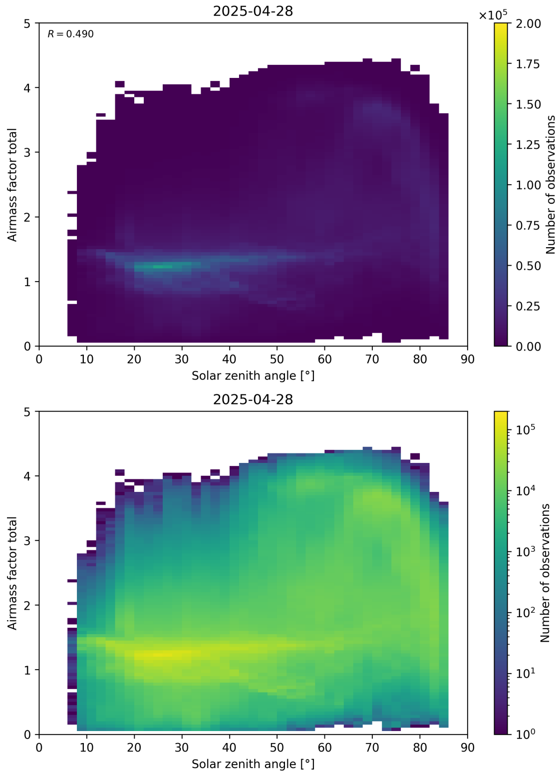
Figure 175: Scatter density plot of “Solar zenith angle” against “Airmass factor total” for 2025-04-27 to 2025-04-29.
