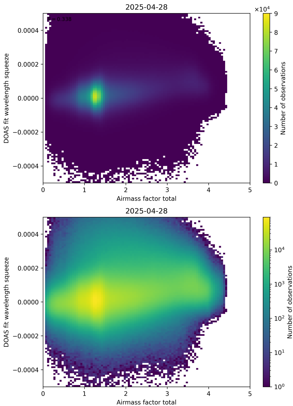
Figure 99: Scatter density plot of “Airmass factor total” against “DOAS fit wavelength squeeze” for 2025-04-27 to 2025-04-29.
