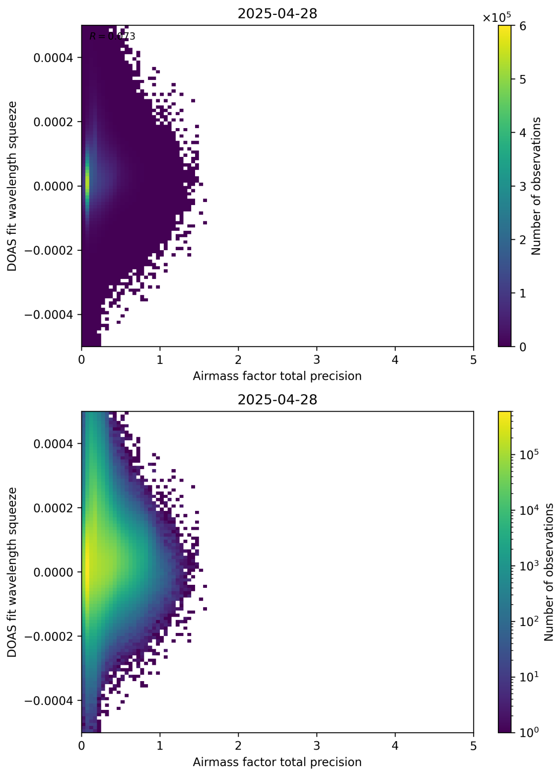
Figure 107: Scatter density plot of “Airmass factor total precision” against “DOAS fit wavelength squeeze” for 2025-04-27 to 2025-04-29.
