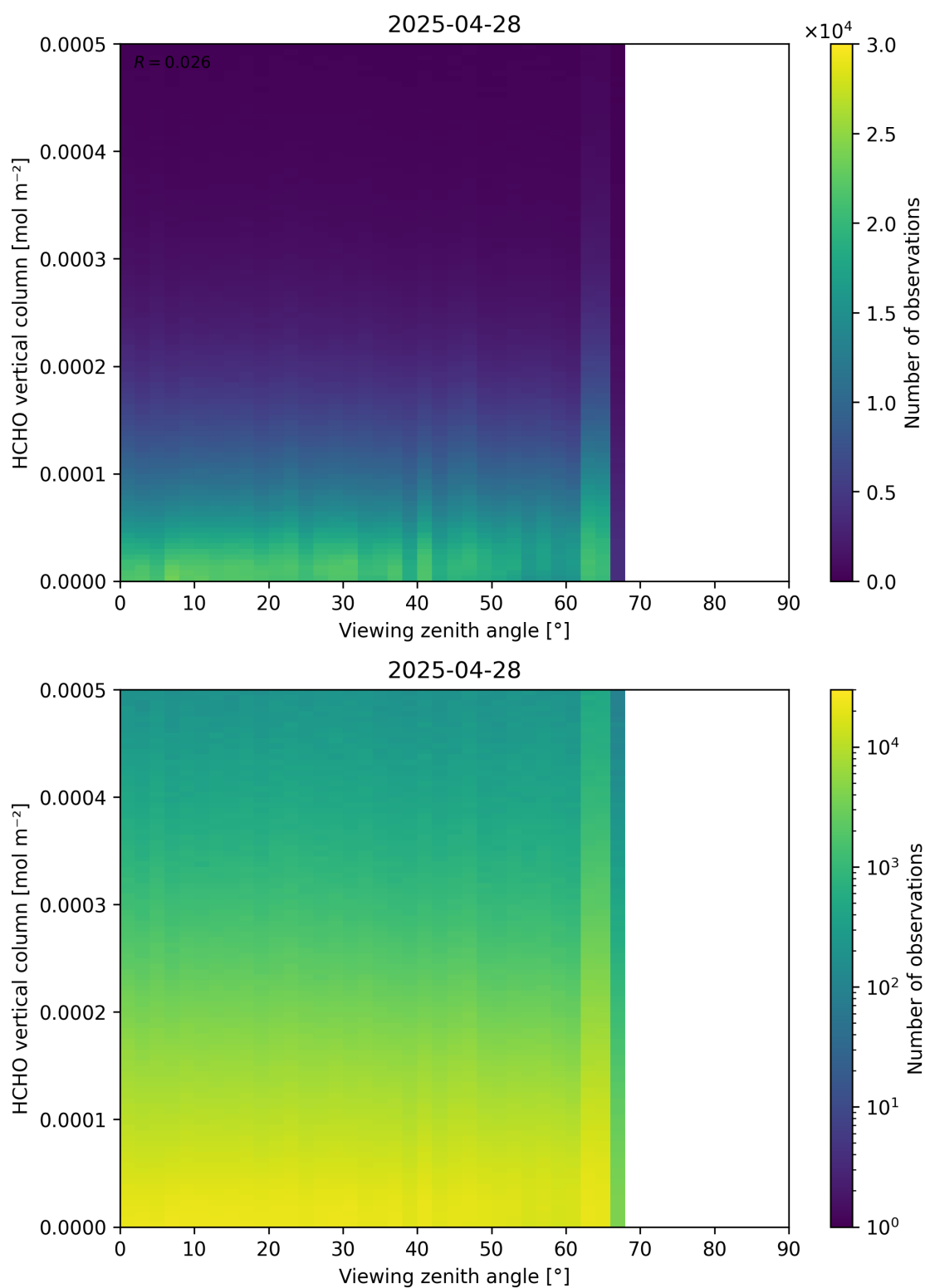
Figure 192: Scatter density plot of “Viewing zenith angle” against “HCHO vertical column” for 2025-04-27 to 2025-04-29.
