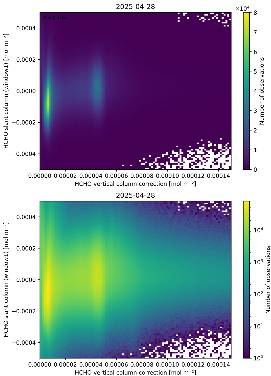
Figure 118: Scatter density plot of “HCHO vertical column correction” against “HCHO slant column (window1)” for 2025-04-27 to 2025-04-29.
