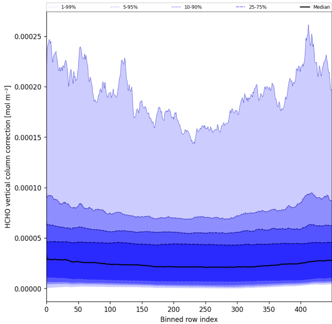
Figure 51: Along track statistics of “HCHO vertical column correction” for 2025-04-27 to 2025-04-29
