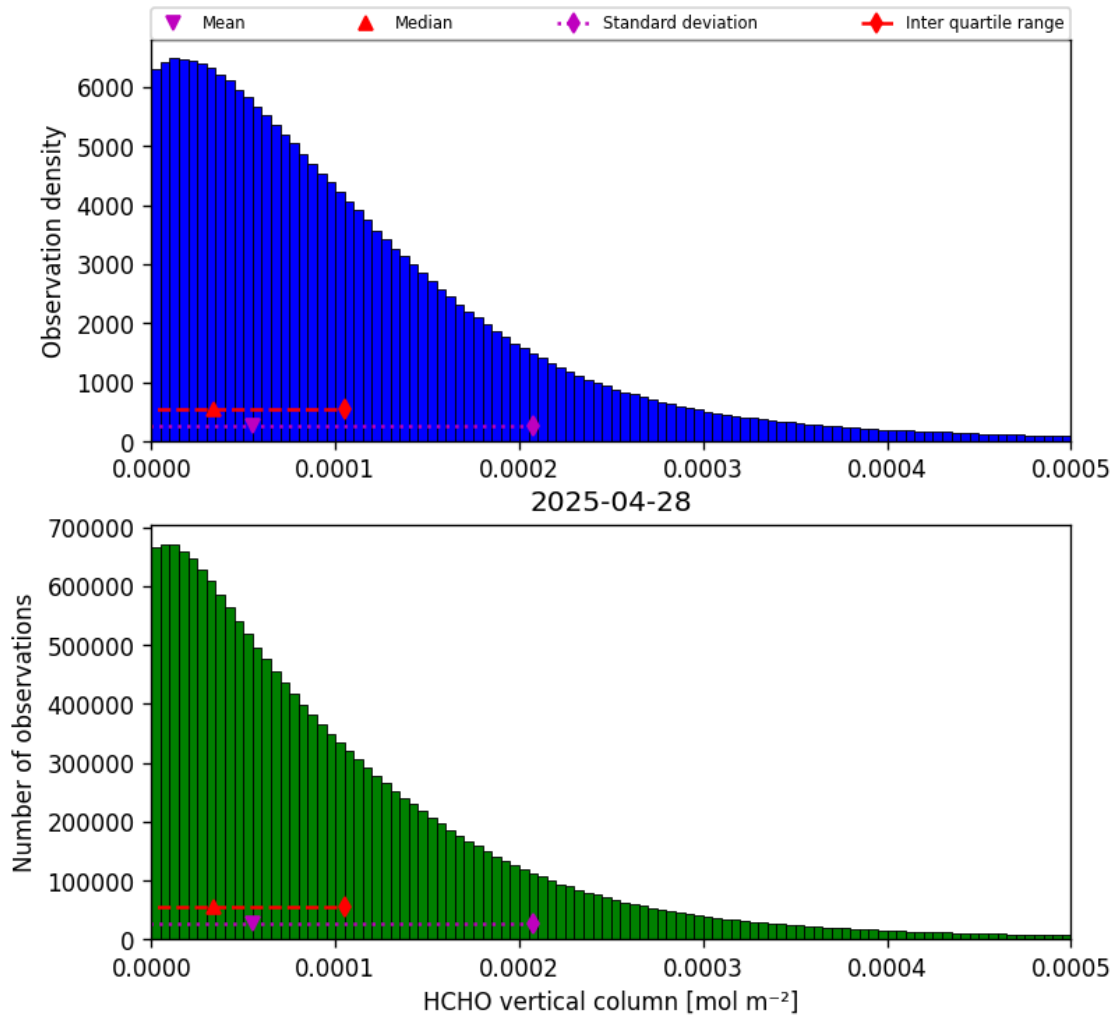
Figure 35: Histogram of “HCHO vertical column” for 2025-04-27 to 2025-04-29
