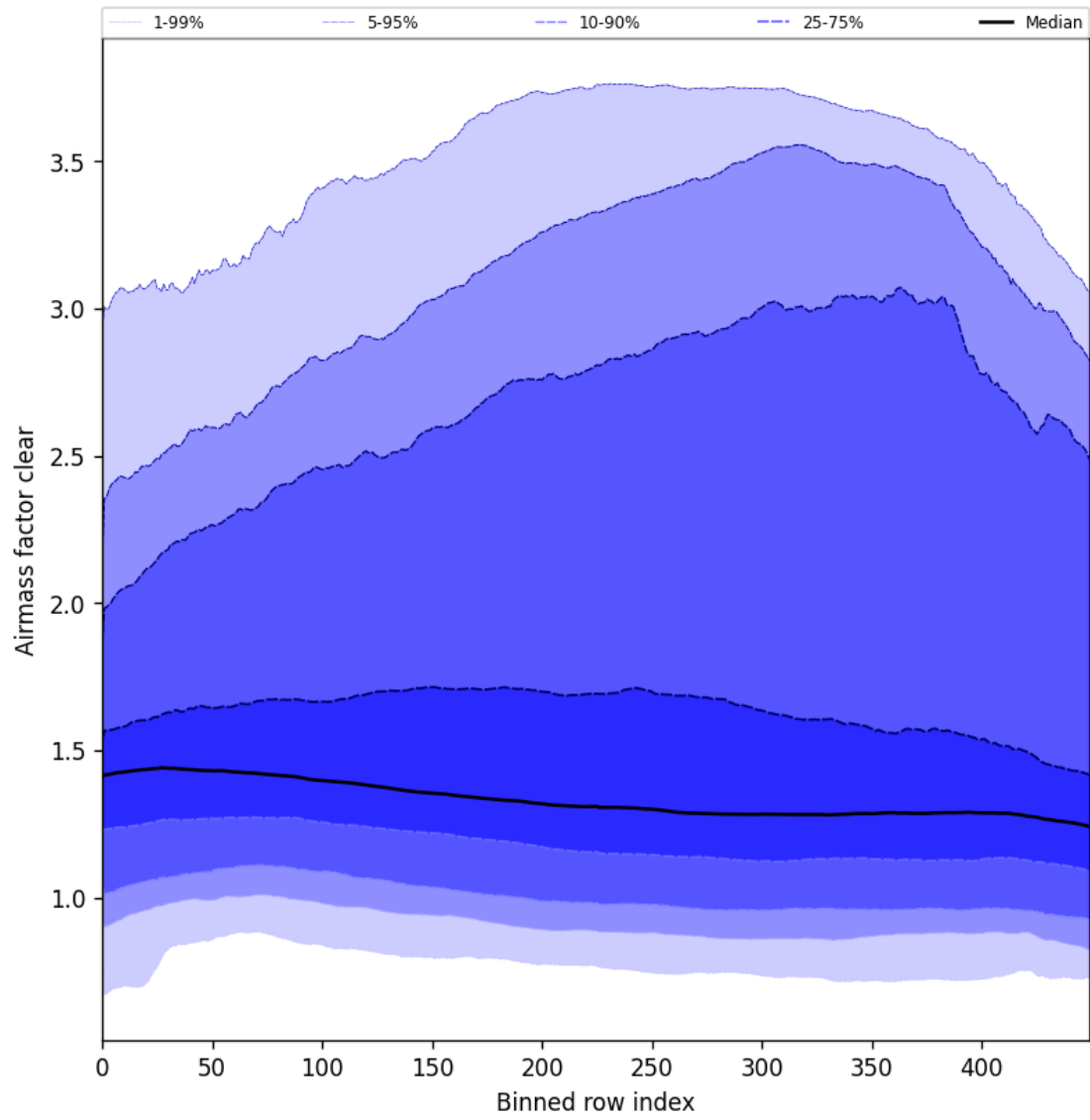
Figure 56: Along track statistics of “Airmass factor clear” for 2025-04-27 to 2025-04-29
