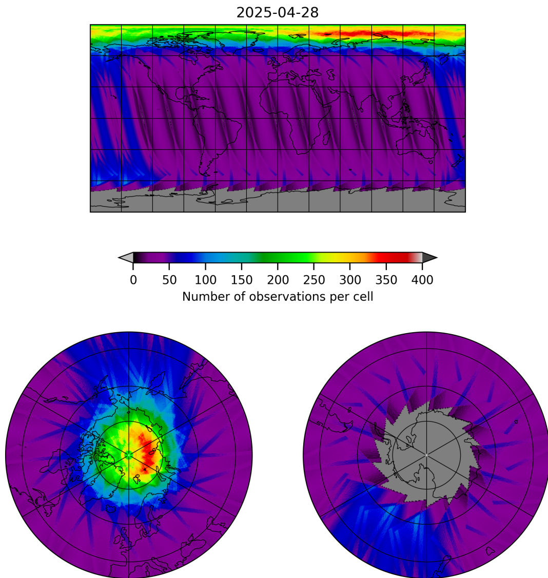
Figure 19: Map of the number of observations for 2025-04-27 to 2025-04-29
