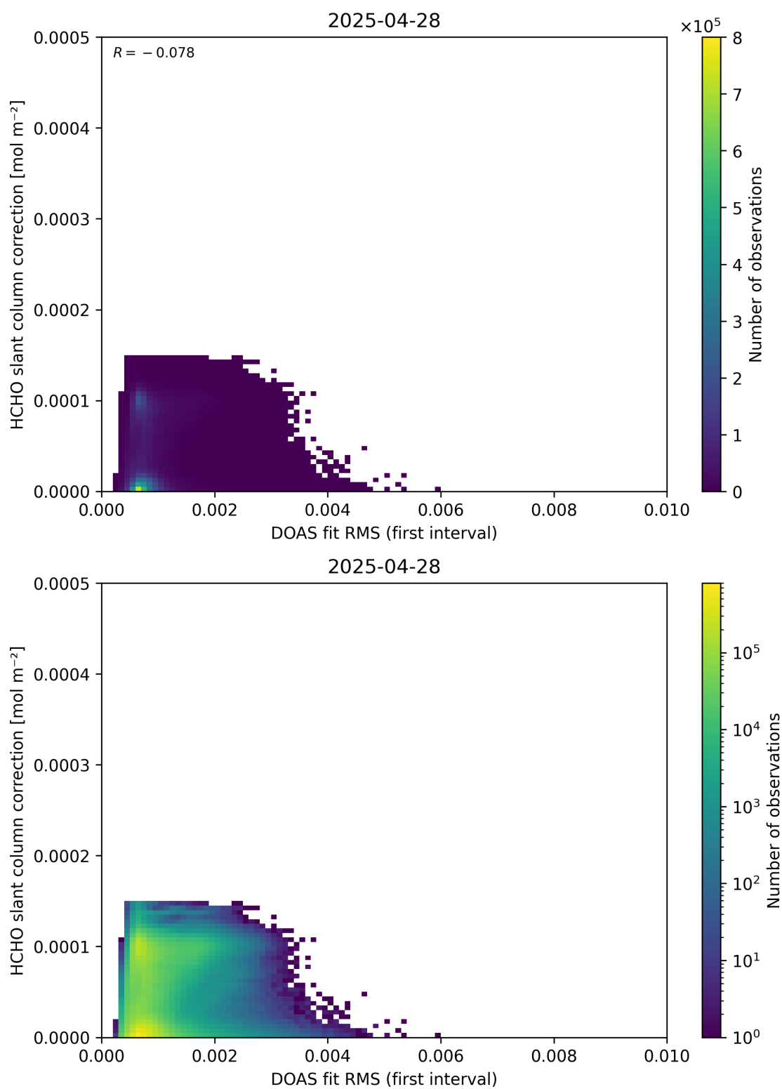
Figure 63: Scatter density plot of “DOAS fit RMS (first interval)” against “HCHO slant column correction” for 2025-04-27 to 2025-04-29.
