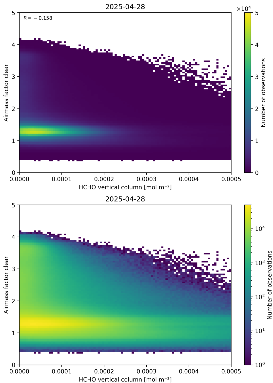
Figure 126: Scatter density plot of “HCHO vertical column” against “Airmass factor clear” for 2025-04-27 to 2025-04-29.
