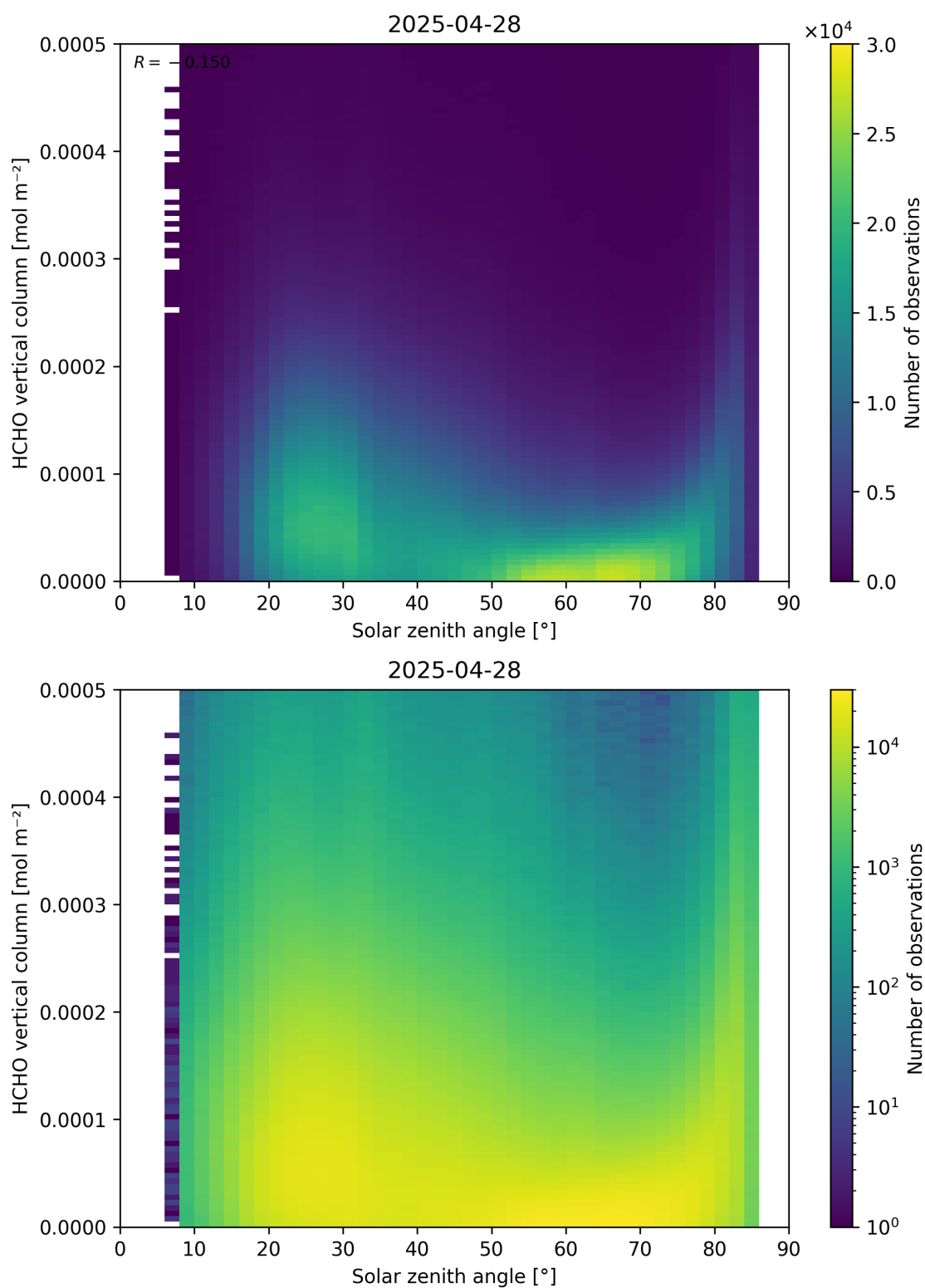
Figure 177: Scatter density plot of “Solar zenith angle” against “HCHO vertical column” for 2025-04-27 to 2025-04-29.
