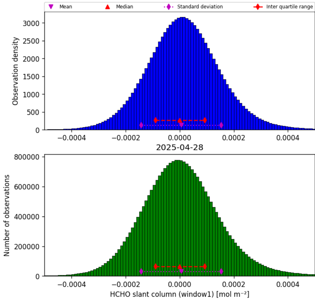
Figure 38: Histogram of “HCHO slant column (window1)” for 2025-04-27 to 2025-04-29
