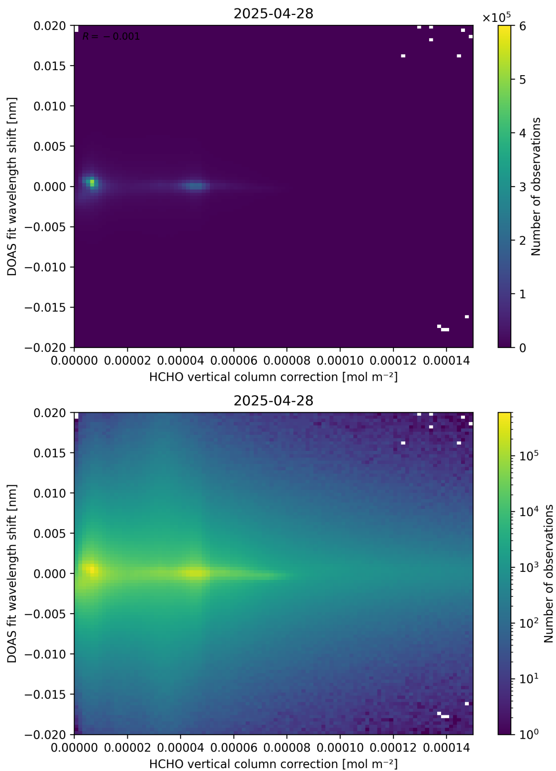
Figure 113: Scatter density plot of “HCHO vertical column correction” against “DOAS fit wavelength shift” for 2025-04-27 to 2025-04-29.
