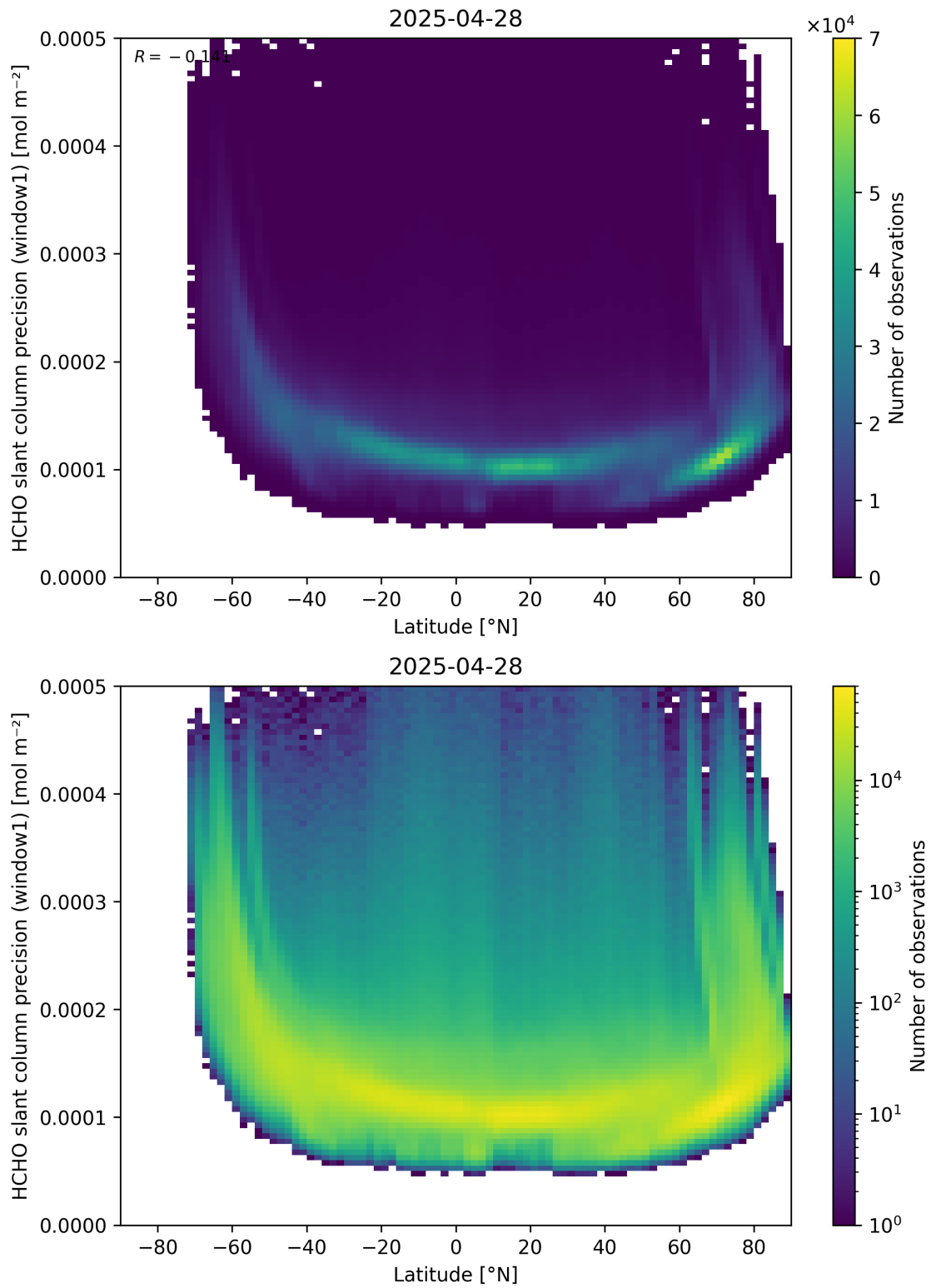
Figure 160: Scatter density plot of “Latitude” against “HCHO slant column precision (window1)” for 2025-04-27 to 2025-04-29.
