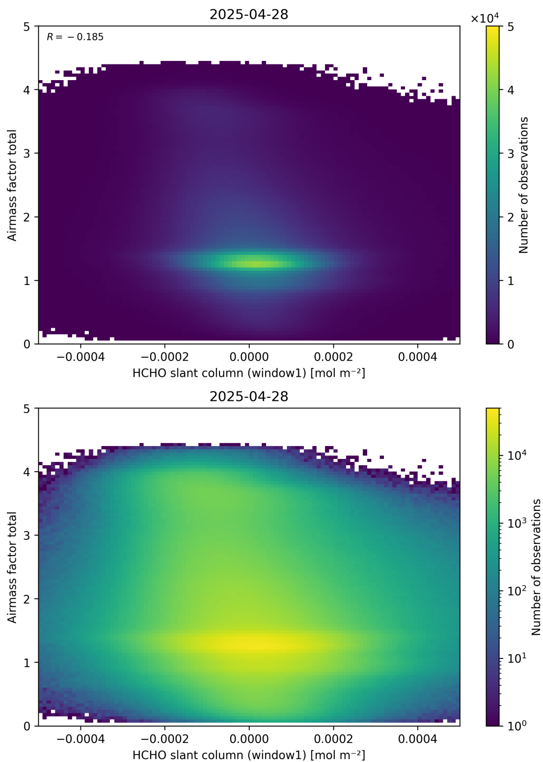
Figure 85: Scatter density plot of “HCHO slant column (window1)” against “Airmass factor total” for 2025-04-27 to 2025-04-29.
