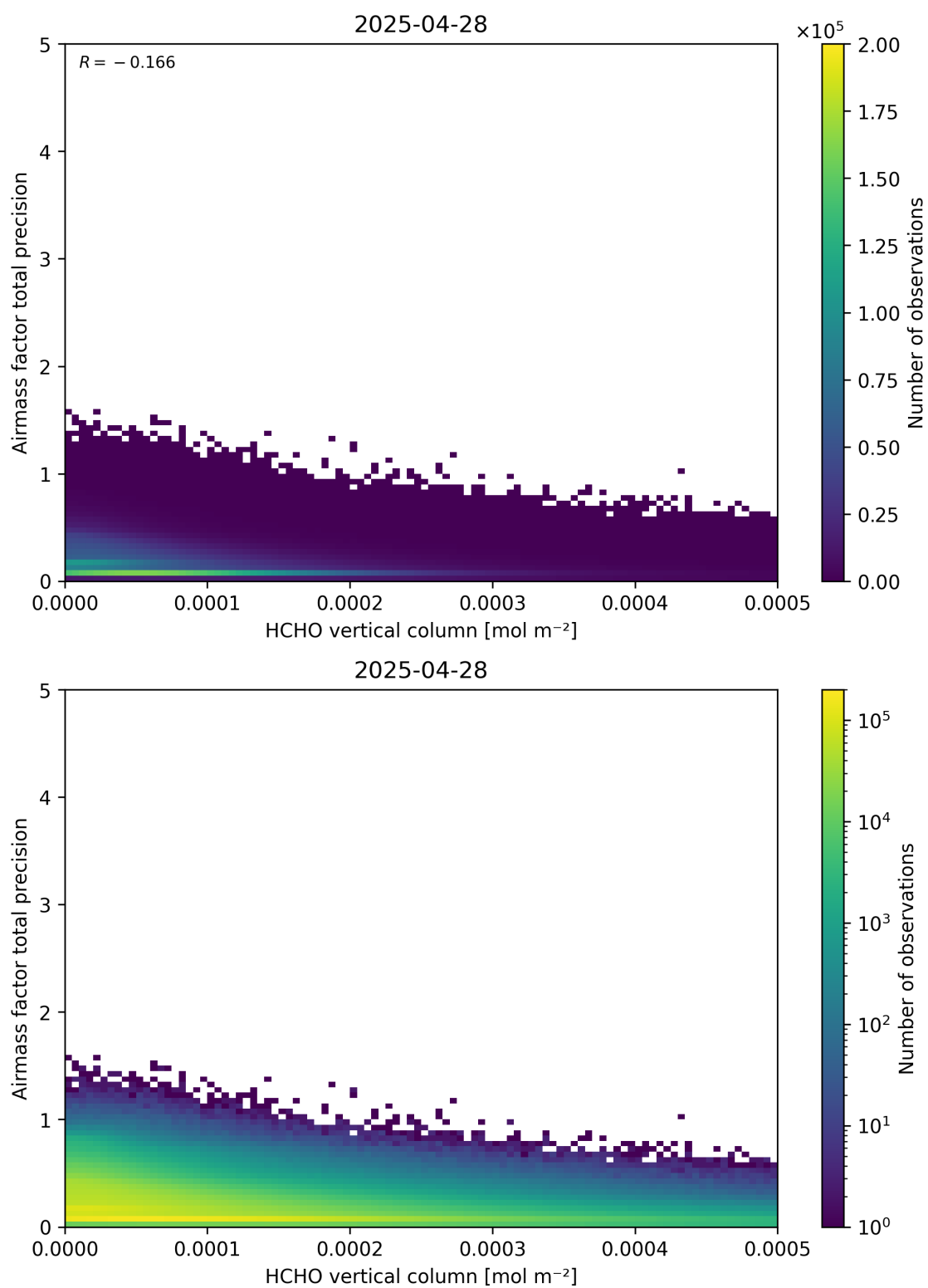
Figure 132: Scatter density plot of “HCHO vertical column” against “Airmass factor total precision” for 2025-04-27 to 2025-04-29.
