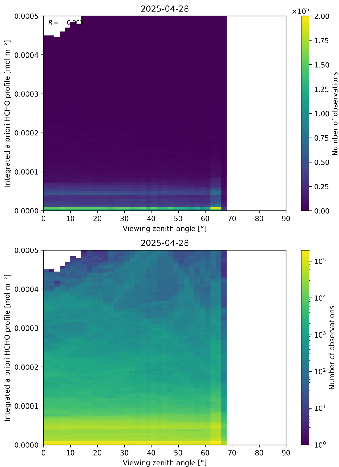
Figure 195: Scatter density plot of “Viewing zenith angle” against “Integrated a priori HCHO profile” for 2025-04-27 to 2025-04-29.
