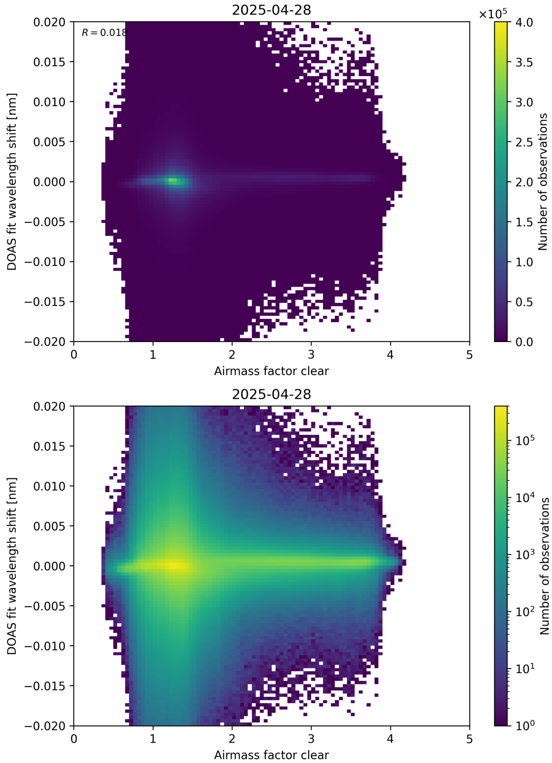
Figure 72: Scatter density plot of “Airmass factor clear” against “DOAS fit wavelength shift” for 2025-04-27 to 2025-04-29.
