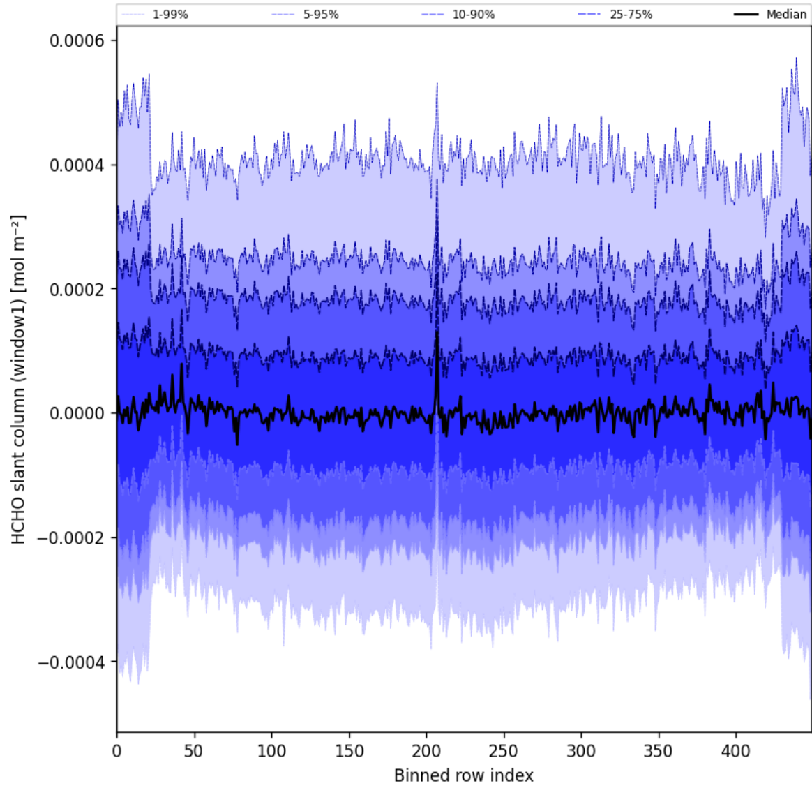
Figure 52: Along track statistics of “HCHO slant column (window1)” for 2025-04-27 to 2025-04-29
