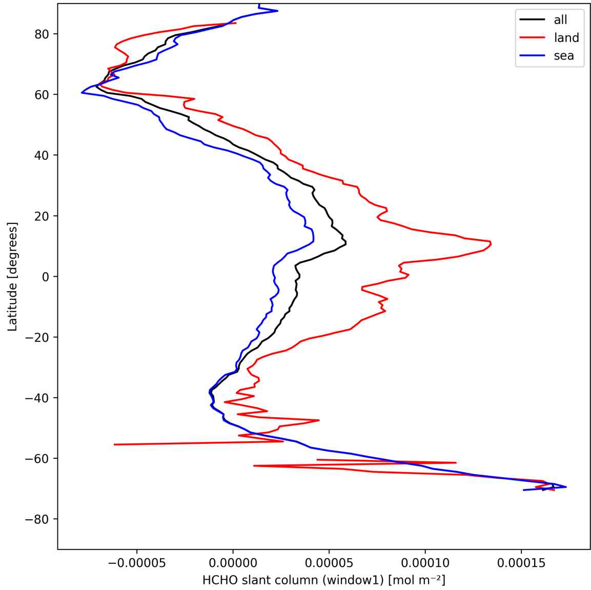
Figure 24: Zonal average of “HCHO slant column (window1)” for 2025-04-27 to 2025-04-29.
