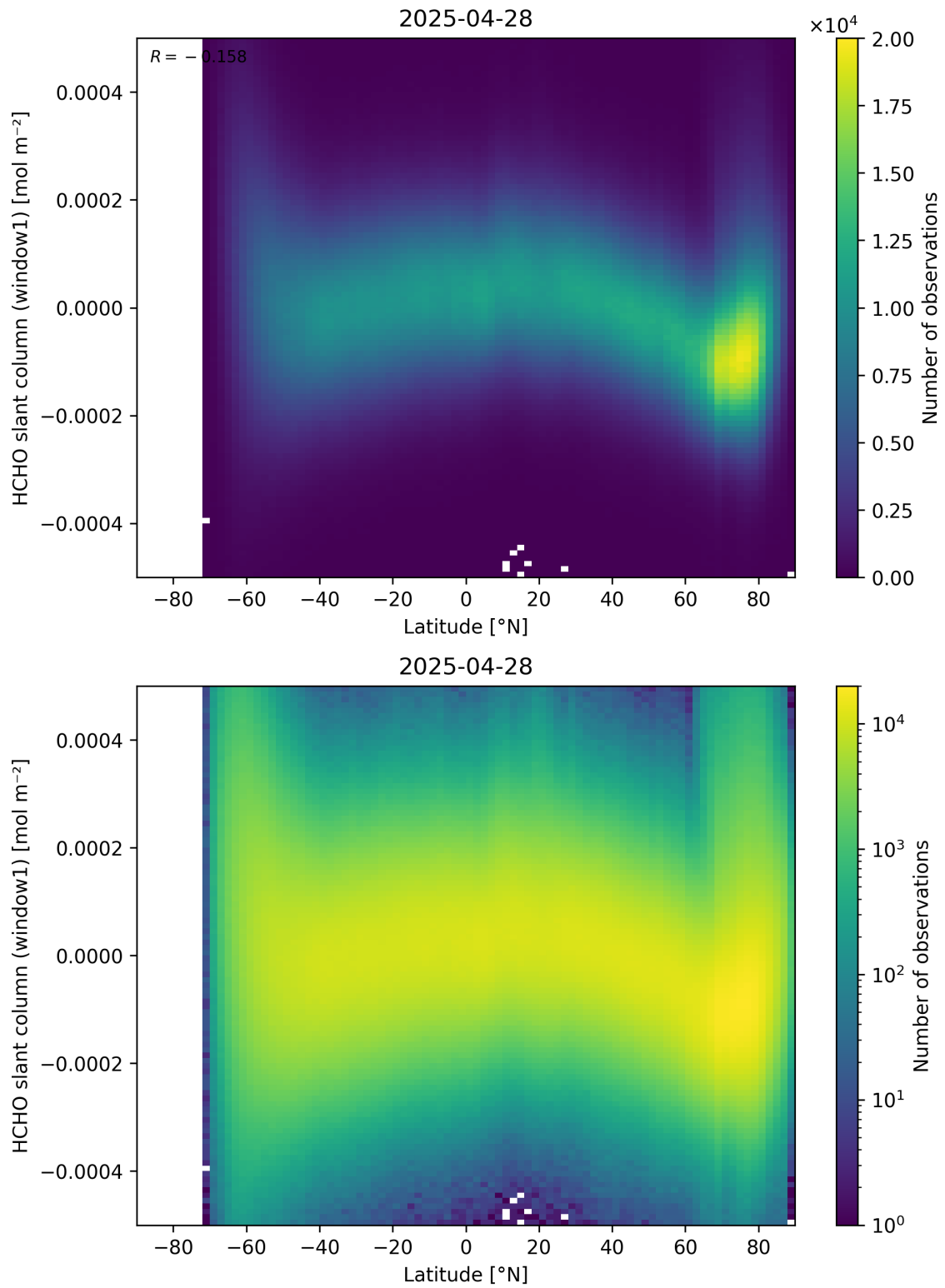
Figure 159: Scatter density plot of “Latitude” against “HCHO slant column (window1)” for 2025-04-27 to 2025-04-29.
