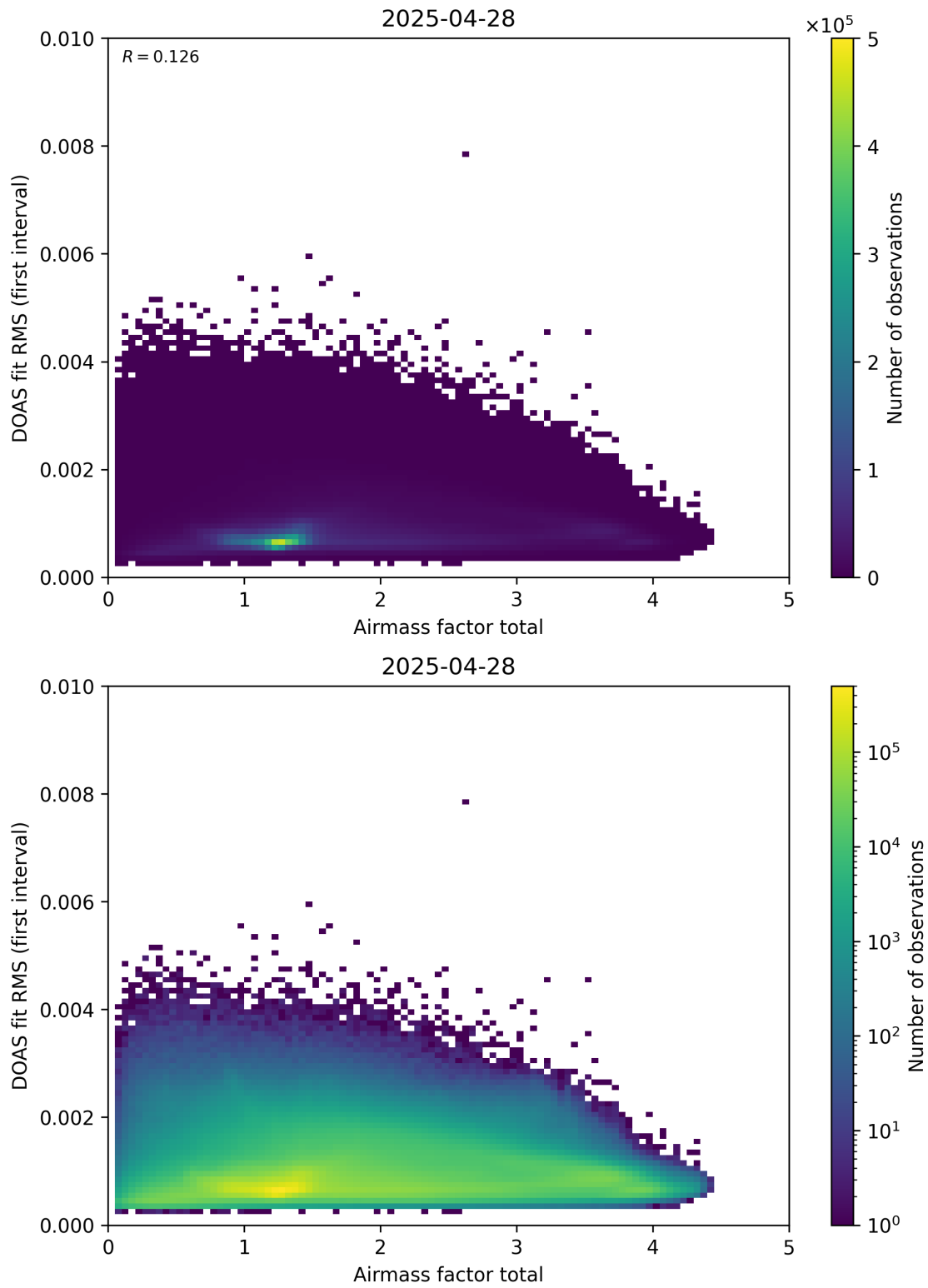
Figure 97: Scatter density plot of “Airmass factor total” against “DOAS fit RMS (first interval)” for 2025-04-27 to 2025-04-29.
