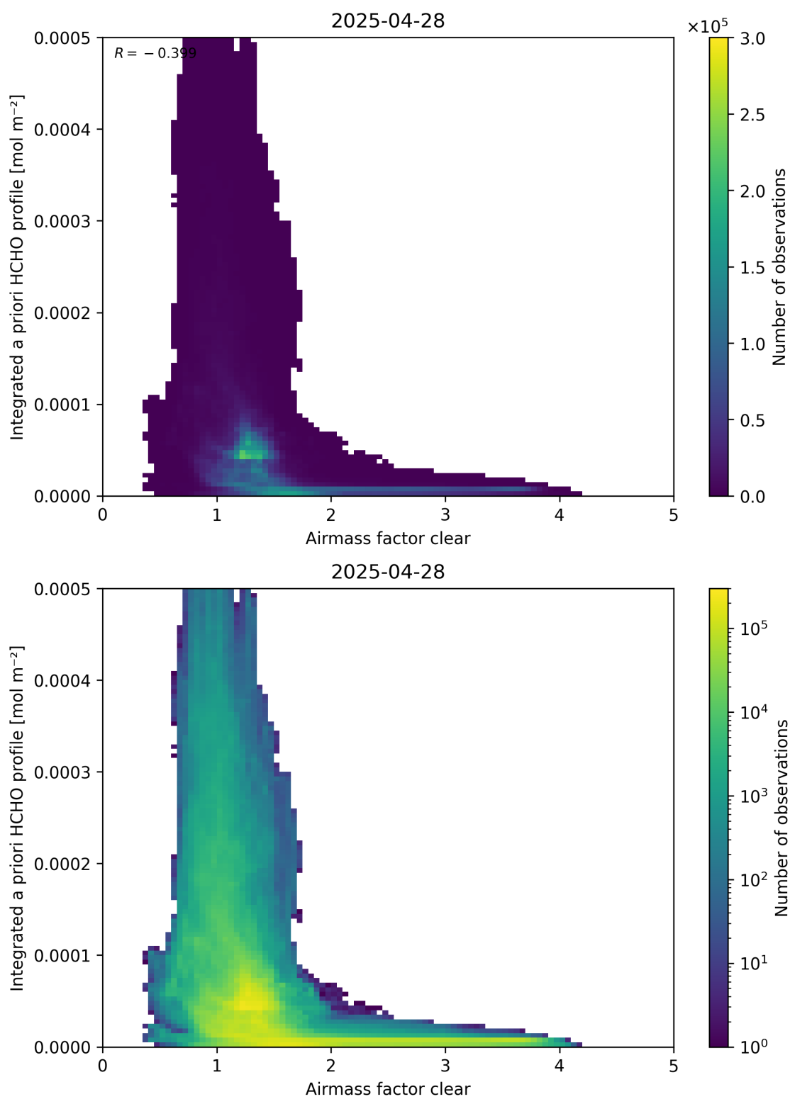
Figure 76: Scatter density plot of “Airmass factor clear” against “Integrated a priori HCHO profile” for 2025-04-27 to 2025-04-29.
