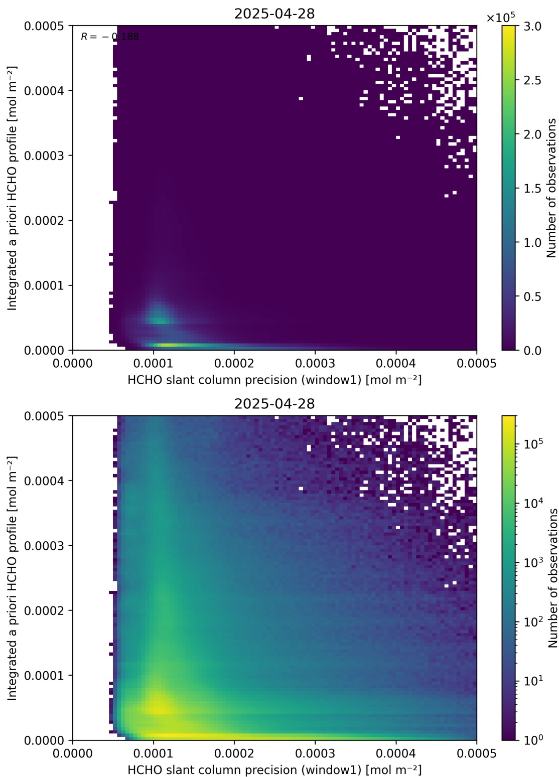
Figure 96: Scatter density plot of “HCHO slant column precision (window1)” against “Integrated a priori HCHO profile” for 2025-04-27 to 2025-04-29.
