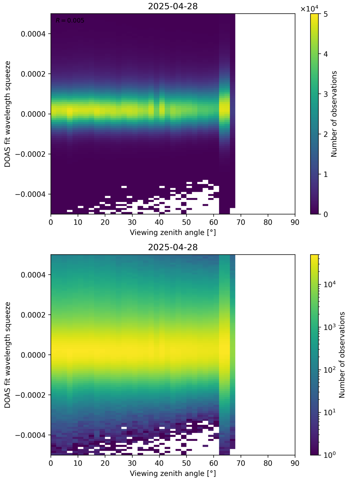
Figure 184: Scatter density plot of “Viewing zenith angle” against “DOAS fit wavelength squeeze” for 2025-04-27 to 2025-04-29.
