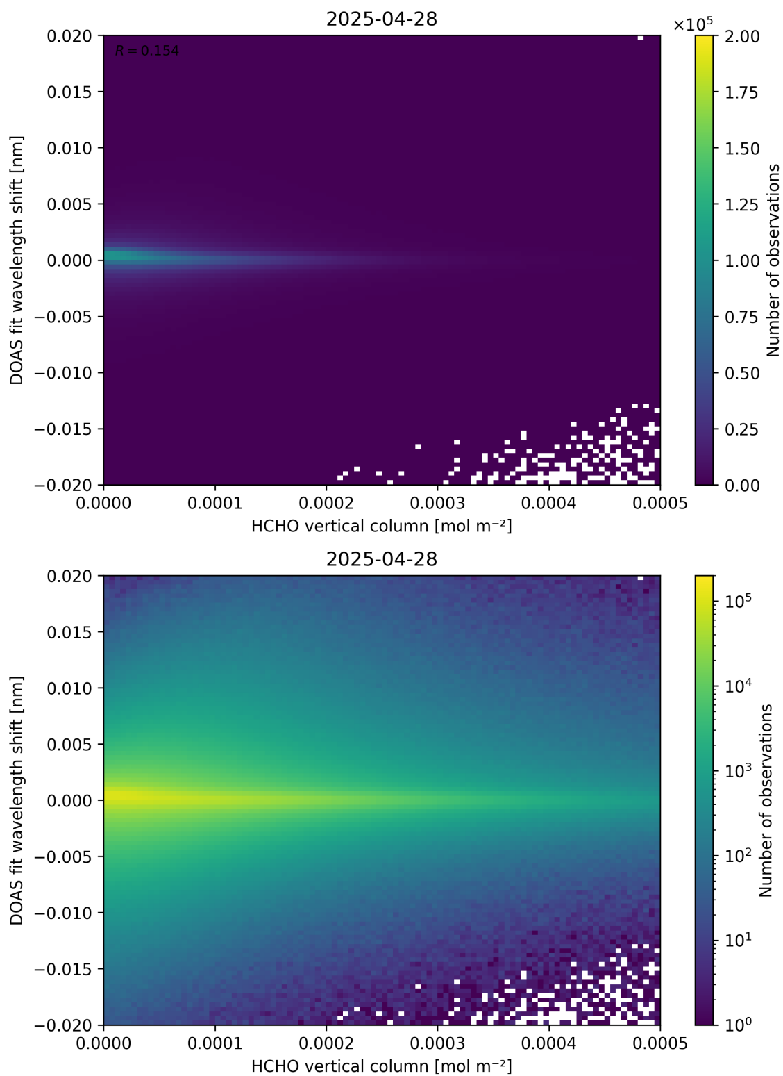
Figure 124: Scatter density plot of “HCHO vertical column” against “DOAS fit wavelength shift” for 2025-04-27 to 2025-04-29.
