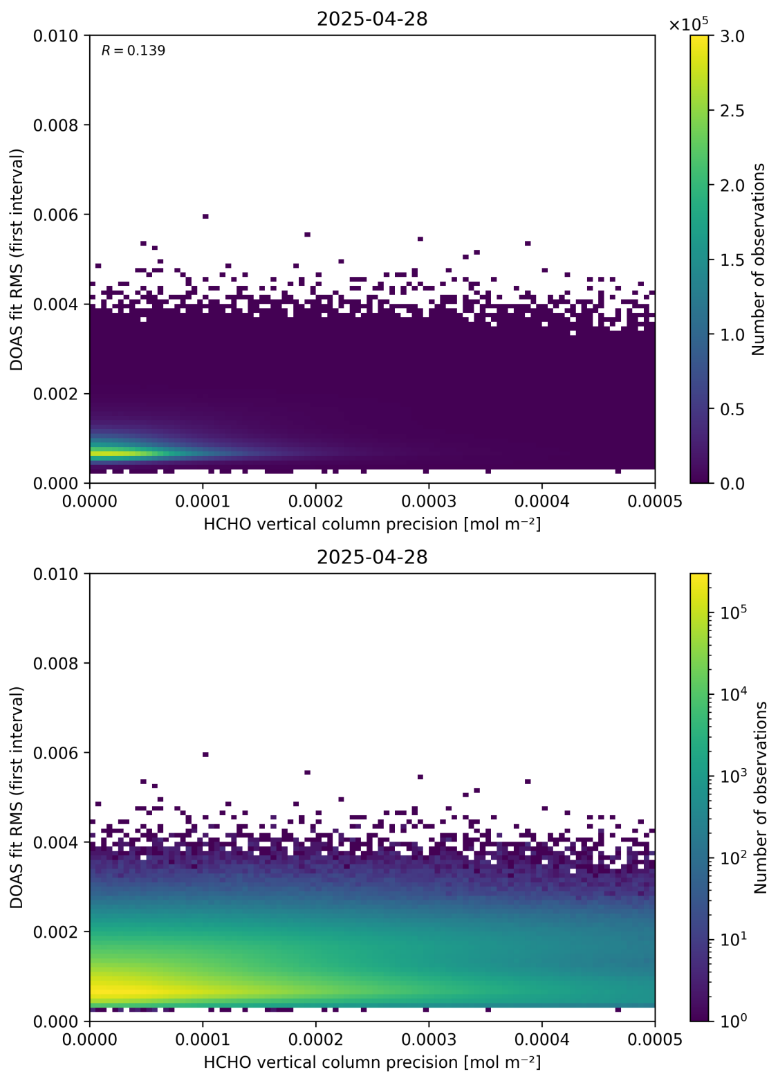
Figure 136: Scatter density plot of “HCHO vertical column precision” against “DOAS fit RMS (first interval)” for 2025-04-27 to 2025-04-29.
