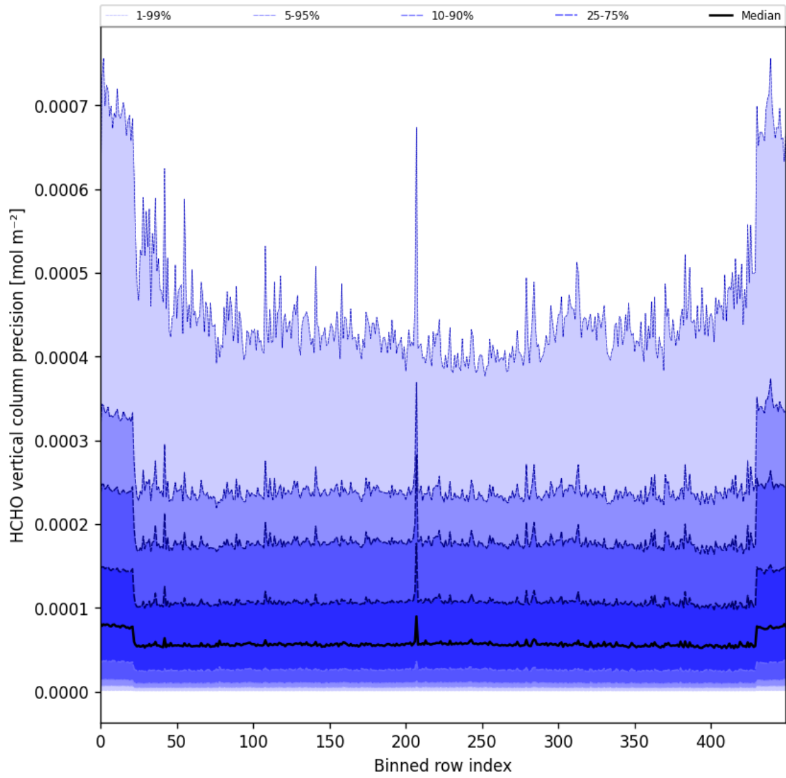
Figure 50: Along track statistics of “HCHO vertical column precision” for 2025-04-27 to 2025-04-29
