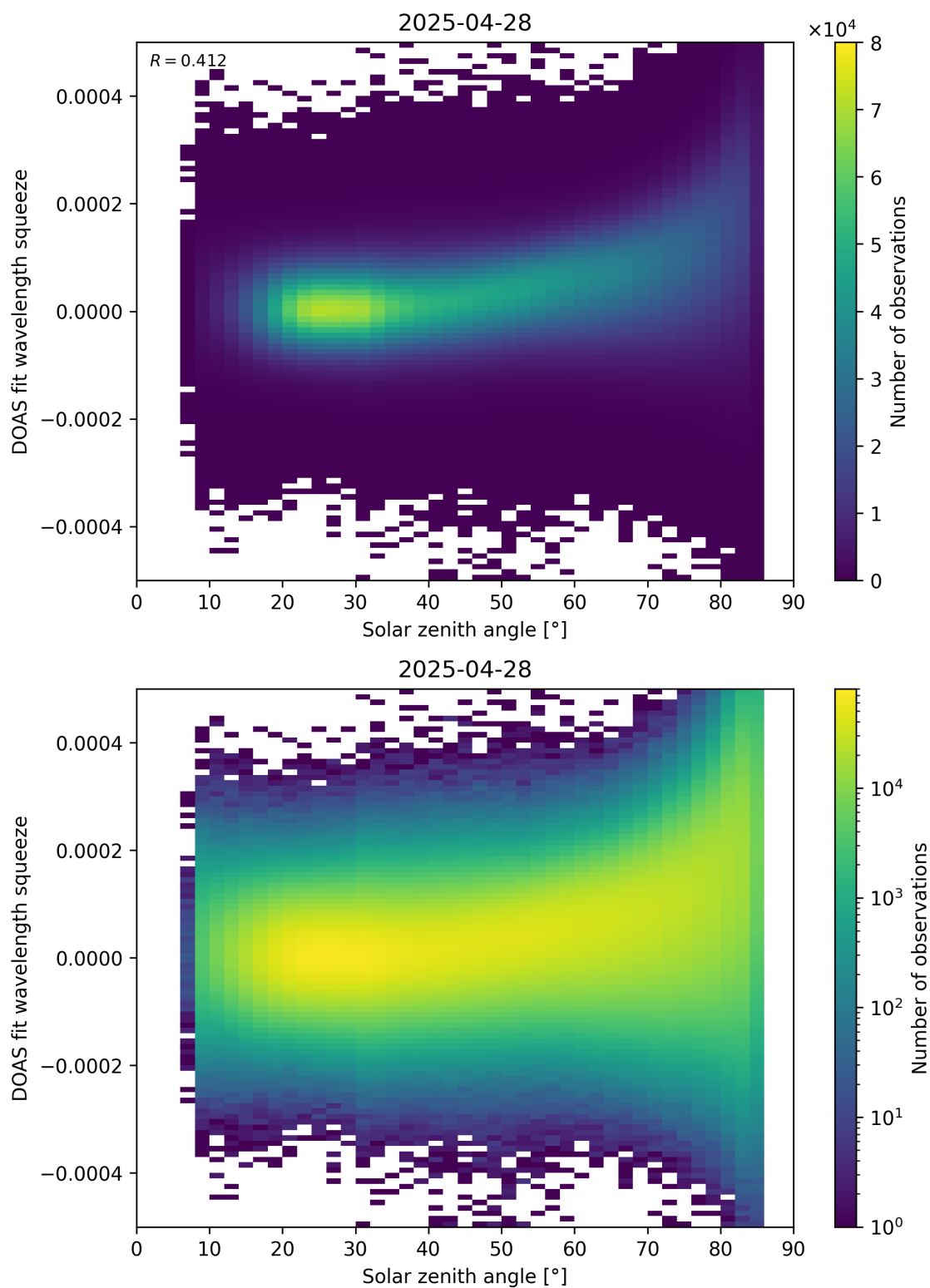
Figure 169: Scatter density plot of “Solar zenith angle” against “DOAS fit wavelength squeeze” for 2025-04-27 to 2025-04-29.
