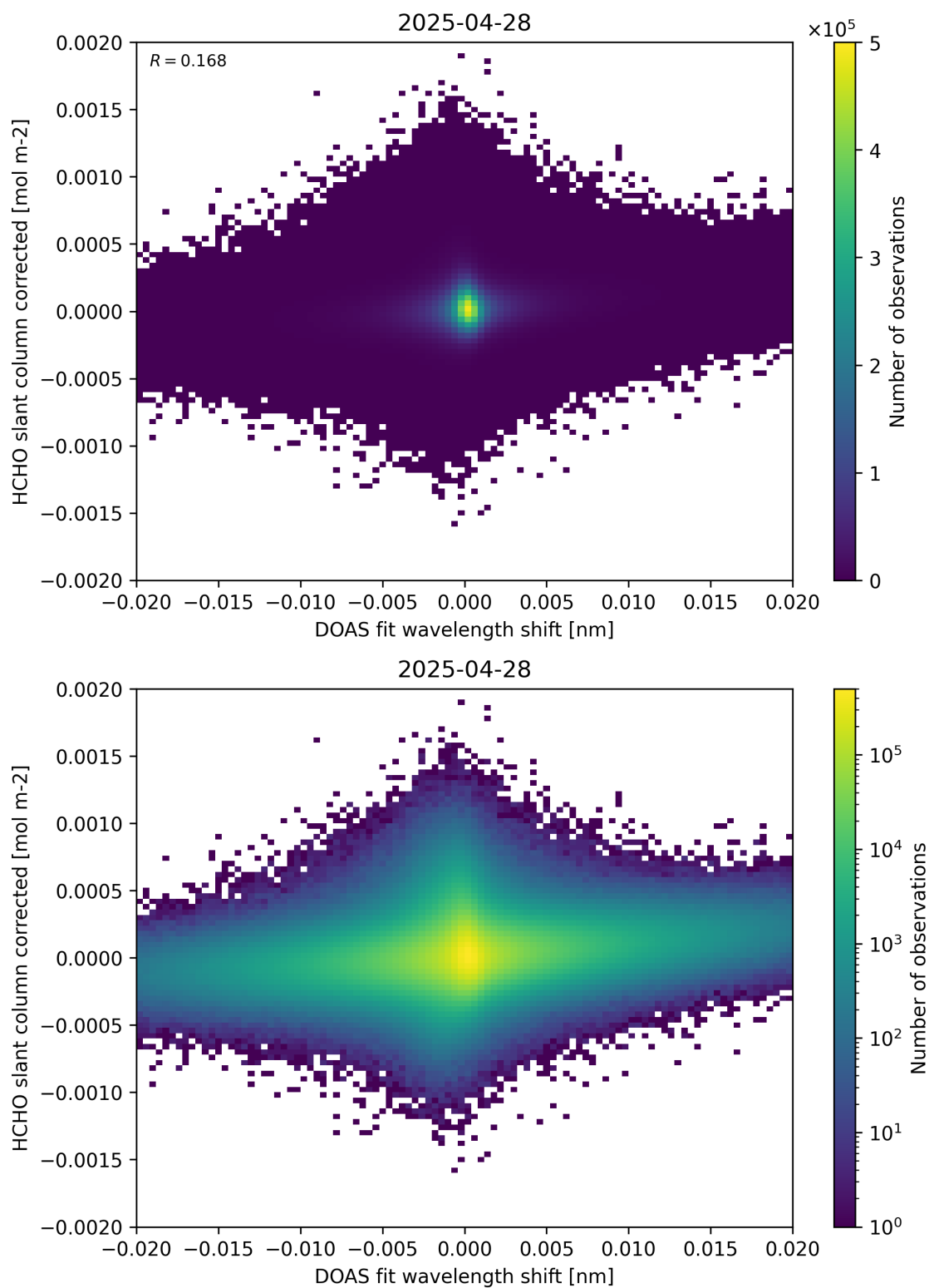
Figure 66: Scatter density plot of “DOAS fit wavelength shift” against “HCHO slant column corrected” for 2025-04-27 to 2025-04-29.
