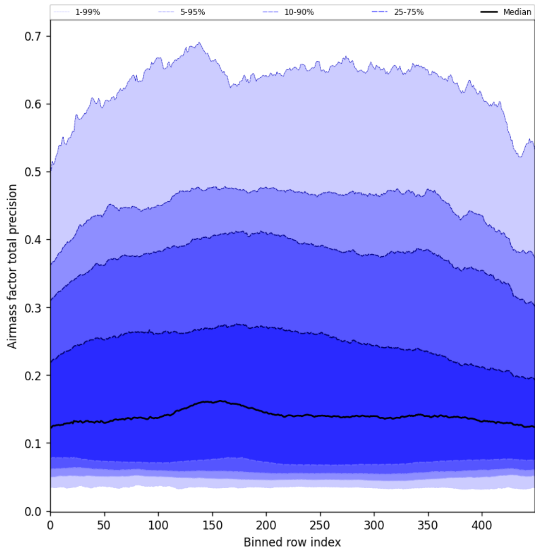
Figure 55: Along track statistics of “Airmass factor total precision” for 2025-04-27 to 2025-04-29
