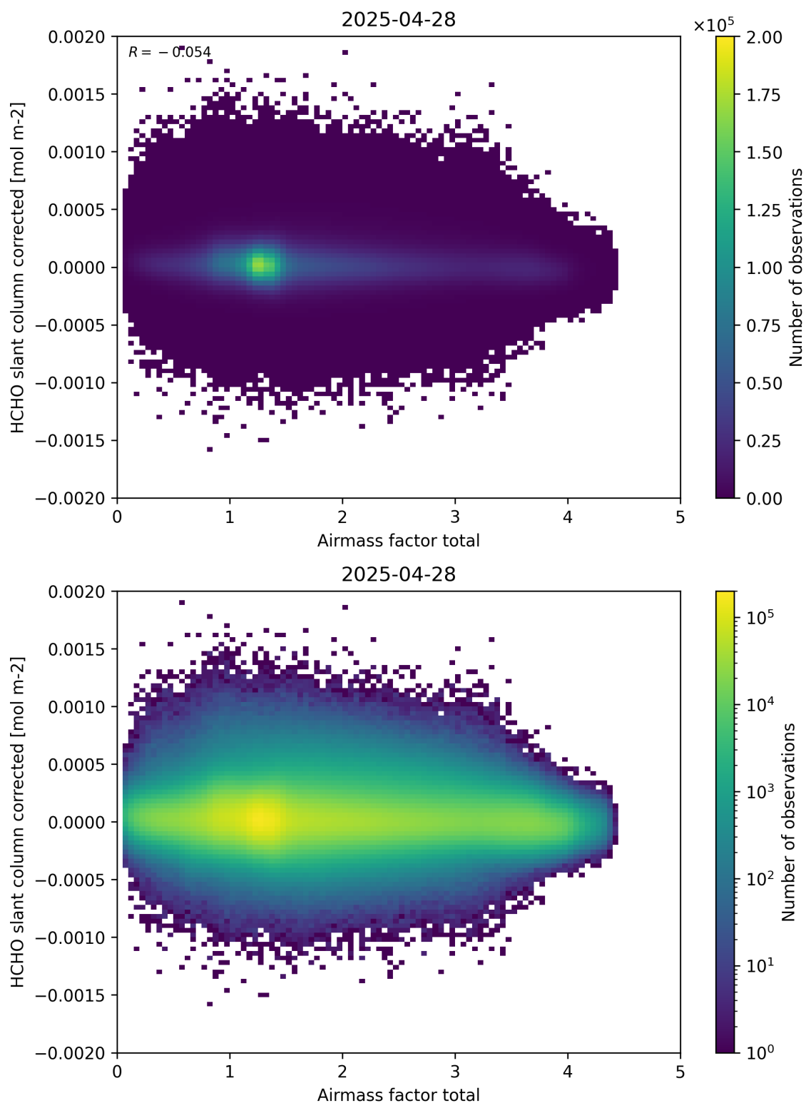
Figure 101: Scatter density plot of “Airmass factor total” against “HCHO slant column corrected” for 2025-04-27 to 2025-04-29.
