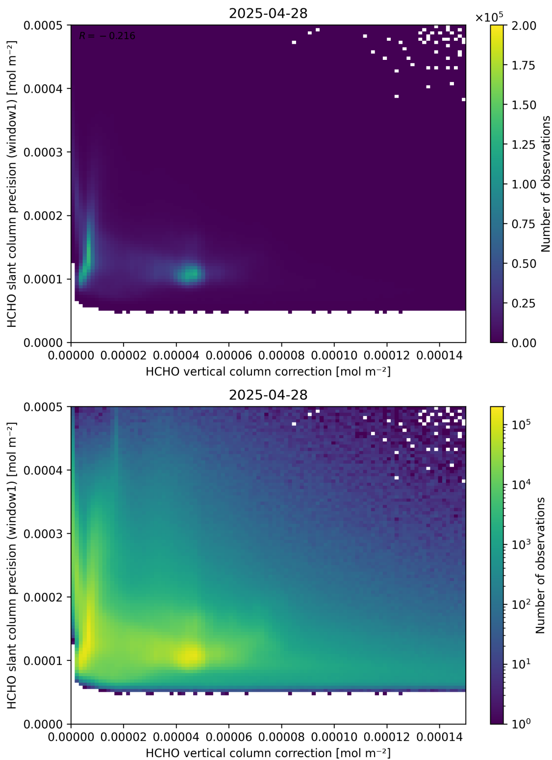
Figure 119: Scatter density plot of “HCHO vertical column correction” against “HCHO slant column precision (window1)” for 2025-04-27 to 2025-04-29.
