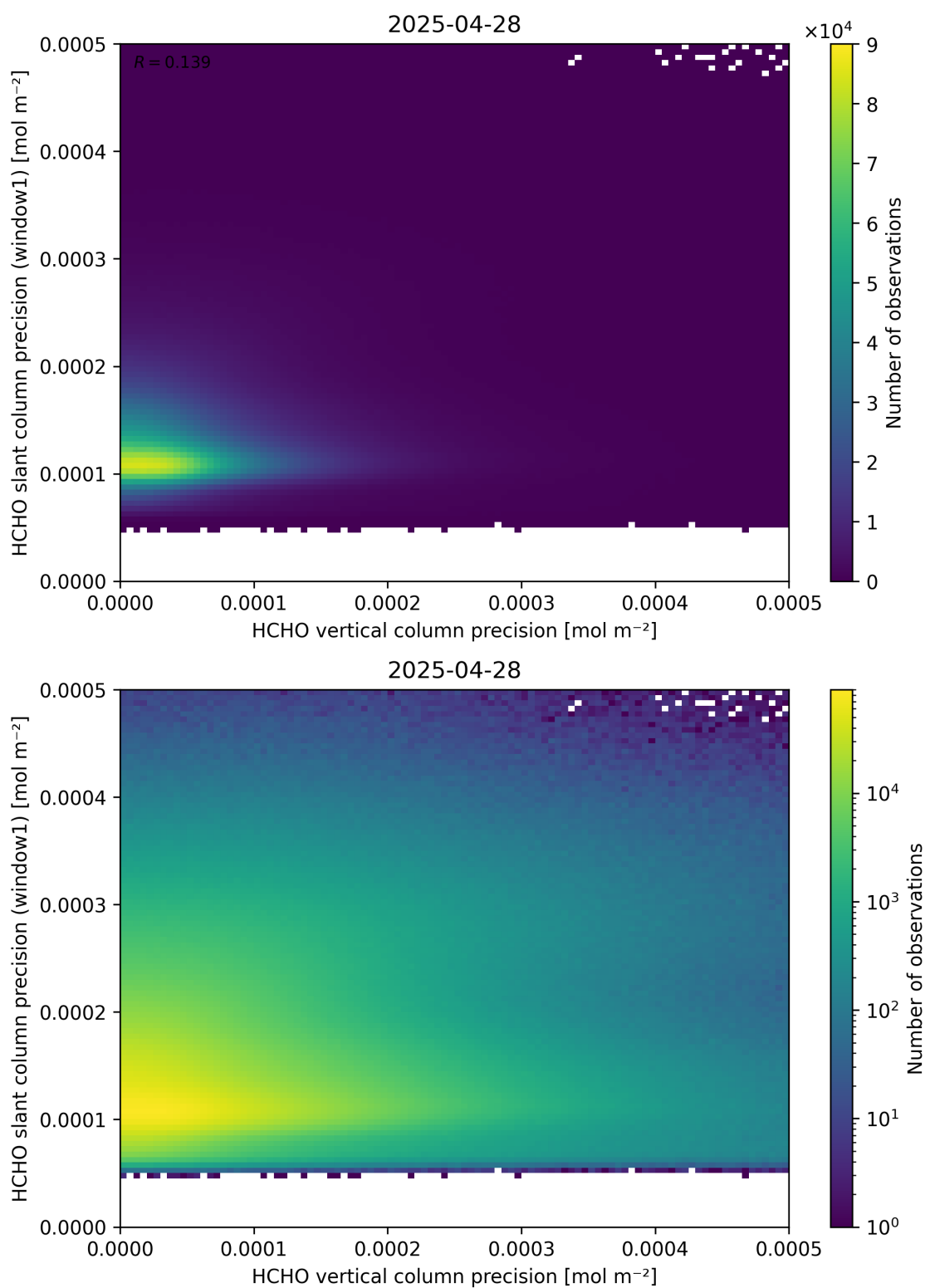
Figure 143: Scatter density plot of “HCHO vertical column precision” against “HCHO slant column precision (window1)” for 2025-04-27 to 2025-04-29.
