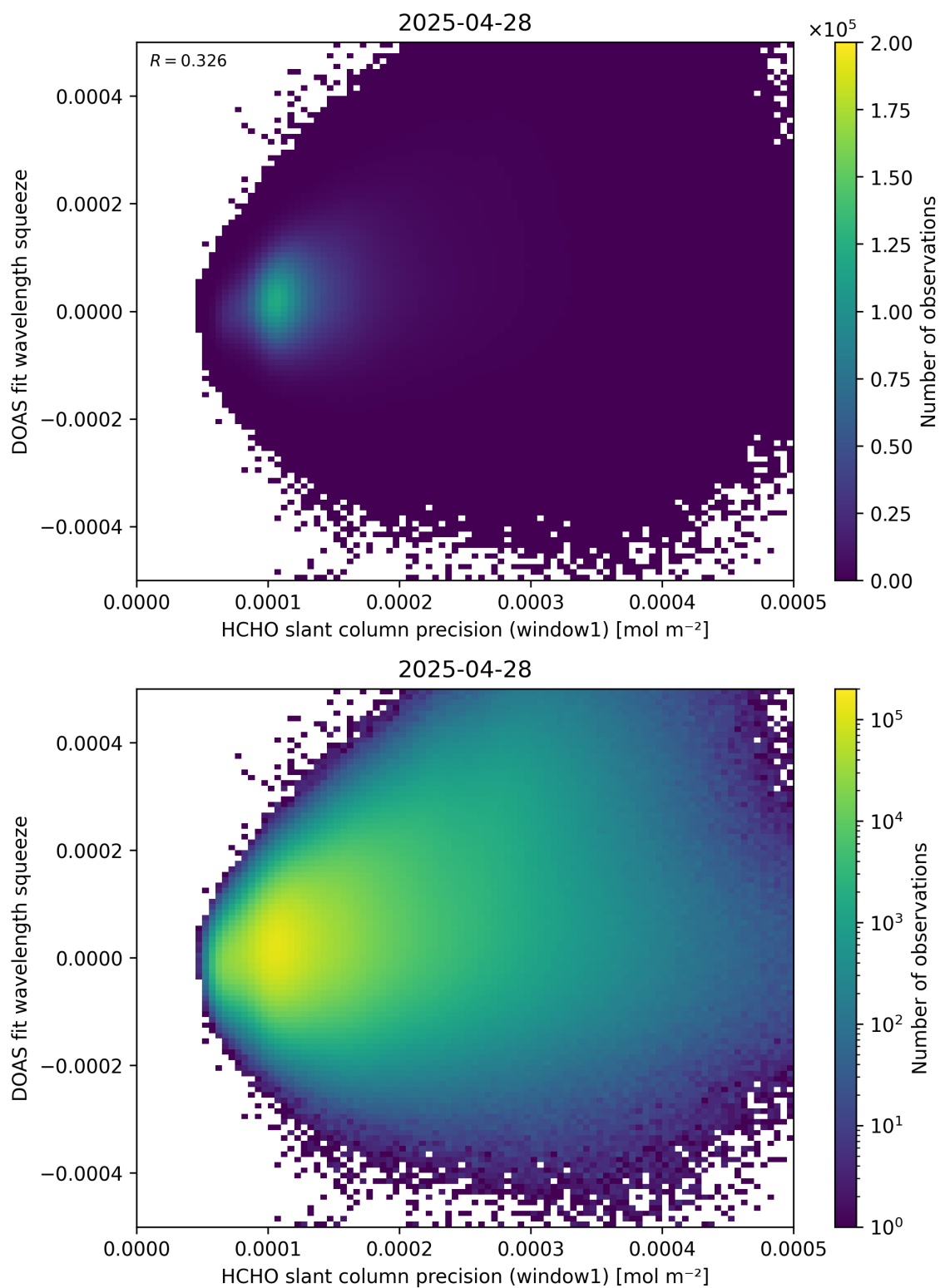
Figure 90: Scatter density plot of “HCHO slant column precision (window1)” against “DOAS fit wavelength squeeze” for 2025-04-27 to 2025-04-29.
