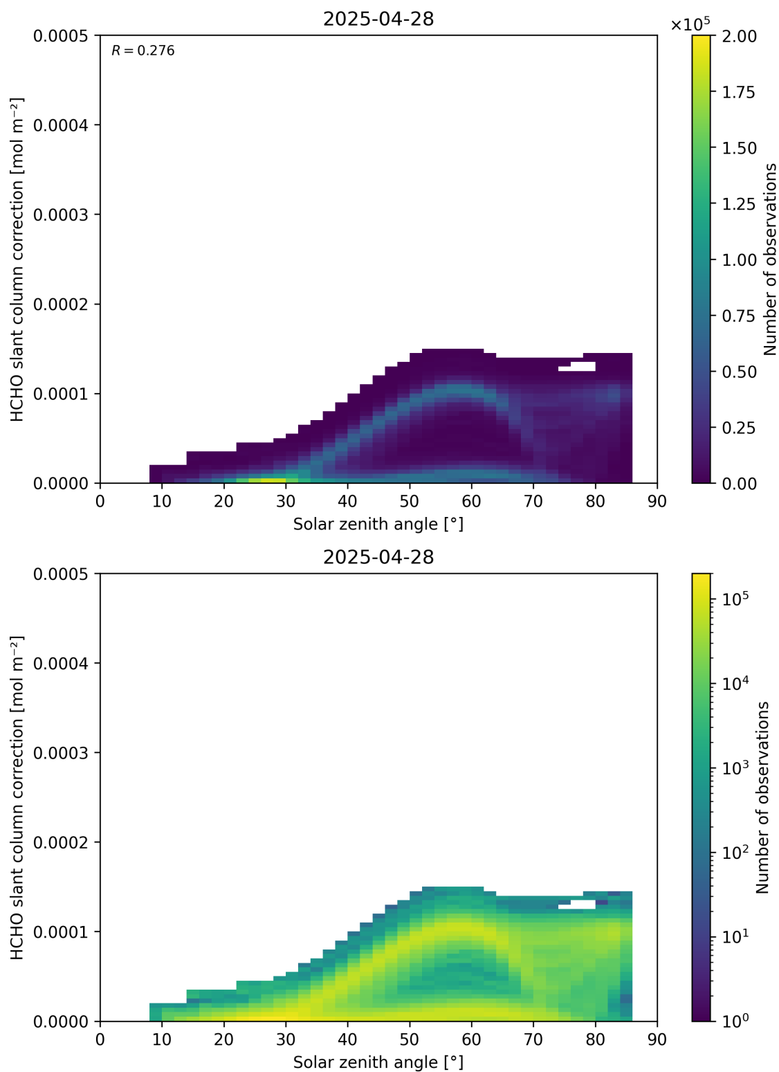
Figure 172: Scatter density plot of “Solar zenith angle” against “HCHO slant column correction” for 2025-04-27 to 2025-04-29.
