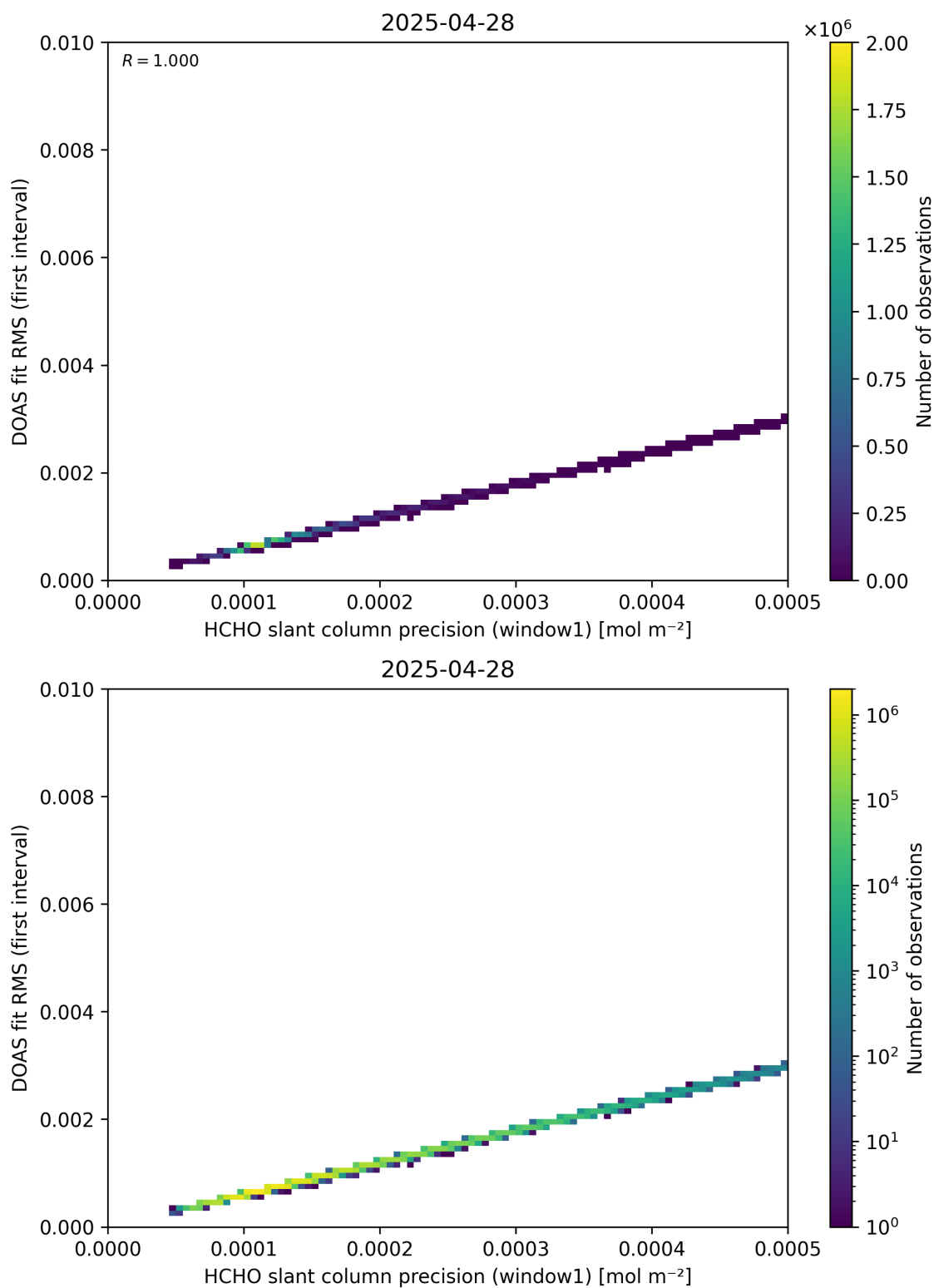
Figure 88: Scatter density plot of “HCHO slant column precision (window1)” against “DOAS fit RMS (first interval)” for 2025-04-27 to 2025-04-29.
