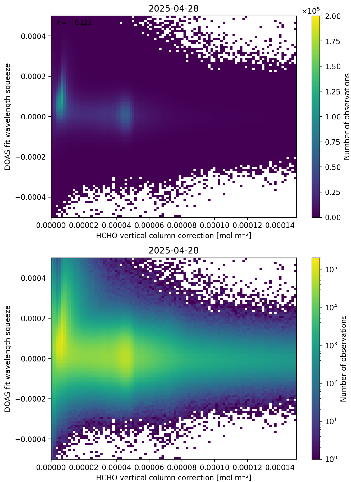
Figure 114: Scatter density plot of “HCHO vertical column correction” against “DOAS fit wavelength squeeze” for 2025-04-27 to 2025-04-29.
