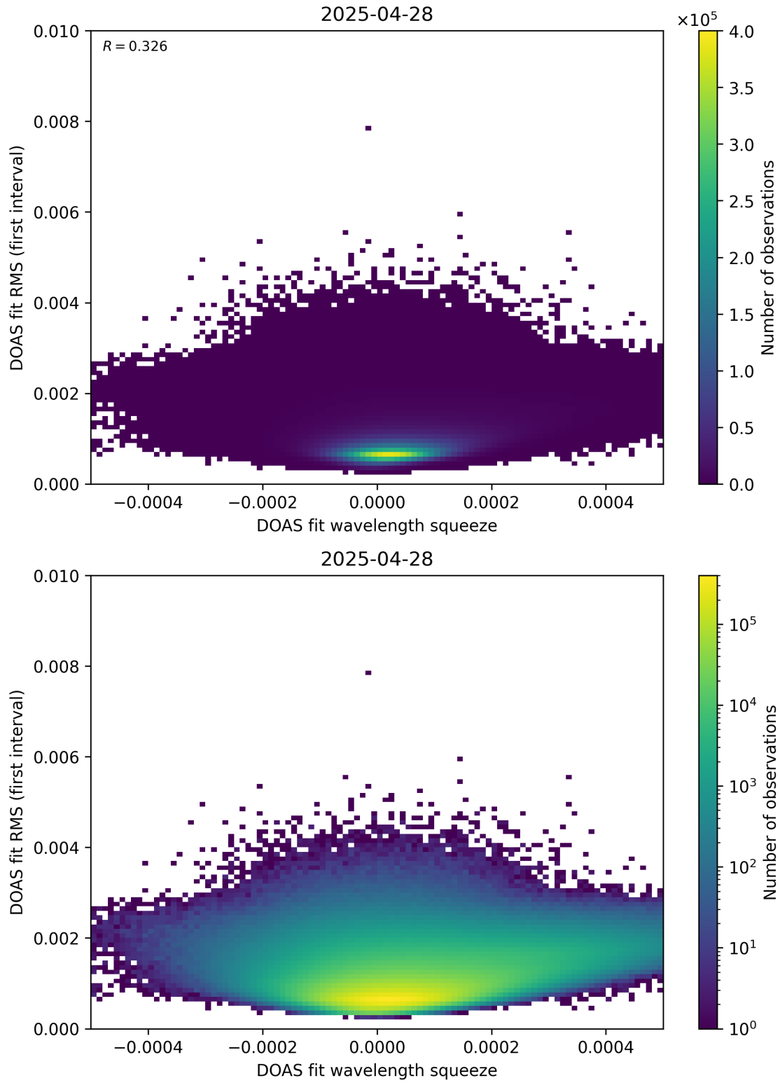
Figure 68: Scatter density plot of “DOAS fit wavelength squeeze” against “DOAS fit RMS (first interval)” for 2025-04-27 to 2025-04-29.
