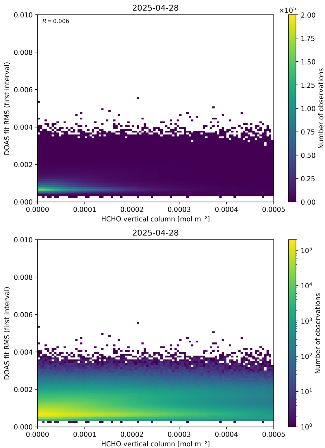
Figure 123: Scatter density plot of “HCHO vertical column” against “DOAS fit RMS (first interval)” for 2025-04-27 to 2025-04-29.
