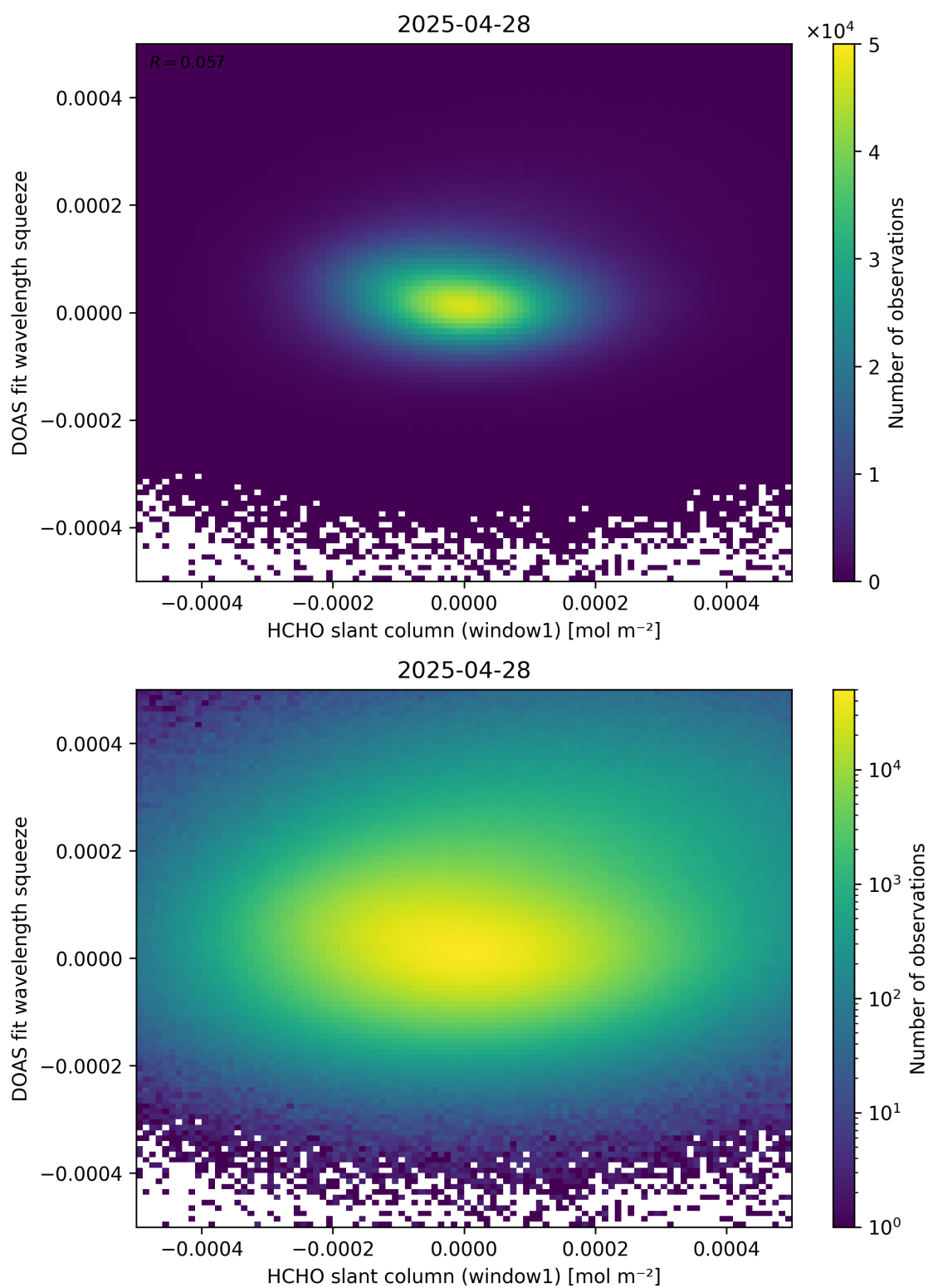
Figure 80: Scatter density plot of “HCHO slant column (window1)” against “DOAS fit wavelength squeeze” for 2025-04-27 to 2025-04-29.
