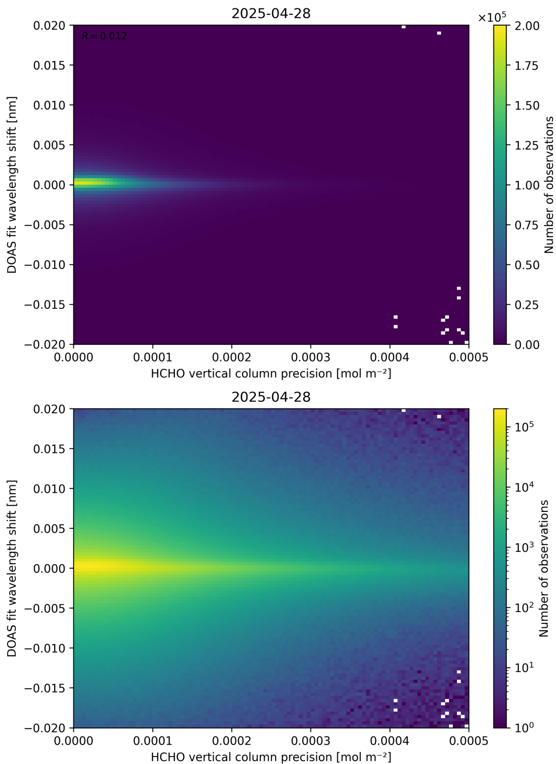
Figure 137: Scatter density plot of “HCHO vertical column precision” against “DOAS fit wavelength shift” for 2025-04-27 to 2025-04-29.
