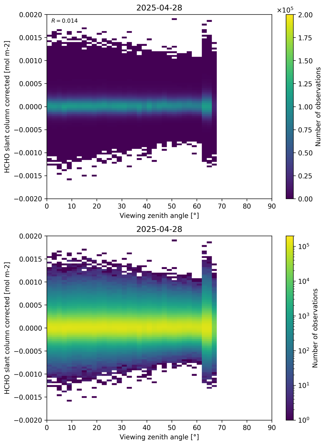
Figure 186: Scatter density plot of “Viewing zenith angle” against “HCHO slant column corrected” for 2025-04-27 to 2025-04-29.
