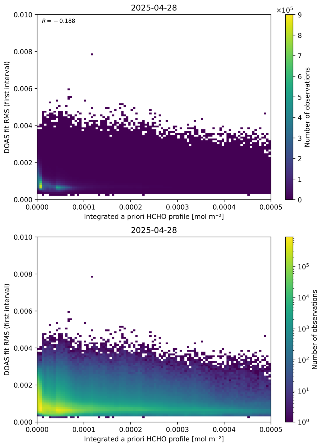
Figure 148: Scatter density plot of “Integrated a priori HCHO profile” against “DOAS fit RMS (first interval)” for 2025-04-27 to 2025-04-29.
