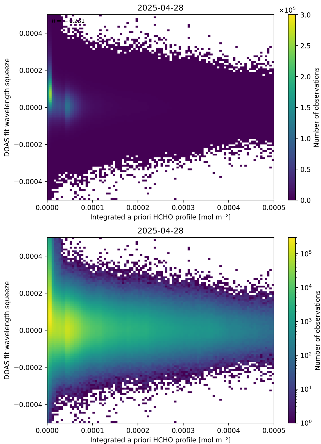
Figure 150: Scatter density plot of “Integrated a priori HCHO profile” against “DOAS fit wavelength squeeze” for 2025-04-27 to 2025-04-29.
