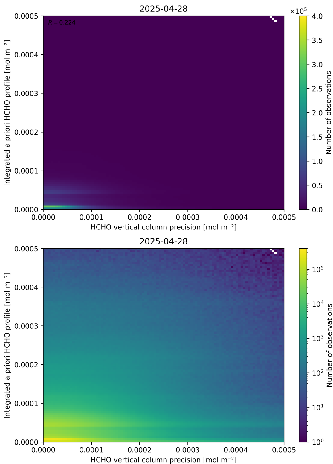
Figure 147: Scatter density plot of “HCHO vertical column precision” against “Integrated a priori HCHO profile” for 2025-04-27 to 2025-04-29.
