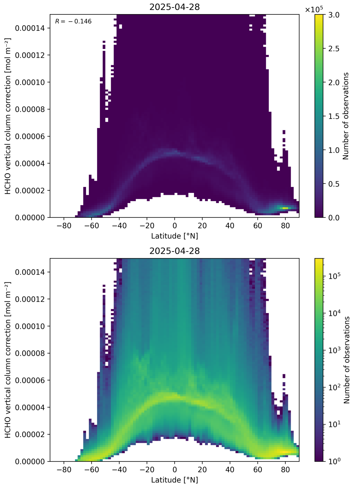
Figure 164: Scatter density plot of “Latitude” against “HCHO vertical column correction” for 2025-04-27 to 2025-04-29.
