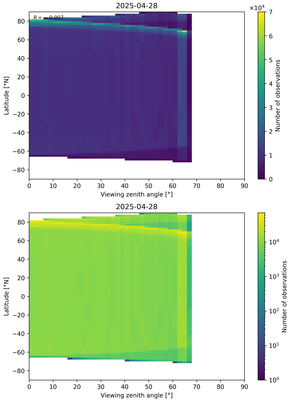
Figure 196: Scatter density plot of “Viewing zenith angle” against “Latitude” for 2025-04-27 to 2025-04-29.
