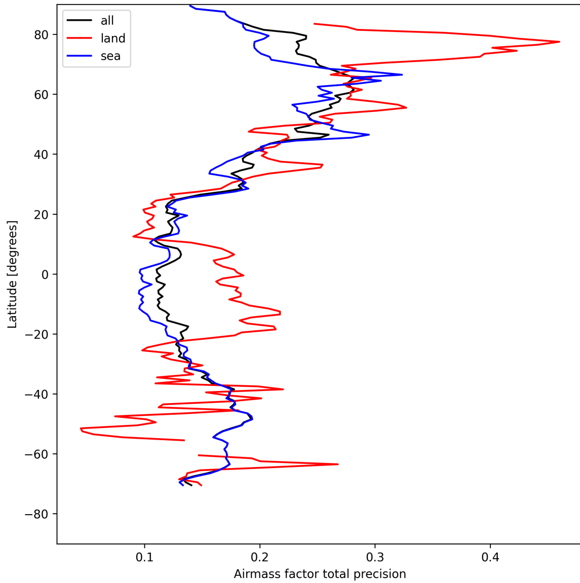
Figure 27: Zonal average of “Airmass factor total precision” for 2025-04-27 to 2025-04-29.
