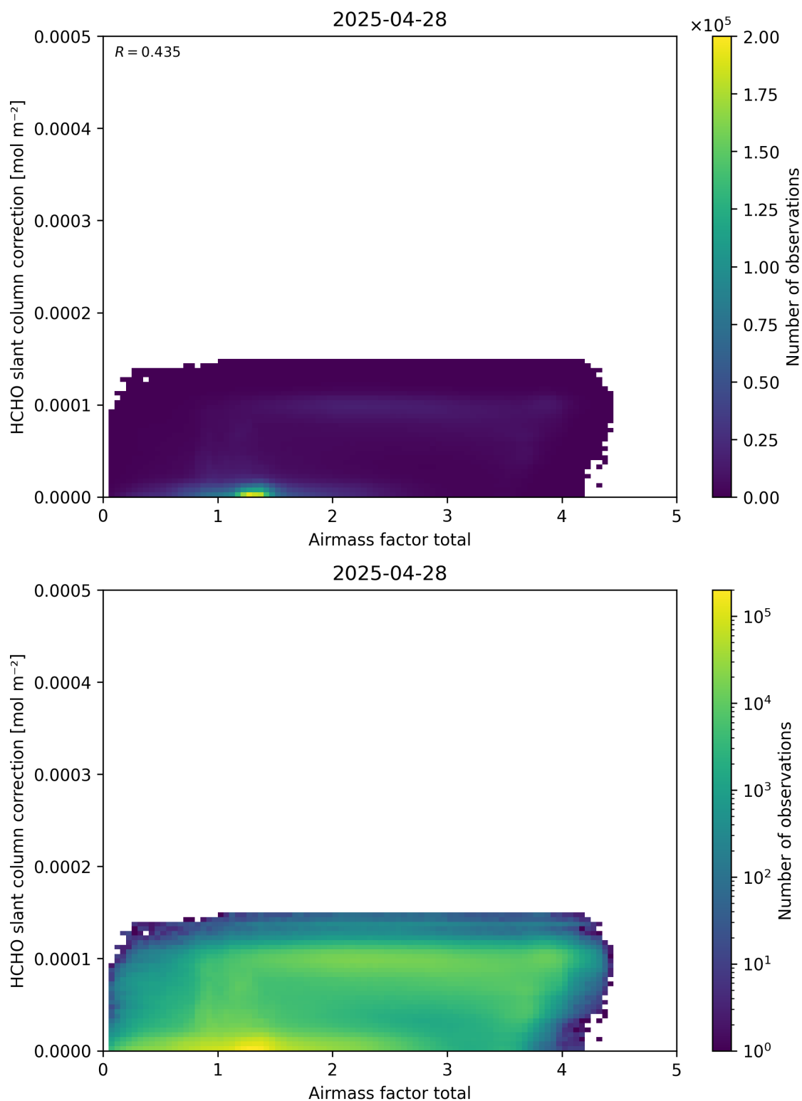
Figure 102: Scatter density plot of “Airmass factor total” against “HCHO slant column correction” for 2025-04-27 to 2025-04-29.
