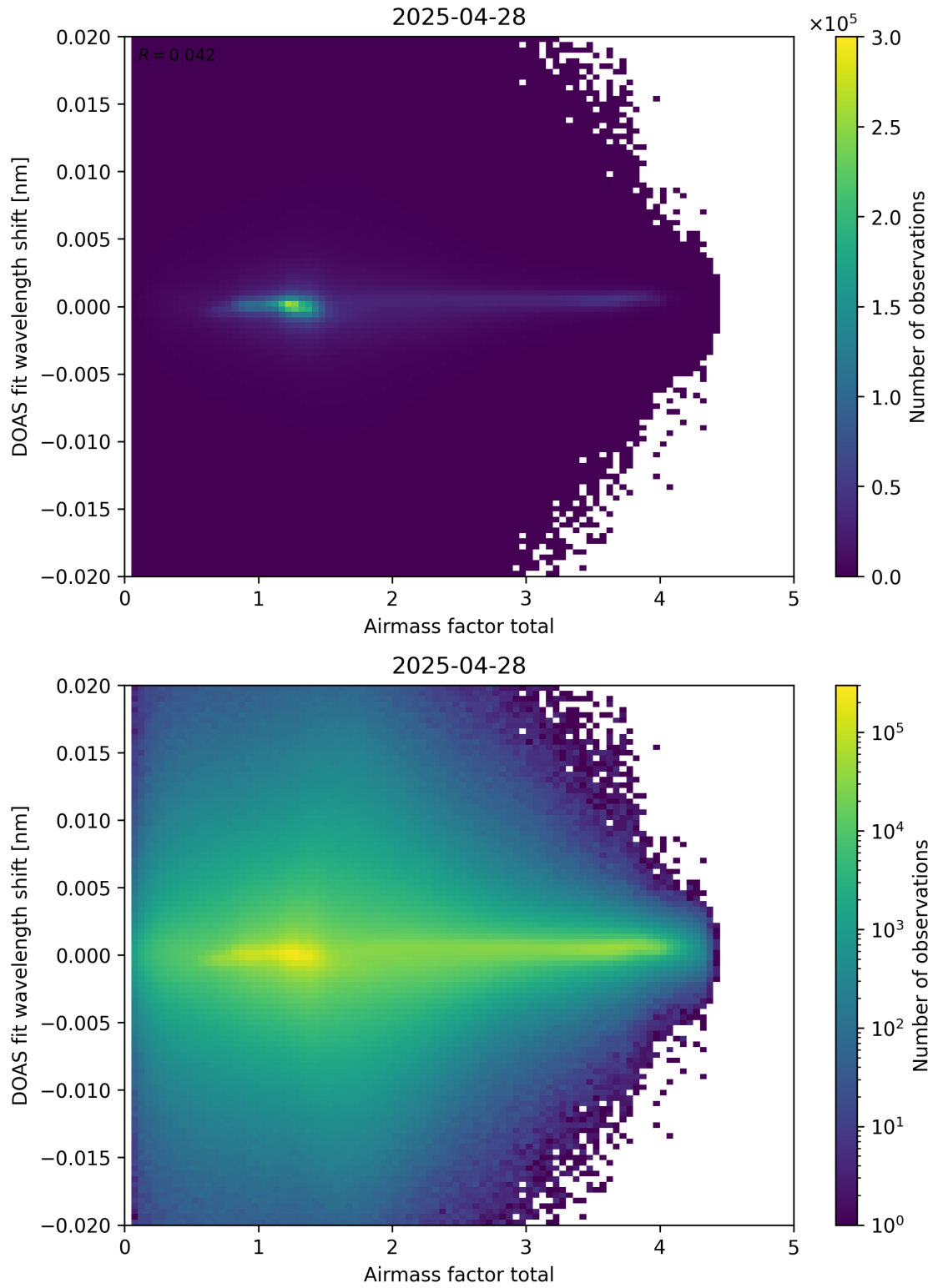
Figure 98: Scatter density plot of “Airmass factor total” against “DOAS fit wavelength shift” for 2025-04-27 to 2025-04-29.
