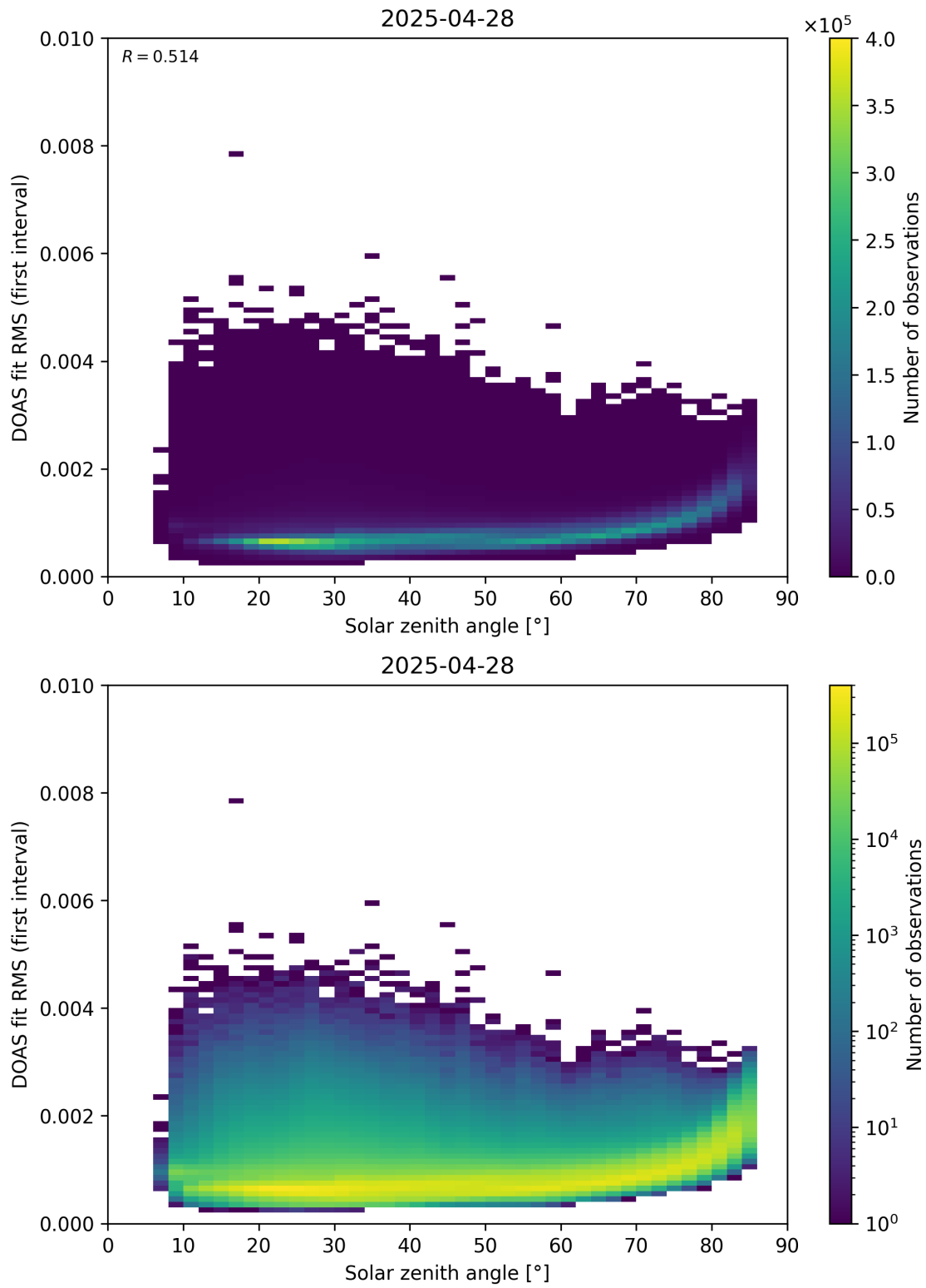
Figure 167: Scatter density plot of “Solar zenith angle” against “DOAS fit RMS (first interval)” for 2025-04-27 to 2025-04-29.
