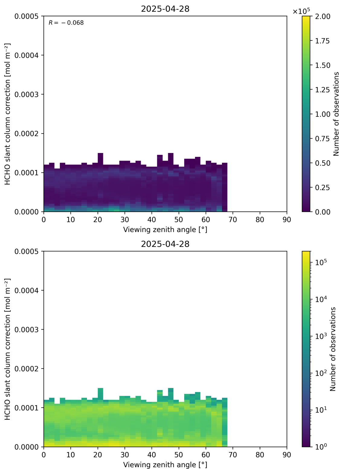
Figure 187: Scatter density plot of “Viewing zenith angle” against “HCHO slant column correction” for 2025-04-27 to 2025-04-29.
