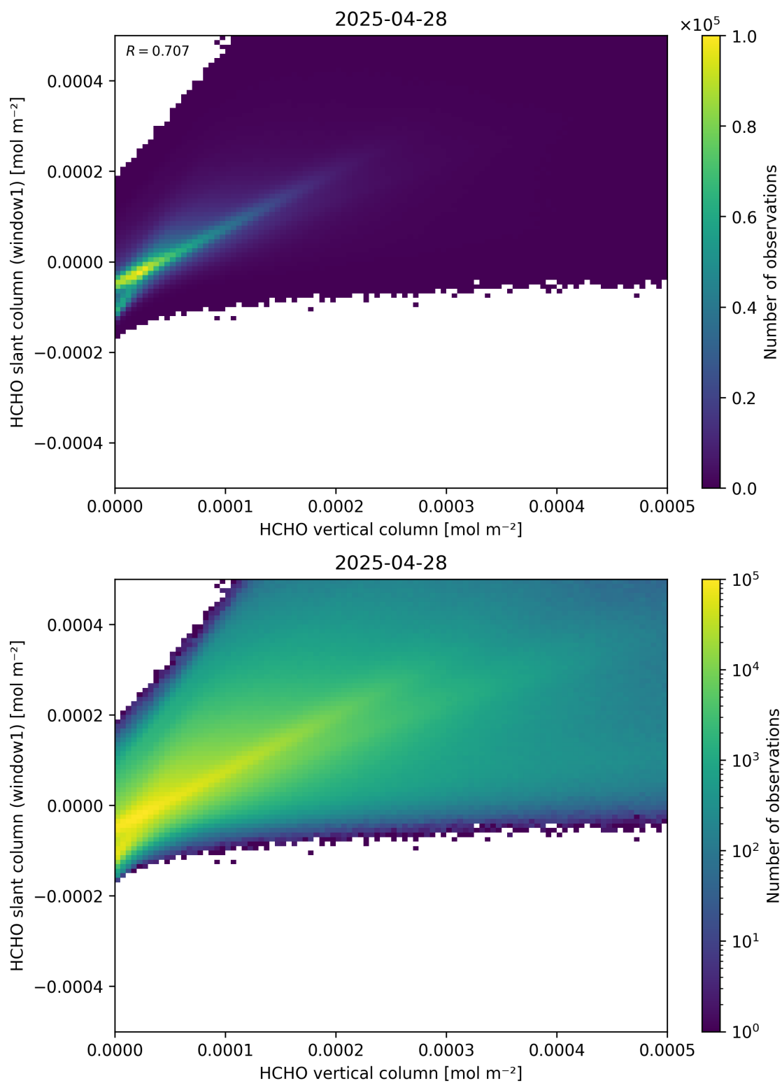
Figure 129: Scatter density plot of “HCHO vertical column” against “HCHO slant column (window1)” for 2025-04-27 to 2025-04-29.
