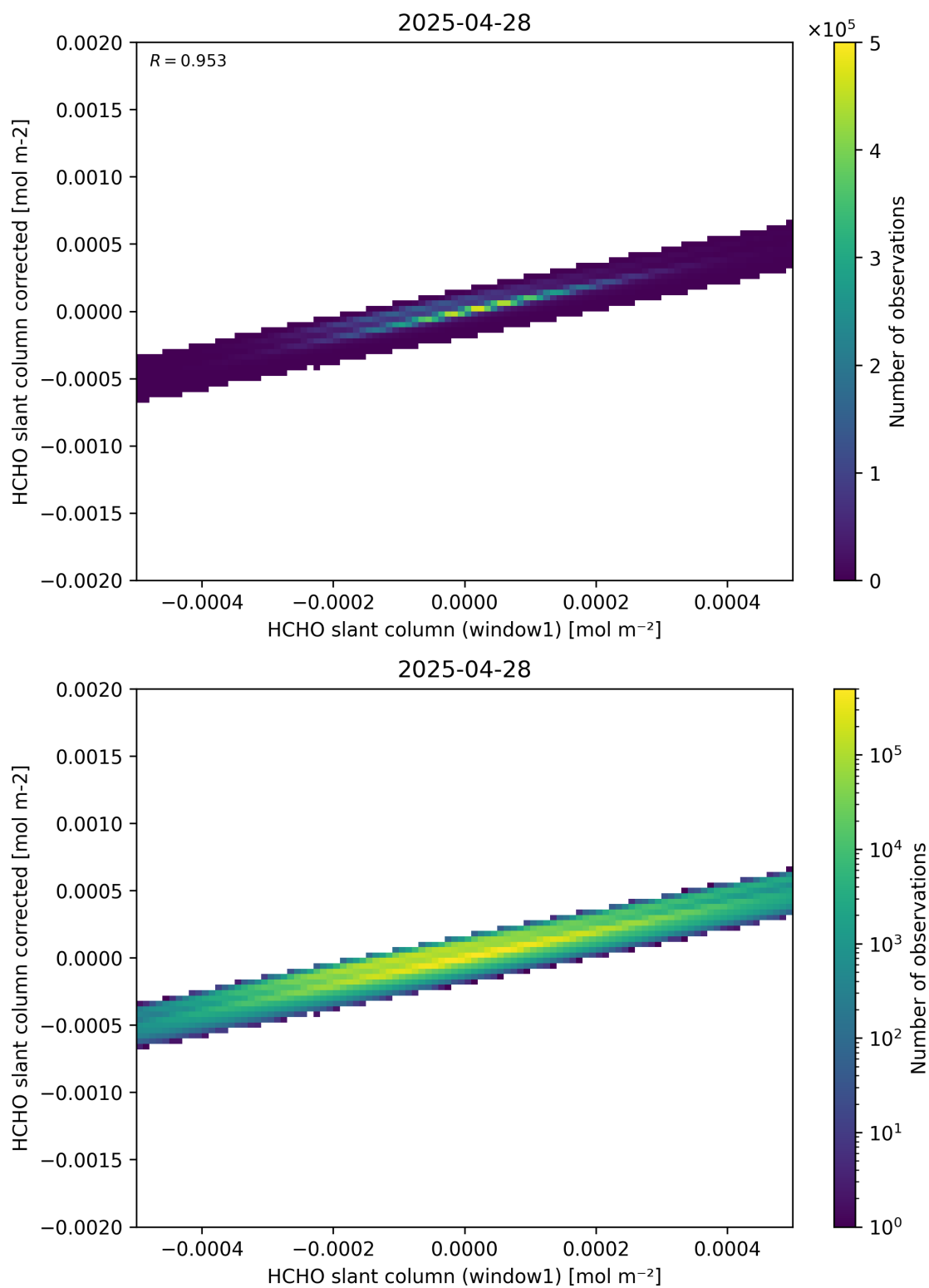
Figure 82: Scatter density plot of “HCHO slant column (window1)” against “HCHO slant column corrected” for 2025-04-27 to 2025-04-29.
