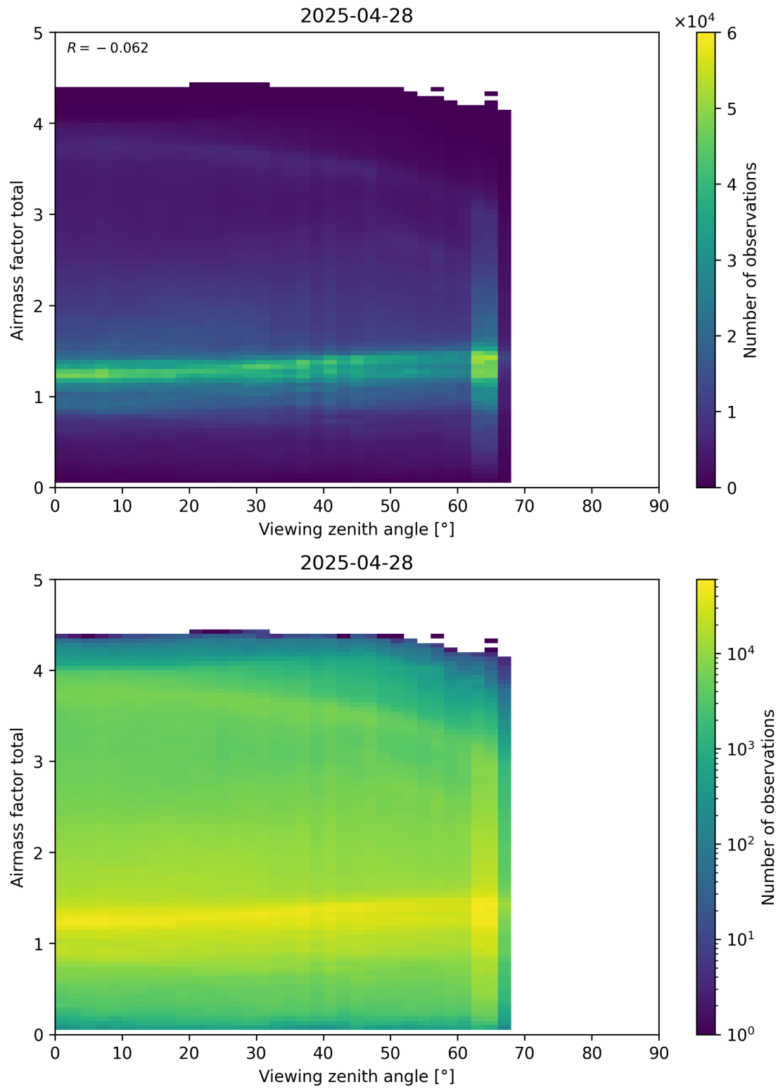
Figure 190: Scatter density plot of “Viewing zenith angle” against “Airmass factor total” for 2025-04-27 to 2025-04-29.
