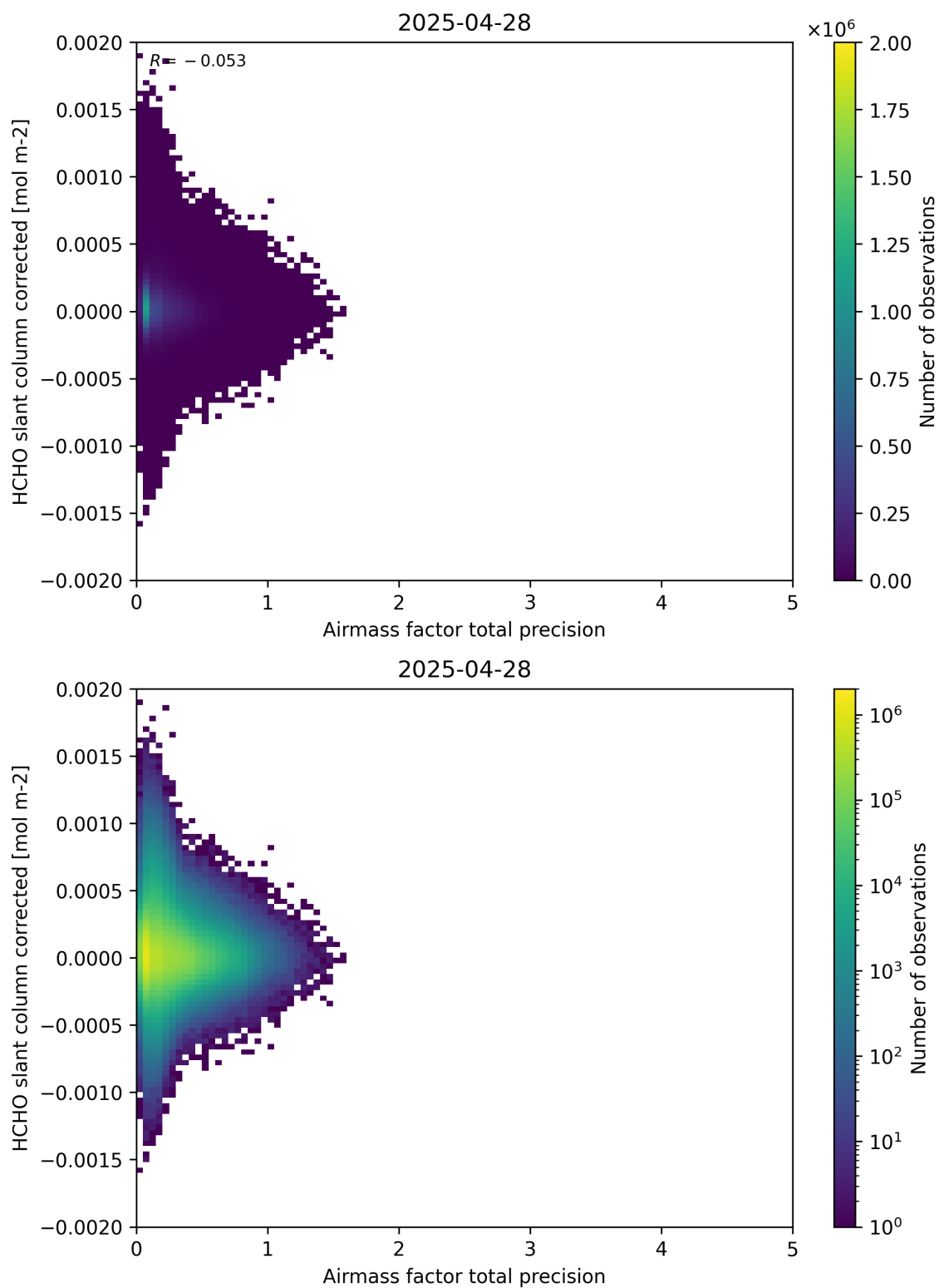
Figure 109: Scatter density plot of “Airmass factor total precision” against “HCHO slant column corrected” for 2025-04-27 to 2025-04-29.
