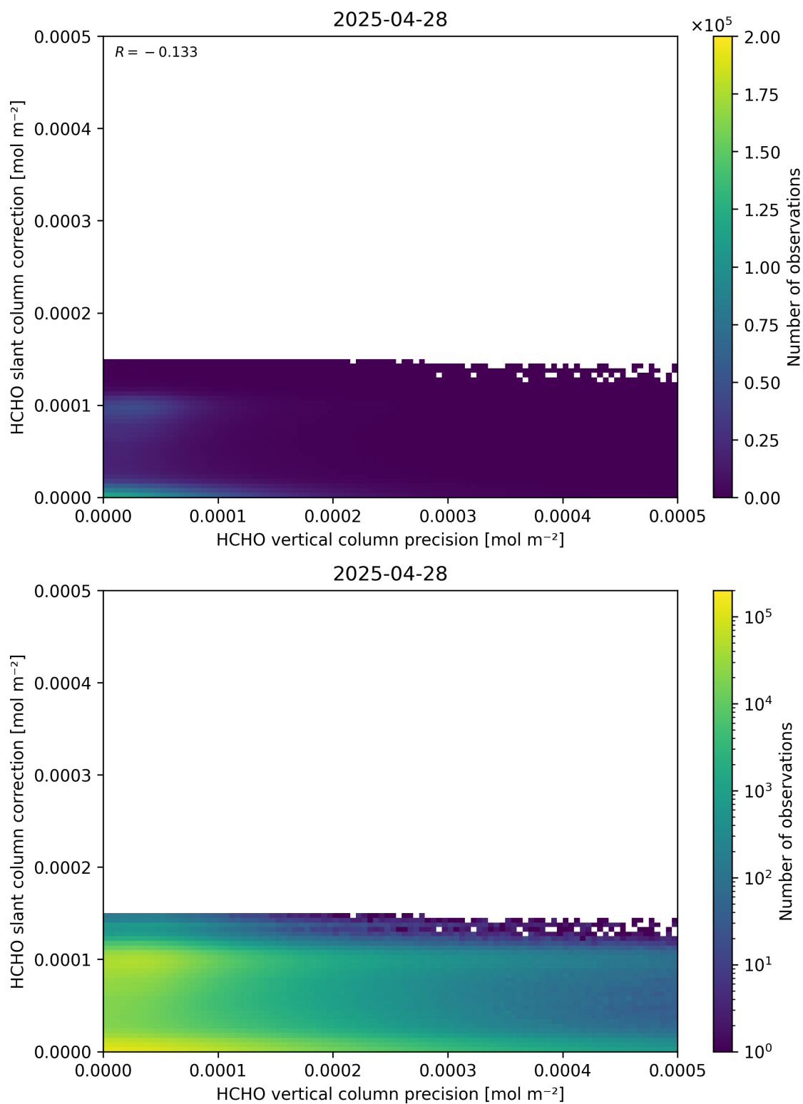
Figure 141: Scatter density plot of “HCHO vertical column precision” against “HCHO slant column correction” for 2025-04-27 to 2025-04-29.
