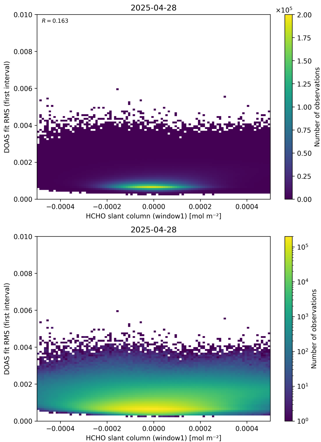
Figure 78: Scatter density plot of “HCHO slant column (window1)” against “DOAS fit RMS (first interval)” for 2025-04-27 to 2025-04-29.
