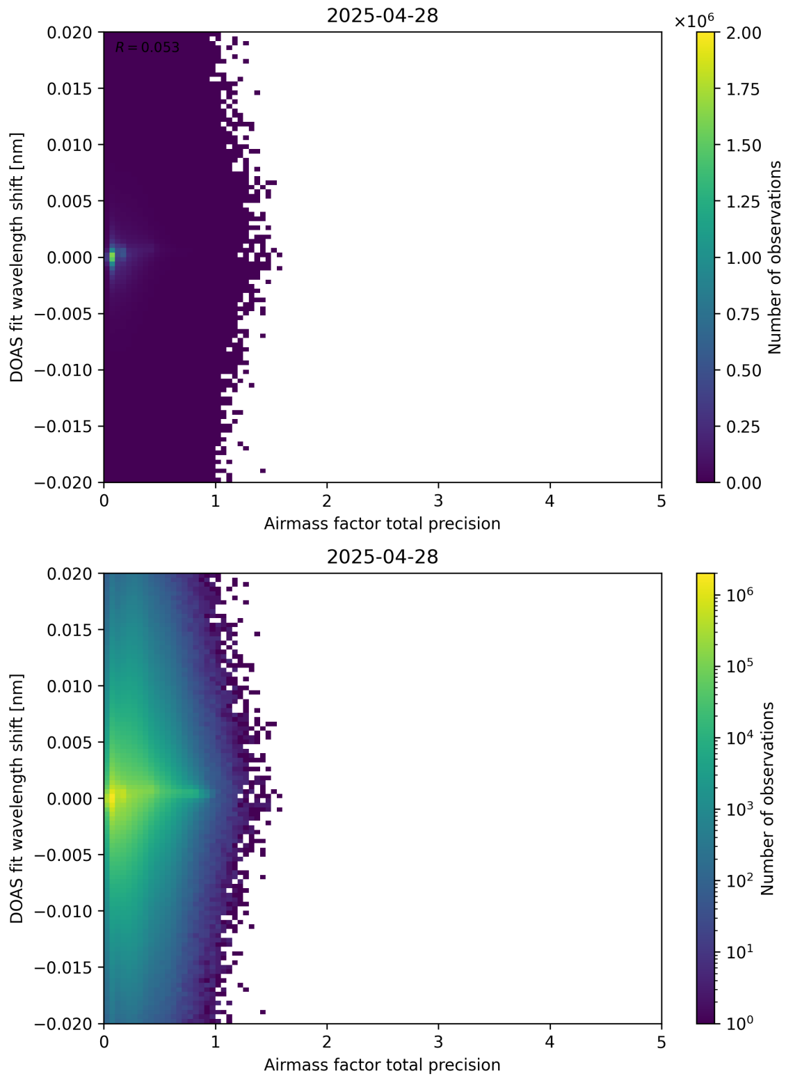
Figure 106: Scatter density plot of “Airmass factor total precision” against “DOAS fit wavelength shift” for 2025-04-27 to 2025-04-29.
