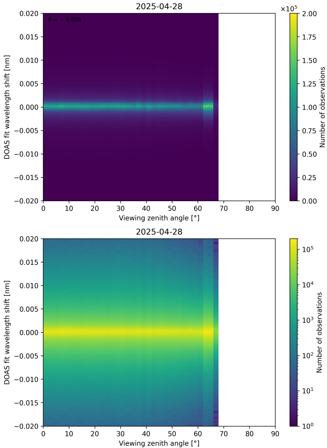
Figure 183: Scatter density plot of “Viewing zenith angle” against “DOAS fit wavelength shift” for 2025-04-27 to 2025-04-29.
