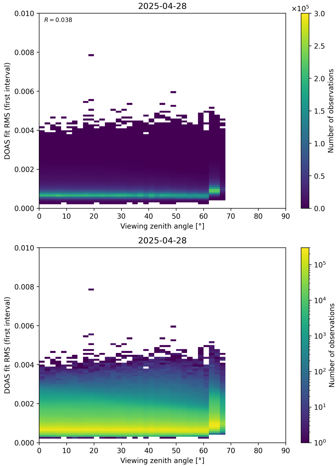
Figure 182: Scatter density plot of “Viewing zenith angle” against “DOAS fit RMS (first interval)” for 2025-04-27 to 2025-04-29.
