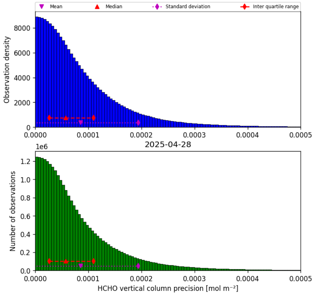
Figure 36: Histogram of “HCHO vertical column precision” for 2025-04-27 to 2025-04-29
