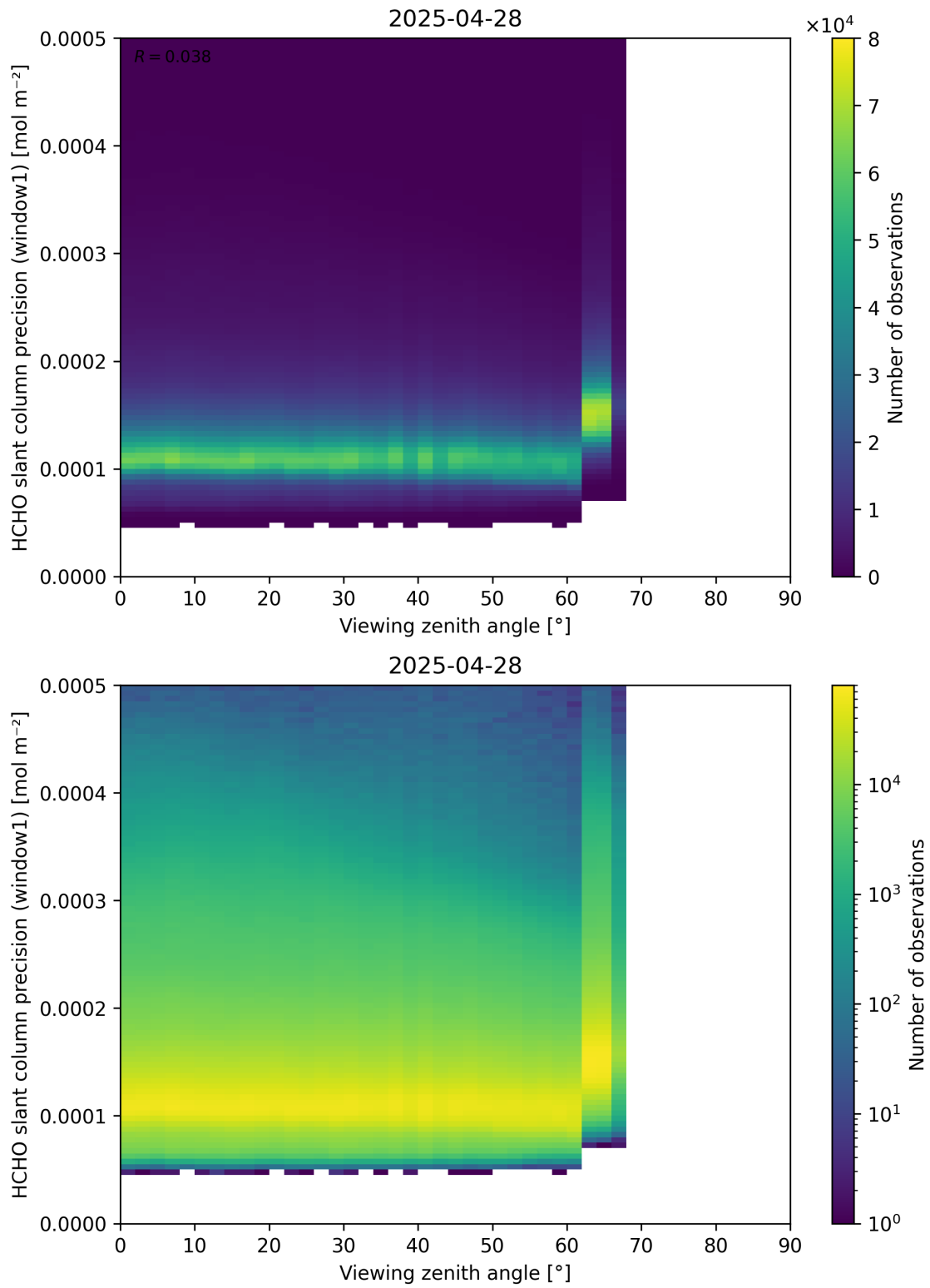
Figure 189: Scatter density plot of “Viewing zenith angle” against “HCHO slant column precision (window1)” for 2025-04-27 to 2025-04-29.
