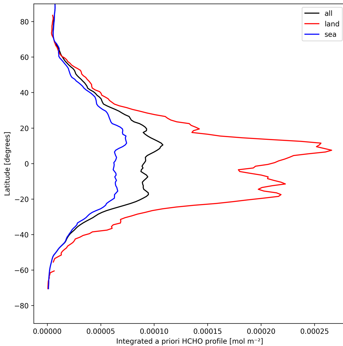
Figure 29: Zonal average of “Integrated a priori HCHO profile” for 2025-04-27 to 2025-04-29.
