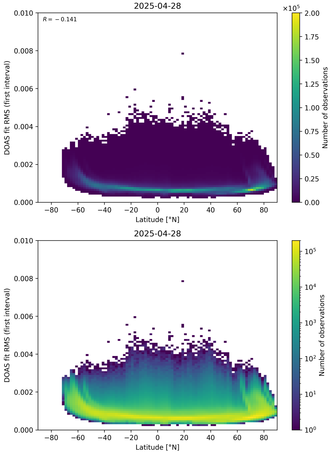
Figure 153: Scatter density plot of “Latitude” against “DOAS fit RMS (first interval)” for 2025-04-27 to 2025-04-29.
