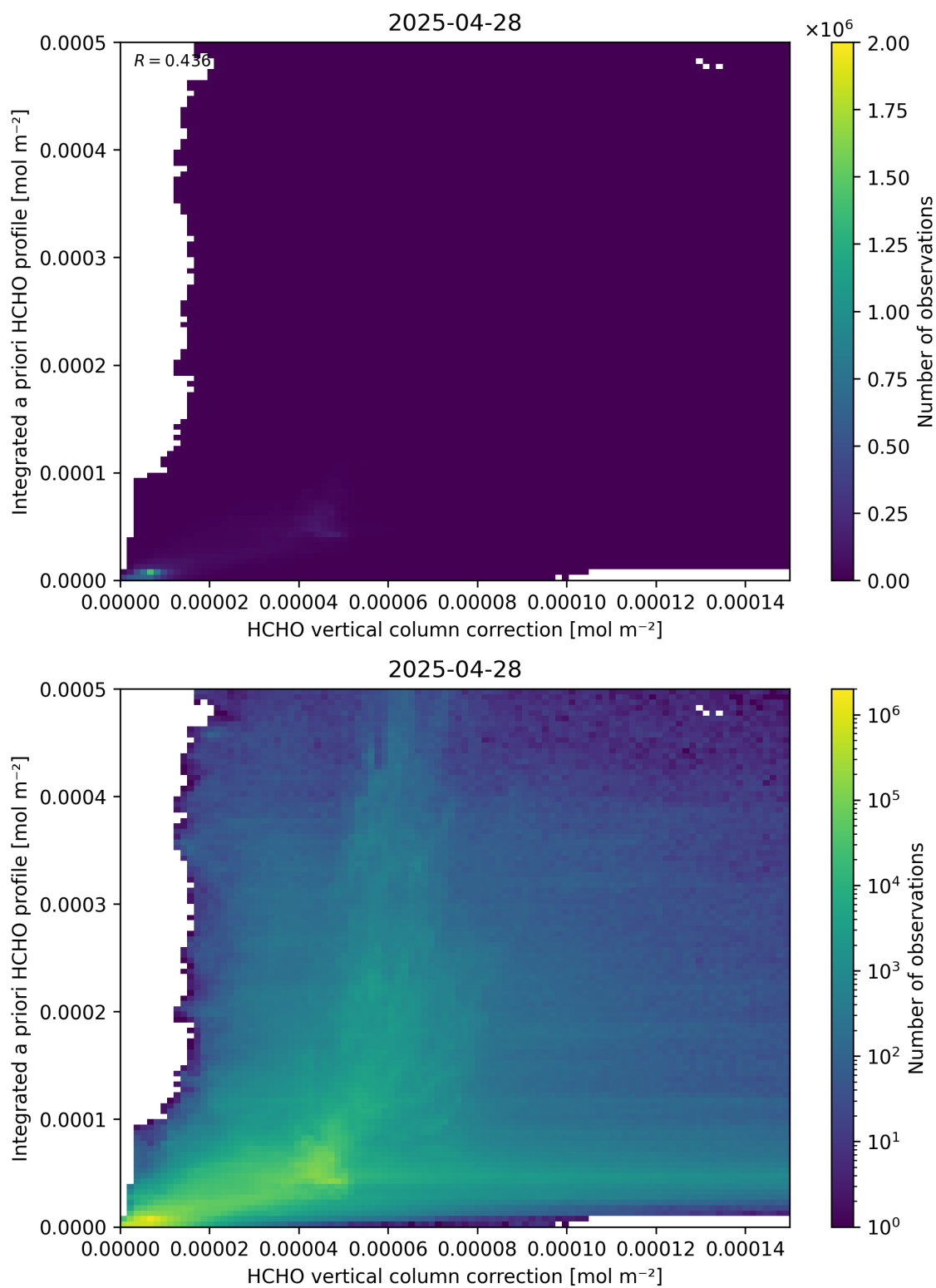
Figure 122: Scatter density plot of “HCHO vertical column correction” against “Integrated a priori HCHO profile” for 2025-04-27 to 2025-04-29.
