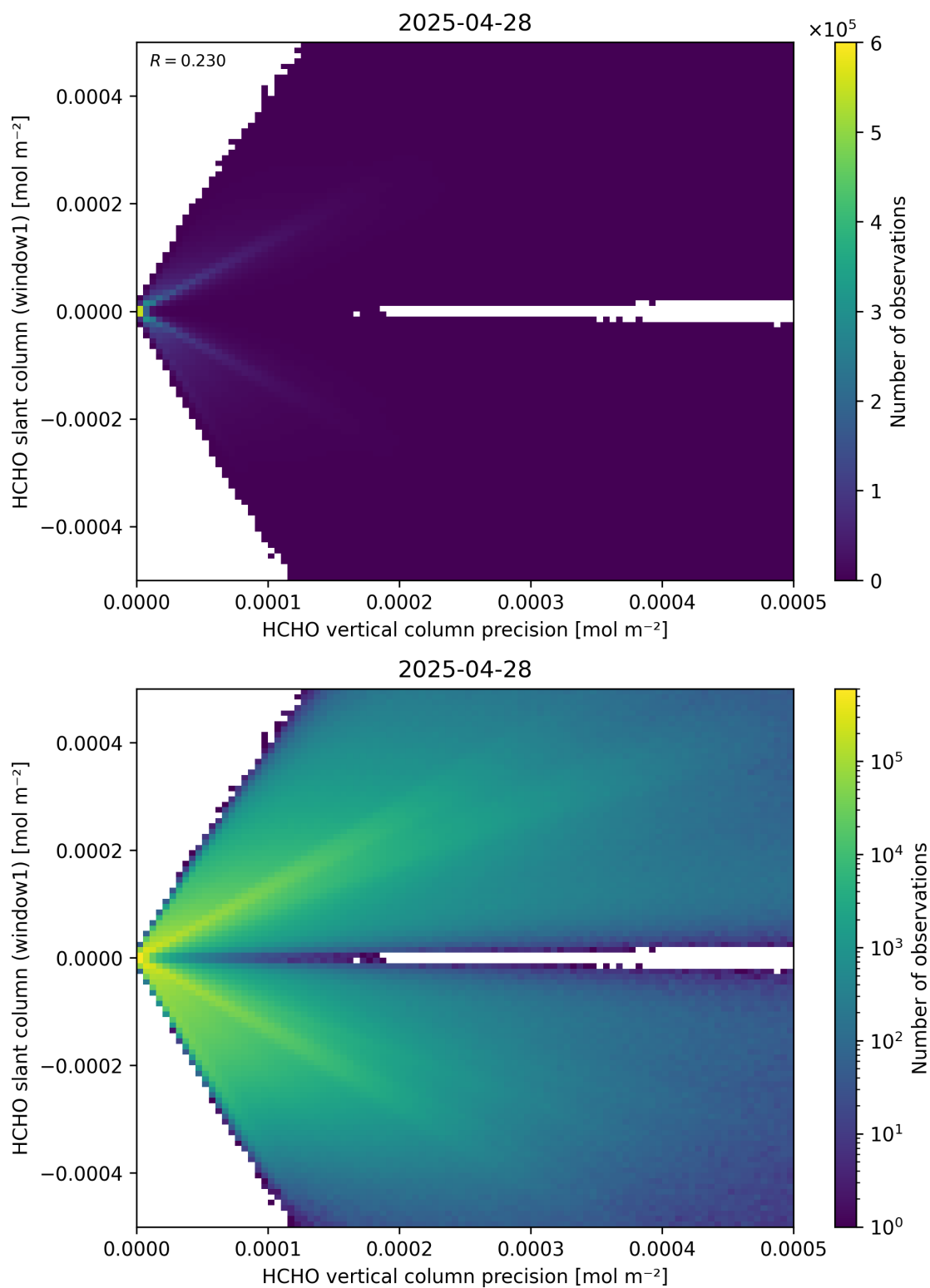
Figure 142: Scatter density plot of “HCHO vertical column precision” against “HCHO slant column (window1)” for 2025-04-27 to 2025-04-29.
