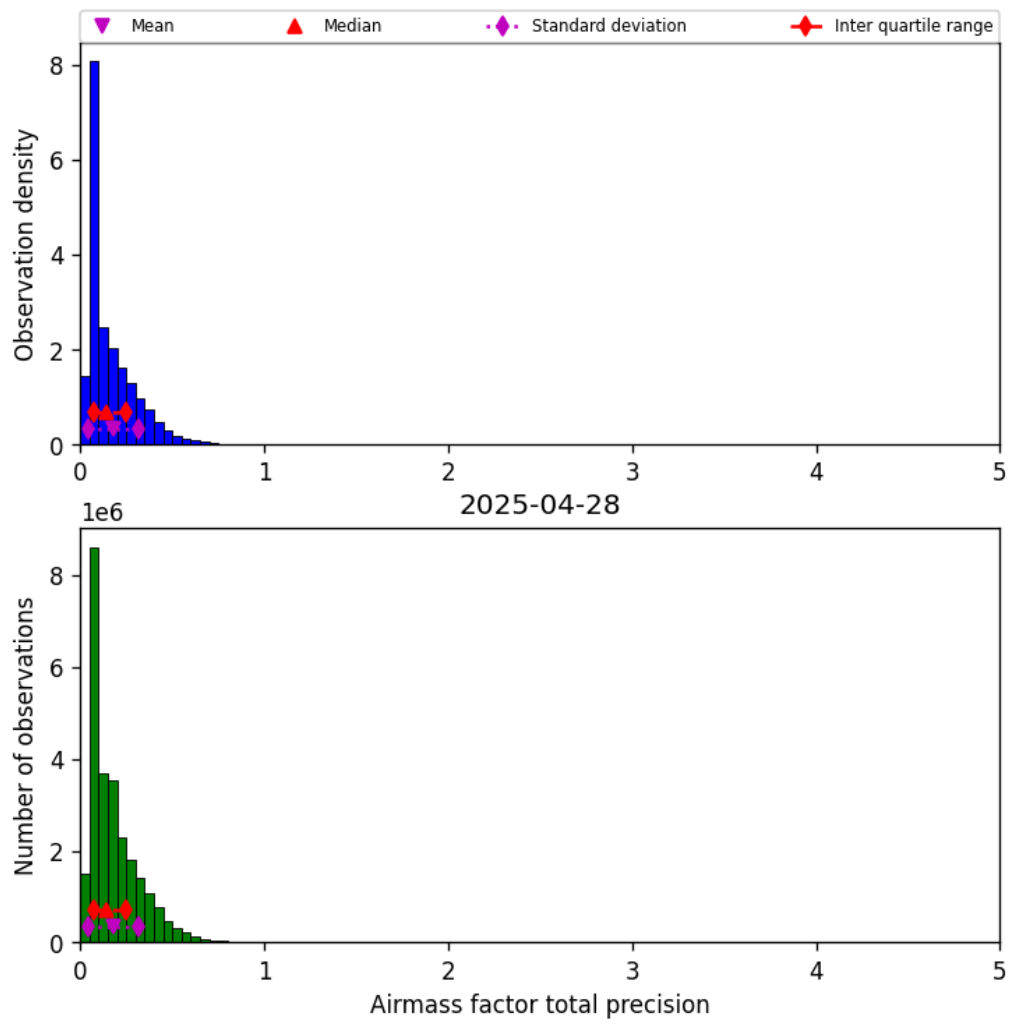
Figure 41: Histogram of “Airmass factor total precision” for 2025-04-27 to 2025-04-29
