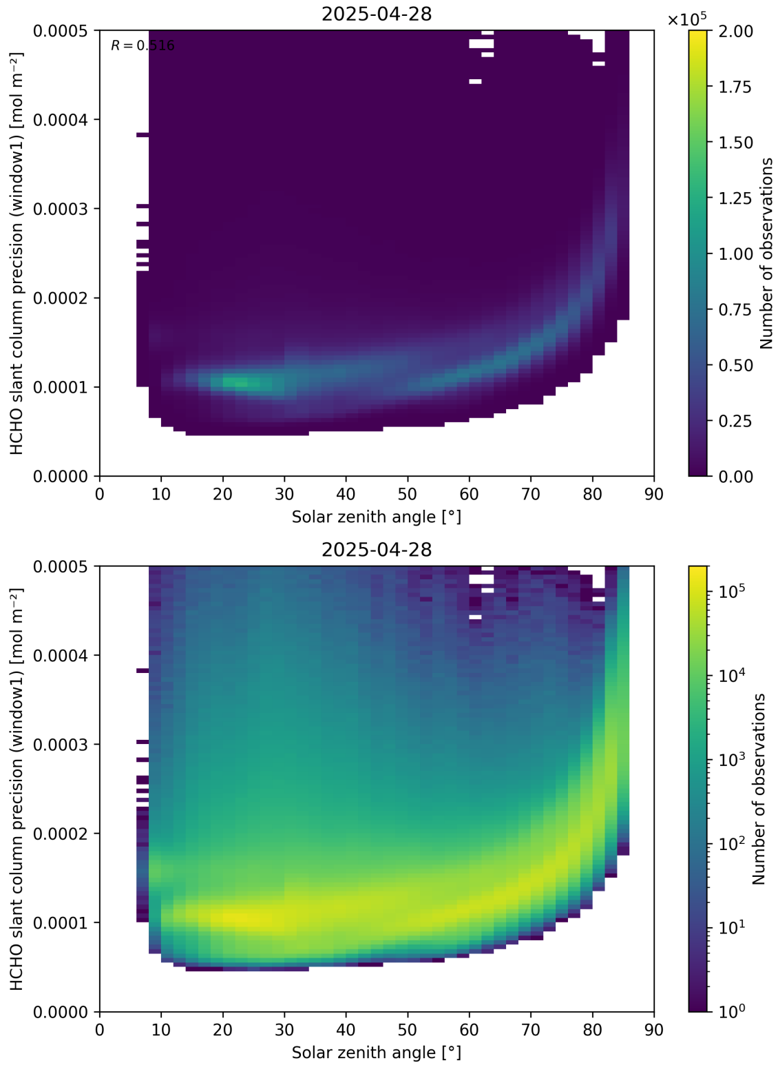
Figure 174: Scatter density plot of “Solar zenith angle” against “HCHO slant column precision (window1)” for 2025-04-27 to 2025-04-29.
