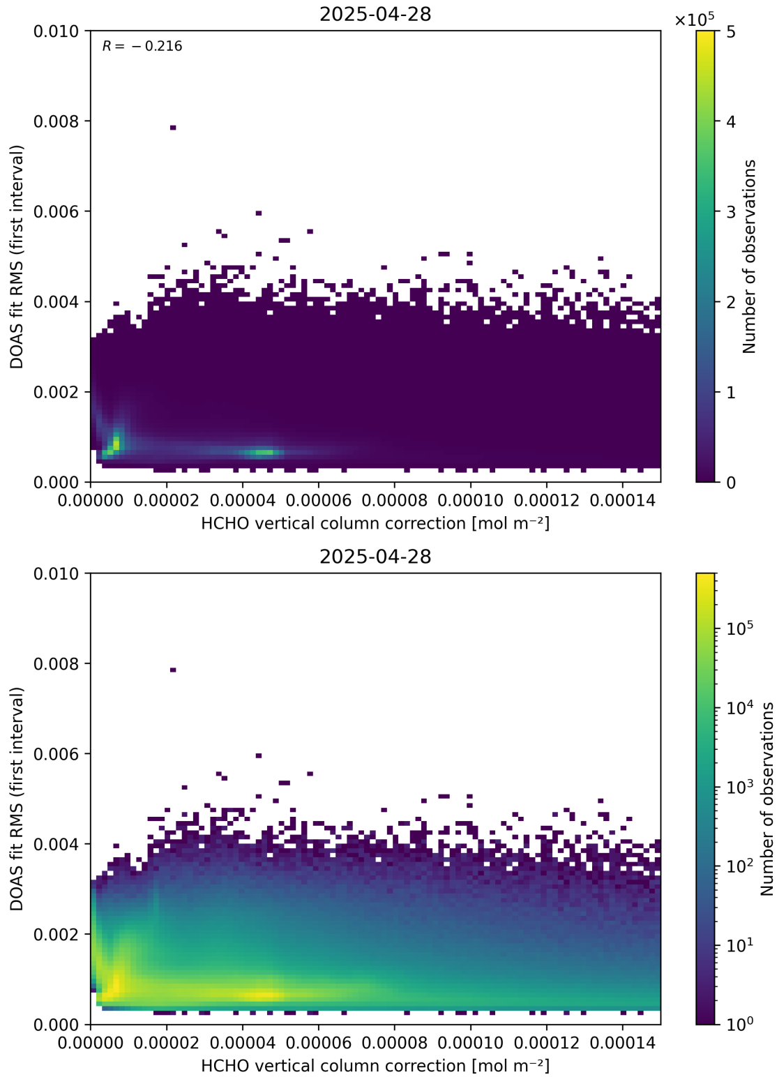
Figure 112: Scatter density plot of “HCHO vertical column correction” against “DOAS fit RMS (first interval)” for 2025-04-27 to 2025-04-29.
