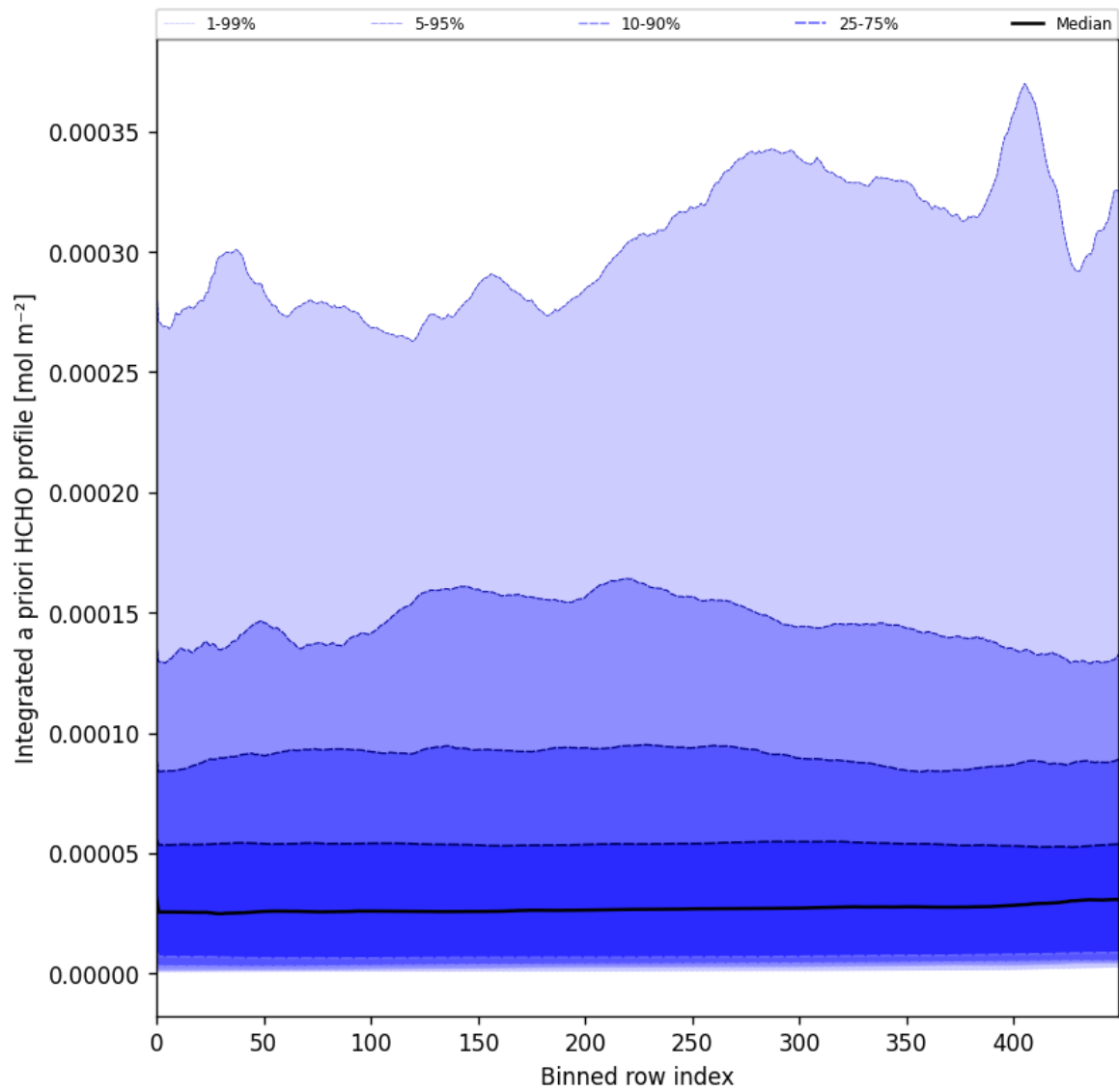
Figure 57: Along track statistics of “Integrated a priori HCHO profile” for 2025-04-27 to 2025-04-29
