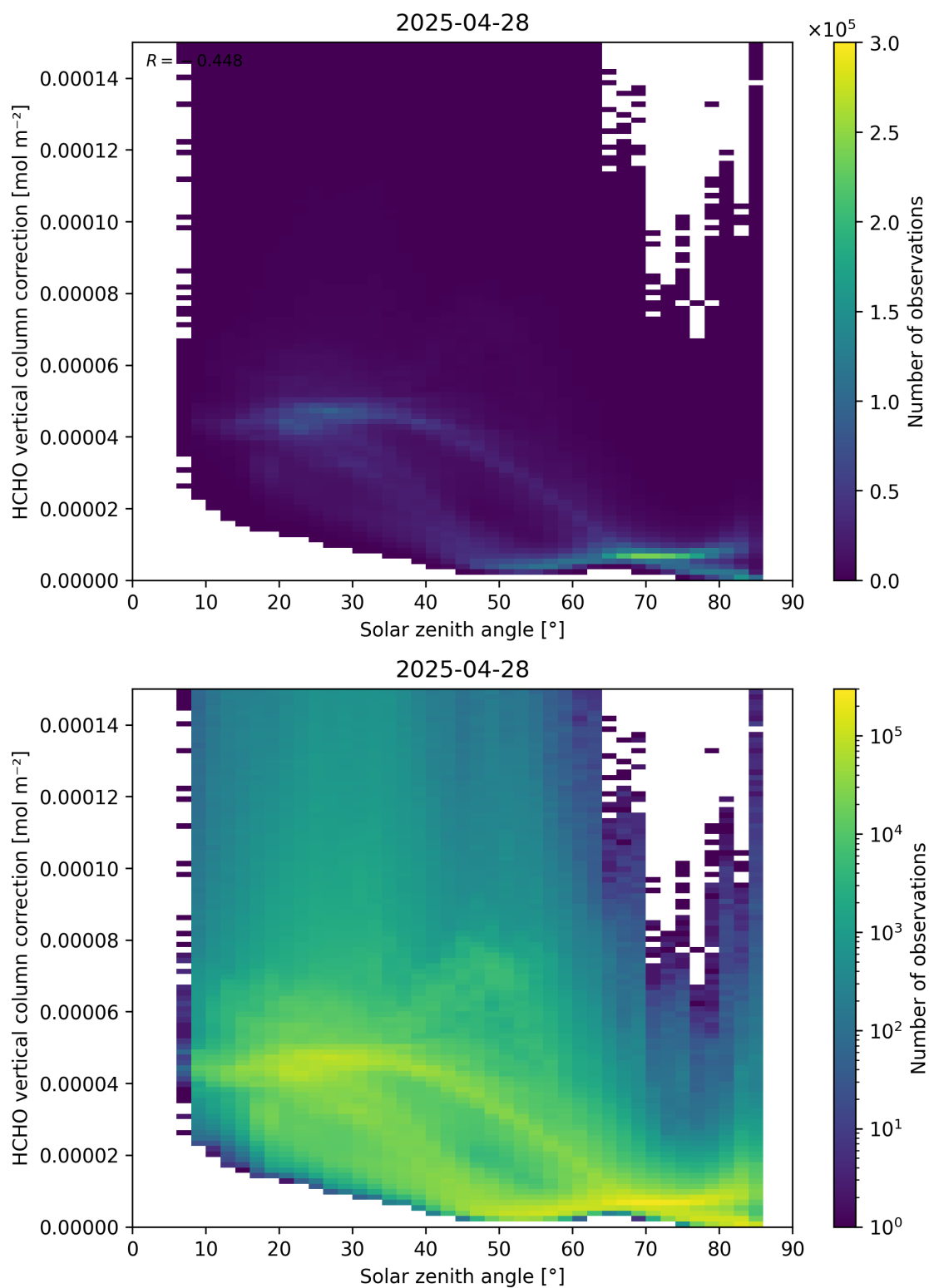
Figure 178: Scatter density plot of “Solar zenith angle” against “HCHO vertical column correction” for 2025-04-27 to 2025-04-29.
