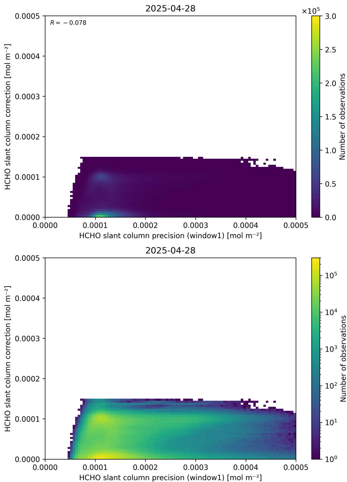
Figure 93: Scatter density plot of “HCHO slant column precision (window1)” against “HCHO slant column correction” for 2025-04-27 to 2025-04-29.
