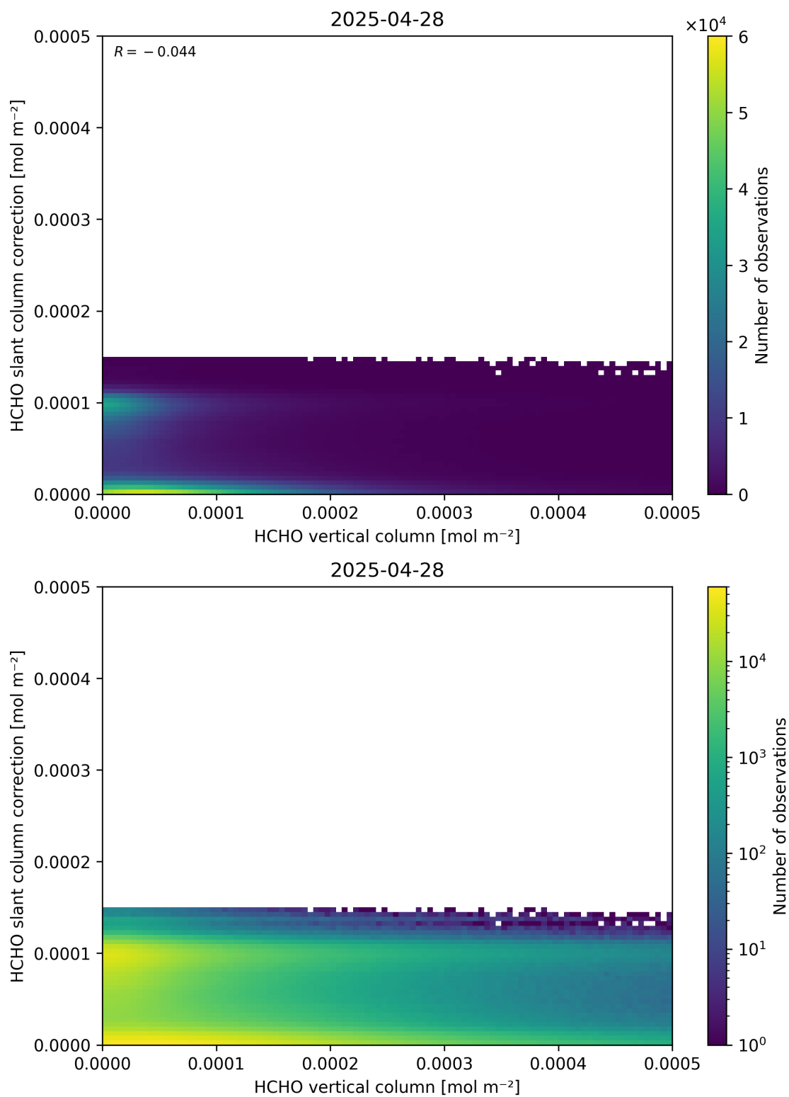
Figure 128: Scatter density plot of “HCHO vertical column” against “HCHO slant column correction” for 2025-04-27 to 2025-04-29.
