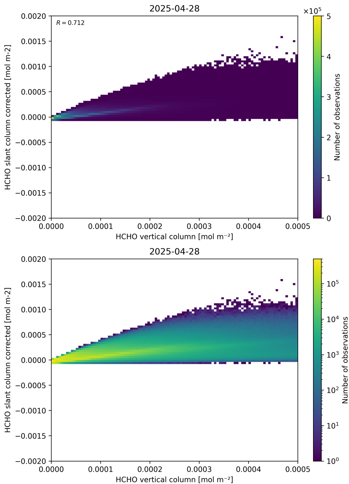
Figure 127: Scatter density plot of “HCHO vertical column” against “HCHO slant column corrected” for 2025-04-27 to 2025-04-29.
