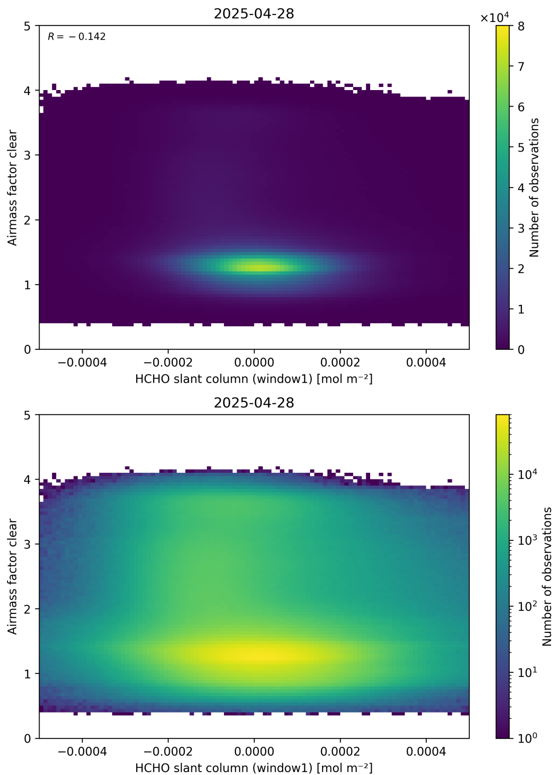
Figure 81: Scatter density plot of “HCHO slant column (window1)” against “Airmass factor clear” for 2025-04-27 to 2025-04-29.
