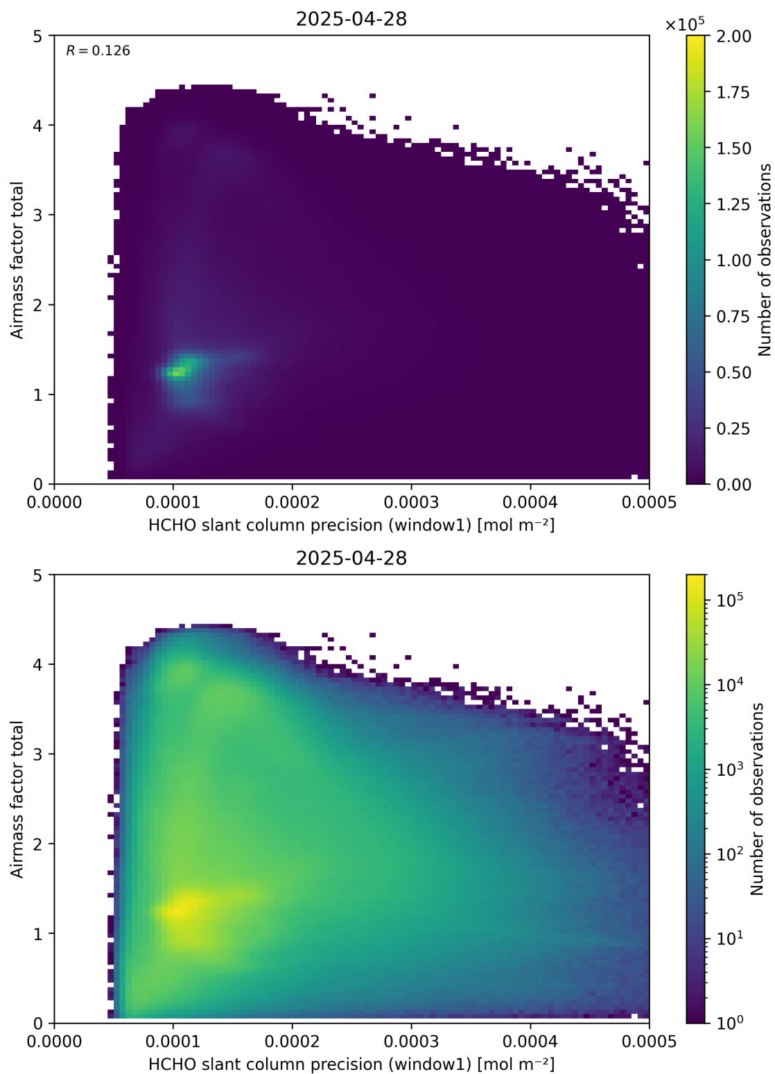
Figure 94: Scatter density plot of “HCHO slant column precision (window1)” against “Airmass factor total” for 2025-04-27 to 2025-04-29.
