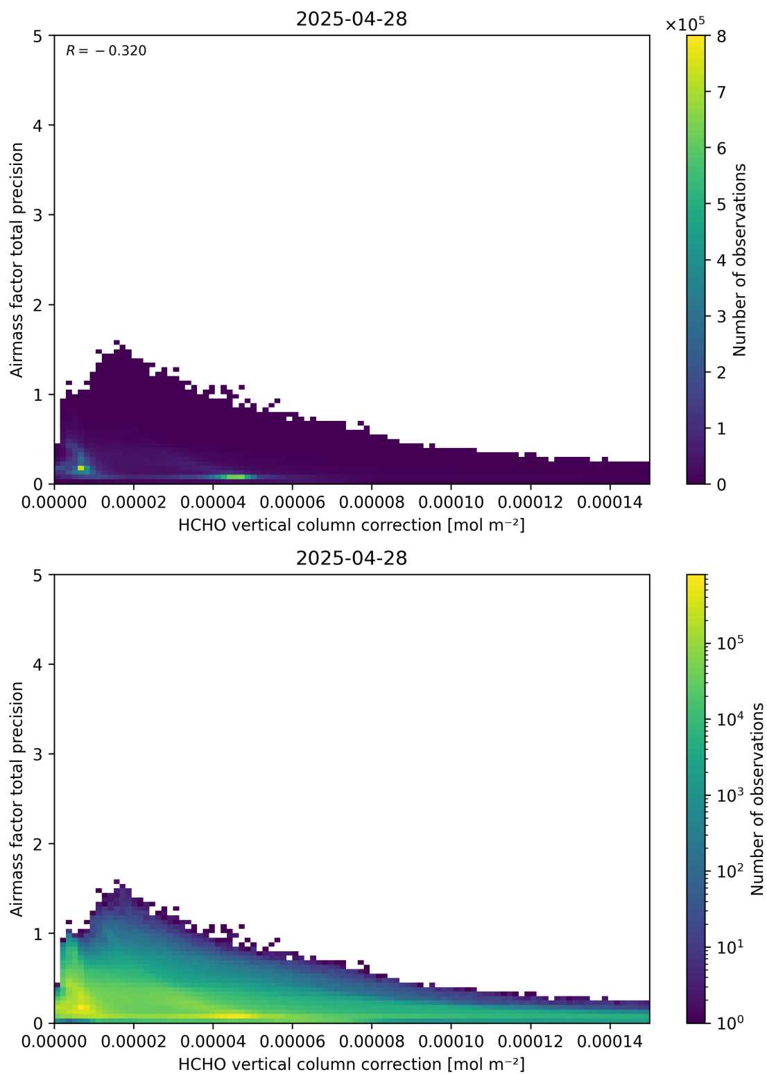
Figure 121: Scatter density plot of “HCHO vertical column correction” against “Airmass factor total precision” for 2025-04-27 to 2025-04-29.
