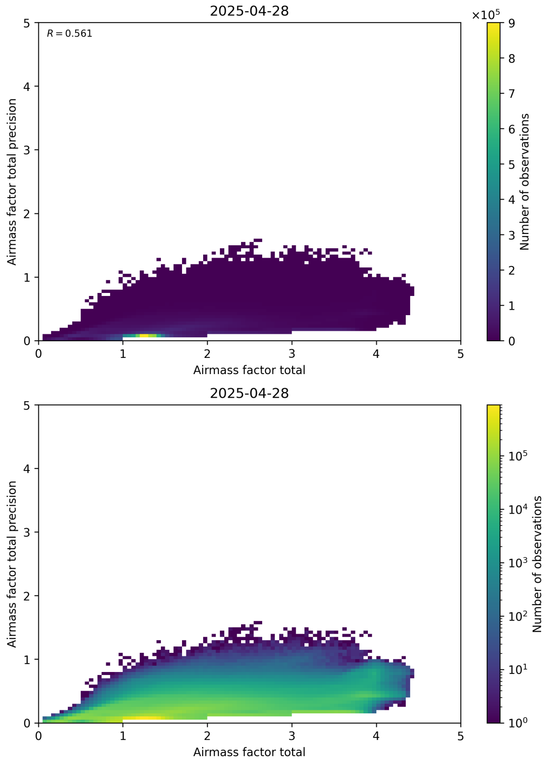
Figure 103: Scatter density plot of “Airmass factor total” against “Airmass factor total precision” for 2025-04-27 to 2025-04-29.
