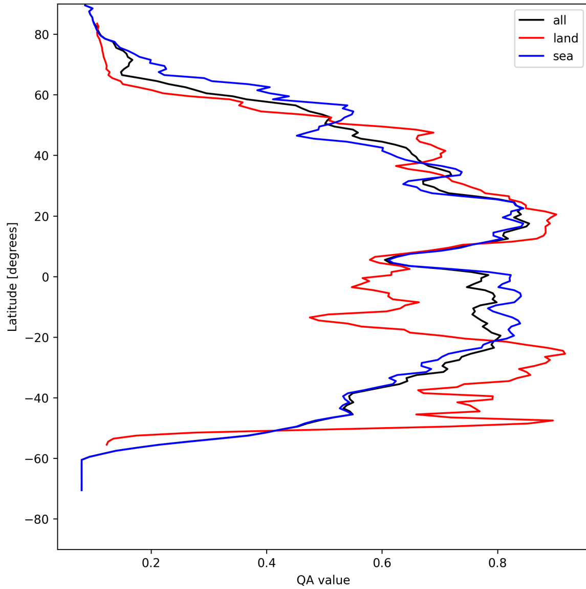
Figure 20: Zonal average of “QA value” for 2025-04-27 to 2025-04-29.
