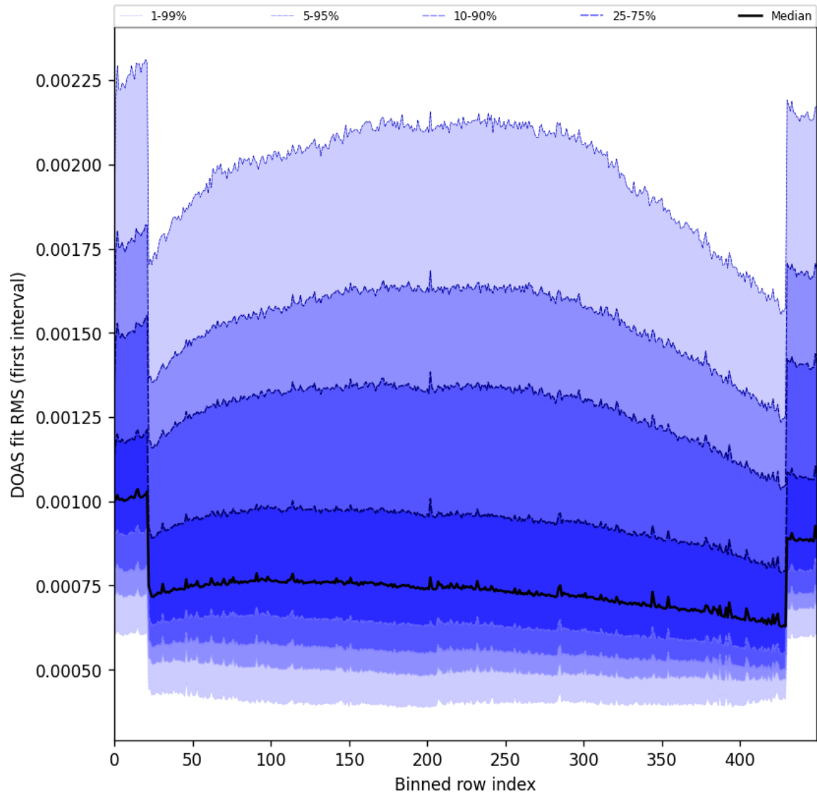
Figure 60: Along track statistics of “DOAS fit RMS (first interval)” for 2025-04-27 to 2025-04-29
