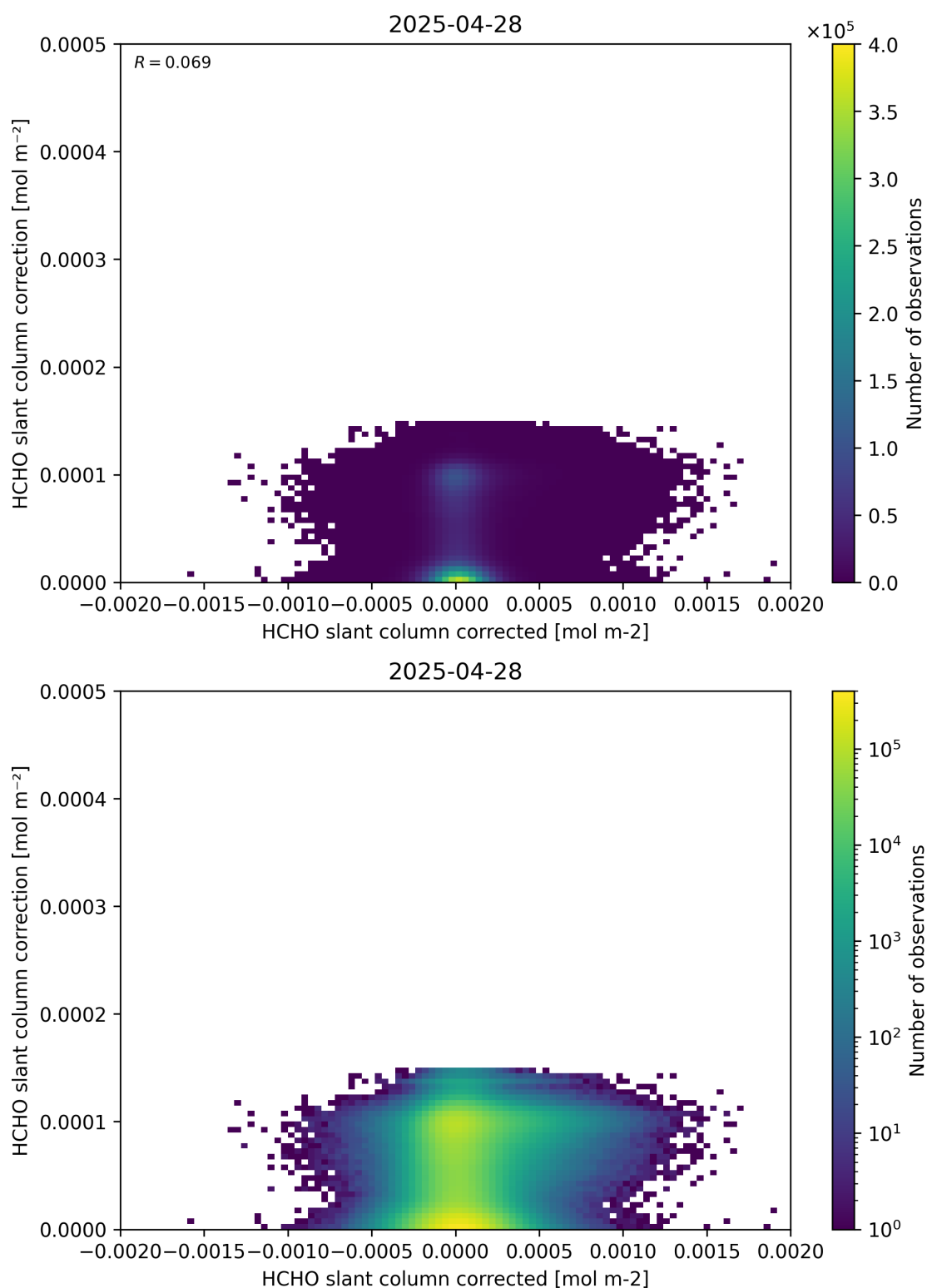
Figure 77: Scatter density plot of “HCHO slant column corrected” against “HCHO slant column correction” for 2025-04-27 to 2025-04-29.
