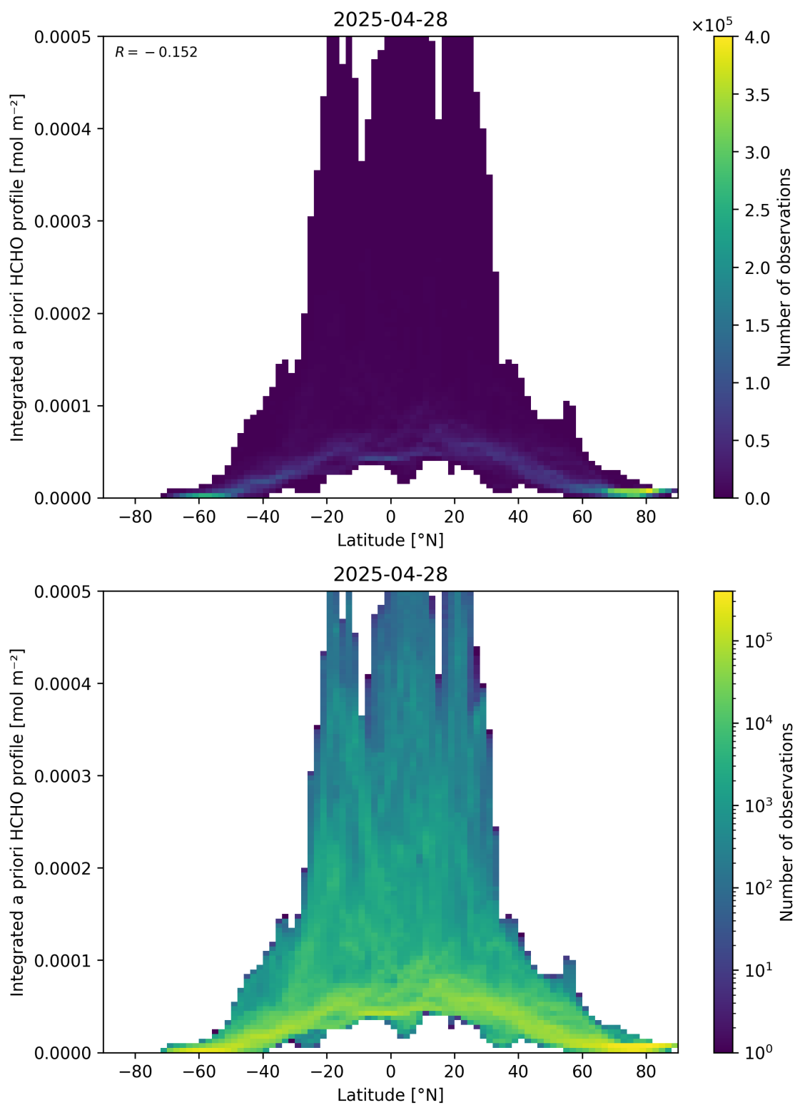
Figure 166: Scatter density plot of “Latitude” against “Integrated a priori HCHO profile” for 2025-04-27 to 2025-04-29.
