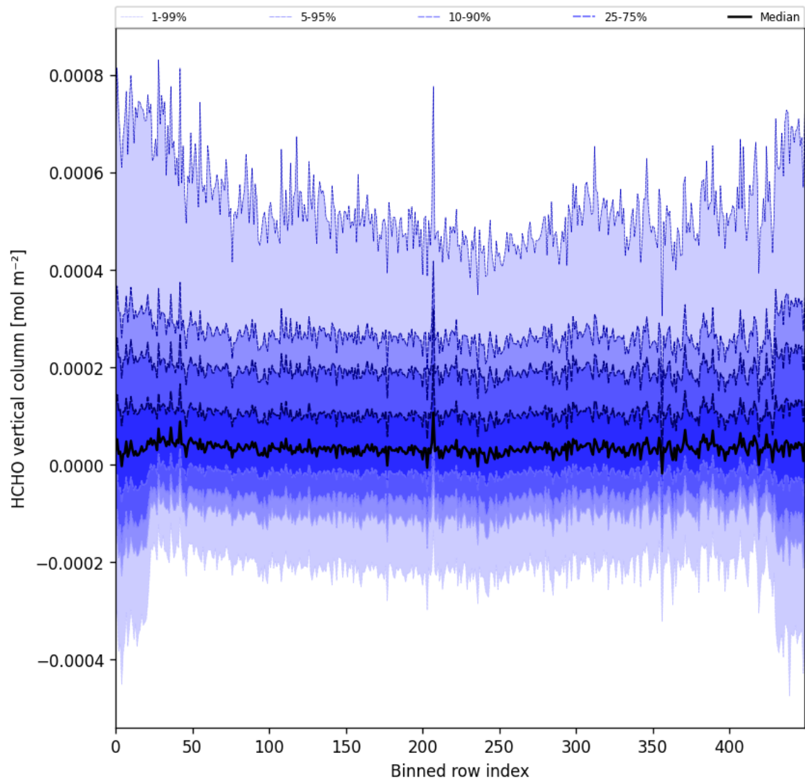
Figure 49: Along track statistics of “HCHO vertical column” for 2025-04-27 to 2025-04-29
