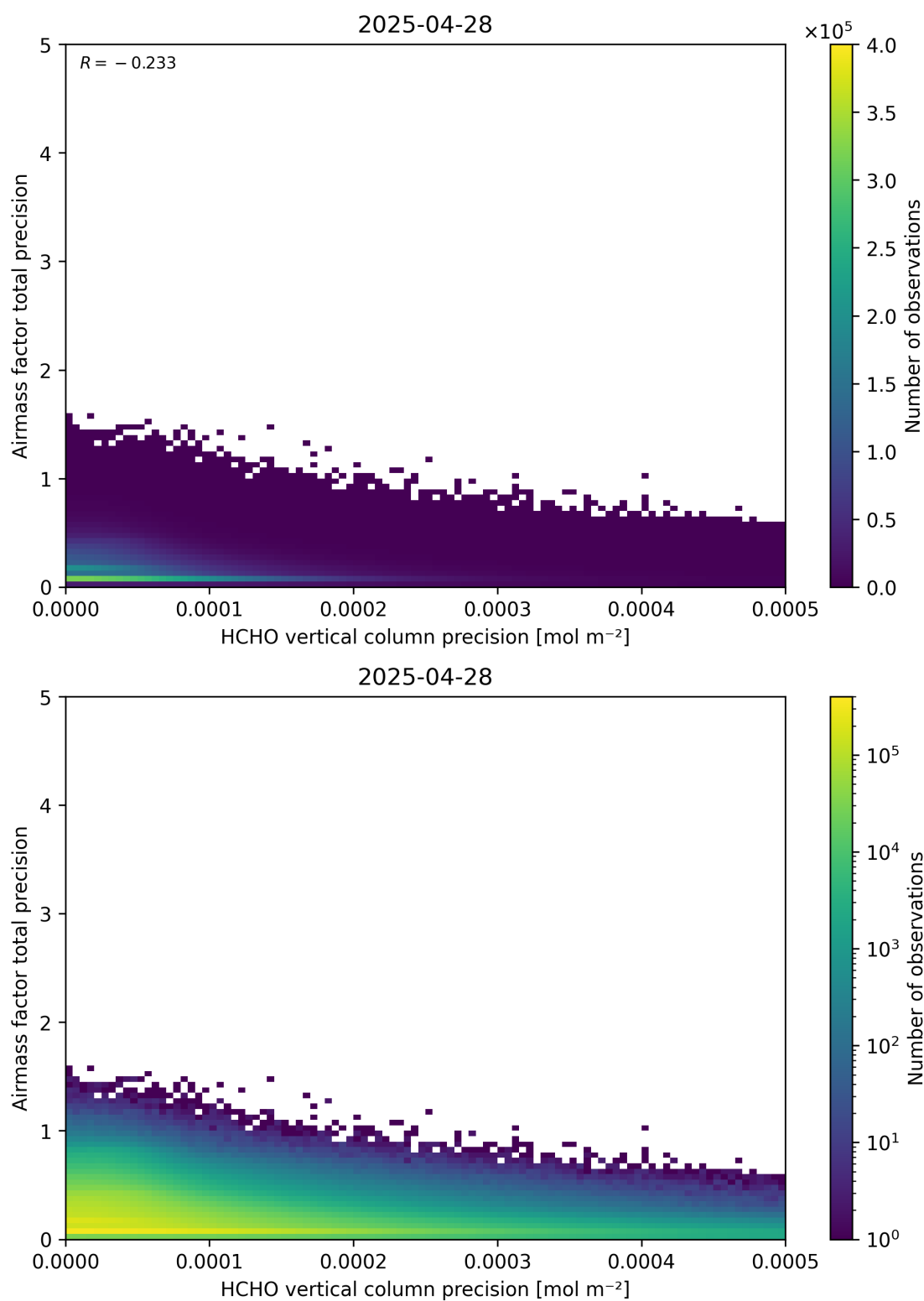
Figure 145: Scatter density plot of “HCHO vertical column precision” against “Airmass factor total precision” for 2025-04-27 to 2025-04-29.
