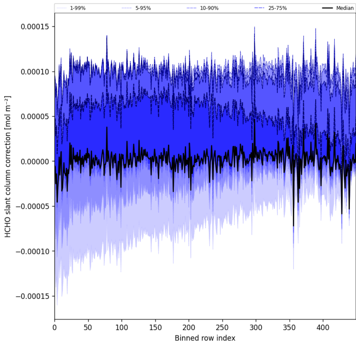
Figure 61: Along track statistics of “HCHO slant column correction” for 2025-04-27 to 2025-04-29
