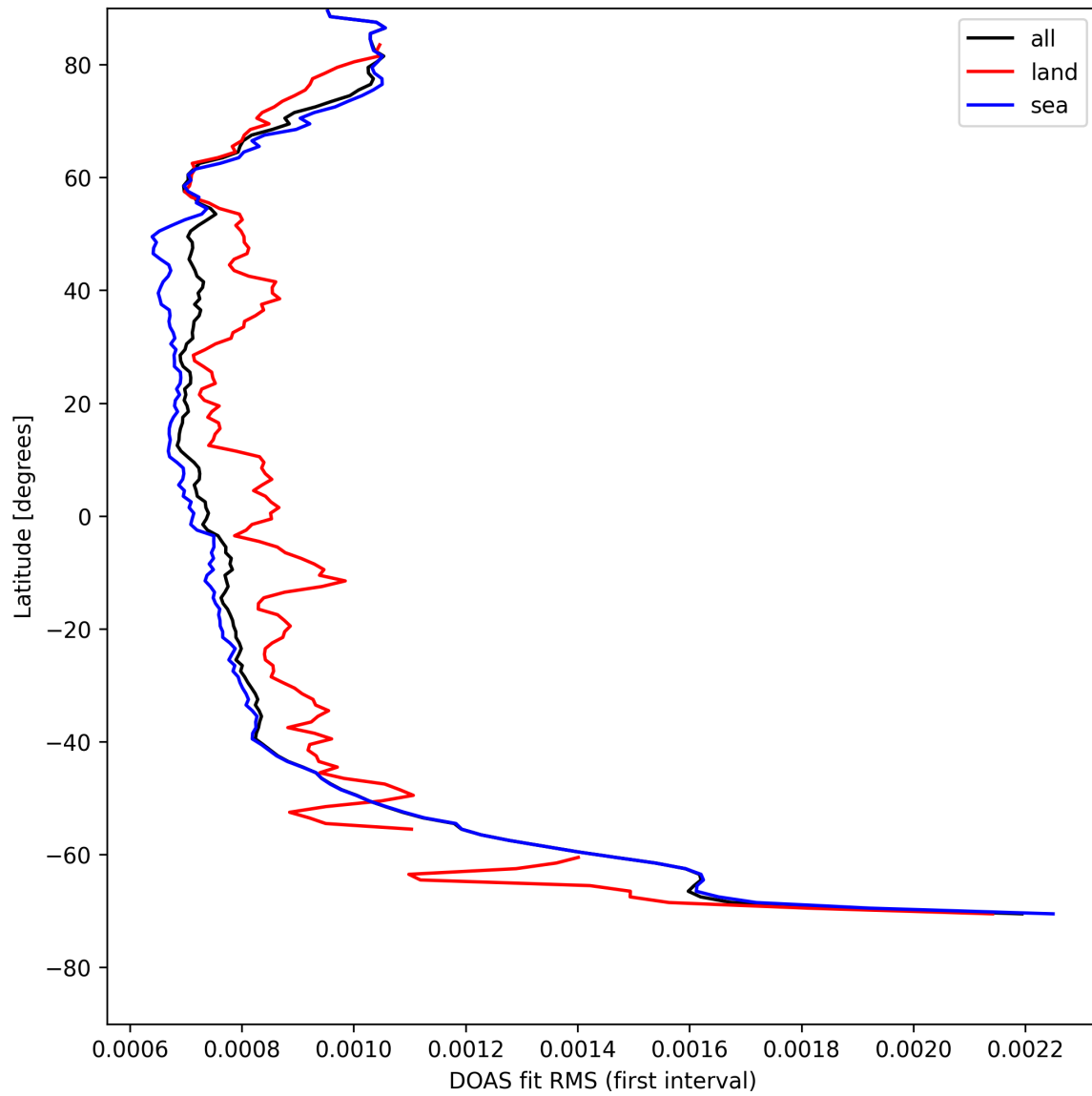
Figure 32: Zonal average of "DOAS fit RMS (first interval)" for 2025-04-27 to 2025-04-29.
