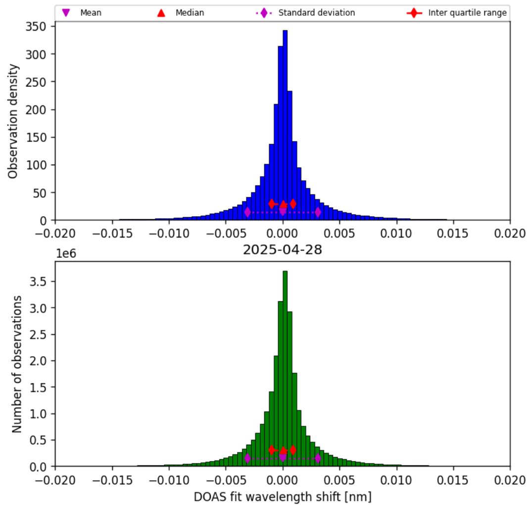
Figure 44: Histogram of “DOAS fit wavelength shift” for 2025-04-27 to 2025-04-29
