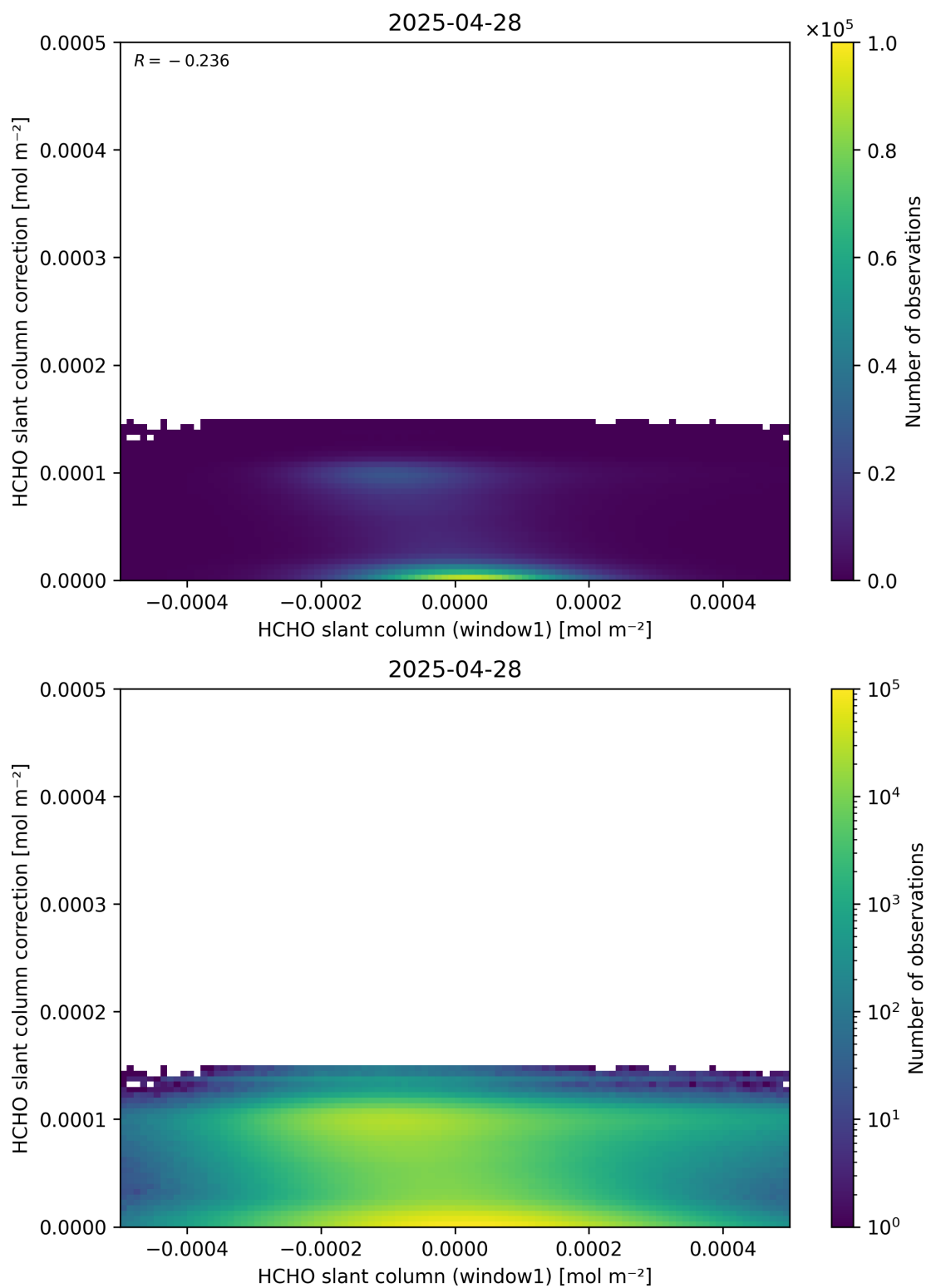
Figure 83: Scatter density plot of “HCHO slant column (window1)” against “HCHO slant column correction” for 2025-04-27 to 2025-04-29.
