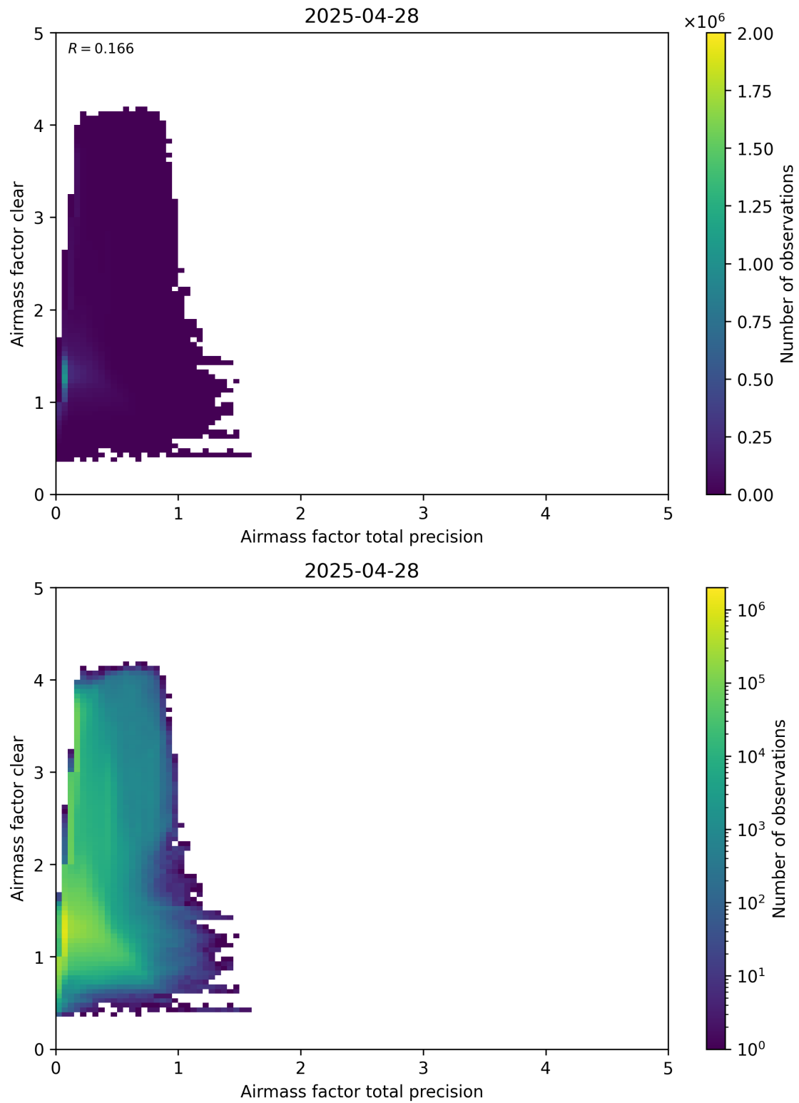
Figure 108: Scatter density plot of “Airmass factor total precision” against “Airmass factor clear” for 2025-04-27 to 2025-04-29.
