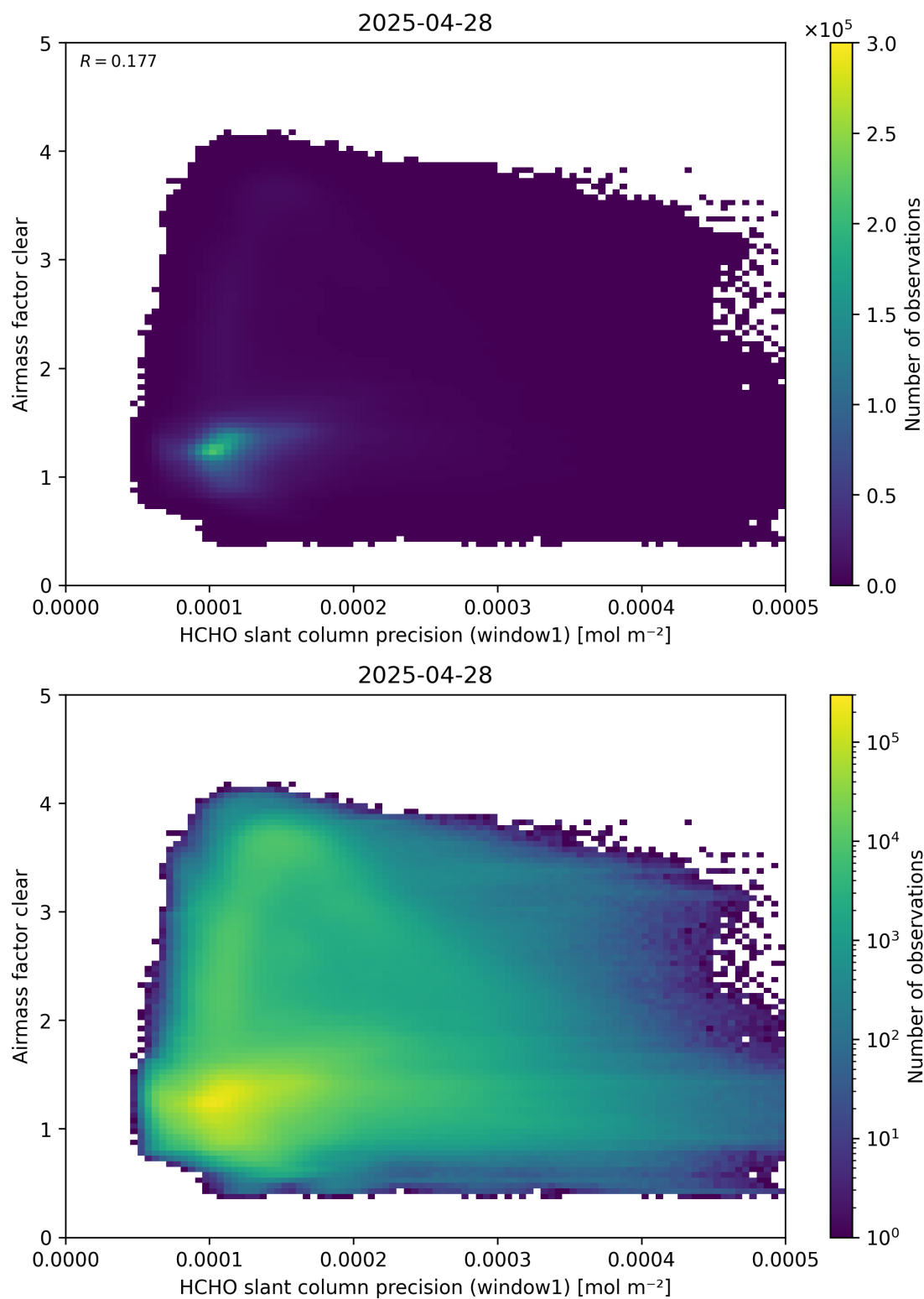
Figure 91: Scatter density plot of “HCHO slant column precision (window1)” against “Airmass factor clear” for 2025-04-27 to 2025-04-29.
