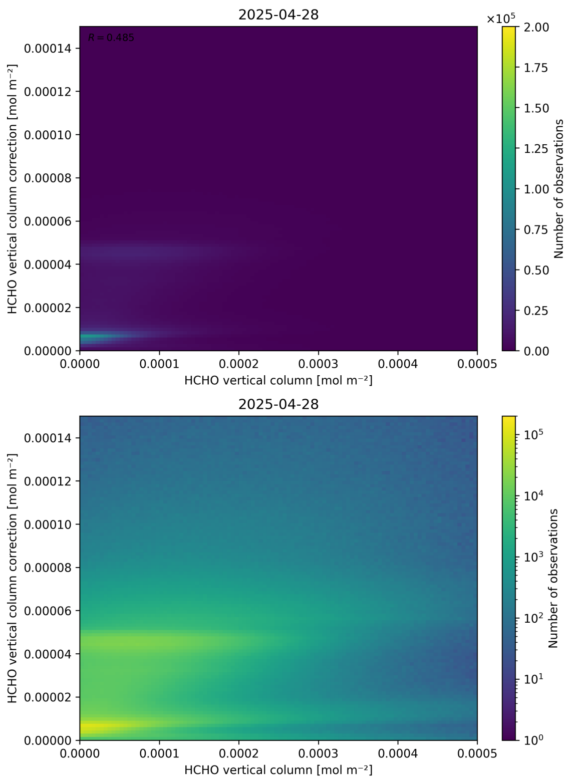
Figure 133: Scatter density plot of “HCHO vertical column” against “HCHO vertical column correction” for 2025-04-27 to 2025-04-29.
