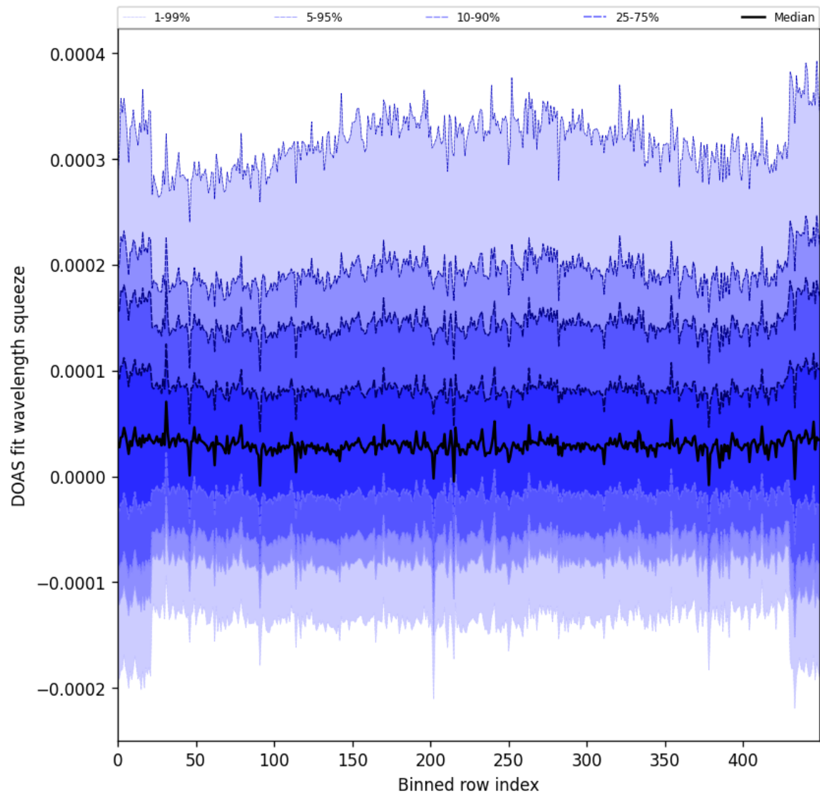
Figure 59: Along track statistics of “DOAS fit wavelength squeeze” for 2025-04-27 to 2025-04-29
