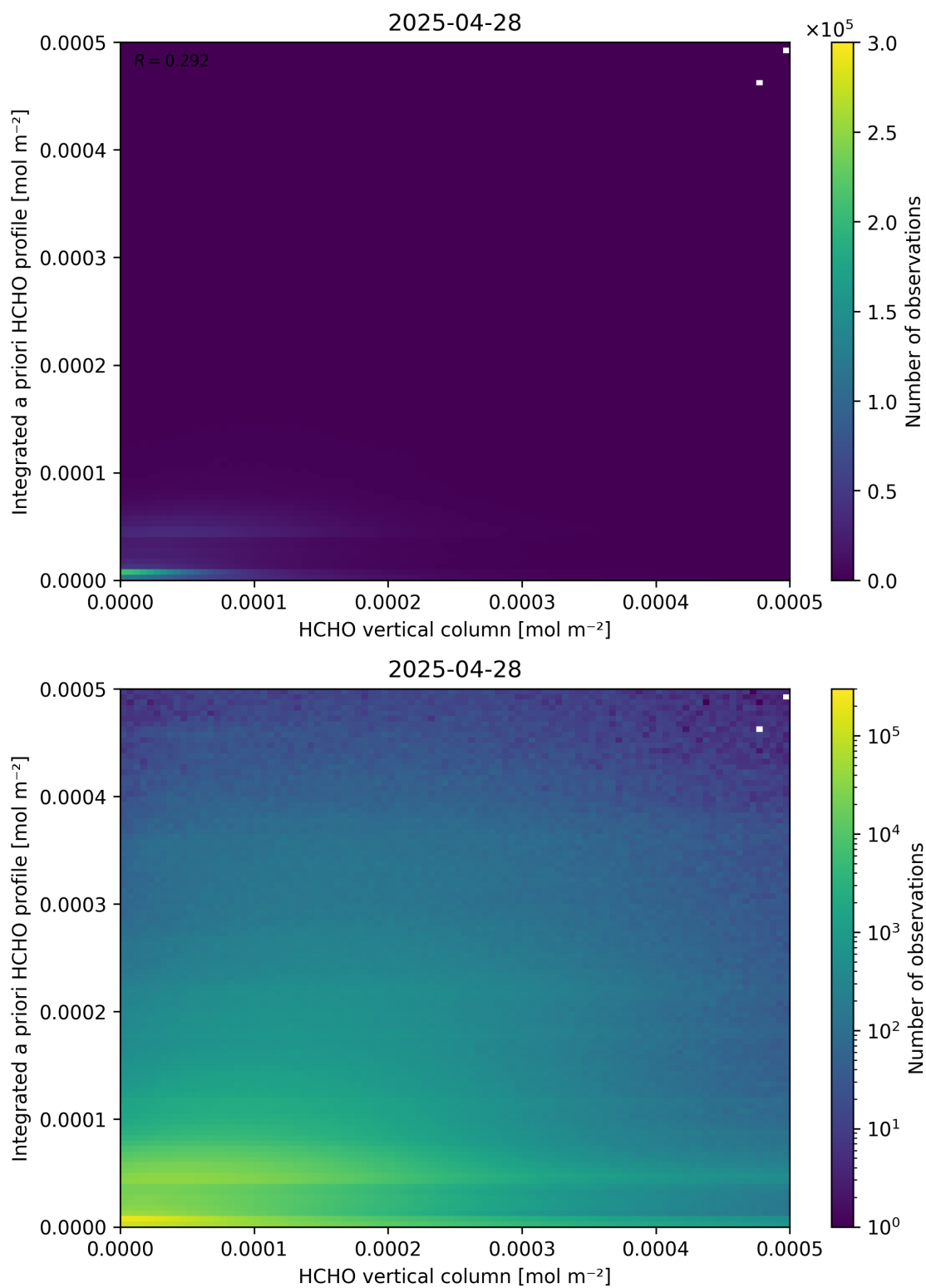
Figure 135: Scatter density plot of “HCHO vertical column” against “Integrated a priori HCHO profile” for 2025-04-27 to 2025-04-29.
