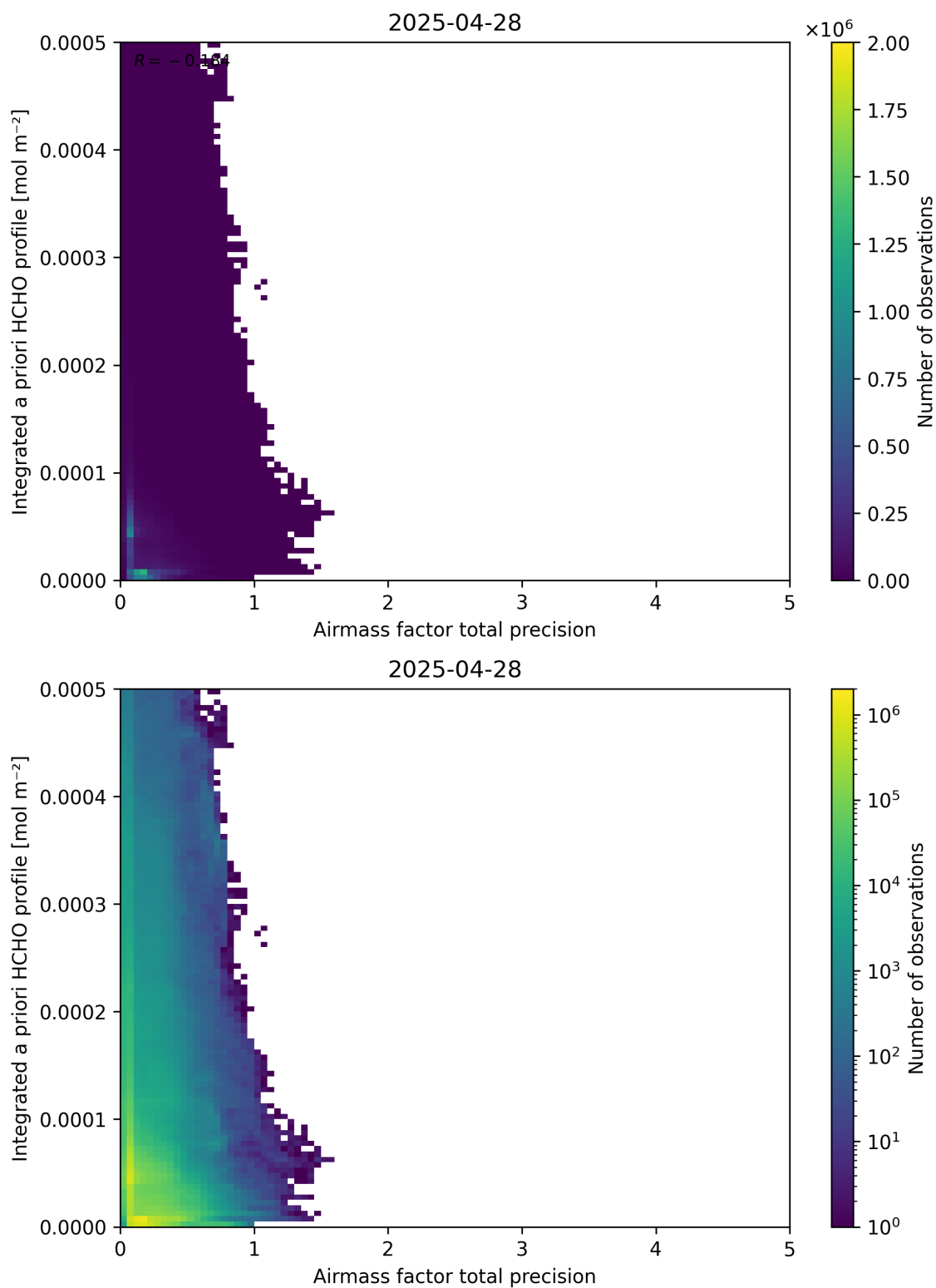
Figure 111: Scatter density plot of “Airmass factor total precision” against “Integrated a priori HCHO profile” for 2025-04-27 to 2025-04-29.
