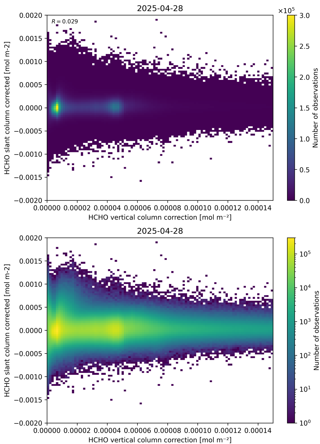
Figure 116: Scatter density plot of “HCHO vertical column correction” against “HCHO slant column corrected” for 2025-04-27 to 2025-04-29.
