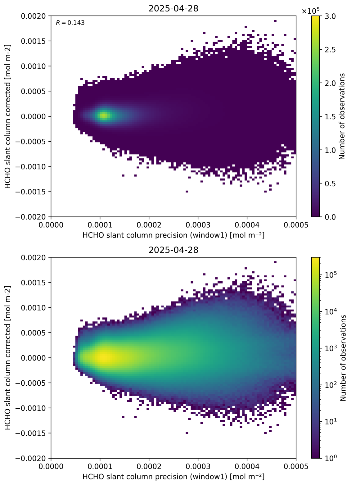
Figure 92: Scatter density plot of “HCHO slant column precision (window1)” against “HCHO slant column corrected” for 2025-04-27 to 2025-04-29.
