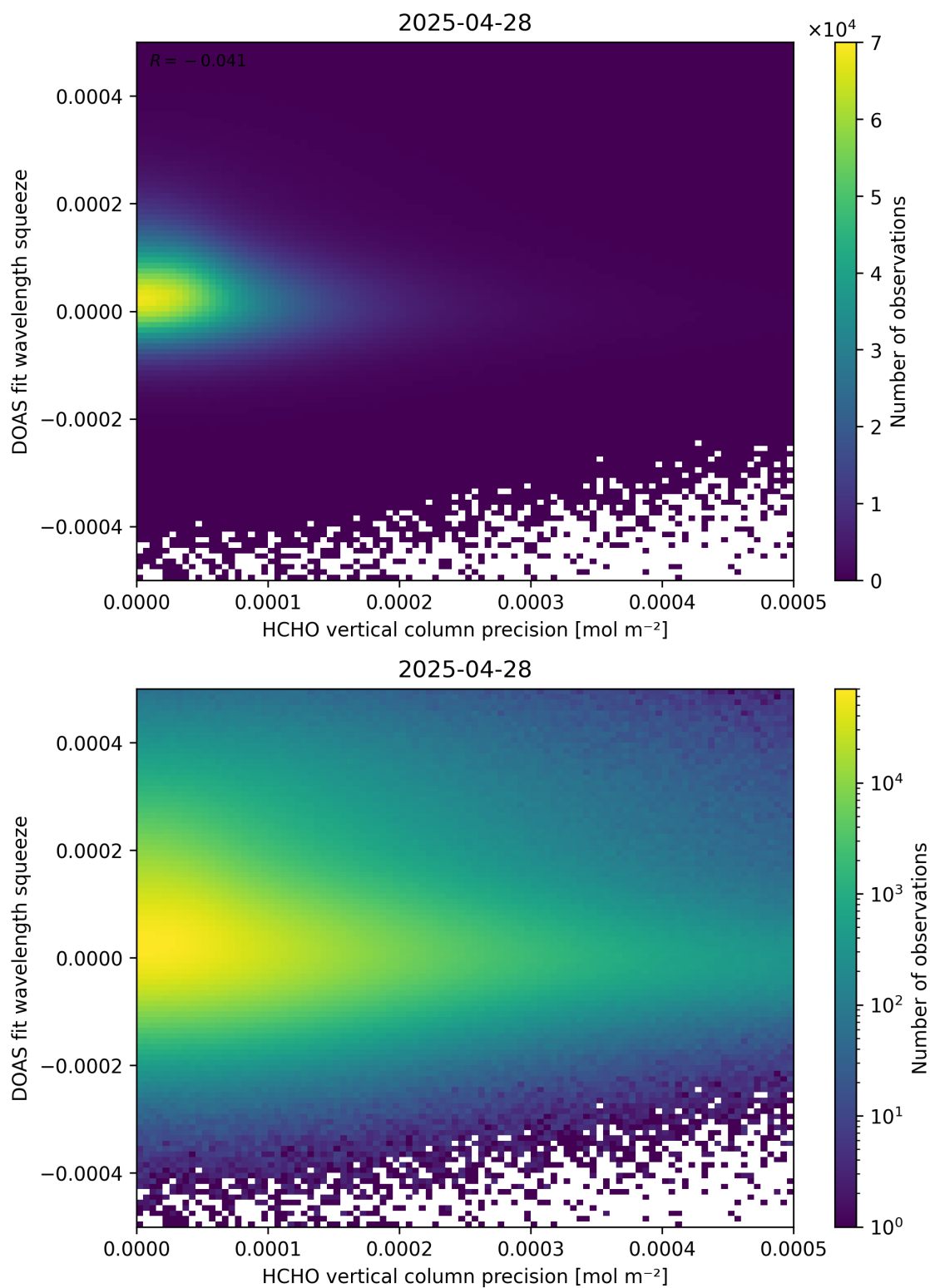
Figure 138: Scatter density plot of “HCHO vertical column precision” against “DOAS fit wavelength squeeze” for 2025-04-27 to 2025-04-29.
