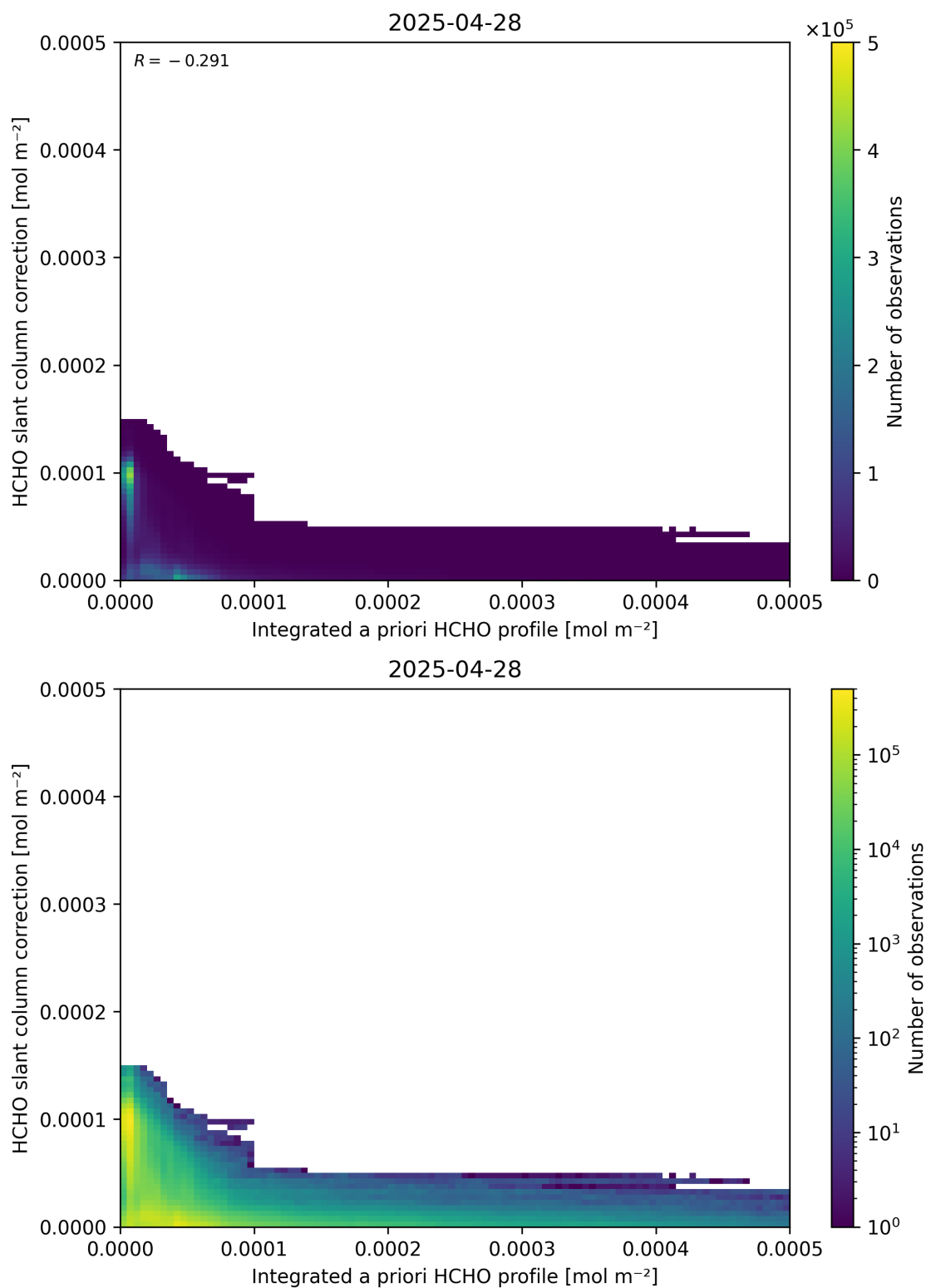
Figure 152: Scatter density plot of “Integrated a priori HCHO profile” against “HCHO slant column correction” for 2025-04-27 to 2025-04-29.
