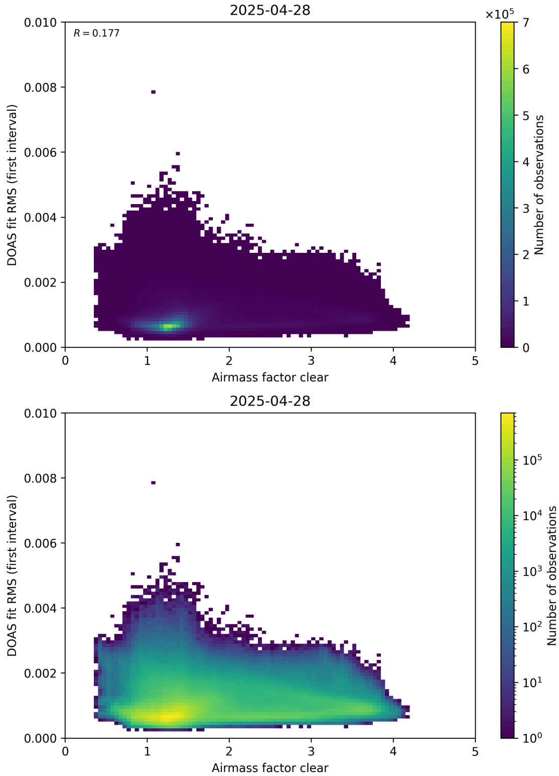
Figure 71: Scatter density plot of “Airmass factor clear” against “DOAS fit RMS (first interval)” for 2025-04-27 to 2025-04-29.
