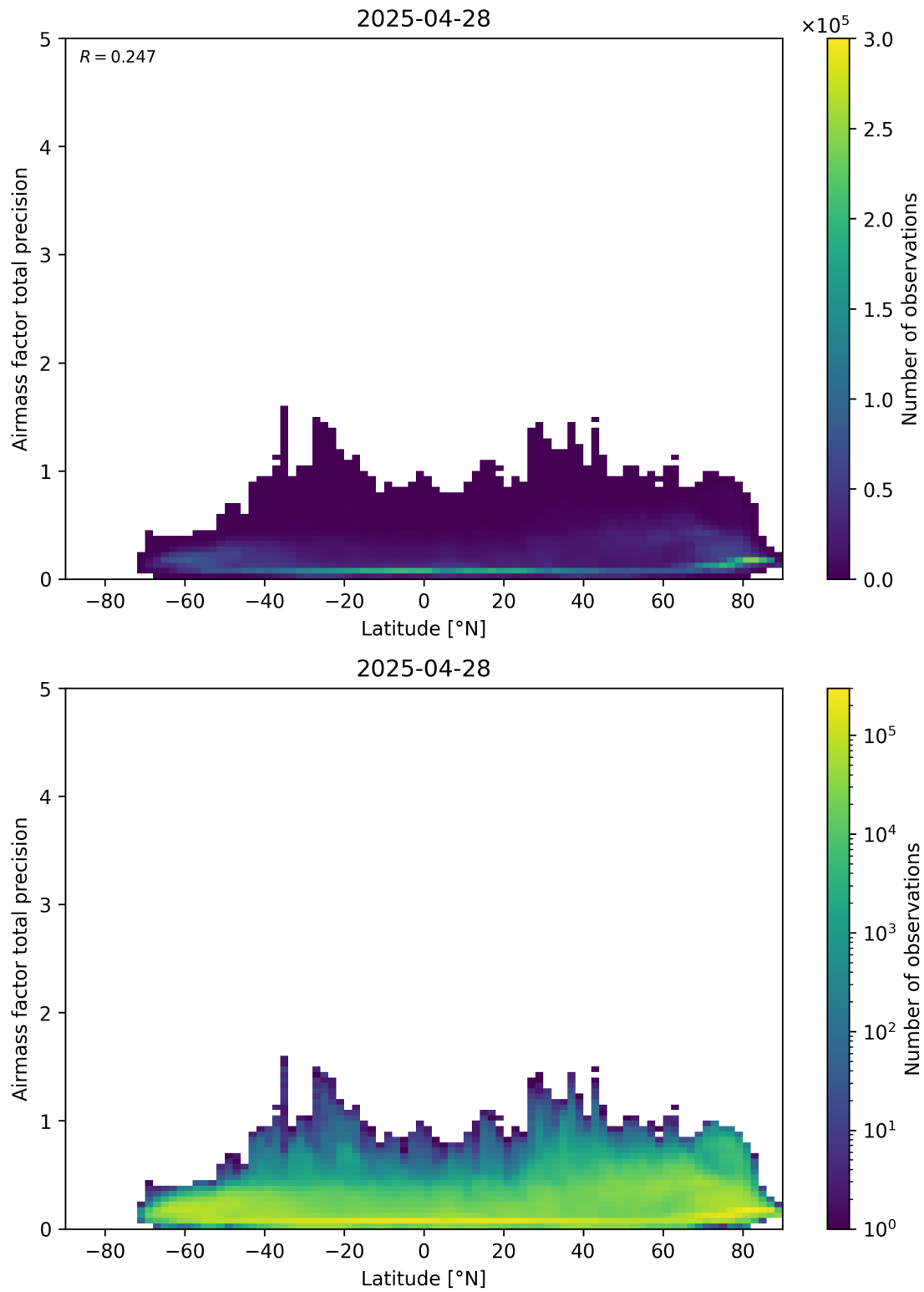
Figure 162: Scatter density plot of “Latitude” against “Airmass factor total precision” for 2025-04-27 to 2025-04-29.
