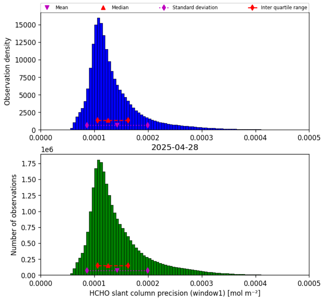
Figure 39: Histogram of “HCHO slant column precision (window1)” for 2025-04-27 to 2025-04-29
