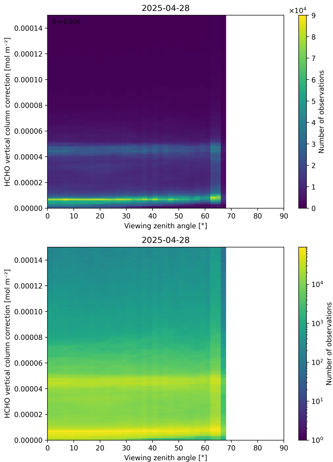
Figure 193: Scatter density plot of “Viewing zenith angle” against “HCHO vertical column correction” for 2025-04-27 to 2025-04-29.
