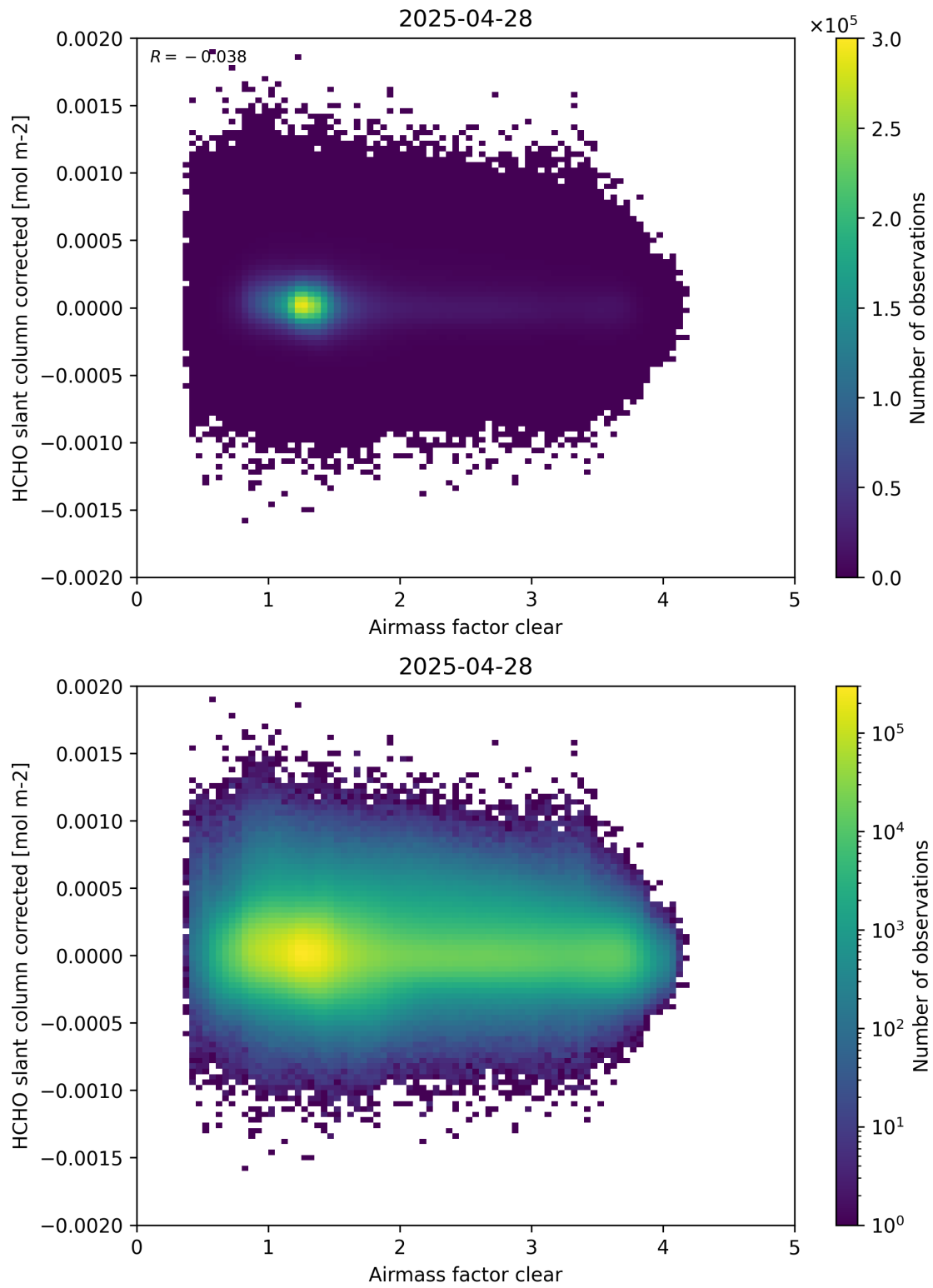
Figure 74: Scatter density plot of “Airmass factor clear” against “HCHO slant column corrected” for 2025-04-27 to 2025-04-29.
