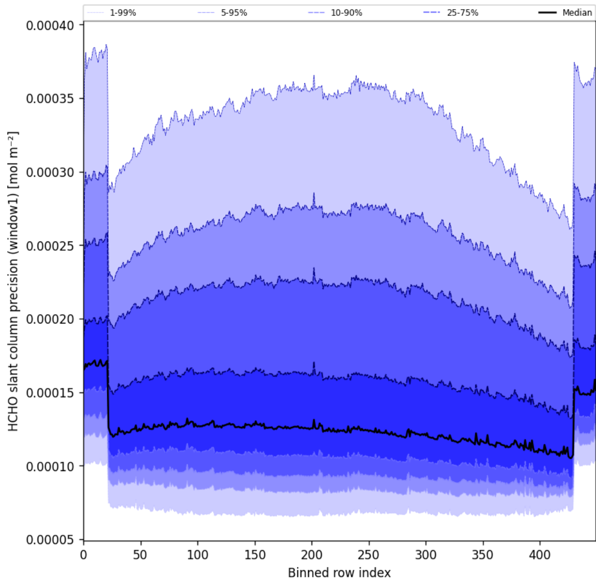
Figure 53: Along track statistics of “HCHO slant column precision (window1)” for 2025-04-27 to 2025-04-29
