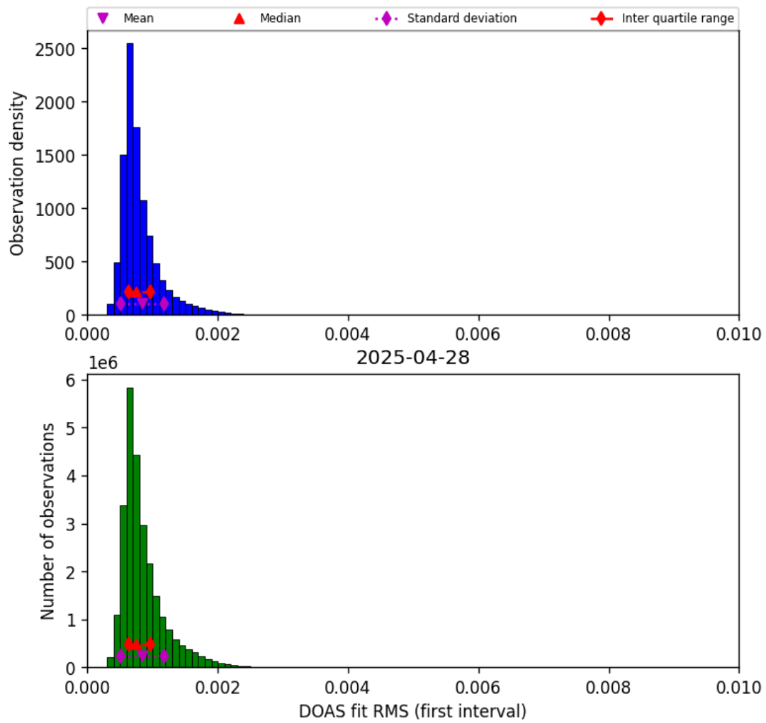
Figure 46: Histogram of “DOAS fit RMS (first interval)” for 2025-04-27 to 2025-04-29
