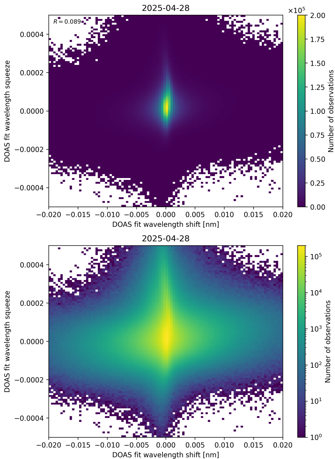
Figure 65: Scatter density plot of “DOAS fit wavelength shift” against “DOAS fit wavelength squeeze” for 2025-04-27 to 2025-04-29.
