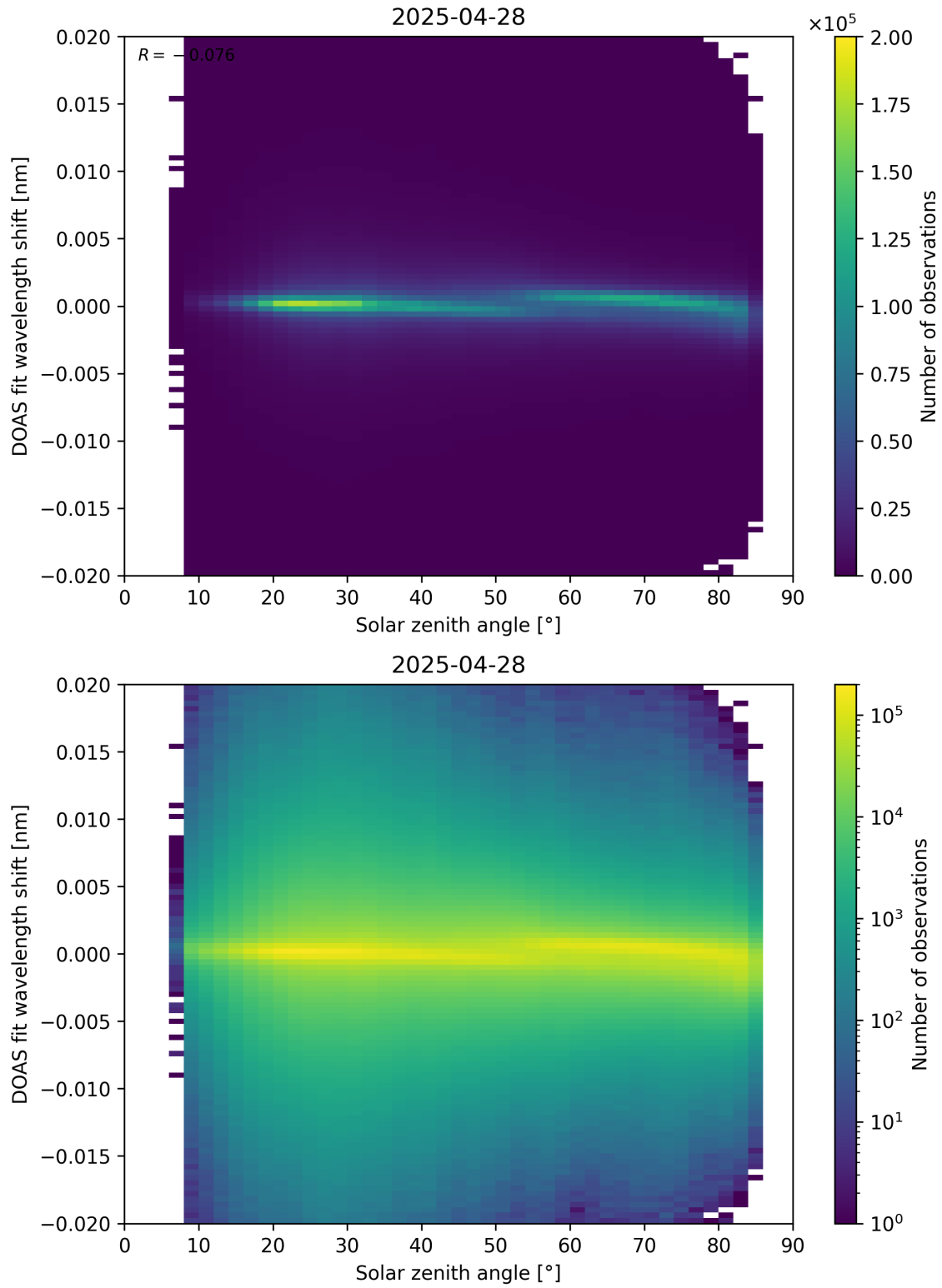
Figure 168: Scatter density plot of “Solar zenith angle” against “DOAS fit wavelength shift” for 2025-04-27 to 2025-04-29.
