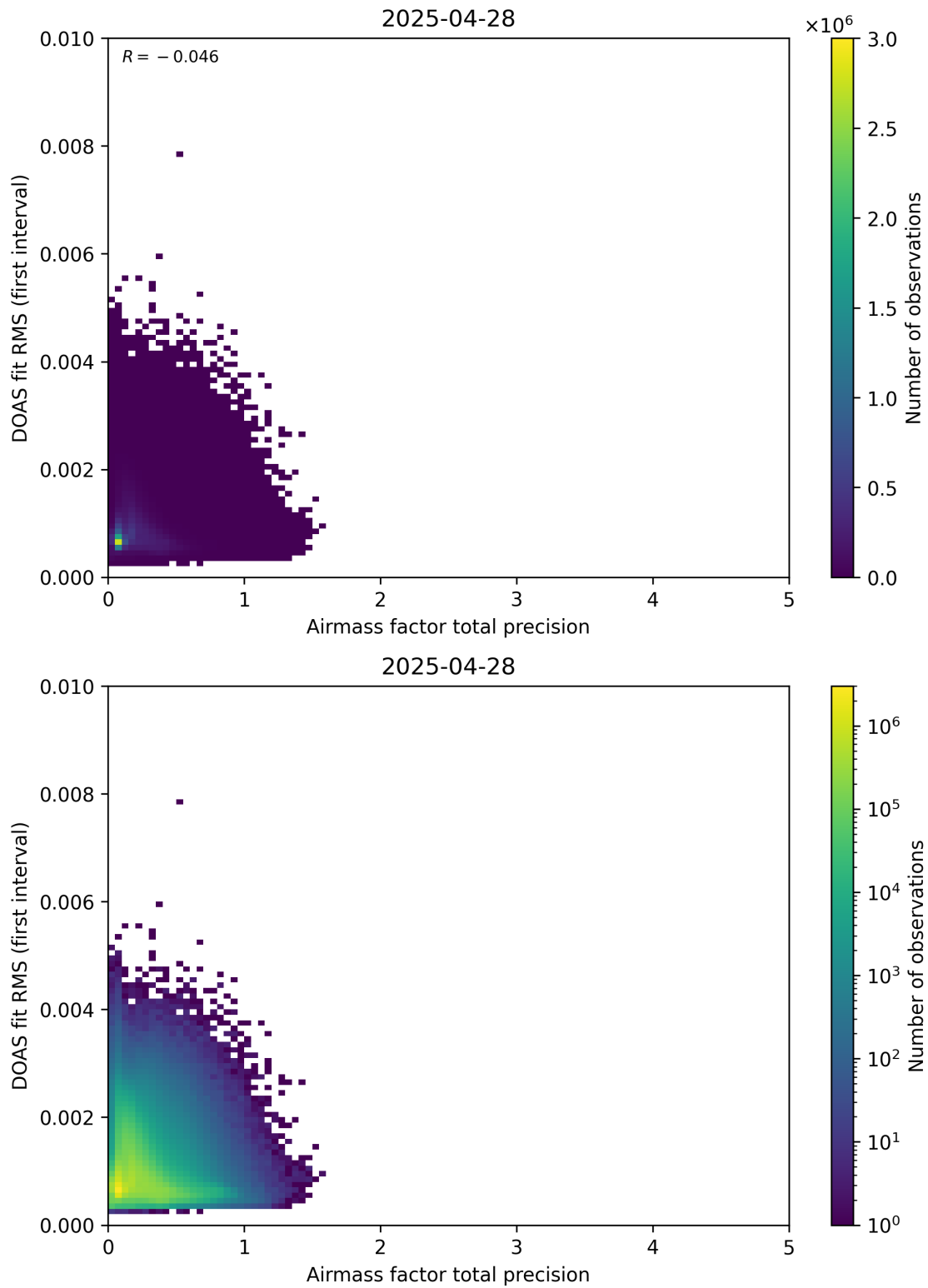
Figure 105: Scatter density plot of “Airmass factor total precision” against “DOAS fit RMS (first interval)” for 2025-04-27 to 2025-04-29.
