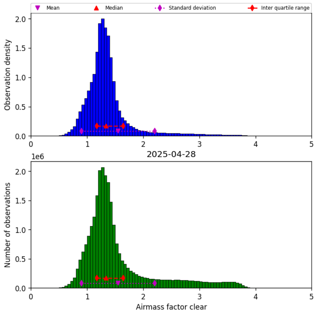
Figure 42: Histogram of “Airmass factor clear” for 2025-04-27 to 2025-04-29
