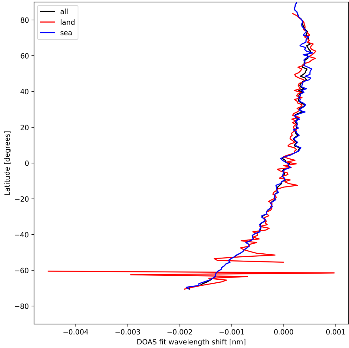
Figure 30: Zonal average of “DOAS fit wavelength shift” for 2025-04-27 to 2025-04-29.
