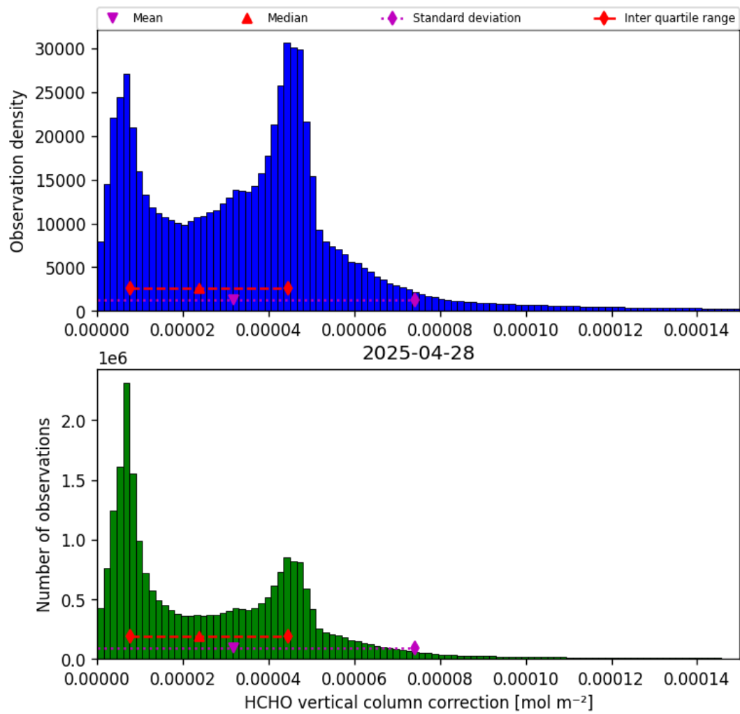
Figure 37: Histogram of “HCHO vertical column correction” for 2025-04-27 to 2025-04-29
