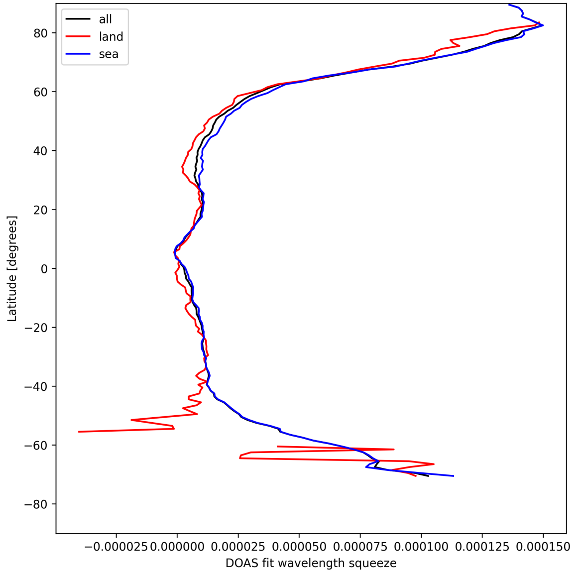
Figure 31: Zonal average of “DOAS fit wavelength squeeze” for 2025-04-27 to 2025-04-29.
