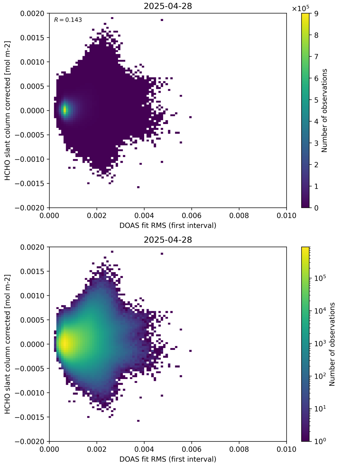
Figure 62: Scatter density plot of “DOAS fit RMS (first interval)” against “HCHO slant column corrected” for 2025-04-27 to 2025-04-29.
