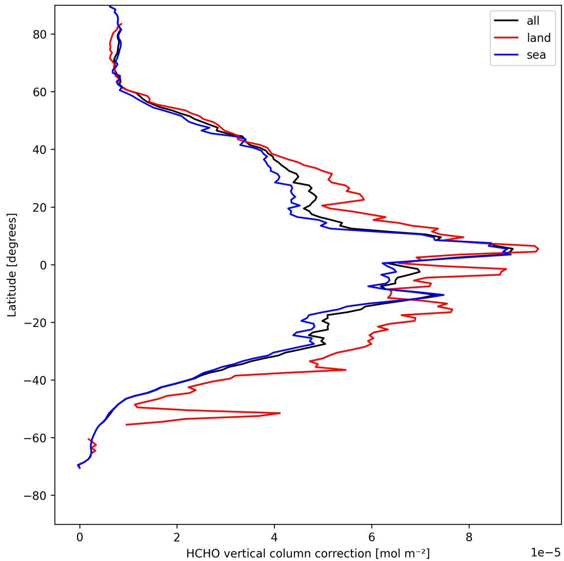
Figure 23: Zonal average of “HCHO vertical column correction” for 2025-04-27 to 2025-04-29.
