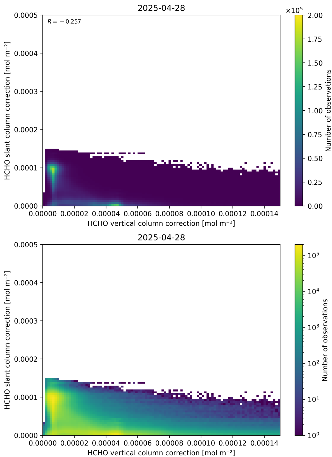
Figure 117: Scatter density plot of “HCHO vertical column correction” against “HCHO slant column correction” for 2025-04-27 to 2025-04-29.
