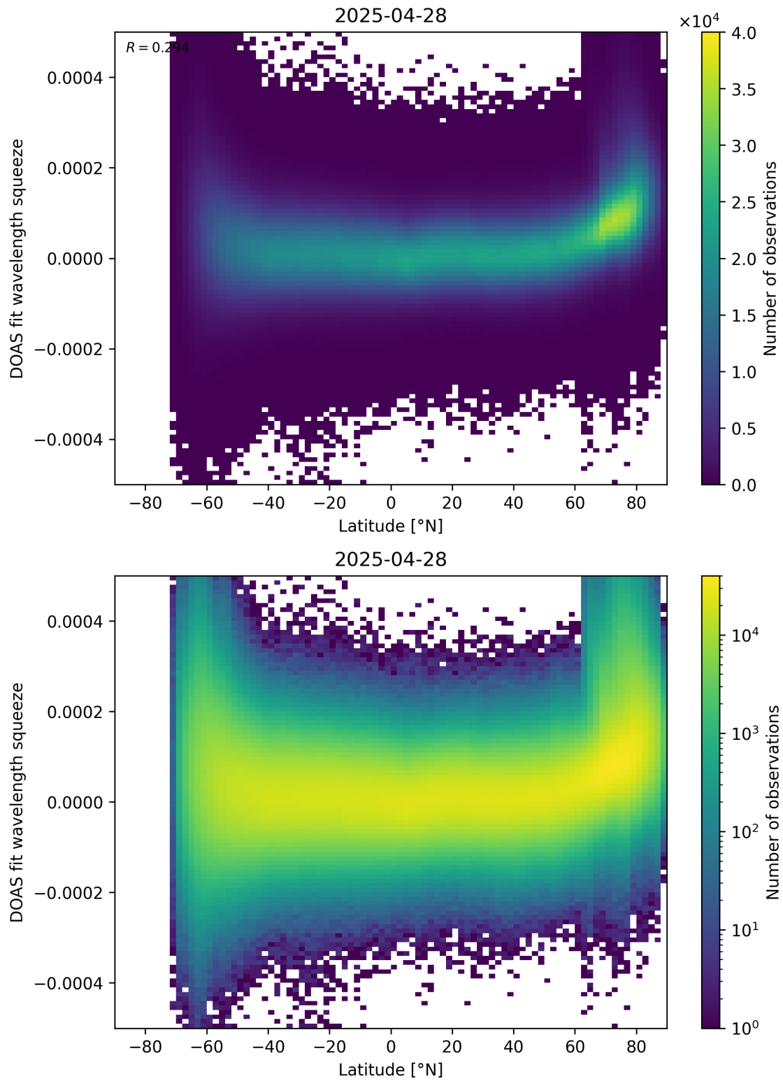
Figure 155: Scatter density plot of “Latitude” against “DOAS fit wavelength squeeze” for 2025-04-27 to 2025-04-29.
