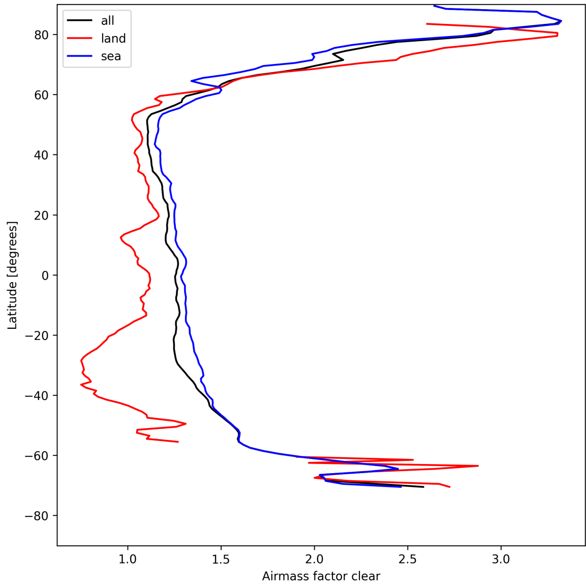
Figure 28: Zonal average of “Airmass factor clear” for 2025-04-27 to 2025-04-29.
