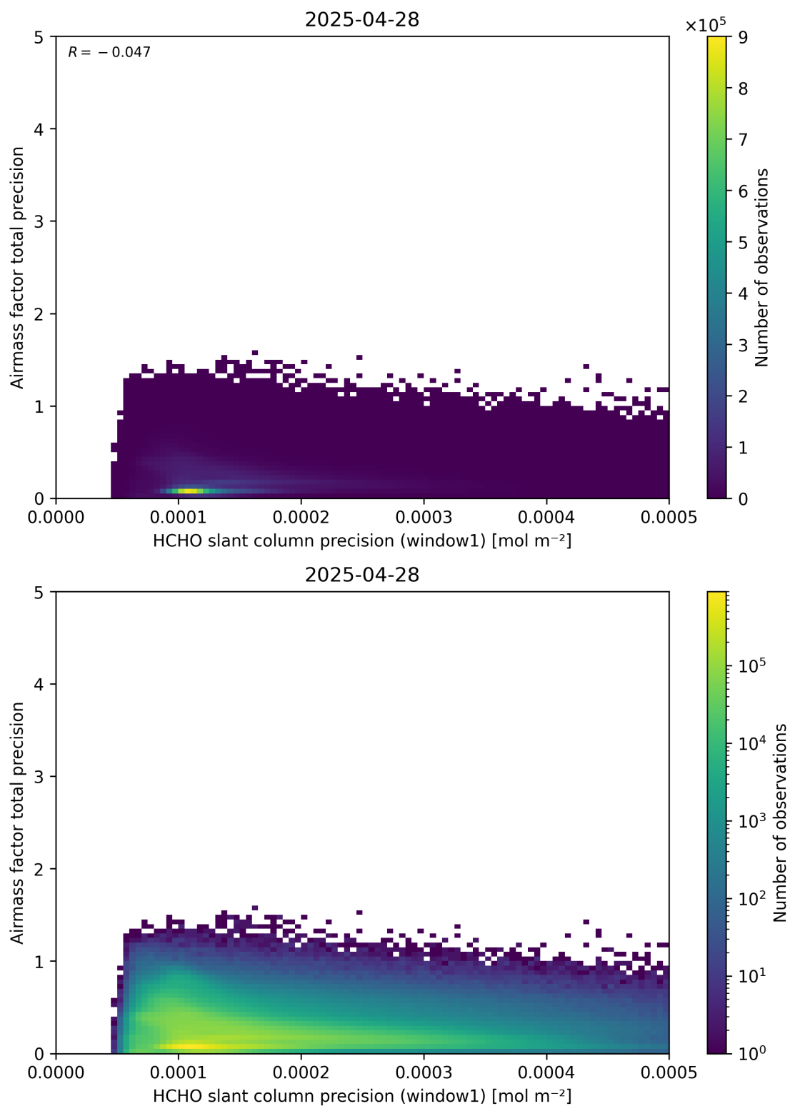
Figure 95: Scatter density plot of “HCHO slant column precision (window1)” against “Airmass factor total precision” for 2025-04-27 to 2025-04-29.
