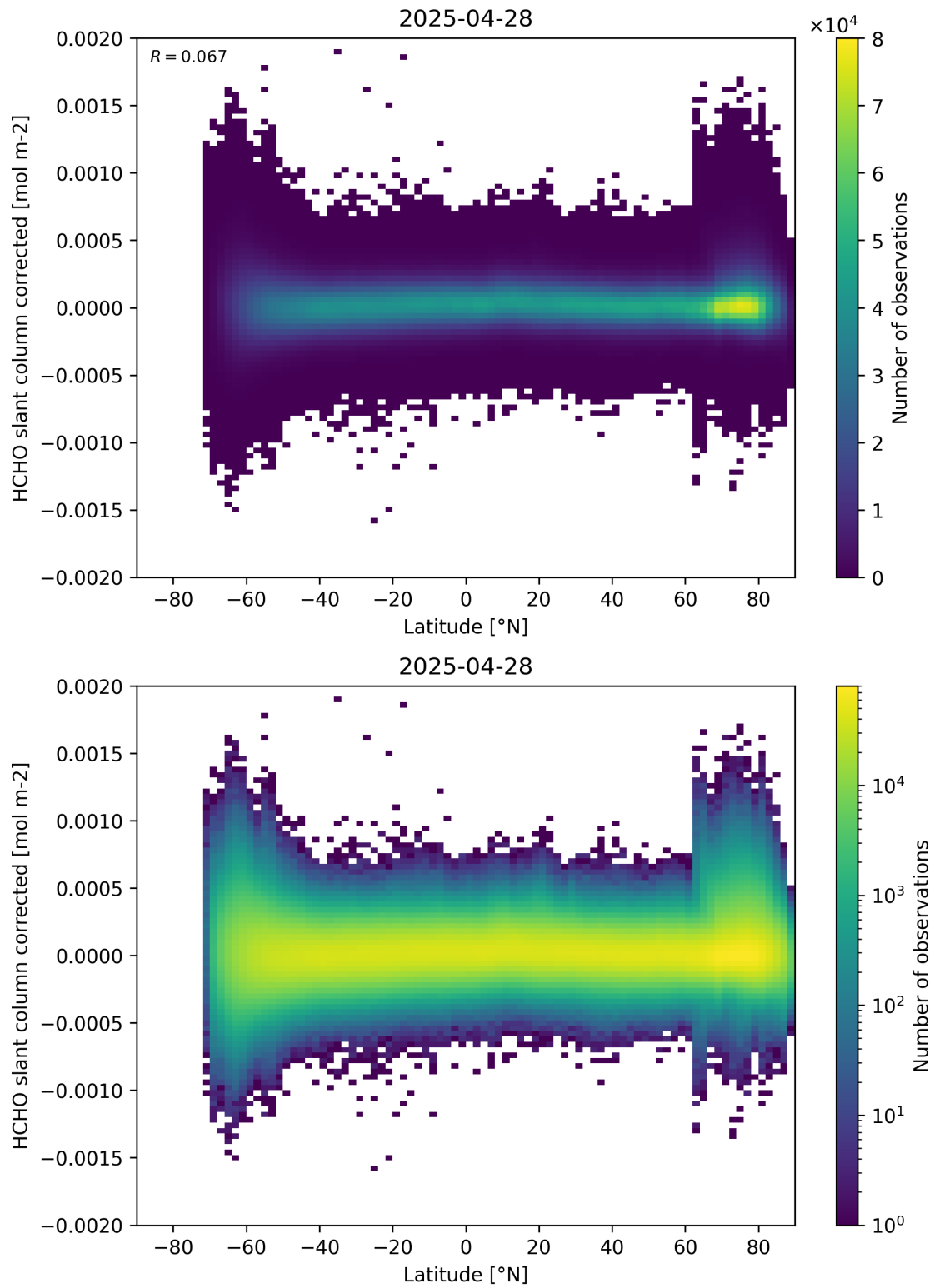
Figure 157: Scatter density plot of “Latitude” against “HCHO slant column corrected” for 2025-04-27 to 2025-04-29.
