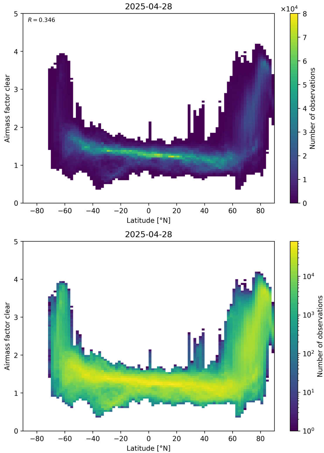
Figure 156: Scatter density plot of “Latitude” against “Airmass factor clear” for 2025-04-27 to 2025-04-29.
