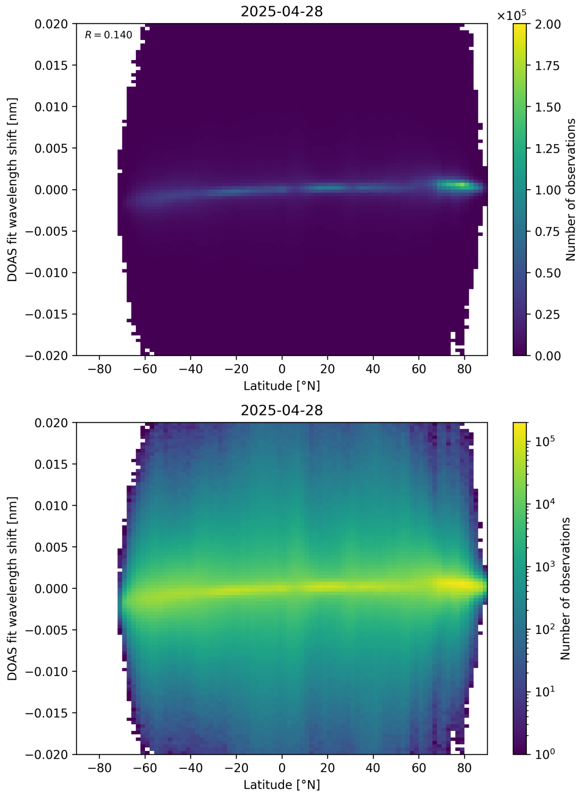
Figure 154: Scatter density plot of “Latitude” against “DOAS fit wavelength shift” for 2025-04-27 to 2025-04-29.
