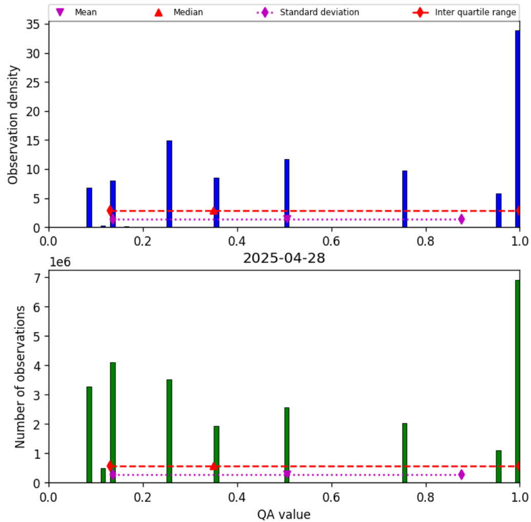
Figure 34: Histogram of “QA value” for 2025-04-27 to 2025-04-29
