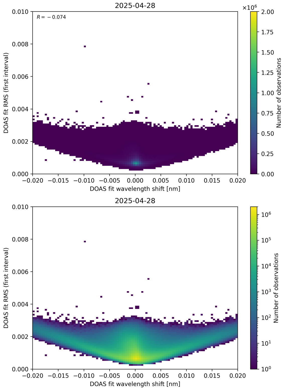
Figure 64: Scatter density plot of “DOAS fit wavelength shift” against “DOAS fit RMS (first interval)” for 2025-04-27 to 2025-04-29.
