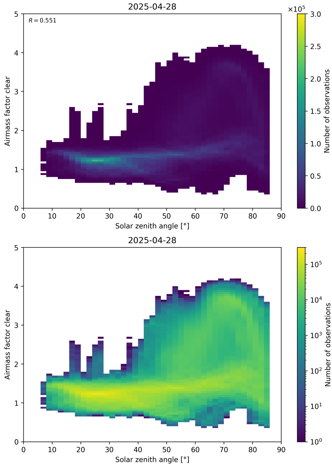
Figure 170: Scatter density plot of “Solar zenith angle” against “Airmass factor clear” for 2025-04-27 to 2025-04-29.
