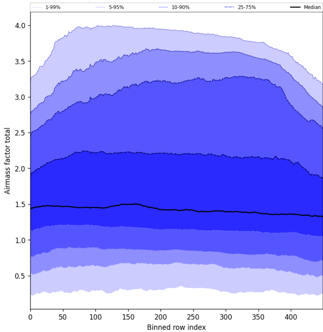
Figure 54: Along track statistics of “Airmass factor total” for 2025-04-27 to 2025-04-29
