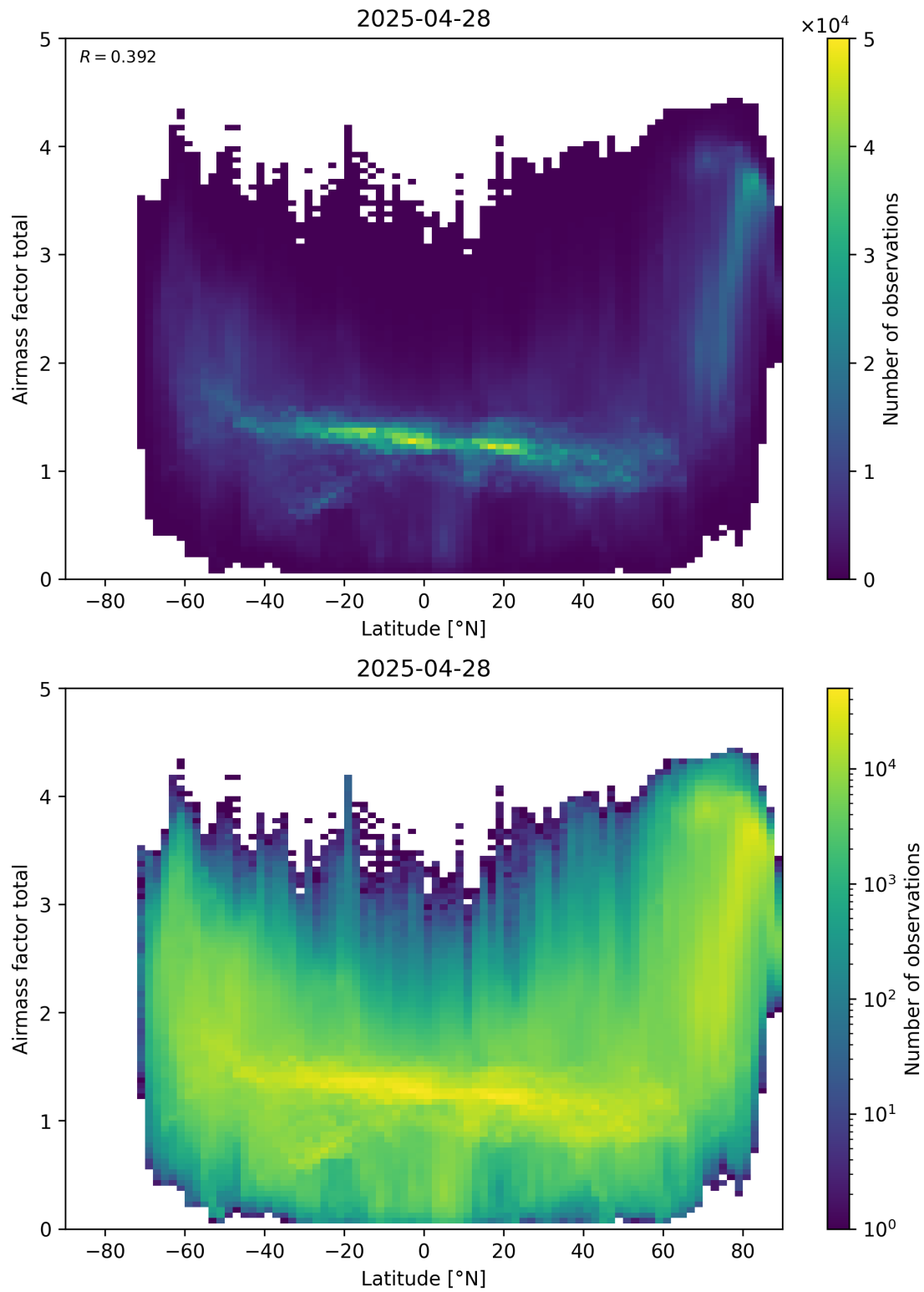
Figure 161: Scatter density plot of “Latitude” against “Airmass factor total” for 2025-04-27 to 2025-04-29.
