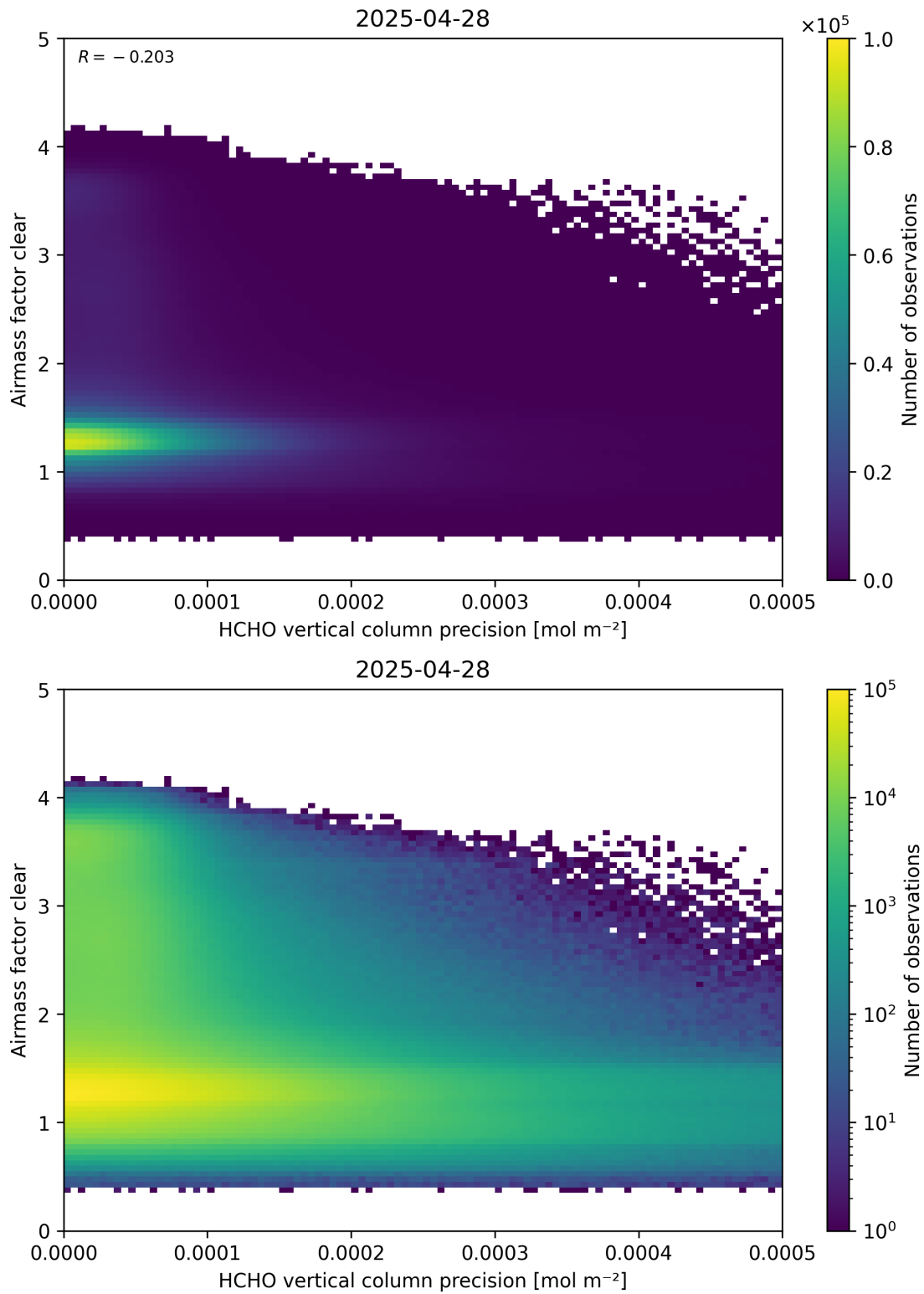
Figure 139: Scatter density plot of “HCHO vertical column precision” against “Airmass factor clear” for 2025-04-27 to 2025-04-29.
