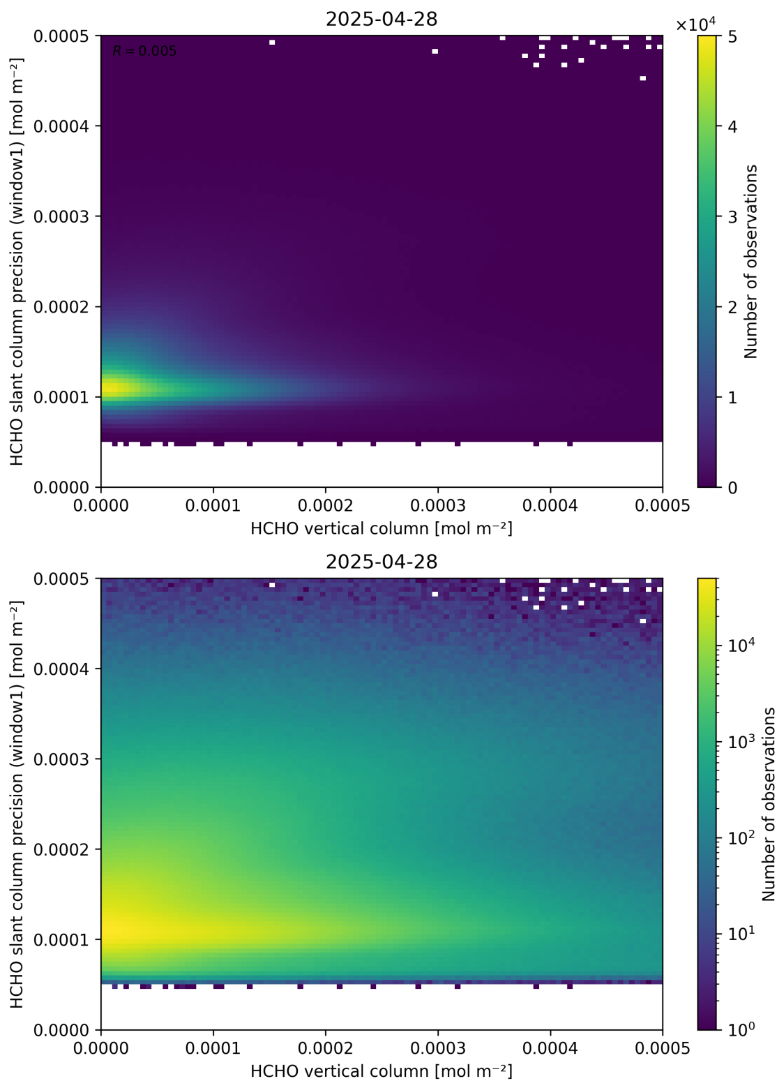
Figure 130: Scatter density plot of “HCHO vertical column” against “HCHO slant column precision (window1)” for 2025-04-27 to 2025-04-29.
