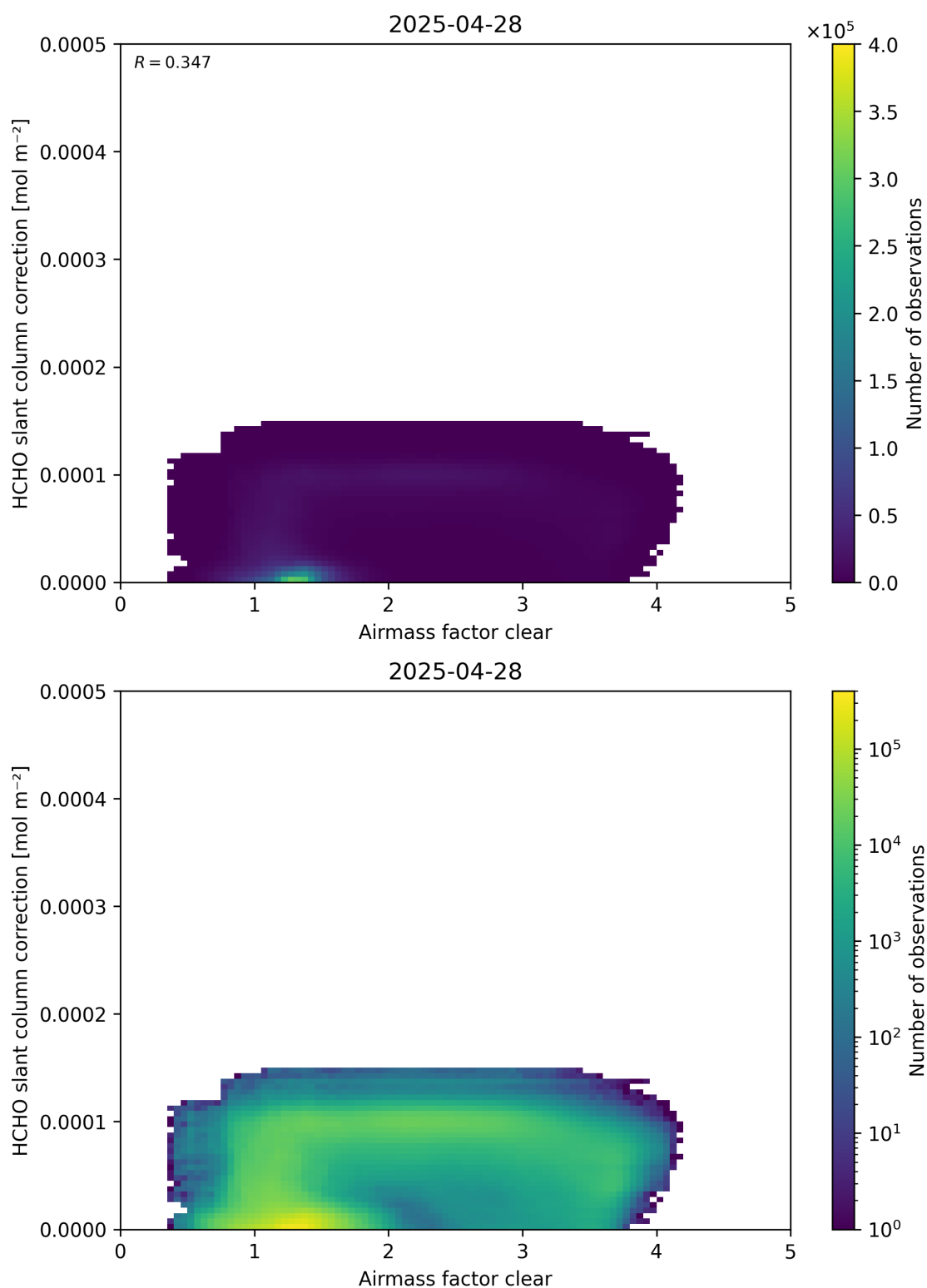
Figure 75: Scatter density plot of “Airmass factor clear” against “HCHO slant column correction” for 2025-04-27 to 2025-04-29.
