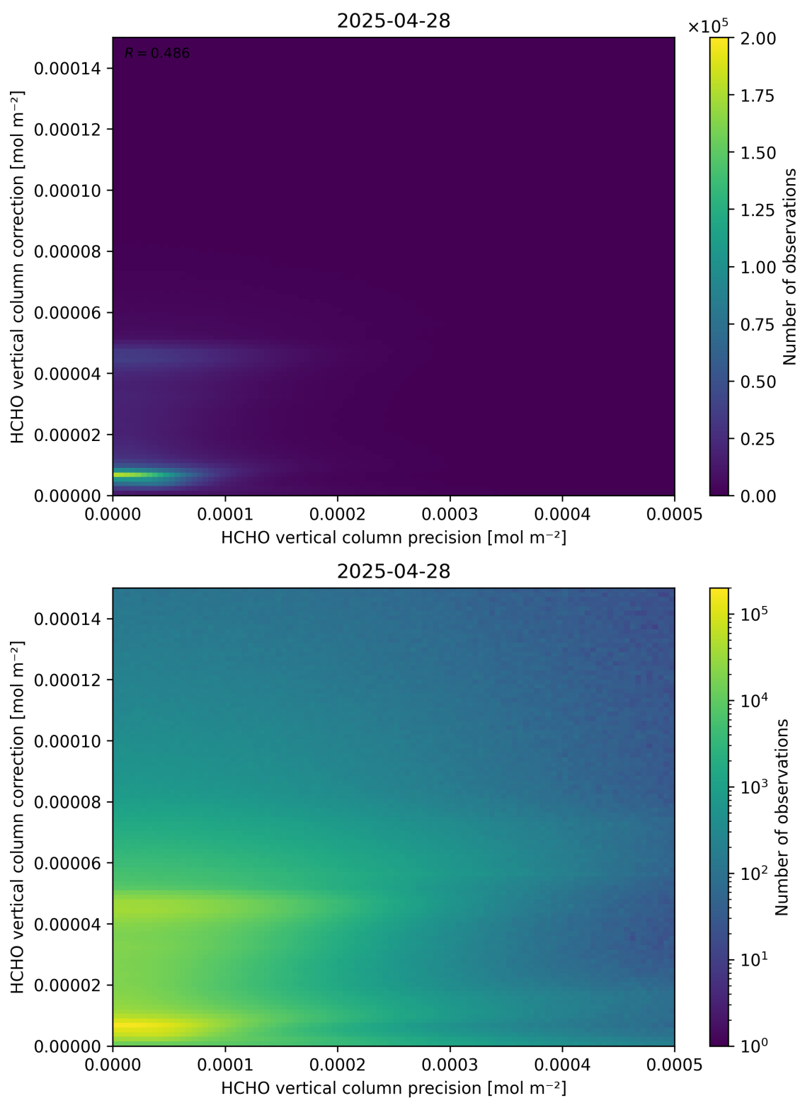
Figure 146: Scatter density plot of “HCHO vertical column precision” against “HCHO vertical column correction” for 2025-04-27 to 2025-04-29.
