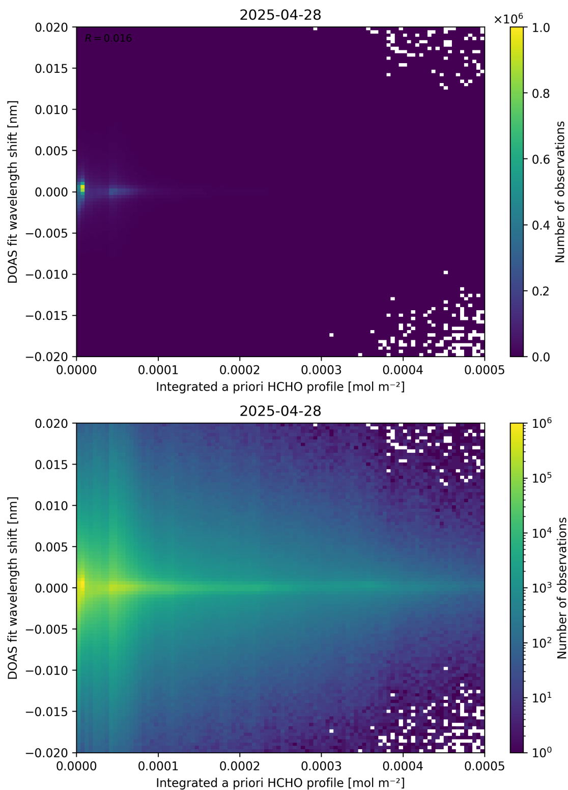
Figure 149: Scatter density plot of “Integrated a priori HCHO profile” against “DOAS fit wavelength shift” for 2025-04-27 to 2025-04-29.
