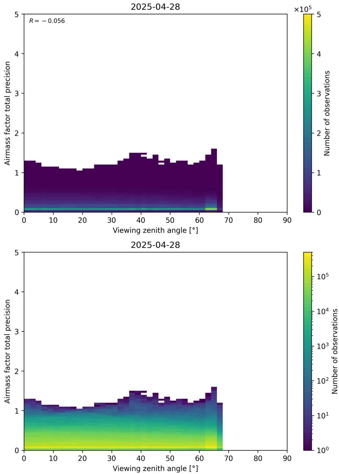
Figure 191: Scatter density plot of “Viewing zenith angle” against “Airmass factor total precision” for 2025-04-27 to 2025-04-29.
