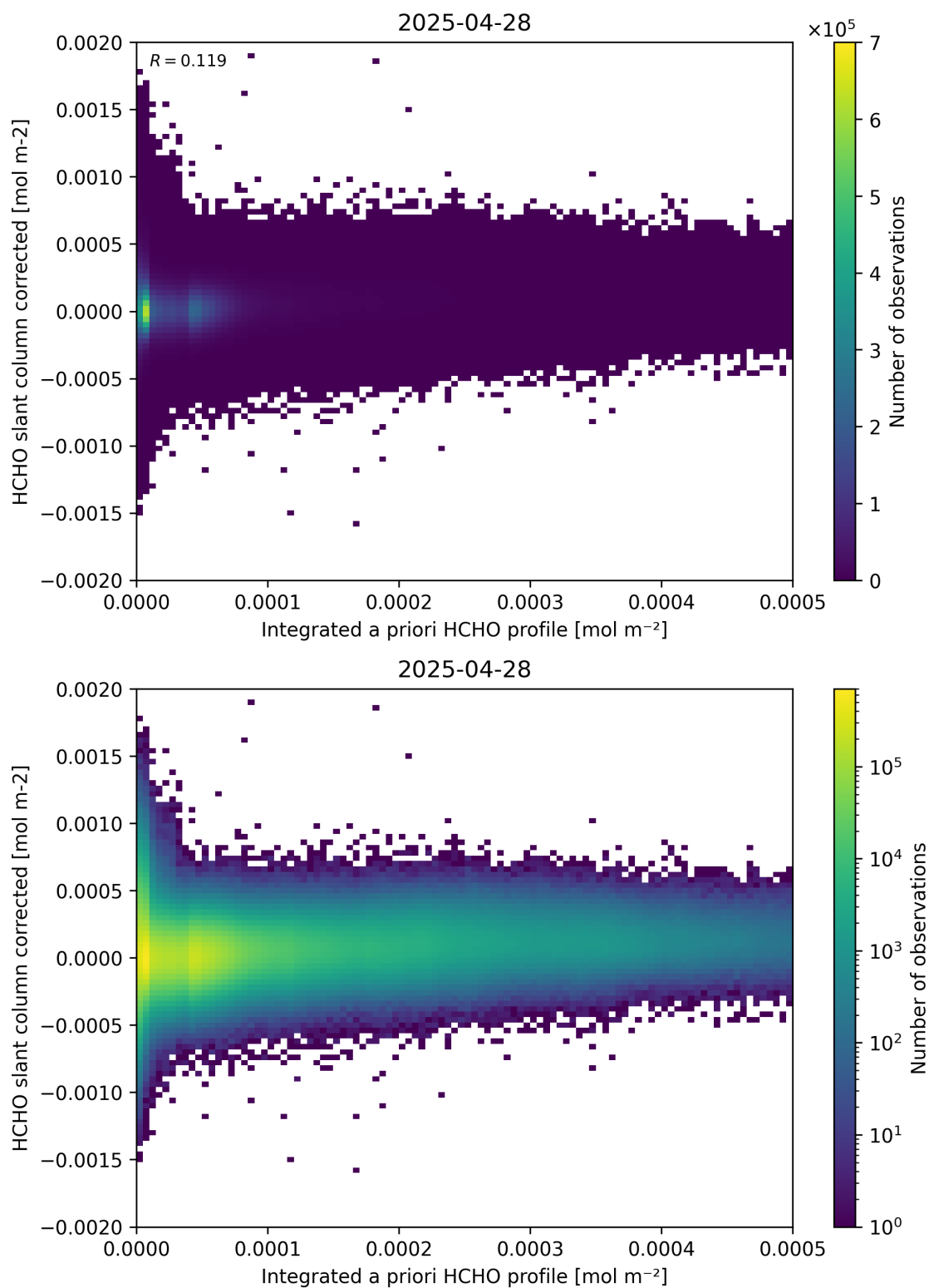
Figure 151: Scatter density plot of “Integrated a priori HCHO profile” against “HCHO slant column corrected” for 2025-04-27 to 2025-04-29.
