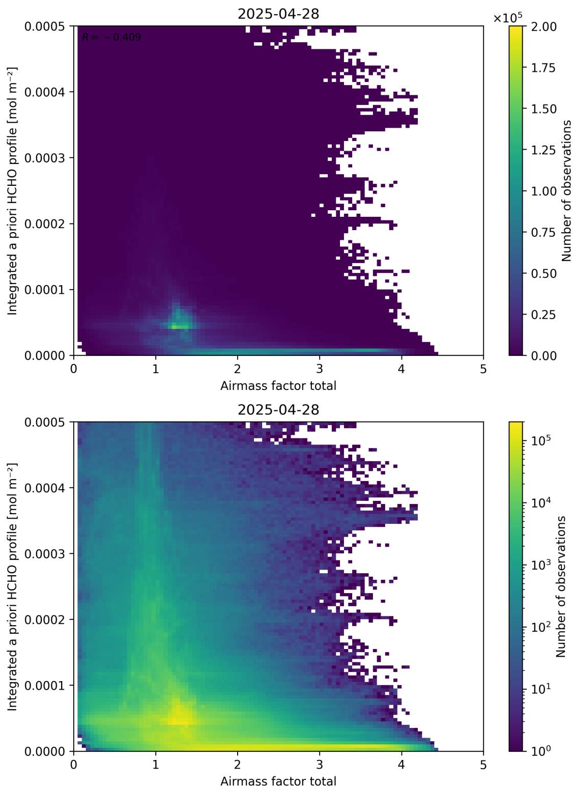
Figure 104: Scatter density plot of “Airmass factor total” against “Integrated a priori HCHO profile” for 2025-04-27 to 2025-04-29.
