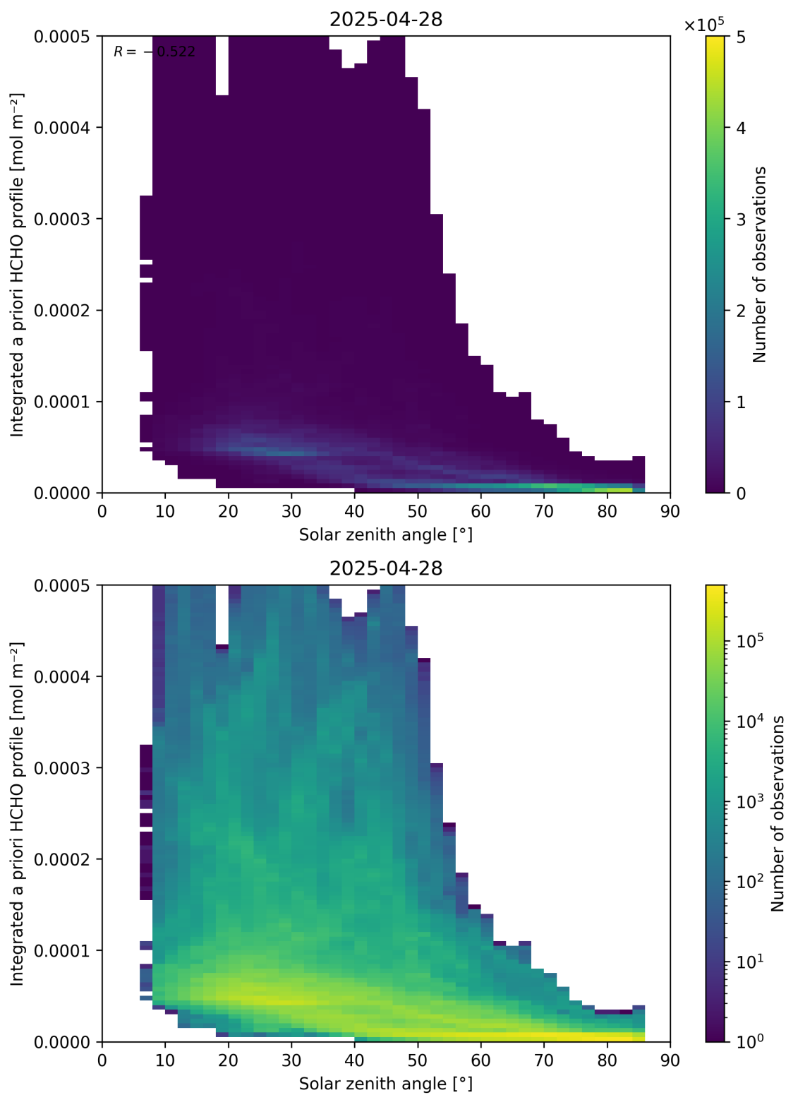
Figure 180: Scatter density plot of “Solar zenith angle” against “Integrated a priori HCHO profile” for 2025-04-27 to 2025-04-29.
