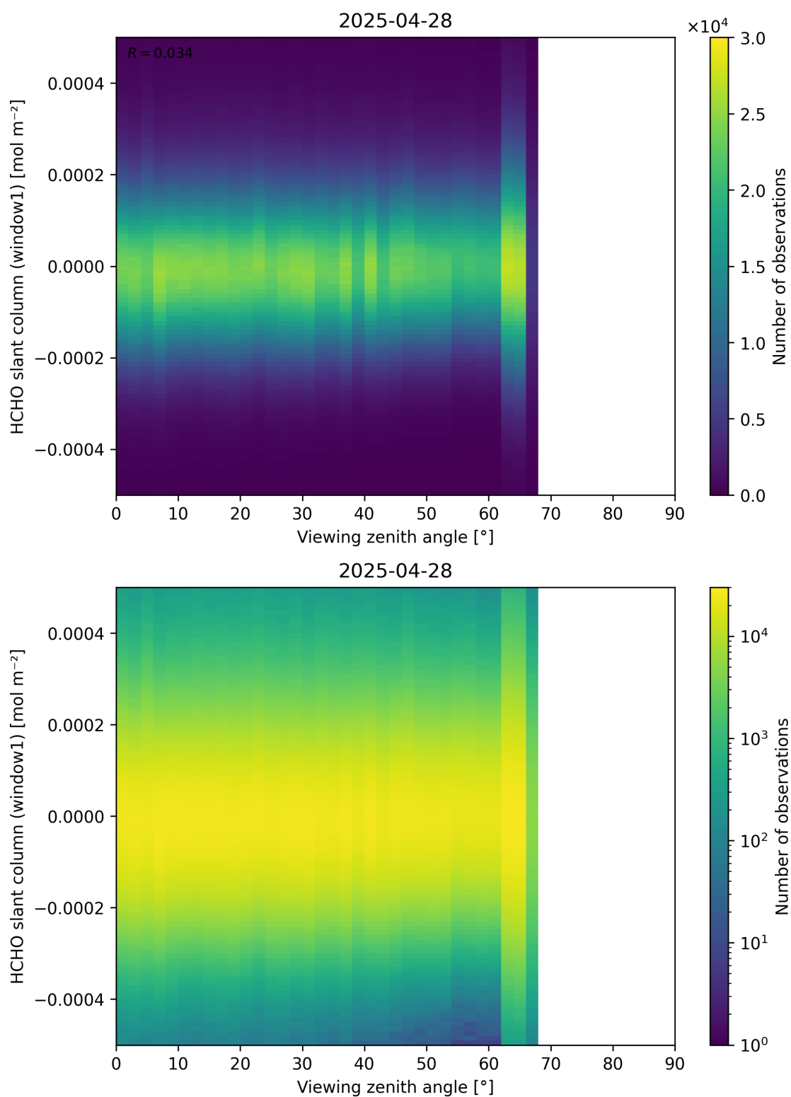
Figure 188: Scatter density plot of “Viewing zenith angle” against “HCHO slant column (window1)” for 2025-04-27 to 2025-04-29.
