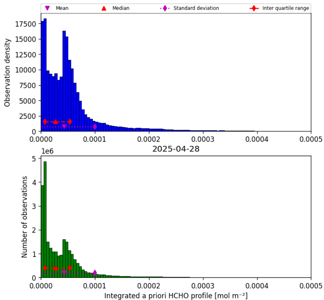
Figure 43: Histogram of “Integrated a priori HCHO profile” for 2025-04-27 to 2025-04-29
