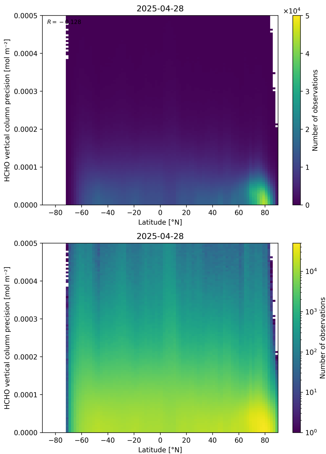
Figure 165: Scatter density plot of “Latitude” against “HCHO vertical column precision” for 2025-04-27 to 2025-04-29.
