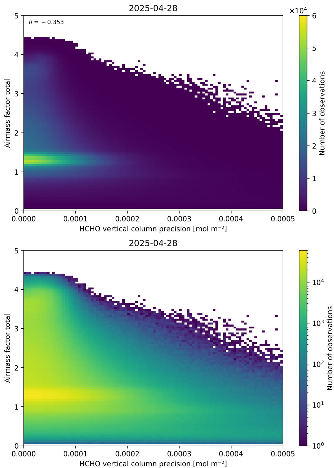
Figure 144: Scatter density plot of “HCHO vertical column precision” against “Airmass factor total” for 2025-04-27 to 2025-04-29.
