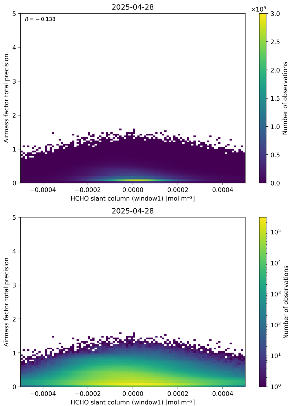
Figure 86: Scatter density plot of “HCHO slant column (window1)” against “Airmass factor total precision” for 2025-04-27 to 2025-04-29.
