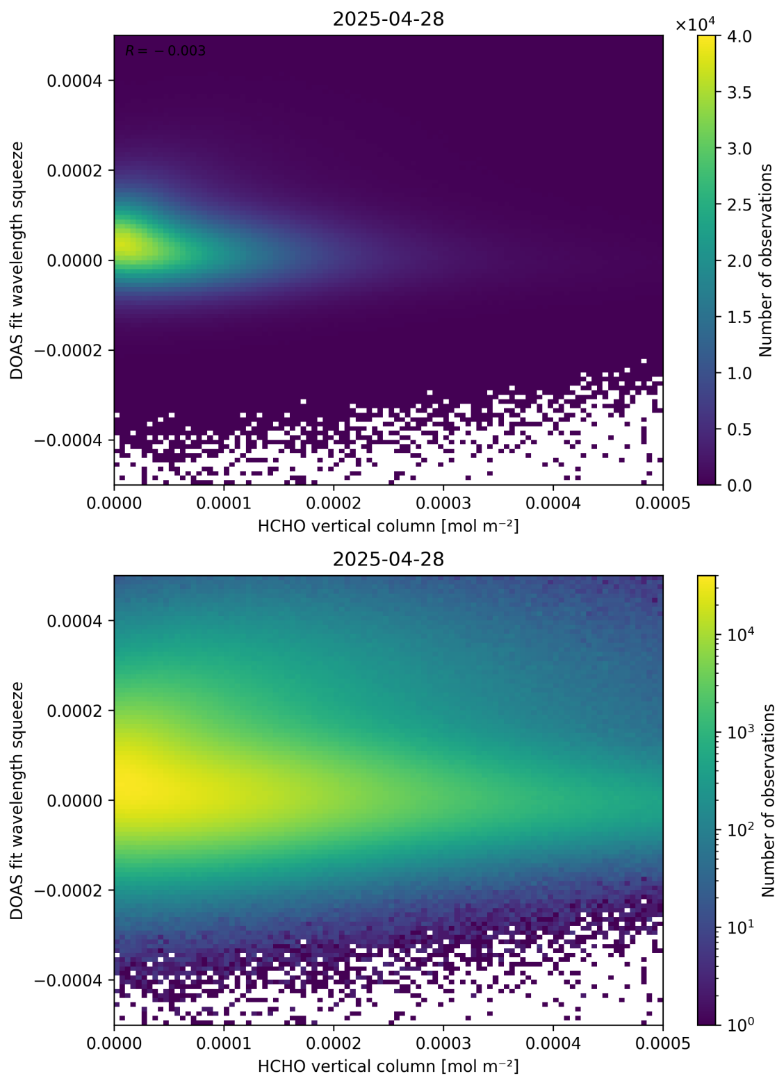
Figure 125: Scatter density plot of “HCHO vertical column” against “DOAS fit wavelength squeeze” for 2025-04-27 to 2025-04-29.
