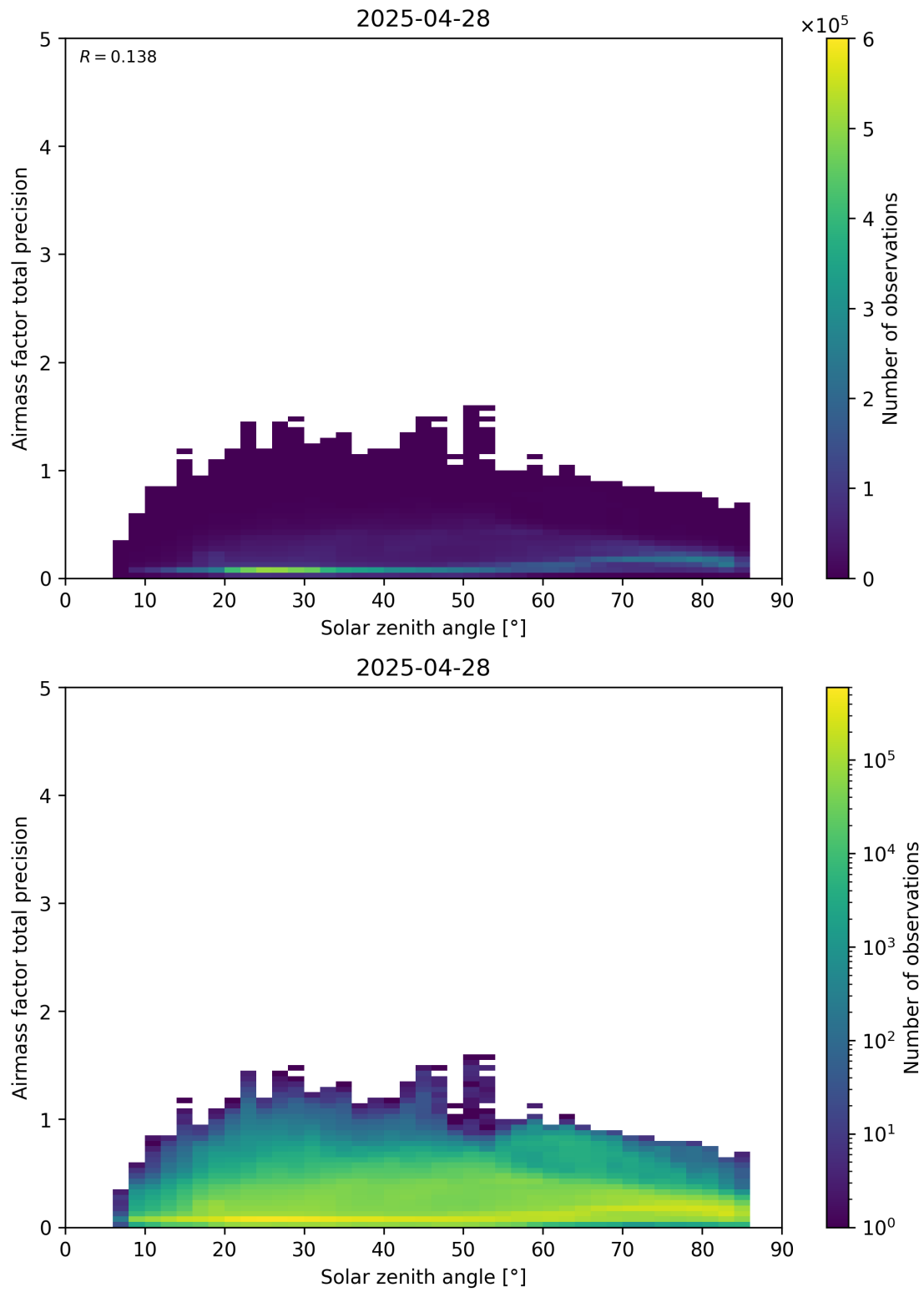
Figure 176: Scatter density plot of “Solar zenith angle” against “Airmass factor total precision” for 2025-04-27 to 2025-04-29.
