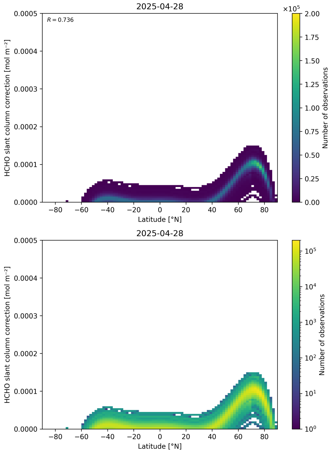
Figure 158: Scatter density plot of “Latitude” against “HCHO slant column correction” for 2025-04-27 to 2025-04-29.
