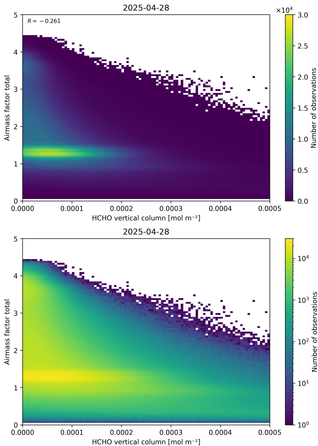
Figure 131: Scatter density plot of “HCHO vertical column” against “Airmass factor total” for 2025-04-27 to 2025-04-29.
