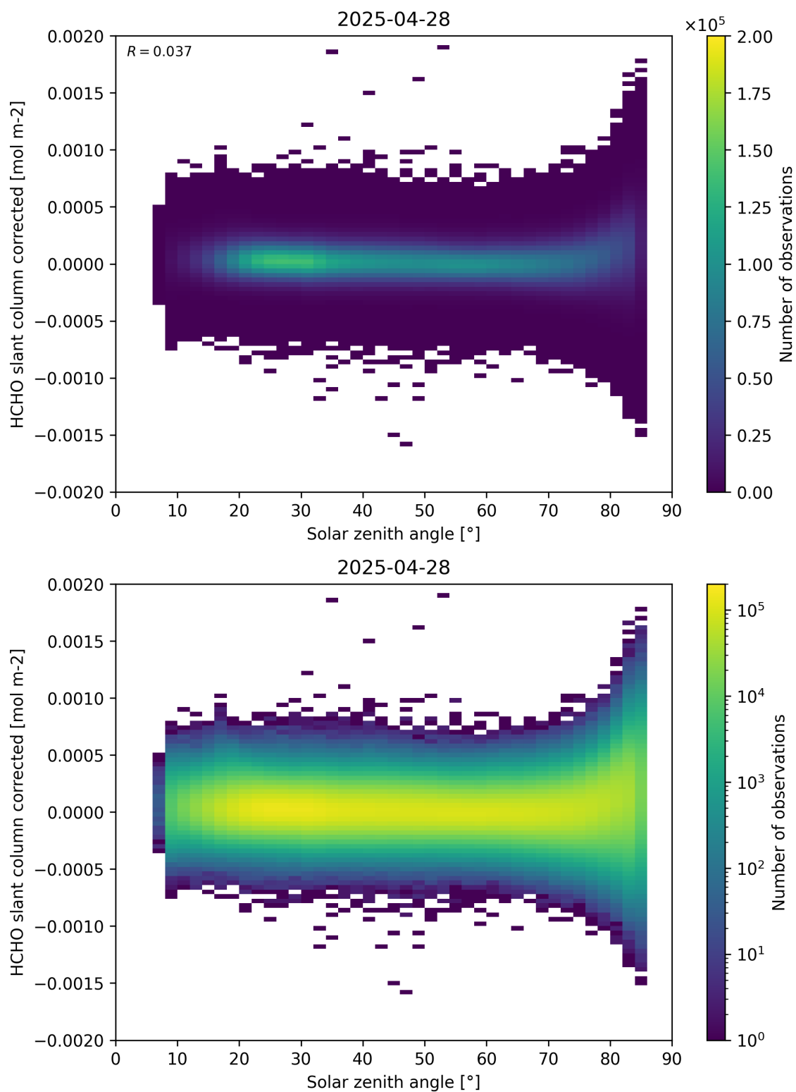
Figure 171: Scatter density plot of “Solar zenith angle” against “HCHO slant column corrected” for 2025-04-27 to 2025-04-29.
