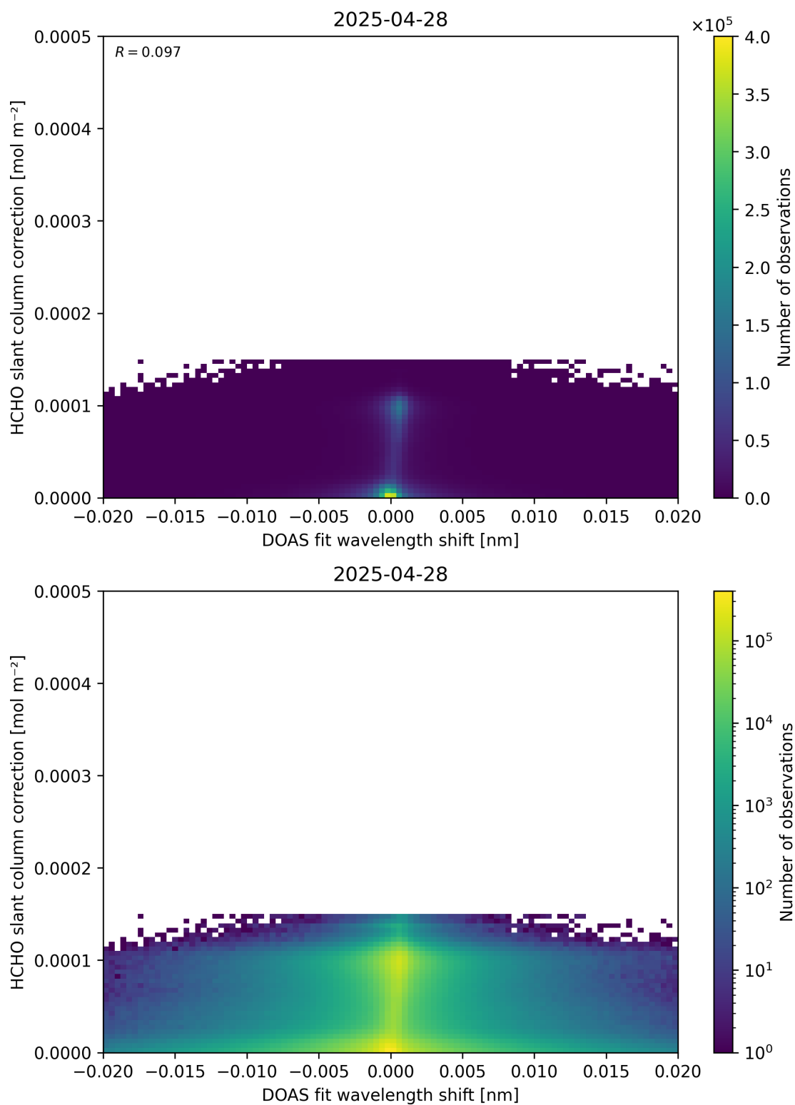
Figure 67: Scatter density plot of “DOAS fit wavelength shift” against “HCHO slant column correction” for 2025-04-27 to 2025-04-29.
