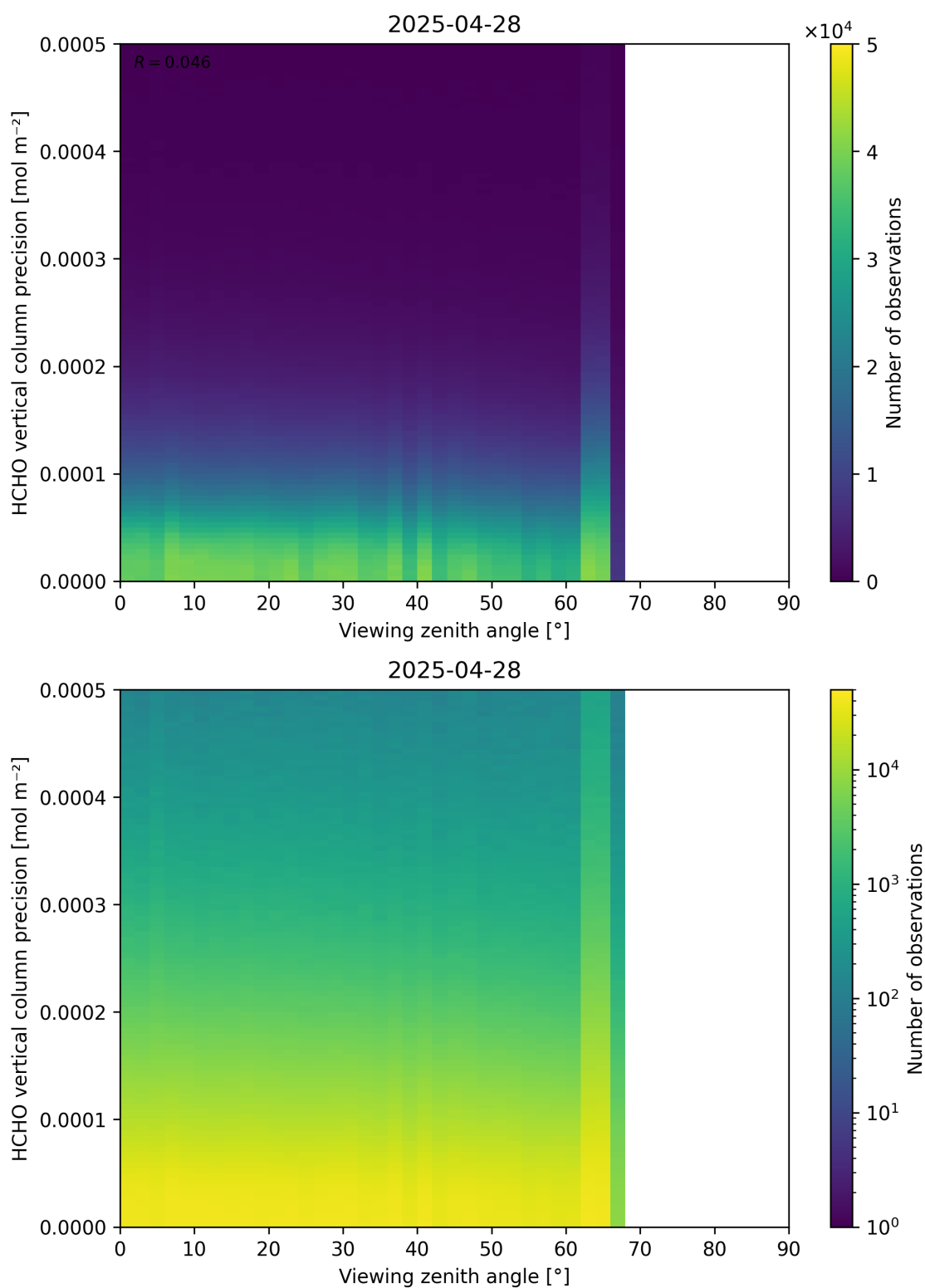
Figure 194: Scatter density plot of “Viewing zenith angle” against “HCHO vertical column precision” for 2025-04-27 to 2025-04-29.
