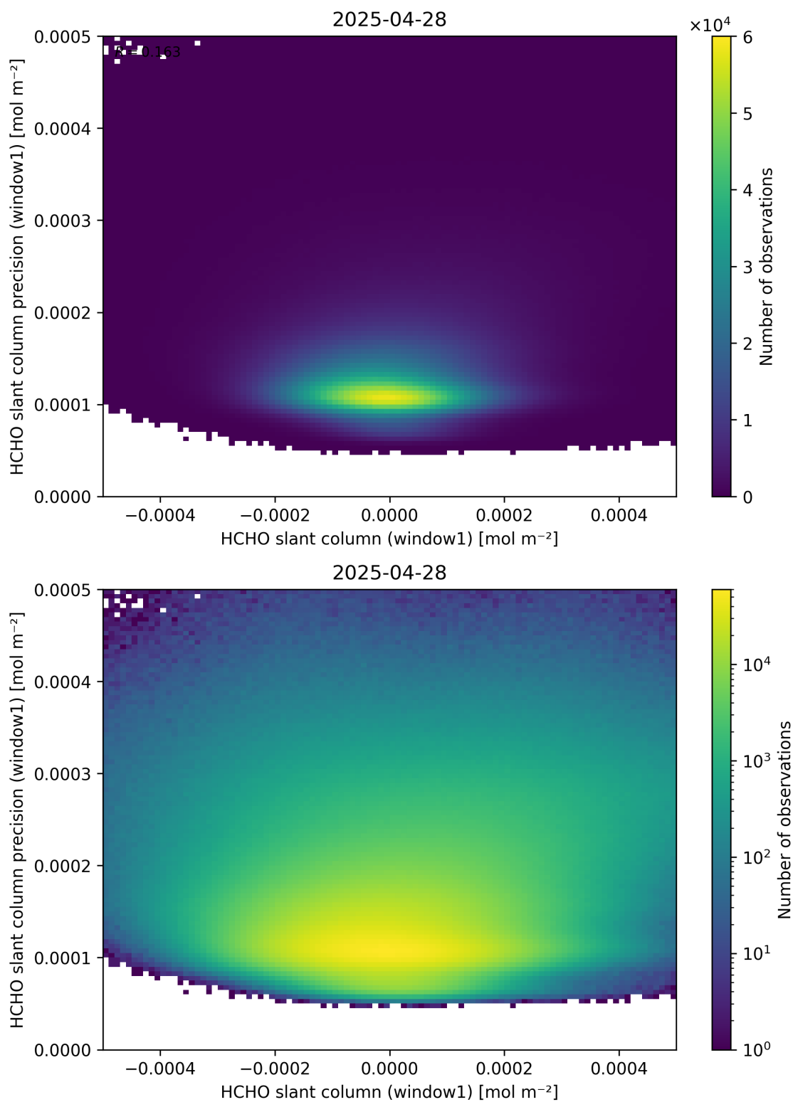
Figure 84: Scatter density plot of “HCHO slant column (window1)” against “HCHO slant column precision (window1)” for 2025-04-27 to 2025-04-29.
