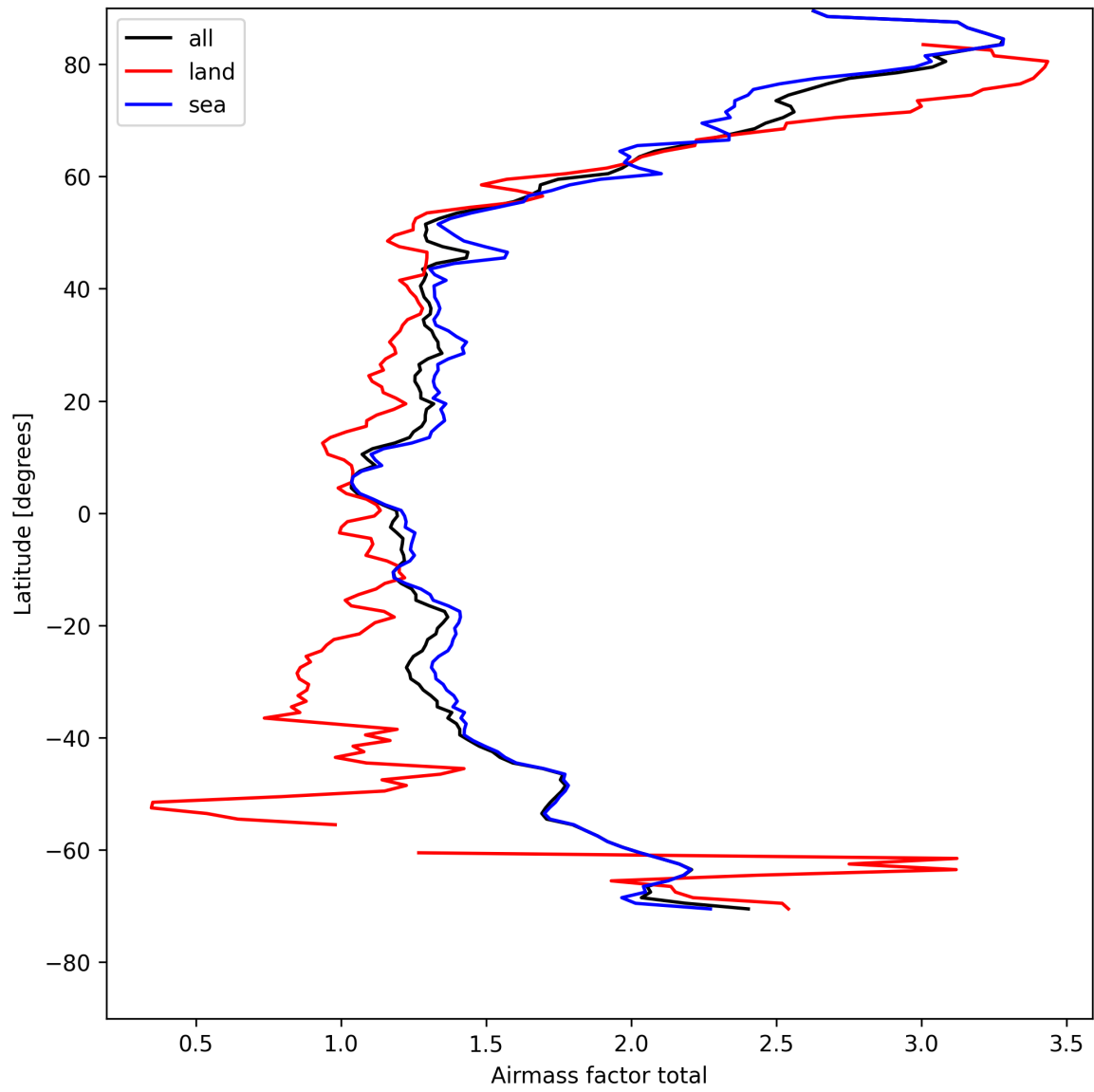
Figure 26: Zonal average of “Airmass factor total” for 2025-04-27 to 2025-04-29.
