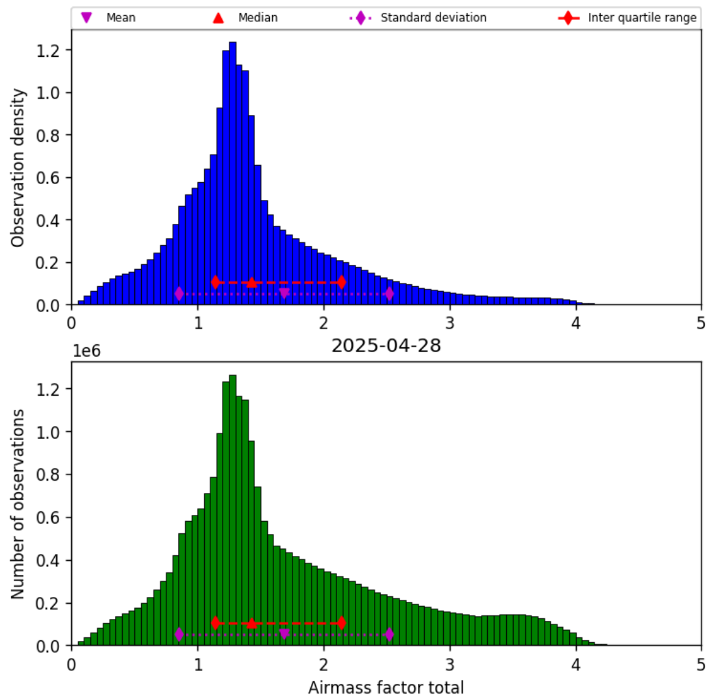
Figure 40: Histogram of “Airmass factor total” for 2025-04-27 to 2025-04-29
