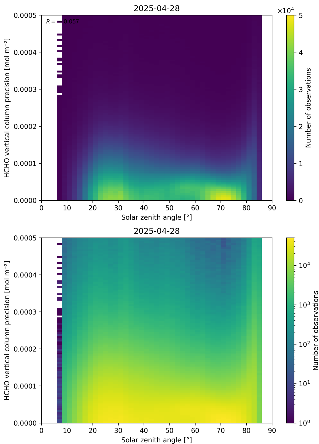
Figure 179: Scatter density plot of “Solar zenith angle” against “HCHO vertical column precision” for 2025-04-27 to 2025-04-29.
