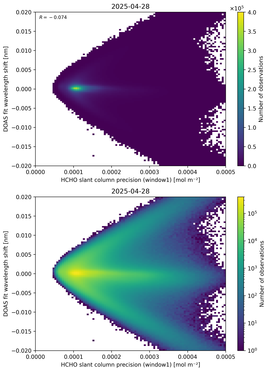
Figure 89: Scatter density plot of “HCHO slant column precision (window1)” against “DOAS fit wavelength shift” for 2025-04-27 to 2025-04-29.
