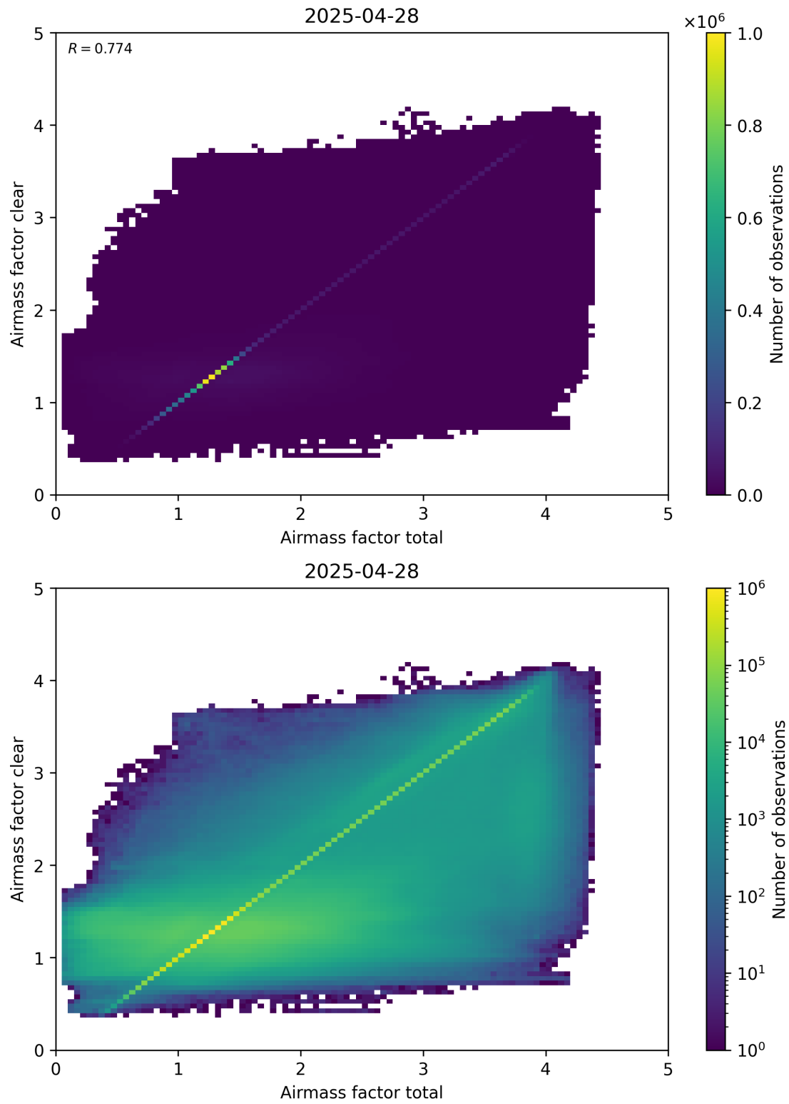
Figure 100: Scatter density plot of “Airmass factor total” against “Airmass factor clear” for 2025-04-27 to 2025-04-29.
