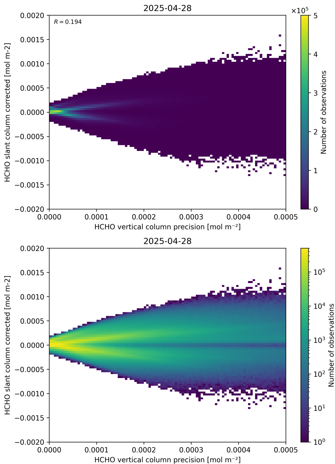
Figure 140: Scatter density plot of “HCHO vertical column precision” against “HCHO slant column corrected” for 2025-04-27 to 2025-04-29.
