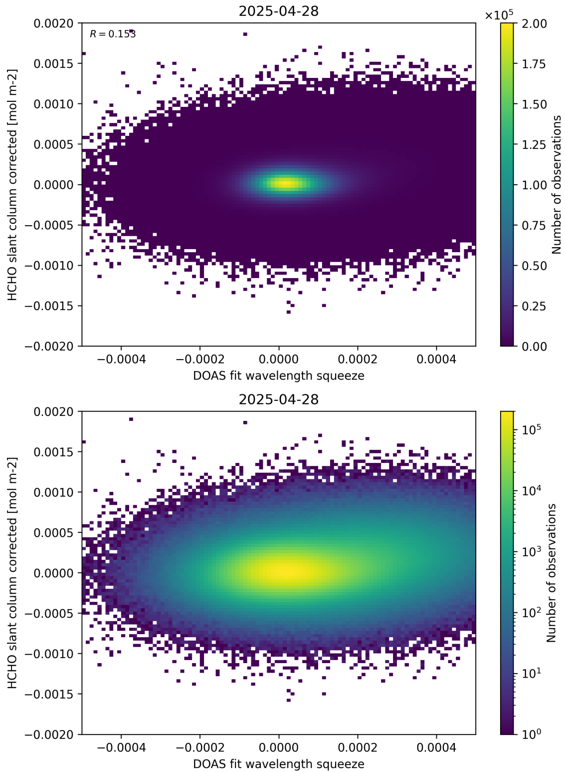
Figure 69: Scatter density plot of “DOAS fit wavelength squeeze” against “HCHO slant column corrected” for 2025-04-27 to 2025-04-29.
