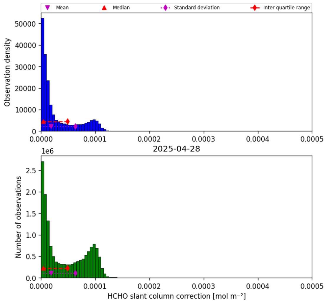
Figure 47: Histogram of “HCHO slant column correction” for 2025-04-27 to 2025-04-29
