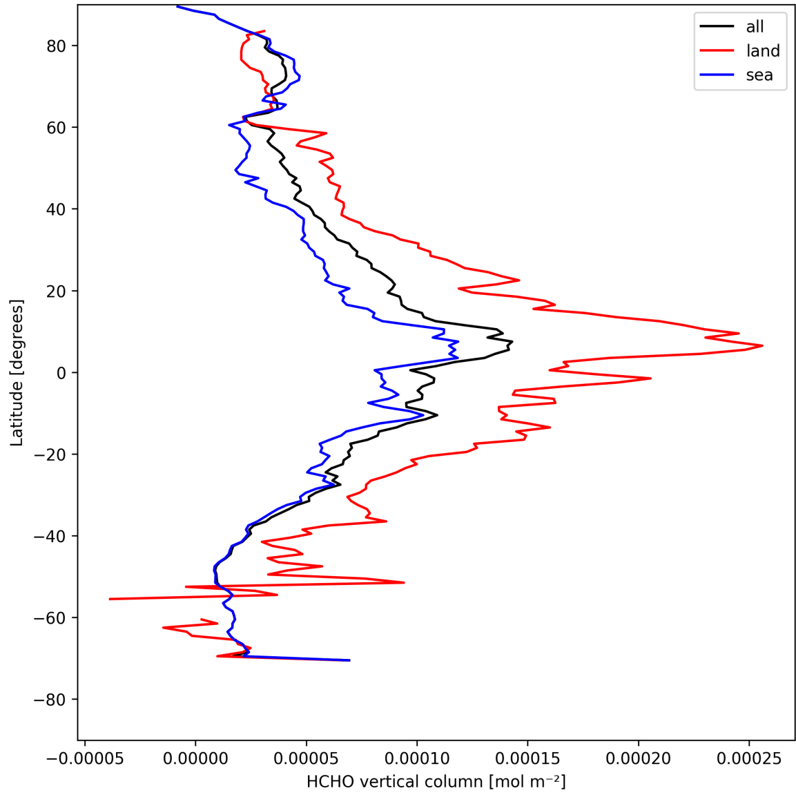
Figure 21: Zonal average of “HCHO vertical column” for 2025-04-27 to 2025-04-29.
