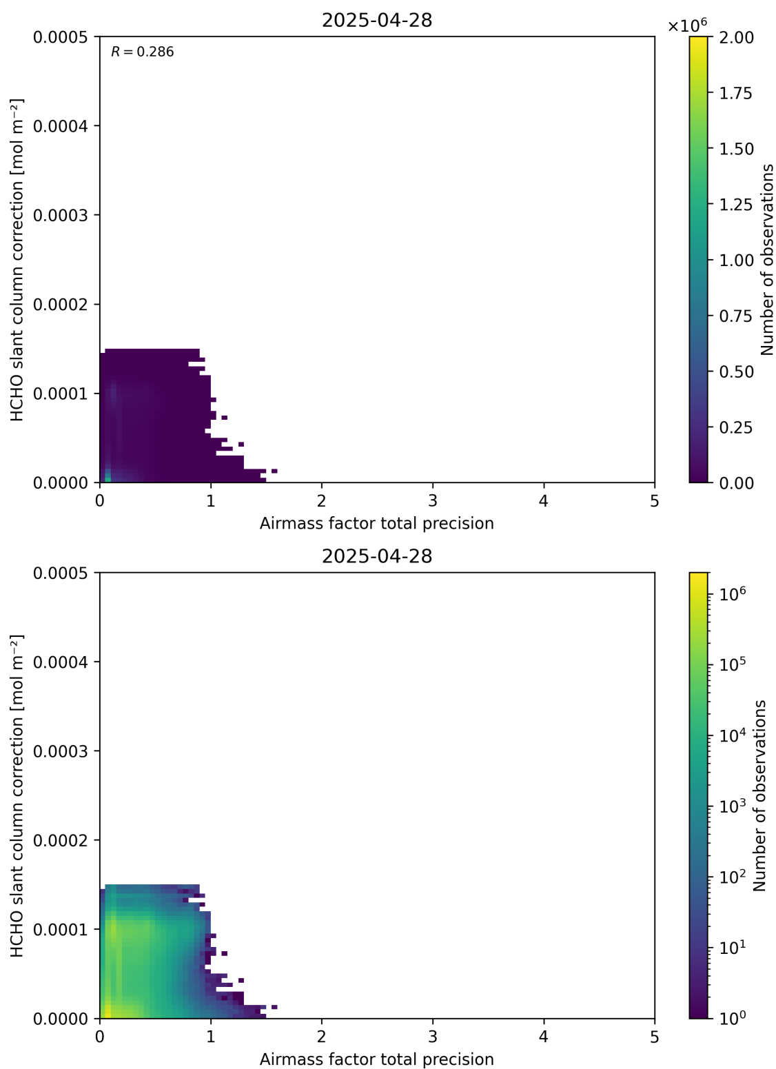
Figure 110: Scatter density plot of “Airmass factor total precision” against “HCHO slant column correction” for 2025-04-27 to 2025-04-29.
