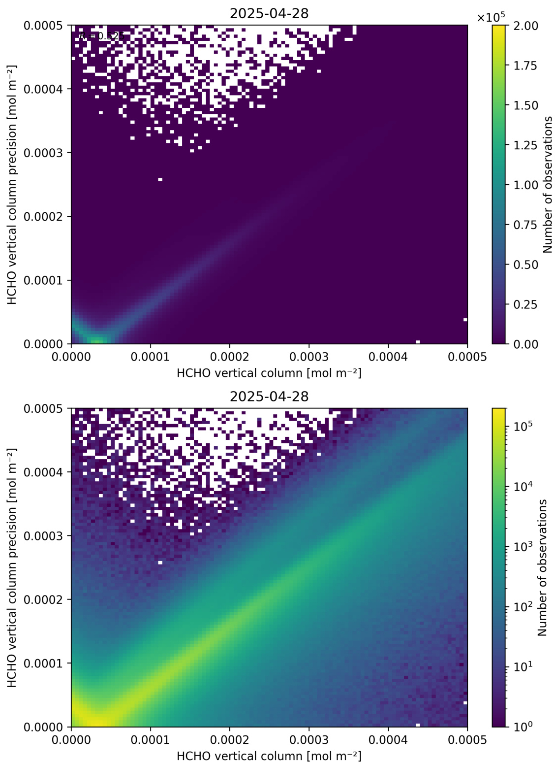
Figure 134: Scatter density plot of “HCHO vertical column” against “HCHO vertical column precision” for 2025-04-27 to 2025-04-29.
