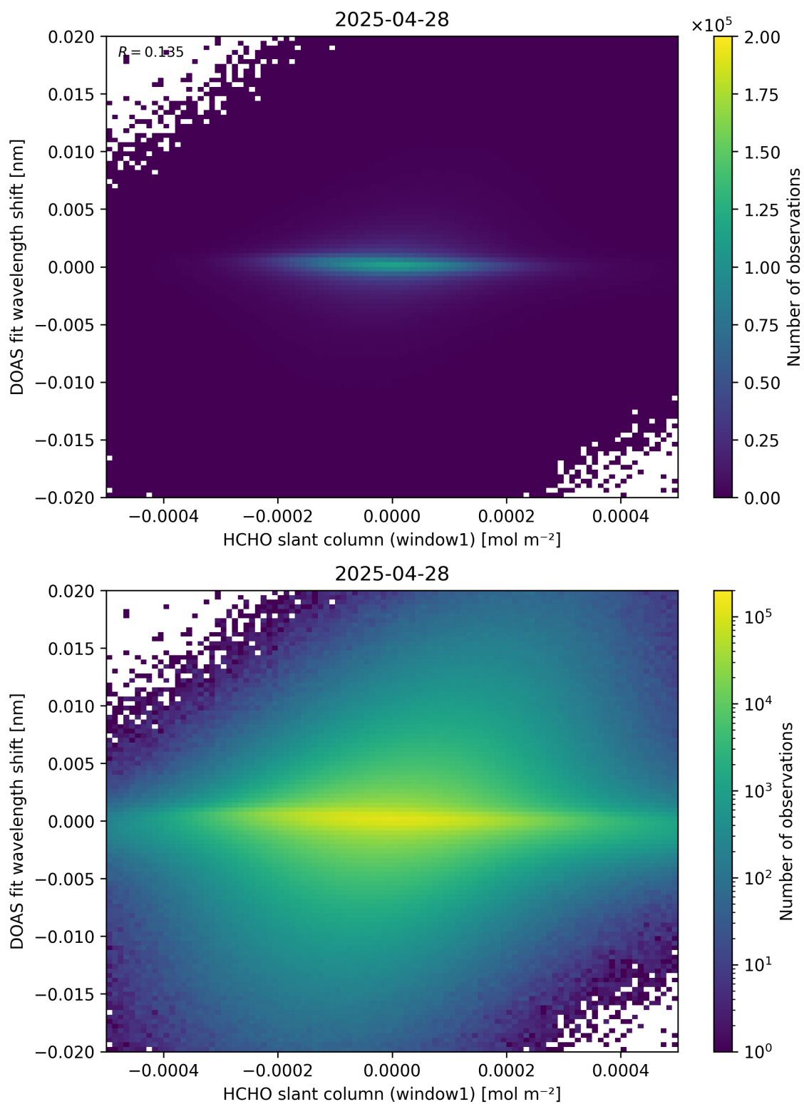
Figure 79: Scatter density plot of “HCHO slant column (window1)” against “DOAS fit wavelength shift” for 2025-04-27 to 2025-04-29.
