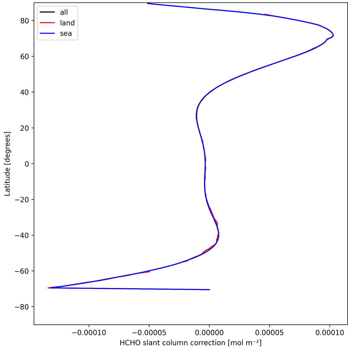
Figure 33: Zonal average of “HCHO slant column correction” for 2025-04-27 to 2025-04-29.
