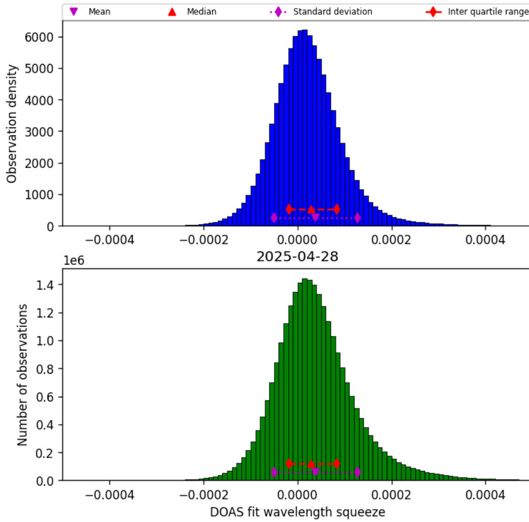
Figure 45: Histogram of “DOAS fit wavelength squeeze” for 2025-04-27 to 2025-04-29
