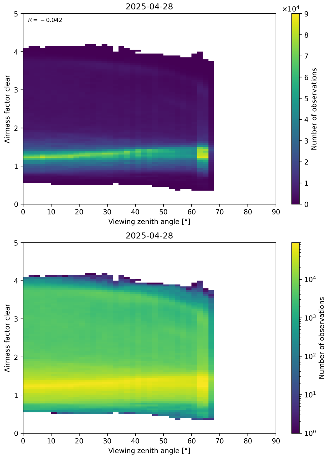
Figure 185: Scatter density plot of “Viewing zenith angle” against “Airmass factor clear” for 2025-04-27 to 2025-04-29.
