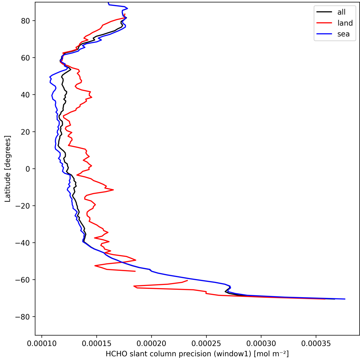
Figure 25: Zonal average of “HCHO slant column precision (window1)” for 2025-04-27 to 2025-04-29.
