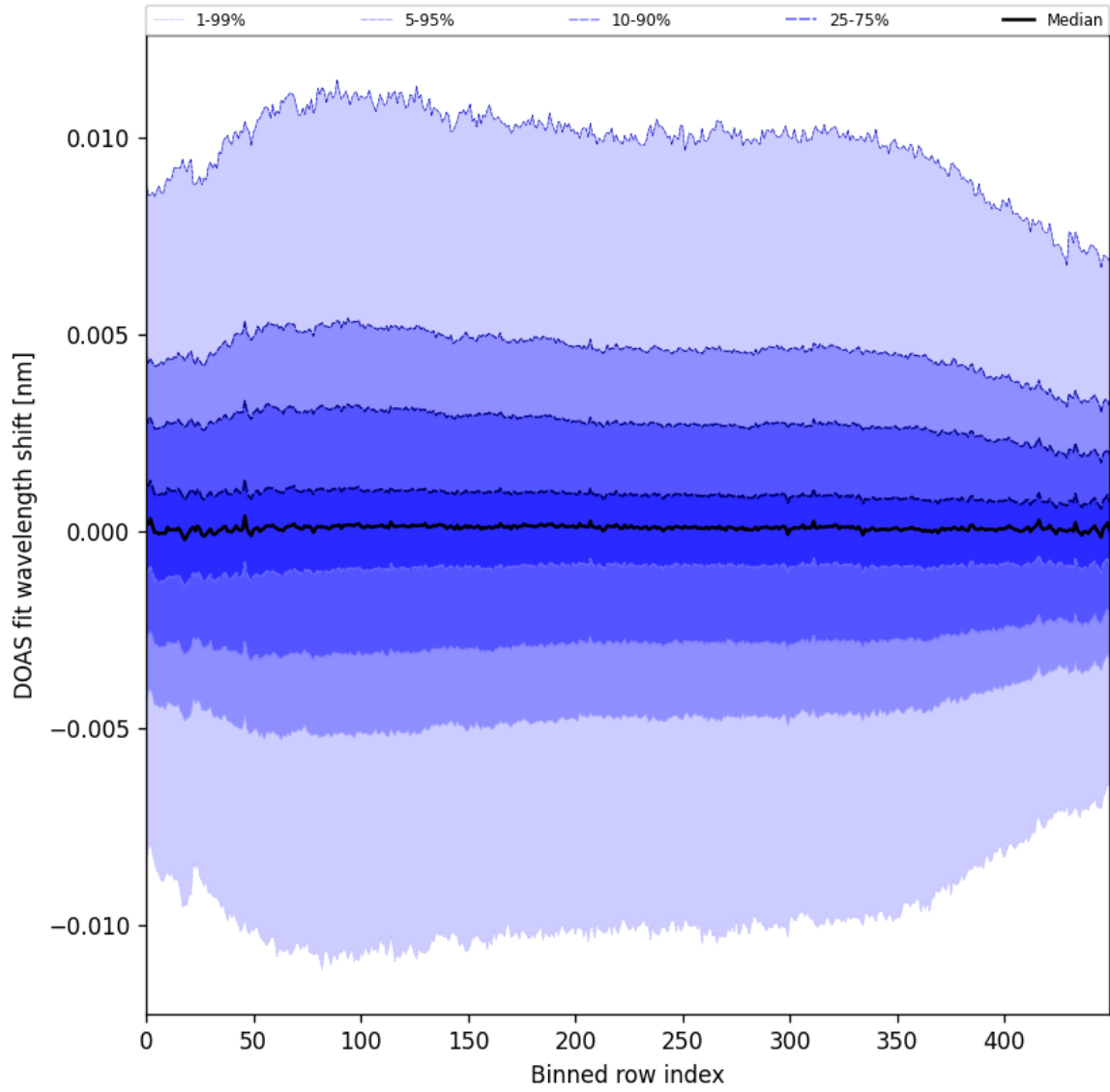
Figure 58: Along track statistics of “DOAS fit wavelength shift” for 2025-04-27 to 2025-04-29
