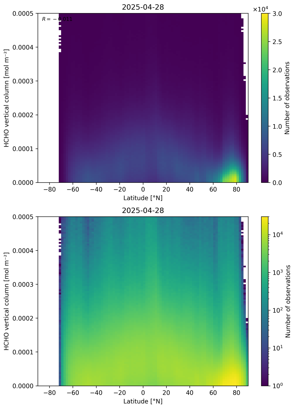
Figure 163: Scatter density plot of “Latitude” against “HCHO vertical column” for 2025-04-27 to 2025-04-29.
