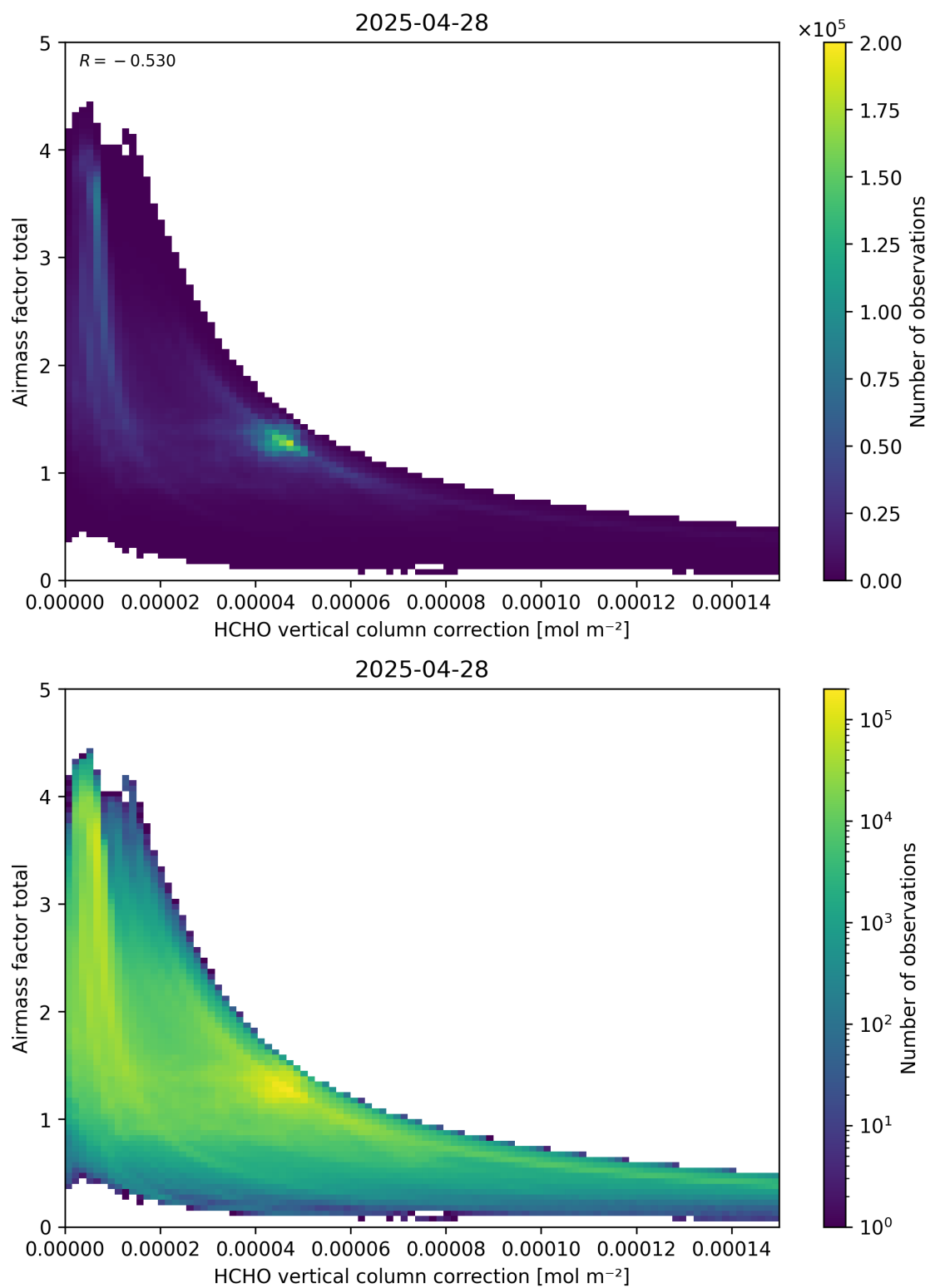
Figure 120: Scatter density plot of “HCHO vertical column correction” against “Airmass factor total” for 2025-04-27 to 2025-04-29.
