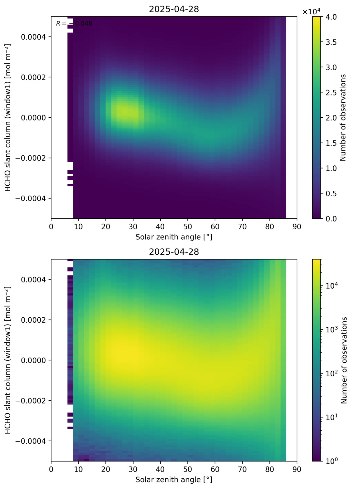
Figure 173: Scatter density plot of “Solar zenith angle” against “HCHO slant column (window1)” for 2025-04-27 to 2025-04-29.
