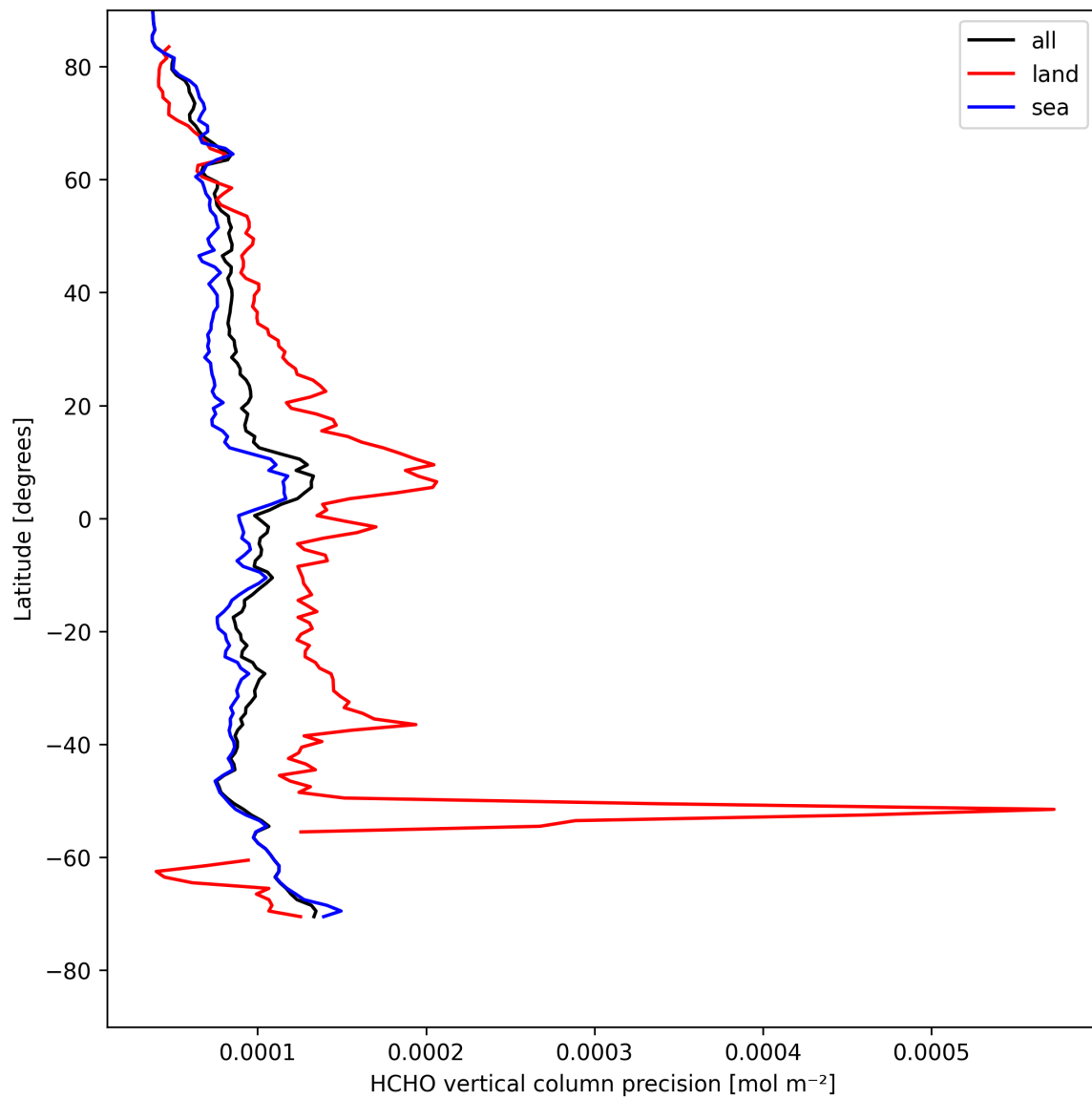
Figure 22: Zonal average of “HCHO vertical column precision” for 2025-04-27 to 2025-04-29.
