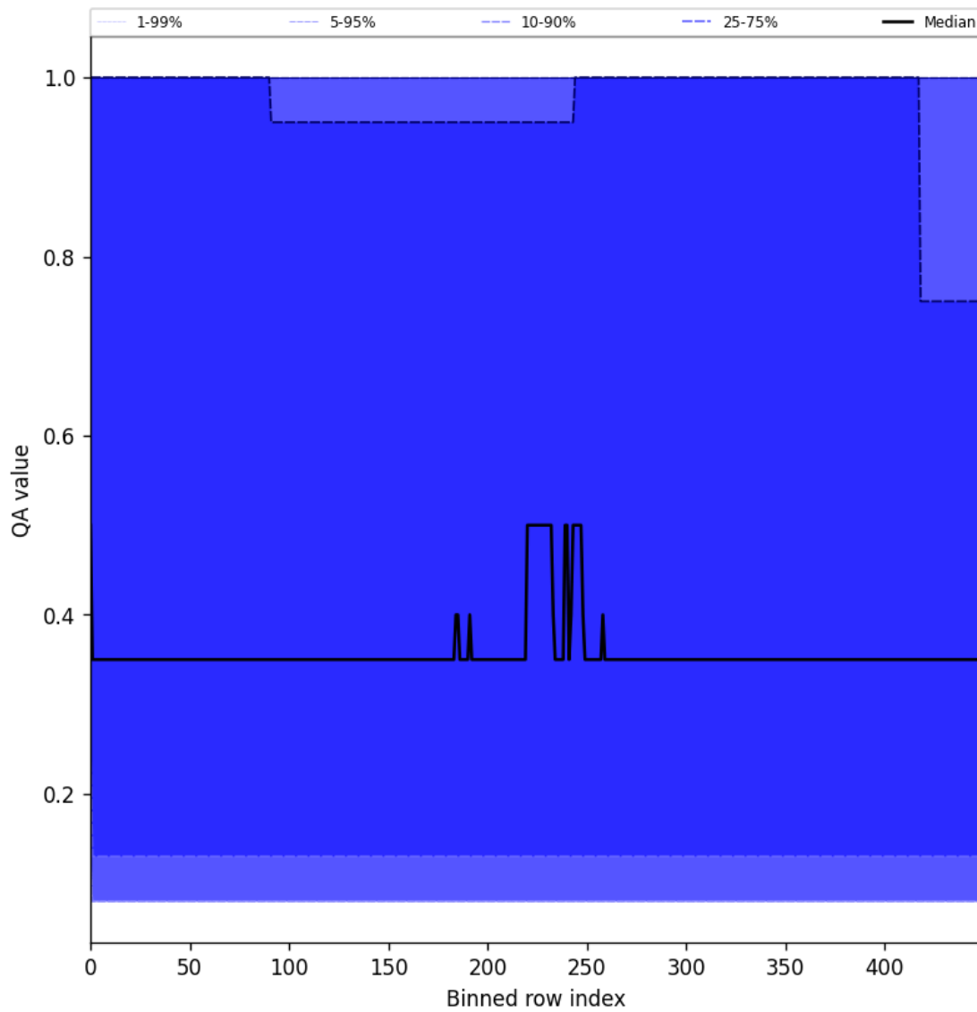
Figure 48: Along track statistics of “QA value” for 2025-04-27 to 2025-04-29
