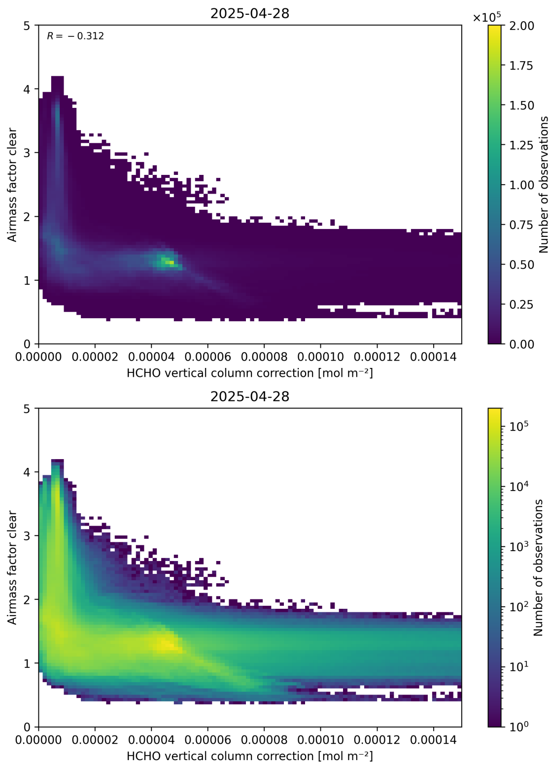
Figure 115: Scatter density plot of “HCHO vertical column correction” against “Airmass factor clear” for 2025-04-27 to 2025-04-29.
