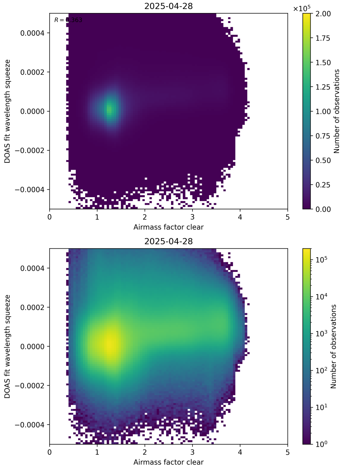
Figure 73: Scatter density plot of “Airmass factor clear” against “DOAS fit wavelength squeeze” for 2025-04-27 to 2025-04-29.
