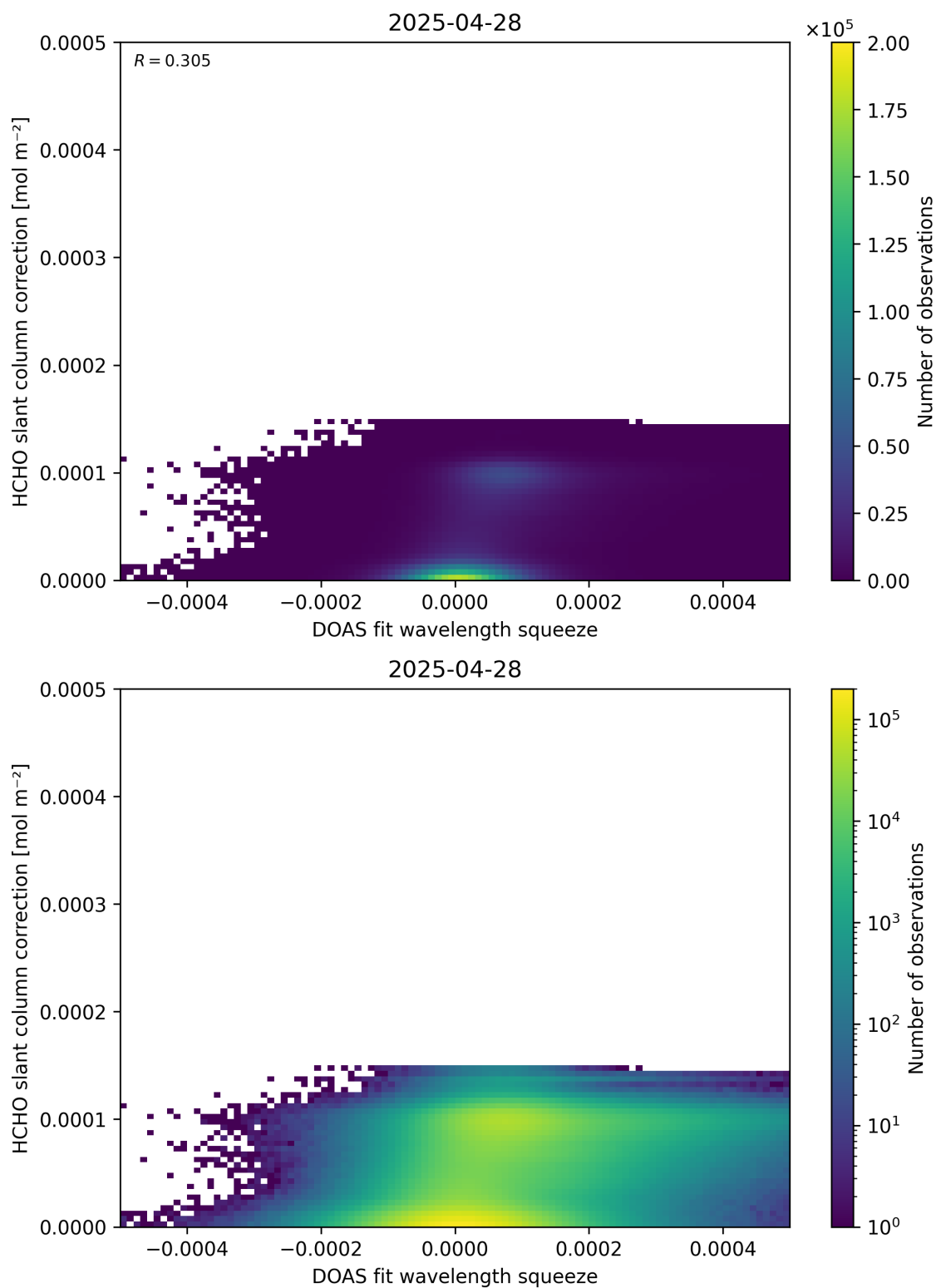
Figure 70: Scatter density plot of “DOAS fit wavelength squeeze” against “HCHO slant column correction” for 2025-04-27 to 2025-04-29.
