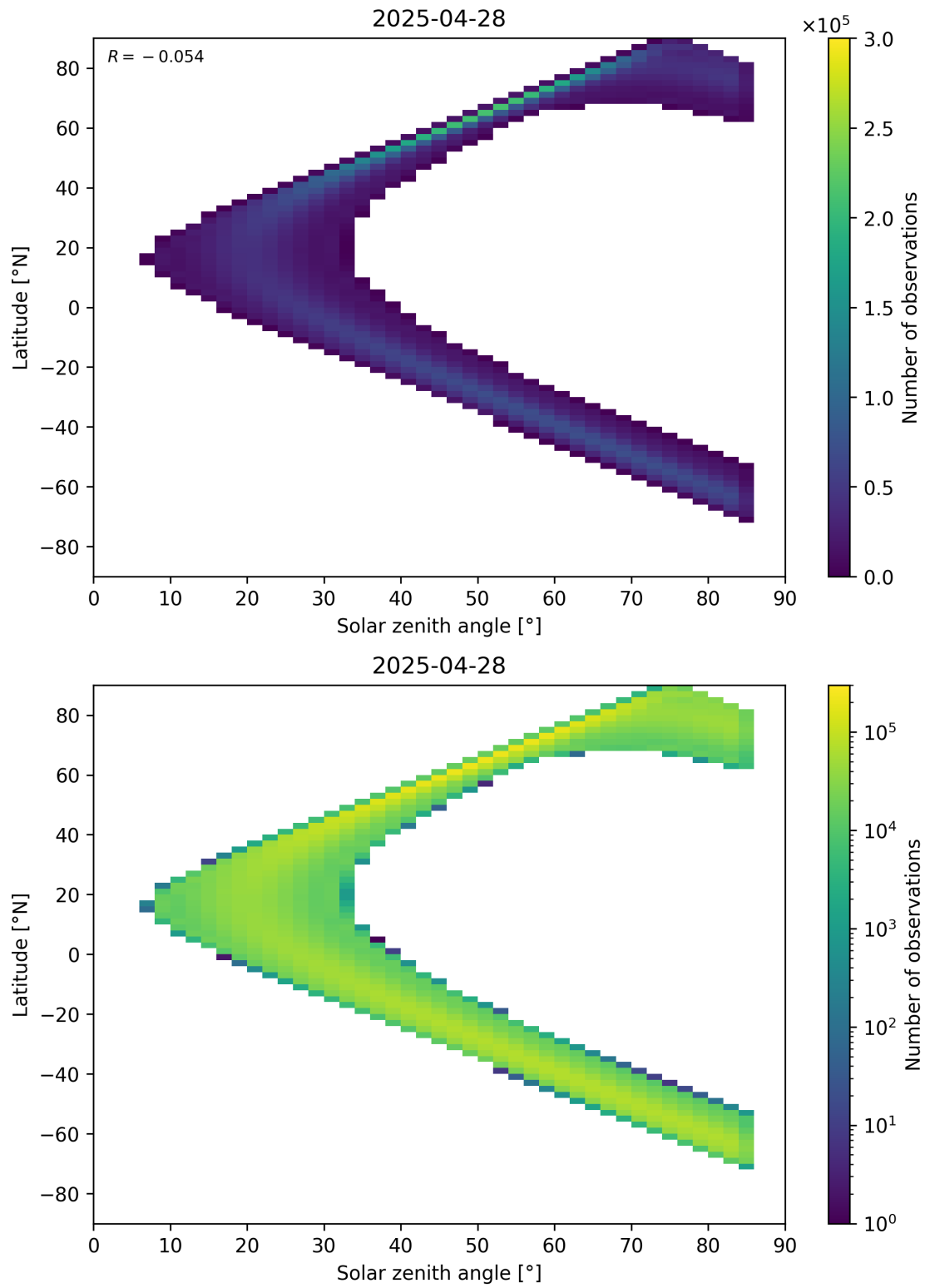
Figure 181: Scatter density plot of “Solar zenith angle” against “Latitude” for 2025-04-27 to 2025-04-29.
