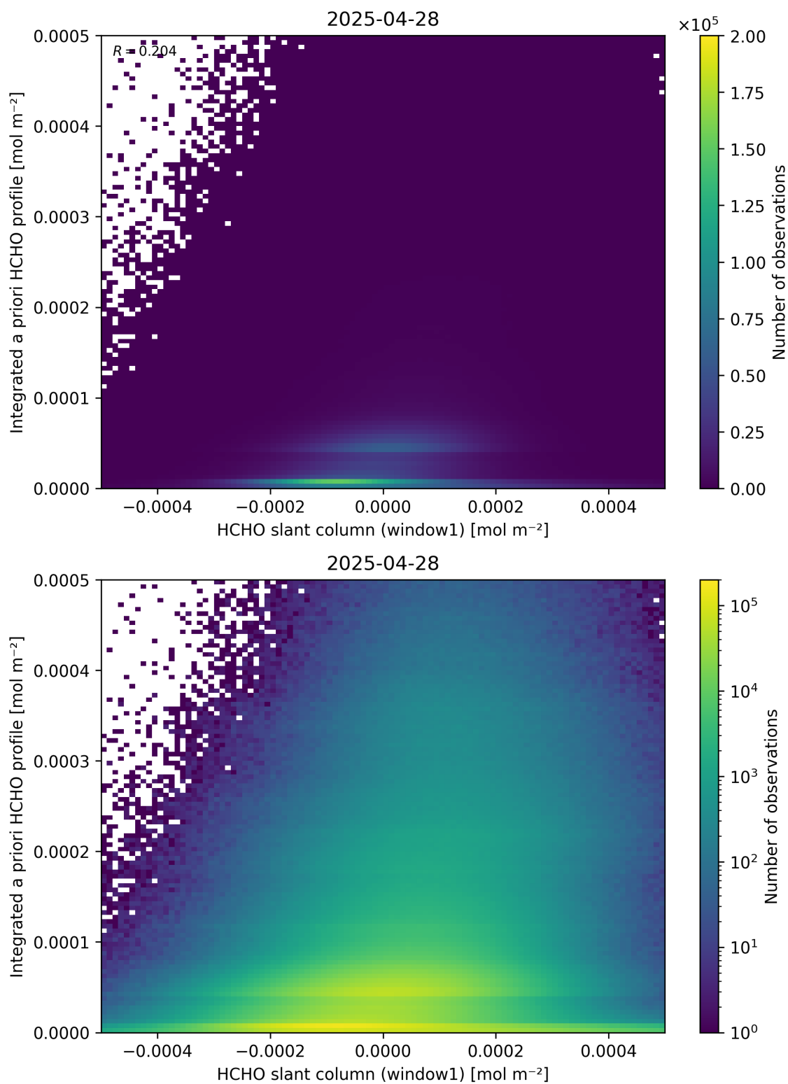
Figure 87: Scatter density plot of “HCHO slant column (window1)” against “Integrated a priori HCHO profile” for 2025-04-27 to 2025-04-29.
