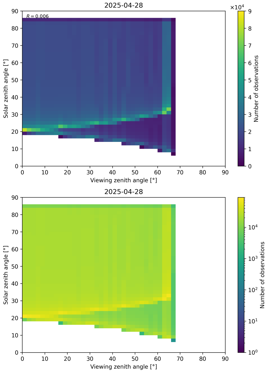
Figure 197: Scatter density plot of “Viewing zenith angle” against “Solar zenith angle” for 2025-04-27 to 2025-04-29.
