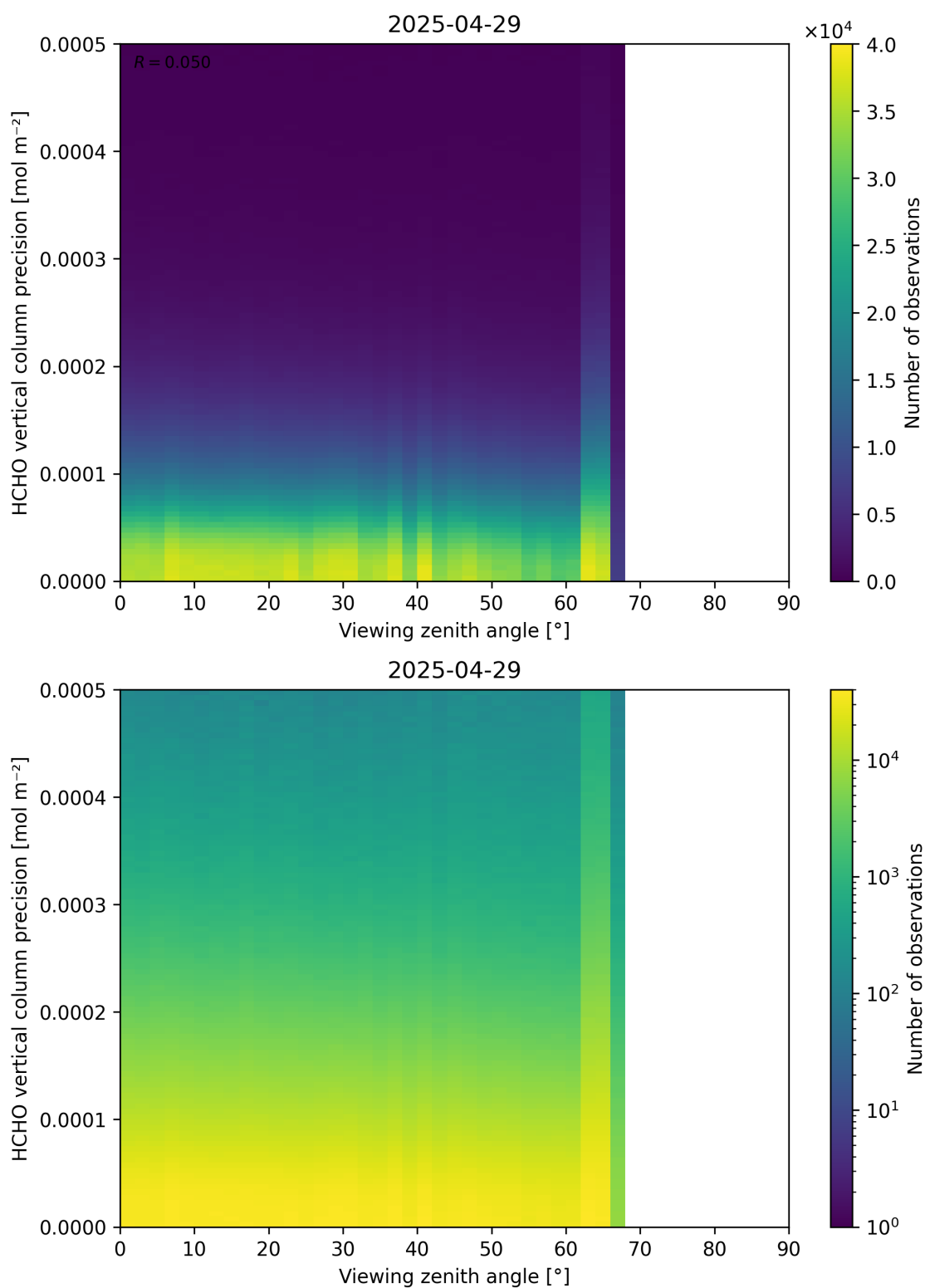
Figure 194: Scatter density plot of “Viewing zenith angle” against “HCHO vertical column precision” for 2025-04-29 to 2025-04-30.
