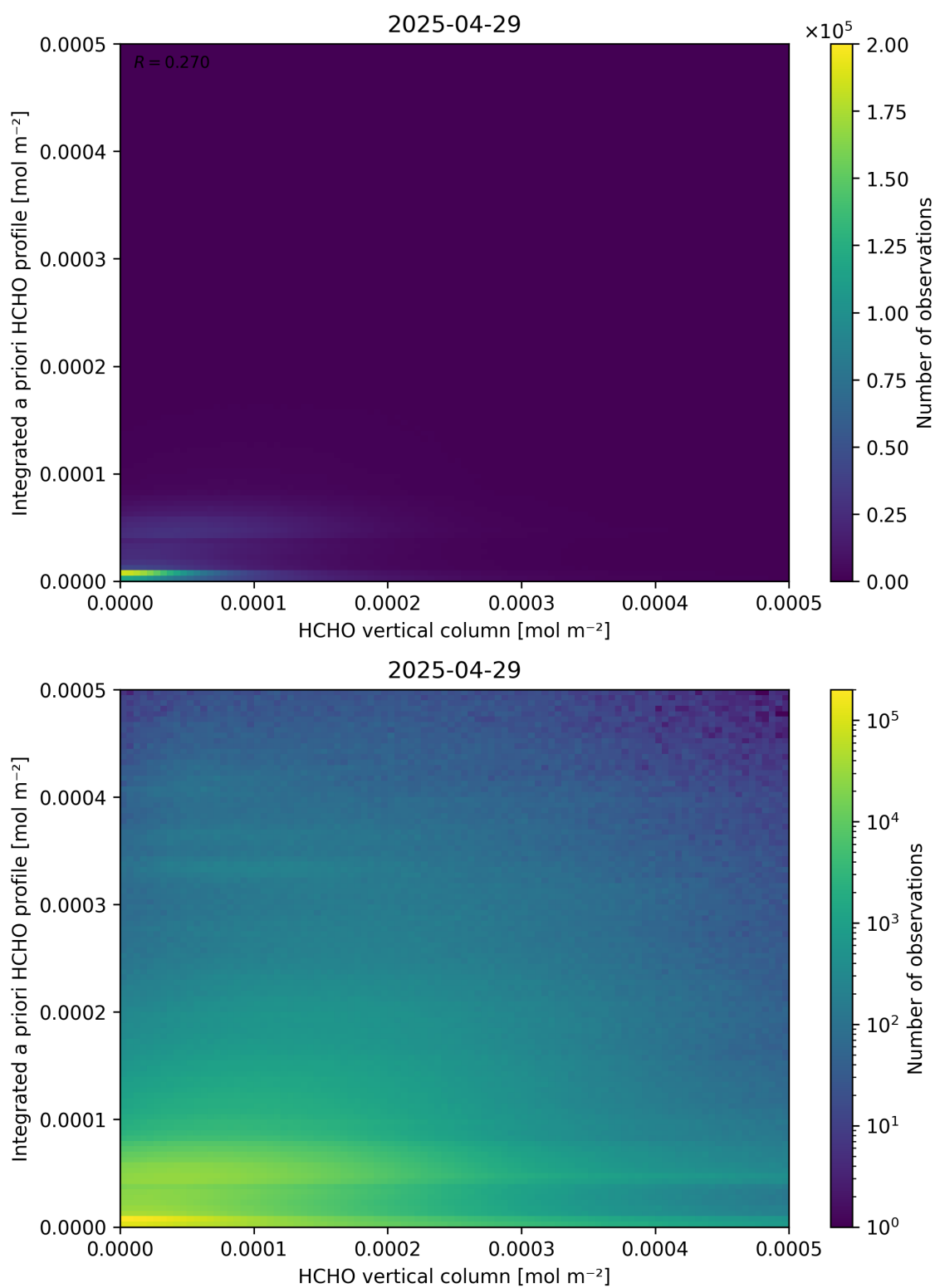
Figure 135: Scatter density plot of “HCHO vertical column” against “Integrated a priori HCHO profile” for 2025-04-29 to 2025-04-30.
