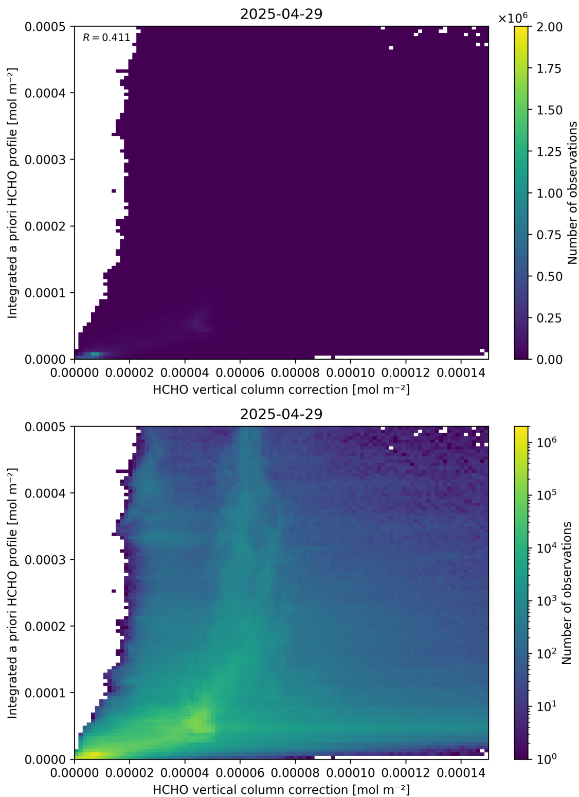
Figure 122: Scatter density plot of “HCHO vertical column correction” against “Integrated a priori HCHO profile” for 2025-04-29 to 2025-04-30.
