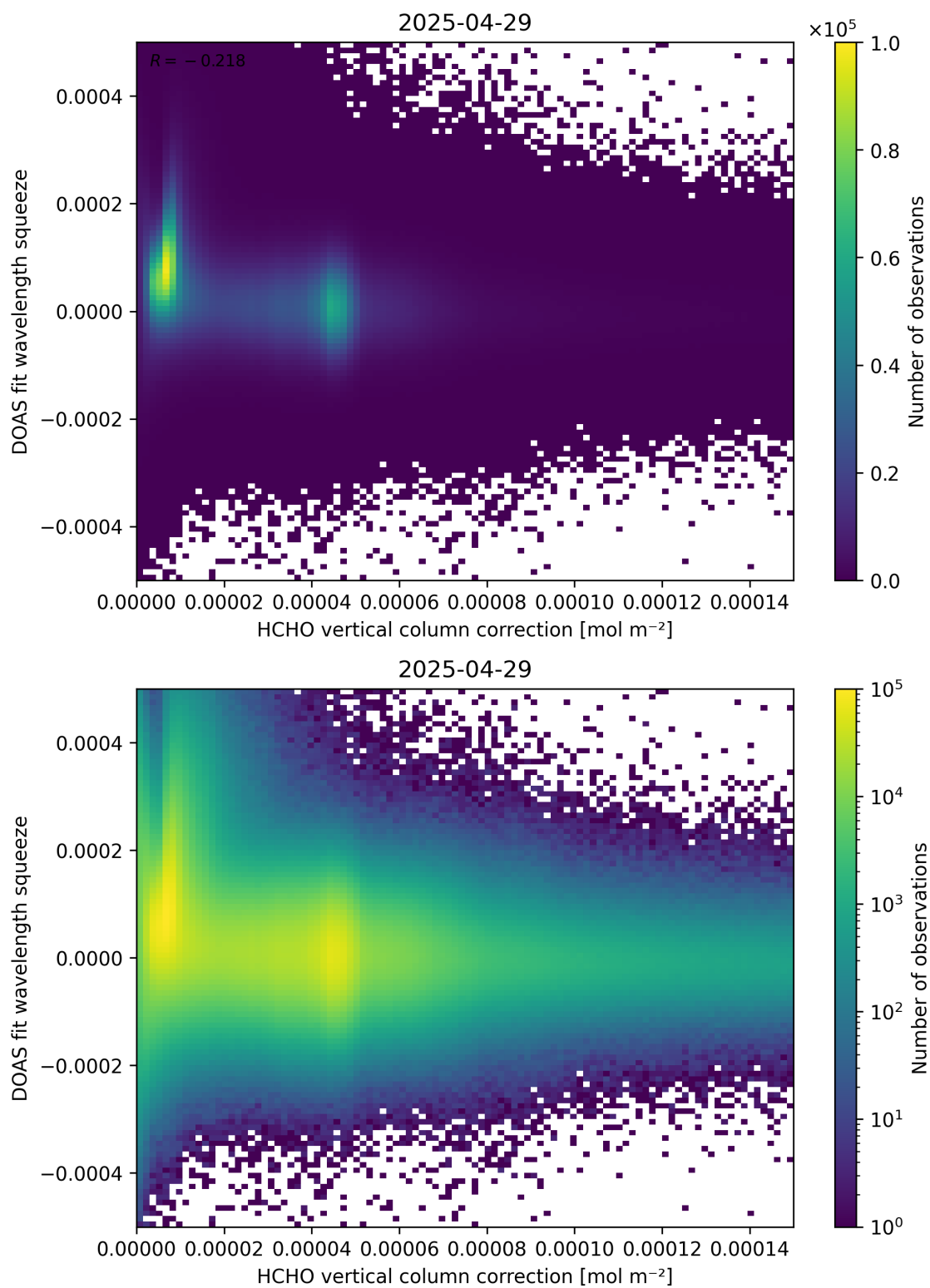
Figure 114: Scatter density plot of “HCHO vertical column correction” against “DOAS fit wavelength squeeze” for 2025-04-29 to 2025-04-30.
