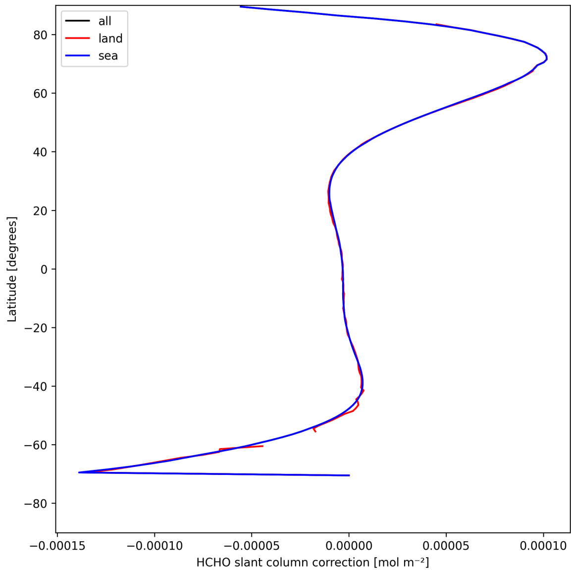
Figure 33: Zonal average of “HCHO slant column correction” for 2025-04-29 to 2025-04-30.
