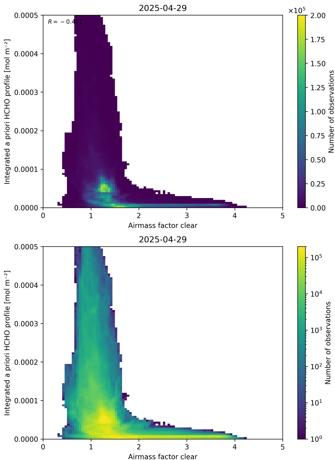
Figure 76: Scatter density plot of “Airmass factor clear” against “Integrated a priori HCHO profile” for 2025-04-29 to 2025-04-30.
