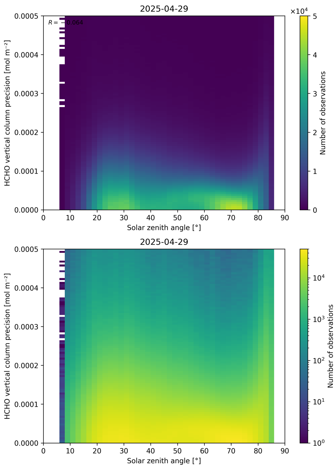
Figure 179: Scatter density plot of “Solar zenith angle” against “HCHO vertical column precision” for 2025-04-29 to 2025-04-30.
