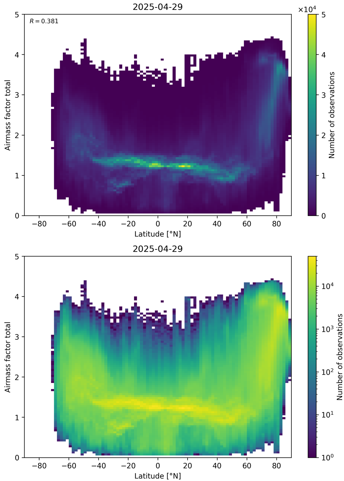
Figure 161: Scatter density plot of “Latitude” against “Airmass factor total” for 2025-04-29 to 2025-04-30.
