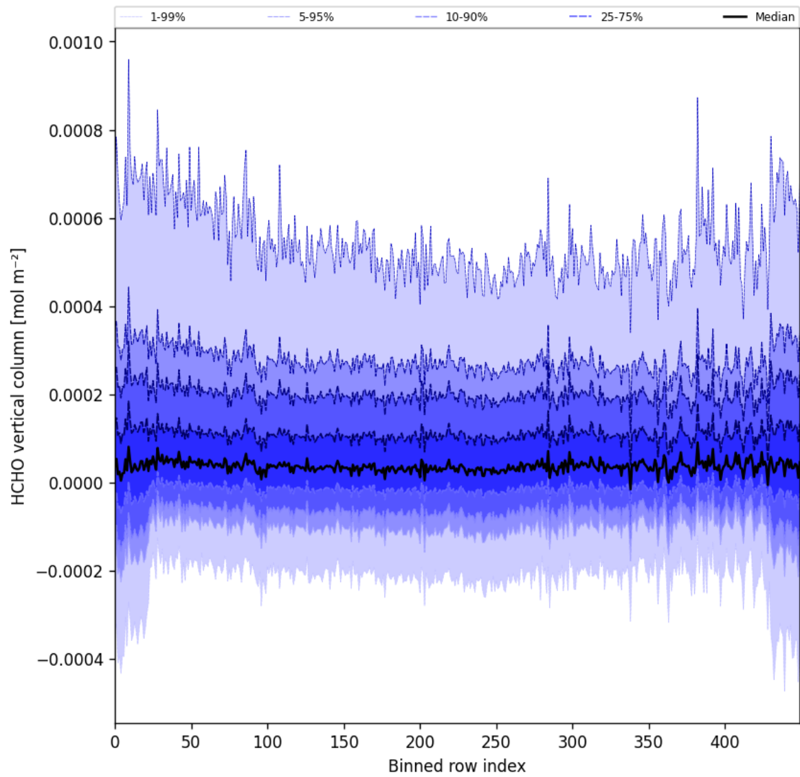
Figure 49: Along track statistics of “HCHO vertical column” for 2025-04-29 to 2025-04-30
