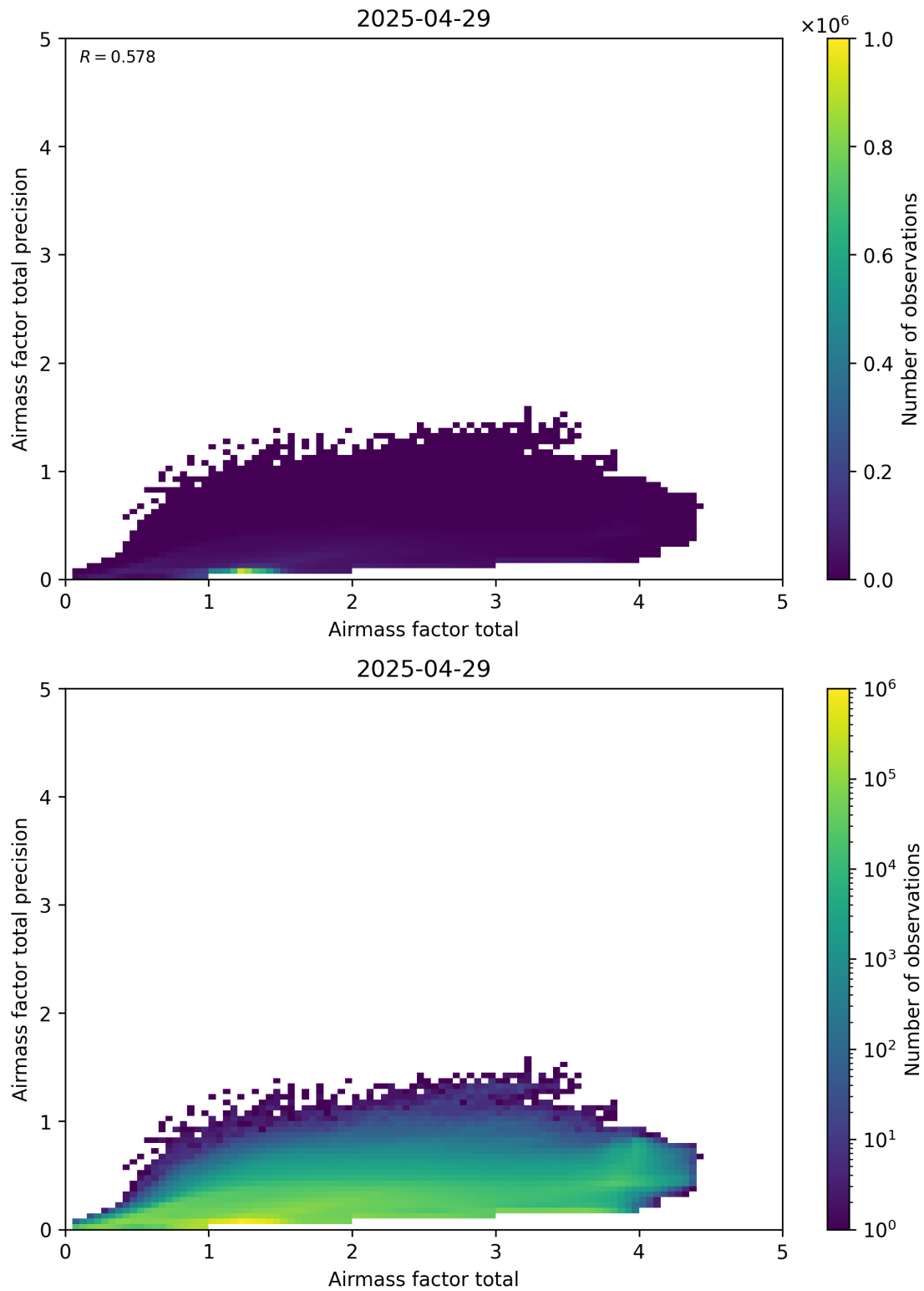
Figure 103: Scatter density plot of “Airmass factor total” against “Airmass factor total precision” for 2025-04-29 to 2025-04-30.
