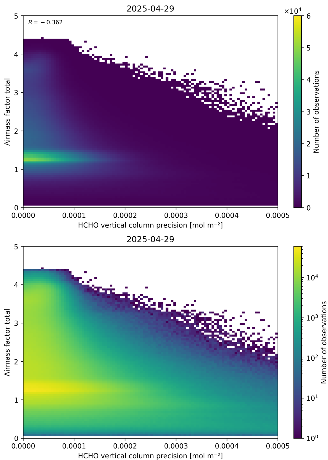
Figure 144: Scatter density plot of “HCHO vertical column precision” against “Airmass factor total” for 2025-04-29 to 2025-04-30.
