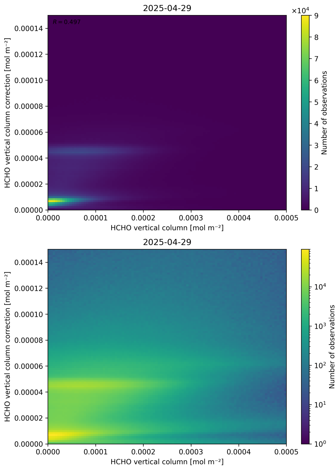
Figure 133: Scatter density plot of “HCHO vertical column” against “HCHO vertical column correction” for 2025-04-29 to 2025-04-30.
