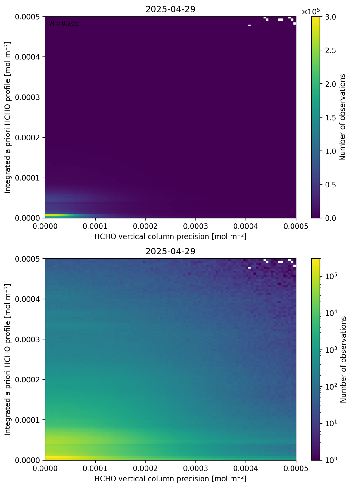
Figure 147: Scatter density plot of “HCHO vertical column precision” against “Integrated a priori HCHO profile” for 2025-04-29 to 2025-04-30.
