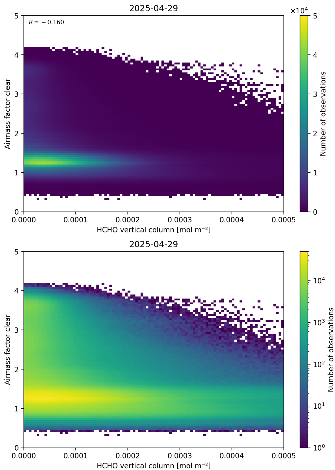
Figure 126: Scatter density plot of “HCHO vertical column” against “Airmass factor clear” for 2025-04-29 to 2025-04-30.
