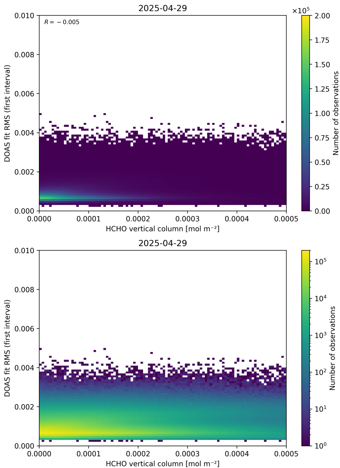
Figure 123: Scatter density plot of “HCHO vertical column” against “DOAS fit RMS (first interval)” for 2025-04-29 to 2025-04-30.
