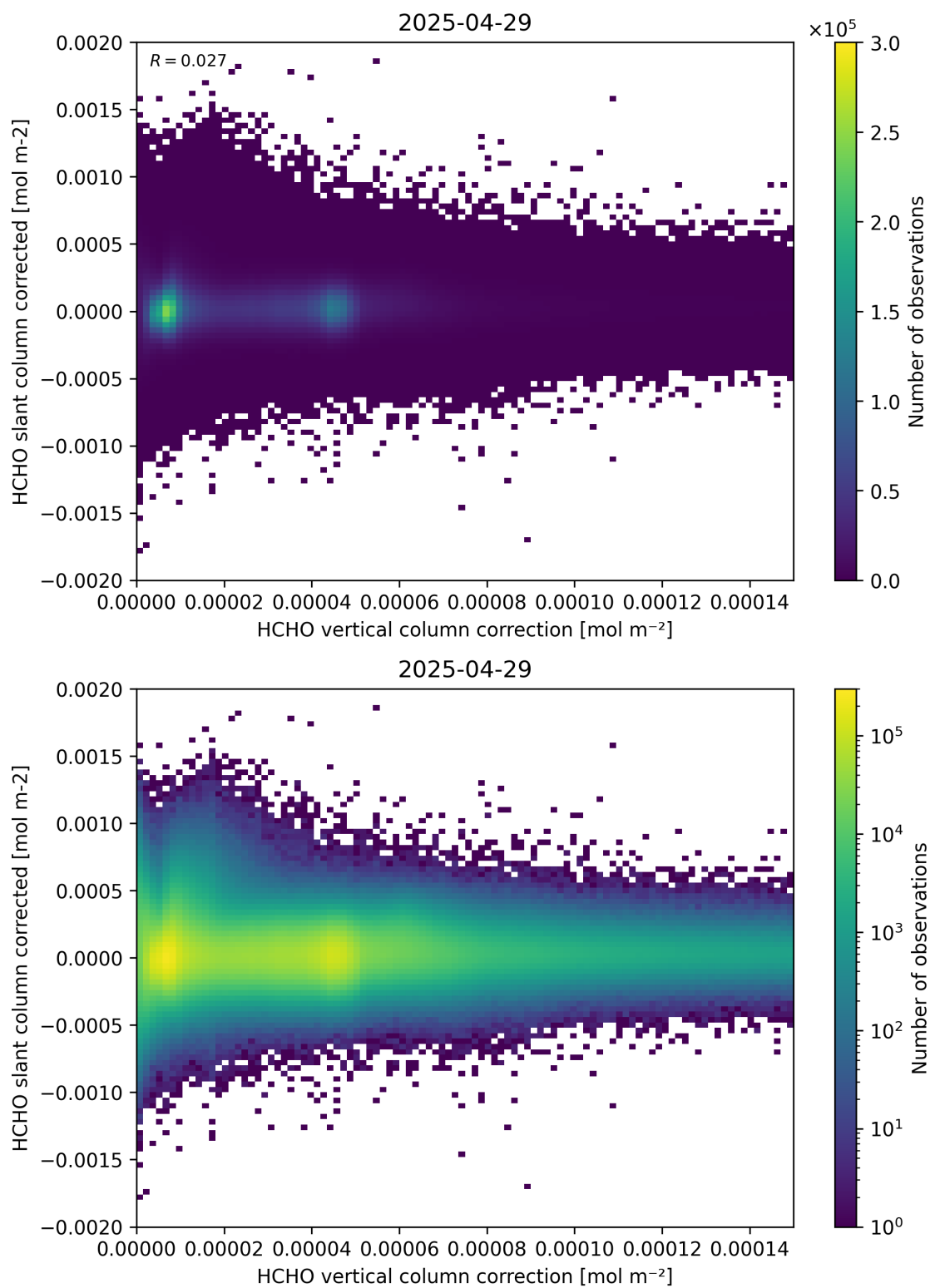
Figure 116: Scatter density plot of “HCHO vertical column correction” against “HCHO slant column corrected” for 2025-04-29 to 2025-04-30.
