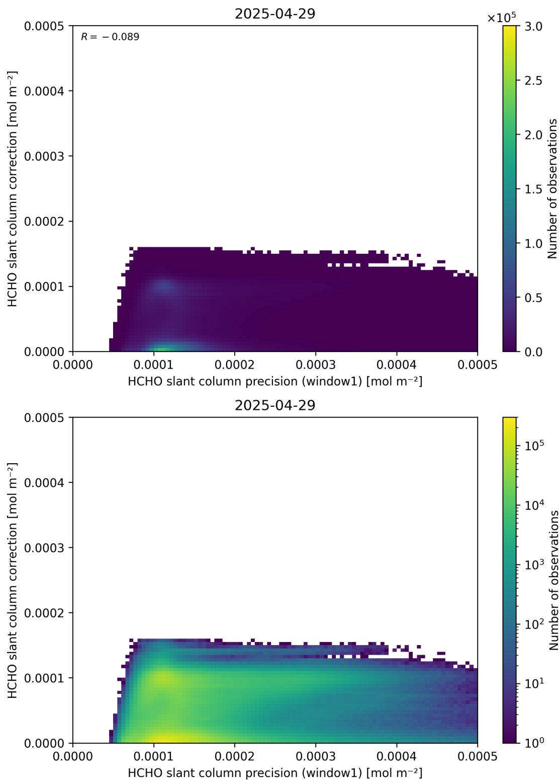
Figure 93: Scatter density plot of “HCHO slant column precision (window1)” against “HCHO slant column correction” for 2025-04-29 to 2025-04-30.
