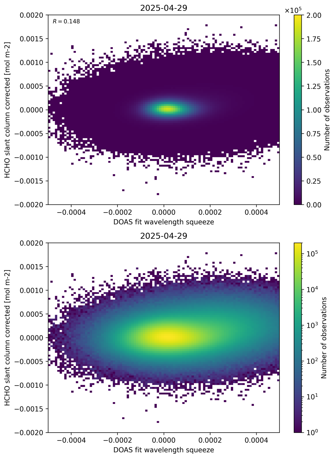
Figure 69: Scatter density plot of “DOAS fit wavelength squeeze” against “HCHO slant column corrected” for 2025-04-29 to 2025-04-30.
