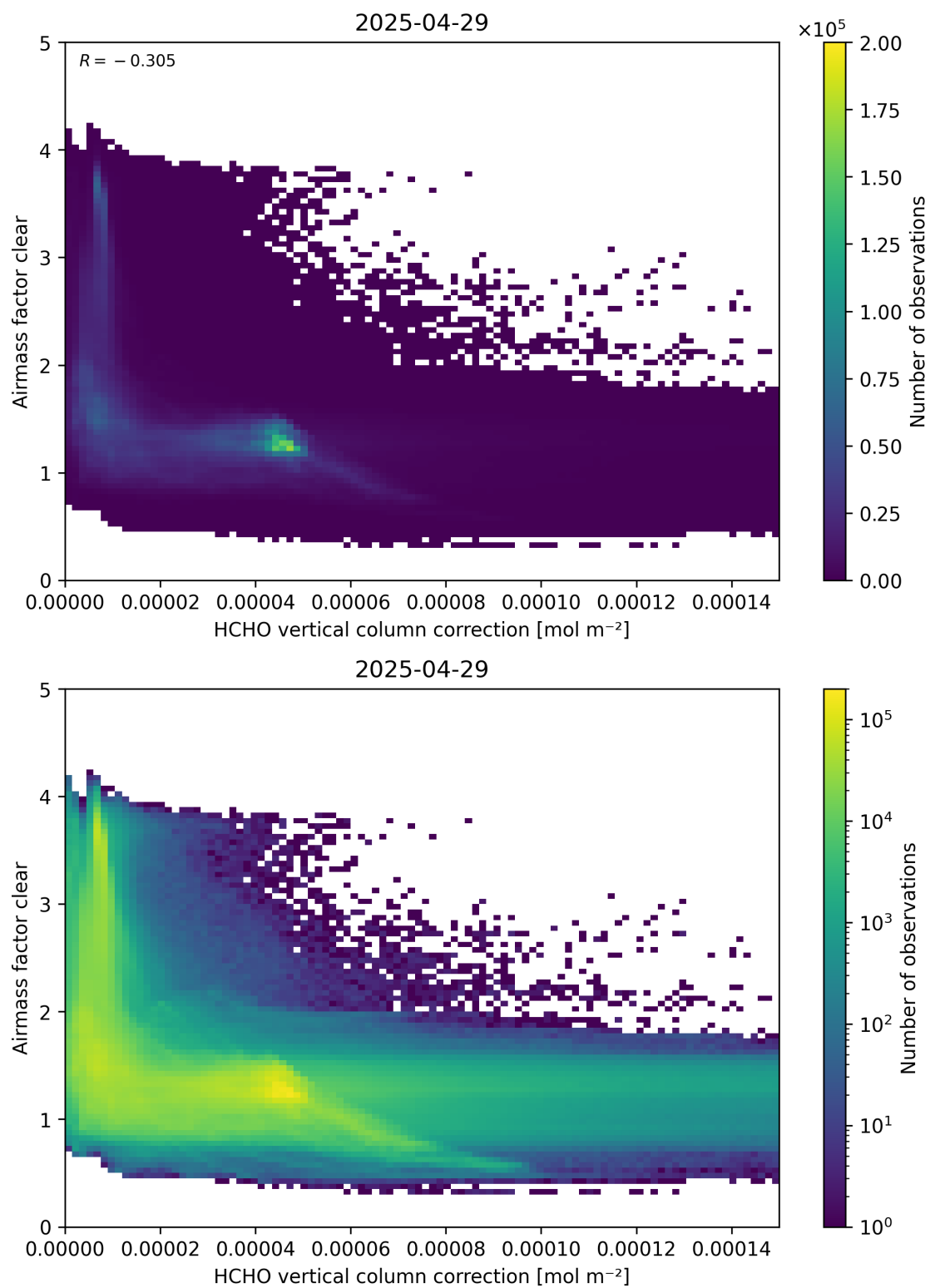
Figure 115: Scatter density plot of “HCHO vertical column correction” against “Airmass factor clear” for 2025-04-29 to 2025-04-30.
