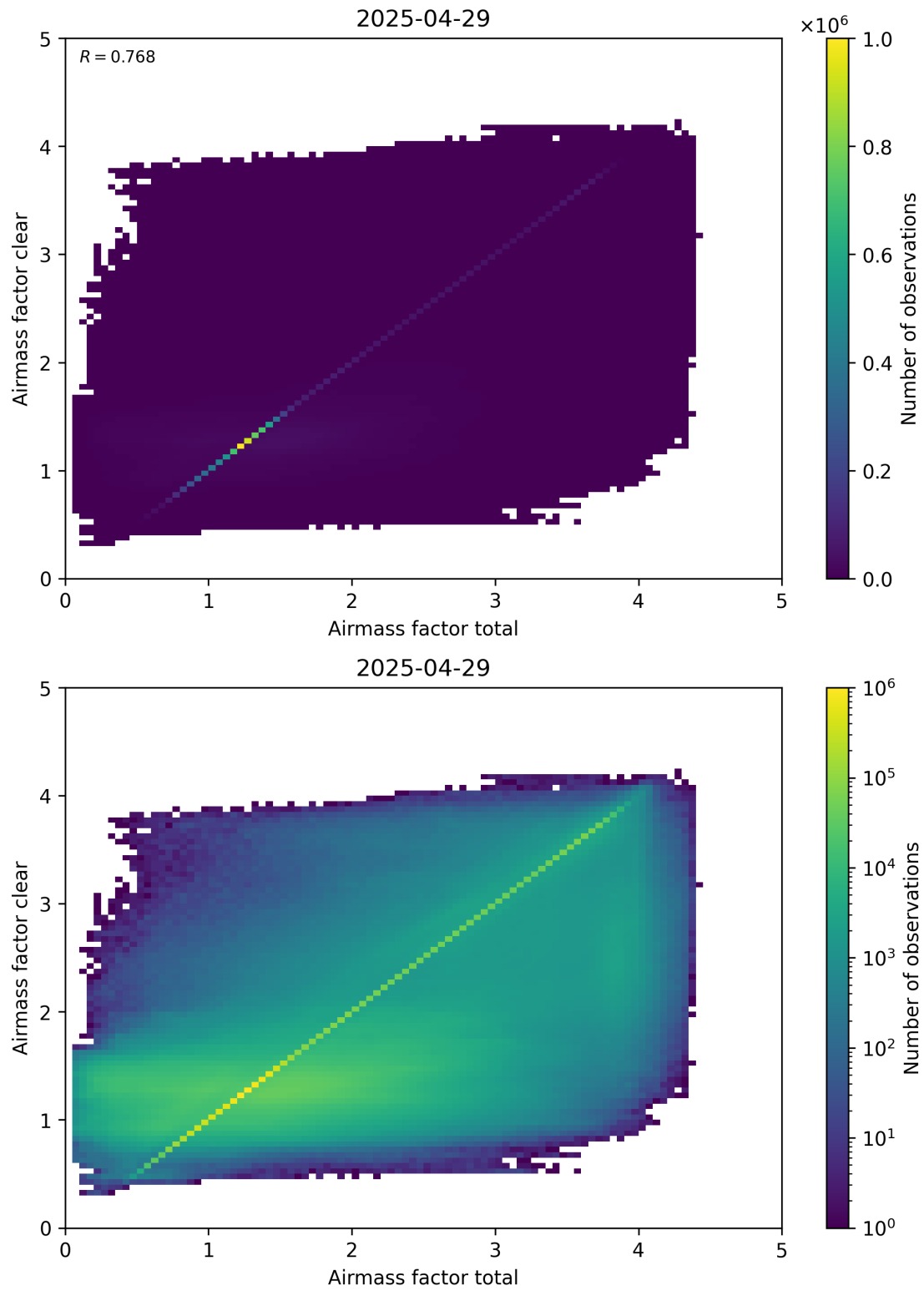
Figure 100: Scatter density plot of “Airmass factor total” against “Airmass factor clear” for 2025-04-29 to 2025-04-30.
