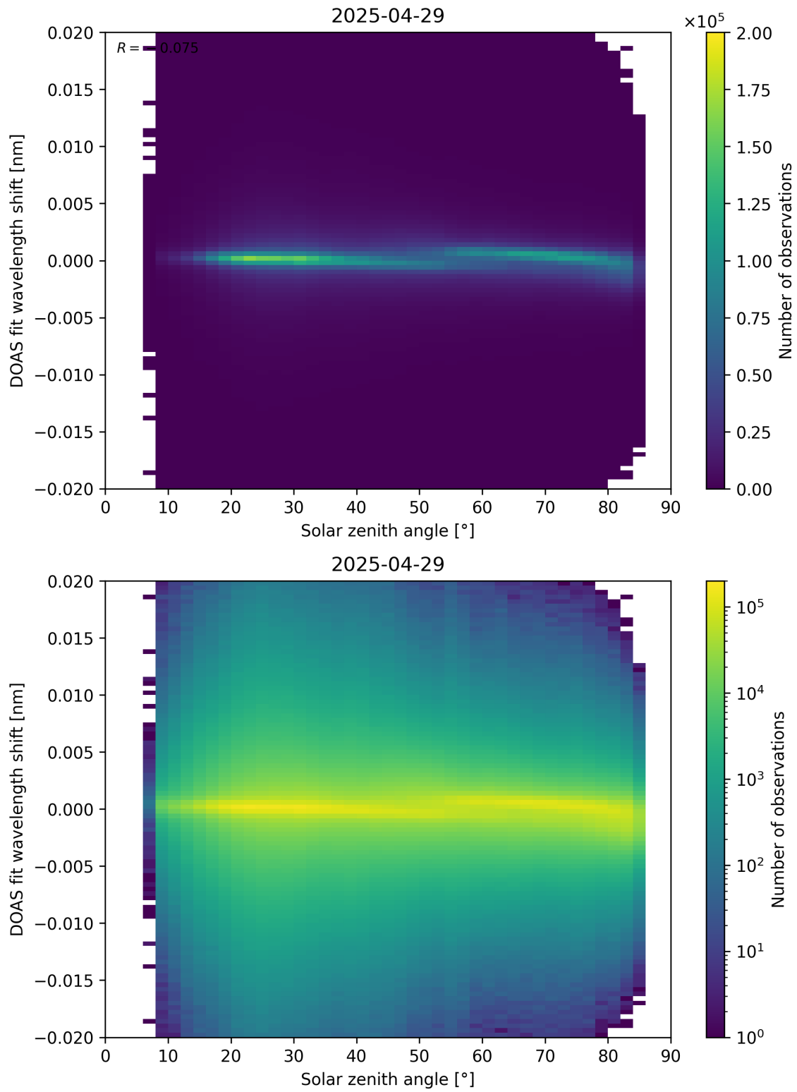
Figure 168: Scatter density plot of “Solar zenith angle” against “DOAS fit wavelength shift” for 2025-04-29 to 2025-04-30.
