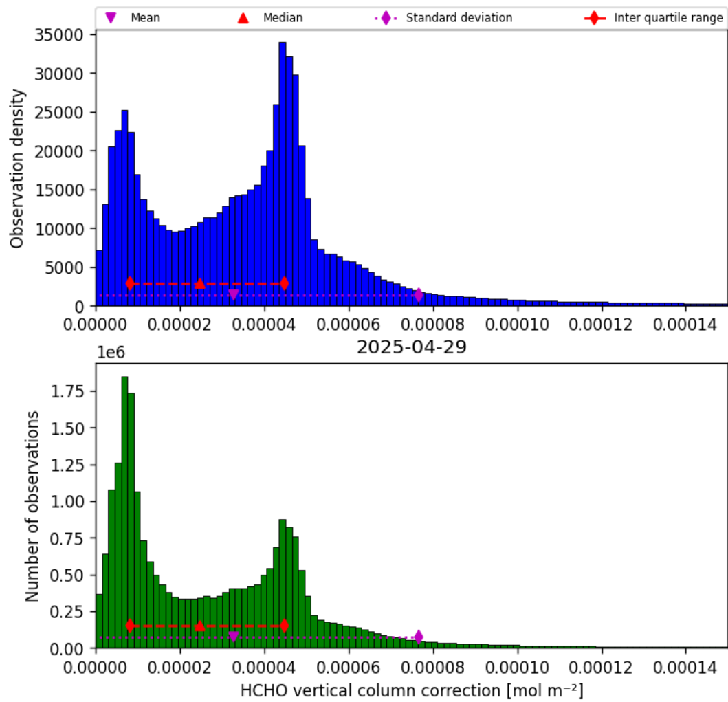
Figure 37: Histogram of “HCHO vertical column correction” for 2025-04-29 to 2025-04-30
