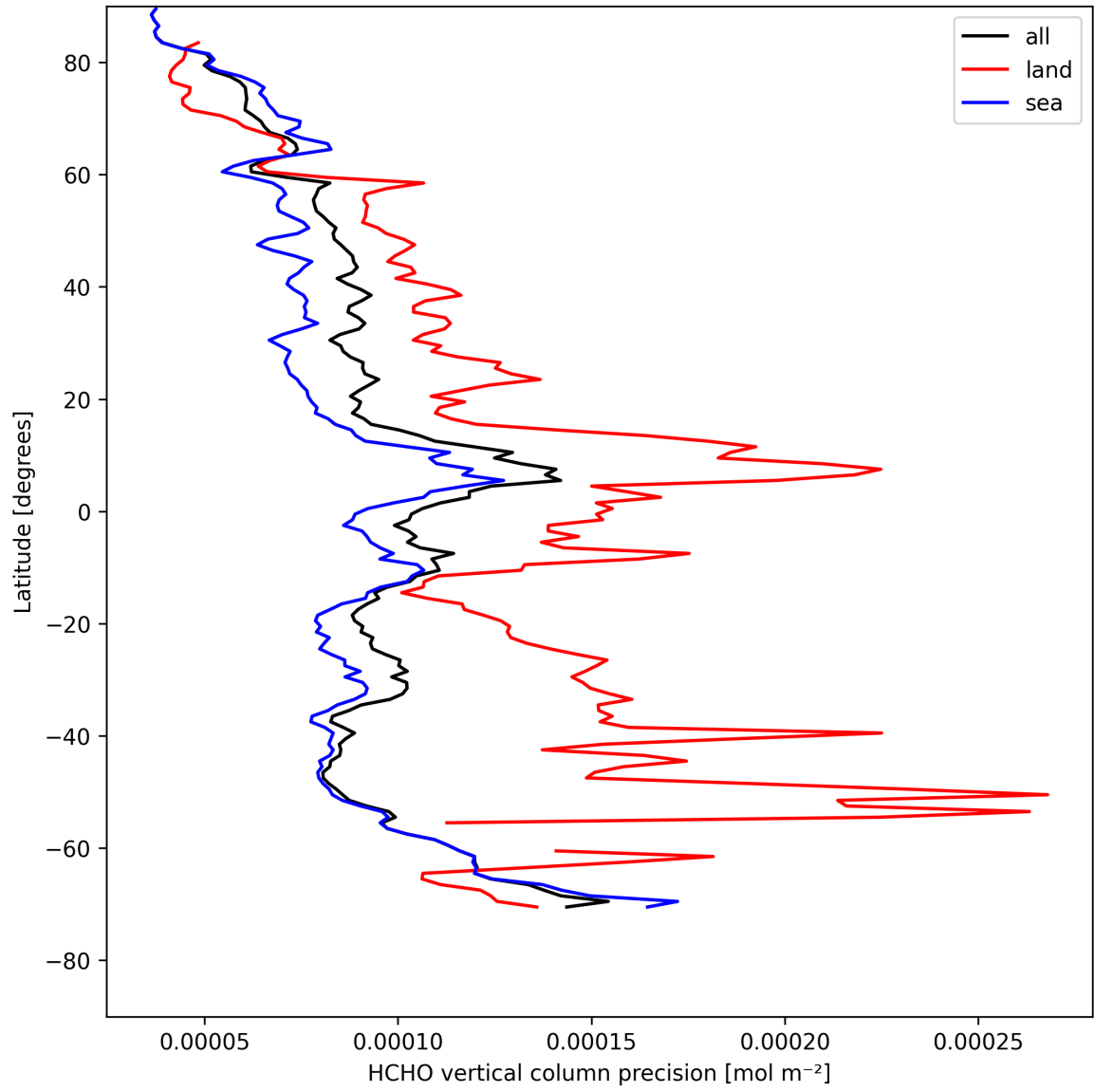
Figure 22: Zonal average of “HCHO vertical column precision” for 2025-04-29 to 2025-04-30.
