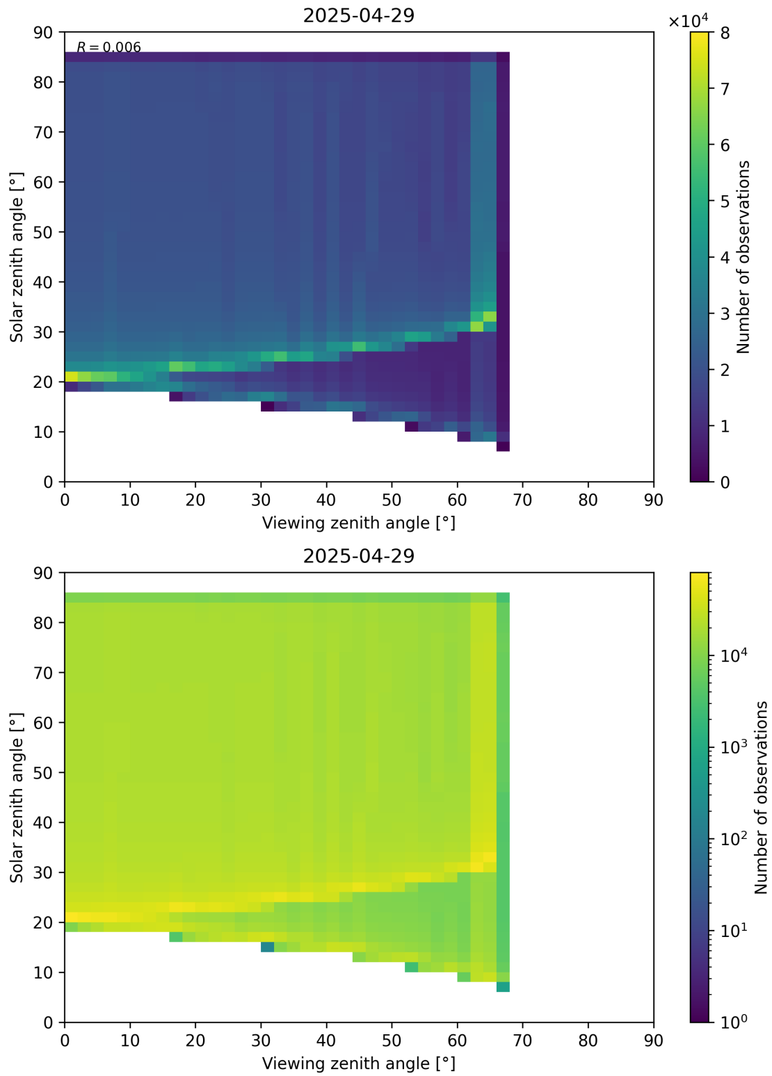
Figure 197: Scatter density plot of “Viewing zenith angle” against “Solar zenith angle” for 2025-04-29 to 2025-04-30.
