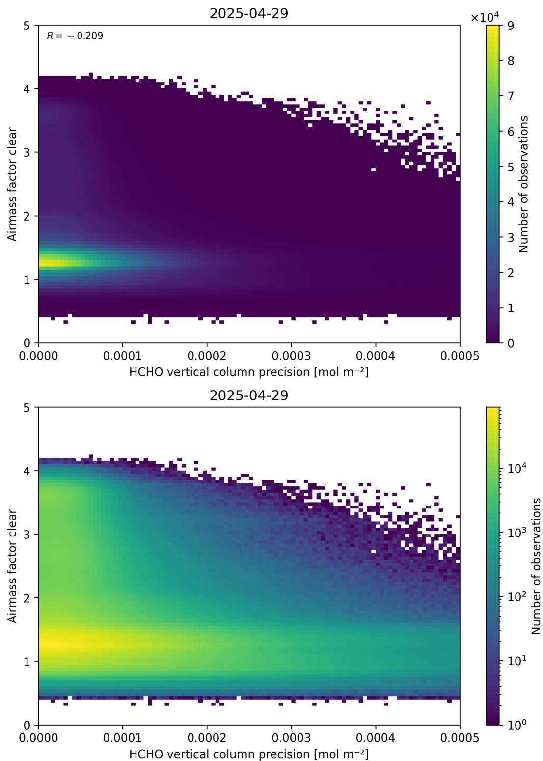
Figure 139: Scatter density plot of “HCHO vertical column precision” against “Airmass factor clear” for 2025-04-29 to 2025-04-30.
