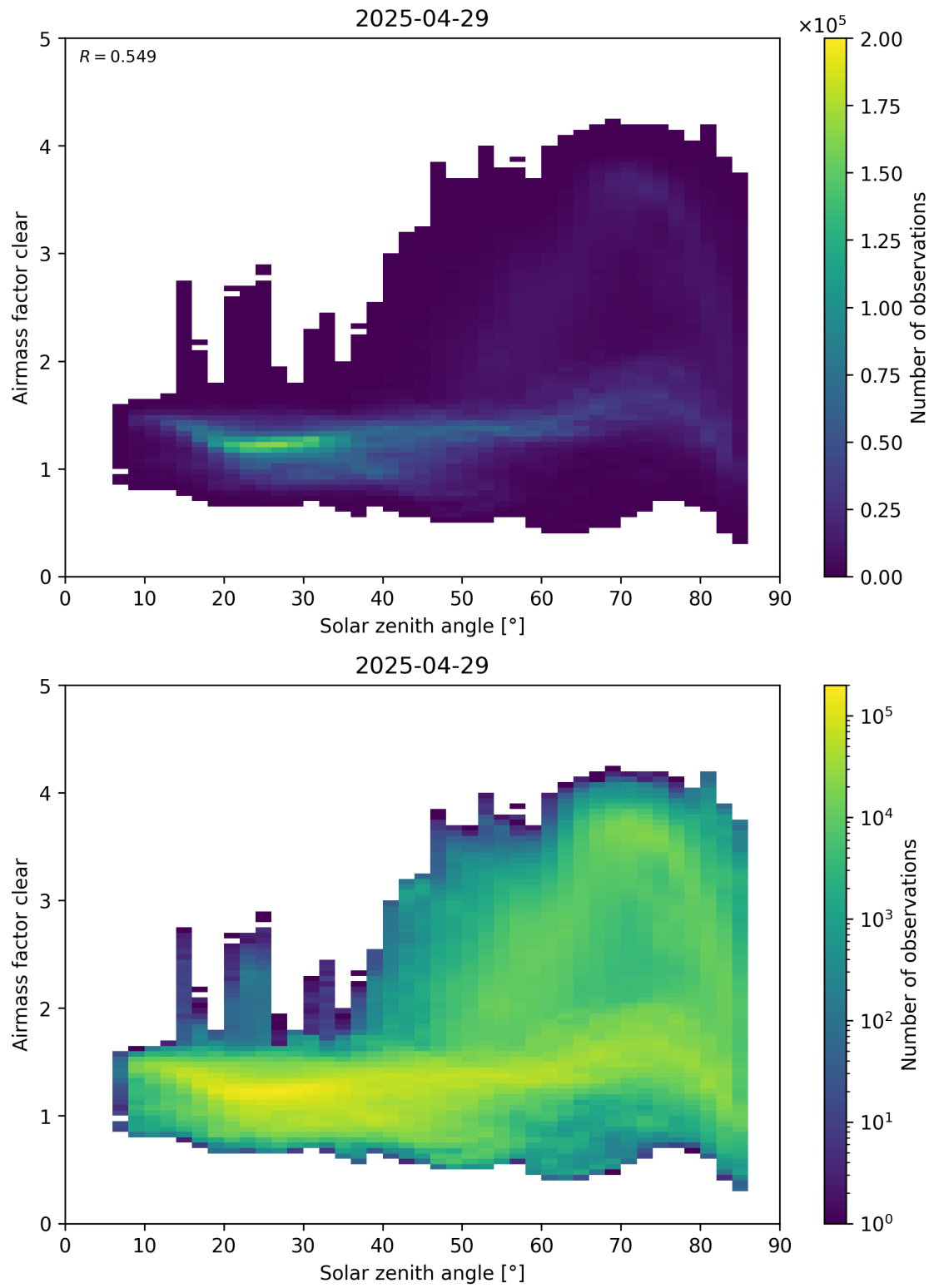
Figure 170: Scatter density plot of “Solar zenith angle” against “Airmass factor clear” for 2025-04-29 to 2025-04-30.
