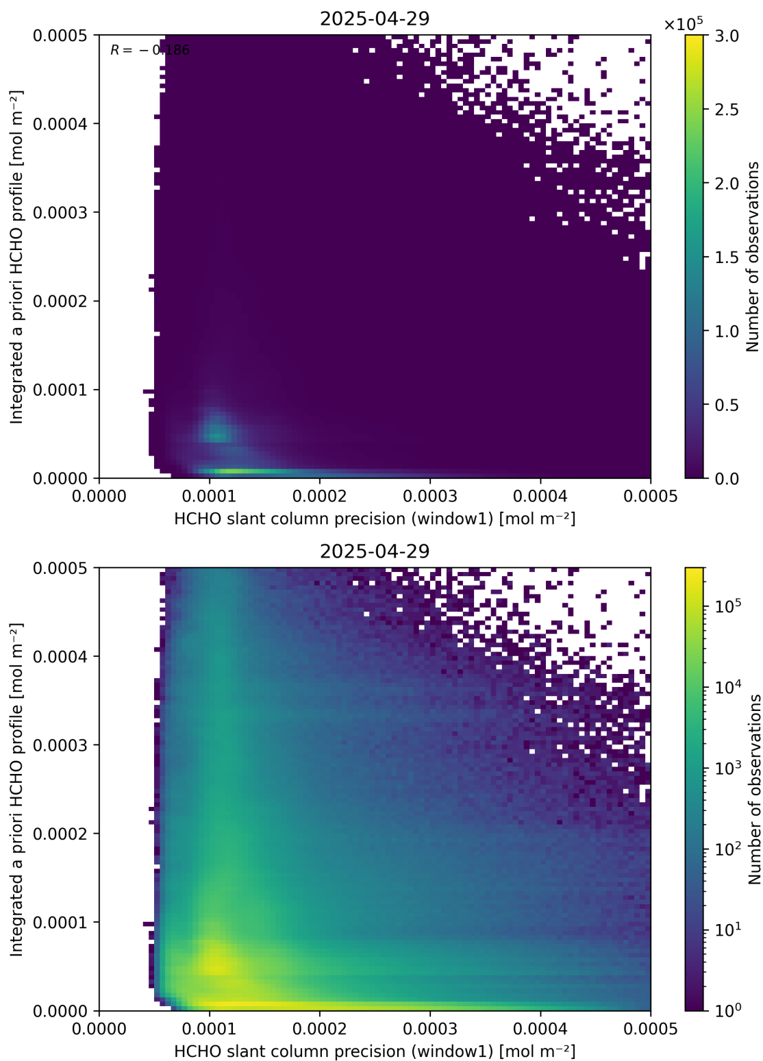
Figure 96: Scatter density plot of “HCHO slant column precision (window1)” against “Integrated a priori HCHO profile” for 2025-04-29 to 2025-04-30.
