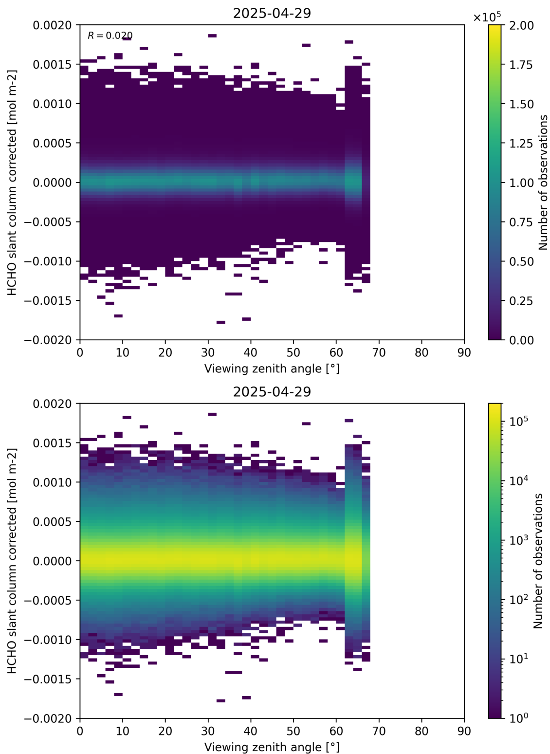
Figure 186: Scatter density plot of “Viewing zenith angle” against “HCHO slant column corrected” for 2025-04-29 to 2025-04-30.
