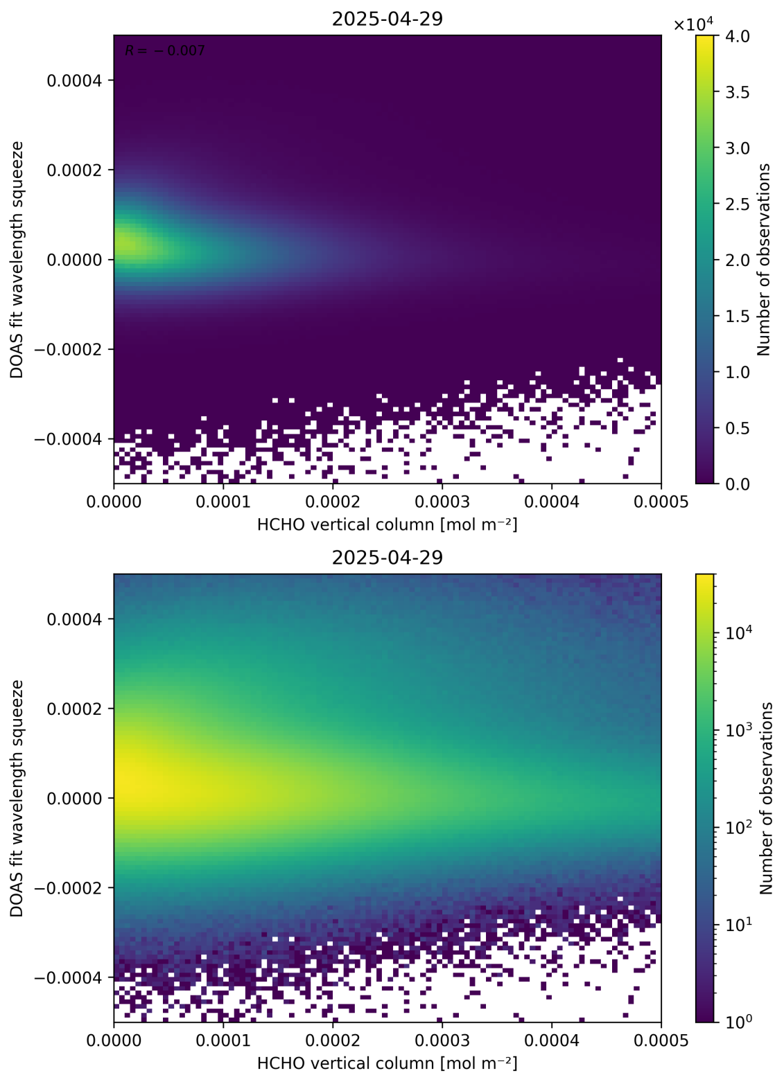
Figure 125: Scatter density plot of “HCHO vertical column” against “DOAS fit wavelength squeeze” for 2025-04-29 to 2025-04-30.
