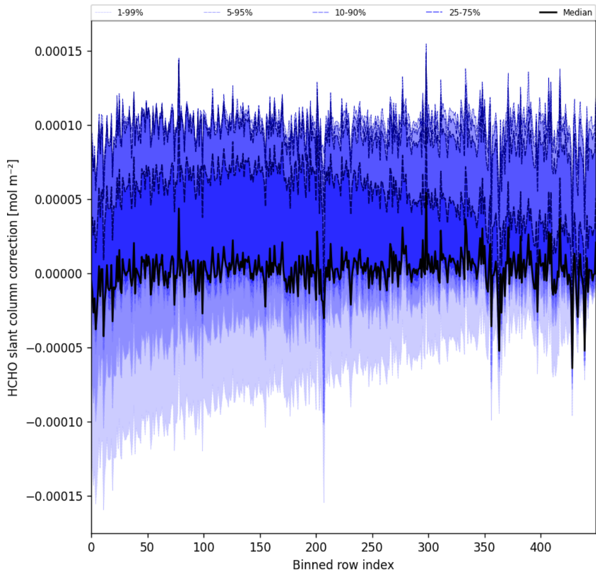
Figure 61: Along track statistics of “HCHO slant column correction” for 2025-04-29 to 2025-04-30
