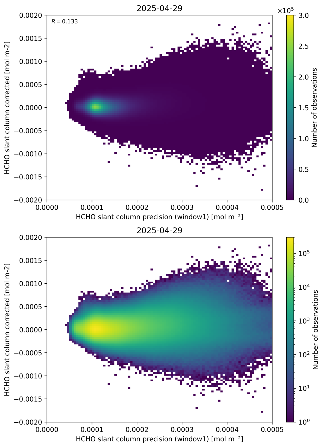
Figure 92: Scatter density plot of “HCHO slant column precision (window1)” against “HCHO slant column corrected” for 2025-04-29 to 2025-04-30.
