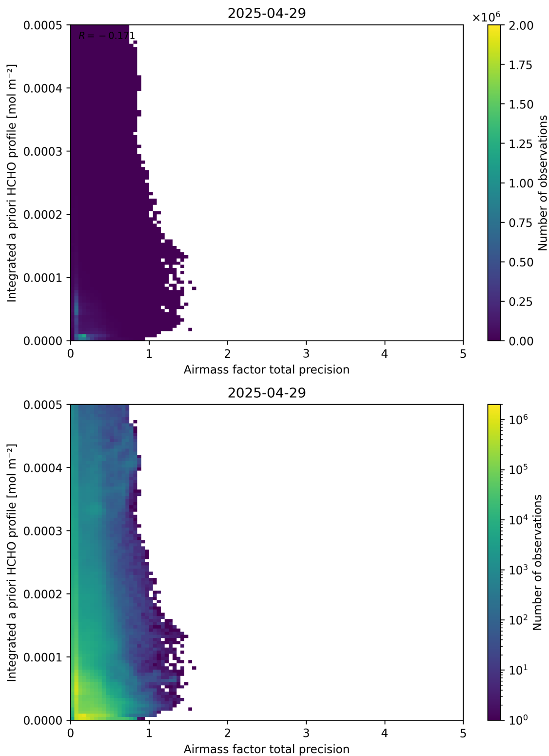
Figure 111: Scatter density plot of “Airmass factor total precision” against “Integrated a priori HCHO profile” for 2025-04-29 to 2025-04-30.
