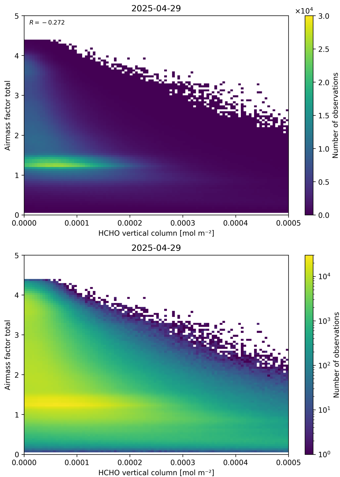
Figure 131: Scatter density plot of “HCHO vertical column” against “Airmass factor total” for 2025-04-29 to 2025-04-30.
