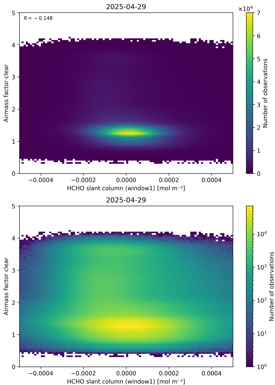
Figure 81: Scatter density plot of “HCHO slant column (window1)” against “Airmass factor clear” for 2025-04-29 to 2025-04-30.
