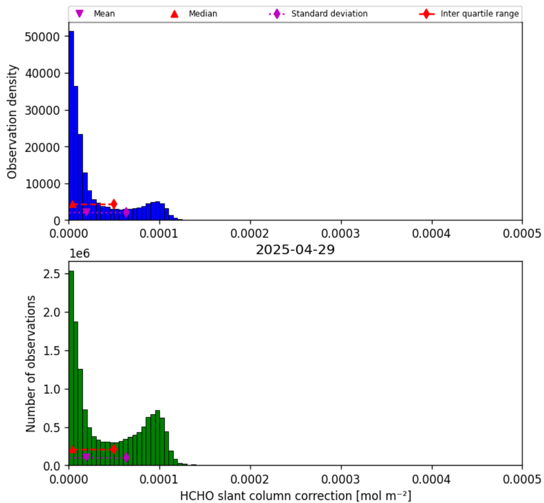
Figure 47: Histogram of “HCHO slant column correction” for 2025-04-29 to 2025-04-30
