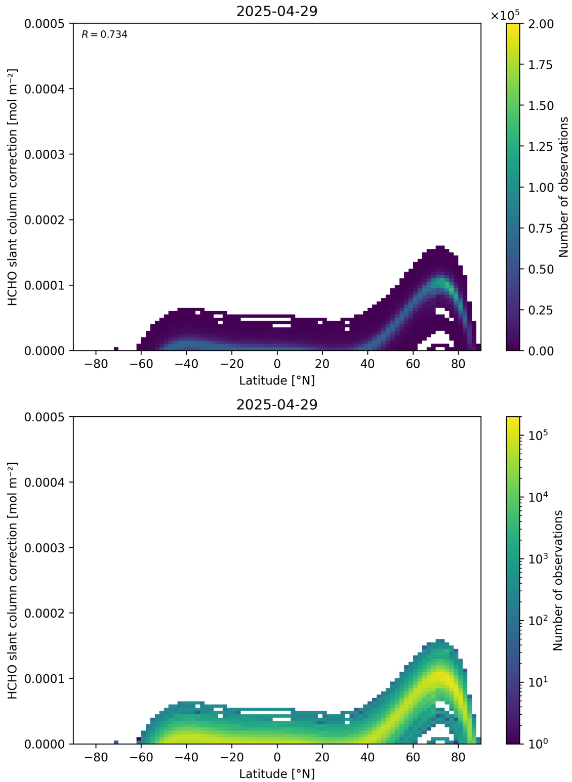
Figure 158: Scatter density plot of “Latitude” against “HCHO slant column correction” for 2025-04-29 to 2025-04-30.
