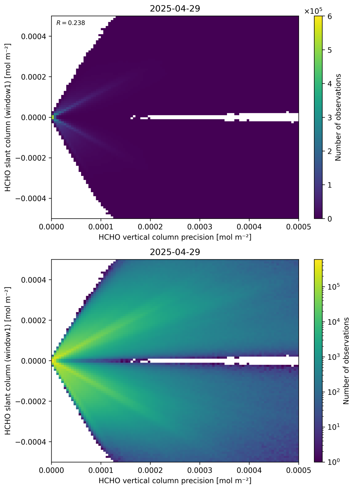
Figure 142: Scatter density plot of “HCHO vertical column precision” against “HCHO slant column (window1)” for 2025-04-29 to 2025-04-30.
