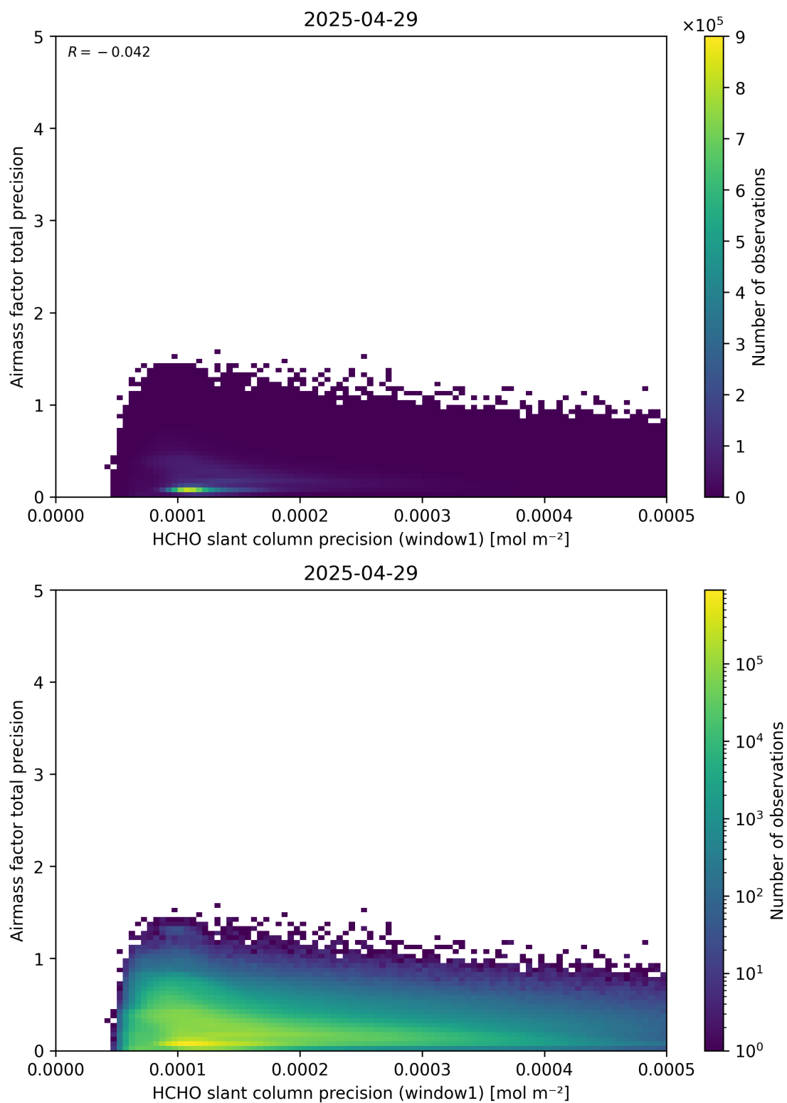
Figure 95: Scatter density plot of “HCHO slant column precision (window1)” against “Airmass factor total precision” for 2025-04-29 to 2025-04-30.
