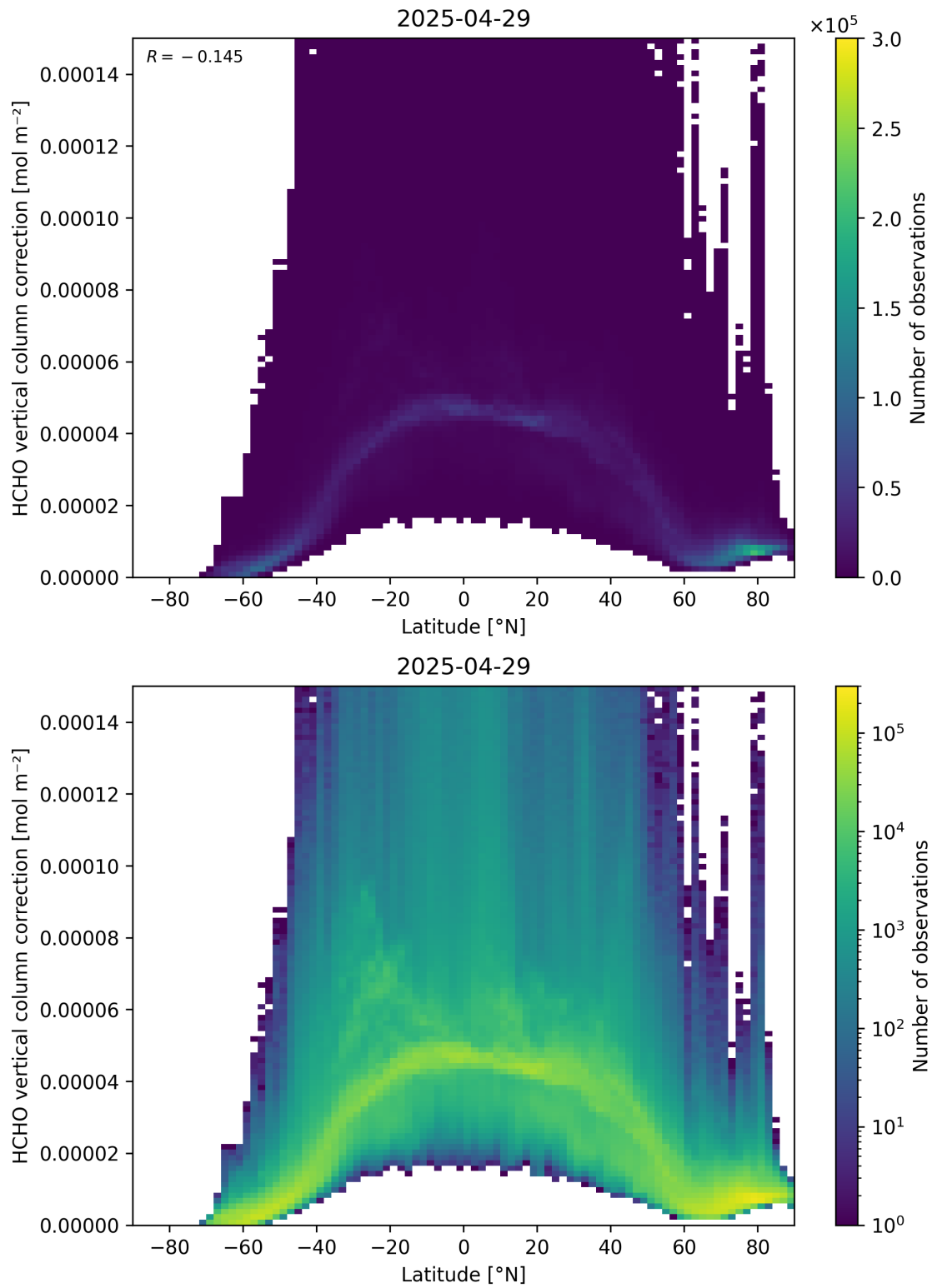
Figure 164: Scatter density plot of “Latitude” against “HCHO vertical column correction” for 2025-04-29 to 2025-04-30.
