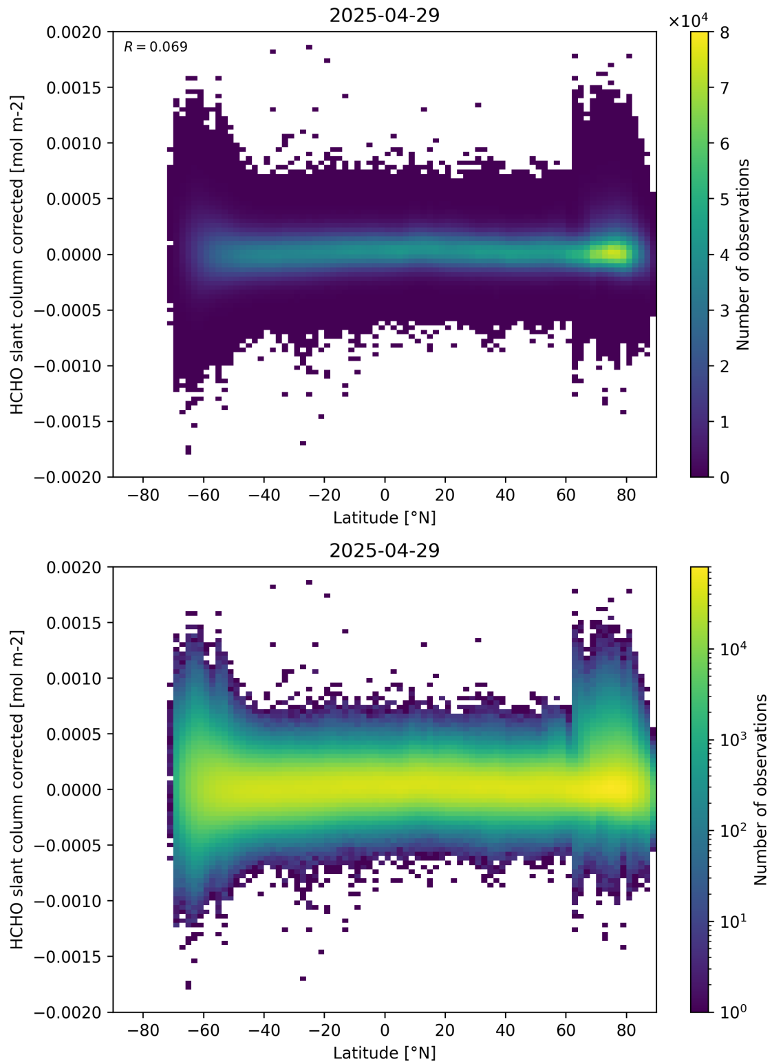
Figure 157: Scatter density plot of “Latitude” against “HCHO slant column corrected” for 2025-04-29 to 2025-04-30.
