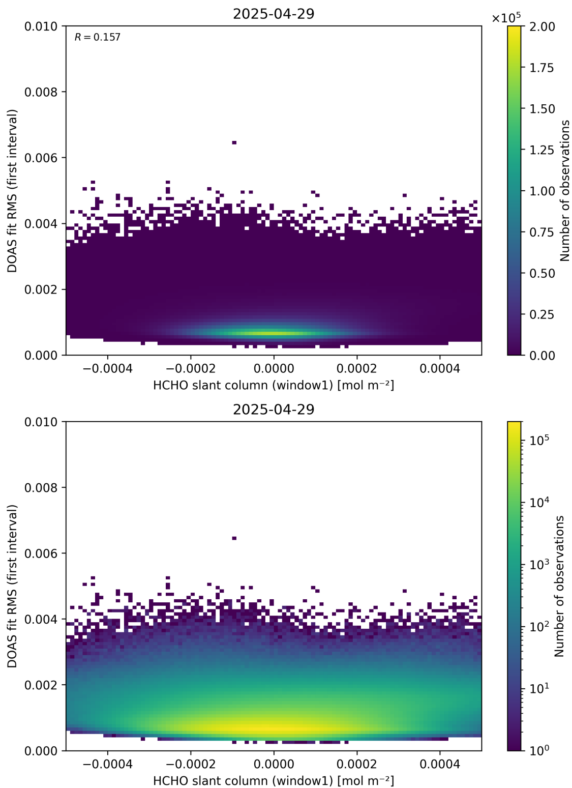
Figure 78: Scatter density plot of “HCHO slant column (window1)” against “DOAS fit RMS (first interval)” for 2025-04-29 to 2025-04-30.
