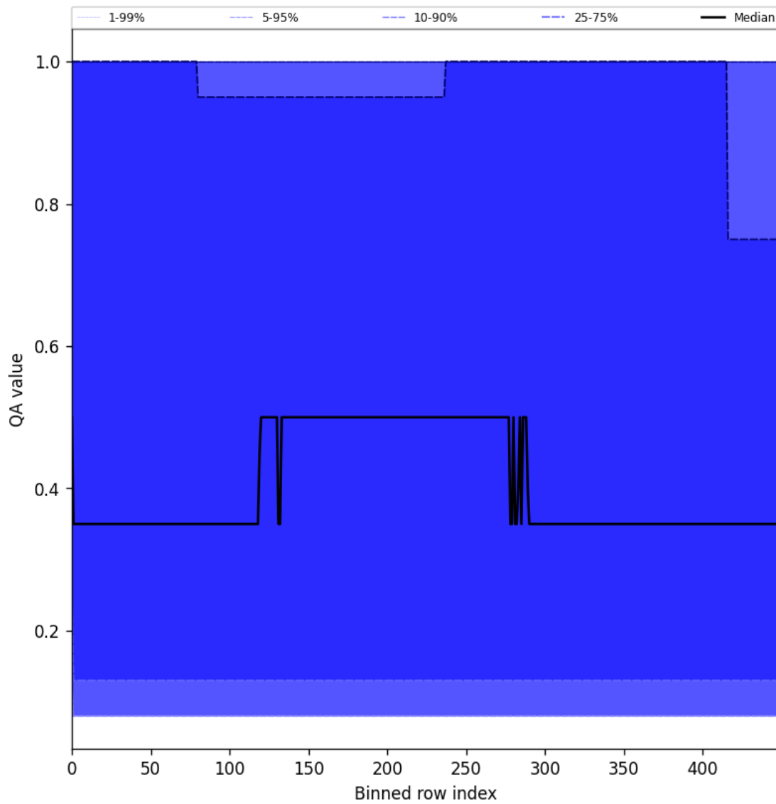
Figure 48: Along track statistics of “QA value” for 2025-04-29 to 2025-04-30
