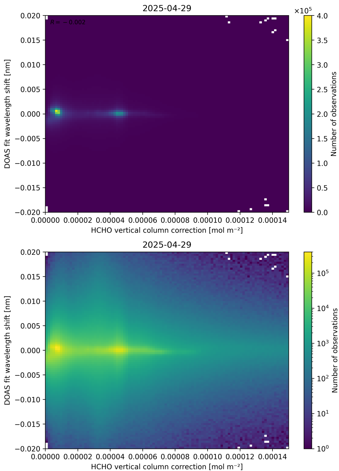
Figure 113: Scatter density plot of “HCHO vertical column correction” against “DOAS fit wavelength shift” for 2025-04-29 to 2025-04-30.
