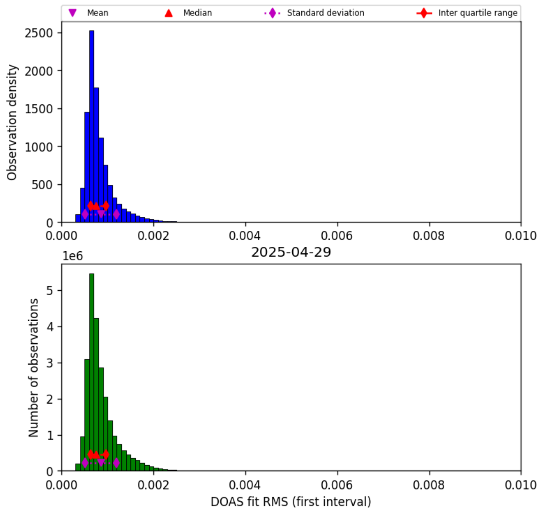
Figure 46: Histogram of “DOAS fit RMS (first interval)” for 2025-04-29 to 2025-04-30
