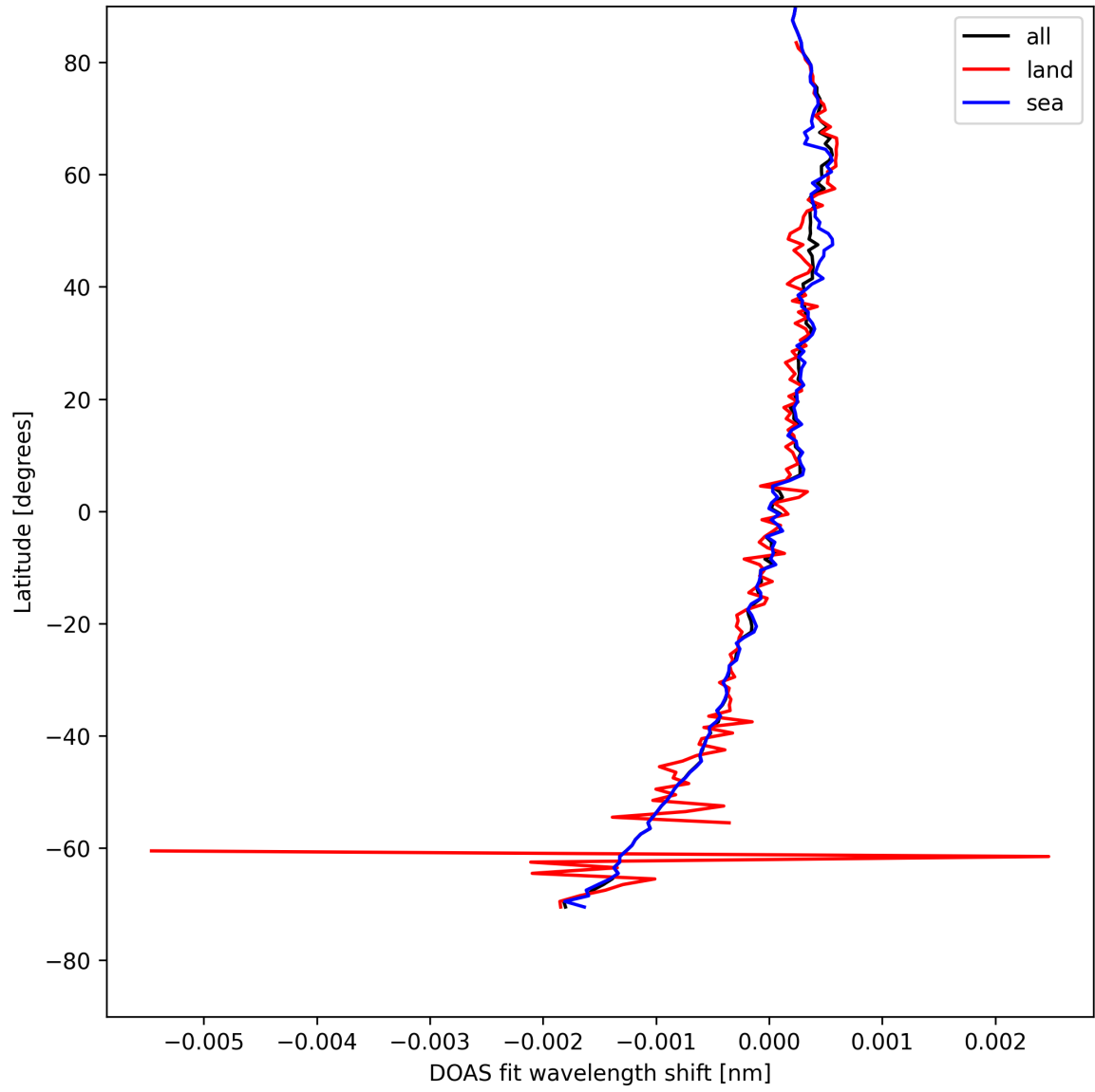
Figure 30: Zonal average of "DOAS fit wavelength shift" for 2025-04-29 to 2025-04-30.
