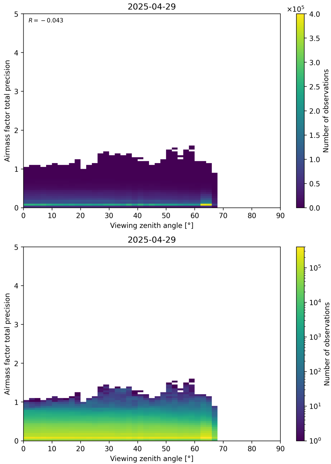
Figure 191: Scatter density plot of “Viewing zenith angle” against “Airmass factor total precision” for 2025-04-29 to 2025-04-30.
