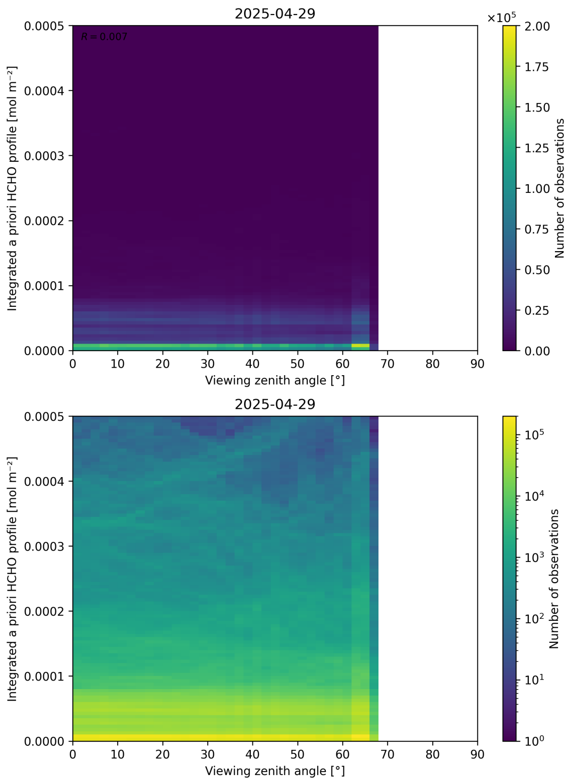
Figure 195: Scatter density plot of “Viewing zenith angle” against “Integrated a priori HCHO profile” for 2025-04-29 to 2025-04-30.
