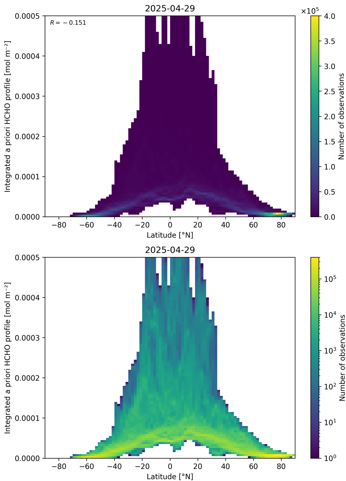
Figure 166: Scatter density plot of “Latitude” against “Integrated a priori HCHO profile” for 2025-04-29 to 2025-04-30.
