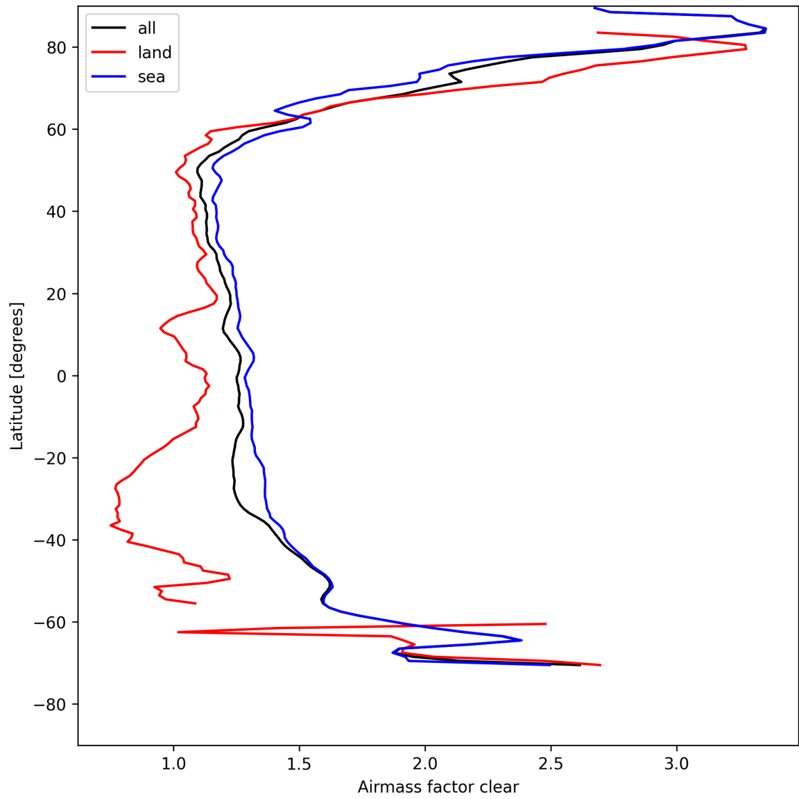
Figure 28: Zonal average of “Airmass factor clear” for 2025-04-29 to 2025-04-30.
