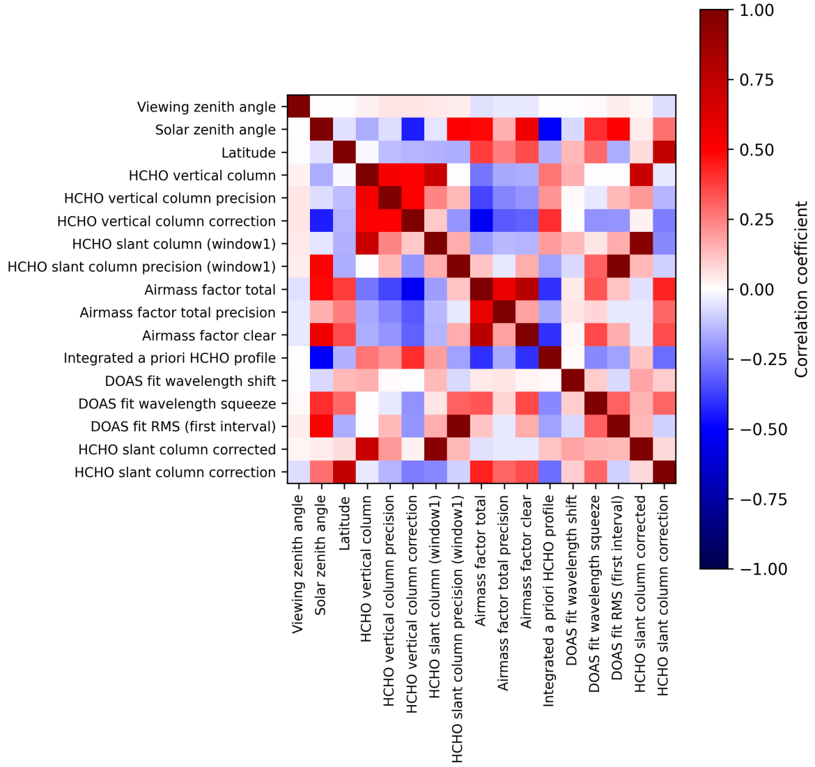
Figure 2: Map of correlation matrix for 2025-04-29 to 2025-04-30.
