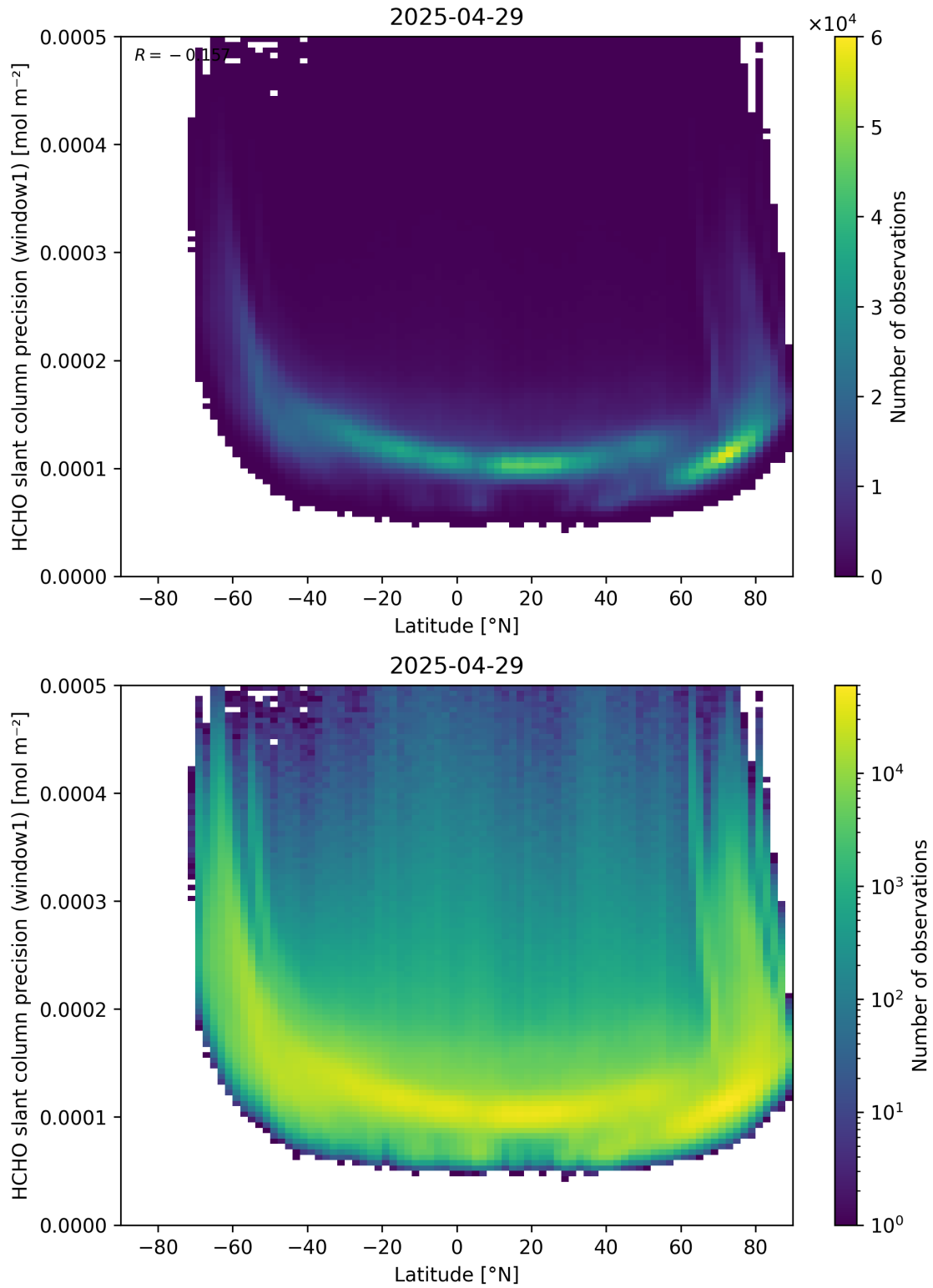
Figure 160: Scatter density plot of “Latitude” against “HCHO slant column precision (window1)” for 2025-04-29 to 2025-04-30.
