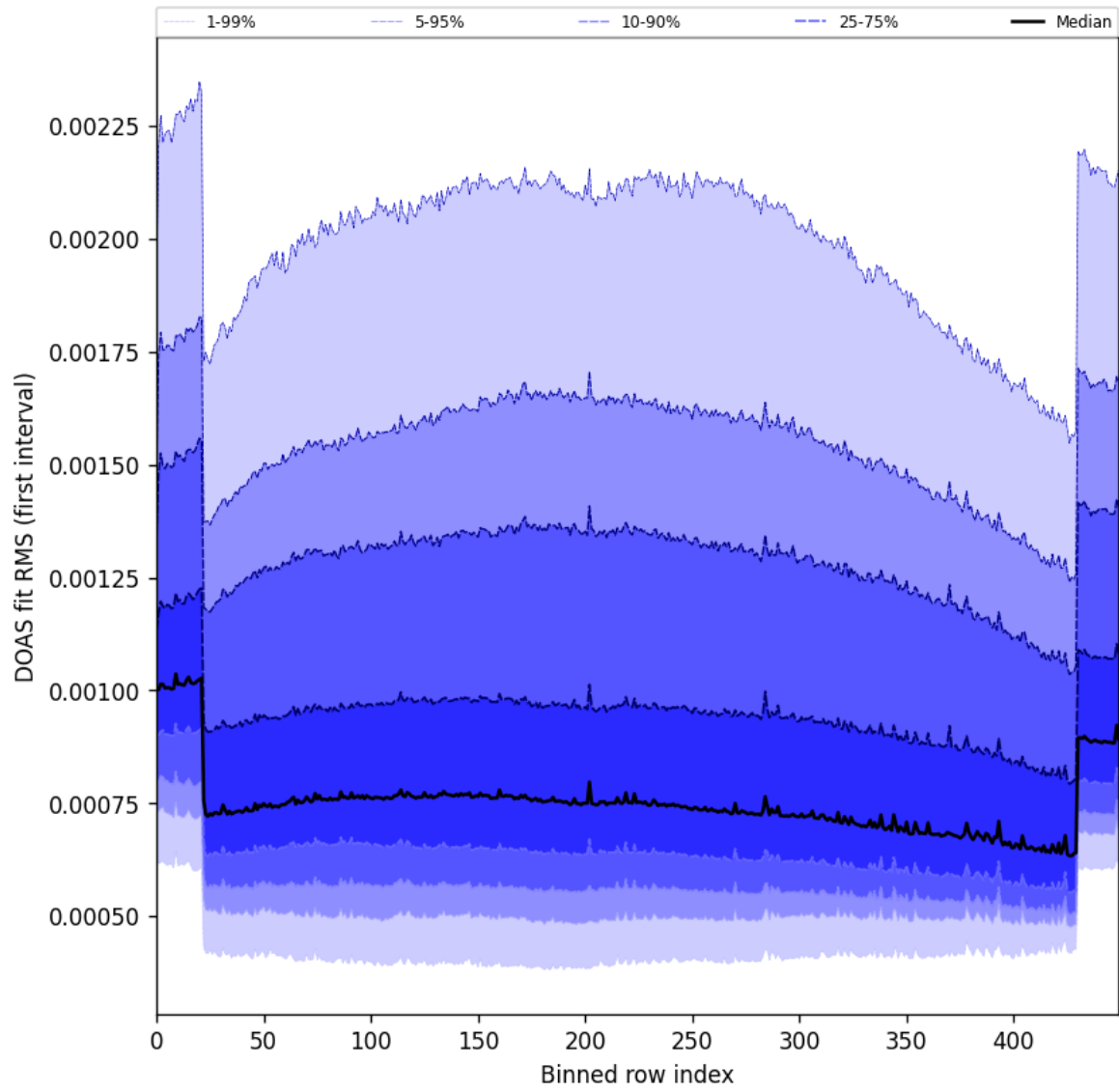
Figure 60: Along track statistics of “DOAS fit RMS (first interval)” for 2025-04-29 to 2025-04-30
