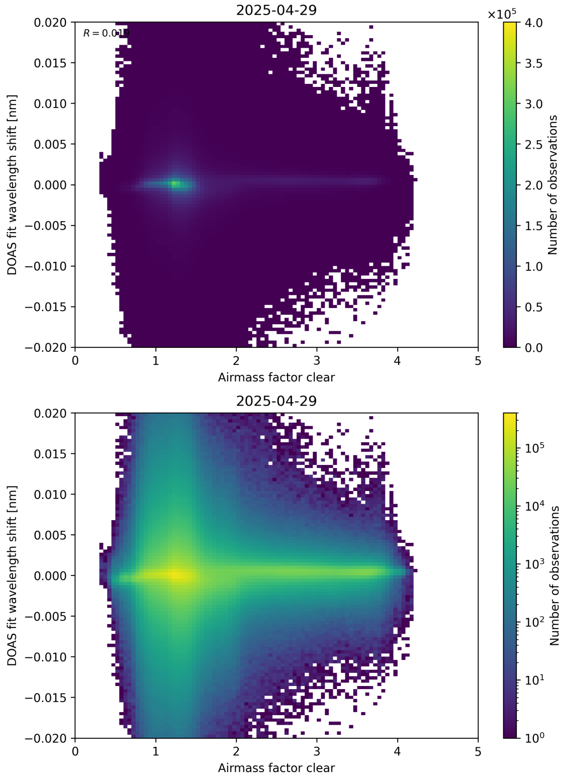
Figure 72: Scatter density plot of “Airmass factor clear” against “DOAS fit wavelength shift” for 2025-04-29 to 2025-04-30.
