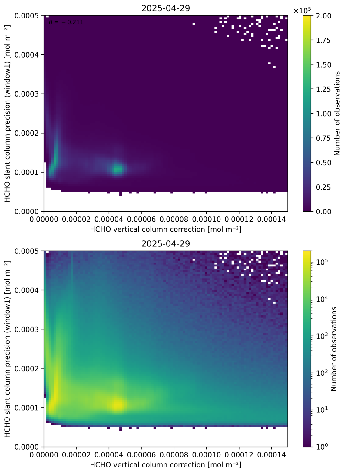
Figure 119: Scatter density plot of “HCHO vertical column correction” against “HCHO slant column precision (window1)” for 2025-04-29 to 2025-04-30.
