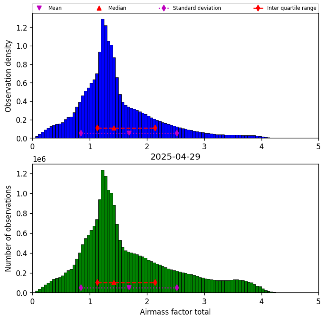
Figure 40: Histogram of “Airmass factor total” for 2025-04-29 to 2025-04-30
