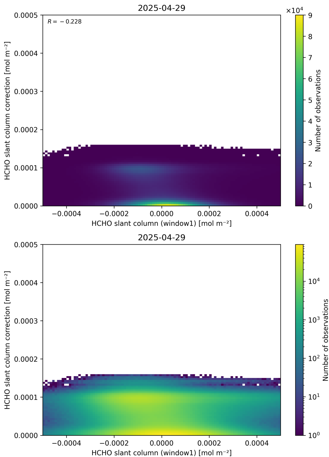
Figure 83: Scatter density plot of “HCHO slant column (window1)” against “HCHO slant column correction” for 2025-04-29 to 2025-04-30.
