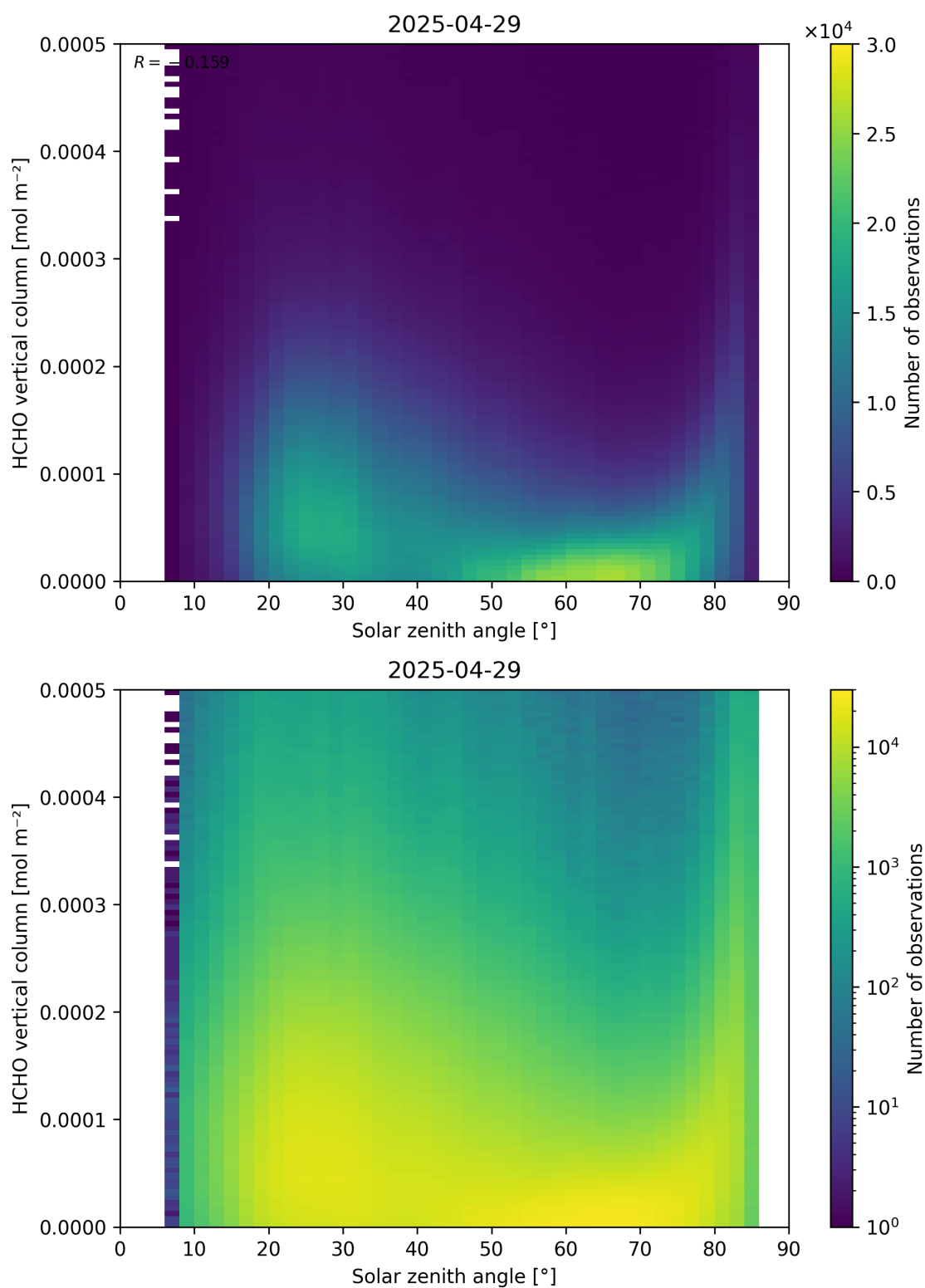
Figure 177: Scatter density plot of “Solar zenith angle” against “HCHO vertical column” for 2025-04-29 to 2025-04-30.
