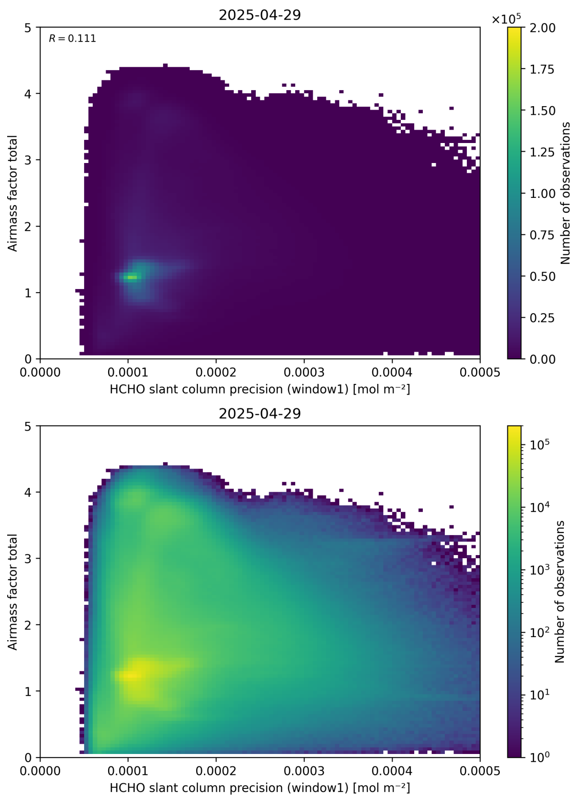
Figure 94: Scatter density plot of “HCHO slant column precision (window1)” against “Airmass factor total” for 2025-04-29 to 2025-04-30.
