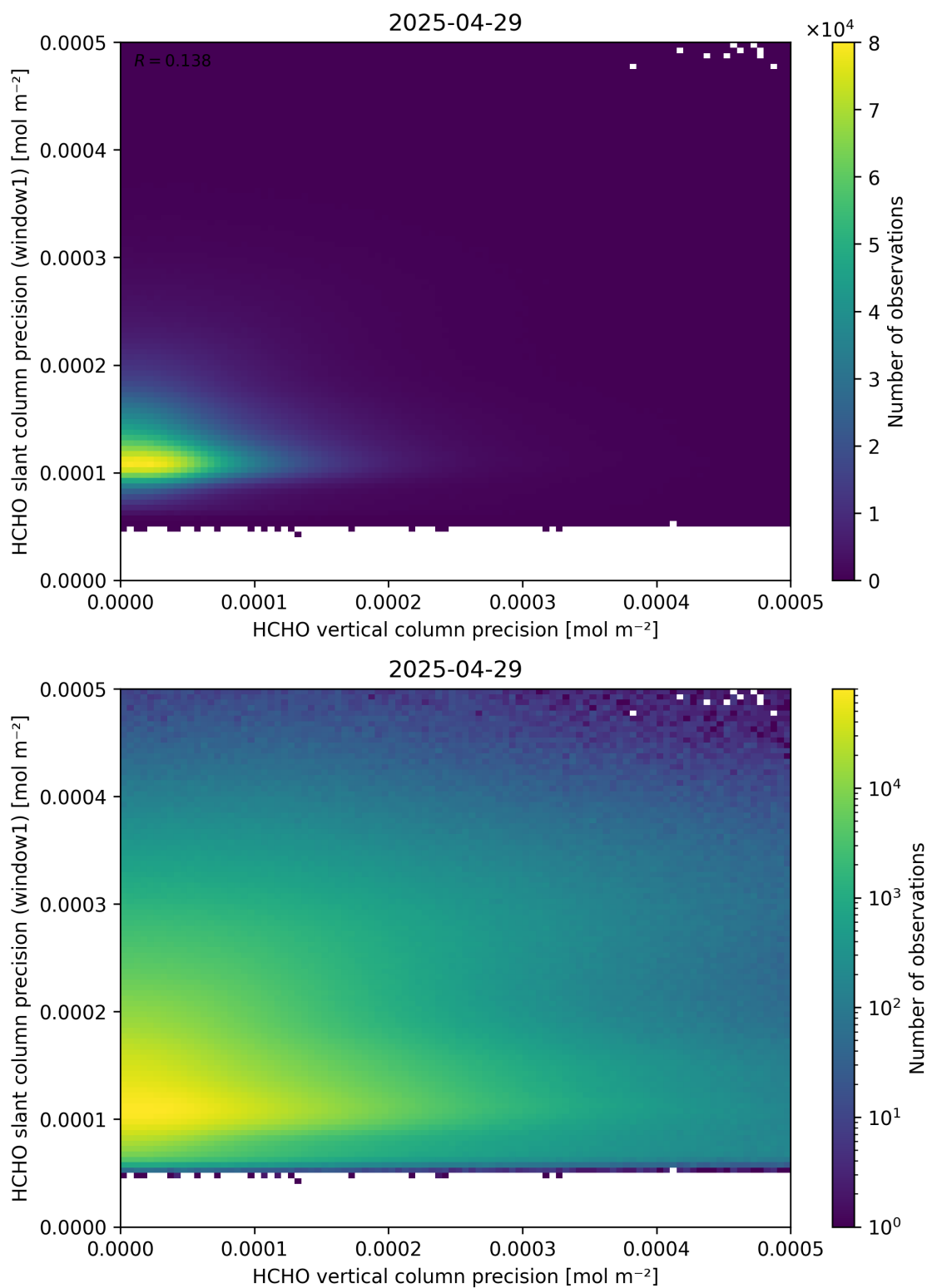
Figure 143: Scatter density plot of “HCHO vertical column precision” against “HCHO slant column precision (window1)” for 2025-04-29 to 2025-04-30.
