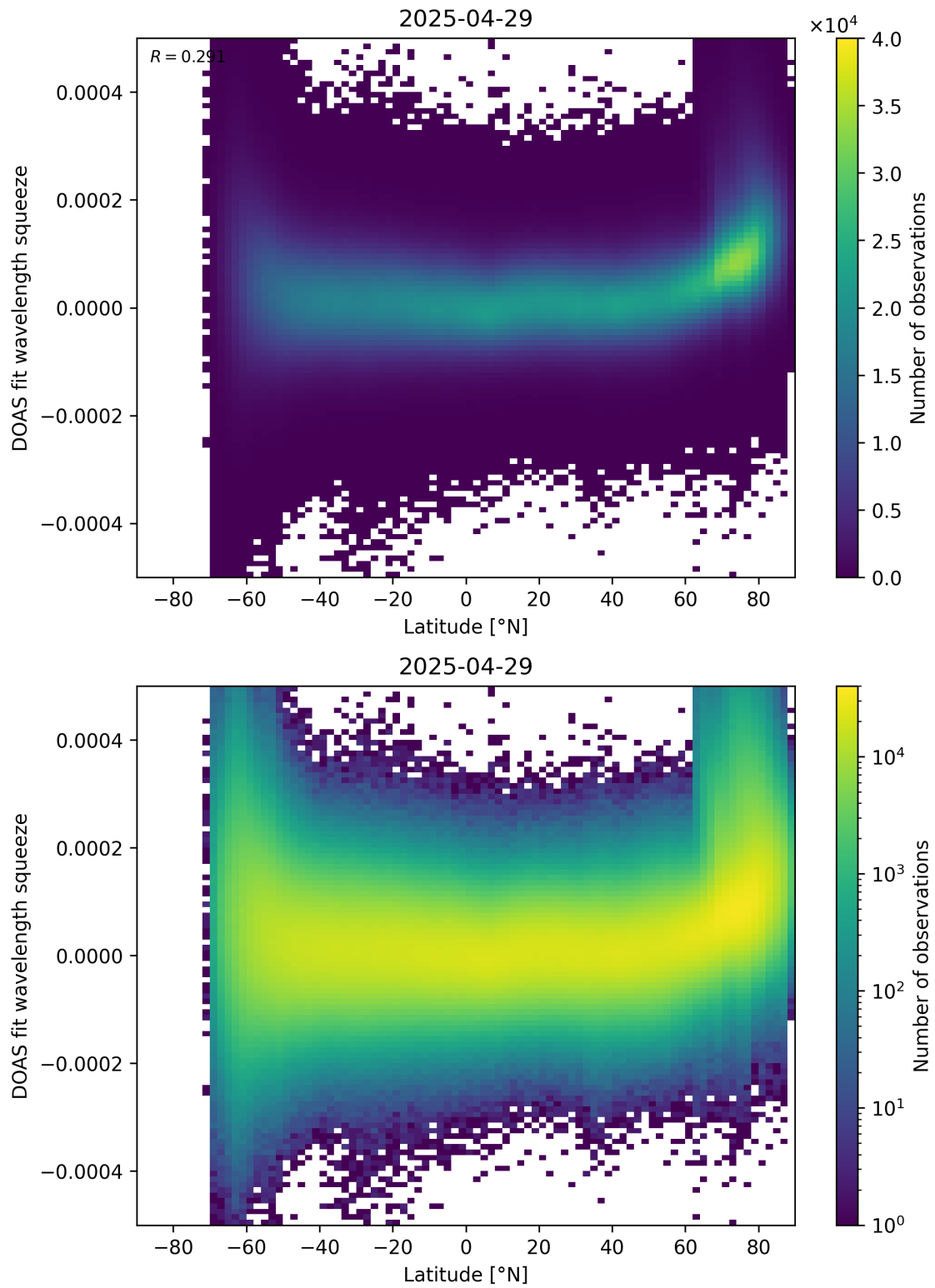
Figure 155: Scatter density plot of “Latitude” against “DOAS fit wavelength squeeze” for 2025-04-29 to 2025-04-30.
