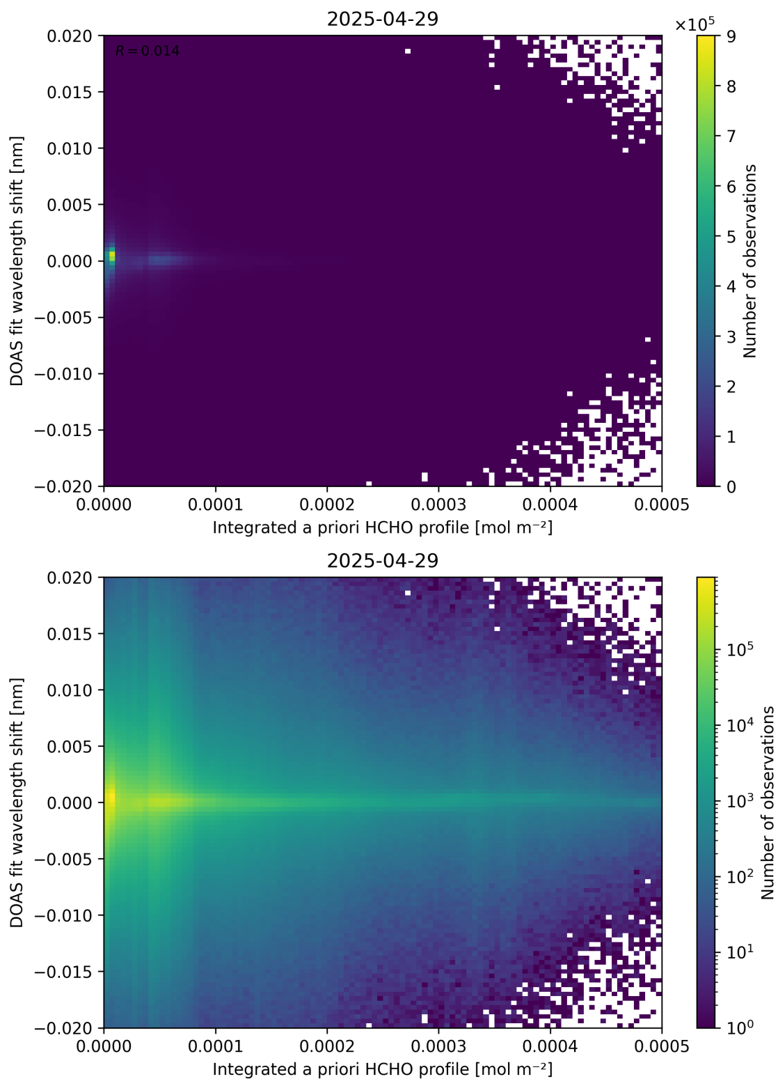
Figure 149: Scatter density plot of “Integrated a priori HCHO profile” against “DOAS fit wavelength shift” for 2025-04-29 to 2025-04-30.
