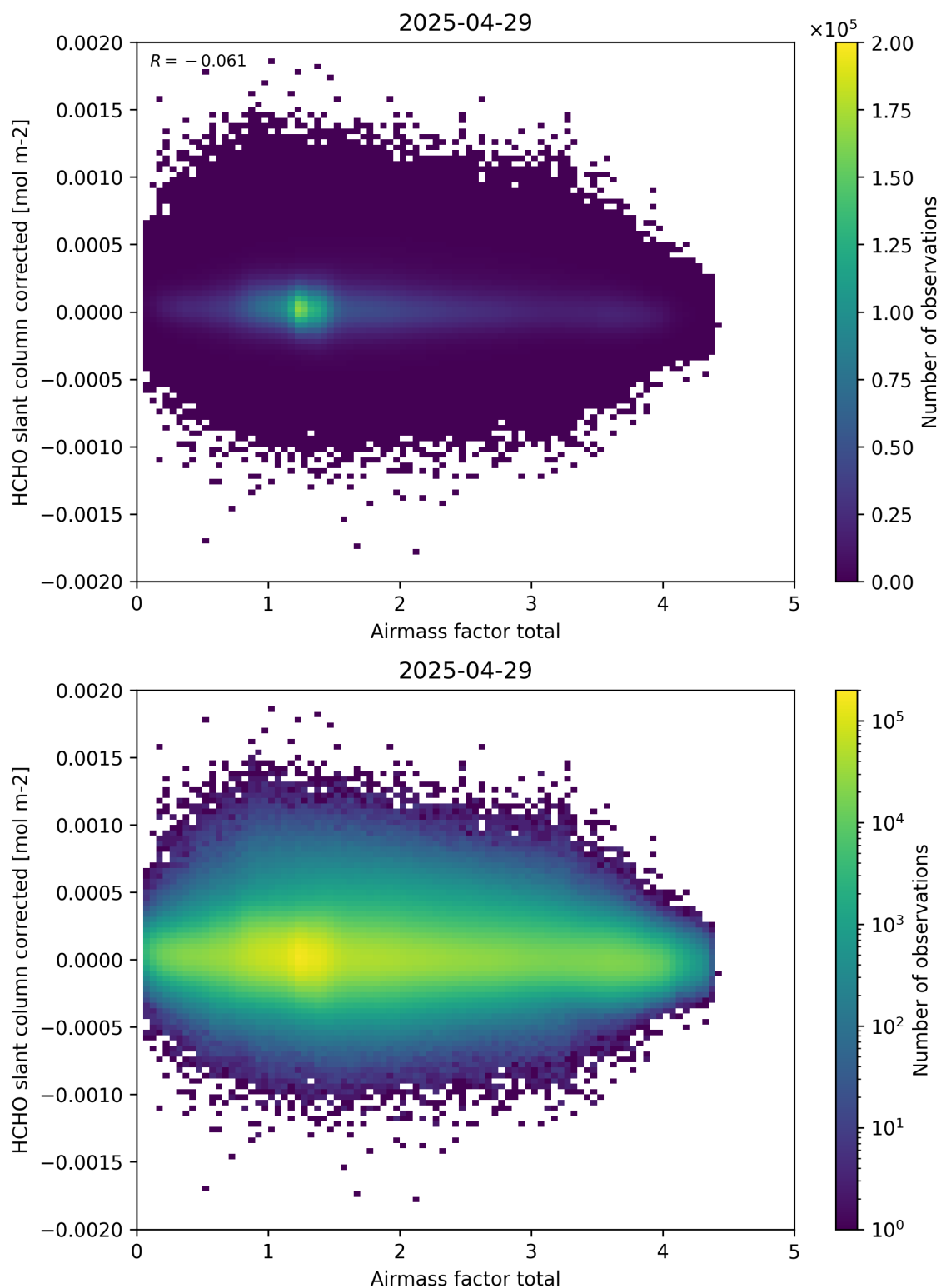
Figure 101: Scatter density plot of “Airmass factor total” against “HCHO slant column corrected” for 2025-04-29 to 2025-04-30.
