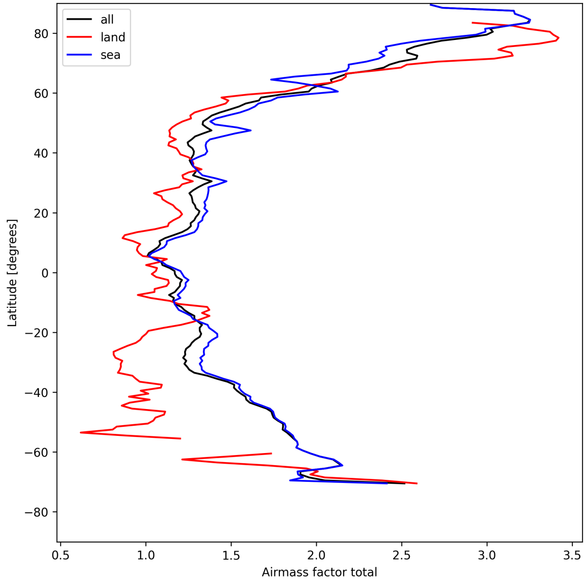
Figure 26: Zonal average of “Airmass factor total” for 2025-04-29 to 2025-04-30.
