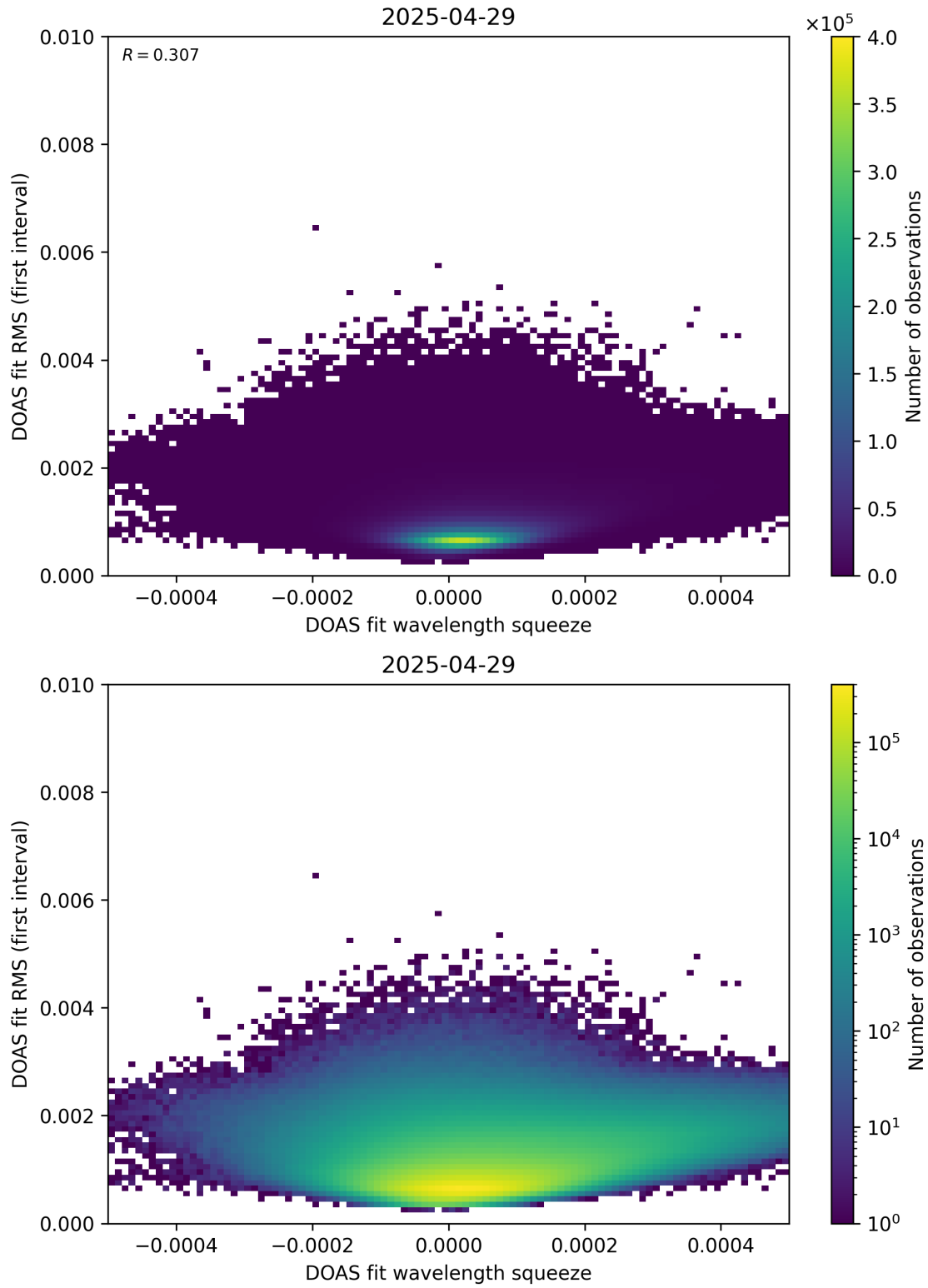
Figure 68: Scatter density plot of “DOAS fit wavelength squeeze” against “DOAS fit RMS (first interval)” for 2025-04-29 to 2025-04-30.
