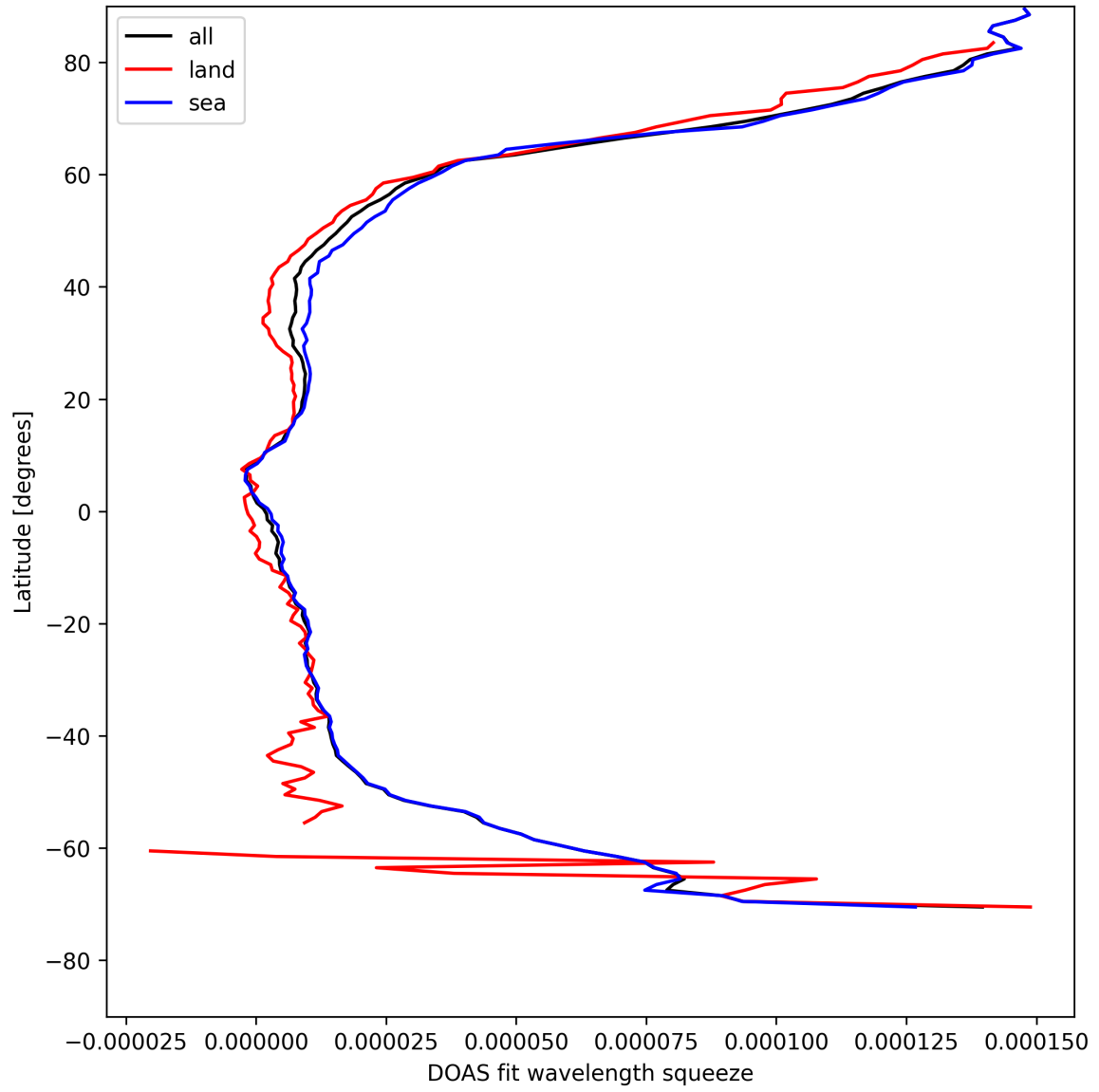
Figure 31: Zonal average of “DOAS fit wavelength squeeze” for 2025-04-29 to 2025-04-30.
