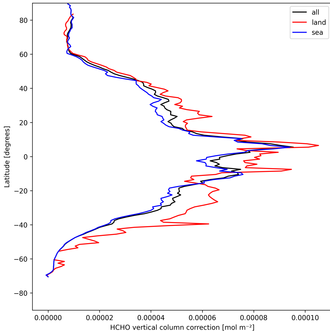
Figure 23: Zonal average of “HCHO vertical column correction” for 2025-04-29 to 2025-04-30.
