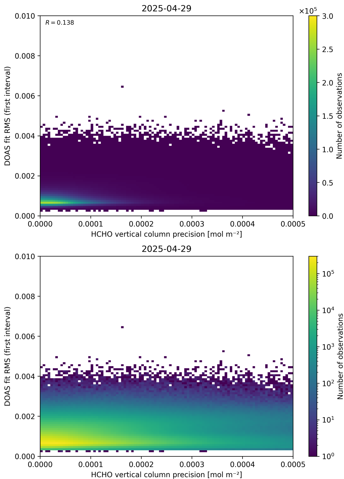
Figure 136: Scatter density plot of “HCHO vertical column precision” against “DOAS fit RMS (first interval)” for 2025-04-29 to 2025-04-30.
