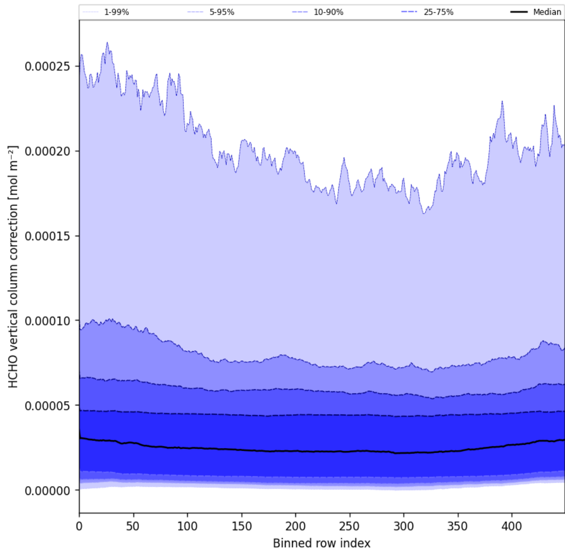
Figure 51: Along track statistics of “HCHO vertical column correction” for 2025-04-29 to 2025-04-30
