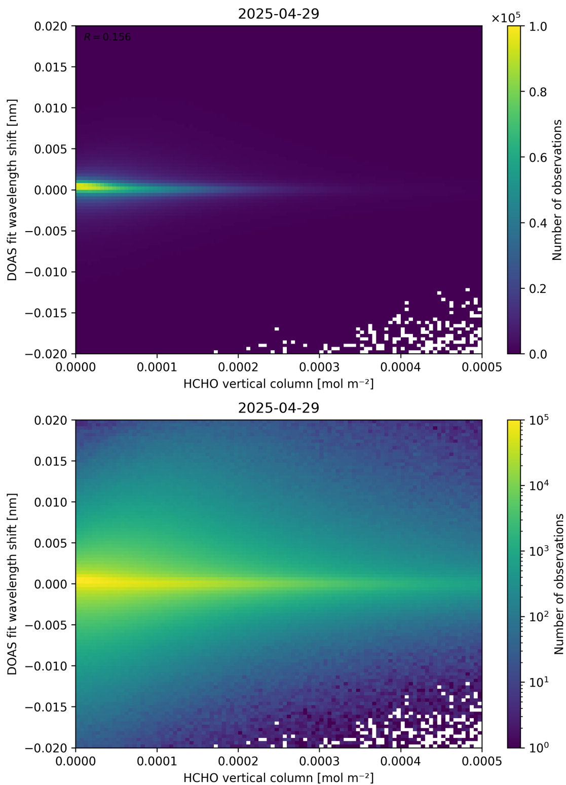
Figure 124: Scatter density plot of “HCHO vertical column” against “DOAS fit wavelength shift” for 2025-04-29 to 2025-04-30.
