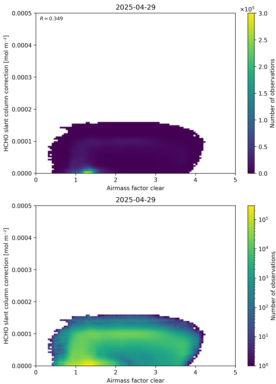
Figure 75: Scatter density plot of “Air mass factor clear” against “HCHO slant column correction” for 2025-04-29 to 2025-04-30.
