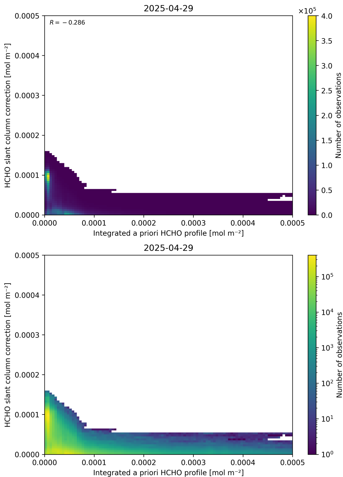
Figure 152: Scatter density plot of “Integrated a priori HCHO profile” against “HCHO slant column correction” for 2025-04-29 to 2025-04-30.
