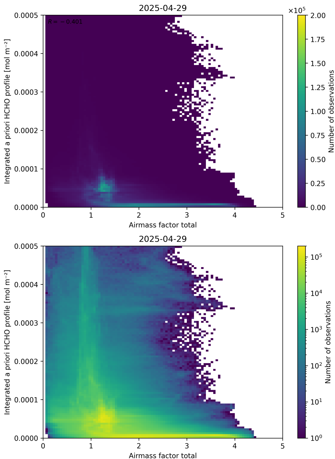
Figure 104: Scatter density plot of “Airmass factor total” against “Integrated a priori HCHO profile” for 2025-04-29 to 2025-04-30.
