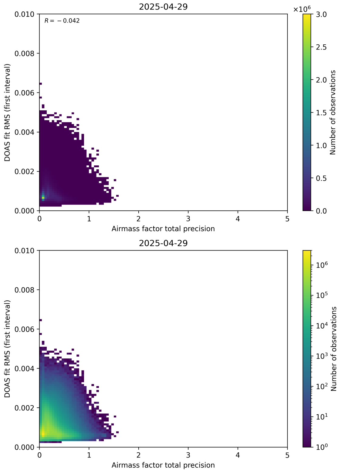
Figure 105: Scatter density plot of “Airmass factor total precision” against “DOAS fit RMS (first interval)” for 2025-04-29 to 2025-04-30.
