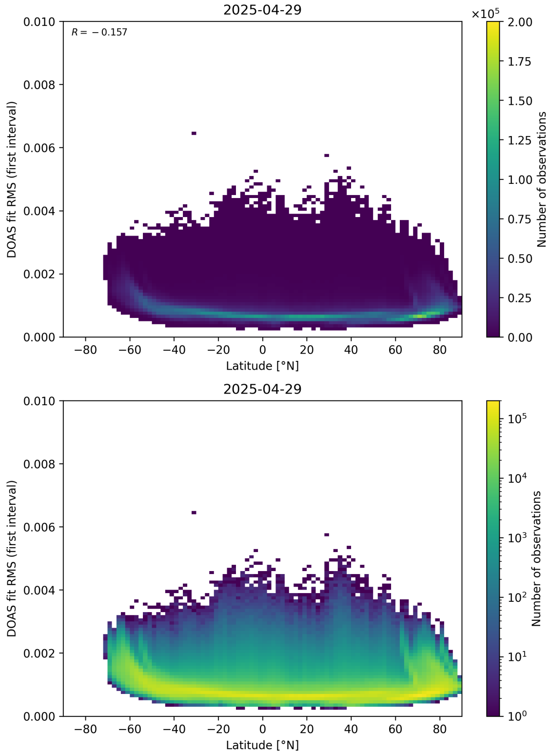
Figure 153: Scatter density plot of “Latitude” against “DOAS fit RMS (first interval)” for 2025-04-29 to 2025-04-30.
