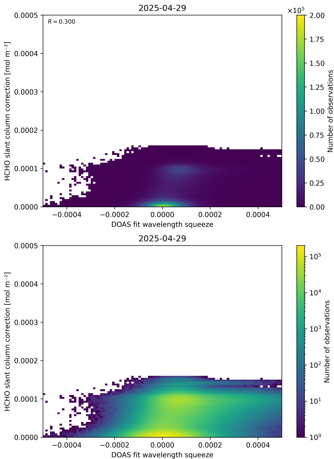
Figure 70: Scatter density plot of “DOAS fit wavelength squeeze” against “HCHO slant column correction” for 2025-04-29 to 2025-04-30.
