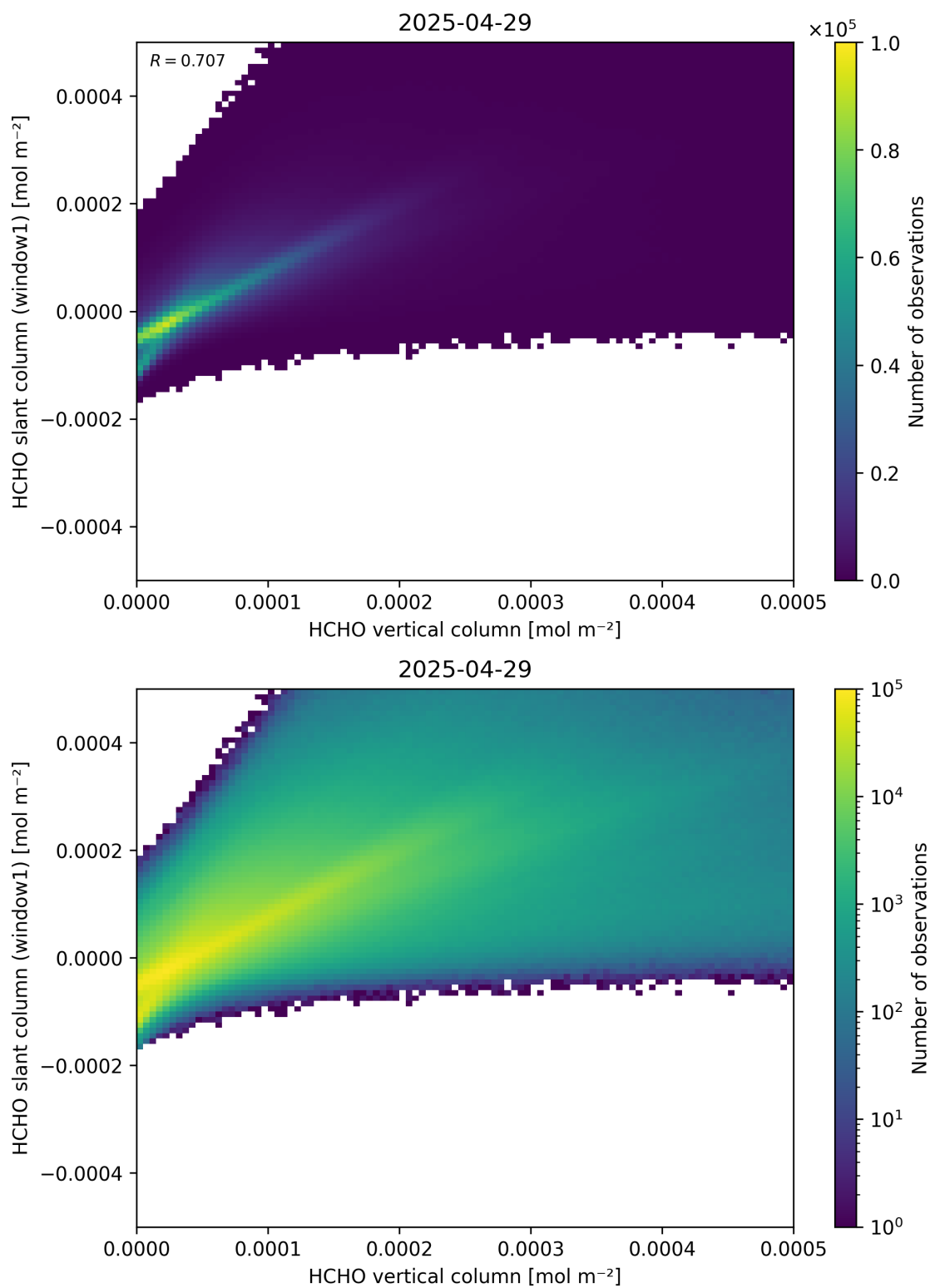
Figure 129: Scatter density plot of “HCHO vertical column” against “HCHO slant column (window1)” for 2025-04-29 to 2025-04-30.
