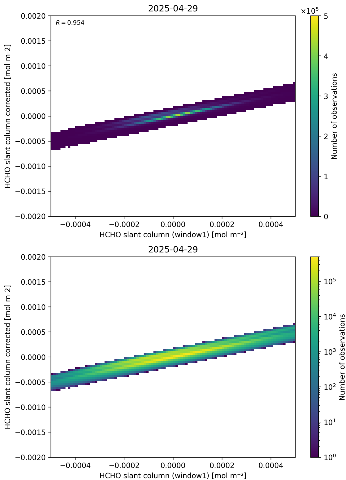
Figure 82: Scatter density plot of “HCHO slant column (window1)” against “HCHO slant column corrected” for 2025-04-29 to 2025-04-30.
