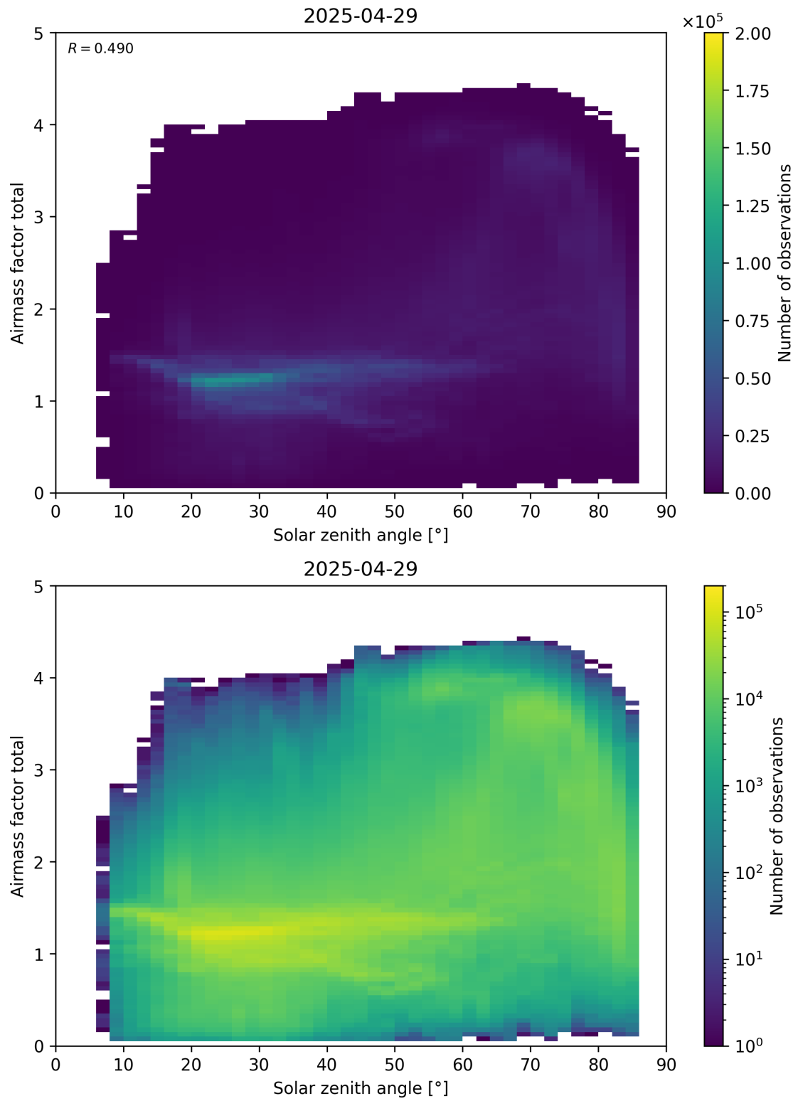
Figure 175: Scatter density plot of “Solar zenith angle” against “Airmass factor total” for 2025-04-29 to 2025-04-30.
