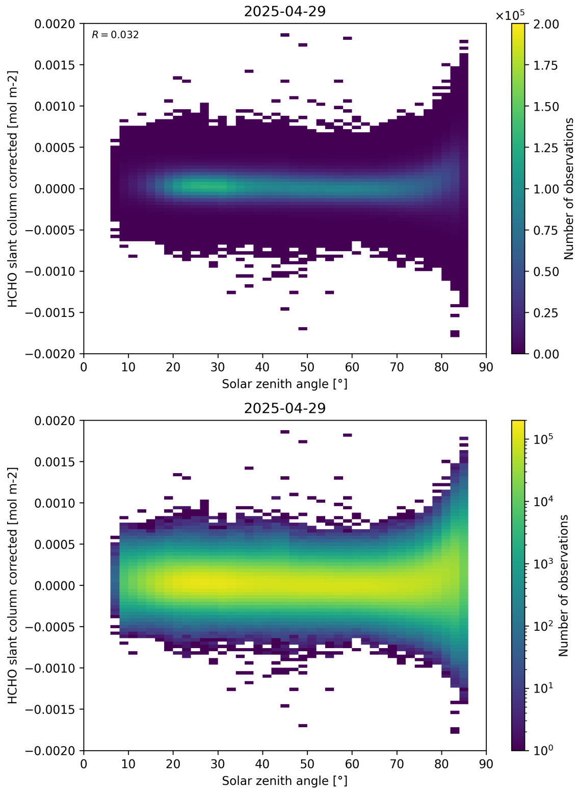
Figure 171: Scatter density plot of “Solar zenith angle” against “HCHO slant column corrected” for 2025-04-29 to 2025-04-30.
