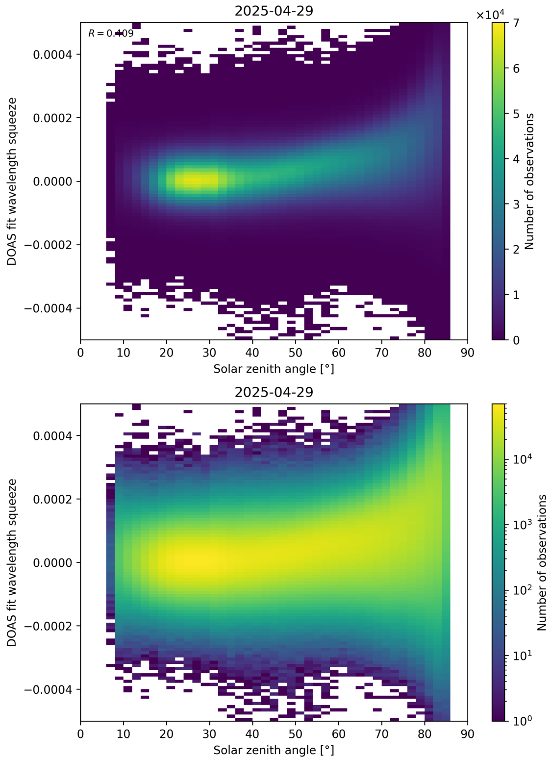
Figure 169: Scatter density plot of “Solar zenith angle” against “DOAS fit wavelength squeeze” for 2025-04-29 to 2025-04-30.
