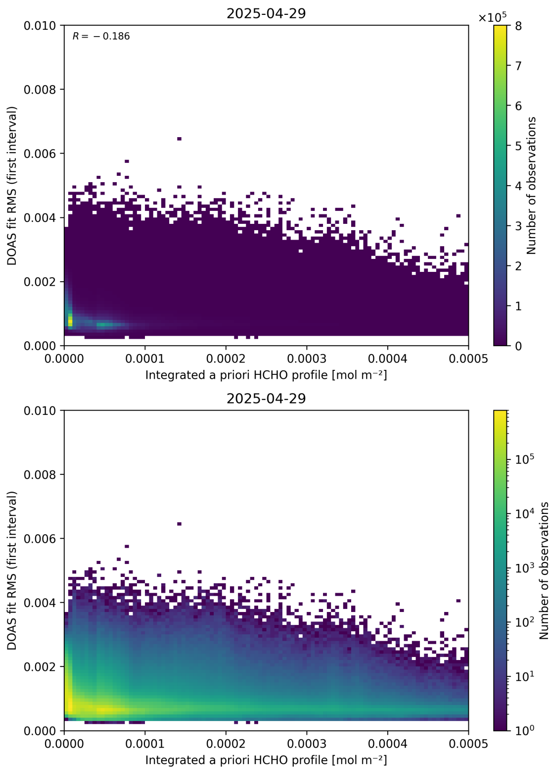
Figure 148: Scatter density plot of “Integrated a priori HCHO profile” against “DOAS fit RMS (first interval)” for 2025-04-29 to 2025-04-30.
