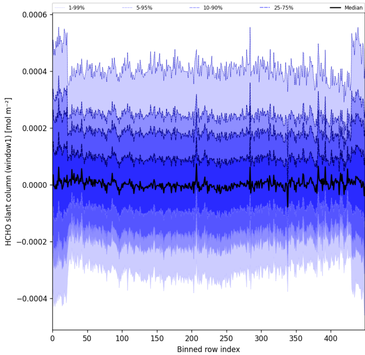
Figure 52: Along track statistics of “HCHO slant column (window1)” for 2025-04-29 to 2025-04-30
