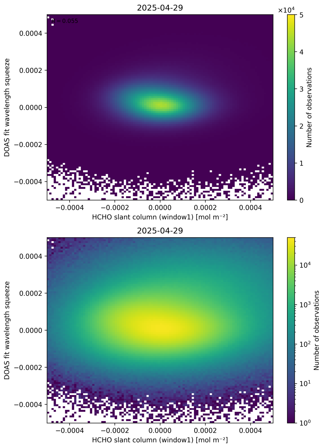
Figure 80: Scatter density plot of “HCHO slant column (window1)” against “DOAS fit wavelength squeeze” for 2025-04-29 to 2025-04-30.
