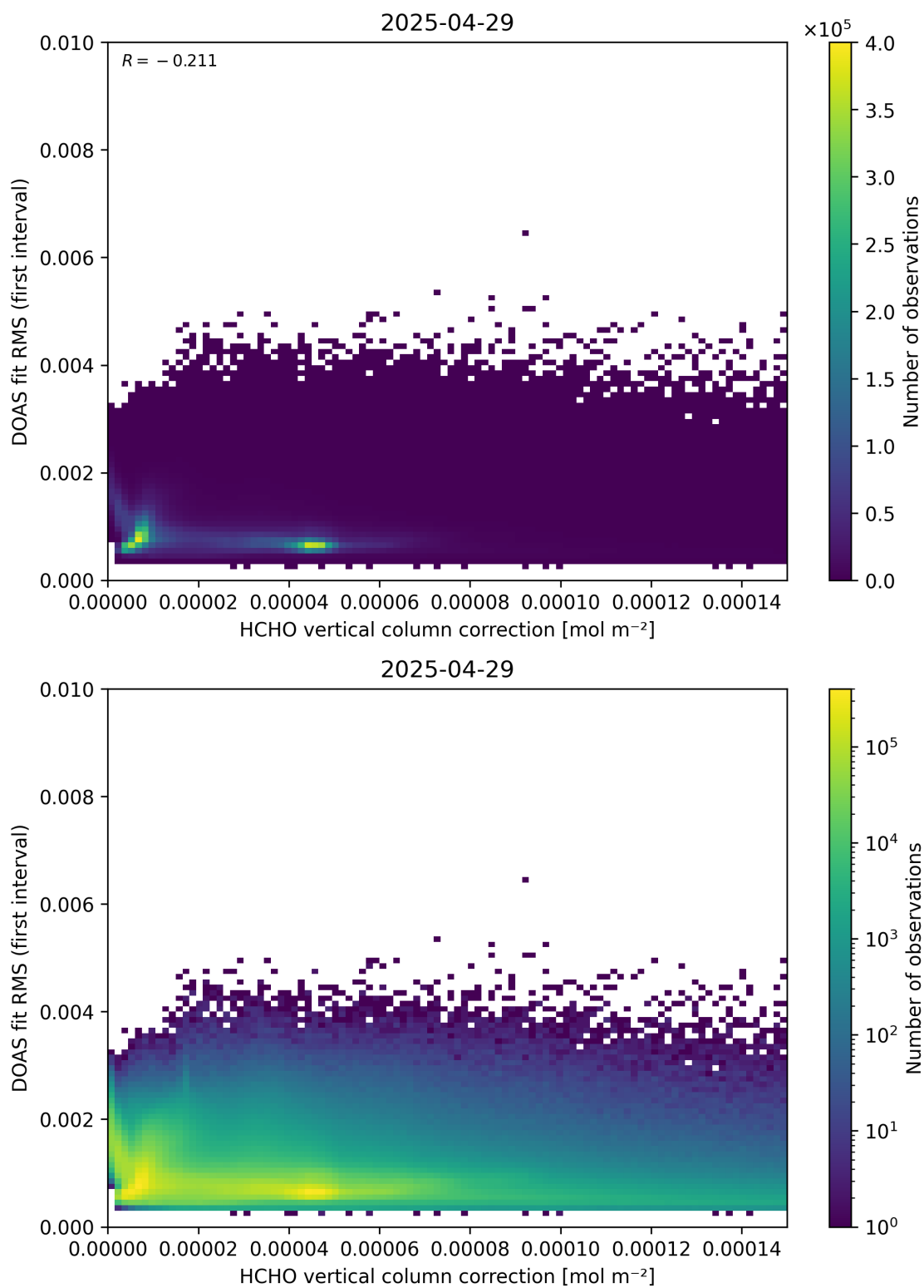
Figure 112: Scatter density plot of “HCHO vertical column correction” against “DOAS fit RMS (first interval)” for 2025-04-29 to 2025-04-30.
