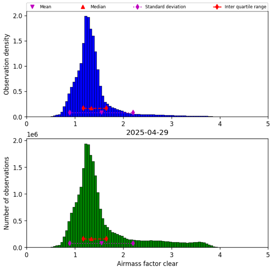
Figure 42: Histogram of “Airmass factor clear” for 2025-04-29 to 2025-04-30
