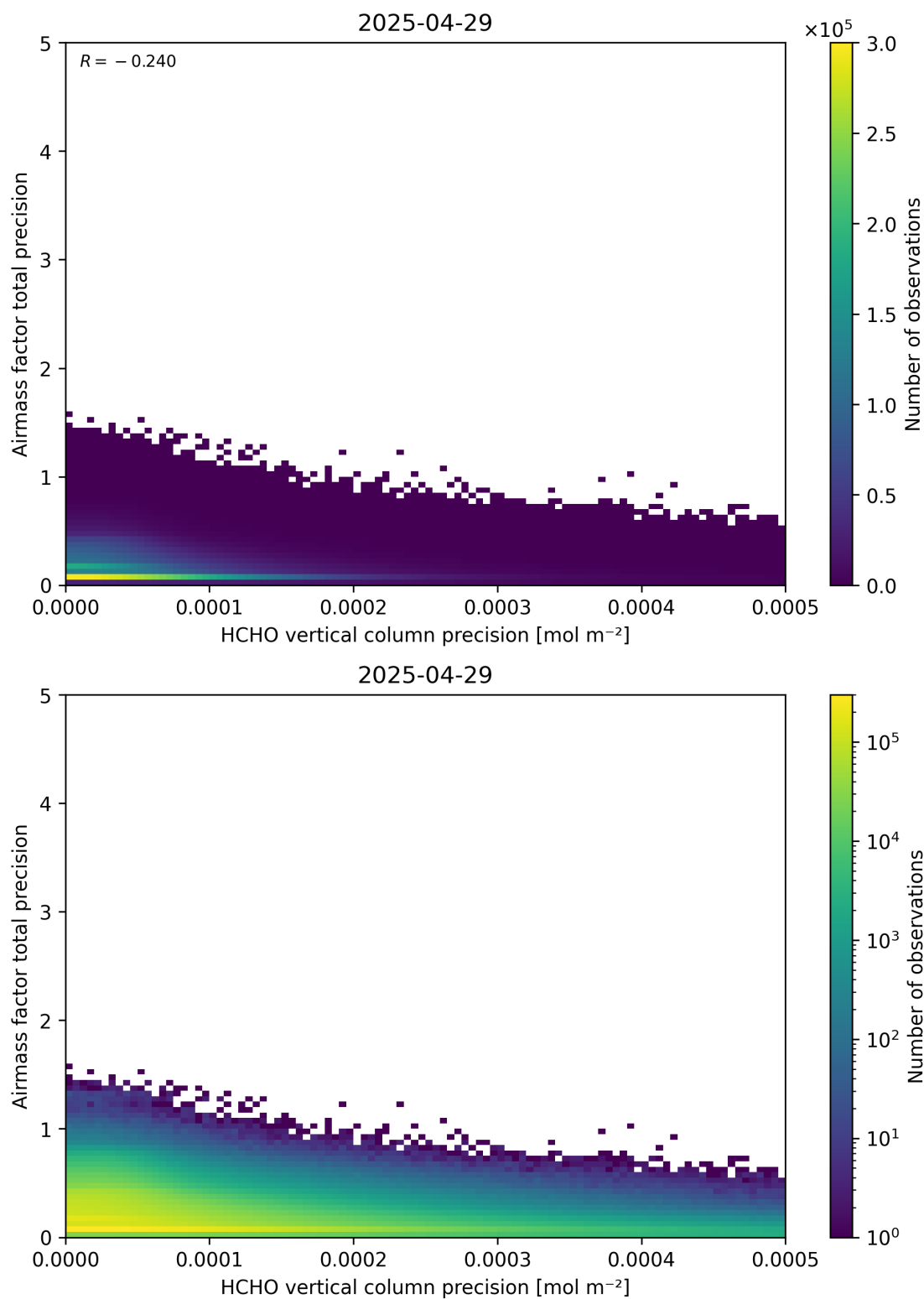
Figure 145: Scatter density plot of “HCHO vertical column precision” against “Airmass factor total precision” for 2025-04-29 to 2025-04-30.
