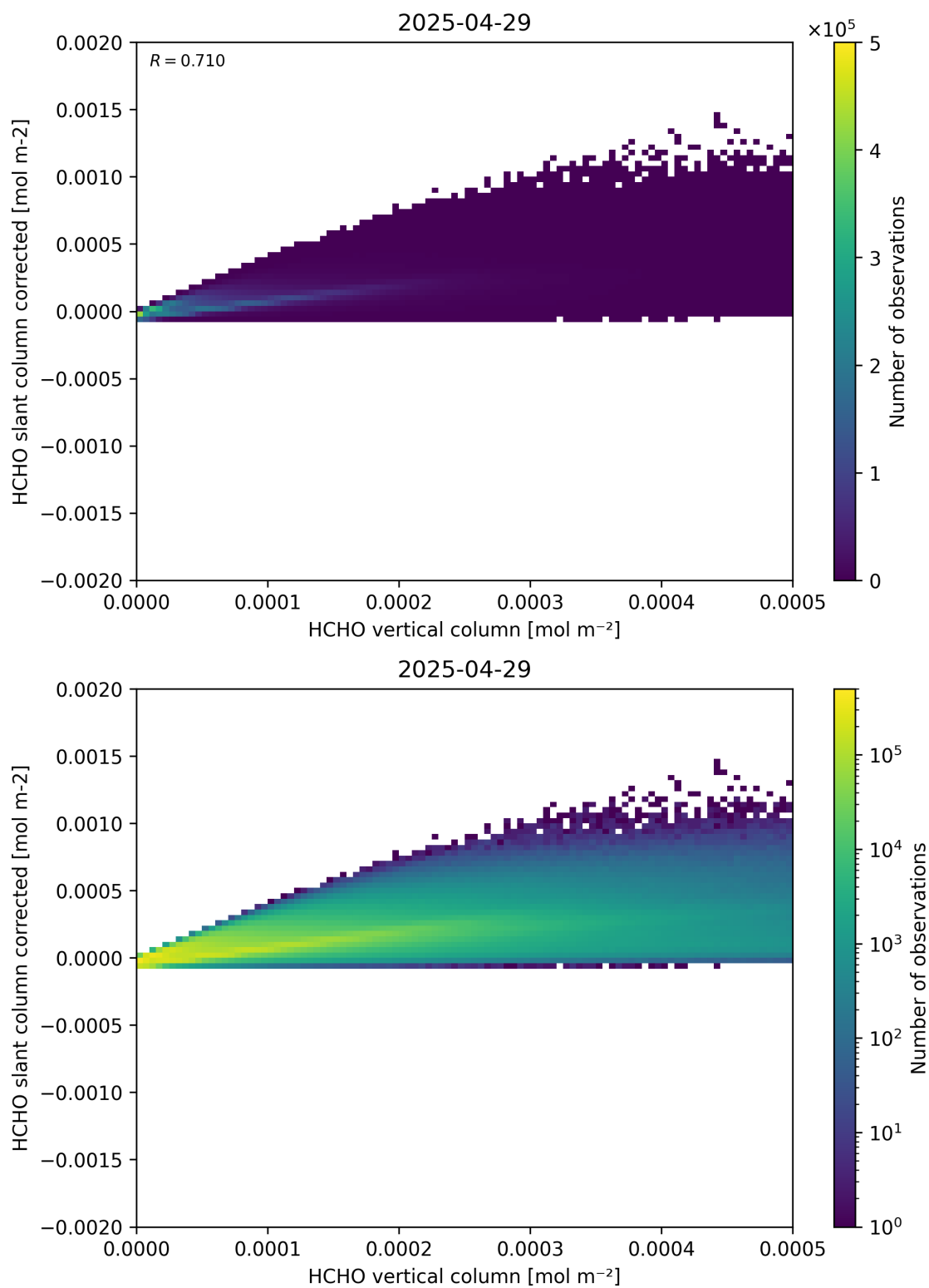
Figure 127: Scatter density plot of “HCHO vertical column” against “HCHO slant column corrected” for 2025-04-29 to 2025-04-30.
