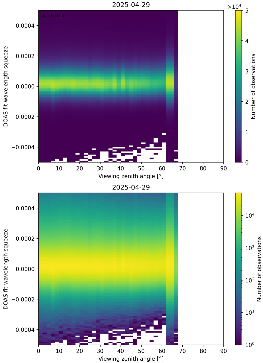
Figure 184: Scatter density plot of “Viewing zenith angle” against “DOAS fit wavelength squeeze” for 2025-04-29 to 2025-04-30.
