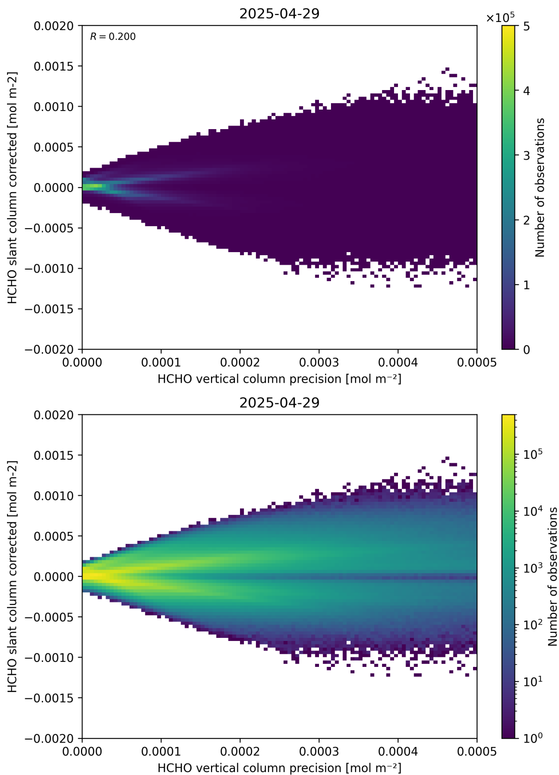
Figure 140: Scatter density plot of “HCHO vertical column precision” against “HCHO slant column corrected” for 2025-04-29 to 2025-04-30.
