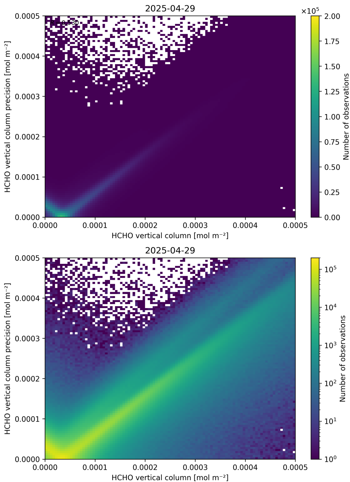
Figure 134: Scatter density plot of “HCHO vertical column” against “HCHO vertical column precision” for 2025-04-29 to 2025-04-30.
