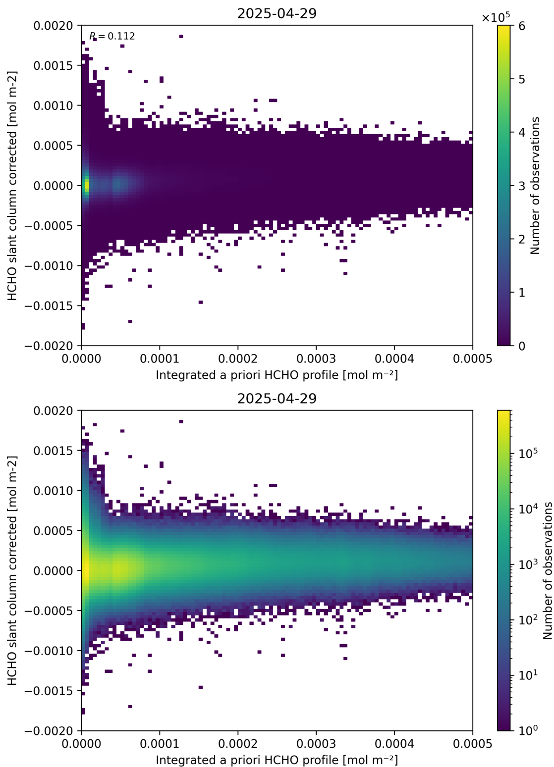
Figure 151: Scatter density plot of “Integrated a priori HCHO profile” against “HCHO slant column corrected” for 2025-04-29 to 2025-04-30.
