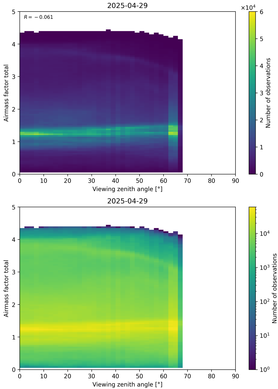
Figure 190: Scatter density plot of “Viewing zenith angle” against “Airmass factor total” for 2025-04-29 to 2025-04-30.
