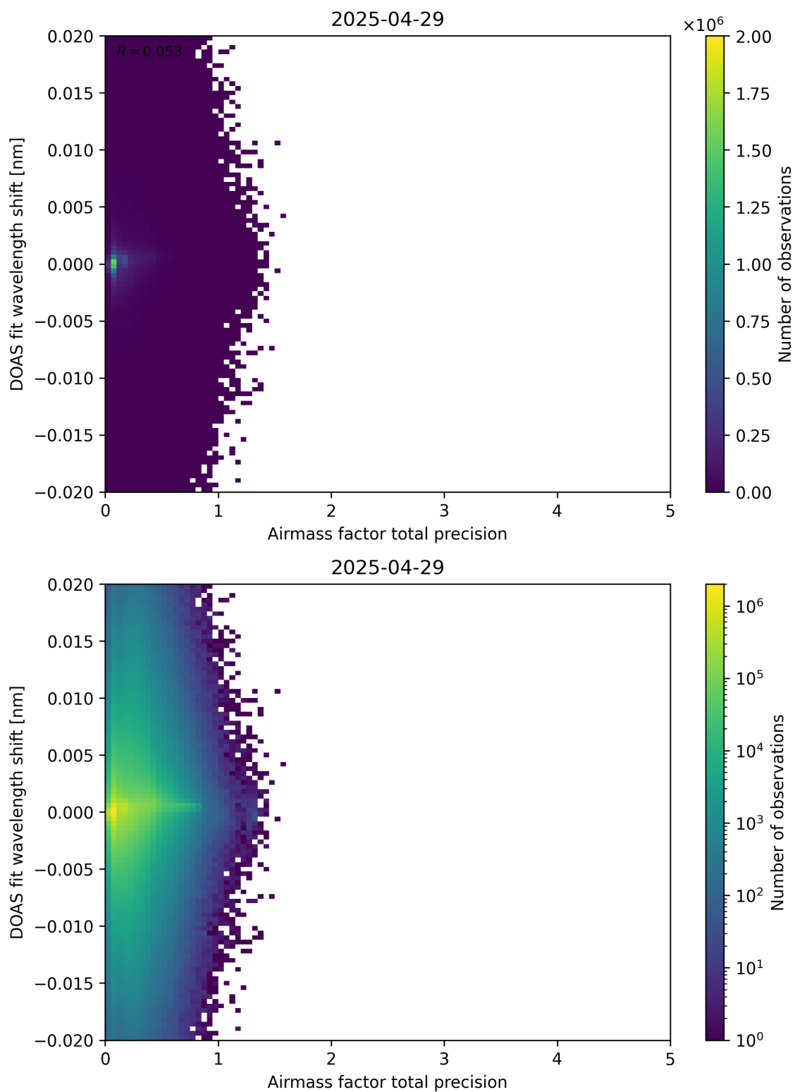
Figure 106: Scatter density plot of “Airmass factor total precision” against “DOAS fit wavelength shift” for 2025-04-29 to 2025-04-30.
