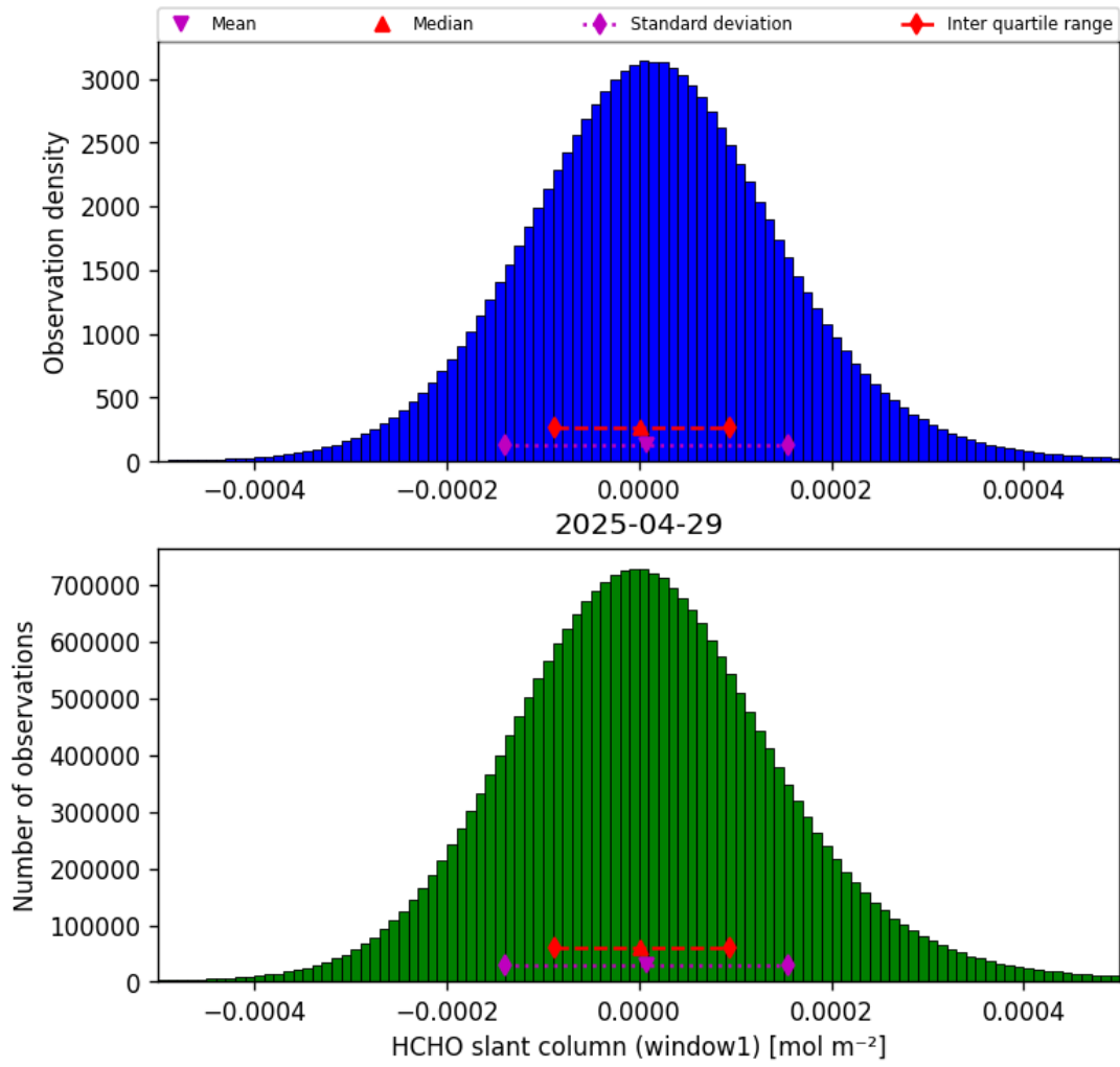
Figure 38: Histogram of “HCHO slant column (window1)” for 2025-04-29 to 2025-04-30
