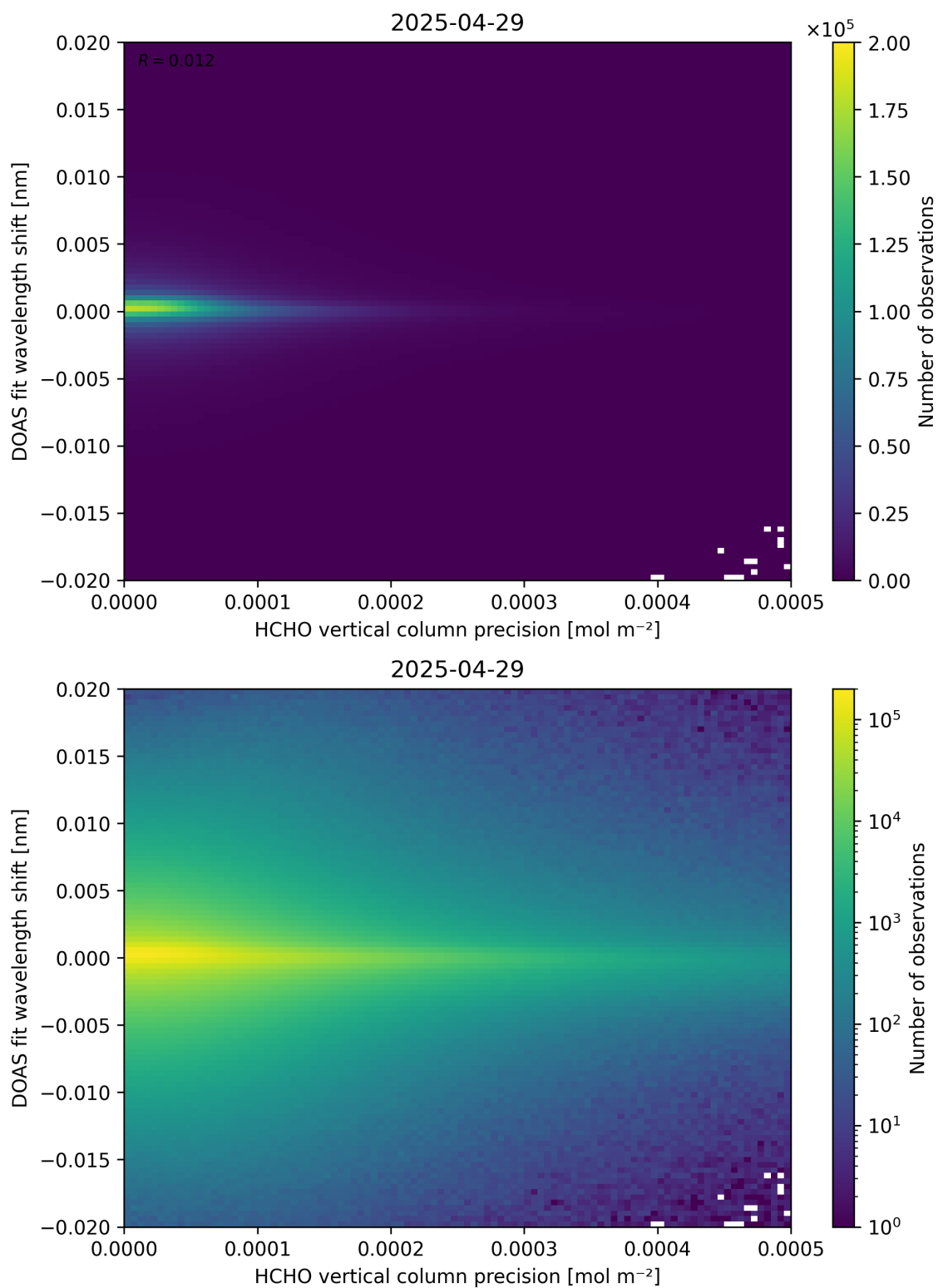
Figure 137: Scatter density plot of “HCHO vertical column precision” against “DOAS fit wavelength shift” for 2025-04-29 to 2025-04-30.
