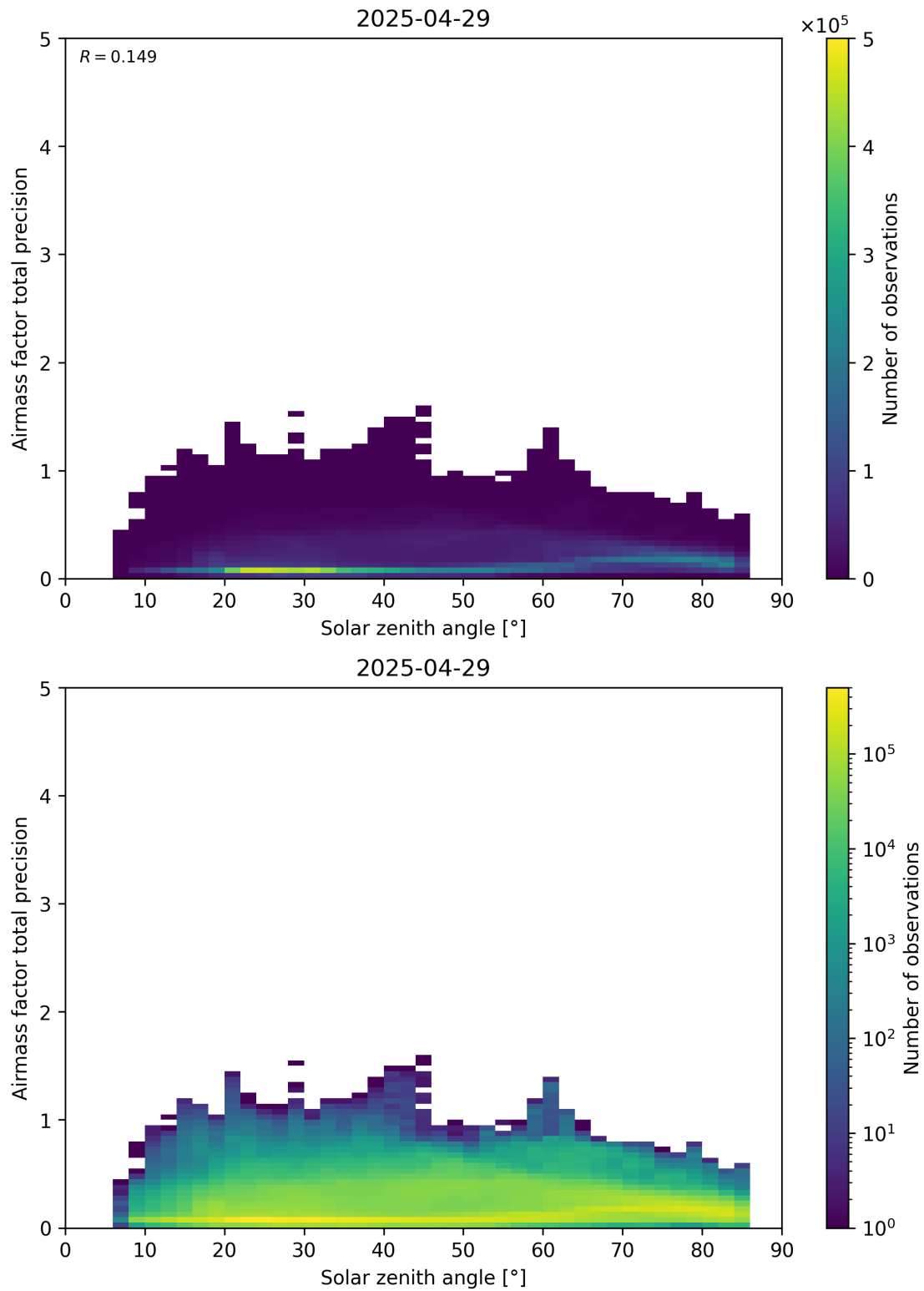
Figure 176: Scatter density plot of “Solar zenith angle” against “Airmass factor total precision” for 2025-04-29 to 2025-04-30.
