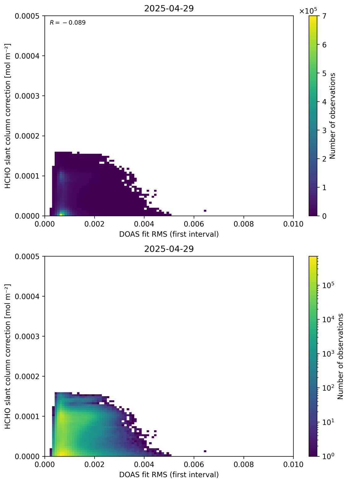
Figure 63: Scatter density plot of “DOAS fit RMS (first interval)” against “HCHO slant column correction” for 2025-04-29 to 2025-04-30.
