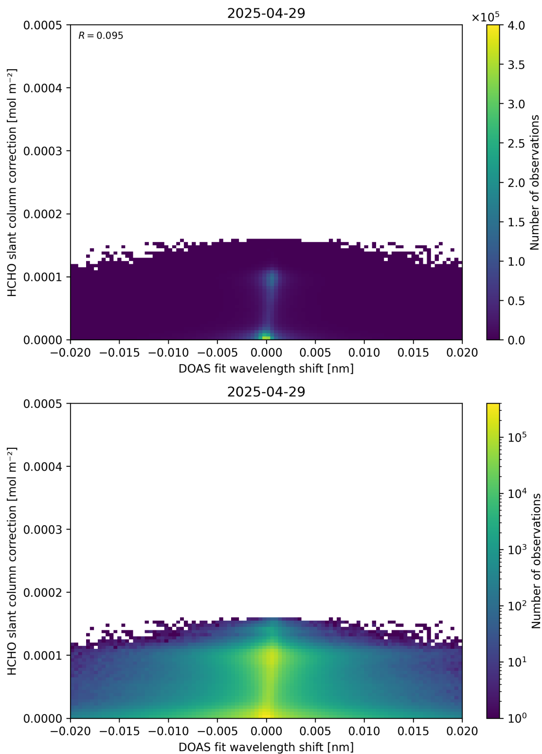
Figure 67: Scatter density plot of “DOAS fit wavelength shift” against “HCHO slant column correction” for 2025-04-29 to 2025-04-30.
