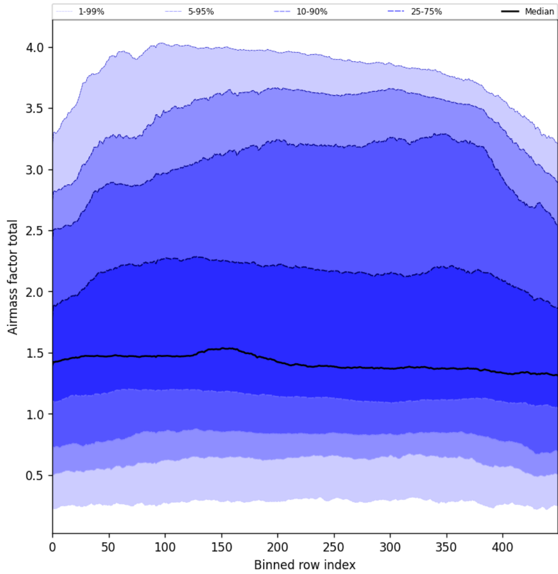
Figure 54: Along track statistics of “Airmass factor total” for 2025-04-29 to 2025-04-30
