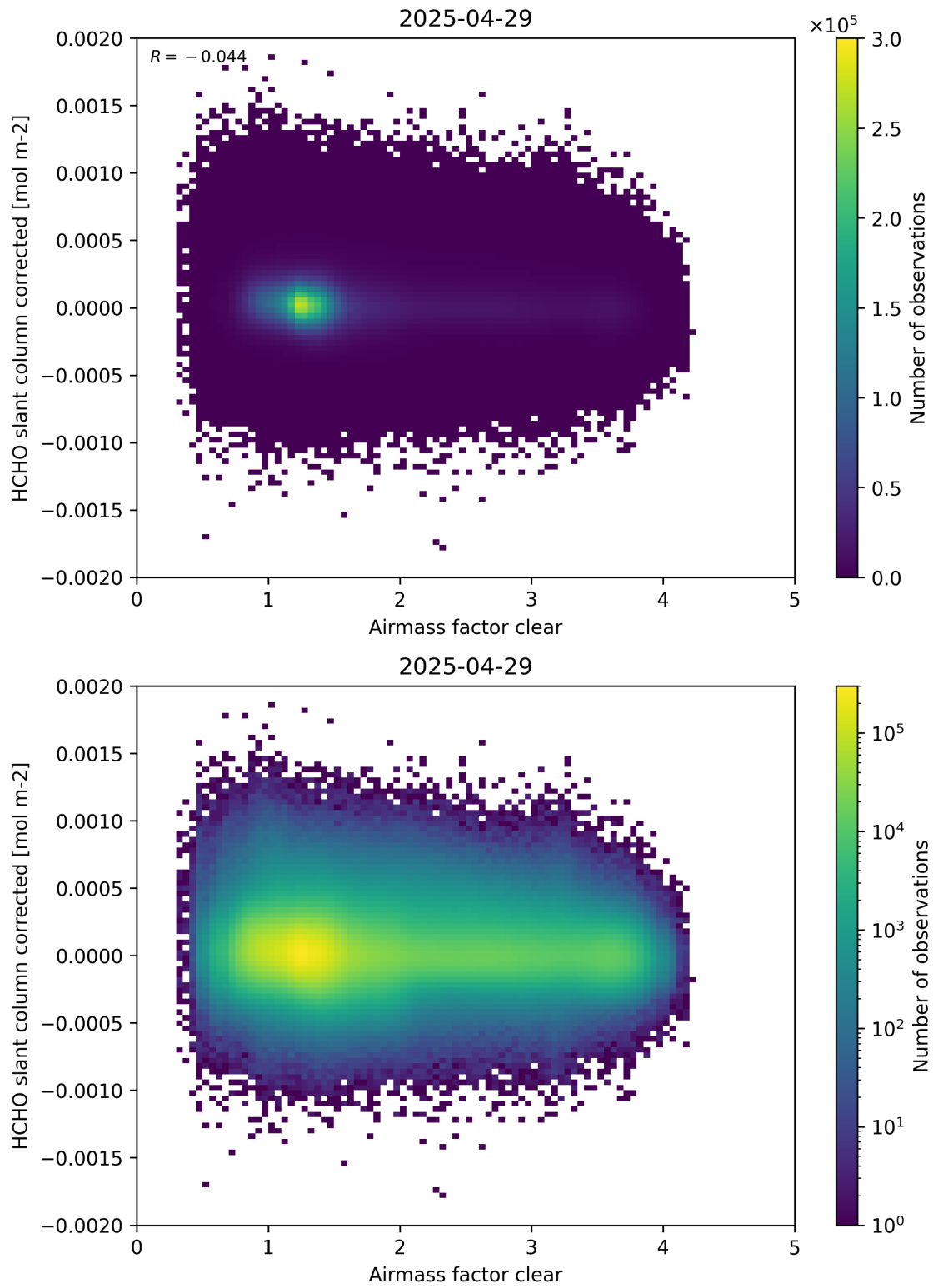
Figure 74: Scatter density plot of “Airmass factor clear” against “HCHO slant column corrected” for 2025-04-29 to 2025-04-30.
