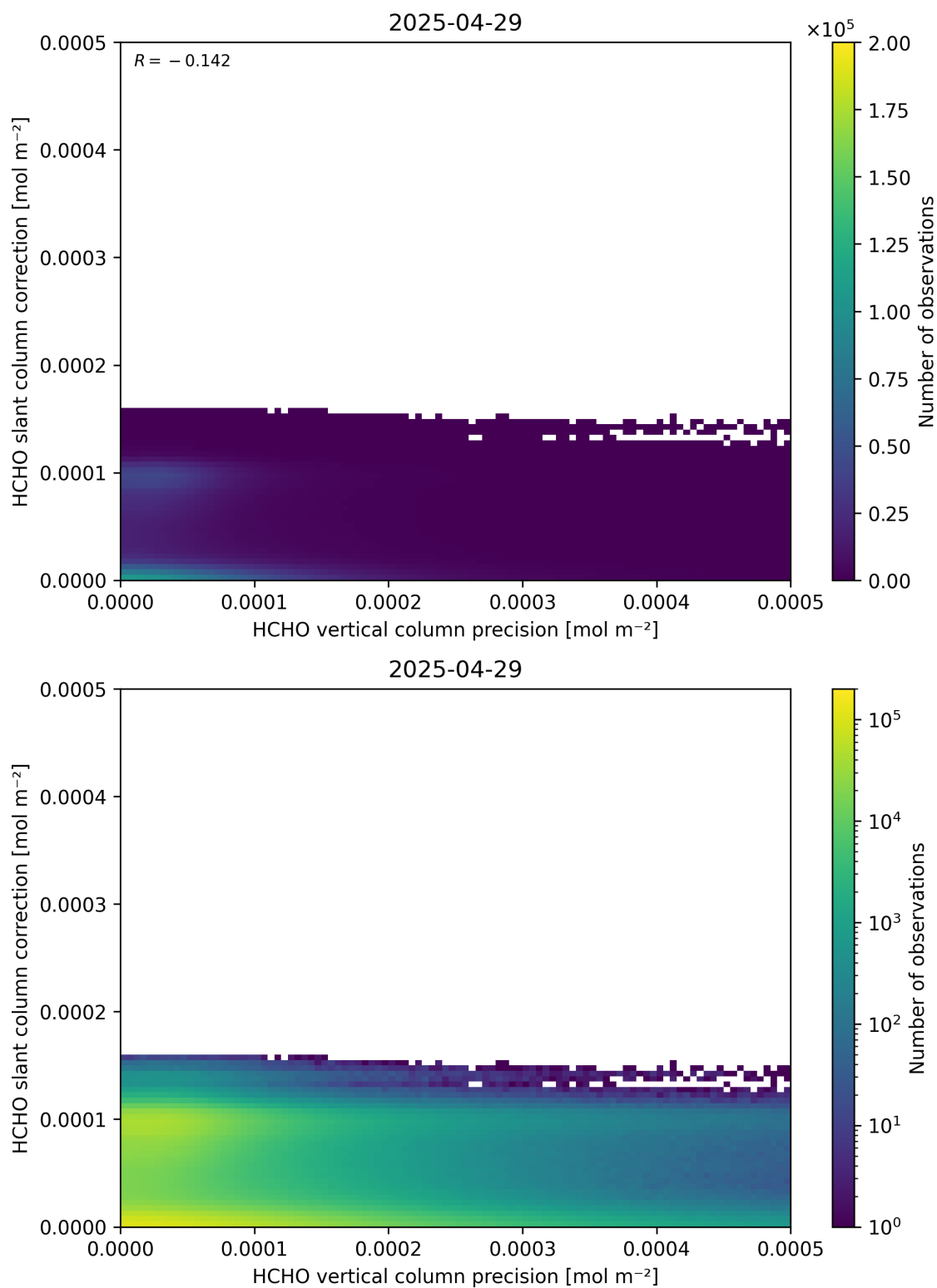
Figure 141: Scatter density plot of “HCHO vertical column precision” against “HCHO slant column correction” for 2025-04-29 to 2025-04-30.
