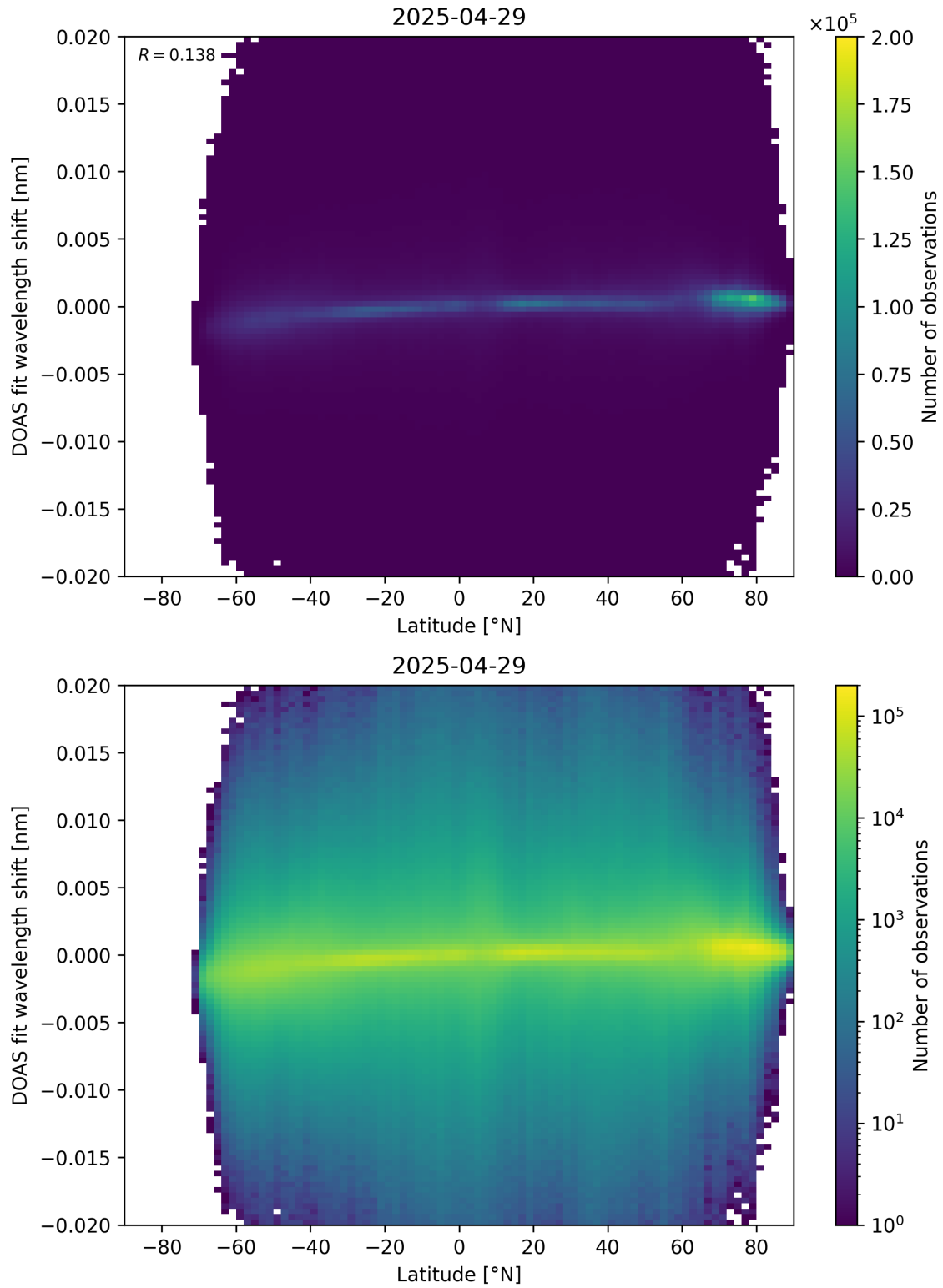
Figure 154: Scatter density plot of “Latitude” against “DOAS fit wavelength shift” for 2025-04-29 to 2025-04-30.
