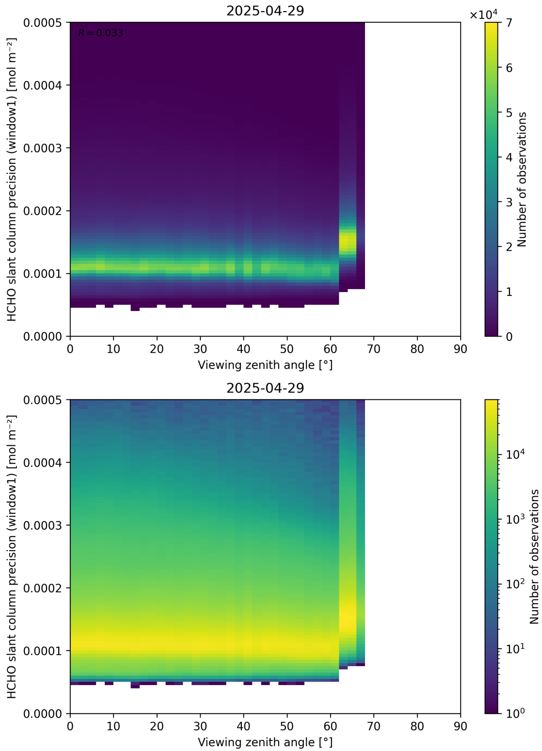
Figure 189: Scatter density plot of “Viewing zenith angle” against “HCHO slant column precision (window1)” for 2025-04-29 to 2025-04-30.
