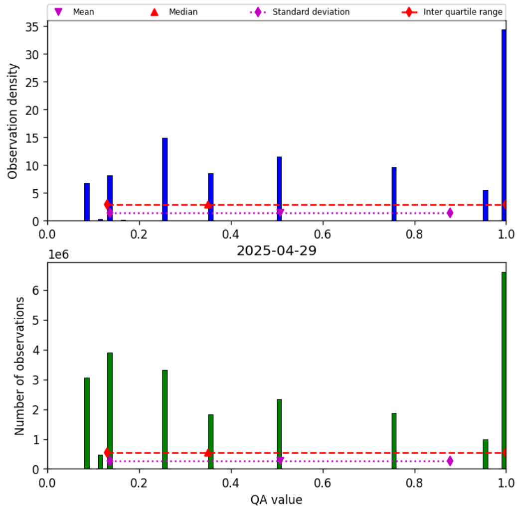
Figure 34: Histogram of “QA value” for 2025-04-29 to 2025-04-30
