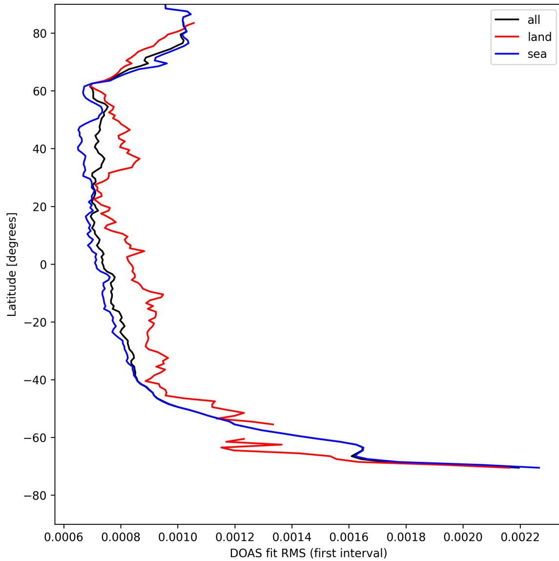
Figure 32: Zonal average of “DOAS fit RMS (first interval)” for 2025-04-29 to 2025-04-30.
