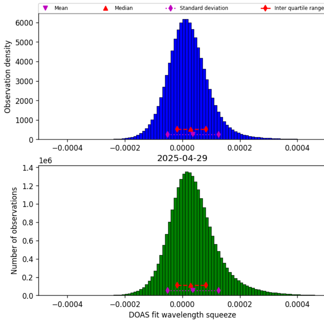
Figure 45: Histogram of “DOAS fit wavelength squeeze” for 2025-04-29 to 2025-04-30
