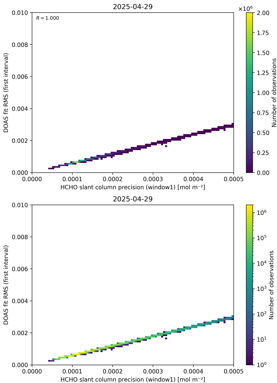
Figure 88: Scatter density plot of “HCHO slant column precision (window1)” against “DOAS fit RMS (first interval)” for 2025-04-29 to 2025-04-30.
