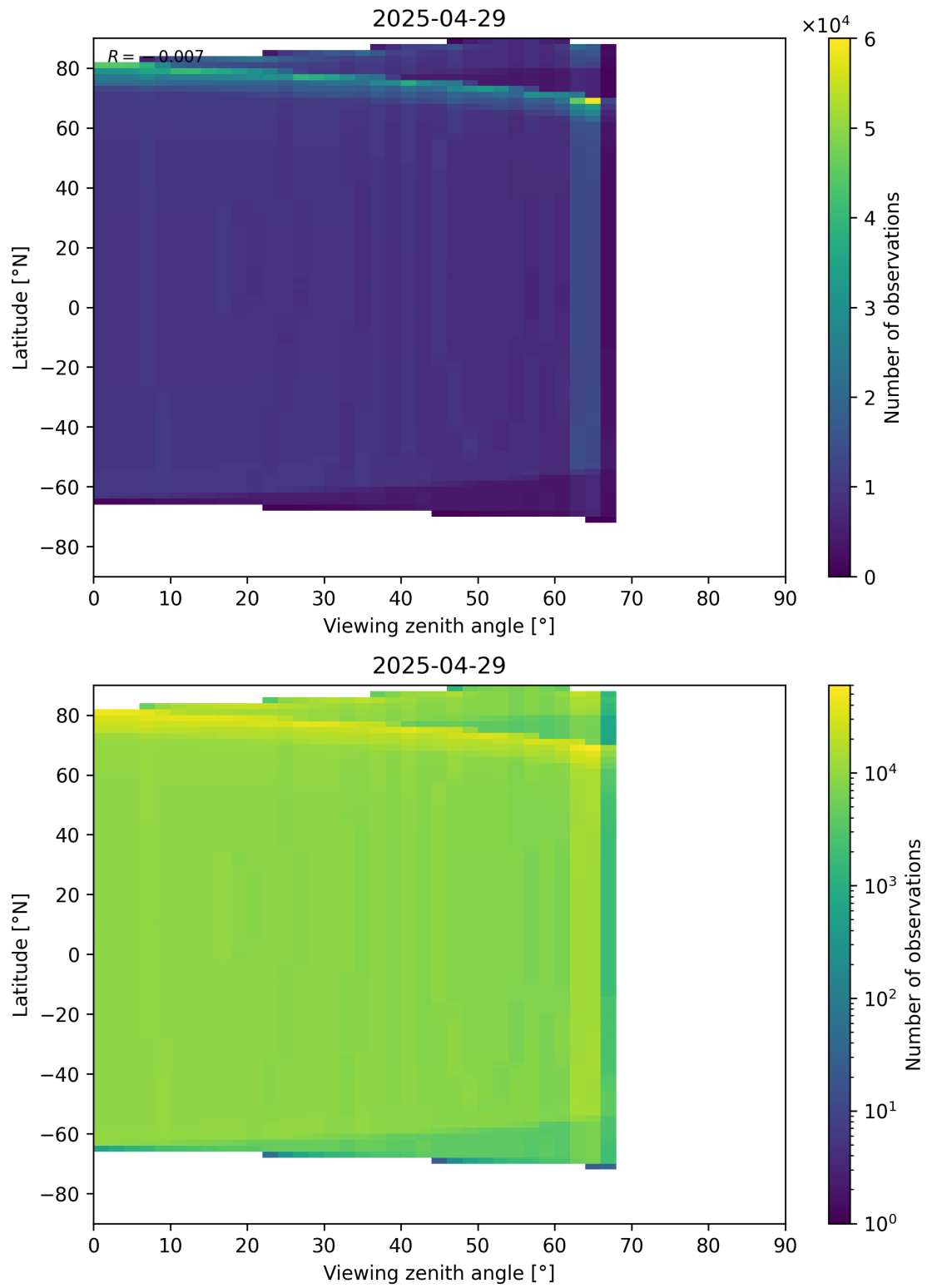
Figure 196: Scatter density plot of “Viewing zenith angle” against “Latitude” for 2025-04-29 to 2025-04-30.
