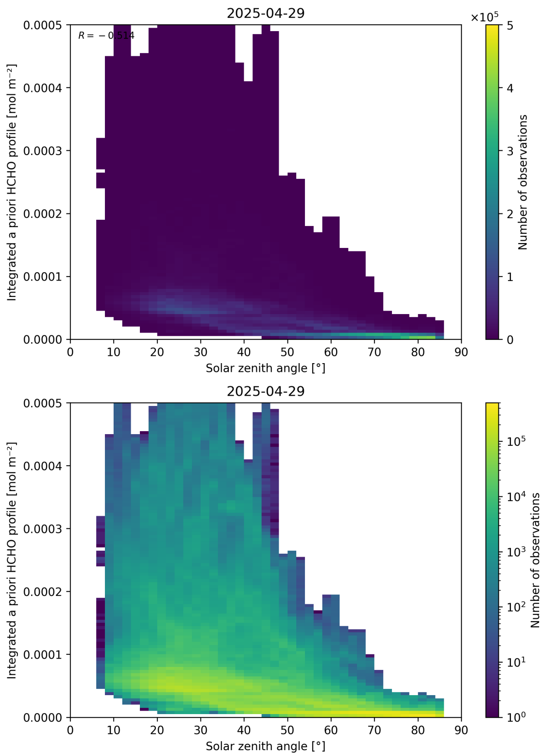
Figure 180: Scatter density plot of “Solar zenith angle” against “Integrated a priori HCHO profile” for 2025-04-29 to 2025-04-30.
