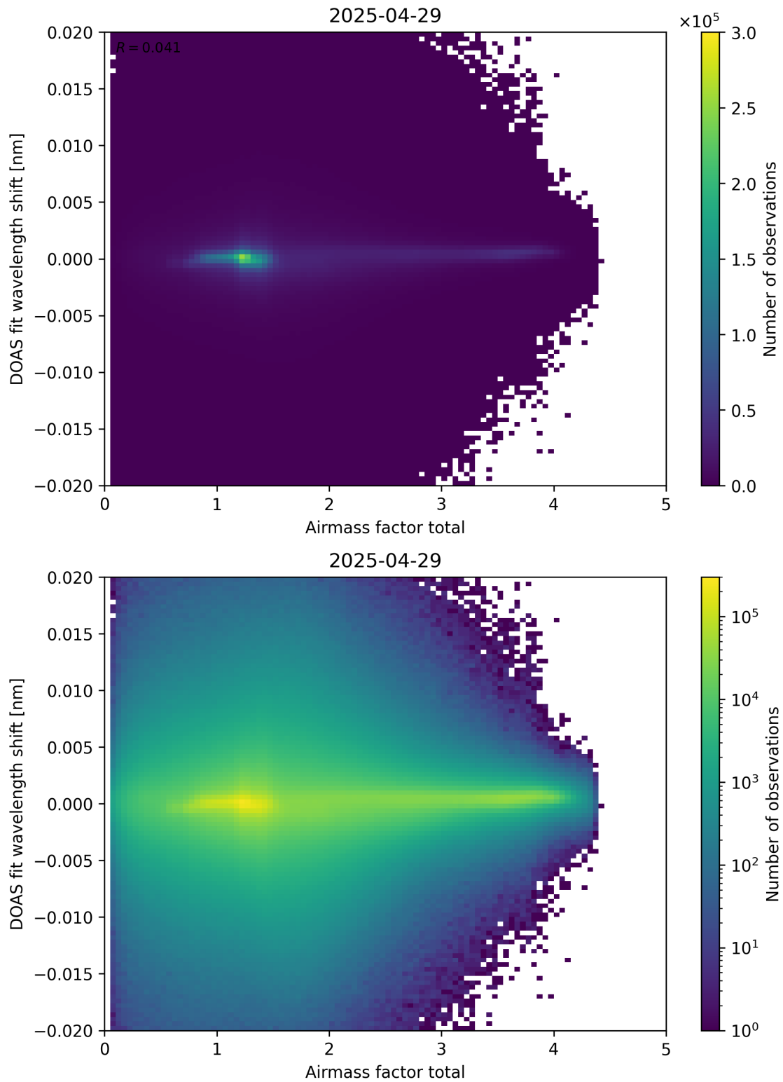
Figure 98: Scatter density plot of “Airmass factor total” against “DOAS fit wavelength shift” for 2025-04-29 to 2025-04-30.
