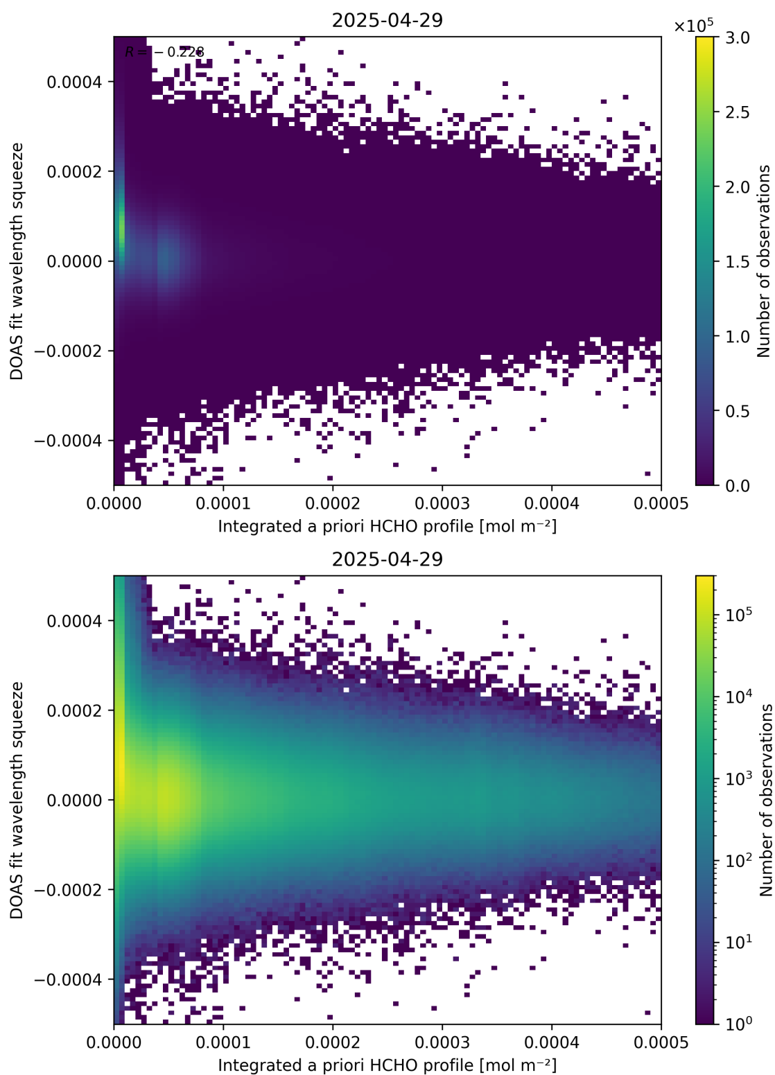
Figure 150: Scatter density plot of “Integrated a priori HCHO profile” against “DOAS fit wavelength squeeze” for 2025-04-29 to 2025-04-30.
