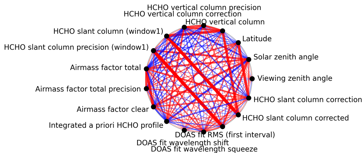
Figure 1: Map of correlation graph for 2025-04-29 to 2025-04-30.
