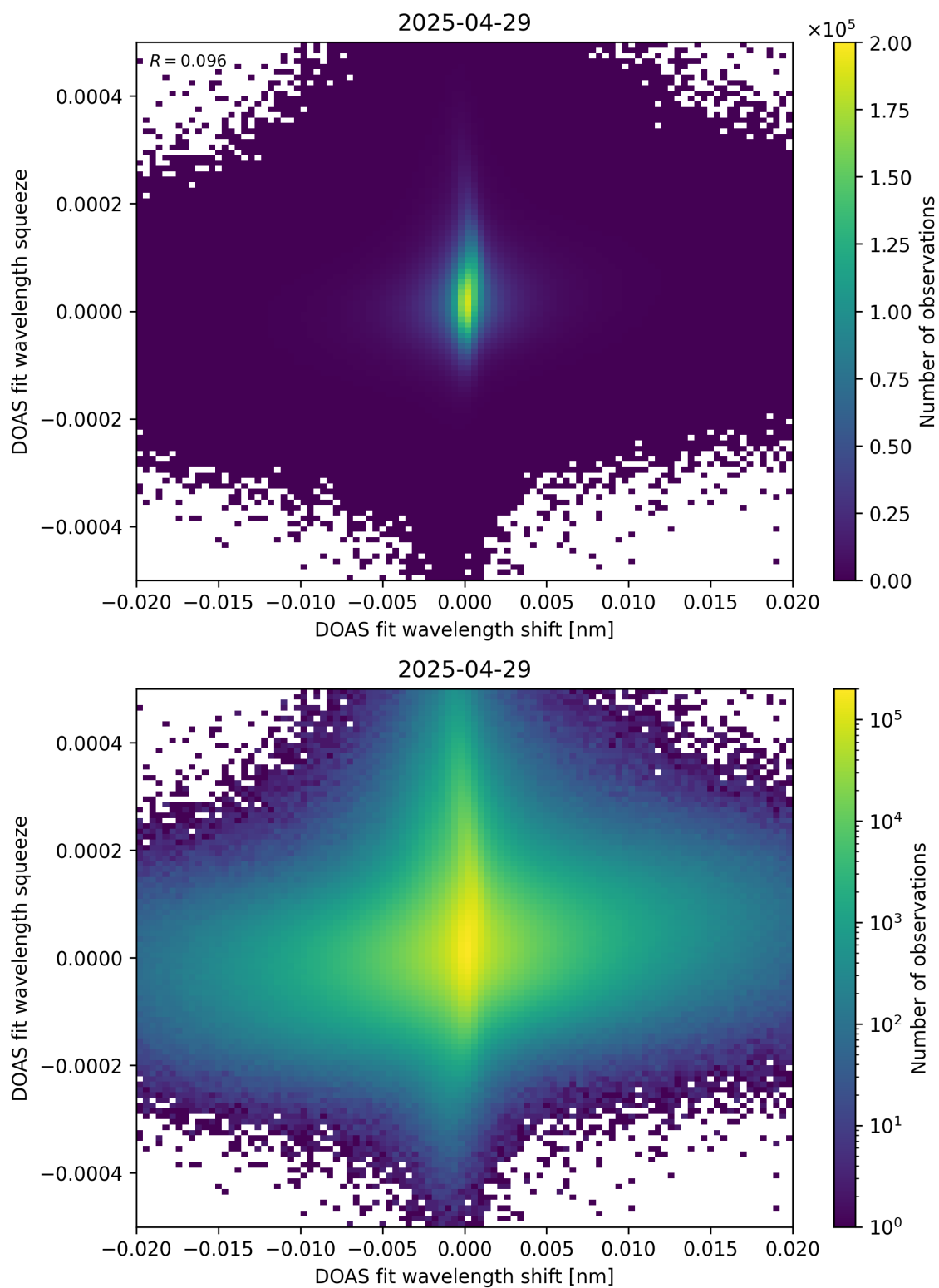
Figure 65: Scatter density plot of “DOAS fit wavelength shift” against “DOAS fit wavelength squeeze” for 2025-04-29 to 2025-04-30.
