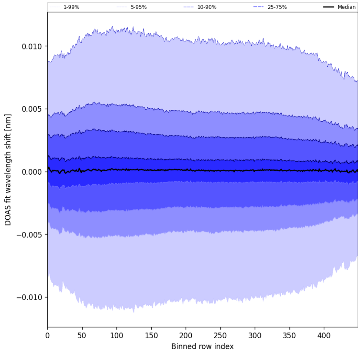
Figure 58: Along track statistics of “DOAS fit wavelength shift” for 2025-04-29 to 2025-04-30
