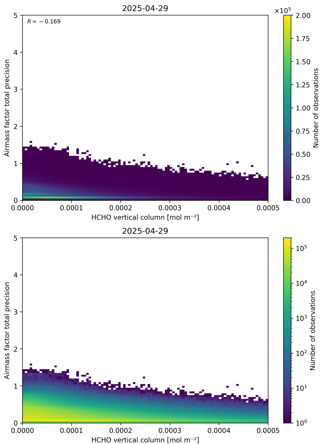
Figure 132: Scatter density plot of “HCHO vertical column” against “Airmass factor total precision” for 2025-04-29 to 2025-04-30.
