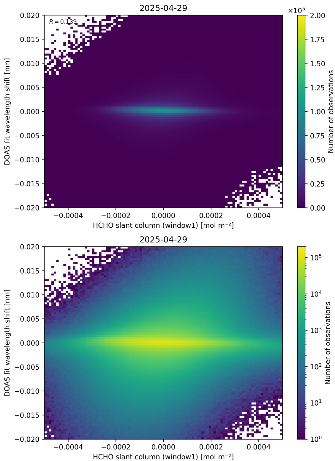
Figure 79: Scatter density plot of “HCHO slant column (window1)” against “DOAS fit wavelength shift” for 2025-04-29 to 2025-04-30.
