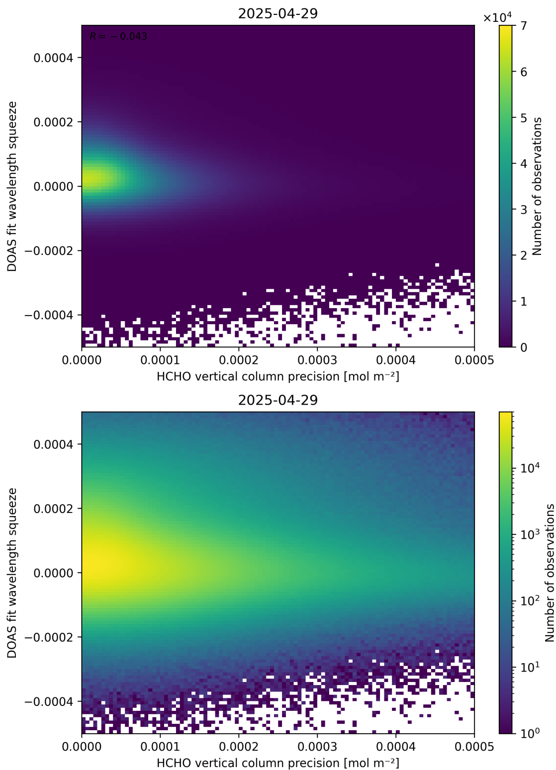
Figure 138: Scatter density plot of “HCHO vertical column precision” against “DOAS fit wavelength squeeze” for 2025-04-29 to 2025-04-30.
