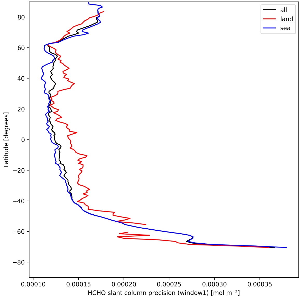
Figure 25: Zonal average of “HCHO slant column precision (window1)” for 2025-04-29 to 2025-04-30.
