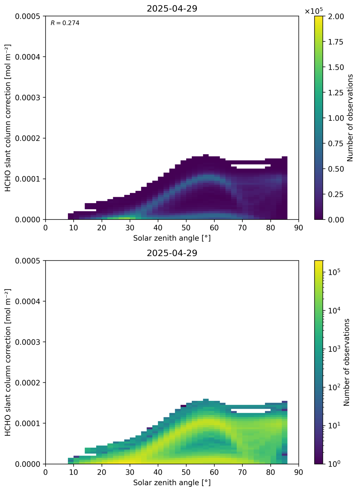
Figure 172: Scatter density plot of “Solar zenith angle” against “HCHO slant column correction” for 2025-04-29 to 2025-04-30.
