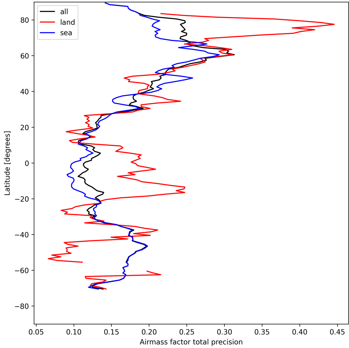
Figure 27: Zonal average of “Airmass factor total precision” for 2025-04-29 to 2025-04-30.
