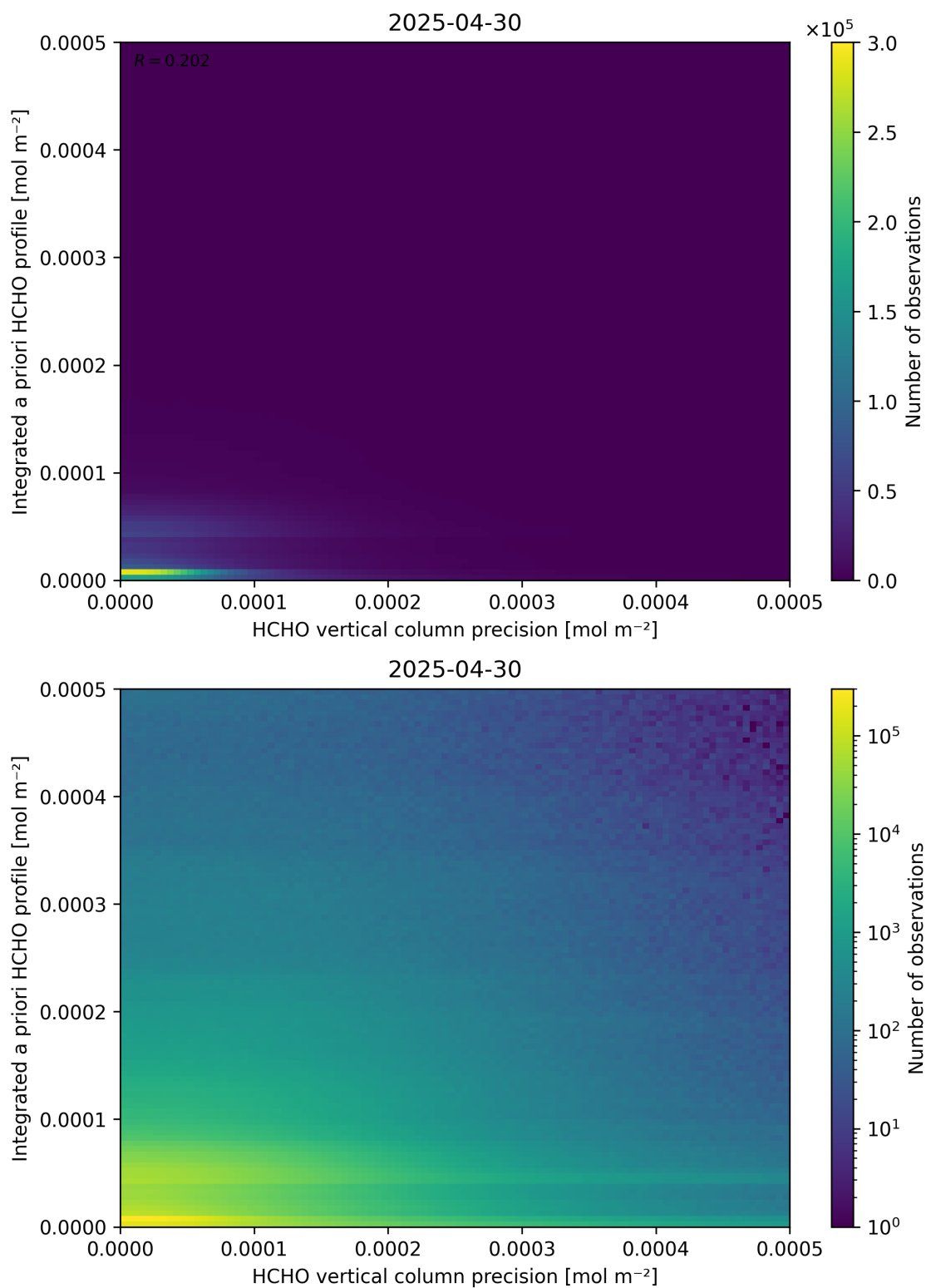
Figure 147: Scatter density plot of “HCHO vertical column precision” against “Integrated a priori HCHO profile” for 2025-04-29 to 2025-05-01.
