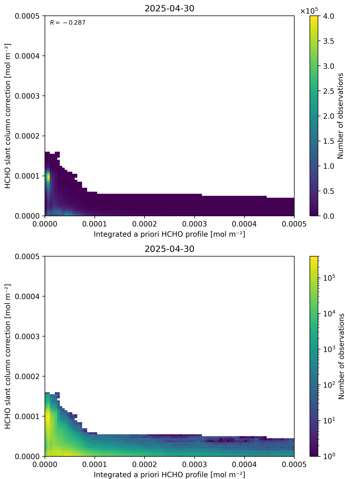
Figure 152: Scatter density plot of “Integrated a priori HCHO profile” against “HCHO slant column correction” for 2025-04-29 to 2025-05-01.
