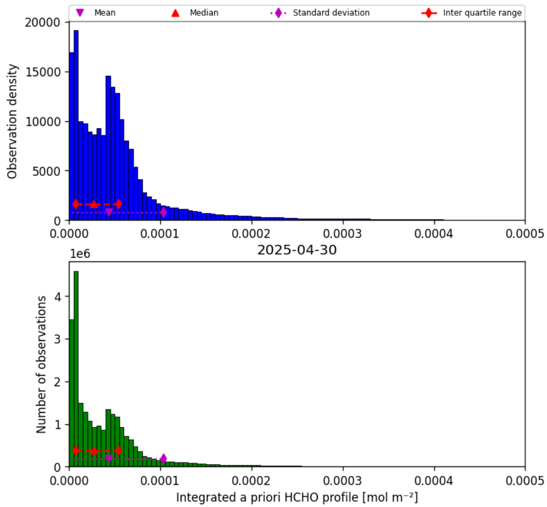
Figure 43: Histogram of “Integrated a priori HCHO profile” for 2025-04-29 to 2025-05-01
