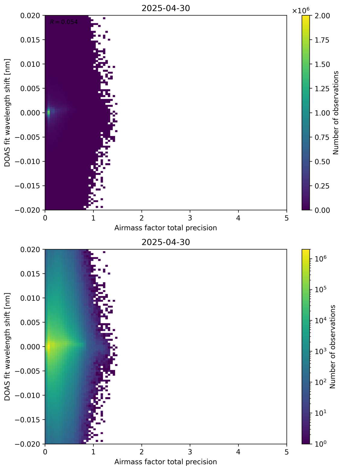
Figure 106: Scatter density plot of “Airmass factor total precision” against “DOAS fit wavelength shift” for 2025-04-29 to 2025-05-01.
