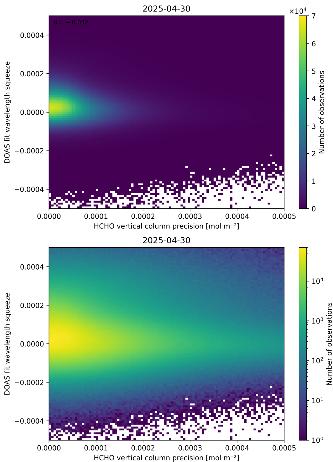
Figure 138: Scatter density plot of “HCHO vertical column precision” against “DOAS fit wavelength squeeze” for 2025-04-29 to 2025-05-01.
