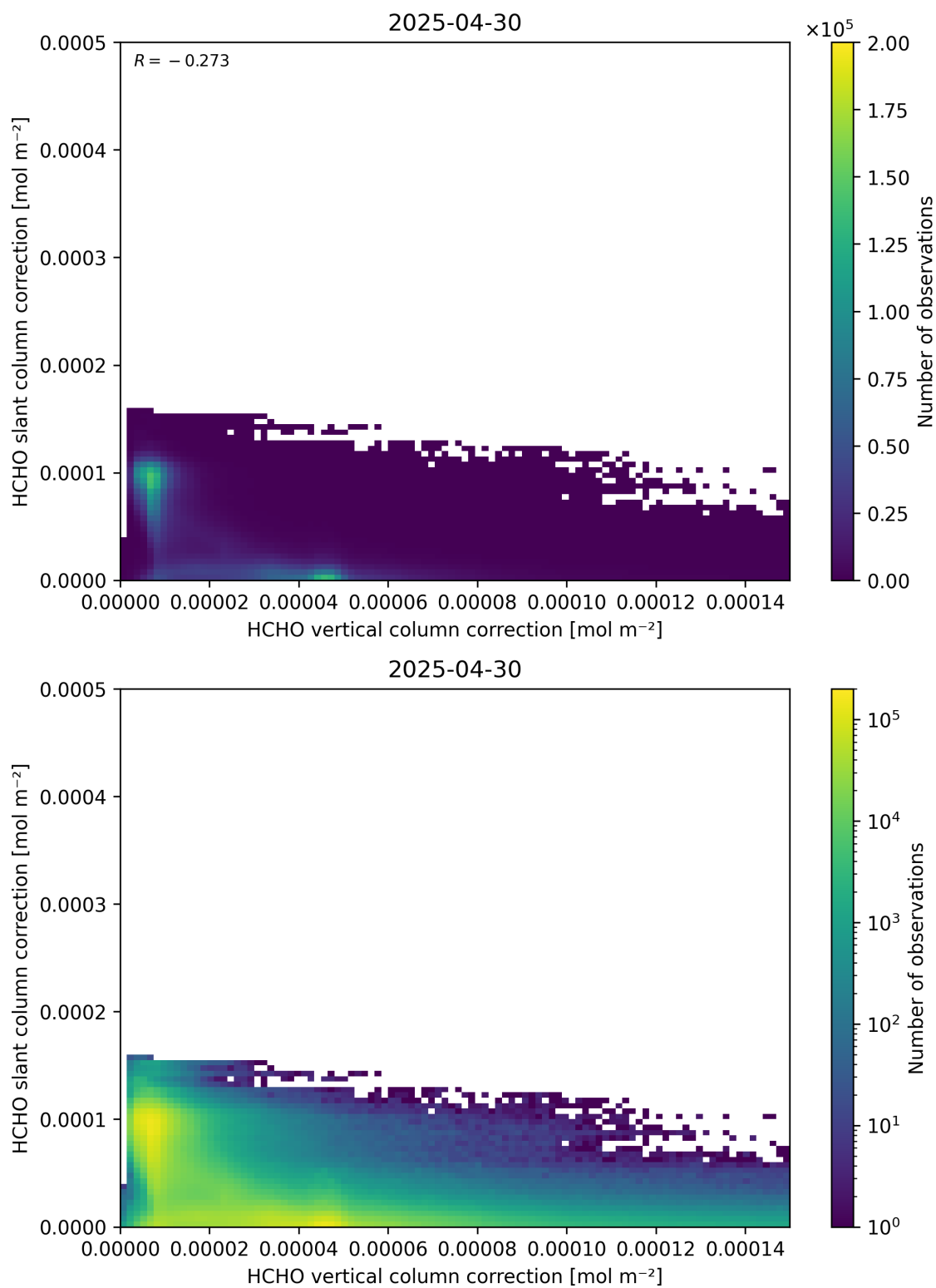
Figure 117: Scatter density plot of “HCHO vertical column correction” against “HCHO slant column correction” for 2025-04-29 to 2025-05-01.
