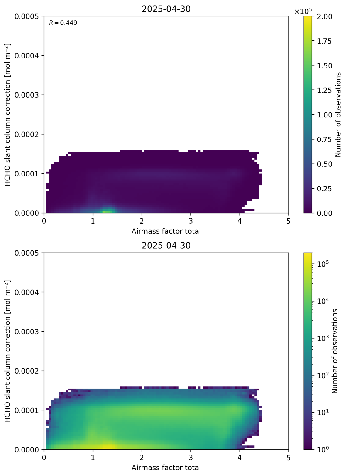
Figure 102: Scatter density plot of “Airmass factor total” against “HCHO slant column correction” for 2025-04-29 to 2025-05-01.
