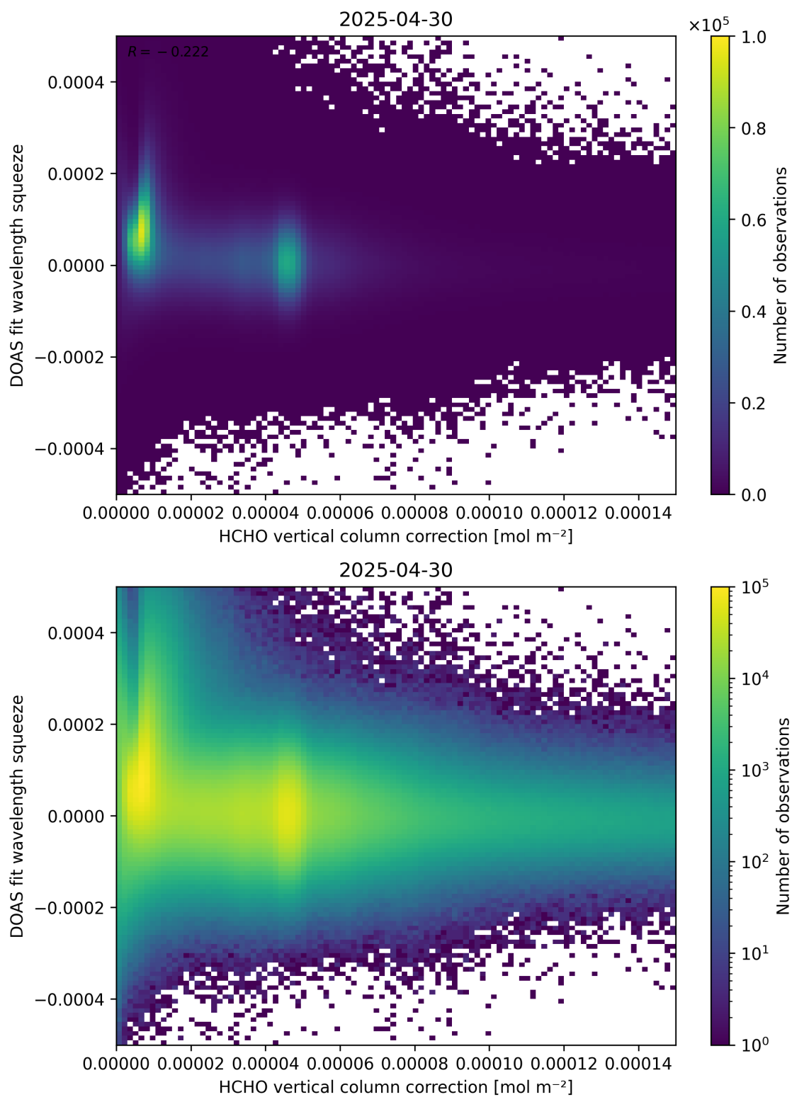
Figure 114: Scatter density plot of “HCHO vertical column correction” against “DOAS fit wavelength squeeze” for 2025-04-29 to 2025-05-01.
