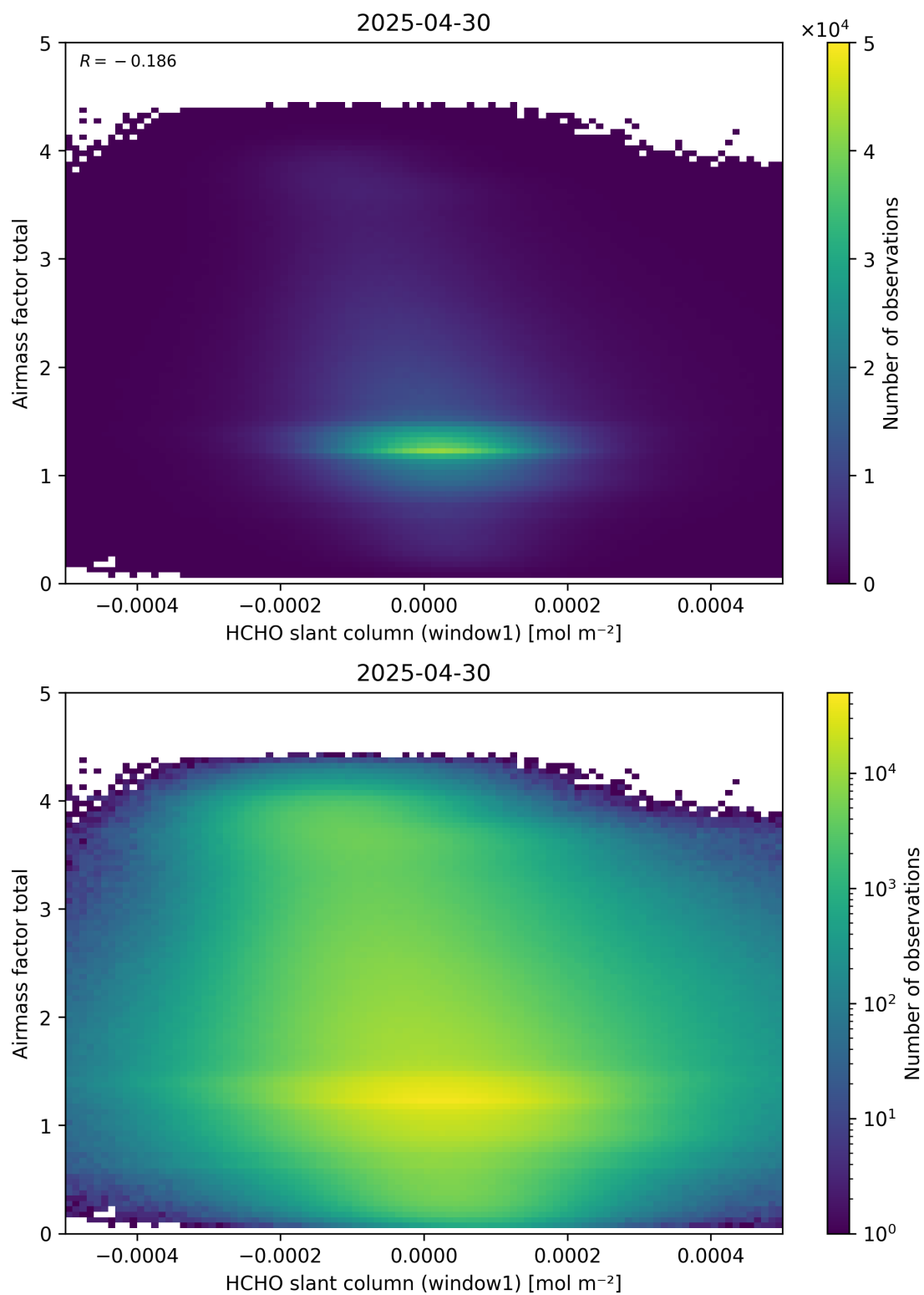
Figure 85: Scatter density plot of “HCHO slant column (window1)” against “Airmass factor total” for 2025-04-29 to 2025-05-01.
