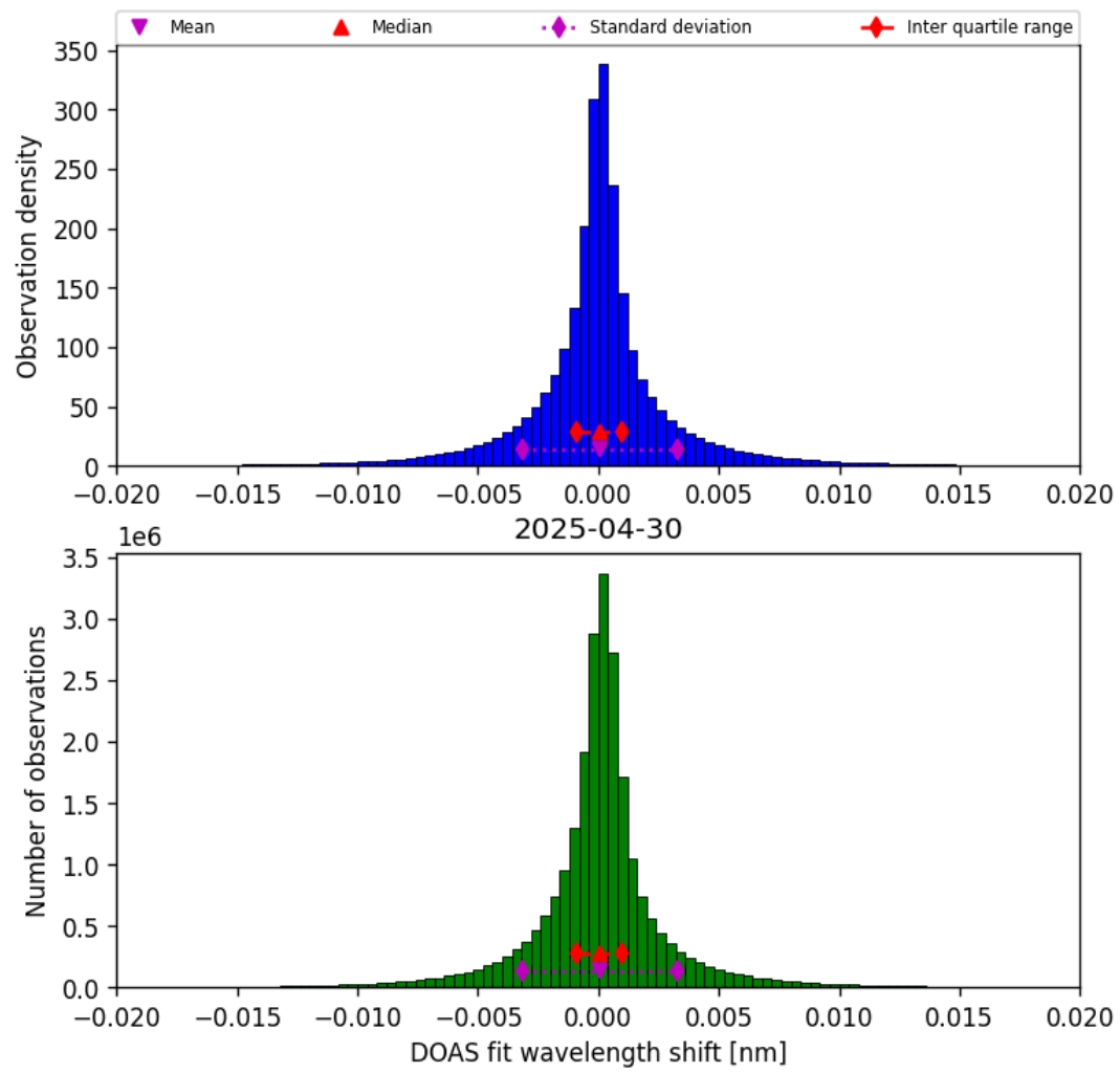
Figure 44: Histogram of “DOAS fit wavelength shift” for 2025-04-29 to 2025-05-01
