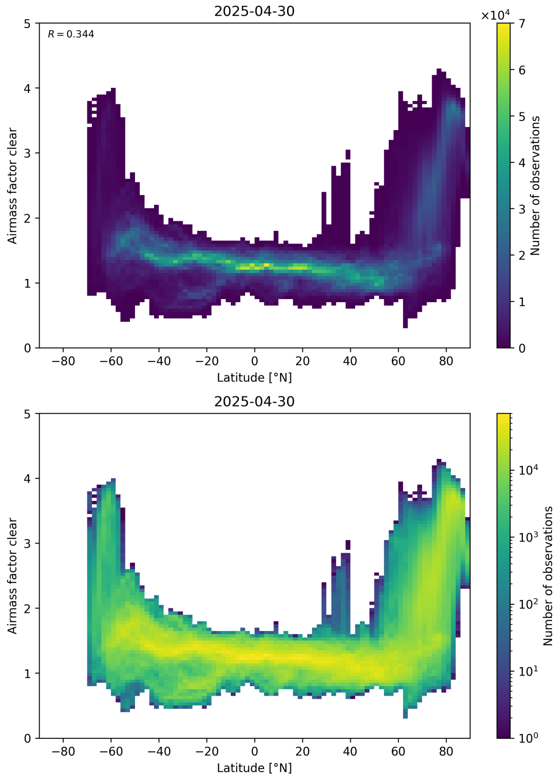
Figure 156: Scatter density plot of “Latitude” against “Airmass factor clear” for 2025-04-29 to 2025-05-01.
