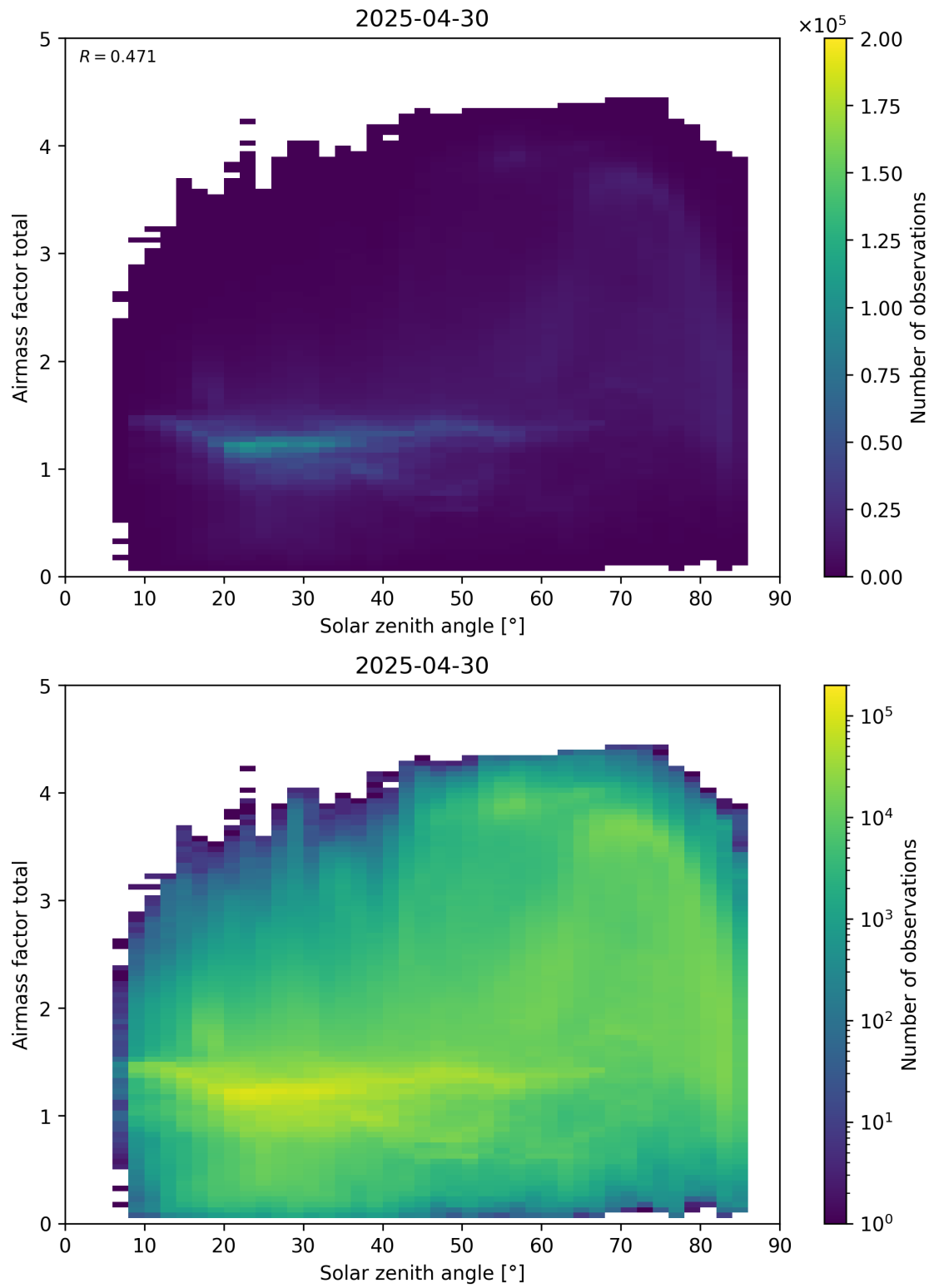
Figure 175: Scatter density plot of “Solar zenith angle” against “Airmass factor total” for 2025-04-29 to 2025-05-01.
