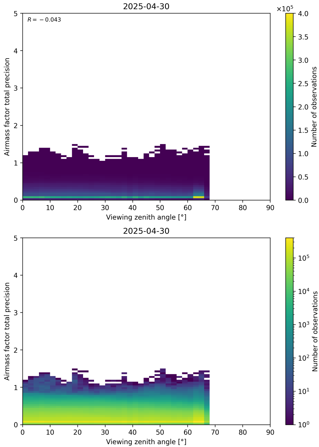
Figure 191: Scatter density plot of “Viewing zenith angle” against “Airmass factor total precision” for 2025-04-29 to 2025-05-01.
