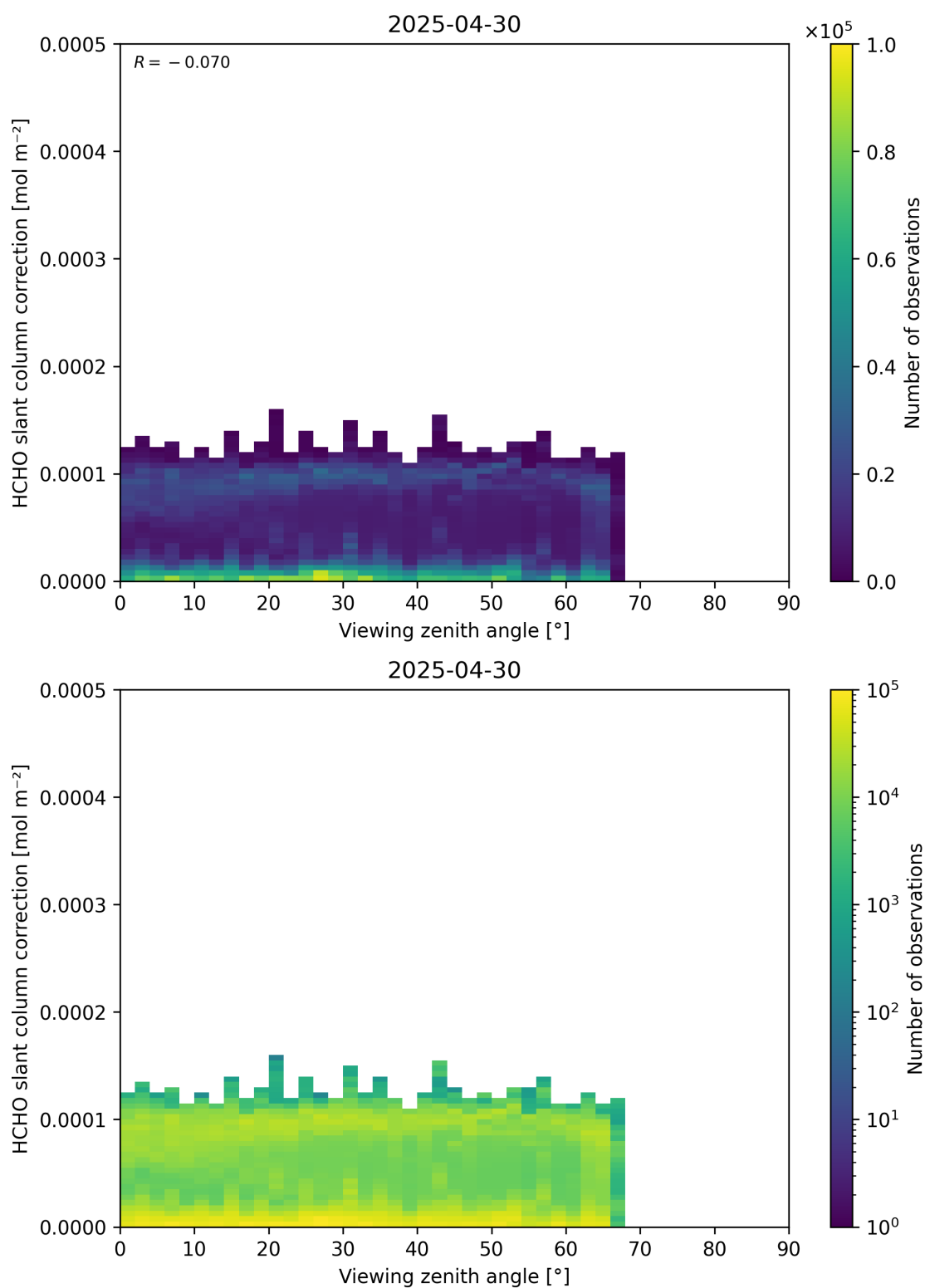
Figure 187: Scatter density plot of “Viewing zenith angle” against “HCHO slant column correction” for 2025-04-29 to 2025-05-01.
