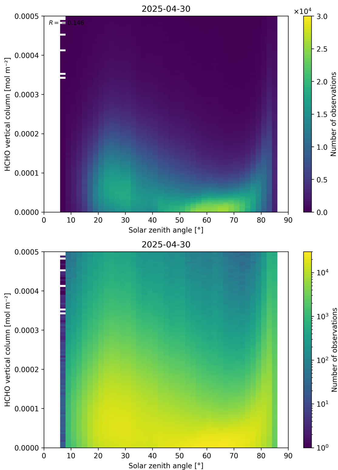
Figure 177: Scatter density plot of “Solar zenith angle” against “HCHO vertical column” for 2025-04-29 to 2025-05-01.
