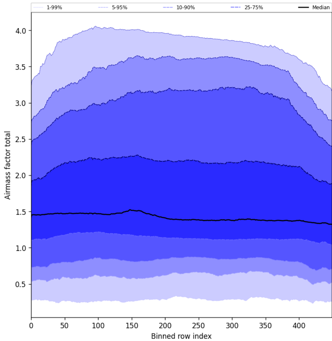
Figure 54: Along track statistics of “Airmass factor total” for 2025-04-29 to 2025-05-01
