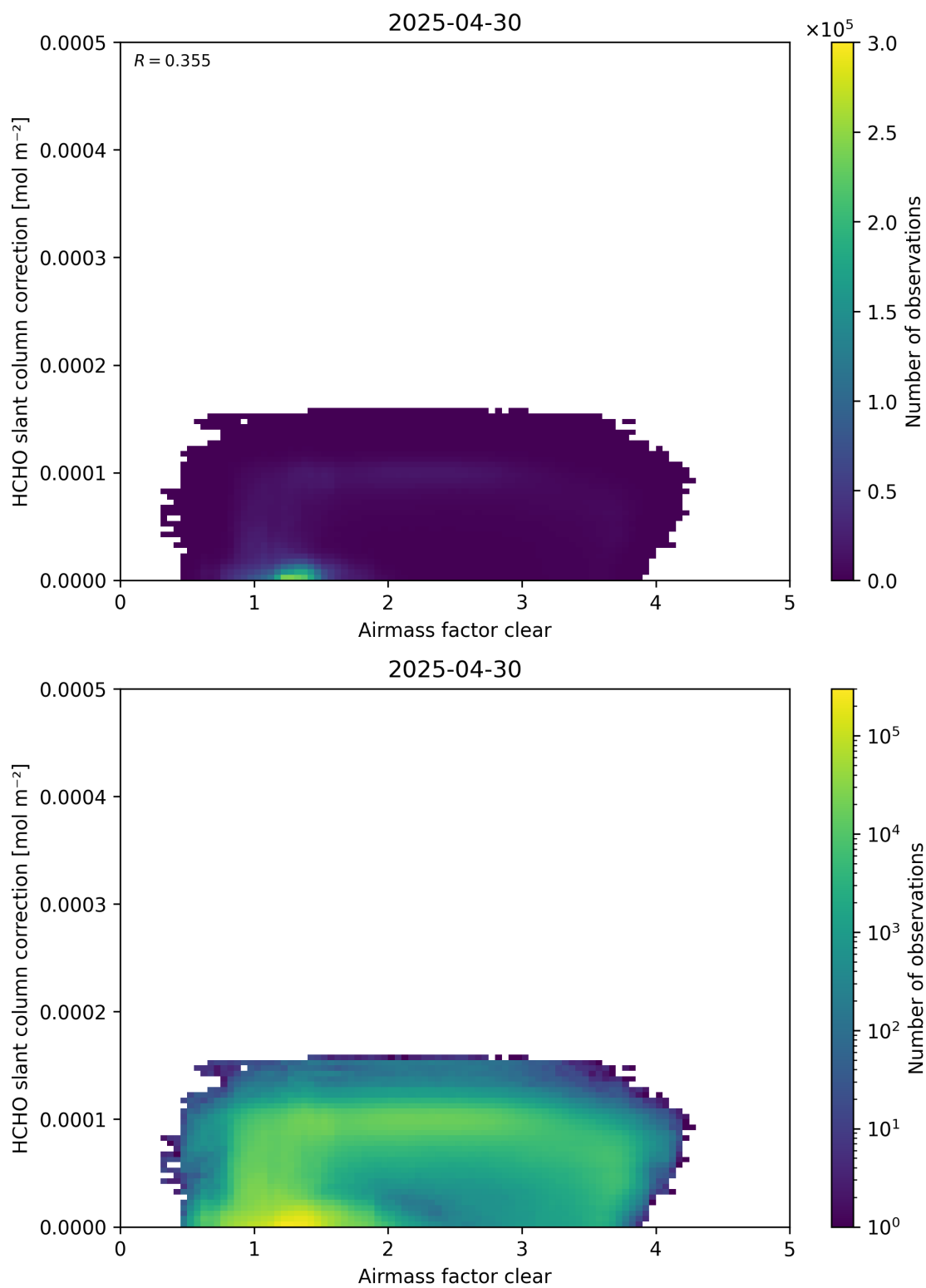
Figure 75: Scatter density plot of “Airmass factor clear” against “HCHO slant column correction” for 2025-04-29 to 2025-05-01.
