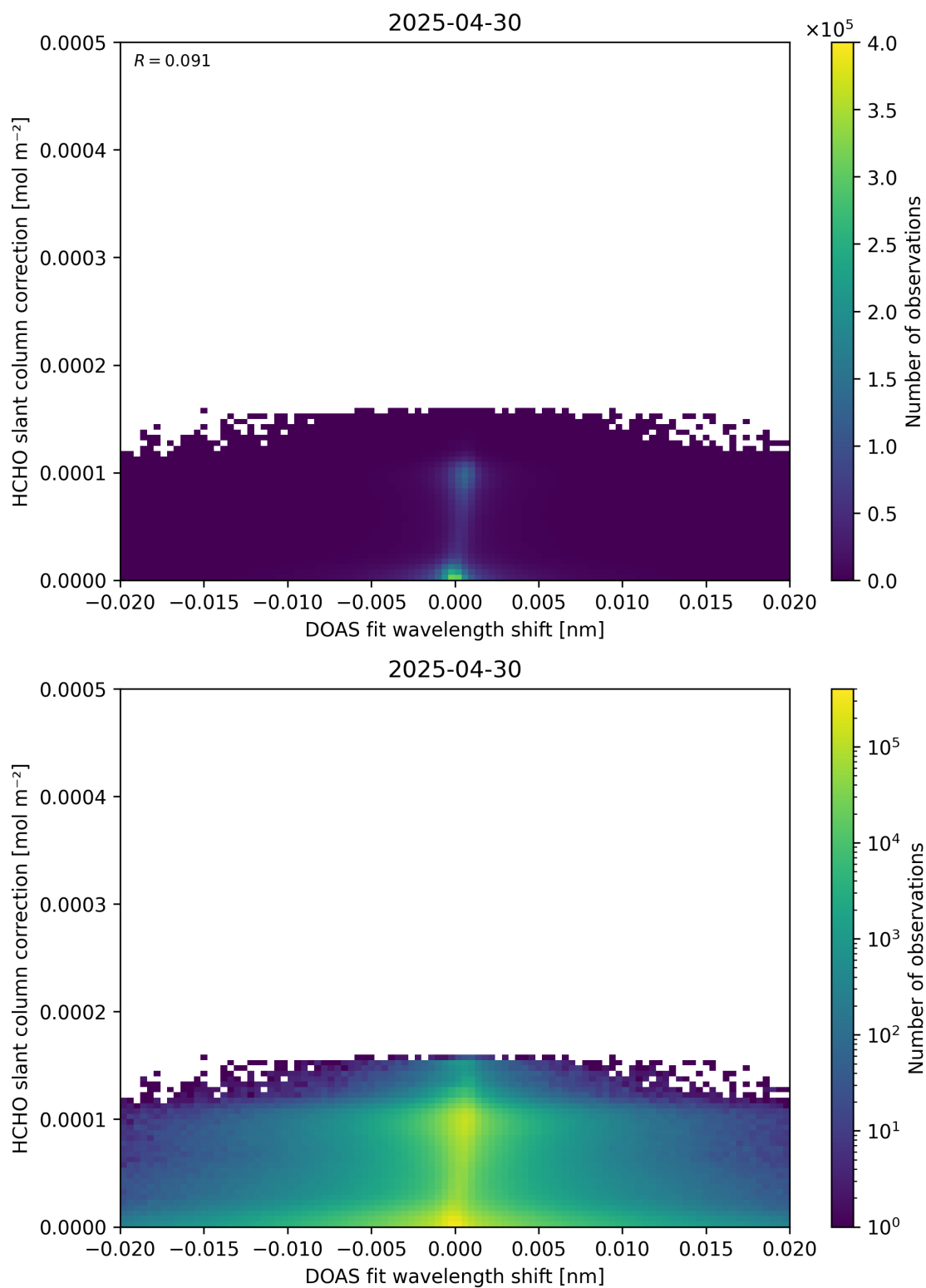
Figure 67: Scatter density plot of “DOAS fit wavelength shift” against “HCHO slant column correction” for 2025-04-29 to 2025-05-01.
