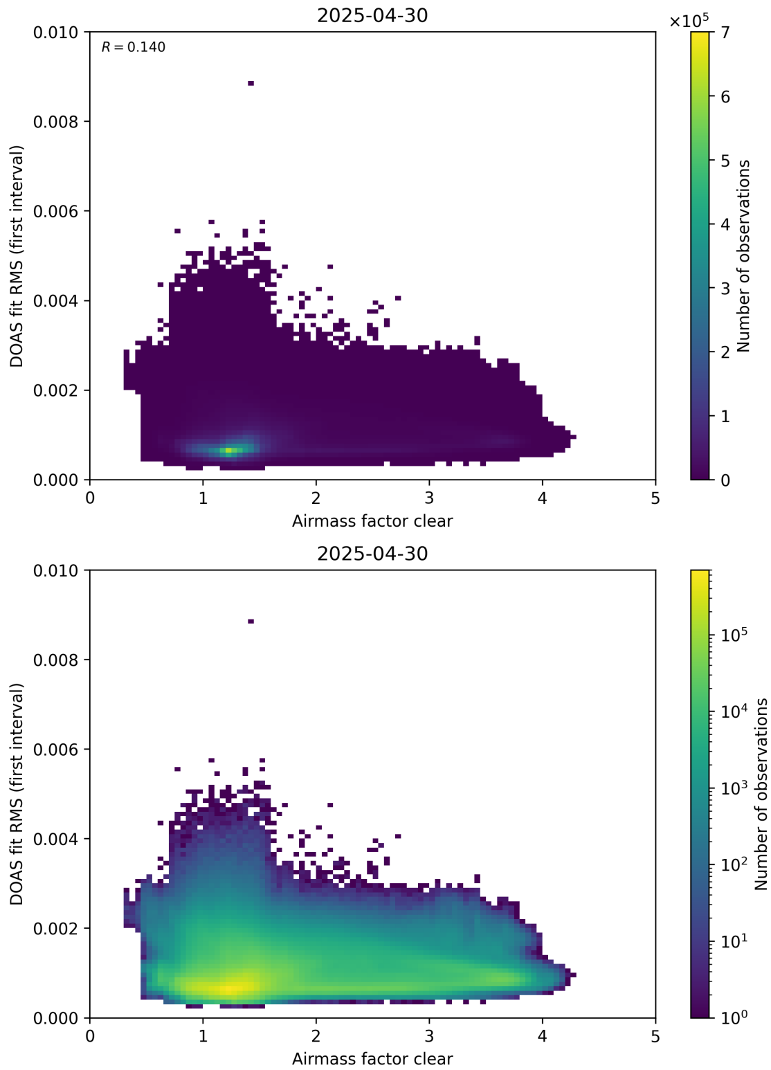
Figure 71: Scatter density plot of “Airmass factor clear” against “DOAS fit RMS (first interval)” for 2025-04-29 to 2025-05-01.
