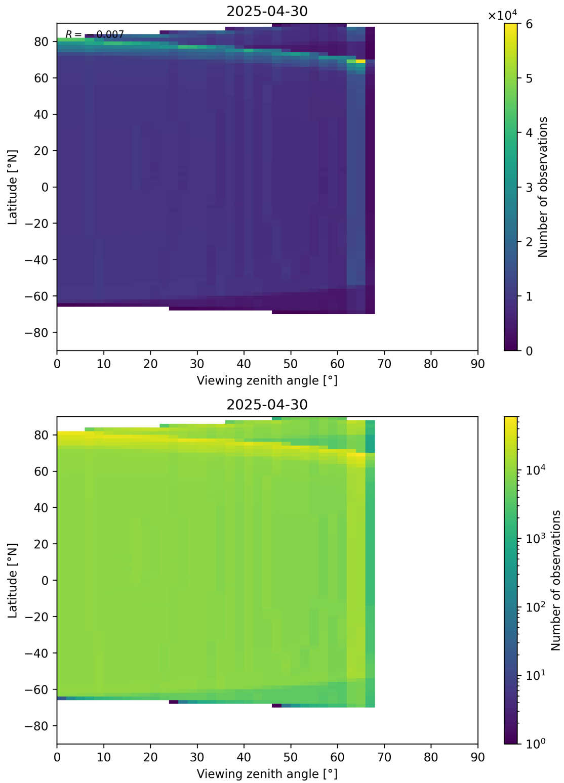
Figure 196: Scatter density plot of “Viewing zenith angle” against “Latitude” for 2025-04-29 to 2025-05-01.
