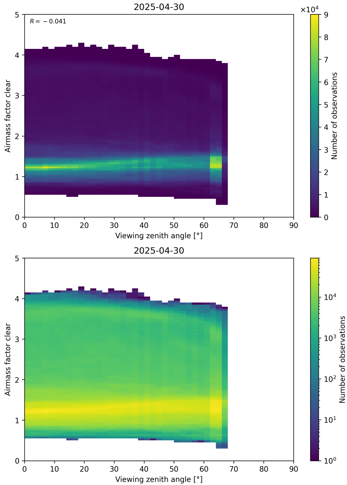
Figure 185: Scatter density plot of “Viewing zenith angle” against “Airmass factor clear” for 2025-04-29 to 2025-05-01.
