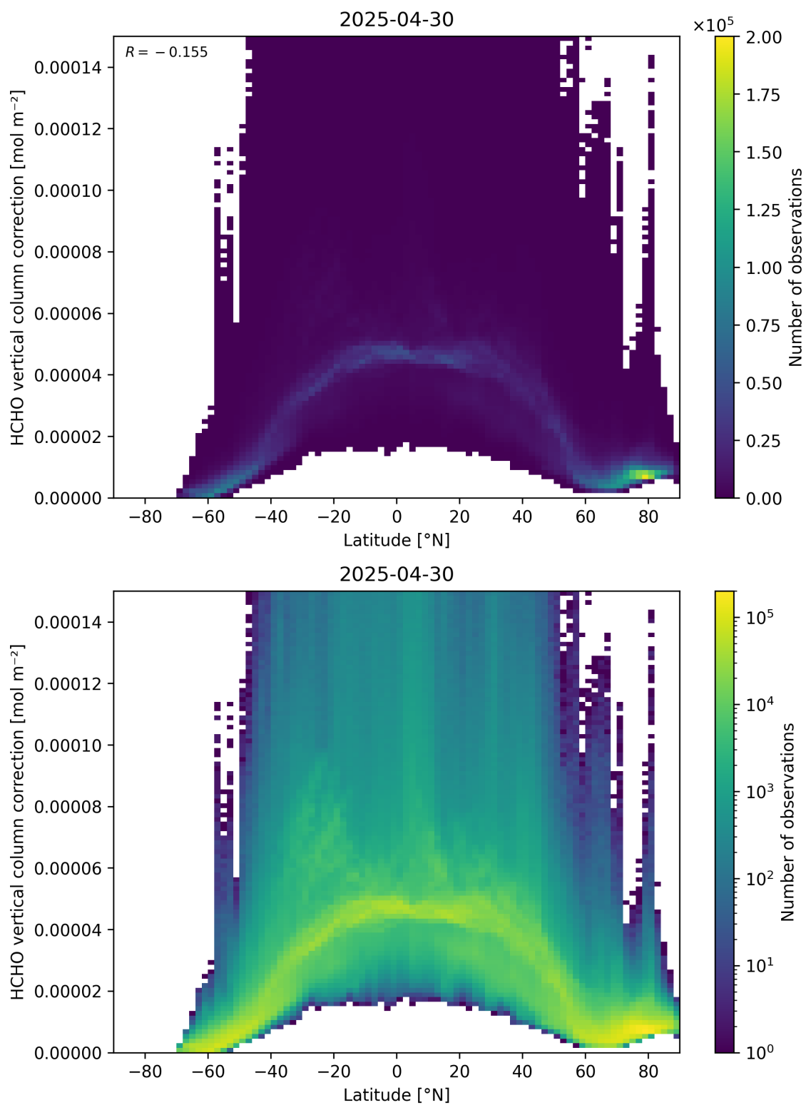
Figure 164: Scatter density plot of “Latitude” against “HCHO vertical column correction” for 2025-04-29 to 2025-05-01.
