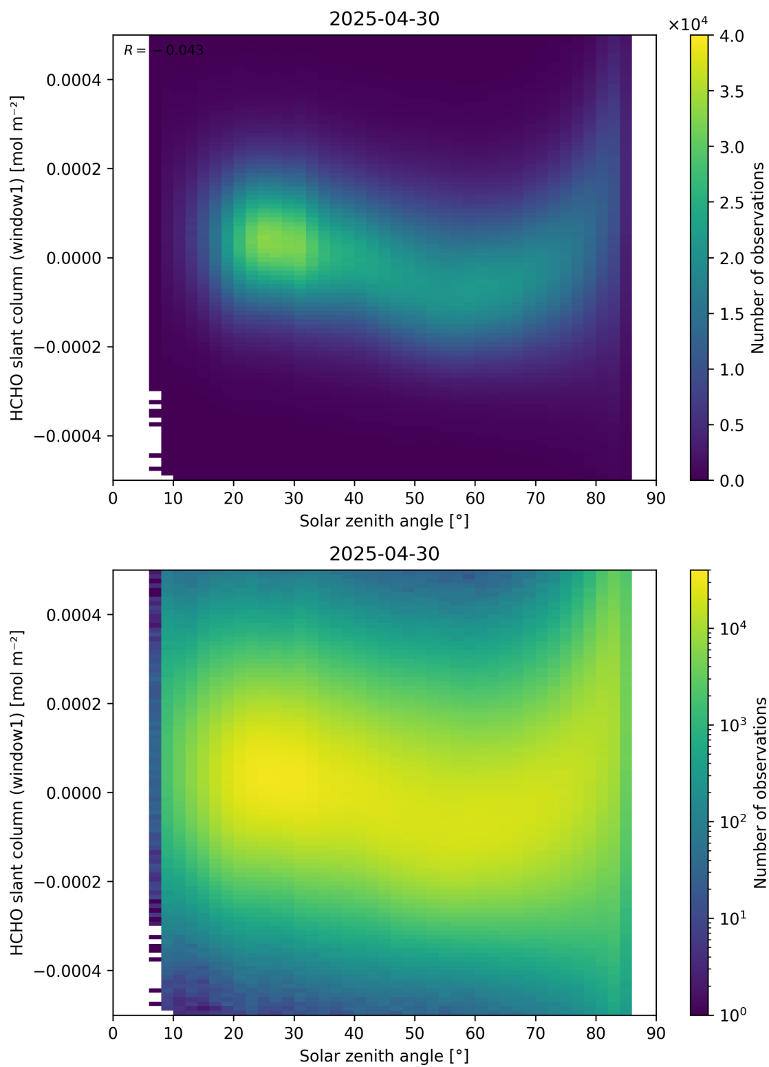
Figure 173: Scatter density plot of “Solar zenith angle” against “HCHO slant column (window1)” for 2025-04-29 to 2025-05-01.
