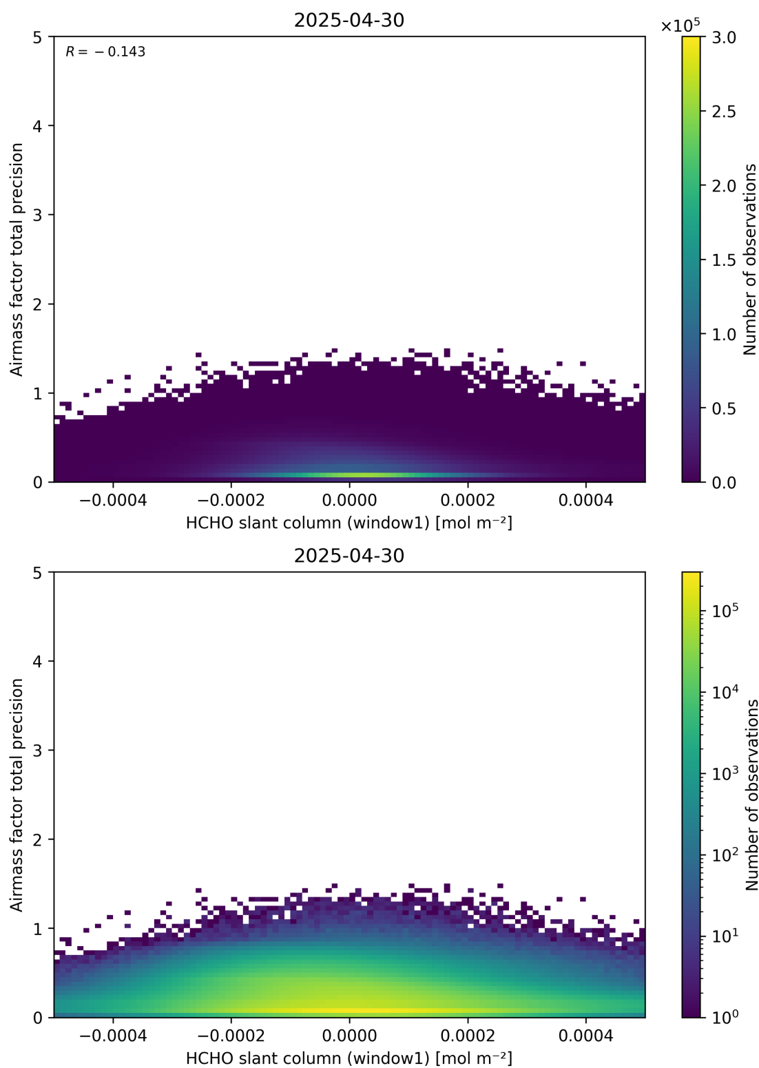
Figure 86: Scatter density plot of “HCHO slant column (window1)” against “Airmass factor total precision” for 2025-04-29 to 2025-05-01.
