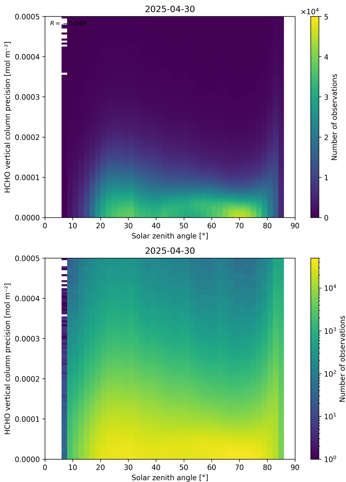
Figure 179: Scatter density plot of “Solar zenith angle” against “HCHO vertical column precision” for 2025-04-29 to 2025-05-01.
