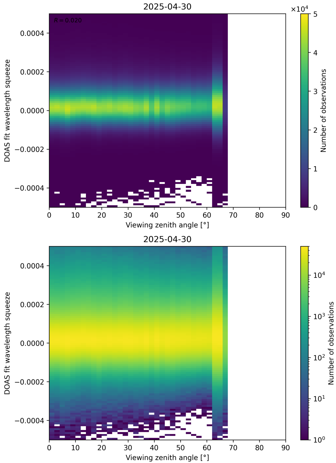
Figure 184: Scatter density plot of “Viewing zenith angle” against “DOAS fit wavelength squeeze” for 2025-04-29 to 2025-05-01.
