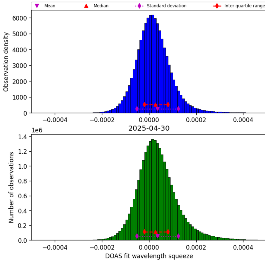
Figure 45: Histogram of “DOAS fit wavelength squeeze” for 2025-04-29 to 2025-05-01
