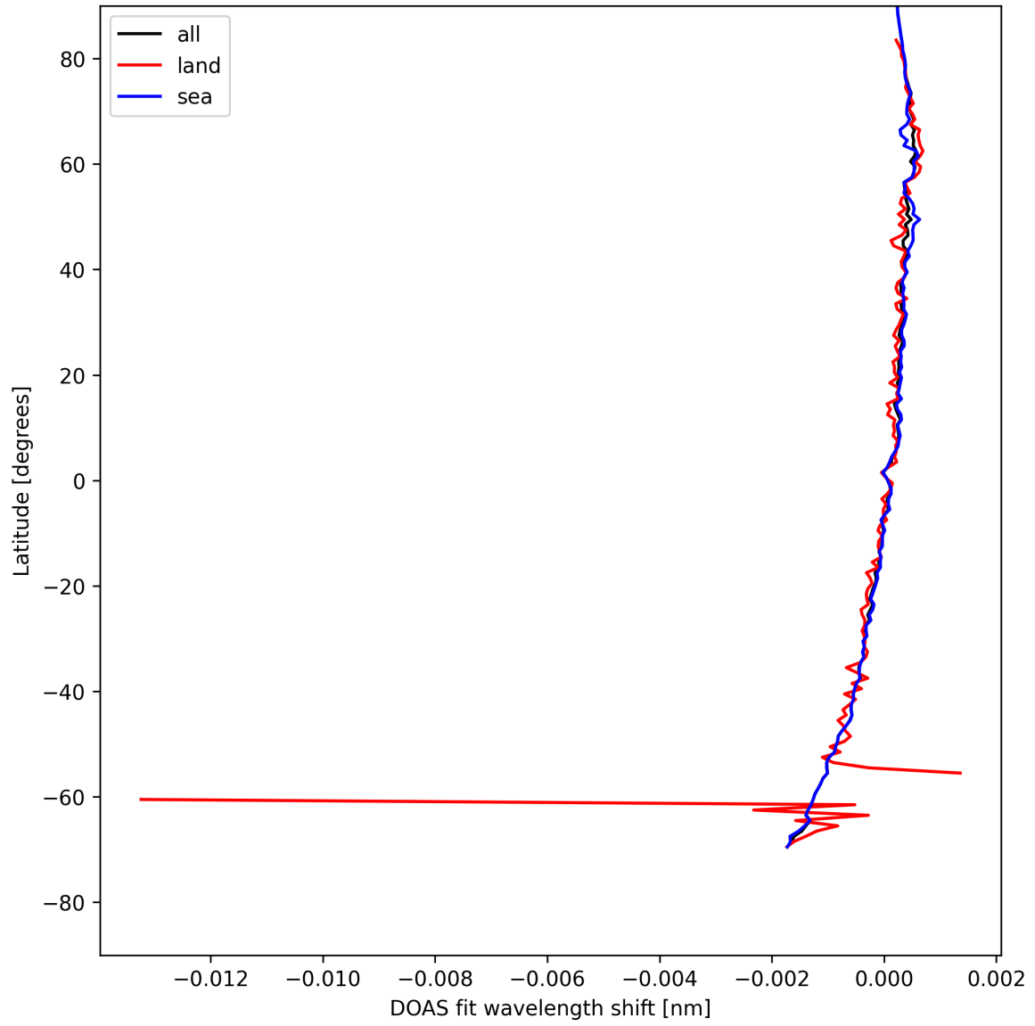
Figure 30: Zonal average of “DOAS fit wavelength shift” for 2025-04-29 to 2025-05-01.
