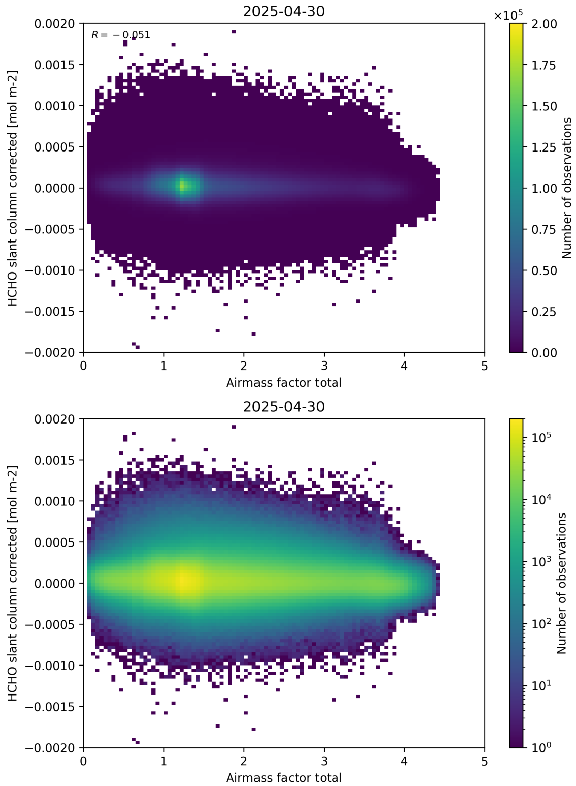
Figure 101: Scatter density plot of “Airmass factor total” against “HCHO slant column corrected” for 2025-04-29 to 2025-05-01.
