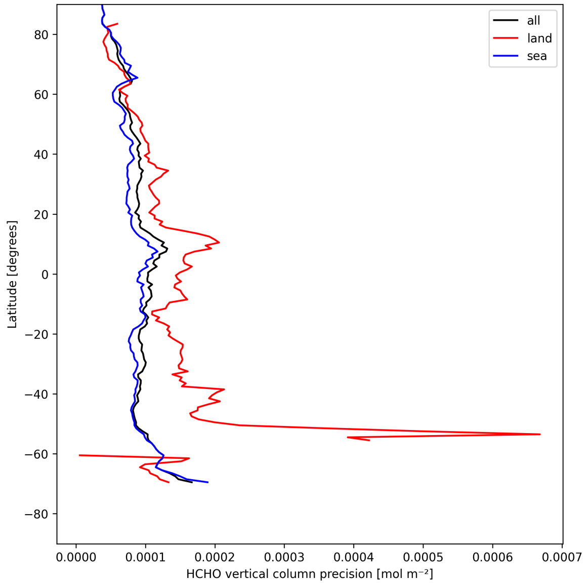
Figure 22: Zonal average of “HCHO vertical column precision” for 2025-04-29 to 2025-05-01.
