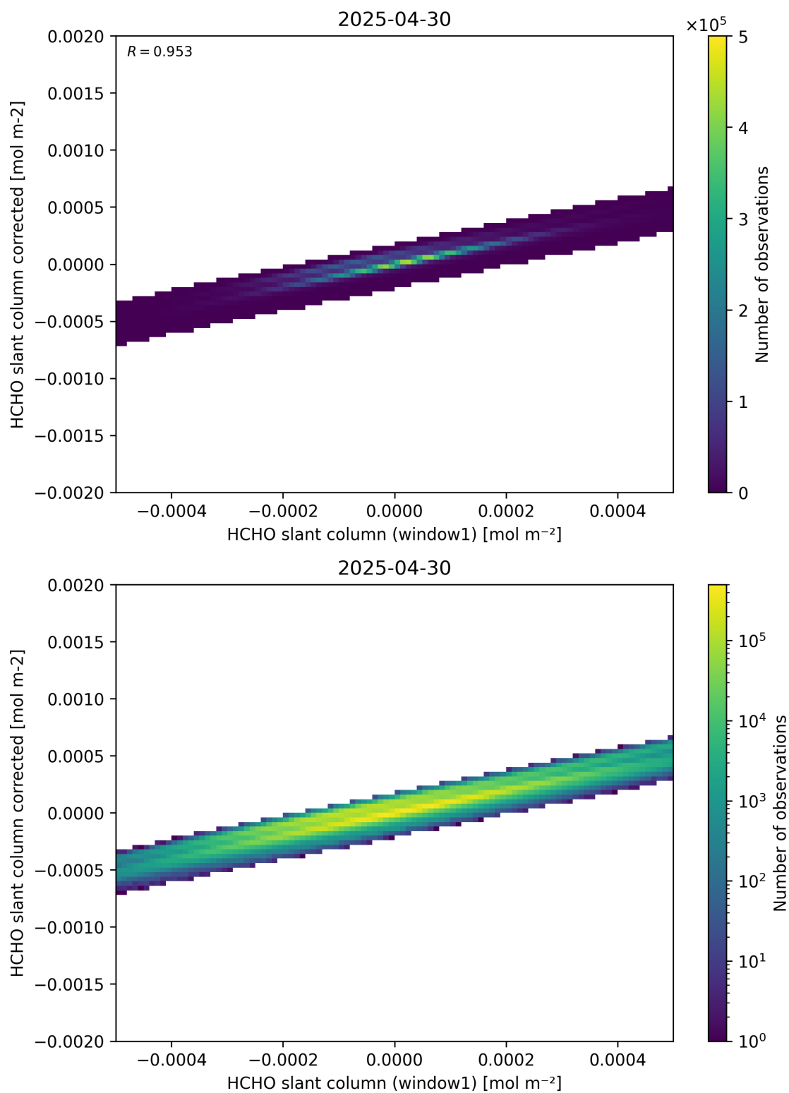
Figure 82: Scatter density plot of “HCHO slant column (window1)” against “HCHO slant column corrected” for 2025-04-29 to 2025-05-01.
