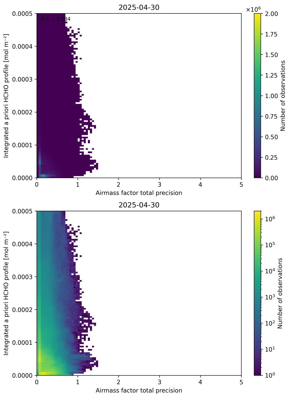
Figure 111: Scatter density plot of “Airmass factor total precision” against “Integrated a priori HCHO profile” for 2025-04-29 to 2025-05-01.
