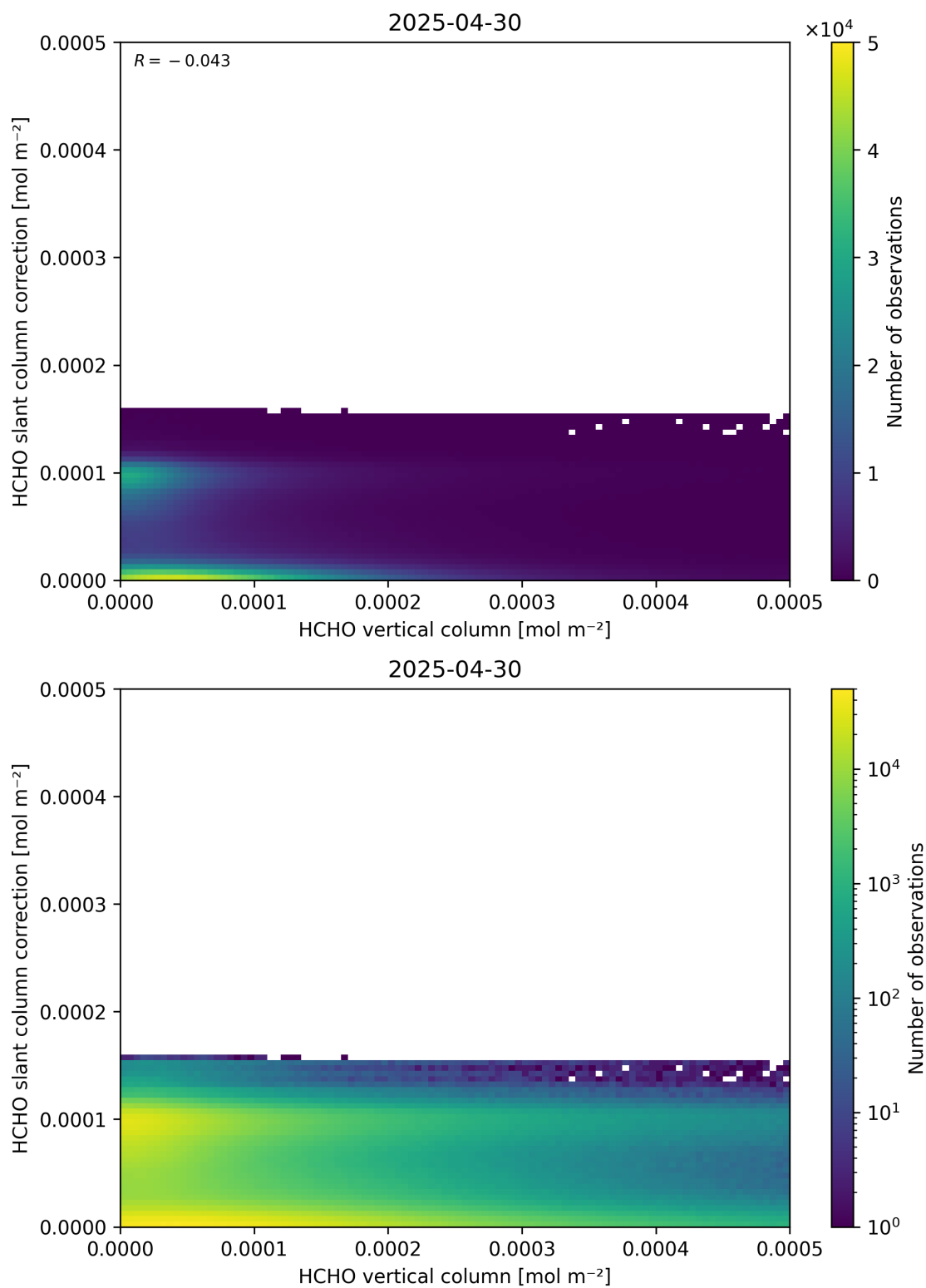
Figure 128: Scatter density plot of “HCHO vertical column” against “HCHO slant column correction” for 2025-04-29 to 2025-05-01.
