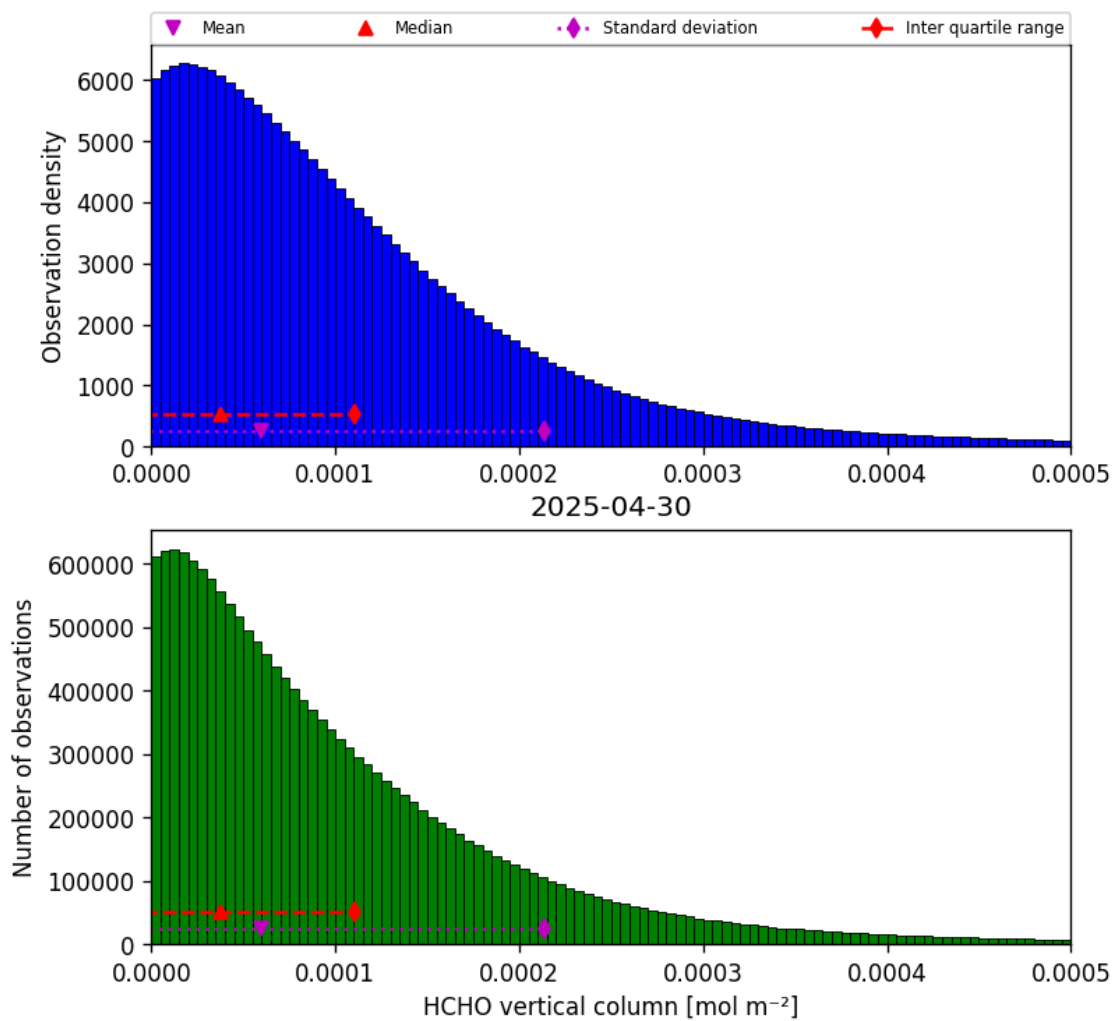
Figure 35: Histogram of “HCHO vertical column” for 2025-04-29 to 2025-05-01
