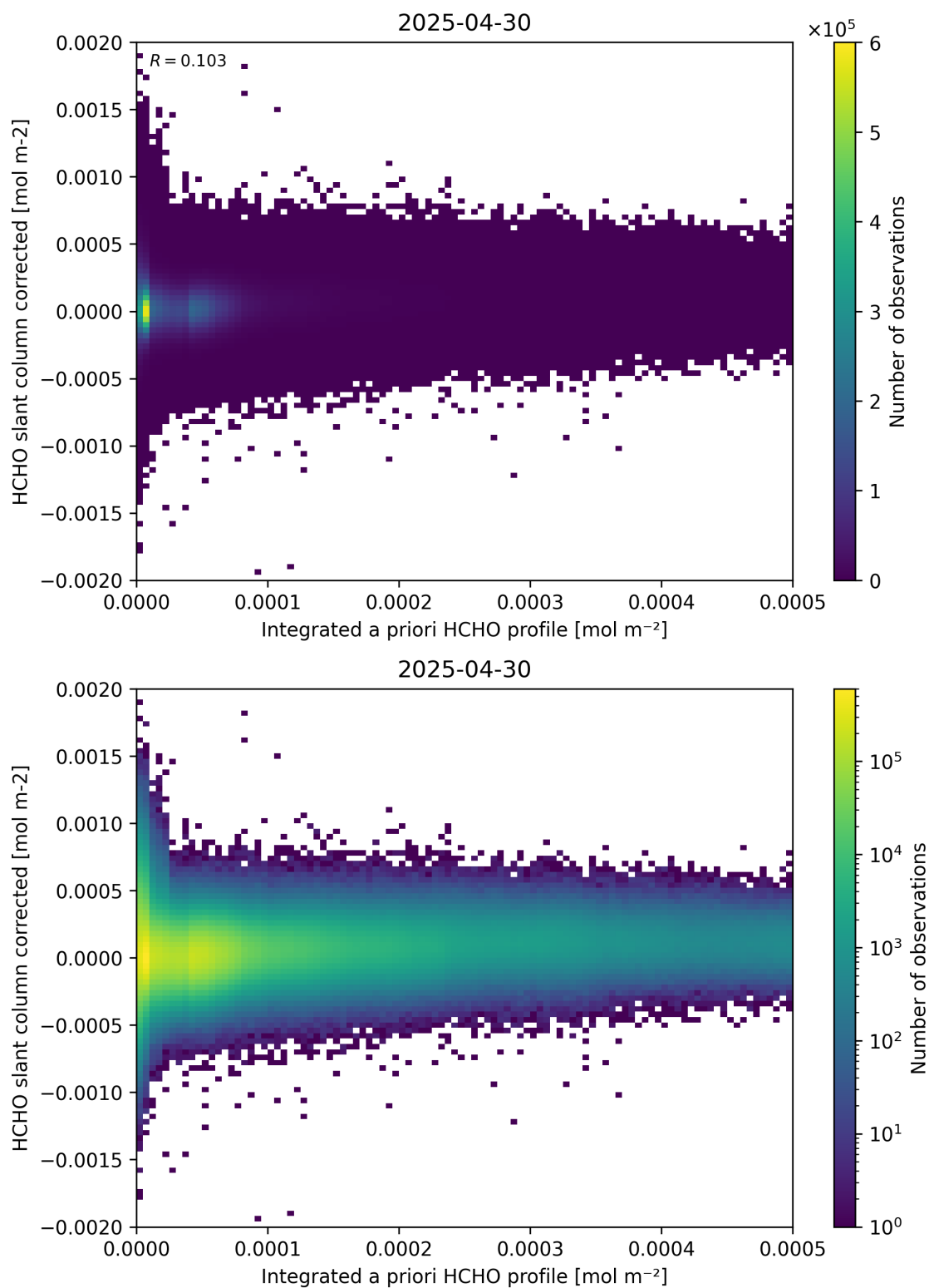
Figure 151: Scatter density plot of “Integrated a priori HCHO profile” against “HCHO slant column corrected” for 2025-04-29 to 2025-05-01.
