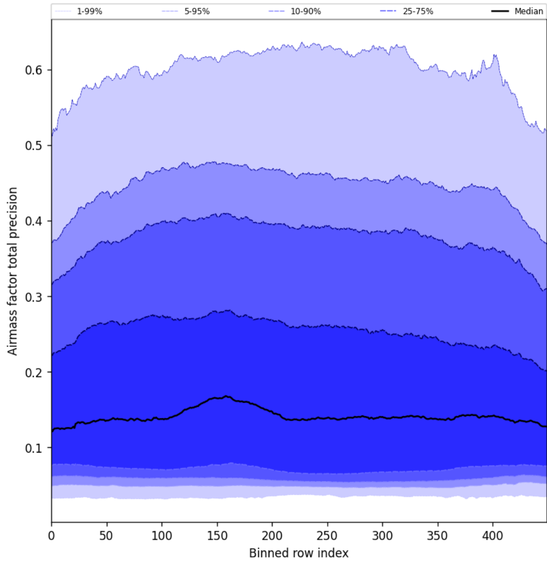
Figure 55: Along track statistics of “Airmass factor total precision” for 2025-04-29 to 2025-05-01
