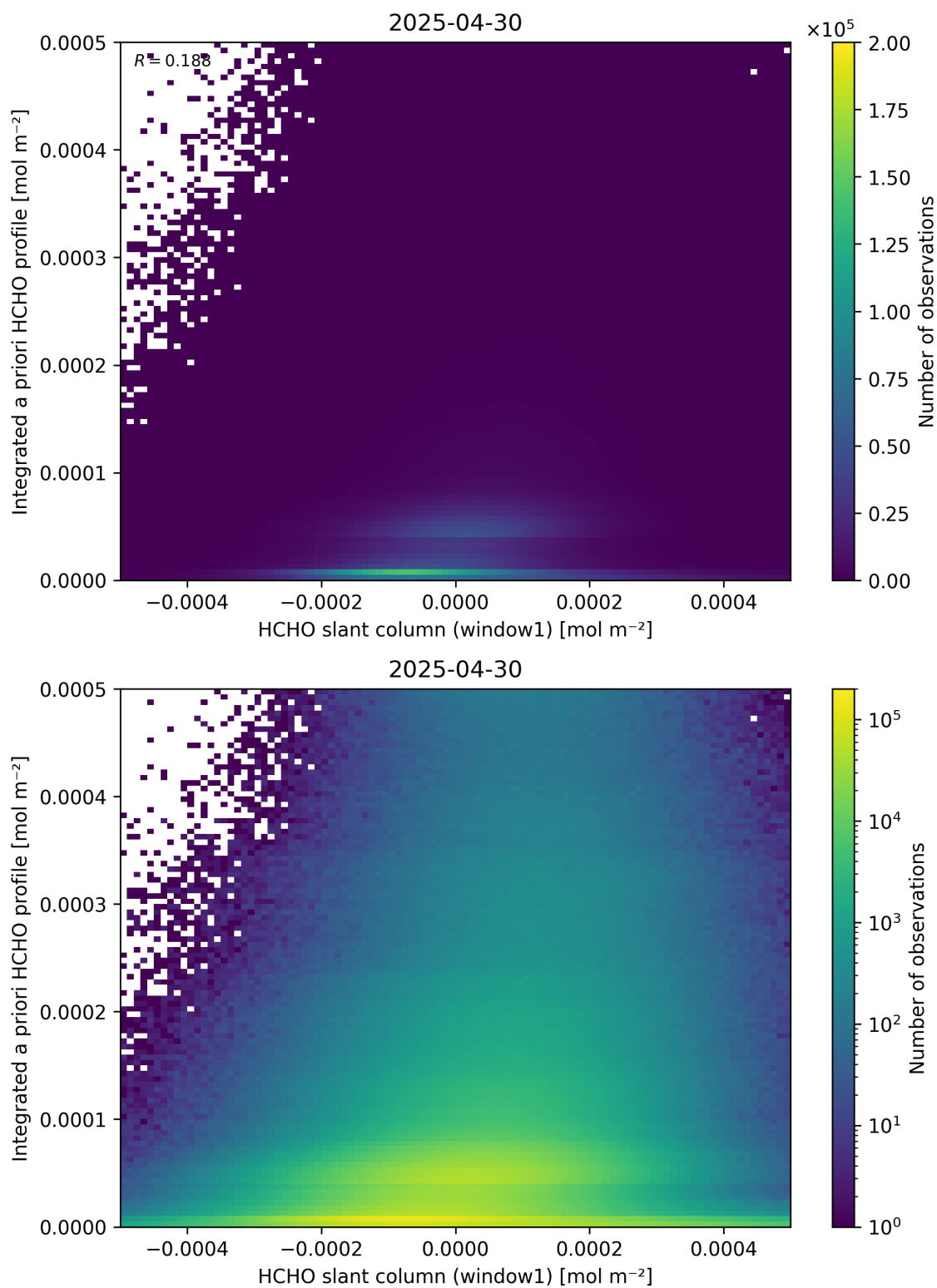
Figure 87: Scatter density plot of “HCHO slant column (window1)” against “Integrated a priori HCHO profile” for 2025-04-29 to 2025-05-01.
