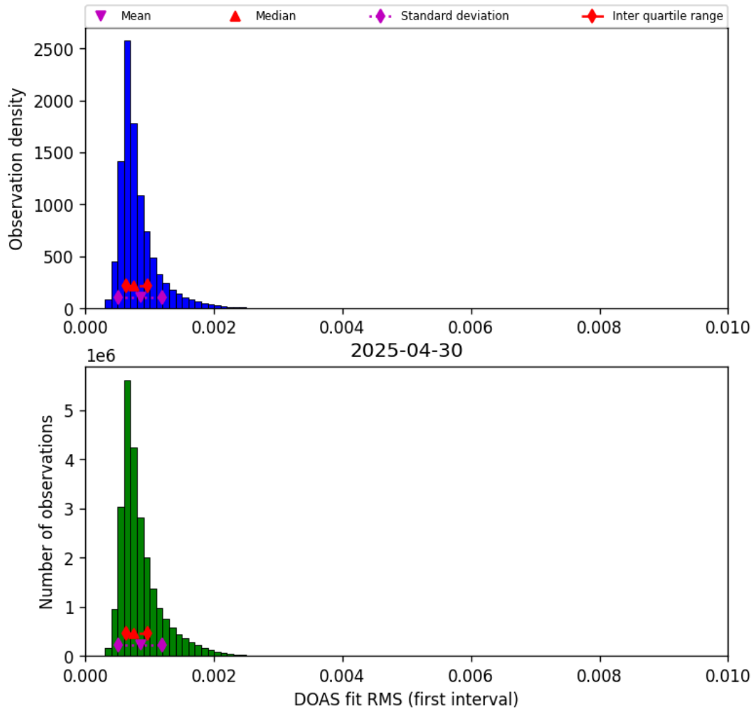
Figure 46: Histogram of “DOAS fit RMS (first interval)” for 2025-04-29 to 2025-05-01
