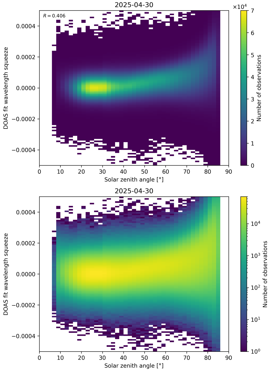
Figure 169: Scatter density plot of “Solar zenith angle” against “DOAS fit wavelength squeeze” for 2025-04-29 to 2025-05-01.
