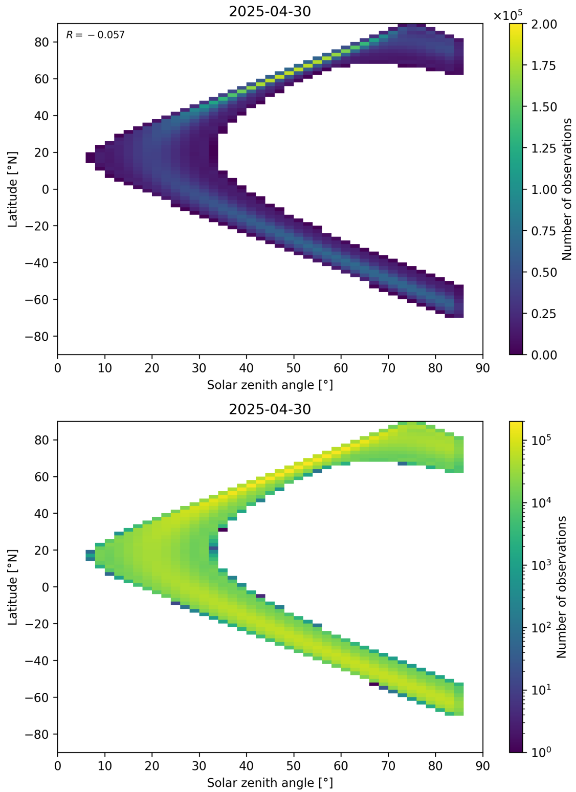
Figure 181: Scatter density plot of “Solar zenith angle” against “Latitude” for 2025-04-29 to 2025-05-01.
