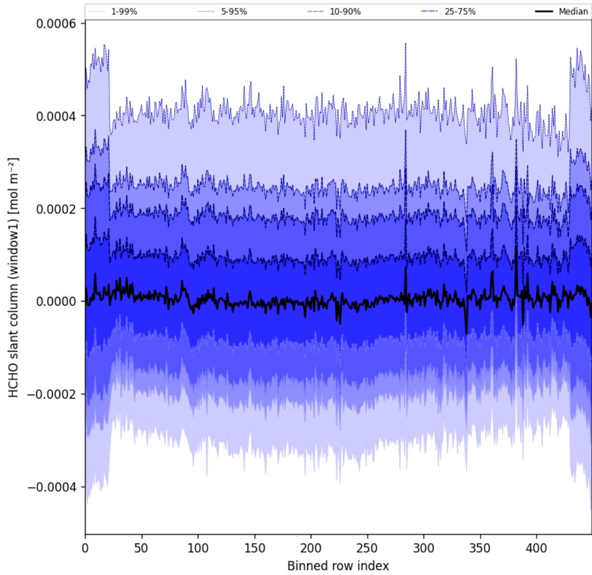
Figure 52: Along track statistics of “HCHO slant column (window1)” for 2025-04-29 to 2025-05-01
