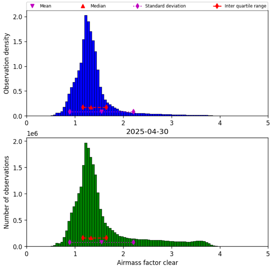
Figure 42: Histogram of “Airmass factor clear” for 2025-04-29 to 2025-05-01
