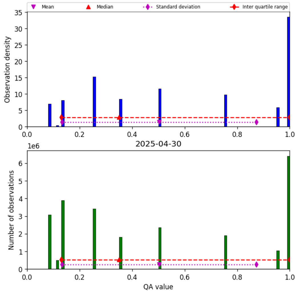
Figure 34: Histogram of “QA value” for 2025-04-29 to 2025-05-01
