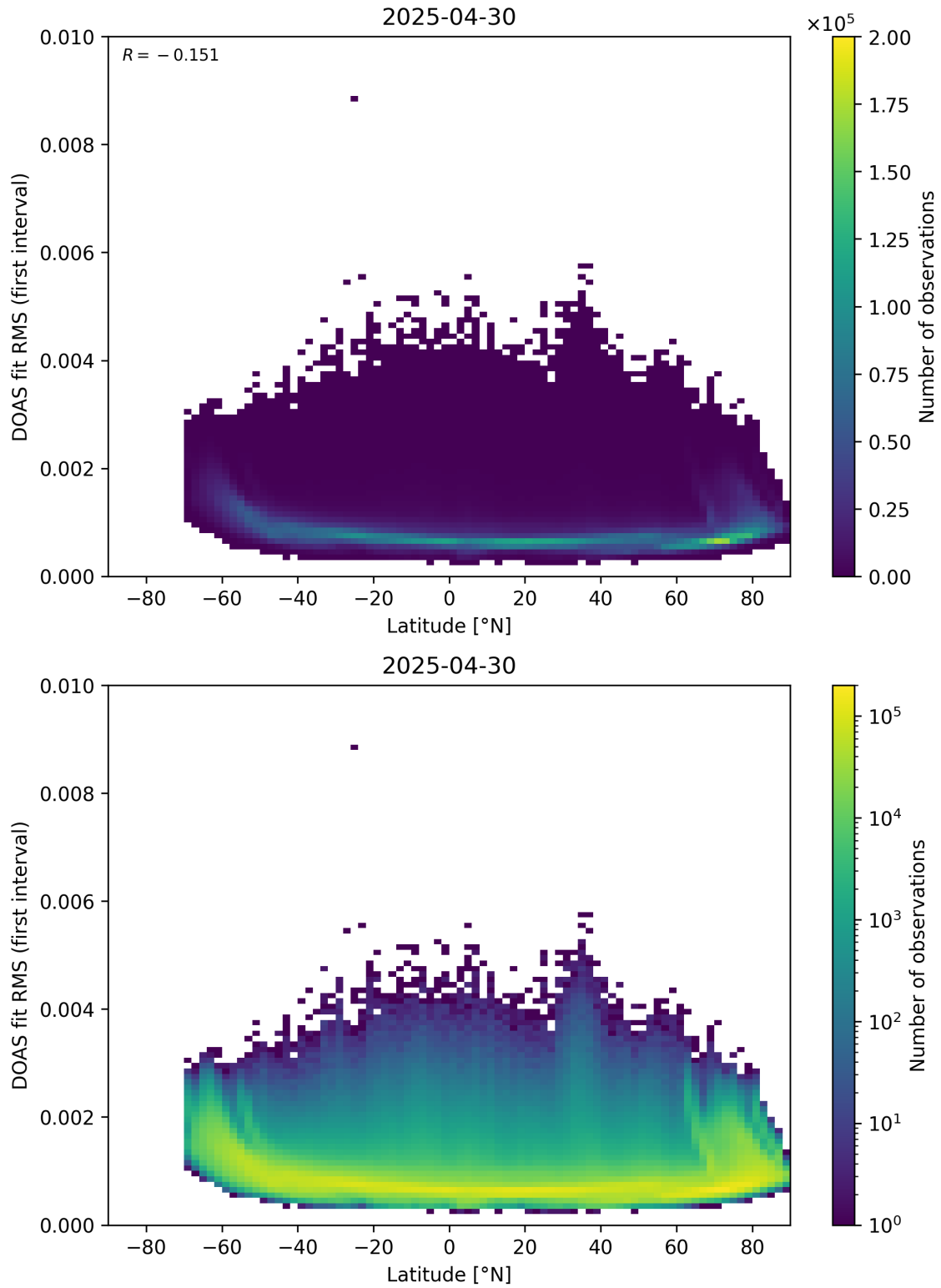
Figure 153: Scatter density plot of “Latitude” against “DOAS fit RMS (first interval)” for 2025-04-29 to 2025-05-01.
