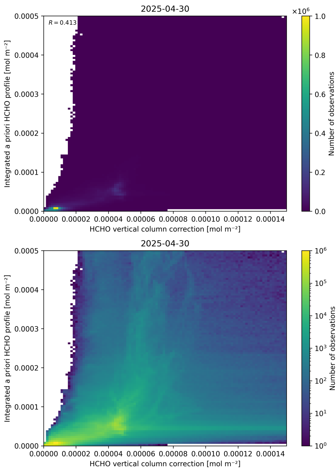
Figure 122: Scatter density plot of “HCHO vertical column correction” against “Integrated a priori HCHO profile” for 2025-04-29 to 2025-05-01.
