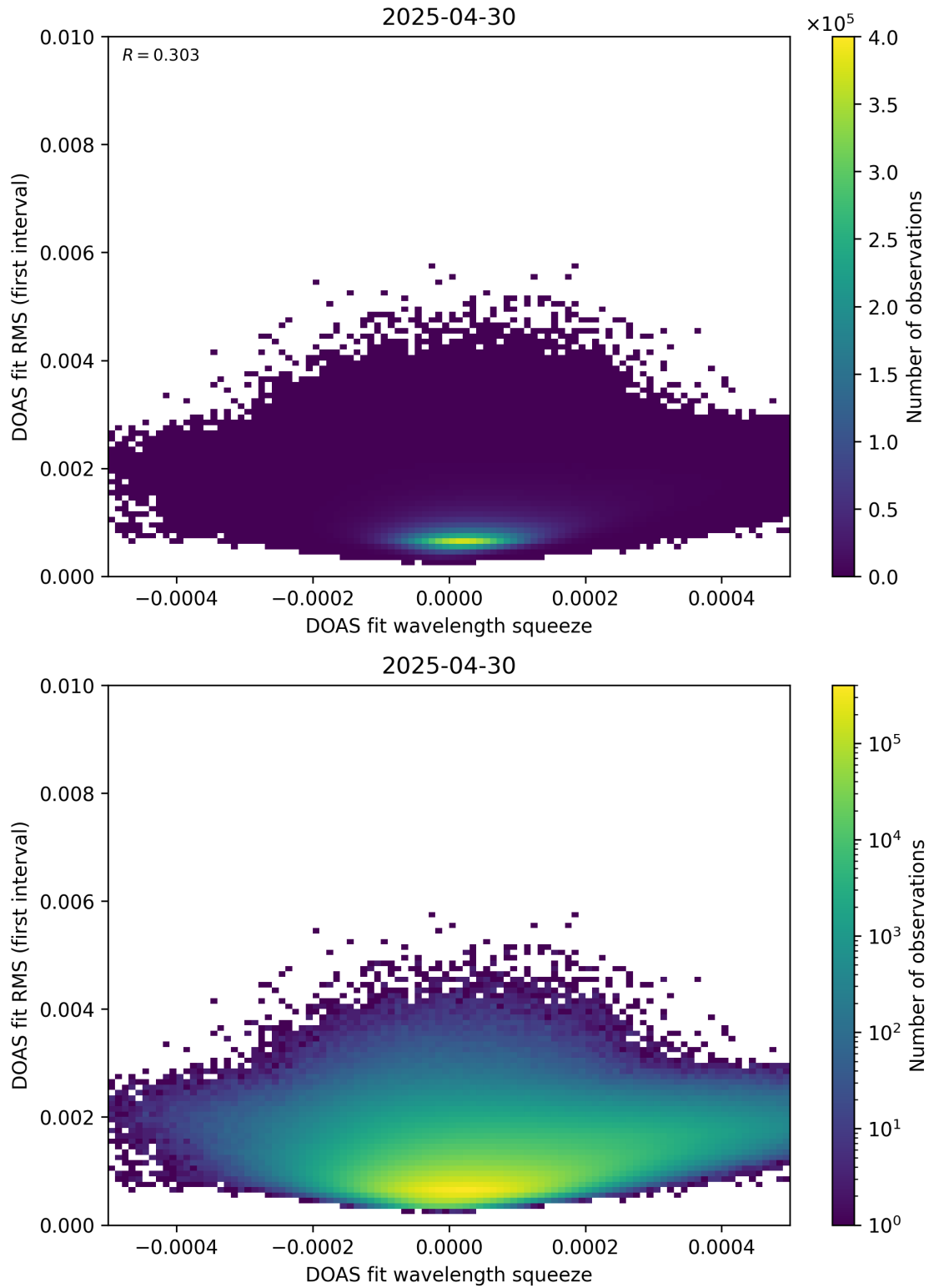
Figure 68: Scatter density plot of “DOAS fit wavelength squeeze” against “DOAS fit RMS (first interval)” for 2025-04-29 to 2025-05-01.
