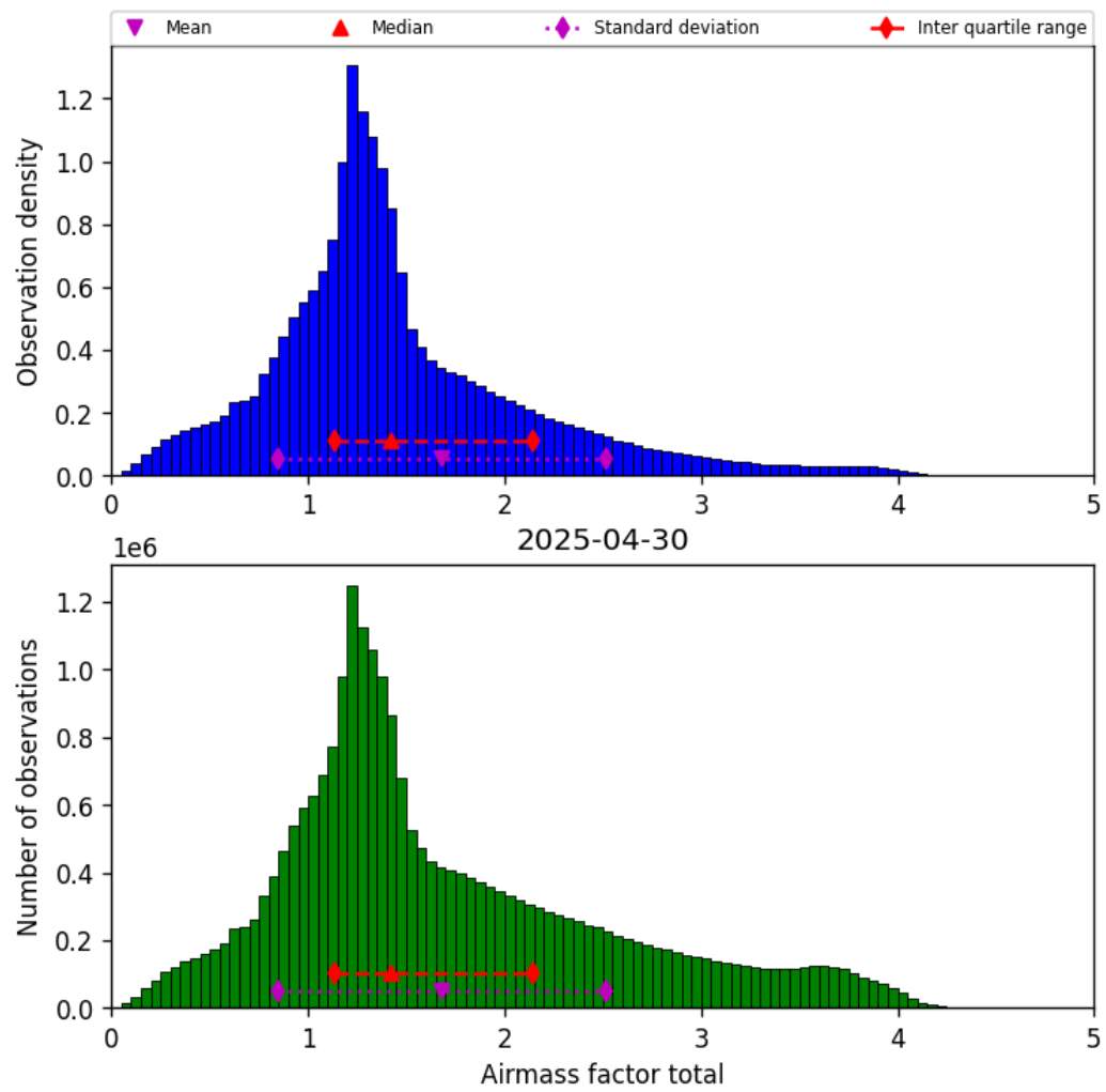
Figure 40: Histogram of “Airmass factor total” for 2025-04-29 to 2025-05-01
