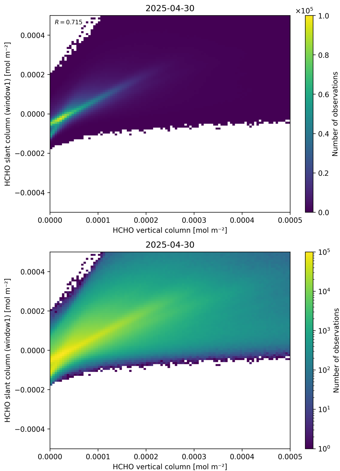
Figure 129: Scatter density plot of “HCHO vertical column” against “HCHO slant column (window1)” for 2025-04-29 to 2025-05-01.
