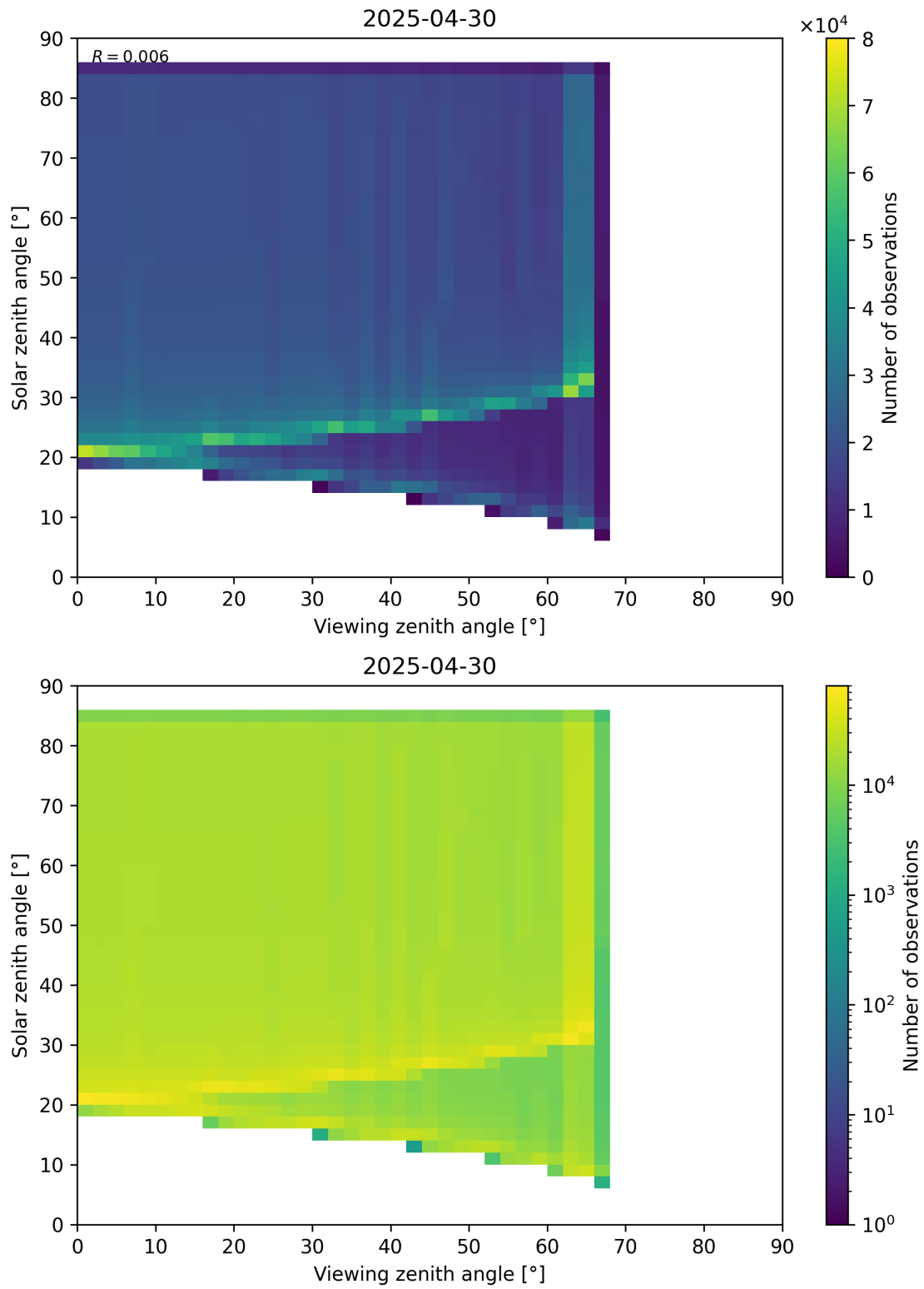
Figure 197: Scatter density plot of “Viewing zenith angle” against “Solar zenith angle” for 2025-04-29 to 2025-05-01.
