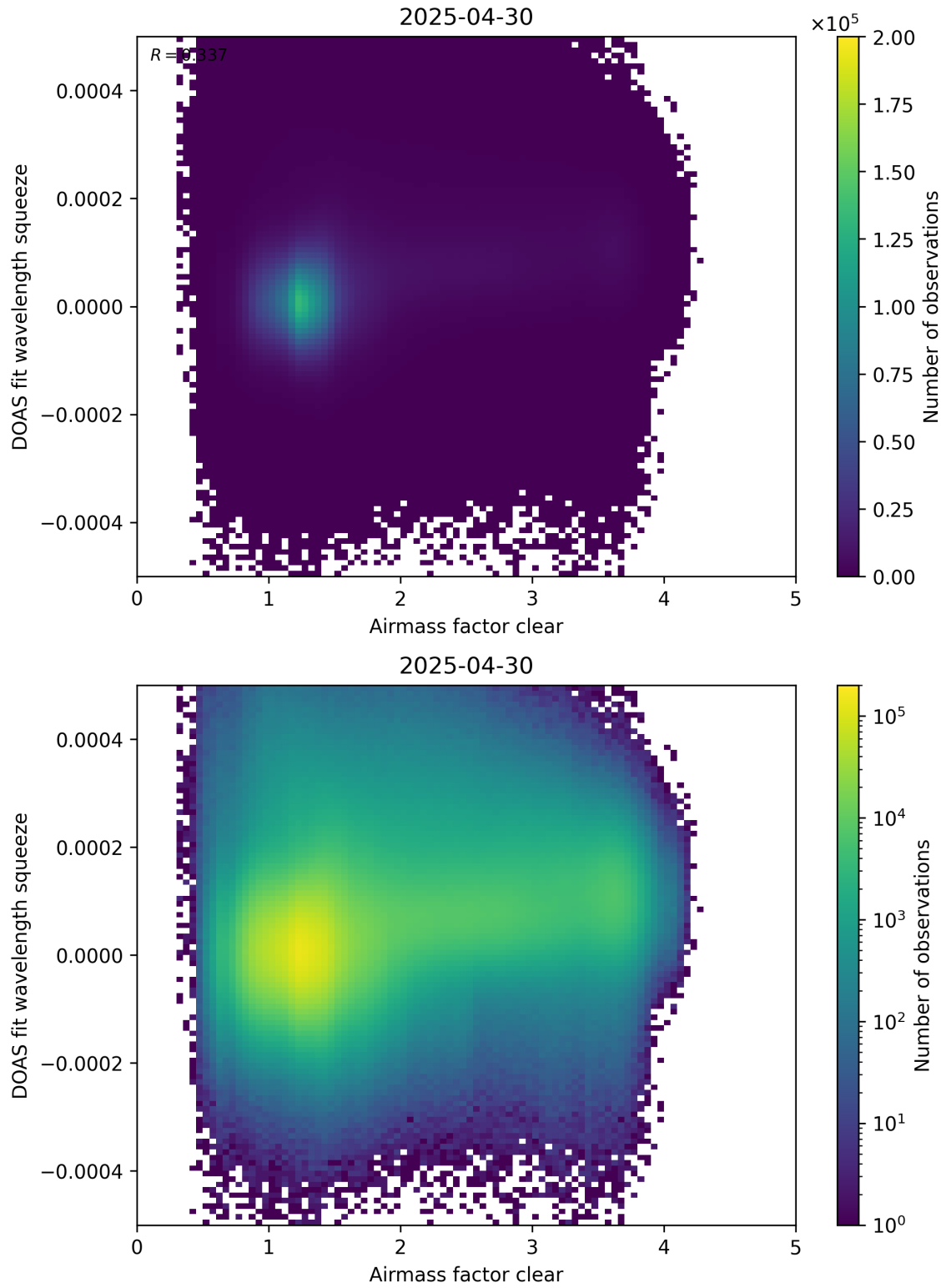
Figure 73: Scatter density plot of “Airmass factor clear” against “DOAS fit wavelength squeeze” for 2025-04-29 to 2025-05-01.
