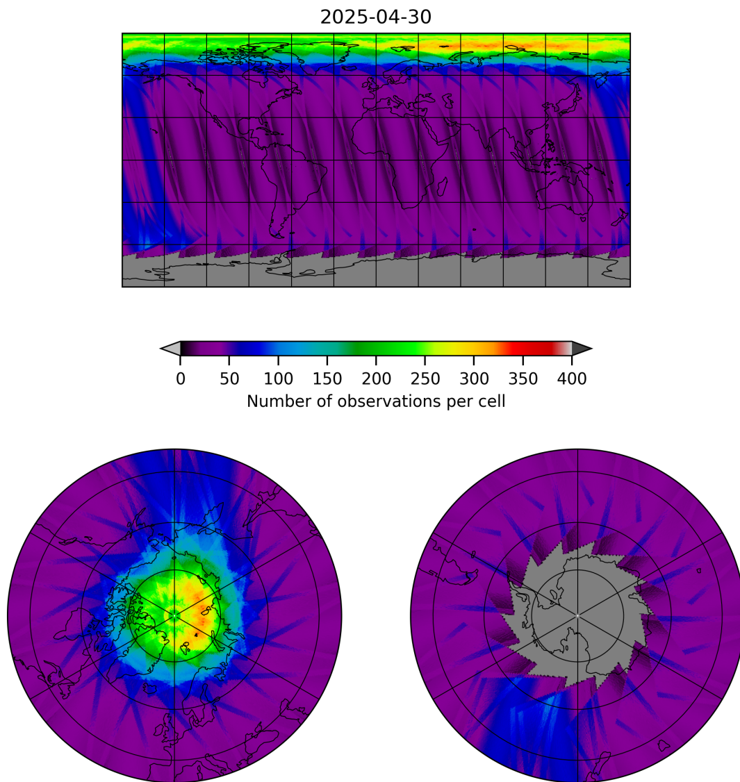
Figure 19: Map of the number of observations for 2025-04-29 to 2025-05-01
