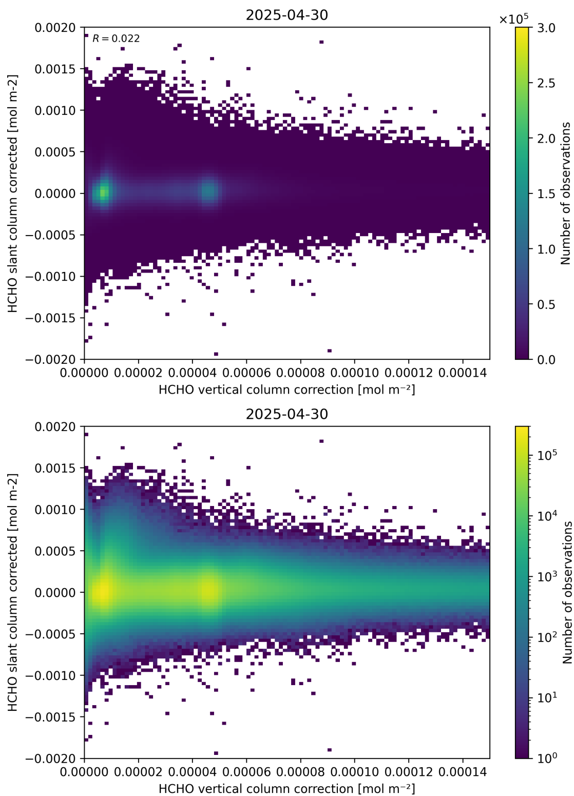
Figure 116: Scatter density plot of “HCHO vertical column correction” against “HCHO slant column corrected” for 2025-04-29 to 2025-05-01.
