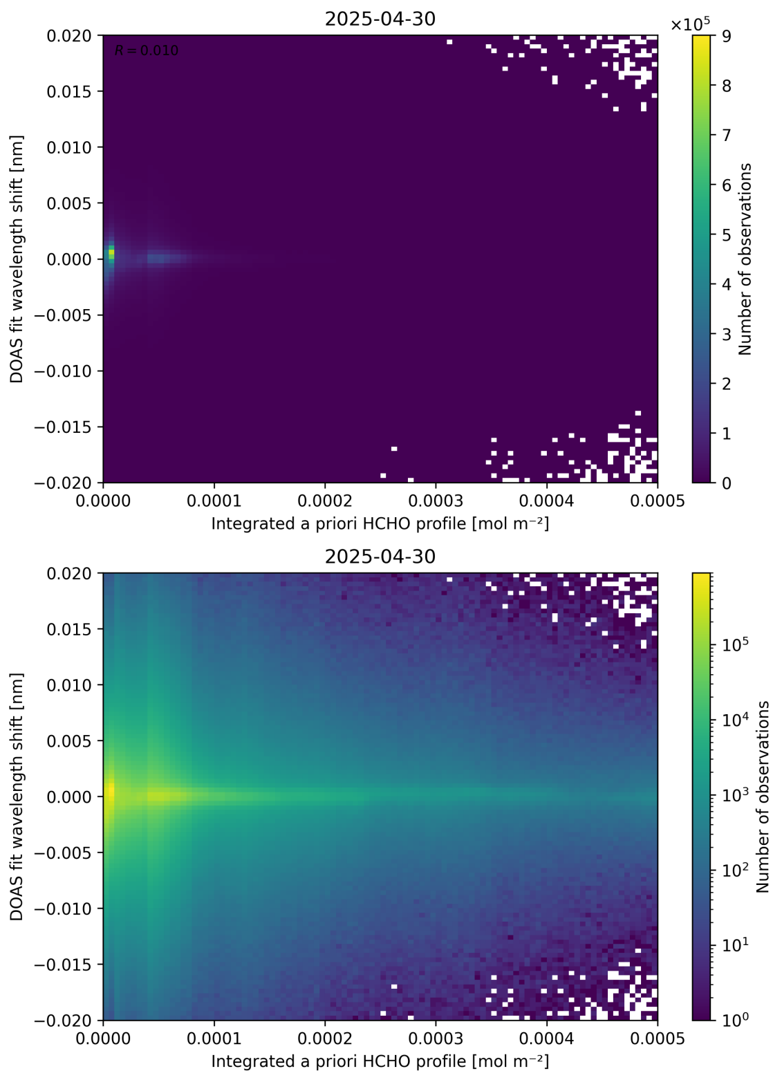
Figure 149: Scatter density plot of “Integrated a priori HCHO profile” against “DOAS fit wavelength shift” for 2025-04-29 to 2025-05-01.
