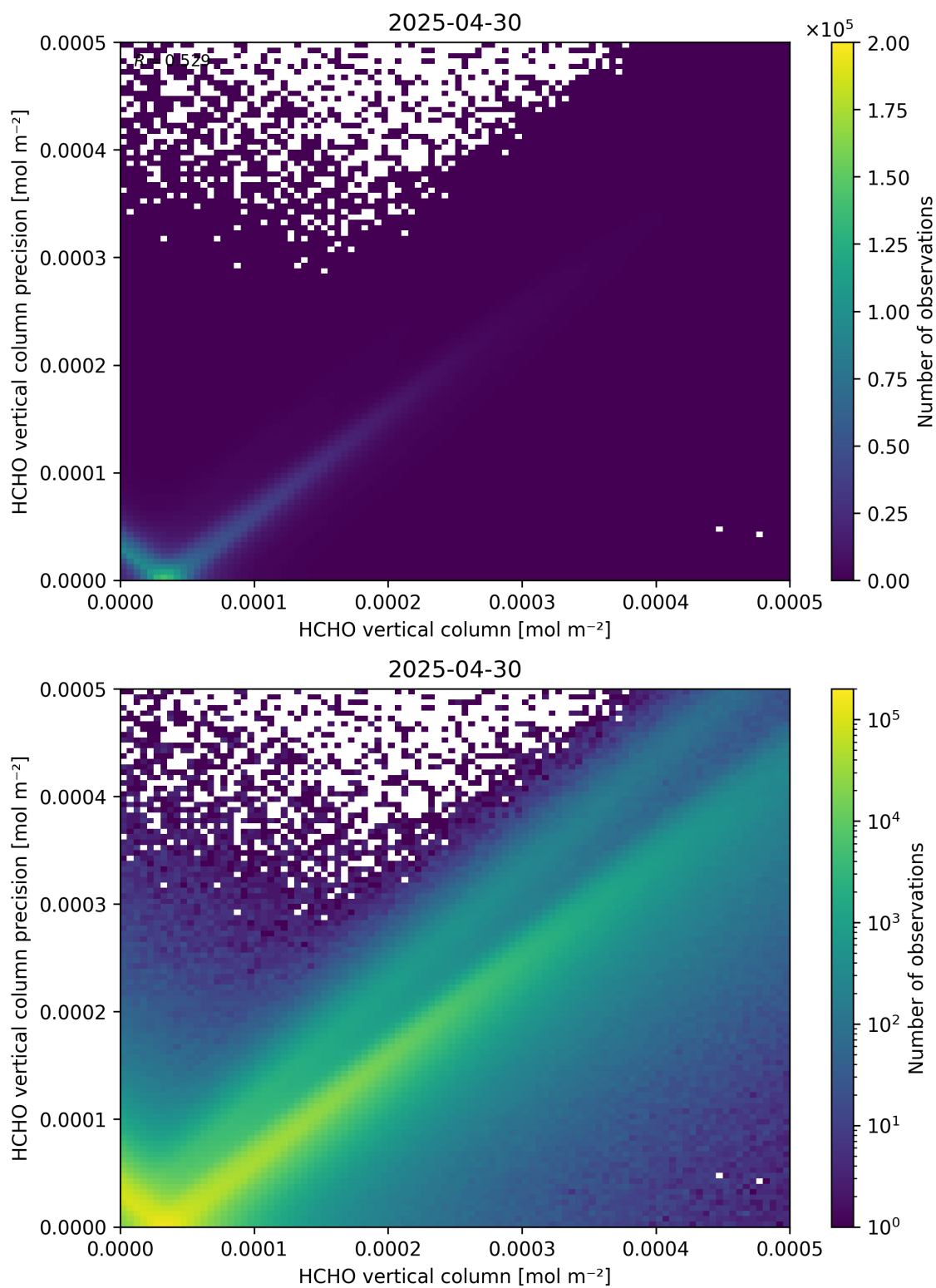
Figure 134: Scatter density plot of “HCHO vertical column” against “HCHO vertical column precision” for 2025-04-29 to 2025-05-01.
