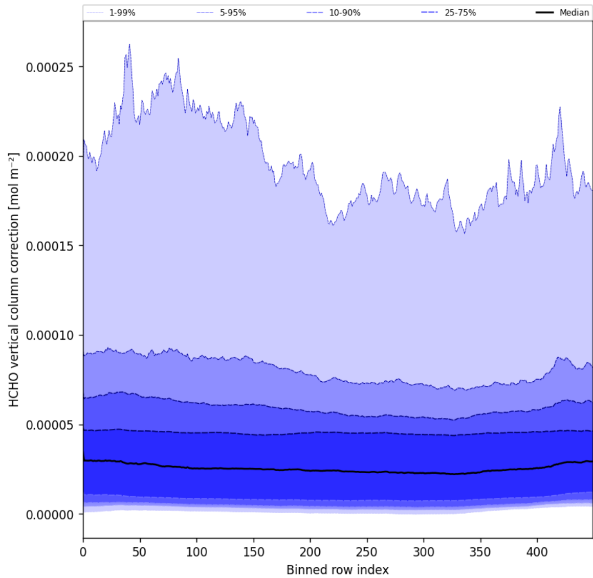
Figure 51: Along track statistics of “HCHO vertical column correction” for 2025-04-29 to 2025-05-01
