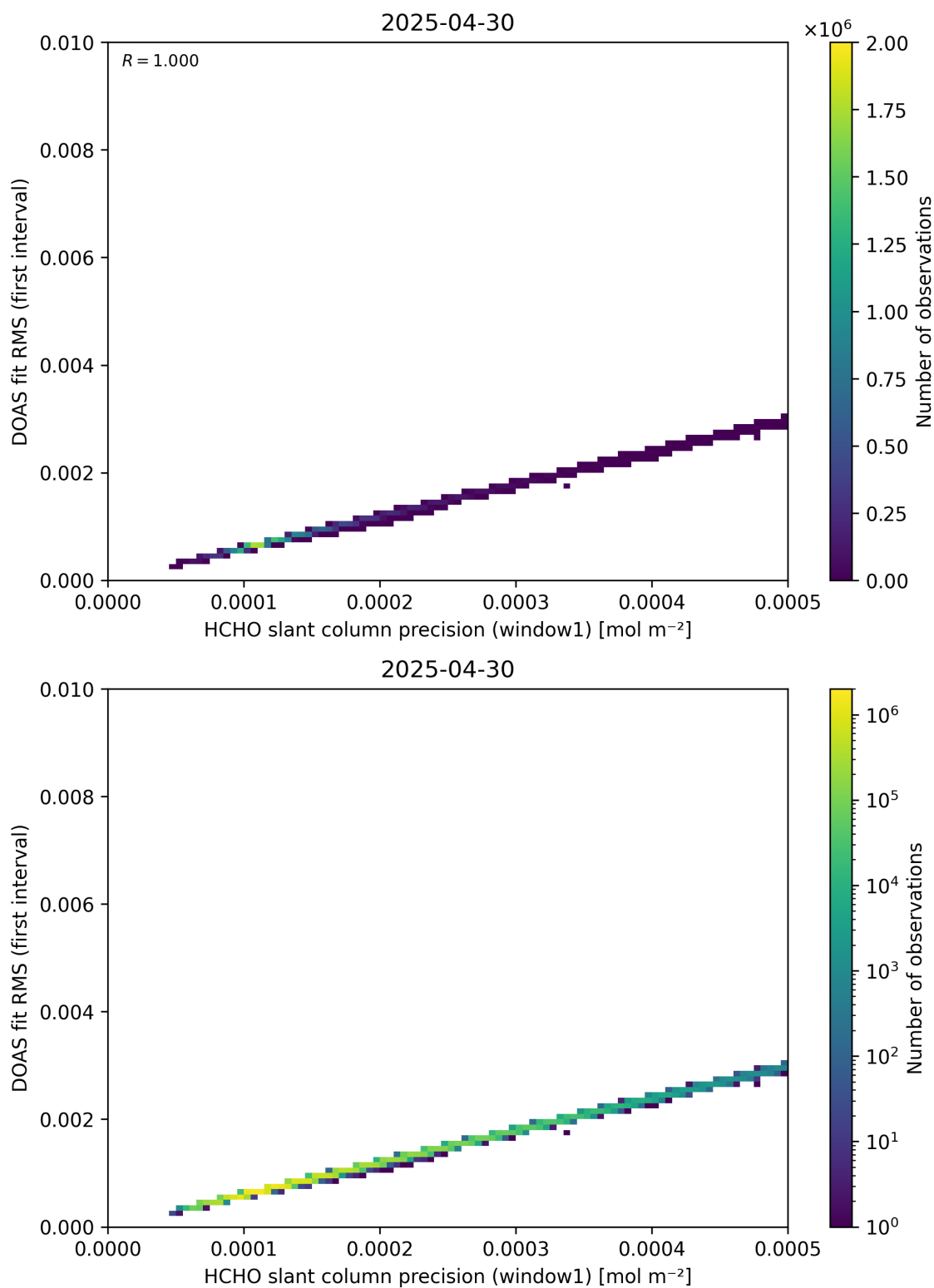
Figure 88: Scatter density plot of “HCHO slant column precision (window1)” against “DOAS fit RMS (first interval)” for 2025-04-29 to 2025-05-01.
