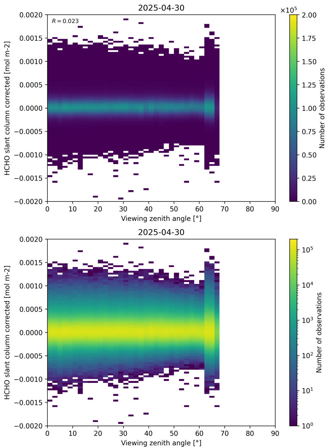
Figure 186: Scatter density plot of “Viewing zenith angle” against “HCHO slant column corrected” for 2025-04-29 to 2025-05-01.
