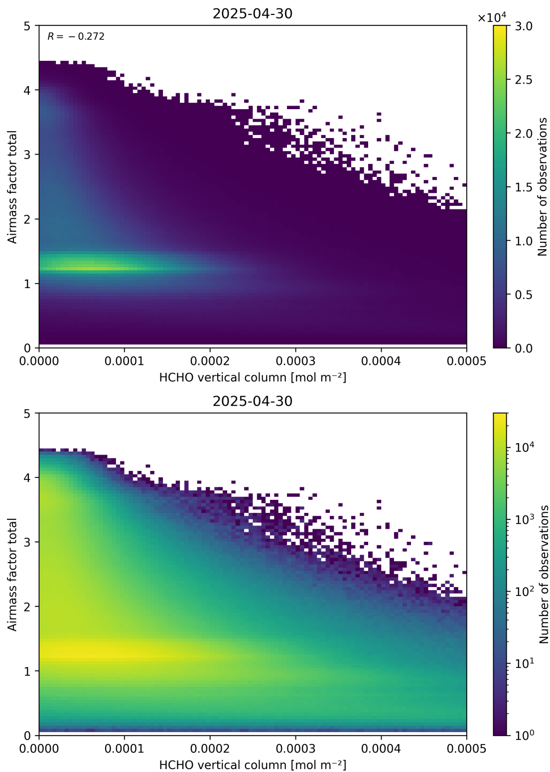
Figure 131: Scatter density plot of “HCHO vertical column” against “Airmass factor total” for 2025-04-29 to 2025-05-01.
