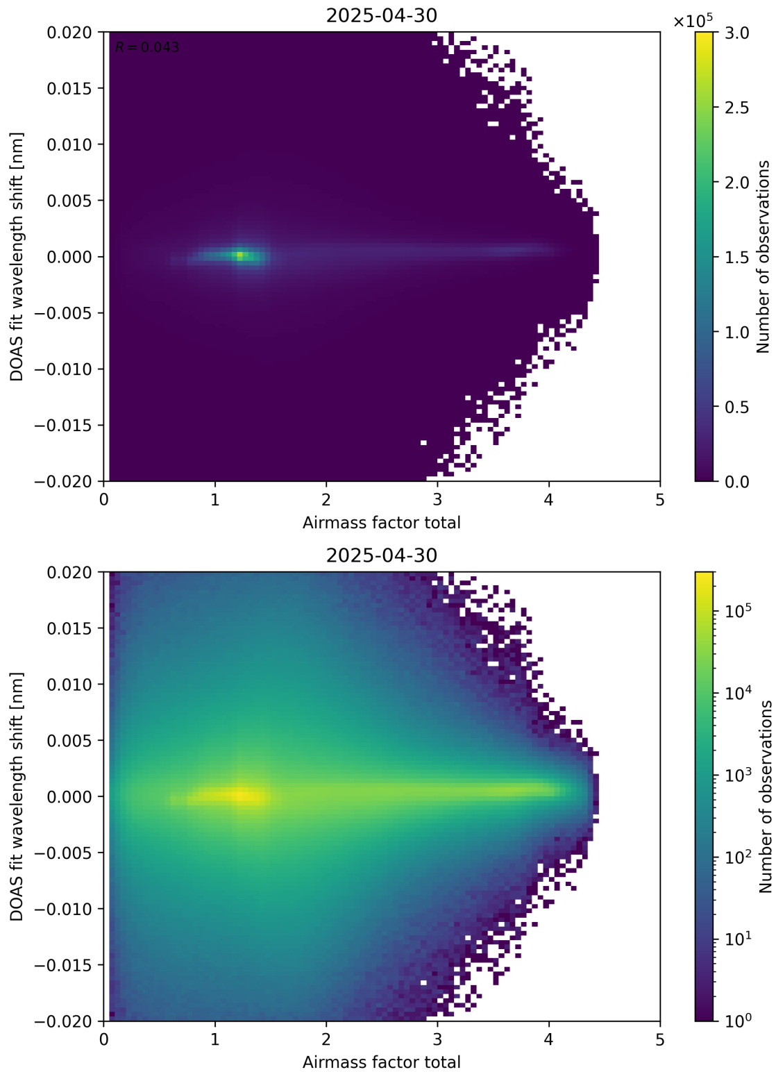
Figure 98: Scatter density plot of “Airmass factor total” against “DOAS fit wavelength shift” for 2025-04-29 to 2025-05-01.
