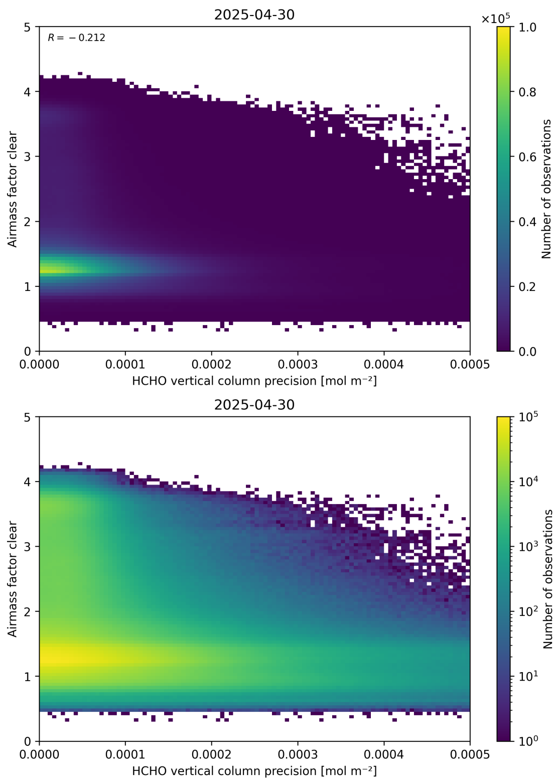
Figure 139: Scatter density plot of “HCHO vertical column precision” against “Airmass factor clear” for 2025-04-29 to 2025-05-01.
