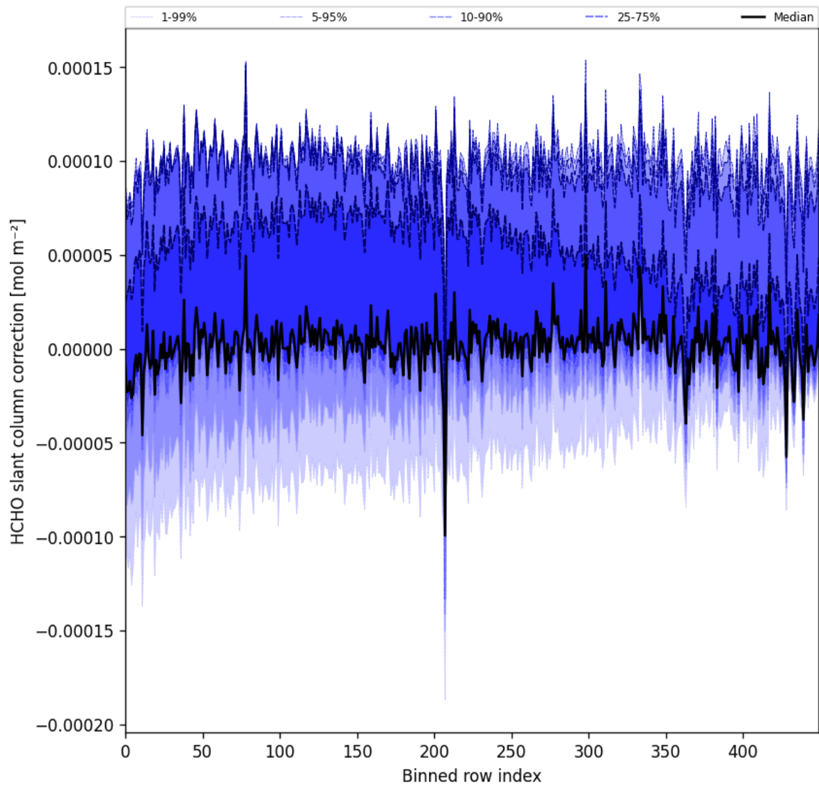
Figure 61: Along track statistics of “HCHO slant column correction” for 2025-04-29 to 2025-05-01
