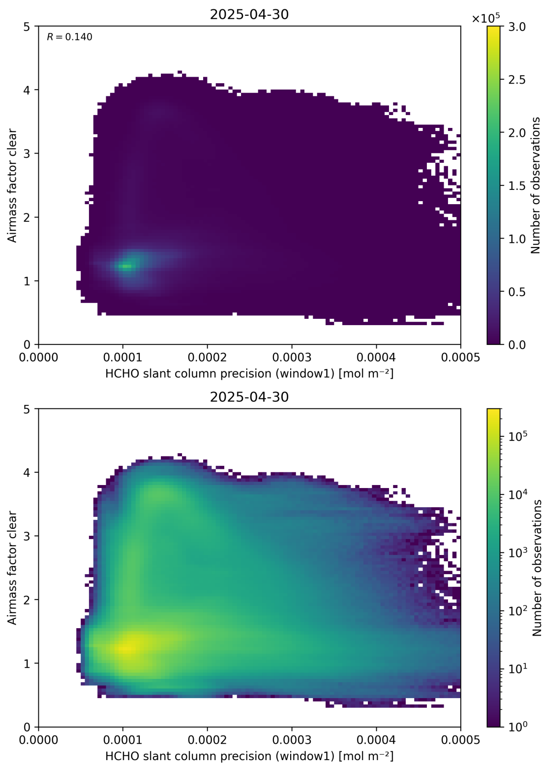
Figure 91: Scatter density plot of “HCHO slant column precision (window1)” against “Airmass factor clear” for 2025-04-29 to 2025-05-01.
