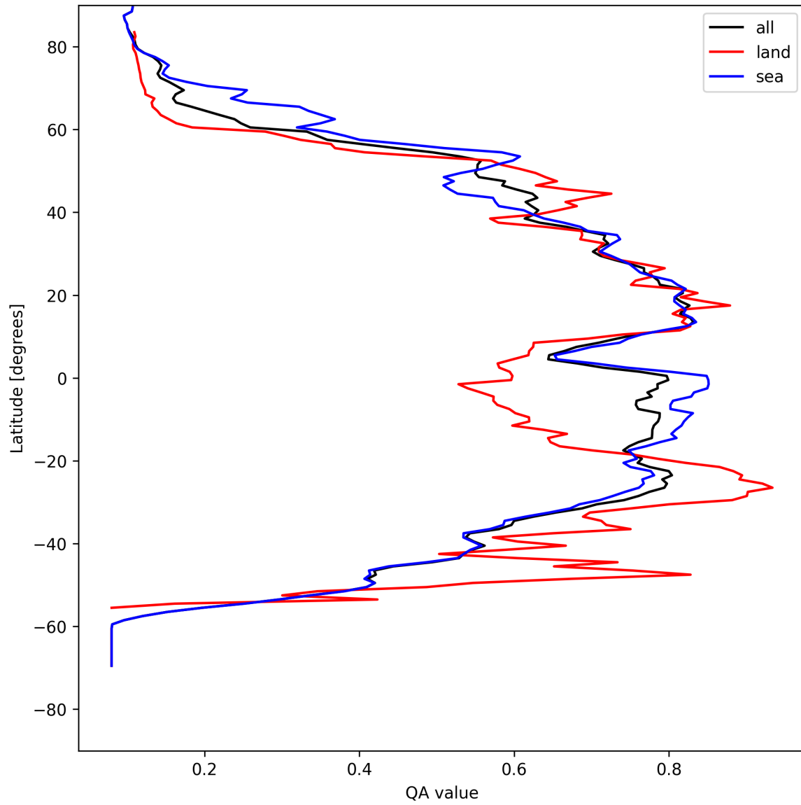
Figure 20: Zonal average of “QA value” for 2025-04-29 to 2025-05-01.
