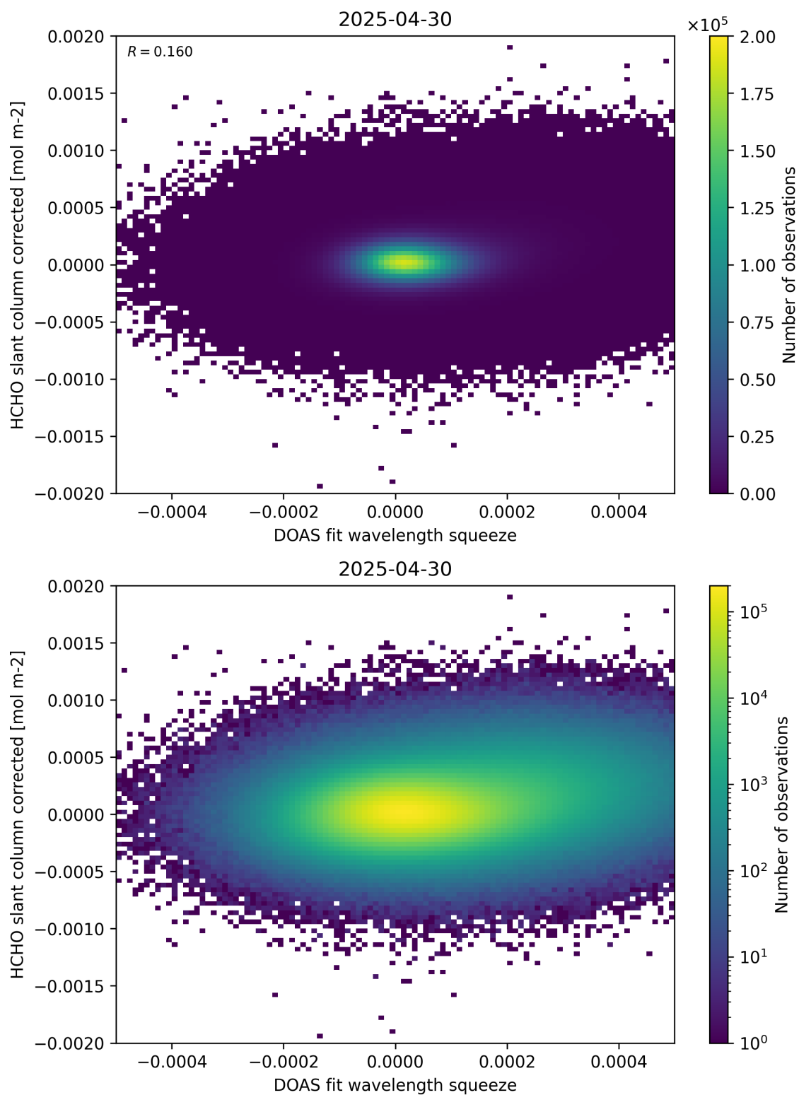
Figure 69: Scatter density plot of “DOAS fit wavelength squeeze” against “HCHO slant column corrected” for 2025-04-29 to 2025-05-01.
