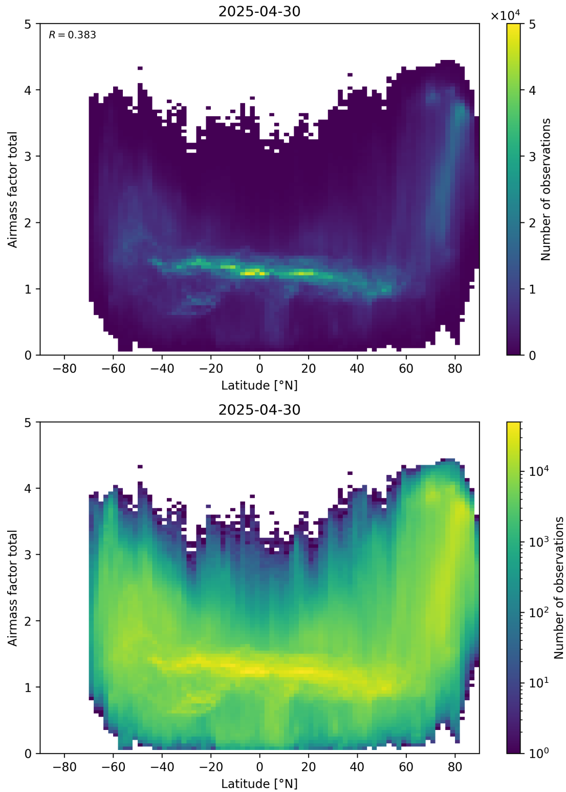
Figure 161: Scatter density plot of “Latitude” against “Airmass factor total” for 2025-04-29 to 2025-05-01.
