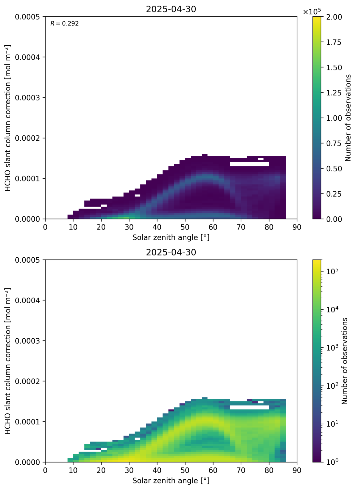
Figure 172: Scatter density plot of “Solar zenith angle” against “HCHO slant column correction” for 2025-04-29 to 2025-05-01.
