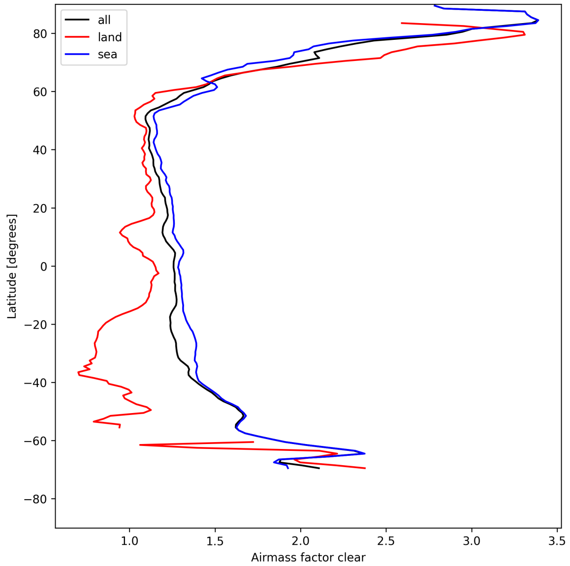
Figure 28: Zonal average of “Airmass factor clear” for 2025-04-29 to 2025-05-01.
