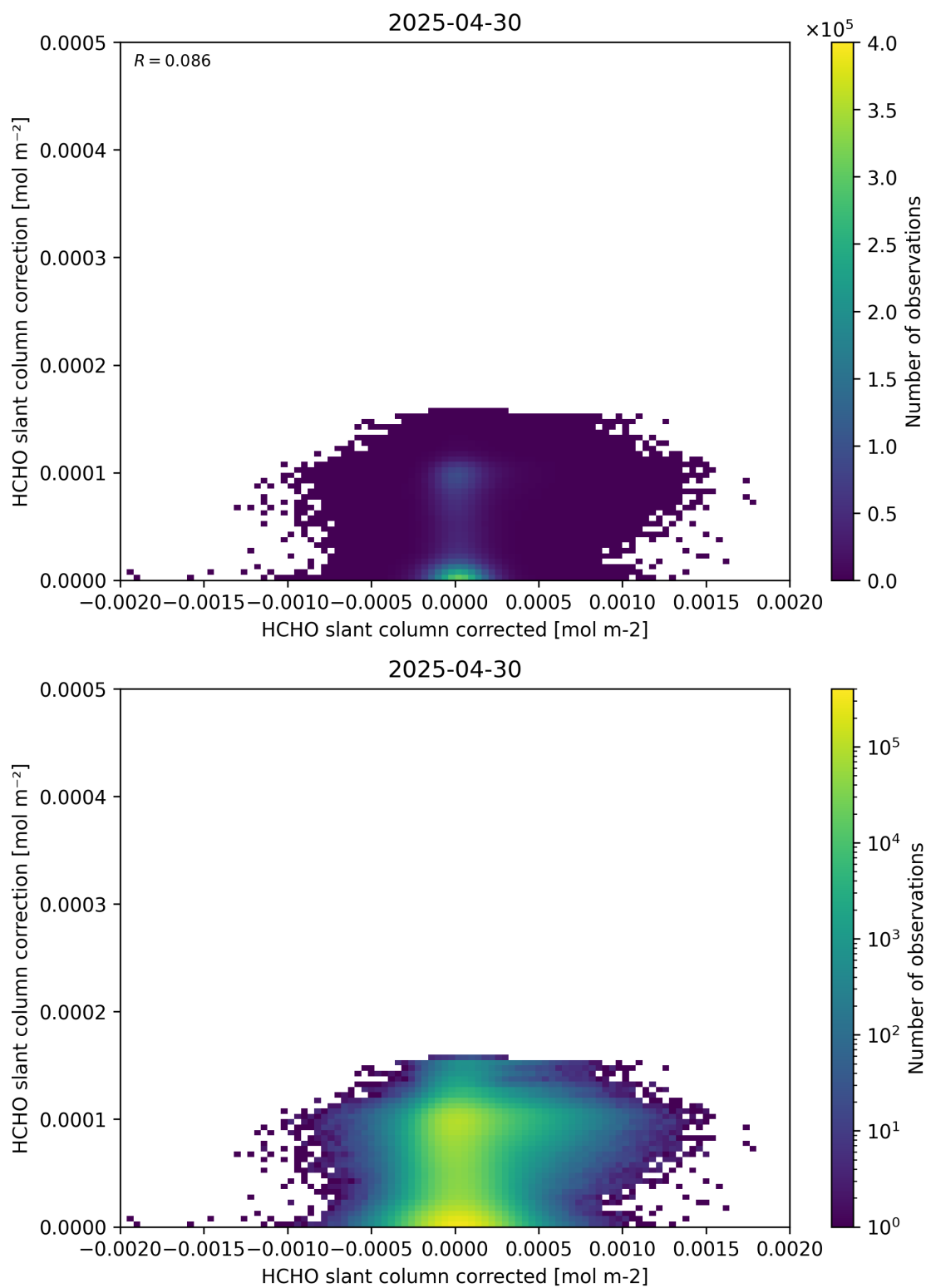
Figure 77: Scatter density plot of “HCHO slant column corrected” against “HCHO slant column correction” for 2025-04-29 to 2025-05-01.
