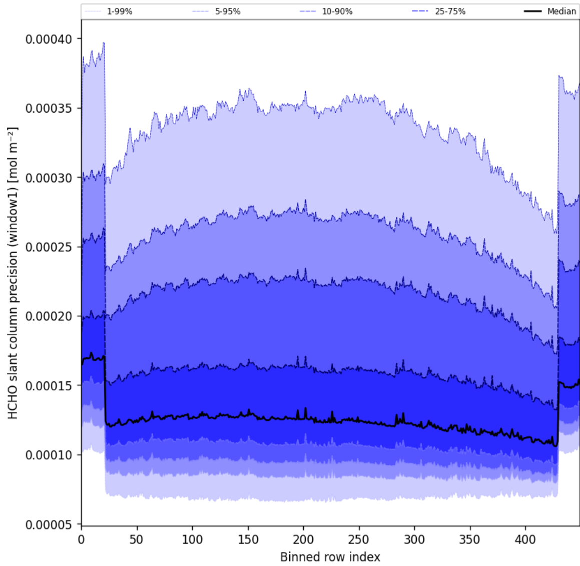
Figure 53: Along track statistics of “HCHO slant column precision (window1)” for 2025-04-29 to 2025-05-01
