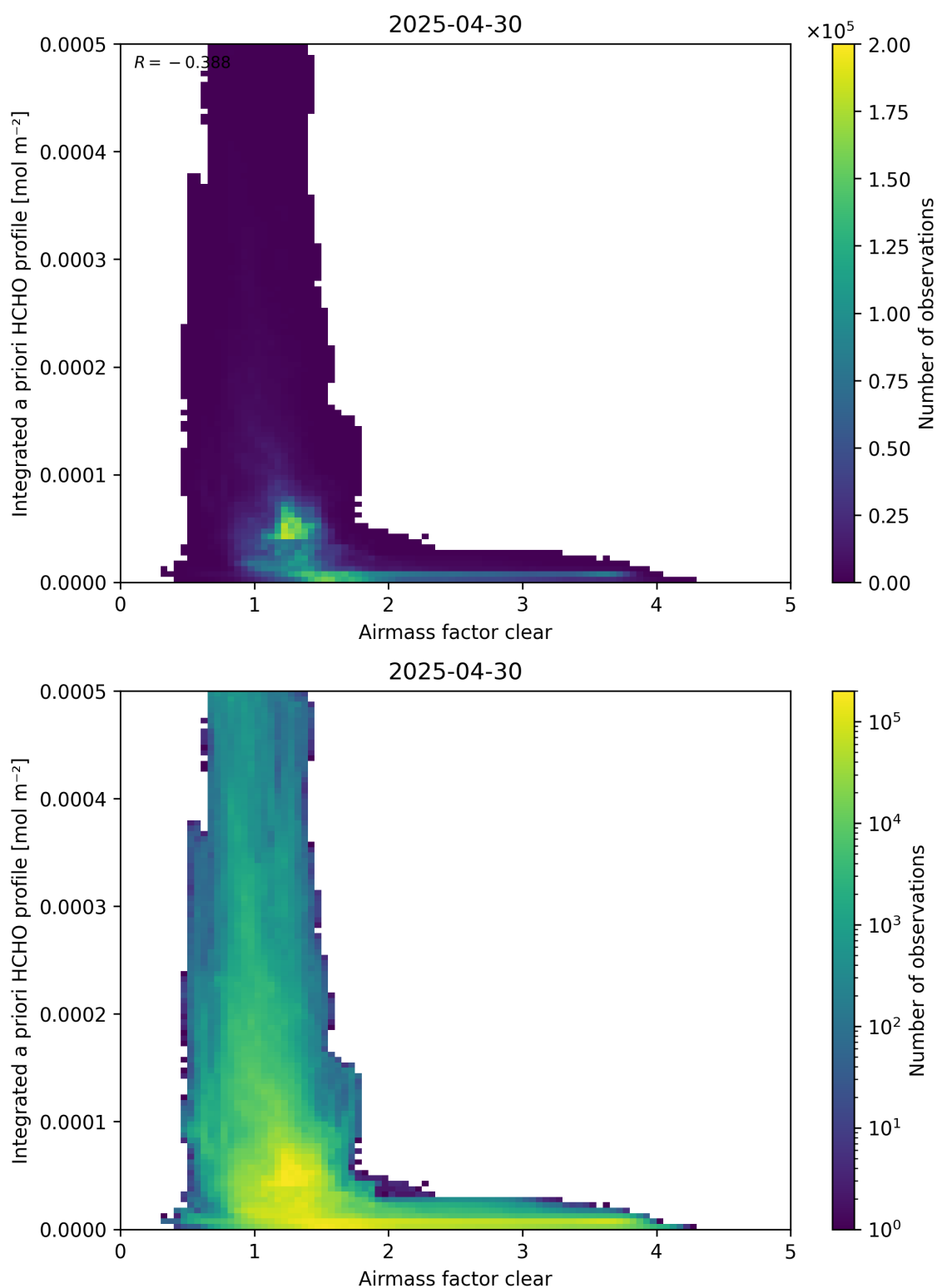
Figure 76: Scatter density plot of “Airmass factor clear” against “Integrated a priori HCHO profile” for 2025-04-29 to 2025-05-01.
