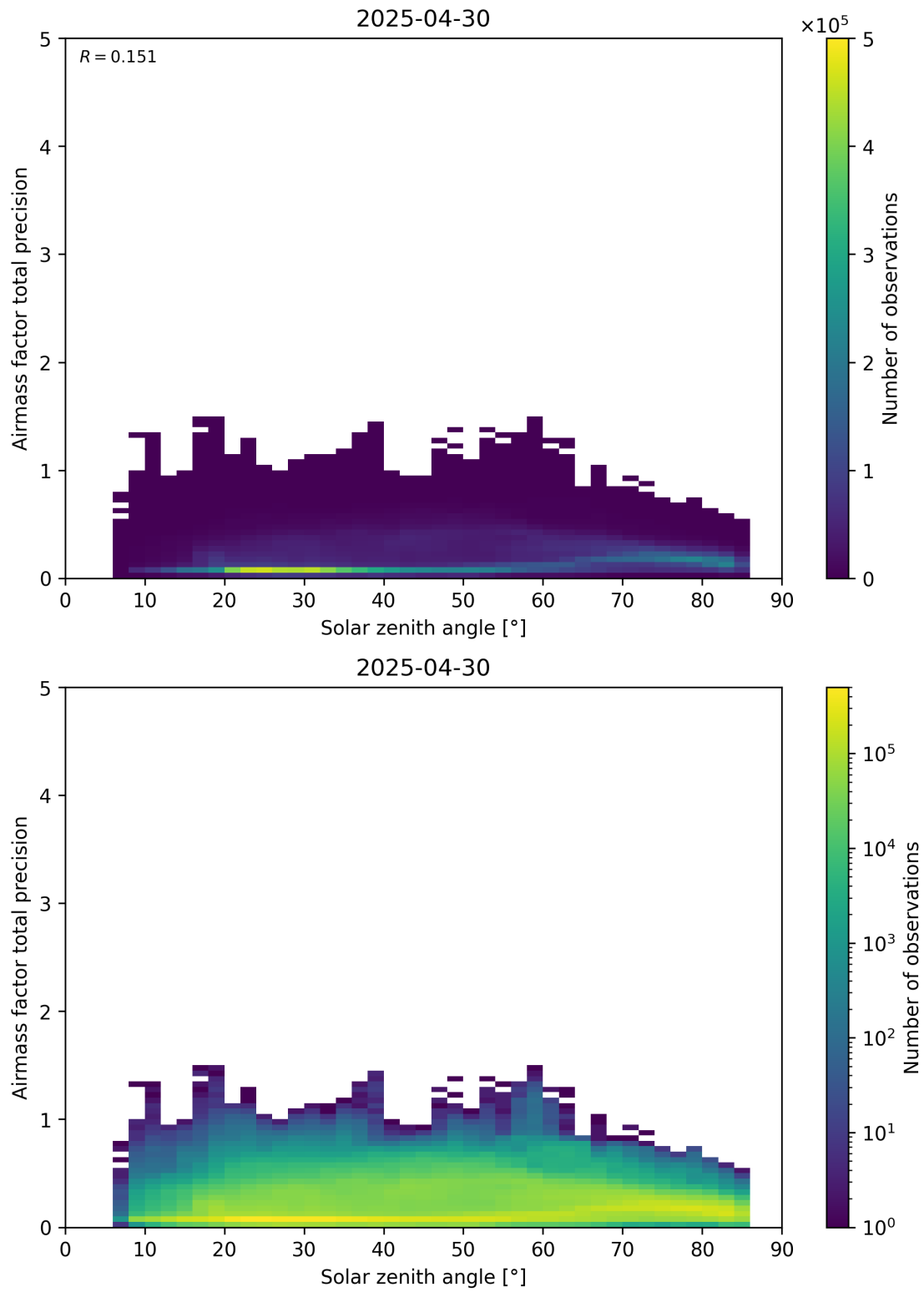
Figure 176: Scatter density plot of “Solar zenith angle” against “Airmass factor total precision” for 2025-04-29 to 2025-05-01.
