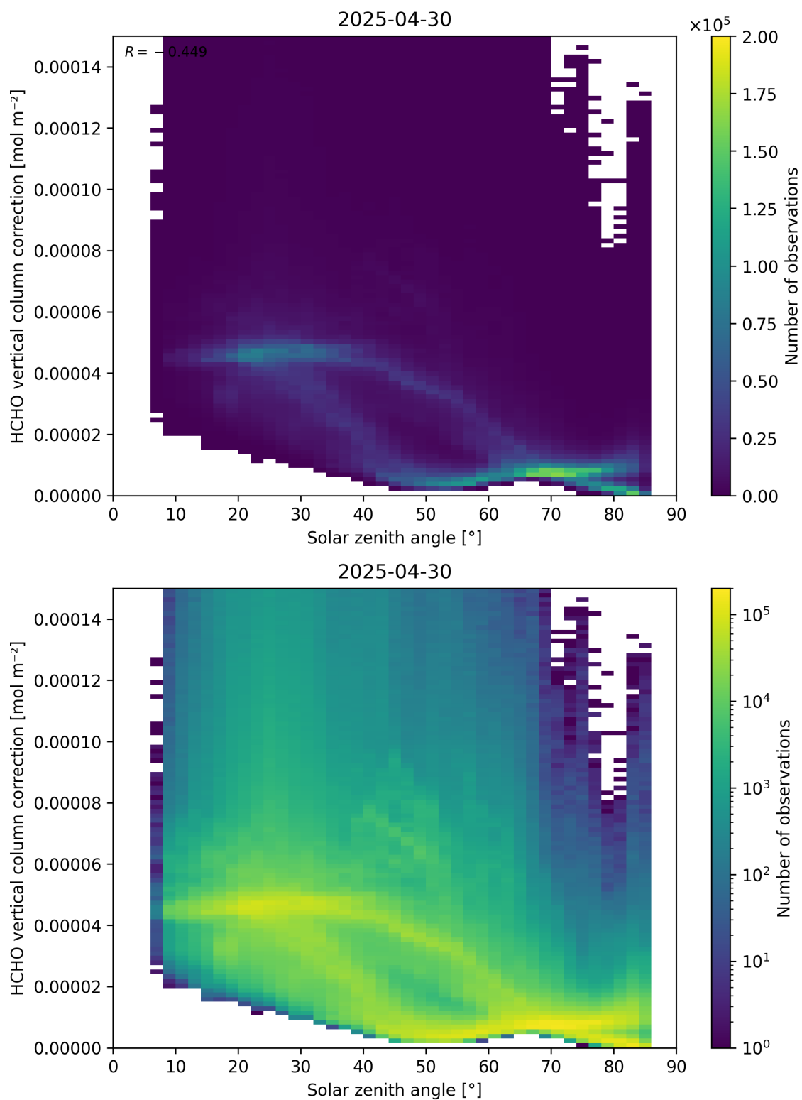
Figure 178: Scatter density plot of “Solar zenith angle” against “HCHO vertical column correction” for 2025-04-29 to 2025-05-01.
