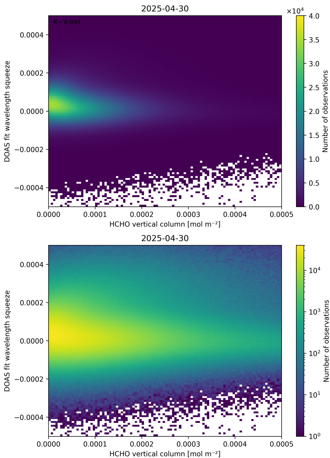
Figure 125: Scatter density plot of “HCHO vertical column” against “DOAS fit wavelength squeeze” for 2025-04-29 to 2025-05-01.
