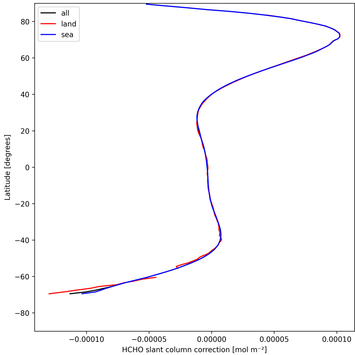
Figure 33: Zonal average of “HCHO slant column correction” for 2025-04-29 to 2025-05-01.
