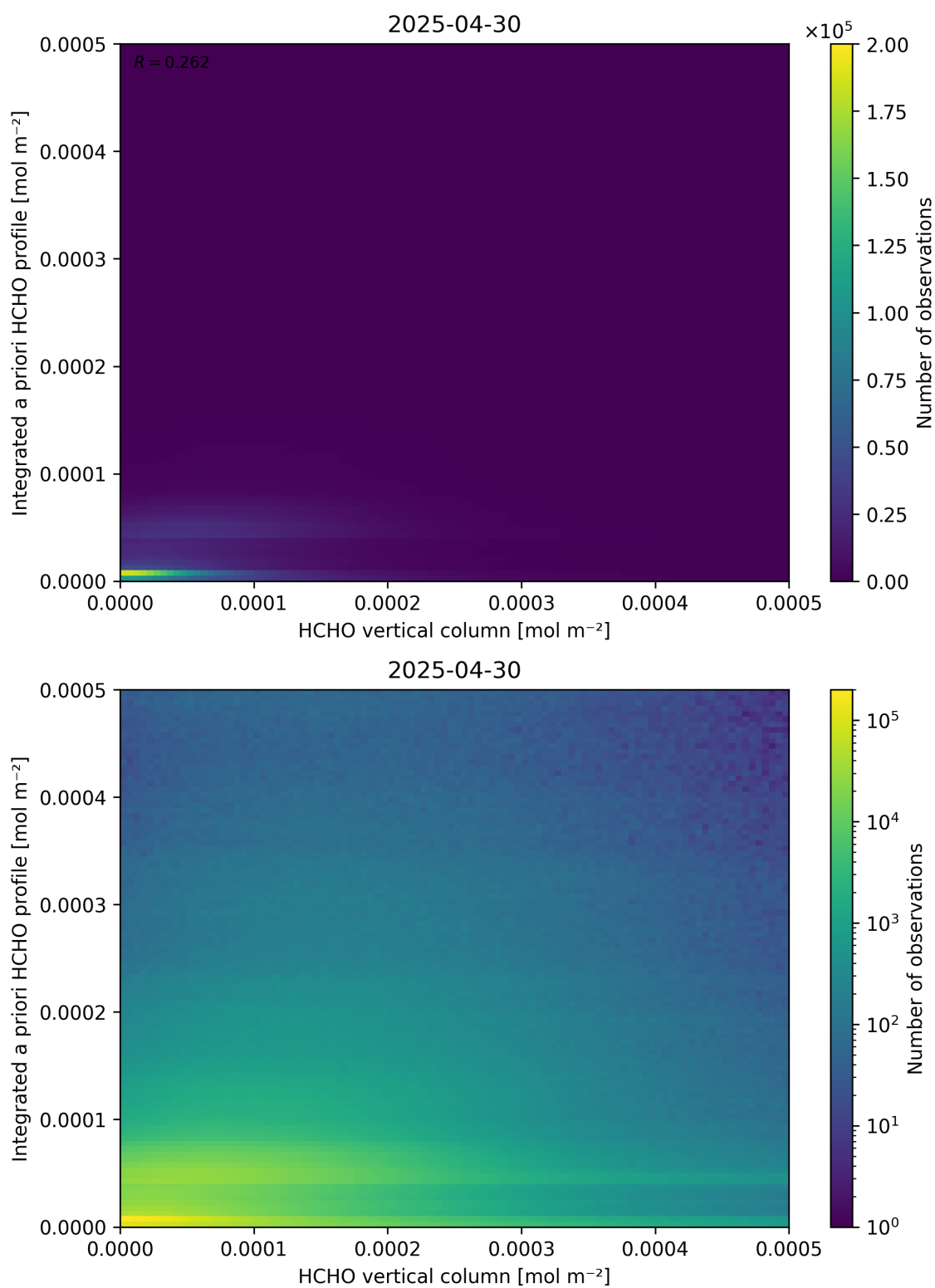
Figure 135: Scatter density plot of “HCHO vertical column” against “Integrated a priori HCHO profile” for 2025-04-29 to 2025-05-01.
