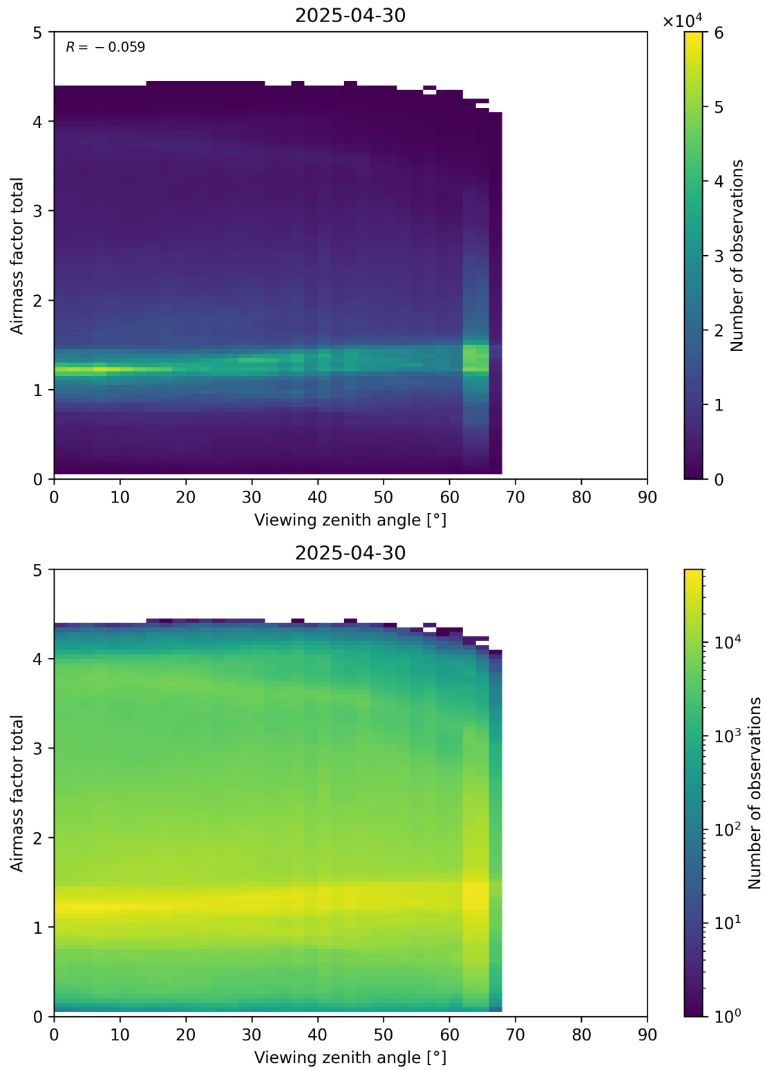
Figure 190: Scatter density plot of “Viewing zenith angle” against “Airmass factor total” for 2025-04-29 to 2025-05-01.
