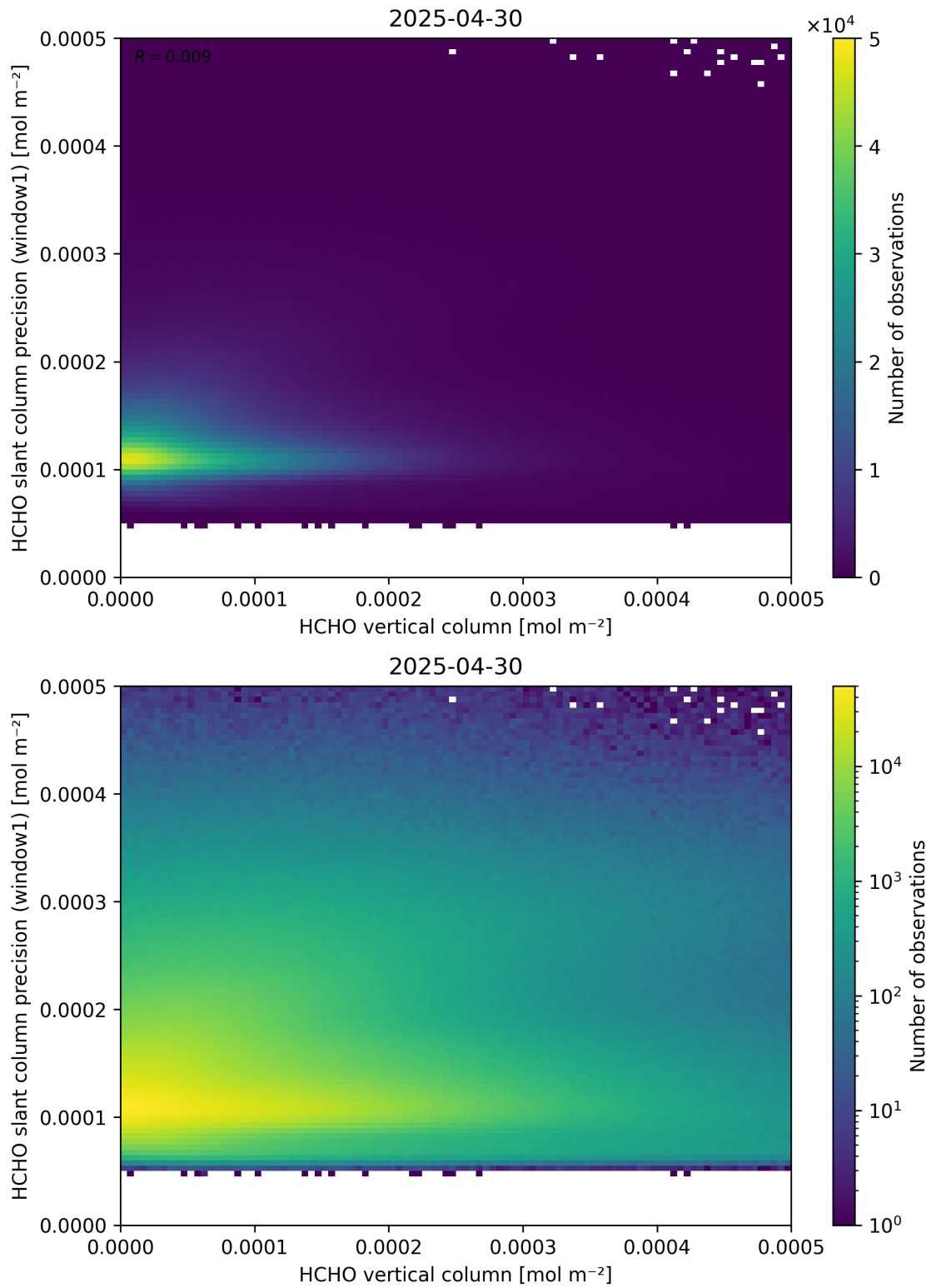
Figure 130: Scatter density plot of “HCHO vertical column” against “HCHO slant column precision (window1)” for 2025-04-29 to 2025-05-01.
