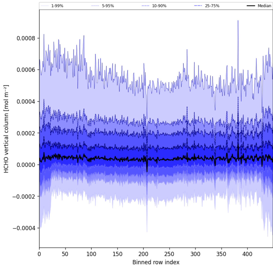
Figure 49: Along track statistics of “HCHO vertical column” for 2025-04-29 to 2025-05-01
