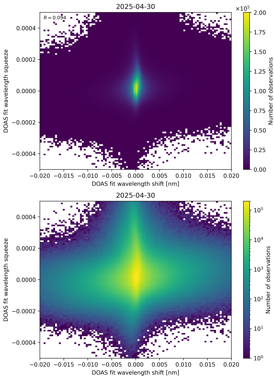
Figure 65: Scatter density plot of “DOAS fit wavelength shift” against “DOAS fit wavelength squeeze” for 2025-04-29 to 2025-05-01.
