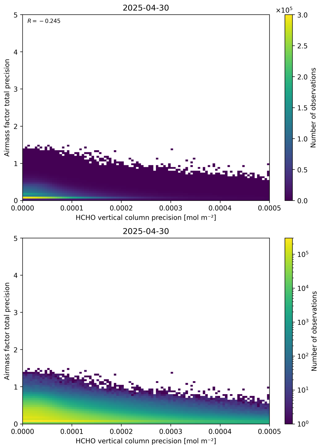
Figure 145: Scatter density plot of “HCHO vertical column precision” against “Airmass factor total precision” for 2025-04-29 to 2025-05-01.
