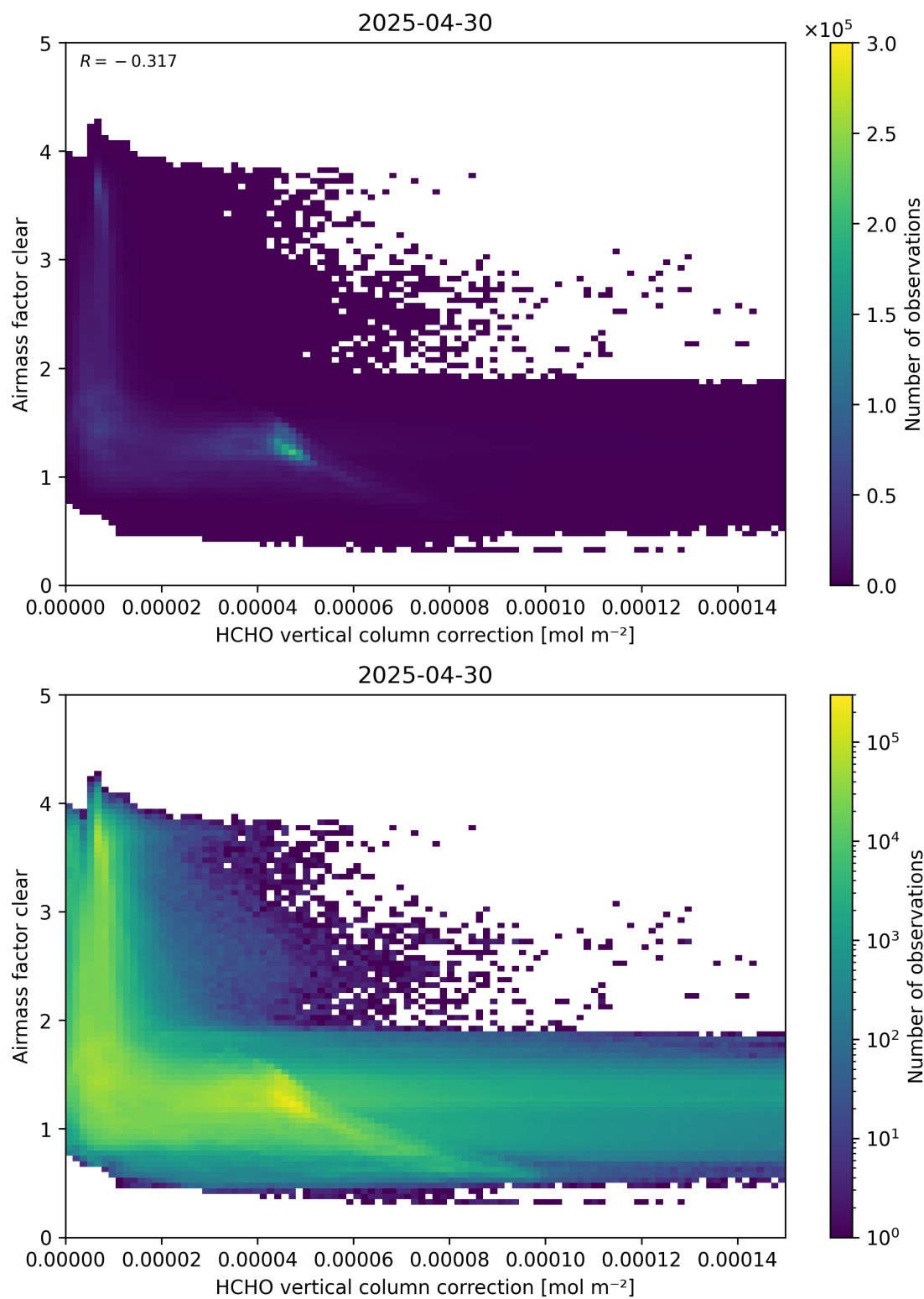
Figure 115: Scatter density plot of “HCHO vertical column correction” against “Airmass factor clear” for 2025-04-29 to 2025-05-01.
