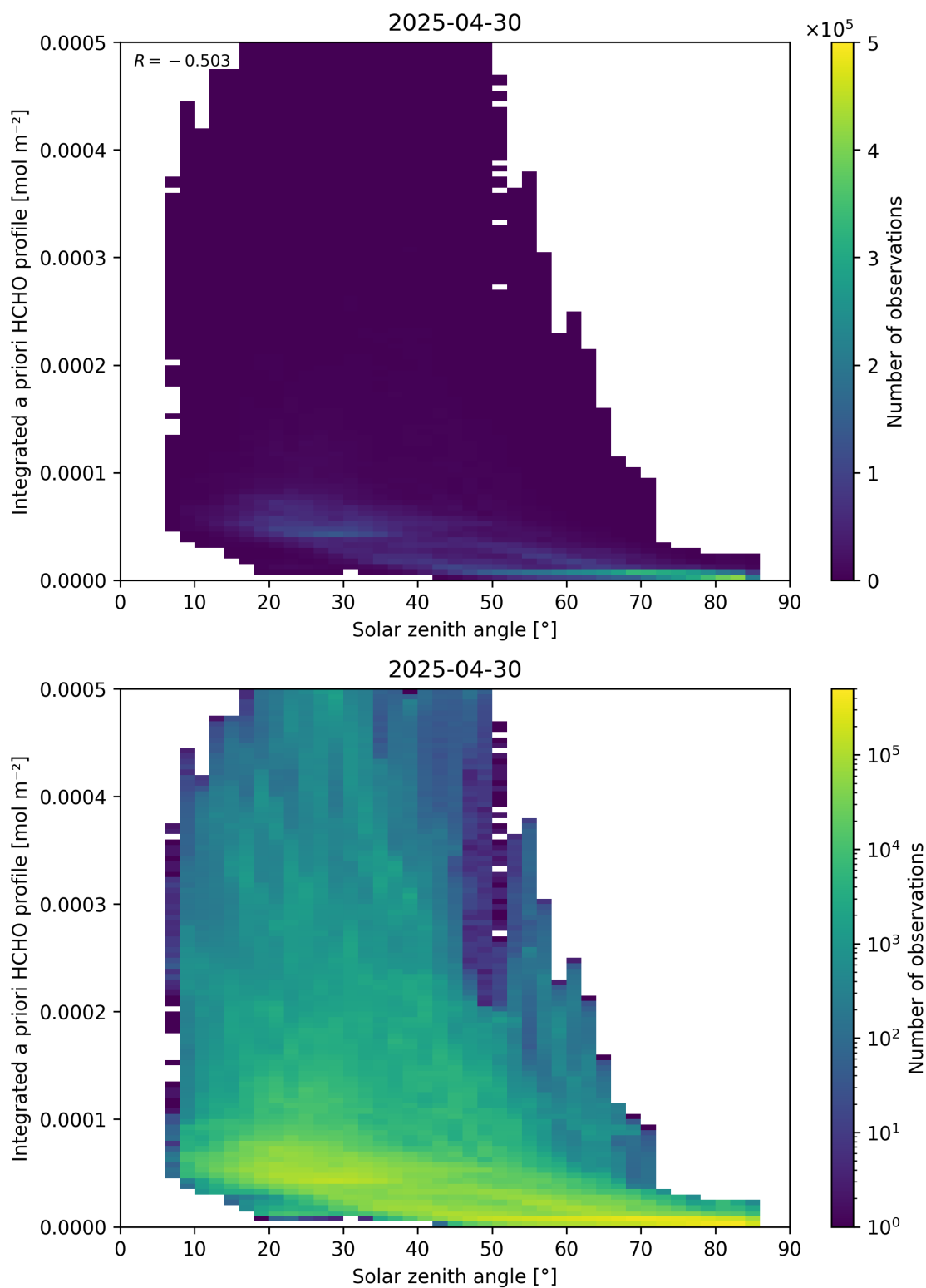
Figure 180: Scatter density plot of “Solar zenith angle” against “Integrated a priori HCHO profile” for 2025-04-29 to 2025-05-01.
