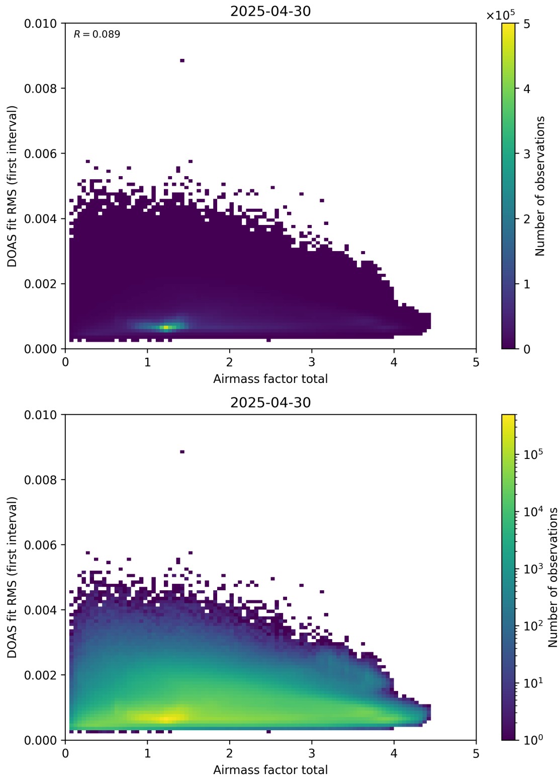
Figure 97: Scatter density plot of “Airmass factor total” against “DOAS fit RMS (first interval)” for 2025-04-29 to 2025-05-01.
