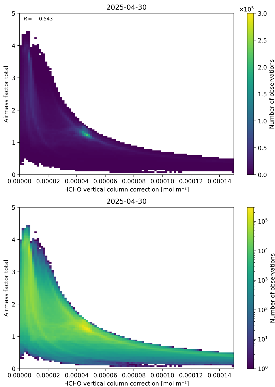
Figure 120: Scatter density plot of “HCHO vertical column correction” against “Airmass factor total” for 2025-04-29 to 2025-05-01.
