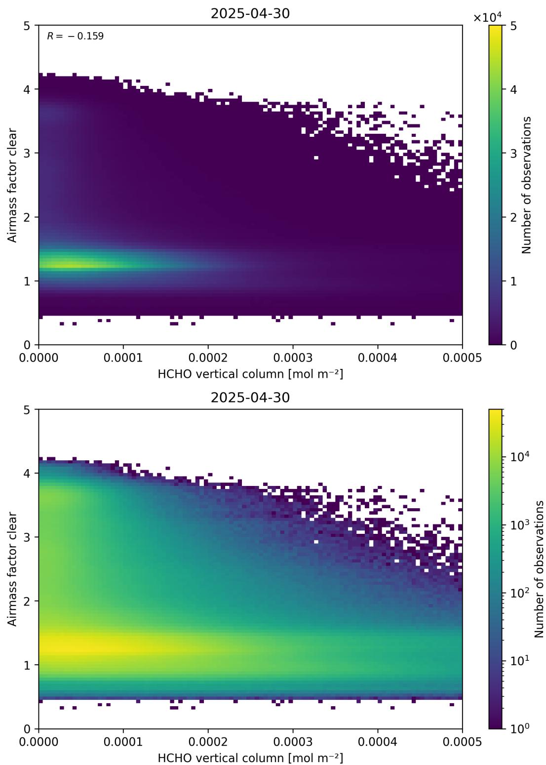
Figure 126: Scatter density plot of “HCHO vertical column” against “Airmass factor clear” for 2025-04-29 to 2025-05-01.
