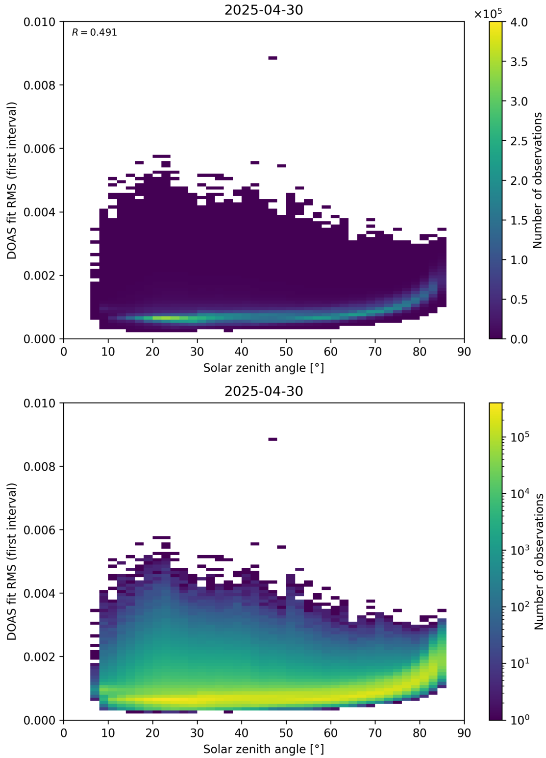
Figure 167: Scatter density plot of “Solar zenith angle” against “DOAS fit RMS (first interval)” for 2025-04-29 to 2025-05-01.
