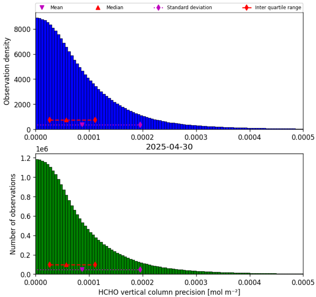
Figure 36: Histogram of “HCHO vertical column precision” for 2025-04-29 to 2025-05-01
