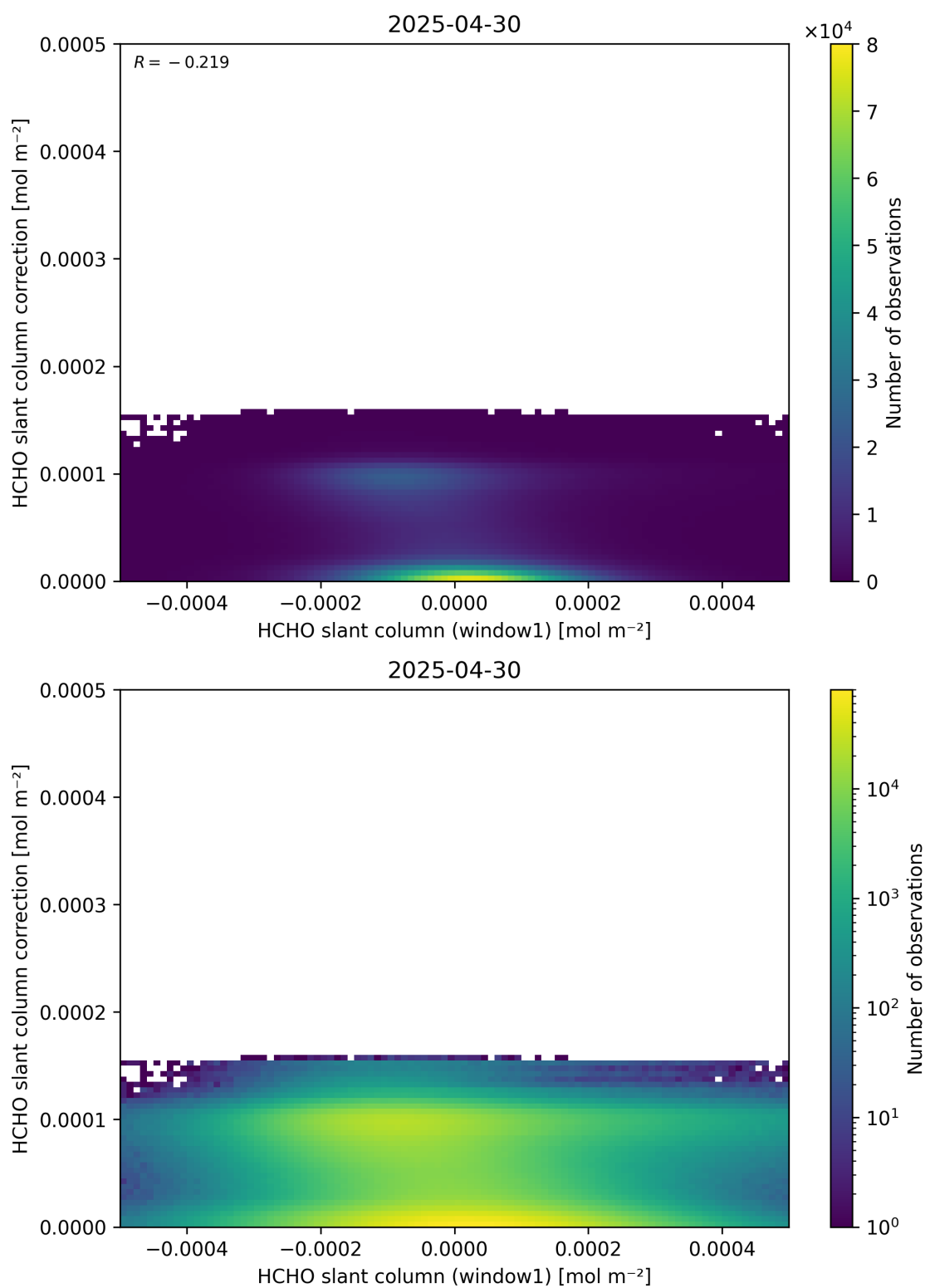
Figure 83: Scatter density plot of “HCHO slant column (window1)” against “HCHO slant column correction” for 2025-04-29 to 2025-05-01.
