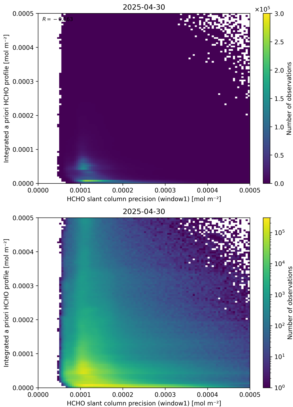
Figure 96: Scatter density plot of “HCHO slant column precision (window1)” against “Integrated a priori HCHO profile” for 2025-04-29 to 2025-05-01.
