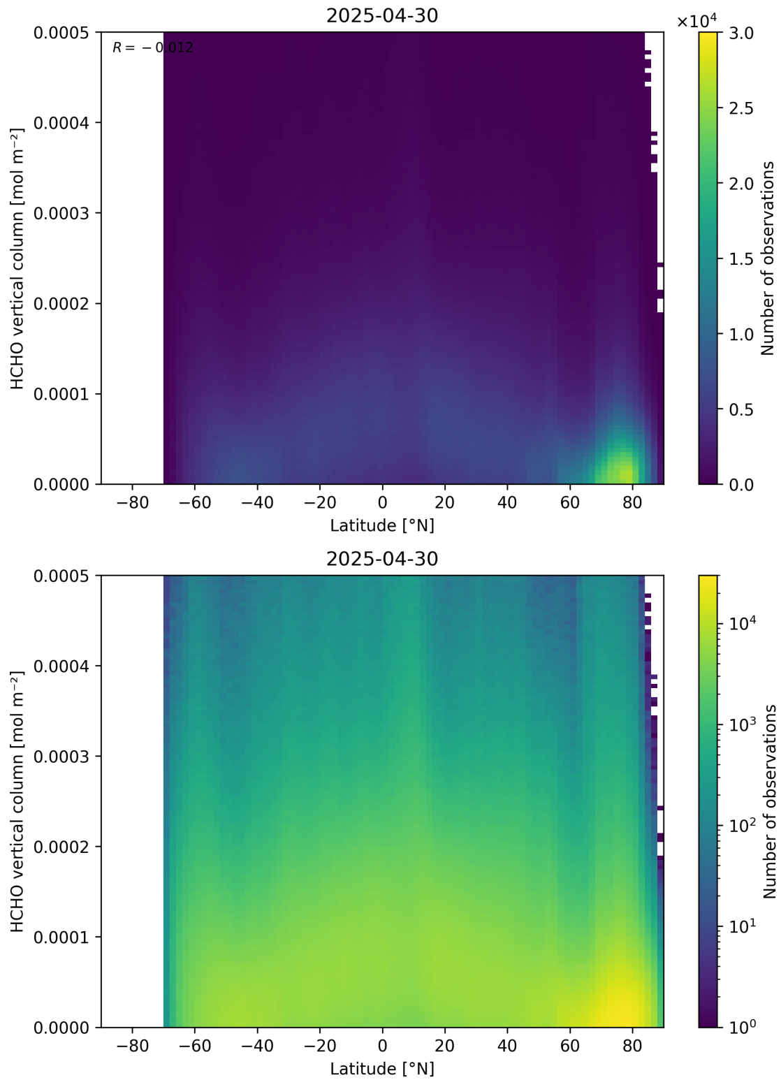
Figure 163: Scatter density plot of “Latitude” against “HCHO vertical column” for 2025-04-29 to 2025-05-01.
