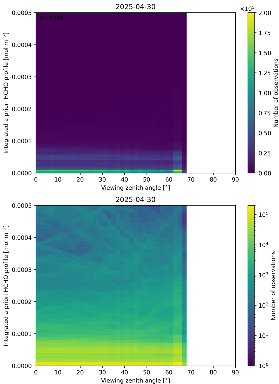
Figure 195: Scatter density plot of “Viewing zenith angle” against “Integrated a priori HCHO profile” for 2025-04-29 to 2025-05-01.
