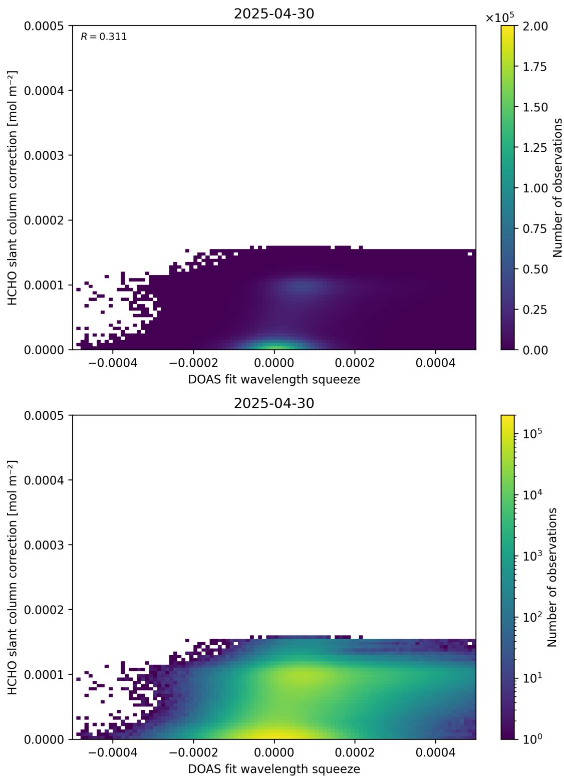
Figure 70: Scatter density plot of “DOAS fit wavelength squeeze” against “HCHO slant column correction” for 2025-04-29 to 2025-05-01.
