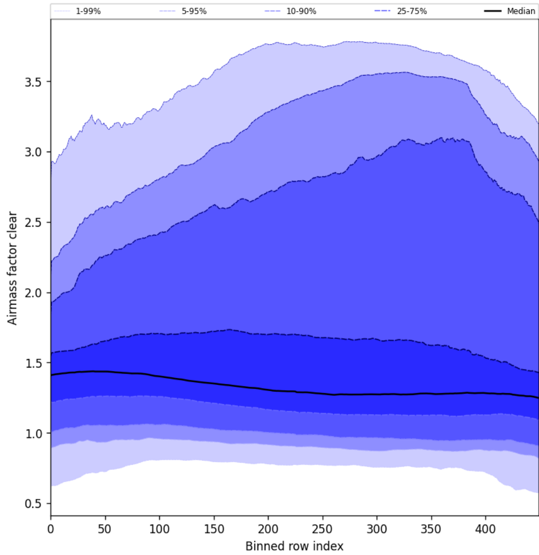
Figure 56: Along track statistics of “Airmass factor clear” for 2025-04-29 to 2025-05-01
