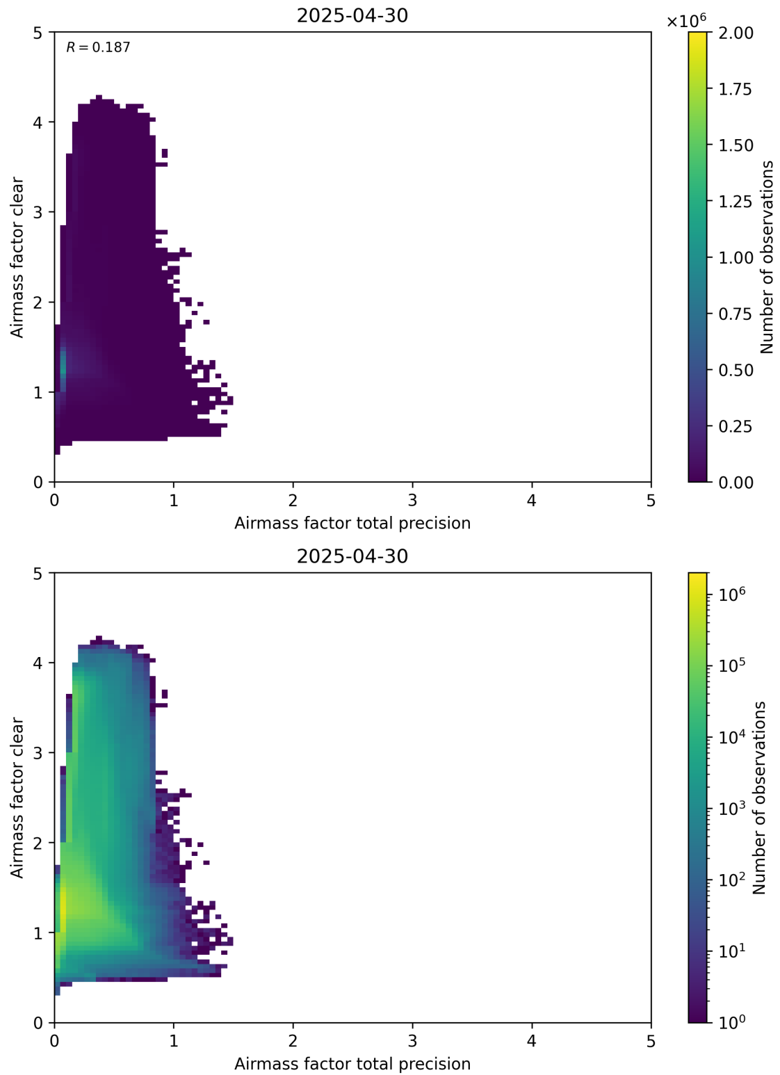
Figure 108: Scatter density plot of “Airmass factor total precision” against “Airmass factor clear” for 2025-04-29 to 2025-05-01.
