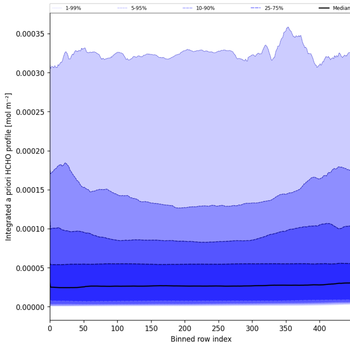
Figure 57: Along track statistics of “Integrated a priori HCHO profile” for 2025-04-29 to 2025-05-01
