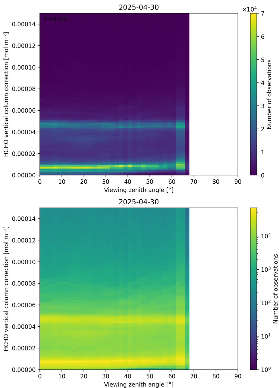
Figure 193: Scatter density plot of “Viewing zenith angle” against “HCHO vertical column correction” for 2025-04-29 to 2025-05-01.
