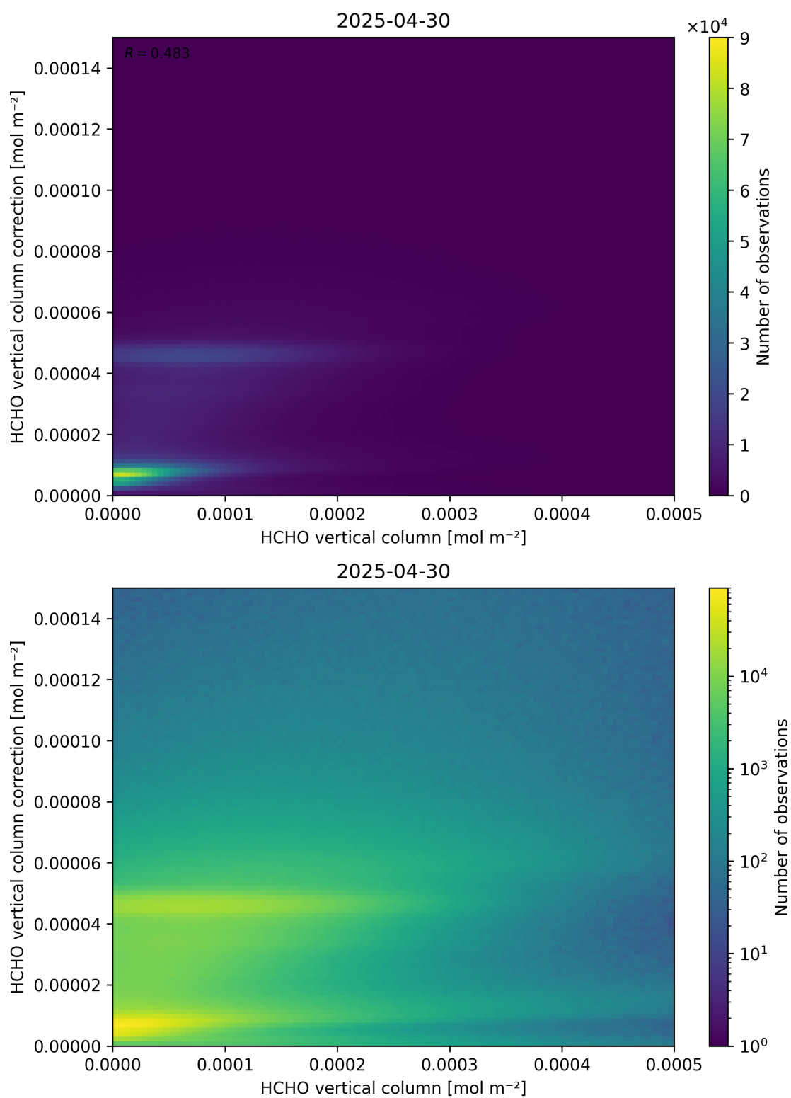
Figure 133: Scatter density plot of “HCHO vertical column” against “HCHO vertical column correction” for 2025-04-29 to 2025-05-01.
