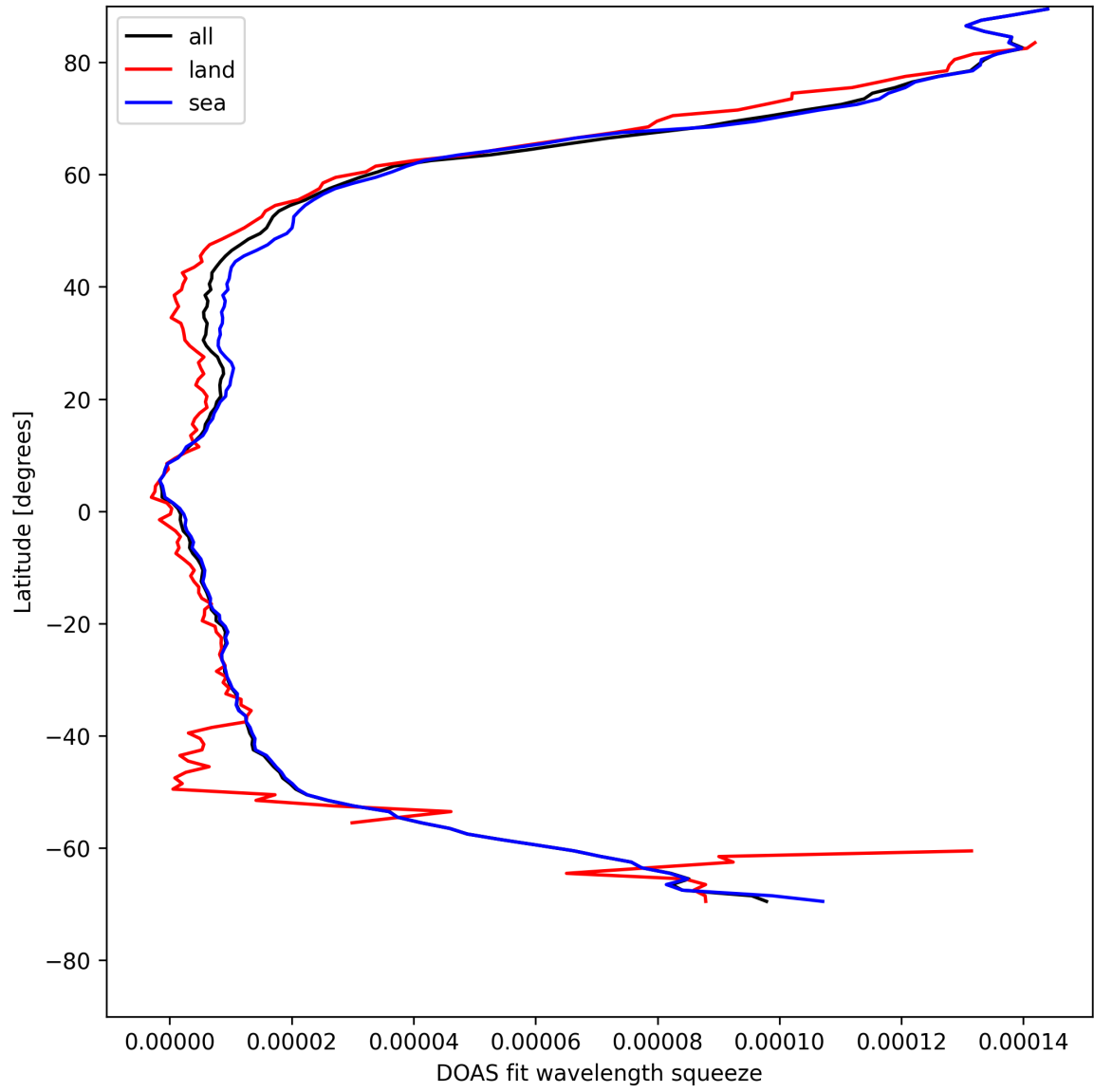
Figure 31: Zonal average of “DOAS fit wavelength squeeze” for 2025-04-29 to 2025-05-01.
