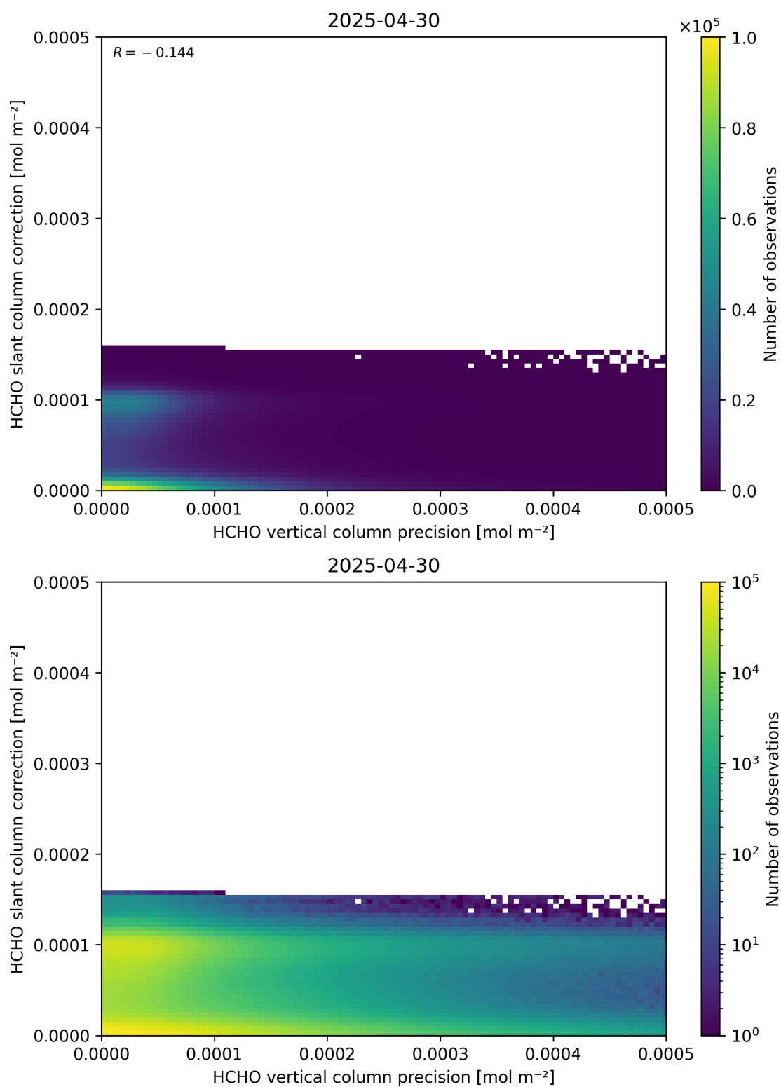
Figure 141: Scatter density plot of “HCHO vertical column precision” against “HCHO slant column correction” for 2025-04-29 to 2025-05-01.
