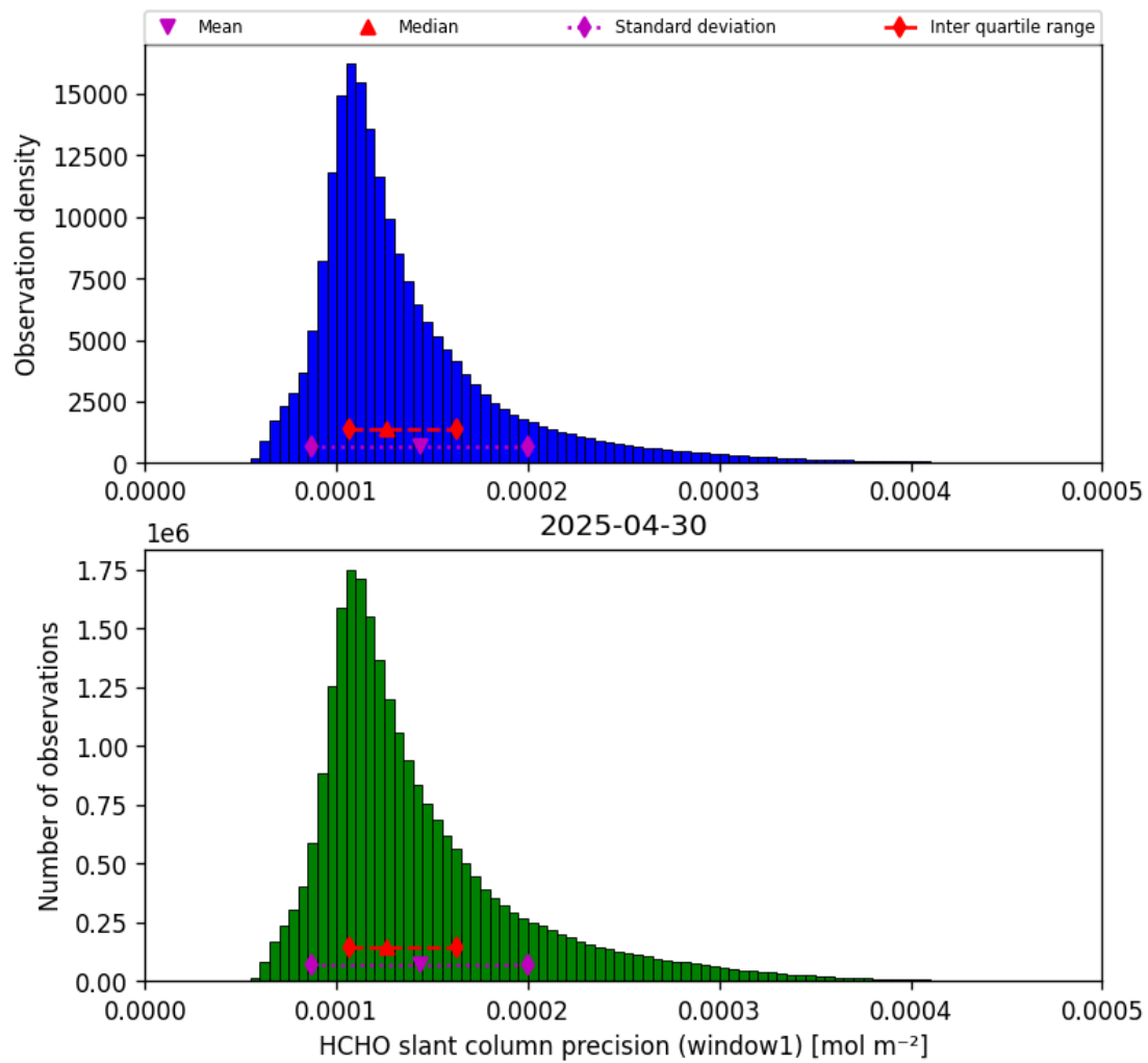
Figure 39: Histogram of “HCHO slant column precision (window1)” for 2025-04-29 to 2025-05-01
