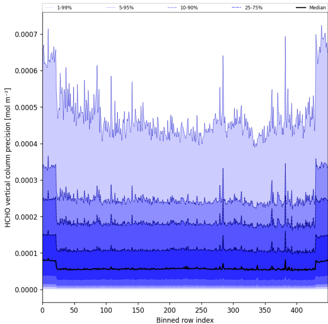
Figure 50: Along track statistics of “HCHO vertical column precision” for 2025-04-29 to 2025-05-01
