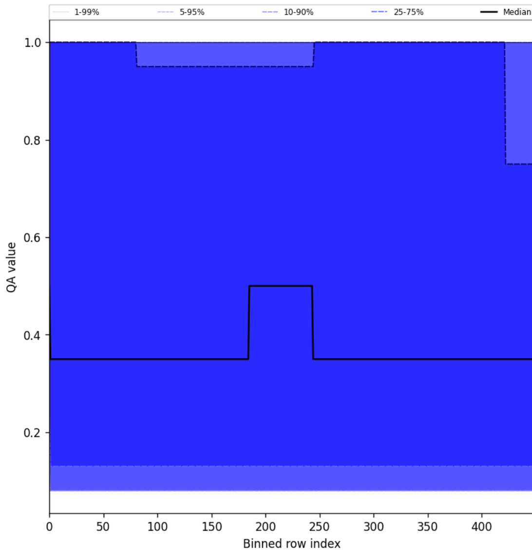
Figure 48: Along track statistics of “QA value” for 2025-04-29 to 2025-05-01
