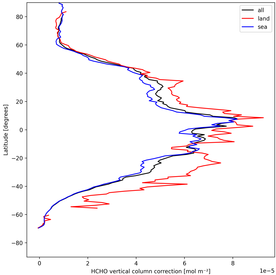
Figure 23: Zonal average of “HCHO vertical column correction” for 2025-04-29 to 2025-05-01.
