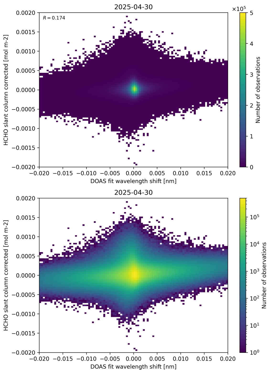
Figure 66: Scatter density plot of “DOAS fit wavelength shift” against “HCHO slant column corrected” for 2025-04-29 to 2025-05-01.
