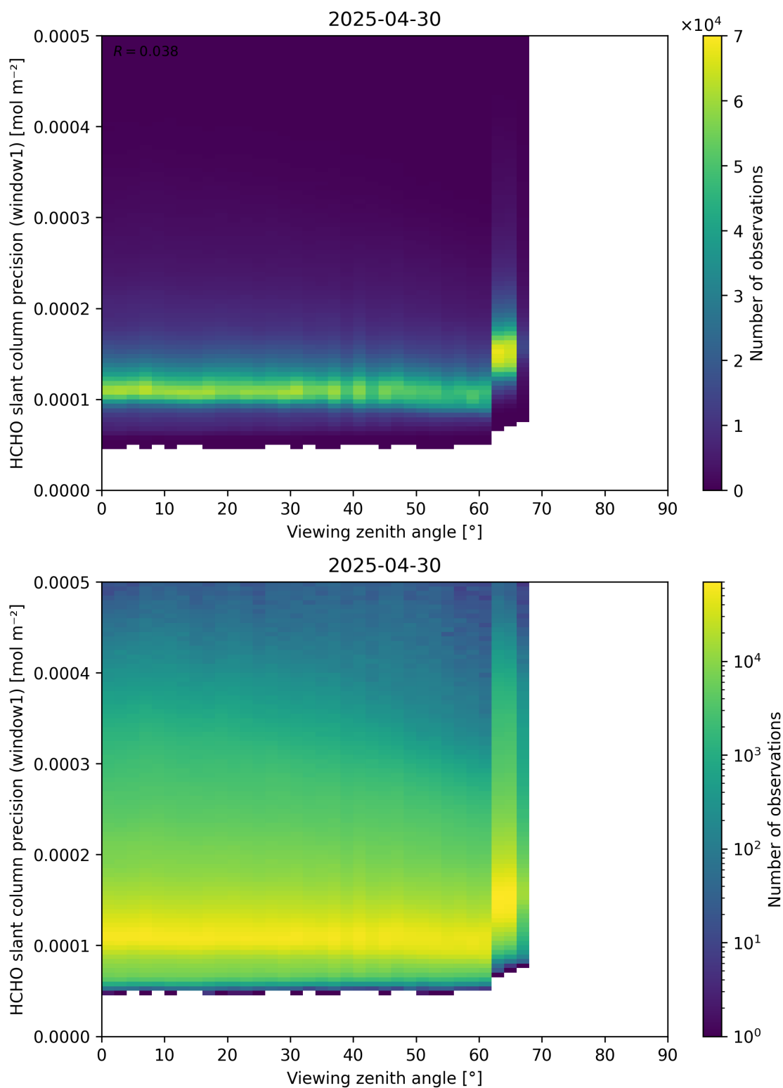
Figure 189: Scatter density plot of “Viewing zenith angle” against “HCHO slant column precision (window1)” for 2025-04-29 to 2025-05-01.
