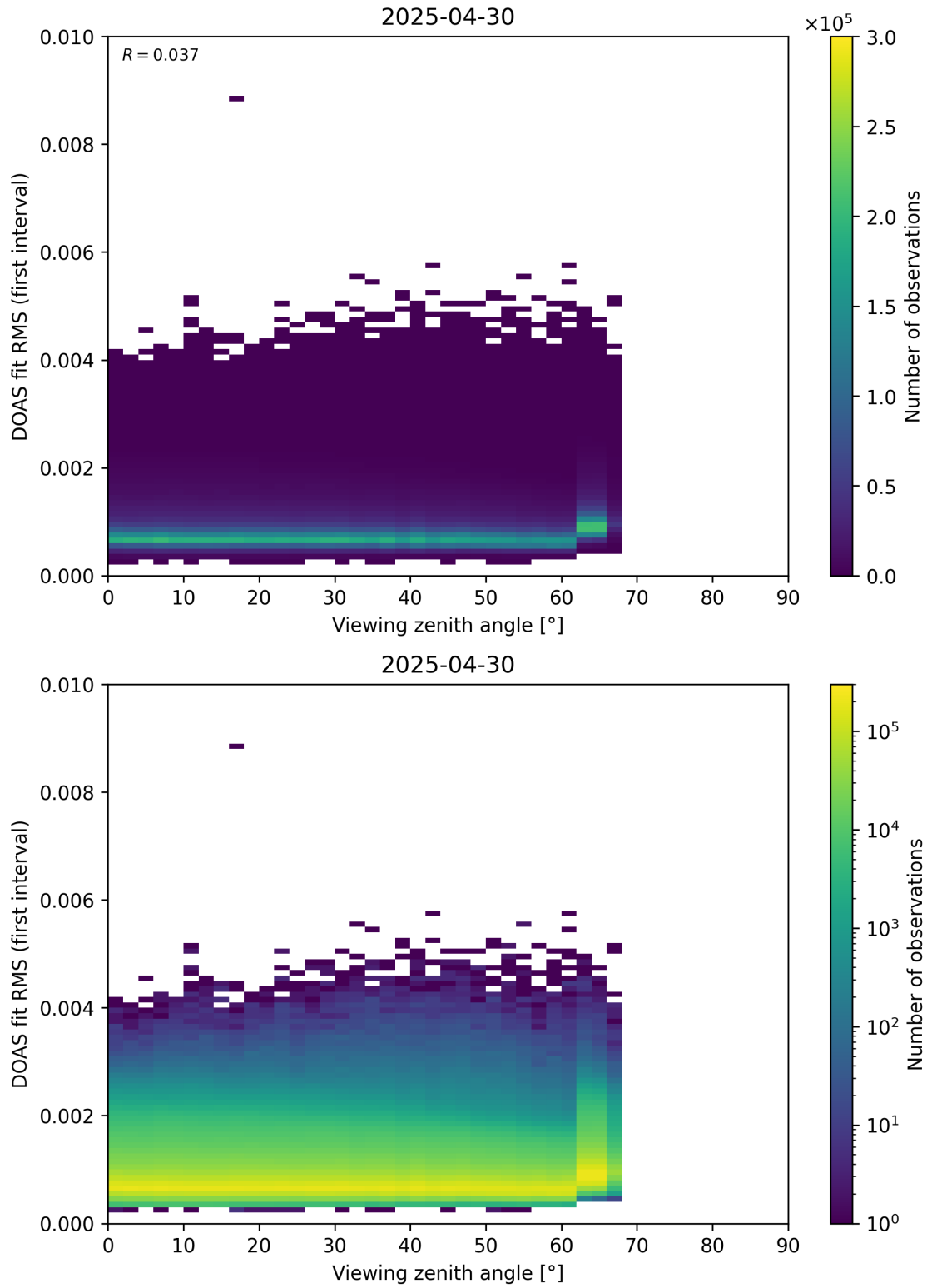
Figure 182: Scatter density plot of “Viewing zenith angle” against “DOAS fit RMS (first interval)” for 2025-04-29 to 2025-05-01.
