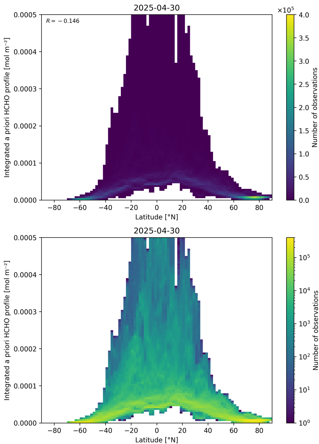
Figure 166: Scatter density plot of “Latitude” against “Integrated a priori HCHO profile” for 2025-04-29 to 2025-05-01.
