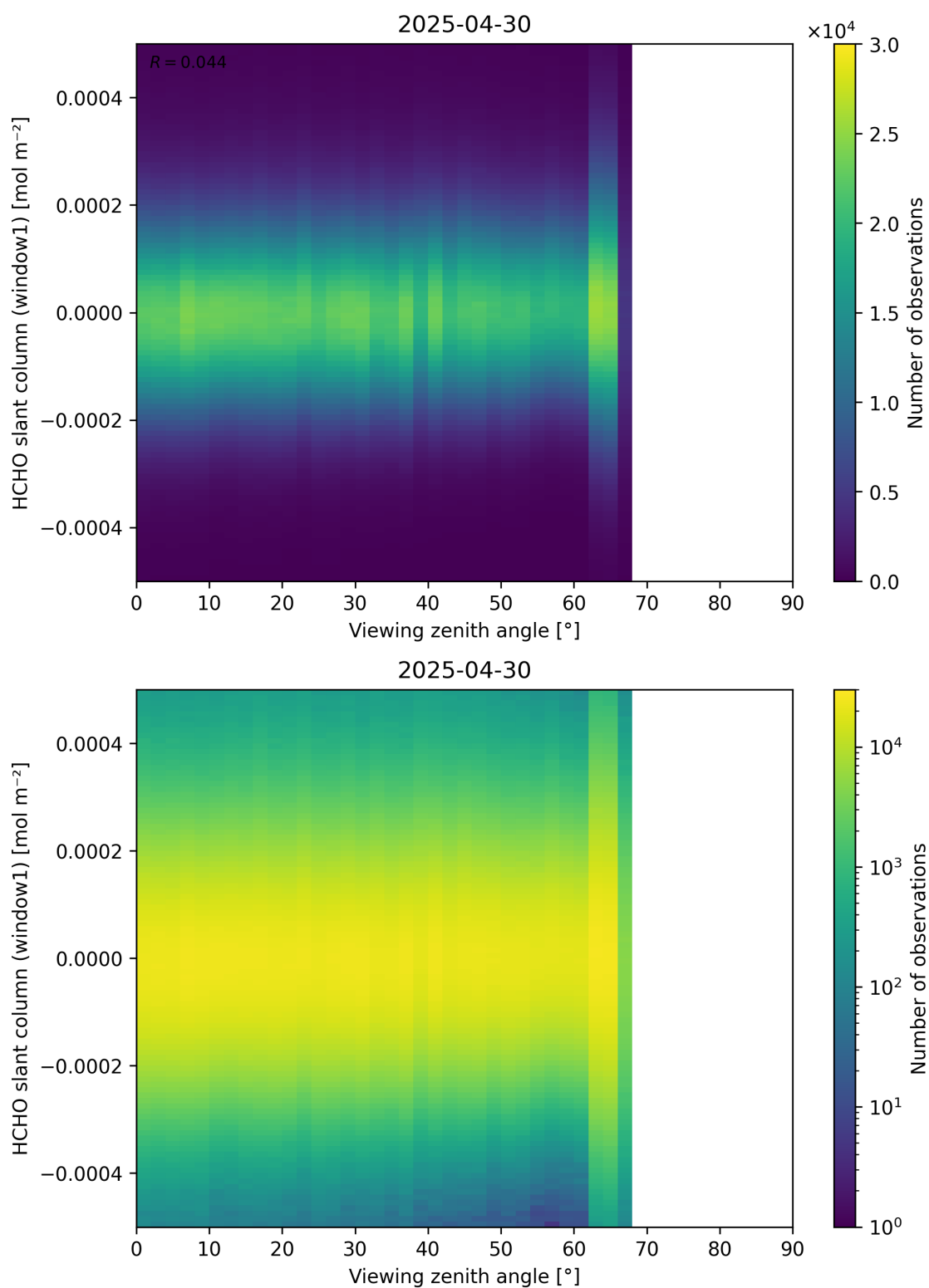
Figure 188: Scatter density plot of “Viewing zenith angle” against “HCHO slant column (window1)” for 2025-04-29 to 2025-05-01.
