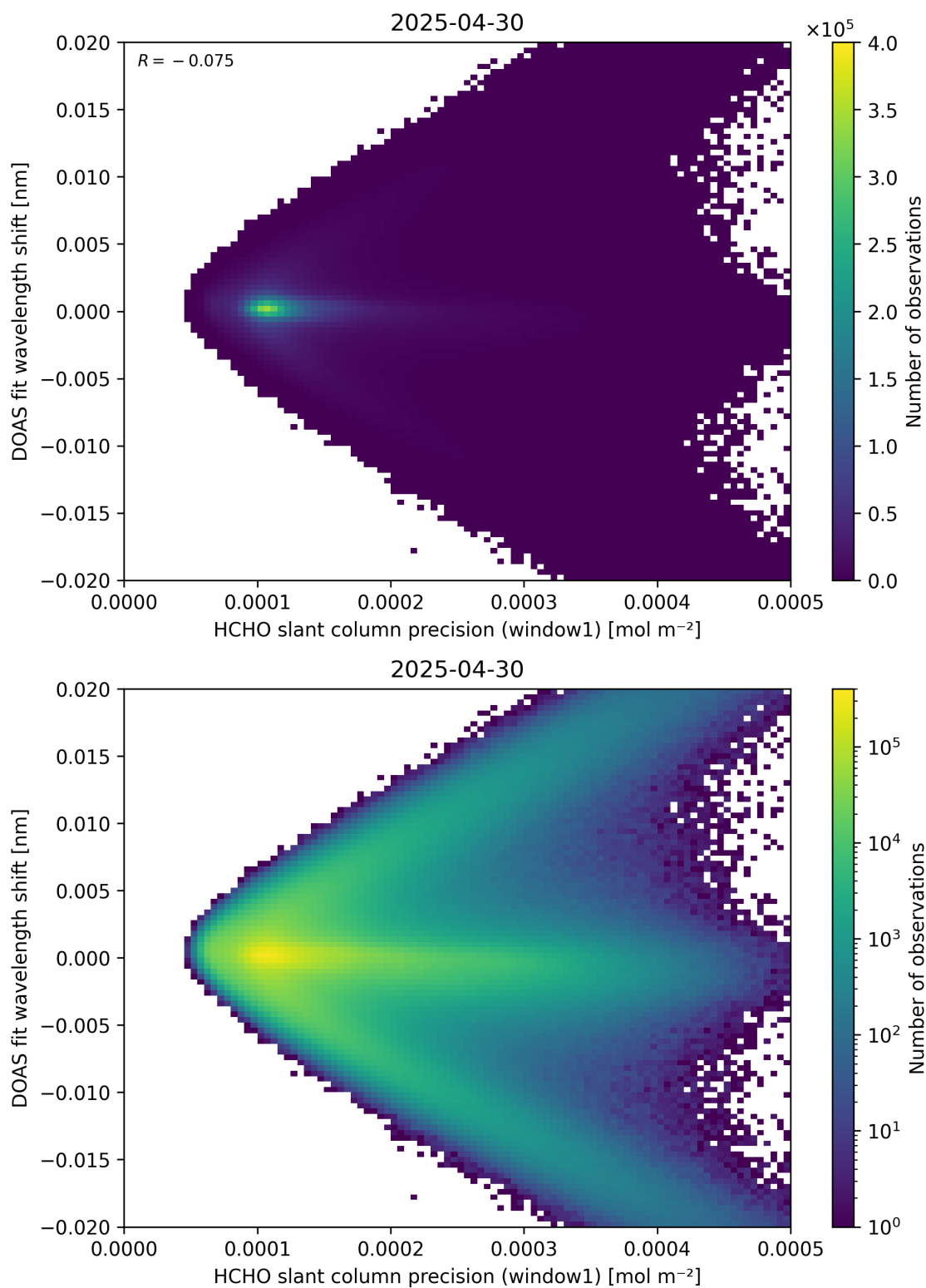
Figure 89: Scatter density plot of “HCHO slant column precision (window1)” against “DOAS fit wavelength shift” for 2025-04-29 to 2025-05-01.
