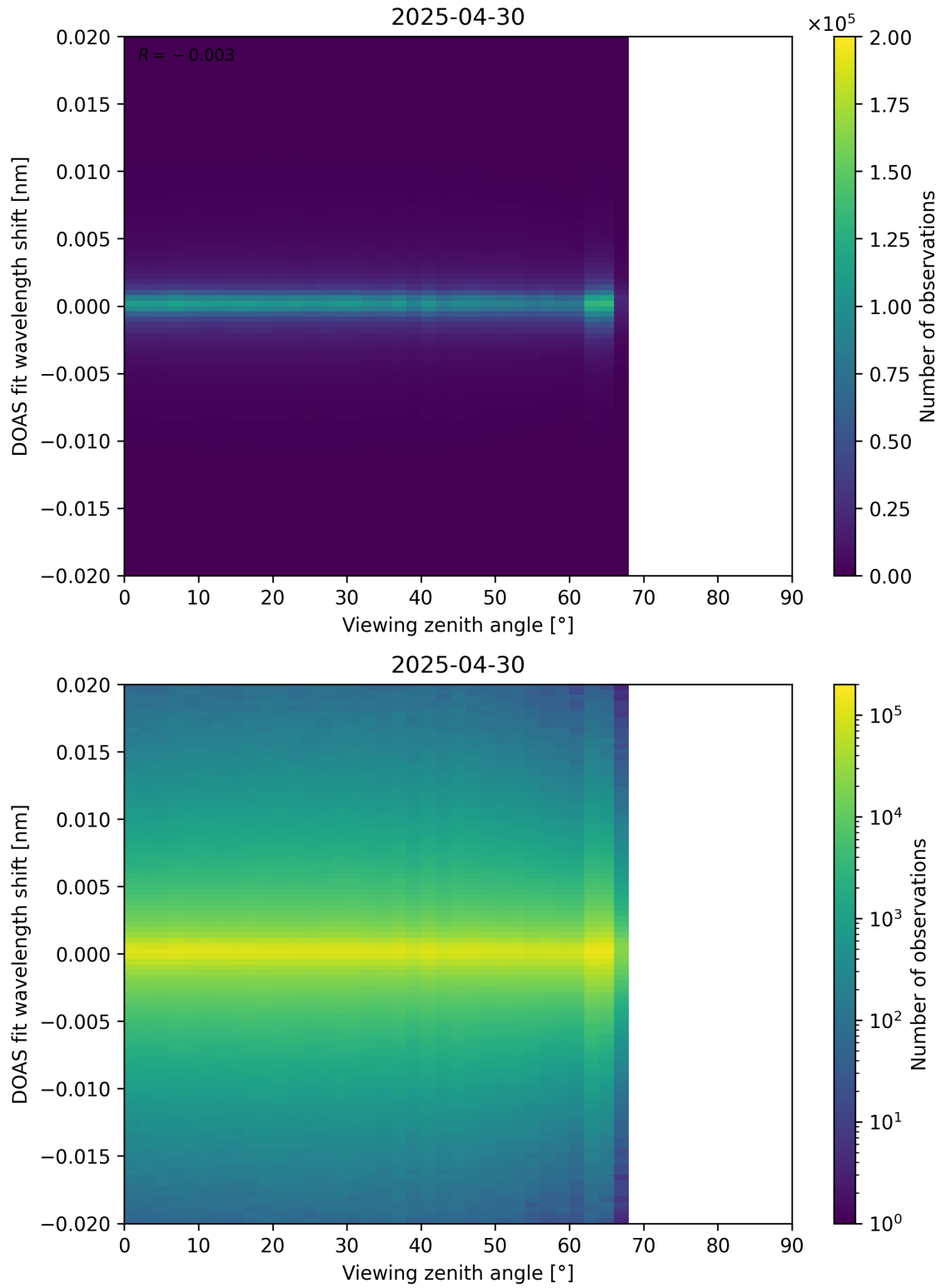
Figure 183: Scatter density plot of “Viewing zenith angle” against “DOAS fit wavelength shift” for 2025-04-29 to 2025-05-01.
