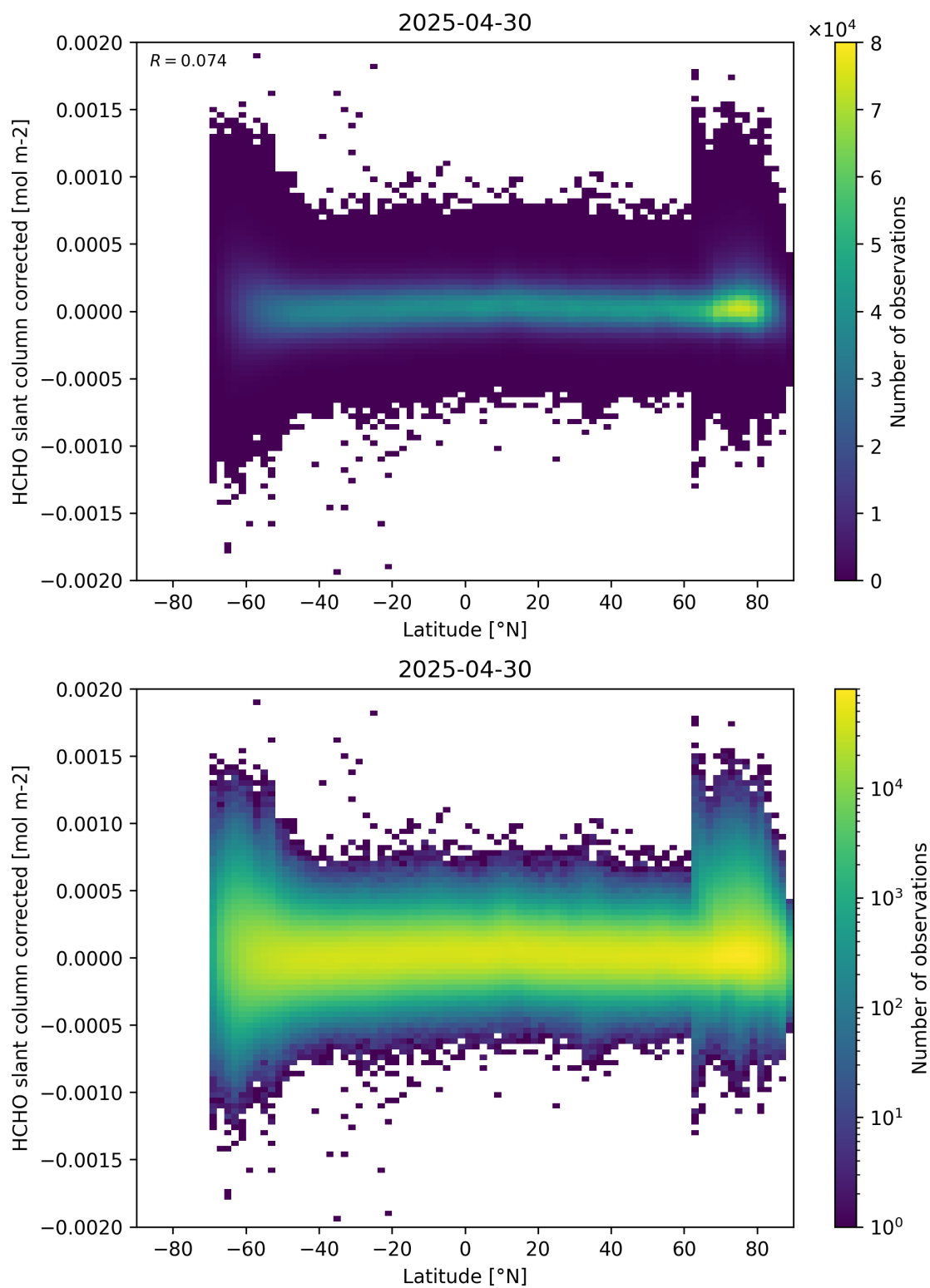
Figure 157: Scatter density plot of “Latitude” against “HCHO slant column corrected” for 2025-04-29 to 2025-05-01.
