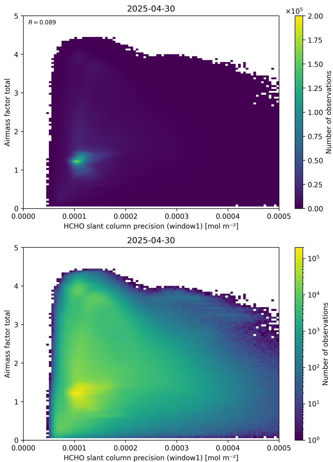
Figure 94: Scatter density plot of “HCHO slant column precision (window1)” against “Airmass factor total” for 2025-04-29 to 2025-05-01.
