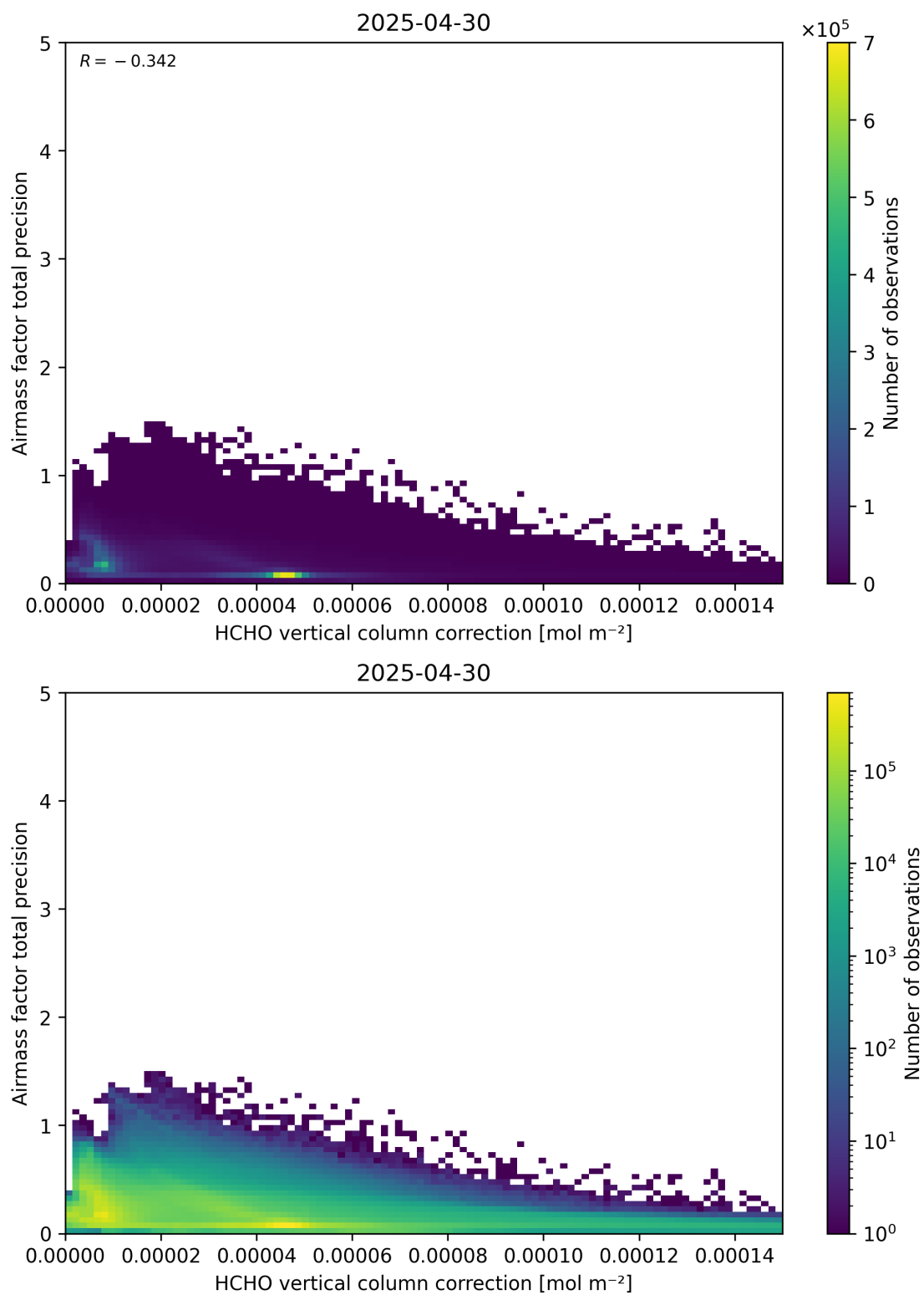
Figure 121: Scatter density plot of “HCHO vertical column correction” against “Airmass factor total precision” for 2025-04-29 to 2025-05-01.
