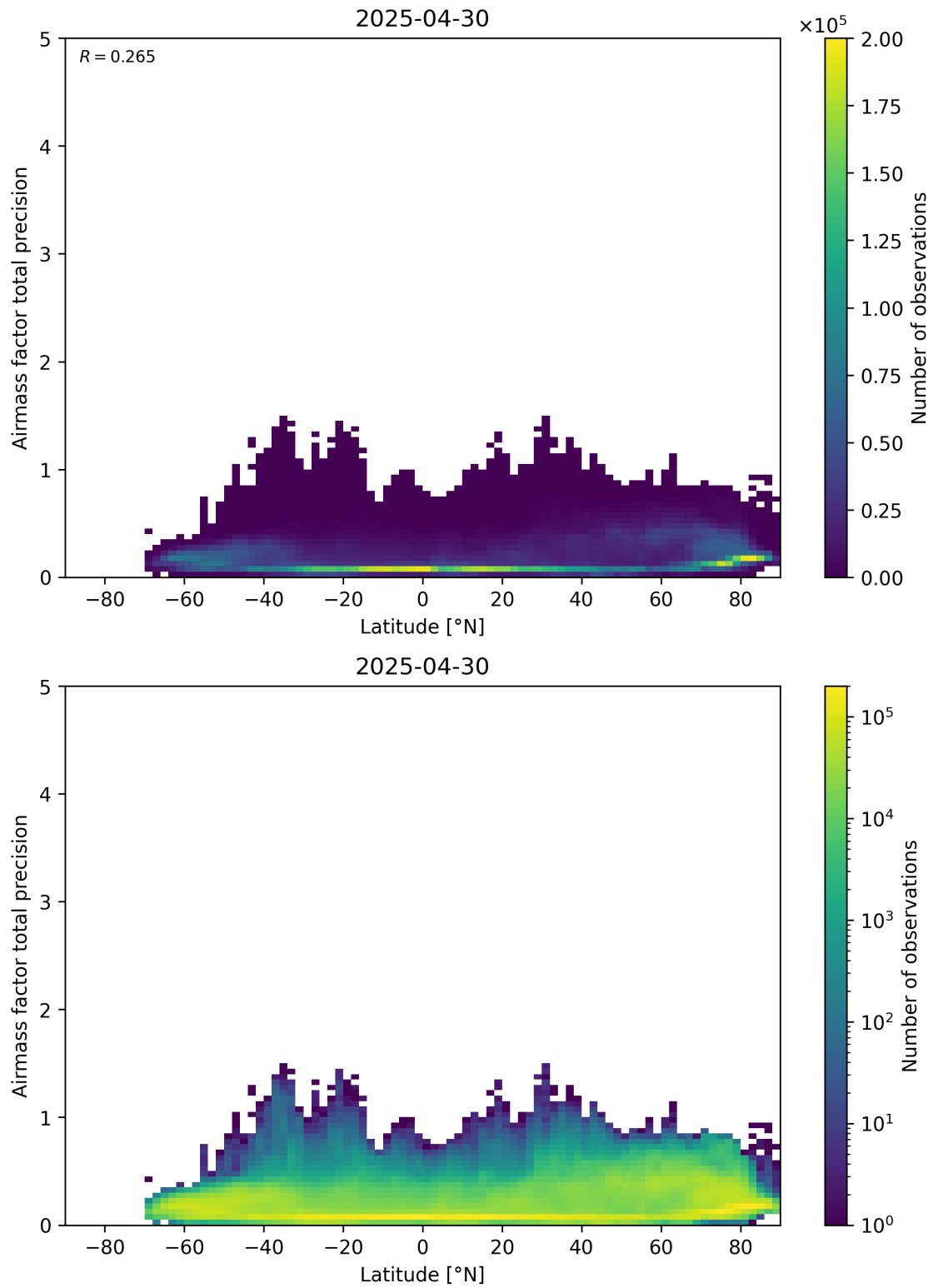
Figure 162: Scatter density plot of “Latitude” against “Airmass factor total precision” for 2025-04-29 to 2025-05-01.
