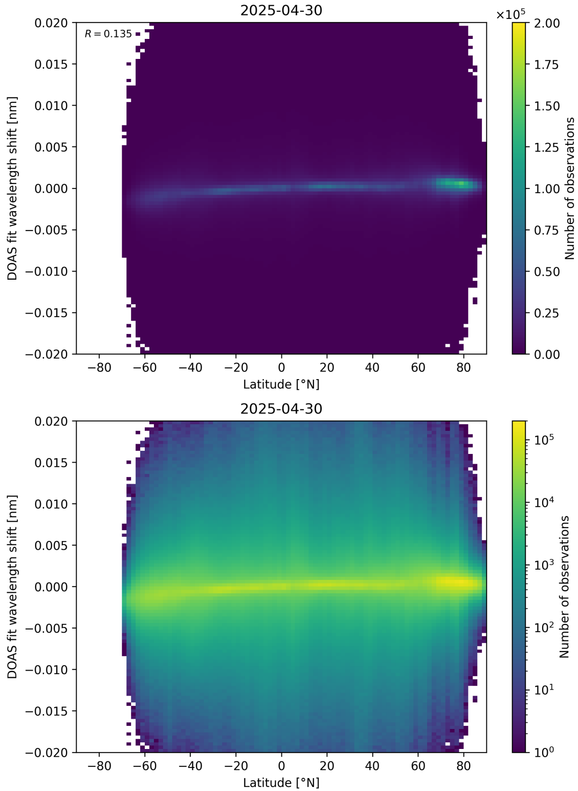
Figure 154: Scatter density plot of “Latitude” against “DOAS fit wavelength shift” for 2025-04-29 to 2025-05-01.
