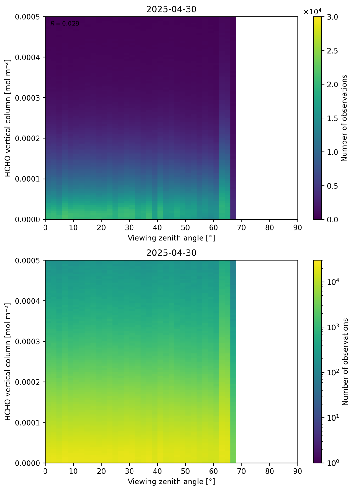
Figure 192: Scatter density plot of “Viewing zenith angle” against “HCHO vertical column” for 2025-04-29 to 2025-05-01.
