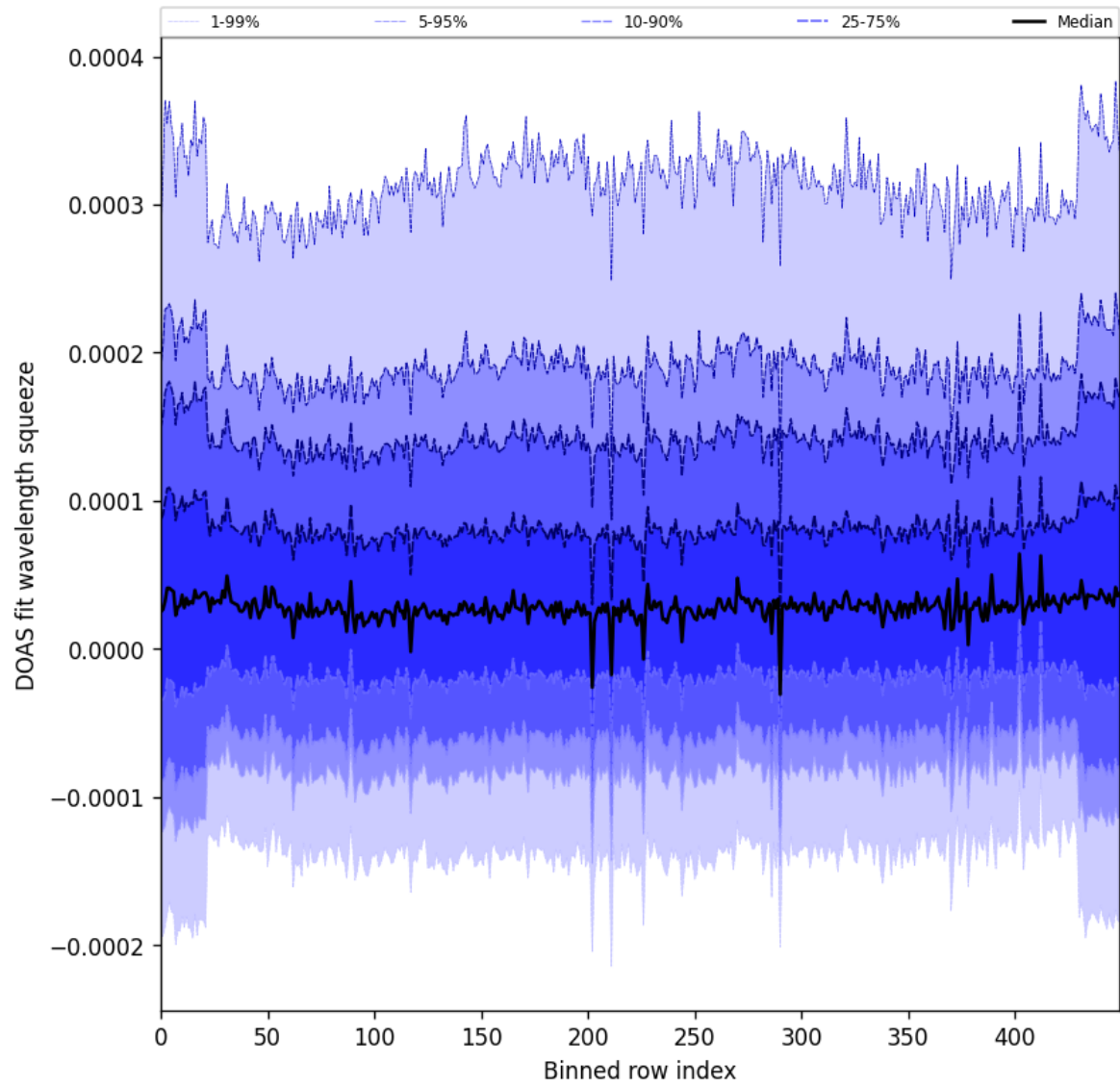
Figure 59: Along track statistics of “DOAS fit wavelength squeeze” for 2025-04-29 to 2025-05-01
