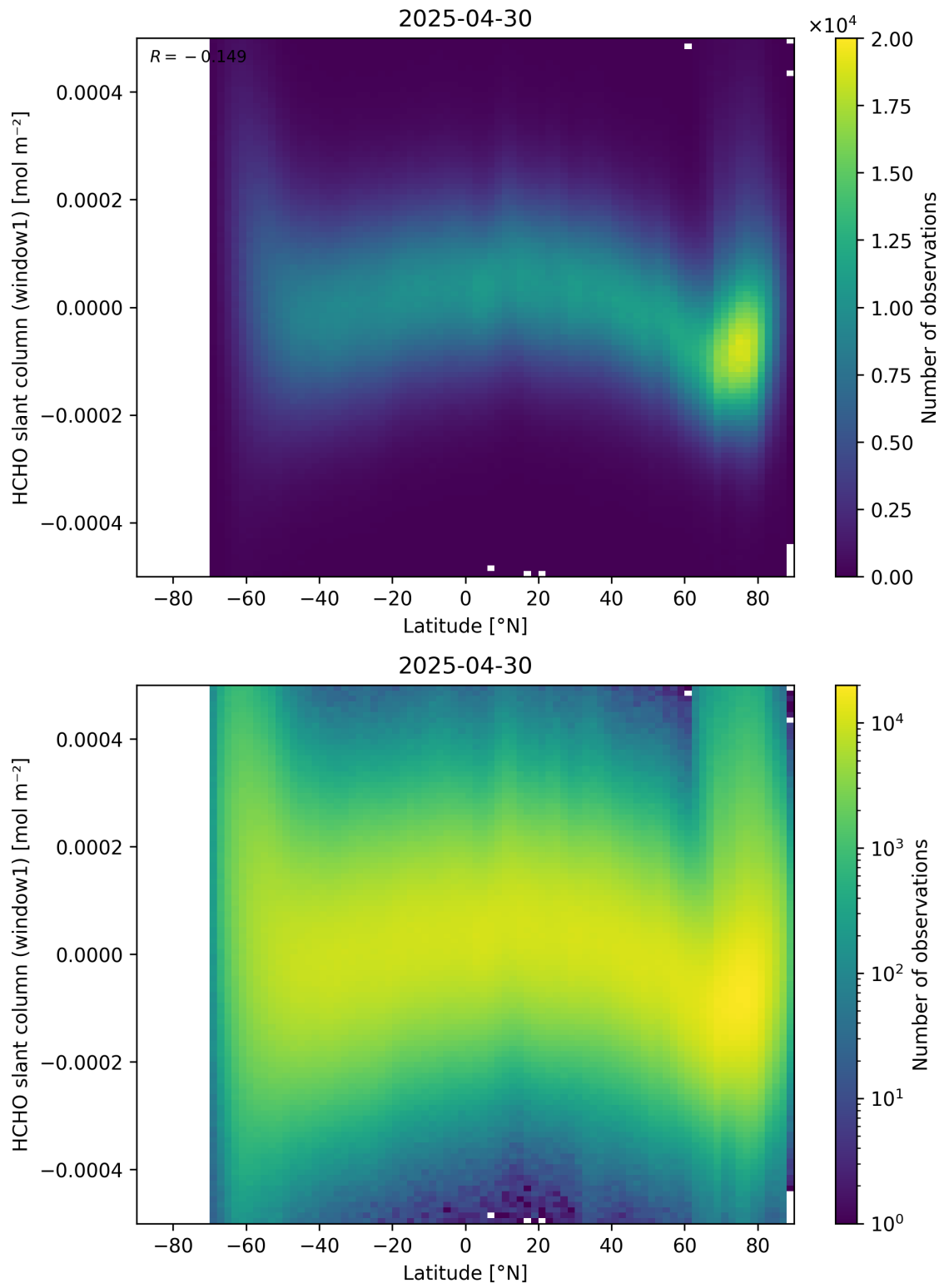
Figure 159: Scatter density plot of “Latitude” against “HCHO slant column (window1)” for 2025-04-29 to 2025-05-01.
