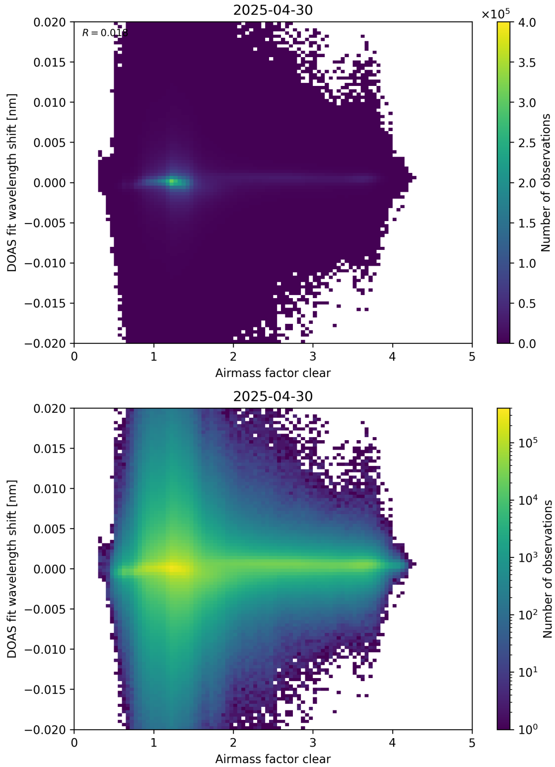
Figure 72: Scatter density plot of “Airmass factor clear” against “DOAS fit wavelength shift” for 2025-04-29 to 2025-05-01.
