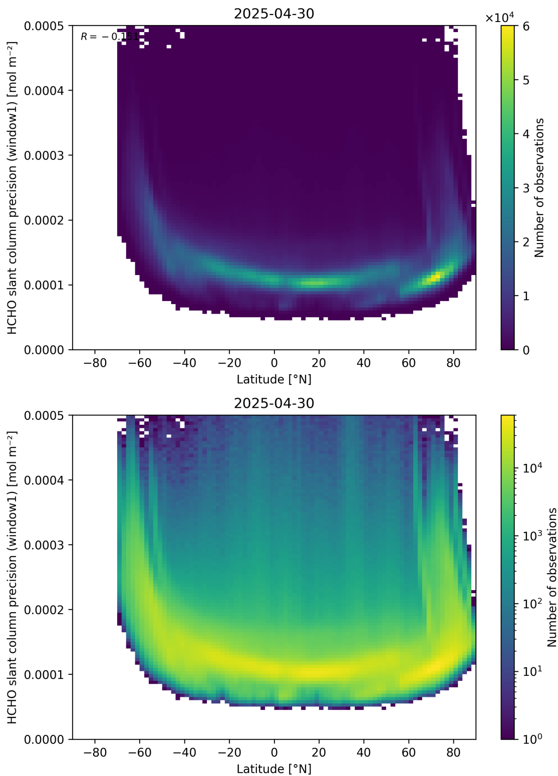
Figure 160: Scatter density plot of “Latitude” against “HCHO slant column precision (window1)” for 2025-04-29 to 2025-05-01.
