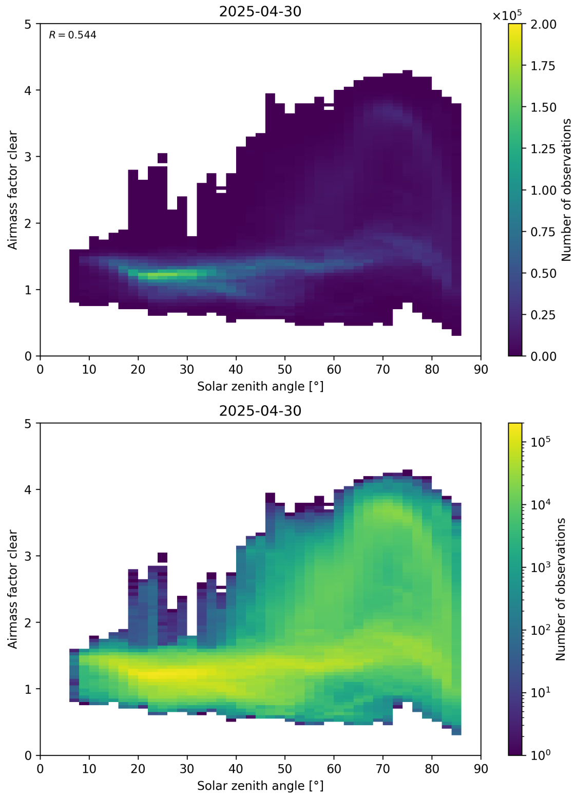
Figure 170: Scatter density plot of “Solar zenith angle” against “Airmass factor clear” for 2025-04-29 to 2025-05-01.
