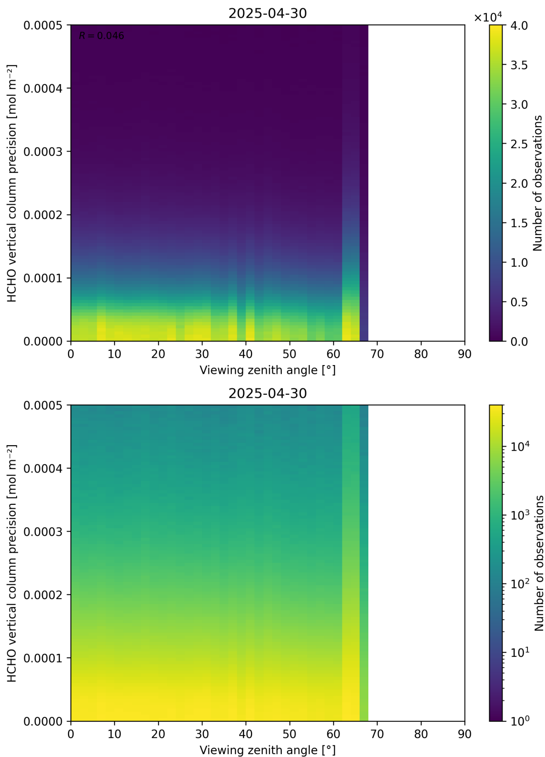
Figure 194: Scatter density plot of “Viewing zenith angle” against “HCHO vertical column precision” for 2025-04-29 to 2025-05-01.
