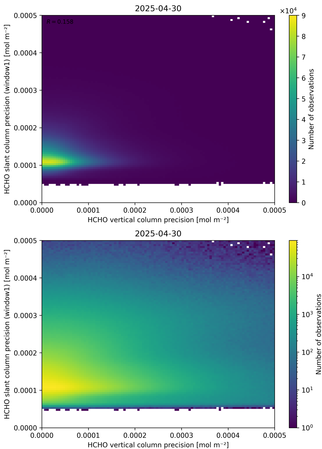
Figure 143: Scatter density plot of “HCHO vertical column precision” against “HCHO slant column precision (window1)” for 2025-04-29 to 2025-05-01.
