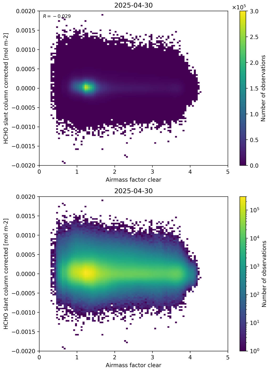
Figure 74: Scatter density plot of “Airmass factor clear” against “HCHO slant column corrected” for 2025-04-29 to 2025-05-01.
