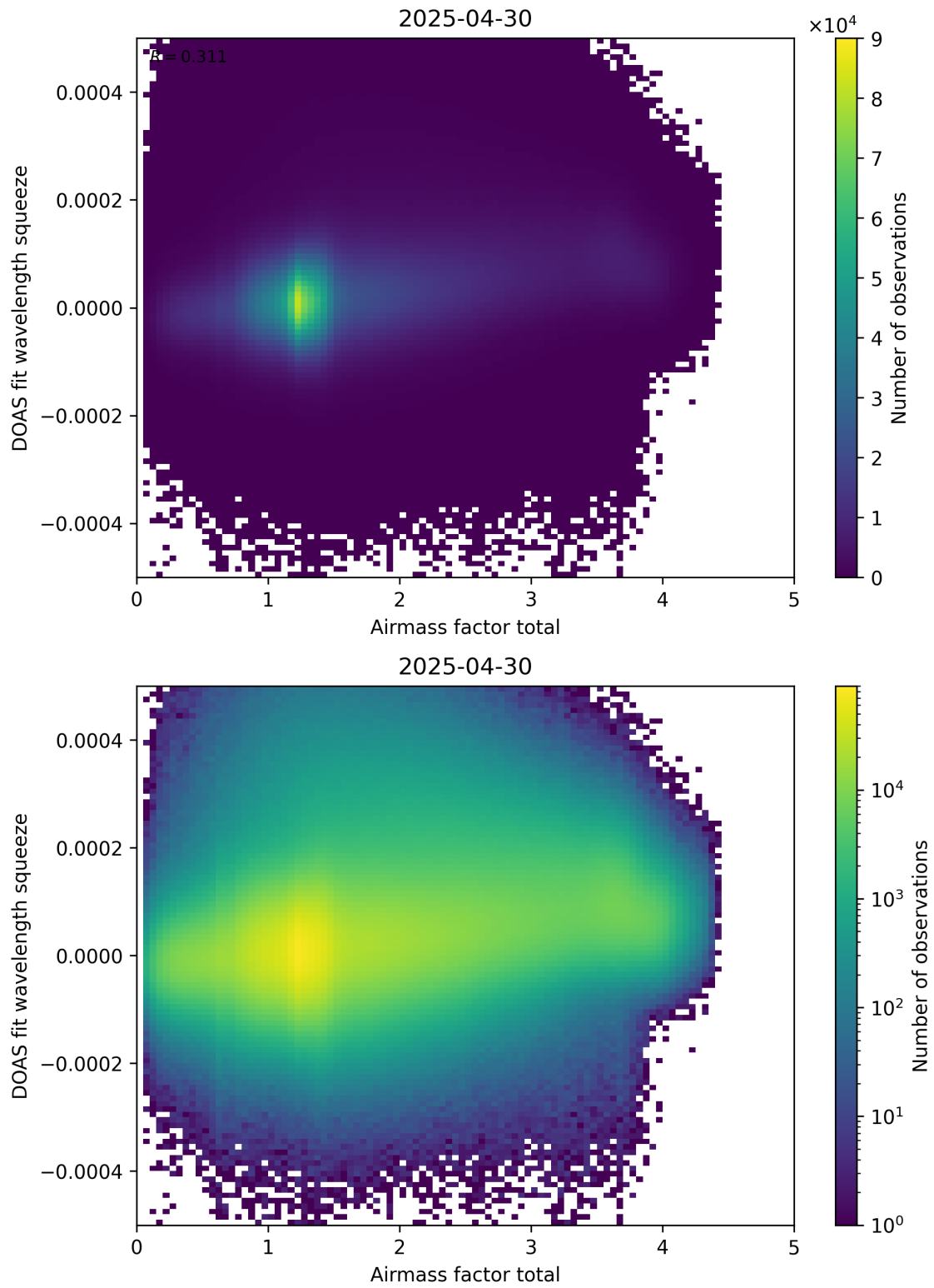
Figure 99: Scatter density plot of “Airmass factor total” against “DOAS fit wavelength squeeze” for 2025-04-29 to 2025-05-01.
