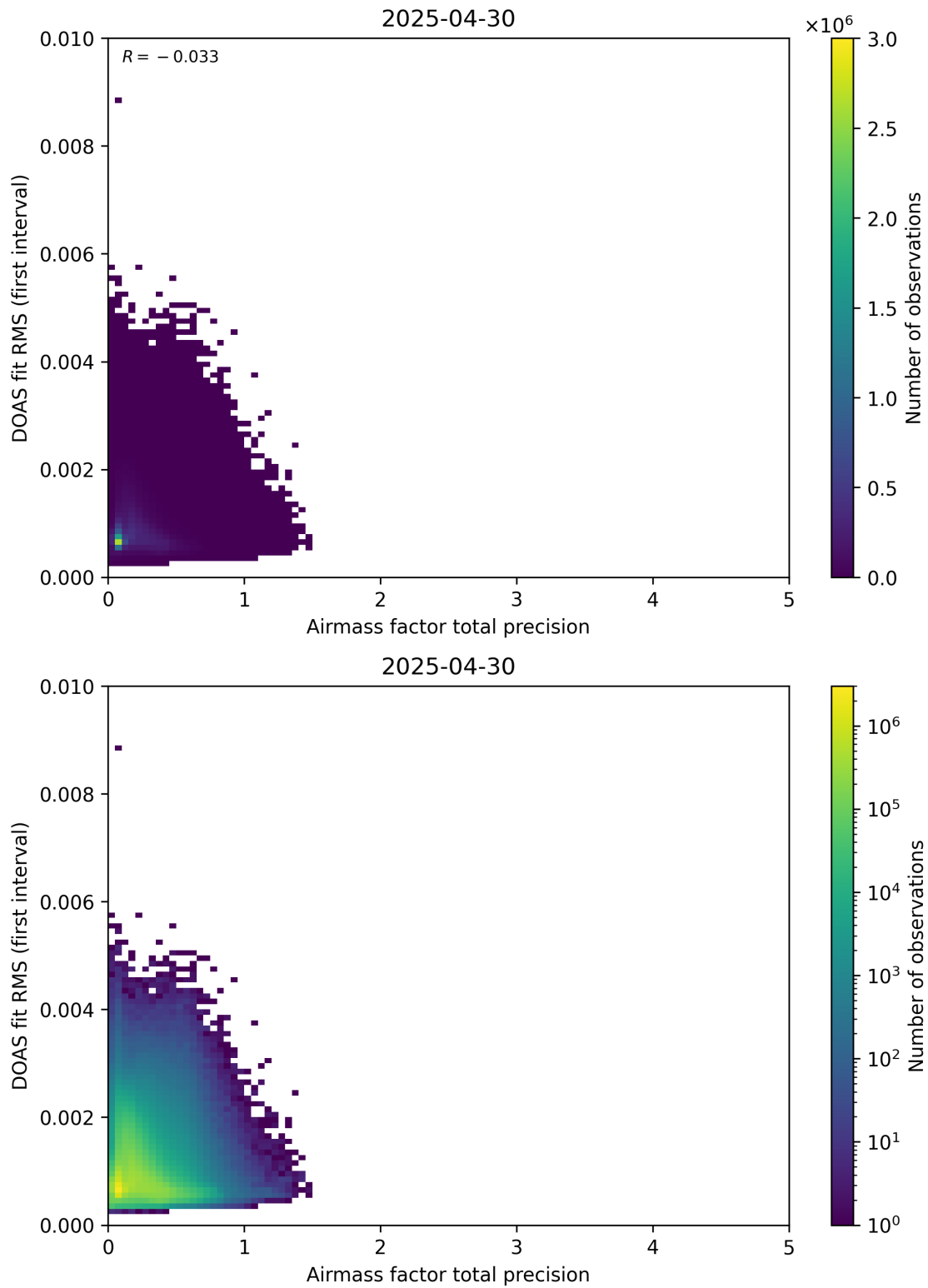
Figure 105: Scatter density plot of “Airmass factor total precision” against “DOAS fit RMS (first interval)” for 2025-04-29 to 2025-05-01.
