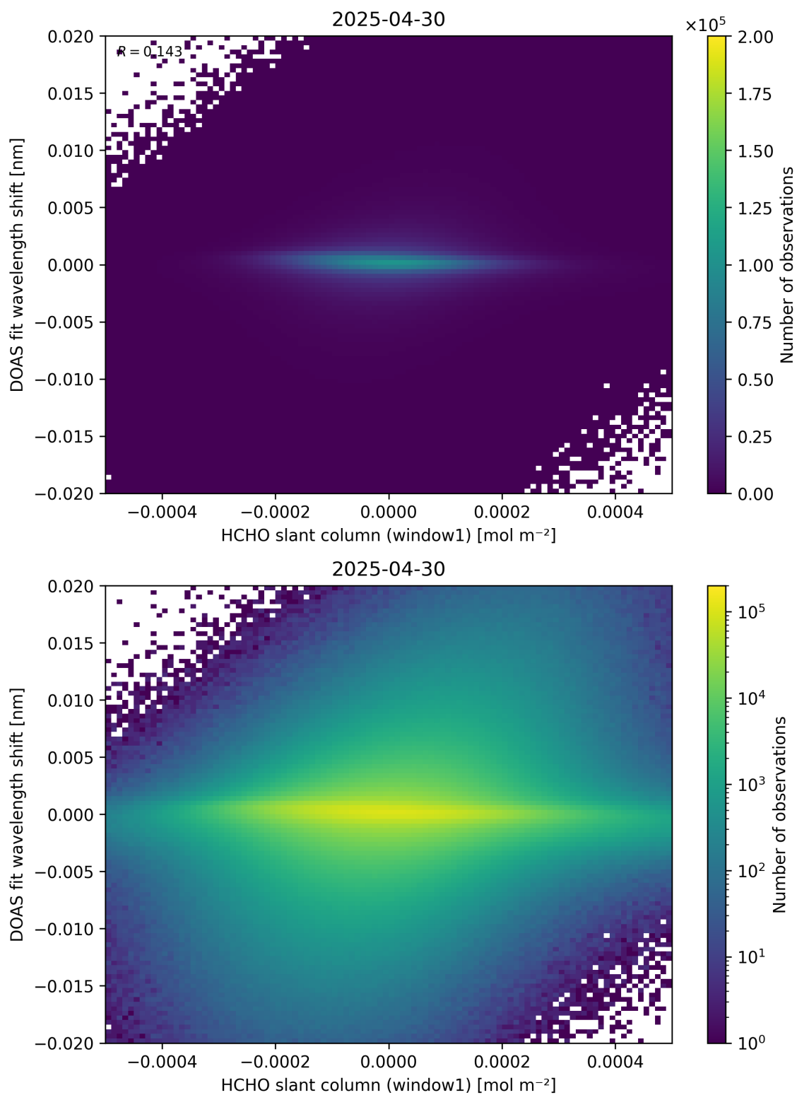
Figure 79: Scatter density plot of “HCHO slant column (window1)” against “DOAS fit wavelength shift” for 2025-04-29 to 2025-05-01.
