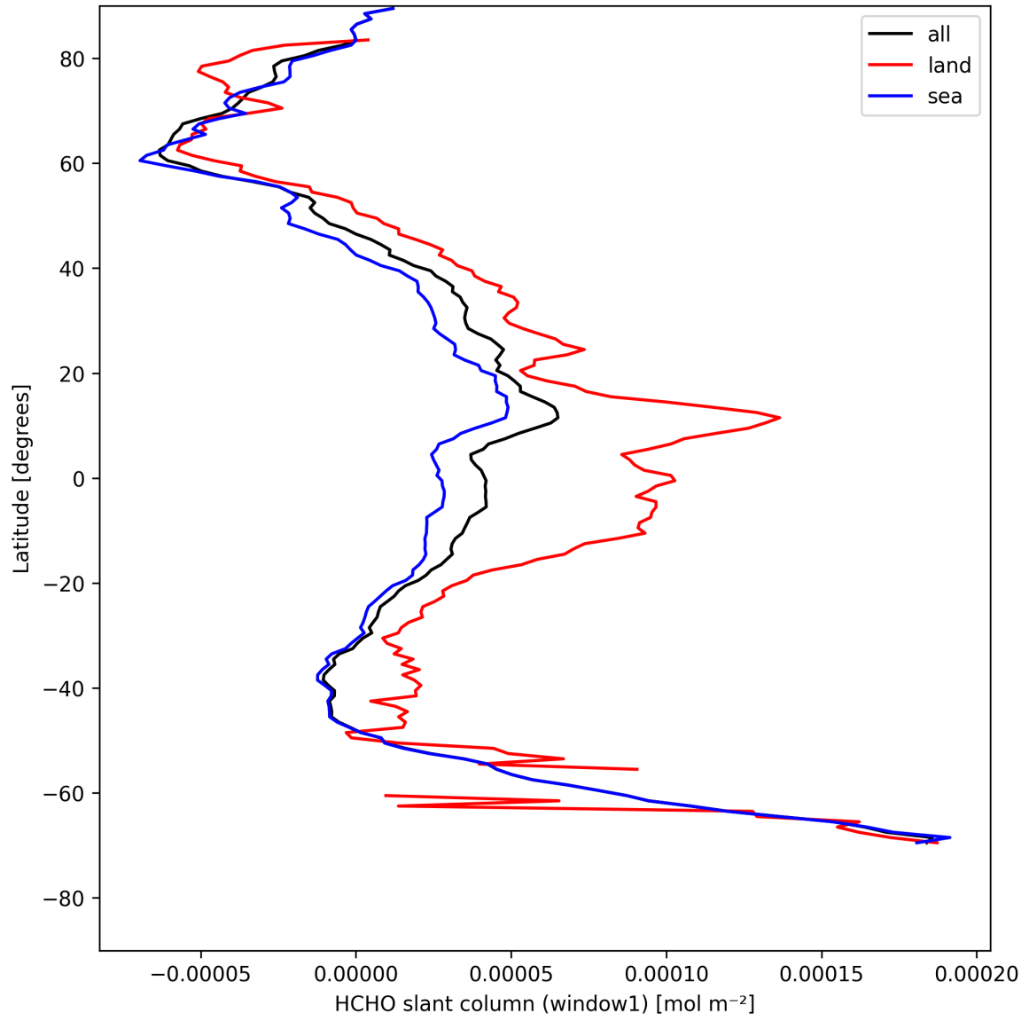
Figure 24: Zonal average of “HCHO slant column (window1)” for 2025-04-29 to 2025-05-01.
