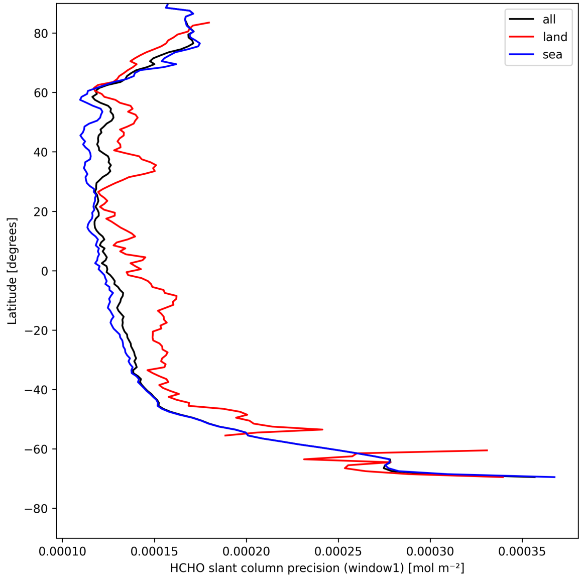
Figure 25: Zonal average of “HCHO slant column precision (window1)” for 2025-04-29 to 2025-05-01.
