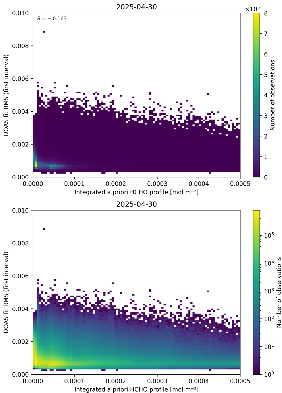
Figure 148: Scatter density plot of “Integrated a priori HCHO profile” against “DOAS fit RMS (first interval)” for 2025-04-29 to 2025-05-01.
