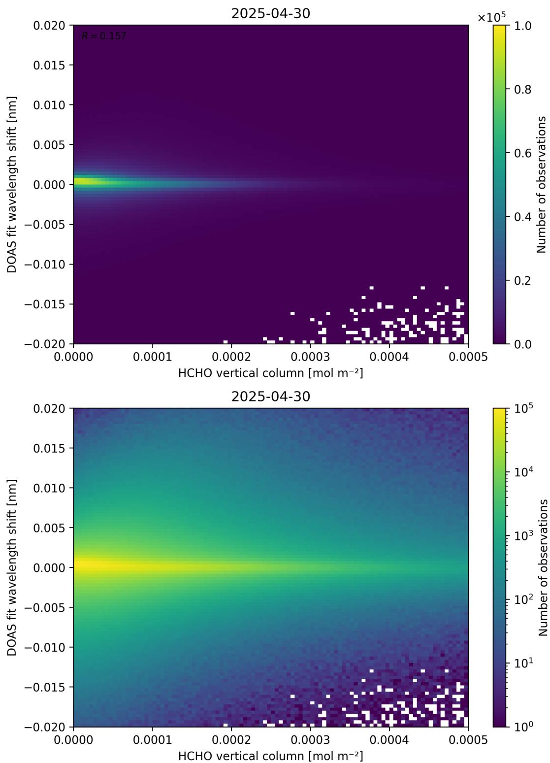
Figure 124: Scatter density plot of “HCHO vertical column” against “DOAS fit wavelength shift” for 2025-04-29 to 2025-05-01.
