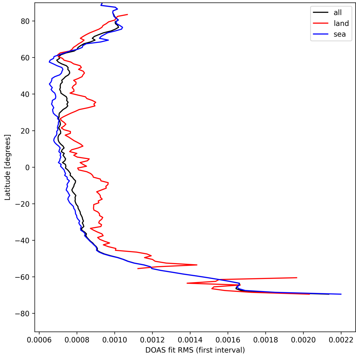
Figure 32: Zonal average of “DOAS fit RMS (first interval)” for 2025-04-29 to 2025-05-01.
