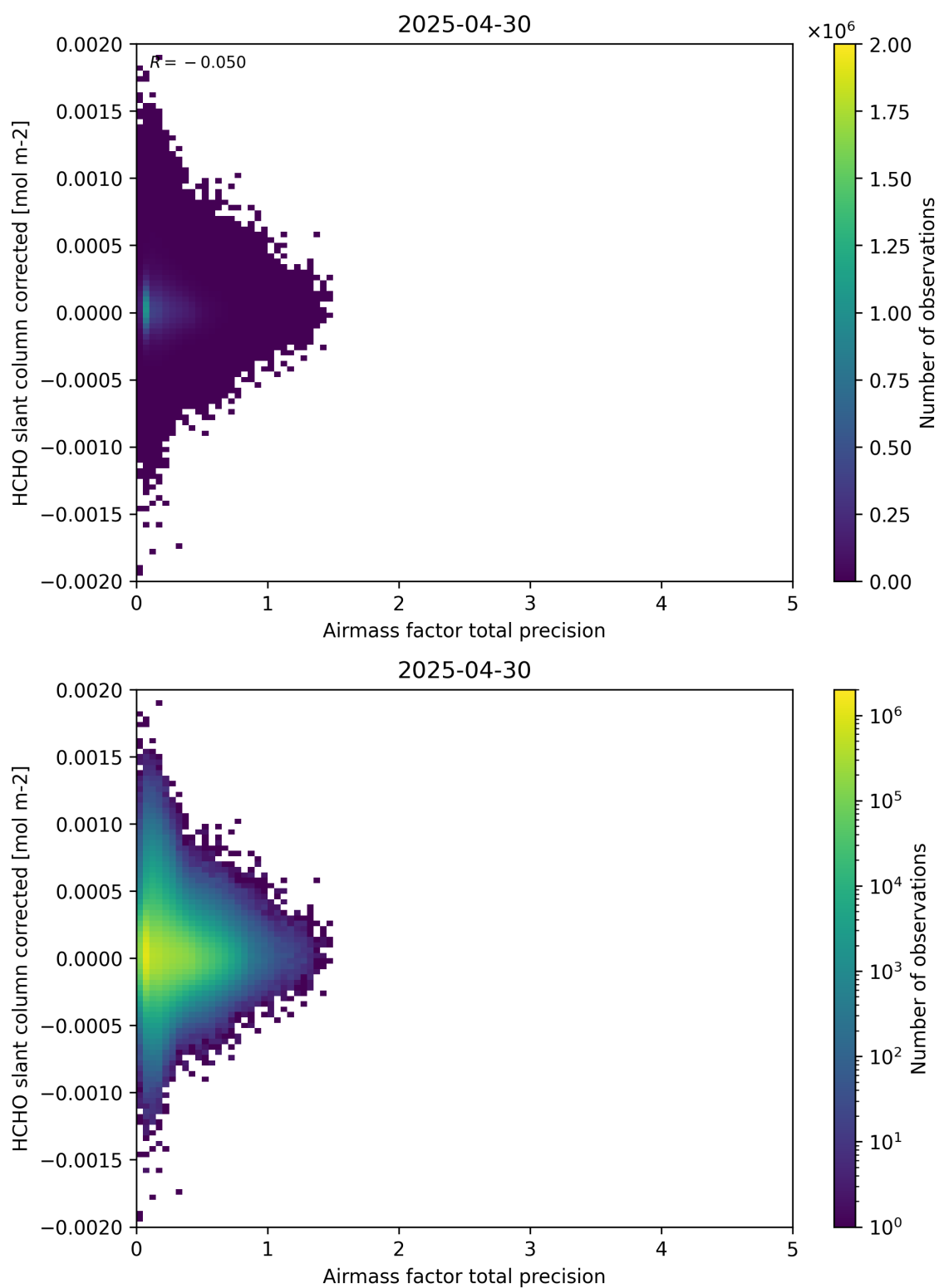
Figure 109: Scatter density plot of “Airmass factor total precision” against “HCHO slant column corrected” for 2025-04-29 to 2025-05-01.
