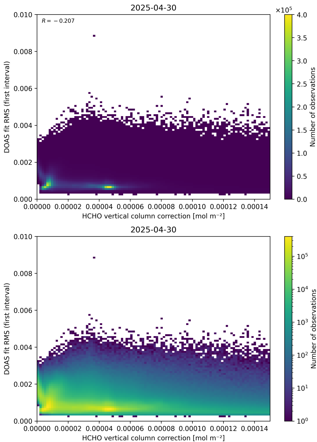
Figure 112: Scatter density plot of “HCHO vertical column correction” against “DOAS fit RMS (first interval)” for 2025-04-29 to 2025-05-01.
