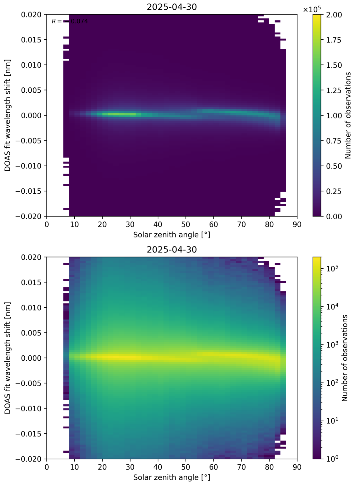
Figure 168: Scatter density plot of “Solar zenith angle” against “DOAS fit wavelength shift” for 2025-04-29 to 2025-05-01.
