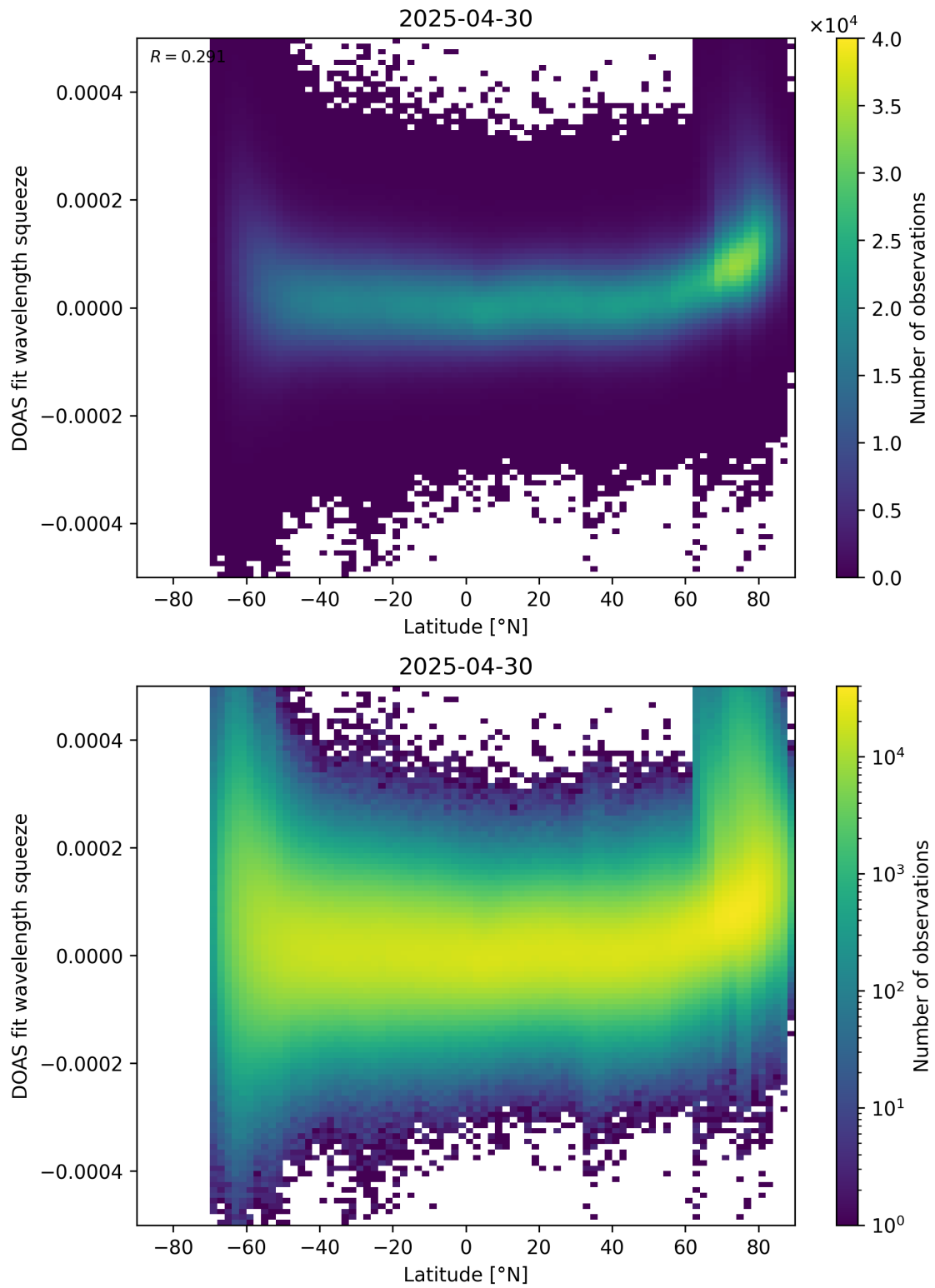
Figure 155: Scatter density plot of “Latitude” against “DOAS fit wavelength squeeze” for 2025-04-29 to 2025-05-01.
