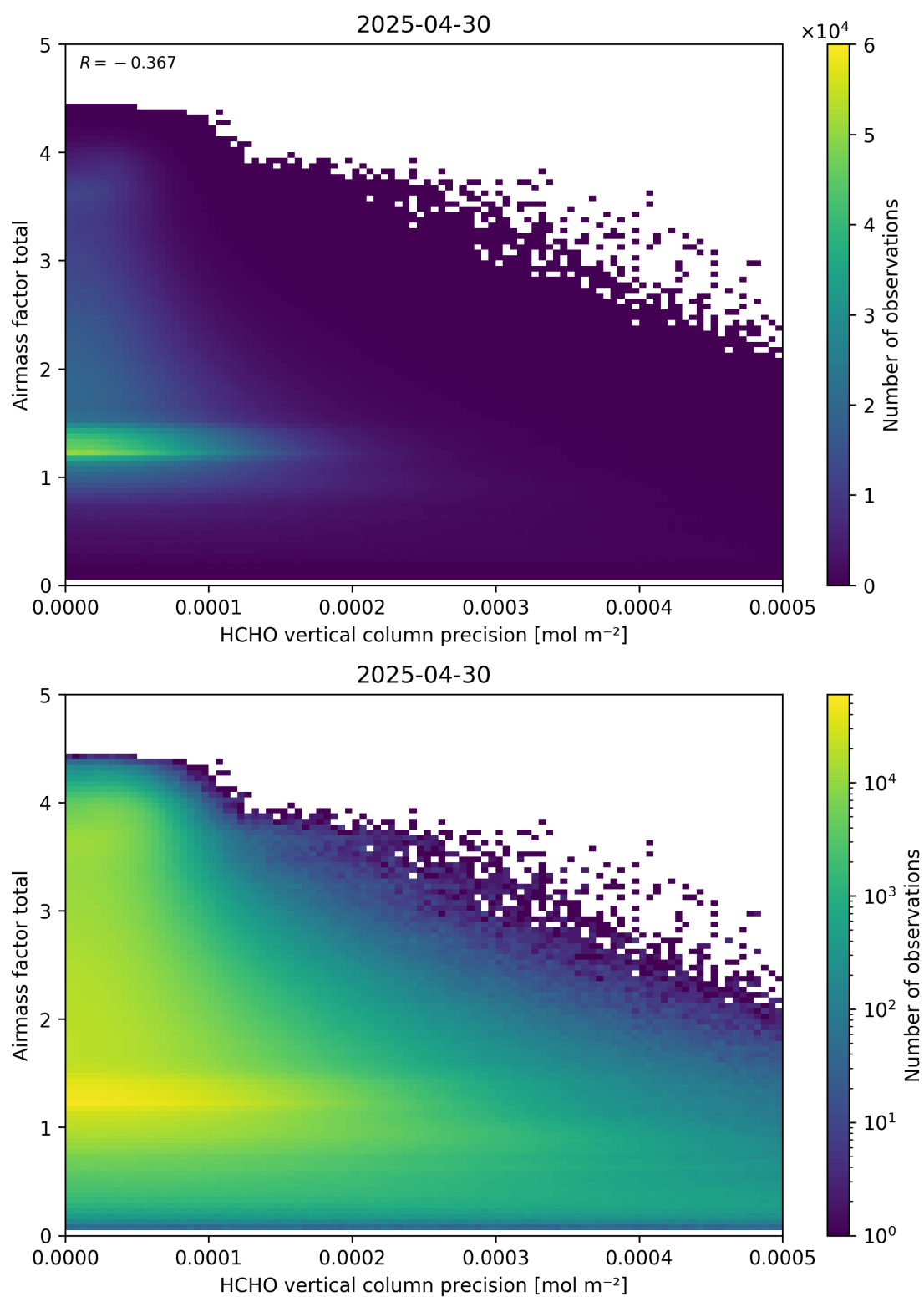
Figure 144: Scatter density plot of “HCHO vertical column precision” against “Airmass factor total” for 2025-04-29 to 2025-05-01.
