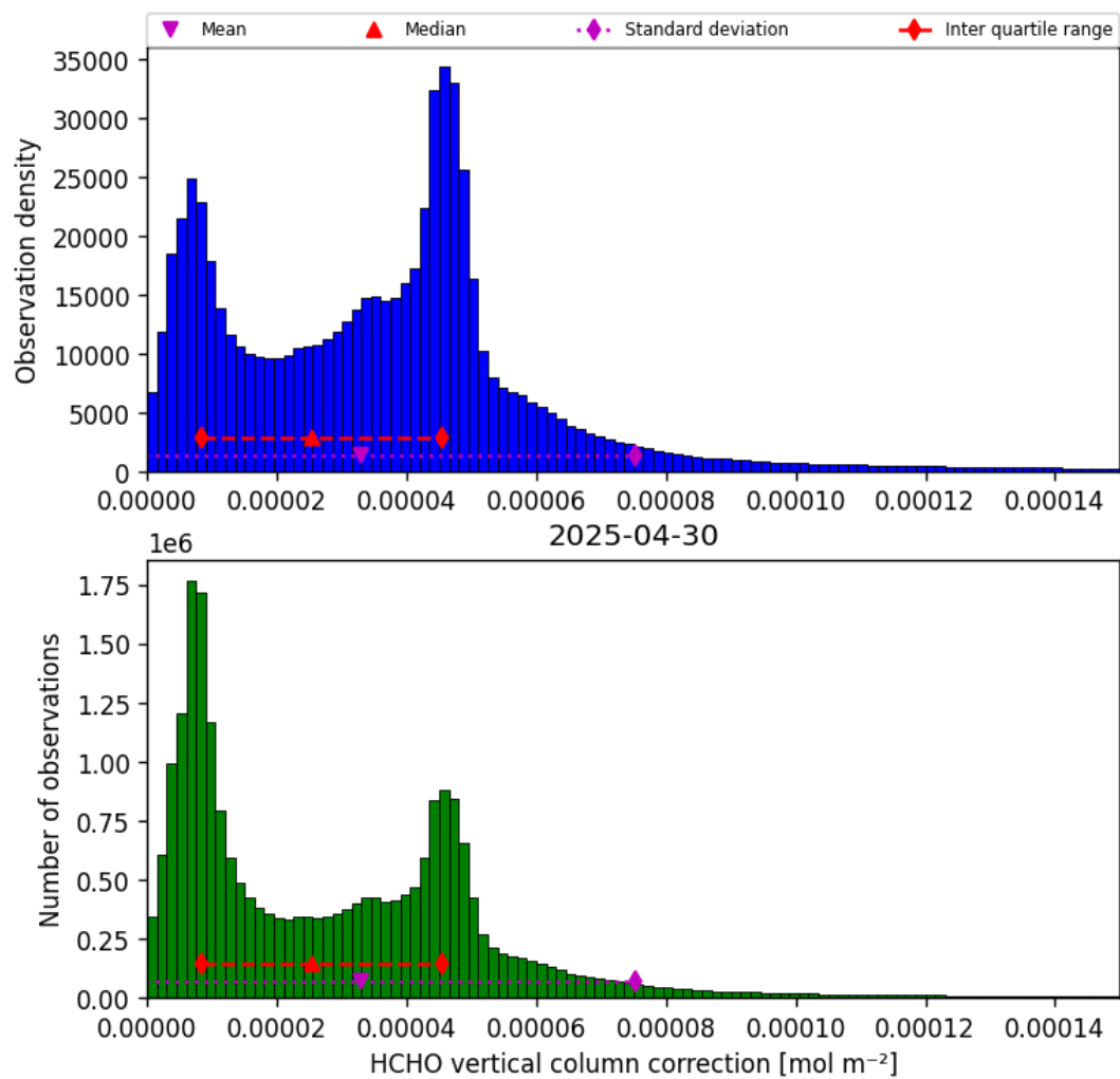
Figure 37: Histogram of “HCHO vertical column correction” for 2025-04-29 to 2025-05-01
