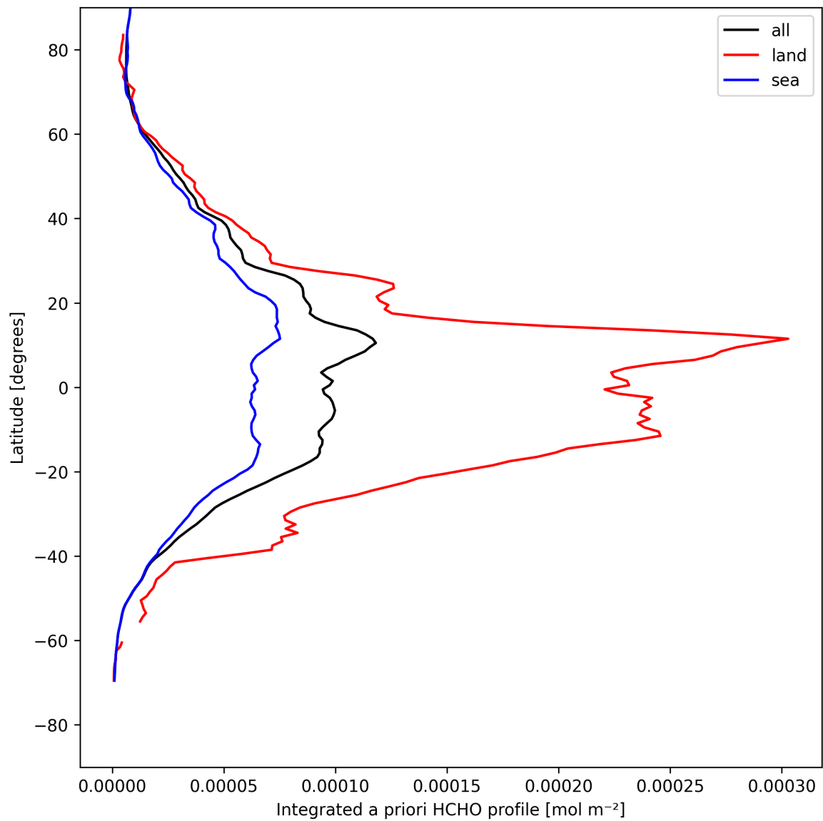
Figure 29: Zonal average of “Integrated a priori HCHO profile” for 2025-04-29 to 2025-05-01.
