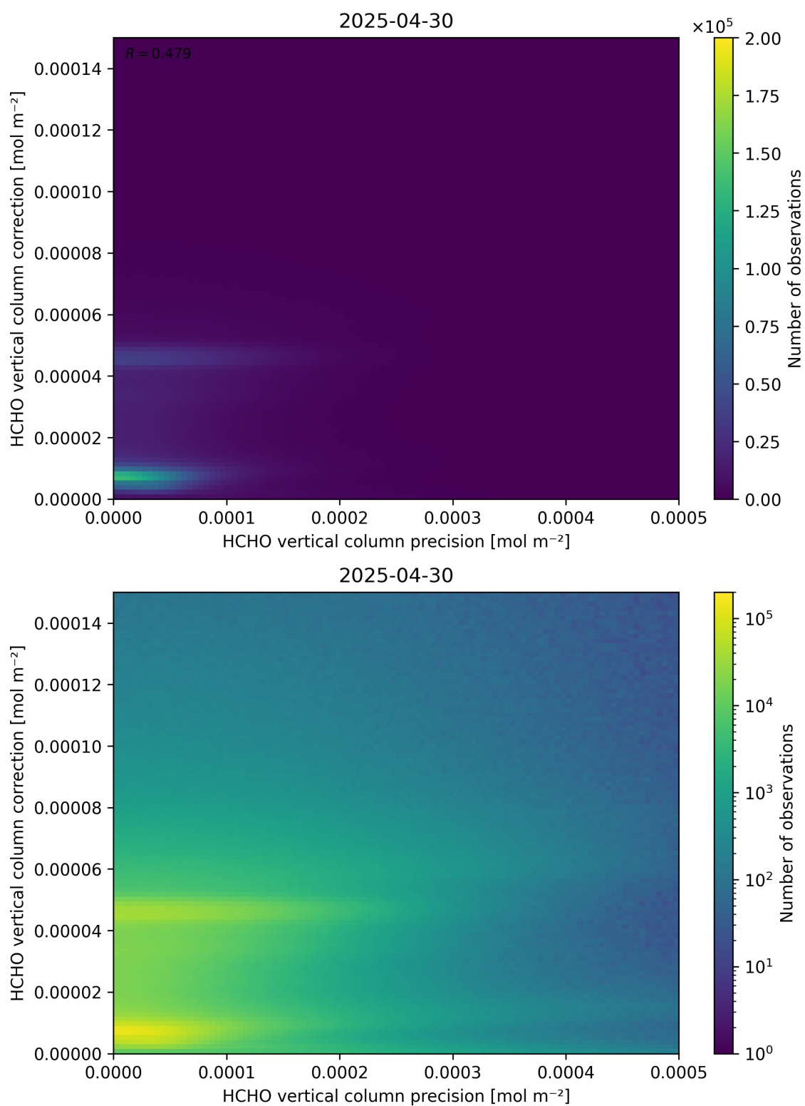
Figure 146: Scatter density plot of “HCHO vertical column precision” against “HCHO vertical column correction” for 2025-04-29 to 2025-05-01.
