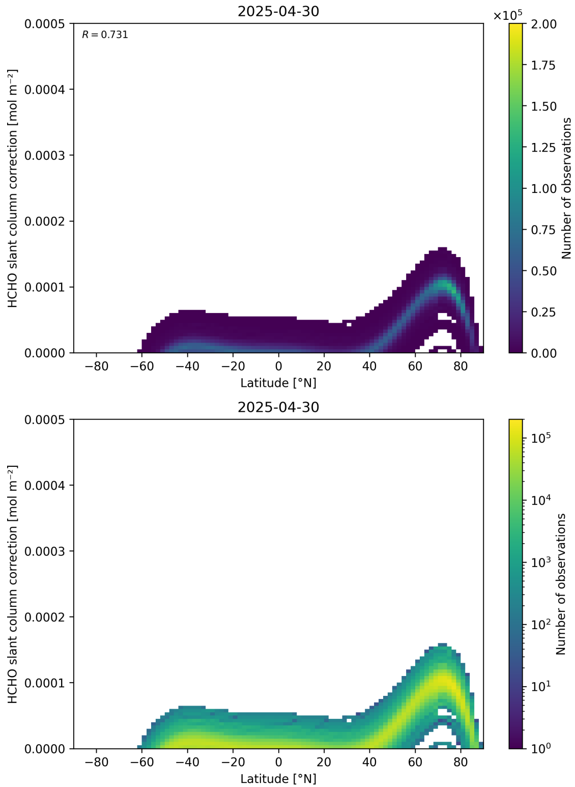
Figure 158: Scatter density plot of “Latitude” against “HCHO slant column correction” for 2025-04-29 to 2025-05-01.
