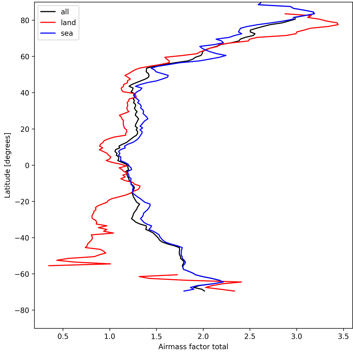
Figure 26: Zonal average of “Airmass factor total” for 2025-04-29 to 2025-05-01.
