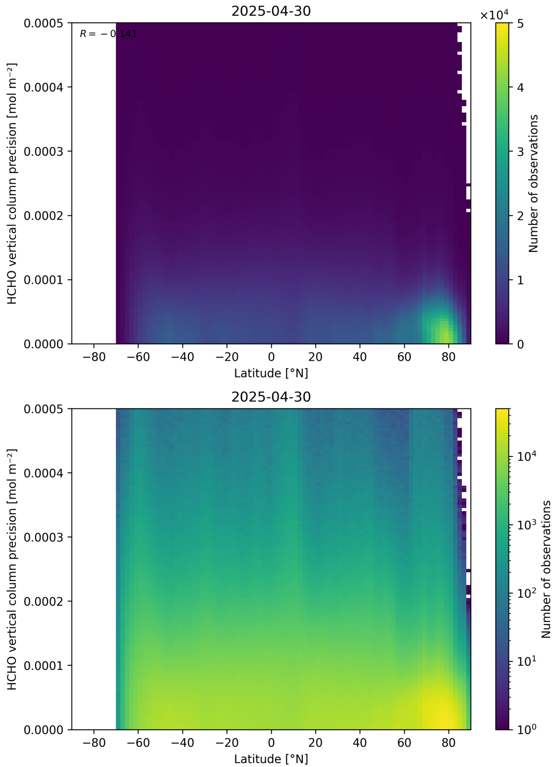
Figure 165: Scatter density plot of “Latitude” against “HCHO vertical column precision” for 2025-04-29 to 2025-05-01.
