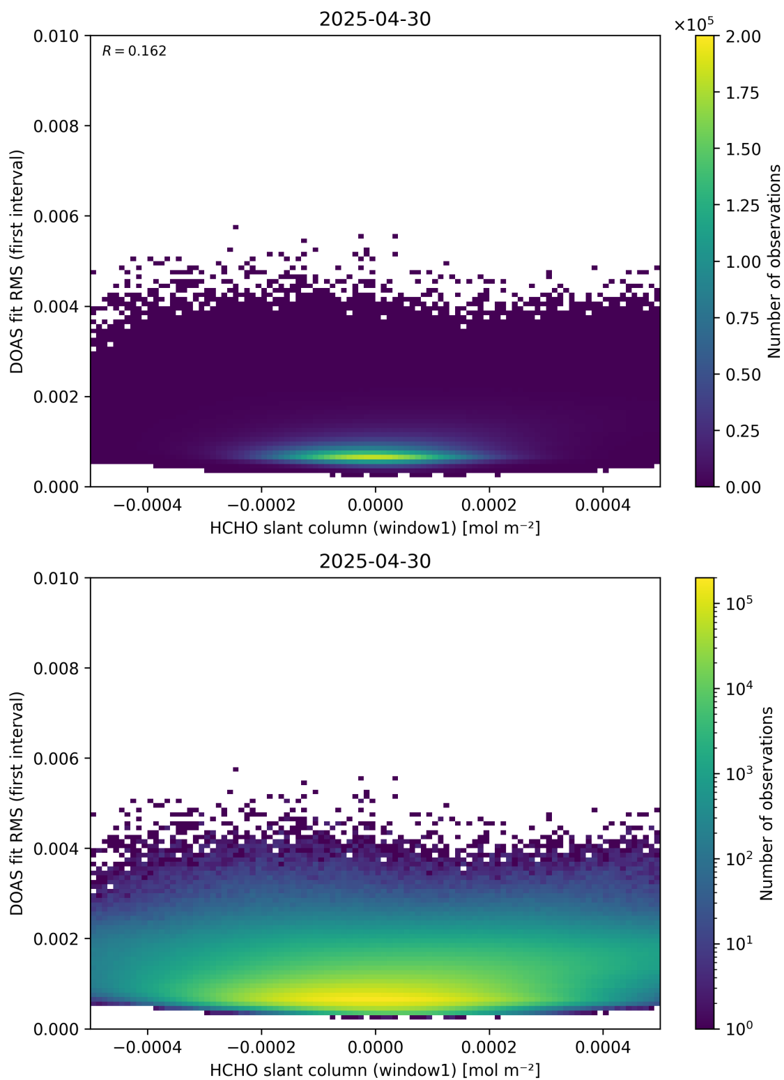
Figure 78: Scatter density plot of “HCHO slant column (window1)” against “DOAS fit RMS (first interval)” for 2025-04-29 to 2025-05-01.
