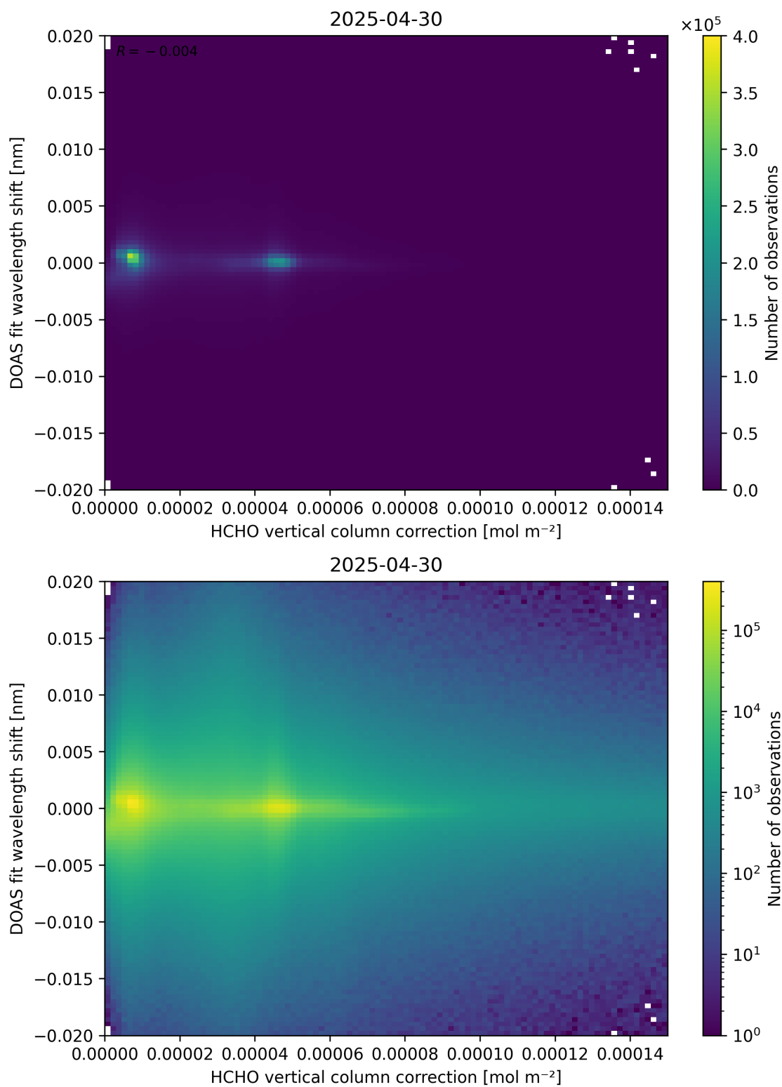
Figure 113: Scatter density plot of “HCHO vertical column correction” against “DOAS fit wavelength shift” for 2025-04-29 to 2025-05-01.
