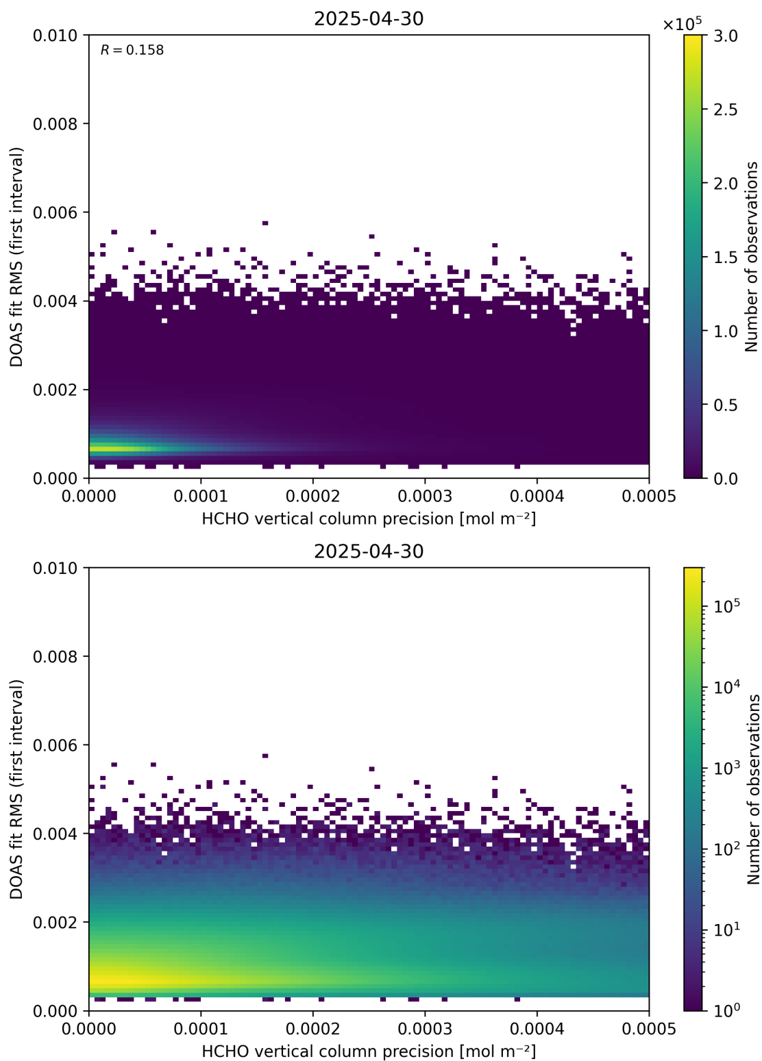
Figure 136: Scatter density plot of “HCHO vertical column precision” against “DOAS fit RMS (first interval)” for 2025-04-29 to 2025-05-01.
