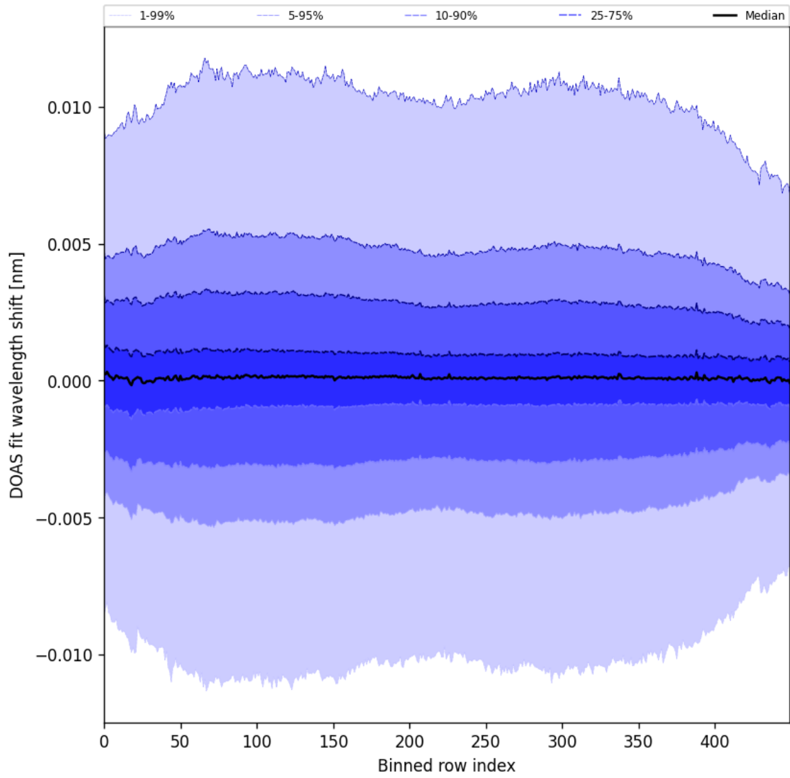
Figure 58: Along track statistics of “DOAS fit wavelength shift” for 2025-04-29 to 2025-05-01
