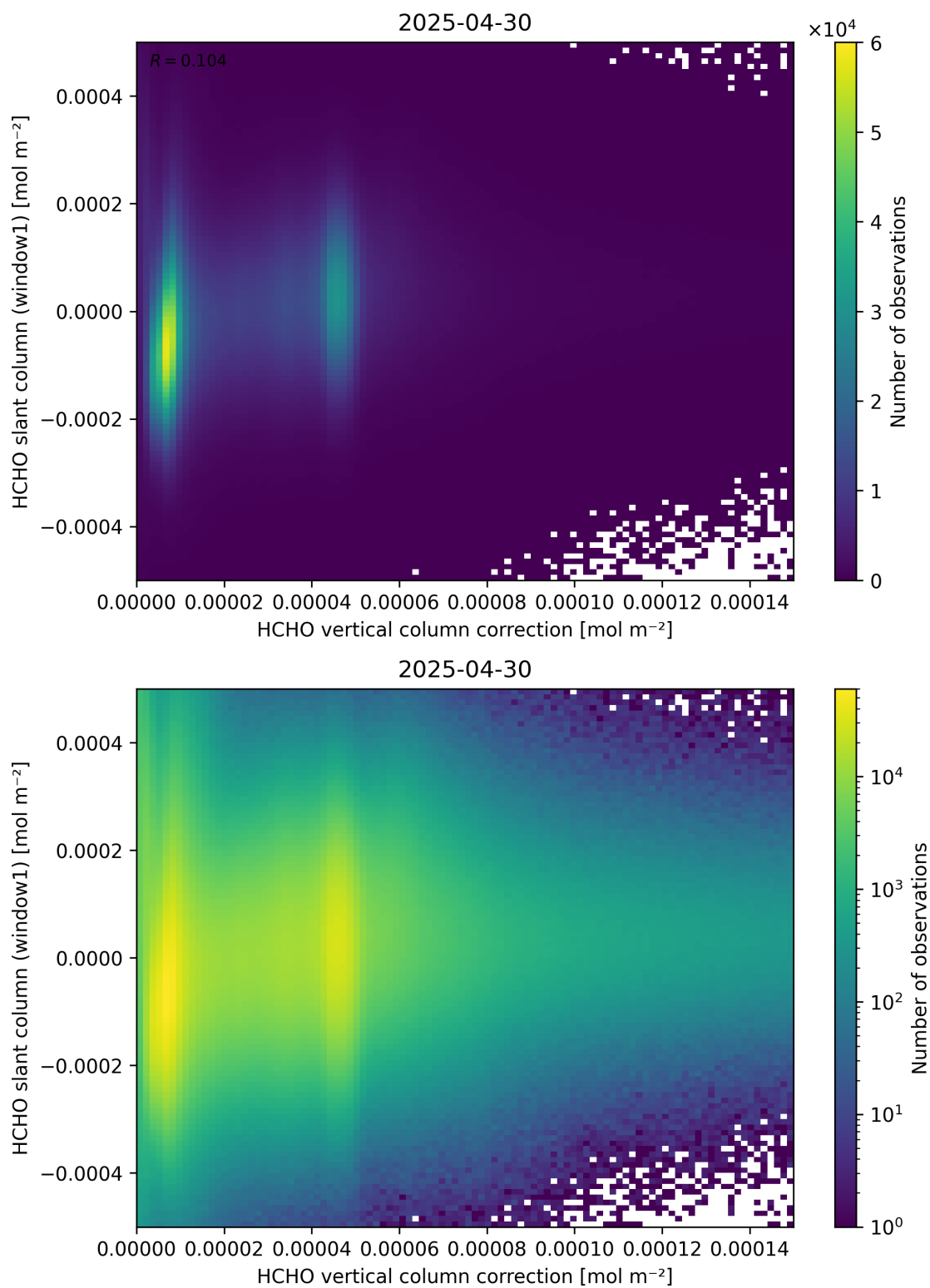
Figure 118: Scatter density plot of “HCHO vertical column correction” against “HCHO slant column (window1)” for 2025-04-29 to 2025-05-01.
