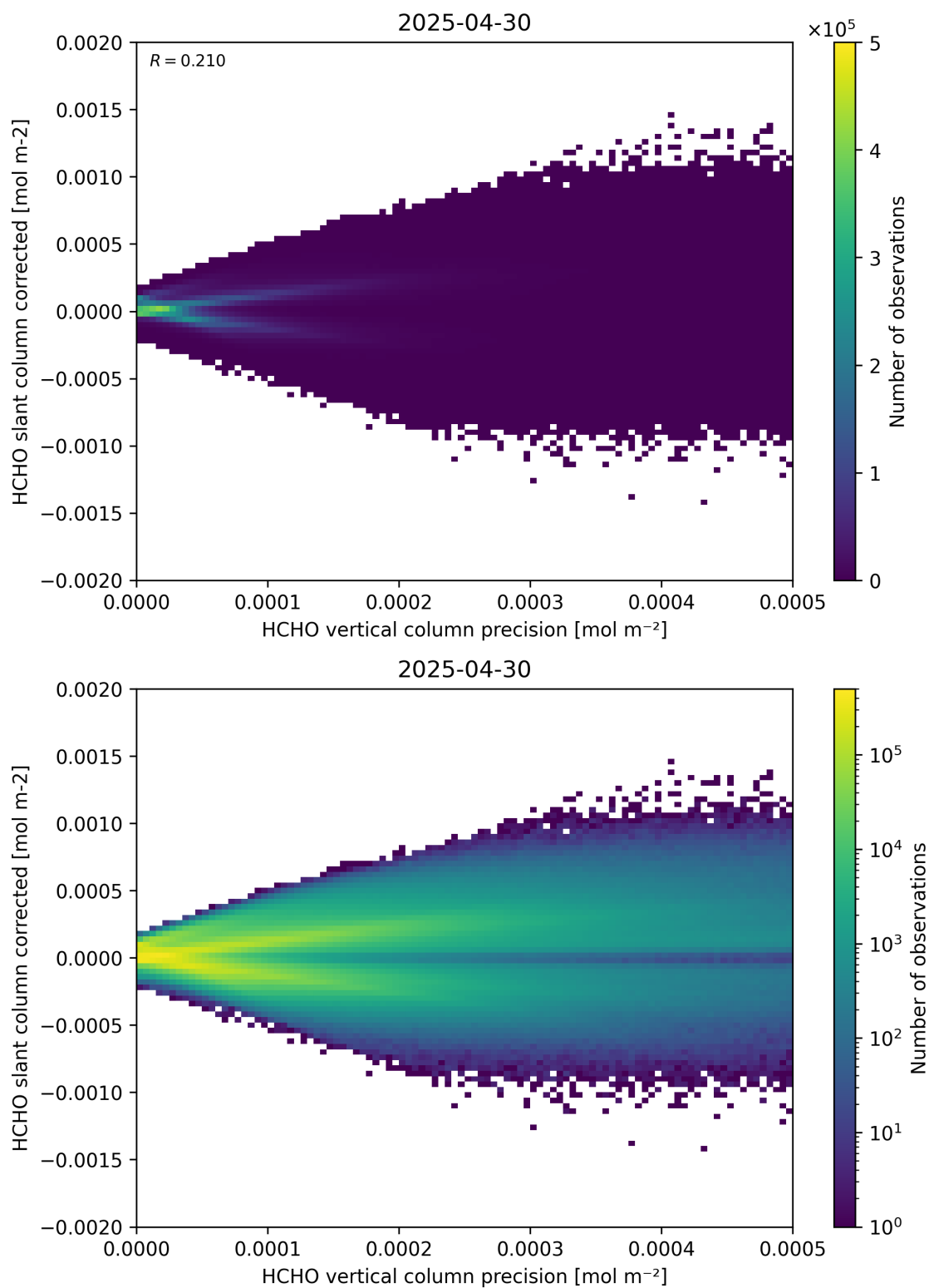
Figure 140: Scatter density plot of “HCHO vertical column precision” against “HCHO slant column corrected” for 2025-04-29 to 2025-05-01.
