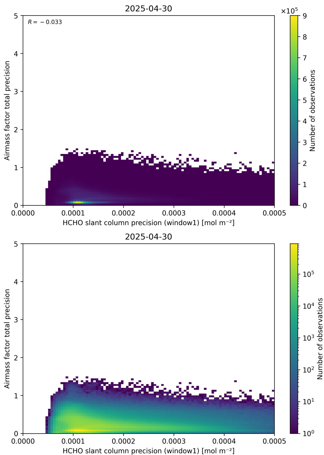
Figure 95: Scatter density plot of “HCHO slant column precision (window1)” against “Airmass factor total precision” for 2025-04-29 to 2025-05-01.
