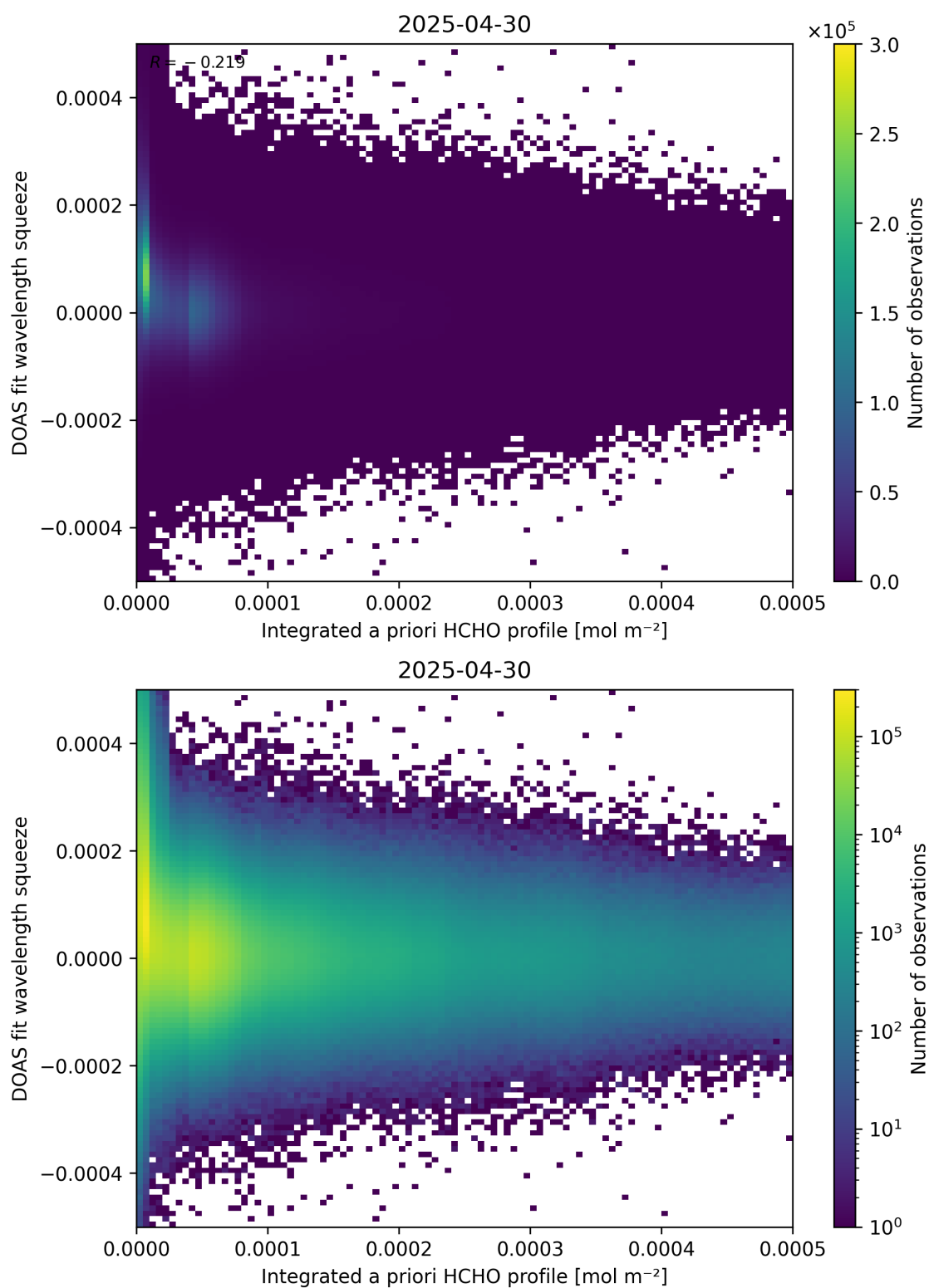
Figure 150: Scatter density plot of “Integrated a priori HCHO profile” against “DOAS fit wavelength squeeze” for 2025-04-29 to 2025-05-01.
