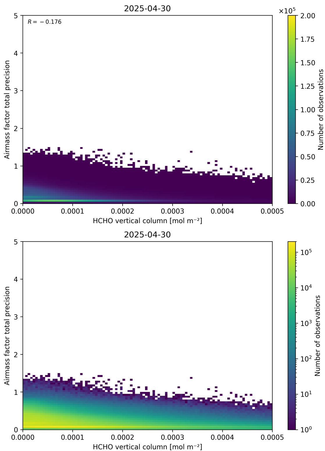
Figure 132: Scatter density plot of “HCHO vertical column” against “Airmass factor total precision” for 2025-04-29 to 2025-05-01.
