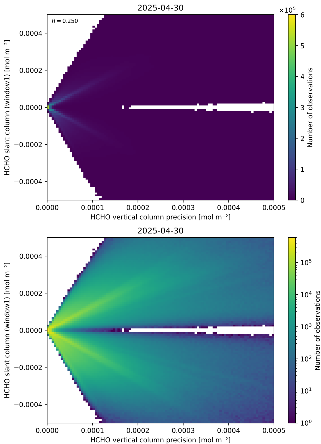
Figure 142: Scatter density plot of “HCHO vertical column precision” against “HCHO slant column (window1)” for 2025-04-29 to 2025-05-01.
