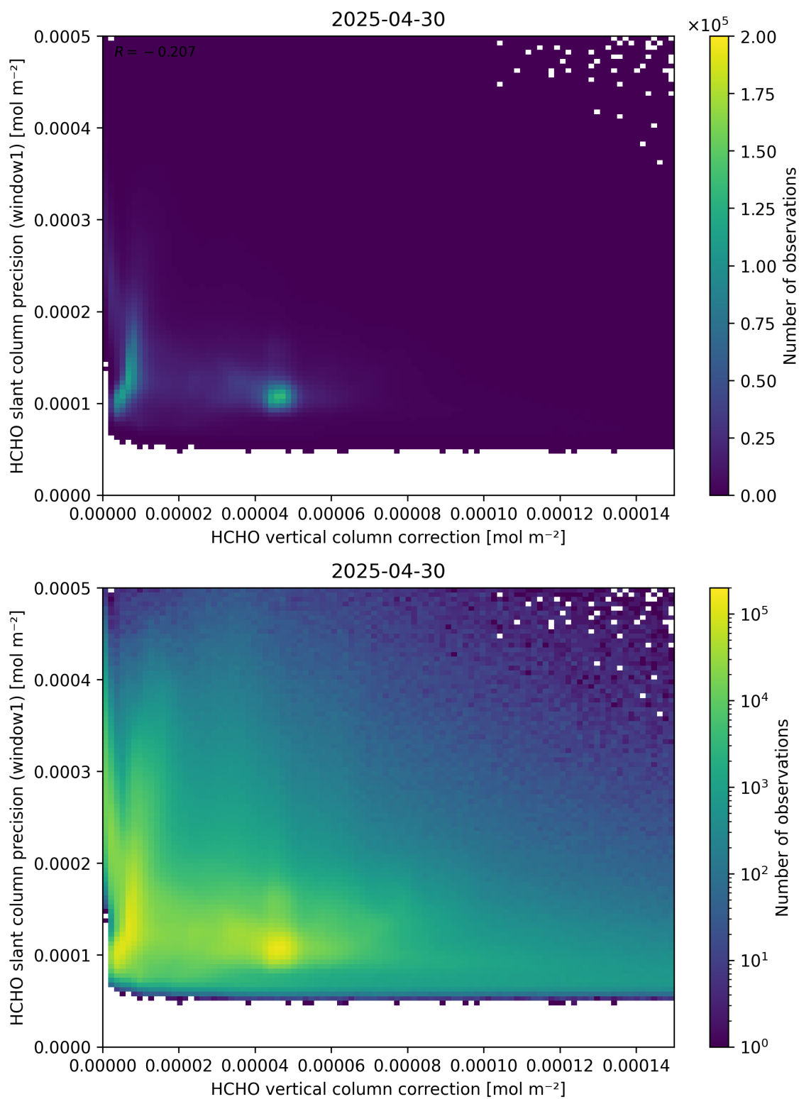
Figure 119: Scatter density plot of “HCHO vertical column correction” against “HCHO slant column precision (window1)” for 2025-04-29 to 2025-05-01.
