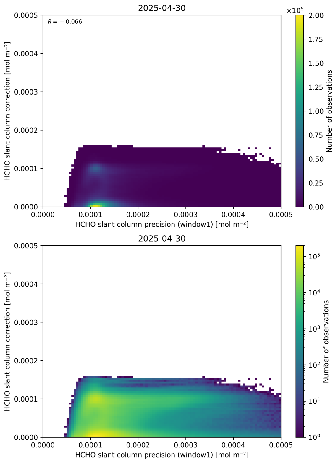
Figure 93: Scatter density plot of “HCHO slant column precision (window1)” against “HCHO slant column correction” for 2025-04-29 to 2025-05-01.
