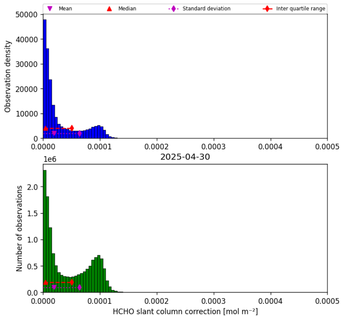
Figure 47: Histogram of “HCHO slant column correction” for 2025-04-29 to 2025-05-01
