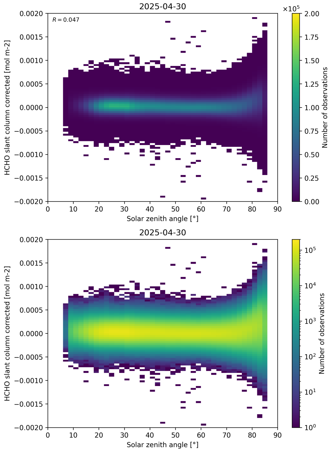
Figure 171: Scatter density plot of “Solar zenith angle” against “HCHO slant column corrected” for 2025-04-29 to 2025-05-01.
