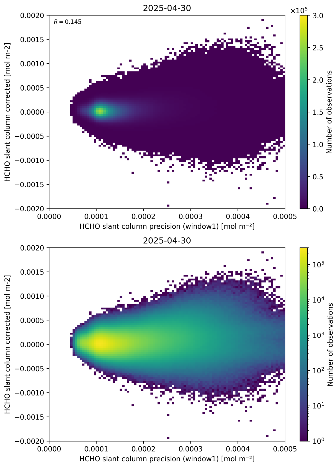
Figure 92: Scatter density plot of “HCHO slant column precision (window1)” against “HCHO slant column corrected” for 2025-04-29 to 2025-05-01.
