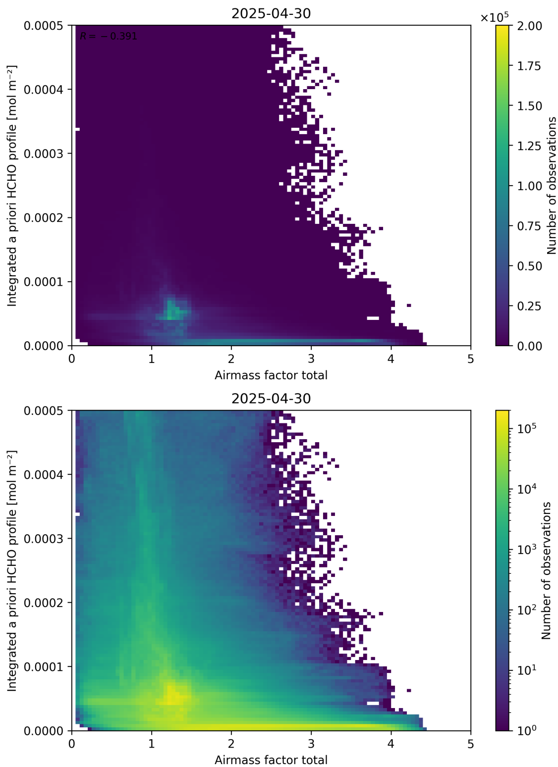
Figure 104: Scatter density plot of “Airmass factor total” against “Integrated a priori HCHO profile” for 2025-04-29 to 2025-05-01.
