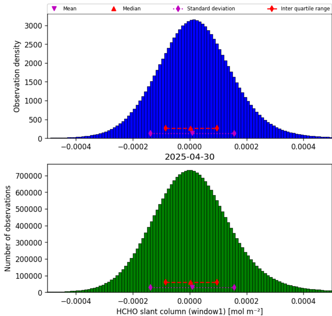
Figure 38: Histogram of “HCHO slant column (window1)” for 2025-04-29 to 2025-05-01
