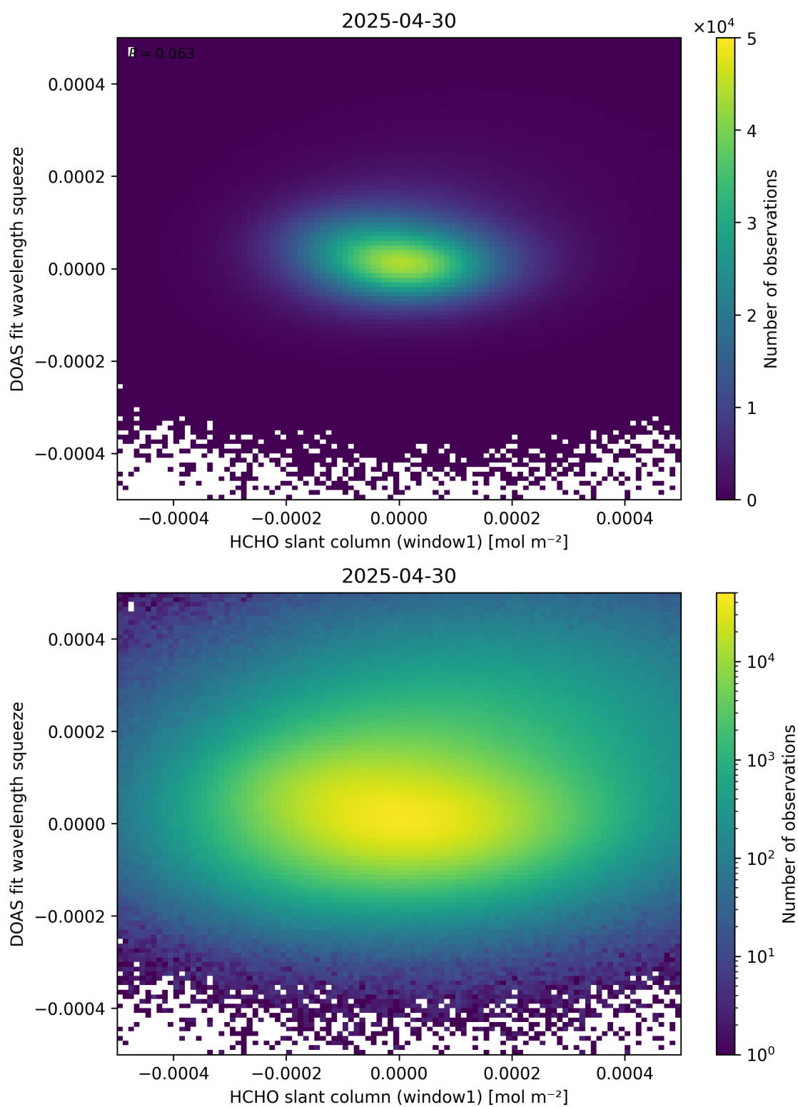
Figure 80: Scatter density plot of “HCHO slant column (window1)” against “DOAS fit wavelength squeeze” for 2025-04-29 to 2025-05-01.
