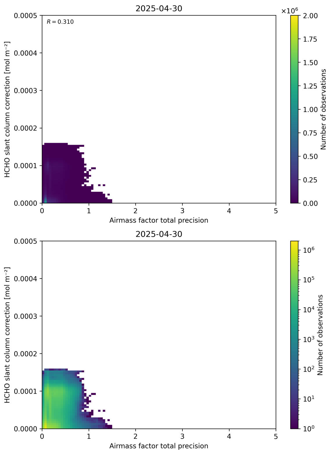
Figure 110: Scatter density plot of “Airmass factor total precision” against “HCHO slant column correction” for 2025-04-29 to 2025-05-01.
