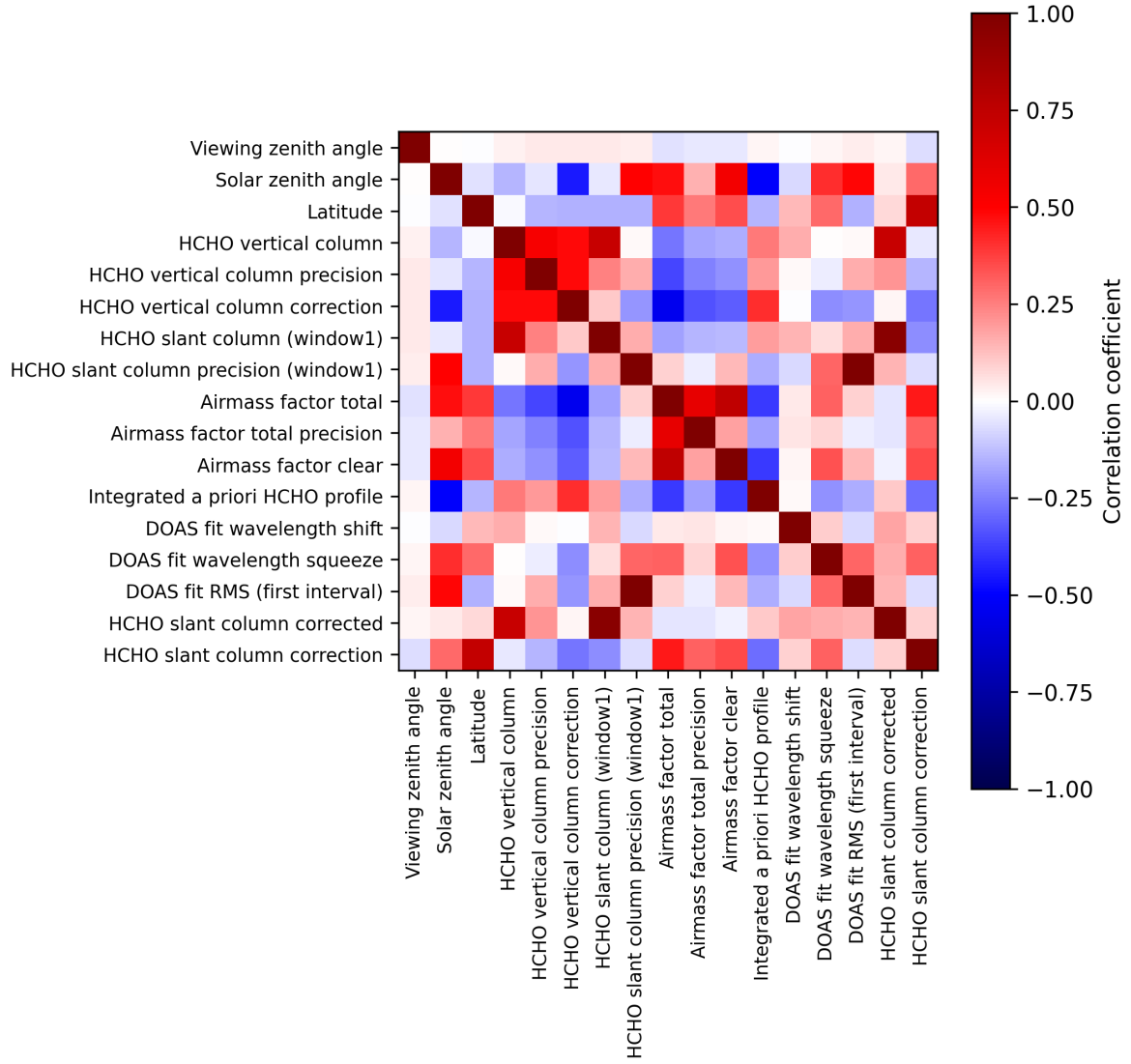
Figure 2: Map of correlation matrix for 2025-04-29 to 2025-05-01.
