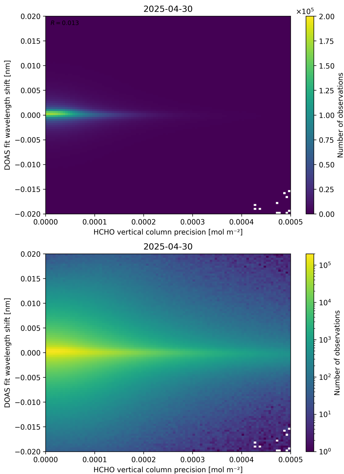
Figure 137: Scatter density plot of “HCHO vertical column precision” against “DOAS fit wavelength shift” for 2025-04-29 to 2025-05-01.
