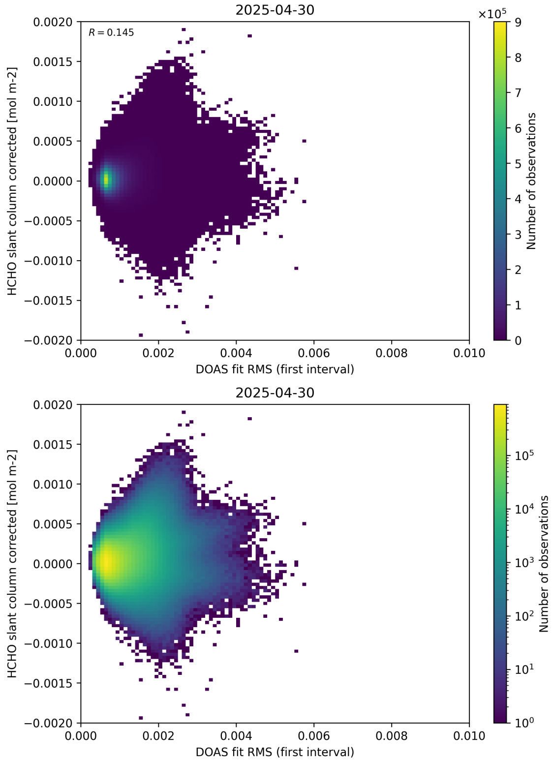
Figure 62: Scatter density plot of “DOAS fit RMS (first interval)” against “HCHO slant column corrected” for 2025-04-29 to 2025-05-01.
