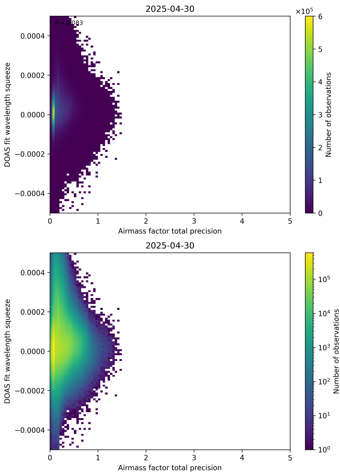
Figure 107: Scatter density plot of “Airmass factor total precision” against “DOAS fit wavelength squeeze” for 2025-04-29 to 2025-05-01.
