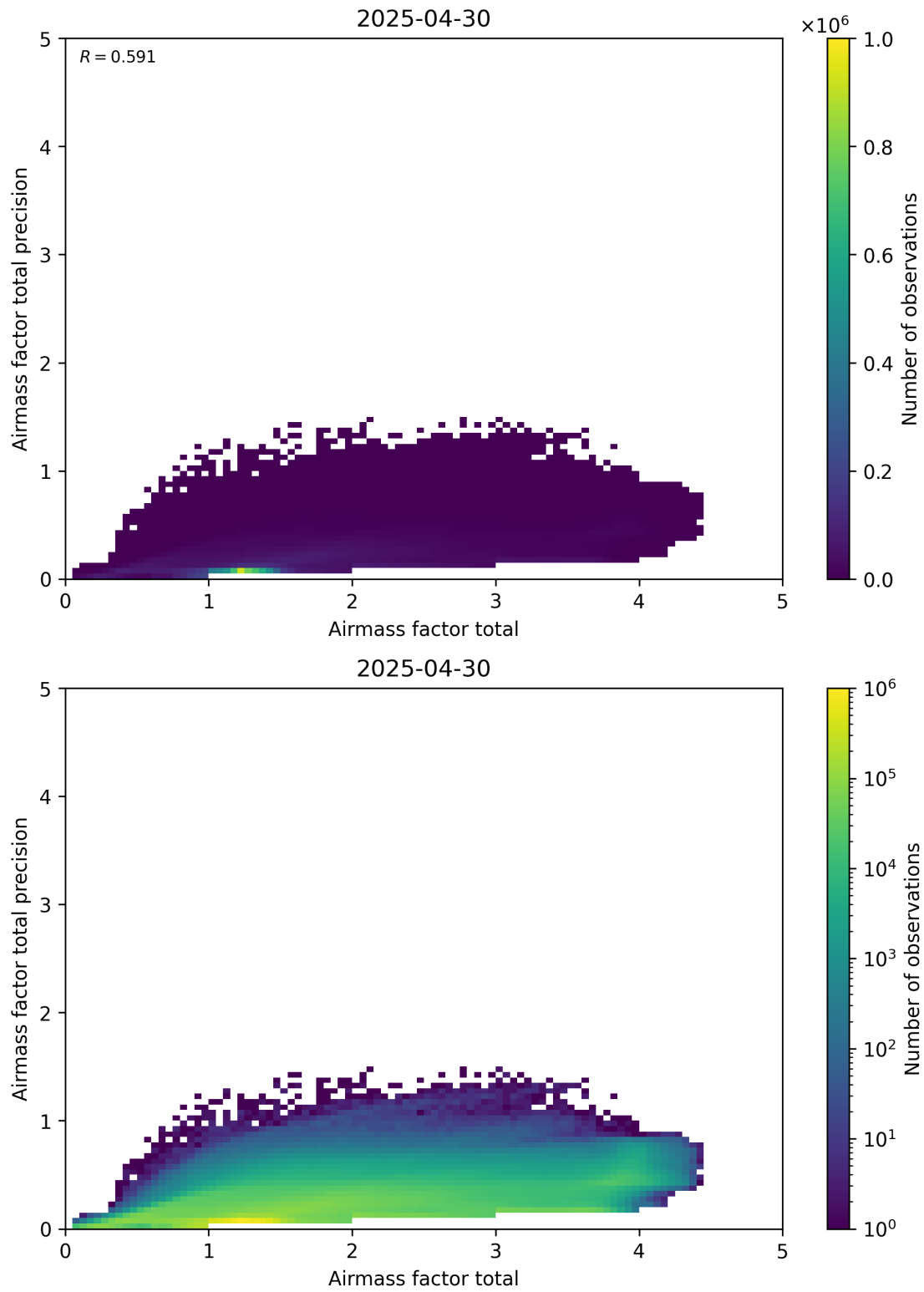
Figure 103: Scatter density plot of “Airmass factor total” against “Airmass factor total precision” for 2025-04-29 to 2025-05-01.
