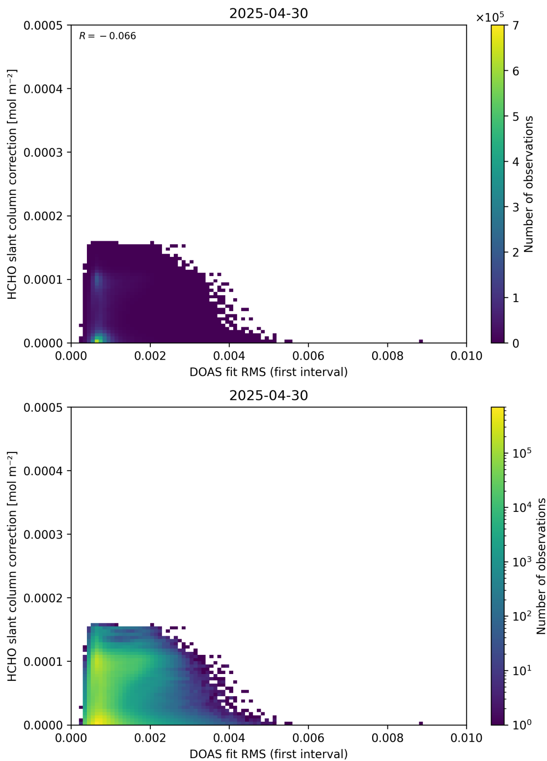
Figure 63: Scatter density plot of “DOAS fit RMS (first interval)” against “HCHO slant column correction” for 2025-04-29 to 2025-05-01.
