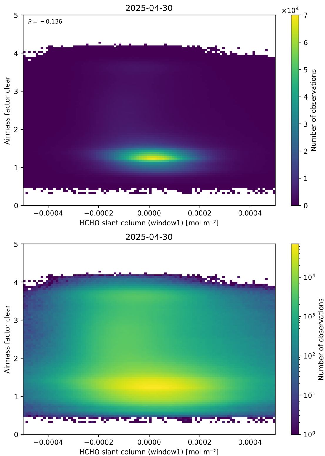
Figure 81: Scatter density plot of “HCHO slant column (window1)” against “Airmass factor clear” for 2025-04-29 to 2025-05-01.
