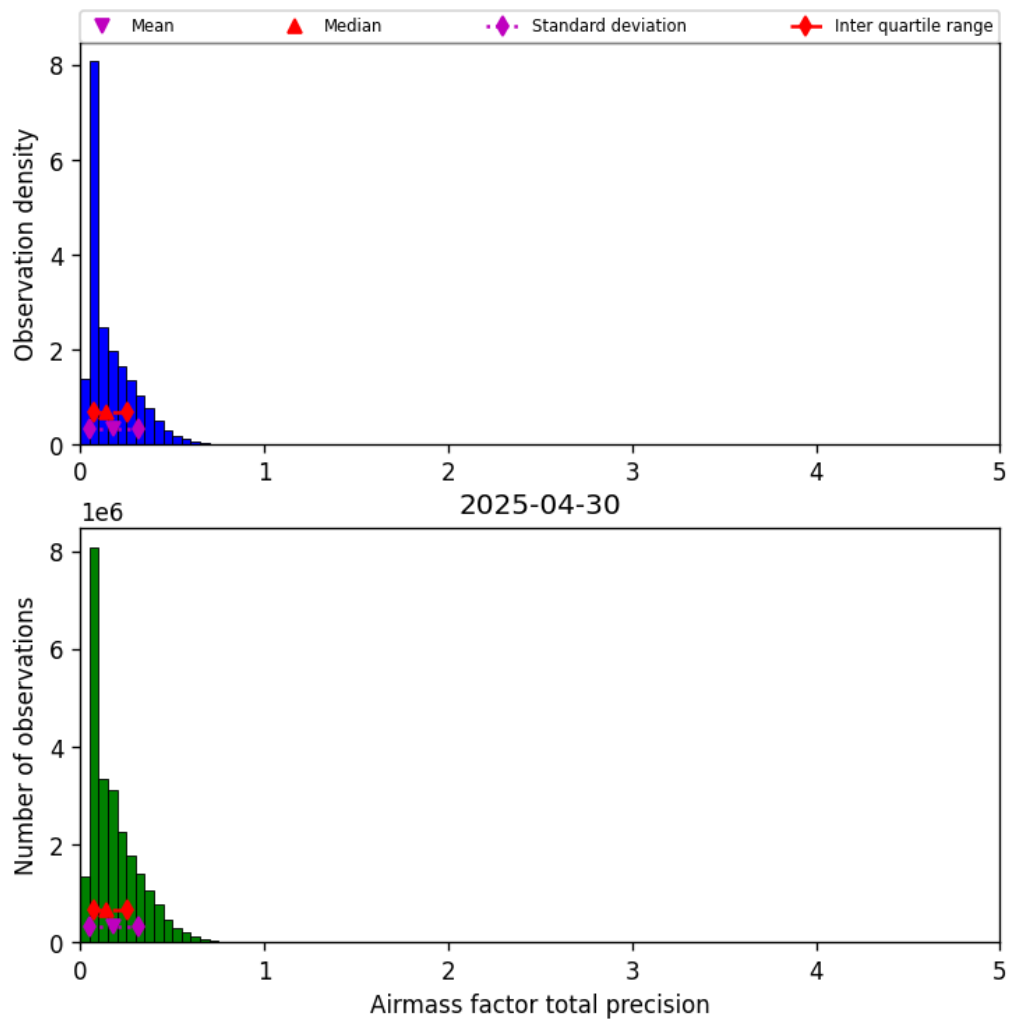
Figure 41: Histogram of “Airmass factor total precision” for 2025-04-29 to 2025-05-01
