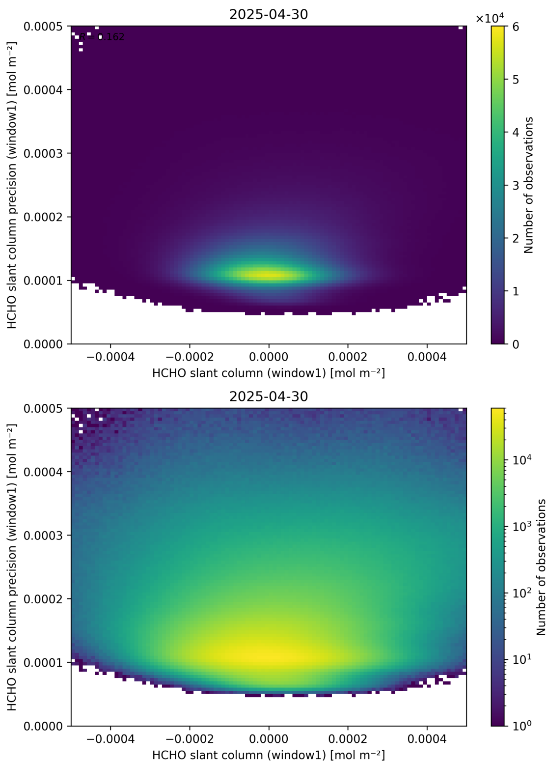
Figure 84: Scatter density plot of “HCHO slant column (window1)” against “HCHO slant column precision (window1)” for 2025-04-29 to 2025-05-01.
