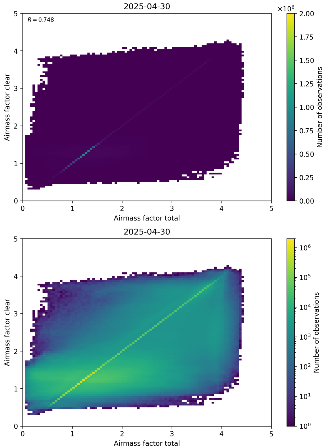
Figure 100: Scatter density plot of “Airmass factor total” against “Airmass factor clear” for 2025-04-29 to 2025-05-01.
