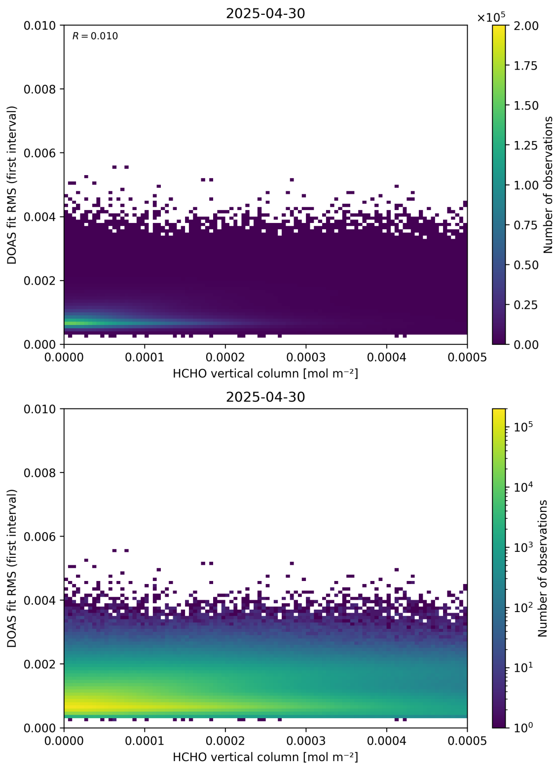
Figure 123: Scatter density plot of “HCHO vertical column” against “DOAS fit RMS (first interval)” for 2025-04-29 to 2025-05-01.
