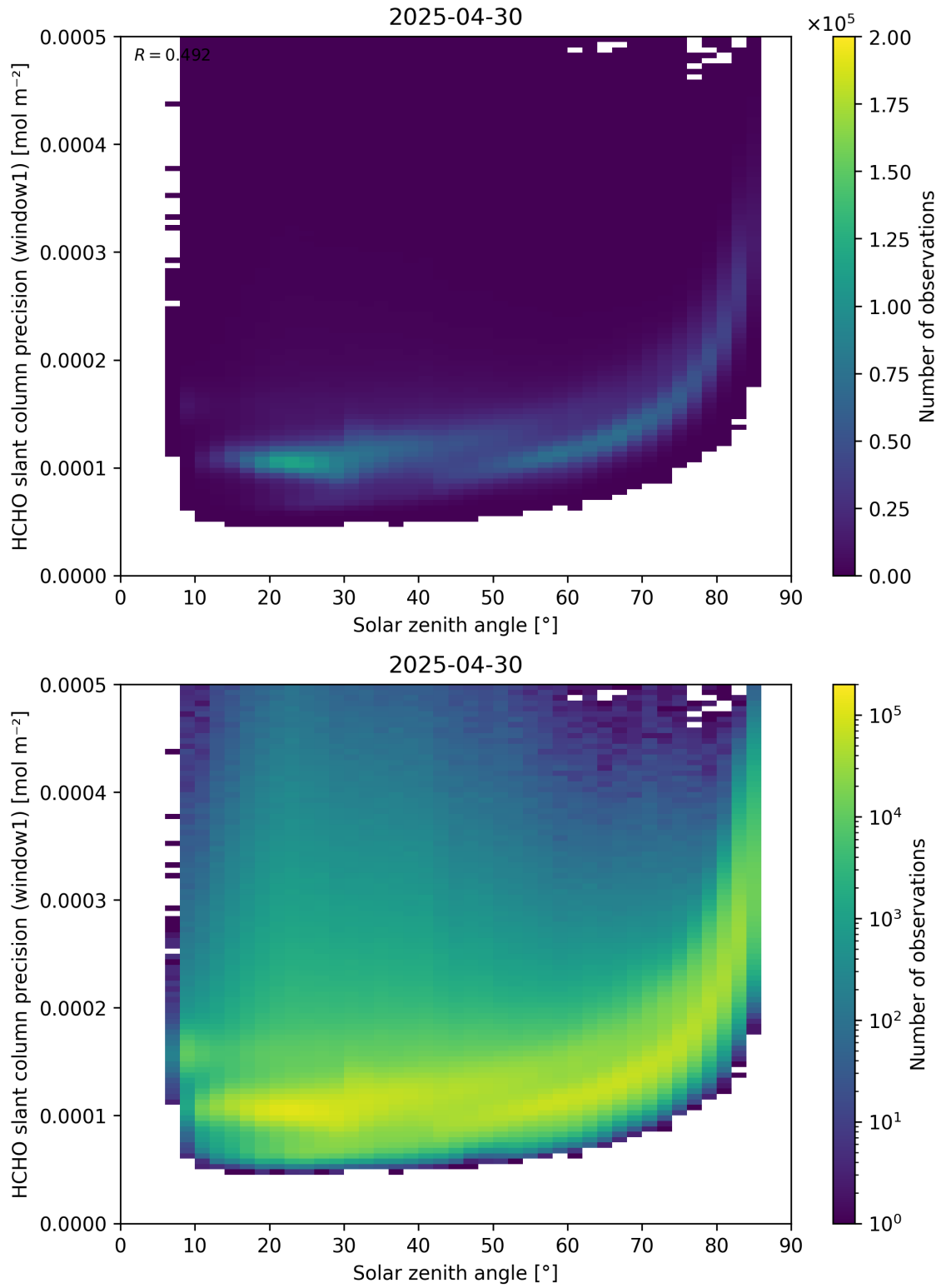
Figure 174: Scatter density plot of “Solar zenith angle” against “HCHO slant column precision (window1)” for 2025-04-29 to 2025-05-01.
