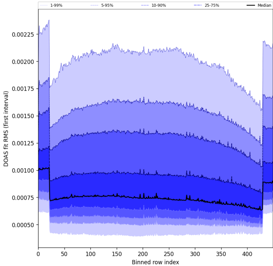
Figure 60: Along track statistics of “DOAS fit RMS (first interval)” for 2025-04-29 to 2025-05-01
