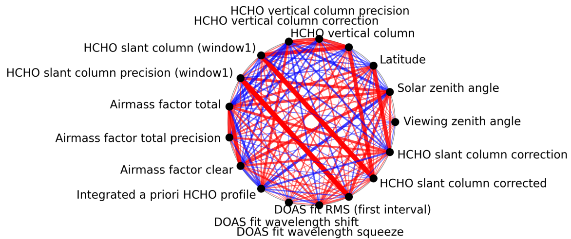
Figure 1: Map of correlation graph for 2025-04-29 to 2025-05-01.
