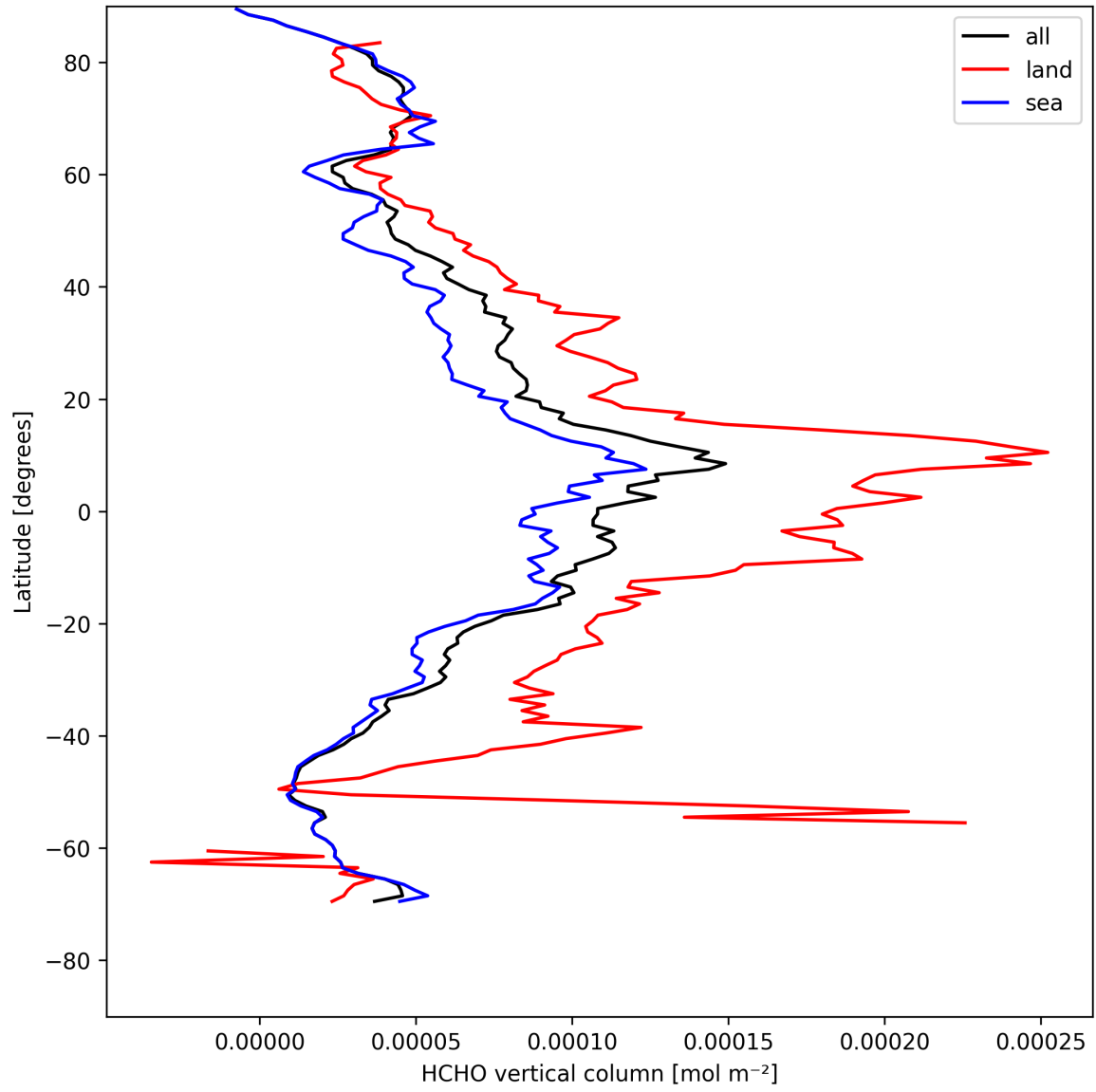
Figure 21: Zonal average of “HCHO vertical column” for 2025-04-29 to 2025-05-01.
