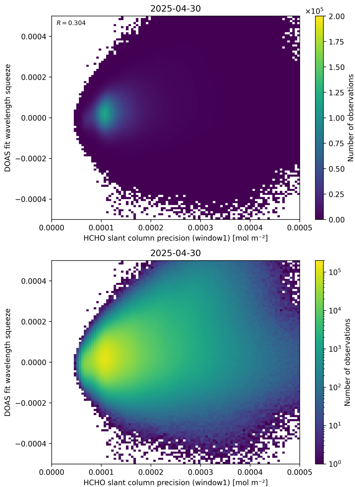
Figure 90: Scatter density plot of “HCHO slant column precision (window1)” against “DOAS fit wavelength squeeze” for 2025-04-29 to 2025-05-01.
