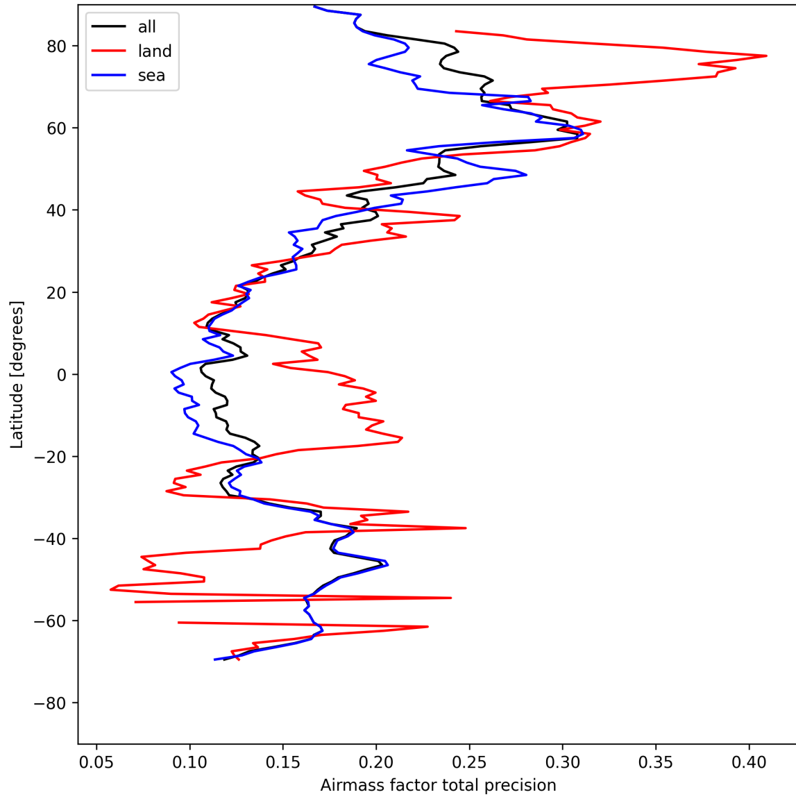
Figure 27: Zonal average of “Airmass factor total precision” for 2025-04-29 to 2025-05-01.
