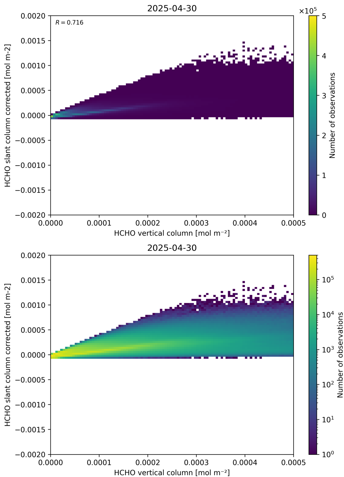
Figure 127: Scatter density plot of “HCHO vertical column” against “HCHO slant column corrected” for 2025-04-29 to 2025-05-01.
