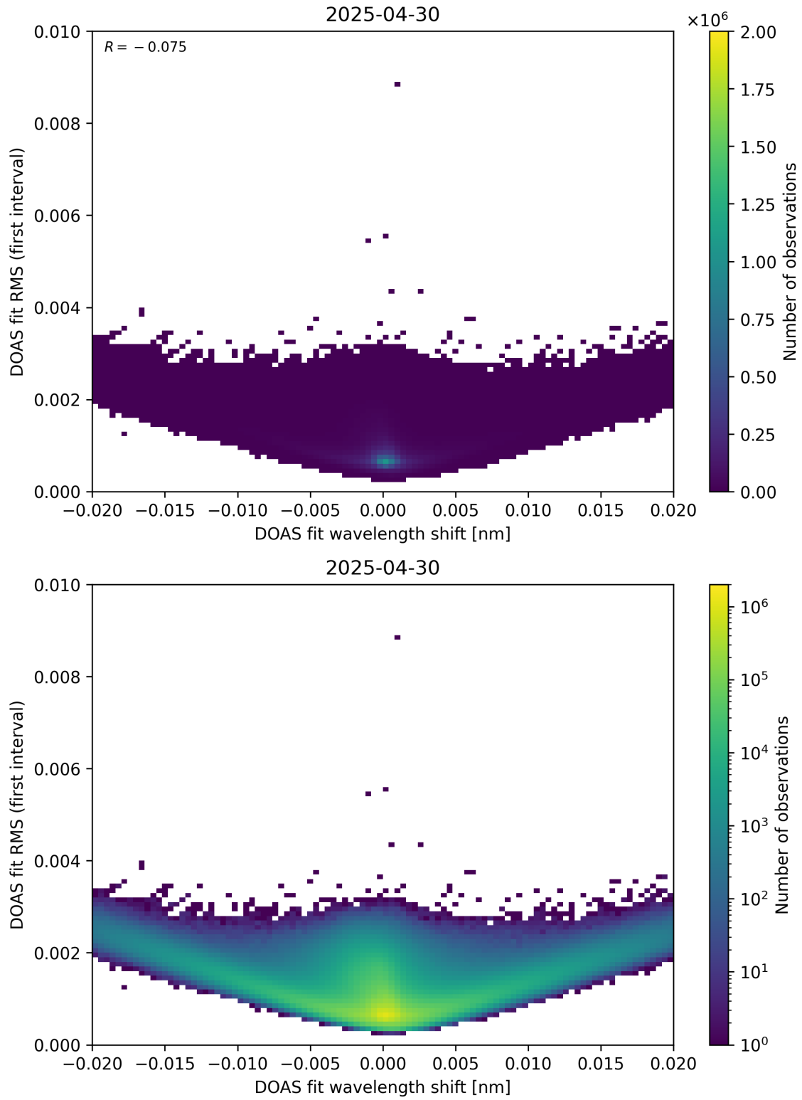
Figure 64: Scatter density plot of “DOAS fit wavelength shift” against “DOAS fit RMS (first interval)” for 2025-04-29 to 2025-05-01.
