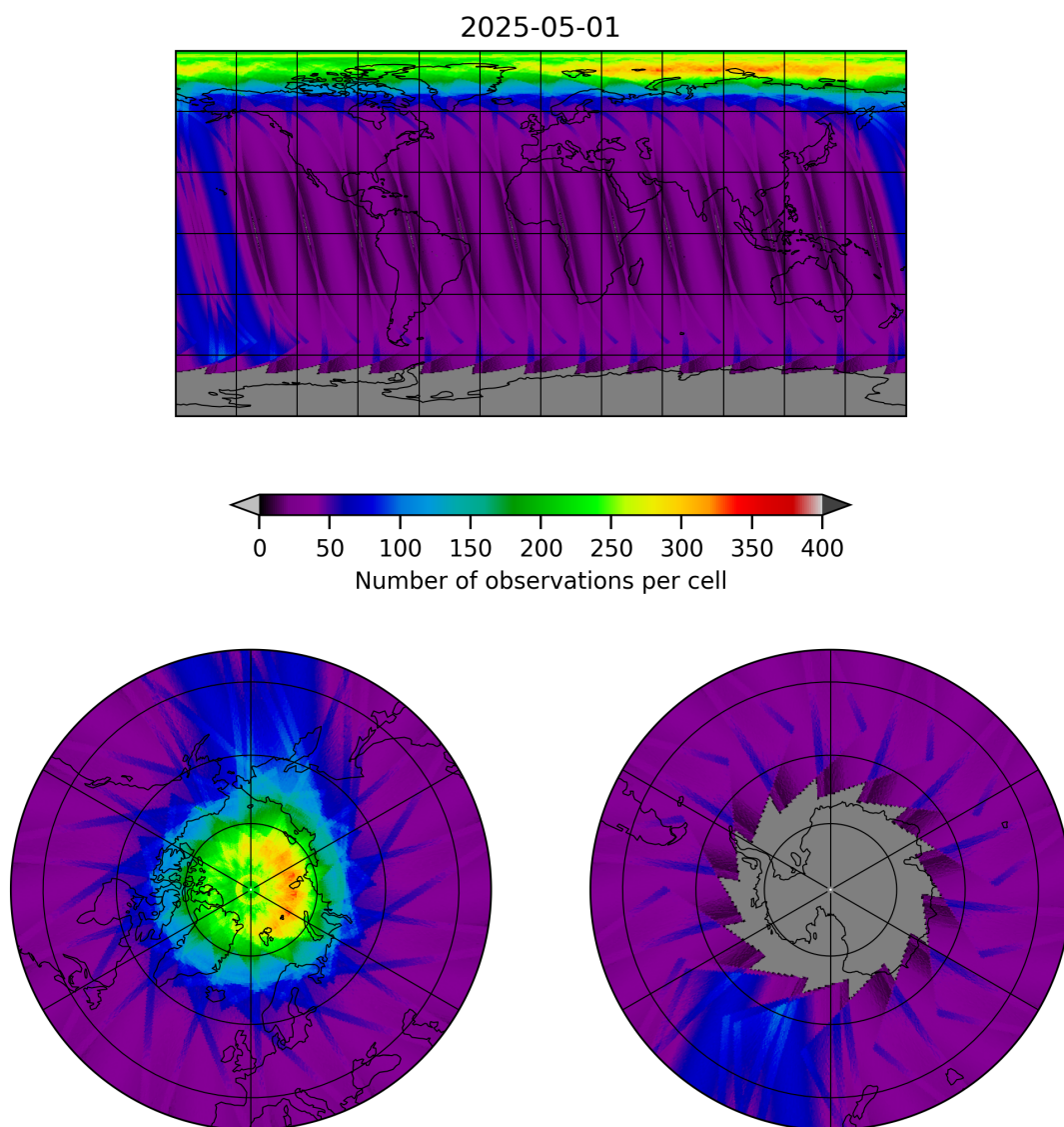
Figure 19: Map of the number of observations for 2025-04-30 to 2025-05-02
