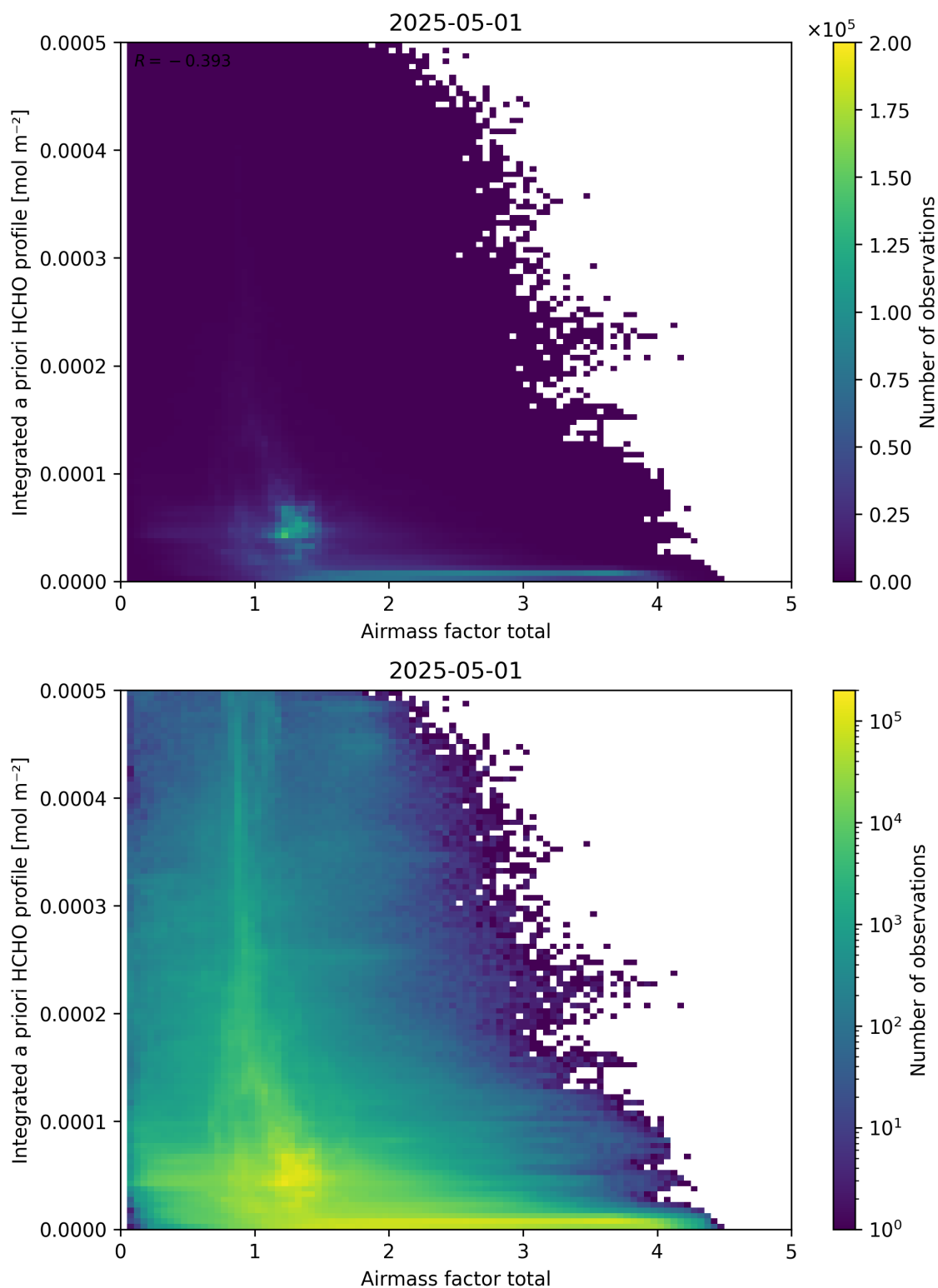
Figure 104: Scatter density plot of “Airmass factor total” against “Integrated a priori HCHO profile” for 2025-04-30 to 2025-05-02.
