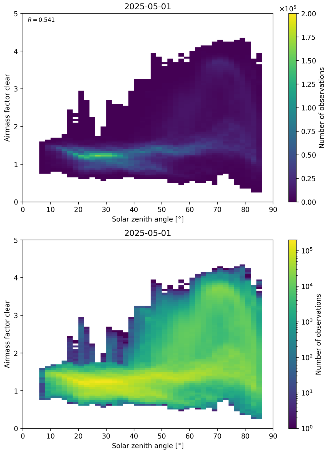
Figure 170: Scatter density plot of “Solar zenith angle” against “Airmass factor clear” for 2025-04-30 to 2025-05-02.
