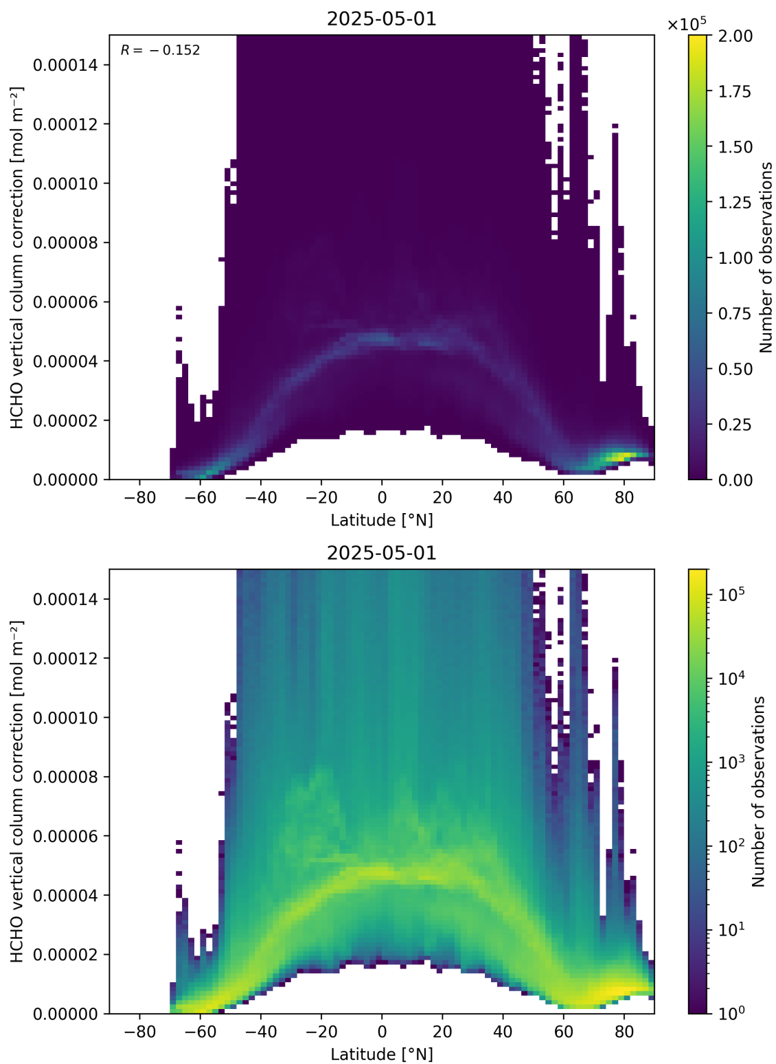
Figure 164: Scatter density plot of “Latitude” against “HCHO vertical column correction” for 2025-04-30 to 2025-05-02.
