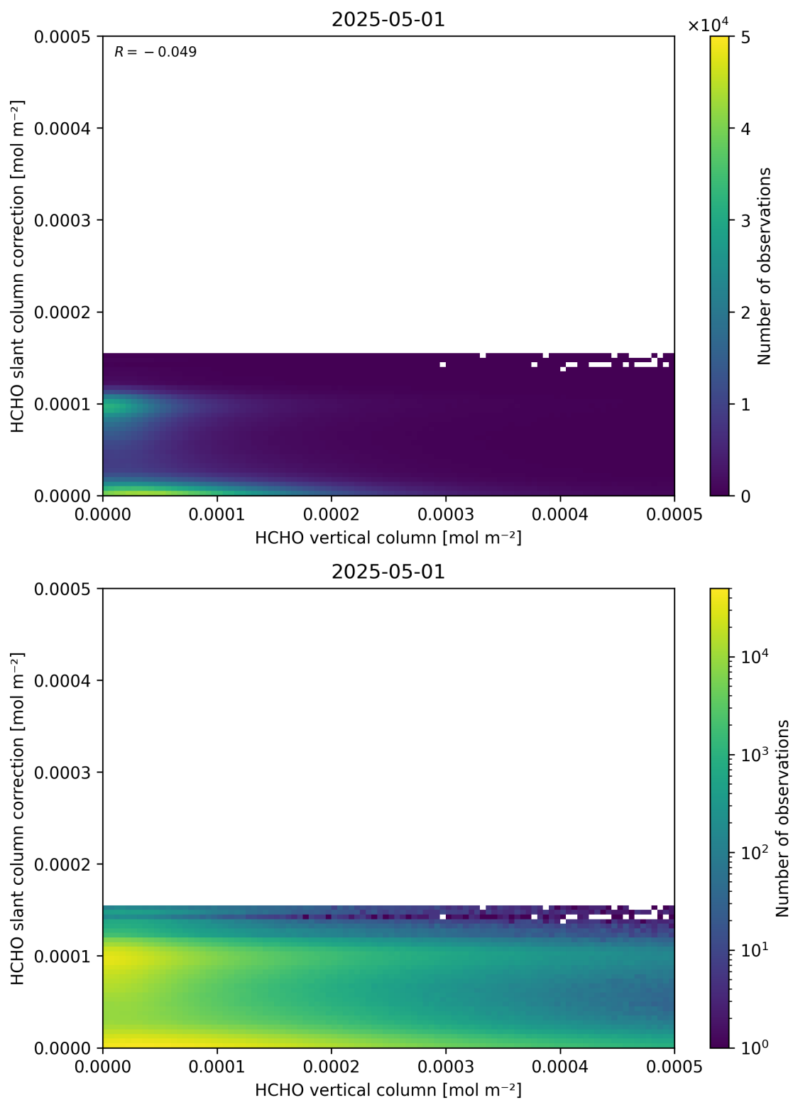
Figure 128: Scatter density plot of “HCHO vertical column” against “HCHO slant column correction” for 2025-04-30 to 2025-05-02.
