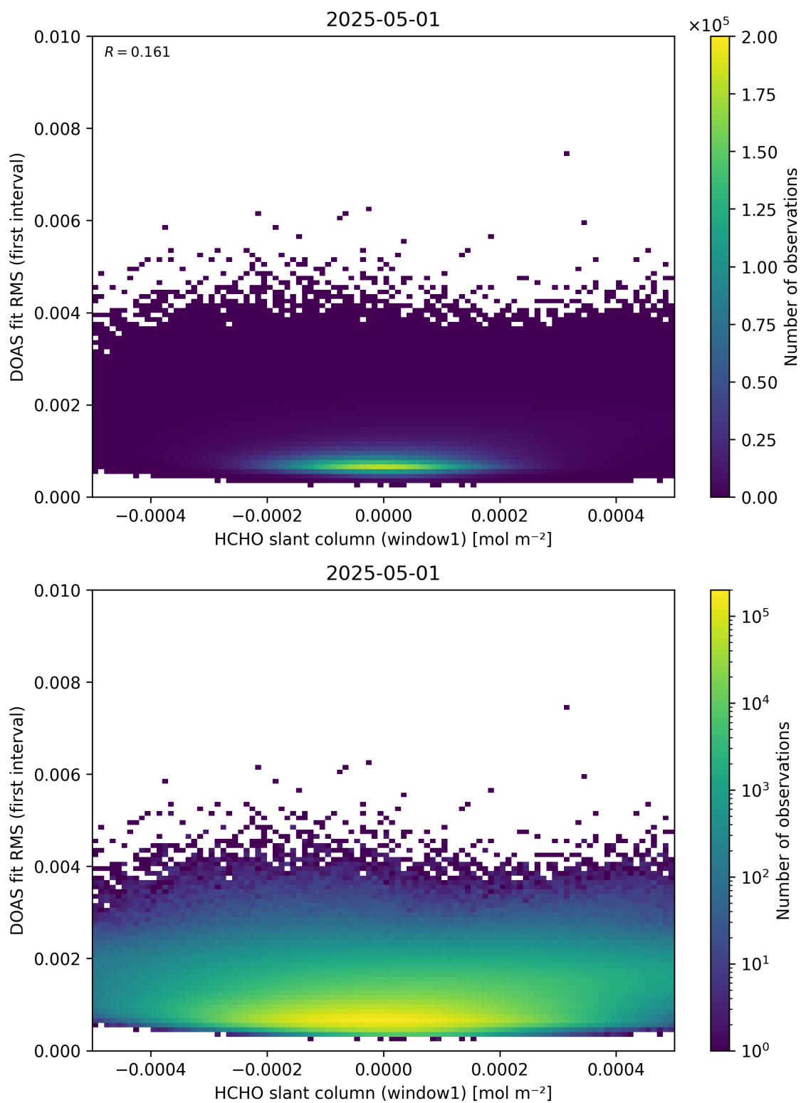
Figure 78: Scatter density plot of “HCHO slant column (window1)” against “DOAS fit RMS (first interval)” for 2025-04-30 to 2025-05-02.
