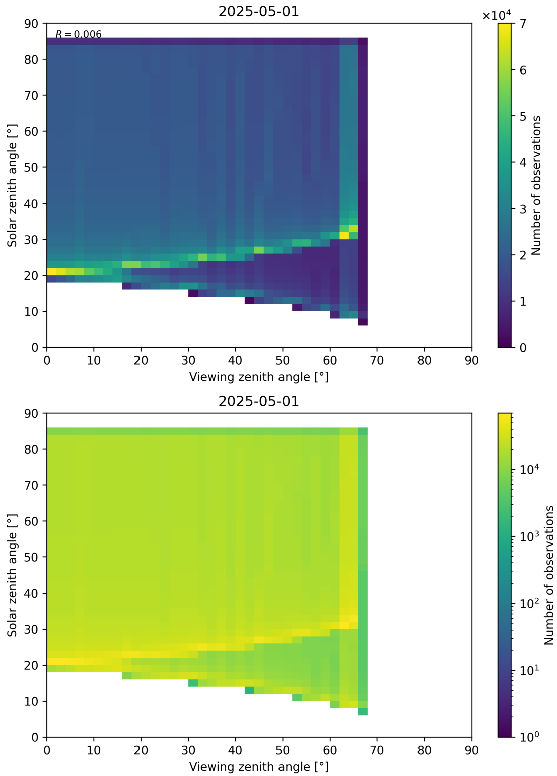
Figure 197: Scatter density plot of “Viewing zenith angle” against “Solar zenith angle” for 2025-04-30 to 2025-05-02.
