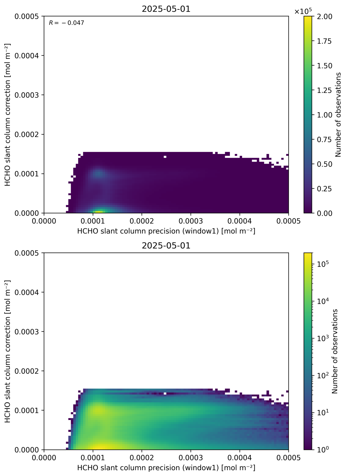
Figure 93: Scatter density plot of “HCHO slant column precision (window1)” against “HCHO slant column correction” for 2025-04-30 to 2025-05-02.
