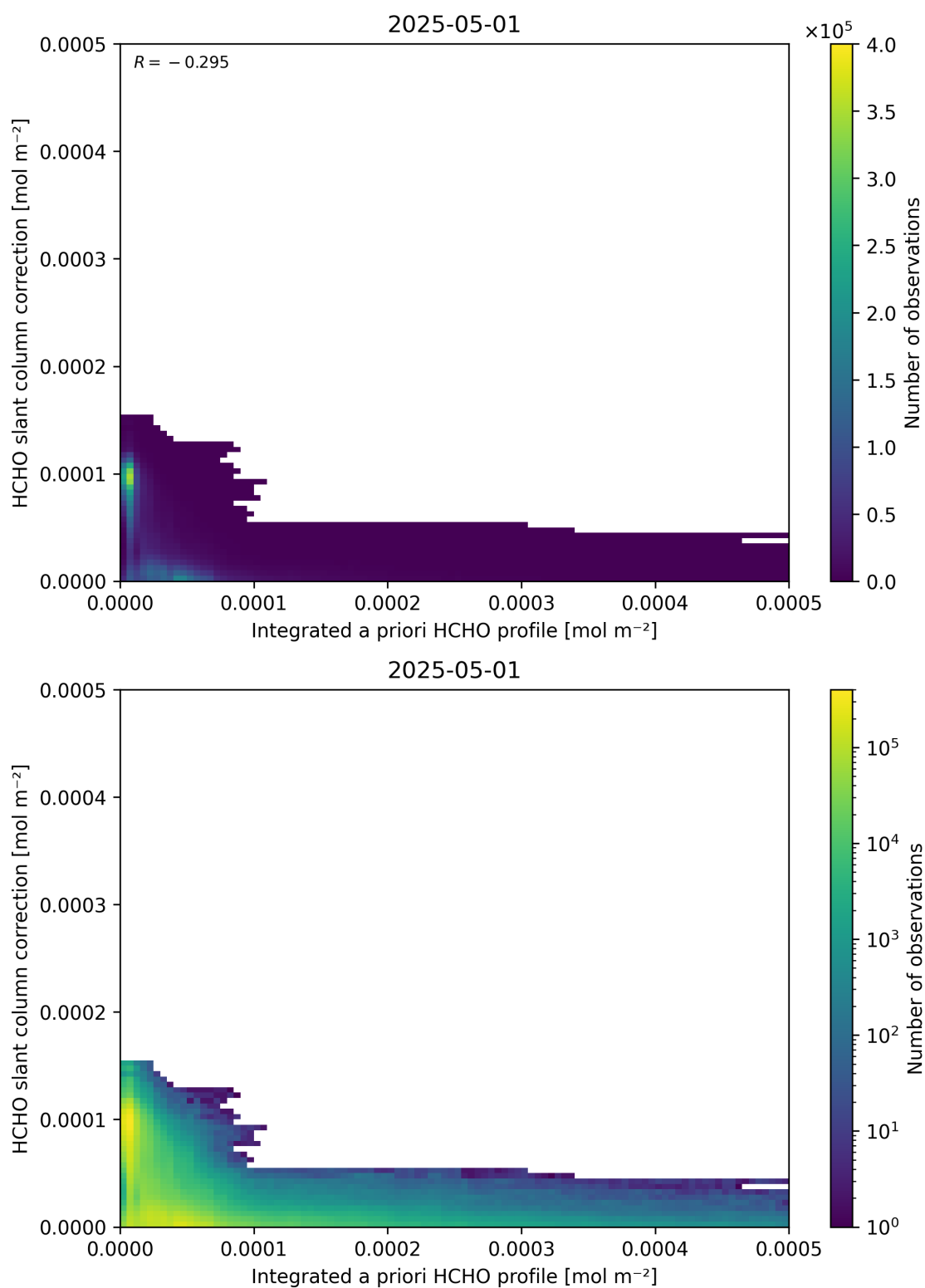
Figure 152: Scatter density plot of “Integrated a priori HCHO profile” against “HCHO slant column correction” for 2025-04-30 to 2025-05-02.
