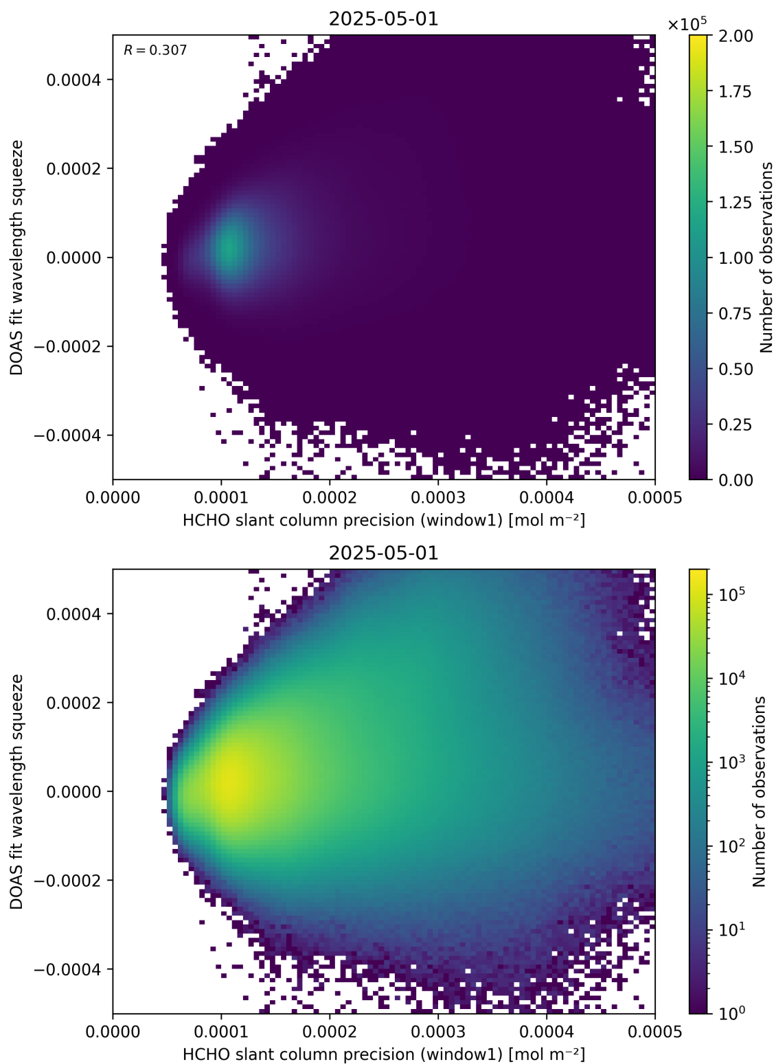
Figure 90: Scatter density plot of “HCHO slant column precision (window1)” against “DOAS fit wavelength squeeze” for 2025-04-30 to 2025-05-02.
