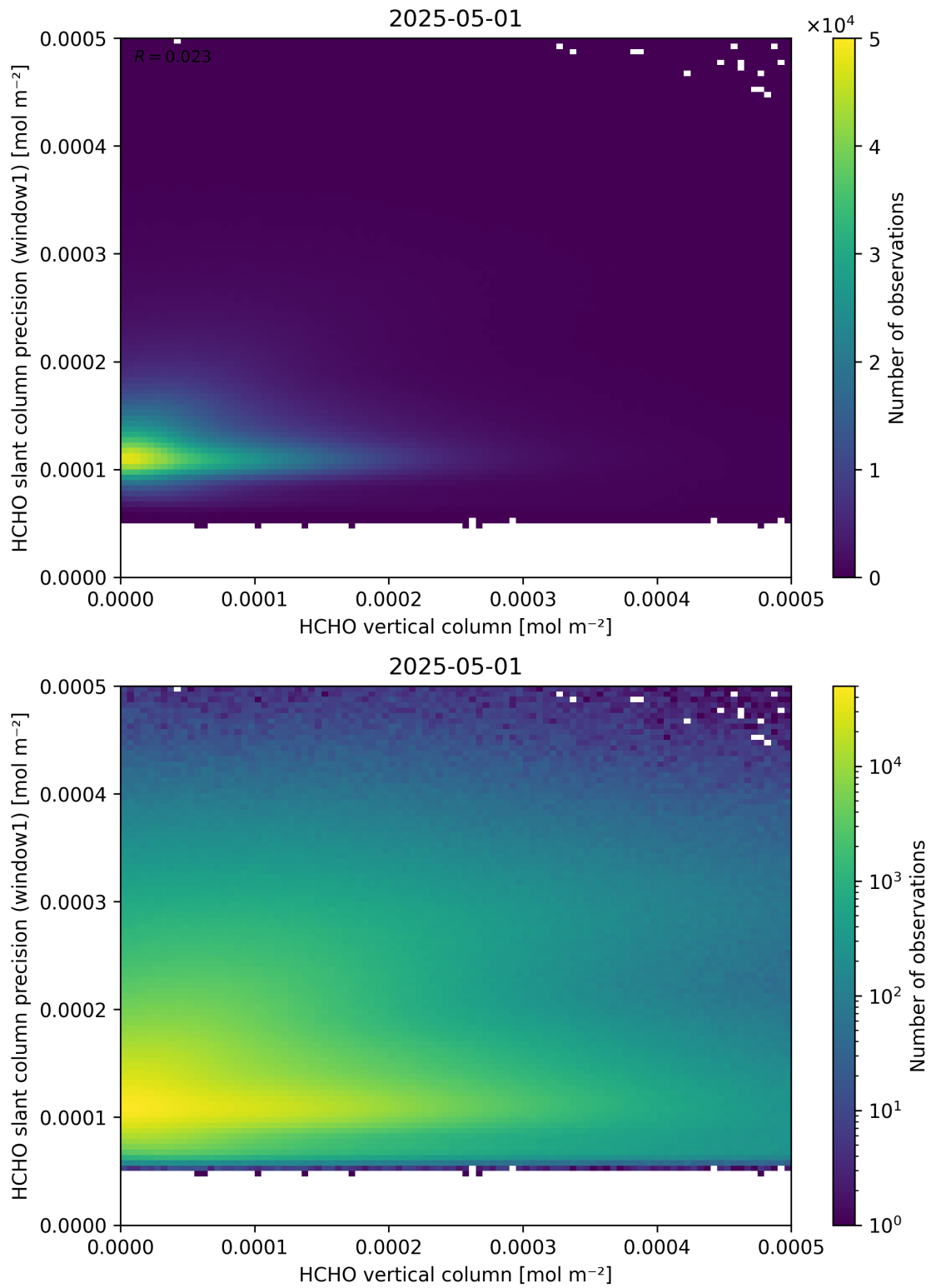
Figure 130: Scatter density plot of “HCHO vertical column” against “HCHO slant column precision (window1)” for 2025-04-30 to 2025-05-02.
