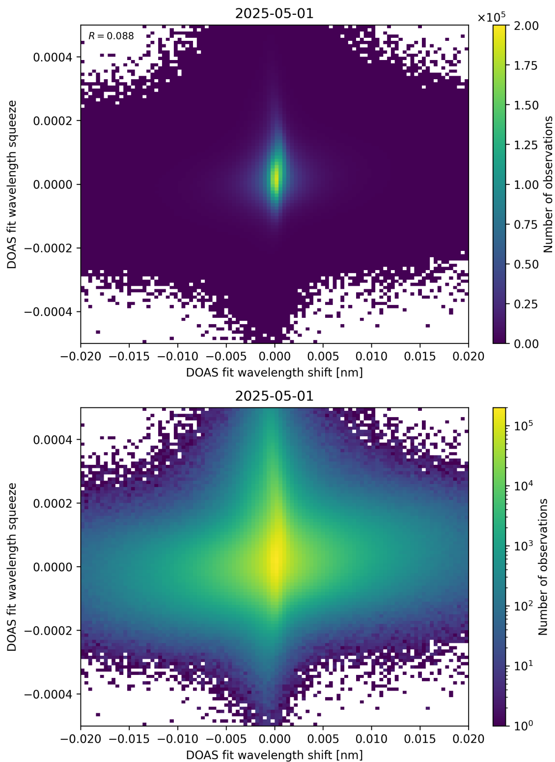
Figure 65: Scatter density plot of “DOAS fit wavelength shift” against “DOAS fit wavelength squeeze” for 2025-04-30 to 2025-05-02.
