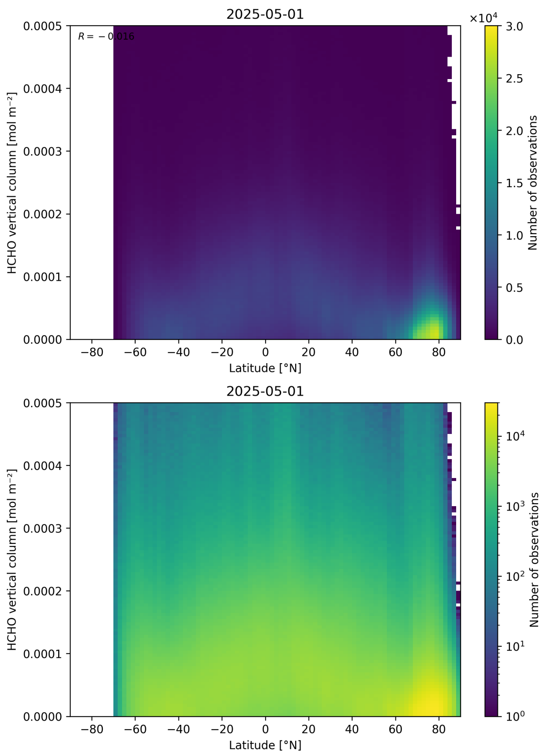
Figure 163: Scatter density plot of “Latitude” against “HCHO vertical column” for 2025-04-30 to 2025-05-02.
