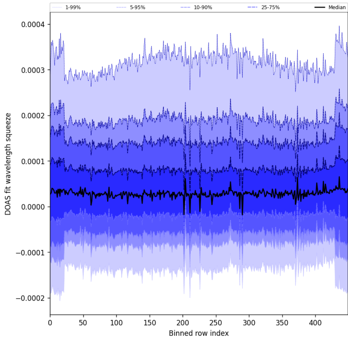
Figure 59: Along track statistics of “DOAS fit wavelength squeeze” for 2025-04-30 to 2025-05-02
