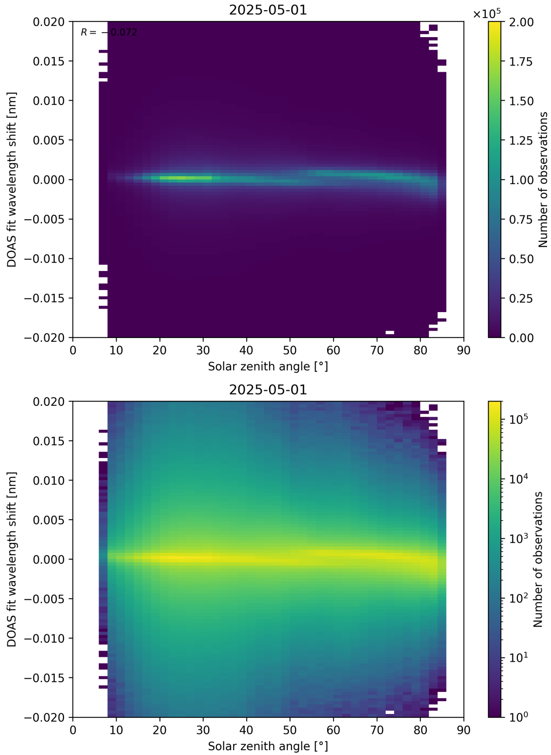
Figure 168: Scatter density plot of “Solar zenith angle” against “DOAS fit wavelength shift” for 2025-04-30 to 2025-05-02.
