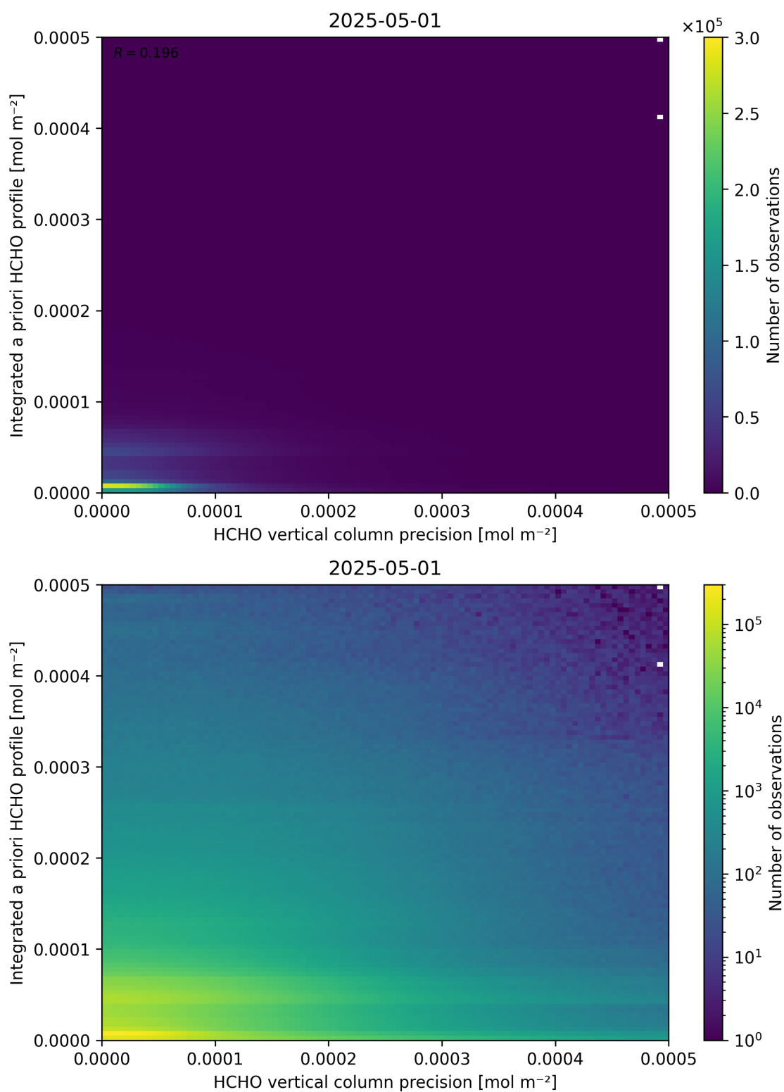
Figure 147: Scatter density plot of “HCHO vertical column precision” against “Integrated a priori HCHO profile” for 2025-04-30 to 2025-05-02.
