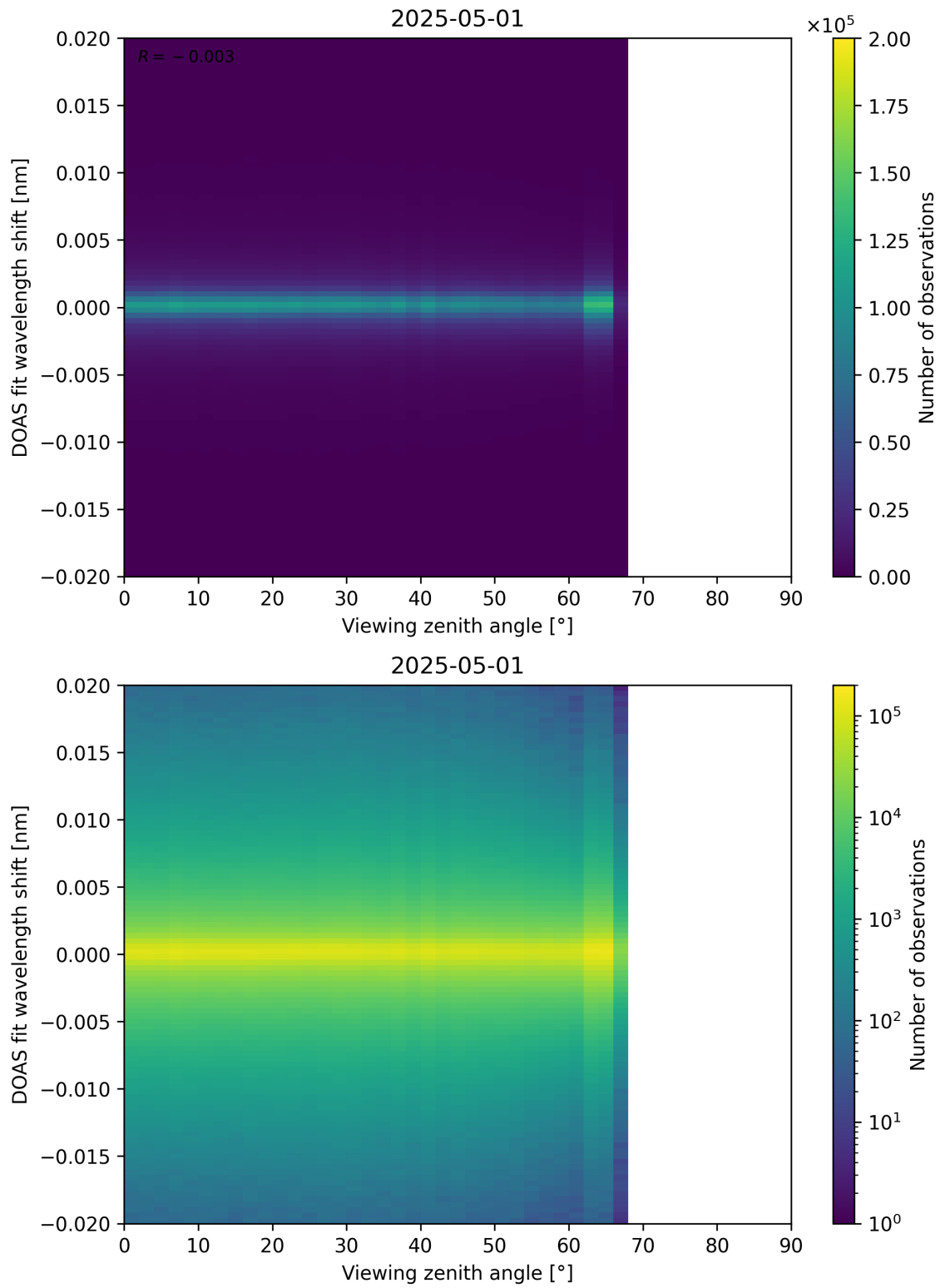
Figure 183: Scatter density plot of “Viewing zenith angle” against “DOAS fit wavelength shift” for 2025-04-30 to 2025-05-02.
