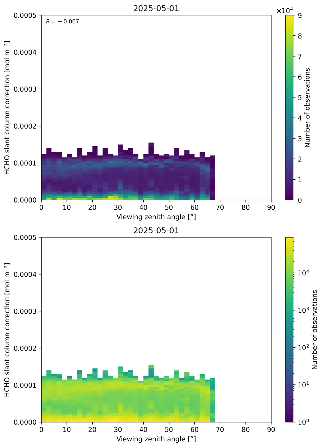
Figure 187: Scatter density plot of “Viewing zenith angle” against “HCHO slant column correction” for 2025-04-30 to 2025-05-02.
