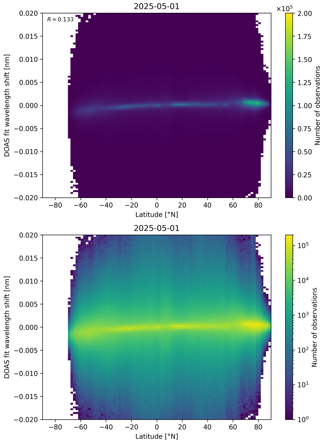
Figure 154: Scatter density plot of “Latitude” against “DOAS fit wavelength shift” for 2025-04-30 to 2025-05-02.
