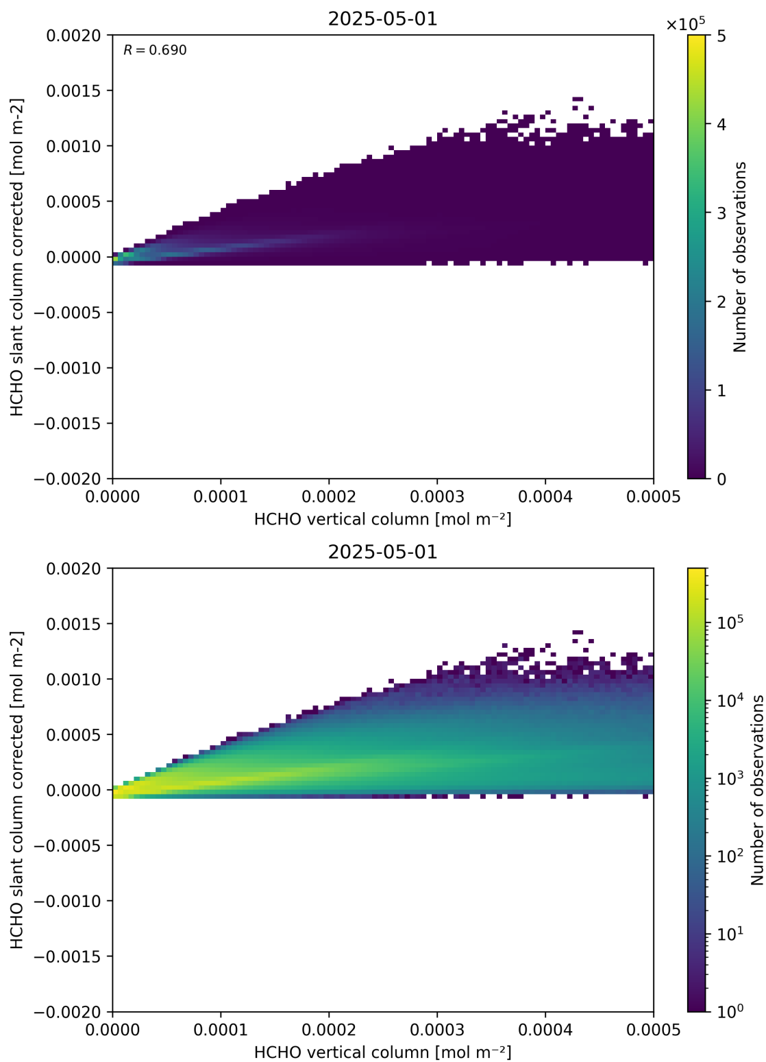
Figure 127: Scatter density plot of “HCHO vertical column” against “HCHO slant column corrected” for 2025-04-30 to 2025-05-02.
