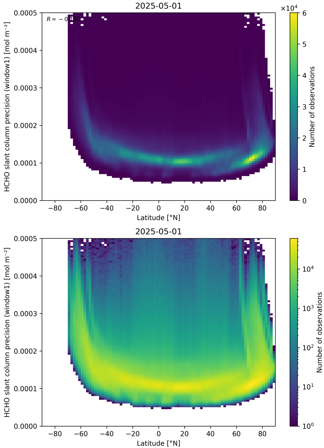
Figure 160: Scatter density plot of “Latitude” against “HCHO slant column precision (window1)” for 2025-04-30 to 2025-05-02.
