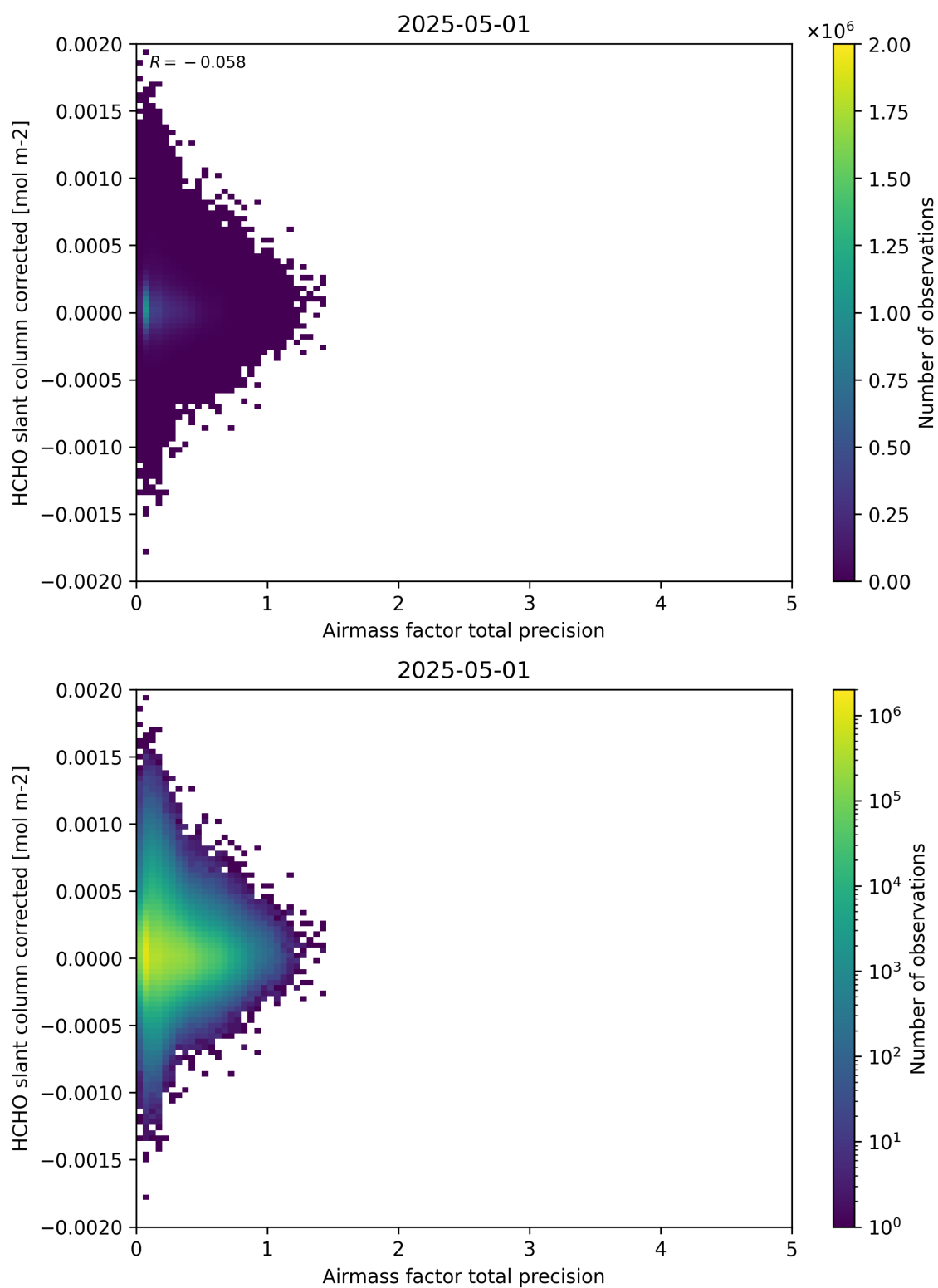
Figure 109: Scatter density plot of “Airmass factor total precision” against “HCHO slant column corrected” for 2025-04-30 to 2025-05-02.
