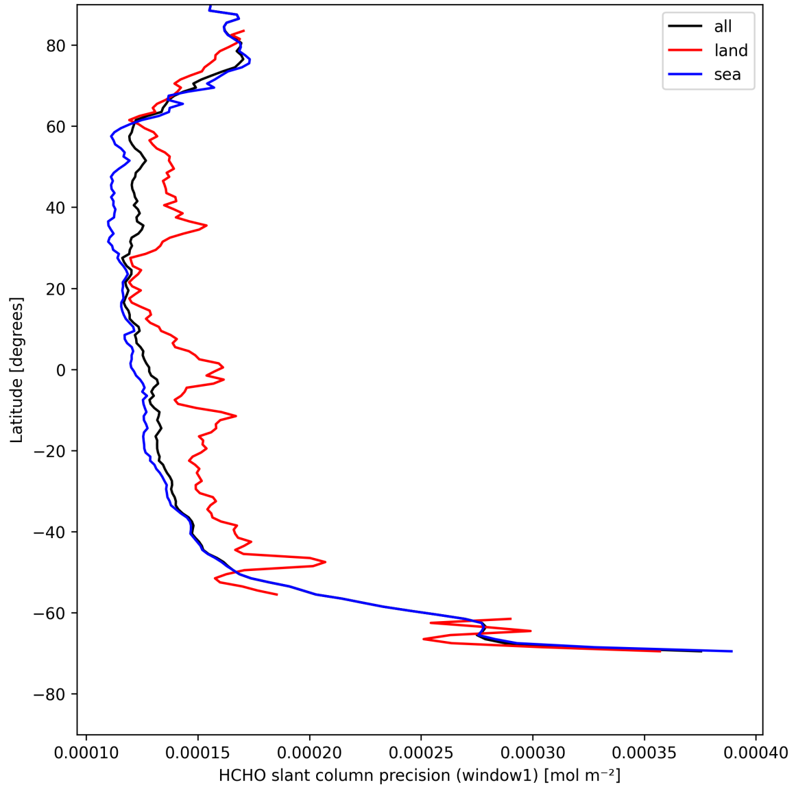
Figure 25: Zonal average of “HCHO slant column precision (window1)” for 2025-04-30 to 2025-05-02.
