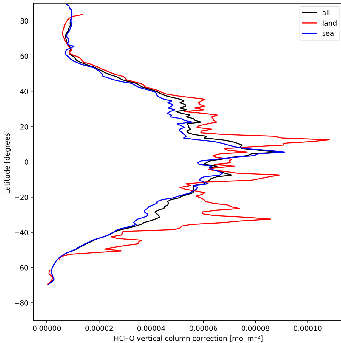
Figure 23: Zonal average of “HCHO vertical column correction” for 2025-04-30 to 2025-05-02.
