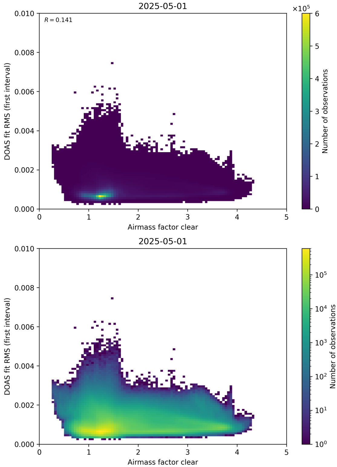
Figure 71: Scatter density plot of “Airmass factor clear” against “DOAS fit RMS (first interval)” for 2025-04-30 to 2025-05-02.
