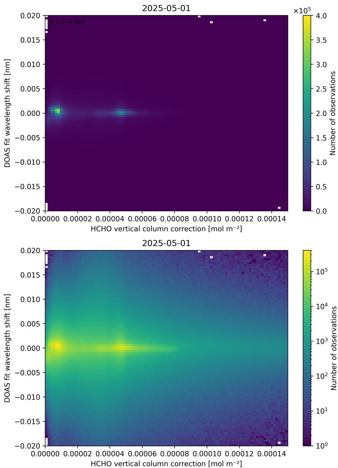
Figure 113: Scatter density plot of “HCHO vertical column correction” against “DOAS fit wavelength shift” for 2025-04-30 to 2025-05-02.
