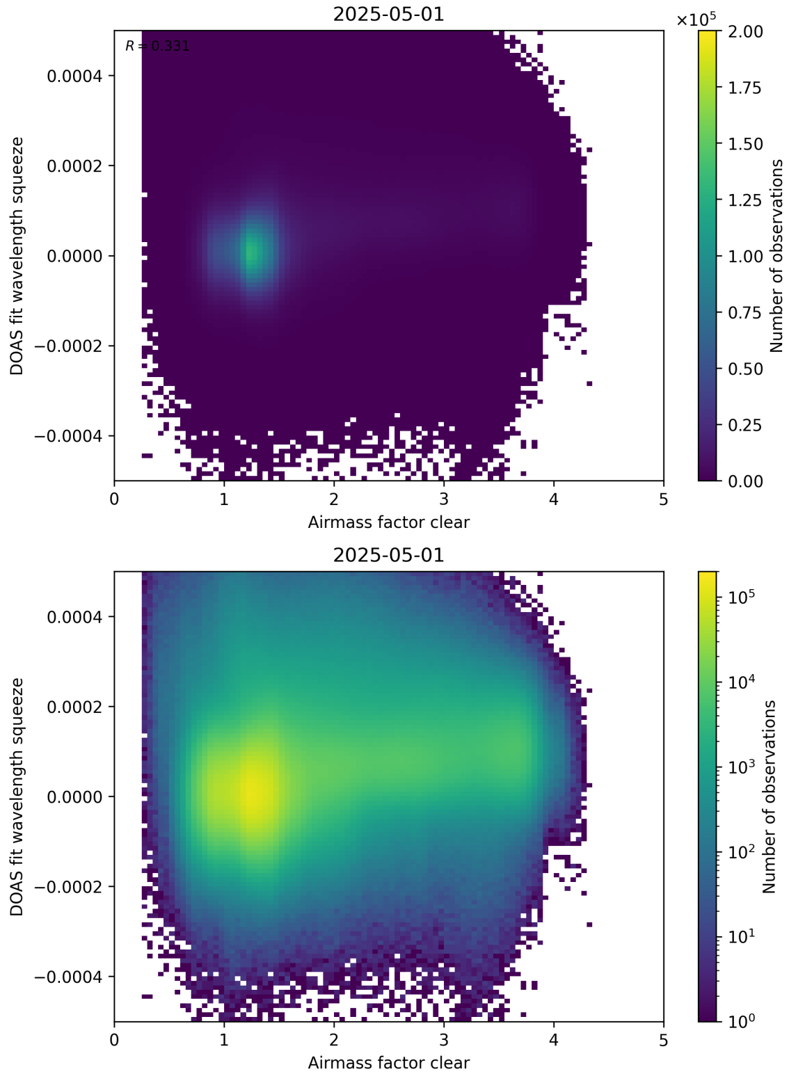
Figure 73: Scatter density plot of “Airmass factor clear” against “DOAS fit wavelength squeeze” for 2025-04-30 to 2025-05-02.
