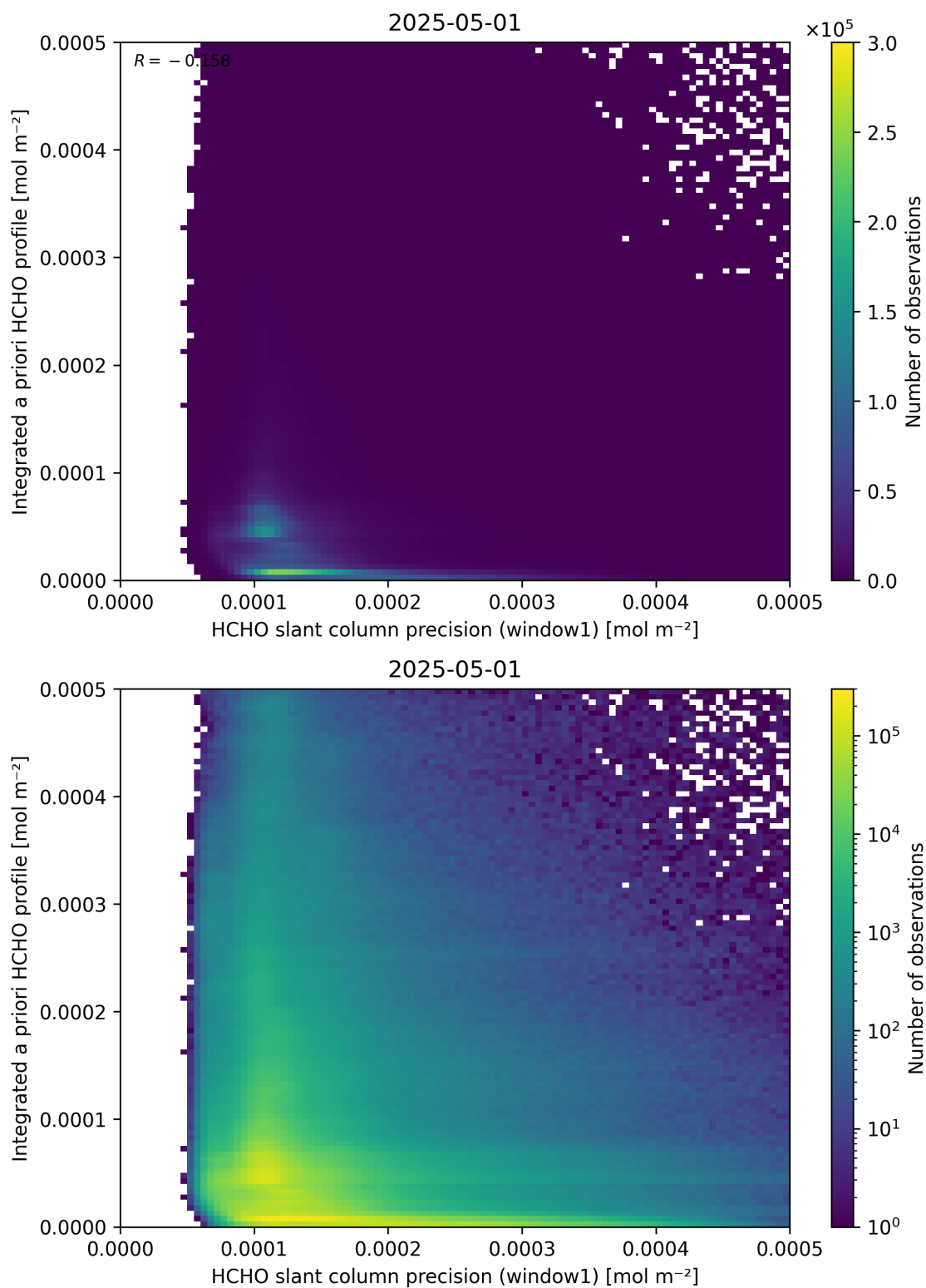
Figure 96: Scatter density plot of “HCHO slant column precision (window1)” against “Integrated a priori HCHO profile” for 2025-04-30 to 2025-05-02.
