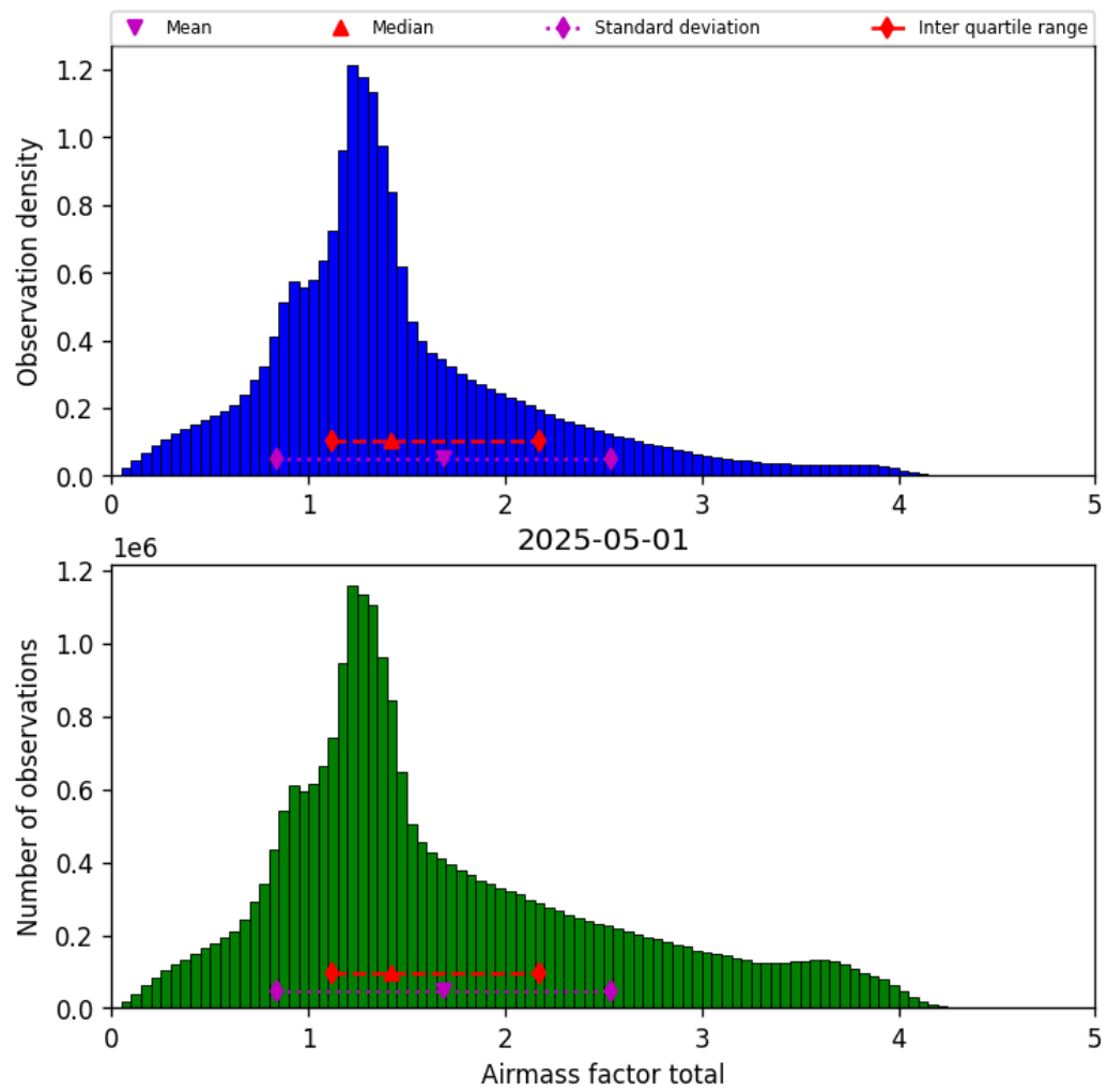
Figure 40: Histogram of “Airmass factor total” for 2025-04-30 to 2025-05-02
