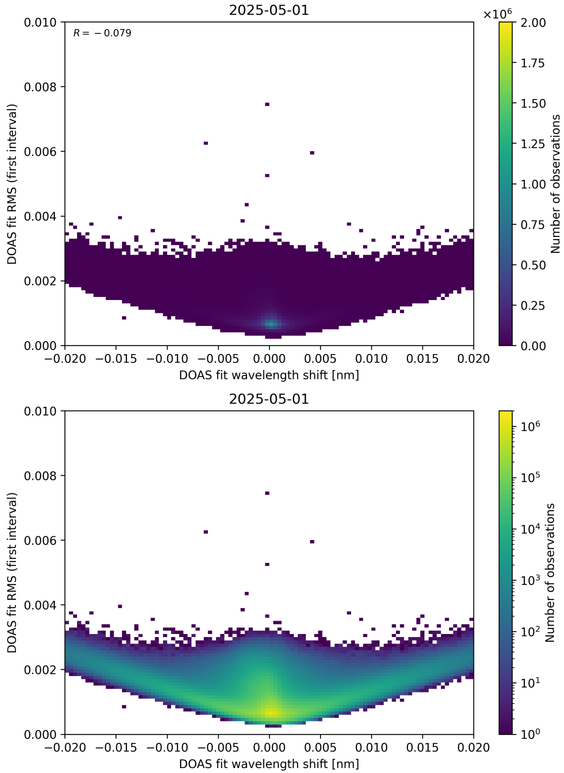
Figure 64: Scatter density plot of “DOAS fit wavelength shift” against “DOAS fit RMS (first interval)” for 2025-04-30 to 2025-05-02.
