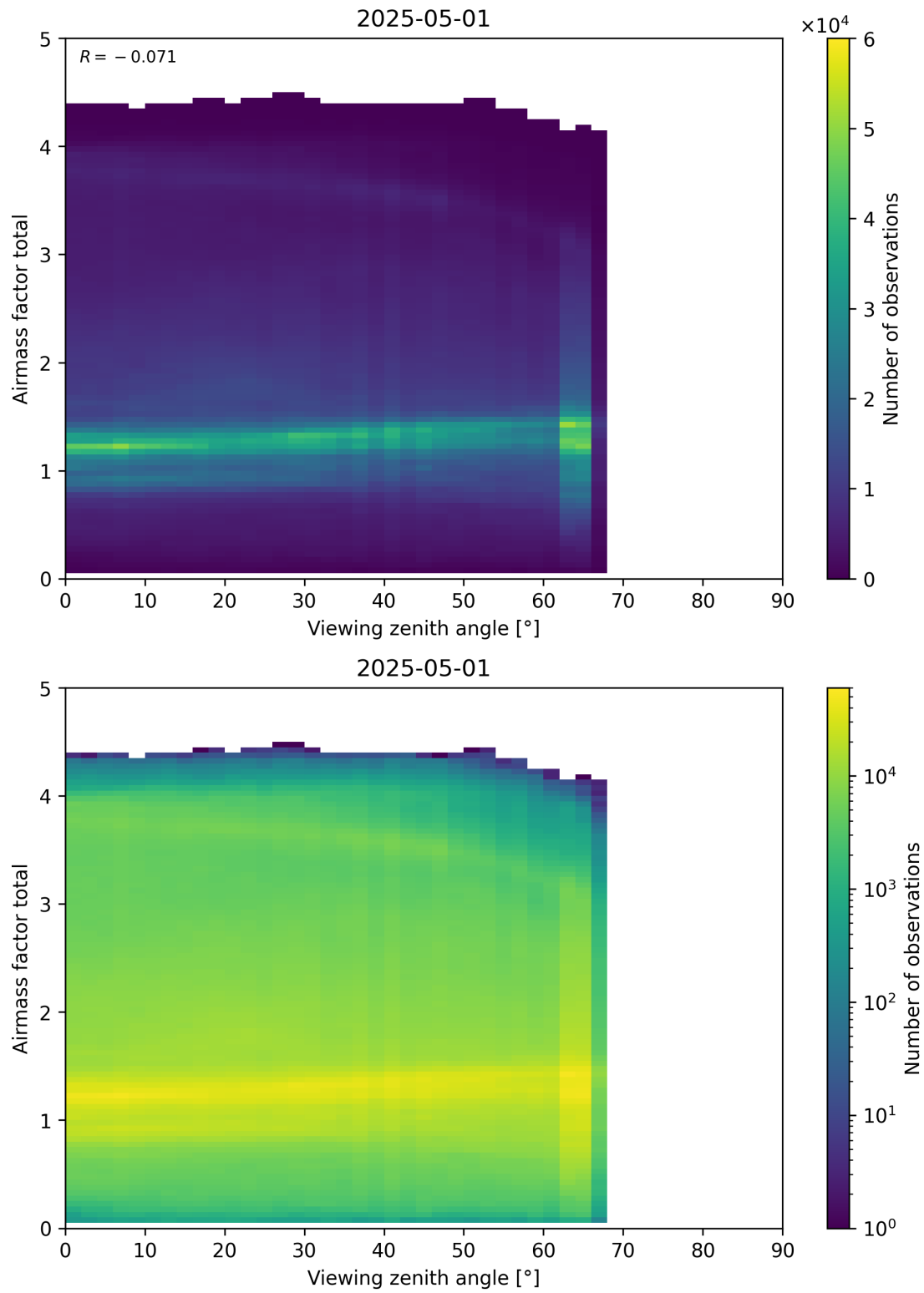
Figure 190: Scatter density plot of “Viewing zenith angle” against “Airmass factor total” for 2025-04-30 to 2025-05-02.
