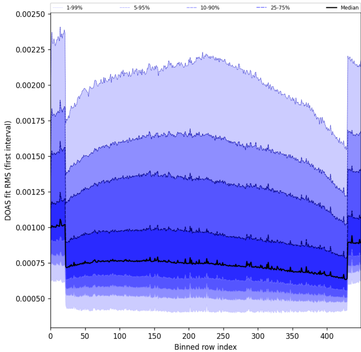
Figure 60: Along track statistics of “DOAS fit RMS (first interval)” for 2025-04-30 to 2025-05-02
