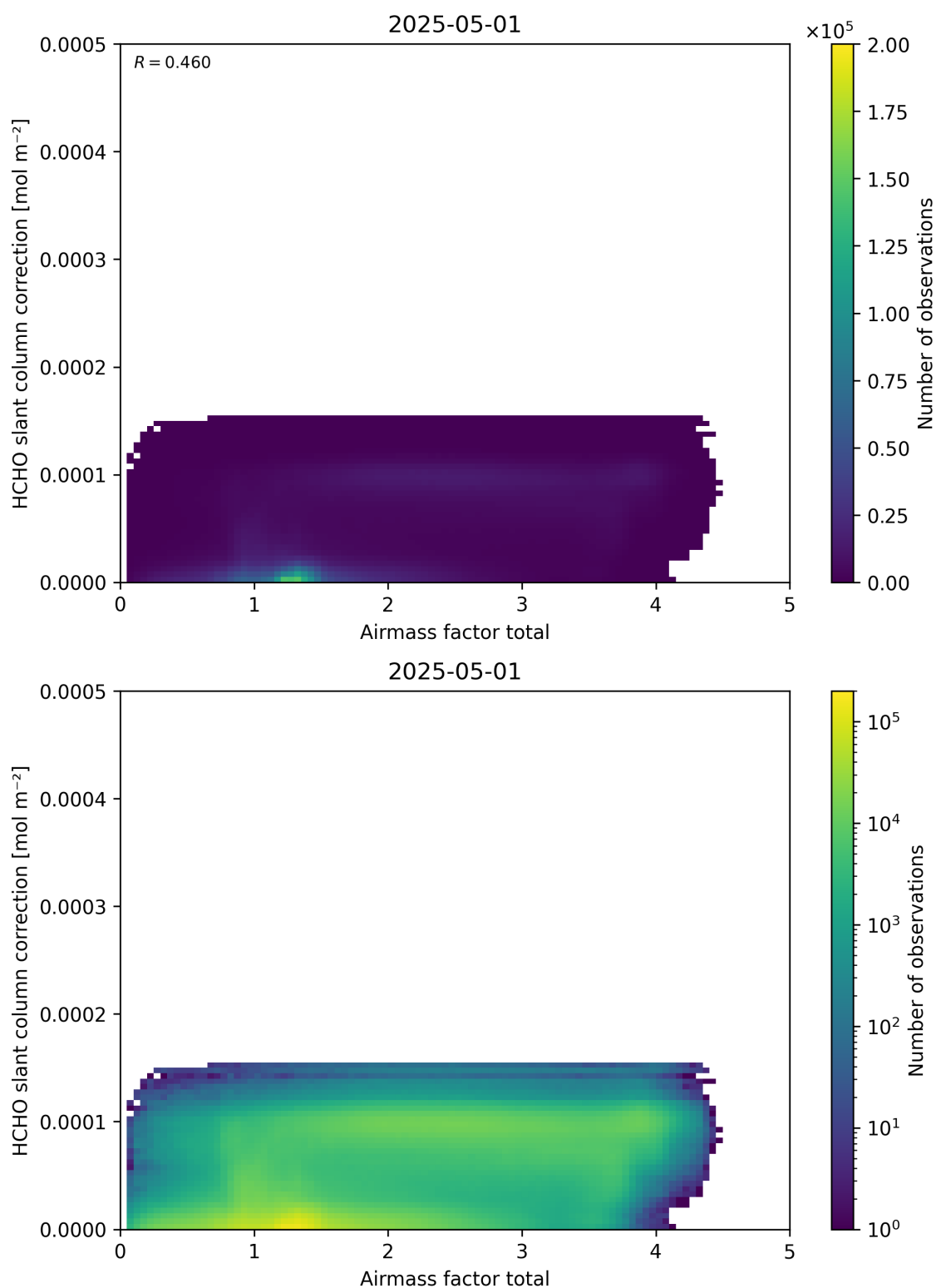
Figure 102: Scatter density plot of “Airmass factor total” against “HCHO slant column correction” for 2025-04-30 to 2025-05-02.
