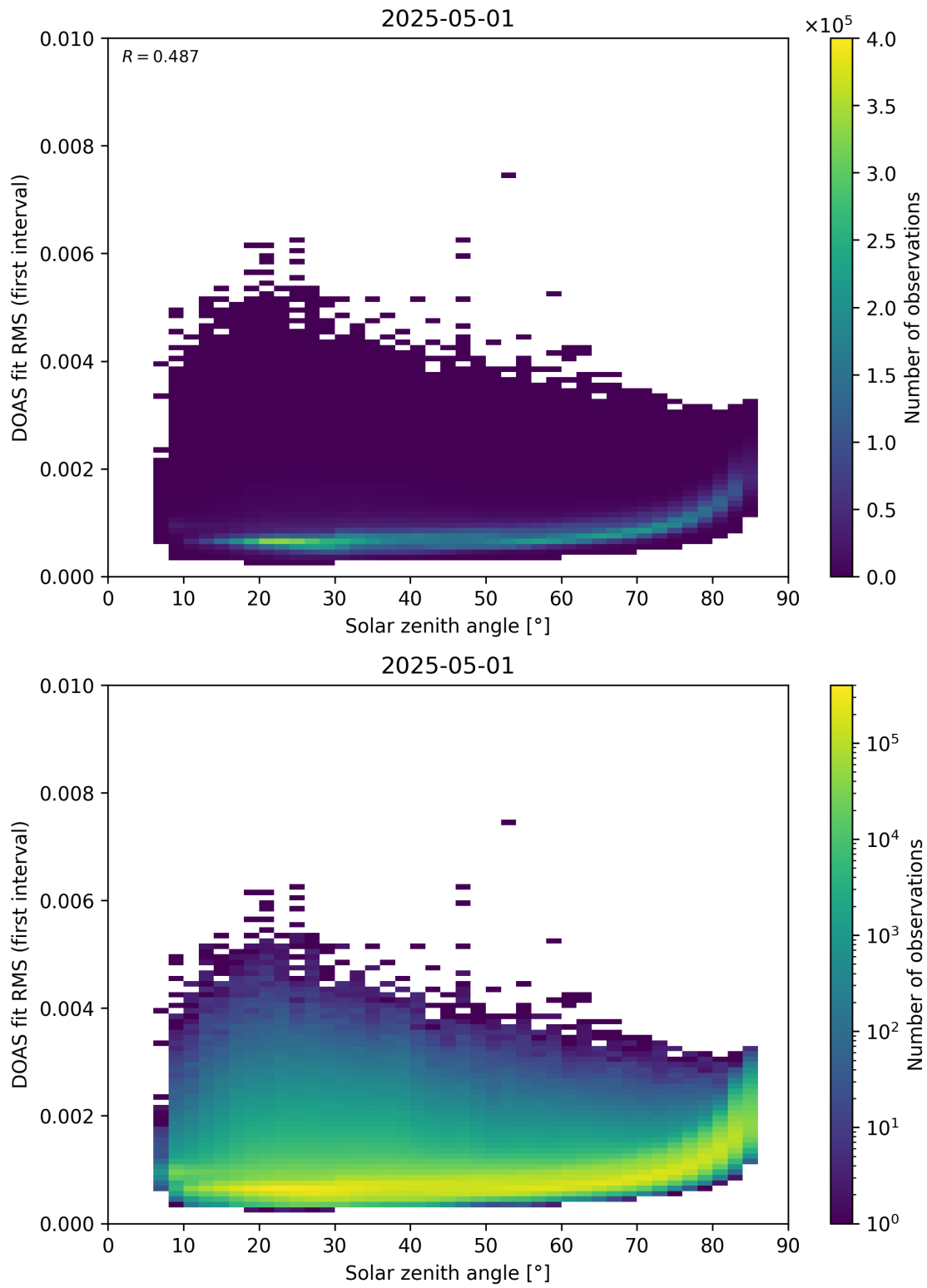
Figure 167: Scatter density plot of “Solar zenith angle” against “DOAS fit RMS (first interval)” for 2025-04-30 to 2025-05-02.
