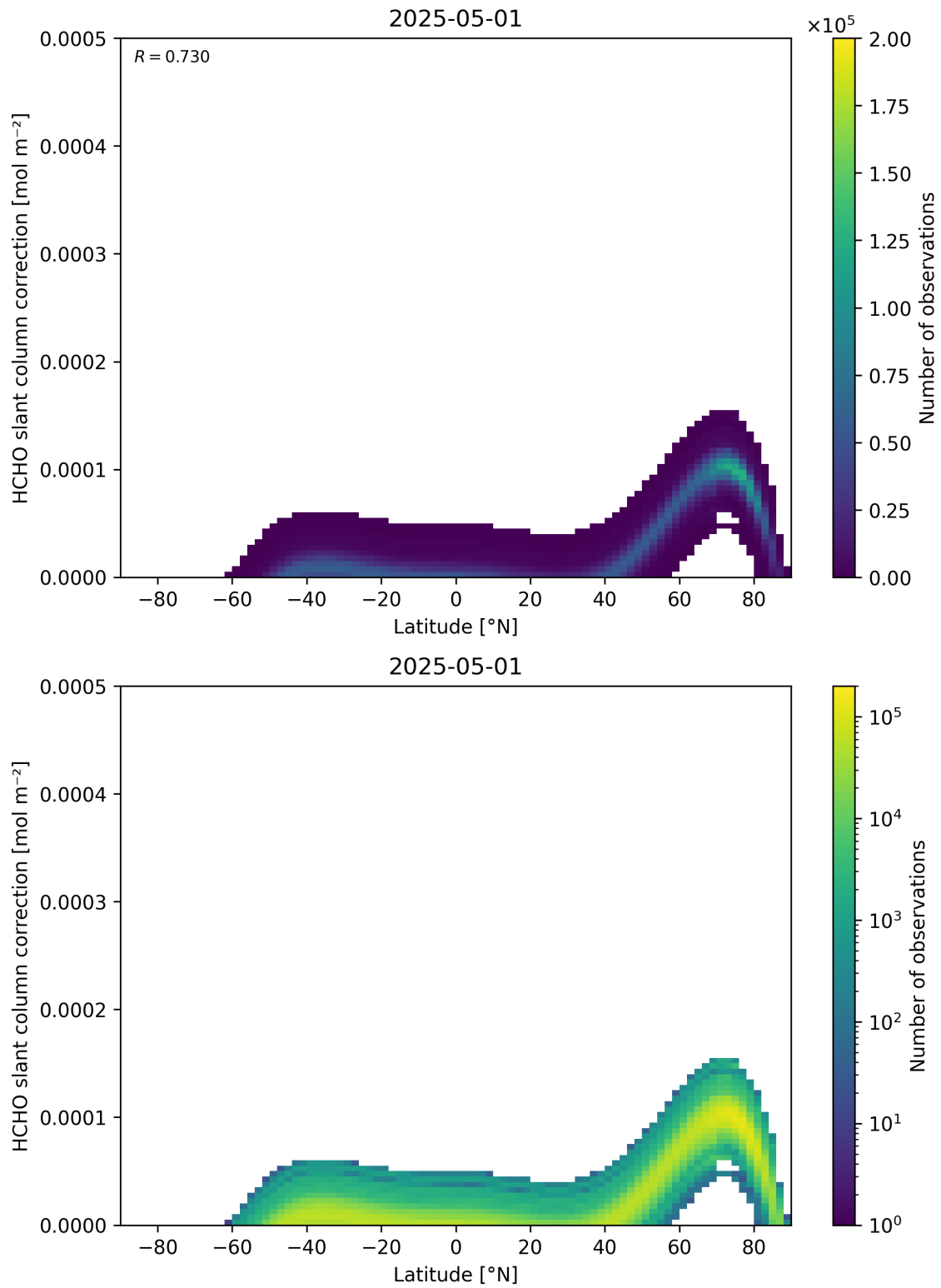
Figure 158: Scatter density plot of “Latitude” against “HCHO slant column correction” for 2025-04-30 to 2025-05-02.
