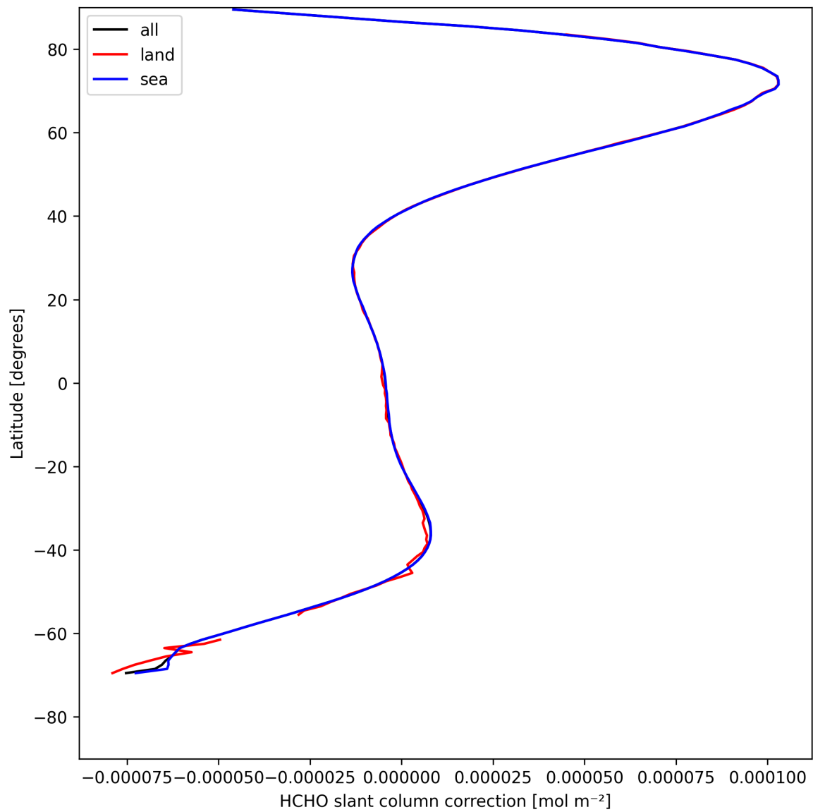
Figure 33: Zonal average of “HCHO slant column correction” for 2025-04-30 to 2025-05-02.
