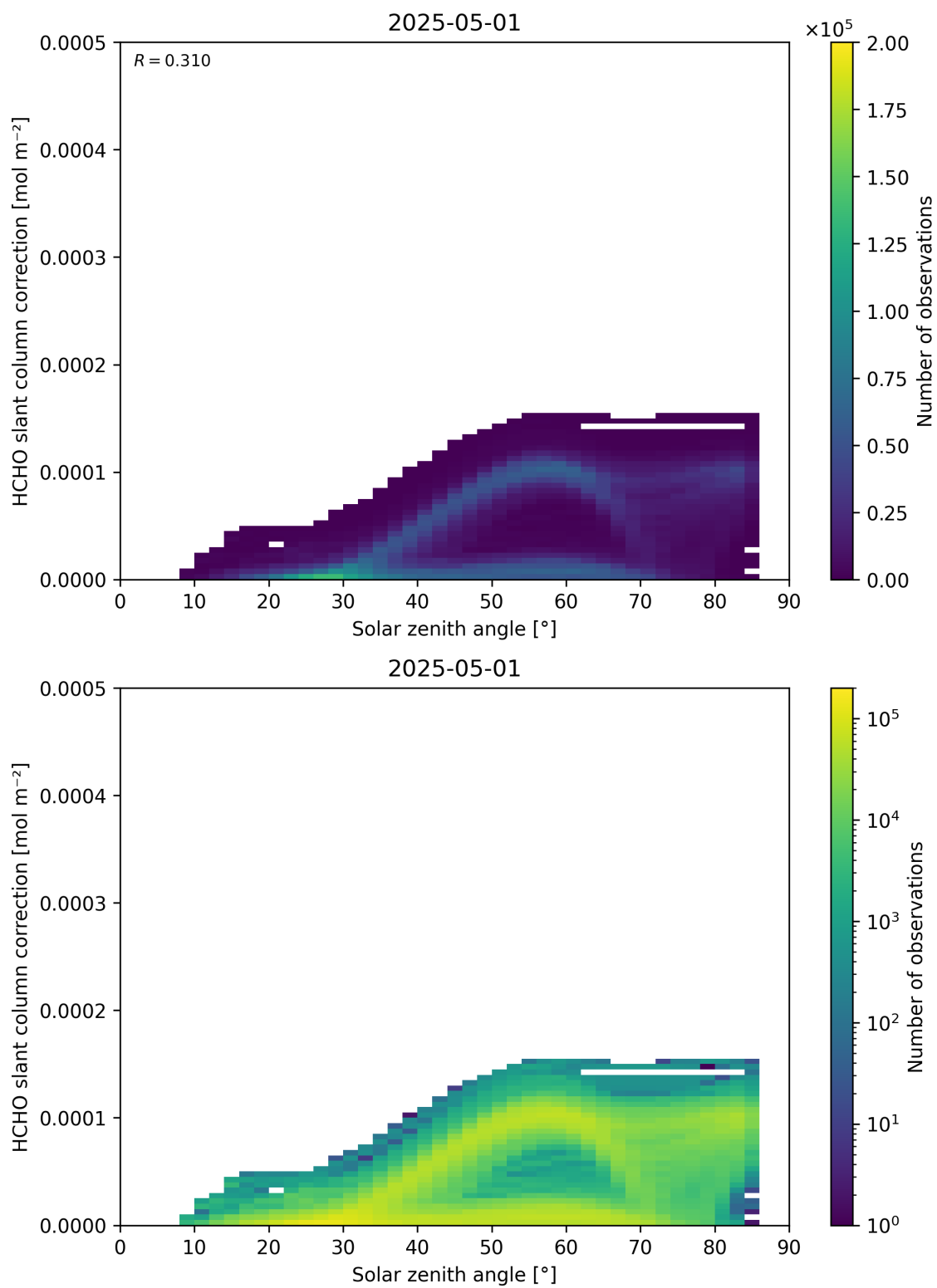
Figure 172: Scatter density plot of “Solar zenith angle” against “HCHO slant column correction” for 2025-04-30 to 2025-05-02.
