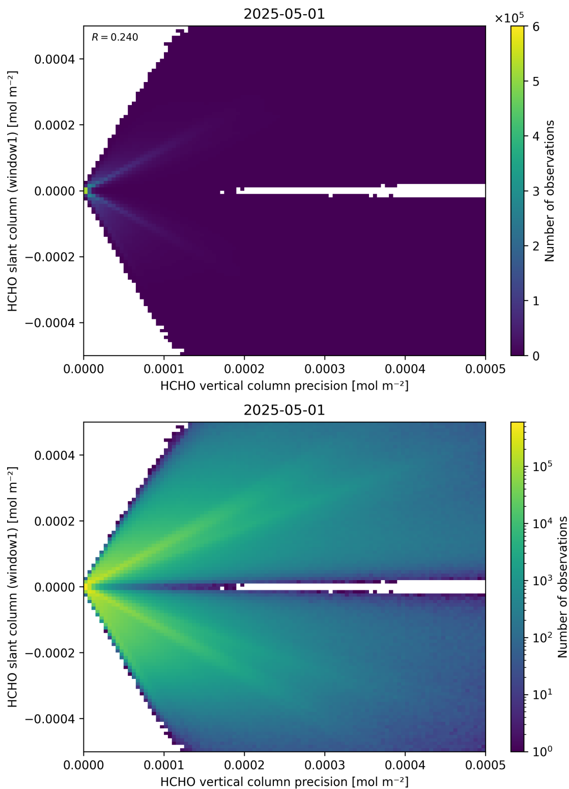
Figure 142: Scatter density plot of “HCHO vertical column precision” against “HCHO slant column (window1)” for 2025-04-30 to 2025-05-02.
