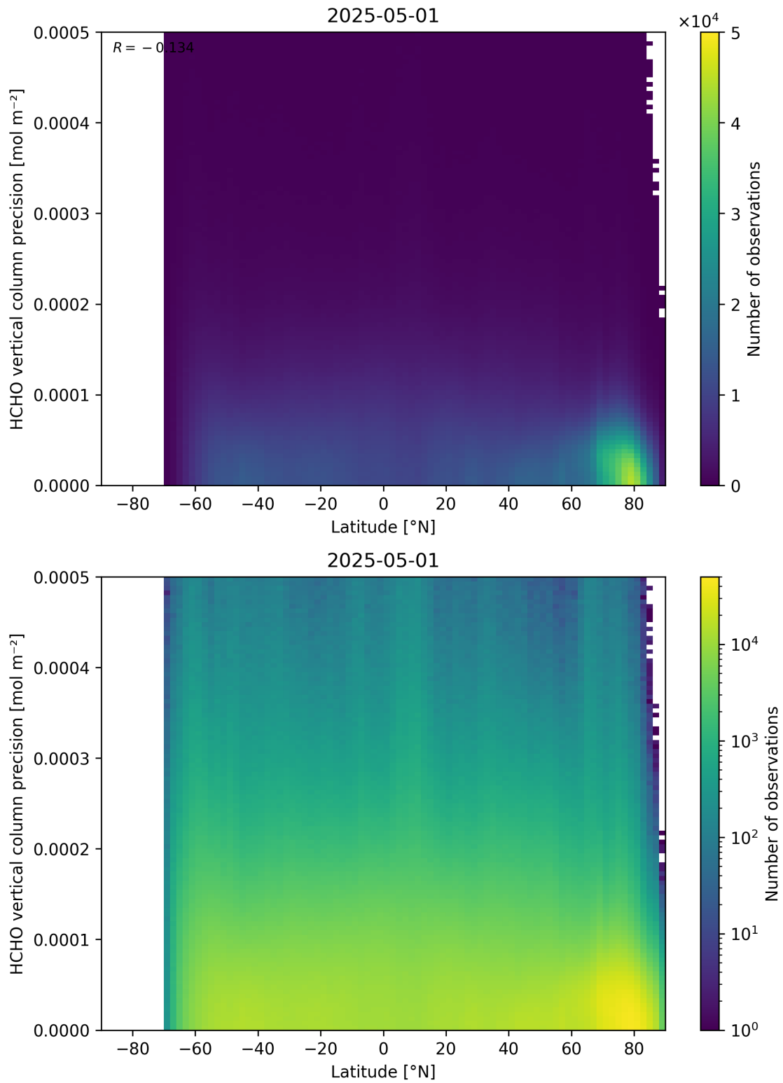
Figure 165: Scatter density plot of “Latitude” against “HCHO vertical column precision” for 2025-04-30 to 2025-05-02.
