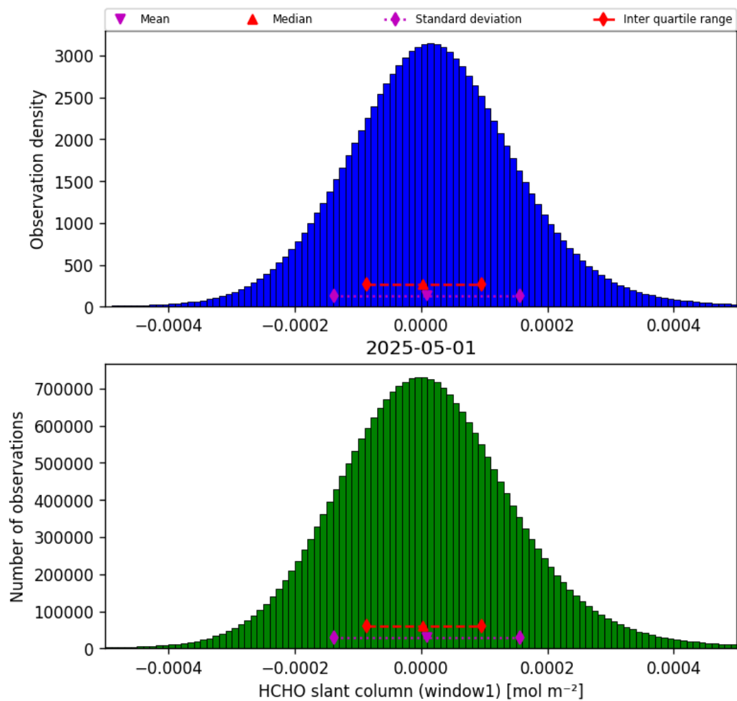
Figure 38: Histogram of “HCHO slant column (window1)” for 2025-04-30 to 2025-05-02
