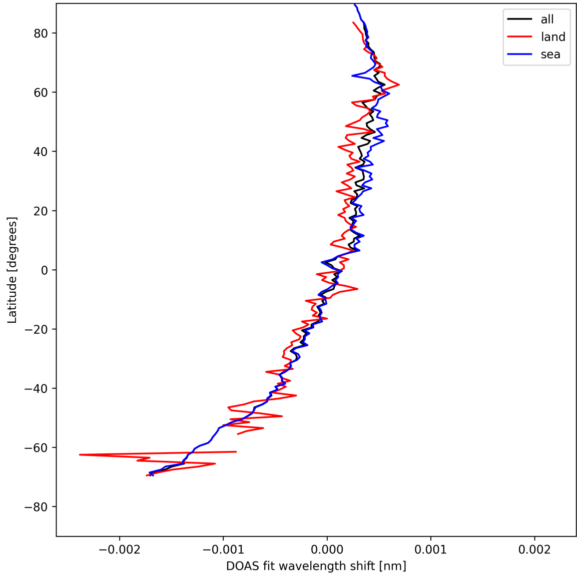
Figure 30: Zonal average of “DOAS fit wavelength shift” for 2025-04-30 to 2025-05-02.
