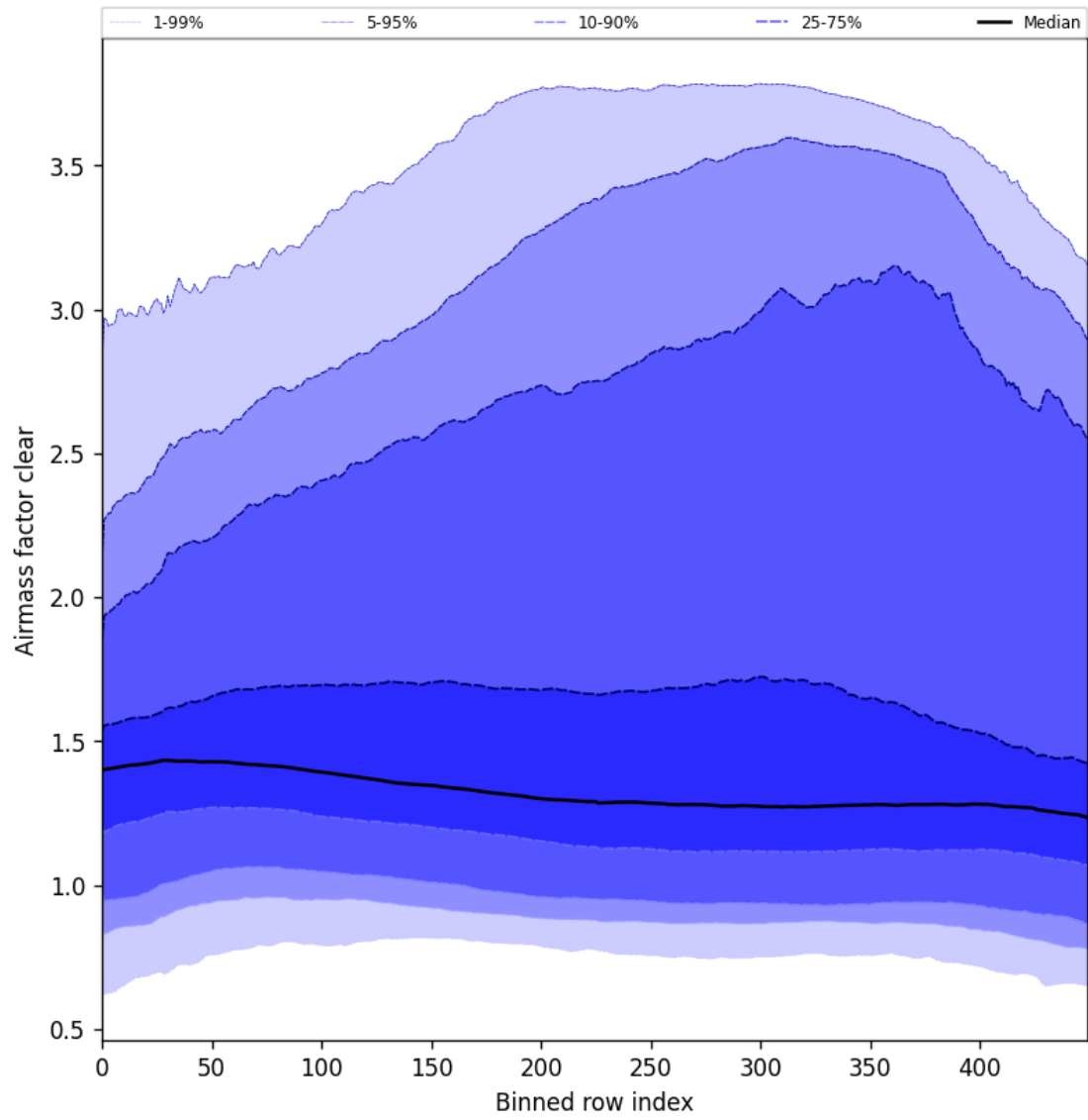
Figure 56: Along track statistics of “Airmass factor clear” for 2025-04-30 to 2025-05-02
