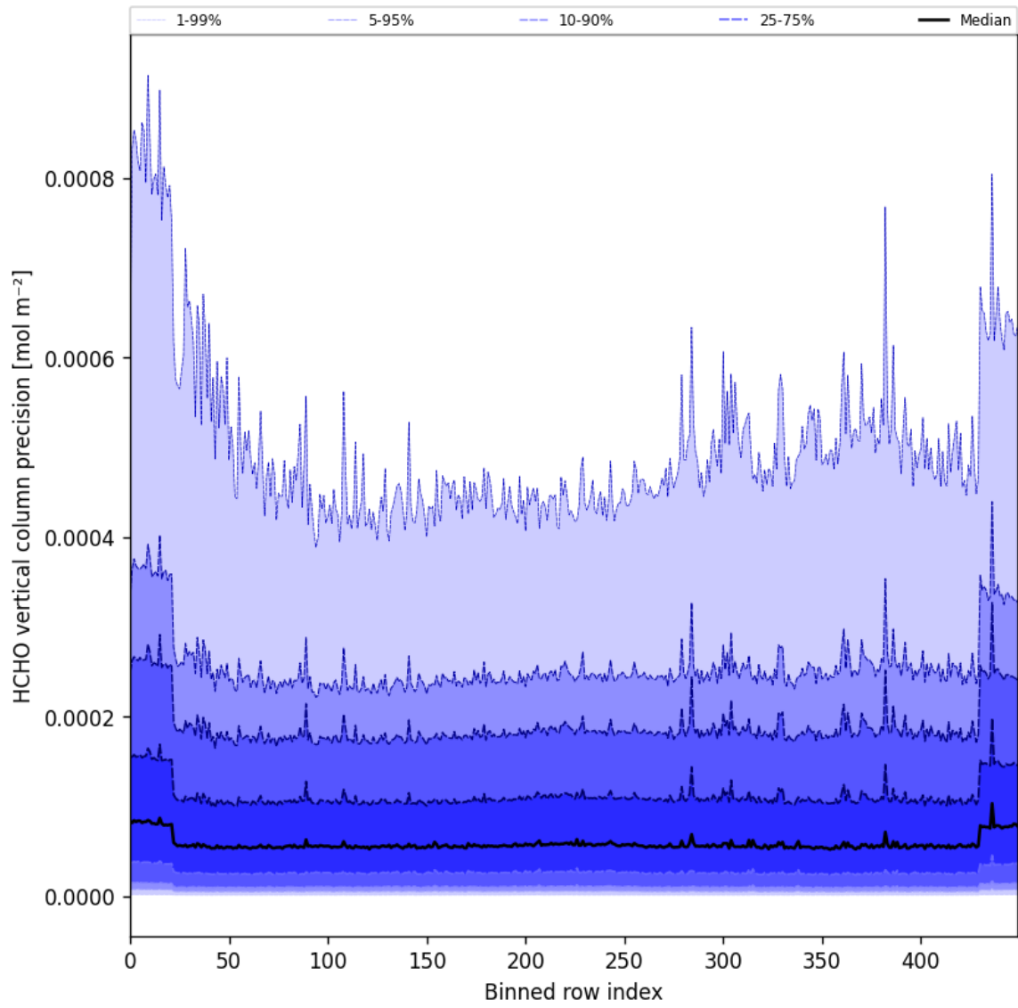
Figure 50: Along track statistics of “HCHO vertical column precision” for 2025-04-30 to 2025-05-02
