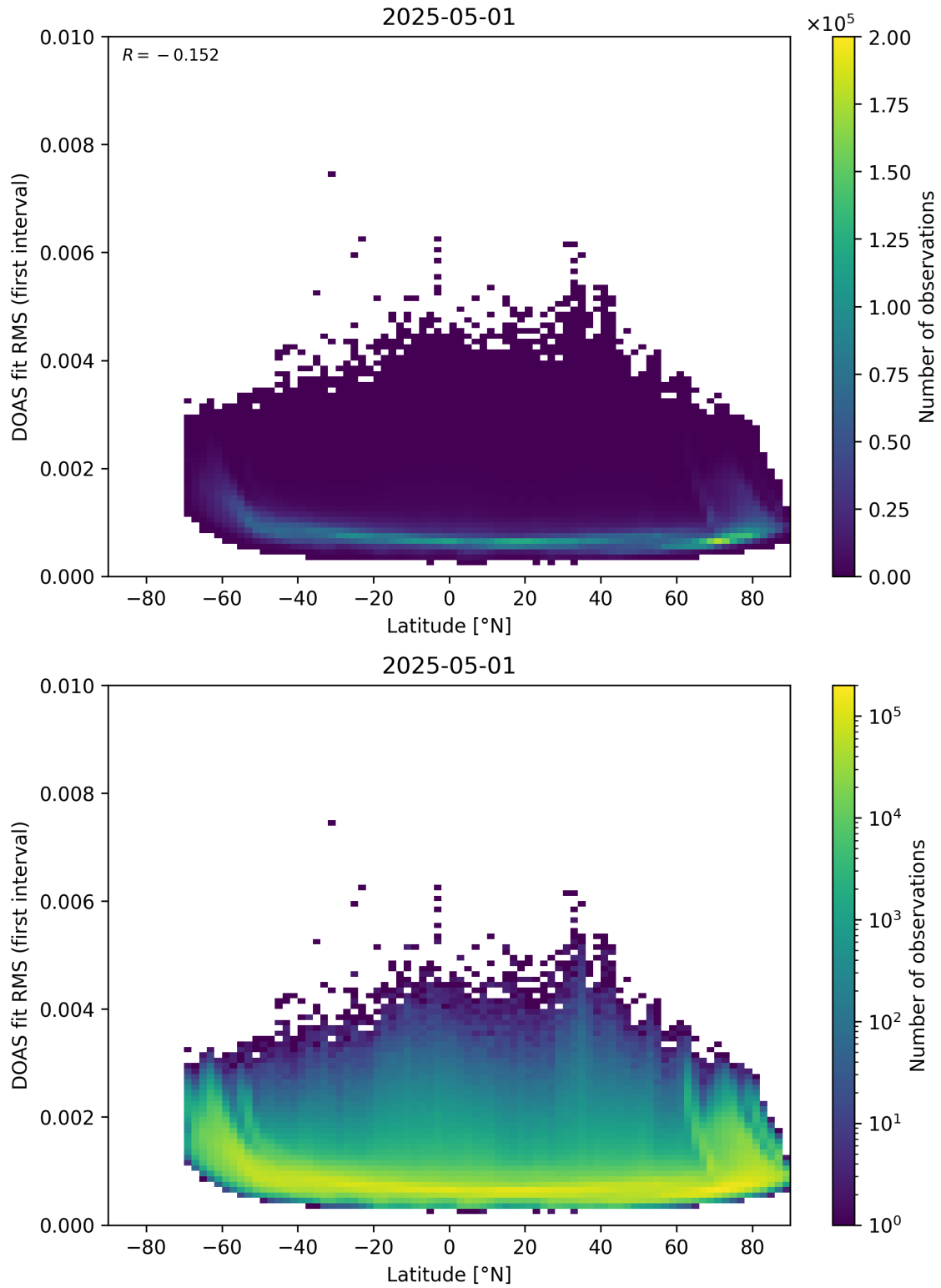
Figure 153: Scatter density plot of “Latitude” against “DOAS fit RMS (first interval)” for 2025-04-30 to 2025-05-02.
