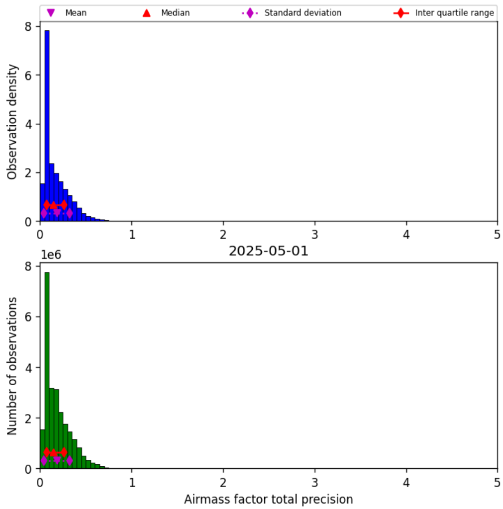
Figure 41: Histogram of “Airmass factor total precision” for 2025-04-30 to 2025-05-02
