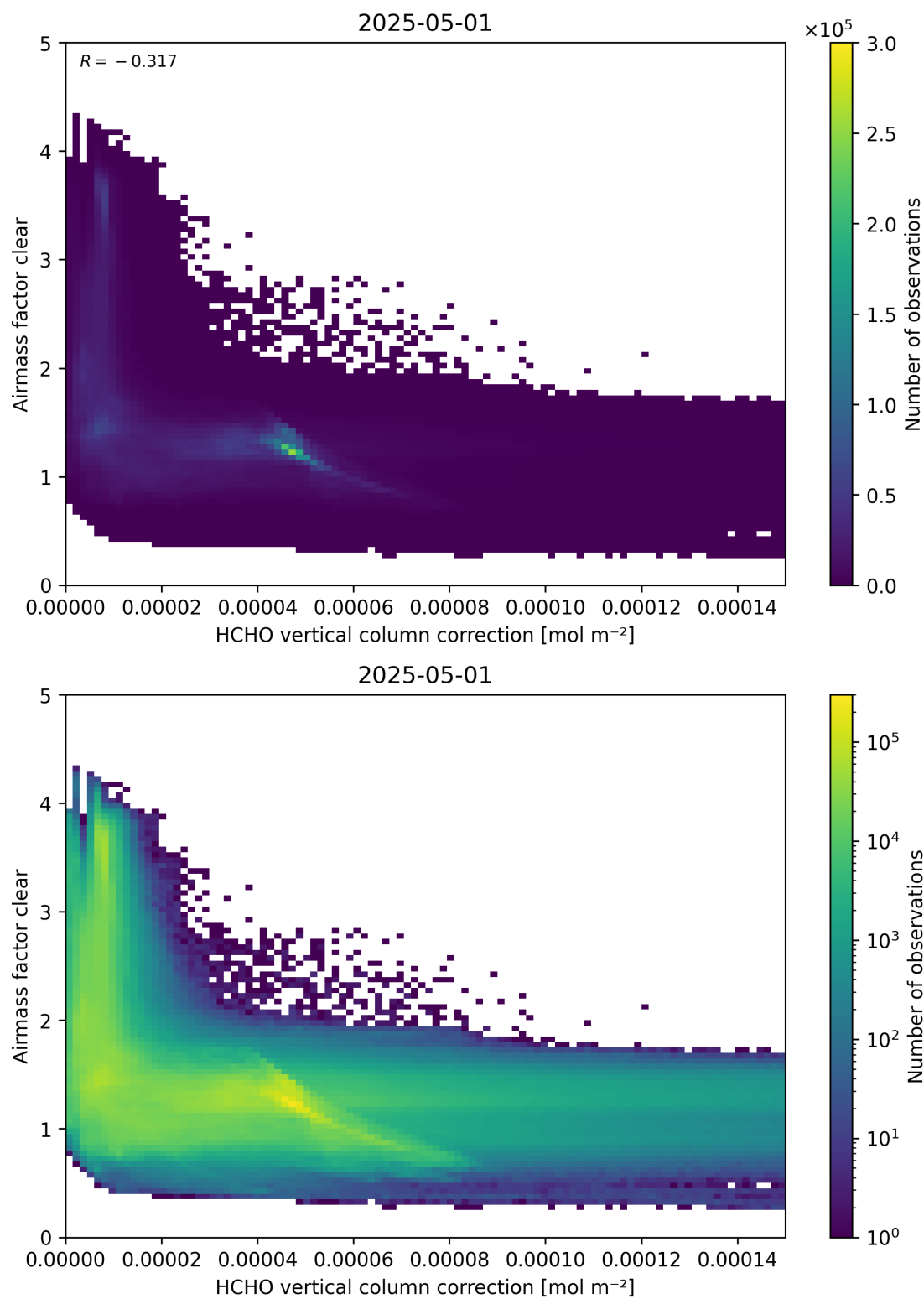
Figure 115: Scatter density plot of “HCHO vertical column correction” against “Airmass factor clear” for 2025-04-30 to 2025-05-02.
