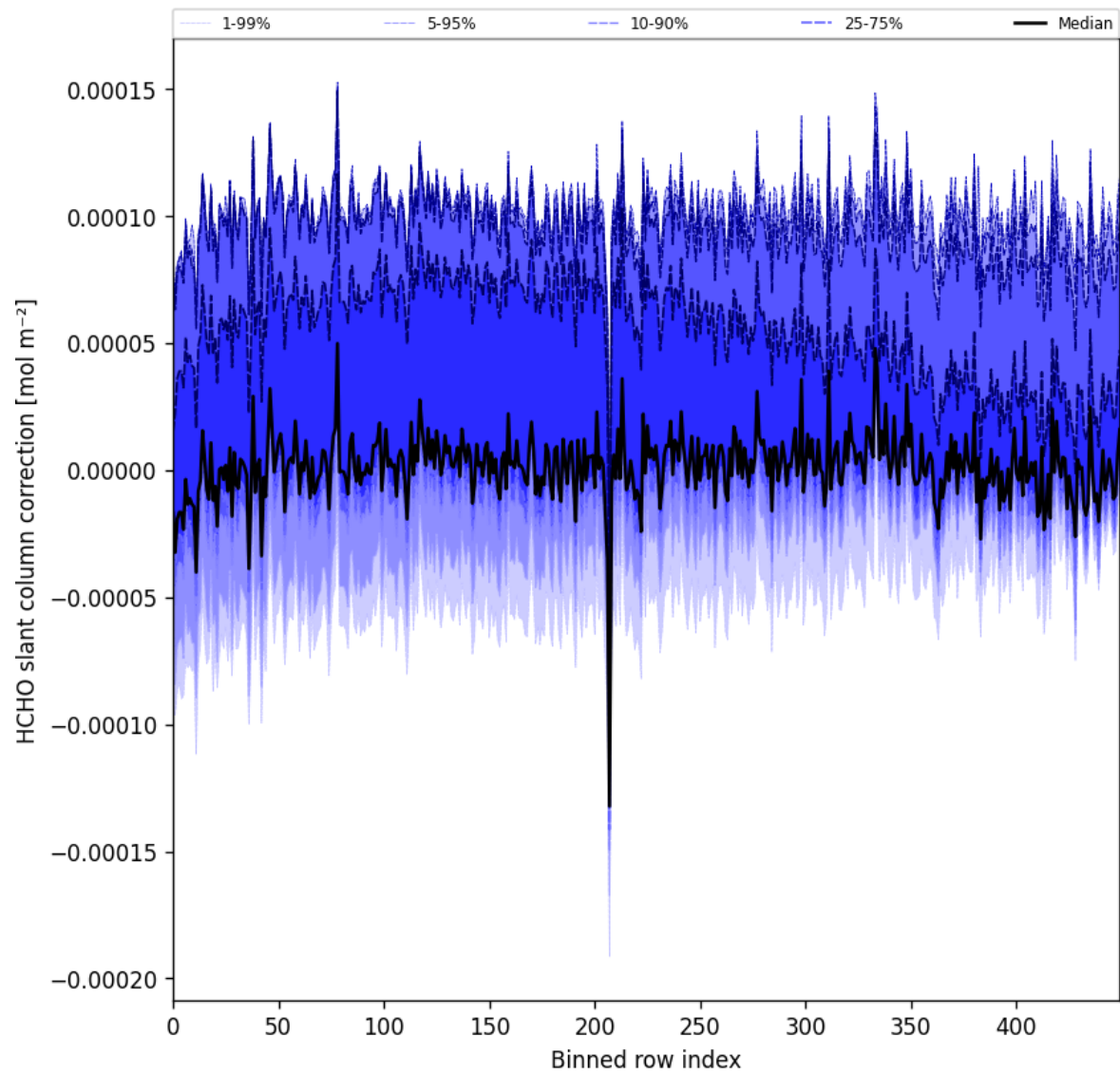
Figure 61: Along track statistics of "HCHO slant column correction" for 2025-04-30 to 2025-05-02
