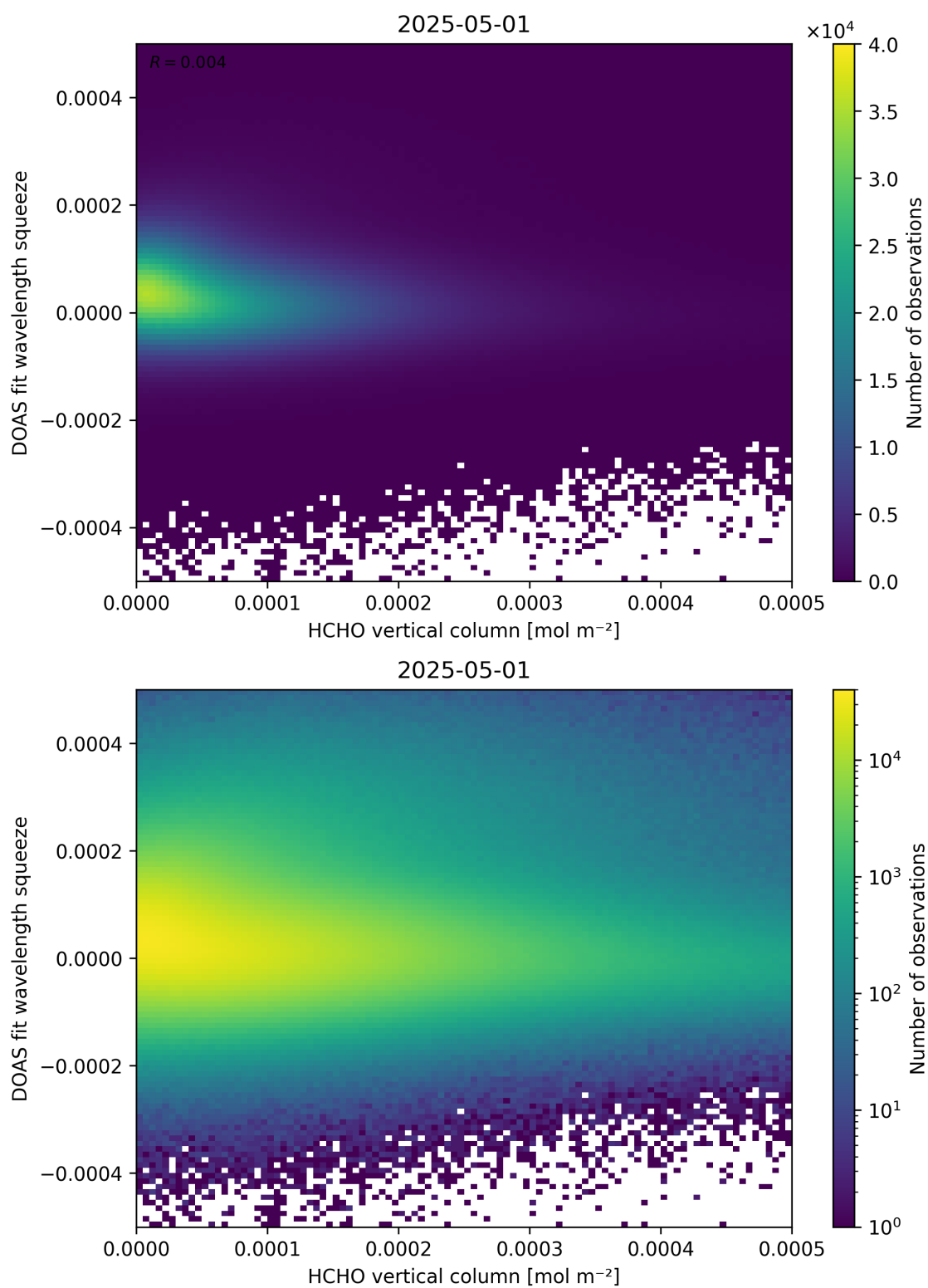
Figure 125: Scatter density plot of “HCHO vertical column” against “DOAS fit wavelength squeeze” for 2025-04-30 to 2025-05-02.
