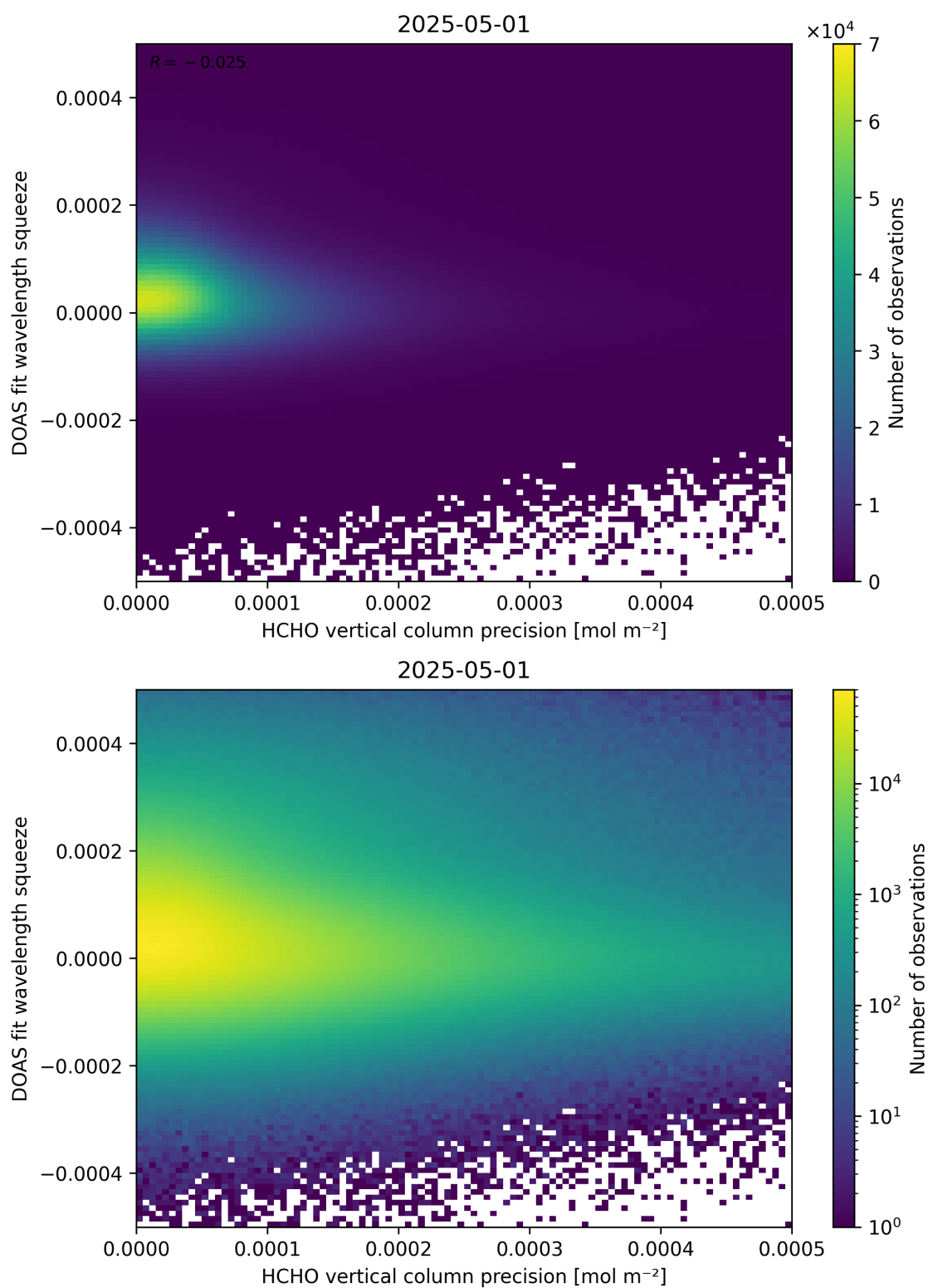
Figure 138: Scatter density plot of “HCHO vertical column precision” against “DOAS fit wavelength squeeze” for 2025-04-30 to 2025-05-02.
