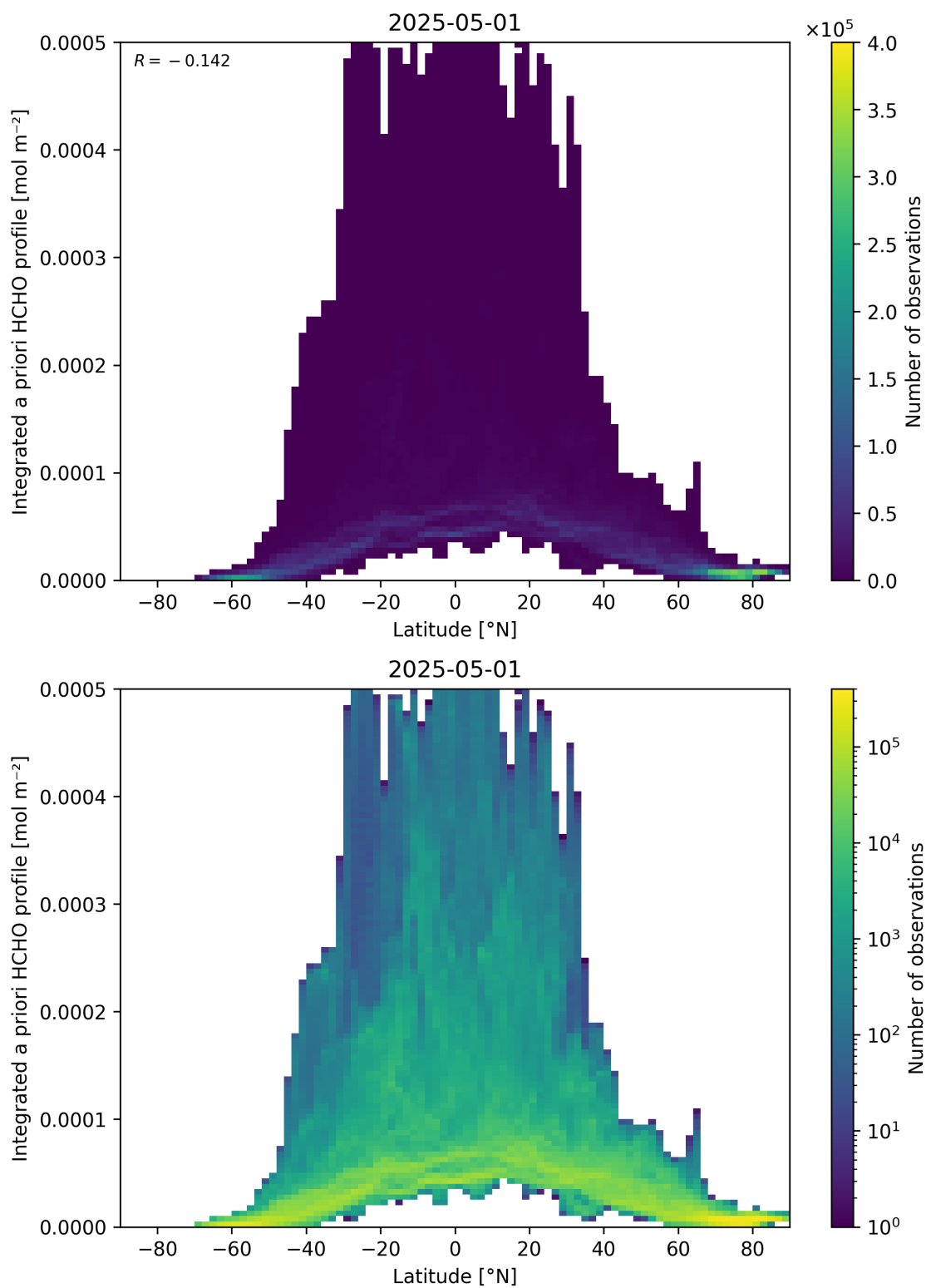
Figure 166: Scatter density plot of “Latitude” against “Integrated a priori HCHO profile” for 2025-04-30 to 2025-05-02.
