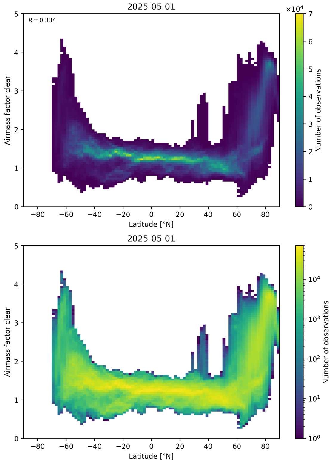
Figure 156: Scatter density plot of “Latitude” against “Airmass factor clear” for 2025-04-30 to 2025-05-02.
