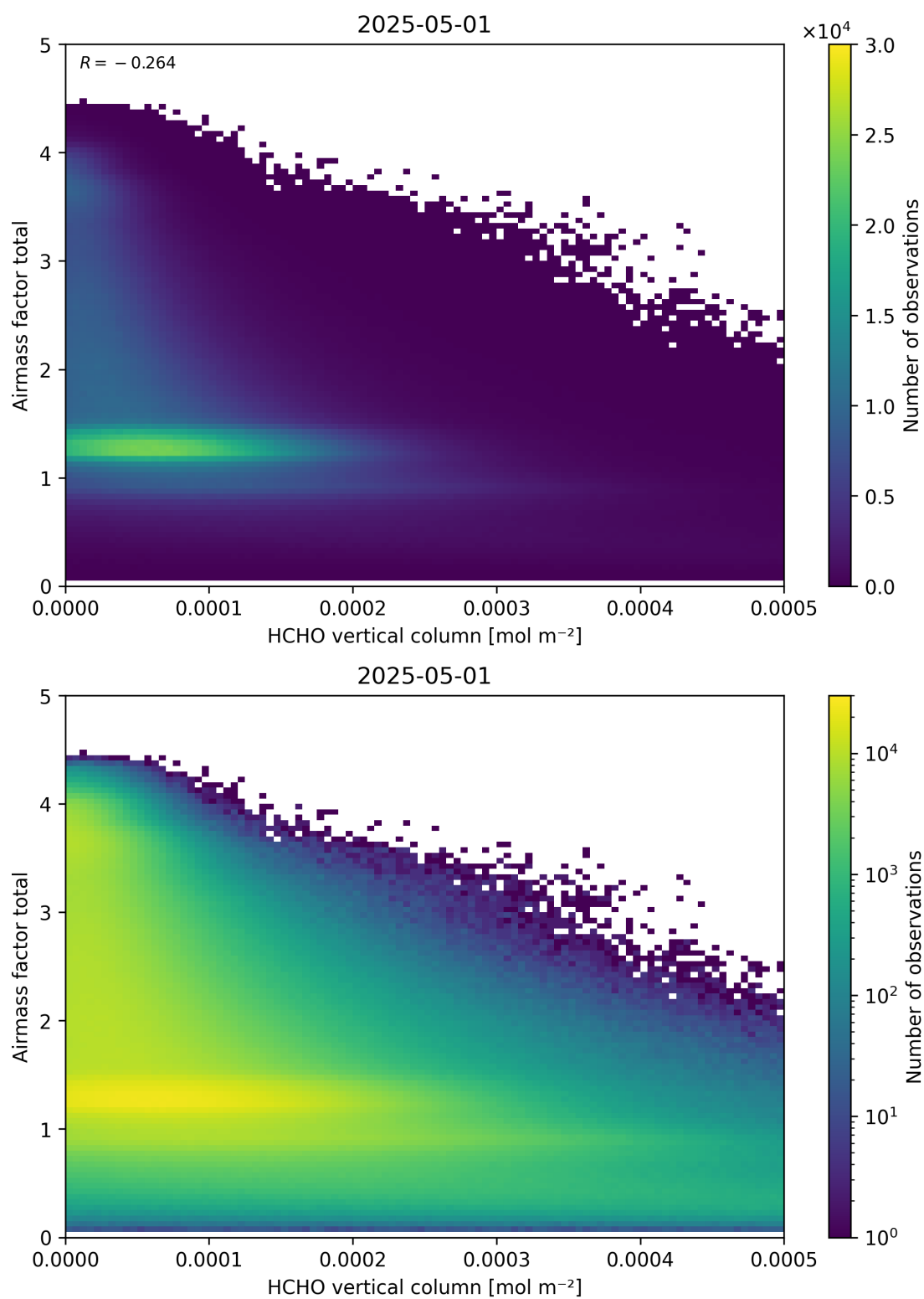
Figure 131: Scatter density plot of “HCHO vertical column” against “Airmass factor total” for 2025-04-30 to 2025-05-02.
