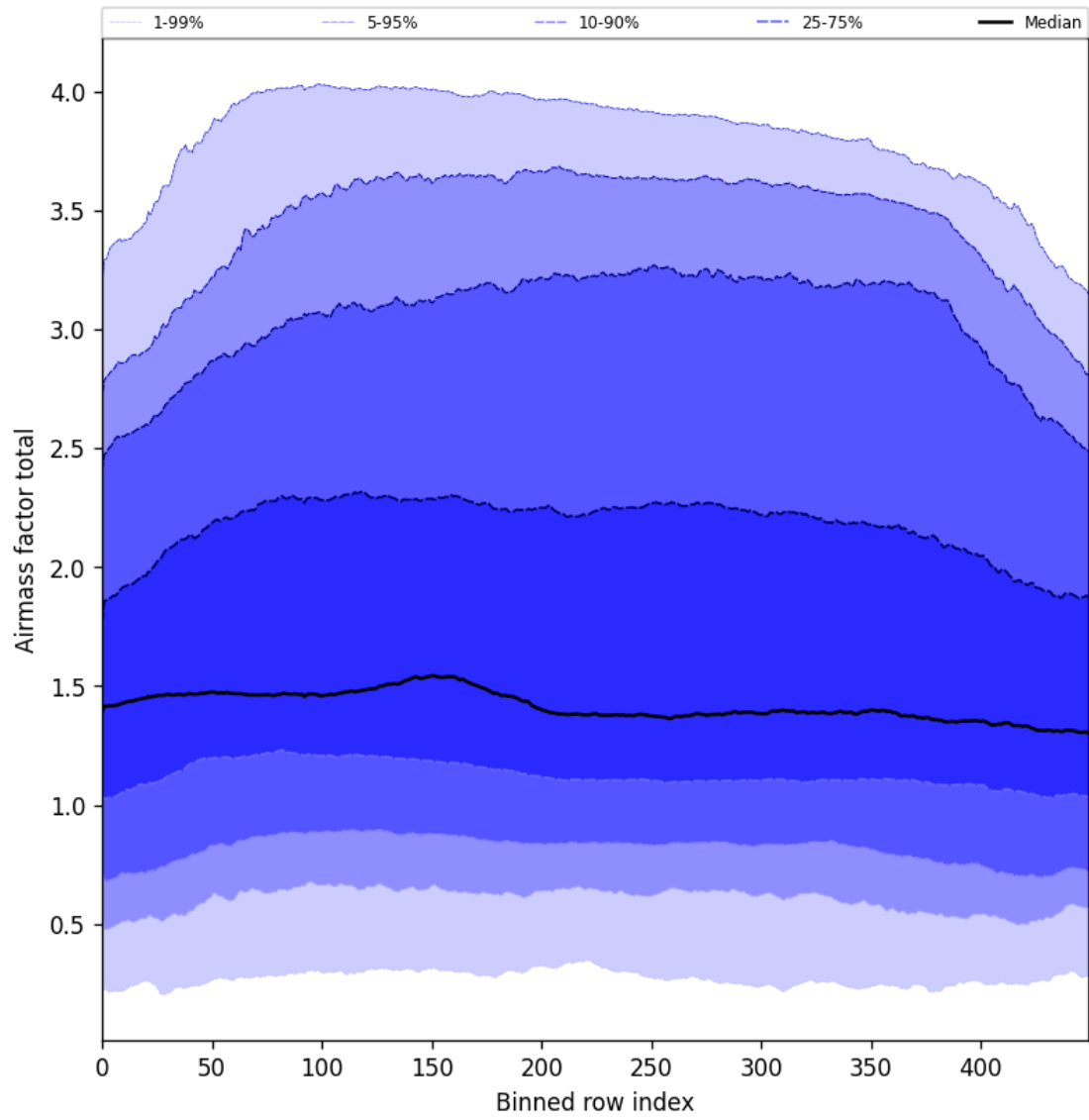
Figure 54: Along track statistics of “Airmass factor total” for 2025-04-30 to 2025-05-02
