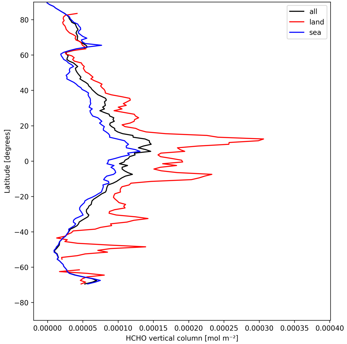
Figure 21: Zonal average of “HCHO vertical column” for 2025-04-30 to 2025-05-02.
