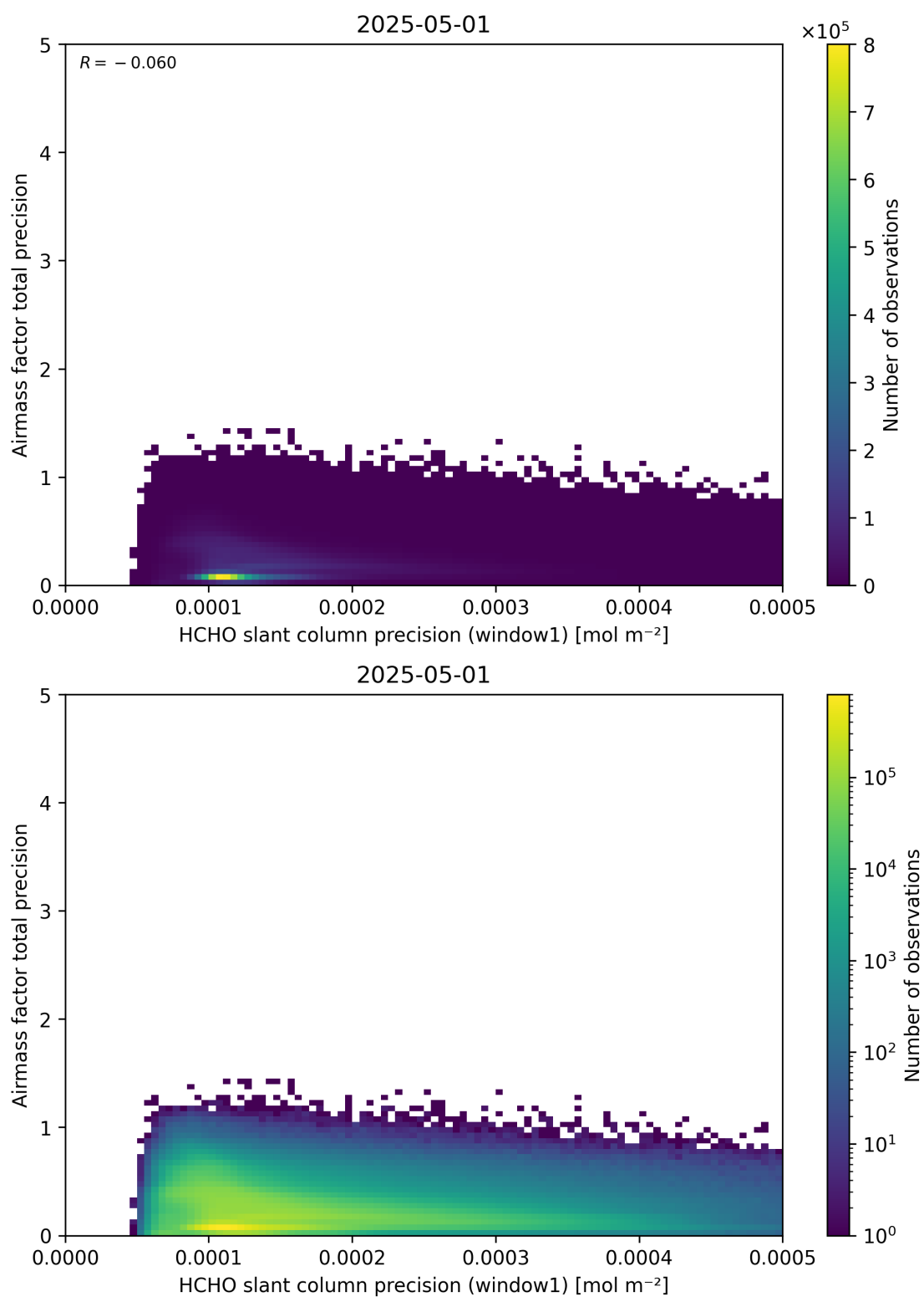
Figure 95: Scatter density plot of “HCHO slant column precision (window1)” against “Airmass factor total precision” for 2025-04-30 to 2025-05-02.
