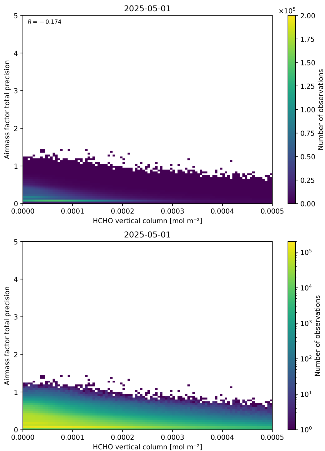
Figure 132: Scatter density plot of “HCHO vertical column” against “Airmass factor total precision” for 2025-04-30 to 2025-05-02.
