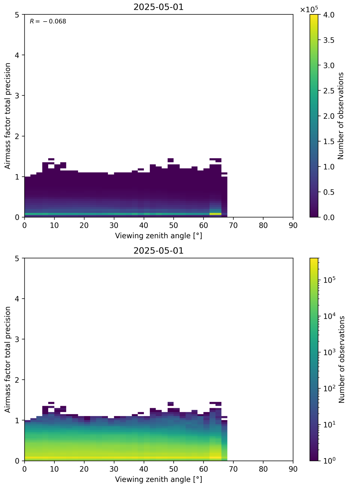
Figure 191: Scatter density plot of “Viewing zenith angle” against “Airmass factor total precision” for 2025-04-30 to 2025-05-02.
