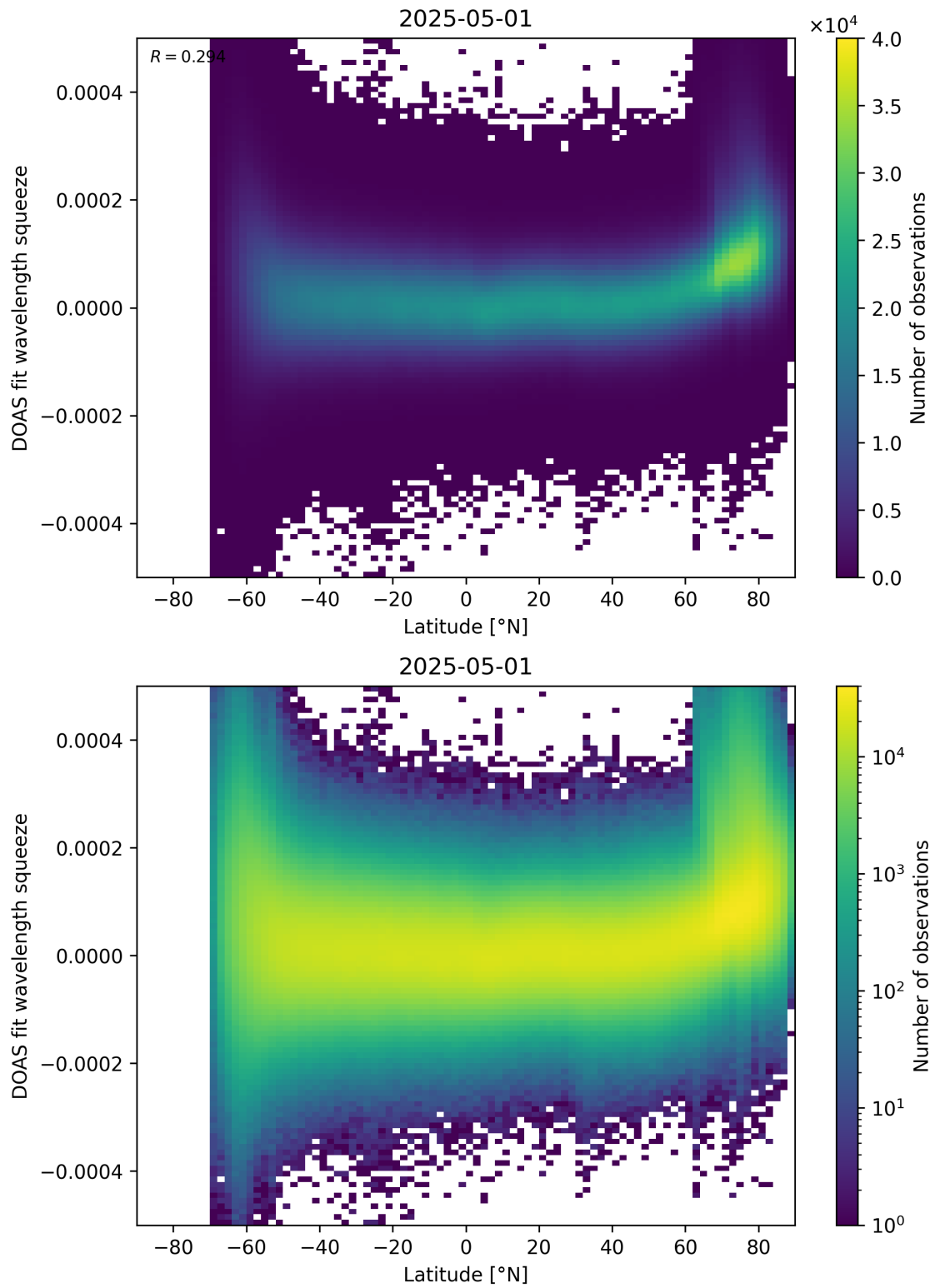
Figure 155: Scatter density plot of “Latitude” against “DOAS fit wavelength squeeze” for 2025-04-30 to 2025-05-02.
