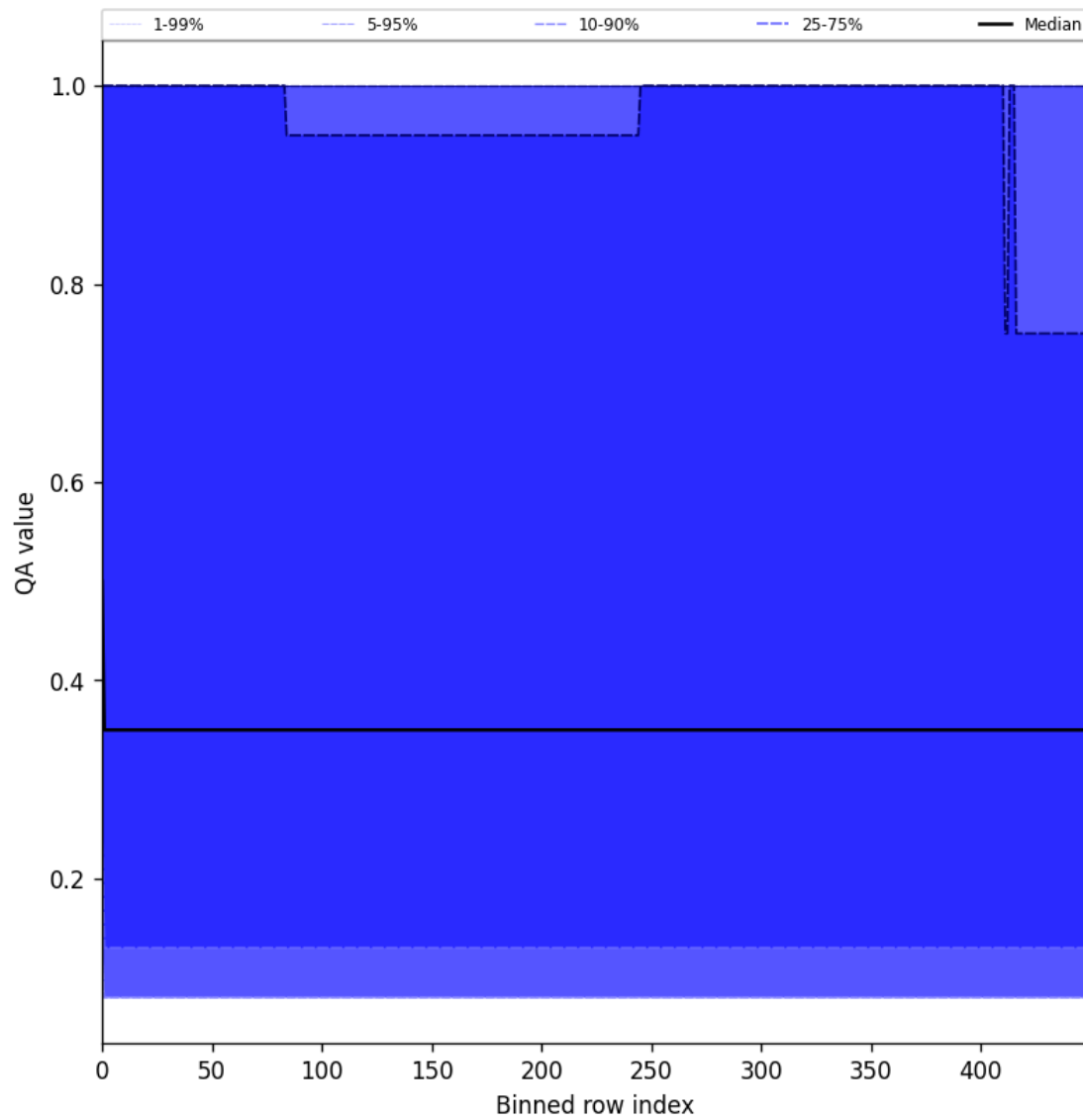
Figure 48: Along track statistics of “QA value” for 2025-04-30 to 2025-05-02
