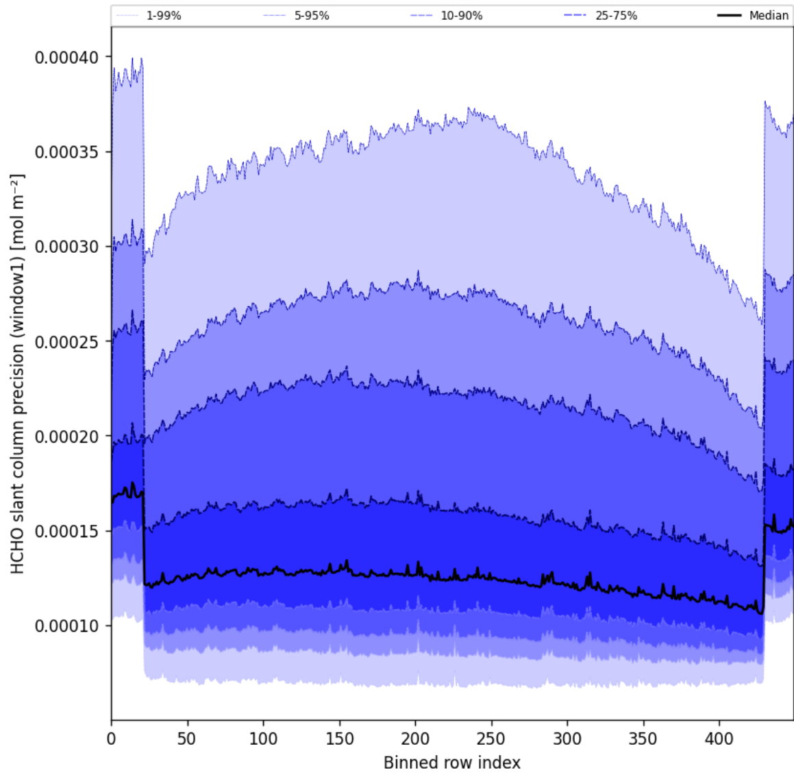
Figure 53: Along track statistics of “HCHO slant column precision (window1)” for 2025-04-30 to 2025-05-02
