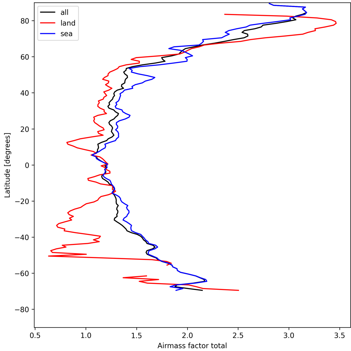
Figure 26: Zonal average of “Airmass factor total” for 2025-04-30 to 2025-05-02.
