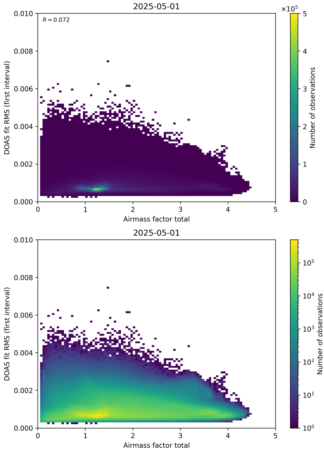
Figure 97: Scatter density plot of “Airmass factor total” against “DOAS fit RMS (first interval)” for 2025-04-30 to 2025-05-02.
