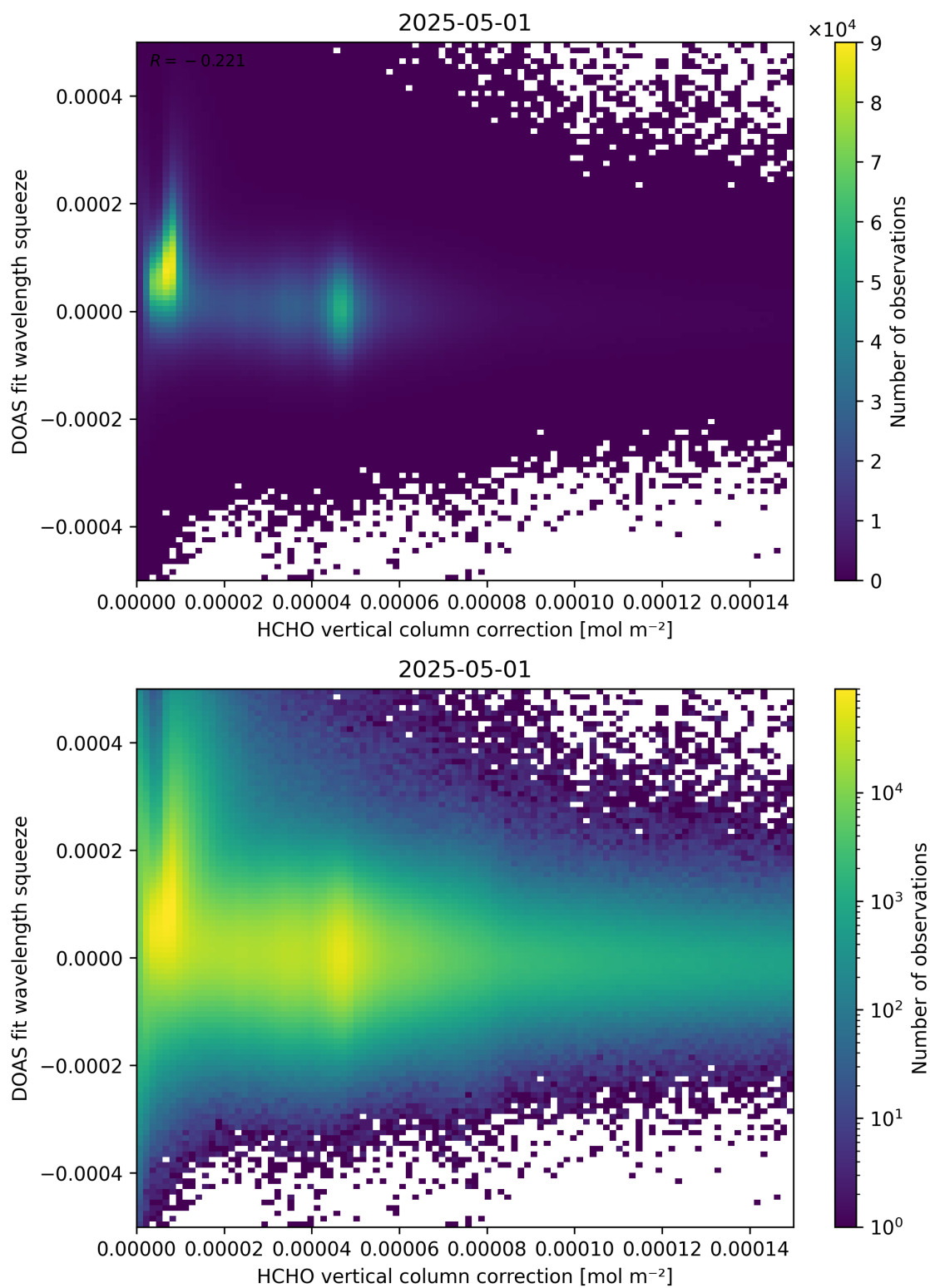
Figure 114: Scatter density plot of “HCHO vertical column correction” against “DOAS fit wavelength squeeze” for 2025-04-30 to 2025-05-02.
