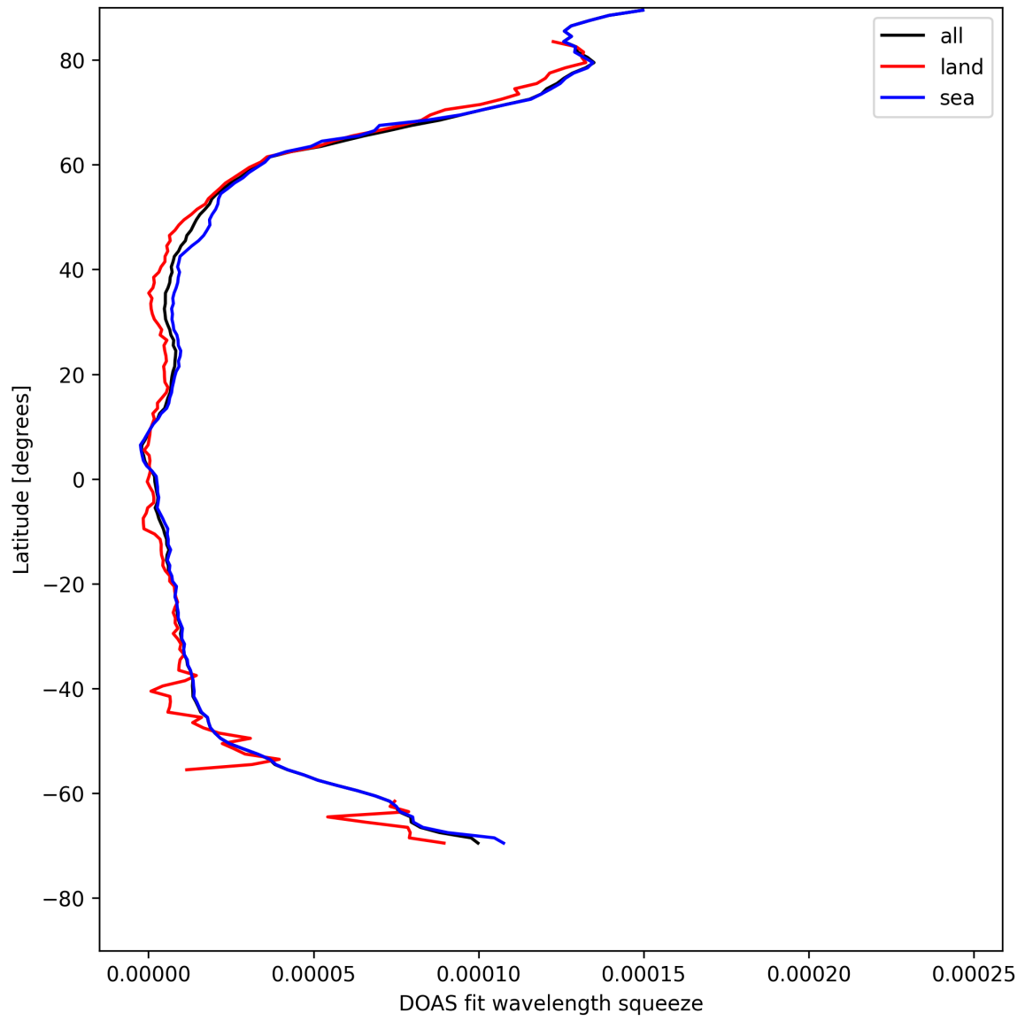
Figure 31: Zonal average of “DOAS fit wavelength squeeze” for 2025-04-30 to 2025-05-02.
