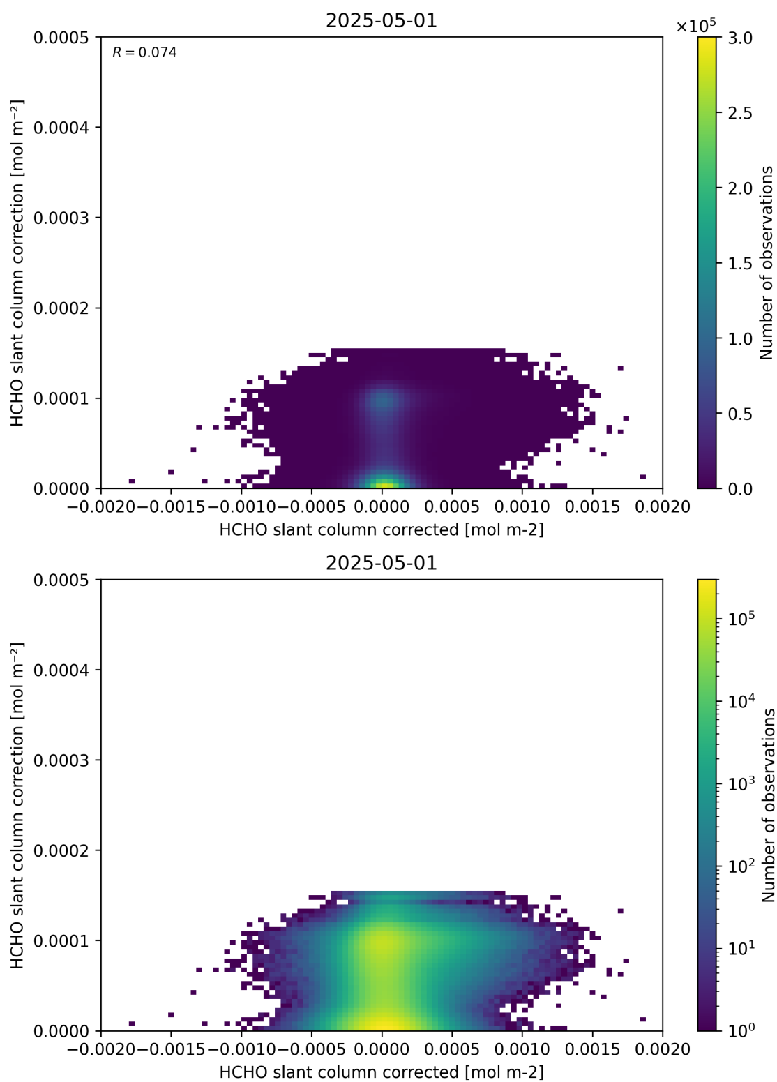
Figure 77: Scatter density plot of “HCHO slant column corrected” against “HCHO slant column correction” for 2025-04-30 to 2025-05-02.
