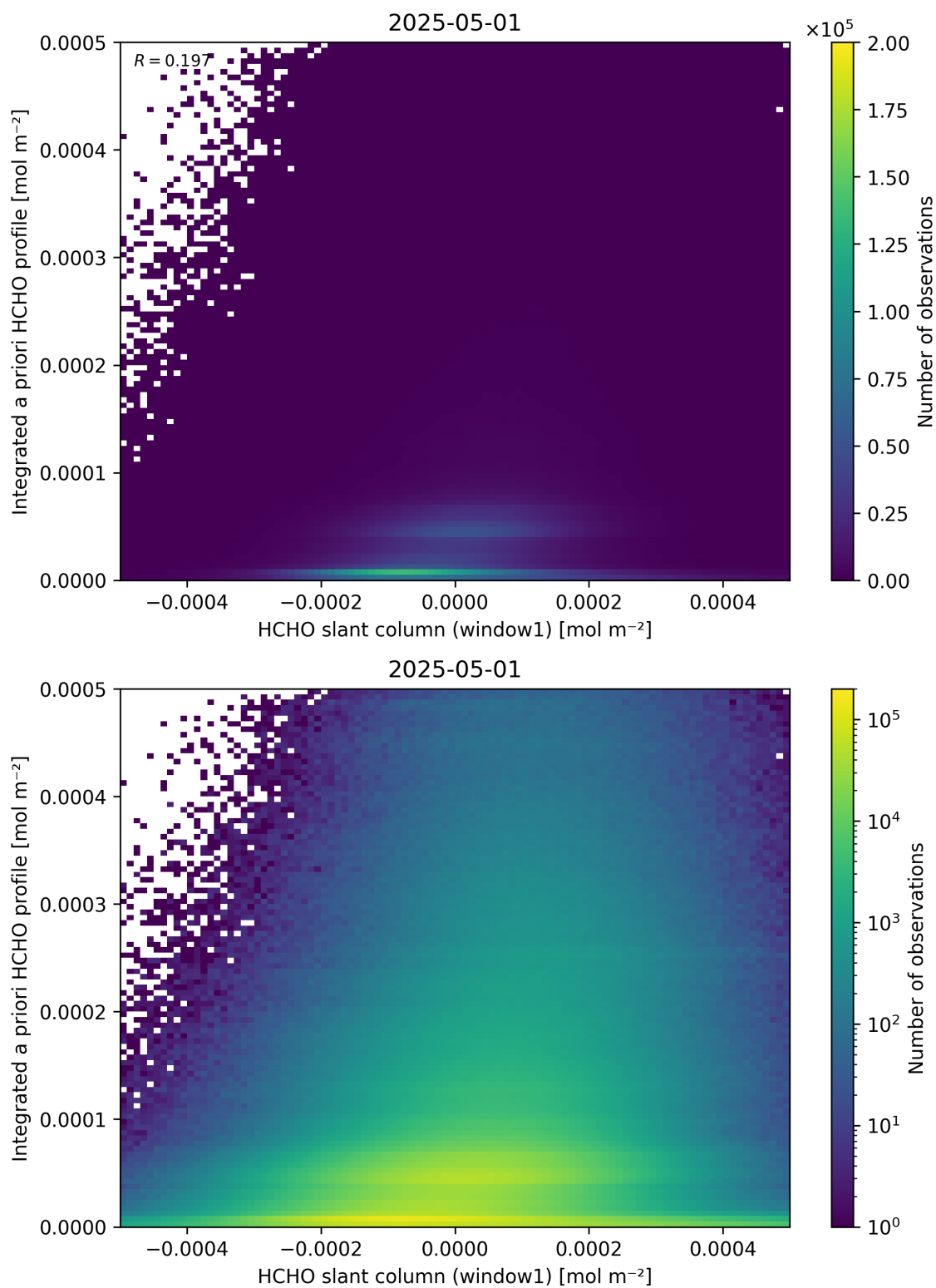
Figure 87: Scatter density plot of “HCHO slant column (window1)” against “Integrated a priori HCHO profile” for 2025-04-30 to 2025-05-02.
