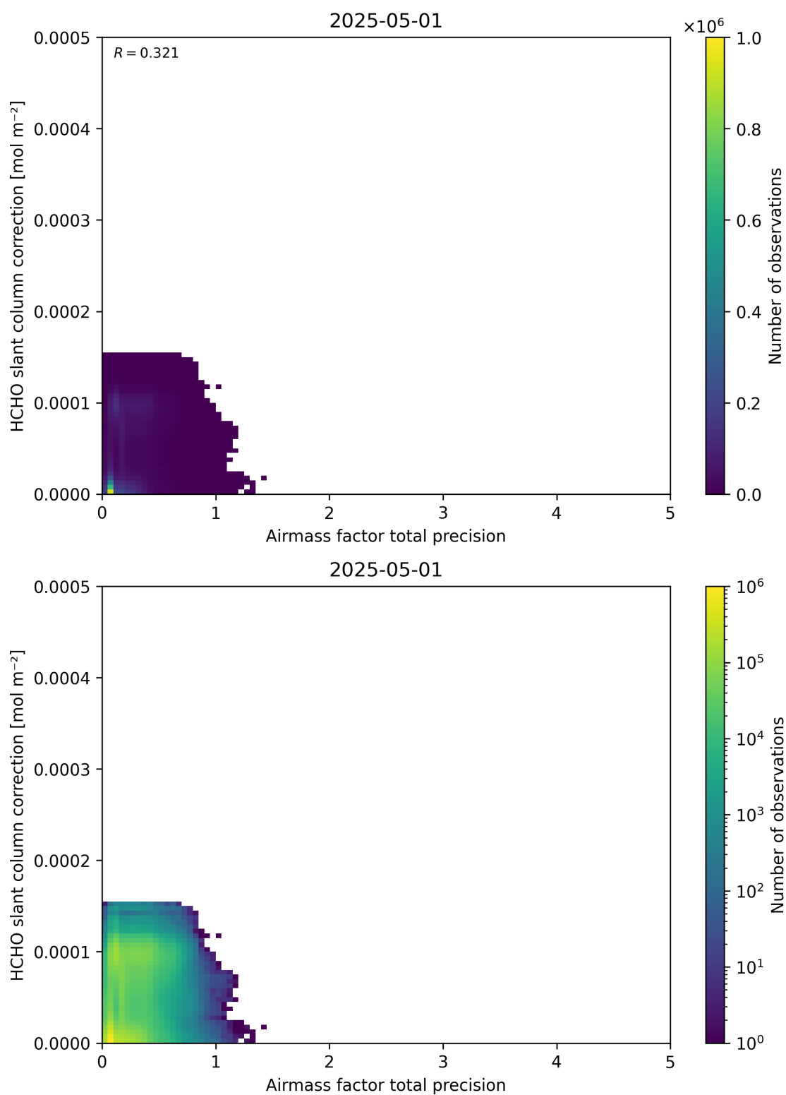
Figure 110: Scatter density plot of “Airmass factor total precision” against “HCHO slant column correction” for 2025-04-30 to 2025-05-02.
