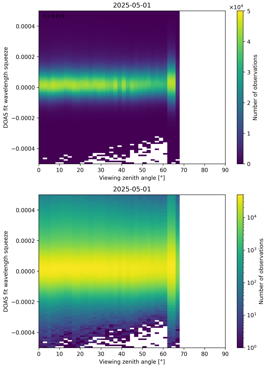
Figure 184: Scatter density plot of “Viewing zenith angle” against “DOAS fit wavelength squeeze” for 2025-04-30 to 2025-05-02.
