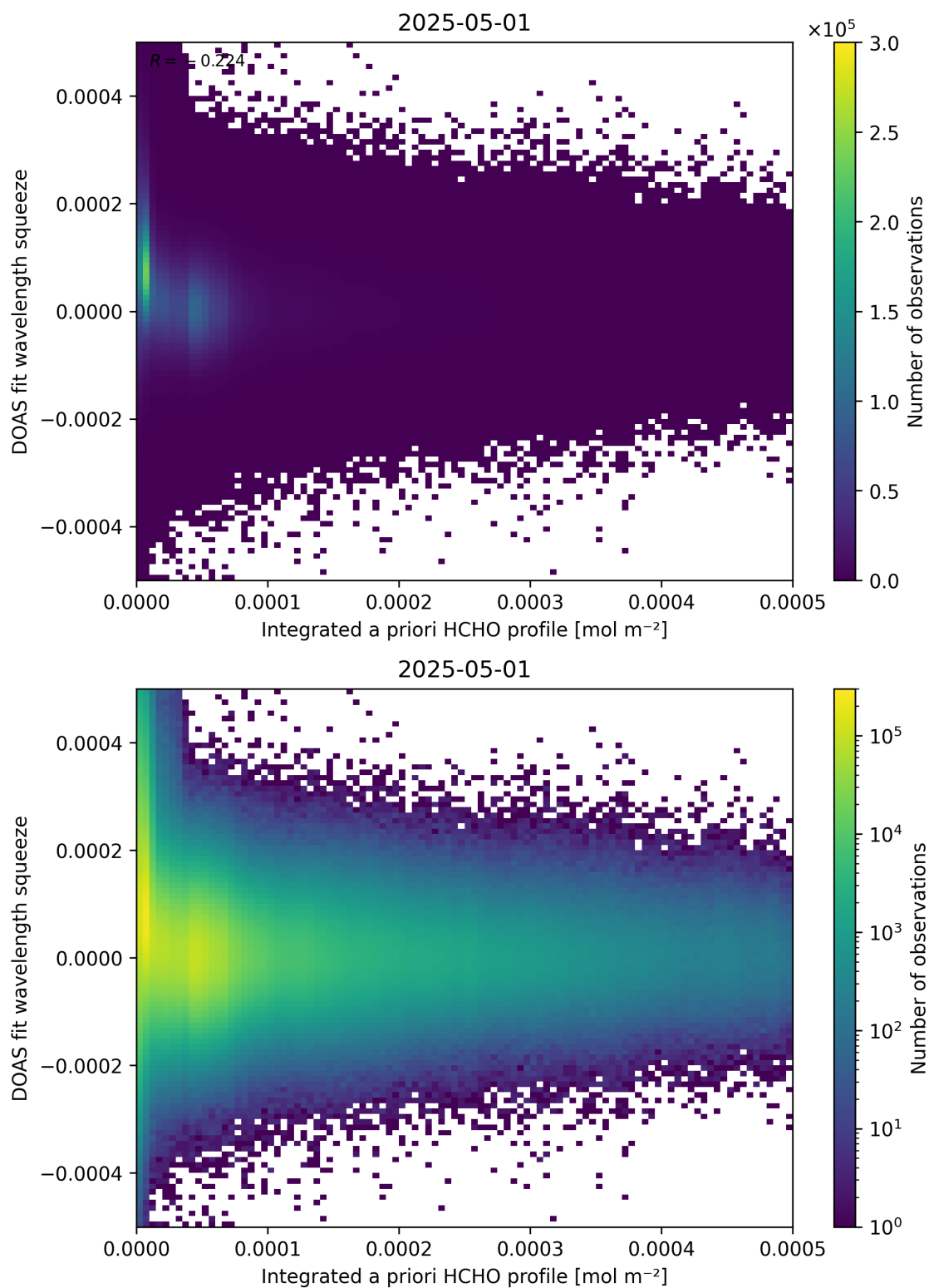
Figure 150: Scatter density plot of “Integrated a priori HCHO profile” against “DOAS fit wavelength squeeze” for 2025-04-30 to 2025-05-02.
