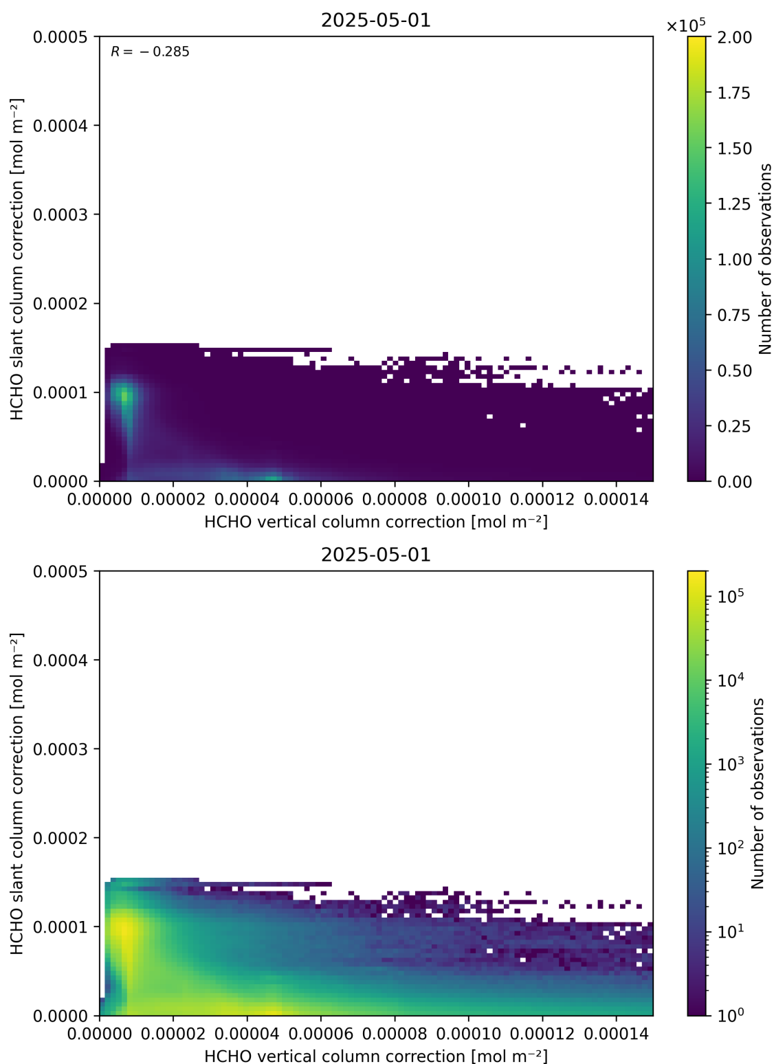
Figure 117: Scatter density plot of “HCHO vertical column correction” against “HCHO slant column correction” for 2025-04-30 to 2025-05-02.
