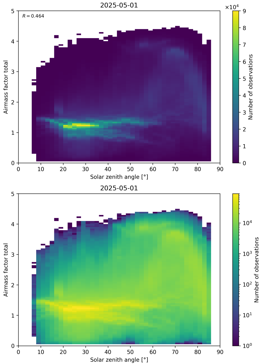
Figure 175: Scatter density plot of “Solar zenith angle” against “Airmass factor total” for 2025-04-30 to 2025-05-02.
