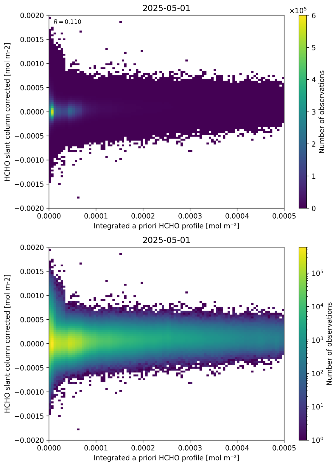
Figure 151: Scatter density plot of “Integrated a priori HCHO profile” against “HCHO slant column corrected” for 2025-04-30 to 2025-05-02.
