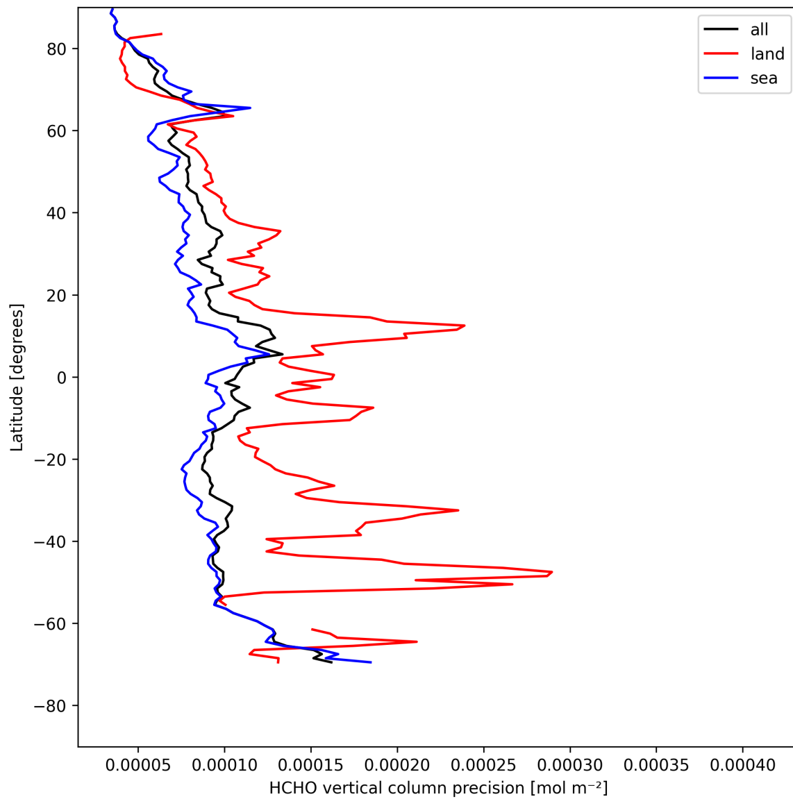
Figure 22: Zonal average of “HCHO vertical column precision” for 2025-04-30 to 2025-05-02.
