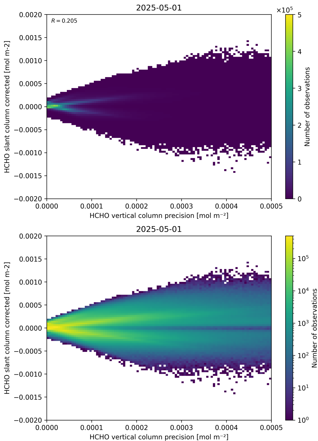
Figure 140: Scatter density plot of “HCHO vertical column precision” against “HCHO slant column corrected” for 2025-04-30 to 2025-05-02.
