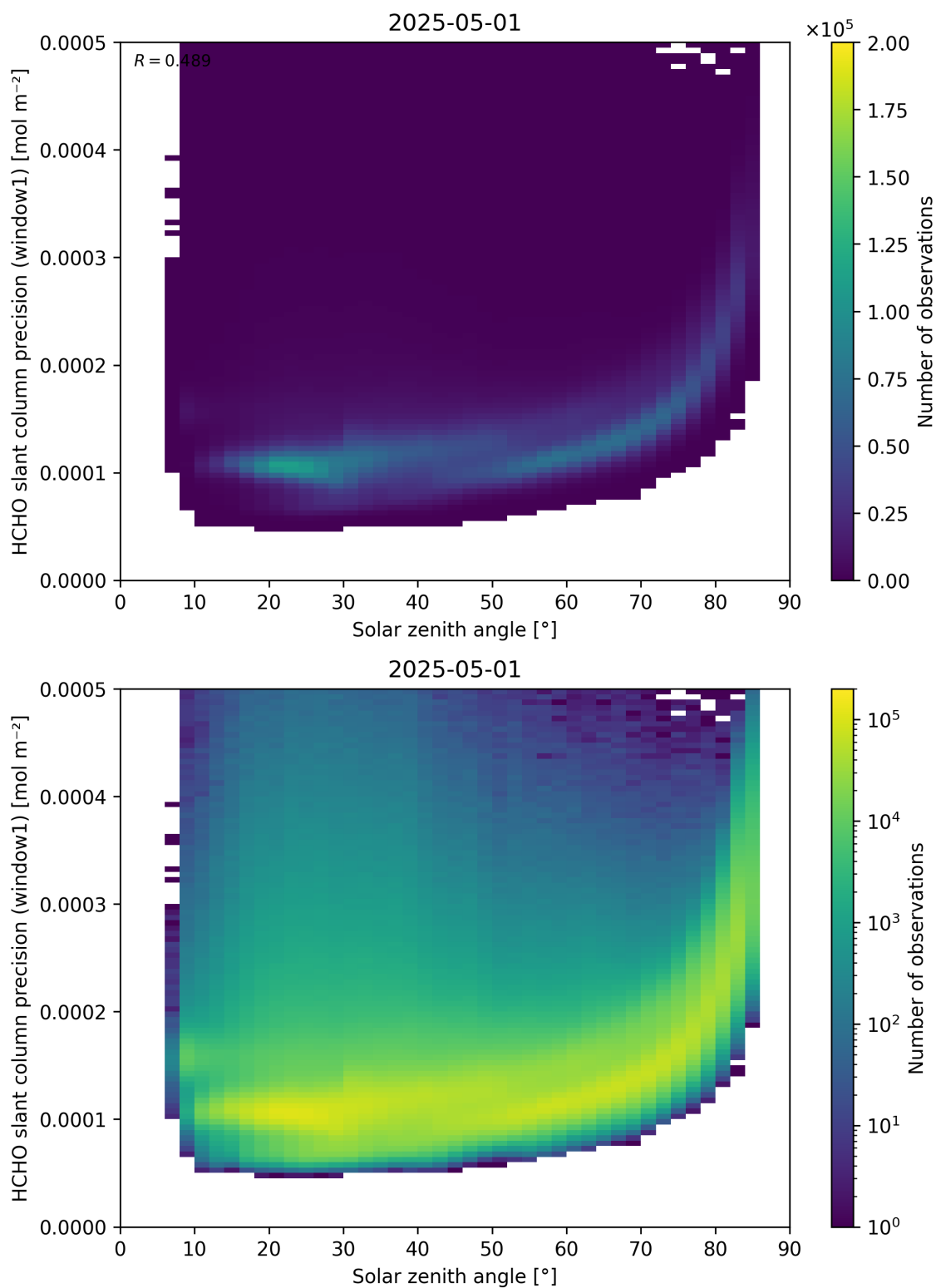
Figure 174: Scatter density plot of “Solar zenith angle” against “HCHO slant column precision (window1)” for 2025-04-30 to 2025-05-02.
