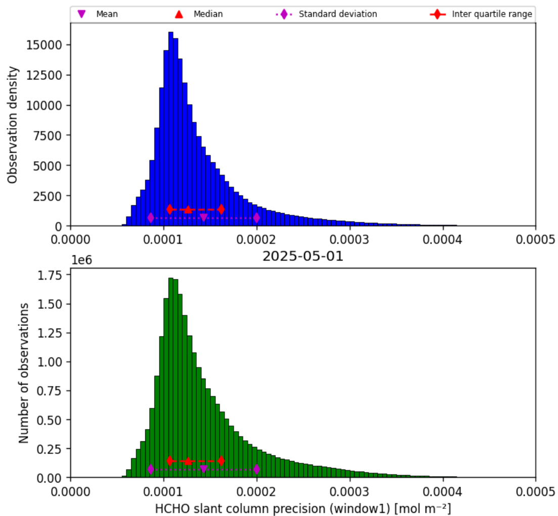
Figure 39: Histogram of “HCHO slant column precision (window1)” for 2025-04-30 to 2025-05-02
