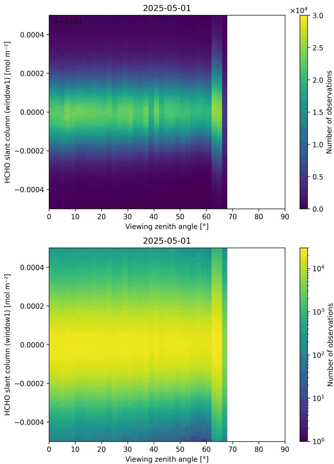
Figure 188: Scatter density plot of “Viewing zenith angle” against “HCHO slant column (window1)” for 2025-04-30 to 2025-05-02.
