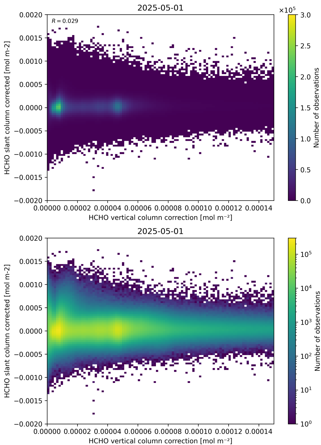
Figure 116: Scatter density plot of “HCHO vertical column correction” against “HCHO slant column corrected” for 2025-04-30 to 2025-05-02.
