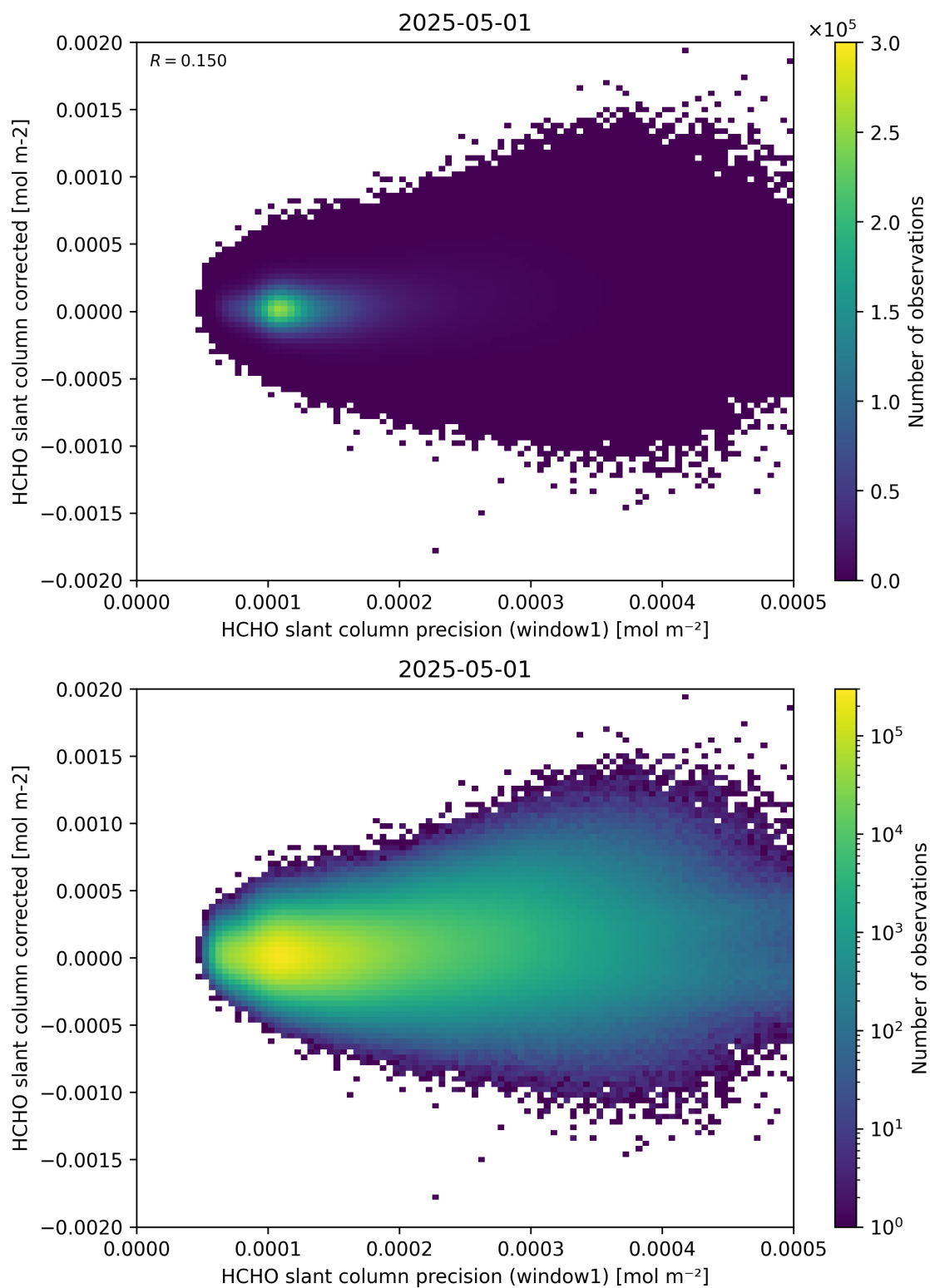
Figure 92: Scatter density plot of “HCHO slant column precision (window1)” against “HCHO slant column corrected” for 2025-04-30 to 2025-05-02.
