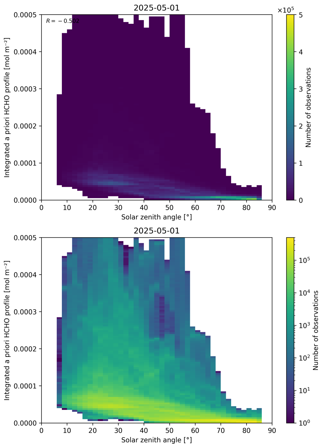
Figure 180: Scatter density plot of “Solar zenith angle” against “Integrated a priori HCHO profile” for 2025-04-30 to 2025-05-02.
