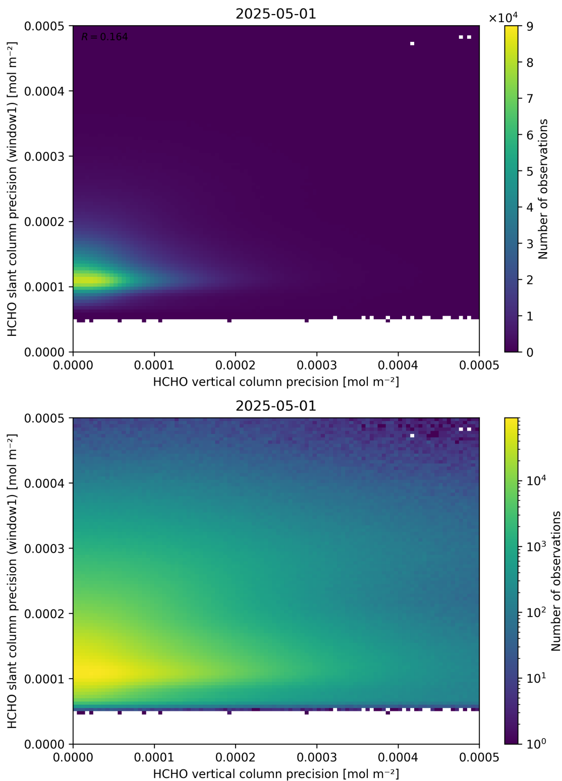
Figure 143: Scatter density plot of “HCHO vertical column precision” against “HCHO slant column precision (window1)” for 2025-04-30 to 2025-05-02.
