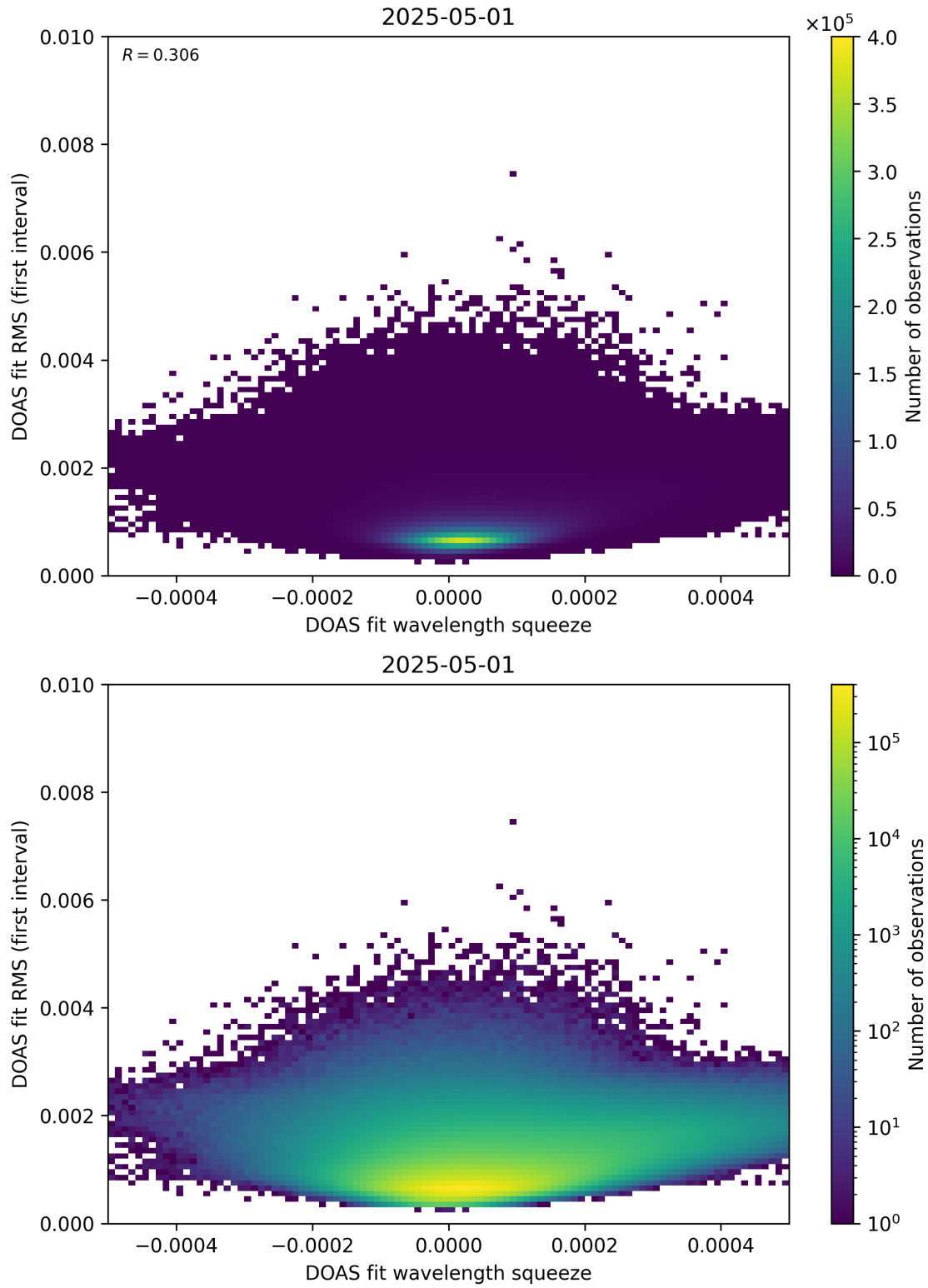
Figure 68: Scatter density plot of “DOAS fit wavelength squeeze” against “DOAS fit RMS (first interval)” for 2025-04-30 to 2025-05-02.
