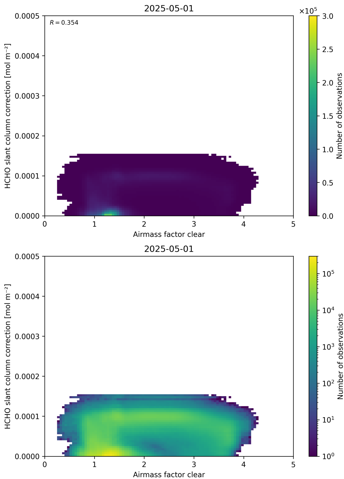
Figure 75: Scatter density plot of “Airmass factor clear” against “HCHO slant column correction” for 2025-04-30 to 2025-05-02.
