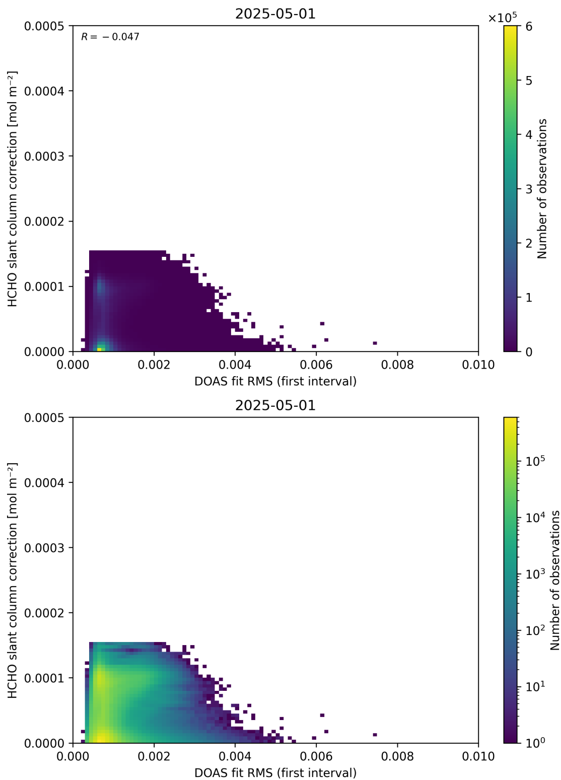
Figure 63: Scatter density plot of “DOAS fit RMS (first interval)” against “HCHO slant column correction” for 2025-04-30 to 2025-05-02.
