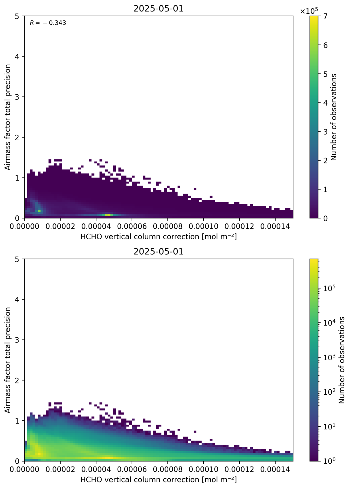
Figure 121: Scatter density plot of “HCHO vertical column correction” against “Airmass factor total precision” for 2025-04-30 to 2025-05-02.
