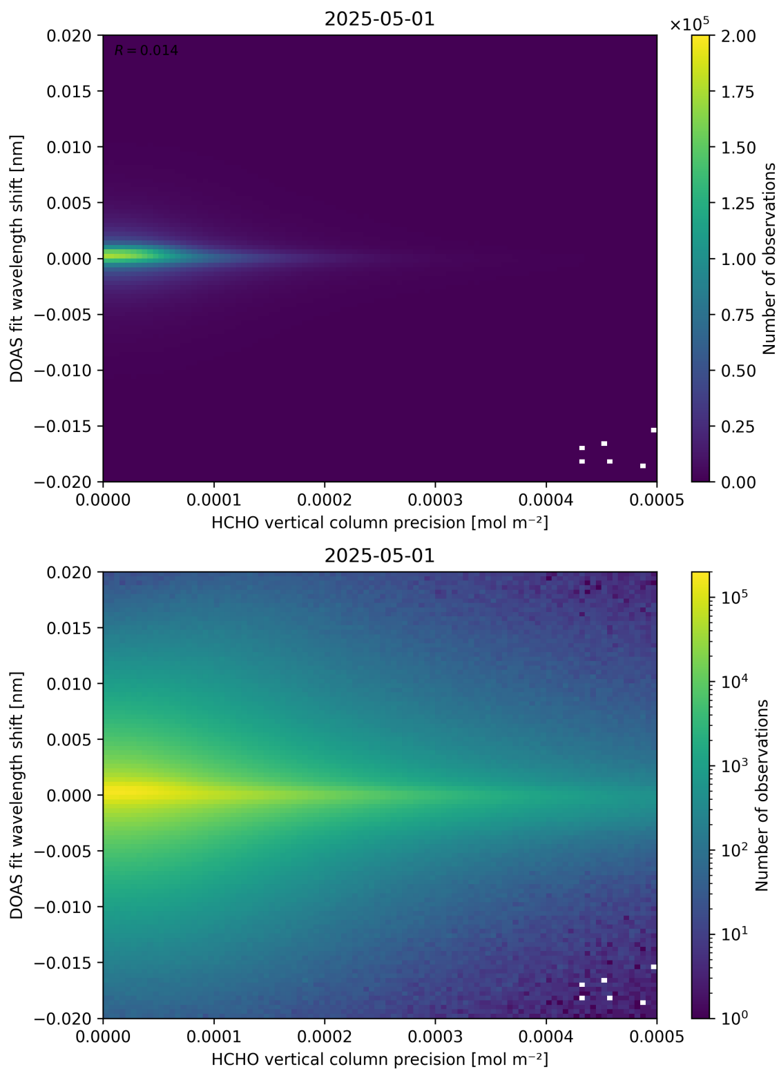
Figure 137: Scatter density plot of “HCHO vertical column precision” against “DOAS fit wavelength shift” for 2025-04-30 to 2025-05-02.
