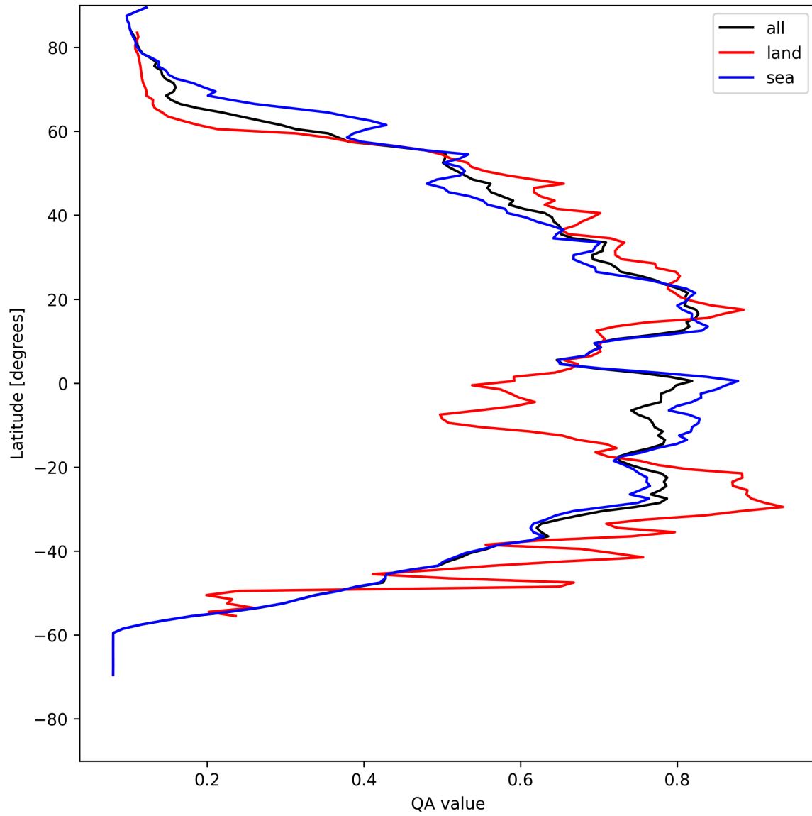
Figure 20: Zonal average of “QA value” for 2025-04-30 to 2025-05-02.
