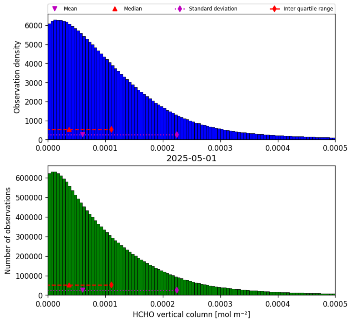
Figure 35: Histogram of “HCHO vertical column” for 2025-04-30 to 2025-05-02
