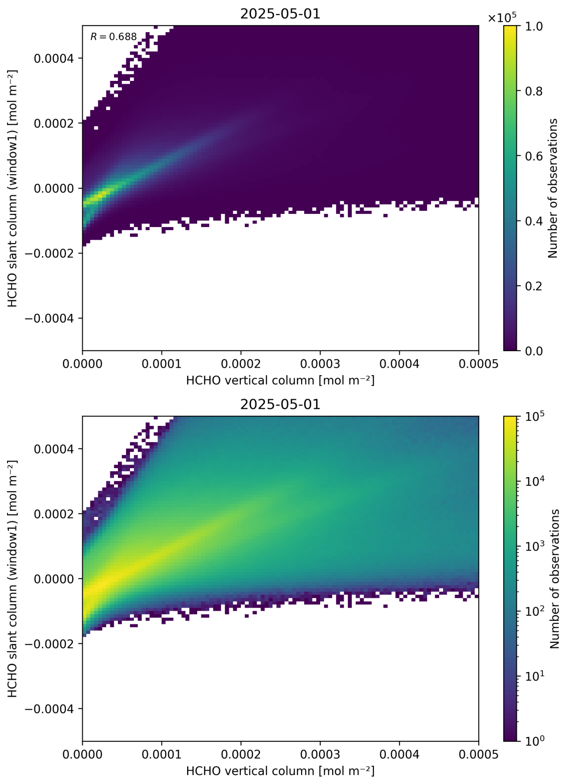
Figure 129: Scatter density plot of “HCHO vertical column” against “HCHO slant column (window1)” for 2025-04-30 to 2025-05-02.
