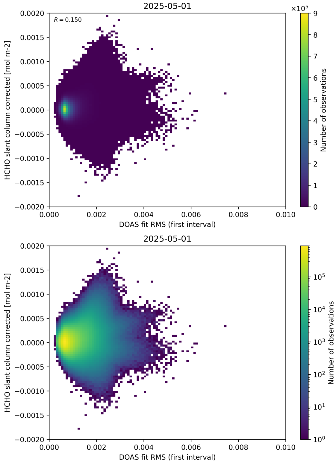
Figure 62: Scatter density plot of “DOAS fit RMS (first interval)” against “HCHO slant column corrected” for 2025-04-30 to 2025-05-02.
