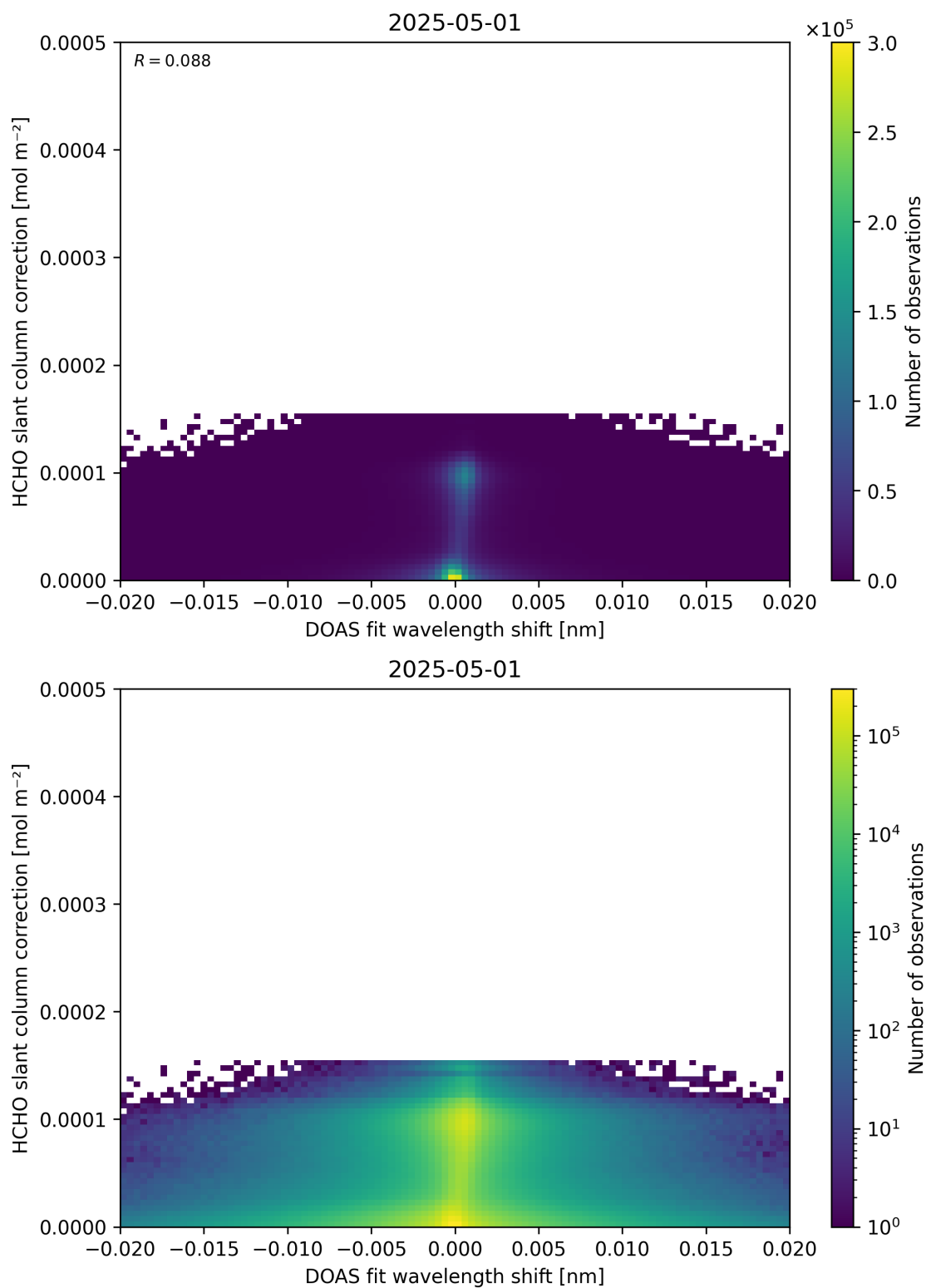
Figure 67: Scatter density plot of “DOAS fit wavelength shift” against “HCHO slant column correction” for 2025-04-30 to 2025-05-02.
