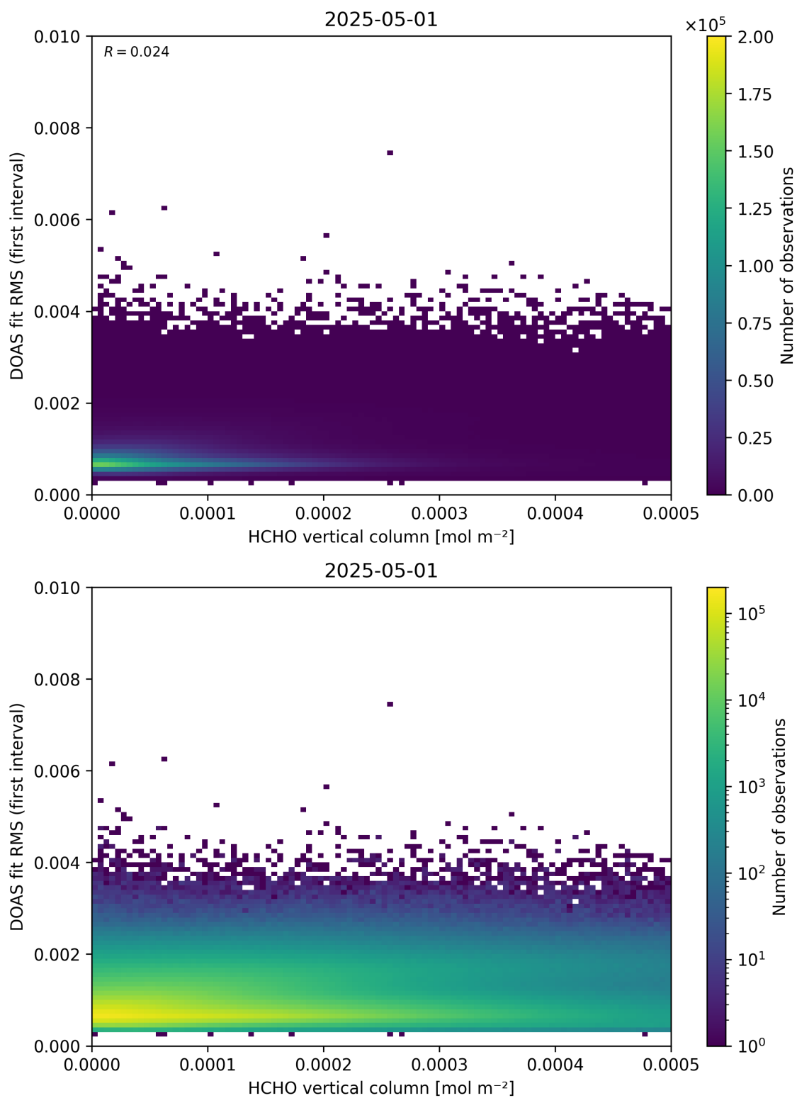
Figure 123: Scatter density plot of “HCHO vertical column” against “DOAS fit RMS (first interval)” for 2025-04-30 to 2025-05-02.
