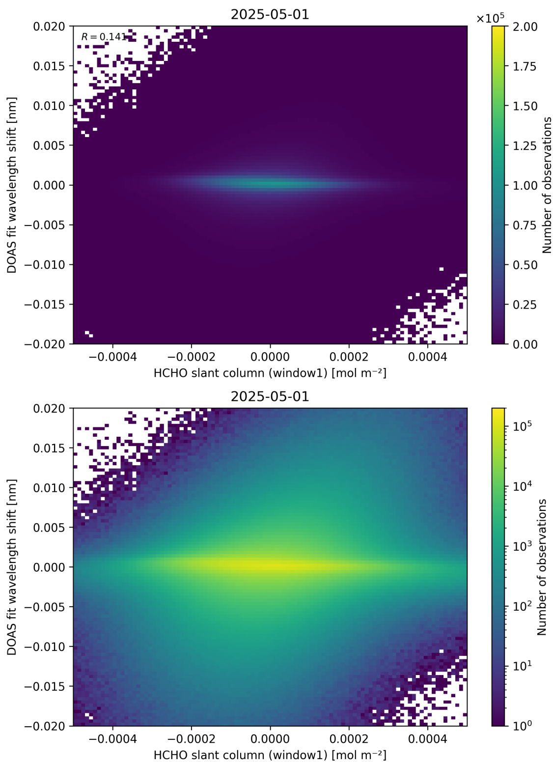
Figure 79: Scatter density plot of “HCHO slant column (window1)” against “DOAS fit wavelength shift” for 2025-04-30 to 2025-05-02.
