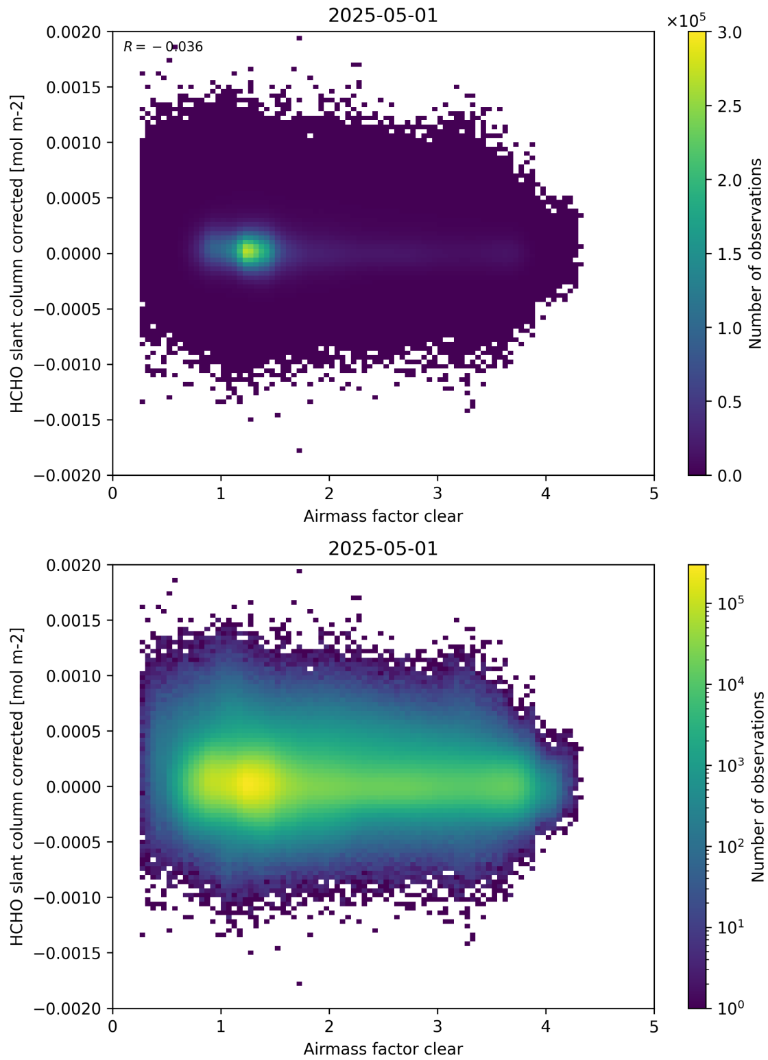
Figure 74: Scatter density plot of “Airmass factor clear” against “HCHO slant column corrected” for 2025-04-30 to 2025-05-02.
