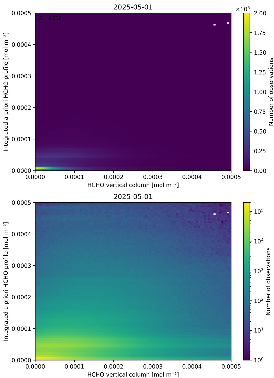
Figure 135: Scatter density plot of “HCHO vertical column” against “Integrated a priori HCHO profile” for 2025-04-30 to 2025-05-02.
