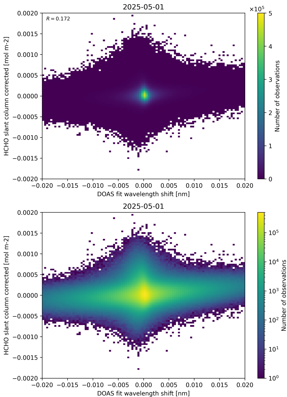
Figure 66: Scatter density plot of “DOAS fit wavelength shift” against “HCHO slant column corrected” for 2025-04-30 to 2025-05-02.
