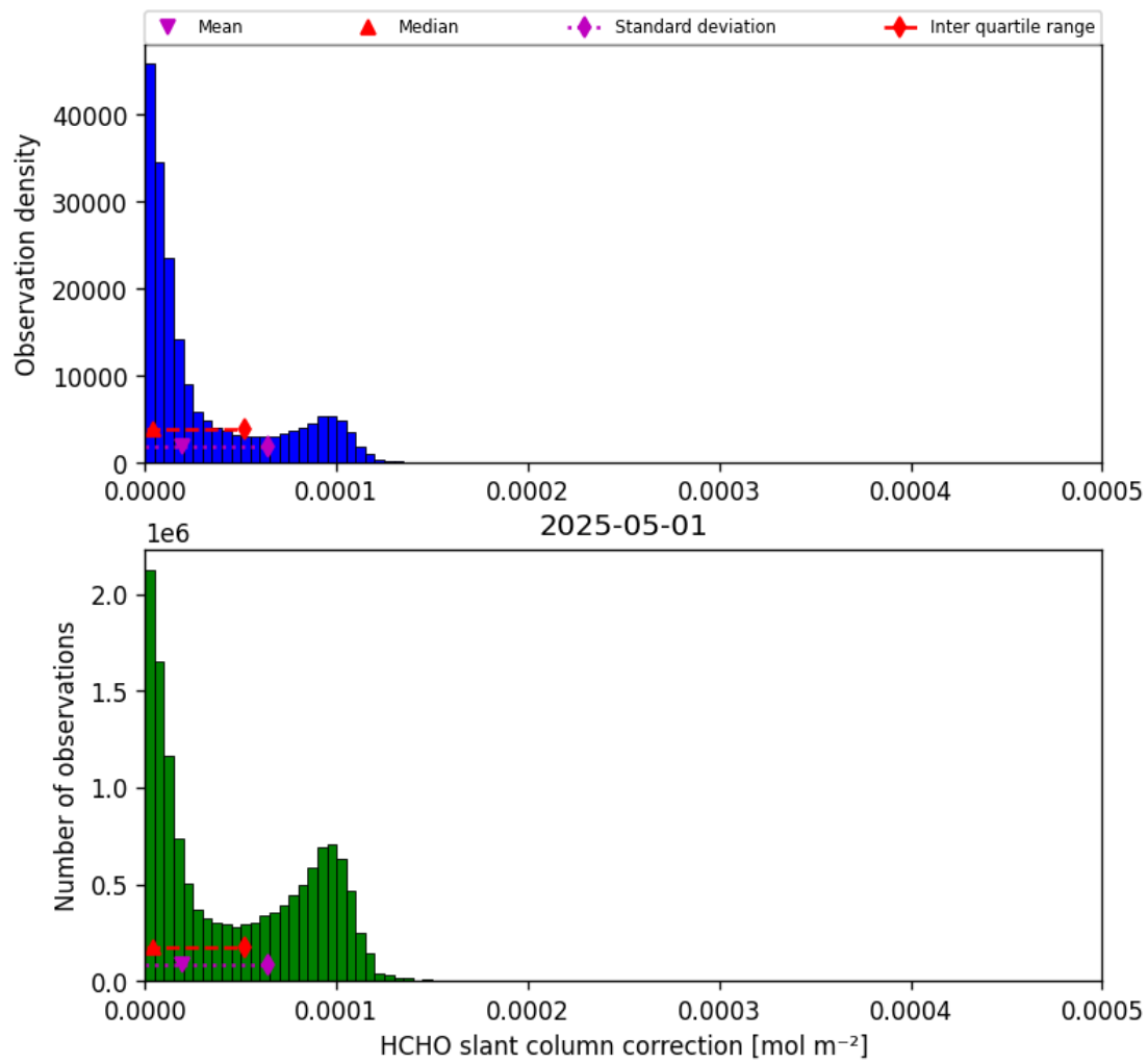
Figure 47: Histogram of “HCHO slant column correction” for 2025-04-30 to 2025-05-02
