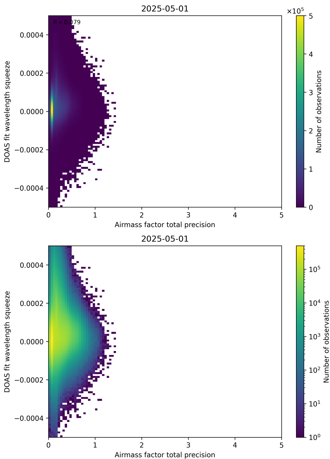
Figure 107: Scatter density plot of “Airmass factor total precision” against “DOAS fit wavelength squeeze” for 2025-04-30 to 2025-05-02.
