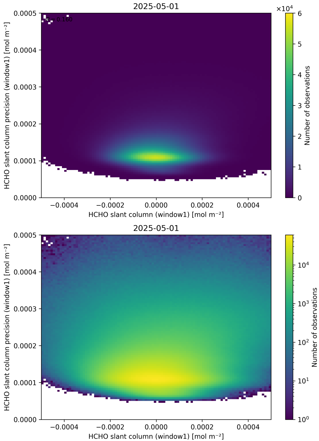
Figure 84: Scatter density plot of “HCHO slant column (window1)” against “HCHO slant column precision (window1)” for 2025-04-30 to 2025-05-02.
