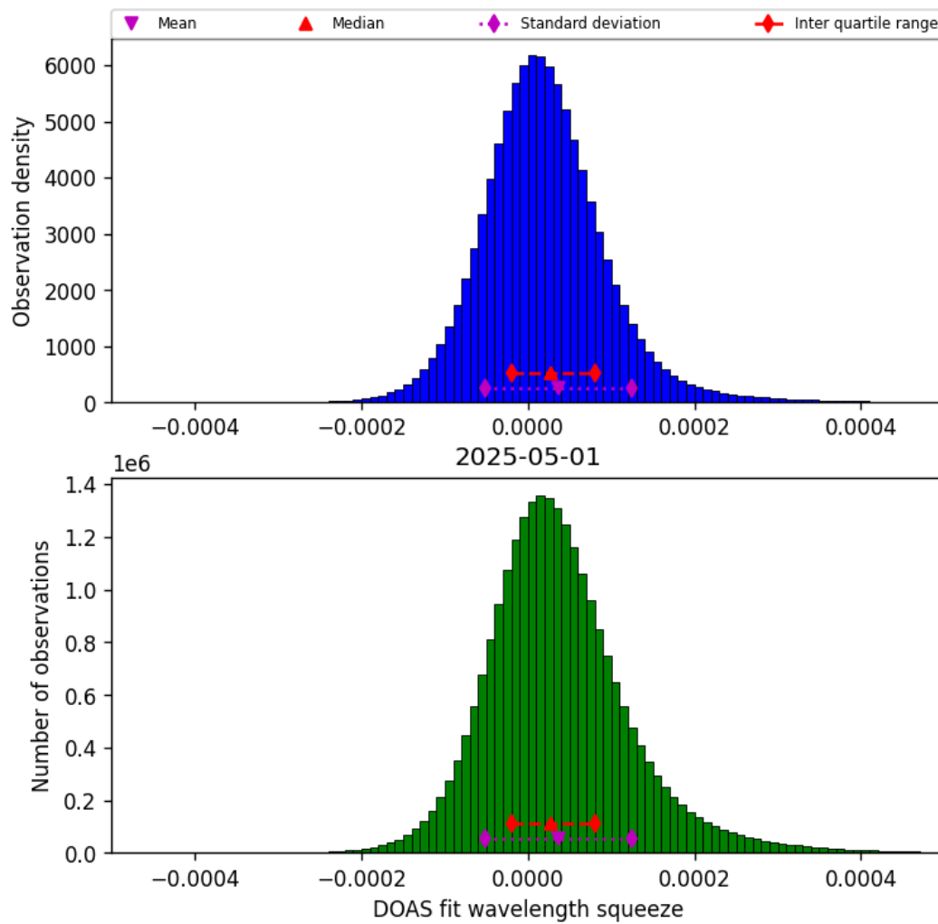
Figure 45: Histogram of “DOAS fit wavelength squeeze” for 2025-04-30 to 2025-05-02
