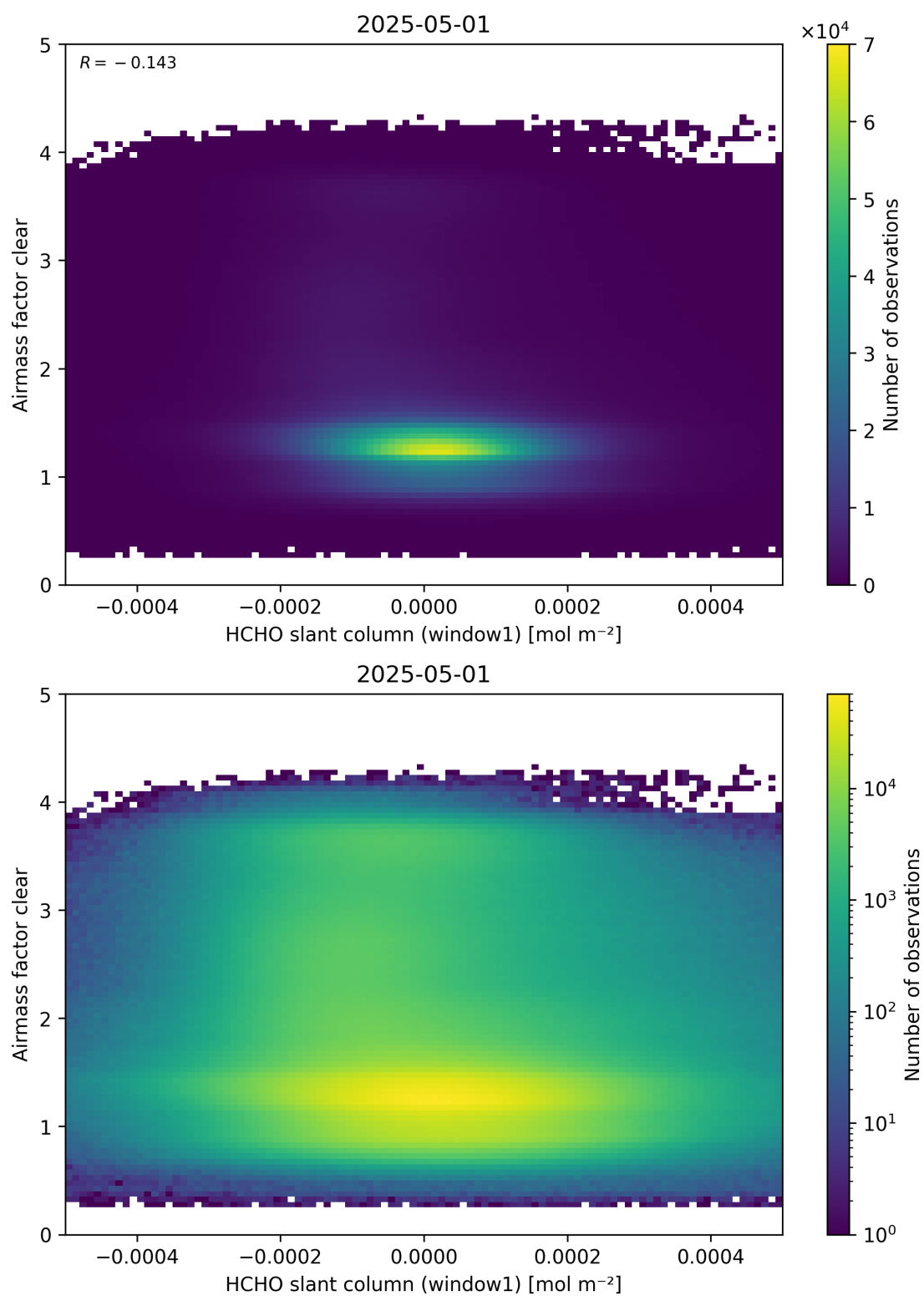
Figure 81: Scatter density plot of “HCHO slant column (window1)” against “Airmass factor clear” for 2025-04-30 to 2025-05-02.
