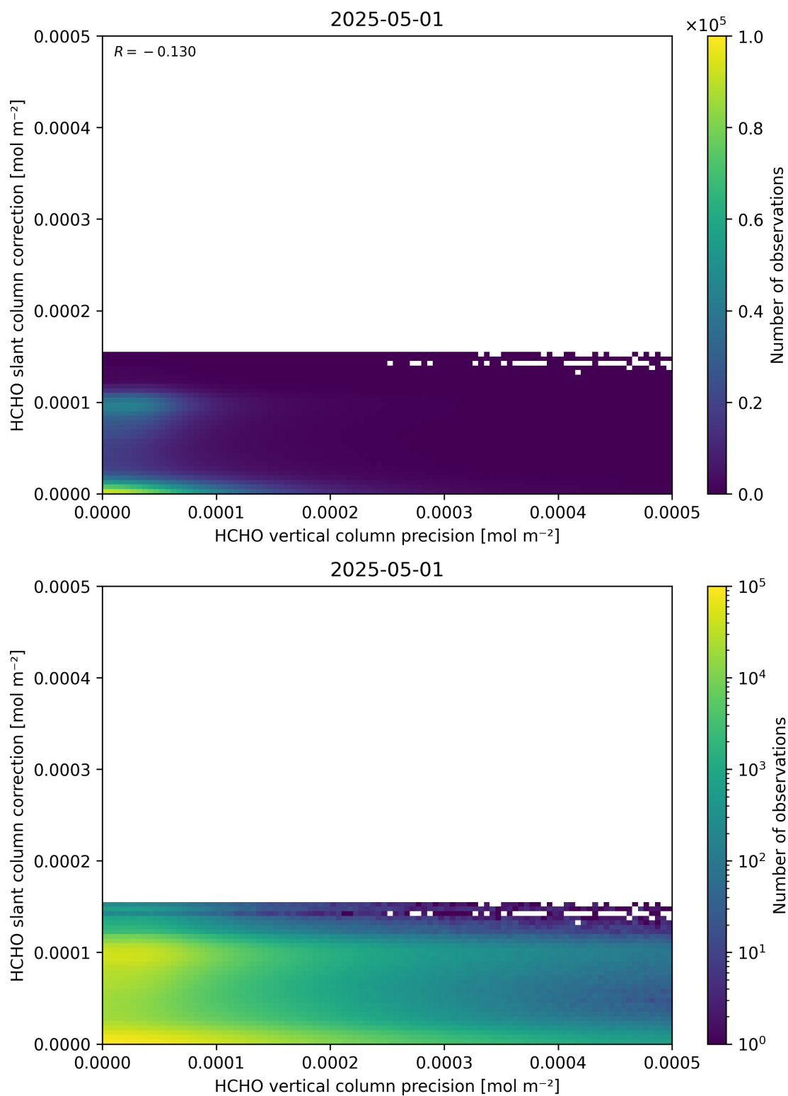
Figure 141: Scatter density plot of “HCHO vertical column precision” against “HCHO slant column correction” for 2025-04-30 to 2025-05-02.
