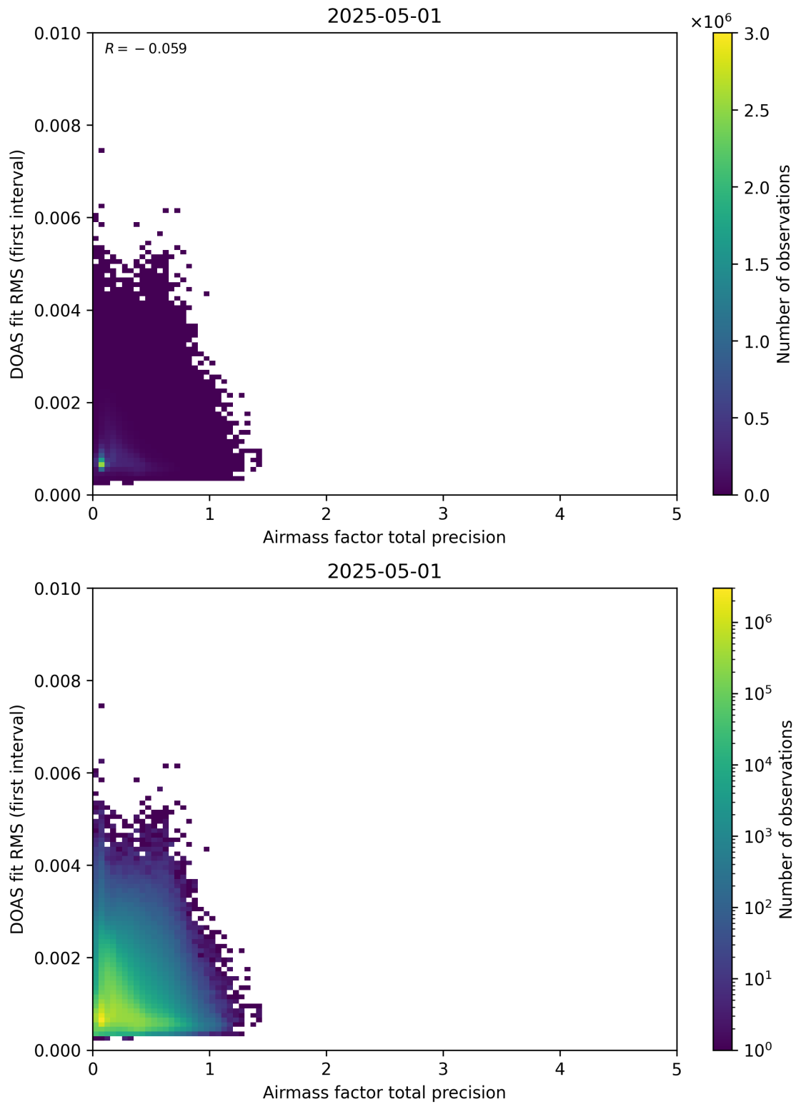
Figure 105: Scatter density plot of “Airmass factor total precision” against “DOAS fit RMS (first interval)” for 2025-04-30 to 2025-05-02.
