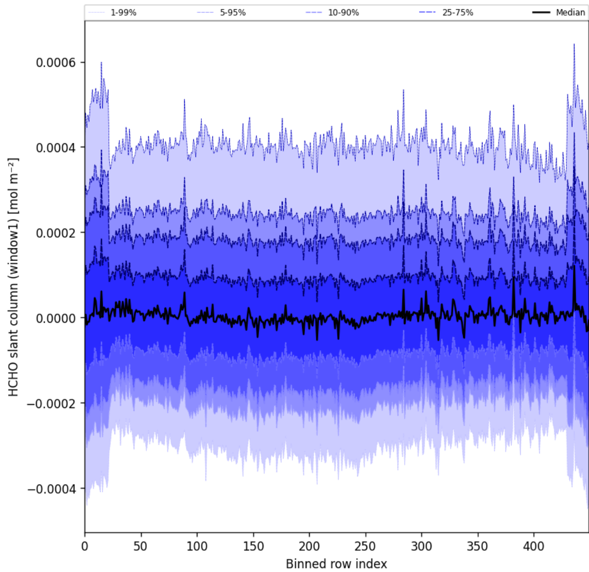
Figure 52: Along track statistics of “HCHO slant column (window1)” for 2025-04-30 to 2025-05-02
