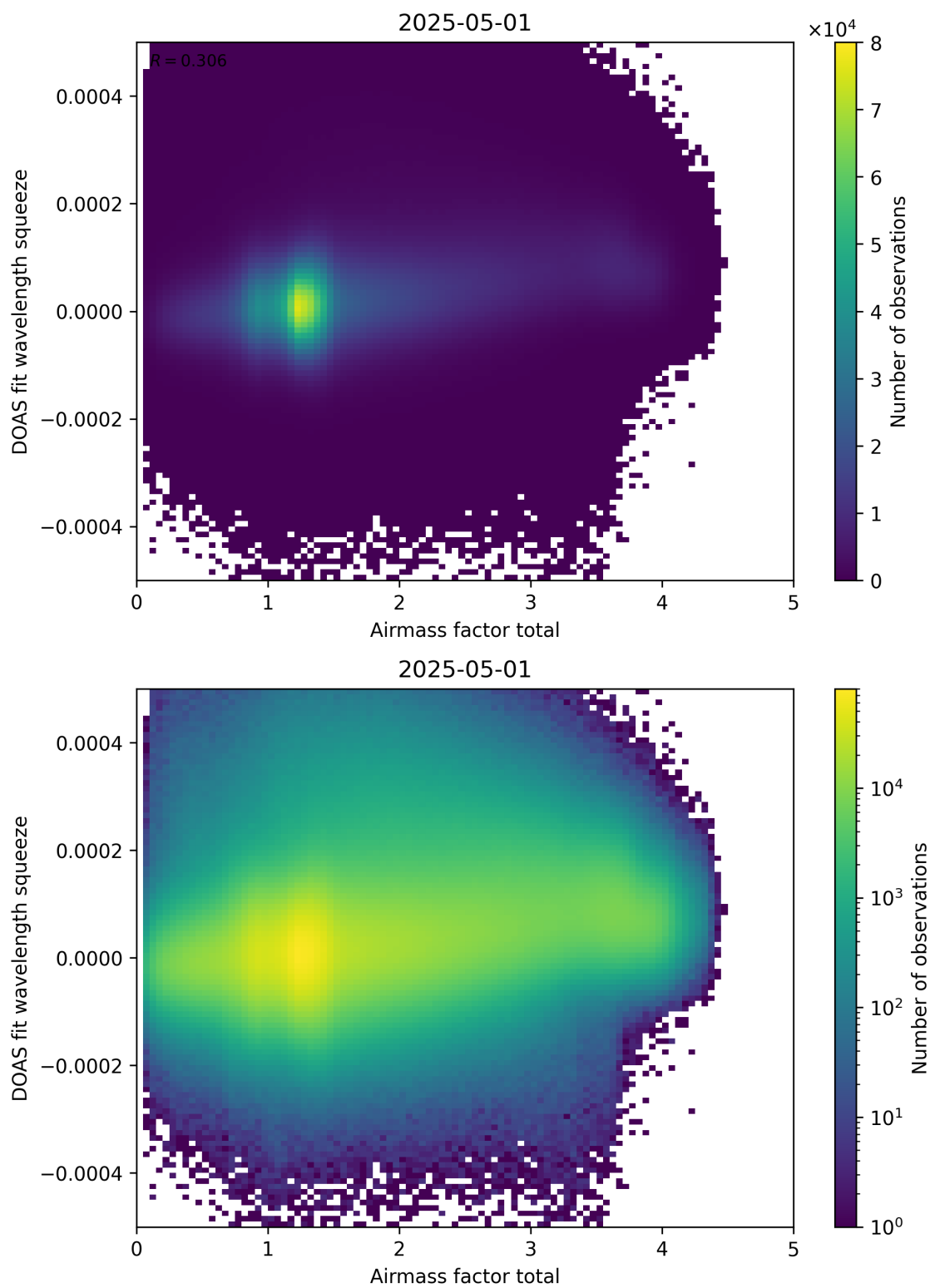
Figure 99: Scatter density plot of “Airmass factor total” against “DOAS fit wavelength squeeze” for 2025-04-30 to 2025-05-02.
