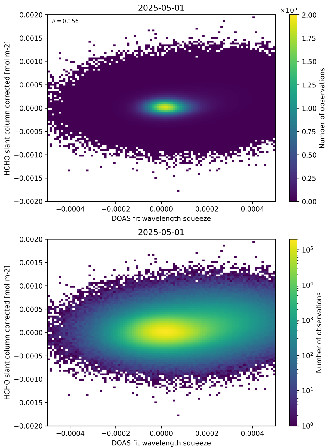
Figure 69: Scatter density plot of “DOAS fit wavelength squeeze” against “HCHO slant column corrected” for 2025-04-30 to 2025-05-02.
