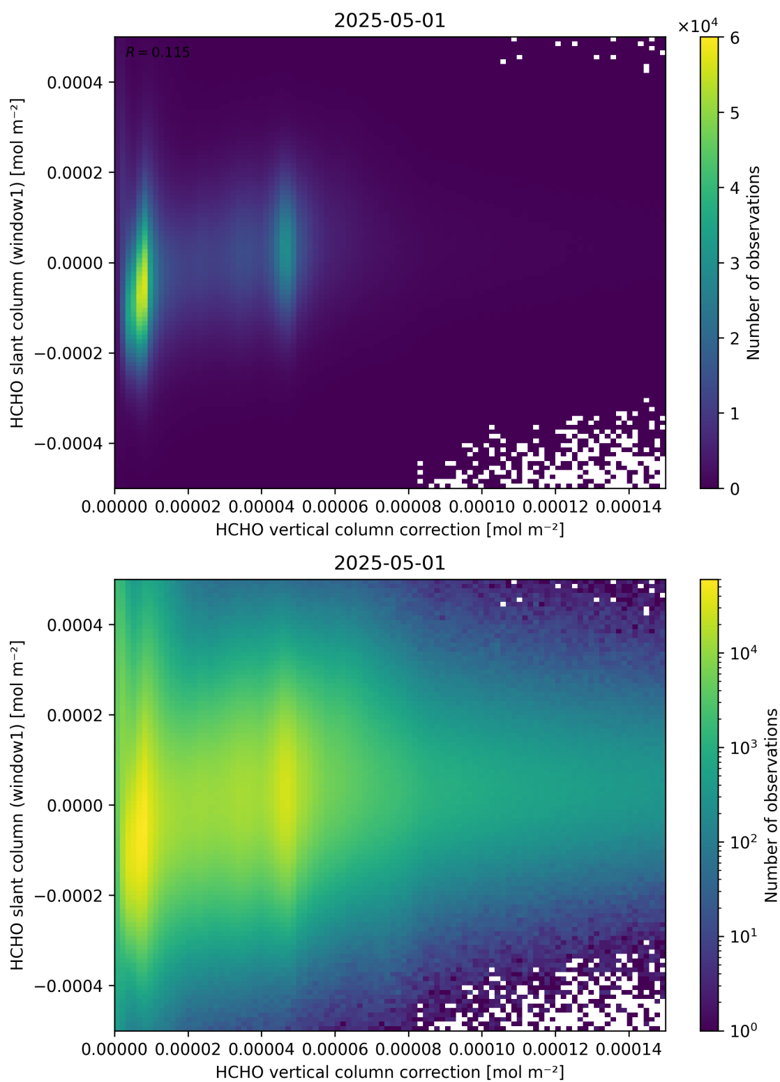
Figure 118: Scatter density plot of “HCHO vertical column correction” against “HCHO slant column (window1)” for 2025-04-30 to 2025-05-02.
