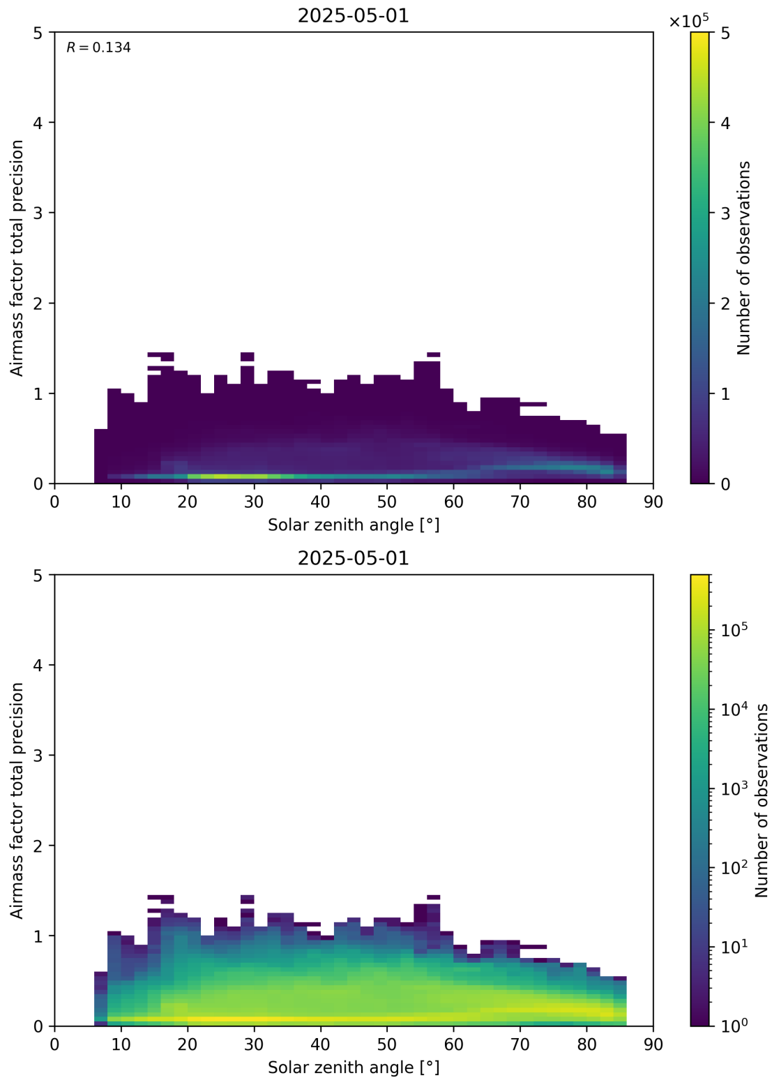
Figure 176: Scatter density plot of “Solar zenith angle” against “Airmass factor total precision” for 2025-04-30 to 2025-05-02.
