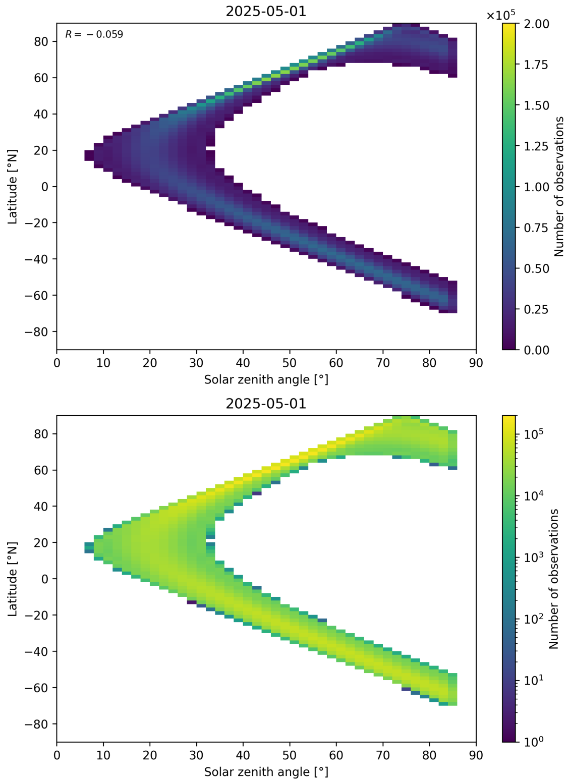
Figure 181: Scatter density plot of “Solar zenith angle” against “Latitude” for 2025-04-30 to 2025-05-02.
