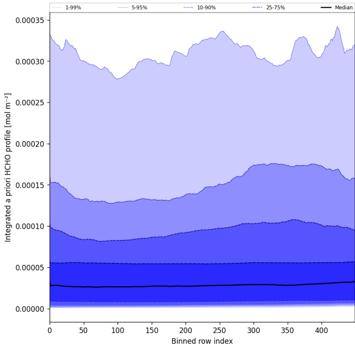
Figure 57: Along track statistics of “Integrated a priori HCHO profile” for 2025-04-30 to 2025-05-02
