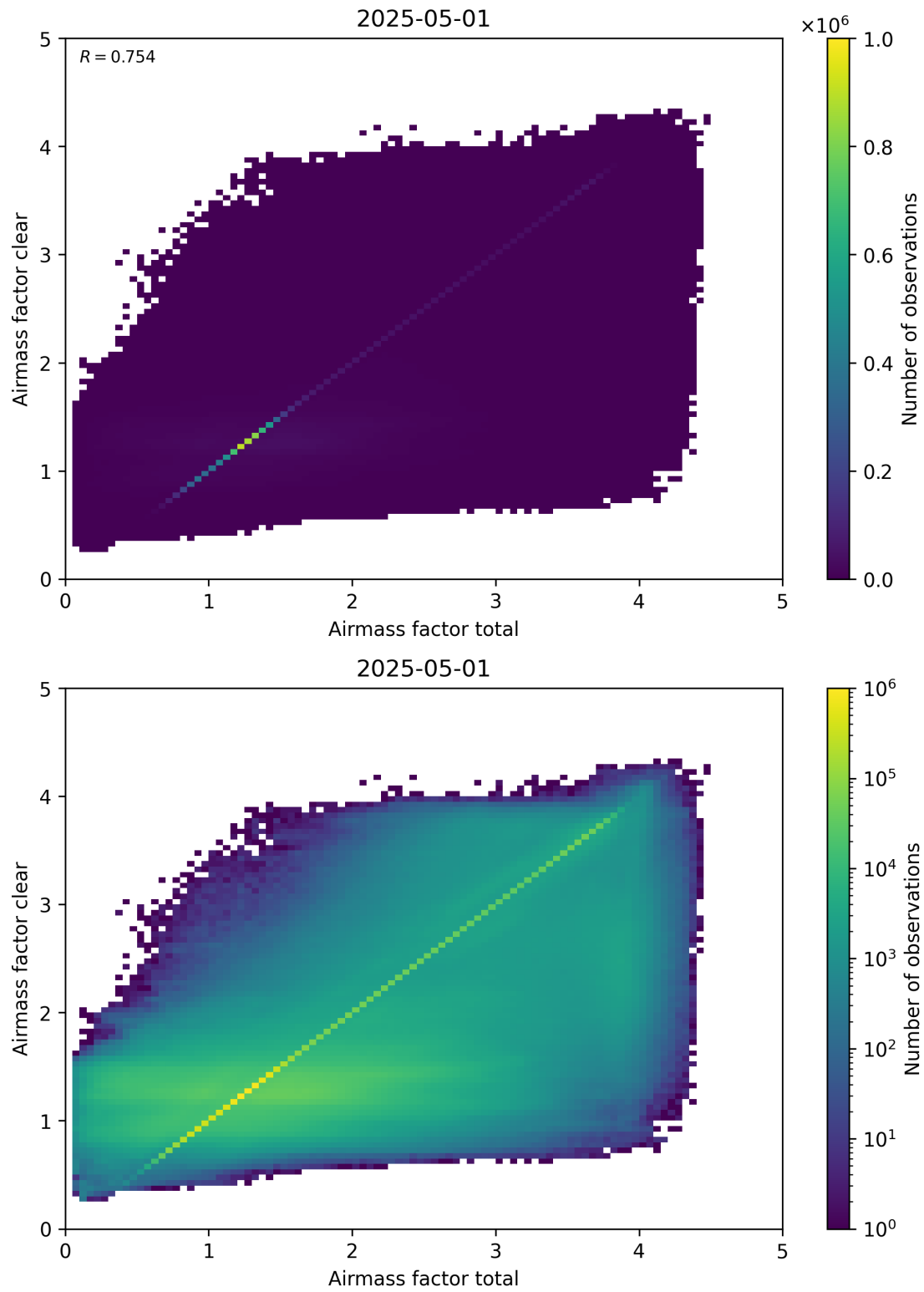
Figure 100: Scatter density plot of “Airmass factor total” against “Airmass factor clear” for 2025-04-30 to 2025-05-02.
