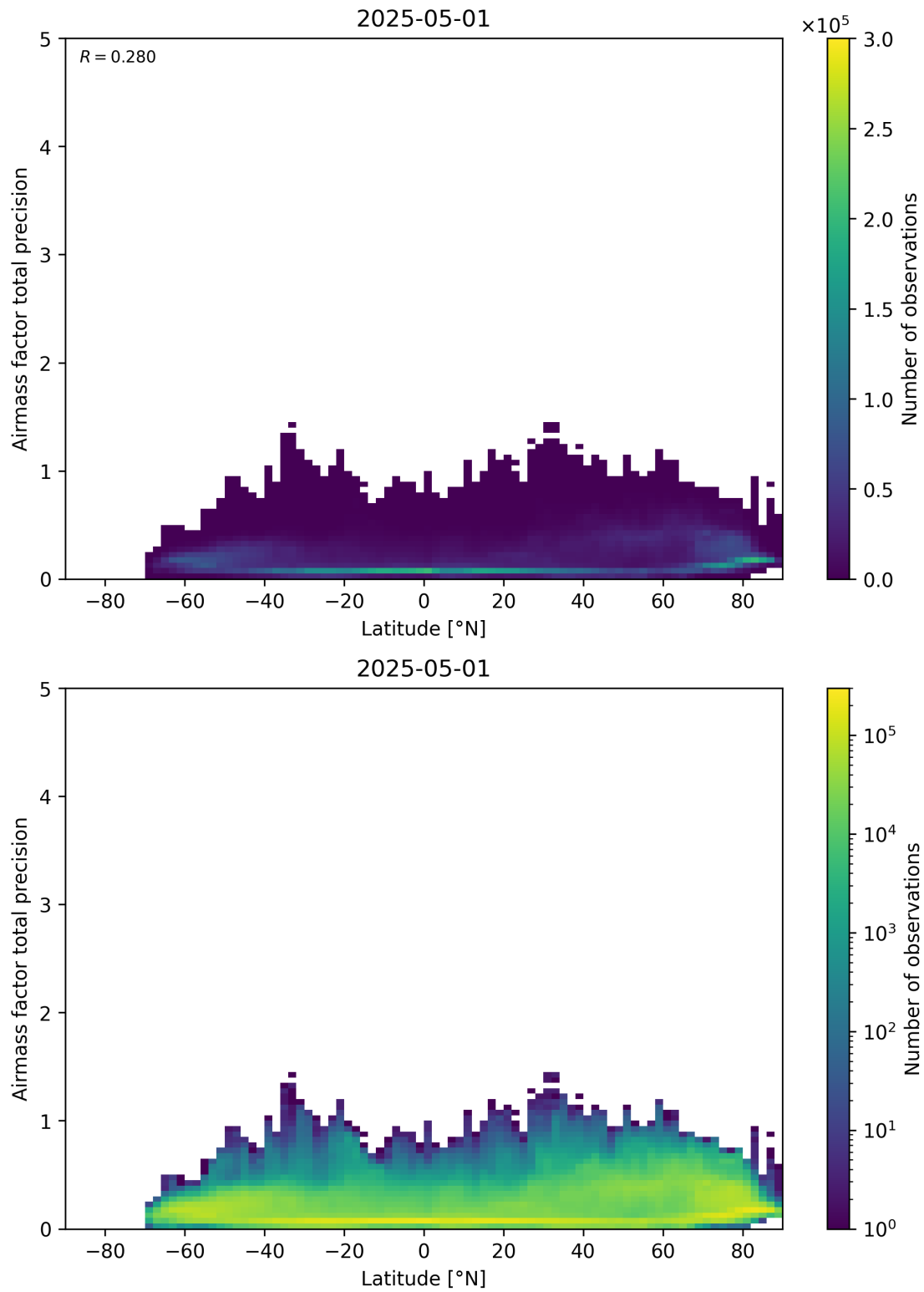
Figure 162: Scatter density plot of “Latitude” against “Airmass factor total precision” for 2025-04-30 to 2025-05-02.
