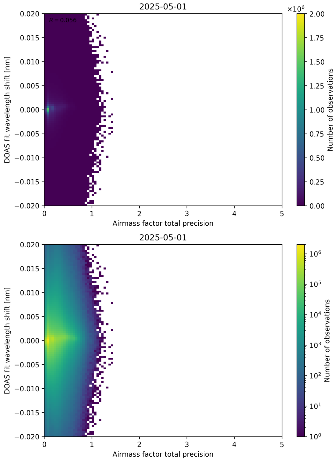
Figure 106: Scatter density plot of “Airmass factor total precision” against “DOAS fit wavelength shift” for 2025-04-30 to 2025-05-02.
