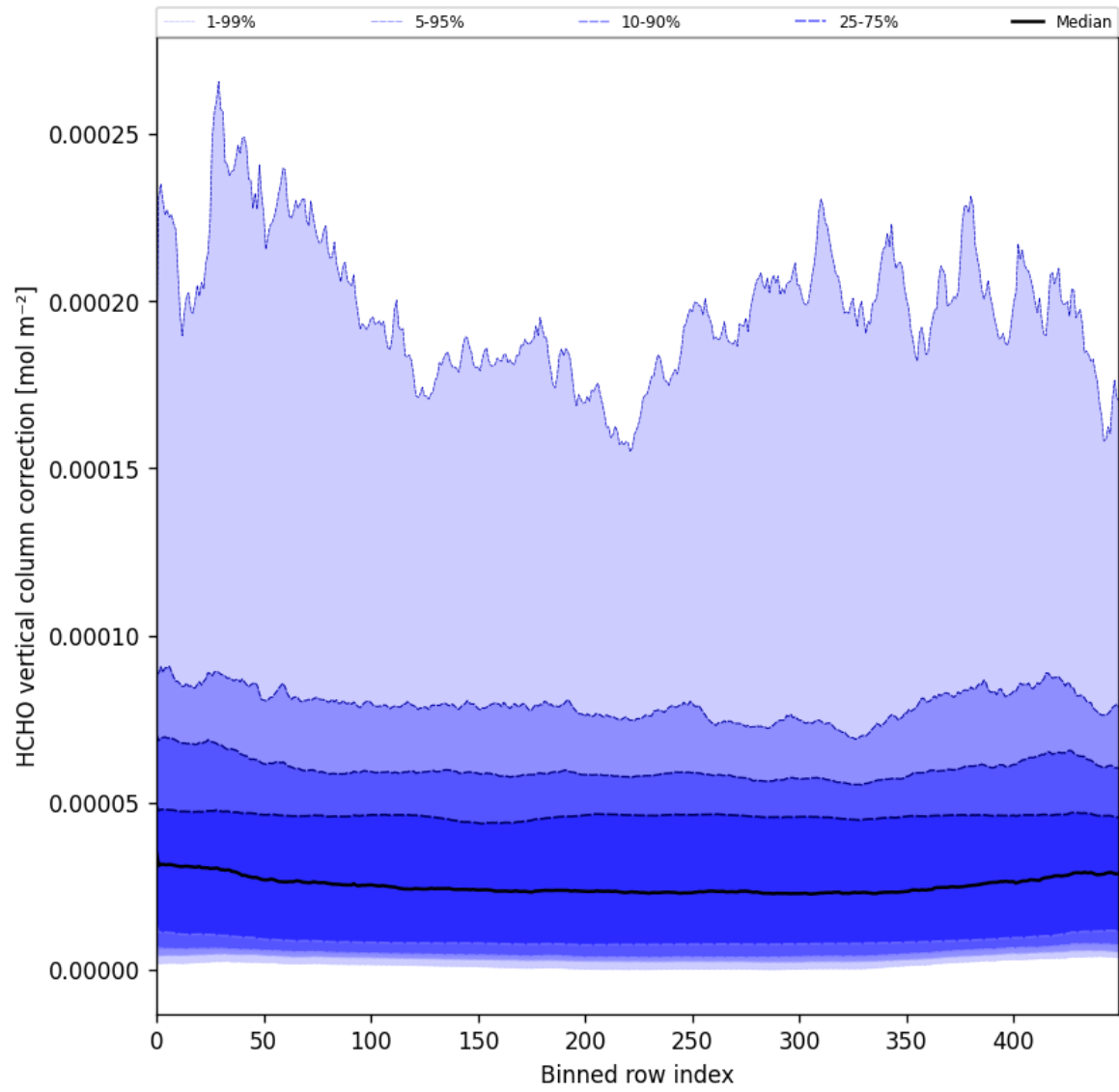
Figure 51: Along track statistics of “HCHO vertical column correction” for 2025-04-30 to 2025-05-02
