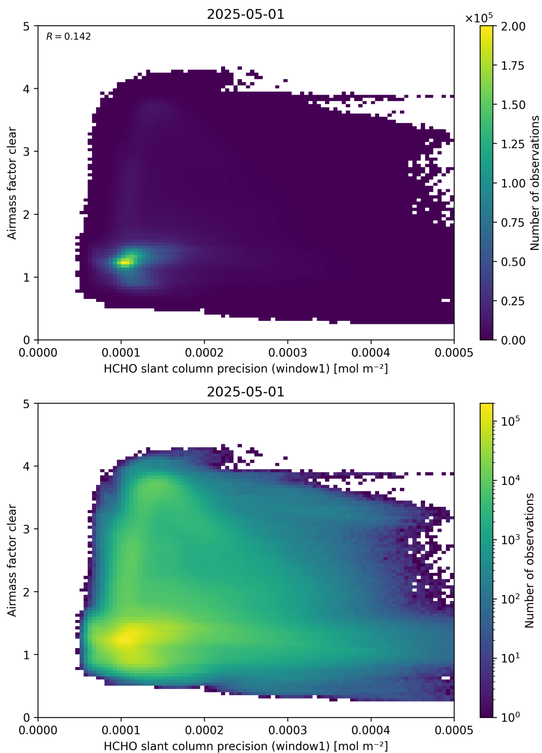
Figure 91: Scatter density plot of “HCHO slant column precision (window1)” against “Airmass factor clear” for 2025-04-30 to 2025-05-02.
