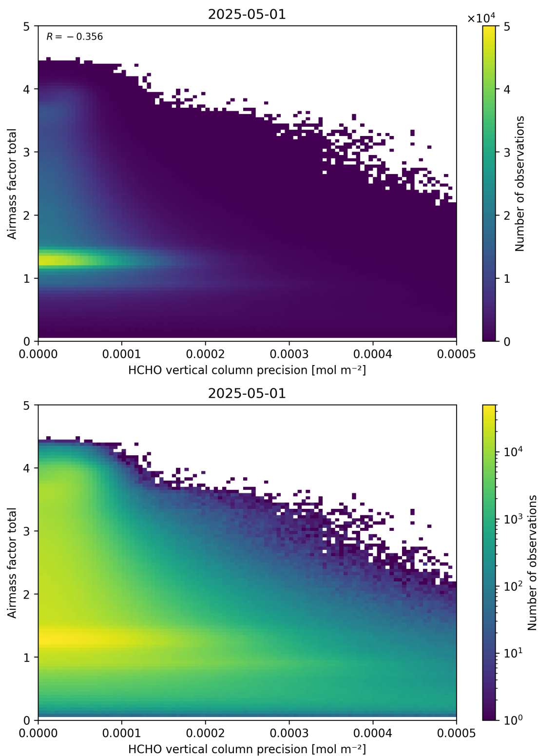
Figure 144: Scatter density plot of “HCHO vertical column precision” against “Airmass factor total” for 2025-04-30 to 2025-05-02.
