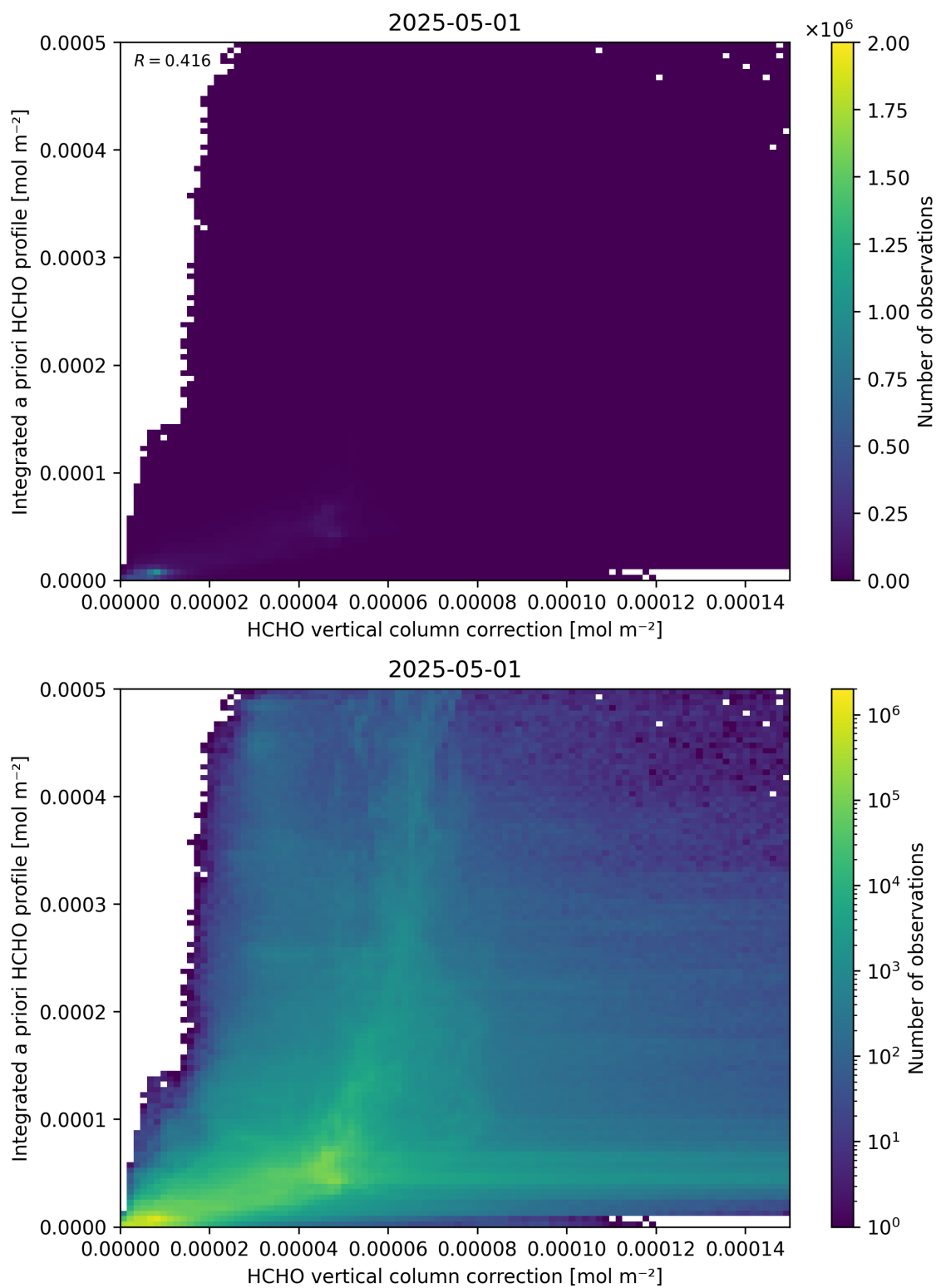
Figure 122: Scatter density plot of “HCHO vertical column correction” against “Integrated a priori HCHO profile” for 2025-04-30 to 2025-05-02.
