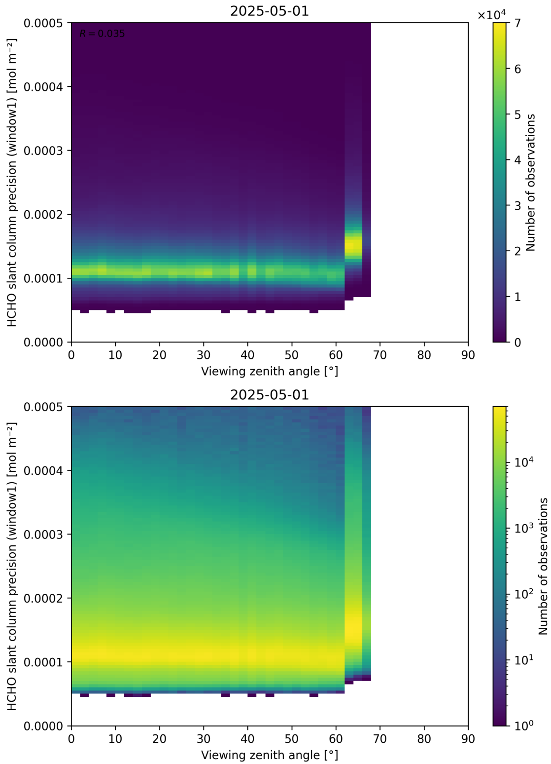
Figure 189: Scatter density plot of “Viewing zenith angle” against “HCHO slant column precision (window1)” for 2025-04-30 to 2025-05-02.
