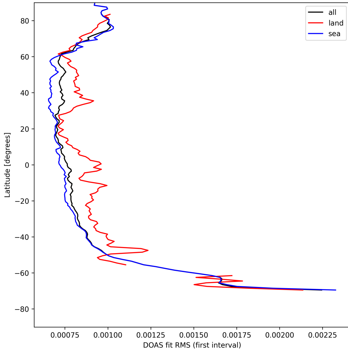
Figure 32: Zonal average of “DOAS fit RMS (first interval)” for 2025-04-30 to 2025-05-02.
