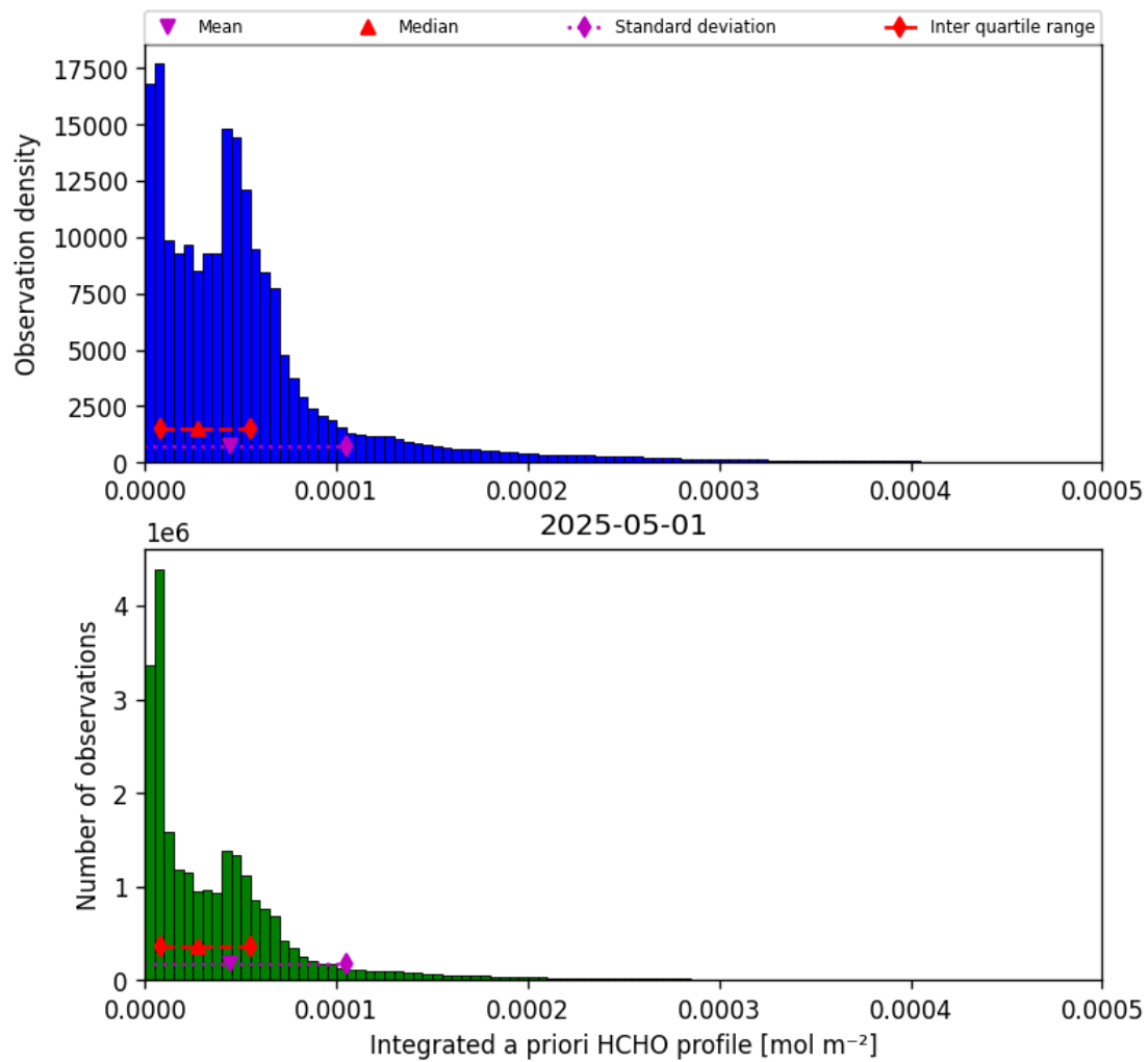
Figure 43: Histogram of “Integrated a priori HCHO profile” for 2025-04-30 to 2025-05-02
