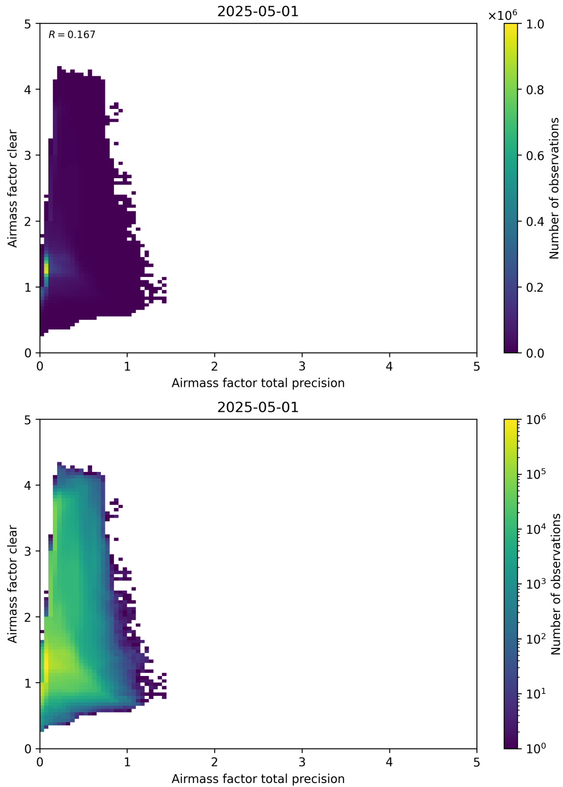
Figure 108: Scatter density plot of “Airmass factor total precision” against “Airmass factor clear” for 2025-04-30 to 2025-05-02.
