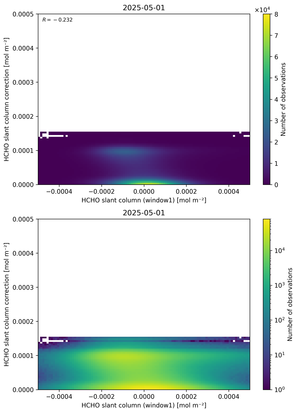
Figure 83: Scatter density plot of “HCHO slant column (window1)” against “HCHO slant column correction” for 2025-04-30 to 2025-05-02.
