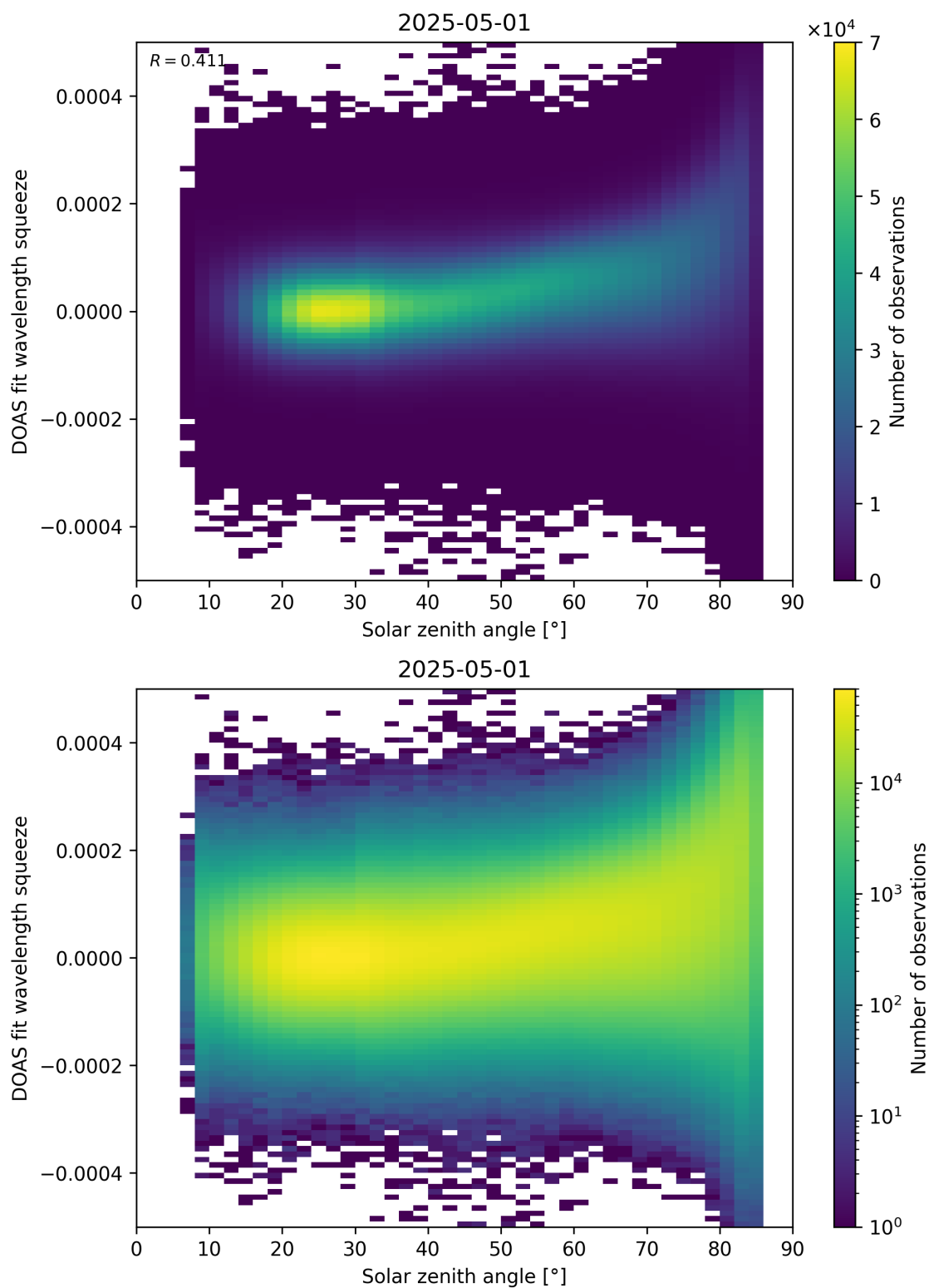
Figure 169: Scatter density plot of “Solar zenith angle” against “DOAS fit wavelength squeeze” for 2025-04-30 to 2025-05-02.
