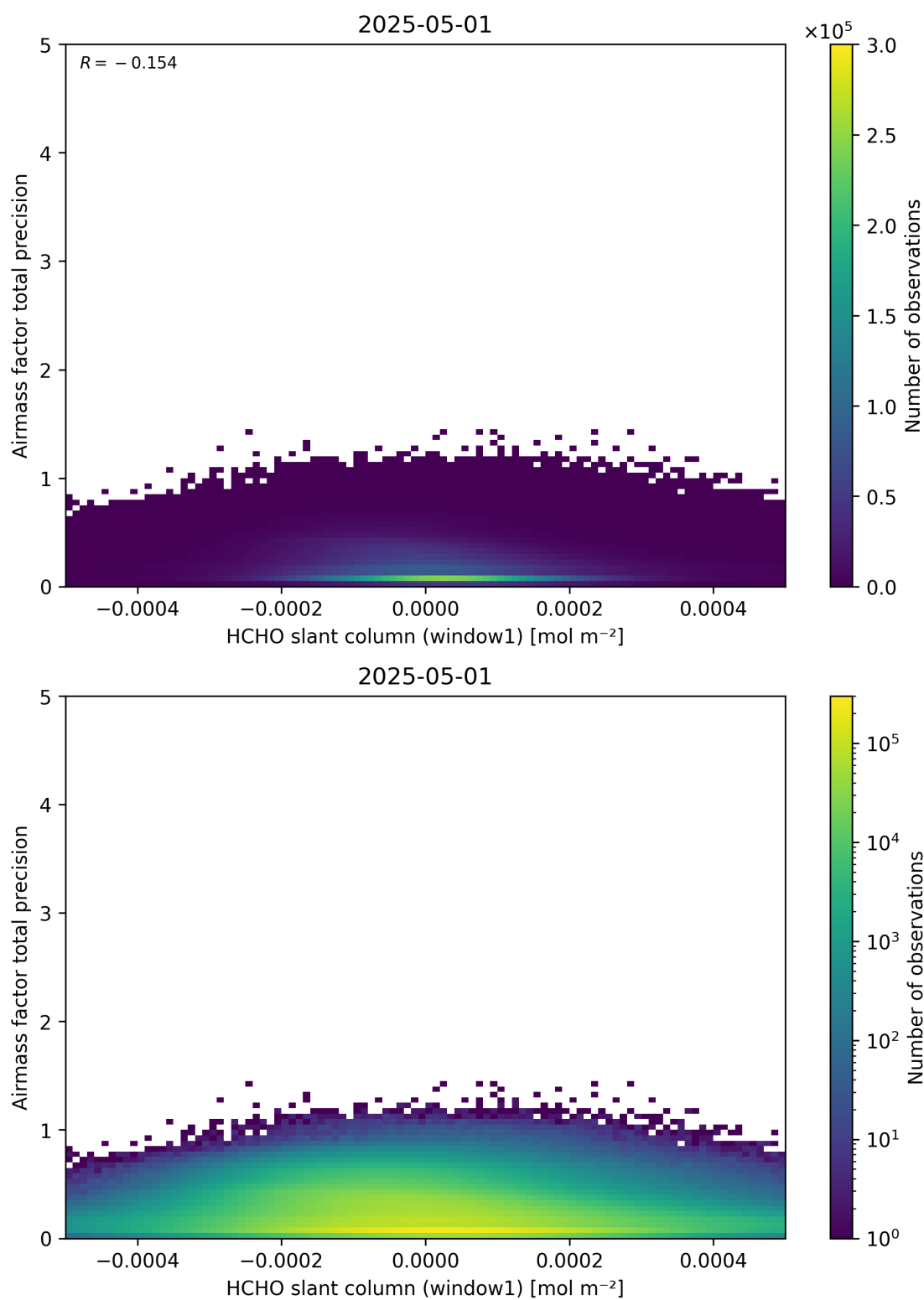
Figure 86: Scatter density plot of “HCHO slant column (window1)” against “Airmass factor total precision” for 2025-04-30 to 2025-05-02.
