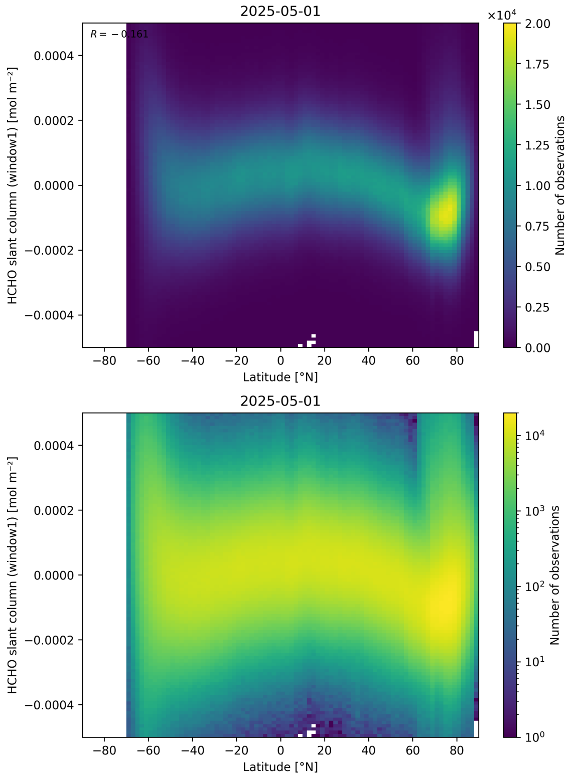
Figure 159: Scatter density plot of “Latitude” against “HCHO slant column (window1)” for 2025-04-30 to 2025-05-02.
