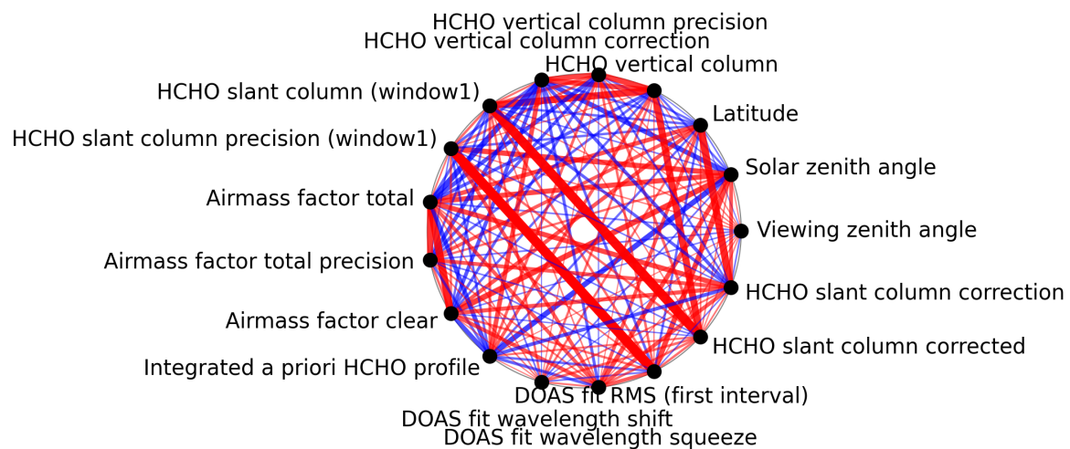
Figure 1: Map of correlation graph for 2025-04-30 to 2025-05-02.
