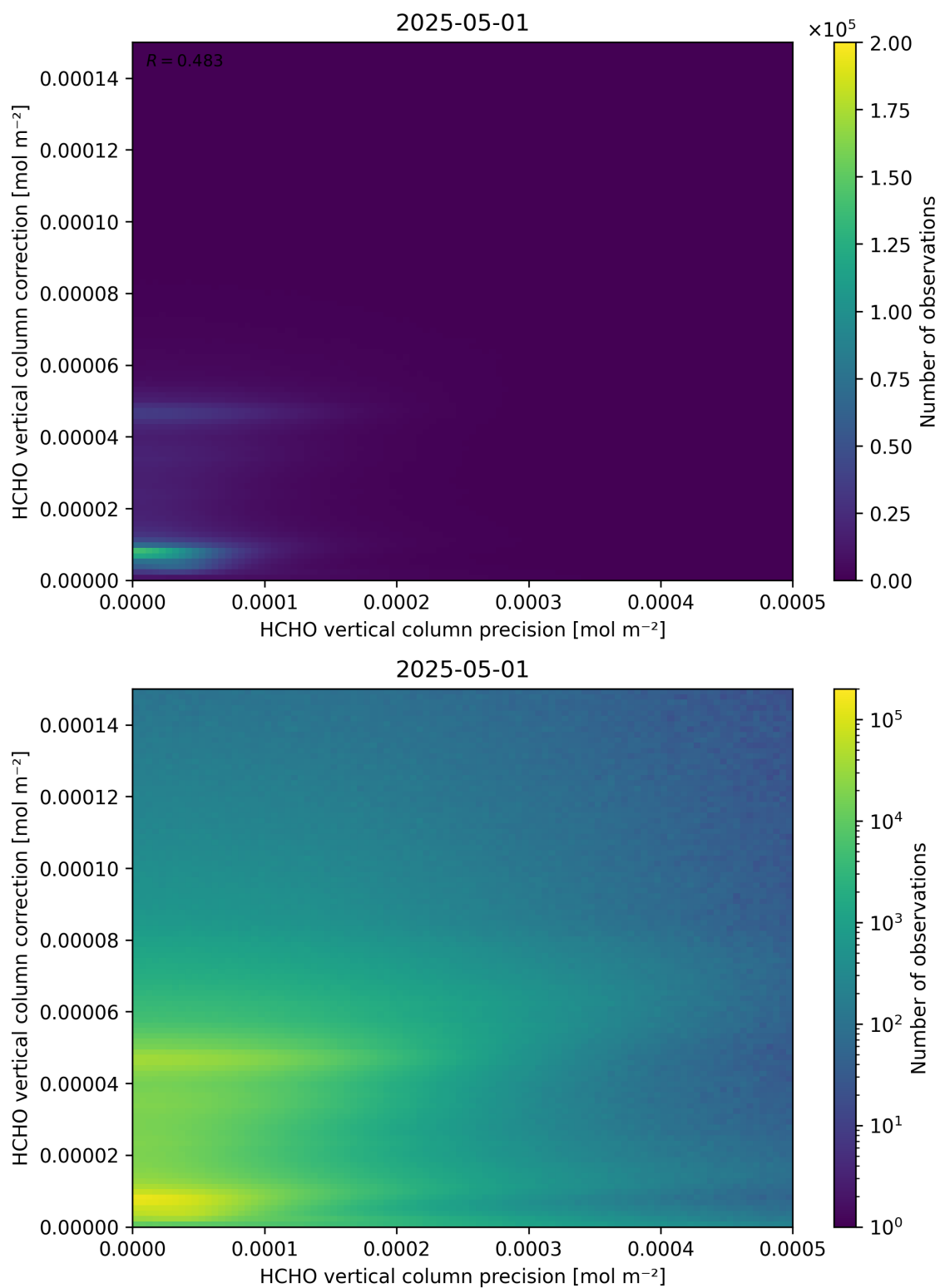
Figure 146: Scatter density plot of “HCHO vertical column precision” against “HCHO vertical column correction” for 2025-04-30 to 2025-05-02.
