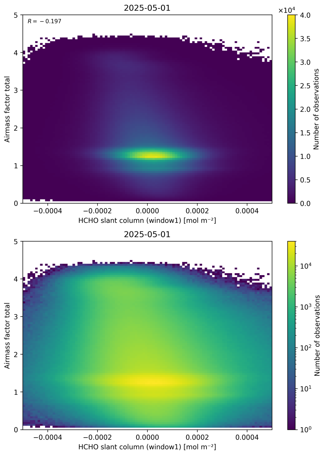
Figure 85: Scatter density plot of “HCHO slant column (window1)” against “Airmass factor total” for 2025-04-30 to 2025-05-02.
