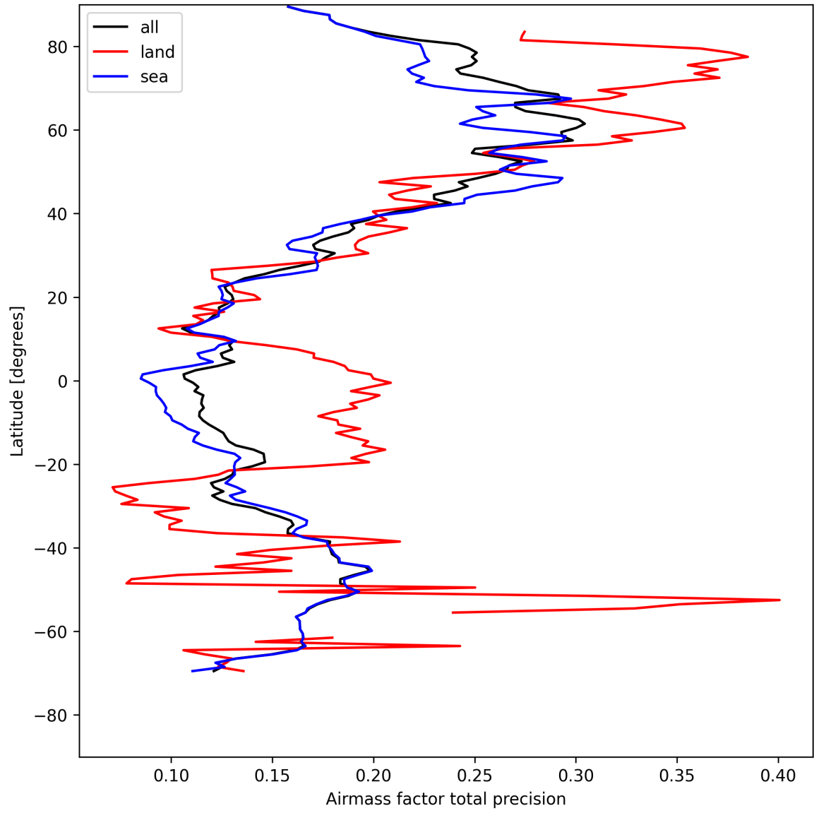
Figure 27: Zonal average of “Airmass factor total precision” for 2025-04-30 to 2025-05-02.
