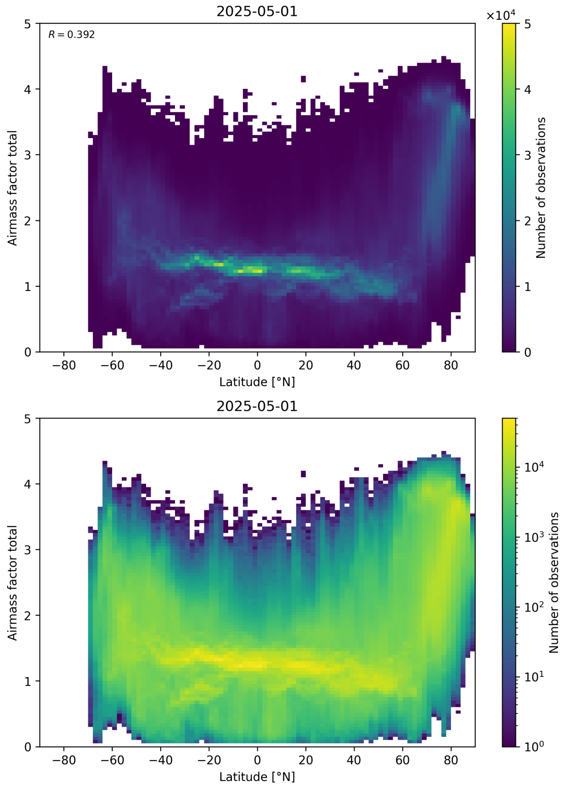
Figure 161: Scatter density plot of “Latitude” against “Airmass factor total” for 2025-04-30 to 2025-05-02.
