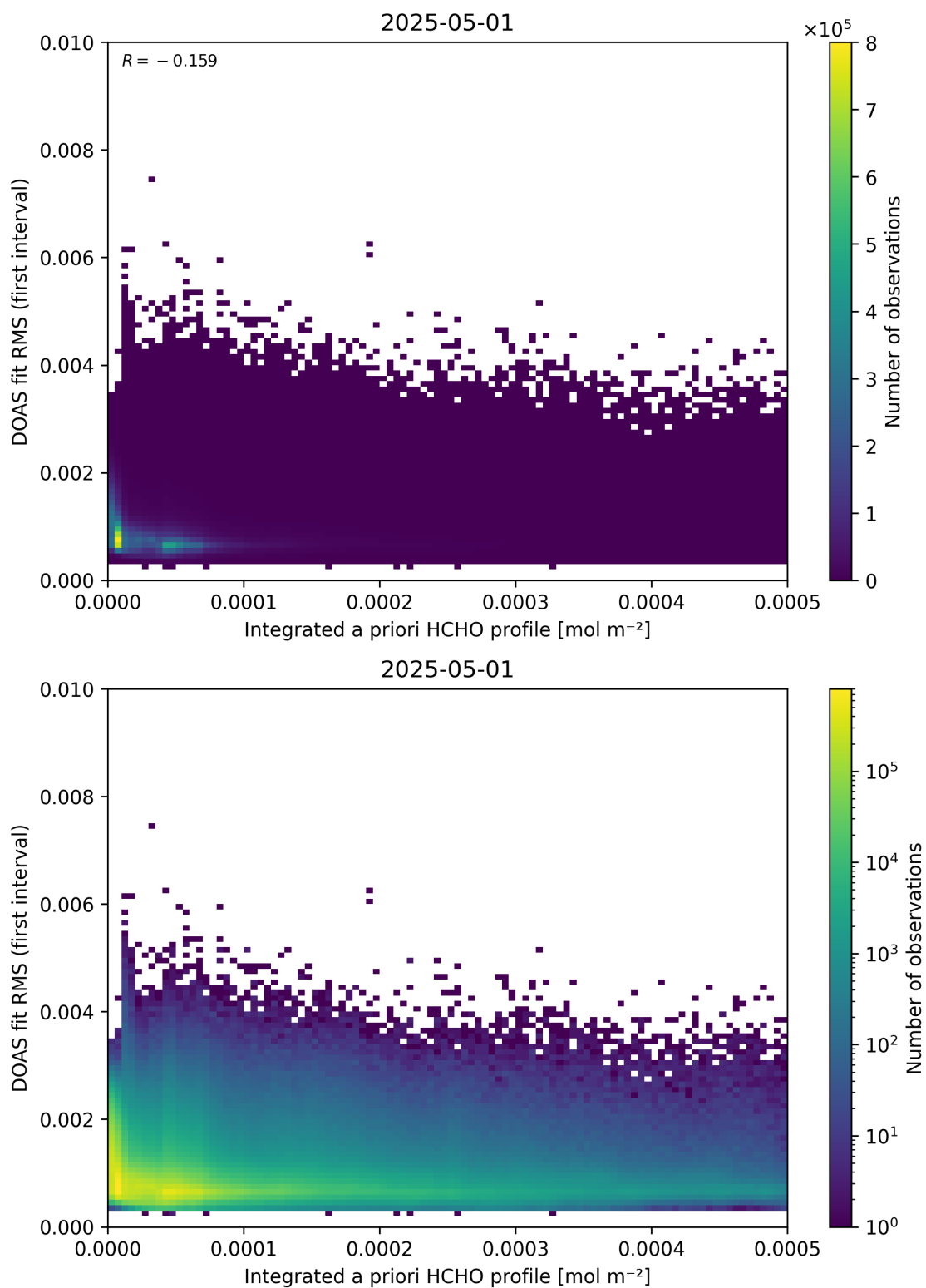
Figure 148: Scatter density plot of “Integrated a priori HCHO profile” against “DOAS fit RMS (first interval)” for 2025-04-30 to 2025-05-02.
