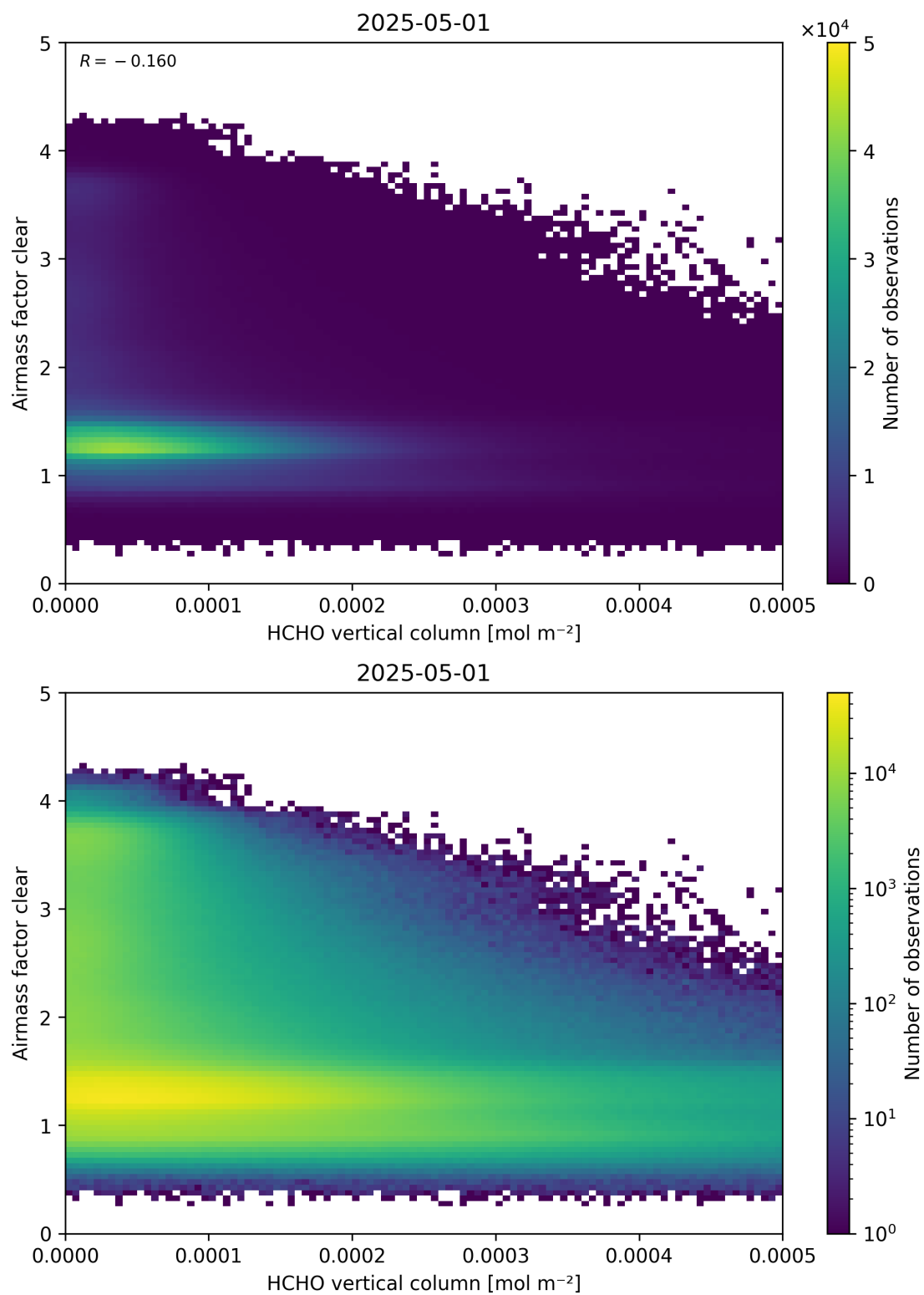
Figure 126: Scatter density plot of “HCHO vertical column” against “Airmass factor clear” for 2025-04-30 to 2025-05-02.
