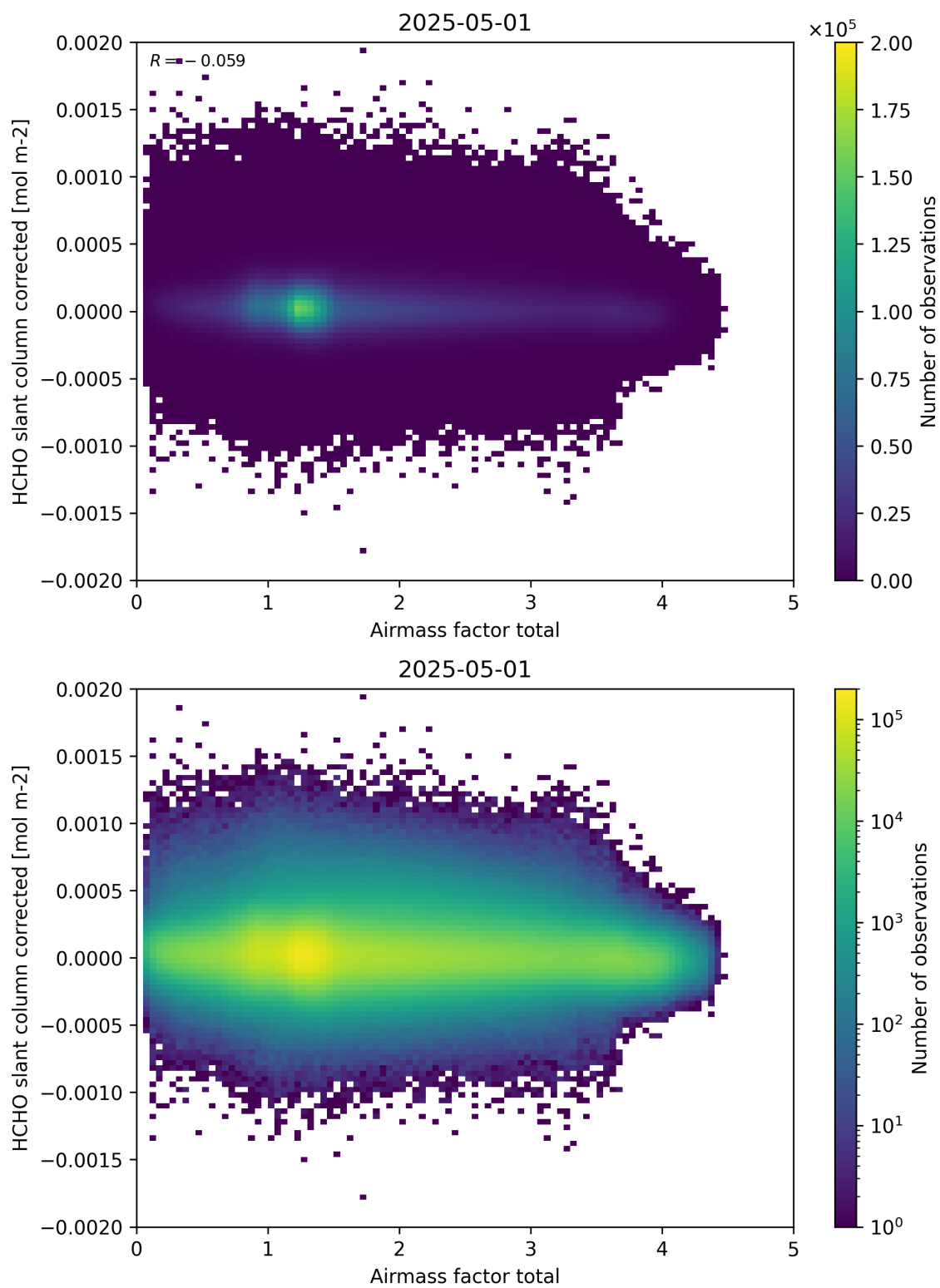
Figure 101: Scatter density plot of “Airmass factor total” against “HCHO slant column corrected” for 2025-04-30 to 2025-05-02.
