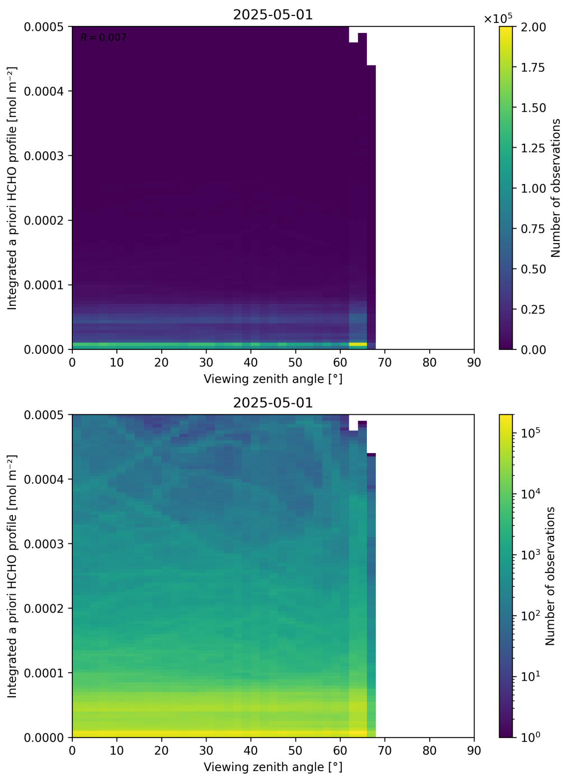
Figure 195: Scatter density plot of “Viewing zenith angle” against “Integrated a priori HCHO profile” for 2025-04-30 to 2025-05-02.
