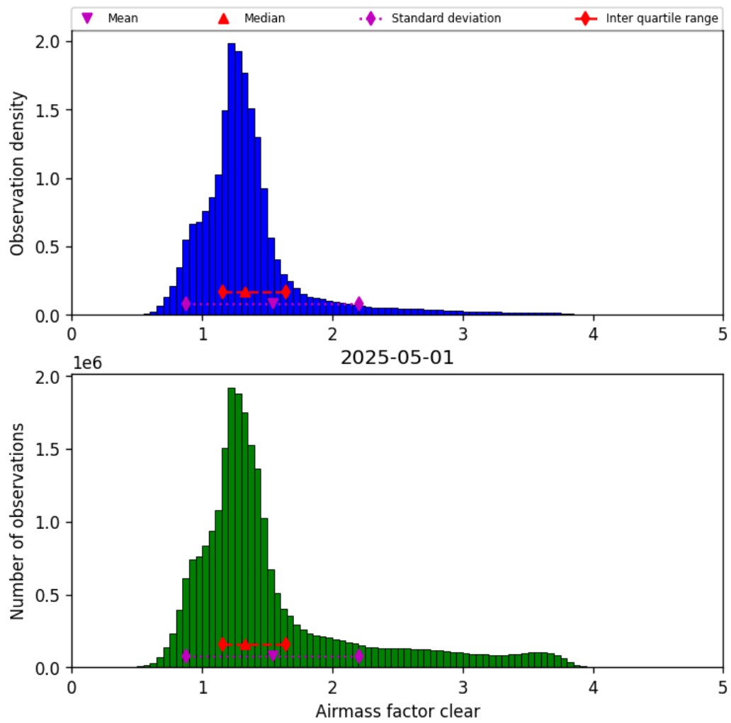
Figure 42: Histogram of “Airmass factor clear” for 2025-04-30 to 2025-05-02
