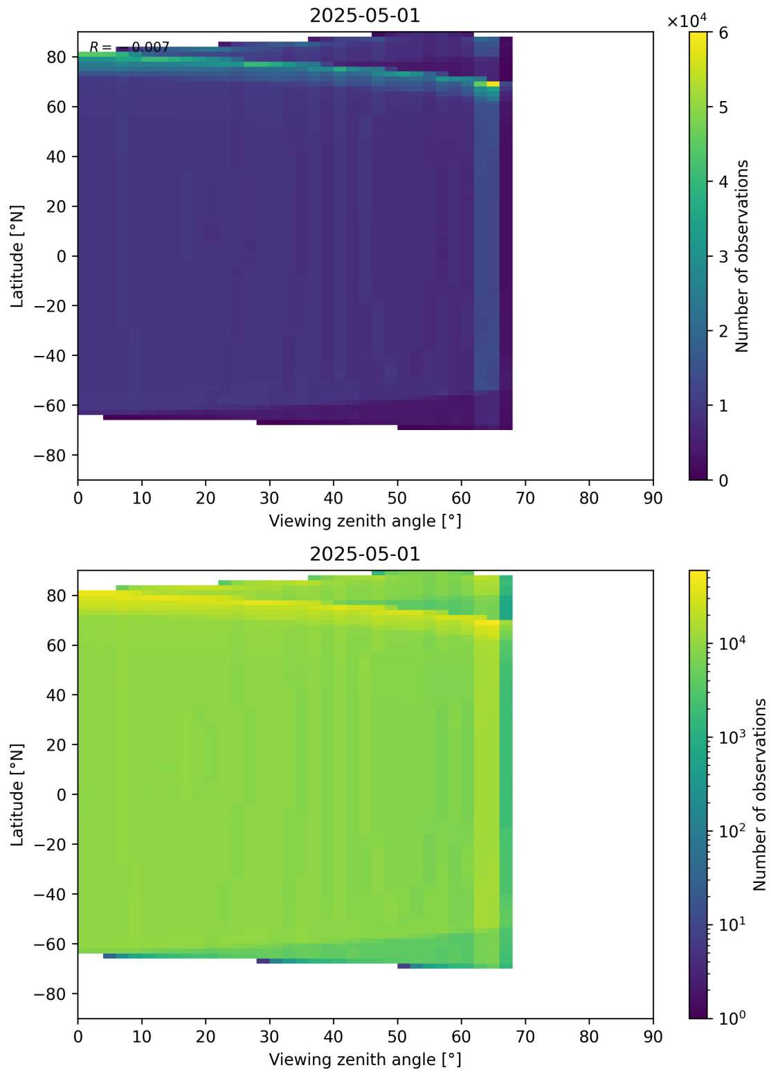
Figure 196: Scatter density plot of “Viewing zenith angle” against “Latitude” for 2025-04-30 to 2025-05-02.
