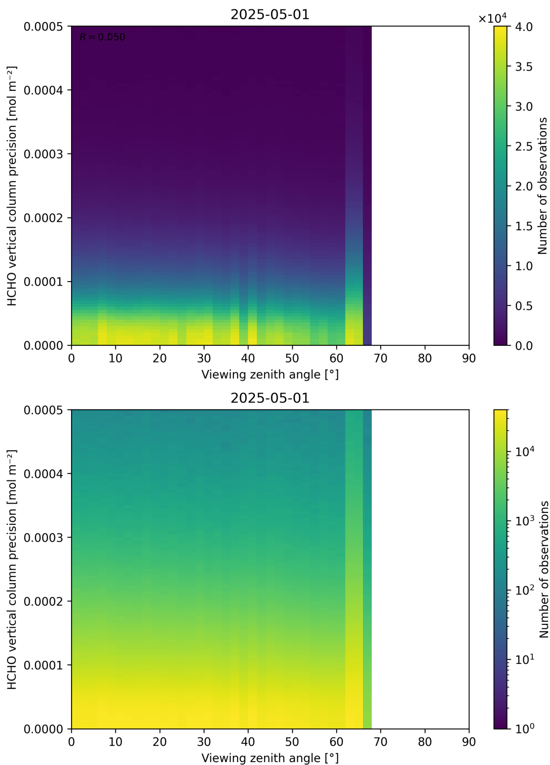
Figure 194: Scatter density plot of “Viewing zenith angle” against “HCHO vertical column precision” for 2025-04-30 to 2025-05-02.
