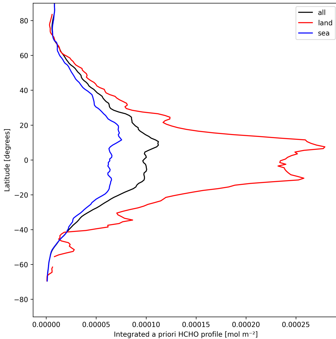
Figure 29: Zonal average of “Integrated a priori HCHO profile” for 2025-04-30 to 2025-05-02.
