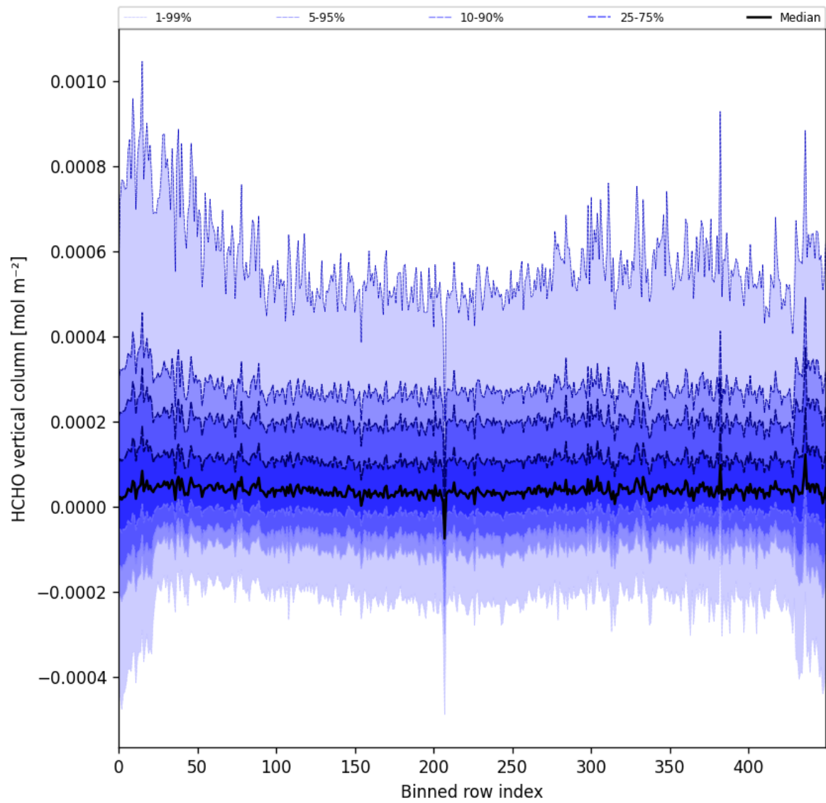
Figure 49: Along track statistics of “HCHO vertical column” for 2025-04-30 to 2025-05-02
