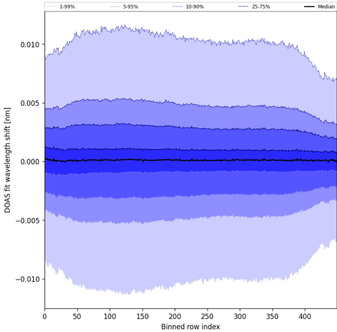
Figure 58: Along track statistics of “DOAS fit wavelength shift” for 2025-04-30 to 2025-05-02
