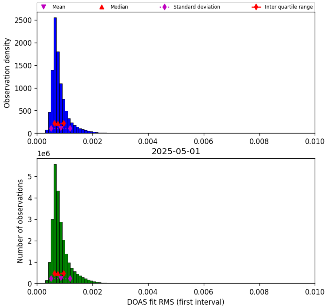
Figure 46: Histogram of “DOAS fit RMS (first interval)” for 2025-04-30 to 2025-05-02
