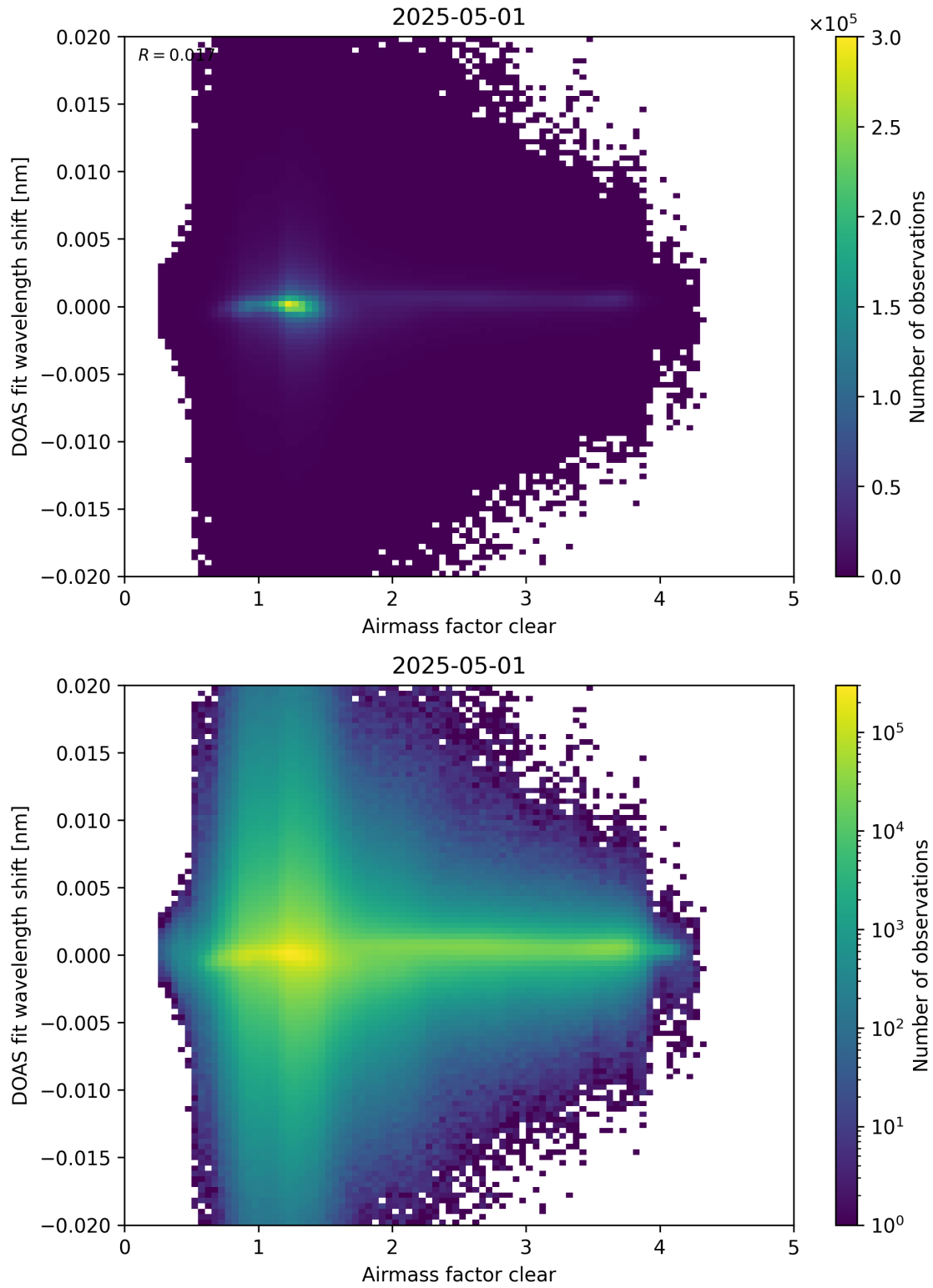
Figure 72: Scatter density plot of “Airmass factor clear” against “DOAS fit wavelength shift” for 2025-04-30 to 2025-05-02.
