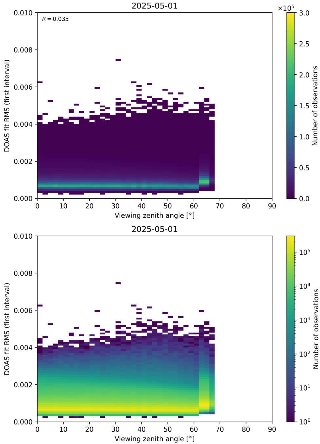
Figure 182: Scatter density plot of “Viewing zenith angle” against “DOAS fit RMS (first interval)” for 2025-04-30 to 2025-05-02.
