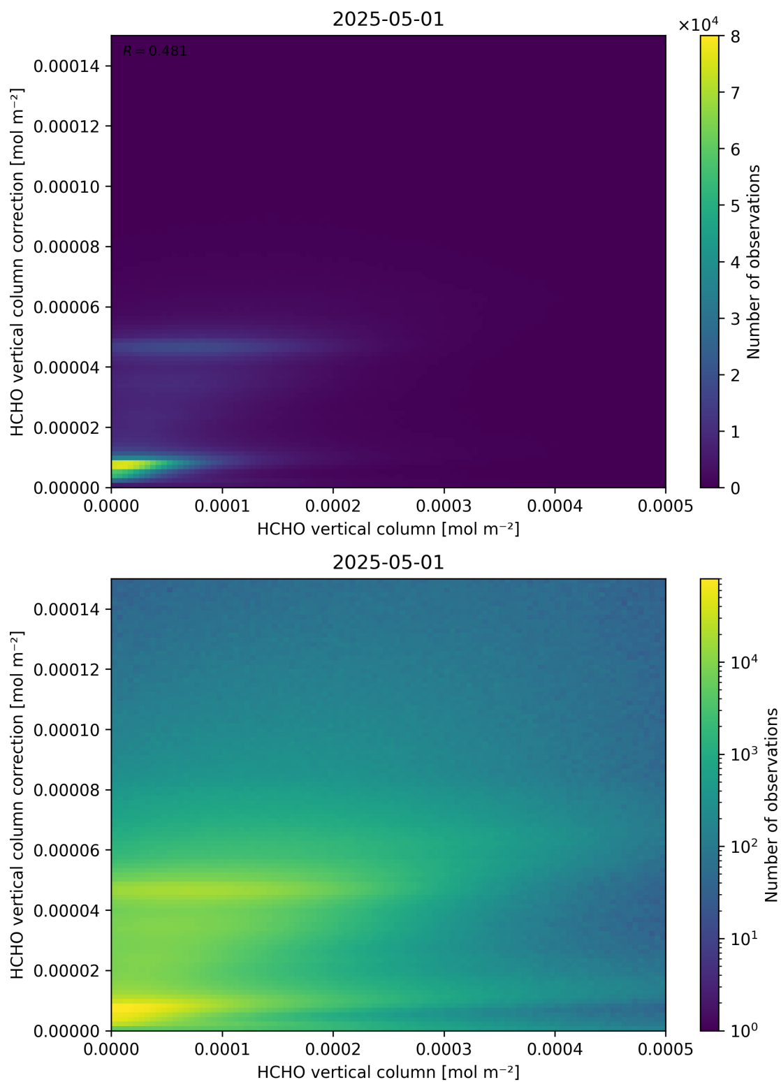
Figure 133: Scatter density plot of “HCHO vertical column” against “HCHO vertical column correction” for 2025-04-30 to 2025-05-02.
