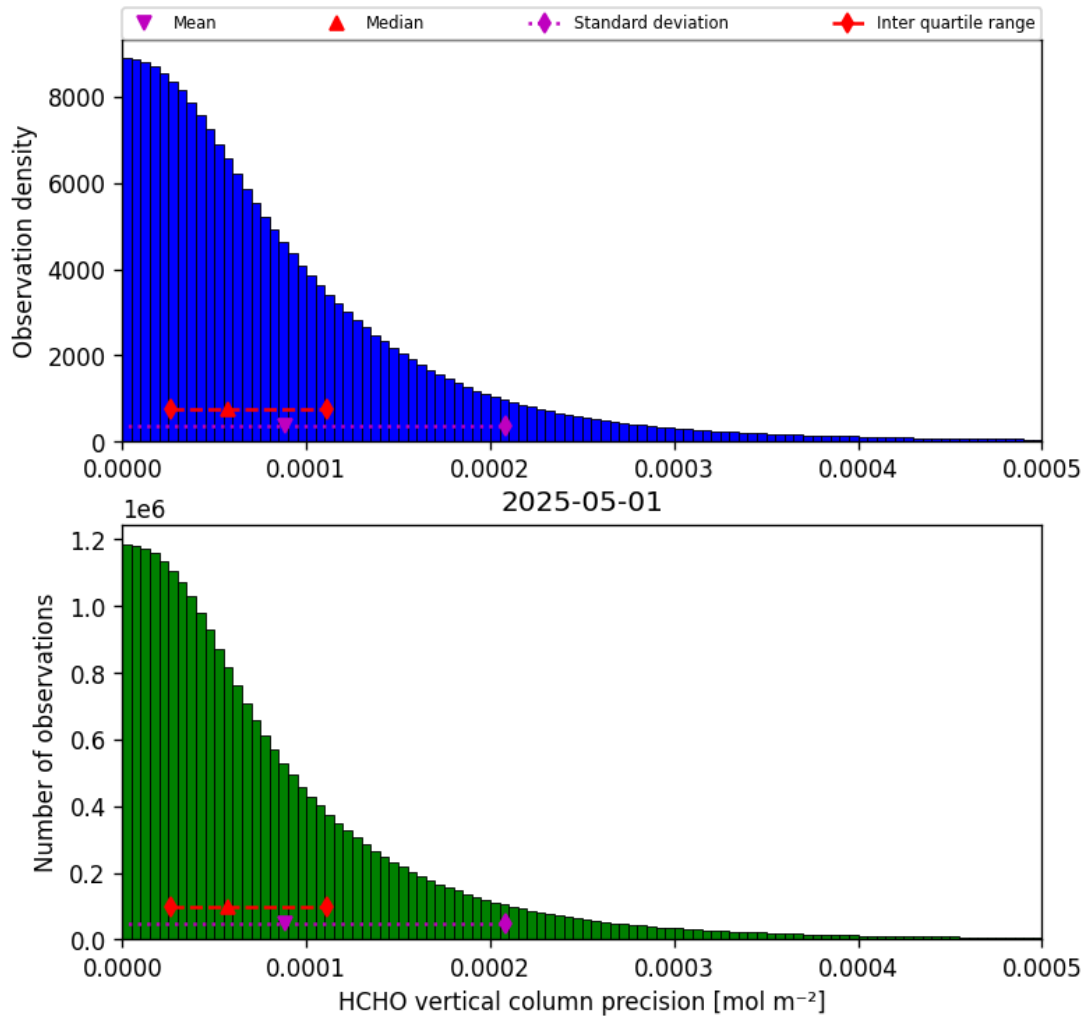
Figure 36: Histogram of “HCHO vertical column precision” for 2025-04-30 to 2025-05-02
