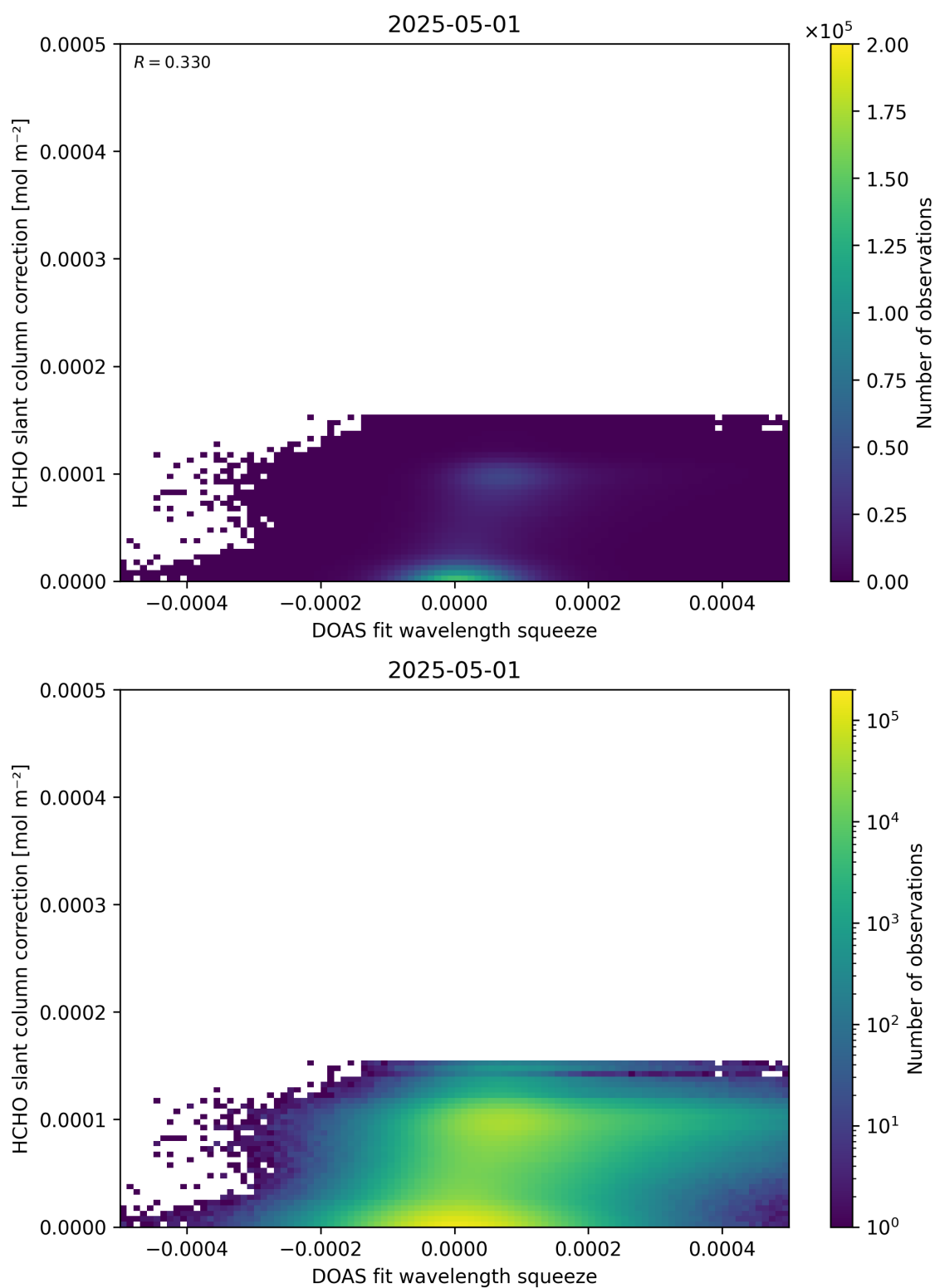
Figure 70: Scatter density plot of “DOAS fit wavelength squeeze” against “HCHO slant column correction” for 2025-04-30 to 2025-05-02.
