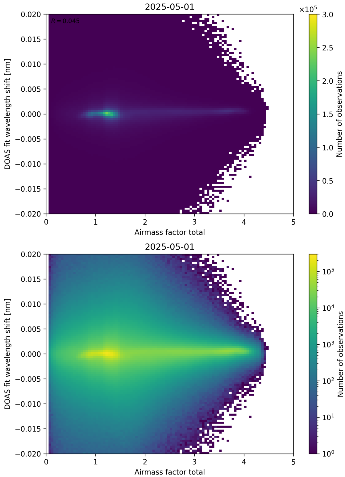
Figure 98: Scatter density plot of “Airmass factor total” against “DOAS fit wavelength shift” for 2025-04-30 to 2025-05-02.
