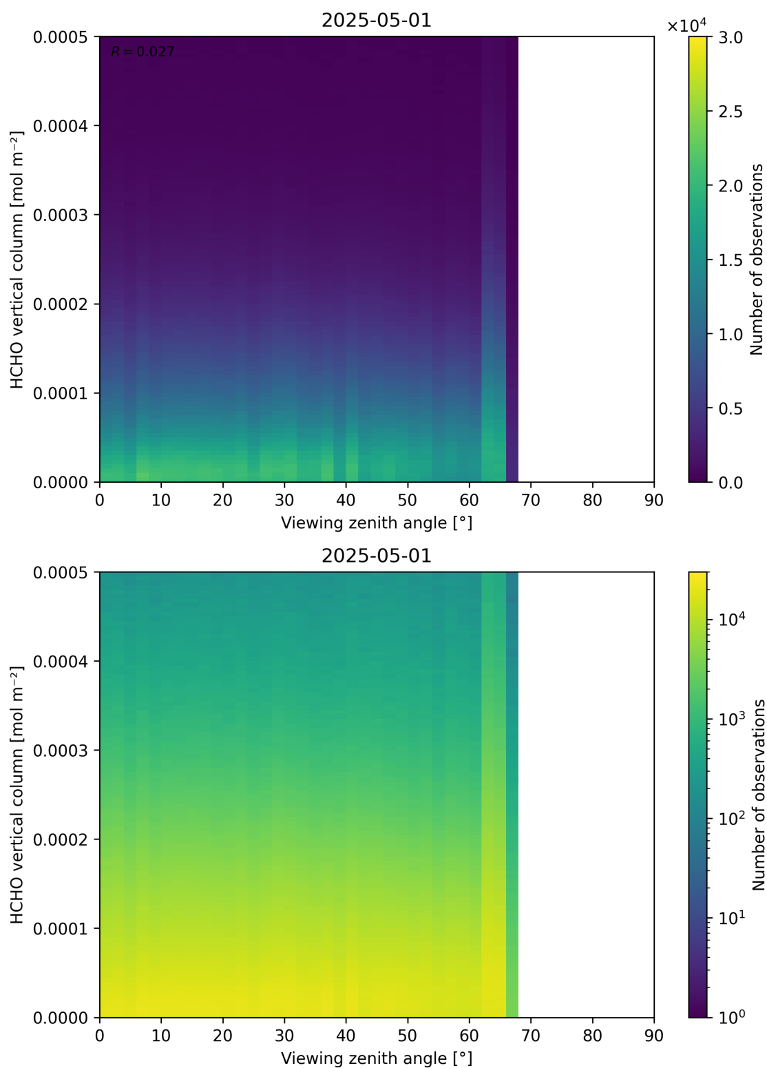
Figure 192: Scatter density plot of “Viewing zenith angle” against “HCHO vertical column” for 2025-04-30 to 2025-05-02.
