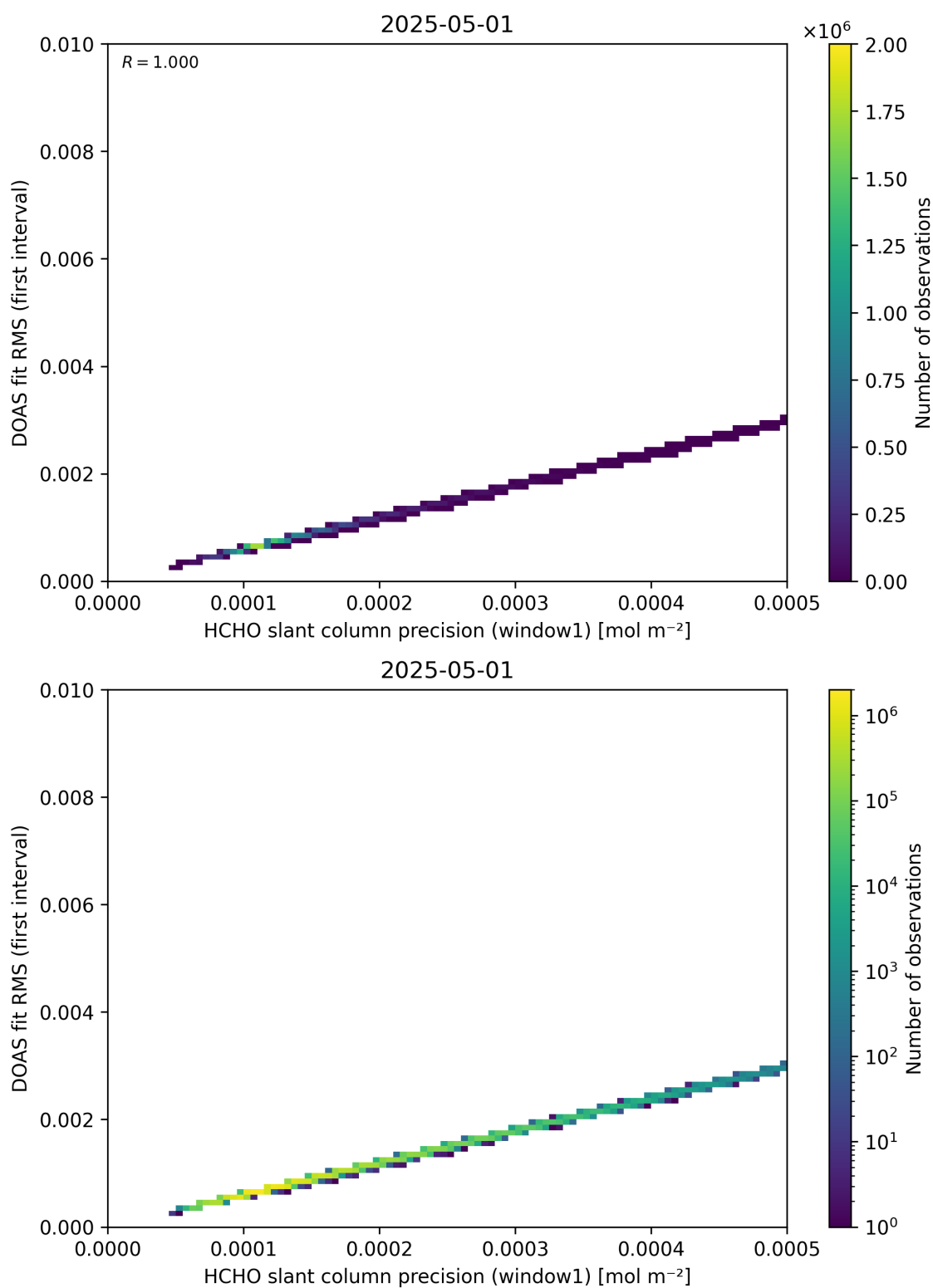
Figure 88: Scatter density plot of “HCHO slant column precision (window1)” against “DOAS fit RMS (first interval)” for 2025-04-30 to 2025-05-02.
