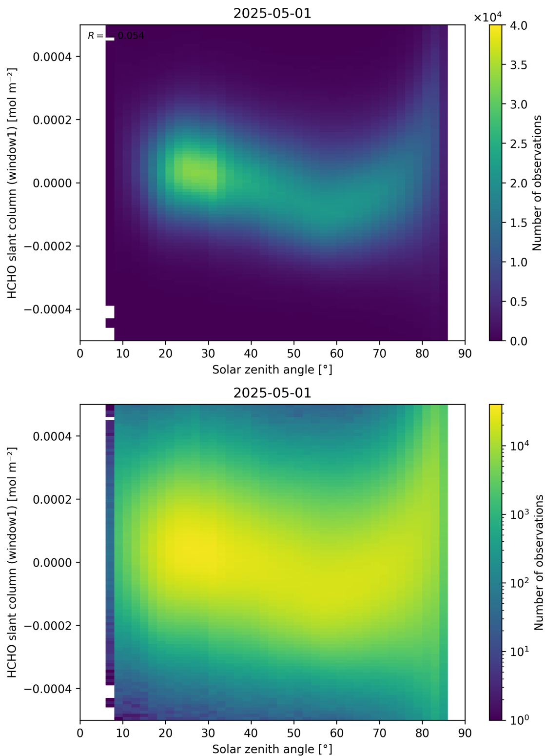
Figure 173: Scatter density plot of “Solar zenith angle” against “HCHO slant column (window1)” for 2025-04-30 to 2025-05-02.
