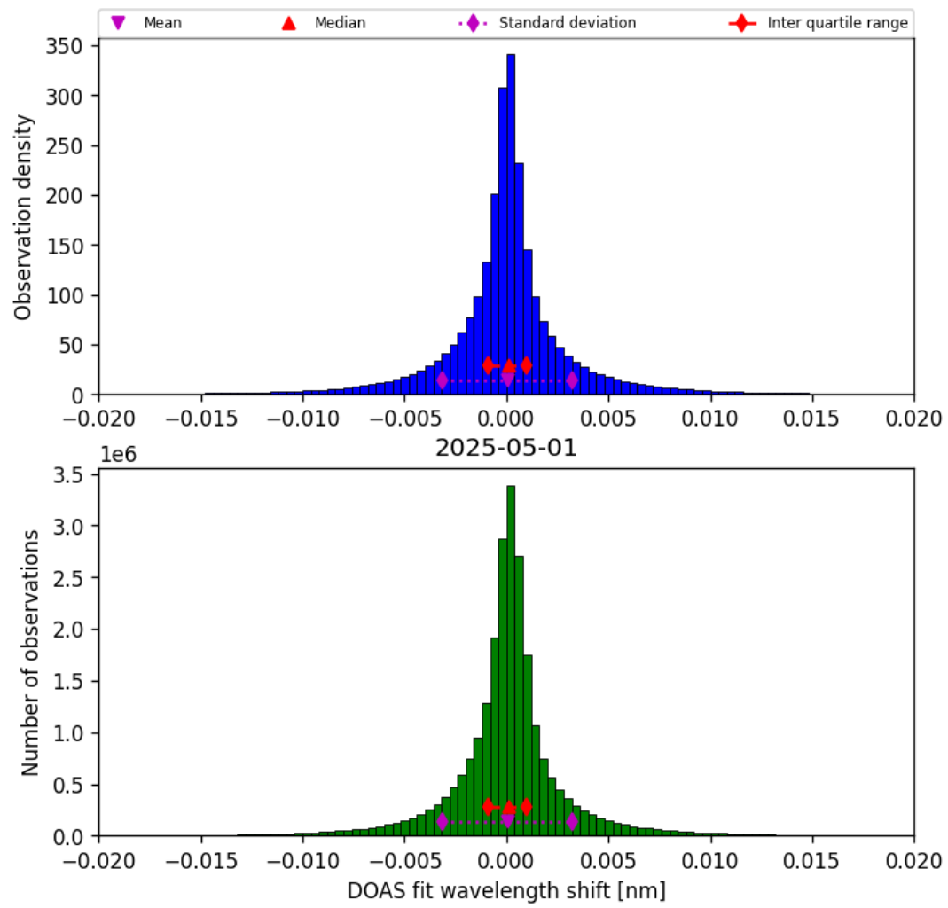
Figure 44: Histogram of “DOAS fit wavelength shift” for 2025-04-30 to 2025-05-02
