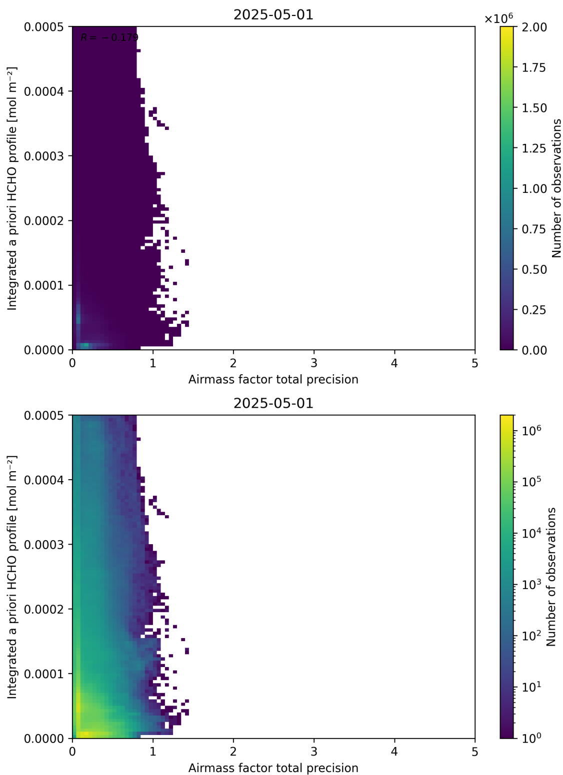
Figure 111: Scatter density plot of “Airmass factor total precision” against “Integrated a priori HCHO profile” for 2025-04-30 to 2025-05-02.
