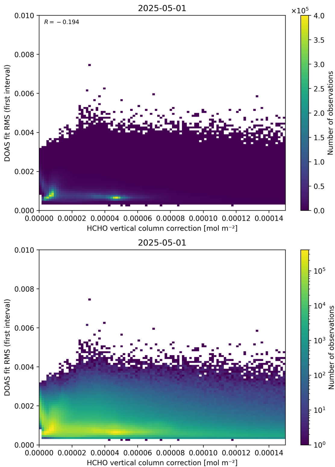
Figure 112: Scatter density plot of “HCHO vertical column correction” against “DOAS fit RMS (first interval)” for 2025-04-30 to 2025-05-02.
