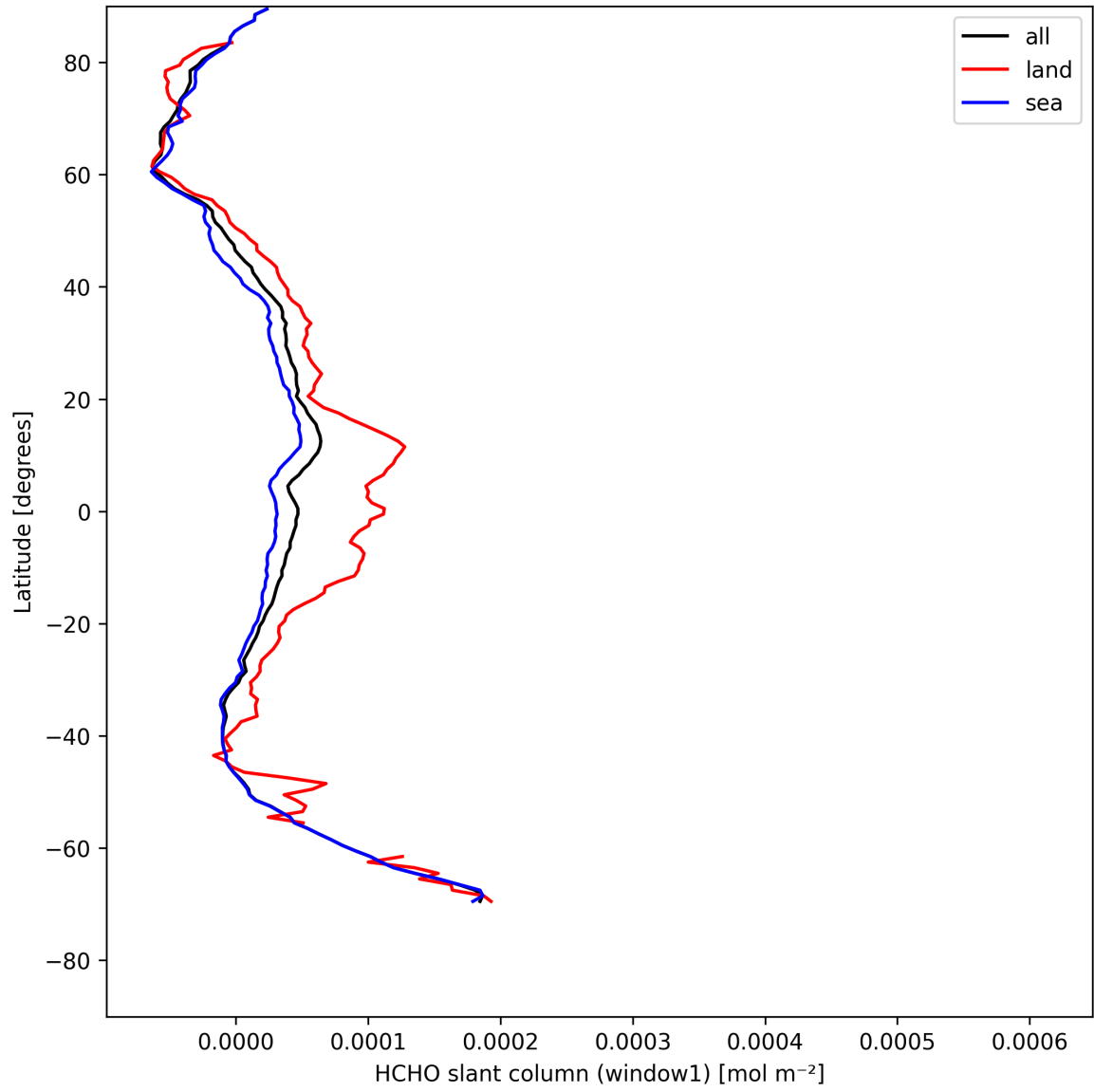
Figure 24: Zonal average of “HCHO slant column (window1)” for 2025-04-30 to 2025-05-02.
