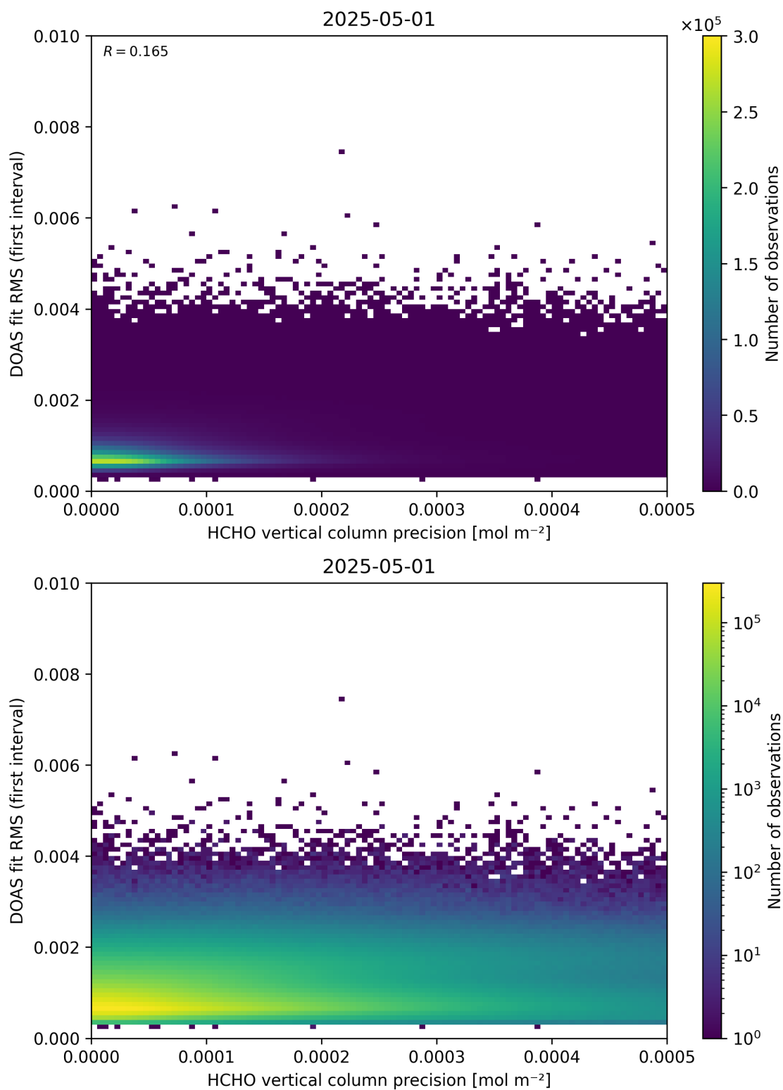
Figure 136: Scatter density plot of “HCHO vertical column precision” against “DOAS fit RMS (first interval)” for 2025-04-30 to 2025-05-02.
