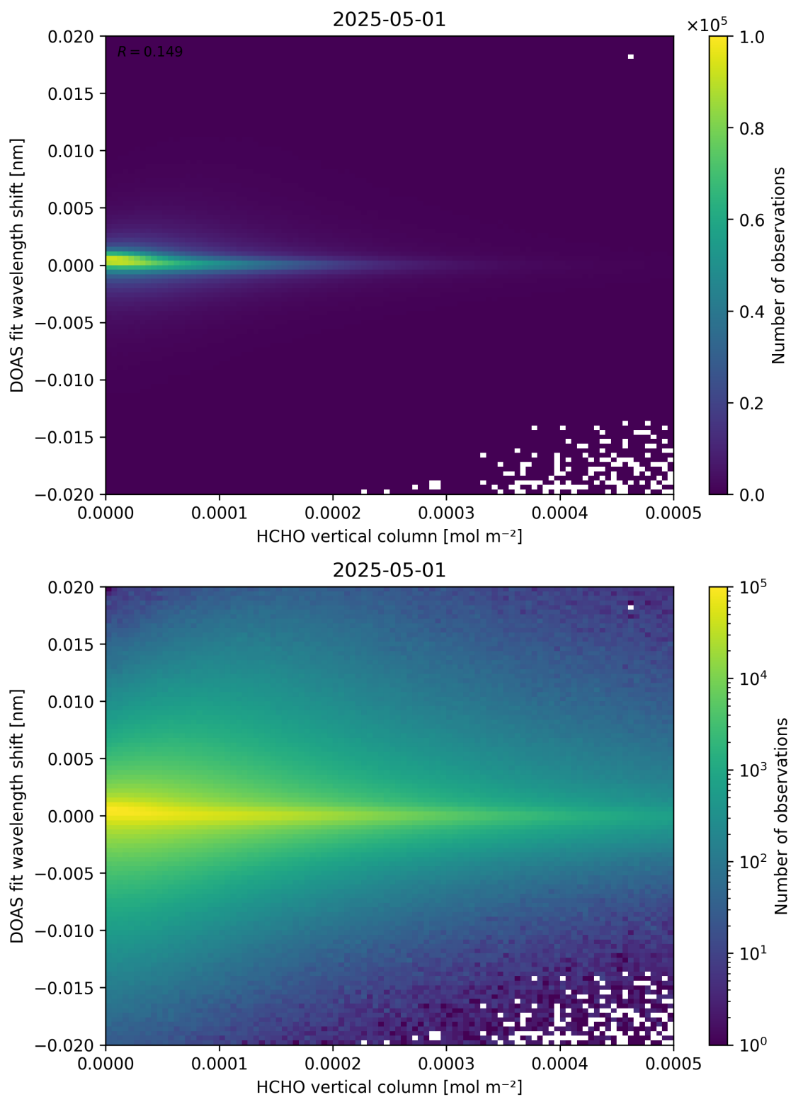
Figure 124: Scatter density plot of “HCHO vertical column” against “DOAS fit wavelength shift” for 2025-04-30 to 2025-05-02.
