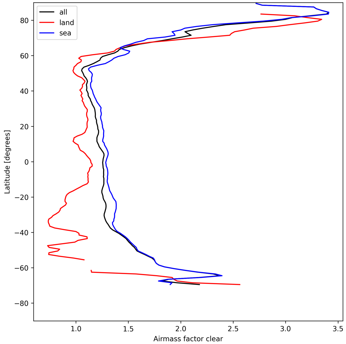
Figure 28: Zonal average of “Airmass factor clear” for 2025-04-30 to 2025-05-02.
