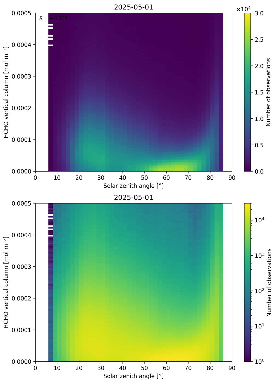
Figure 177: Scatter density plot of “Solar zenith angle” against “HCHO vertical column” for 2025-04-30 to 2025-05-02.
