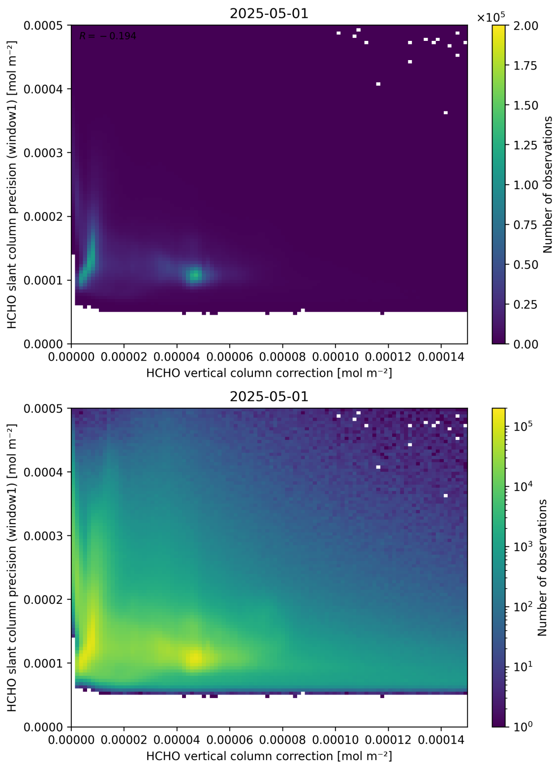
Figure 119: Scatter density plot of “HCHO vertical column correction” against “HCHO slant column precision (window1)” for 2025-04-30 to 2025-05-02.
