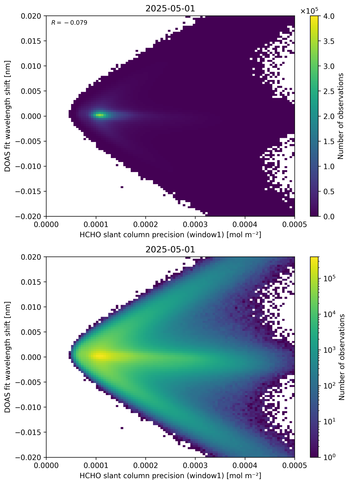
Figure 89: Scatter density plot of “HCHO slant column precision (window1)” against “DOAS fit wavelength shift” for 2025-04-30 to 2025-05-02.
