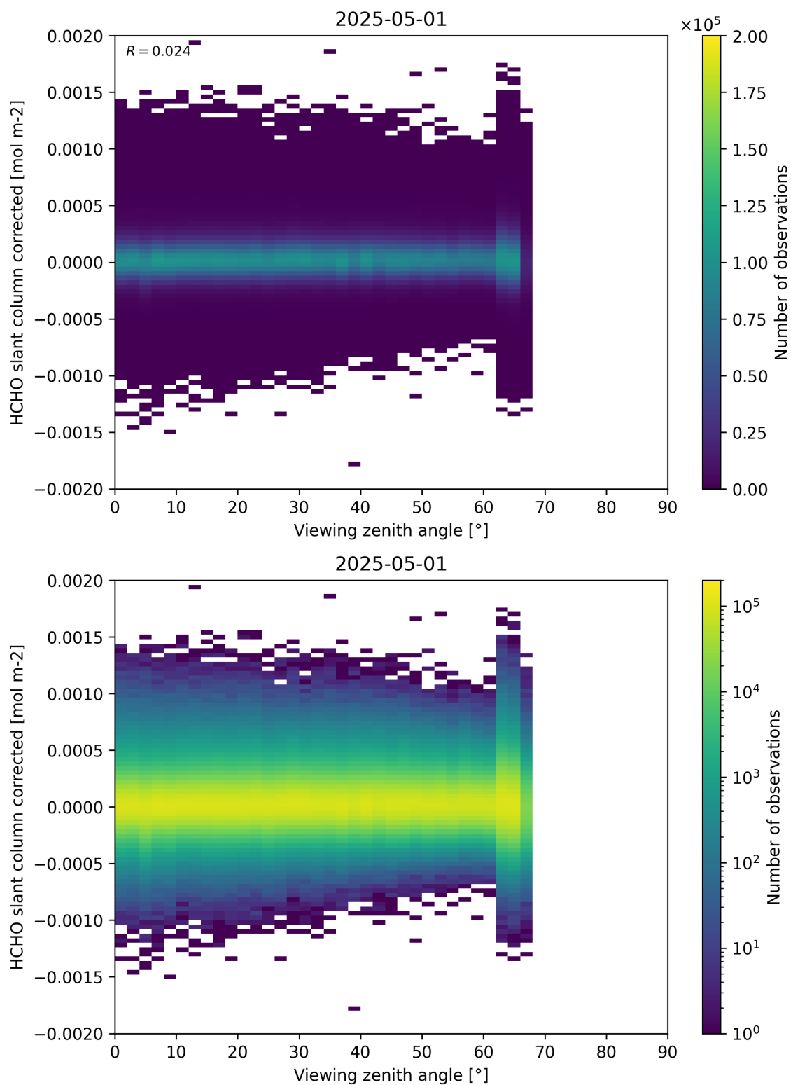
Figure 186: Scatter density plot of “Viewing zenith angle” against “HCHO slant column corrected” for 2025-04-30 to 2025-05-02.
