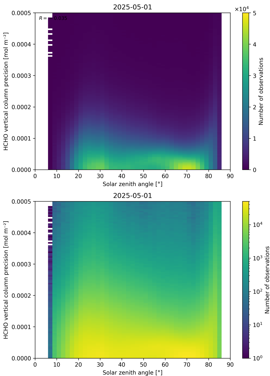
Figure 179: Scatter density plot of “Solar zenith angle” against “HCHO vertical column precision” for 2025-04-30 to 2025-05-02.
