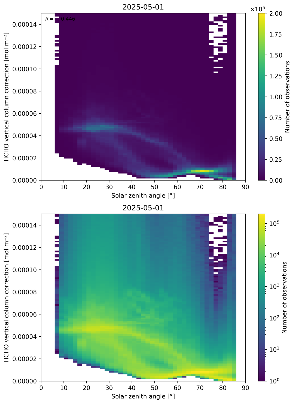
Figure 178: Scatter density plot of “Solar zenith angle” against “HCHO vertical column correction” for 2025-04-30 to 2025-05-02.
