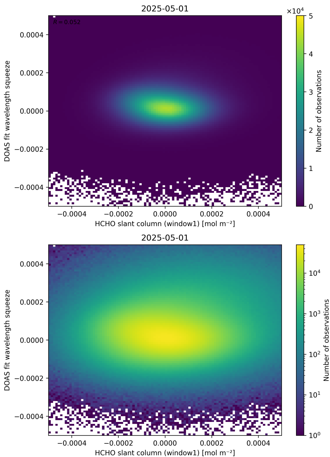
Figure 80: Scatter density plot of “HCHO slant column (window1)” against “DOAS fit wavelength squeeze” for 2025-04-30 to 2025-05-02.
