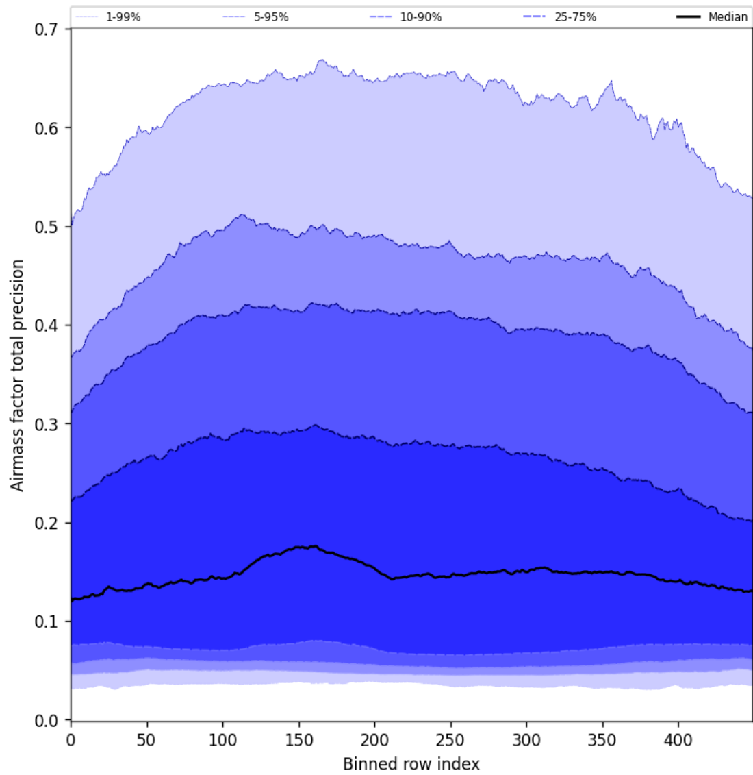
Figure 55: Along track statistics of “Airmass factor total precision” for 2025-04-30 to 2025-05-02
