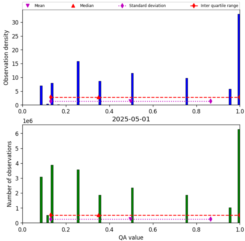
Figure 34: Histogram of “QA value” for 2025-04-30 to 2025-05-02
