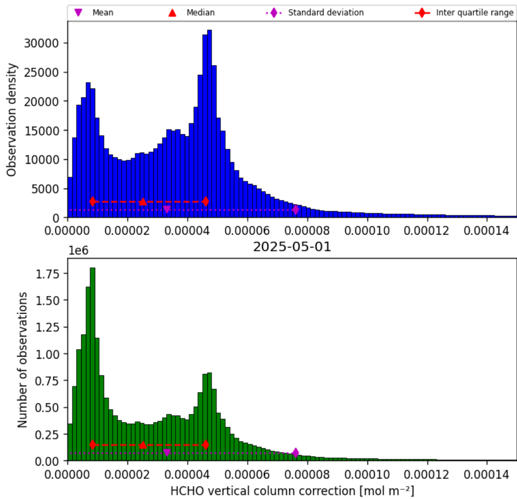
Figure 37: Histogram of “HCHO vertical column correction” for 2025-04-30 to 2025-05-02
