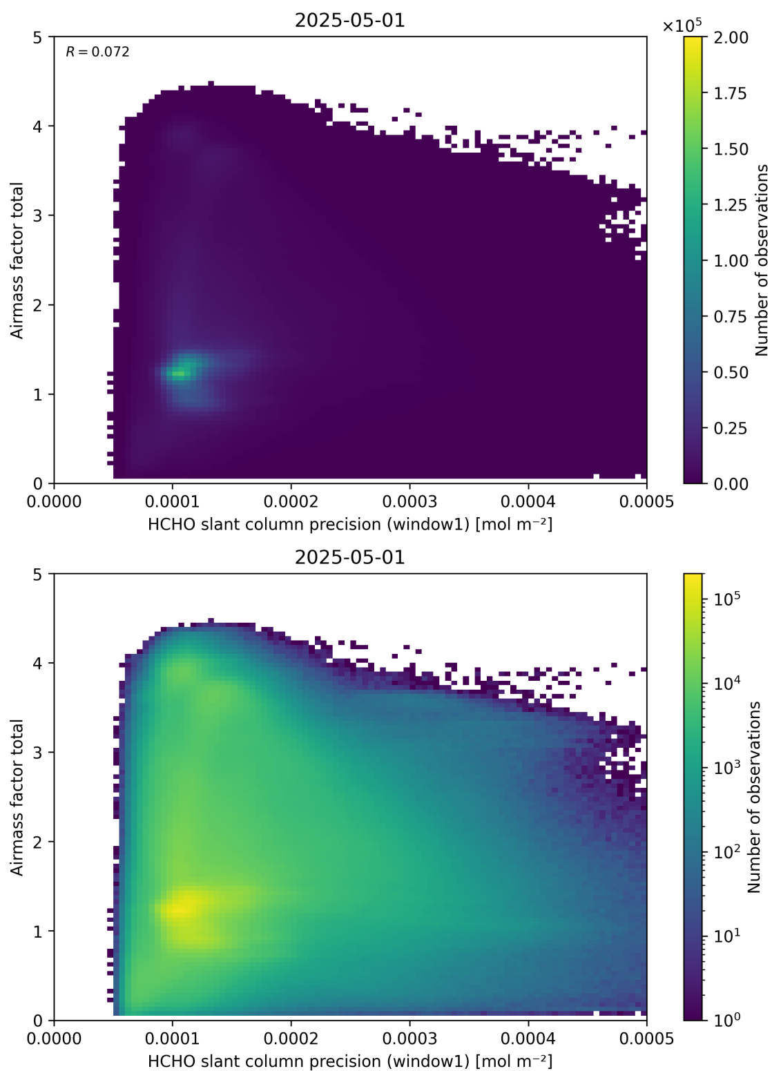
Figure 94: Scatter density plot of “HCHO slant column precision (window1)” against “Airmass factor total” for 2025-04-30 to 2025-05-02.
