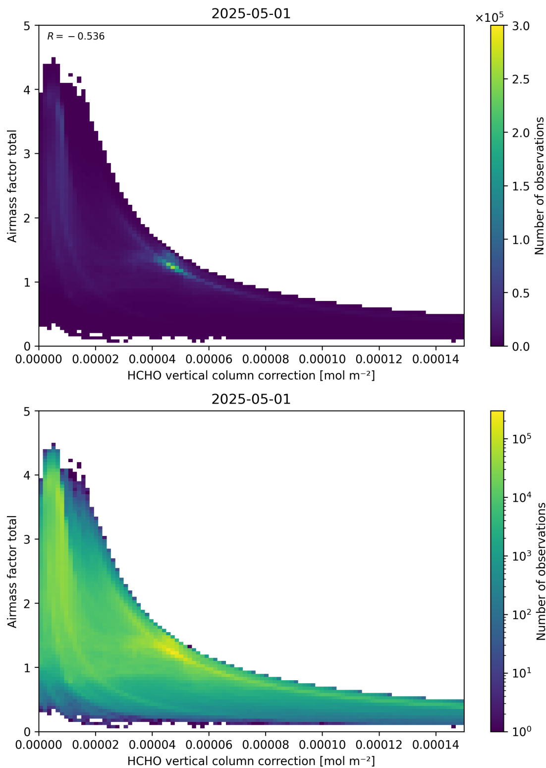
Figure 120: Scatter density plot of “HCHO vertical column correction” against “Airmass factor total” for 2025-04-30 to 2025-05-02.
