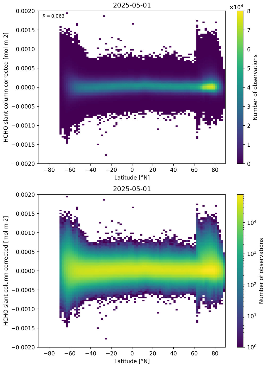
Figure 157: Scatter density plot of “Latitude” against “HCHO slant column corrected” for 2025-04-30 to 2025-05-02.
