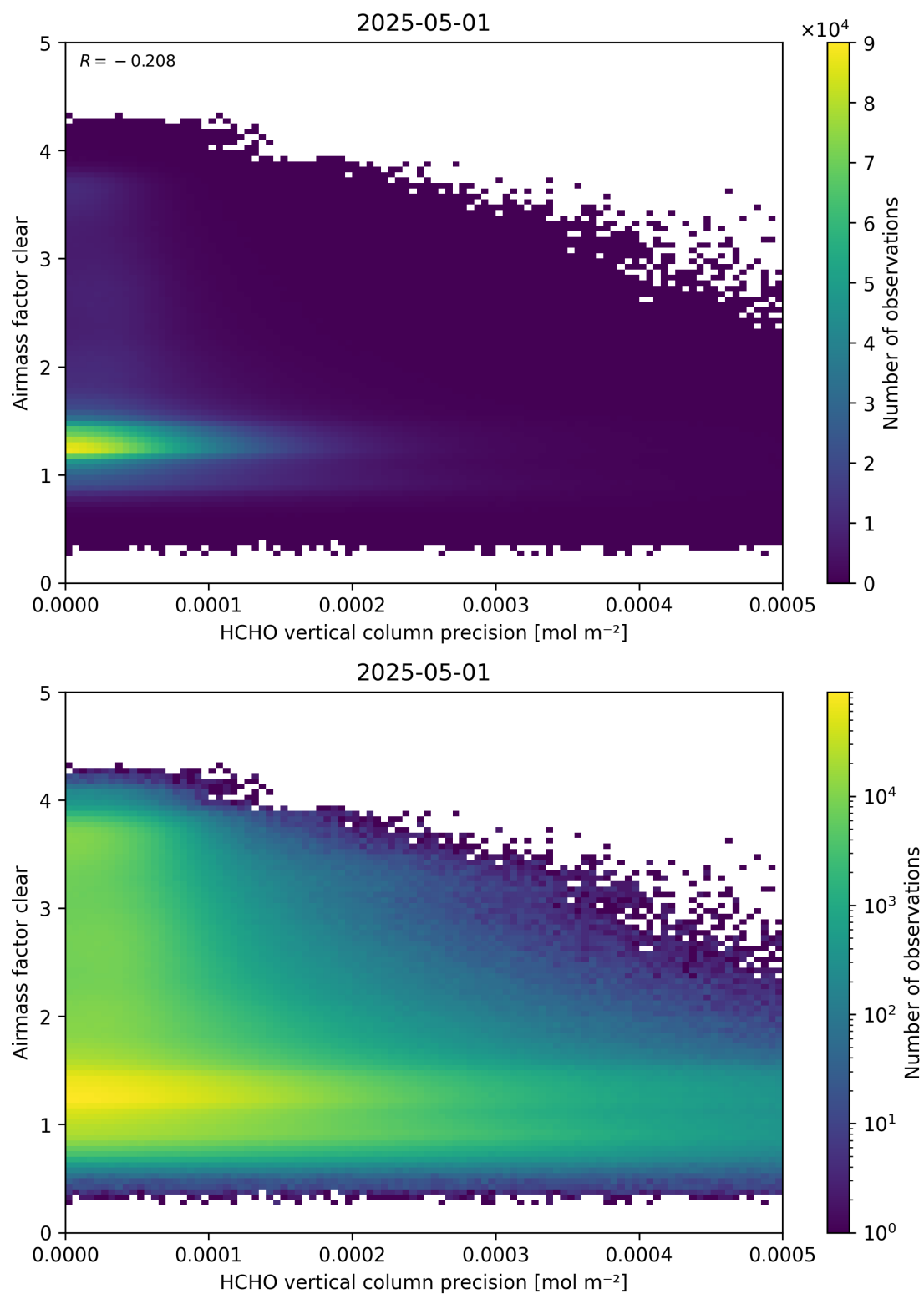
Figure 139: Scatter density plot of “HCHO vertical column precision” against “Airmass factor clear” for 2025-04-30 to 2025-05-02.
