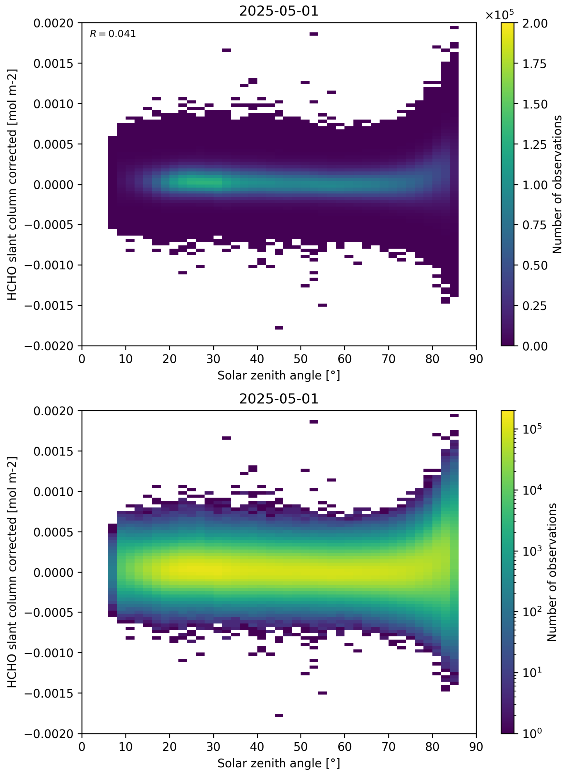
Figure 171: Scatter density plot of “Solar zenith angle” against “HCHO slant column corrected” for 2025-04-30 to 2025-05-02.
