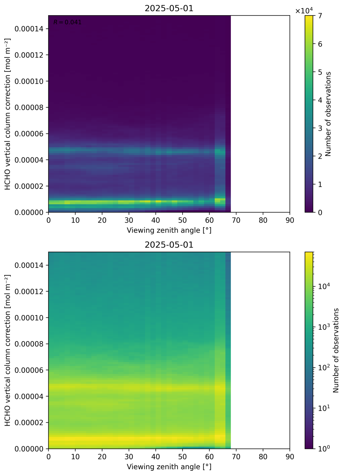
Figure 193: Scatter density plot of “Viewing zenith angle” against “HCHO vertical column correction” for 2025-04-30 to 2025-05-02.
