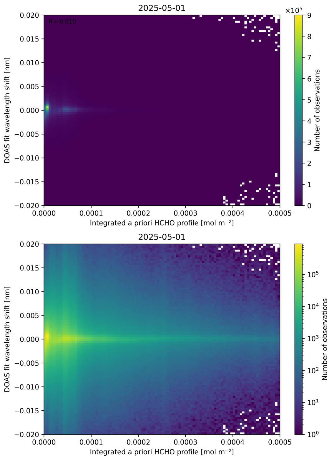
Figure 149: Scatter density plot of “Integrated a priori HCHO profile” against “DOAS fit wavelength shift” for 2025-04-30 to 2025-05-02.
