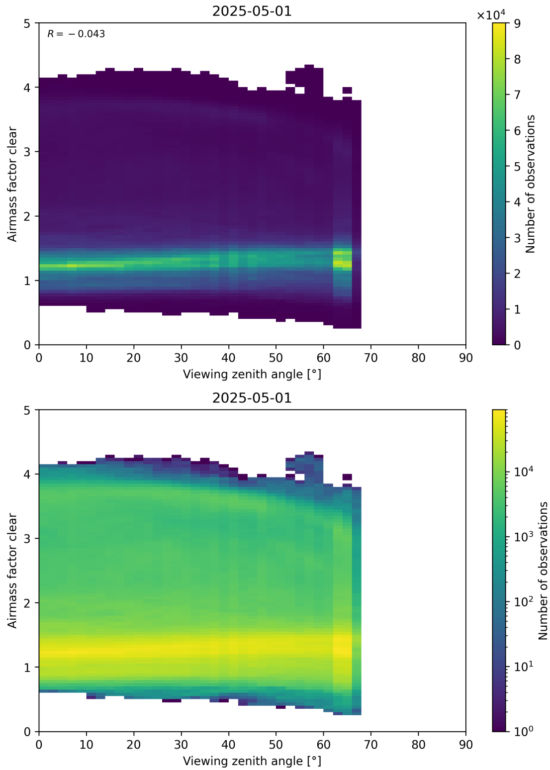
Figure 185: Scatter density plot of “Viewing zenith angle” against “Airmass factor clear” for 2025-04-30 to 2025-05-02.
