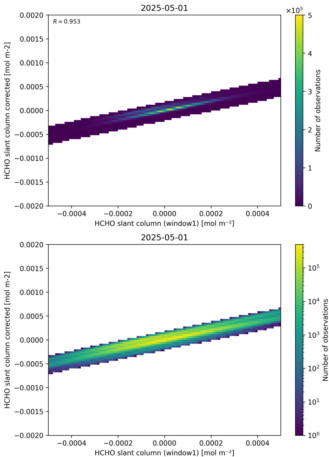
Figure 82: Scatter density plot of “HCHO slant column (window1)” against “HCHO slant column corrected” for 2025-04-30 to 2025-05-02.
