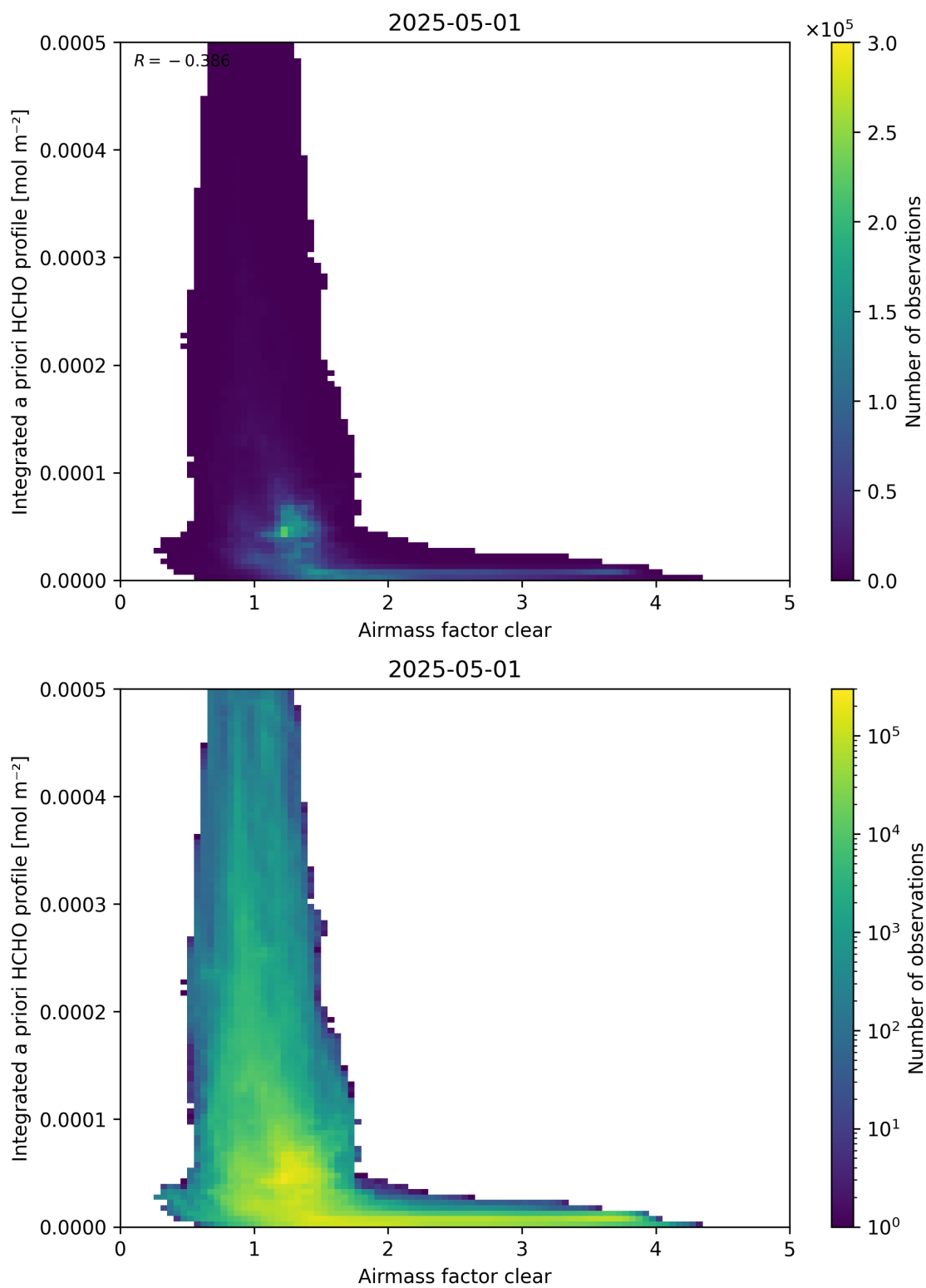
Figure 76: Scatter density plot of “Airmass factor clear” against “Integrated a priori HCHO profile” for 2025-04-30 to 2025-05-02.
