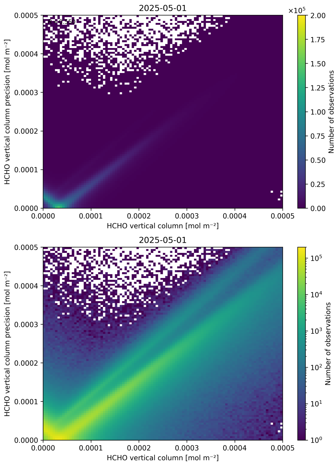
Figure 134: Scatter density plot of “HCHO vertical column” against “HCHO vertical column precision” for 2025-04-30 to 2025-05-02.
