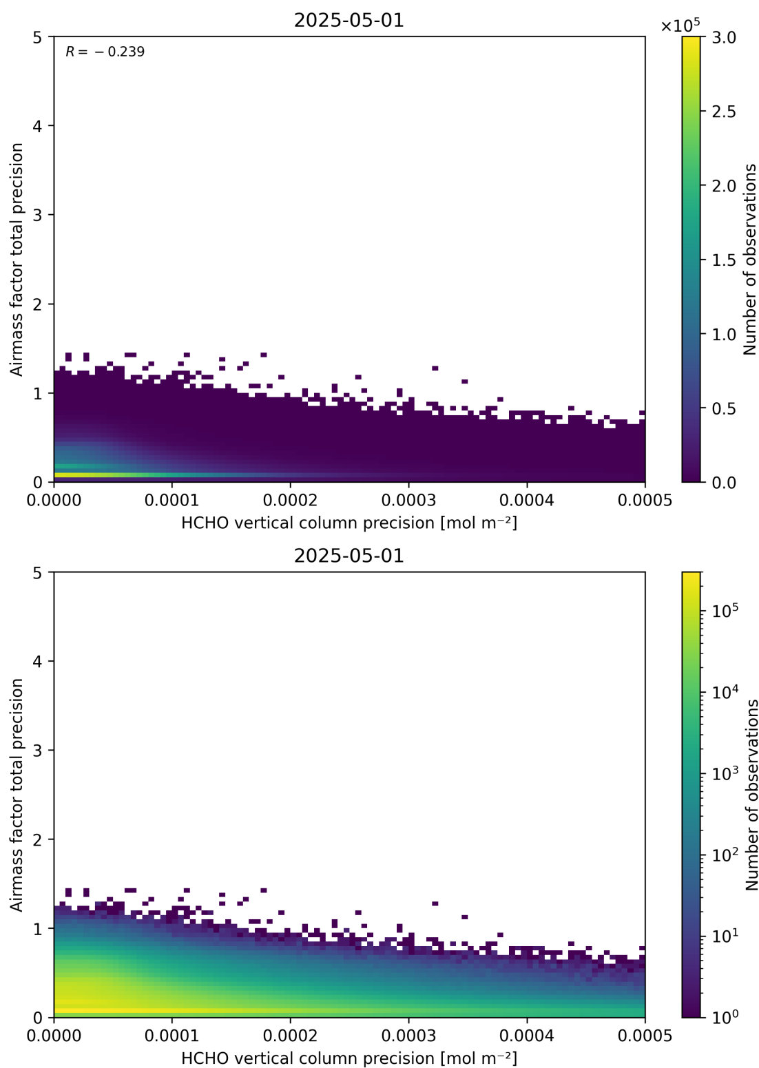
Figure 145: Scatter density plot of “HCHO vertical column precision” against “Airmass factor total precision” for 2025-04-30 to 2025-05-02.
