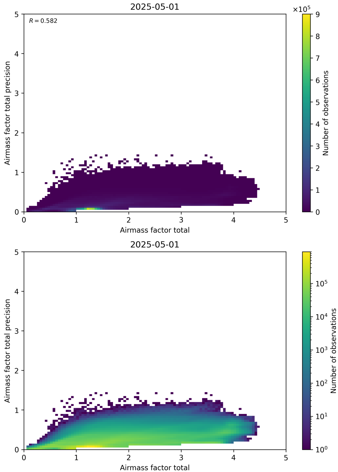
Figure 103: Scatter density plot of “Airmass factor total” against “Airmass factor total precision” for 2025-04-30 to 2025-05-02.
