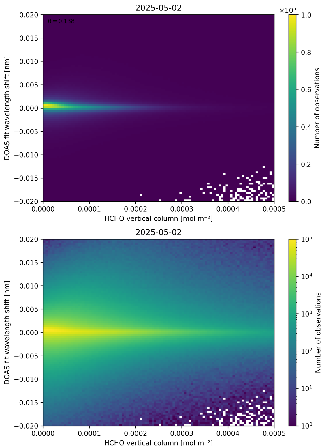
Figure 124: Scatter density plot of “HCHO vertical column” against “DOAS fit wavelength shift” for 2025-05-01 to 2025-05-03.
