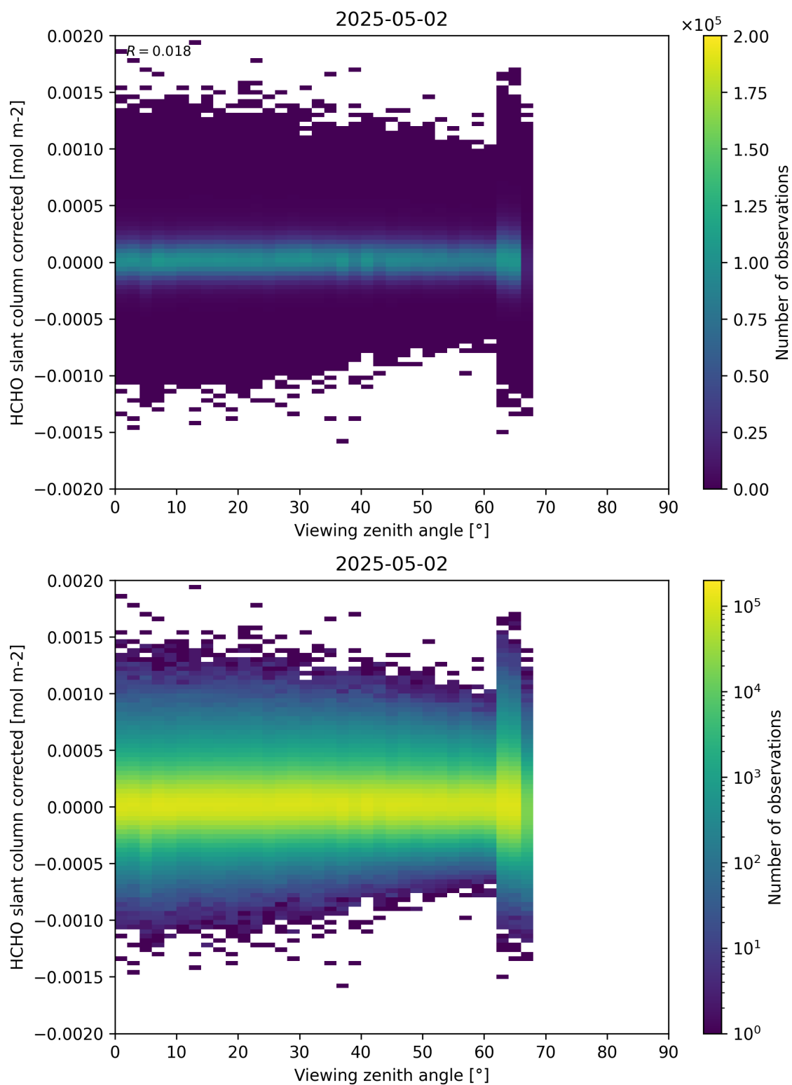
Figure 186: Scatter density plot of “Viewing zenith angle” against “HCHO slant column corrected” for 2025-05-01 to 2025-05-03.
