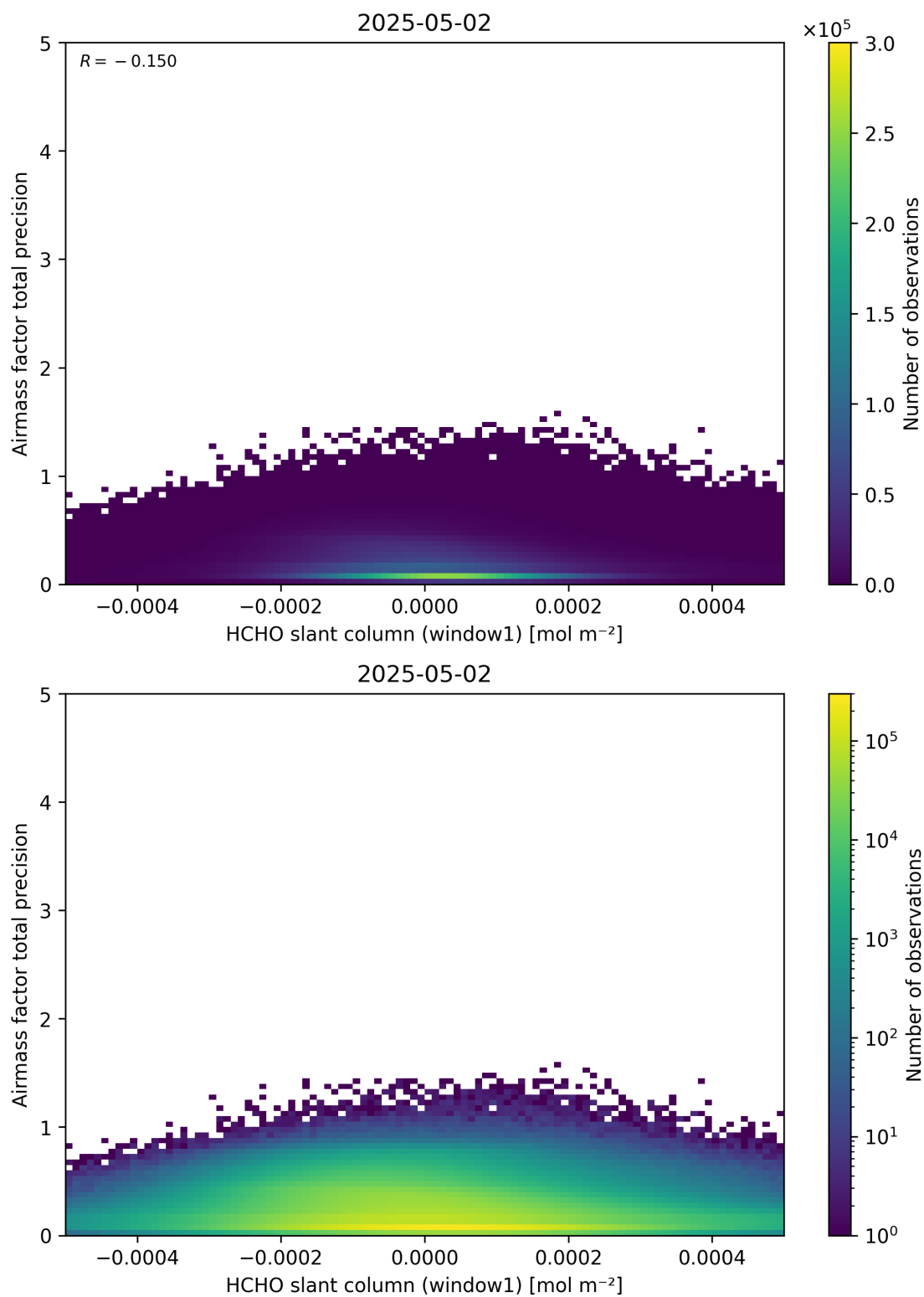
Figure 86: Scatter density plot of “HCHO slant column (window1)” against “Airmass factor total precision” for 2025-05-01 to 2025-05-03.
