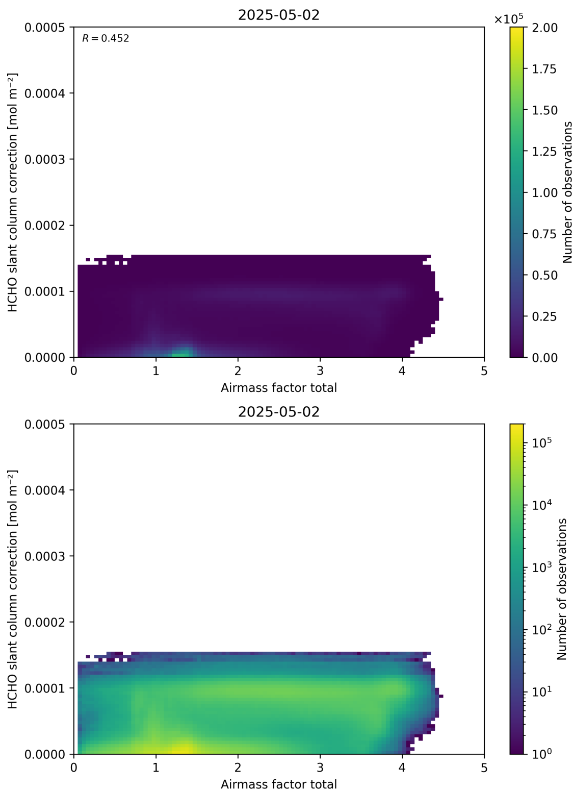
Figure 102: Scatter density plot of “Airmass factor total” against “HCHO slant column correction” for 2025-05-01 to 2025-05-03.
