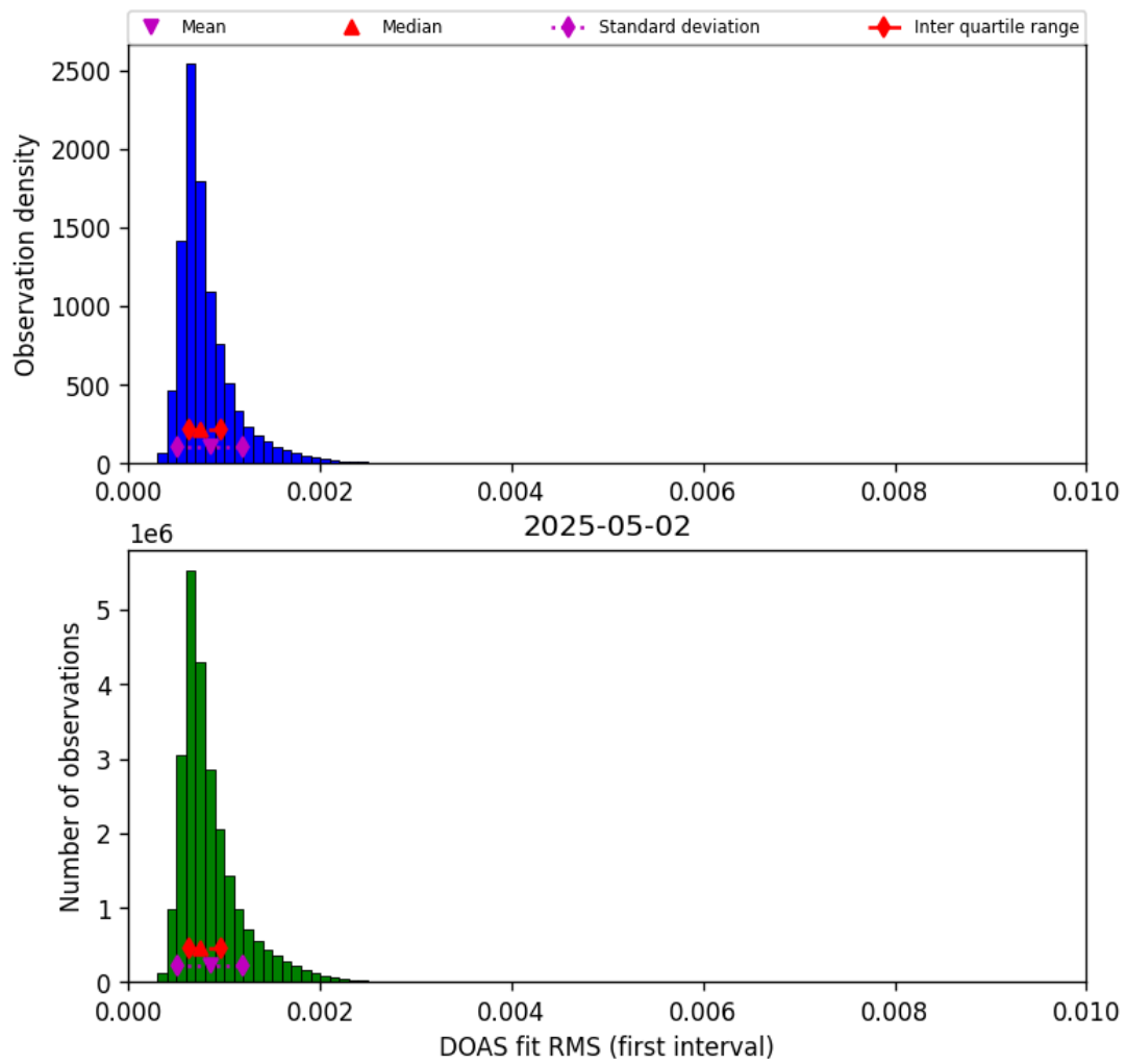
Figure 46: Histogram of “DOAS fit RMS (first interval)” for 2025-05-01 to 2025-05-03
