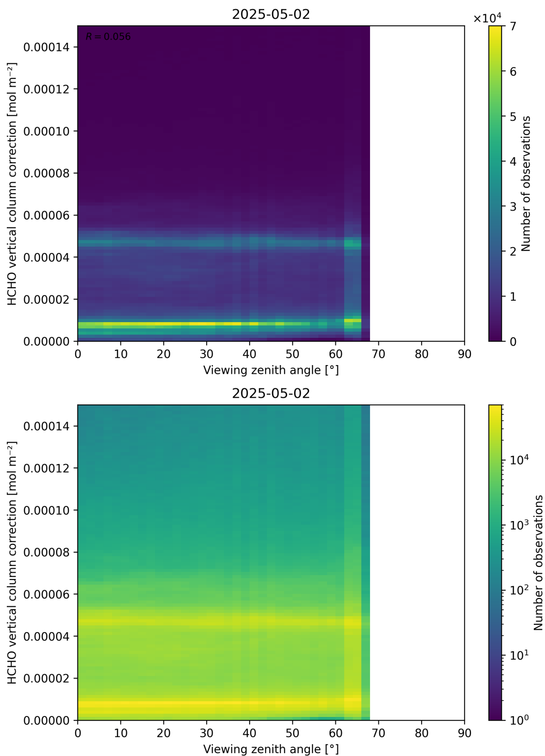
Figure 193: Scatter density plot of “Viewing zenith angle” against “HCHO vertical column correction” for 2025-05-01 to 2025-05-03.
