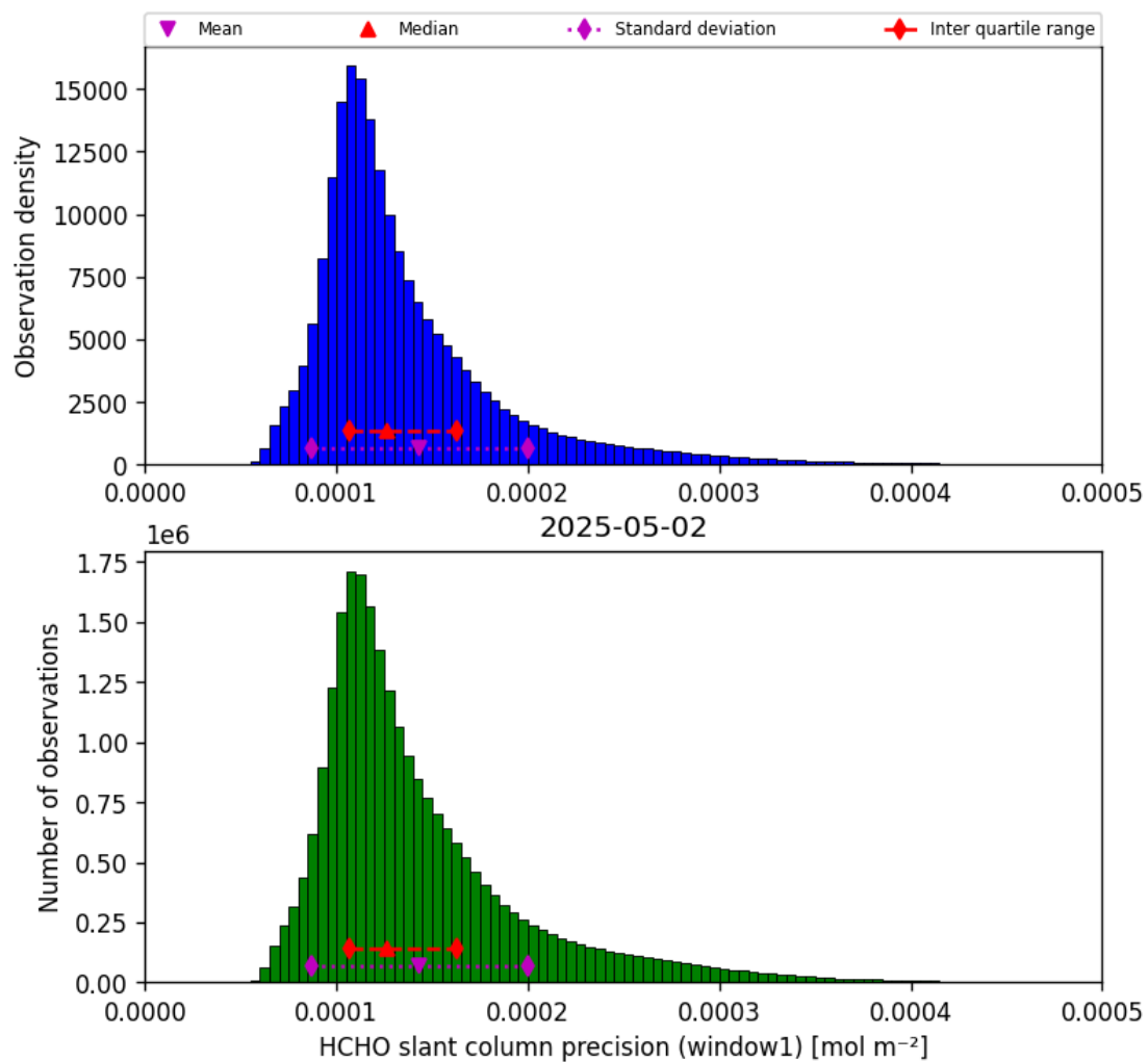
Figure 39: Histogram of “HCHO slant column precision (window1)” for 2025-05-01 to 2025-05-03
