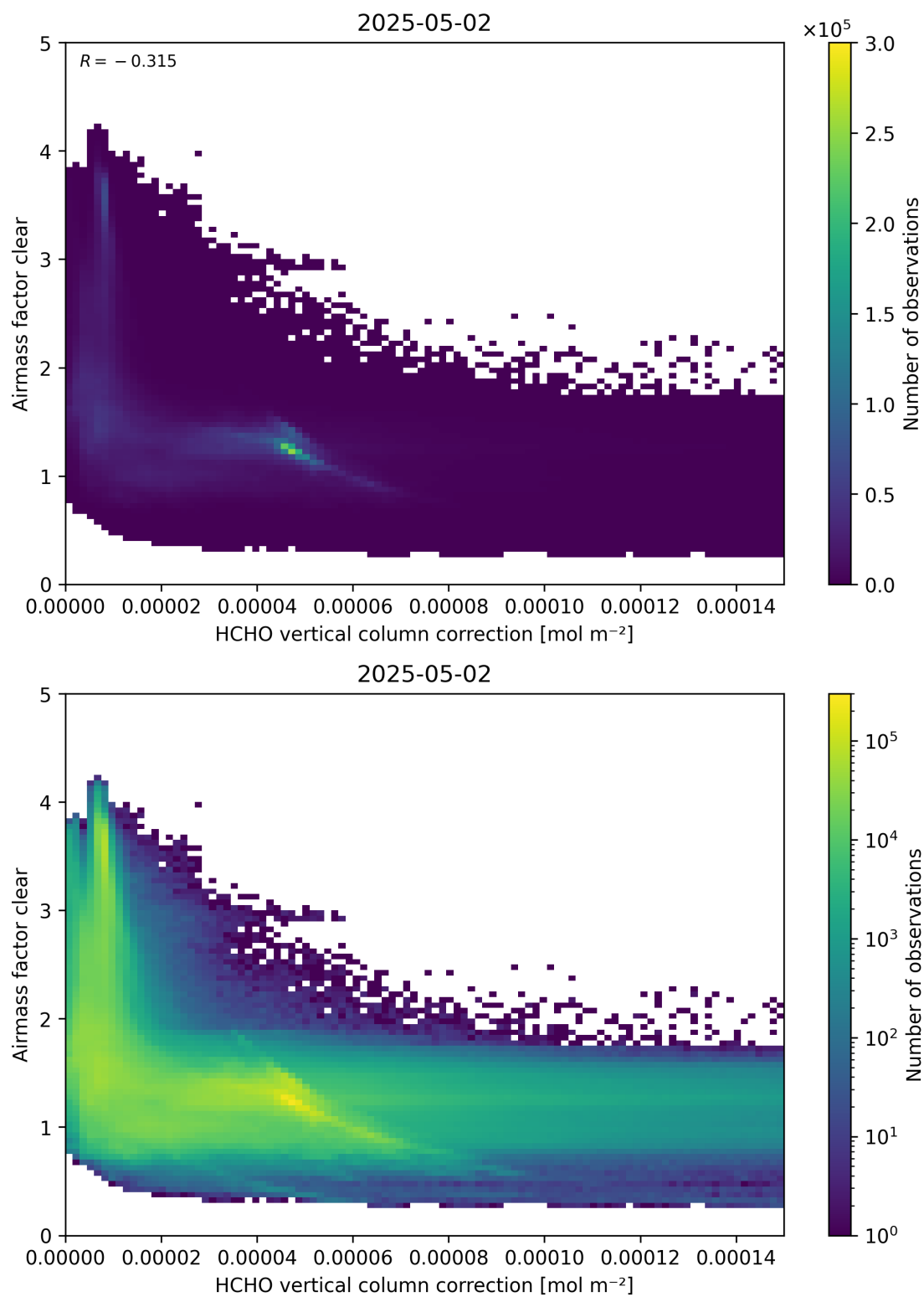
Figure 115: Scatter density plot of “HCHO vertical column correction” against “Airmass factor clear” for 2025-05-01 to 2025-05-03.
