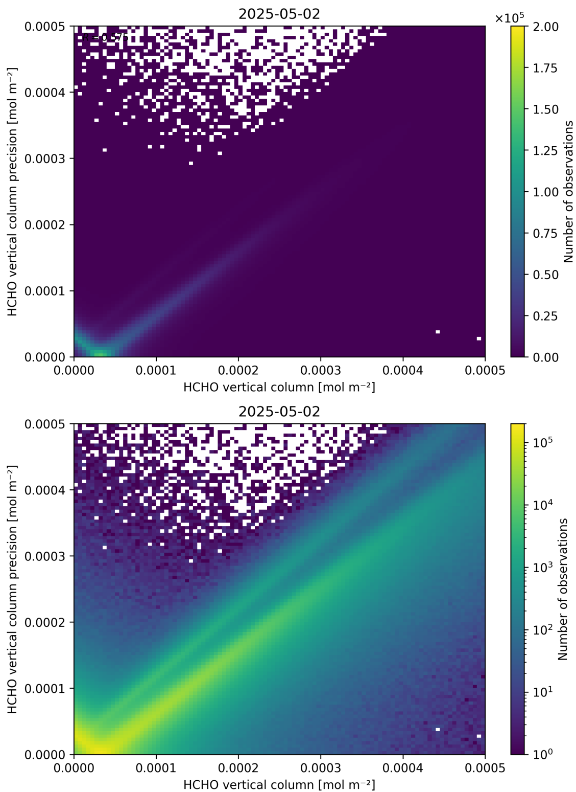
Figure 134: Scatter density plot of “HCHO vertical column” against “HCHO vertical column precision” for 2025-05-01 to 2025-05-03.
