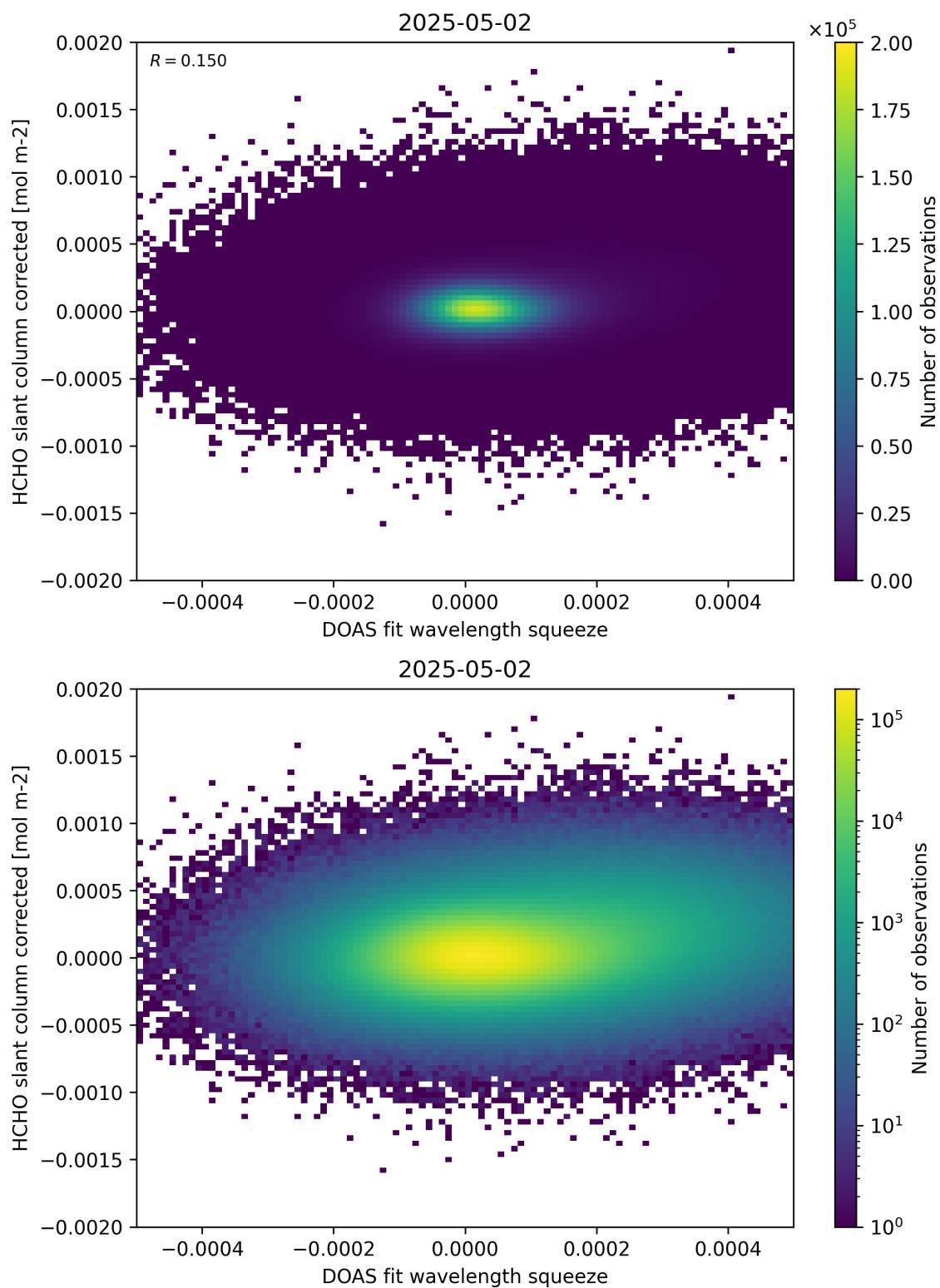
Figure 69: Scatter density plot of “DOAS fit wavelength squeeze” against “HCHO slant column corrected” for 2025-05-01 to 2025-05-03.
