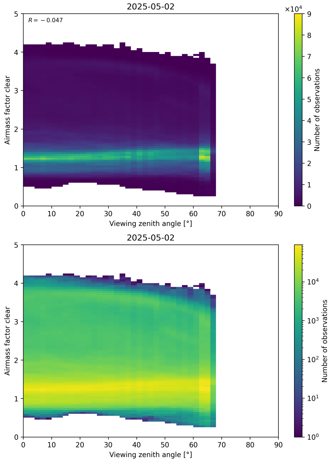
Figure 185: Scatter density plot of “Viewing zenith angle” against “Airmass factor clear” for 2025-05-01 to 2025-05-03.
