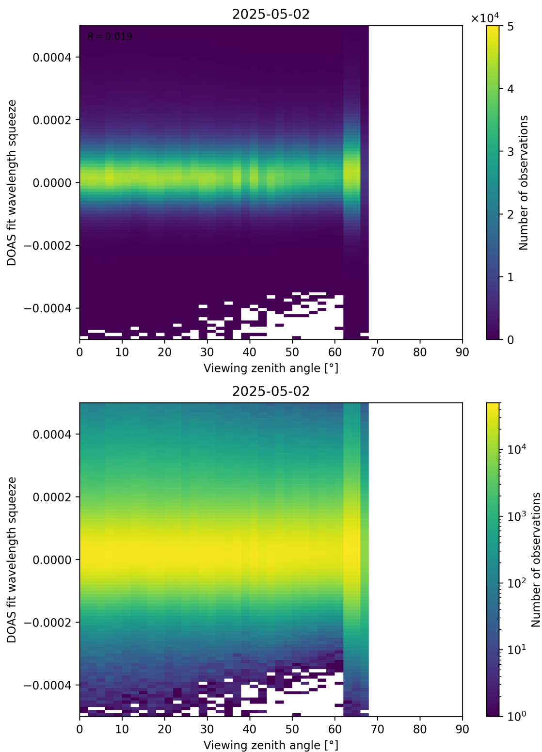
Figure 184: Scatter density plot of “Viewing zenith angle” against “DOAS fit wavelength squeeze” for 2025-05-01 to 2025-05-03.
