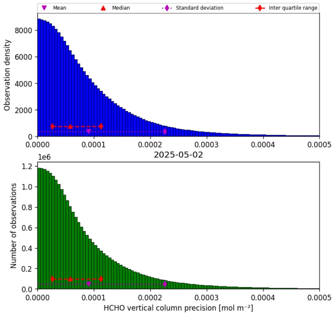
Figure 36: Histogram of “HCHO vertical column precision” for 2025-05-01 to 2025-05-03
