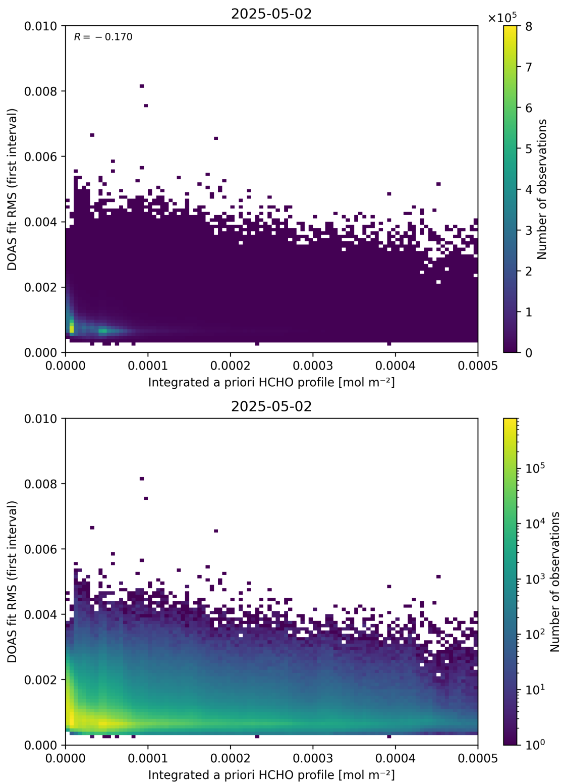
Figure 148: Scatter density plot of “Integrated a priori HCHO profile” against “DOAS fit RMS (first interval)” for 2025-05-01 to 2025-05-03.
