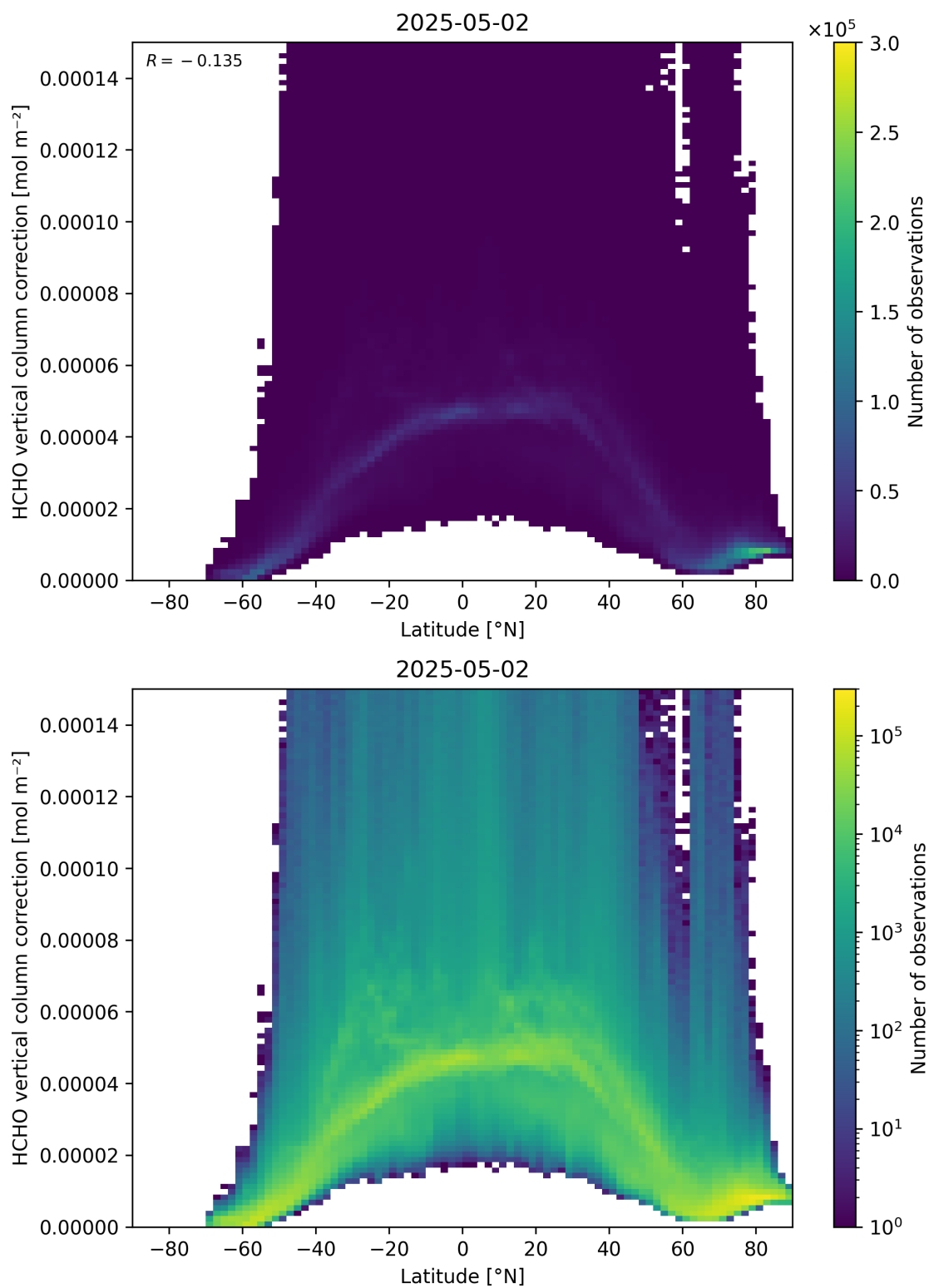
Figure 164: Scatter density plot of “Latitude” against “HCHO vertical column correction” for 2025-05-01 to 2025-05-03.
