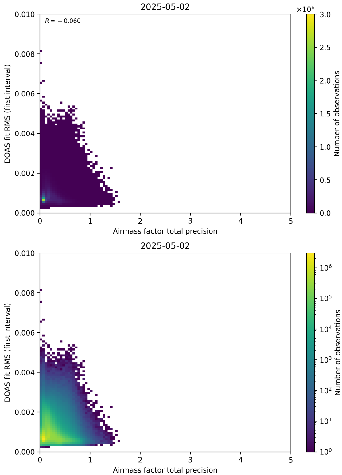
Figure 105: Scatter density plot of “Airmass factor total precision” against “DOAS fit RMS (first interval)” for 2025-05-01 to 2025-05-03.
