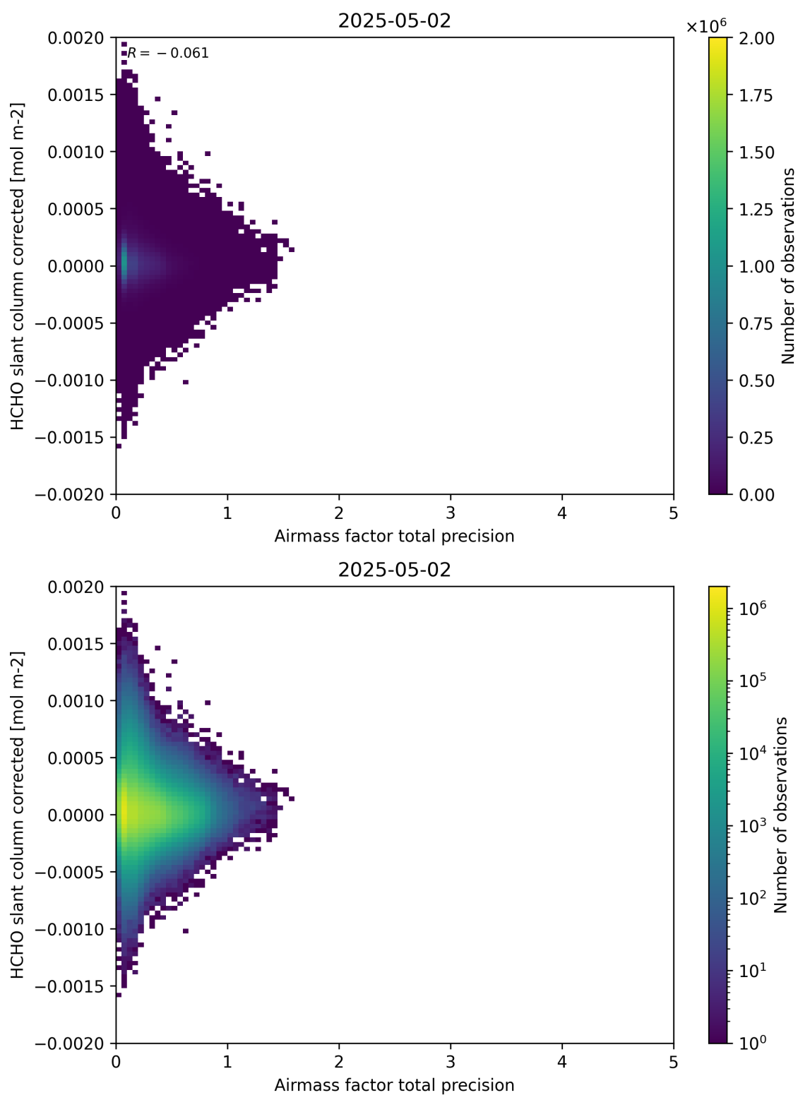
Figure 109: Scatter density plot of “Airmass factor total precision” against “HCHO slant column corrected” for 2025-05-01 to 2025-05-03.
