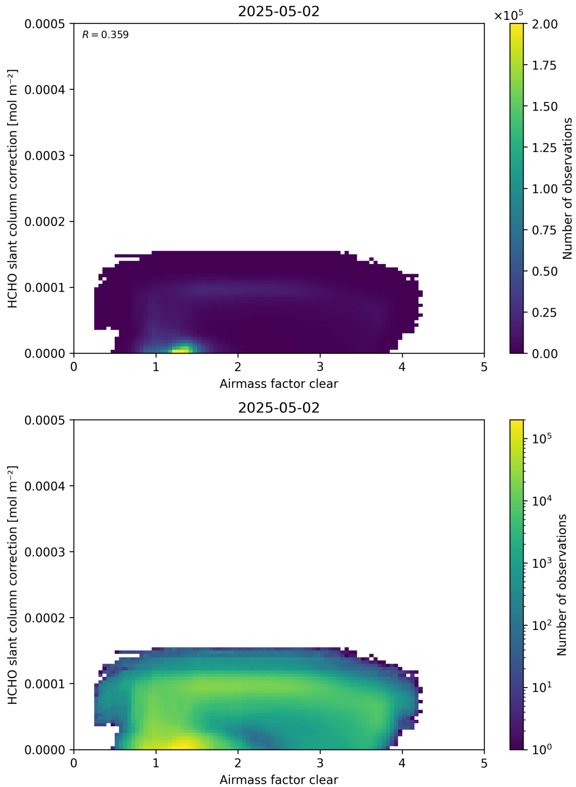
Figure 75: Scatter density plot of “Airmass factor clear” against “HCHO slant column correction” for 2025-05-01 to 2025-05-03.
