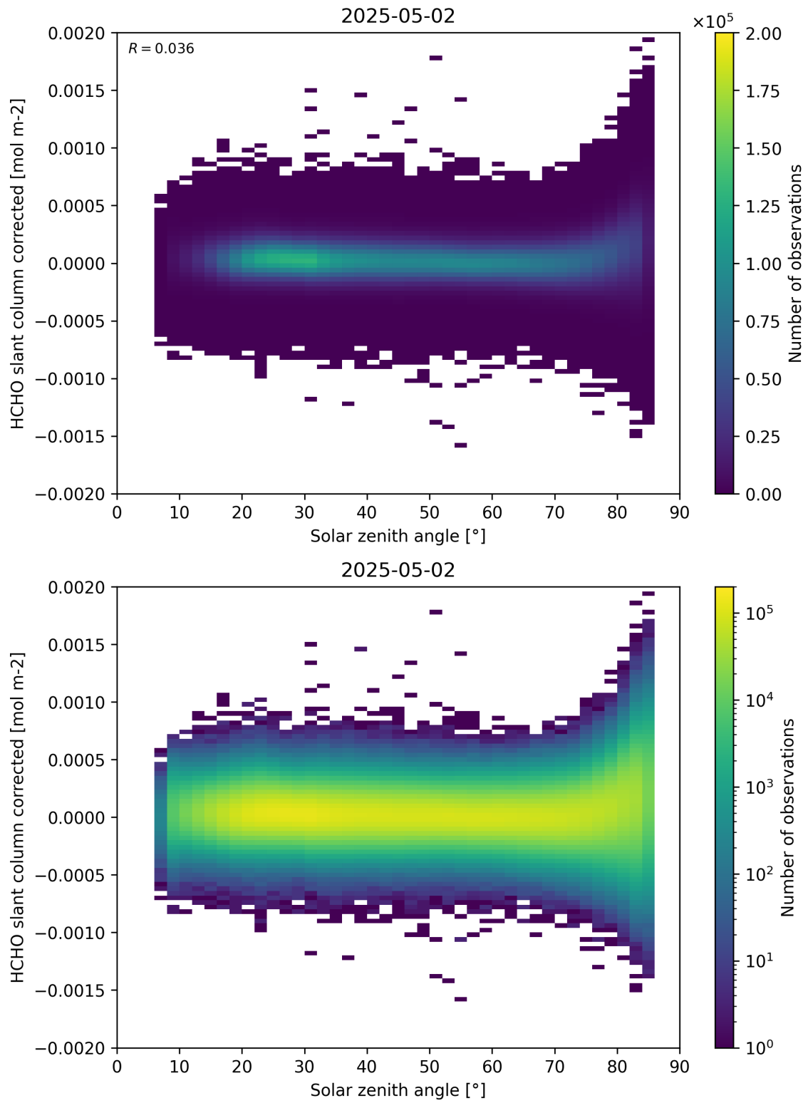
Figure 171: Scatter density plot of “Solar zenith angle” against “HCHO slant column corrected” for 2025-05-01 to 2025-05-03.
