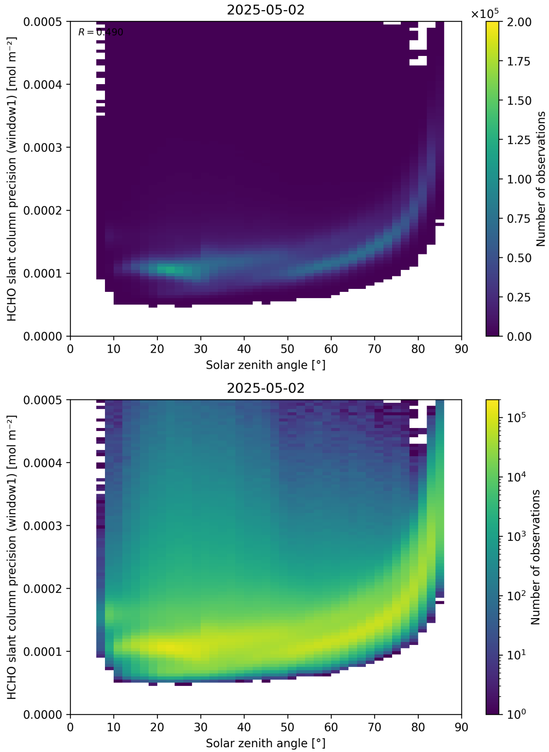
Figure 174: Scatter density plot of “Solar zenith angle” against “HCHO slant column precision (window1)” for 2025-05-01 to 2025-05-03.
