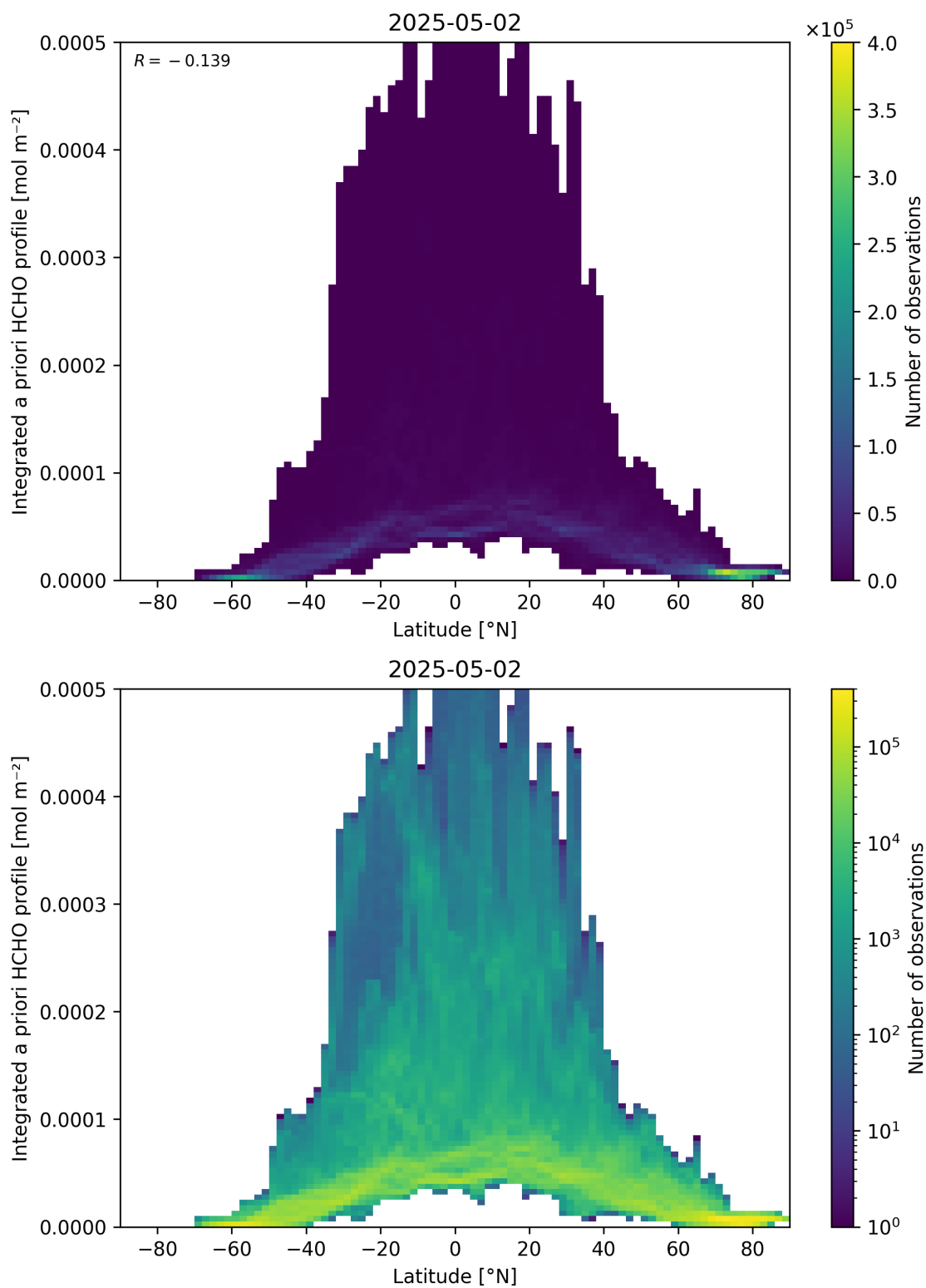
Figure 166: Scatter density plot of “Latitude” against “Integrated a priori HCHO profile” for 2025-05-01 to 2025-05-03.
