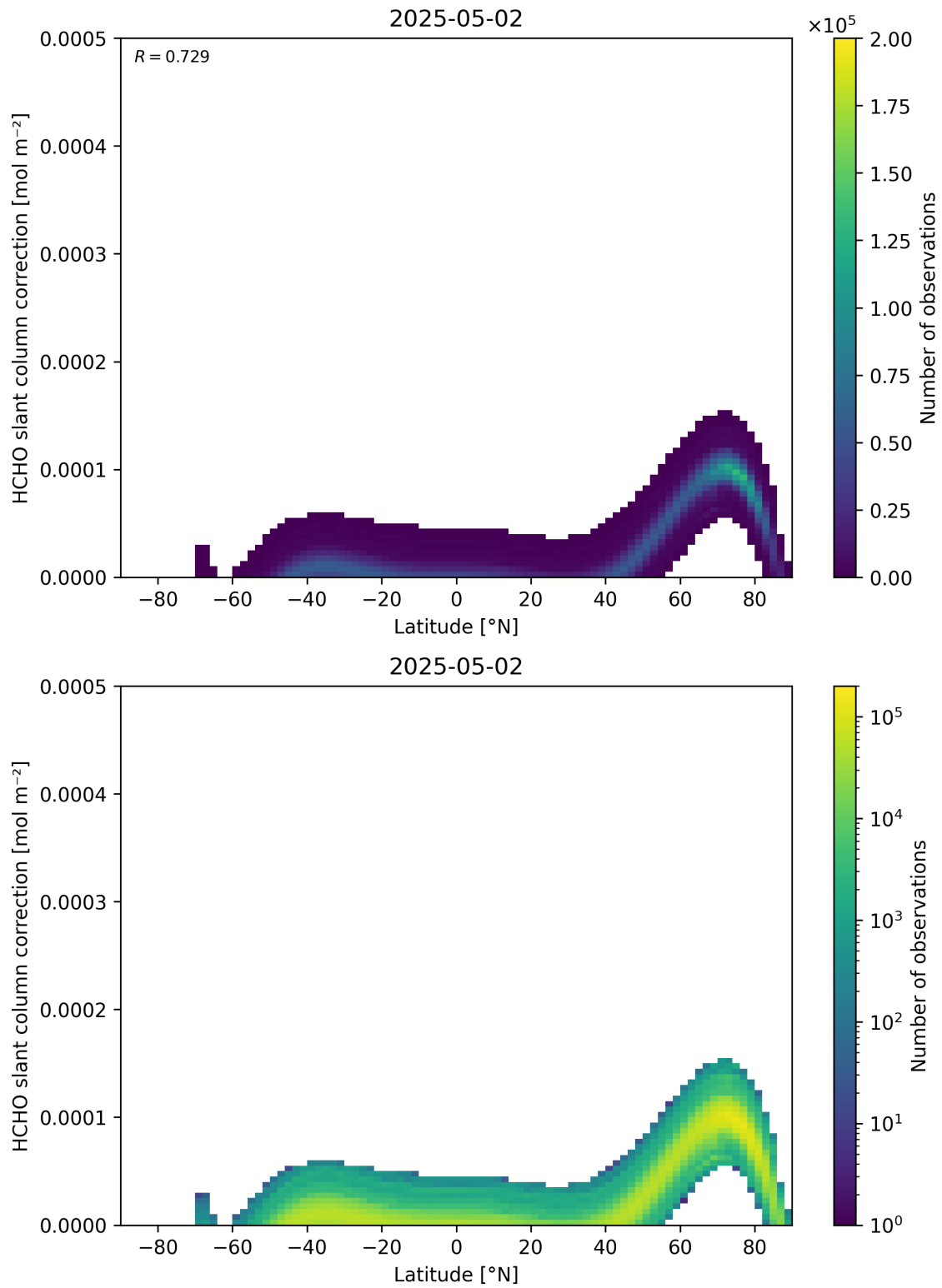
Figure 158: Scatter density plot of “Latitude” against “HCHO slant column correction” for 2025-05-01 to 2025-05-03.
