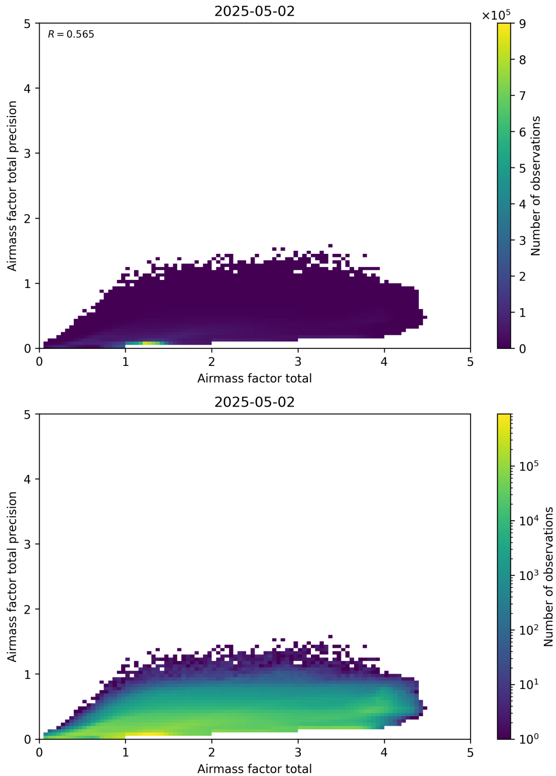
Figure 103: Scatter density plot of “Airmass factor total” against “Airmass factor total precision” for 2025-05-01 to 2025-05-03.
