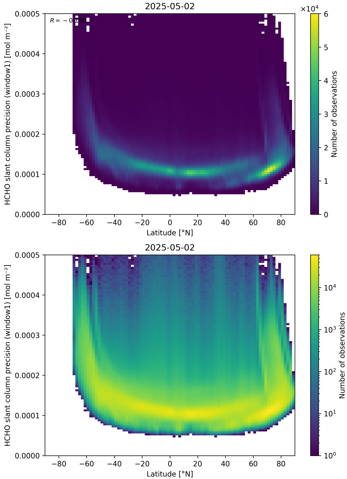
Figure 160: Scatter density plot of “Latitude” against “HCHO slant column precision (window1)” for 2025-05-01 to 2025-05-03.
