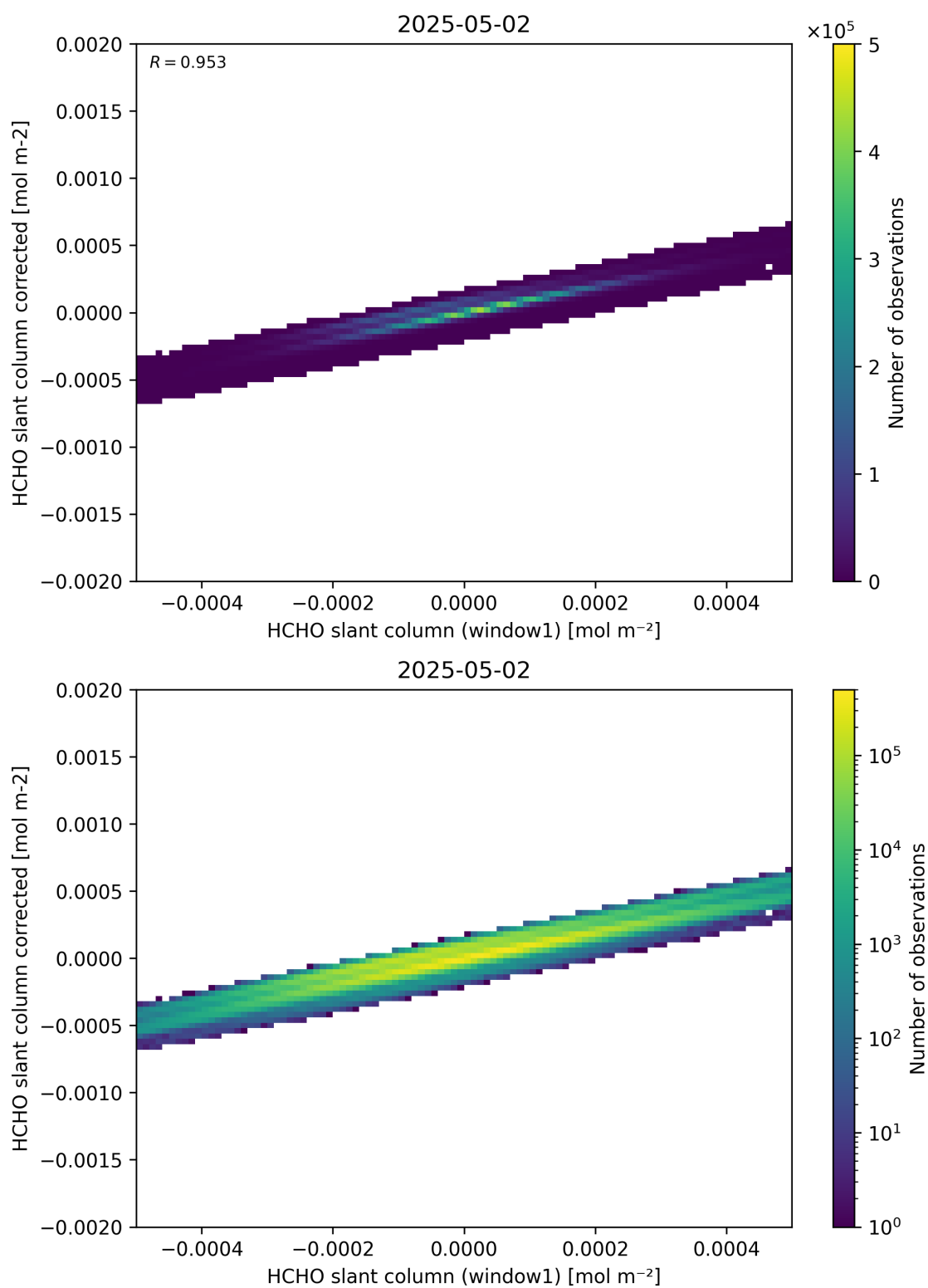
Figure 82: Scatter density plot of “HCHO slant column (window1)” against “HCHO slant column corrected” for 2025-05-01 to 2025-05-03.
