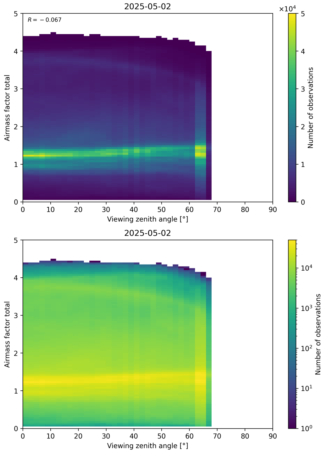
Figure 190: Scatter density plot of “Viewing zenith angle” against “Airmass factor total” for 2025-05-01 to 2025-05-03.
