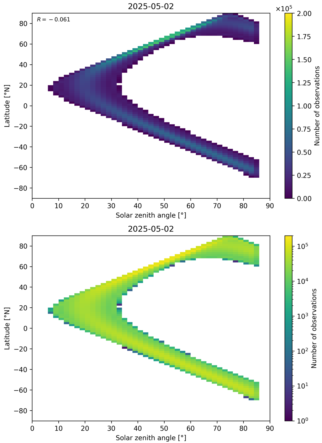
Figure 181: Scatter density plot of “Solar zenith angle” against “Latitude” for 2025-05-01 to 2025-05-03.
