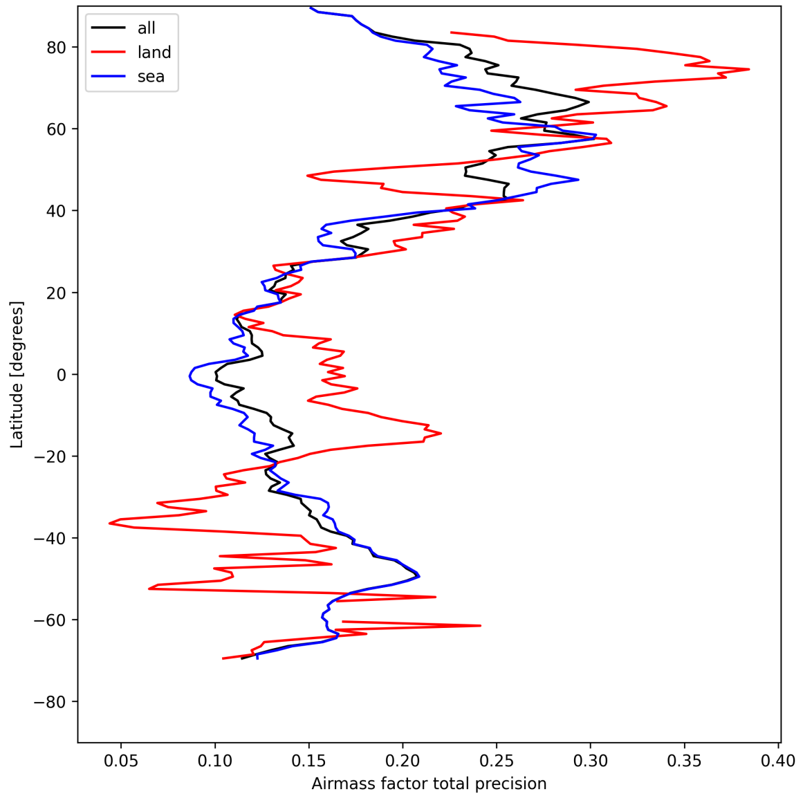
Figure 27: Zonal average of “Airmass factor total precision” for 2025-05-01 to 2025-05-03.
