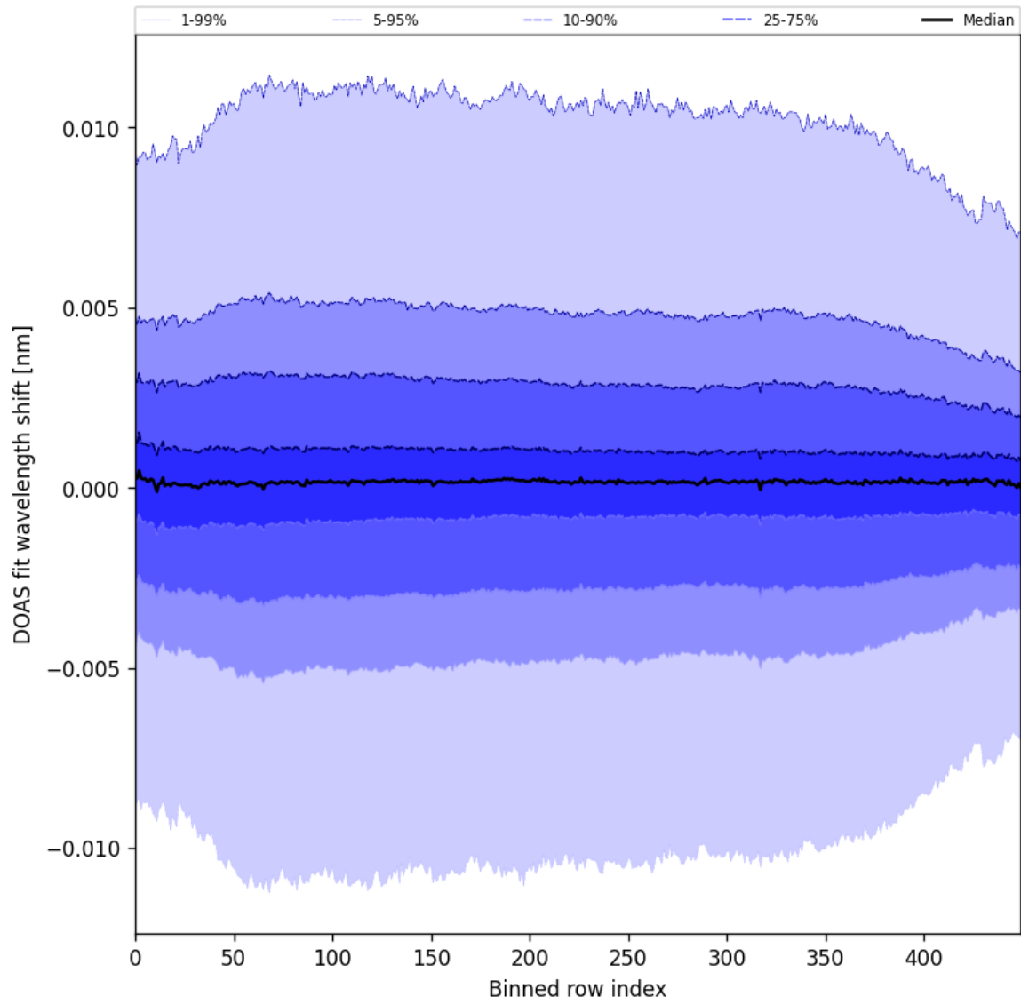
Figure 58: Along track statistics of “DOAS fit wavelength shift” for 2025-05-01 to 2025-05-03
