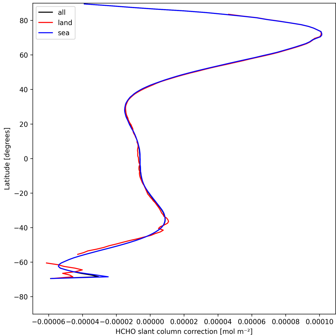
Figure 33: Zonal average of “HCHO slant column correction” for 2025-05-01 to 2025-05-03.
