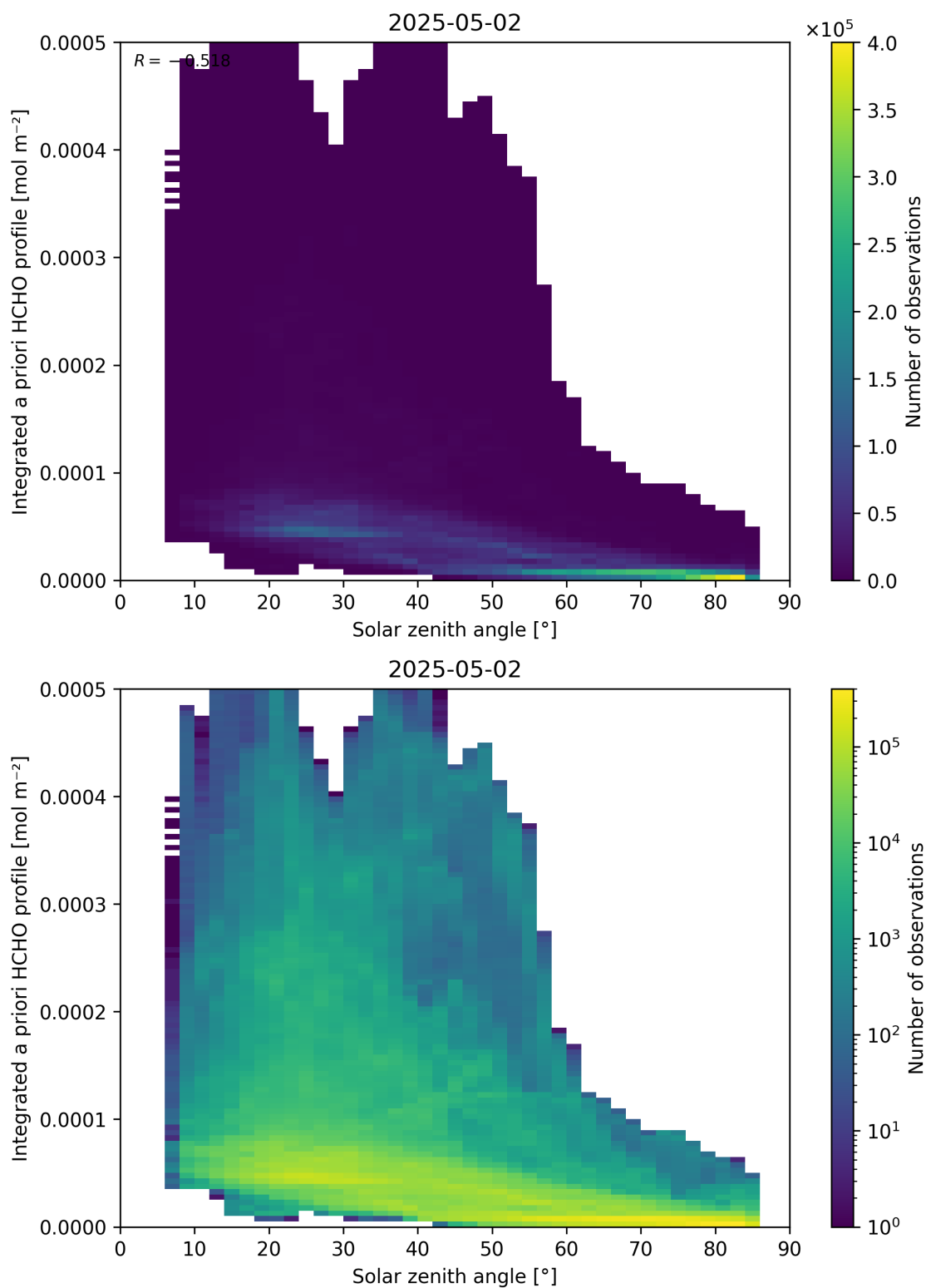
Figure 180: Scatter density plot of “Solar zenith angle” against “Integrated a priori HCHO profile” for 2025-05-01 to 2025-05-03.
