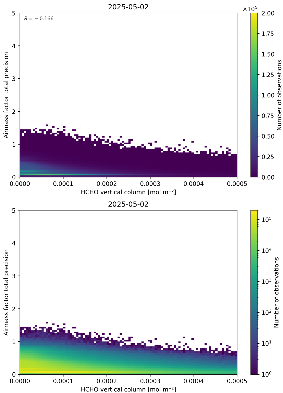
Figure 132: Scatter density plot of “HCHO vertical column” against “Airmass factor total precision” for 2025-05-01 to 2025-05-03.
