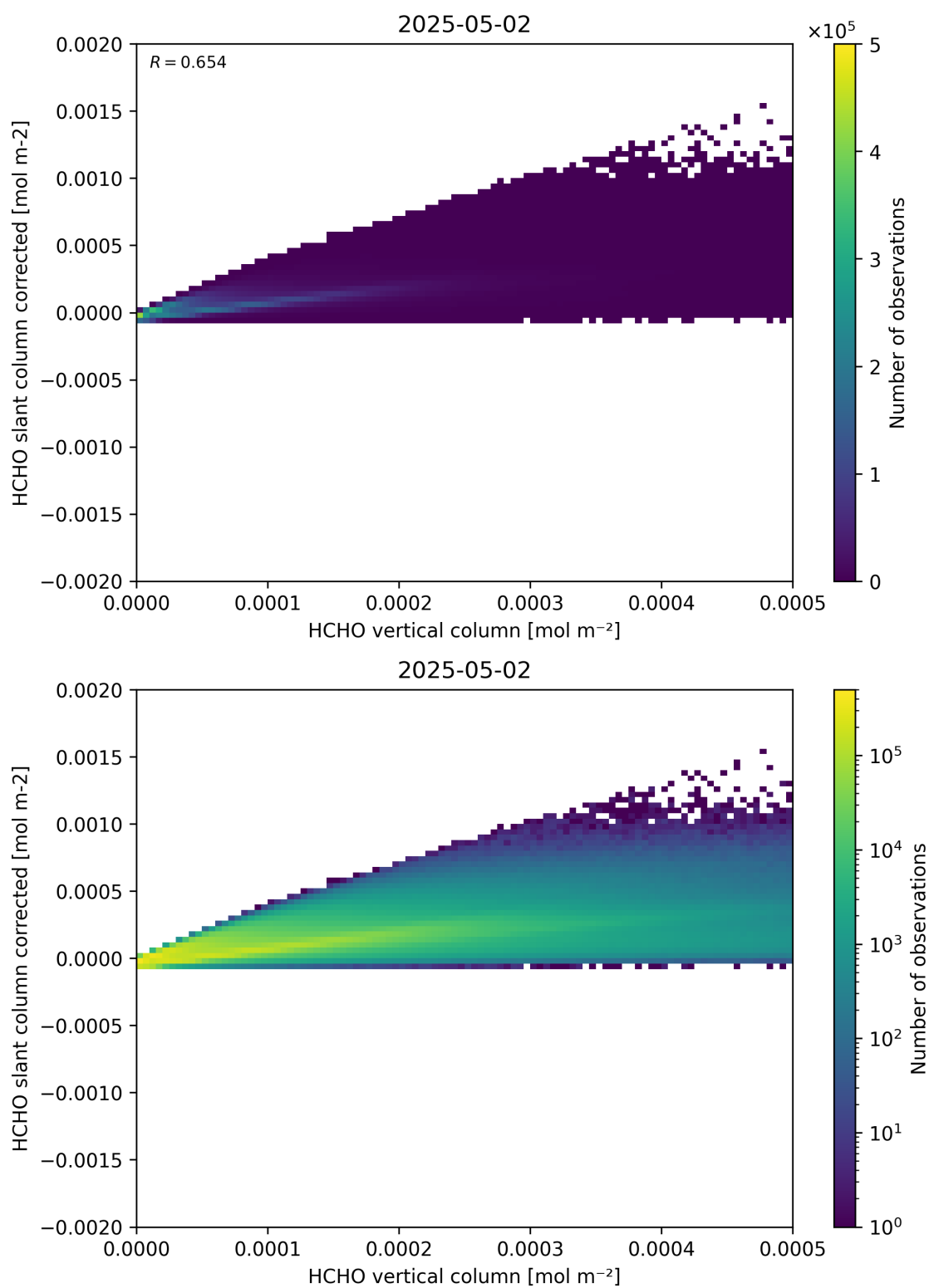
Figure 127: Scatter density plot of “HCHO vertical column” against “HCHO slant column corrected” for 2025-05-01 to 2025-05-03.
