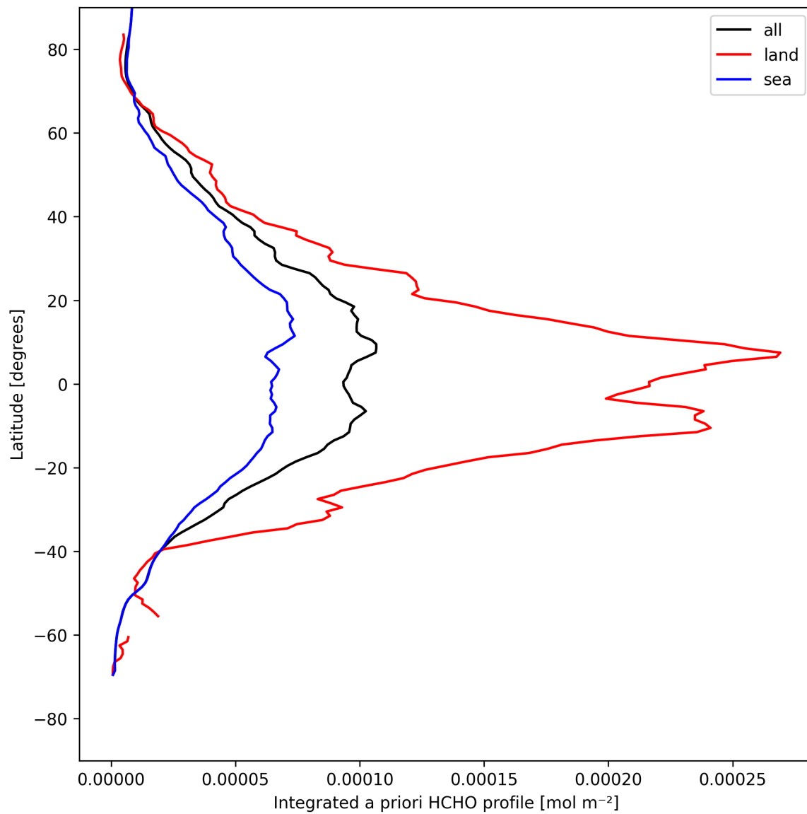
Figure 29: Zonal average of “Integrated a priori HCHO profile” for 2025-05-01 to 2025-05-03.
