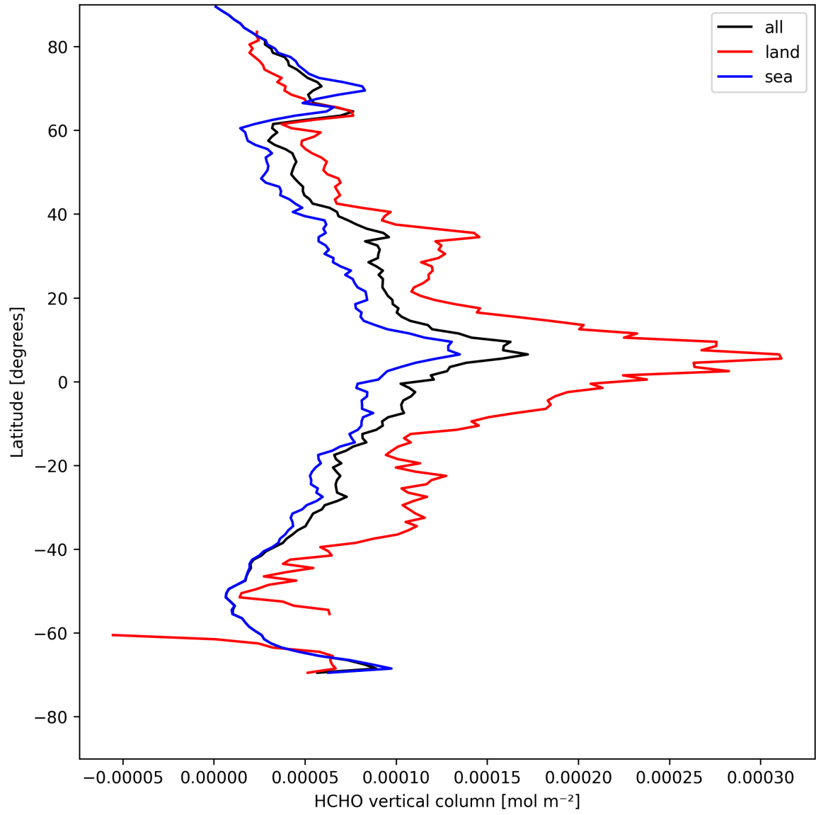
Figure 21: Zonal average of “HCHO vertical column” for 2025-05-01 to 2025-05-03.
