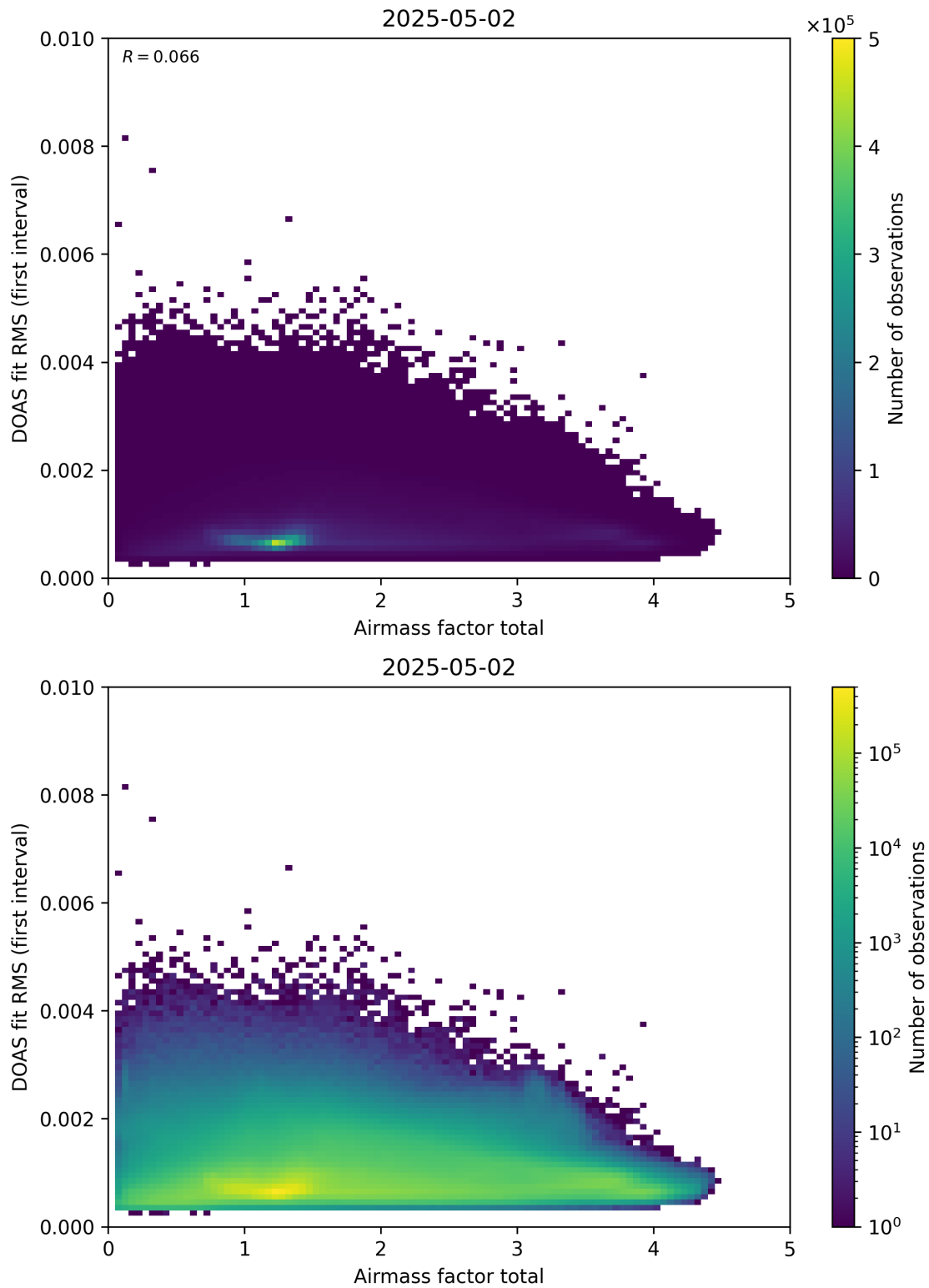
Figure 97: Scatter density plot of “Airmass factor total” against “DOAS fit RMS (first interval)” for 2025-05-01 to 2025-05-03.
