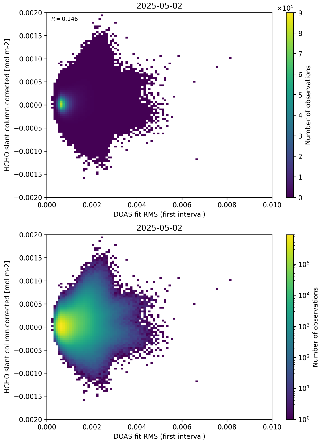
Figure 62: Scatter density plot of “DOAS fit RMS (first interval)” against “HCHO slant column corrected” for 2025-05-01 to 2025-05-03.
