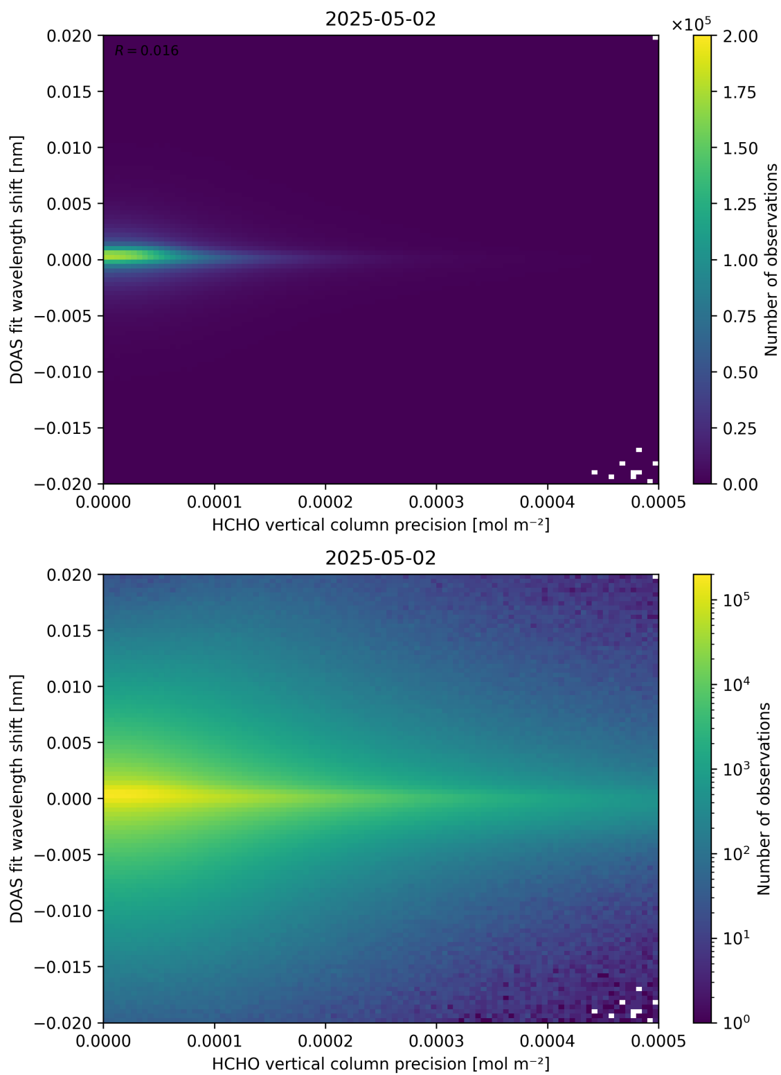
Figure 137: Scatter density plot of “HCHO vertical column precision” against “DOAS fit wavelength shift” for 2025-05-01 to 2025-05-03.
