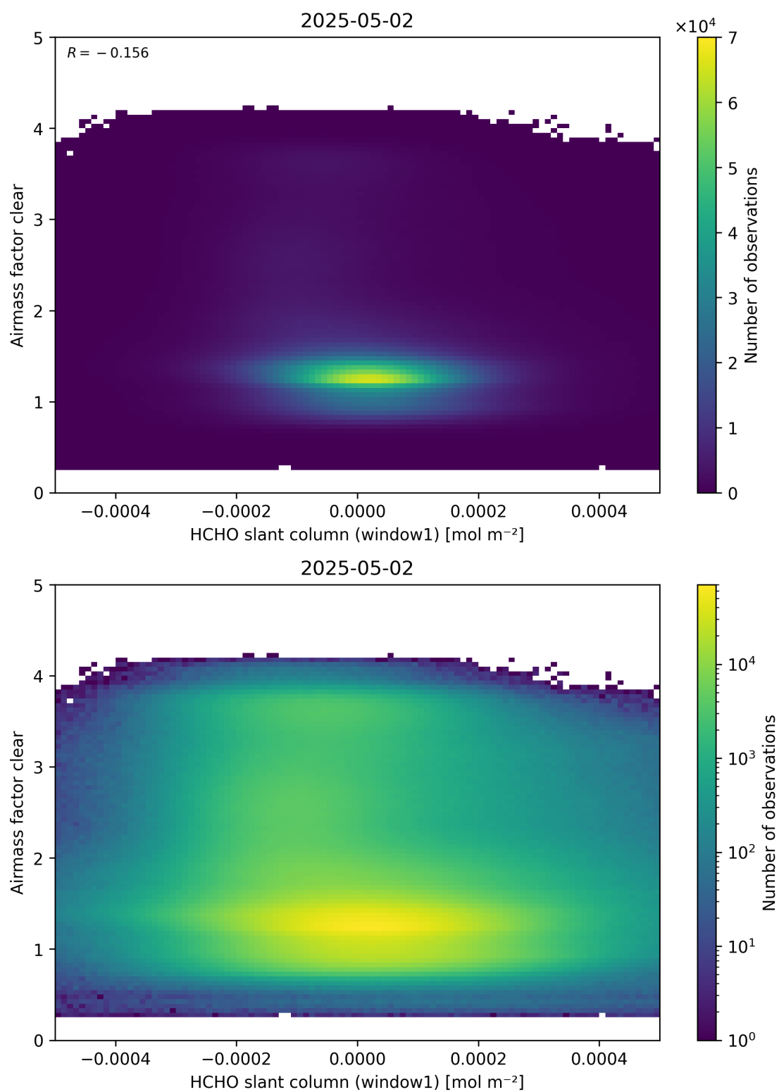
Figure 81: Scatter density plot of “HCHO slant column (window1)” against “Airmass factor clear” for 2025-05-01 to 2025-05-03.
