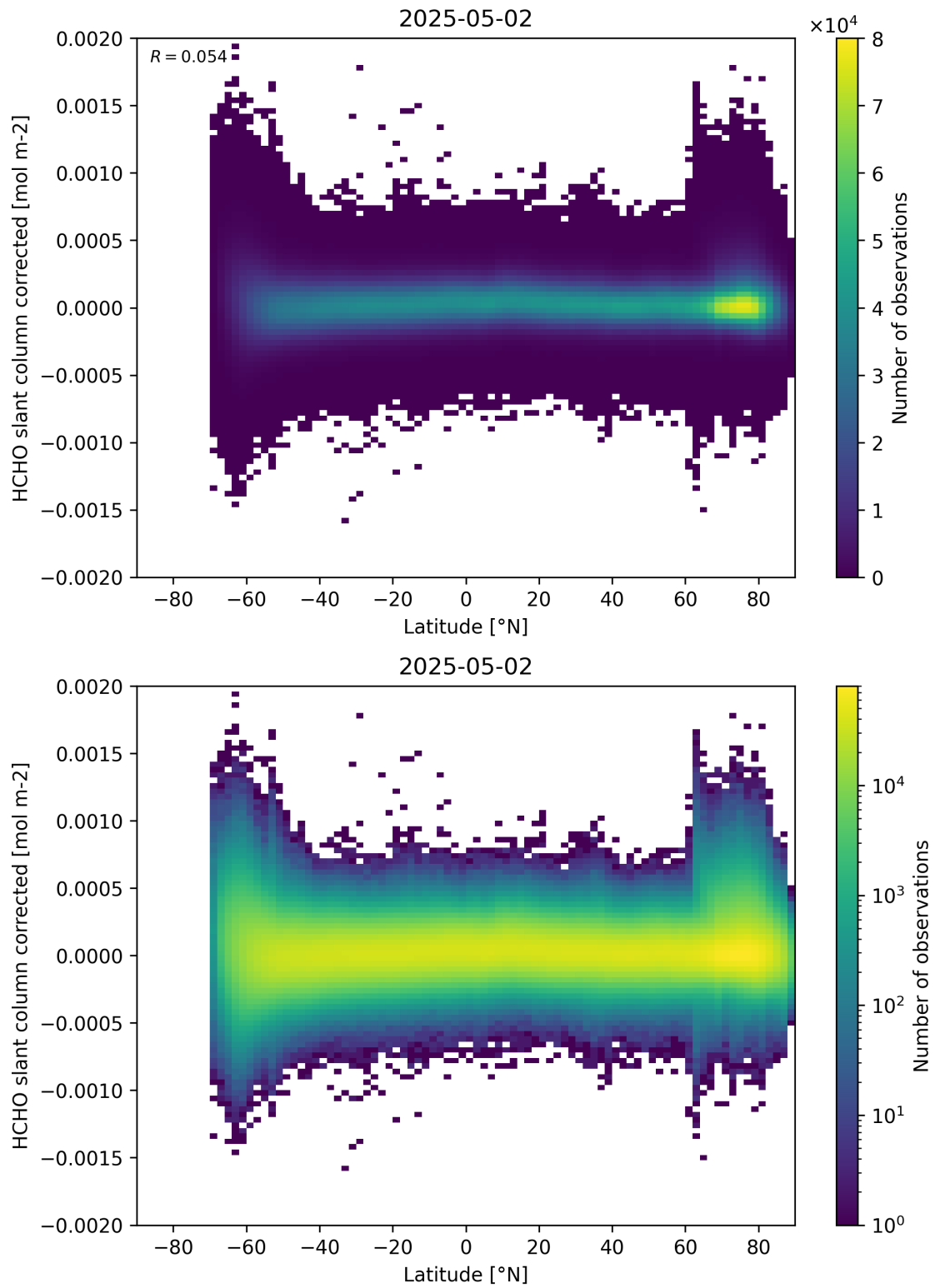
Figure 157: Scatter density plot of “Latitude” against “HCHO slant column corrected” for 2025-05-01 to 2025-05-03.
