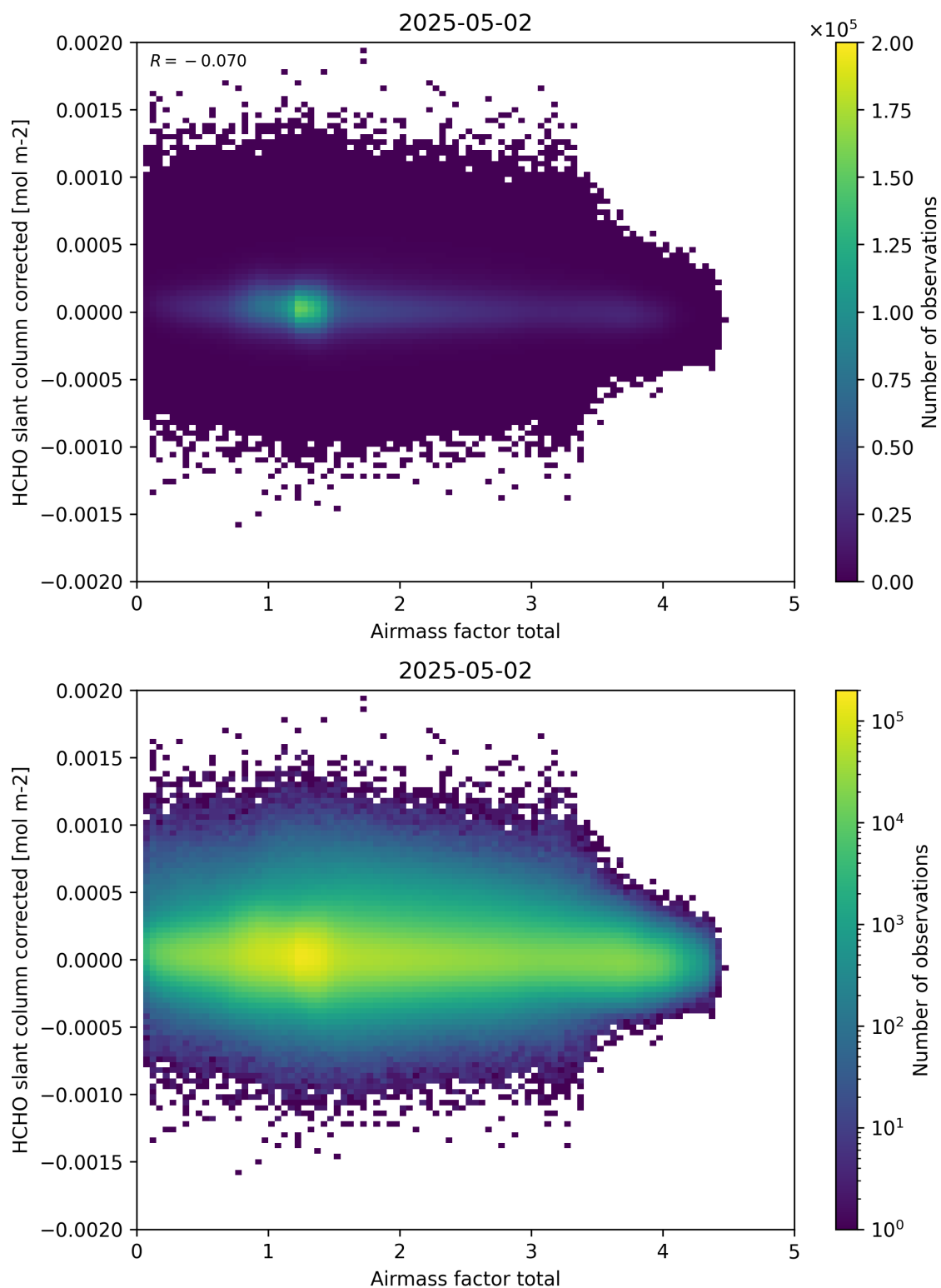
Figure 101: Scatter density plot of “Airmass factor total” against “HCHO slant column corrected” for 2025-05-01 to 2025-05-03.
