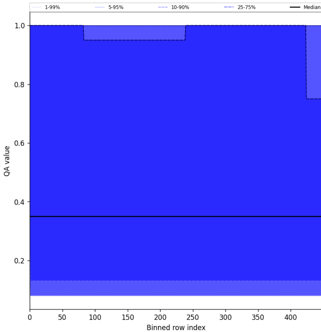
Figure 48: Along track statistics of “QA value” for 2025-05-01 to 2025-05-03
