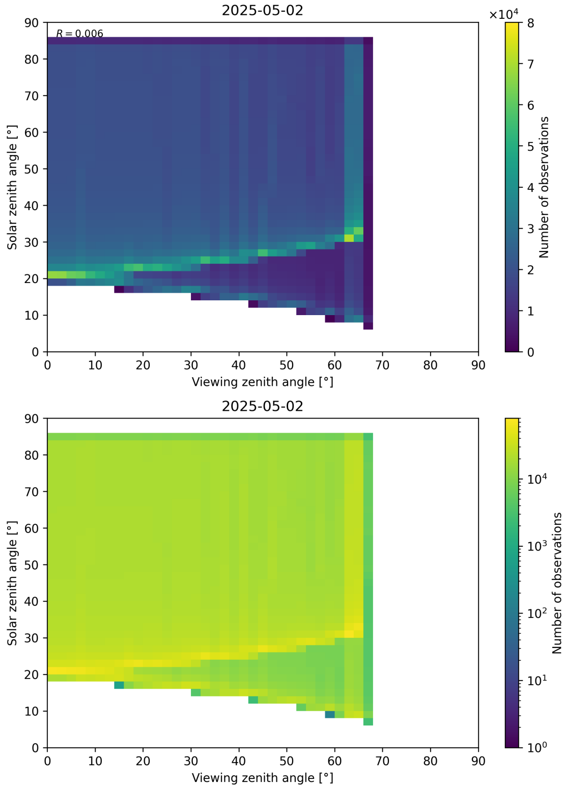
Figure 197: Scatter density plot of “Viewing zenith angle” against “Solar zenith angle” for 2025-05-01 to 2025-05-03.
