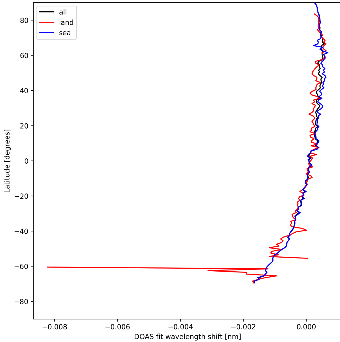
Figure 30: Zonal average of “DOAS fit wavelength shift” for 2025-05-01 to 2025-05-03.
