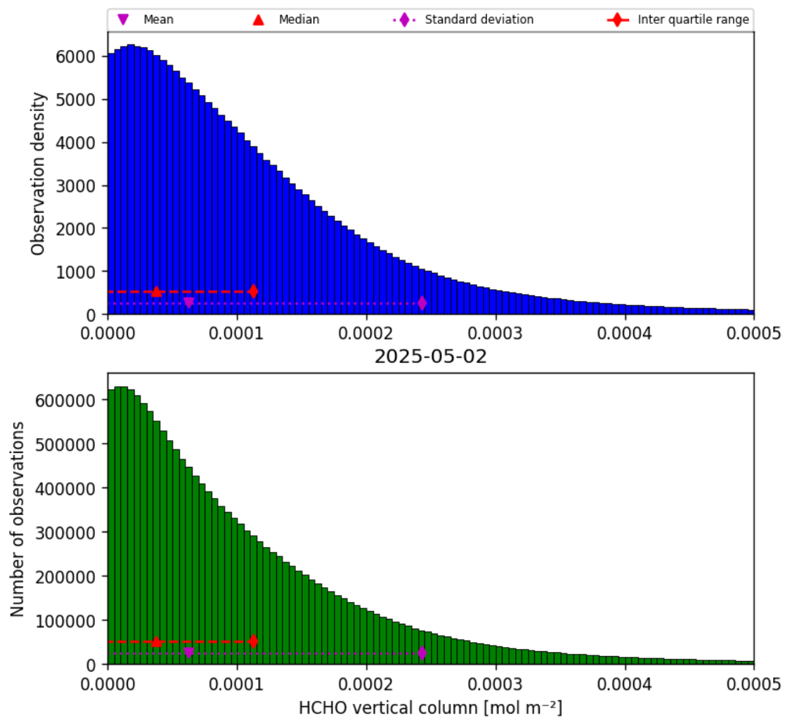
Figure 35: Histogram of “HCHO vertical column” for 2025-05-01 to 2025-05-03
