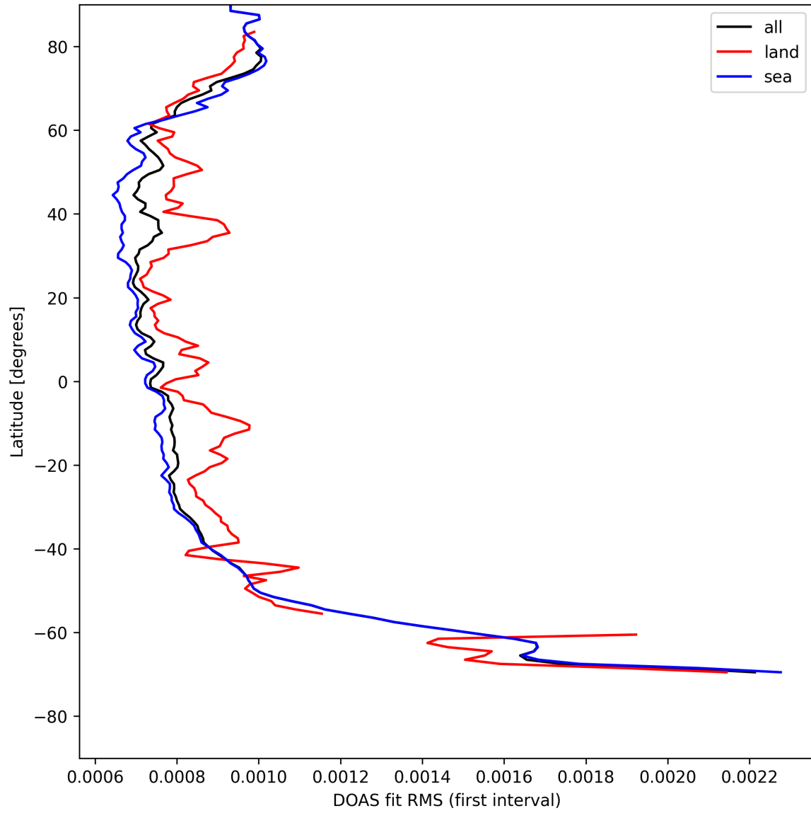
Figure 32: Zonal average of “DOAS fit RMS (first interval)” for 2025-05-01 to 2025-05-03.
