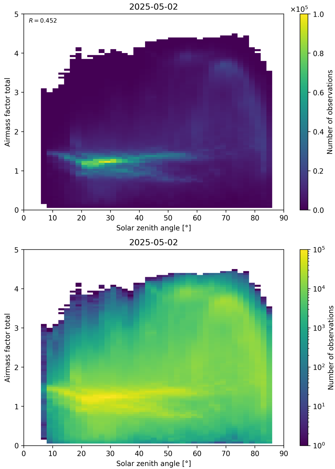
Figure 175: Scatter density plot of “Solar zenith angle” against “Airmass factor total” for 2025-05-01 to 2025-05-03.
