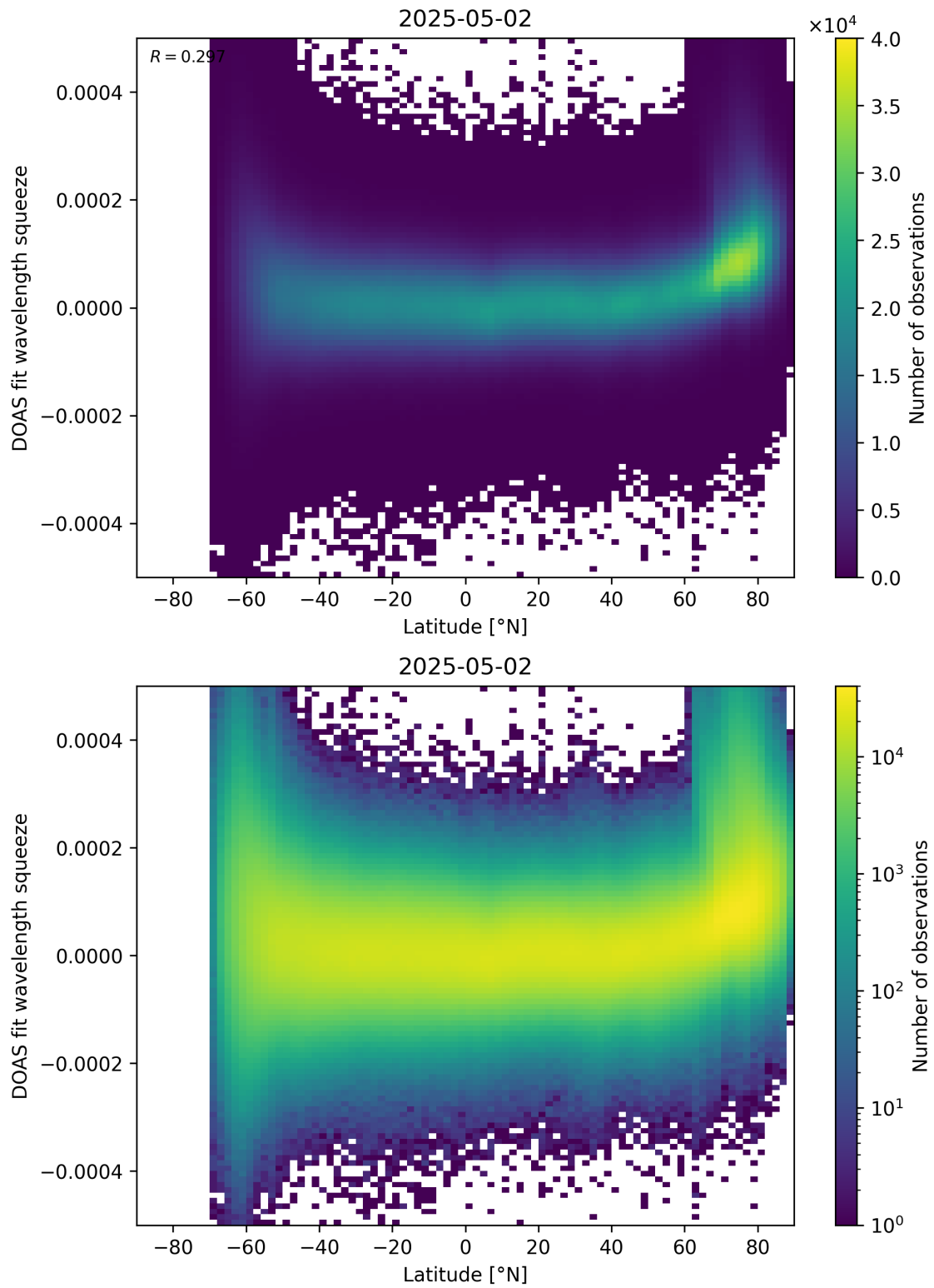
Figure 155: Scatter density plot of “Latitude” against “DOAS fit wavelength squeeze” for 2025-05-01 to 2025-05-03.
