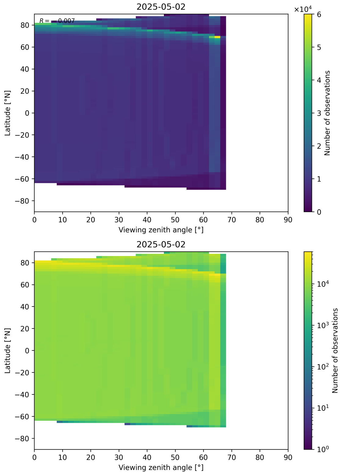
Figure 196: Scatter density plot of “Viewing zenith angle” against “Latitude” for 2025-05-01 to 2025-05-03.
