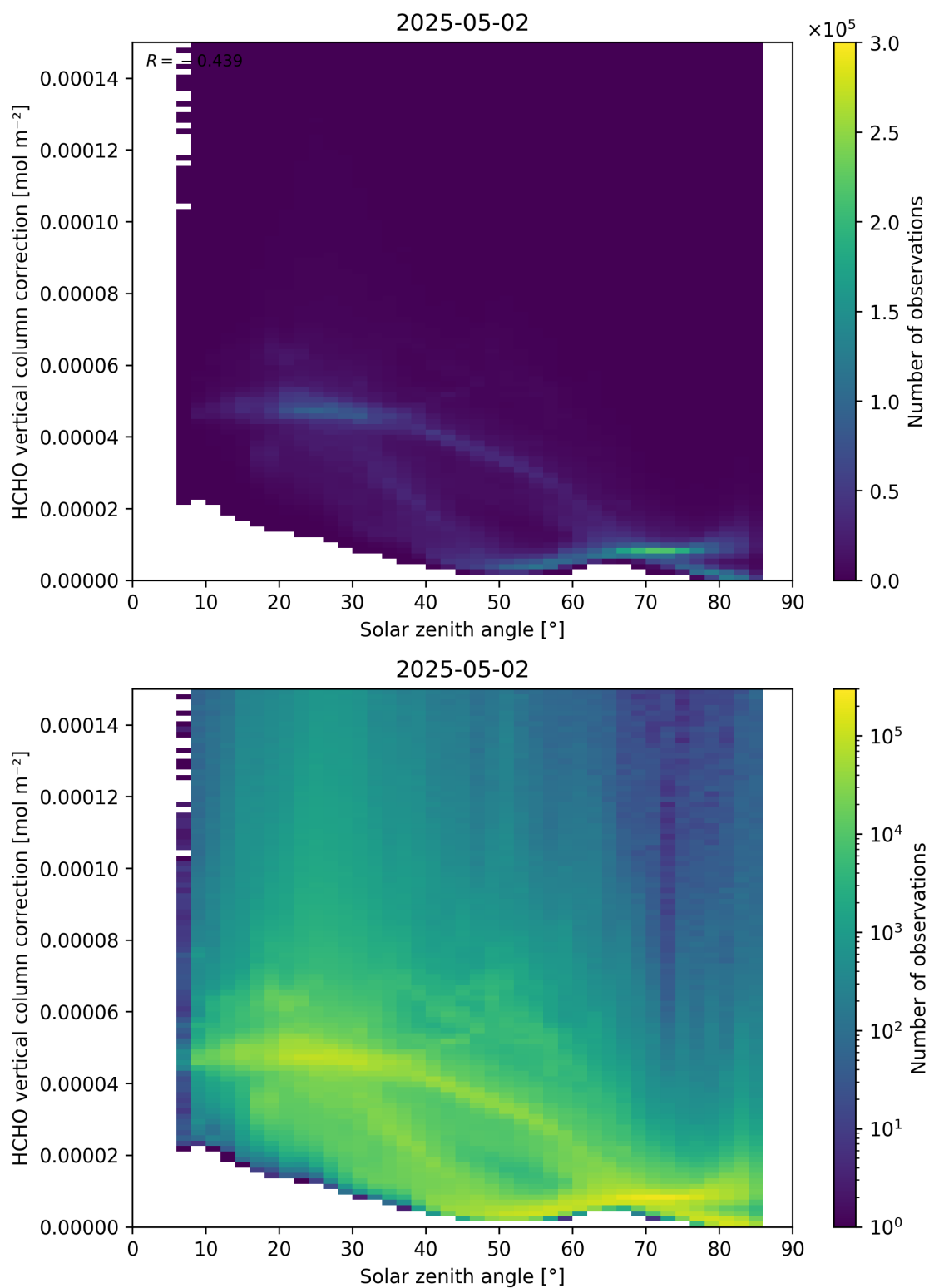
Figure 178: Scatter density plot of “Solar zenith angle” against “HCHO vertical column correction” for 2025-05-01 to 2025-05-03.
