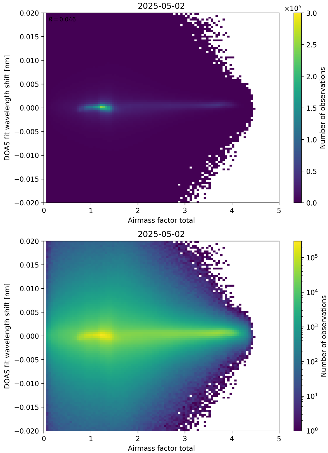
Figure 98: Scatter density plot of “Airmass factor total” against “DOAS fit wavelength shift” for 2025-05-01 to 2025-05-03.
