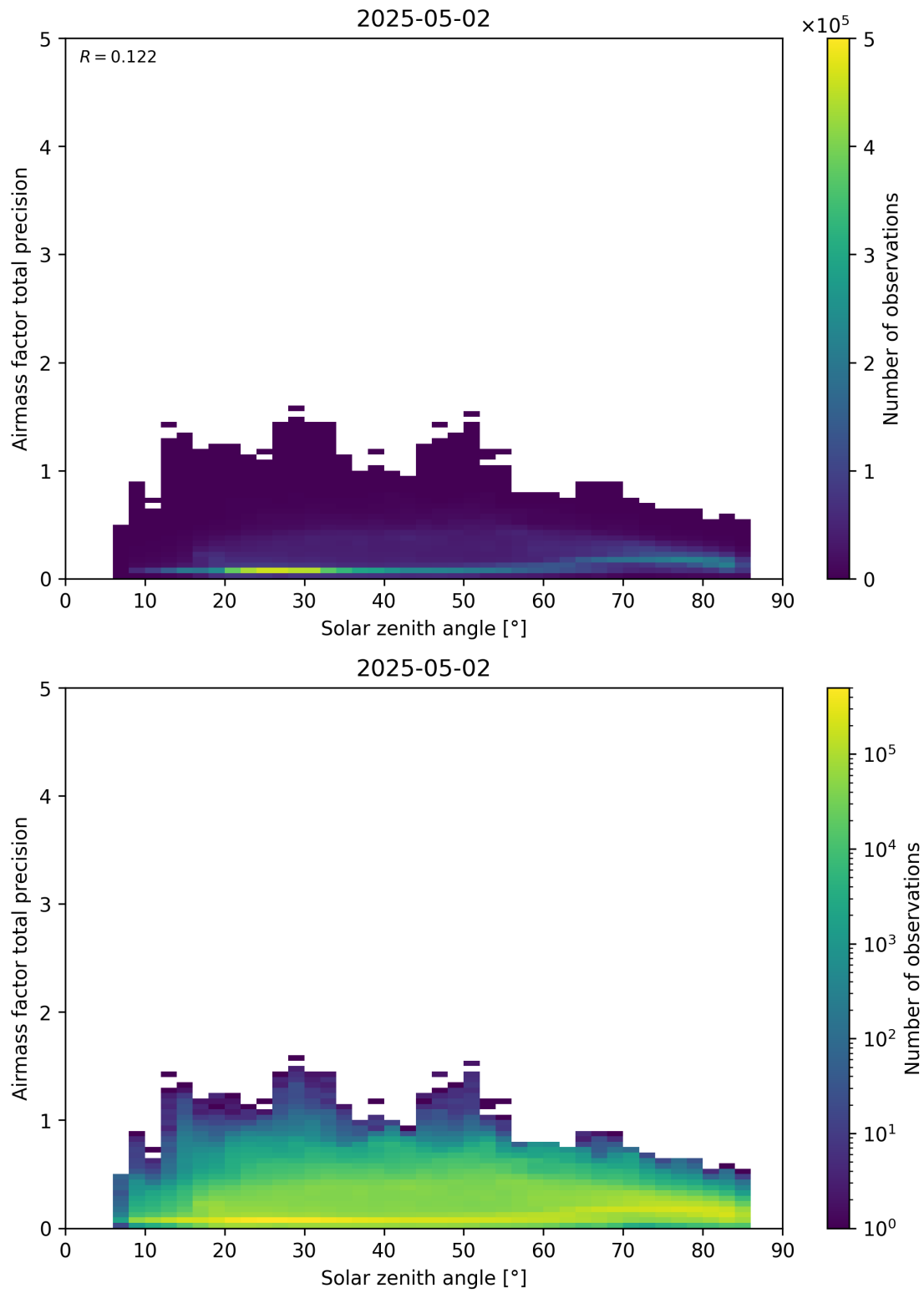
Figure 176: Scatter density plot of “Solar zenith angle” against “Airmass factor total precision” for 2025-05-01 to 2025-05-03.
