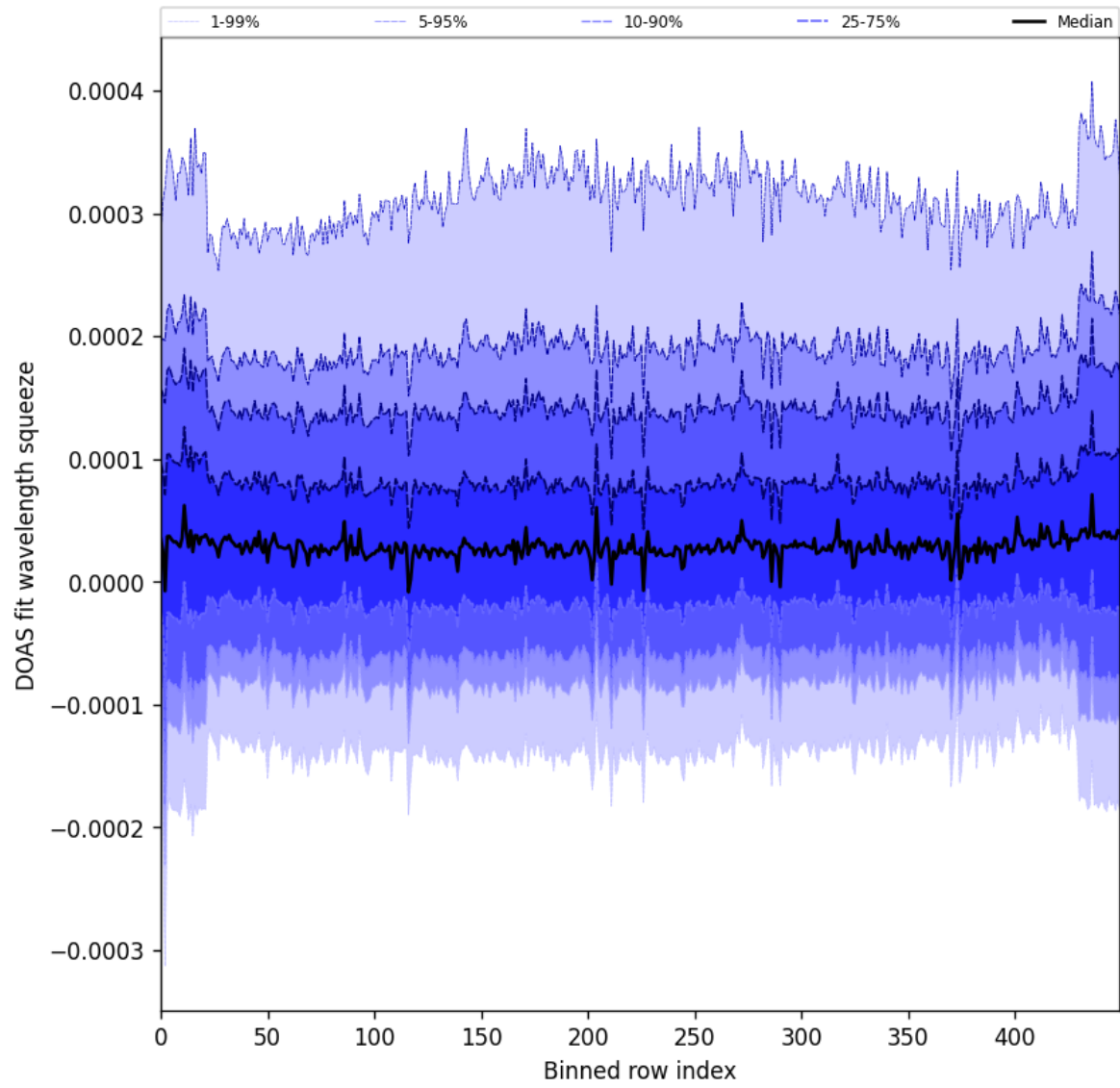
Figure 59: Along track statistics of “DOAS fit wavelength squeeze” for 2025-05-01 to 2025-05-03
