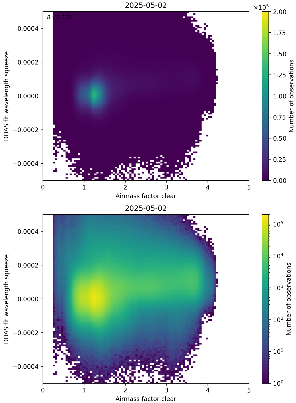
Figure 73: Scatter density plot of “Airmass factor clear” against “DOAS fit wavelength squeeze” for 2025-05-01 to 2025-05-03.
