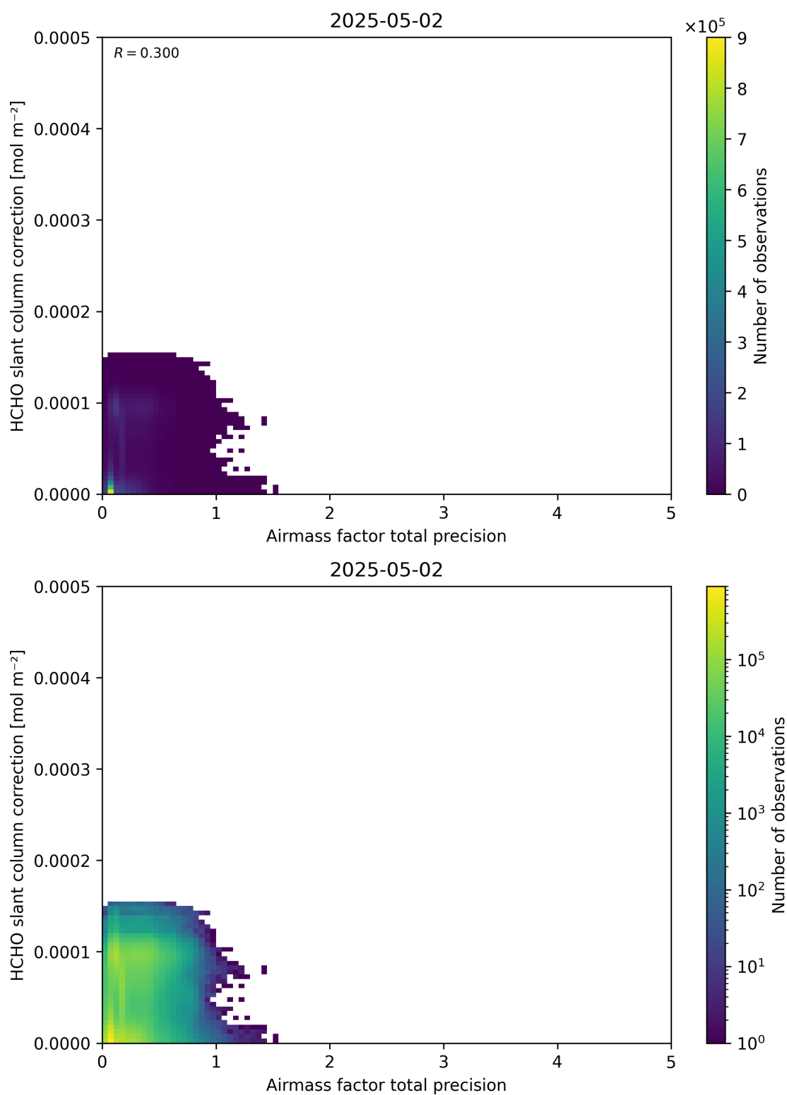
Figure 110: Scatter density plot of “Airmass factor total precision” against “HCHO slant column correction” for 2025-05-01 to 2025-05-03.
