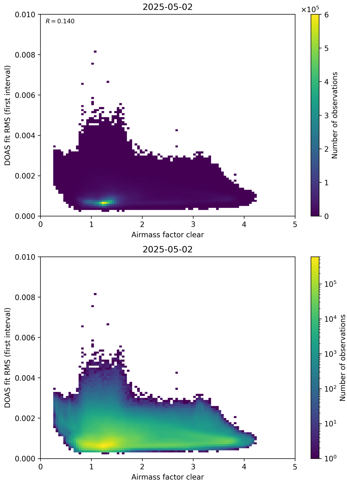
Figure 71: Scatter density plot of “Airmass factor clear” against “DOAS fit RMS (first interval)” for 2025-05-01 to 2025-05-03.
