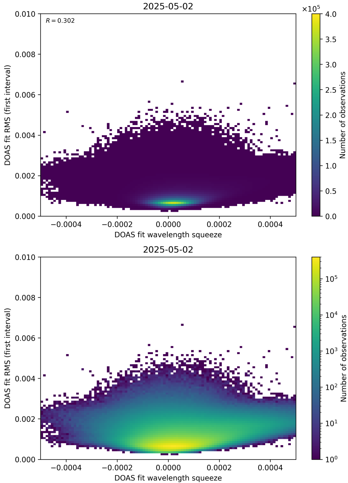
Figure 68: Scatter density plot of “DOAS fit wavelength squeeze” against “DOAS fit RMS (first interval)” for 2025-05-01 to 2025-05-03.
