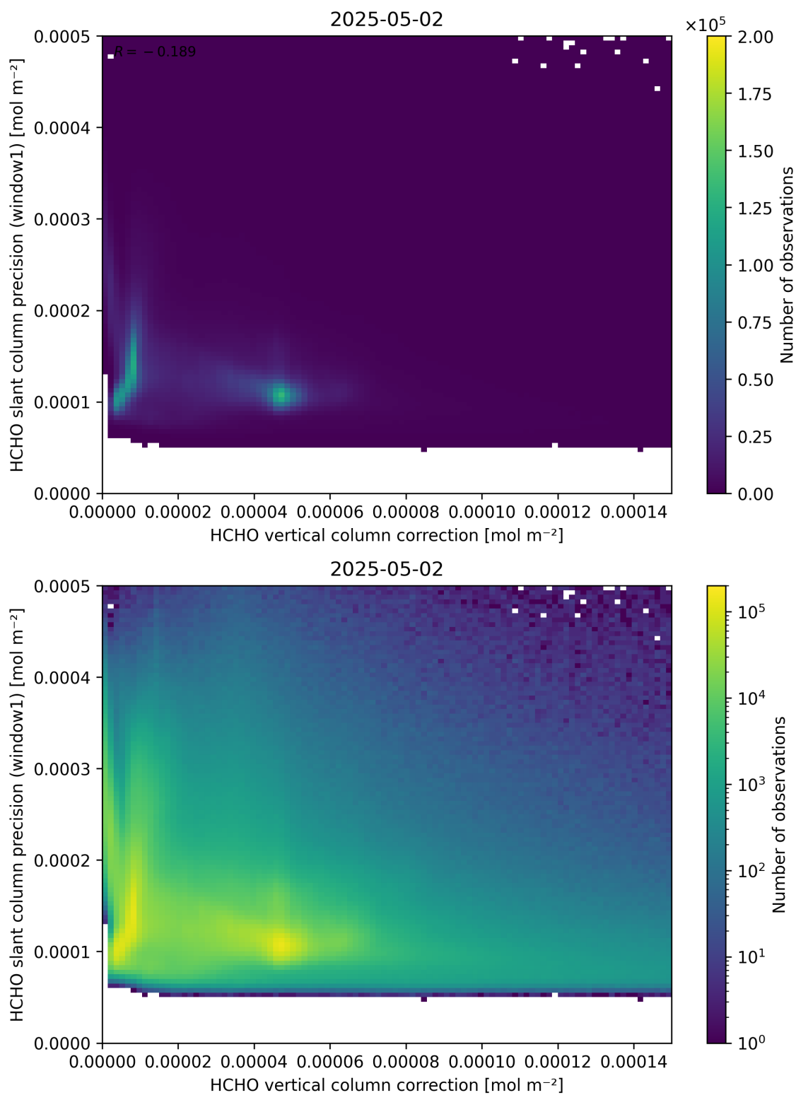
Figure 119: Scatter density plot of “HCHO vertical column correction” against “HCHO slant column precision (window1)” for 2025-05-01 to 2025-05-03.
