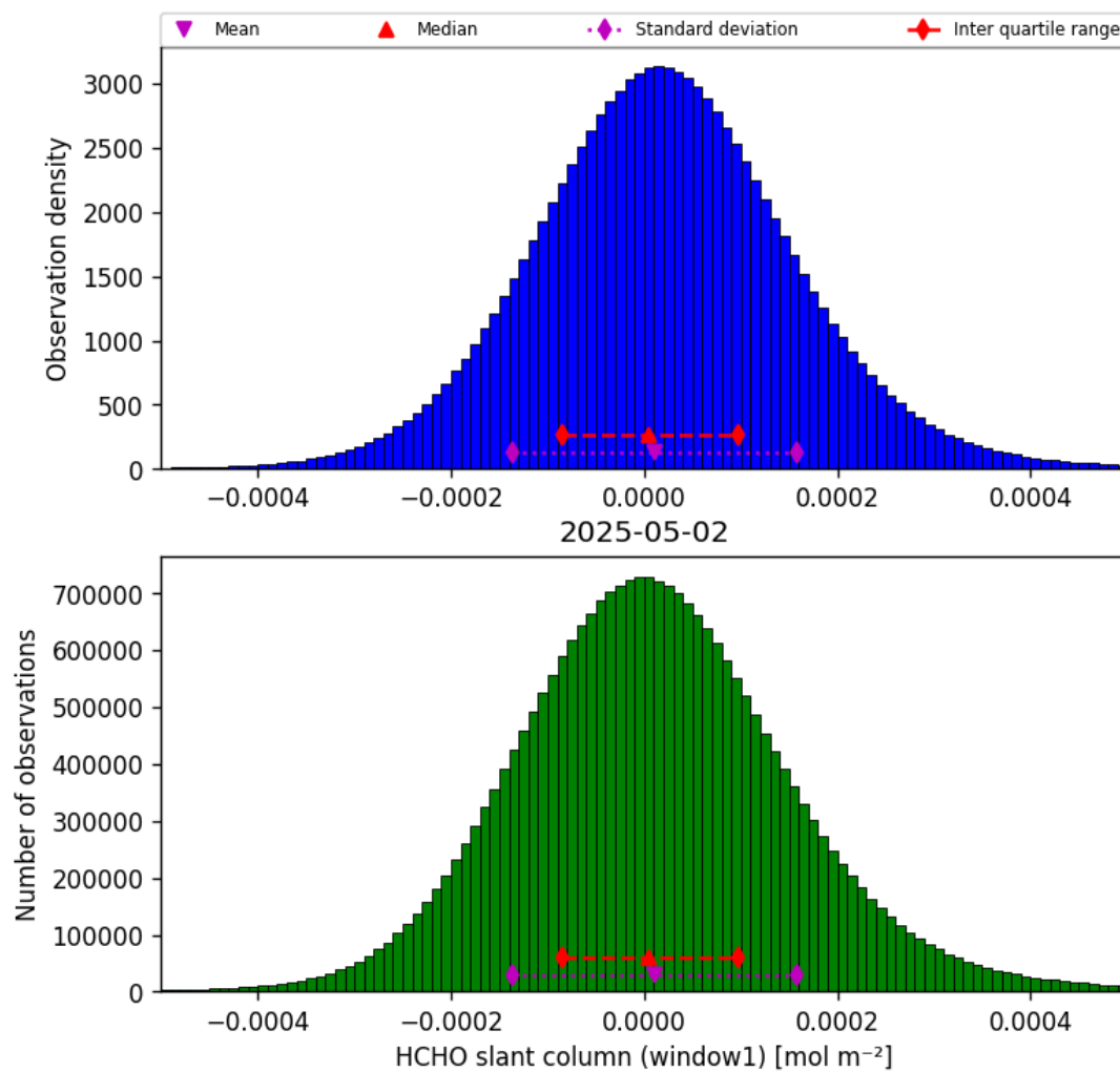
Figure 38: Histogram of “HCHO slant column (window1)” for 2025-05-01 to 2025-05-03
