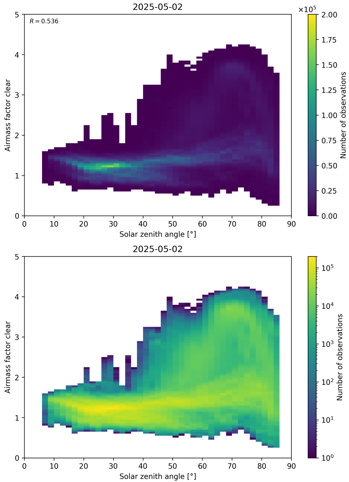
Figure 170: Scatter density plot of “Solar zenith angle” against “Airmass factor clear” for 2025-05-01 to 2025-05-03.
