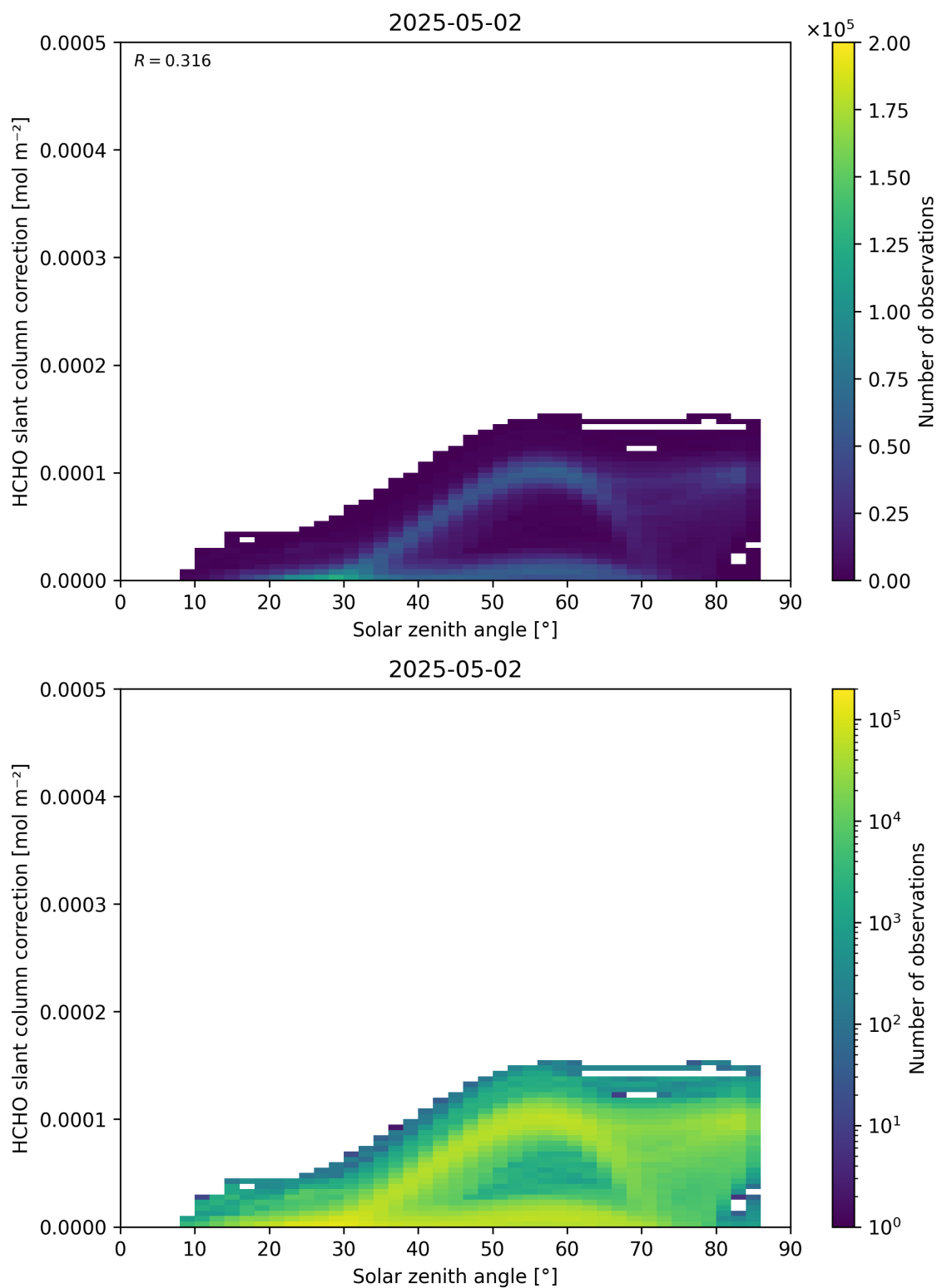
Figure 172: Scatter density plot of “Solar zenith angle” against “HCHO slant column correction” for 2025-05-01 to 2025-05-03.
