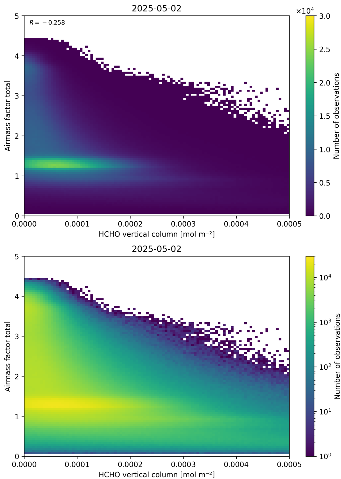
Figure 131: Scatter density plot of “HCHO vertical column” against “Airmass factor total” for 2025-05-01 to 2025-05-03.
