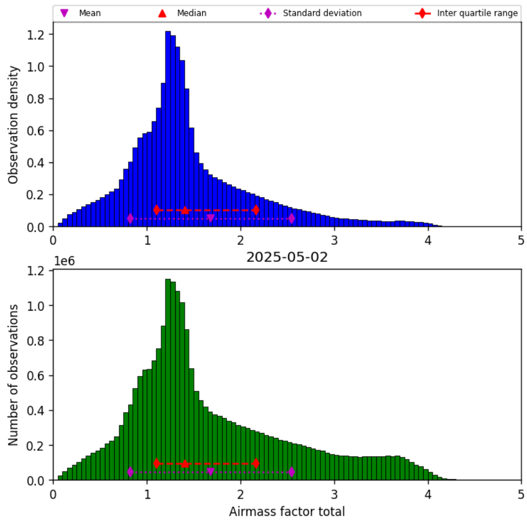
Figure 40: Histogram of “Airmass factor total” for 2025-05-01 to 2025-05-03
