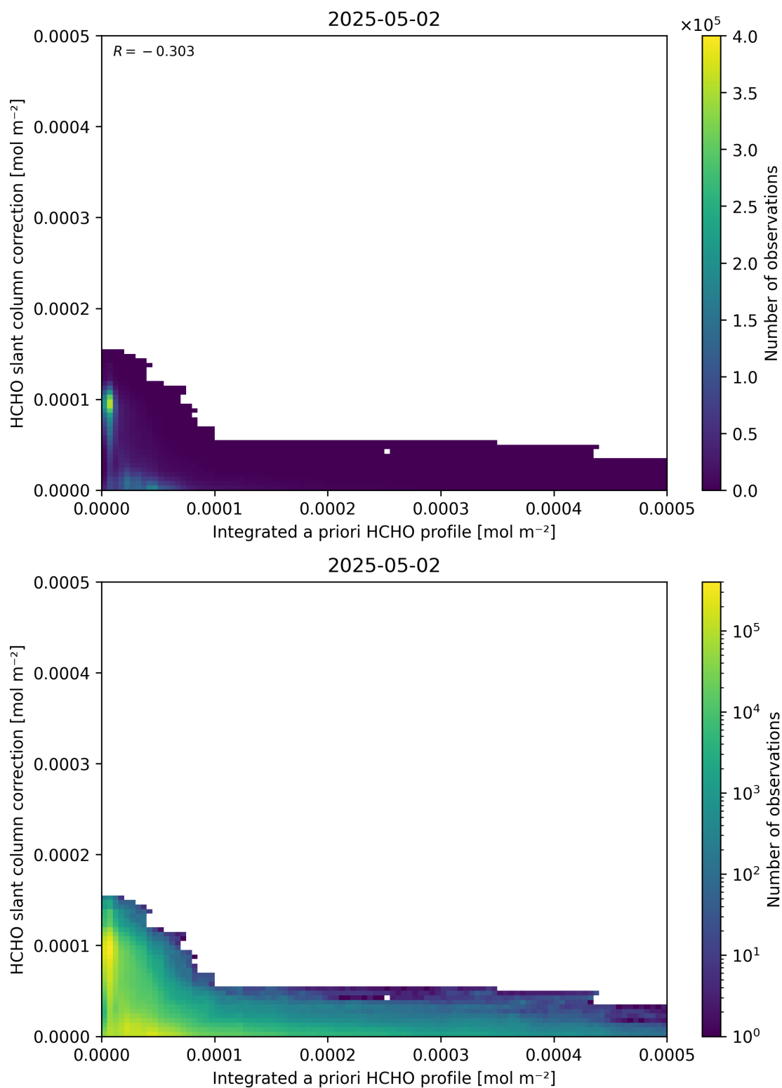
Figure 152: Scatter density plot of “Integrated a priori HCHO profile” against “HCHO slant column correction” for 2025-05-01 to 2025-05-03.
