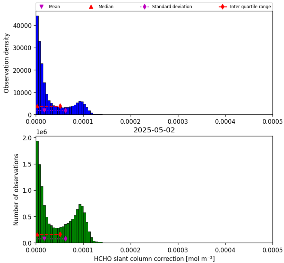
Figure 47: Histogram of “HCHO slant column correction” for 2025-05-01 to 2025-05-03
