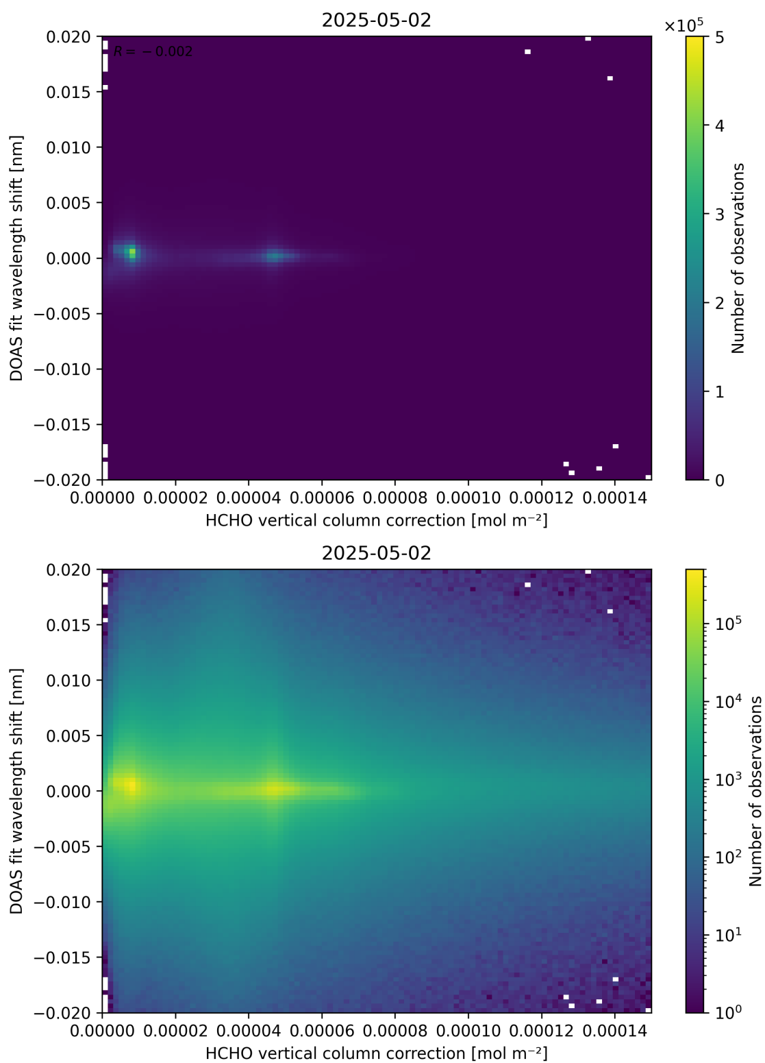
Figure 113: Scatter density plot of “HCHO vertical column correction” against “DOAS fit wavelength shift” for 2025-05-01 to 2025-05-03.
