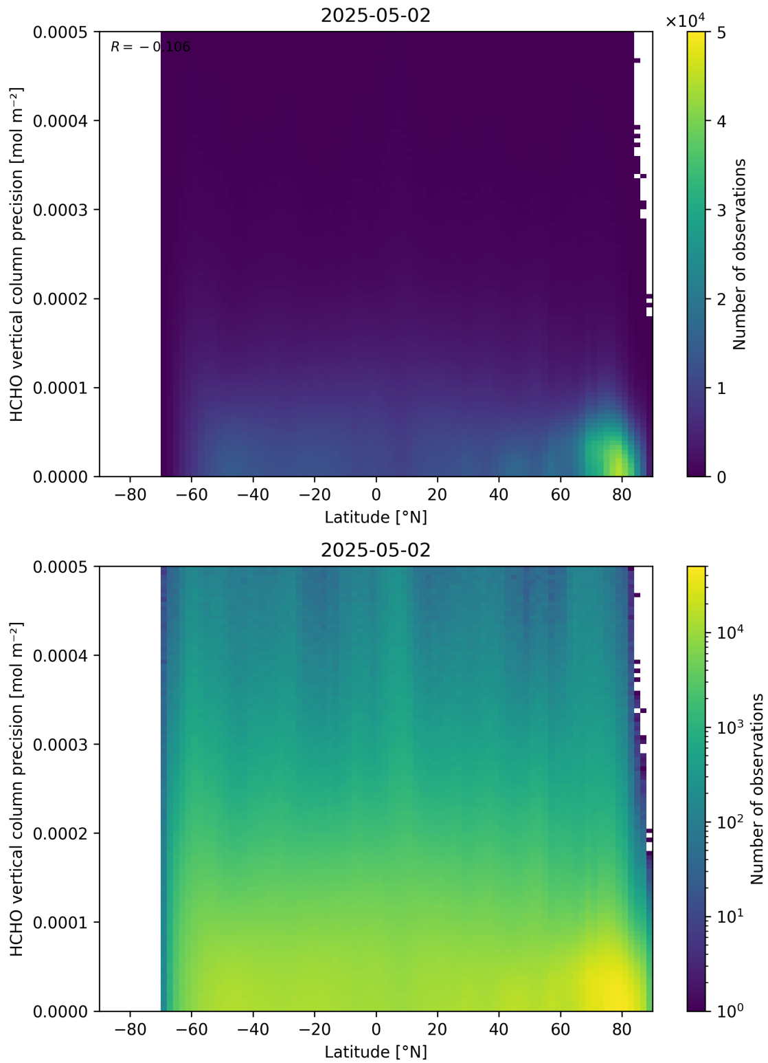
Figure 165: Scatter density plot of “Latitude” against “HCHO vertical column precision” for 2025-05-01 to 2025-05-03.
