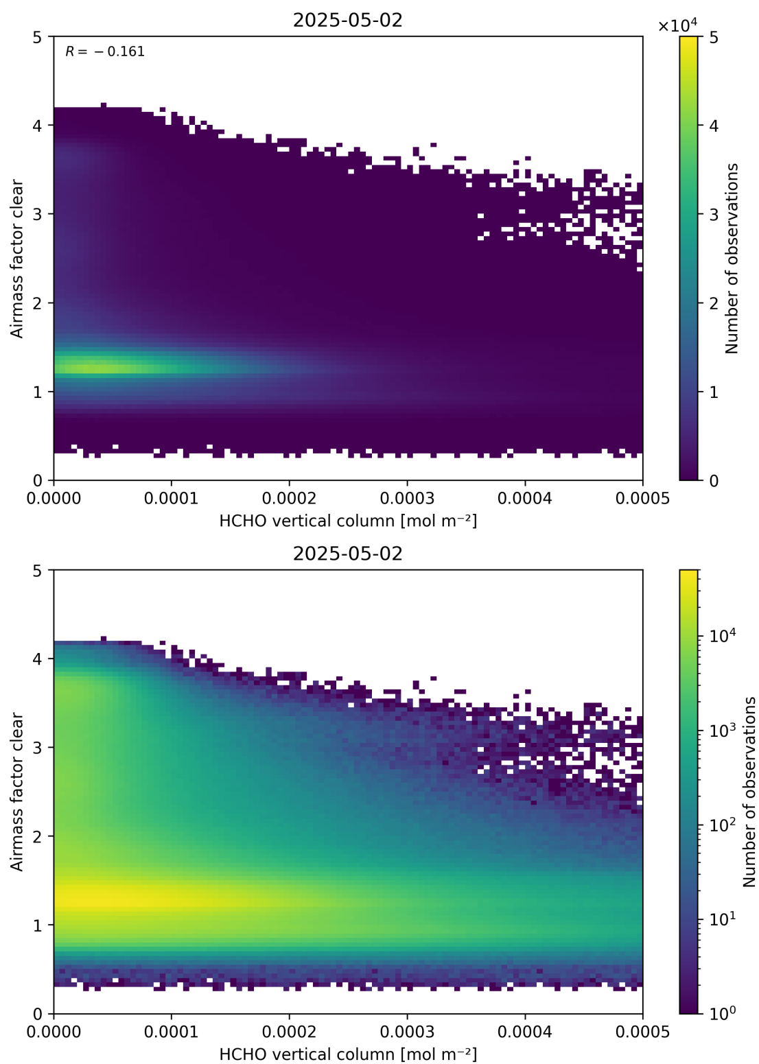
Figure 126: Scatter density plot of “HCHO vertical column” against “Airmass factor clear” for 2025-05-01 to 2025-05-03.
