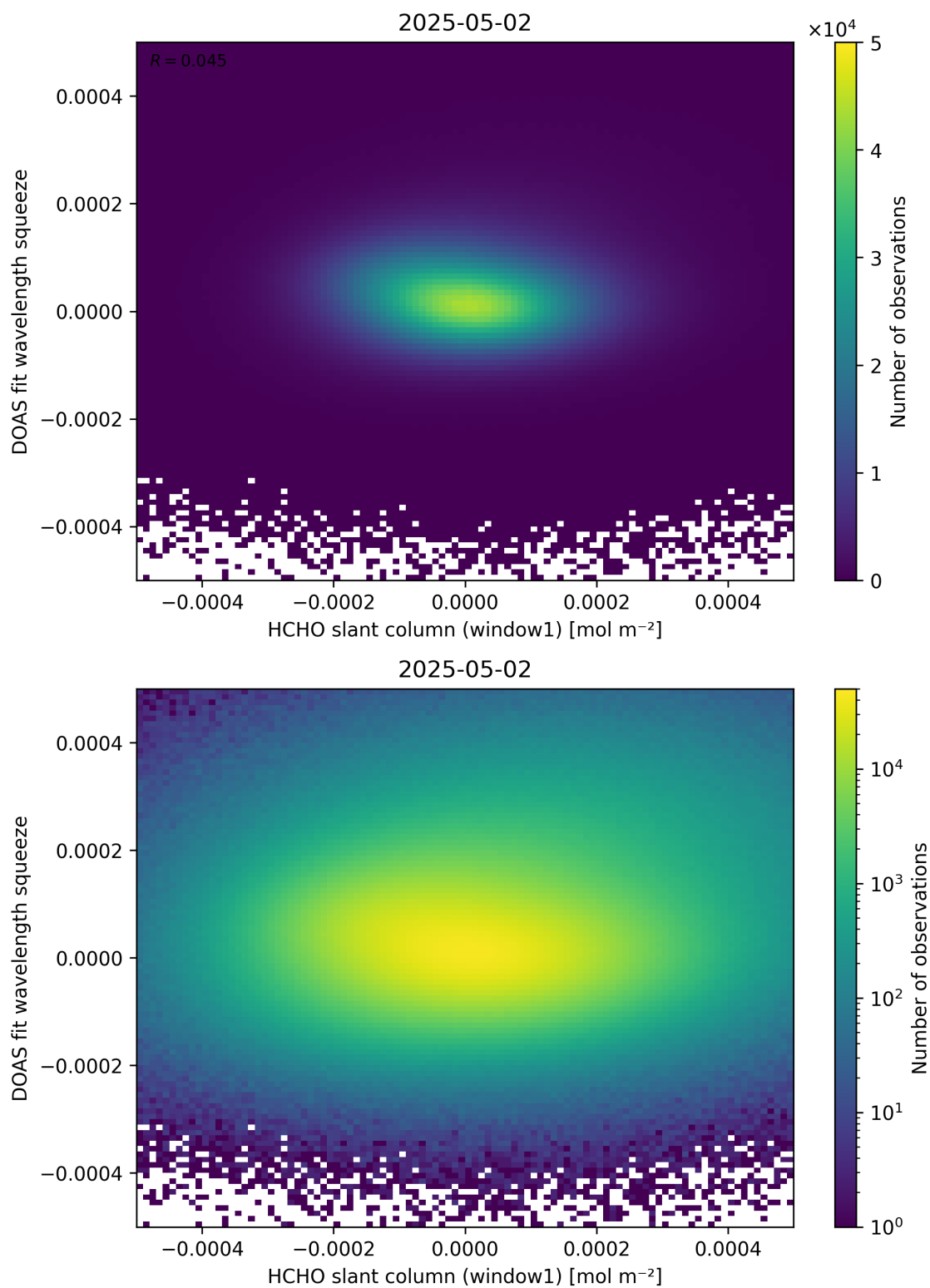
Figure 80: Scatter density plot of “HCHO slant column (window1)” against “DOAS fit wavelength squeeze” for 2025-05-01 to 2025-05-03.
