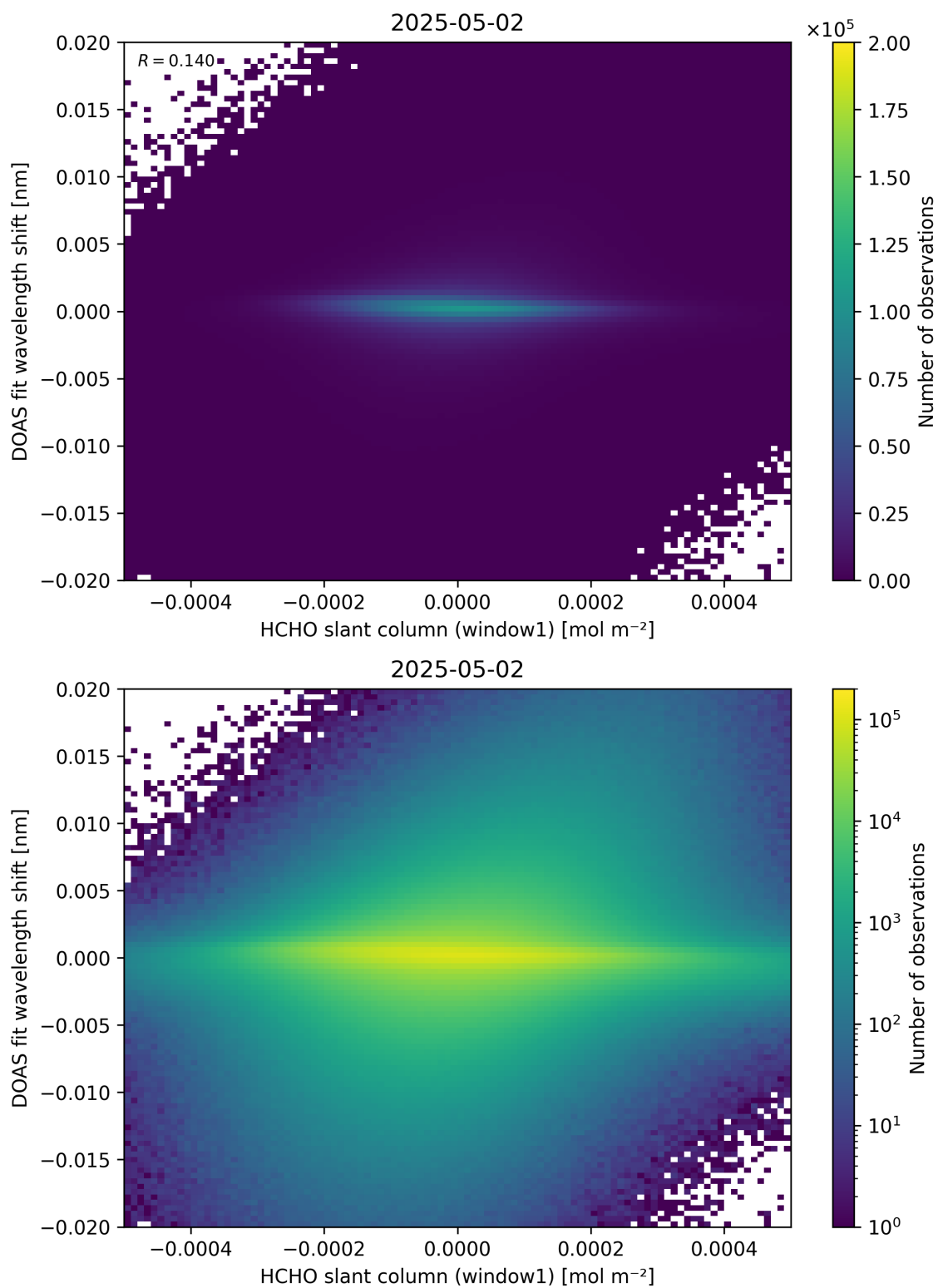
Figure 79: Scatter density plot of “HCHO slant column (window1)” against “DOAS fit wavelength shift” for 2025-05-01 to 2025-05-03.
