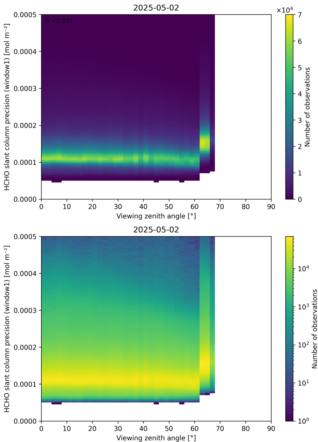
Figure 189: Scatter density plot of “Viewing zenith angle” against “HCHO slant column precision (window1)” for 2025-05-01 to 2025-05-03.
