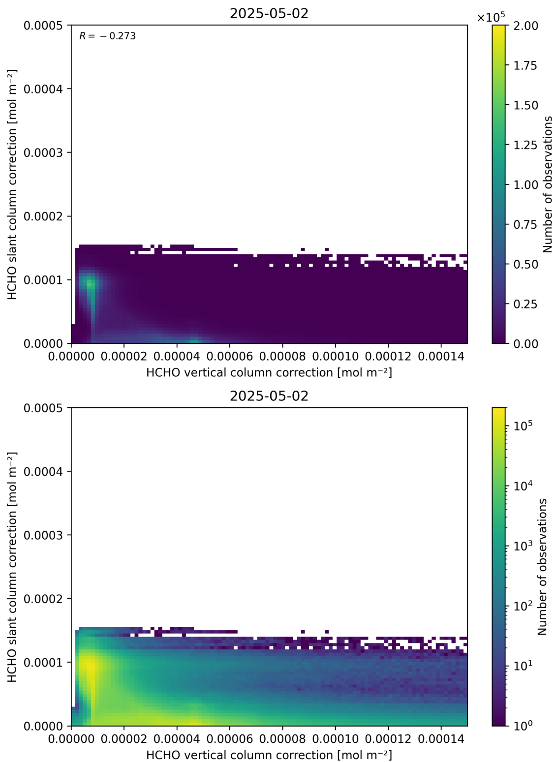
Figure 117: Scatter density plot of “HCHO vertical column correction” against “HCHO slant column correction” for 2025-05-01 to 2025-05-03.
