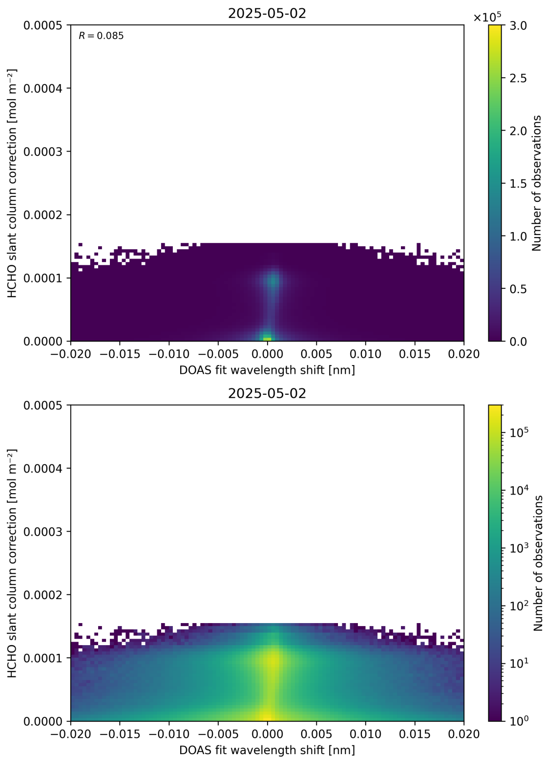
Figure 67: Scatter density plot of “DOAS fit wavelength shift” against “HCHO slant column correction” for 2025-05-01 to 2025-05-03.
