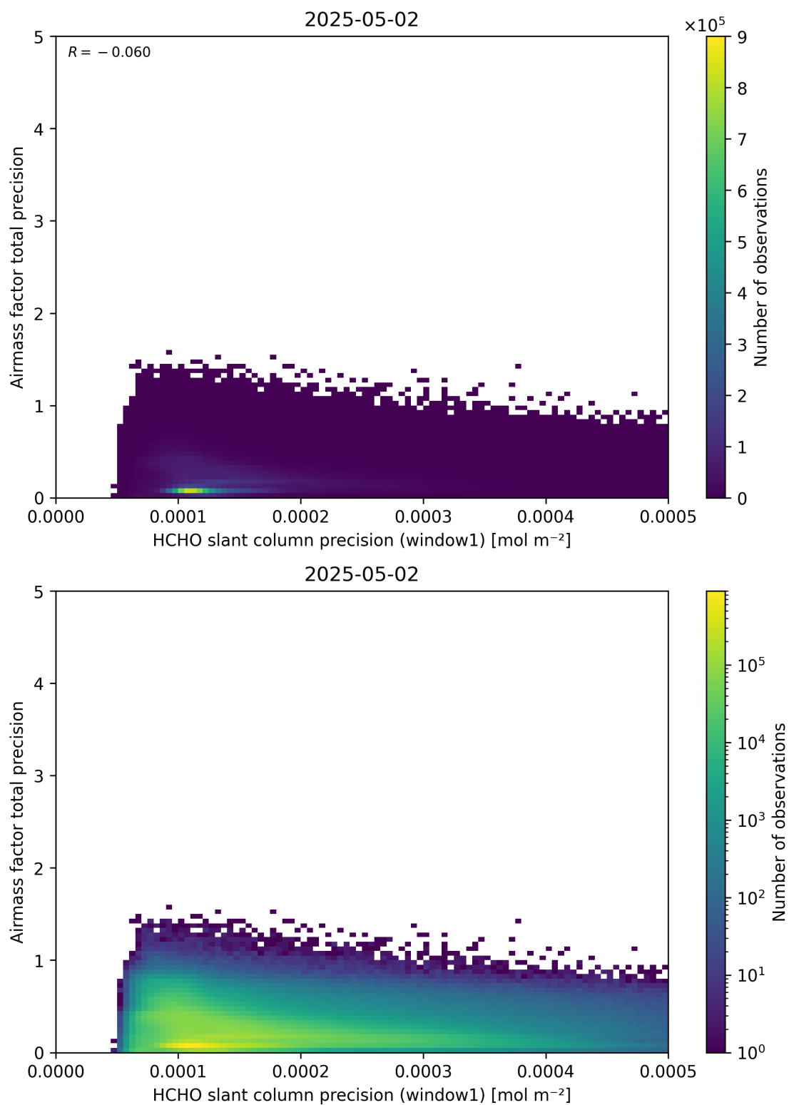
Figure 95: Scatter density plot of “HCHO slant column precision (window1)” against “Airmass factor total precision” for 2025-05-01 to 2025-05-03.
