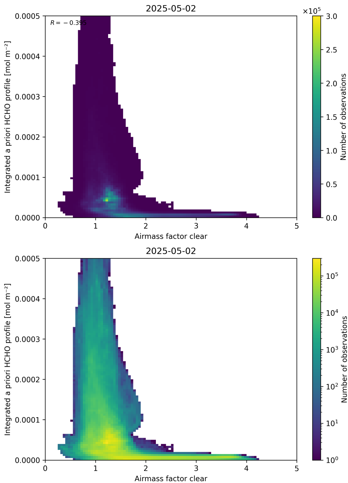
Figure 76: Scatter density plot of “Airmass factor clear” against “Integrated a priori HCHO profile” for 2025-05-01 to 2025-05-03.
