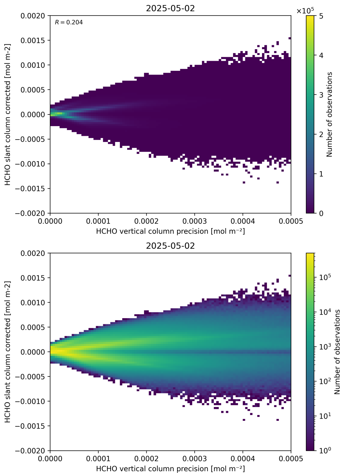
Figure 140: Scatter density plot of “HCHO vertical column precision” against “HCHO slant column corrected” for 2025-05-01 to 2025-05-03.
