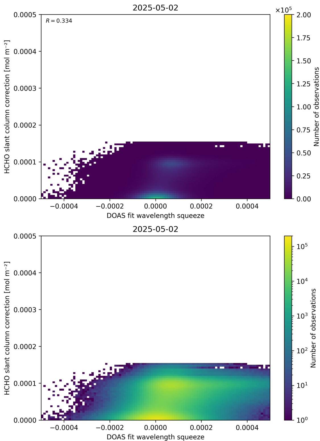
Figure 70: Scatter density plot of “DOAS fit wavelength squeeze” against “HCHO slant column correction” for 2025-05-01 to 2025-05-03.
