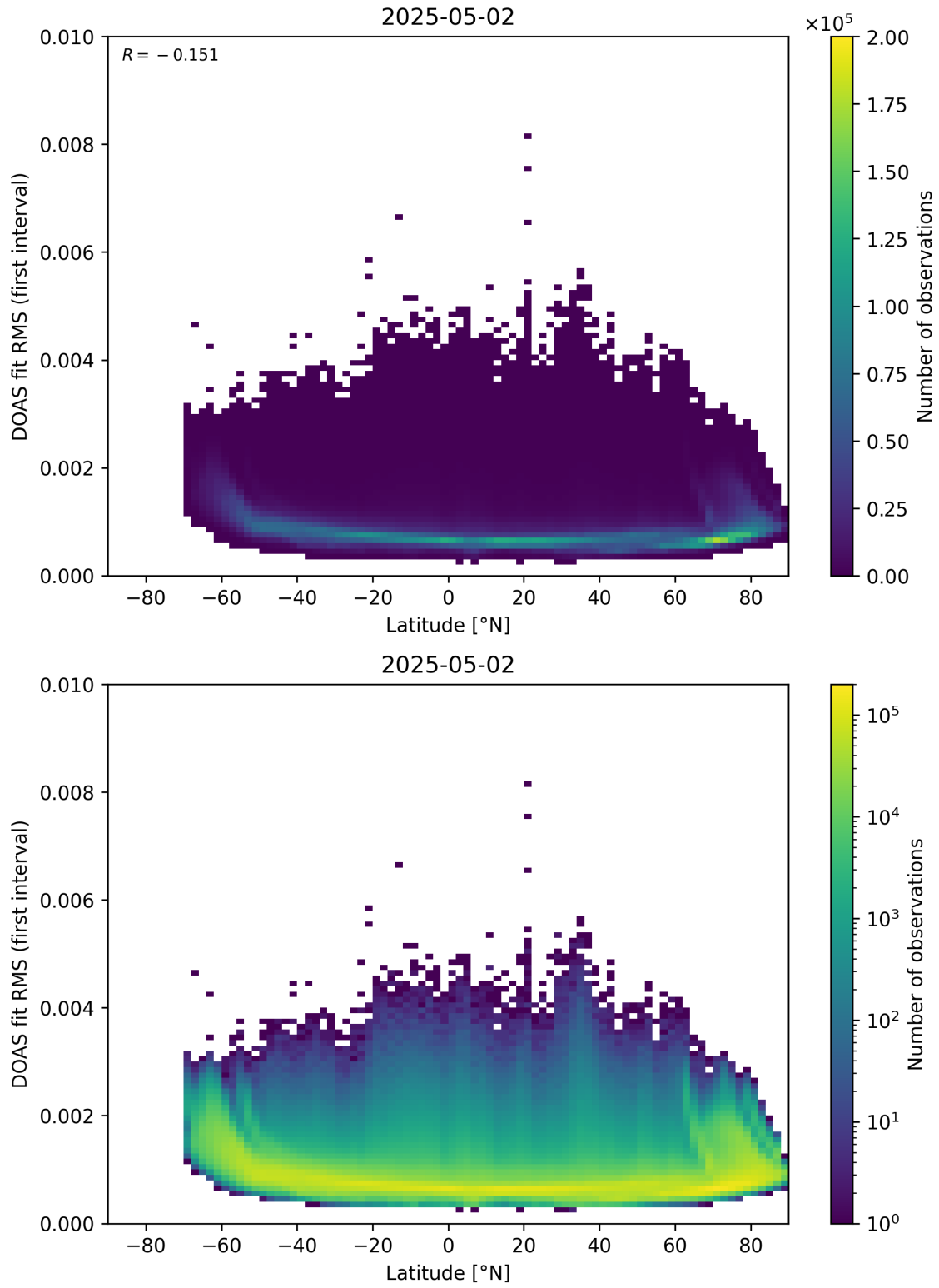
Figure 153: Scatter density plot of “Latitude” against “DOAS fit RMS (first interval)” for 2025-05-01 to 2025-05-03.
