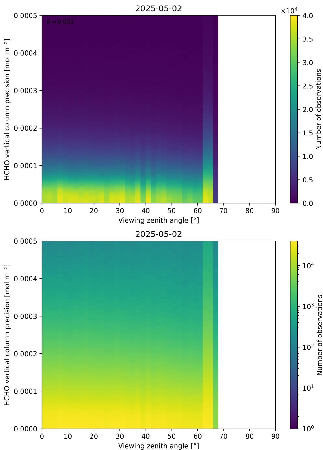
Figure 194: Scatter density plot of “Viewing zenith angle” against “HCHO vertical column precision” for 2025-05-01 to 2025-05-03.
