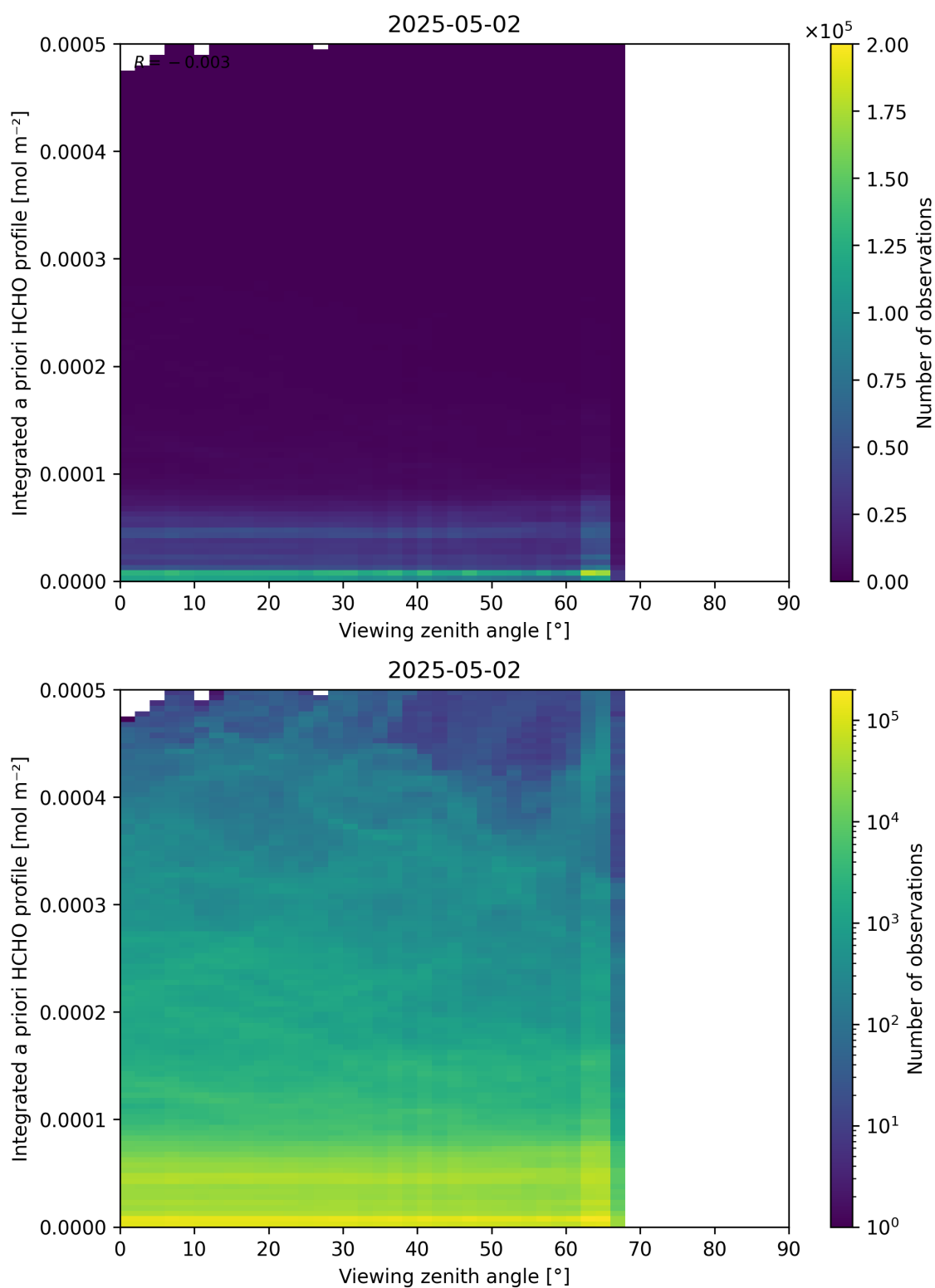
Figure 195: Scatter density plot of “Viewing zenith angle” against “Integrated a priori HCHO profile” for 2025-05-01 to 2025-05-03.
