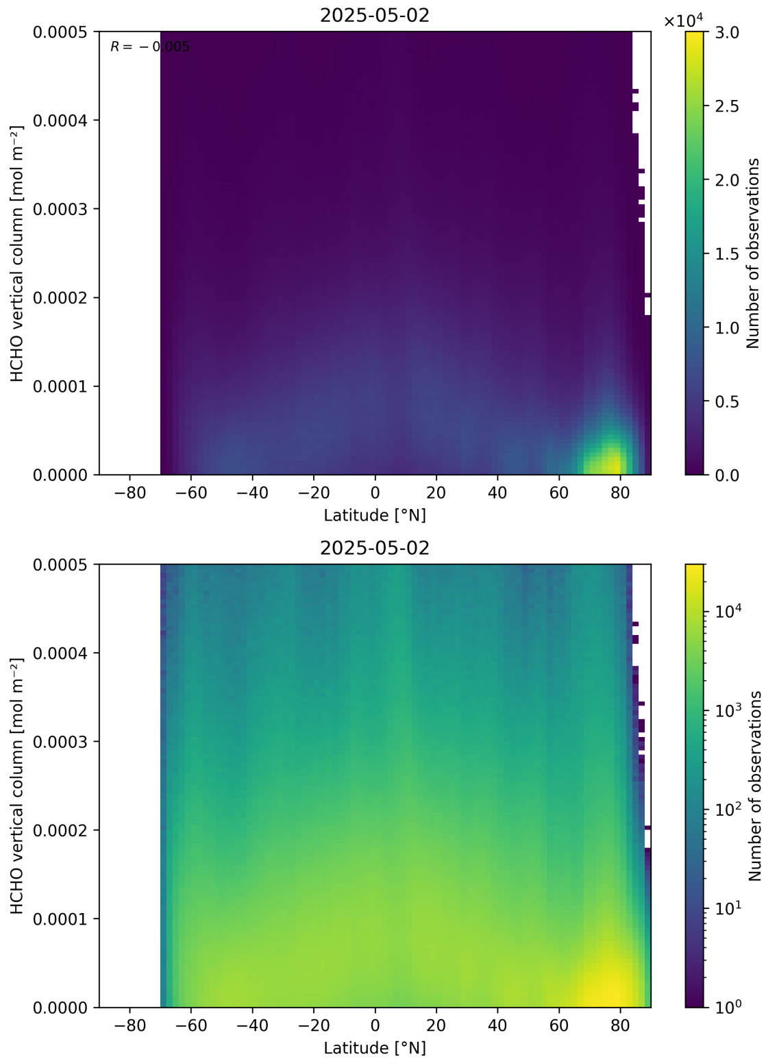
Figure 163: Scatter density plot of “Latitude” against “HCHO vertical column” for 2025-05-01 to 2025-05-03.
