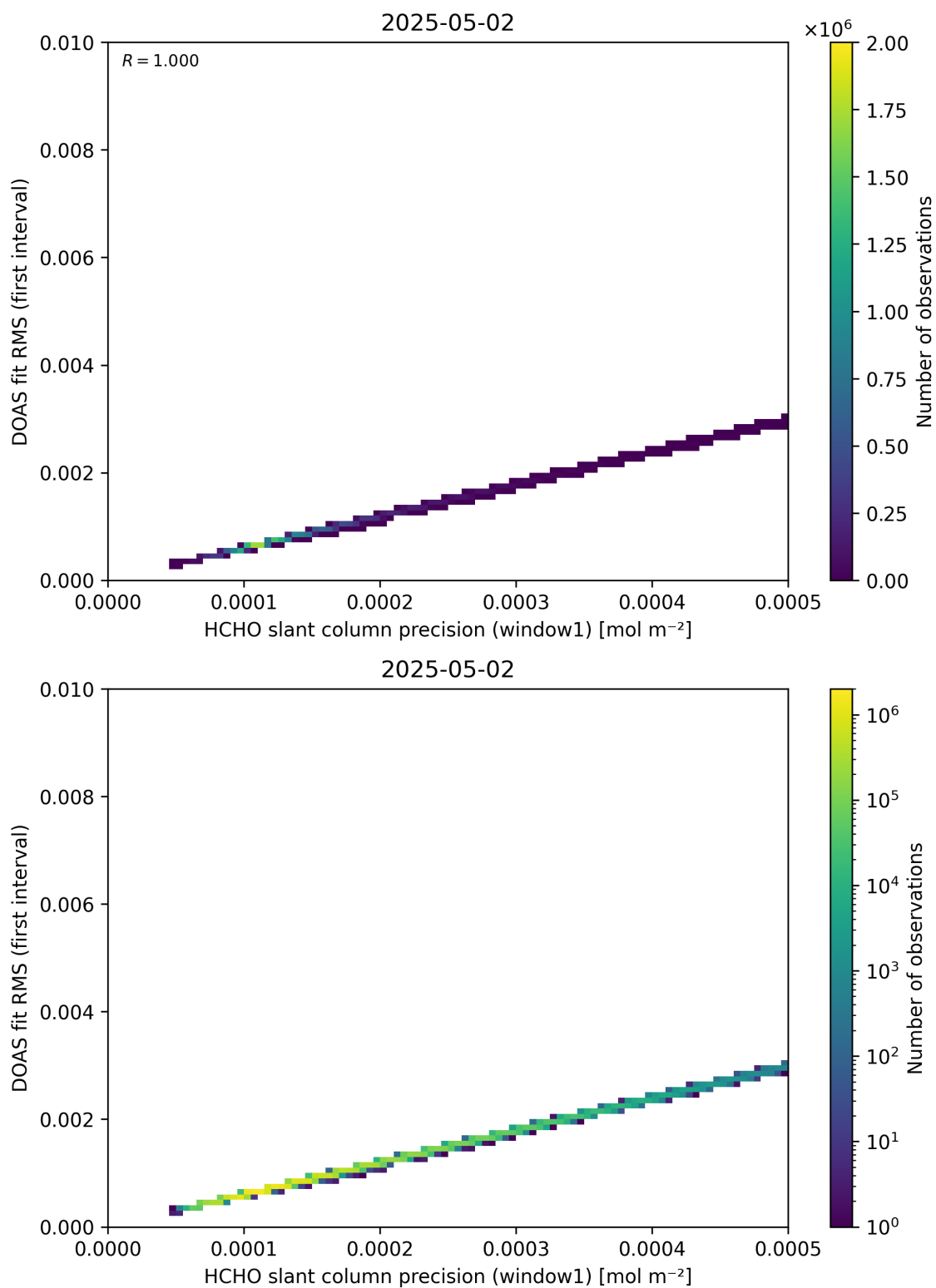
Figure 88: Scatter density plot of “HCHO slant column precision (window1)” against “DOAS fit RMS (first interval)” for 2025-05-01 to 2025-05-03.
