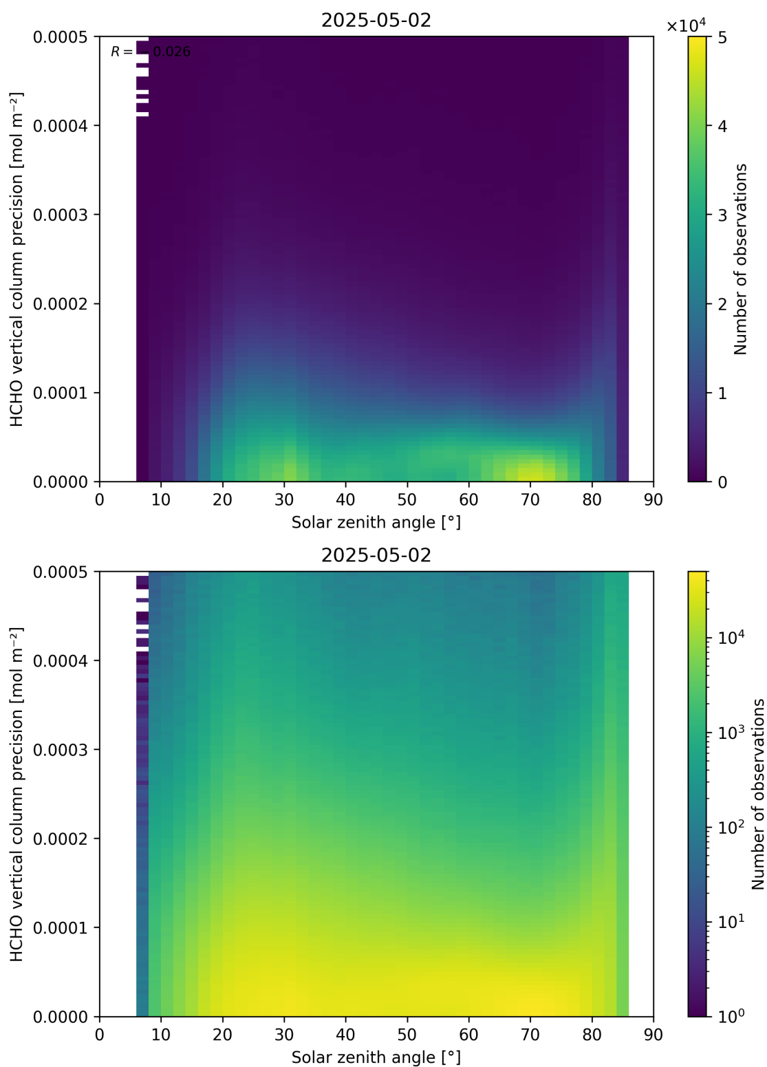
Figure 179: Scatter density plot of “Solar zenith angle” against “HCHO vertical column precision” for 2025-05-01 to 2025-05-03.
