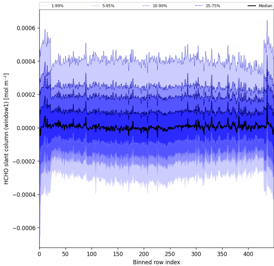
Figure 52: Along track statistics of “HCHO slant column (window1)” for 2025-05-01 to 2025-05-03
