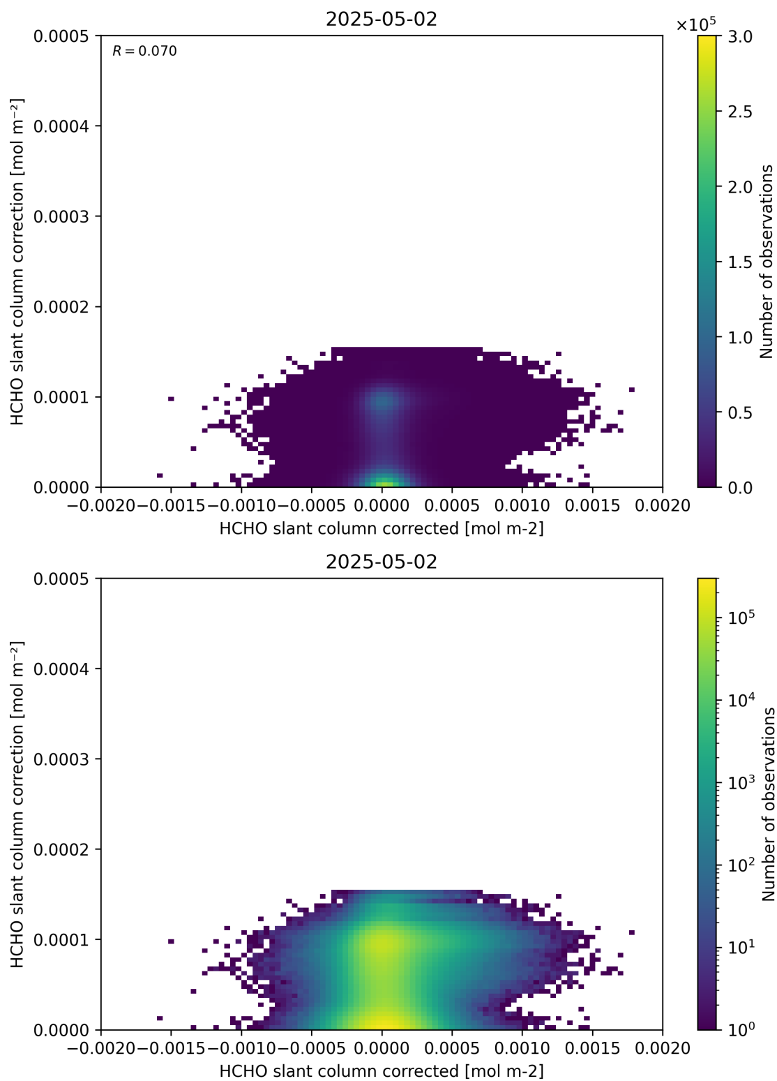
Figure 77: Scatter density plot of “HCHO slant column corrected” against “HCHO slant column correction” for 2025-05-01 to 2025-05-03.
