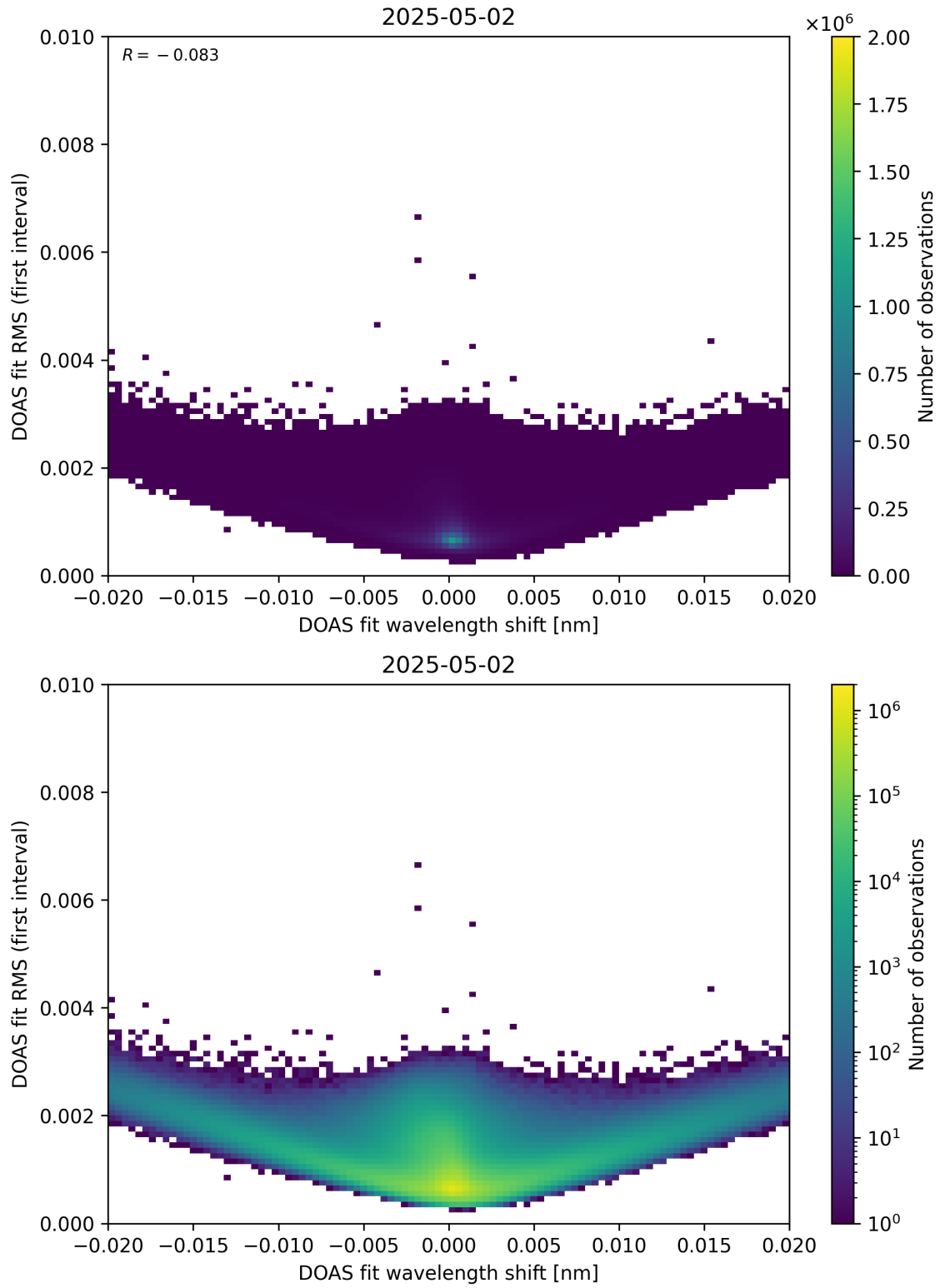
Figure 64: Scatter density plot of “DOAS fit wavelength shift” against “DOAS fit RMS (first interval)” for 2025-05-01 to 2025-05-03.
