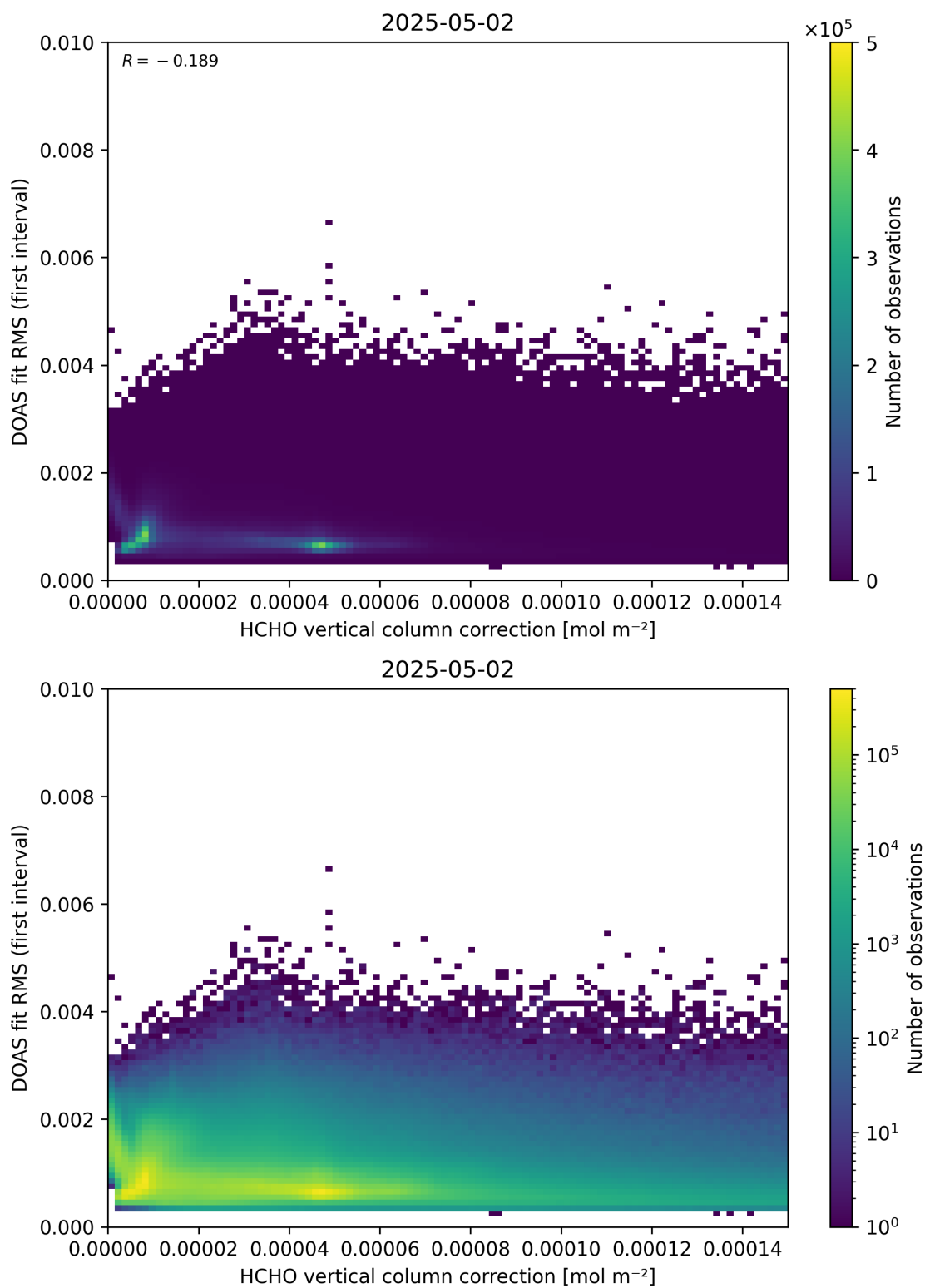
Figure 112: Scatter density plot of “HCHO vertical column correction” against “DOAS fit RMS (first interval)” for 2025-05-01 to 2025-05-03.
