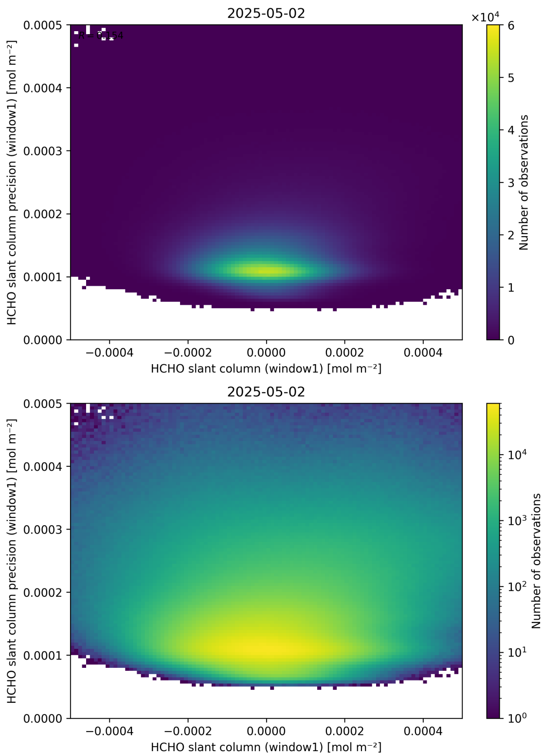
Figure 84: Scatter density plot of “HCHO slant column (window1)” against “HCHO slant column precision (window1)” for 2025-05-01 to 2025-05-03.
