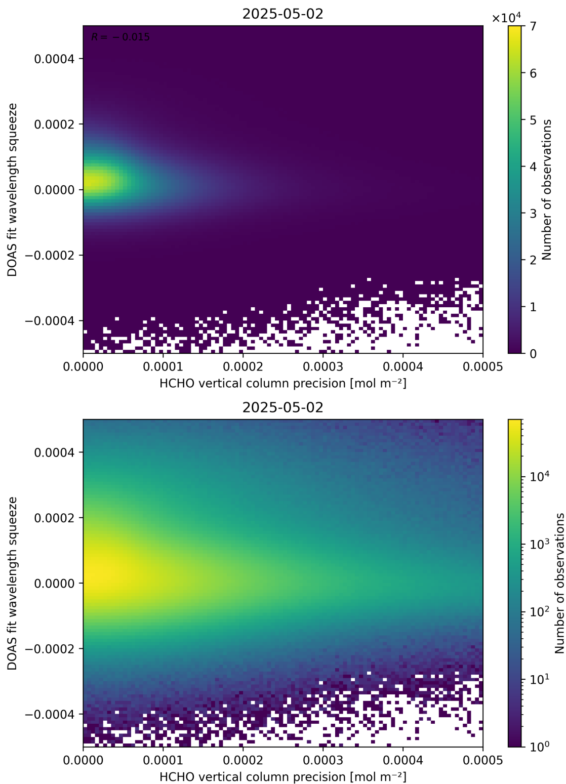
Figure 138: Scatter density plot of “HCHO vertical column precision” against “DOAS fit wavelength squeeze” for 2025-05-01 to 2025-05-03.
