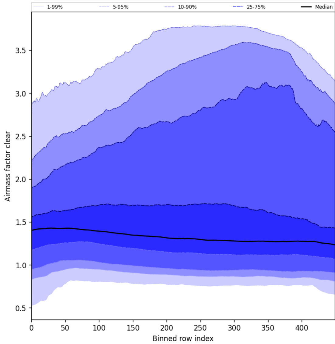
Figure 56: Along track statistics of “Airmass factor clear” for 2025-05-01 to 2025-05-03
