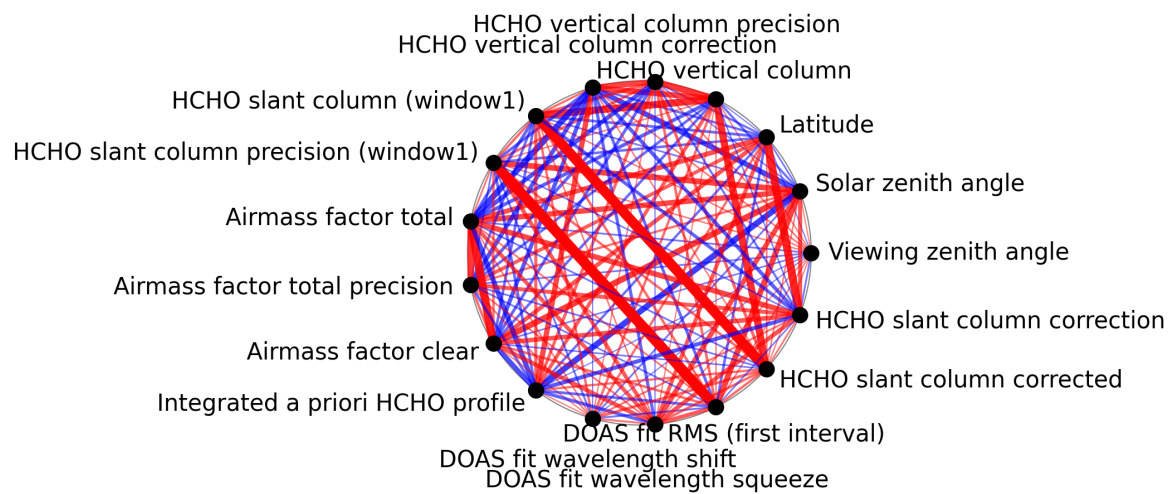
Figure 1: Map of correlation graph for 2025-05-01 to 2025-05-03.
