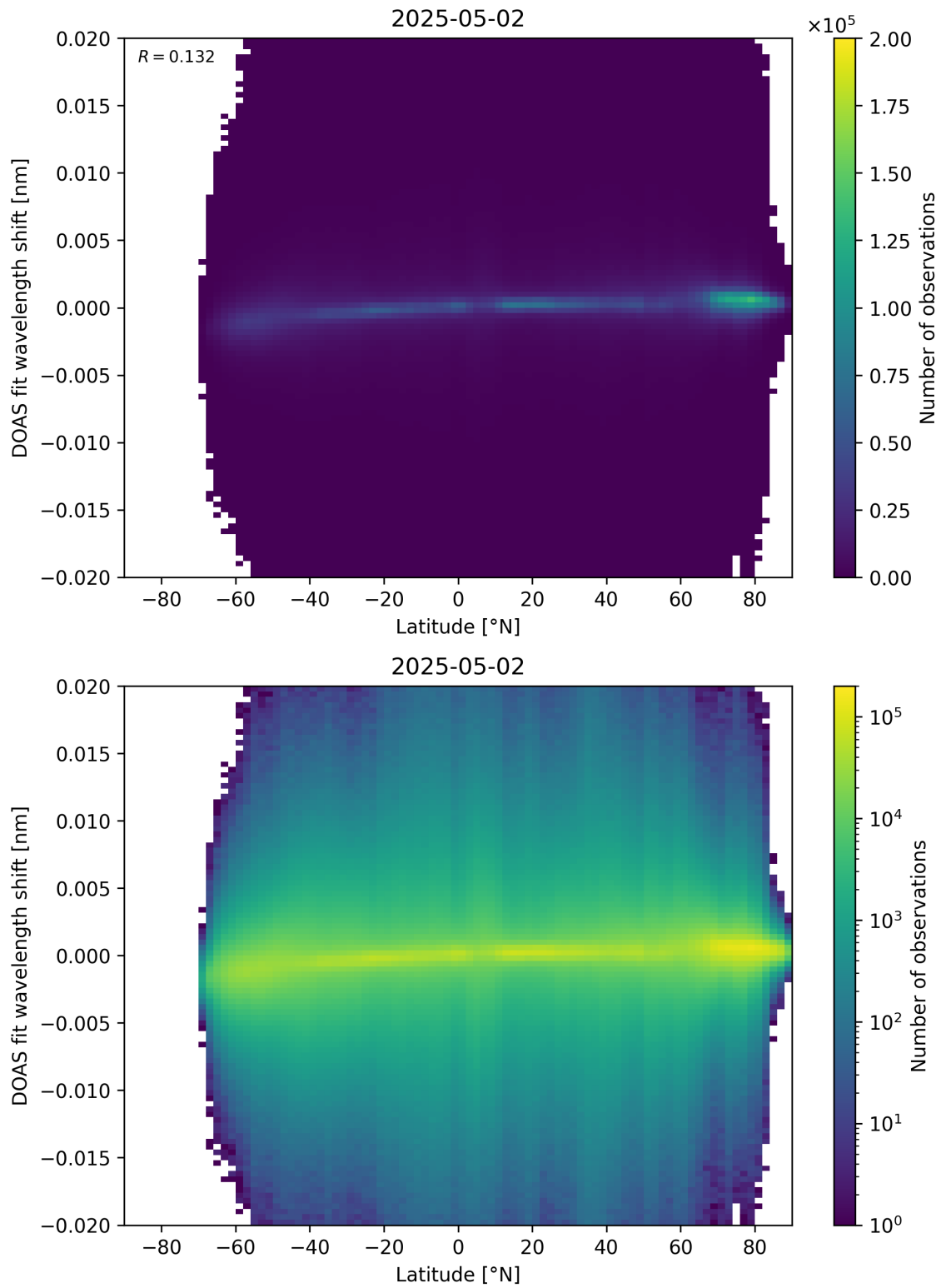
Figure 154: Scatter density plot of “Latitude” against “DOAS fit wavelength shift” for 2025-05-01 to 2025-05-03.
