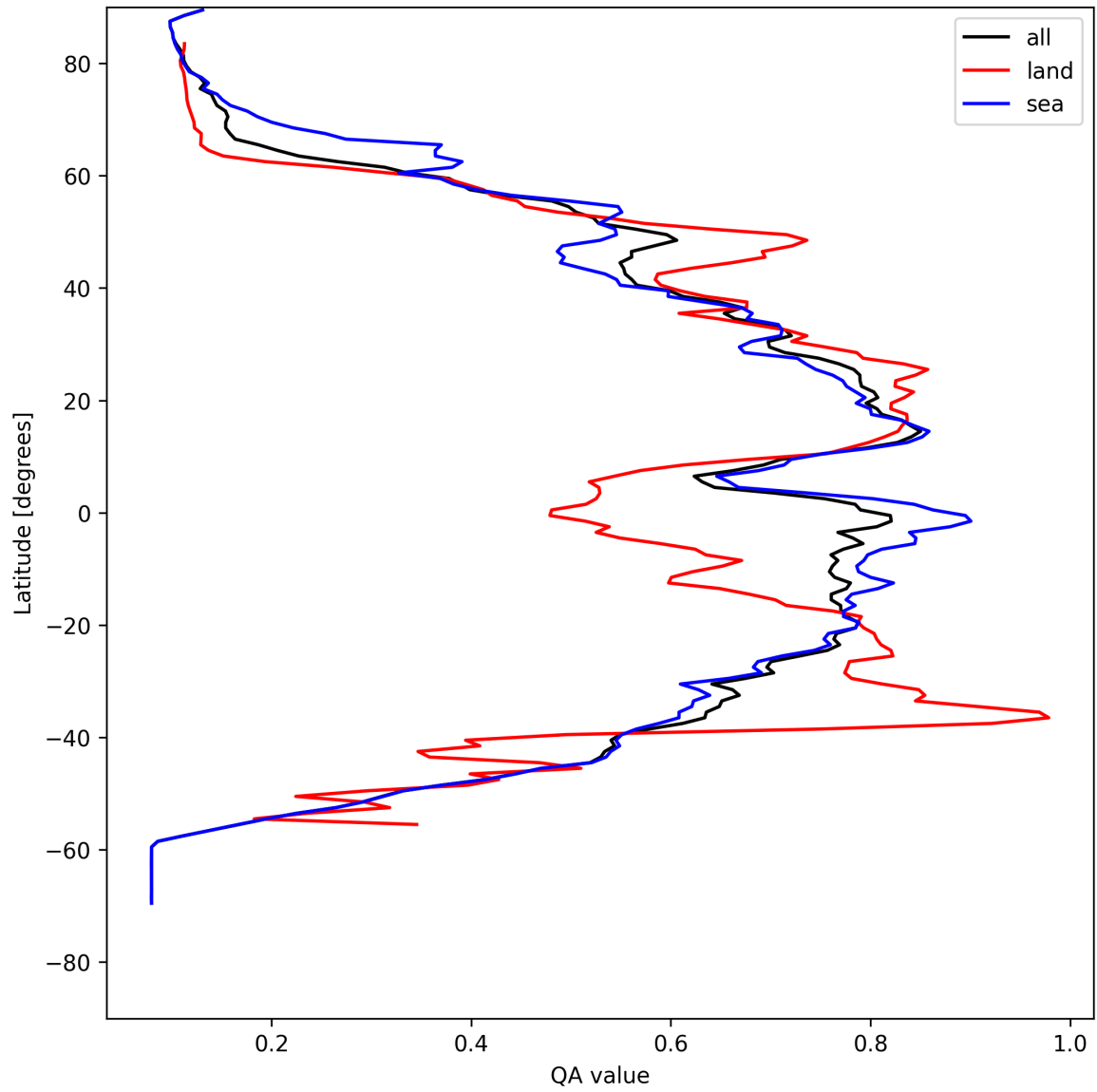
Figure 20: Zonal average of “QA value” for 2025-05-01 to 2025-05-03.
