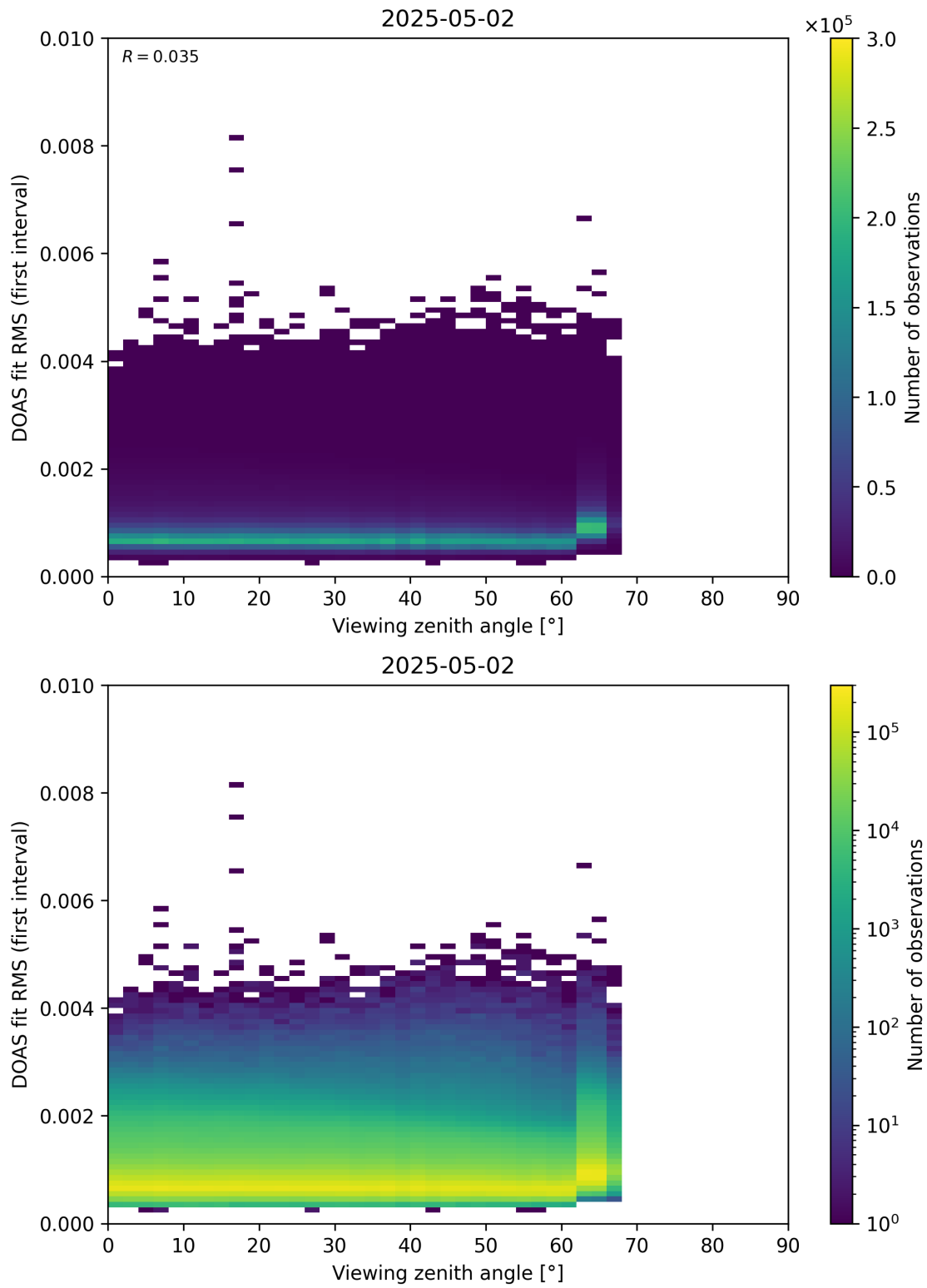
Figure 182: Scatter density plot of “Viewing zenith angle” against “DOAS fit RMS (first interval)” for 2025-05-01 to 2025-05-03.
