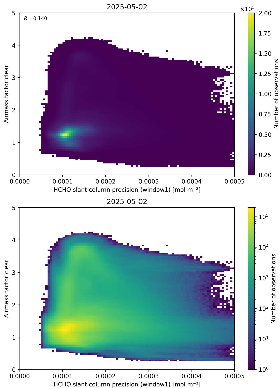
Figure 91: Scatter density plot of “HCHO slant column precision (window1)” against “Airmass factor clear” for 2025-05-01 to 2025-05-03.
