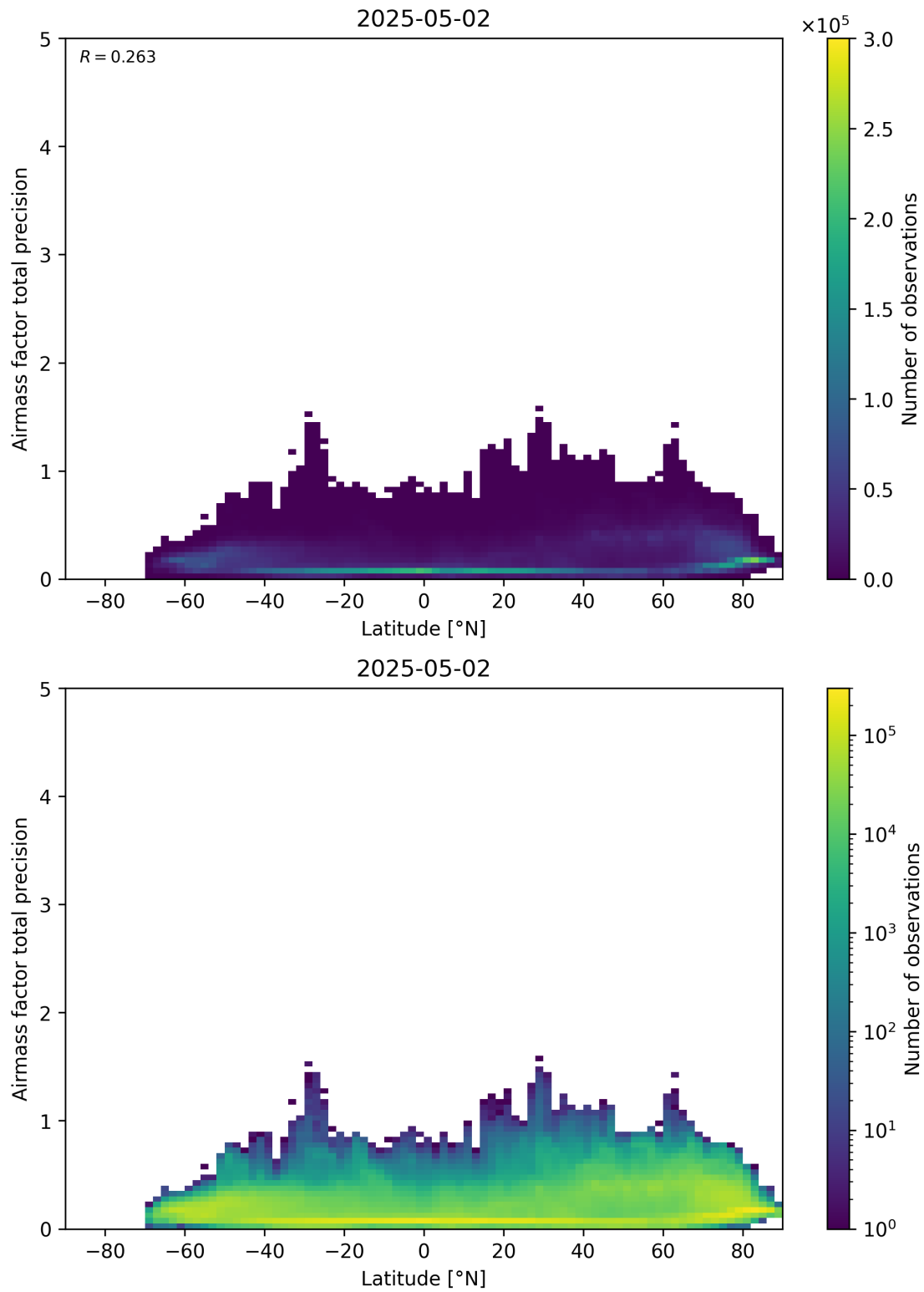
Figure 162: Scatter density plot of “Latitude” against “Airmass factor total precision” for 2025-05-01 to 2025-05-03.
