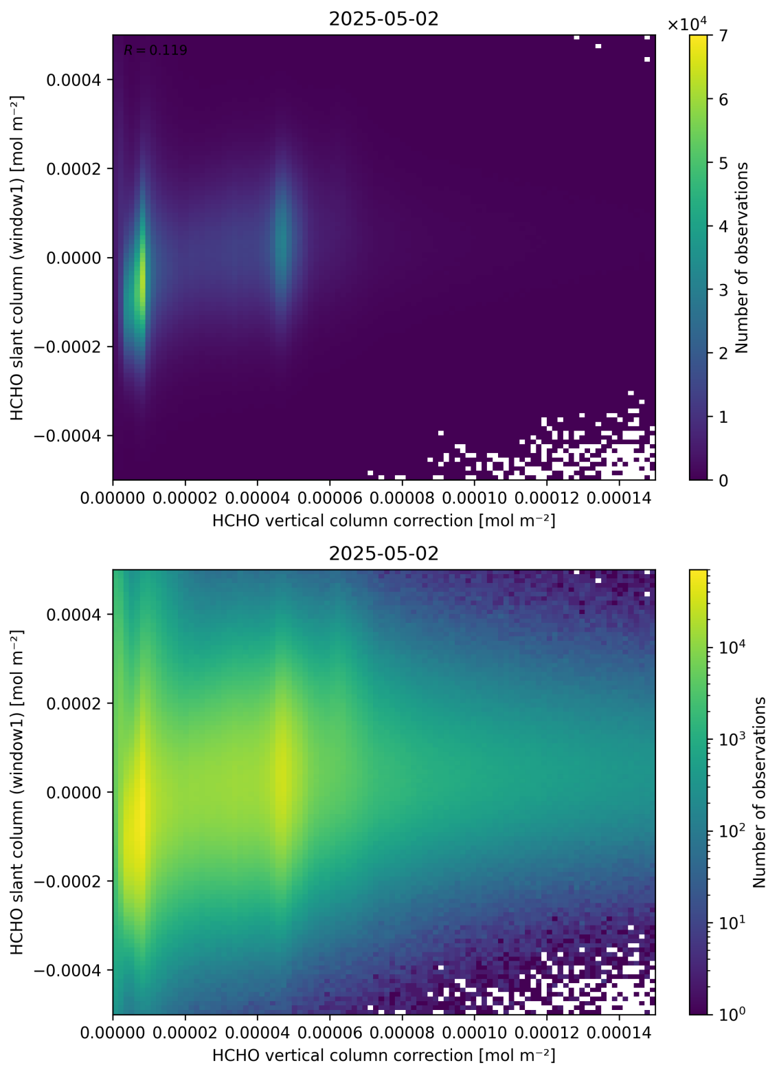
Figure 118: Scatter density plot of “HCHO vertical column correction” against “HCHO slant column (window1)” for 2025-05-01 to 2025-05-03.
