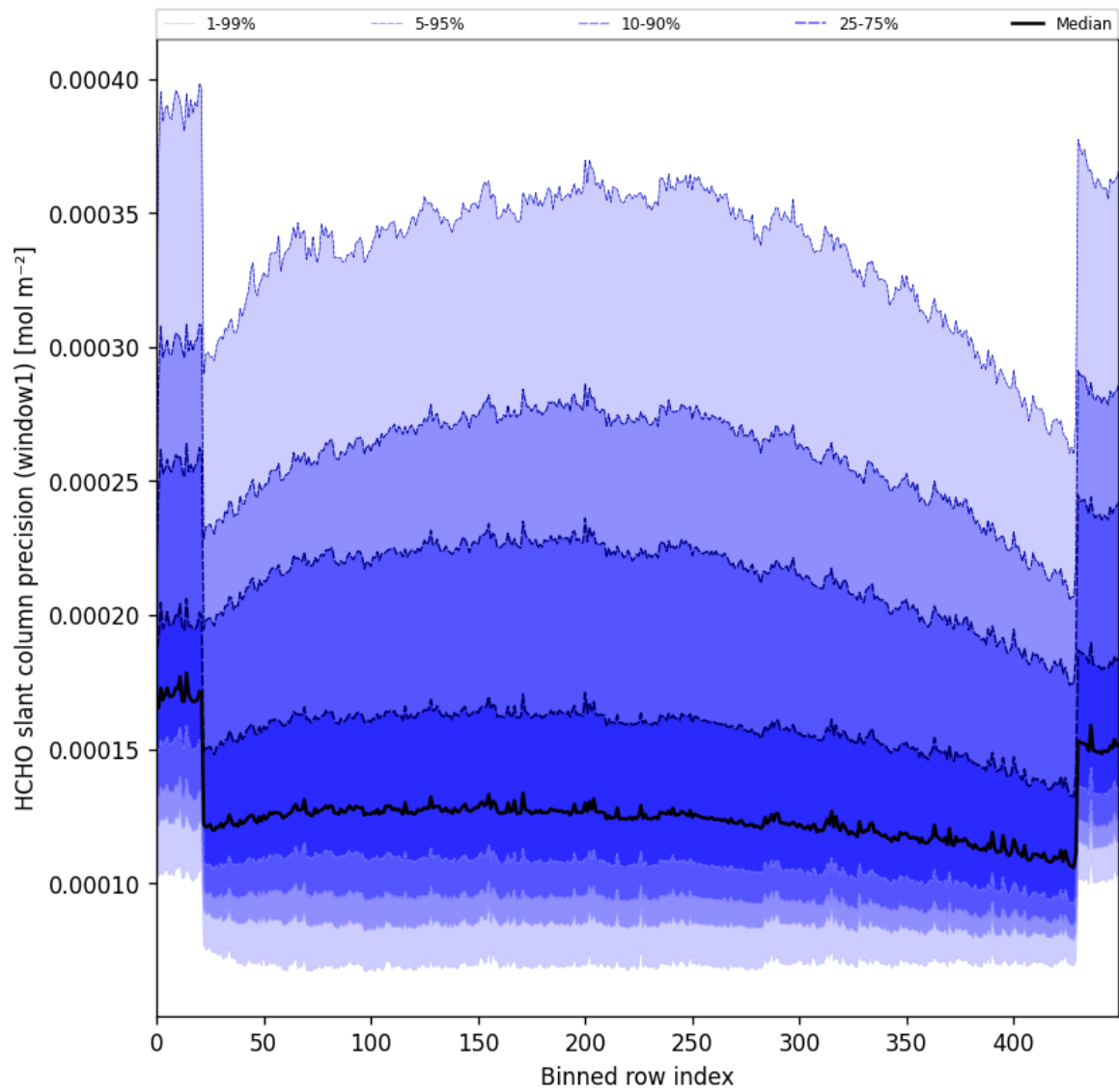
Figure 53: Along track statistics of “HCHO slant column precision (window1)” for 2025-05-01 to 2025-05-03
