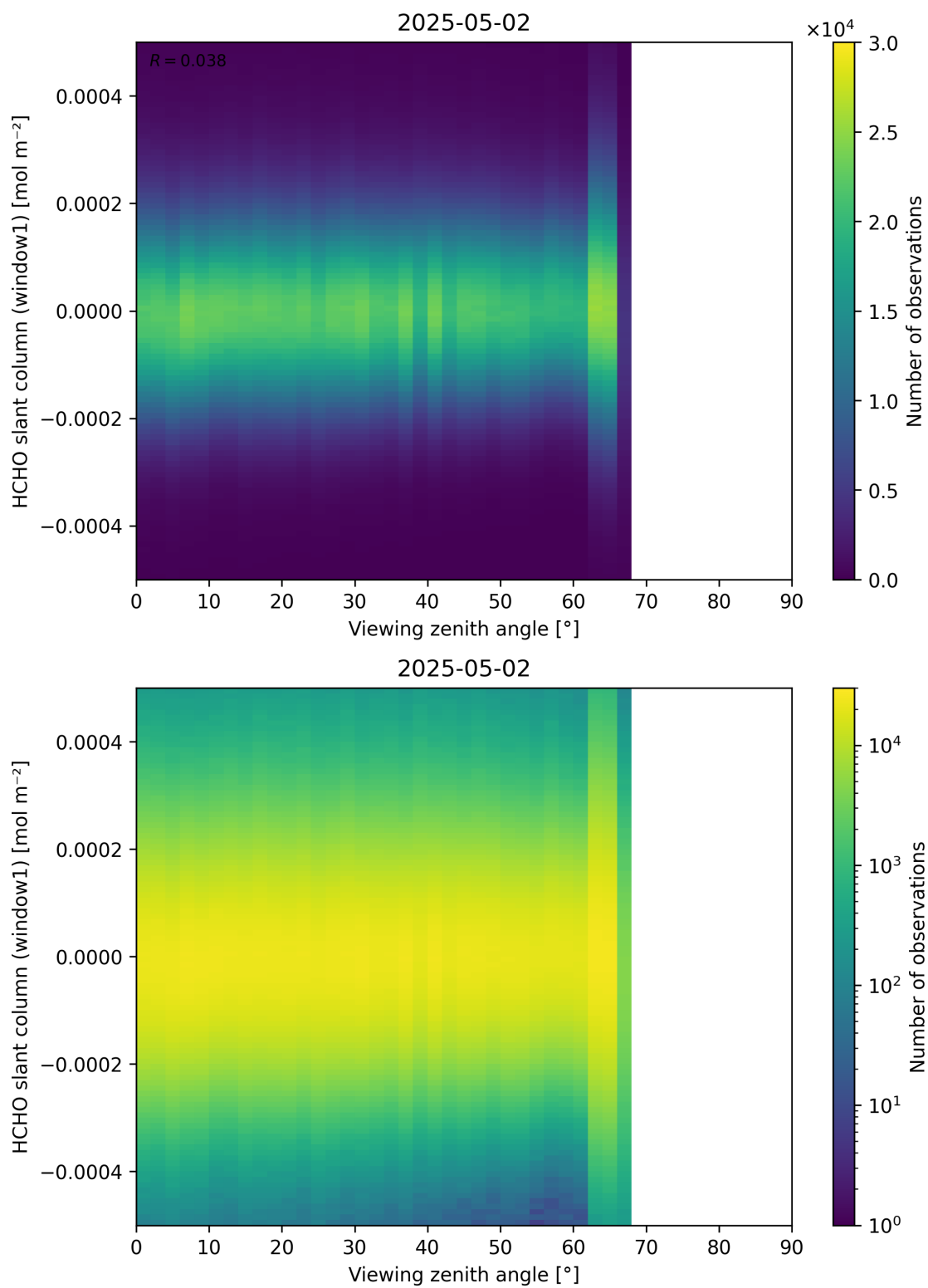
Figure 188: Scatter density plot of “Viewing zenith angle” against “HCHO slant column (window1)” for 2025-05-01 to 2025-05-03.
