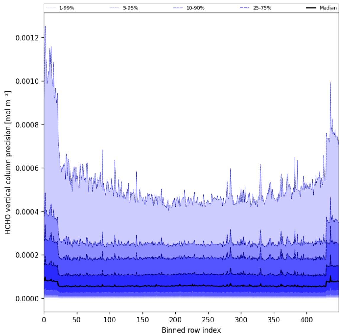
Figure 50: Along track statistics of “HCHO vertical column precision” for 2025-05-01 to 2025-05-03
