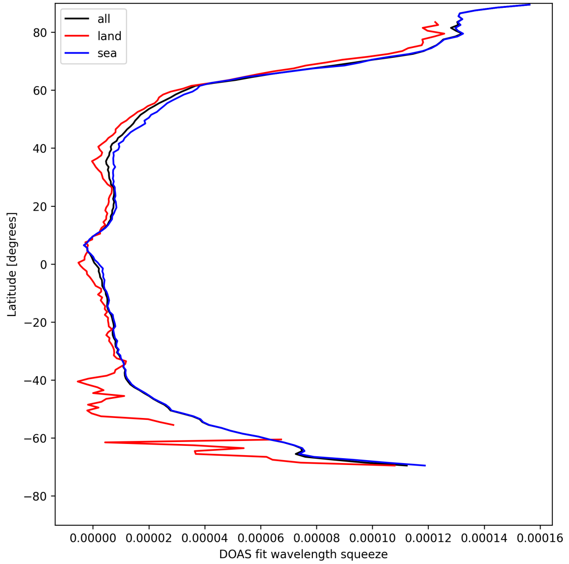
Figure 31: Zonal average of “DOAS fit wavelength squeeze” for 2025-05-01 to 2025-05-03.
