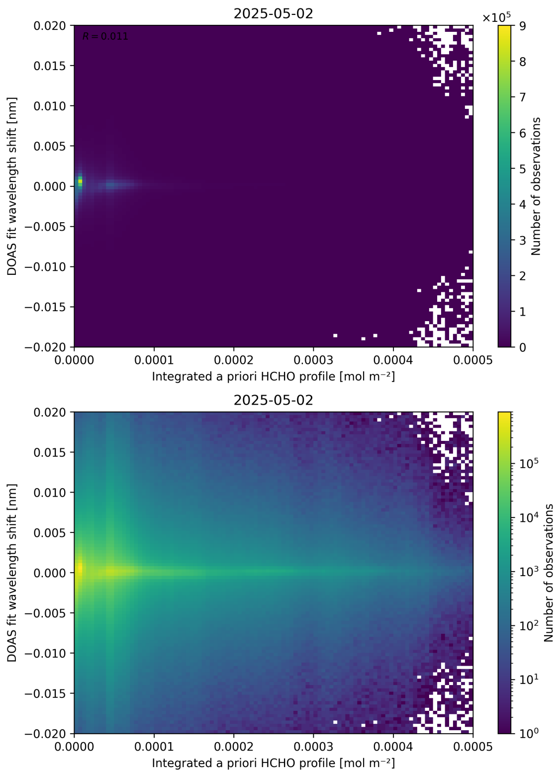
Figure 149: Scatter density plot of “Integrated a priori HCHO profile” against “DOAS fit wavelength shift” for 2025-05-01 to 2025-05-03.
