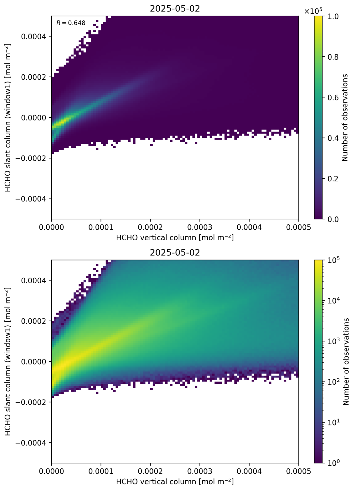
Figure 129: Scatter density plot of “HCHO vertical column” against “HCHO slant column (window1)” for 2025-05-01 to 2025-05-03.
