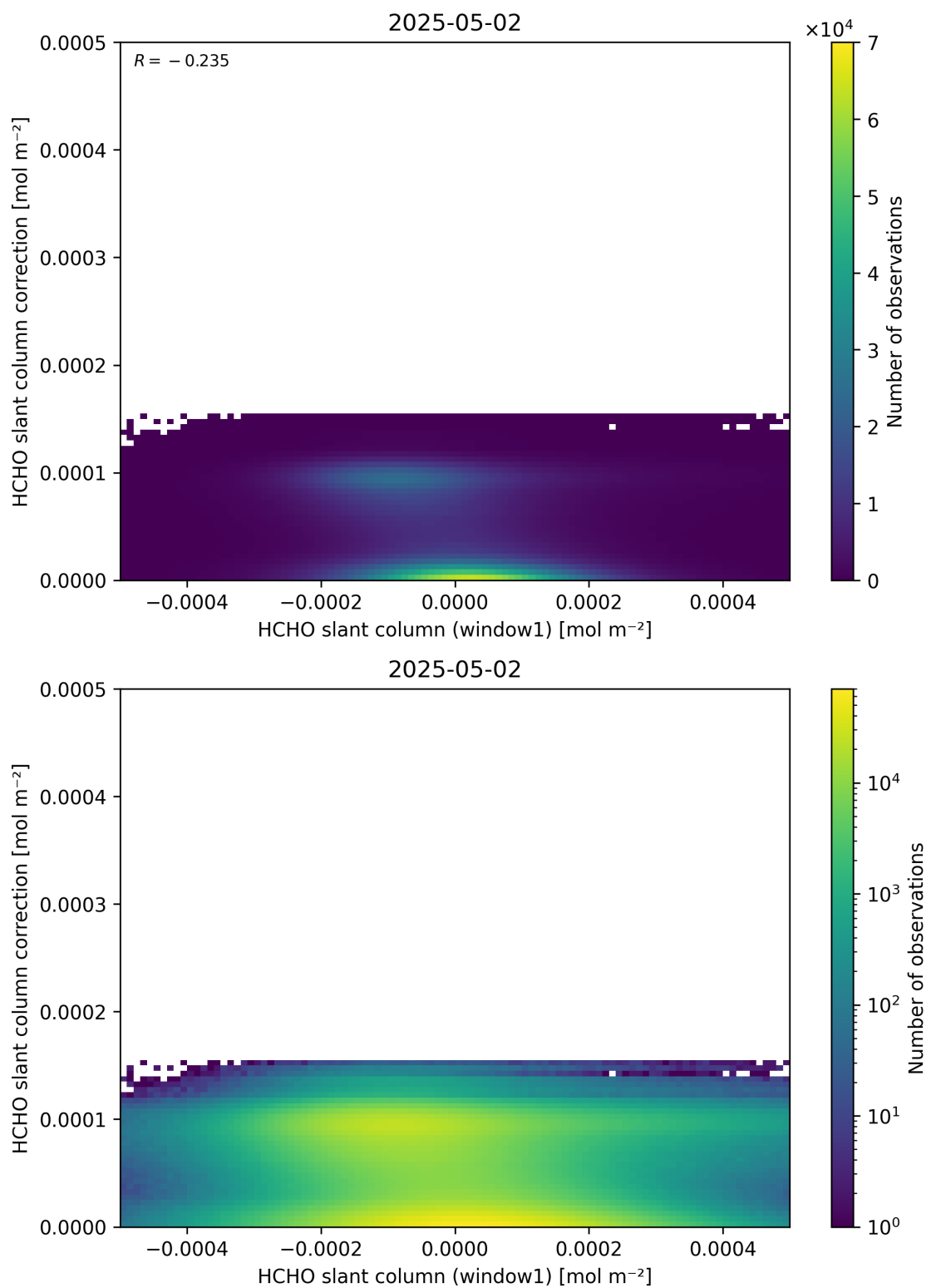
Figure 83: Scatter density plot of “HCHO slant column (window1)” against “HCHO slant column correction” for 2025-05-01 to 2025-05-03.
