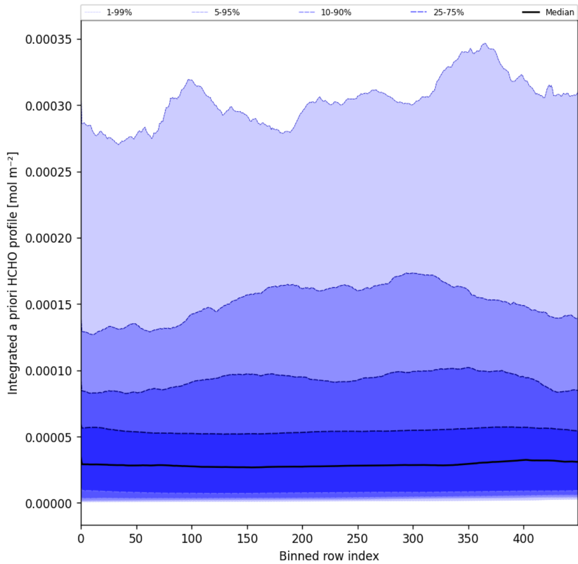
Figure 57: Along track statistics of "Integrated a priori HCHO profile" for 2025-05-01 to 2025-05-03
