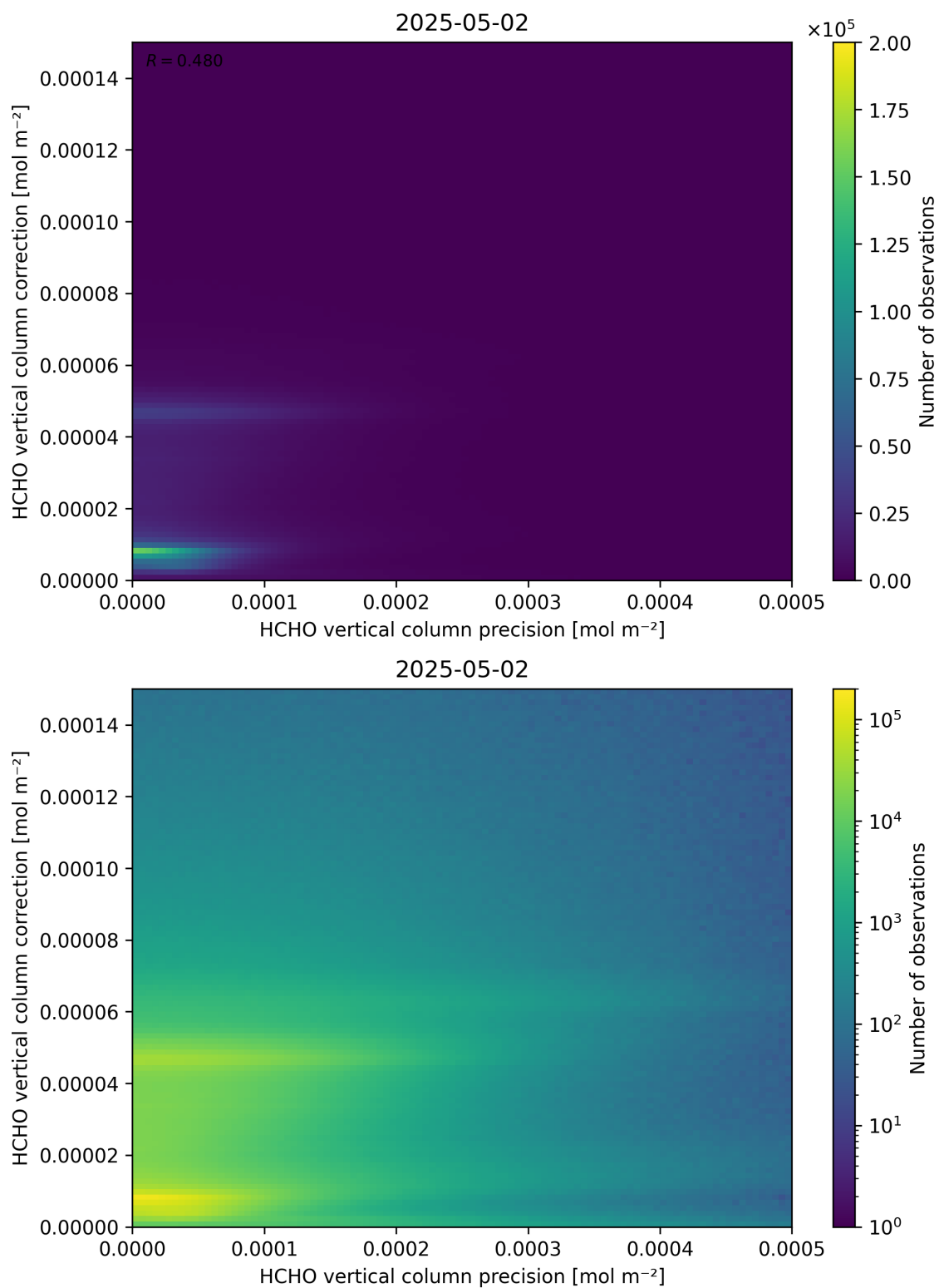
Figure 146: Scatter density plot of “HCHO vertical column precision” against “HCHO vertical column correction” for 2025-05-01 to 2025-05-03.
