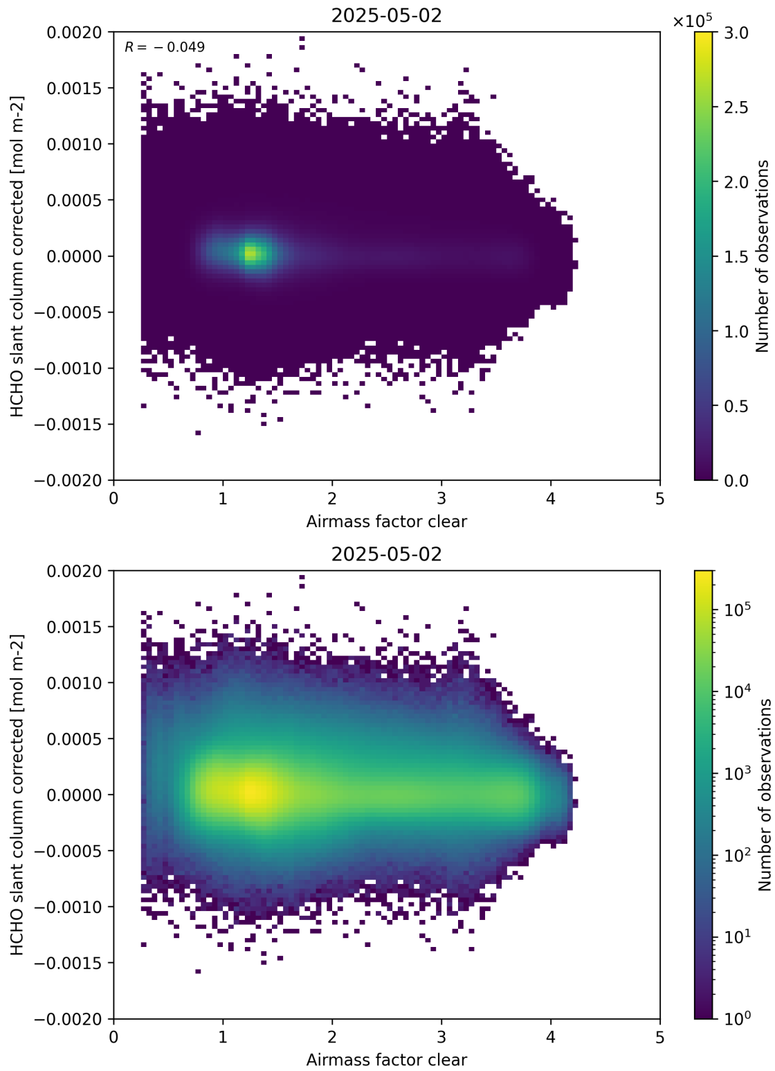
Figure 74: Scatter density plot of “Airmass factor clear” against “HCHO slant column corrected” for 2025-05-01 to 2025-05-03.
