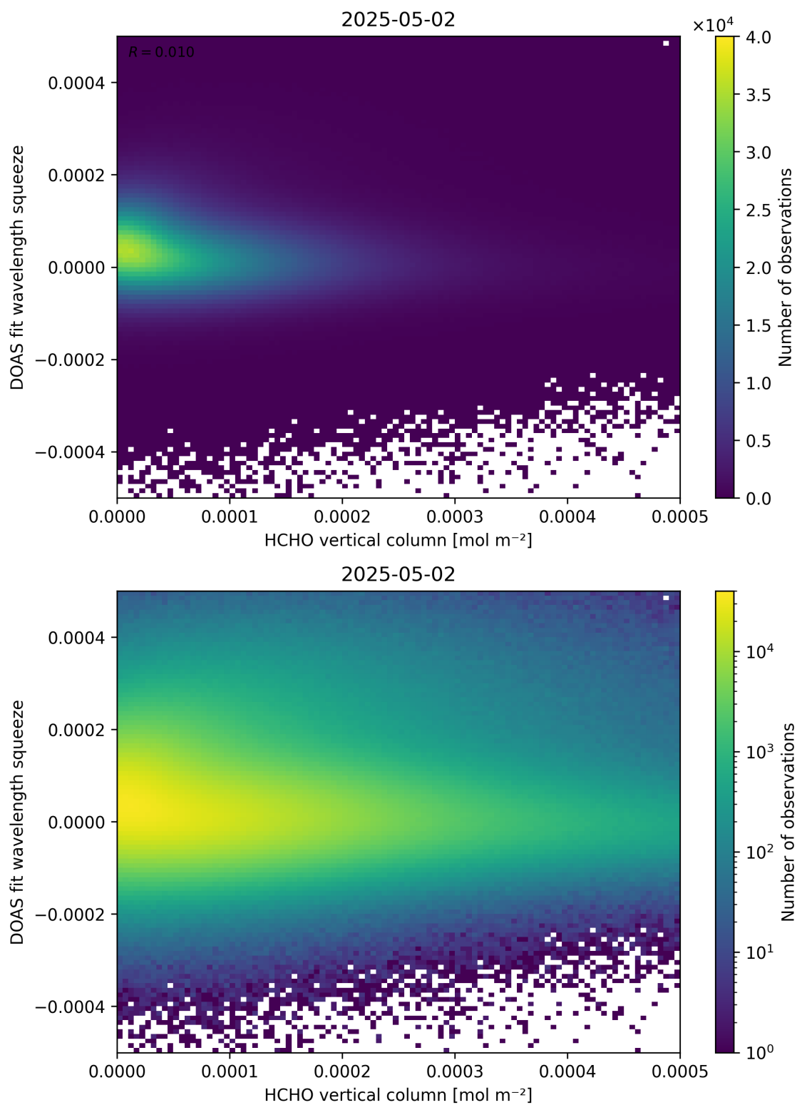
Figure 125: Scatter density plot of “HCHO vertical column” against “DOAS fit wavelength squeeze” for 2025-05-01 to 2025-05-03.
