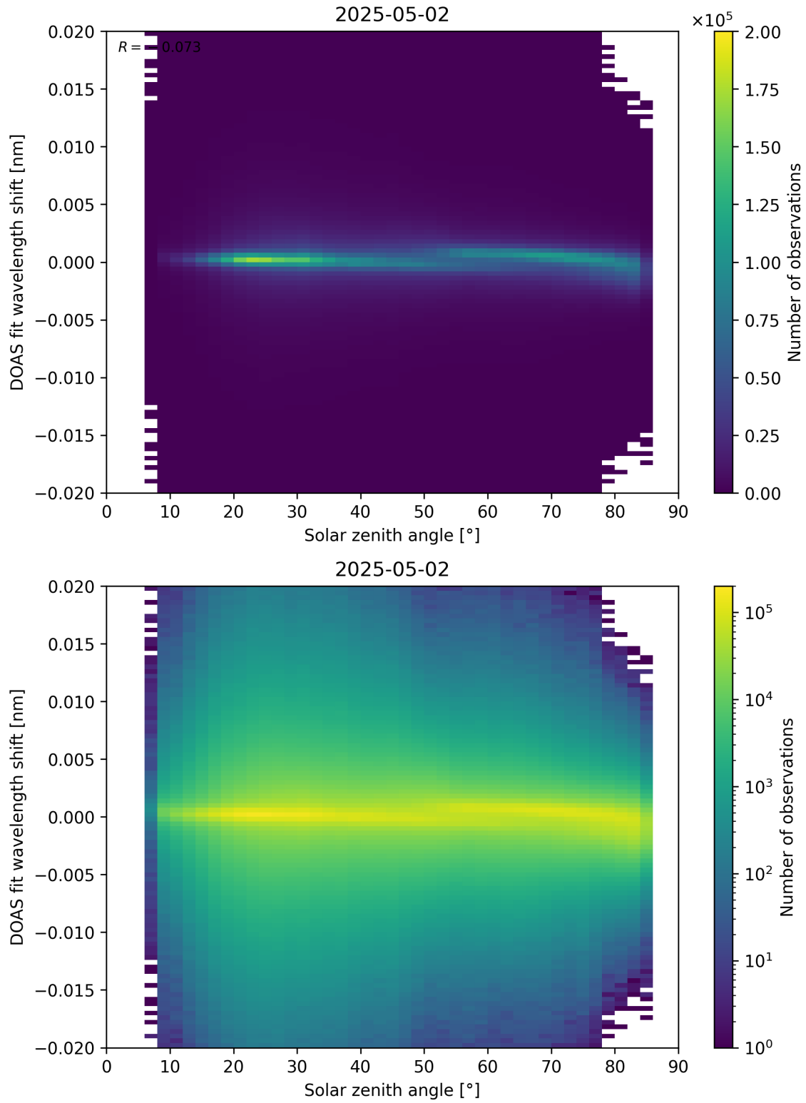
Figure 168: Scatter density plot of “Solar zenith angle” against “DOAS fit wavelength shift” for 2025-05-01 to 2025-05-03.
