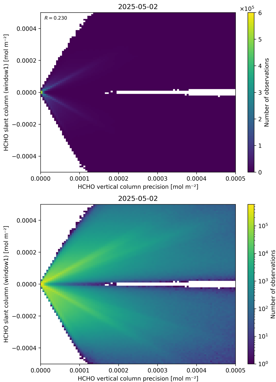
Figure 142: Scatter density plot of “HCHO vertical column precision” against “HCHO slant column (window1)” for 2025-05-01 to 2025-05-03.
