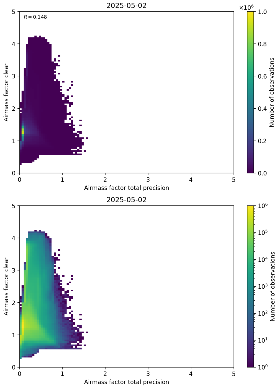
Figure 108: Scatter density plot of “Airmass factor total precision” against “Airmass factor clear” for 2025-05-01 to 2025-05-03.
