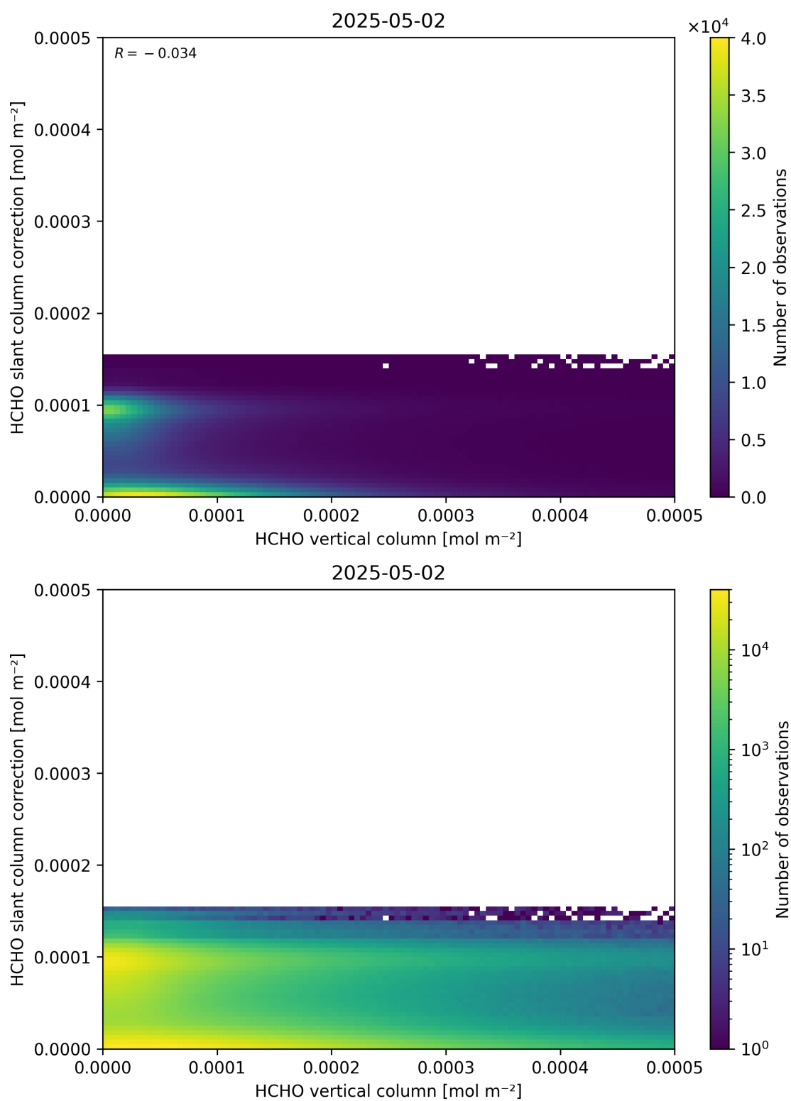
Figure 128: Scatter density plot of “HCHO vertical column” against “HCHO slant column correction” for 2025-05-01 to 2025-05-03.
