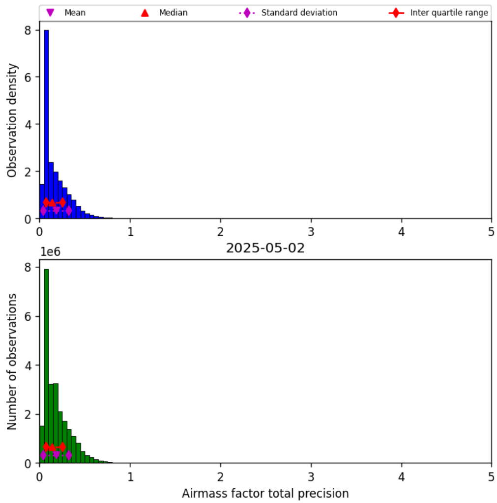
Figure 41: Histogram of “Airmass factor total precision” for 2025-05-01 to 2025-05-03
