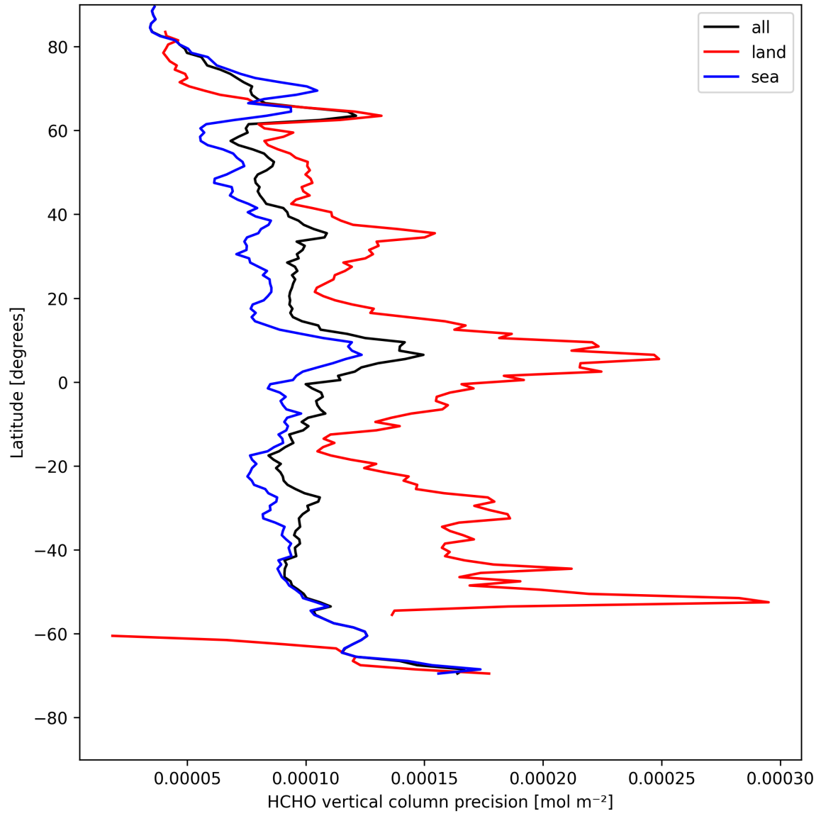
Figure 22: Zonal average of “HCHO vertical column precision” for 2025-05-01 to 2025-05-03.
