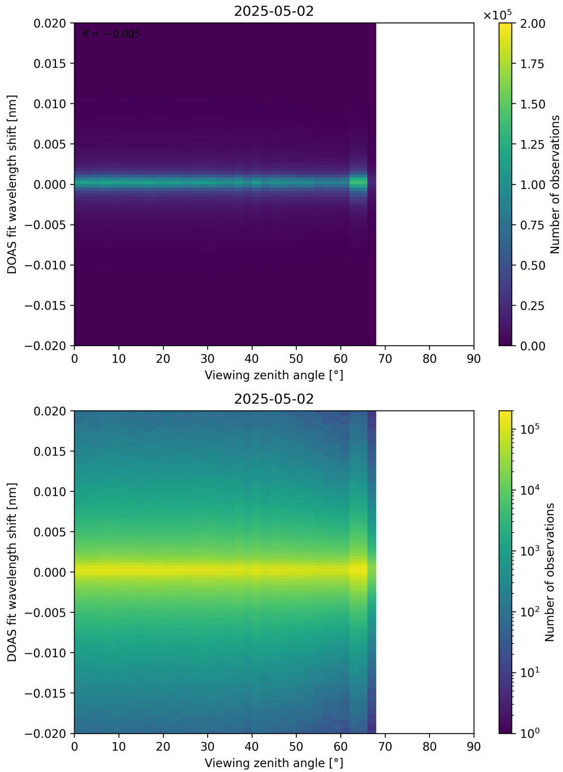
Figure 183: Scatter density plot of “Viewing zenith angle” against “DOAS fit wavelength shift” for 2025-05-01 to 2025-05-03.
