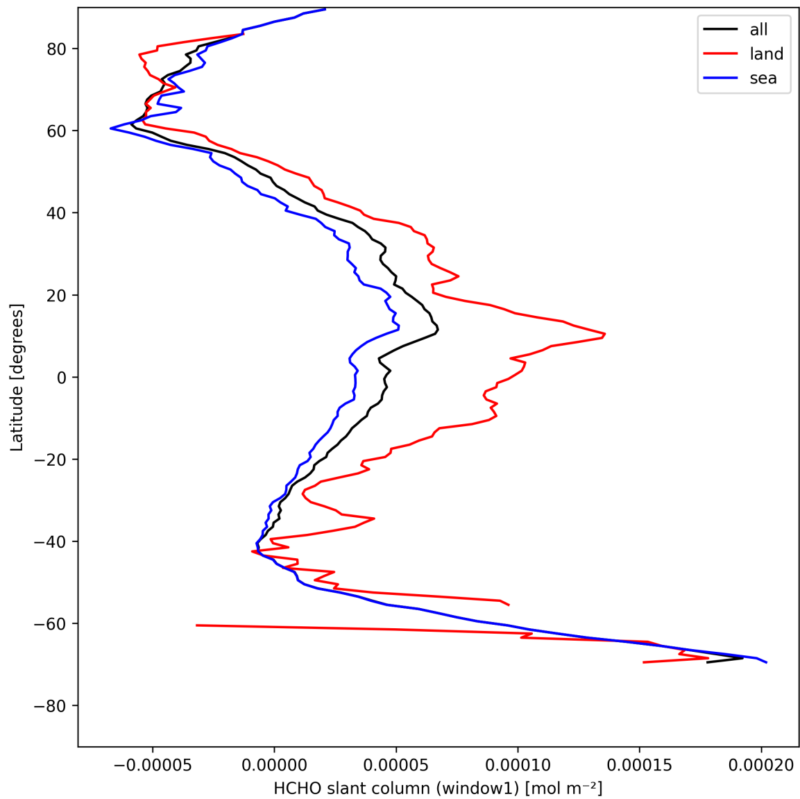
Figure 24: Zonal average of “HCHO slant column (window1)” for 2025-05-01 to 2025-05-03.
