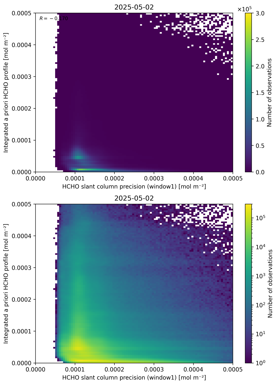
Figure 96: Scatter density plot of “HCHO slant column precision (window1)” against “Integrated a priori HCHO profile” for 2025-05-01 to 2025-05-03.
