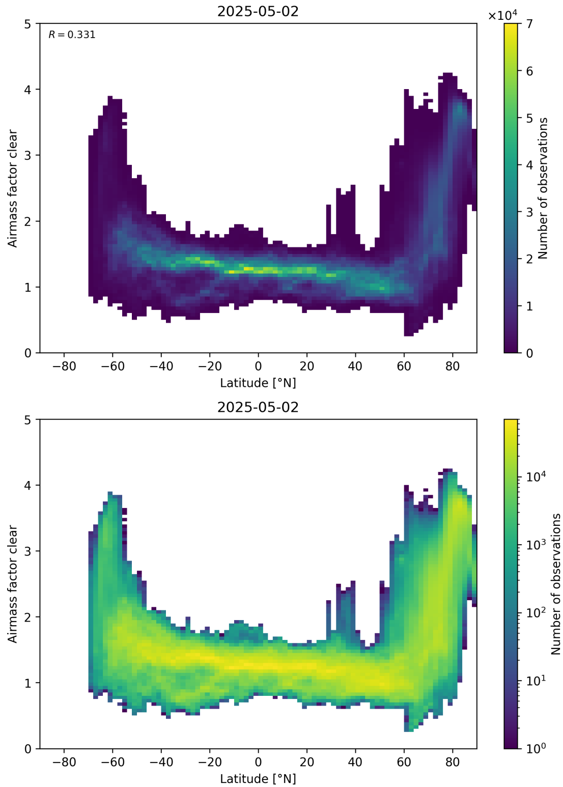
Figure 156: Scatter density plot of “Latitude” against “Airmass factor clear” for 2025-05-01 to 2025-05-03.
