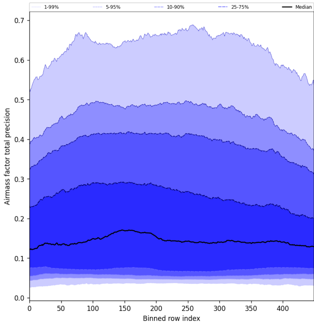
Figure 55: Along track statistics of “Airmass factor total precision” for 2025-05-01 to 2025-05-03
