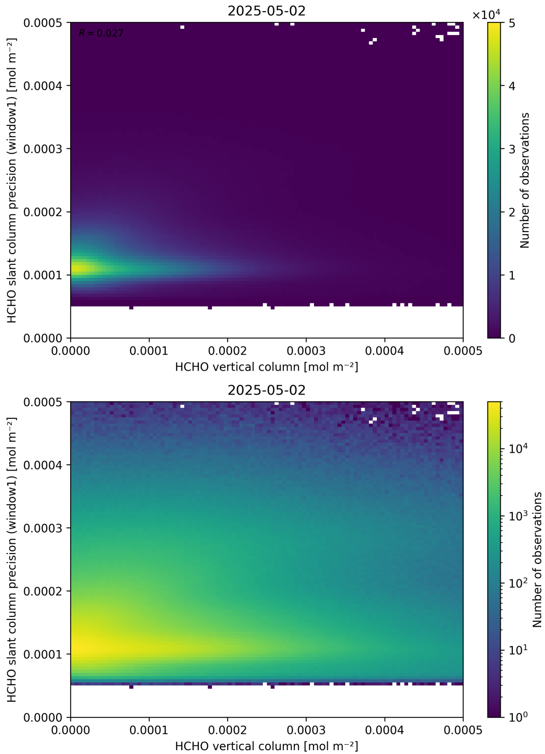
Figure 130: Scatter density plot of “HCHO vertical column” against “HCHO slant column precision (window1)” for 2025-05-01 to 2025-05-03.
