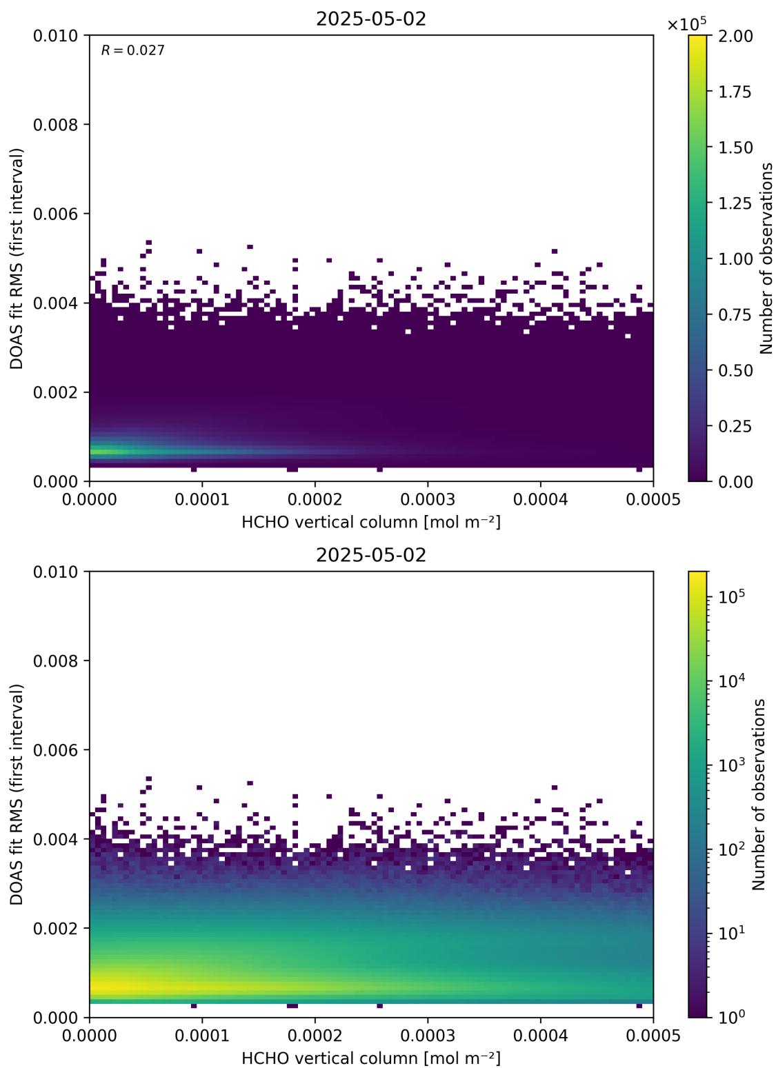
Figure 123: Scatter density plot of “HCHO vertical column” against “DOAS fit RMS (first interval)” for 2025-05-01 to 2025-05-03.
