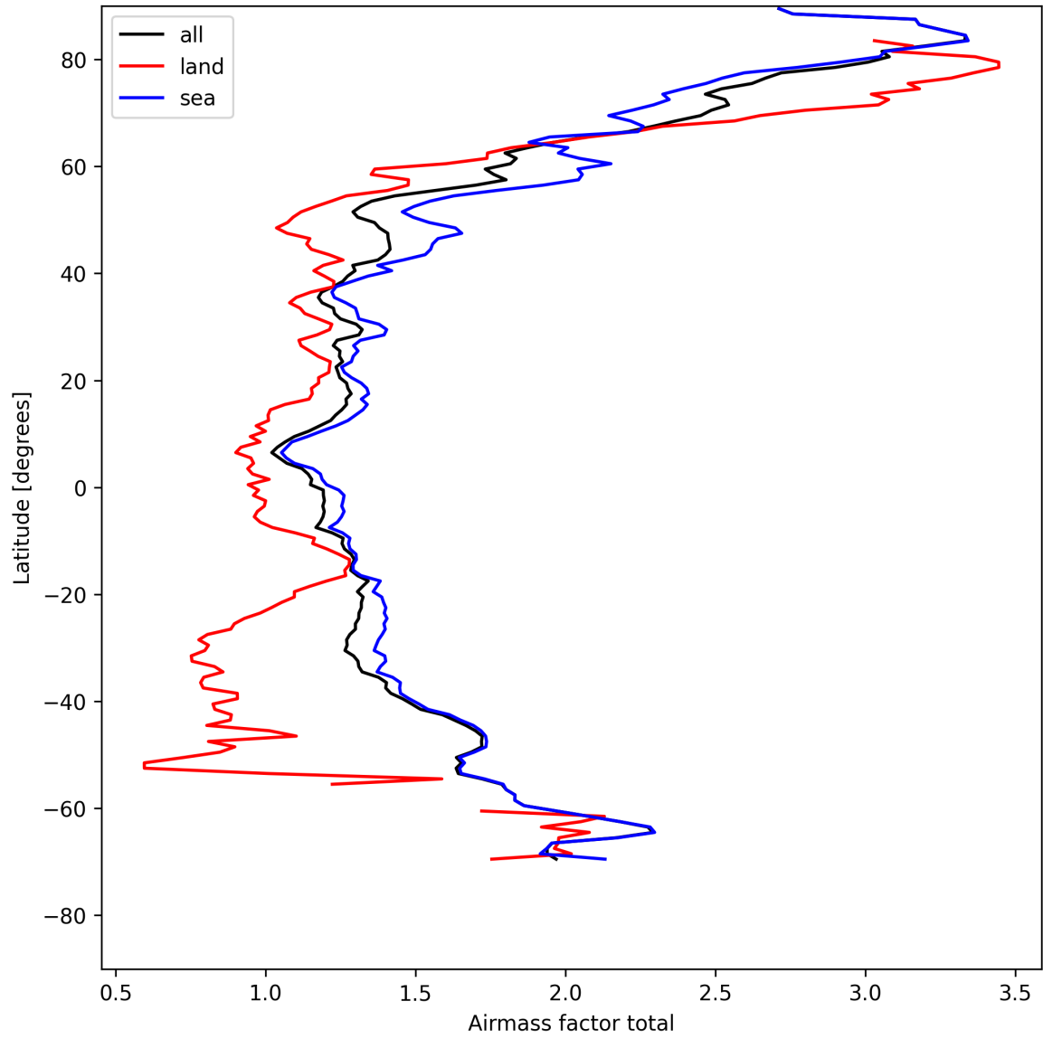
Figure 26: Zonal average of “Airmass factor total” for 2025-05-01 to 2025-05-03.
