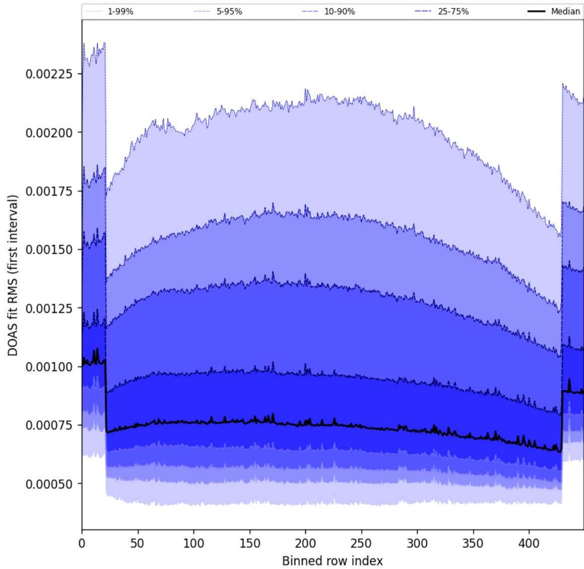
Figure 60: Along track statistics of “DOAS fit RMS (first interval)” for 2025-05-01 to 2025-05-03
