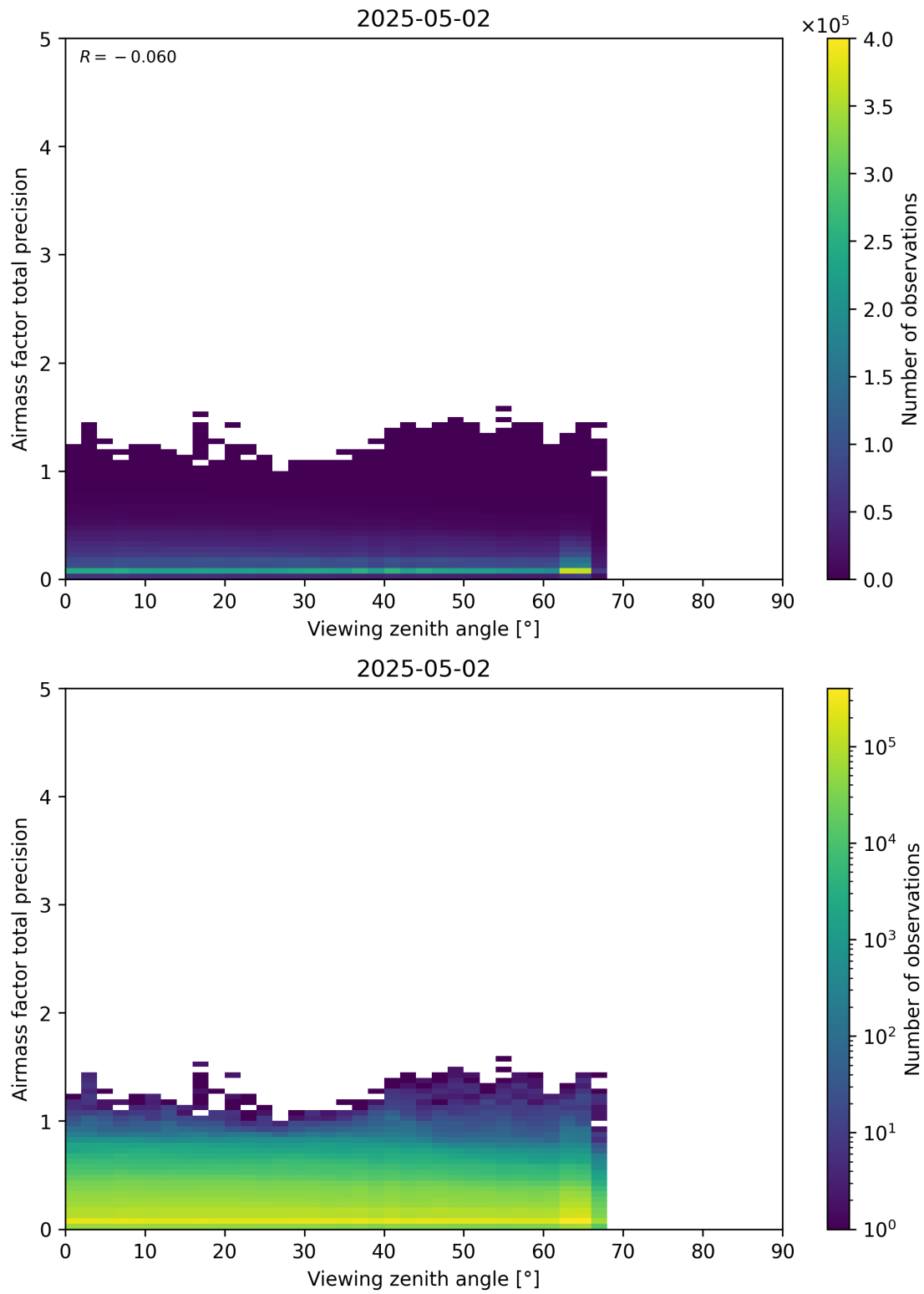
Figure 191: Scatter density plot of “Viewing zenith angle” against “Airmass factor total precision” for 2025-05-01 to 2025-05-03.
