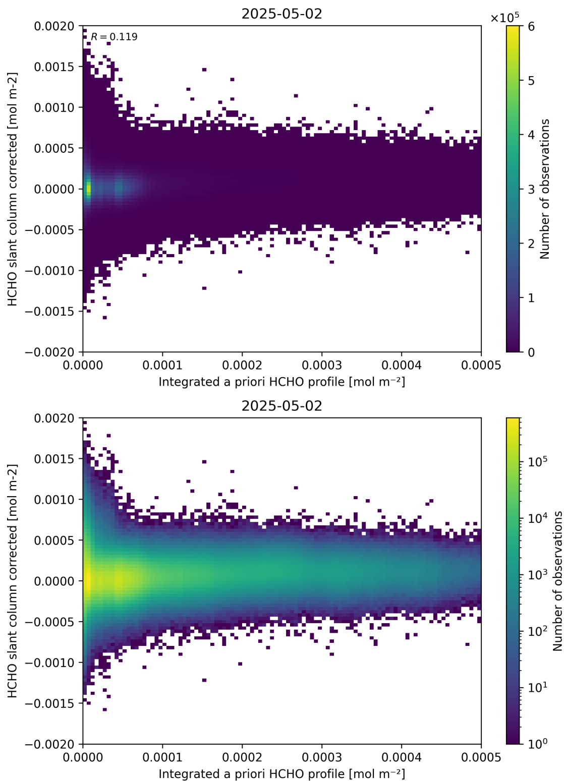
Figure 151: Scatter density plot of “Integrated a priori HCHO profile” against “HCHO slant column corrected” for 2025-05-01 to 2025-05-03.
