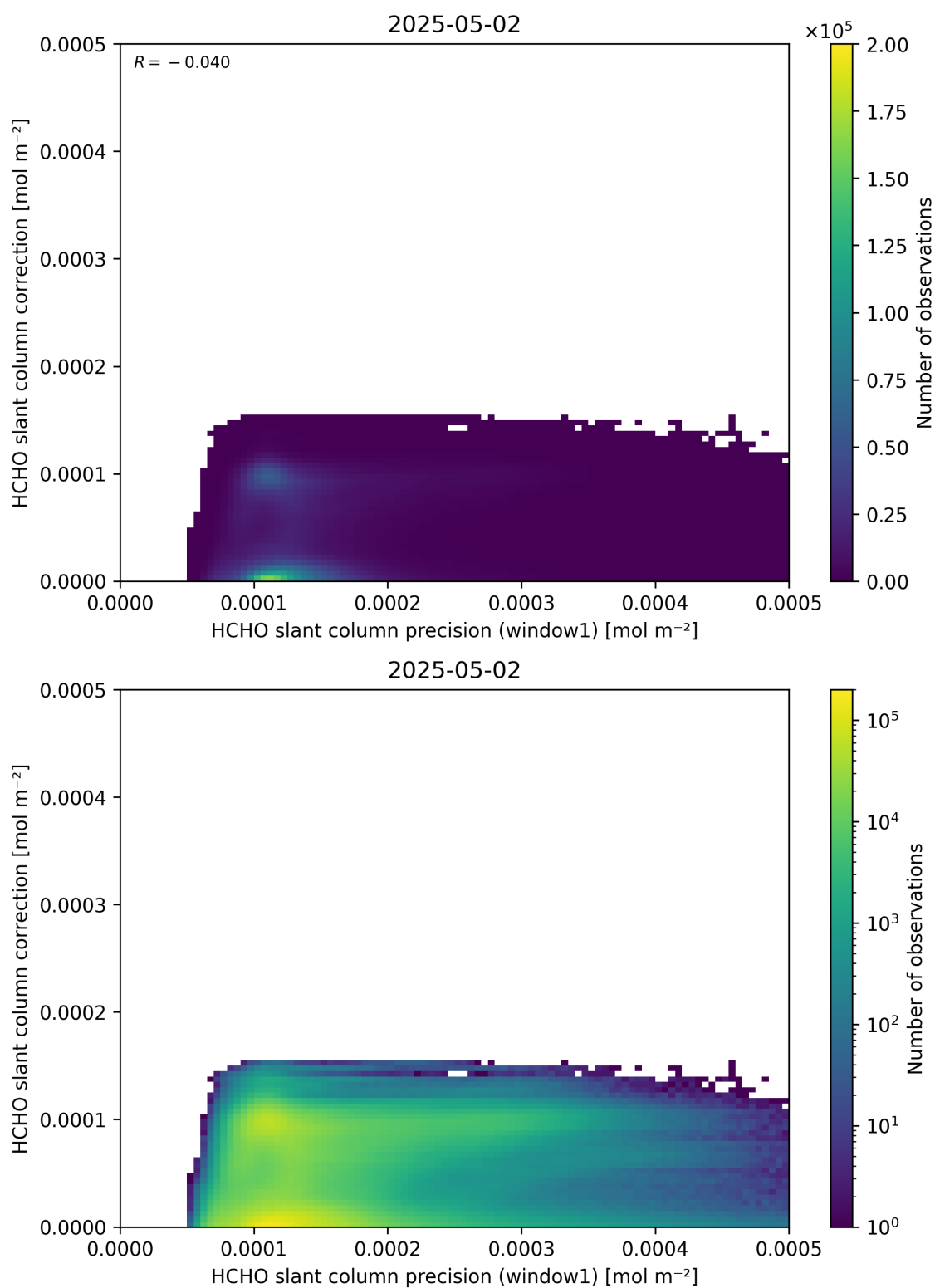
Figure 93: Scatter density plot of “HCHO slant column precision (window1)” against “HCHO slant column correction” for 2025-05-01 to 2025-05-03.
