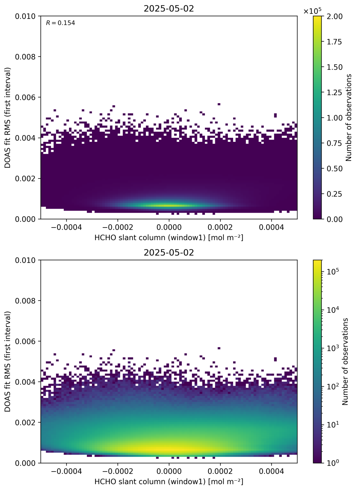
Figure 78: Scatter density plot of “HCHO slant column (window1)” against “DOAS fit RMS (first interval)” for 2025-05-01 to 2025-05-03.
