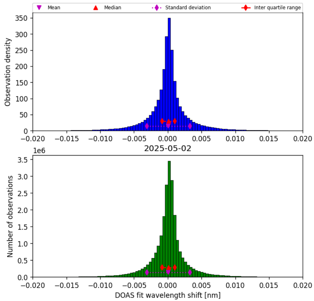
Figure 44: Histogram of “DOAS fit wavelength shift” for 2025-05-01 to 2025-05-03
