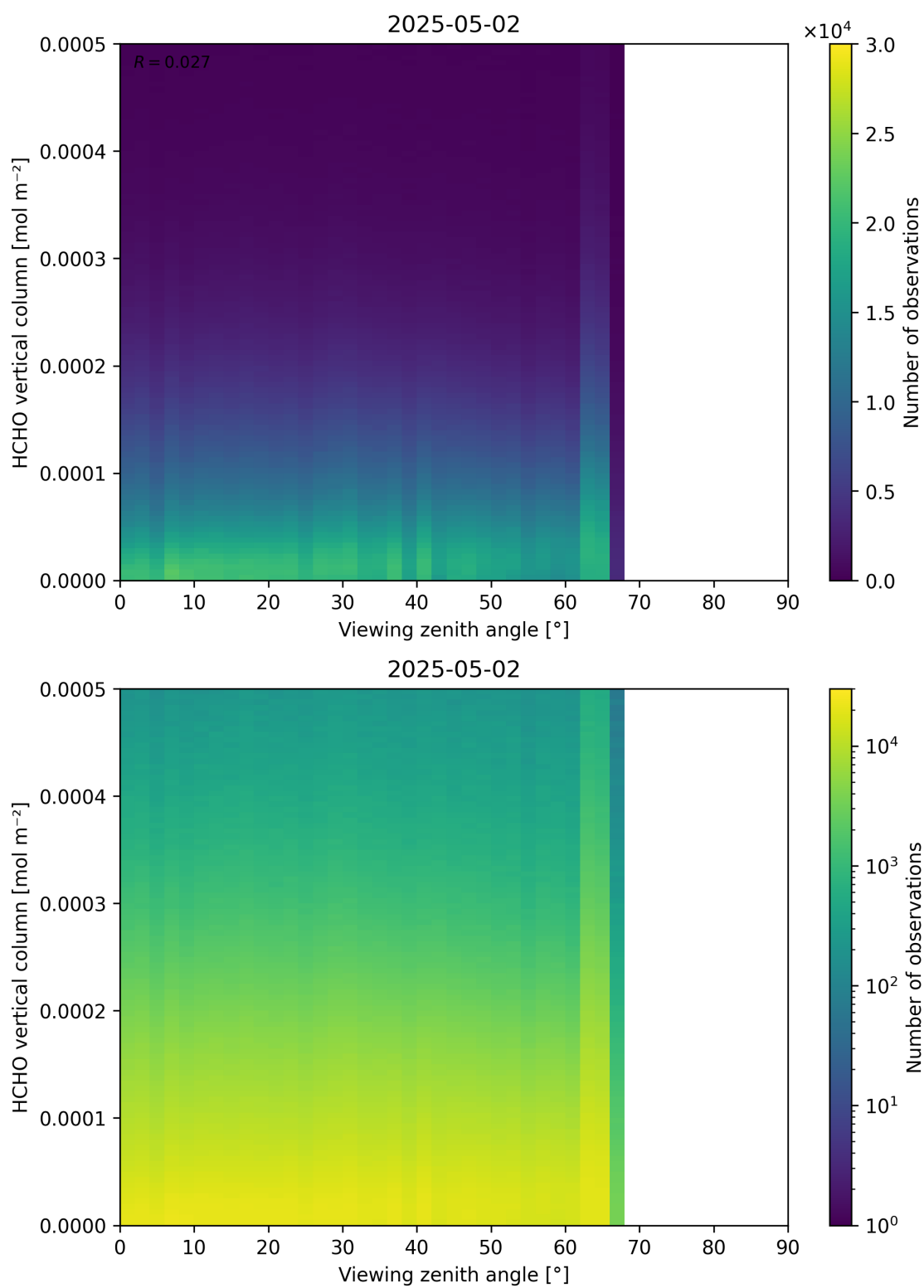
Figure 192: Scatter density plot of “Viewing zenith angle” against “HCHO vertical column” for 2025-05-01 to 2025-05-03.
