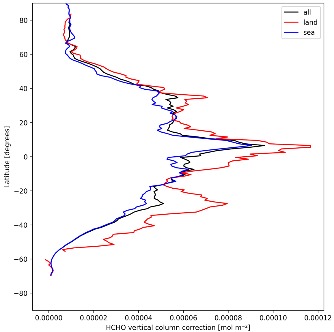
Figure 23: Zonal average of “HCHO vertical column correction” for 2025-05-01 to 2025-05-03.
