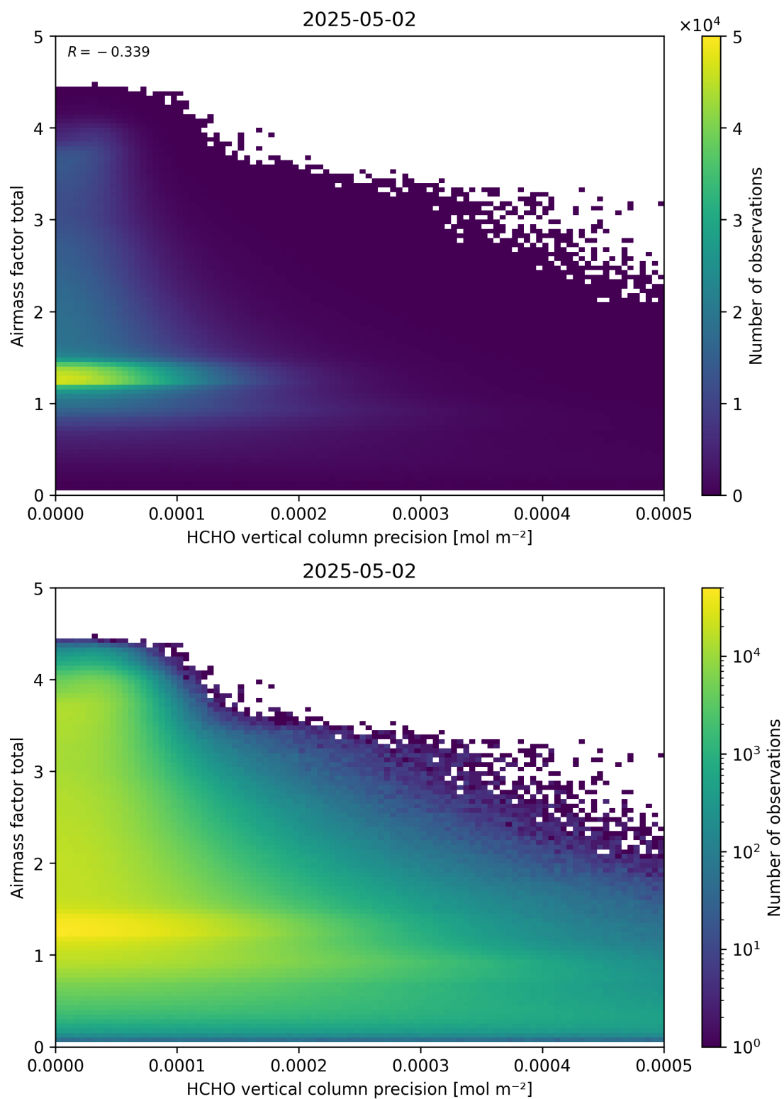
Figure 144: Scatter density plot of “HCHO vertical column precision” against “Airmass factor total” for 2025-05-01 to 2025-05-03.
