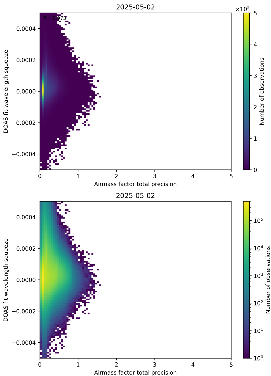
Figure 107: Scatter density plot of “Airmass factor total precision” against “DOAS fit wavelength squeeze” for 2025-05-01 to 2025-05-03.
