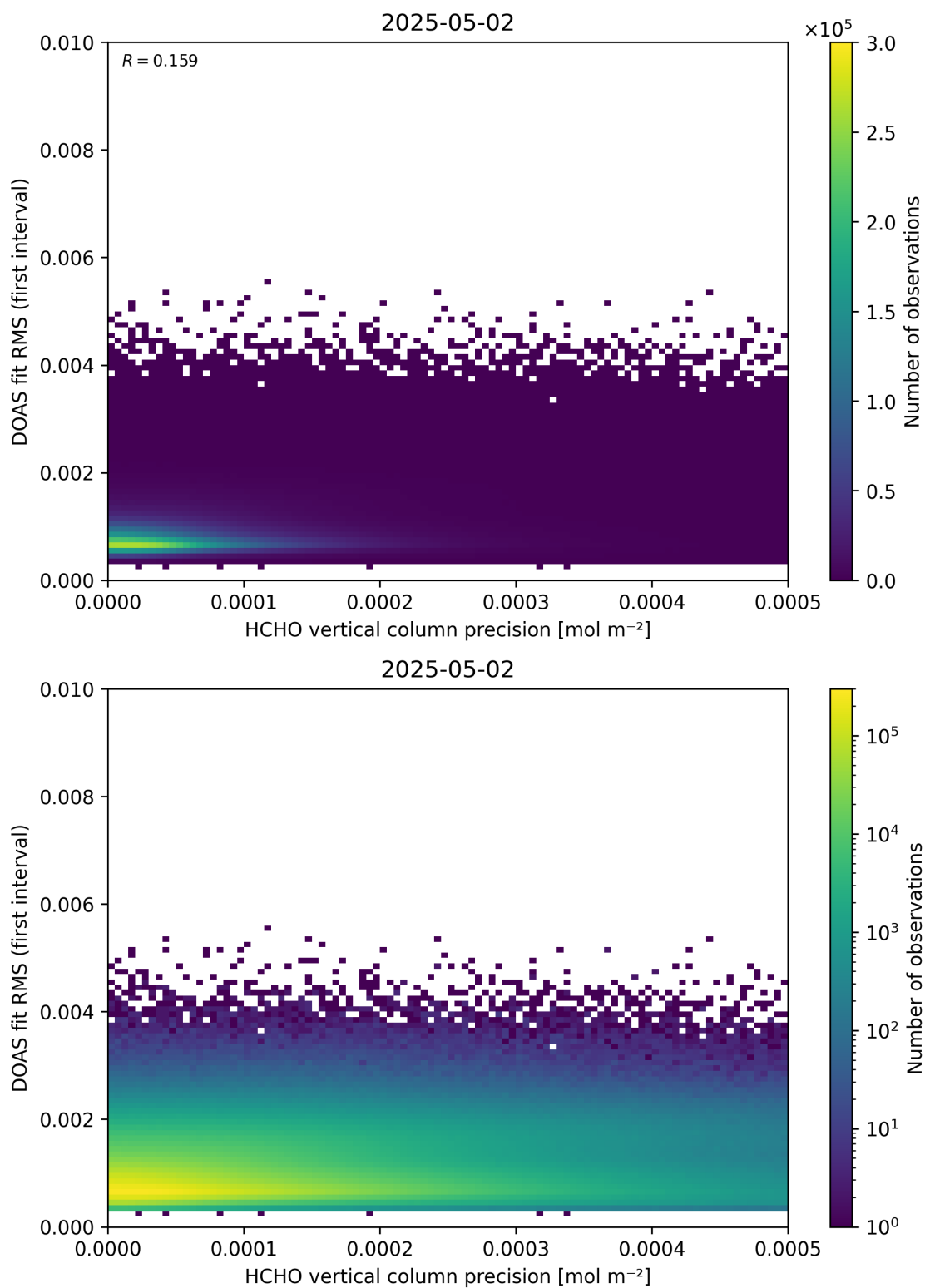
Figure 136: Scatter density plot of “HCHO vertical column precision” against “DOAS fit RMS (first interval)” for 2025-05-01 to 2025-05-03.
