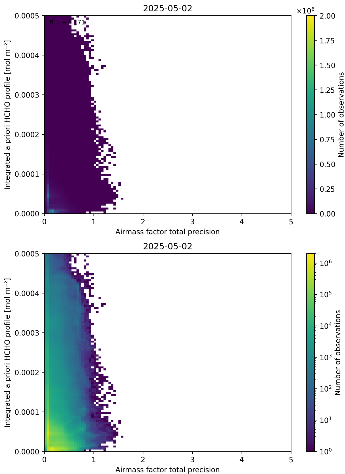
Figure 111: Scatter density plot of “Airmass factor total precision” against “Integrated a priori HCHO profile” for 2025-05-01 to 2025-05-03.
