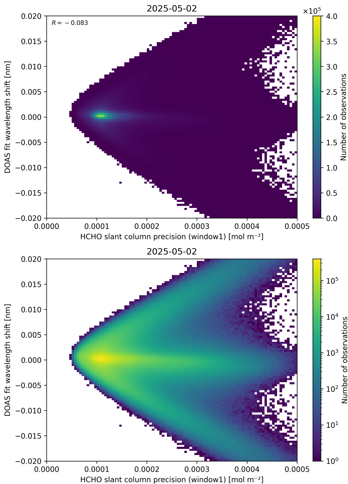
Figure 89: Scatter density plot of “HCHO slant column precision (window1)” against “DOAS fit wavelength shift” for 2025-05-01 to 2025-05-03.
