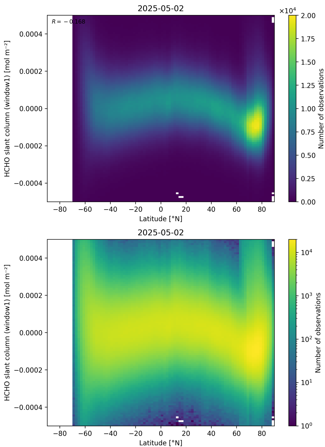
Figure 159: Scatter density plot of “Latitude” against “HCHO slant column (window1)” for 2025-05-01 to 2025-05-03.
