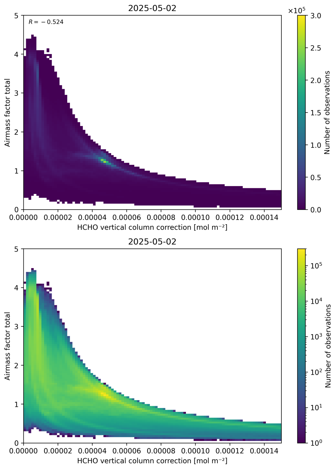
Figure 120: Scatter density plot of “HCHO vertical column correction” against “Airmass factor total” for 2025-05-01 to 2025-05-03.
