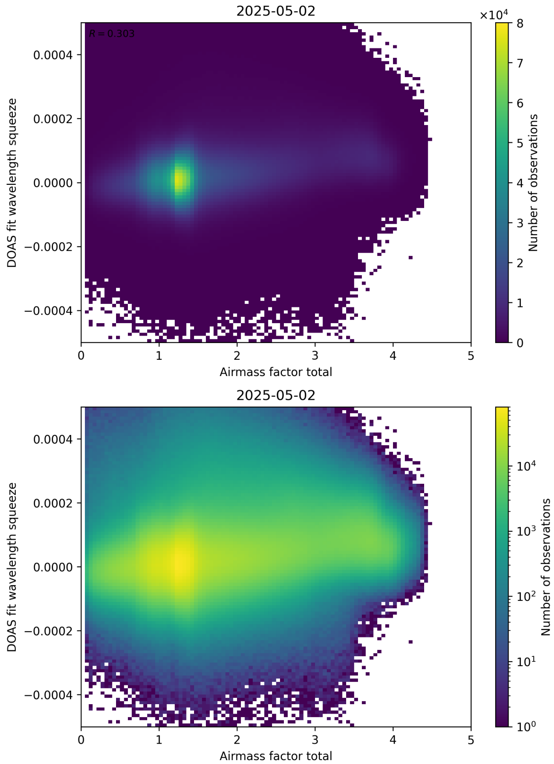
Figure 99: Scatter density plot of “Airmass factor total” against “DOAS fit wavelength squeeze” for 2025-05-01 to 2025-05-03.
