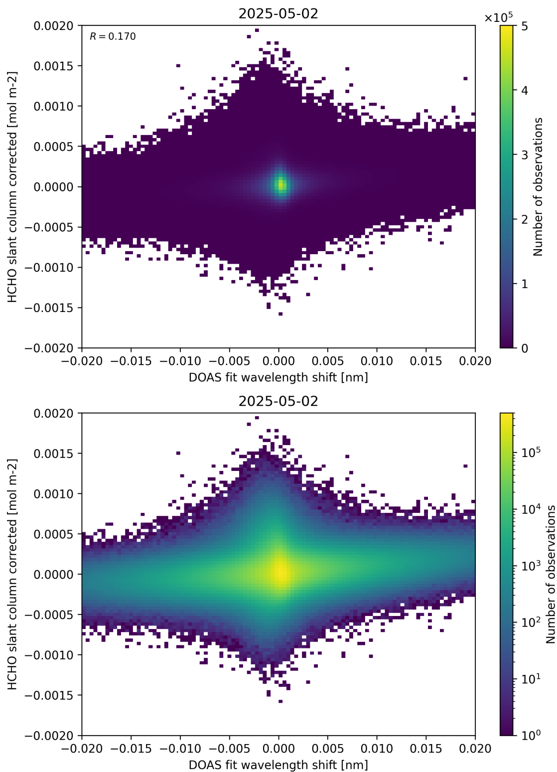
Figure 66: Scatter density plot of “DOAS fit wavelength shift” against “HCHO slant column corrected” for 2025-05-01 to 2025-05-03.
