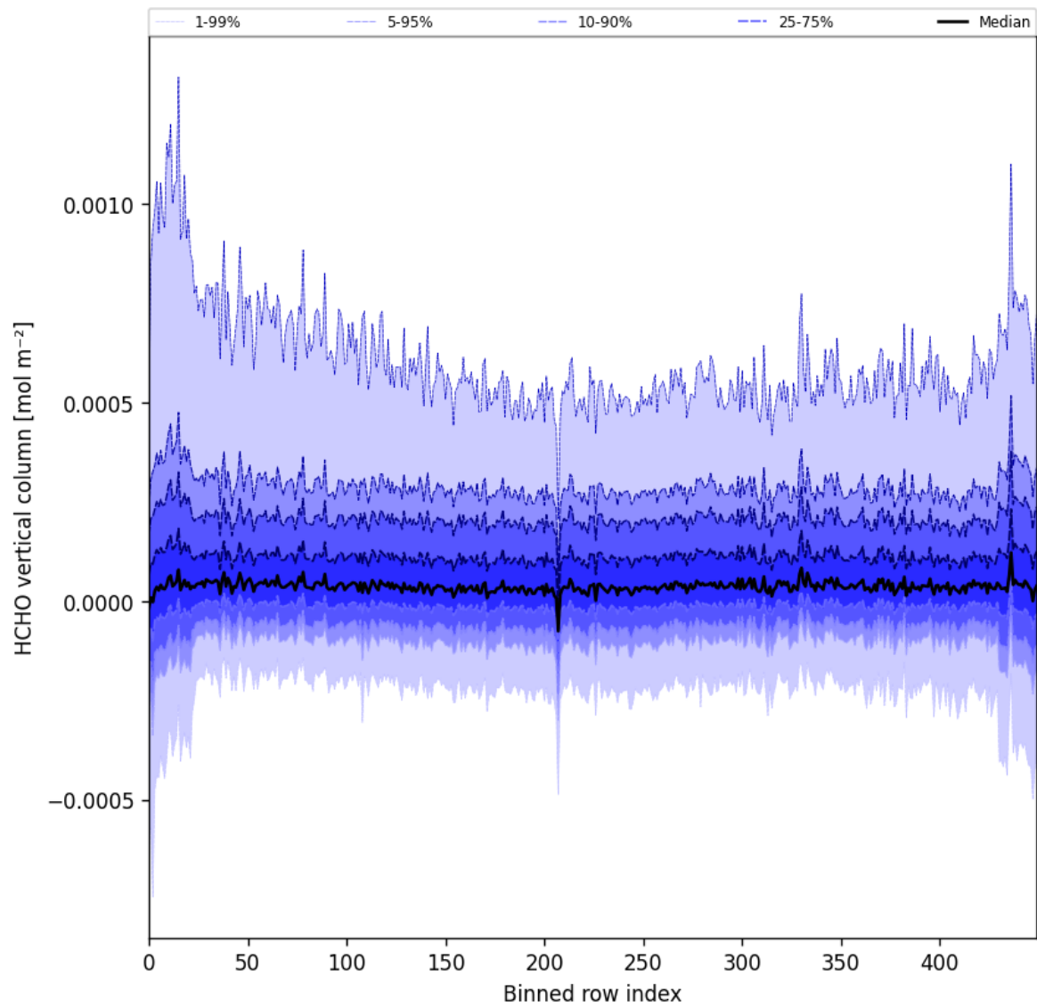
Figure 49: Along track statistics of “HCHO vertical column” for 2025-05-01 to 2025-05-03
