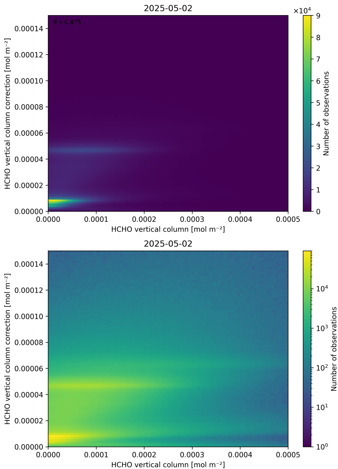
Figure 133: Scatter density plot of “HCHO vertical column” against “HCHO vertical column correction” for 2025-05-01 to 2025-05-03.
