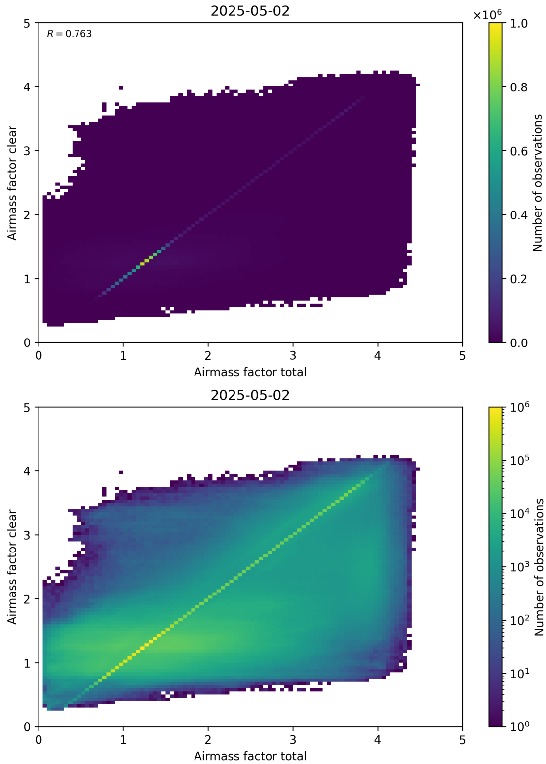
Figure 100: Scatter density plot of “Airmass factor total” against “Airmass factor clear” for 2025-05-01 to 2025-05-03.
