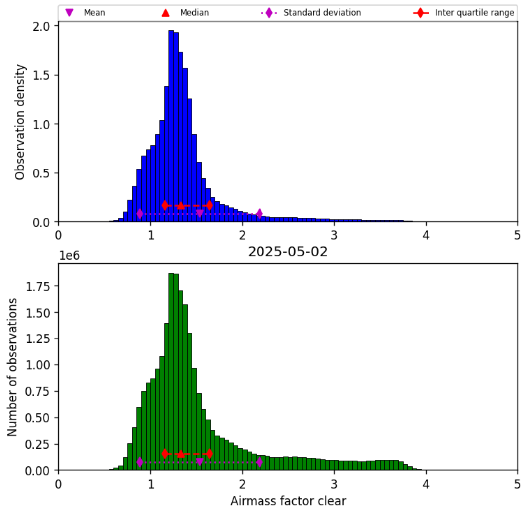
Figure 42: Histogram of “Airmass factor clear” for 2025-05-01 to 2025-05-03
