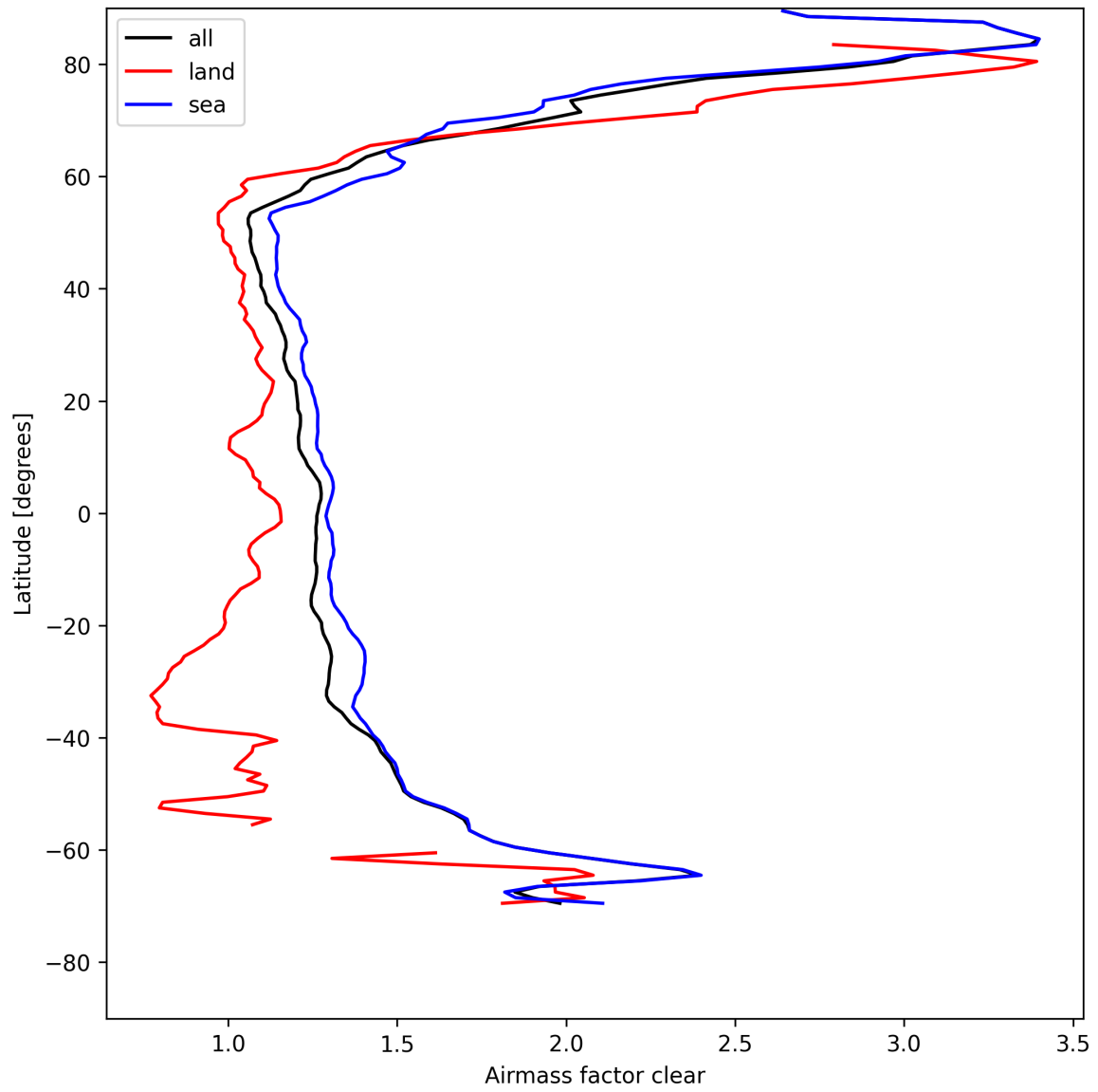
Figure 28: Zonal average of “Airmass factor clear” for 2025-05-01 to 2025-05-03.
