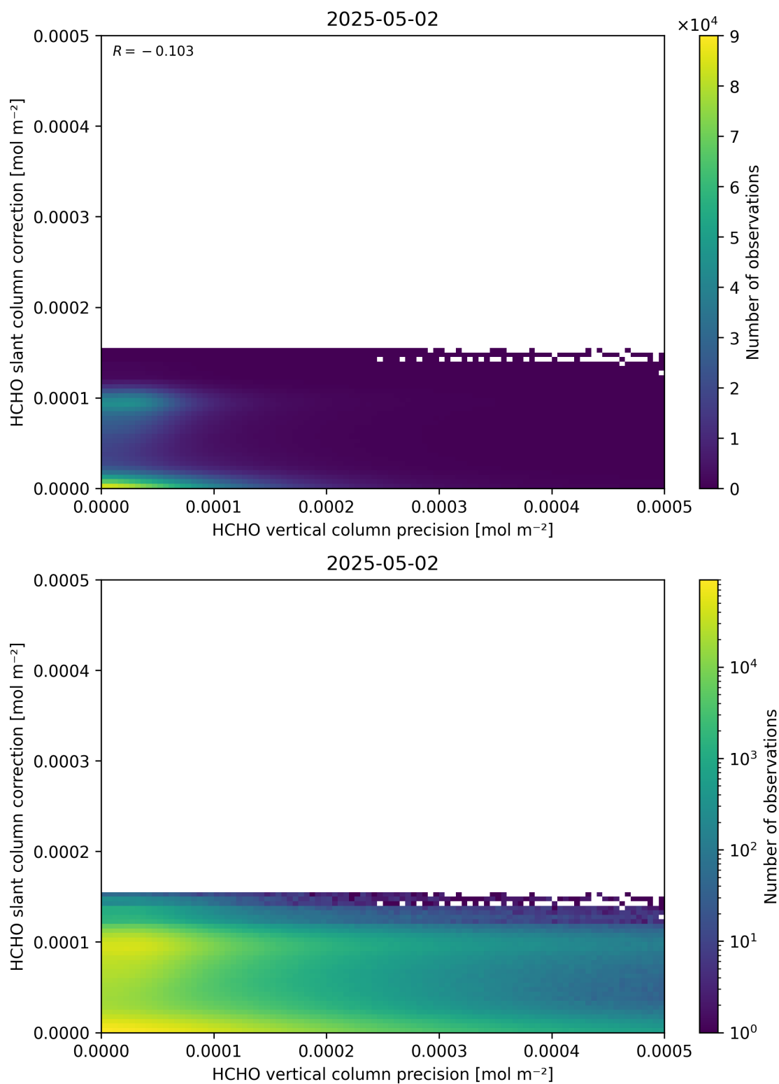
Figure 141: Scatter density plot of “HCHO vertical column precision” against “HCHO slant column correction” for 2025-05-01 to 2025-05-03.
