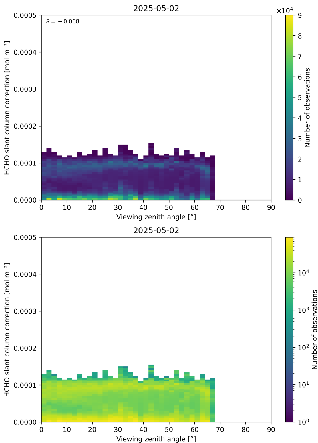
Figure 187: Scatter density plot of “Viewing zenith angle” against “HCHO slant column correction” for 2025-05-01 to 2025-05-03.
