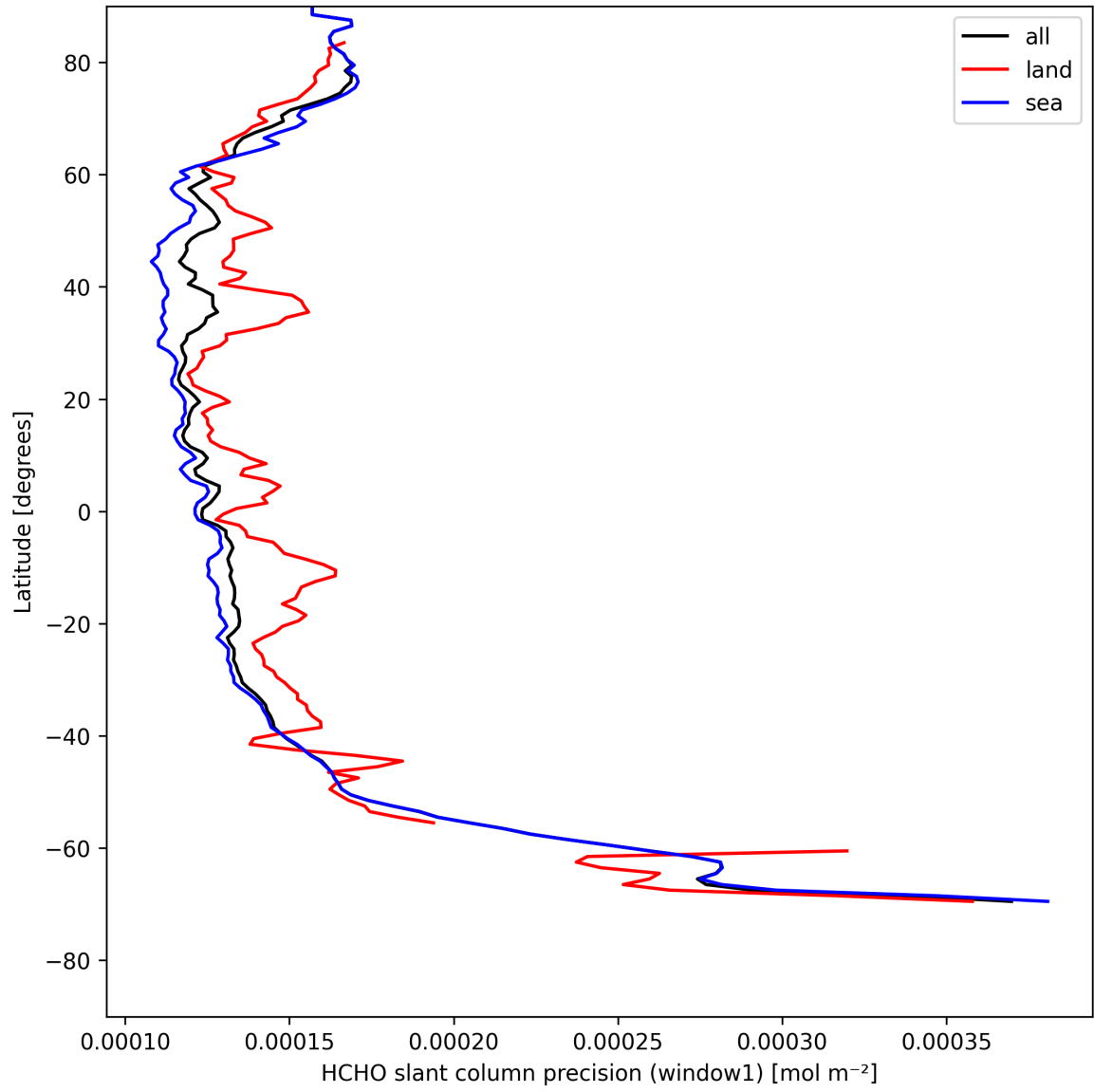
Figure 25: Zonal average of “HCHO slant column precision (window1)” for 2025-05-01 to 2025-05-03.
