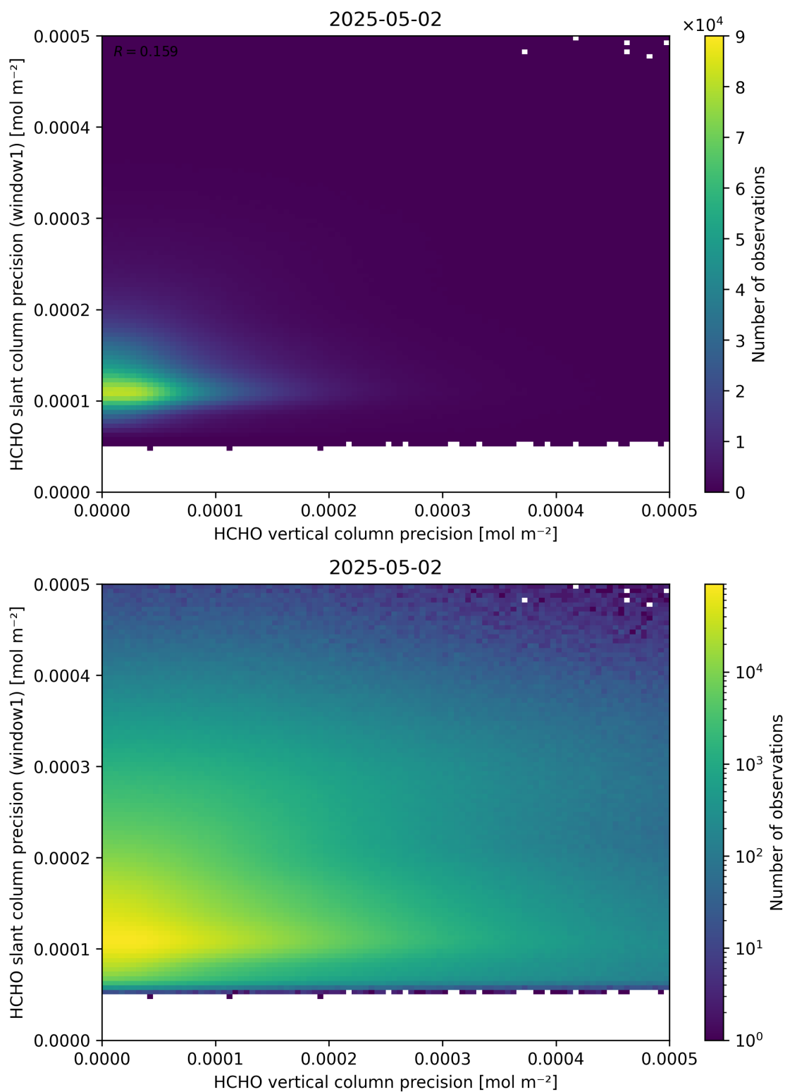
Figure 143: Scatter density plot of “HCHO vertical column precision” against “HCHO slant column precision (window1)” for 2025-05-01 to 2025-05-03.
