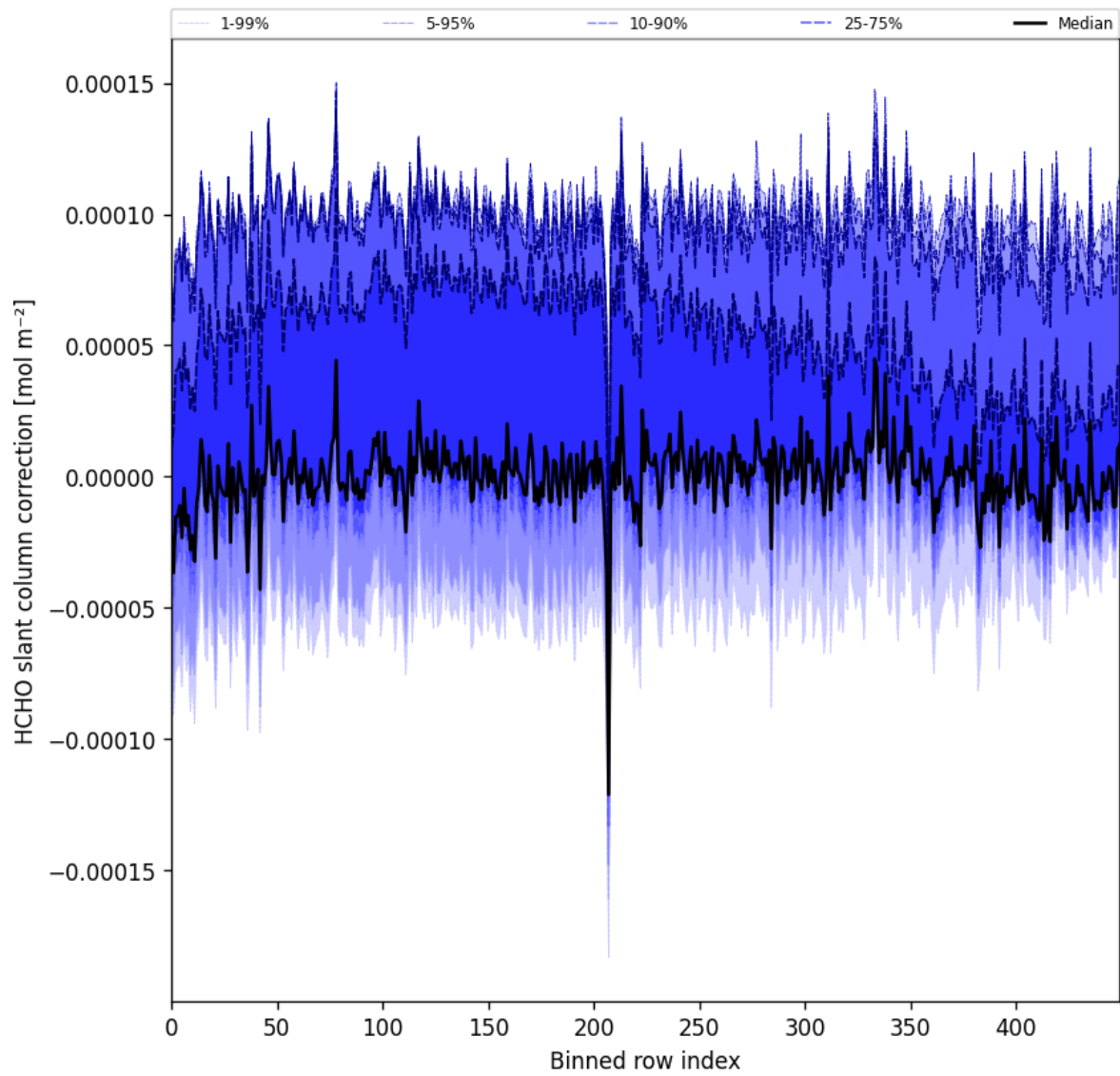
Figure 61: Along track statistics of “HCHO slant column correction” for 2025-05-01 to 2025-05-03
