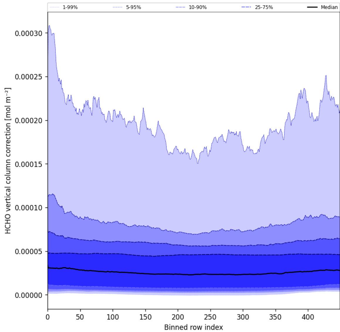
Figure 51: Along track statistics of “HCHO vertical column correction” for 2025-05-01 to 2025-05-03
