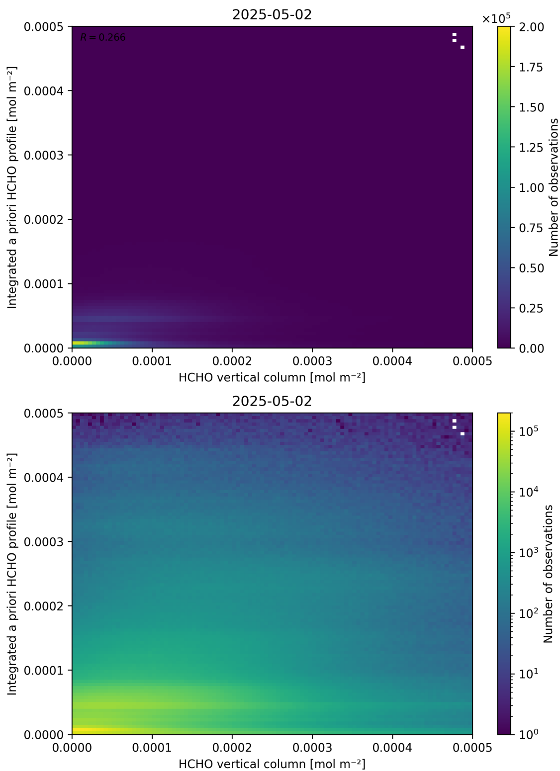
Figure 135: Scatter density plot of “HCHO vertical column” against “Integrated a priori HCHO profile” for 2025-05-01 to 2025-05-03.
