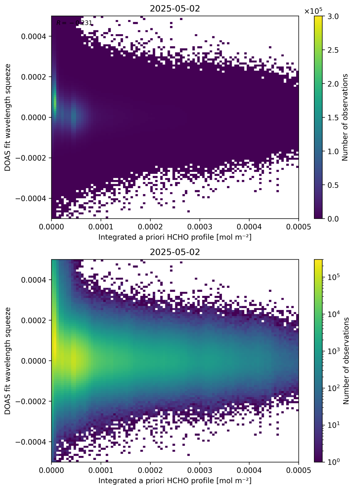
Figure 150: Scatter density plot of “Integrated a priori HCHO profile” against “DOAS fit wavelength squeeze” for 2025-05-01 to 2025-05-03.
