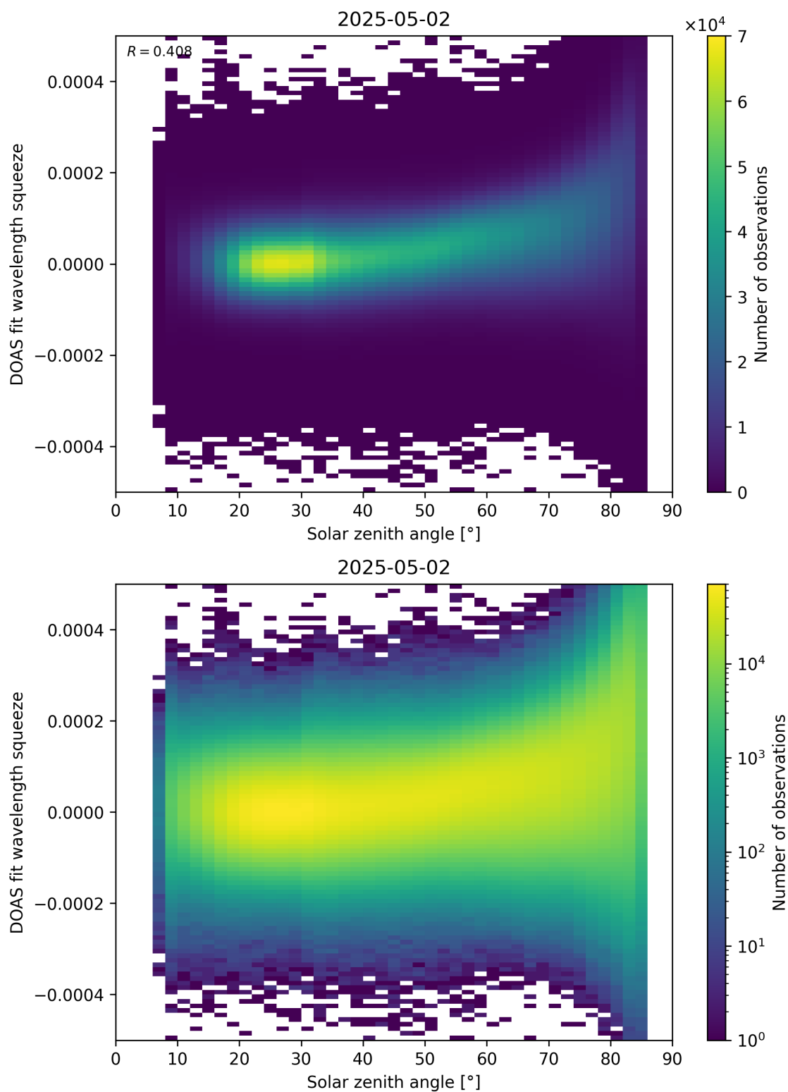
Figure 169: Scatter density plot of “Solar zenith angle” against “DOAS fit wavelength squeeze” for 2025-05-01 to 2025-05-03.
