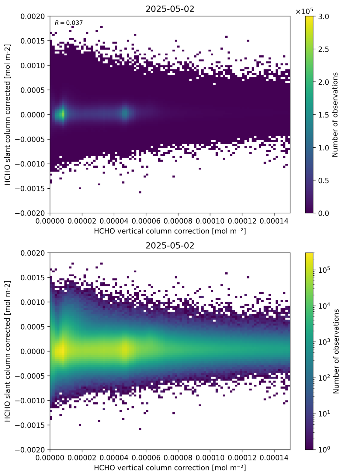
Figure 116: Scatter density plot of “HCHO vertical column correction” against “HCHO slant column corrected” for 2025-05-01 to 2025-05-03.
