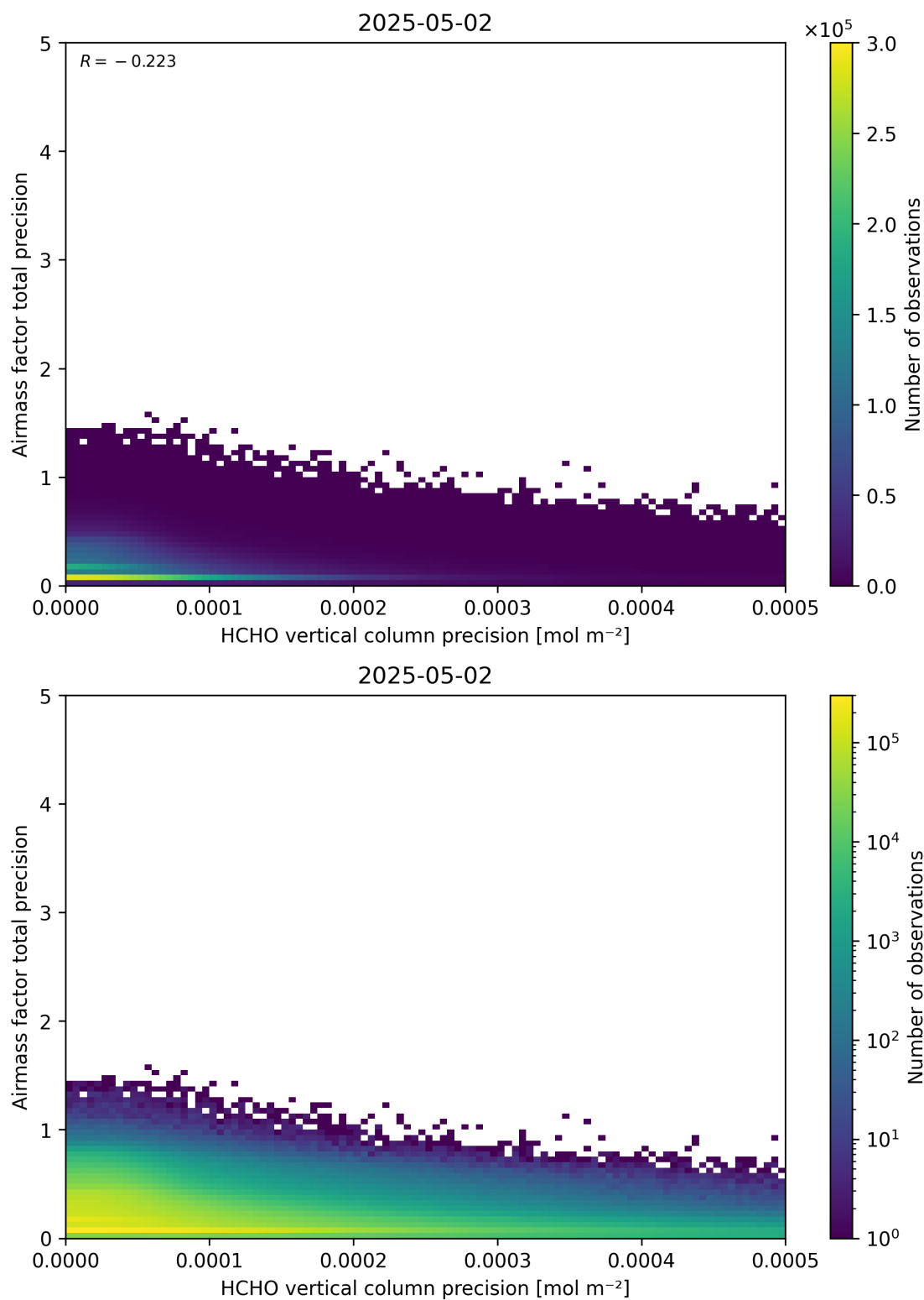
Figure 145: Scatter density plot of “HCHO vertical column precision” against “Airmass factor total precision” for 2025-05-01 to 2025-05-03.
