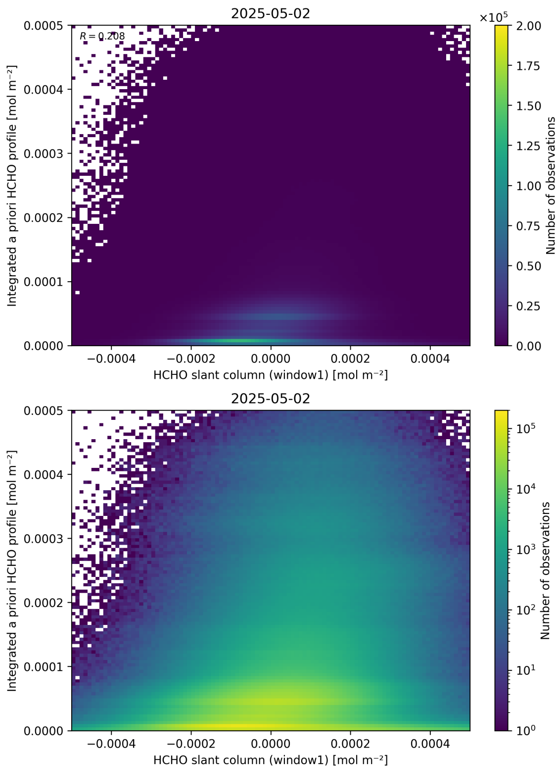
Figure 87: Scatter density plot of “HCHO slant column (window1)” against “Integrated a priori HCHO profile” for 2025-05-01 to 2025-05-03.
