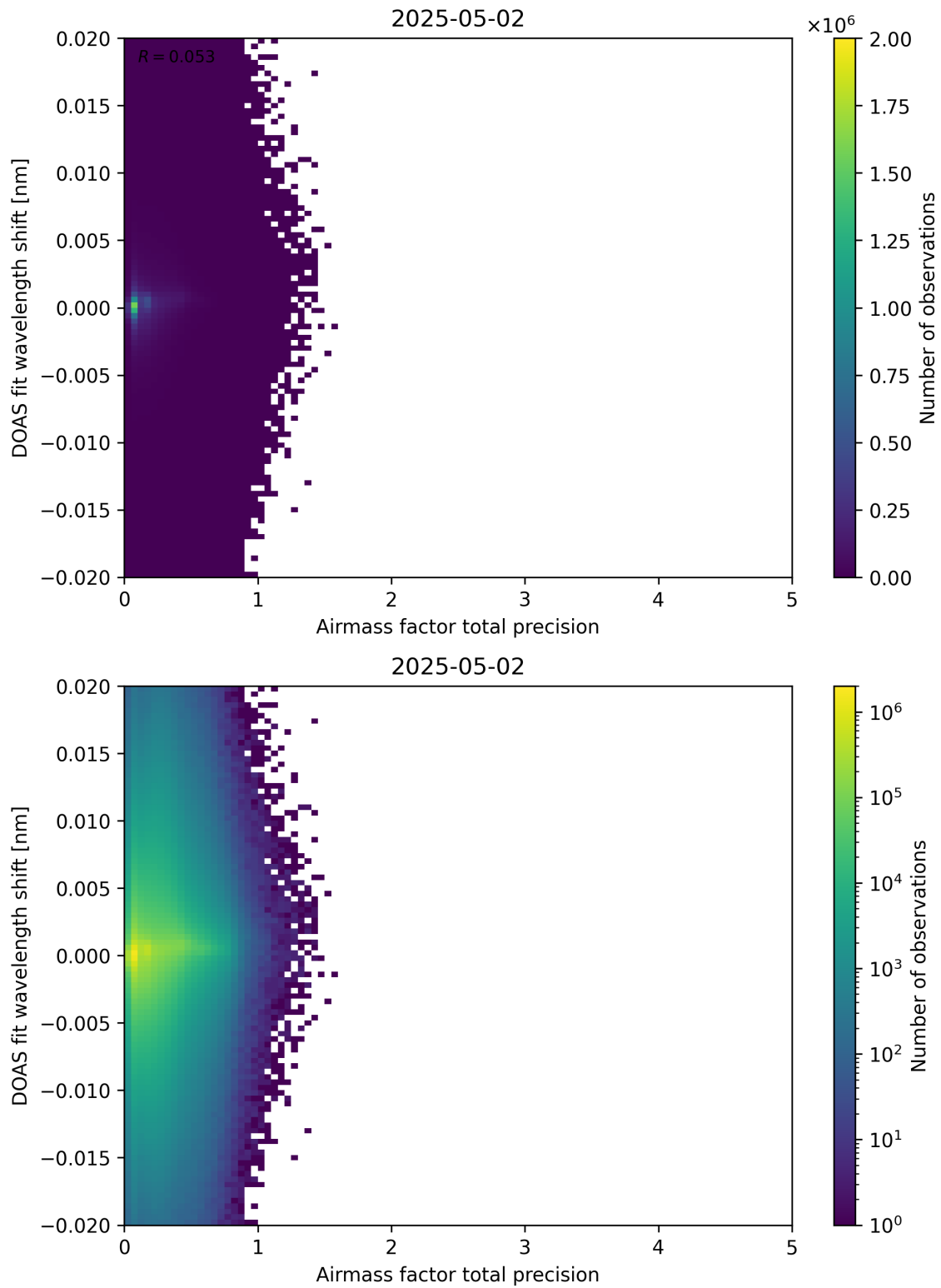
Figure 106: Scatter density plot of “Airmass factor total precision” against “DOAS fit wavelength shift” for 2025-05-01 to 2025-05-03.
