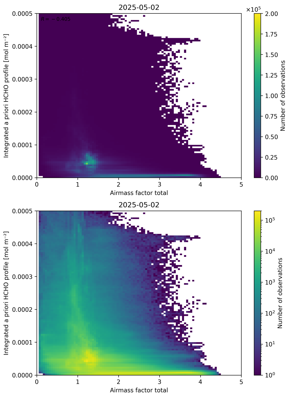
Figure 104: Scatter density plot of “Airmass factor total” against “Integrated a priori HCHO profile” for 2025-05-01 to 2025-05-03.
