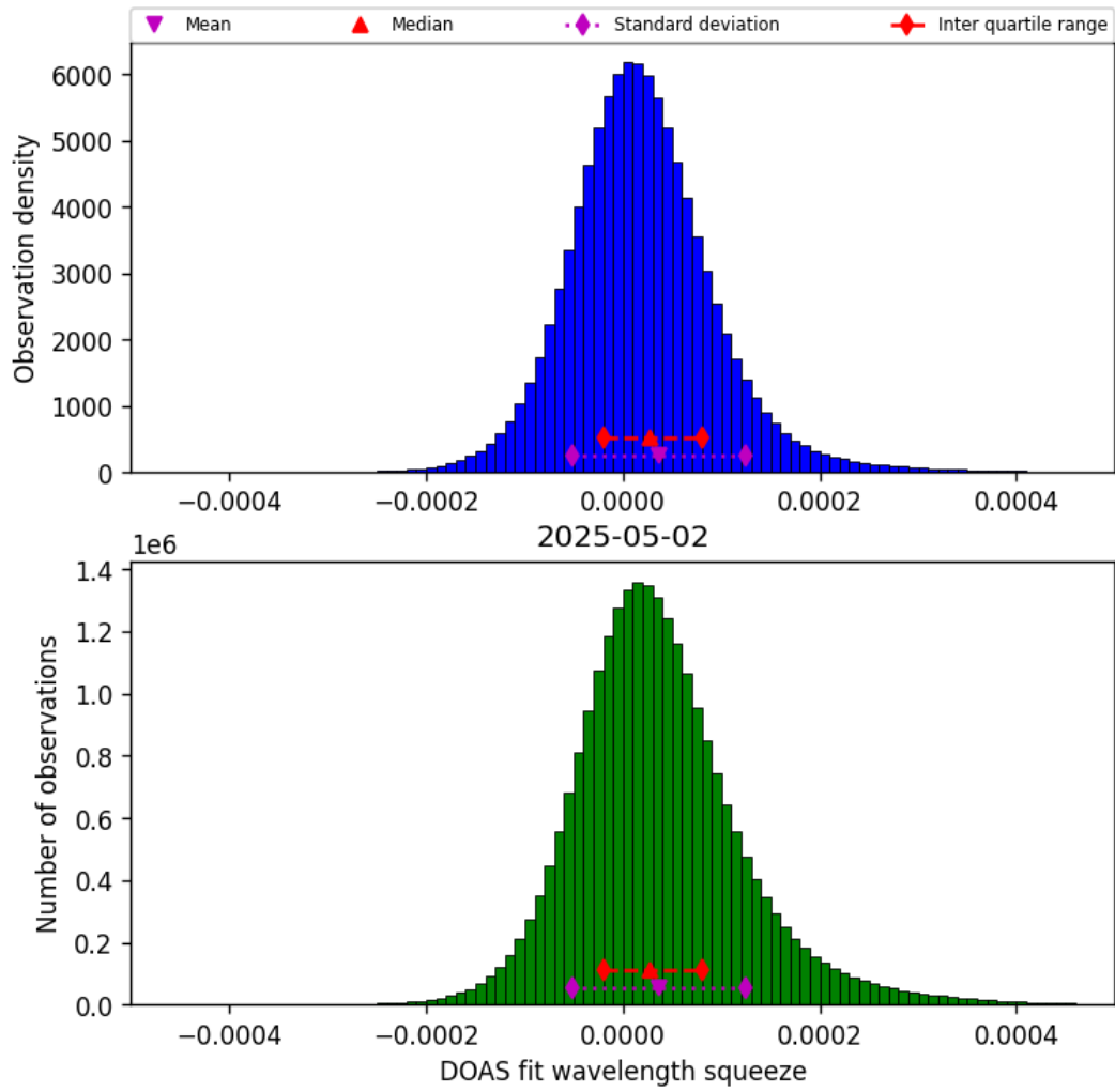
Figure 45: Histogram of “DOAS fit wavelength squeeze” for 2025-05-01 to 2025-05-03
