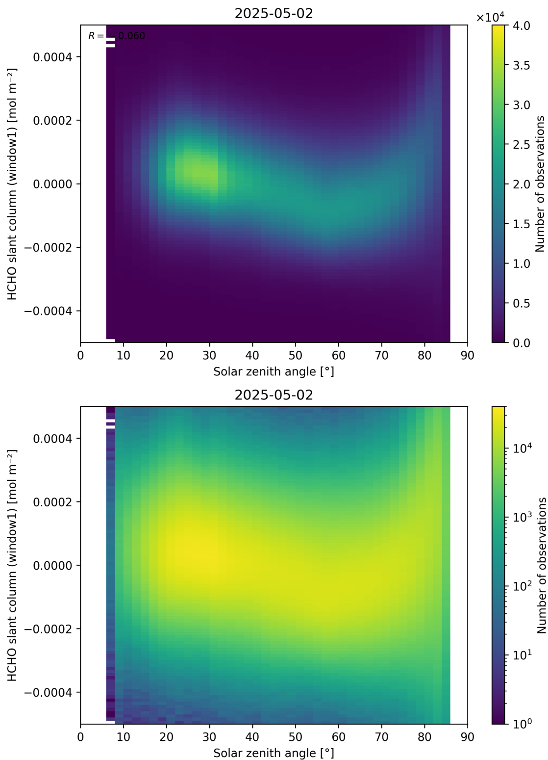
Figure 173: Scatter density plot of “Solar zenith angle” against “HCHO slant column (window1)” for 2025-05-01 to 2025-05-03.
