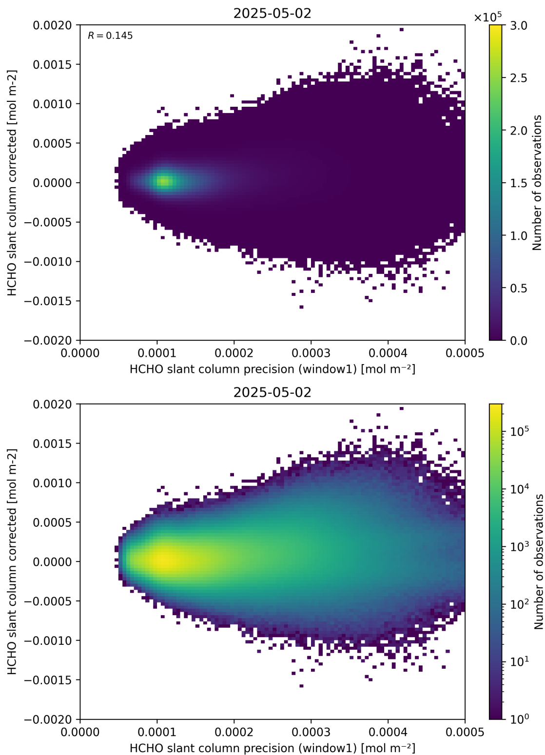
Figure 92: Scatter density plot of “HCHO slant column precision (window1)” against “HCHO slant column corrected” for 2025-05-01 to 2025-05-03.
