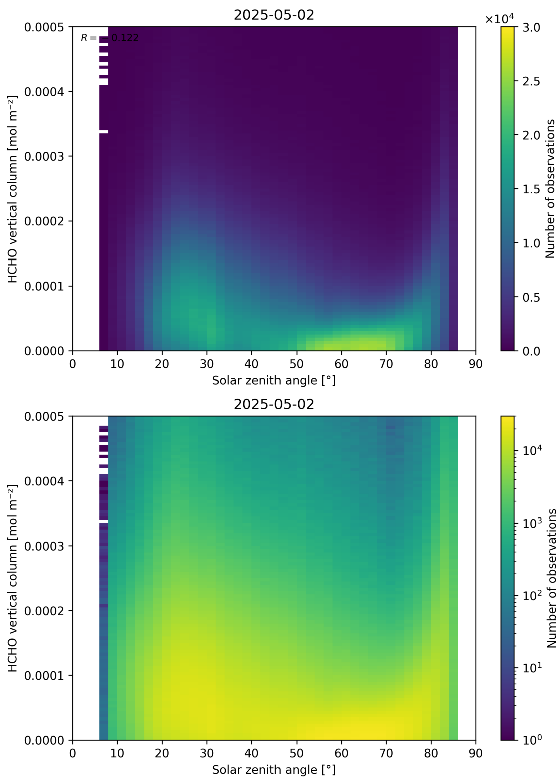
Figure 177: Scatter density plot of “Solar zenith angle” against “HCHO vertical column” for 2025-05-01 to 2025-05-03.
