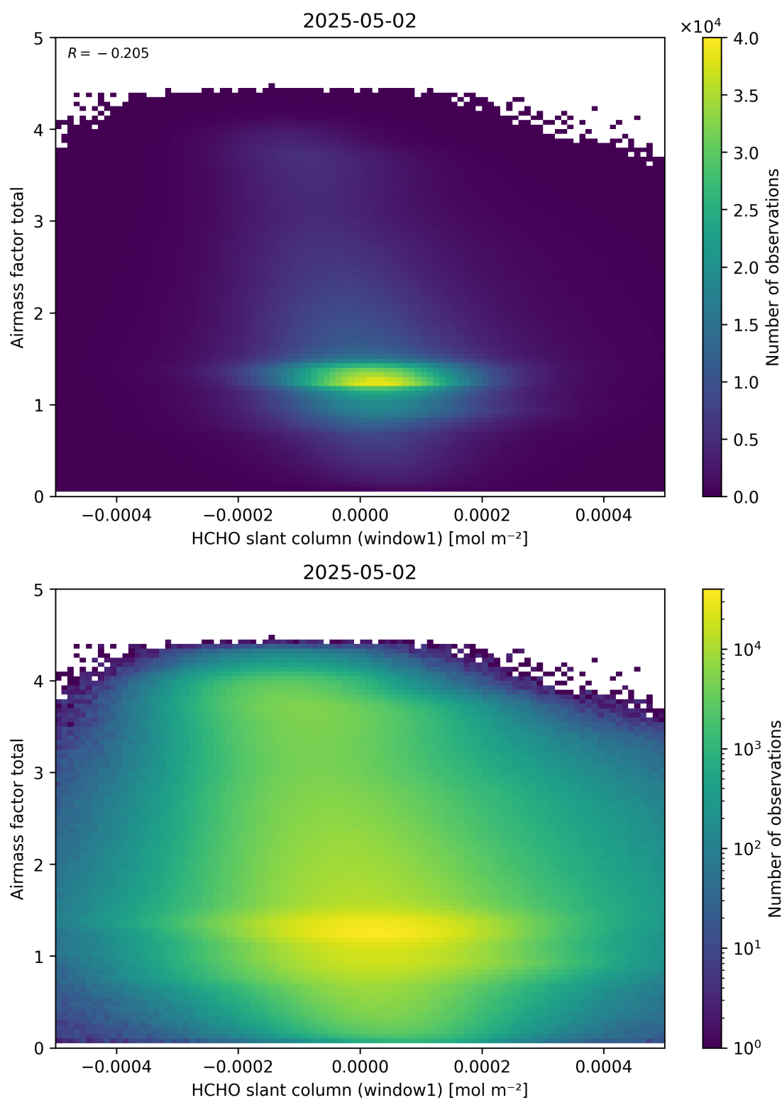
Figure 85: Scatter density plot of “HCHO slant column (window1)” against “Airmass factor total” for 2025-05-01 to 2025-05-03.
