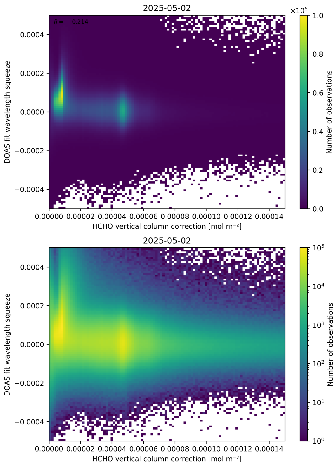
Figure 114: Scatter density plot of “HCHO vertical column correction” against “DOAS fit wavelength squeeze” for 2025-05-01 to 2025-05-03.
