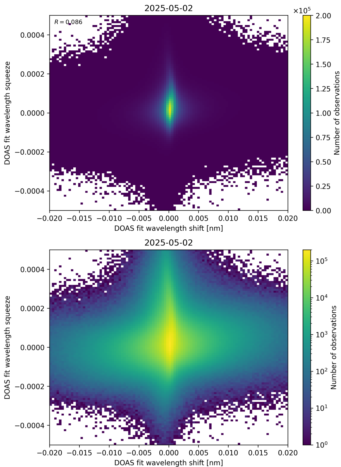
Figure 65: Scatter density plot of “DOAS fit wavelength shift” against “DOAS fit wavelength squeeze” for 2025-05-01 to 2025-05-03.
