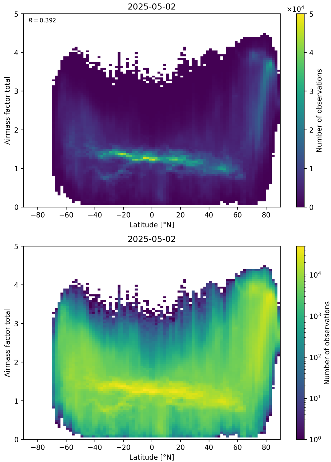
Figure 161: Scatter density plot of “Latitude” against “Airmass factor total” for 2025-05-01 to 2025-05-03.
