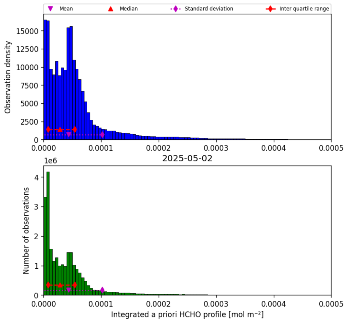
Figure 43: Histogram of “Integrated a priori HCHO profile” for 2025-05-01 to 2025-05-03
