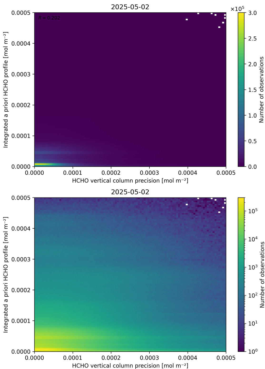
Figure 147: Scatter density plot of “HCHO vertical column precision” against “Integrated a priori HCHO profile” for 2025-05-01 to 2025-05-03.
