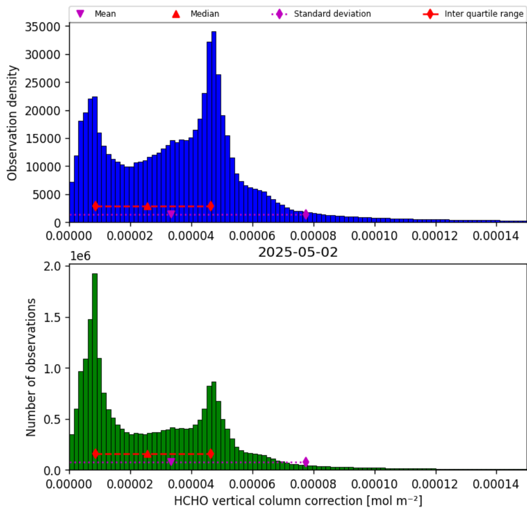
Figure 37: Histogram of “HCHO vertical column correction” for 2025-05-01 to 2025-05-03
