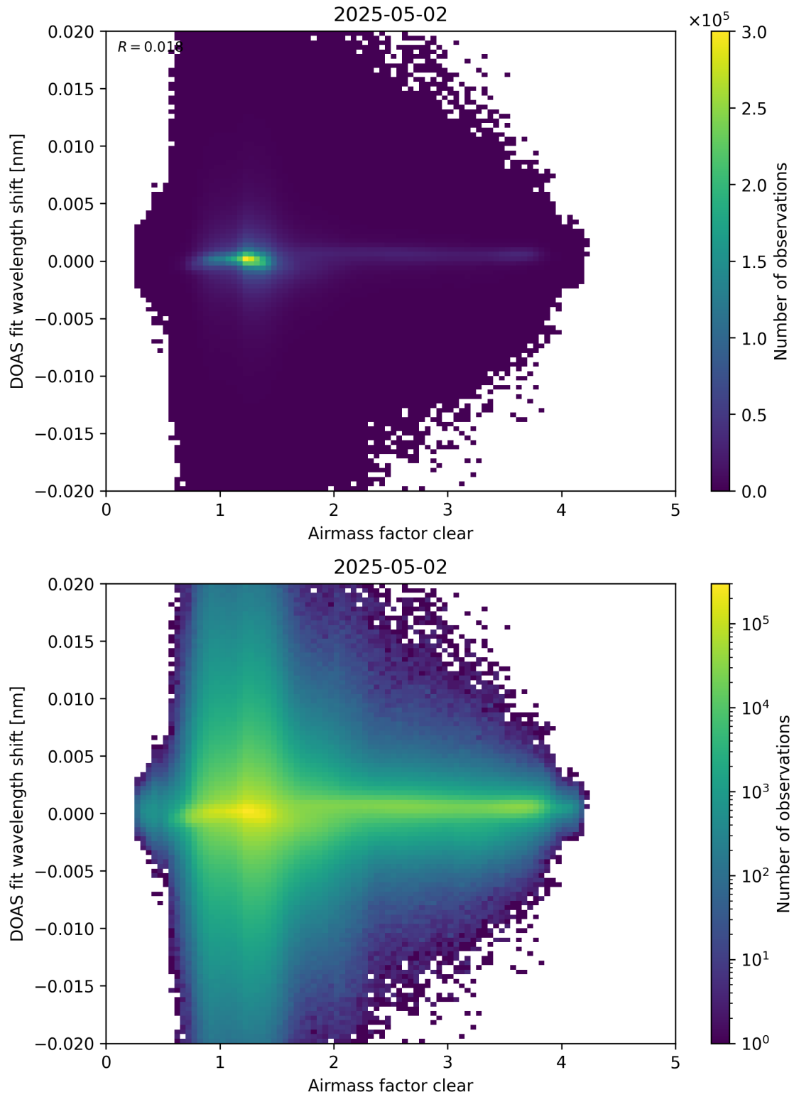
Figure 72: Scatter density plot of “Airmass factor clear” against “DOAS fit wavelength shift” for 2025-05-01 to 2025-05-03.
