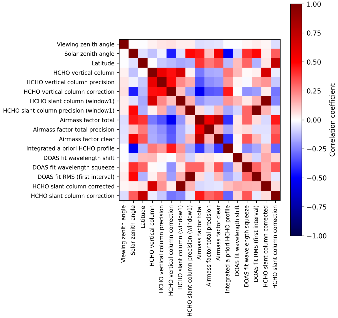
Figure 2: Map of correlation matrix for 2025-05-01 to 2025-05-03.
