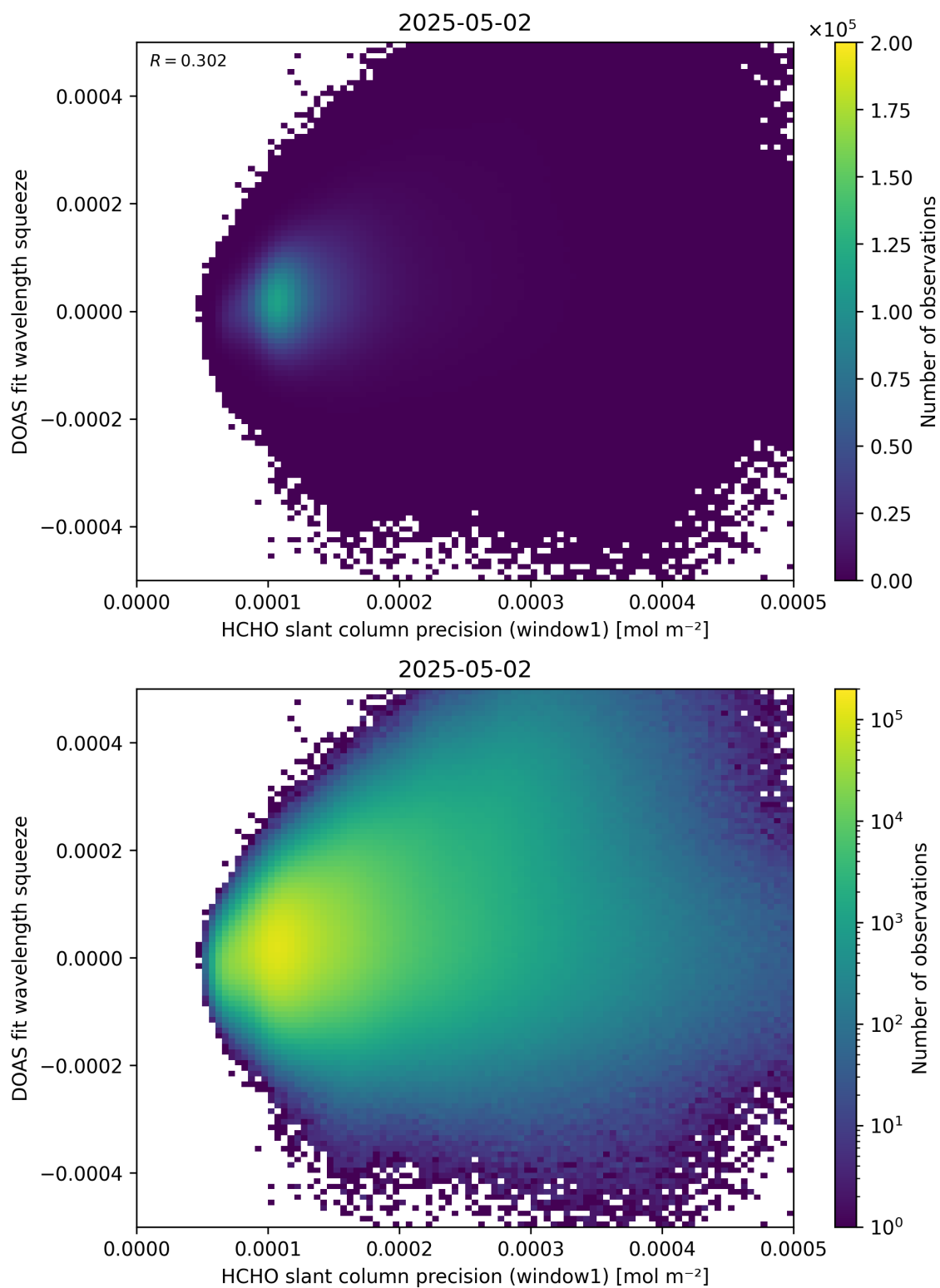
Figure 90: Scatter density plot of “HCHO slant column precision (window1)” against “DOAS fit wavelength squeeze” for 2025-05-01 to 2025-05-03.
