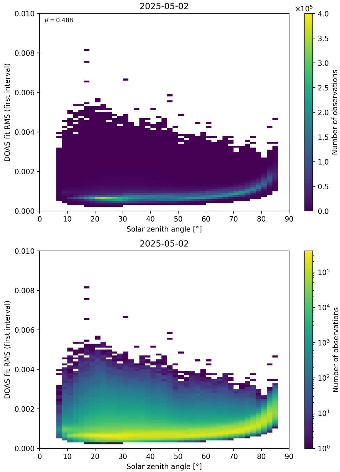
Figure 167: Scatter density plot of “Solar zenith angle” against “DOAS fit RMS (first interval)” for 2025-05-01 to 2025-05-03.
