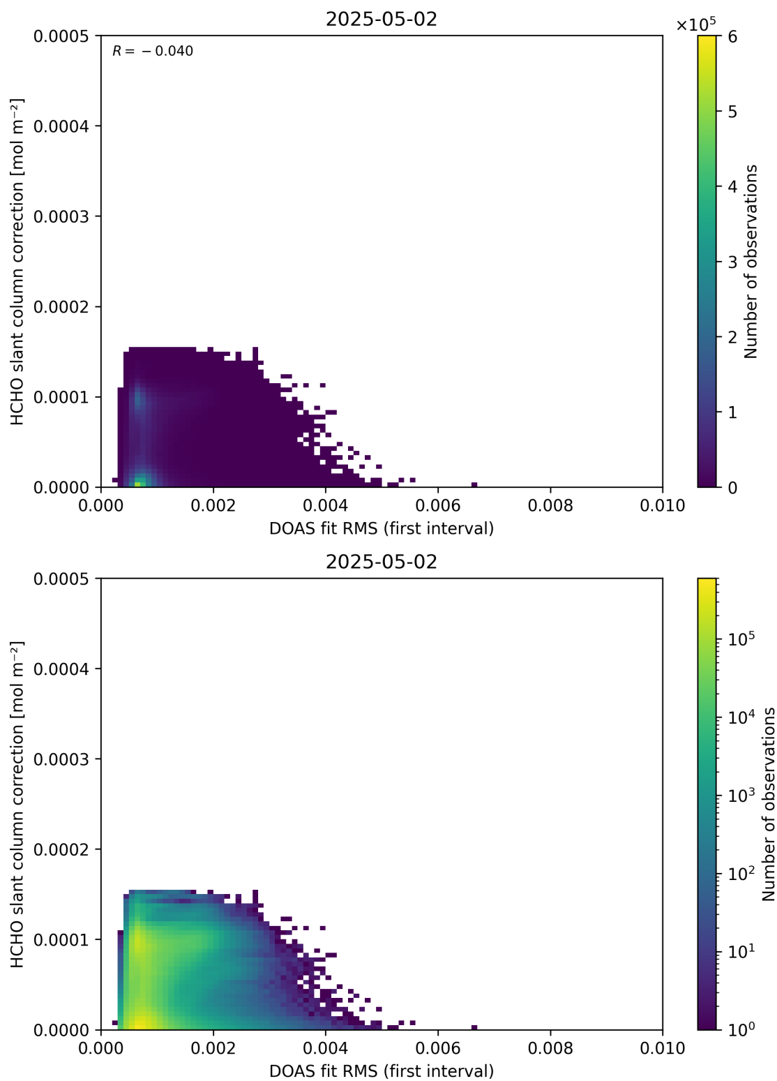
Figure 63: Scatter density plot of “DOAS fit RMS (first interval)” against “HCHO slant column correction” for 2025-05-01 to 2025-05-03.
