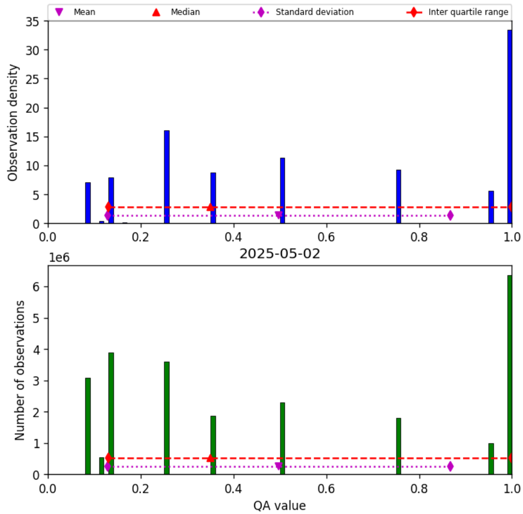
Figure 34: Histogram of “QA value” for 2025-05-01 to 2025-05-03
