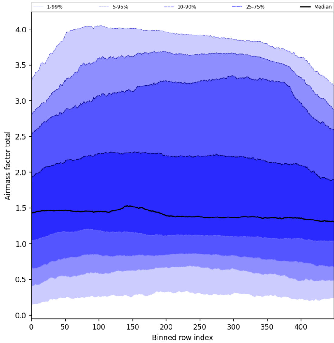
Figure 54: Along track statistics of “Airmass factor total” for 2025-05-01 to 2025-05-03
