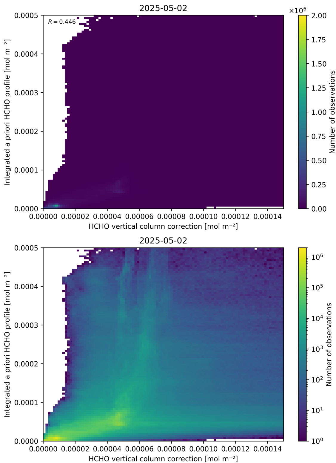
Figure 122: Scatter density plot of “HCHO vertical column correction” against “Integrated a priori HCHO profile” for 2025-05-01 to 2025-05-03.
