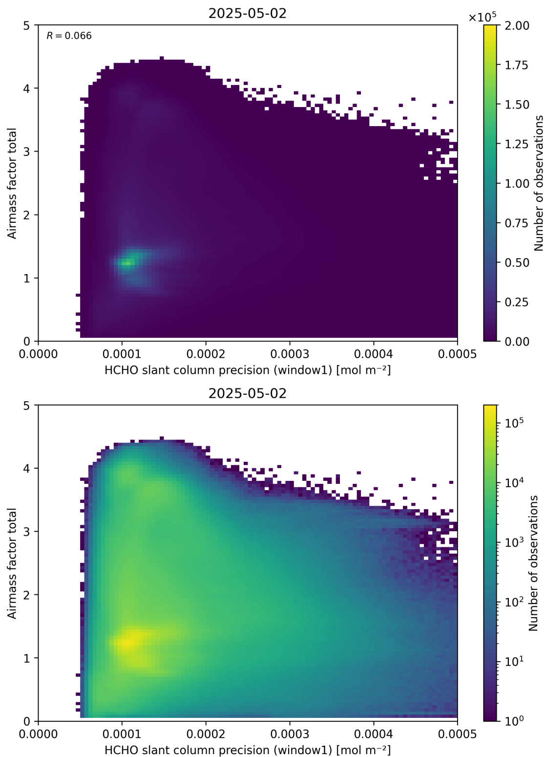
Figure 94: Scatter density plot of “HCHO slant column precision (window1)” against “Airmass factor total” for 2025-05-01 to 2025-05-03.
