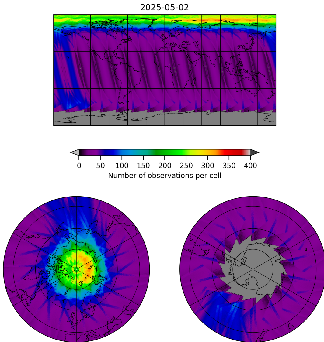
Figure 19: Map of the number of observations for 2025-05-01 to 2025-05-03
