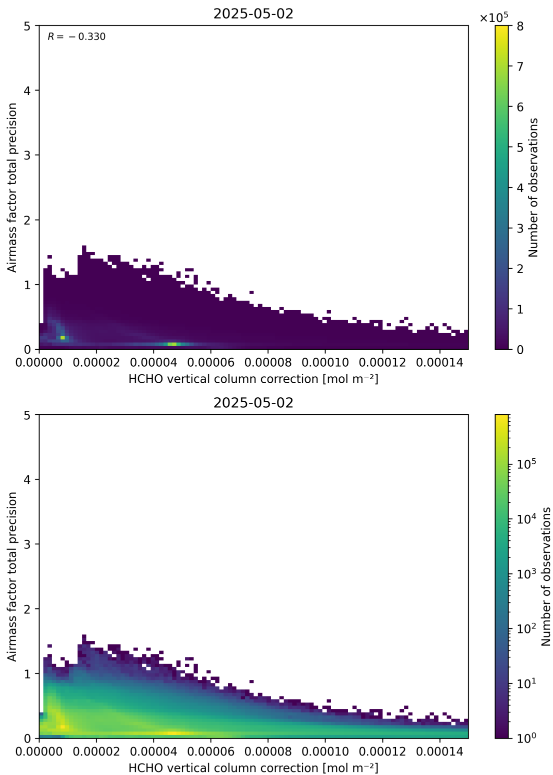
Figure 121: Scatter density plot of “HCHO vertical column correction” against “Airmass factor total precision” for 2025-05-01 to 2025-05-03.
