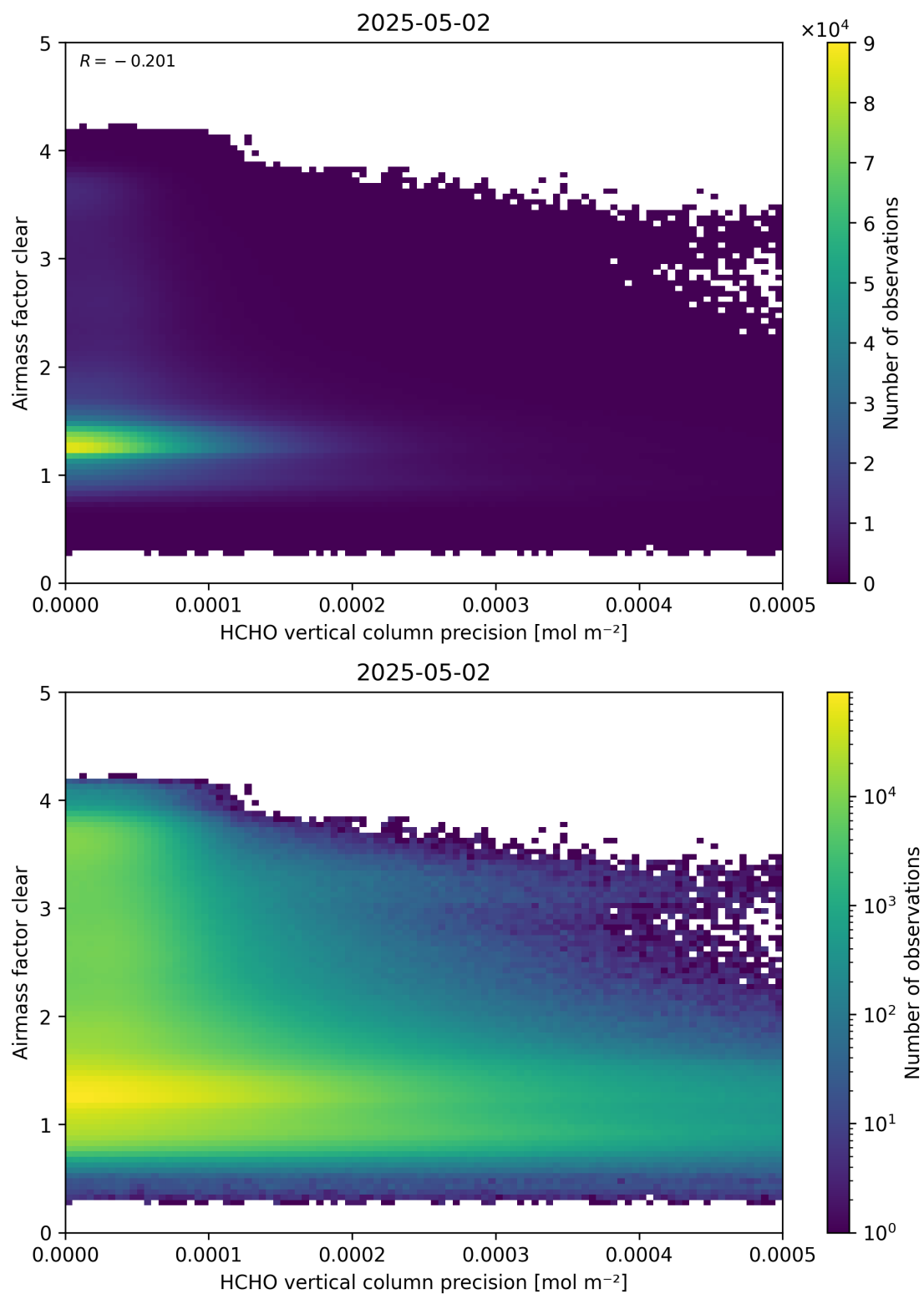
Figure 139: Scatter density plot of “HCHO vertical column precision” against “Airmass factor clear” for 2025-05-01 to 2025-05-03.
