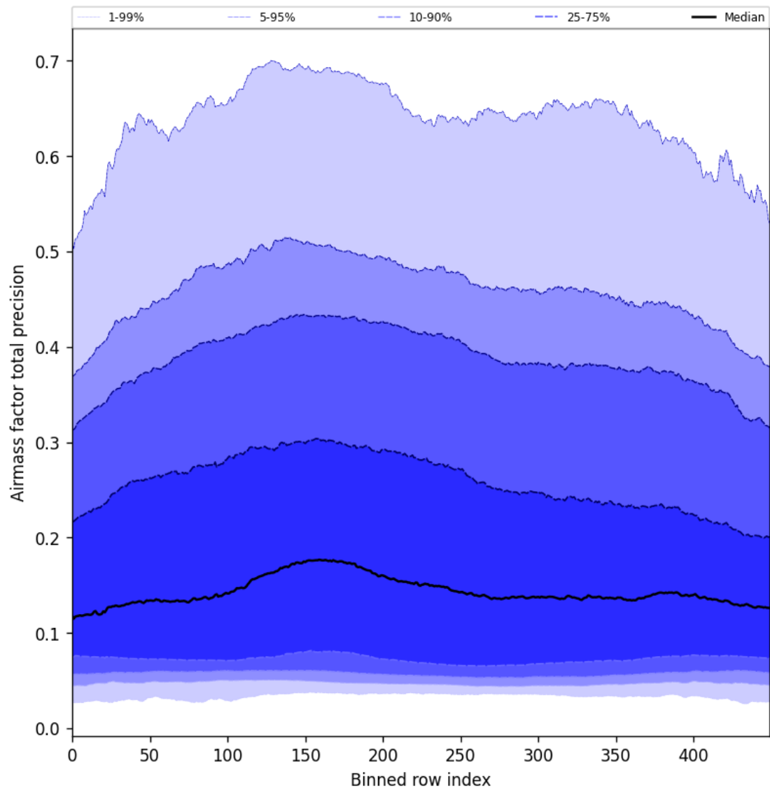
Figure 55: Along track statistics of “Airmass factor total precision” for 2025-05-02 to 2025-05-04
