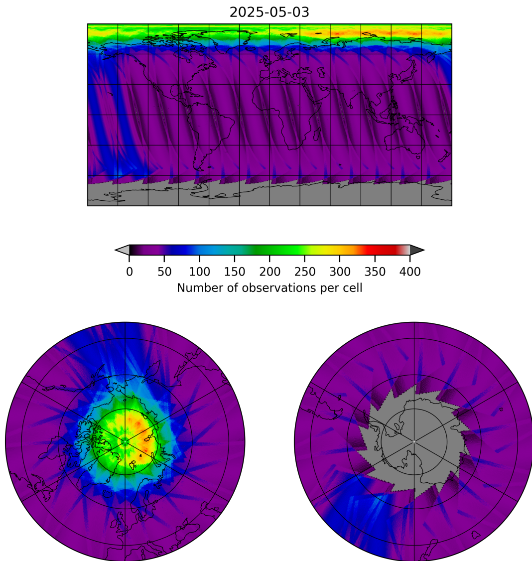
Figure 19: Map of the number of observations for 2025-05-02 to 2025-05-04
