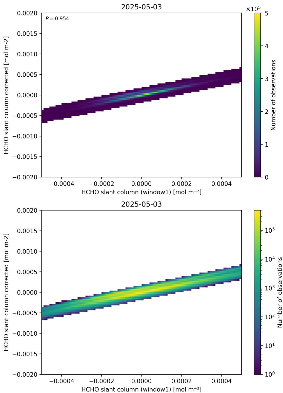
Figure 82: Scatter density plot of “HCHO slant column (window1)” against “HCHO slant column corrected” for 2025-05-02 to 2025-05-04.
