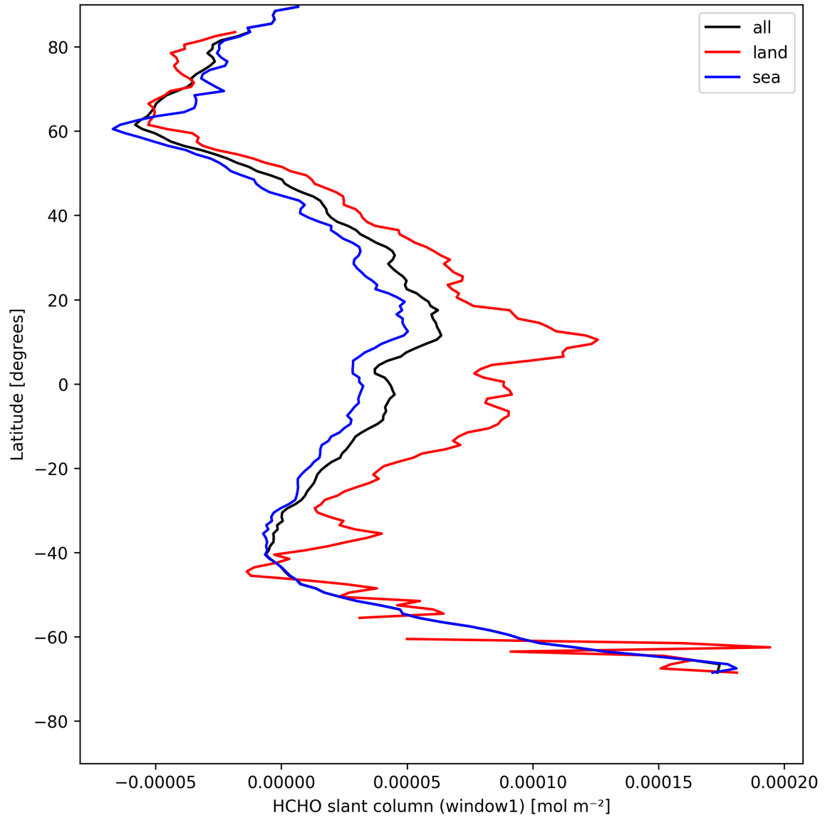
Figure 24: Zonal average of “HCHO slant column (window1)” for 2025-05-02 to 2025-05-04.
