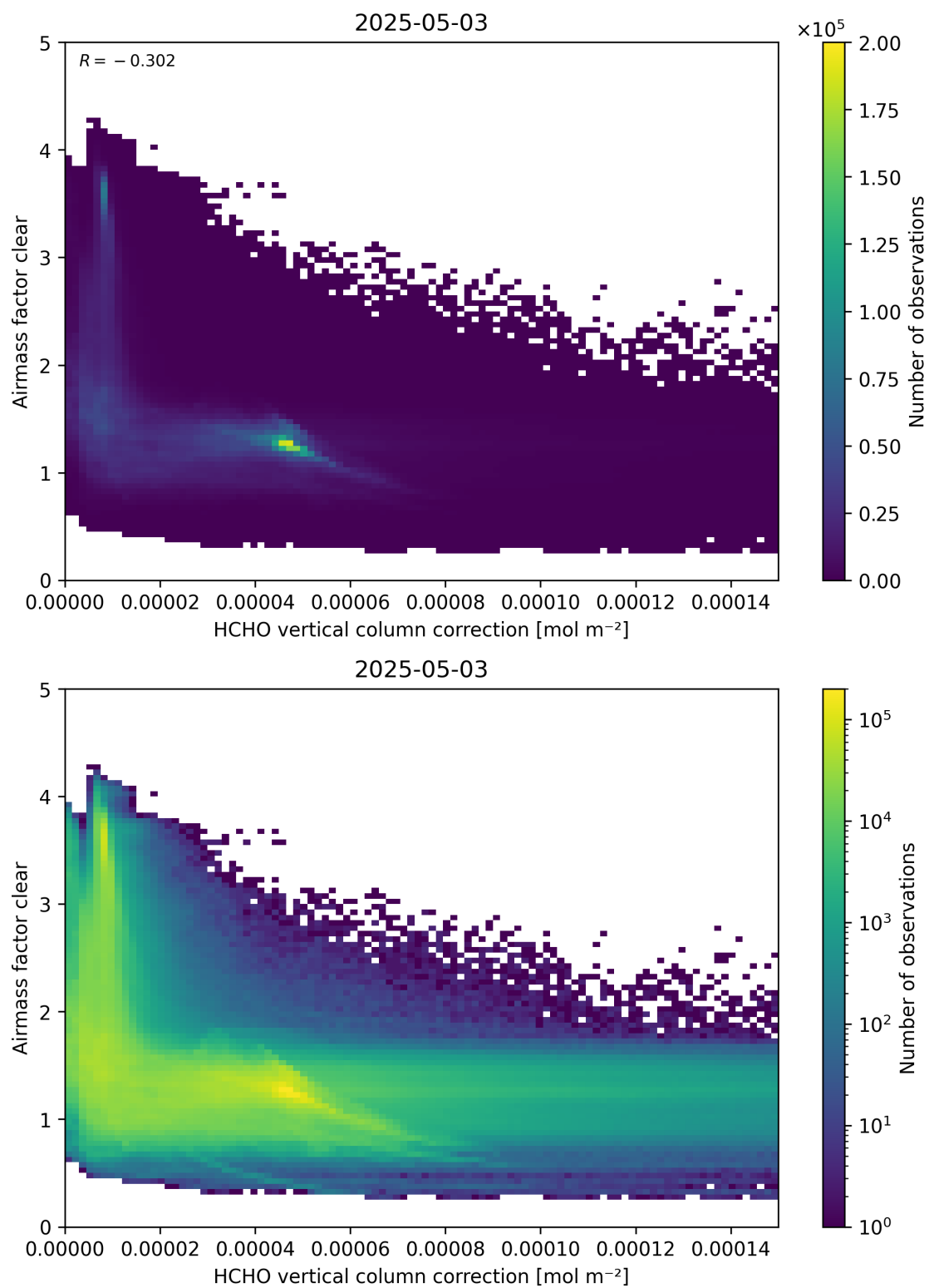
Figure 115: Scatter density plot of “HCHO vertical column correction” against “Airmass factor clear” for 2025-05-02 to 2025-05-04.
