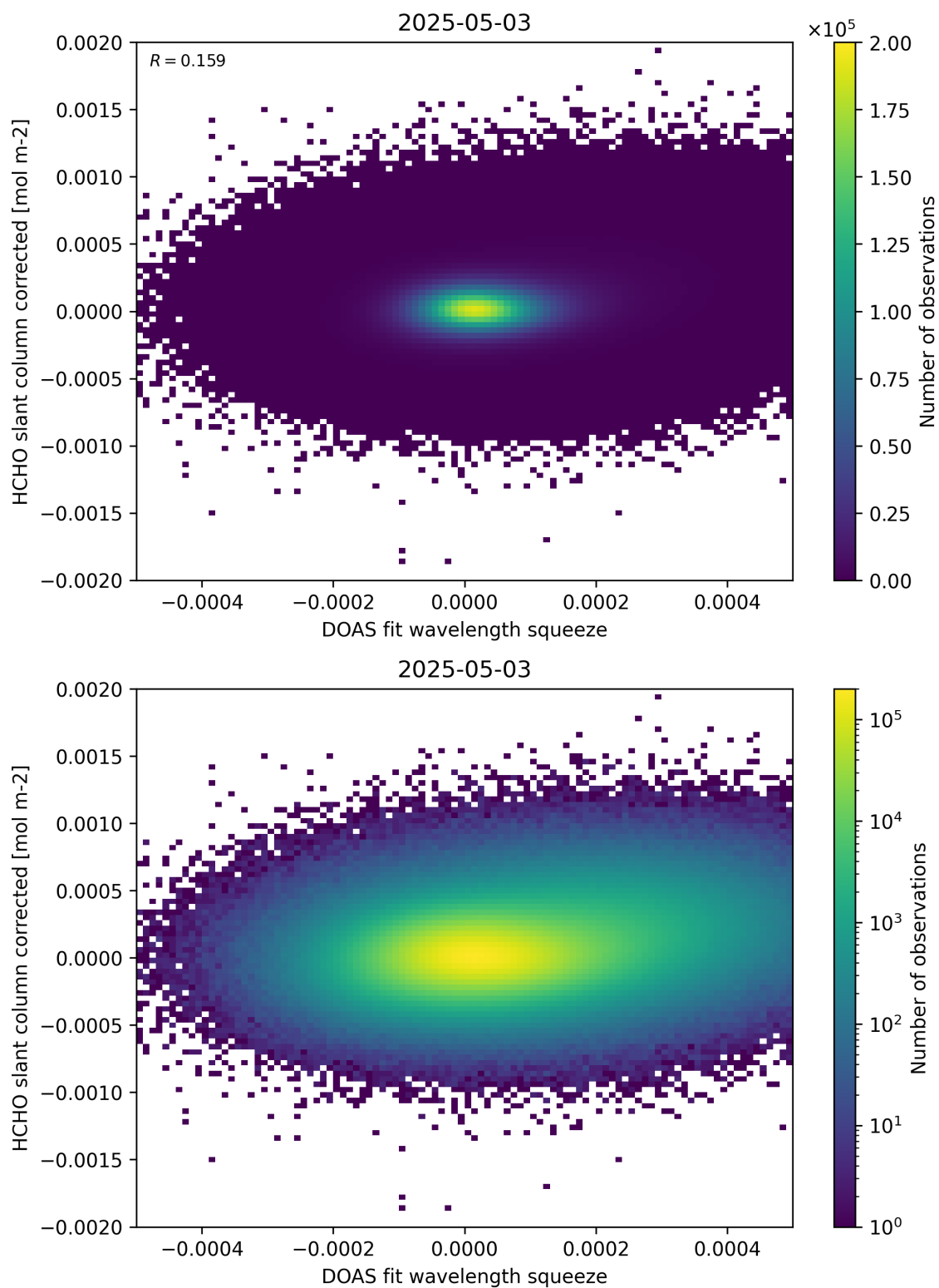
Figure 69: Scatter density plot of “DOAS fit wavelength squeeze” against “HCHO slant column corrected” for 2025-05-02 to 2025-05-04.
