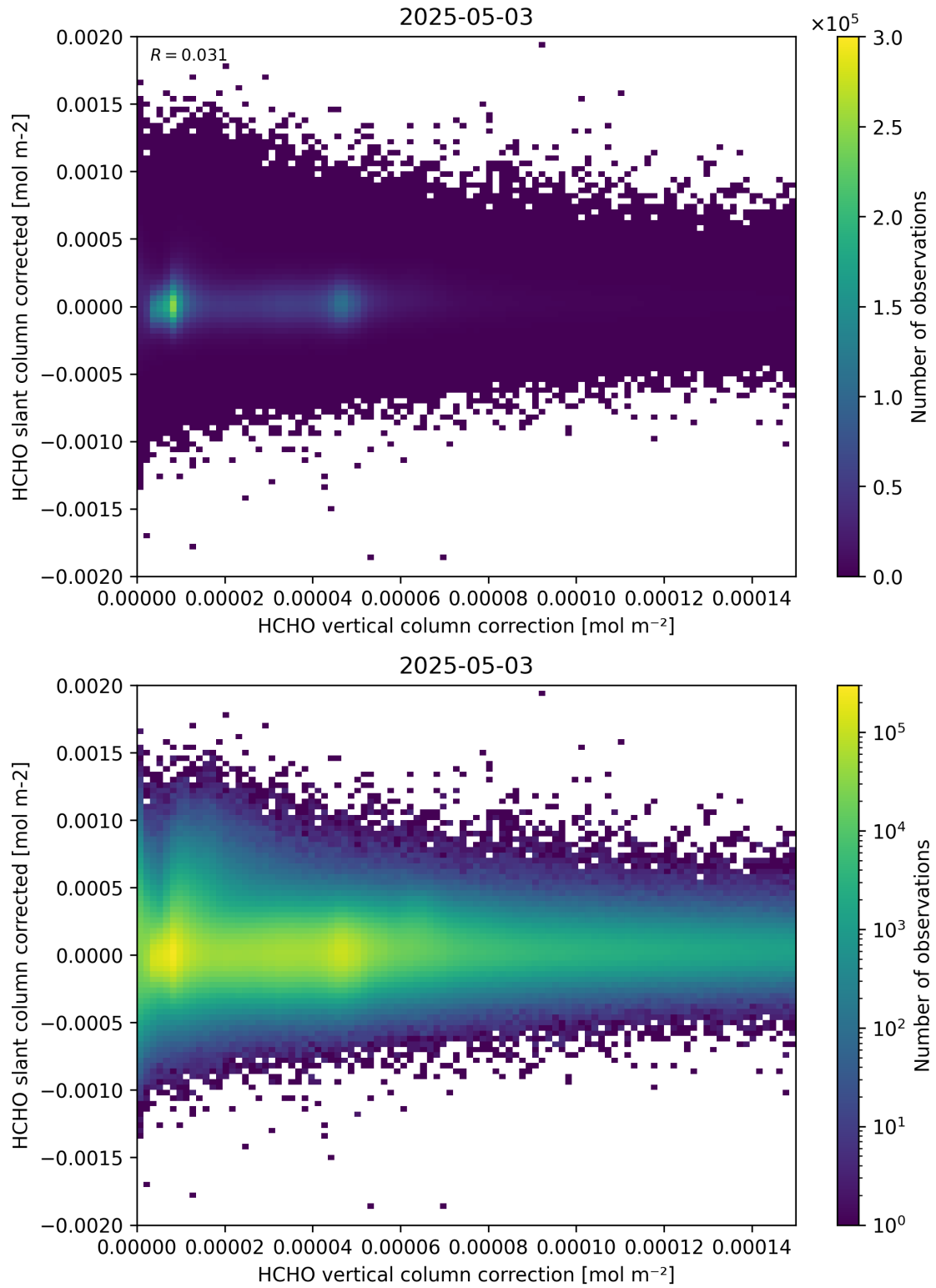
Figure 116: Scatter density plot of “HCHO vertical column correction” against “HCHO slant column corrected” for 2025-05-02 to 2025-05-04.
