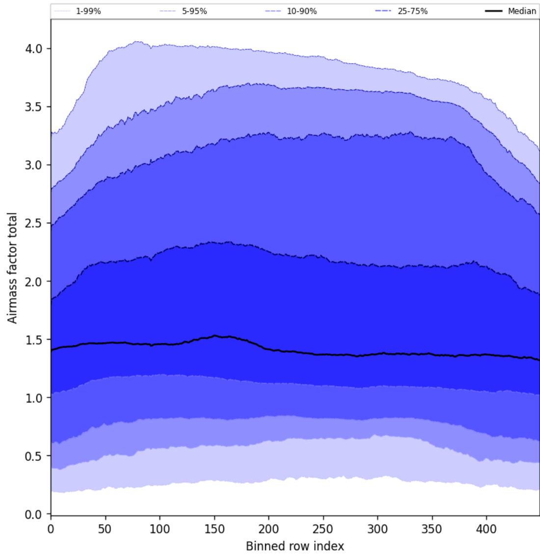
Figure 54: Along track statistics of “Airmass factor total” for 2025-05-02 to 2025-05-04
