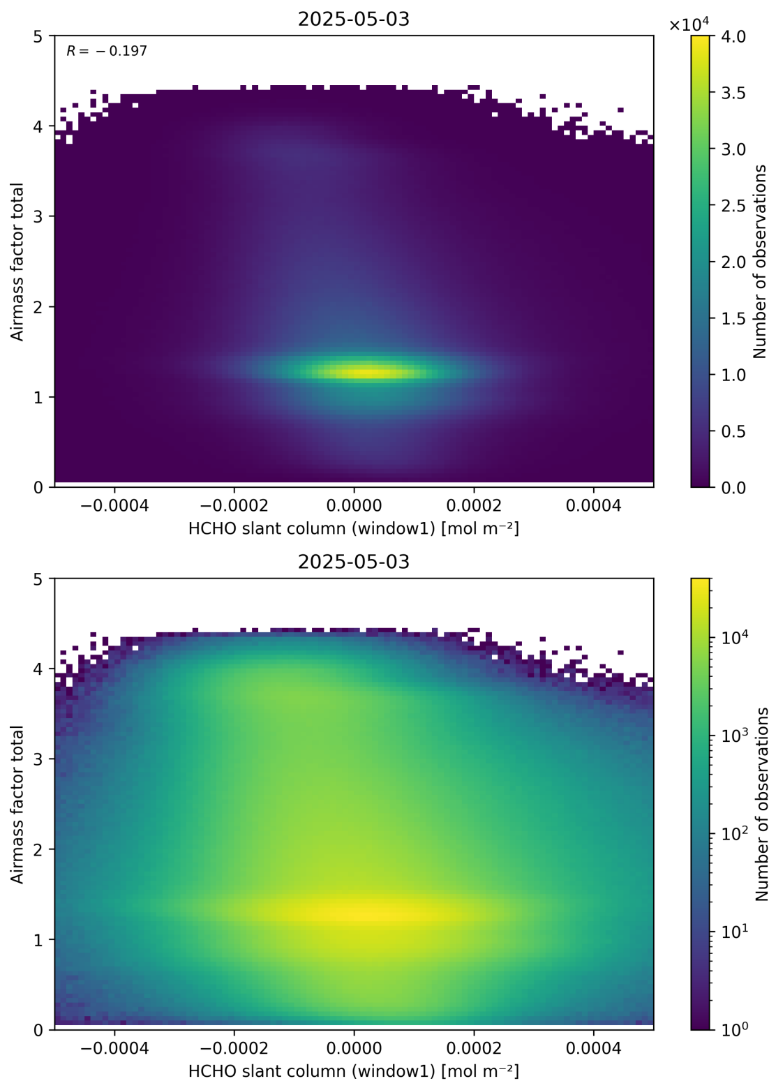
Figure 85: Scatter density plot of “HCHO slant column (window1)” against “Airmass factor total” for 2025-05-02 to 2025-05-04.
