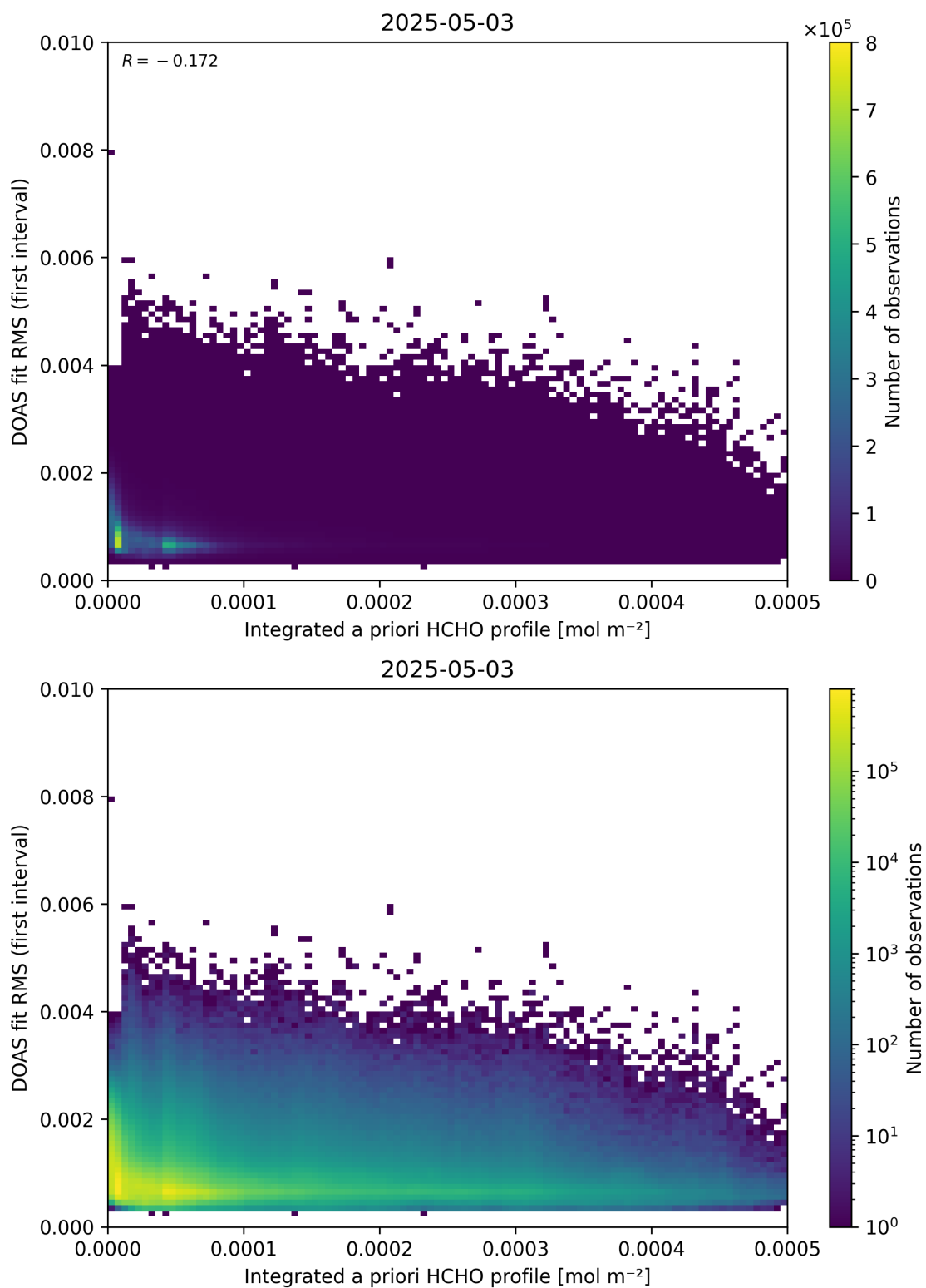
Figure 148: Scatter density plot of “Integrated a priori HCHO profile” against “DOAS fit RMS (first interval)” for 2025-05-02 to 2025-05-04.
