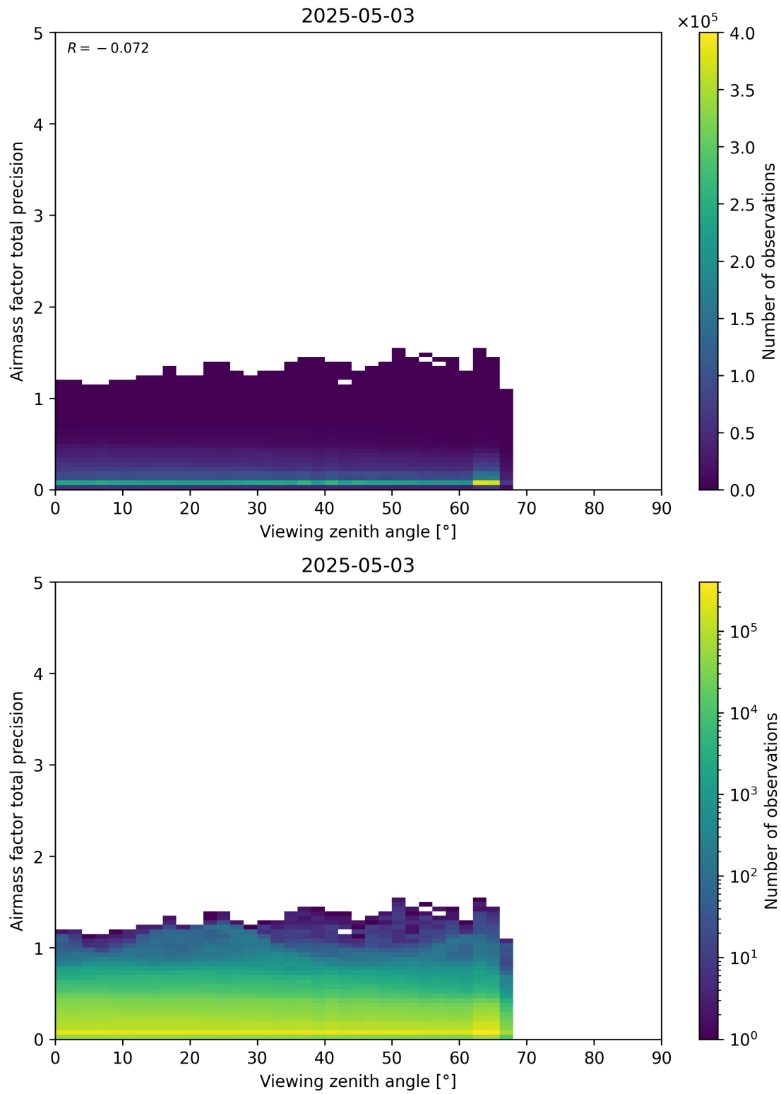
Figure 191: Scatter density plot of “Viewing zenith angle” against “Airmass factor total precision” for 2025-05-02 to 2025-05-04.
