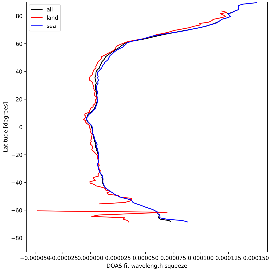
Figure 31: Zonal average of “DOAS fit wavelength squeeze” for 2025-05-02 to 2025-05-04.
