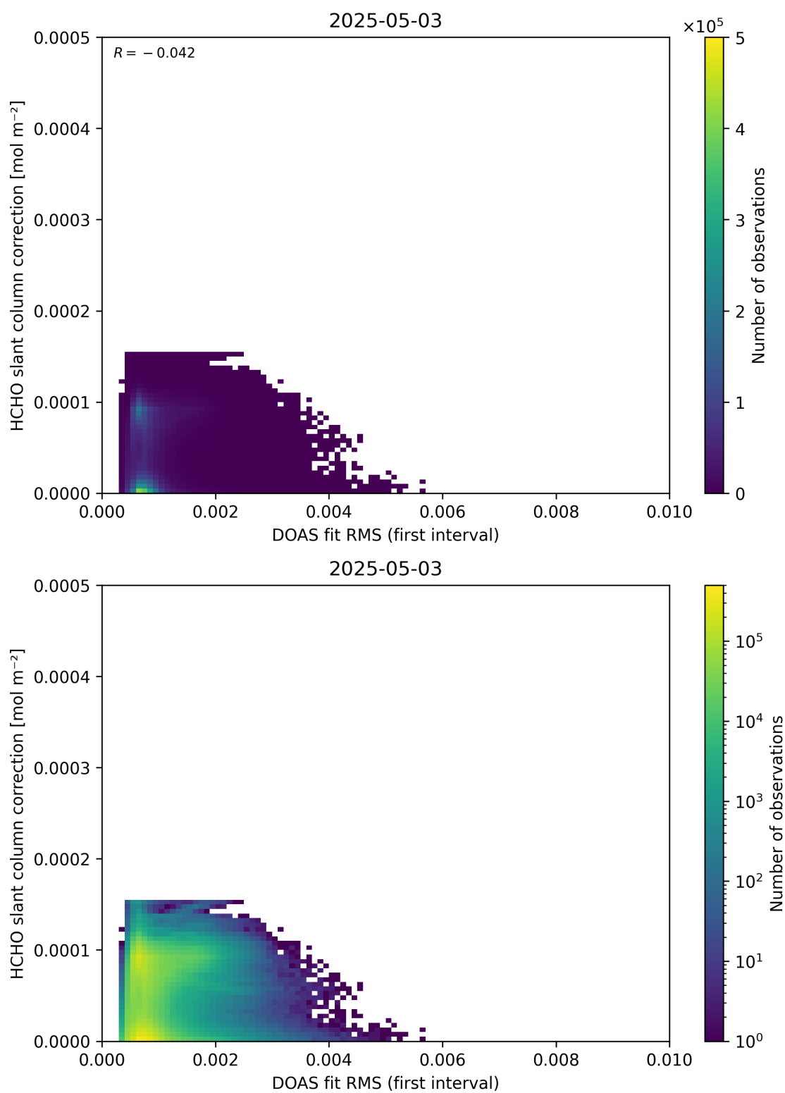
Figure 63: Scatter density plot of “DOAS fit RMS (first interval)” against “HCHO slant column correction” for 2025-05-02 to 2025-05-04.
