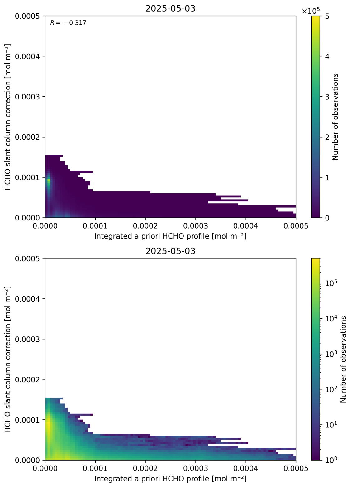
Figure 152: Scatter density plot of “Integrated a priori HCHO profile” against “HCHO slant column correction” for 2025-05-02 to 2025-05-04.
