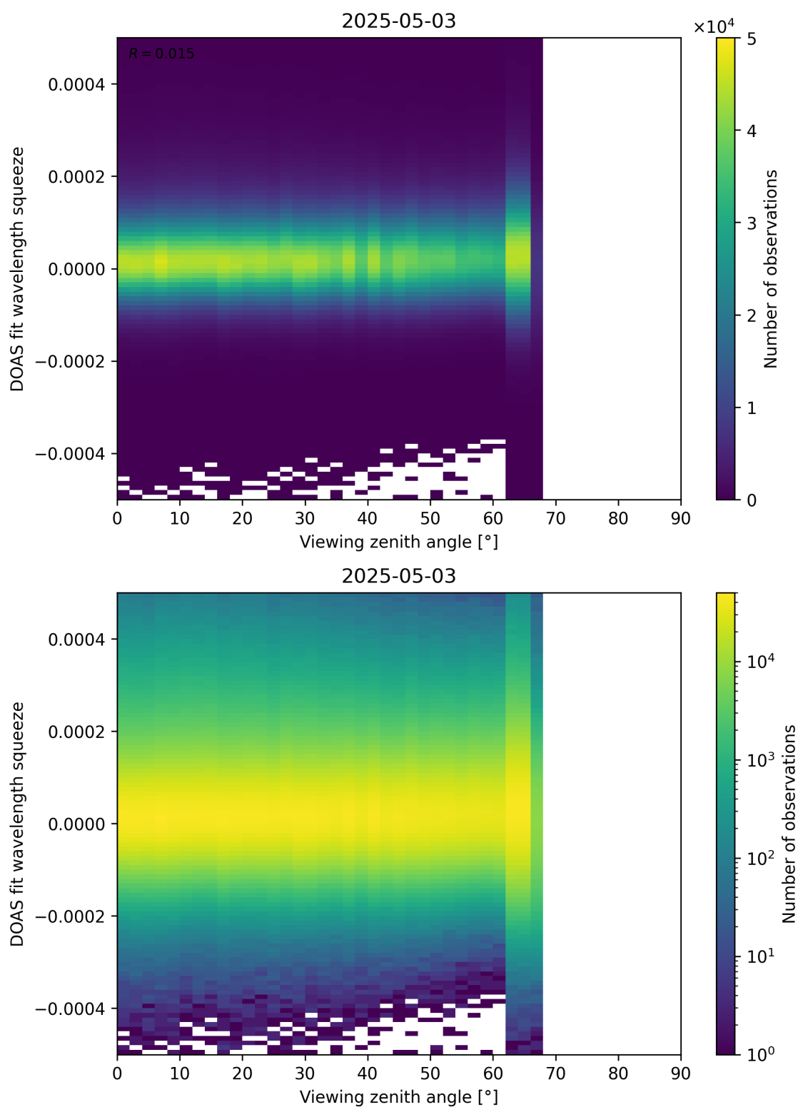
Figure 184: Scatter density plot of “Viewing zenith angle” against “DOAS fit wavelength squeeze” for 2025-05-02 to 2025-05-04.
