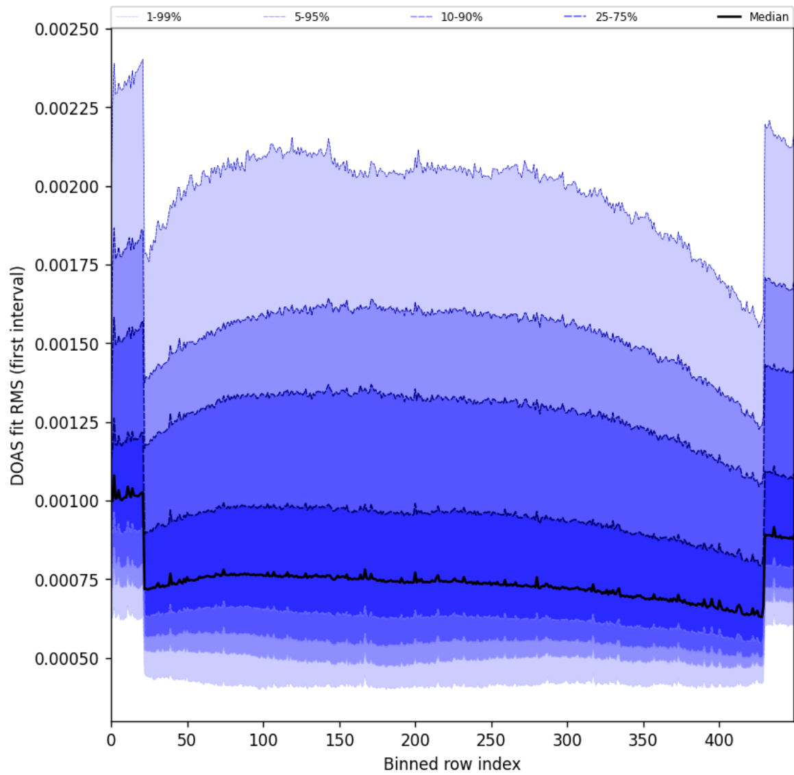
Figure 60: Along track statistics of “DOAS fit RMS (first interval)” for 2025-05-02 to 2025-05-04
