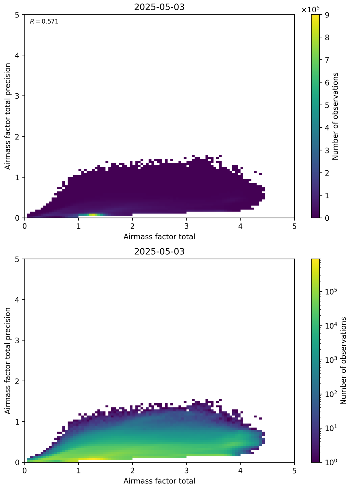
Figure 103: Scatter density plot of “Airmass factor total” against “Airmass factor total precision” for 2025-05-02 to 2025-05-04.
