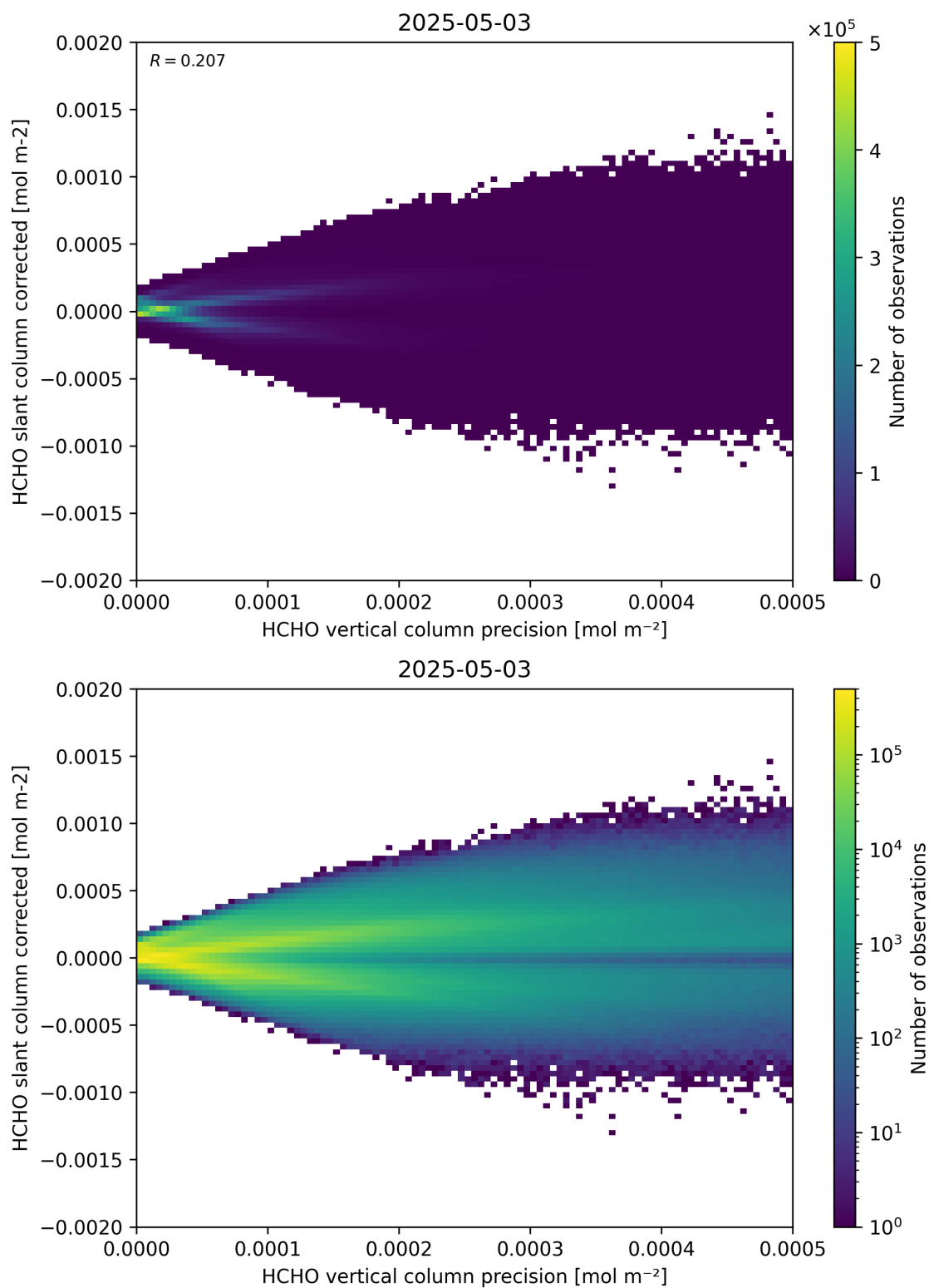
Figure 140: Scatter density plot of “HCHO vertical column precision” against “HCHO slant column corrected” for 2025-05-02 to 2025-05-04.
