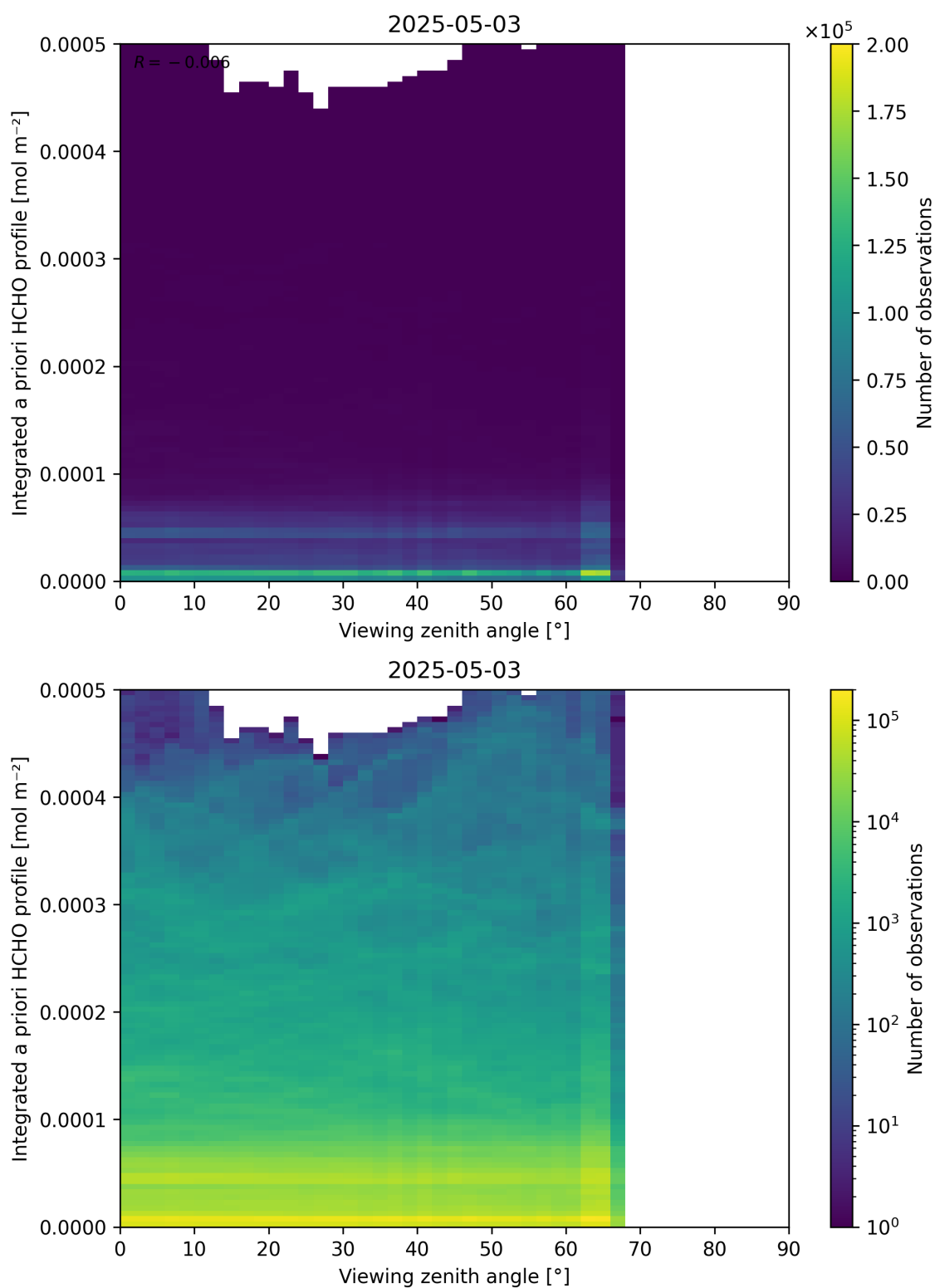
Figure 195: Scatter density plot of “Viewing zenith angle” against “Integrated a priori HCHO profile” for 2025-05-02 to 2025-05-04.
