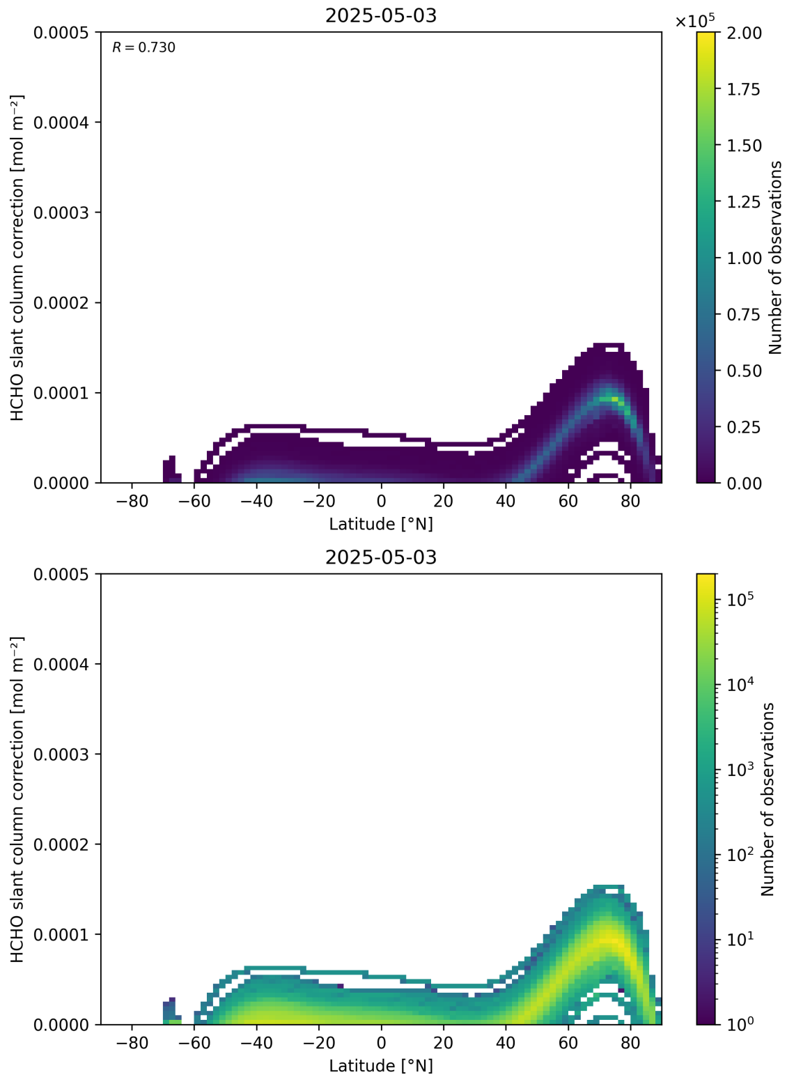
Figure 158: Scatter density plot of “Latitude” against “HCHO slant column correction” for 2025-05-02 to 2025-05-04.
