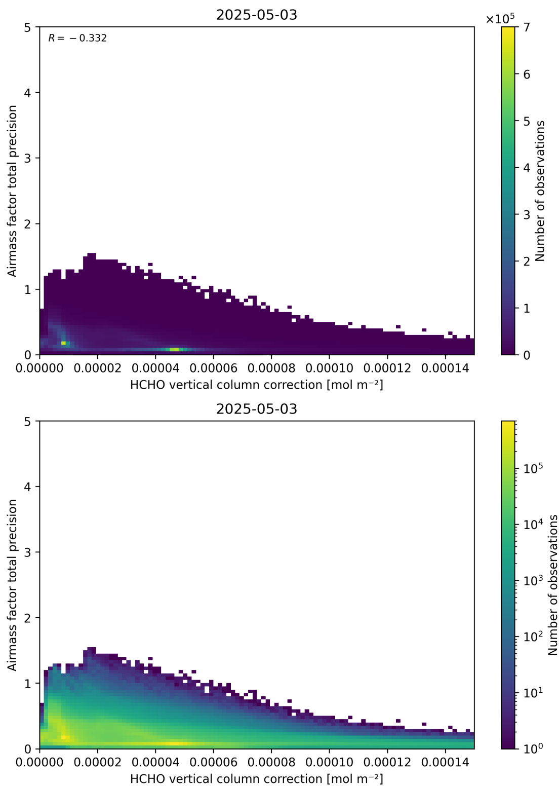
Figure 121: Scatter density plot of “HCHO vertical column correction” against “Airmass factor total precision” for 2025-05-02 to 2025-05-04.
