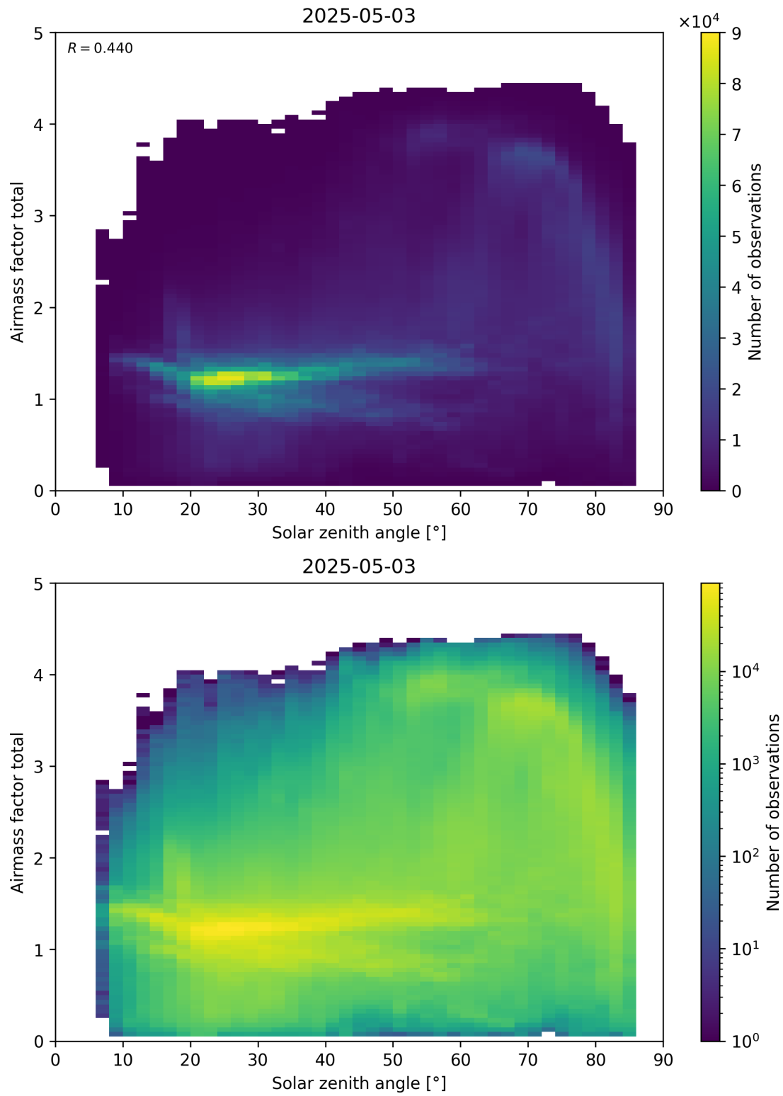
Figure 175: Scatter density plot of “Solar zenith angle” against “Airmass factor total” for 2025-05-02 to 2025-05-04.
