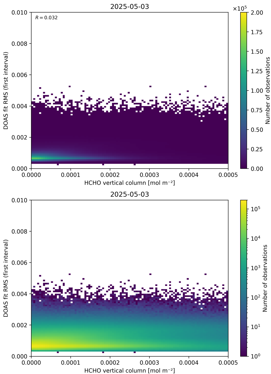
Figure 123: Scatter density plot of “HCHO vertical column” against “DOAS fit RMS (first interval)” for 2025-05-02 to 2025-05-04.
