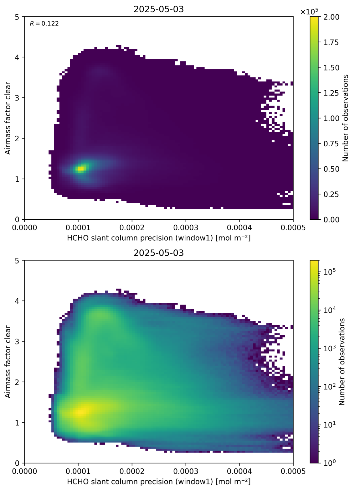
Figure 91: Scatter density plot of “HCHO slant column precision (window1)” against “Airmass factor clear” for 2025-05-02 to 2025-05-04.
