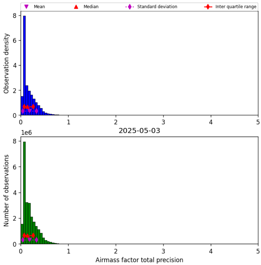
Figure 41: Histogram of “Airmass factor total precision” for 2025-05-02 to 2025-05-04
