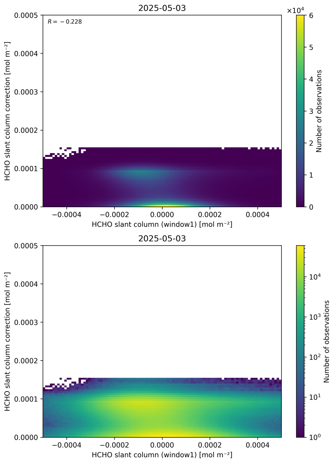
Figure 83: Scatter density plot of “HCHO slant column (window1)” against “HCHO slant column correction” for 2025-05-02 to 2025-05-04.
