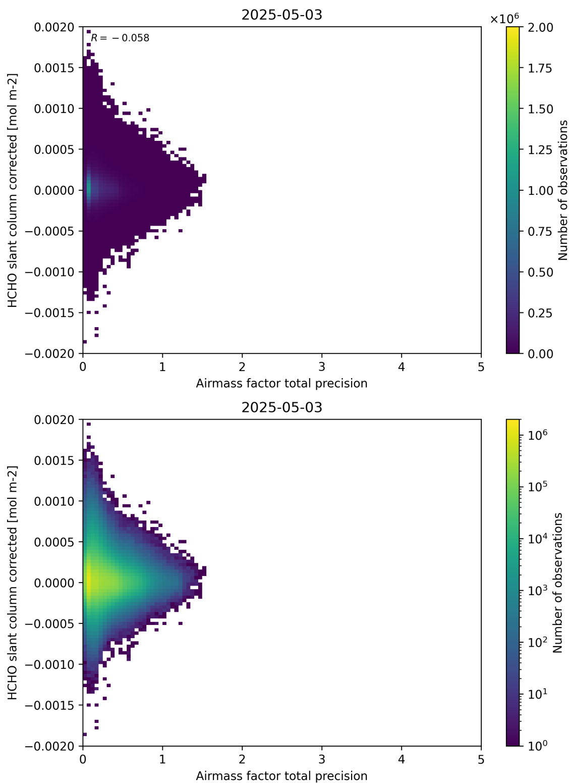
Figure 109: Scatter density plot of “Airmass factor total precision” against “HCHO slant column corrected” for 2025-05-02 to 2025-05-04.
