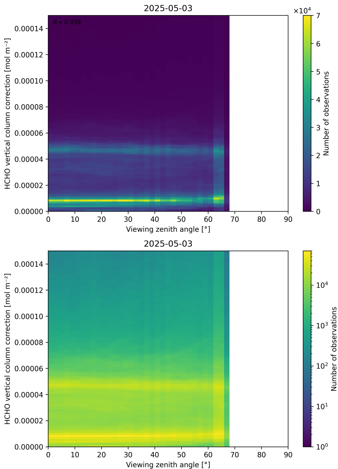
Figure 193: Scatter density plot of “Viewing zenith angle” against “HCHO vertical column correction” for 2025-05-02 to 2025-05-04.
