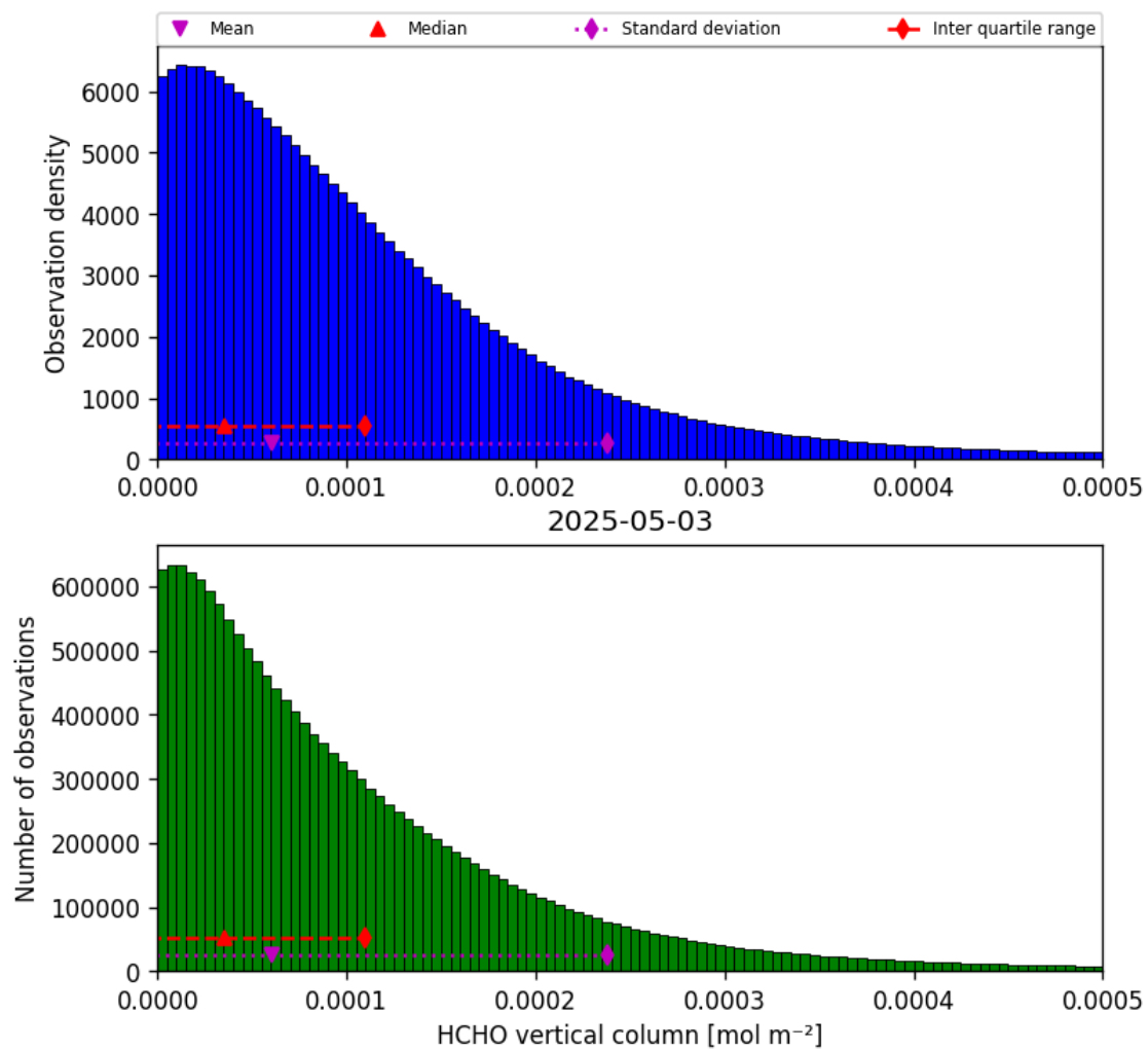
Figure 35: Histogram of “HCHO vertical column” for 2025-05-02 to 2025-05-04
