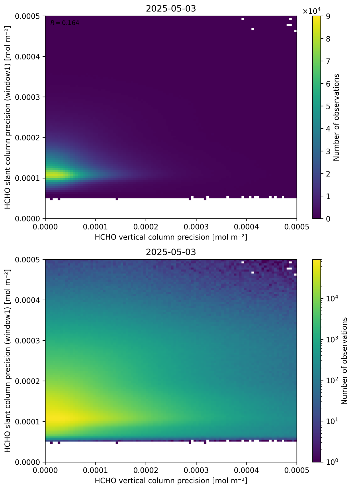
Figure 143: Scatter density plot of “HCHO vertical column precision” against “HCHO slant column precision (window1)” for 2025-05-02 to 2025-05-04.
