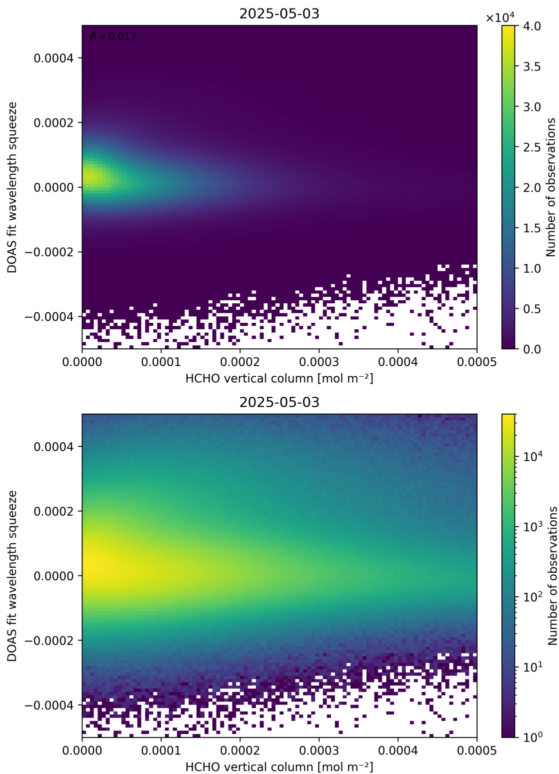
Figure 125: Scatter density plot of “HCHO vertical column” against “DOAS fit wavelength squeeze” for 2025-05-02 to 2025-05-04.
