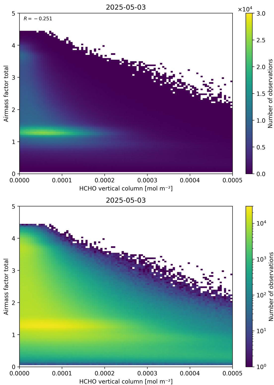
Figure 131: Scatter density plot of “HCHO vertical column” against “Airmass factor total” for 2025-05-02 to 2025-05-04.
