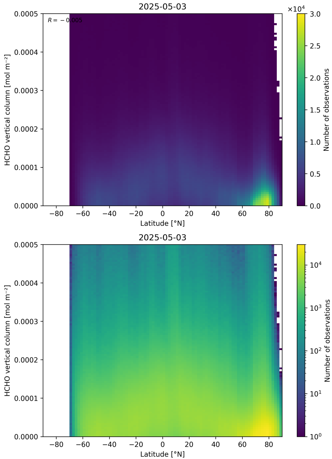
Figure 163: Scatter density plot of “Latitude” against “HCHO vertical column” for 2025-05-02 to 2025-05-04.
