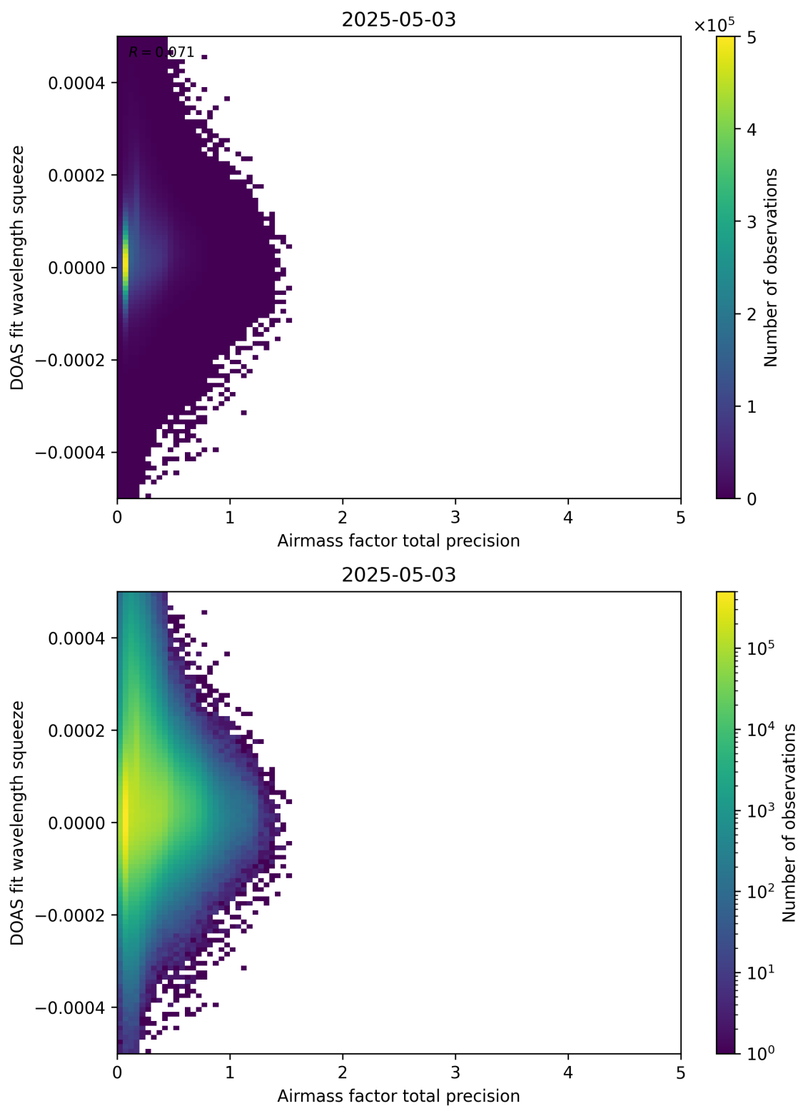
Figure 107: Scatter density plot of “Airmass factor total precision” against “DOAS fit wavelength squeeze” for 2025-05-02 to 2025-05-04.
