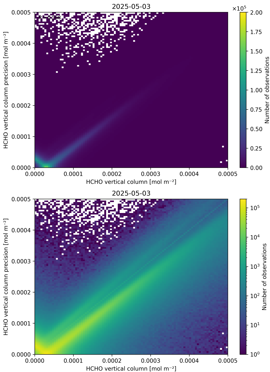
Figure 134: Scatter density plot of “HCHO vertical column” against “HCHO vertical column precision” for 2025-05-02 to 2025-05-04.
