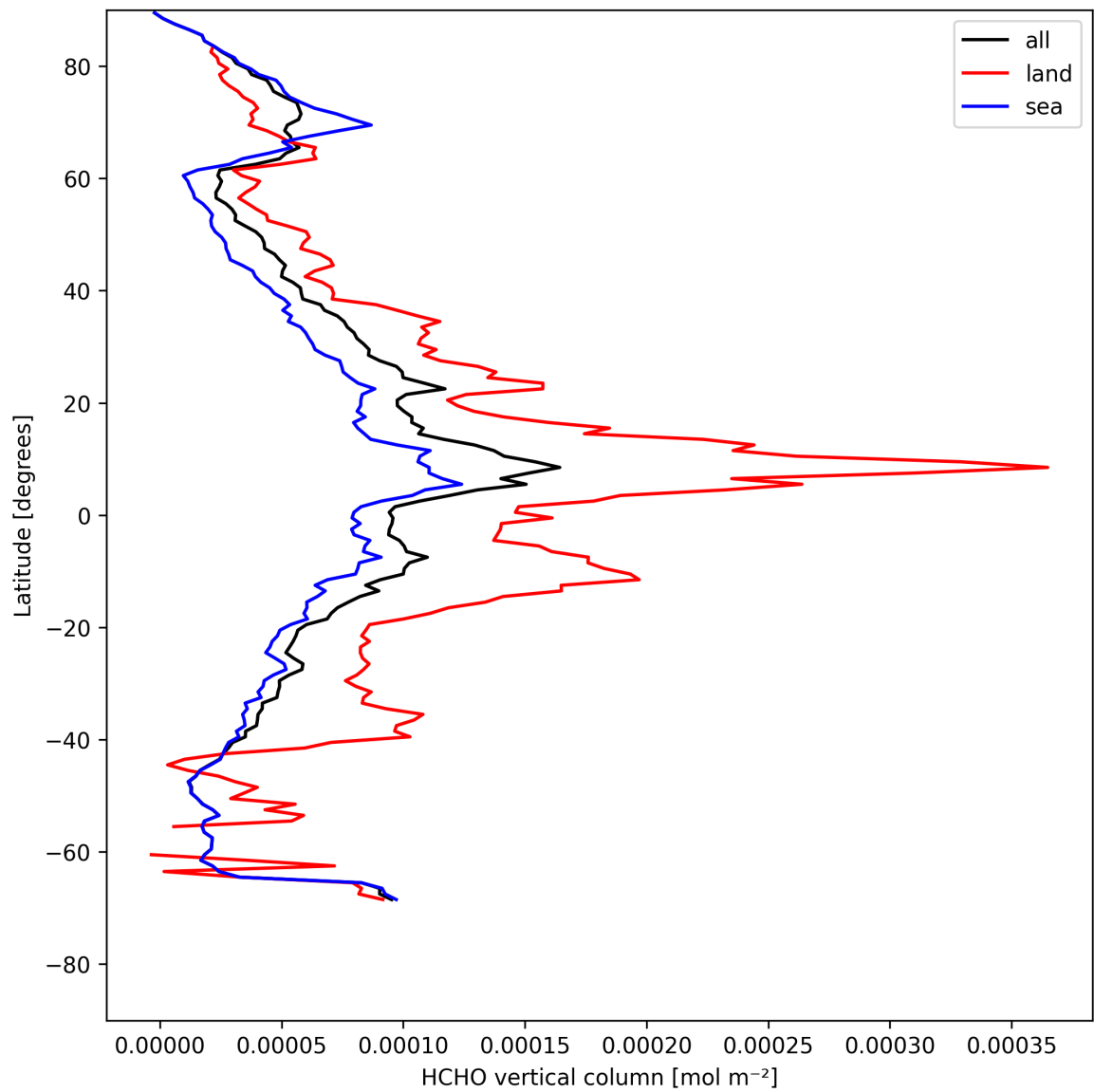
Figure 21: Zonal average of “HCHO vertical column” for 2025-05-02 to 2025-05-04.
