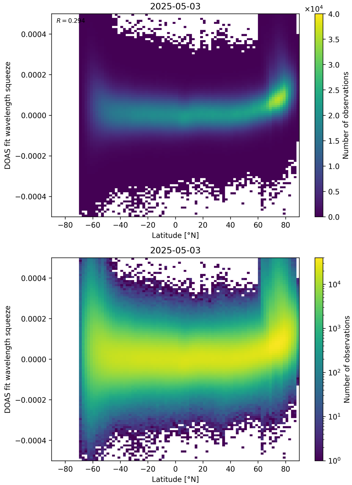
Figure 155: Scatter density plot of “Latitude” against “DOAS fit wavelength squeeze” for 2025-05-02 to 2025-05-04.
