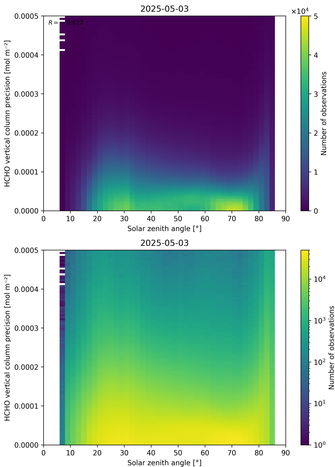
Figure 179: Scatter density plot of “Solar zenith angle” against “HCHO vertical column precision” for 2025-05-02 to 2025-05-04.
