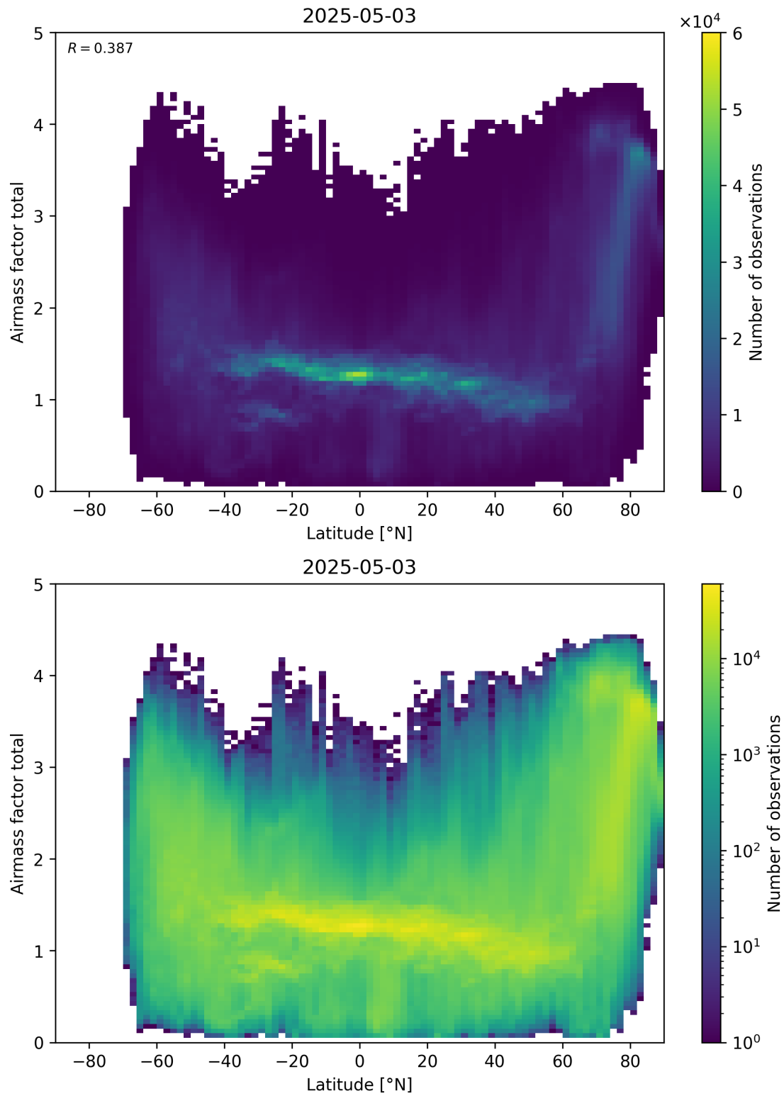
Figure 161: Scatter density plot of “Latitude” against “Airmass factor total” for 2025-05-02 to 2025-05-04.
