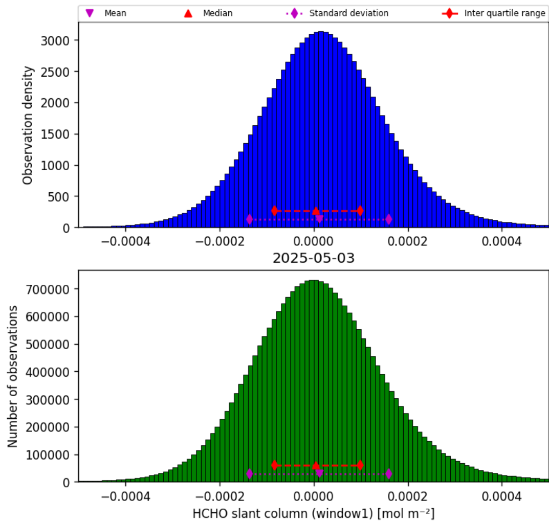
Figure 38: Histogram of “HCHO slant column (window1)” for 2025-05-02 to 2025-05-04
