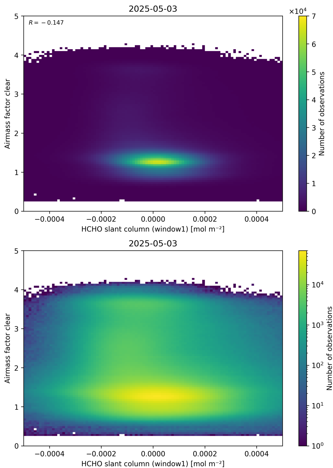
Figure 81: Scatter density plot of “HCHO slant column (window1)” against “Airmass factor clear” for 2025-05-02 to 2025-05-04.
