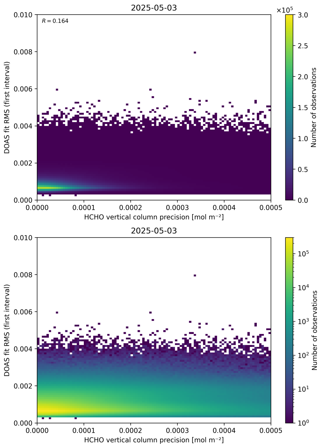
Figure 136: Scatter density plot of “HCHO vertical column precision” against “DOAS fit RMS (first interval)” for 2025-05-02 to 2025-05-04.
