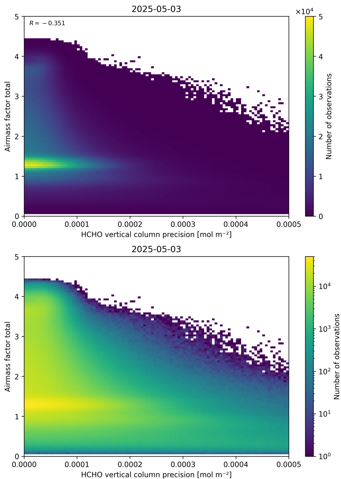
Figure 144: Scatter density plot of “HCHO vertical column precision” against “Airmass factor total” for 2025-05-02 to 2025-05-04.
