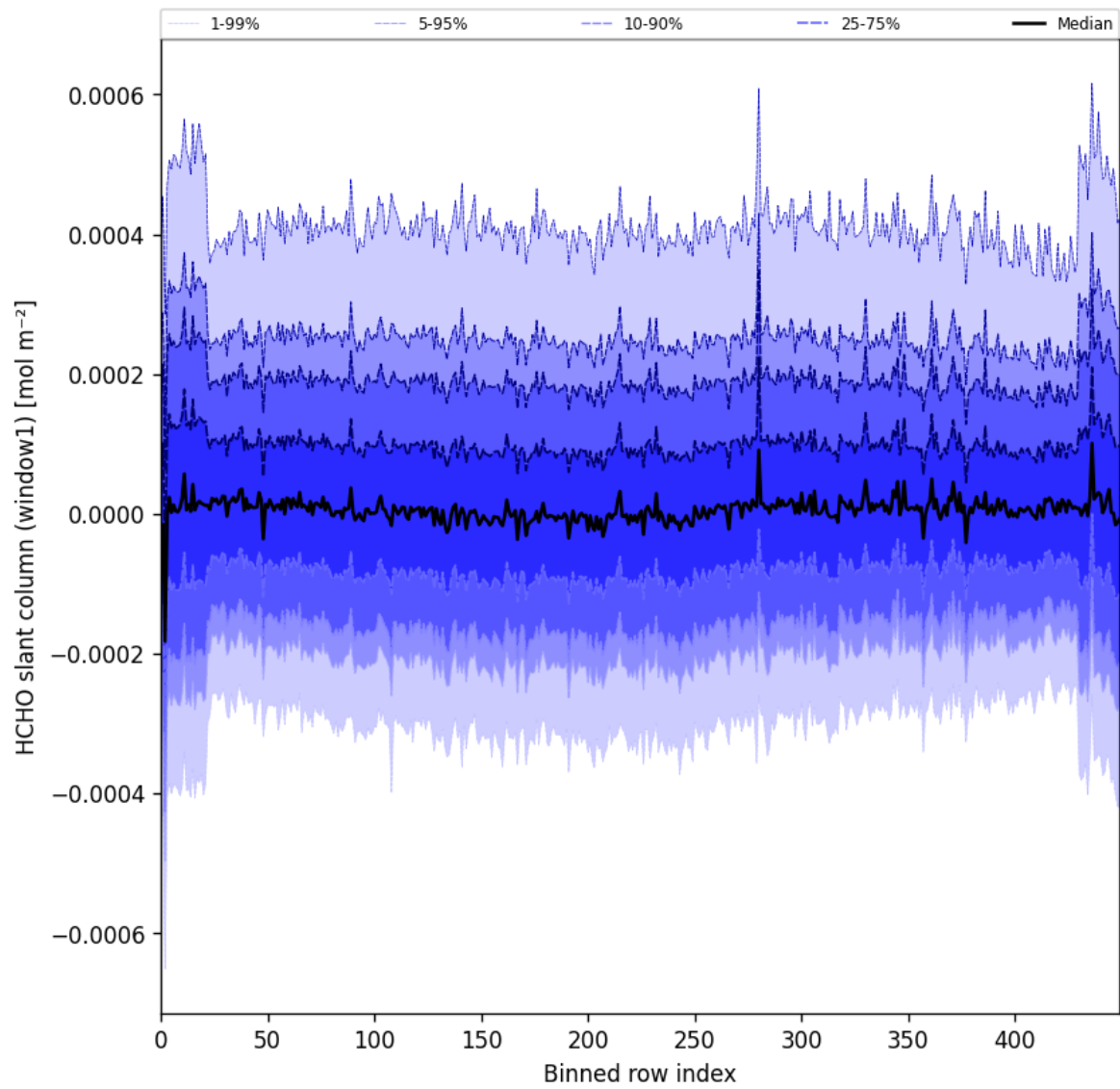
Figure 52: Along track statistics of “HCHO slant column (window1)” for 2025-05-02 to 2025-05-04
