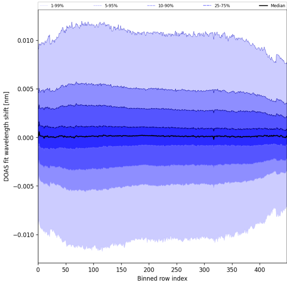
Figure 58: Along track statistics of “DOAS fit wavelength shift” for 2025-05-02 to 2025-05-04
