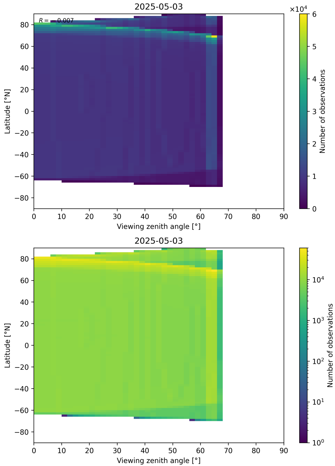
Figure 196: Scatter density plot of “Viewing zenith angle” against “Latitude” for 2025-05-02 to 2025-05-04.
