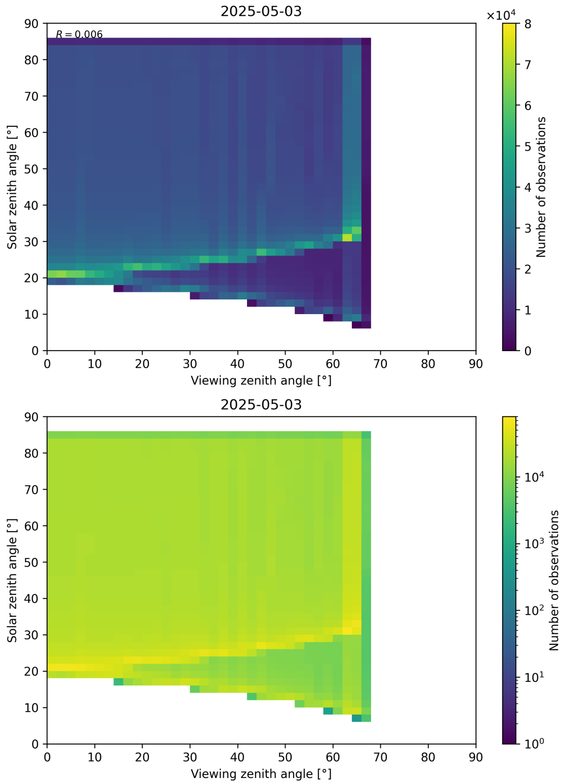
Figure 197: Scatter density plot of “Viewing zenith angle” against “Solar zenith angle” for 2025-05-02 to 2025-05-04.
