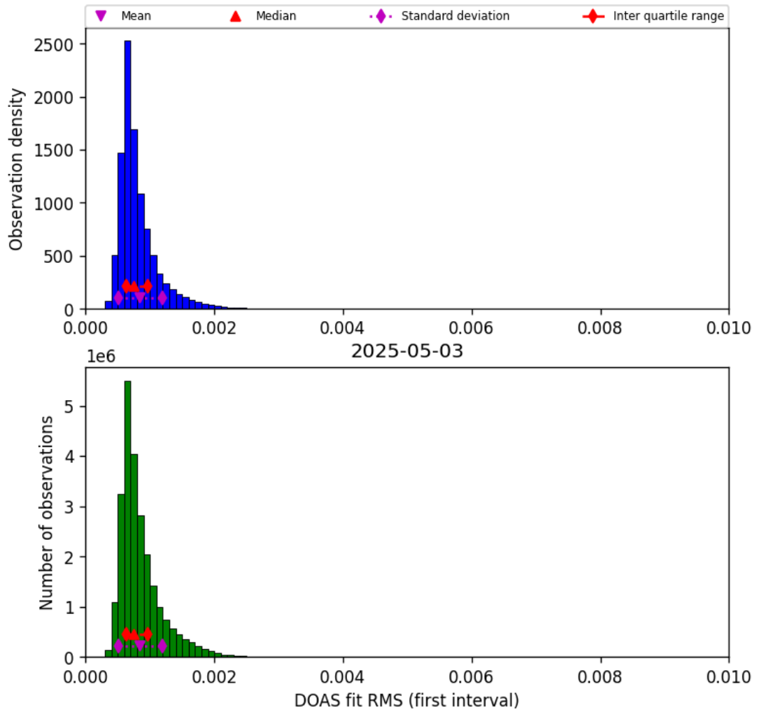
Figure 46: Histogram of “DOAS fit RMS (first interval)” for 2025-05-02 to 2025-05-04
