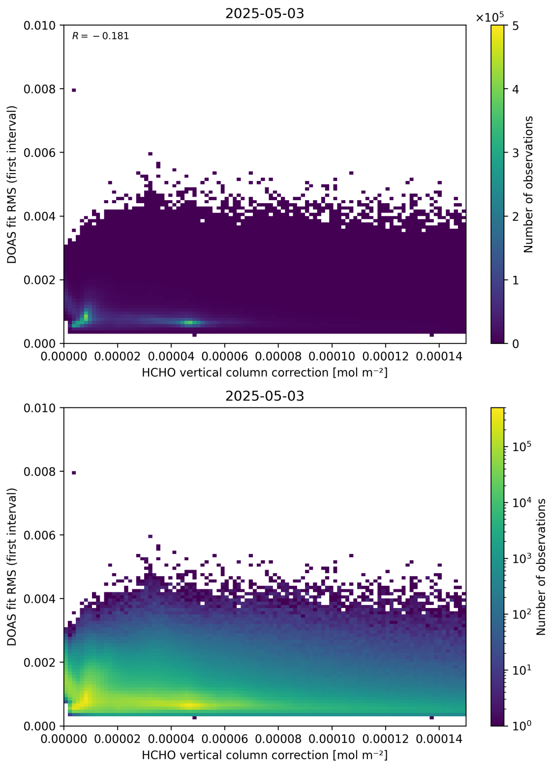
Figure 112: Scatter density plot of “HCHO vertical column correction” against “DOAS fit RMS (first interval)” for 2025-05-02 to 2025-05-04.
