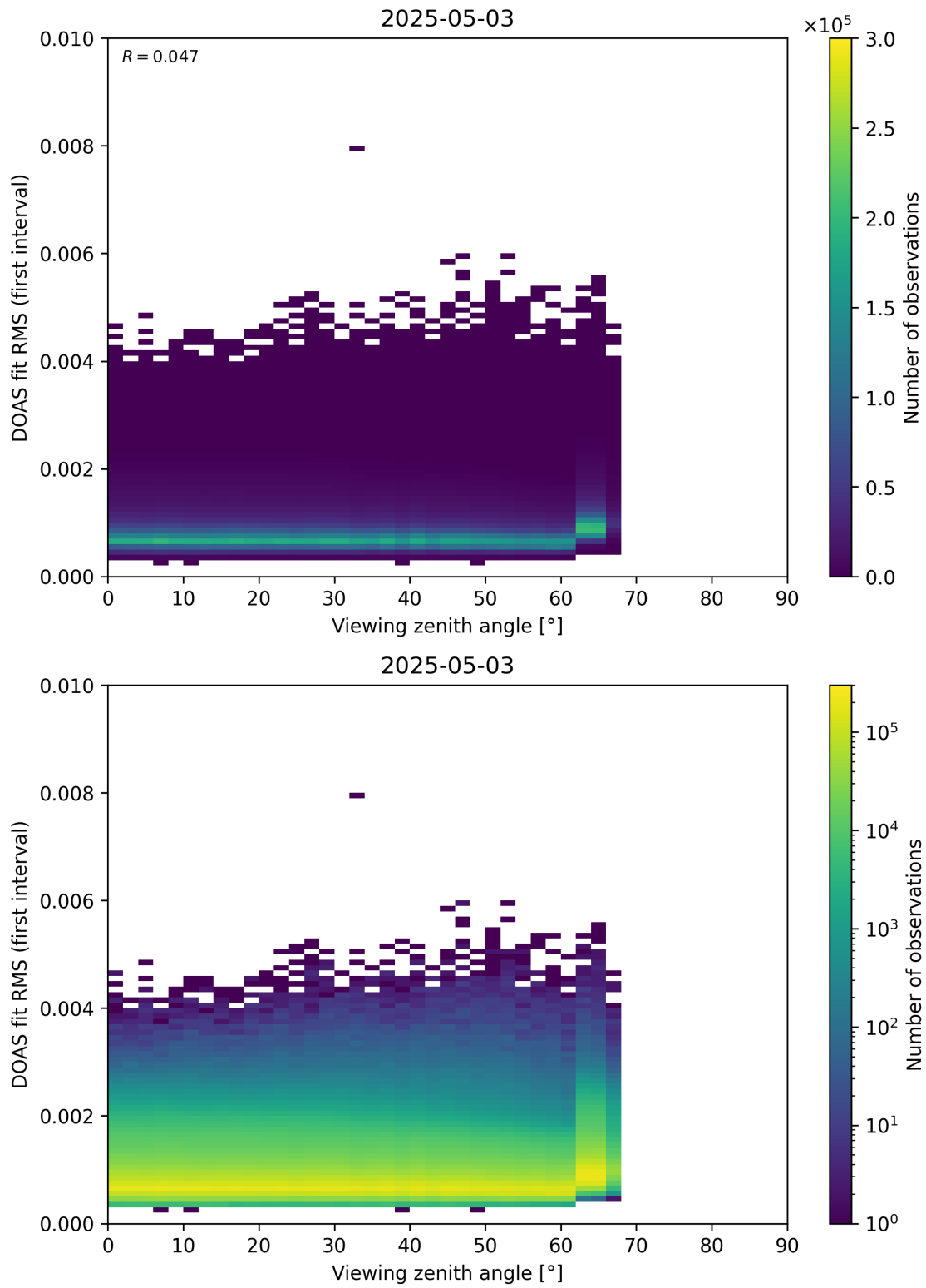
Figure 182: Scatter density plot of “Viewing zenith angle” against “DOAS fit RMS (first interval)” for 2025-05-02 to 2025-05-04.
