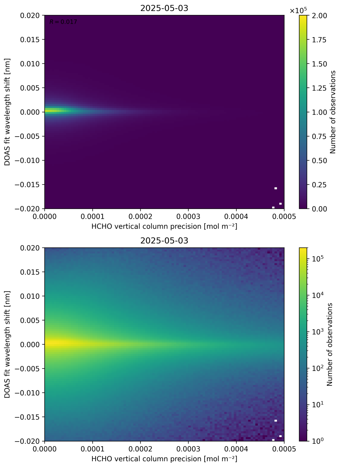
Figure 137: Scatter density plot of “HCHO vertical column precision” against “DOAS fit wavelength shift” for 2025-05-02 to 2025-05-04.
