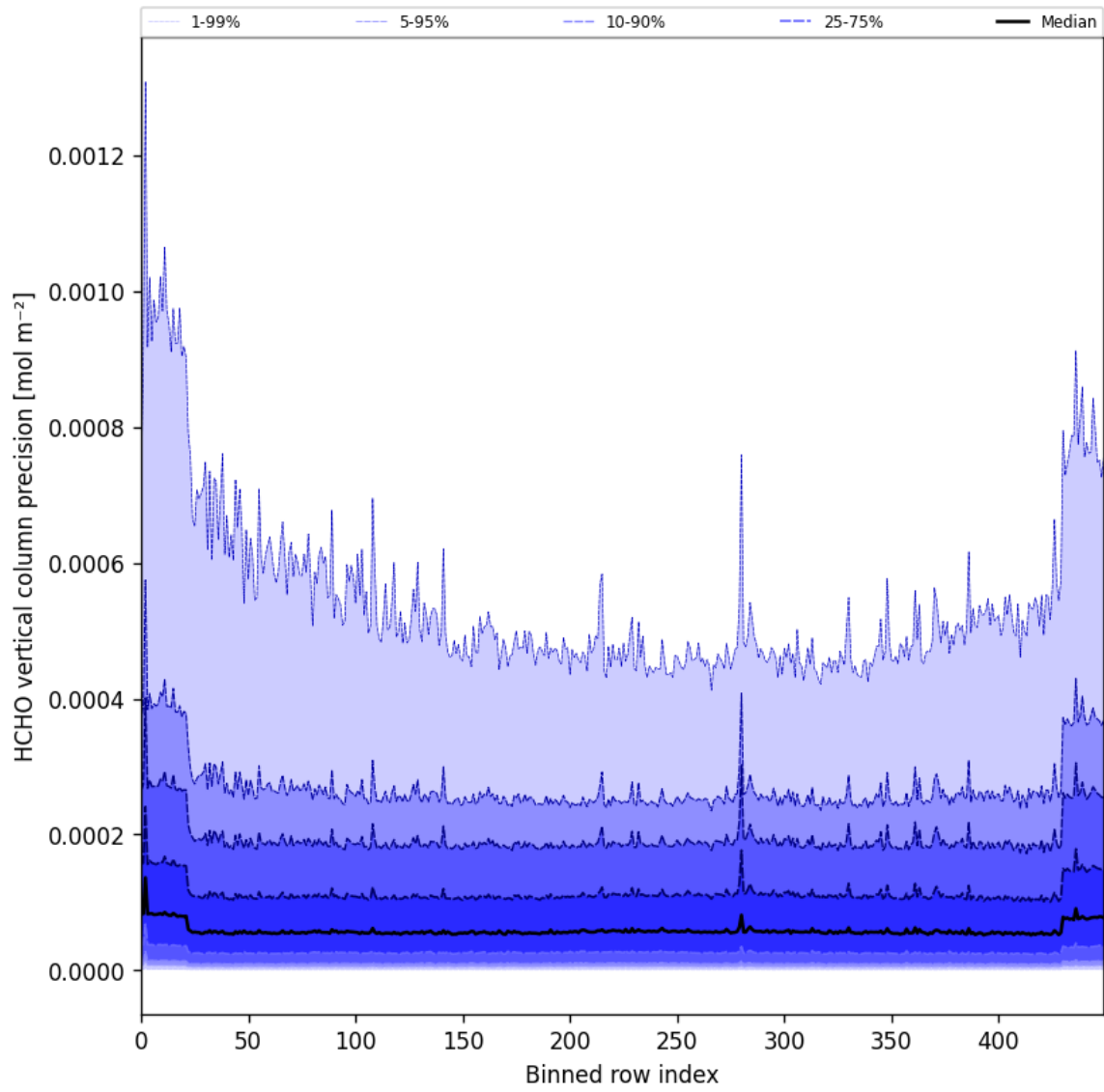
Figure 50: Along track statistics of “HCHO vertical column precision” for 2025-05-02 to 2025-05-04
