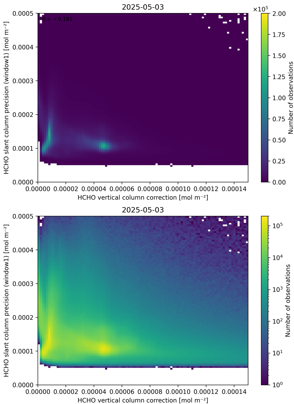
Figure 119: Scatter density plot of “HCHO vertical column correction” against “HCHO slant column precision (window1)” for 2025-05-02 to 2025-05-04.
