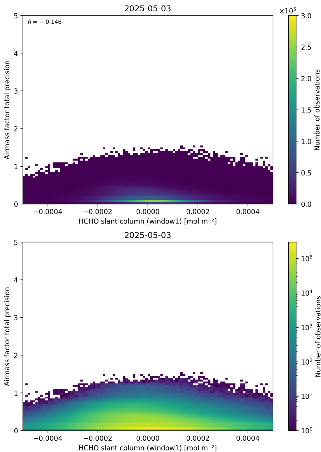
Figure 86: Scatter density plot of “HCHO slant column (window1)” against “Airmass factor total precision” for 2025-05-02 to 2025-05-04.
