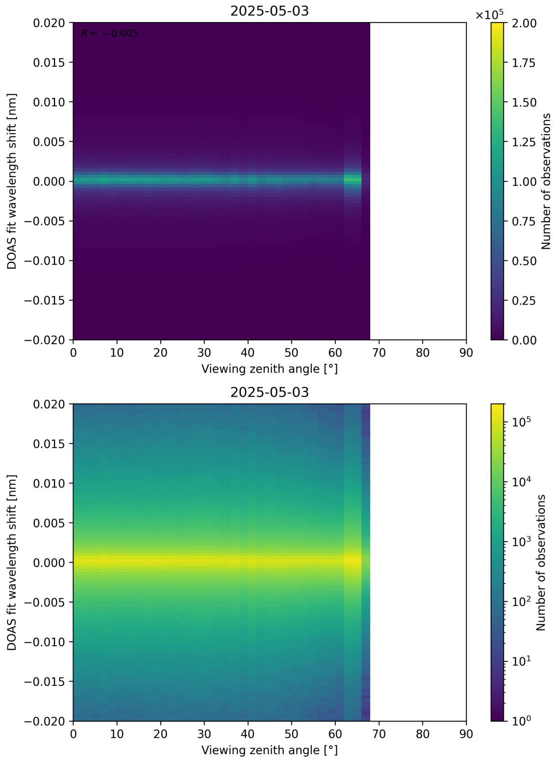
Figure 183: Scatter density plot of “Viewing zenith angle” against “DOAS fit wavelength shift” for 2025-05-02 to 2025-05-04.
