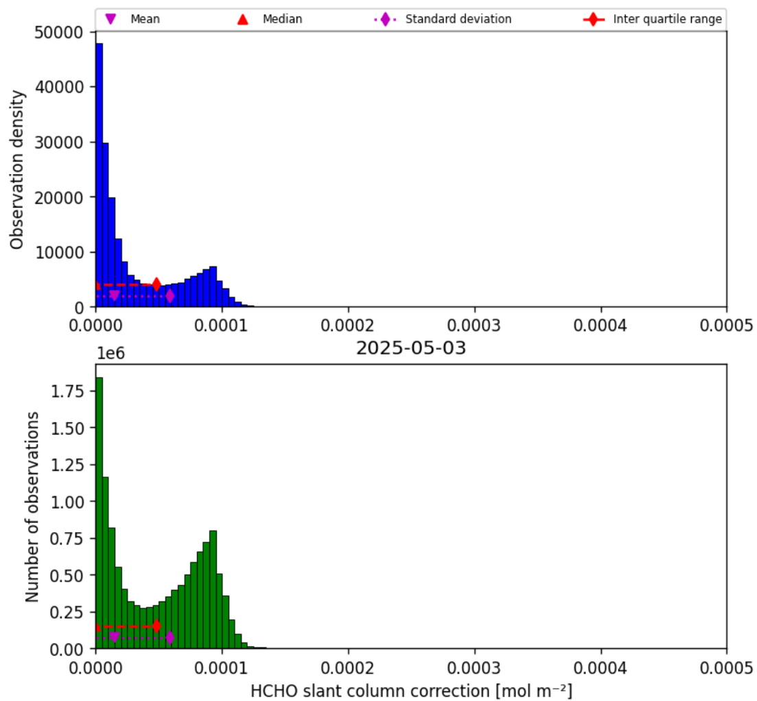
Figure 47: Histogram of “HCHO slant column correction” for 2025-05-02 to 2025-05-04
