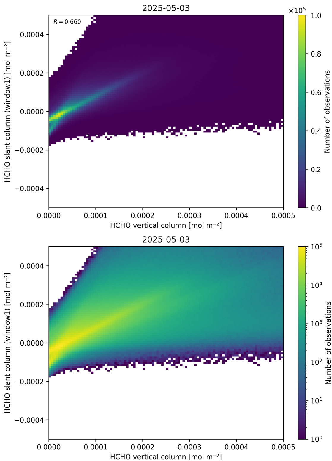
Figure 129: Scatter density plot of “HCHO vertical column” against “HCHO slant column (window1)” for 2025-05-02 to 2025-05-04.
