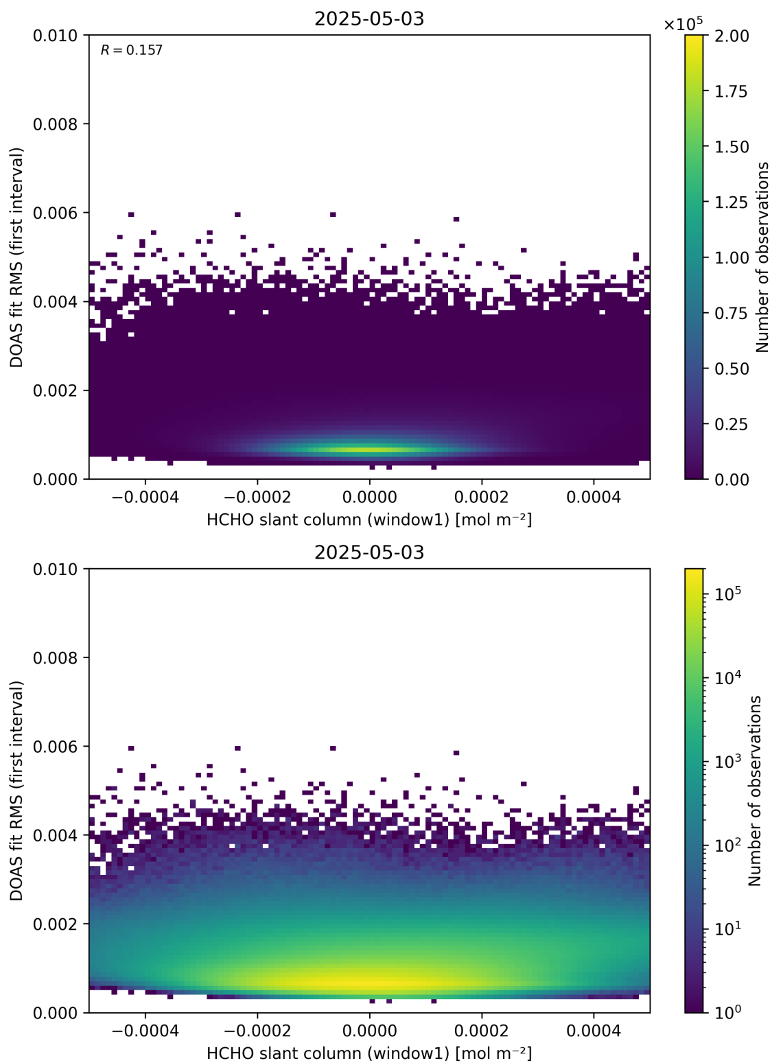
Figure 78: Scatter density plot of “HCHO slant column (window1)” against “DOAS fit RMS (first interval)” for 2025-05-02 to 2025-05-04.
