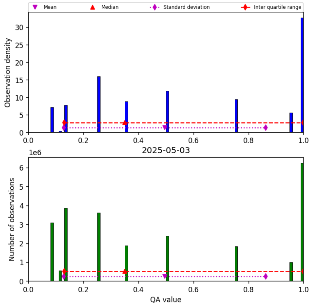
Figure 34: Histogram of “QA value” for 2025-05-02 to 2025-05-04
