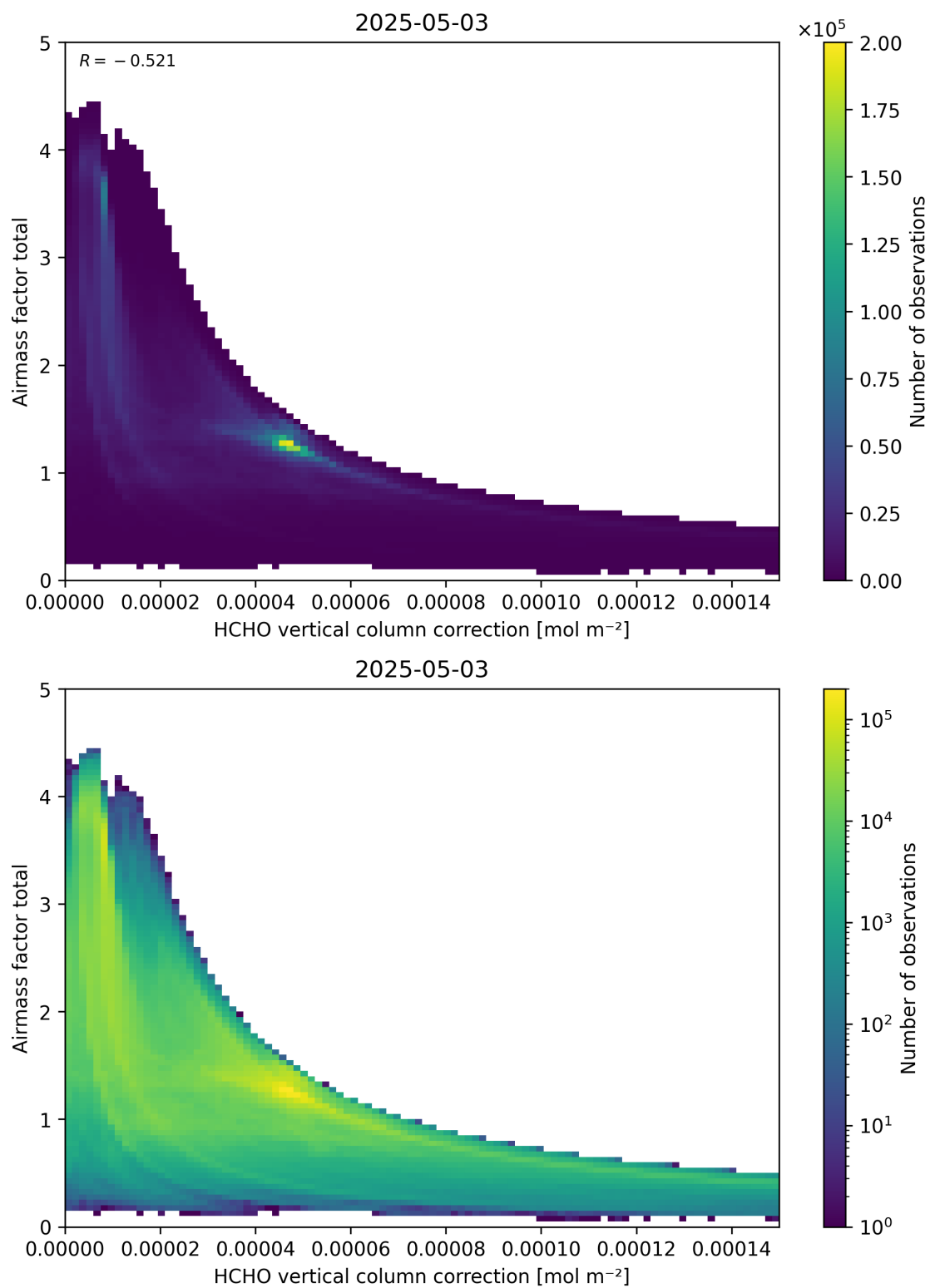
Figure 120: Scatter density plot of “HCHO vertical column correction” against “Airmass factor total” for 2025-05-02 to 2025-05-04.
