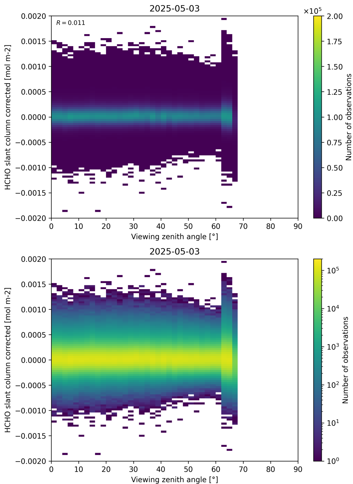
Figure 186: Scatter density plot of “Viewing zenith angle” against “HCHO slant column corrected” for 2025-05-02 to 2025-05-04.
