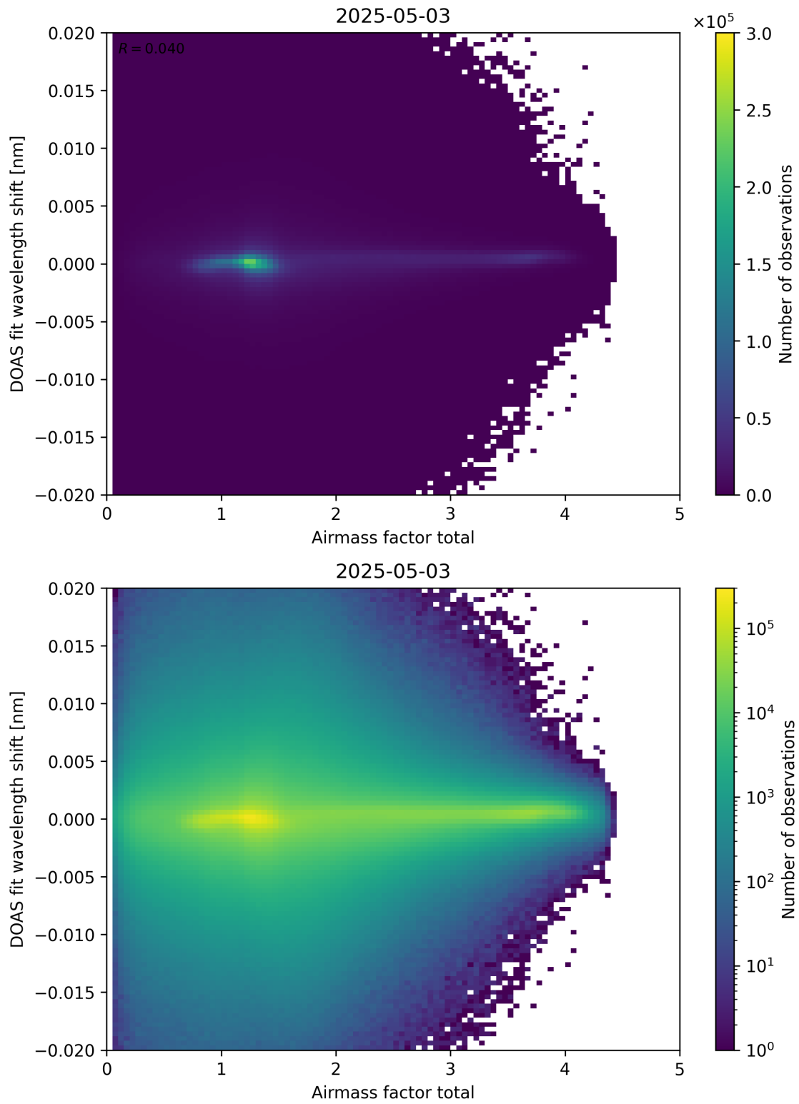
Figure 98: Scatter density plot of “Airmass factor total” against “DOAS fit wavelength shift” for 2025-05-02 to 2025-05-04.
