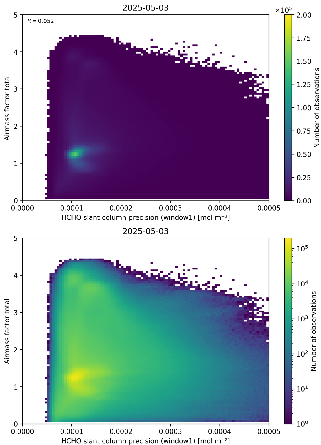
Figure 94: Scatter density plot of “HCHO slant column precision (window1)” against “Airmass factor total” for 2025-05-02 to 2025-05-04.
