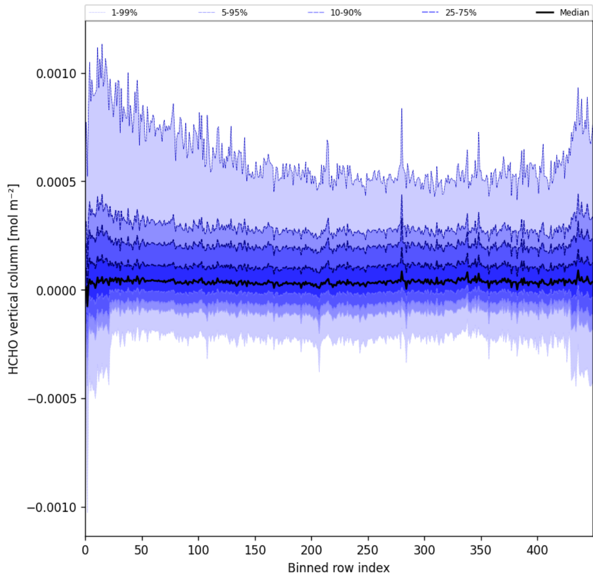
Figure 49: Along track statistics of “HCHO vertical column” for 2025-05-02 to 2025-05-04
