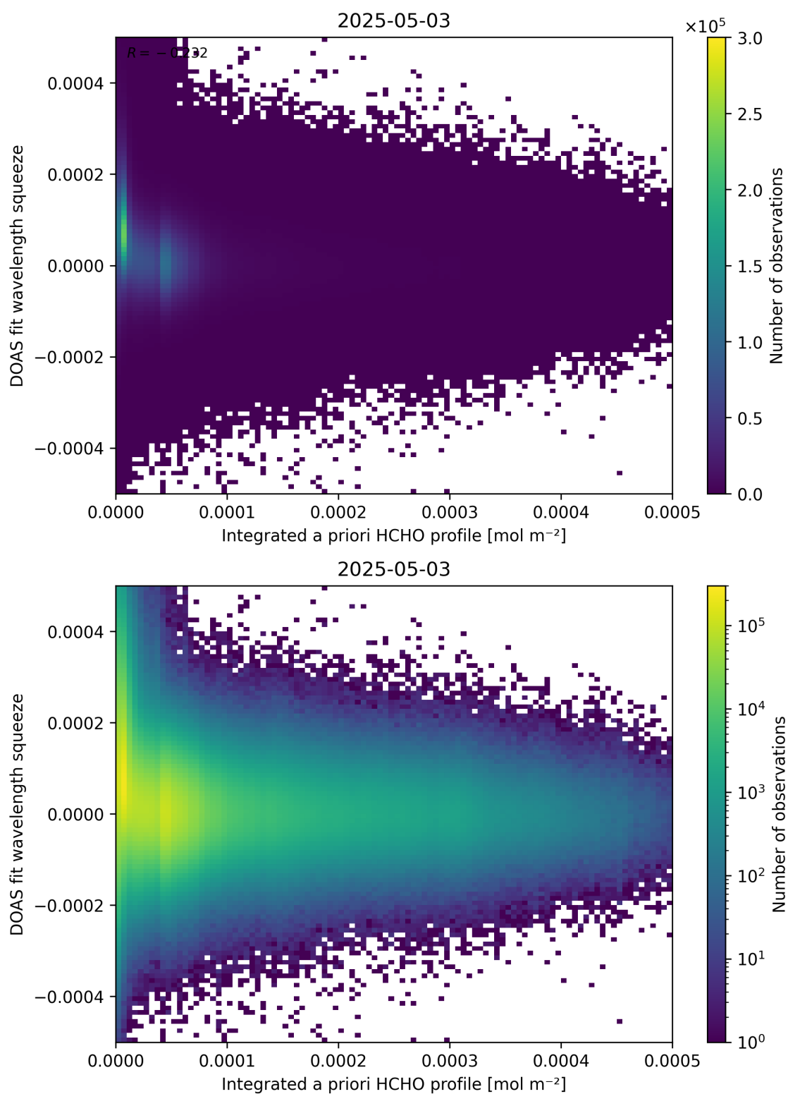
Figure 150: Scatter density plot of “Integrated a priori HCHO profile” against “DOAS fit wavelength squeeze” for 2025-05-02 to 2025-05-04.
