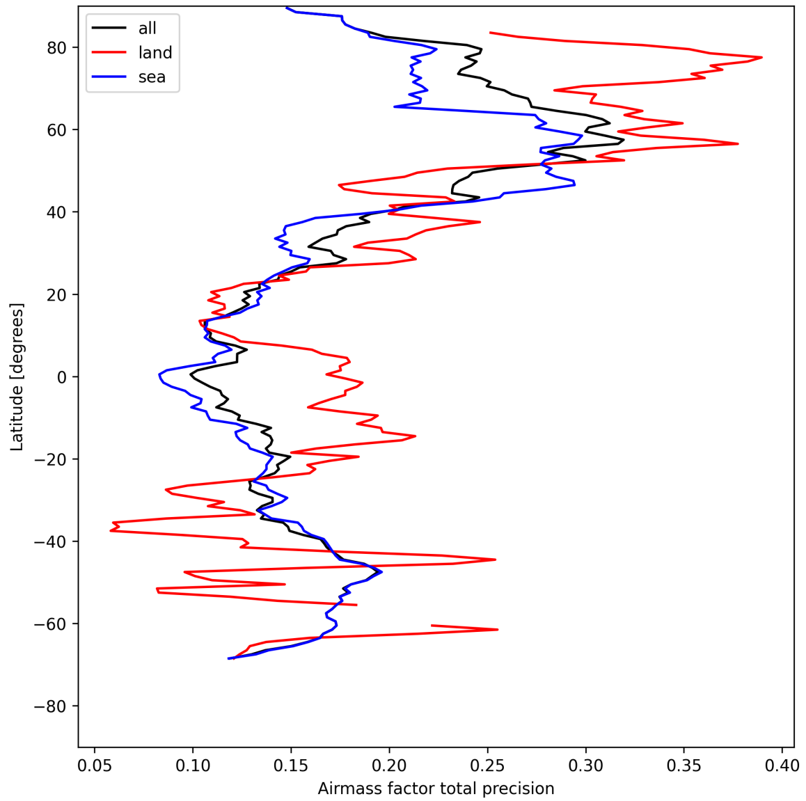
Figure 27: Zonal average of “Airmass factor total precision” for 2025-05-02 to 2025-05-04.
