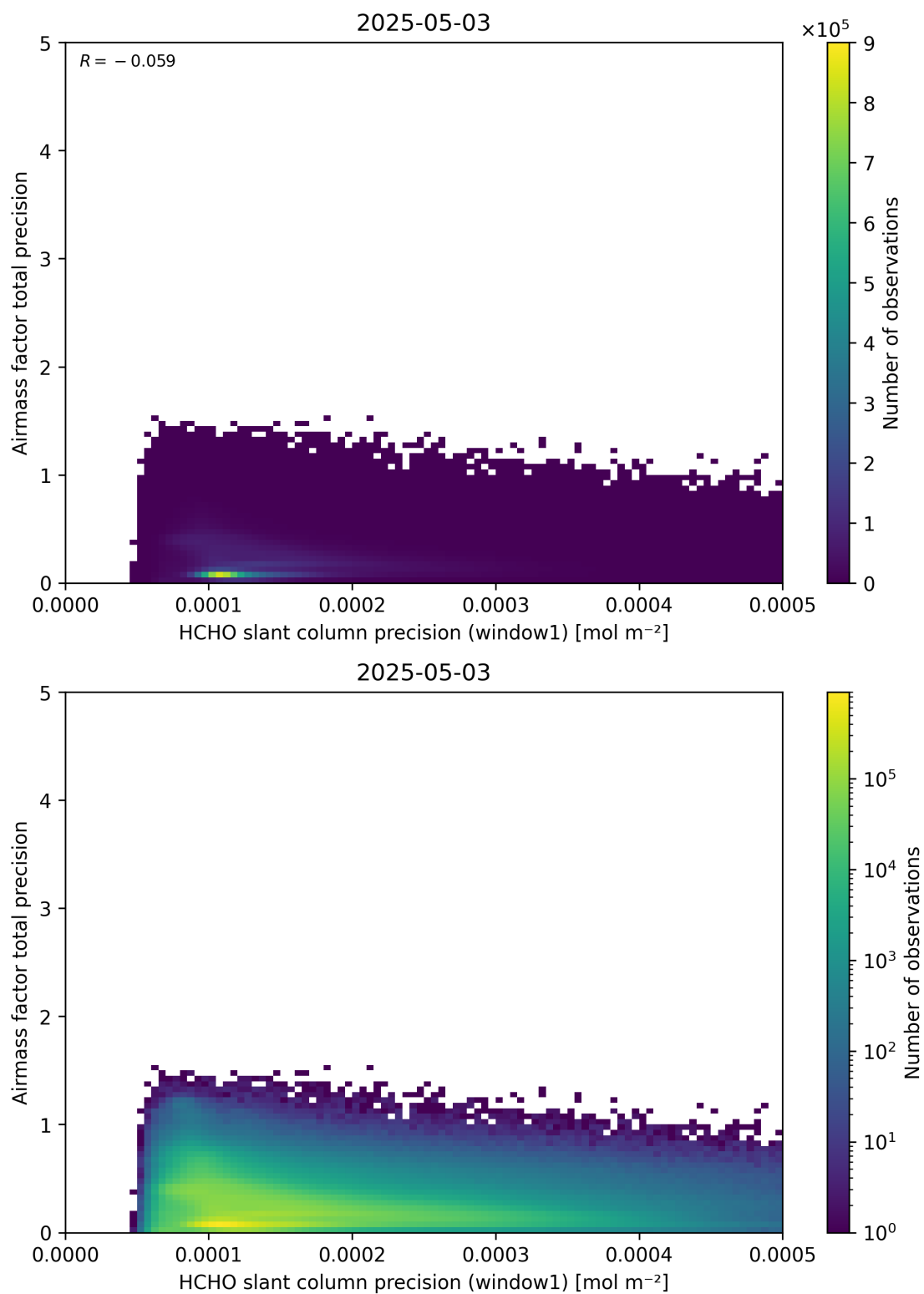
Figure 95: Scatter density plot of “HCHO slant column precision (window1)” against “Airmass factor total precision” for 2025-05-02 to 2025-05-04.
