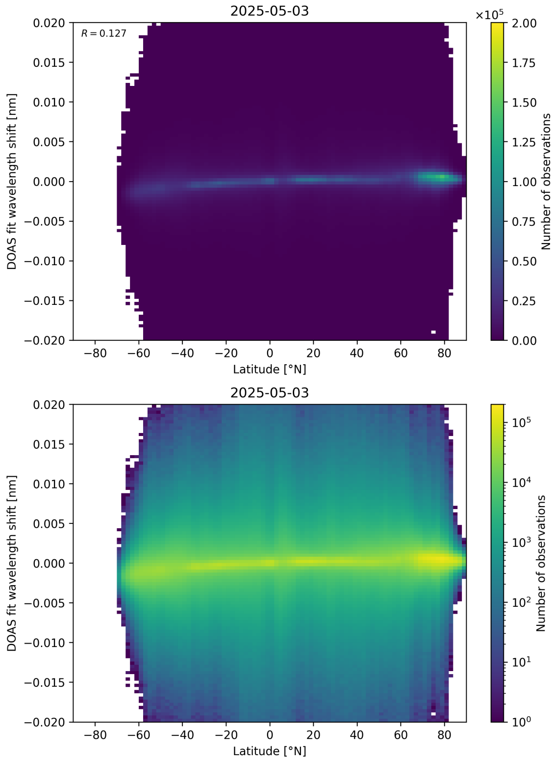
Figure 154: Scatter density plot of “Latitude” against “DOAS fit wavelength shift” for 2025-05-02 to 2025-05-04.
