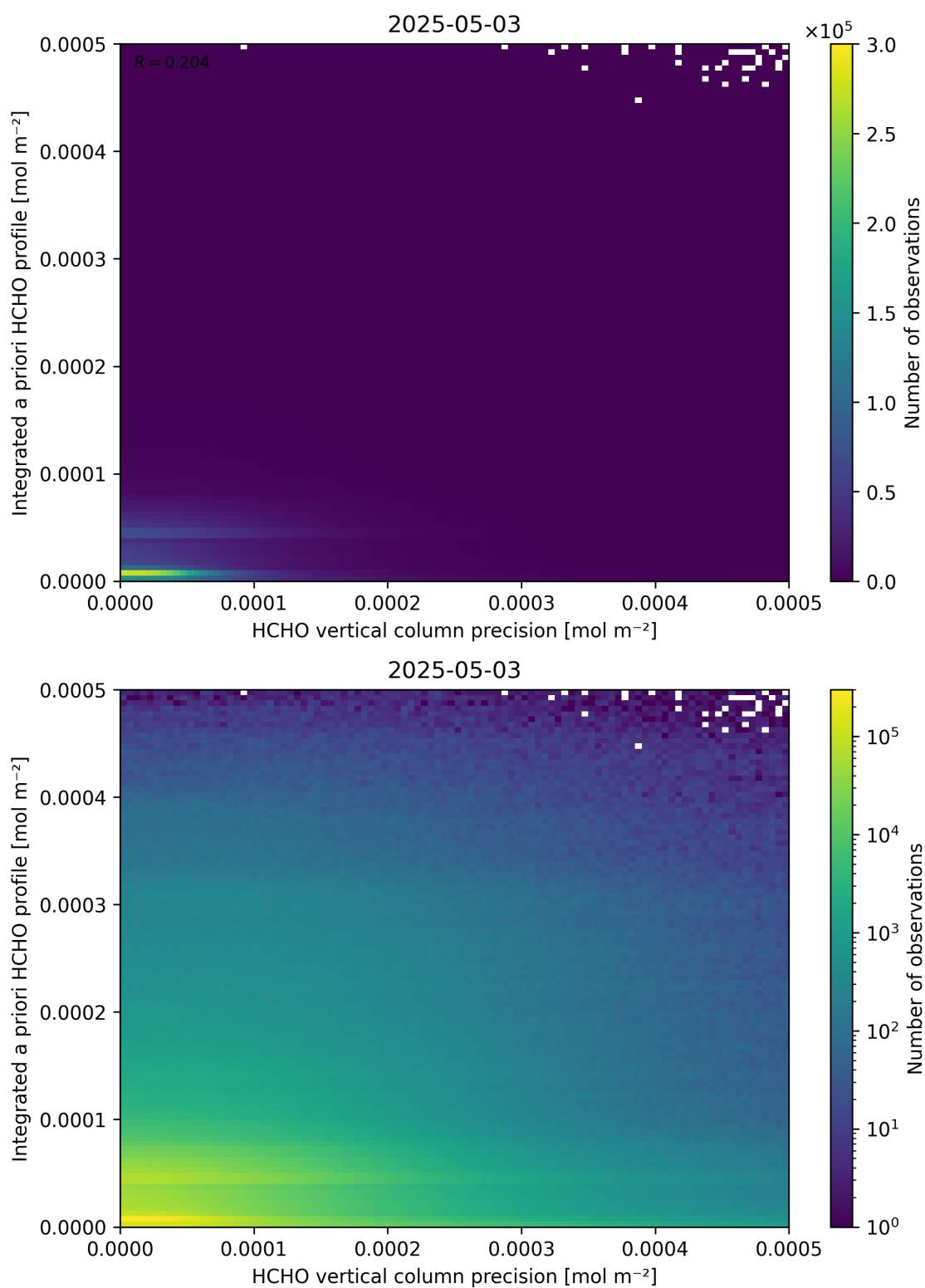
Figure 147: Scatter density plot of “HCHO vertical column precision” against “Integrated a priori HCHO profile” for 2025-05-02 to 2025-05-04.
