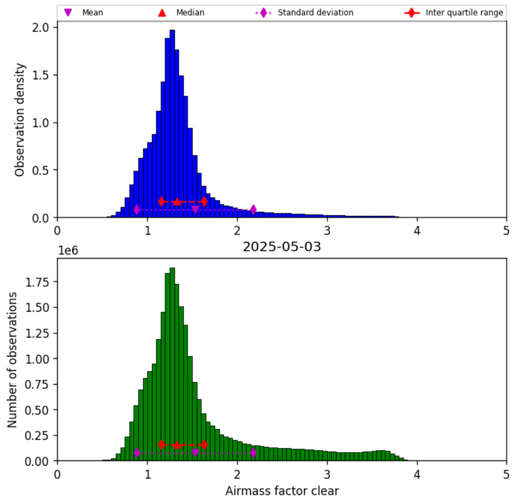
Figure 42: Histogram of “Airmass factor clear” for 2025-05-02 to 2025-05-04
