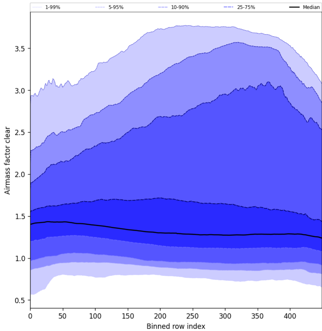
Figure 56: Along track statistics of “Airmass factor clear” for 2025-05-02 to 2025-05-04
