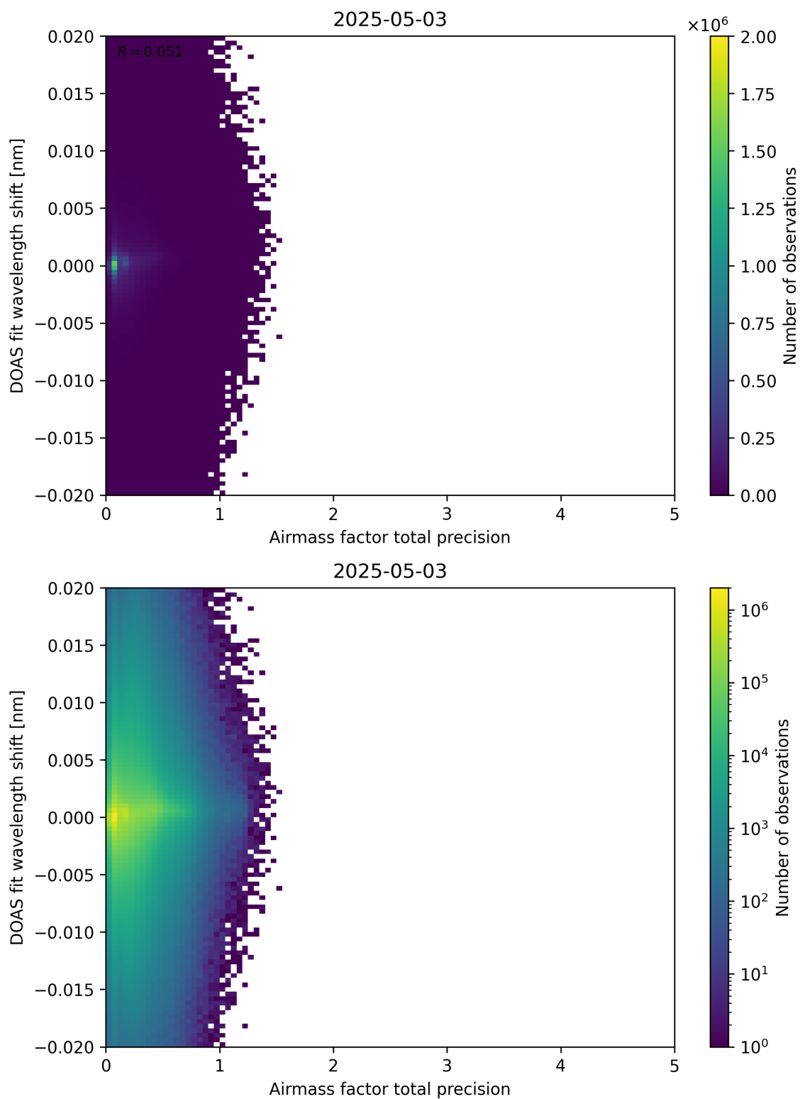
Figure 106: Scatter density plot of “Airmass factor total precision” against “DOAS fit wavelength shift” for 2025-05-02 to 2025-05-04.
