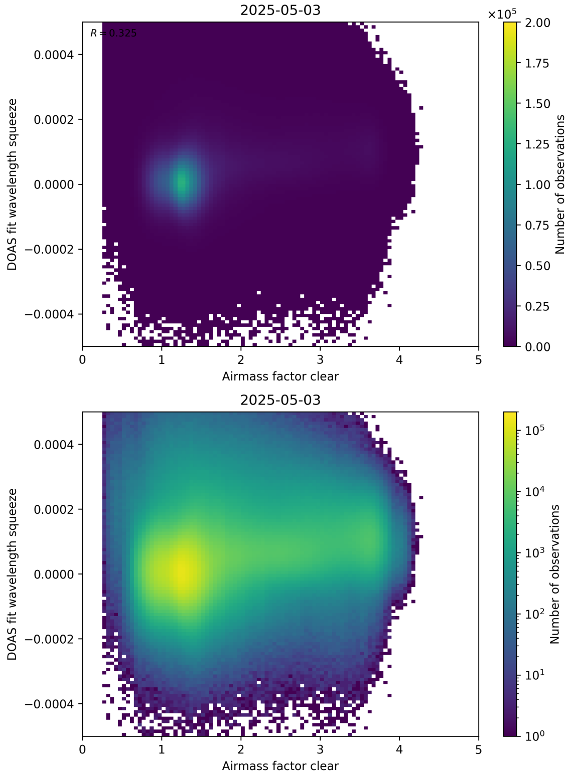
Figure 73: Scatter density plot of “Airmass factor clear” against “DOAS fit wavelength squeeze” for 2025-05-02 to 2025-05-04.
