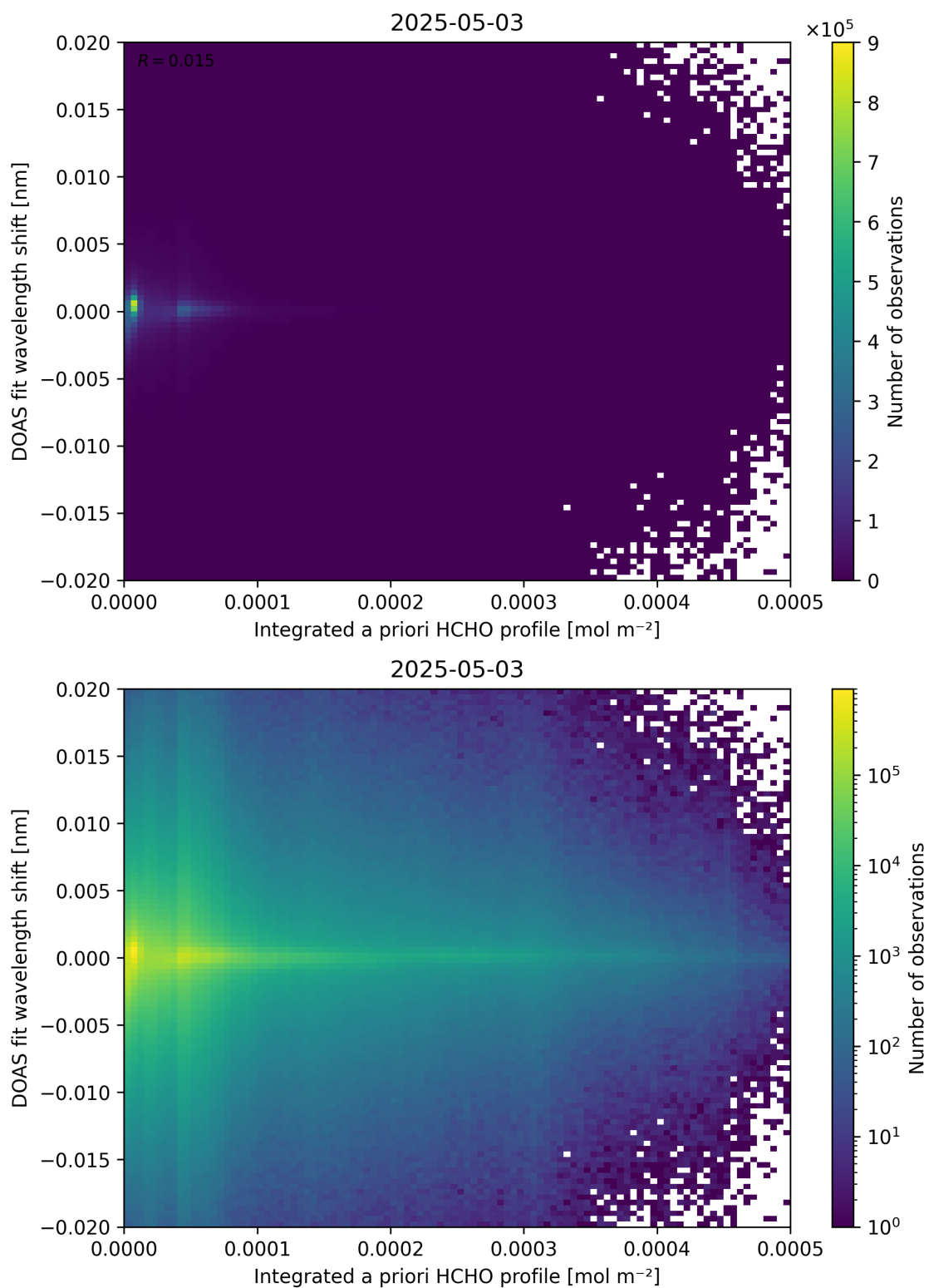
Figure 149: Scatter density plot of “Integrated a priori HCHO profile” against “DOAS fit wavelength shift” for 2025-05-02 to 2025-05-04.
