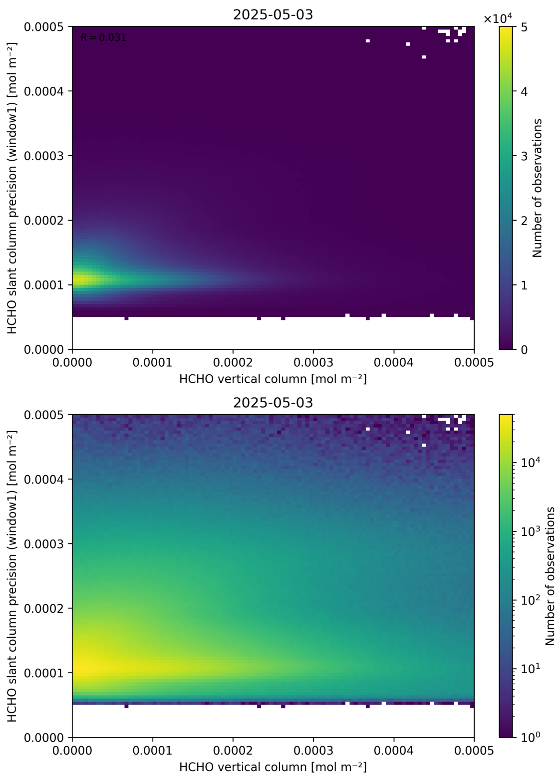
Figure 130: Scatter density plot of “HCHO vertical column” against “HCHO slant column precision (window1)” for 2025-05-02 to 2025-05-04.
