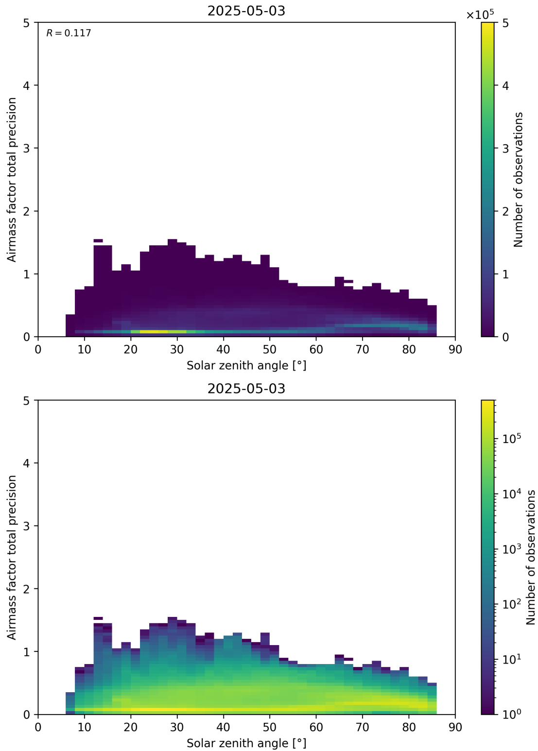
Figure 176: Scatter density plot of “Solar zenith angle” against “Airmass factor total precision” for 2025-05-02 to 2025-05-04.
