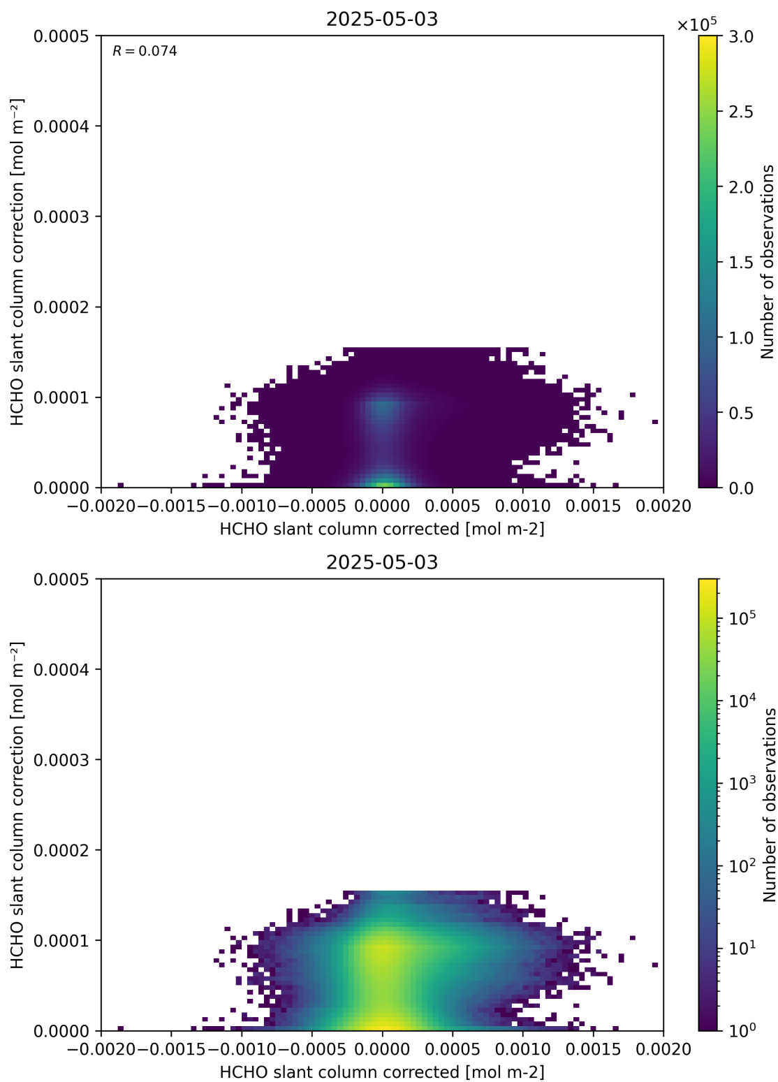
Figure 77: Scatter density plot of “HCHO slant column corrected” against “HCHO slant column correction” for 2025-05-02 to 2025-05-04.
