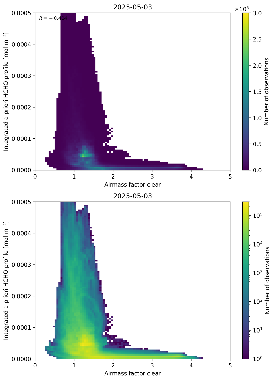
Figure 76: Scatter density plot of “Airmass factor clear” against “Integrated a priori HCHO profile” for 2025-05-02 to 2025-05-04.
