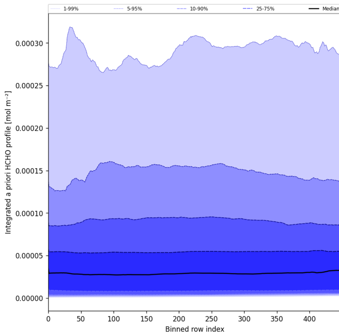
Figure 57: Along track statistics of "Integrated a priori HCHO profile" for 2025-05-02 to 2025-05-04
