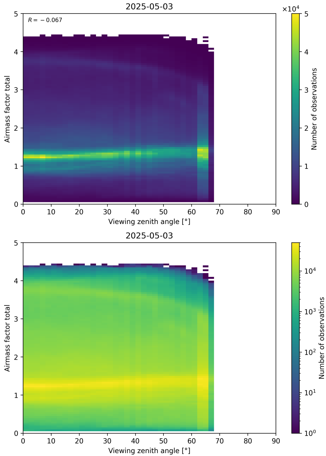
Figure 190: Scatter density plot of “Viewing zenith angle” against “Airmass factor total” for 2025-05-02 to 2025-05-04.
