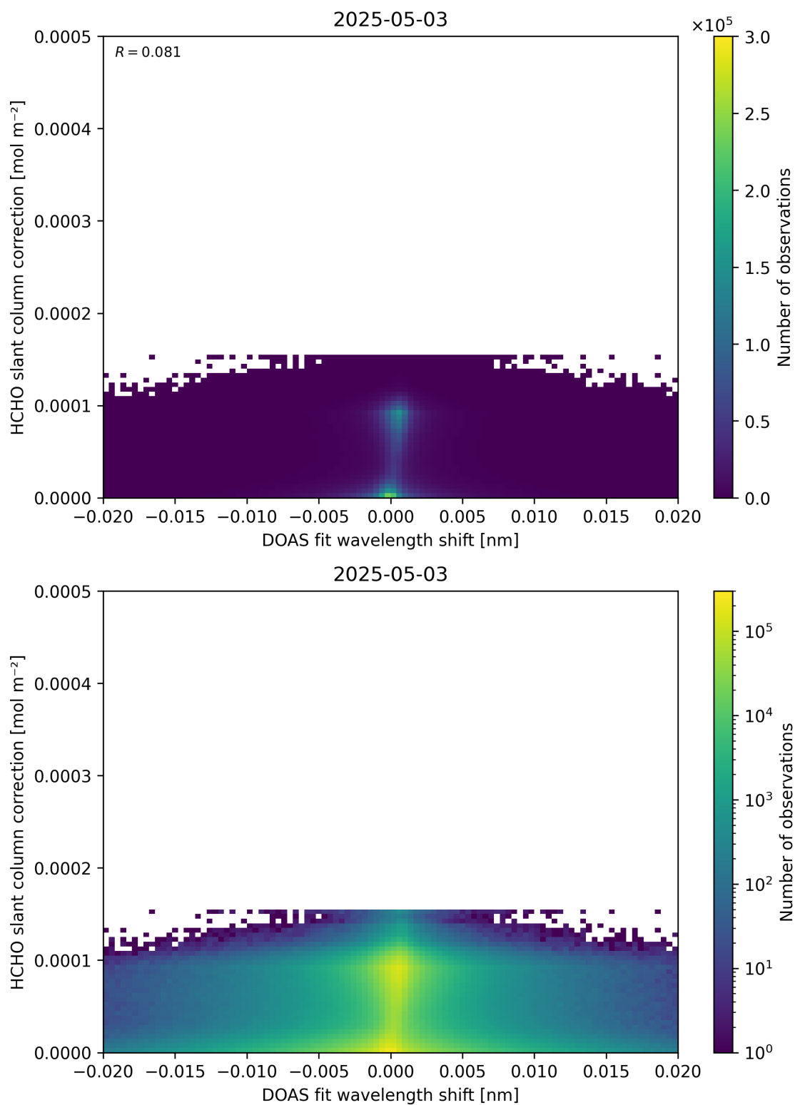
Figure 67: Scatter density plot of “DOAS fit wavelength shift” against “HCHO slant column correction” for 2025-05-02 to 2025-05-04.
