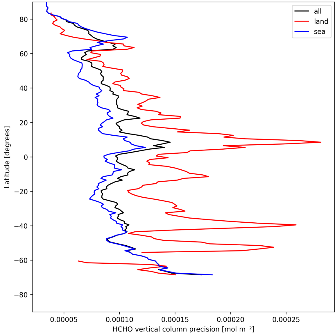
Figure 22: Zonal average of “HCHO vertical column precision” for 2025-05-02 to 2025-05-04.
