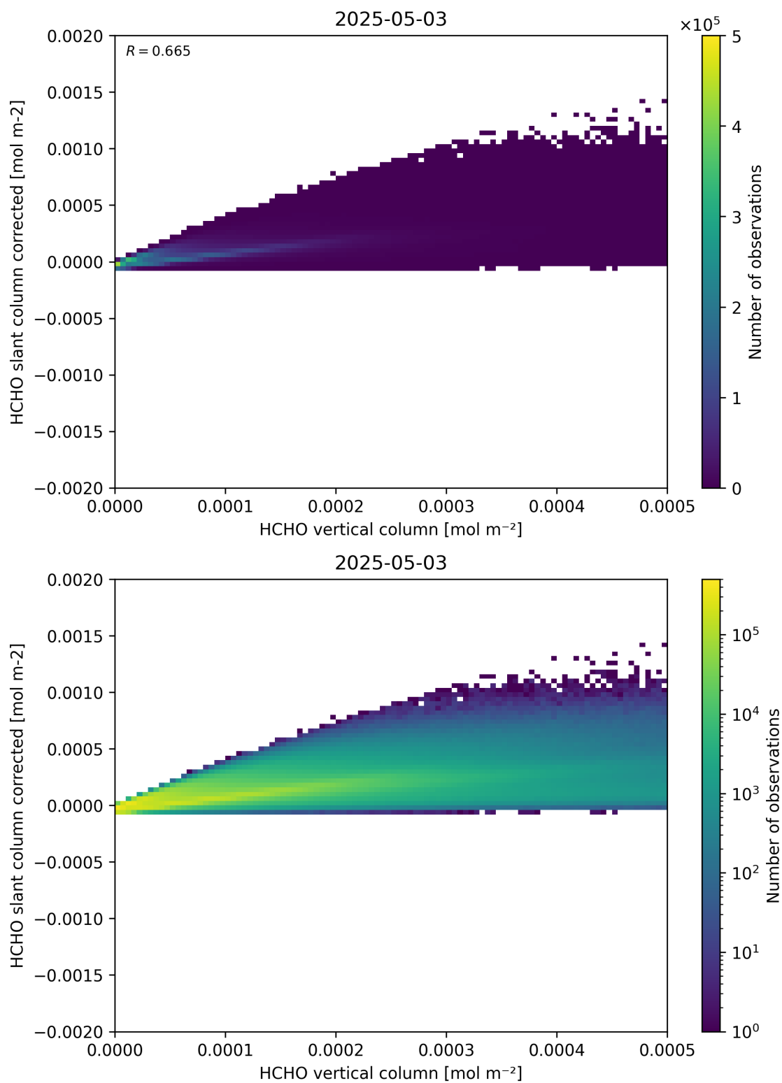
Figure 127: Scatter density plot of “HCHO vertical column” against “HCHO slant column corrected” for 2025-05-02 to 2025-05-04.
