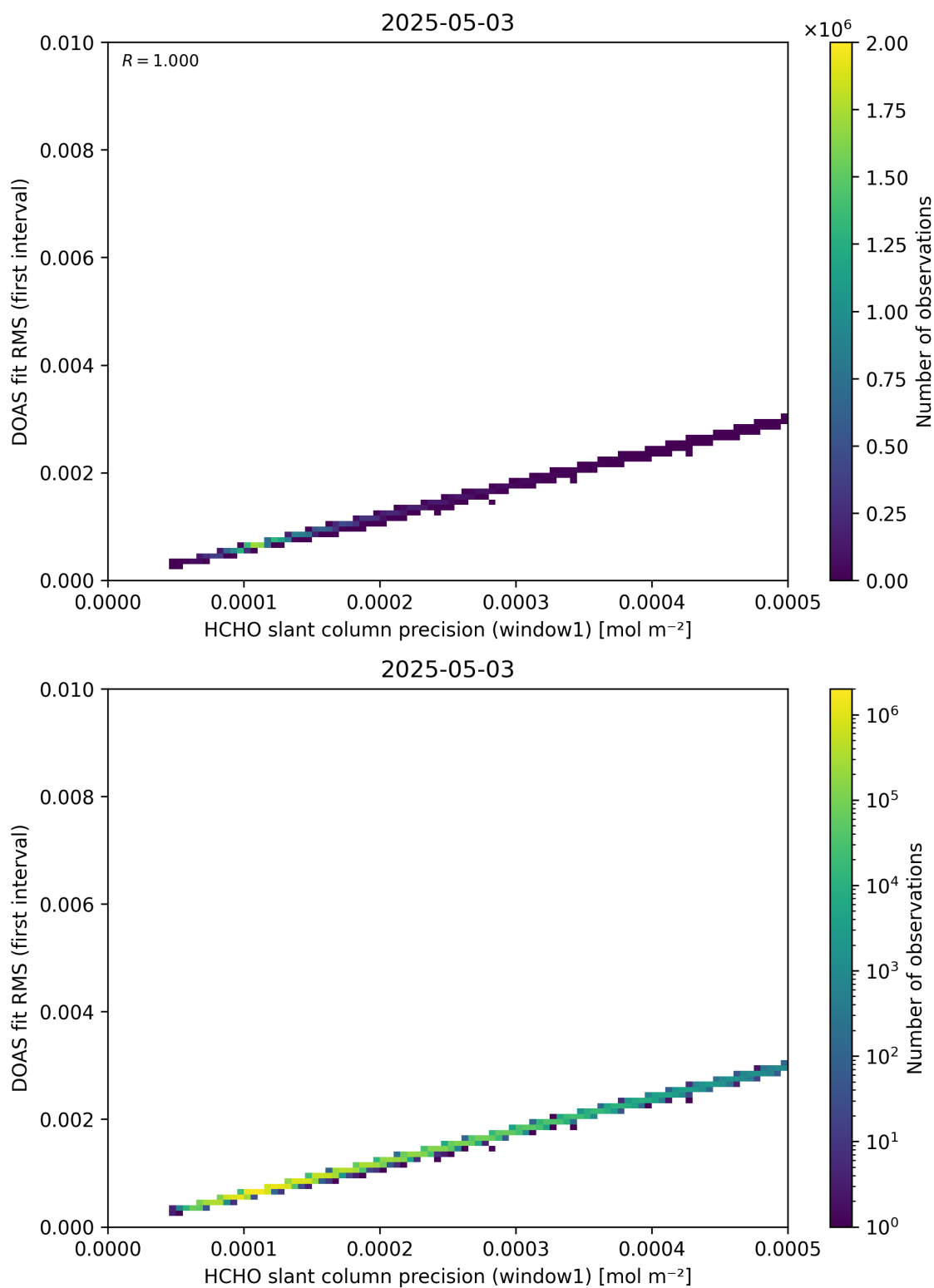
Figure 88: Scatter density plot of “HCHO slant column precision (window1)” against “DOAS fit RMS (first interval)” for 2025-05-02 to 2025-05-04.
