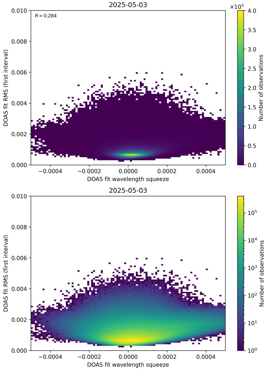
Figure 68: Scatter density plot of “DOAS fit wavelength squeeze” against “DOAS fit RMS (first interval)” for 2025-05-02 to 2025-05-04.
