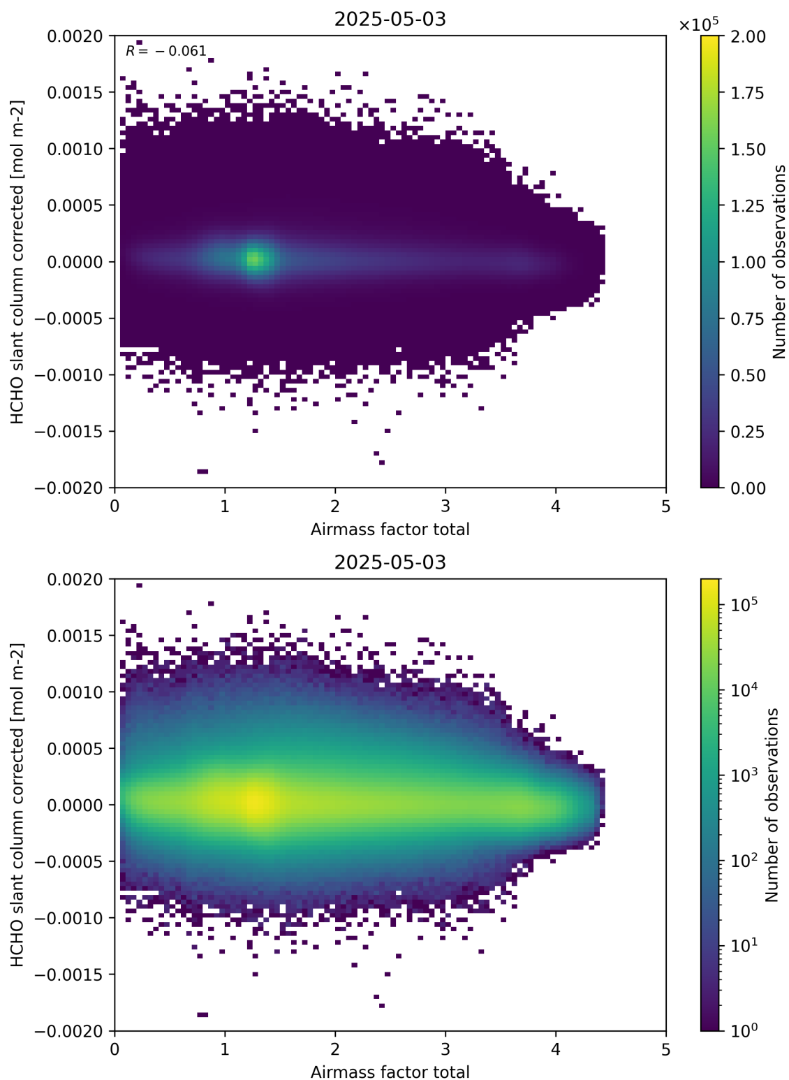
Figure 101: Scatter density plot of “Airmass factor total” against “HCHO slant column corrected” for 2025-05-02 to 2025-05-04.
