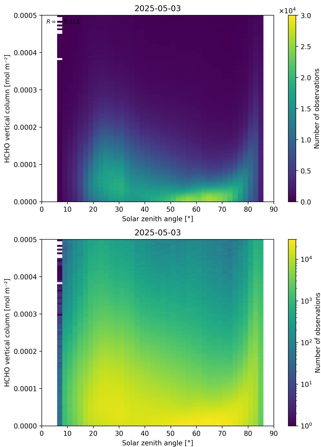
Figure 177: Scatter density plot of “Solar zenith angle” against “HCHO vertical column” for 2025-05-02 to 2025-05-04.
