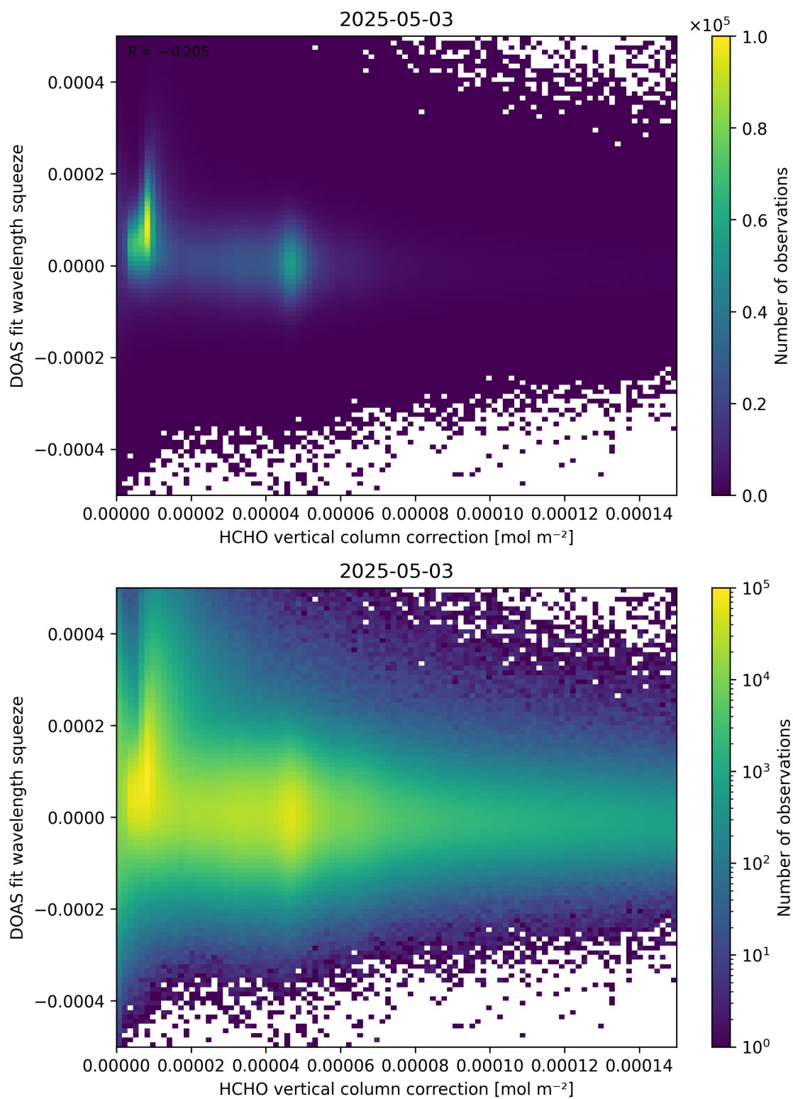
Figure 114: Scatter density plot of “HCHO vertical column correction” against “DOAS fit wavelength squeeze” for 2025-05-02 to 2025-05-04.
