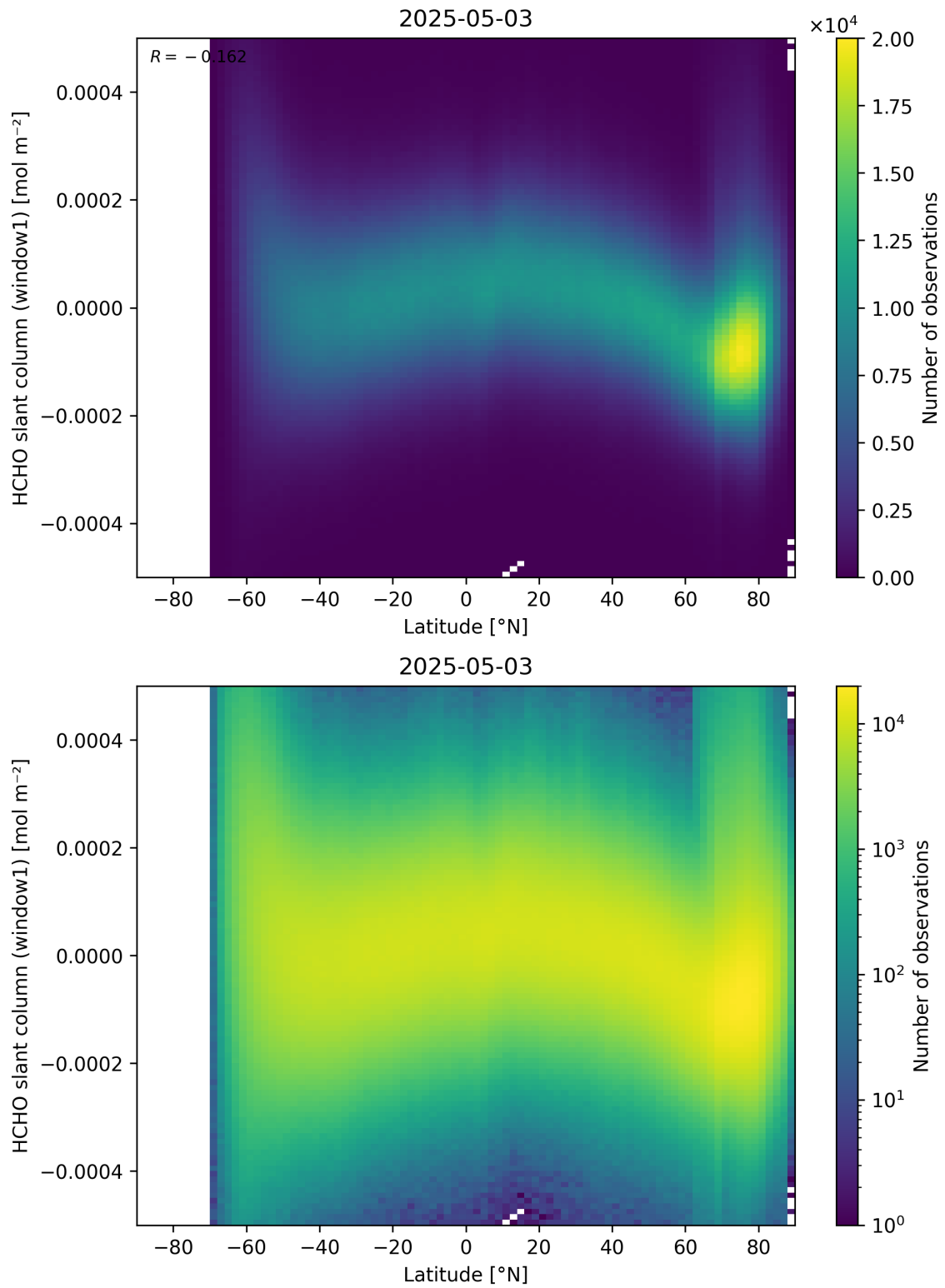
Figure 159: Scatter density plot of “Latitude” against “HCHO slant column (window1)” for 2025-05-02 to 2025-05-04.
