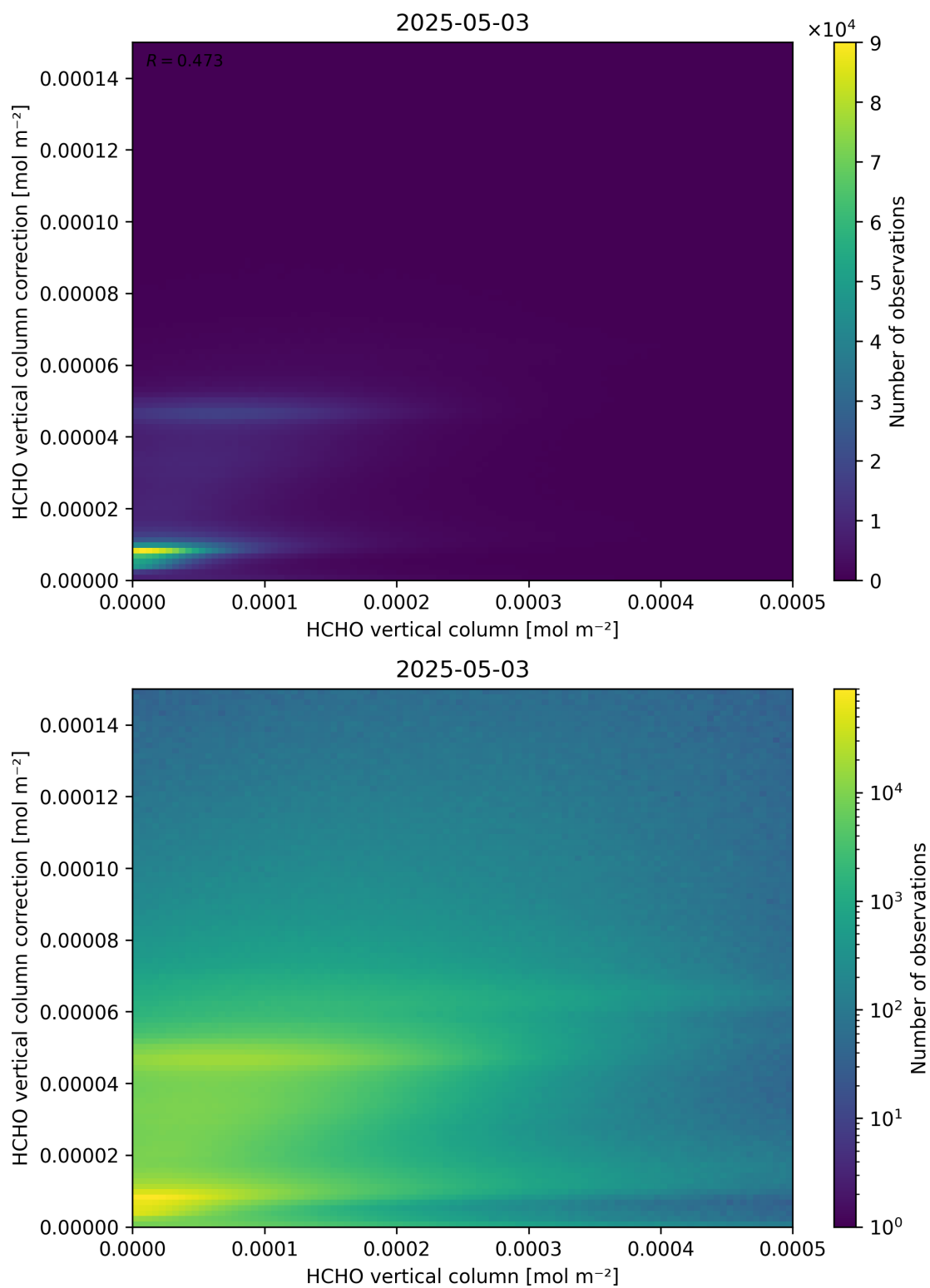
Figure 133: Scatter density plot of “HCHO vertical column” against “HCHO vertical column correction” for 2025-05-02 to 2025-05-04.
