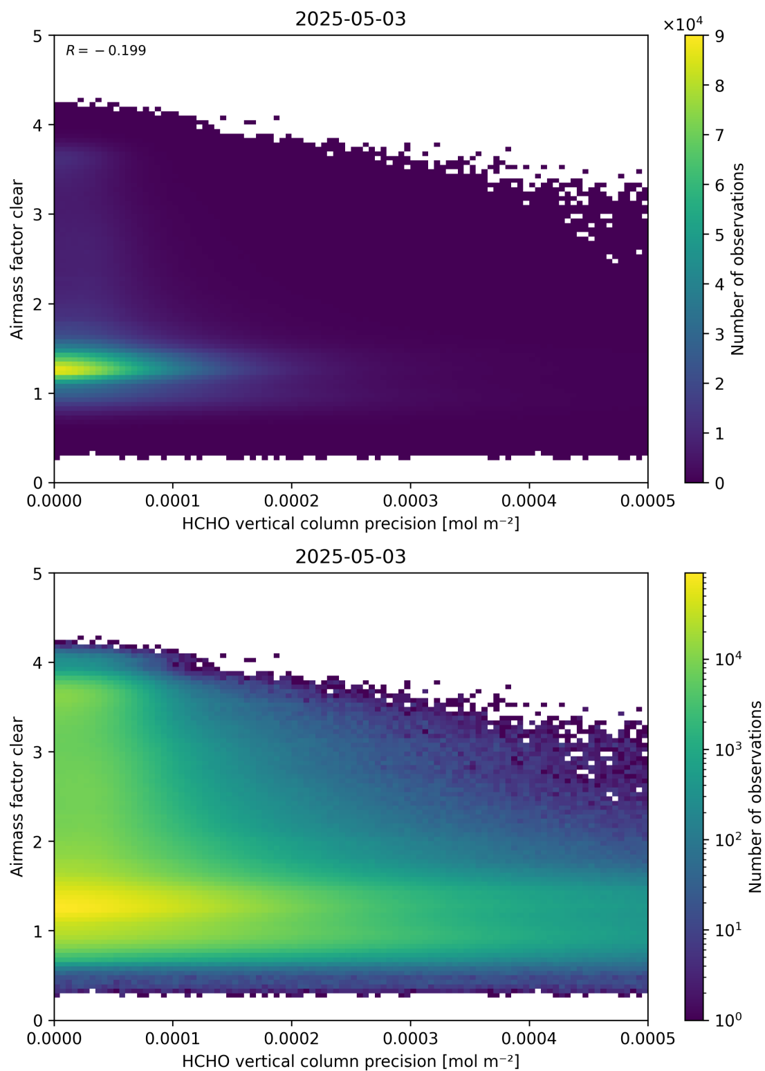
Figure 139: Scatter density plot of “HCHO vertical column precision” against “Airmass factor clear” for 2025-05-02 to 2025-05-04.
