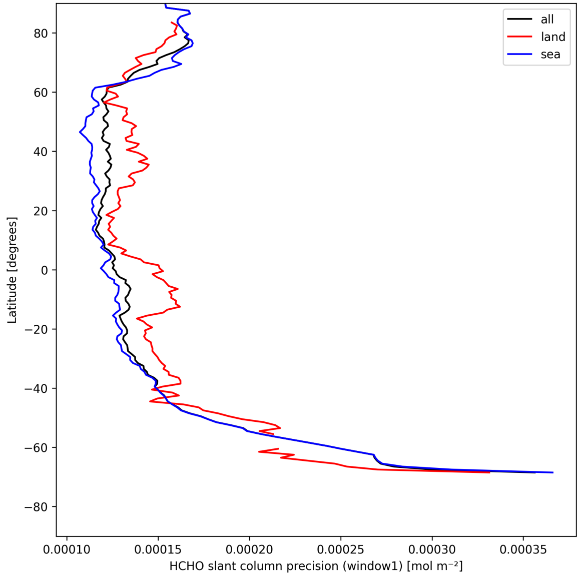
Figure 25: Zonal average of “HCHO slant column precision (window1)” for 2025-05-02 to 2025-05-04.
