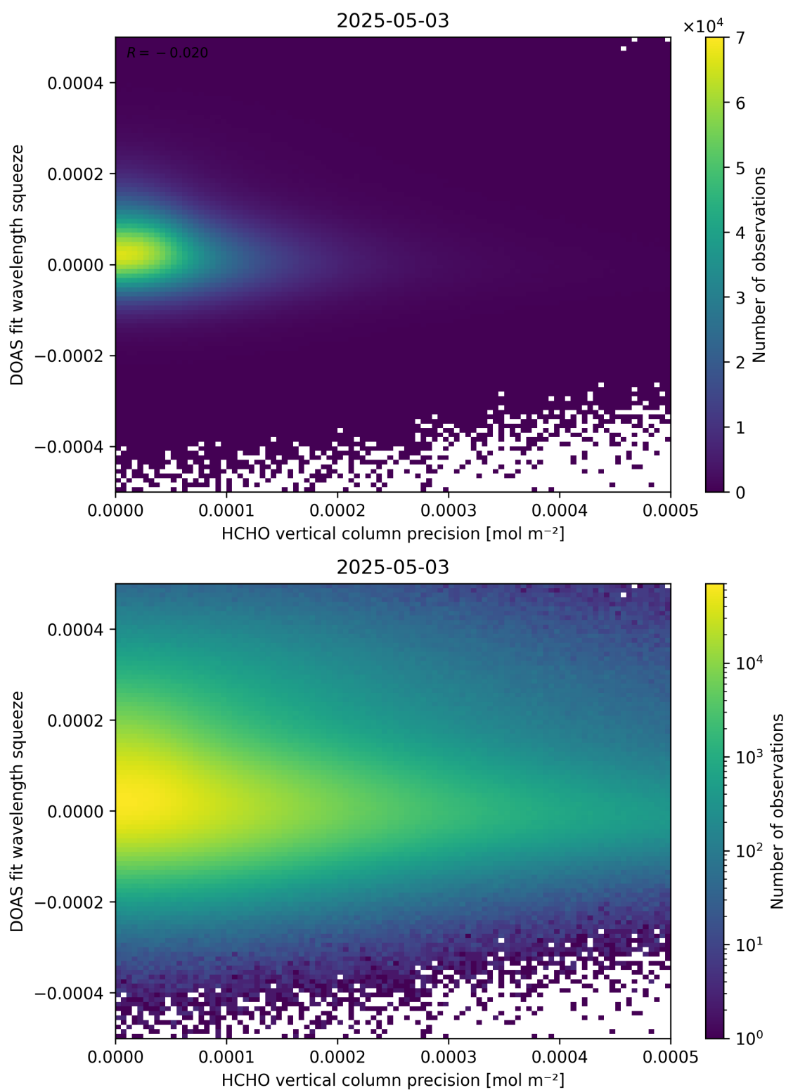
Figure 138: Scatter density plot of “HCHO vertical column precision” against “DOAS fit wavelength squeeze” for 2025-05-02 to 2025-05-04.
