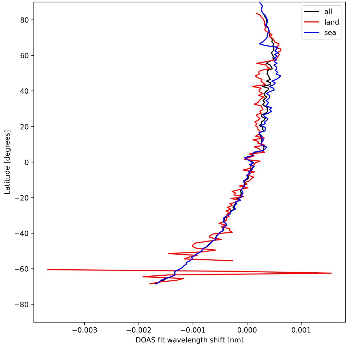
Figure 30: Zonal average of “DOAS fit wavelength shift” for 2025-05-02 to 2025-05-04.
