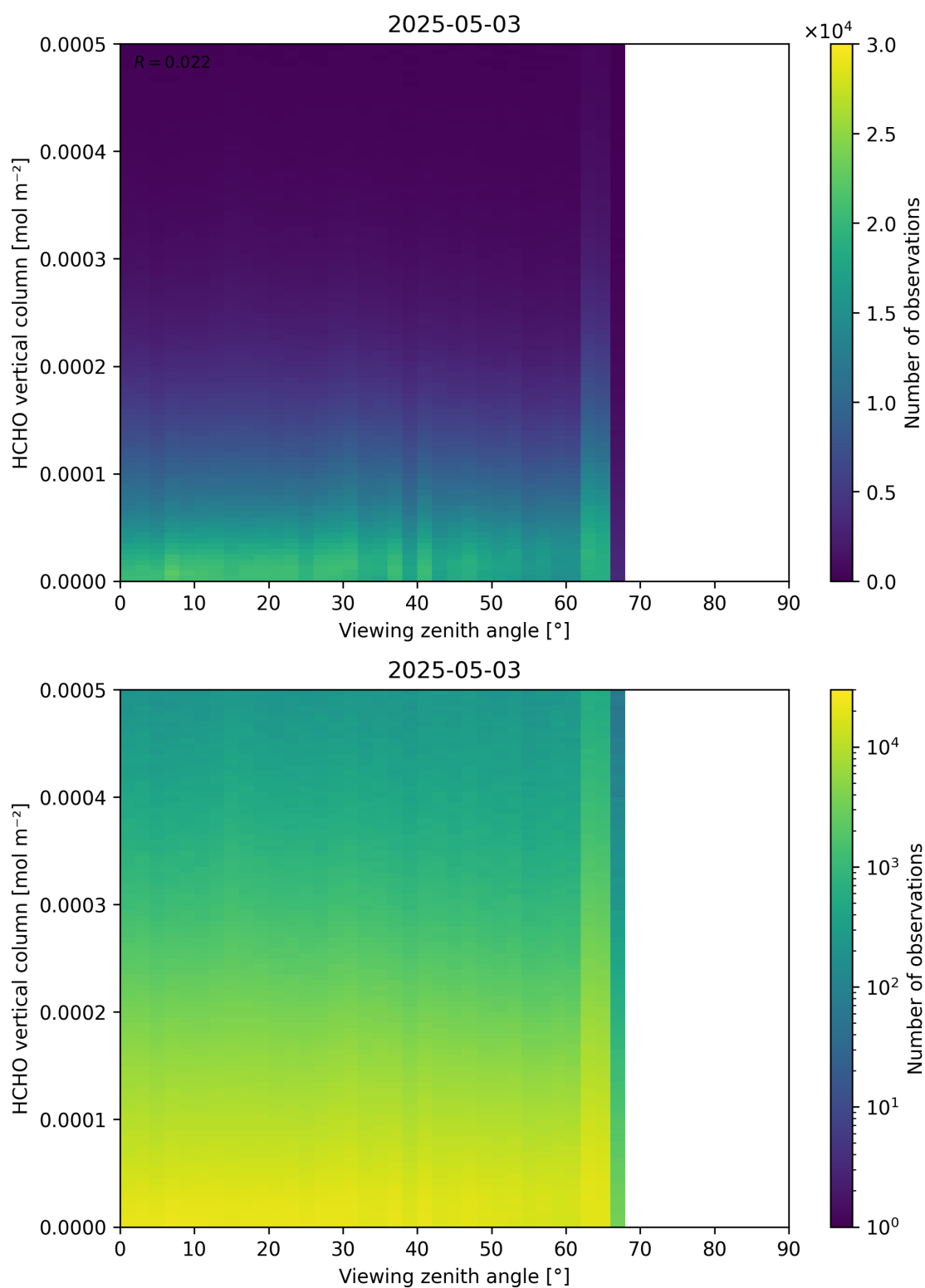
Figure 192: Scatter density plot of “Viewing zenith angle” against “HCHO vertical column” for 2025-05-02 to 2025-05-04.
