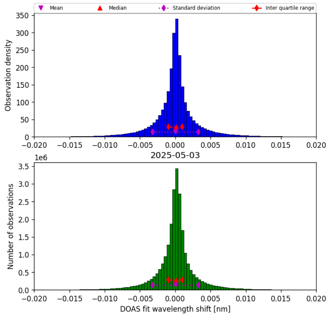
Figure 44: Histogram of “DOAS fit wavelength shift” for 2025-05-02 to 2025-05-04
