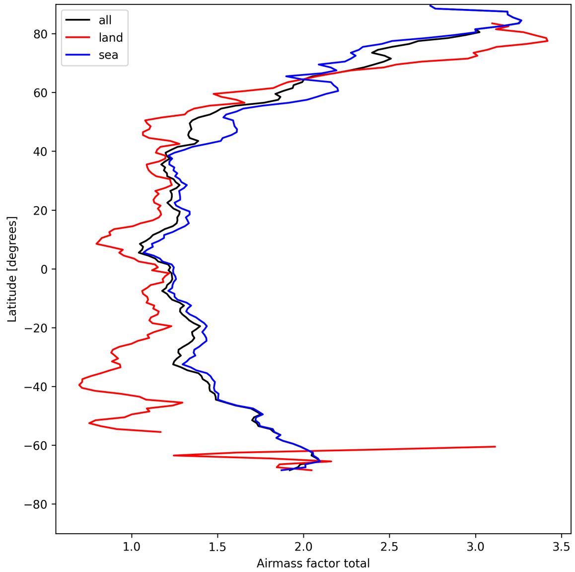
Figure 26: Zonal average of “Airmass factor total” for 2025-05-02 to 2025-05-04.
