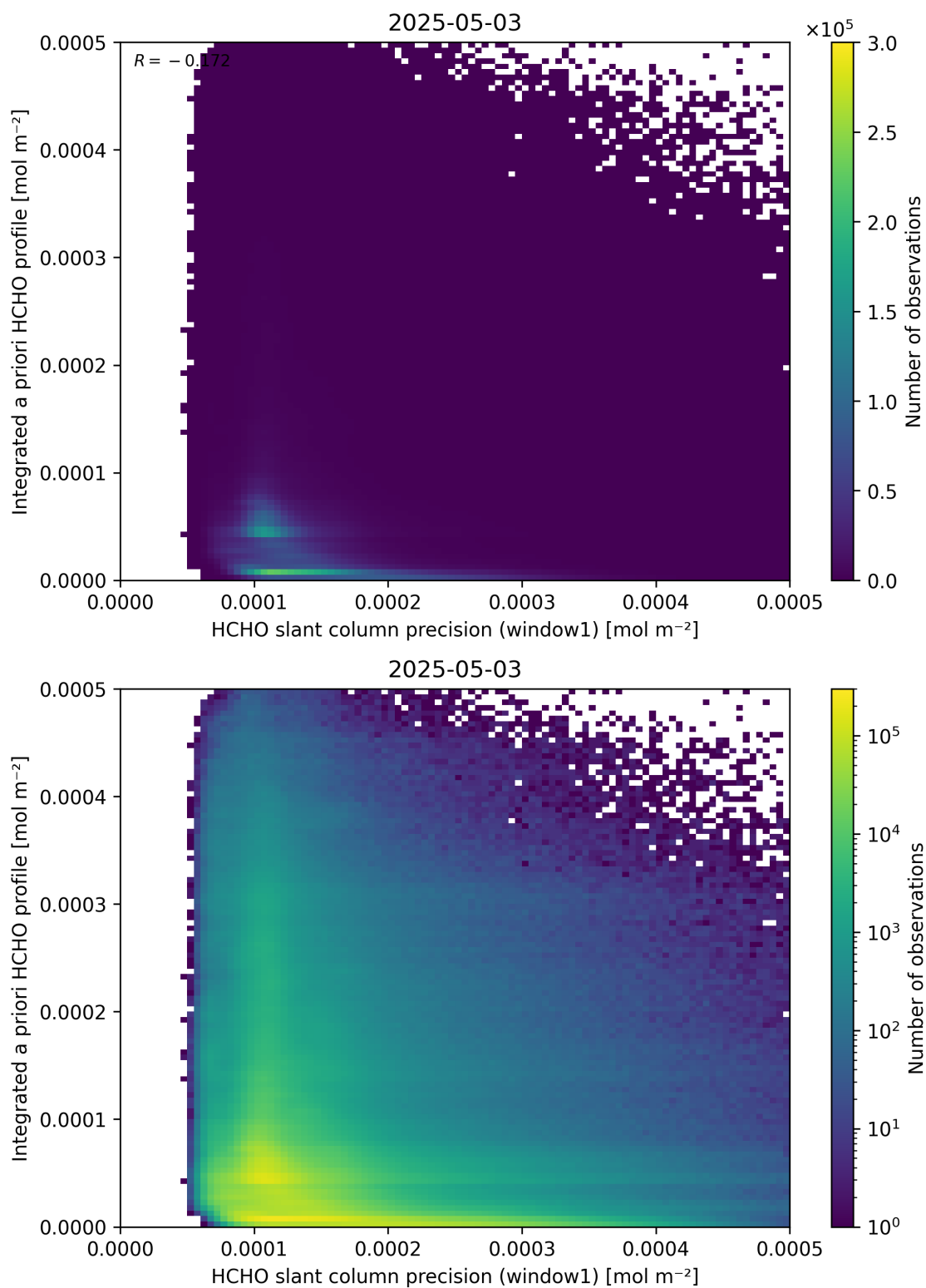
Figure 96: Scatter density plot of “HCHO slant column precision (window1)” against “Integrated a priori HCHO profile” for 2025-05-02 to 2025-05-04.
