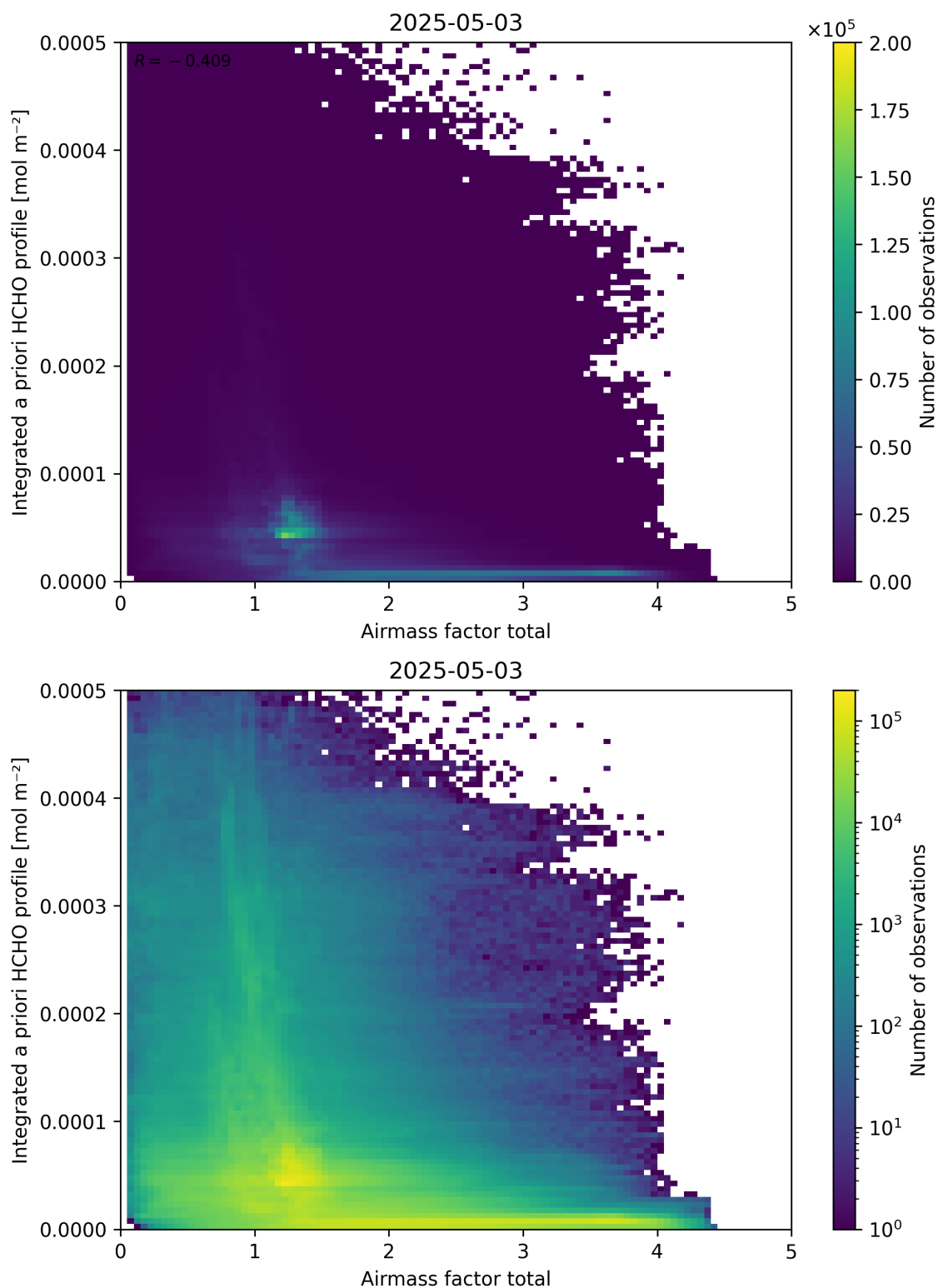
Figure 104: Scatter density plot of “Airmass factor total” against “Integrated a priori HCHO profile” for 2025-05-02 to 2025-05-04.
