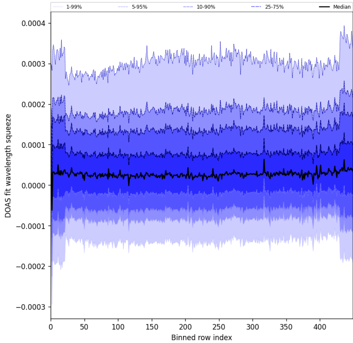
Figure 59: Along track statistics of “DOAS fit wavelength squeeze” for 2025-05-02 to 2025-05-04
