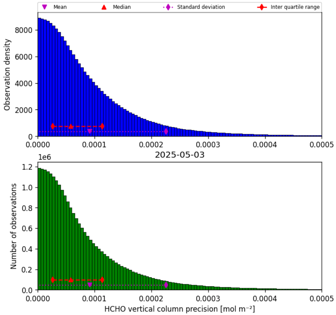
Figure 36: Histogram of “HCHO vertical column precision” for 2025-05-02 to 2025-05-04
