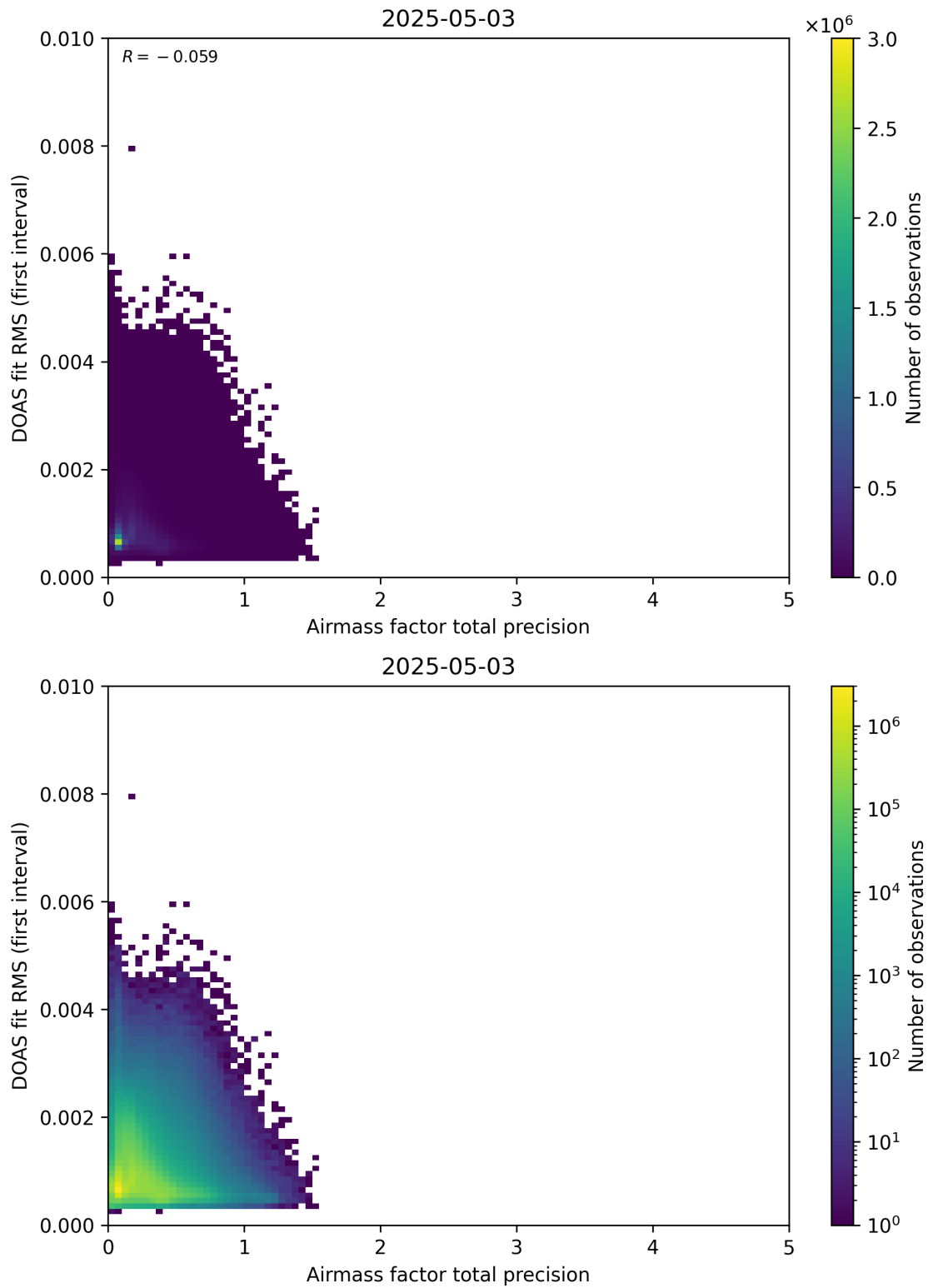
Figure 105: Scatter density plot of “Airmass factor total precision” against “DOAS fit RMS (first interval)” for 2025-05-02 to 2025-05-04.
