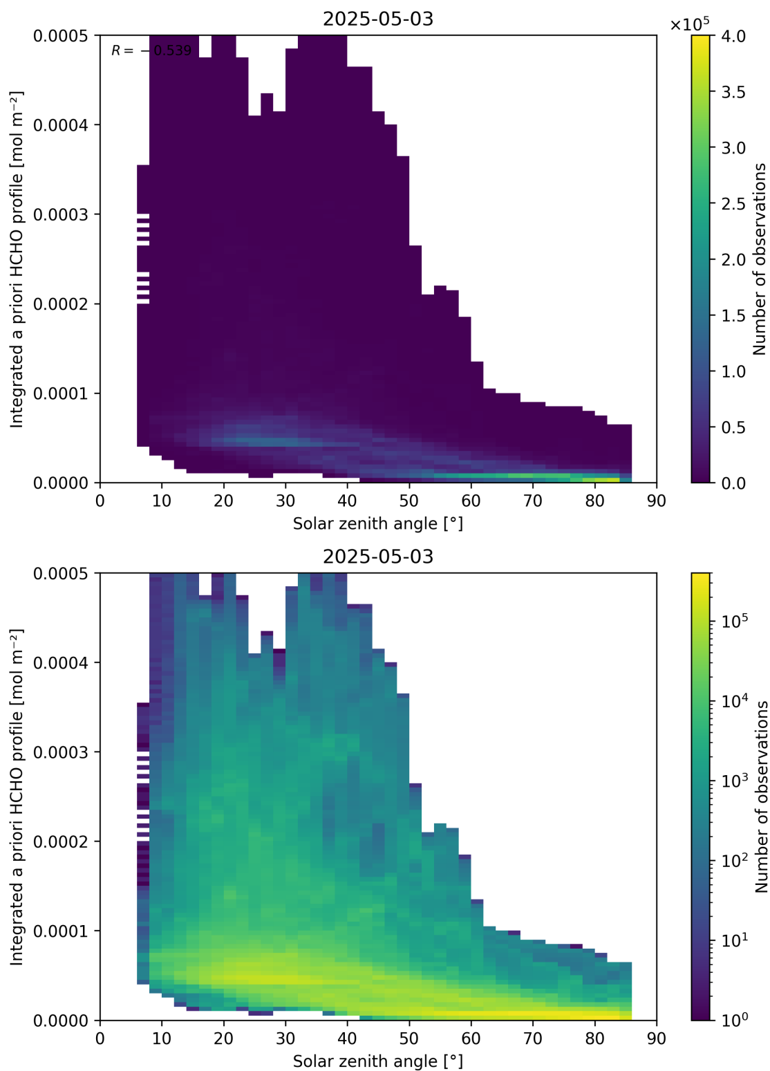
Figure 180: Scatter density plot of “Solar zenith angle” against “Integrated a priori HCHO profile” for 2025-05-02 to 2025-05-04.
