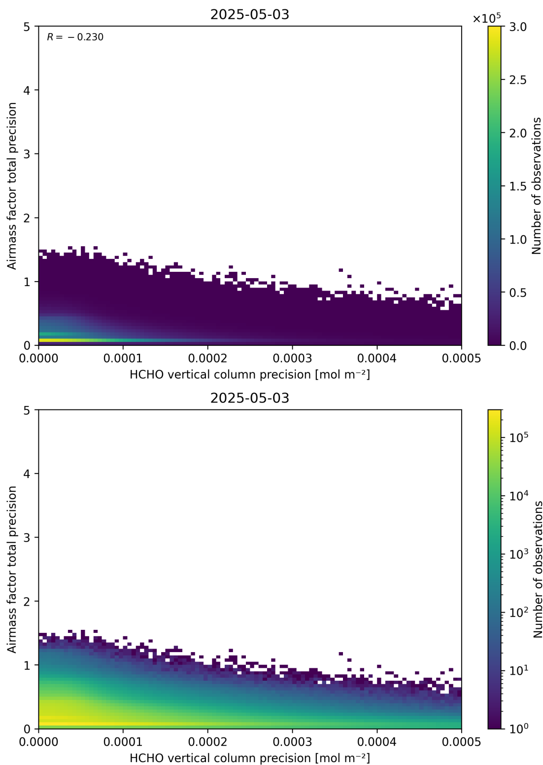
Figure 145: Scatter density plot of “HCHO vertical column precision” against “Airmass factor total precision” for 2025-05-02 to 2025-05-04.
