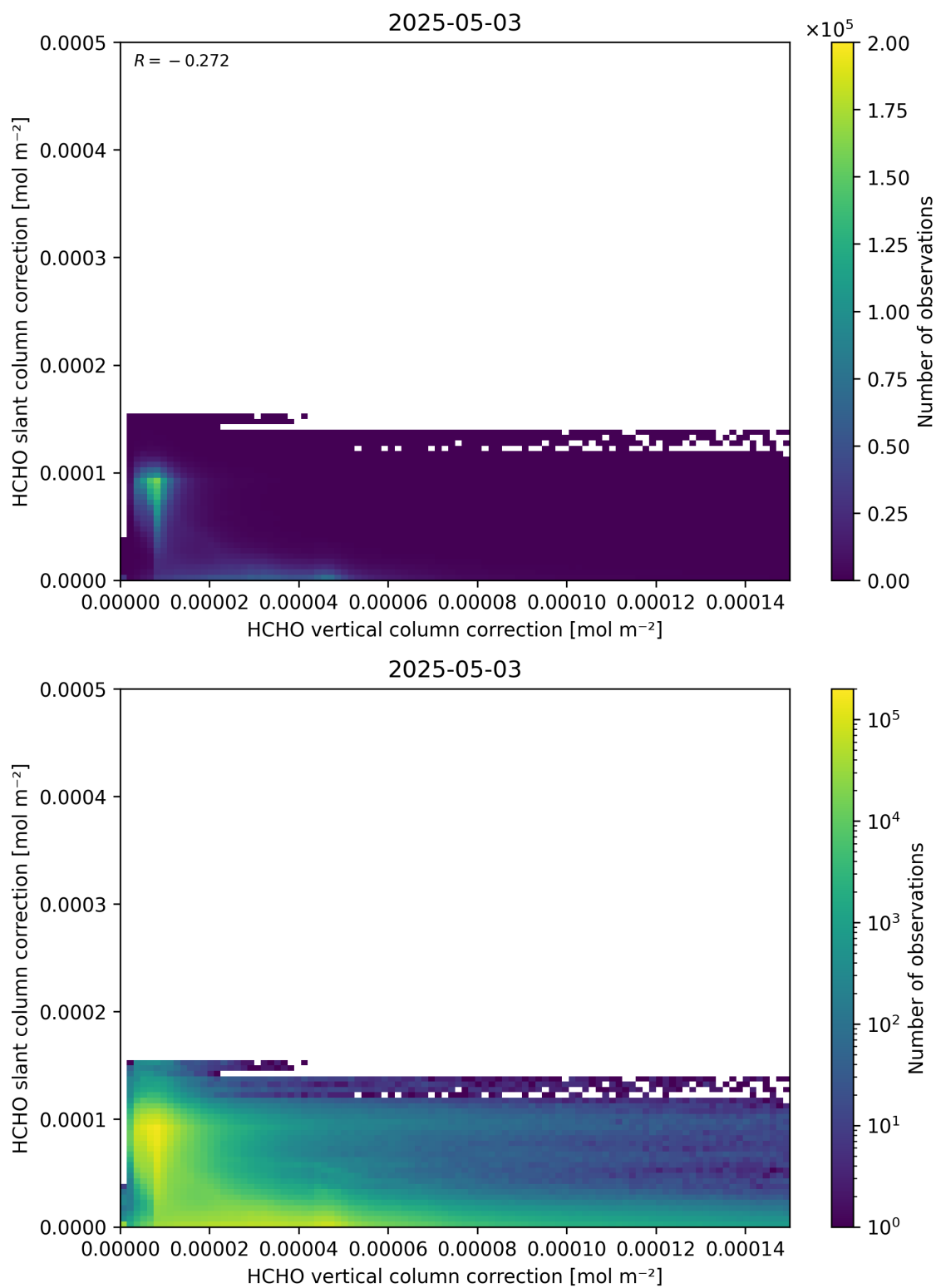
Figure 117: Scatter density plot of “HCHO vertical column correction” against “HCHO slant column correction” for 2025-05-02 to 2025-05-04.
