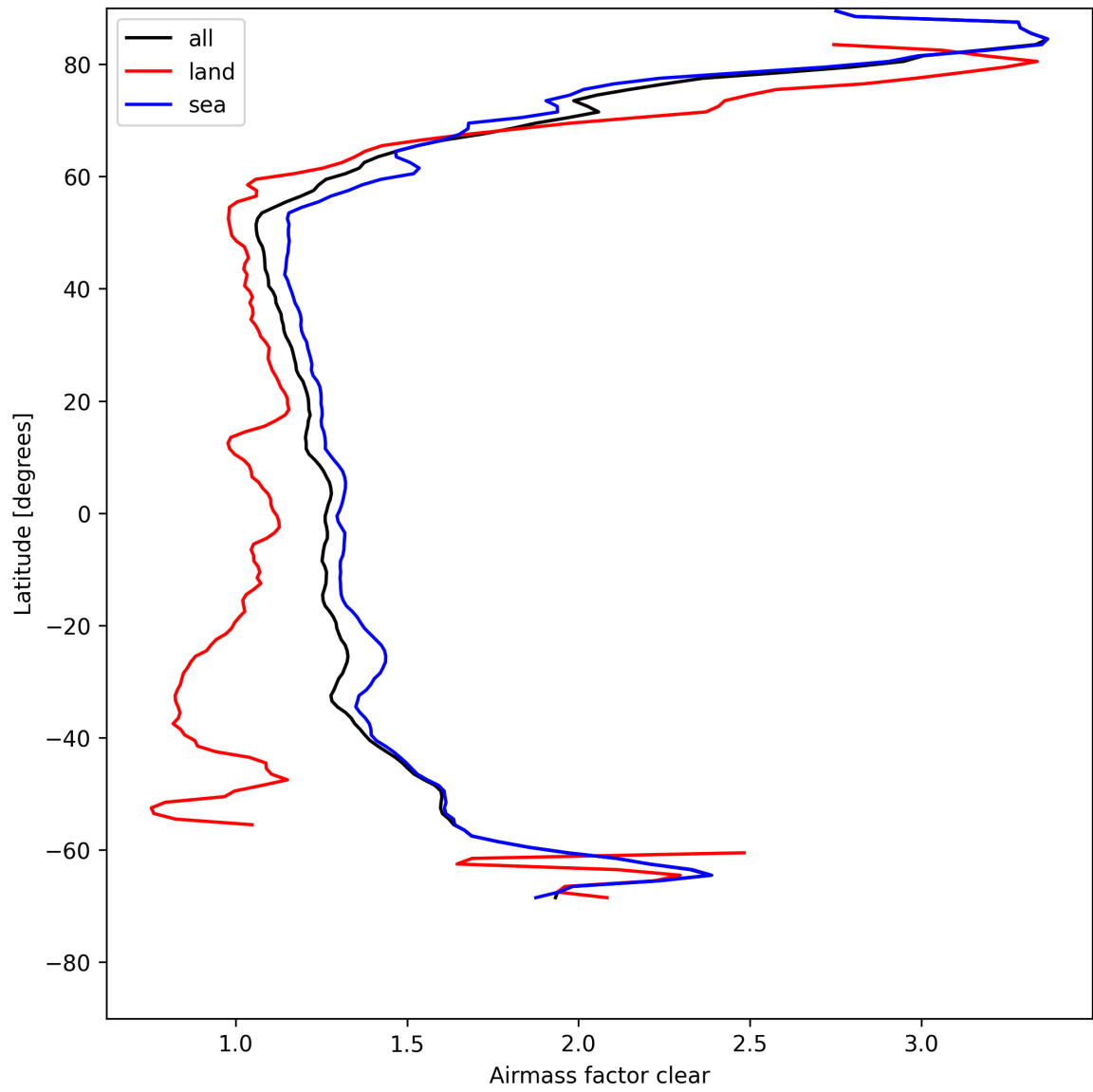
Figure 28: Zonal average of “Airmass factor clear” for 2025-05-02 to 2025-05-04.
