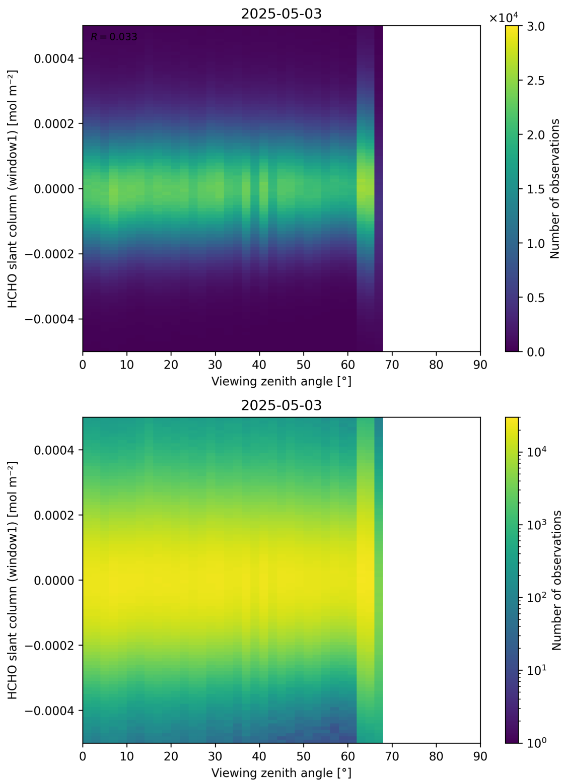
Figure 188: Scatter density plot of “Viewing zenith angle” against “HCHO slant column (window1)” for 2025-05-02 to 2025-05-04.
