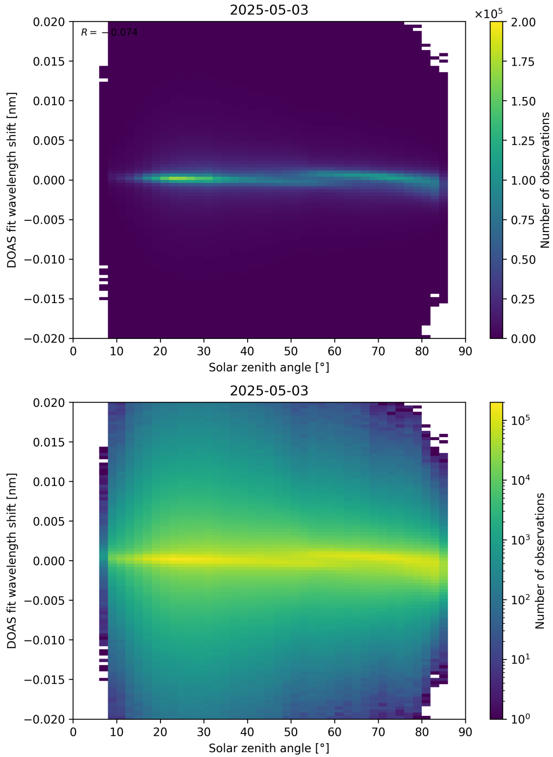
Figure 168: Scatter density plot of “Solar zenith angle” against “DOAS fit wavelength shift” for 2025-05-02 to 2025-05-04.
