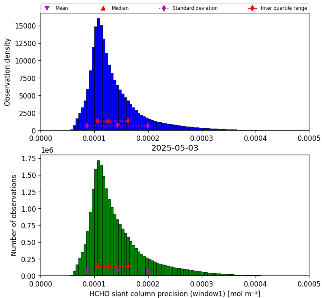
Figure 39: Histogram of “HCHO slant column precision (window1)” for 2025-05-02 to 2025-05-04
