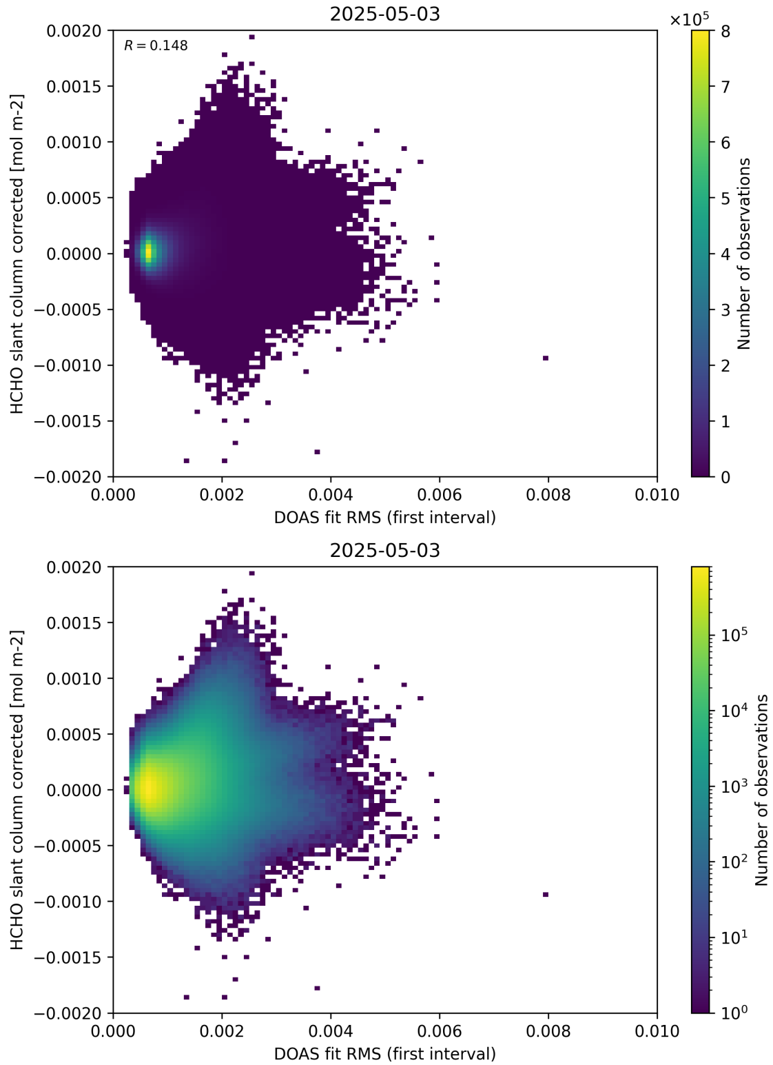
Figure 62: Scatter density plot of “DOAS fit RMS (first interval)” against “HCHO slant column corrected” for 2025-05-02 to 2025-05-04.
