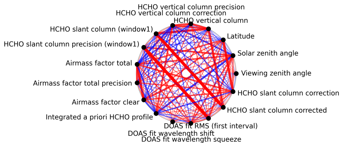
Figure 1: Map of correlation graph for 2025-05-02 to 2025-05-04.
