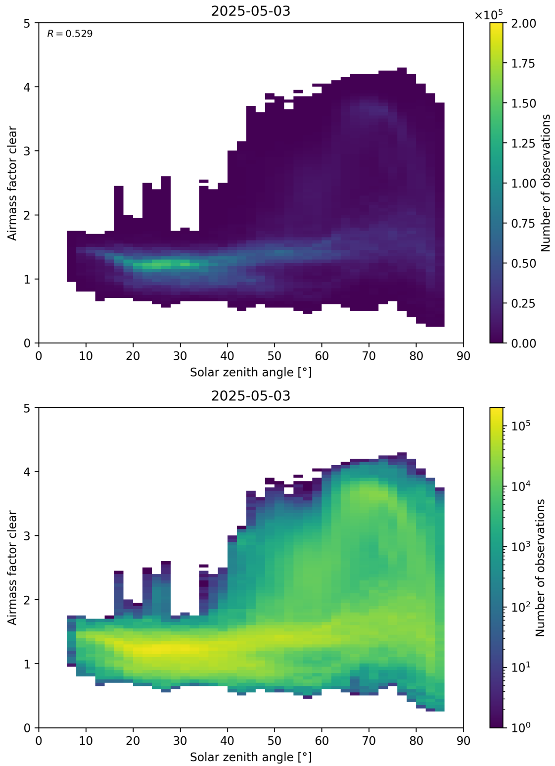
Figure 170: Scatter density plot of “Solar zenith angle” against “Airmass factor clear” for 2025-05-02 to 2025-05-04.
