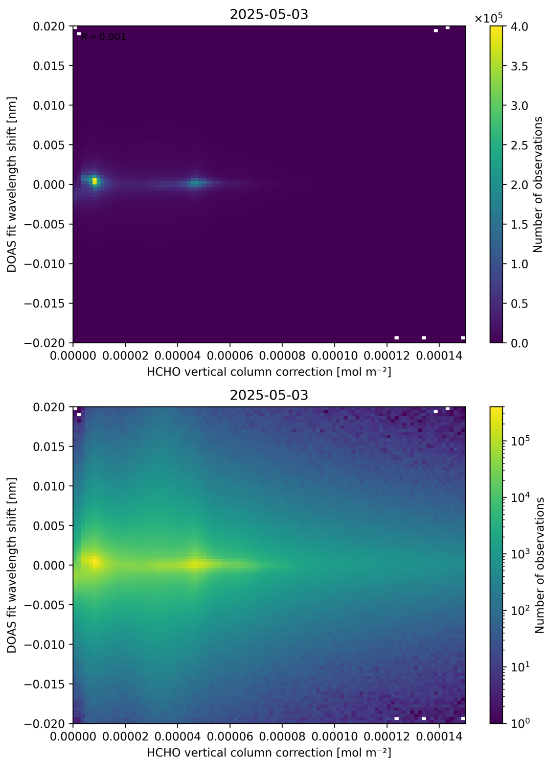
Figure 113: Scatter density plot of “HCHO vertical column correction” against “DOAS fit wavelength shift” for 2025-05-02 to 2025-05-04.
