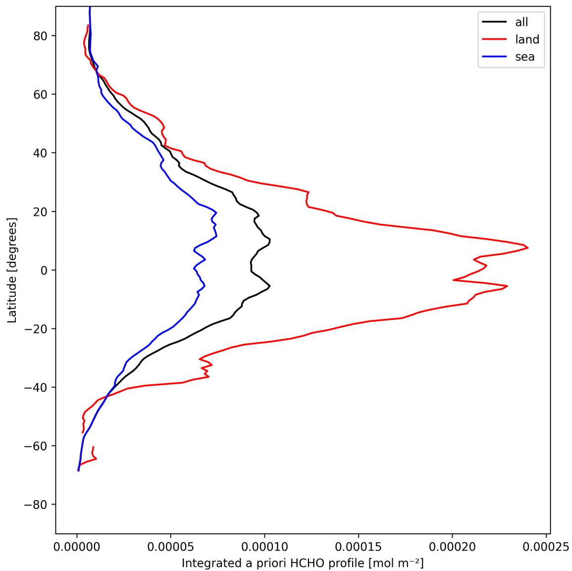
Figure 29: Zonal average of “Integrated a priori HCHO profile” for 2025-05-02 to 2025-05-04.
