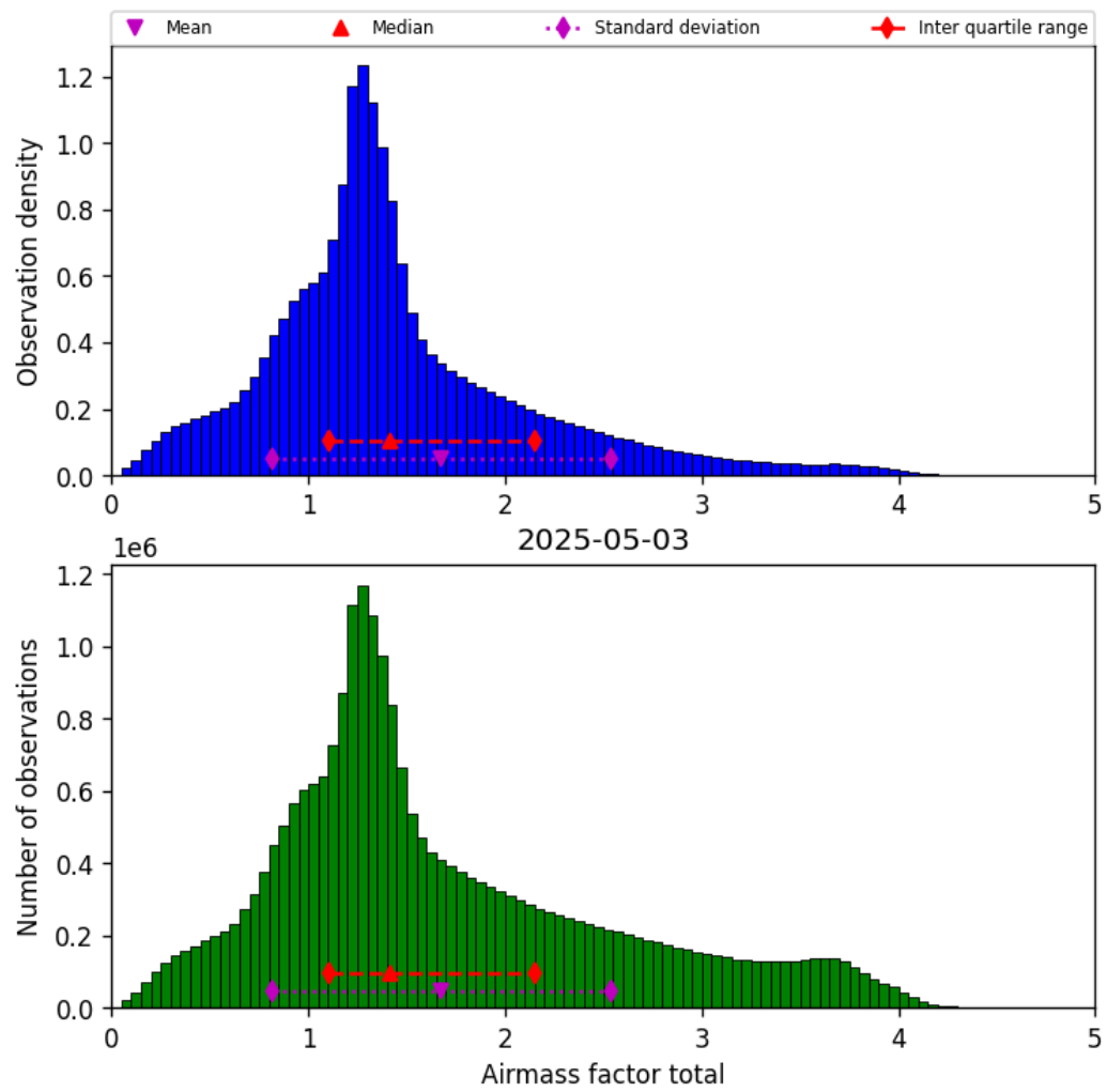
Figure 40: Histogram of “Airmass factor total” for 2025-05-02 to 2025-05-04
