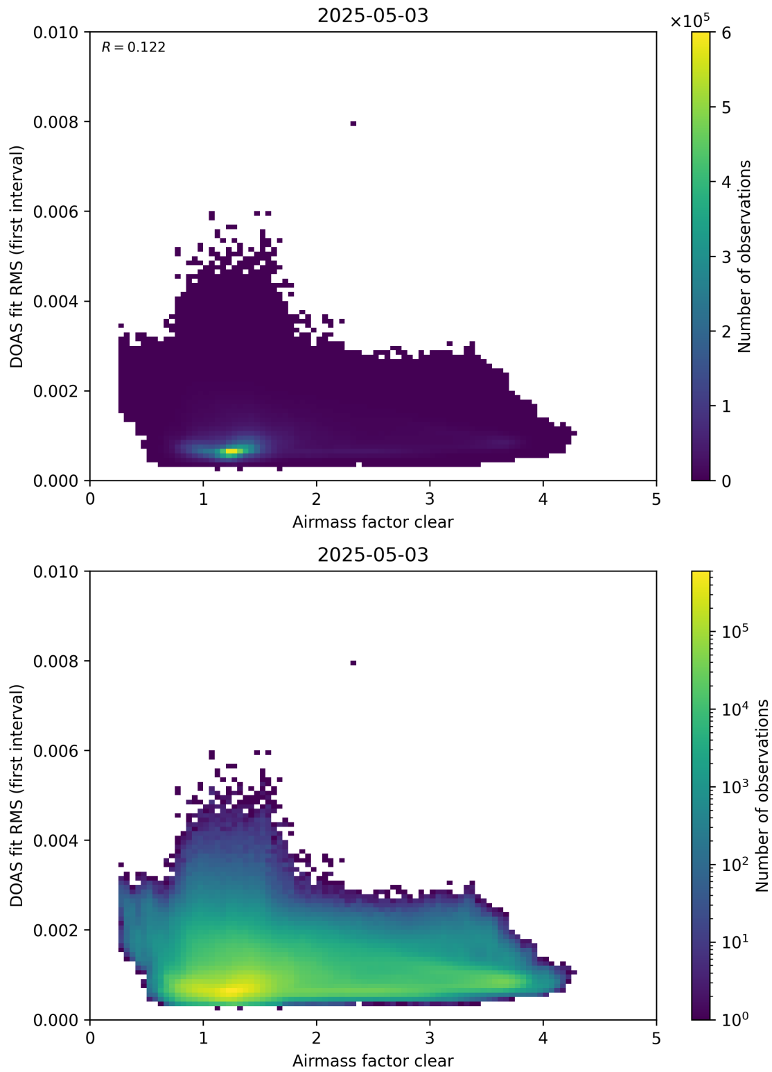
Figure 71: Scatter density plot of “Airmass factor clear” against “DOAS fit RMS (first interval)” for 2025-05-02 to 2025-05-04.
