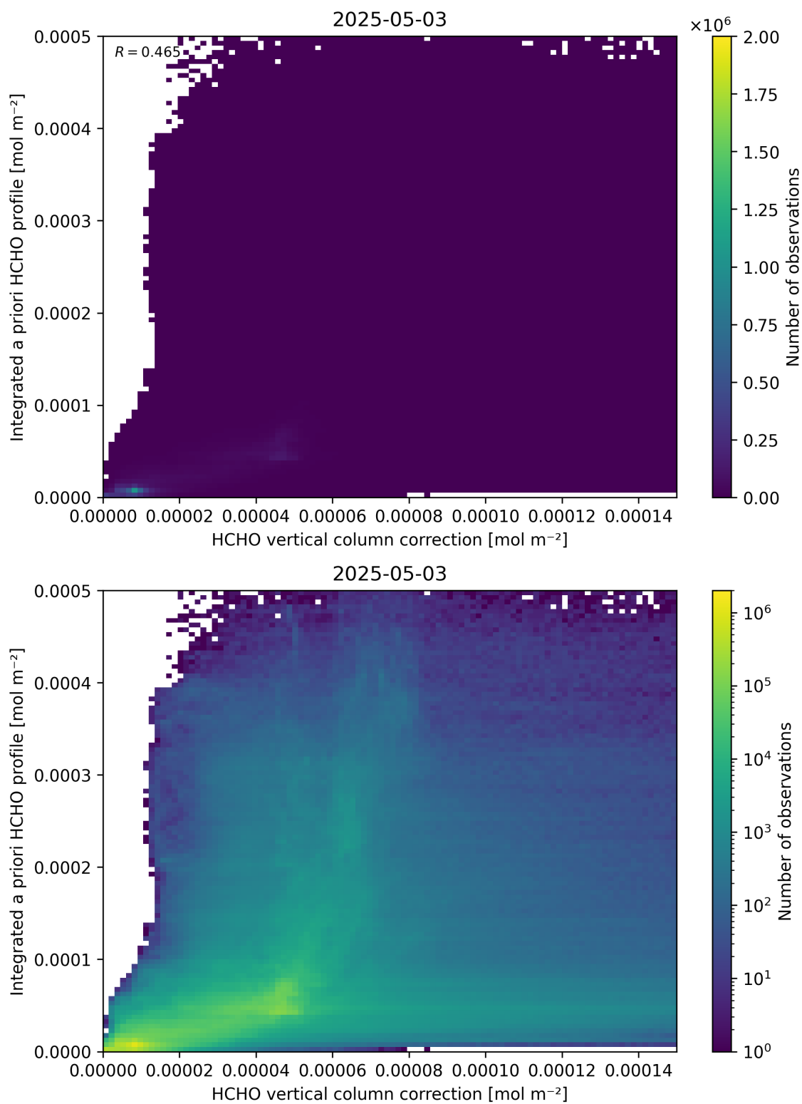
Figure 122: Scatter density plot of “HCHO vertical column correction” against “Integrated a priori HCHO profile” for 2025-05-02 to 2025-05-04.
