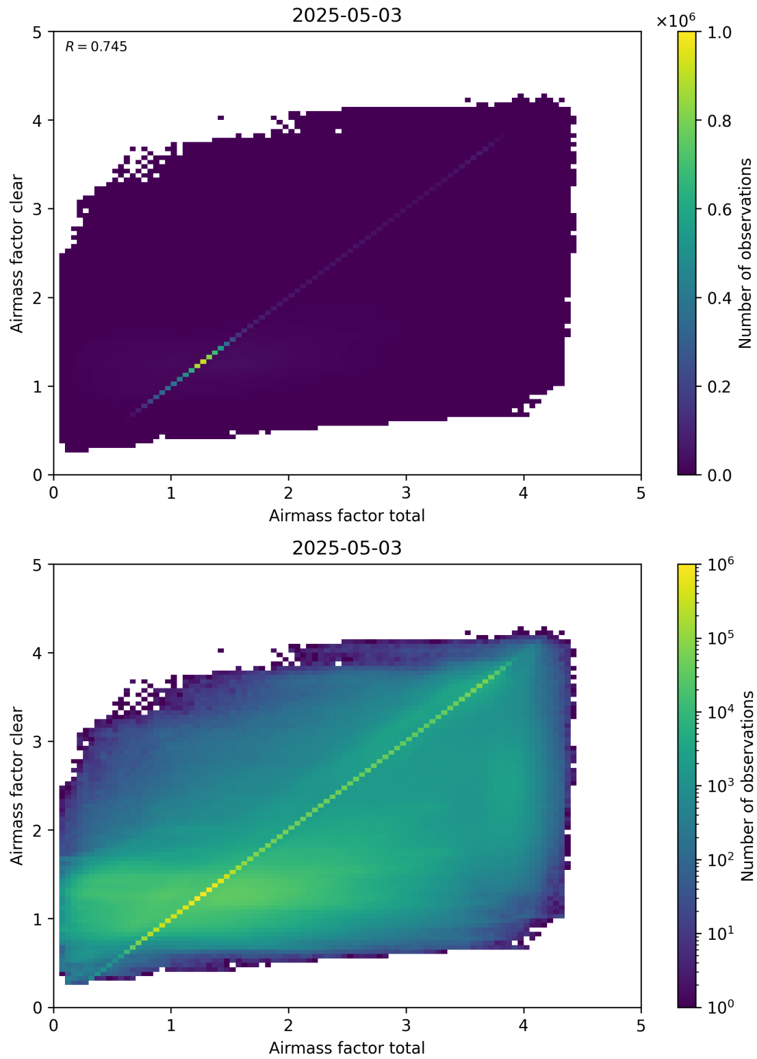
Figure 100: Scatter density plot of “Airmass factor total” against “Airmass factor clear” for 2025-05-02 to 2025-05-04.
