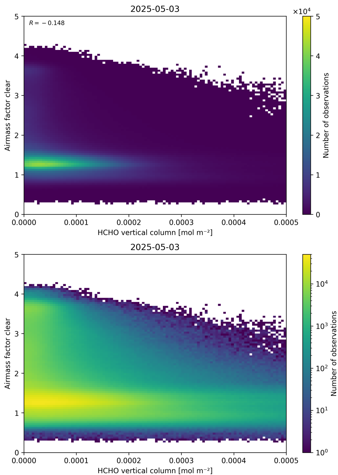
Figure 126: Scatter density plot of “HCHO vertical column” against “Airmass factor clear” for 2025-05-02 to 2025-05-04.
