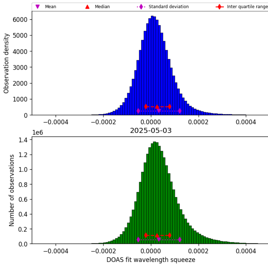
Figure 45: Histogram of “DOAS fit wavelength squeeze” for 2025-05-02 to 2025-05-04
