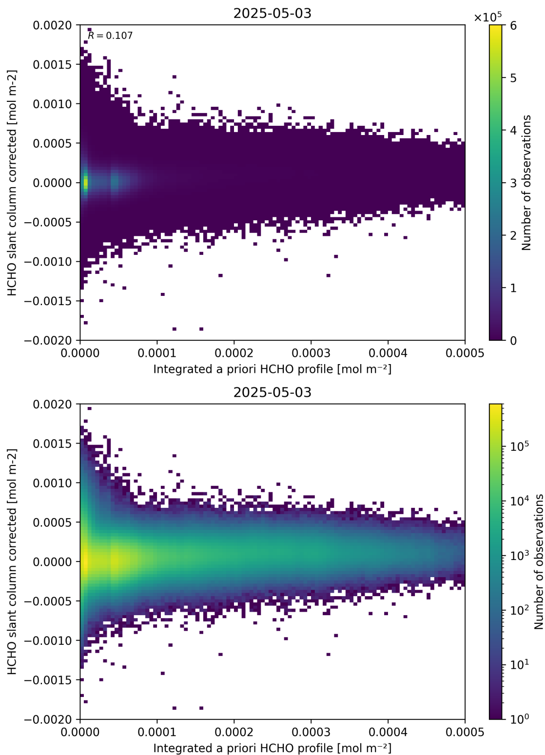
Figure 151: Scatter density plot of “Integrated a priori HCHO profile” against “HCHO slant column corrected” for 2025-05-02 to 2025-05-04.
