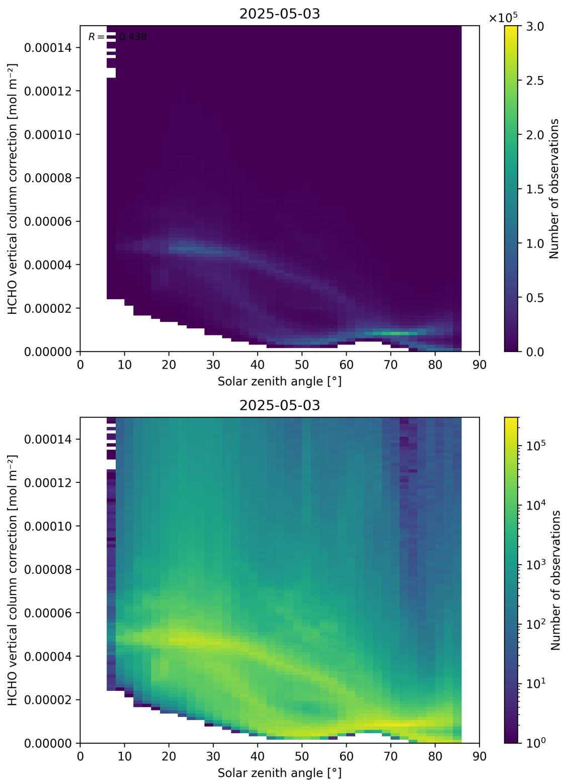
Figure 178: Scatter density plot of “Solar zenith angle” against “HCHO vertical column correction” for 2025-05-02 to 2025-05-04.
