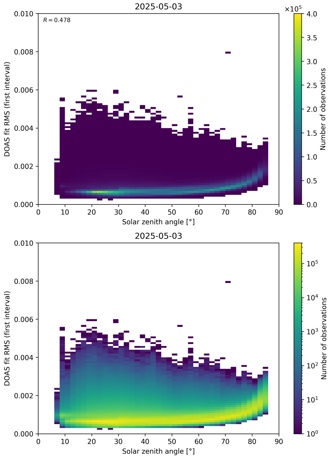
Figure 167: Scatter density plot of “Solar zenith angle” against “DOAS fit RMS (first interval)” for 2025-05-02 to 2025-05-04.
