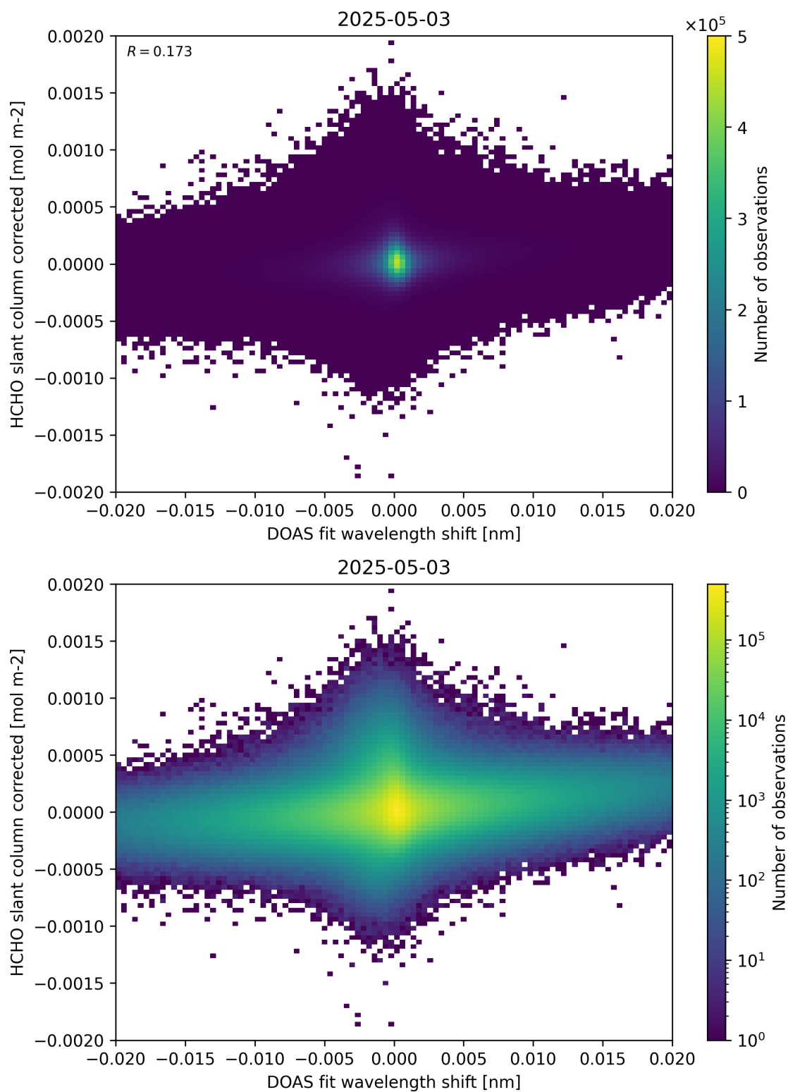
Figure 66: Scatter density plot of “DOAS fit wavelength shift” against “HCHO slant column corrected” for 2025-05-02 to 2025-05-04.
