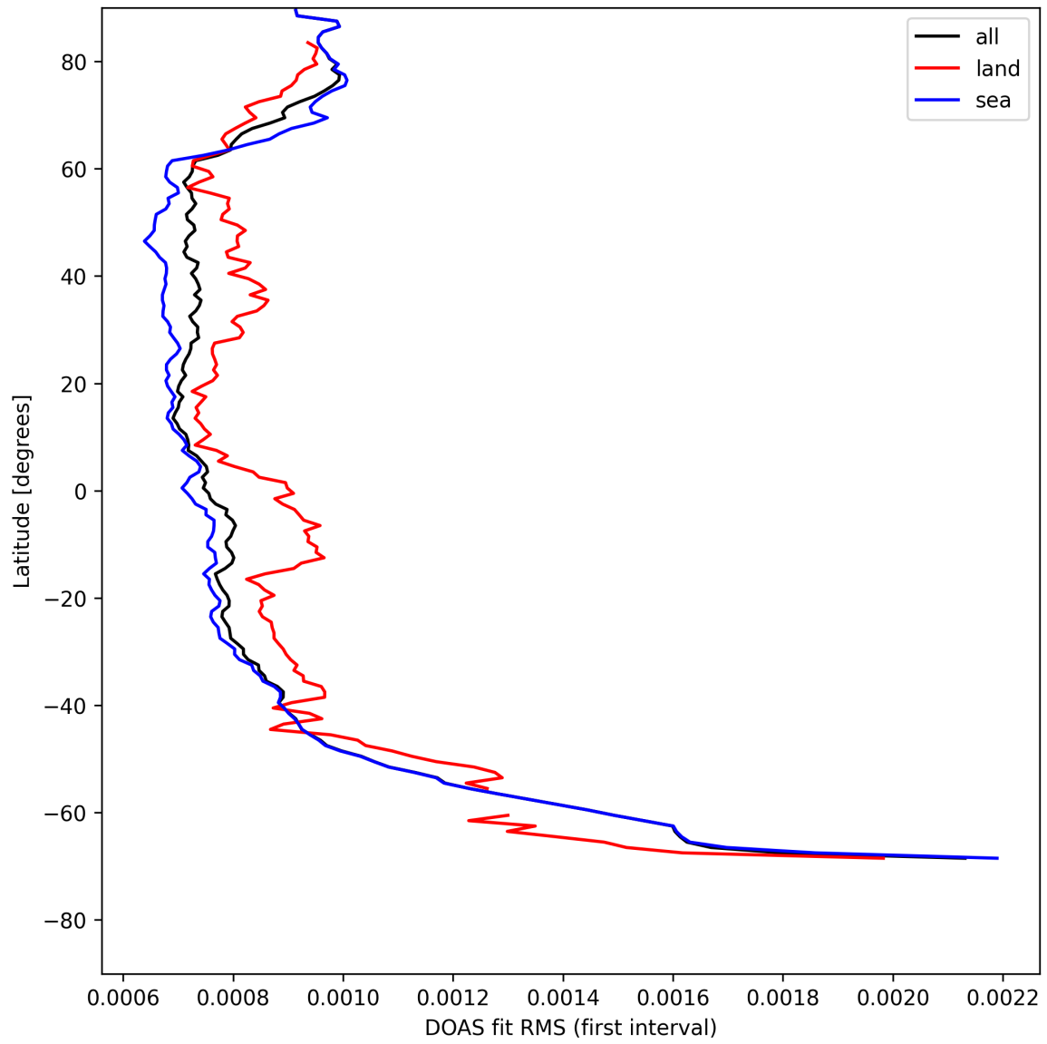
Figure 32: Zonal average of “DOAS fit RMS (first interval)” for 2025-05-02 to 2025-05-04.
