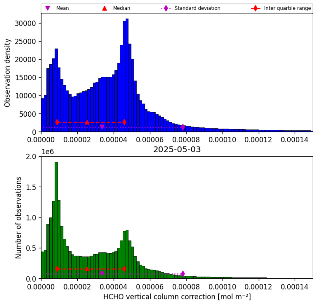
Figure 37: Histogram of “HCHO vertical column correction” for 2025-05-02 to 2025-05-04
