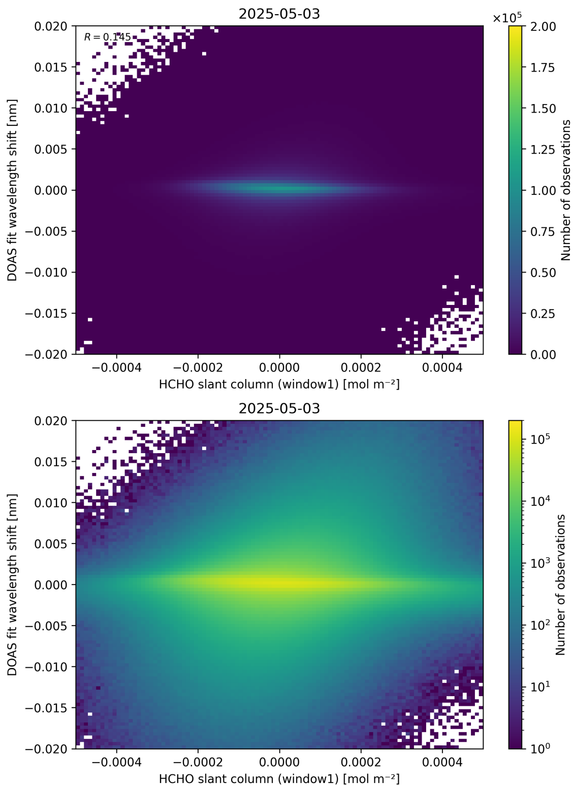
Figure 79: Scatter density plot of “HCHO slant column (window1)” against “DOAS fit wavelength shift” for 2025-05-02 to 2025-05-04.
