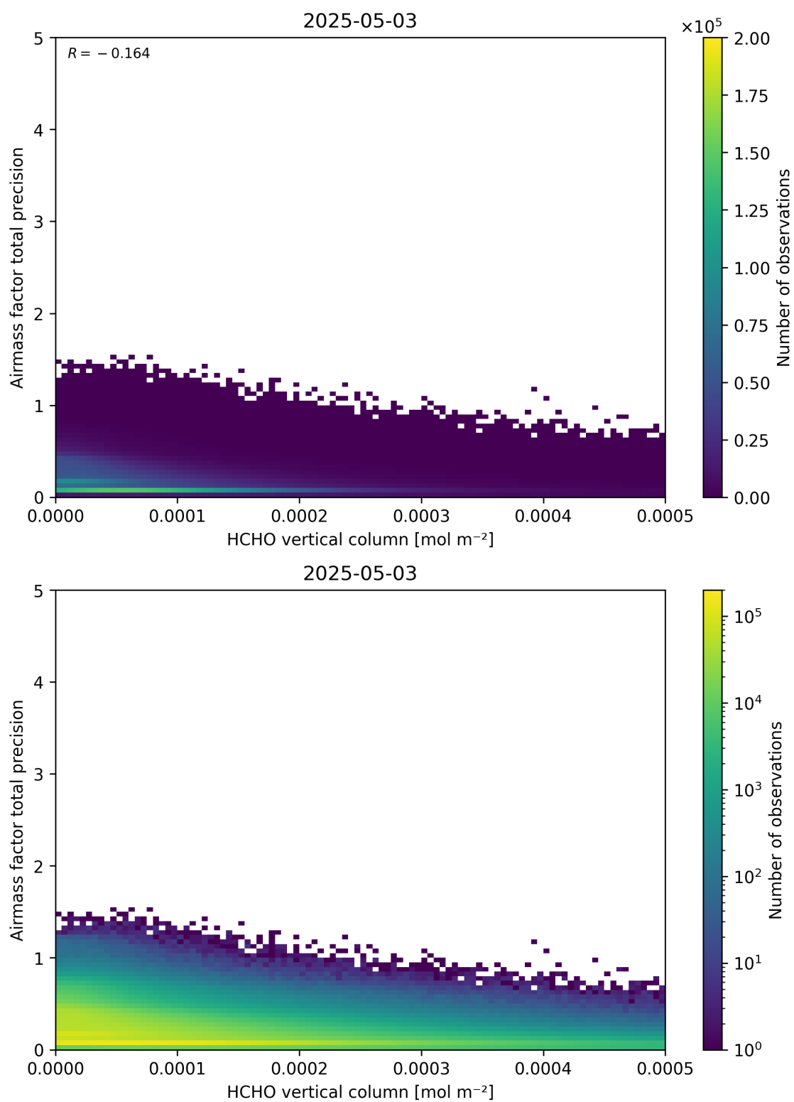
Figure 132: Scatter density plot of “HCHO vertical column” against “Airmass factor total precision” for 2025-05-02 to 2025-05-04.
