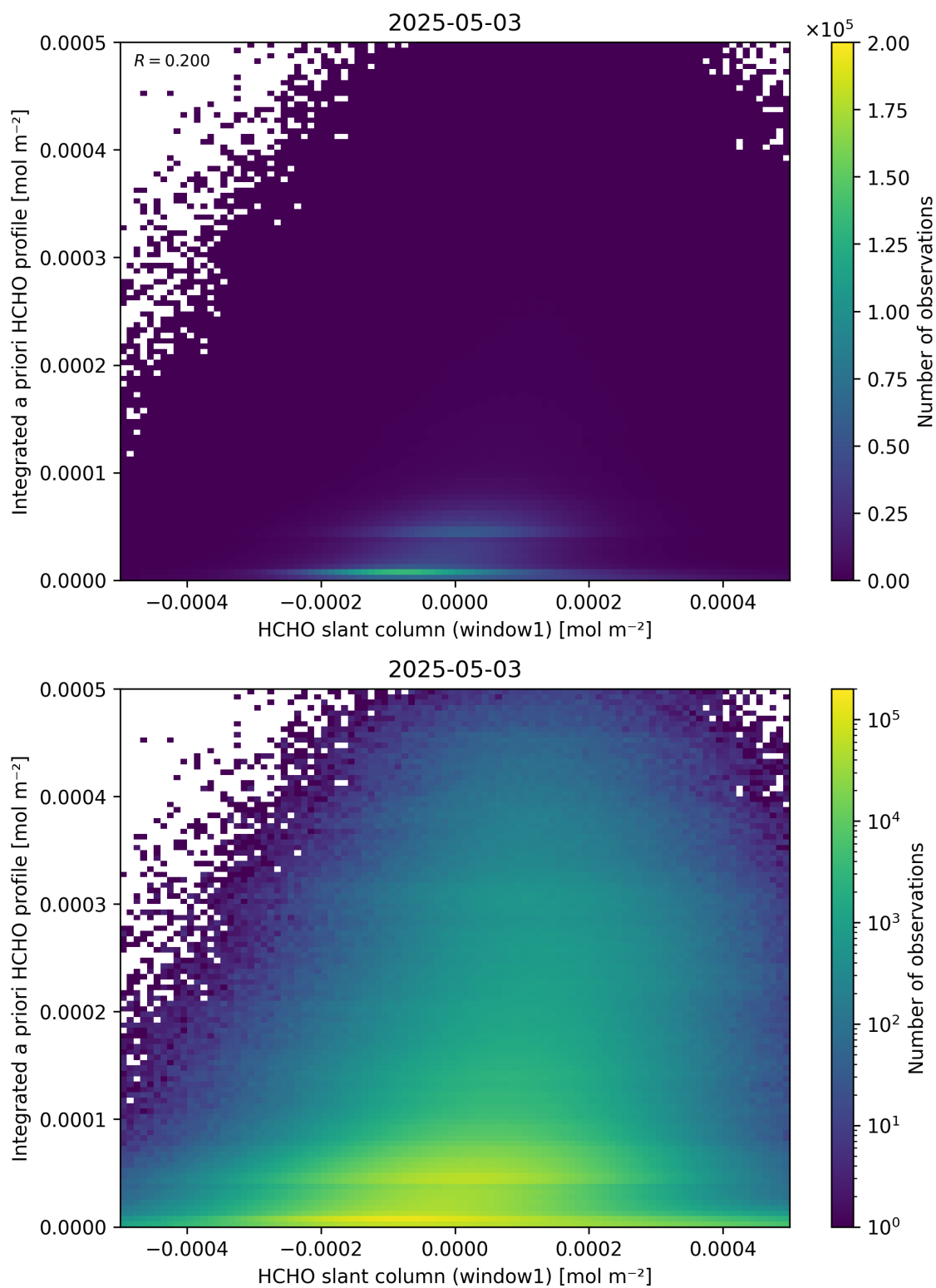
Figure 87: Scatter density plot of “HCHO slant column (window1)” against “Integrated a priori HCHO profile” for 2025-05-02 to 2025-05-04.
