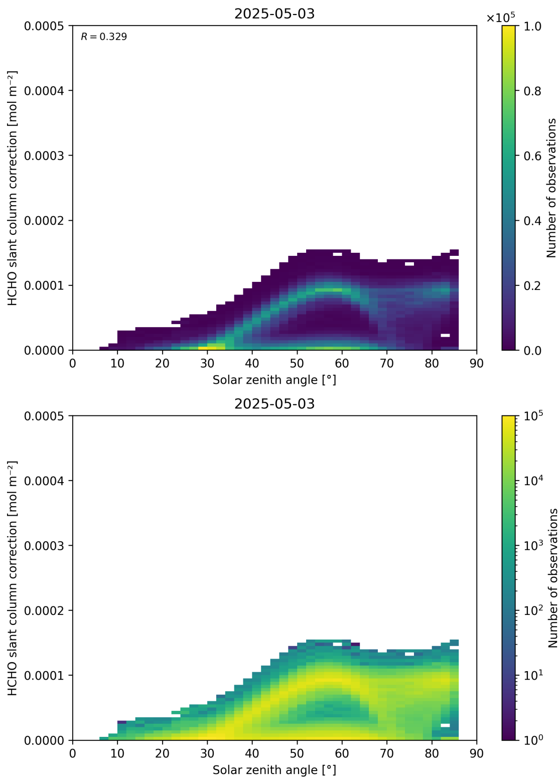
Figure 172: Scatter density plot of “Solar zenith angle” against “HCHO slant column correction” for 2025-05-02 to 2025-05-04.
