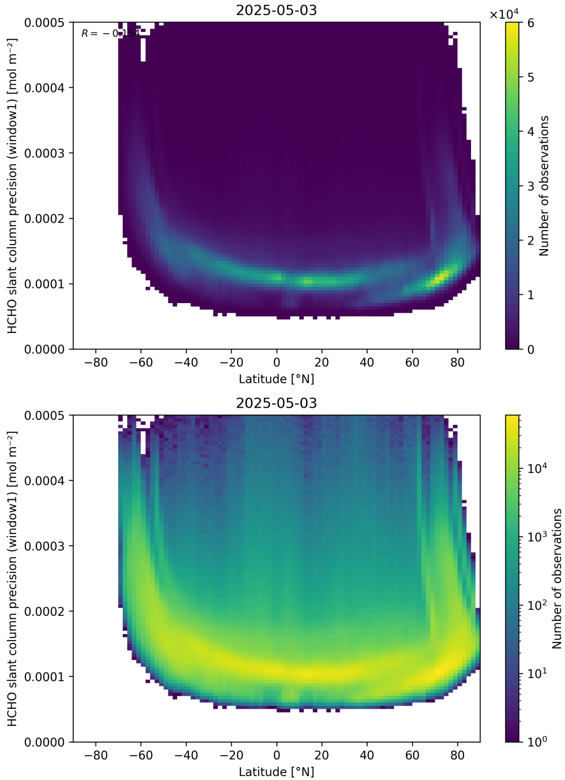
Figure 160: Scatter density plot of “Latitude” against “HCHO slant column precision (window1)” for 2025-05-02 to 2025-05-04.
