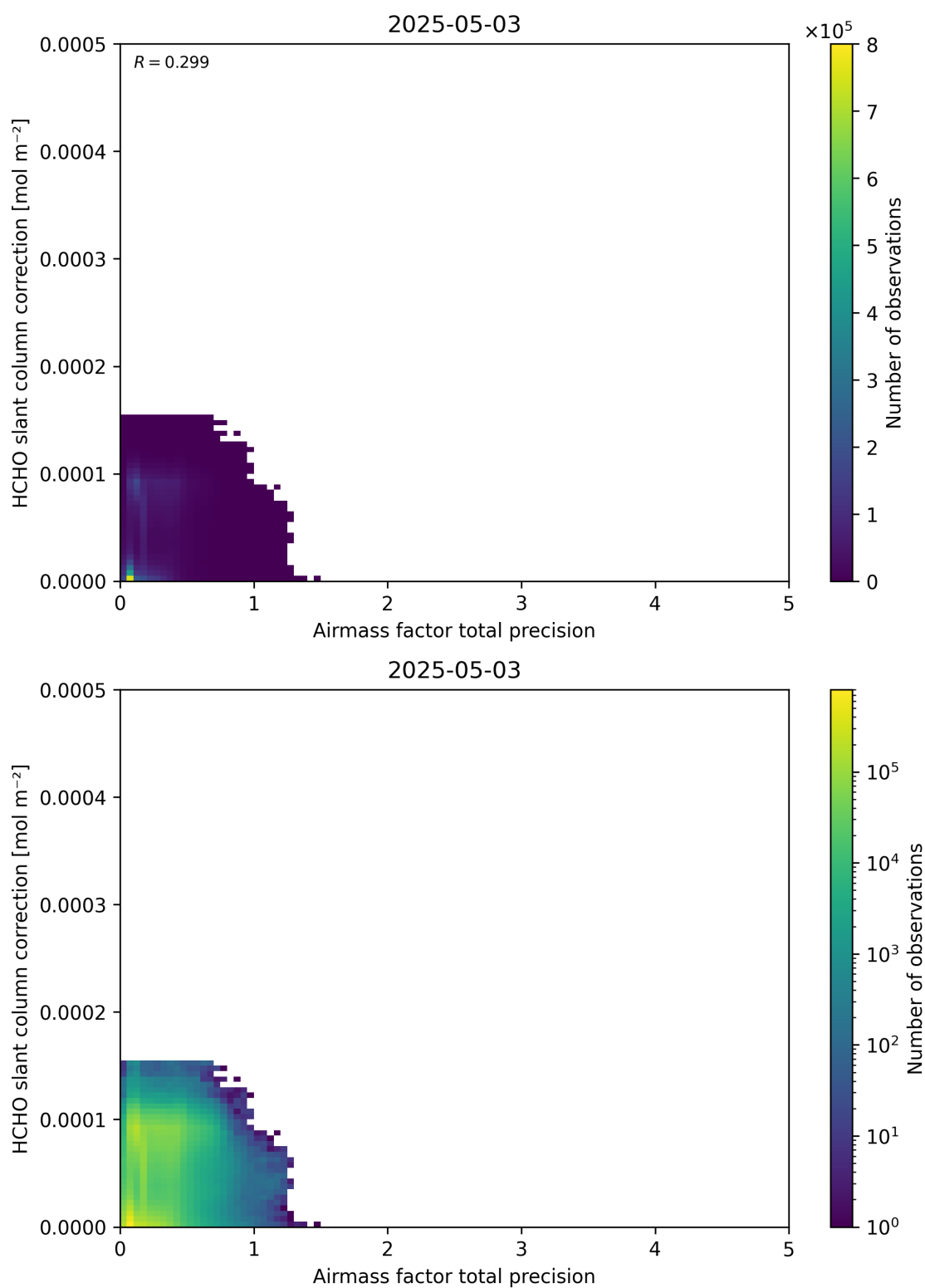
Figure 110: Scatter density plot of “Airmass factor total precision” against “HCHO slant column correction” for 2025-05-02 to 2025-05-04.
