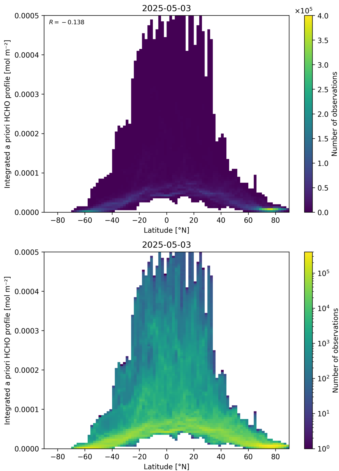
Figure 166: Scatter density plot of “Latitude” against “Integrated a priori HCHO profile” for 2025-05-02 to 2025-05-04.
