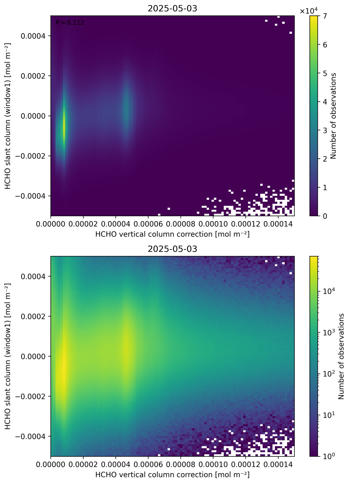
Figure 118: Scatter density plot of “HCHO vertical column correction” against “HCHO slant column (window1)” for 2025-05-02 to 2025-05-04.
