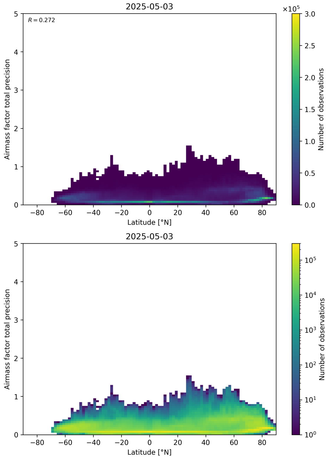
Figure 162: Scatter density plot of “Latitude” against “Airmass factor total precision” for 2025-05-02 to 2025-05-04.
