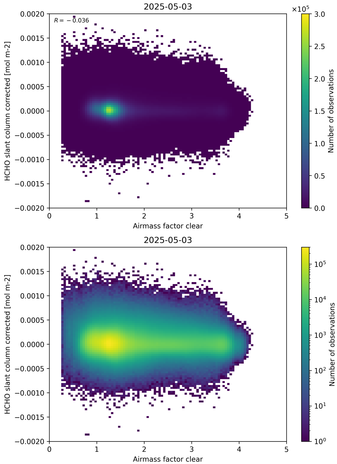
Figure 74: Scatter density plot of “Airmass factor clear” against “HCHO slant column corrected” for 2025-05-02 to 2025-05-04.
