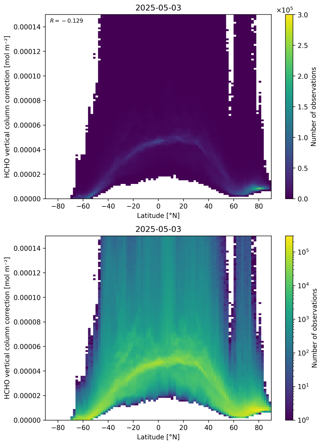
Figure 164: Scatter density plot of “Latitude” against “HCHO vertical column correction” for 2025-05-02 to 2025-05-04.
