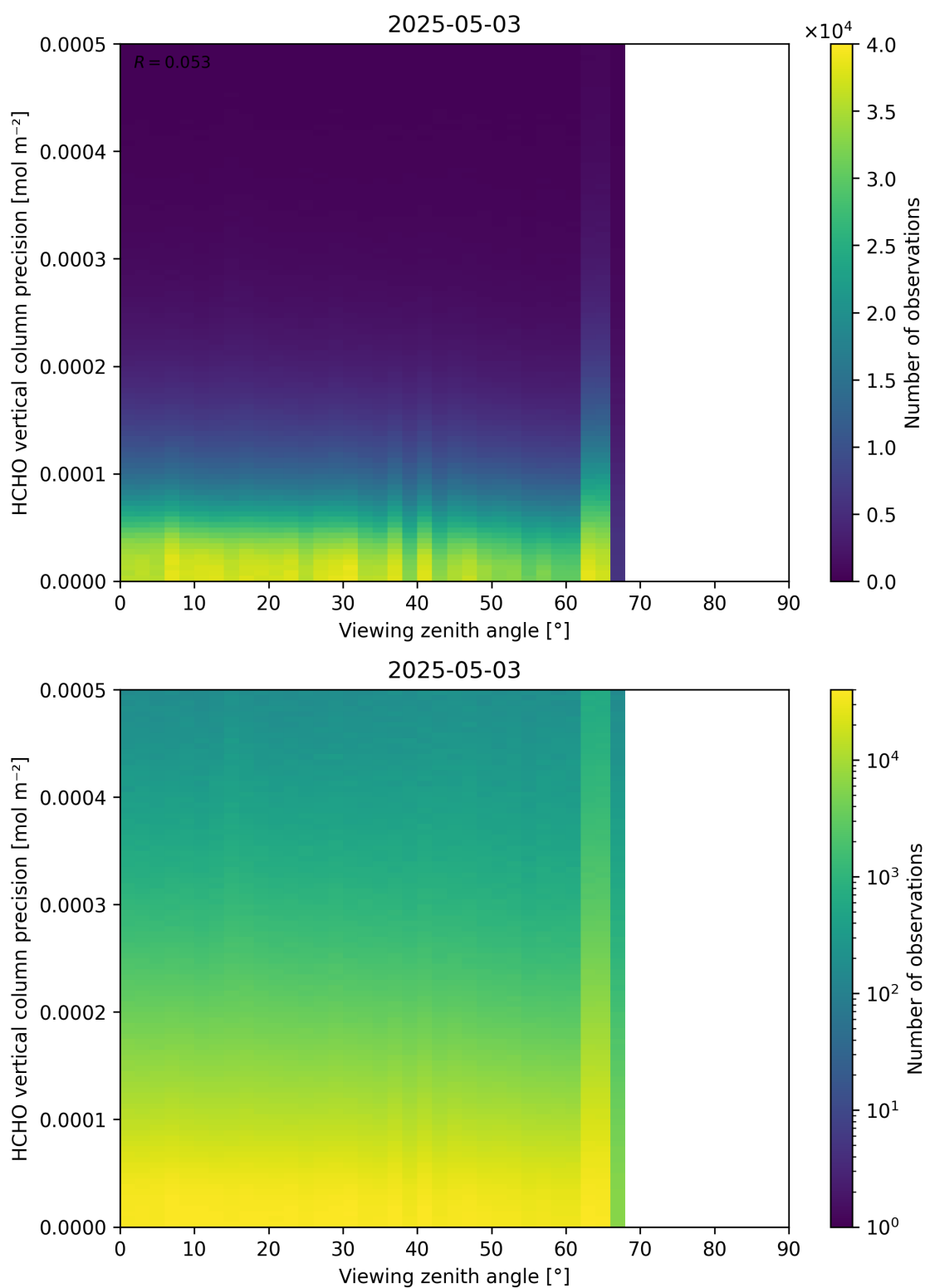
Figure 194: Scatter density plot of “Viewing zenith angle” against “HCHO vertical column precision” for 2025-05-02 to 2025-05-04.
