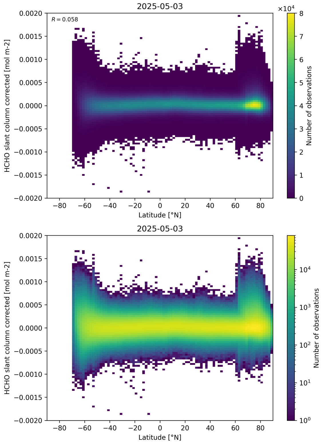
Figure 157: Scatter density plot of “Latitude” against “HCHO slant column corrected” for 2025-05-02 to 2025-05-04.
