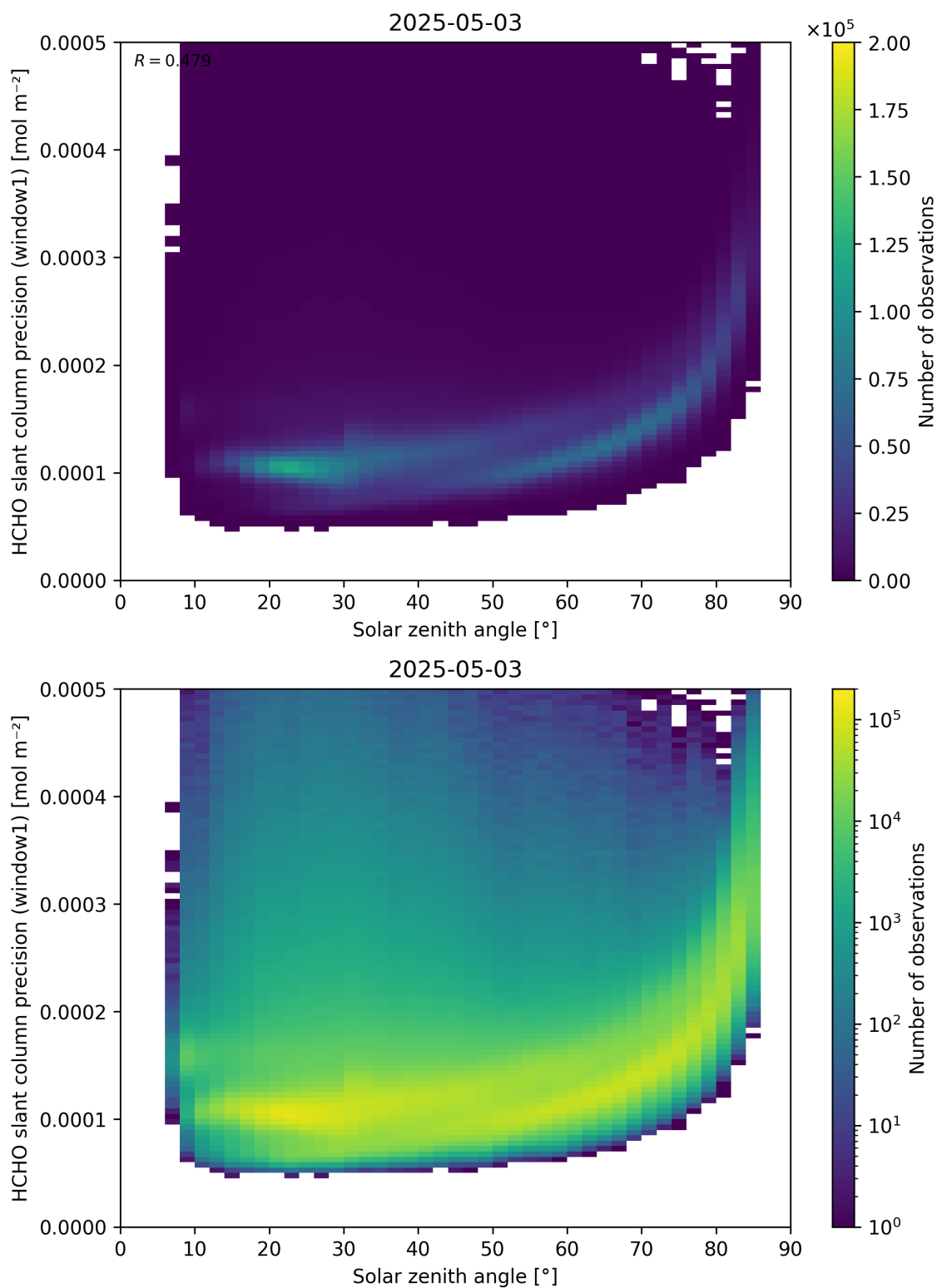
Figure 174: Scatter density plot of “Solar zenith angle” against “HCHO slant column precision (window1)” for 2025-05-02 to 2025-05-04.
