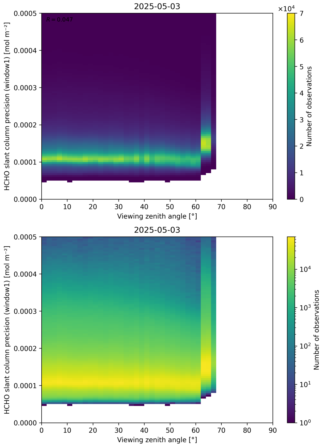
Figure 189: Scatter density plot of “Viewing zenith angle” against “HCHO slant column precision (window1)” for 2025-05-02 to 2025-05-04.
