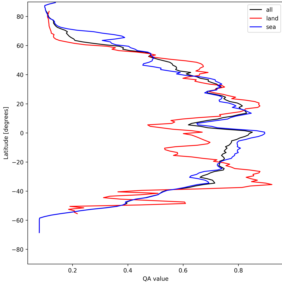
Figure 20: Zonal average of “QA value” for 2025-05-02 to 2025-05-04.
