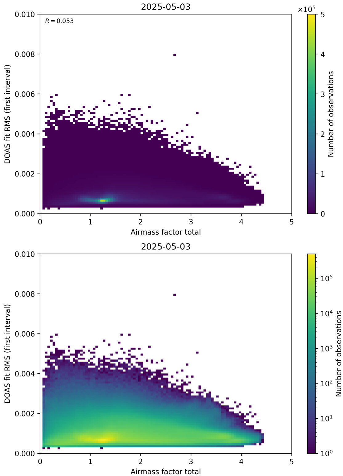
Figure 97: Scatter density plot of “Airmass factor total” against “DOAS fit RMS (first interval)” for 2025-05-02 to 2025-05-04.
