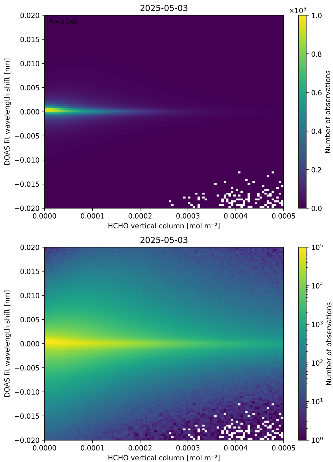
Figure 124: Scatter density plot of “HCHO vertical column” against “DOAS fit wavelength shift” for 2025-05-02 to 2025-05-04.
