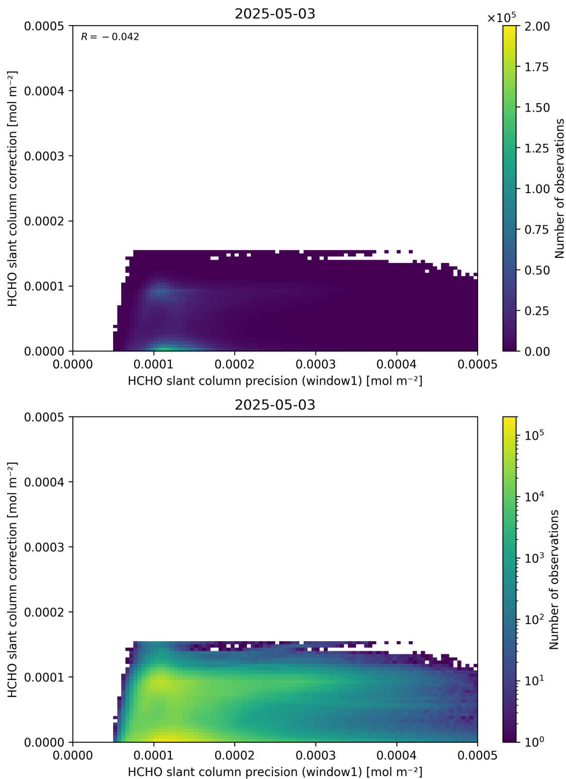
Figure 93: Scatter density plot of “HCHO slant column precision (window1)” against “HCHO slant column correction” for 2025-05-02 to 2025-05-04.
