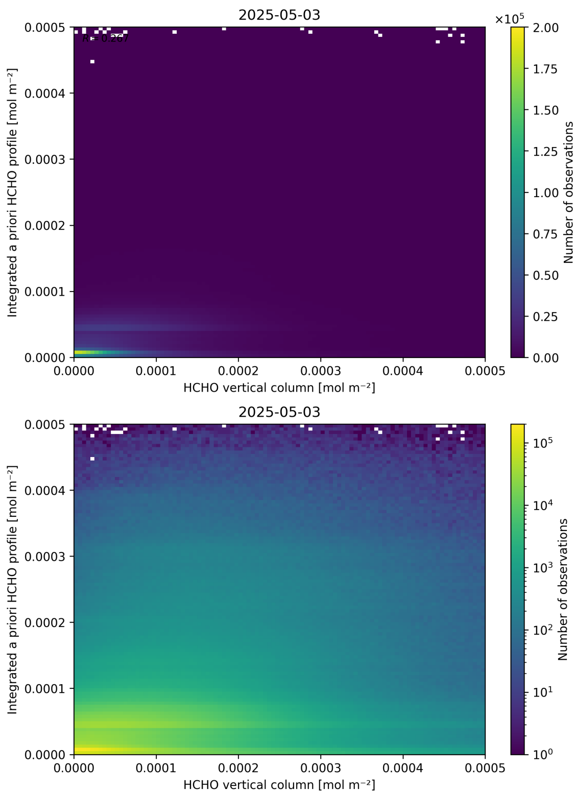
Figure 135: Scatter density plot of “HCHO vertical column” against “Integrated a priori HCHO profile” for 2025-05-02 to 2025-05-04.
