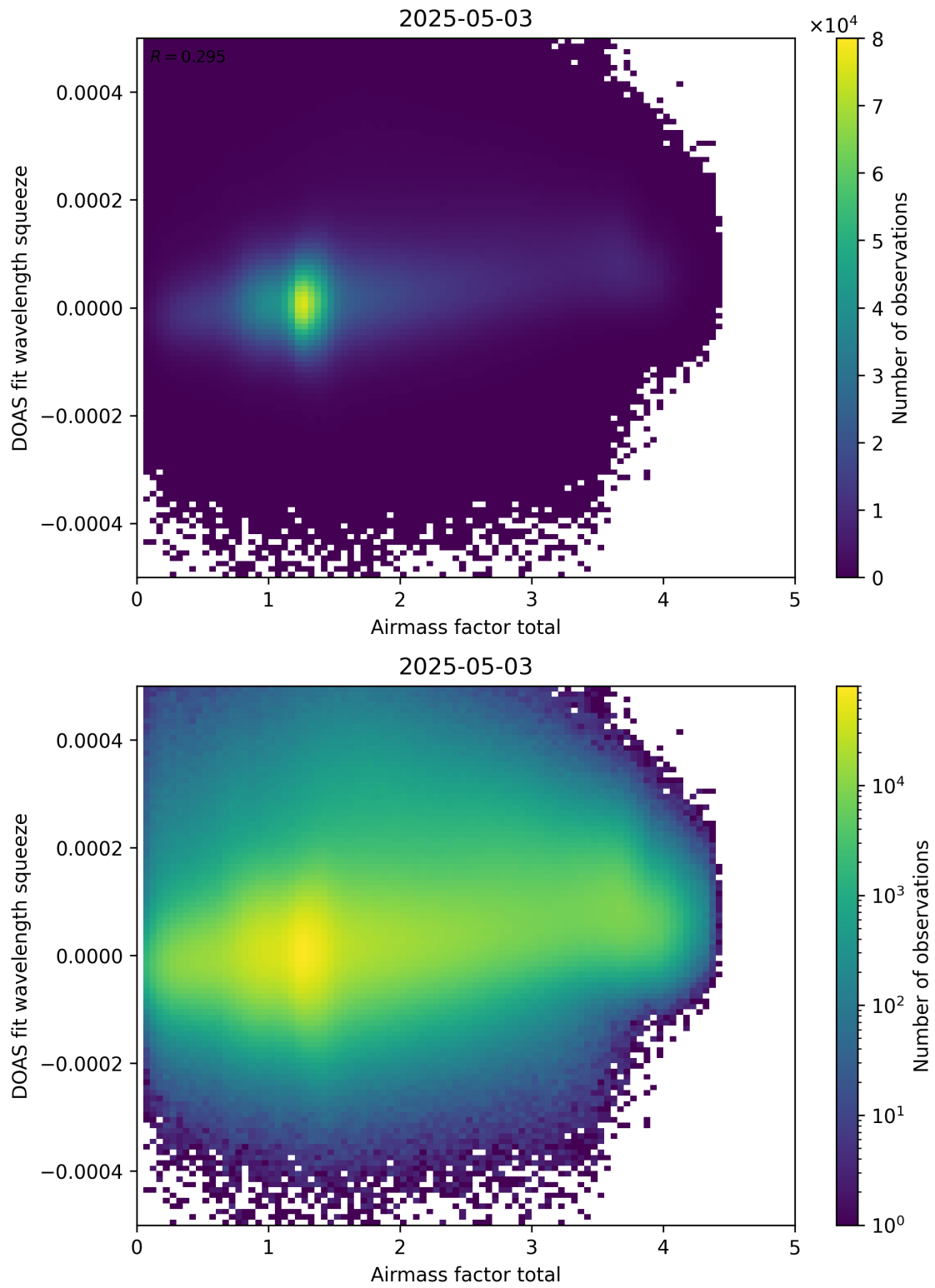
Figure 99: Scatter density plot of “Airmass factor total” against “DOAS fit wavelength squeeze” for 2025-05-02 to 2025-05-04.
