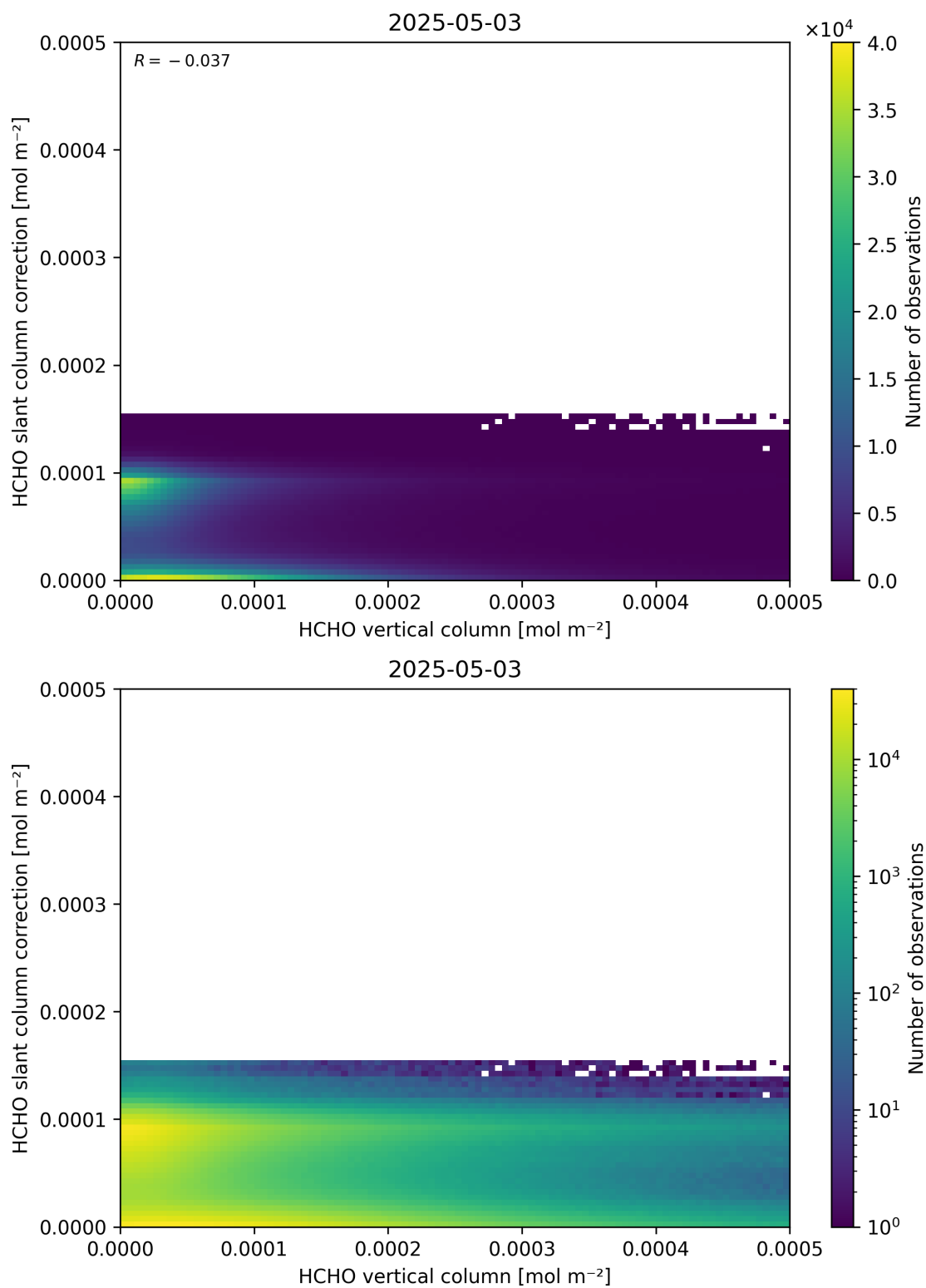
Figure 128: Scatter density plot of “HCHO vertical column” against “HCHO slant column correction” for 2025-05-02 to 2025-05-04.
