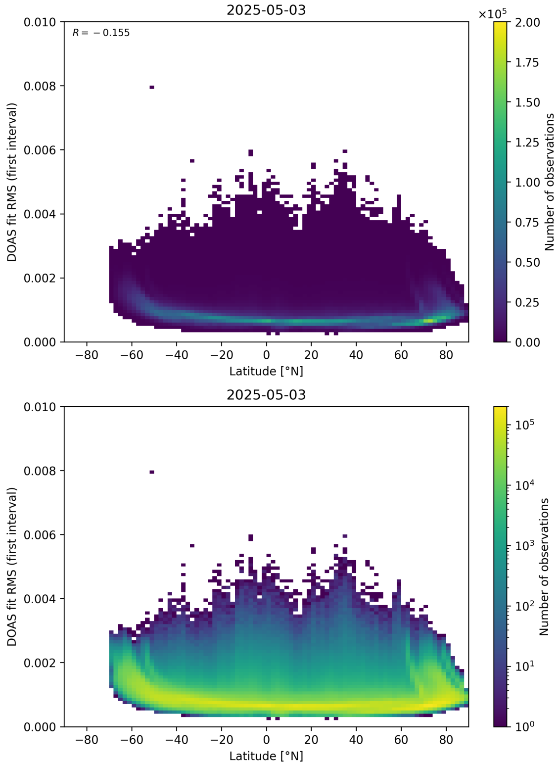
Figure 153: Scatter density plot of “Latitude” against “DOAS fit RMS (first interval)” for 2025-05-02 to 2025-05-04.
