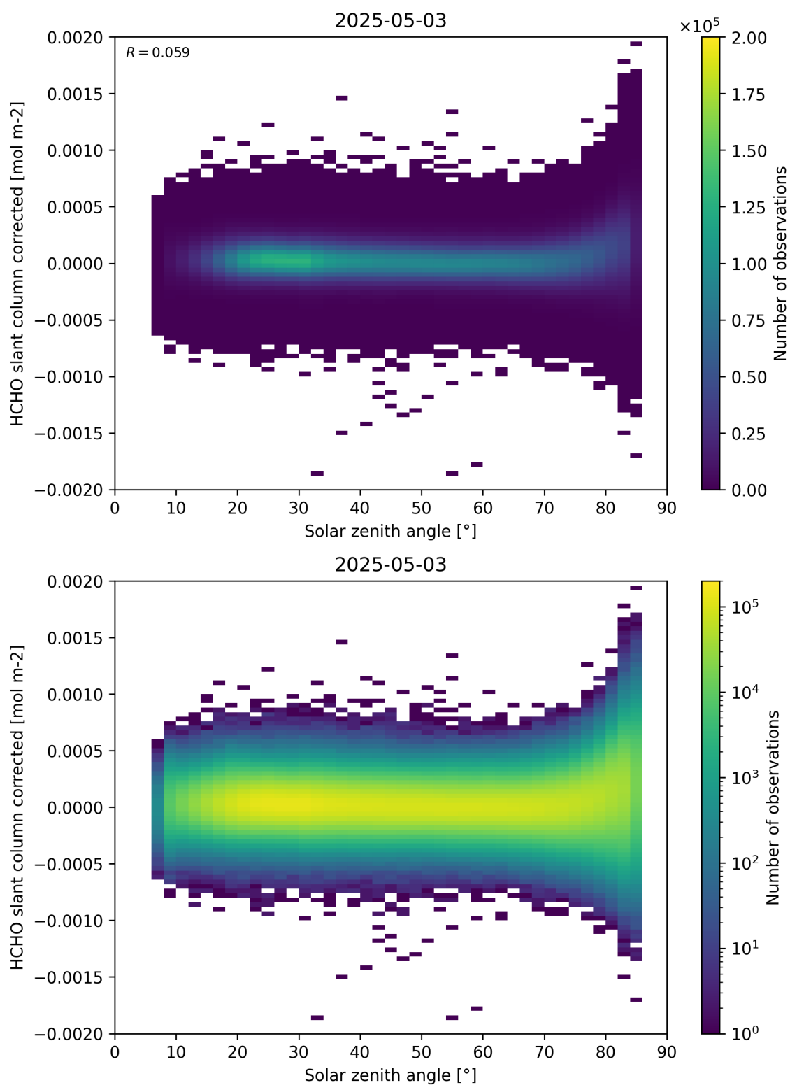
Figure 171: Scatter density plot of “Solar zenith angle” against “HCHO slant column corrected” for 2025-05-02 to 2025-05-04.
