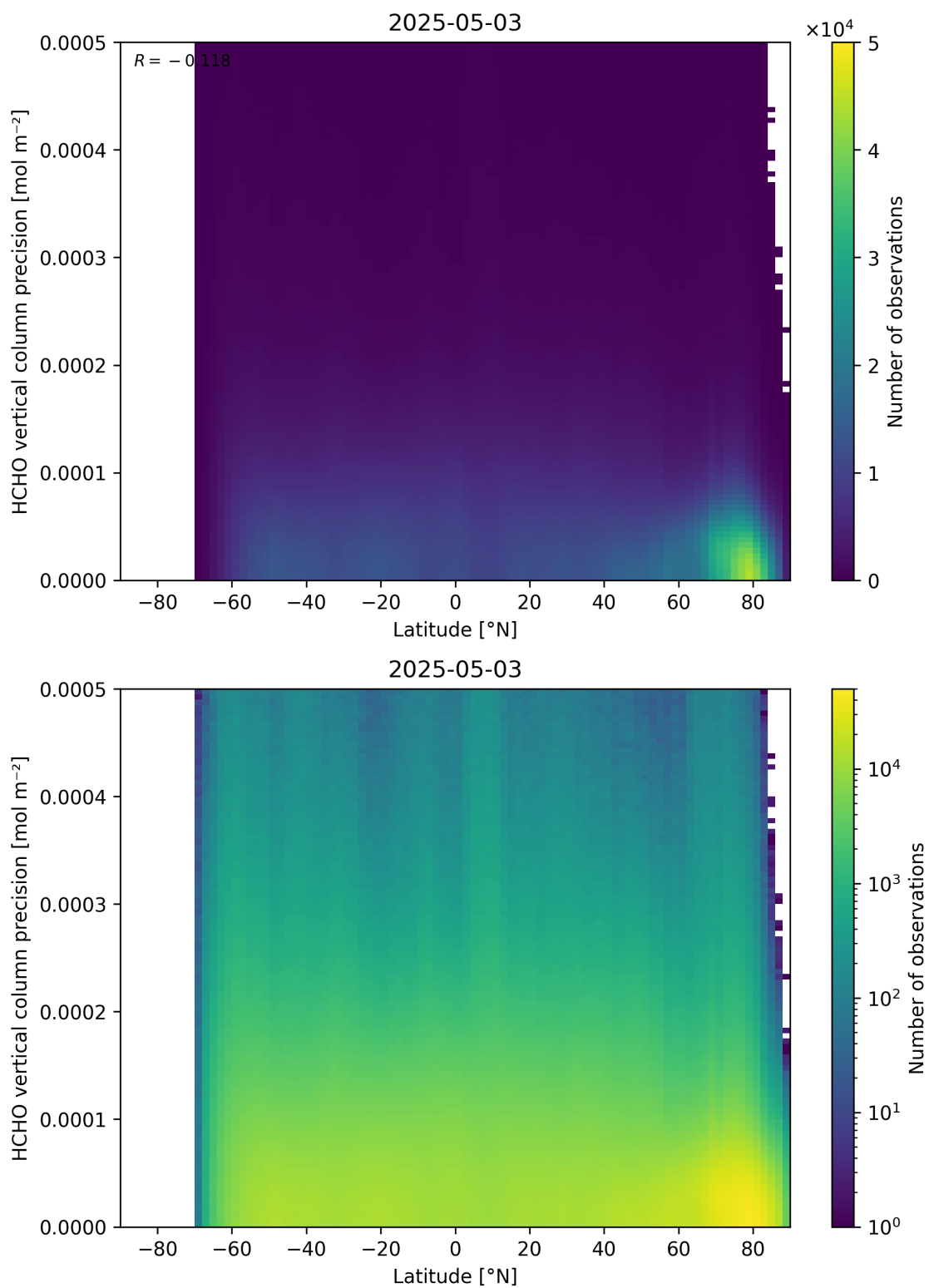
Figure 165: Scatter density plot of “Latitude” against “HCHO vertical column precision” for 2025-05-02 to 2025-05-04.
