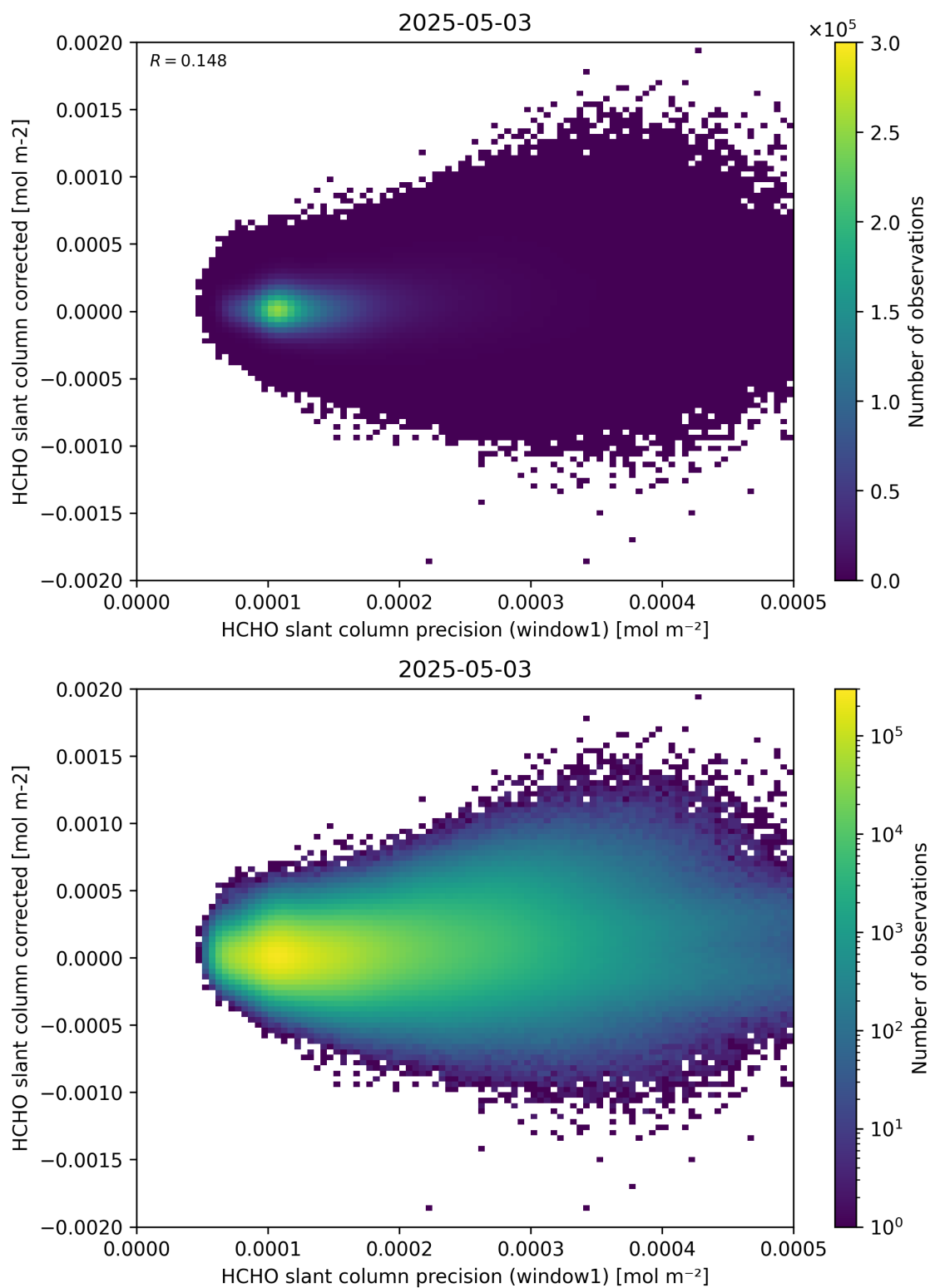
Figure 92: Scatter density plot of “HCHO slant column precision (window1)” against “HCHO slant column corrected” for 2025-05-02 to 2025-05-04.
