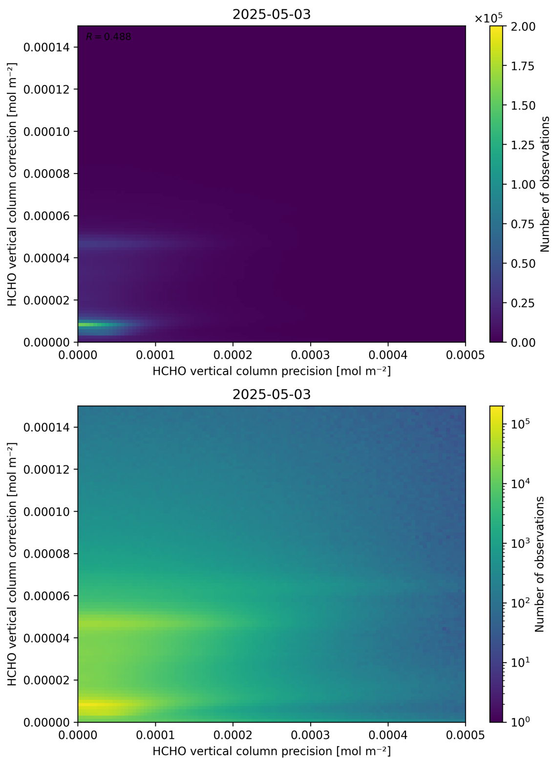
Figure 146: Scatter density plot of “HCHO vertical column precision” against “HCHO vertical column correction” for 2025-05-02 to 2025-05-04.
