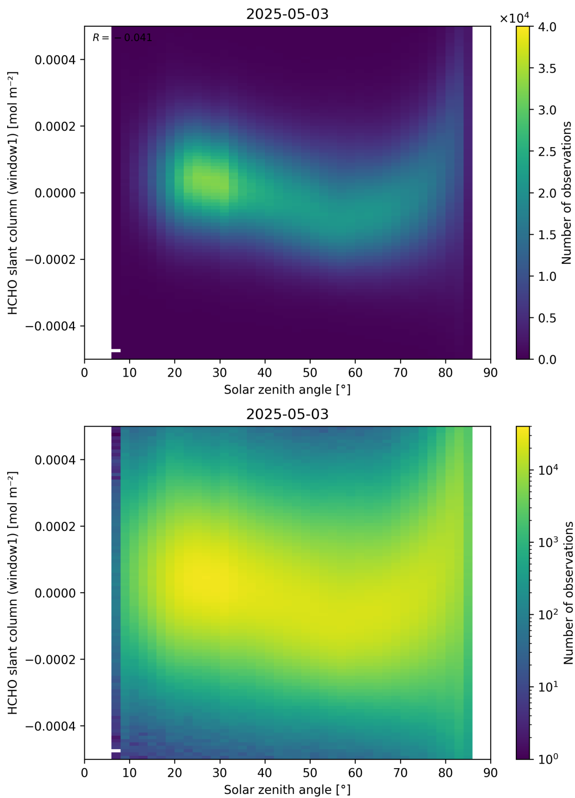
Figure 173: Scatter density plot of “Solar zenith angle” against “HCHO slant column (window1)” for 2025-05-02 to 2025-05-04.
