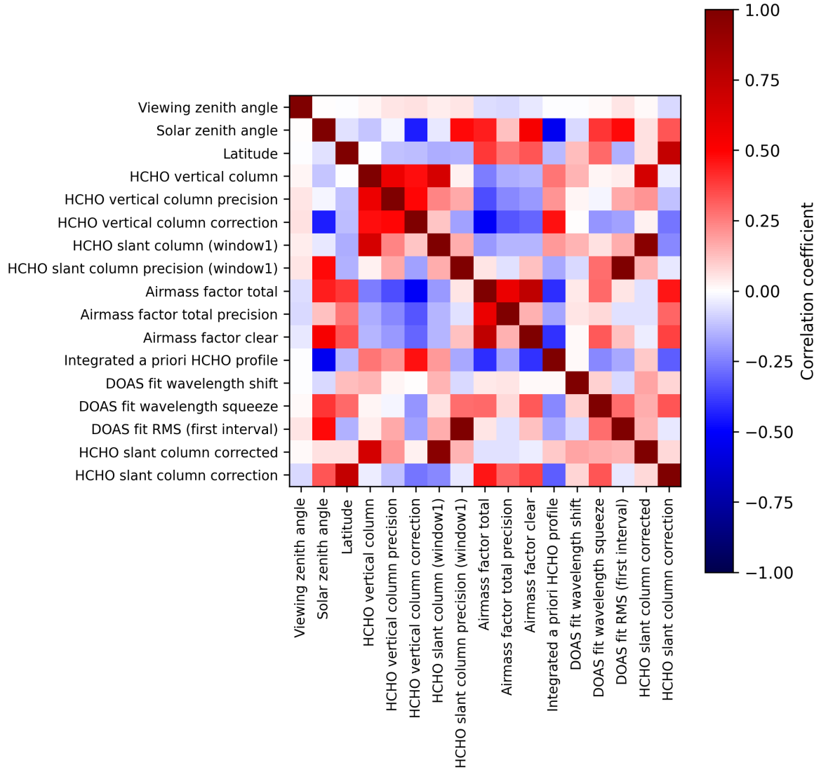
Figure 2: Map of correlation matrix for 2025-05-02 to 2025-05-04.
