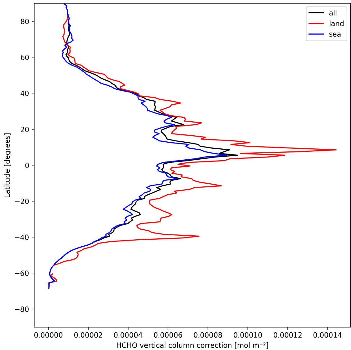
Figure 23: Zonal average of “HCHO vertical column correction” for 2025-05-02 to 2025-05-04.
