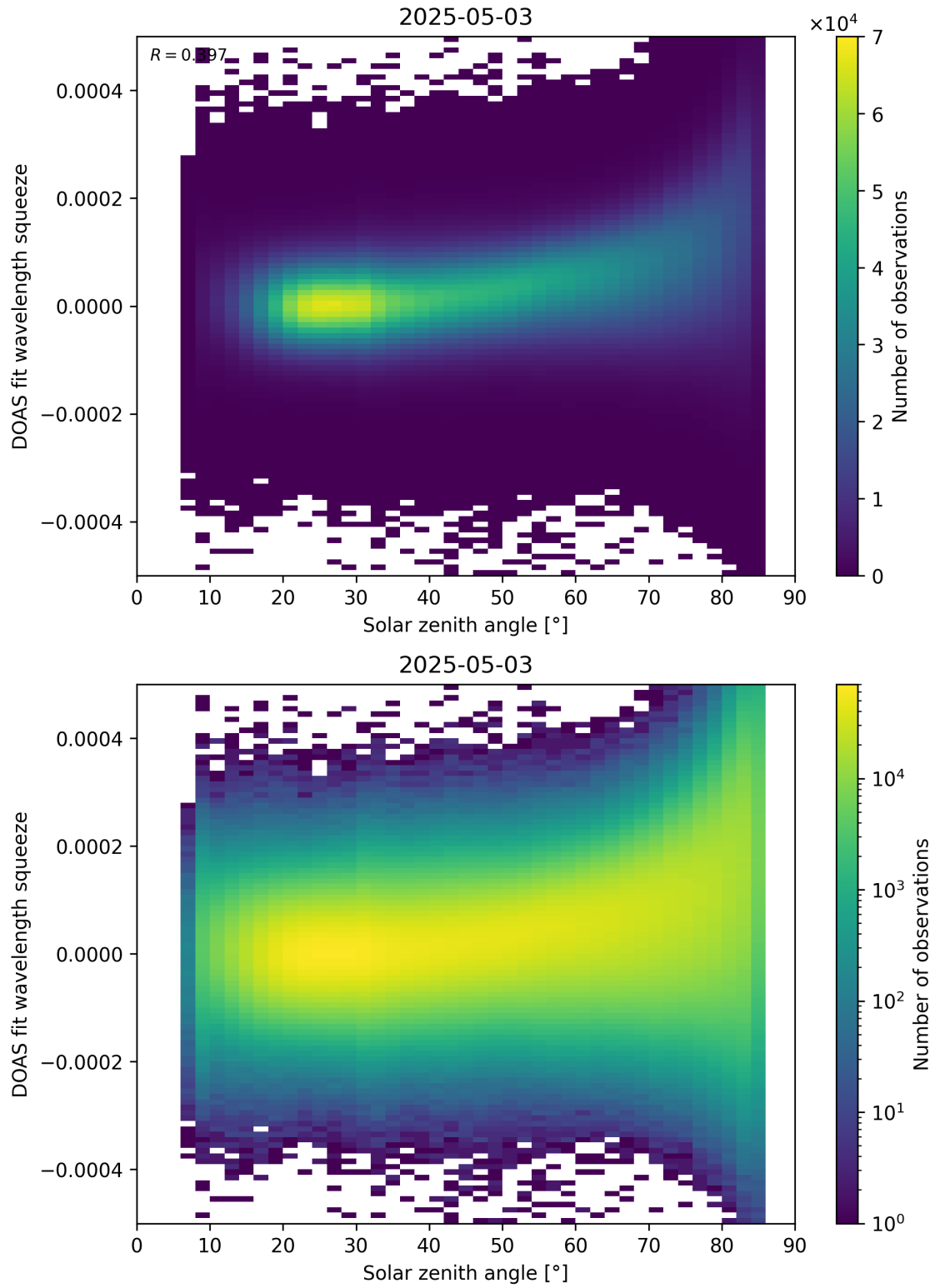
Figure 169: Scatter density plot of “Solar zenith angle” against “DOAS fit wavelength squeeze” for 2025-05-02 to 2025-05-04.
