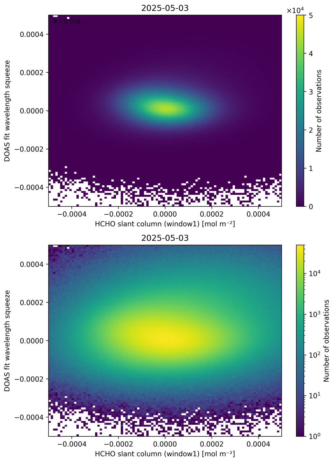
Figure 80: Scatter density plot of “HCHO slant column (window1)” against “DOAS fit wavelength squeeze” for 2025-05-02 to 2025-05-04.
