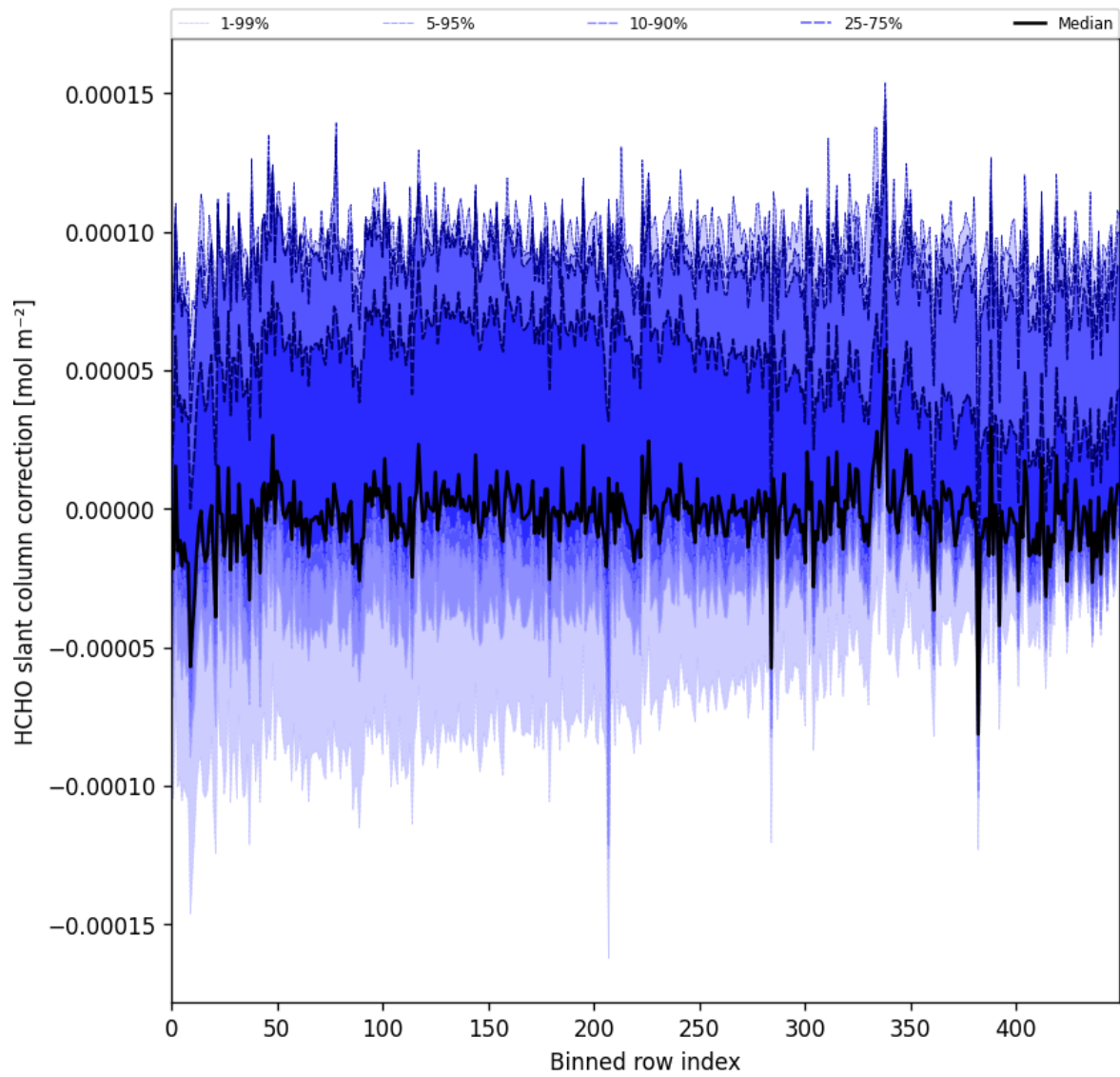
Figure 61: Along track statistics of “HCHO slant column correction” for 2025-05-02 to 2025-05-04
