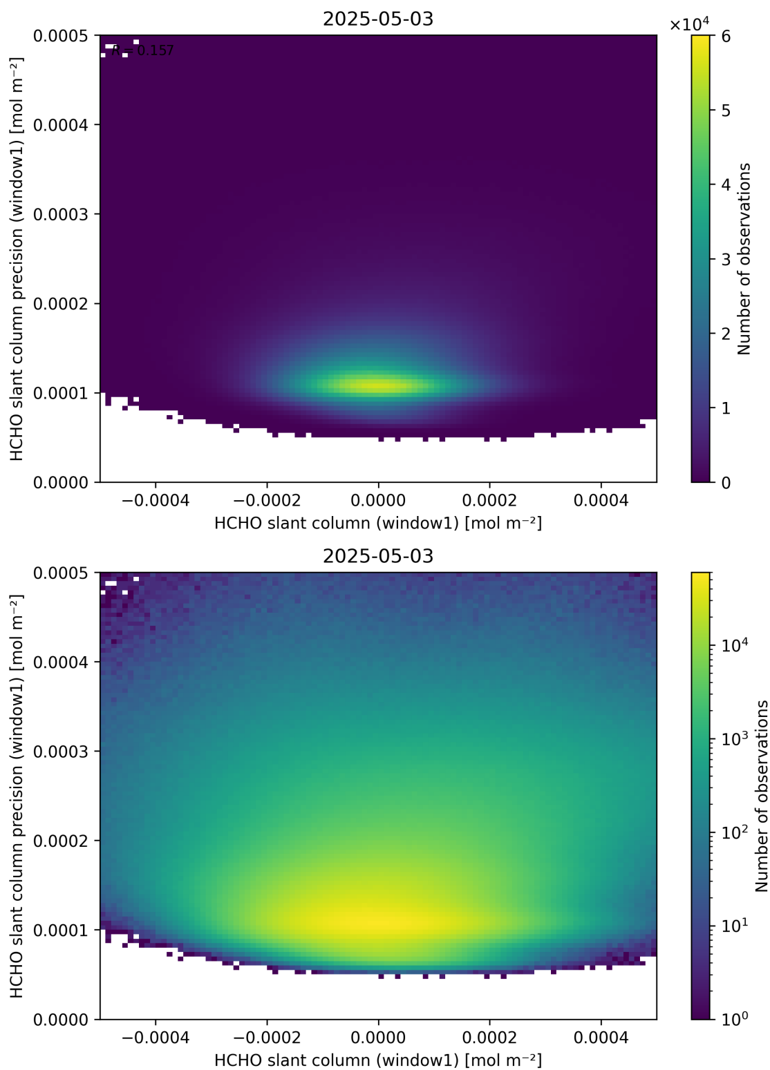
Figure 84: Scatter density plot of “HCHO slant column (window1)” against “HCHO slant column precision (window1)” for 2025-05-02 to 2025-05-04.
