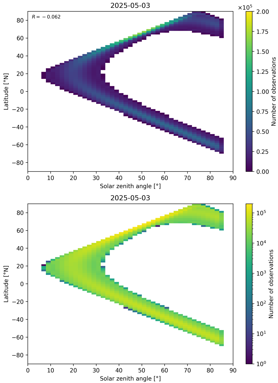
Figure 181: Scatter density plot of “Solar zenith angle” against “Latitude” for 2025-05-02 to 2025-05-04.
