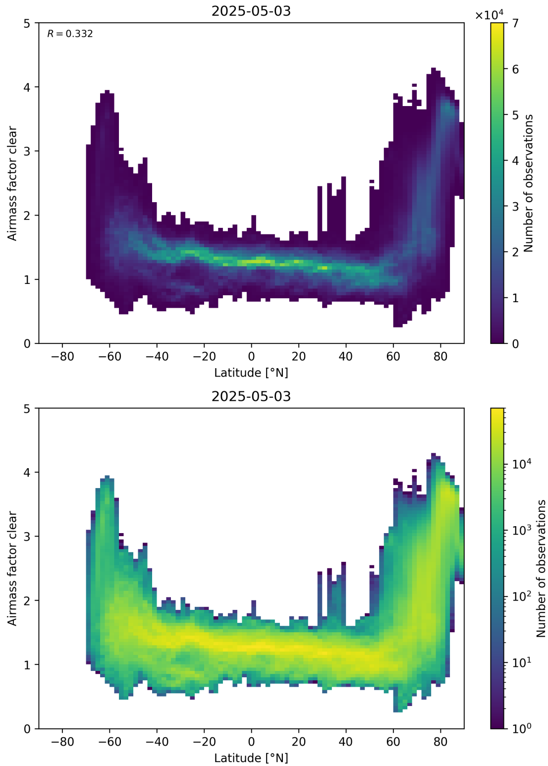
Figure 156: Scatter density plot of “Latitude” against “Airmass factor clear” for 2025-05-02 to 2025-05-04.
