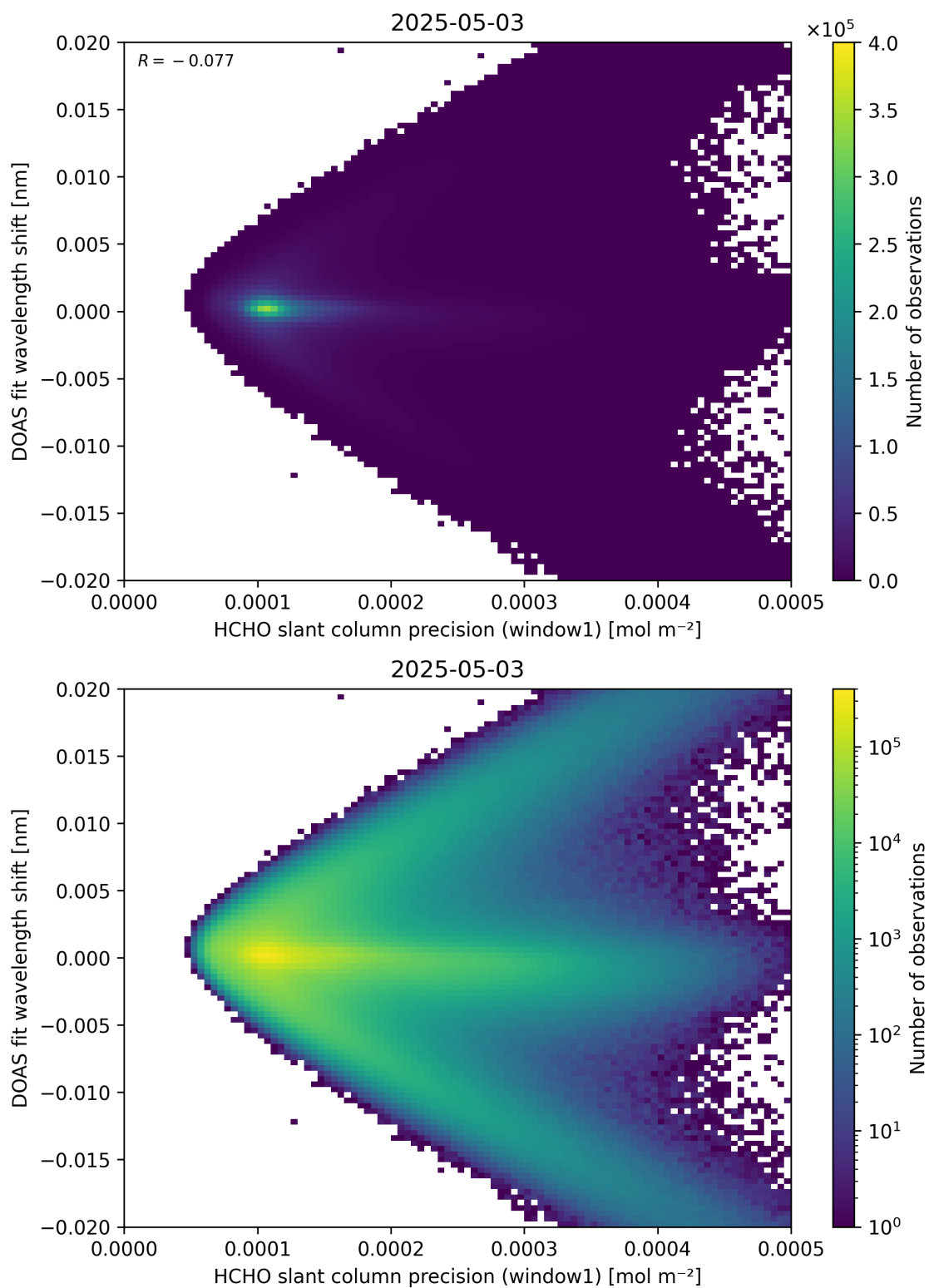
Figure 89: Scatter density plot of “HCHO slant column precision (window1)” against “DOAS fit wavelength shift” for 2025-05-02 to 2025-05-04.
