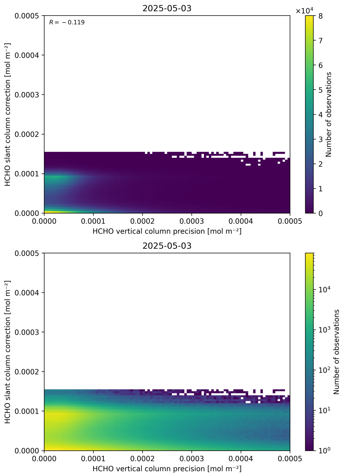
Figure 141: Scatter density plot of “HCHO vertical column precision” against “HCHO slant column correction” for 2025-05-02 to 2025-05-04.
