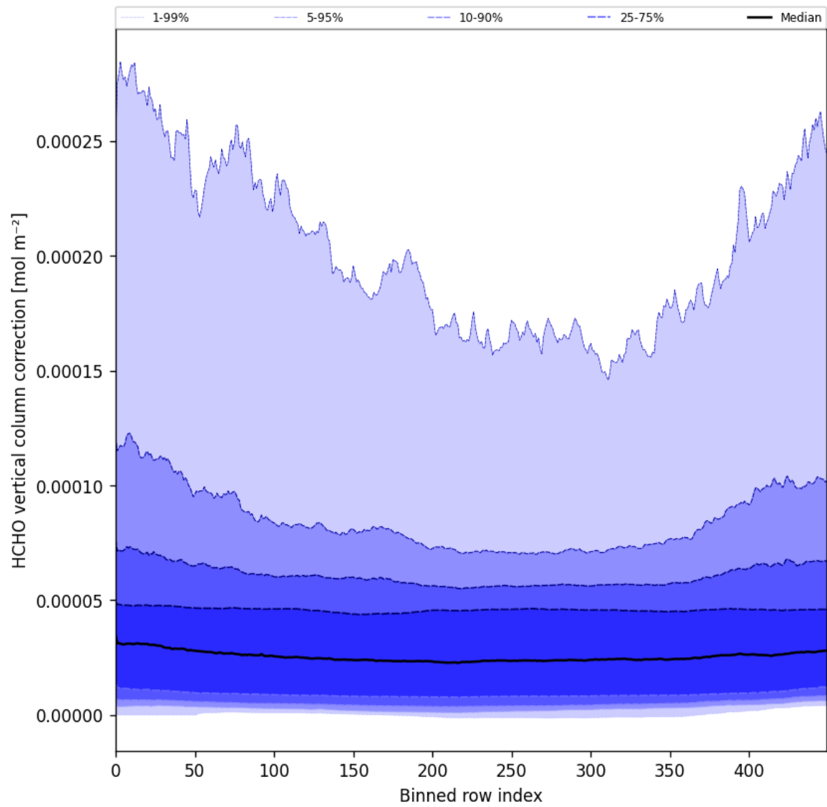
Figure 51: Along track statistics of “HCHO vertical column correction” for 2025-05-02 to 2025-05-04
