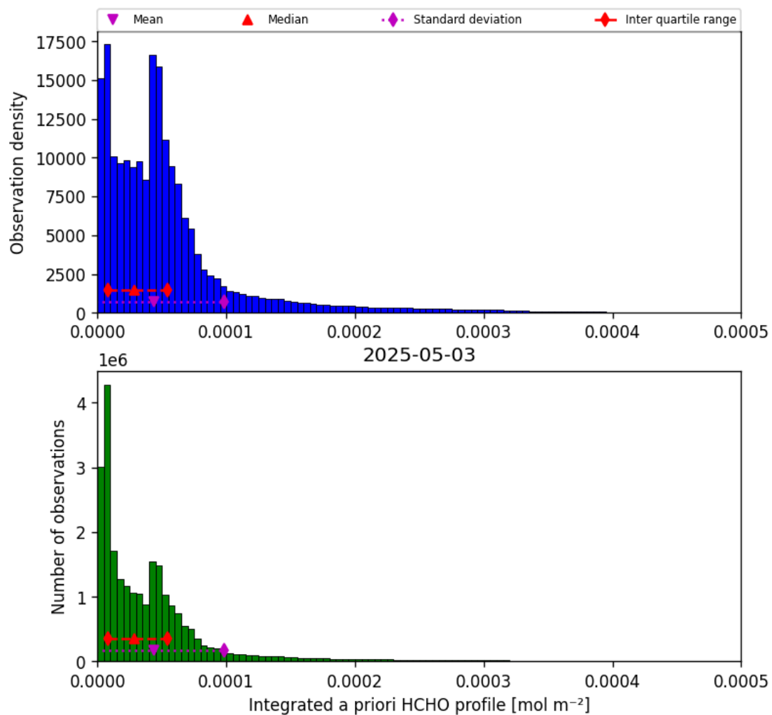
Figure 43: Histogram of “Integrated a priori HCHO profile” for 2025-05-02 to 2025-05-04
