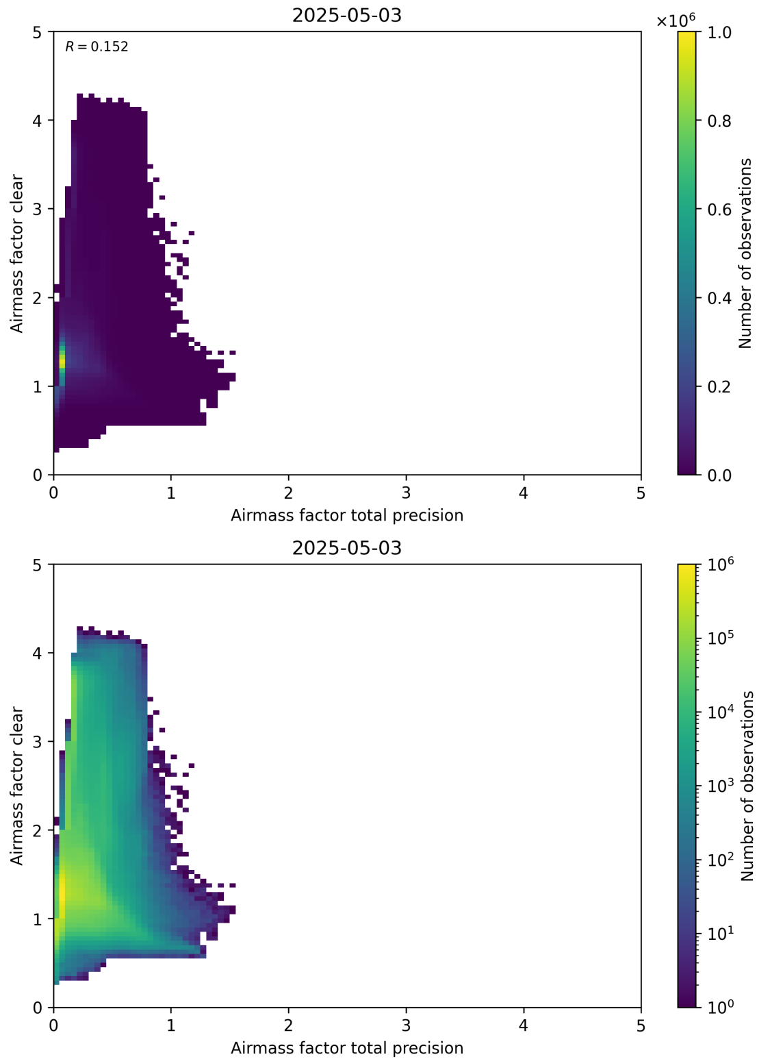
Figure 108: Scatter density plot of “Airmass factor total precision” against “Airmass factor clear” for 2025-05-02 to 2025-05-04.
