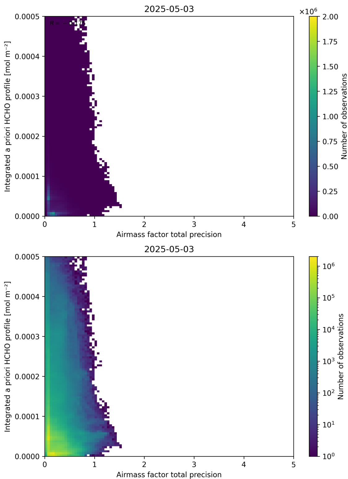
Figure 111: Scatter density plot of “Airmass factor total precision” against “Integrated a priori HCHO profile” for 2025-05-02 to 2025-05-04.
