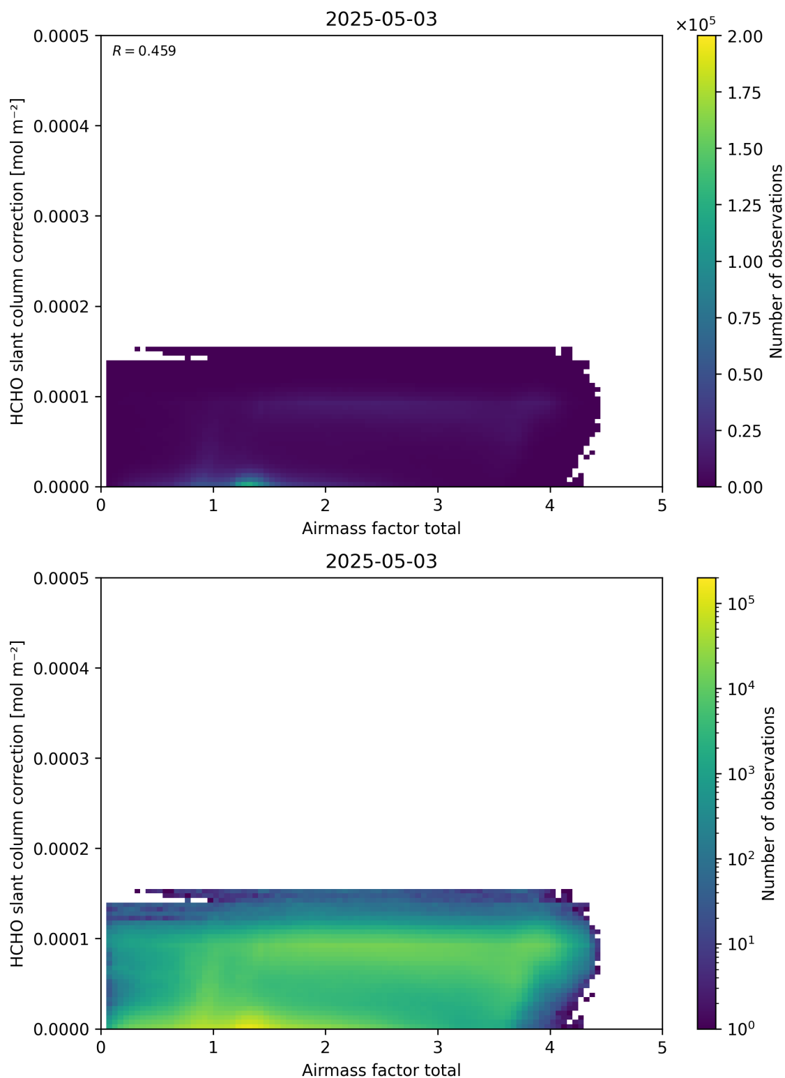
Figure 102: Scatter density plot of “Airmass factor total” against “HCHO slant column correction” for 2025-05-02 to 2025-05-04.
