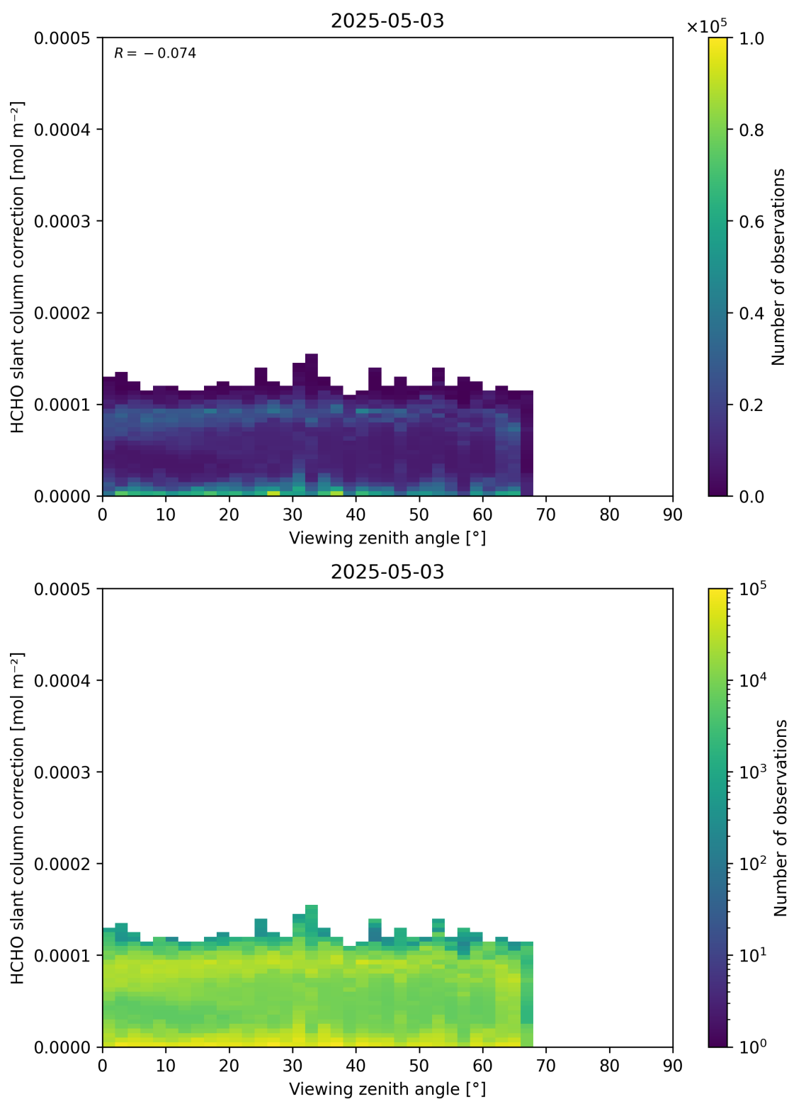
Figure 187: Scatter density plot of “Viewing zenith angle” against “HCHO slant column correction” for 2025-05-02 to 2025-05-04.
