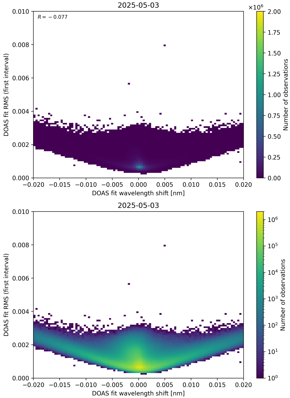
Figure 64: Scatter density plot of “DOAS fit wavelength shift” against “DOAS fit RMS (first interval)” for 2025-05-02 to 2025-05-04.
