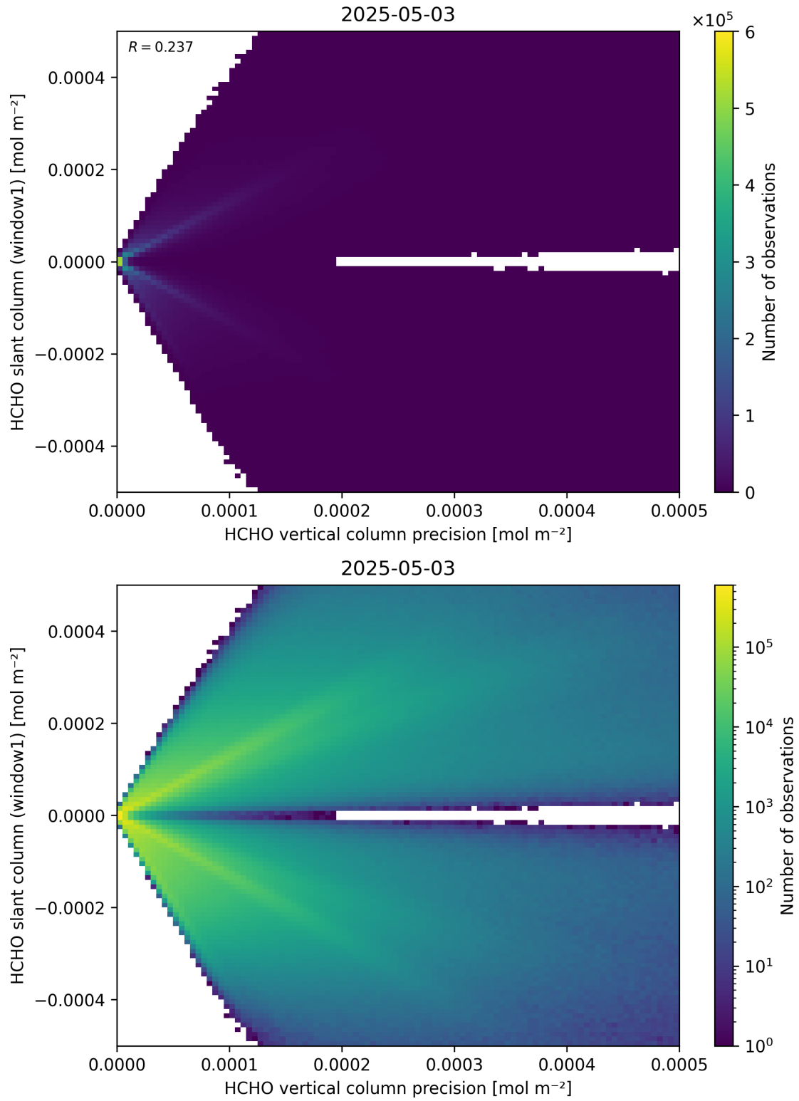
Figure 142: Scatter density plot of “HCHO vertical column precision” against “HCHO slant column (window1)” for 2025-05-02 to 2025-05-04.
