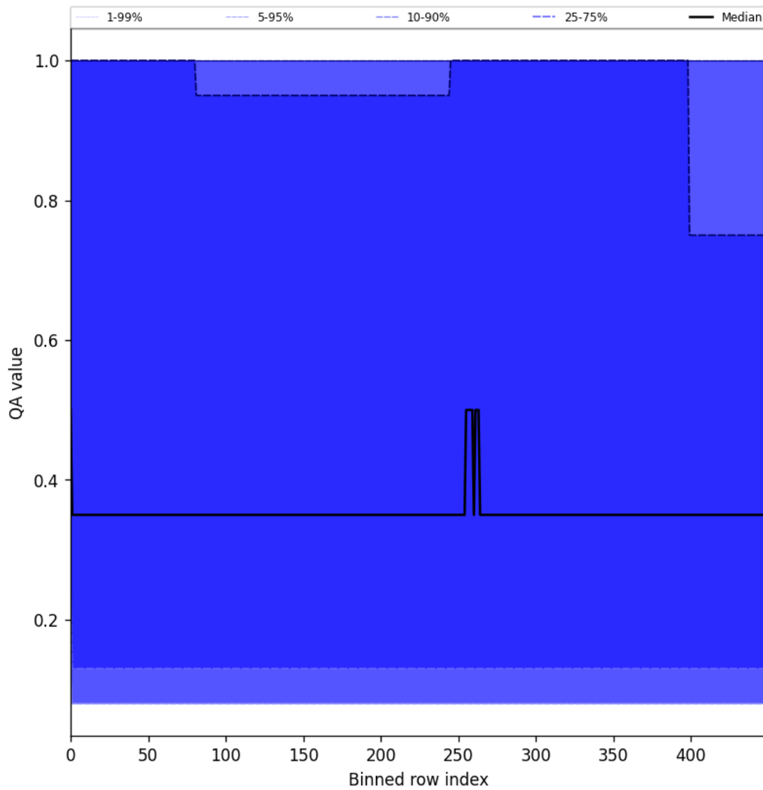
Figure 48: Along track statistics of “QA value” for 2025-05-02 to 2025-05-04
