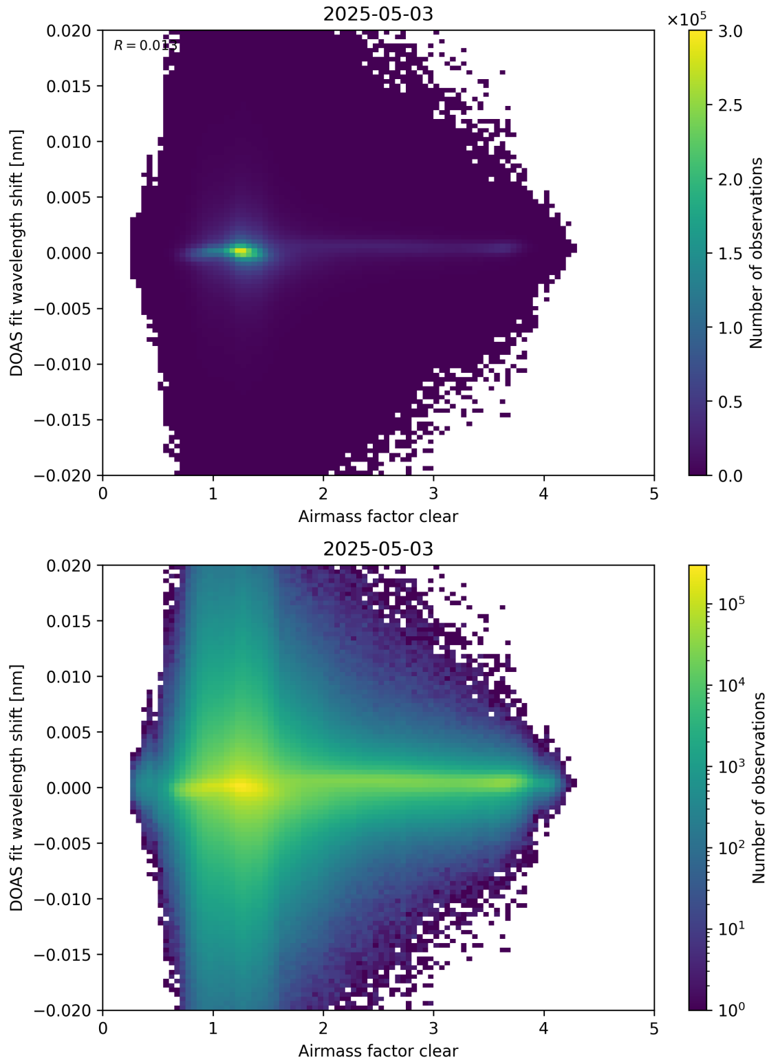
Figure 72: Scatter density plot of “Airmass factor clear” against “DOAS fit wavelength shift” for 2025-05-02 to 2025-05-04.
