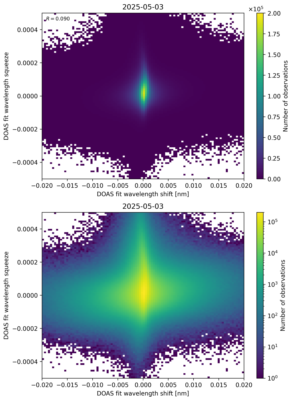
Figure 65: Scatter density plot of “DOAS fit wavelength shift” against “DOAS fit wavelength squeeze” for 2025-05-02 to 2025-05-04.
