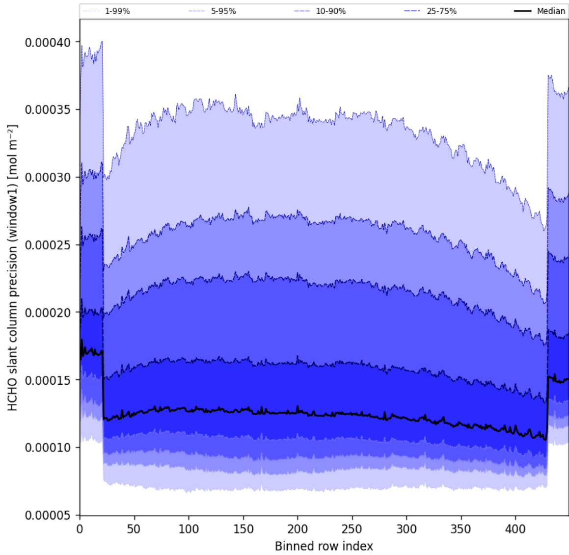
Figure 53: Along track statistics of “HCHO slant column precision (window1)” for 2025-05-02 to 2025-05-04
