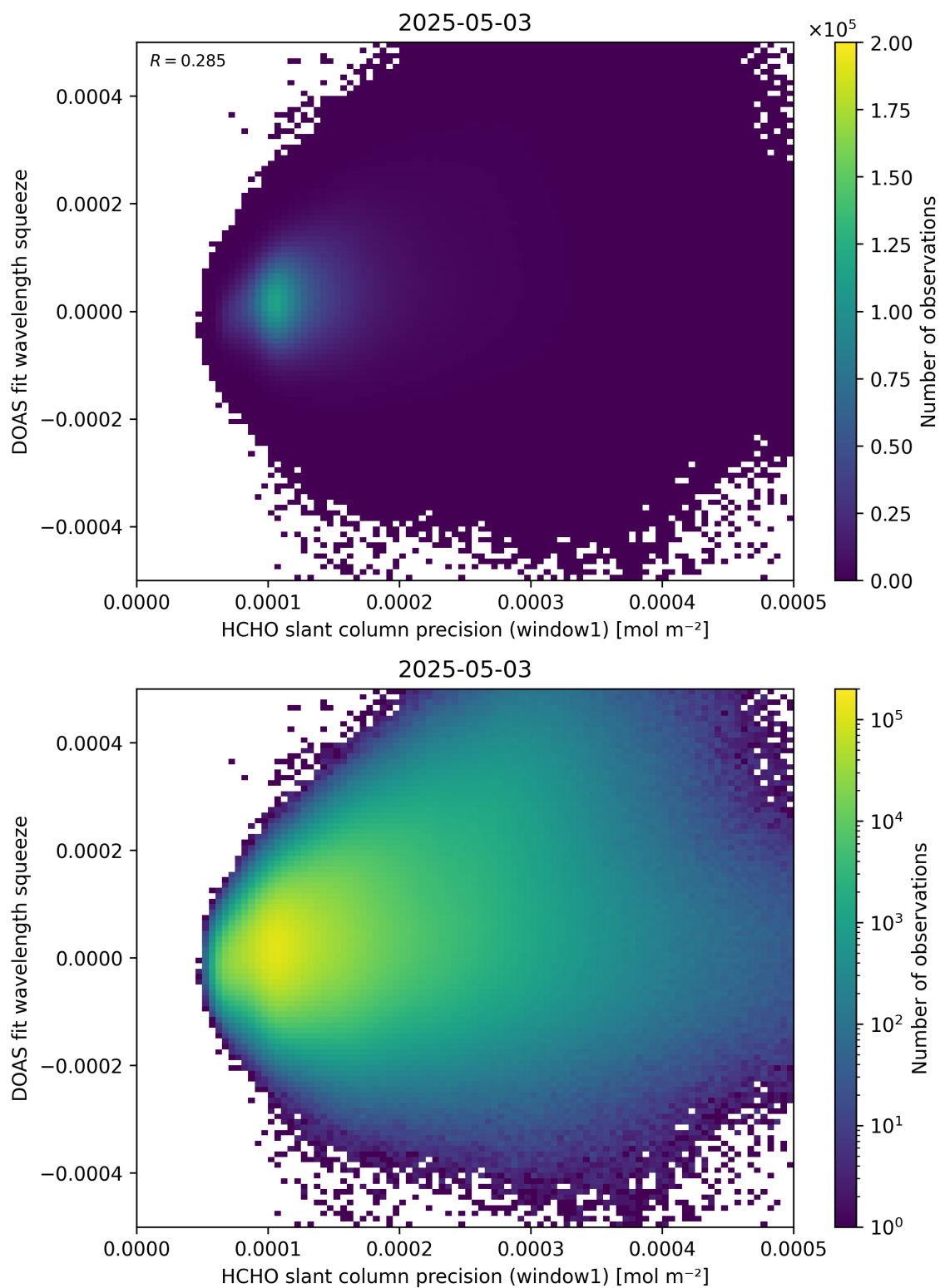
Figure 90: Scatter density plot of “HCHO slant column precision (window1)” against “DOAS fit wavelength squeeze” for 2025-05-02 to 2025-05-04.
