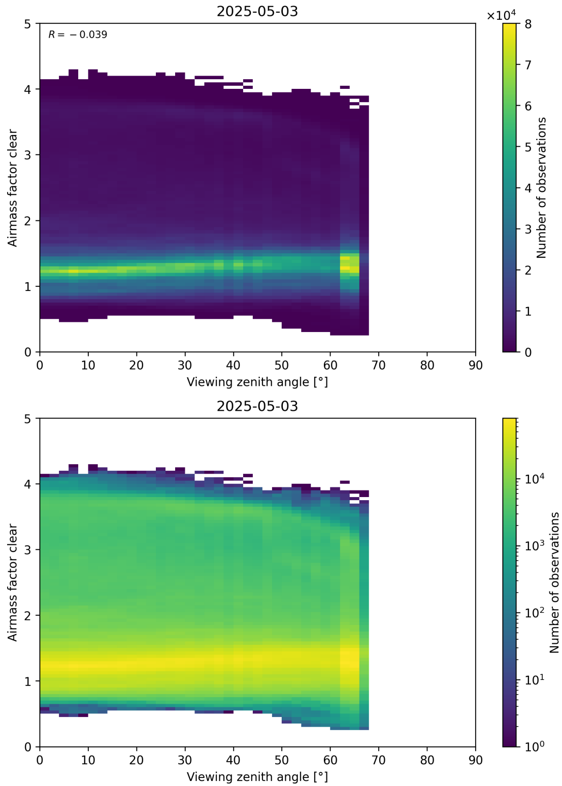
Figure 185: Scatter density plot of “Viewing zenith angle” against “Airmass factor clear” for 2025-05-02 to 2025-05-04.
