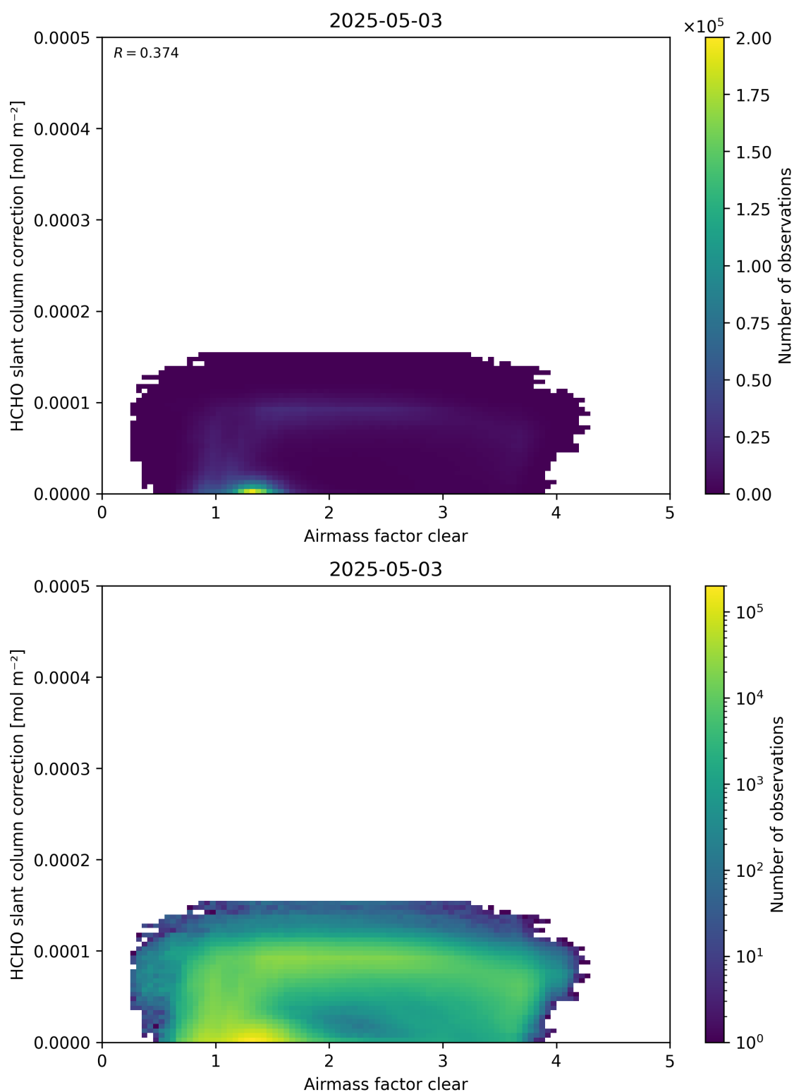
Figure 75: Scatter density plot of “Airmass factor clear” against “HCHO slant column correction” for 2025-05-02 to 2025-05-04.
