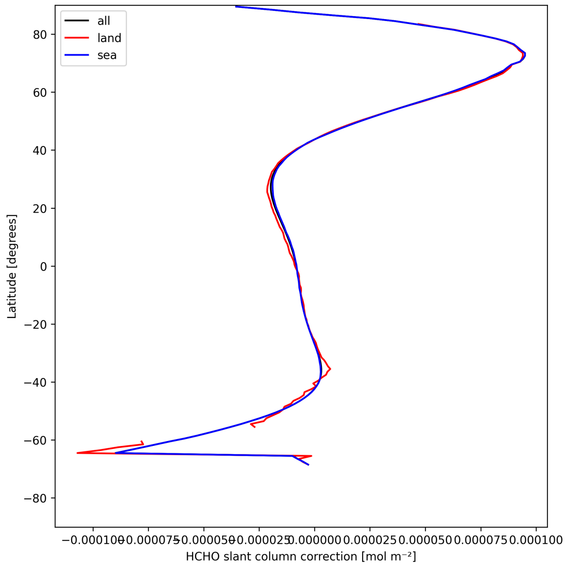
Figure 33: Zonal average of “HCHO slant column correction” for 2025-05-02 to 2025-05-04.
