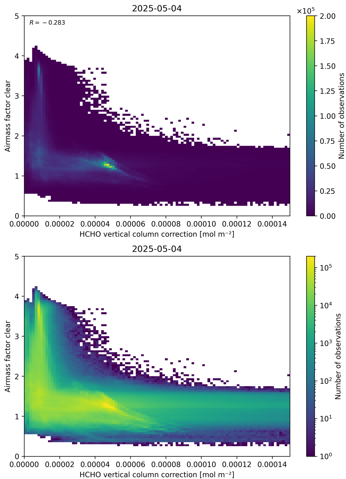
Figure 115: Scatter density plot of “HCHO vertical column correction” against “Airmass factor clear” for 2025-05-03 to 2025-05-05.
