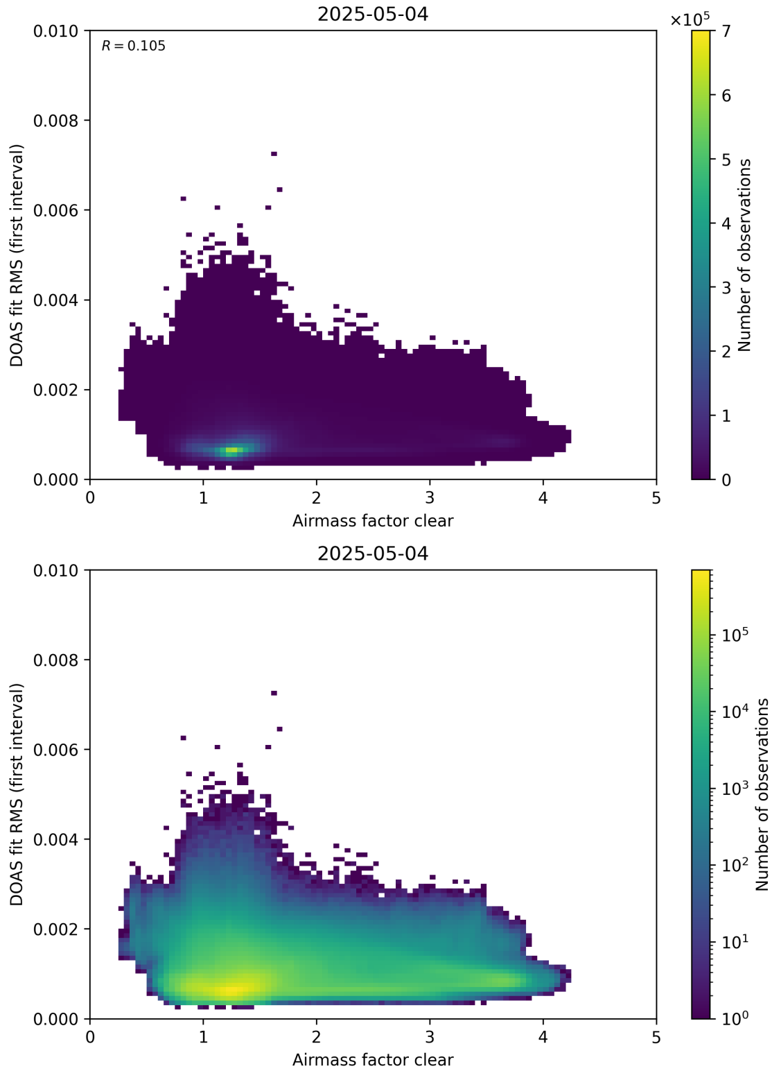
Figure 71: Scatter density plot of “Airmass factor clear” against “DOAS fit RMS (first interval)” for 2025-05-03 to 2025-05-05.
