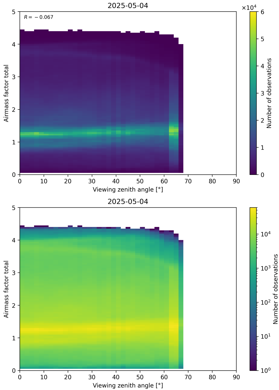
Figure 190: Scatter density plot of “Viewing zenith angle” against “Airmass factor total” for 2025-05-03 to 2025-05-05.
