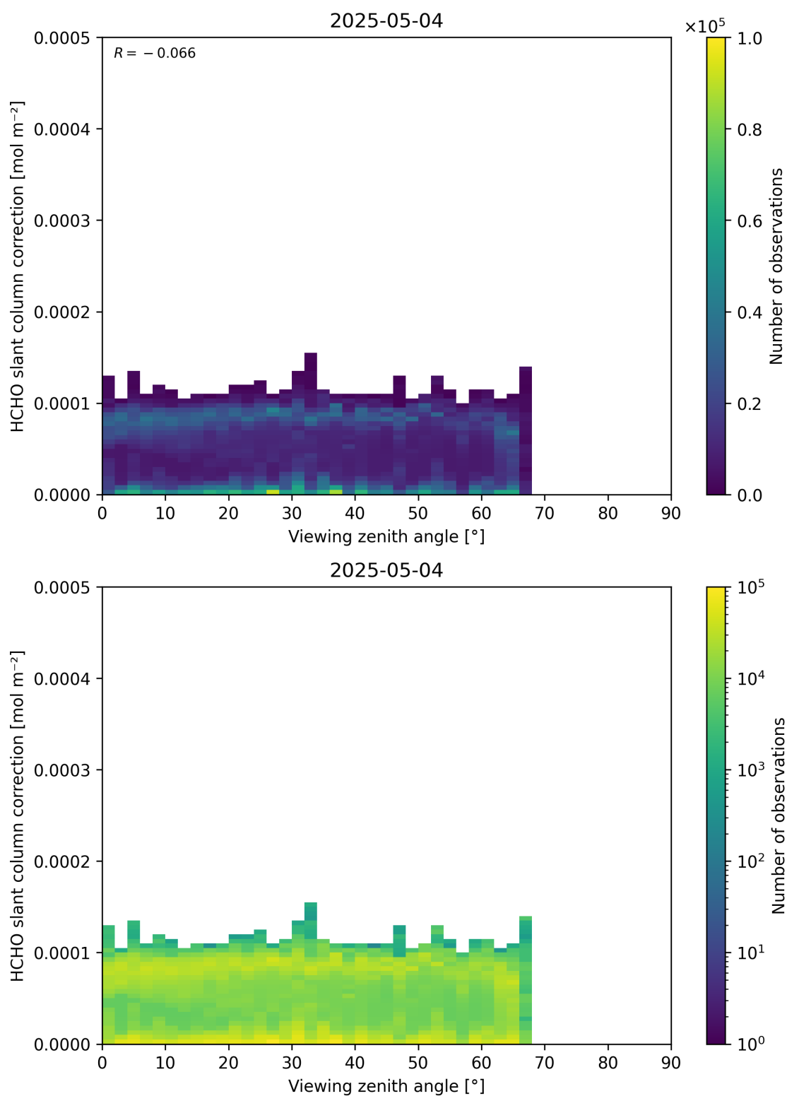
Figure 187: Scatter density plot of “Viewing zenith angle” against “HCHO slant column correction” for 2025-05-03 to 2025-05-05.
