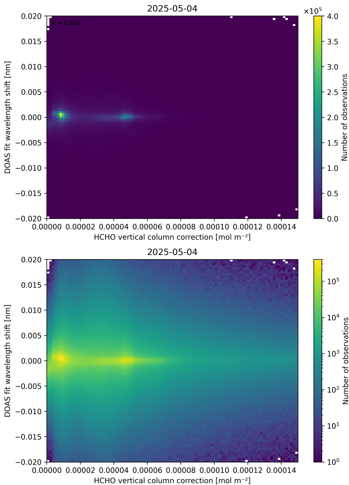
Figure 113: Scatter density plot of “HCHO vertical column correction” against “DOAS fit wavelength shift” for 2025-05-03 to 2025-05-05.
