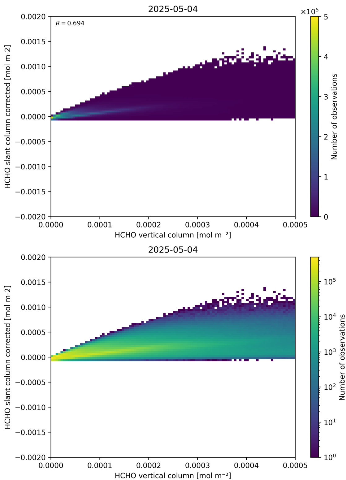
Figure 127: Scatter density plot of “HCHO vertical column” against “HCHO slant column corrected” for 2025-05-03 to 2025-05-05.
