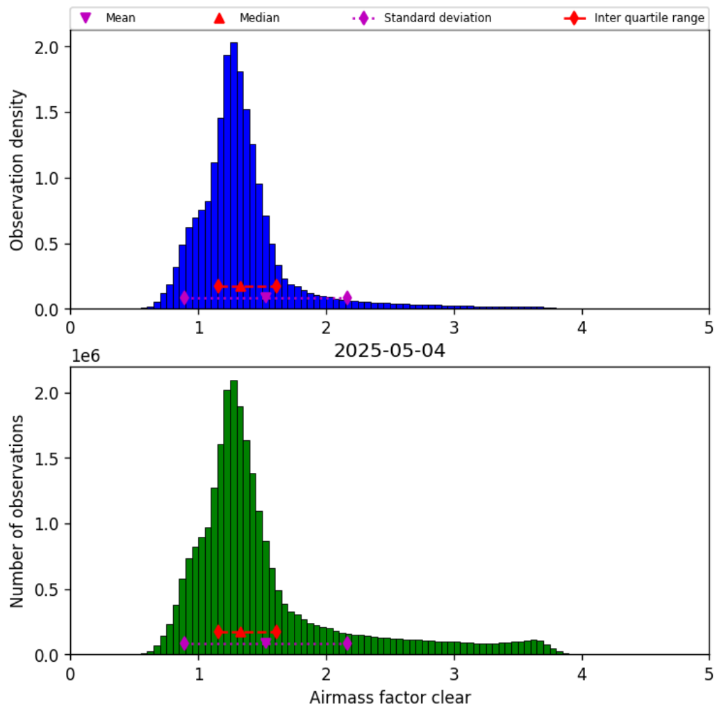
Figure 42: Histogram of “Airmass factor clear” for 2025-05-03 to 2025-05-05
