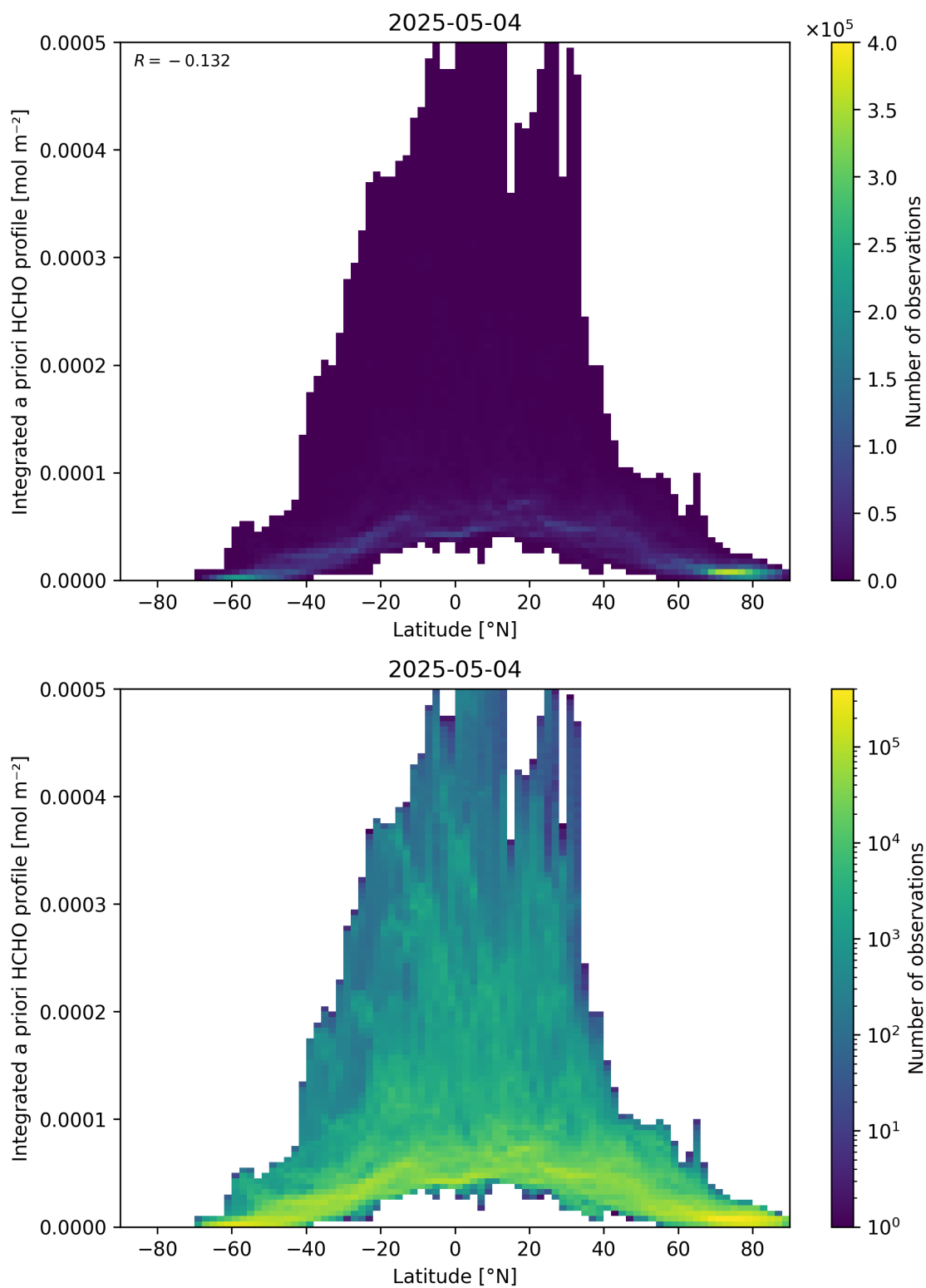
Figure 166: Scatter density plot of “Latitude” against “Integrated a priori HCHO profile” for 2025-05-03 to 2025-05-05.
