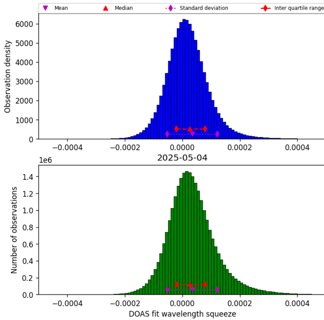
Figure 45: Histogram of “DOAS fit wavelength squeeze” for 2025-05-03 to 2025-05-05
