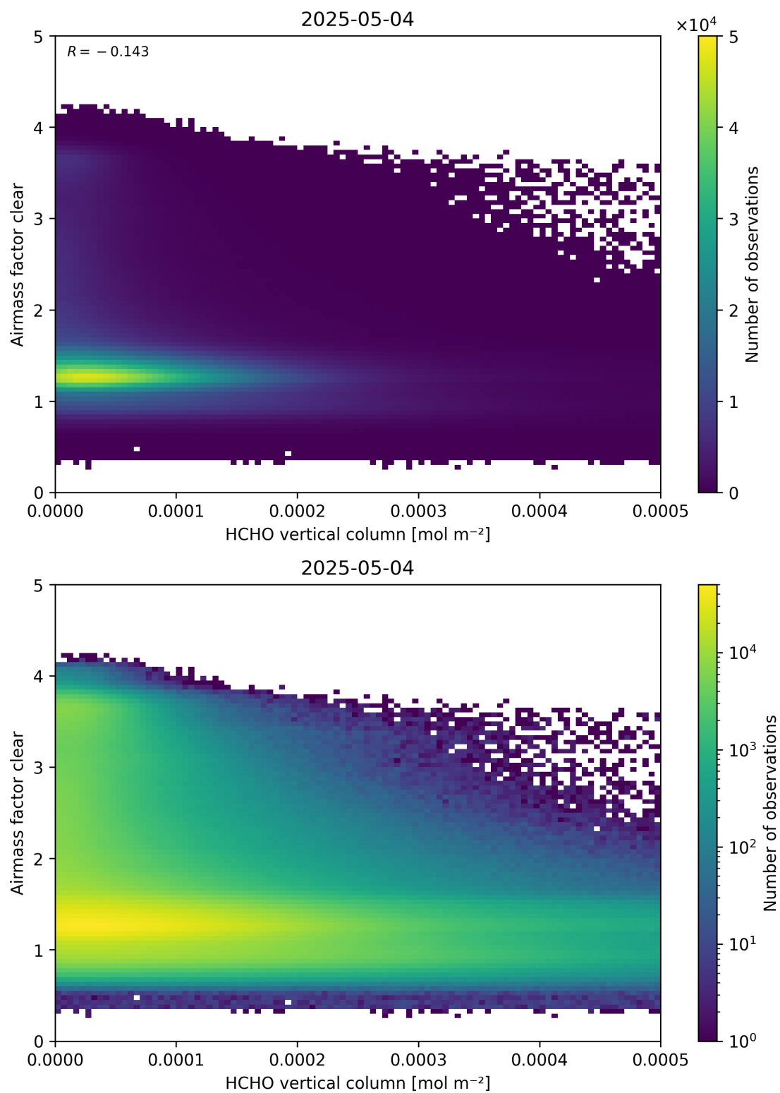
Figure 126: Scatter density plot of “HCHO vertical column” against “Airmass factor clear” for 2025-05-03 to 2025-05-05.
