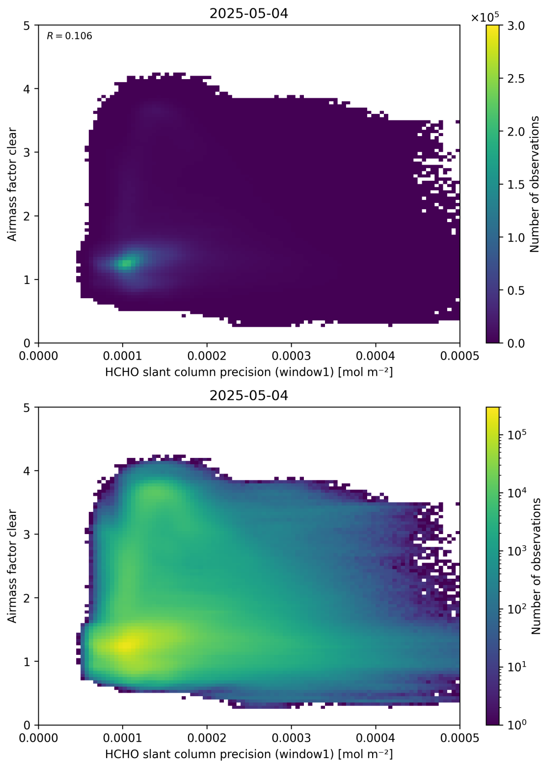
Figure 91: Scatter density plot of “HCHO slant column precision (window1)” against “Airmass factor clear” for 2025-05-03 to 2025-05-05.
