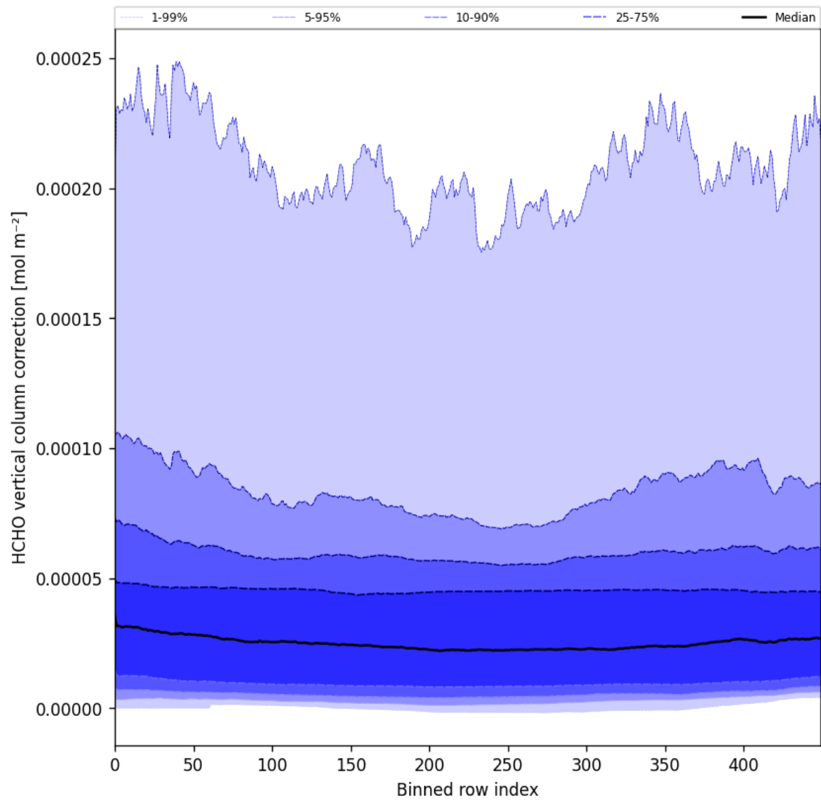
Figure 51: Along track statistics of “HCHO vertical column correction” for 2025-05-03 to 2025-05-05
