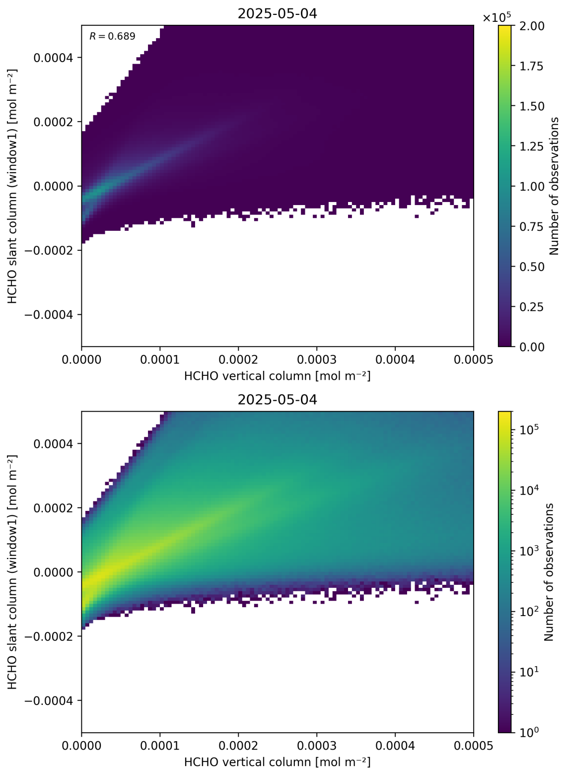
Figure 129: Scatter density plot of “HCHO vertical column” against “HCHO slant column (window1)” for 2025-05-03 to 2025-05-05.
