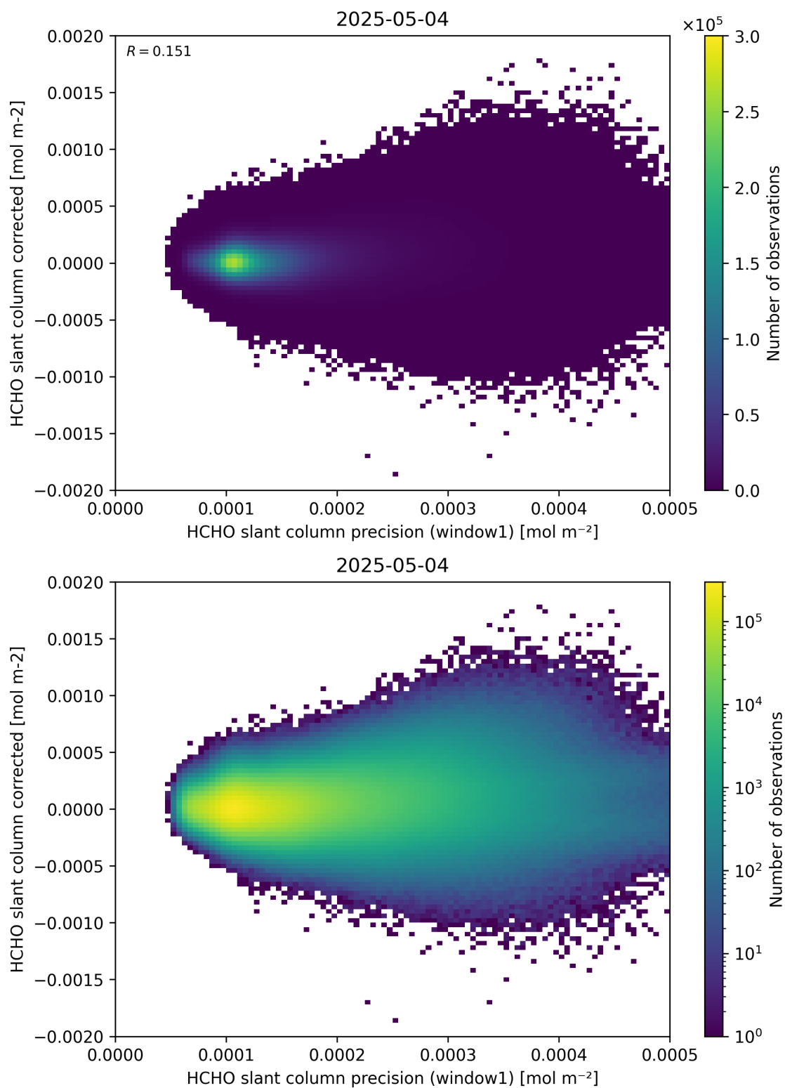
Figure 92: Scatter density plot of “HCHO slant column precision (window1)” against “HCHO slant column corrected” for 2025-05-03 to 2025-05-05.
