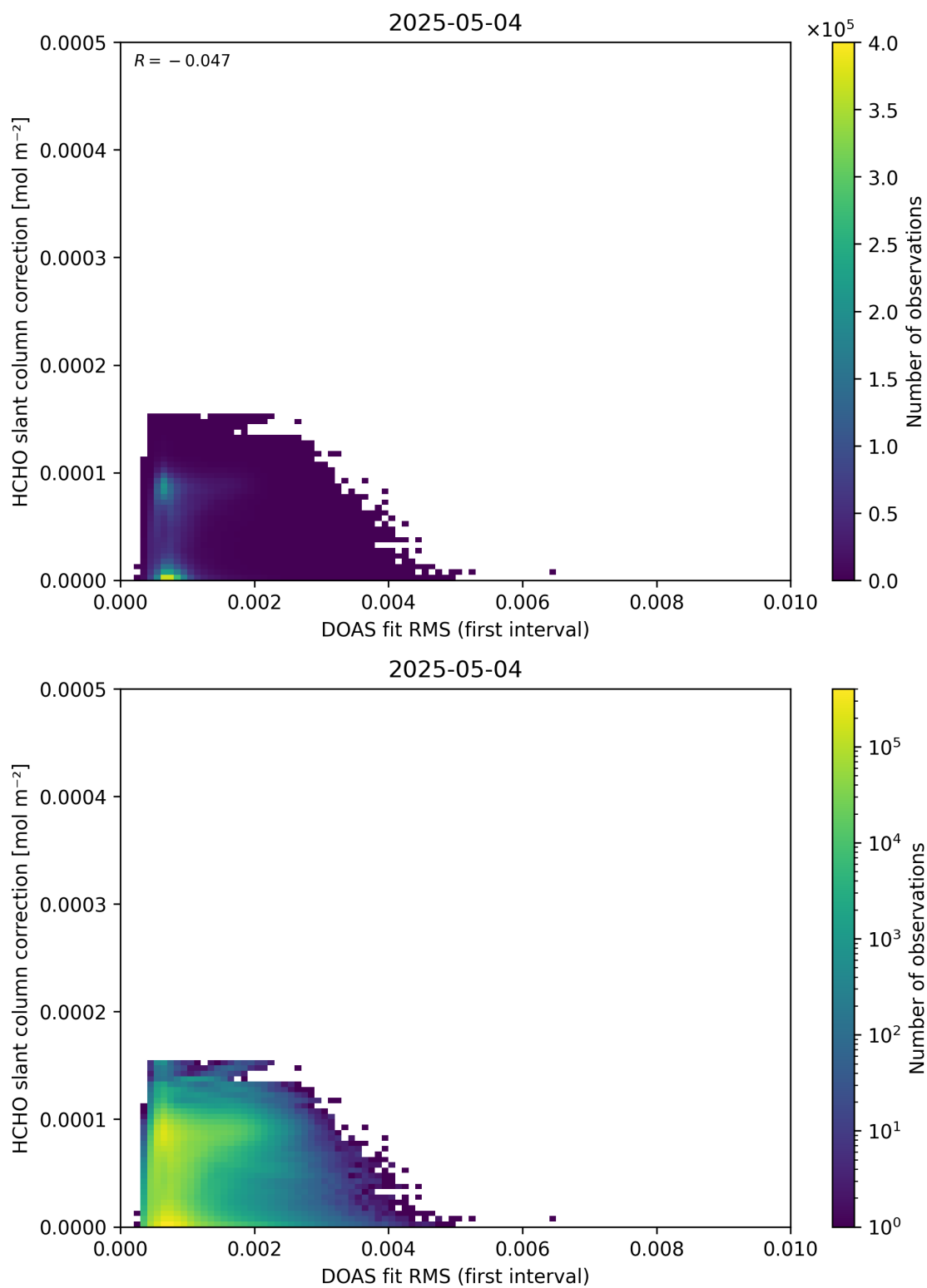
Figure 63: Scatter density plot of “DOAS fit RMS (first interval)” against “HCHO slant column correction” for 2025-05-03 to 2025-05-05.
