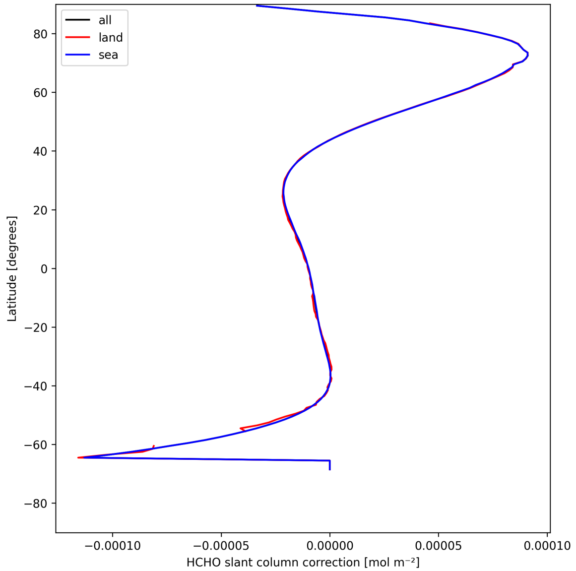
Figure 33: Zonal average of “HCHO slant column correction” for 2025-05-03 to 2025-05-05.
