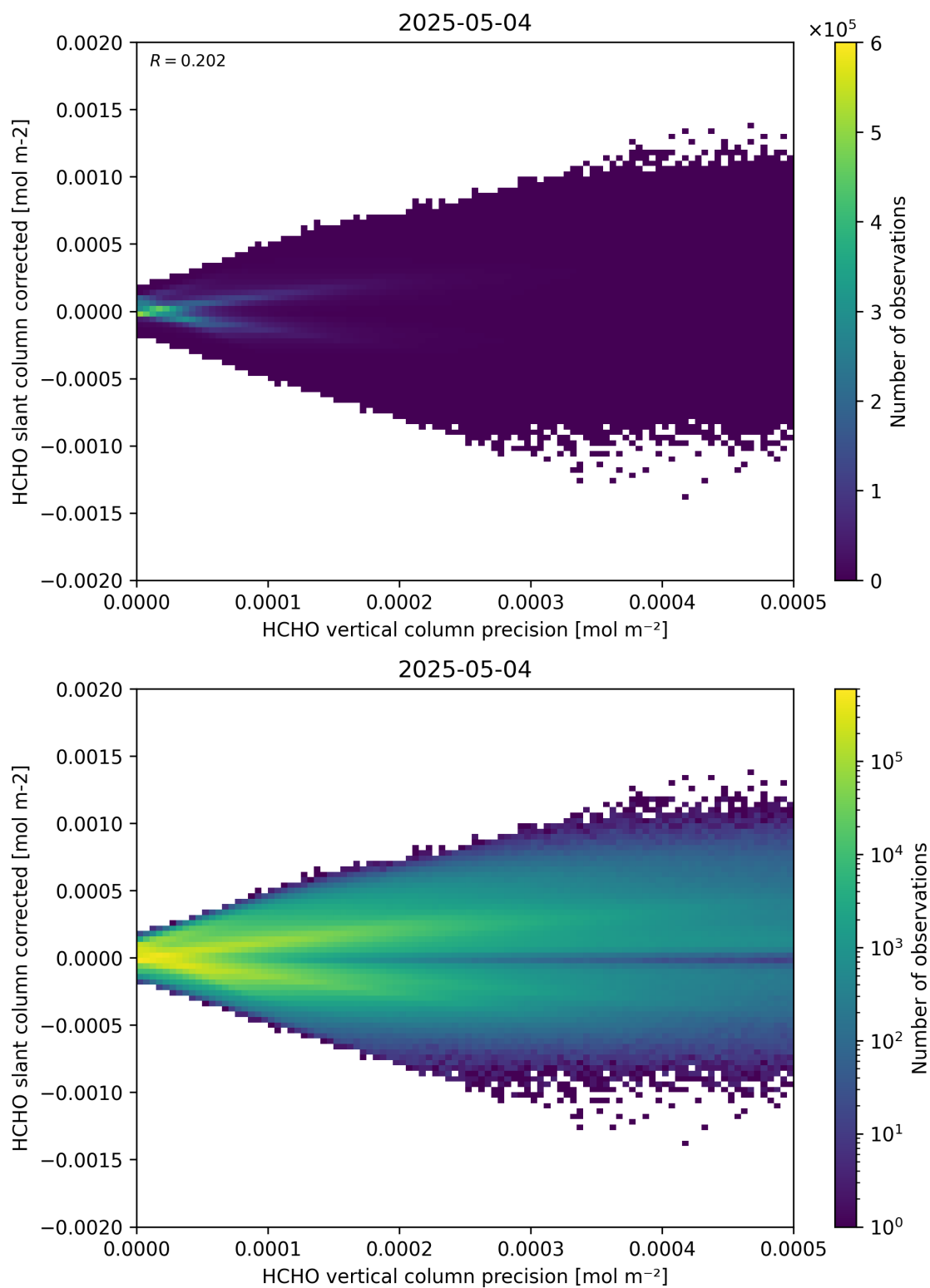
Figure 140: Scatter density plot of “HCHO vertical column precision” against “HCHO slant column corrected” for 2025-05-03 to 2025-05-05.
