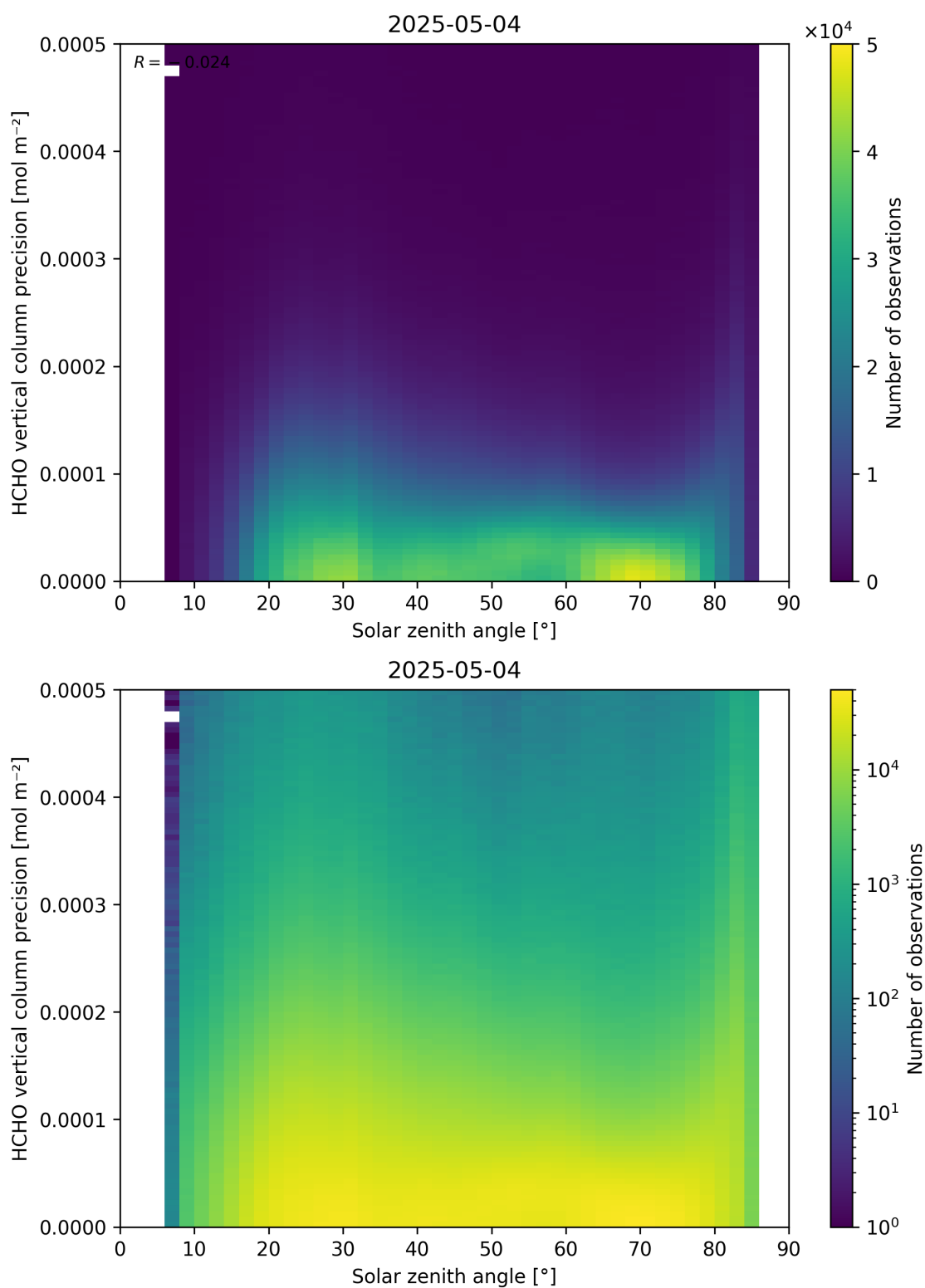
Figure 179: Scatter density plot of “Solar zenith angle” against “HCHO vertical column precision” for 2025-05-03 to 2025-05-05.
