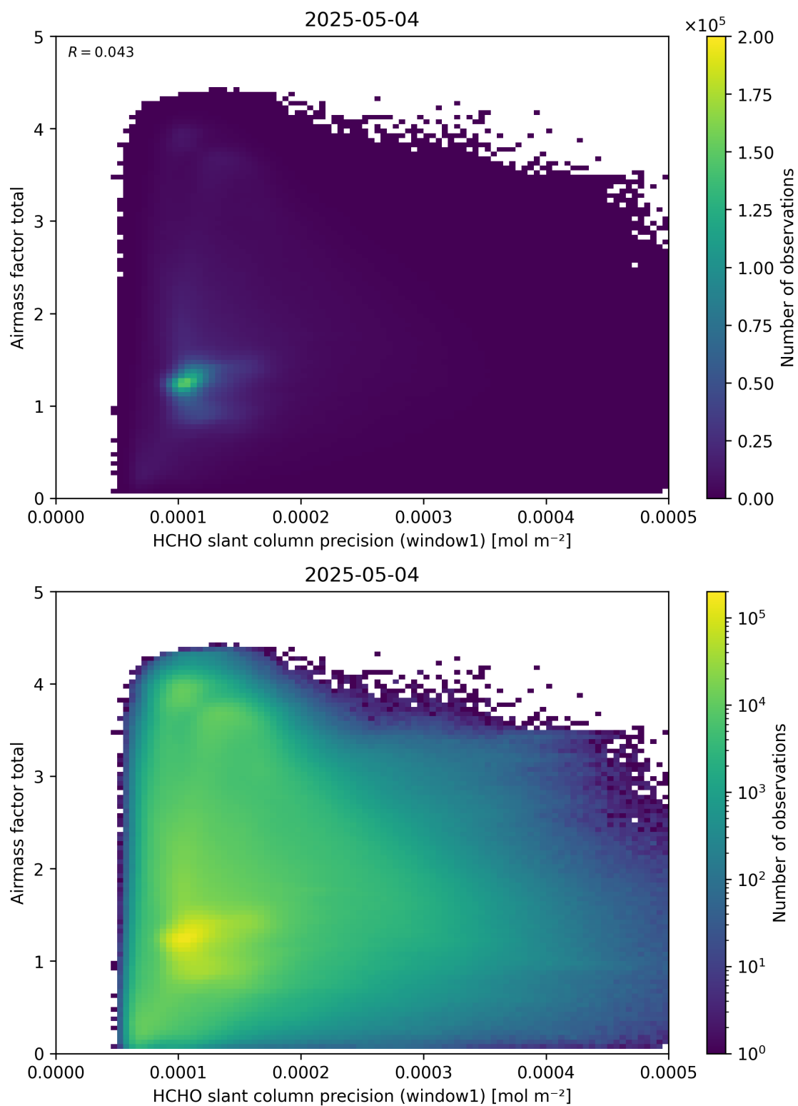
Figure 94: Scatter density plot of “HCHO slant column precision (window1)” against “Airmass factor total” for 2025-05-03 to 2025-05-05.
