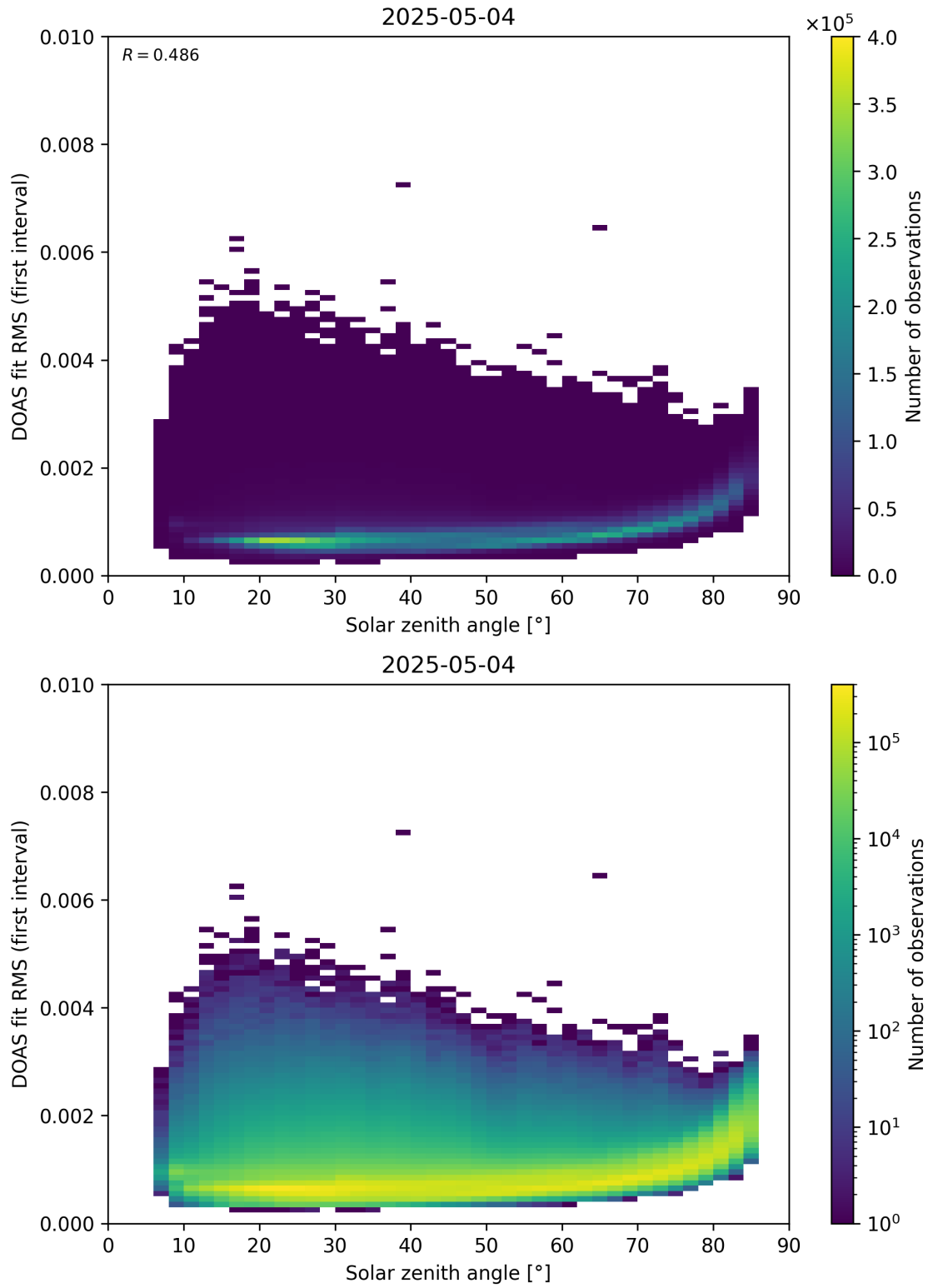
Figure 167: Scatter density plot of “Solar zenith angle” against “DOAS fit RMS (first interval)” for 2025-05-03 to 2025-05-05.
