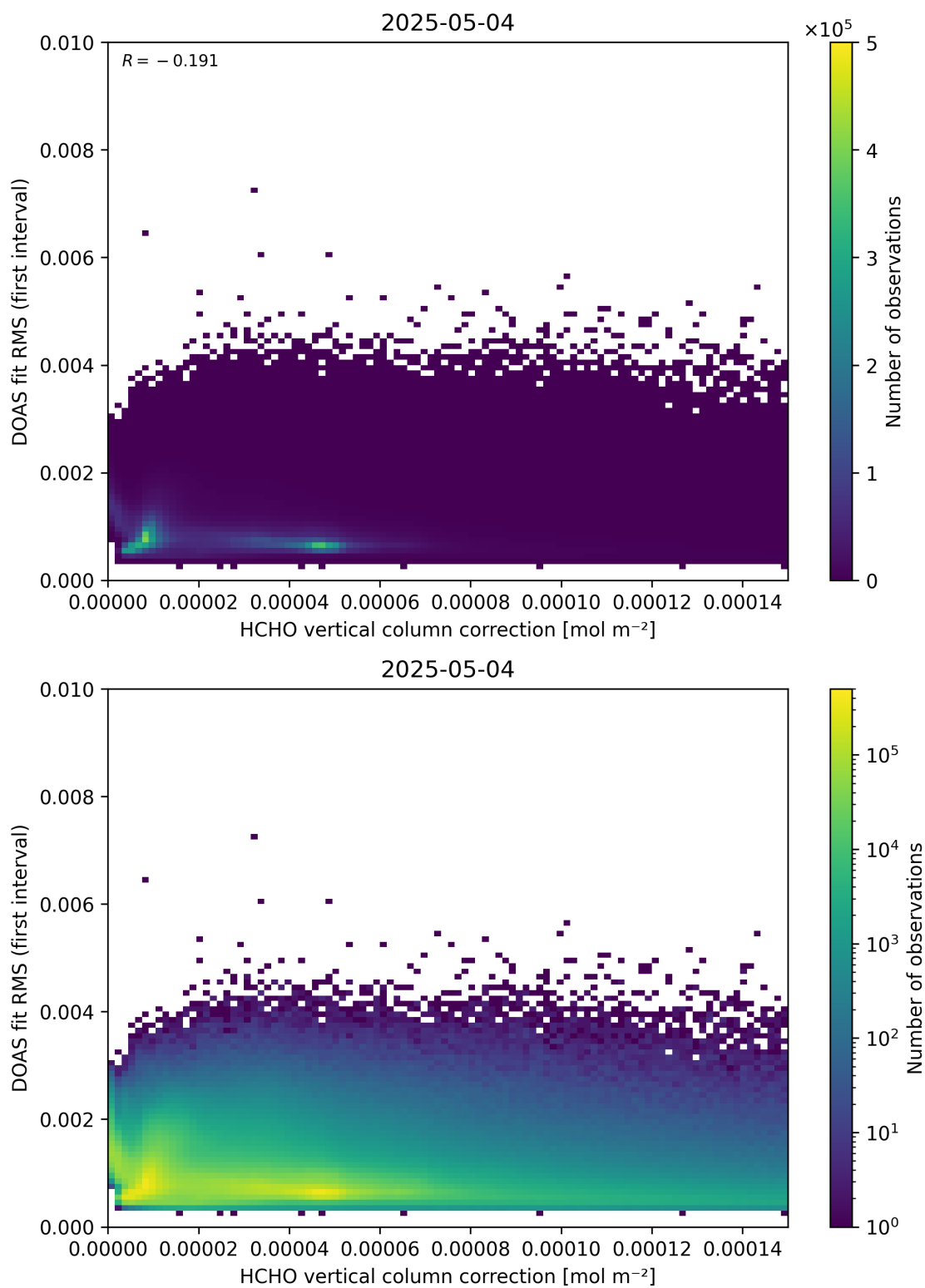
Figure 112: Scatter density plot of “HCHO vertical column correction” against “DOAS fit RMS (first interval)” for 2025-05-03 to 2025-05-05.
