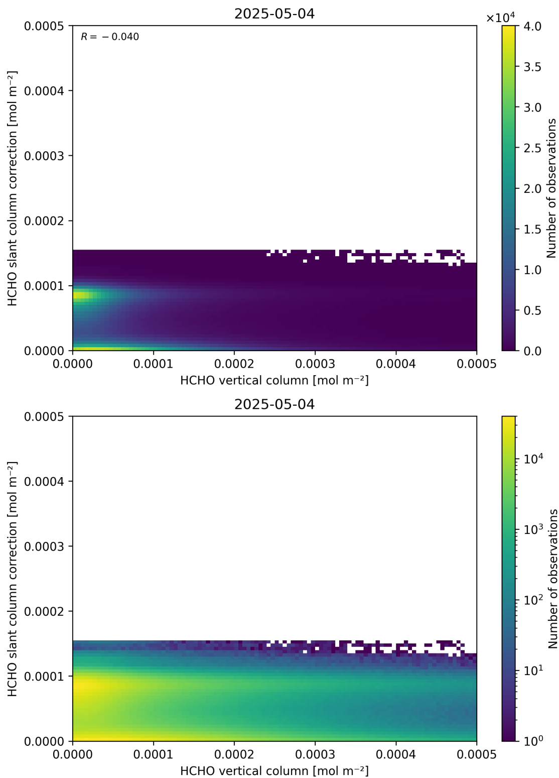
Figure 128: Scatter density plot of “HCHO vertical column” against “HCHO slant column correction” for 2025-05-03 to 2025-05-05.
