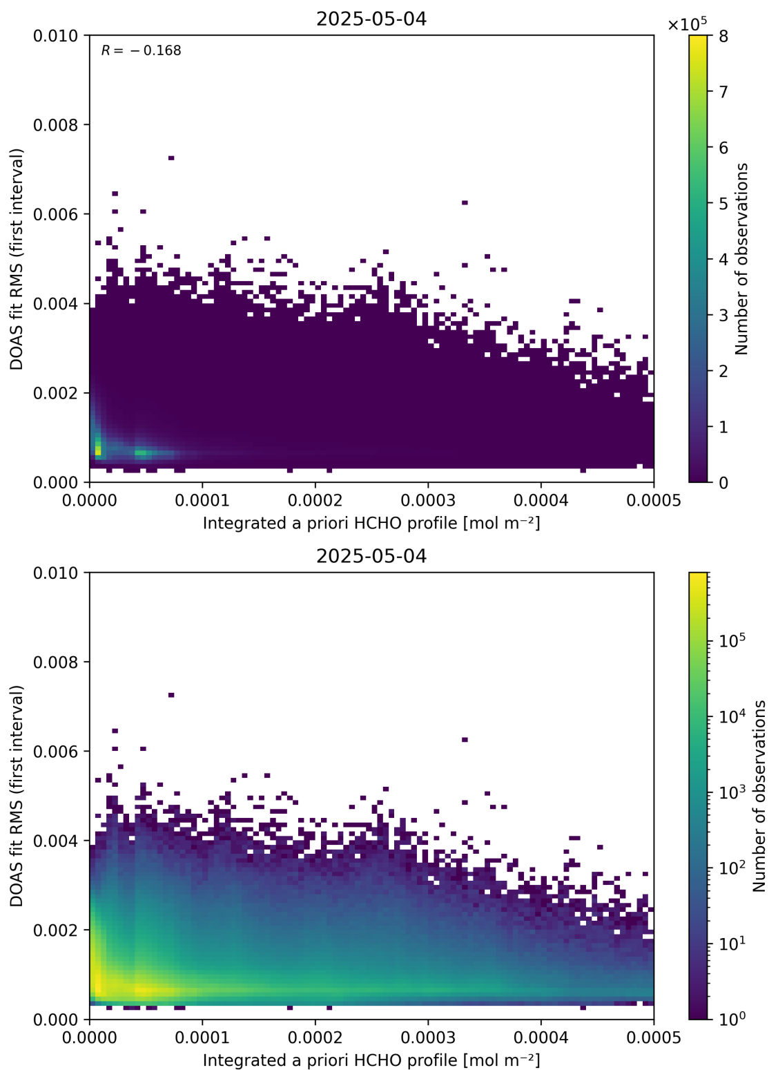
Figure 148: Scatter density plot of “Integrated a priori HCHO profile” against “DOAS fit RMS (first interval)” for 2025-05-03 to 2025-05-05.
