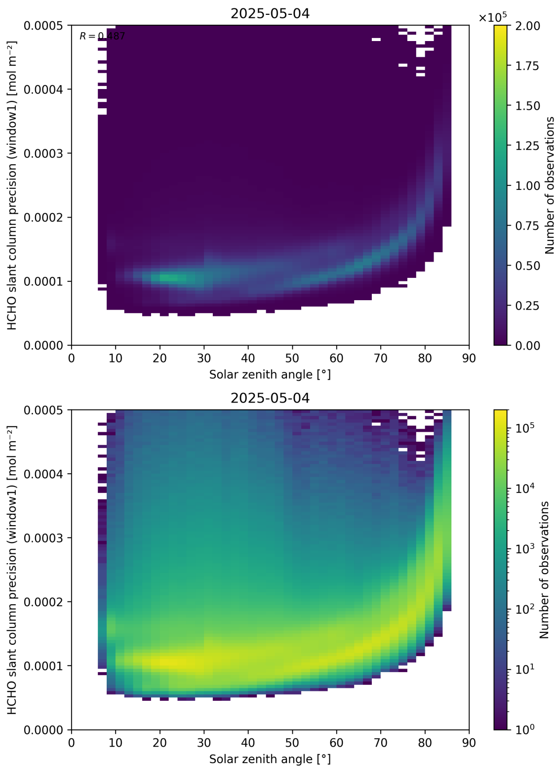
Figure 174: Scatter density plot of “Solar zenith angle” against “HCHO slant column precision (window1)” for 2025-05-03 to 2025-05-05.
