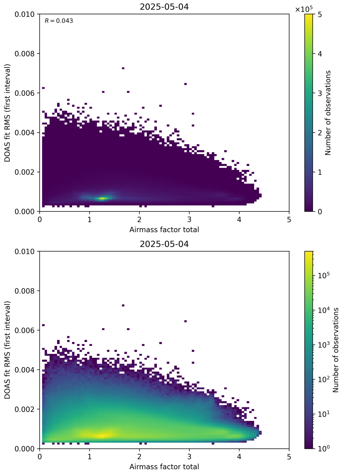
Figure 97: Scatter density plot of “Airmass factor total” against “DOAS fit RMS (first interval)” for 2025-05-03 to 2025-05-05.
