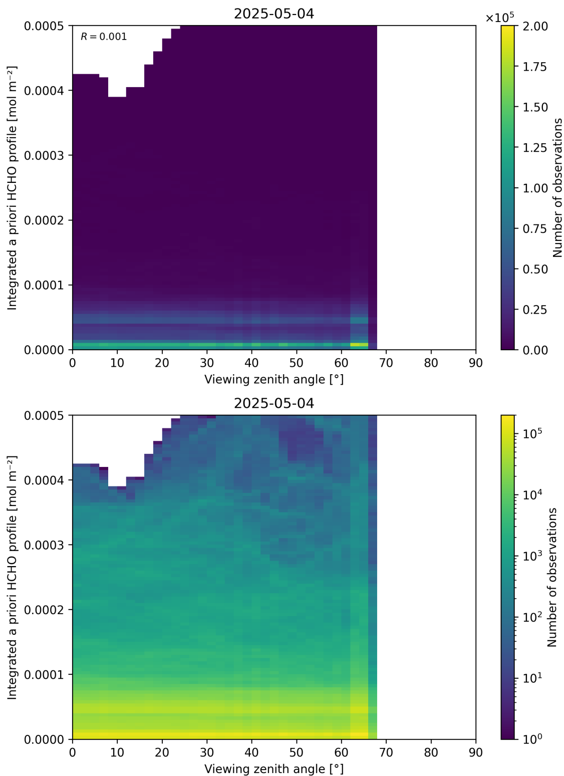
Figure 195: Scatter density plot of “Viewing zenith angle” against “Integrated a priori HCHO profile” for 2025-05-03 to 2025-05-05.
