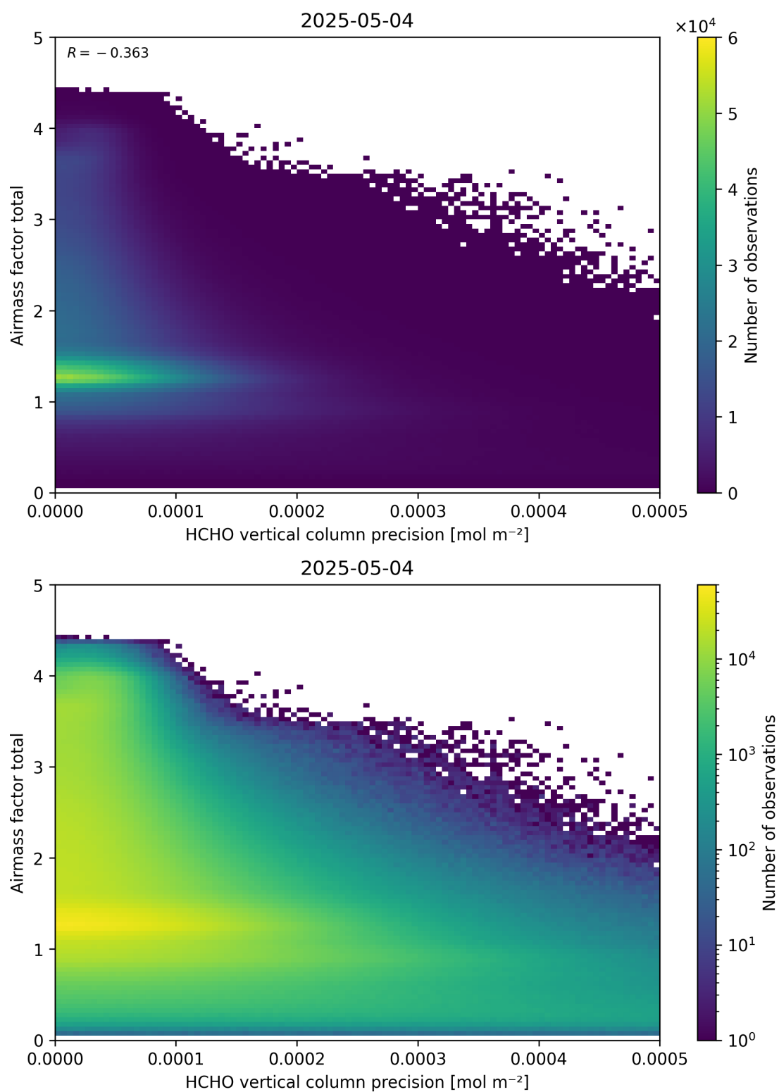
Figure 144: Scatter density plot of “HCHO vertical column precision” against “Airmass factor total” for 2025-05-03 to 2025-05-05.
