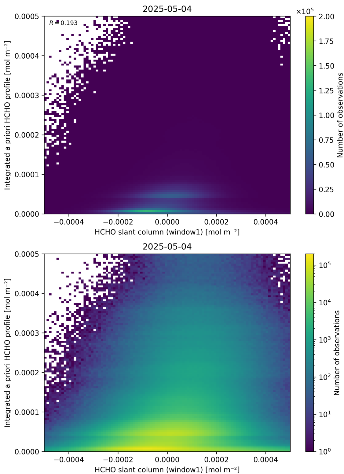
Figure 87: Scatter density plot of “HCHO slant column (window1)” against “Integrated a priori HCHO profile” for 2025-05-03 to 2025-05-05.
