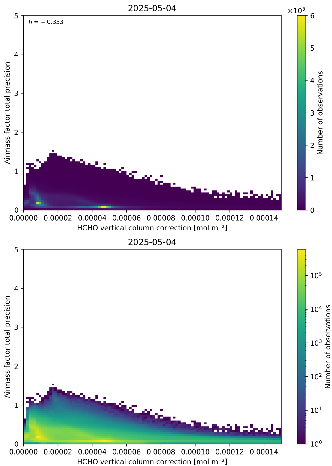
Figure 121: Scatter density plot of “HCHO vertical column correction” against “Airmass factor total precision” for 2025-05-03 to 2025-05-05.
