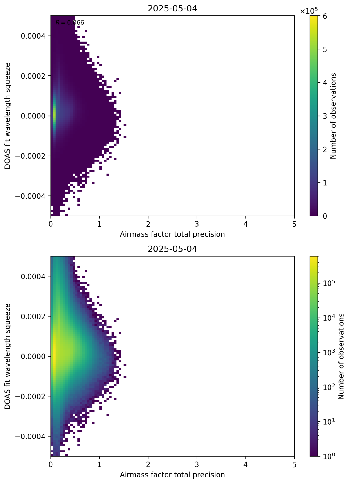
Figure 107: Scatter density plot of “Airmass factor total precision” against “DOAS fit wavelength squeeze” for 2025-05-03 to 2025-05-05.
