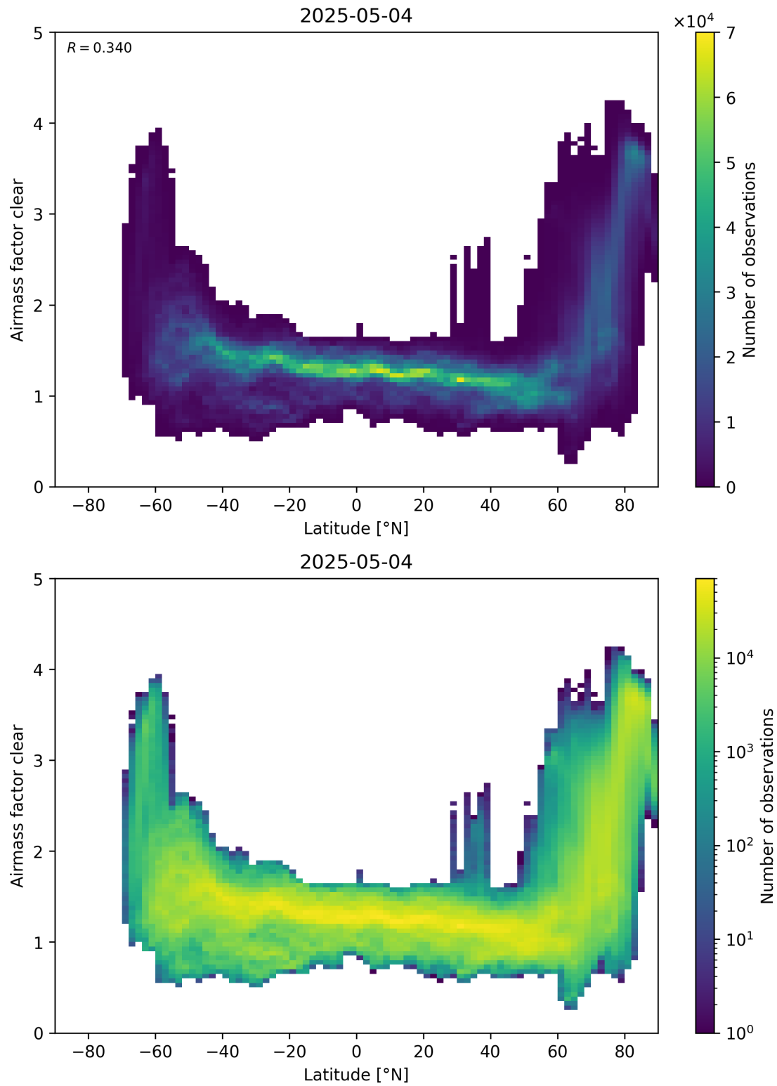
Figure 156: Scatter density plot of “Latitude” against “Airmass factor clear” for 2025-05-03 to 2025-05-05.
