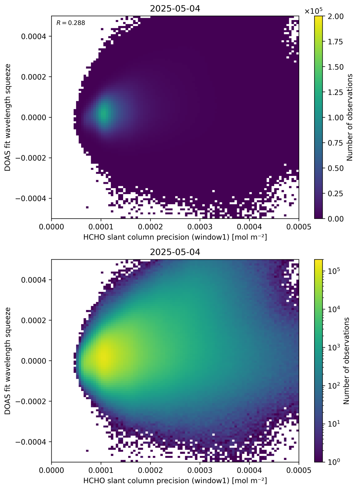
Figure 90: Scatter density plot of “HCHO slant column precision (window1)” against “DOAS fit wavelength squeeze” for 2025-05-03 to 2025-05-05.
