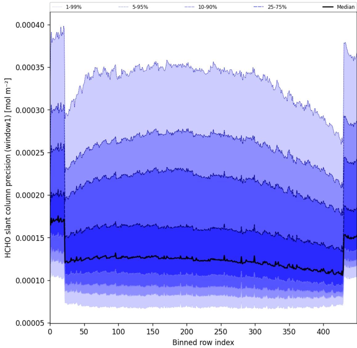
Figure 53: Along track statistics of “HCHO slant column precision (window1)” for 2025-05-03 to 2025-05-05
