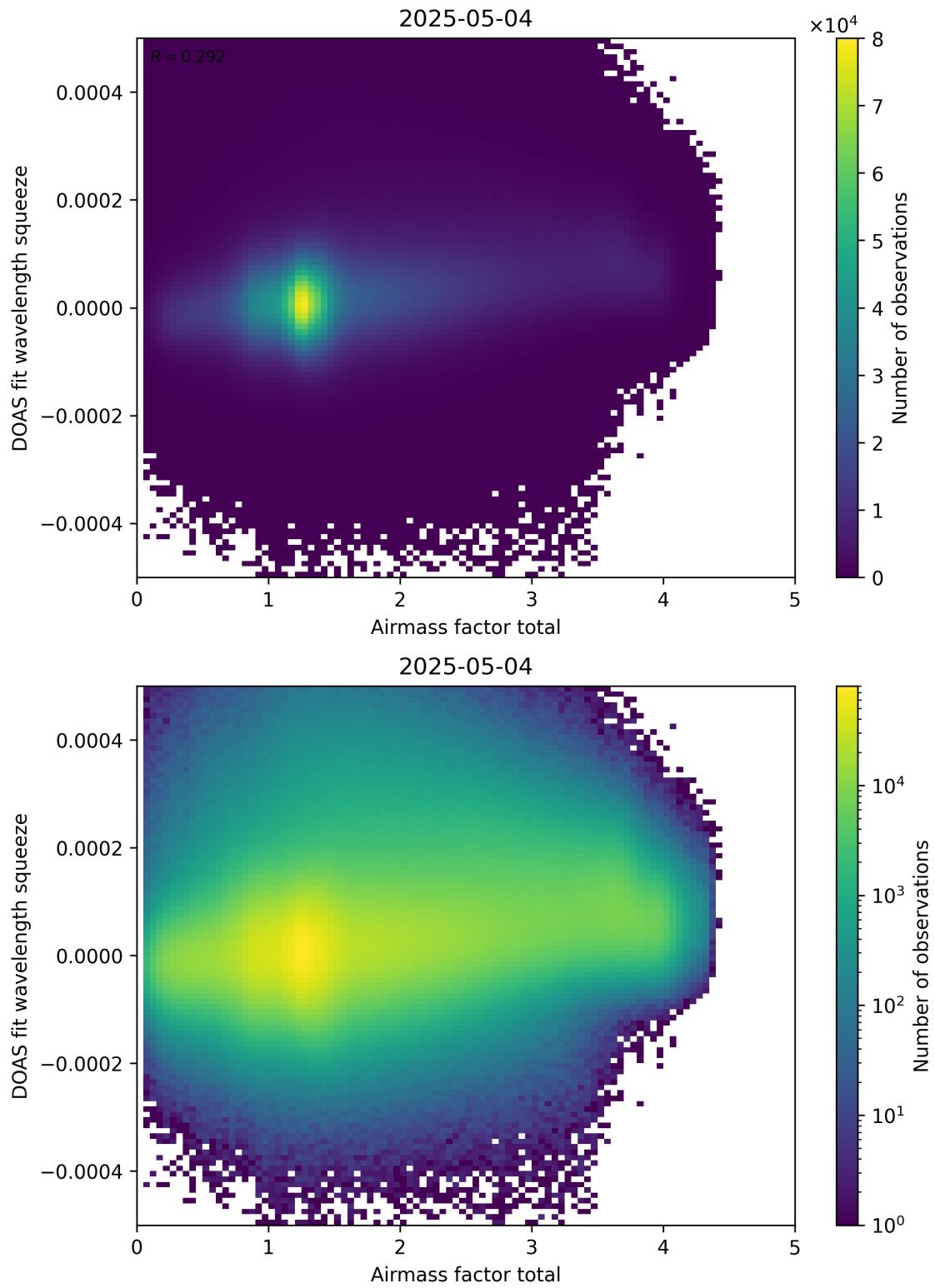
Figure 99: Scatter density plot of “Airmass factor total” against “DOAS fit wavelength squeeze” for 2025-05-03 to 2025-05-05.
