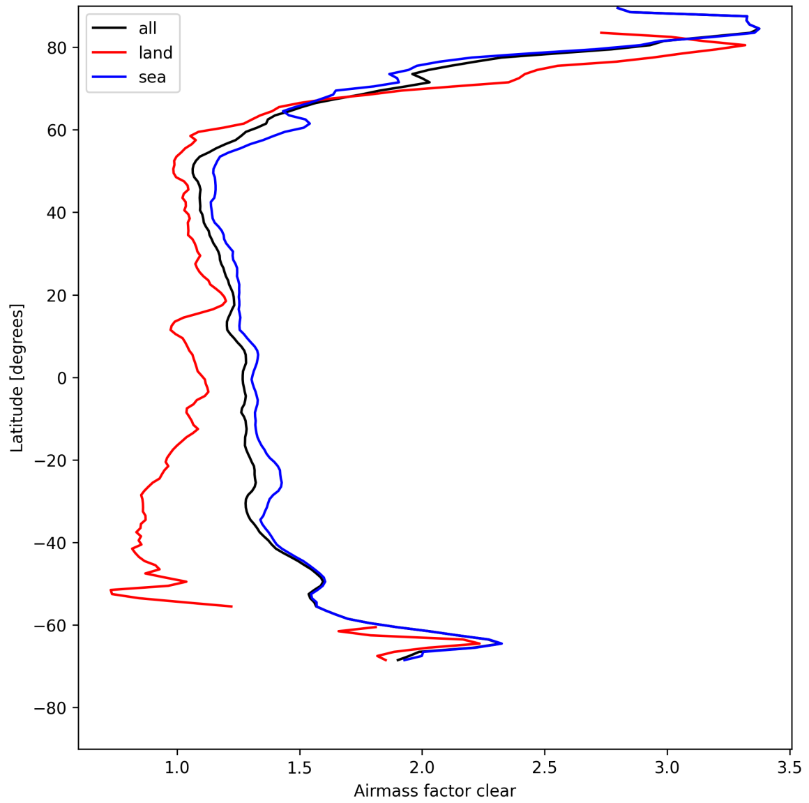
Figure 28: Zonal average of “Airmass factor clear” for 2025-05-03 to 2025-05-05.
