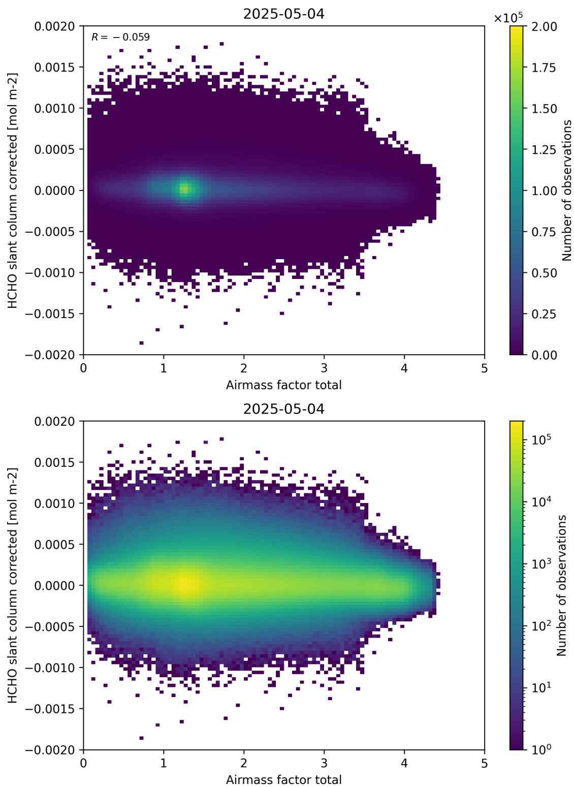
Figure 101: Scatter density plot of “Airmass factor total” against “HCHO slant column corrected” for 2025-05-03 to 2025-05-05.
