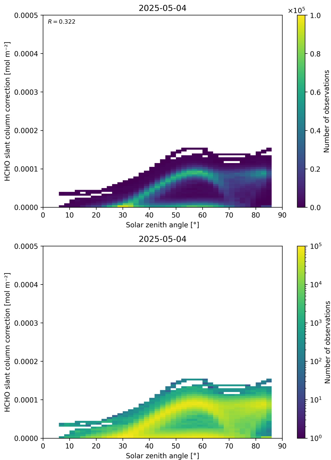
Figure 172: Scatter density plot of “Solar zenith angle” against “HCHO slant column correction” for 2025-05-03 to 2025-05-05.
