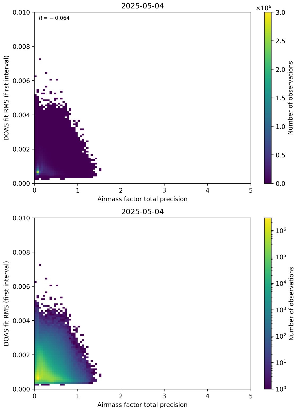
Figure 105: Scatter density plot of “Airmass factor total precision” against “DOAS fit RMS (first interval)” for 2025-05-03 to 2025-05-05.
