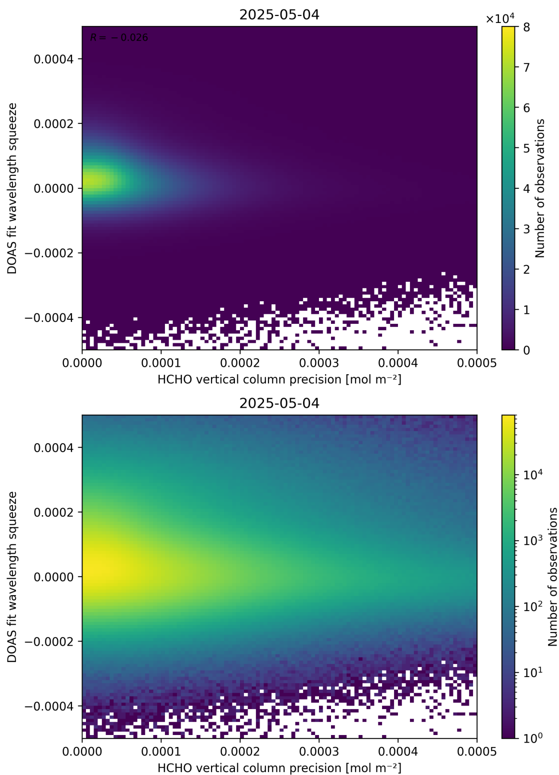
Figure 138: Scatter density plot of “HCHO vertical column precision” against “DOAS fit wavelength squeeze” for 2025-05-03 to 2025-05-05.
