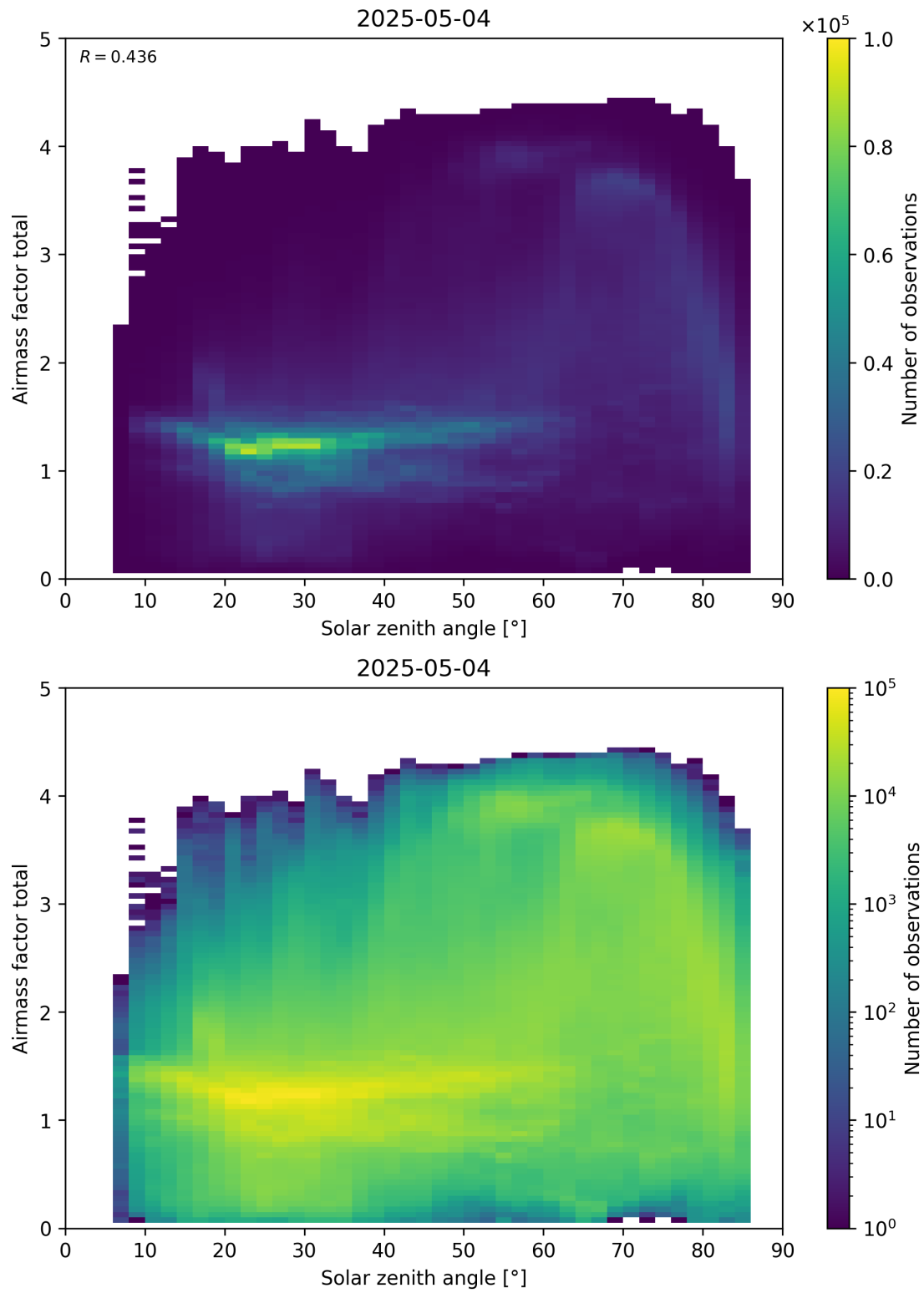
Figure 175: Scatter density plot of “Solar zenith angle” against “Airmass factor total” for 2025-05-03 to 2025-05-05.
