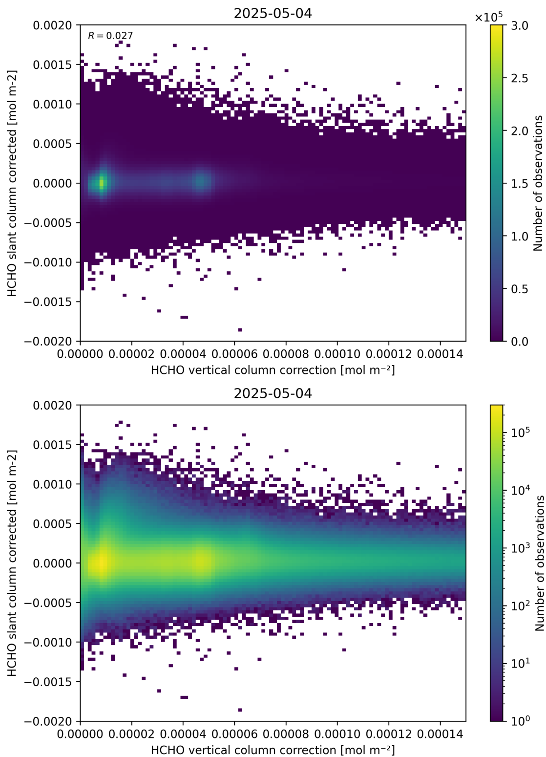
Figure 116: Scatter density plot of “HCHO vertical column correction” against “HCHO slant column corrected” for 2025-05-03 to 2025-05-05.
