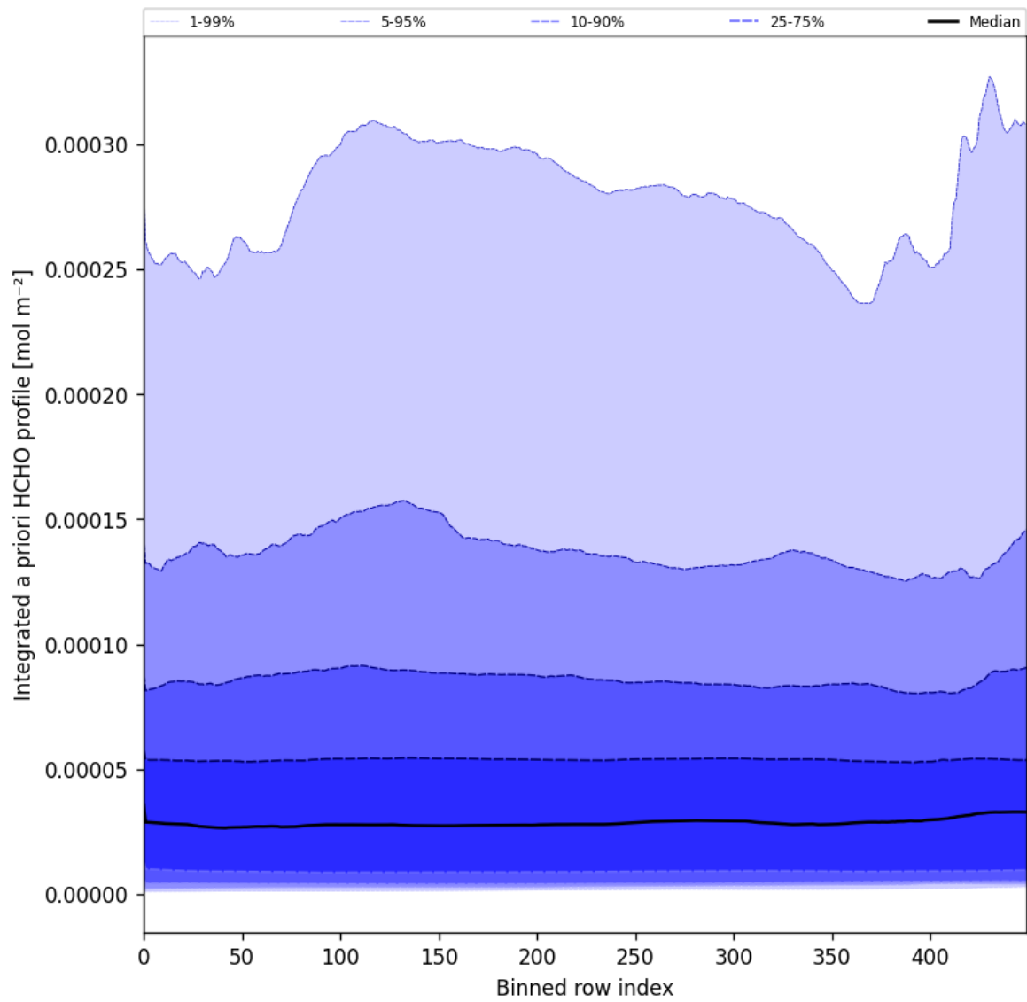
Figure 57: Along track statistics of “Integrated a priori HCHO profile” for 2025-05-03 to 2025-05-05
