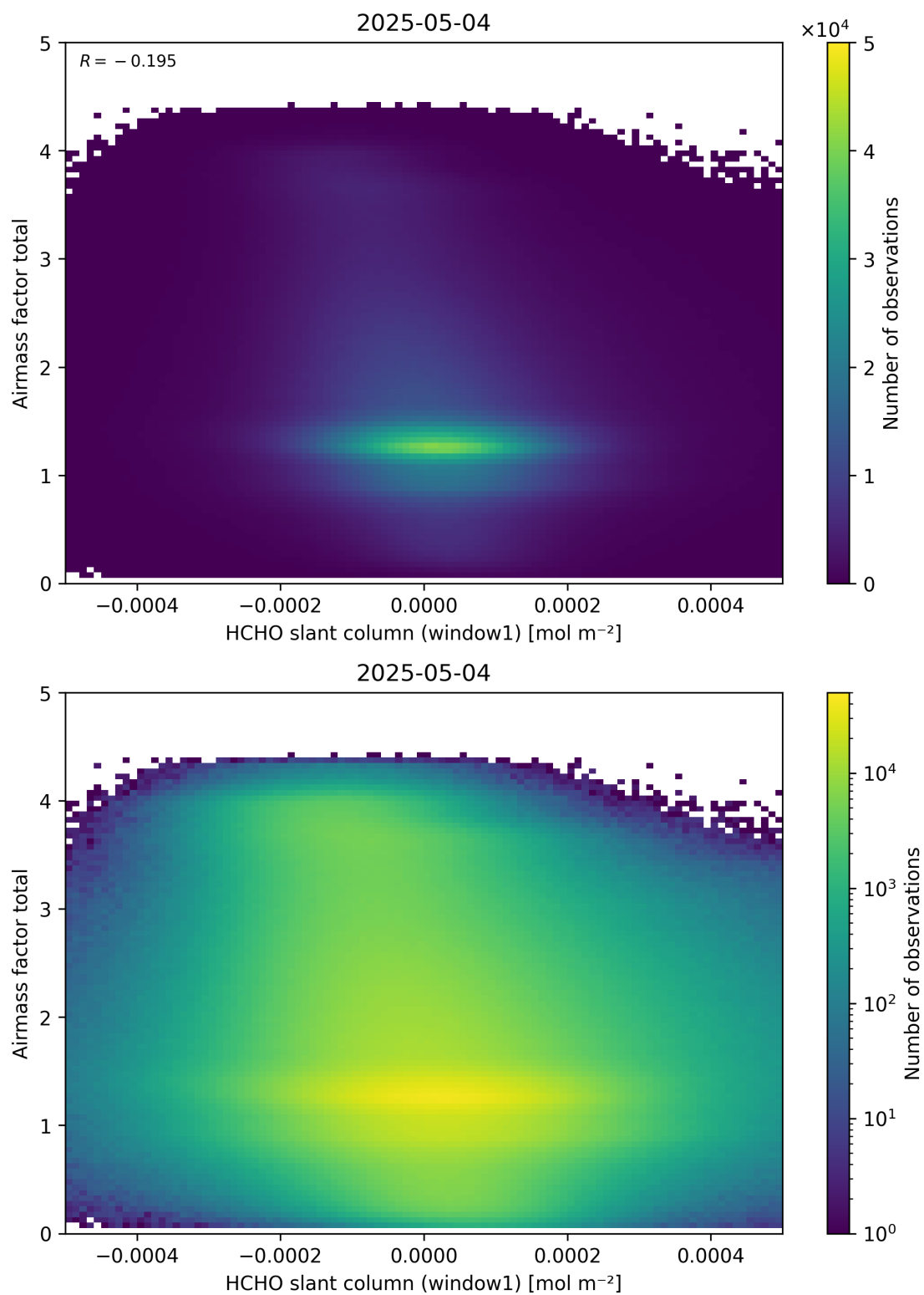
Figure 85: Scatter density plot of “HCHO slant column (window1)” against “Airmass factor total” for 2025-05-03 to 2025-05-05.
