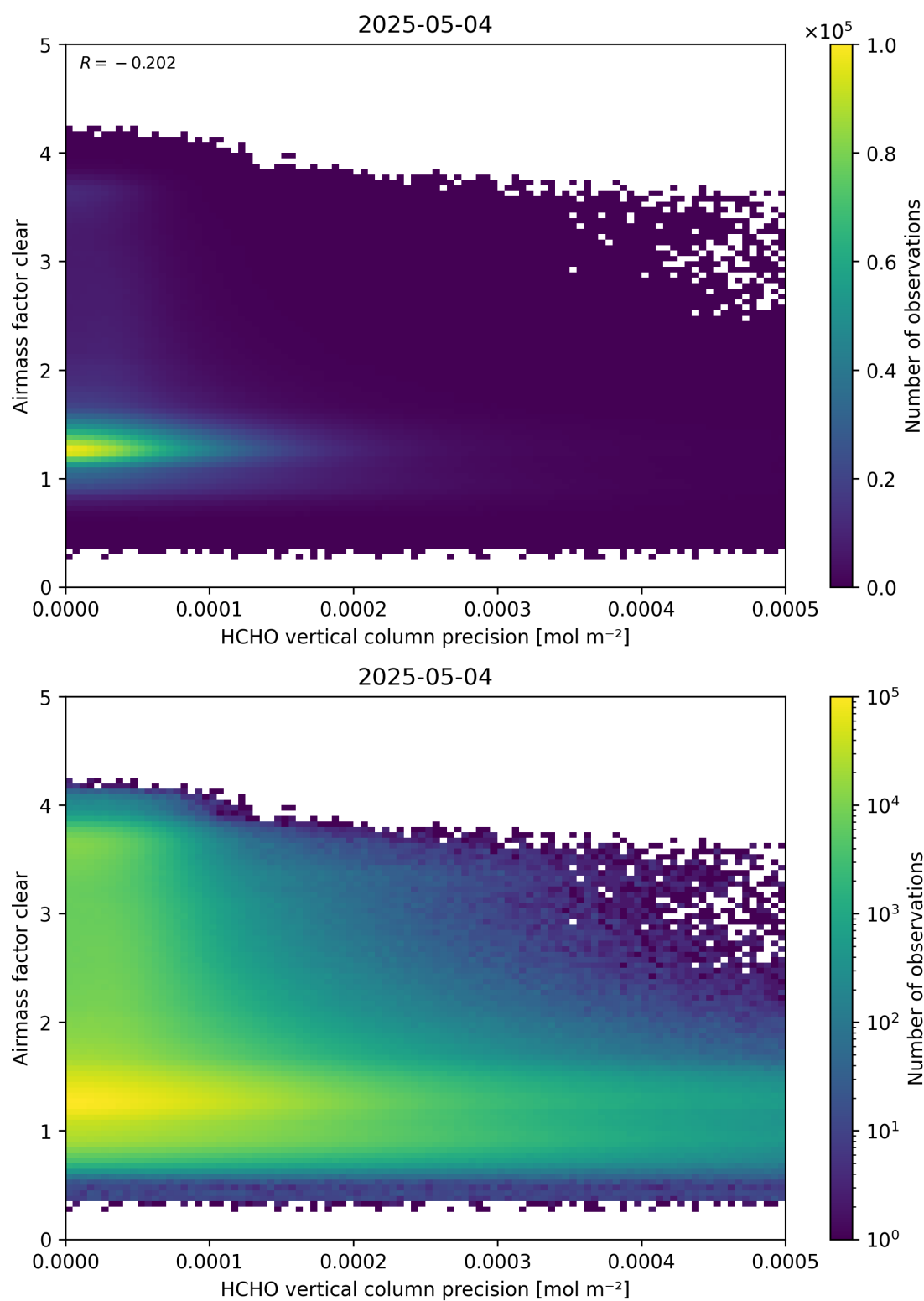
Figure 139: Scatter density plot of “HCHO vertical column precision” against “Airmass factor clear” for 2025-05-03 to 2025-05-05.
