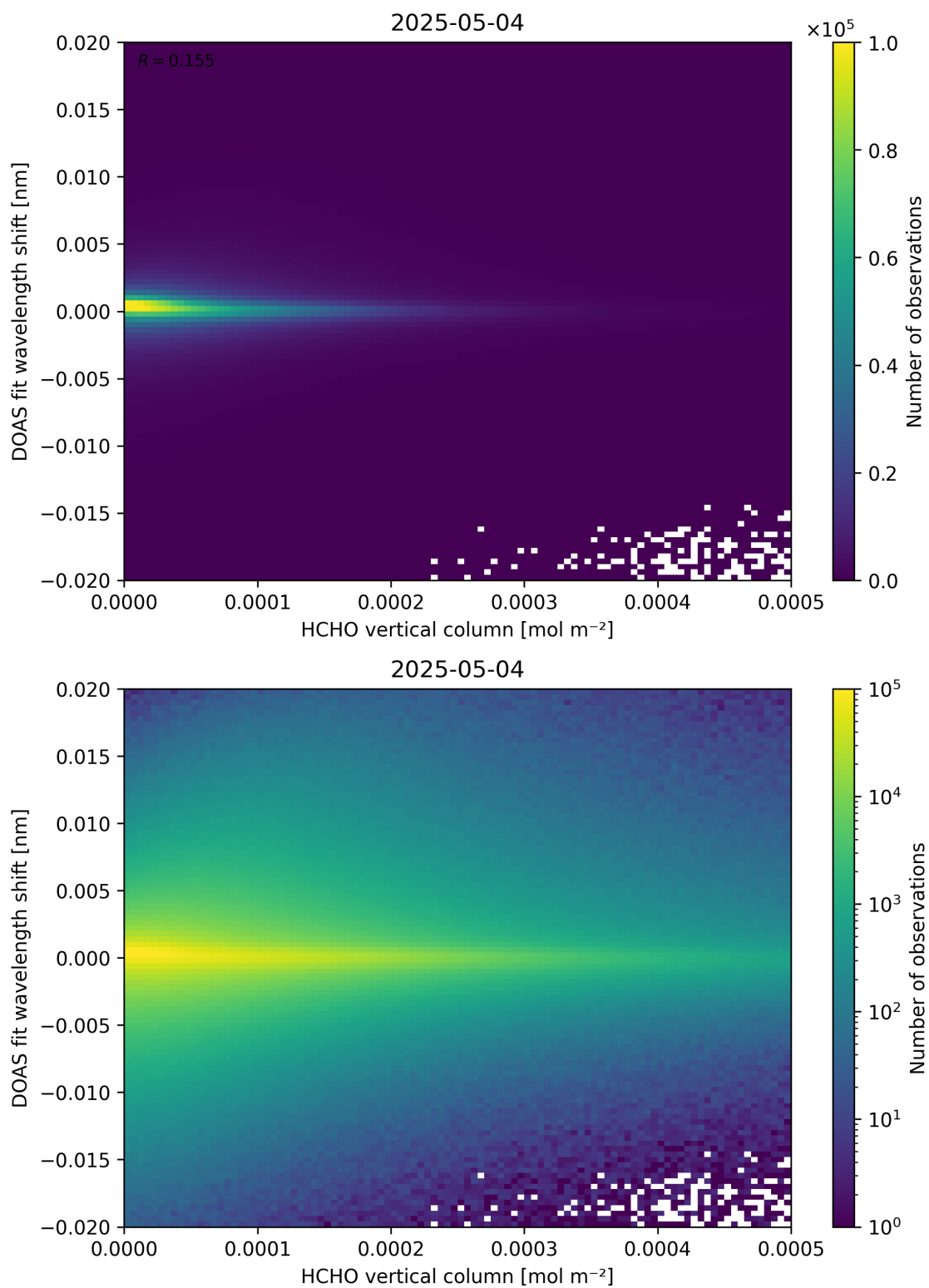
Figure 124: Scatter density plot of “HCHO vertical column” against “DOAS fit wavelength shift” for 2025-05-03 to 2025-05-05.
