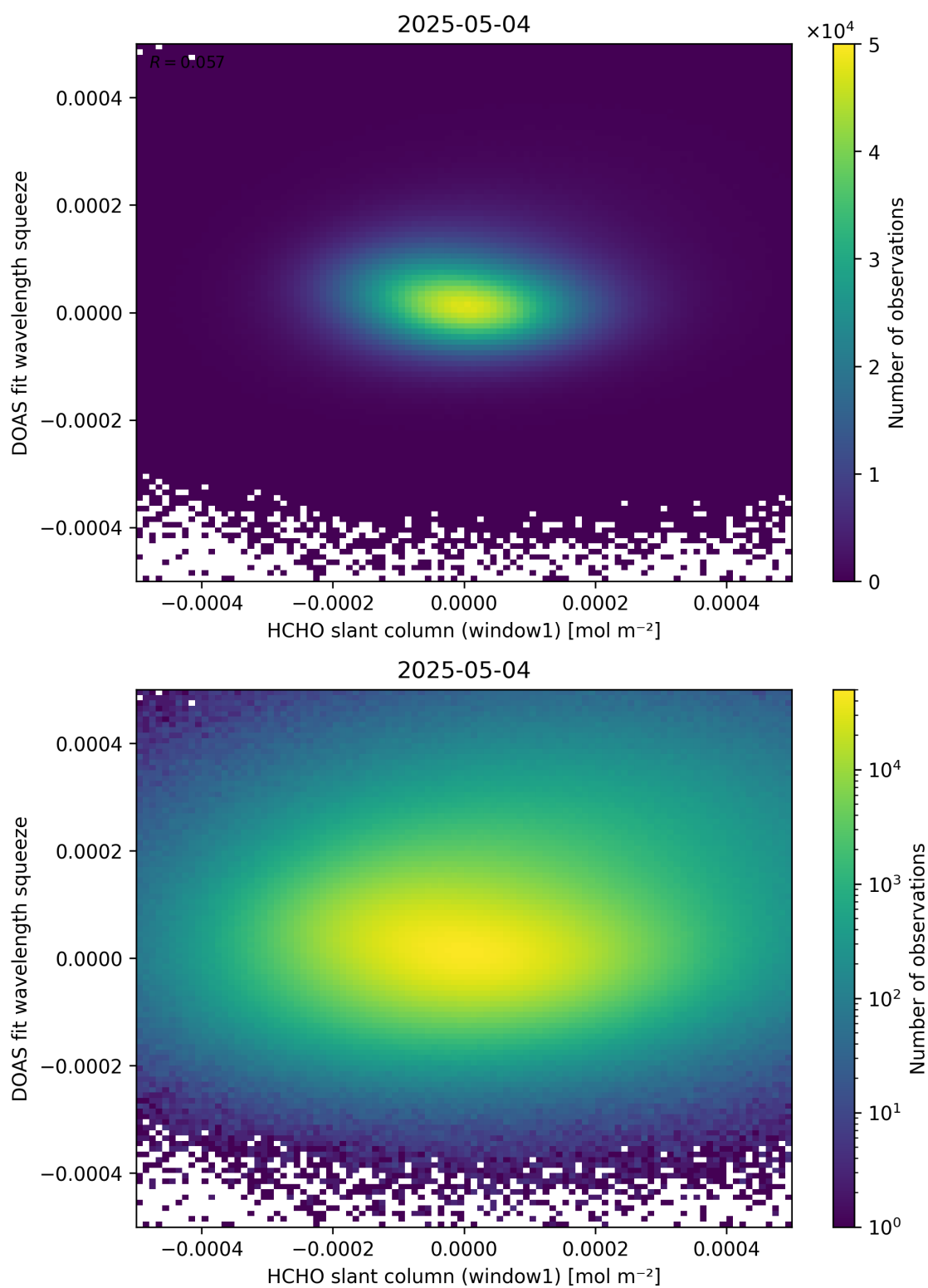
Figure 80: Scatter density plot of “HCHO slant column (window1)” against “DOAS fit wavelength squeeze” for 2025-05-03 to 2025-05-05.
