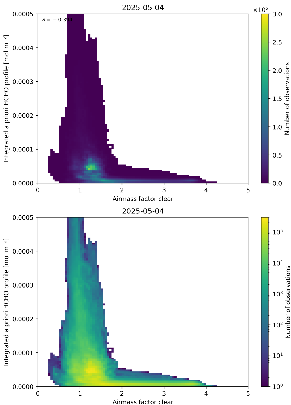
Figure 76: Scatter density plot of “Airmass factor clear” against “Integrated a priori HCHO profile” for 2025-05-03 to 2025-05-05.
