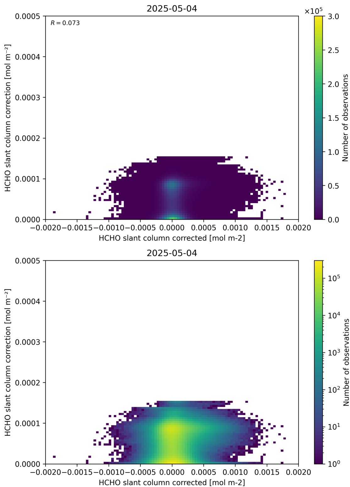
Figure 77: Scatter density plot of “HCHO slant column corrected” against “HCHO slant column correction” for 2025-05-03 to 2025-05-05.
