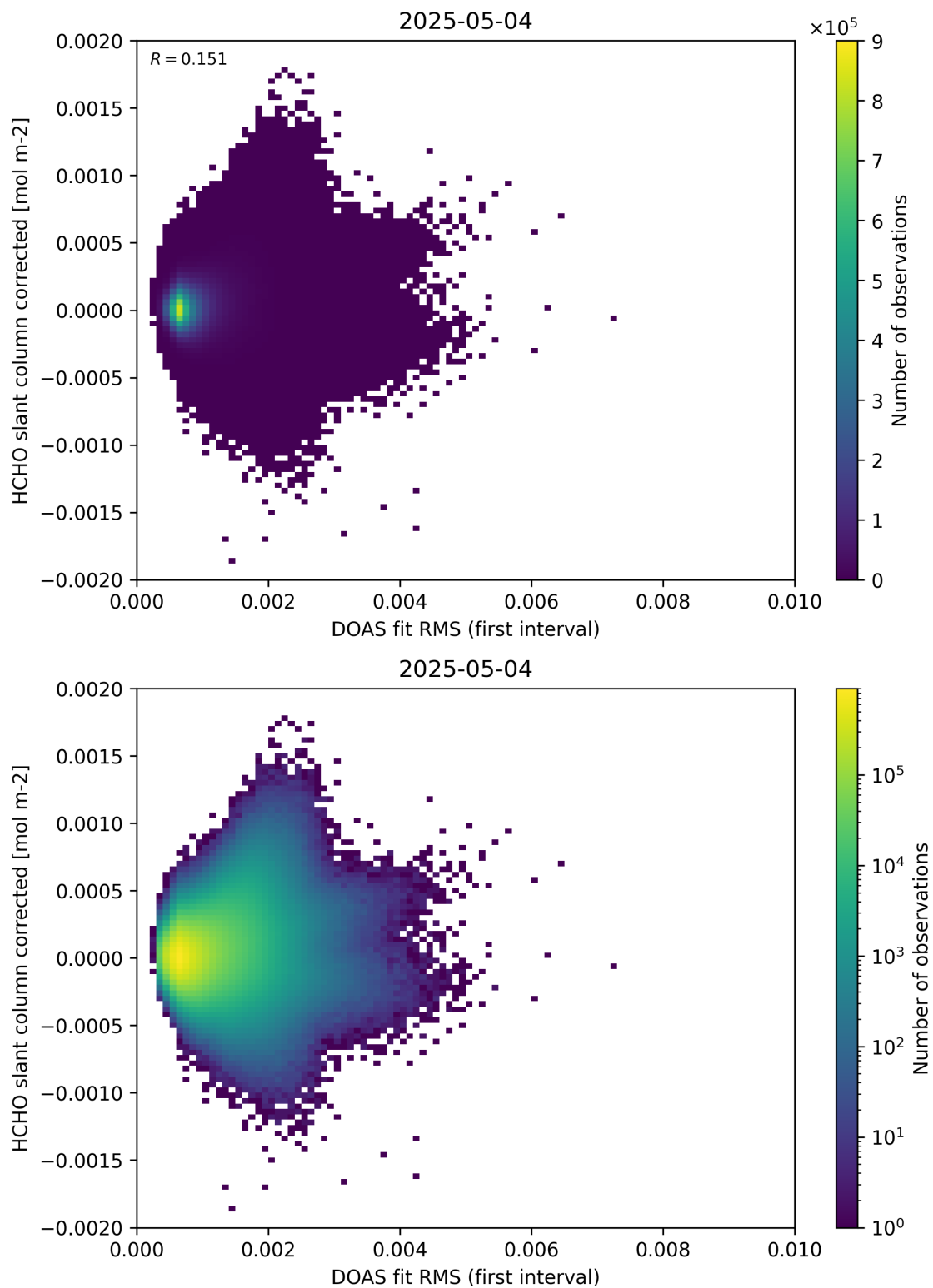
Figure 62: Scatter density plot of “DOAS fit RMS (first interval)” against “HCHO slant column corrected” for 2025-05-03 to 2025-05-05.
