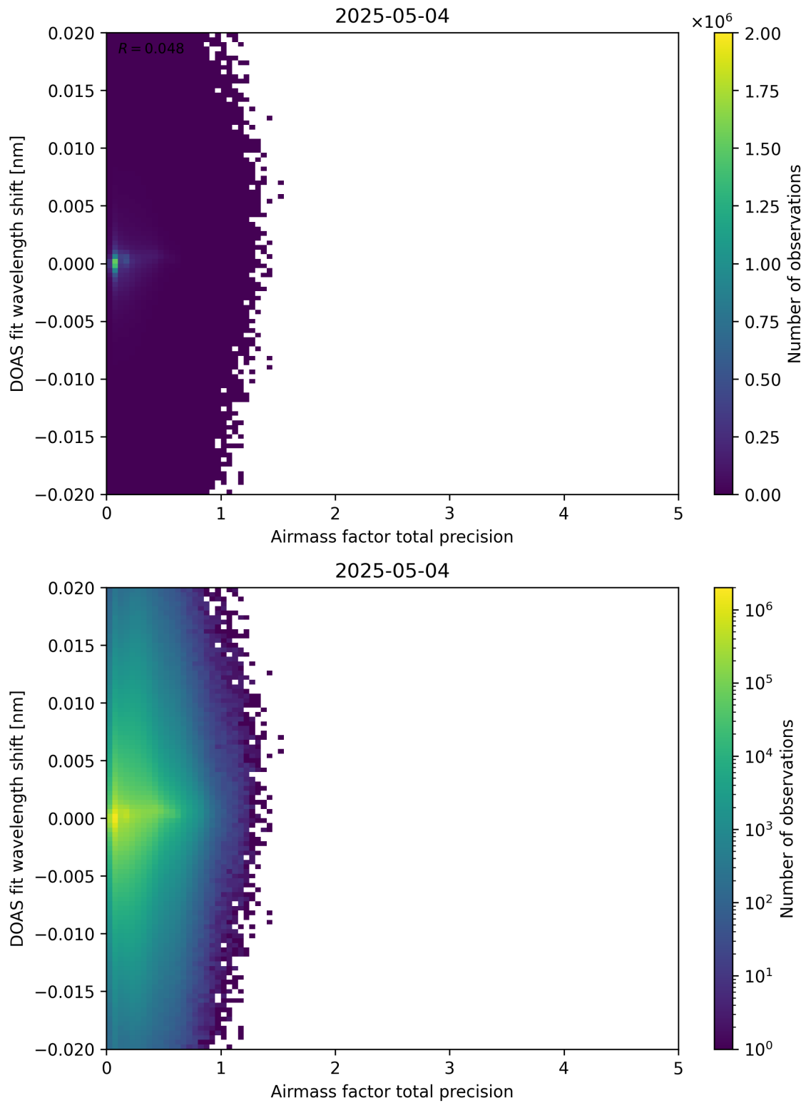
Figure 106: Scatter density plot of “Airmass factor total precision” against “DOAS fit wavelength shift” for 2025-05-03 to 2025-05-05.
