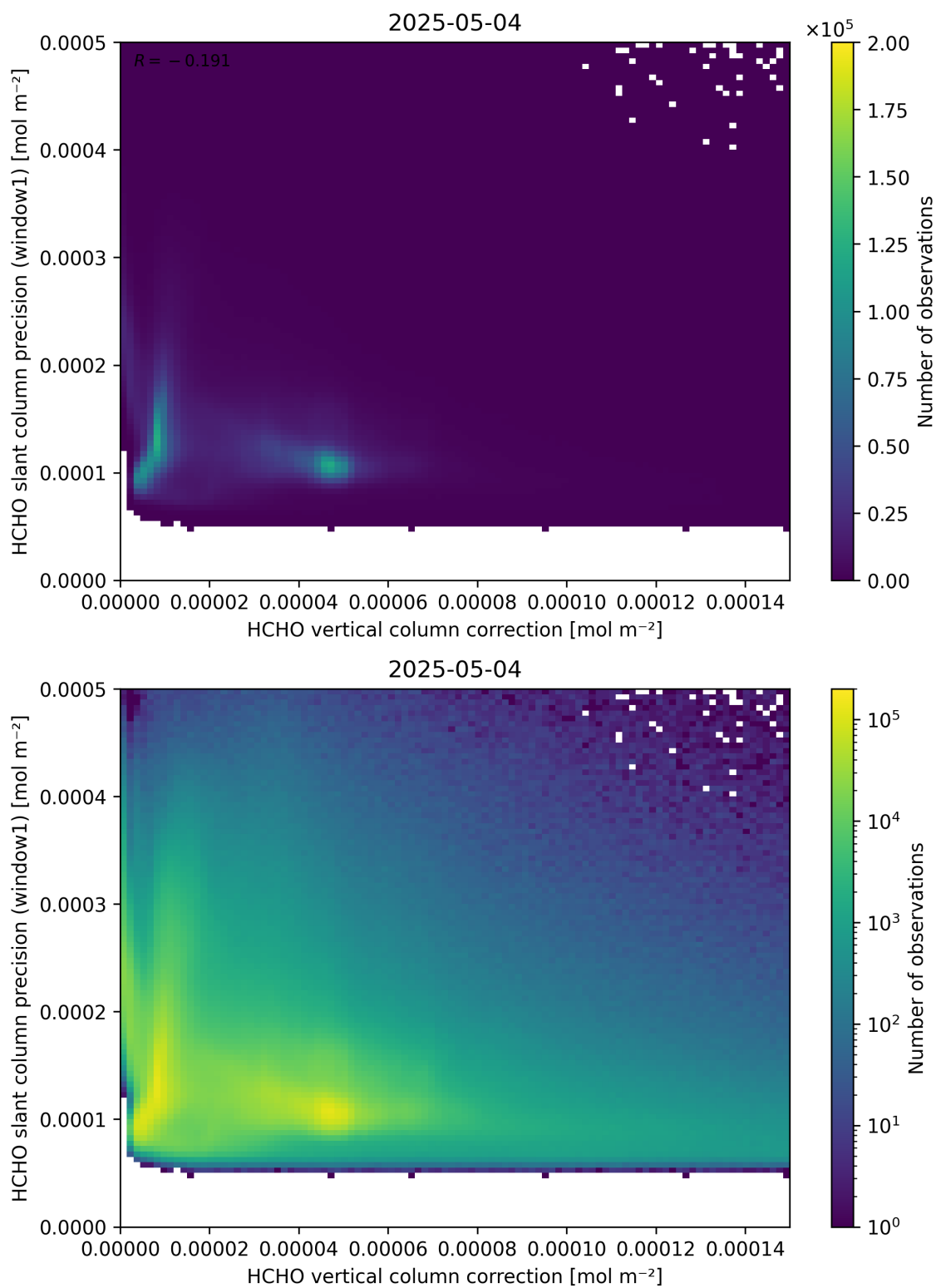
Figure 119: Scatter density plot of “HCHO vertical column correction” against “HCHO slant column precision (window1)” for 2025-05-03 to 2025-05-05.
