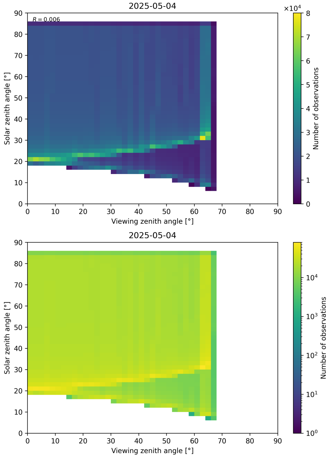
Figure 197: Scatter density plot of “Viewing zenith angle” against “Solar zenith angle” for 2025-05-03 to 2025-05-05.
