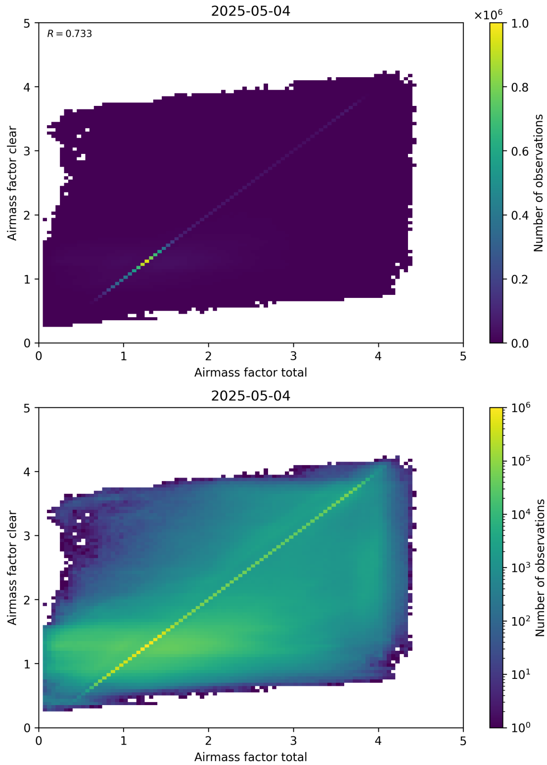
Figure 100: Scatter density plot of “Airmass factor total” against “Airmass factor clear” for 2025-05-03 to 2025-05-05.
