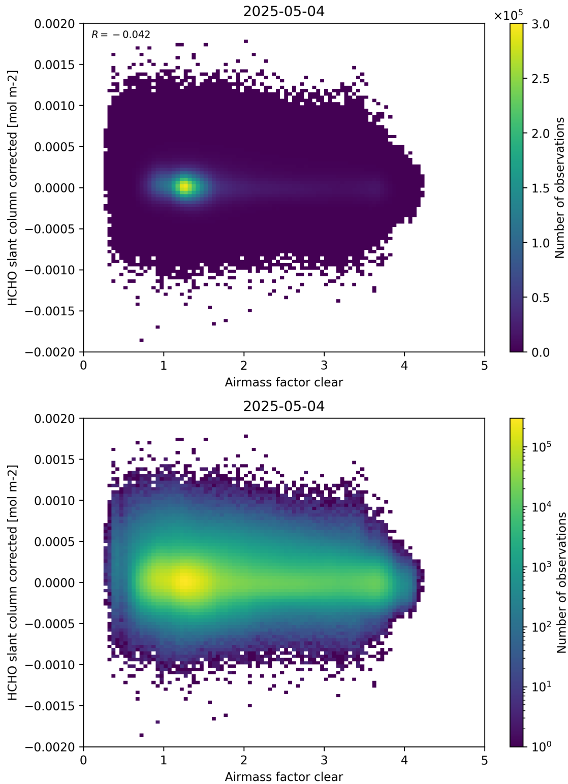
Figure 74: Scatter density plot of “Airmass factor clear” against “HCHO slant column corrected” for 2025-05-03 to 2025-05-05.
