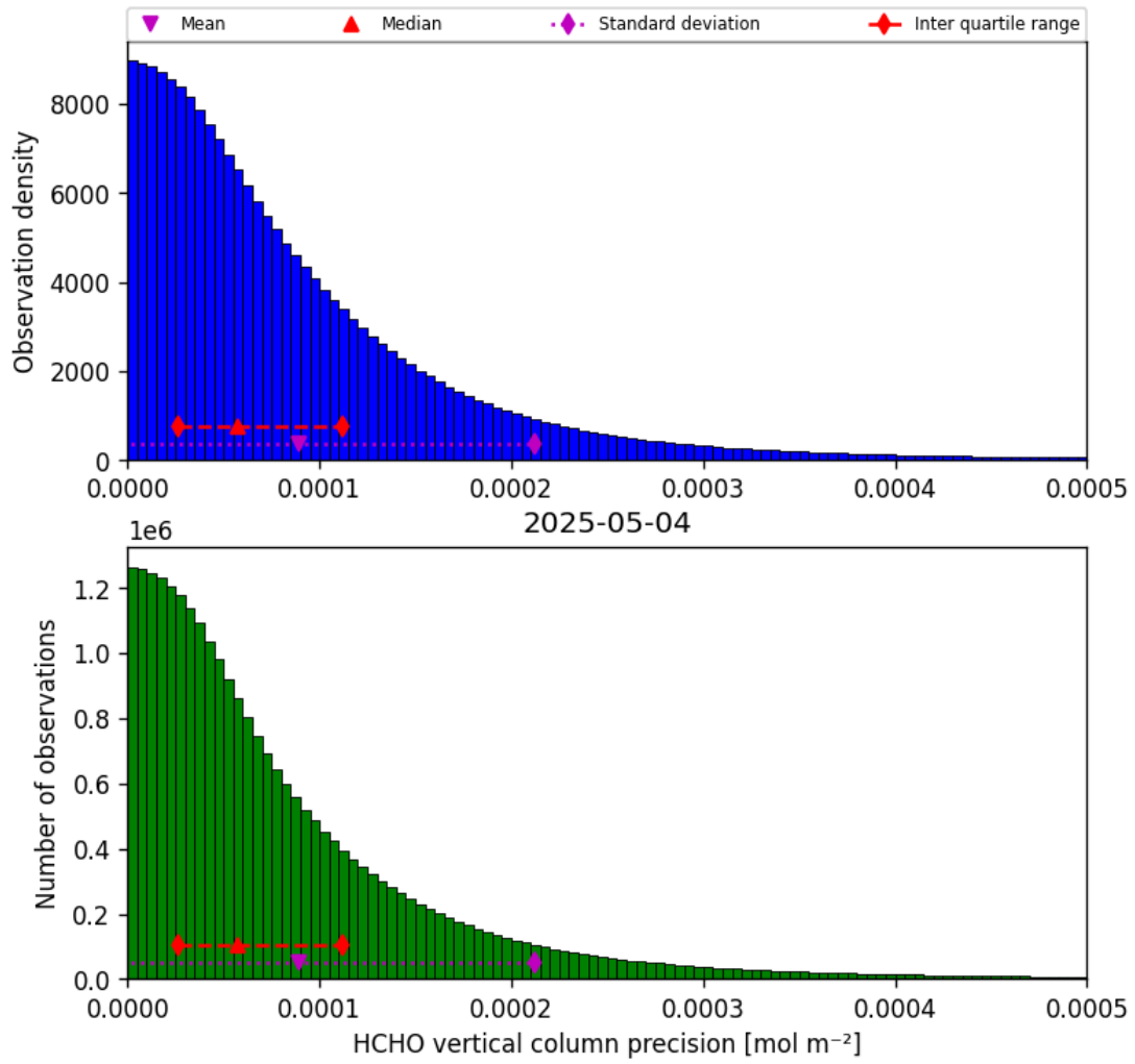
Figure 36: Histogram of “HCHO vertical column precision” for 2025-05-03 to 2025-05-05
