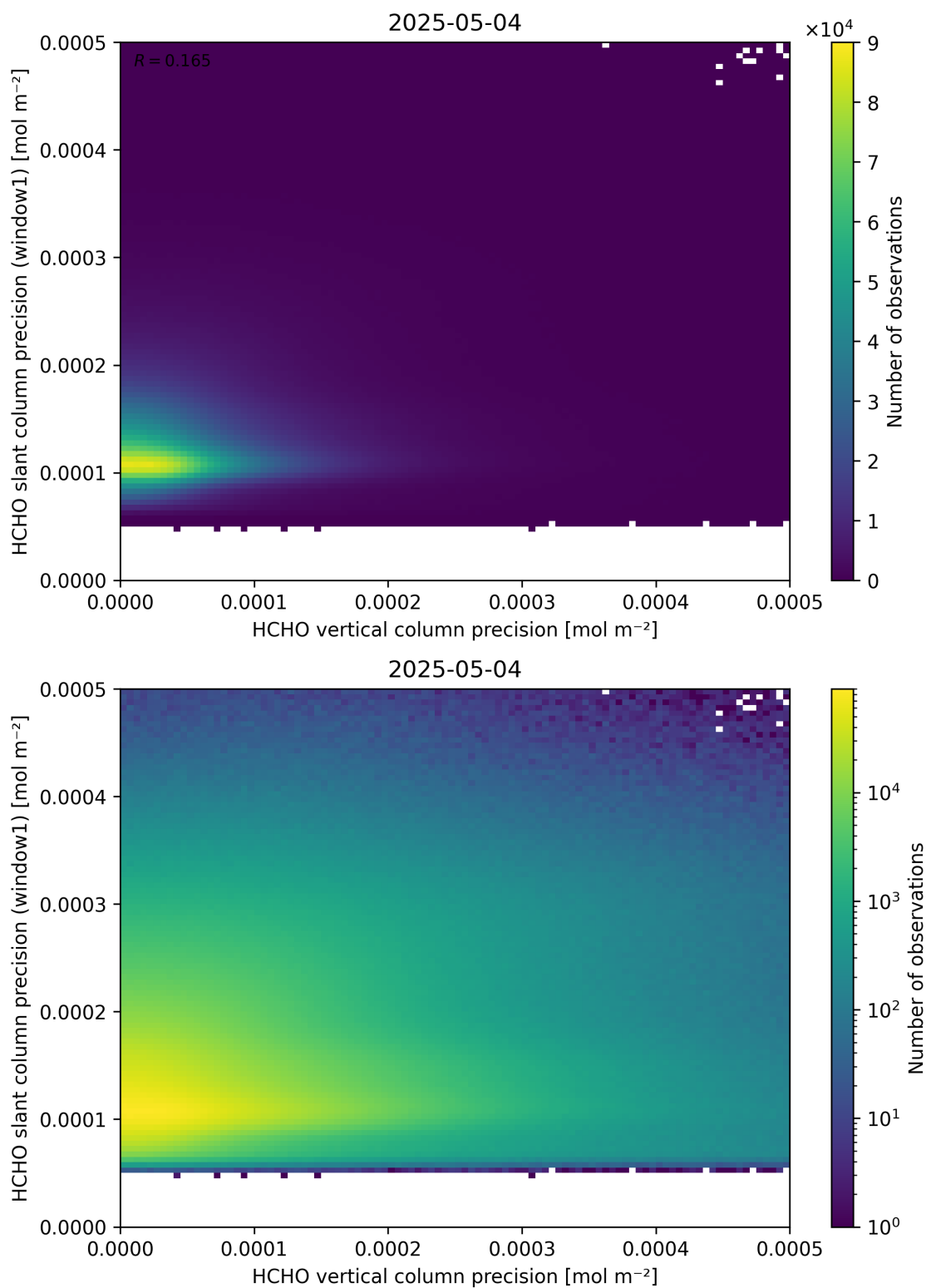
Figure 143: Scatter density plot of “HCHO vertical column precision” against “HCHO slant column precision (window1)” for 2025-05-03 to 2025-05-05.
