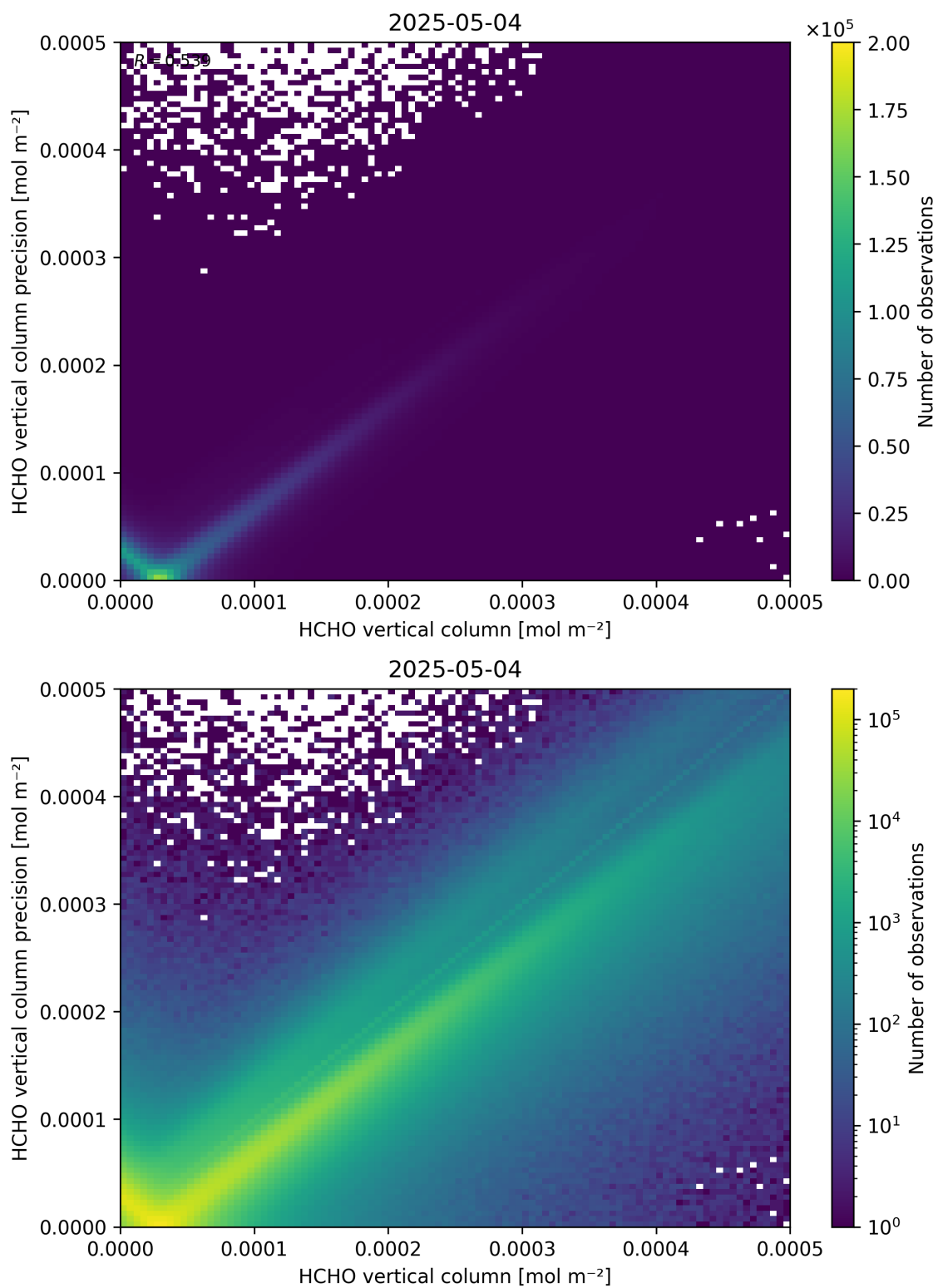
Figure 134: Scatter density plot of “HCHO vertical column” against “HCHO vertical column precision” for 2025-05-03 to 2025-05-05.
