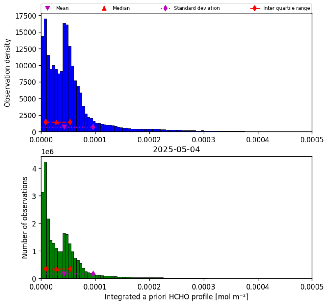
Figure 43: Histogram of “Integrated a priori HCHO profile” for 2025-05-03 to 2025-05-05
