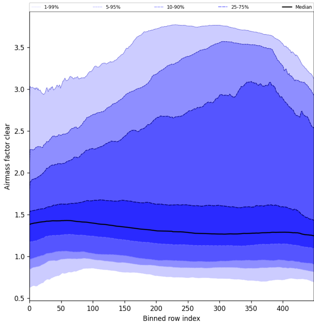
Figure 56: Along track statistics of “Airmass factor clear” for 2025-05-03 to 2025-05-05
