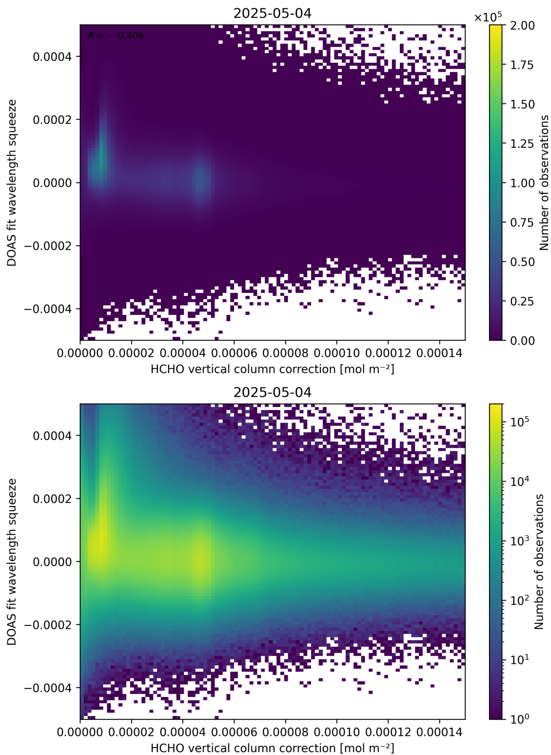
Figure 114: Scatter density plot of “HCHO vertical column correction” against “DOAS fit wavelength squeeze” for 2025-05-03 to 2025-05-05.
