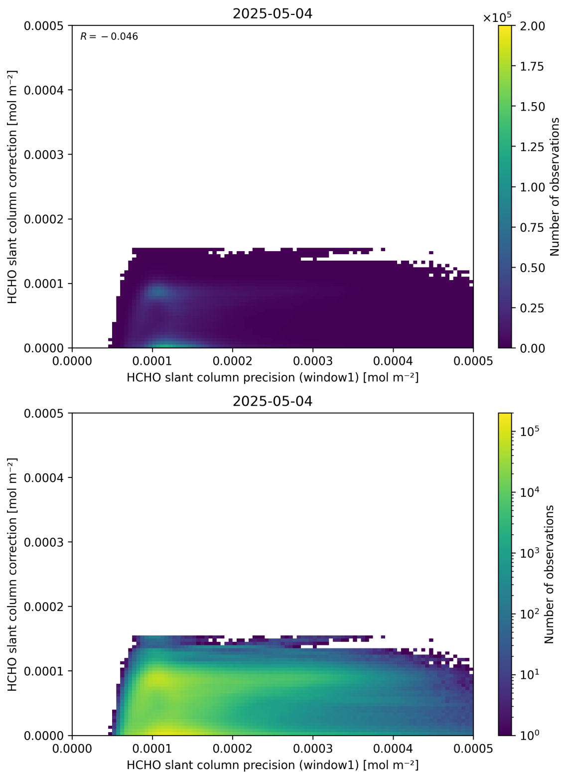
Figure 93: Scatter density plot of “HCHO slant column precision (window1)” against “HCHO slant column correction” for 2025-05-03 to 2025-05-05.
