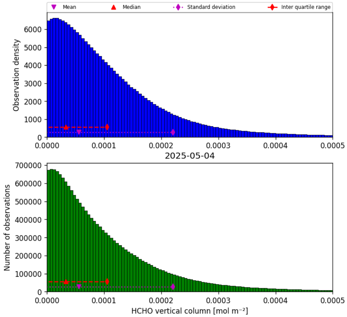
Figure 35: Histogram of “HCHO vertical column” for 2025-05-03 to 2025-05-05
