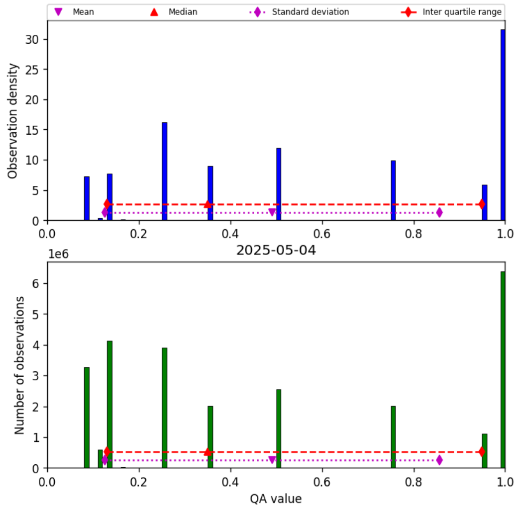
Figure 34: Histogram of “QA value” for 2025-05-03 to 2025-05-05
