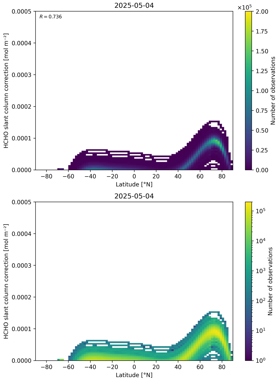
Figure 158: Scatter density plot of “Latitude” against “HCHO slant column correction” for 2025-05-03 to 2025-05-05.
