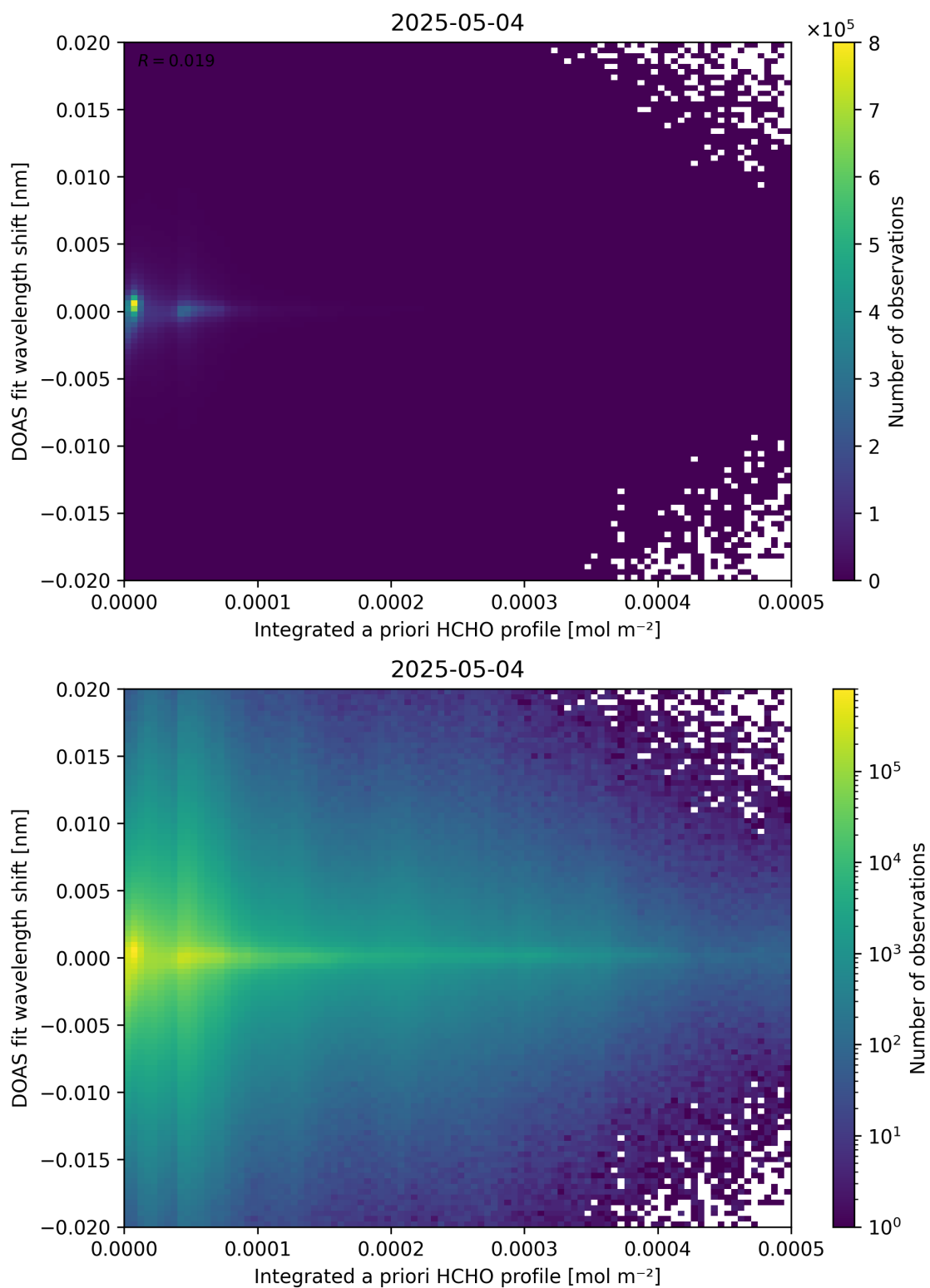
Figure 149: Scatter density plot of “Integrated a priori HCHO profile” against “DOAS fit wavelength shift” for 2025-05-03 to 2025-05-05.
