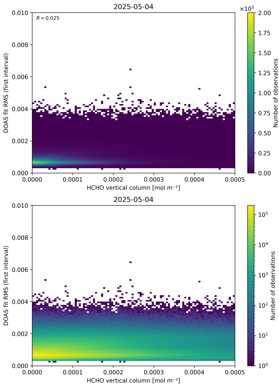
Figure 123: Scatter density plot of “HCHO vertical column” against “DOAS fit RMS (first interval)” for 2025-05-03 to 2025-05-05.
