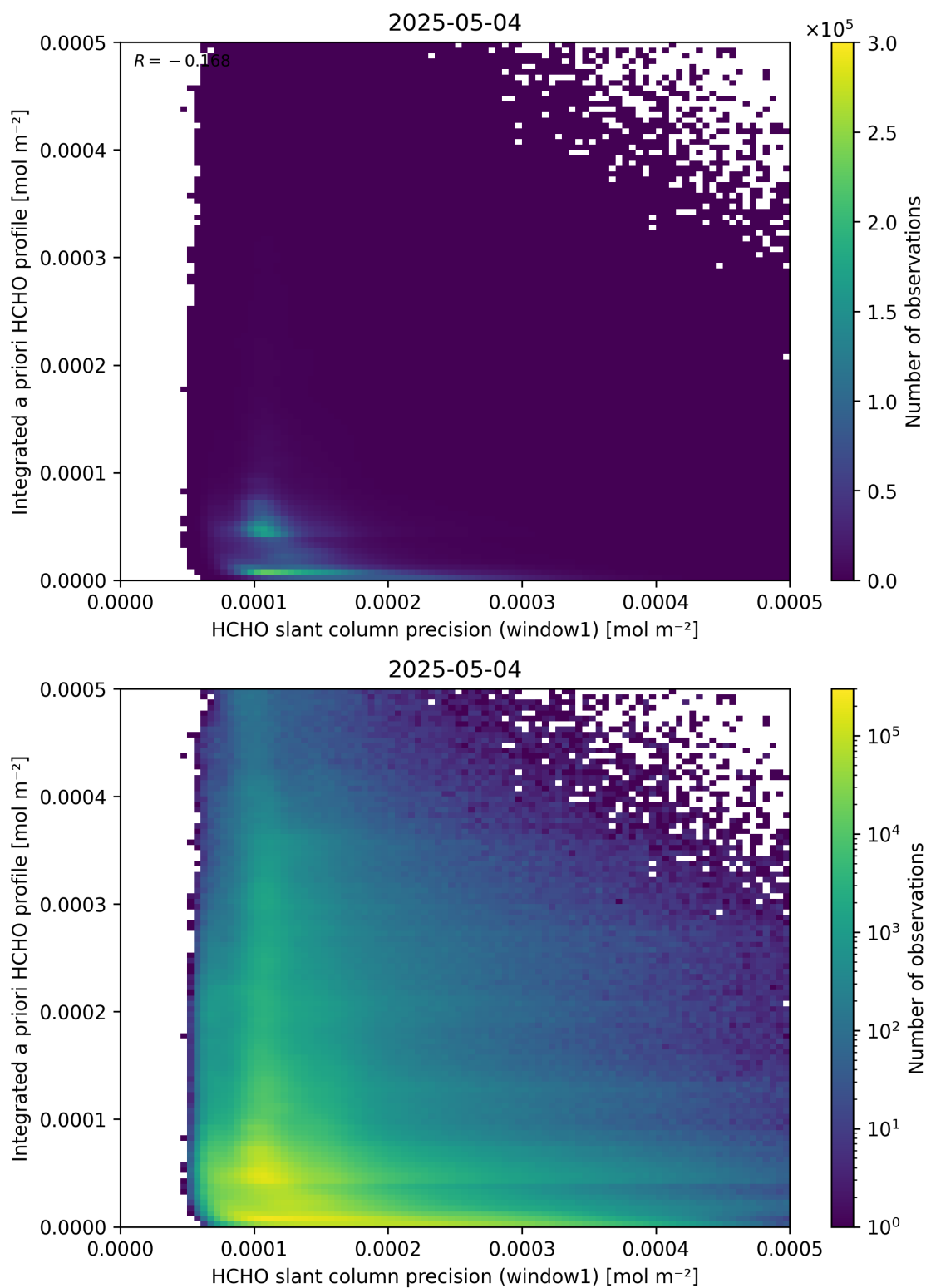
Figure 96: Scatter density plot of “HCHO slant column precision (window1)” against “Integrated a priori HCHO profile” for 2025-05-03 to 2025-05-05.
