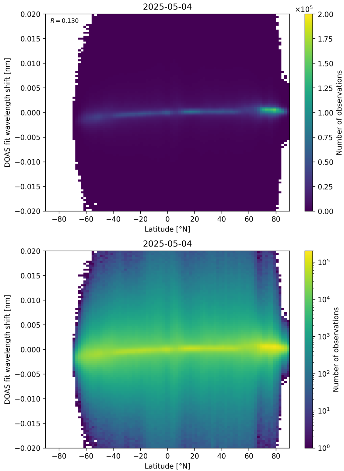
Figure 154: Scatter density plot of “Latitude” against “DOAS fit wavelength shift” for 2025-05-03 to 2025-05-05.
