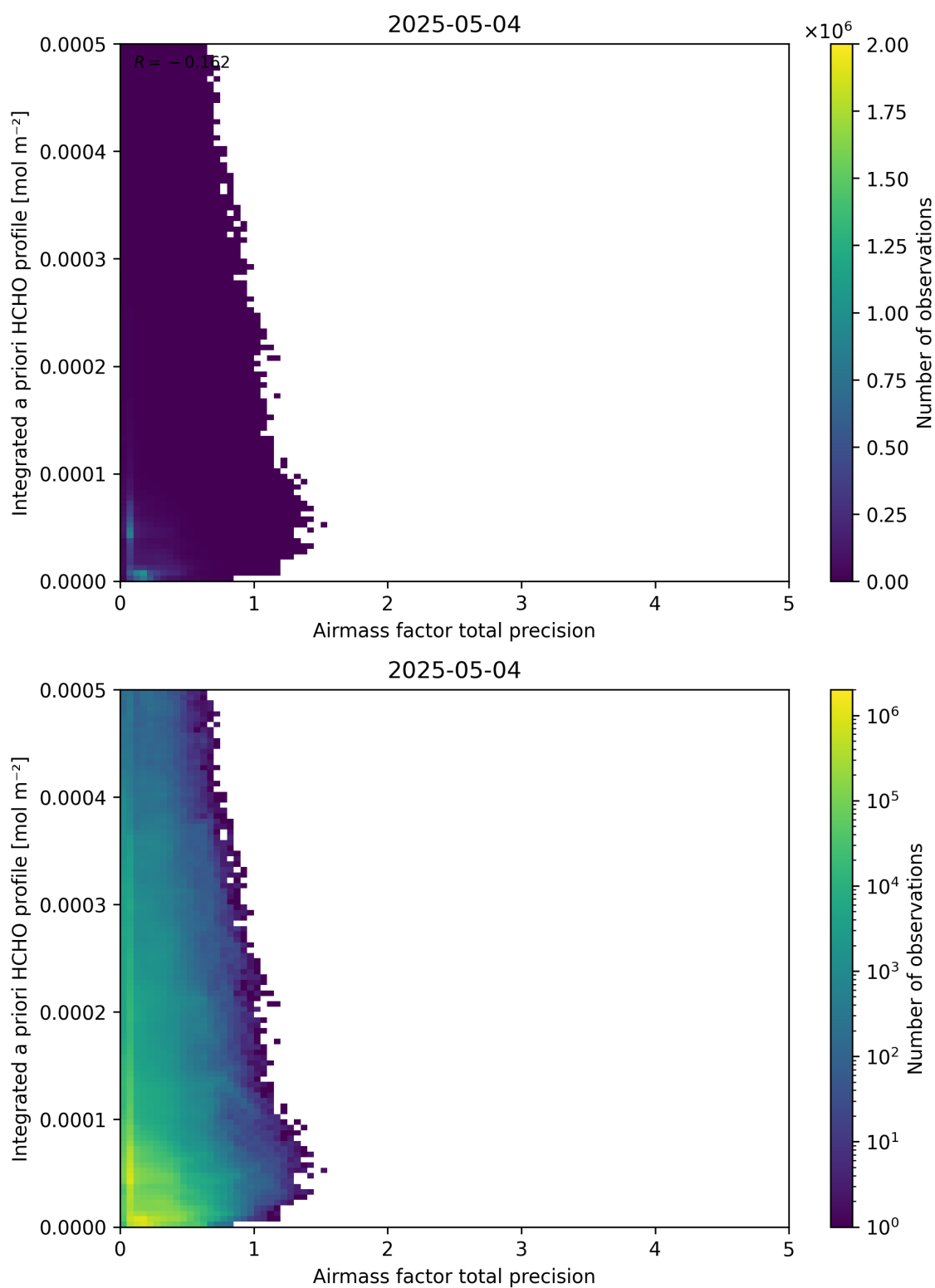
Figure 111: Scatter density plot of “Airmass factor total precision” against “Integrated a priori HCHO profile” for 2025-05-03 to 2025-05-05.
