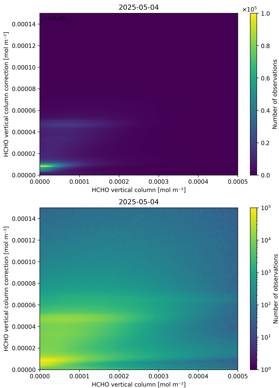
Figure 133: Scatter density plot of “HCHO vertical column” against “HCHO vertical column correction” for 2025-05-03 to 2025-05-05.
