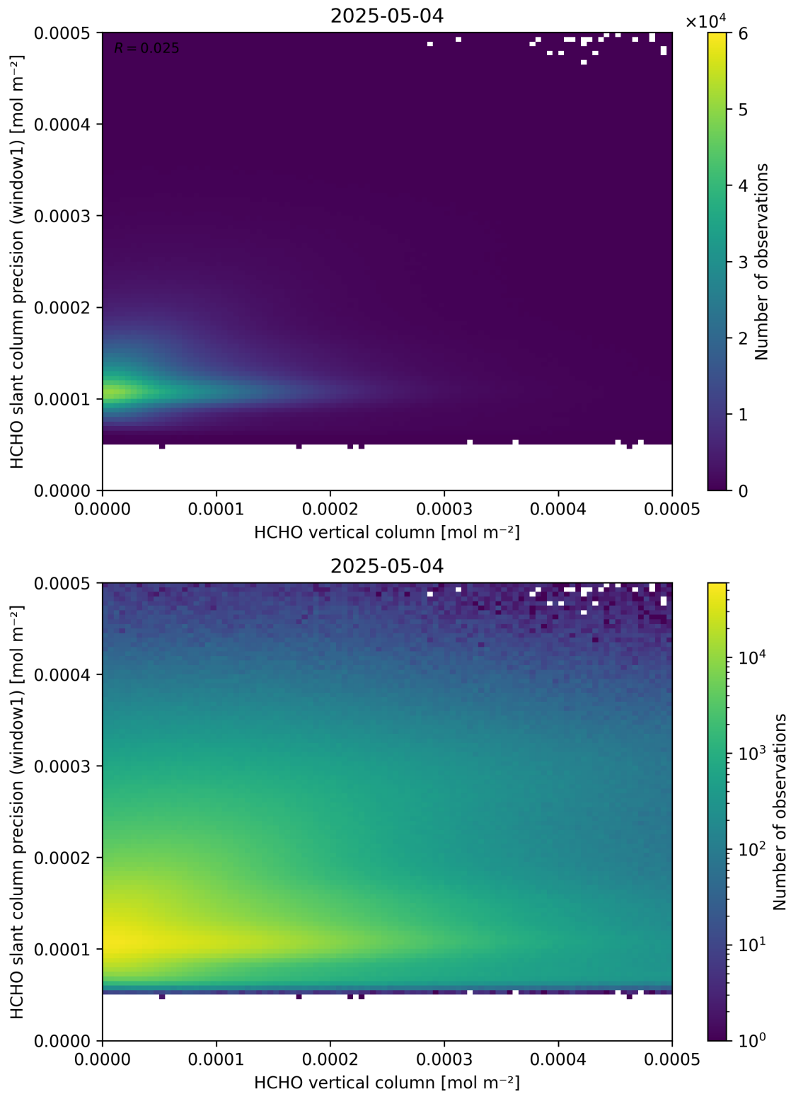
Figure 130: Scatter density plot of “HCHO vertical column” against “HCHO slant column precision (window1)” for 2025-05-03 to 2025-05-05.
