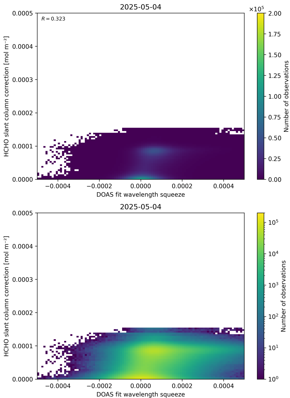
Figure 70: Scatter density plot of “DOAS fit wavelength squeeze” against “HCHO slant column correction” for 2025-05-03 to 2025-05-05.
