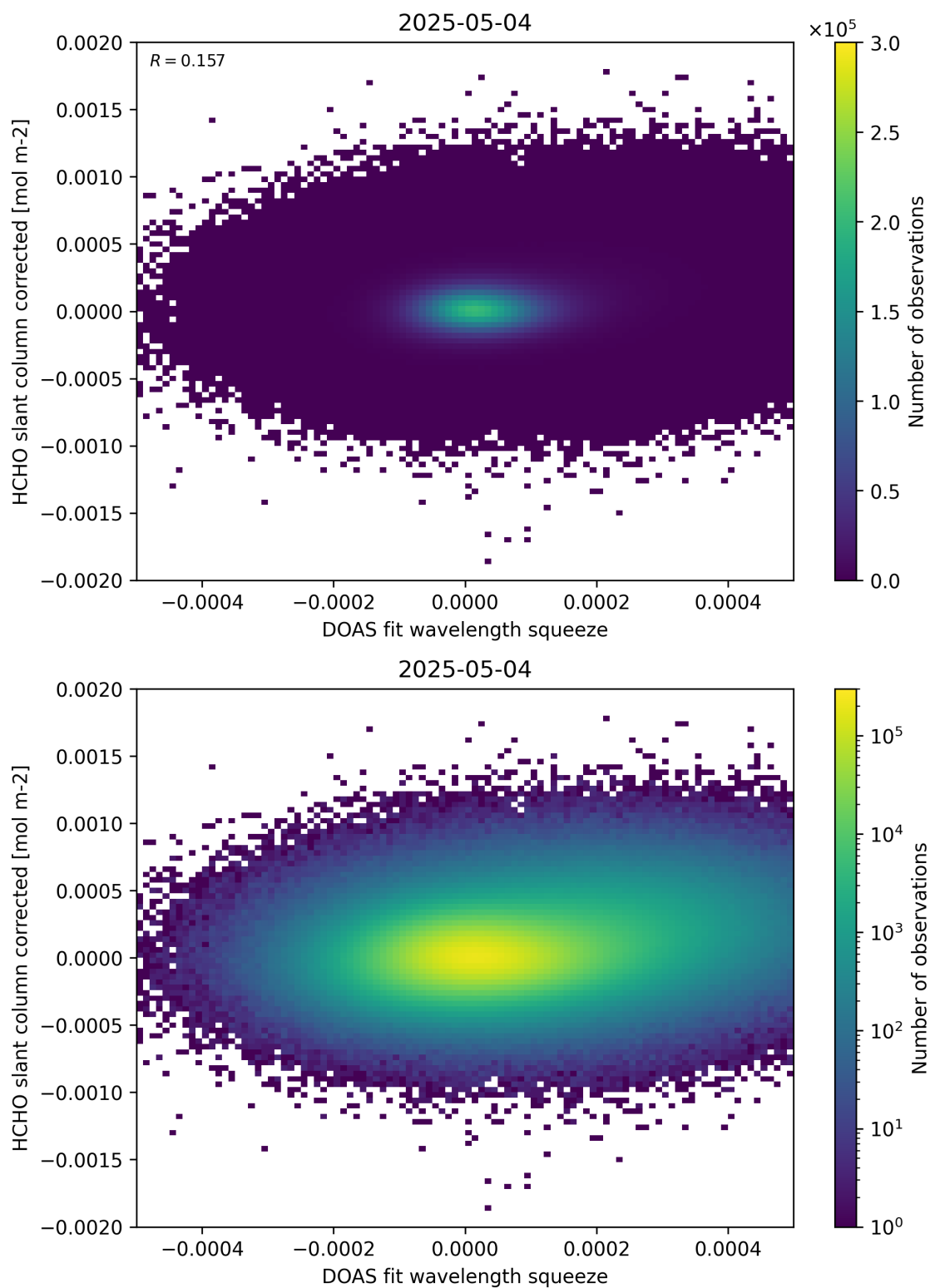
Figure 69: Scatter density plot of “DOAS fit wavelength squeeze” against “HCHO slant column corrected” for 2025-05-03 to 2025-05-05.
