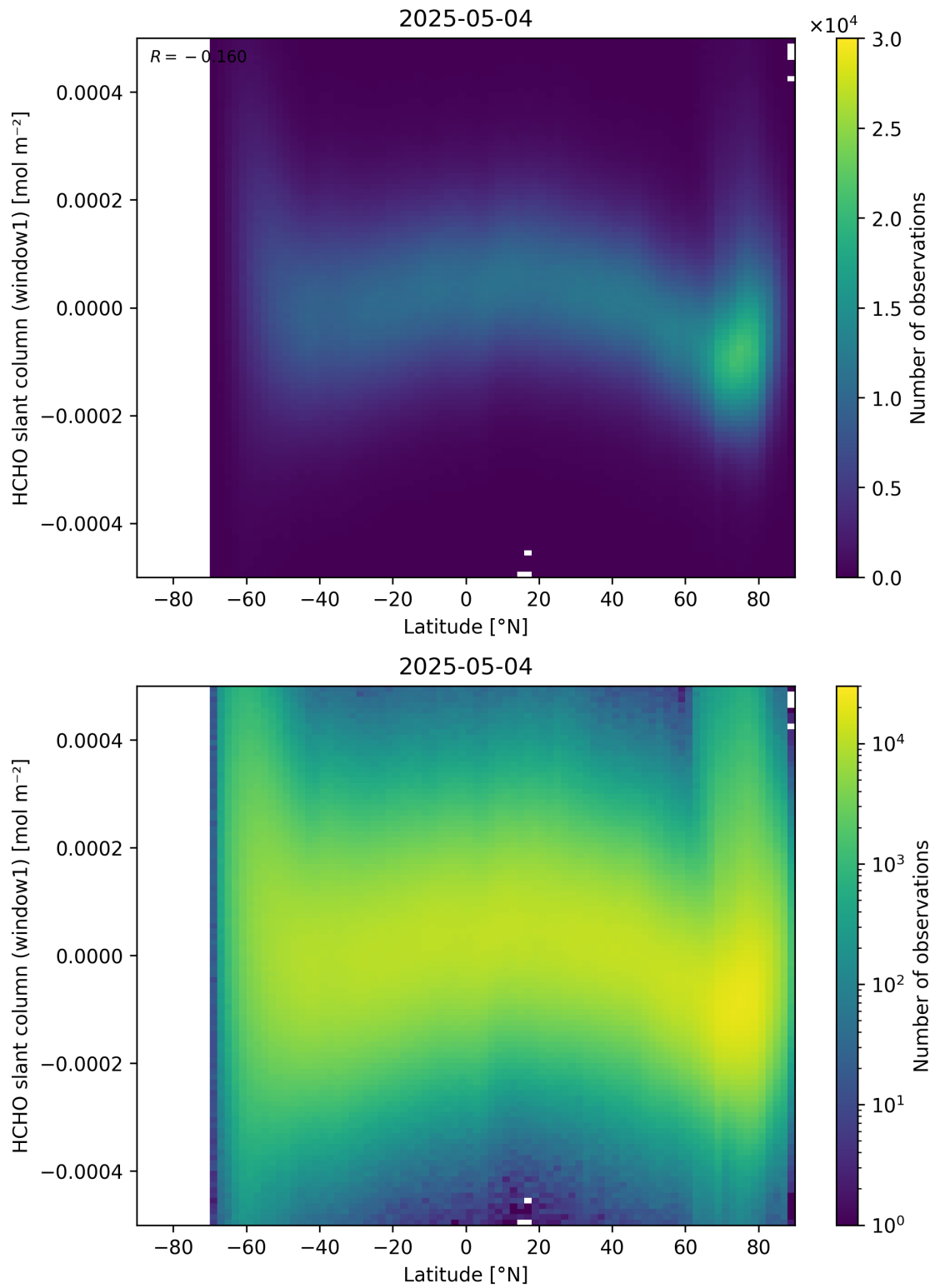
Figure 159: Scatter density plot of “Latitude” against “HCHO slant column (window1)” for 2025-05-03 to 2025-05-05.
