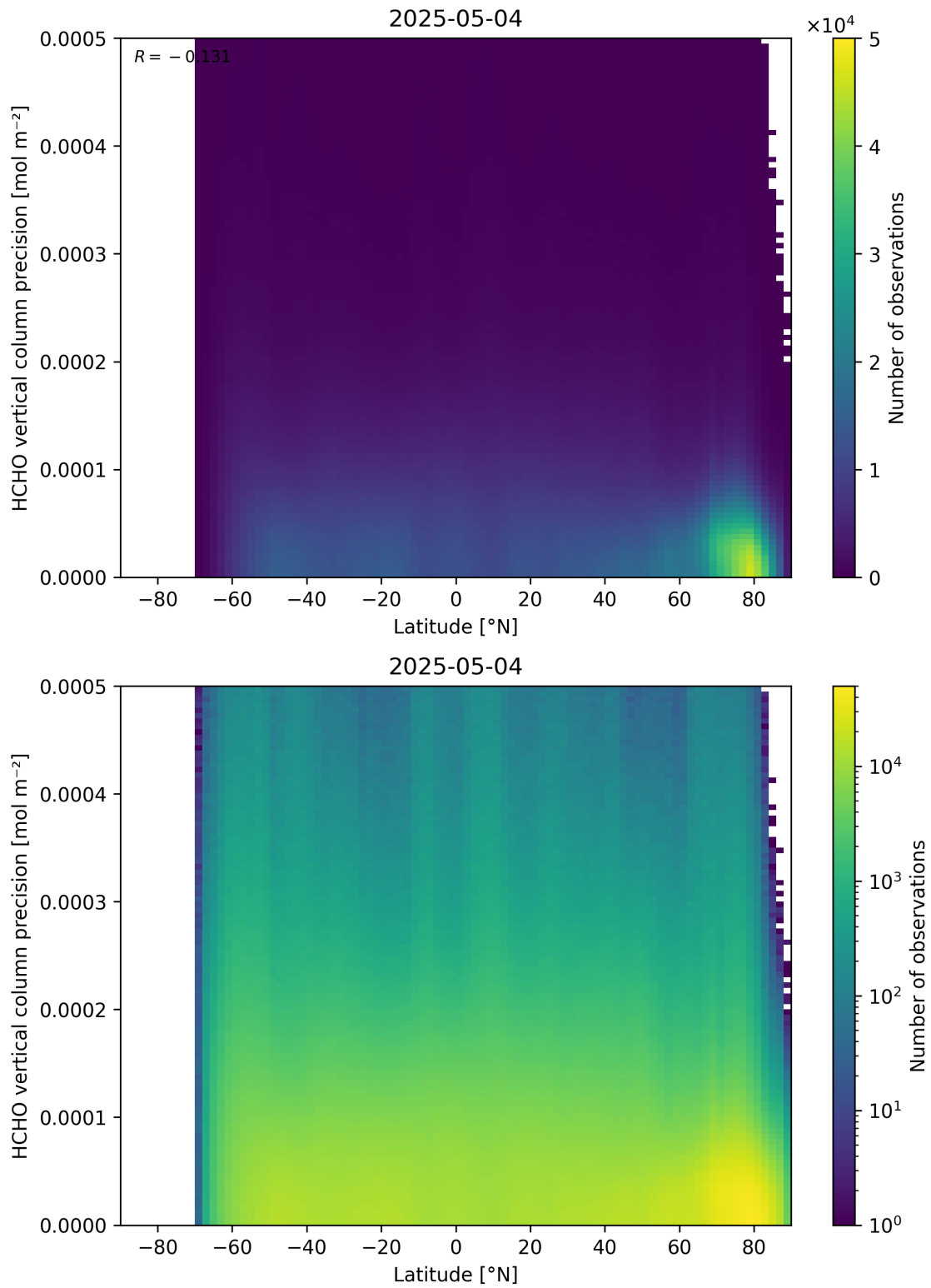
Figure 165: Scatter density plot of “Latitude” against “HCHO vertical column precision” for 2025-05-03 to 2025-05-05.
