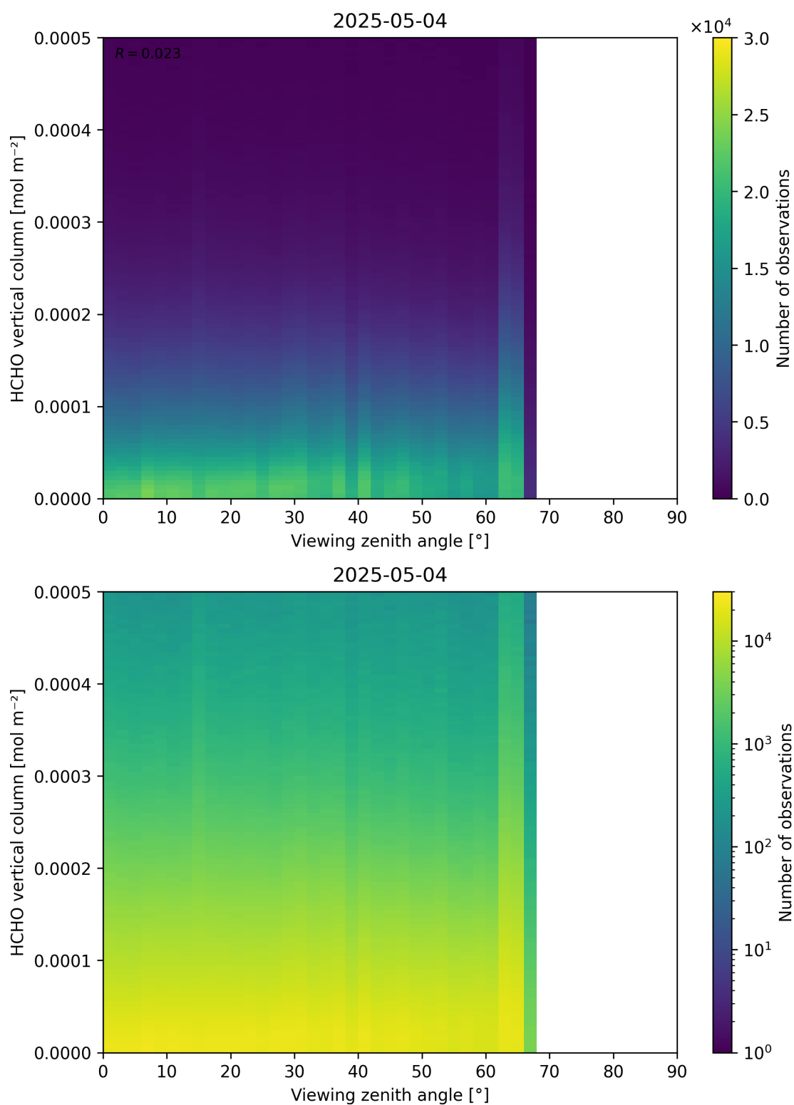
Figure 192: Scatter density plot of “Viewing zenith angle” against “HCHO vertical column” for 2025-05-03 to 2025-05-05.
