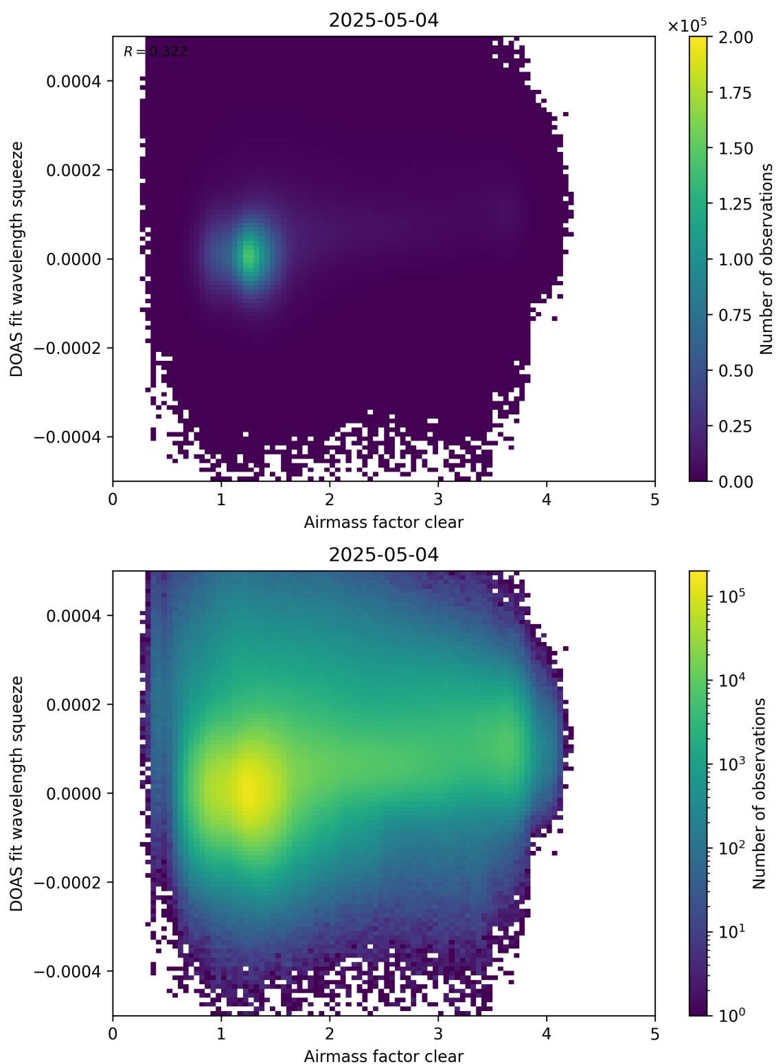
Figure 73: Scatter density plot of “Airmass factor clear” against “DOAS fit wavelength squeeze” for 2025-05-03 to 2025-05-05.
