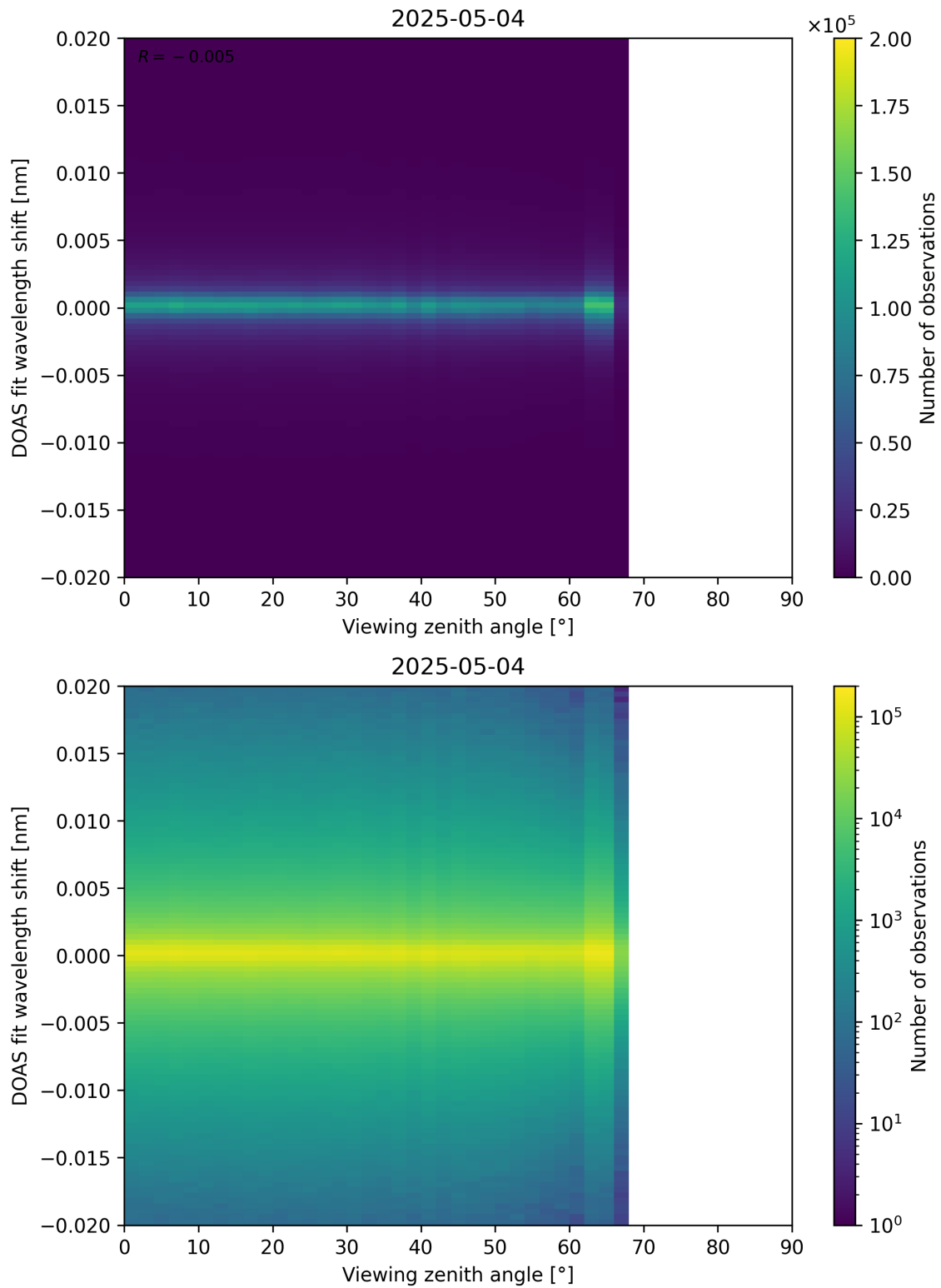
Figure 183: Scatter density plot of “Viewing zenith angle” against “DOAS fit wavelength shift” for 2025-05-03 to 2025-05-05.
