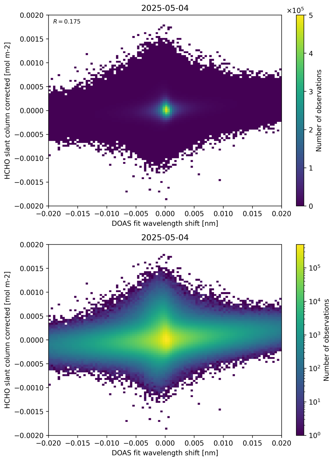
Figure 66: Scatter density plot of “DOAS fit wavelength shift” against “HCHO slant column corrected” for 2025-05-03 to 2025-05-05.
