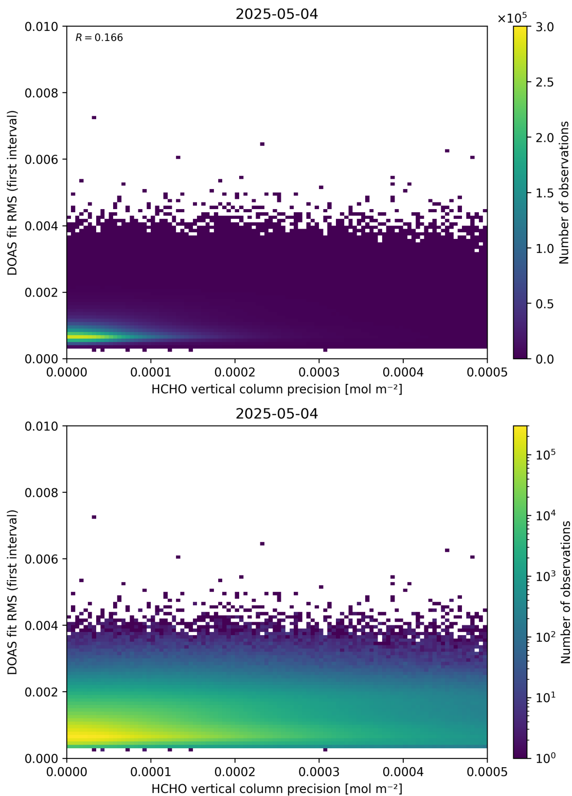
Figure 136: Scatter density plot of “HCHO vertical column precision” against “DOAS fit RMS (first interval)” for 2025-05-03 to 2025-05-05.
