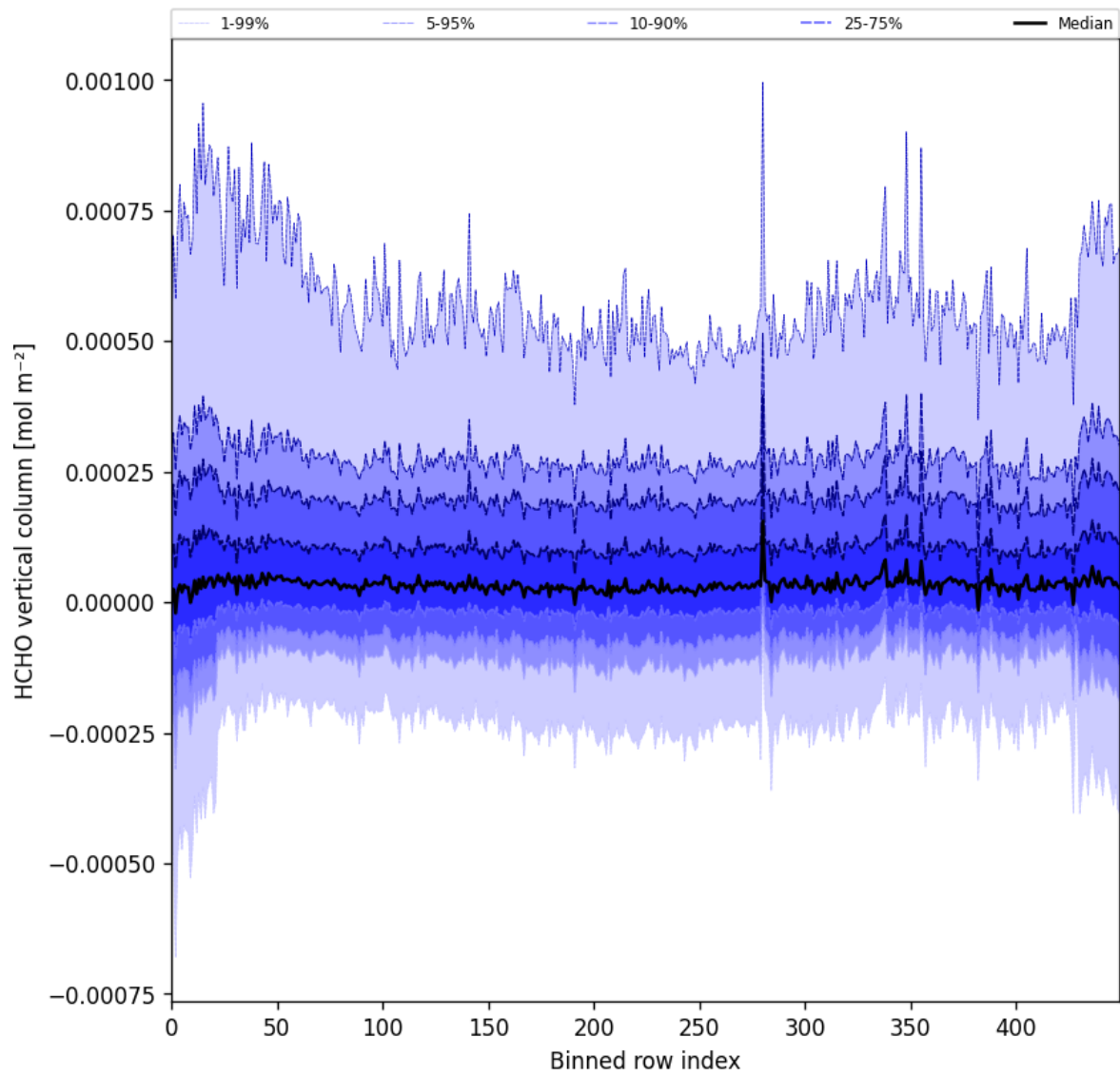
Figure 49: Along track statistics of “HCHO vertical column” for 2025-05-03 to 2025-05-05
