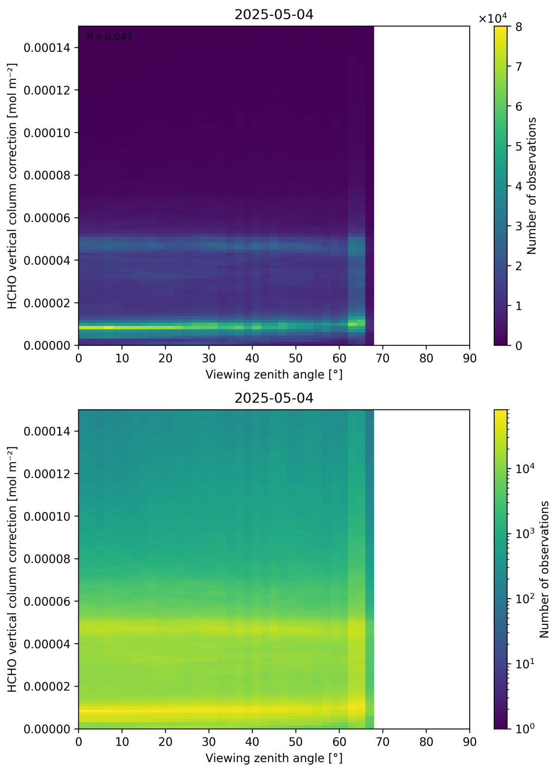
Figure 193: Scatter density plot of “Viewing zenith angle” against “HCHO vertical column correction” for 2025-05-03 to 2025-05-05.
