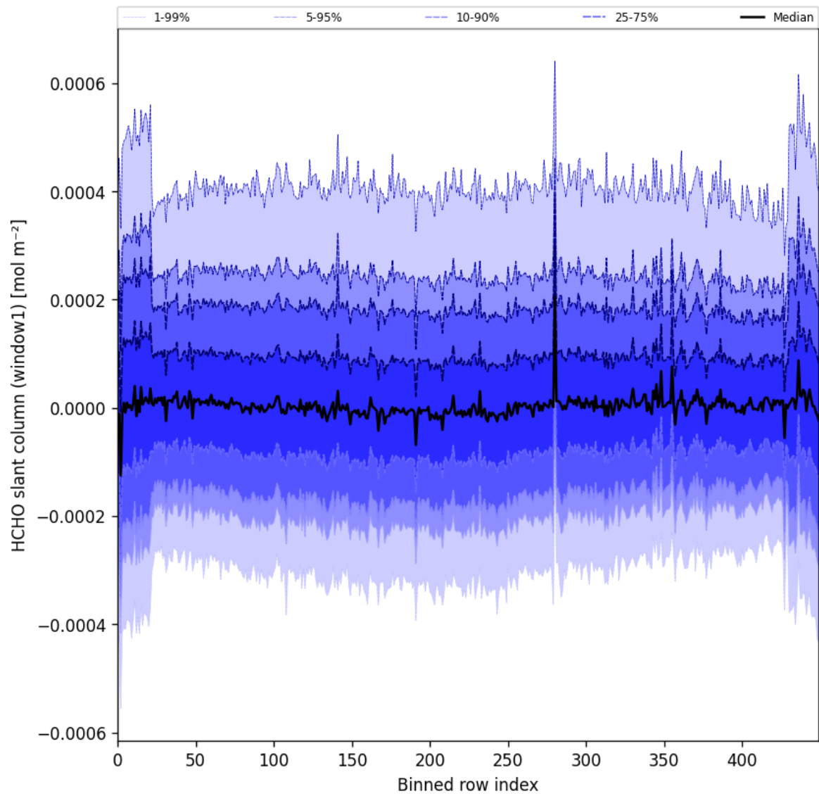
Figure 52: Along track statistics of “HCHO slant column (window1)” for 2025-05-03 to 2025-05-05
