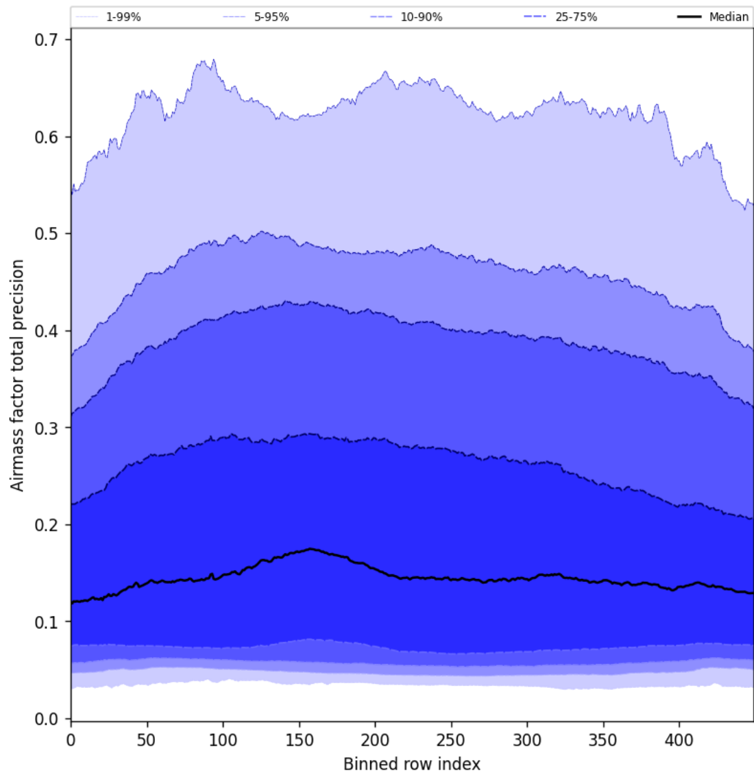
Figure 55: Along track statistics of “Airmass factor total precision” for 2025-05-03 to 2025-05-05
