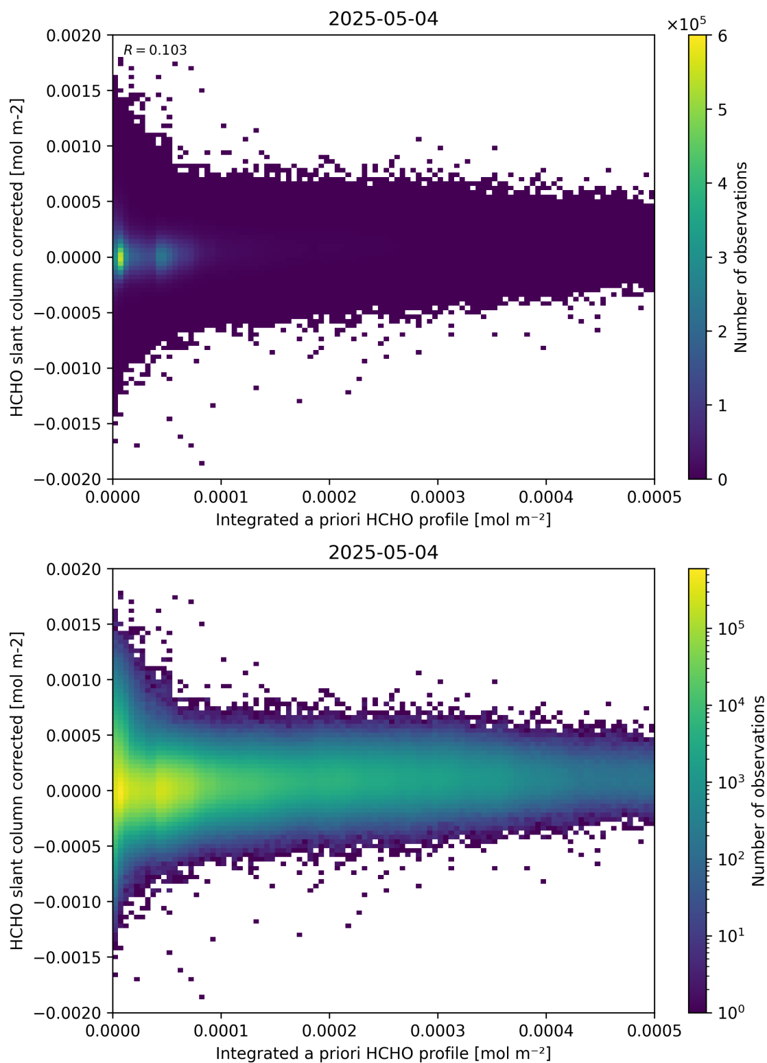
Figure 151: Scatter density plot of “Integrated a priori HCHO profile” against “HCHO slant column corrected” for 2025-05-03 to 2025-05-05.
