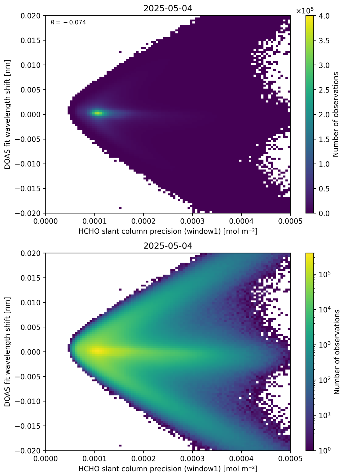
Figure 89: Scatter density plot of “HCHO slant column precision (window1)” against “DOAS fit wavelength shift” for 2025-05-03 to 2025-05-05.
