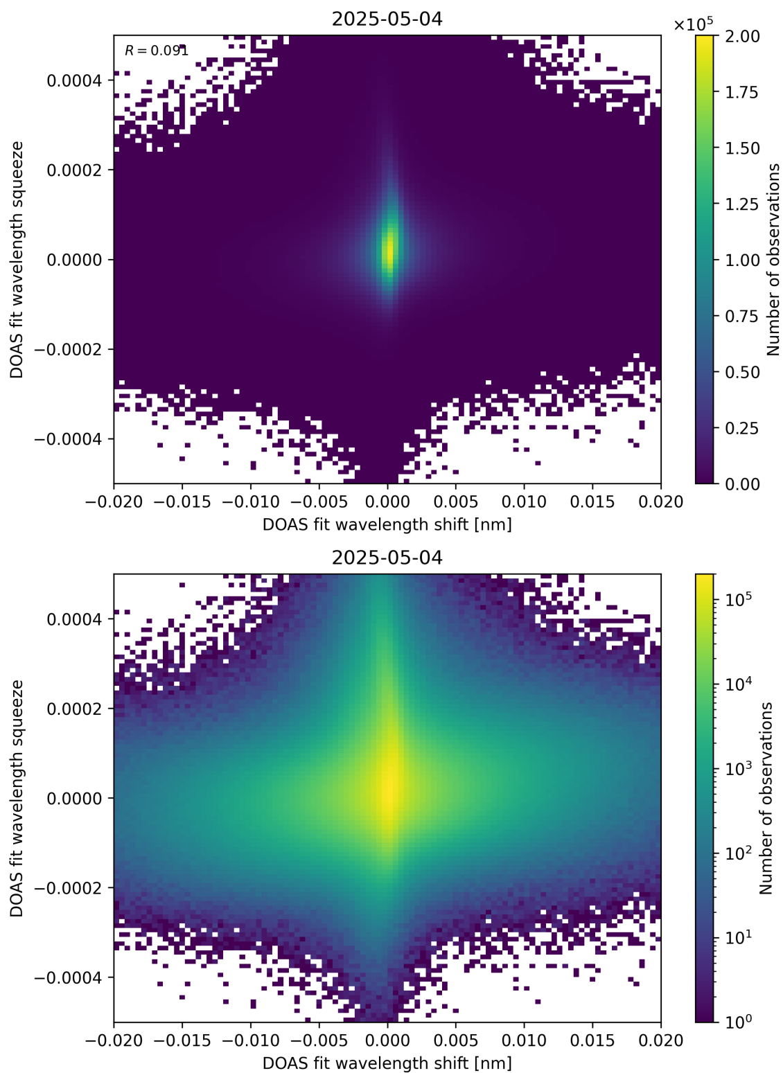
Figure 65: Scatter density plot of “DOAS fit wavelength shift” against “DOAS fit wavelength squeeze” for 2025-05-03 to 2025-05-05.
