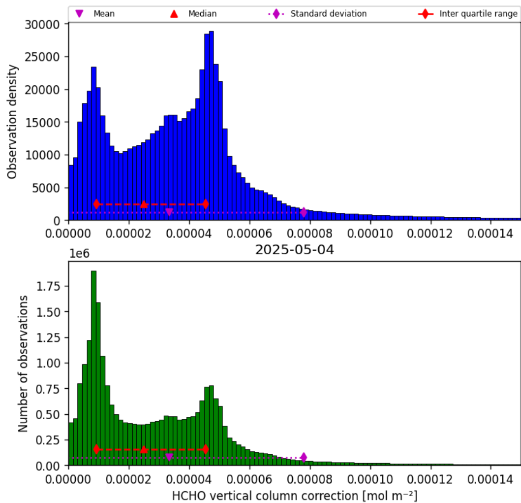
Figure 37: Histogram of “HCHO vertical column correction” for 2025-05-03 to 2025-05-05
