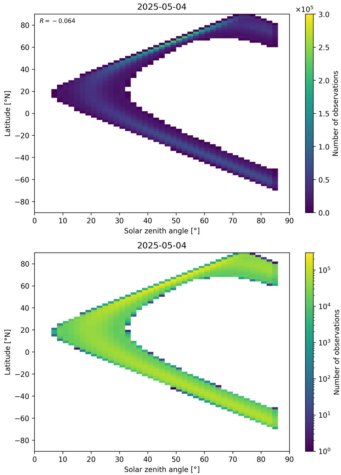
Figure 181: Scatter density plot of “Solar zenith angle” against “Latitude” for 2025-05-03 to 2025-05-05.
