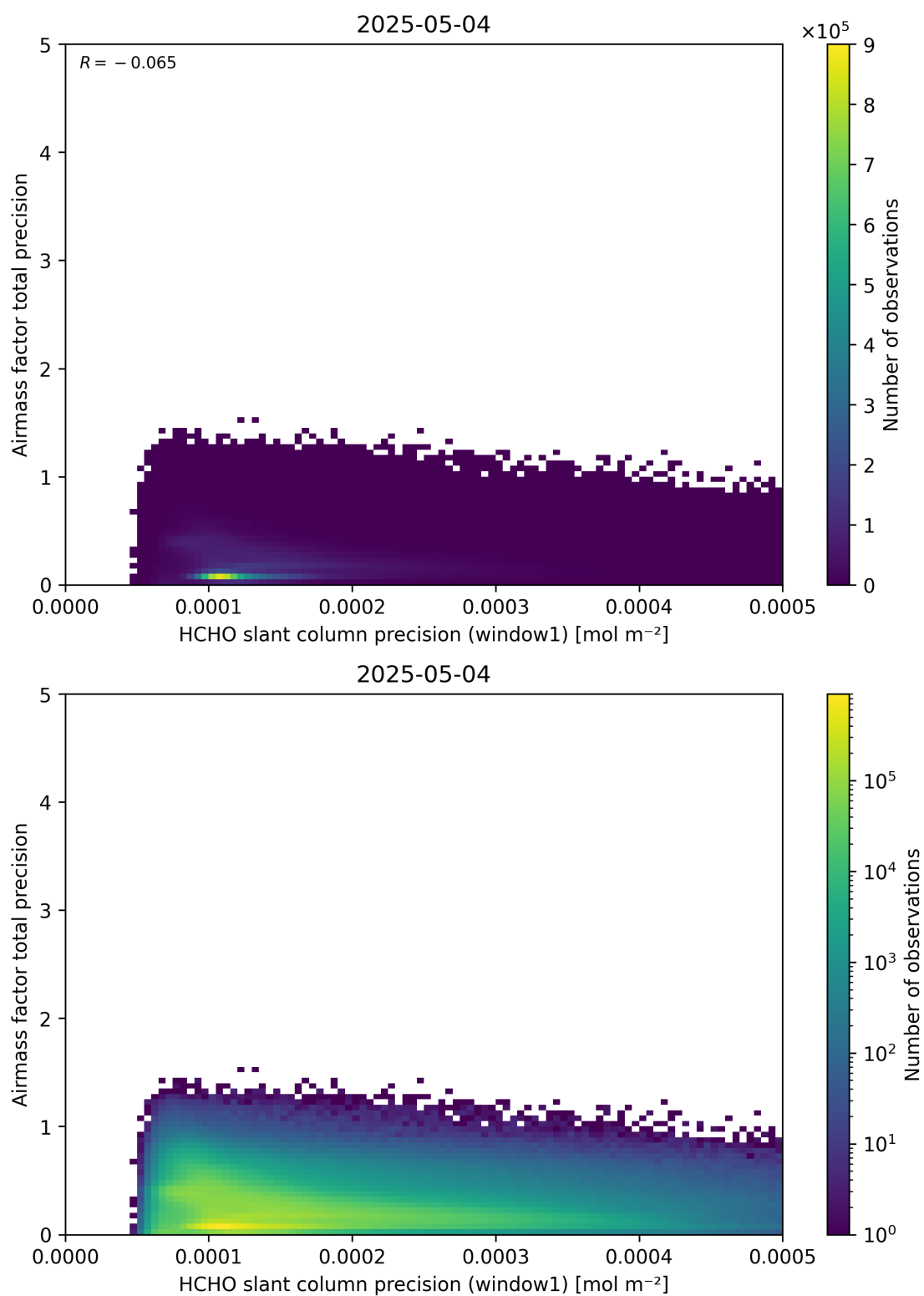
Figure 95: Scatter density plot of “HCHO slant column precision (window1)” against “Airmass factor total precision” for 2025-05-03 to 2025-05-05.
