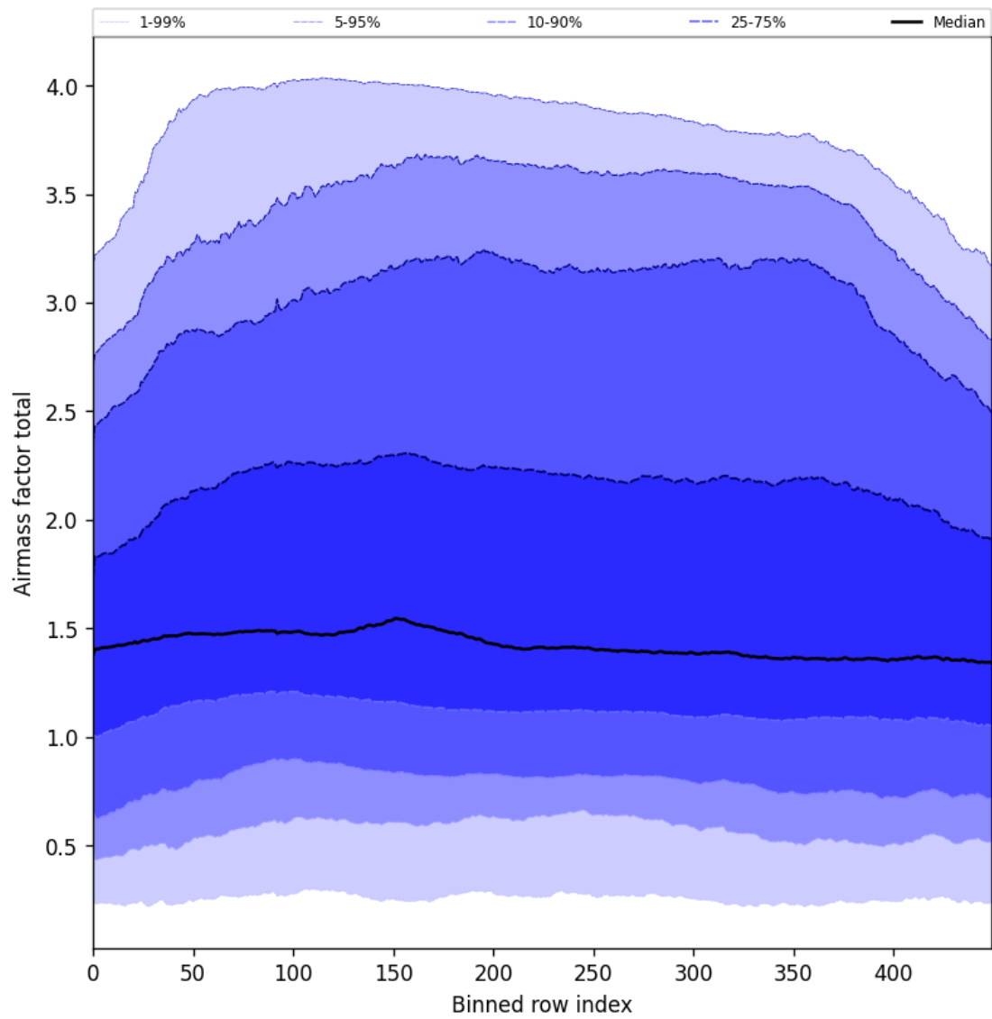
Figure 54: Along track statistics of “Airmass factor total” for 2025-05-03 to 2025-05-05
