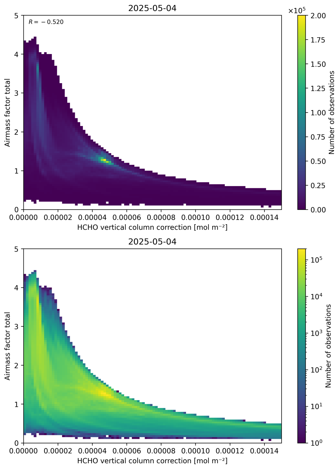
Figure 120: Scatter density plot of “HCHO vertical column correction” against “Airmass factor total” for 2025-05-03 to 2025-05-05.
