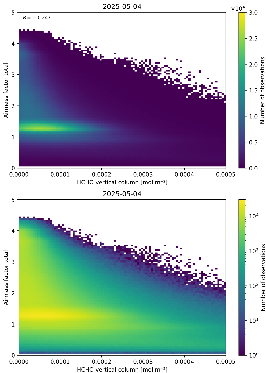
Figure 131: Scatter density plot of “HCHO vertical column” against “Airmass factor total” for 2025-05-03 to 2025-05-05.
