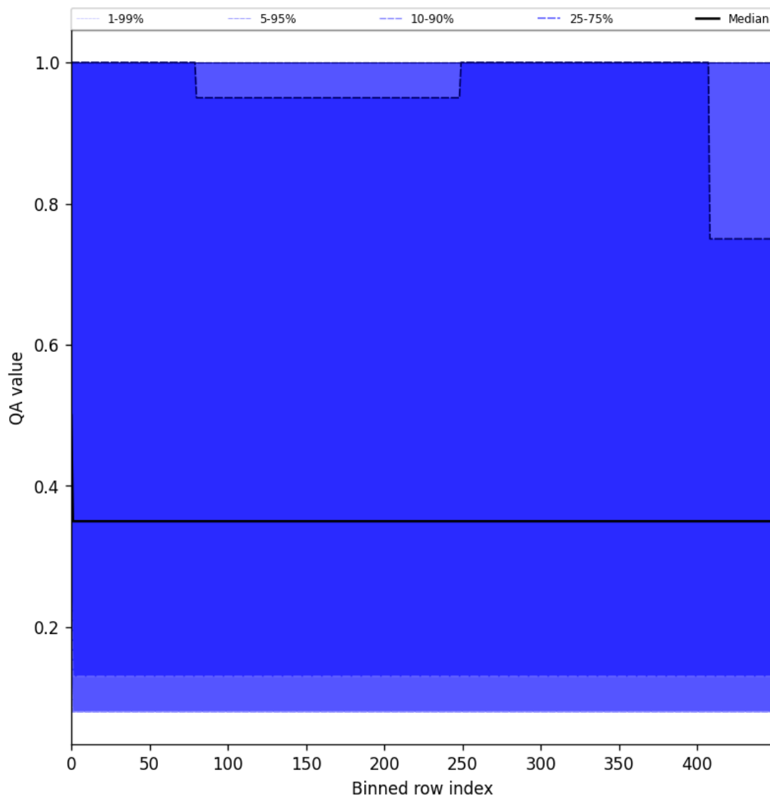
Figure 48: Along track statistics of “QA value” for 2025-05-03 to 2025-05-05
