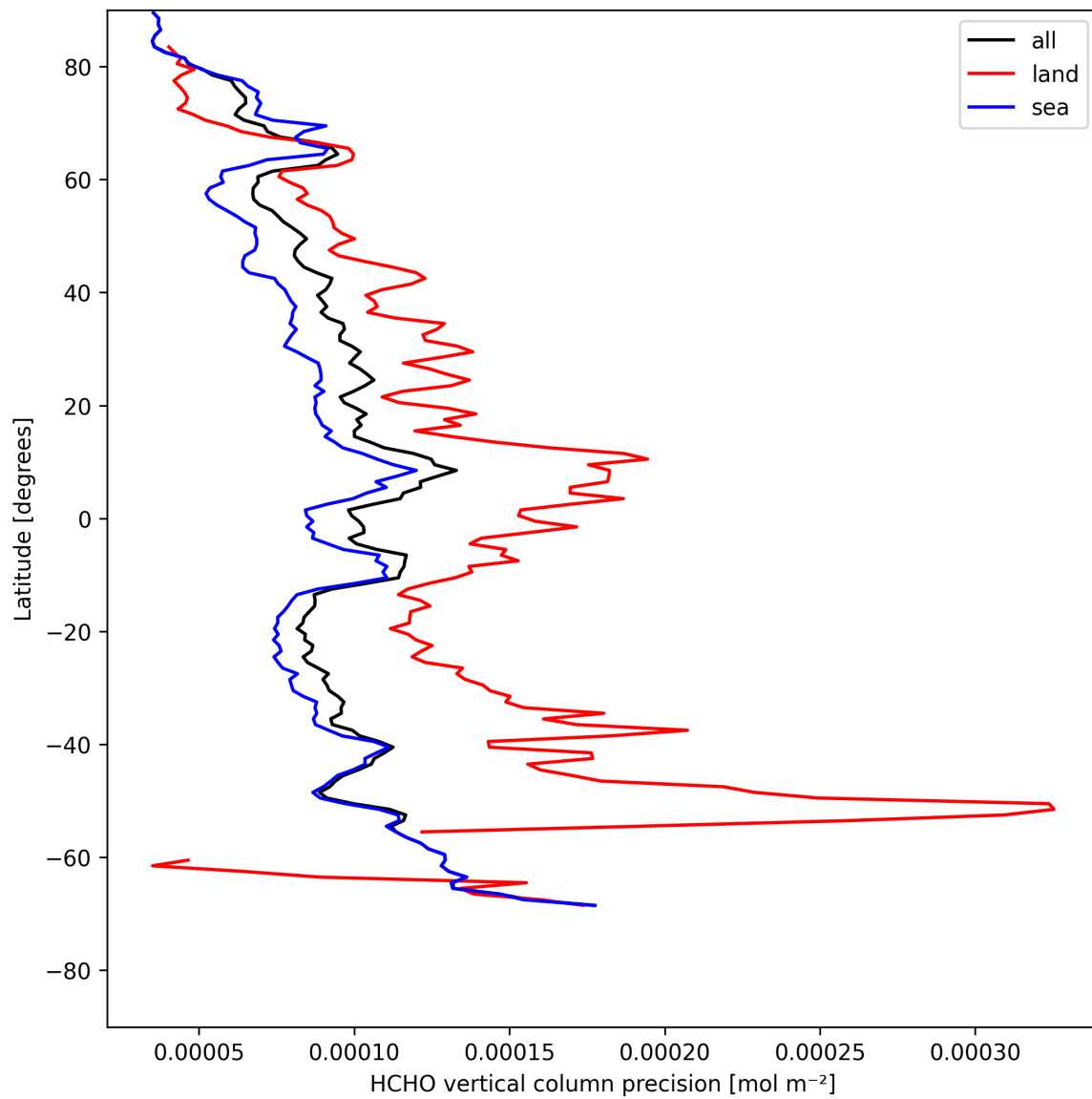
Figure 22: Zonal average of “HCHO vertical column precision” for 2025-05-03 to 2025-05-05.
