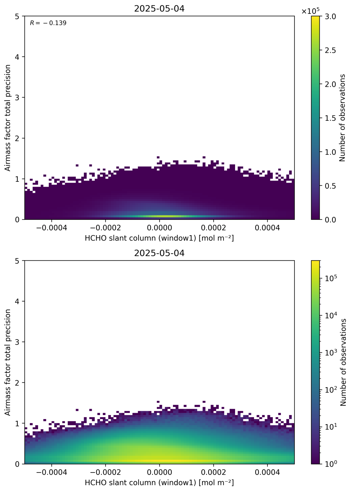
Figure 86: Scatter density plot of “HCHO slant column (window1)” against “Airmass factor total precision” for 2025-05-03 to 2025-05-05.
