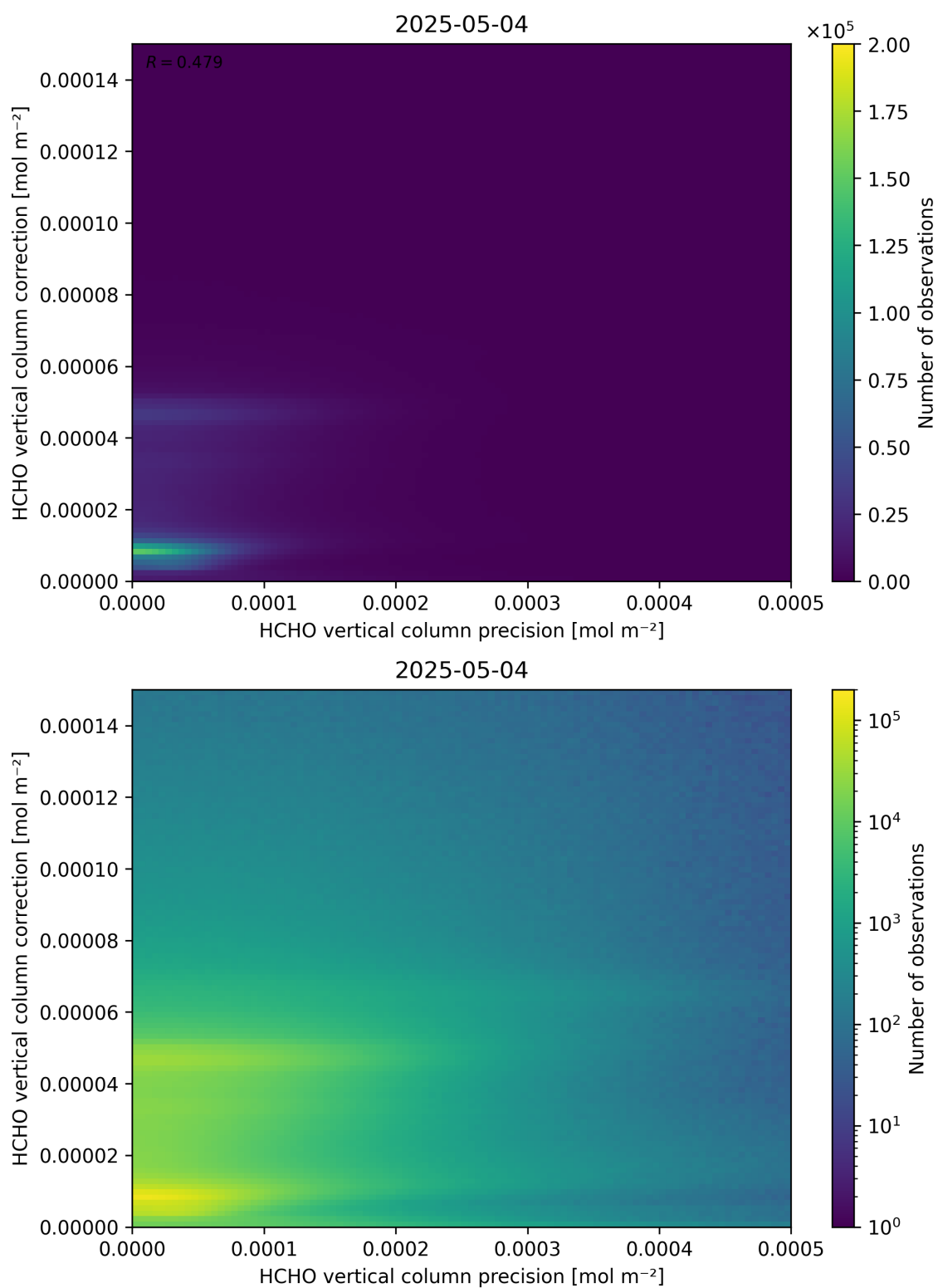
Figure 146: Scatter density plot of “HCHO vertical column precision” against “HCHO vertical column correction” for 2025-05-03 to 2025-05-05.
