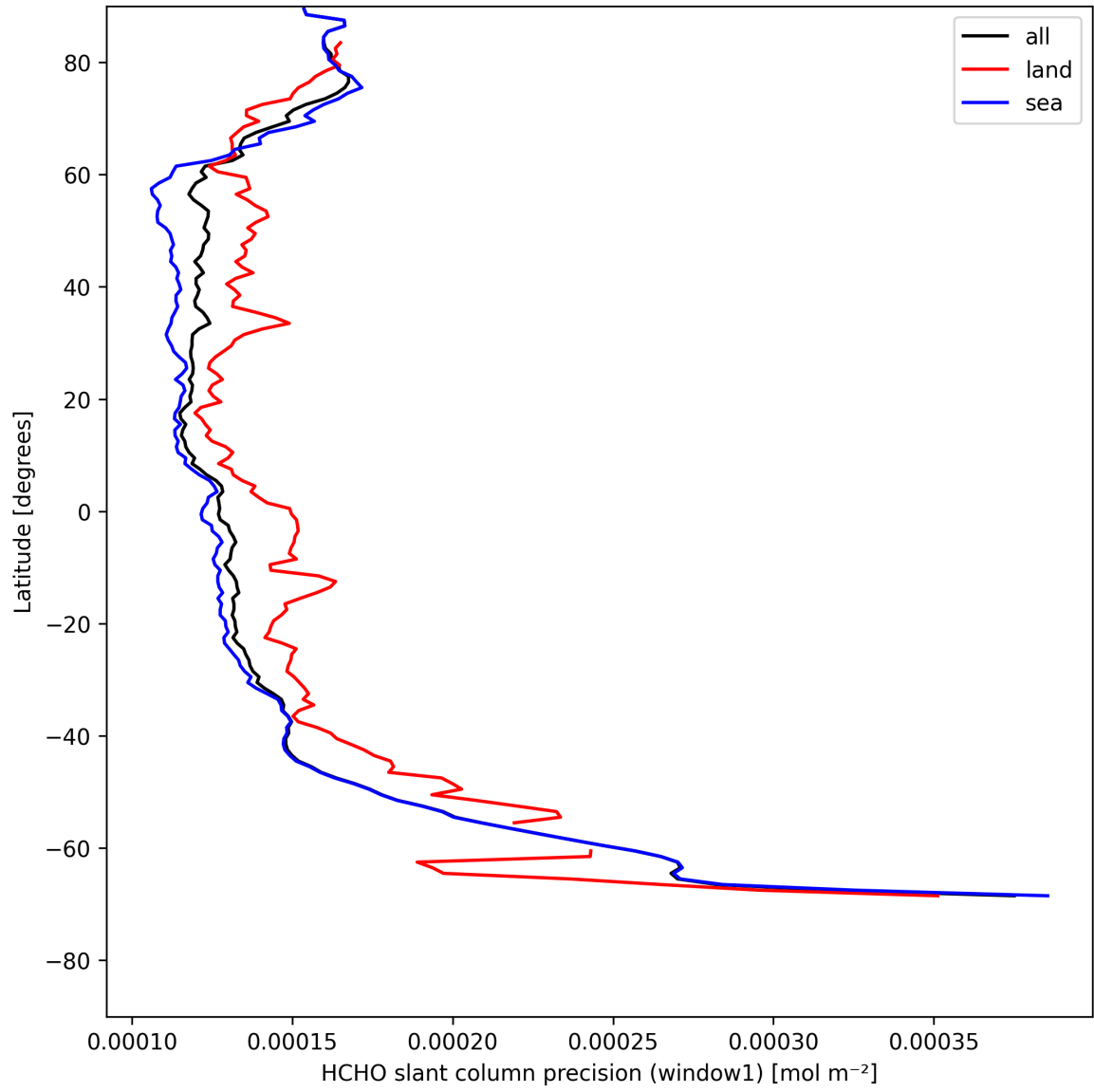
Figure 25: Zonal average of “HCHO slant column precision (window1)” for 2025-05-03 to 2025-05-05.
