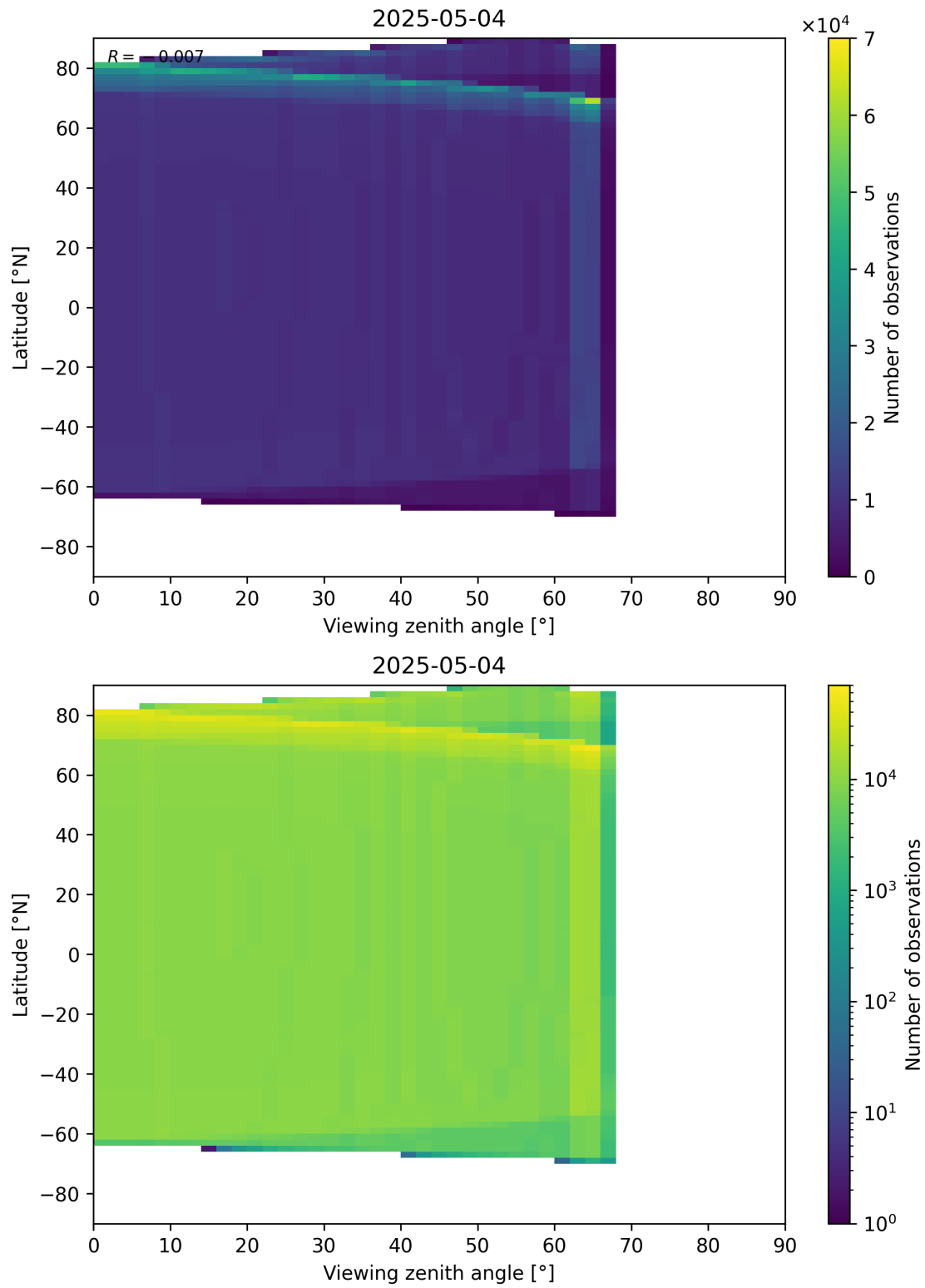
Figure 196: Scatter density plot of “Viewing zenith angle” against “Latitude” for 2025-05-03 to 2025-05-05.
