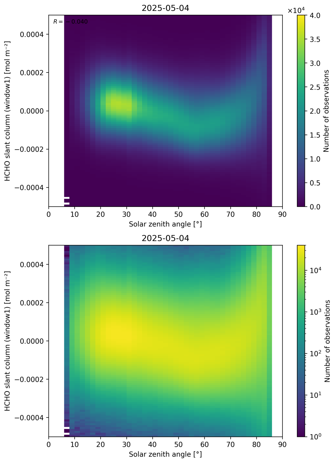
Figure 173: Scatter density plot of “Solar zenith angle” against “HCHO slant column (window1)” for 2025-05-03 to 2025-05-05.
