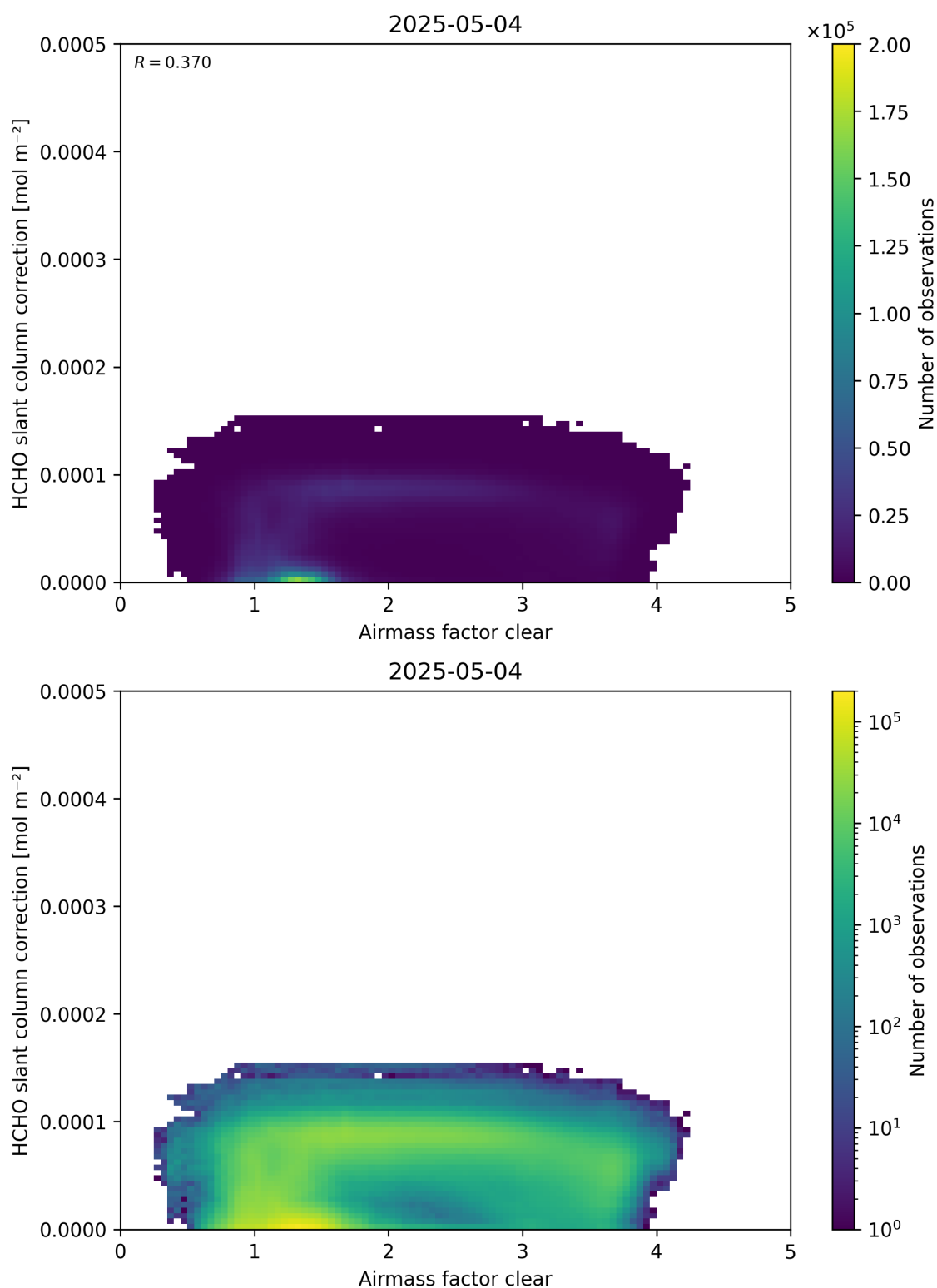
Figure 75: Scatter density plot of “Airmass factor clear” against “HCHO slant column correction” for 2025-05-03 to 2025-05-05.
