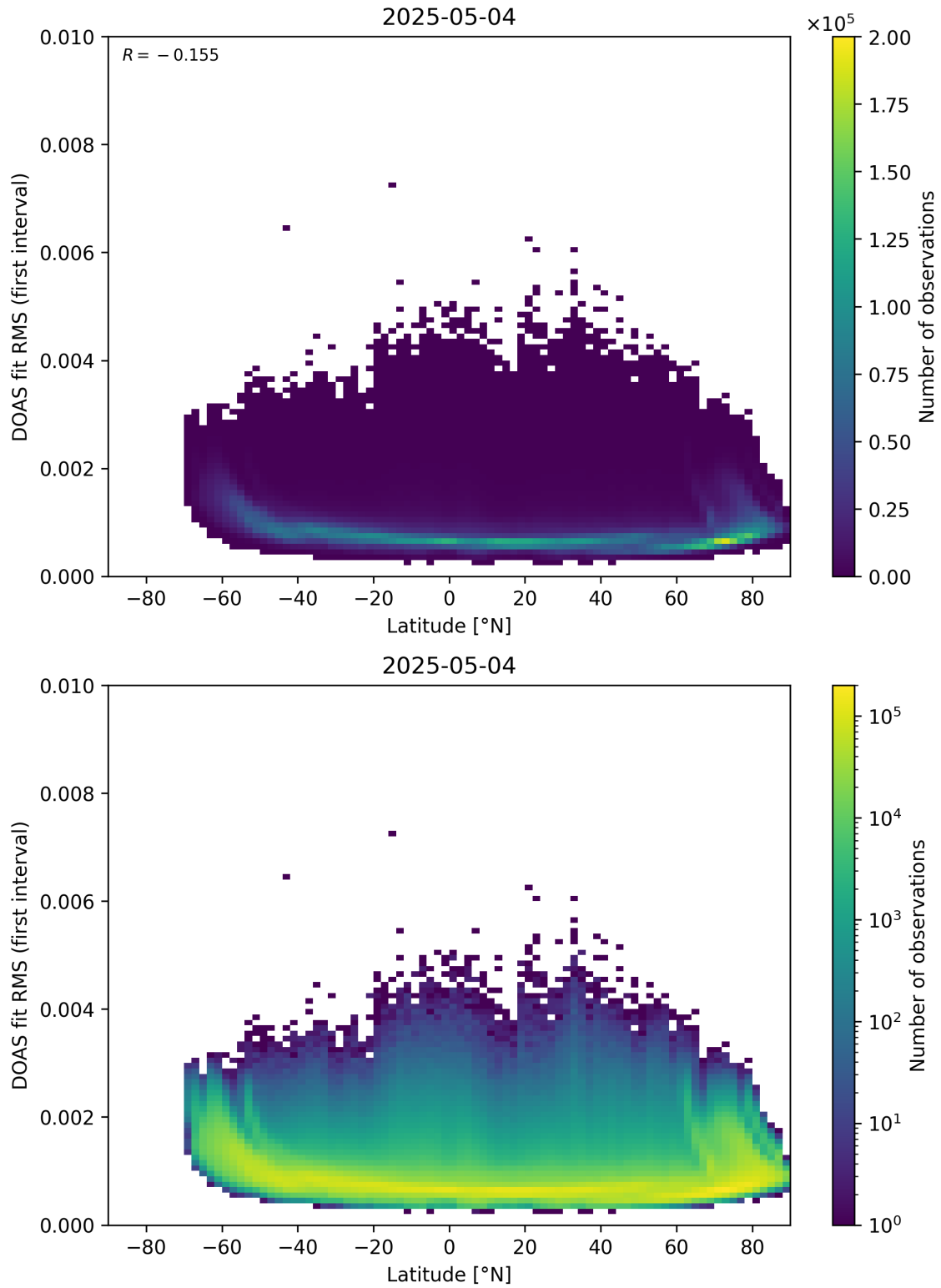
Figure 153: Scatter density plot of “Latitude” against “DOAS fit RMS (first interval)” for 2025-05-03 to 2025-05-05.
