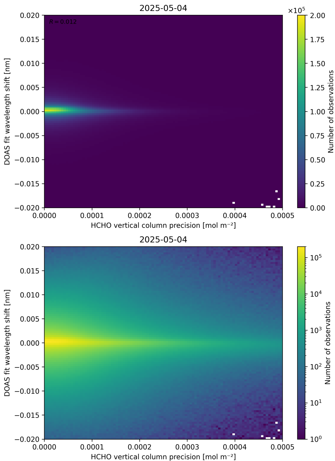
Figure 137: Scatter density plot of “HCHO vertical column precision” against “DOAS fit wavelength shift” for 2025-05-03 to 2025-05-05.
