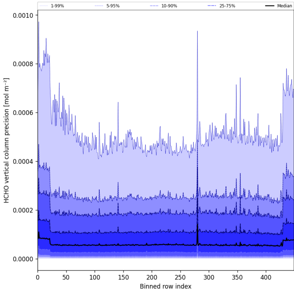
Figure 50: Along track statistics of “HCHO vertical column precision” for 2025-05-03 to 2025-05-05
