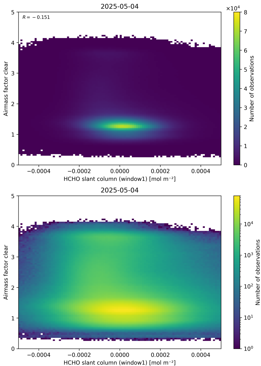
Figure 81: Scatter density plot of “HCHO slant column (window1)” against “Airmass factor clear” for 2025-05-03 to 2025-05-05.
