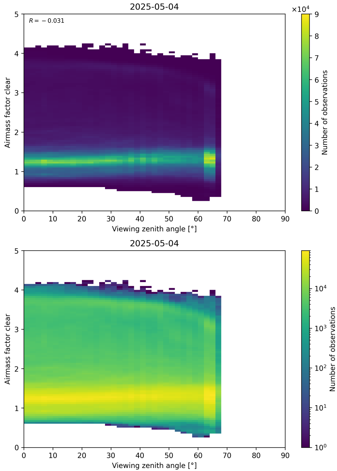
Figure 185: Scatter density plot of “Viewing zenith angle” against “Airmass factor clear” for 2025-05-03 to 2025-05-05.
