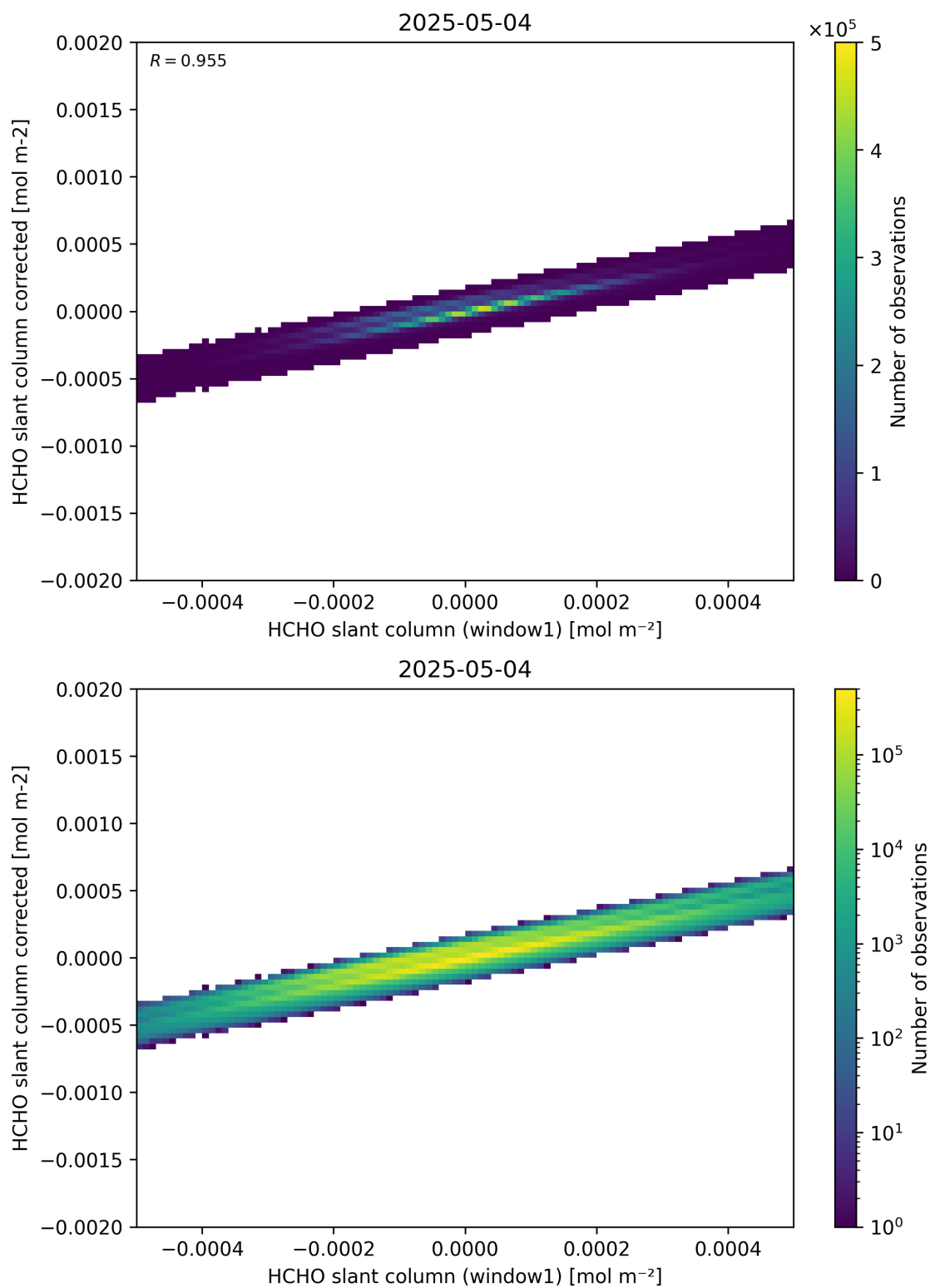
Figure 82: Scatter density plot of “HCHO slant column (window1)” against “HCHO slant column corrected” for 2025-05-03 to 2025-05-05.
