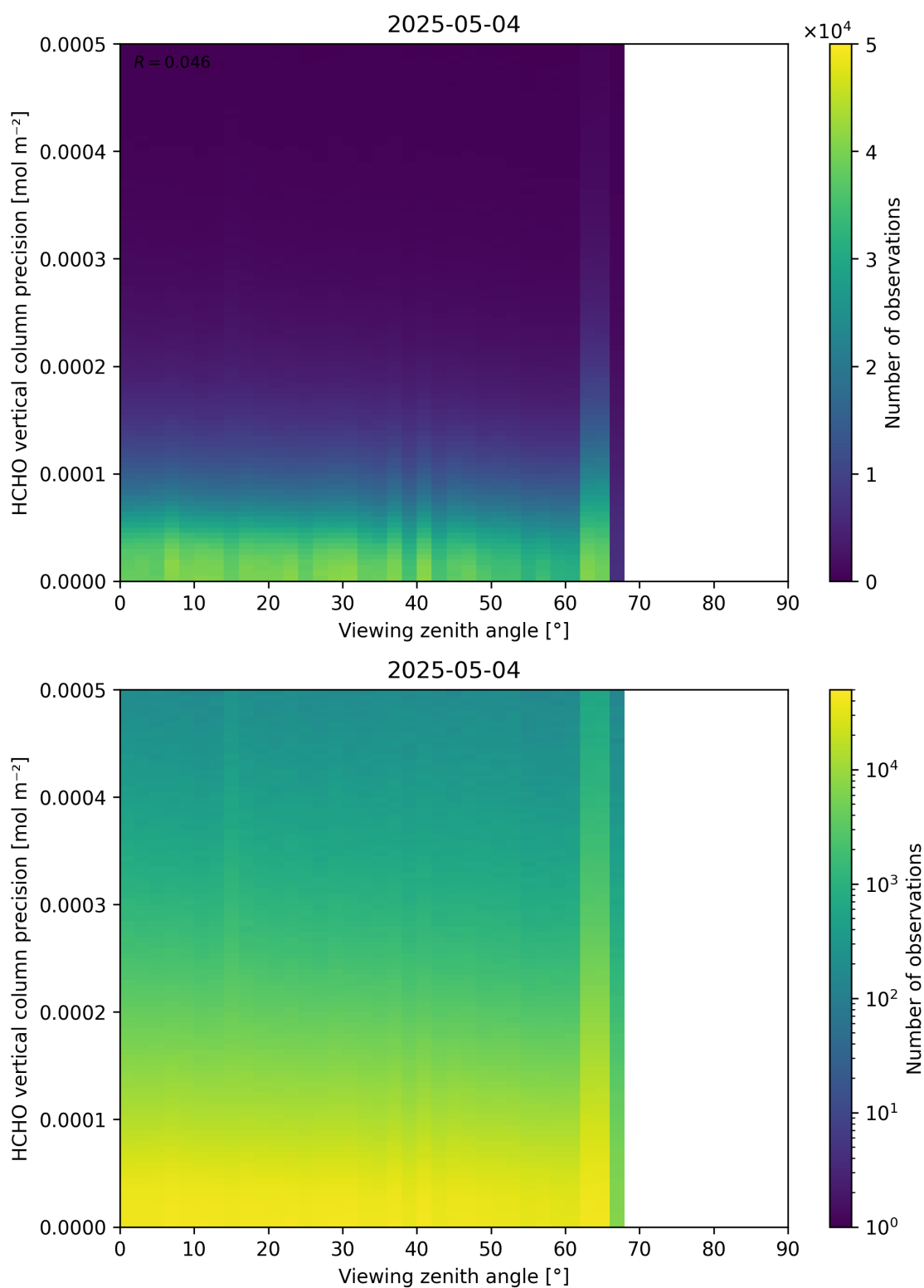
Figure 194: Scatter density plot of “Viewing zenith angle” against “HCHO vertical column precision” for 2025-05-03 to 2025-05-05.
