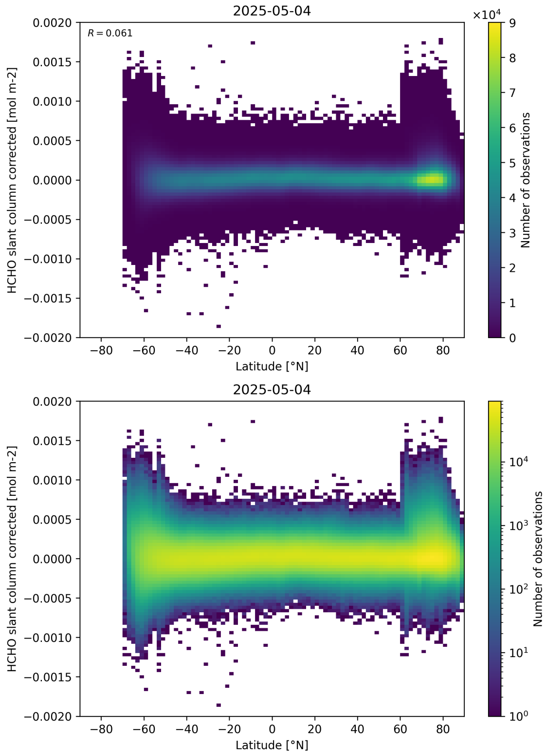
Figure 157: Scatter density plot of “Latitude” against “HCHO slant column corrected” for 2025-05-03 to 2025-05-05.
