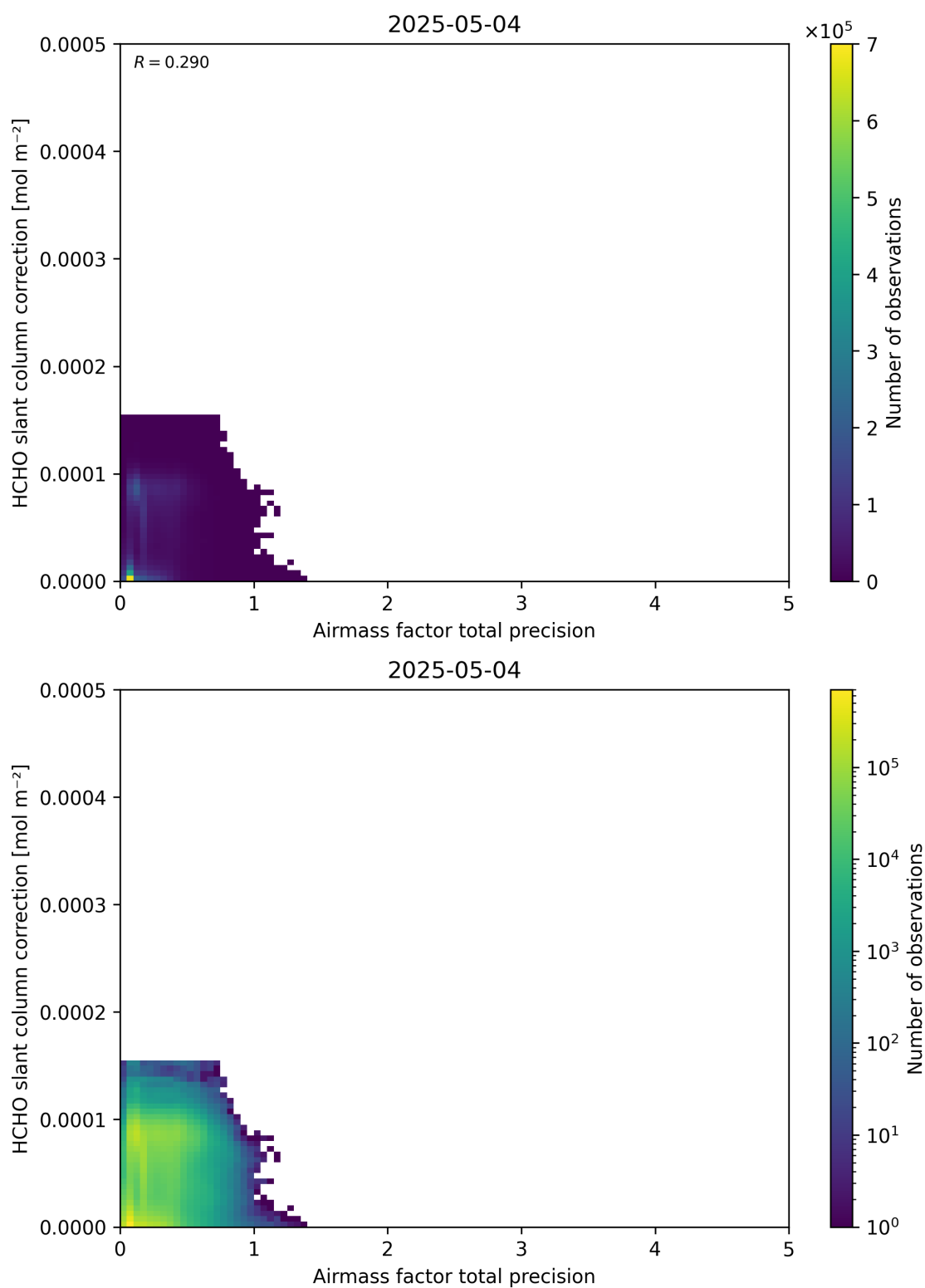
Figure 110: Scatter density plot of “Airmass factor total precision” against “HCHO slant column correction” for 2025-05-03 to 2025-05-05.
