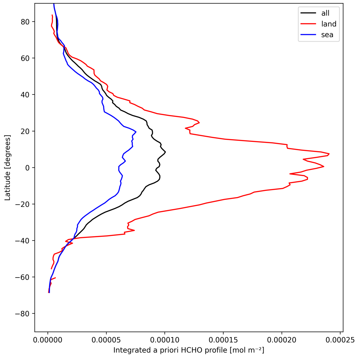
Figure 29: Zonal average of “Integrated a priori HCHO profile” for 2025-05-03 to 2025-05-05.
