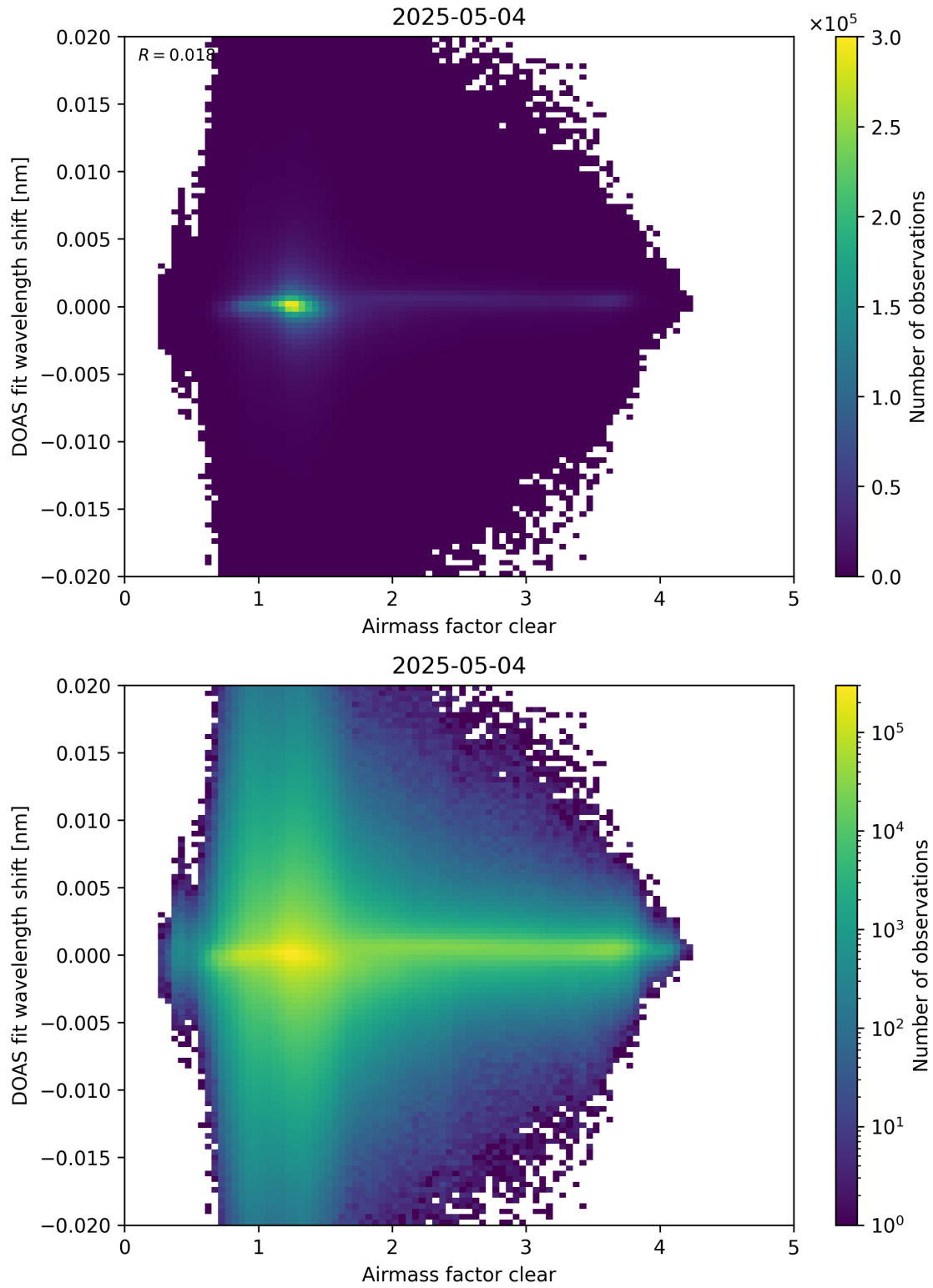
Figure 72: Scatter density plot of “Airmass factor clear” against “DOAS fit wavelength shift” for 2025-05-03 to 2025-05-05.
