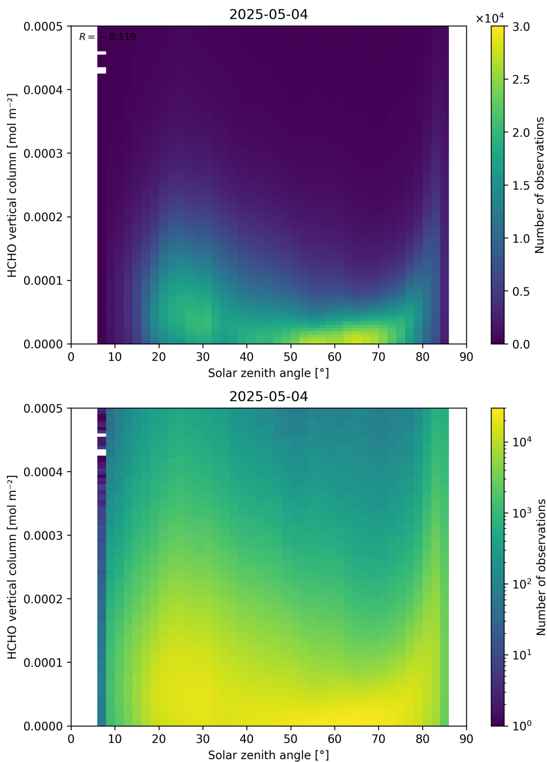
Figure 177: Scatter density plot of “Solar zenith angle” against “HCHO vertical column” for 2025-05-03 to 2025-05-05.
