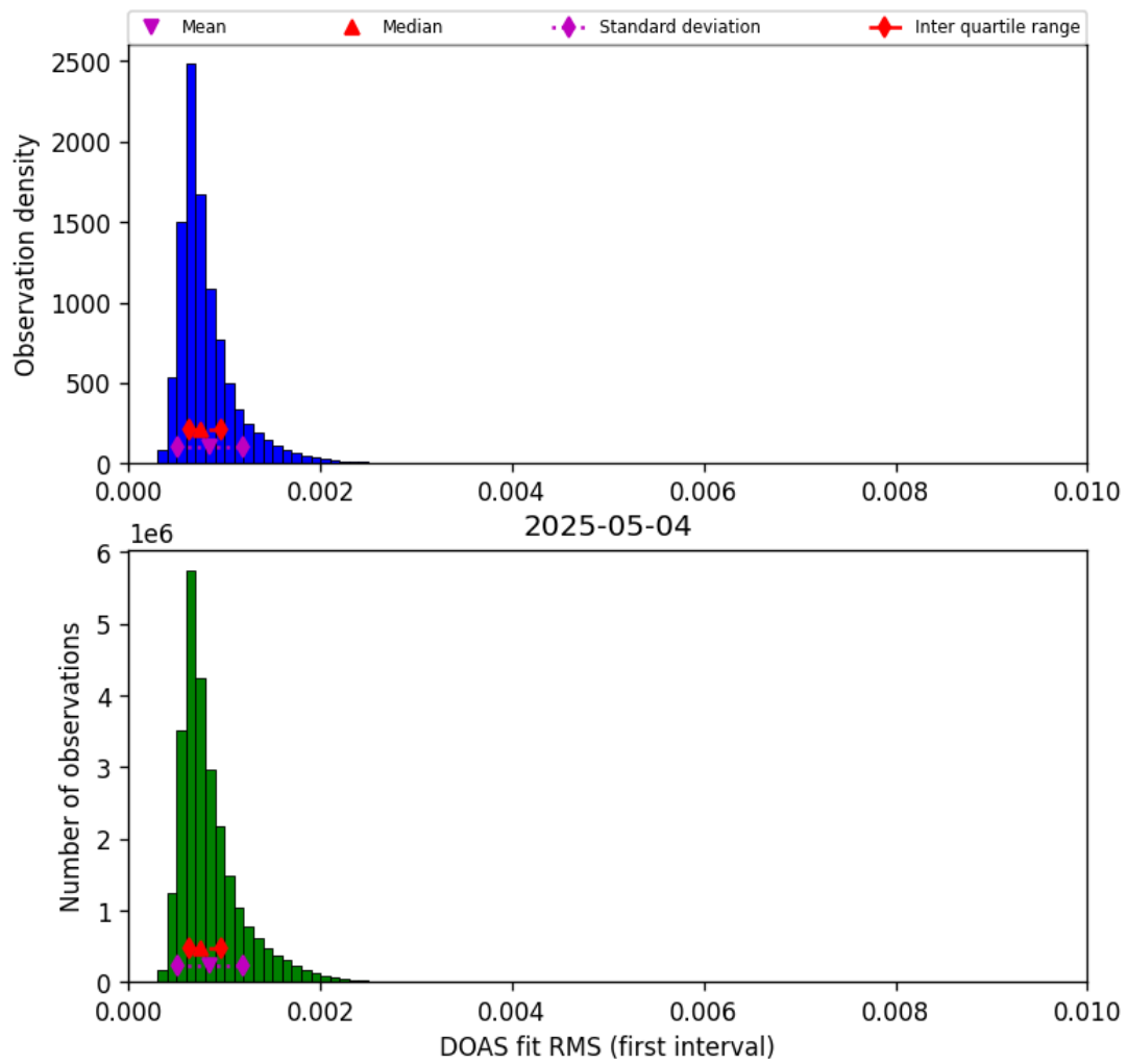
Figure 46: Histogram of “DOAS fit RMS (first interval)” for 2025-05-03 to 2025-05-05
