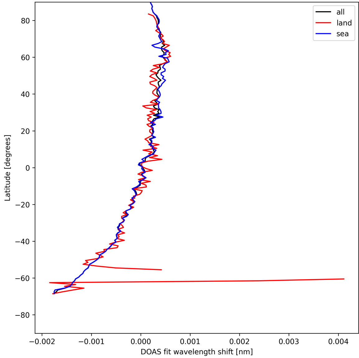
Figure 30: Zonal average of “DOAS fit wavelength shift” for 2025-05-03 to 2025-05-05.
