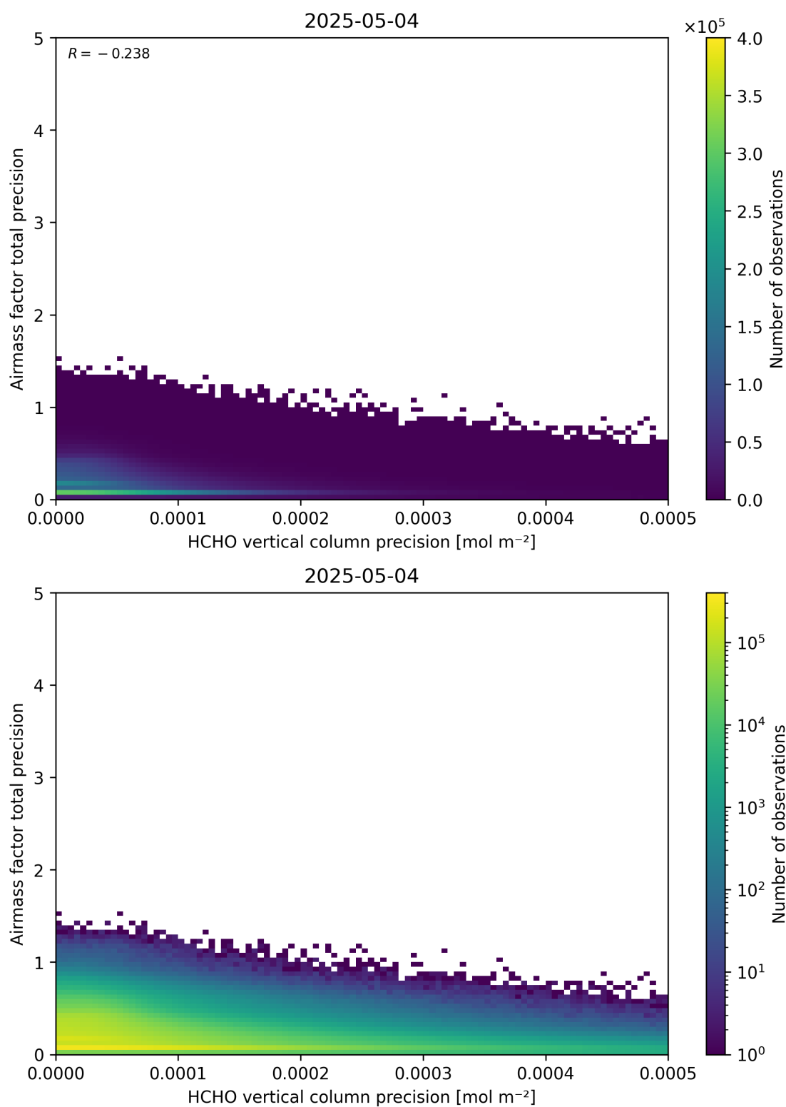
Figure 145: Scatter density plot of “HCHO vertical column precision” against “Airmass factor total precision” for 2025-05-03 to 2025-05-05.
