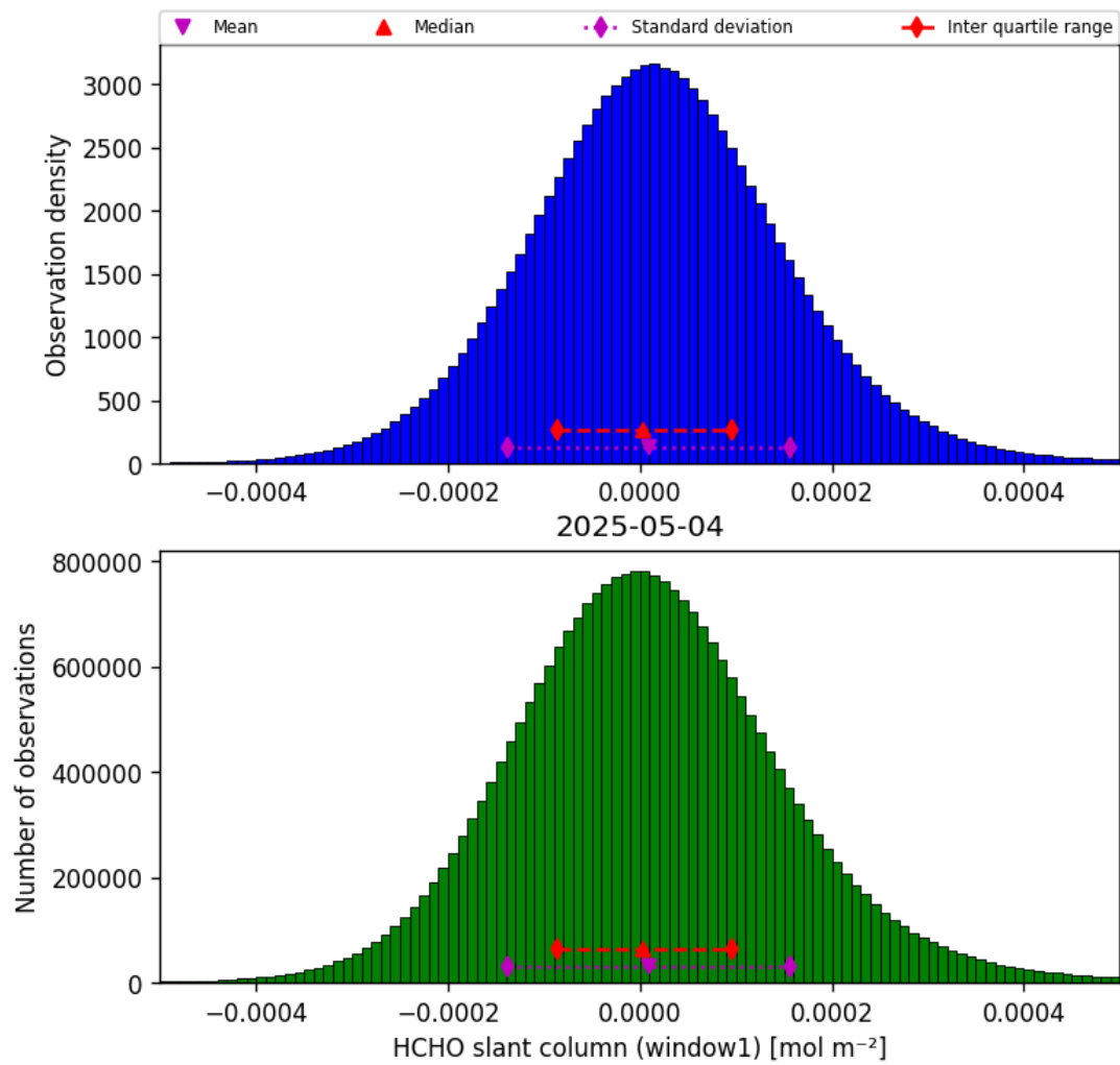
Figure 38: Histogram of “HCHO slant column (window1)” for 2025-05-03 to 2025-05-05
