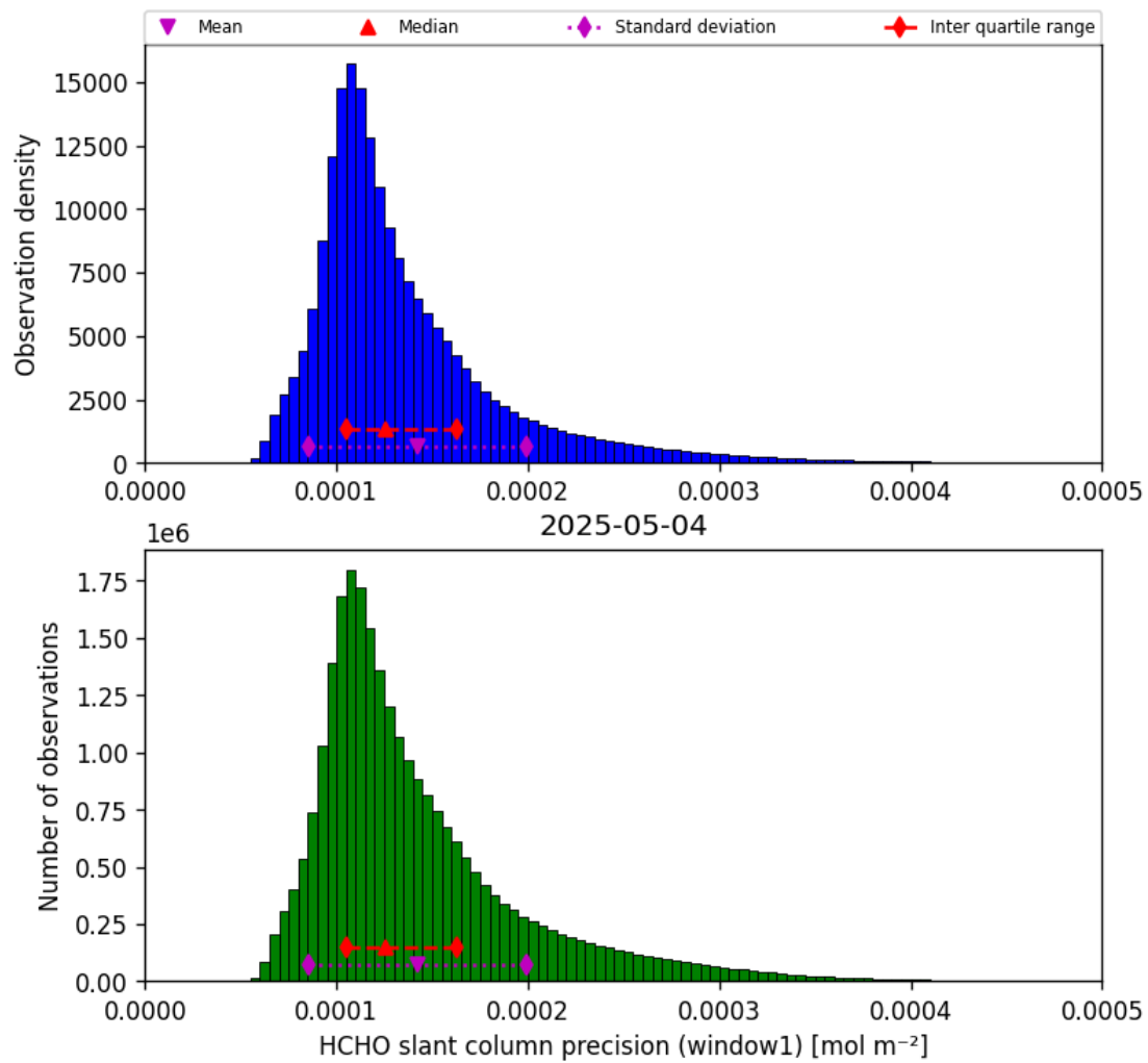
Figure 39: Histogram of “HCHO slant column precision (window1)” for 2025-05-03 to 2025-05-05
