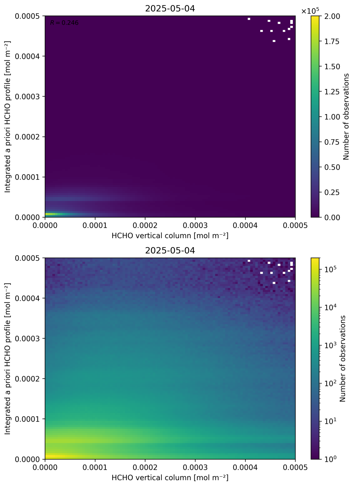
Figure 135: Scatter density plot of “HCHO vertical column” against “Integrated a priori HCHO profile” for 2025-05-03 to 2025-05-05.
