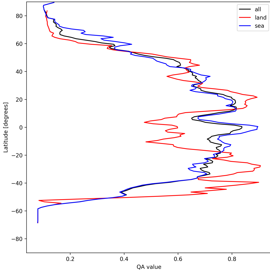
Figure 20: Zonal average of “QA value” for 2025-05-03 to 2025-05-05.
