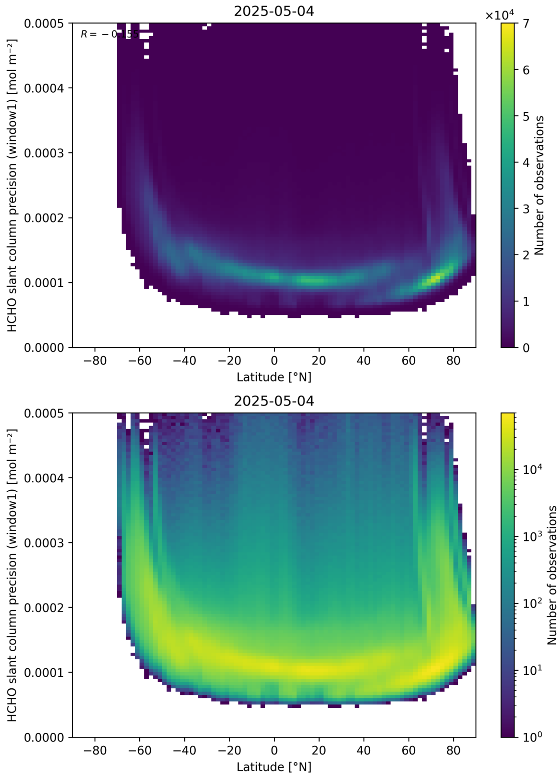
Figure 160: Scatter density plot of “Latitude” against “HCHO slant column precision (window1)” for 2025-05-03 to 2025-05-05.
