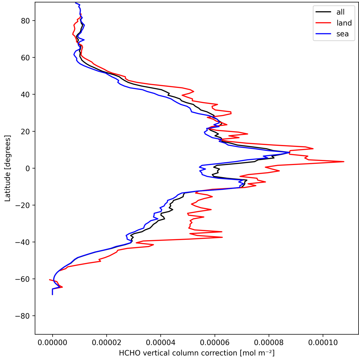
Figure 23: Zonal average of “HCHO vertical column correction” for 2025-05-03 to 2025-05-05.
