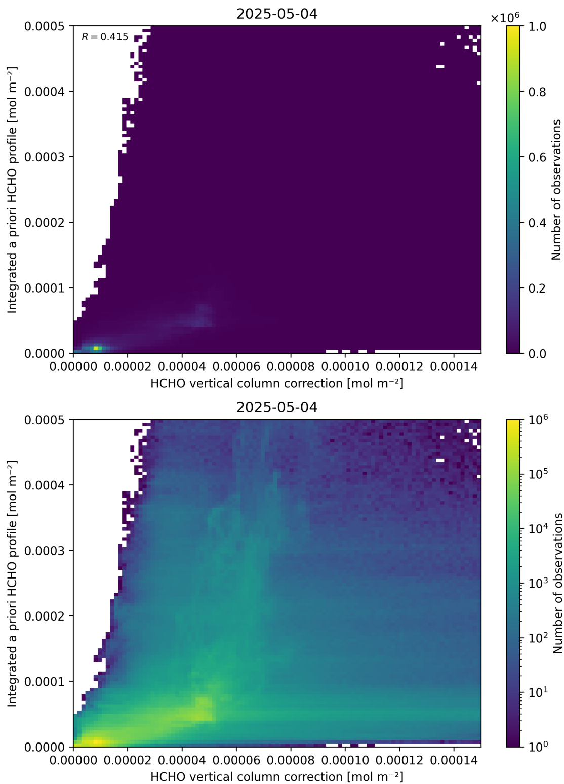
Figure 122: Scatter density plot of “HCHO vertical column correction” against “Integrated a priori HCHO profile” for 2025-05-03 to 2025-05-05.
