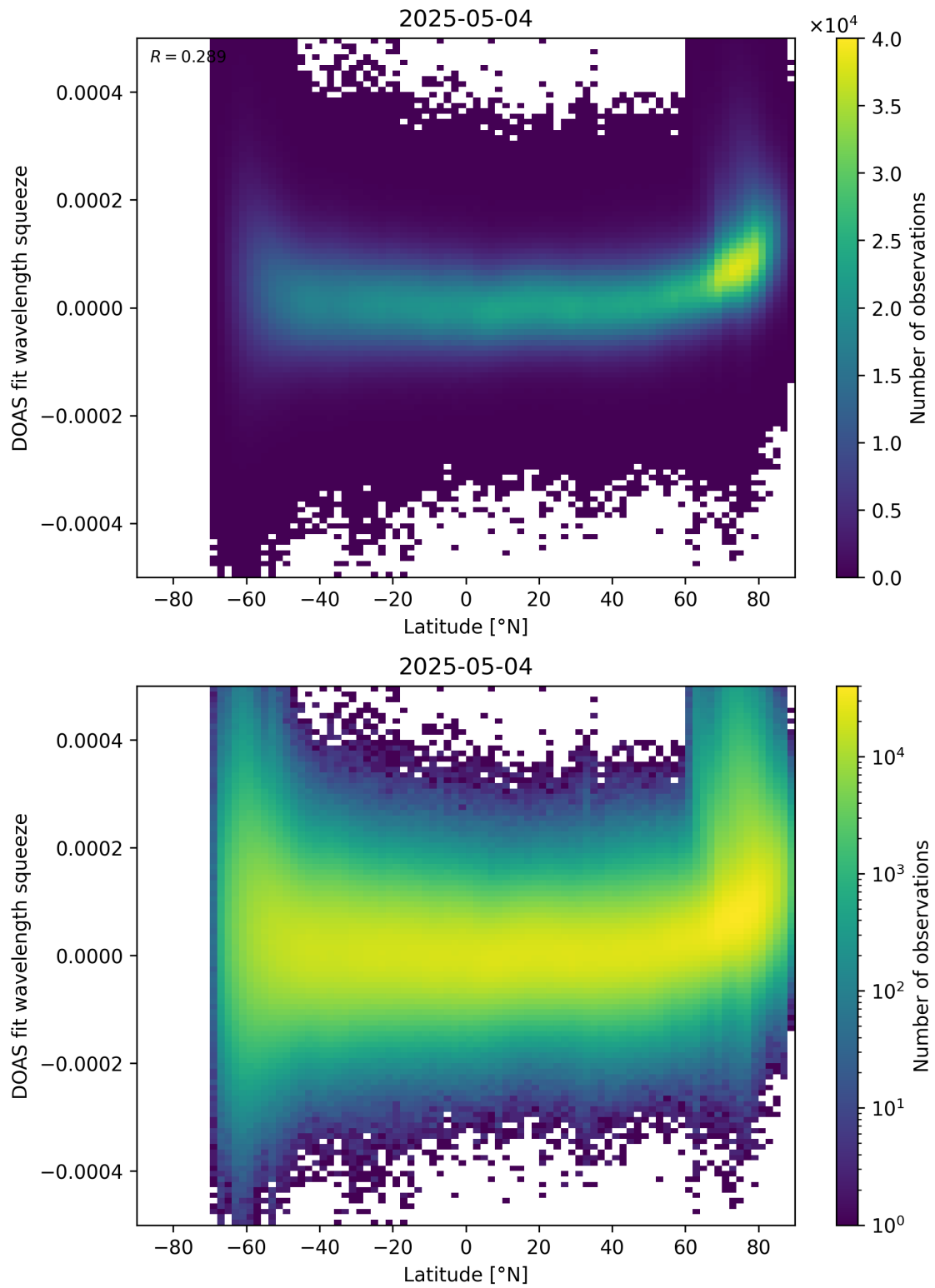
Figure 155: Scatter density plot of “Latitude” against “DOAS fit wavelength squeeze” for 2025-05-03 to 2025-05-05.
