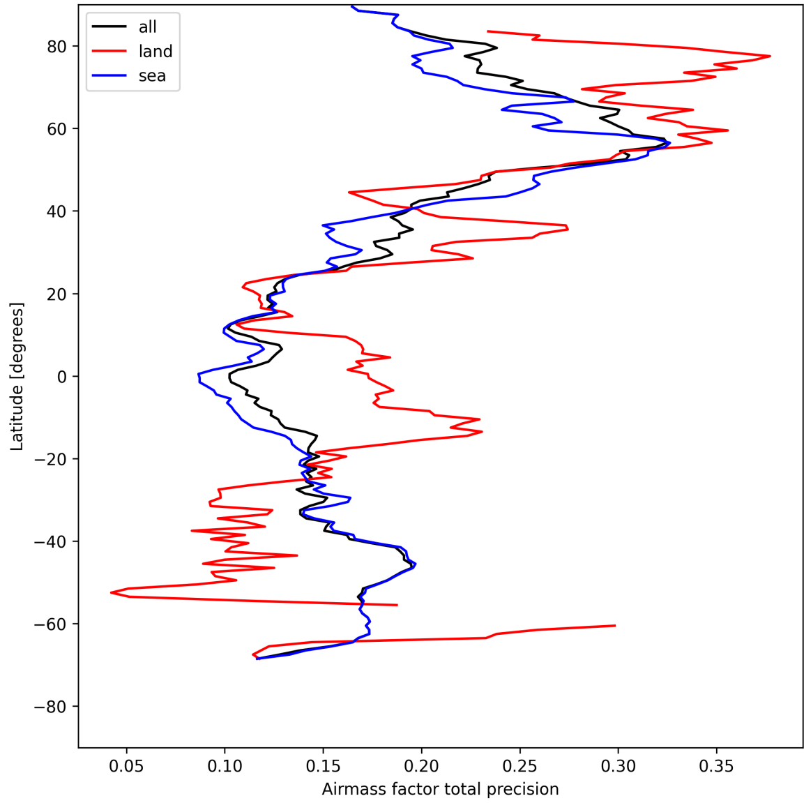
Figure 27: Zonal average of “Airmass factor total precision” for 2025-05-03 to 2025-05-05.
