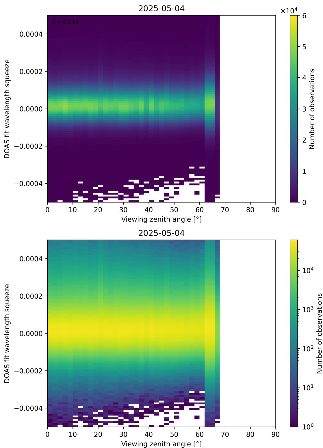
Figure 184: Scatter density plot of “Viewing zenith angle” against “DOAS fit wavelength squeeze” for 2025-05-03 to 2025-05-05.
