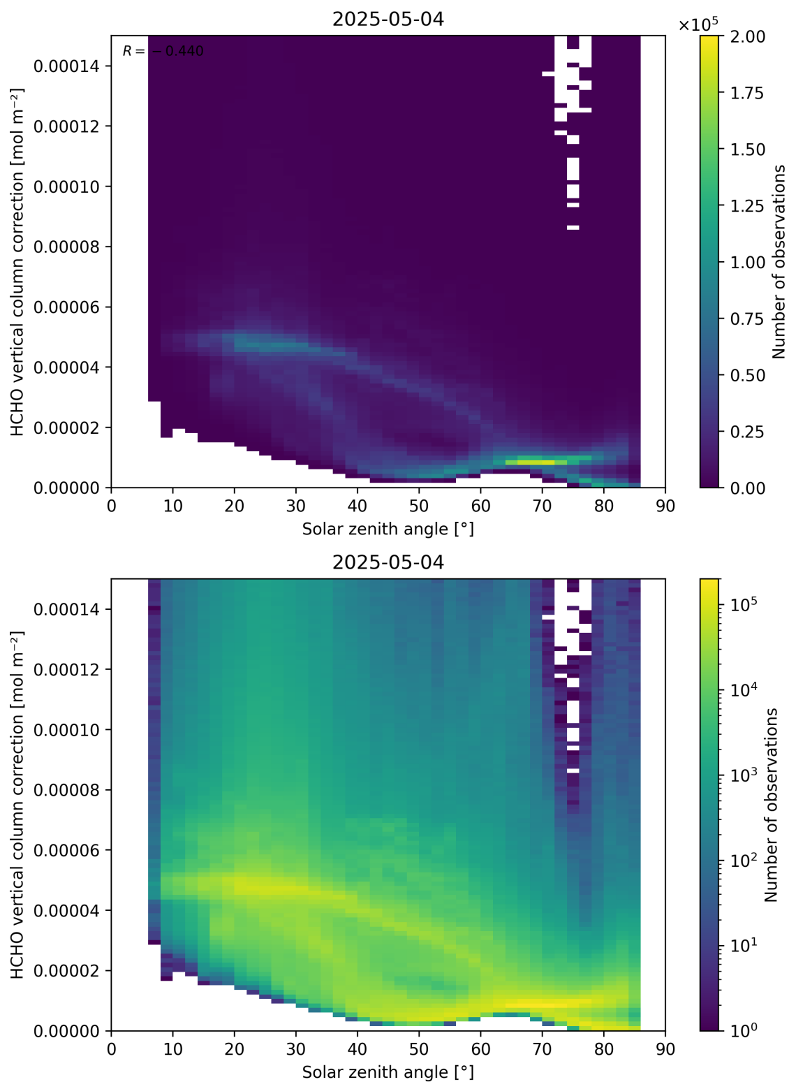
Figure 178: Scatter density plot of “Solar zenith angle” against “HCHO vertical column correction” for 2025-05-03 to 2025-05-05.
