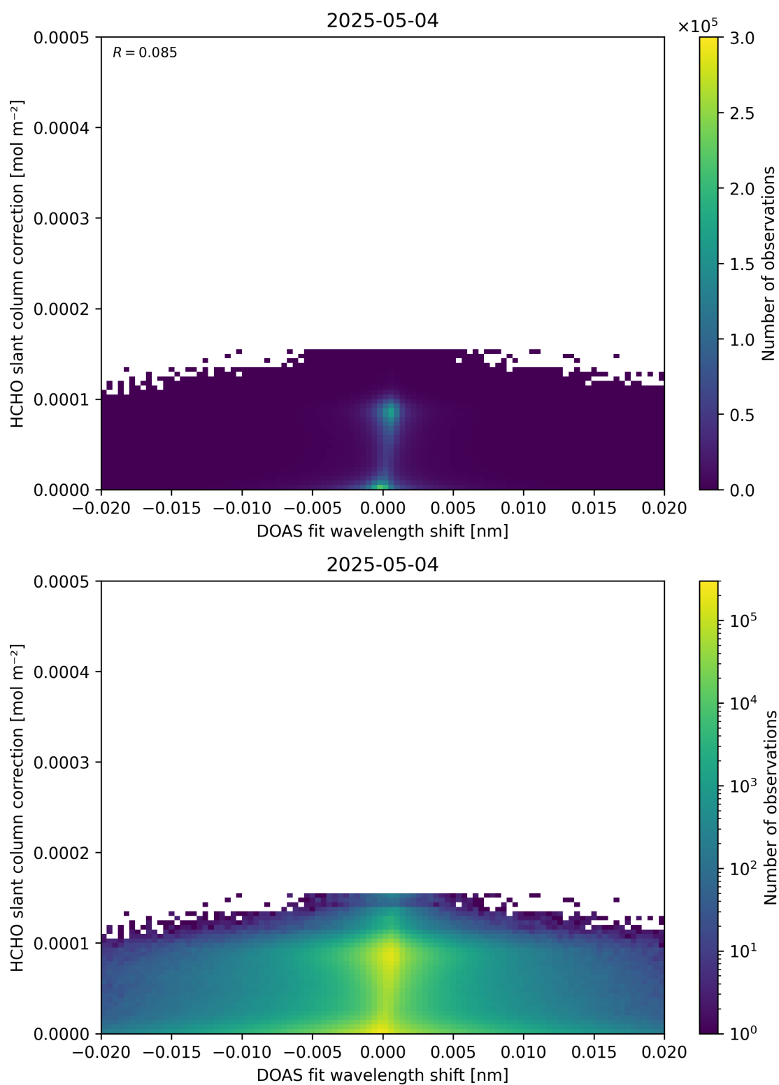
Figure 67: Scatter density plot of “DOAS fit wavelength shift” against “HCHO slant column correction” for 2025-05-03 to 2025-05-05.
