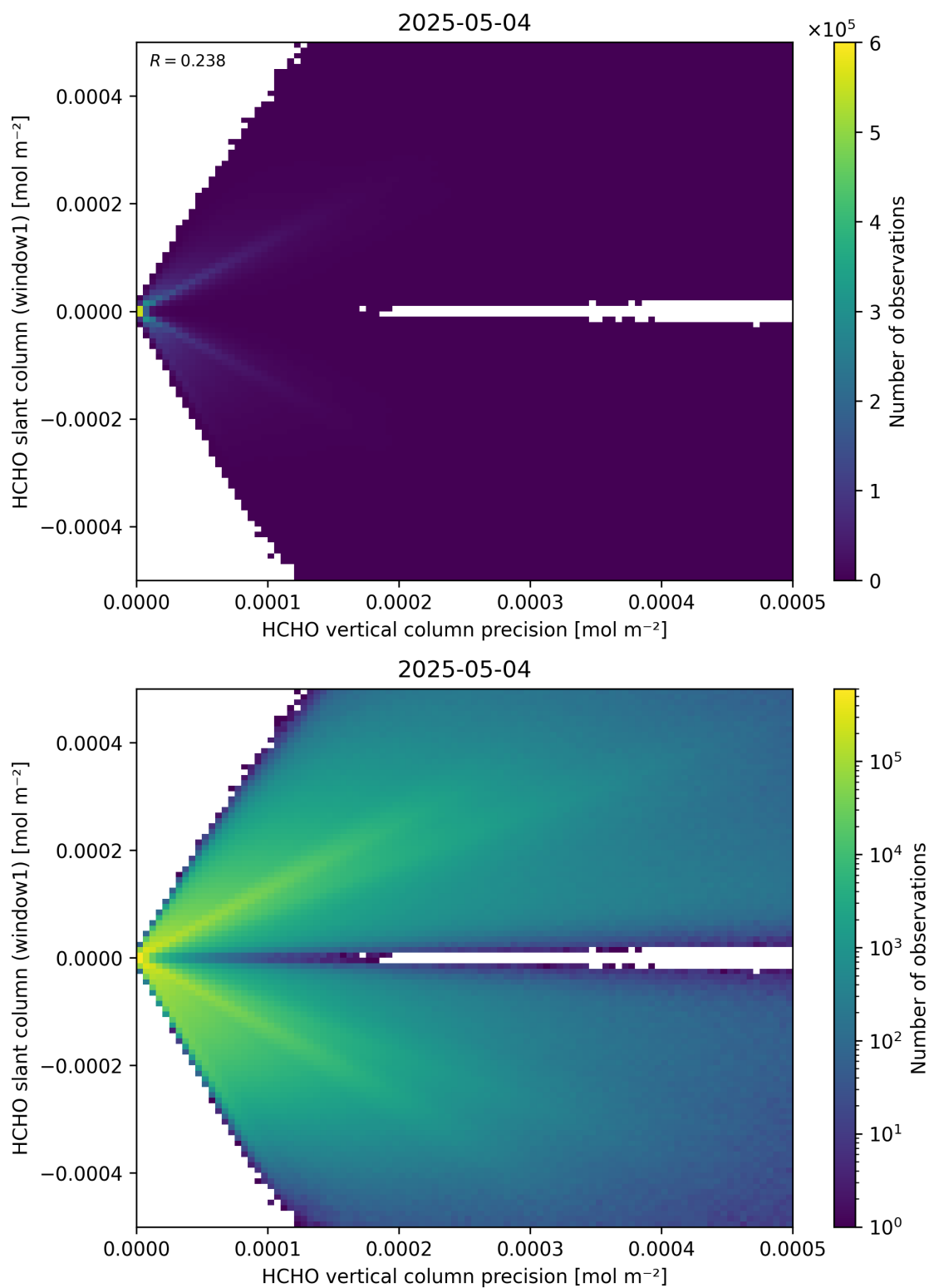
Figure 142: Scatter density plot of “HCHO vertical column precision” against “HCHO slant column (window1)” for 2025-05-03 to 2025-05-05.
