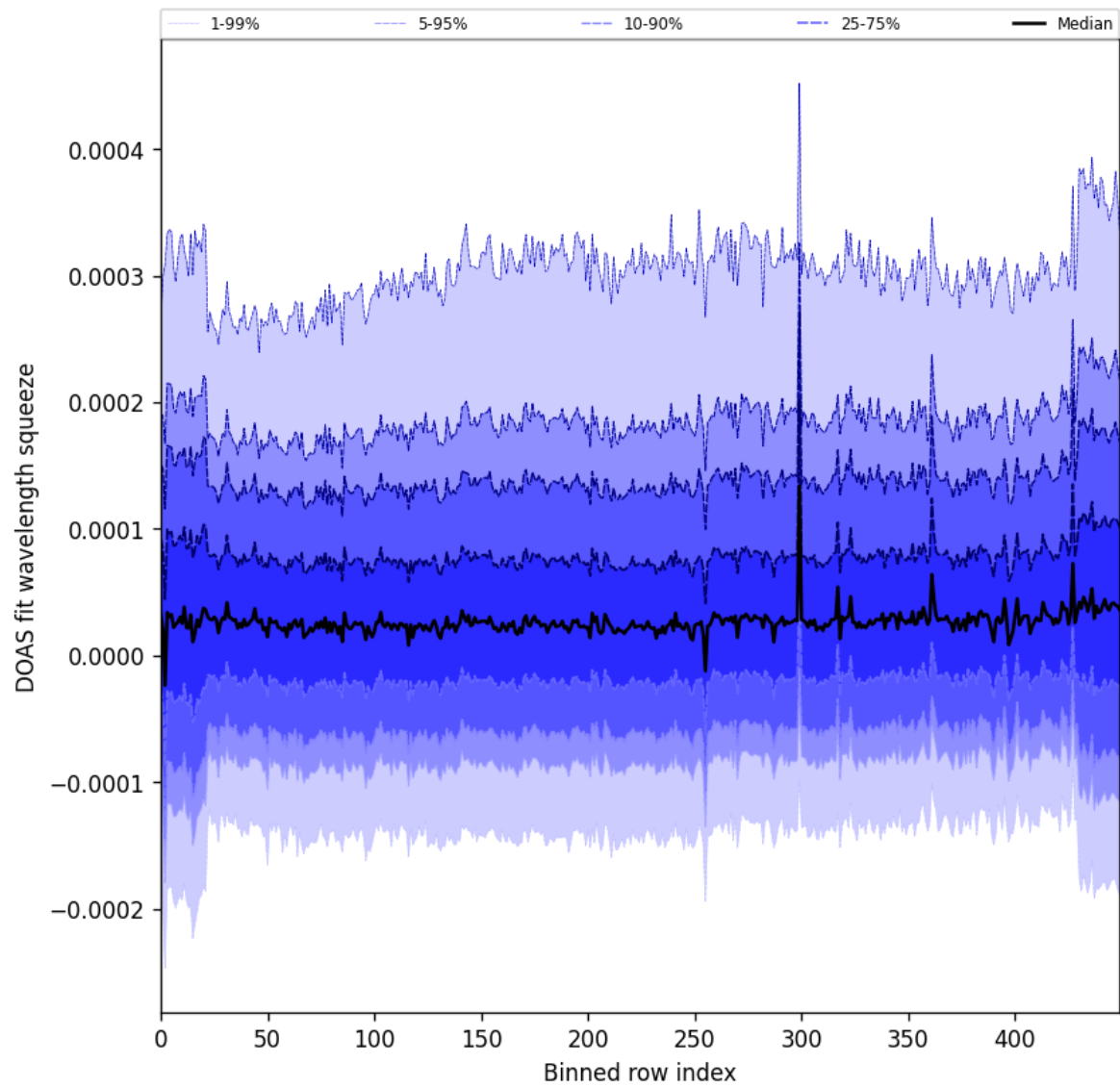
Figure 59: Along track statistics of “DOAS fit wavelength squeeze” for 2025-05-03 to 2025-05-05
