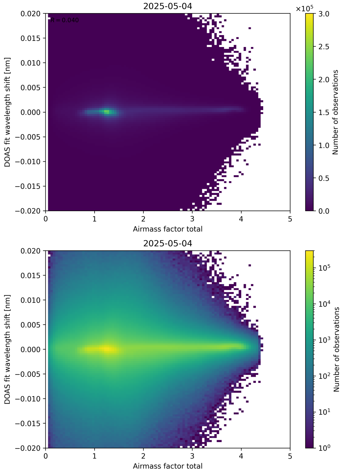
Figure 98: Scatter density plot of “Airmass factor total” against “DOAS fit wavelength shift” for 2025-05-03 to 2025-05-05.
