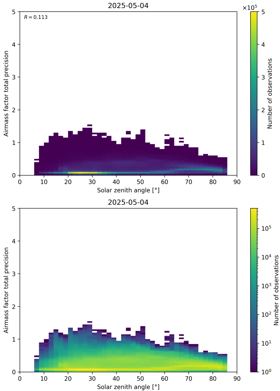
Figure 176: Scatter density plot of “Solar zenith angle” against “Airmass factor total precision” for 2025-05-03 to 2025-05-05.
