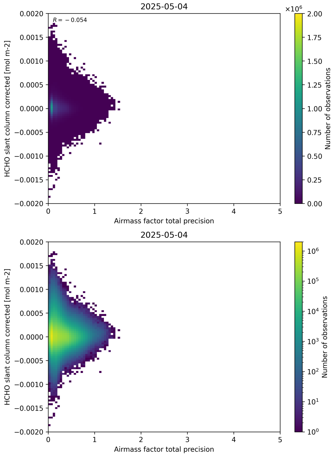
Figure 109: Scatter density plot of “Airmass factor total precision” against “HCHO slant column corrected” for 2025-05-03 to 2025-05-05.
