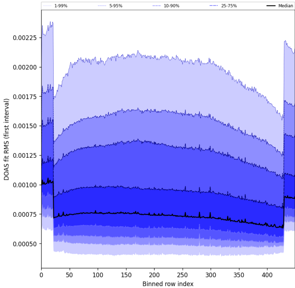
Figure 60: Along track statistics of “DOAS fit RMS (first interval)” for 2025-05-03 to 2025-05-05
