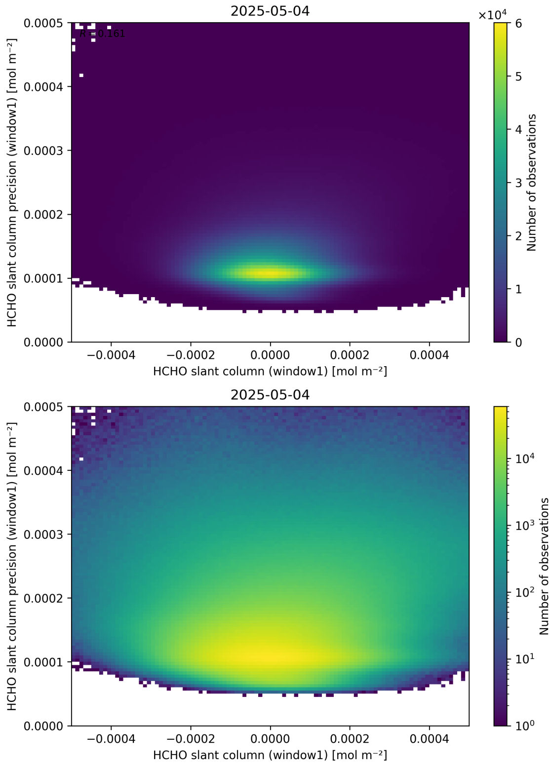
Figure 84: Scatter density plot of “HCHO slant column (window1)” against “HCHO slant column precision (window1)” for 2025-05-03 to 2025-05-05.
