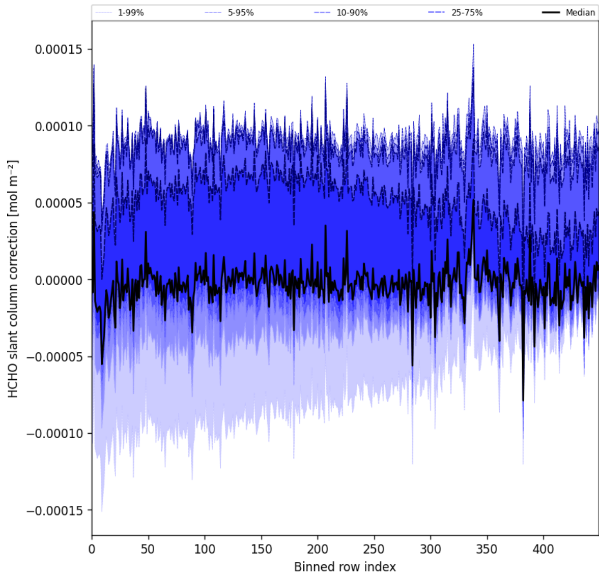
Figure 61: Along track statistics of “HCHO slant column correction” for 2025-05-03 to 2025-05-05
