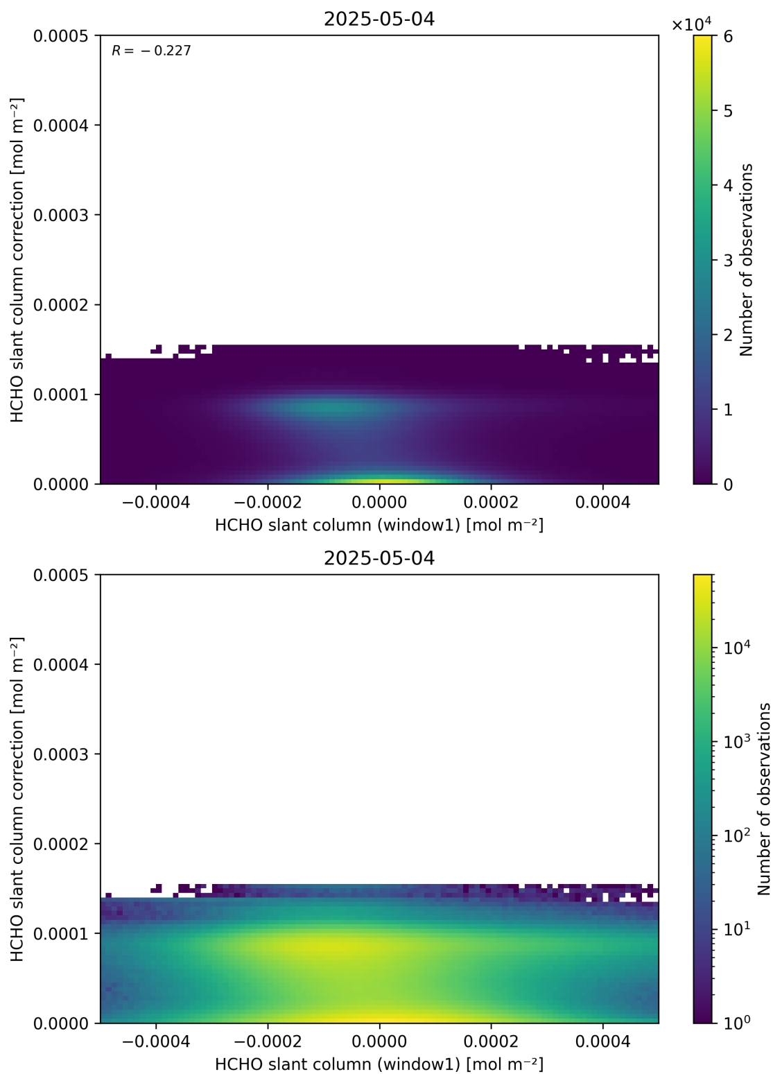
Figure 83: Scatter density plot of “HCHO slant column (window1)” against “HCHO slant column correction” for 2025-05-03 to 2025-05-05.
