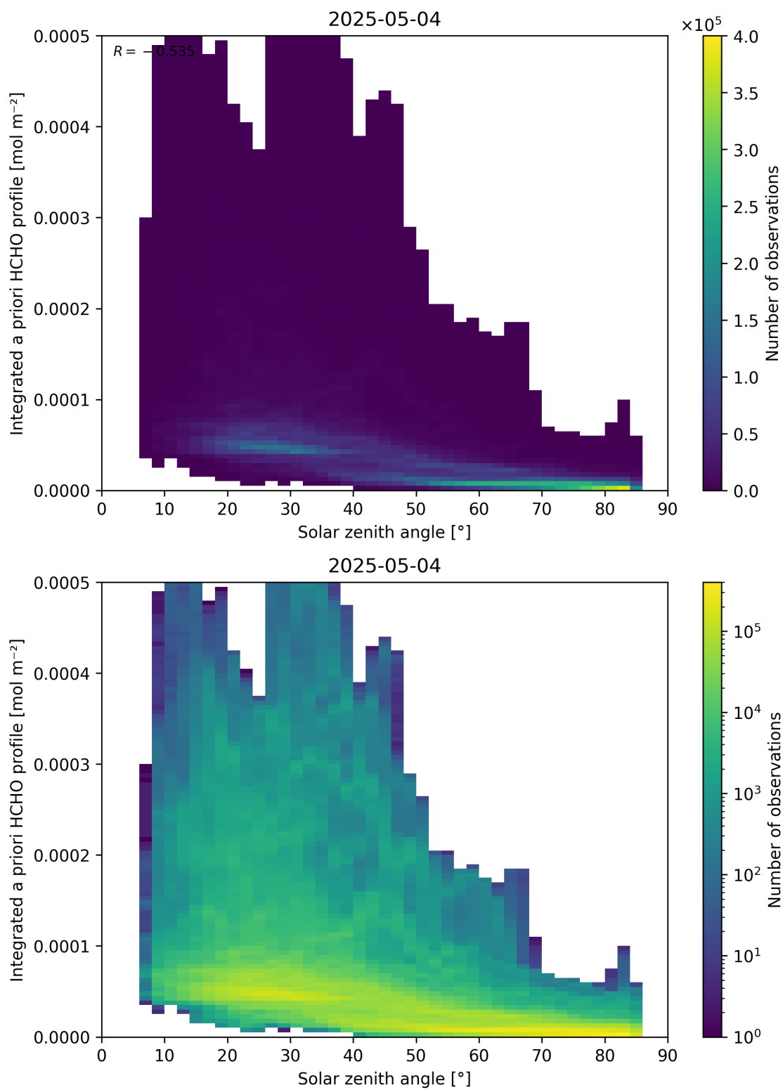
Figure 180: Scatter density plot of “Solar zenith angle” against “Integrated a priori HCHO profile” for 2025-05-03 to 2025-05-05.
