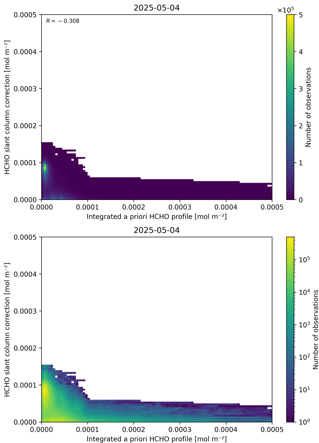
Figure 152: Scatter density plot of “Integrated a priori HCHO profile” against “HCHO slant column correction” for 2025-05-03 to 2025-05-05.
