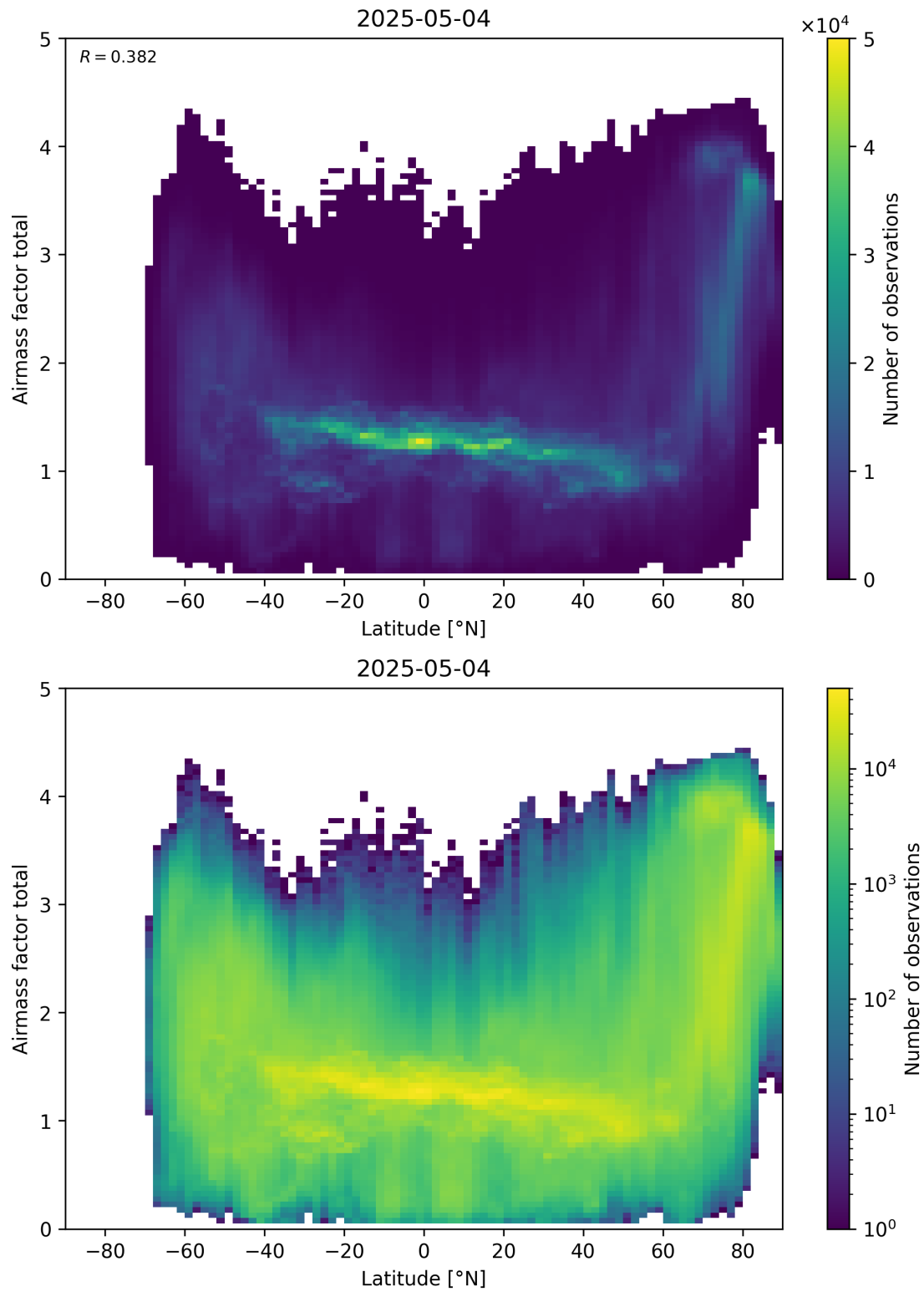
Figure 161: Scatter density plot of “Latitude” against “Airmass factor total” for 2025-05-03 to 2025-05-05.
