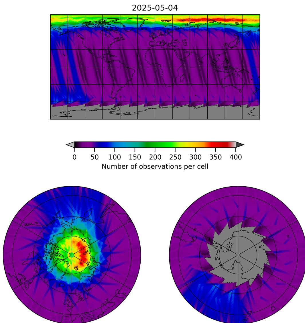
Figure 19: Map of the number of observations for 2025-05-03 to 2025-05-05
