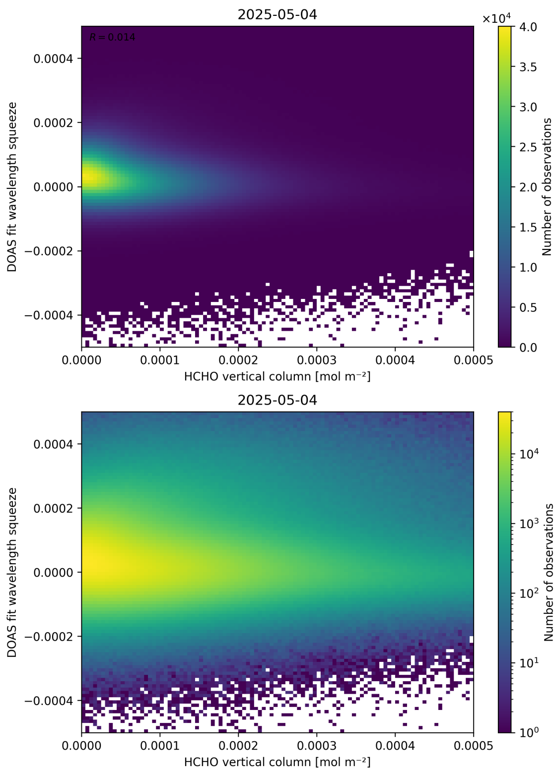
Figure 125: Scatter density plot of “HCHO vertical column” against “DOAS fit wavelength squeeze” for 2025-05-03 to 2025-05-05.
