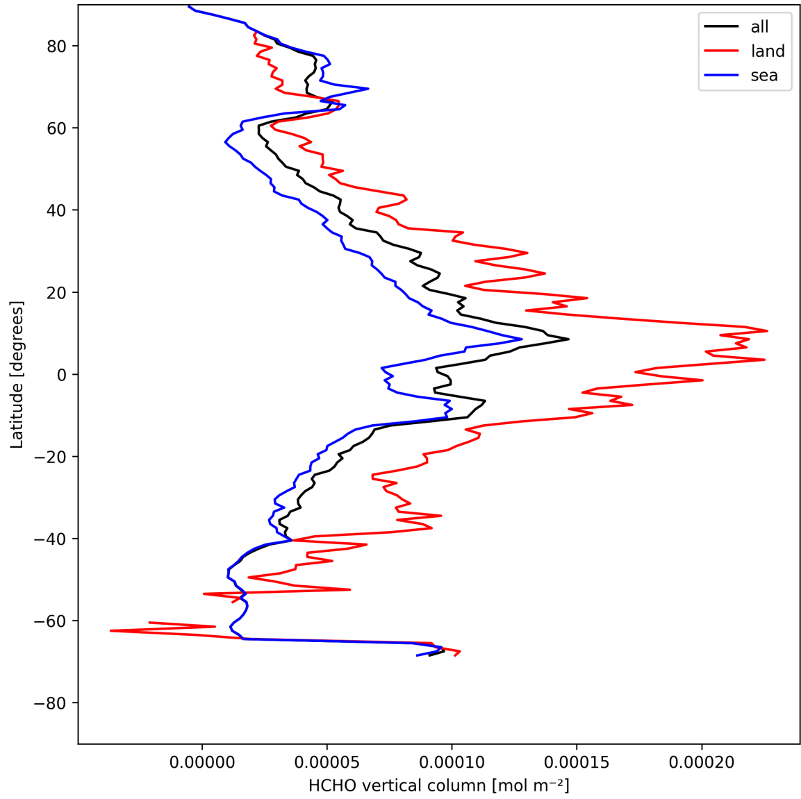
Figure 21: Zonal average of “HCHO vertical column” for 2025-05-03 to 2025-05-05.
