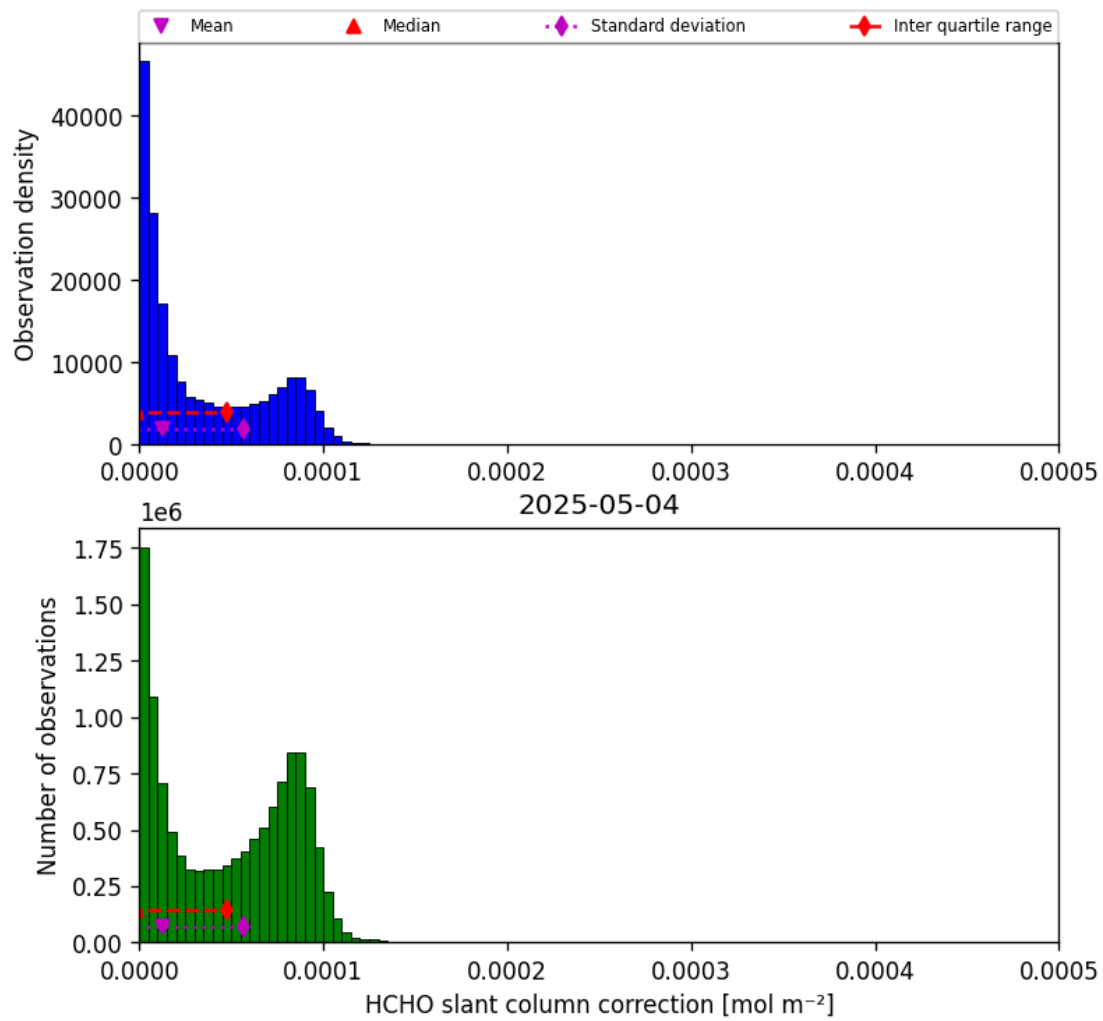
Figure 47: Histogram of “HCHO slant column correction” for 2025-05-03 to 2025-05-05
