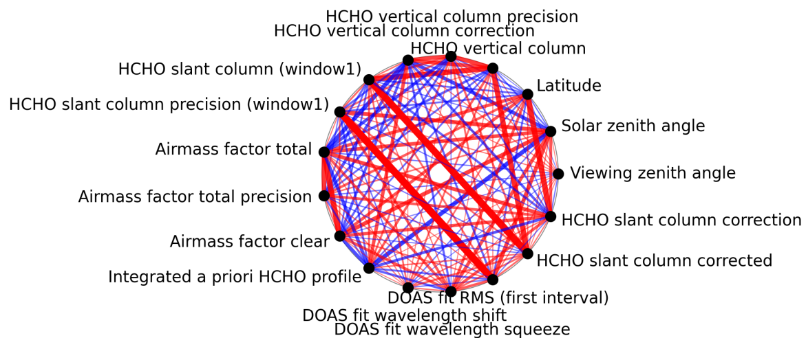
Figure 1: Map of correlation graph for 2025-05-03 to 2025-05-05.
