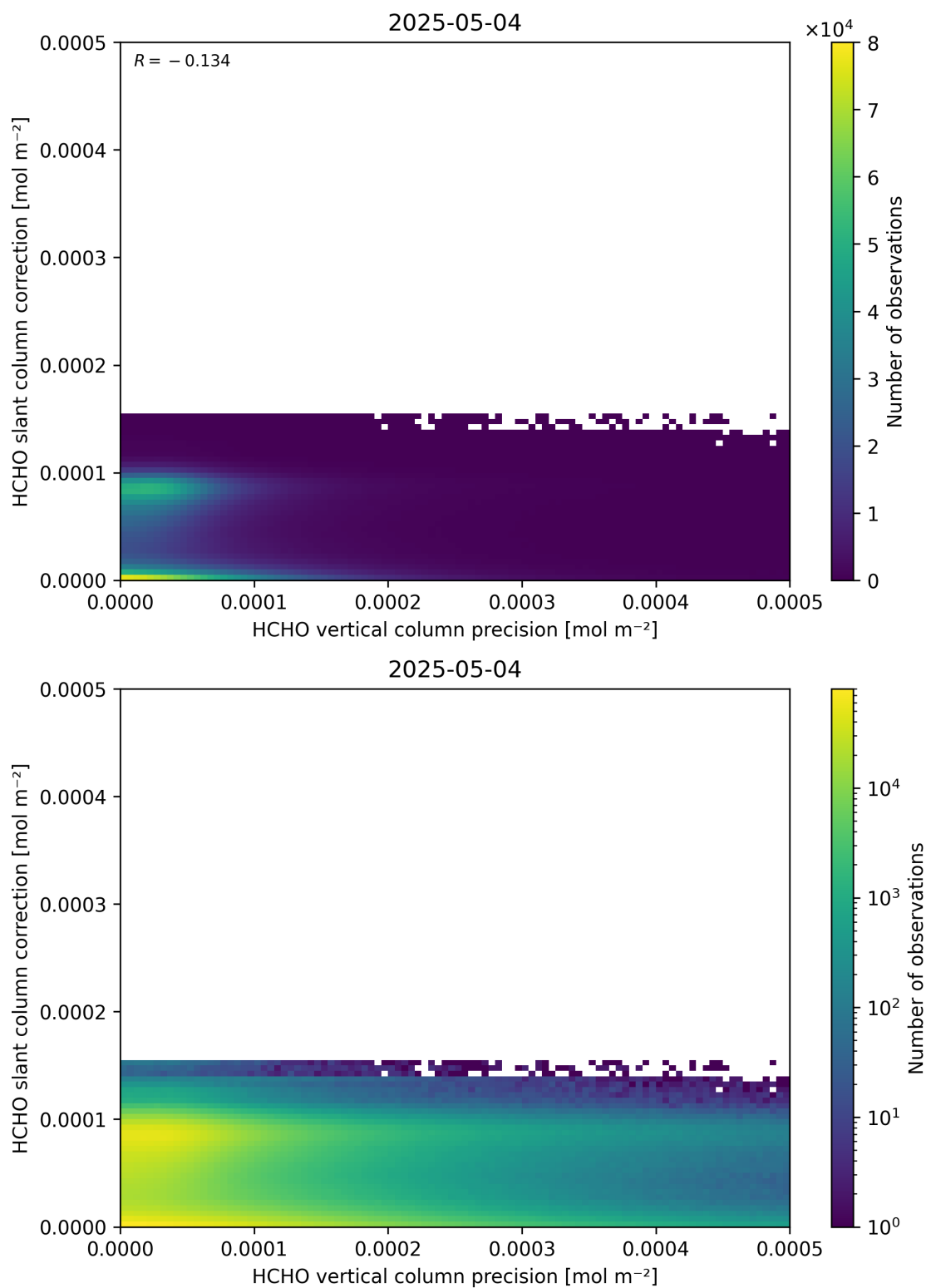
Figure 141: Scatter density plot of “HCHO vertical column precision” against “HCHO slant column correction” for 2025-05-03 to 2025-05-05.
