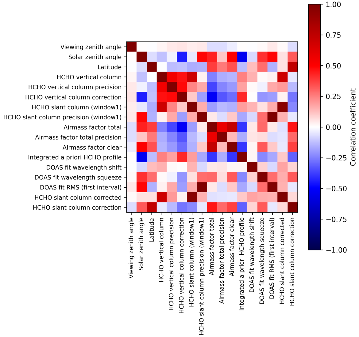
Figure 2: Map of correlation matrix for 2025-05-03 to 2025-05-05.
