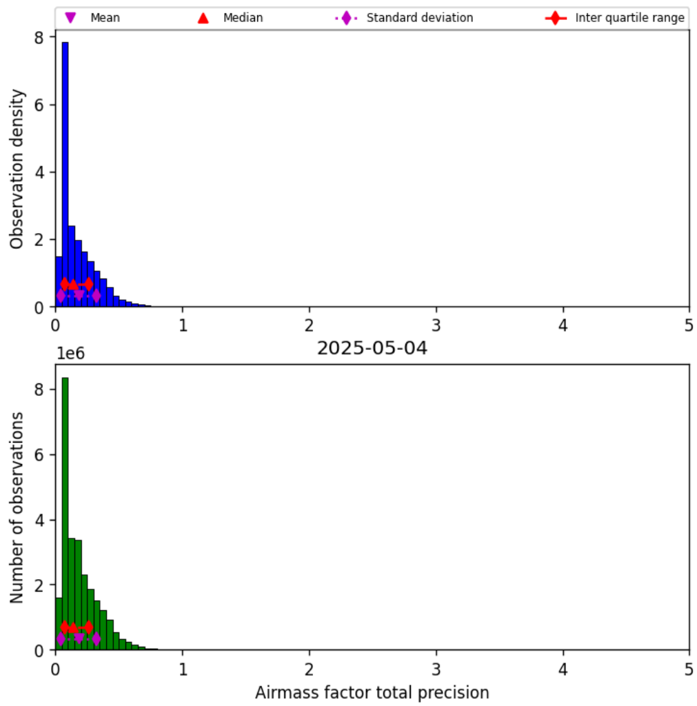
Figure 41: Histogram of “Airmass factor total precision” for 2025-05-03 to 2025-05-05
