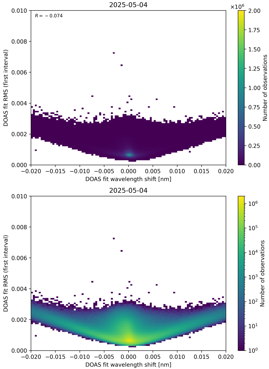
Figure 64: Scatter density plot of “DOAS fit wavelength shift” against “DOAS fit RMS (first interval)” for 2025-05-03 to 2025-05-05.
