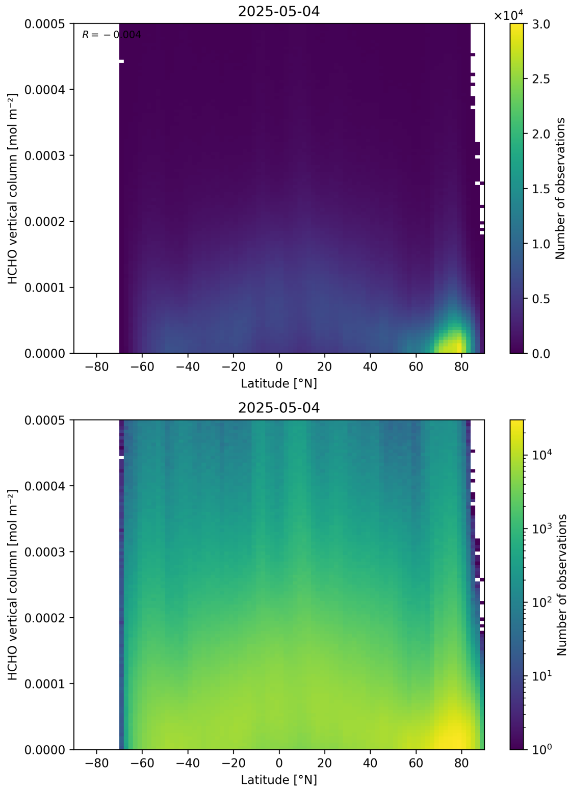
Figure 163: Scatter density plot of “Latitude” against “HCHO vertical column” for 2025-05-03 to 2025-05-05.
