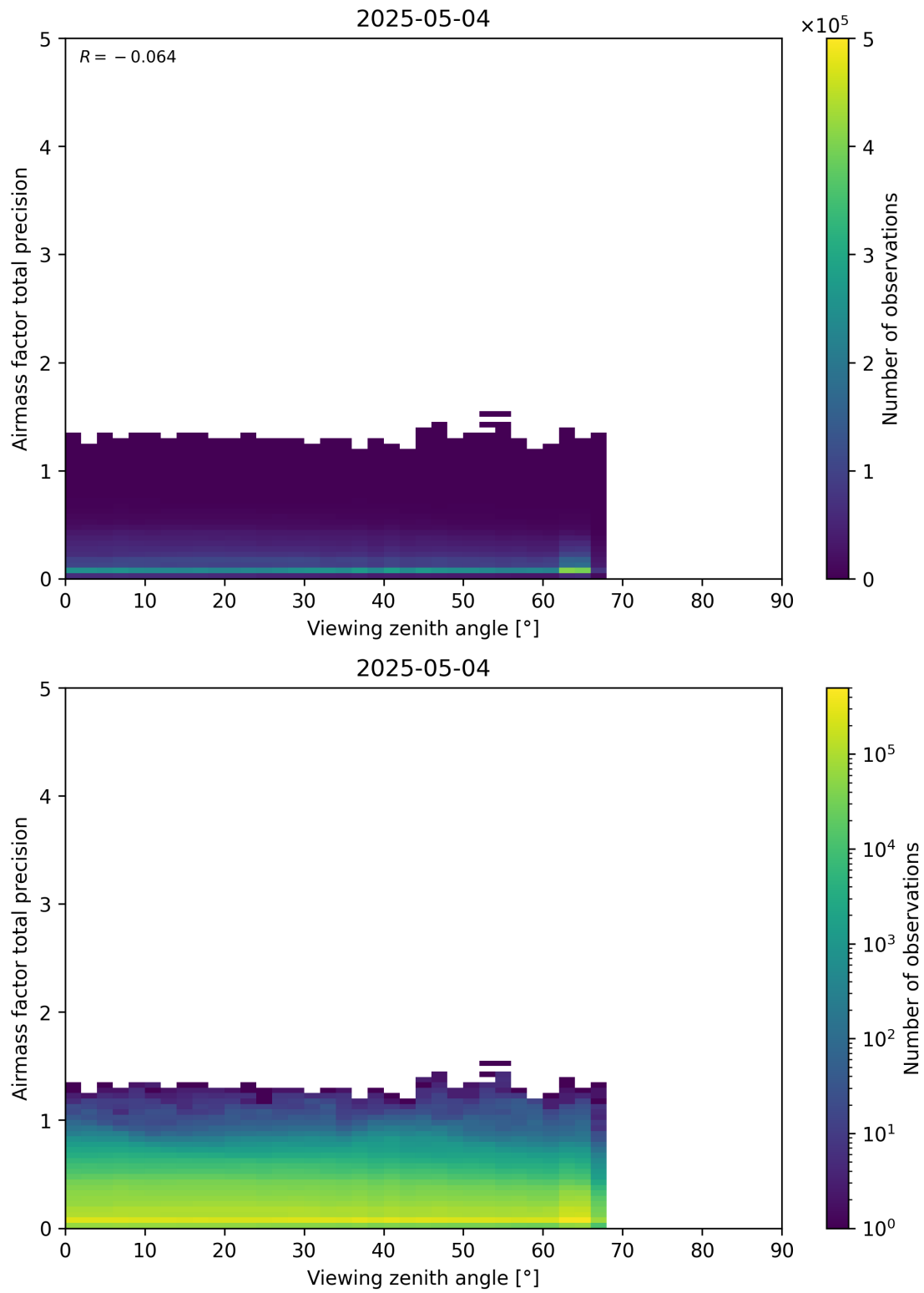
Figure 191: Scatter density plot of “Viewing zenith angle” against “Airmass factor total precision” for 2025-05-03 to 2025-05-05.
