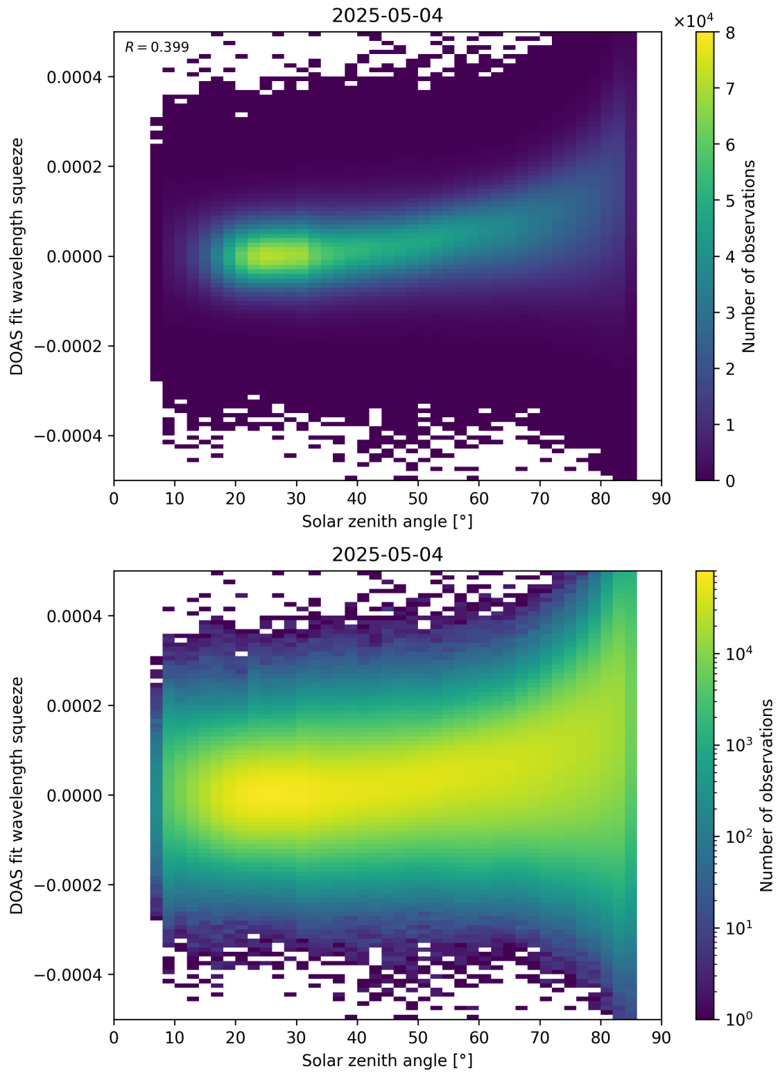
Figure 169: Scatter density plot of “Solar zenith angle” against “DOAS fit wavelength squeeze” for 2025-05-03 to 2025-05-05.
