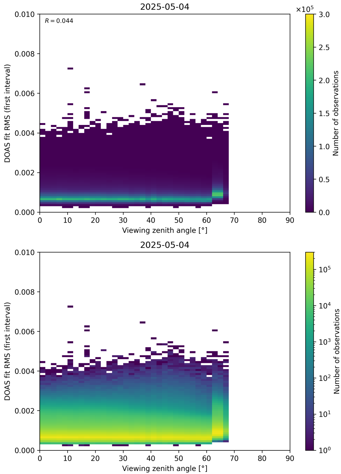
Figure 182: Scatter density plot of “Viewing zenith angle” against “DOAS fit RMS (first interval)” for 2025-05-03 to 2025-05-05.
