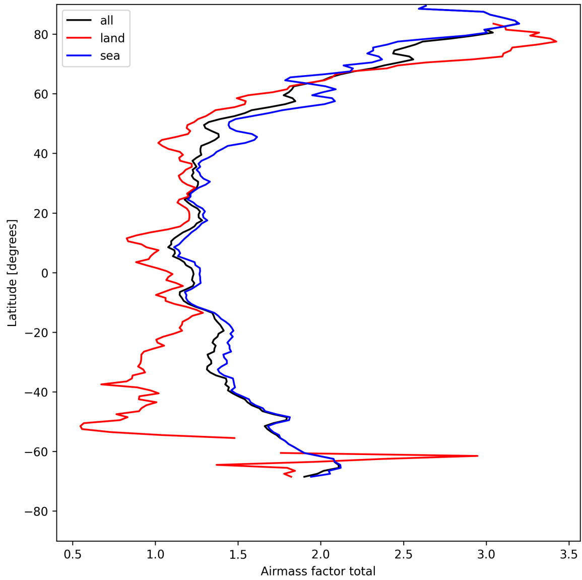
Figure 26: Zonal average of “Airmass factor total” for 2025-05-03 to 2025-05-05.
