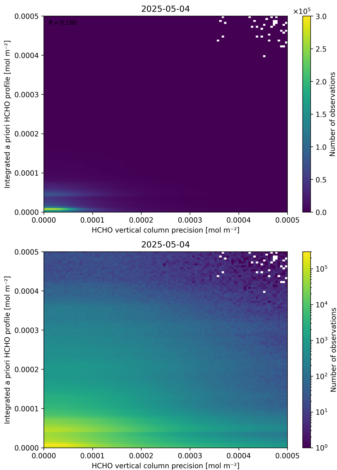
Figure 147: Scatter density plot of “HCHO vertical column precision” against “Integrated a priori HCHO profile” for 2025-05-03 to 2025-05-05.
