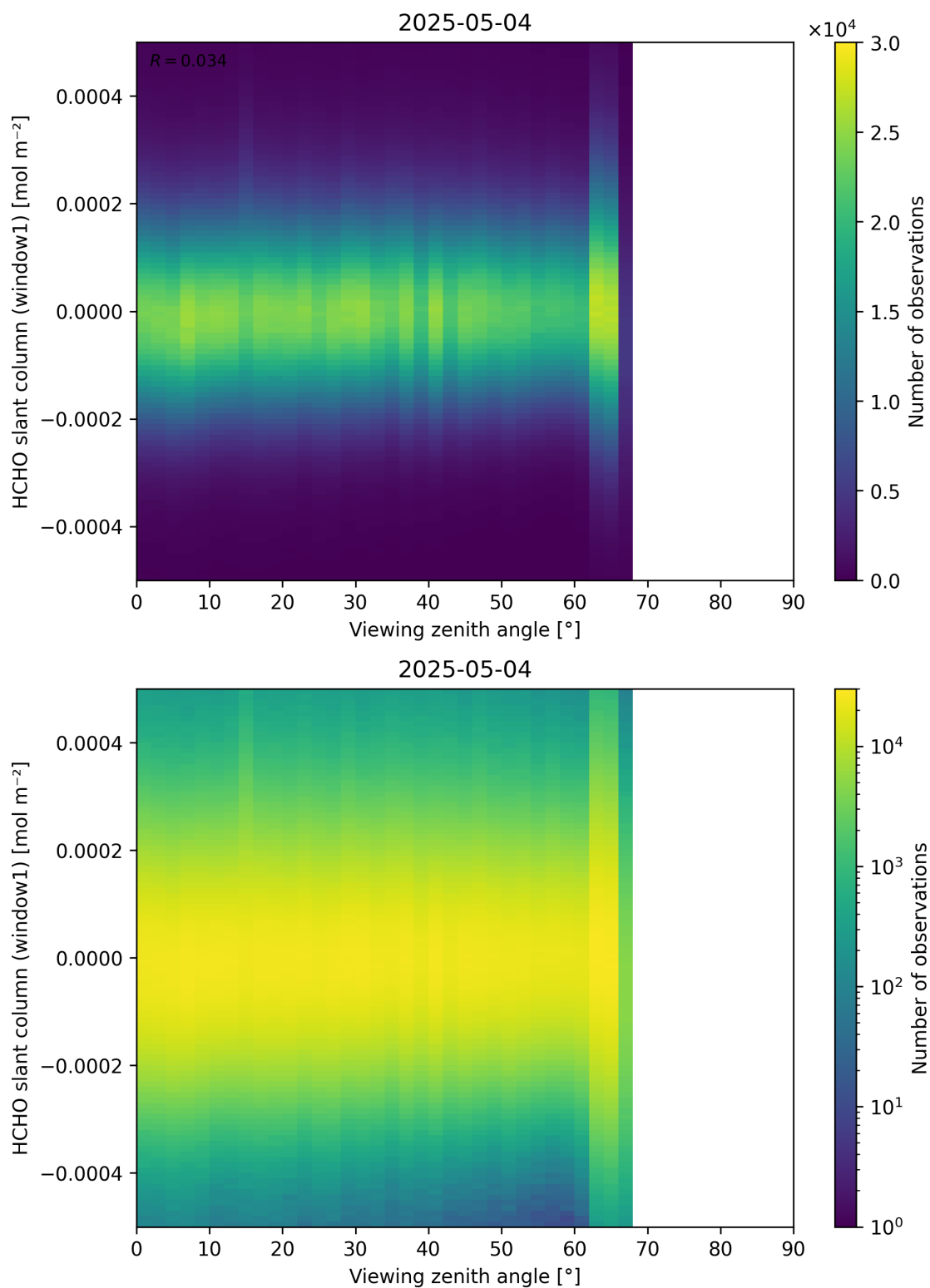
Figure 188: Scatter density plot of “Viewing zenith angle” against “HCHO slant column (window1)” for 2025-05-03 to 2025-05-05.
