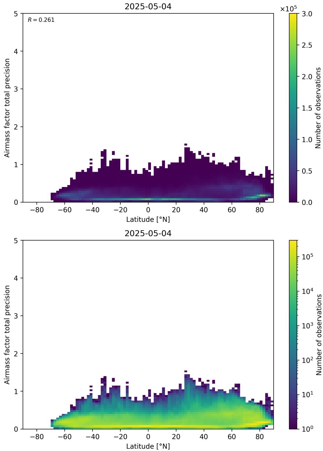
Figure 162: Scatter density plot of “Latitude” against “Airmass factor total precision” for 2025-05-03 to 2025-05-05.
