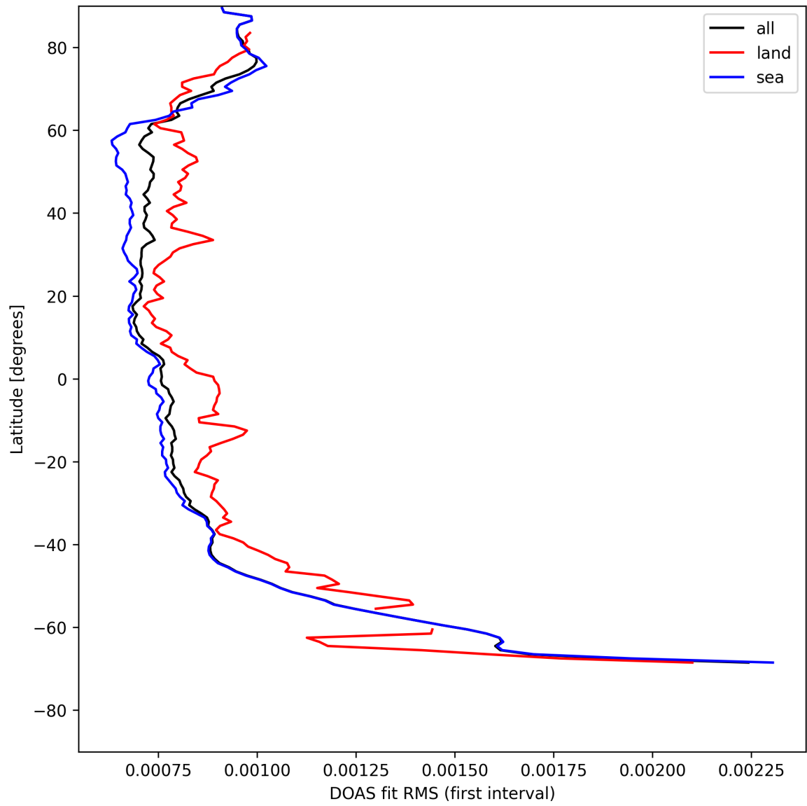
Figure 32: Zonal average of "DOAS fit RMS (first interval)" for 2025-05-03 to 2025-05-05.
