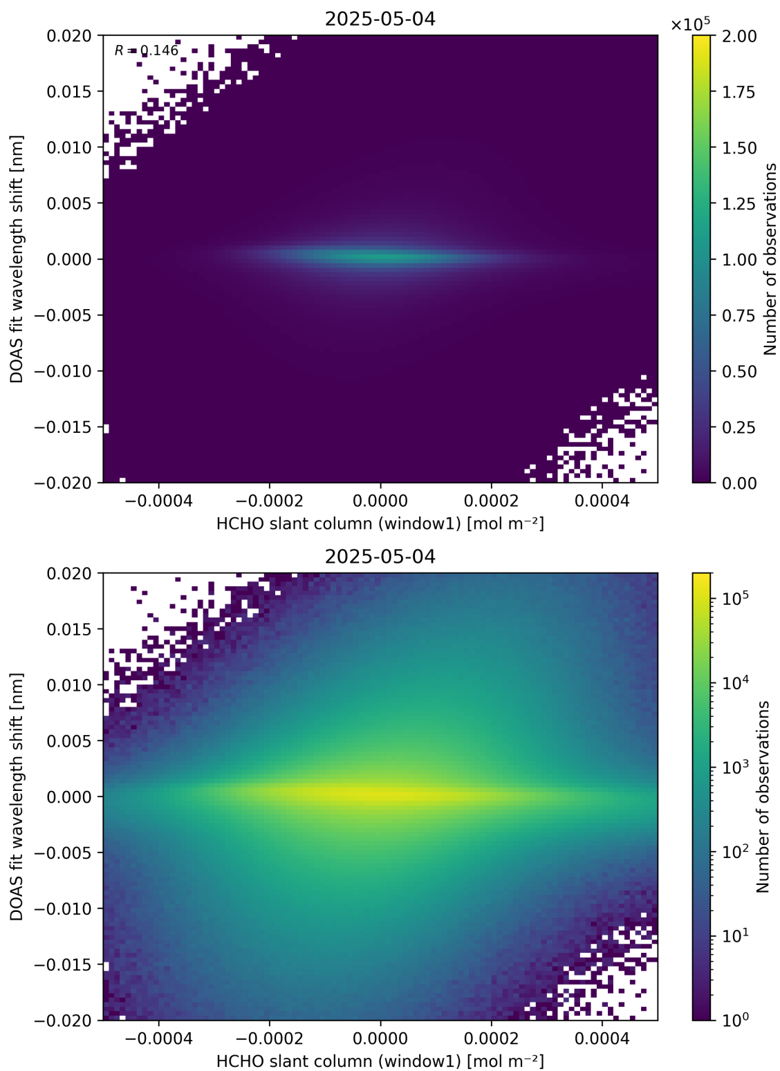
Figure 79: Scatter density plot of “HCHO slant column (window1)” against “DOAS fit wavelength shift” for 2025-05-03 to 2025-05-05.
