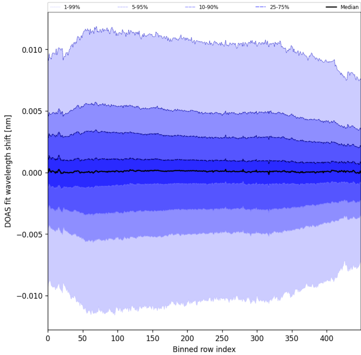
Figure 58: Along track statistics of “DOAS fit wavelength shift” for 2025-05-03 to 2025-05-05
