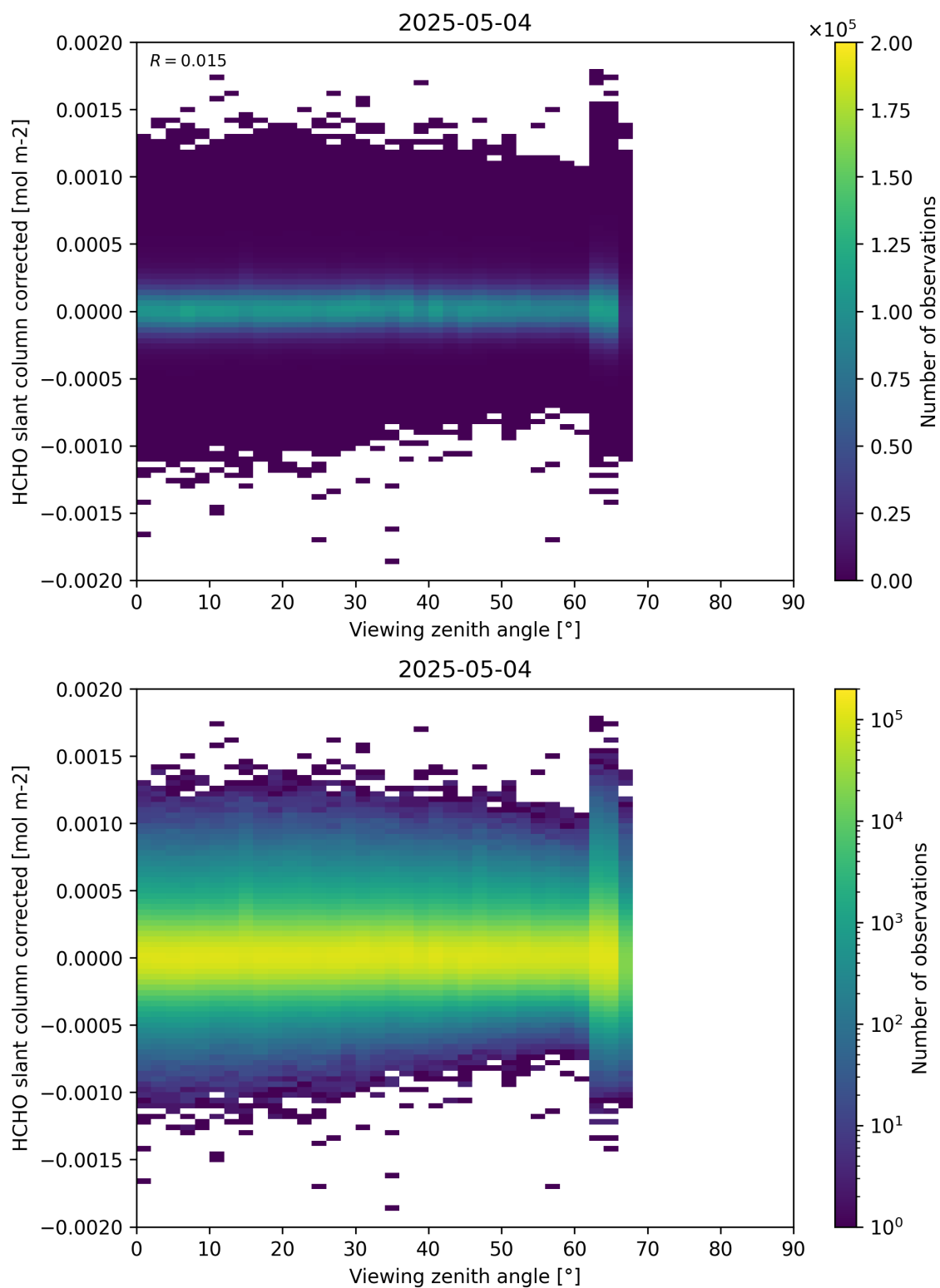
Figure 186: Scatter density plot of “Viewing zenith angle” against “HCHO slant column corrected” for 2025-05-03 to 2025-05-05.
