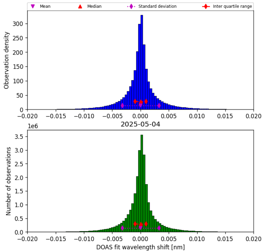
Figure 44: Histogram of “DOAS fit wavelength shift” for 2025-05-03 to 2025-05-05
