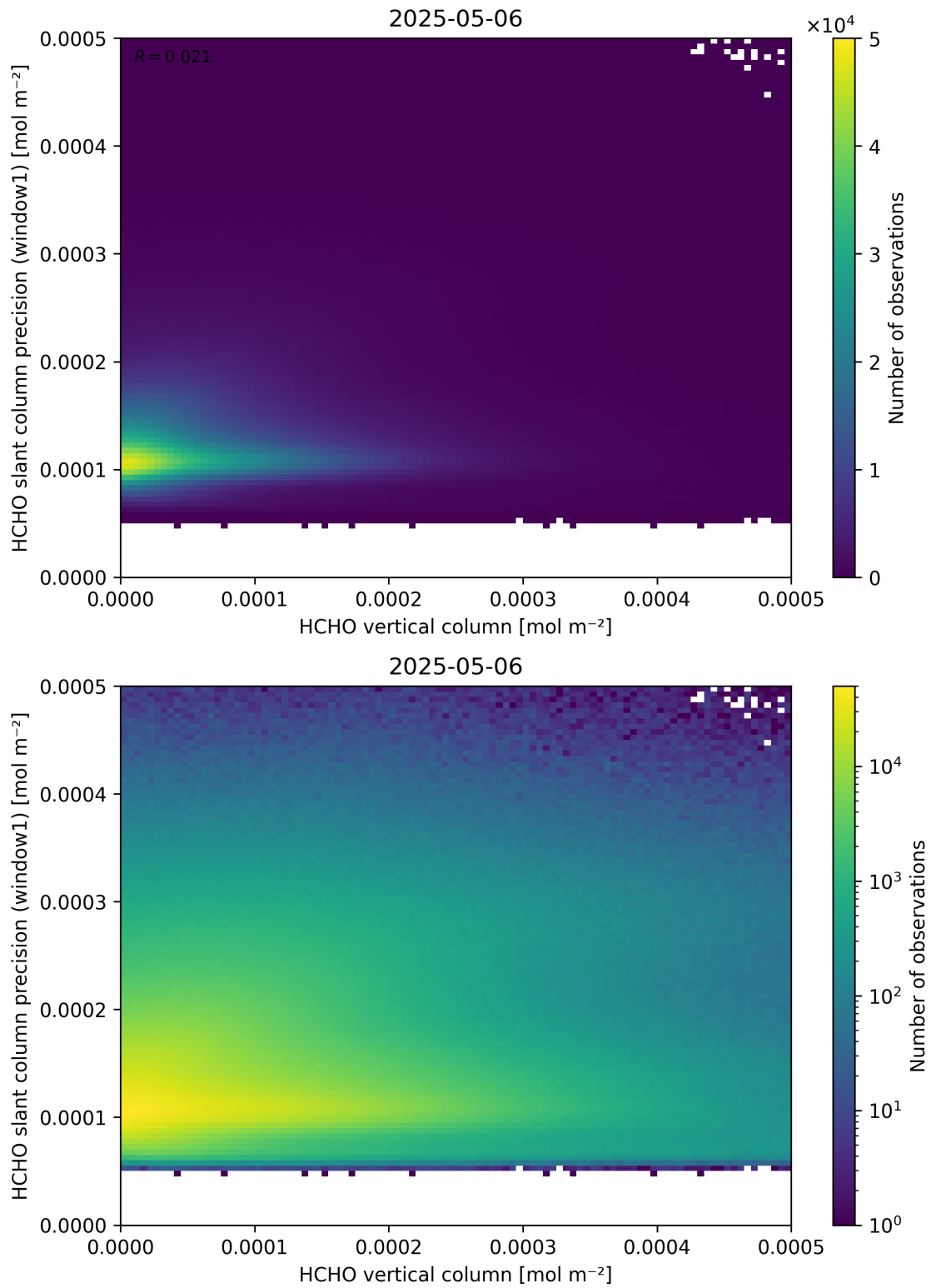
Figure 130: Scatter density plot of “HCHO vertical column” against “HCHO slant column precision (window1)” for 2025-05-05 to 2025-05-07.
