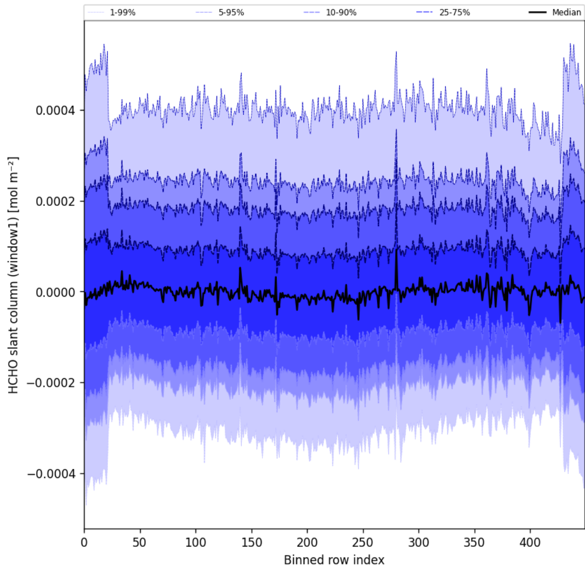
Figure 52: Along track statistics of “HCHO slant column (window1)” for 2025-05-05 to 2025-05-07
