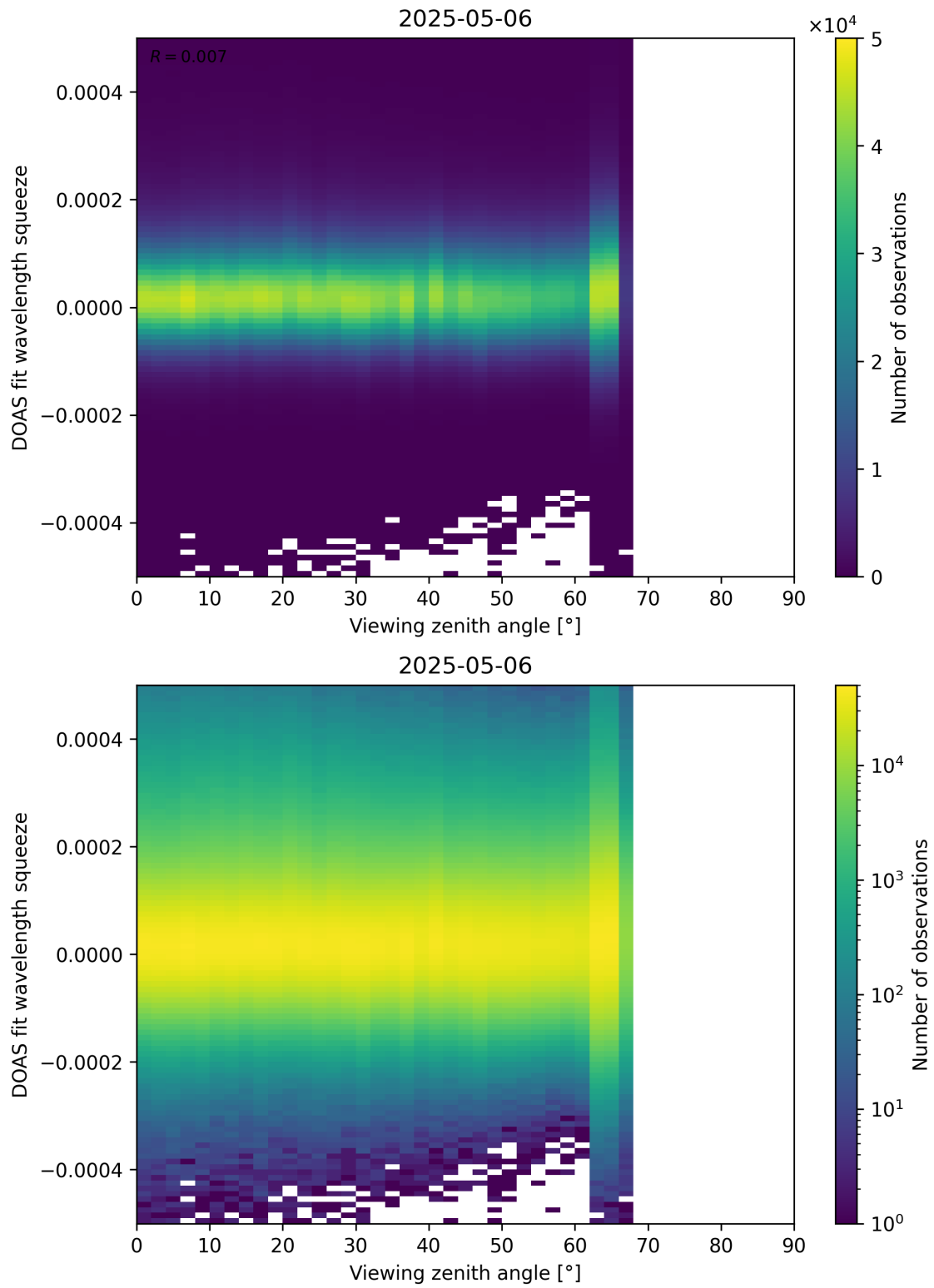
Figure 184: Scatter density plot of “Viewing zenith angle” against “DOAS fit wavelength squeeze” for 2025-05-05 to 2025-05-07.
