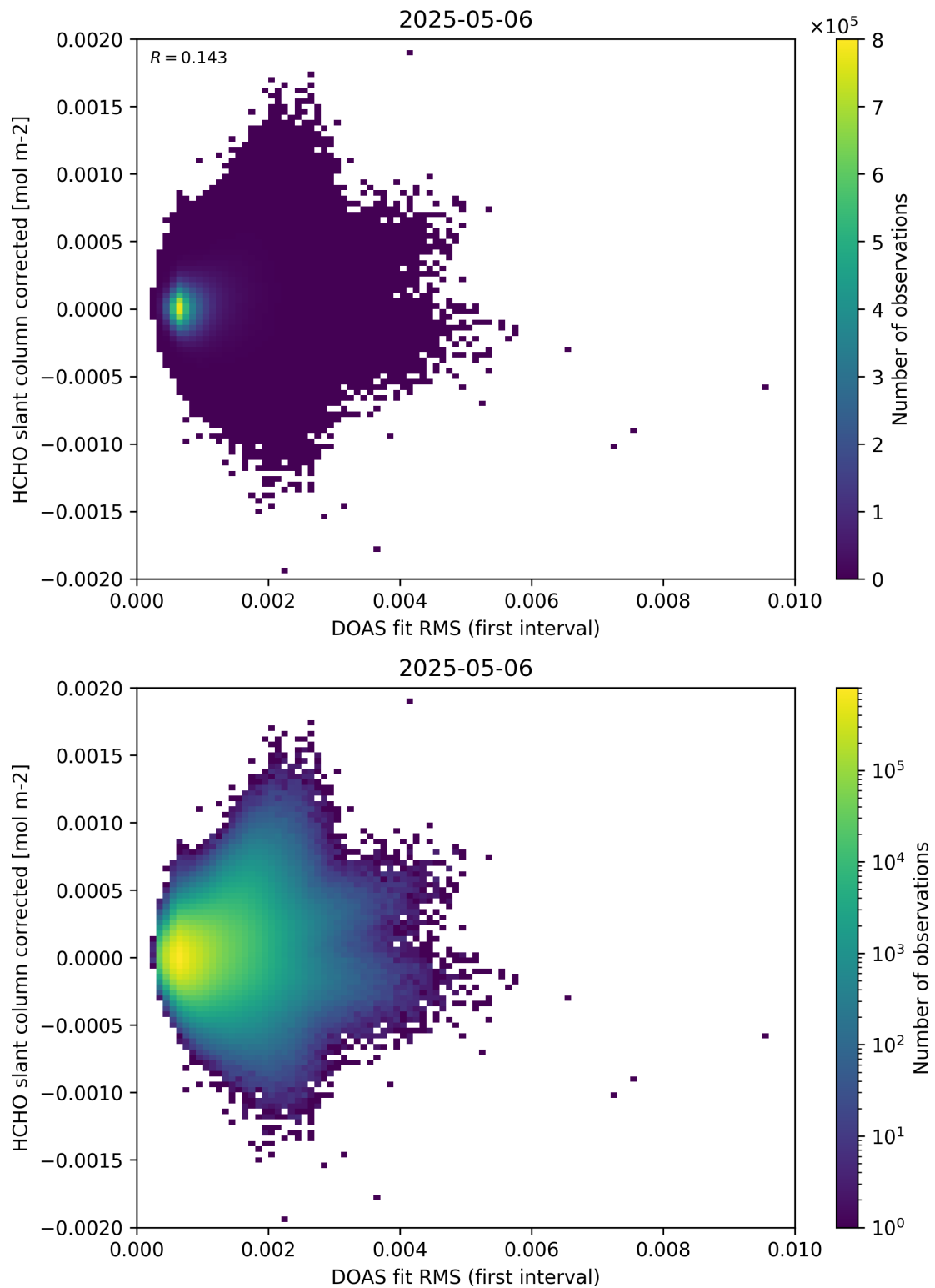
Figure 62: Scatter density plot of “DOAS fit RMS (first interval)” against “HCHO slant column corrected” for 2025-05-05 to 2025-05-07.
