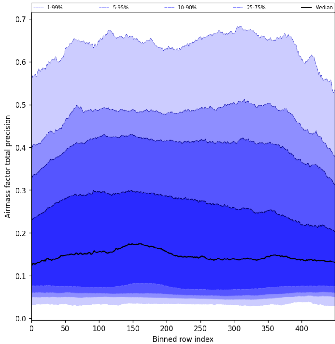
Figure 55: Along track statistics of “Airmass factor total precision” for 2025-05-05 to 2025-05-07
