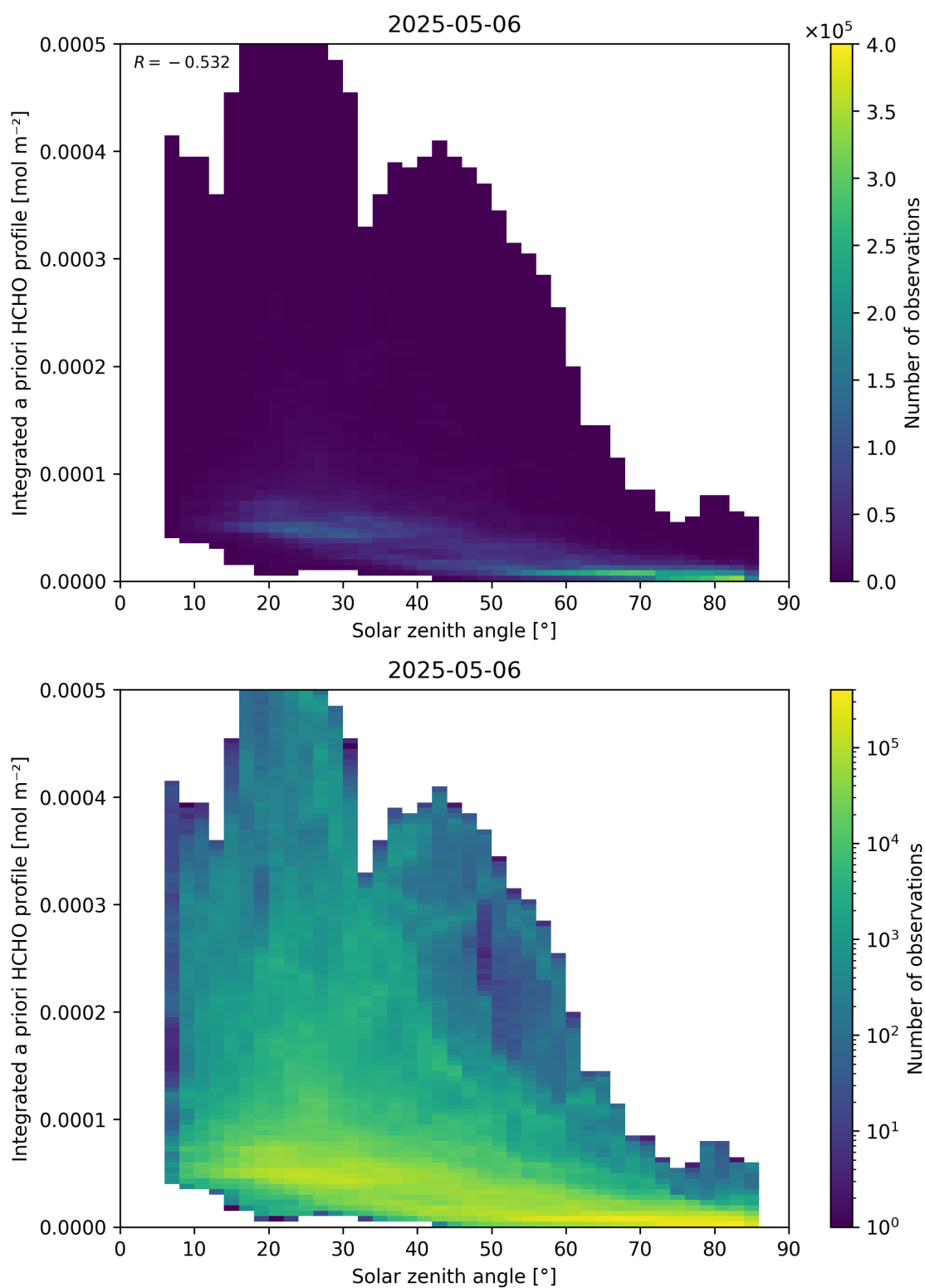
Figure 180: Scatter density plot of “Solar zenith angle” against “Integrated a priori HCHO profile” for 2025-05-05 to 2025-05-07.
