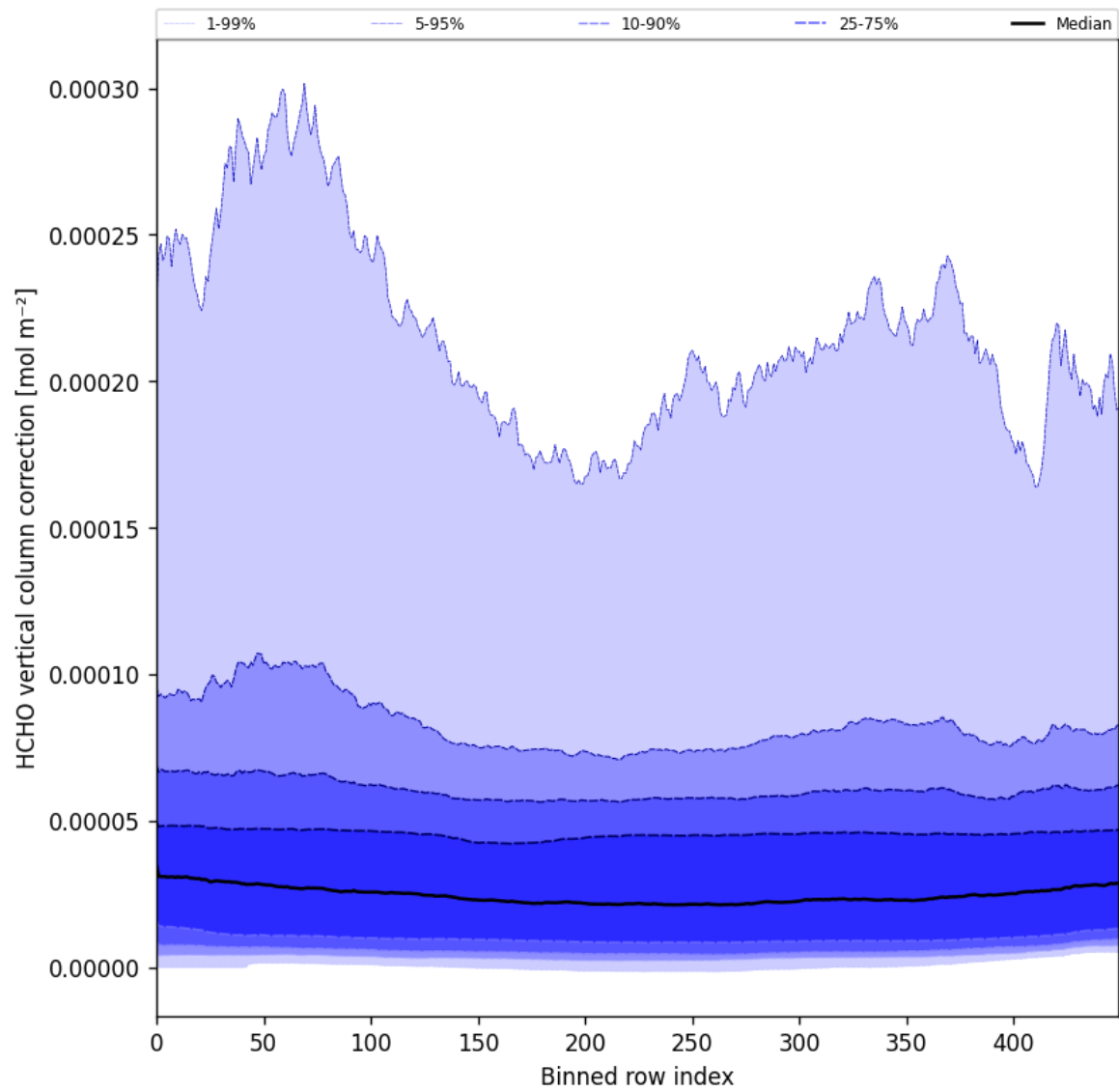
Figure 51: Along track statistics of “HCHO vertical column correction” for 2025-05-05 to 2025-05-07
