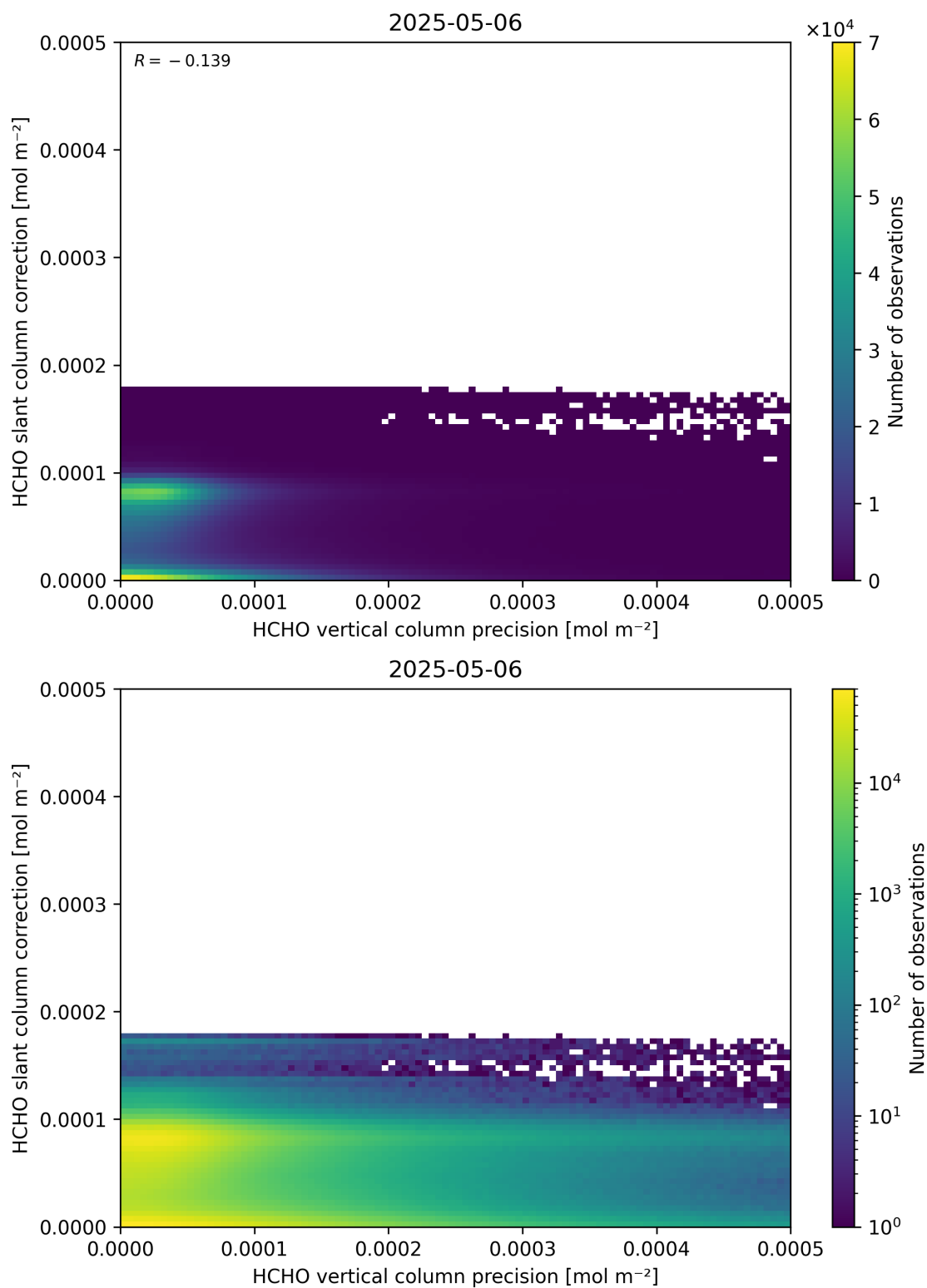
Figure 141: Scatter density plot of “HCHO vertical column precision” against “HCHO slant column correction” for 2025-05-05 to 2025-05-07.
