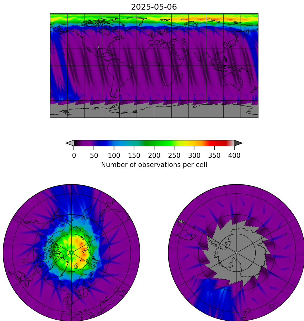
Figure 19: Map of the number of observations for 2025-05-05 to 2025-05-07
