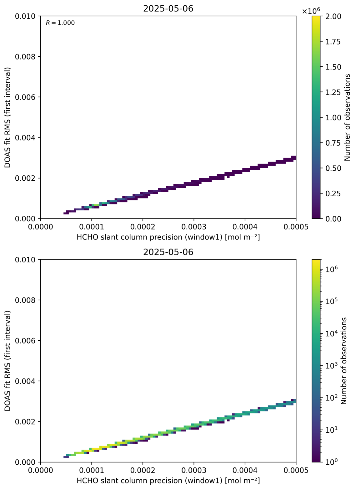
Figure 88: Scatter density plot of “HCHO slant column precision (window1)” against “DOAS fit RMS (first interval)” for 2025-05-05 to 2025-05-07.
