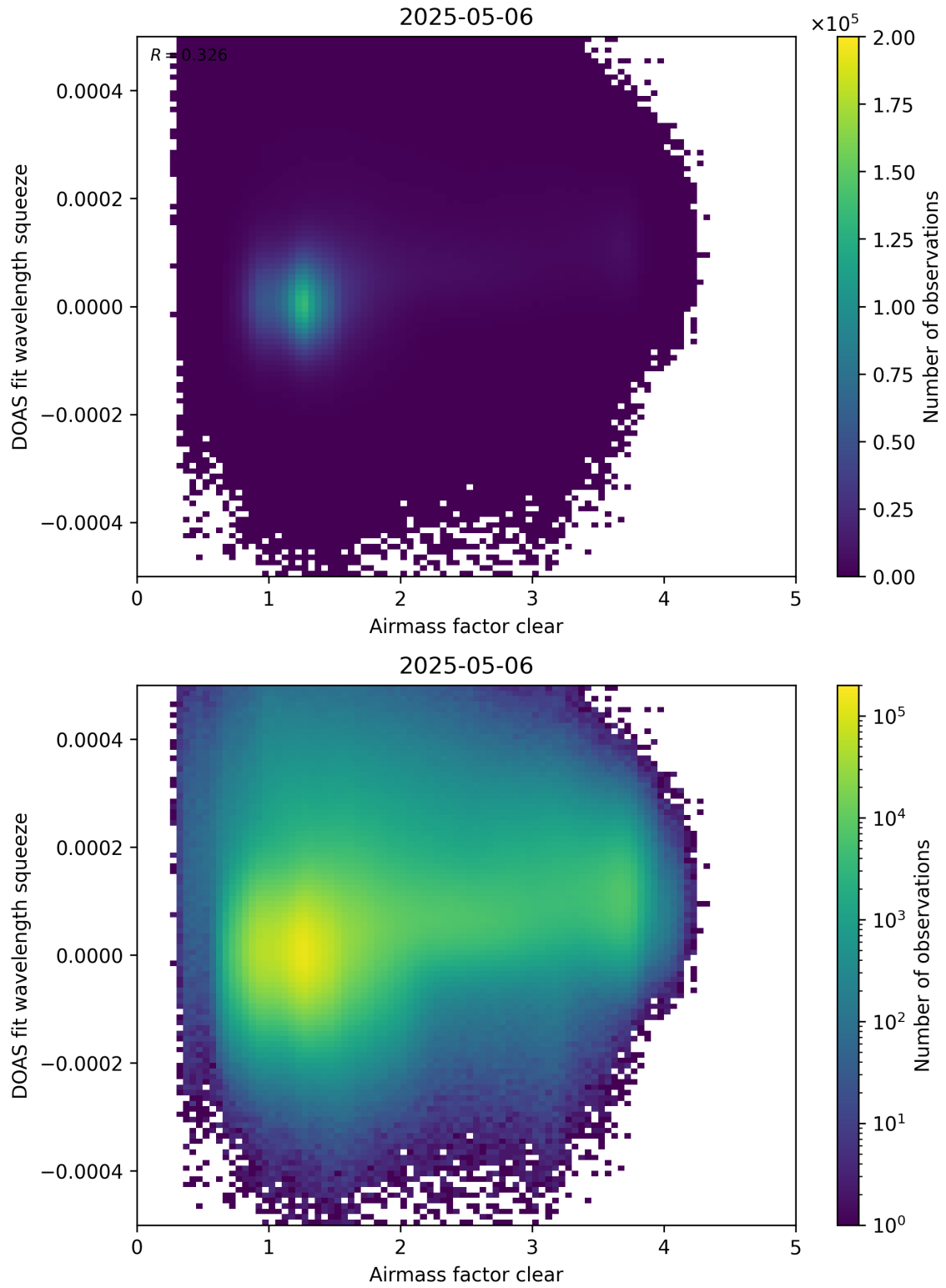
Figure 73: Scatter density plot of “Airmass factor clear” against “DOAS fit wavelength squeeze” for 2025-05-05 to 2025-05-07.
