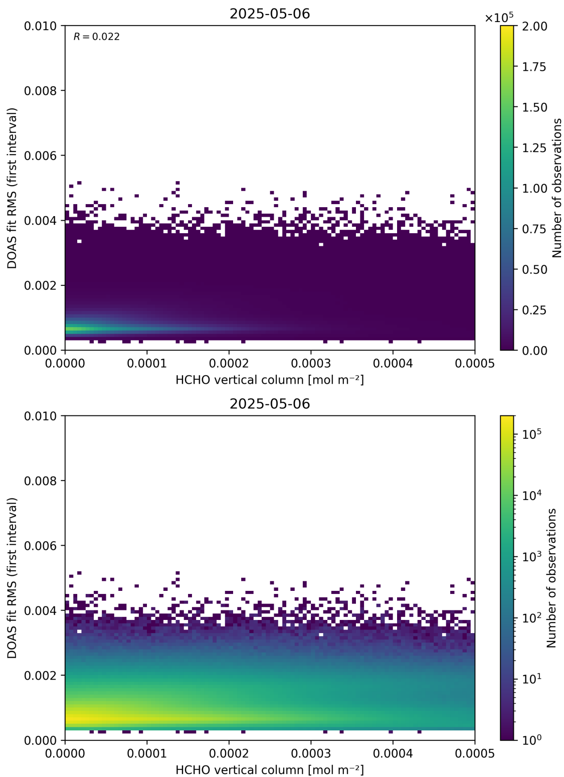
Figure 123: Scatter density plot of “HCHO vertical column” against “DOAS fit RMS (first interval)” for 2025-05-05 to 2025-05-07.
