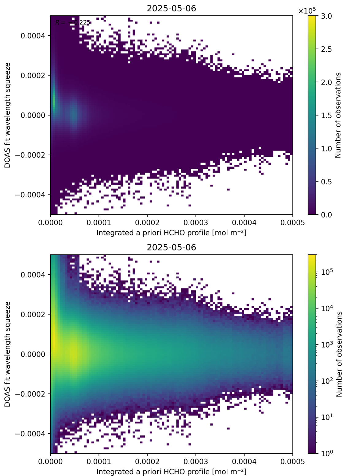
Figure 150: Scatter density plot of “Integrated a priori HCHO profile” against “DOAS fit wavelength squeeze” for 2025-05-05 to 2025-05-07.
