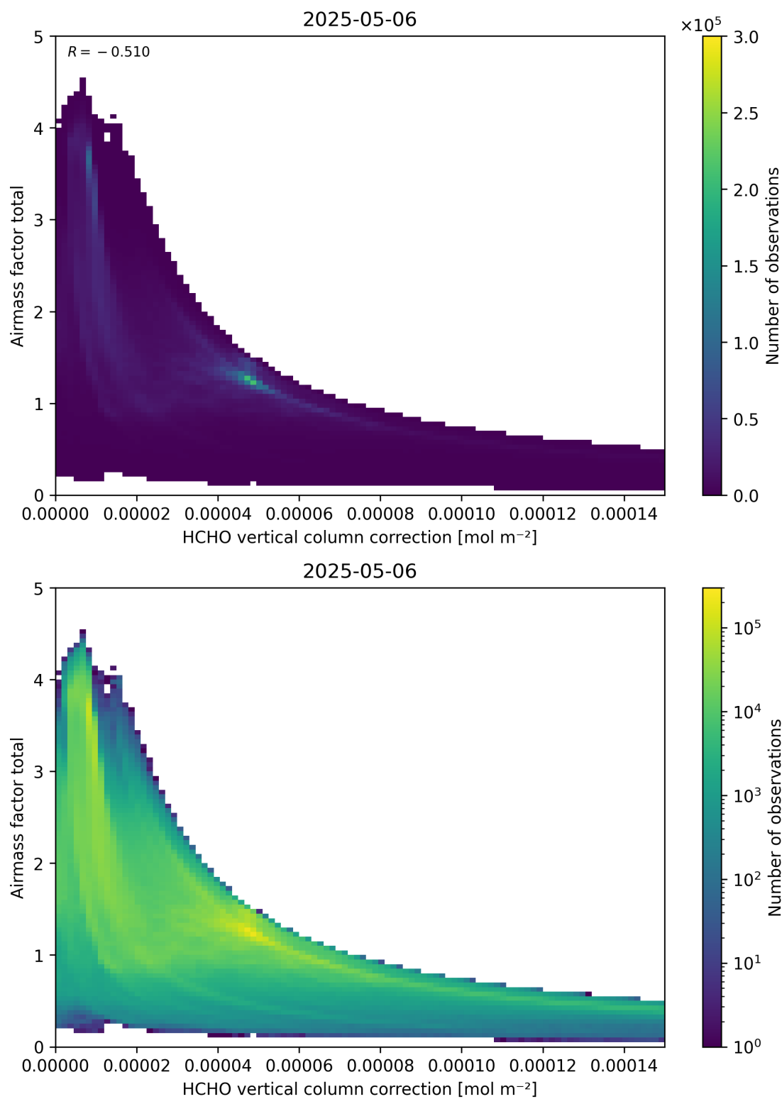
Figure 120: Scatter density plot of “HCHO vertical column correction” against “Airmass factor total” for 2025-05-05 to 2025-05-07.
