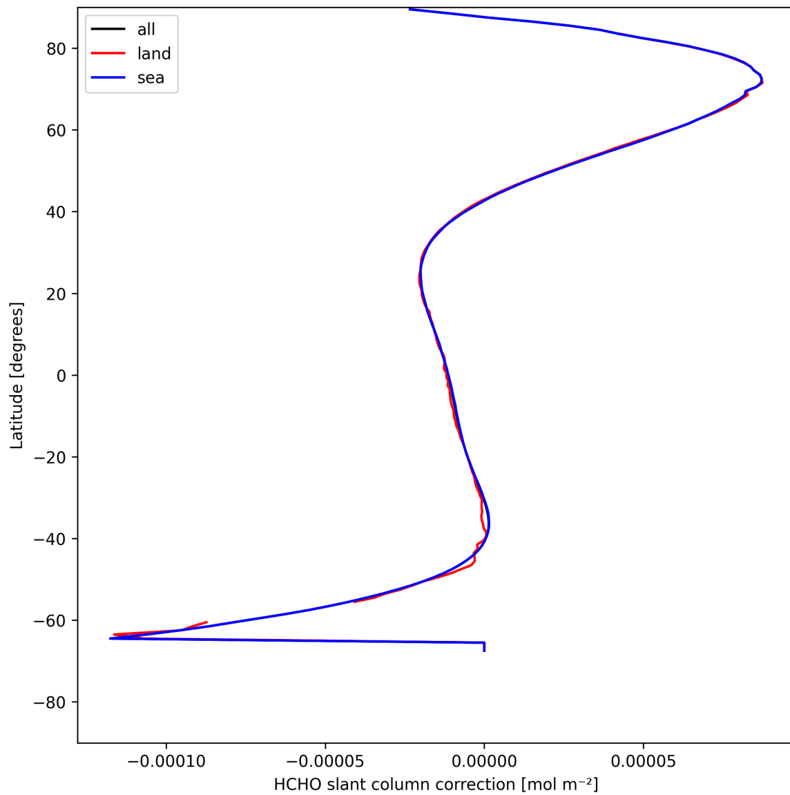
Figure 33: Zonal average of “HCHO slant column correction” for 2025-05-05 to 2025-05-07.
