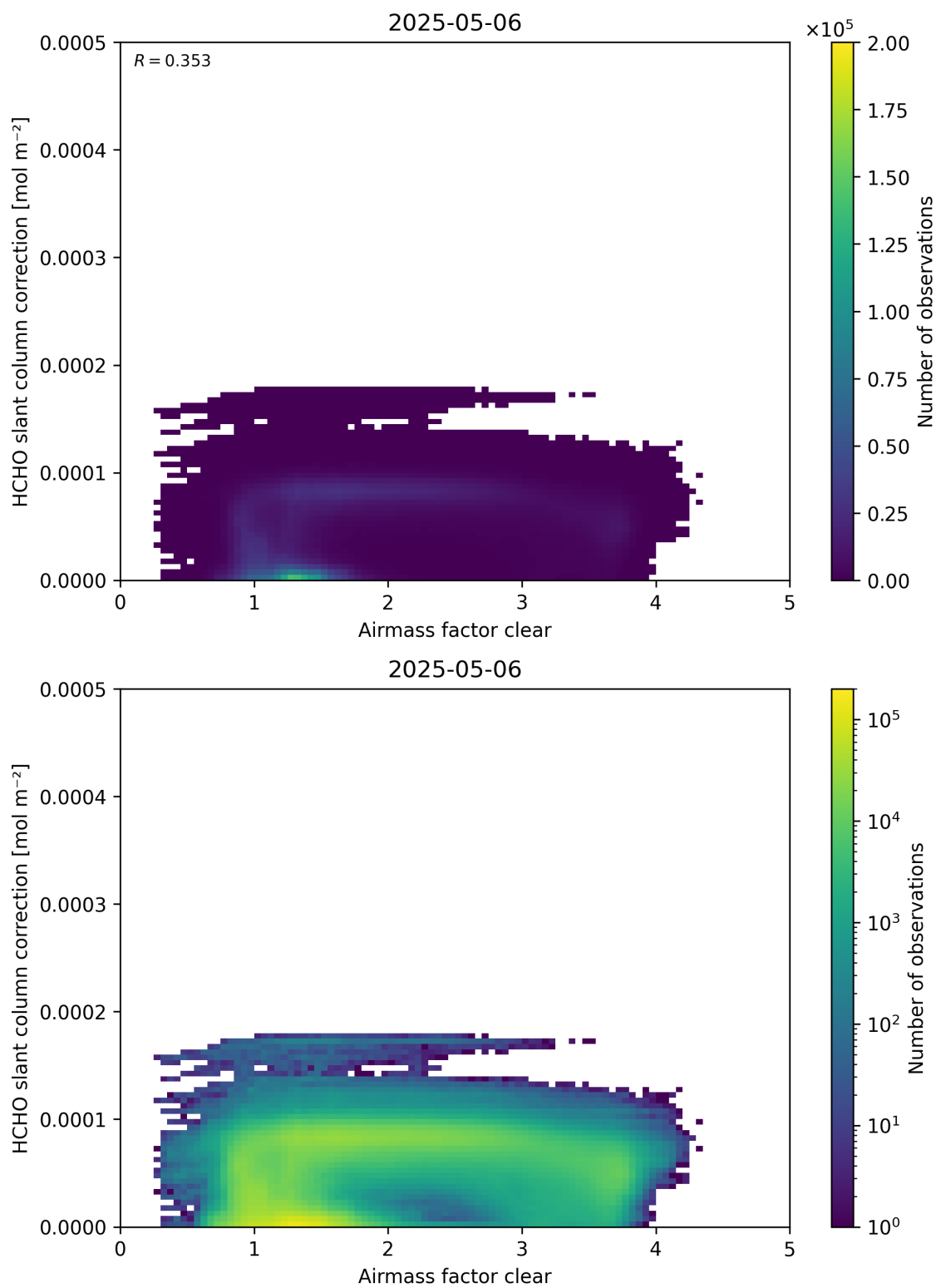
Figure 75: Scatter density plot of “Airmass factor clear” against “HCHO slant column correction” for 2025-05-05 to 2025-05-07.
