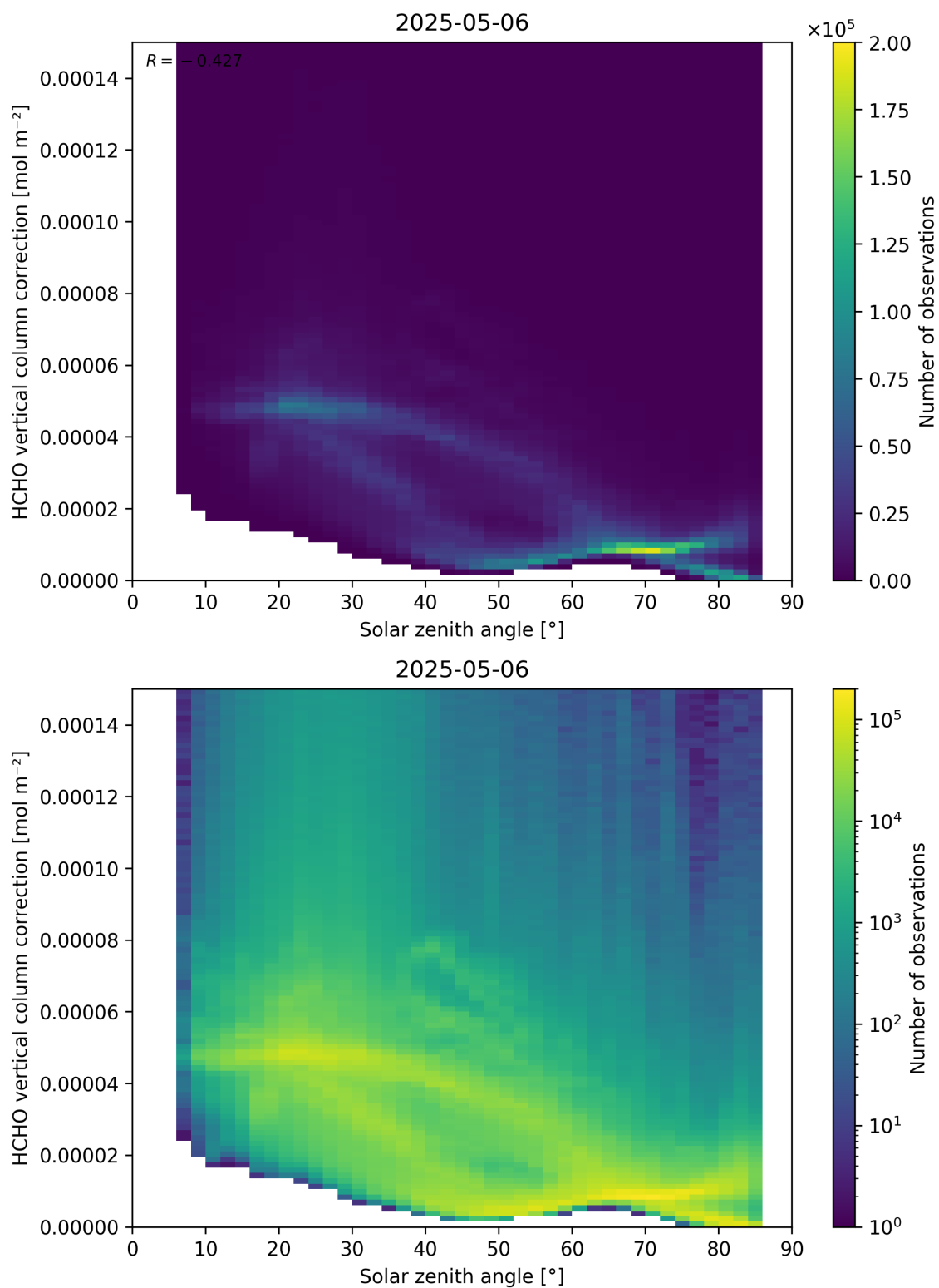
Figure 178: Scatter density plot of “Solar zenith angle” against “HCHO vertical column correction” for 2025-05-05 to 2025-05-07.
