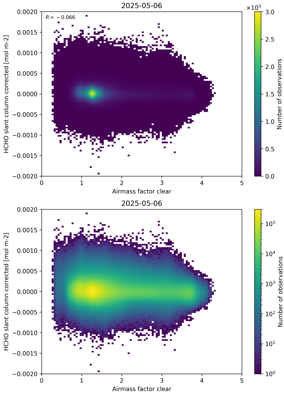
Figure 74: Scatter density plot of “Airmass factor clear” against “HCHO slant column corrected” for 2025-05-05 to 2025-05-07.
