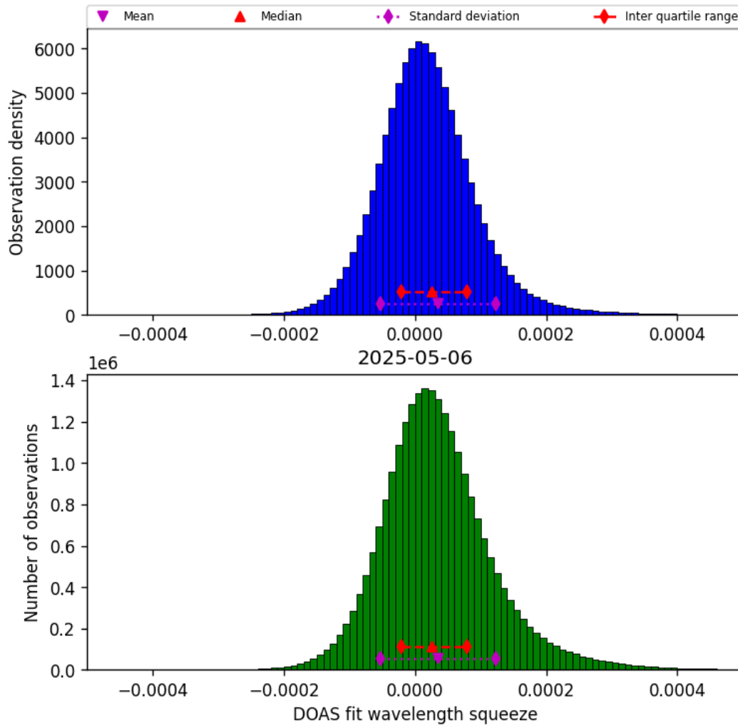
Figure 45: Histogram of “DOAS fit wavelength squeeze” for 2025-05-05 to 2025-05-07
