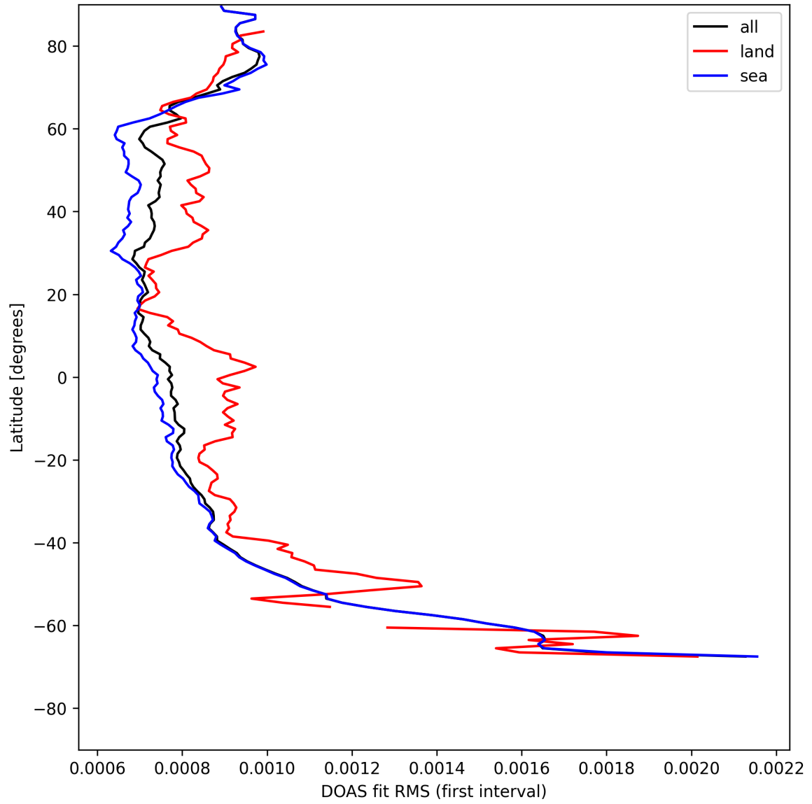
Figure 32: Zonal average of “DOAS fit RMS (first interval)” for 2025-05-05 to 2025-05-07.
