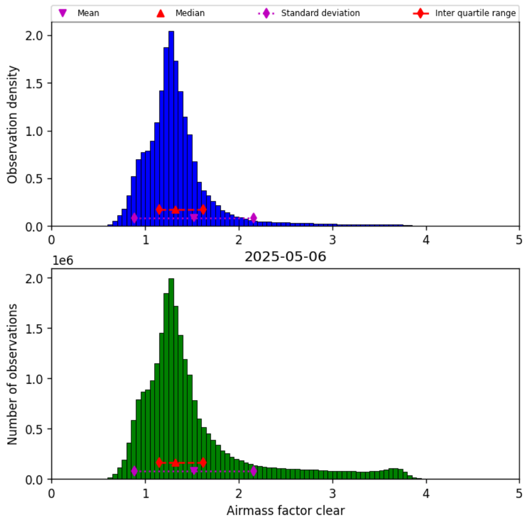
Figure 42: Histogram of “Airmass factor clear” for 2025-05-05 to 2025-05-07
