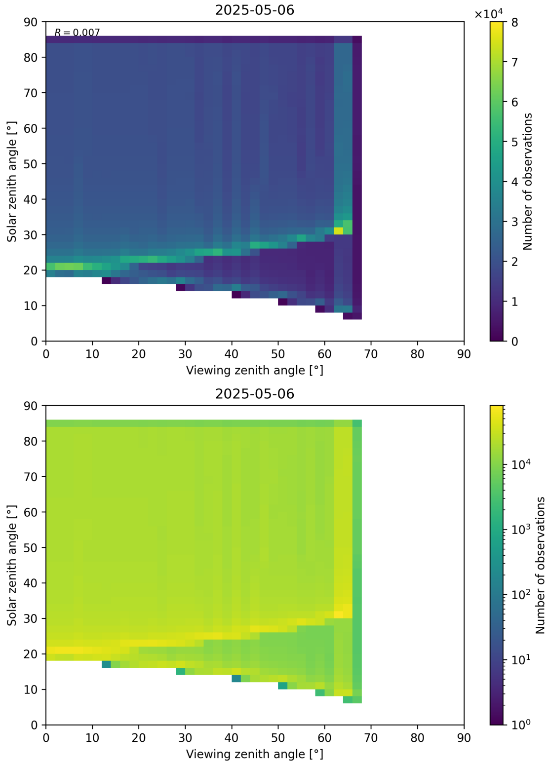
Figure 197: Scatter density plot of “Viewing zenith angle” against “Solar zenith angle” for 2025-05-05 to 2025-05-07.
