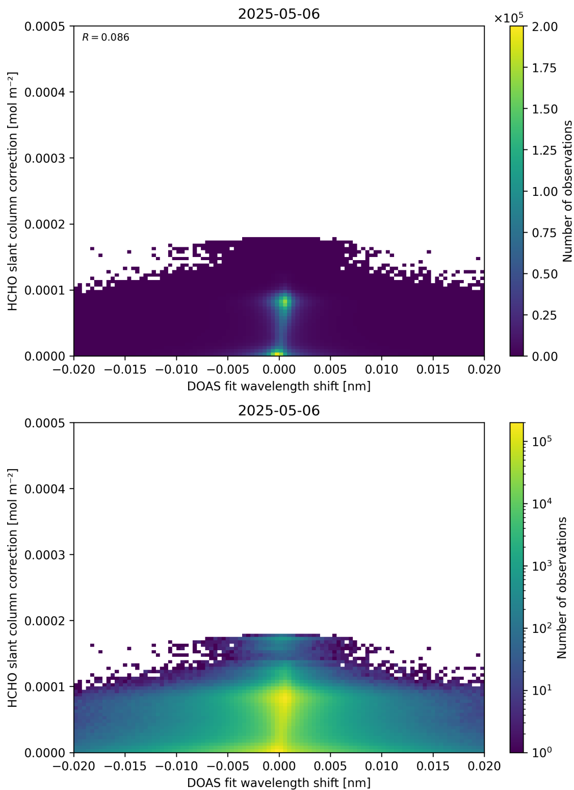
Figure 67: Scatter density plot of “DOAS fit wavelength shift” against “HCHO slant column correction” for 2025-05-05 to 2025-05-07.
