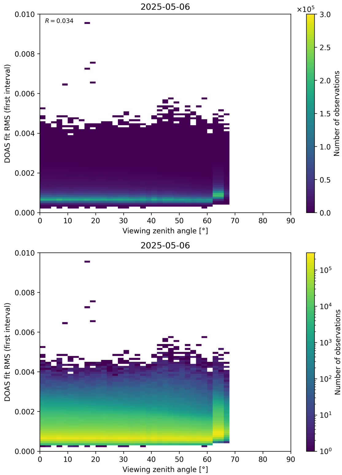
Figure 182: Scatter density plot of “Viewing zenith angle” against “DOAS fit RMS (first interval)” for 2025-05-05 to 2025-05-07.
