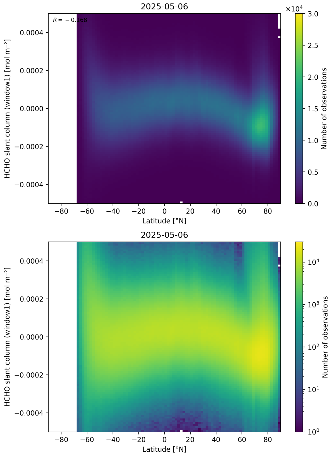
Figure 159: Scatter density plot of “Latitude” against “HCHO slant column (window1)” for 2025-05-05 to 2025-05-07.
