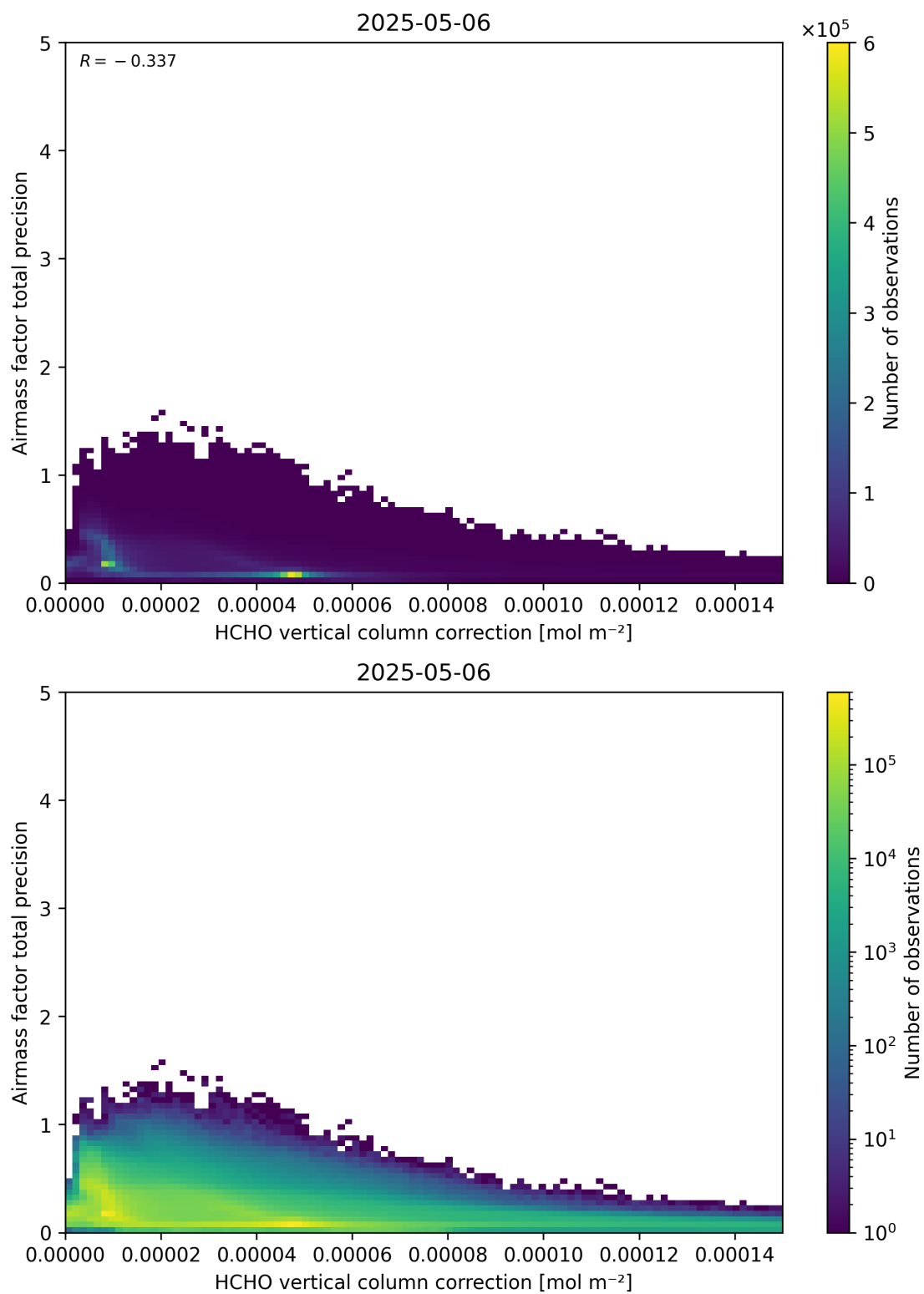
Figure 121: Scatter density plot of “HCHO vertical column correction” against “Airmass factor total precision” for 2025-05-05 to 2025-05-07.
