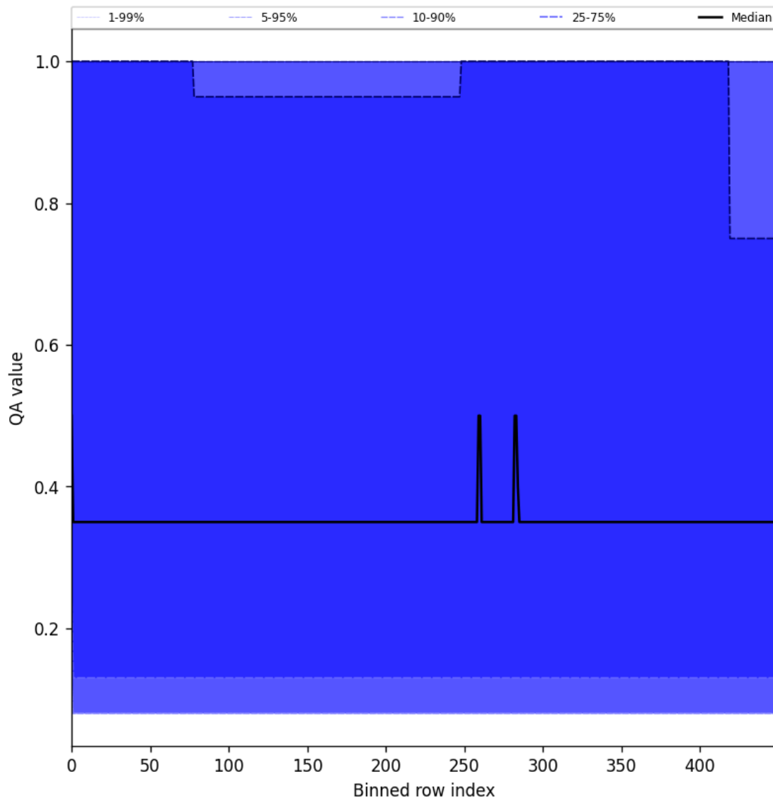
Figure 48: Along track statistics of “QA value” for 2025-05-05 to 2025-05-07
