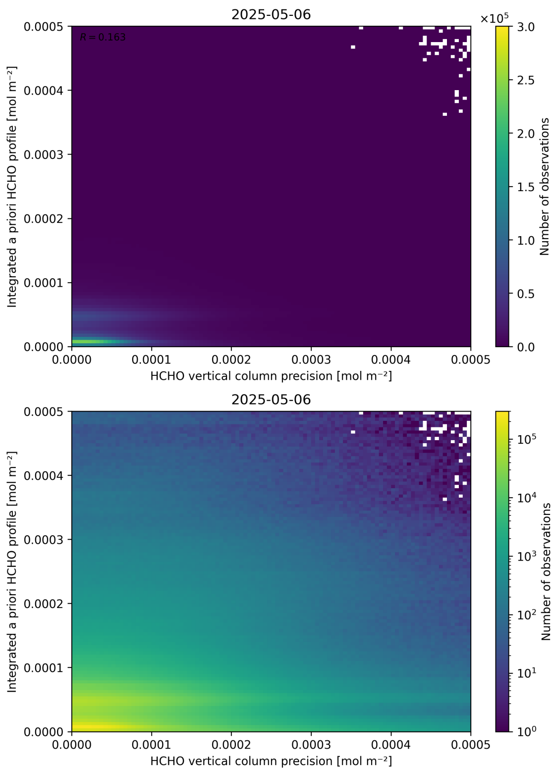
Figure 147: Scatter density plot of “HCHO vertical column precision” against “Integrated a priori HCHO profile” for 2025-05-05 to 2025-05-07.
