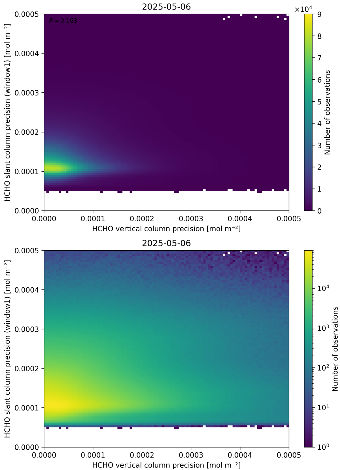
Figure 143: Scatter density plot of “HCHO vertical column precision” against “HCHO slant column precision (window1)” for 2025-05-05 to 2025-05-07.
