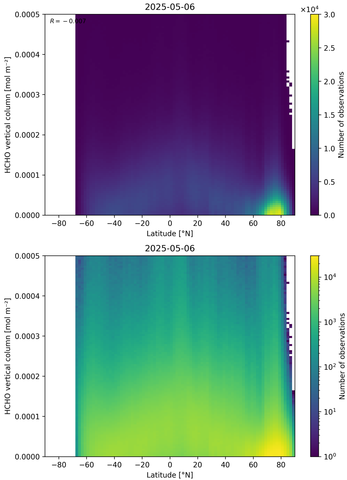
Figure 163: Scatter density plot of “Latitude” against “HCHO vertical column” for 2025-05-05 to 2025-05-07.
