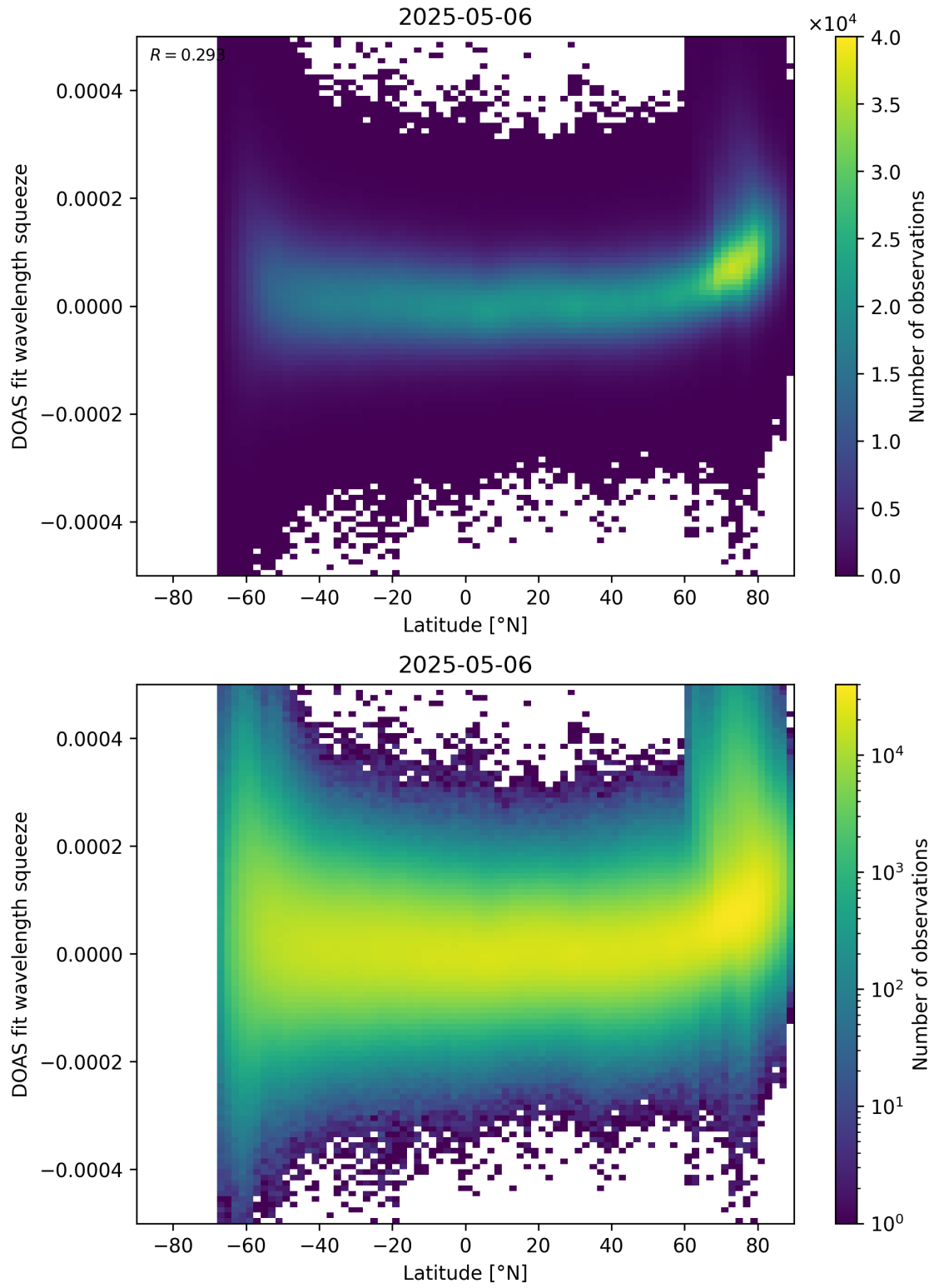
Figure 155: Scatter density plot of “Latitude” against “DOAS fit wavelength squeeze” for 2025-05-05 to 2025-05-07.
