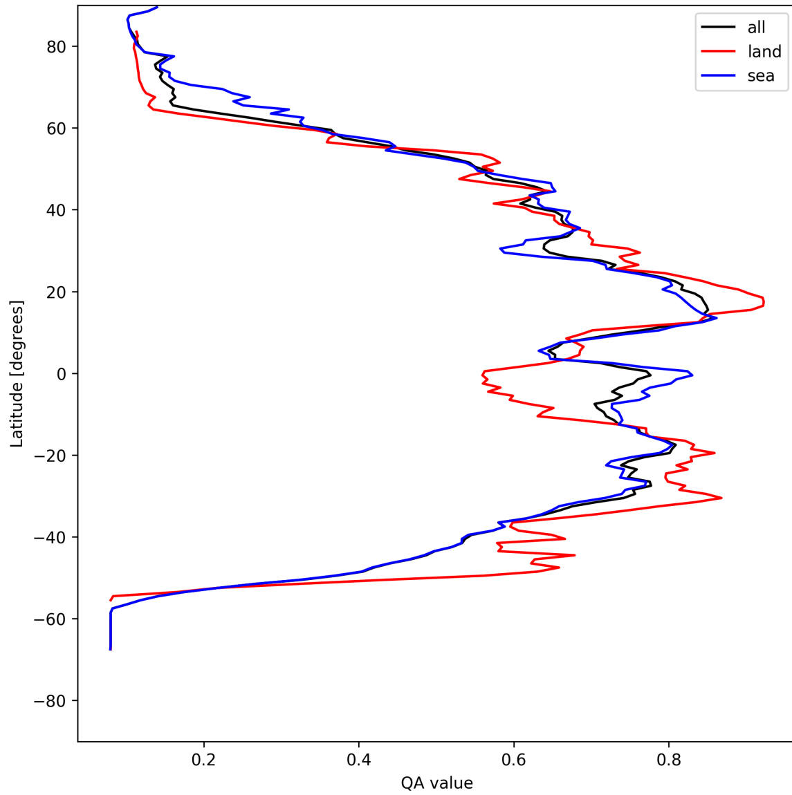
Figure 20: Zonal average of “QA value” for 2025-05-05 to 2025-05-07.
