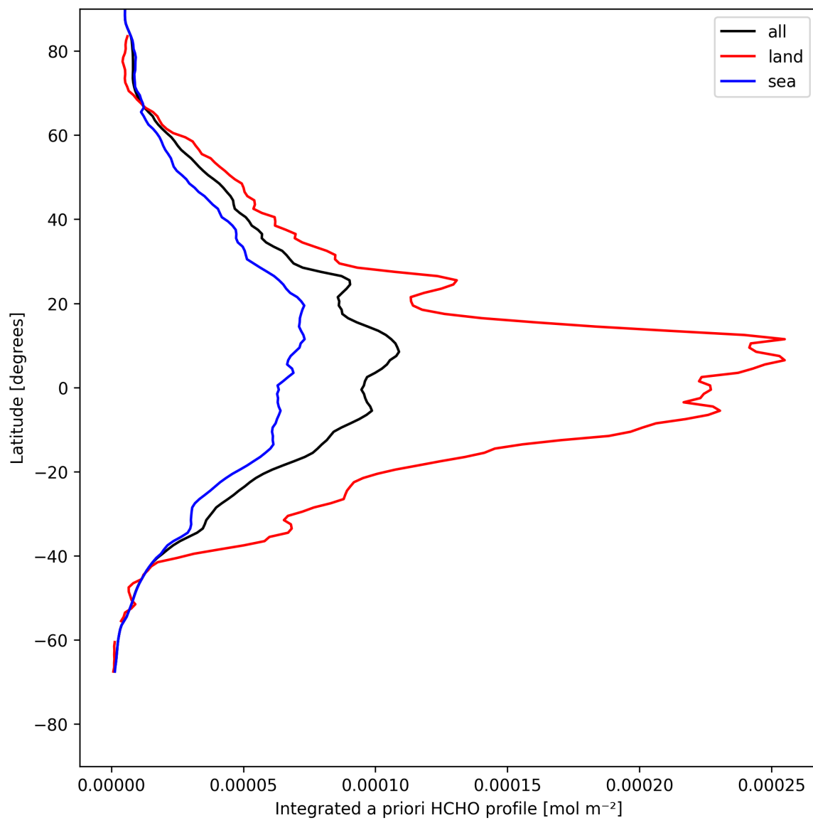
Figure 29: Zonal average of “Integrated a priori HCHO profile” for 2025-05-05 to 2025-05-07.
