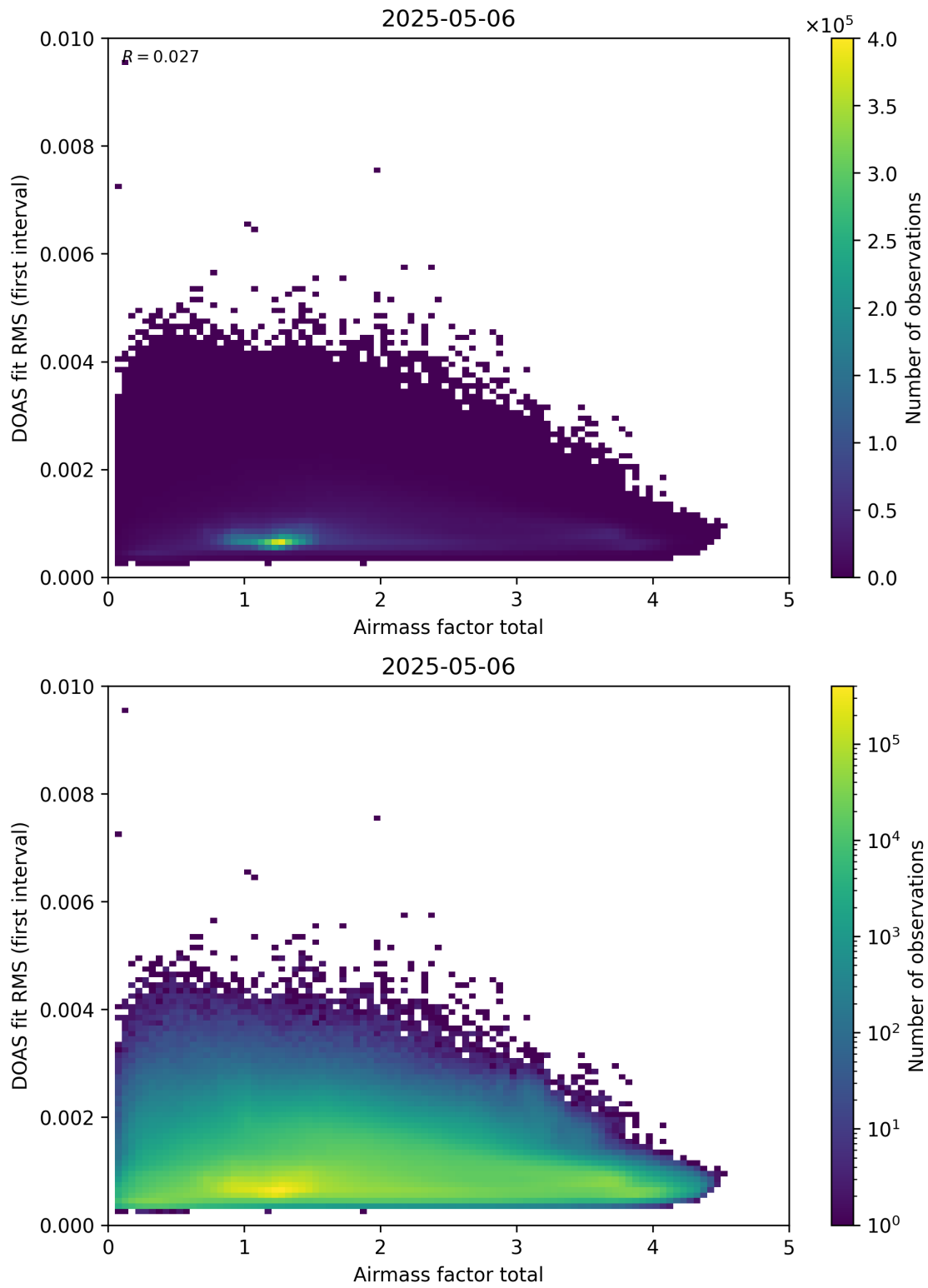
Figure 97: Scatter density plot of “Airmass factor total” against “DOAS fit RMS (first interval)” for 2025-05-05 to 2025-05-07.
