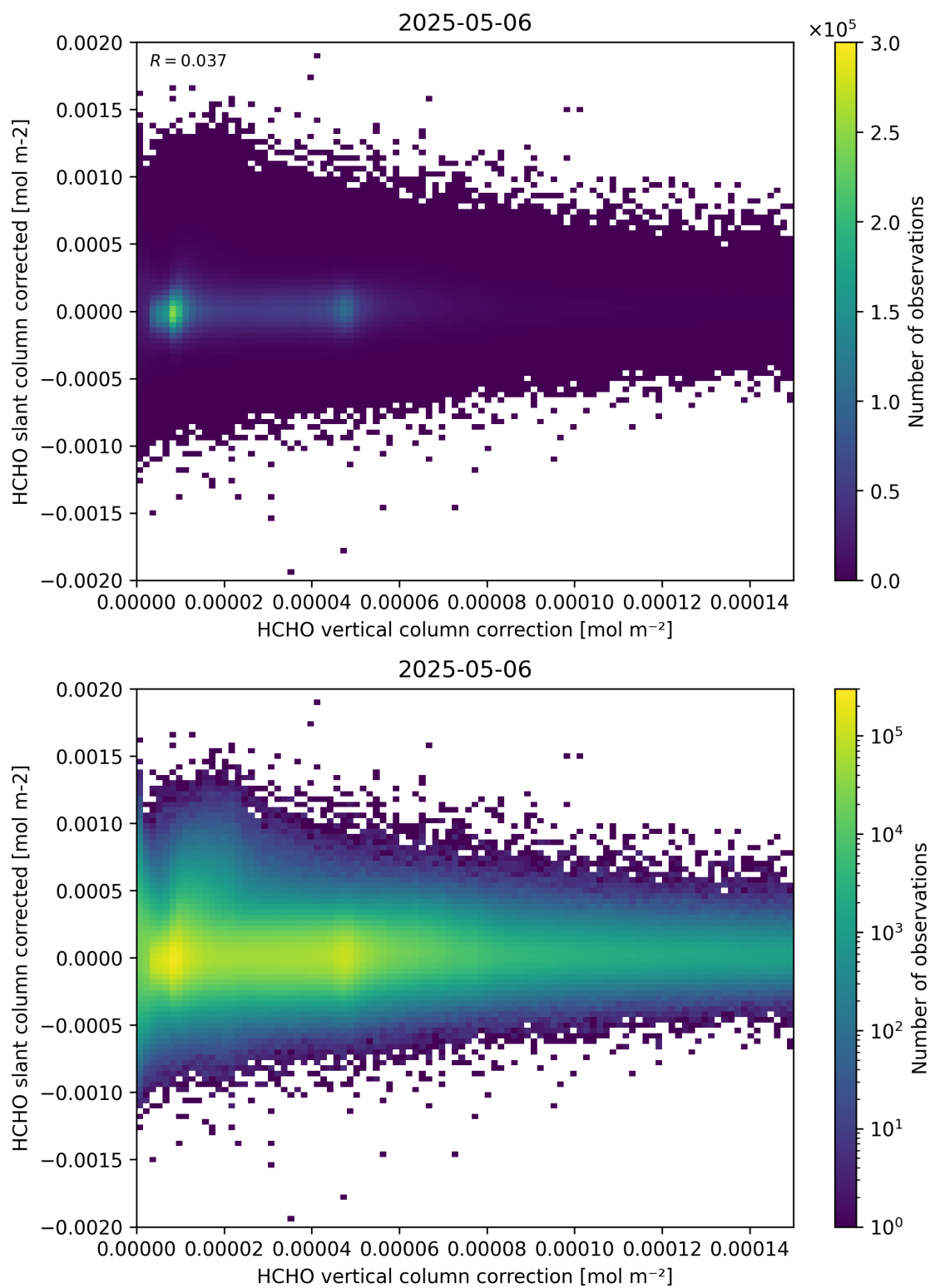
Figure 116: Scatter density plot of “HCHO vertical column correction” against “HCHO slant column corrected” for 2025-05-05 to 2025-05-07.
