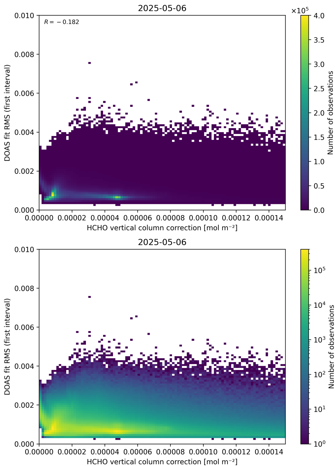
Figure 112: Scatter density plot of “HCHO vertical column correction” against “DOAS fit RMS (first interval)” for 2025-05-05 to 2025-05-07.
