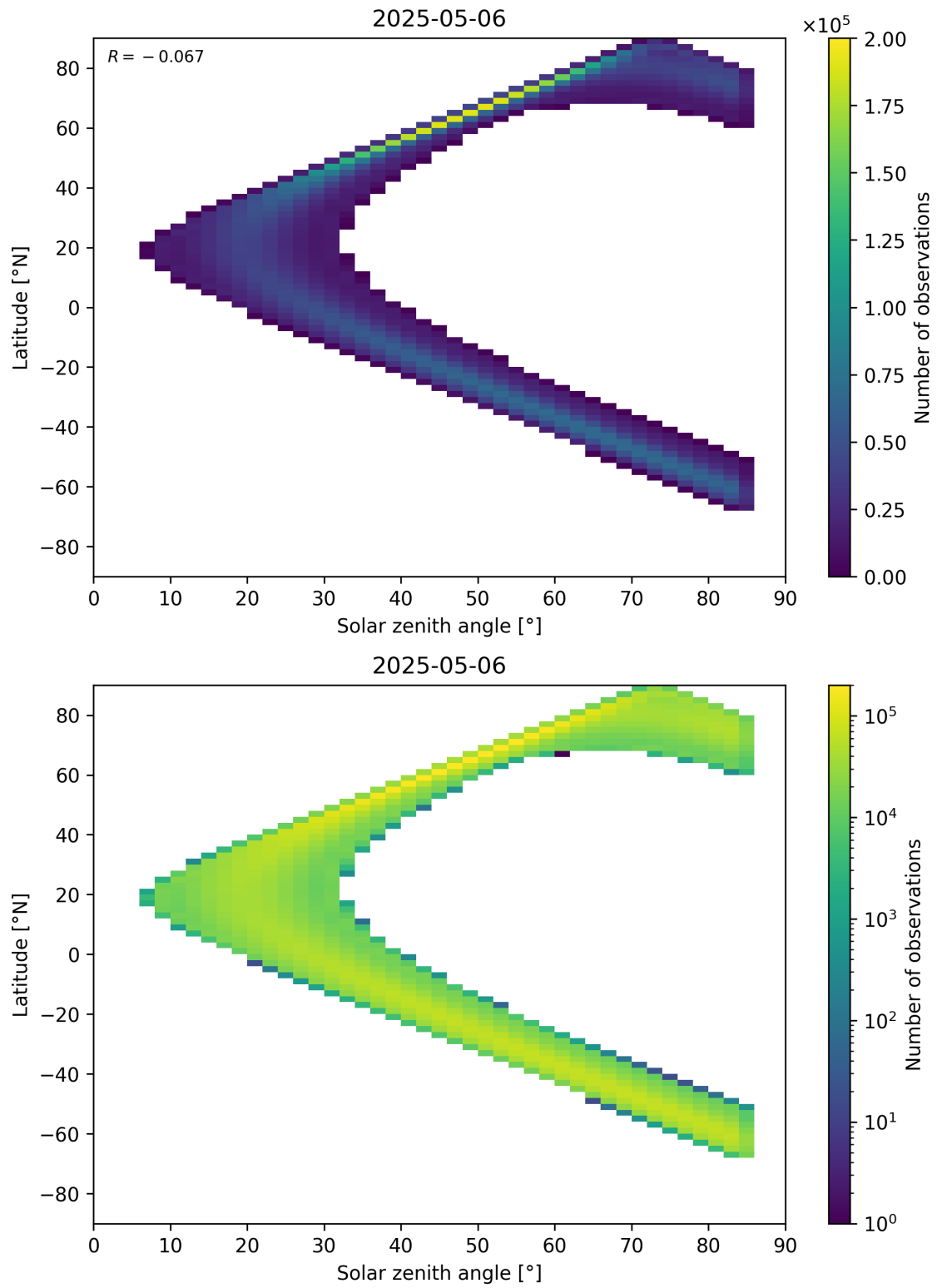
Figure 181: Scatter density plot of “Solar zenith angle” against “Latitude” for 2025-05-05 to 2025-05-07.
