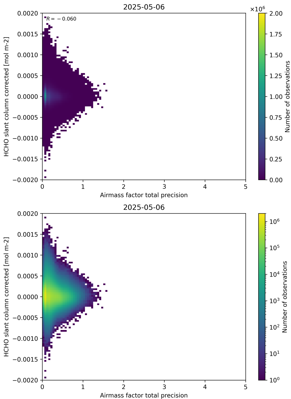
Figure 109: Scatter density plot of “Airmass factor total precision” against “HCHO slant column corrected” for 2025-05-05 to 2025-05-07.
