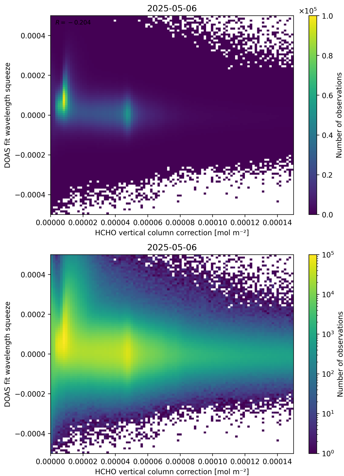
Figure 114: Scatter density plot of “HCHO vertical column correction” against “DOAS fit wavelength squeeze” for 2025-05-05 to 2025-05-07.
