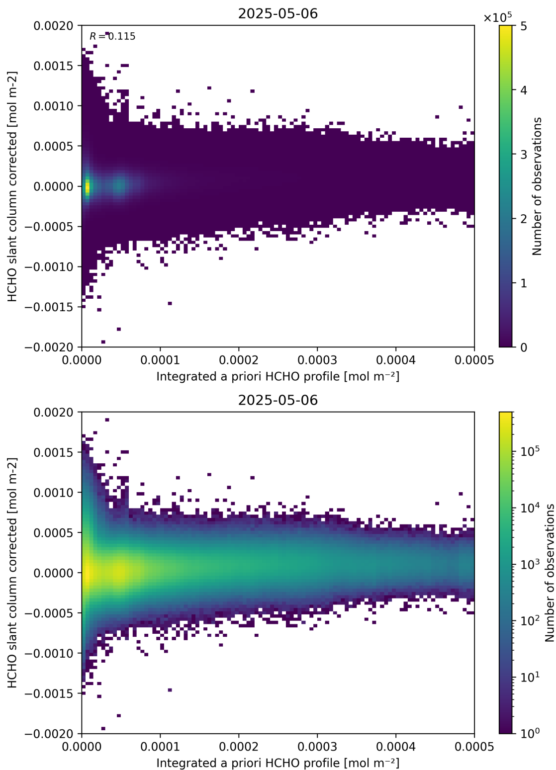
Figure 151: Scatter density plot of “Integrated a priori HCHO profile” against “HCHO slant column corrected” for 2025-05-05 to 2025-05-07.
