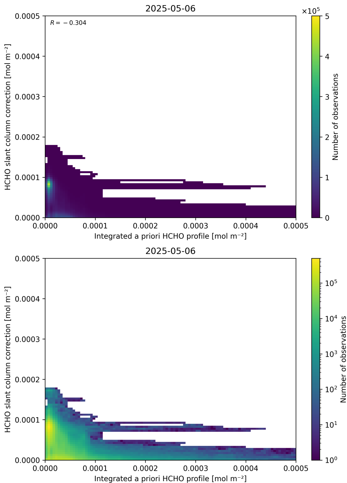
Figure 152: Scatter density plot of “Integrated a priori HCHO profile” against “HCHO slant column correction” for 2025-05-05 to 2025-05-07.
