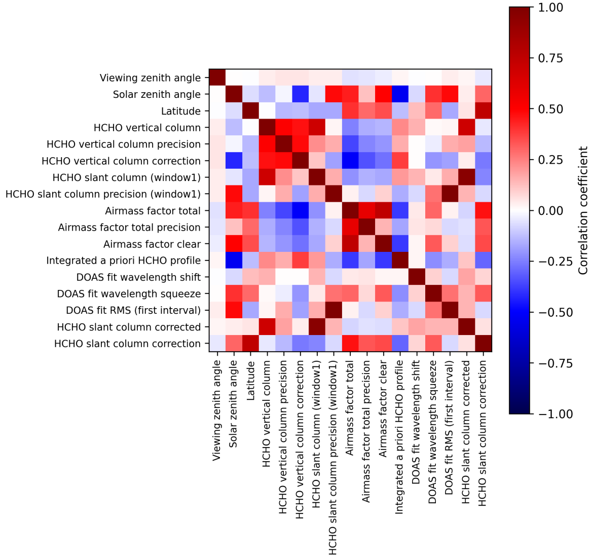
Figure 2: Map of correlation matrix for 2025-05-05 to 2025-05-07.
