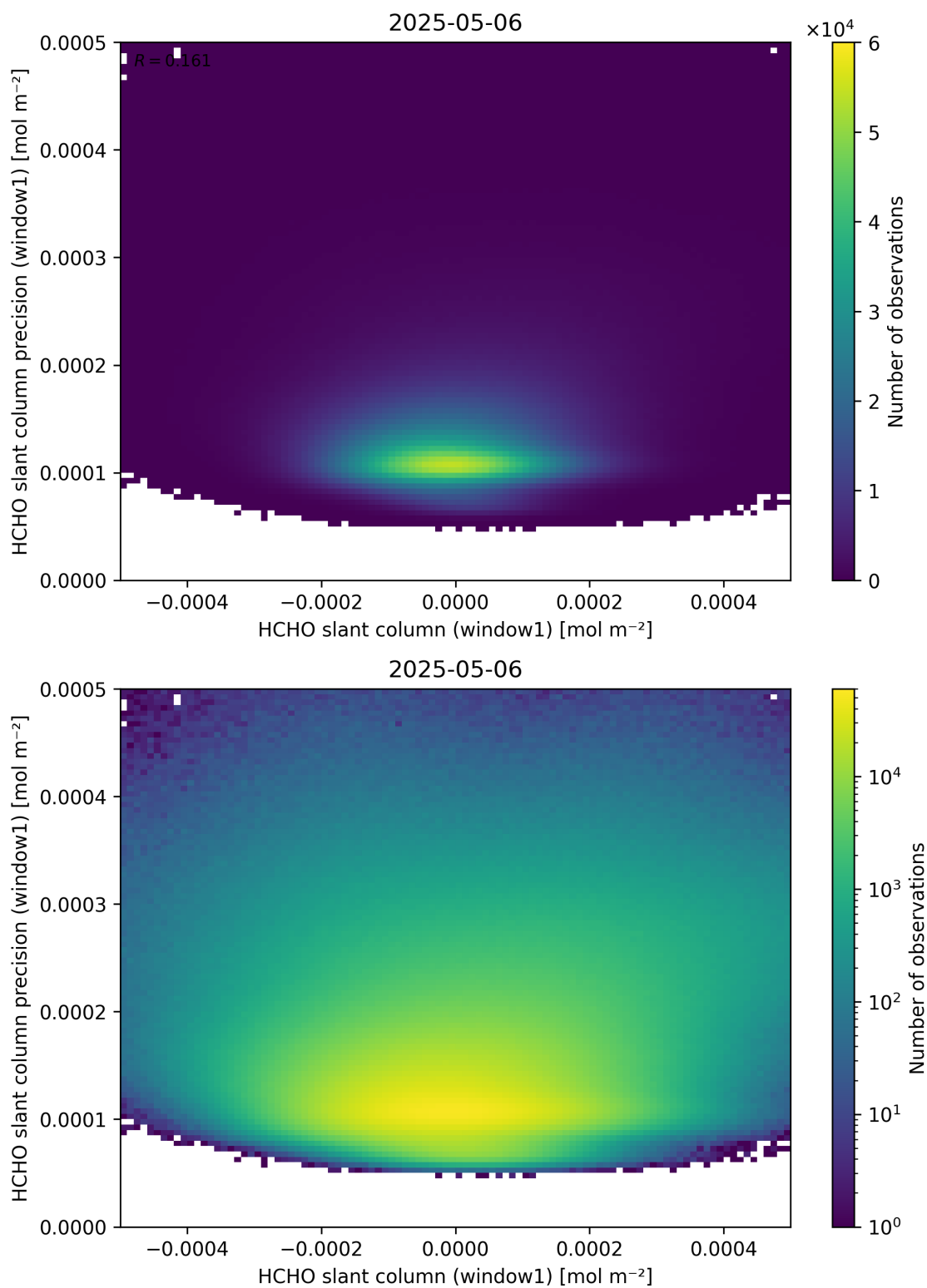
Figure 84: Scatter density plot of “HCHO slant column (window1)” against “HCHO slant column precision (window1)” for 2025-05-05 to 2025-05-07.
