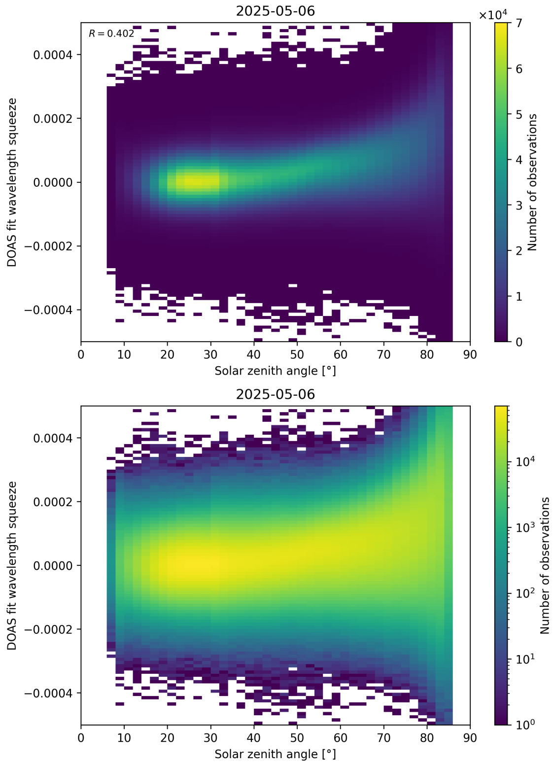
Figure 169: Scatter density plot of “Solar zenith angle” against “DOAS fit wavelength squeeze” for 2025-05-05 to 2025-05-07.
