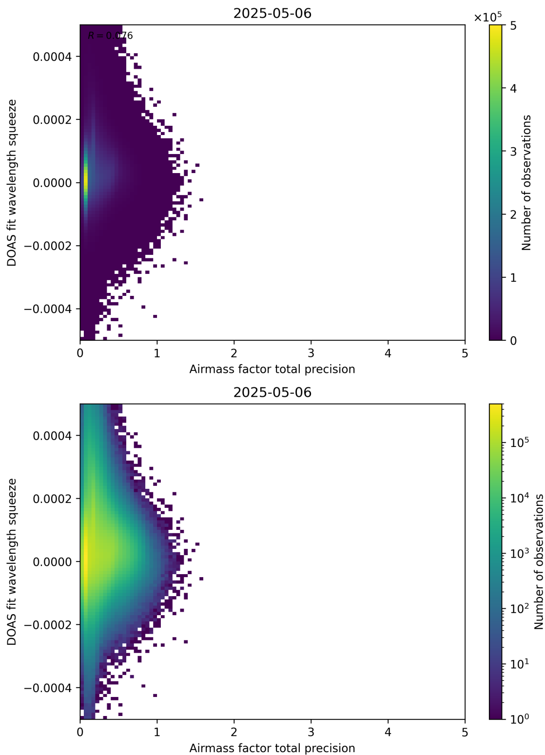
Figure 107: Scatter density plot of “Airmass factor total precision” against “DOAS fit wavelength squeeze” for 2025-05-05 to 2025-05-07.
