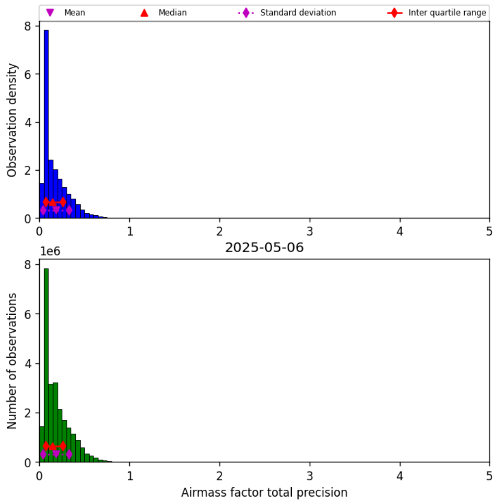
Figure 41: Histogram of “Airmass factor total precision” for 2025-05-05 to 2025-05-07
