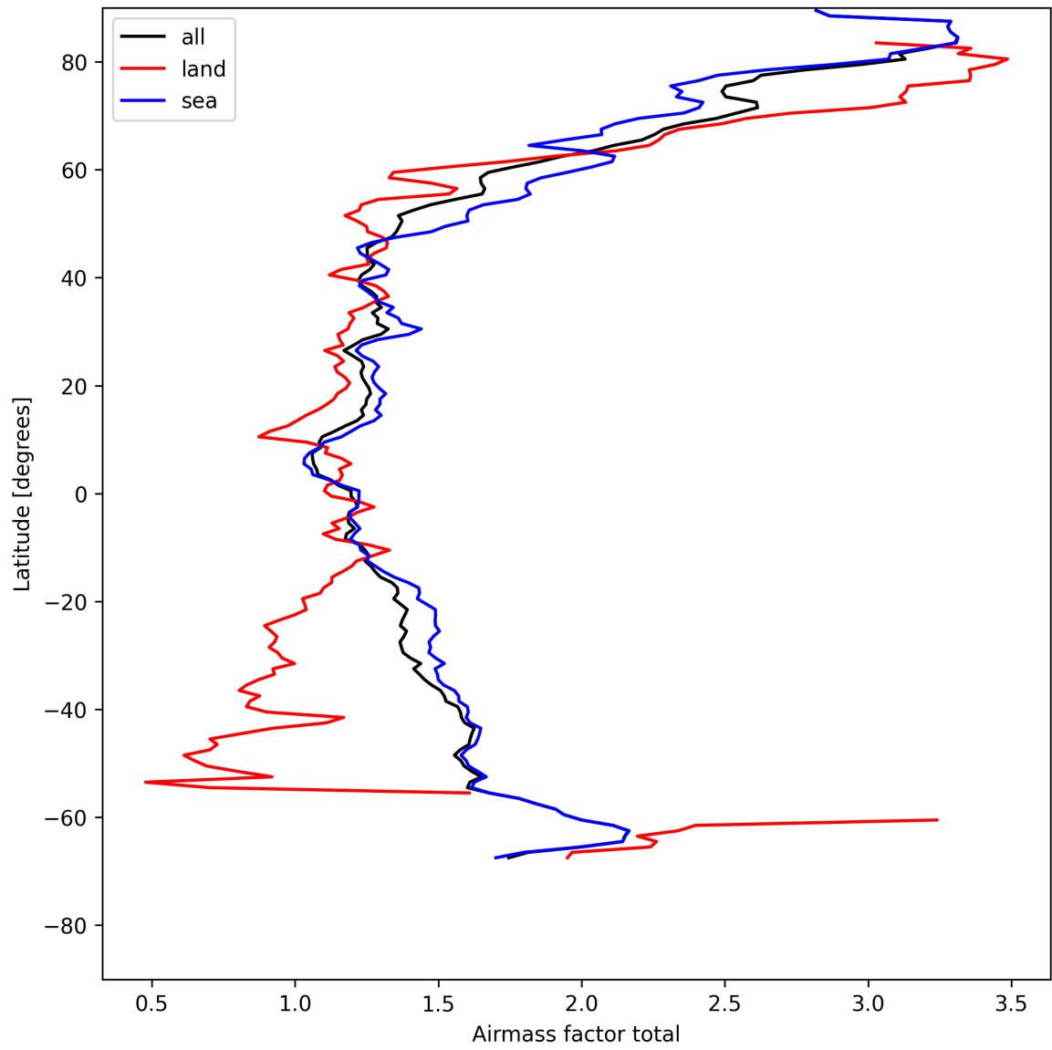
Figure 26: Zonal average of “Airmass factor total” for 2025-05-05 to 2025-05-07.
