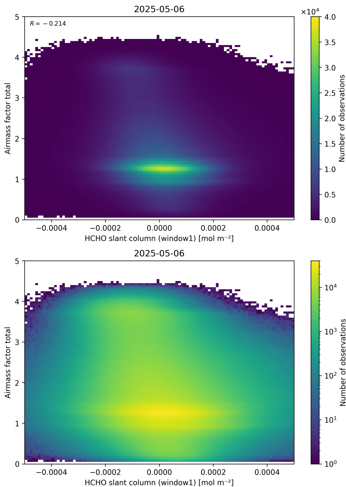
Figure 85: Scatter density plot of “HCHO slant column (window1)” against “Airmass factor total” for 2025-05-05 to 2025-05-07.
