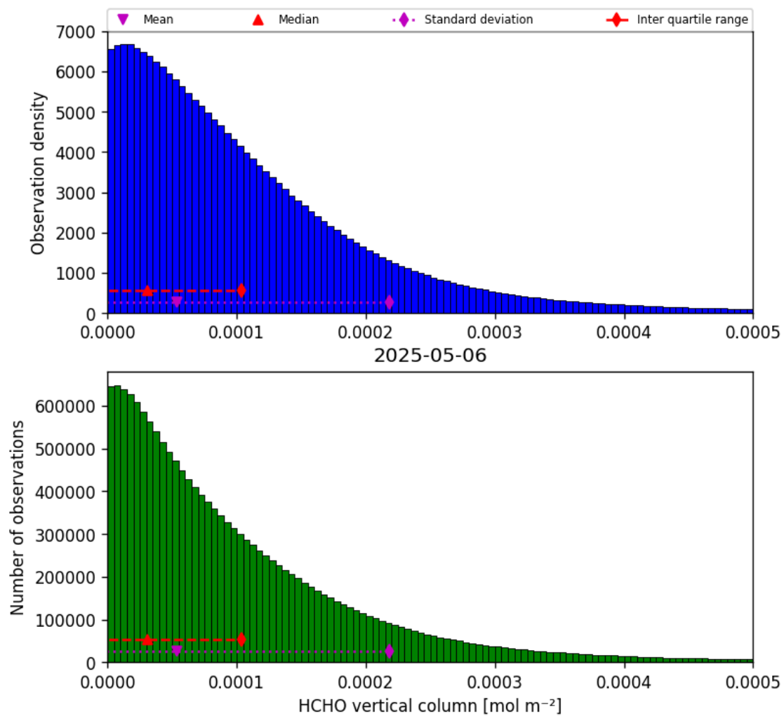
Figure 35: Histogram of “HCHO vertical column” for 2025-05-05 to 2025-05-07
