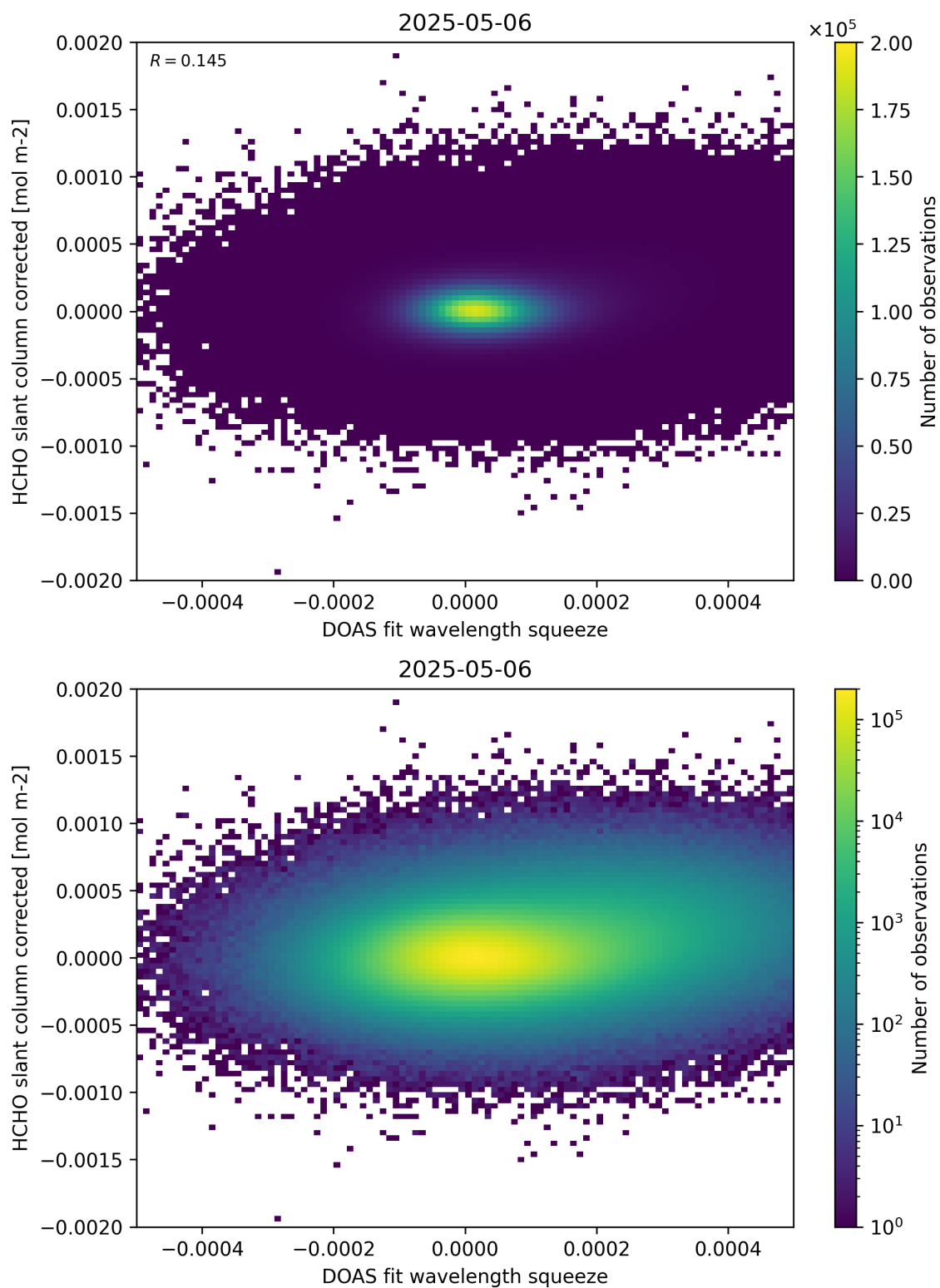
Figure 69: Scatter density plot of “DOAS fit wavelength squeeze” against “HCHO slant column corrected” for 2025-05-05 to 2025-05-07.
