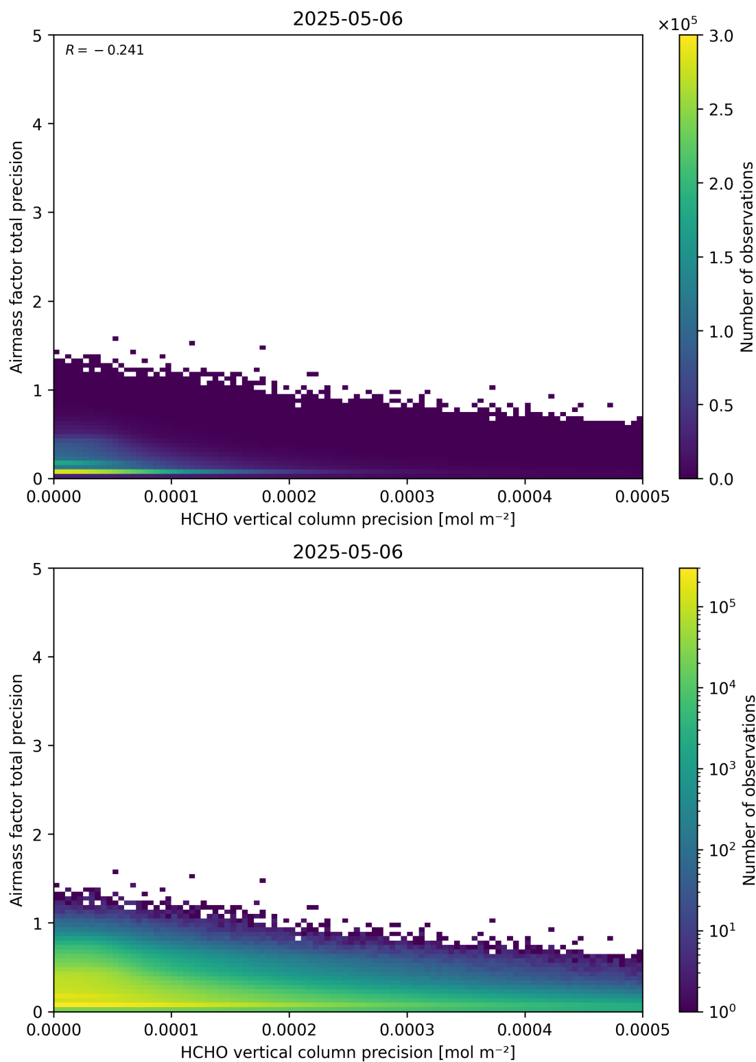
Figure 145: Scatter density plot of “HCHO vertical column precision” against “Airmass factor total precision” for 2025-05-05 to 2025-05-07.
