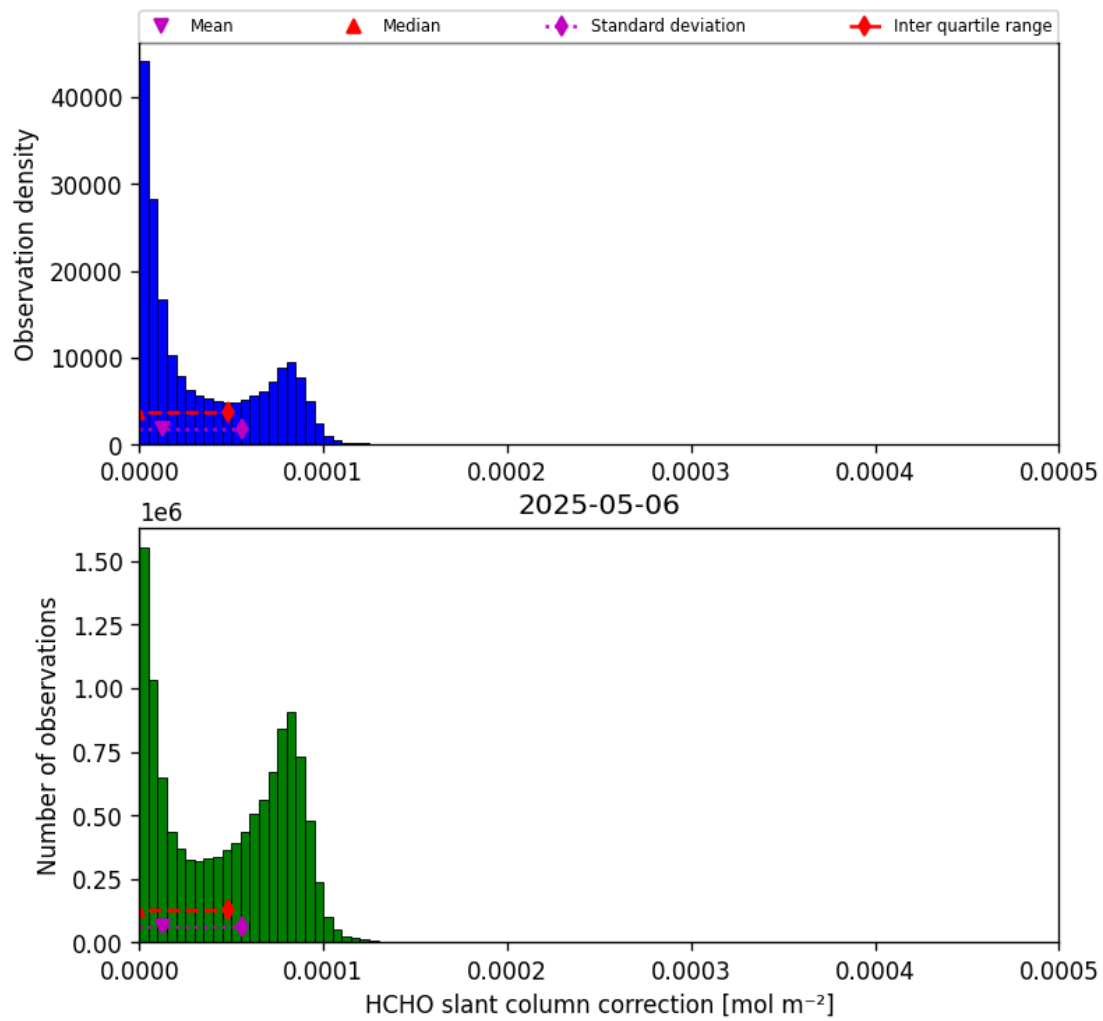
Figure 47: Histogram of “HCHO slant column correction” for 2025-05-05 to 2025-05-07
