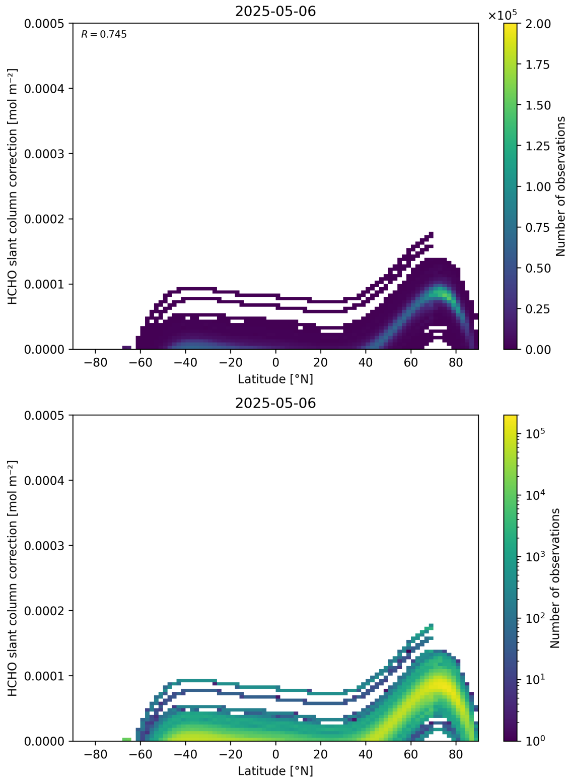
Figure 158: Scatter density plot of “Latitude” against “HCHO slant column correction” for 2025-05-05 to 2025-05-07.
