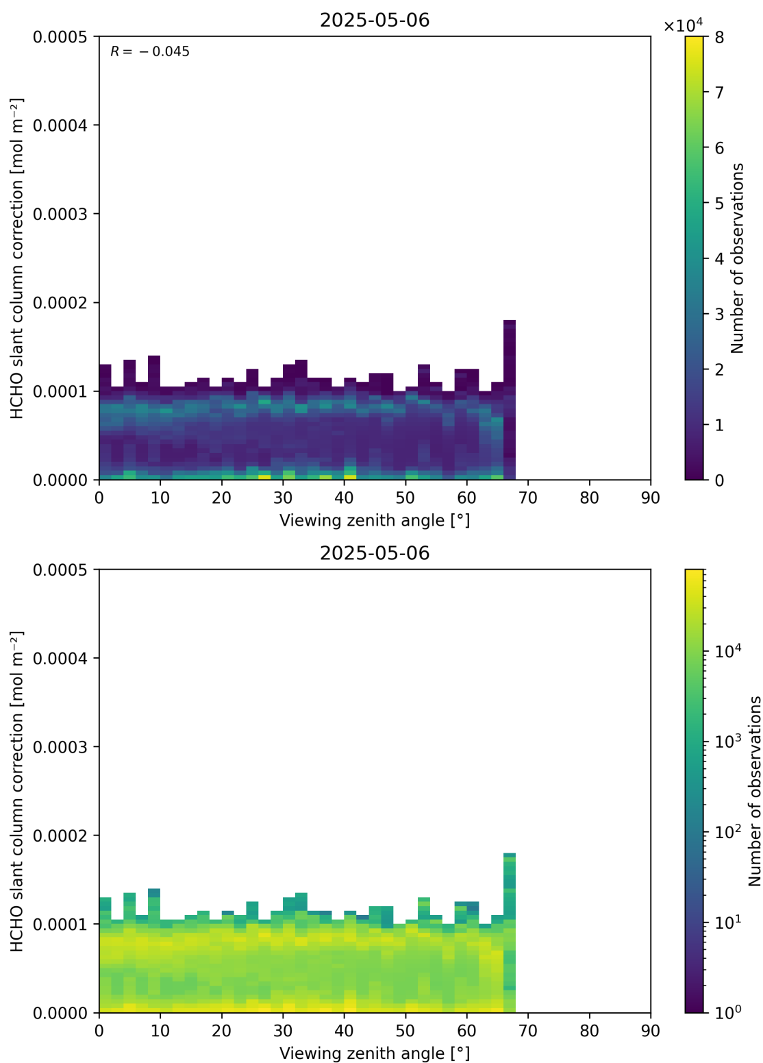
Figure 187: Scatter density plot of “Viewing zenith angle” against “HCHO slant column correction” for 2025-05-05 to 2025-05-07.
