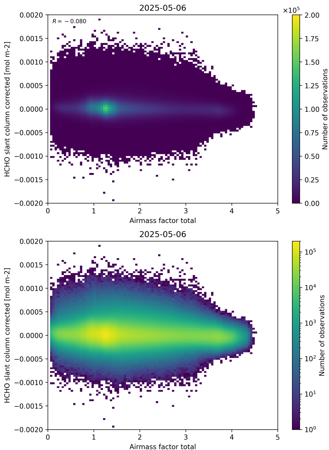
Figure 101: Scatter density plot of “Airmass factor total” against “HCHO slant column corrected” for 2025-05-05 to 2025-05-07.
