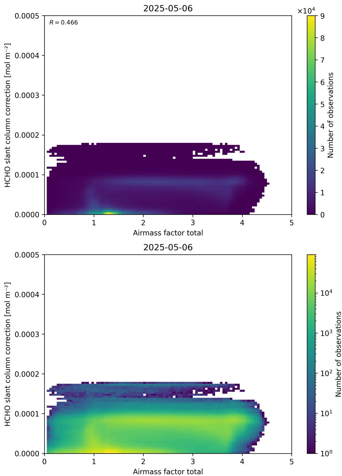
Figure 102: Scatter density plot of “Airmass factor total” against “HCHO slant column correction” for 2025-05-05 to 2025-05-07.
