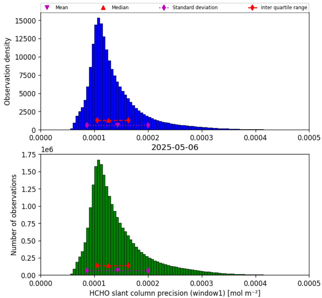
Figure 39: Histogram of “HCHO slant column precision (window1)” for 2025-05-05 to 2025-05-07
