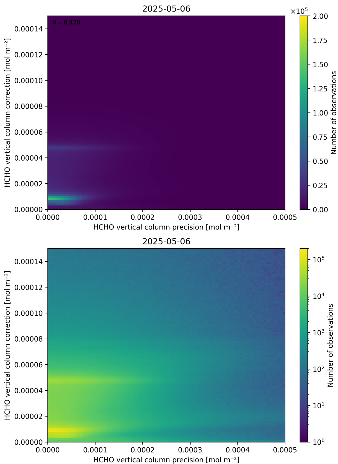
Figure 146: Scatter density plot of “HCHO vertical column precision” against “HCHO vertical column correction” for 2025-05-05 to 2025-05-07.
