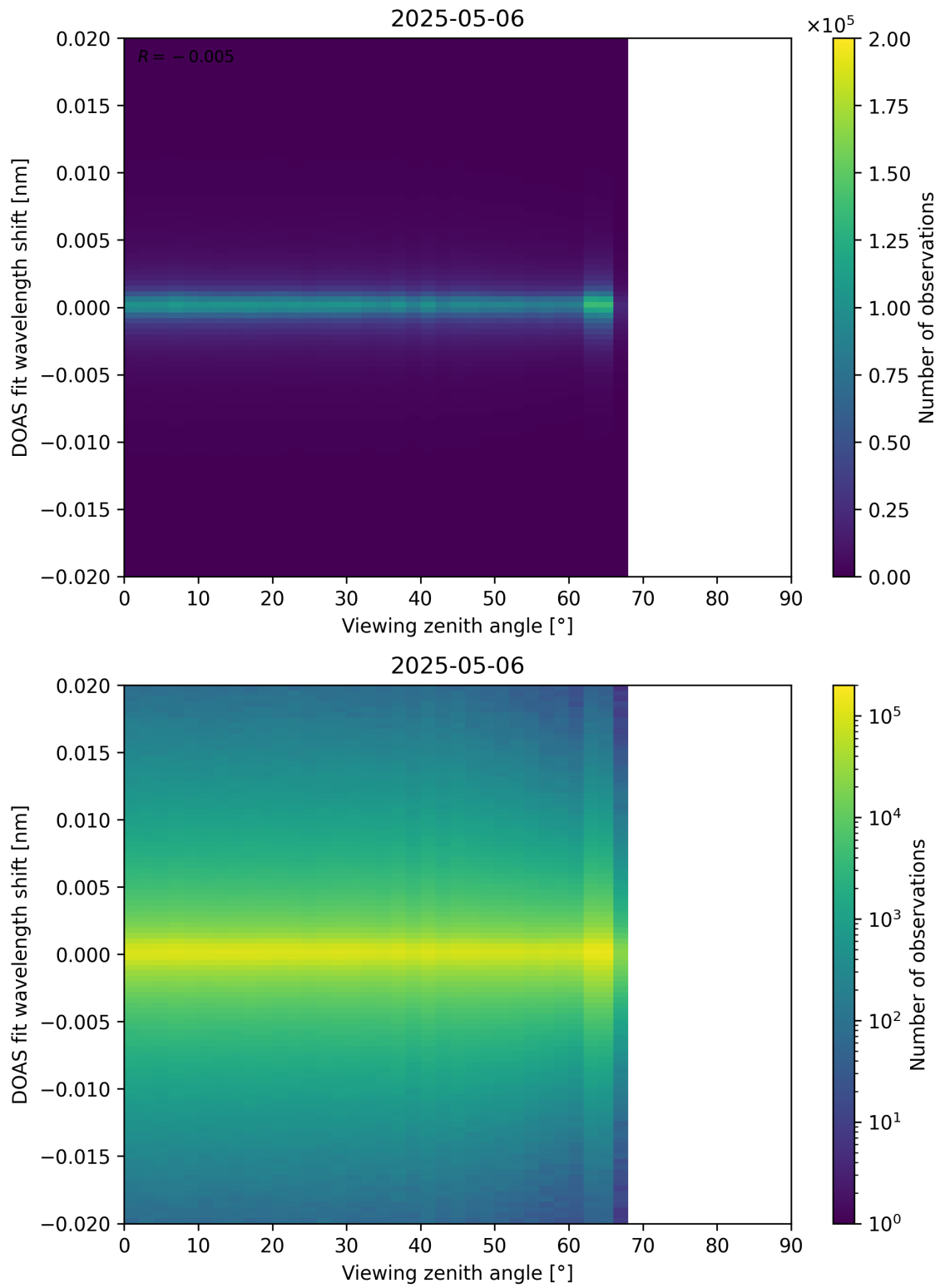
Figure 183: Scatter density plot of “Viewing zenith angle” against “DOAS fit wavelength shift” for 2025-05-05 to 2025-05-07.
