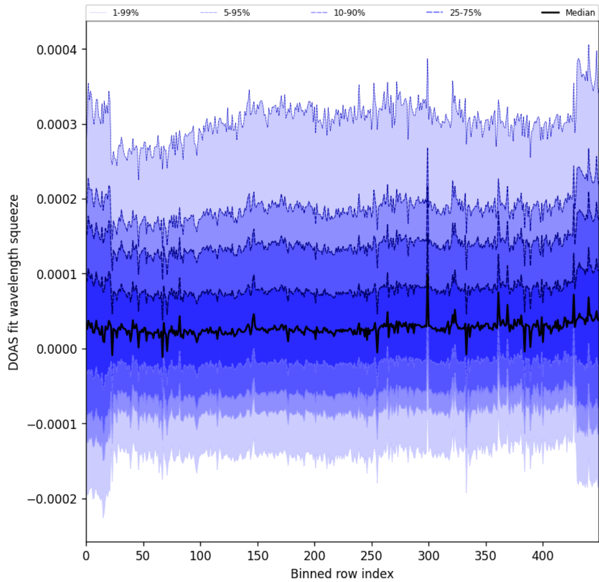
Figure 59: Along track statistics of “DOAS fit wavelength squeeze” for 2025-05-05 to 2025-05-07
