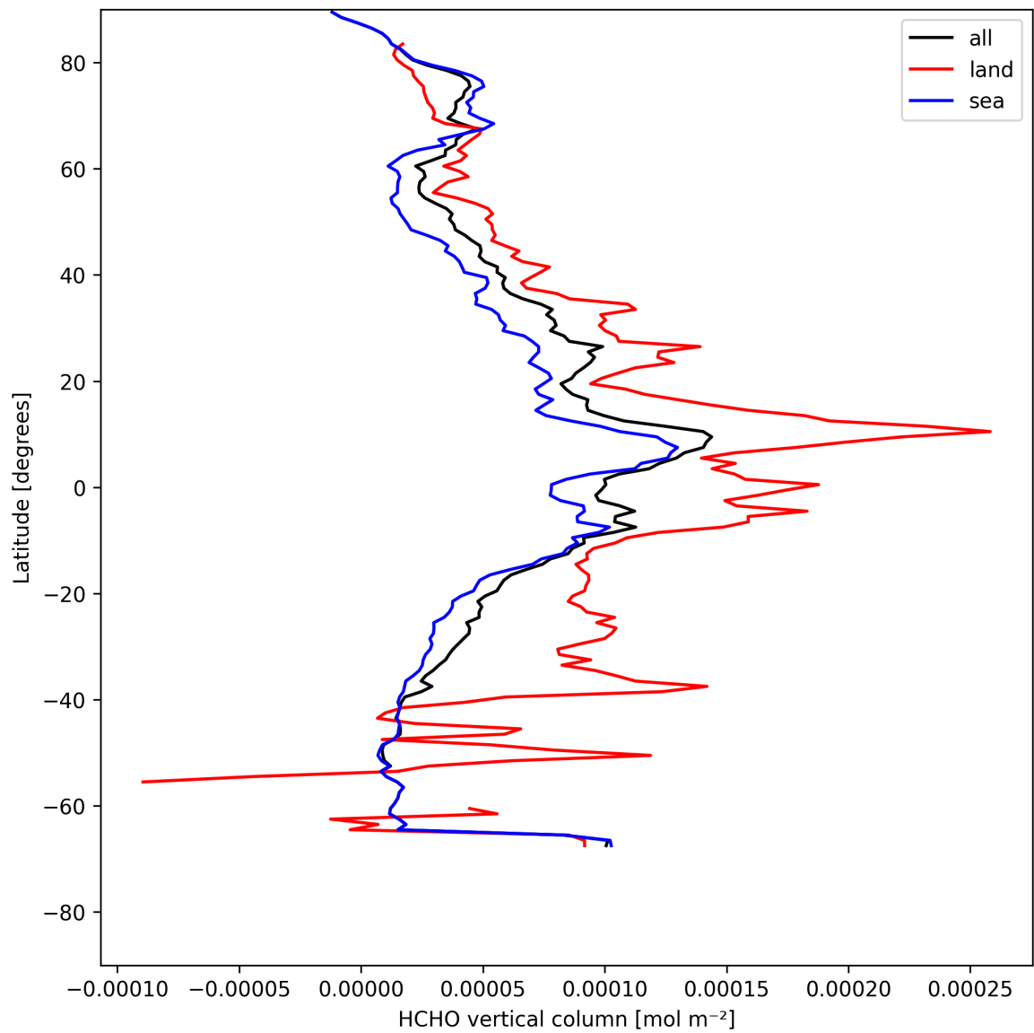
Figure 21: Zonal average of “HCHO vertical column” for 2025-05-05 to 2025-05-07.
