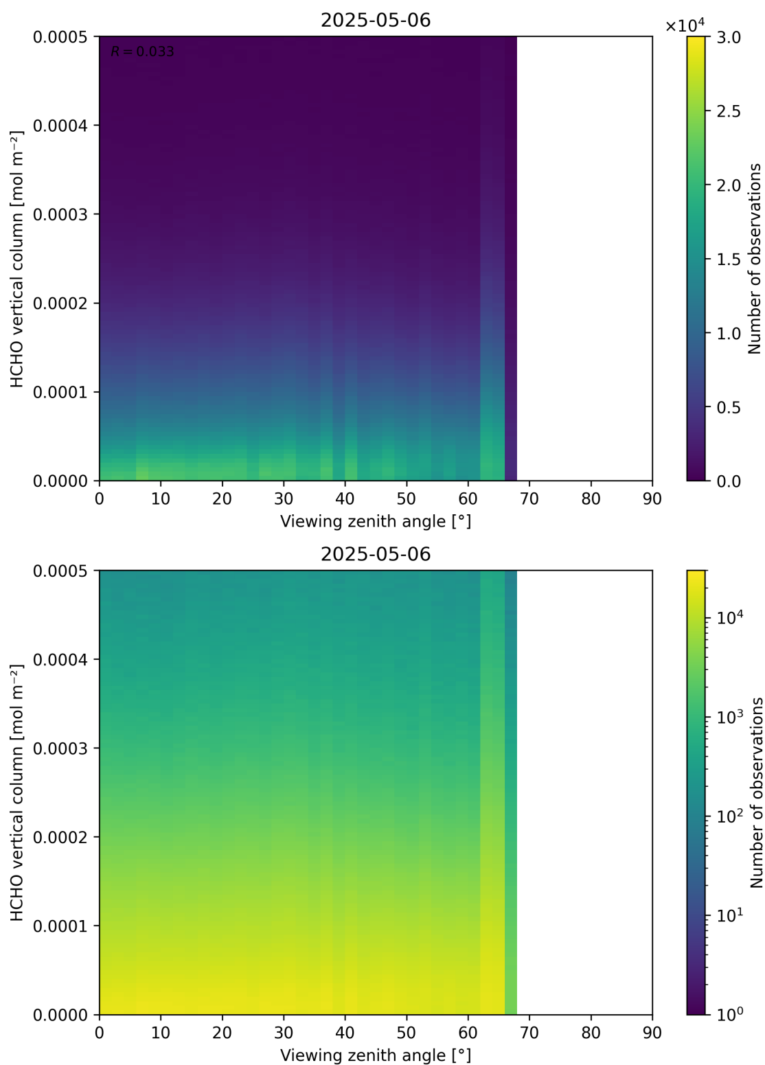
Figure 192: Scatter density plot of “Viewing zenith angle” against “HCHO vertical column” for 2025-05-05 to 2025-05-07.
