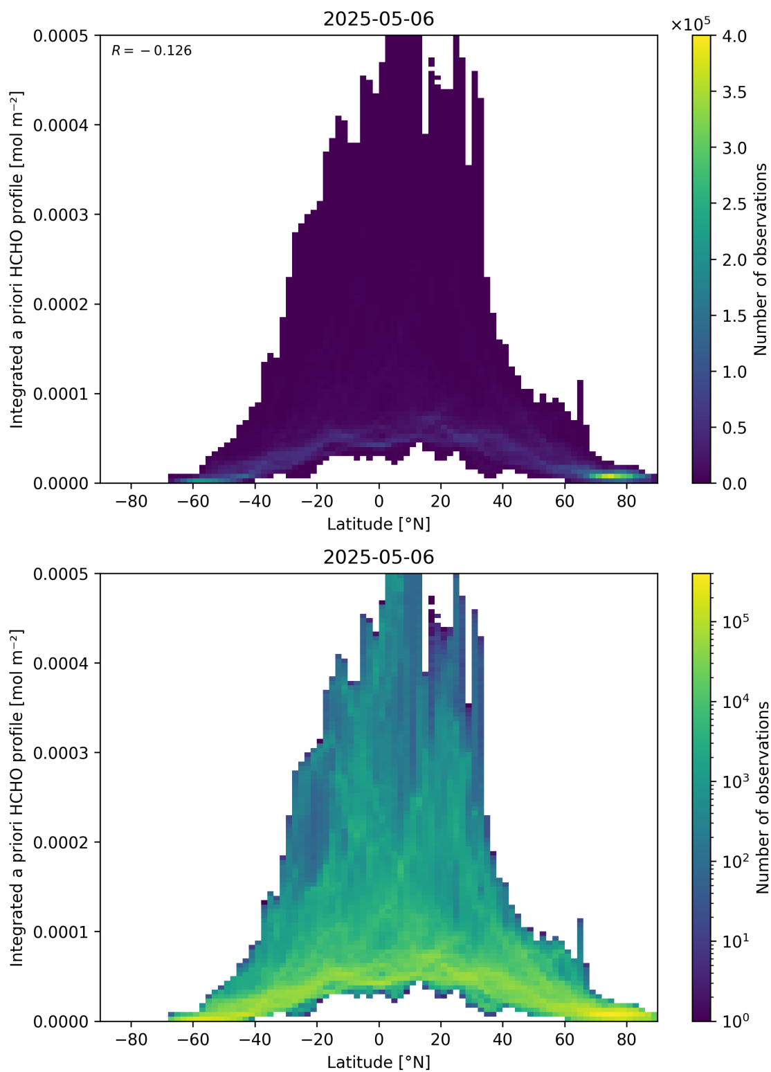
Figure 166: Scatter density plot of “Latitude” against “Integrated a priori HCHO profile” for 2025-05-05 to 2025-05-07.
