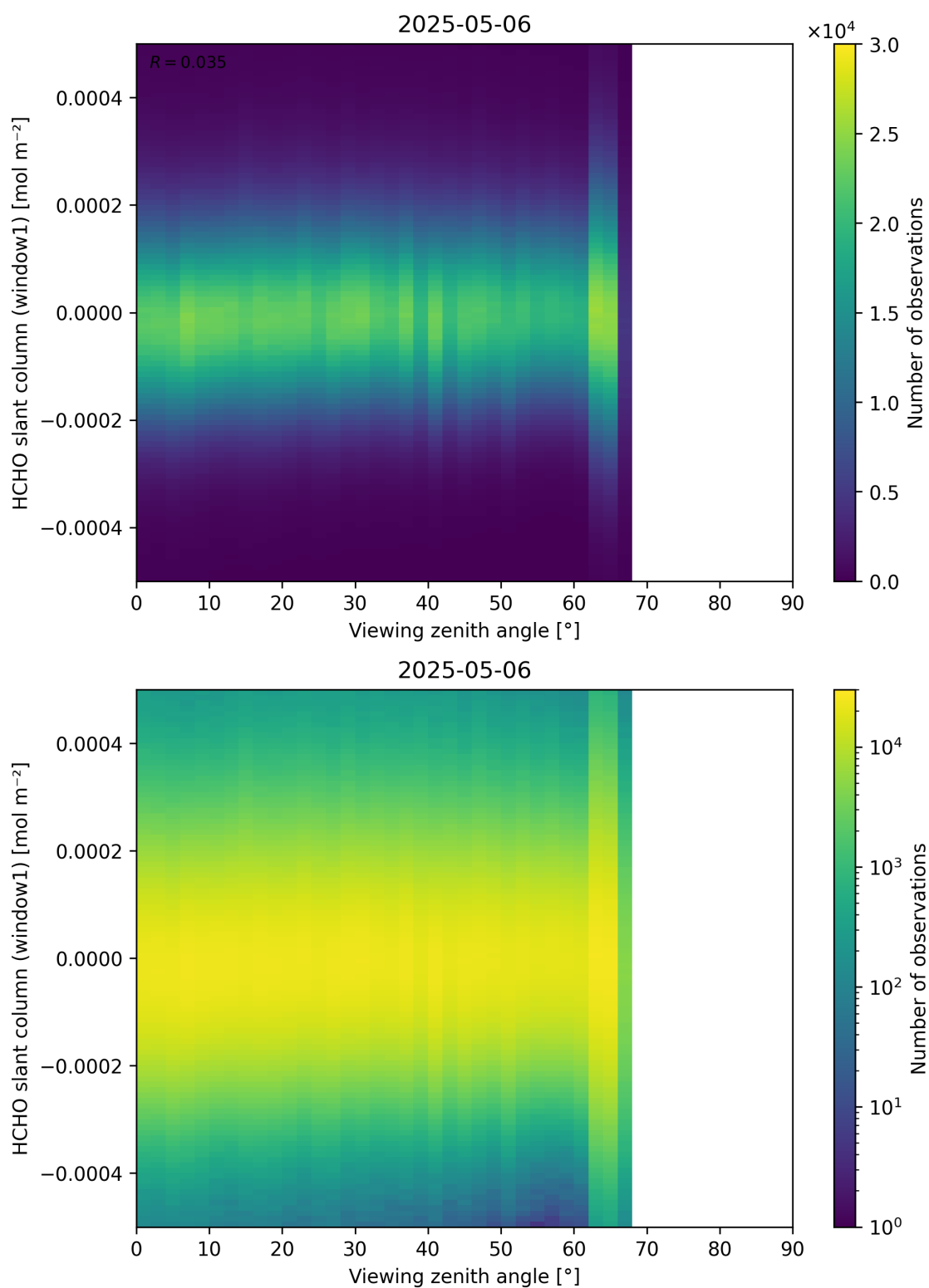
Figure 188: Scatter density plot of “Viewing zenith angle” against “HCHO slant column (window1)” for 2025-05-05 to 2025-05-07.
