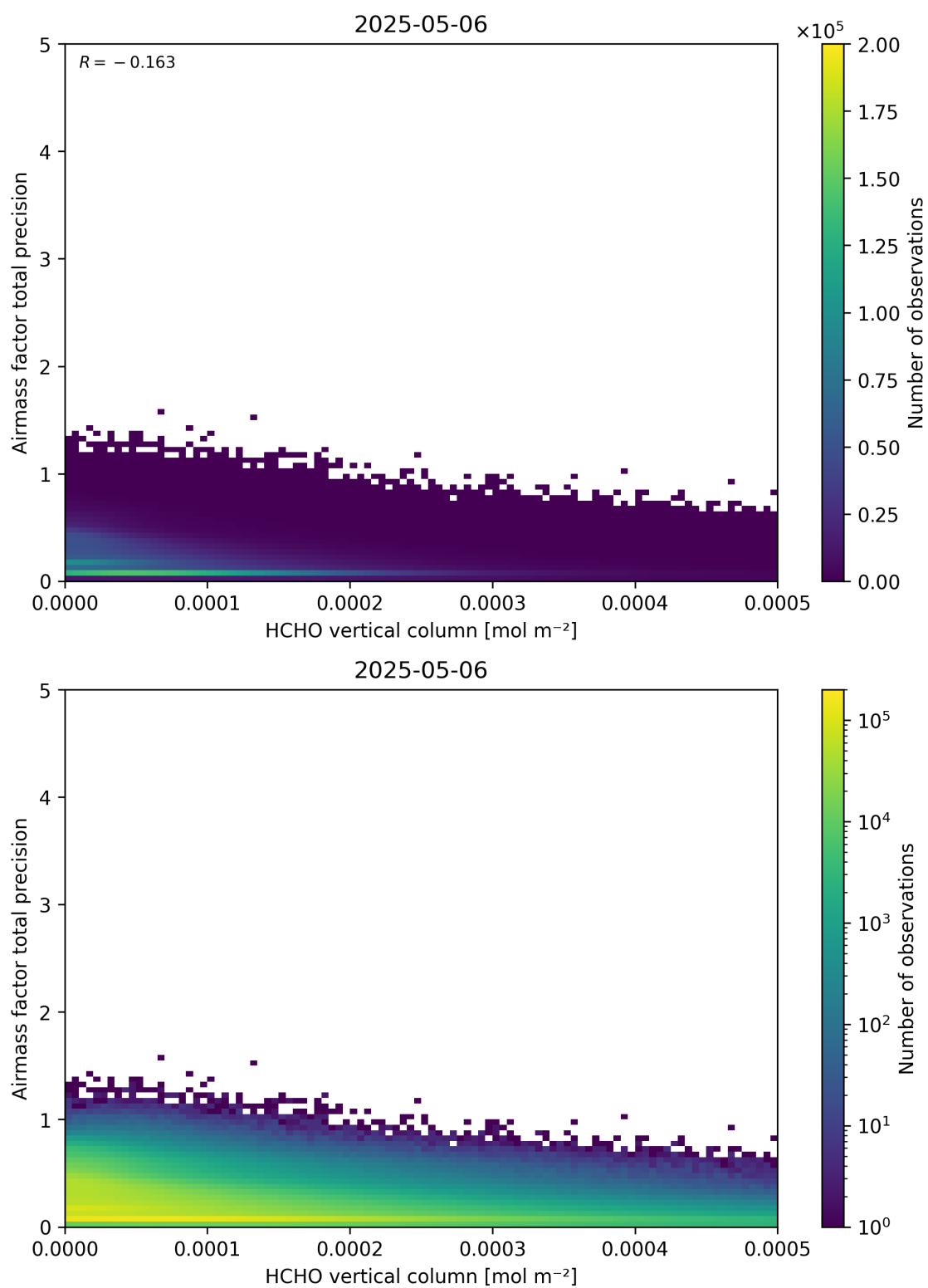
Figure 132: Scatter density plot of “HCHO vertical column” against “Airmass factor total precision” for 2025-05-05 to 2025-05-07.
