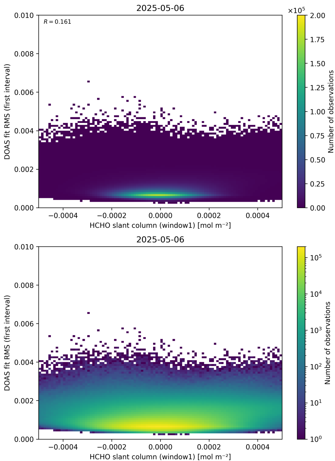
Figure 78: Scatter density plot of “HCHO slant column (window1)” against “DOAS fit RMS (first interval)” for 2025-05-05 to 2025-05-07.
