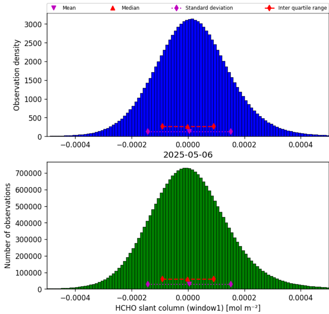
Figure 38: Histogram of “HCHO slant column (window1)” for 2025-05-05 to 2025-05-07
