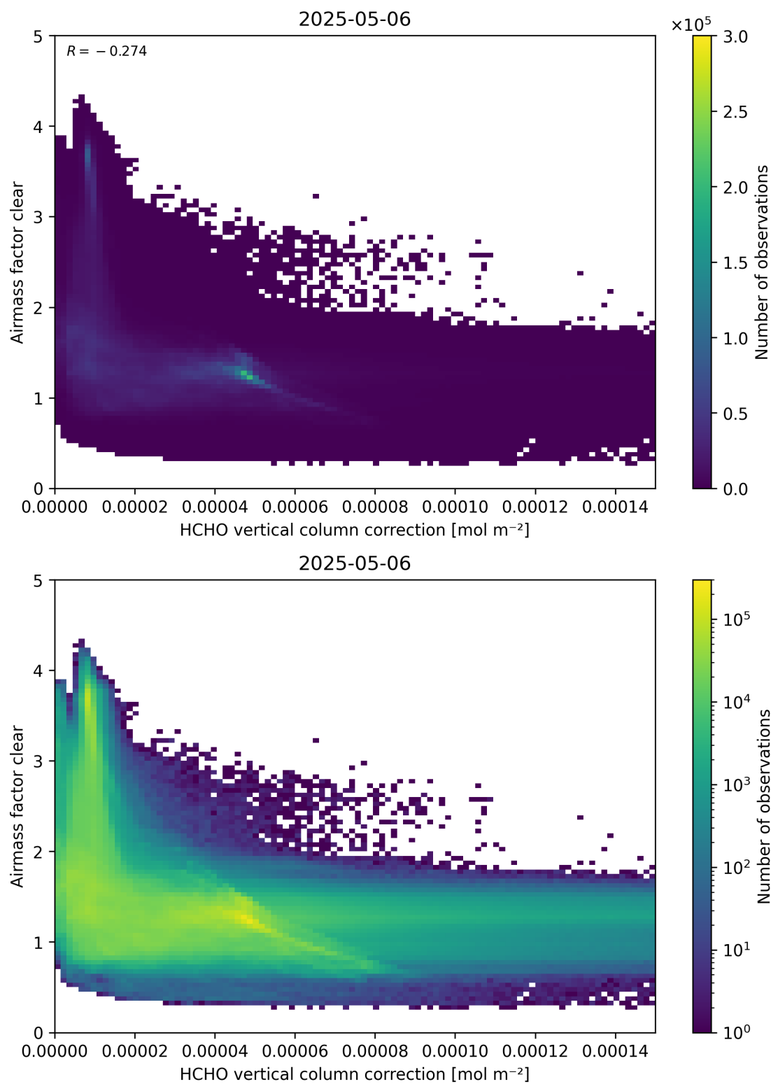
Figure 115: Scatter density plot of “HCHO vertical column correction” against “Airmass factor clear” for 2025-05-05 to 2025-05-07.
