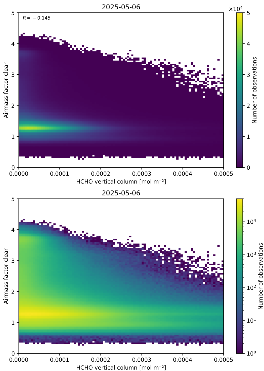
Figure 126: Scatter density plot of “HCHO vertical column” against “Airmass factor clear” for 2025-05-05 to 2025-05-07.
