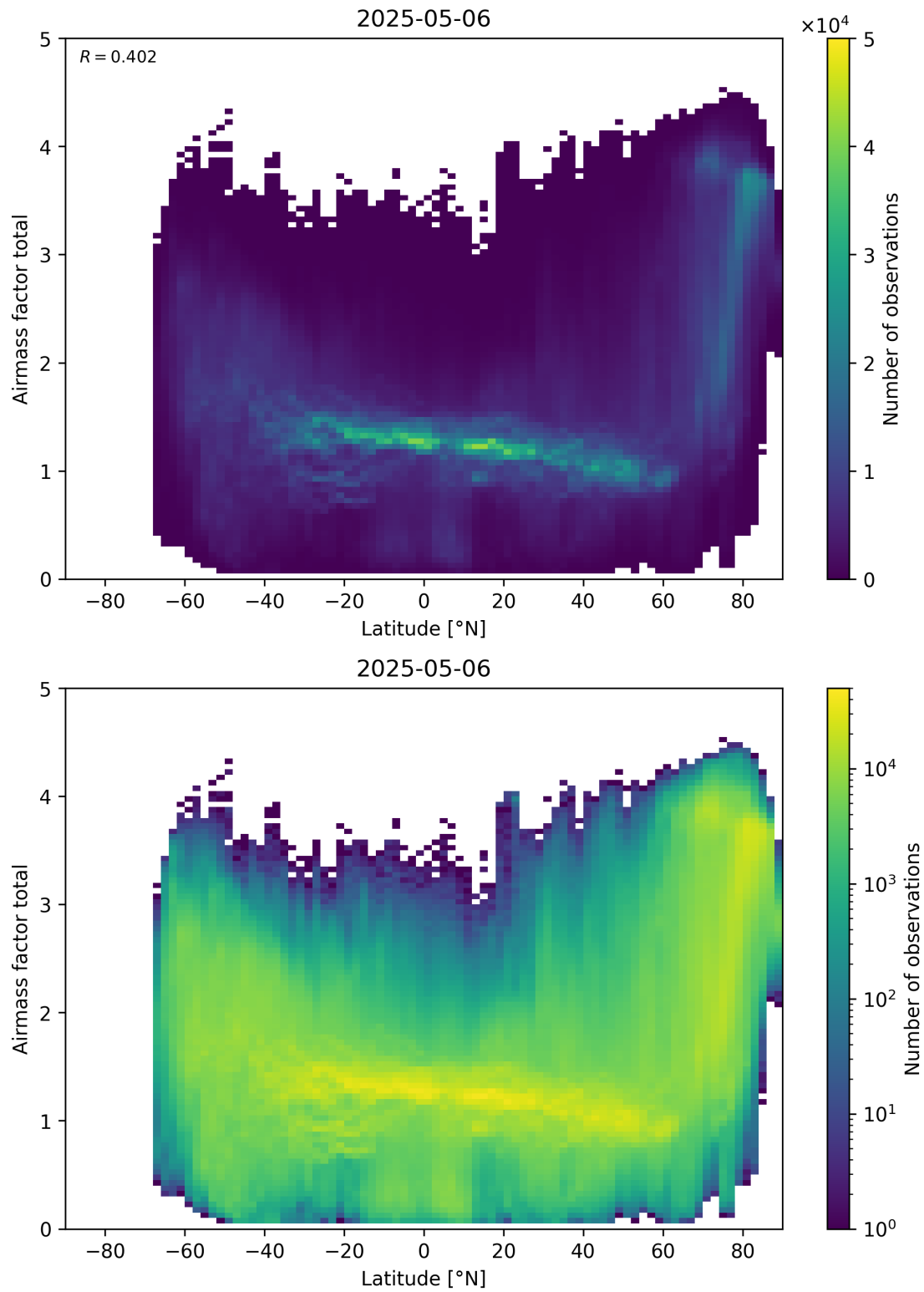
Figure 161: Scatter density plot of “Latitude” against “Airmass factor total” for 2025-05-05 to 2025-05-07.
