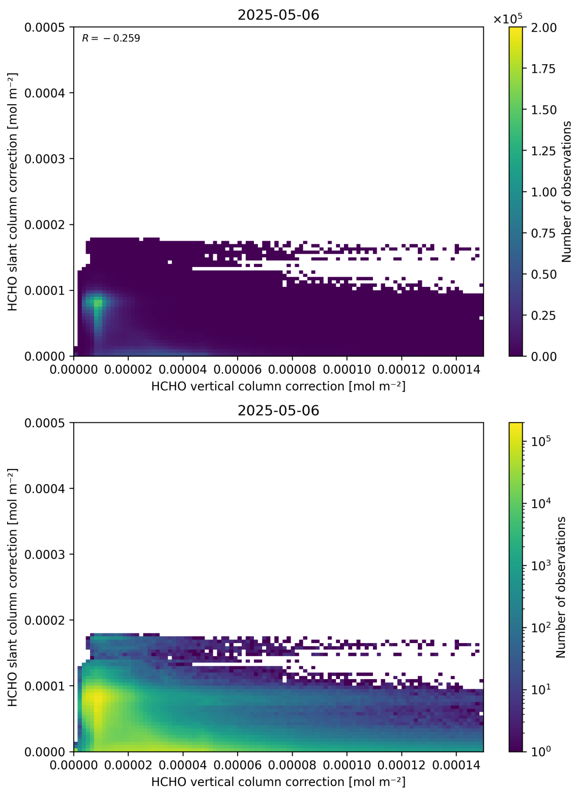
Figure 117: Scatter density plot of “HCHO vertical column correction” against “HCHO slant column correction” for 2025-05-05 to 2025-05-07.
