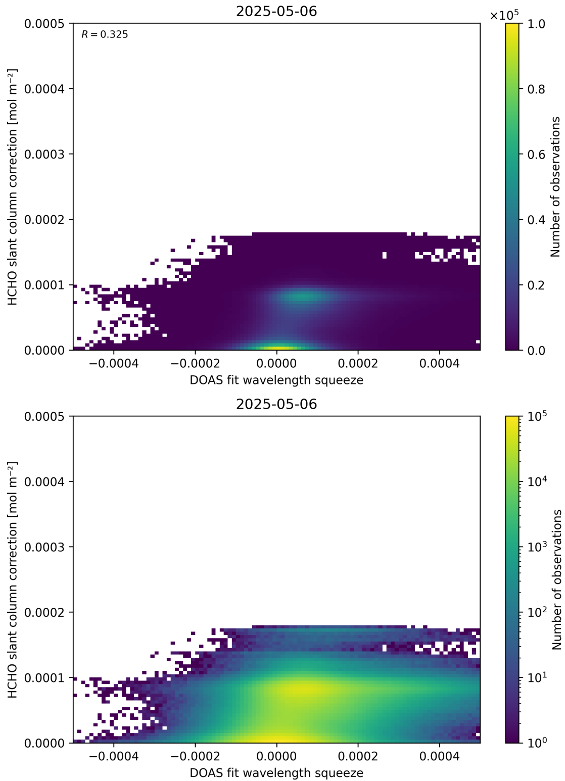
Figure 70: Scatter density plot of “DOAS fit wavelength squeeze” against “HCHO slant column correction” for 2025-05-05 to 2025-05-07.
