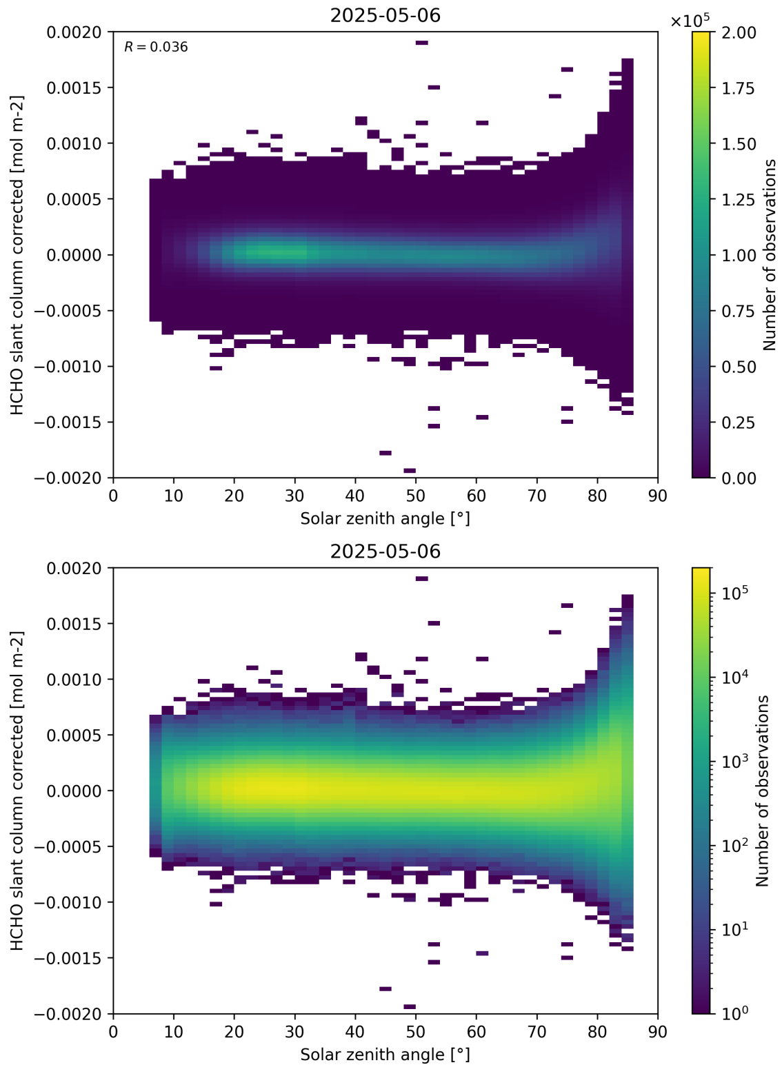
Figure 171: Scatter density plot of “Solar zenith angle” against “HCHO slant column corrected” for 2025-05-05 to 2025-05-07.
