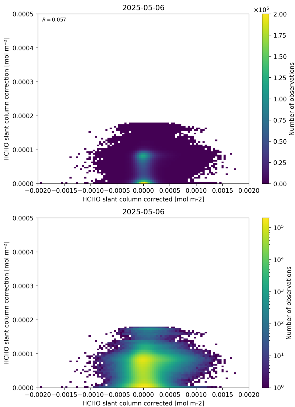
Figure 77: Scatter density plot of “HCHO slant column corrected” against “HCHO slant column correction” for 2025-05-05 to 2025-05-07.
