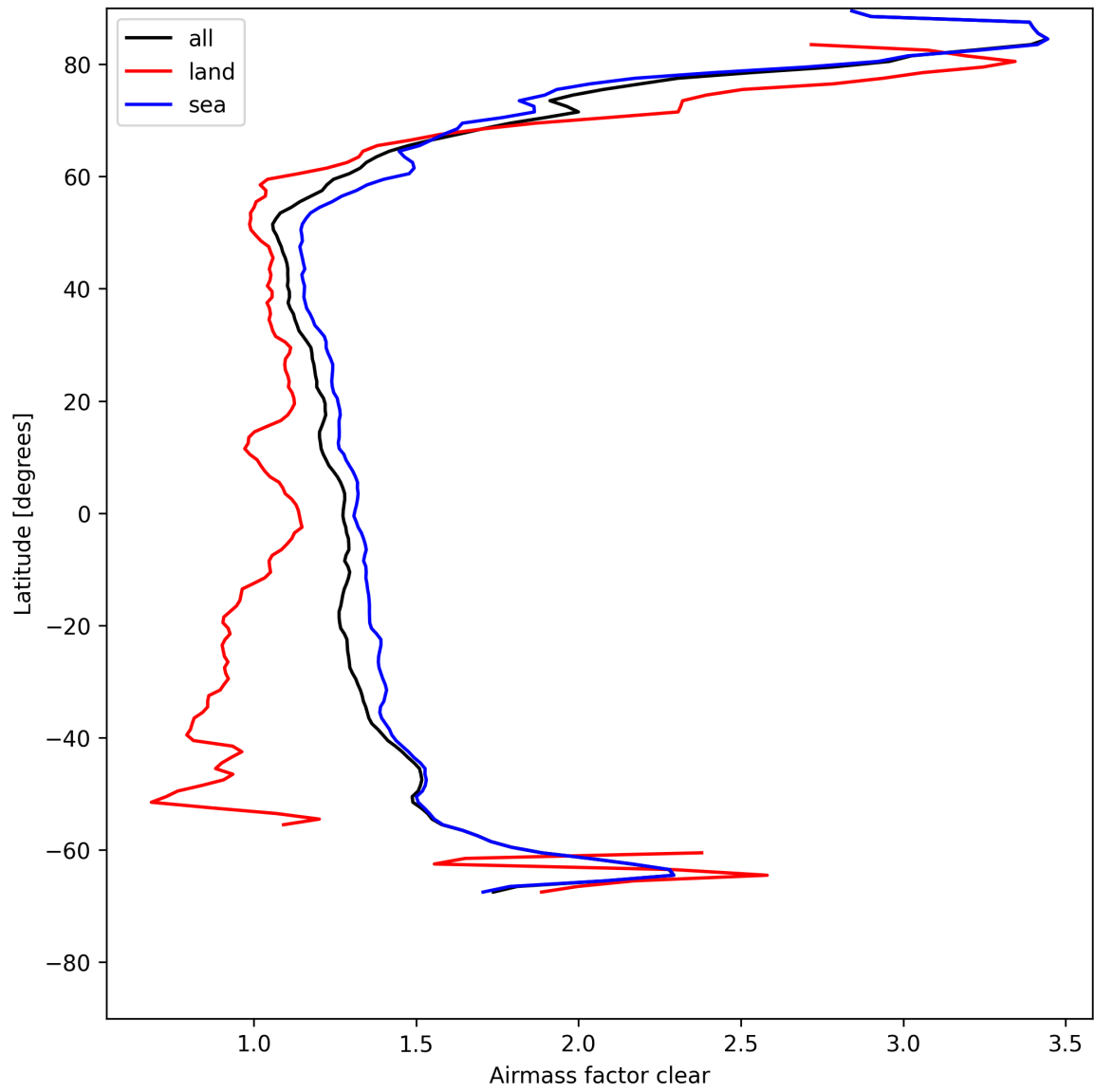
Figure 28: Zonal average of “Airmass factor clear” for 2025-05-05 to 2025-05-07.
