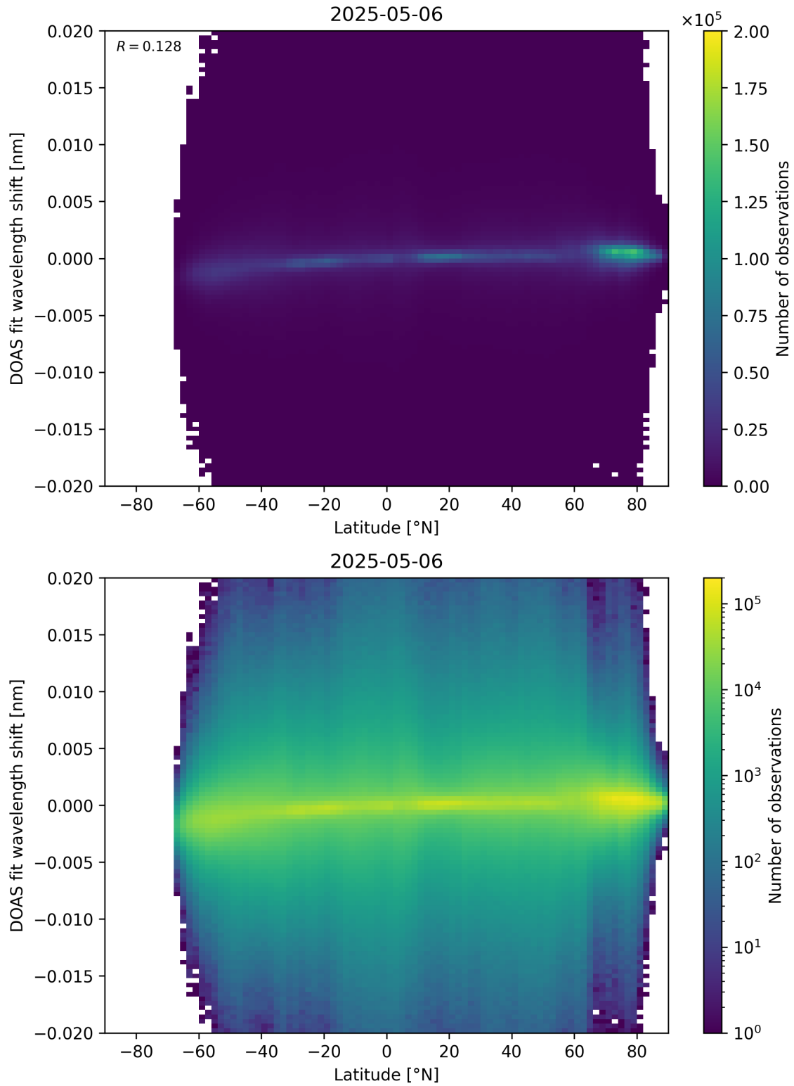
Figure 154: Scatter density plot of “Latitude” against “DOAS fit wavelength shift” for 2025-05-05 to 2025-05-07.
