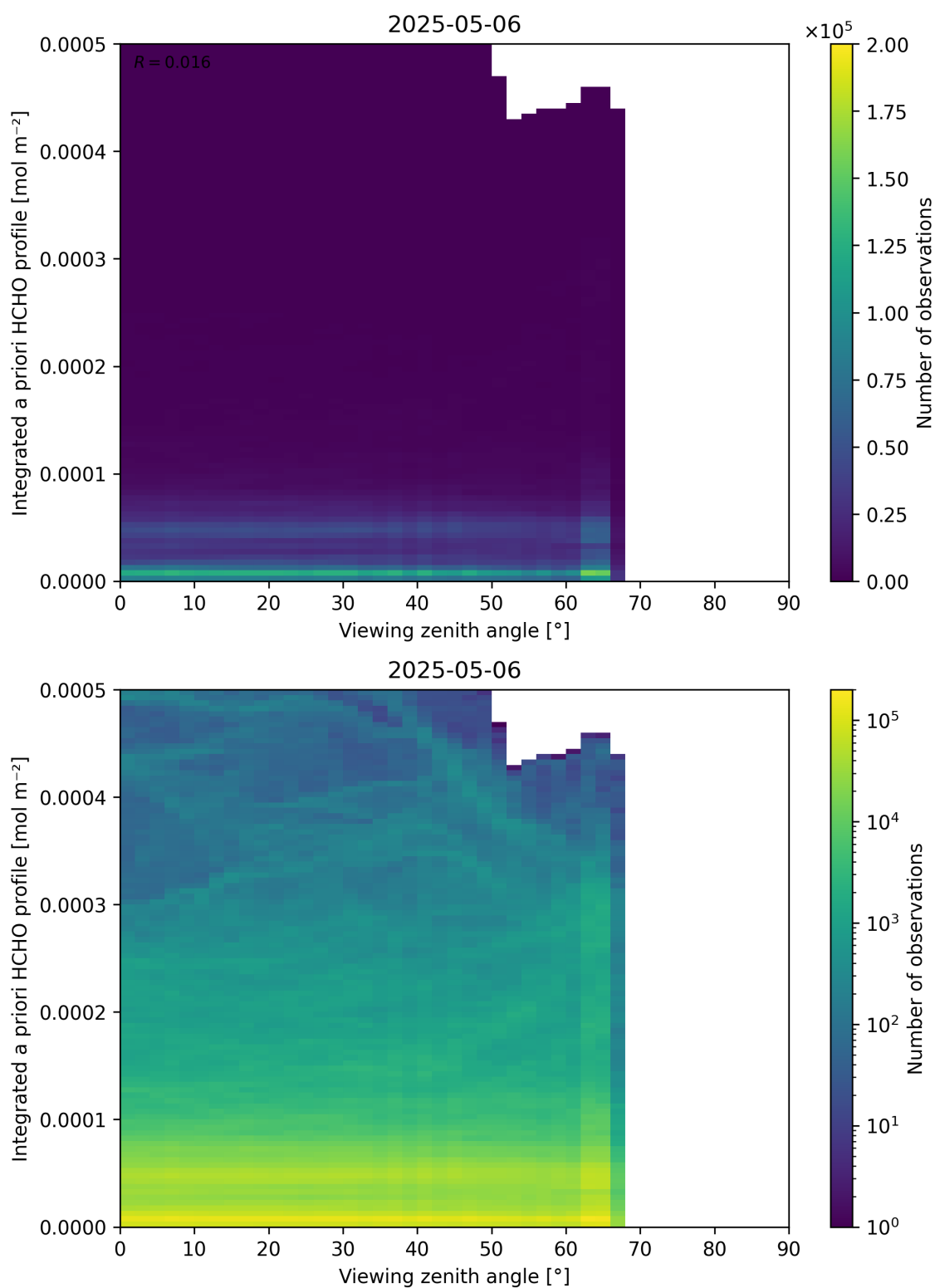
Figure 195: Scatter density plot of “Viewing zenith angle” against “Integrated a priori HCHO profile” for 2025-05-05 to 2025-05-07.
