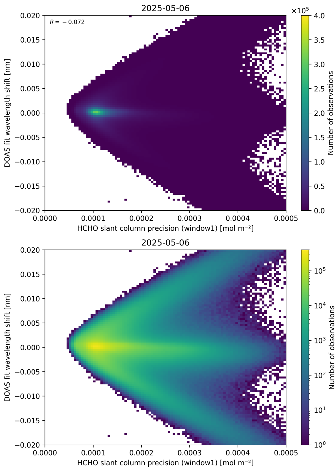
Figure 89: Scatter density plot of “HCHO slant column precision (window1)” against “DOAS fit wavelength shift” for 2025-05-05 to 2025-05-07.
