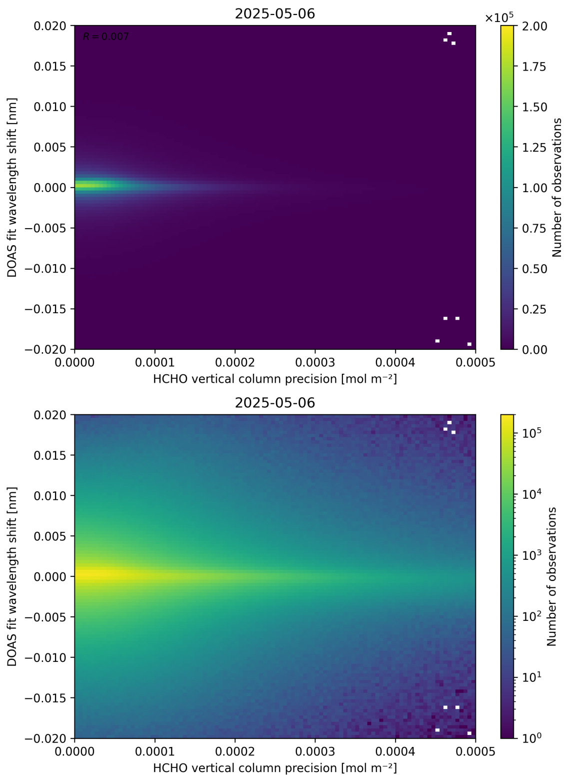
Figure 137: Scatter density plot of “HCHO vertical column precision” against “DOAS fit wavelength shift” for 2025-05-05 to 2025-05-07.
