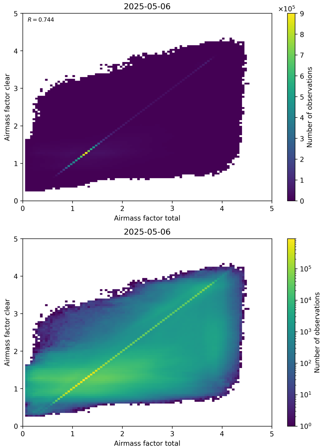
Figure 100: Scatter density plot of “Airmass factor total” against “Airmass factor clear” for 2025-05-05 to 2025-05-07.
