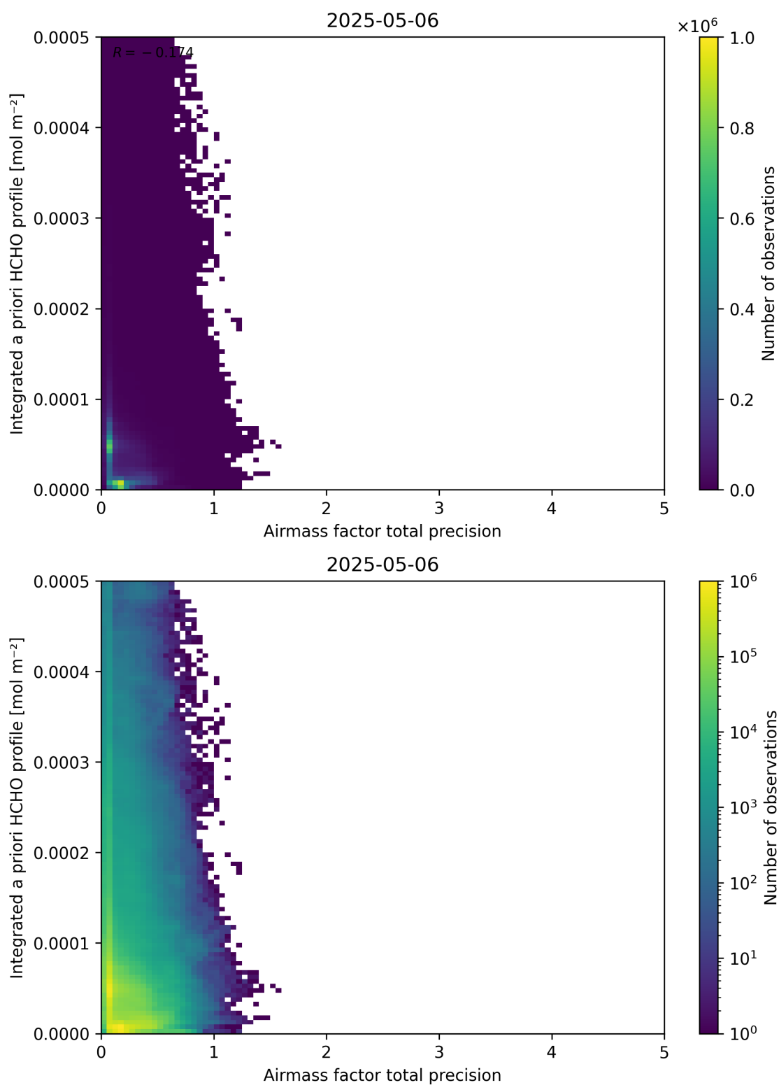
Figure 111: Scatter density plot of “Airmass factor total precision” against “Integrated a priori HCHO profile” for 2025-05-05 to 2025-05-07.
