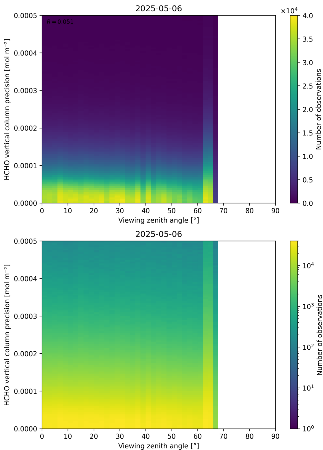
Figure 194: Scatter density plot of “Viewing zenith angle” against “HCHO vertical column precision” for 2025-05-05 to 2025-05-07.
