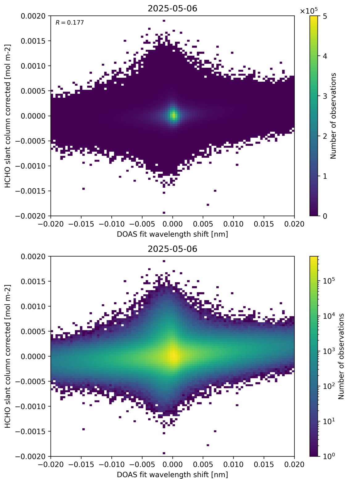
Figure 66: Scatter density plot of “DOAS fit wavelength shift” against “HCHO slant column corrected” for 2025-05-05 to 2025-05-07.
