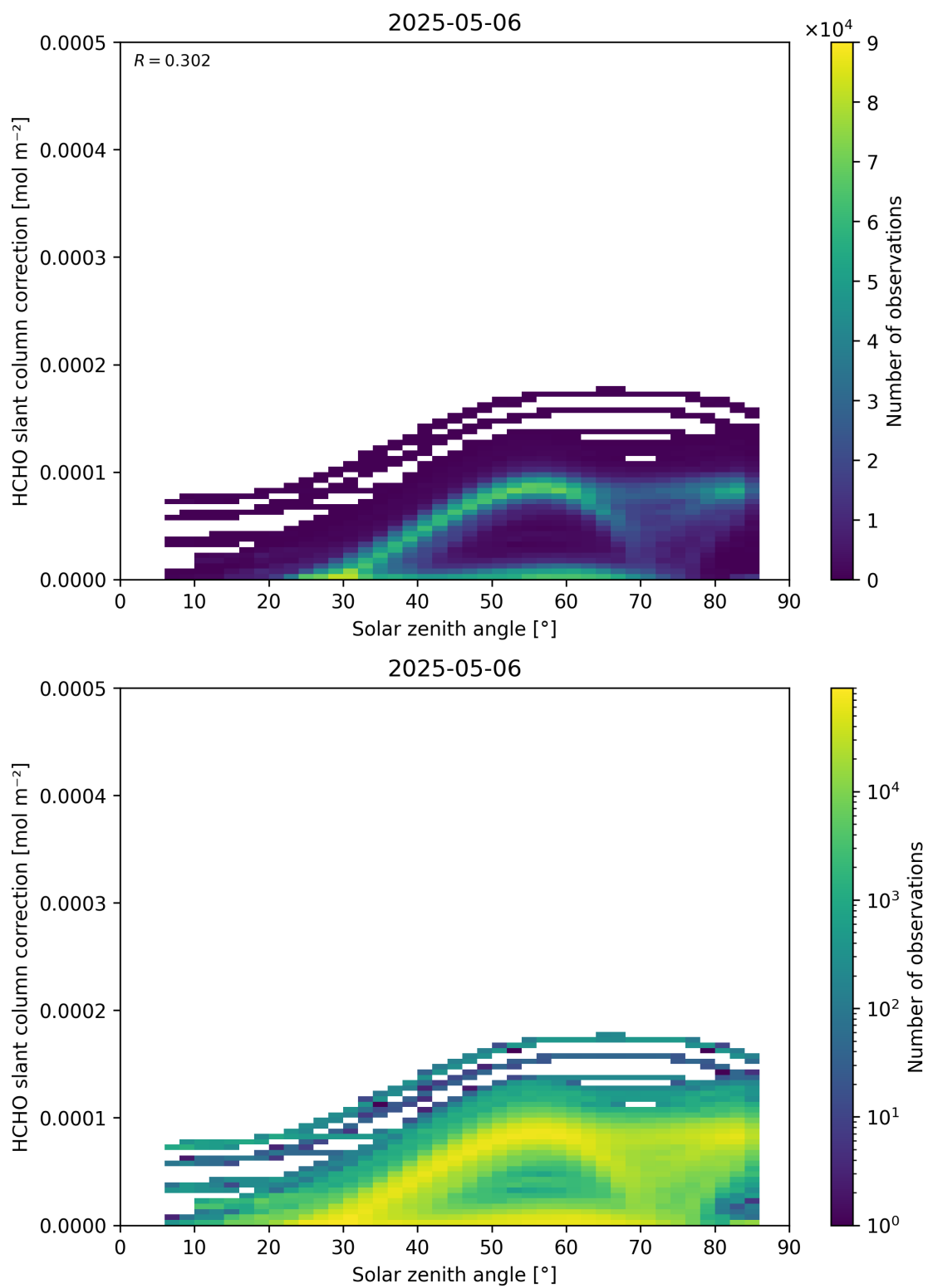
Figure 172: Scatter density plot of “Solar zenith angle” against “HCHO slant column correction” for 2025-05-05 to 2025-05-07.
