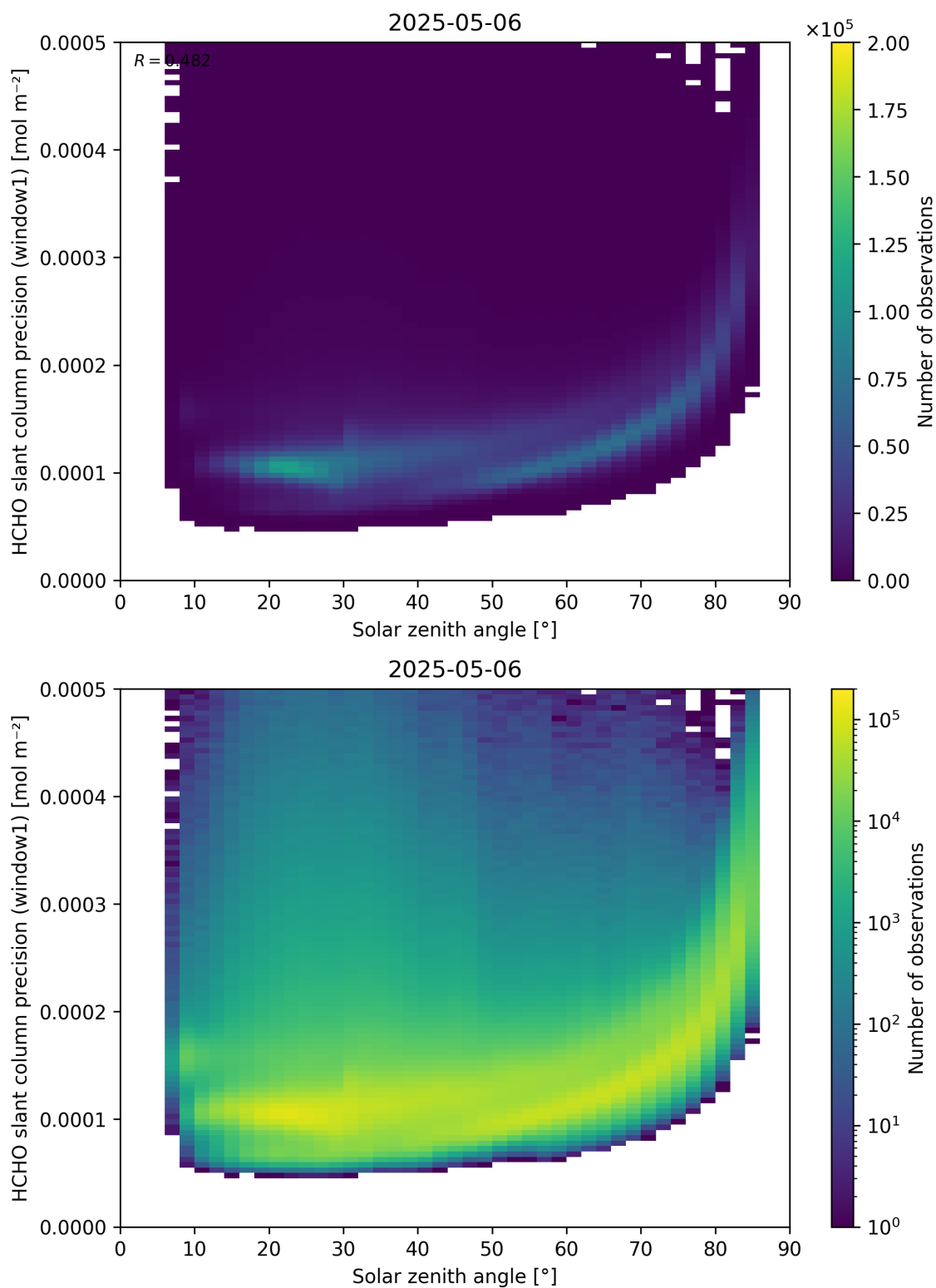
Figure 174: Scatter density plot of “Solar zenith angle” against “HCHO slant column precision (window1)” for 2025-05-05 to 2025-05-07.
