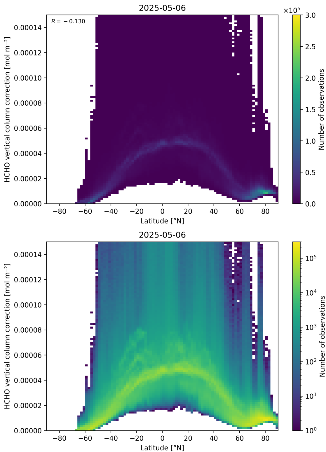
Figure 164: Scatter density plot of “Latitude” against “HCHO vertical column correction” for 2025-05-05 to 2025-05-07.
