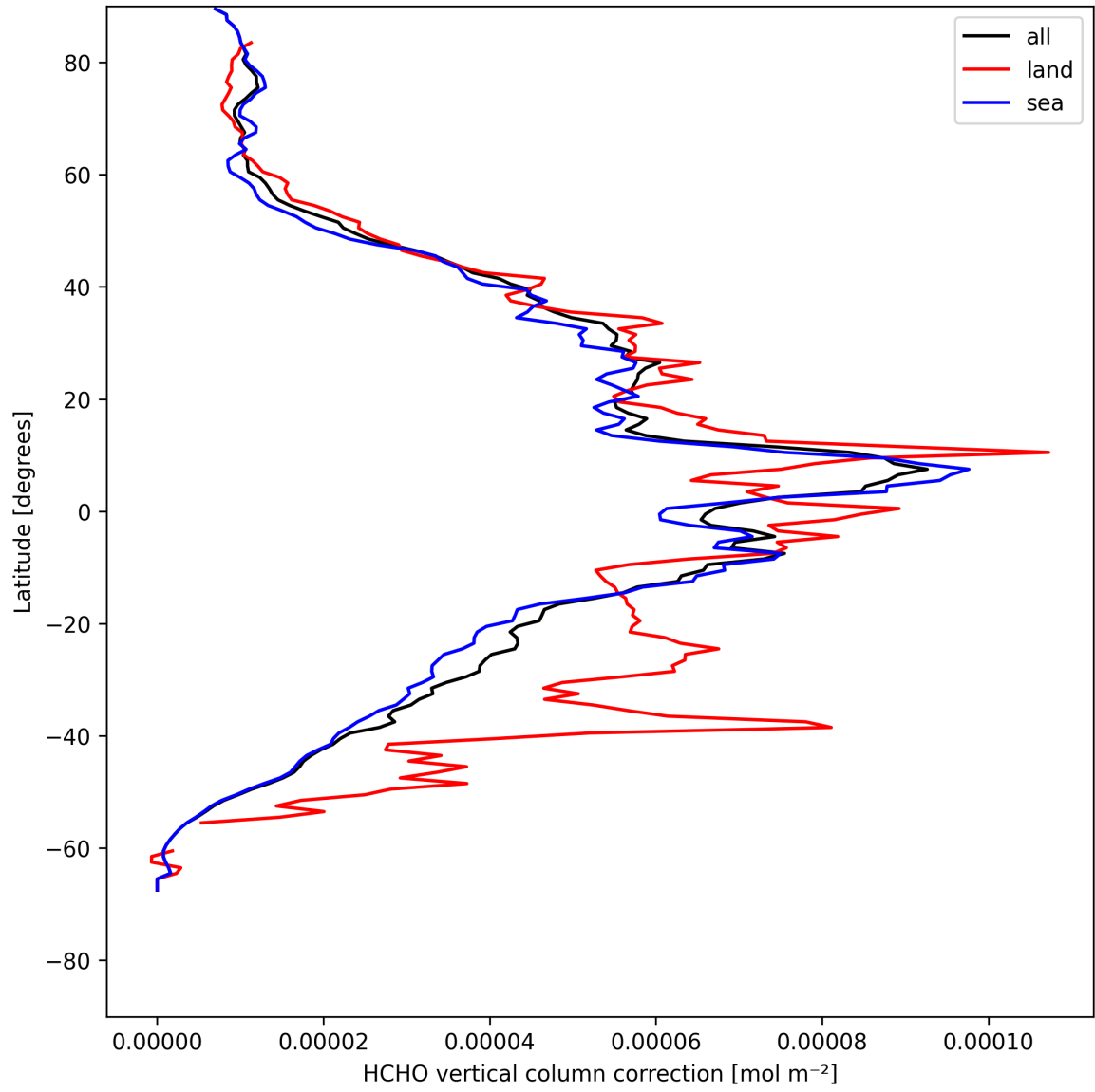
Figure 23: Zonal average of “HCHO vertical column correction” for 2025-05-05 to 2025-05-07.
