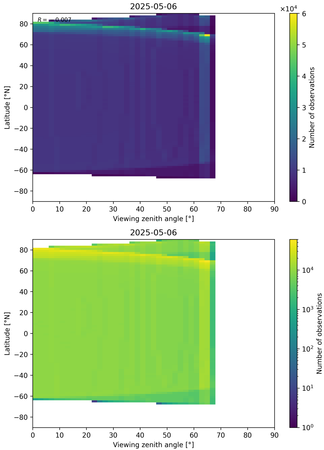
Figure 196: Scatter density plot of “Viewing zenith angle” against “Latitude” for 2025-05-05 to 2025-05-07.
