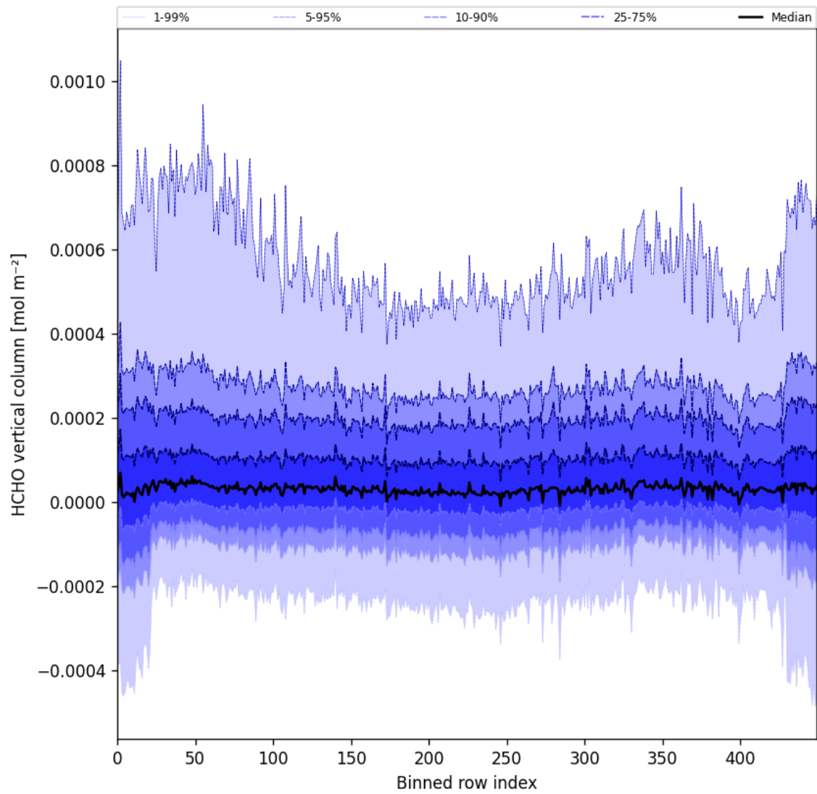
Figure 49: Along track statistics of “HCHO vertical column” for 2025-05-05 to 2025-05-07
