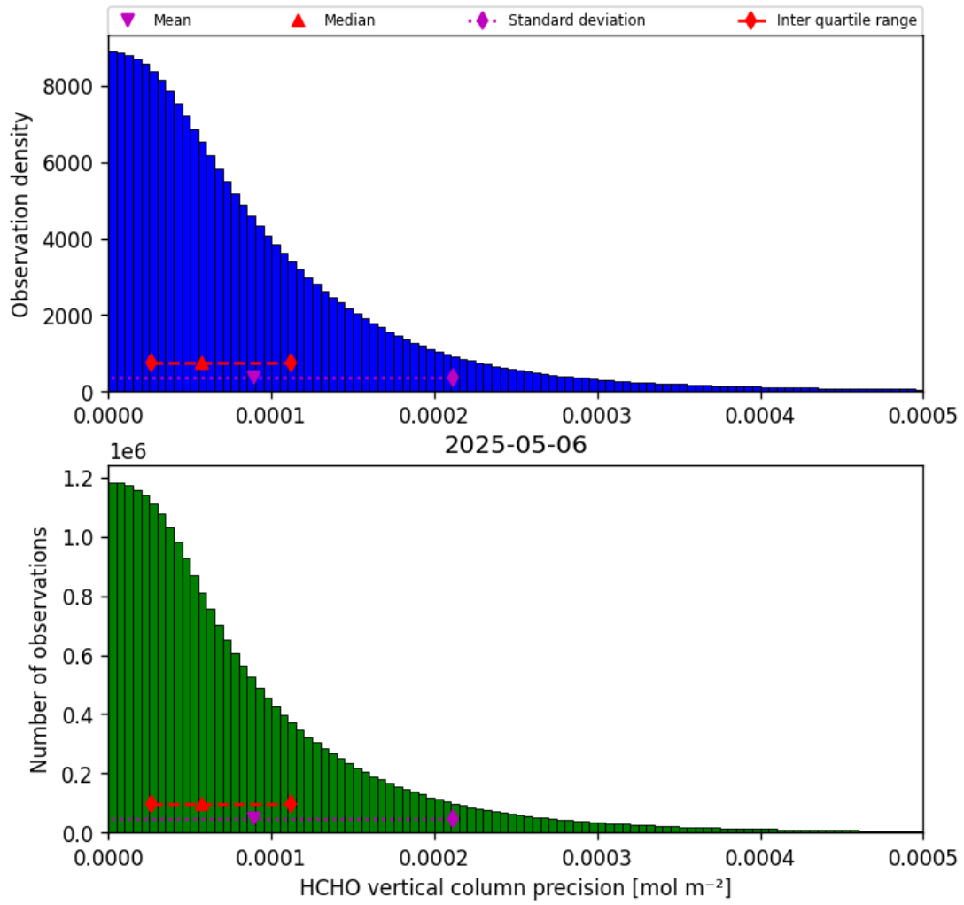
Figure 36: Histogram of “HCHO vertical column precision” for 2025-05-05 to 2025-05-07
