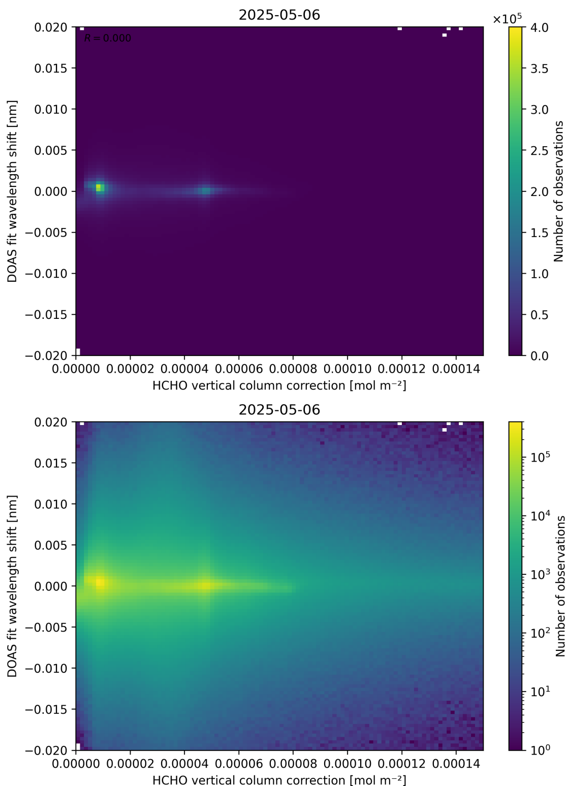
Figure 113: Scatter density plot of “HCHO vertical column correction” against “DOAS fit wavelength shift” for 2025-05-05 to 2025-05-07.
