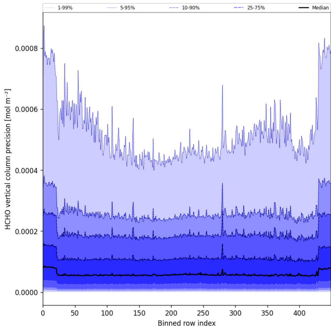
Figure 50: Along track statistics of “HCHO vertical column precision” for 2025-05-05 to 2025-05-07
