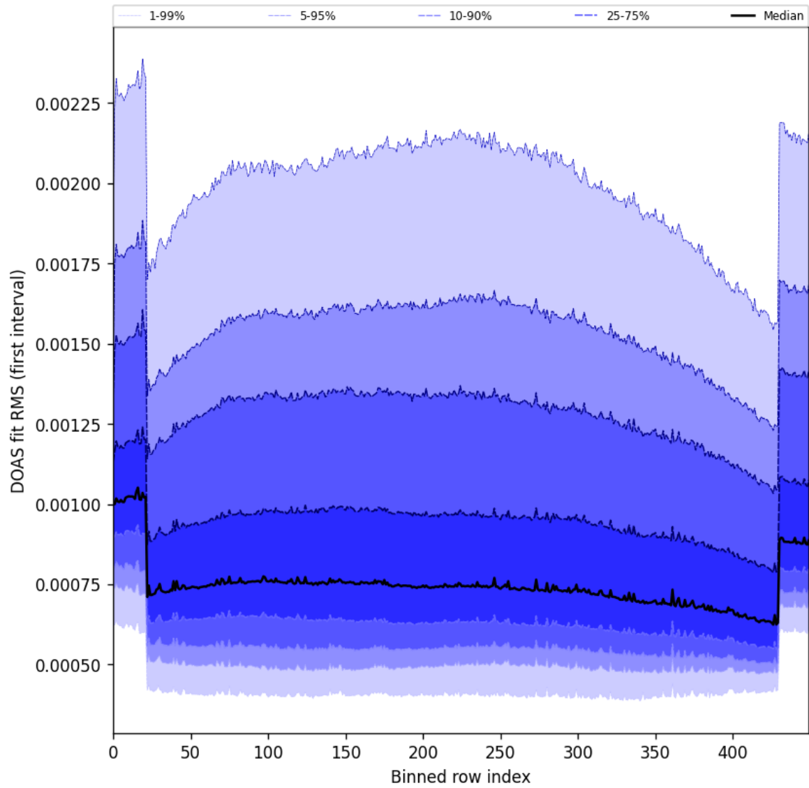
Figure 60: Along track statistics of “DOAS fit RMS (first interval)” for 2025-05-05 to 2025-05-07
