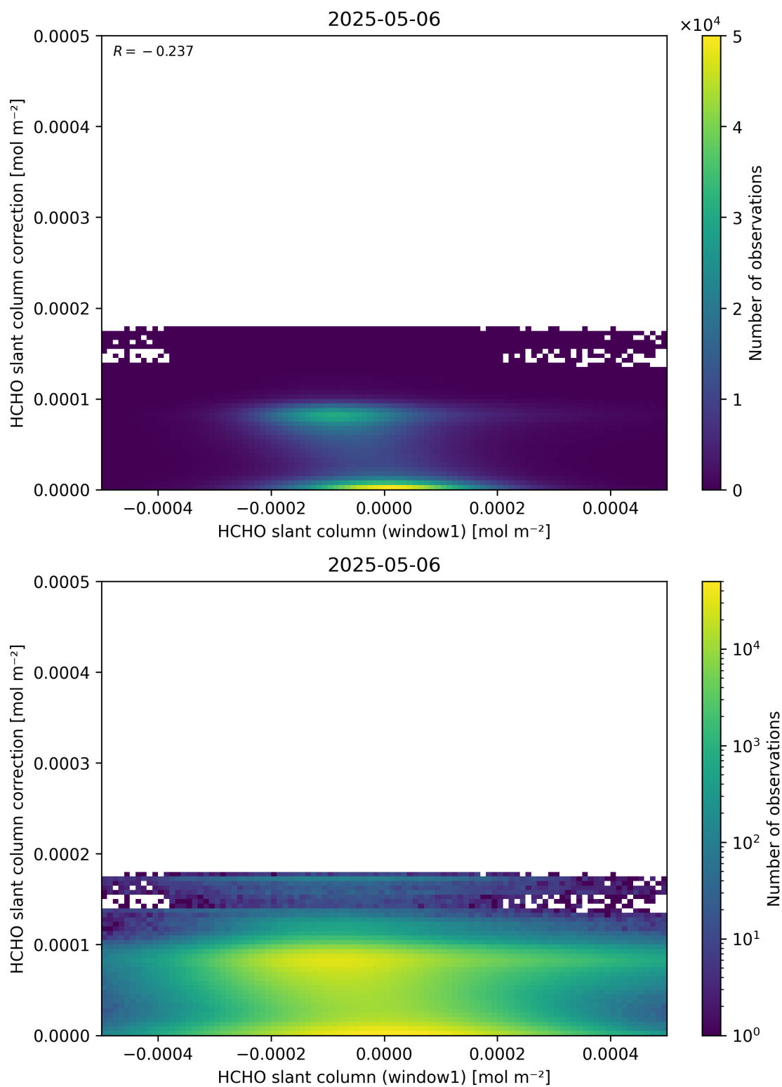
Figure 83: Scatter density plot of “HCHO slant column (window1)” against “HCHO slant column correction” for 2025-05-05 to 2025-05-07.
