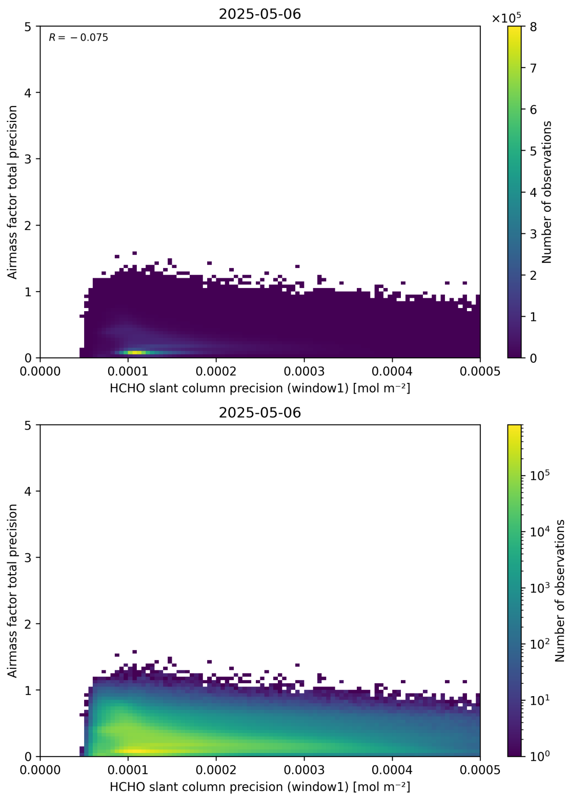
Figure 95: Scatter density plot of “HCHO slant column precision (window1)” against “Airmass factor total precision” for 2025-05-05 to 2025-05-07.
