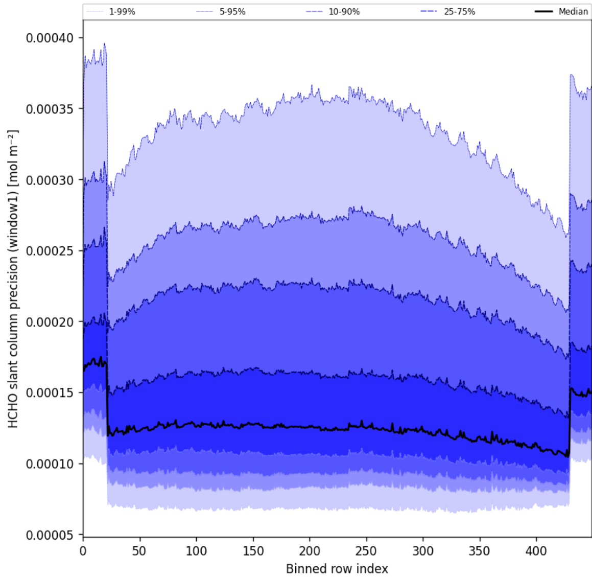
Figure 53: Along track statistics of “HCHO slant column precision (window1)” for 2025-05-05 to 2025-05-07
