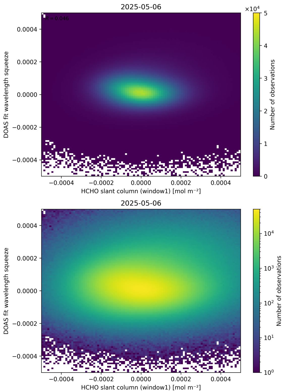
Figure 80: Scatter density plot of “HCHO slant column (window1)” against “DOAS fit wavelength squeeze” for 2025-05-05 to 2025-05-07.
