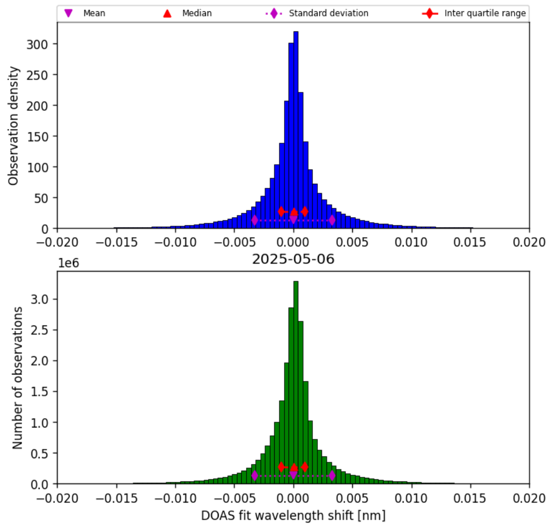
Figure 44: Histogram of “DOAS fit wavelength shift” for 2025-05-05 to 2025-05-07
