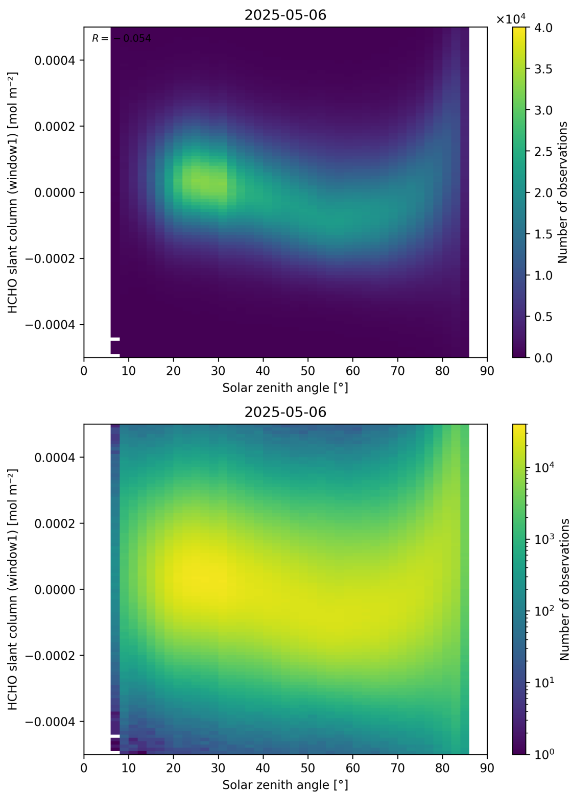
Figure 173: Scatter density plot of “Solar zenith angle” against “HCHO slant column (window1)” for 2025-05-05 to 2025-05-07.
