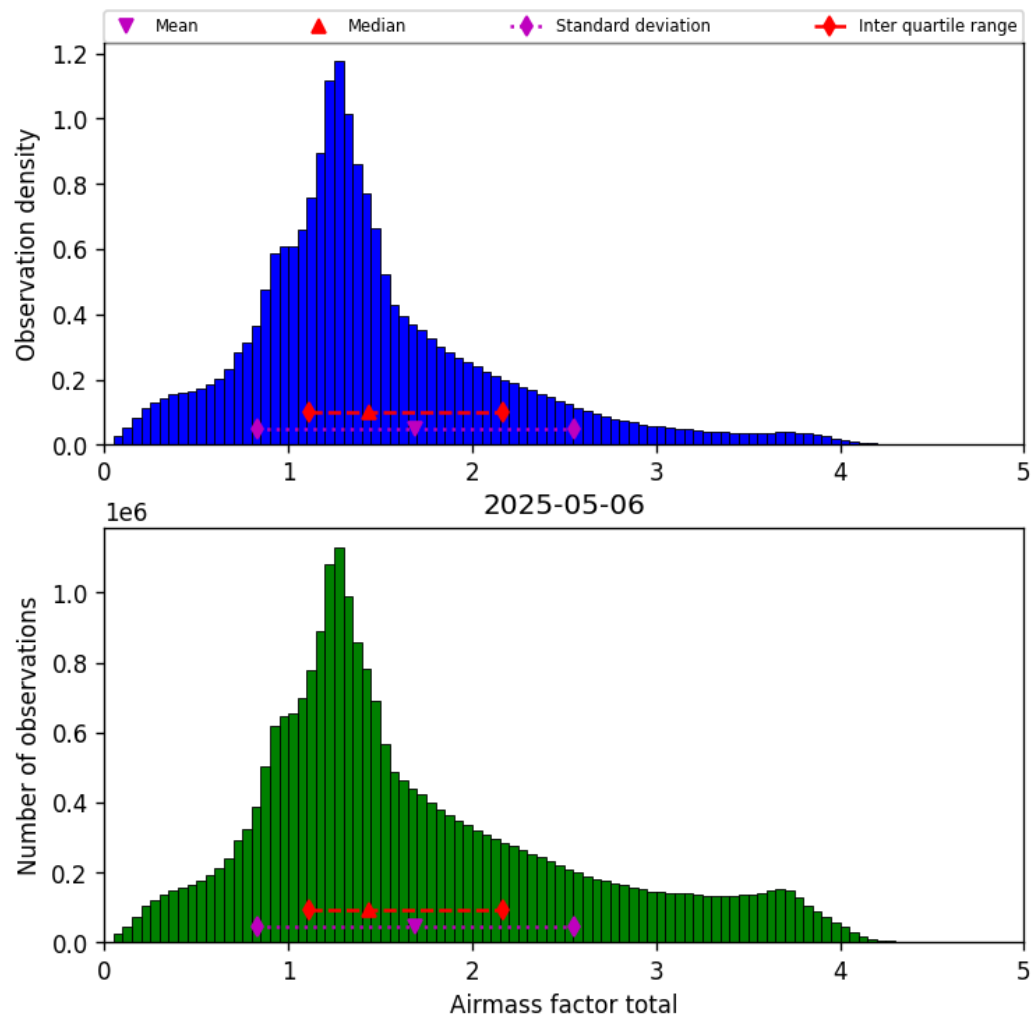
Figure 40: Histogram of “Airmass factor total” for 2025-05-05 to 2025-05-07
