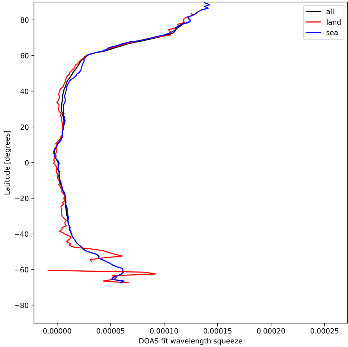
Figure 31: Zonal average of “DOAS fit wavelength squeeze” for 2025-05-05 to 2025-05-07.
