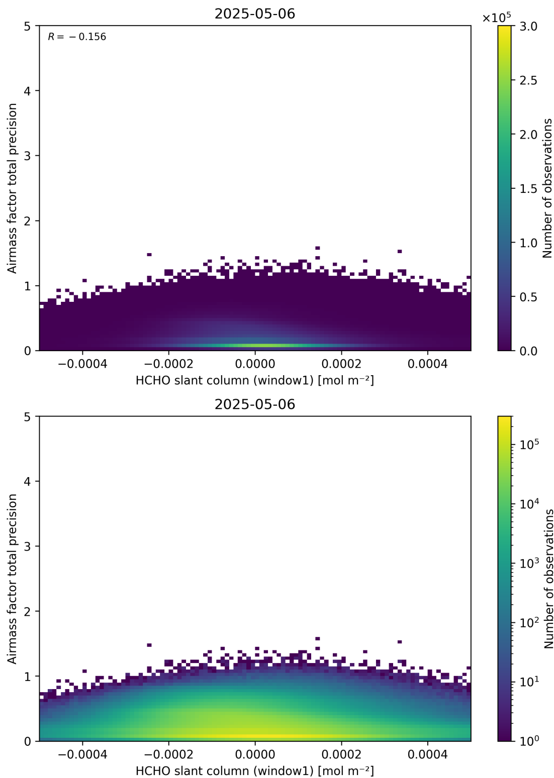
Figure 86: Scatter density plot of “HCHO slant column (window1)” against “Airmass factor total precision” for 2025-05-05 to 2025-05-07.
