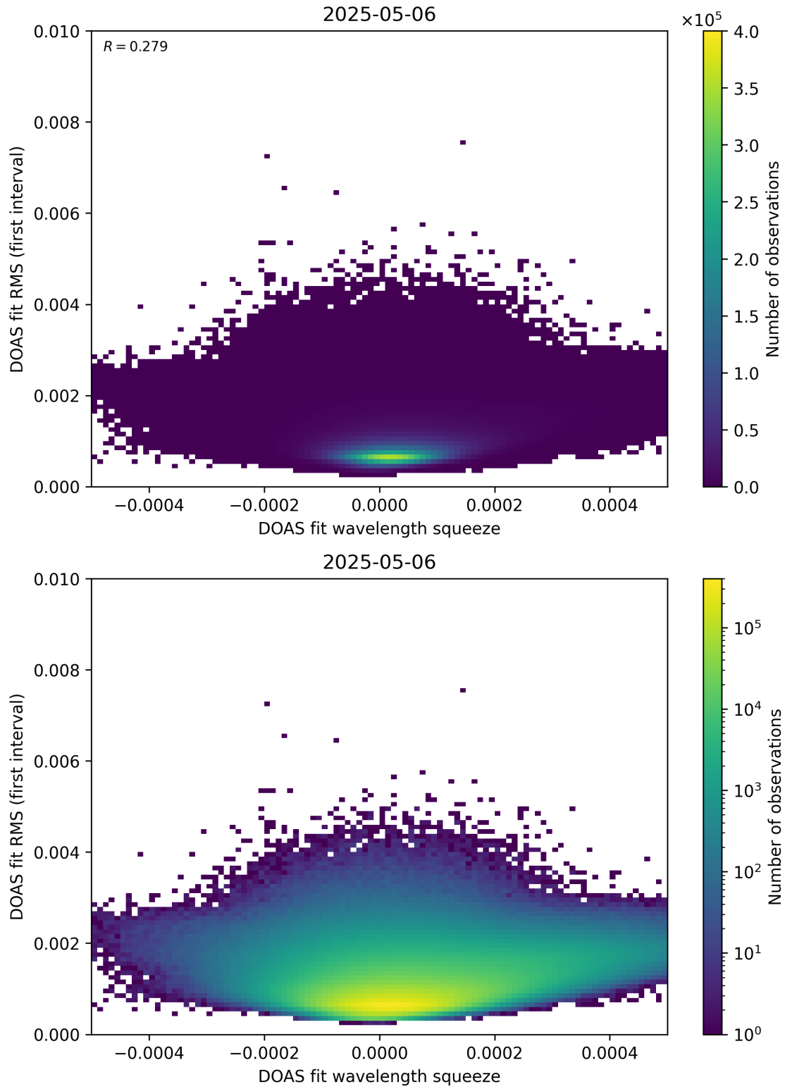
Figure 68: Scatter density plot of “DOAS fit wavelength squeeze” against “DOAS fit RMS (first interval)” for 2025-05-05 to 2025-05-07.
