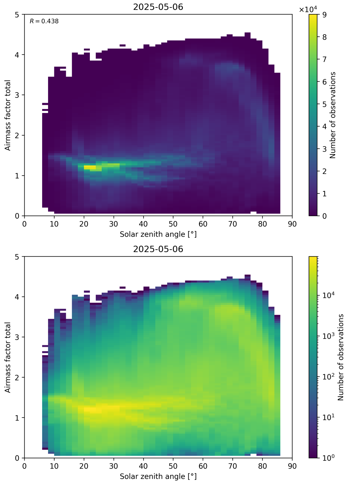
Figure 175: Scatter density plot of “Solar zenith angle” against “Airmass factor total” for 2025-05-05 to 2025-05-07.
