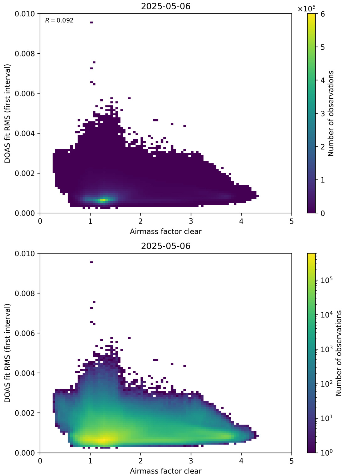
Figure 71: Scatter density plot of “Airmass factor clear” against “DOAS fit RMS (first interval)” for 2025-05-05 to 2025-05-07.
