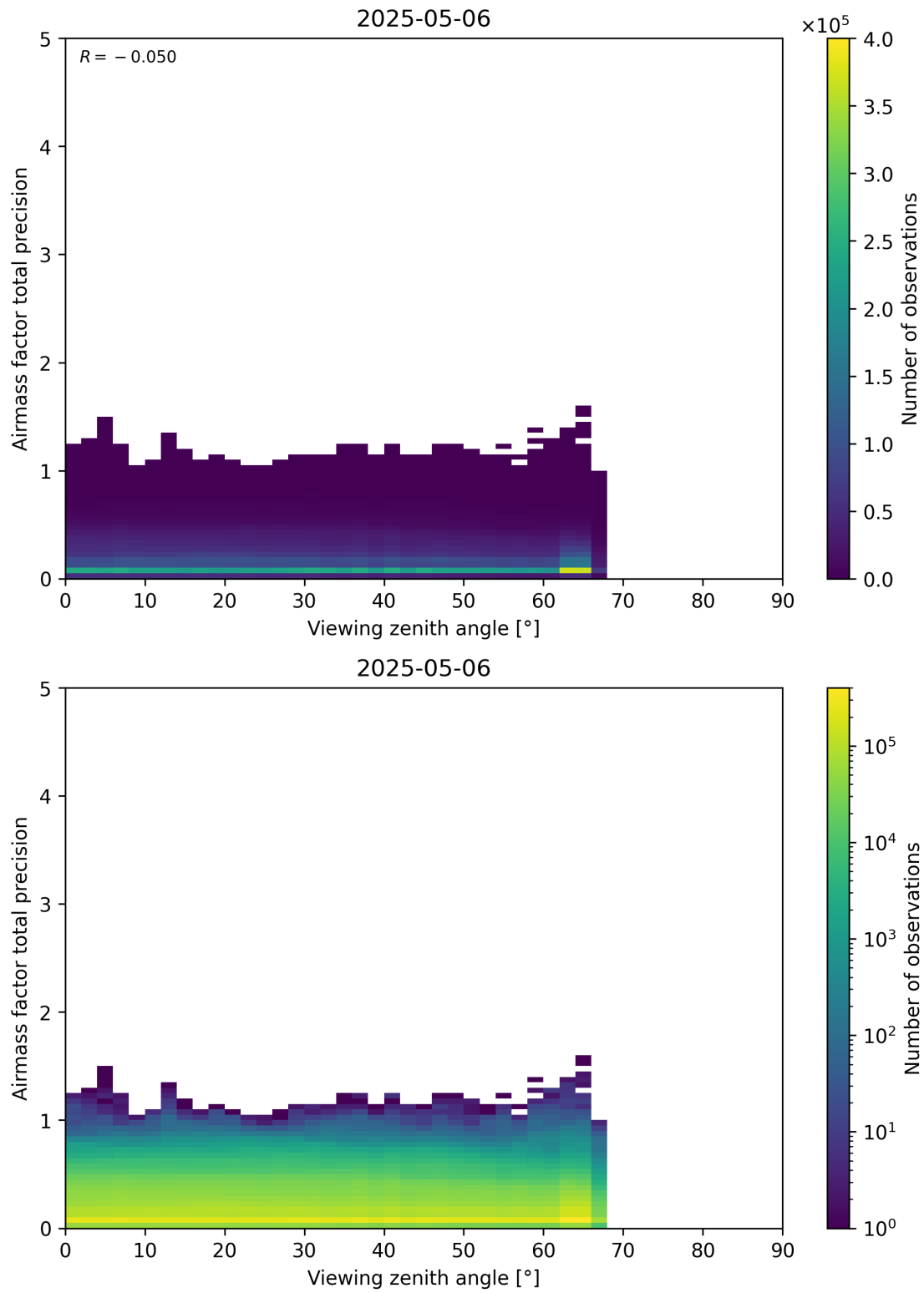
Figure 191: Scatter density plot of “Viewing zenith angle” against “Airmass factor total precision” for 2025-05-05 to 2025-05-07.
