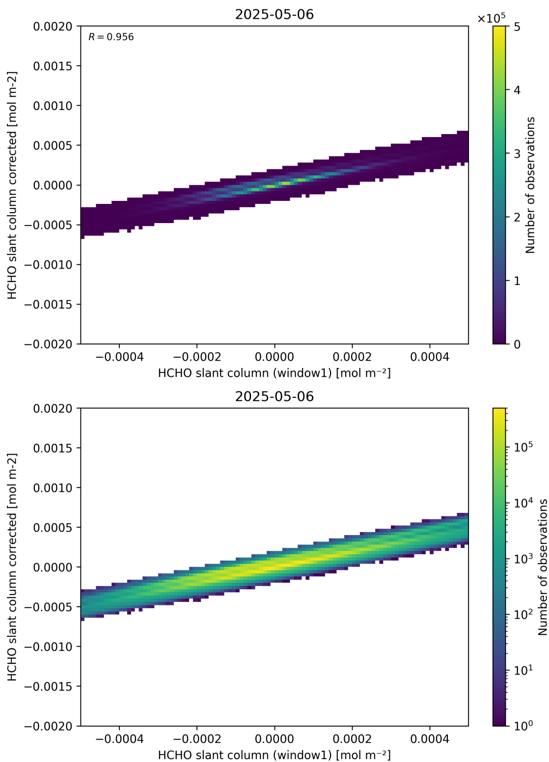
Figure 82: Scatter density plot of “HCHO slant column (window1)” against “HCHO slant column corrected” for 2025-05-05 to 2025-05-07.
