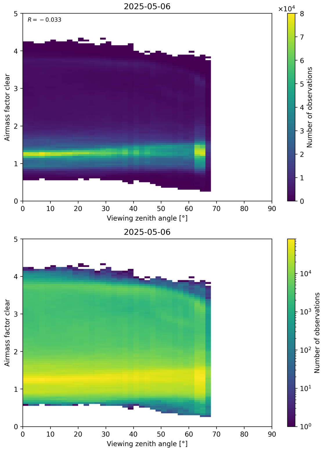
Figure 185: Scatter density plot of “Viewing zenith angle” against “Airmass factor clear” for 2025-05-05 to 2025-05-07.
