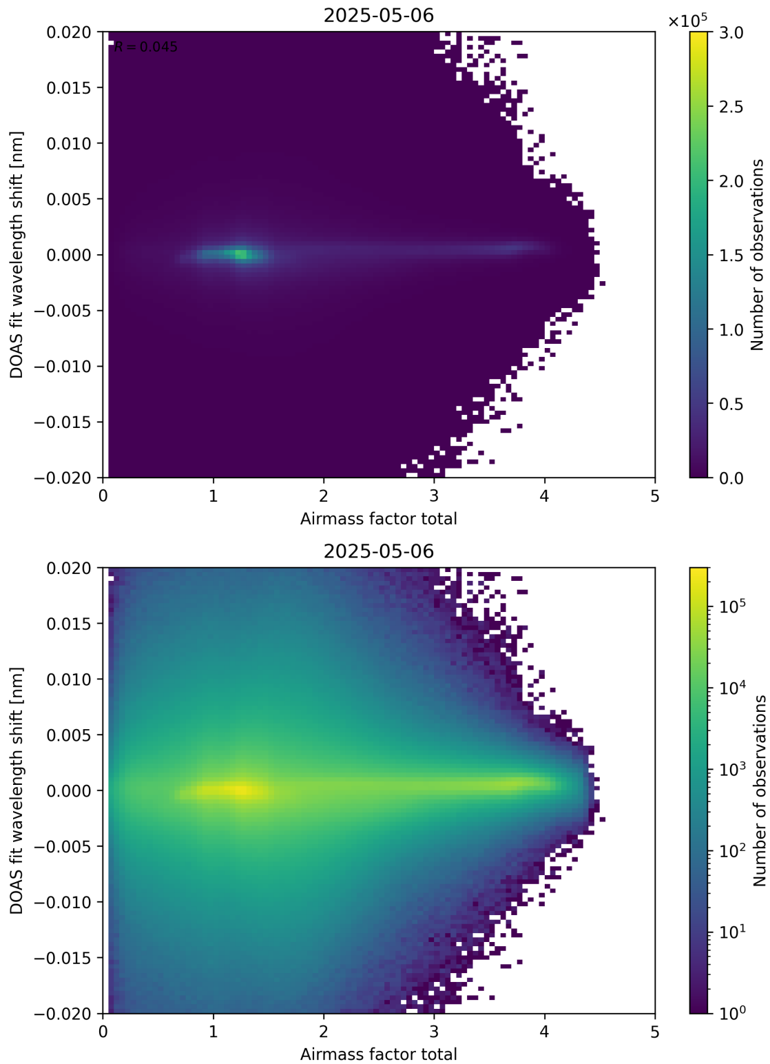
Figure 98: Scatter density plot of “Airmass factor total” against “DOAS fit wavelength shift” for 2025-05-05 to 2025-05-07.
