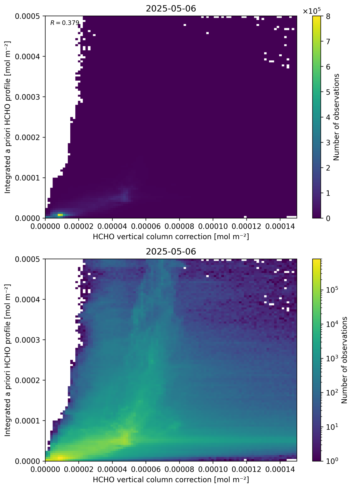
Figure 122: Scatter density plot of “HCHO vertical column correction” against “Integrated a priori HCHO profile” for 2025-05-05 to 2025-05-07.
