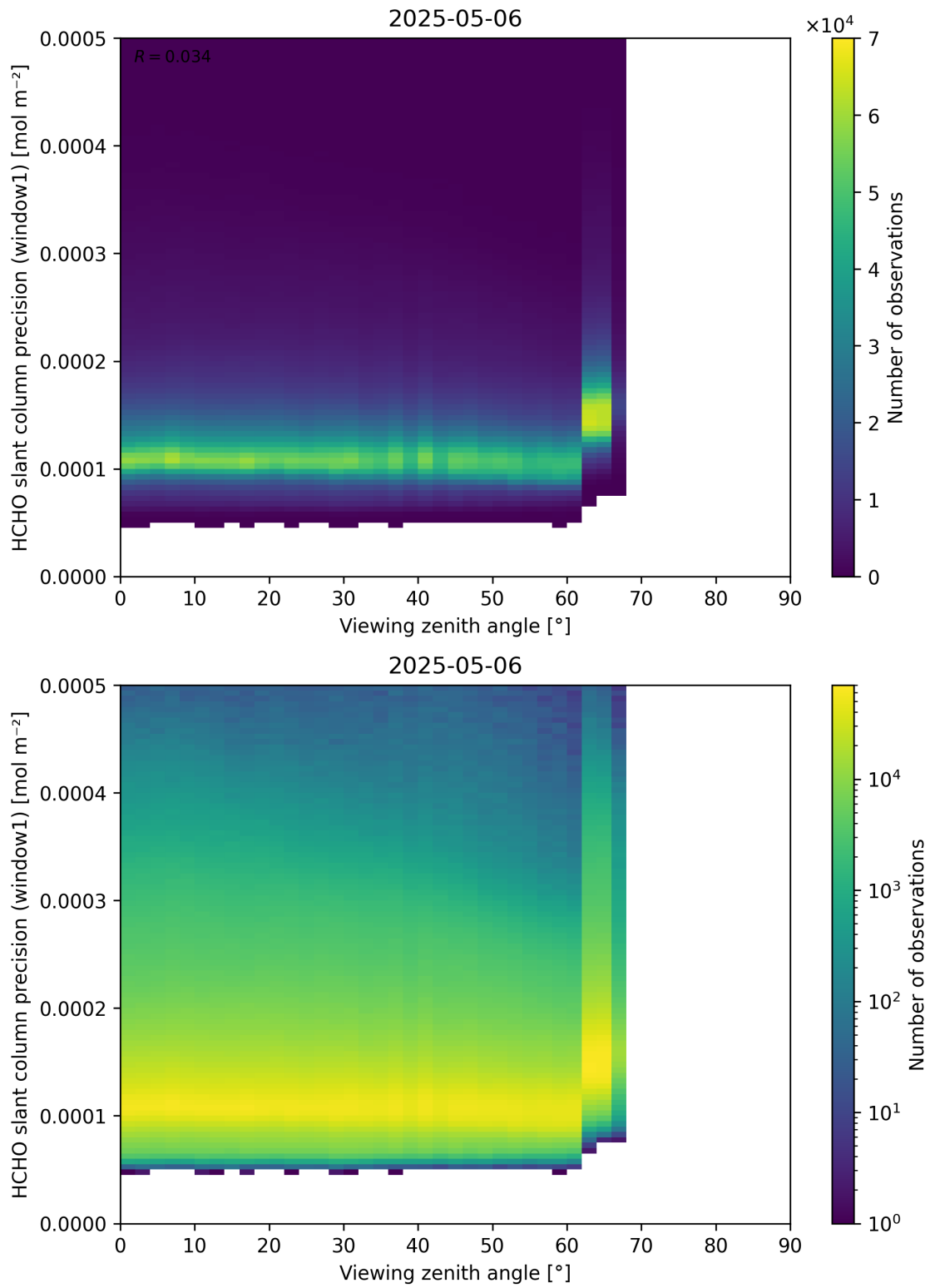
Figure 189: Scatter density plot of “Viewing zenith angle” against “HCHO slant column precision (window1)” for 2025-05-05 to 2025-05-07.
