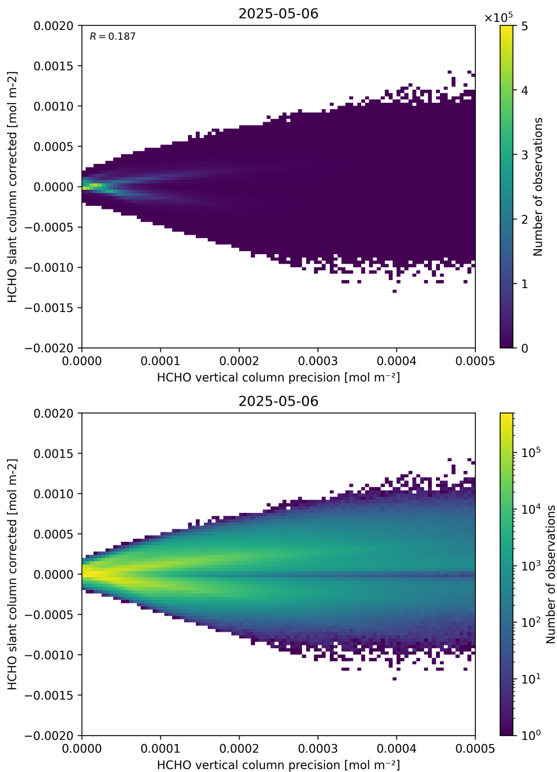
Figure 140: Scatter density plot of “HCHO vertical column precision” against “HCHO slant column corrected” for 2025-05-05 to 2025-05-07.
