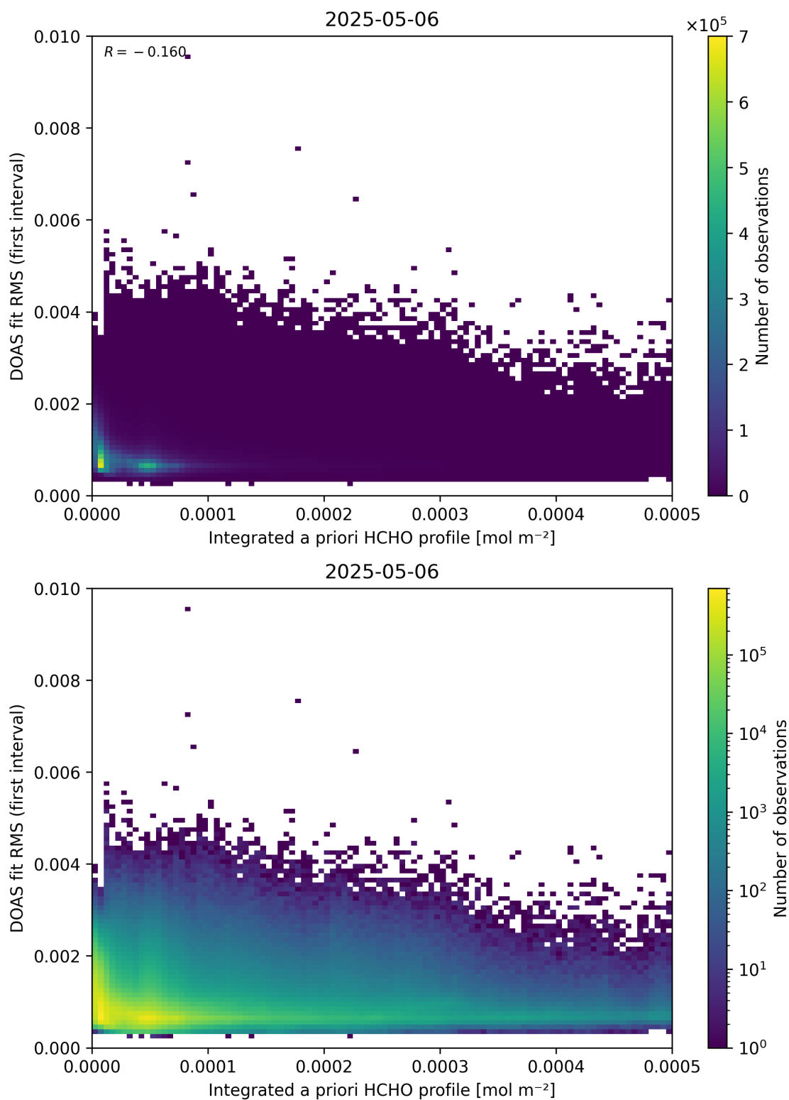
Figure 148: Scatter density plot of “Integrated a priori HCHO profile” against “DOAS fit RMS (first interval)” for 2025-05-05 to 2025-05-07.
