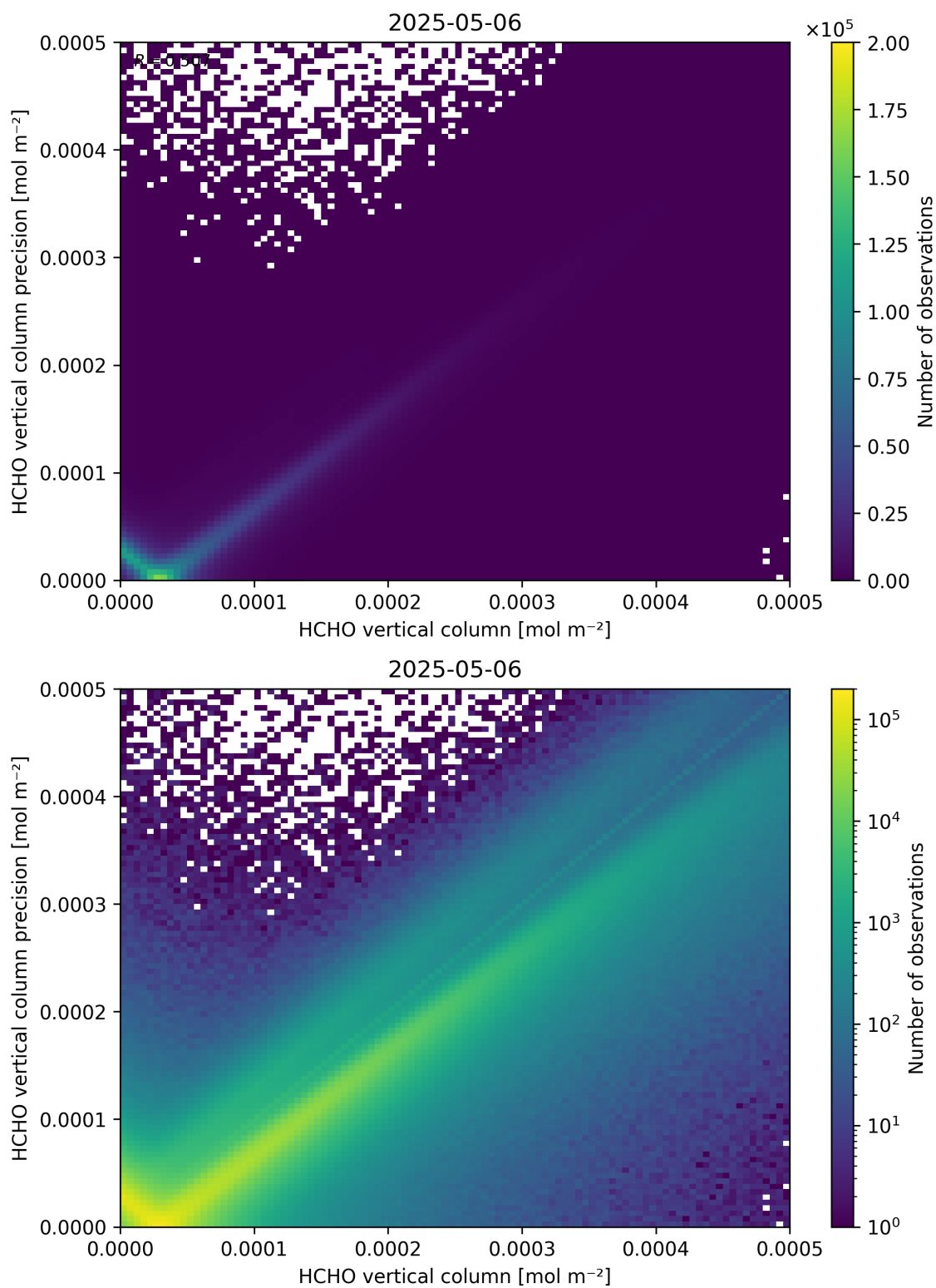
Figure 134: Scatter density plot of “HCHO vertical column” against “HCHO vertical column precision” for 2025-05-05 to 2025-05-07.
