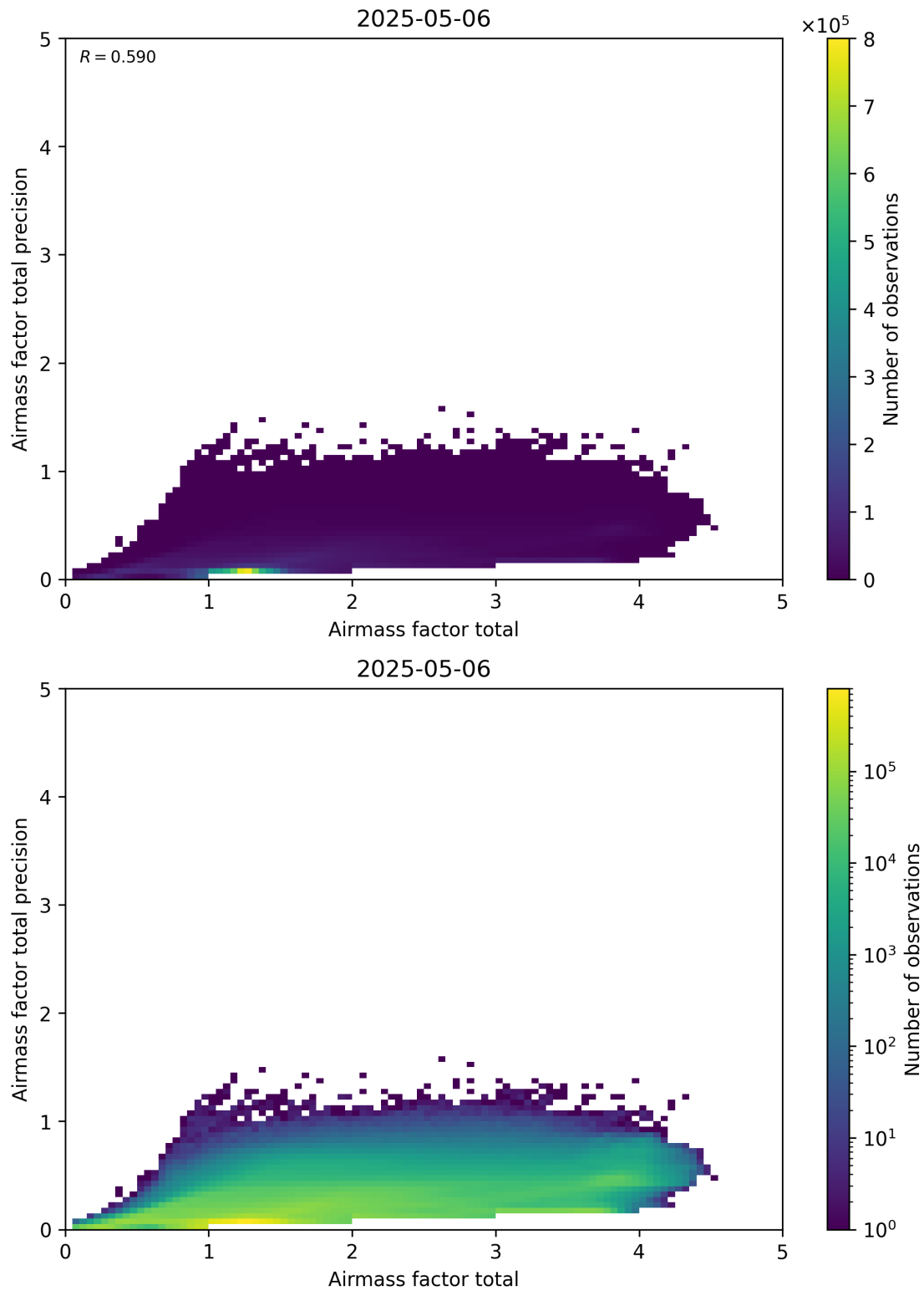
Figure 103: Scatter density plot of “Airmass factor total” against “Airmass factor total precision” for 2025-05-05 to 2025-05-07.
