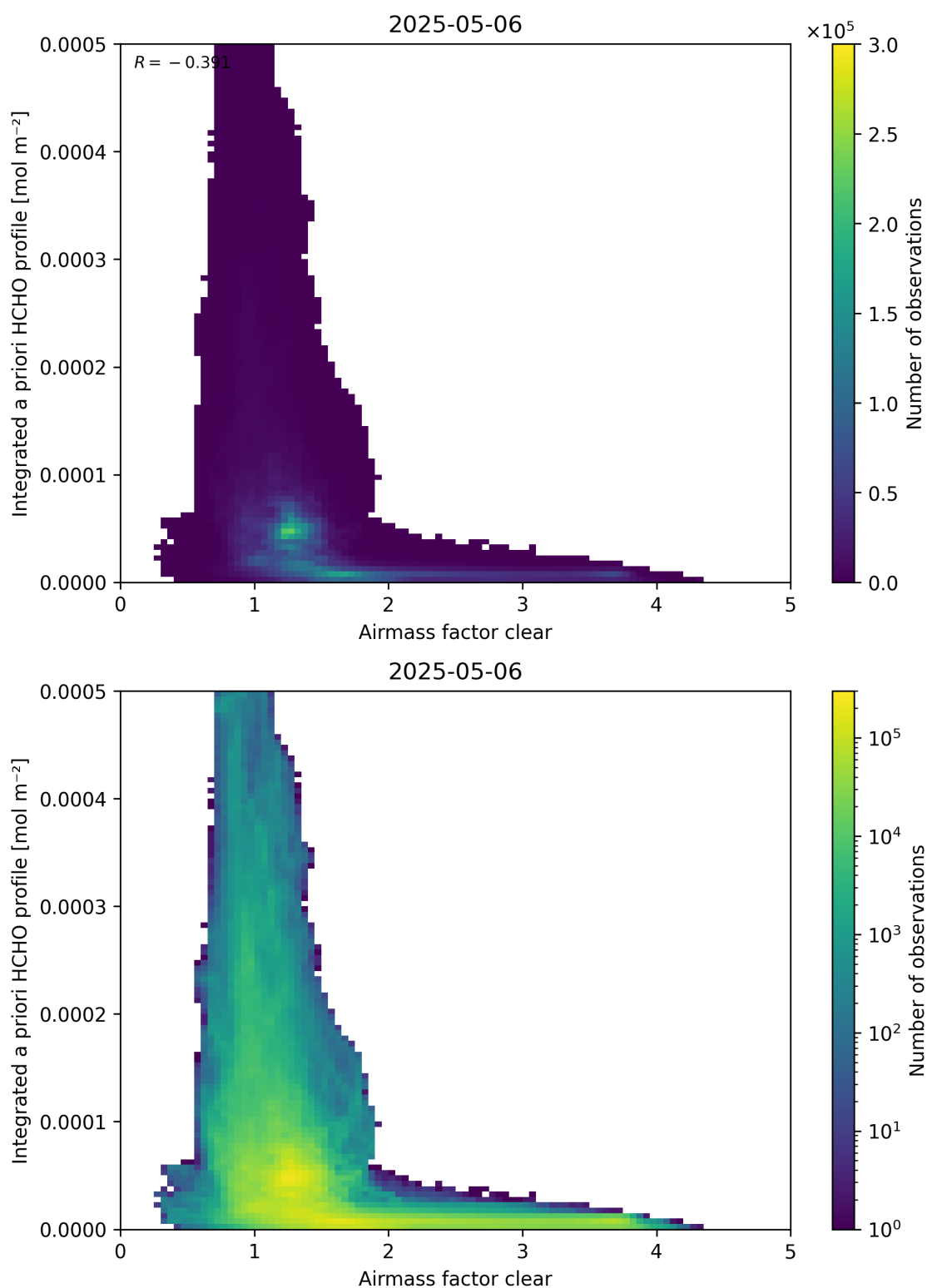
Figure 76: Scatter density plot of “Airmass factor clear” against “Integrated a priori HCHO profile” for 2025-05-05 to 2025-05-07.
