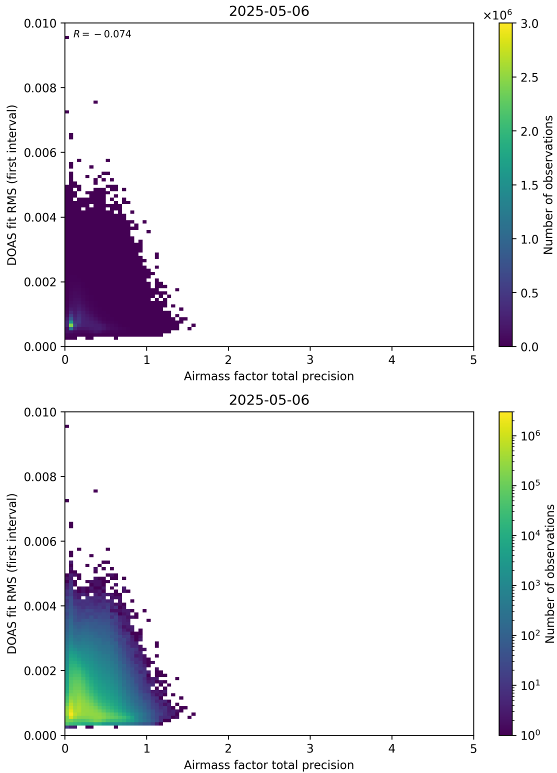
Figure 105: Scatter density plot of “Airmass factor total precision” against “DOAS fit RMS (first interval)” for 2025-05-05 to 2025-05-07.
