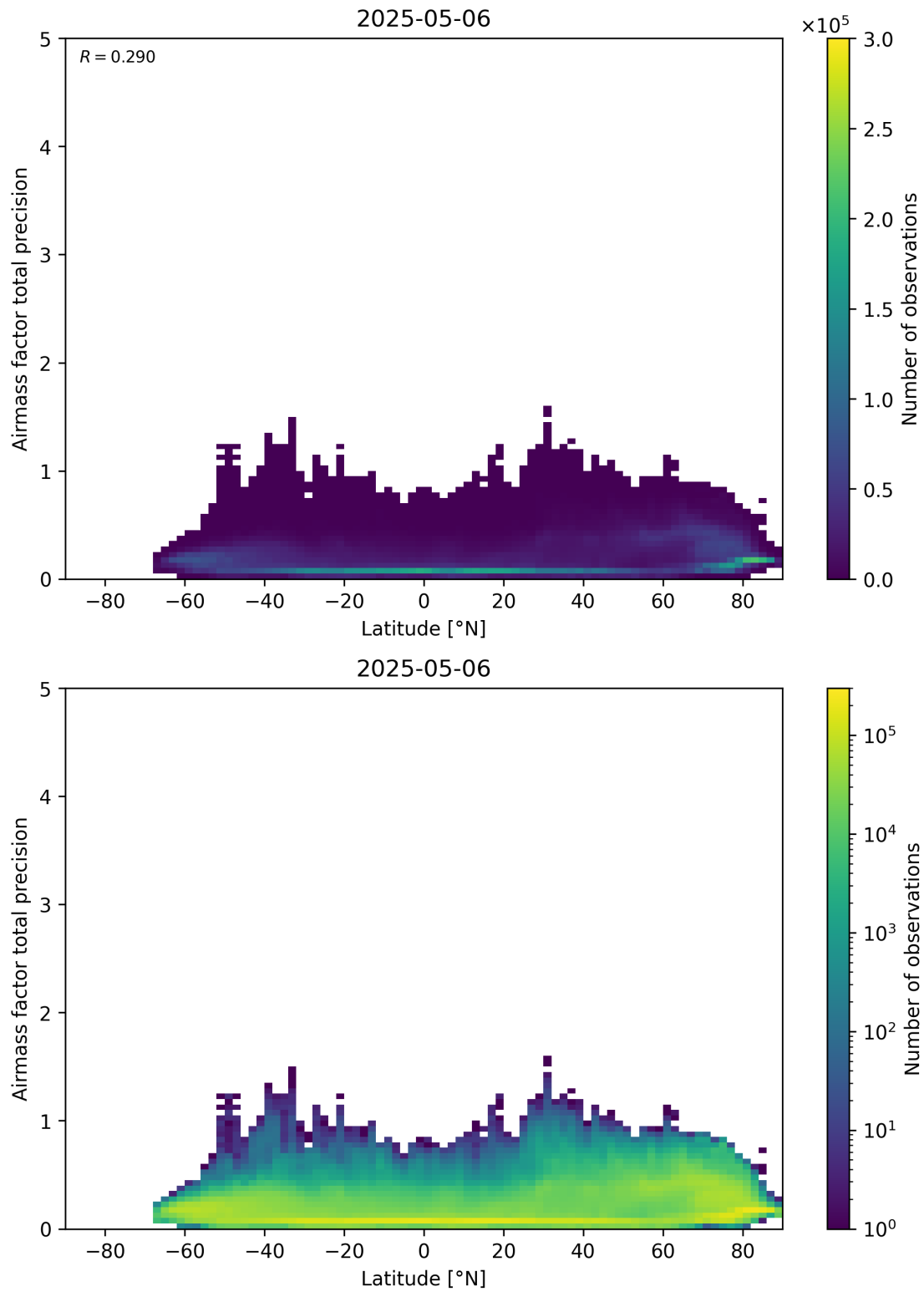
Figure 162: Scatter density plot of “Latitude” against “Airmass factor total precision” for 2025-05-05 to 2025-05-07.
