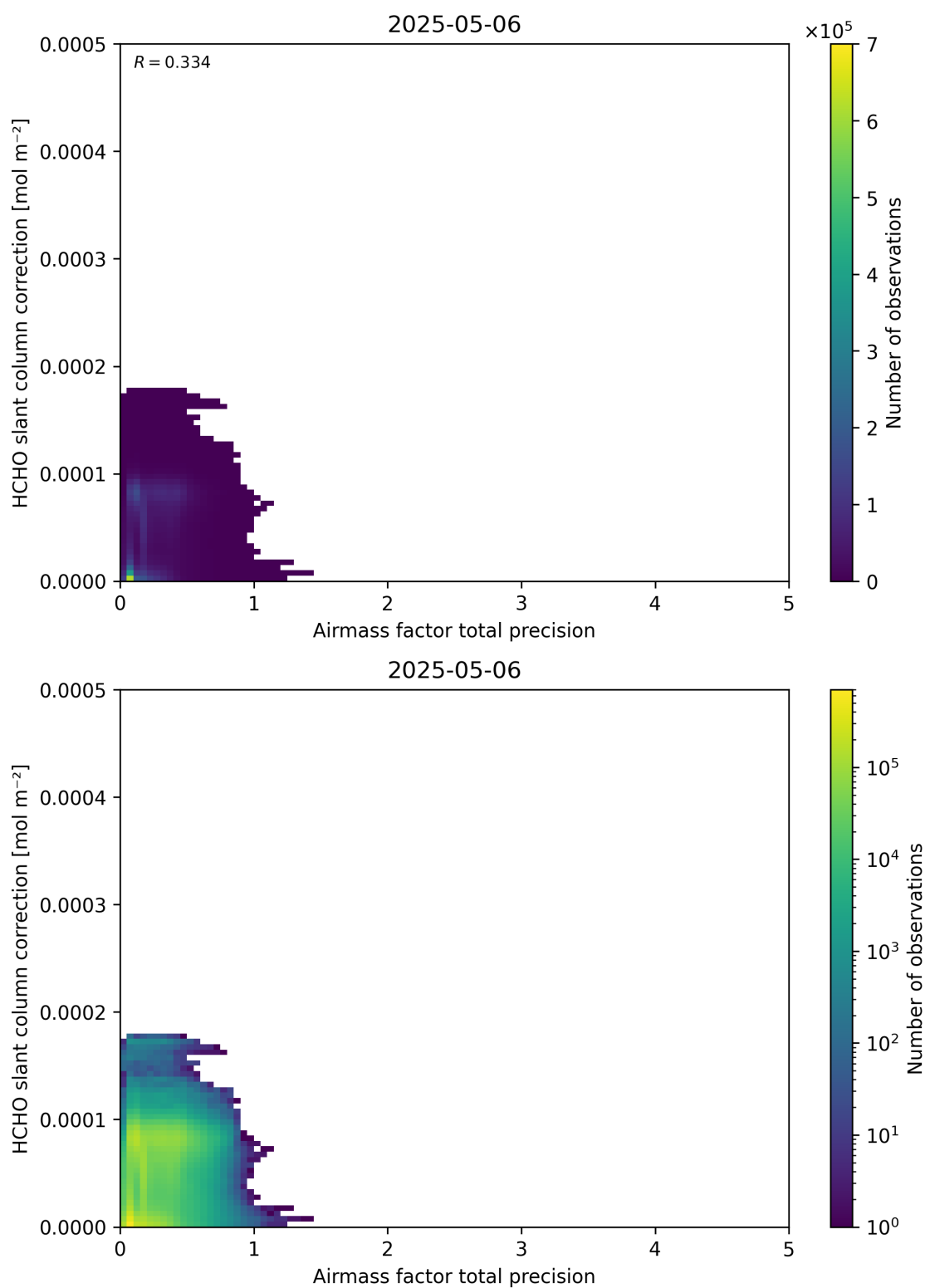
Figure 110: Scatter density plot of “Airmass factor total precision” against “HCHO slant column correction” for 2025-05-05 to 2025-05-07.
