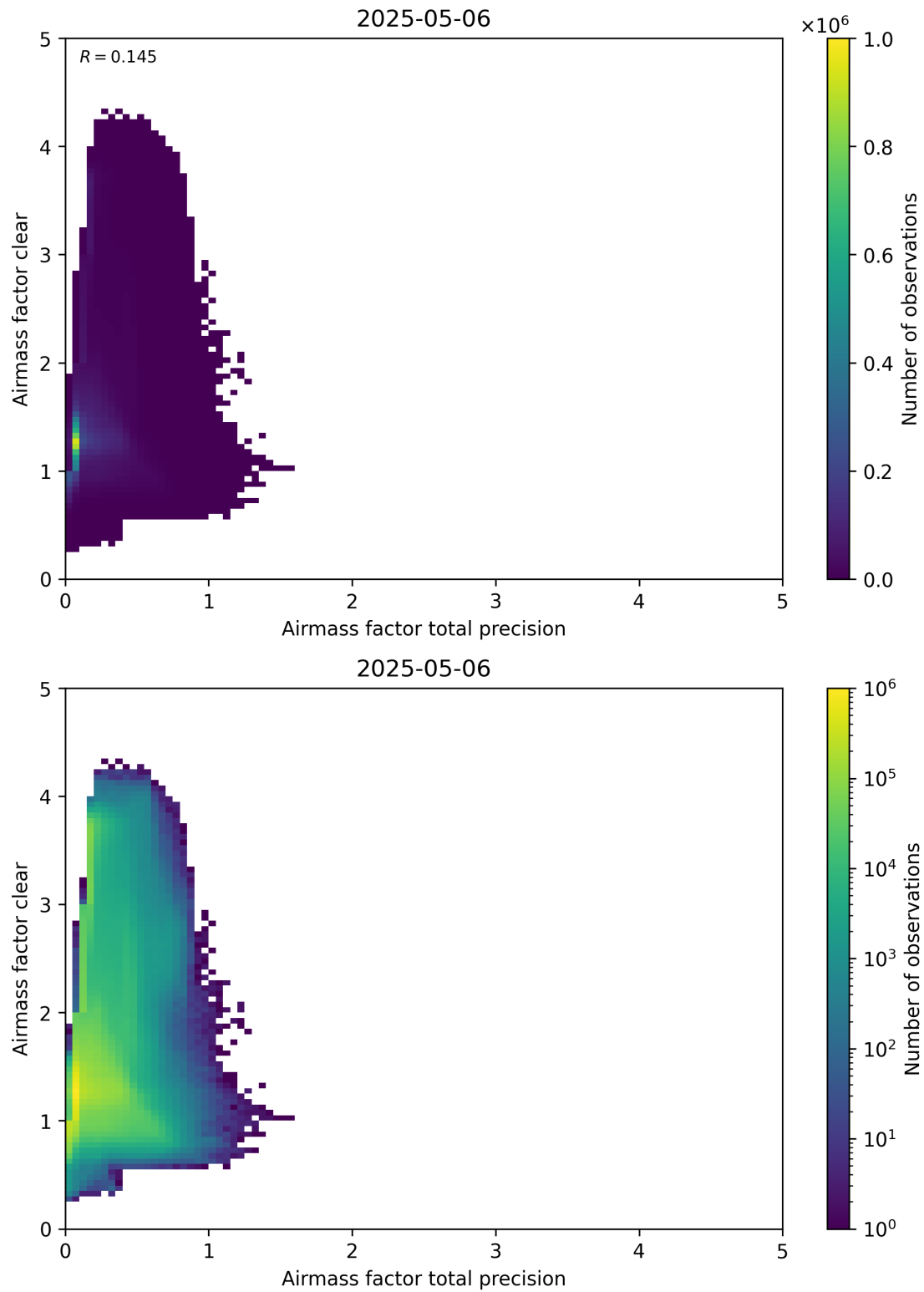
Figure 108: Scatter density plot of “Airmass factor total precision” against “Airmass factor clear” for 2025-05-05 to 2025-05-07.
