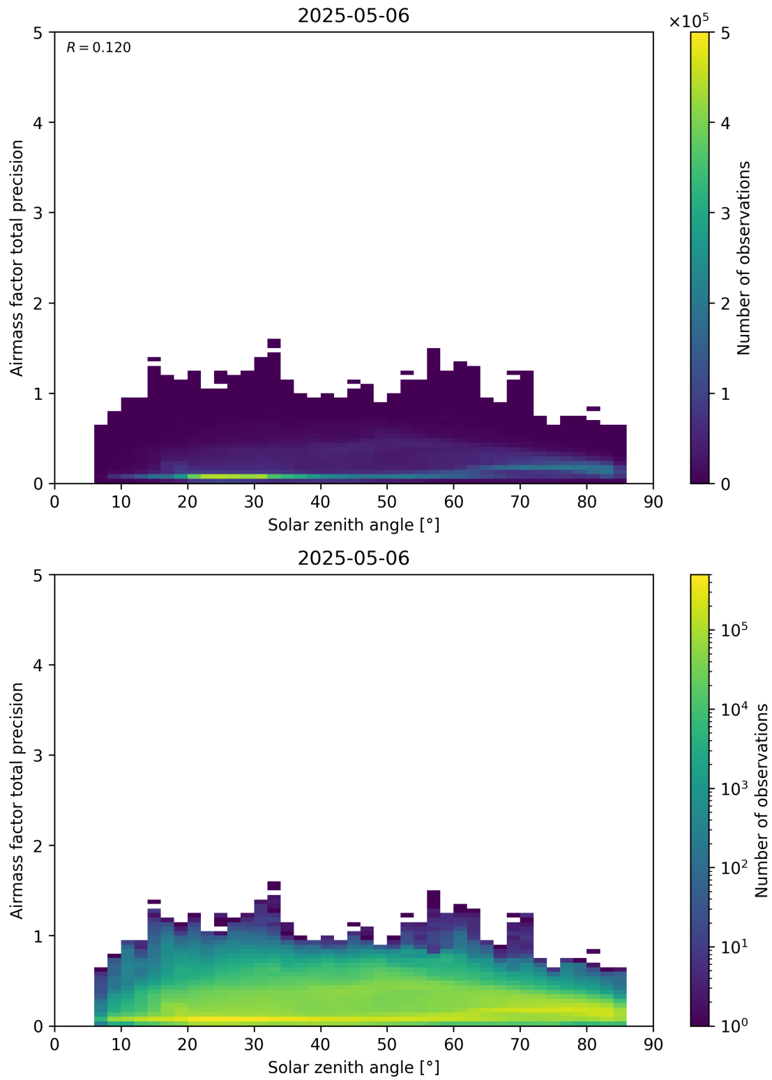
Figure 176: Scatter density plot of “Solar zenith angle” against “Airmass factor total precision” for 2025-05-05 to 2025-05-07.
