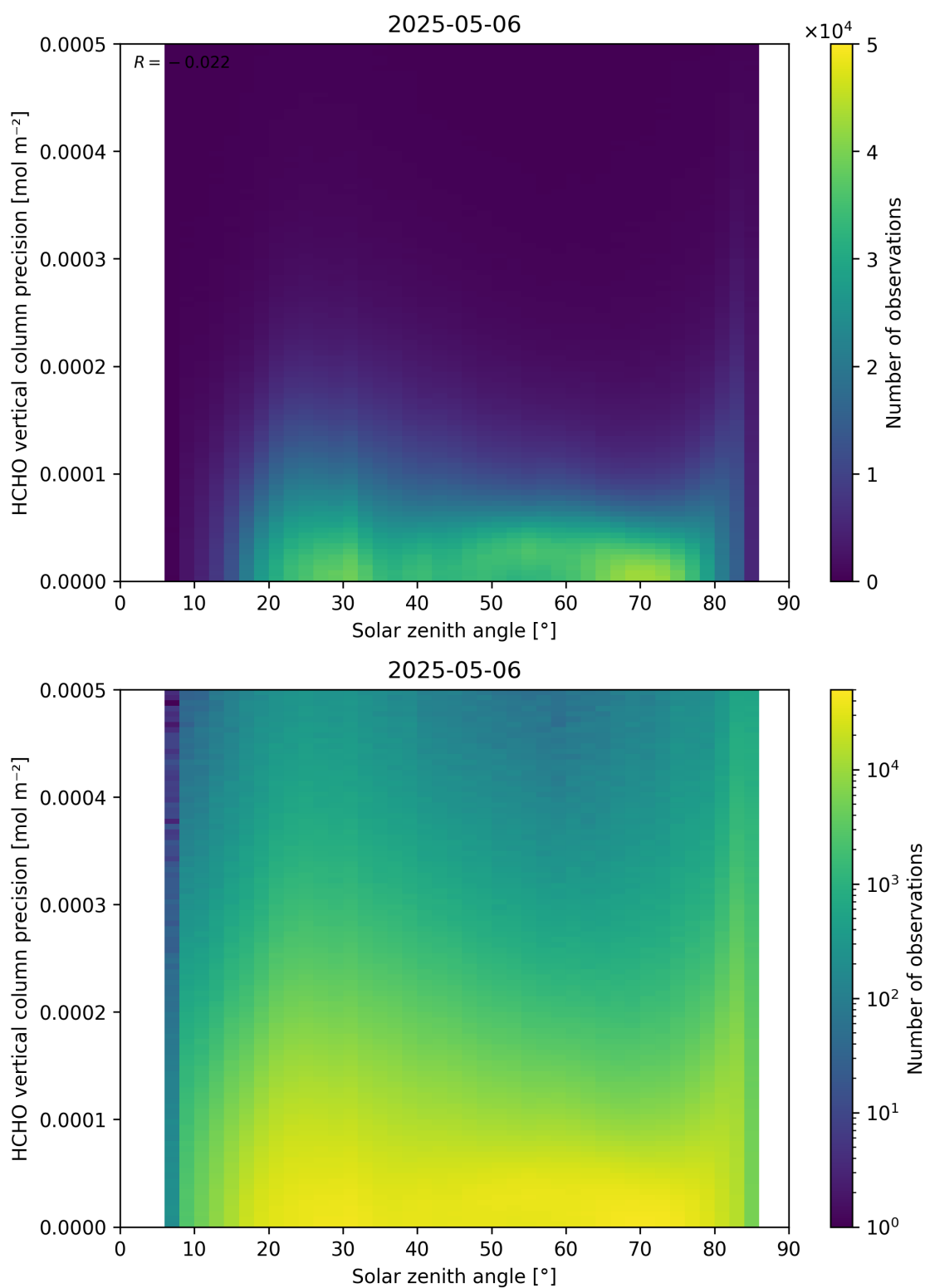
Figure 179: Scatter density plot of “Solar zenith angle” against “HCHO vertical column precision” for 2025-05-05 to 2025-05-07.
