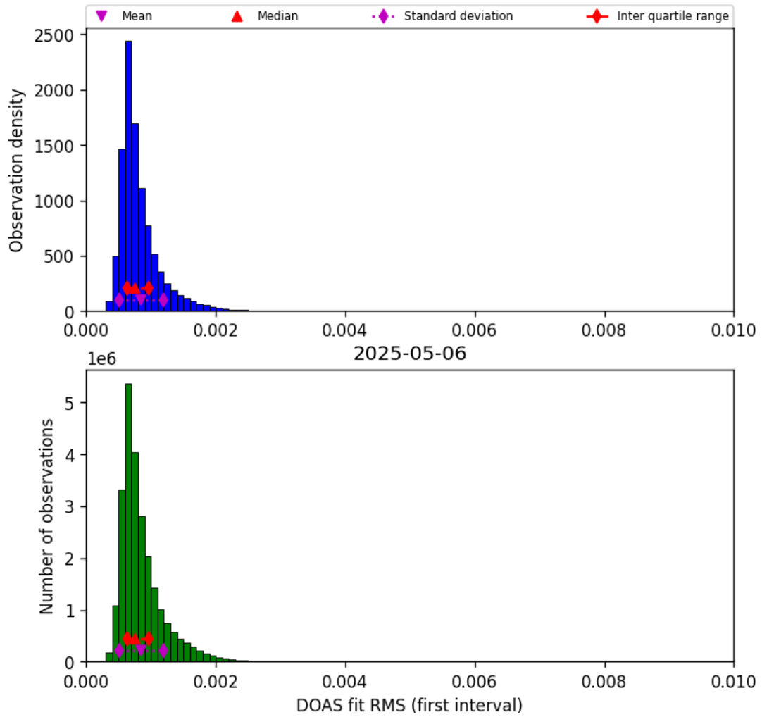
Figure 46: Histogram of “DOAS fit RMS (first interval)” for 2025-05-05 to 2025-05-07
