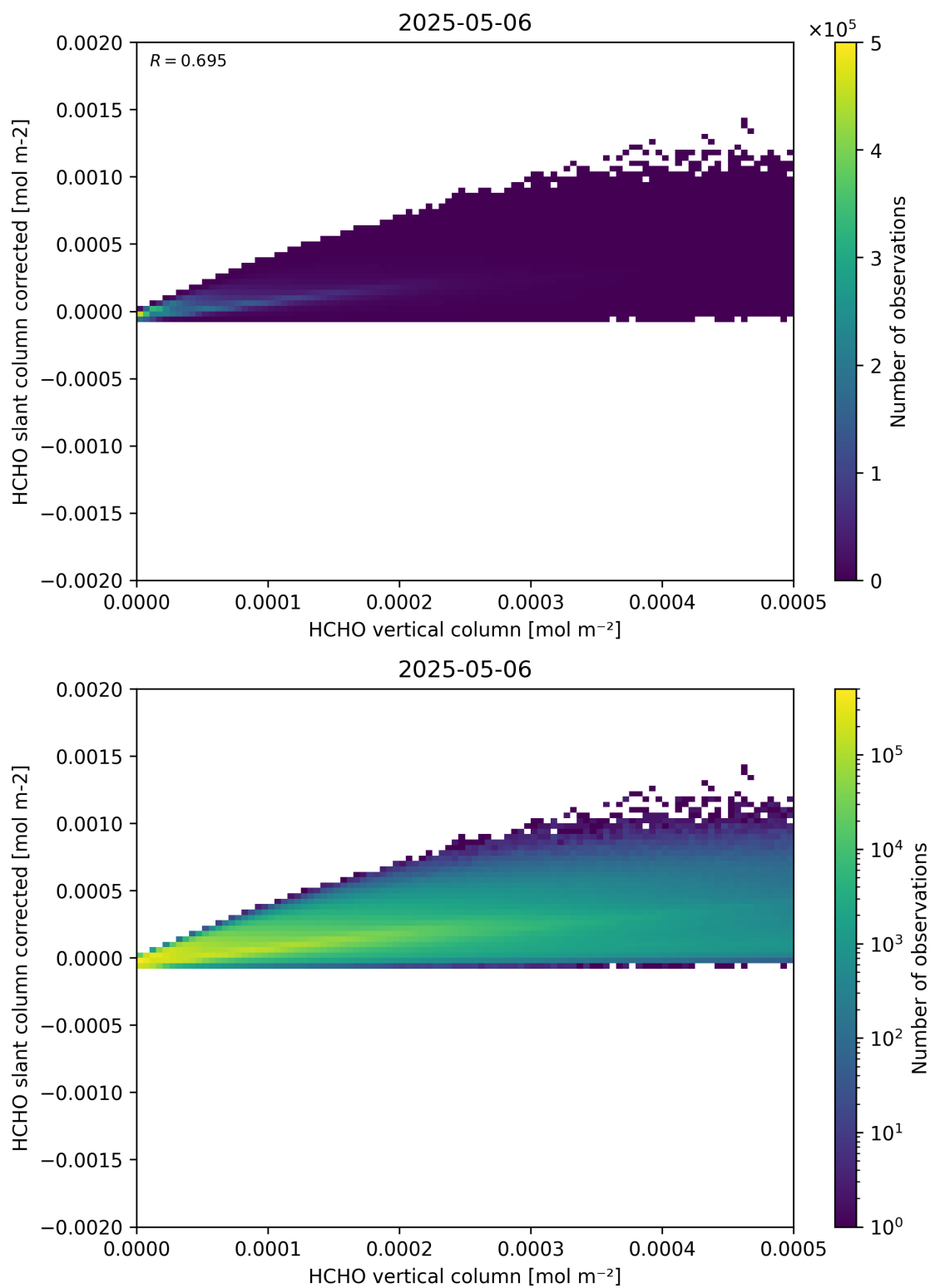
Figure 127: Scatter density plot of “HCHO vertical column” against “HCHO slant column corrected” for 2025-05-05 to 2025-05-07.
