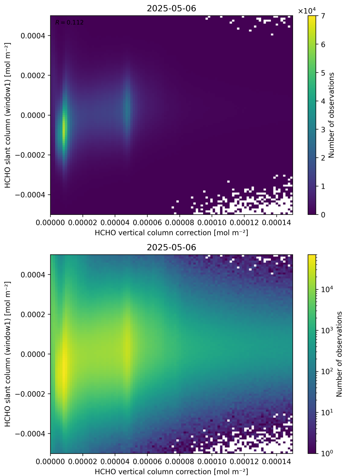
Figure 118: Scatter density plot of “HCHO vertical column correction” against “HCHO slant column (window1)” for 2025-05-05 to 2025-05-07.
