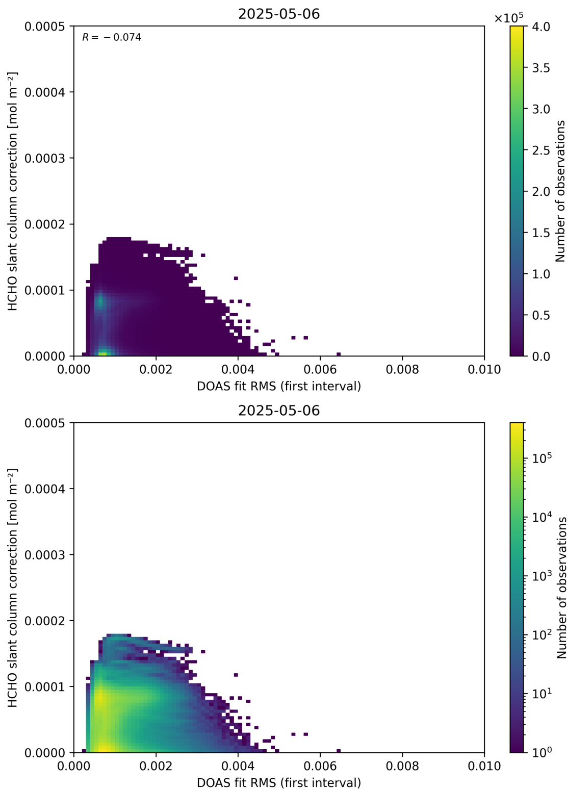
Figure 63: Scatter density plot of “DOAS fit RMS (first interval)” against “HCHO slant column correction” for 2025-05-05 to 2025-05-07.
