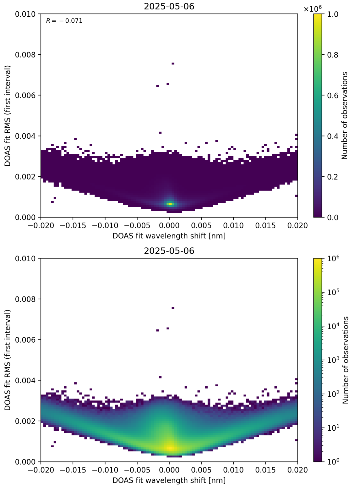
Figure 64: Scatter density plot of “DOAS fit wavelength shift” against “DOAS fit RMS (first interval)” for 2025-05-05 to 2025-05-07.
