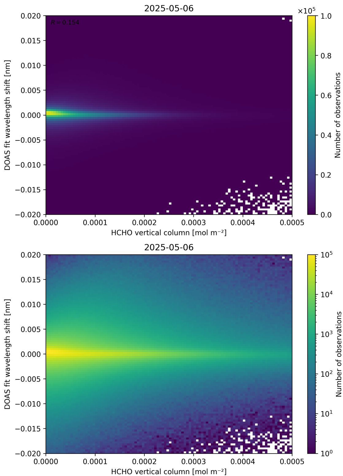
Figure 124: Scatter density plot of “HCHO vertical column” against “DOAS fit wavelength shift” for 2025-05-05 to 2025-05-07.
