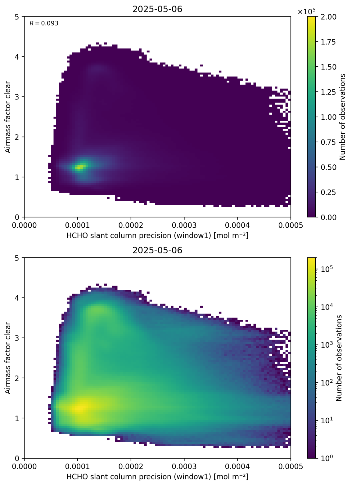
Figure 91: Scatter density plot of “HCHO slant column precision (window1)” against “Airmass factor clear” for 2025-05-05 to 2025-05-07.
