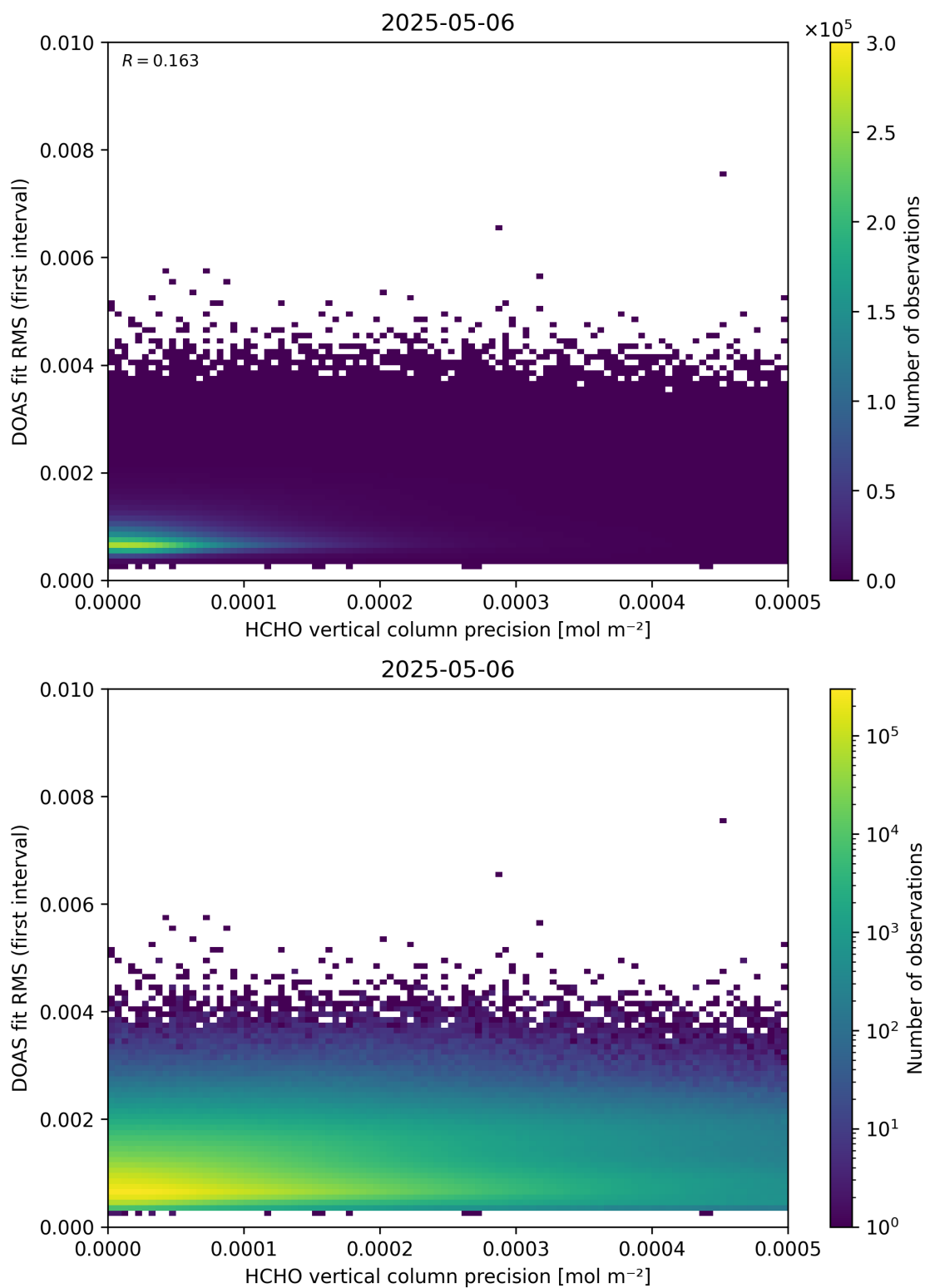
Figure 136: Scatter density plot of “HCHO vertical column precision” against “DOAS fit RMS (first interval)” for 2025-05-05 to 2025-05-07.
