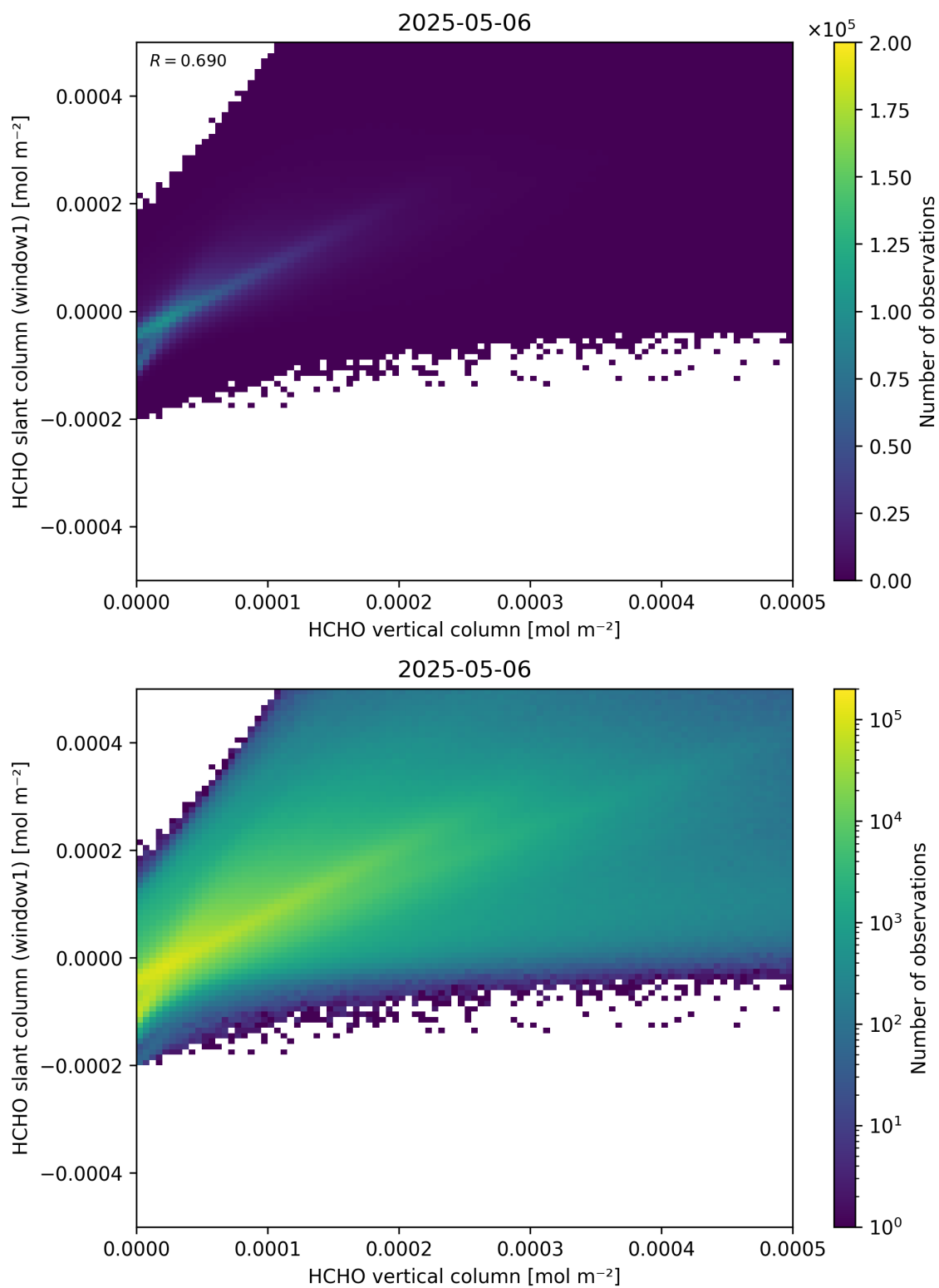
Figure 129: Scatter density plot of “HCHO vertical column” against “HCHO slant column (window1)” for 2025-05-05 to 2025-05-07.
