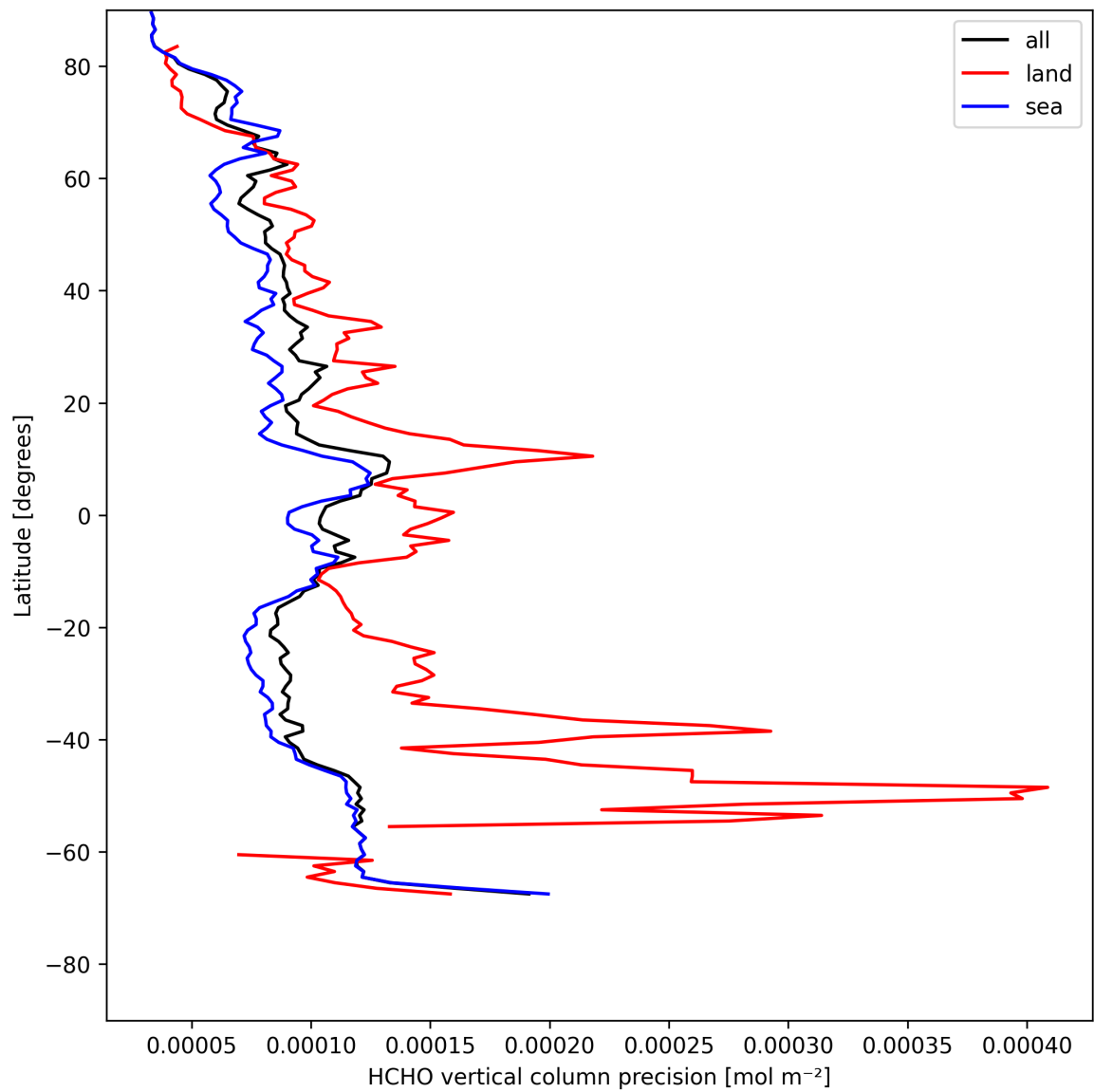
Figure 22: Zonal average of “HCHO vertical column precision” for 2025-05-05 to 2025-05-07.
