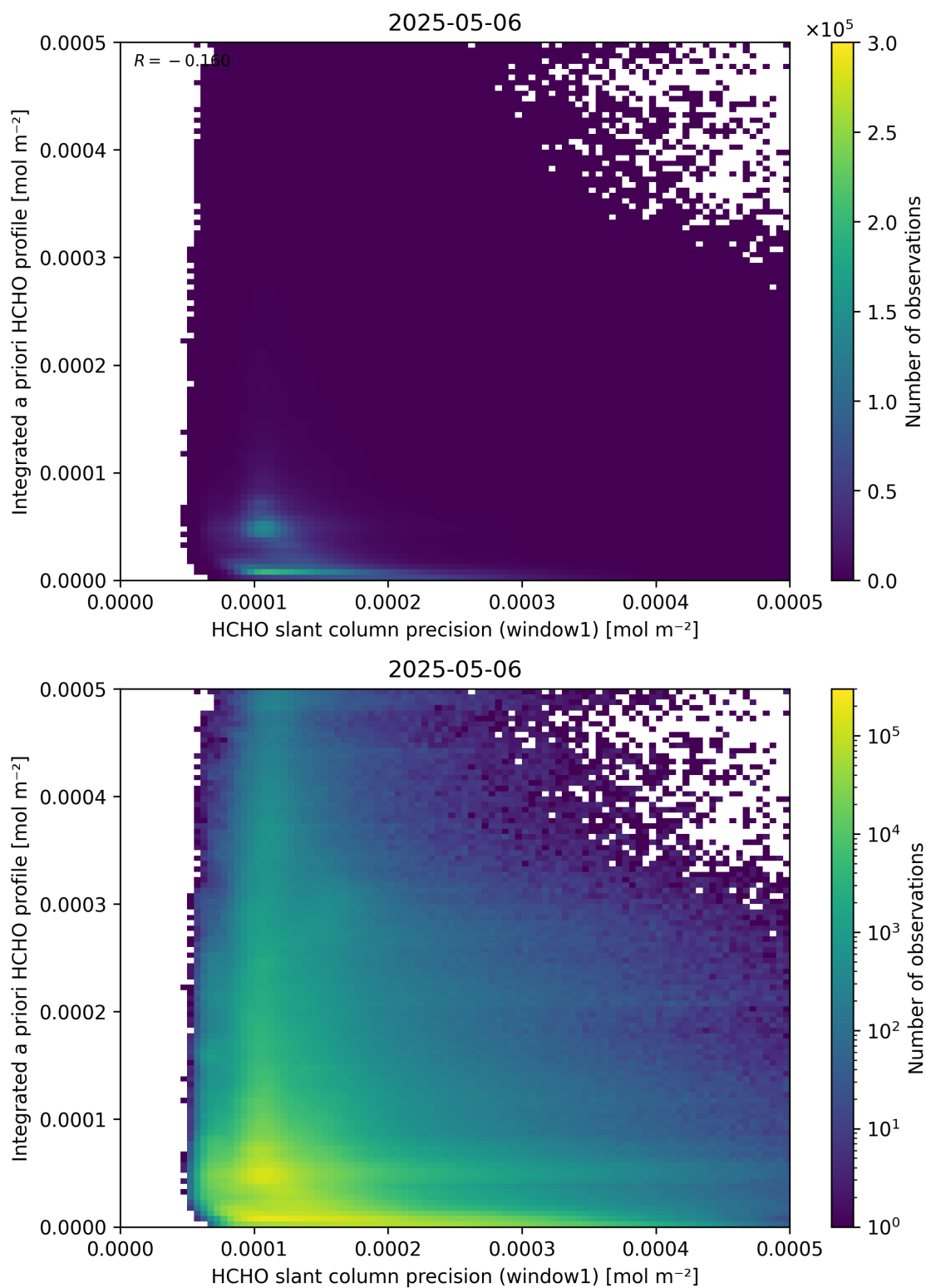
Figure 96: Scatter density plot of “HCHO slant column precision (window1)” against “Integrated a priori HCHO profile” for 2025-05-05 to 2025-05-07.
