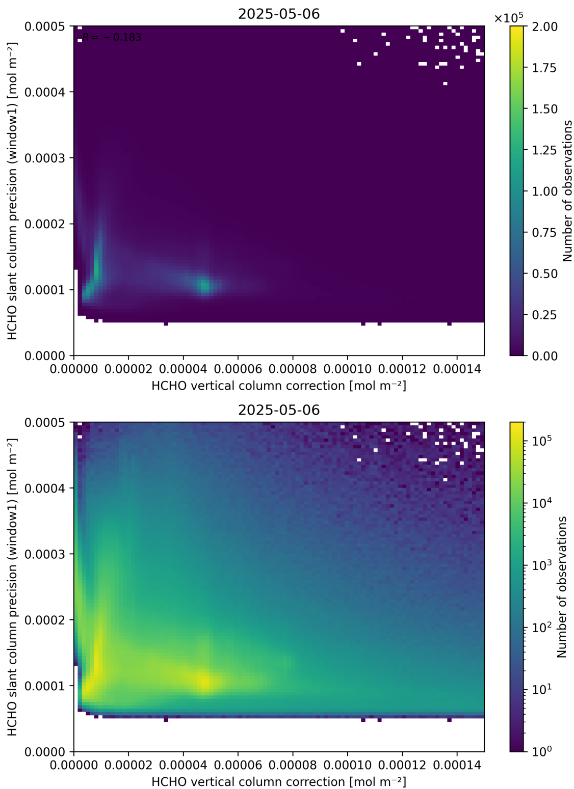
Figure 119: Scatter density plot of “HCHO vertical column correction” against “HCHO slant column precision (window1)” for 2025-05-05 to 2025-05-07.
