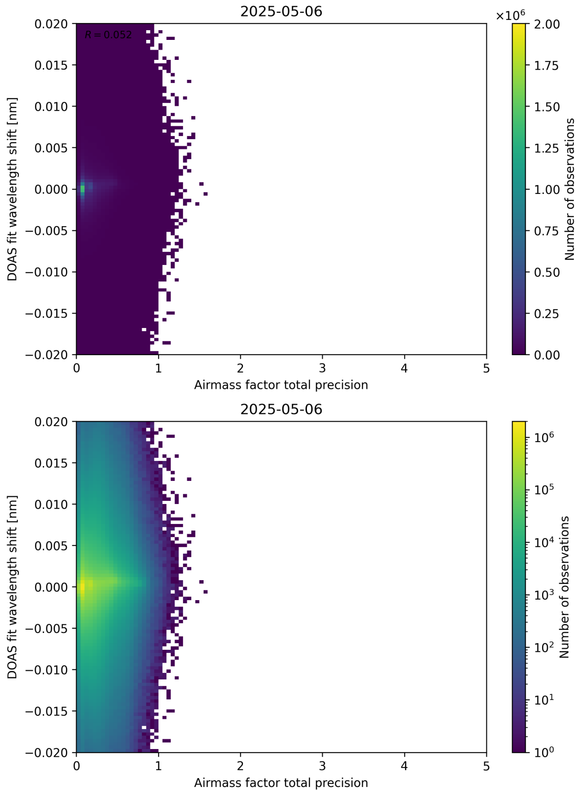
Figure 106: Scatter density plot of “Airmass factor total precision” against “DOAS fit wavelength shift” for 2025-05-05 to 2025-05-07.
