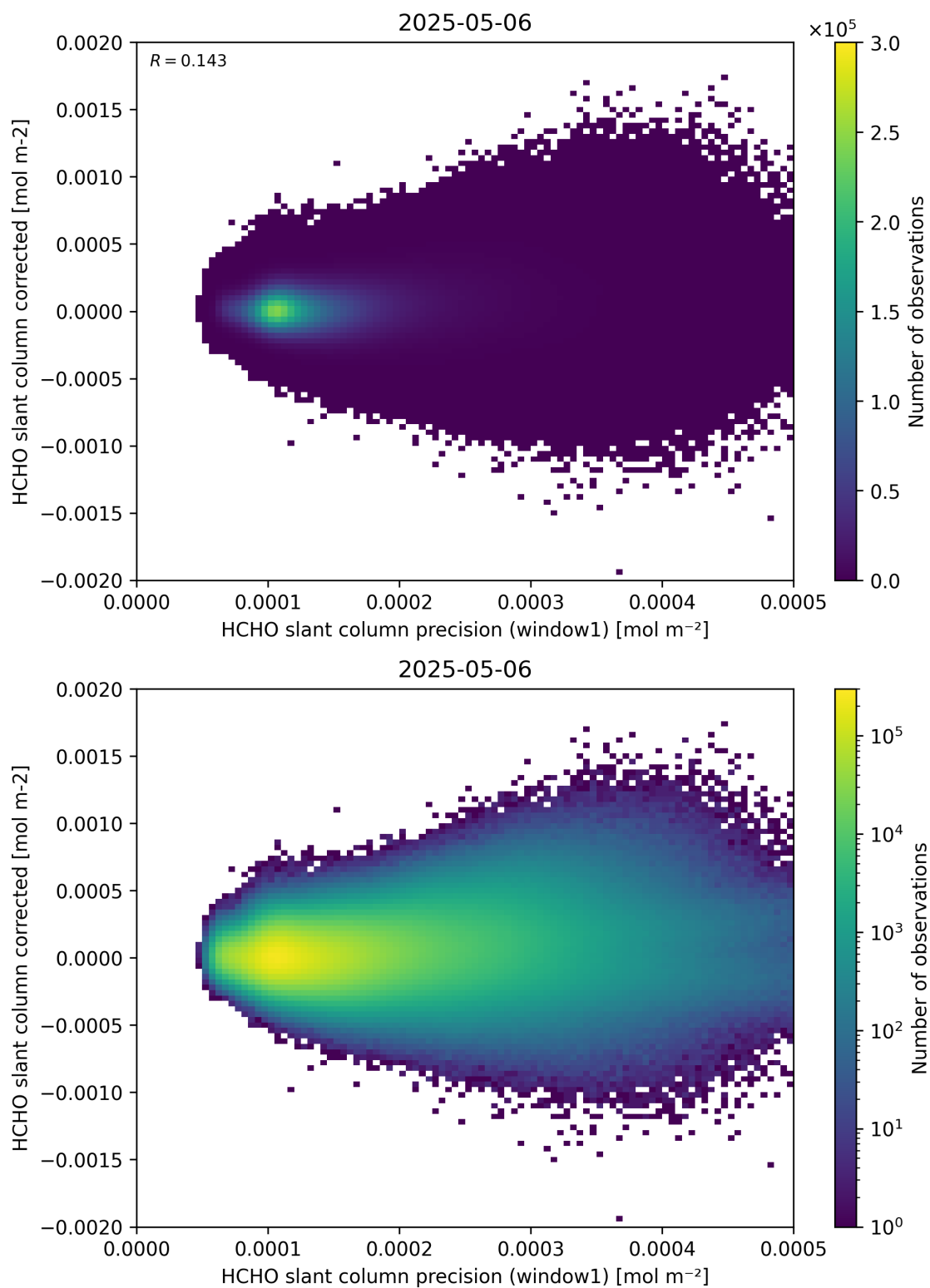
Figure 92: Scatter density plot of “HCHO slant column precision (window1)” against “HCHO slant column corrected” for 2025-05-05 to 2025-05-07.
