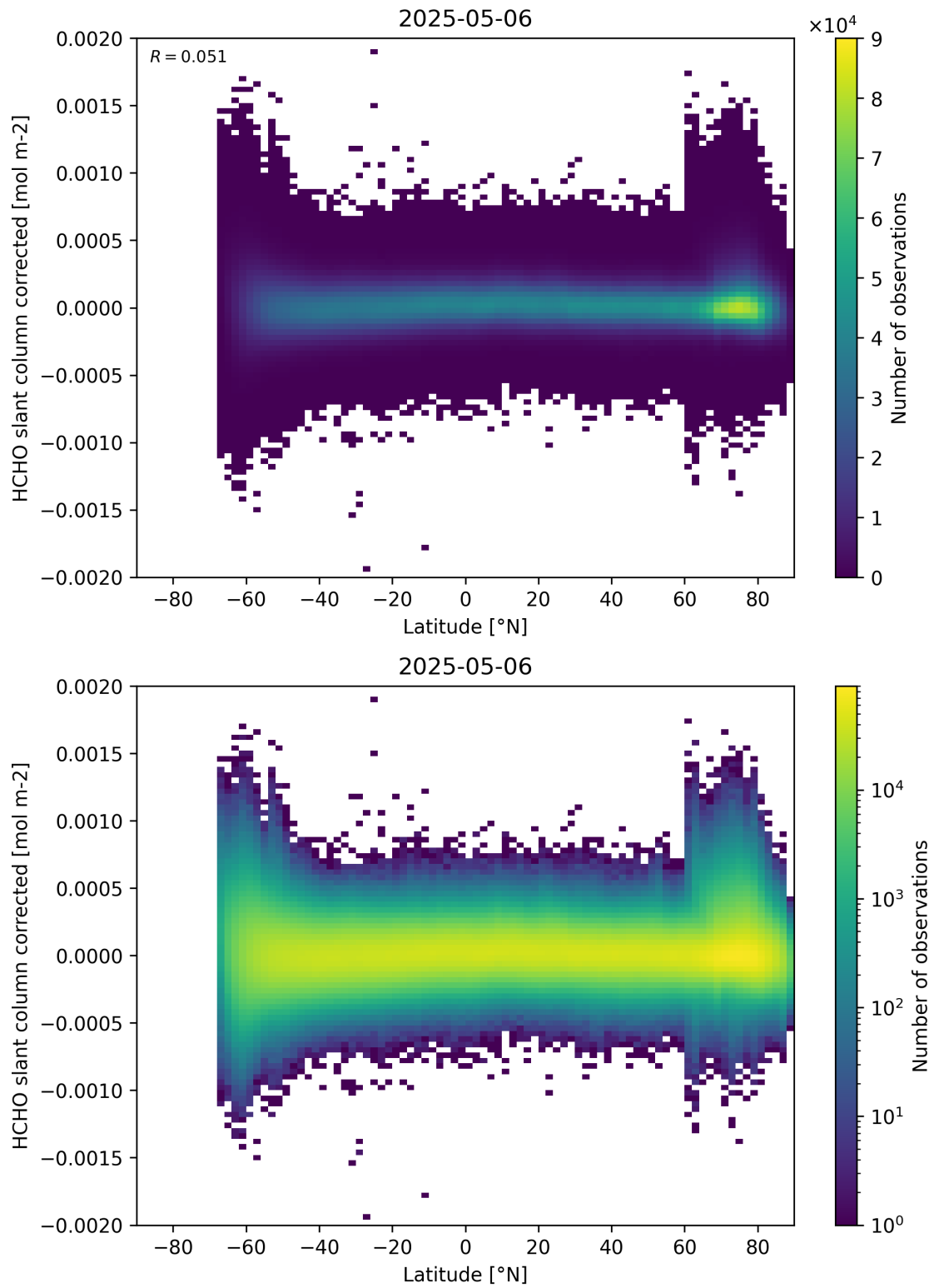
Figure 157: Scatter density plot of “Latitude” against “HCHO slant column corrected” for 2025-05-05 to 2025-05-07.
