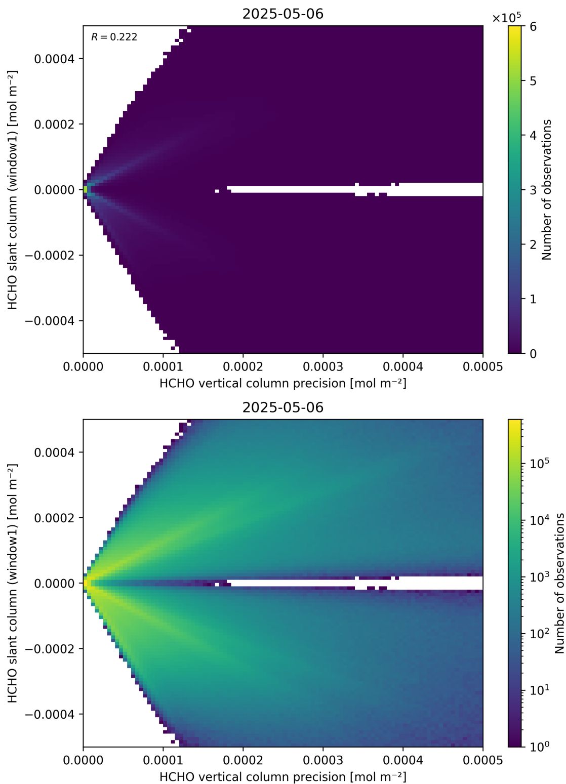
Figure 142: Scatter density plot of “HCHO vertical column precision” against “HCHO slant column (window1)” for 2025-05-05 to 2025-05-07.
