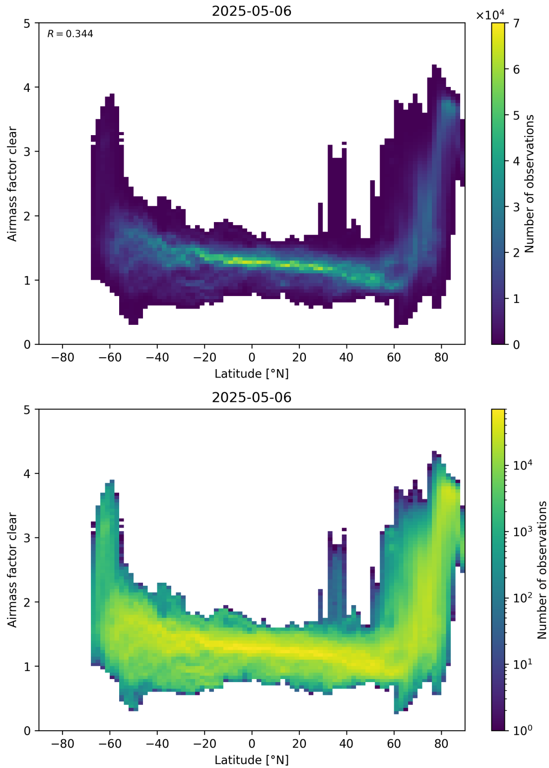
Figure 156: Scatter density plot of “Latitude” against “Airmass factor clear” for 2025-05-05 to 2025-05-07.
