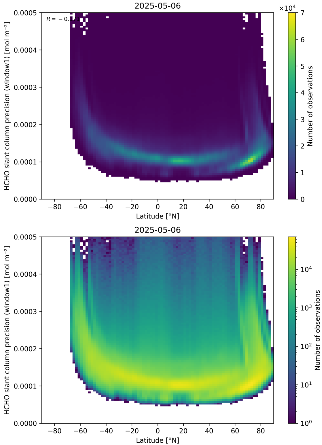
Figure 160: Scatter density plot of “Latitude” against “HCHO slant column precision (window1)” for 2025-05-05 to 2025-05-07.
