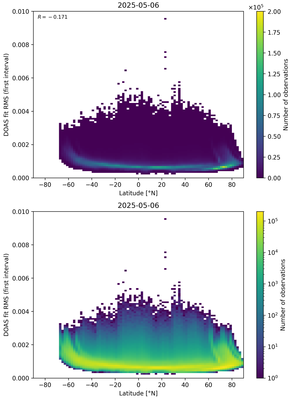
Figure 153: Scatter density plot of “Latitude” against “DOAS fit RMS (first interval)” for 2025-05-05 to 2025-05-07.
