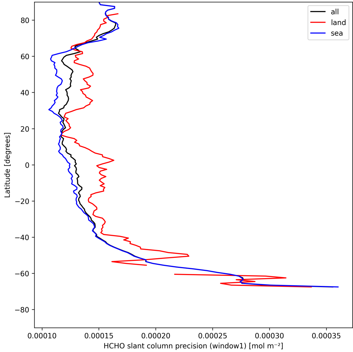
Figure 25: Zonal average of "HCHO slant column precision (window1)" for 2025-05-05 to 2025-05-07.
