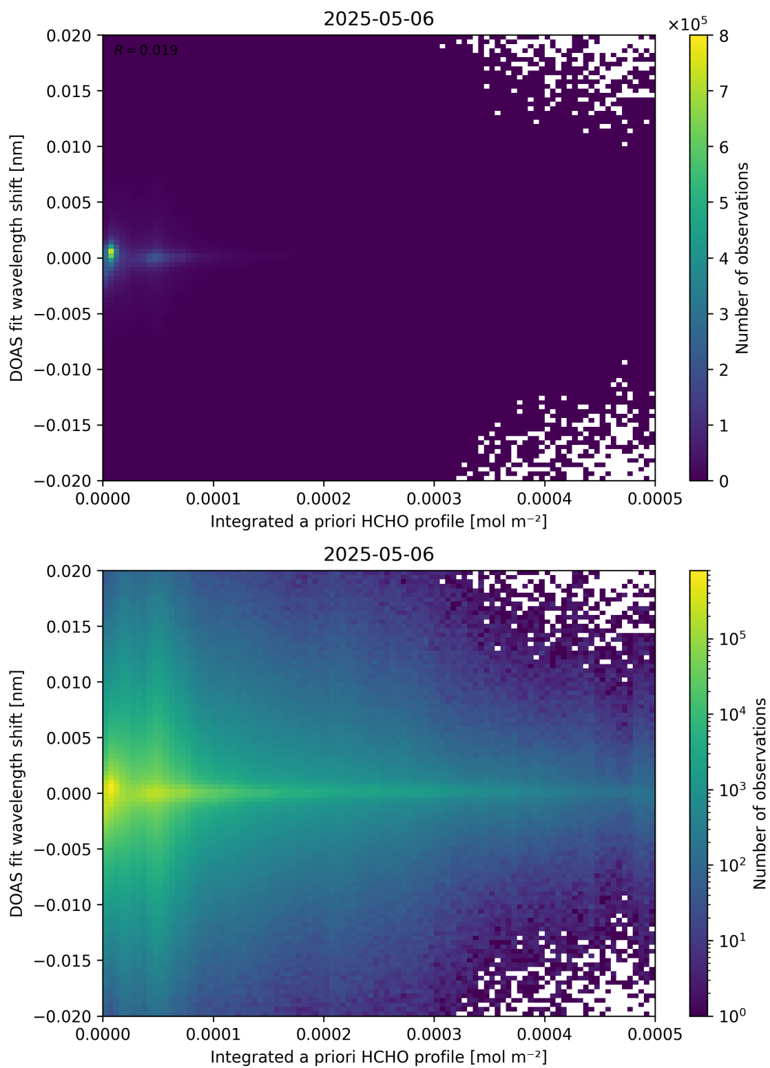
Figure 149: Scatter density plot of “Integrated a priori HCHO profile” against “DOAS fit wavelength shift” for 2025-05-05 to 2025-05-07.
