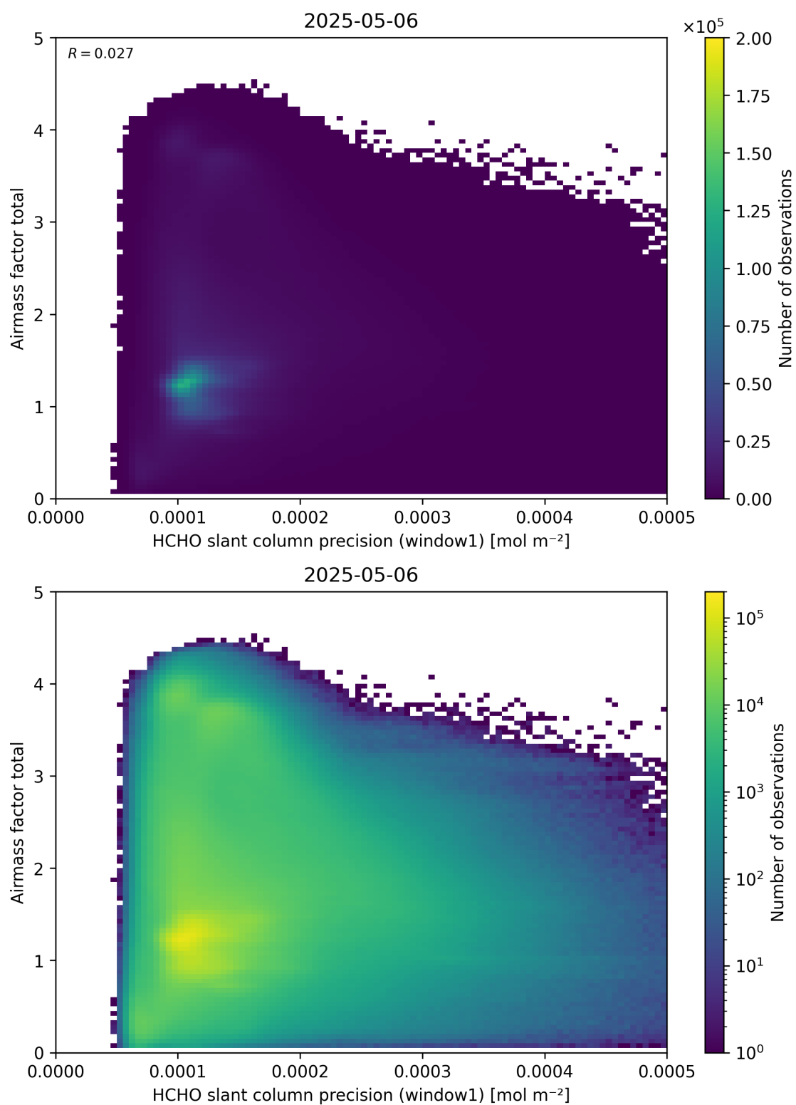
Figure 94: Scatter density plot of “HCHO slant column precision (window1)” against “Airmass factor total” for 2025-05-05 to 2025-05-07.
