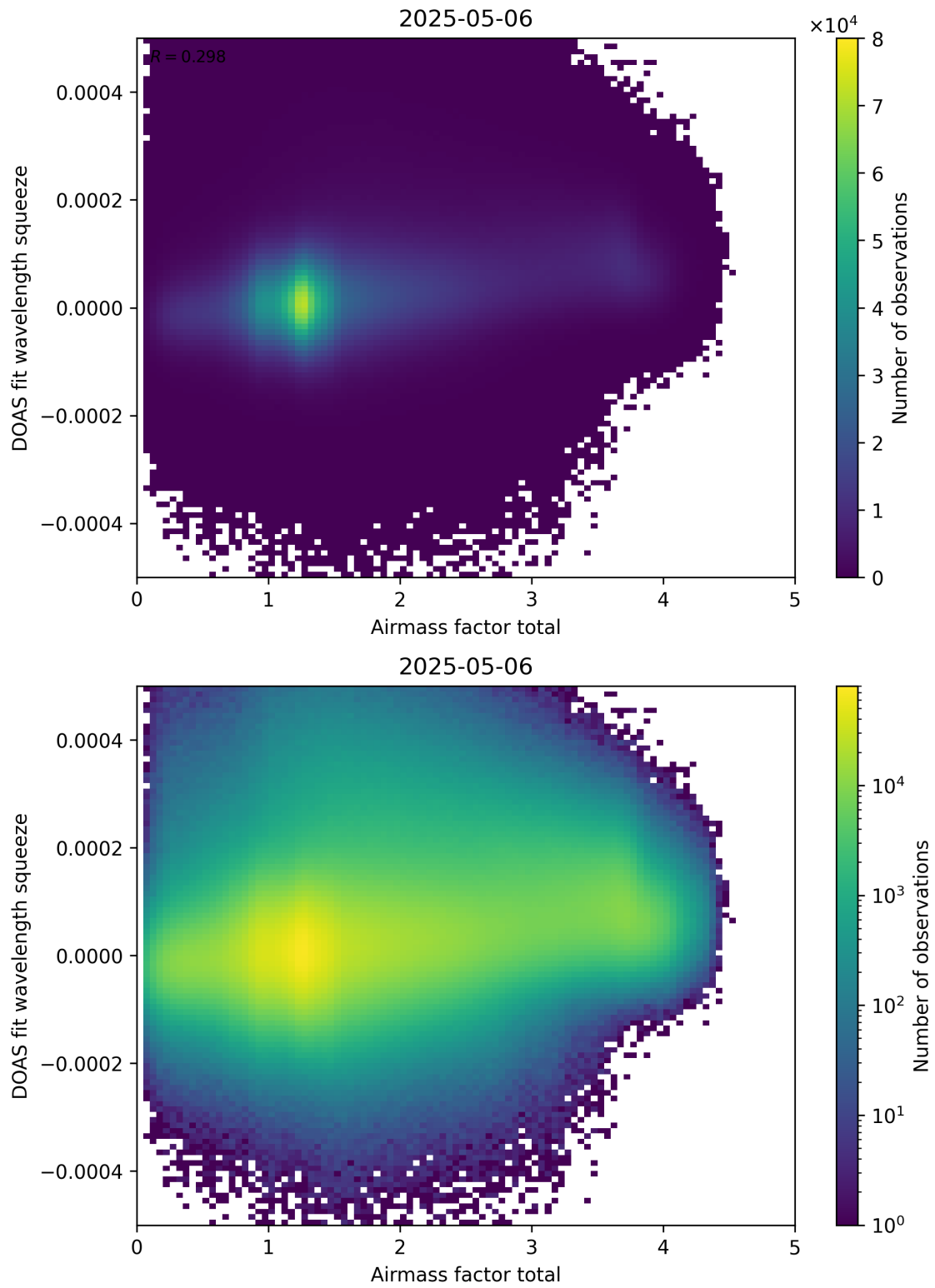
Figure 99: Scatter density plot of “Airmass factor total” against “DOAS fit wavelength squeeze” for 2025-05-05 to 2025-05-07.
