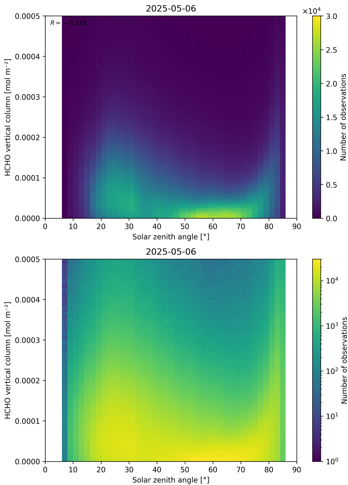
Figure 177: Scatter density plot of “Solar zenith angle” against “HCHO vertical column” for 2025-05-05 to 2025-05-07.
