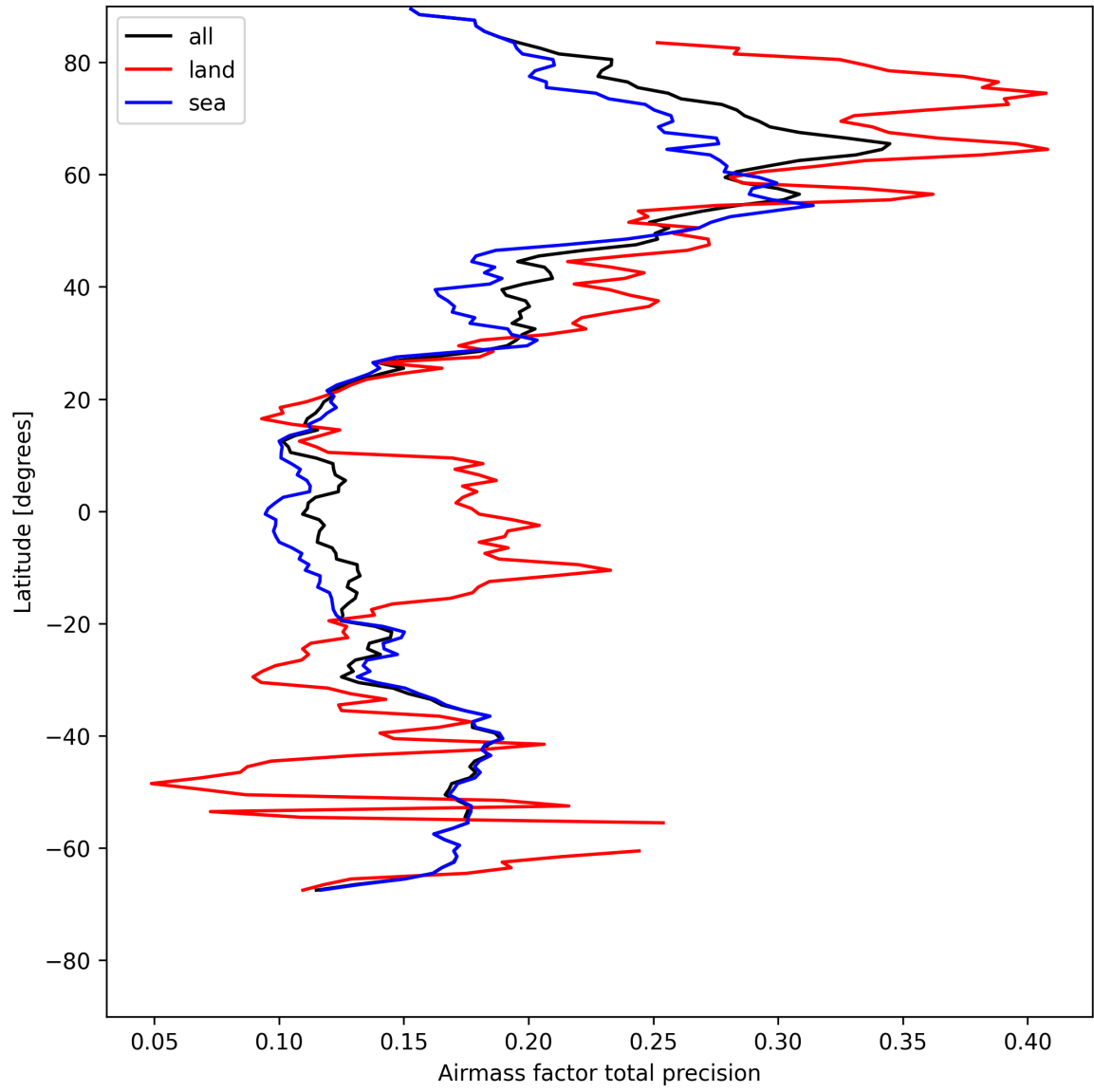
Figure 27: Zonal average of “Airmass factor total precision” for 2025-05-05 to 2025-05-07.
