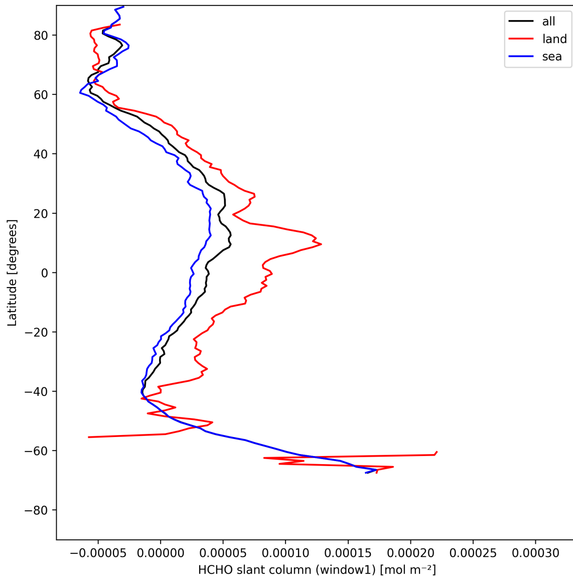
Figure 24: Zonal average of “HCHO slant column (window1)” for 2025-05-05 to 2025-05-07.
