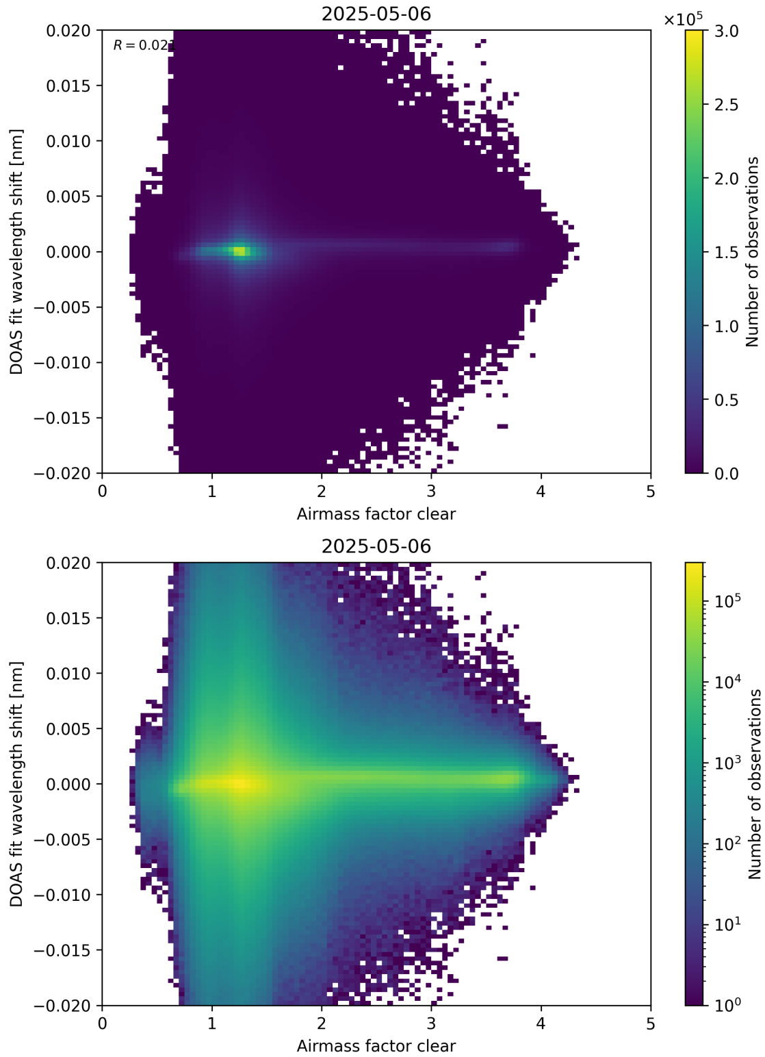
Figure 72: Scatter density plot of “Airmass factor clear” against “DOAS fit wavelength shift” for 2025-05-05 to 2025-05-07.
