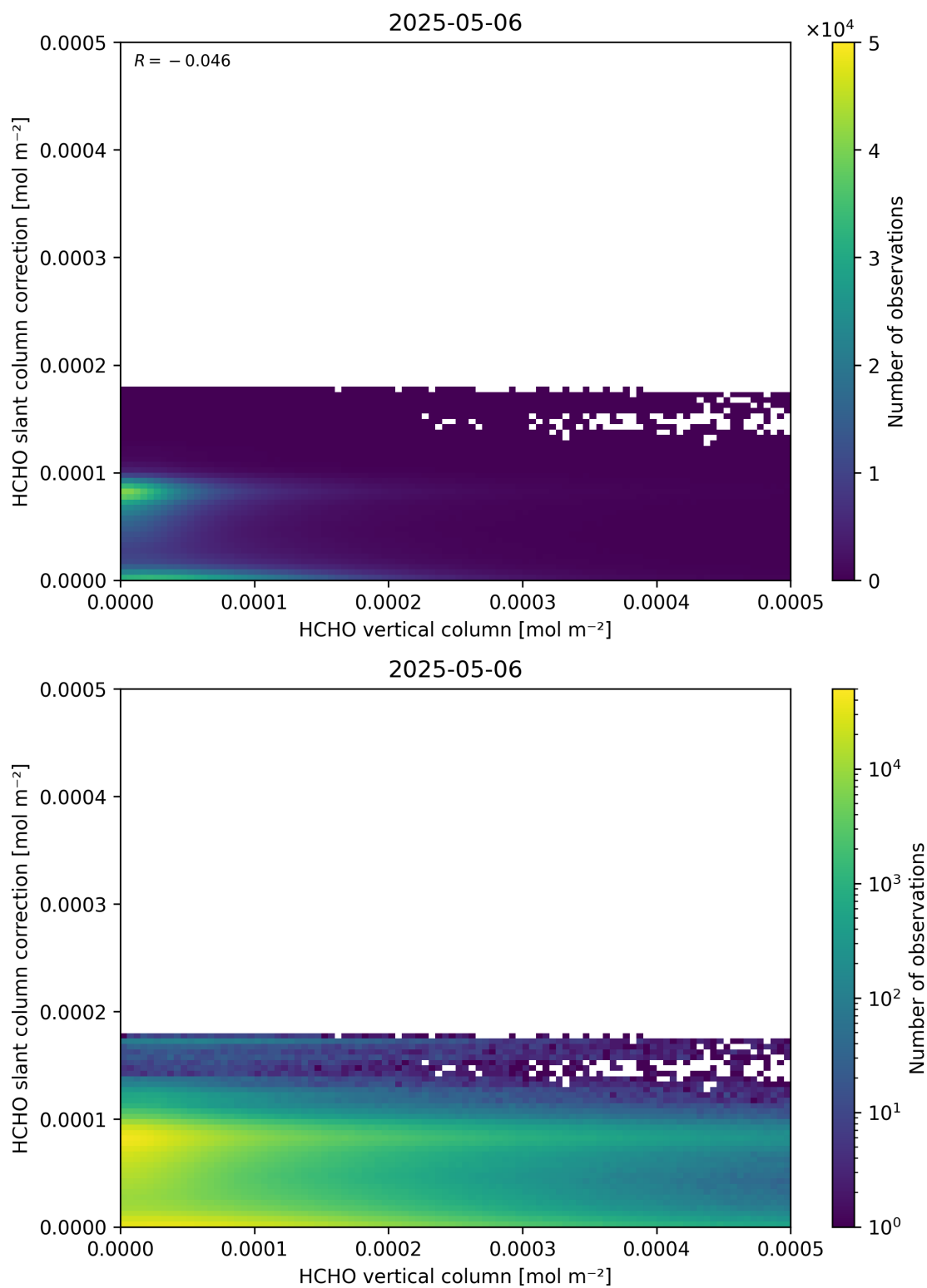
Figure 128: Scatter density plot of “HCHO vertical column” against “HCHO slant column correction” for 2025-05-05 to 2025-05-07.
