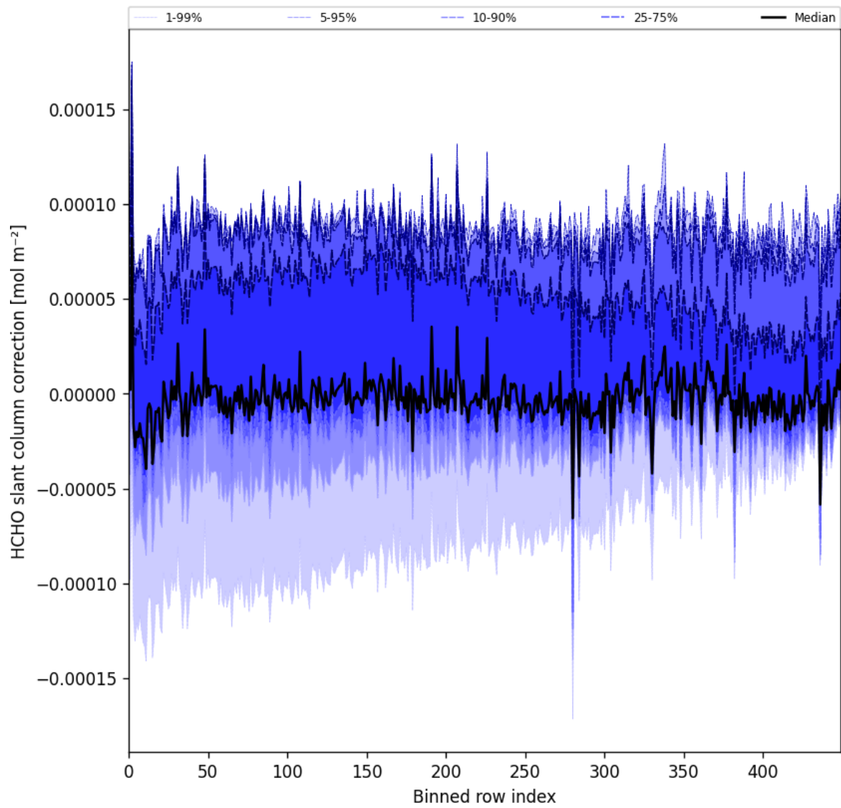
Figure 61: Along track statistics of “HCHO slant column correction” for 2025-05-05 to 2025-05-07
