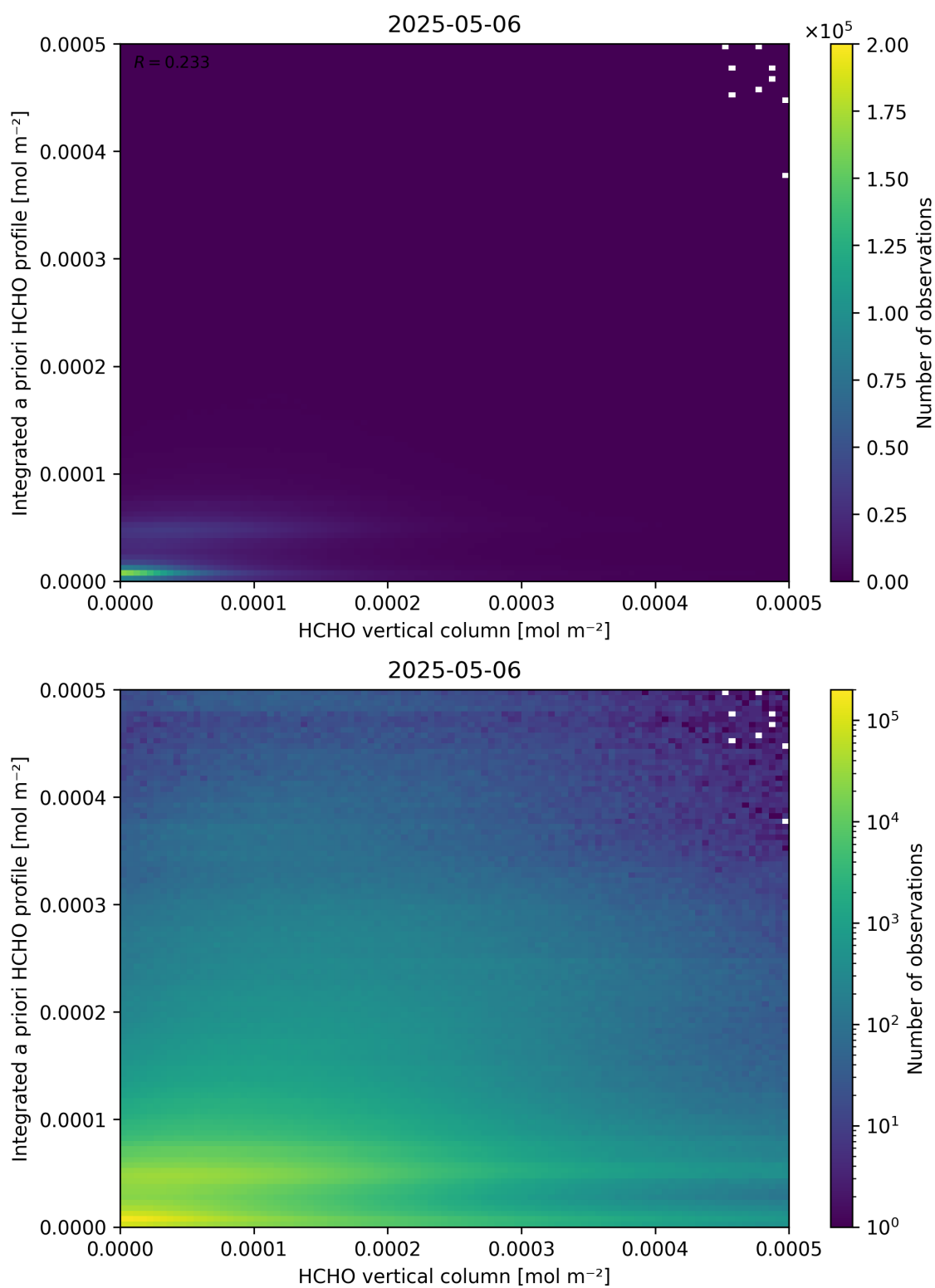
Figure 135: Scatter density plot of “HCHO vertical column” against “Integrated a priori HCHO profile” for 2025-05-05 to 2025-05-07.
