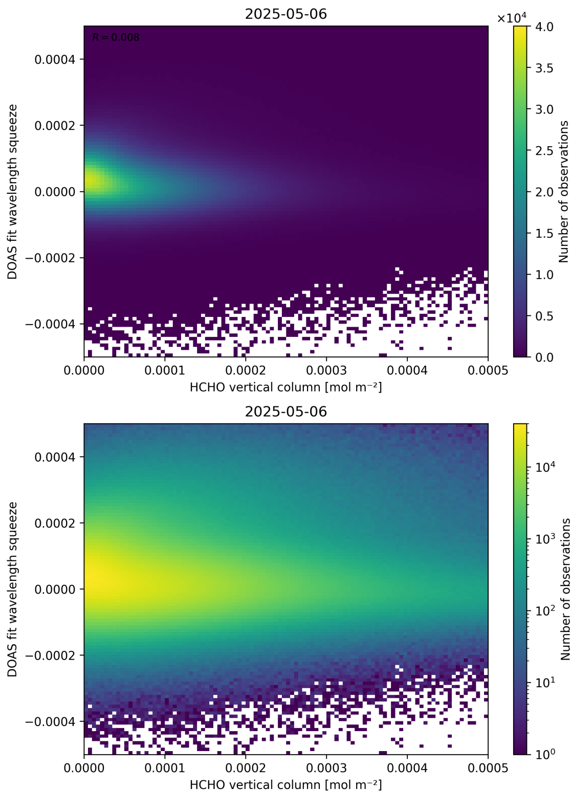
Figure 125: Scatter density plot of “HCHO vertical column” against “DOAS fit wavelength squeeze” for 2025-05-05 to 2025-05-07.
