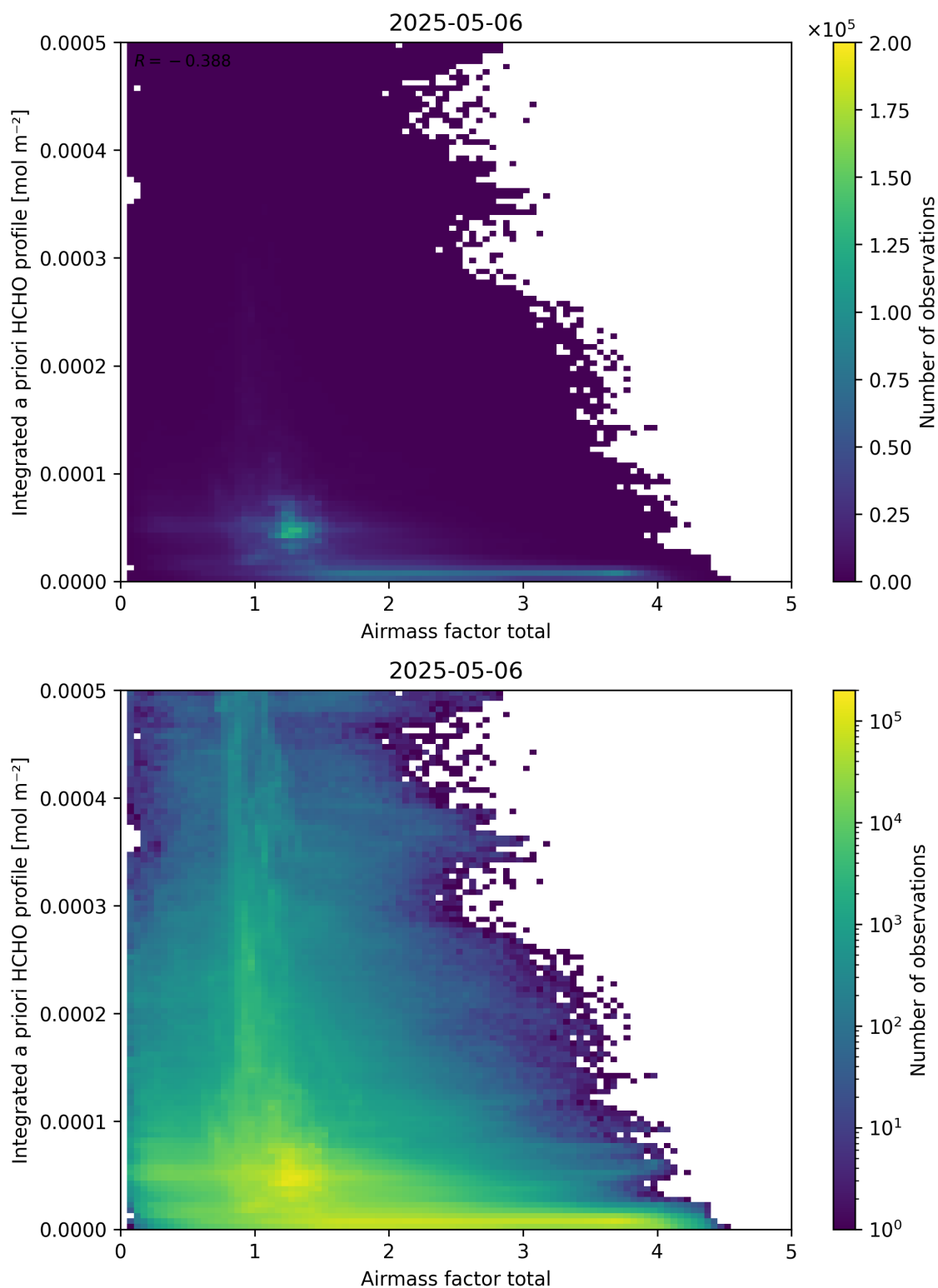
Figure 104: Scatter density plot of “Airmass factor total” against “Integrated a priori HCHO profile” for 2025-05-05 to 2025-05-07.
