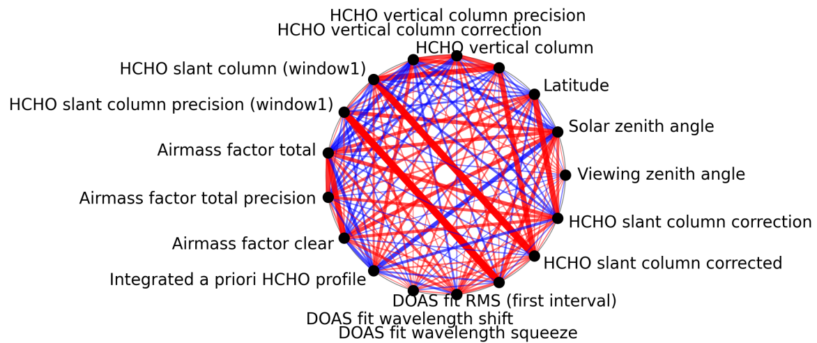
Figure 1: Map of correlation graph for 2025-05-05 to 2025-05-07.
