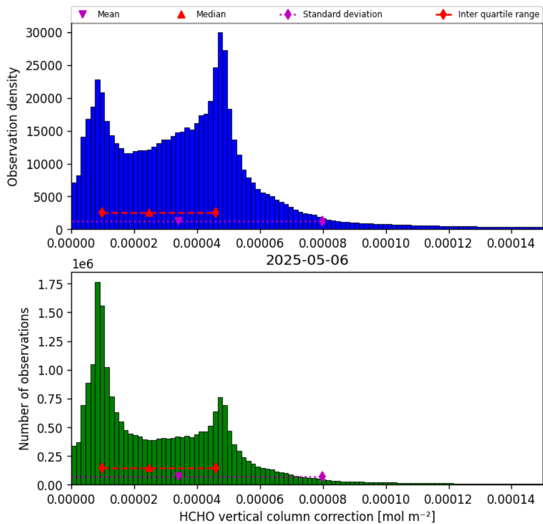
Figure 37: Histogram of “HCHO vertical column correction” for 2025-05-05 to 2025-05-07
