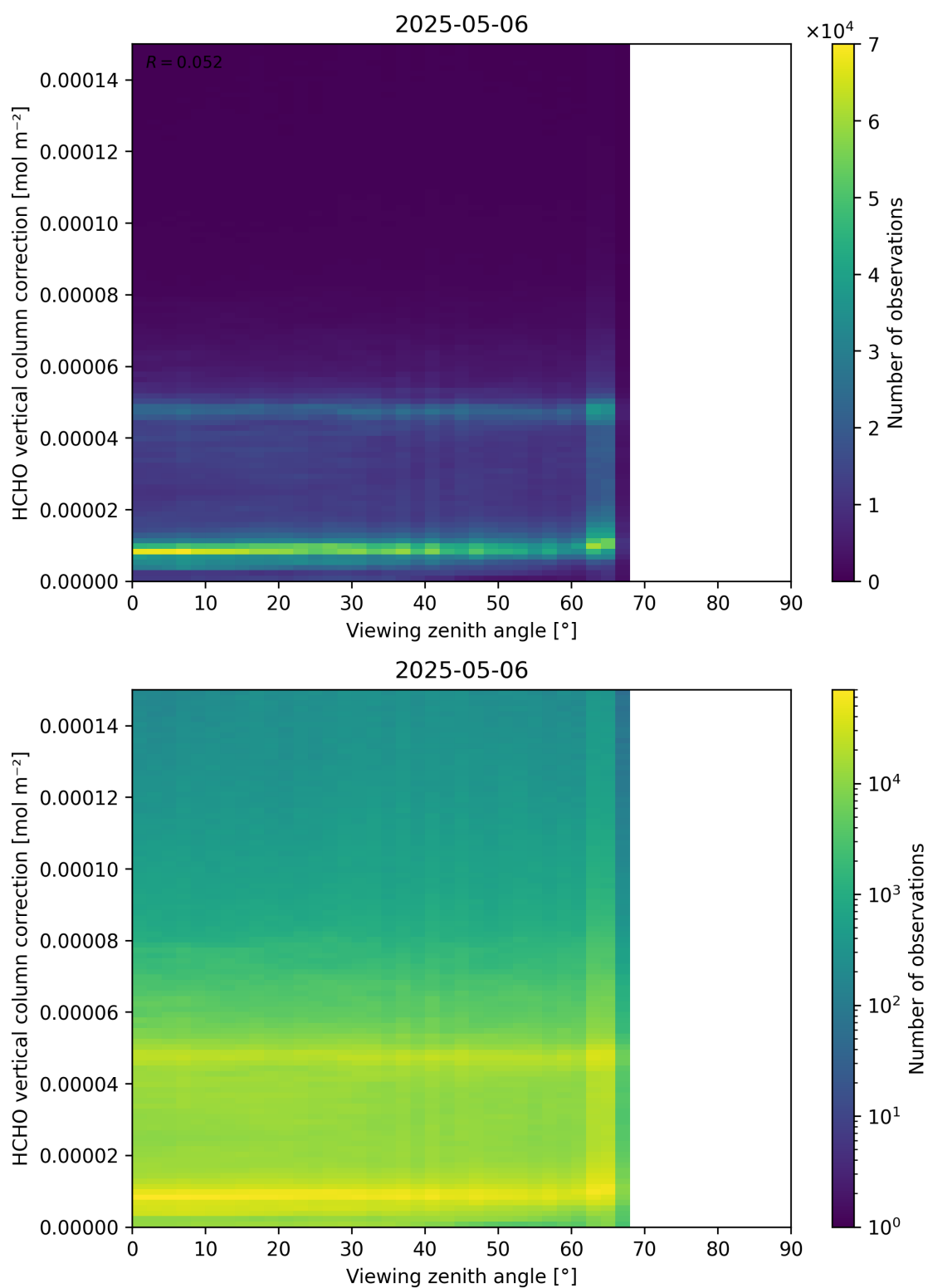
Figure 193: Scatter density plot of “Viewing zenith angle” against “HCHO vertical column correction” for 2025-05-05 to 2025-05-07.
