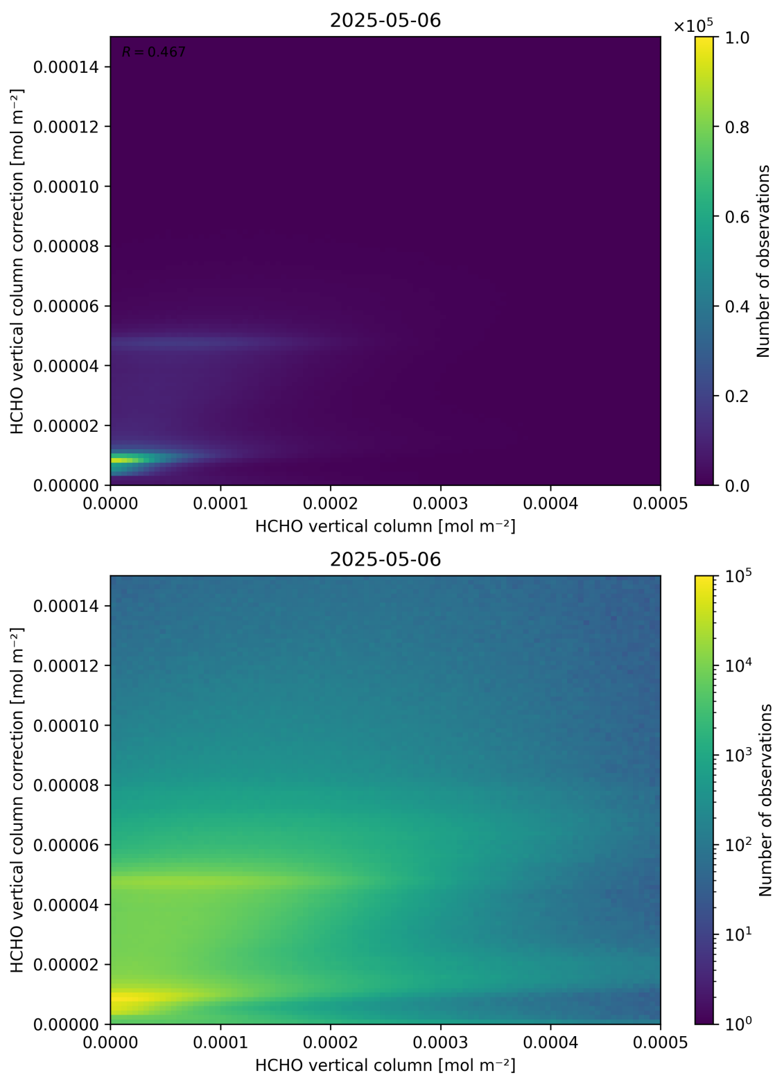
Figure 133: Scatter density plot of “HCHO vertical column” against “HCHO vertical column correction” for 2025-05-05 to 2025-05-07.
