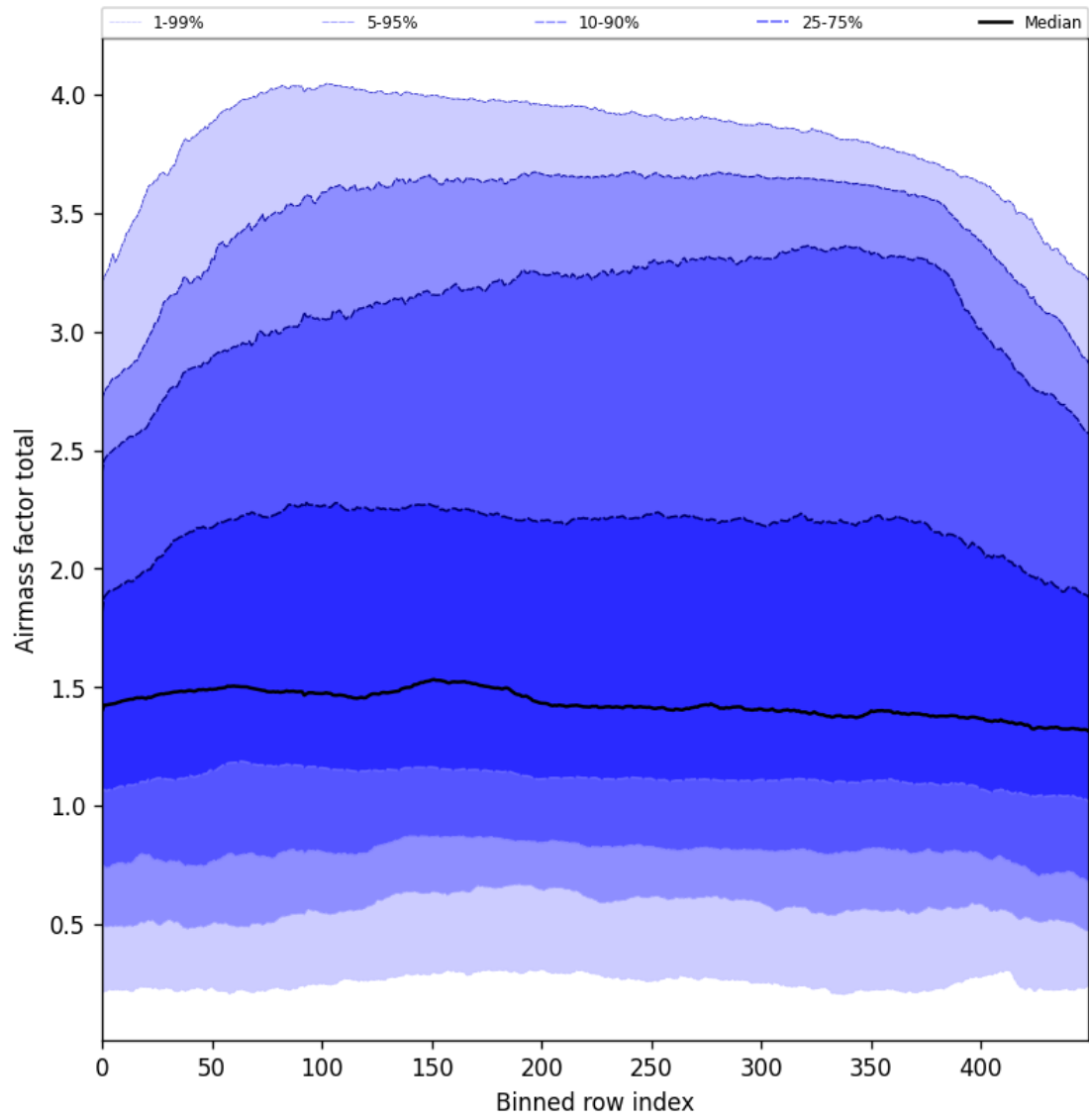
Figure 54: Along track statistics of “Airmass factor total” for 2025-05-05 to 2025-05-07
