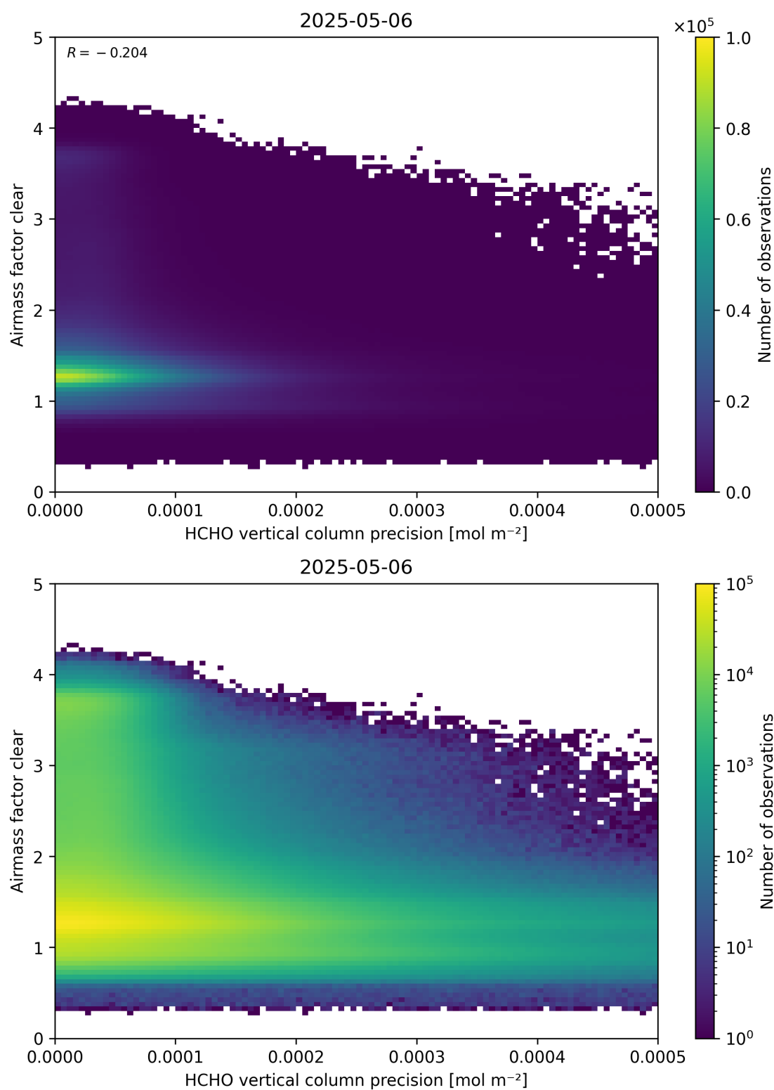
Figure 139: Scatter density plot of “HCHO vertical column precision” against “Airmass factor clear” for 2025-05-05 to 2025-05-07.
