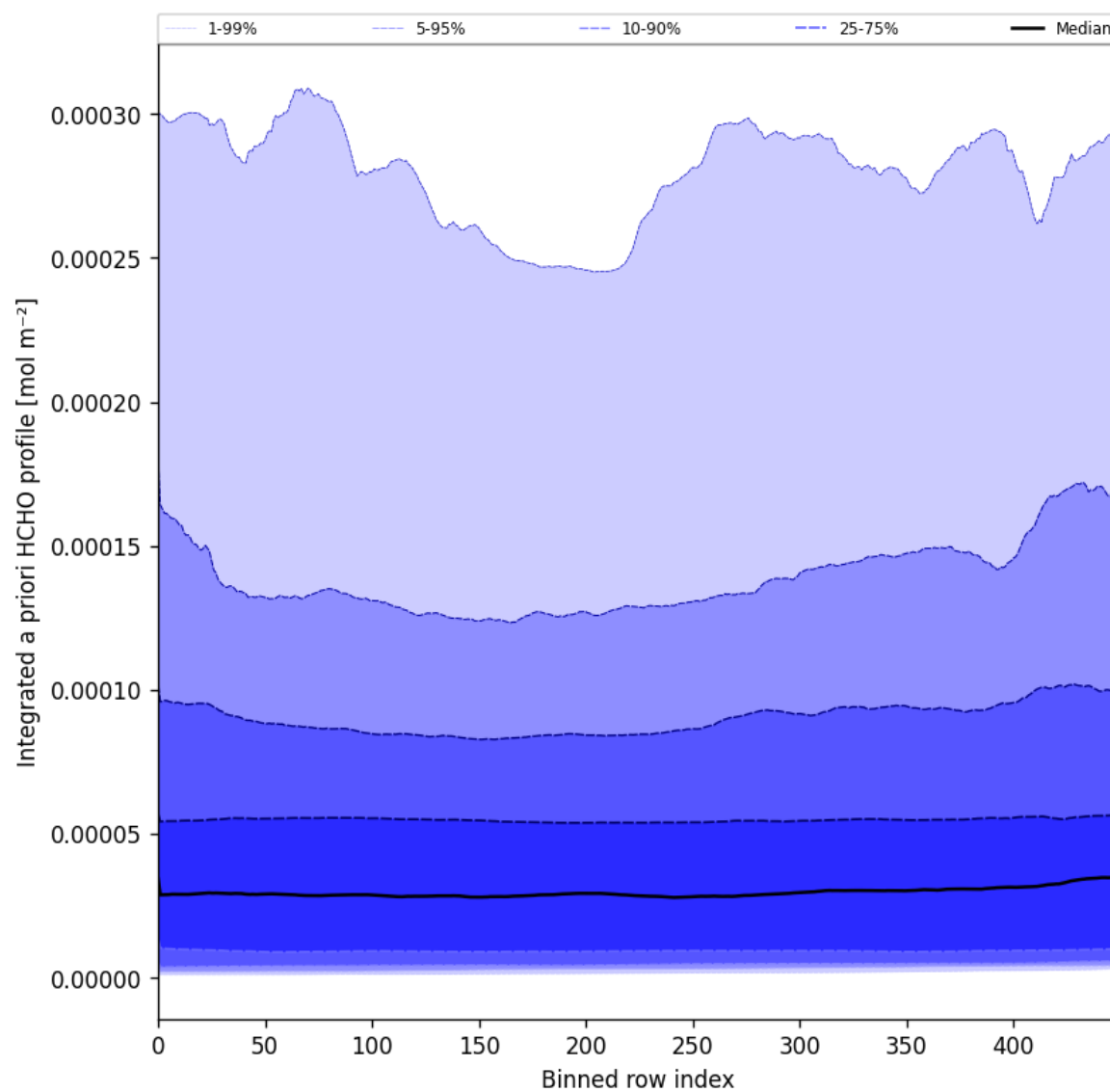
Figure 57: Along track statistics of "Integrated a priori HCHO profile" for 2025-05-05 to 2025-05-07
