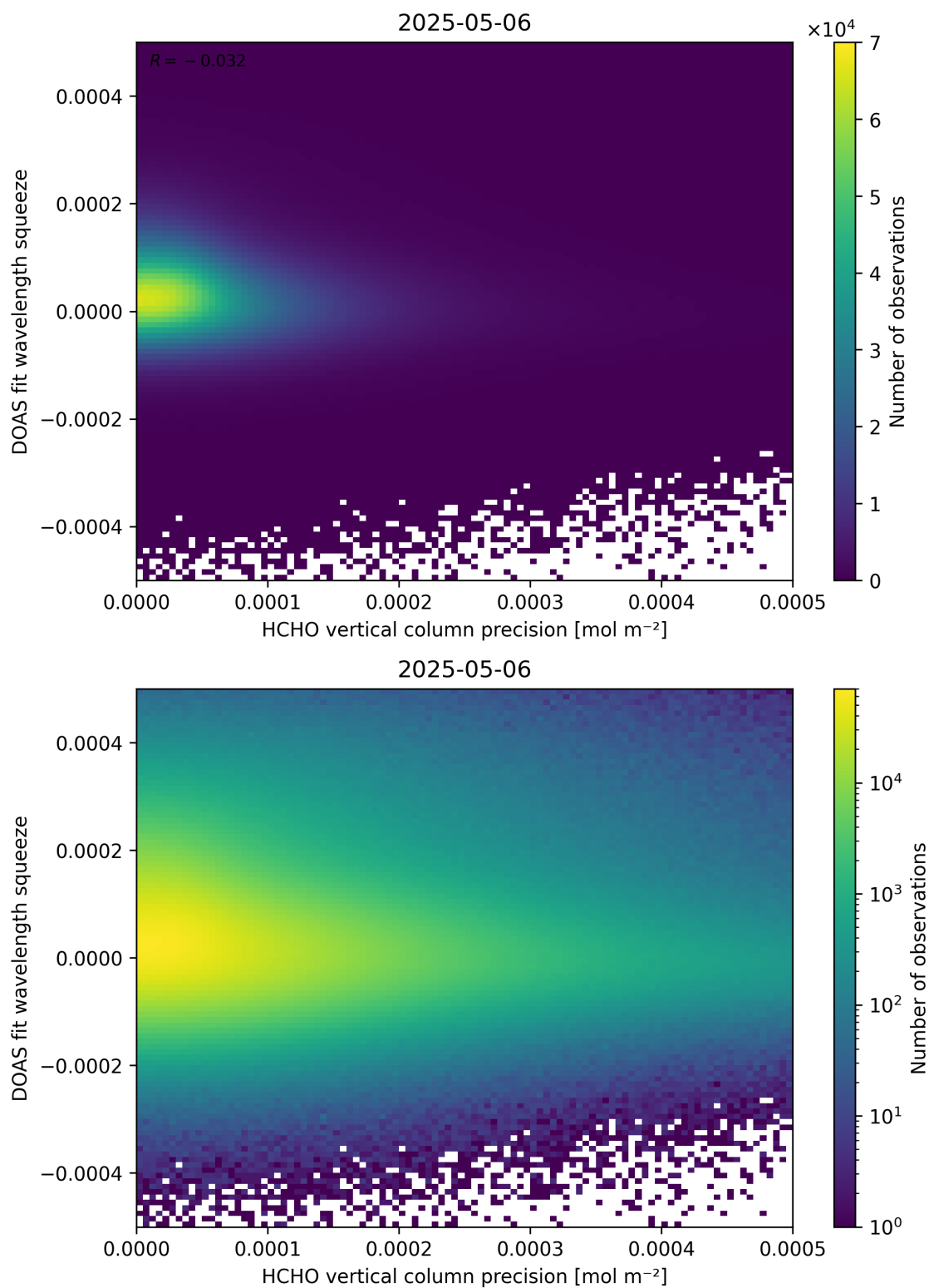
Figure 138: Scatter density plot of “HCHO vertical column precision” against “DOAS fit wavelength squeeze” for 2025-05-05 to 2025-05-07.
