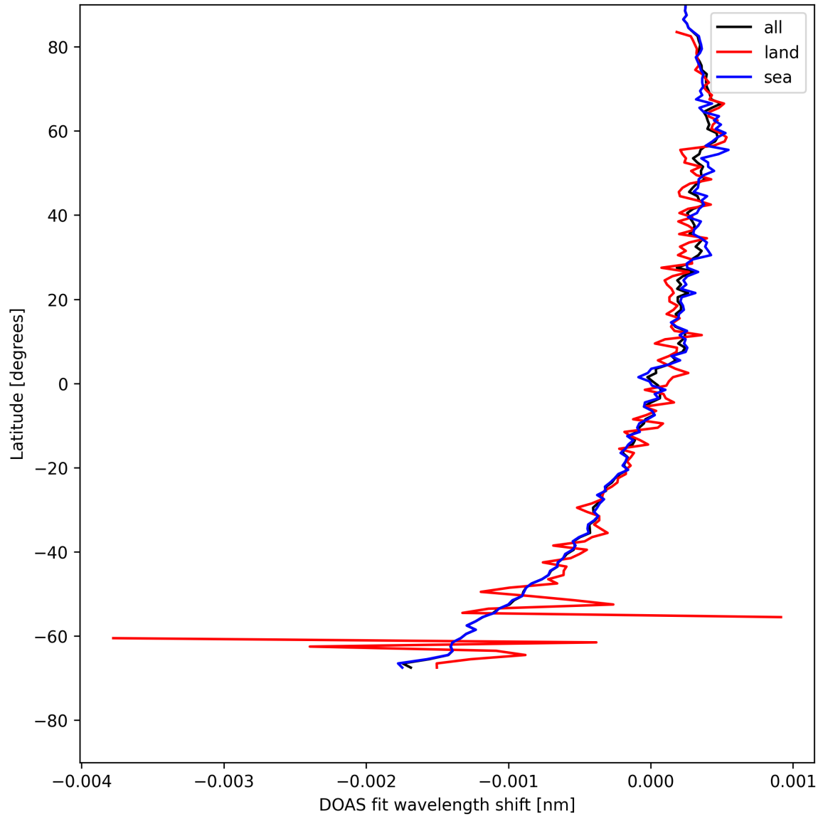
Figure 30: Zonal average of “DOAS fit wavelength shift” for 2025-05-05 to 2025-05-07.
