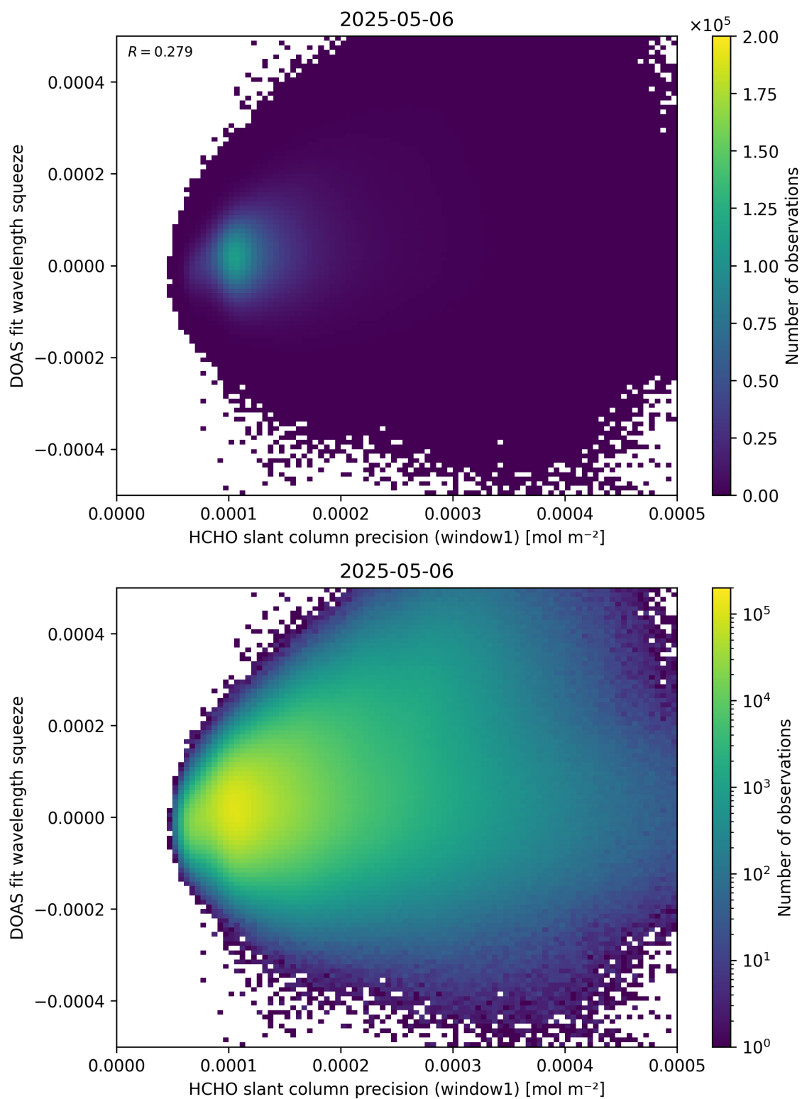
Figure 90: Scatter density plot of “HCHO slant column precision (window1)” against “DOAS fit wavelength squeeze” for 2025-05-05 to 2025-05-07.
