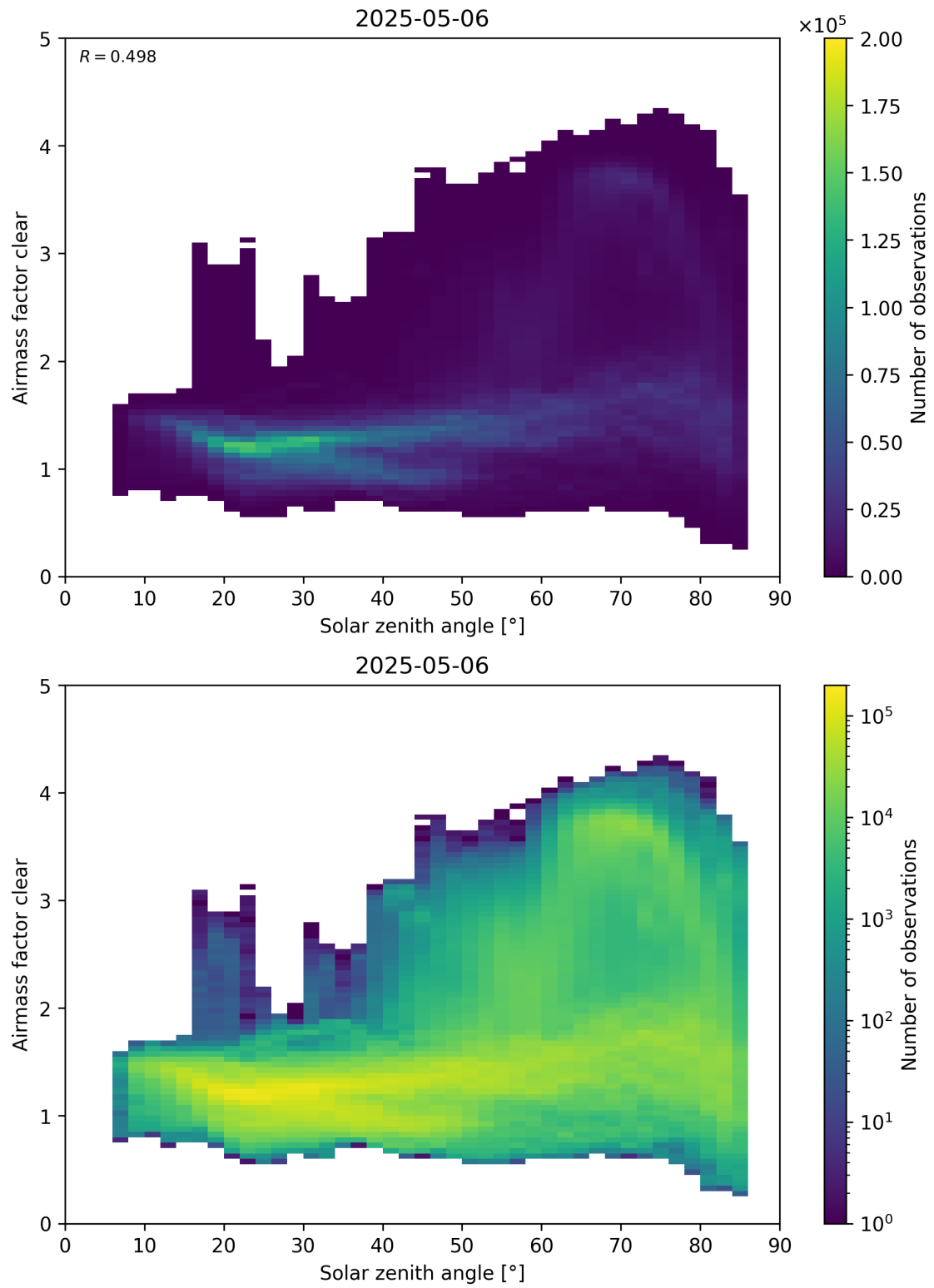
Figure 170: Scatter density plot of “Solar zenith angle” against “Airmass factor clear” for 2025-05-05 to 2025-05-07.
