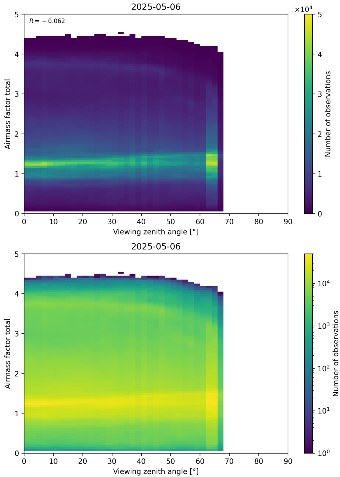
Figure 190: Scatter density plot of “Viewing zenith angle” against “Airmass factor total” for 2025-05-05 to 2025-05-07.
