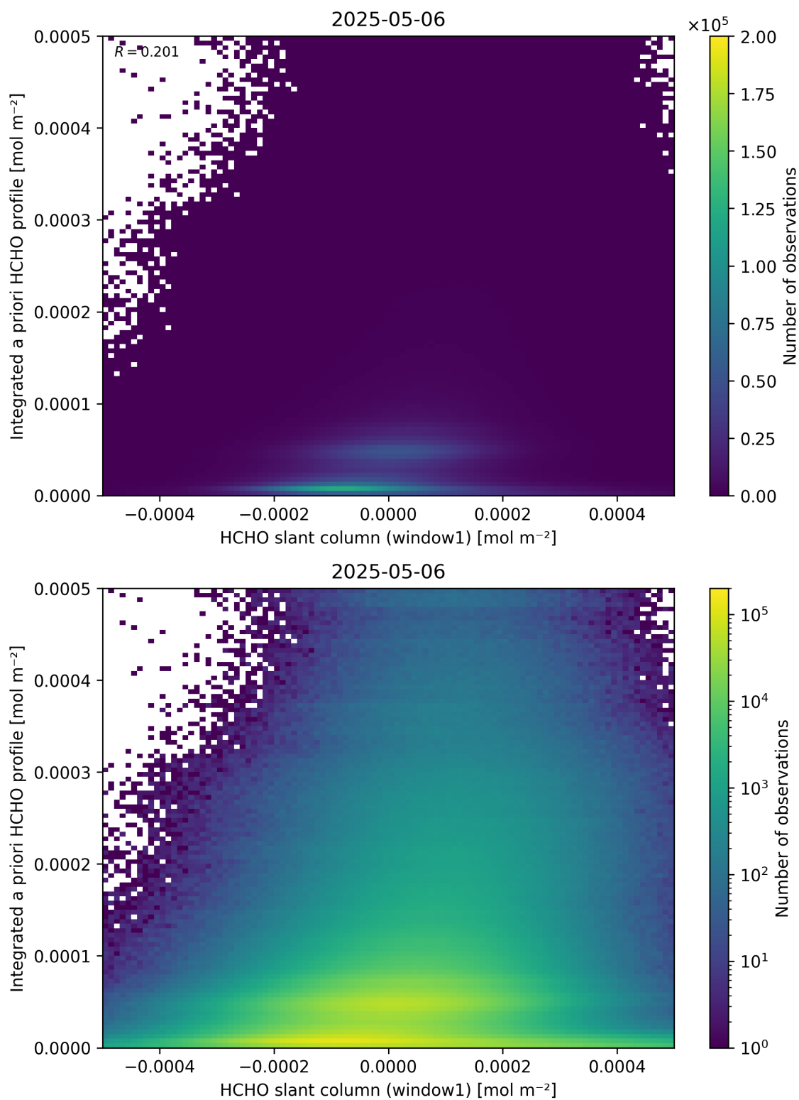
Figure 87: Scatter density plot of “HCHO slant column (window1)” against “Integrated a priori HCHO profile” for 2025-05-05 to 2025-05-07.
