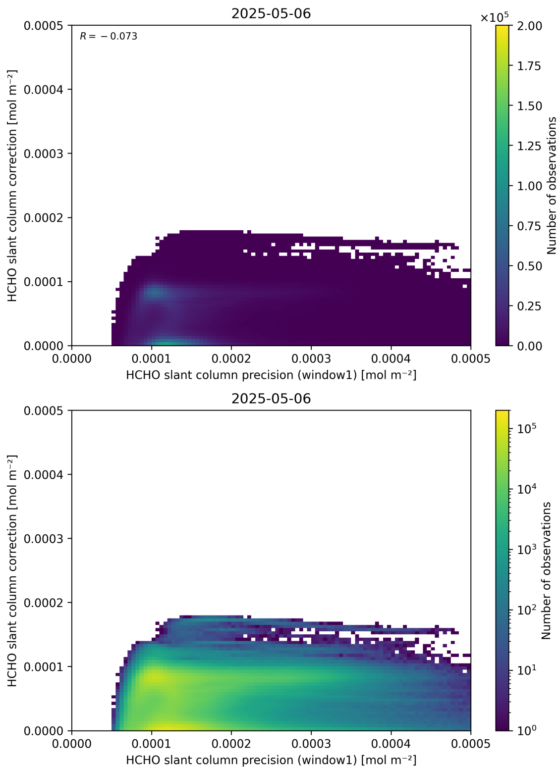
Figure 93: Scatter density plot of “HCHO slant column precision (window1)” against “HCHO slant column correction” for 2025-05-05 to 2025-05-07.
