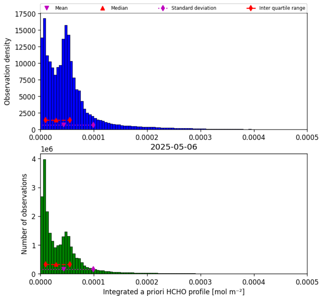
Figure 43: Histogram of “Integrated a priori HCHO profile” for 2025-05-05 to 2025-05-07
