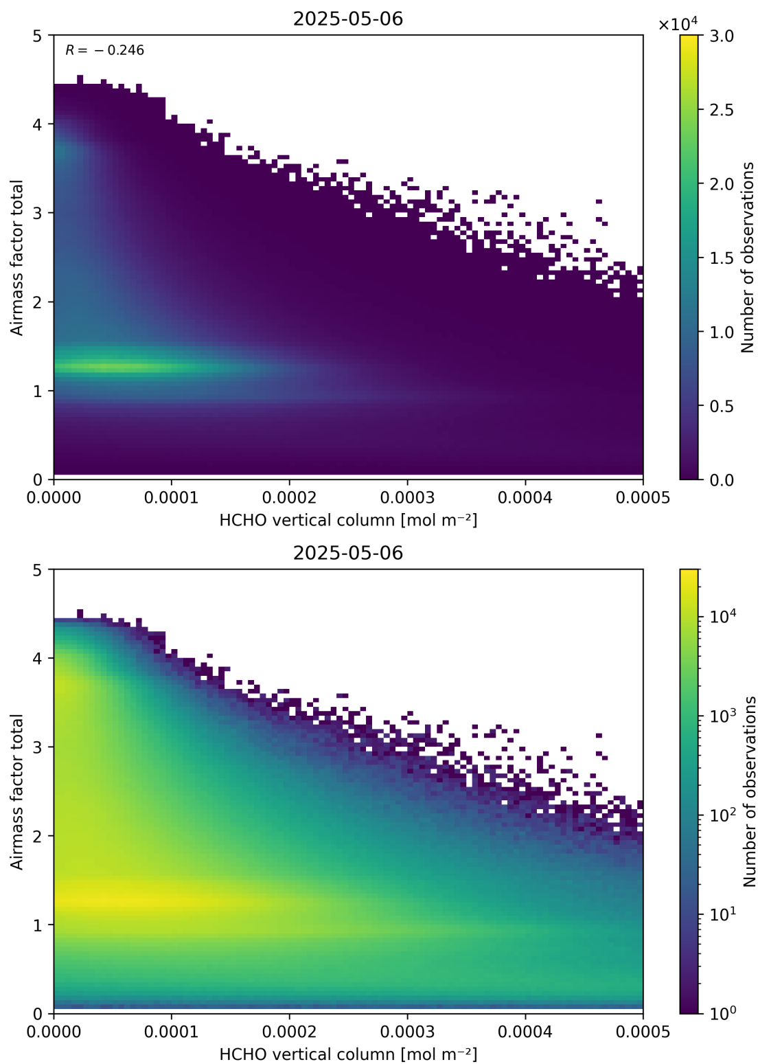
Figure 131: Scatter density plot of “HCHO vertical column” against “Airmass factor total” for 2025-05-05 to 2025-05-07.
