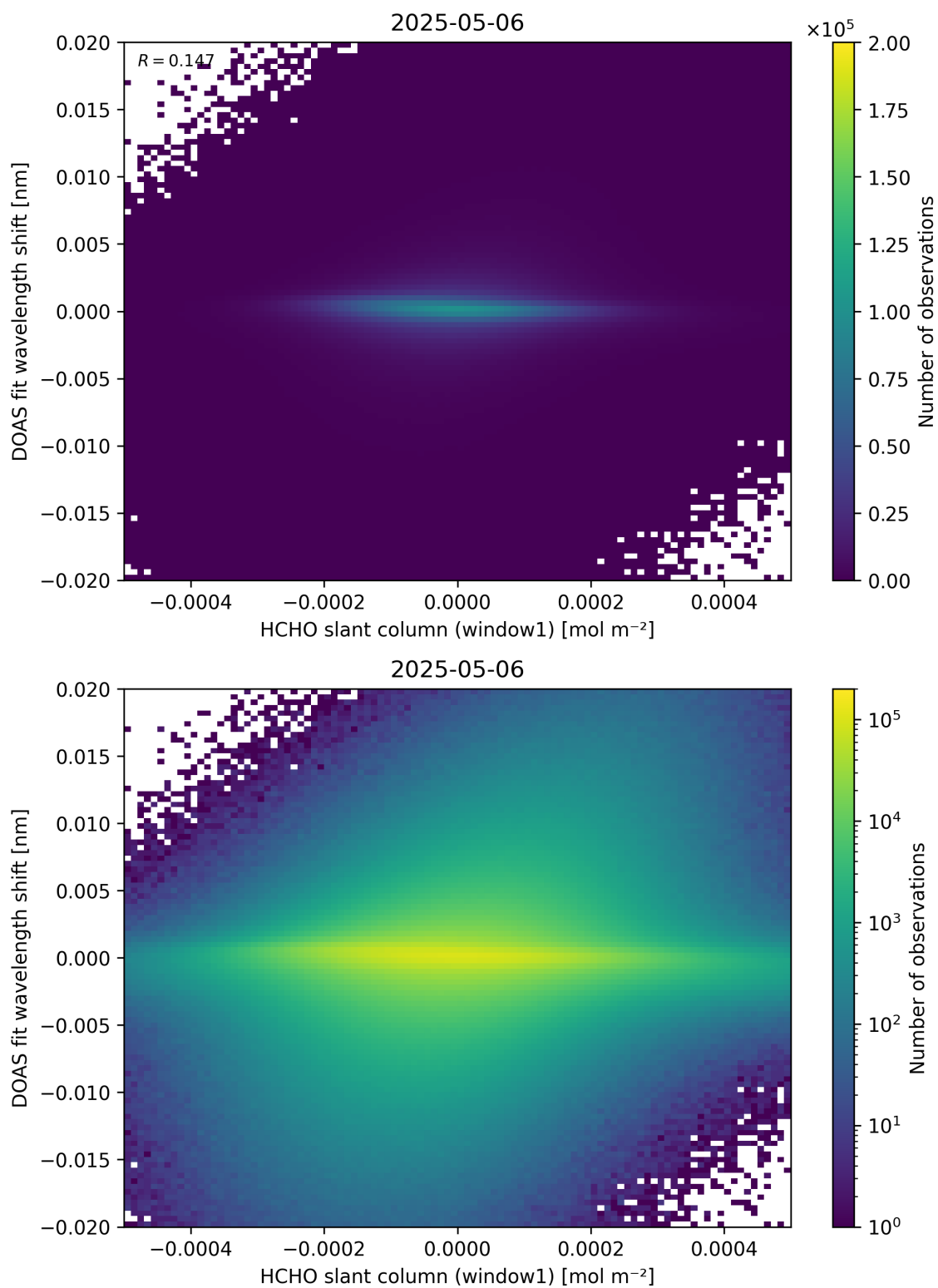
Figure 79: Scatter density plot of “HCHO slant column (window1)” against “DOAS fit wavelength shift” for 2025-05-05 to 2025-05-07.
