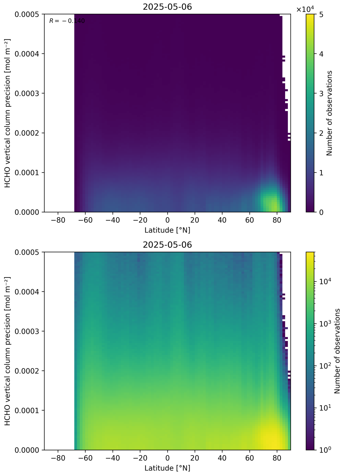
Figure 165: Scatter density plot of “Latitude” against “HCHO vertical column precision” for 2025-05-05 to 2025-05-07.
