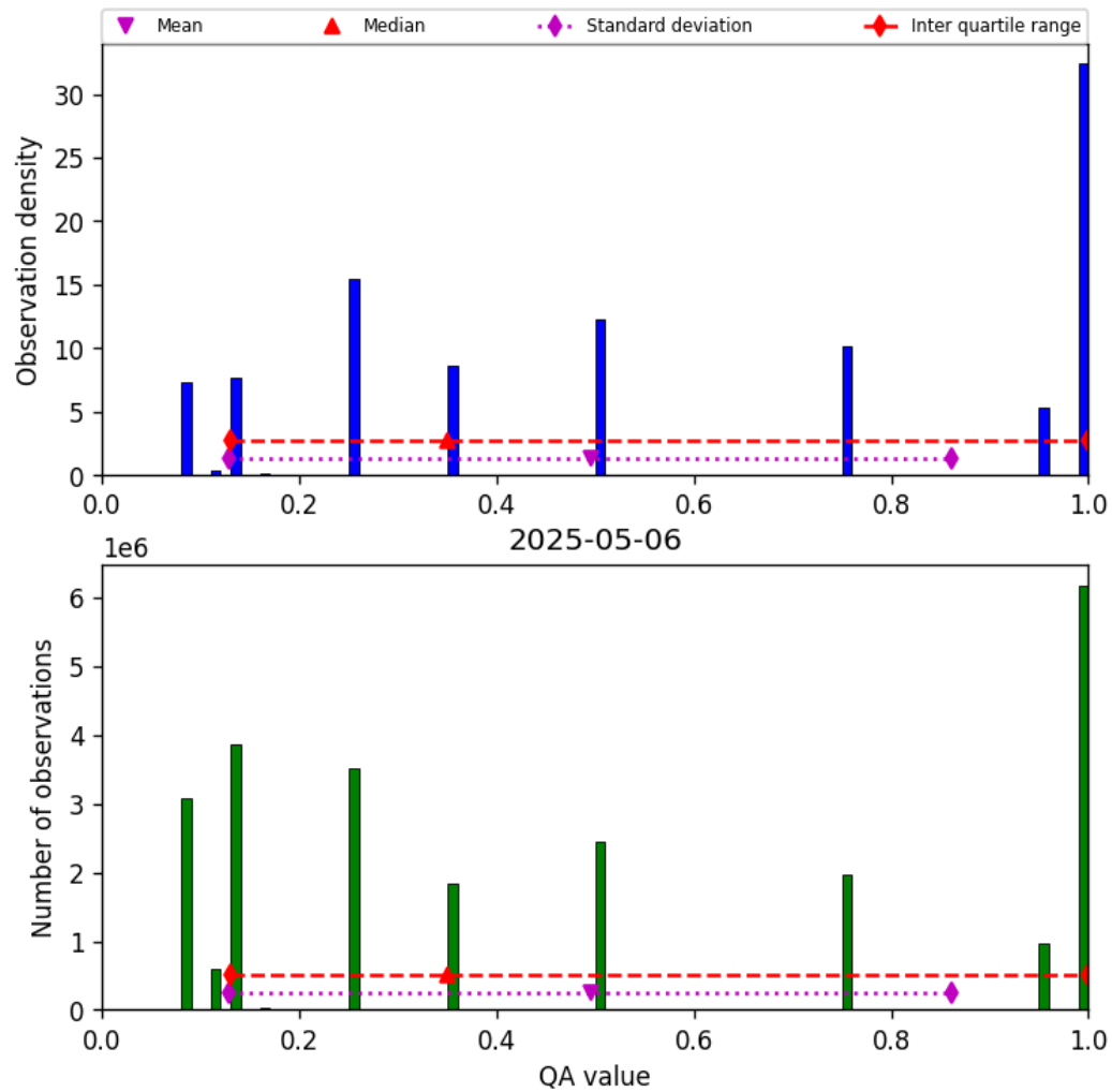
Figure 34: Histogram of “QA value” for 2025-05-05 to 2025-05-07
