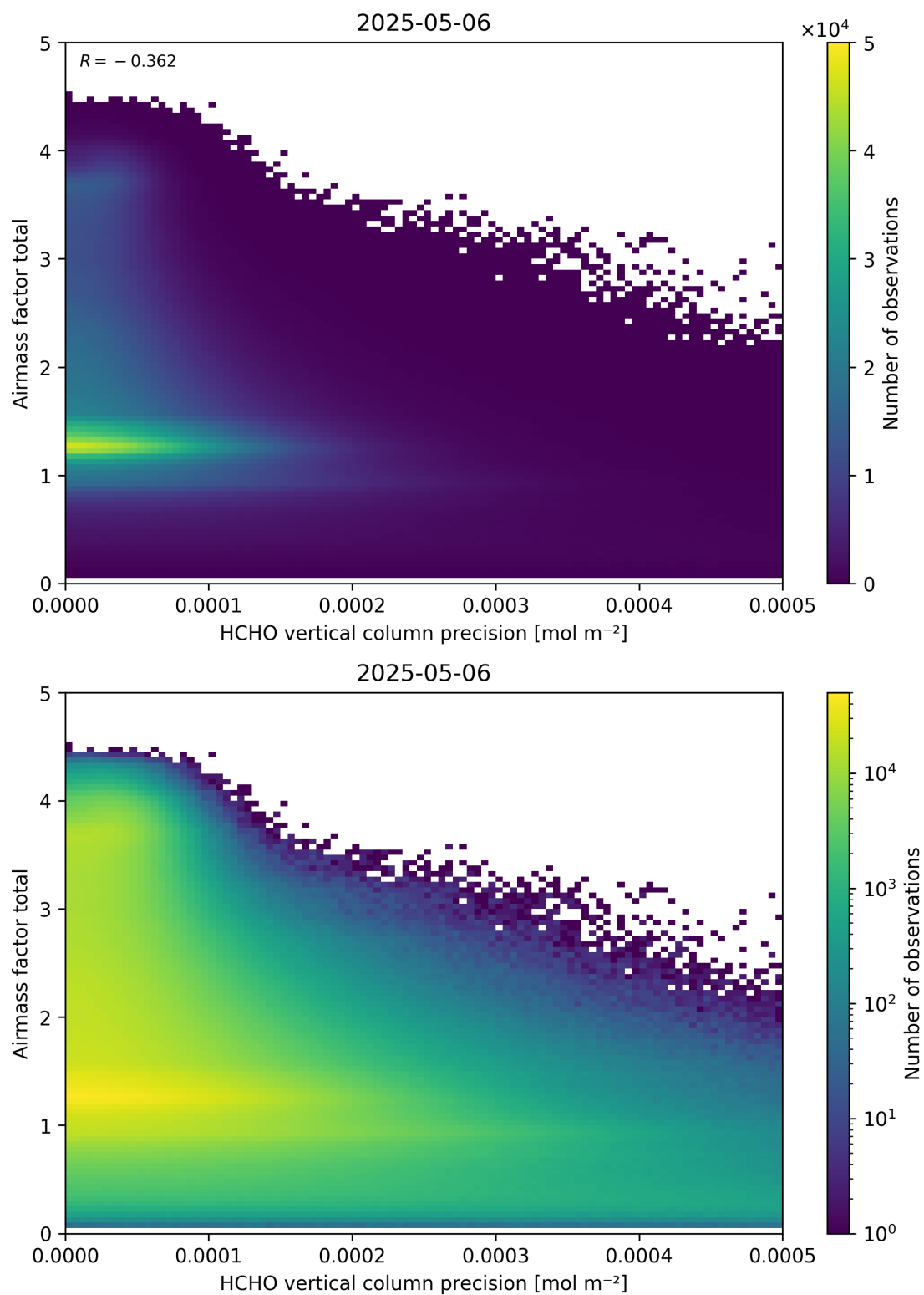
Figure 144: Scatter density plot of “HCHO vertical column precision” against “Airmass factor total” for 2025-05-05 to 2025-05-07.
