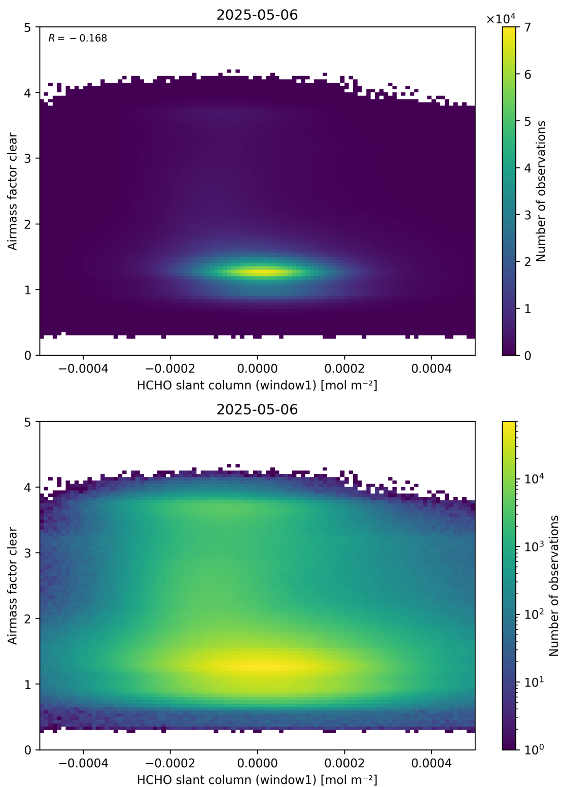
Figure 81: Scatter density plot of “HCHO slant column (window1)” against “Airmass factor clear” for 2025-05-05 to 2025-05-07.
