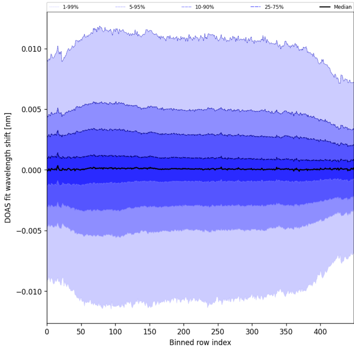
Figure 58: Along track statistics of “DOAS fit wavelength shift” for 2025-05-05 to 2025-05-07
