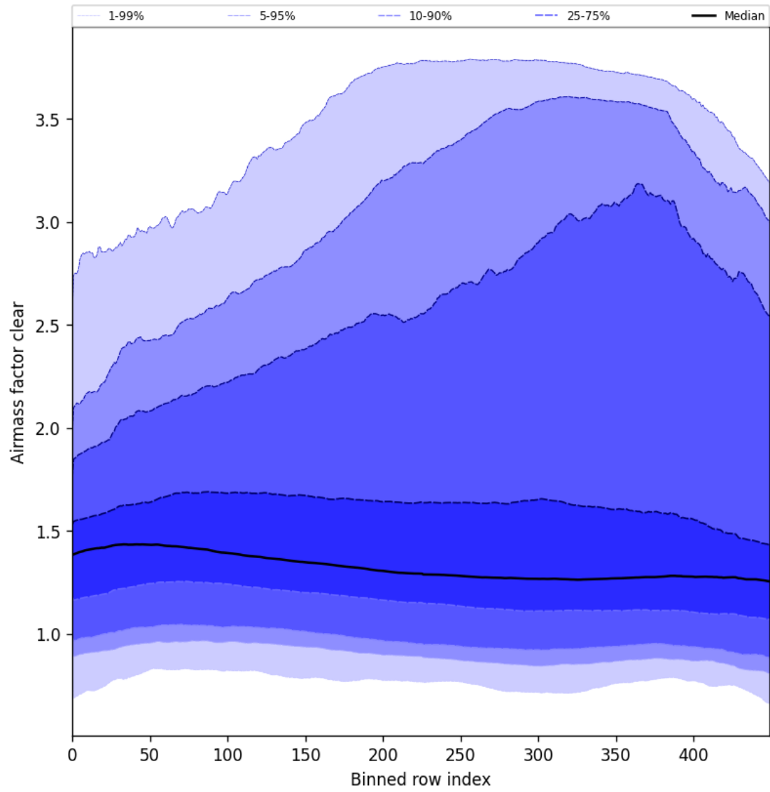
Figure 56: Along track statistics of “Airmass factor clear” for 2025-05-05 to 2025-05-07
