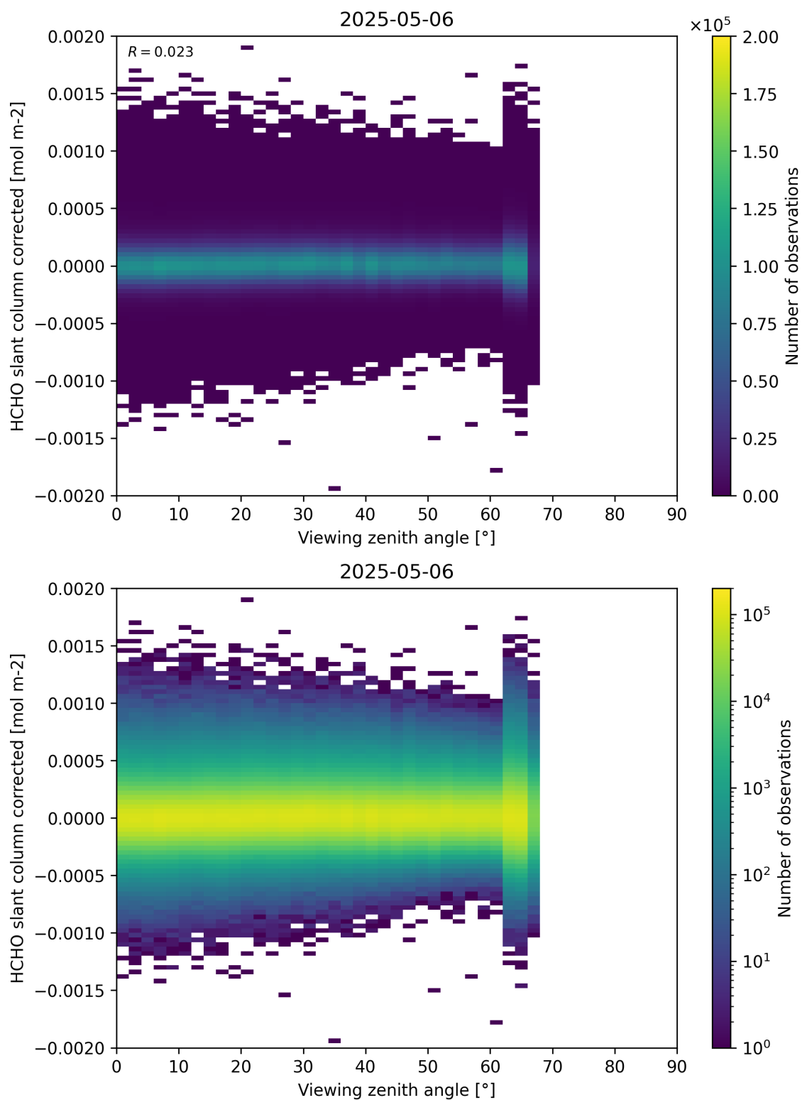
Figure 186: Scatter density plot of “Viewing zenith angle” against “HCHO slant column corrected” for 2025-05-05 to 2025-05-07.
