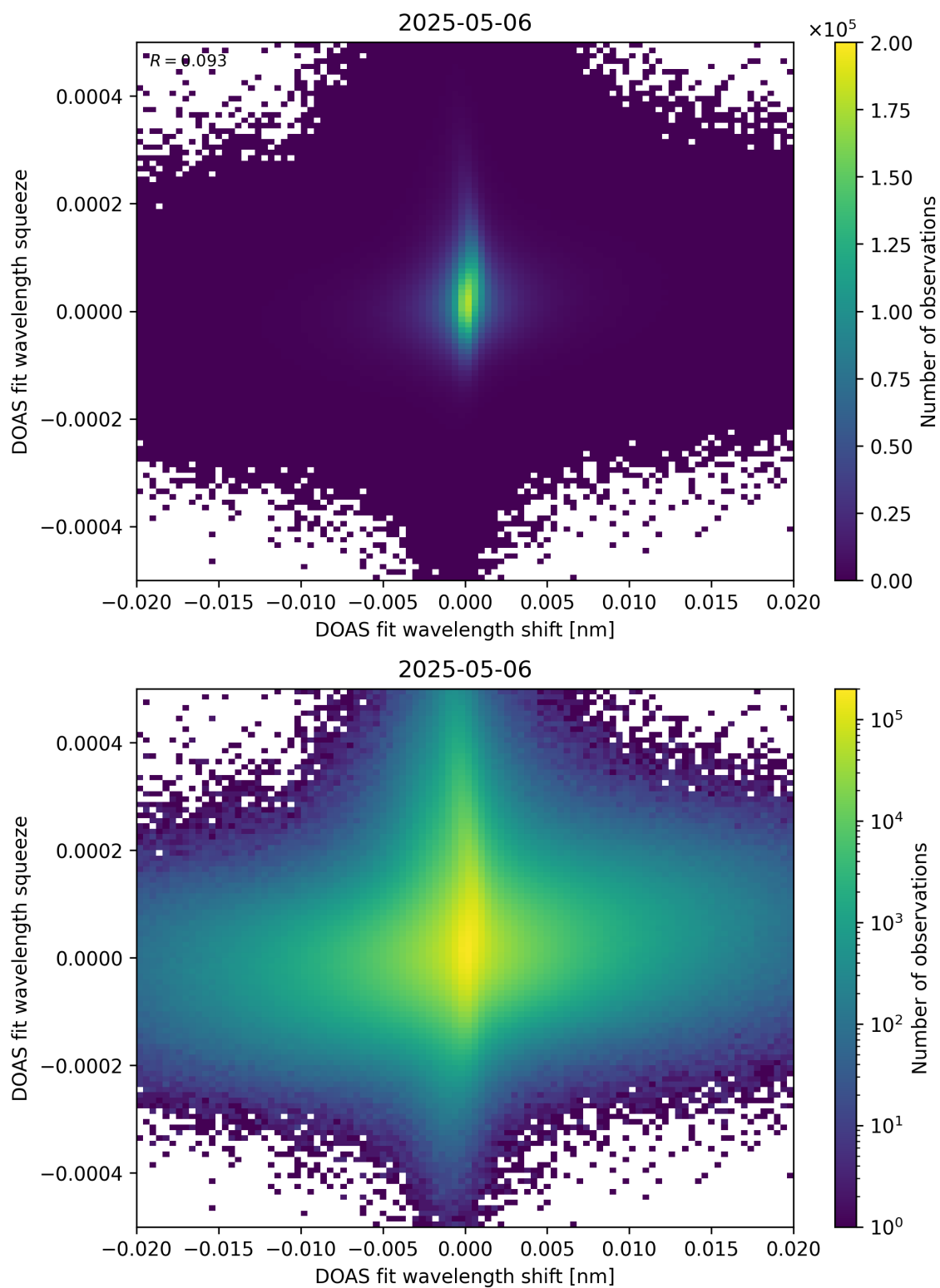
Figure 65: Scatter density plot of “DOAS fit wavelength shift” against “DOAS fit wavelength squeeze” for 2025-05-05 to 2025-05-07.
