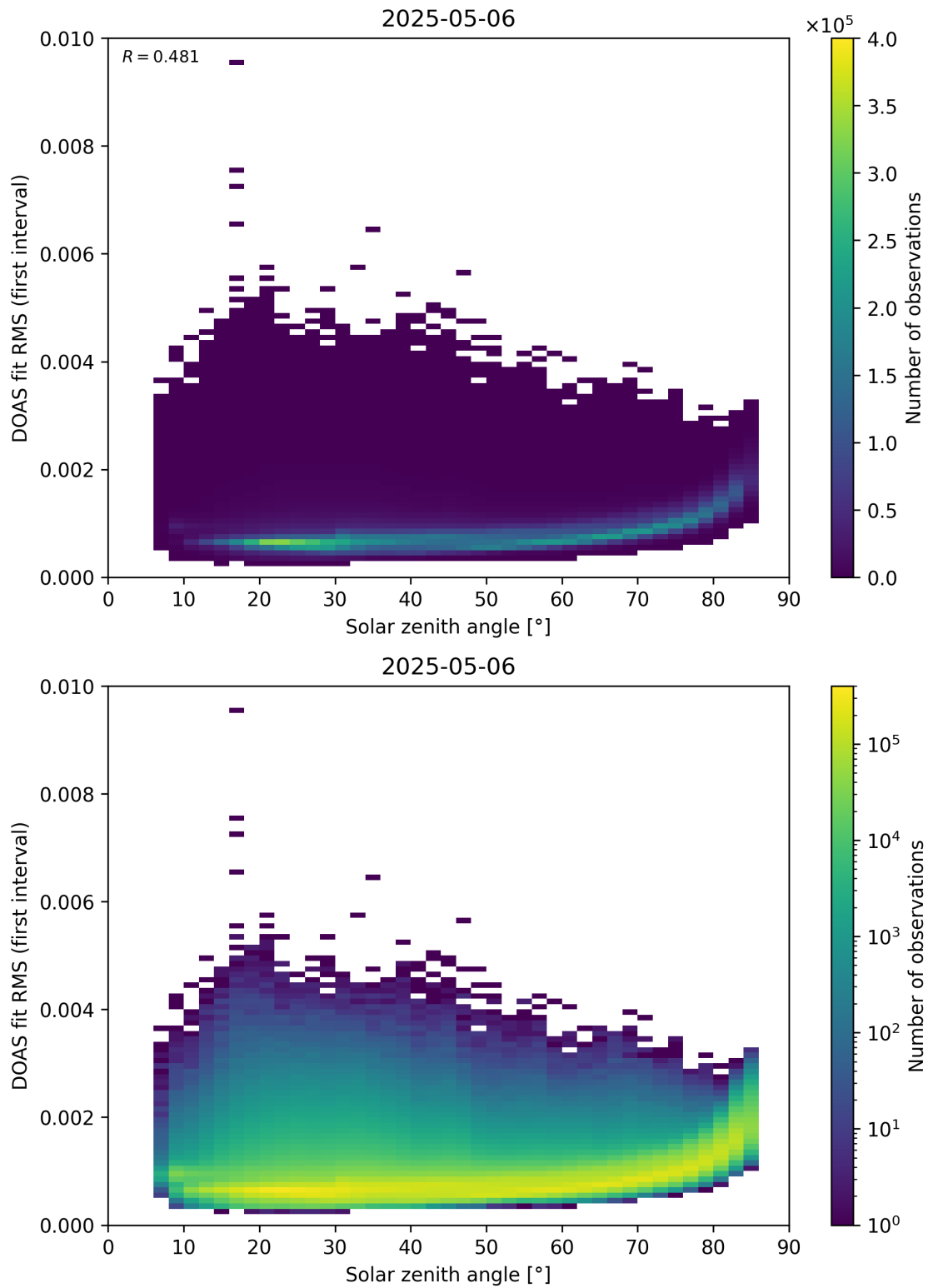
Figure 167: Scatter density plot of “Solar zenith angle” against “DOAS fit RMS (first interval)” for 2025-05-05 to 2025-05-07.
