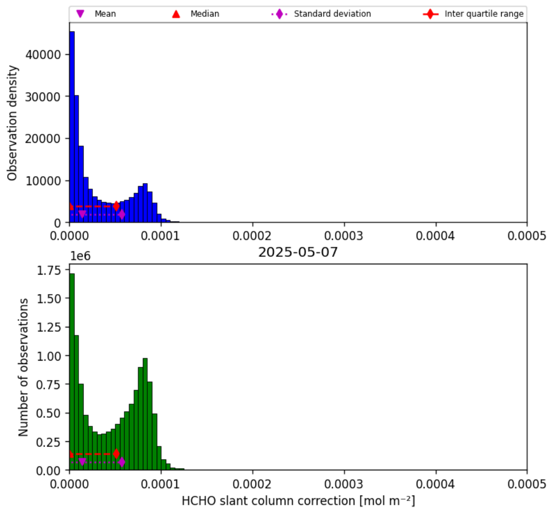
Figure 47: Histogram of “HCHO slant column correction” for 2025-05-06 to 2025-05-08
