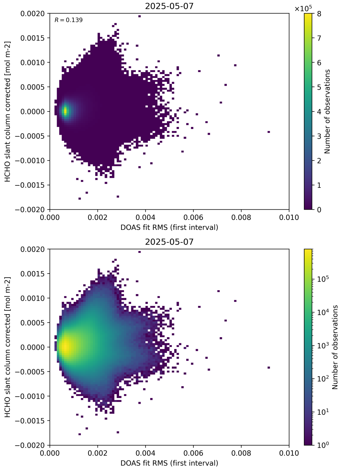
Figure 62: Scatter density plot of “DOAS fit RMS (first interval)” against “HCHO slant column corrected” for 2025-05-06 to 2025-05-08.
