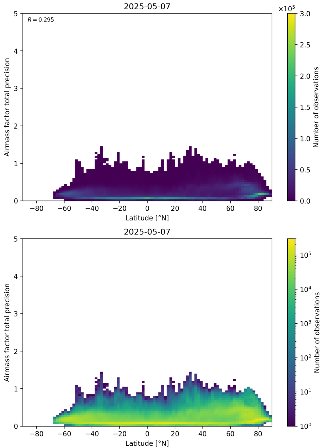
Figure 162: Scatter density plot of “Latitude” against “Airmass factor total precision” for 2025-05-06 to 2025-05-08.
