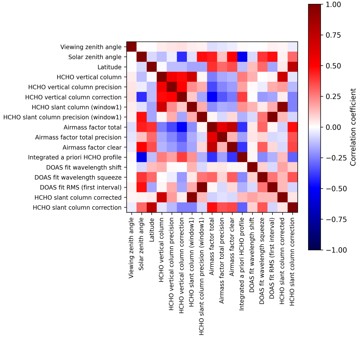
Figure 2: Map of correlation matrix for 2025-05-06 to 2025-05-08.
