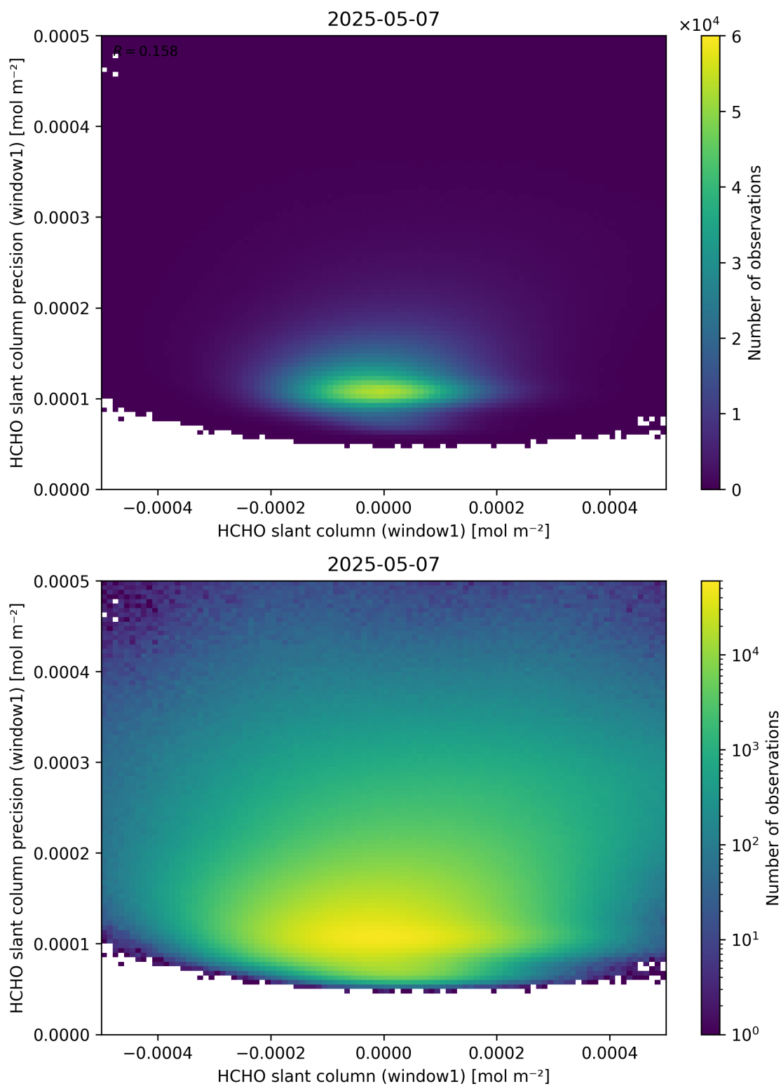
Figure 84: Scatter density plot of “HCHO slant column (window1)” against “HCHO slant column precision (window1)” for 2025-05-06 to 2025-05-08.
