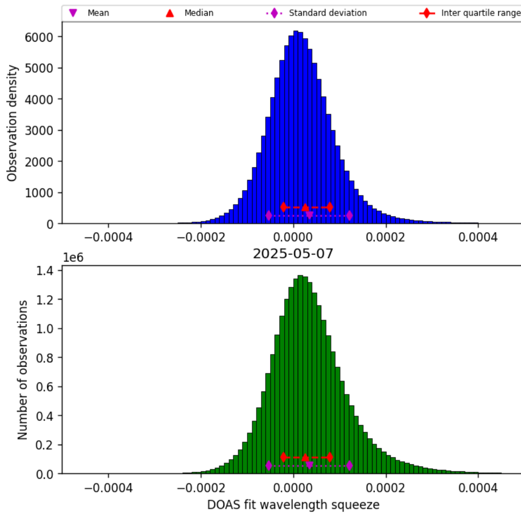
Figure 45: Histogram of “DOAS fit wavelength squeeze” for 2025-05-06 to 2025-05-08
