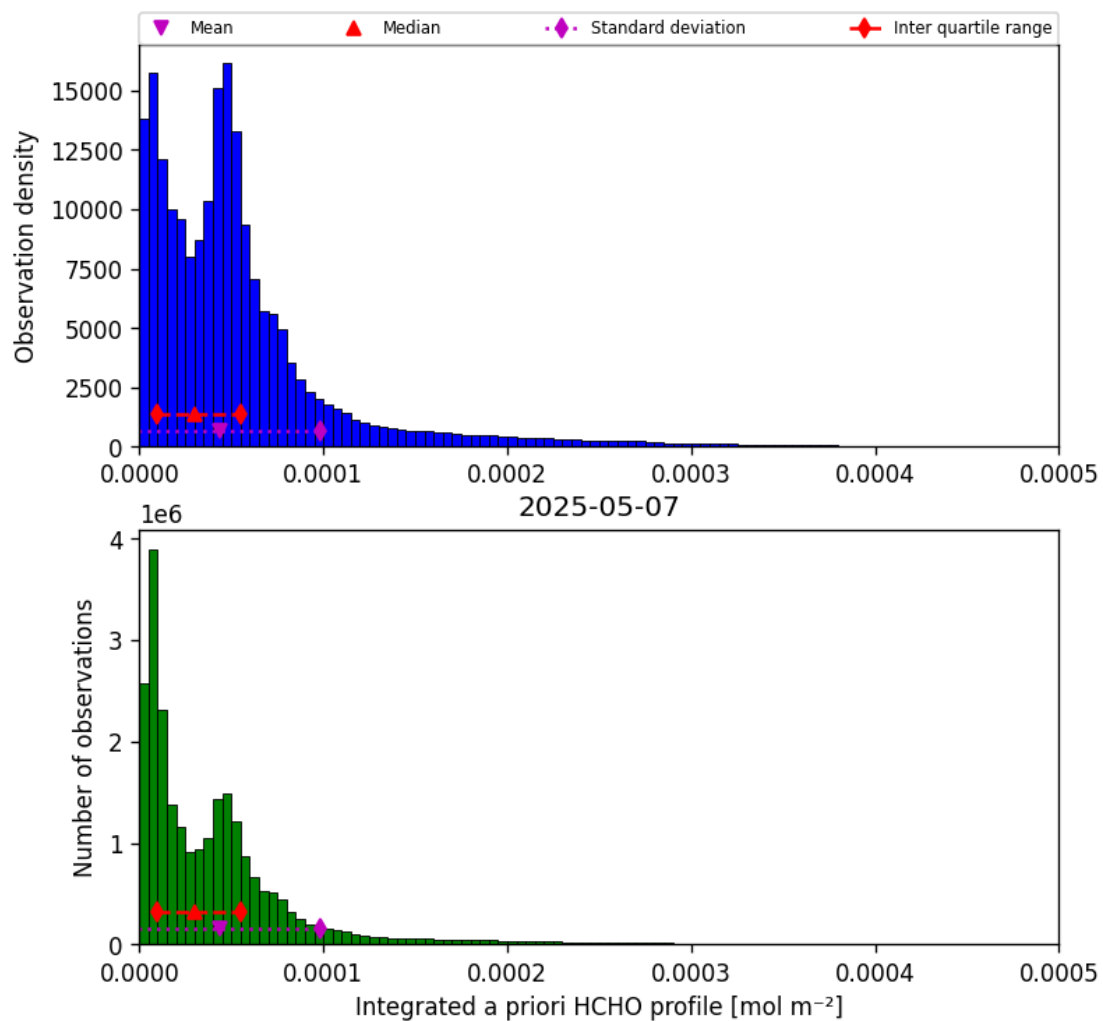
Figure 43: Histogram of “Integrated a priori HCHO profile” for 2025-05-06 to 2025-05-08
