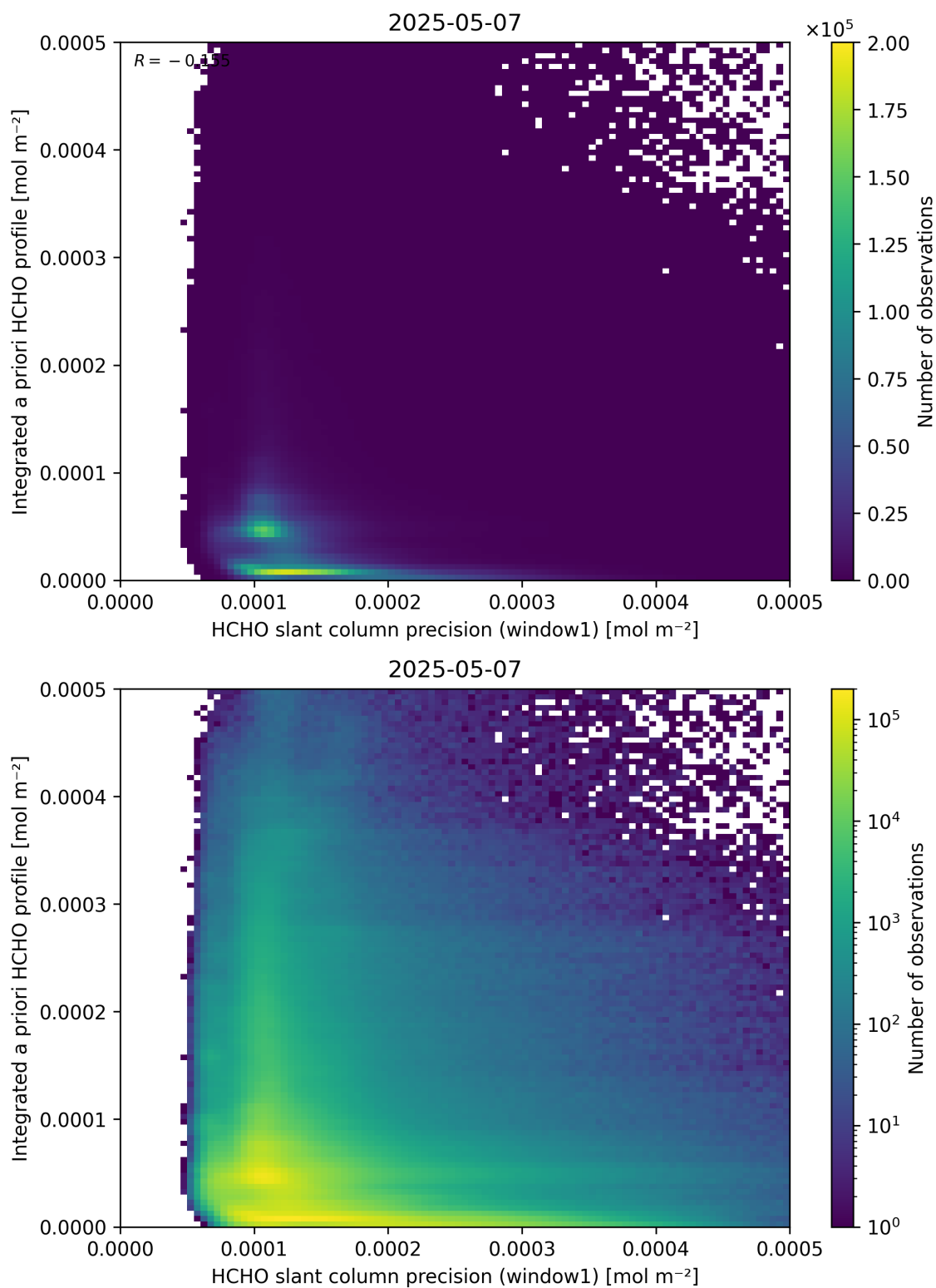
Figure 96: Scatter density plot of “HCHO slant column precision (window1)” against “Integrated a priori HCHO profile” for 2025-05-06 to 2025-05-08.
