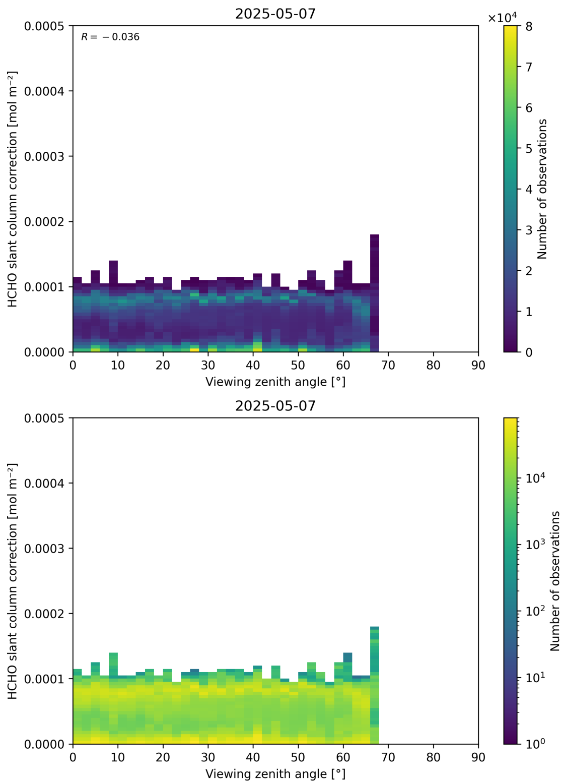
Figure 187: Scatter density plot of “Viewing zenith angle” against “HCHO slant column correction” for 2025-05-06 to 2025-05-08.
