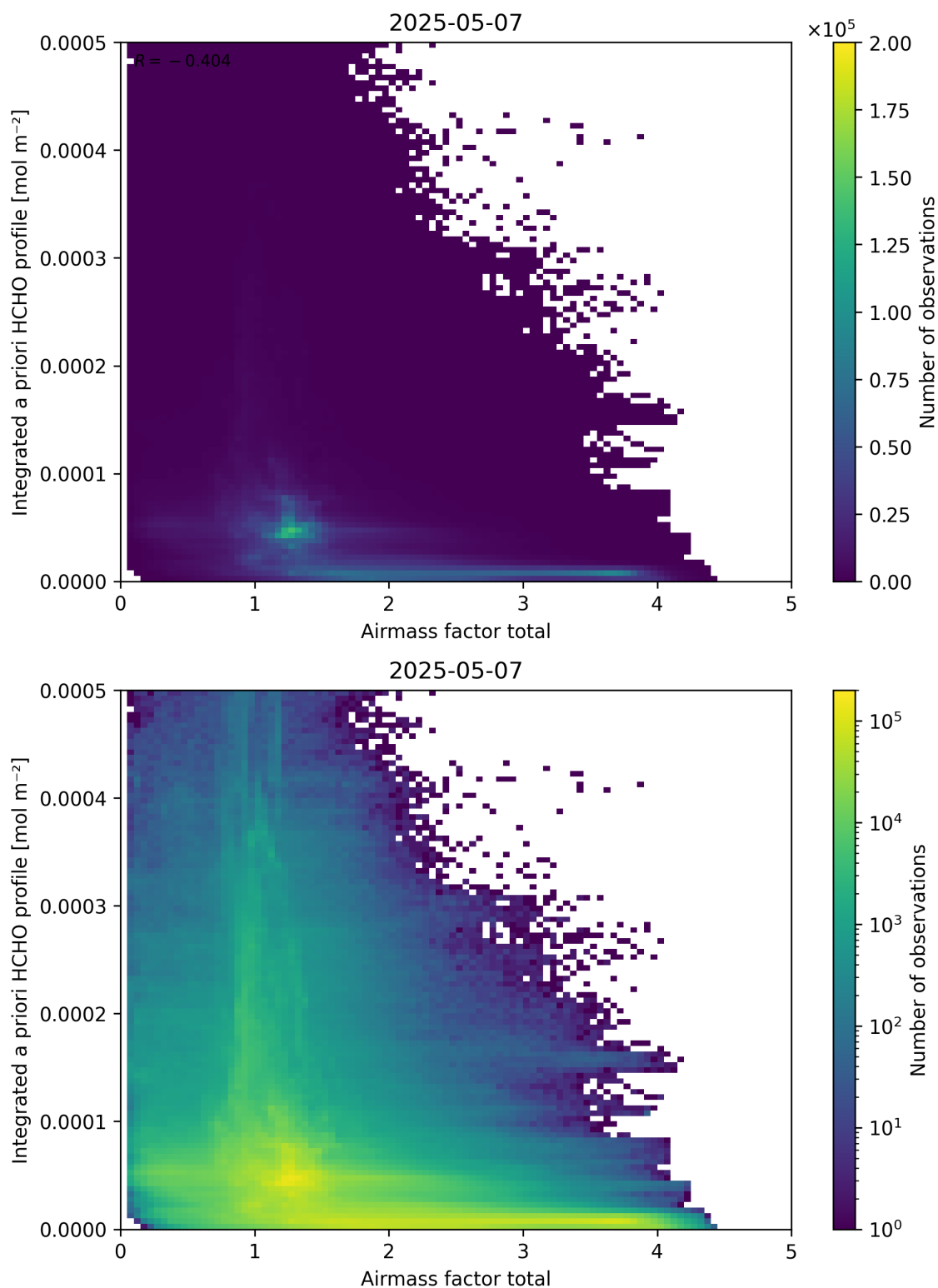
Figure 104: Scatter density plot of “Airmass factor total” against “Integrated a priori HCHO profile” for 2025-05-06 to 2025-05-08.
