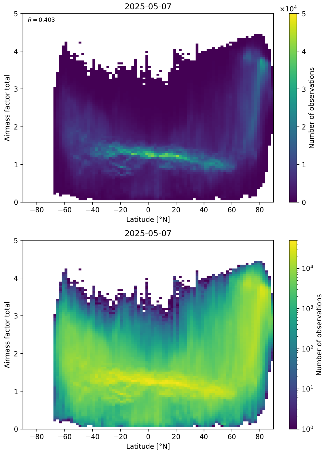
Figure 161: Scatter density plot of “Latitude” against “Airmass factor total” for 2025-05-06 to 2025-05-08.
