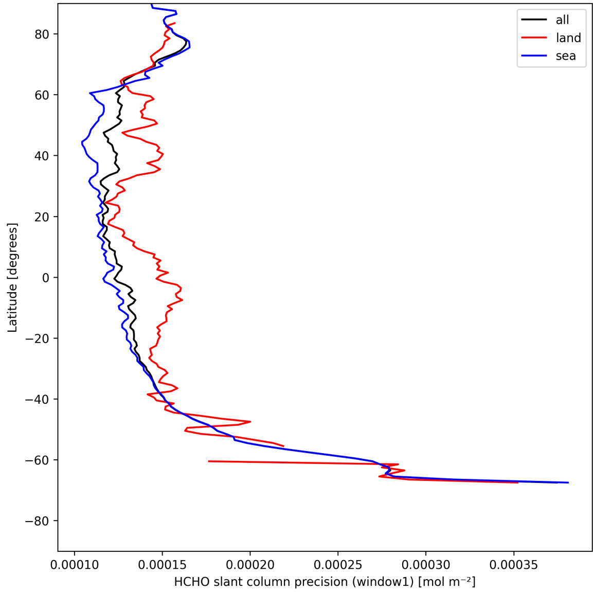
Figure 25: Zonal average of "HCHO slant column precision (window1)" for 2025-05-06 to 2025-05-08.
