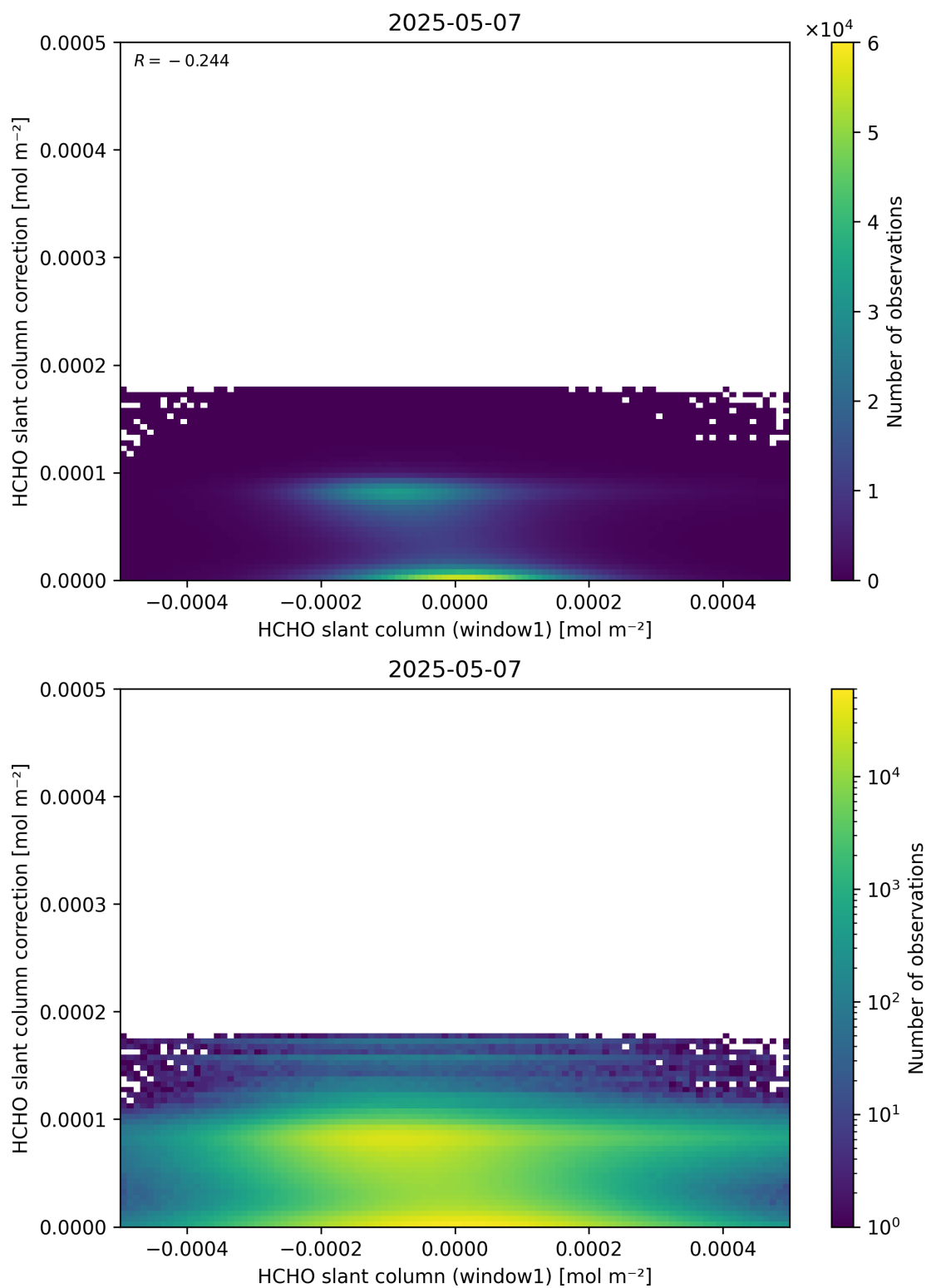
Figure 83: Scatter density plot of “HCHO slant column (window1)” against “HCHO slant column correction” for 2025-05-06 to 2025-05-08.
