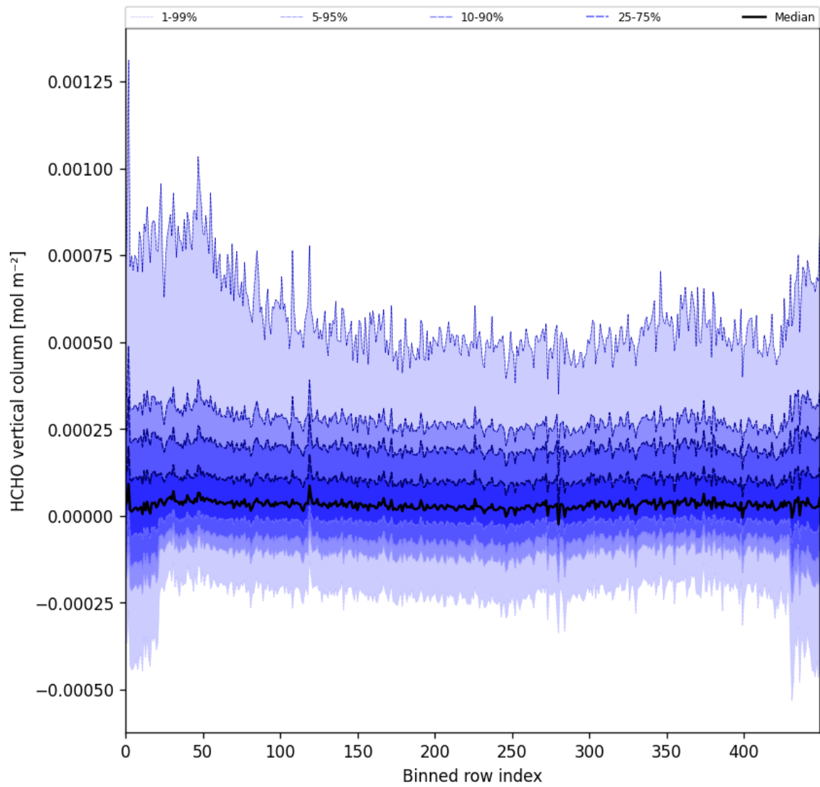
Figure 49: Along track statistics of “HCHO vertical column” for 2025-05-06 to 2025-05-08
