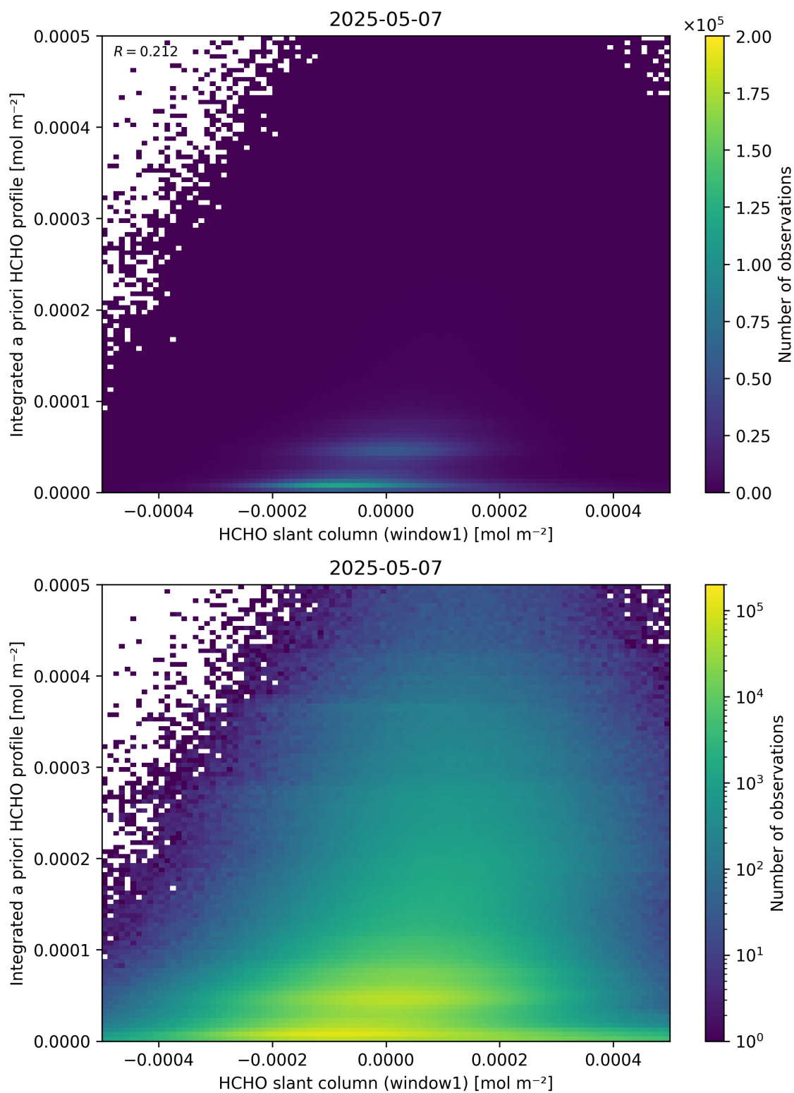
Figure 87: Scatter density plot of “HCHO slant column (window1)” against “Integrated a priori HCHO profile” for 2025-05-06 to 2025-05-08.
