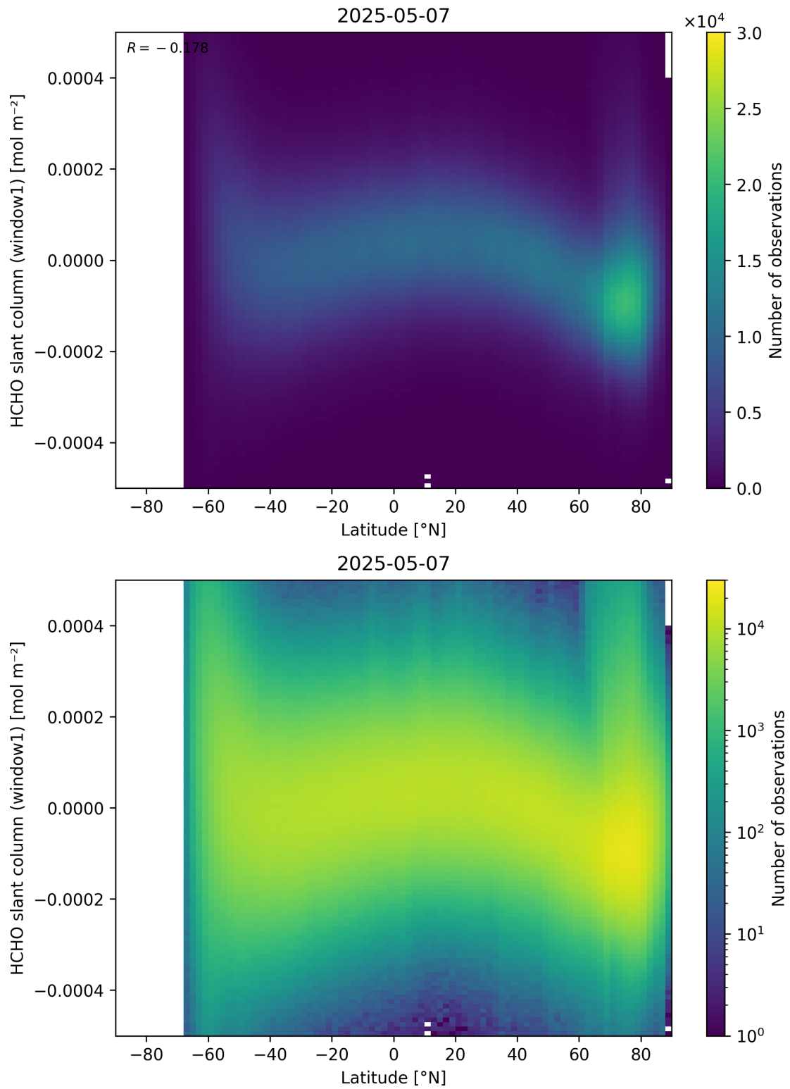
Figure 159: Scatter density plot of “Latitude” against “HCHO slant column (window1)” for 2025-05-06 to 2025-05-08.
