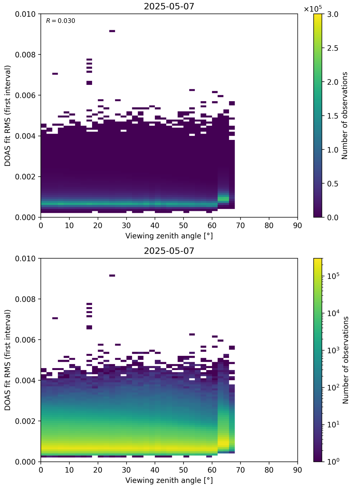
Figure 182: Scatter density plot of “Viewing zenith angle” against “DOAS fit RMS (first interval)” for 2025-05-06 to 2025-05-08.
