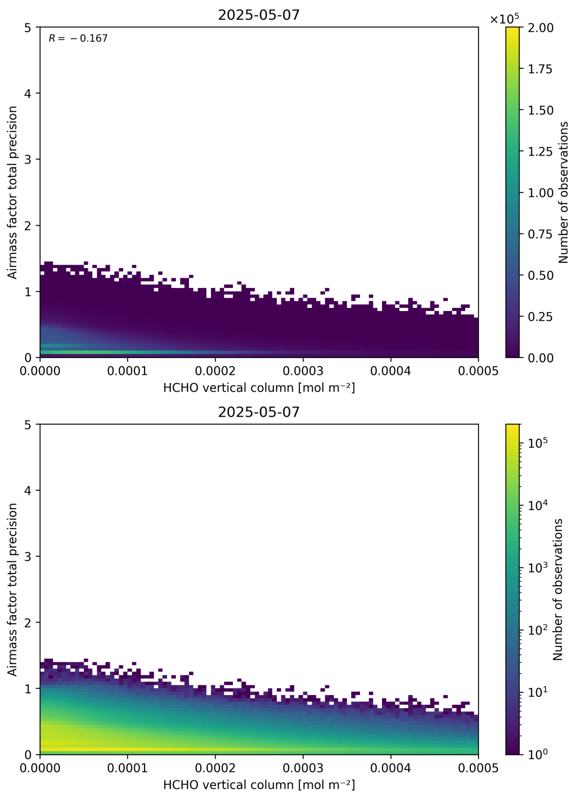
Figure 132: Scatter density plot of “HCHO vertical column” against “Airmass factor total precision” for 2025-05-06 to 2025-05-08.
