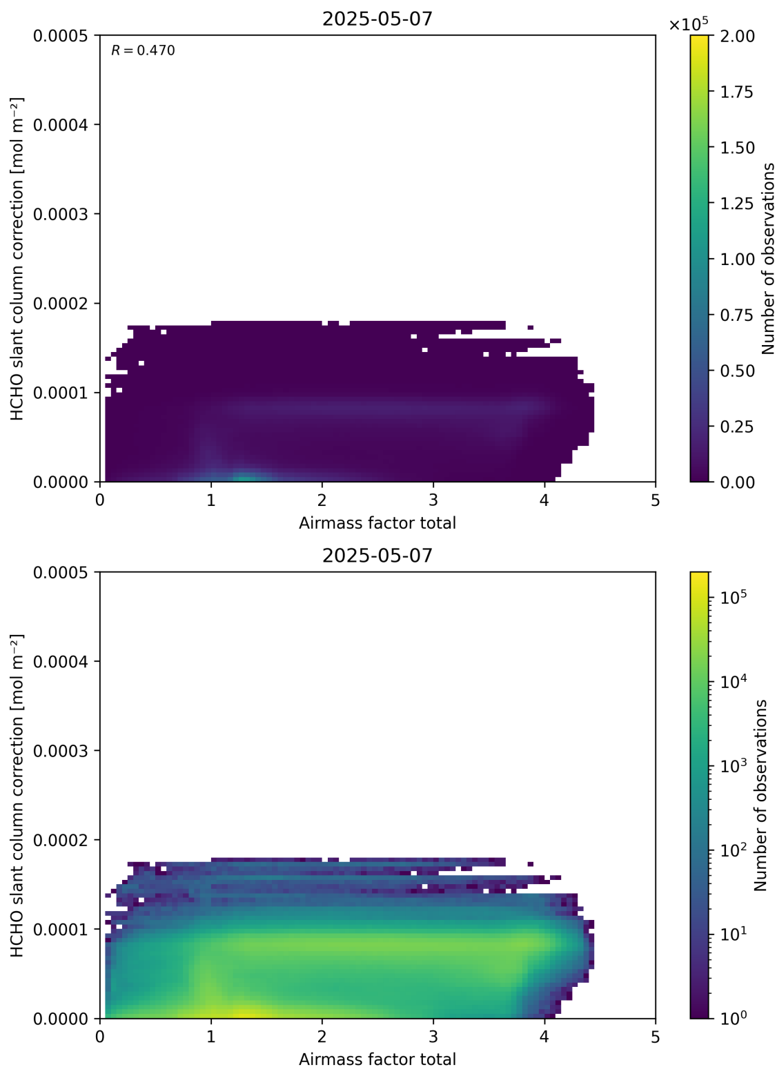
Figure 102: Scatter density plot of “Airmass factor total” against “HCHO slant column correction” for 2025-05-06 to 2025-05-08.
