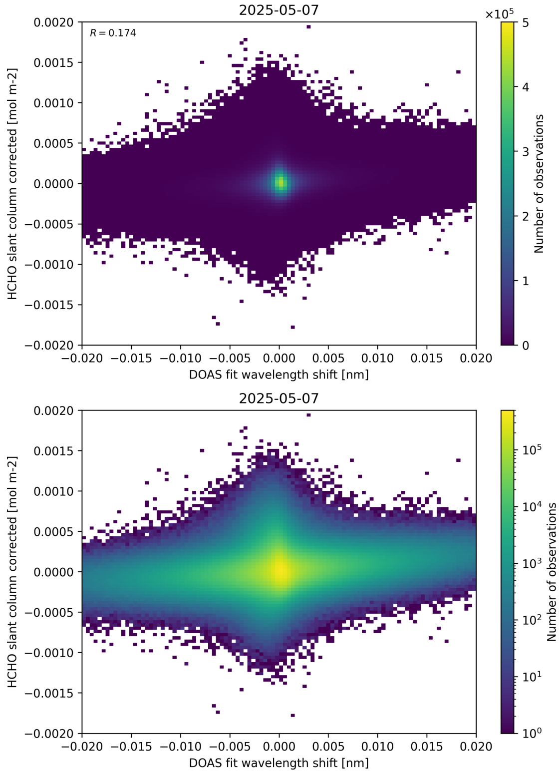
Figure 66: Scatter density plot of “DOAS fit wavelength shift” against “HCHO slant column corrected” for 2025-05-06 to 2025-05-08.
