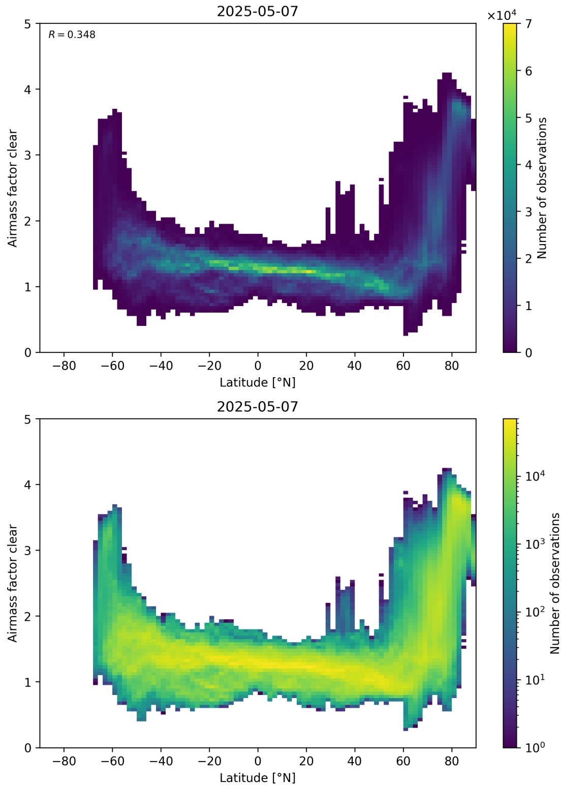
Figure 156: Scatter density plot of “Latitude” against “Airmass factor clear” for 2025-05-06 to 2025-05-08.
