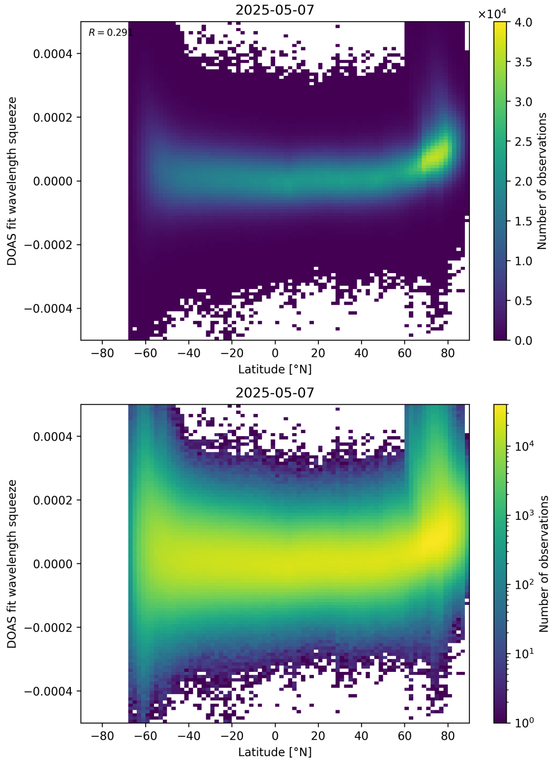
Figure 155: Scatter density plot of “Latitude” against “DOAS fit wavelength squeeze” for 2025-05-06 to 2025-05-08.
