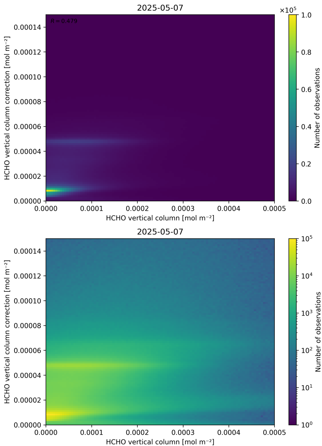
Figure 133: Scatter density plot of “HCHO vertical column” against “HCHO vertical column correction” for 2025-05-06 to 2025-05-08.
