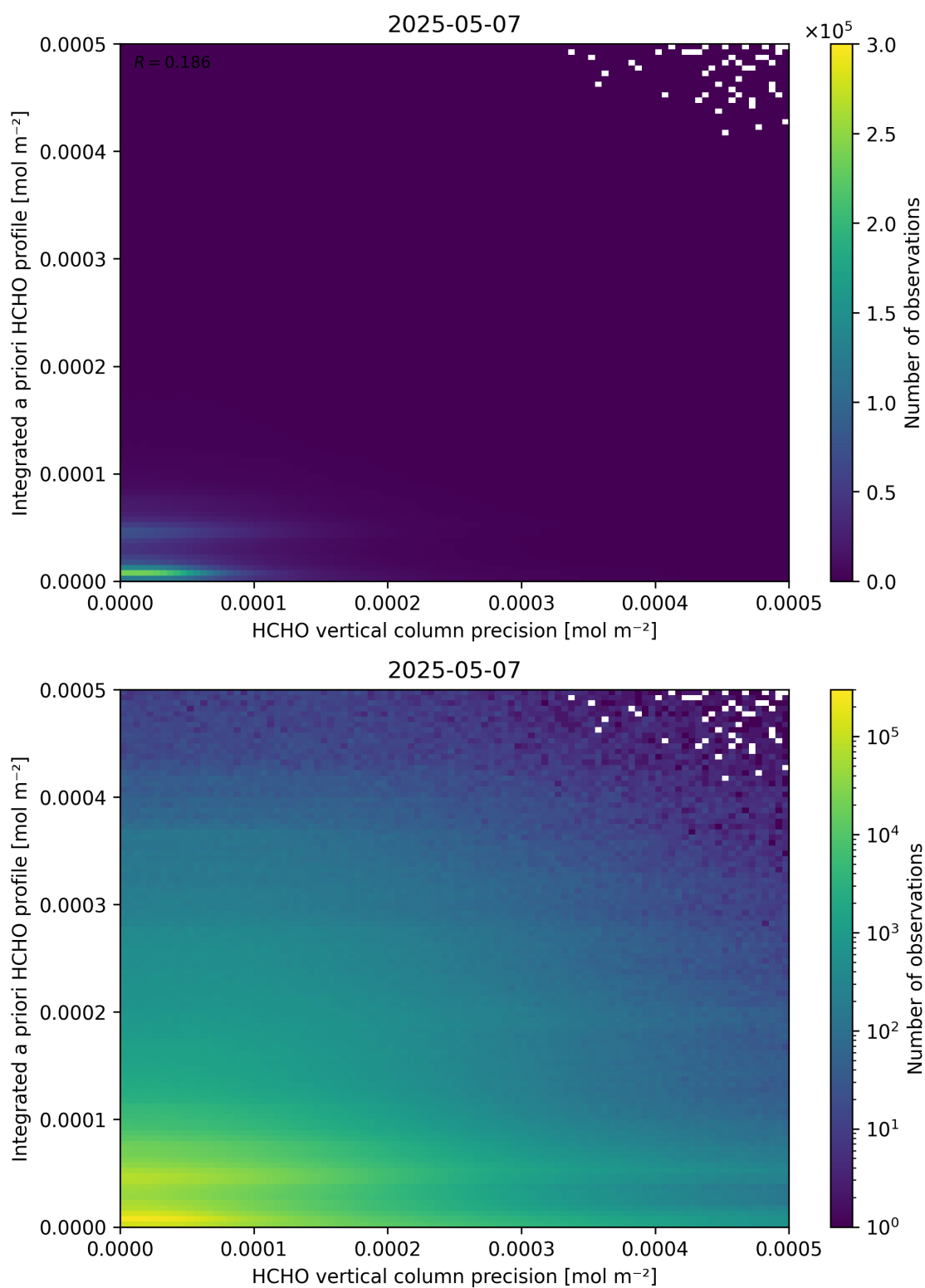
Figure 147: Scatter density plot of “HCHO vertical column precision” against “Integrated a priori HCHO profile” for 2025-05-06 to 2025-05-08.
