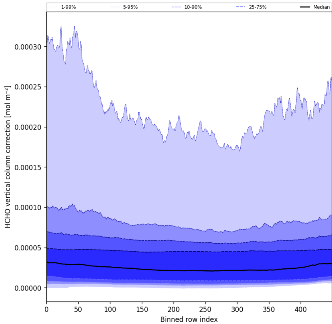
Figure 51: Along track statistics of “HCHO vertical column correction” for 2025-05-06 to 2025-05-08
