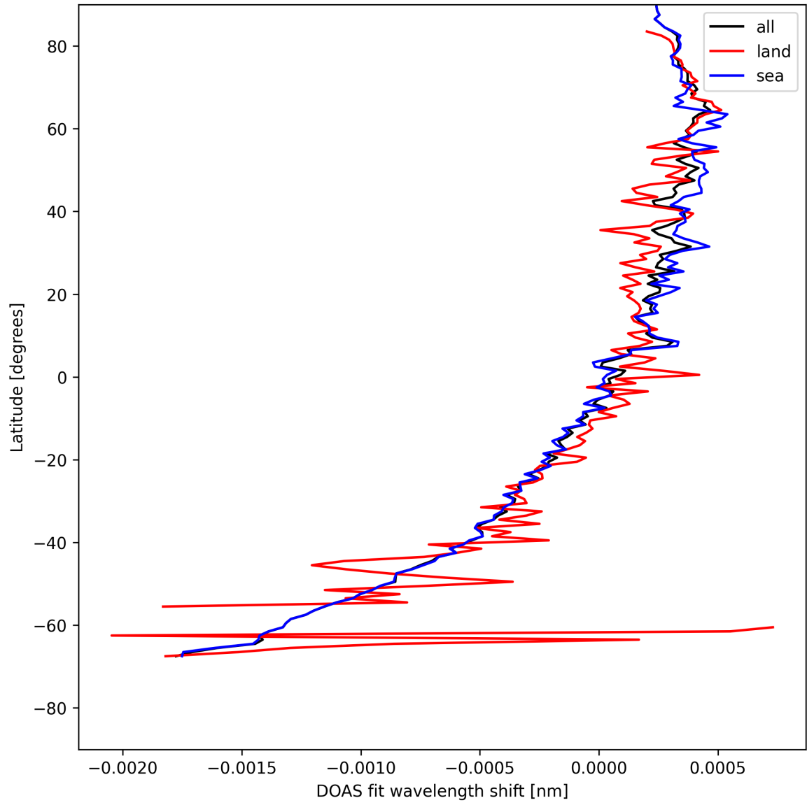
Figure 30: Zonal average of “DOAS fit wavelength shift” for 2025-05-06 to 2025-05-08.
