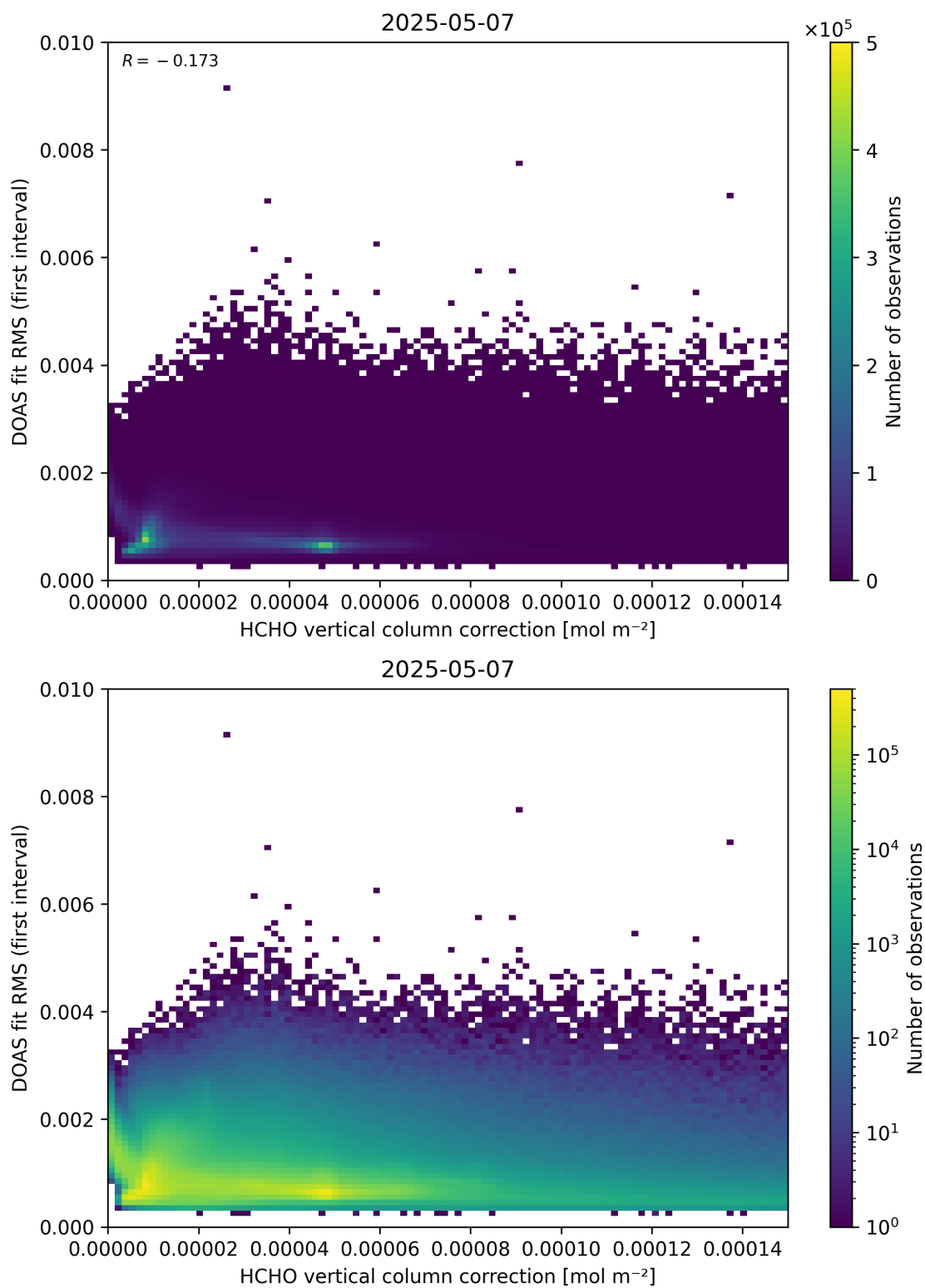
Figure 112: Scatter density plot of “HCHO vertical column correction” against “DOAS fit RMS (first interval)” for 2025-05-06 to 2025-05-08.
