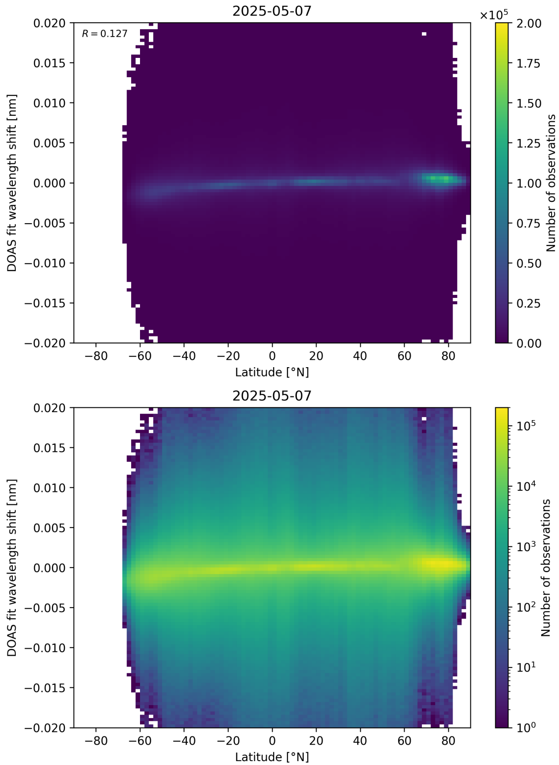
Figure 154: Scatter density plot of “Latitude” against “DOAS fit wavelength shift” for 2025-05-06 to 2025-05-08.
