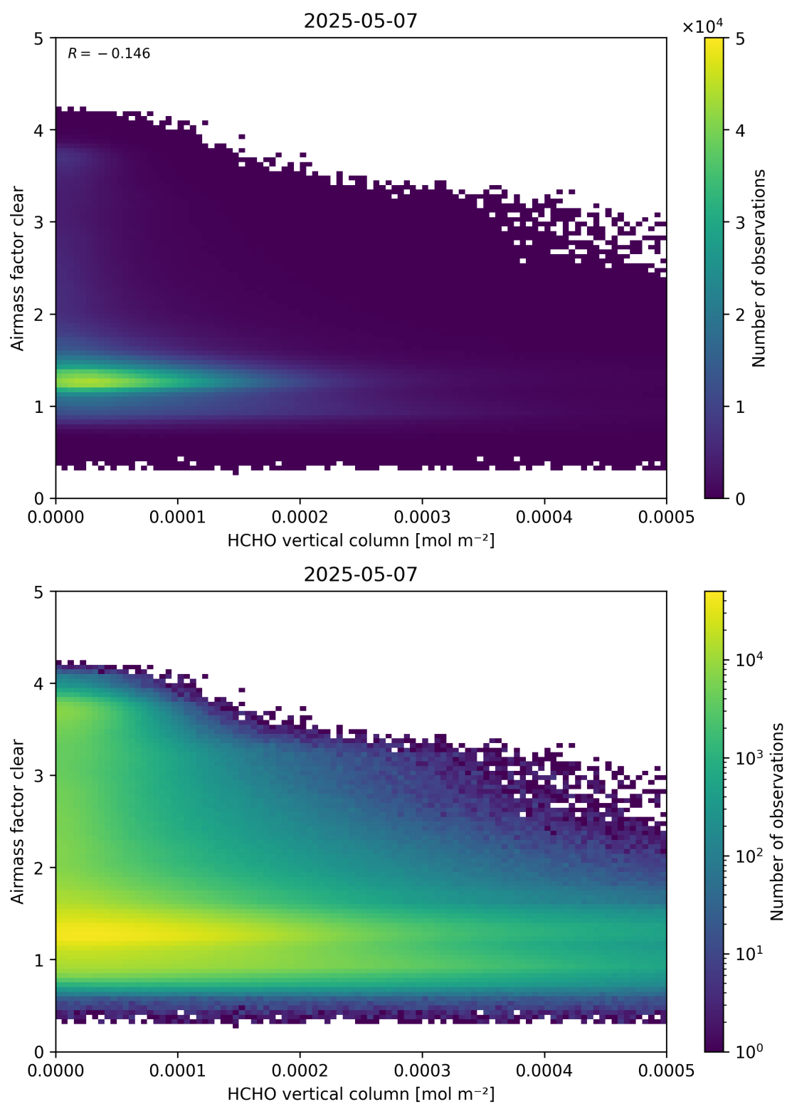
Figure 126: Scatter density plot of “HCHO vertical column” against “Airmass factor clear” for 2025-05-06 to 2025-05-08.
