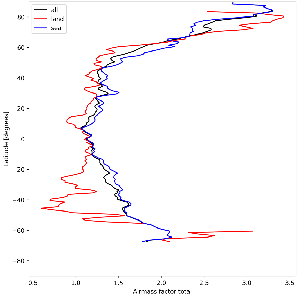
Figure 26: Zonal average of “Airmass factor total” for 2025-05-06 to 2025-05-08.
