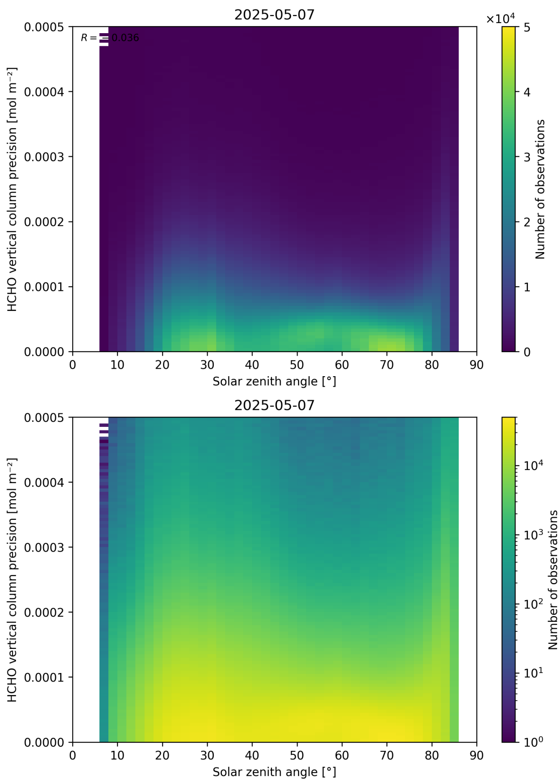
Figure 179: Scatter density plot of “Solar zenith angle” against “HCHO vertical column precision” for 2025-05-06 to 2025-05-08.
