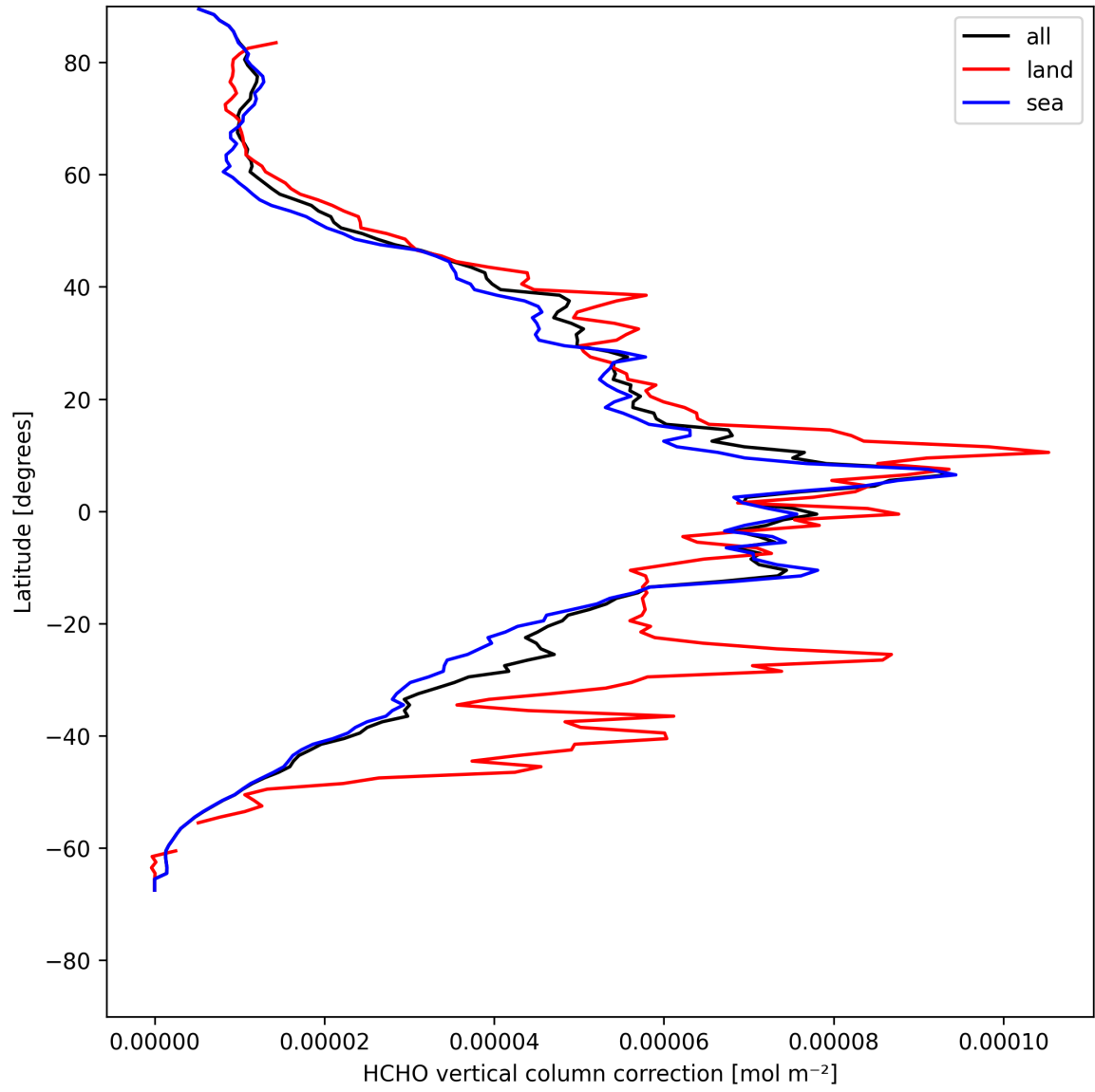
Figure 23: Zonal average of “HCHO vertical column correction” for 2025-05-06 to 2025-05-08.
