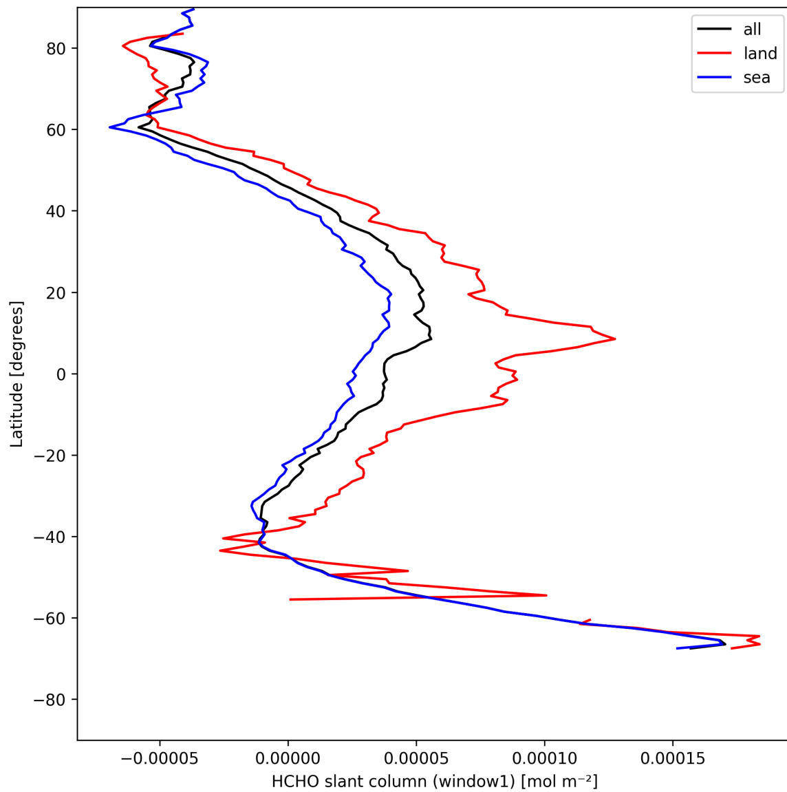
Figure 24: Zonal average of “HCHO slant column (window1)” for 2025-05-06 to 2025-05-08.
