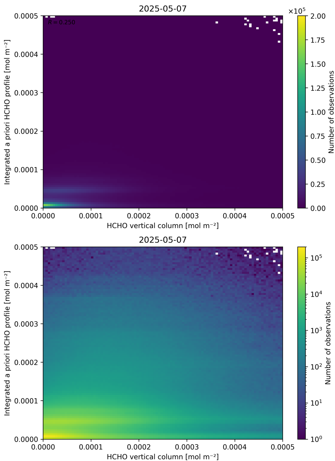
Figure 135: Scatter density plot of “HCHO vertical column” against “Integrated a priori HCHO profile” for 2025-05-06 to 2025-05-08.
