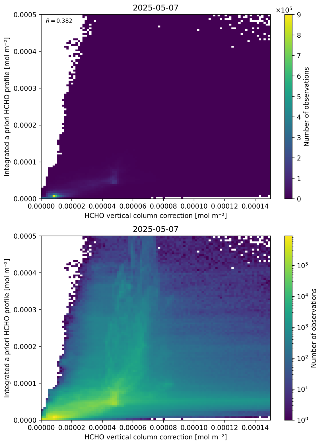
Figure 122: Scatter density plot of “HCHO vertical column correction” against “Integrated a priori HCHO profile” for 2025-05-06 to 2025-05-08.
