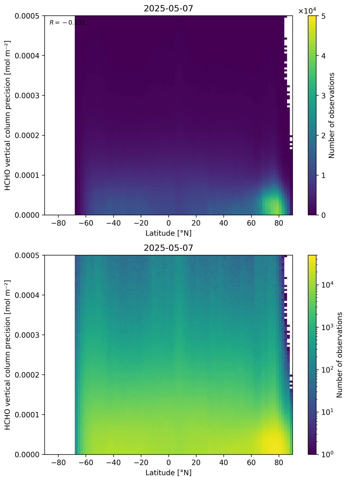
Figure 165: Scatter density plot of “Latitude” against “HCHO vertical column precision” for 2025-05-06 to 2025-05-08.
