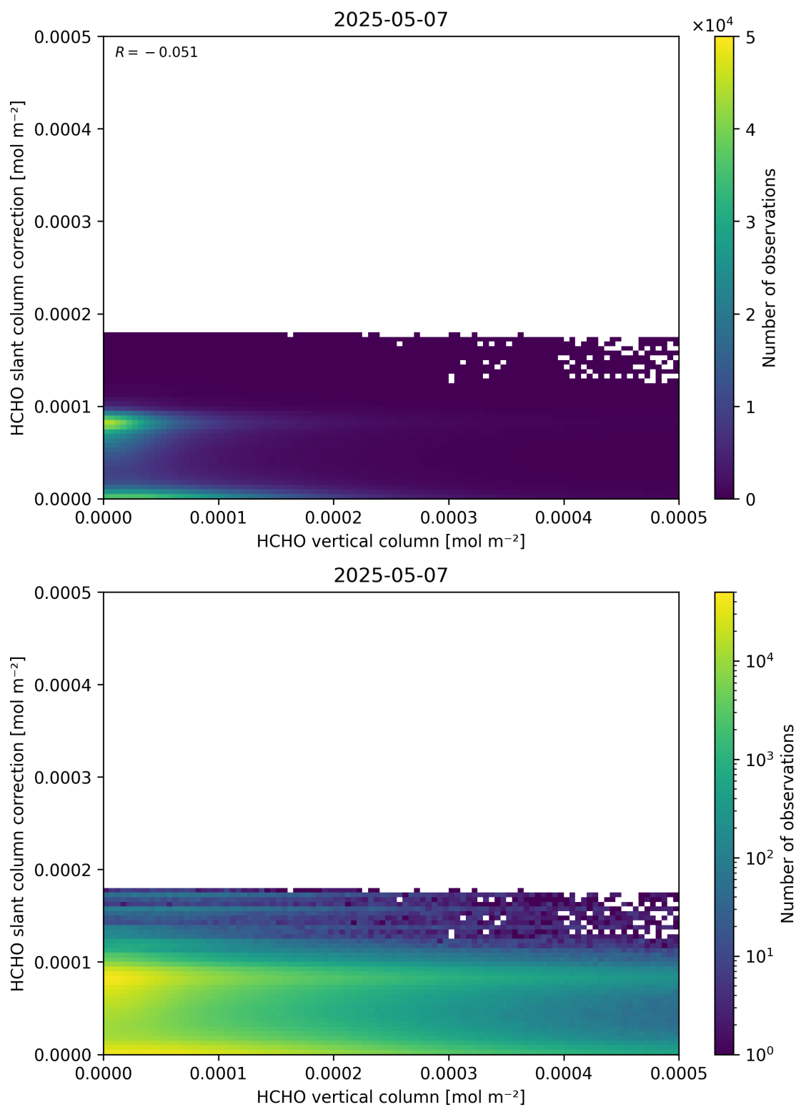
Figure 128: Scatter density plot of “HCHO vertical column” against “HCHO slant column correction” for 2025-05-06 to 2025-05-08.
