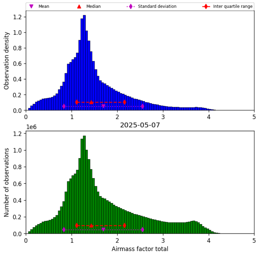
Figure 40: Histogram of “Airmass factor total” for 2025-05-06 to 2025-05-08
