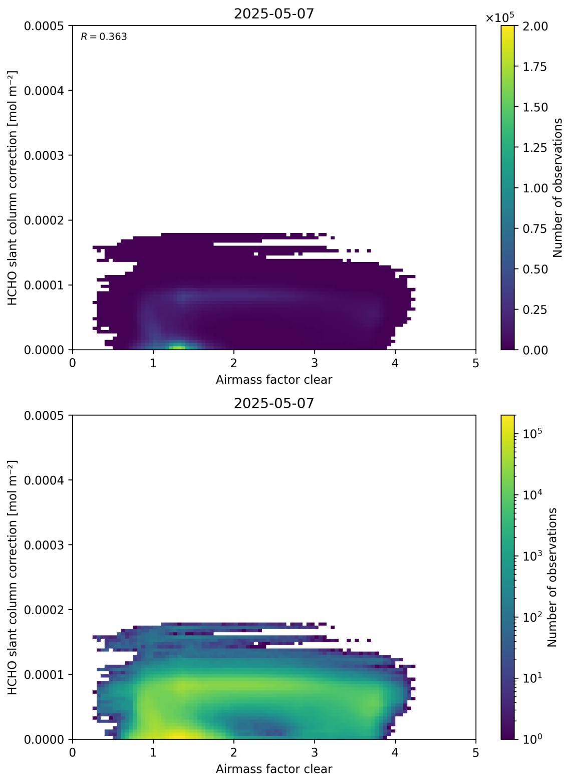
Figure 75: Scatter density plot of “Airmass factor clear” against “HCHO slant column correction” for 2025-05-06 to 2025-05-08.
