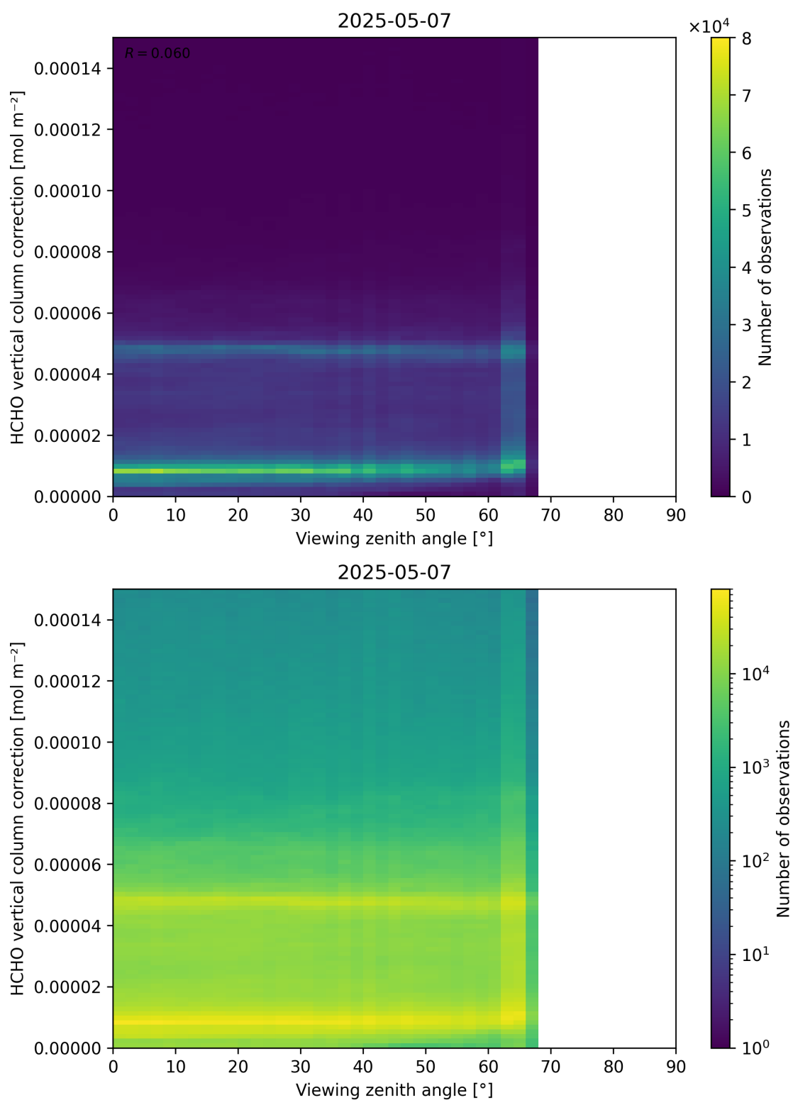
Figure 193: Scatter density plot of “Viewing zenith angle” against “HCHO vertical column correction” for 2025-05-06 to 2025-05-08.
