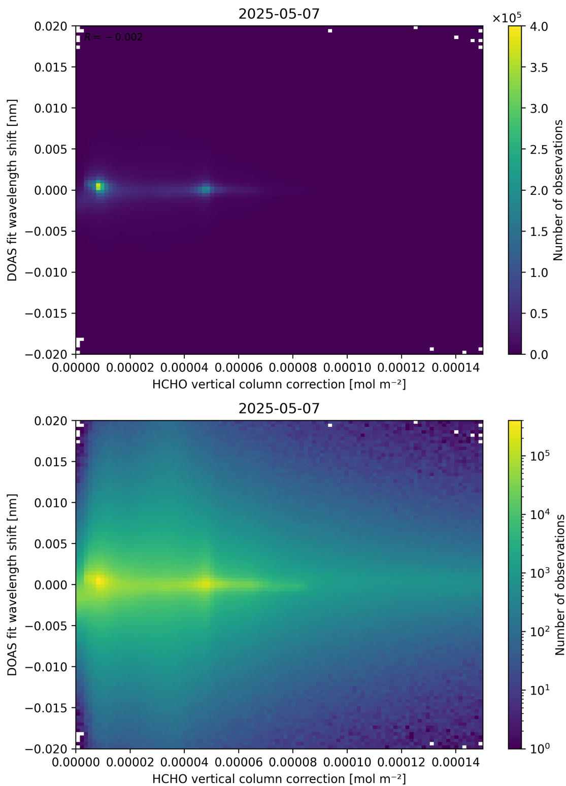
Figure 113: Scatter density plot of “HCHO vertical column correction” against “DOAS fit wavelength shift” for 2025-05-06 to 2025-05-08.
