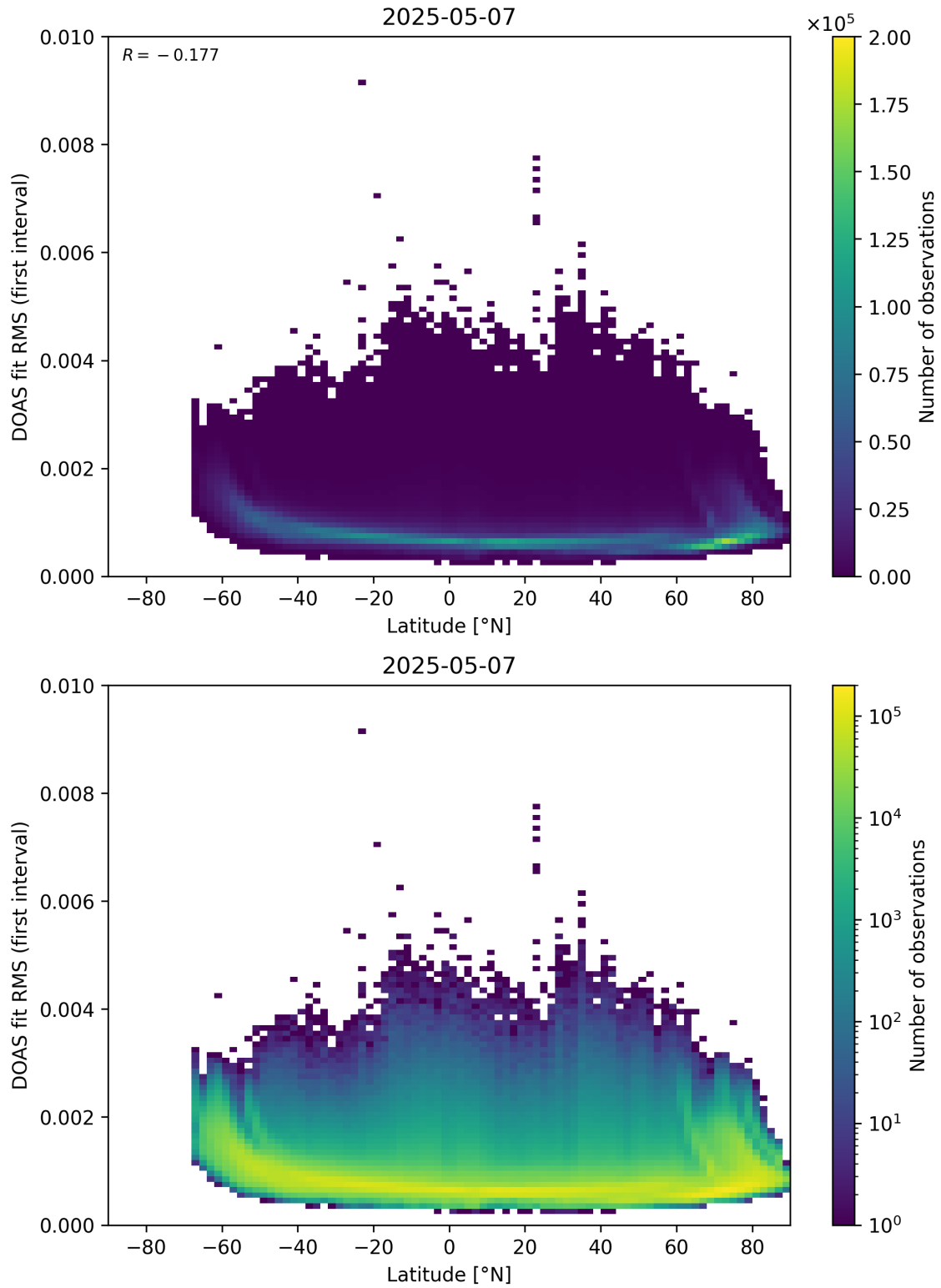
Figure 153: Scatter density plot of “Latitude” against “DOAS fit RMS (first interval)” for 2025-05-06 to 2025-05-08.
