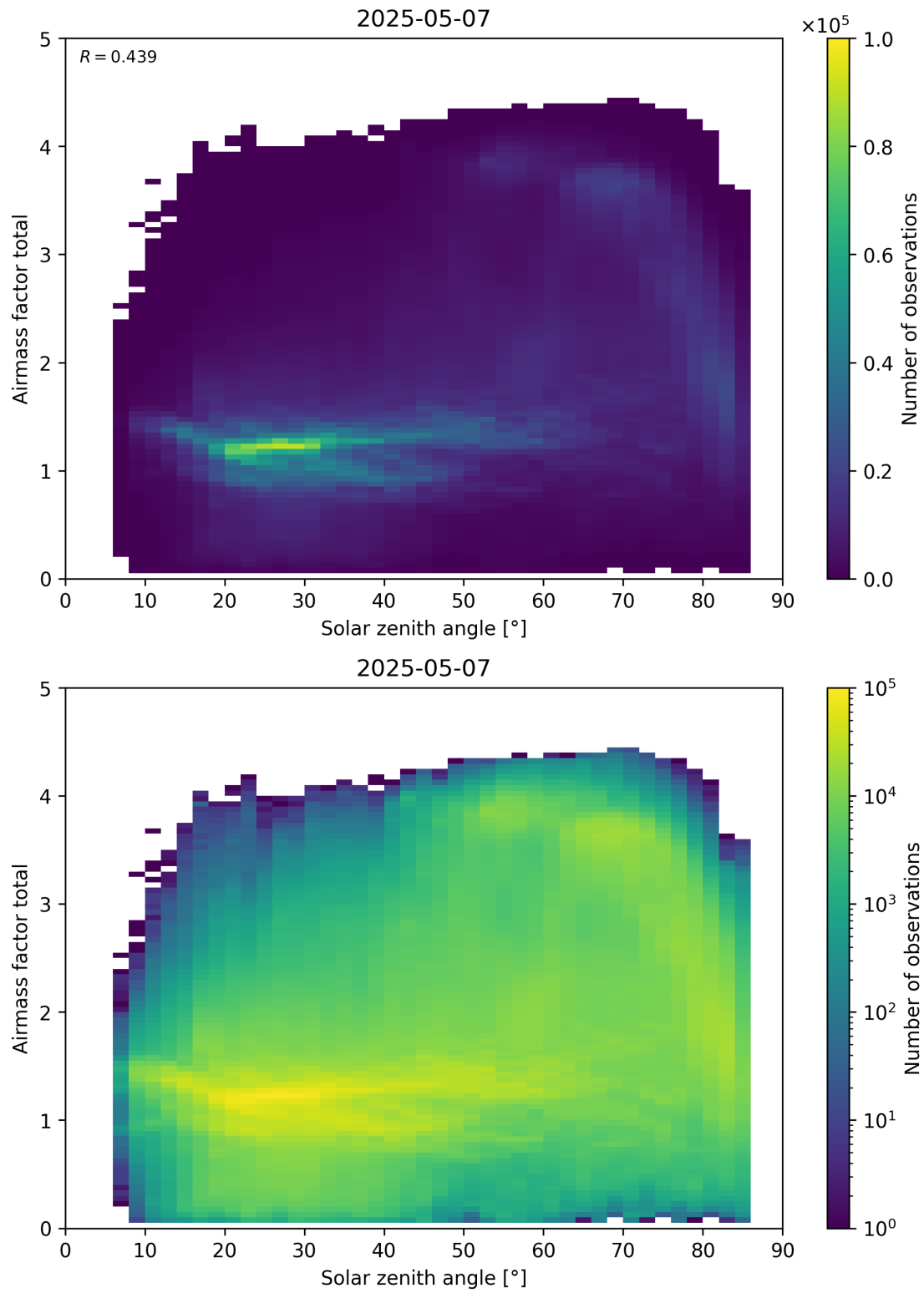
Figure 175: Scatter density plot of “Solar zenith angle” against “Airmass factor total” for 2025-05-06 to 2025-05-08.
