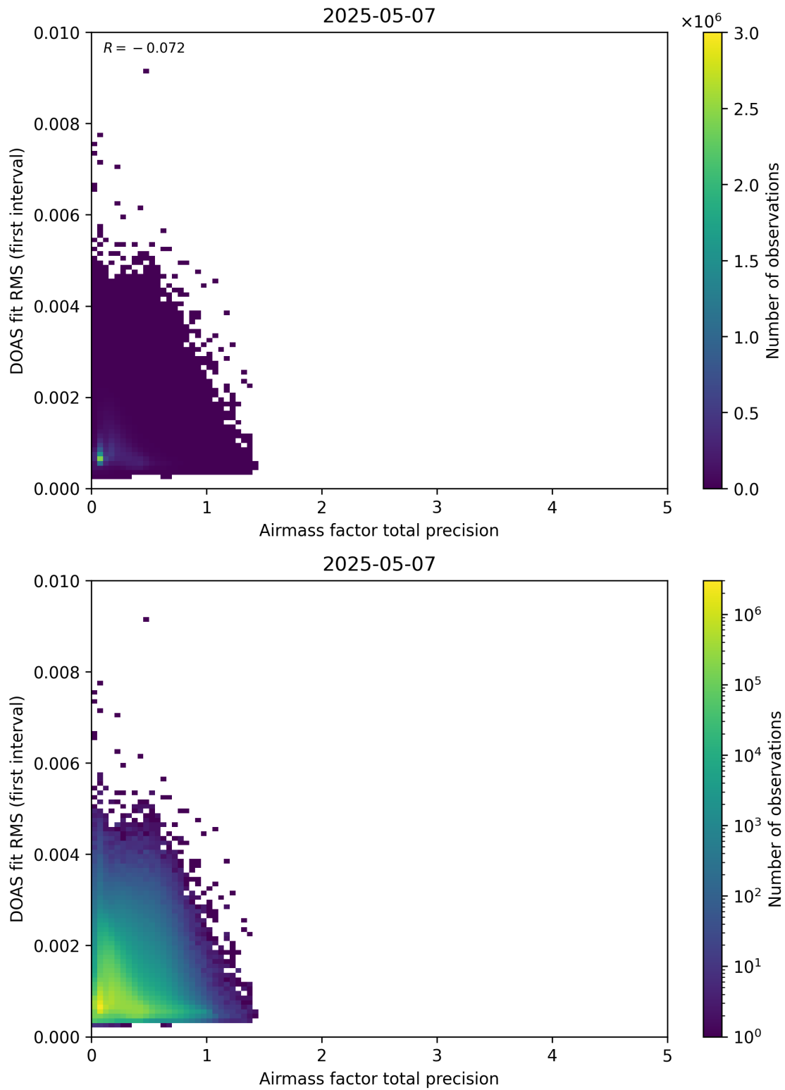
Figure 105: Scatter density plot of “Airmass factor total precision” against “DOAS fit RMS (first interval)” for 2025-05-06 to 2025-05-08.
