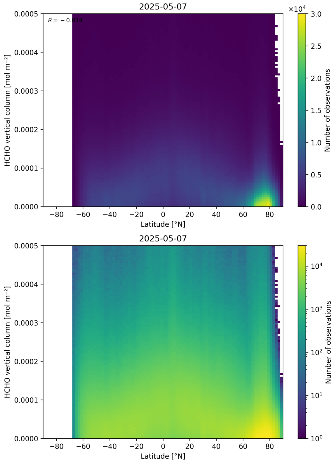
Figure 163: Scatter density plot of “Latitude” against “HCHO vertical column” for 2025-05-06 to 2025-05-08.
