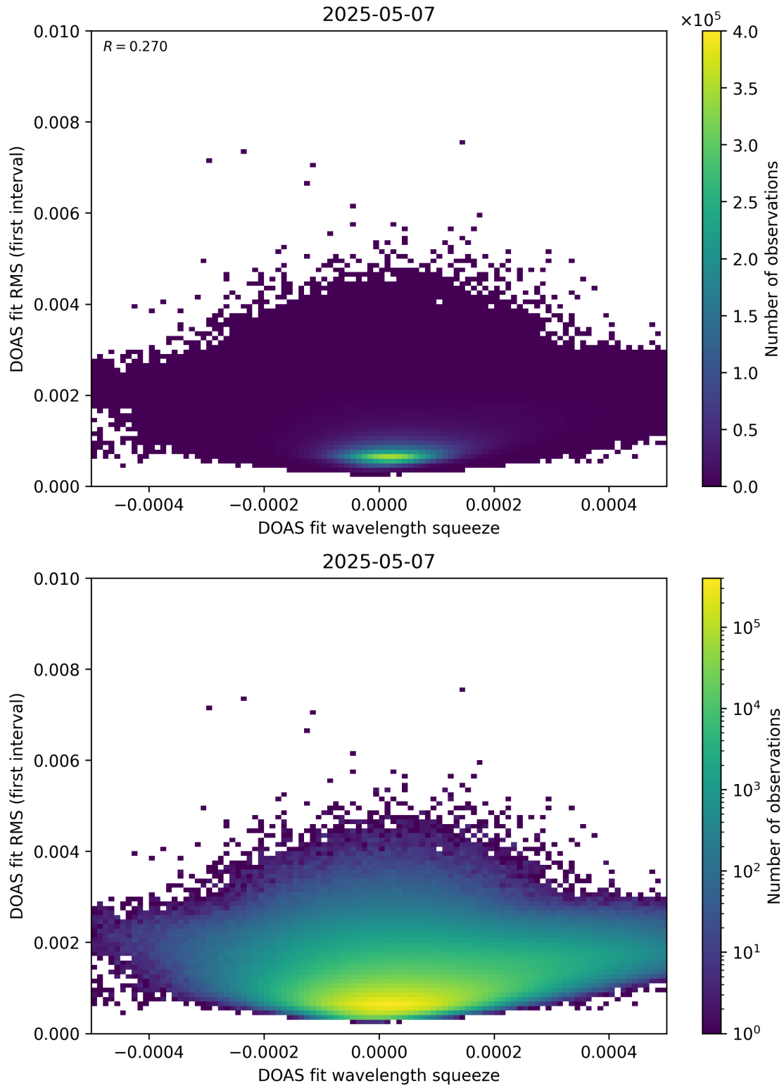
Figure 68: Scatter density plot of “DOAS fit wavelength squeeze” against “DOAS fit RMS (first interval)” for 2025-05-06 to 2025-05-08.
