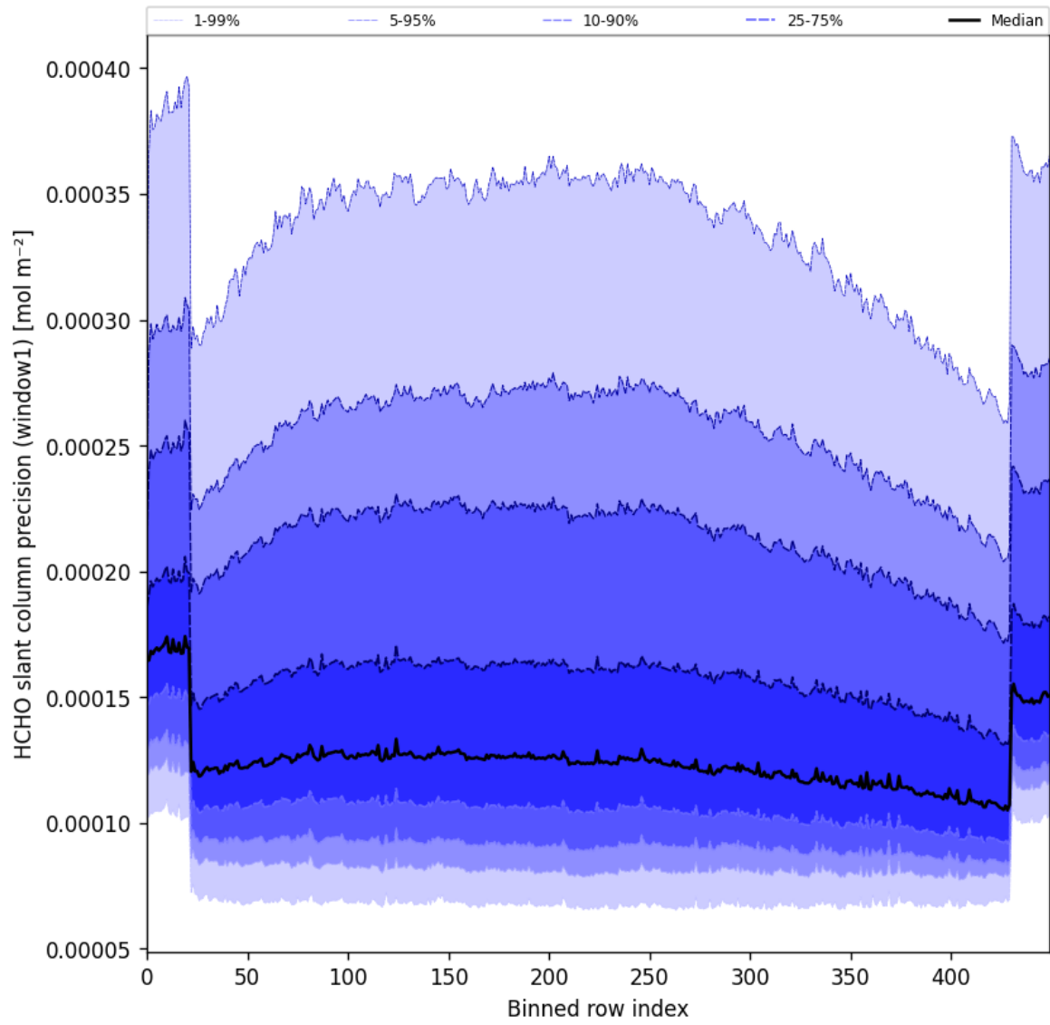
Figure 53: Along track statistics of “HCHO slant column precision (window1)” for 2025-05-06 to 2025-05-08
