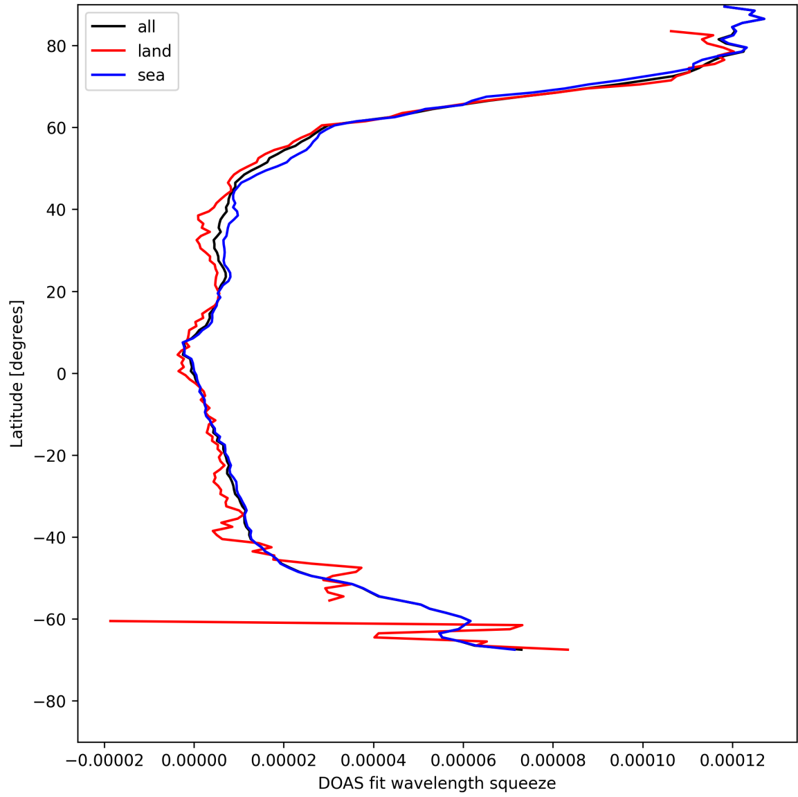
Figure 31: Zonal average of “DOAS fit wavelength squeeze” for 2025-05-06 to 2025-05-08.
