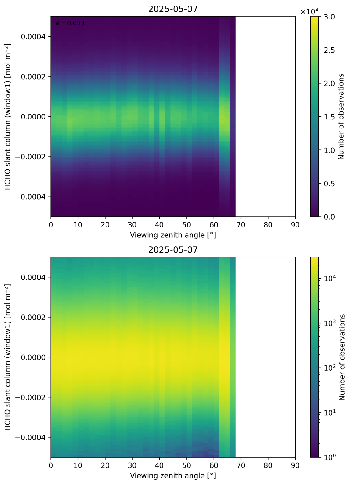
Figure 188: Scatter density plot of “Viewing zenith angle” against “HCHO slant column (window1)” for 2025-05-06 to 2025-05-08.
