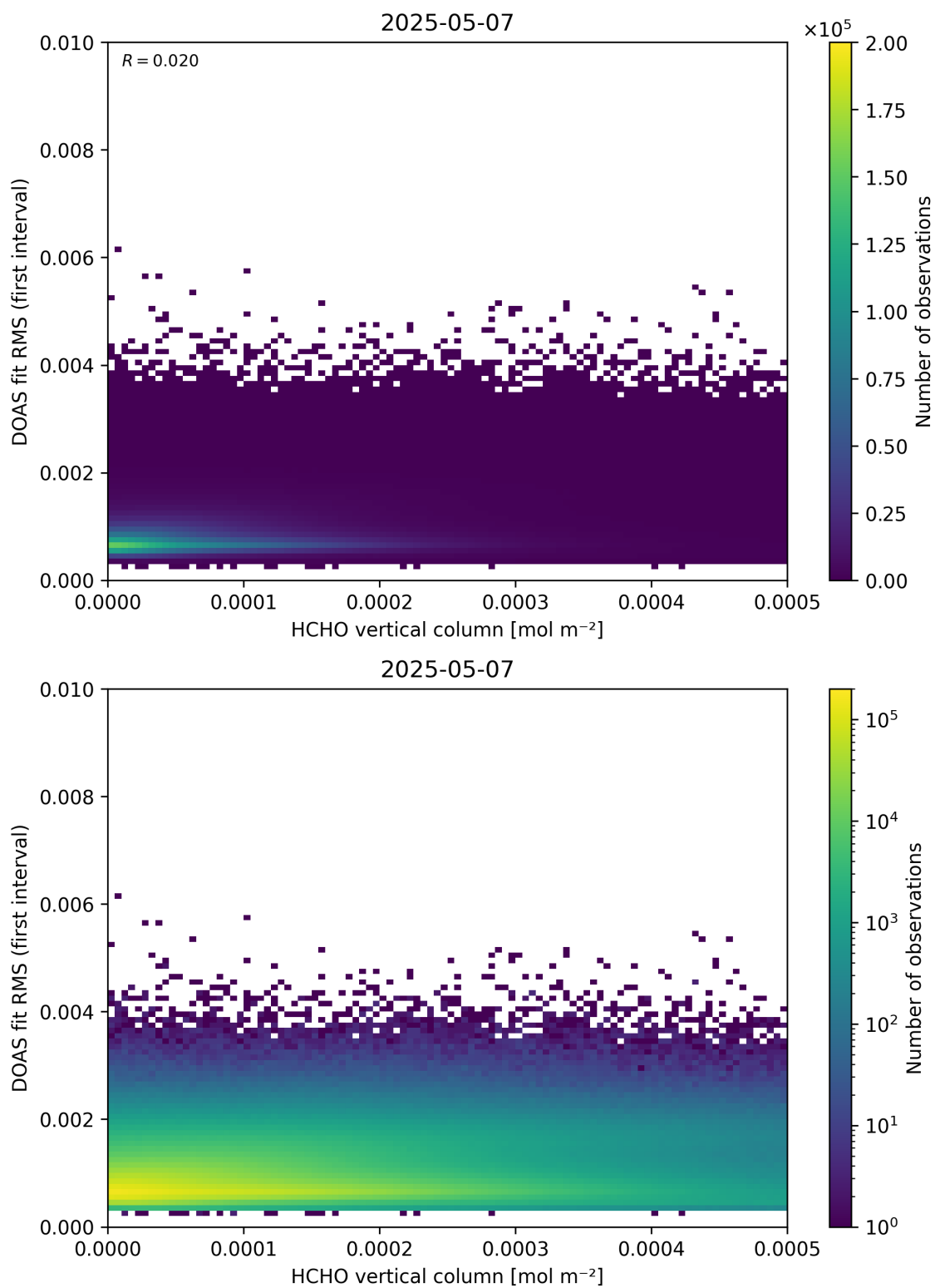
Figure 123: Scatter density plot of “HCHO vertical column” against “DOAS fit RMS (first interval)” for 2025-05-06 to 2025-05-08.
