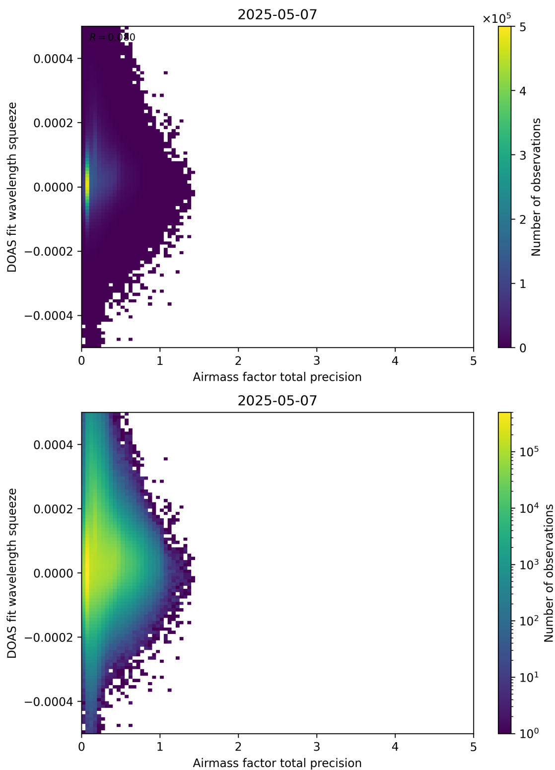
Figure 107: Scatter density plot of “Airmass factor total precision” against “DOAS fit wavelength squeeze” for 2025-05-06 to 2025-05-08.
