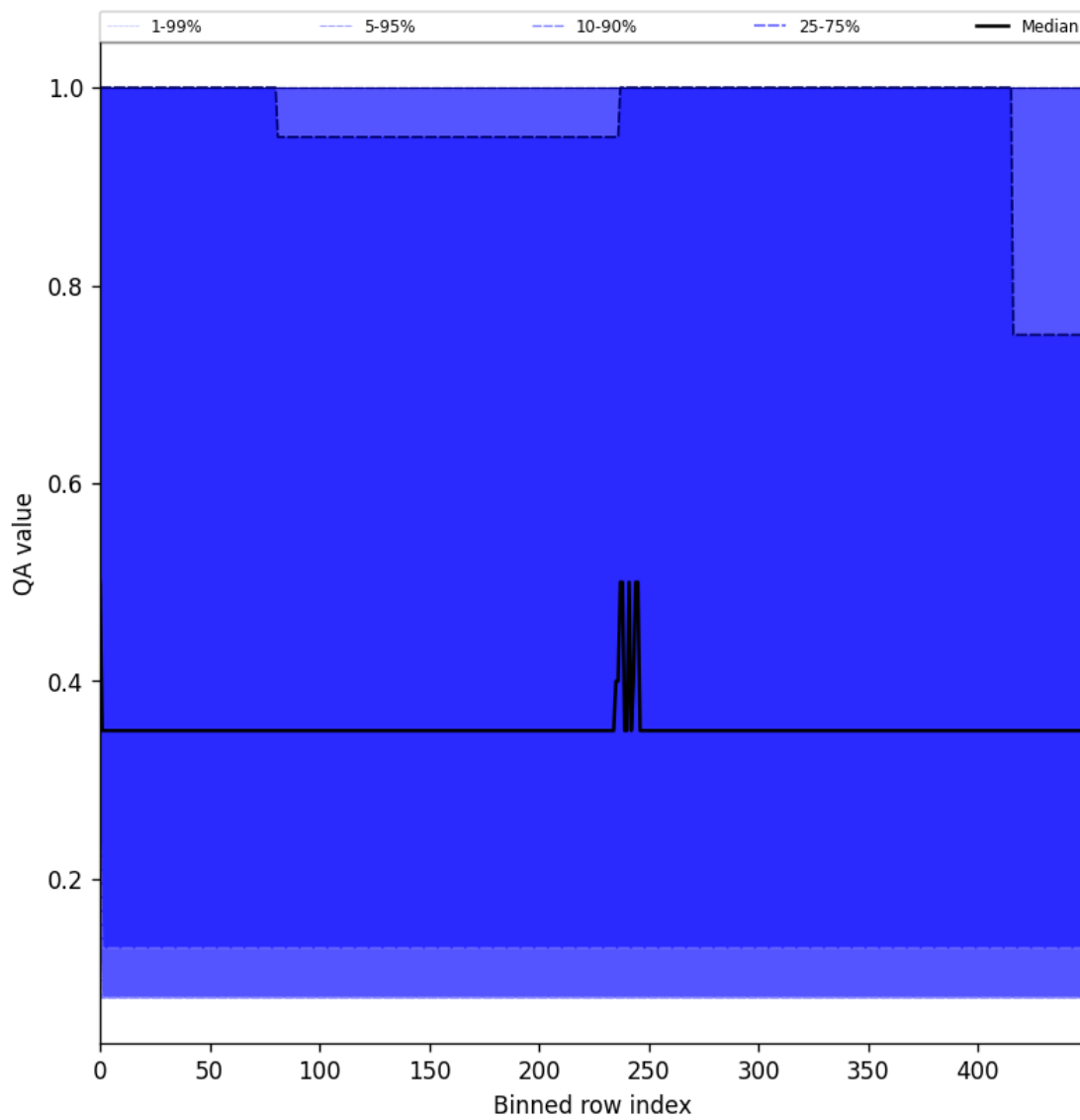
Figure 48: Along track statistics of “QA value” for 2025-05-06 to 2025-05-08
