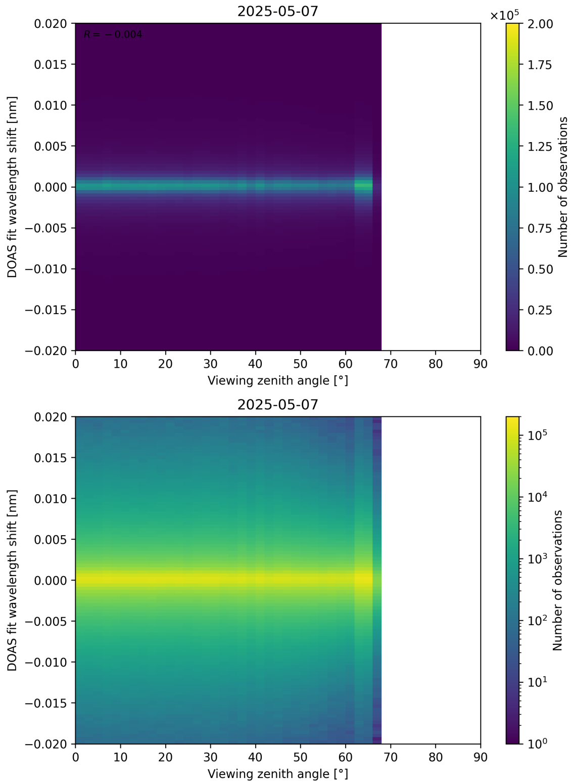
Figure 183: Scatter density plot of “Viewing zenith angle” against “DOAS fit wavelength shift” for 2025-05-06 to 2025-05-08.
