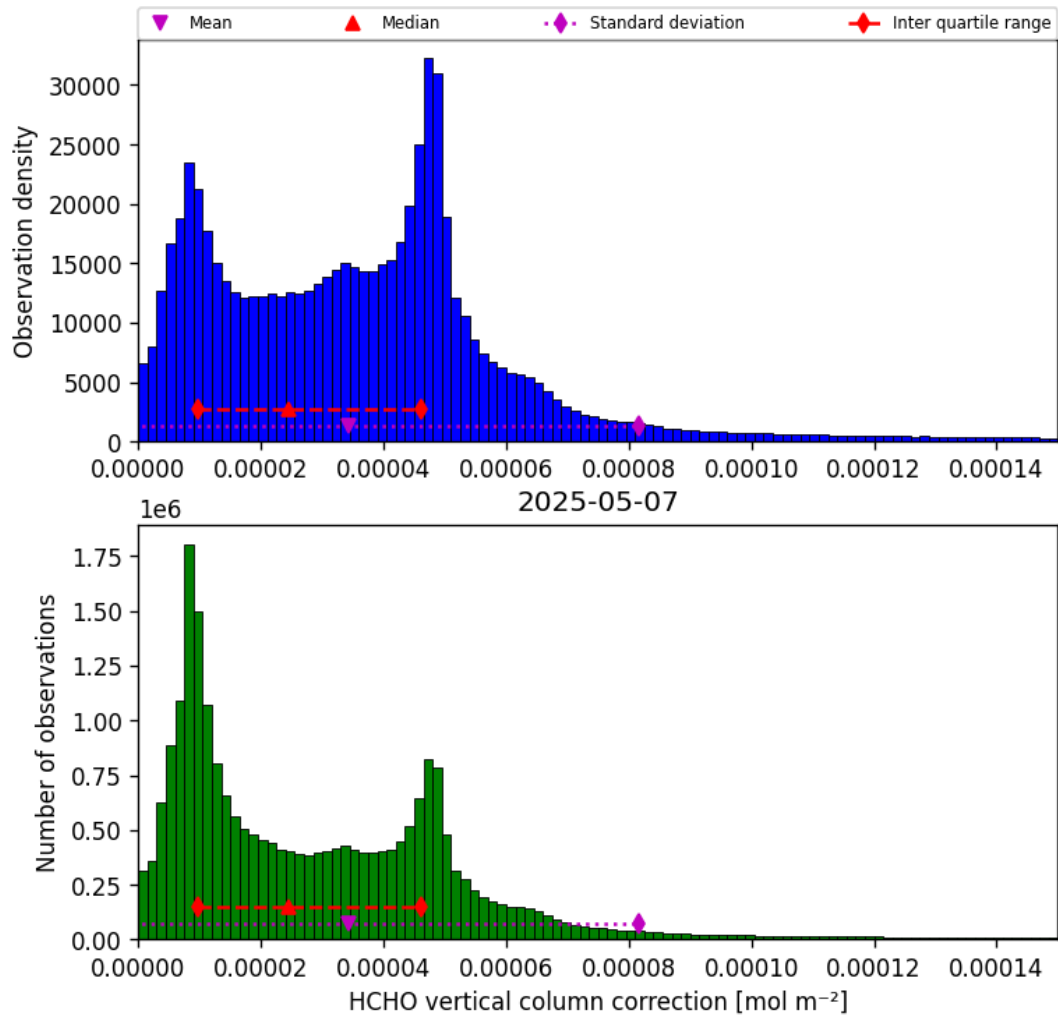
Figure 37: Histogram of “HCHO vertical column correction” for 2025-05-06 to 2025-05-08
