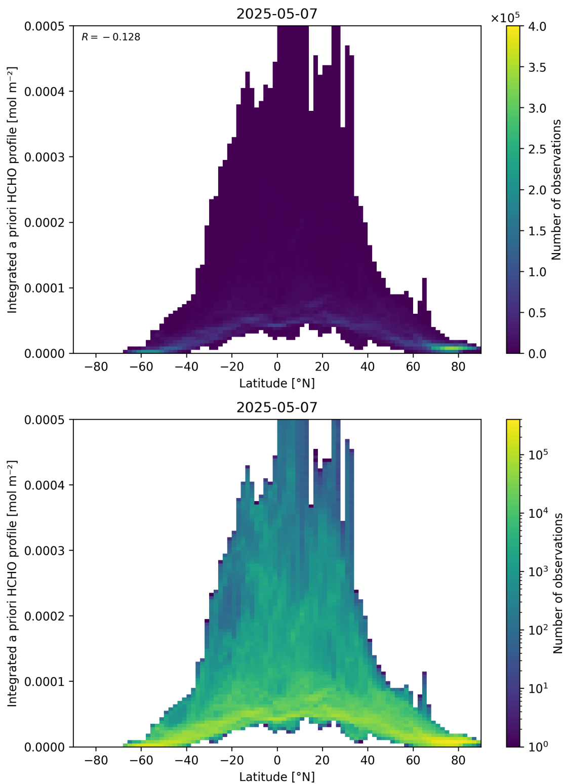
Figure 166: Scatter density plot of “Latitude” against “Integrated a priori HCHO profile” for 2025-05-06 to 2025-05-08.
