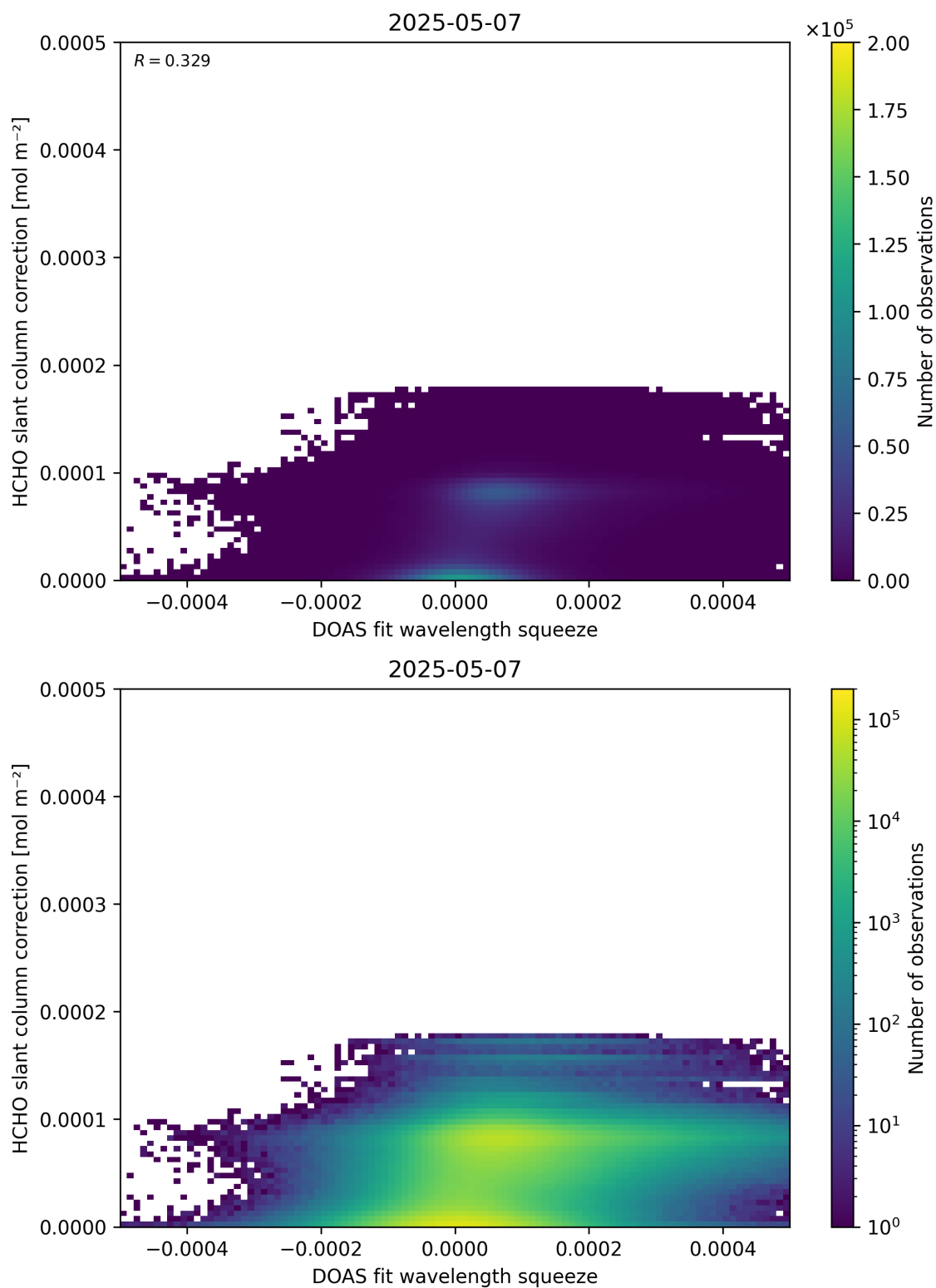
Figure 70: Scatter density plot of “DOAS fit wavelength squeeze” against “HCHO slant column correction” for 2025-05-06 to 2025-05-08.
