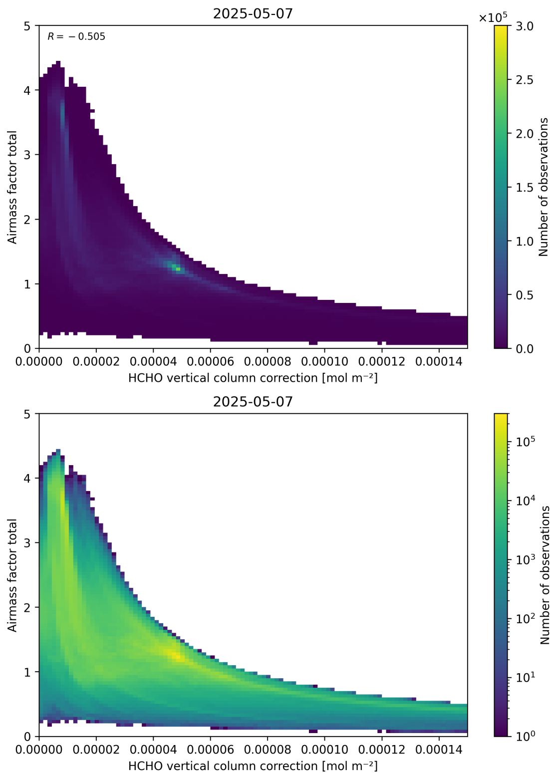
Figure 120: Scatter density plot of “HCHO vertical column correction” against “Airmass factor total” for 2025-05-06 to 2025-05-08.
