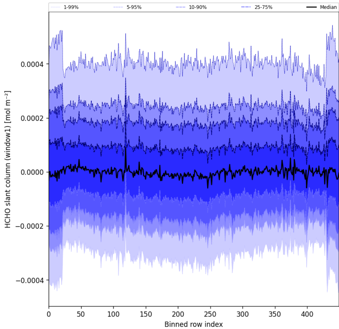
Figure 52: Along track statistics of “HCHO slant column (window1)” for 2025-05-06 to 2025-05-08
