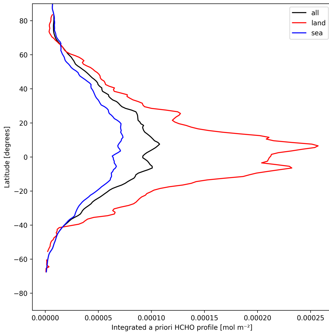
Figure 29: Zonal average of “Integrated a priori HCHO profile” for 2025-05-06 to 2025-05-08.
