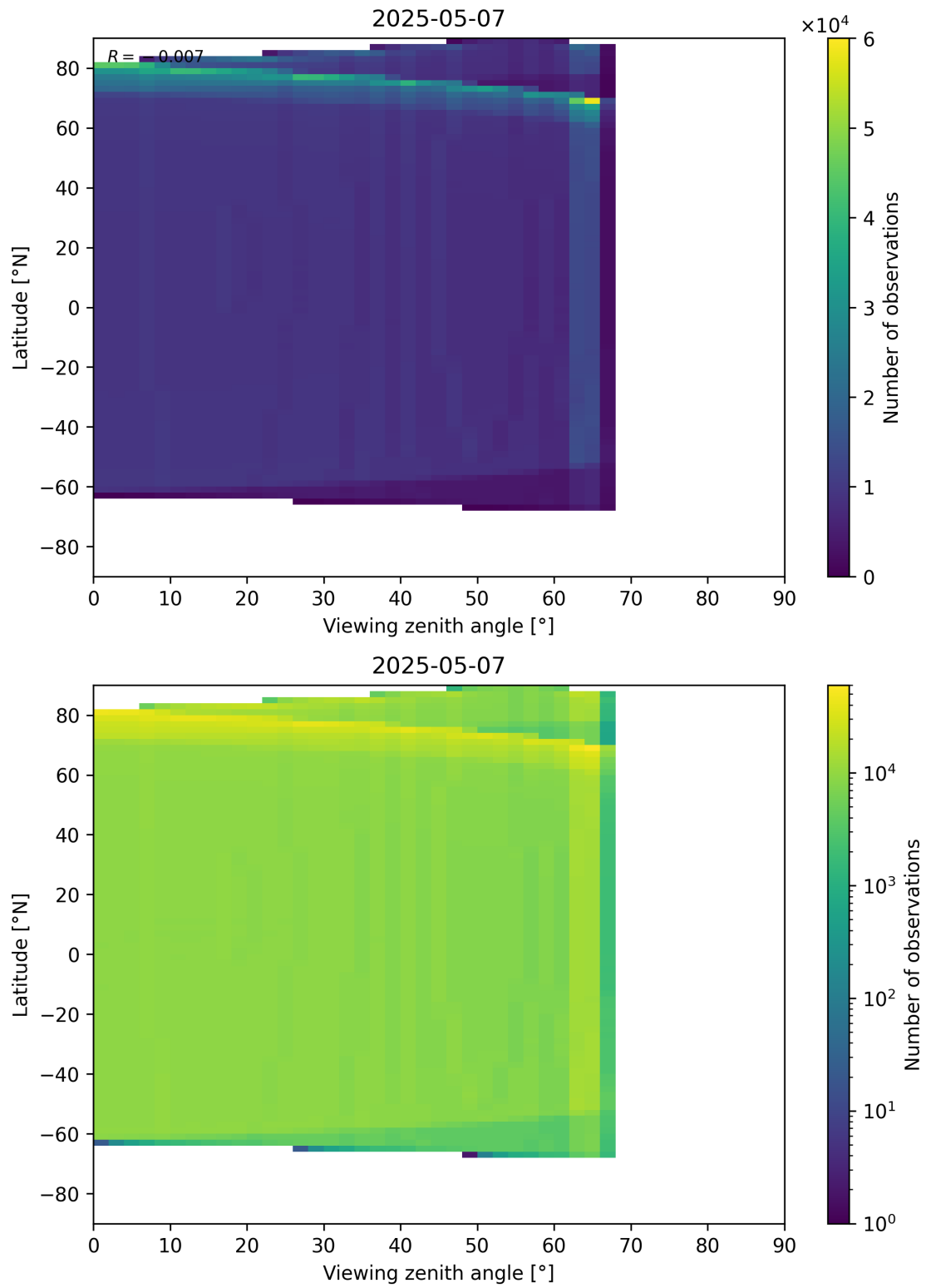
Figure 196: Scatter density plot of “Viewing zenith angle” against “Latitude” for 2025-05-06 to 2025-05-08.
