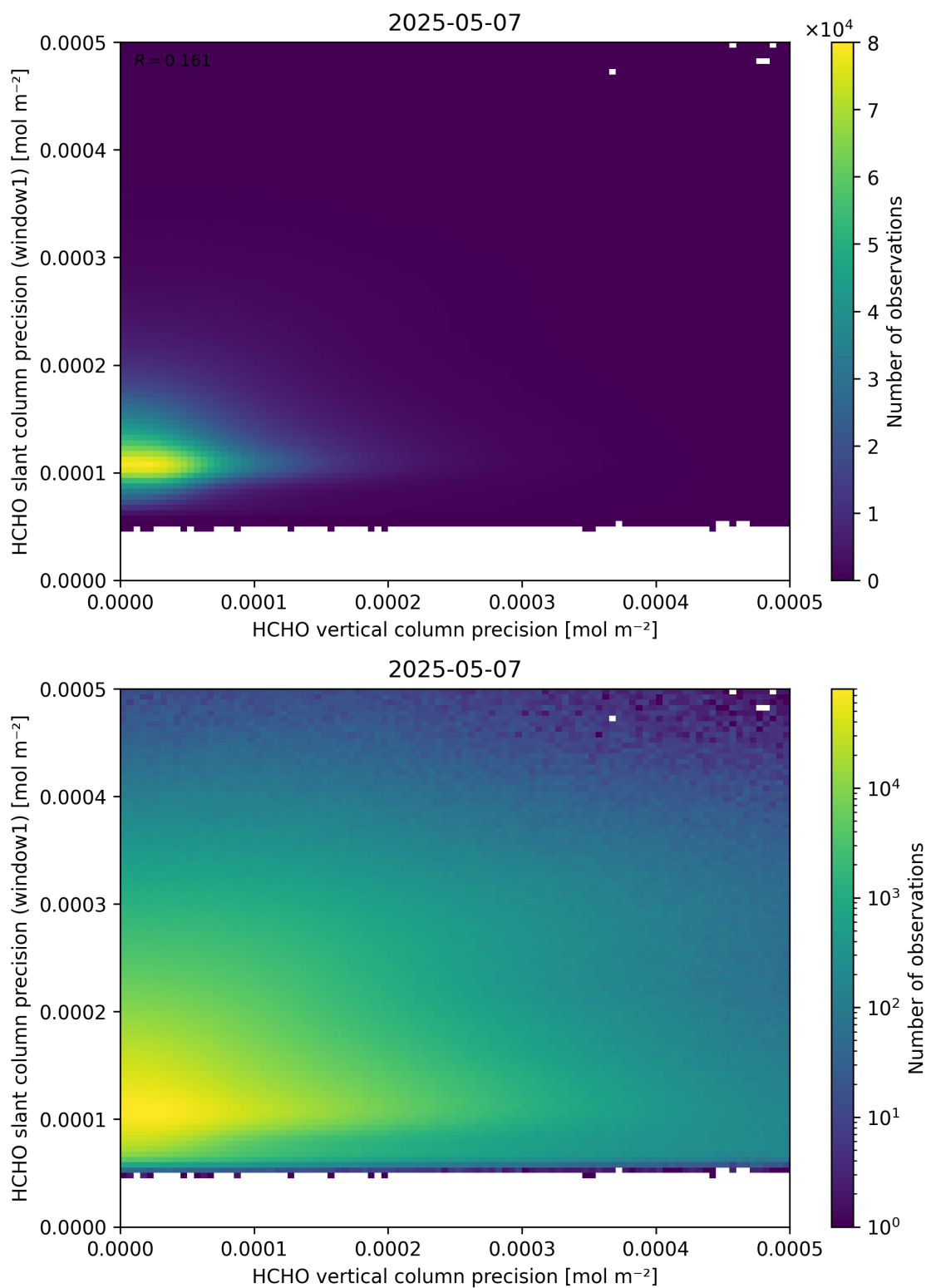
Figure 143: Scatter density plot of “HCHO vertical column precision” against “HCHO slant column precision (window1)” for 2025-05-06 to 2025-05-08.
