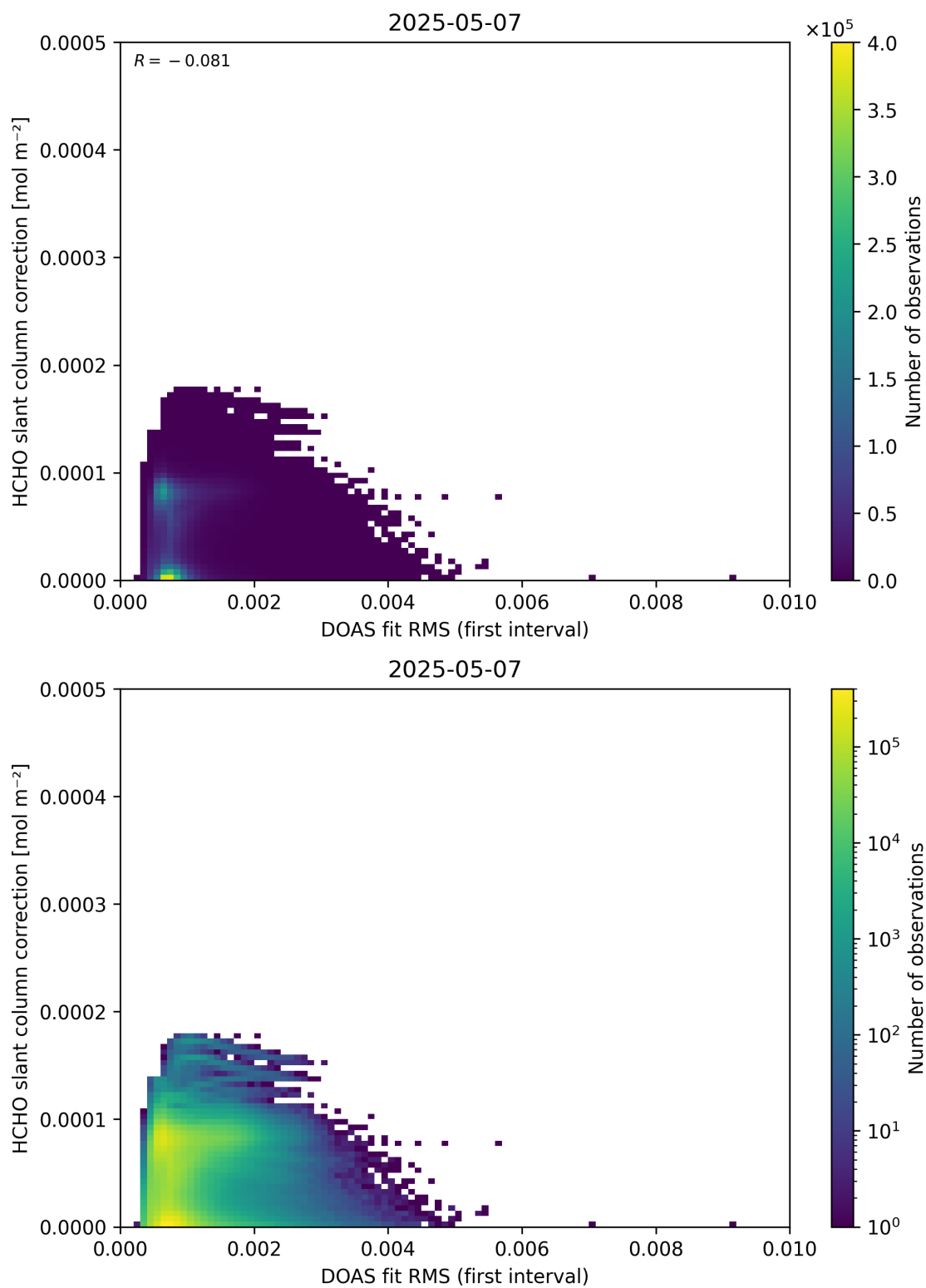
Figure 63: Scatter density plot of “DOAS fit RMS (first interval)” against “HCHO slant column correction” for 2025-05-06 to 2025-05-08.
