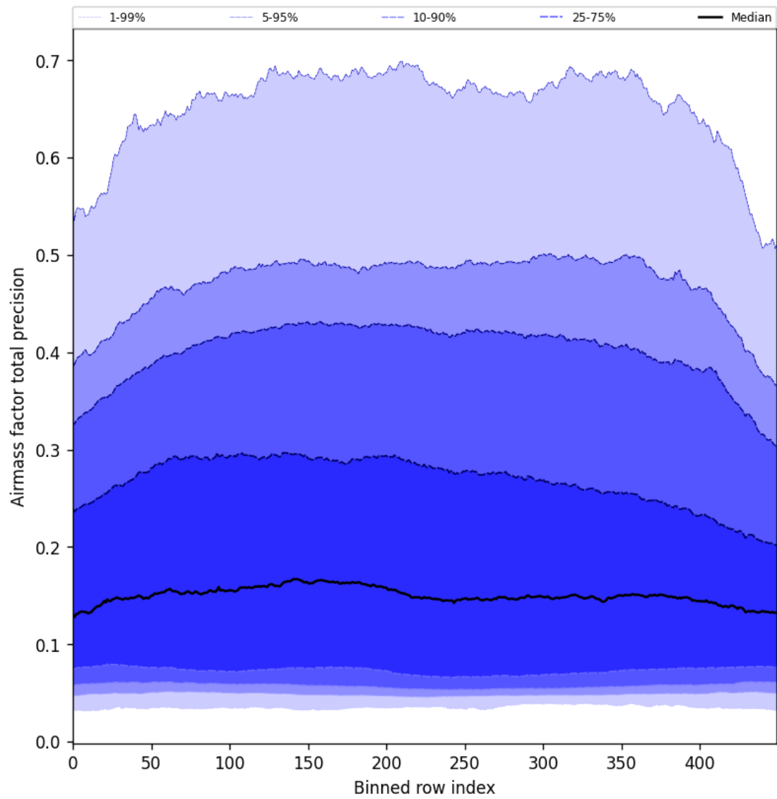
Figure 55: Along track statistics of “Airmass factor total precision” for 2025-05-06 to 2025-05-08
