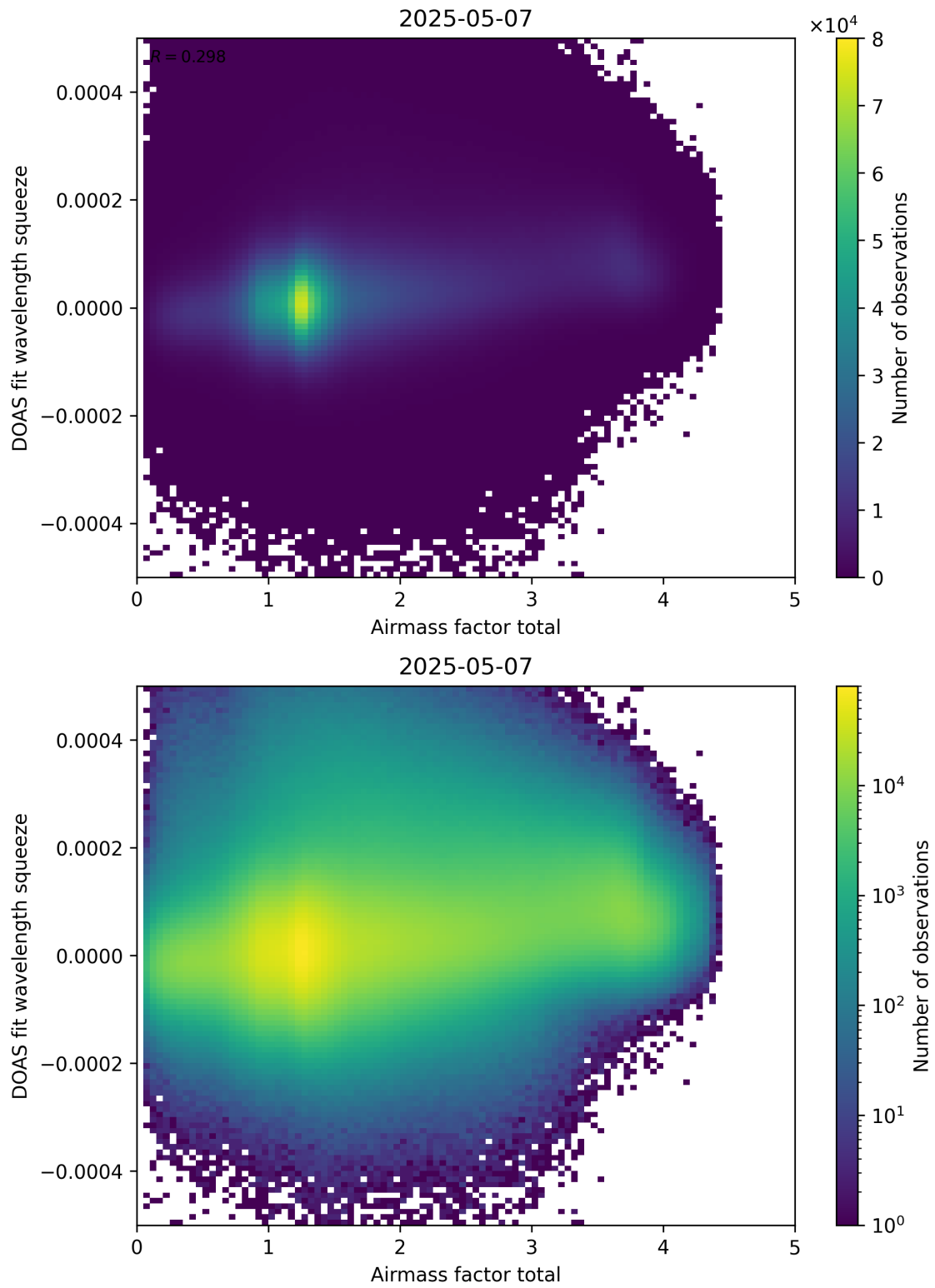
Figure 99: Scatter density plot of “Airmass factor total” against “DOAS fit wavelength squeeze” for 2025-05-06 to 2025-05-08.
