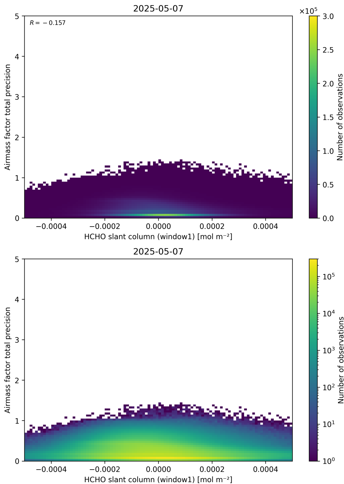
Figure 86: Scatter density plot of “HCHO slant column (window1)” against “Airmass factor total precision” for 2025-05-06 to 2025-05-08.
