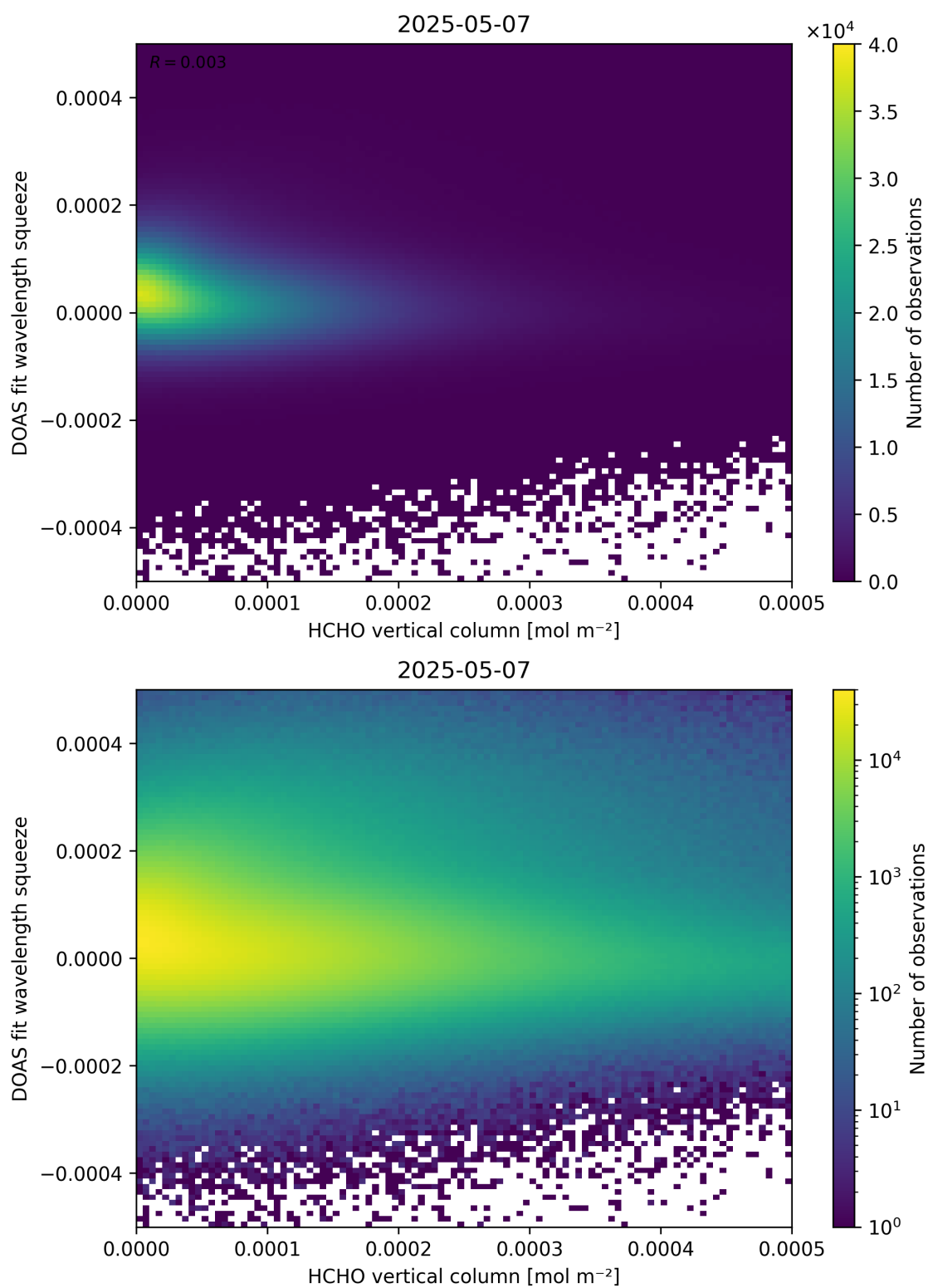
Figure 125: Scatter density plot of “HCHO vertical column” against “DOAS fit wavelength squeeze” for 2025-05-06 to 2025-05-08.
