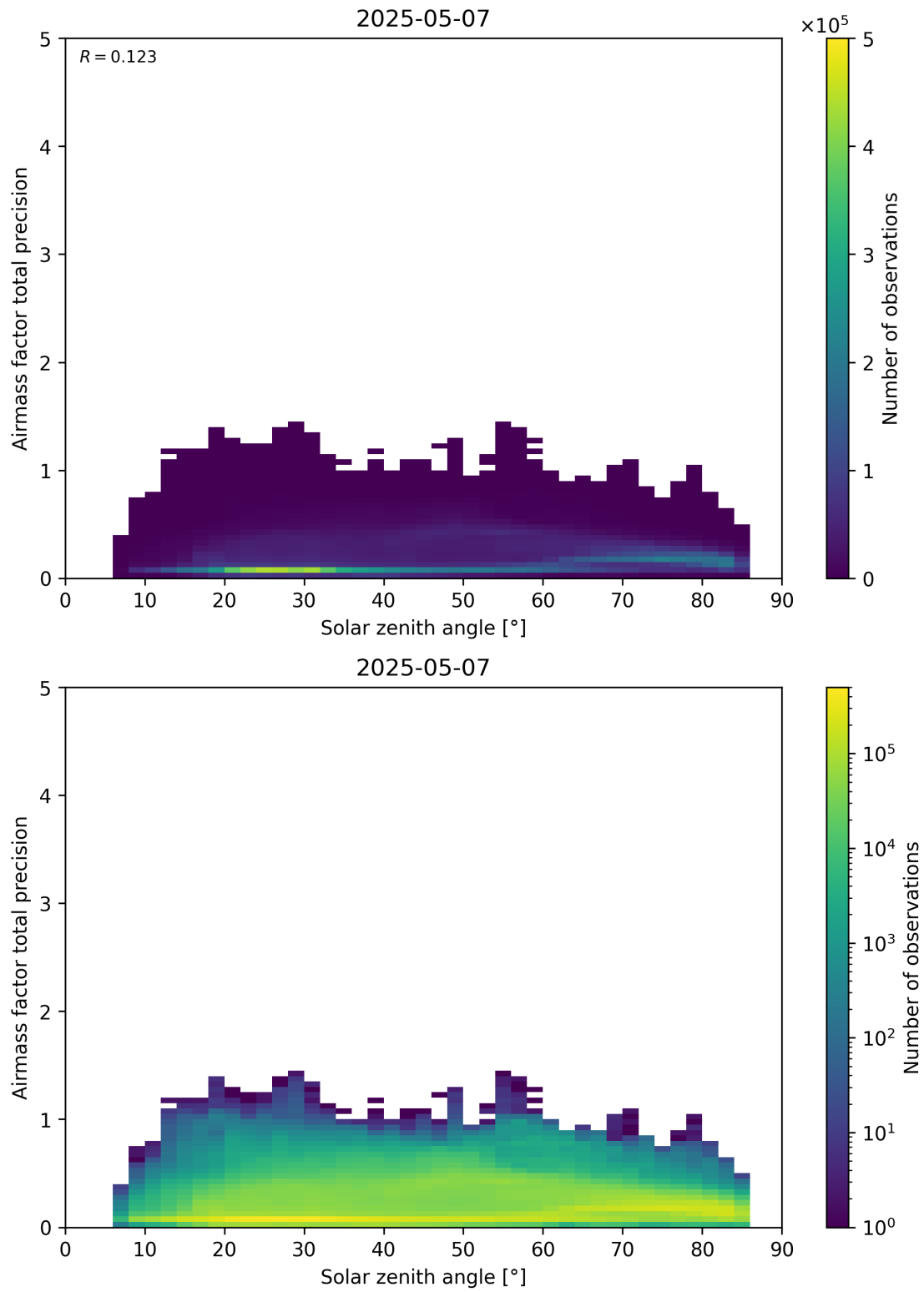
Figure 176: Scatter density plot of “Solar zenith angle” against “Airmass factor total precision” for 2025-05-06 to 2025-05-08.
