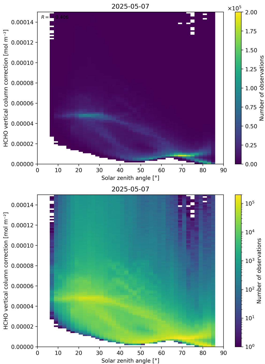
Figure 178: Scatter density plot of “Solar zenith angle” against “HCHO vertical column correction” for 2025-05-06 to 2025-05-08.
