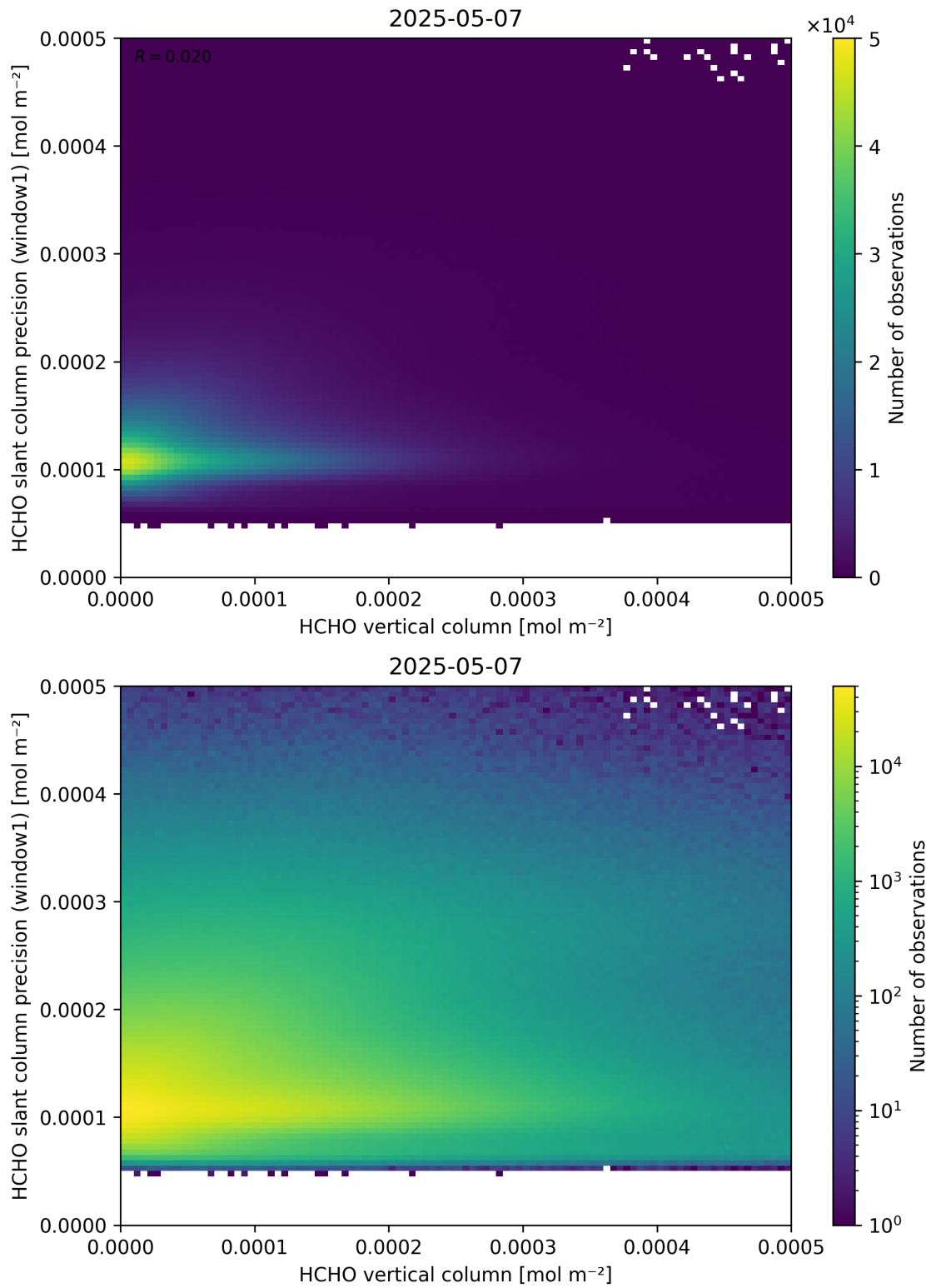
Figure 130: Scatter density plot of “HCHO vertical column” against “HCHO slant column precision (window1)” for 2025-05-06 to 2025-05-08.
