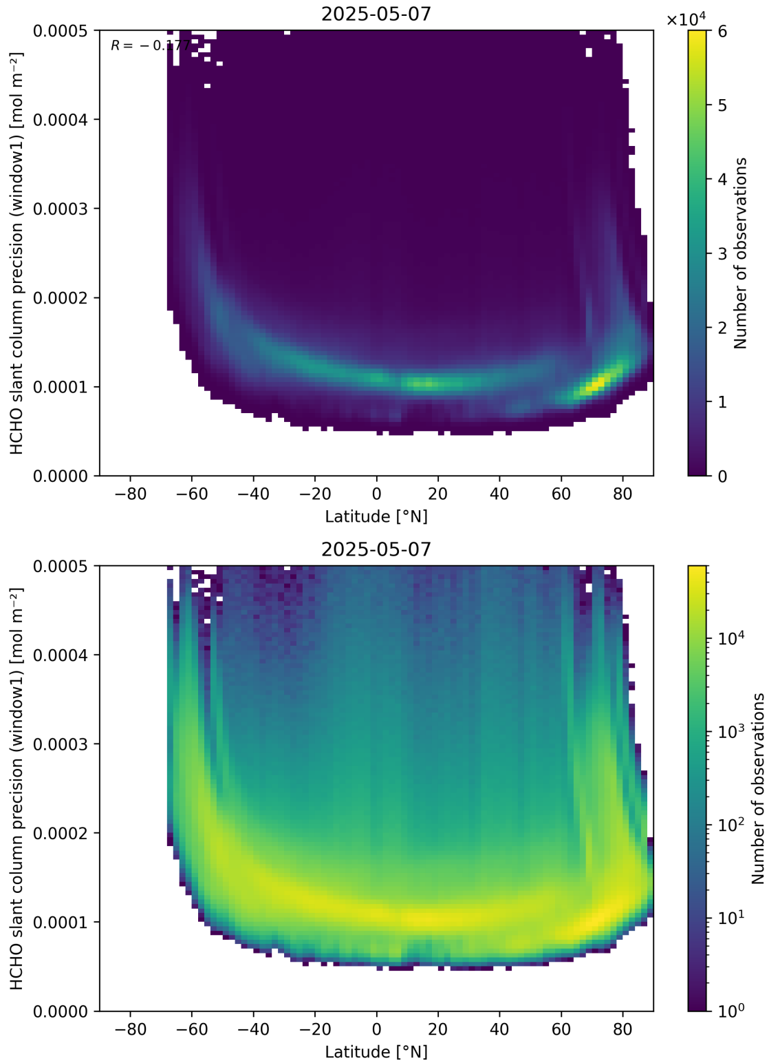
Figure 160: Scatter density plot of “Latitude” against “HCHO slant column precision (window1)” for 2025-05-06 to 2025-05-08.
