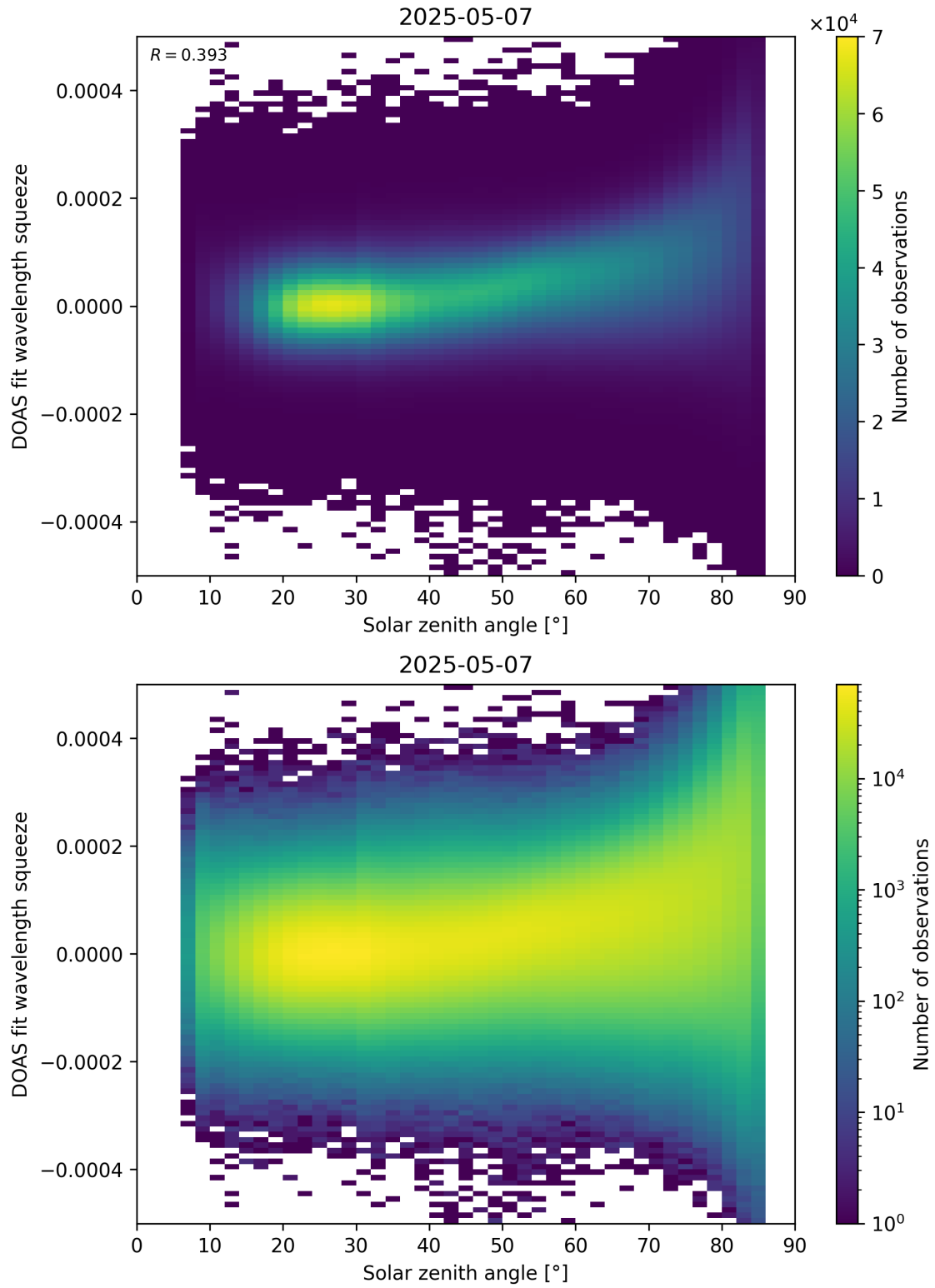
Figure 169: Scatter density plot of “Solar zenith angle” against “DOAS fit wavelength squeeze” for 2025-05-06 to 2025-05-08.
