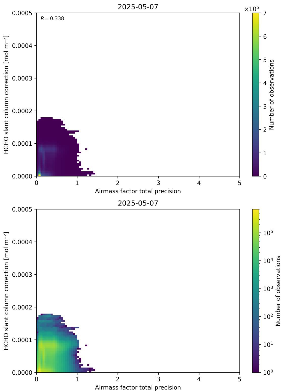
Figure 110: Scatter density plot of “Airmass factor total precision” against “HCHO slant column correction” for 2025-05-06 to 2025-05-08.
