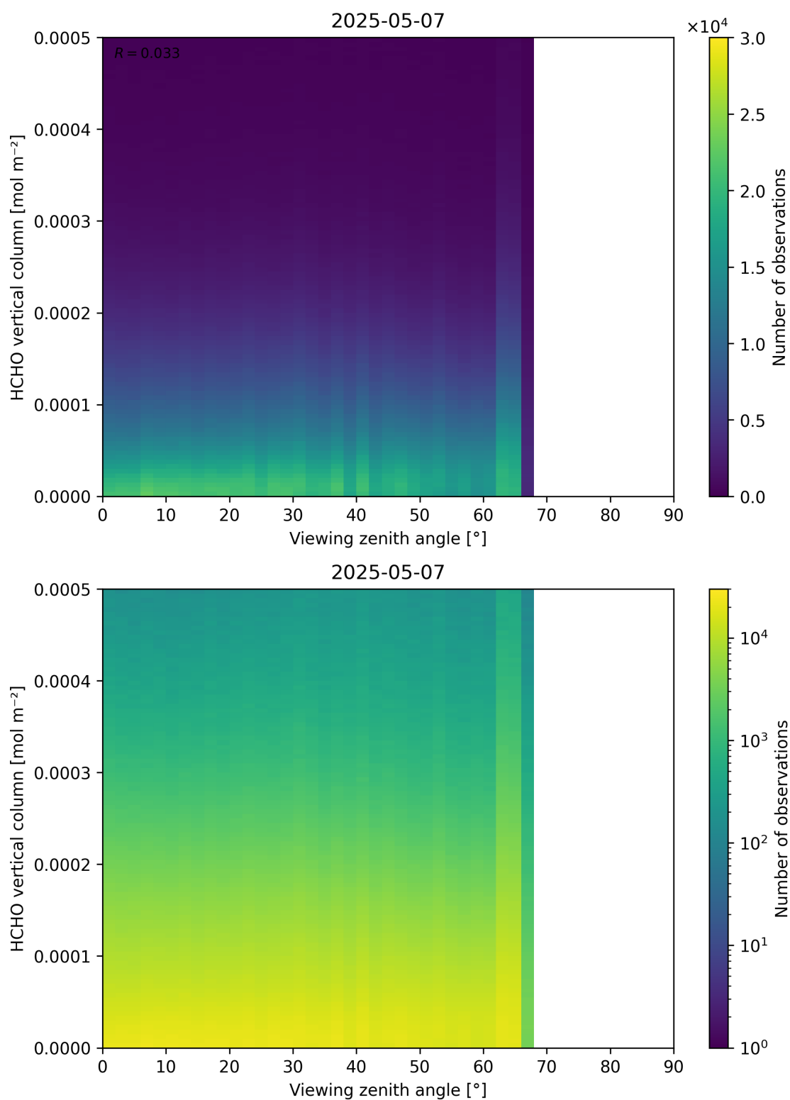
Figure 192: Scatter density plot of “Viewing zenith angle” against “HCHO vertical column” for 2025-05-06 to 2025-05-08.
