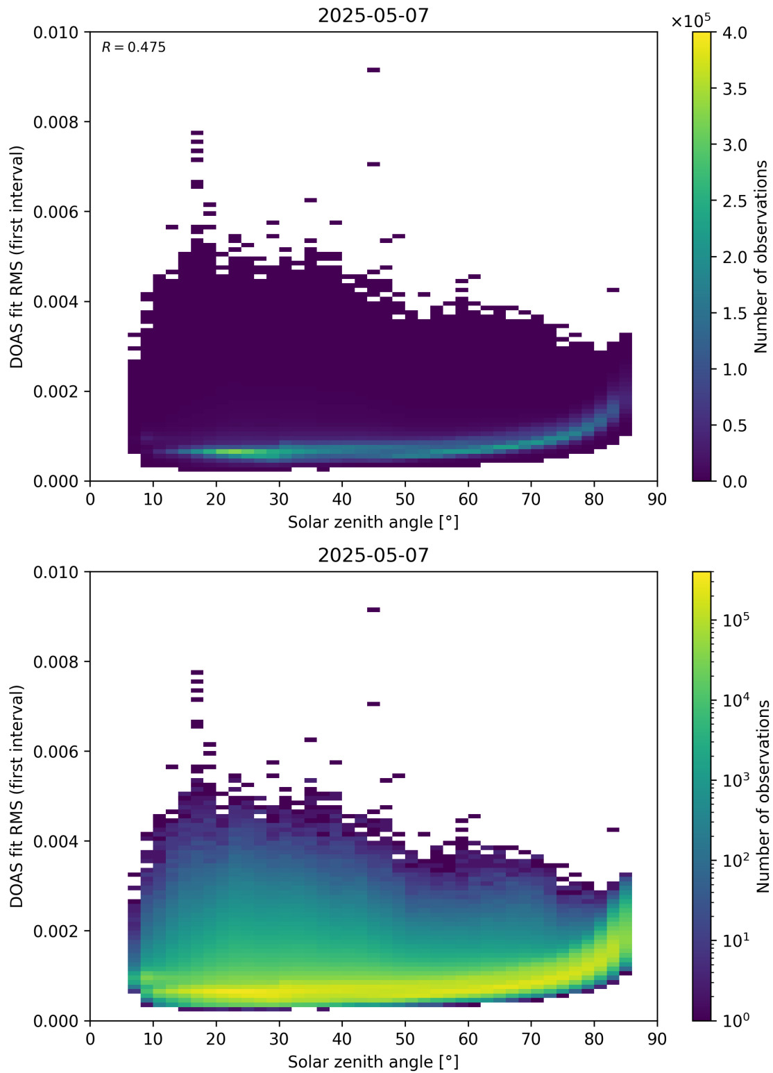
Figure 167: Scatter density plot of “Solar zenith angle” against “DOAS fit RMS (first interval)” for 2025-05-06 to 2025-05-08.
