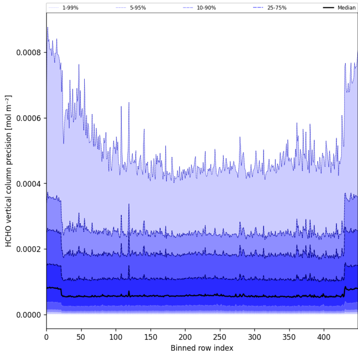
Figure 50: Along track statistics of “HCHO vertical column precision” for 2025-05-06 to 2025-05-08
