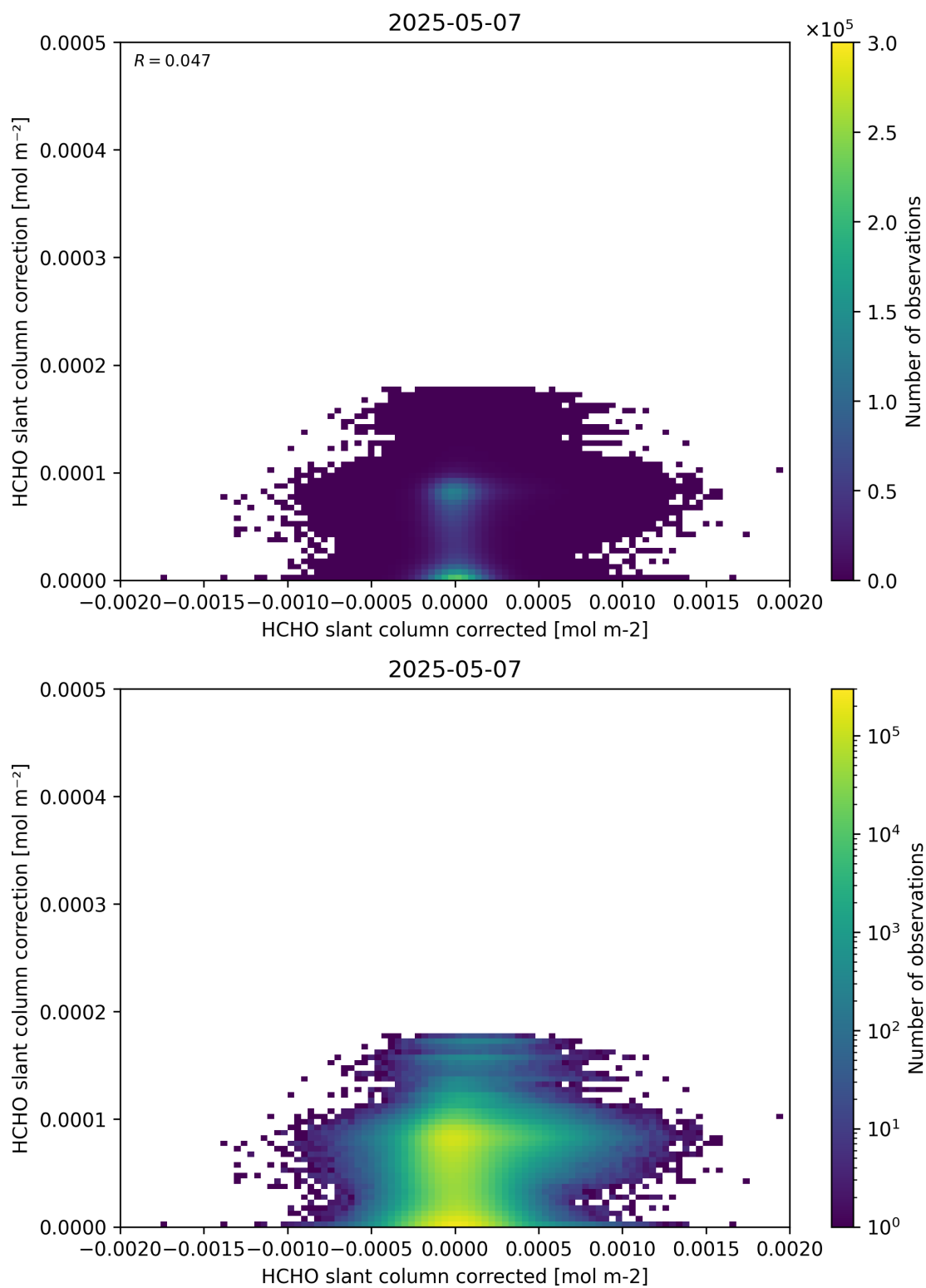
Figure 77: Scatter density plot of “HCHO slant column corrected” against “HCHO slant column correction” for 2025-05-06 to 2025-05-08.
