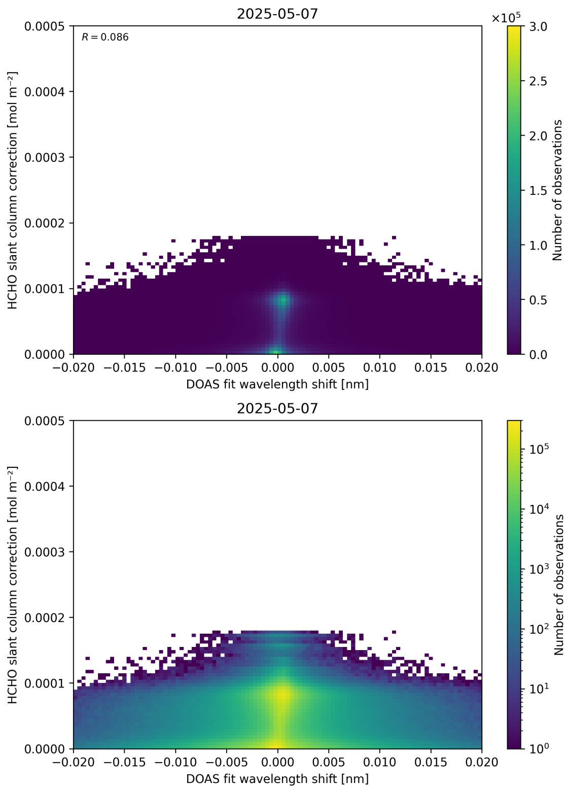
Figure 67: Scatter density plot of “DOAS fit wavelength shift” against “HCHO slant column correction” for 2025-05-06 to 2025-05-08.
