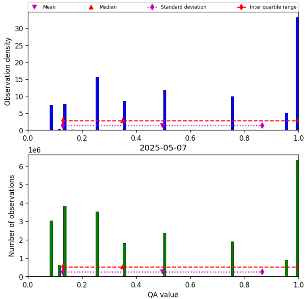
Figure 34: Histogram of “QA value” for 2025-05-06 to 2025-05-08
