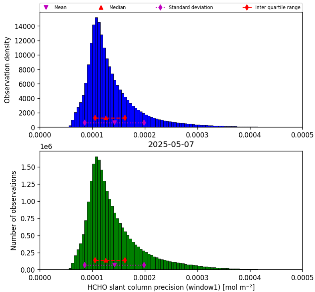
Figure 39: Histogram of “HCHO slant column precision (window1)” for 2025-05-06 to 2025-05-08
