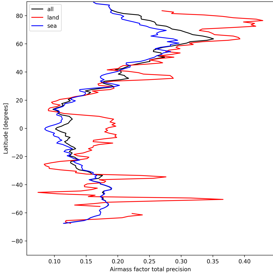
Figure 27: Zonal average of “Airmass factor total precision” for 2025-05-06 to 2025-05-08.
