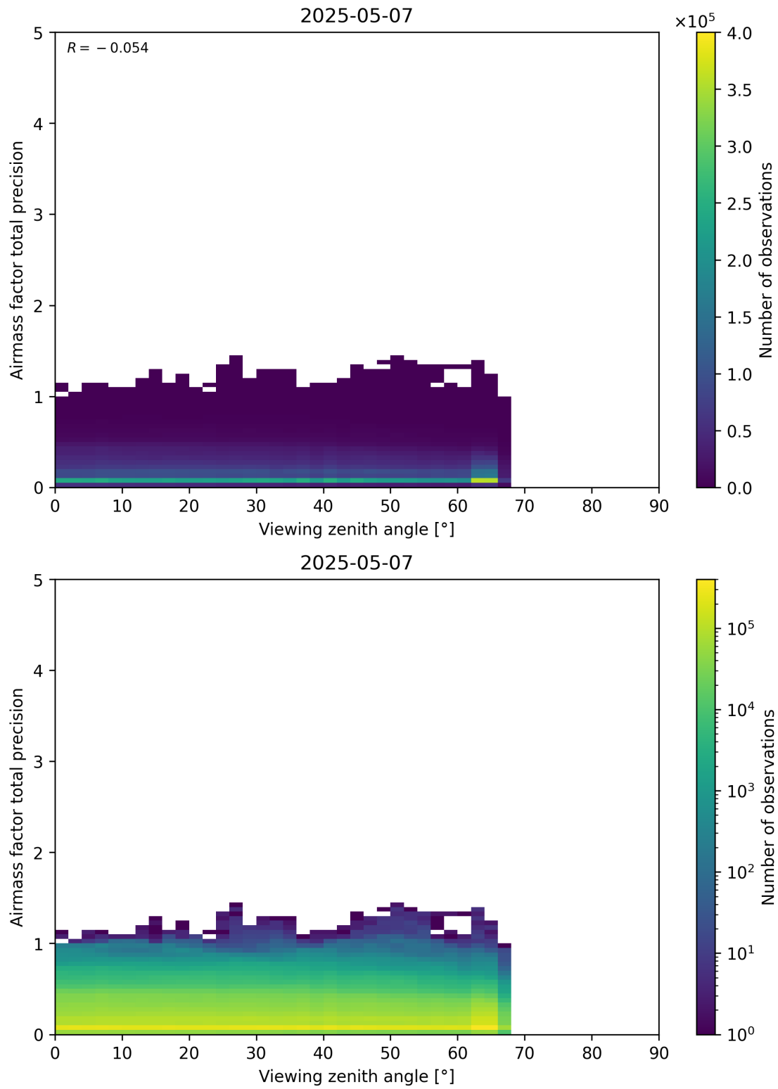
Figure 191: Scatter density plot of “Viewing zenith angle” against “Airmass factor total precision” for 2025-05-06 to 2025-05-08.
