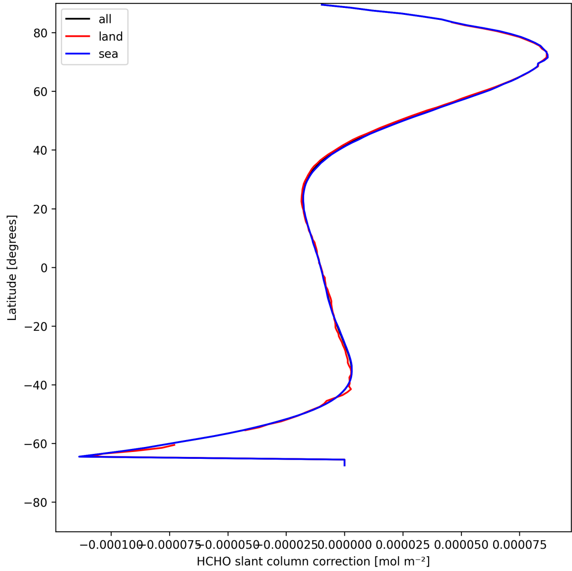
Figure 33: Zonal average of “HCHO slant column correction” for 2025-05-06 to 2025-05-08.
