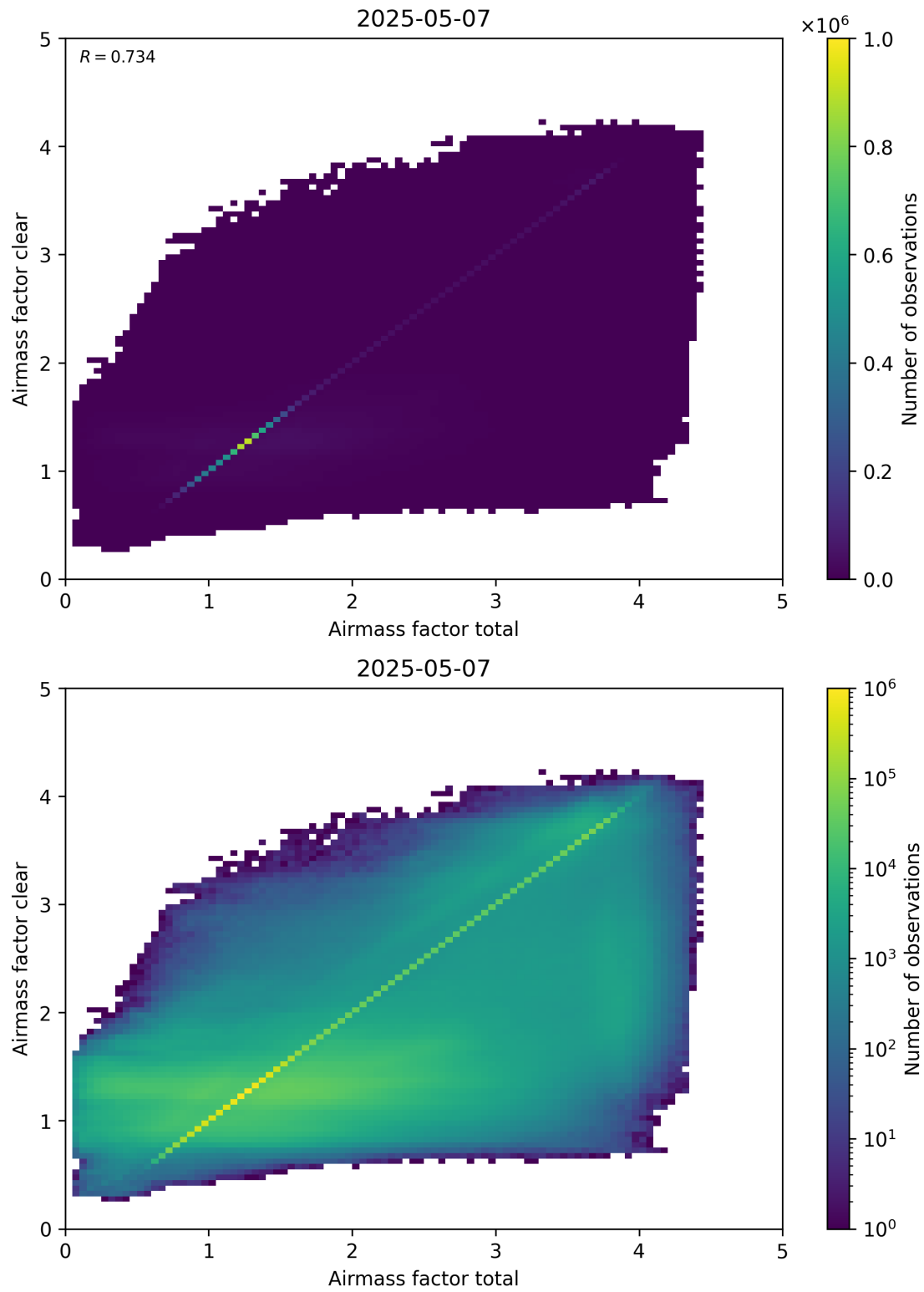
Figure 100: Scatter density plot of “Airmass factor total” against “Airmass factor clear” for 2025-05-06 to 2025-05-08.
