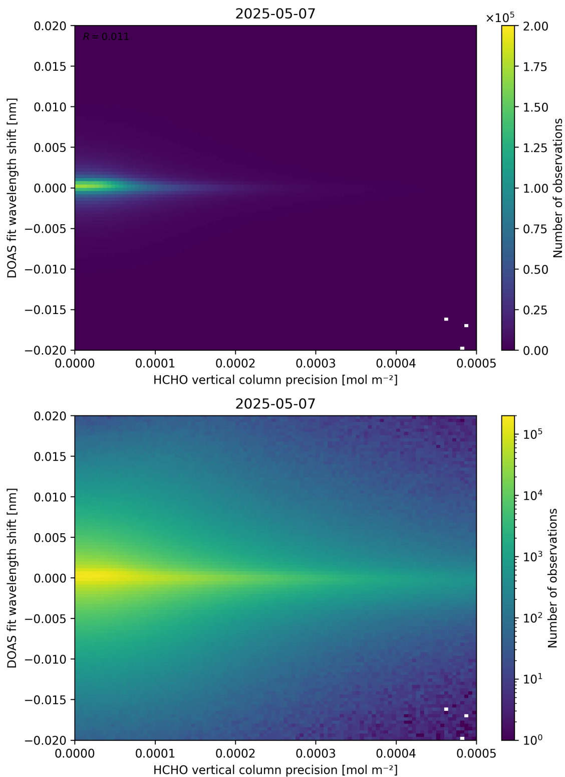
Figure 137: Scatter density plot of “HCHO vertical column precision” against “DOAS fit wavelength shift” for 2025-05-06 to 2025-05-08.
