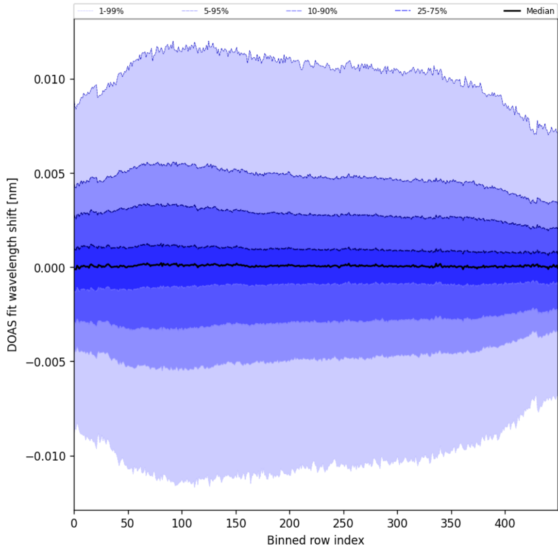
Figure 58: Along track statistics of “DOAS fit wavelength shift” for 2025-05-06 to 2025-05-08
