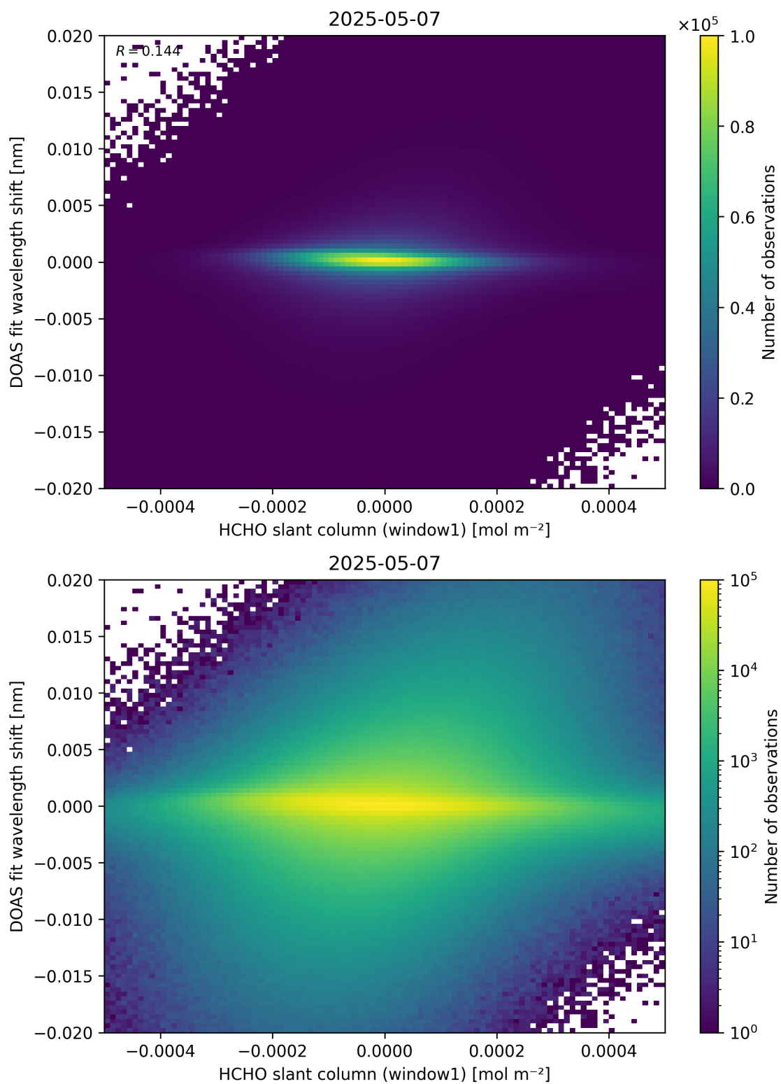
Figure 79: Scatter density plot of “HCHO slant column (window1)” against “DOAS fit wavelength shift” for 2025-05-06 to 2025-05-08.
