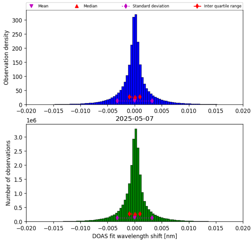
Figure 44: Histogram of “DOAS fit wavelength shift” for 2025-05-06 to 2025-05-08
