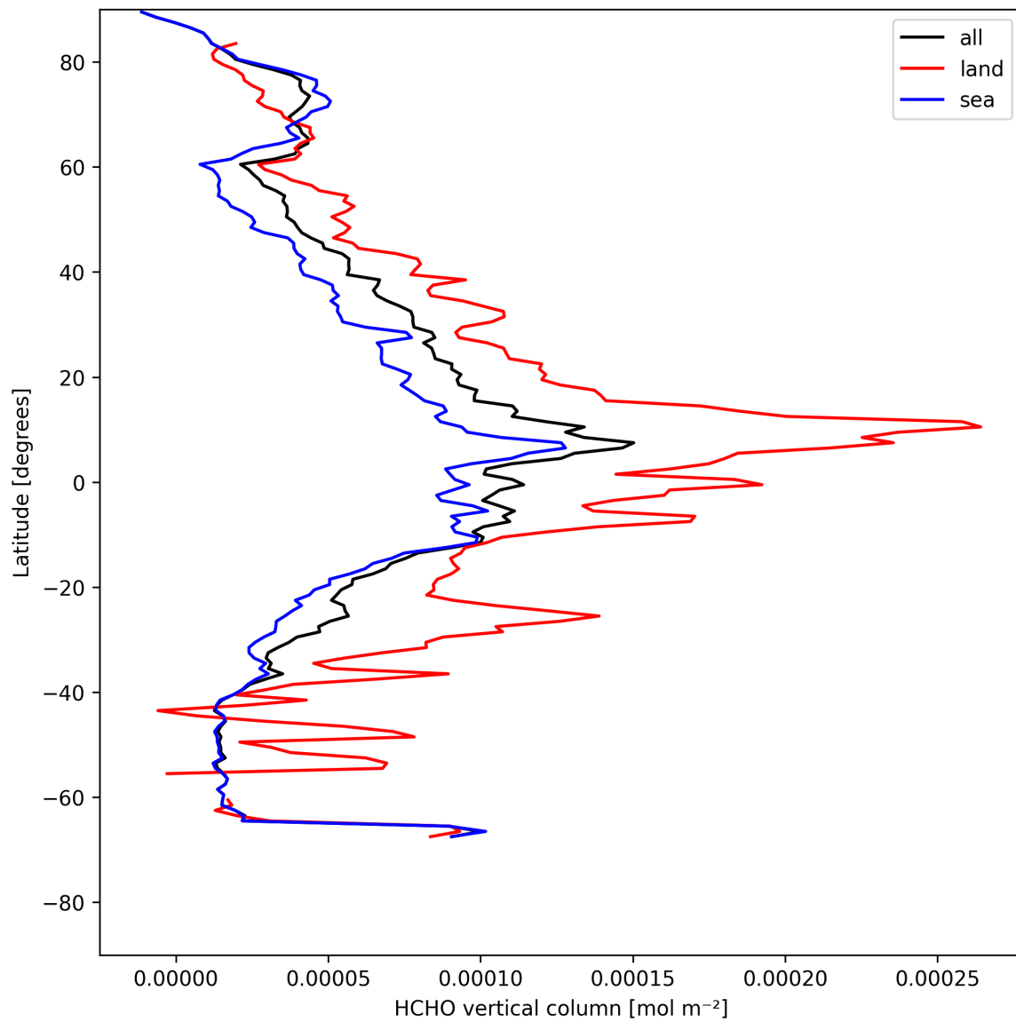
Figure 21: Zonal average of “HCHO vertical column” for 2025-05-06 to 2025-05-08.
