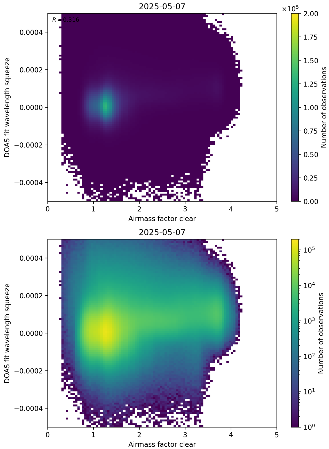
Figure 73: Scatter density plot of “Airmass factor clear” against “DOAS fit wavelength squeeze” for 2025-05-06 to 2025-05-08.
