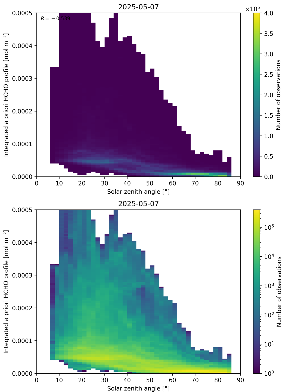
Figure 180: Scatter density plot of “Solar zenith angle” against “Integrated a priori HCHO profile” for 2025-05-06 to 2025-05-08.
