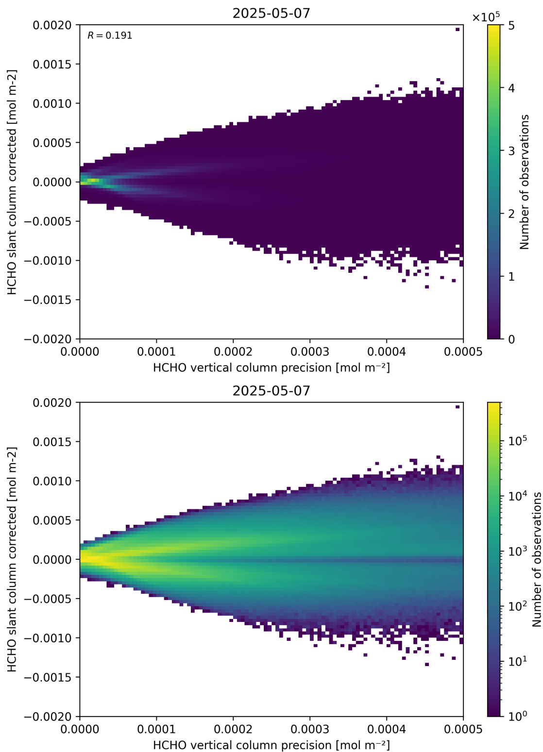
Figure 140: Scatter density plot of “HCHO vertical column precision” against “HCHO slant column corrected” for 2025-05-06 to 2025-05-08.
