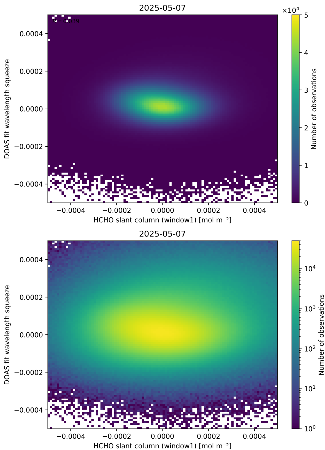
Figure 80: Scatter density plot of “HCHO slant column (window1)” against “DOAS fit wavelength squeeze” for 2025-05-06 to 2025-05-08.
