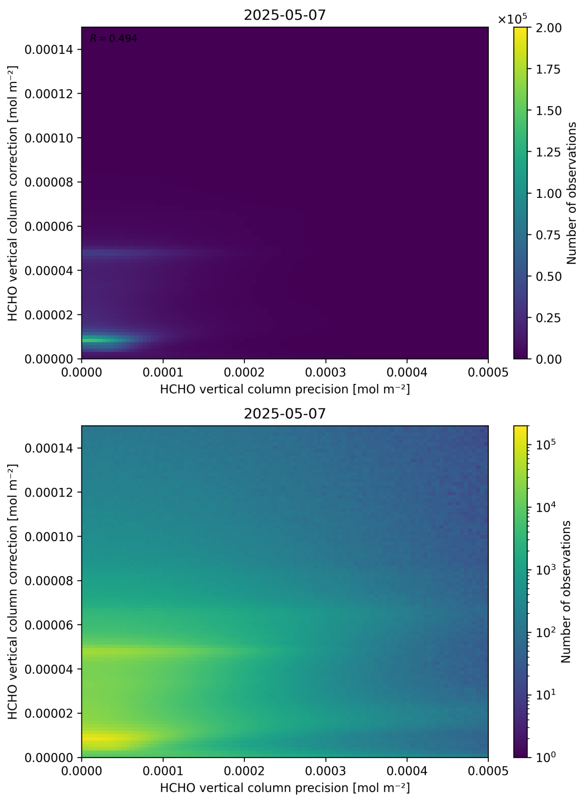
Figure 146: Scatter density plot of “HCHO vertical column precision” against “HCHO vertical column correction” for 2025-05-06 to 2025-05-08.
