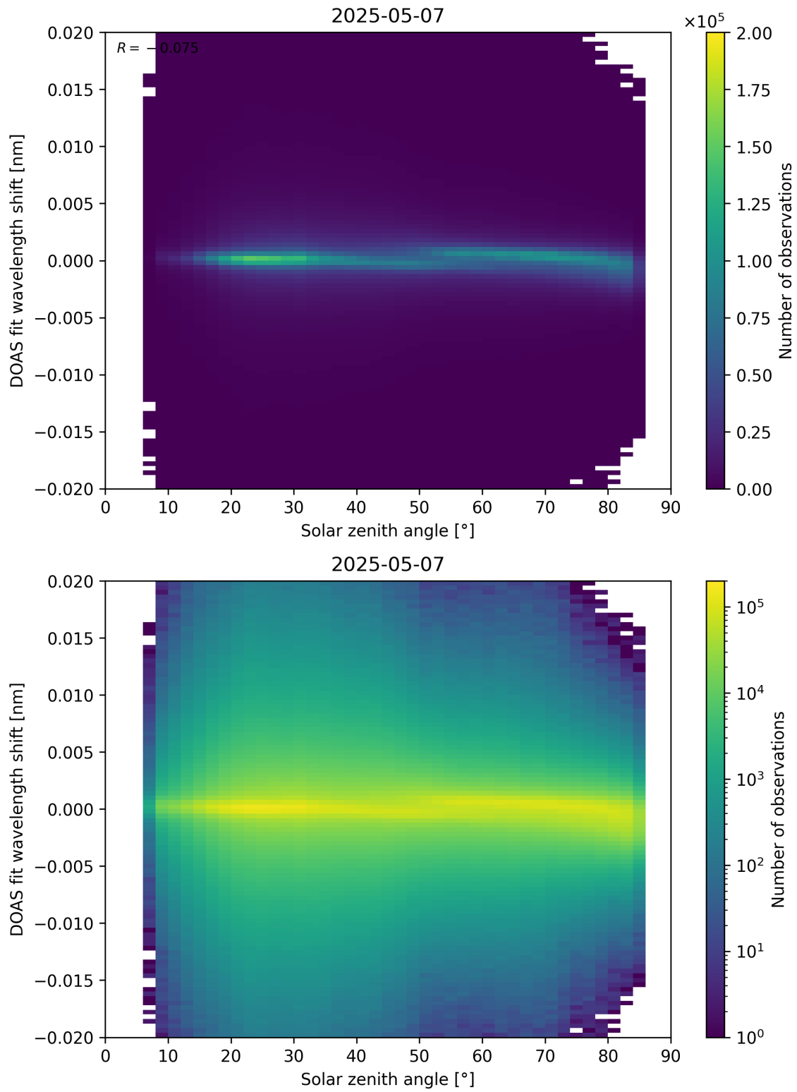
Figure 168: Scatter density plot of “Solar zenith angle” against “DOAS fit wavelength shift” for 2025-05-06 to 2025-05-08.
