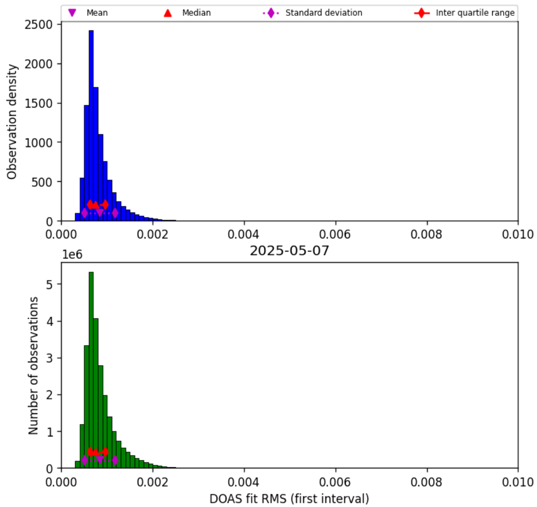
Figure 46: Histogram of “DOAS fit RMS (first interval)” for 2025-05-06 to 2025-05-08
