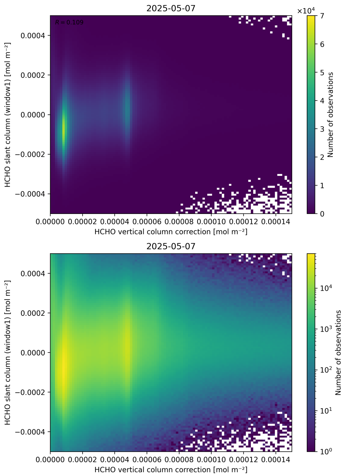
Figure 118: Scatter density plot of “HCHO vertical column correction” against “HCHO slant column (window1)” for 2025-05-06 to 2025-05-08.
