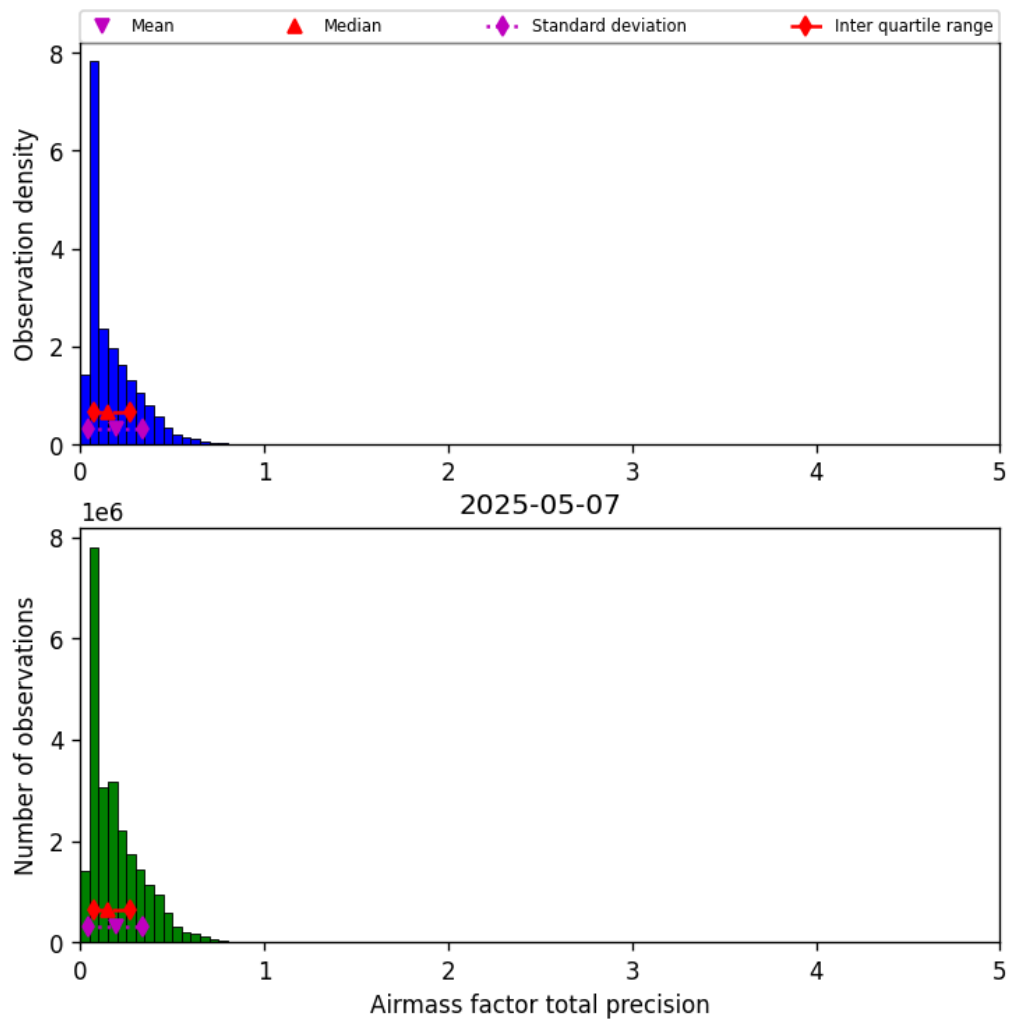
Figure 41: Histogram of “Airmass factor total precision” for 2025-05-06 to 2025-05-08
