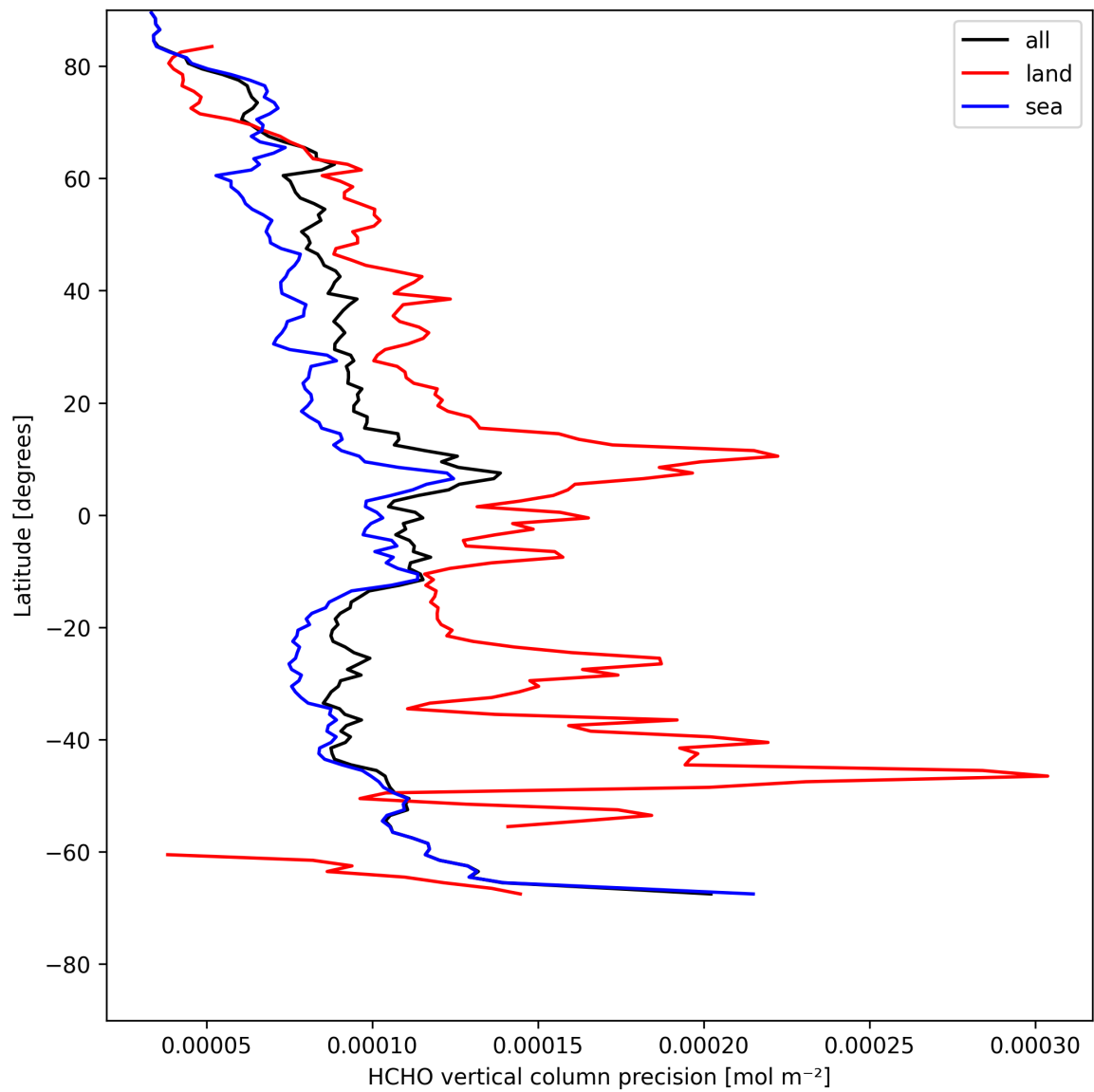
Figure 22: Zonal average of “HCHO vertical column precision” for 2025-05-06 to 2025-05-08.
