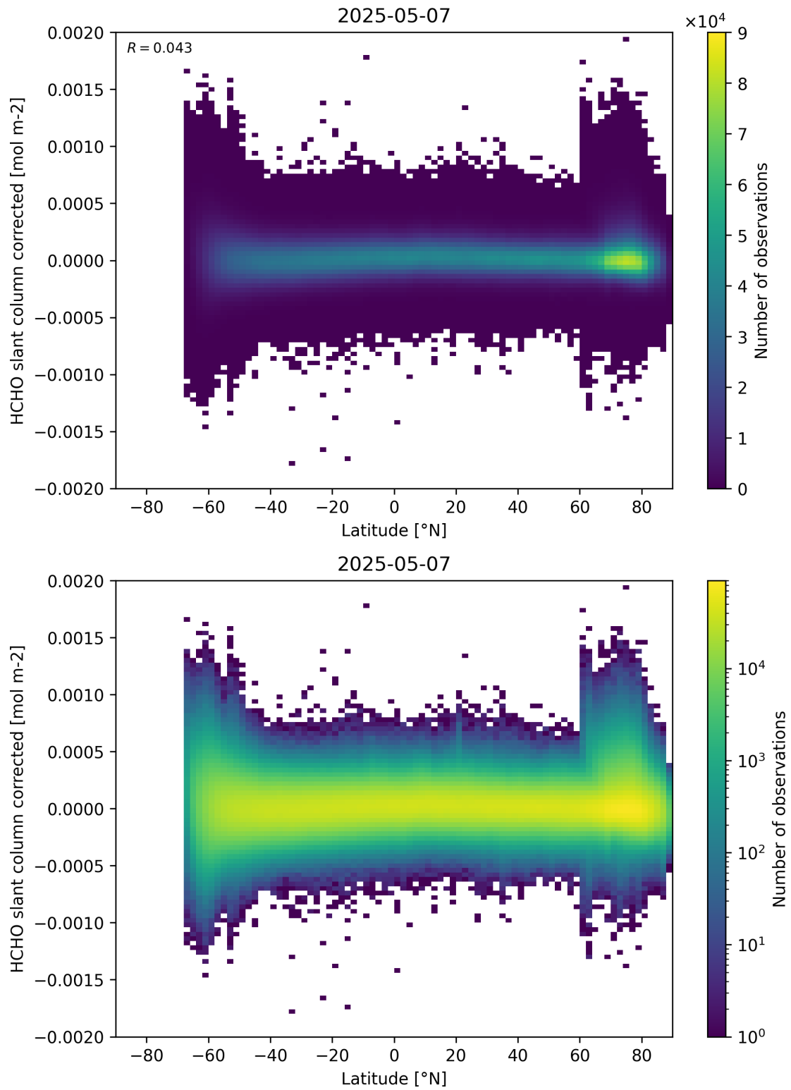
Figure 157: Scatter density plot of “Latitude” against “HCHO slant column corrected” for 2025-05-06 to 2025-05-08.
