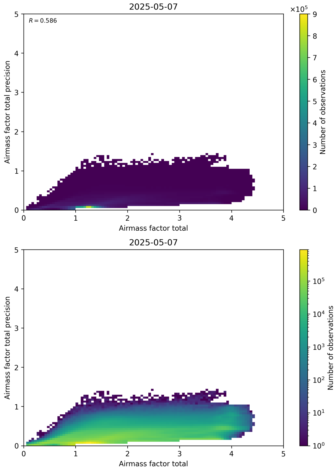
Figure 103: Scatter density plot of “Airmass factor total” against “Airmass factor total precision” for 2025-05-06 to 2025-05-08.
