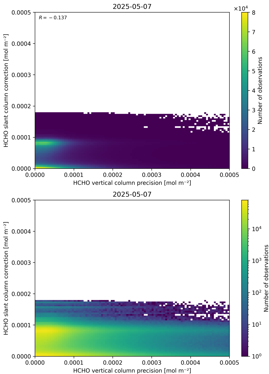
Figure 141: Scatter density plot of “HCHO vertical column precision” against “HCHO slant column correction” for 2025-05-06 to 2025-05-08.
