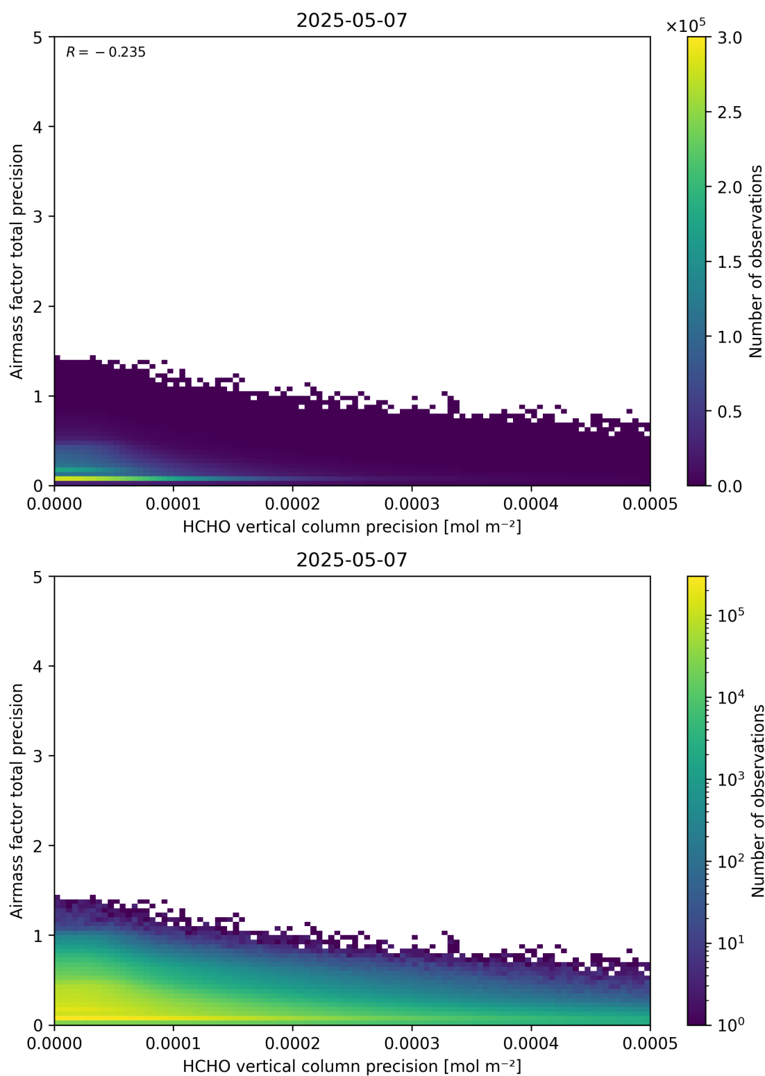
Figure 145: Scatter density plot of “HCHO vertical column precision” against “Airmass factor total precision” for 2025-05-06 to 2025-05-08.
