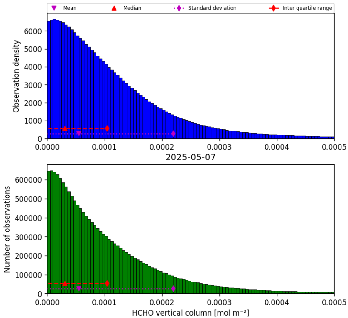
Figure 35: Histogram of “HCHO vertical column” for 2025-05-06 to 2025-05-08
