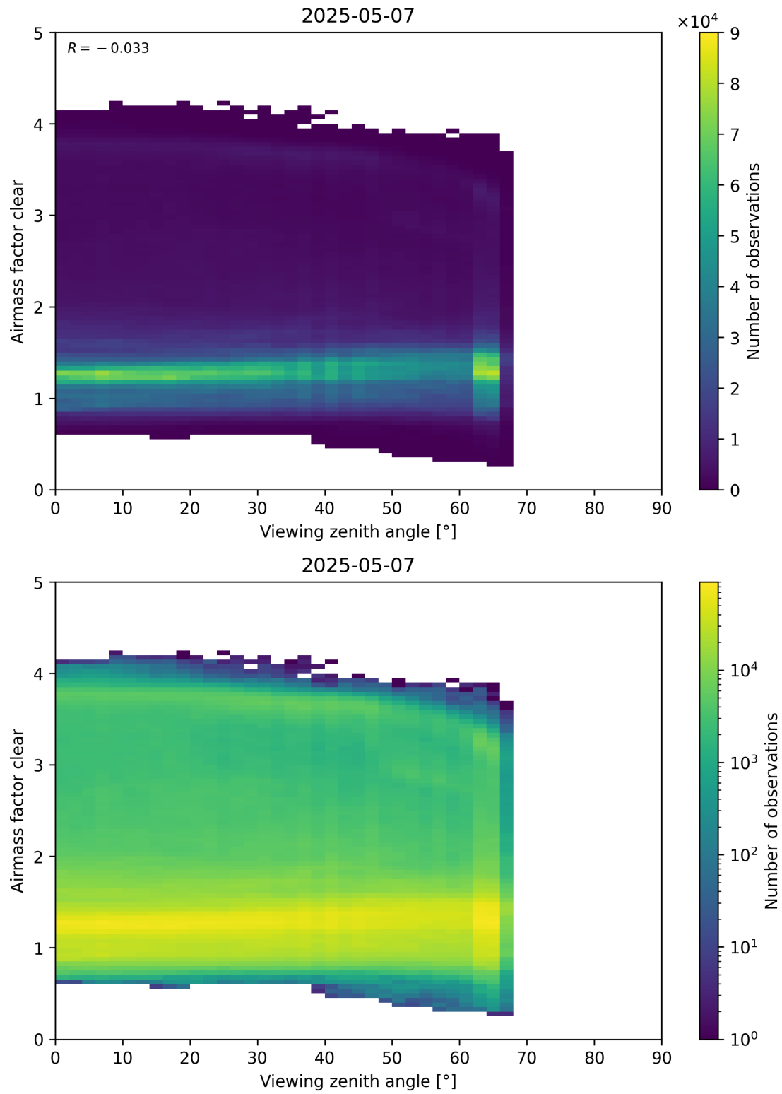
Figure 185: Scatter density plot of “Viewing zenith angle” against “Airmass factor clear” for 2025-05-06 to 2025-05-08.
