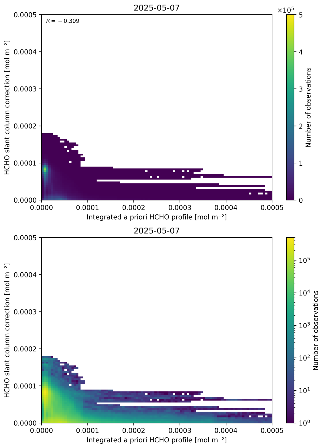
Figure 152: Scatter density plot of “Integrated a priori HCHO profile” against “HCHO slant column correction” for 2025-05-06 to 2025-05-08.
