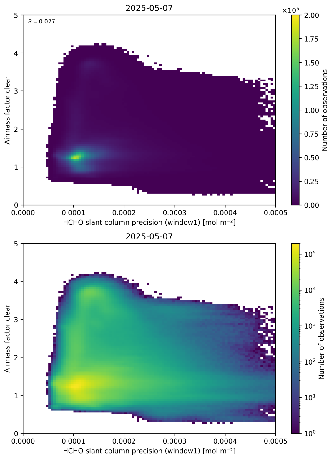
Figure 91: Scatter density plot of “HCHO slant column precision (window1)” against “Airmass factor clear” for 2025-05-06 to 2025-05-08.
