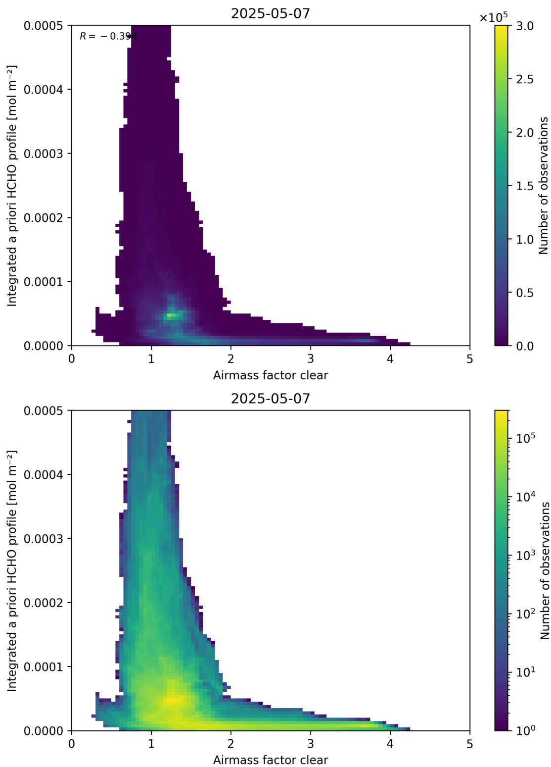
Figure 76: Scatter density plot of “Airmass factor clear” against “Integrated a priori HCHO profile” for 2025-05-06 to 2025-05-08.
