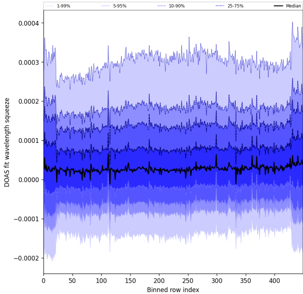
Figure 59: Along track statistics of “DOAS fit wavelength squeeze” for 2025-05-06 to 2025-05-08
