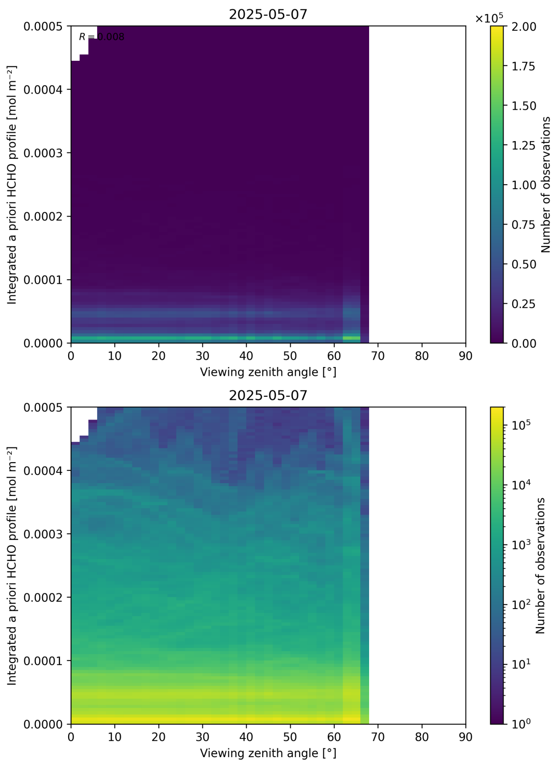
Figure 195: Scatter density plot of “Viewing zenith angle” against “Integrated a priori HCHO profile” for 2025-05-06 to 2025-05-08.
