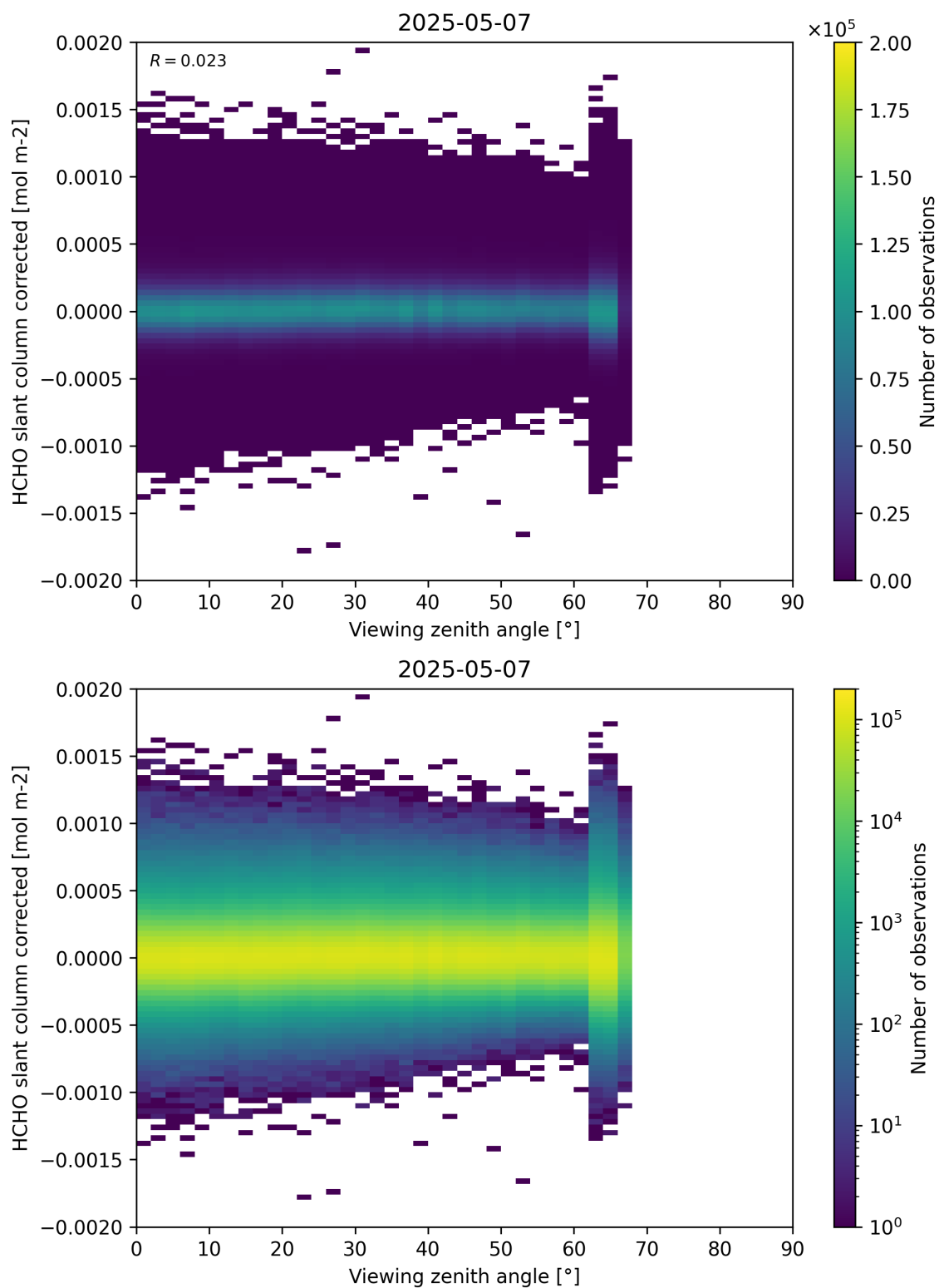
Figure 186: Scatter density plot of “Viewing zenith angle” against “HCHO slant column corrected” for 2025-05-06 to 2025-05-08.
