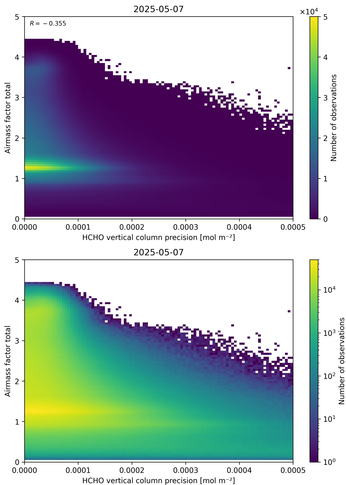
Figure 144: Scatter density plot of “HCHO vertical column precision” against “Airmass factor total” for 2025-05-06 to 2025-05-08.
