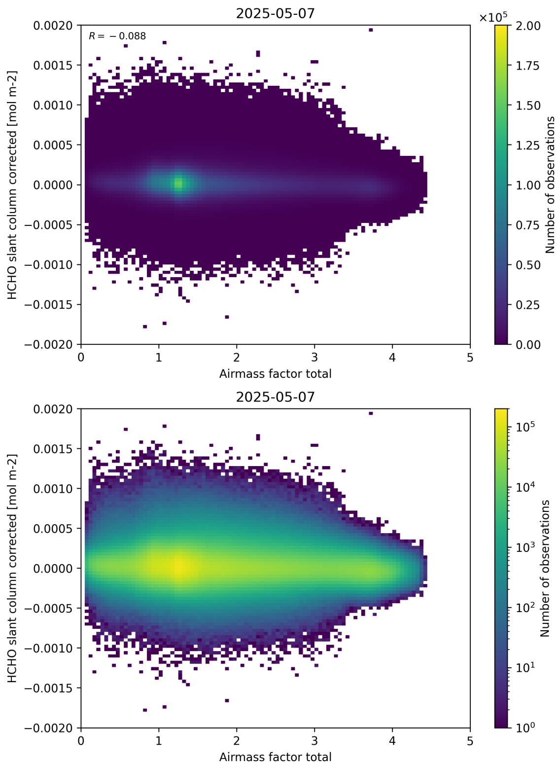
Figure 101: Scatter density plot of “Airmass factor total” against “HCHO slant column corrected” for 2025-05-06 to 2025-05-08.
