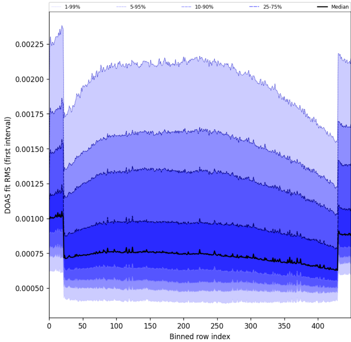
Figure 60: Along track statistics of “DOAS fit RMS (first interval)” for 2025-05-06 to 2025-05-08
