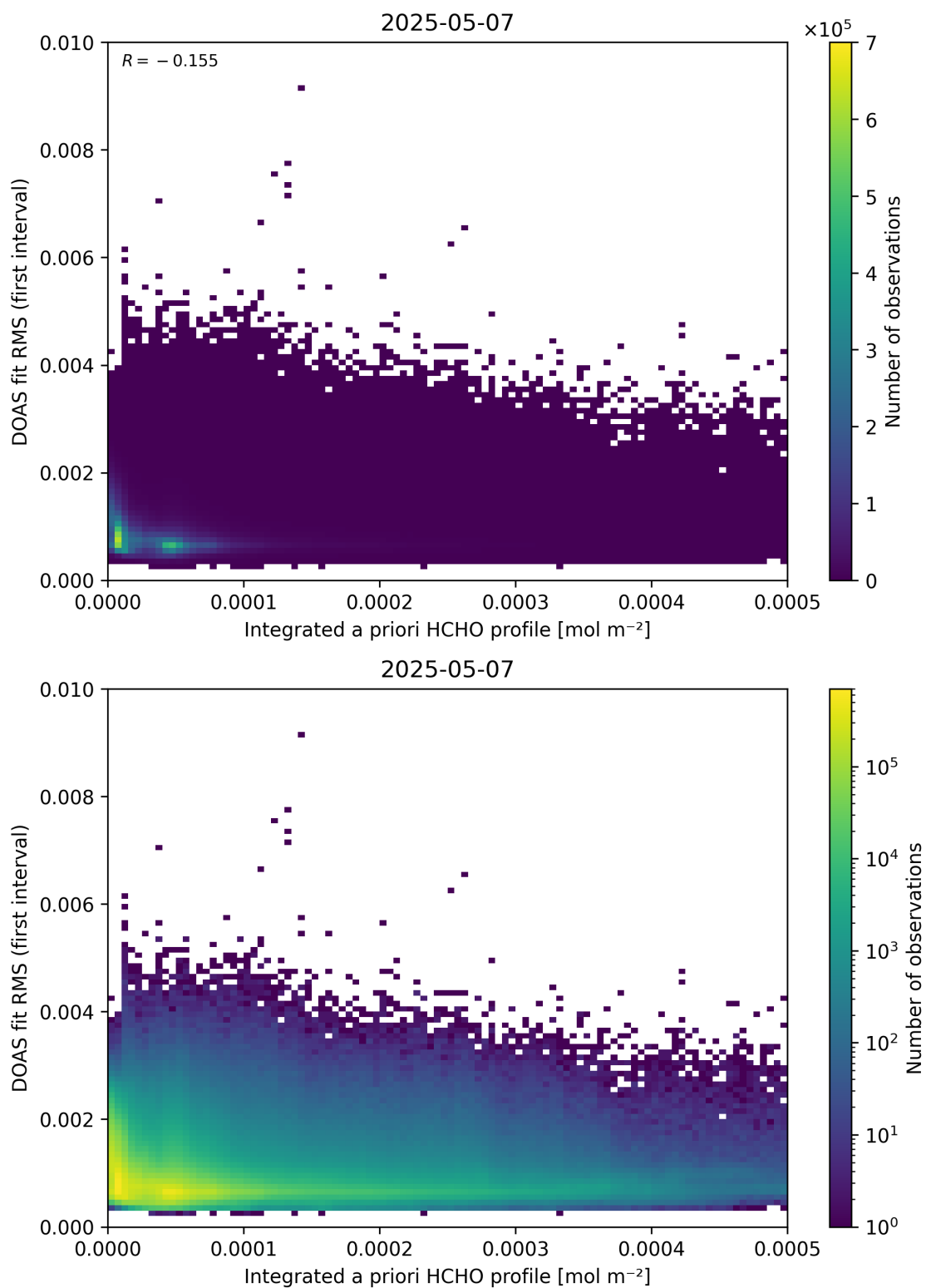
Figure 148: Scatter density plot of “Integrated a priori HCHO profile” against “DOAS fit RMS (first interval)” for 2025-05-06 to 2025-05-08.
