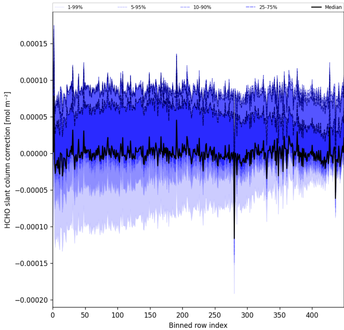
Figure 61: Along track statistics of “HCHO slant column correction” for 2025-05-06 to 2025-05-08
