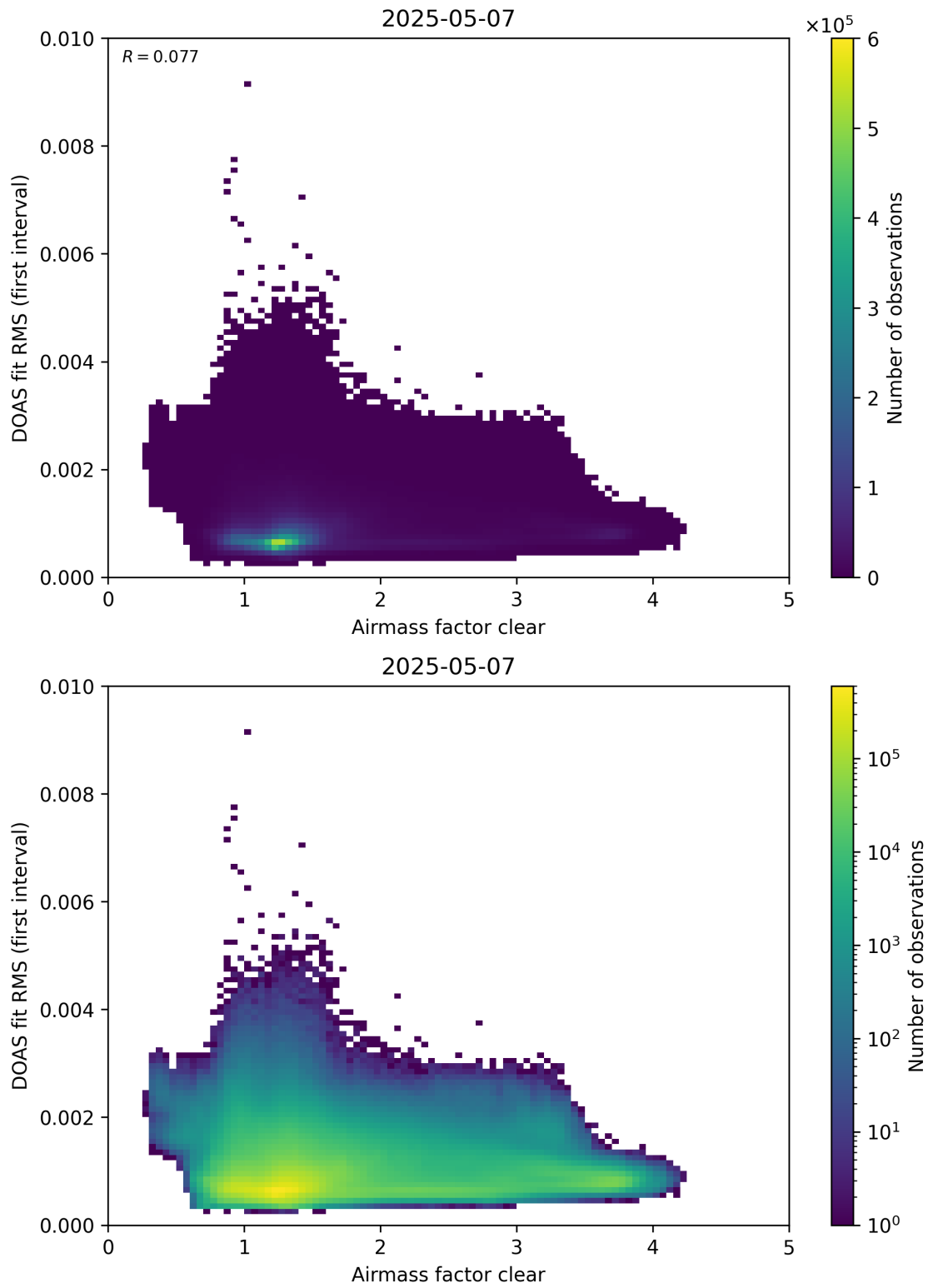
Figure 71: Scatter density plot of “Airmass factor clear” against “DOAS fit RMS (first interval)” for 2025-05-06 to 2025-05-08.
