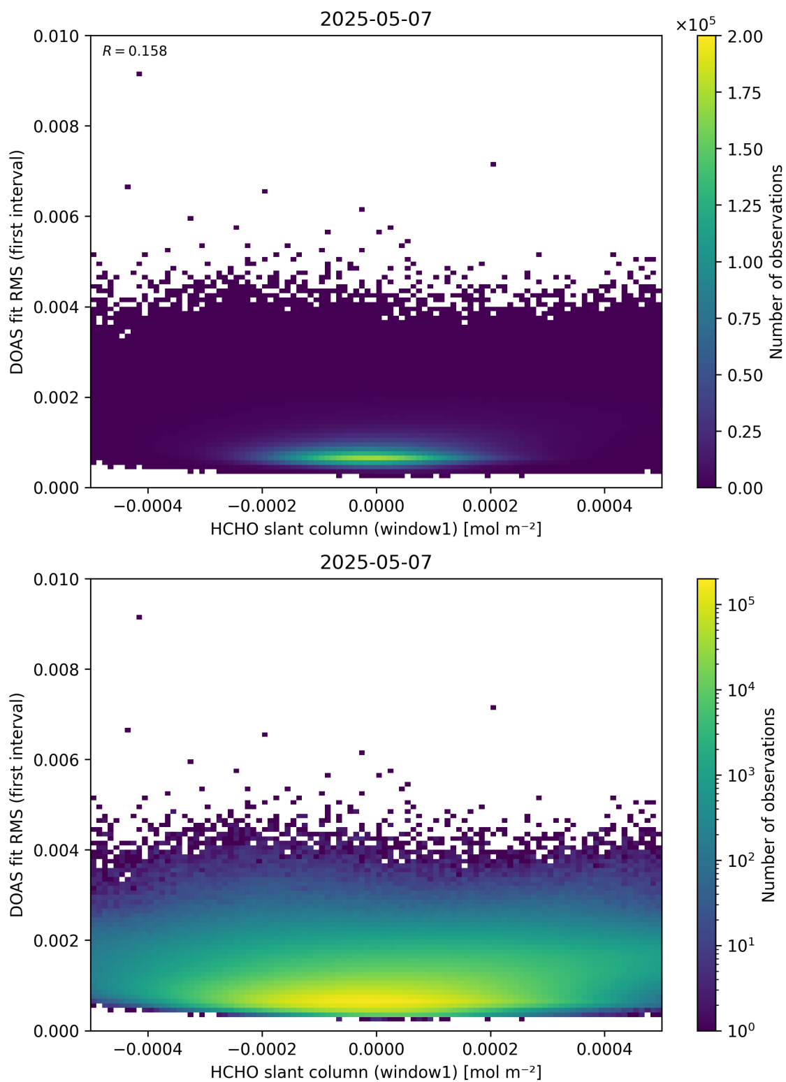
Figure 78: Scatter density plot of “HCHO slant column (window1)” against “DOAS fit RMS (first interval)” for 2025-05-06 to 2025-05-08.
