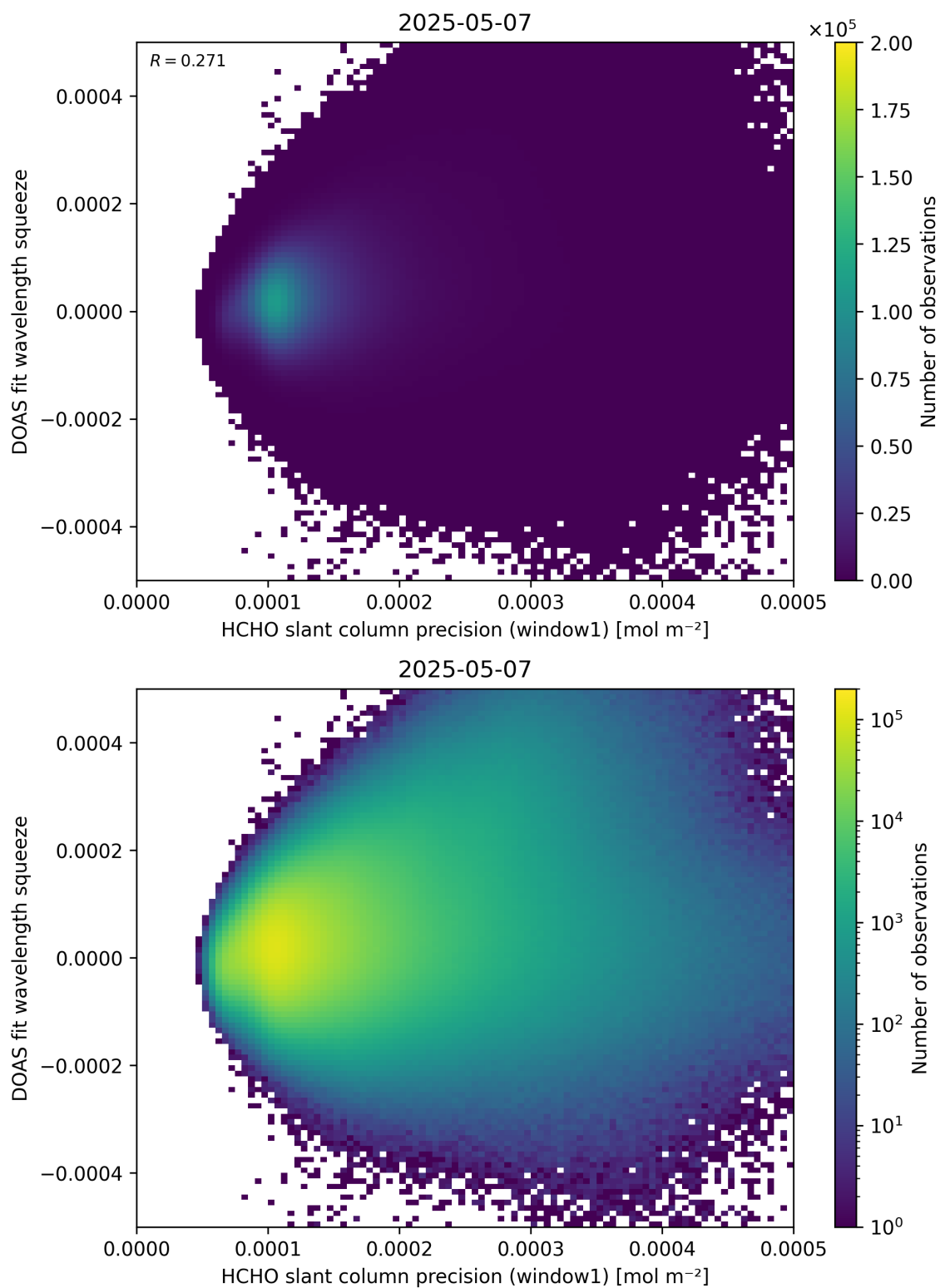
Figure 90: Scatter density plot of “HCHO slant column precision (window1)” against “DOAS fit wavelength squeeze” for 2025-05-06 to 2025-05-08.
