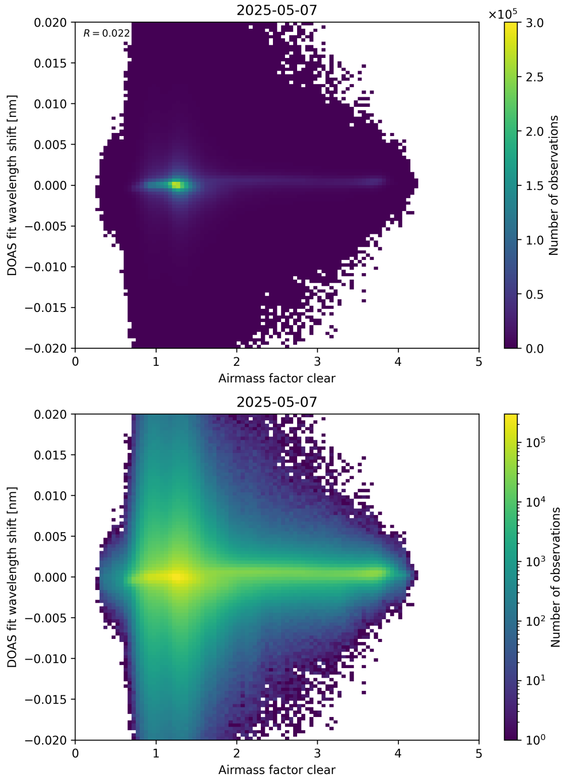
Figure 72: Scatter density plot of “Airmass factor clear” against “DOAS fit wavelength shift” for 2025-05-06 to 2025-05-08.
