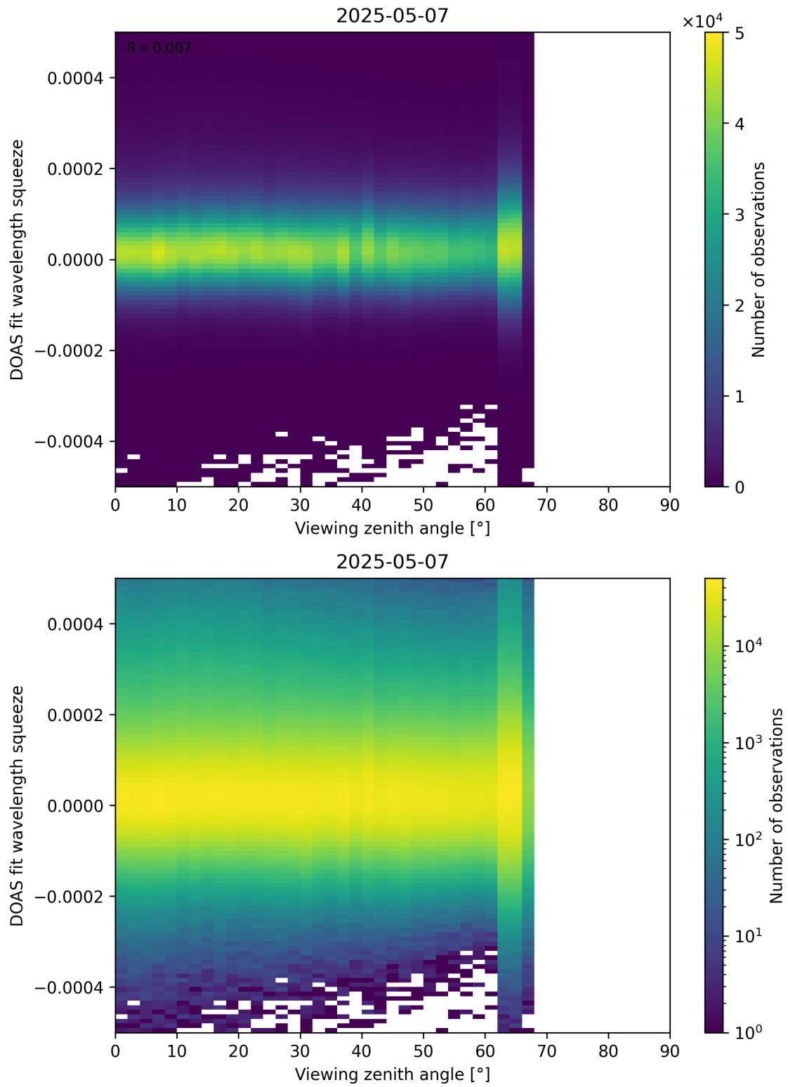
Figure 184: Scatter density plot of “Viewing zenith angle” against “DOAS fit wavelength squeeze” for 2025-05-06 to 2025-05-08.
