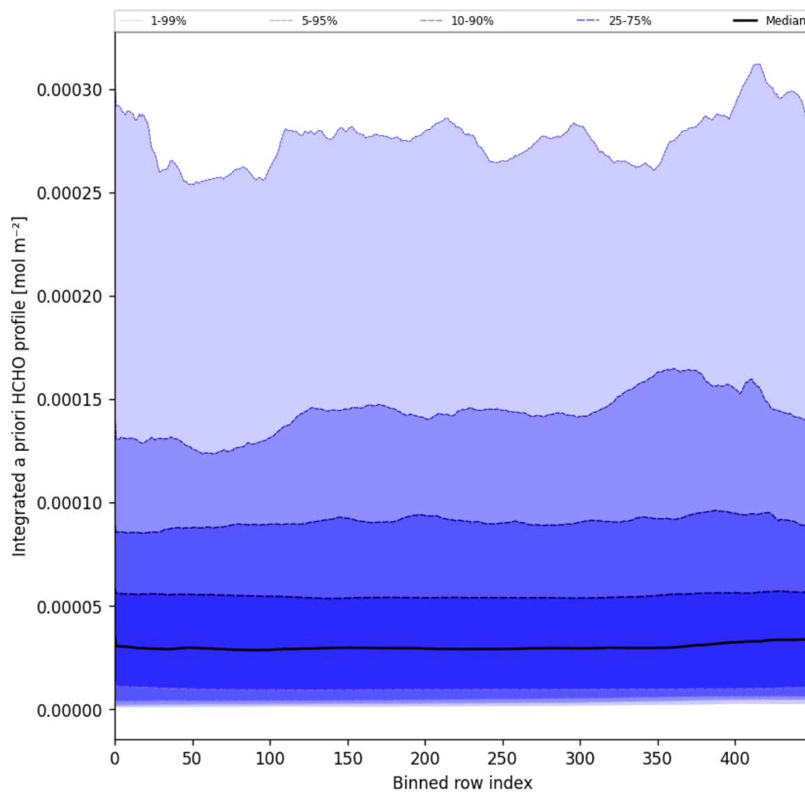
Figure 57: Along track statistics of "Integrated a priori HCHO profile" for 2025-05-06 to 2025-05-08
