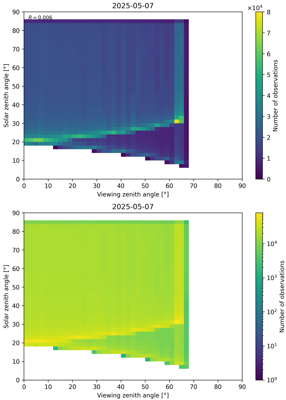
Figure 197: Scatter density plot of “Viewing zenith angle” against “Solar zenith angle” for 2025-05-06 to 2025-05-08.
