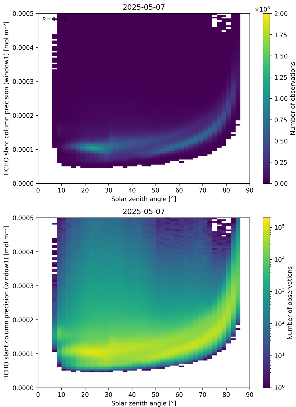
Figure 174: Scatter density plot of “Solar zenith angle” against “HCHO slant column precision (window1)” for 2025-05-06 to 2025-05-08.
