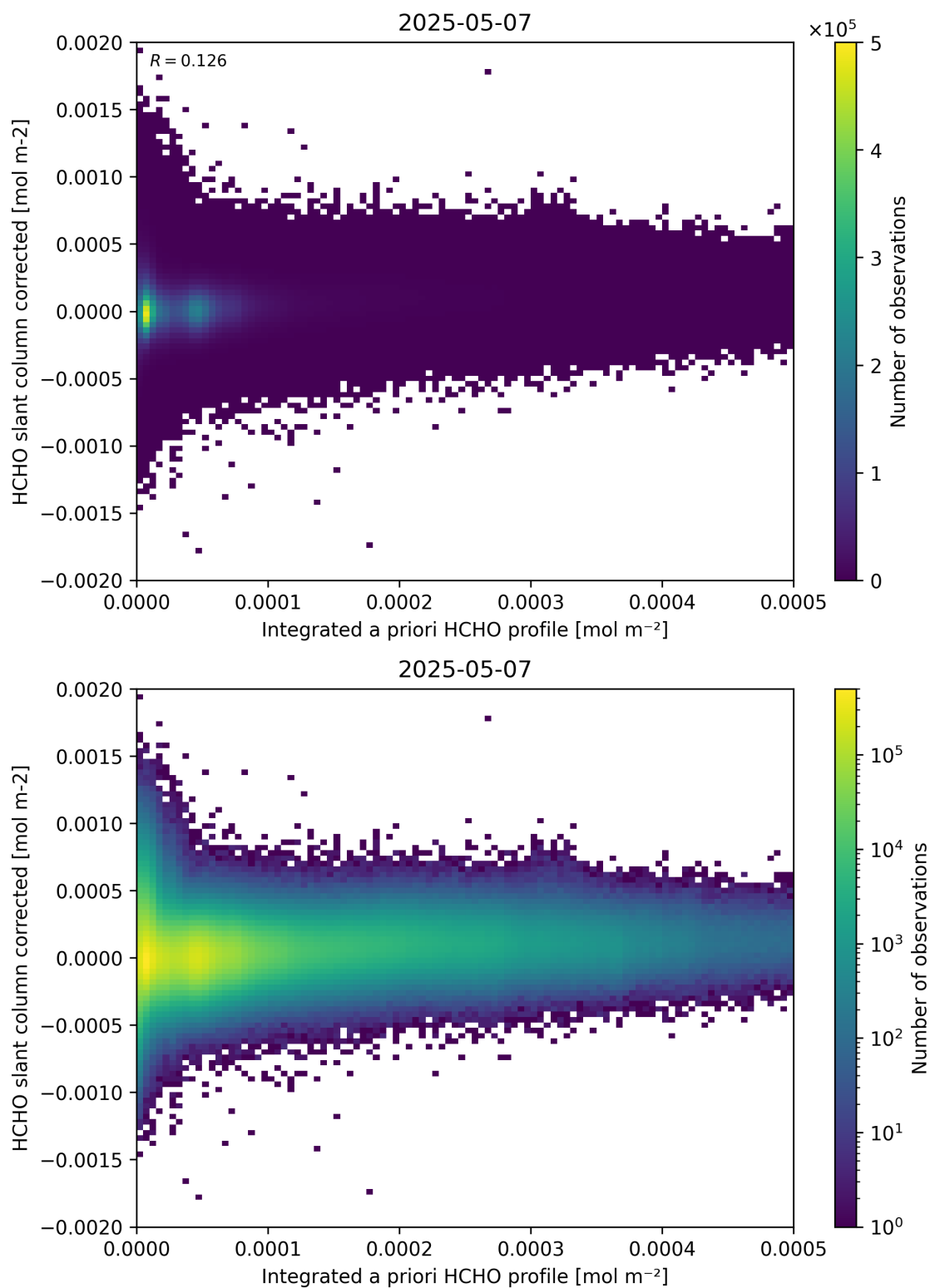
Figure 151: Scatter density plot of “Integrated a priori HCHO profile” against “HCHO slant column corrected” for 2025-05-06 to 2025-05-08.
