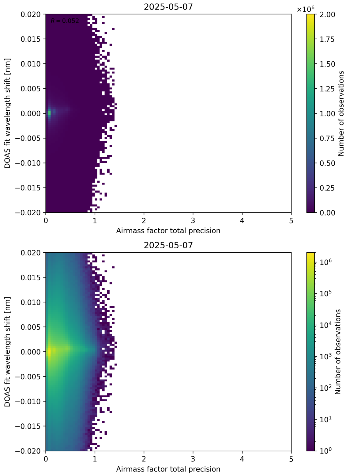
Figure 106: Scatter density plot of “Airmass factor total precision” against “DOAS fit wavelength shift” for 2025-05-06 to 2025-05-08.
