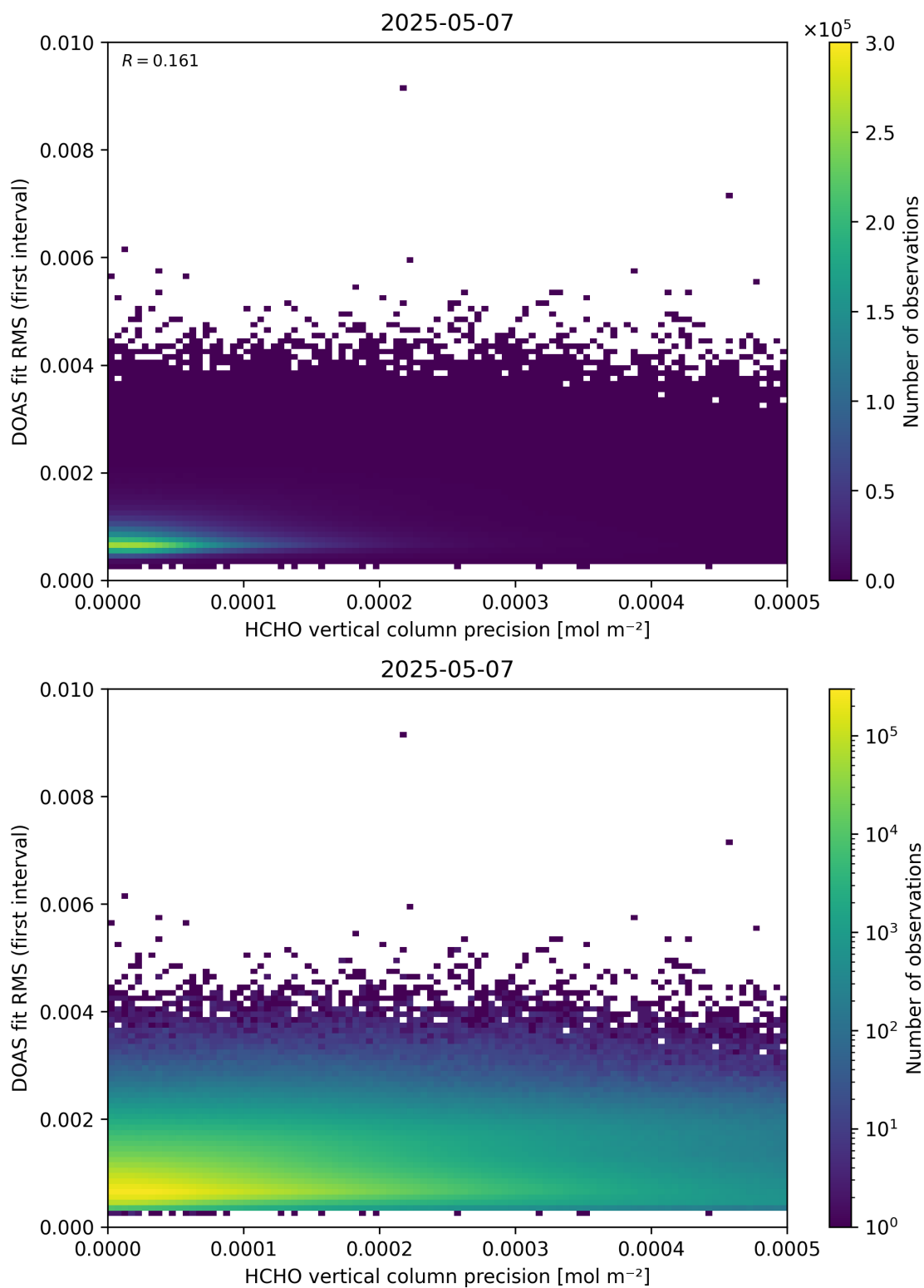
Figure 136: Scatter density plot of “HCHO vertical column precision” against “DOAS fit RMS (first interval)” for 2025-05-06 to 2025-05-08.
