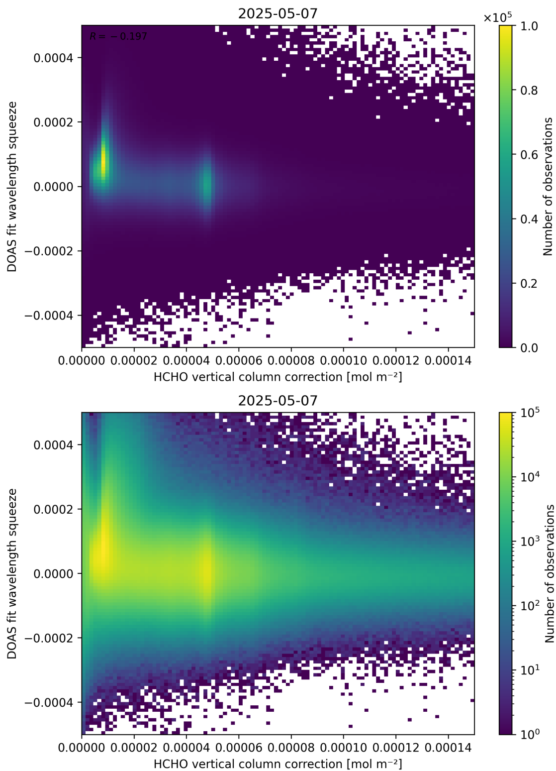
Figure 114: Scatter density plot of “HCHO vertical column correction” against “DOAS fit wavelength squeeze” for 2025-05-06 to 2025-05-08.
