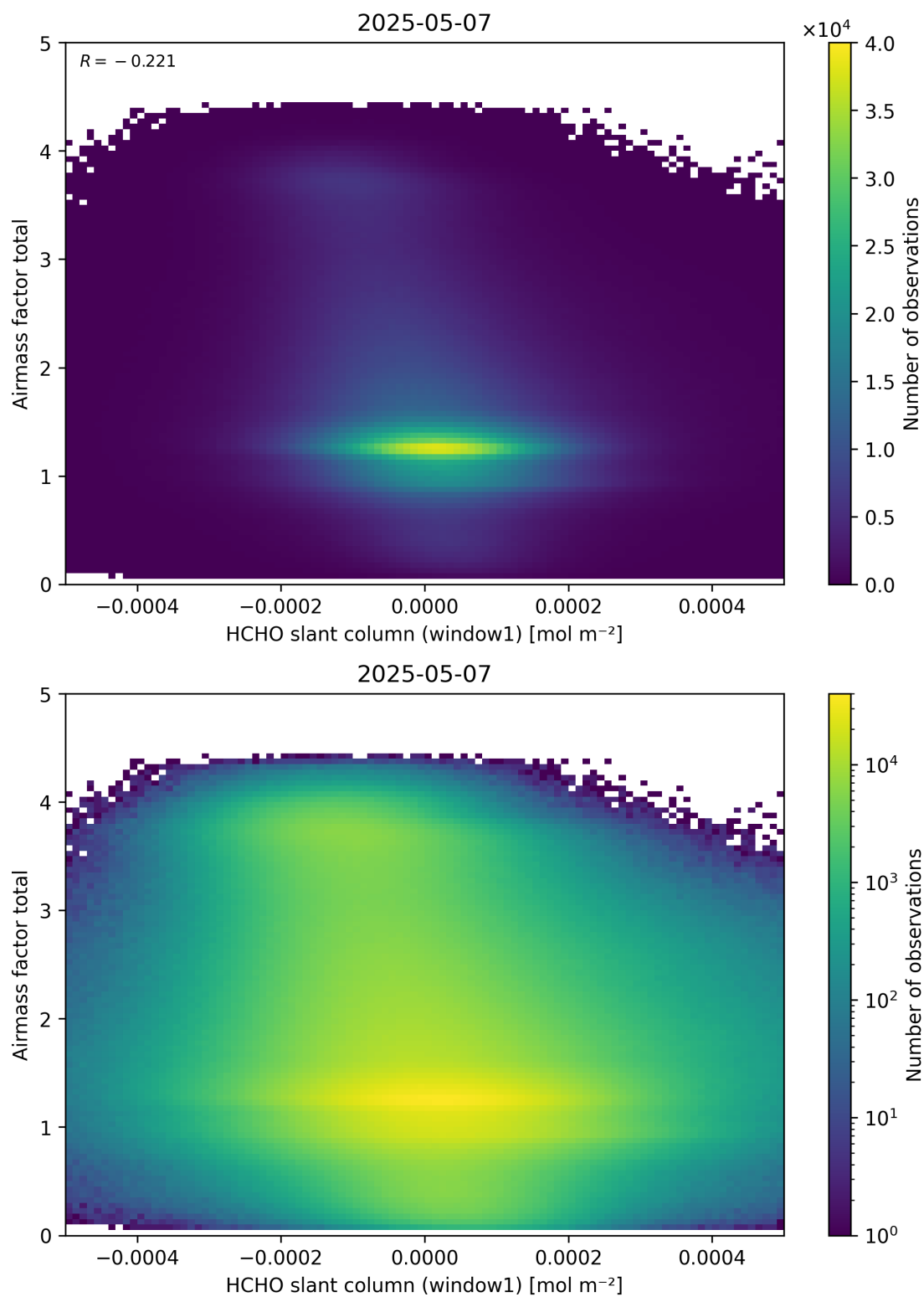
Figure 85: Scatter density plot of “HCHO slant column (window1)” against “Airmass factor total” for 2025-05-06 to 2025-05-08.
