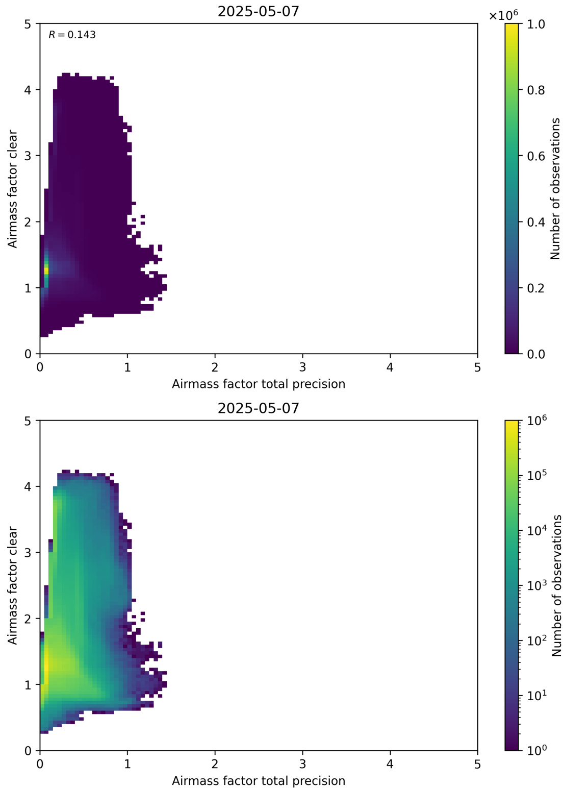
Figure 108: Scatter density plot of “Airmass factor total precision” against “Airmass factor clear” for 2025-05-06 to 2025-05-08.
