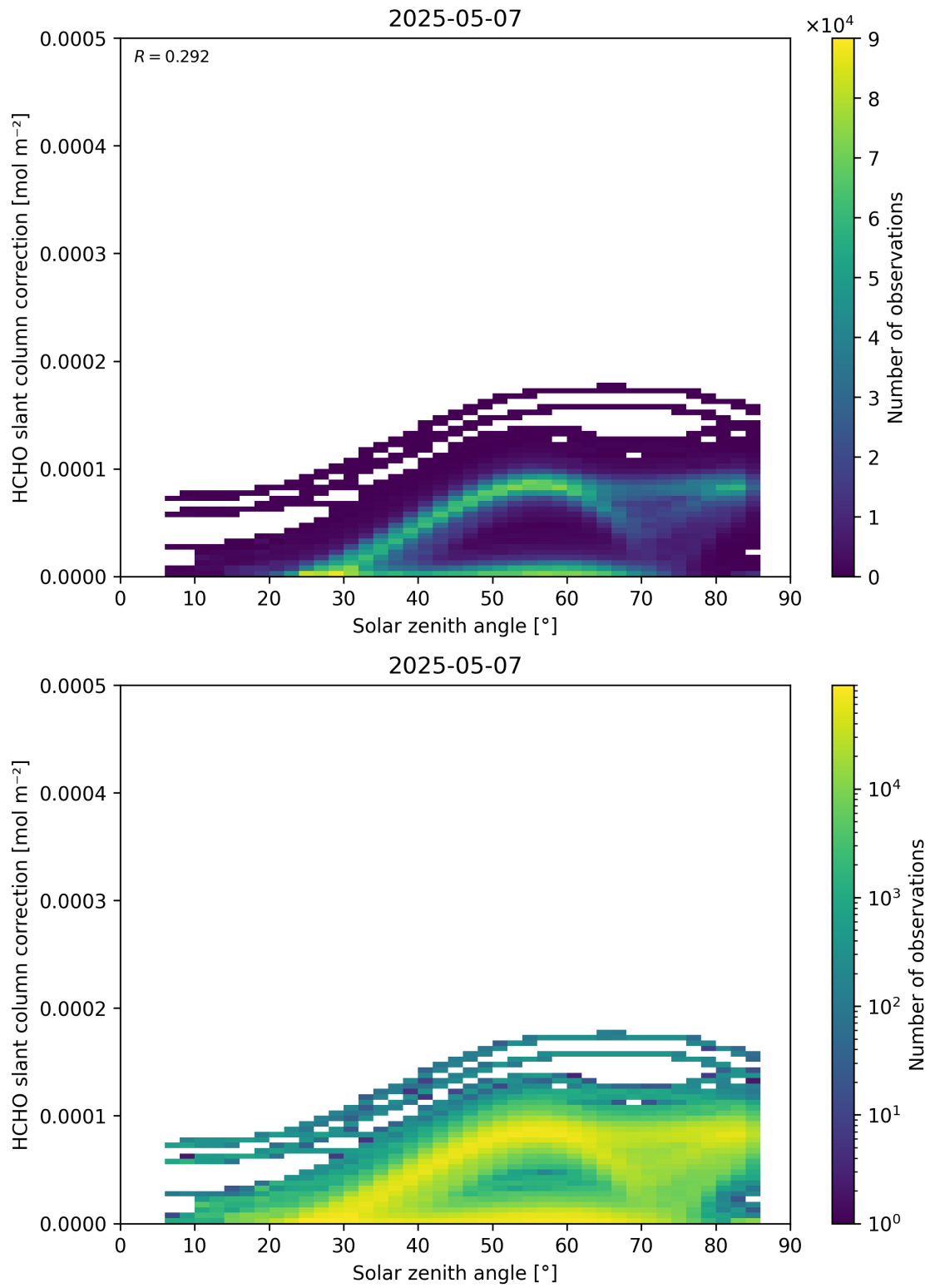
Figure 172: Scatter density plot of “Solar zenith angle” against “HCHO slant column correction” for 2025-05-06 to 2025-05-08.
