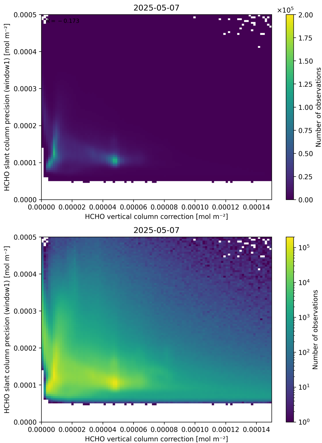
Figure 119: Scatter density plot of “HCHO vertical column correction” against “HCHO slant column precision (window1)” for 2025-05-06 to 2025-05-08.
