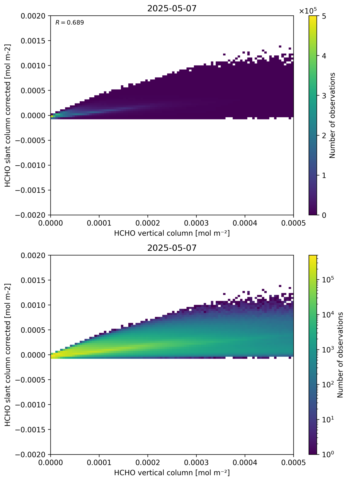
Figure 127: Scatter density plot of “HCHO vertical column” against “HCHO slant column corrected” for 2025-05-06 to 2025-05-08.
