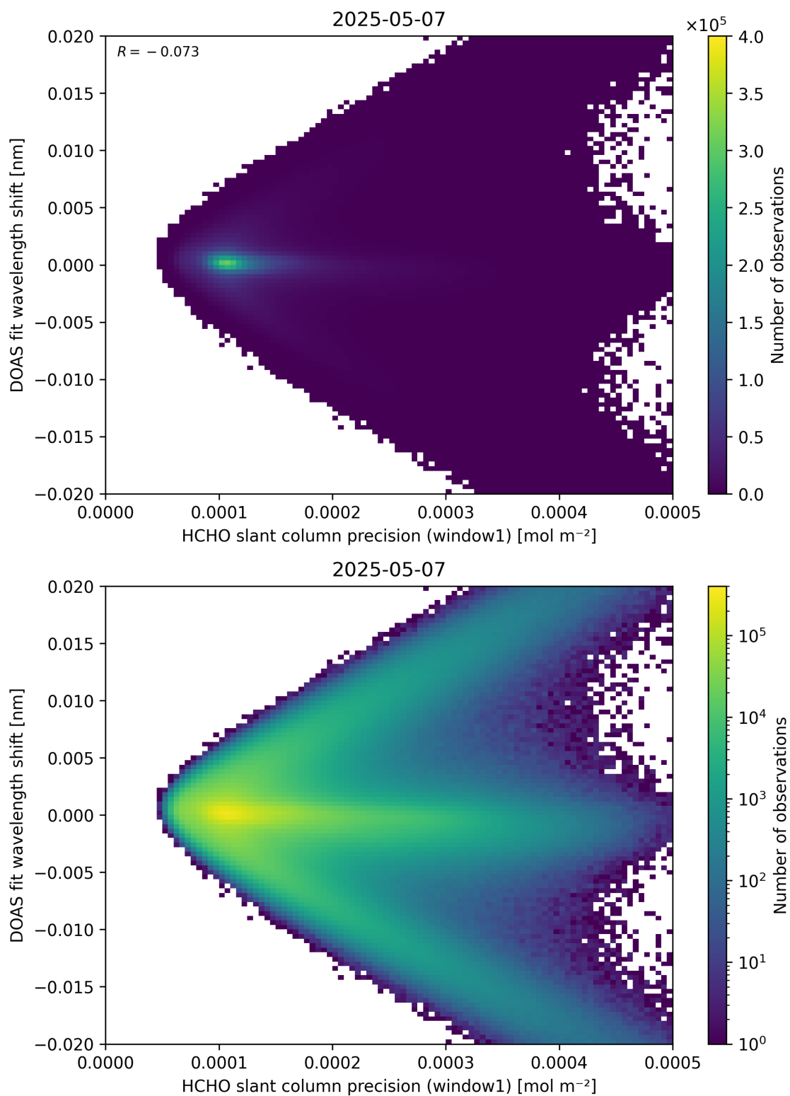
Figure 89: Scatter density plot of “HCHO slant column precision (window1)” against “DOAS fit wavelength shift” for 2025-05-06 to 2025-05-08.
