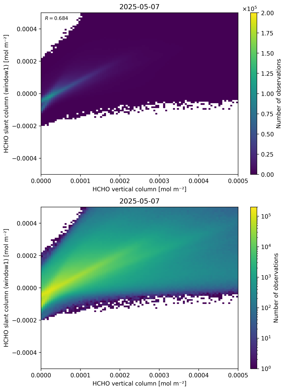
Figure 129: Scatter density plot of “HCHO vertical column” against “HCHO slant column (window1)” for 2025-05-06 to 2025-05-08.
