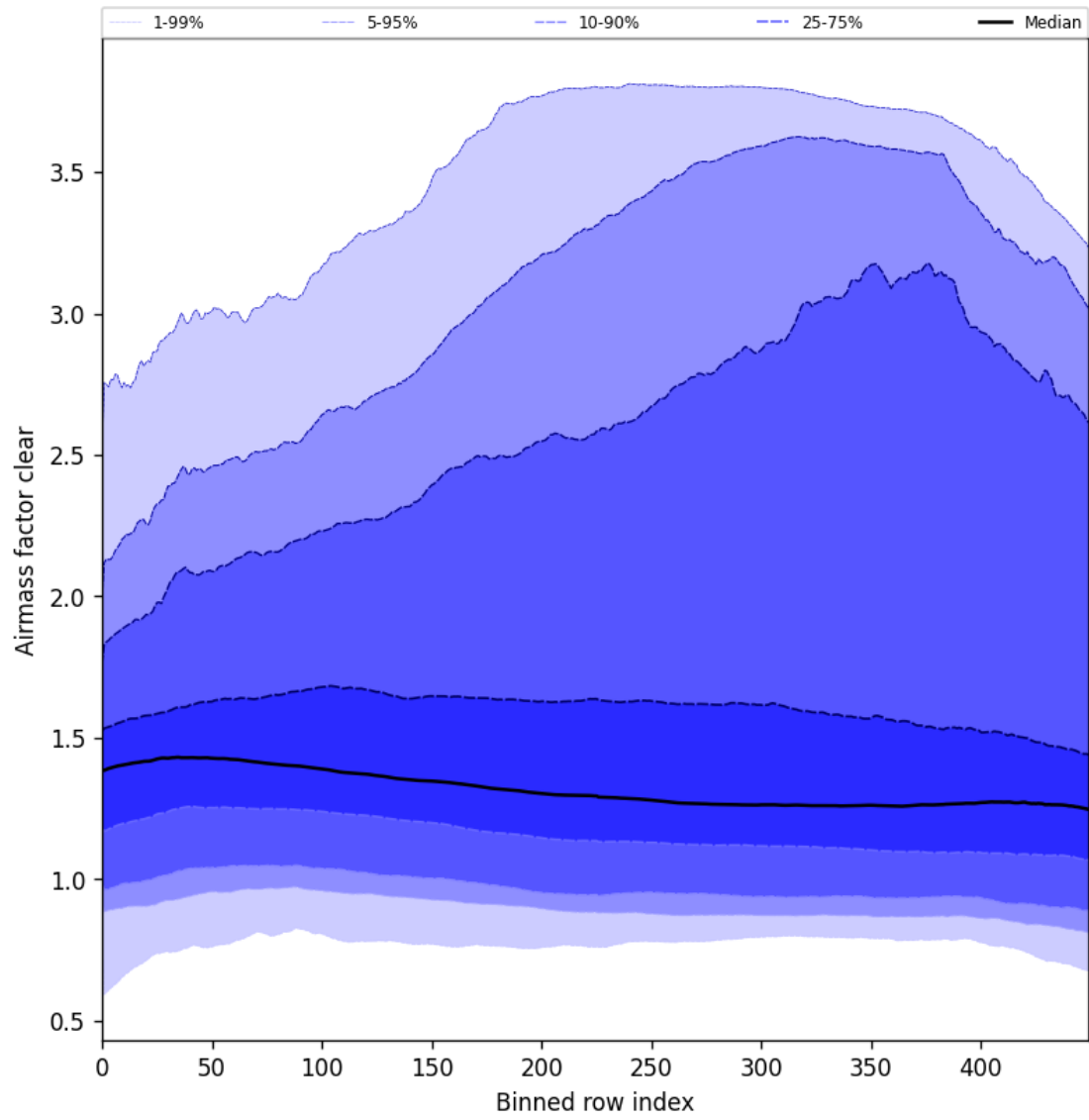
Figure 56: Along track statistics of “Airmass factor clear” for 2025-05-06 to 2025-05-08
