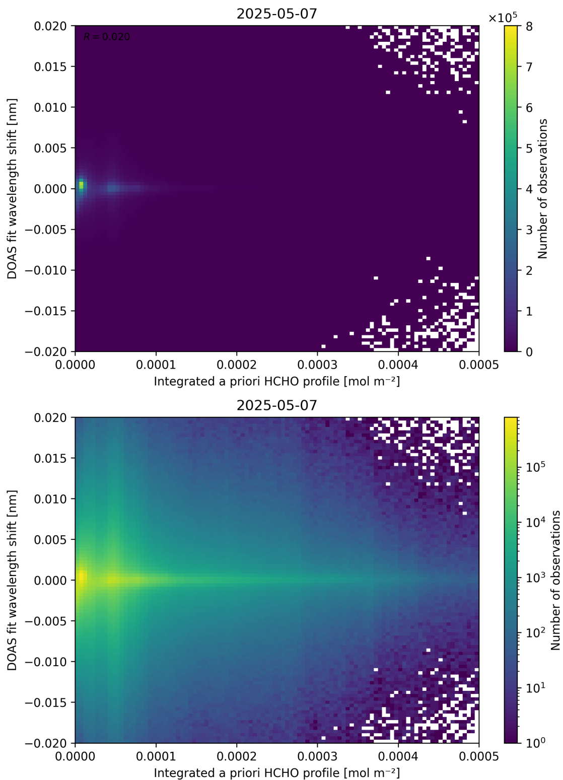
Figure 149: Scatter density plot of “Integrated a priori HCHO profile” against “DOAS fit wavelength shift” for 2025-05-06 to 2025-05-08.
