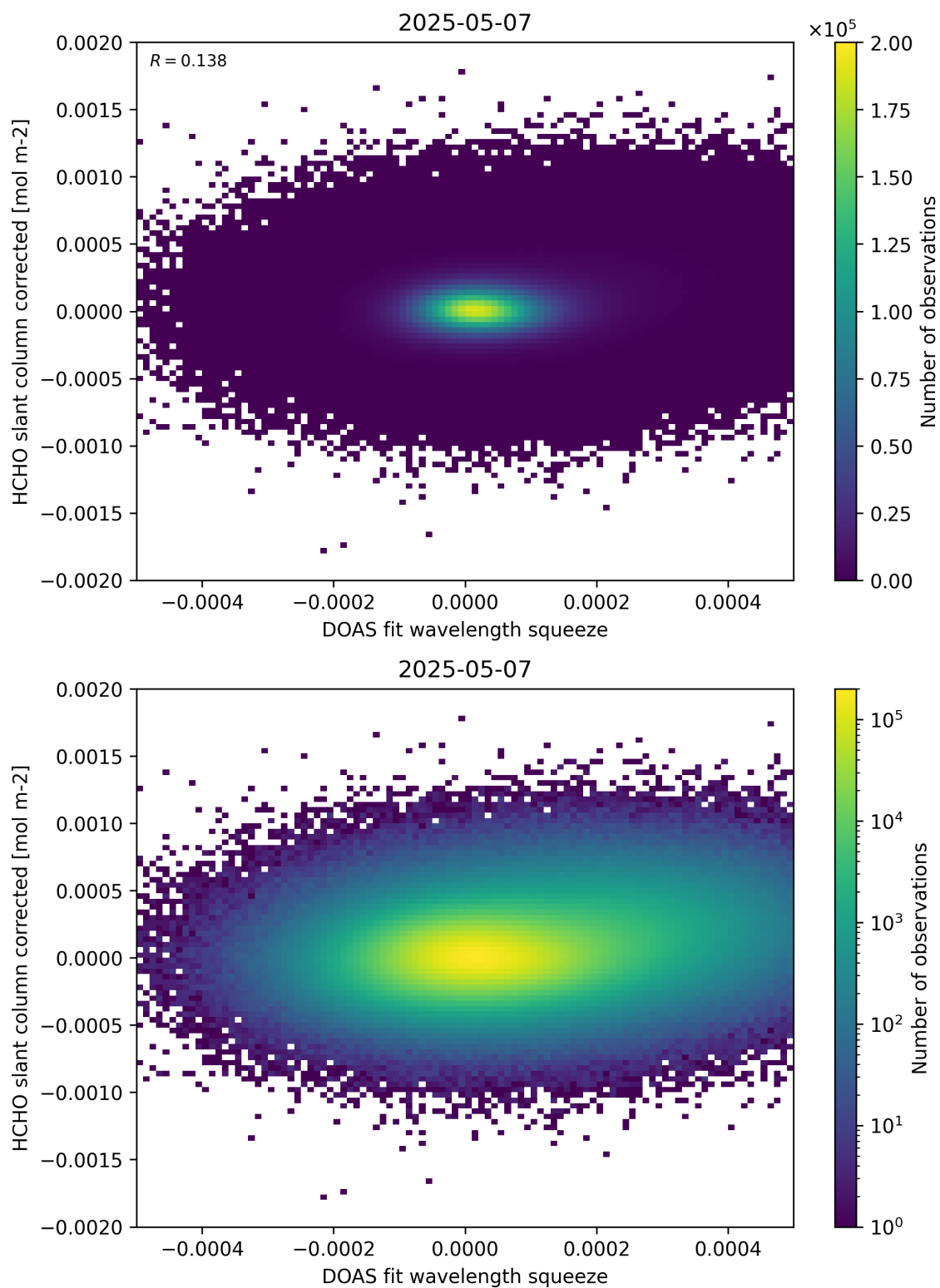
Figure 69: Scatter density plot of “DOAS fit wavelength squeeze” against “HCHO slant column corrected” for 2025-05-06 to 2025-05-08.
