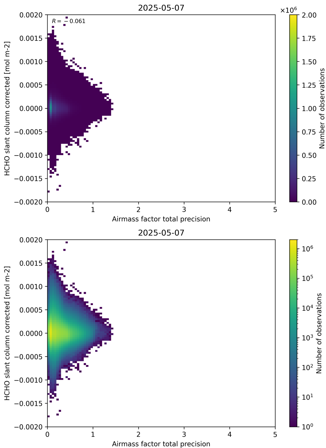
Figure 109: Scatter density plot of “Airmass factor total precision” against “HCHO slant column corrected” for 2025-05-06 to 2025-05-08.
