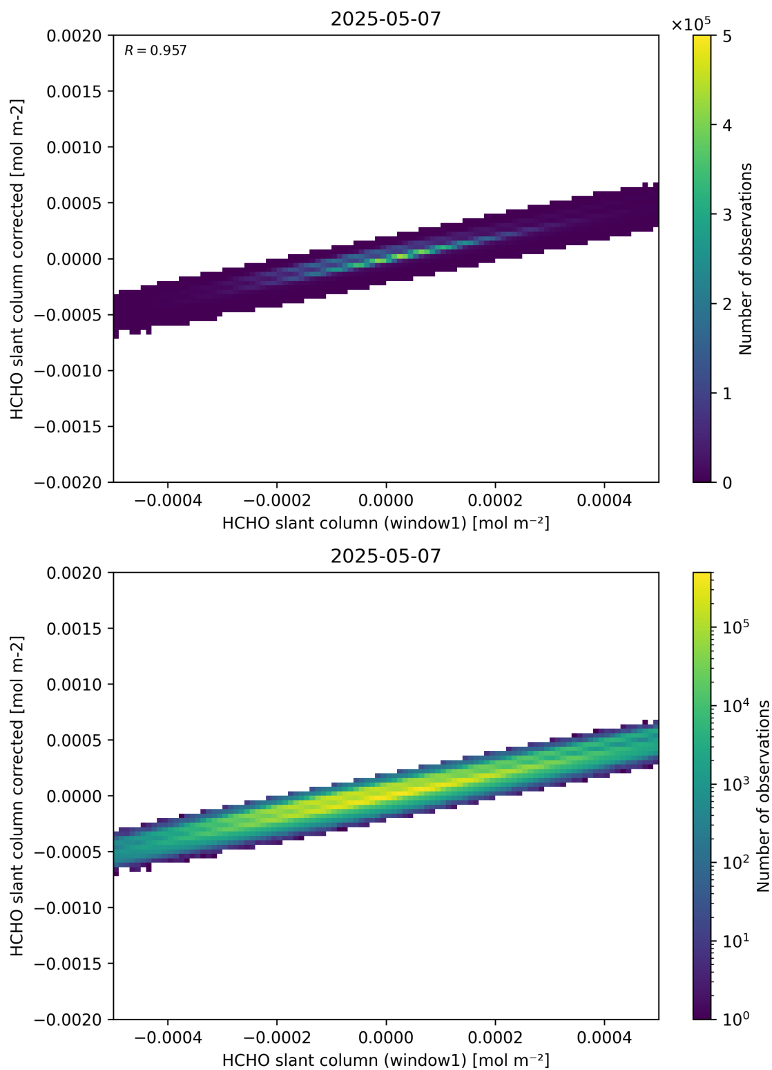
Figure 82: Scatter density plot of “HCHO slant column (window1)” against “HCHO slant column corrected” for 2025-05-06 to 2025-05-08.
