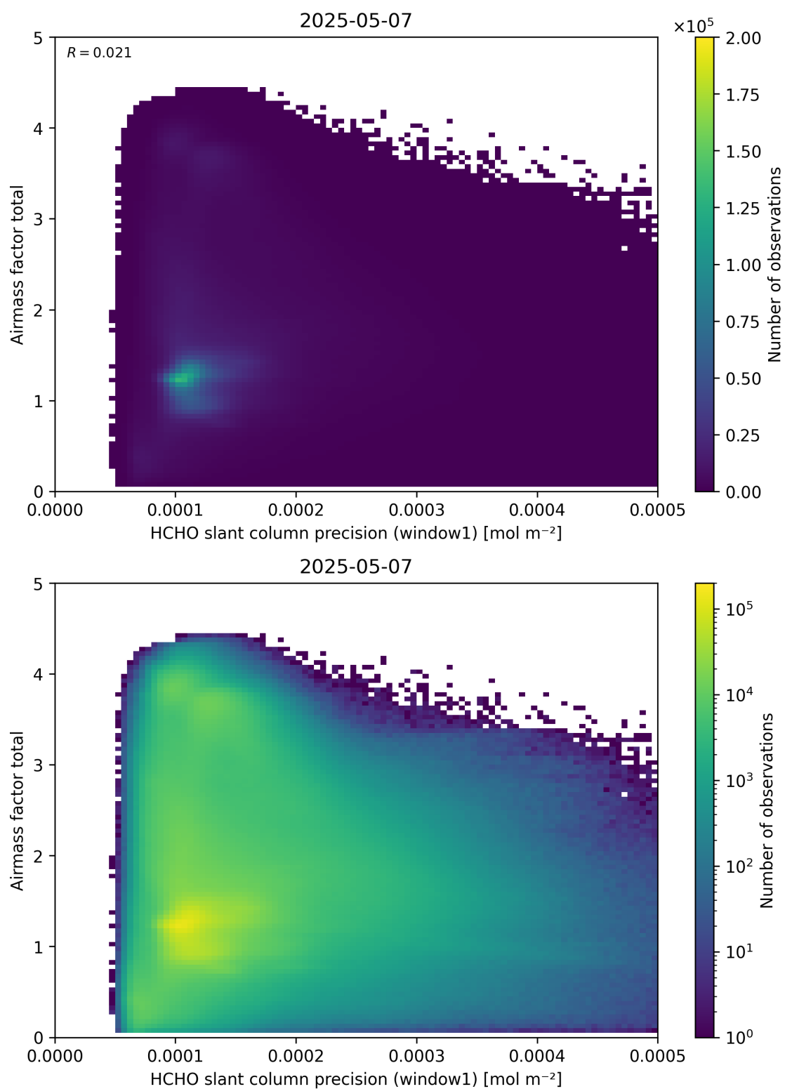
Figure 94: Scatter density plot of “HCHO slant column precision (window1)” against “Airmass factor total” for 2025-05-06 to 2025-05-08.
