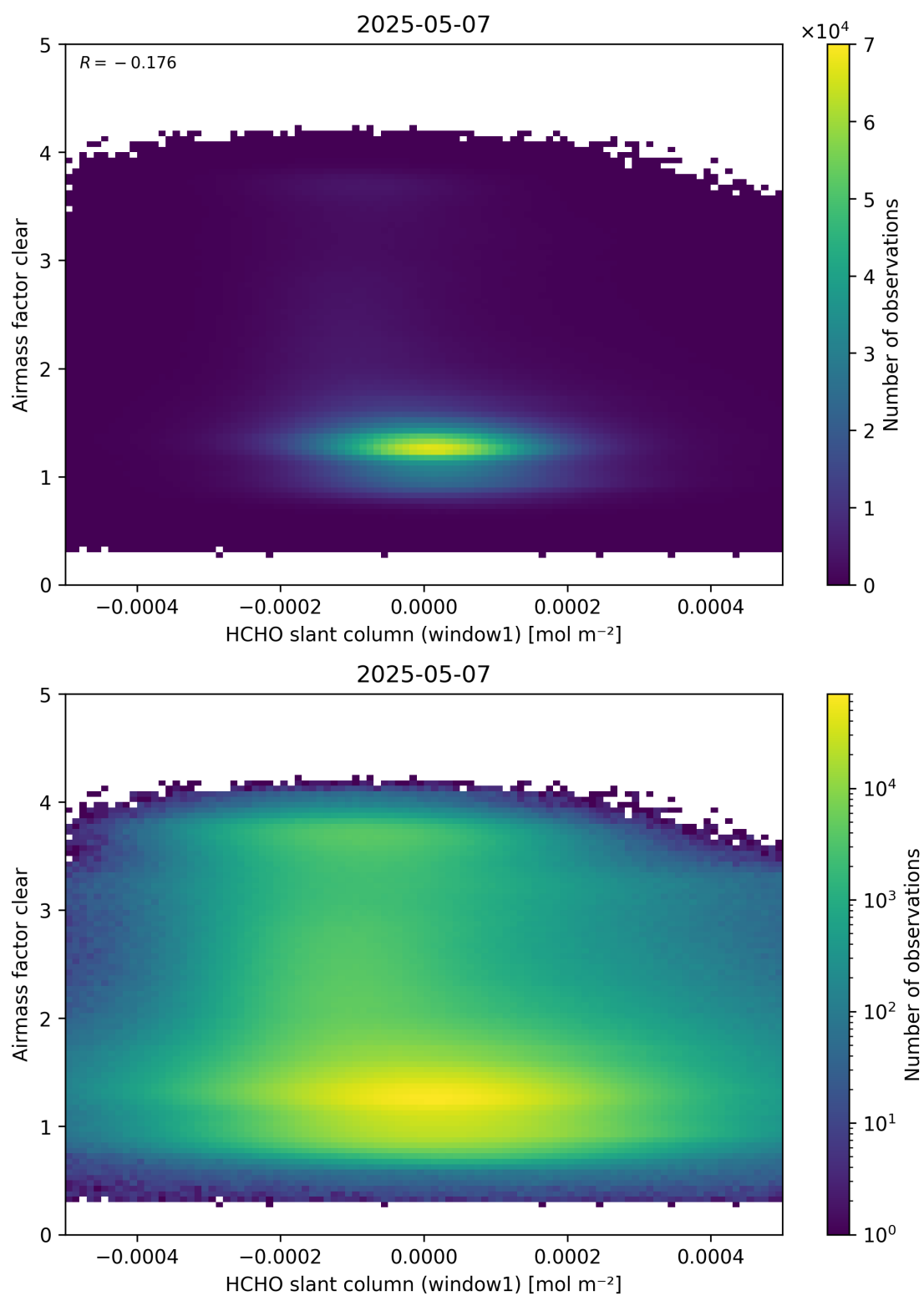
Figure 81: Scatter density plot of “HCHO slant column (window1)” against “Airmass factor clear” for 2025-05-06 to 2025-05-08.
