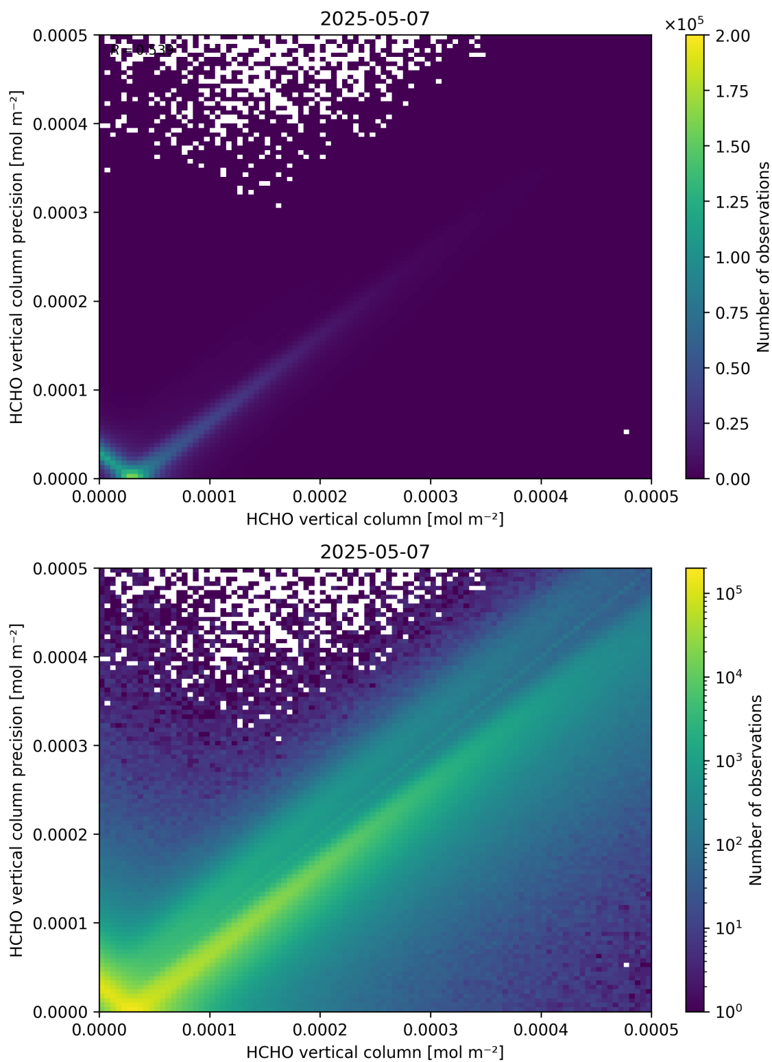
Figure 134: Scatter density plot of “HCHO vertical column” against “HCHO vertical column precision” for 2025-05-06 to 2025-05-08.
