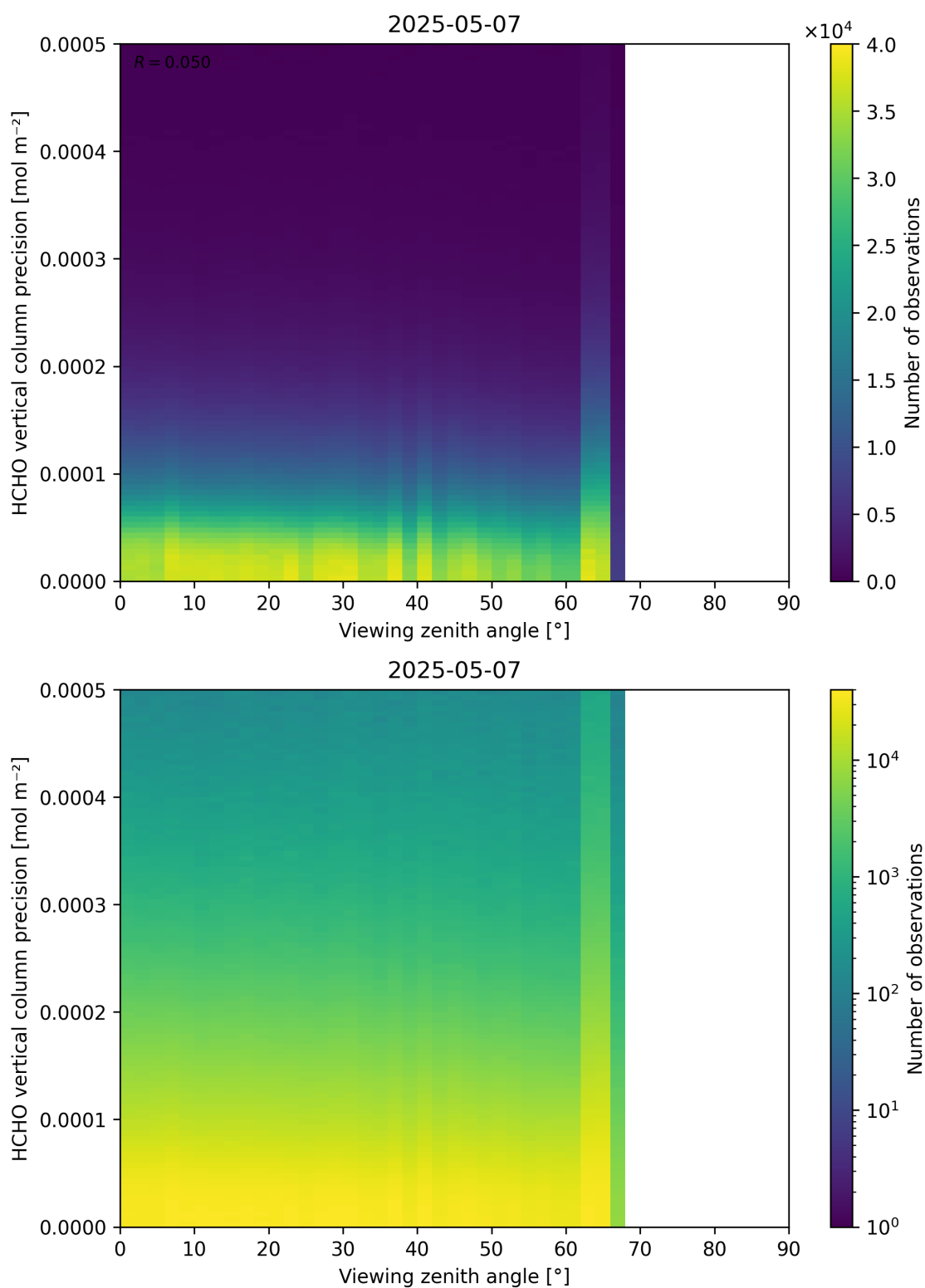
Figure 194: Scatter density plot of “Viewing zenith angle” against “HCHO vertical column precision” for 2025-05-06 to 2025-05-08.
