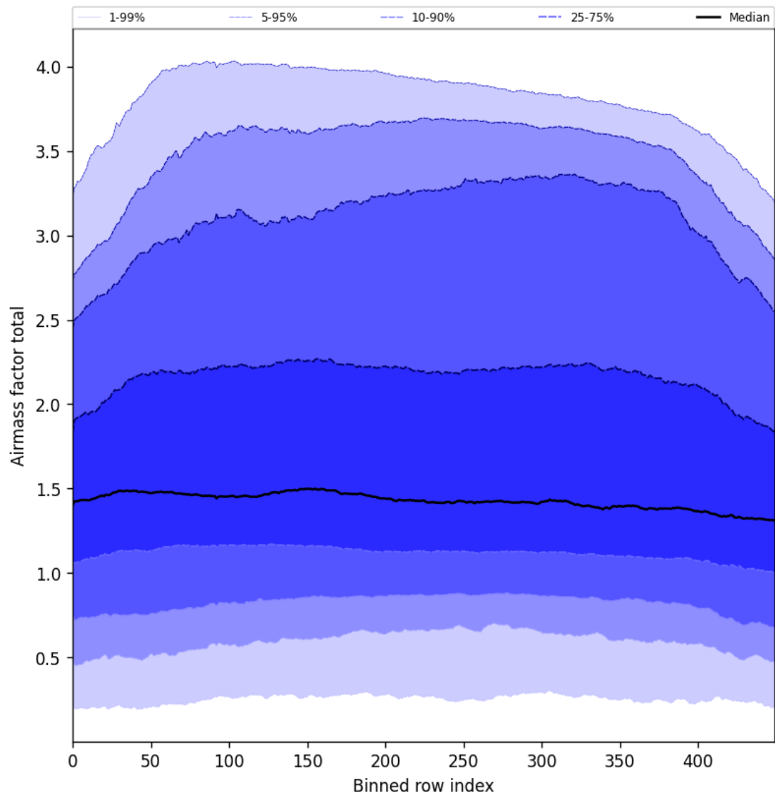
Figure 54: Along track statistics of “Airmass factor total” for 2025-05-06 to 2025-05-08
