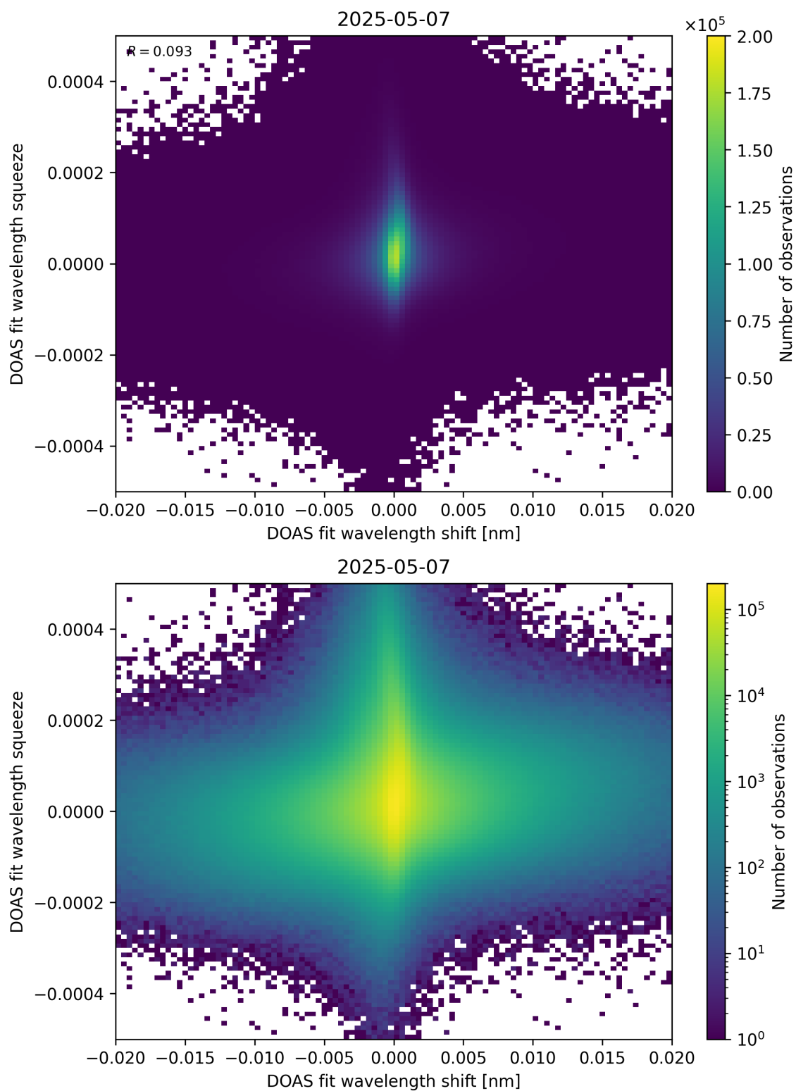
Figure 65: Scatter density plot of “DOAS fit wavelength shift” against “DOAS fit wavelength squeeze” for 2025-05-06 to 2025-05-08.
