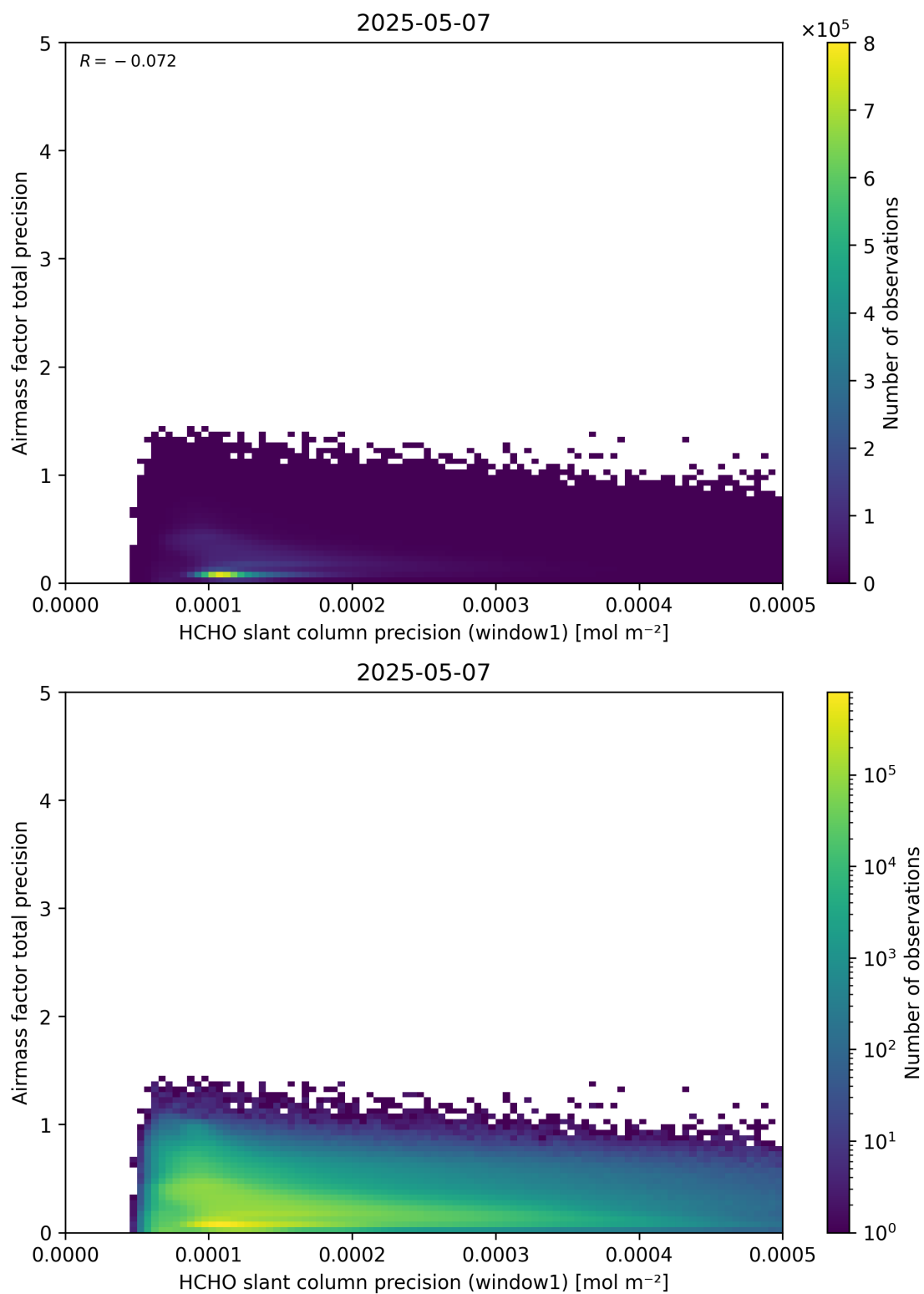
Figure 95: Scatter density plot of “HCHO slant column precision (window1)” against “Airmass factor total precision” for 2025-05-06 to 2025-05-08.
