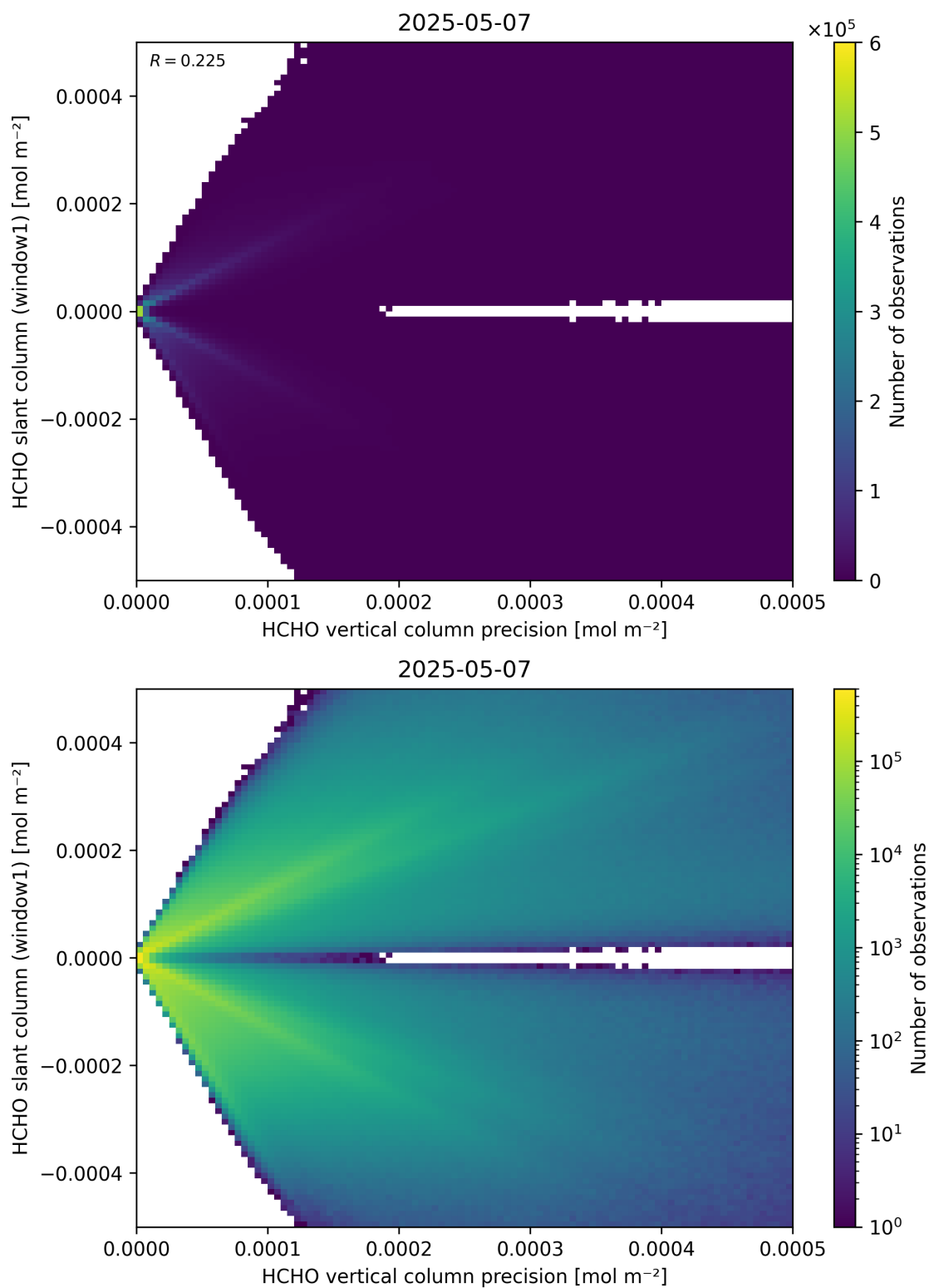
Figure 142: Scatter density plot of “HCHO vertical column precision” against “HCHO slant column (window1)” for 2025-05-06 to 2025-05-08.
