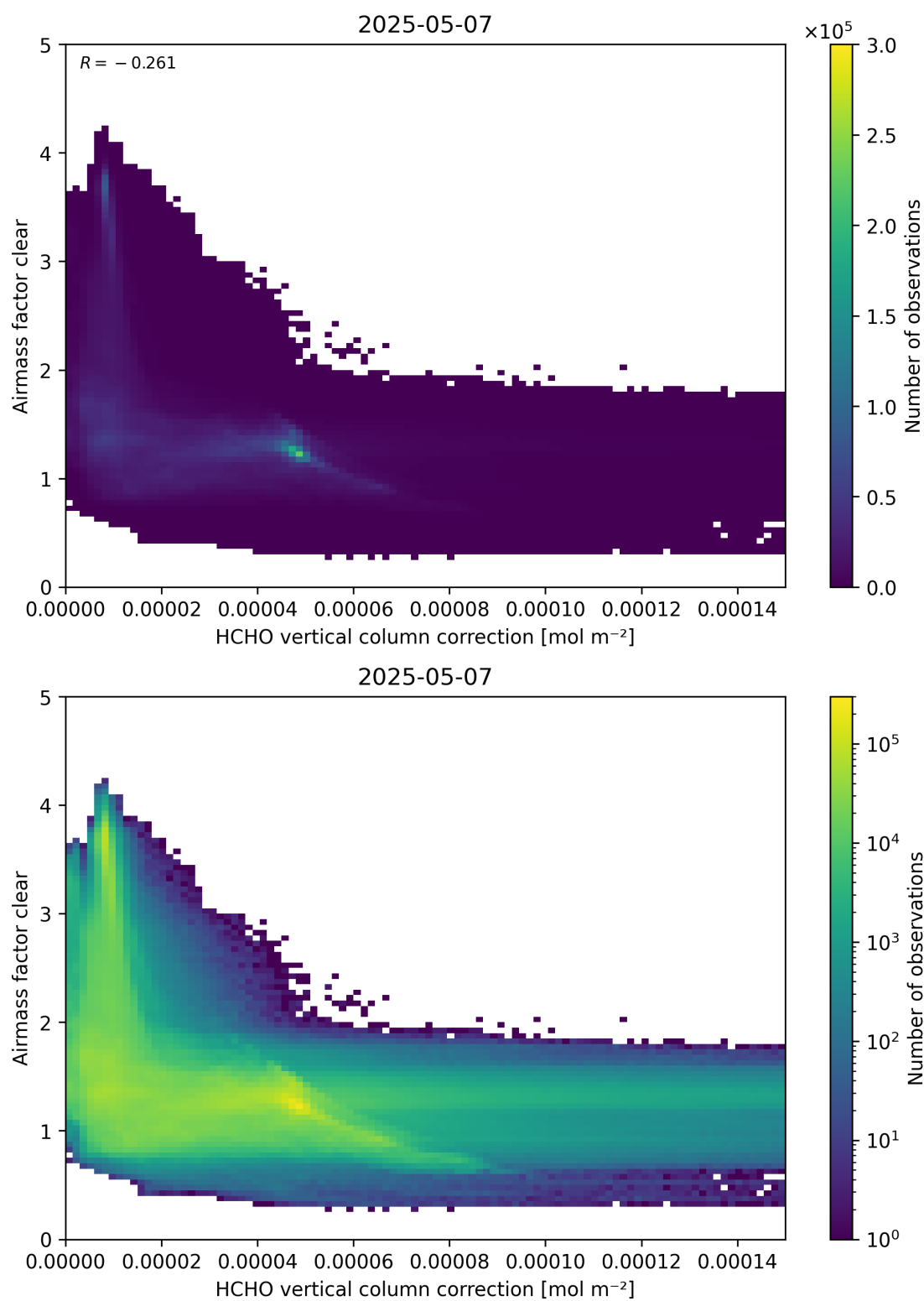
Figure 115: Scatter density plot of “HCHO vertical column correction” against “Airmass factor clear” for 2025-05-06 to 2025-05-08.
