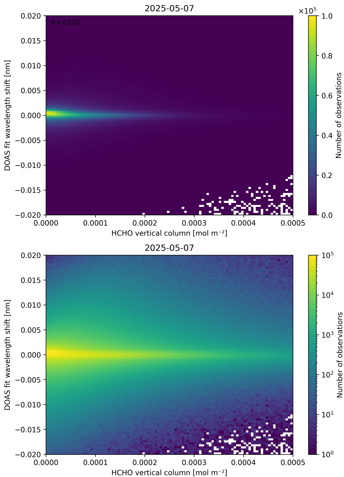
Figure 124: Scatter density plot of “HCHO vertical column” against “DOAS fit wavelength shift” for 2025-05-06 to 2025-05-08.
