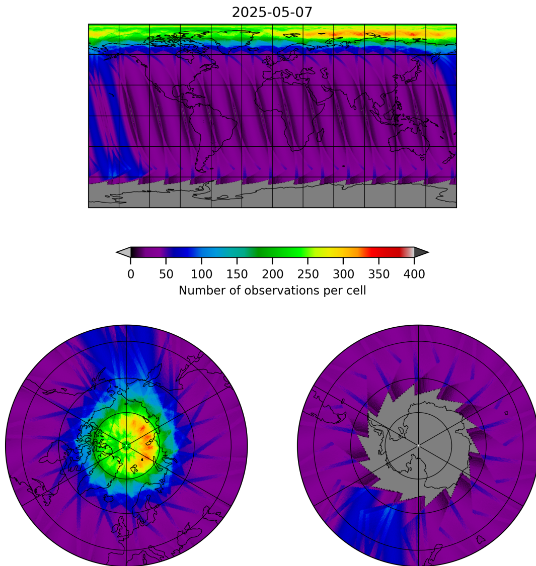
Figure 19: Map of the number of observations for 2025-05-06 to 2025-05-08
