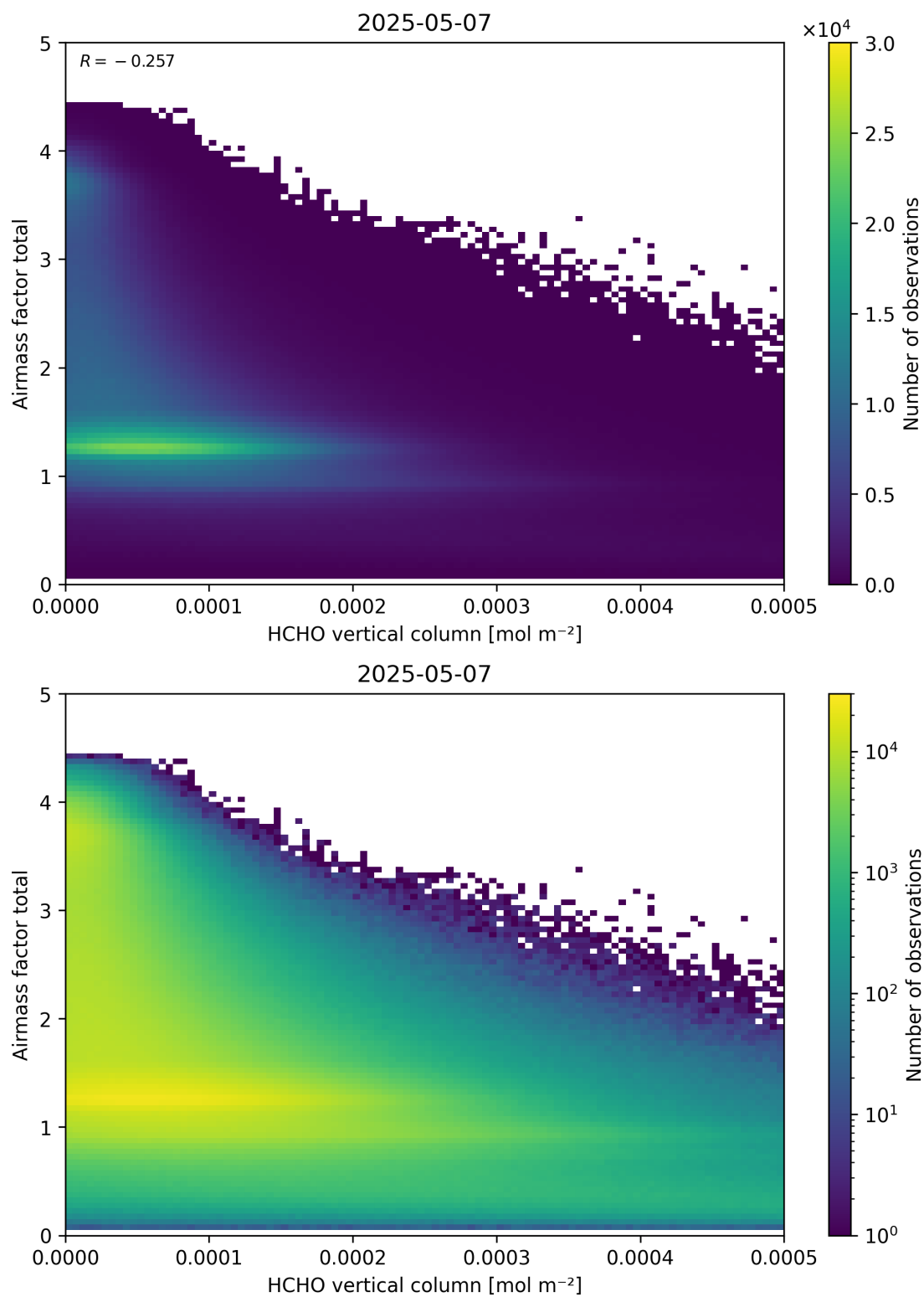
Figure 131: Scatter density plot of “HCHO vertical column” against “Airmass factor total” for 2025-05-06 to 2025-05-08.
