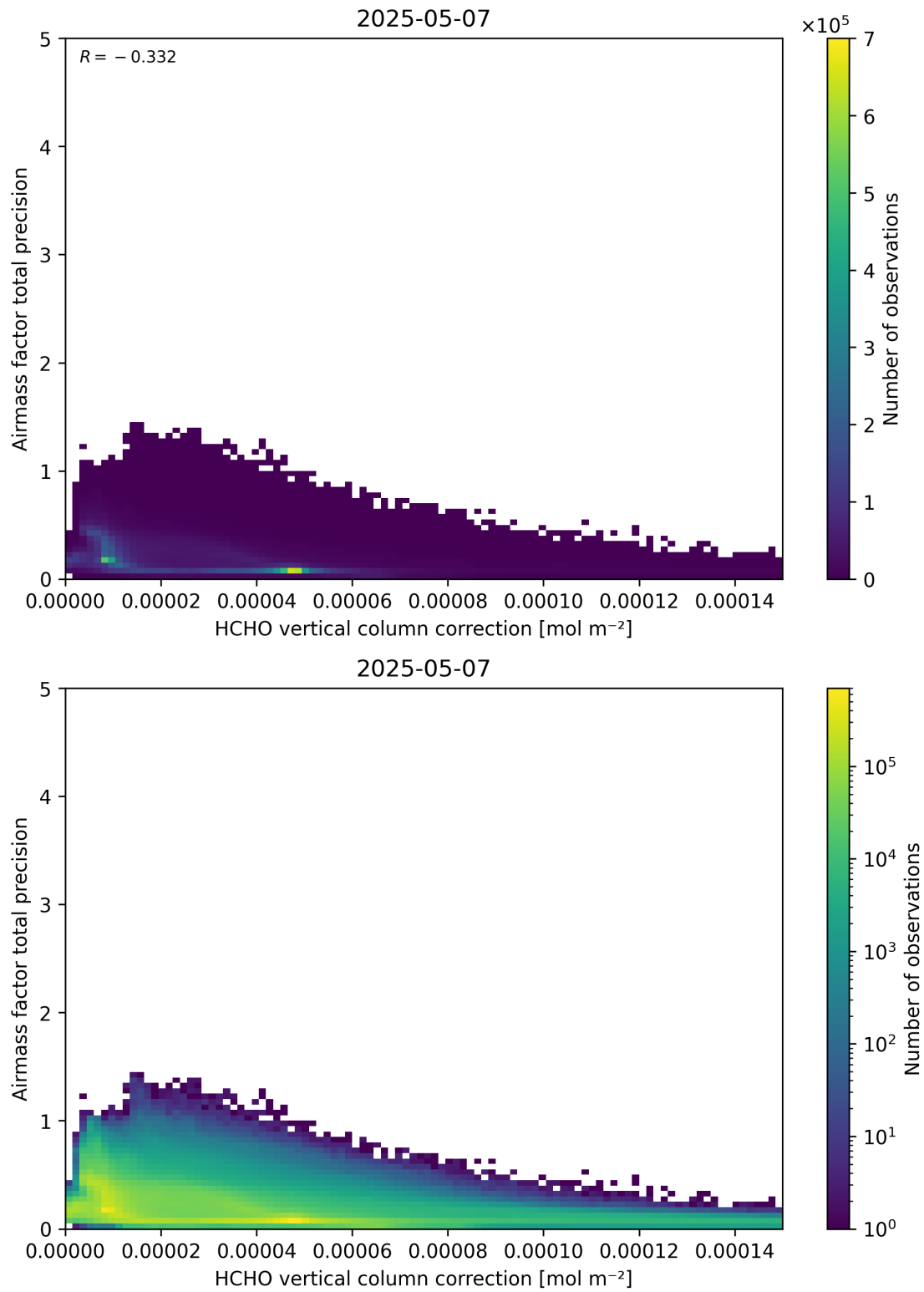
Figure 121: Scatter density plot of “HCHO vertical column correction” against “Airmass factor total precision” for 2025-05-06 to 2025-05-08.
