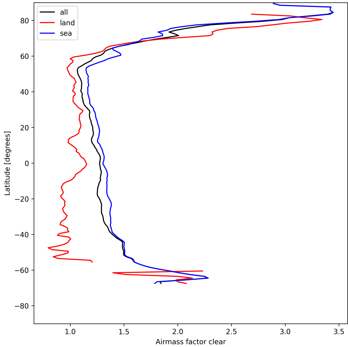
Figure 28: Zonal average of “Airmass factor clear” for 2025-05-06 to 2025-05-08.
