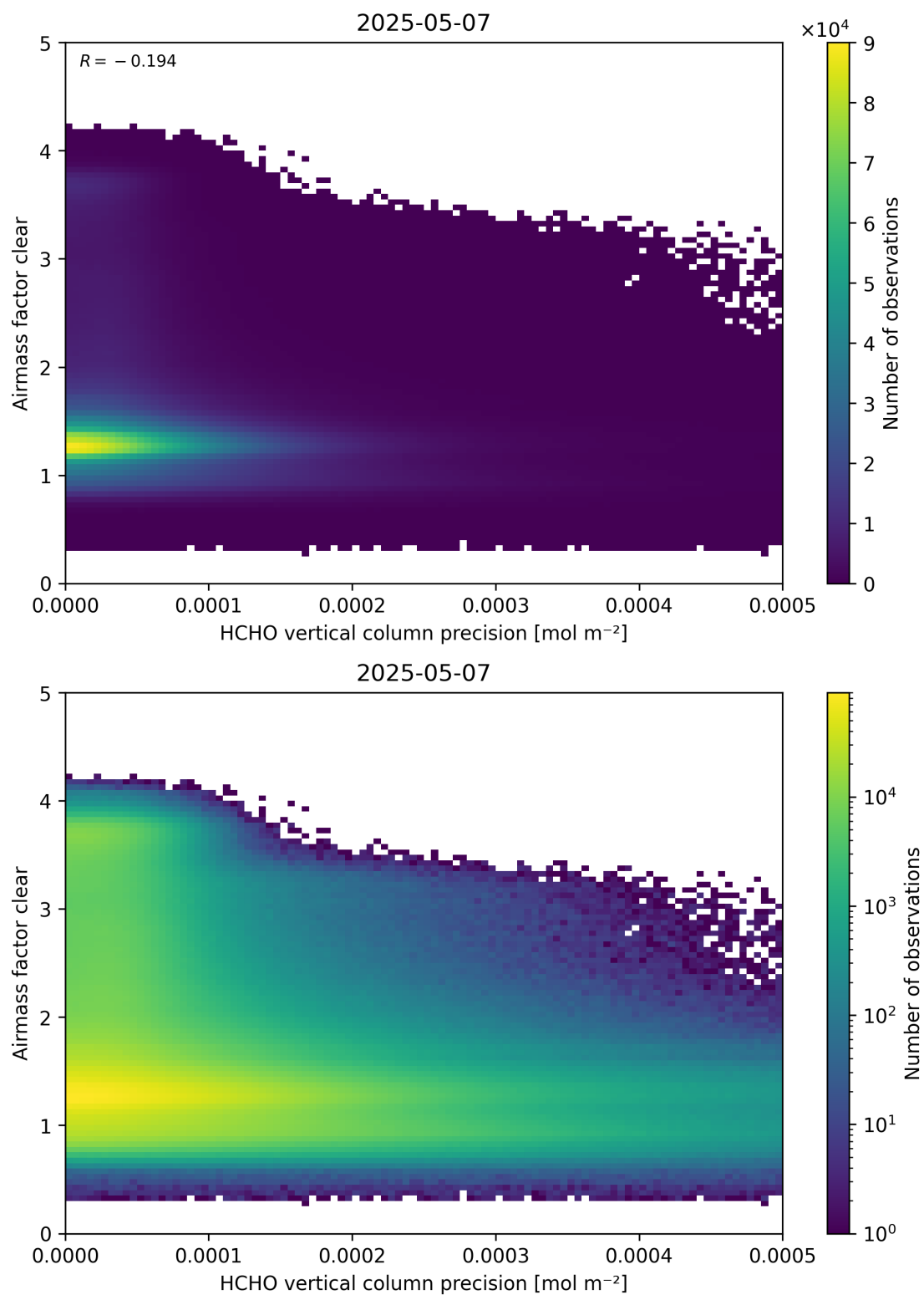
Figure 139: Scatter density plot of “HCHO vertical column precision” against “Airmass factor clear” for 2025-05-06 to 2025-05-08.
