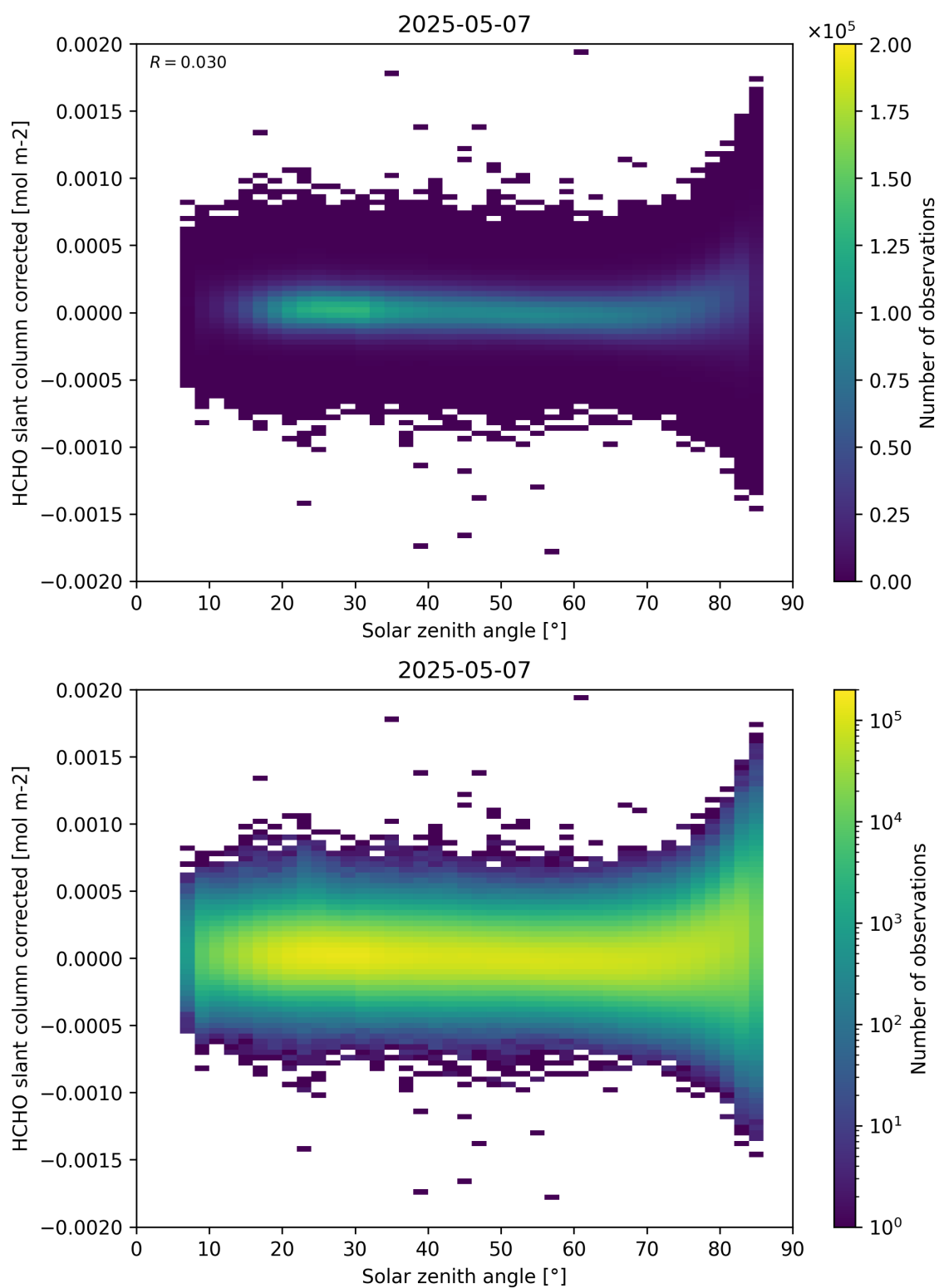
Figure 171: Scatter density plot of “Solar zenith angle” against “HCHO slant column corrected” for 2025-05-06 to 2025-05-08.
