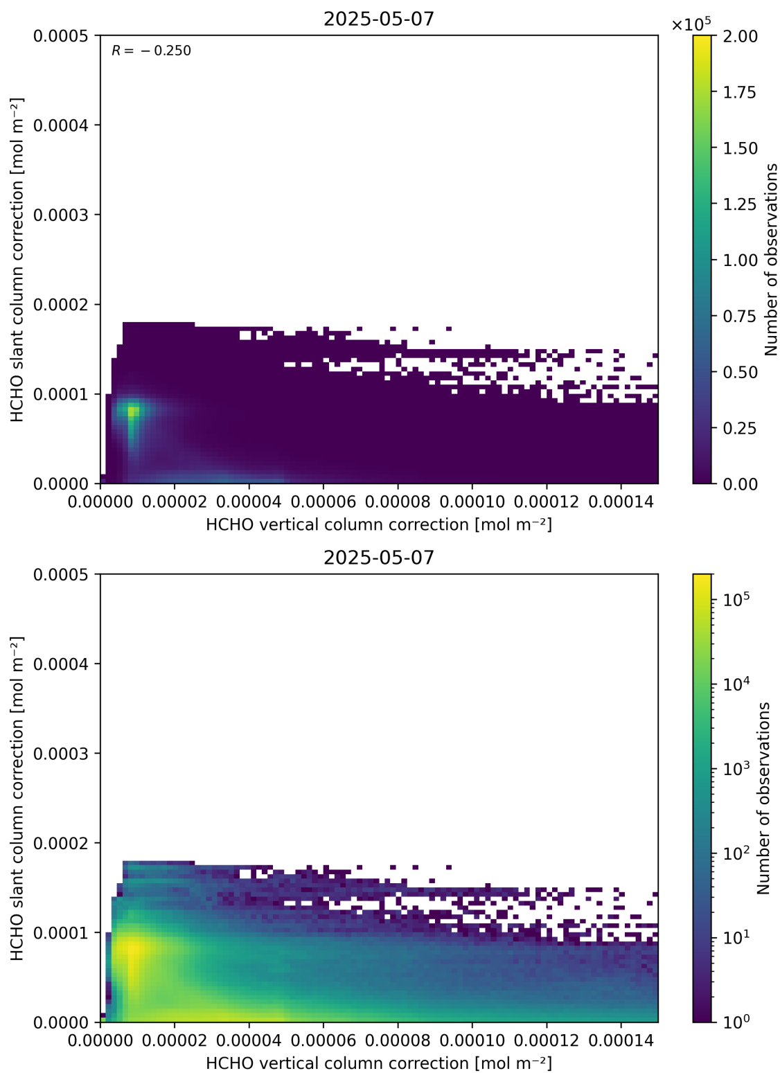
Figure 117: Scatter density plot of “HCHO vertical column correction” against “HCHO slant column correction” for 2025-05-06 to 2025-05-08.
