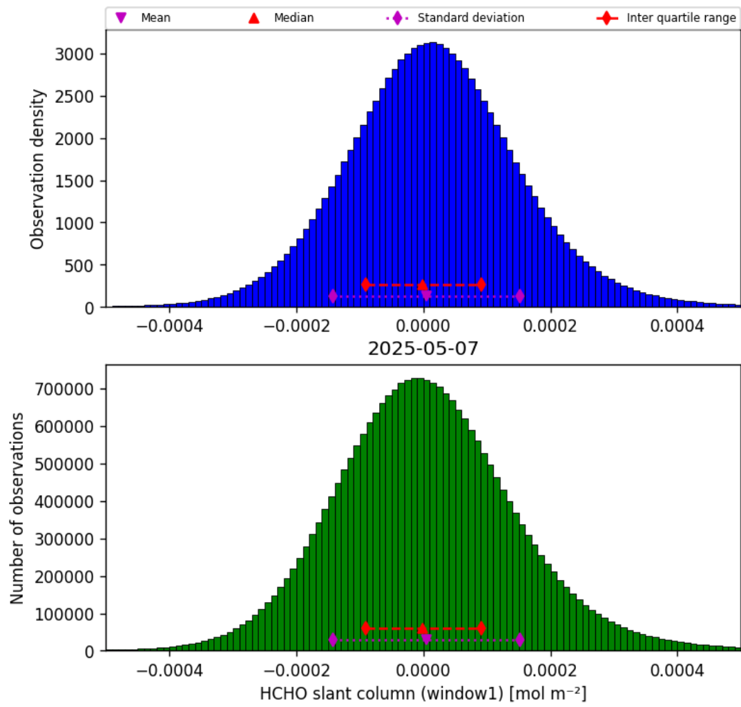
Figure 38: Histogram of “HCHO slant column (window1)” for 2025-05-06 to 2025-05-08
