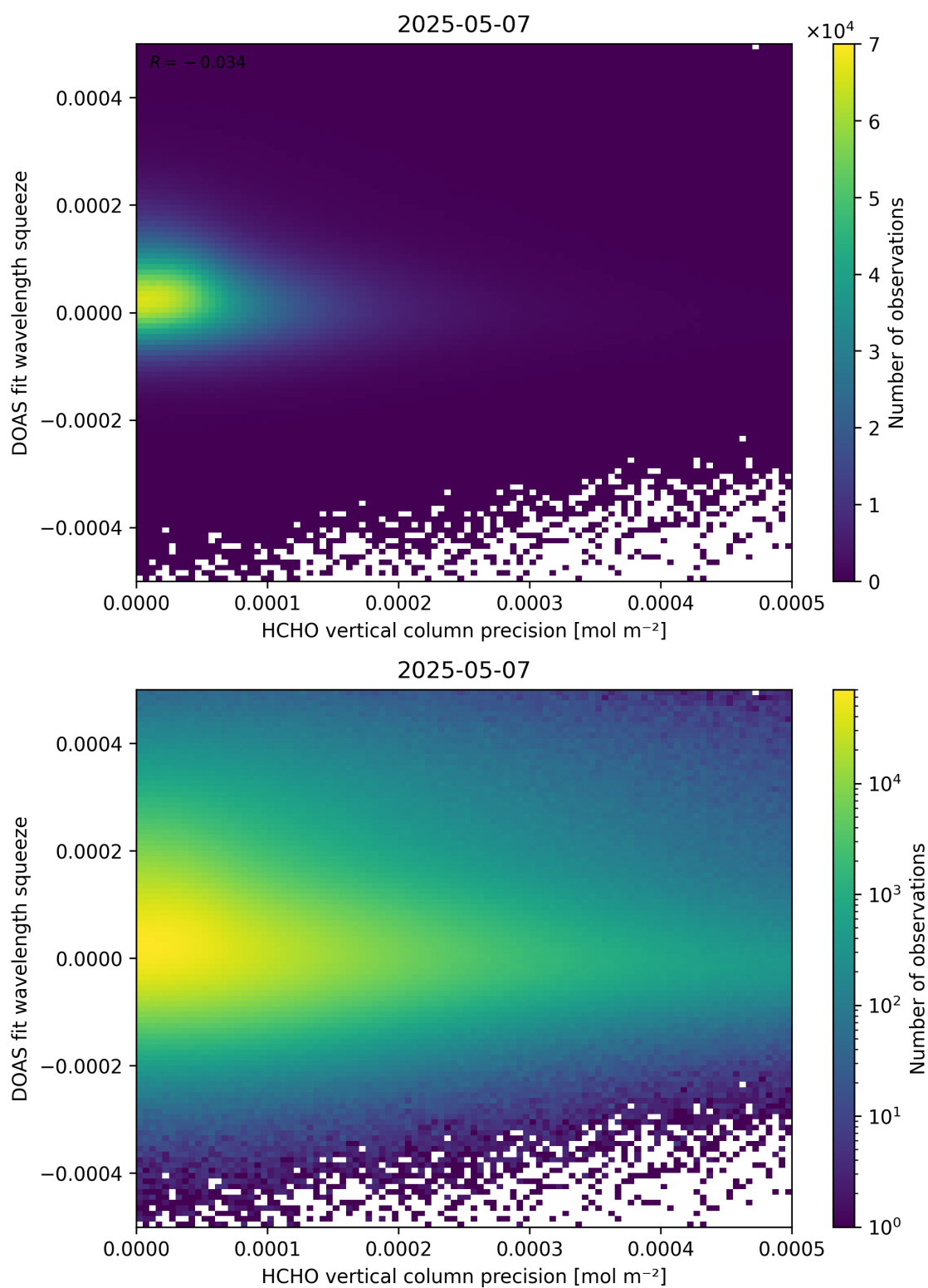
Figure 138: Scatter density plot of “HCHO vertical column precision” against “DOAS fit wavelength squeeze” for 2025-05-06 to 2025-05-08.
