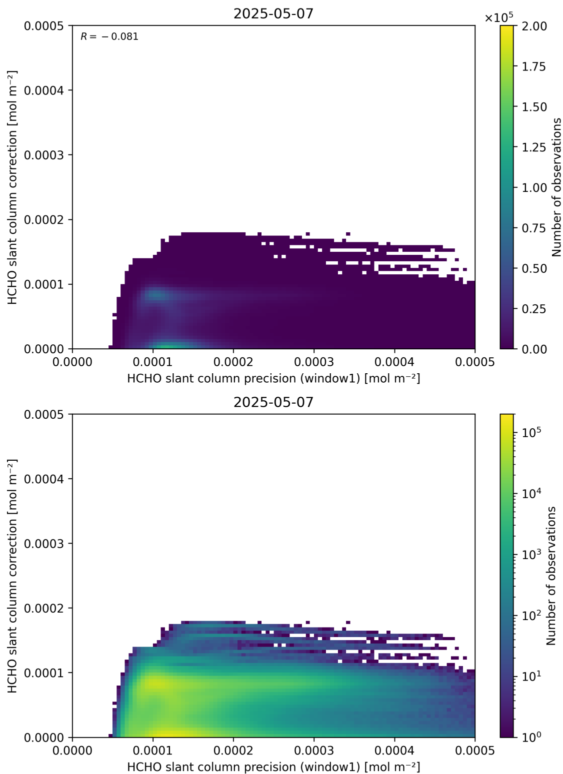
Figure 93: Scatter density plot of “HCHO slant column precision (window1)” against “HCHO slant column correction” for 2025-05-06 to 2025-05-08.
