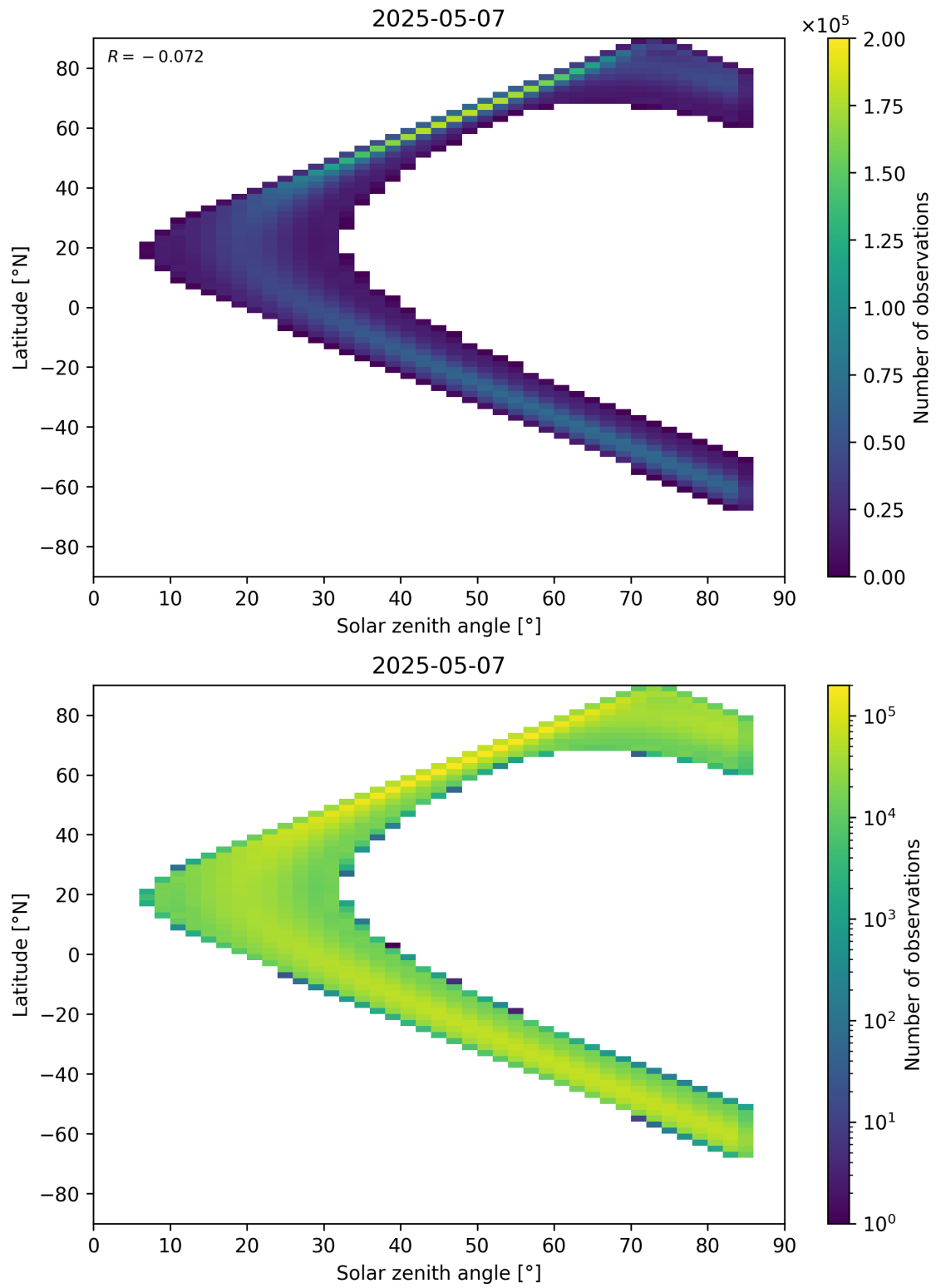
Figure 181: Scatter density plot of “Solar zenith angle” against “Latitude” for 2025-05-06 to 2025-05-08.
