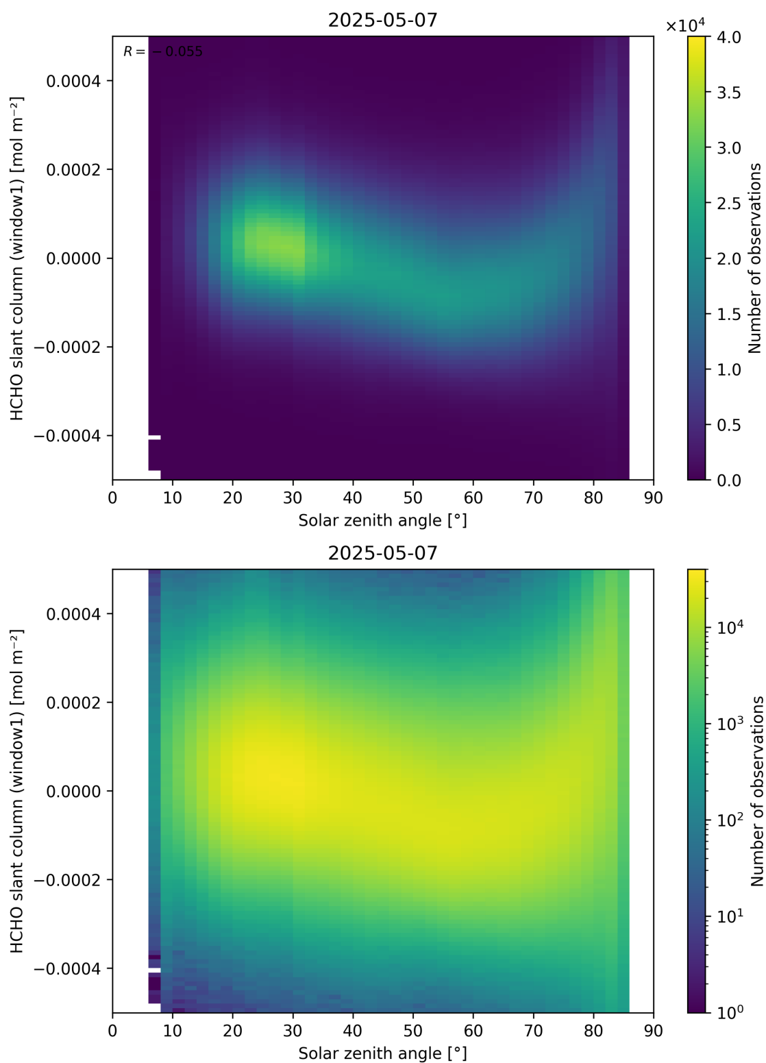
Figure 173: Scatter density plot of “Solar zenith angle” against “HCHO slant column (window1)” for 2025-05-06 to 2025-05-08.
