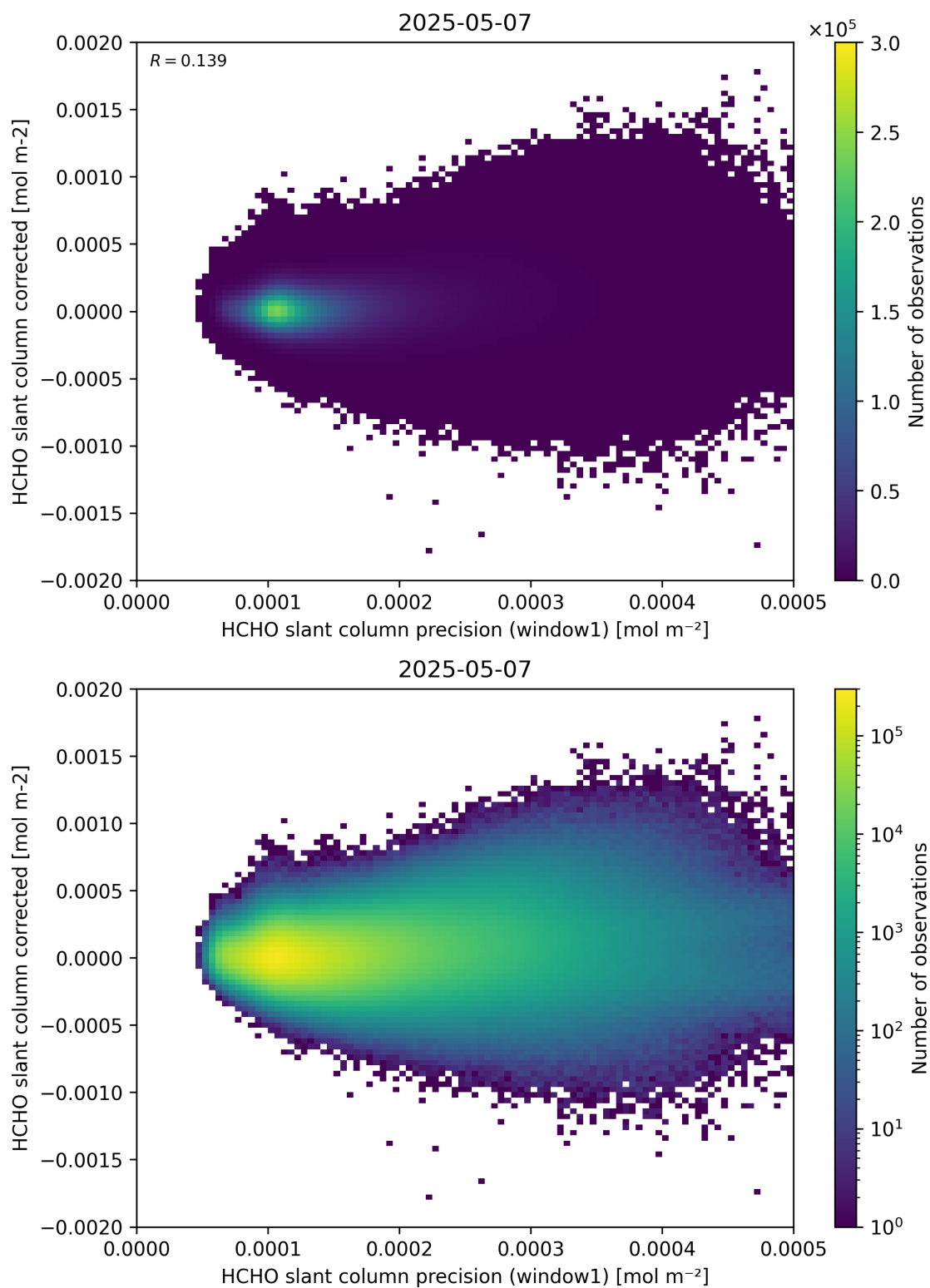
Figure 92: Scatter density plot of “HCHO slant column precision (window1)” against “HCHO slant column corrected” for 2025-05-06 to 2025-05-08.
