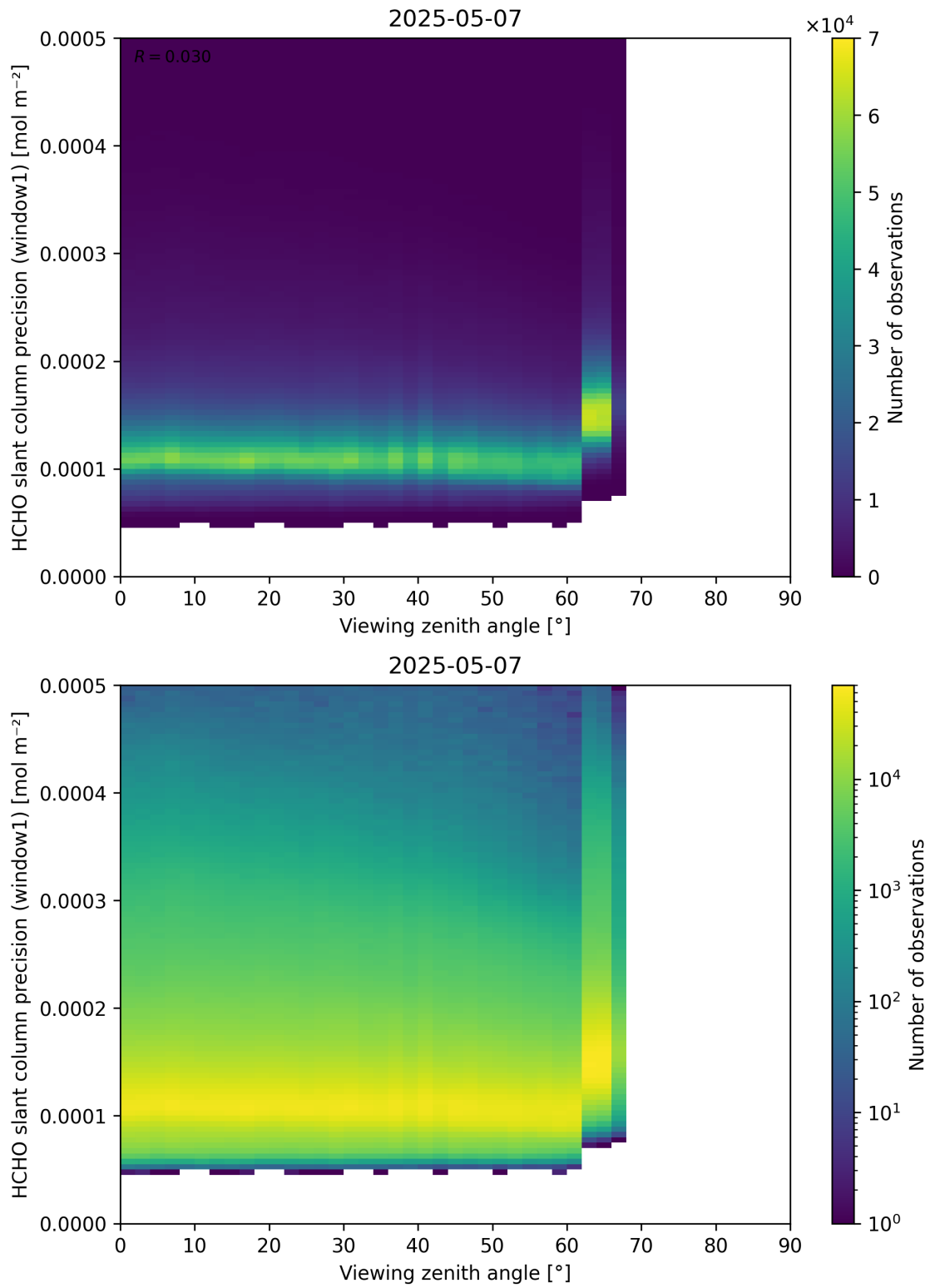
Figure 189: Scatter density plot of “Viewing zenith angle” against “HCHO slant column precision (window1)” for 2025-05-06 to 2025-05-08.
