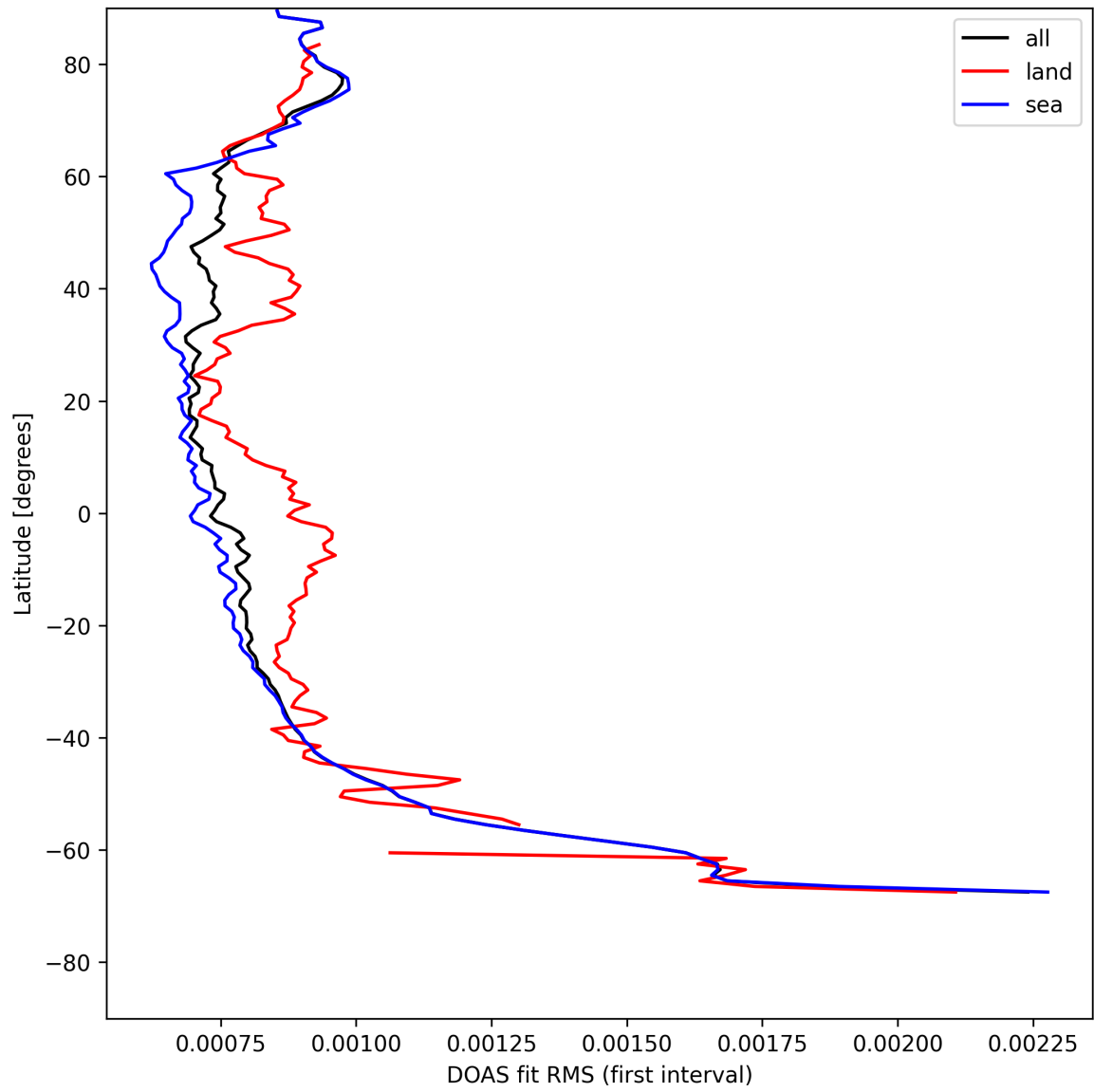
Figure 32: Zonal average of "DOAS fit RMS (first interval)" for 2025-05-06 to 2025-05-08.
