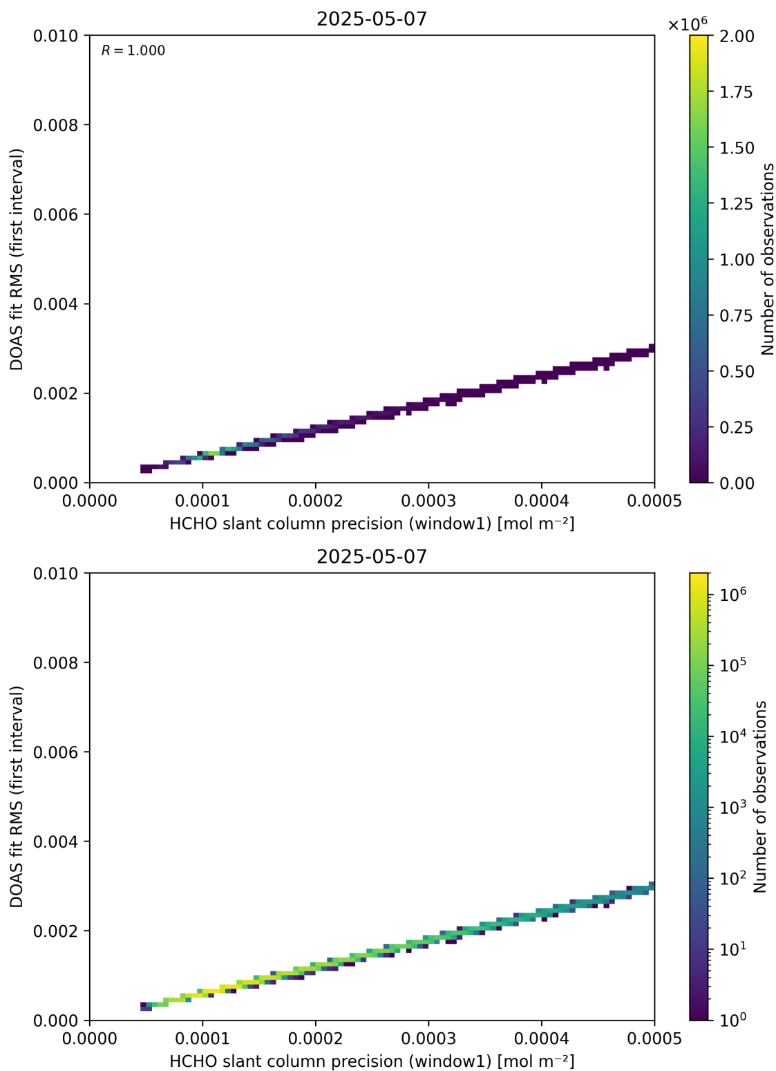
Figure 88: Scatter density plot of “HCHO slant column precision (window1)” against “DOAS fit RMS (first interval)” for 2025-05-06 to 2025-05-08.
