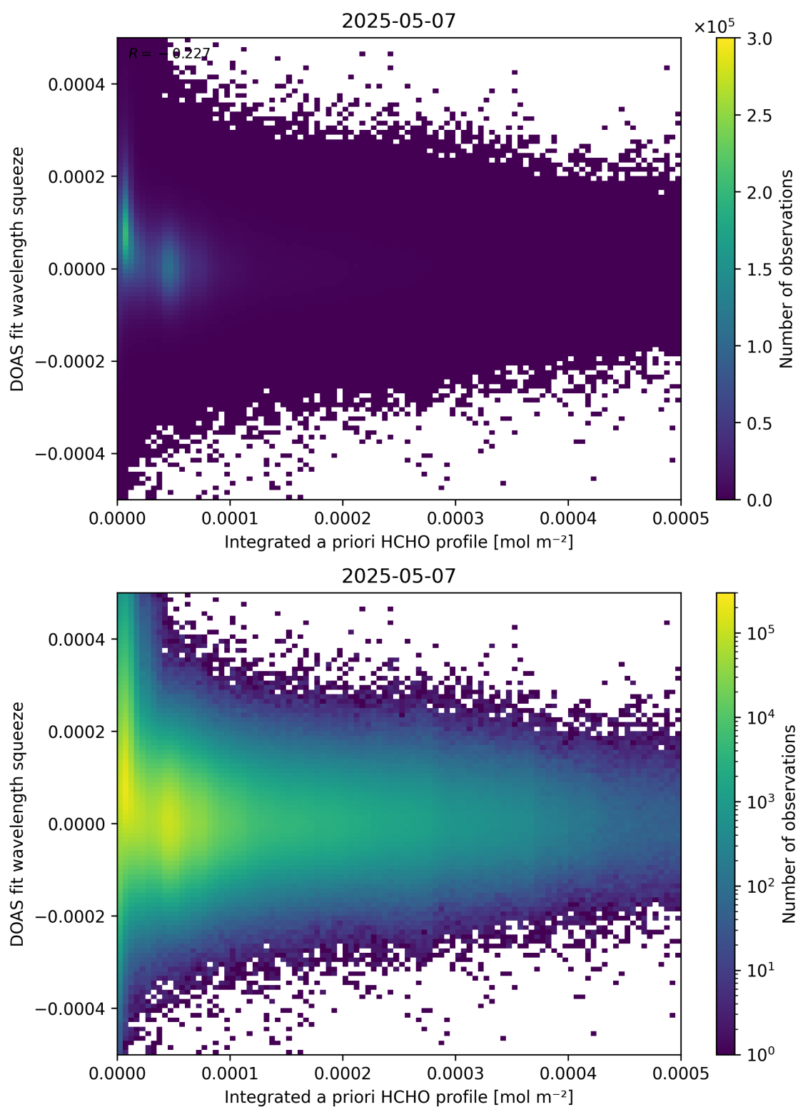
Figure 150: Scatter density plot of “Integrated a priori HCHO profile” against “DOAS fit wavelength squeeze” for 2025-05-06 to 2025-05-08.
