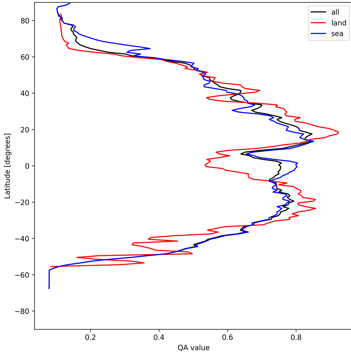
Figure 20: Zonal average of “QA value” for 2025-05-06 to 2025-05-08.
