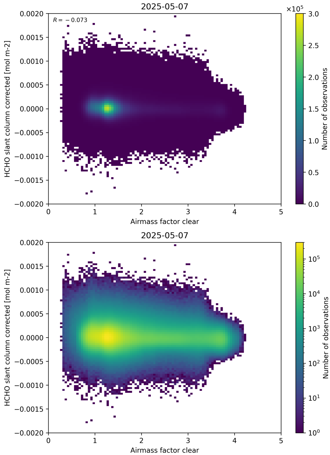
Figure 74: Scatter density plot of “Airmass factor clear” against “HCHO slant column corrected” for 2025-05-06 to 2025-05-08.
