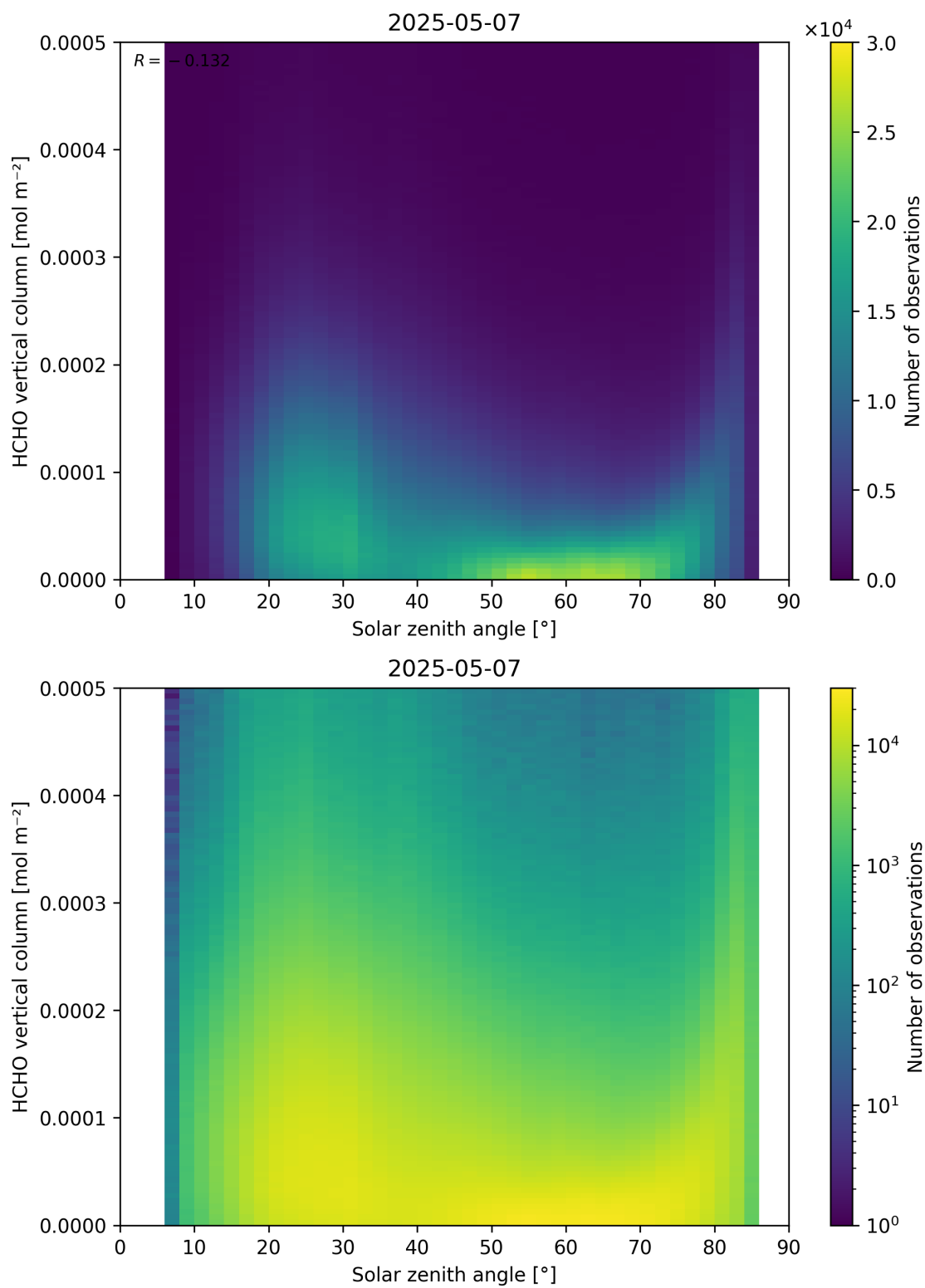
Figure 177: Scatter density plot of “Solar zenith angle” against “HCHO vertical column” for 2025-05-06 to 2025-05-08.
