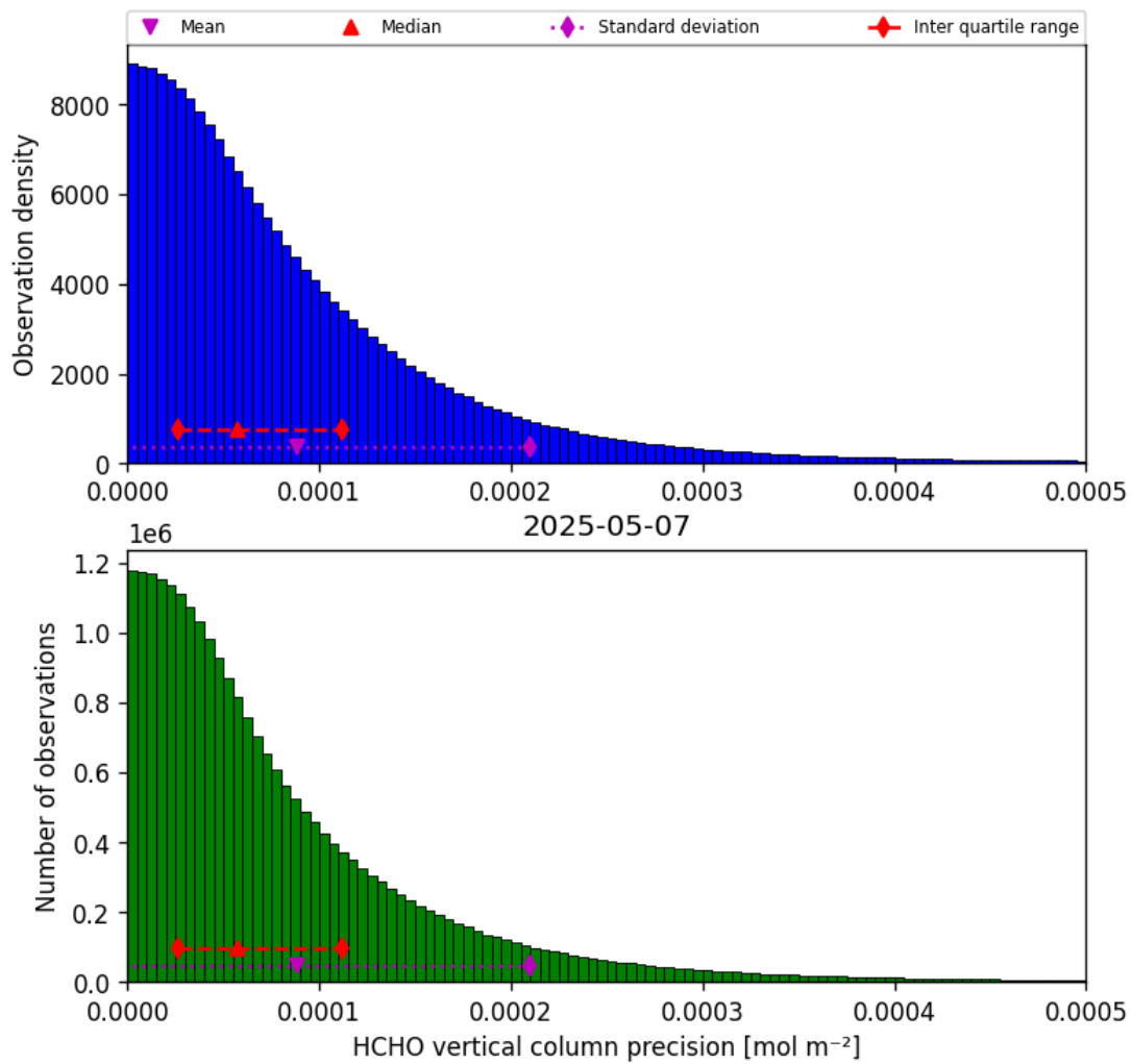
Figure 36: Histogram of “HCHO vertical column precision” for 2025-05-06 to 2025-05-08
