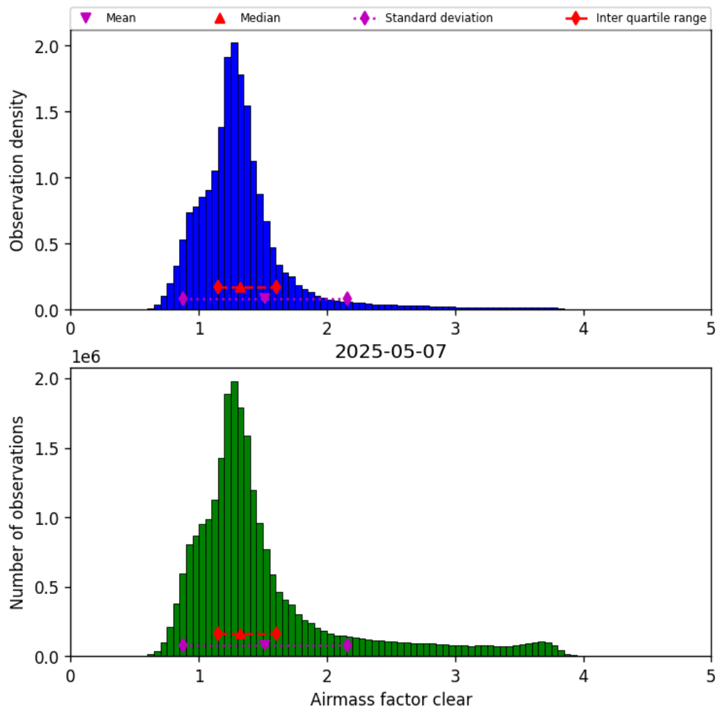
Figure 42: Histogram of “Airmass factor clear” for 2025-05-06 to 2025-05-08
