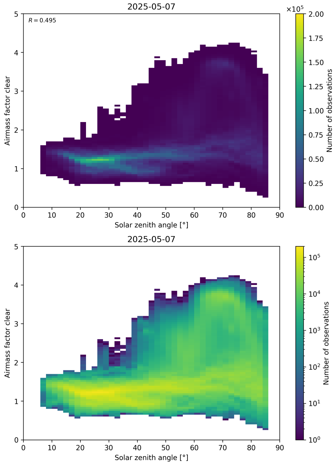
Figure 170: Scatter density plot of “Solar zenith angle” against “Airmass factor clear” for 2025-05-06 to 2025-05-08.
