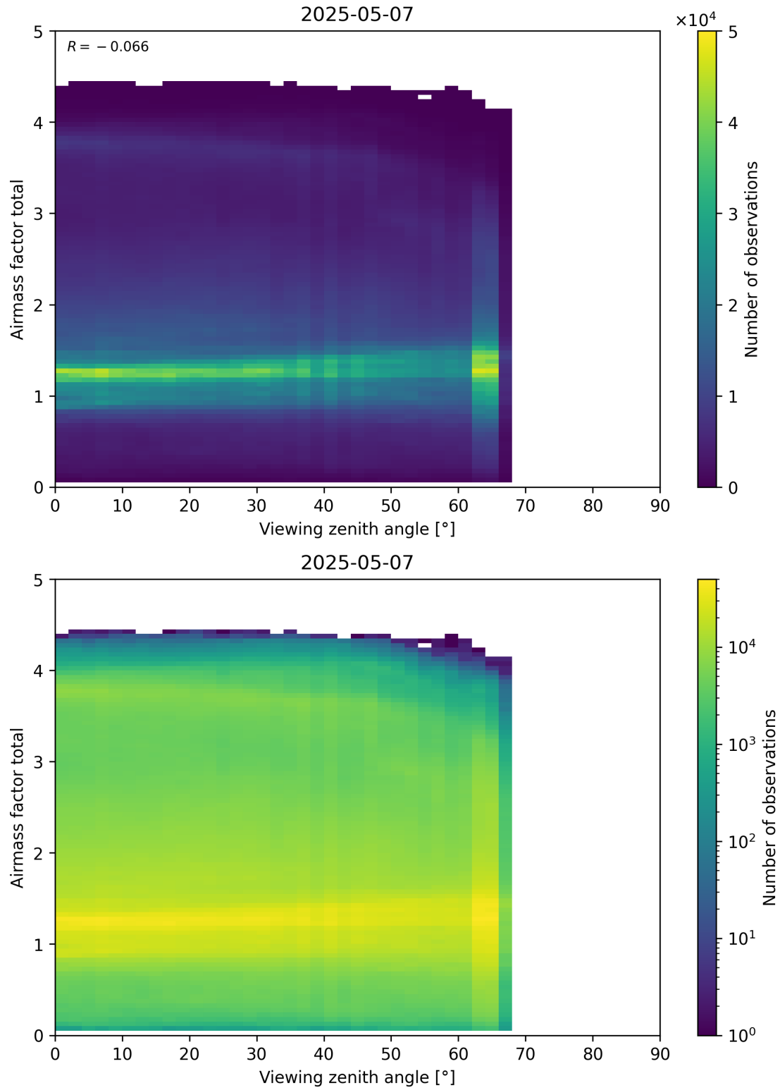
Figure 190: Scatter density plot of “Viewing zenith angle” against “Airmass factor total” for 2025-05-06 to 2025-05-08.
