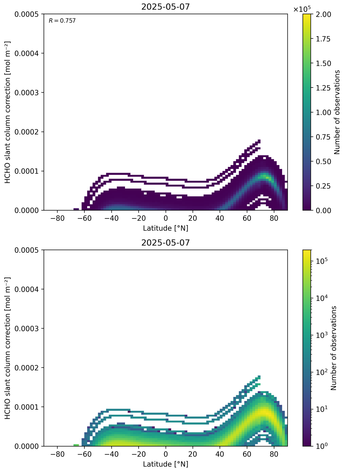
Figure 158: Scatter density plot of “Latitude” against “HCHO slant column correction” for 2025-05-06 to 2025-05-08.
