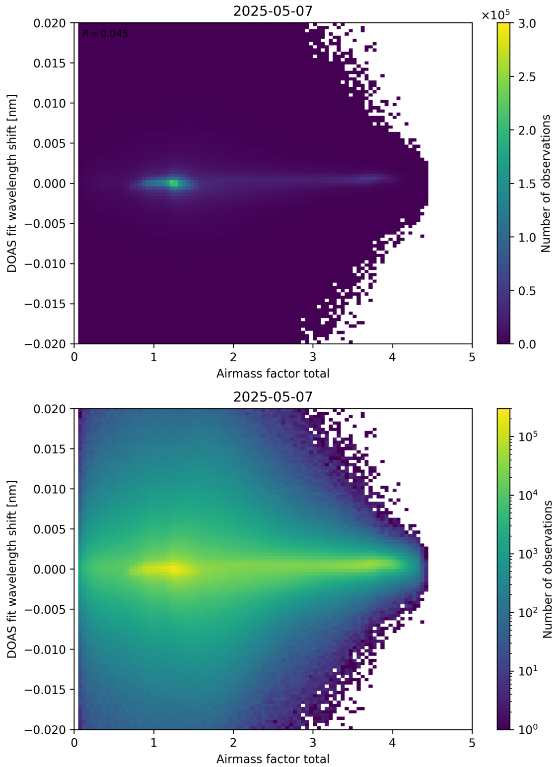
Figure 98: Scatter density plot of “Airmass factor total” against “DOAS fit wavelength shift” for 2025-05-06 to 2025-05-08.
