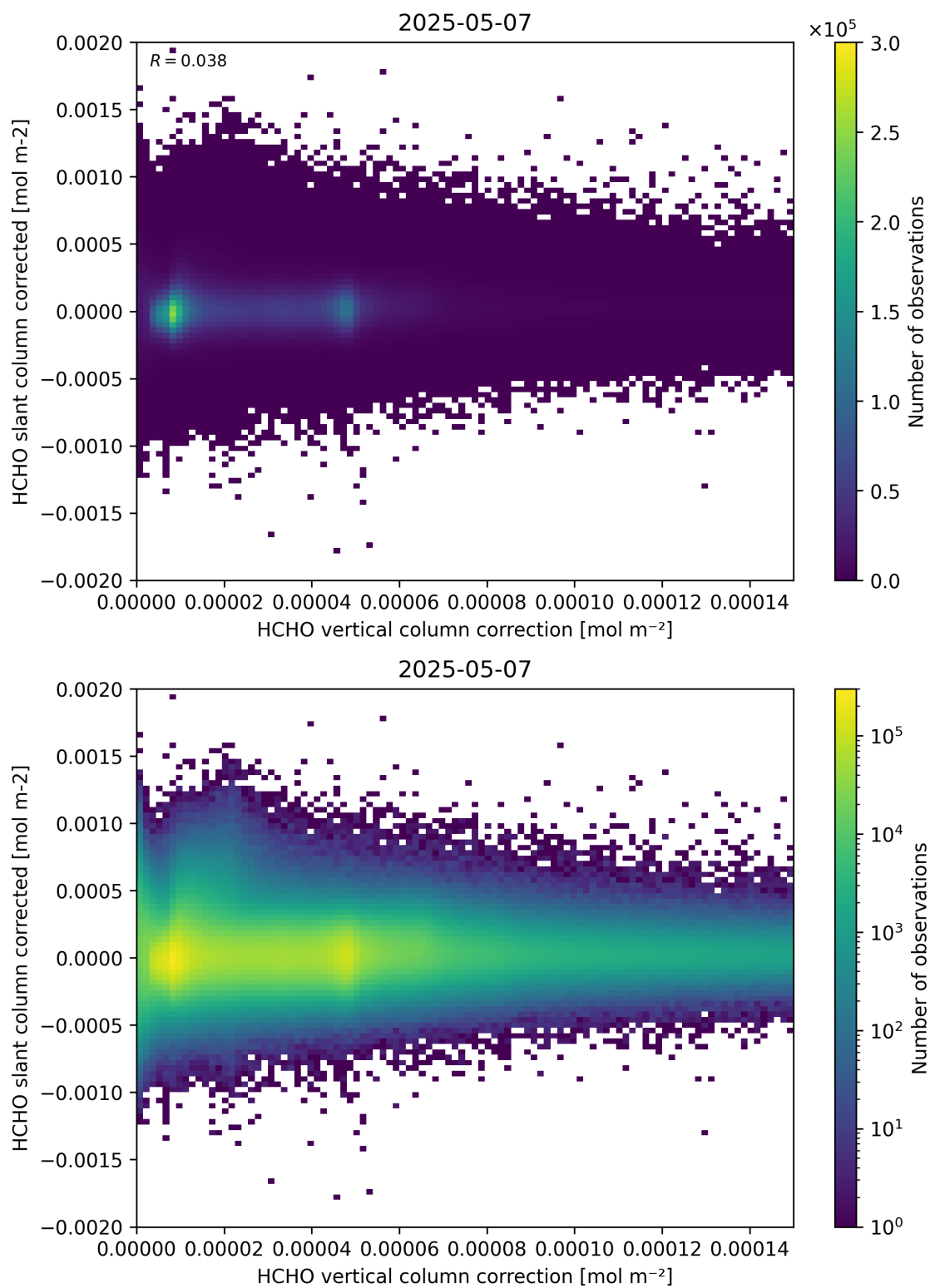
Figure 116: Scatter density plot of “HCHO vertical column correction” against “HCHO slant column corrected” for 2025-05-06 to 2025-05-08.
