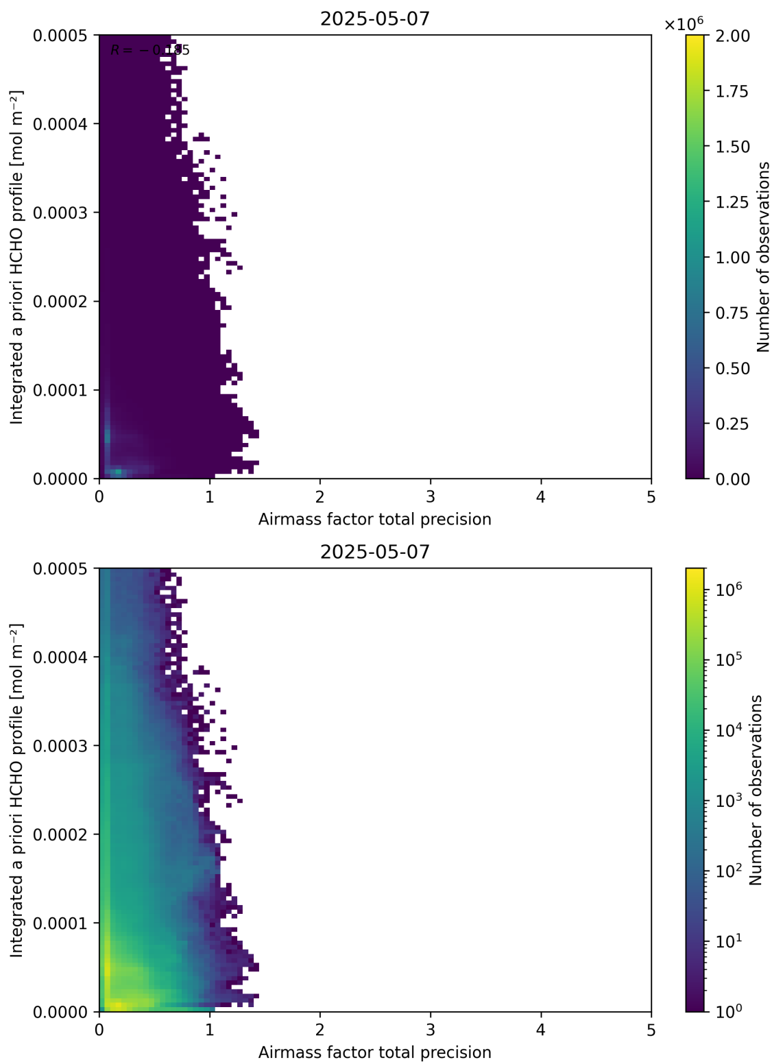
Figure 111: Scatter density plot of “Airmass factor total precision” against “Integrated a priori HCHO profile” for 2025-05-06 to 2025-05-08.
