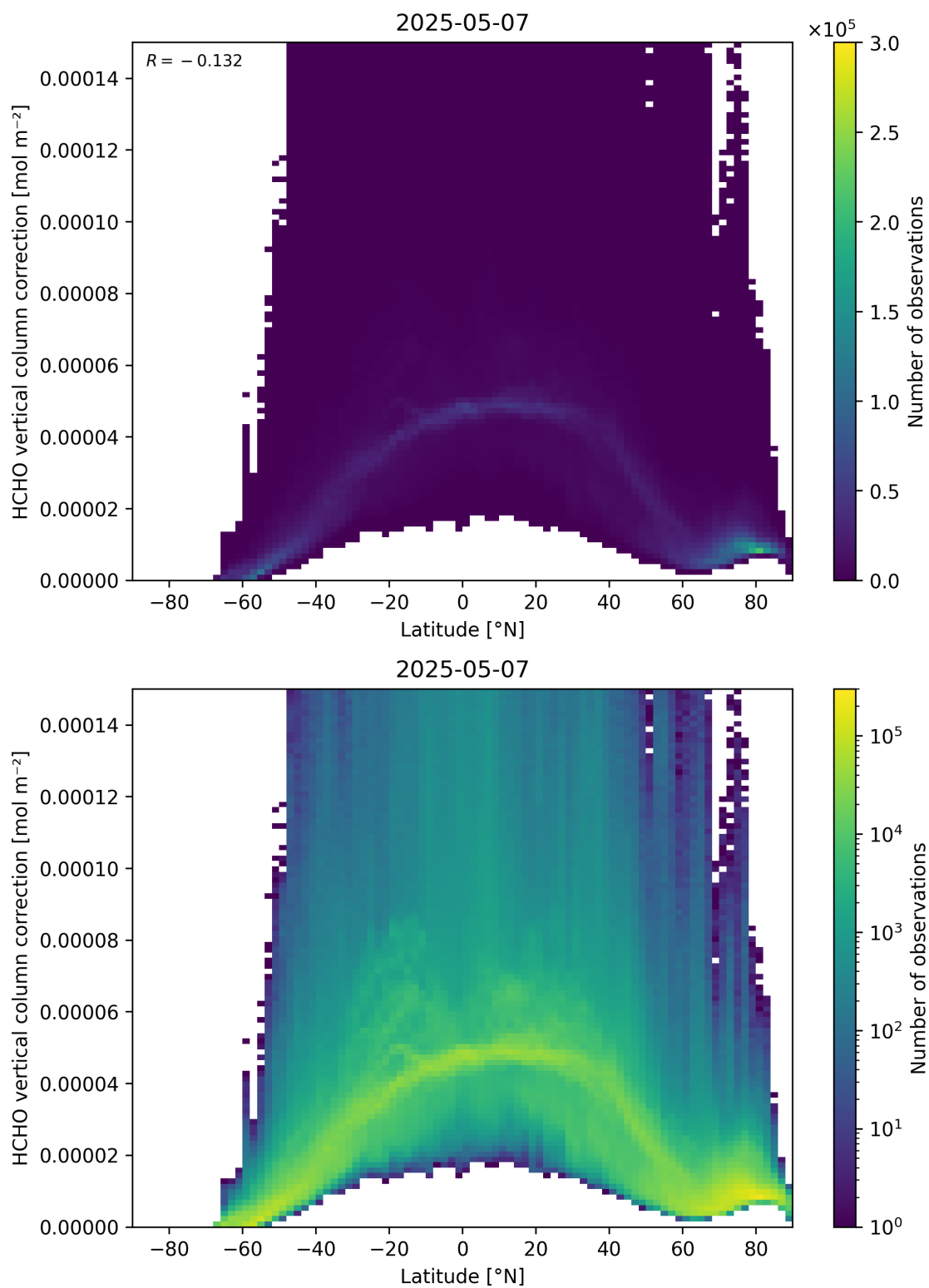
Figure 164: Scatter density plot of “Latitude” against “HCHO vertical column correction” for 2025-05-06 to 2025-05-08.
