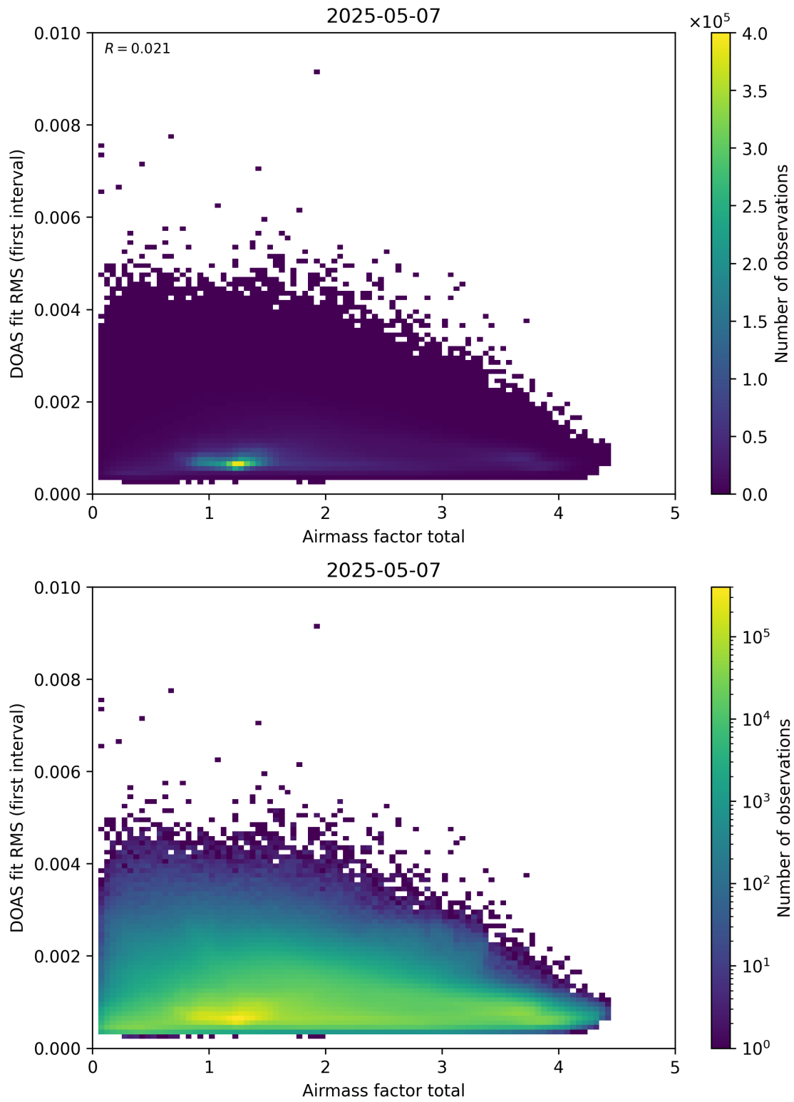
Figure 97: Scatter density plot of “Airmass factor total” against “DOAS fit RMS (first interval)” for 2025-05-06 to 2025-05-08.
