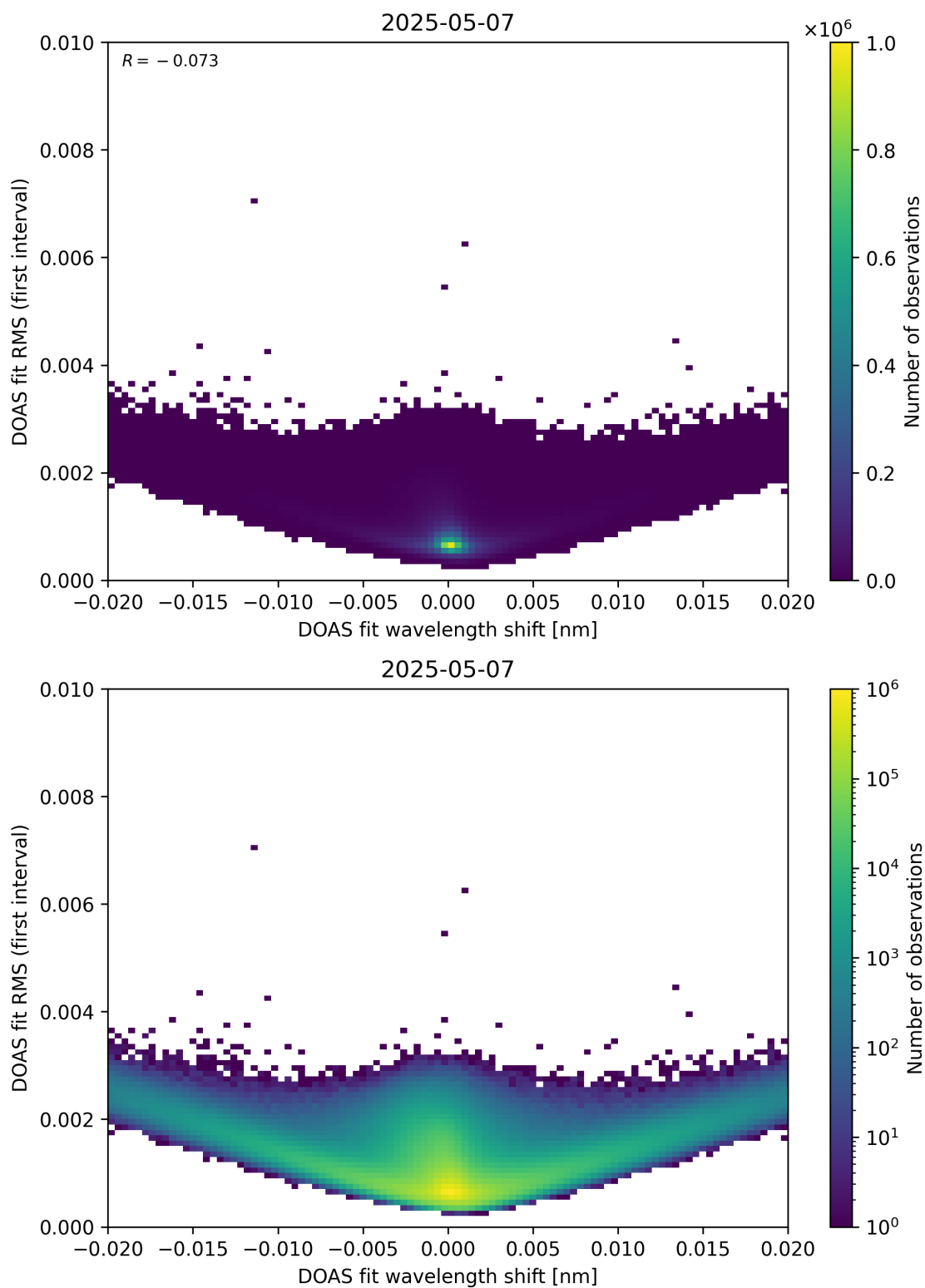
Figure 64: Scatter density plot of “DOAS fit wavelength shift” against “DOAS fit RMS (first interval)” for 2025-05-06 to 2025-05-08.
