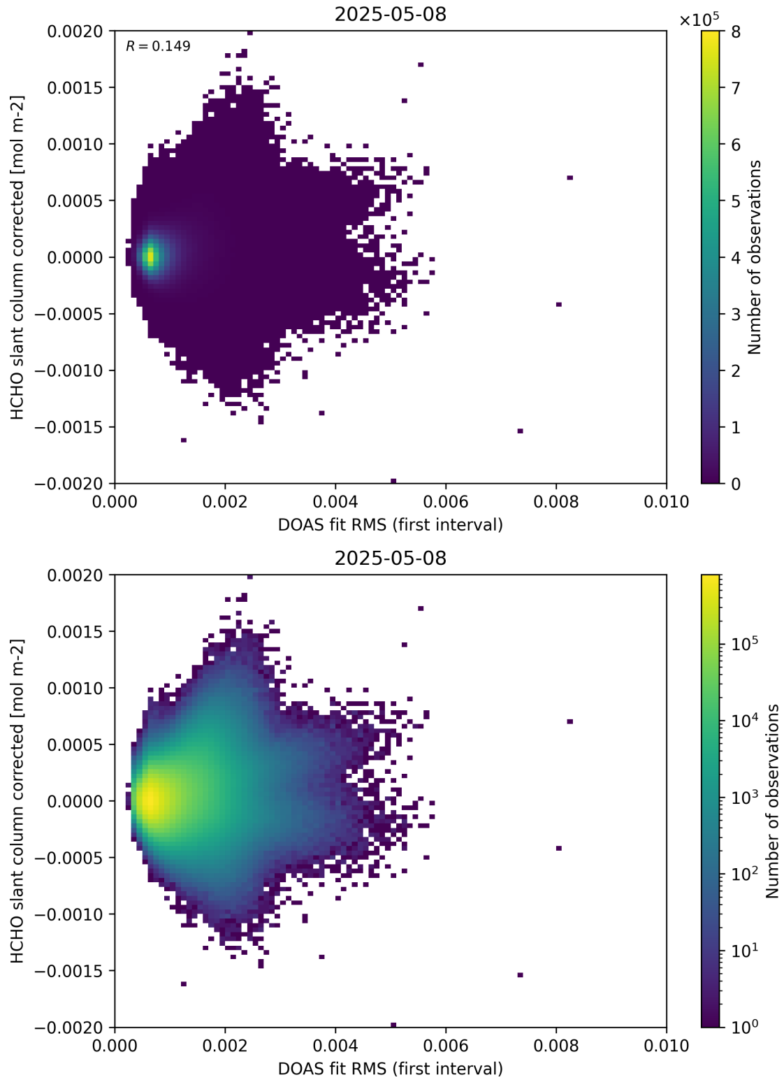
Figure 62: Scatter density plot of “DOAS fit RMS (first interval)” against “HCHO slant column corrected” for 2025-05-07 to 2025-05-09.
