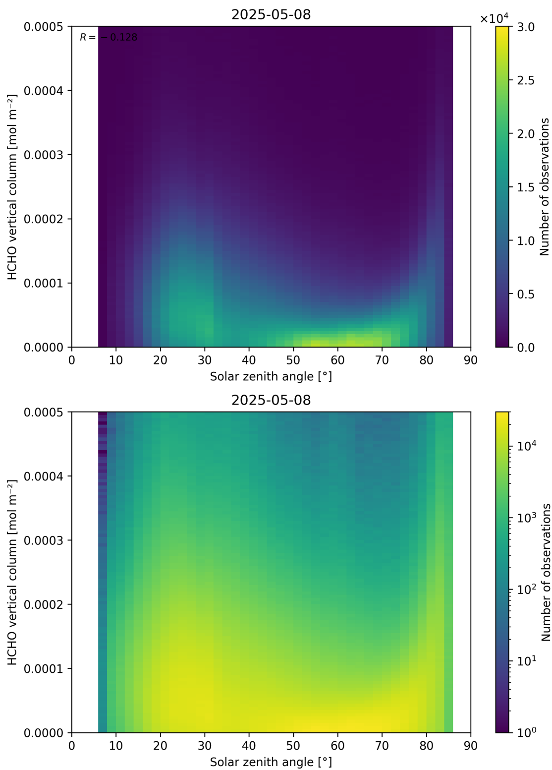
Figure 177: Scatter density plot of “Solar zenith angle” against “HCHO vertical column” for 2025-05-07 to 2025-05-09.
