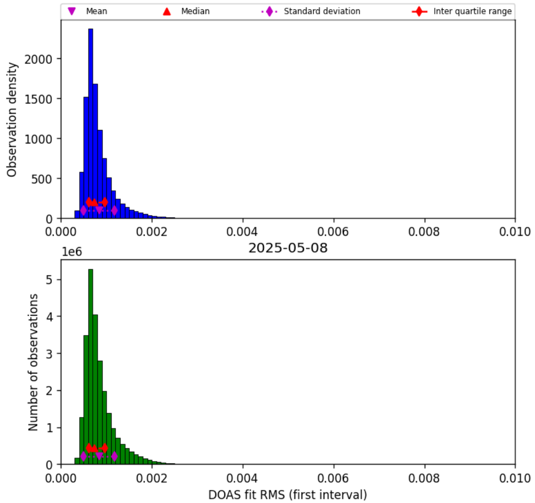
Figure 46: Histogram of “DOAS fit RMS (first interval)” for 2025-05-07 to 2025-05-09
