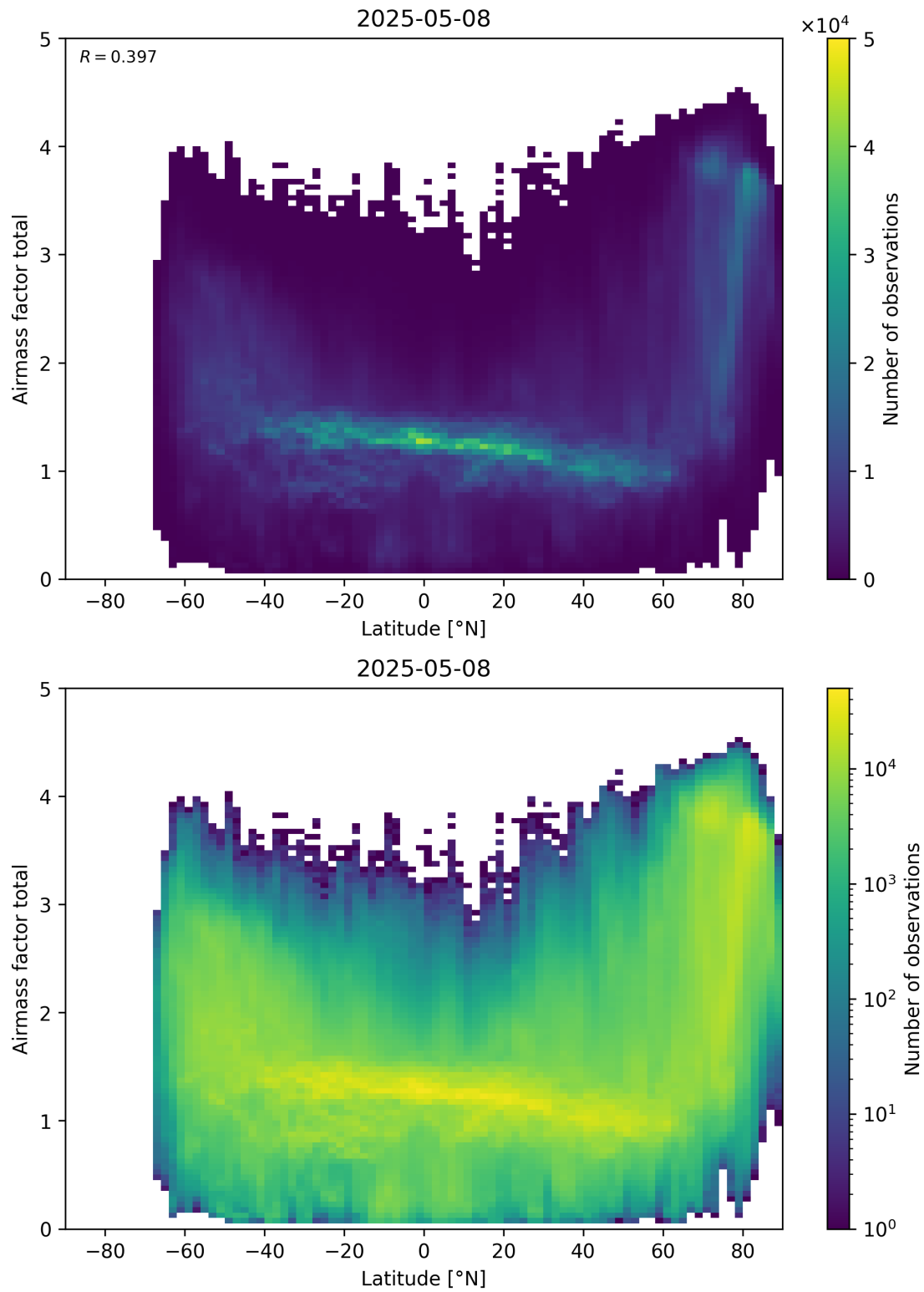
Figure 161: Scatter density plot of “Latitude” against “Airmass factor total” for 2025-05-07 to 2025-05-09.
