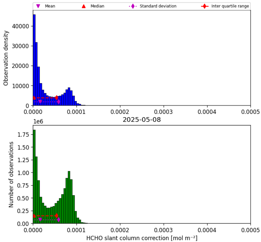
Figure 47: Histogram of “HCHO slant column correction” for 2025-05-07 to 2025-05-09
