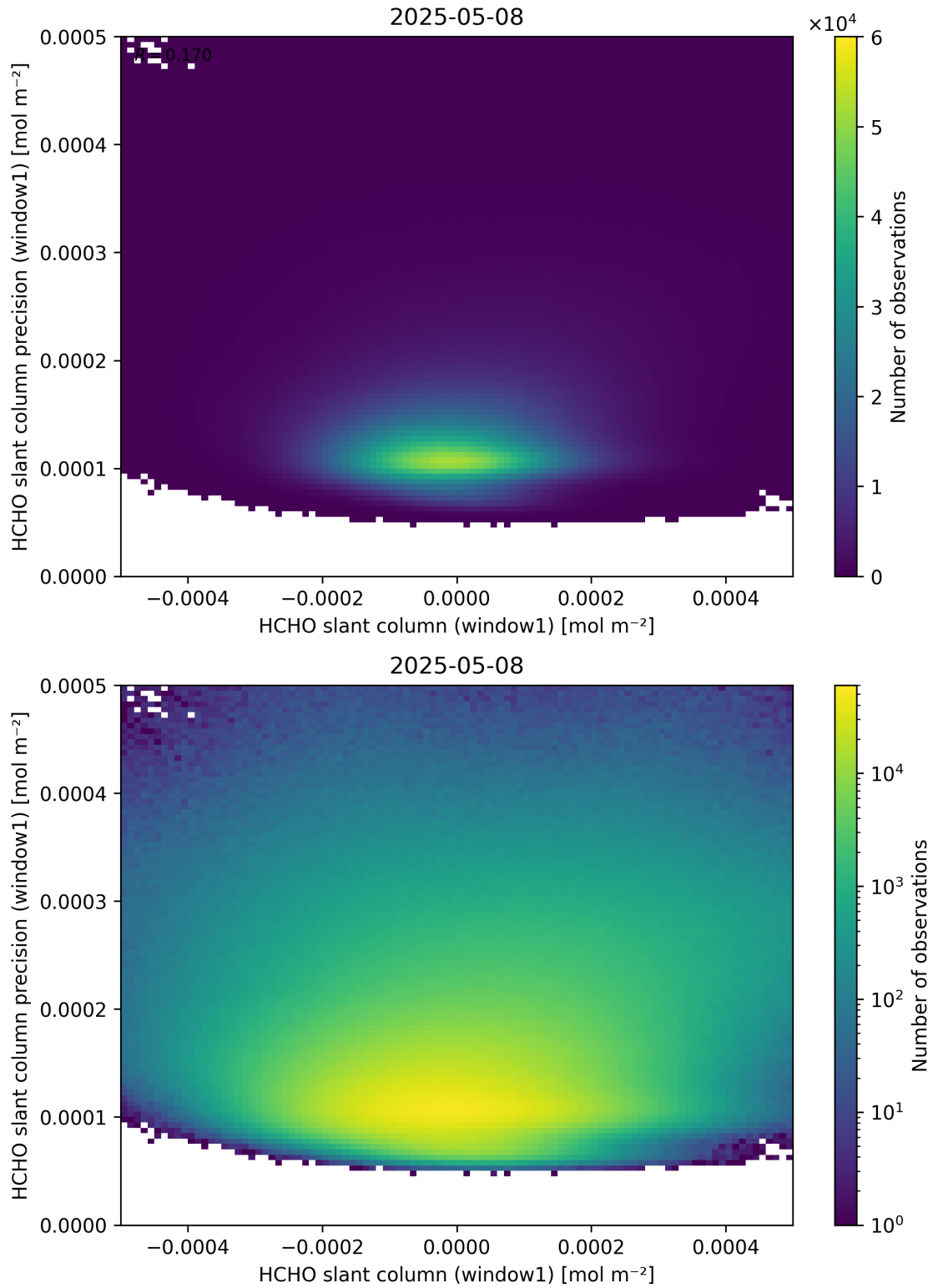
Figure 84: Scatter density plot of “HCHO slant column (window1)” against “HCHO slant column precision (window1)” for 2025-05-07 to 2025-05-09.
