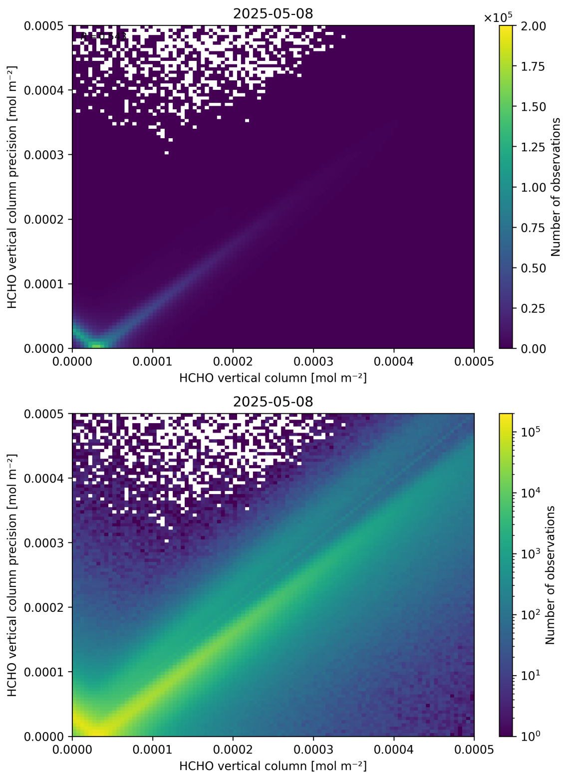
Figure 134: Scatter density plot of “HCHO vertical column” against “HCHO vertical column precision” for 2025-05-07 to 2025-05-09.
