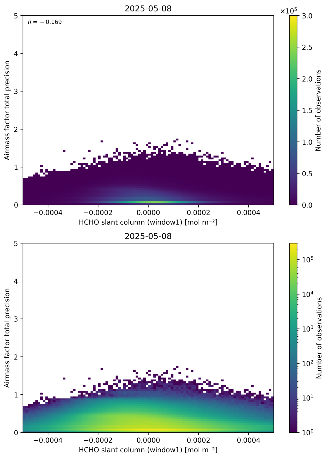
Figure 86: Scatter density plot of “HCHO slant column (window1)” against “Airmass factor total precision” for 2025-05-07 to 2025-05-09.
