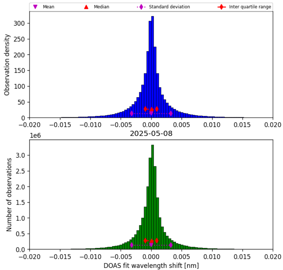
Figure 44: Histogram of “DOAS fit wavelength shift” for 2025-05-07 to 2025-05-09
