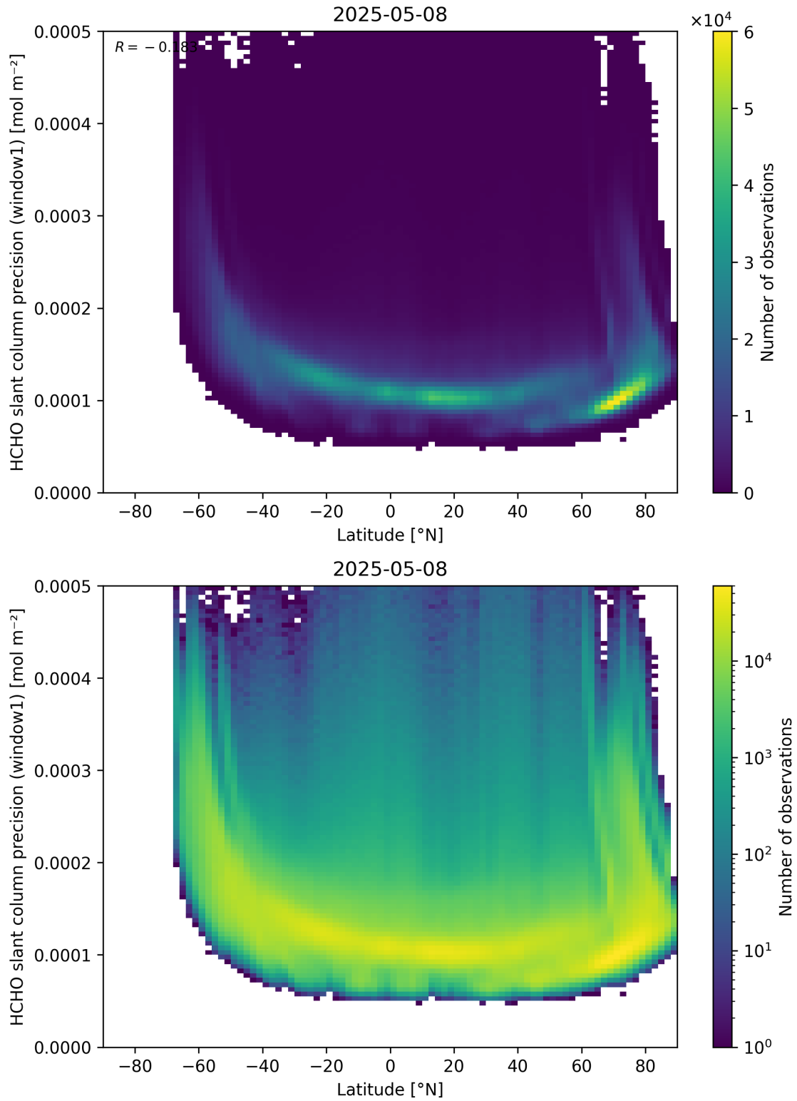
Figure 160: Scatter density plot of “Latitude” against “HCHO slant column precision (window1)” for 2025-05-07 to 2025-05-09.
