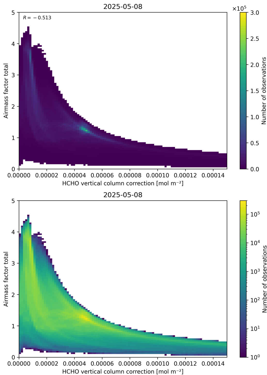
Figure 120: Scatter density plot of “HCHO vertical column correction” against “Airmass factor total” for 2025-05-07 to 2025-05-09.
