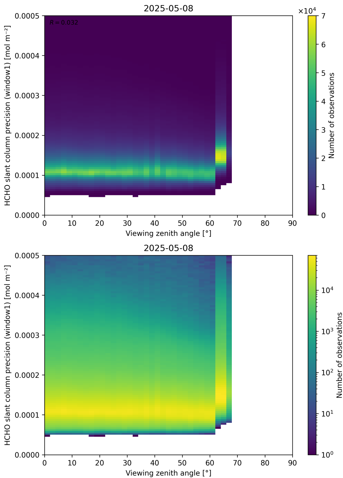
Figure 189: Scatter density plot of “Viewing zenith angle” against “HCHO slant column precision (window1)” for 2025-05-07 to 2025-05-09.
