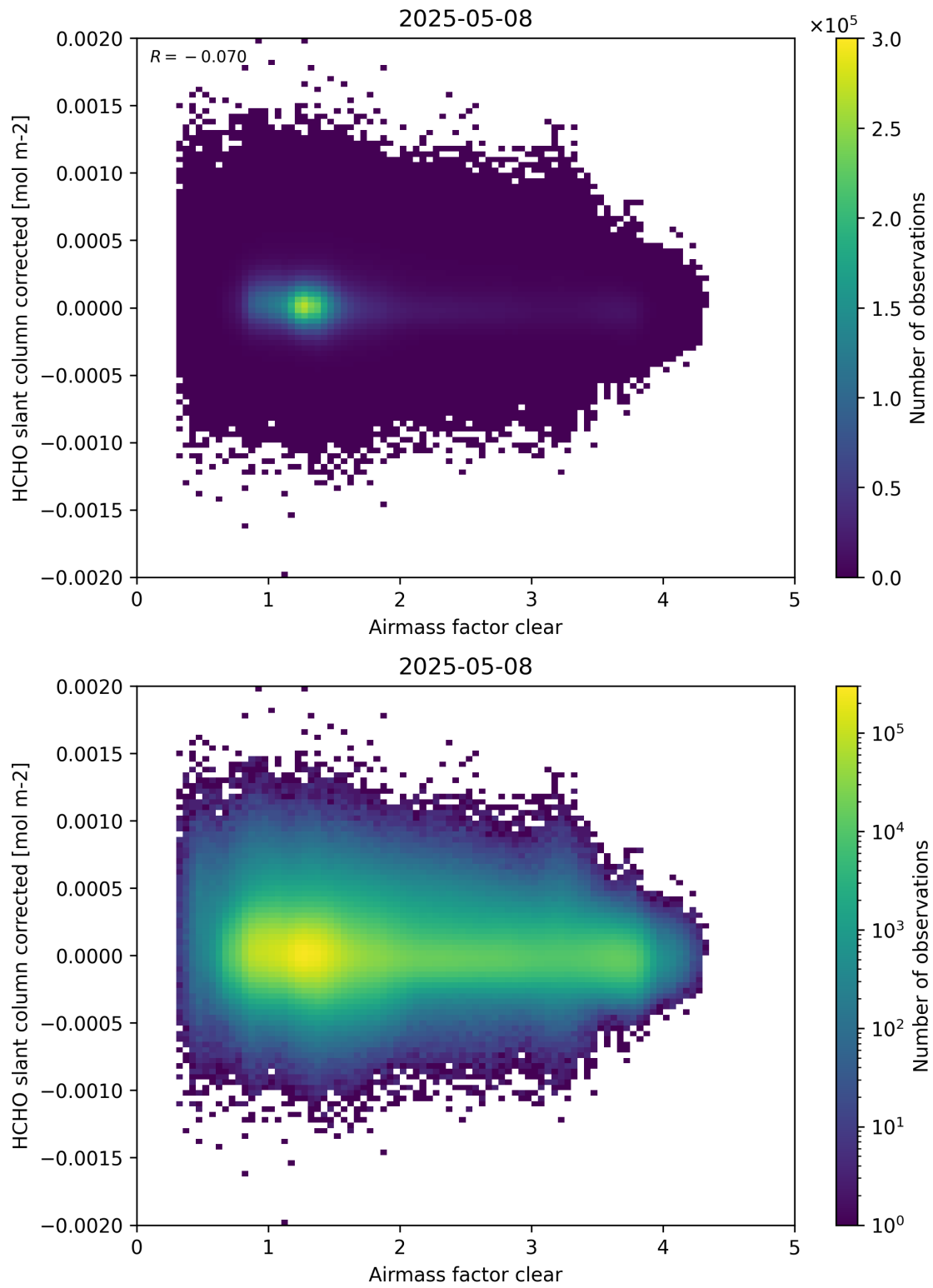
Figure 74: Scatter density plot of “Airmass factor clear” against “HCHO slant column corrected” for 2025-05-07 to 2025-05-09.
