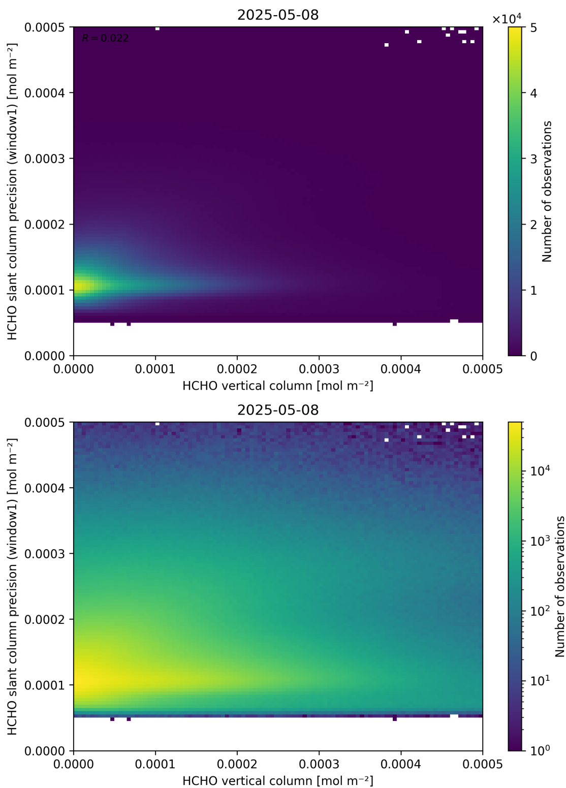
Figure 130: Scatter density plot of “HCHO vertical column” against “HCHO slant column precision (window1)” for 2025-05-07 to 2025-05-09.
