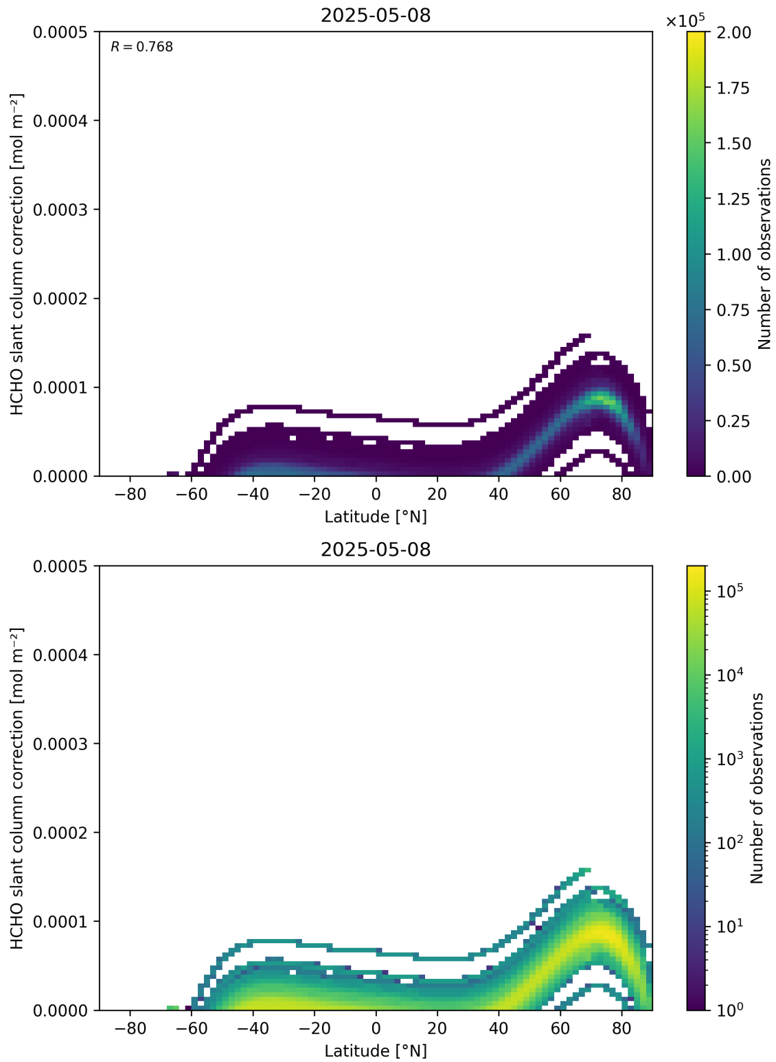
Figure 158: Scatter density plot of “Latitude” against “HCHO slant column correction” for 2025-05-07 to 2025-05-09.
