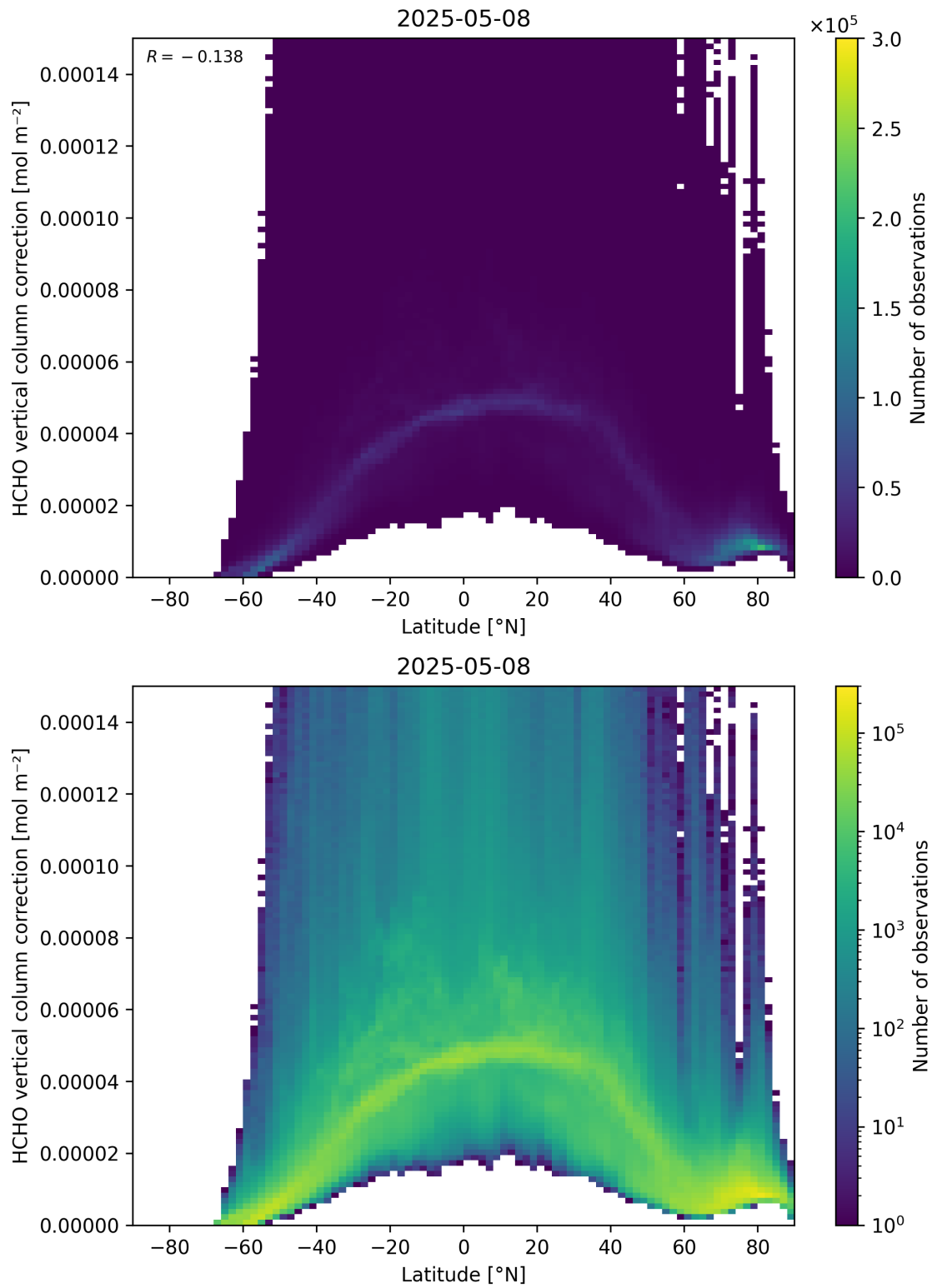
Figure 164: Scatter density plot of “Latitude” against “HCHO vertical column correction” for 2025-05-07 to 2025-05-09.
