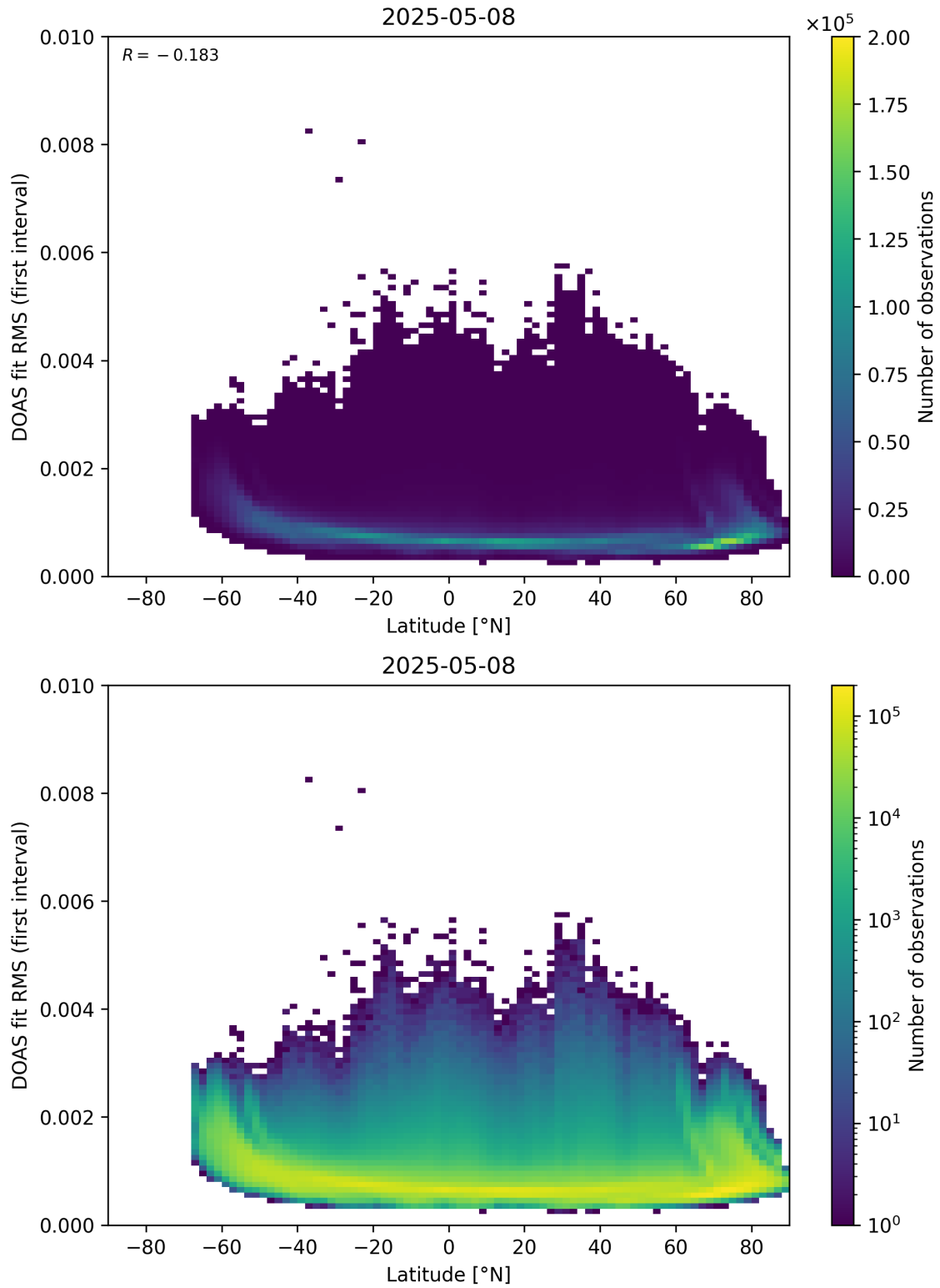
Figure 153: Scatter density plot of “Latitude” against “DOAS fit RMS (first interval)” for 2025-05-07 to 2025-05-09.
