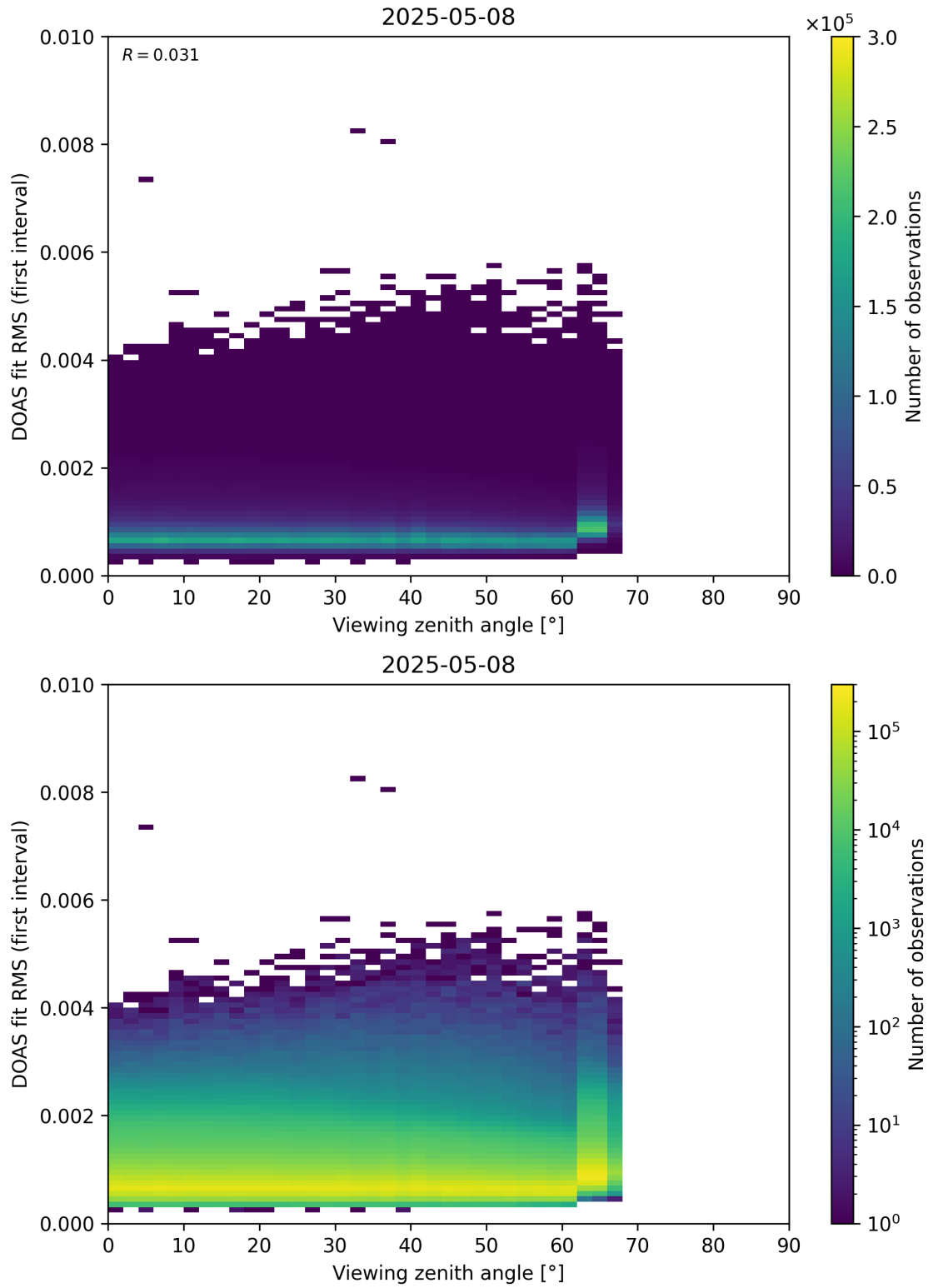
Figure 182: Scatter density plot of “Viewing zenith angle” against “DOAS fit RMS (first interval)” for 2025-05-07 to 2025-05-09.
