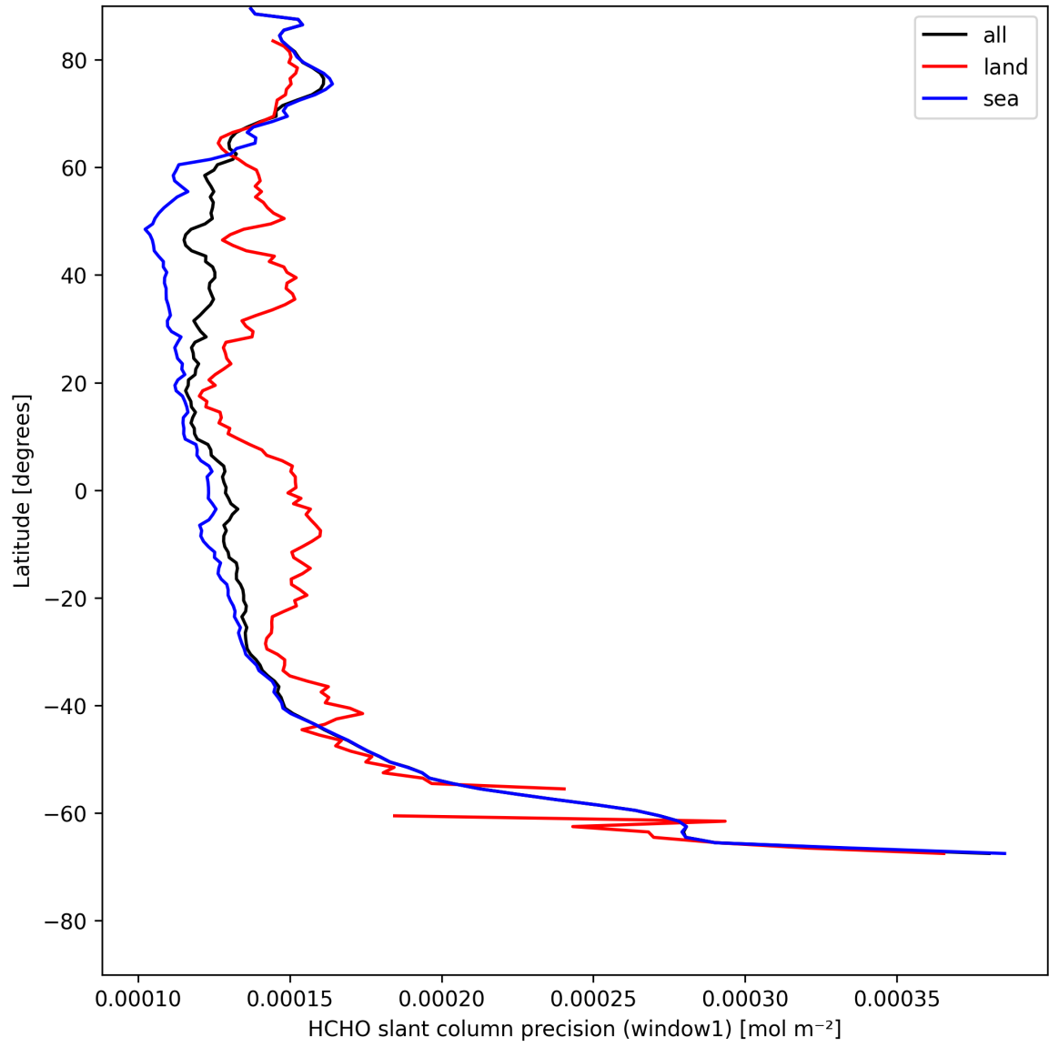
Figure 25: Zonal average of “HCHO slant column precision (window1)” for 2025-05-07 to 2025-05-09.
