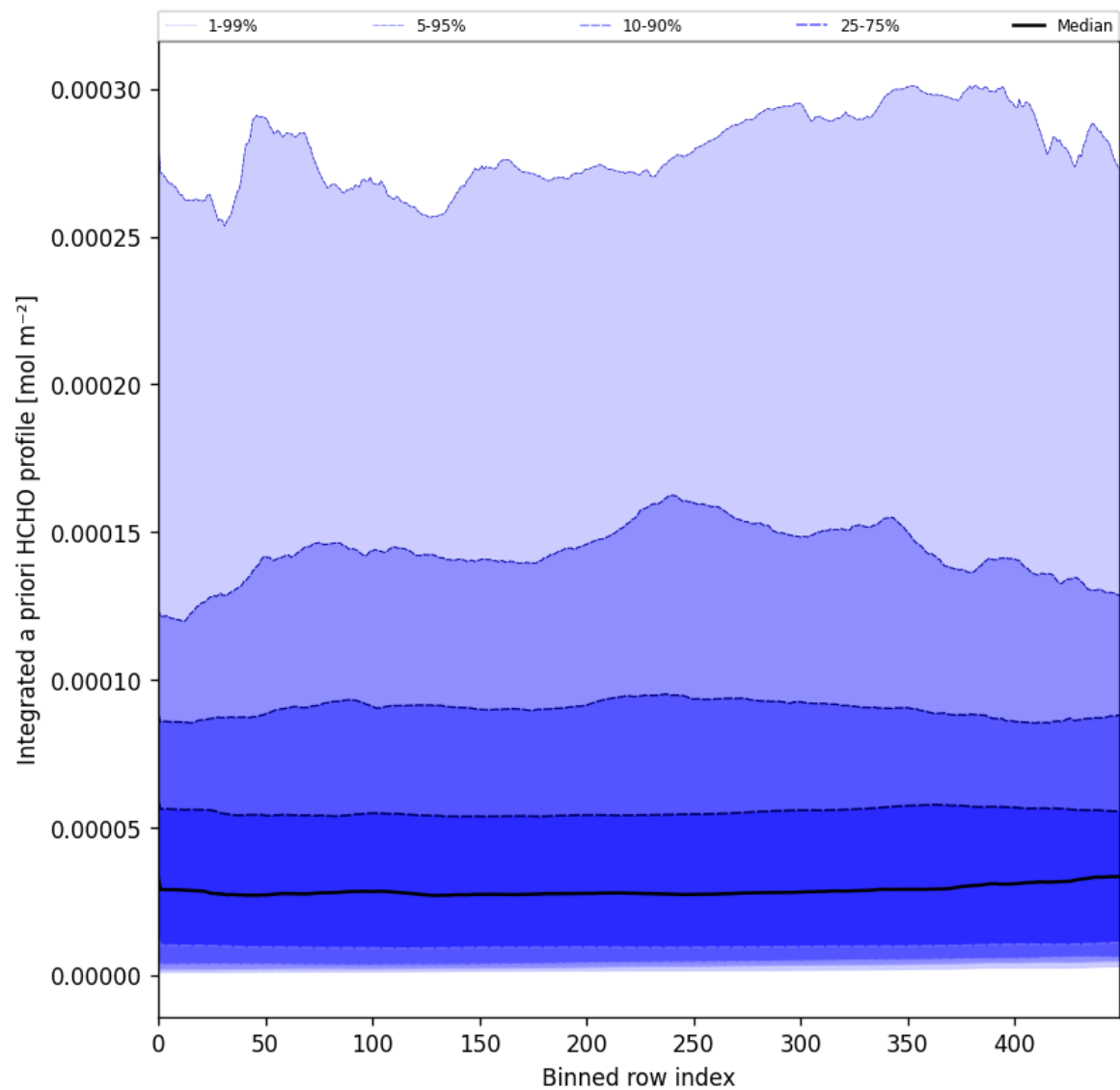
Figure 57: Along track statistics of "Integrated a priori HCHO profile" for 2025-05-07 to 2025-05-09
