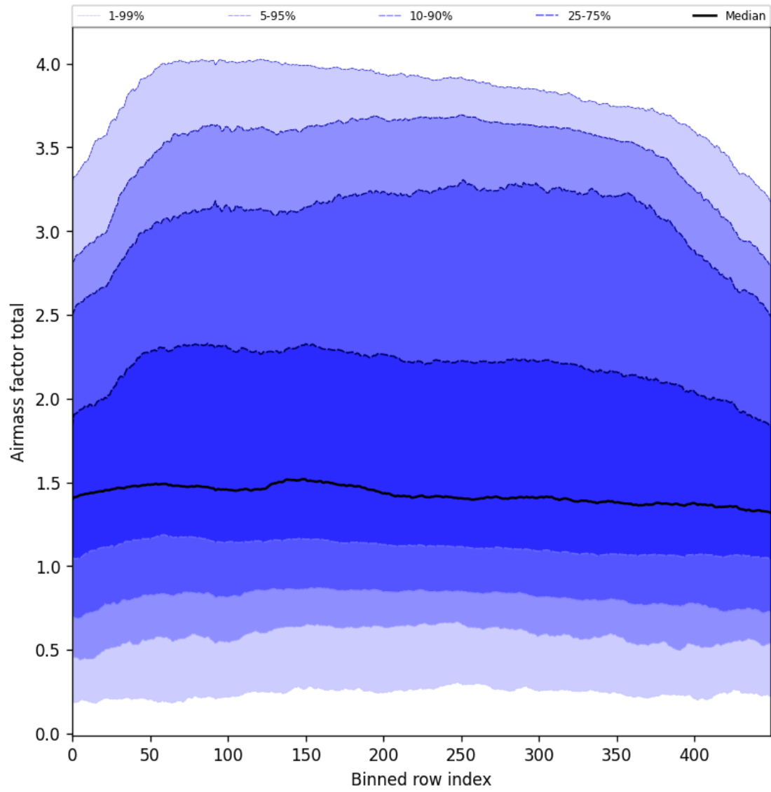
Figure 54: Along track statistics of “Airmass factor total” for 2025-05-07 to 2025-05-09
