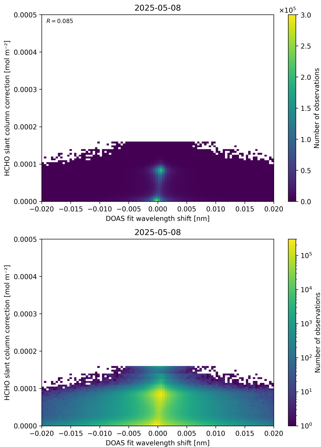
Figure 67: Scatter density plot of “DOAS fit wavelength shift” against “HCHO slant column correction” for 2025-05-07 to 2025-05-09.
