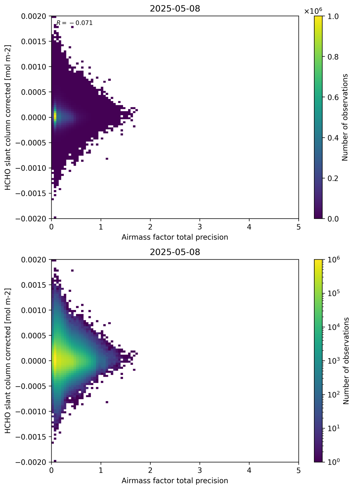
Figure 109: Scatter density plot of “Airmass factor total precision” against “HCHO slant column corrected” for 2025-05-07 to 2025-05-09.
