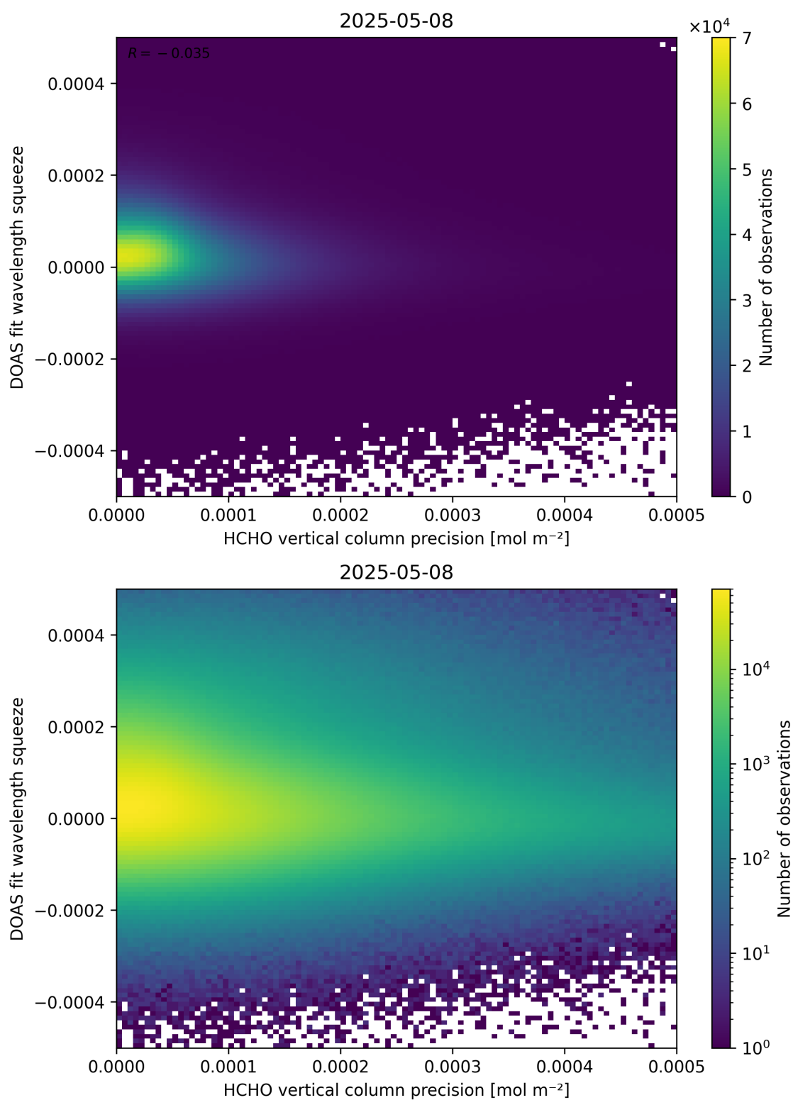
Figure 138: Scatter density plot of “HCHO vertical column precision” against “DOAS fit wavelength squeeze” for 2025-05-07 to 2025-05-09.
