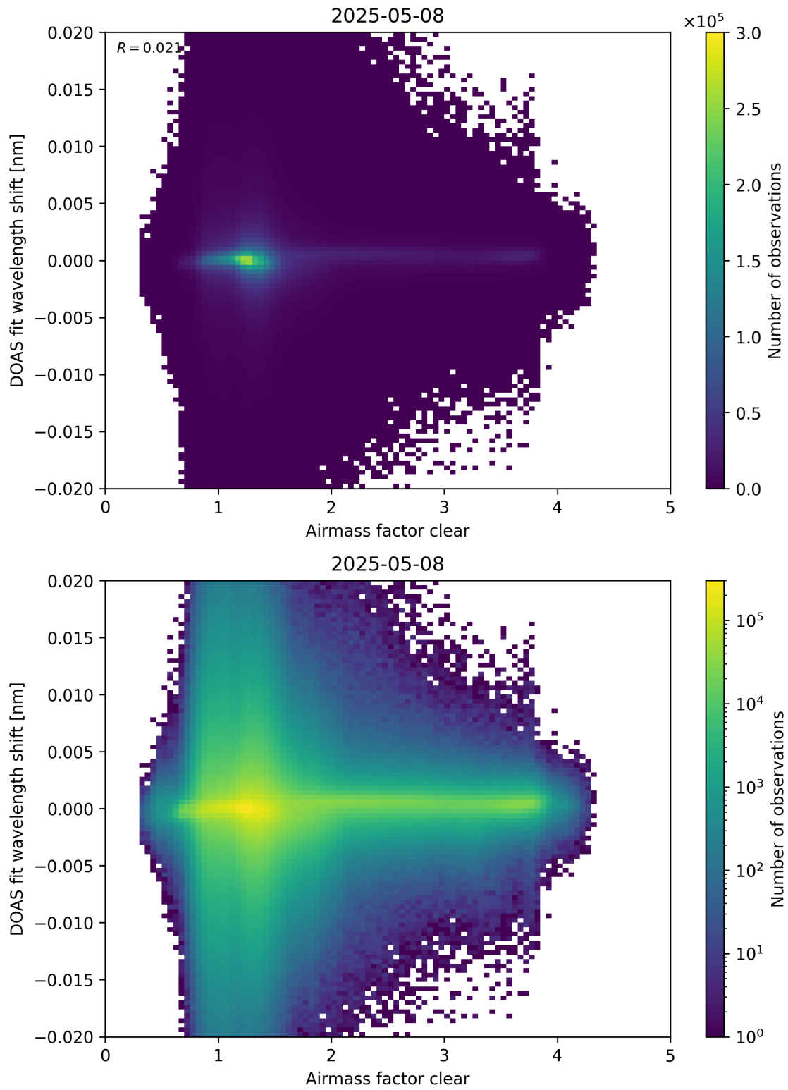
Figure 72: Scatter density plot of “Airmass factor clear” against “DOAS fit wavelength shift” for 2025-05-07 to 2025-05-09.
