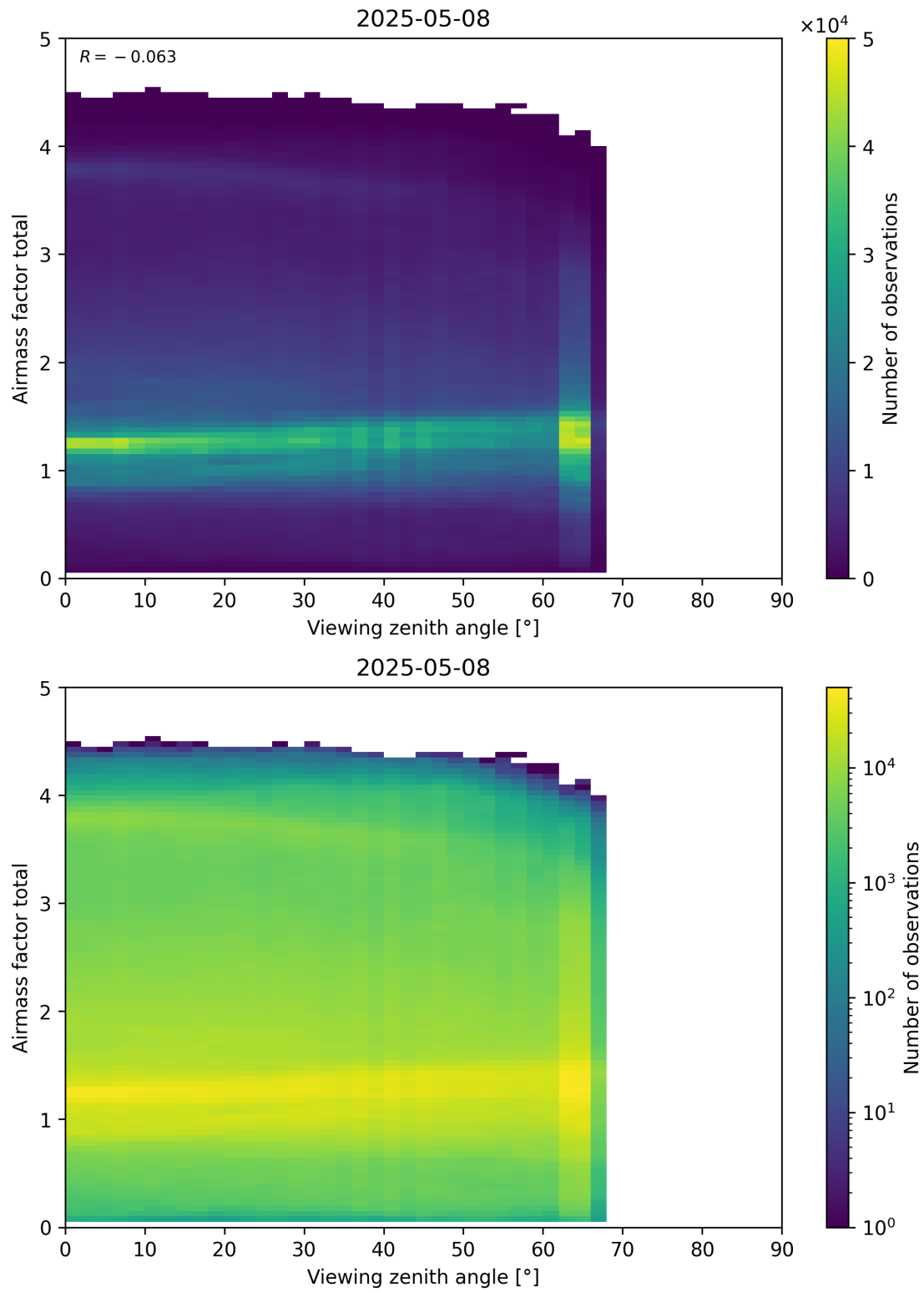
Figure 190: Scatter density plot of “Viewing zenith angle” against “Airmass factor total” for 2025-05-07 to 2025-05-09.
