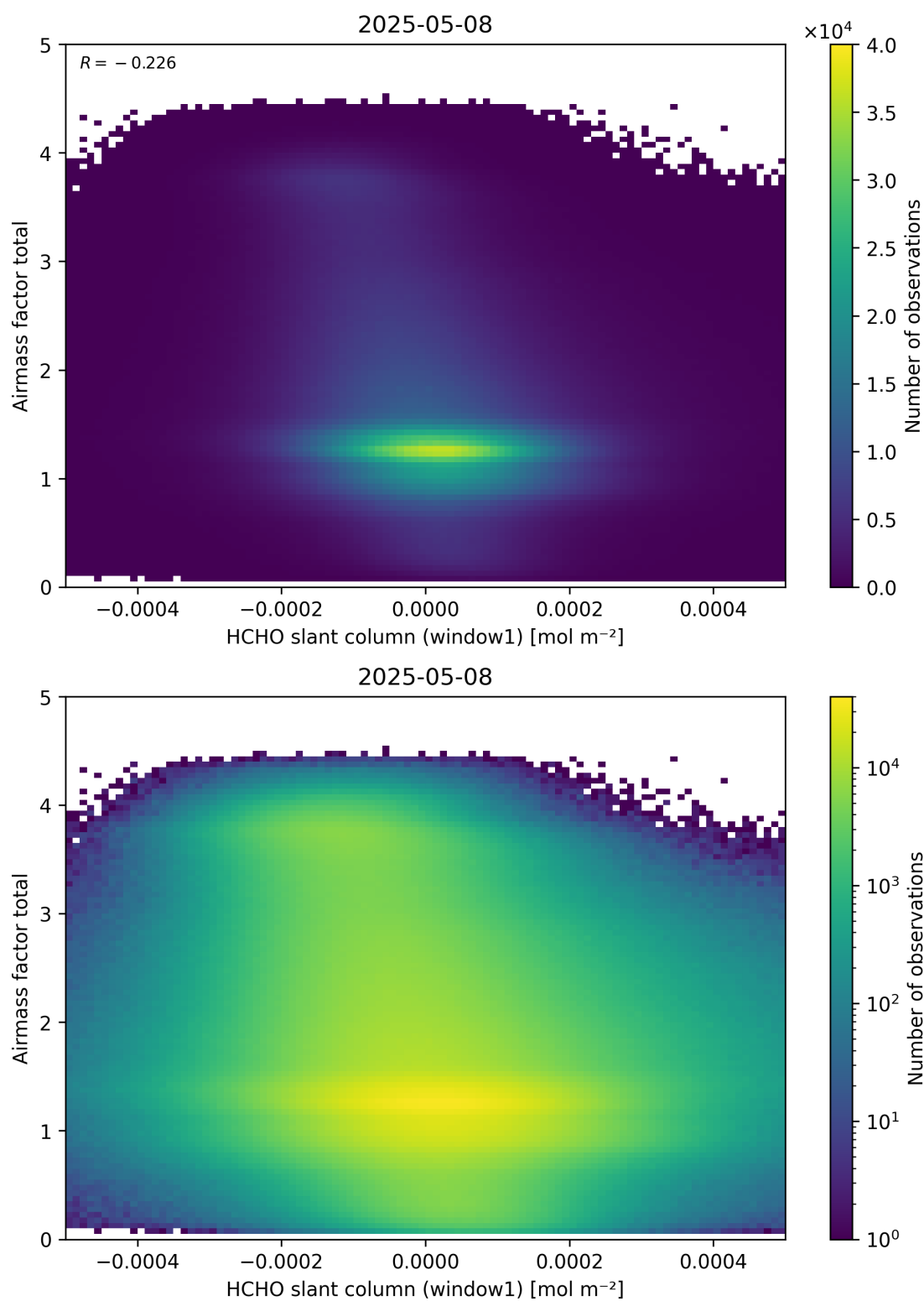
Figure 85: Scatter density plot of “HCHO slant column (window1)” against “Airmass factor total” for 2025-05-07 to 2025-05-09.
