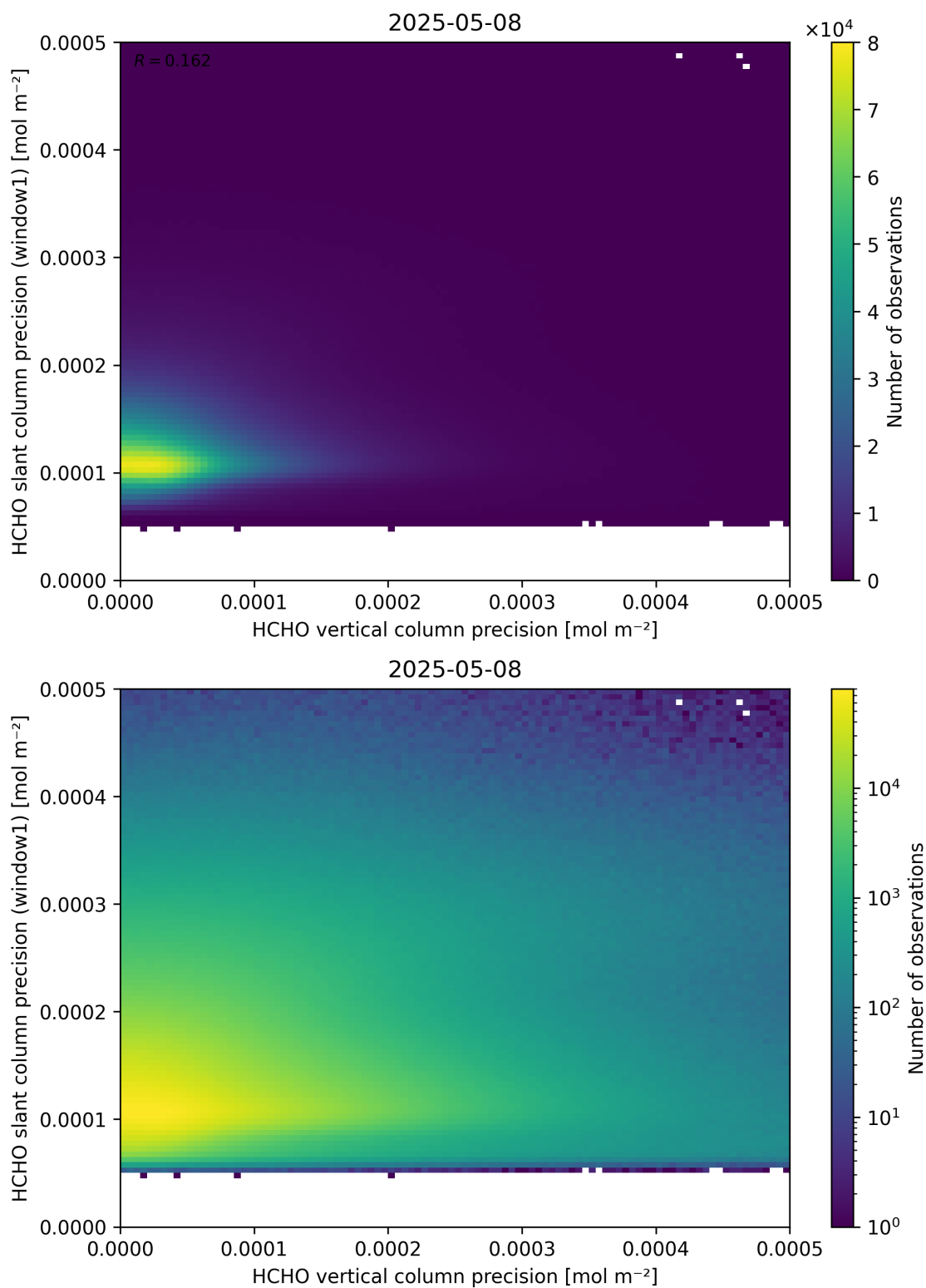
Figure 143: Scatter density plot of “HCHO vertical column precision” against “HCHO slant column precision (window1)” for 2025-05-07 to 2025-05-09.
