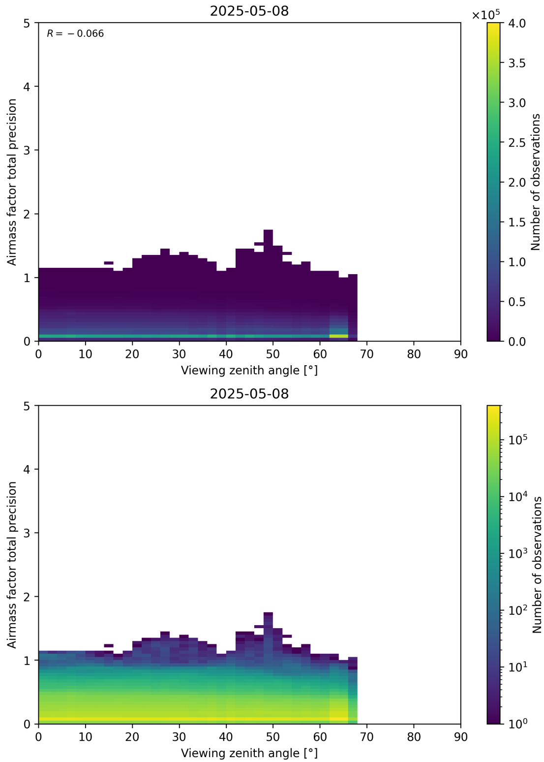
Figure 191: Scatter density plot of “Viewing zenith angle” against “Airmass factor total precision” for 2025-05-07 to 2025-05-09.
