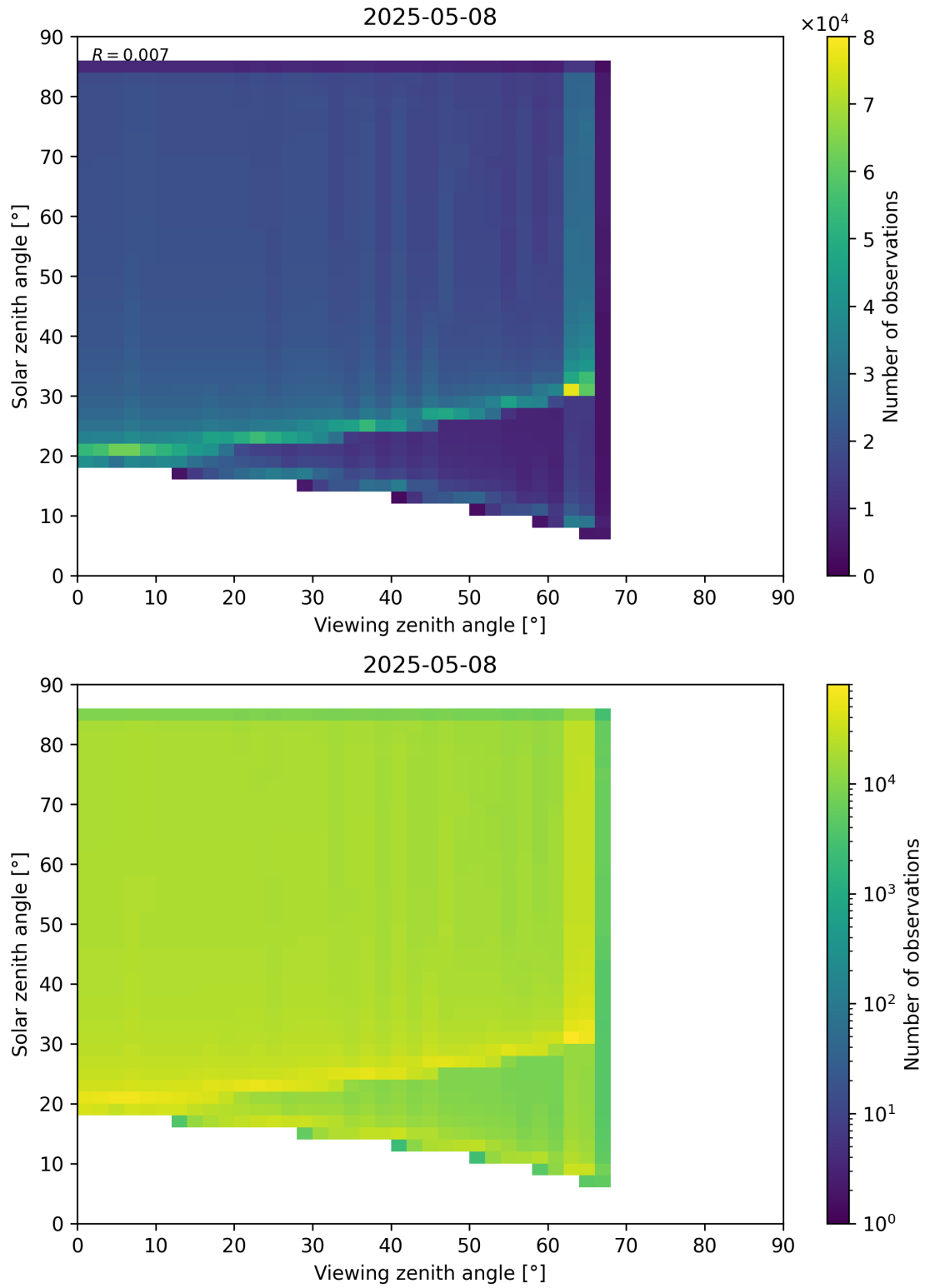
Figure 197: Scatter density plot of “Viewing zenith angle” against “Solar zenith angle” for 2025-05-07 to 2025-05-09.
