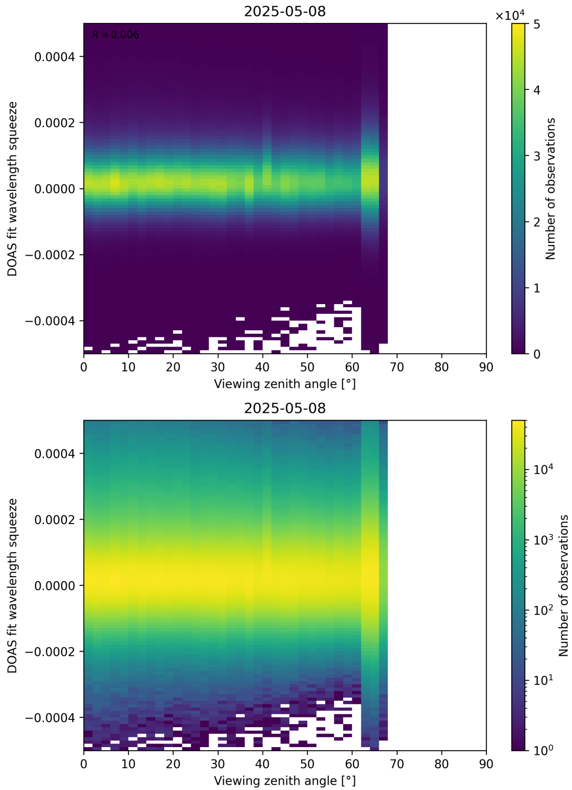
Figure 184: Scatter density plot of “Viewing zenith angle” against “DOAS fit wavelength squeeze” for 2025-05-07 to 2025-05-09.
