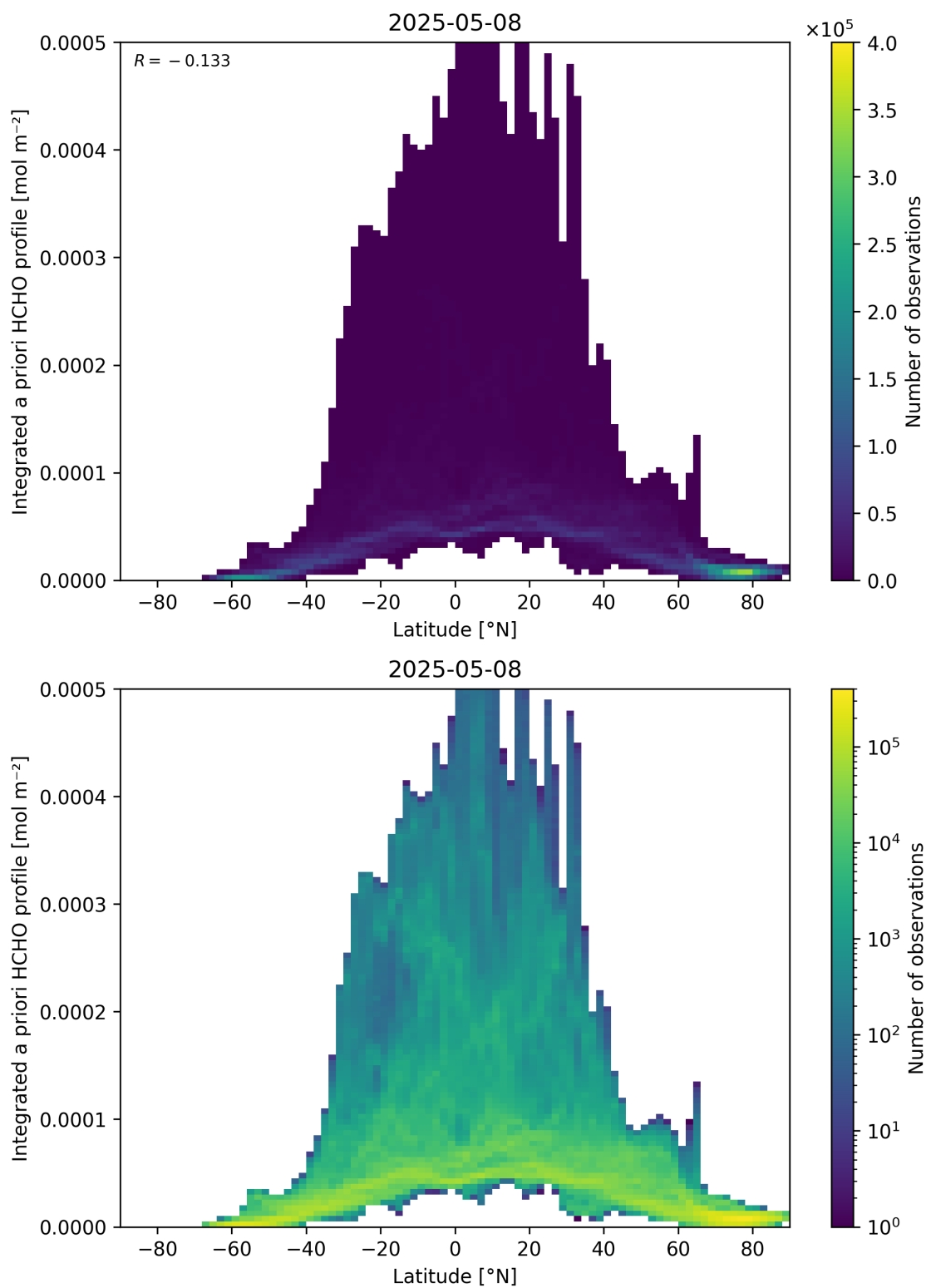
Figure 166: Scatter density plot of “Latitude” against “Integrated a priori HCHO profile” for 2025-05-07 to 2025-05-09.
