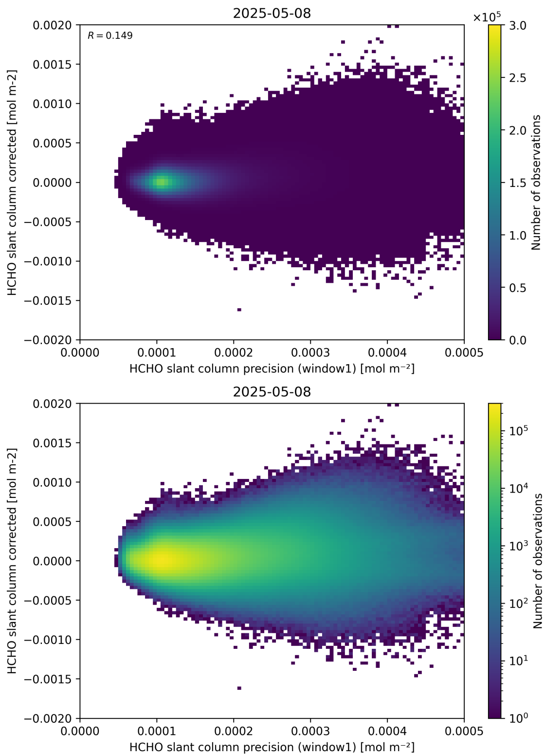
Figure 92: Scatter density plot of “HCHO slant column precision (window1)” against “HCHO slant column corrected” for 2025-05-07 to 2025-05-09.
