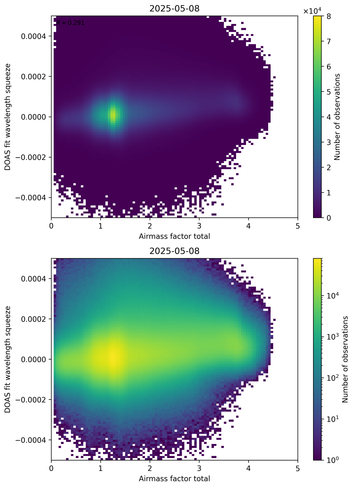
Figure 99: Scatter density plot of “Airmass factor total” against “DOAS fit wavelength squeeze” for 2025-05-07 to 2025-05-09.
