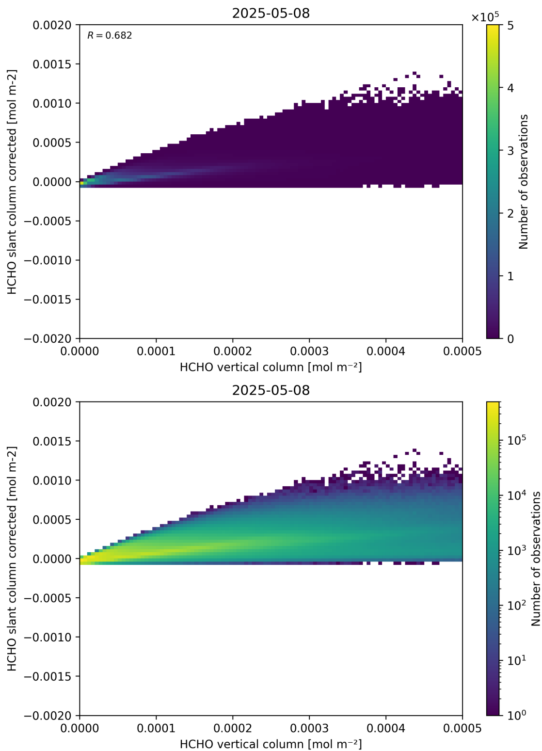
Figure 127: Scatter density plot of “HCHO vertical column” against “HCHO slant column corrected” for 2025-05-07 to 2025-05-09.
