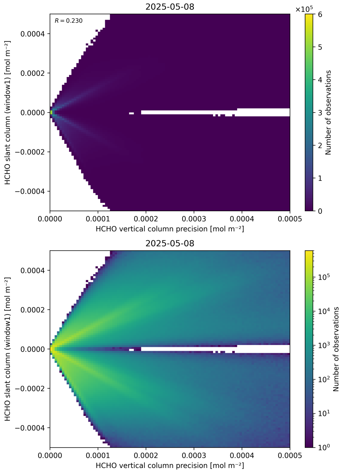
Figure 142: Scatter density plot of “HCHO vertical column precision” against “HCHO slant column (window1)” for 2025-05-07 to 2025-05-09.
