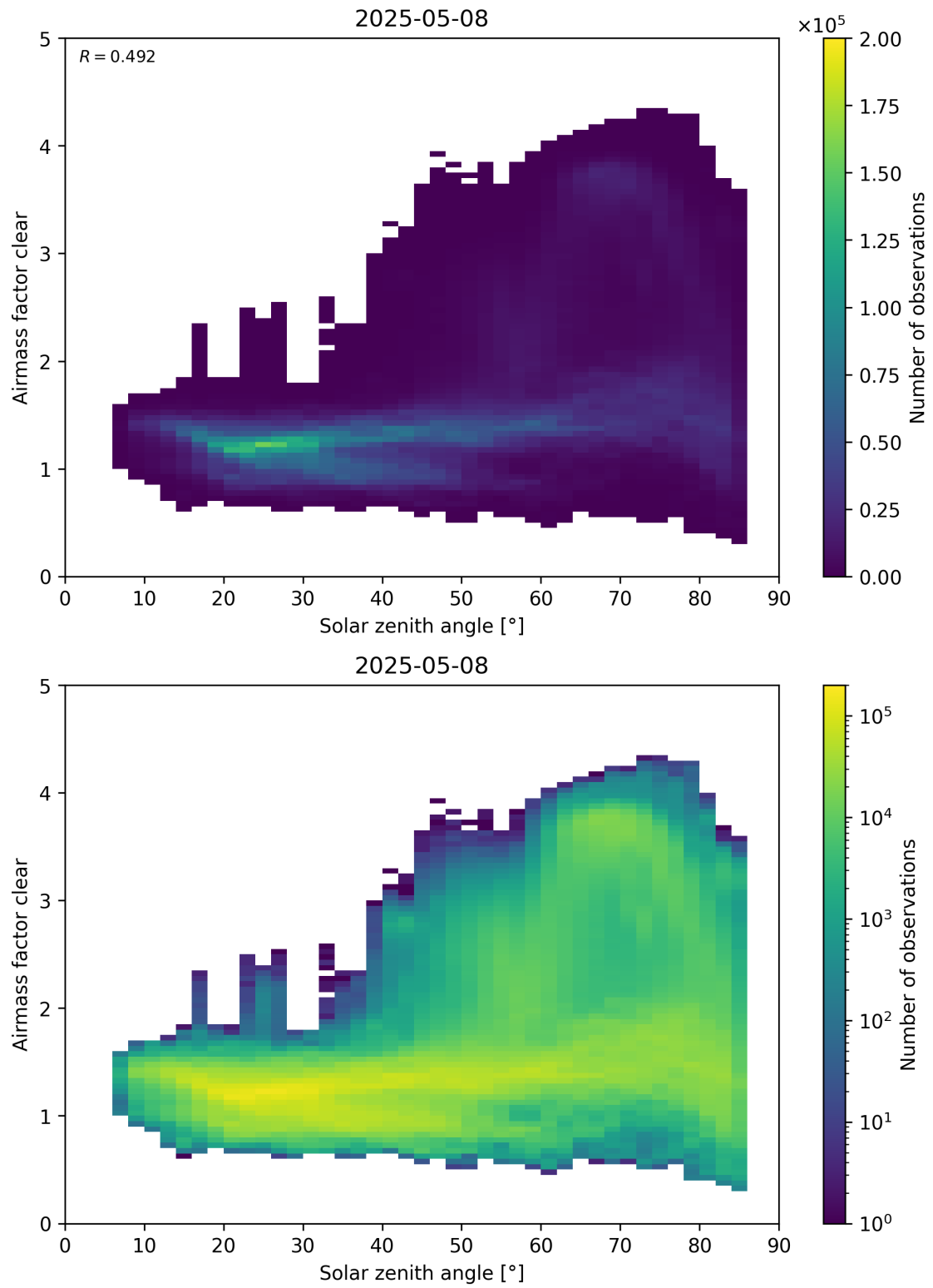
Figure 170: Scatter density plot of “Solar zenith angle” against “Airmass factor clear” for 2025-05-07 to 2025-05-09.
