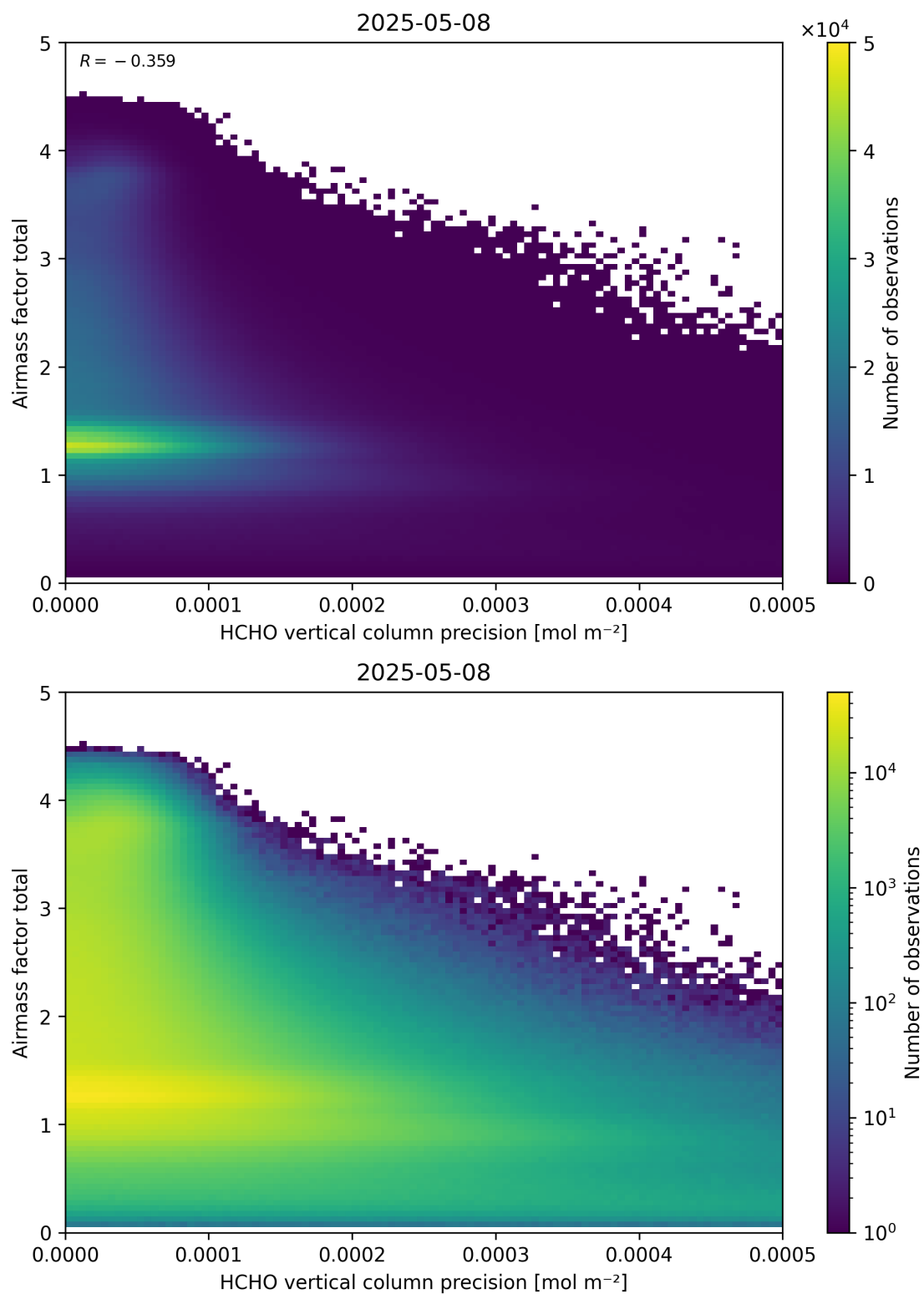
Figure 144: Scatter density plot of “HCHO vertical column precision” against “Airmass factor total” for 2025-05-07 to 2025-05-09.
