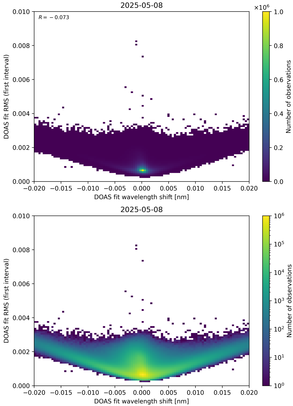
Figure 64: Scatter density plot of “DOAS fit wavelength shift” against “DOAS fit RMS (first interval)” for 2025-05-07 to 2025-05-09.
