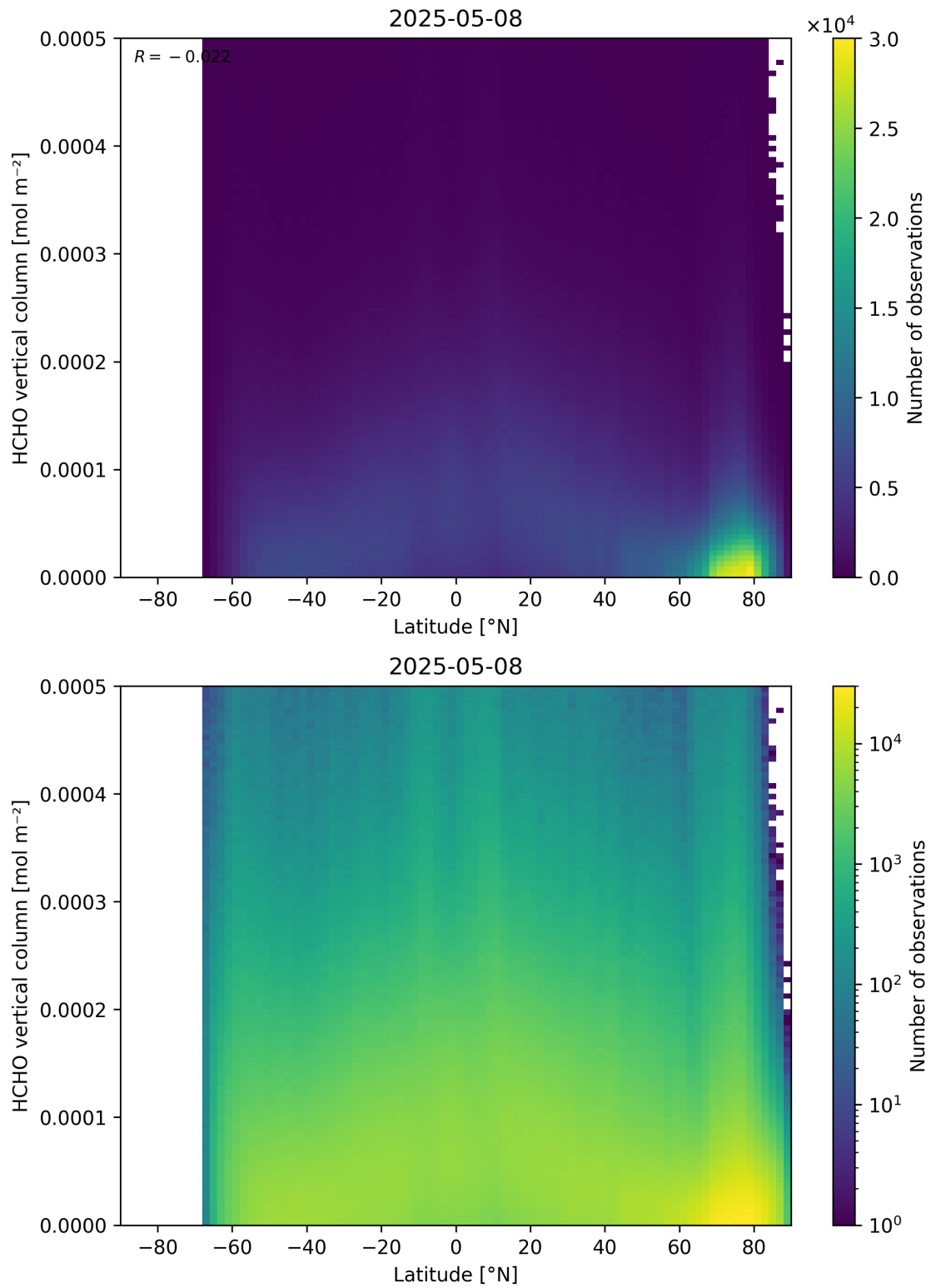
Figure 163: Scatter density plot of “Latitude” against “HCHO vertical column” for 2025-05-07 to 2025-05-09.
