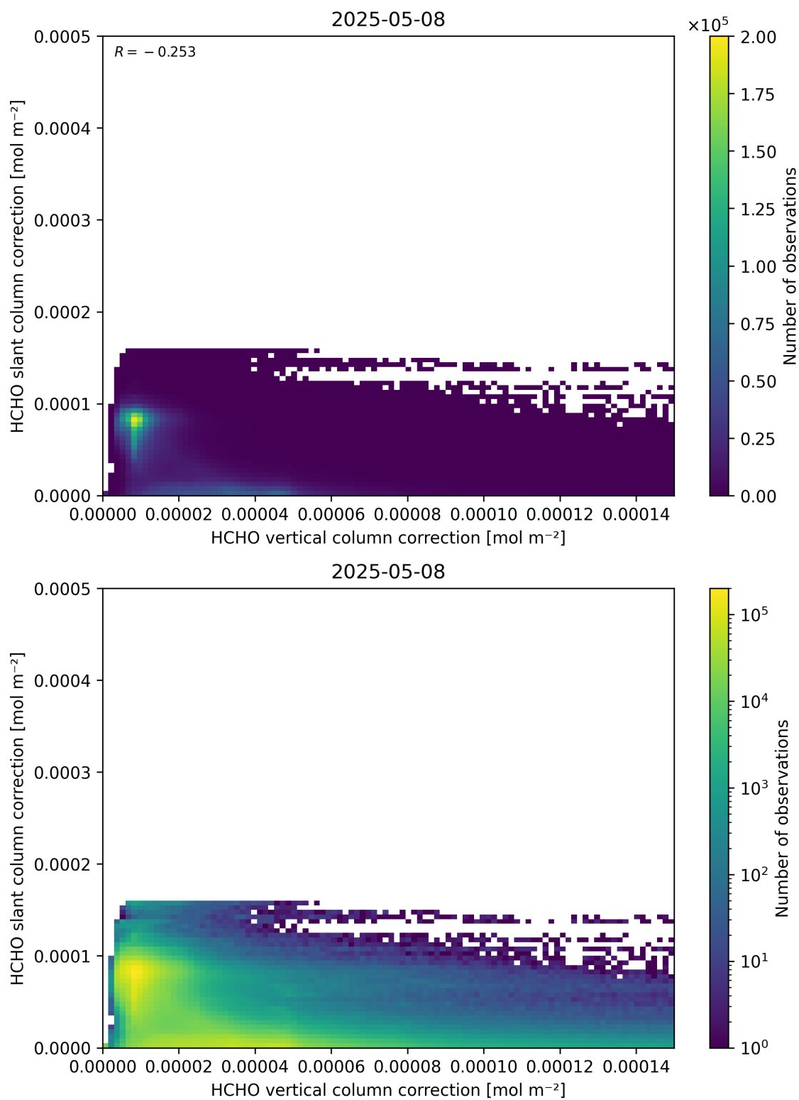
Figure 117: Scatter density plot of “HCHO vertical column correction” against “HCHO slant column correction” for 2025-05-07 to 2025-05-09.
