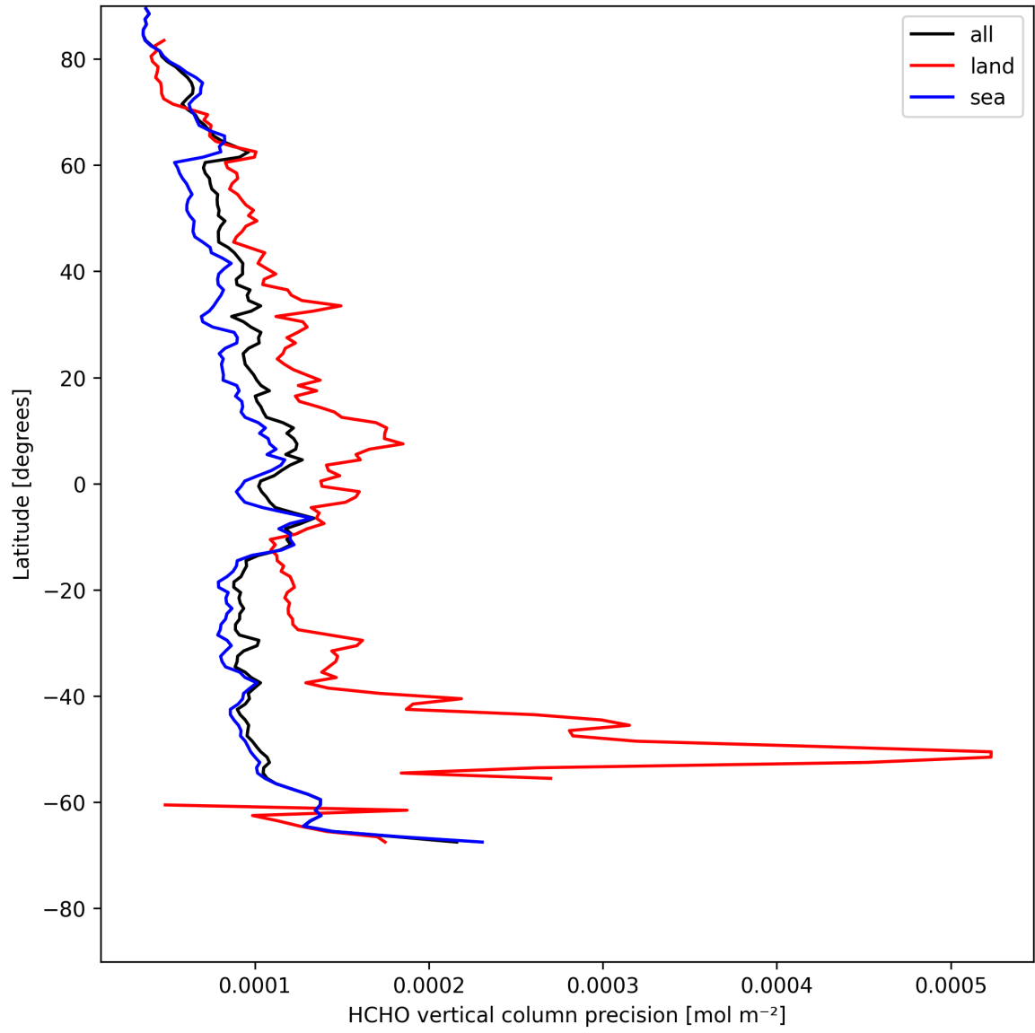
Figure 22: Zonal average of “HCHO vertical column precision” for 2025-05-07 to 2025-05-09.
