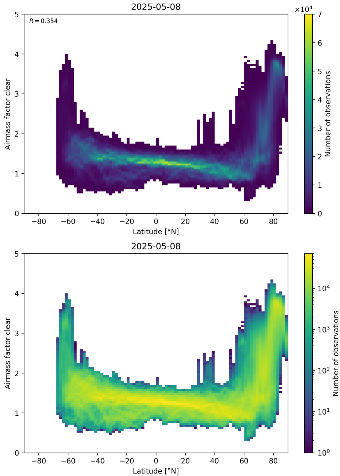
Figure 156: Scatter density plot of “Latitude” against “Airmass factor clear” for 2025-05-07 to 2025-05-09.
