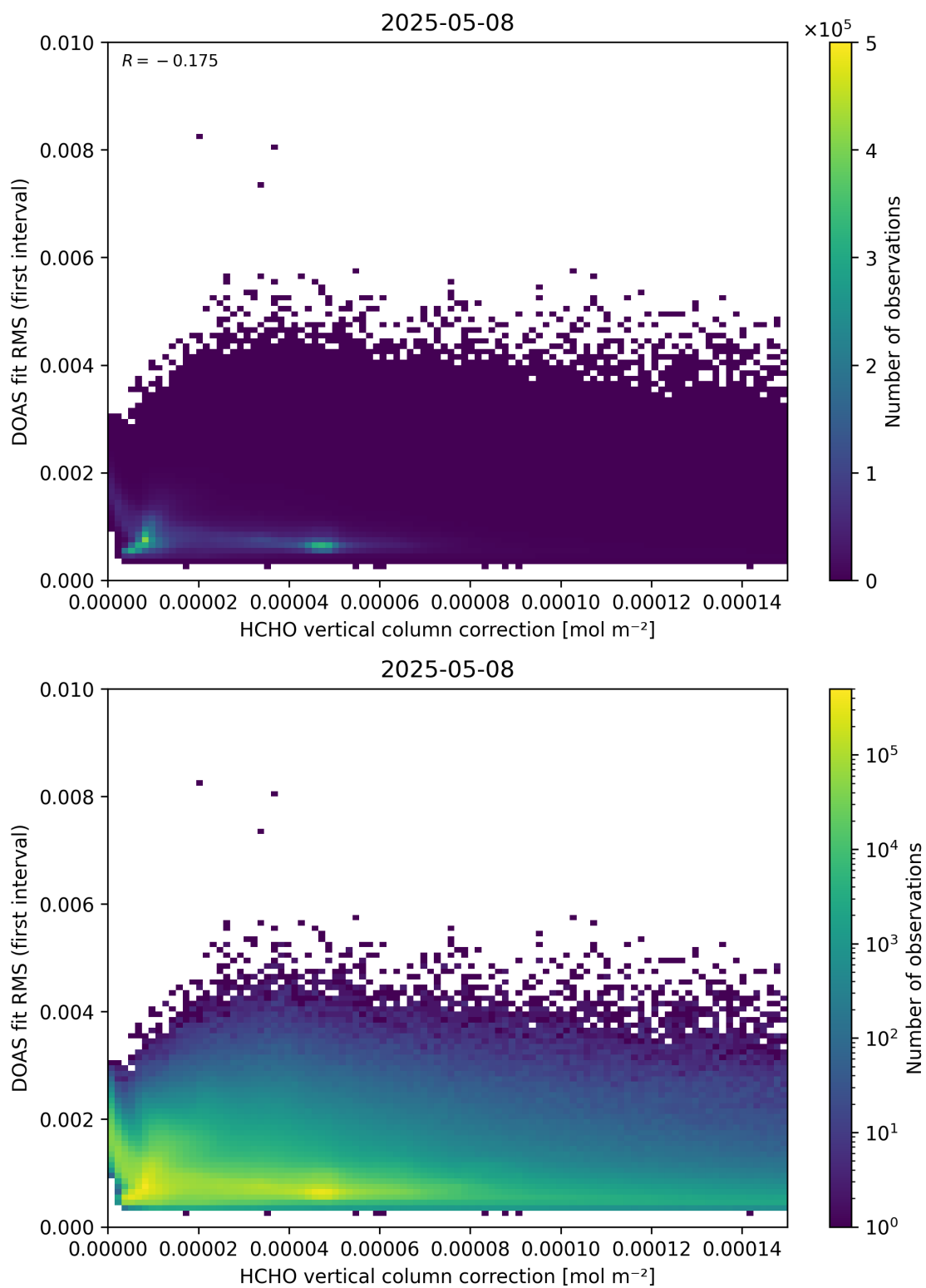
Figure 112: Scatter density plot of “HCHO vertical column correction” against “DOAS fit RMS (first interval)” for 2025-05-07 to 2025-05-09.
