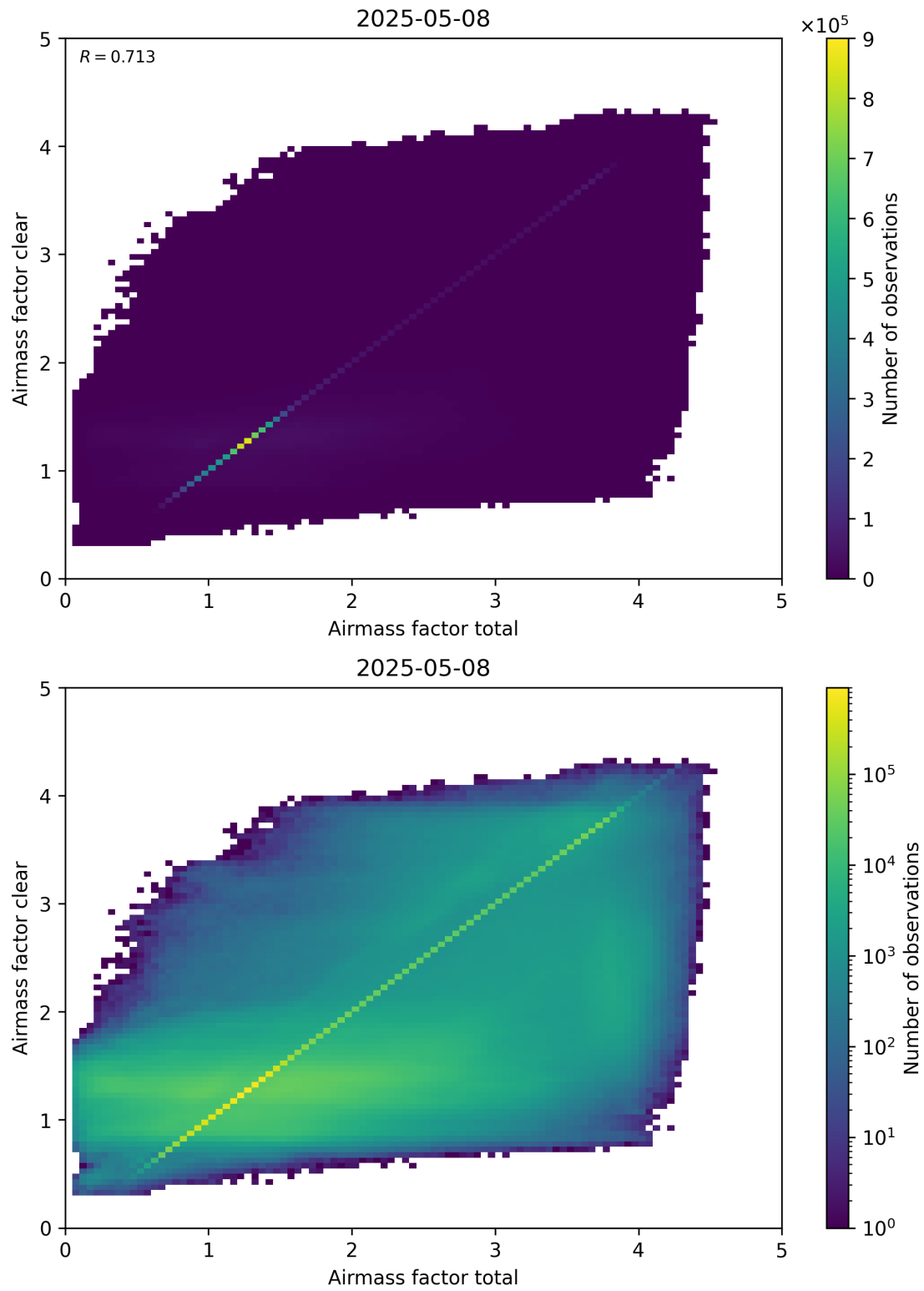
Figure 100: Scatter density plot of “Airmass factor total” against “Airmass factor clear” for 2025-05-07 to 2025-05-09.
