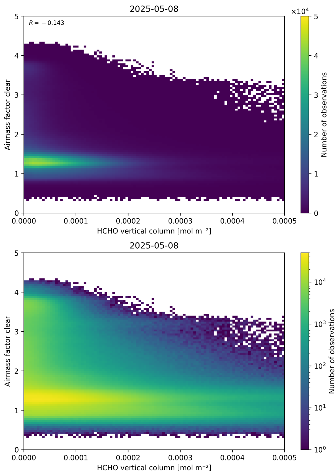
Figure 126: Scatter density plot of “HCHO vertical column” against “Airmass factor clear” for 2025-05-07 to 2025-05-09.
