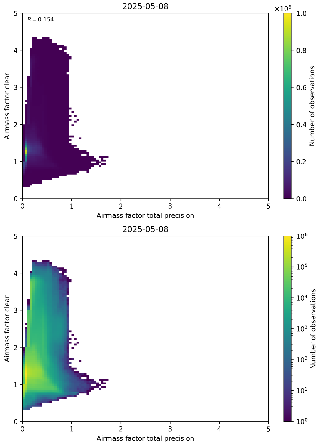
Figure 108: Scatter density plot of “Airmass factor total precision” against “Airmass factor clear” for 2025-05-07 to 2025-05-09.
