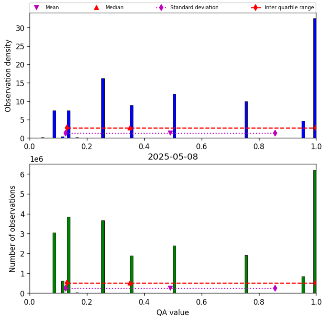
Figure 34: Histogram of “QA value” for 2025-05-07 to 2025-05-09
