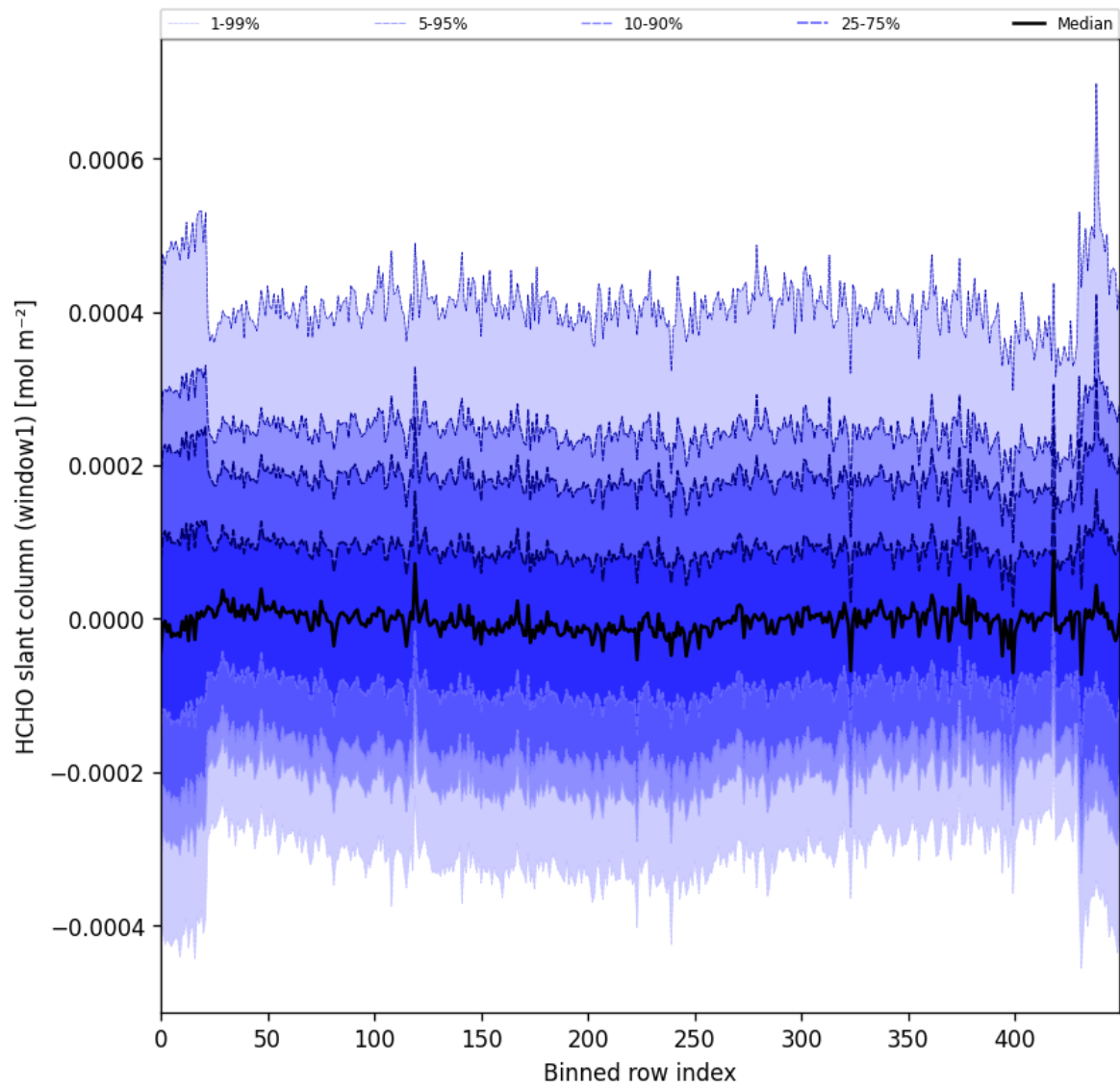
Figure 52: Along track statistics of “HCHO slant column (window1)” for 2025-05-07 to 2025-05-09
