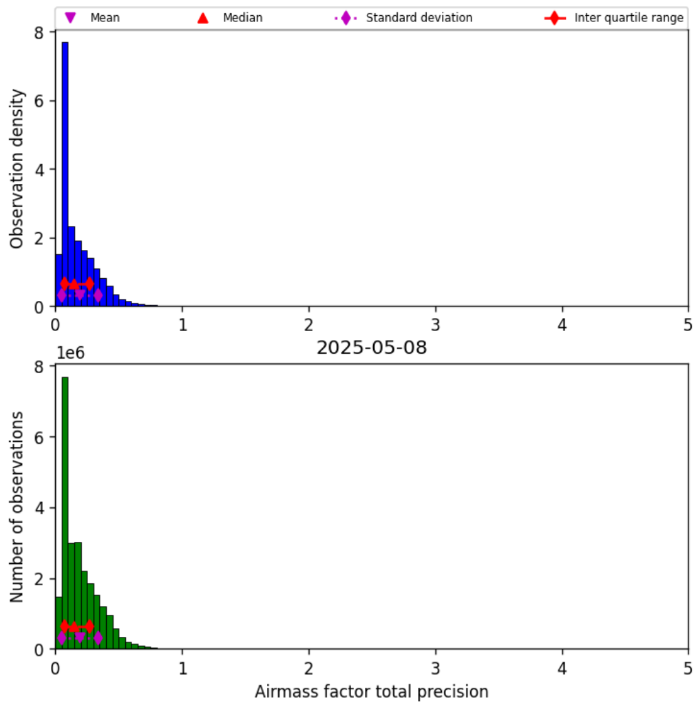
Figure 41: Histogram of “Airmass factor total precision” for 2025-05-07 to 2025-05-09
