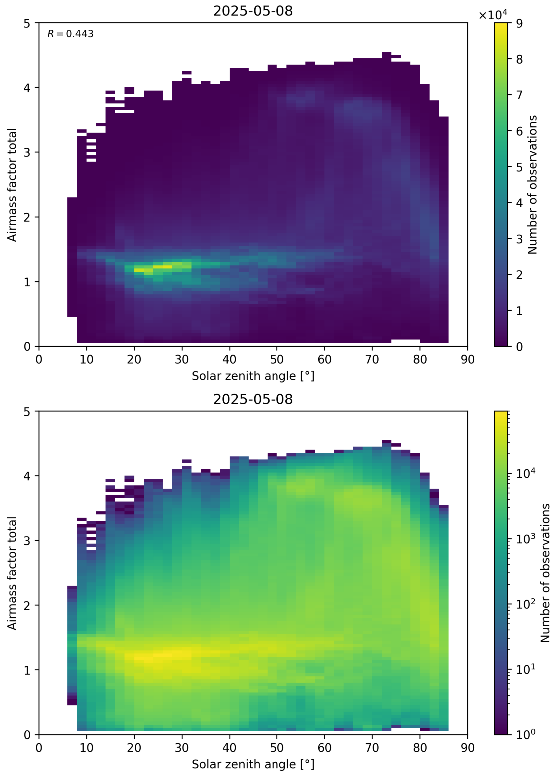
Figure 175: Scatter density plot of “Solar zenith angle” against “Airmass factor total” for 2025-05-07 to 2025-05-09.
