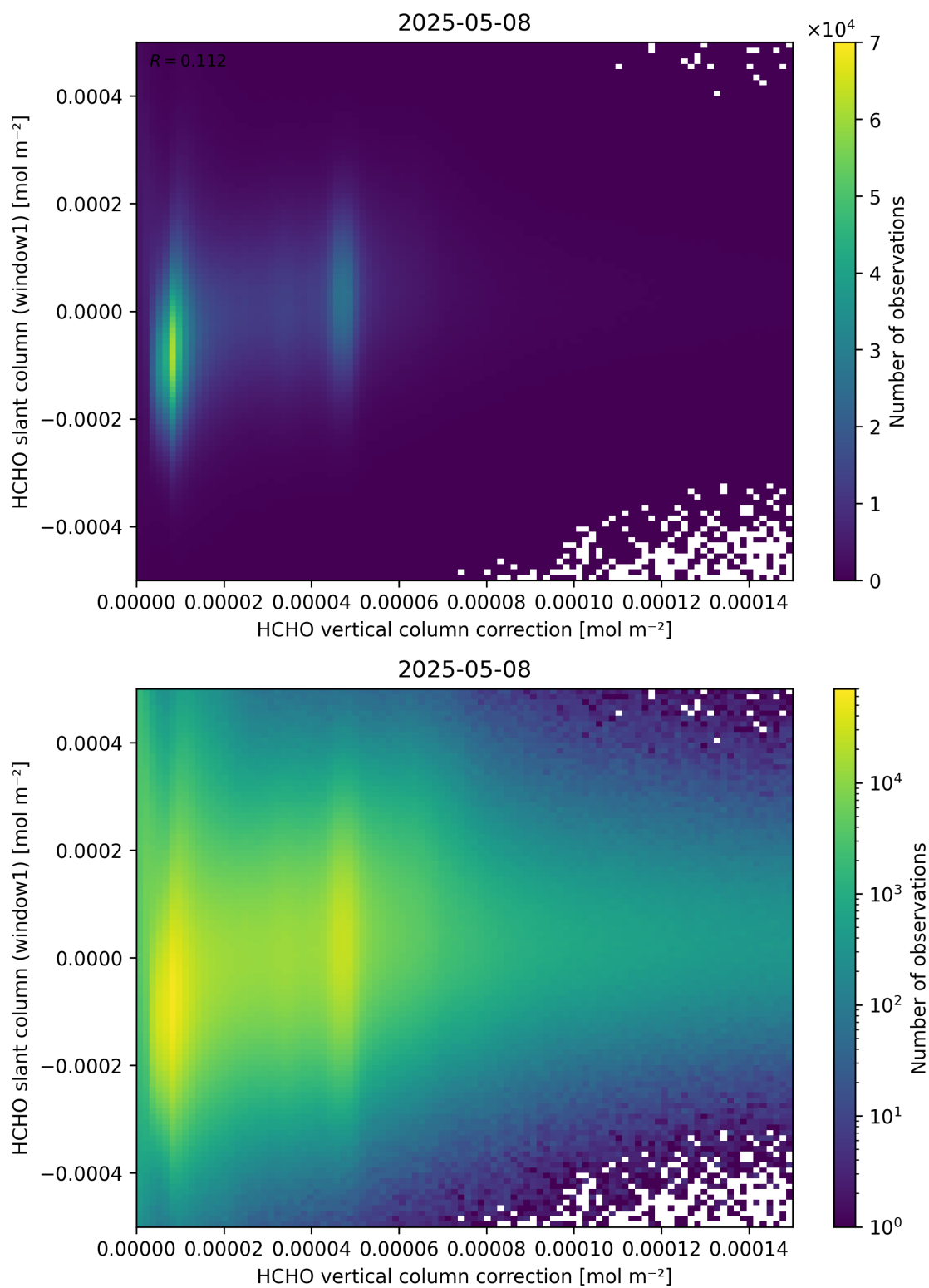
Figure 118: Scatter density plot of “HCHO vertical column correction” against “HCHO slant column (window1)” for 2025-05-07 to 2025-05-09.
