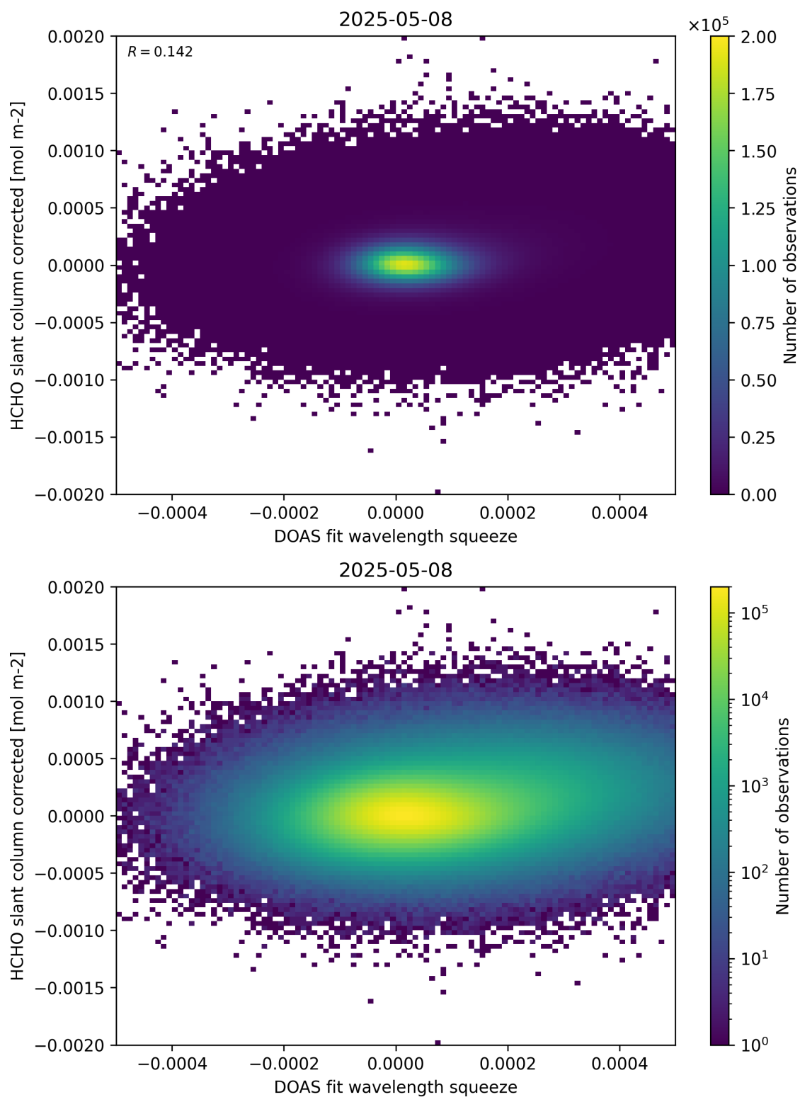
Figure 69: Scatter density plot of “DOAS fit wavelength squeeze” against “HCHO slant column corrected” for 2025-05-07 to 2025-05-09.
