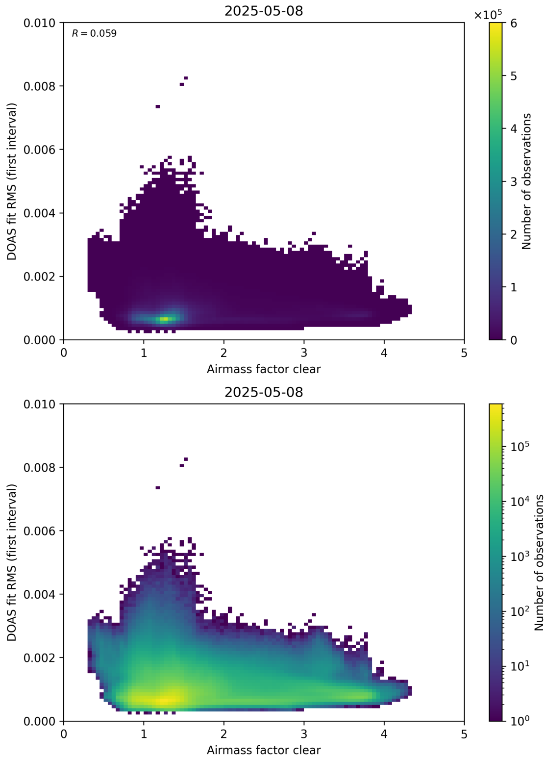
Figure 71: Scatter density plot of “Airmass factor clear” against “DOAS fit RMS (first interval)” for 2025-05-07 to 2025-05-09.
