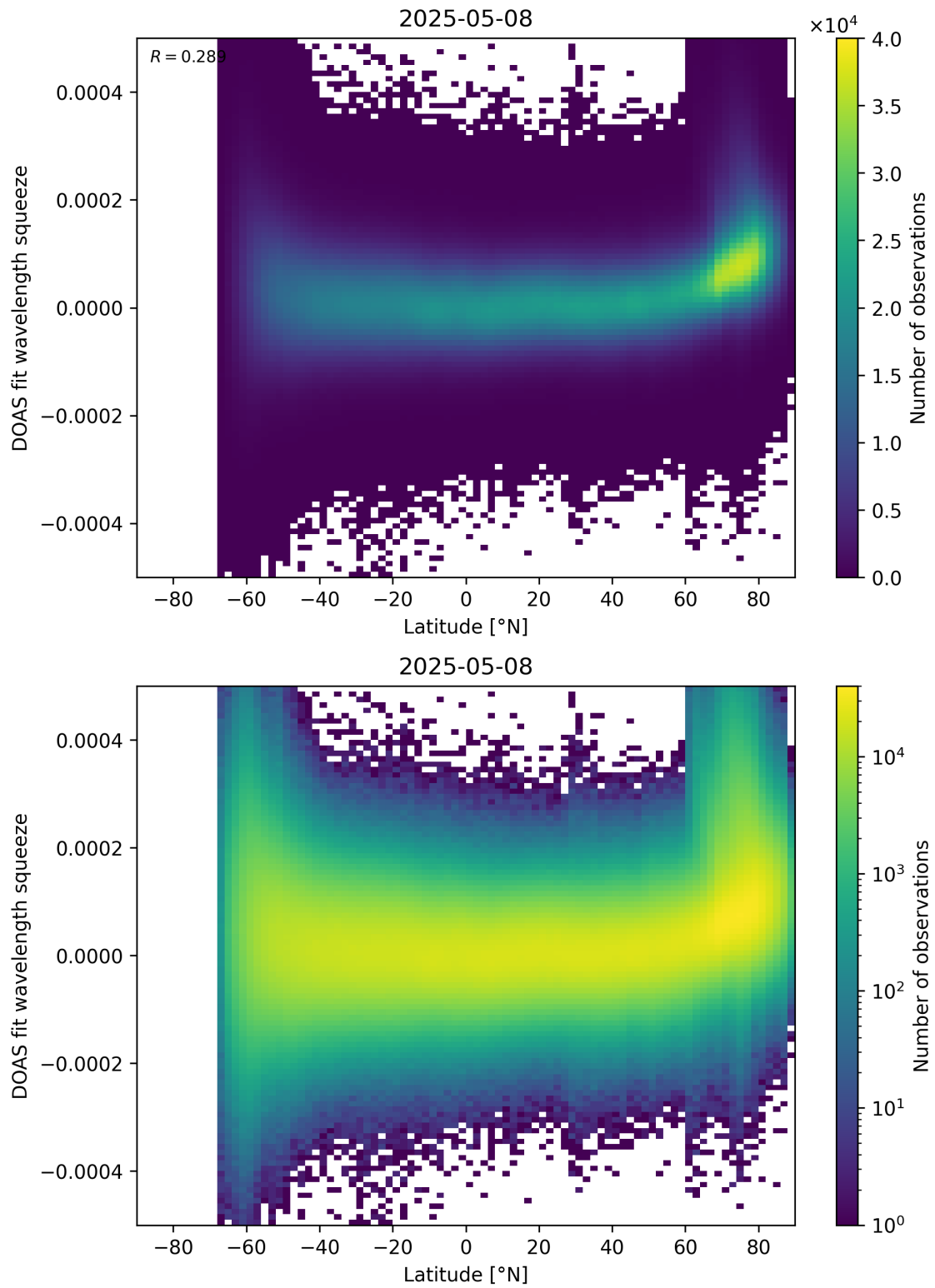
Figure 155: Scatter density plot of “Latitude” against “DOAS fit wavelength squeeze” for 2025-05-07 to 2025-05-09.
