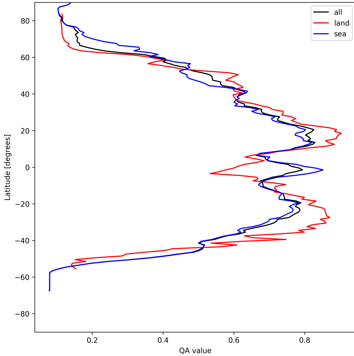
Figure 20: Zonal average of “QA value” for 2025-05-07 to 2025-05-09.
