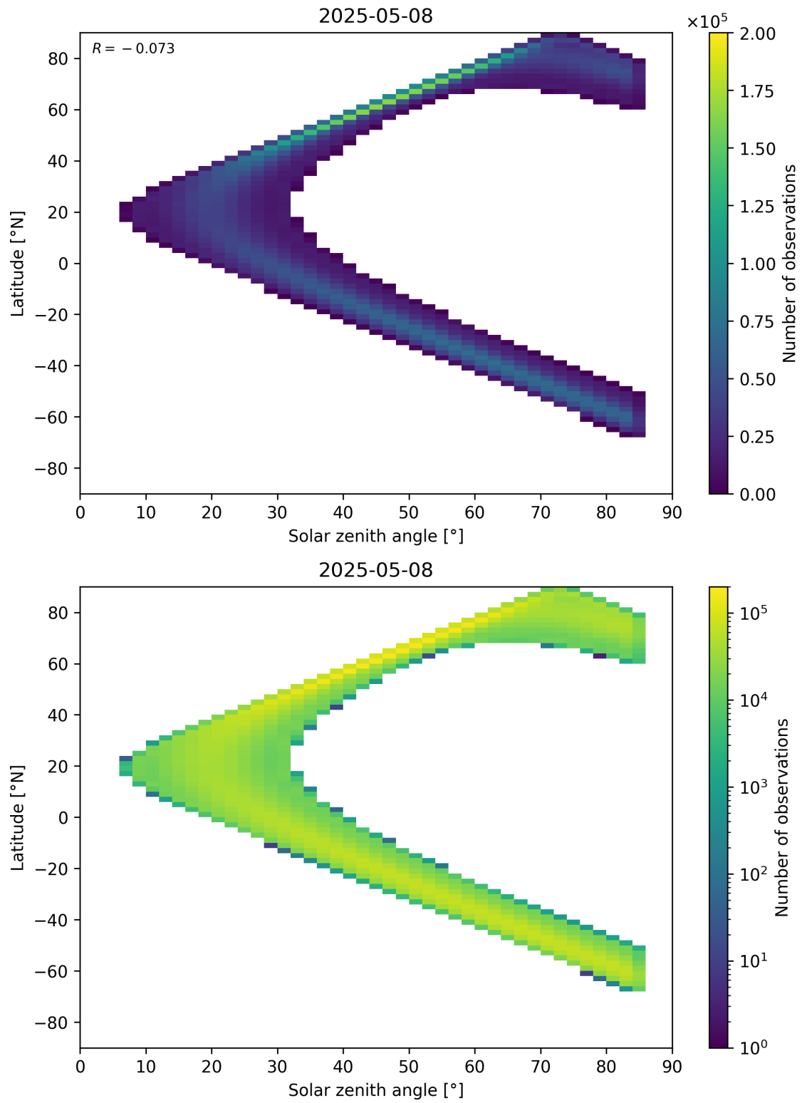
Figure 181: Scatter density plot of “Solar zenith angle” against “Latitude” for 2025-05-07 to 2025-05-09.
