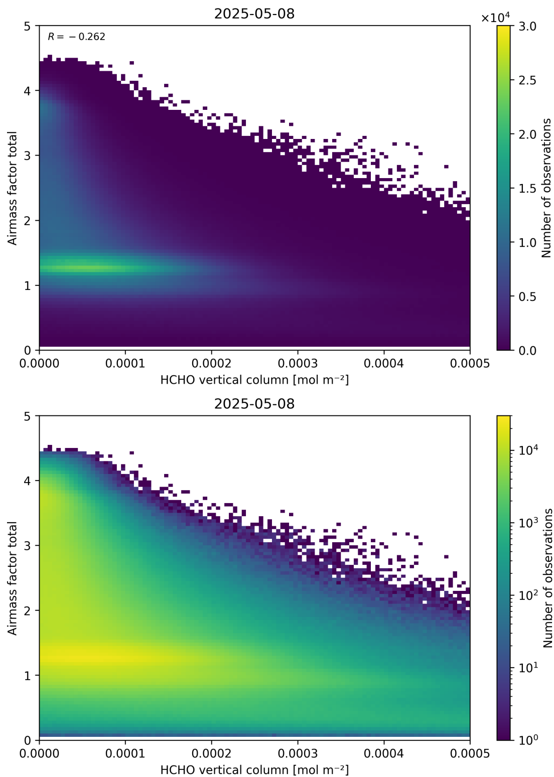
Figure 131: Scatter density plot of “HCHO vertical column” against “Airmass factor total” for 2025-05-07 to 2025-05-09.
