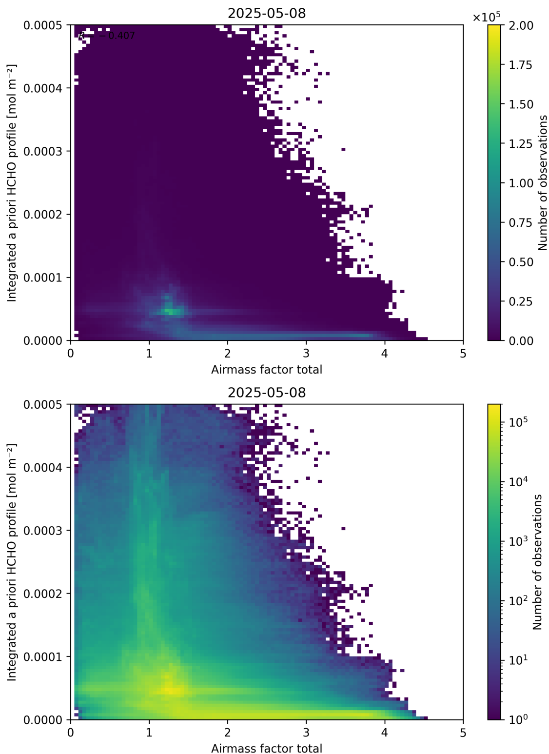
Figure 104: Scatter density plot of “Airmass factor total” against “Integrated a priori HCHO profile” for 2025-05-07 to 2025-05-09.
