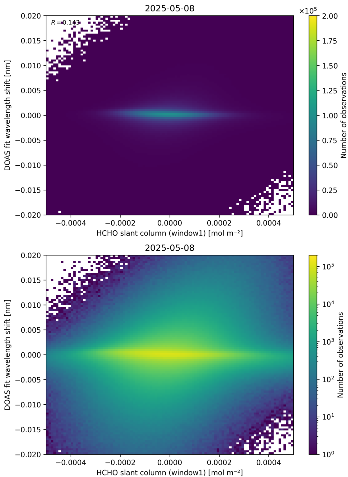
Figure 79: Scatter density plot of “HCHO slant column (window1)” against “DOAS fit wavelength shift” for 2025-05-07 to 2025-05-09.
