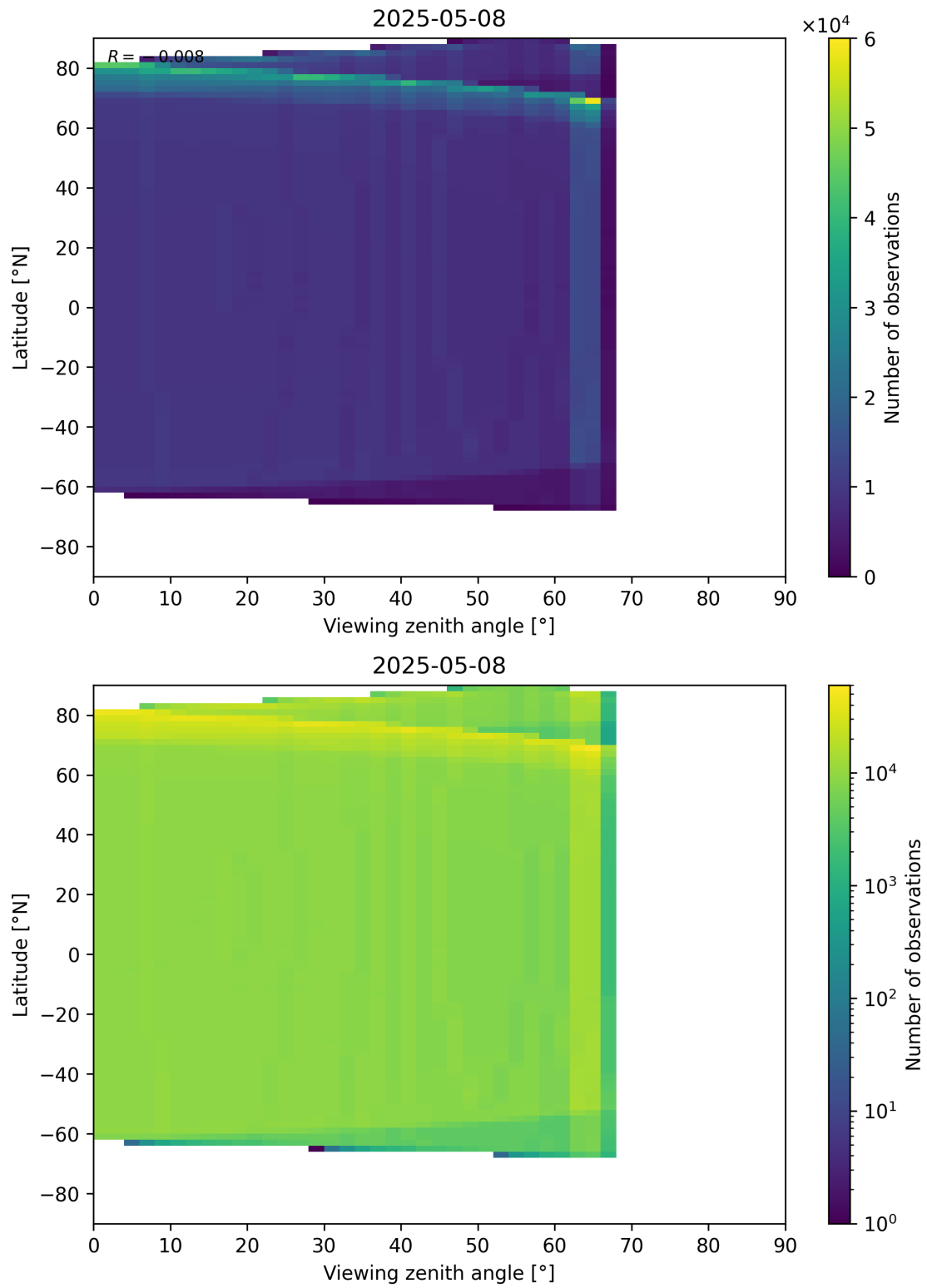
Figure 196: Scatter density plot of “Viewing zenith angle” against “Latitude” for 2025-05-07 to 2025-05-09.
