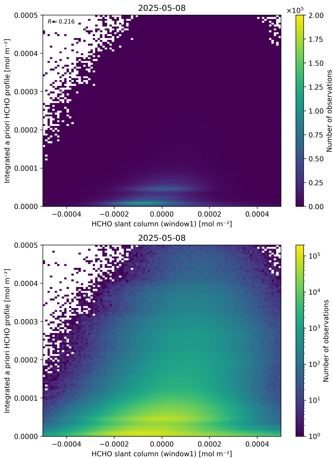
Figure 87: Scatter density plot of “HCHO slant column (window1)” against “Integrated a priori HCHO profile” for 2025-05-07 to 2025-05-09.
