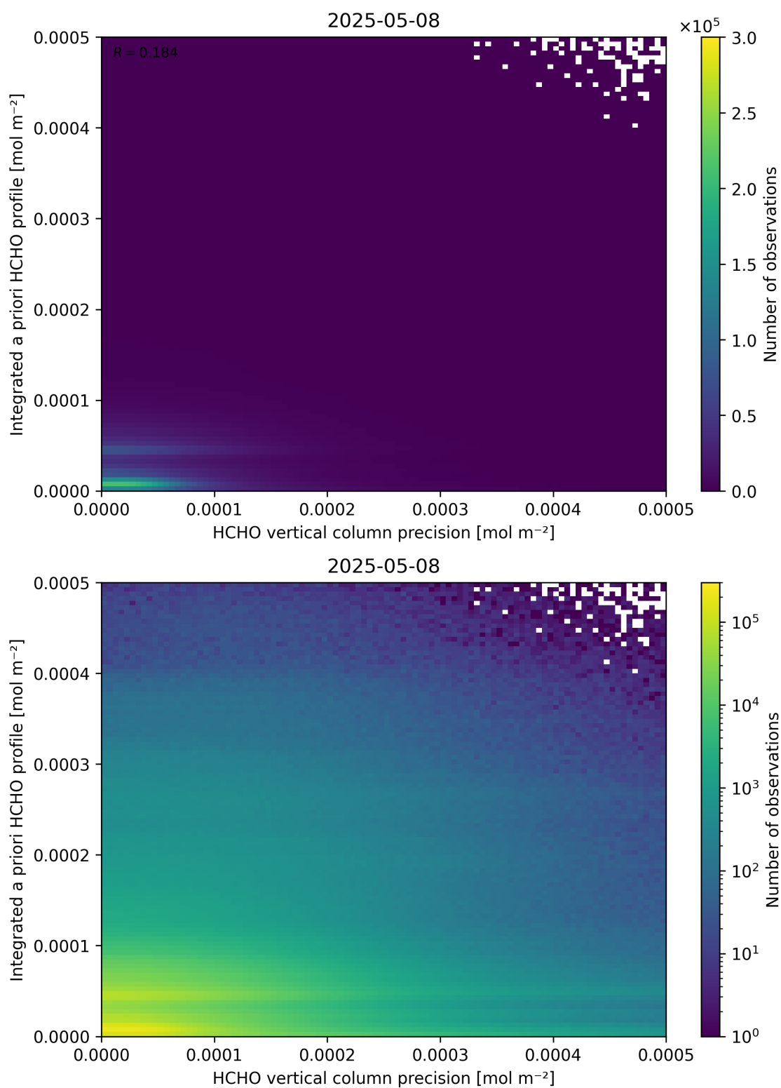
Figure 147: Scatter density plot of “HCHO vertical column precision” against “Integrated a priori HCHO profile” for 2025-05-07 to 2025-05-09.
