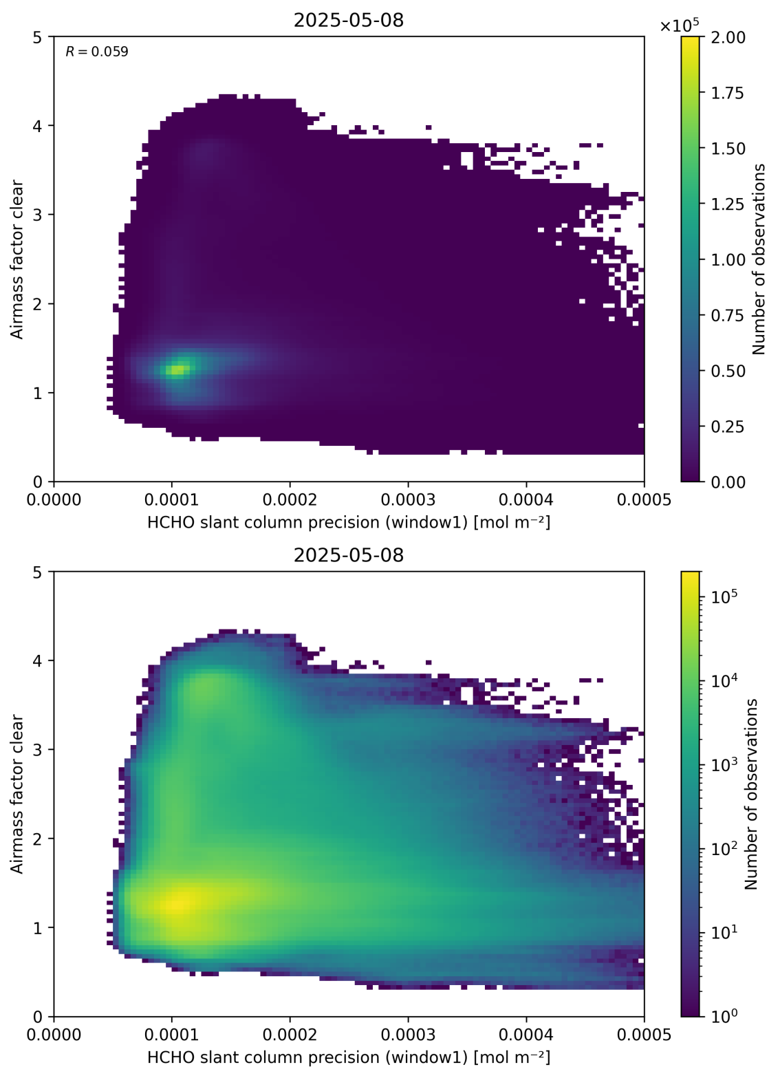
Figure 91: Scatter density plot of “HCHO slant column precision (window1)” against “Airmass factor clear” for 2025-05-07 to 2025-05-09.
