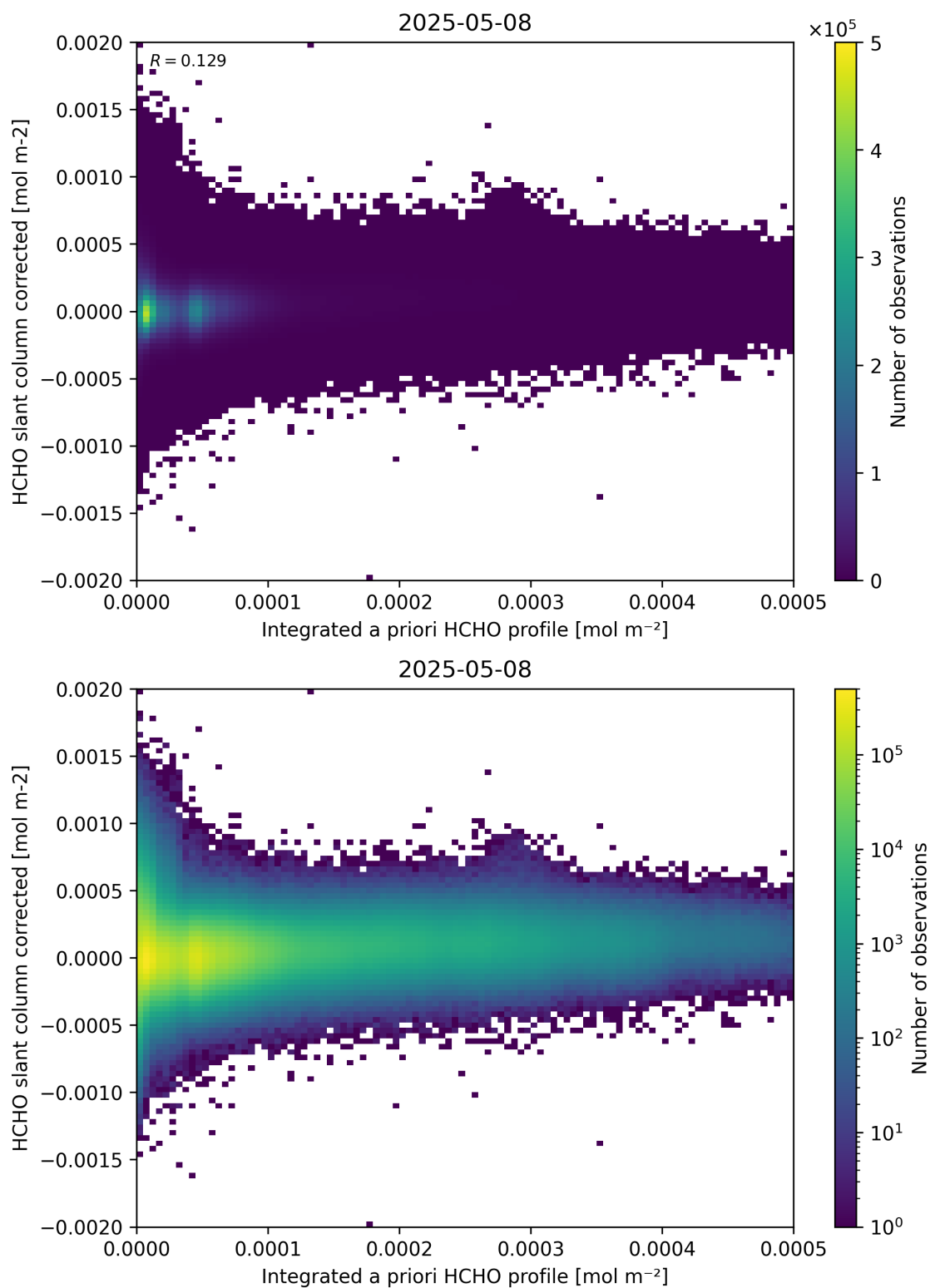
Figure 151: Scatter density plot of “Integrated a priori HCHO profile” against “HCHO slant column corrected” for 2025-05-07 to 2025-05-09.
