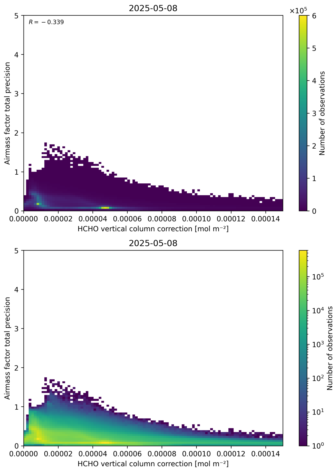
Figure 121: Scatter density plot of “HCHO vertical column correction” against “Airmass factor total precision” for 2025-05-07 to 2025-05-09.
