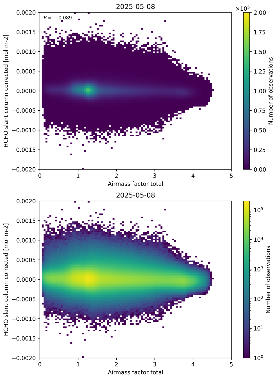
Figure 101: Scatter density plot of “Airmass factor total” against “HCHO slant column corrected” for 2025-05-07 to 2025-05-09.
