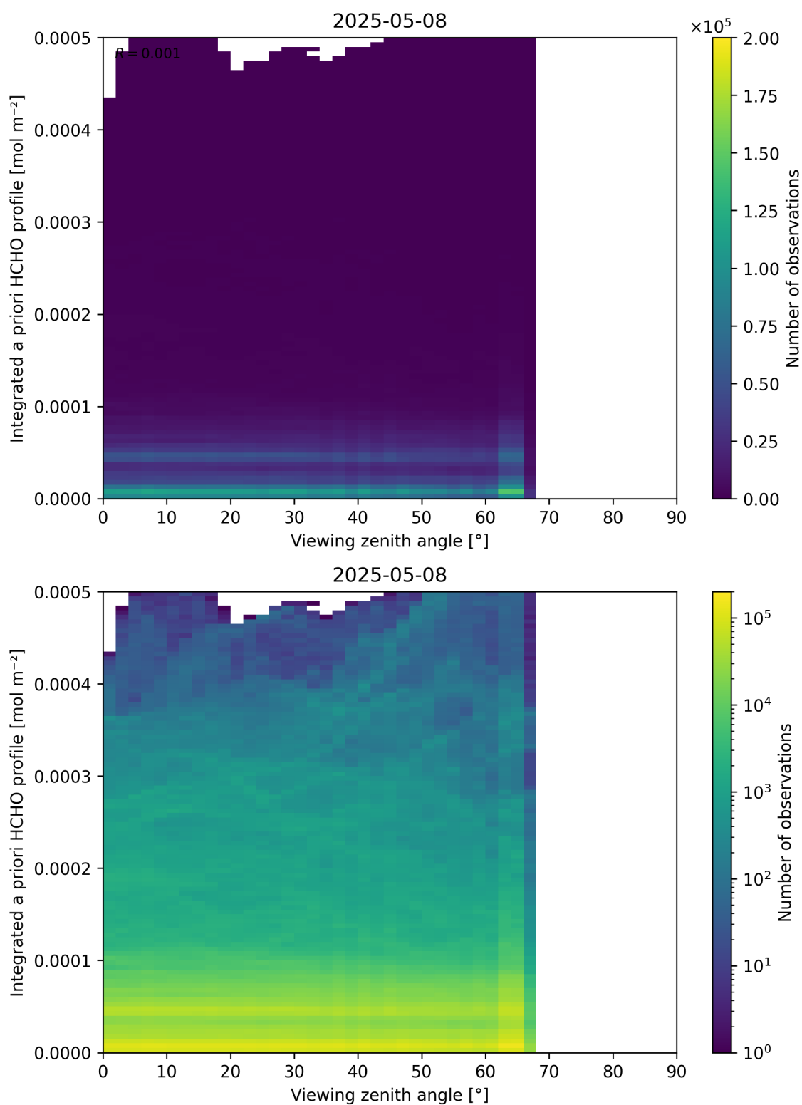
Figure 195: Scatter density plot of “Viewing zenith angle” against “Integrated a priori HCHO profile” for 2025-05-07 to 2025-05-09.
