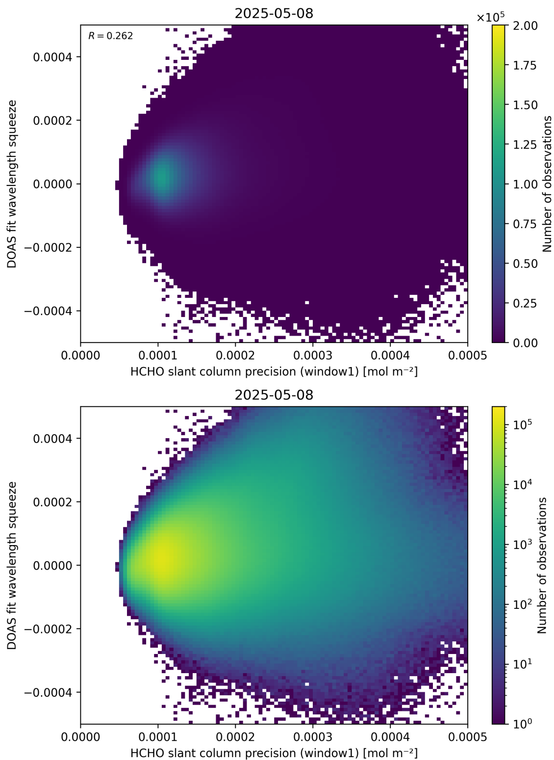
Figure 90: Scatter density plot of “HCHO slant column precision (window1)” against “DOAS fit wavelength squeeze” for 2025-05-07 to 2025-05-09.
