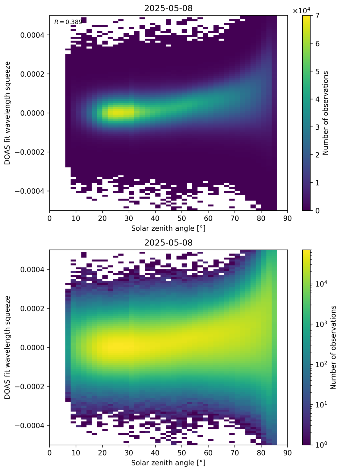
Figure 169: Scatter density plot of “Solar zenith angle” against “DOAS fit wavelength squeeze” for 2025-05-07 to 2025-05-09.
