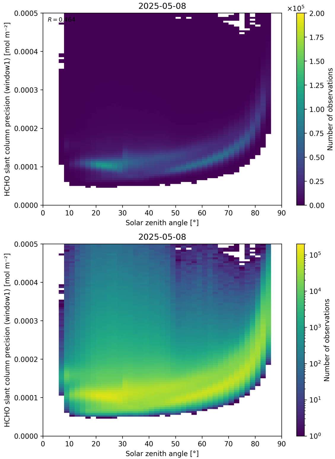
Figure 174: Scatter density plot of “Solar zenith angle” against “HCHO slant column precision (window1)” for 2025-05-07 to 2025-05-09.
