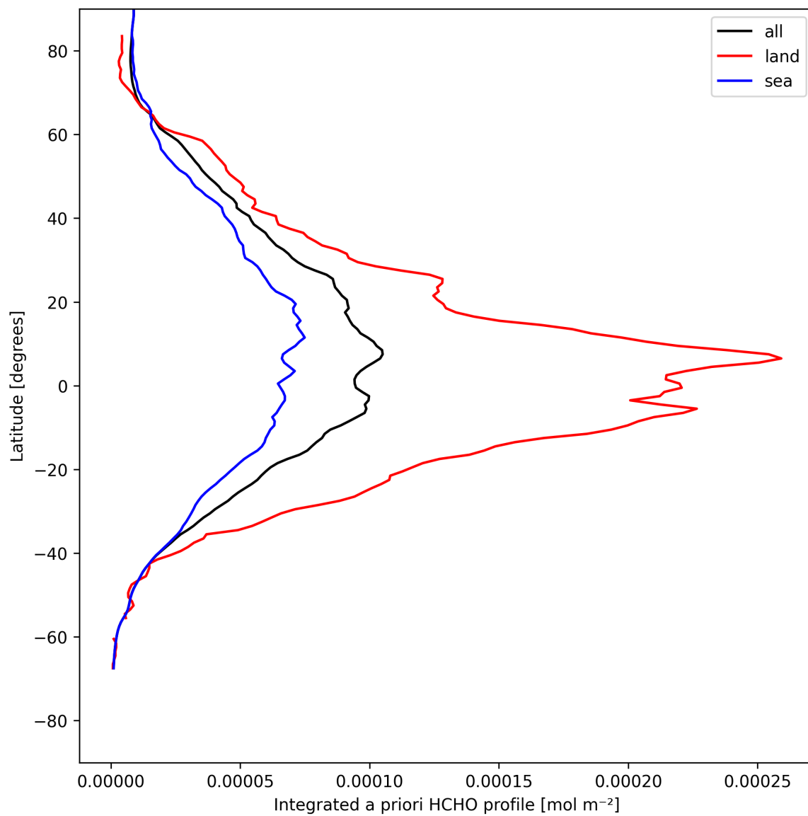
Figure 29: Zonal average of “Integrated a priori HCHO profile” for 2025-05-07 to 2025-05-09.
