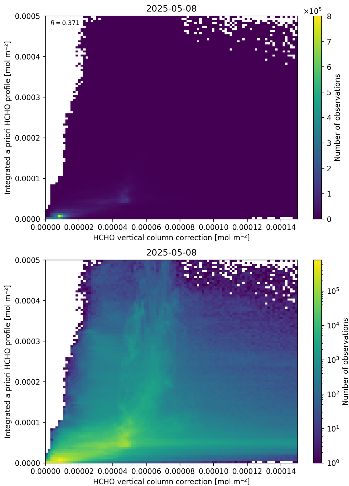
Figure 122: Scatter density plot of “HCHO vertical column correction” against “Integrated a priori HCHO profile” for 2025-05-07 to 2025-05-09.
