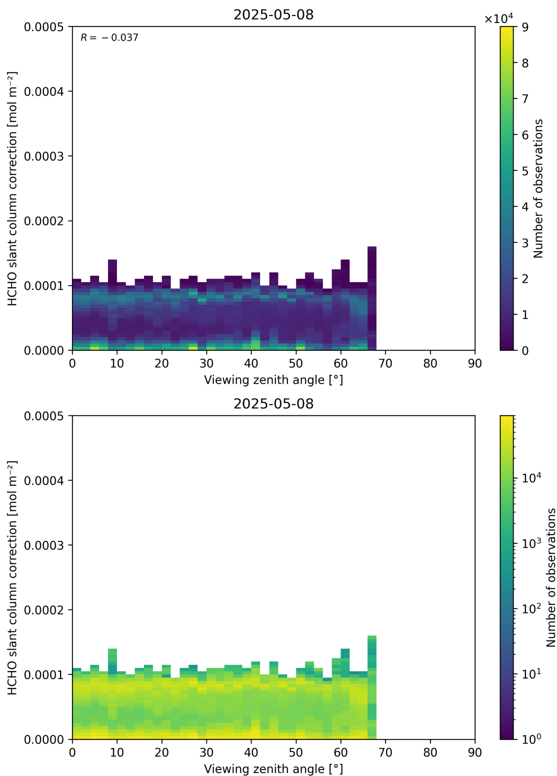
Figure 187: Scatter density plot of “Viewing zenith angle” against “HCHO slant column correction” for 2025-05-07 to 2025-05-09.
