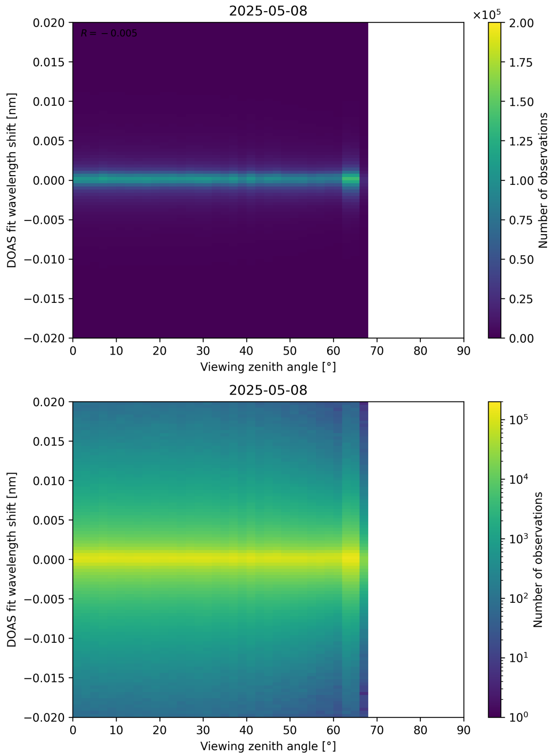
Figure 183: Scatter density plot of “Viewing zenith angle” against “DOAS fit wavelength shift” for 2025-05-07 to 2025-05-09.
