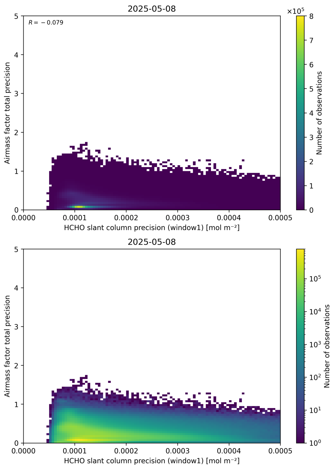
Figure 95: Scatter density plot of “HCHO slant column precision (window1)” against “Airmass factor total precision” for 2025-05-07 to 2025-05-09.
