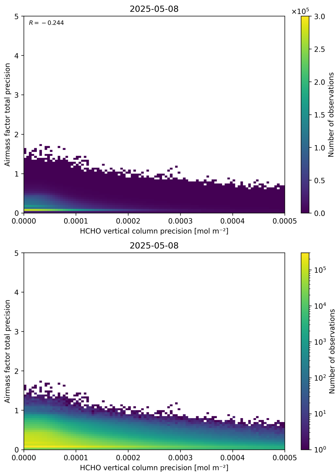
Figure 145: Scatter density plot of “HCHO vertical column precision” against “Airmass factor total precision” for 2025-05-07 to 2025-05-09.
