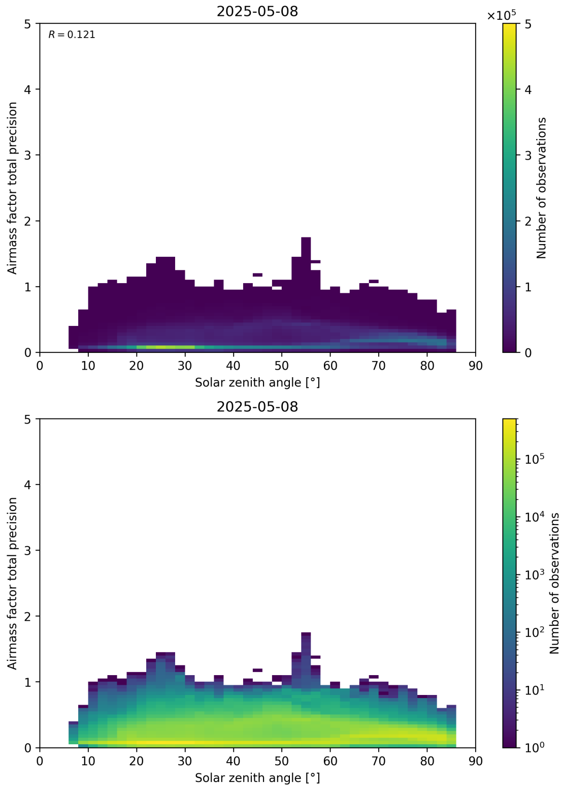
Figure 176: Scatter density plot of “Solar zenith angle” against “Airmass factor total precision” for 2025-05-07 to 2025-05-09.
