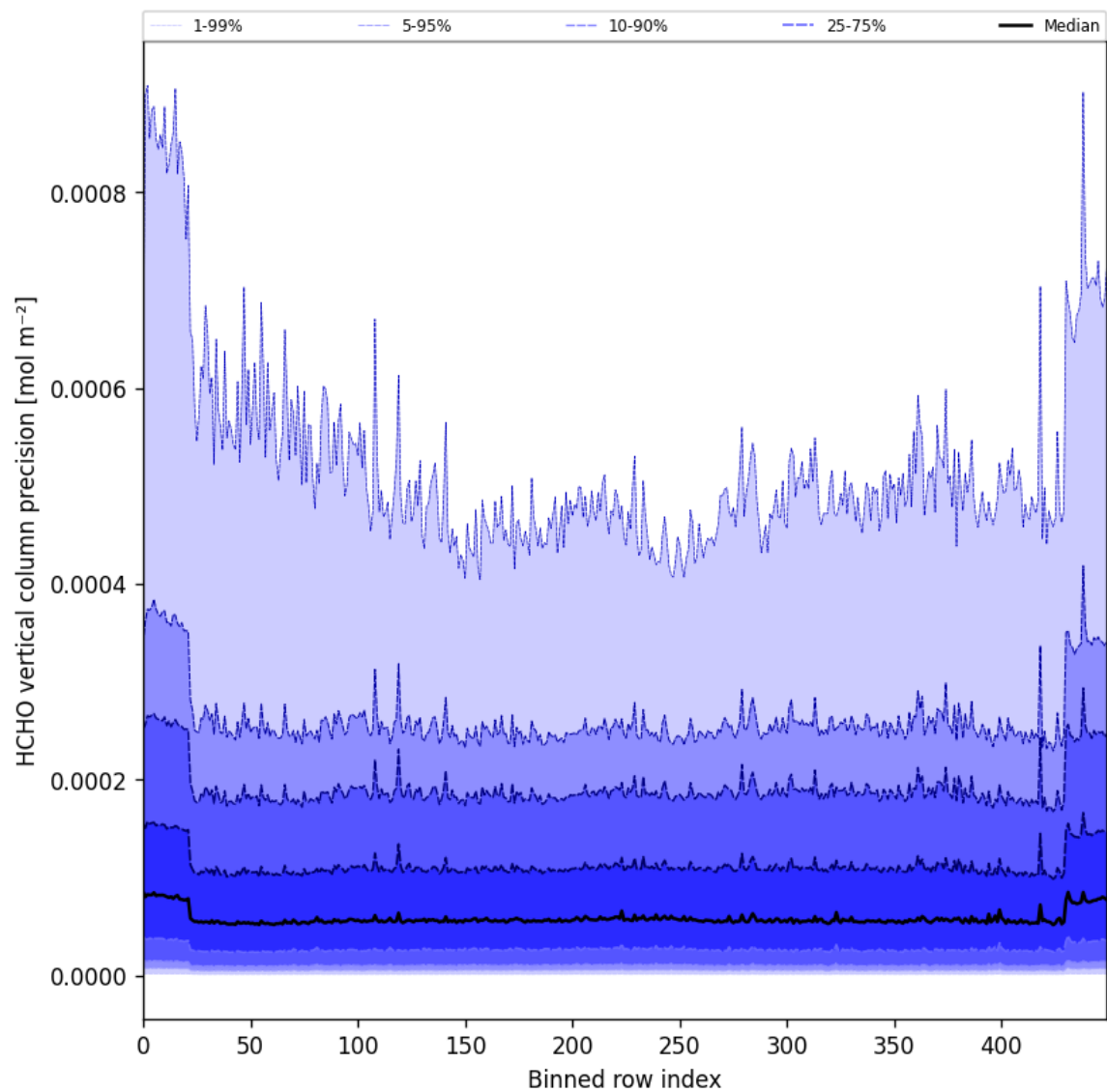
Figure 50: Along track statistics of “HCHO vertical column precision” for 2025-05-07 to 2025-05-09
