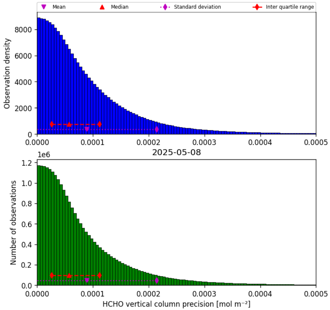
Figure 36: Histogram of “HCHO vertical column precision” for 2025-05-07 to 2025-05-09
