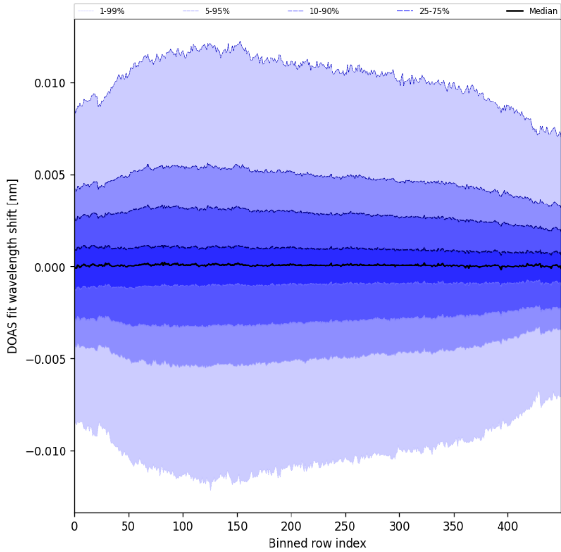
Figure 58: Along track statistics of “DOAS fit wavelength shift” for 2025-05-07 to 2025-05-09
