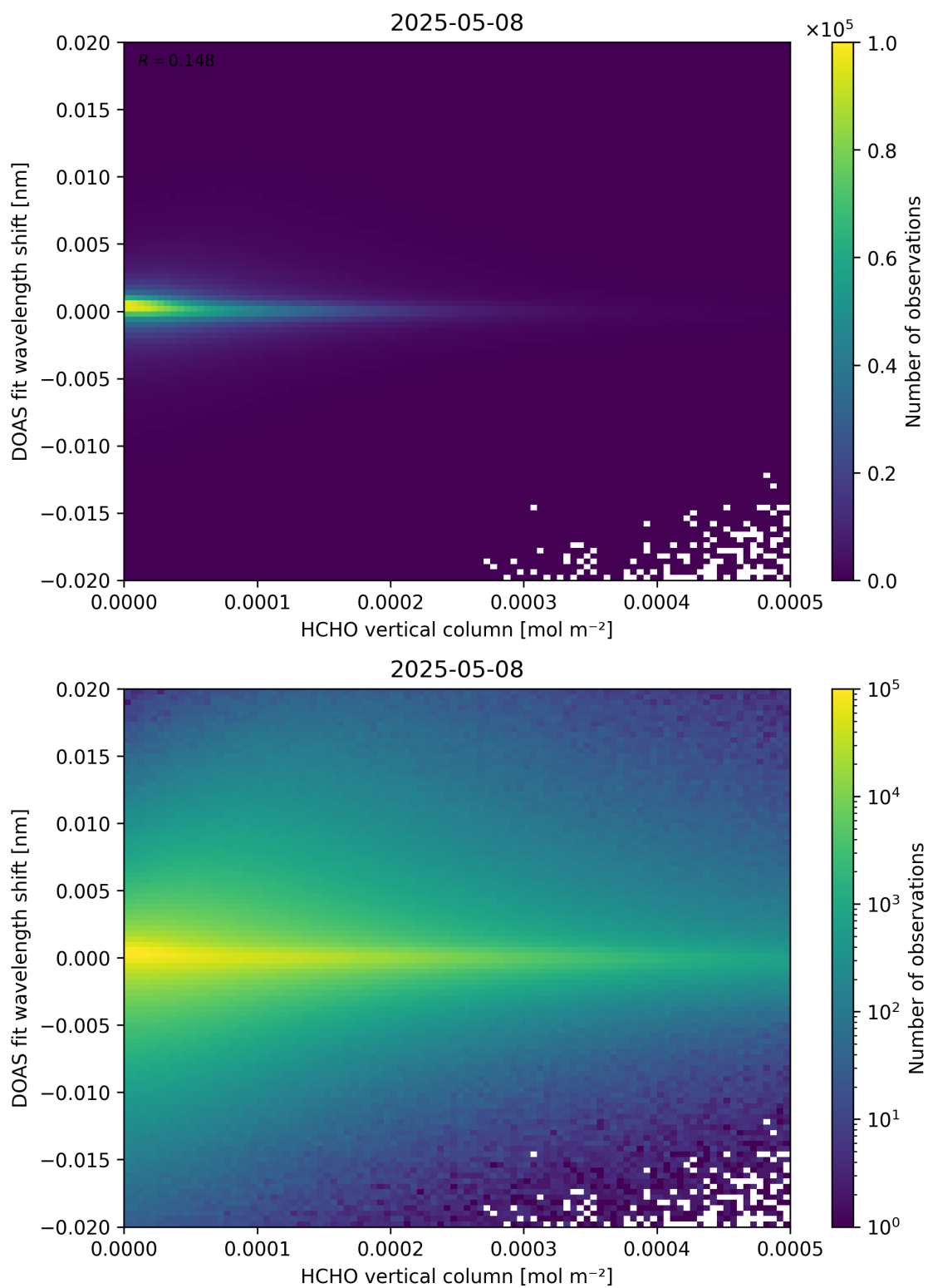
Figure 124: Scatter density plot of “HCHO vertical column” against “DOAS fit wavelength shift” for 2025-05-07 to 2025-05-09.
