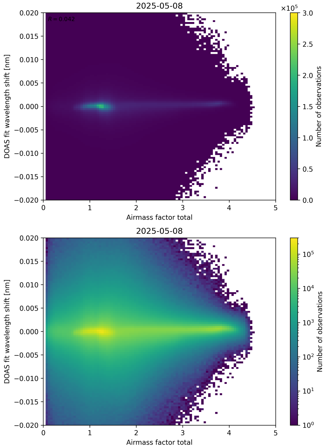
Figure 98: Scatter density plot of “Airmass factor total” against “DOAS fit wavelength shift” for 2025-05-07 to 2025-05-09.
