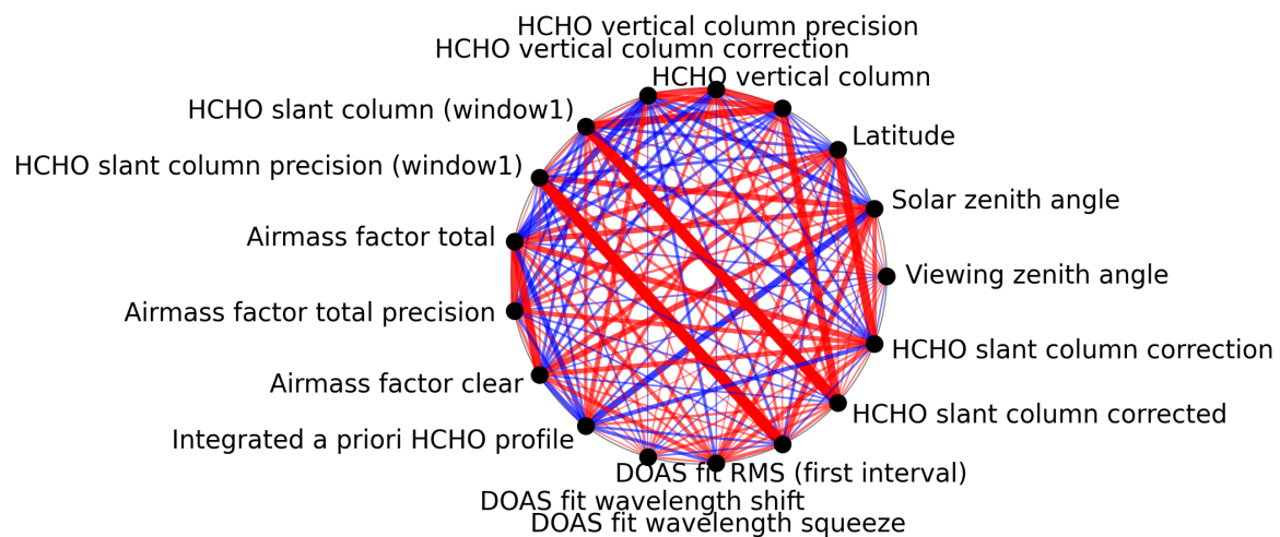
Figure 1: Map of correlation graph for 2025-05-07 to 2025-05-09.
