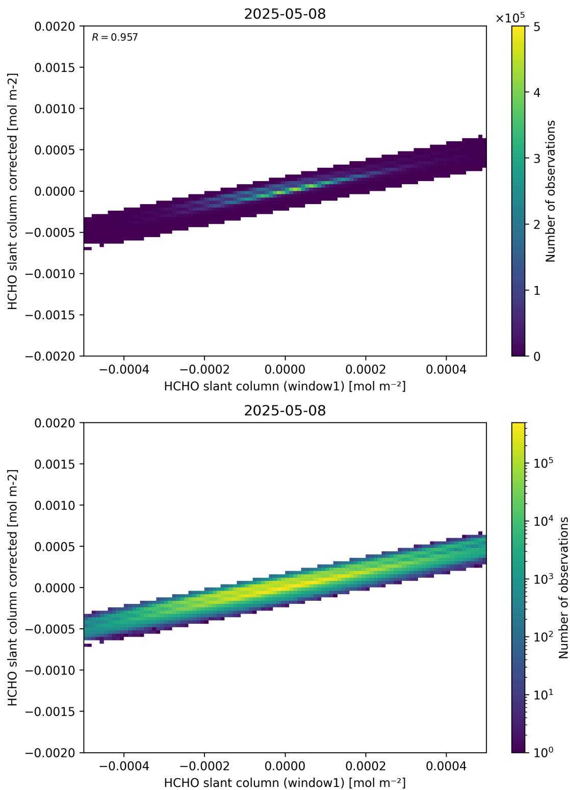
Figure 82: Scatter density plot of “HCHO slant column (window1)” against “HCHO slant column corrected” for 2025-05-07 to 2025-05-09.
