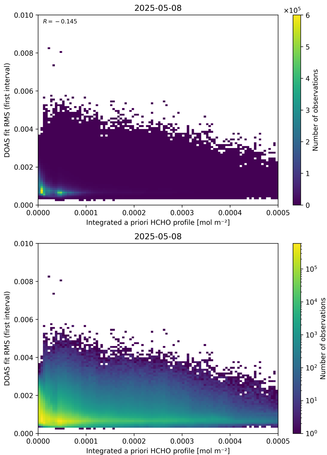
Figure 148: Scatter density plot of “Integrated a priori HCHO profile” against “DOAS fit RMS (first interval)” for 2025-05-07 to 2025-05-09.
