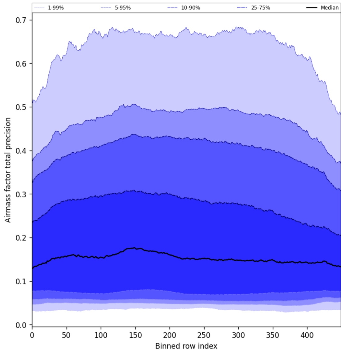
Figure 55: Along track statistics of “Airmass factor total precision” for 2025-05-07 to 2025-05-09
