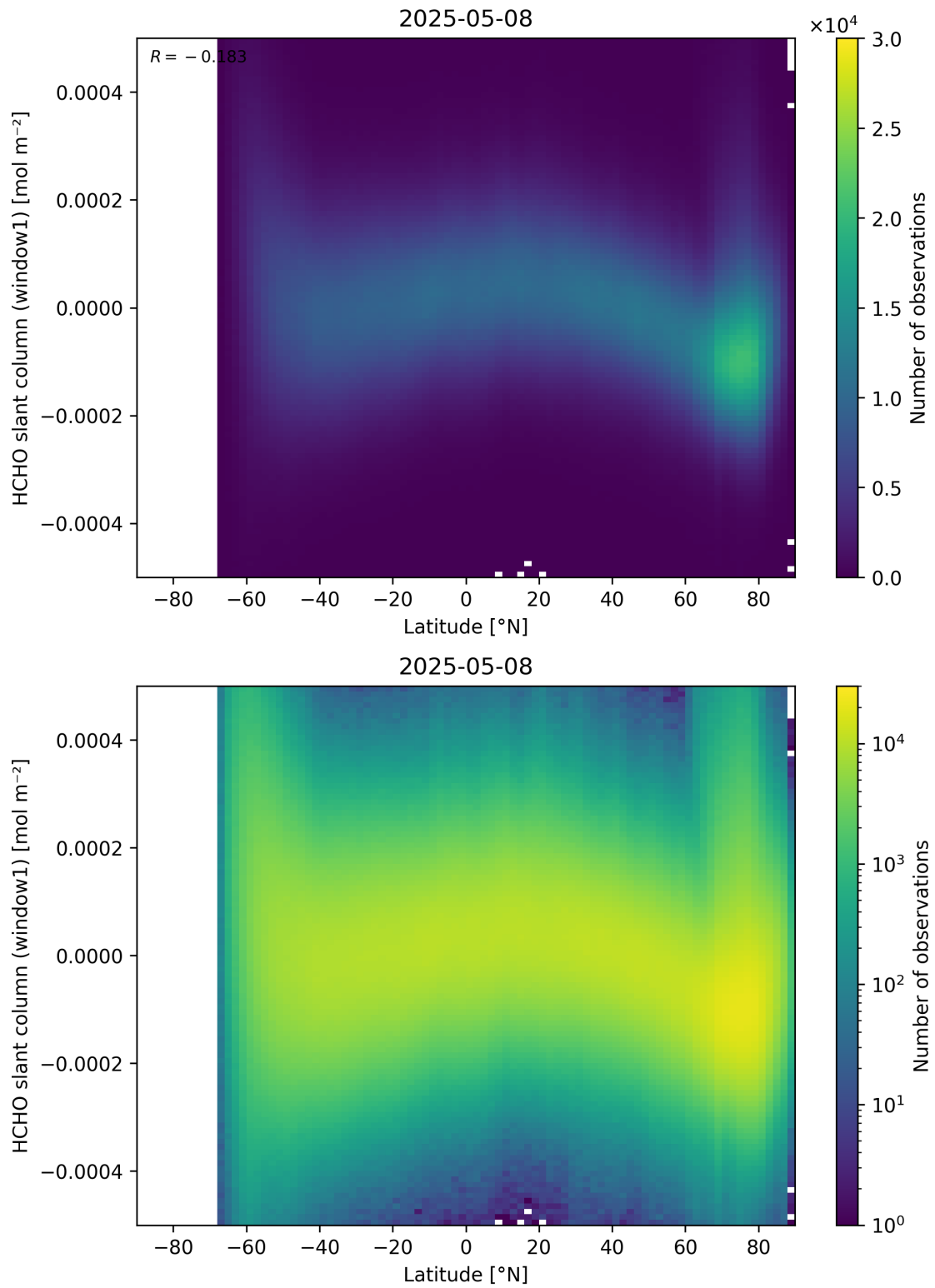
Figure 159: Scatter density plot of “Latitude” against “HCHO slant column (window1)” for 2025-05-07 to 2025-05-09.
