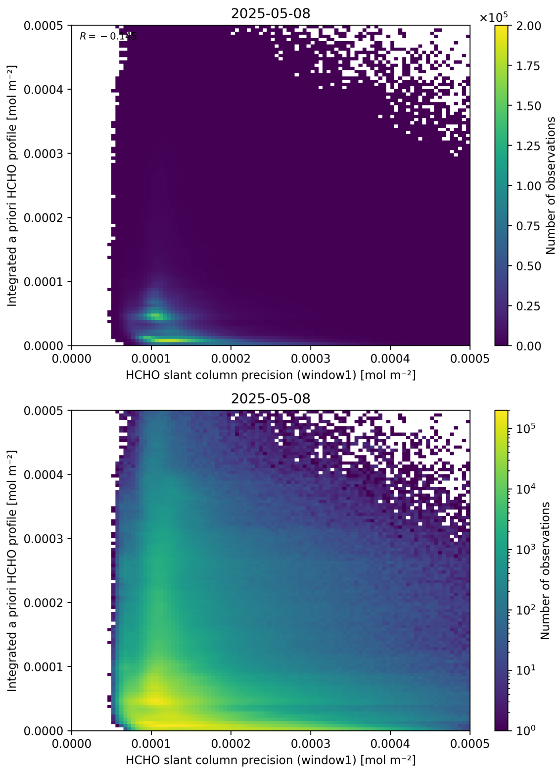
Figure 96: Scatter density plot of “HCHO slant column precision (window1)” against “Integrated a priori HCHO profile” for 2025-05-07 to 2025-05-09.
