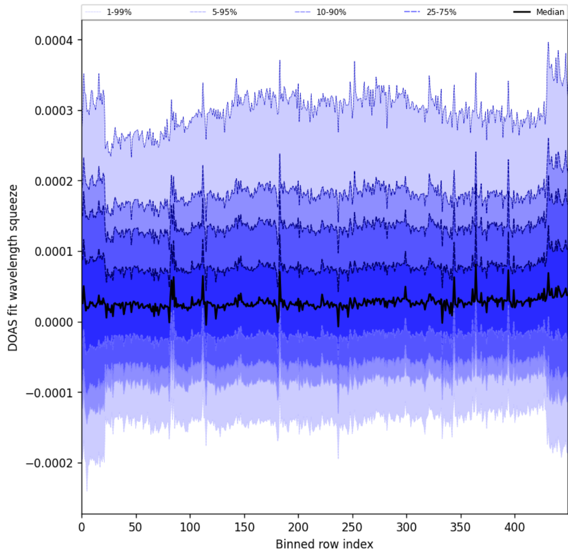
Figure 59: Along track statistics of “DOAS fit wavelength squeeze” for 2025-05-07 to 2025-05-09
