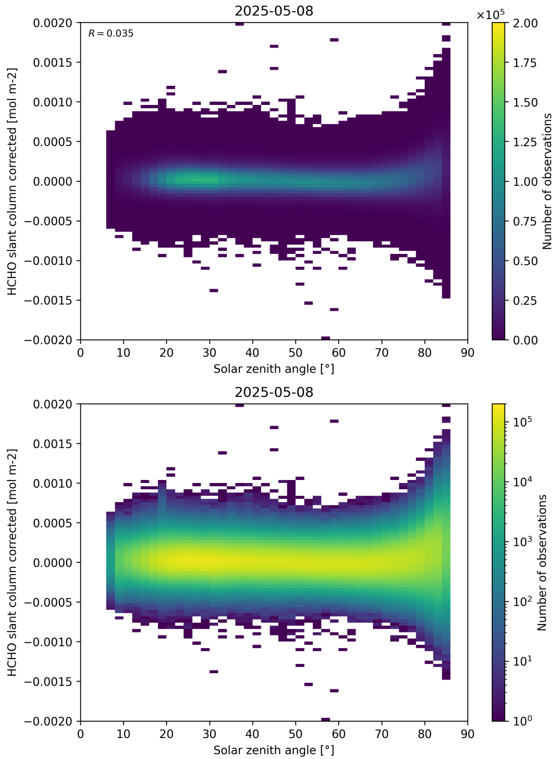
Figure 171: Scatter density plot of “Solar zenith angle” against “HCHO slant column corrected” for 2025-05-07 to 2025-05-09.
