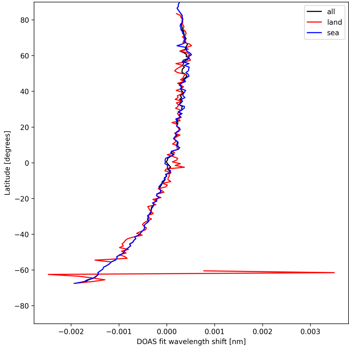
Figure 30: Zonal average of “DOAS fit wavelength shift” for 2025-05-07 to 2025-05-09.
