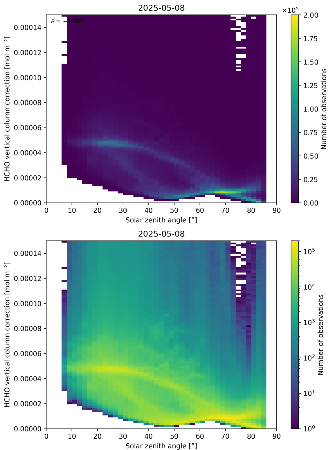
Figure 178: Scatter density plot of “Solar zenith angle” against “HCHO vertical column correction” for 2025-05-07 to 2025-05-09.
