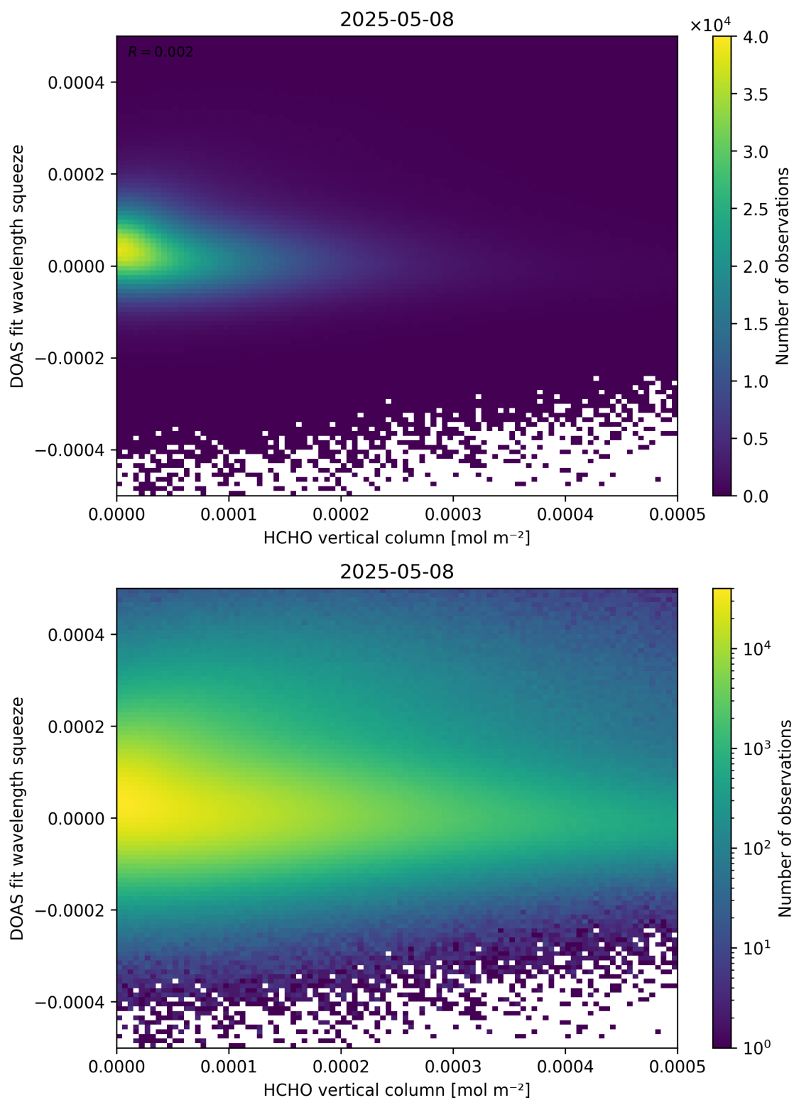
Figure 125: Scatter density plot of “HCHO vertical column” against “DOAS fit wavelength squeeze” for 2025-05-07 to 2025-05-09.
