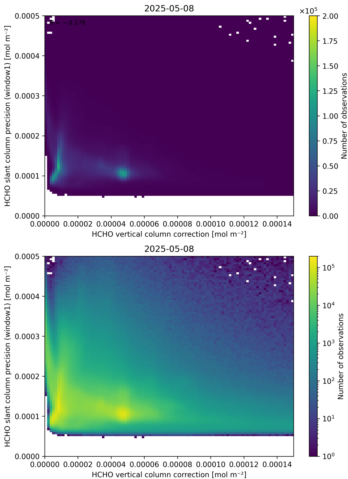
Figure 119: Scatter density plot of “HCHO vertical column correction” against “HCHO slant column precision (window1)” for 2025-05-07 to 2025-05-09.
