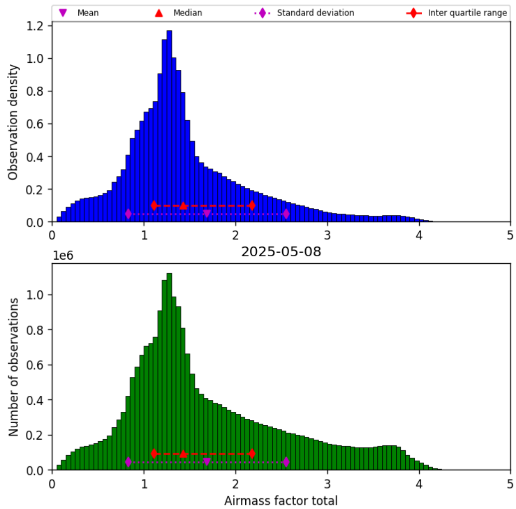
Figure 40: Histogram of “Airmass factor total” for 2025-05-07 to 2025-05-09
