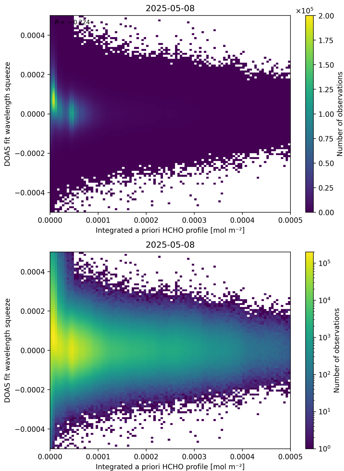
Figure 150: Scatter density plot of “Integrated a priori HCHO profile” against “DOAS fit wavelength squeeze” for 2025-05-07 to 2025-05-09.
