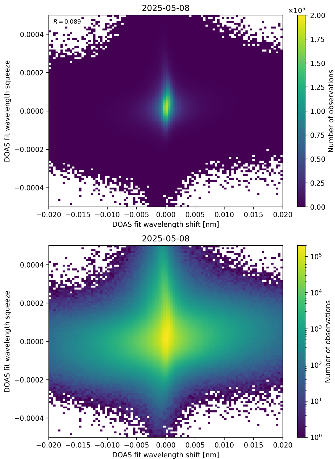
Figure 65: Scatter density plot of “DOAS fit wavelength shift” against “DOAS fit wavelength squeeze” for 2025-05-07 to 2025-05-09.
