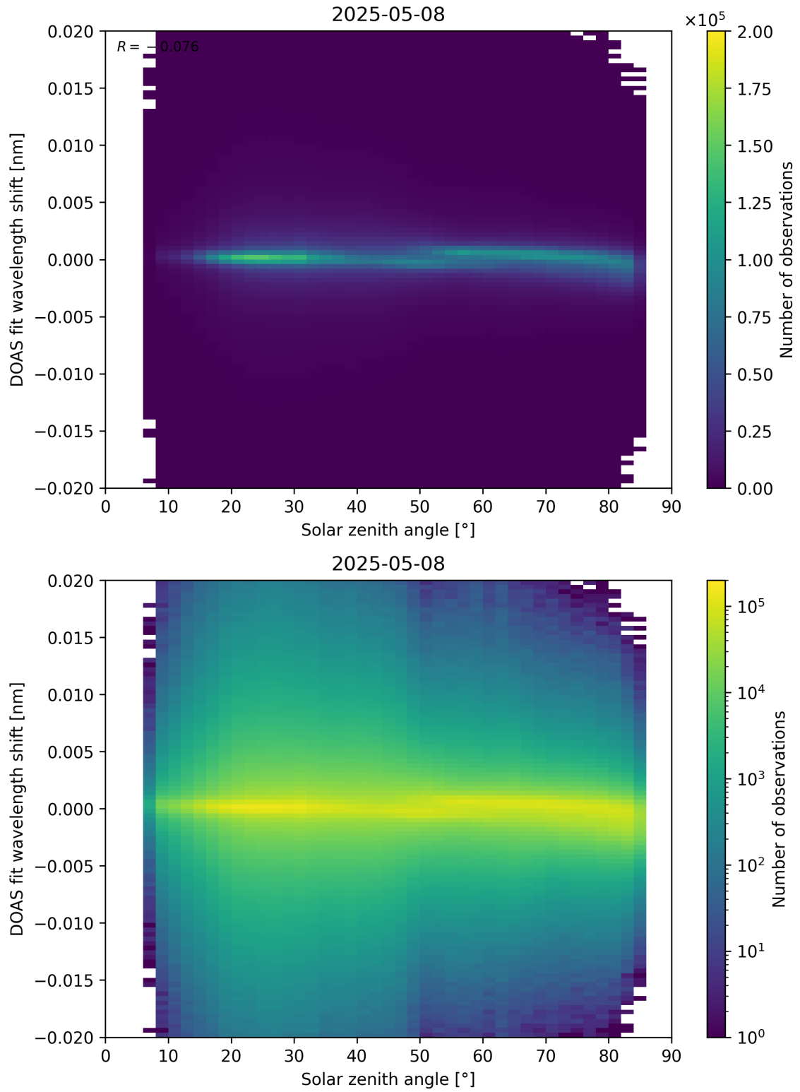
Figure 168: Scatter density plot of “Solar zenith angle” against “DOAS fit wavelength shift” for 2025-05-07 to 2025-05-09.
