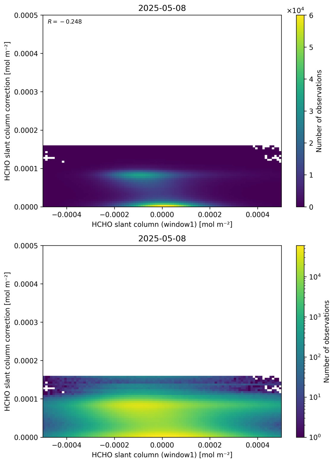
Figure 83: Scatter density plot of “HCHO slant column (window1)” against “HCHO slant column correction” for 2025-05-07 to 2025-05-09.
