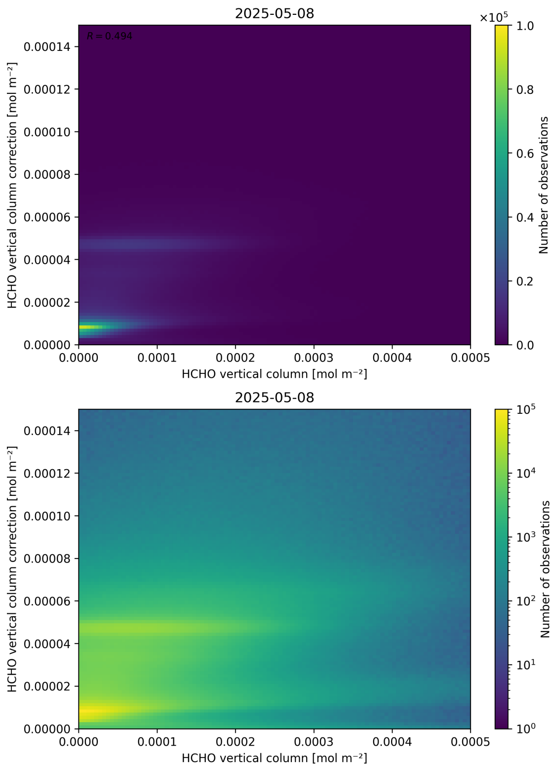
Figure 133: Scatter density plot of “HCHO vertical column” against “HCHO vertical column correction” for 2025-05-07 to 2025-05-09.
