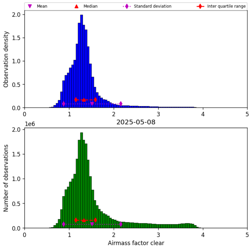
Figure 42: Histogram of “Airmass factor clear” for 2025-05-07 to 2025-05-09
