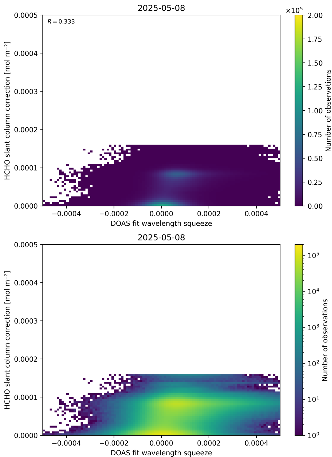
Figure 70: Scatter density plot of “DOAS fit wavelength squeeze” against “HCHO slant column correction” for 2025-05-07 to 2025-05-09.
