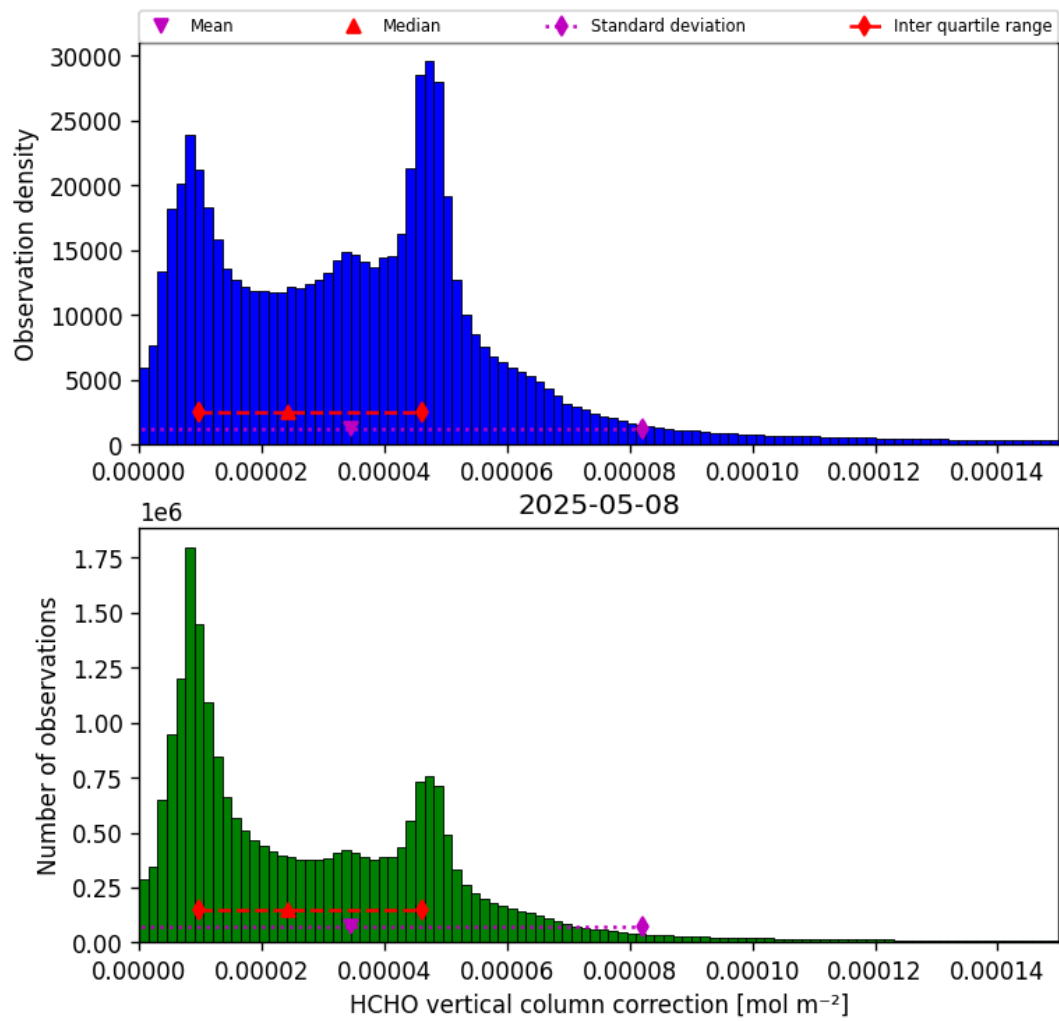
Figure 37: Histogram of “HCHO vertical column correction” for 2025-05-07 to 2025-05-09
