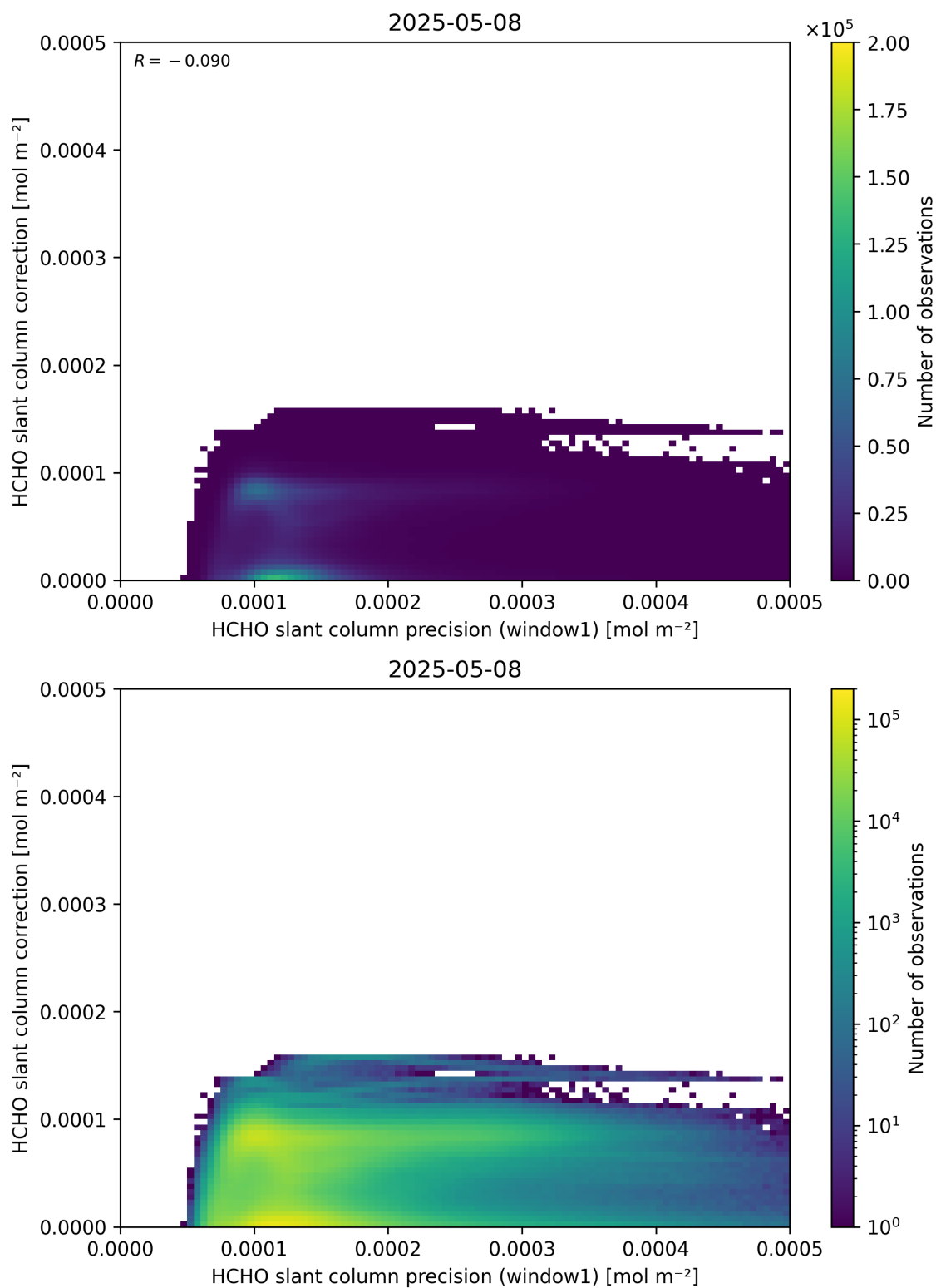
Figure 93: Scatter density plot of “HCHO slant column precision (window1)” against “HCHO slant column correction” for 2025-05-07 to 2025-05-09.
