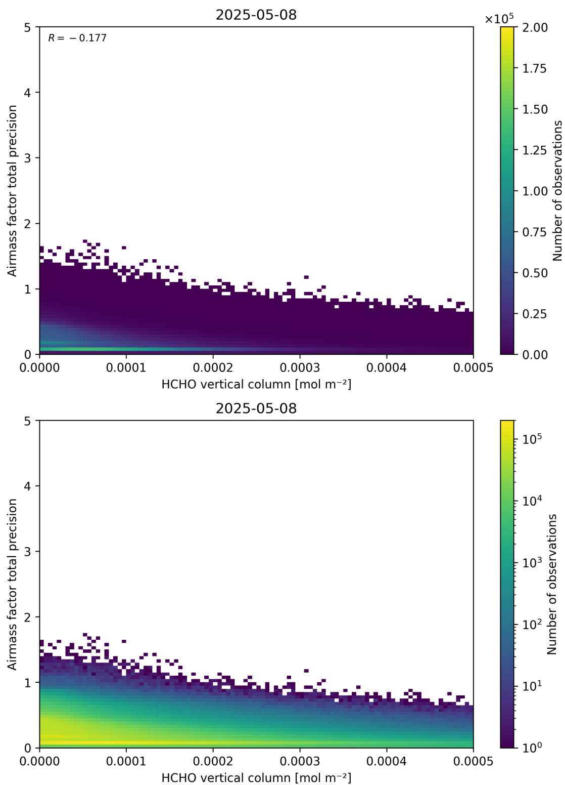
Figure 132: Scatter density plot of “HCHO vertical column” against “Airmass factor total precision” for 2025-05-07 to 2025-05-09.
