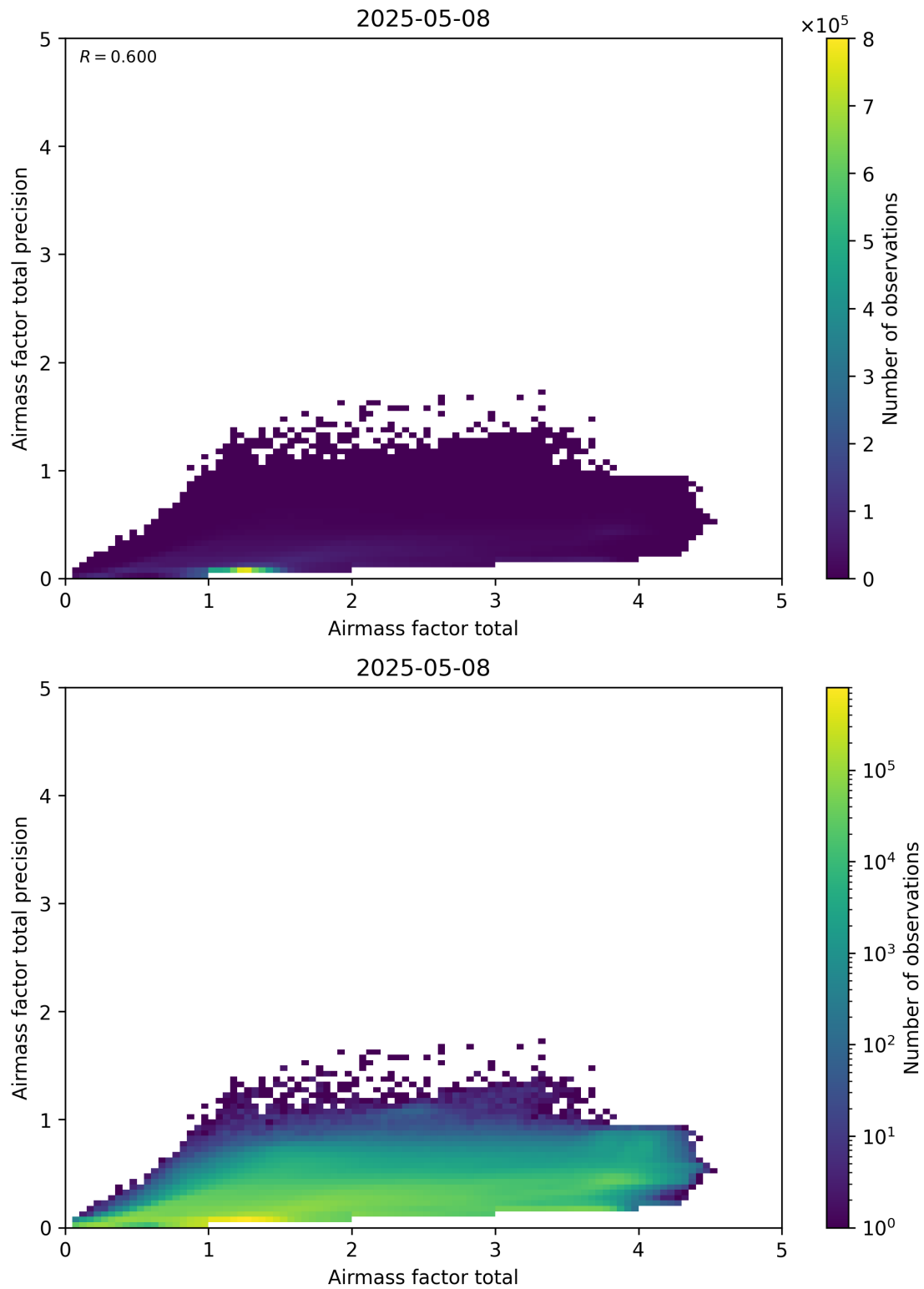
Figure 103: Scatter density plot of “Airmass factor total” against “Airmass factor total precision” for 2025-05-07 to 2025-05-09.
