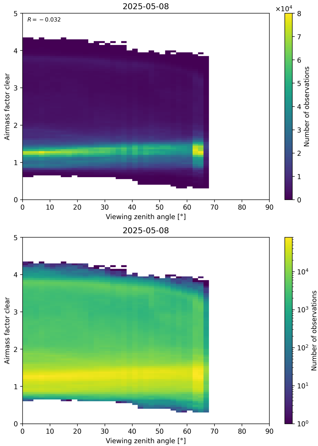
Figure 185: Scatter density plot of “Viewing zenith angle” against “Airmass factor clear” for 2025-05-07 to 2025-05-09.
