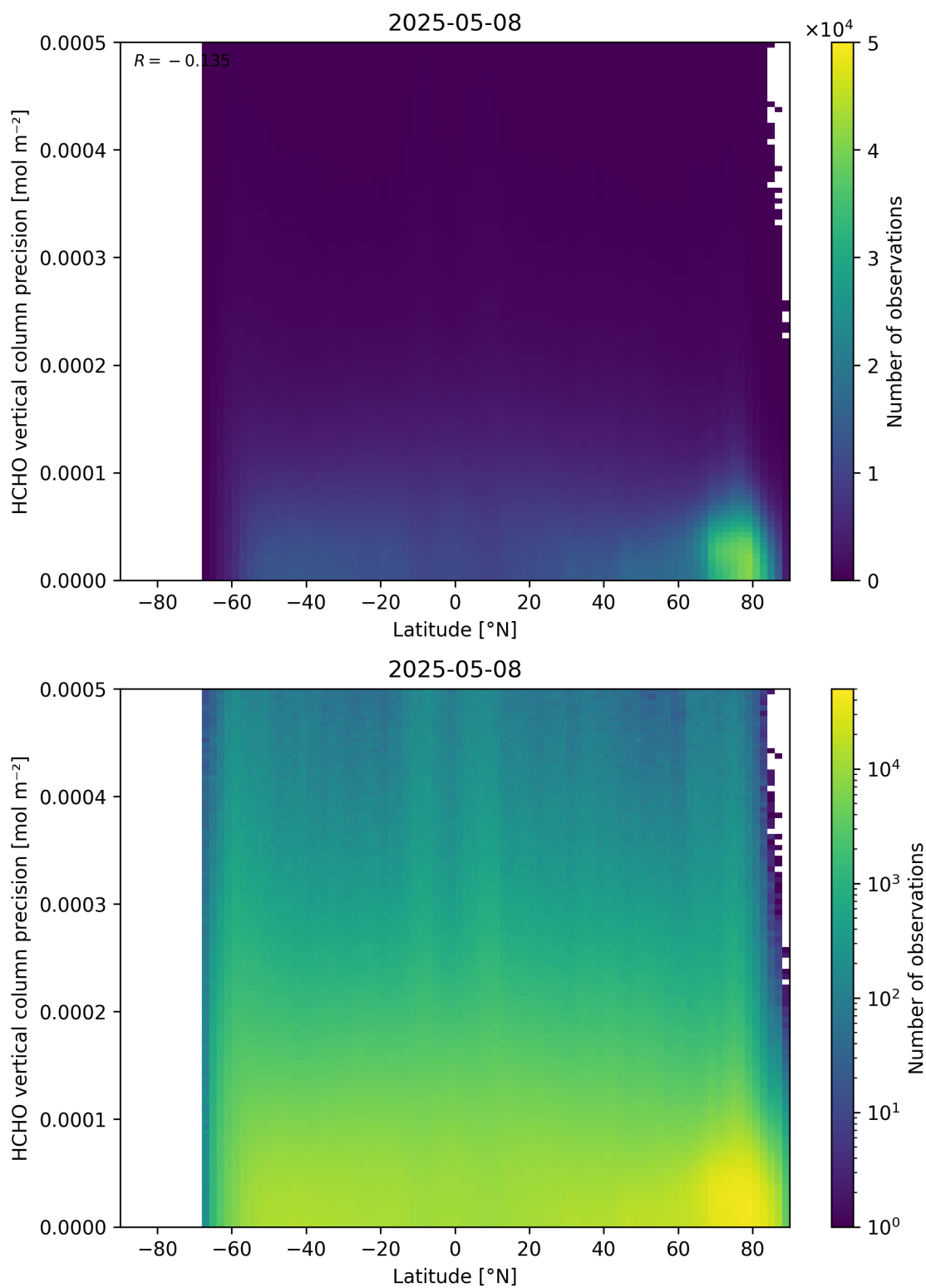
Figure 165: Scatter density plot of “Latitude” against “HCHO vertical column precision” for 2025-05-07 to 2025-05-09.
