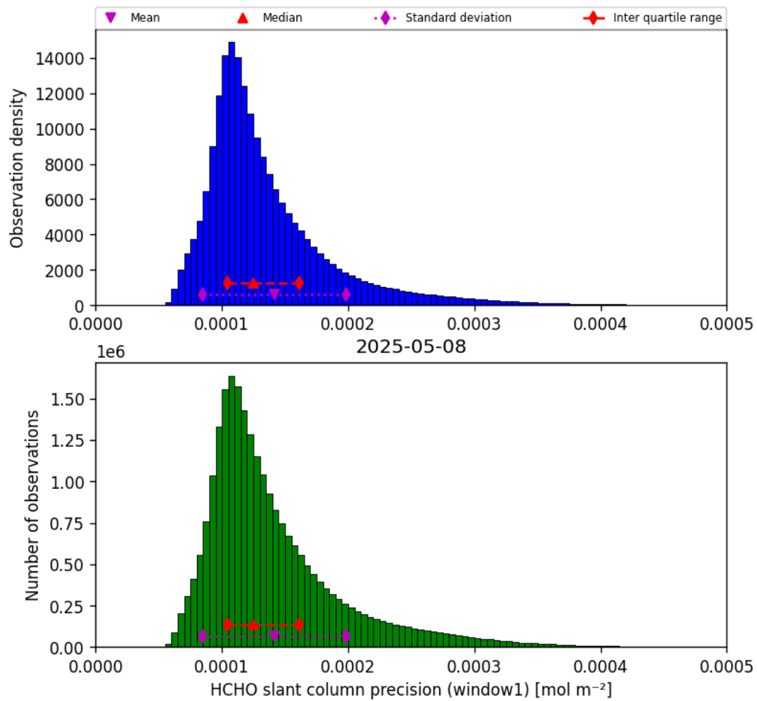
Figure 39: Histogram of “HCHO slant column precision (window1)” for 2025-05-07 to 2025-05-09
