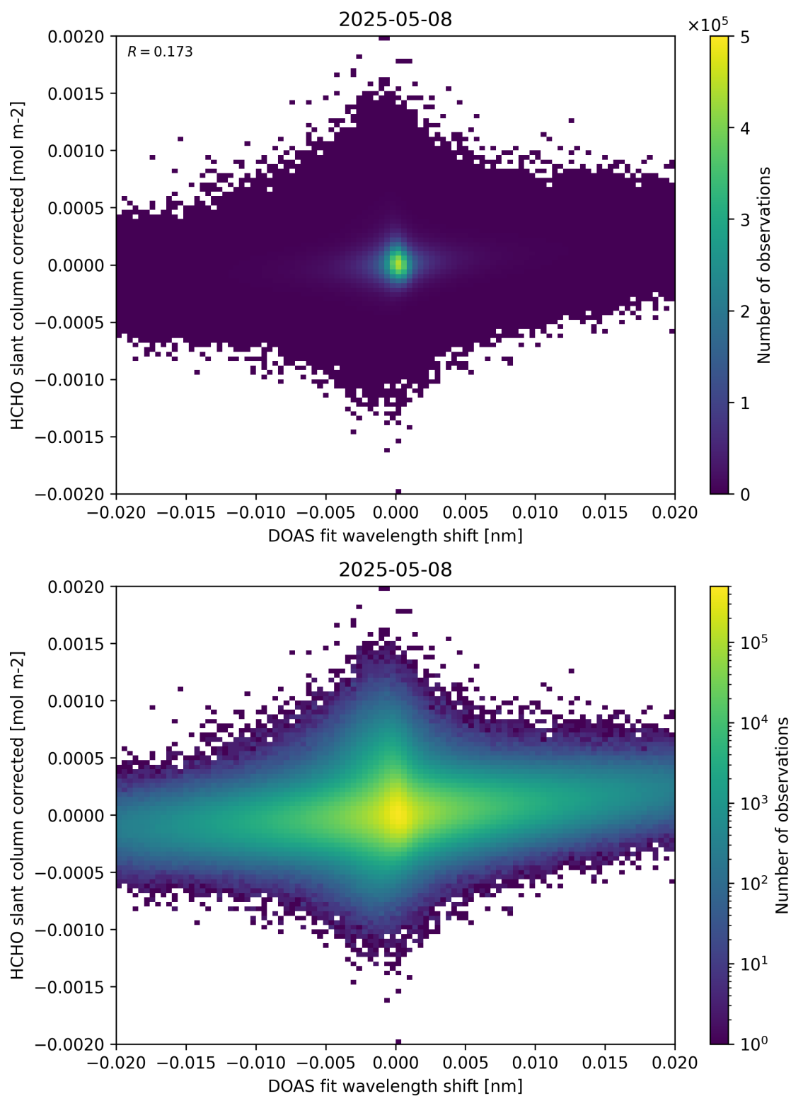
Figure 66: Scatter density plot of “DOAS fit wavelength shift” against “HCHO slant column corrected” for 2025-05-07 to 2025-05-09.
