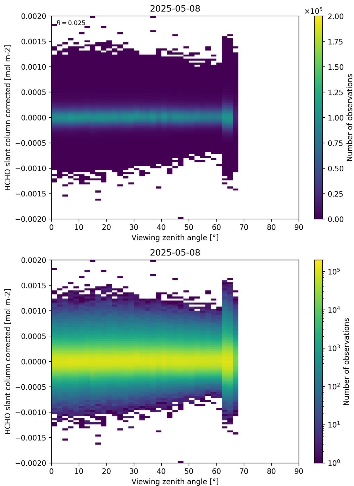
Figure 186: Scatter density plot of “Viewing zenith angle” against “HCHO slant column corrected” for 2025-05-07 to 2025-05-09.
