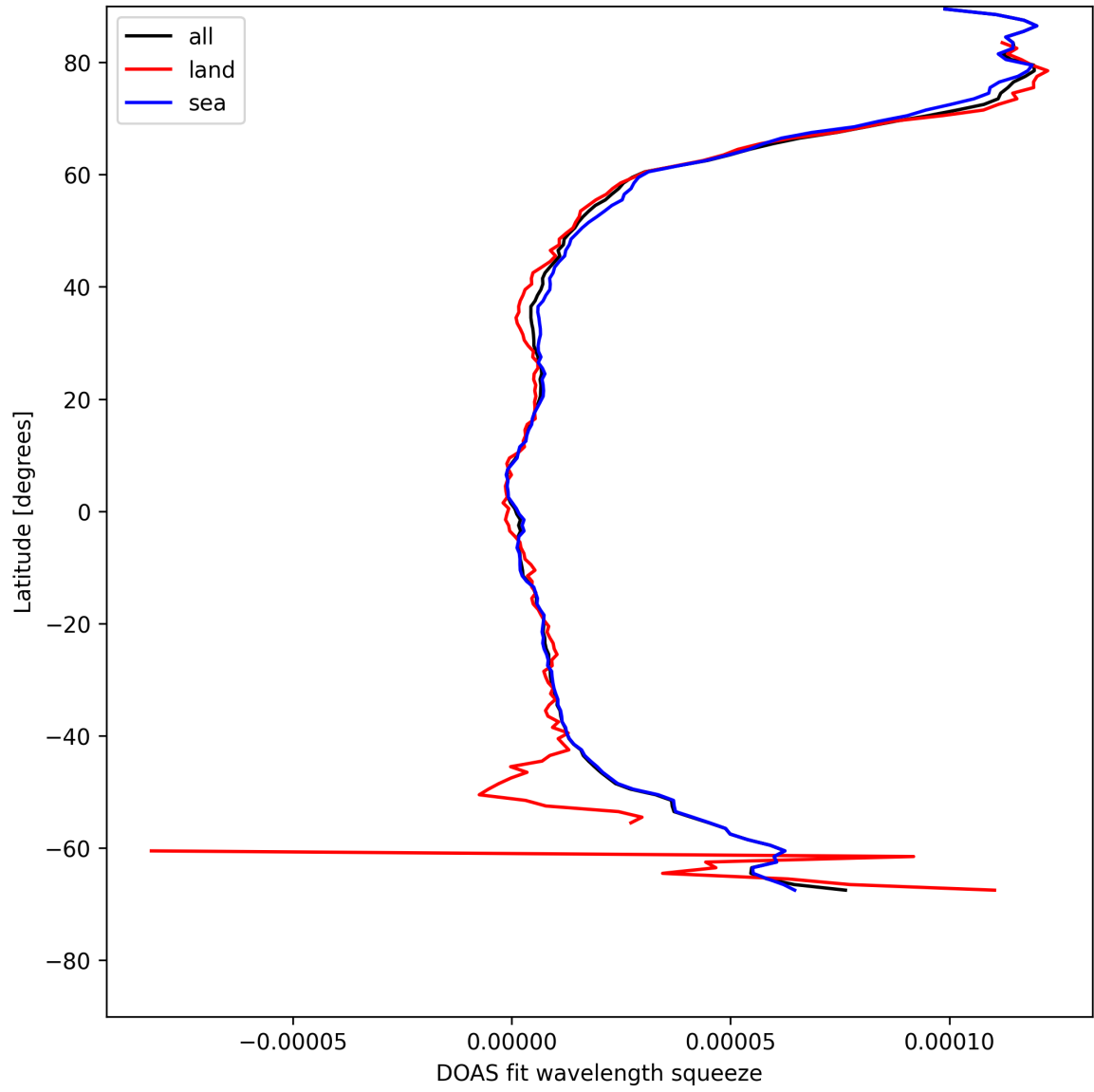
Figure 31: Zonal average of “DOAS fit wavelength squeeze” for 2025-05-07 to 2025-05-09.
