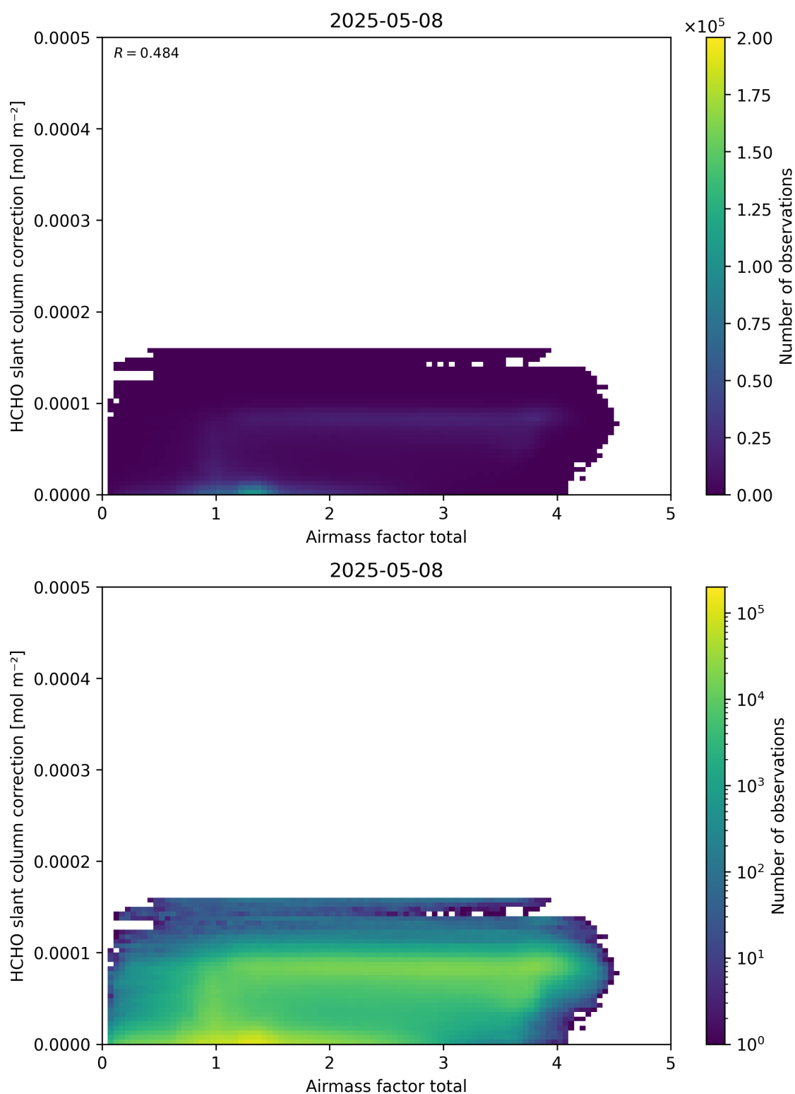
Figure 102: Scatter density plot of “Airmass factor total” against “HCHO slant column correction” for 2025-05-07 to 2025-05-09.
