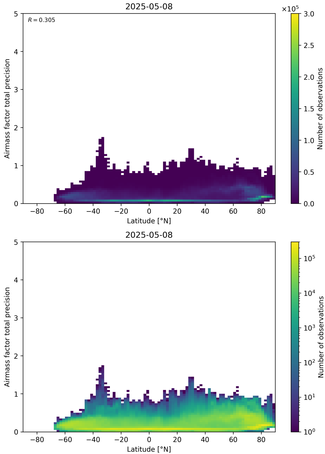
Figure 162: Scatter density plot of “Latitude” against “Airmass factor total precision” for 2025-05-07 to 2025-05-09.
