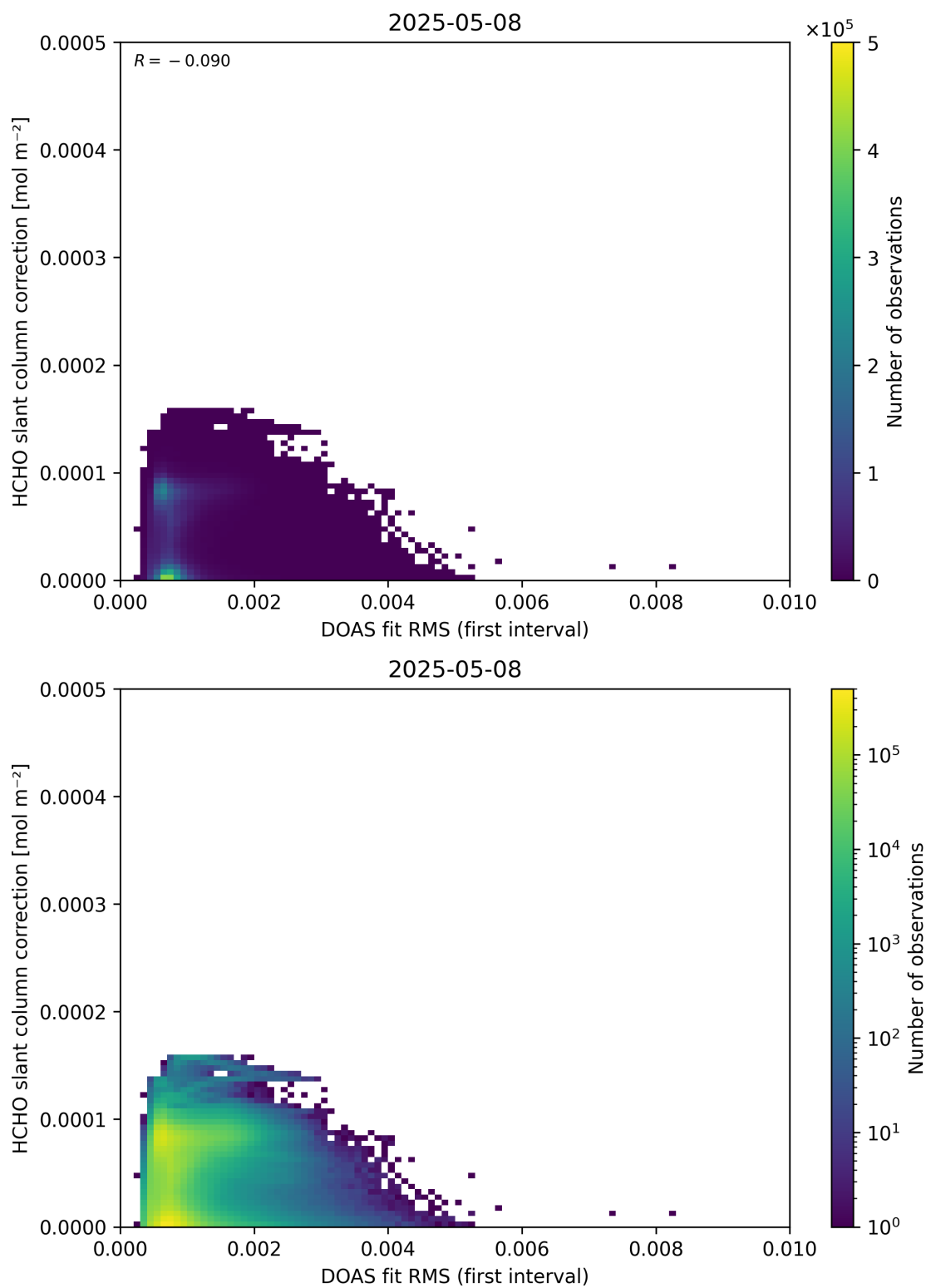
Figure 63: Scatter density plot of “DOAS fit RMS (first interval)” against “HCHO slant column correction” for 2025-05-07 to 2025-05-09.
