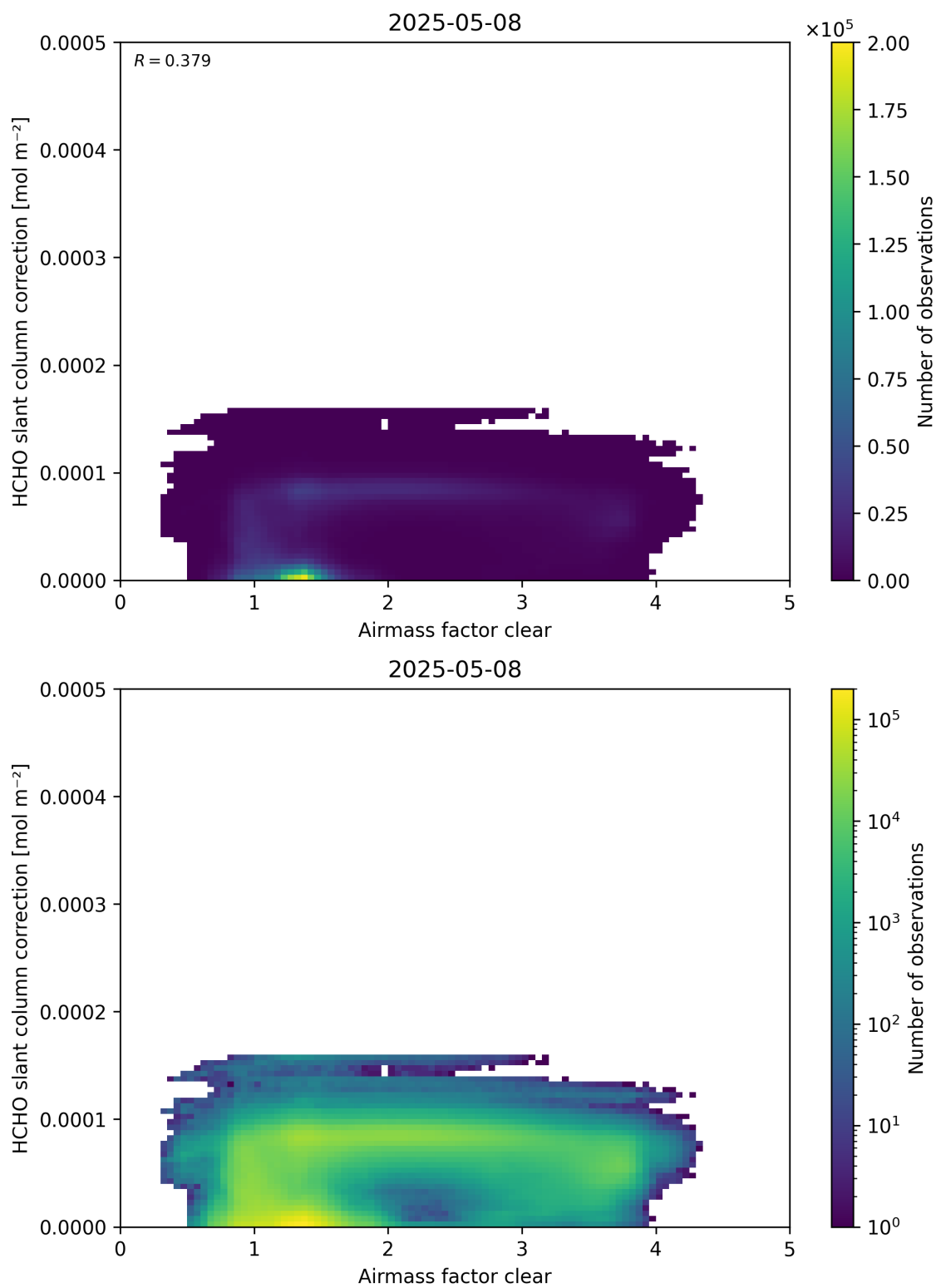
Figure 75: Scatter density plot of “Air mass factor clear” against “HCHO slant column correction” for 2025-05-07 to 2025-05-09.
