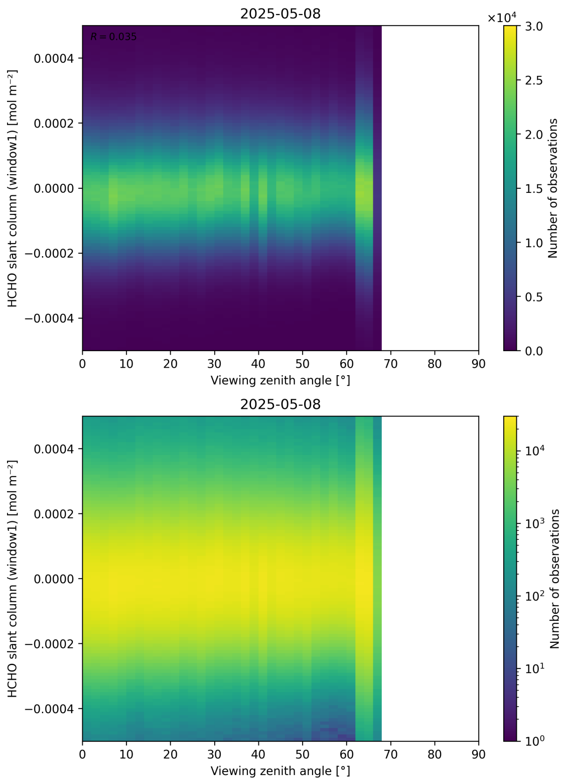
Figure 188: Scatter density plot of “Viewing zenith angle” against “HCHO slant column (window1)” for 2025-05-07 to 2025-05-09.
