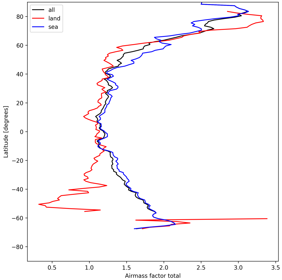
Figure 26: Zonal average of “Airmass factor total” for 2025-05-07 to 2025-05-09.
