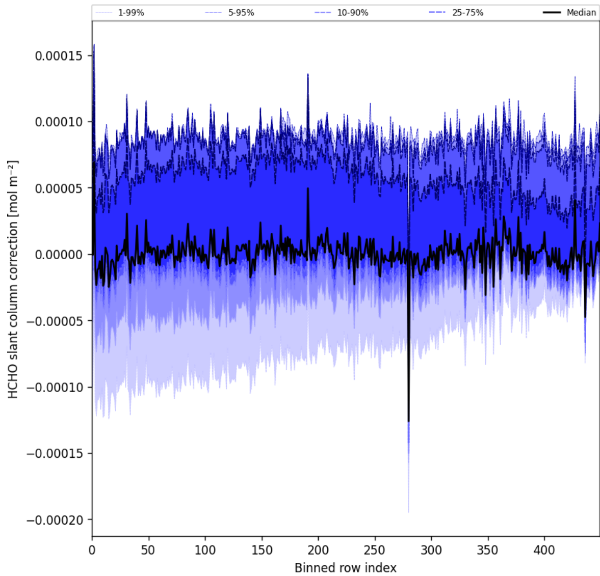
Figure 61: Along track statistics of “HCHO slant column correction” for 2025-05-07 to 2025-05-09
