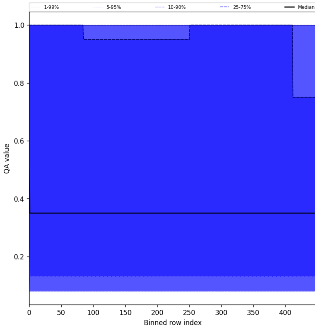
Figure 48: Along track statistics of “QA value” for 2025-05-07 to 2025-05-09
