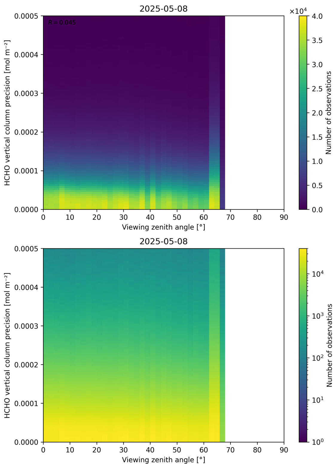
Figure 194: Scatter density plot of “Viewing zenith angle” against “HCHO vertical column precision” for 2025-05-07 to 2025-05-09.
