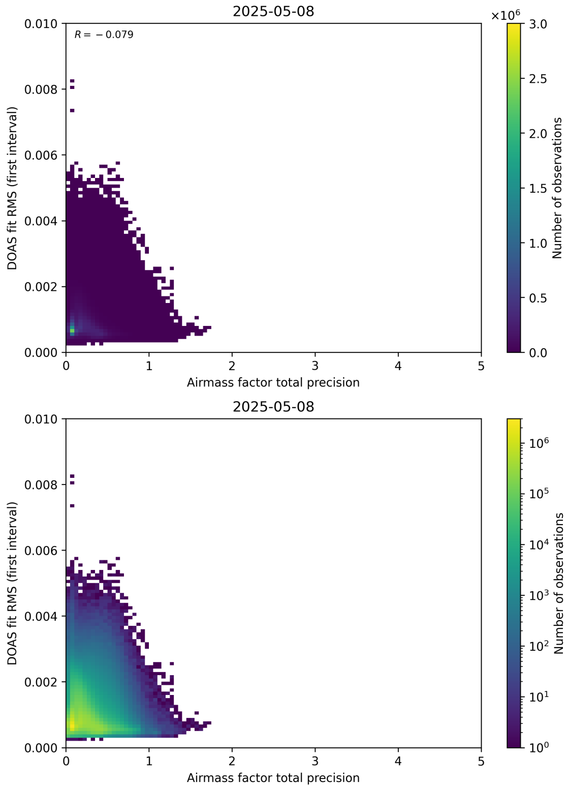
Figure 105: Scatter density plot of “Airmass factor total precision” against “DOAS fit RMS (first interval)” for 2025-05-07 to 2025-05-09.
