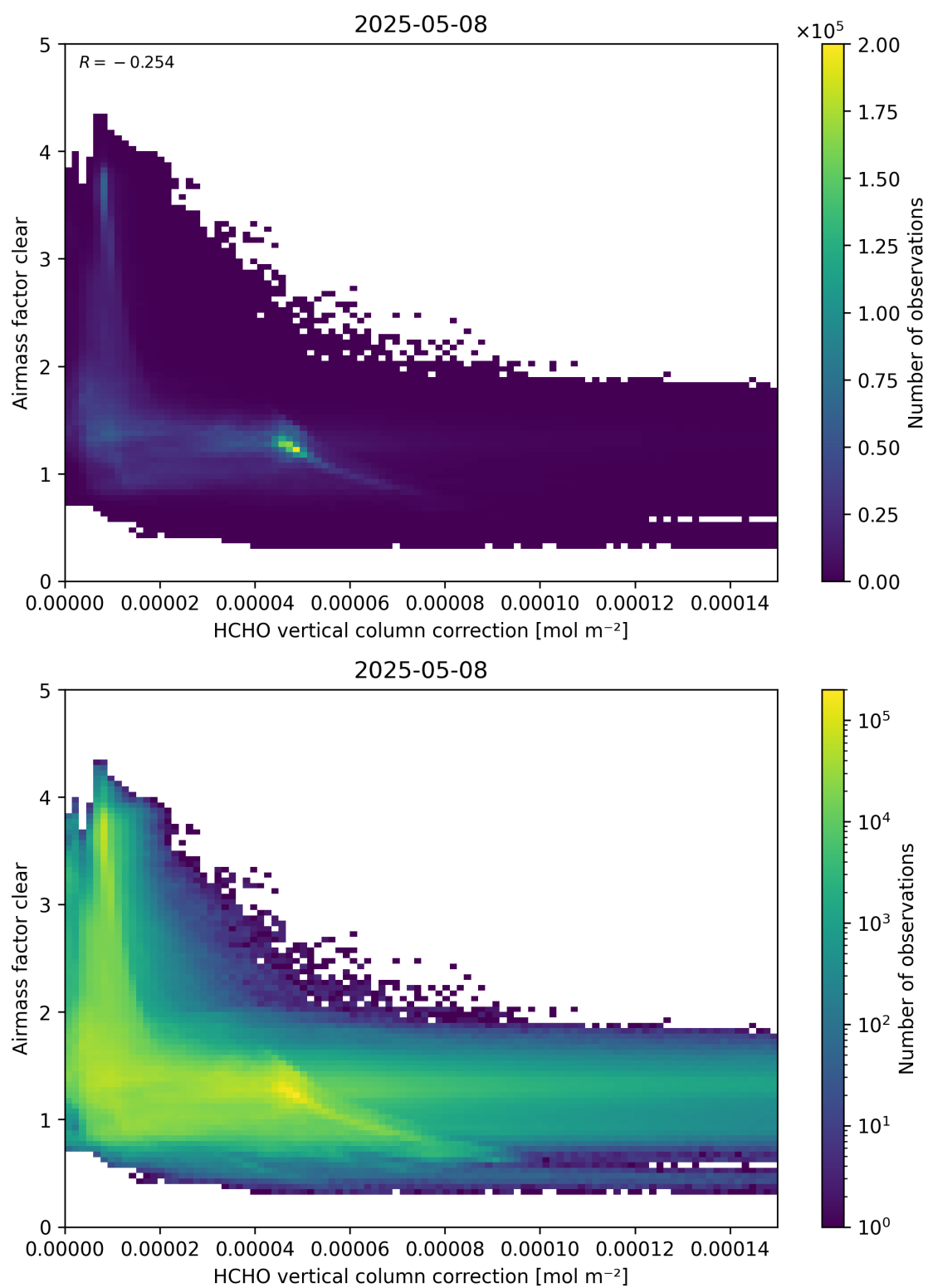
Figure 115: Scatter density plot of “HCHO vertical column correction” against “Airmass factor clear” for 2025-05-07 to 2025-05-09.
