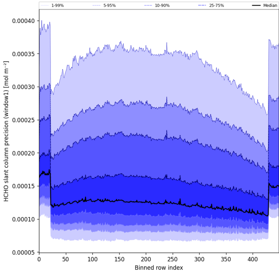
Figure 53: Along track statistics of “HCHO slant column precision (window1)” for 2025-05-07 to 2025-05-09
