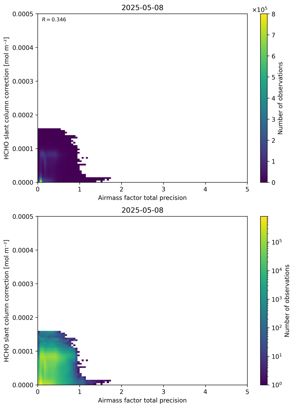
Figure 110: Scatter density plot of “Airmass factor total precision” against “HCHO slant column correction” for 2025-05-07 to 2025-05-09.
