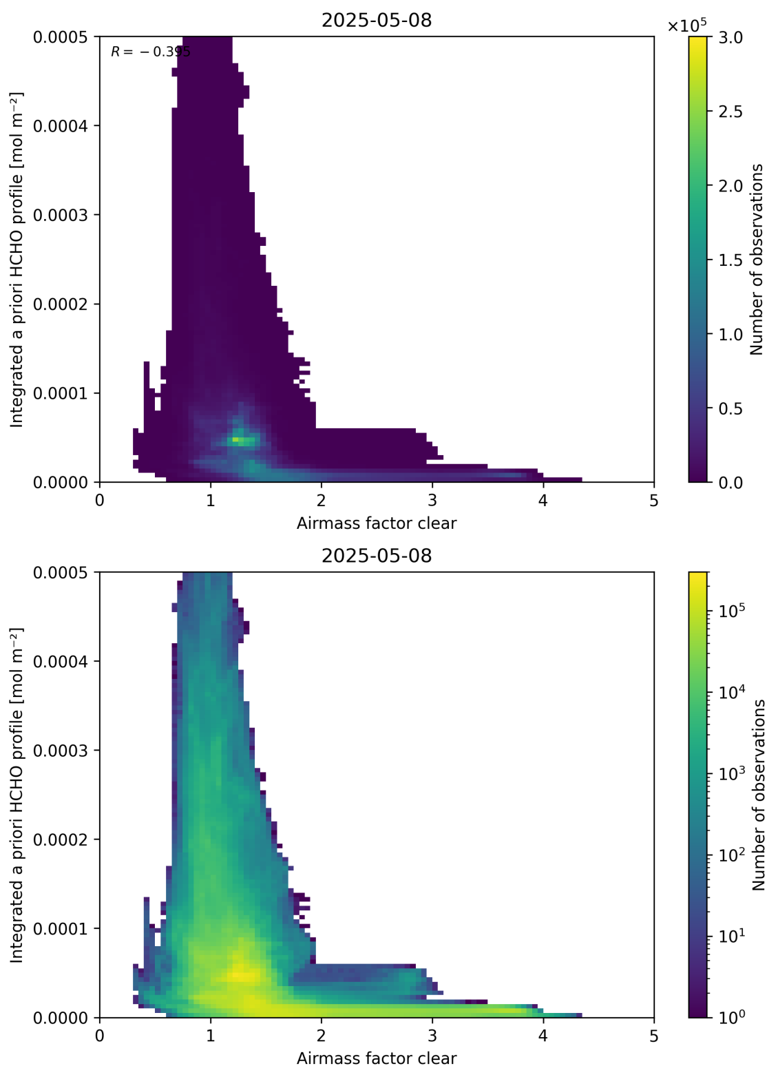
Figure 76: Scatter density plot of “Airmass factor clear” against “Integrated a priori HCHO profile” for 2025-05-07 to 2025-05-09.
