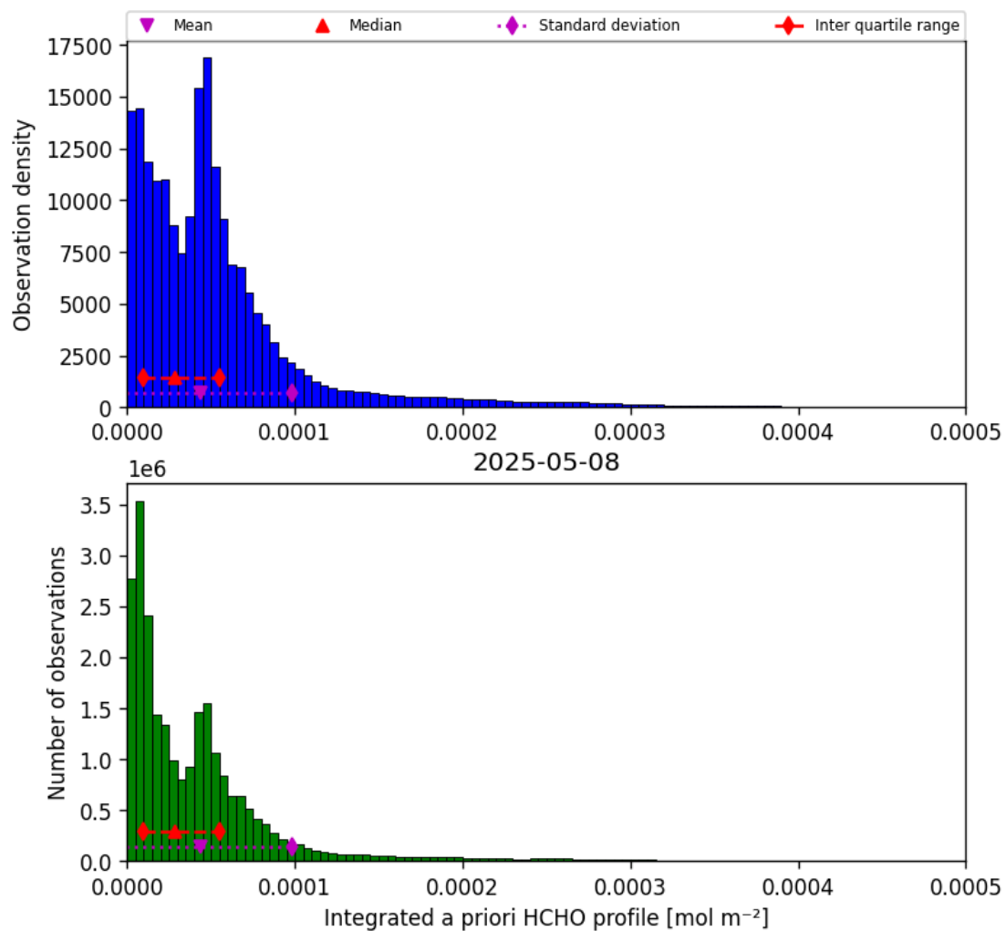
Figure 43: Histogram of “Integrated a priori HCHO profile” for 2025-05-07 to 2025-05-09
