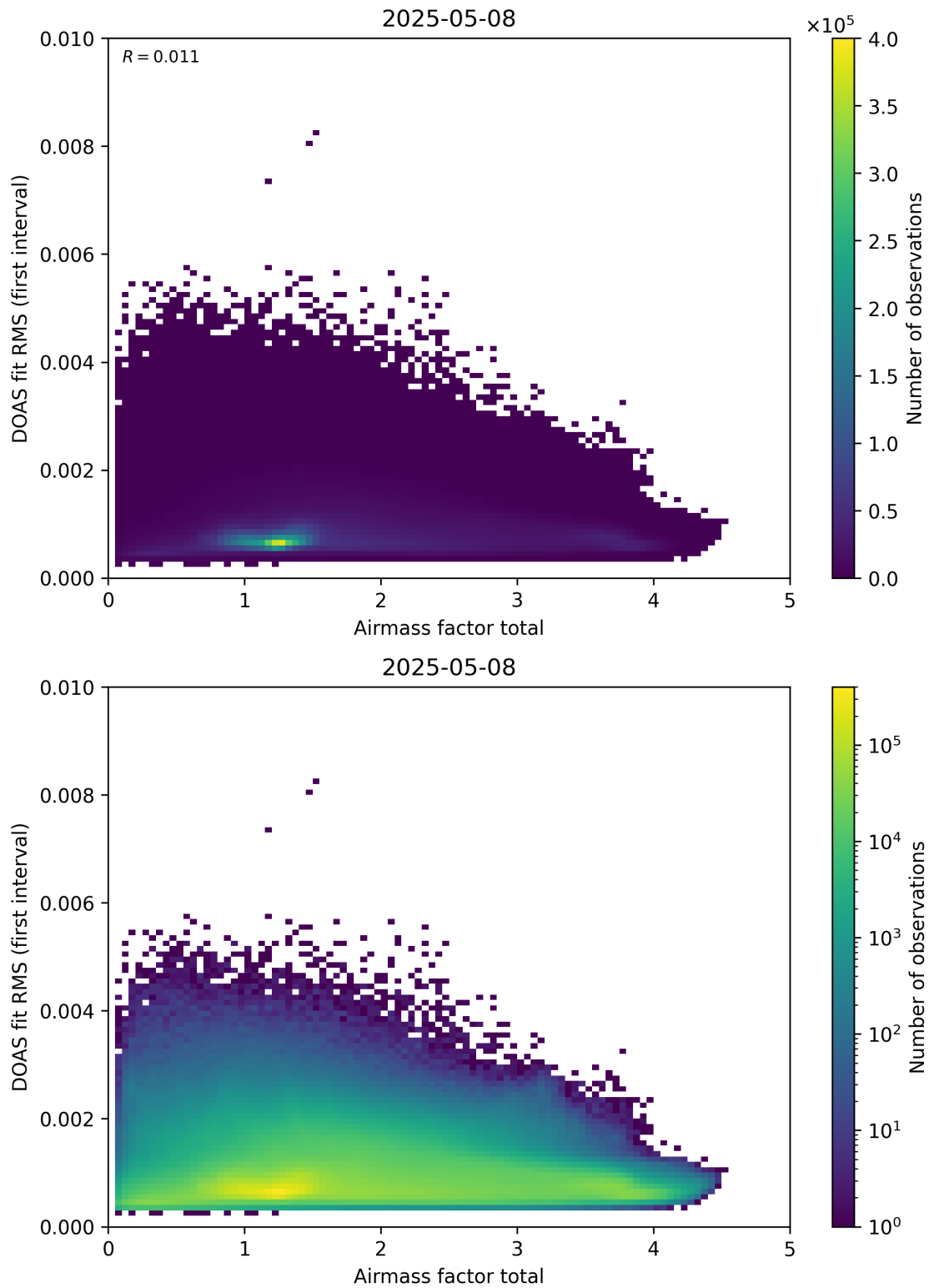
Figure 97: Scatter density plot of “Airmass factor total” against “DOAS fit RMS (first interval)” for 2025-05-07 to 2025-05-09.
