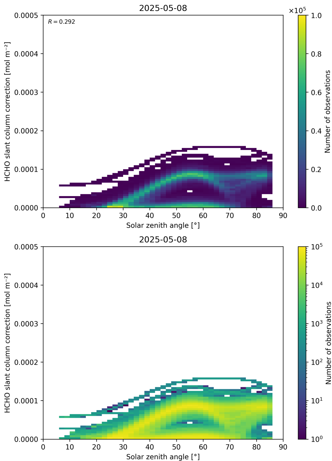
Figure 172: Scatter density plot of “Solar zenith angle” against “HCHO slant column correction” for 2025-05-07 to 2025-05-09.
