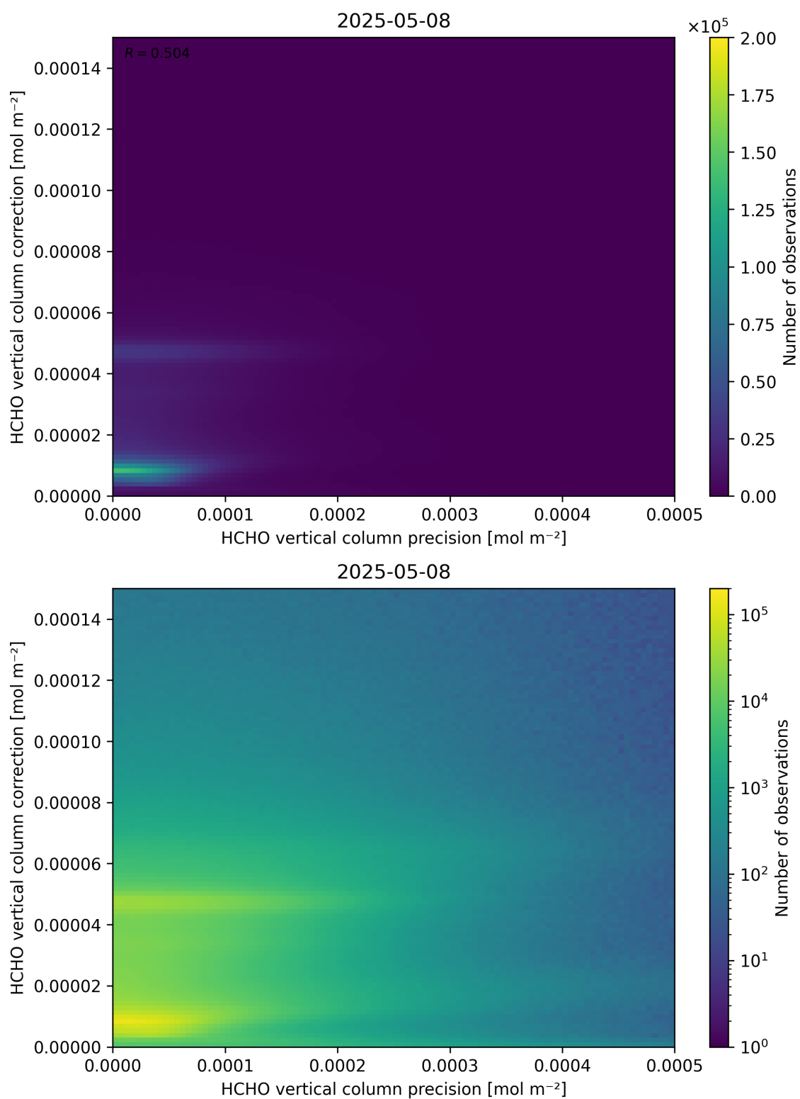
Figure 146: Scatter density plot of “HCHO vertical column precision” against “HCHO vertical column correction” for 2025-05-07 to 2025-05-09.
