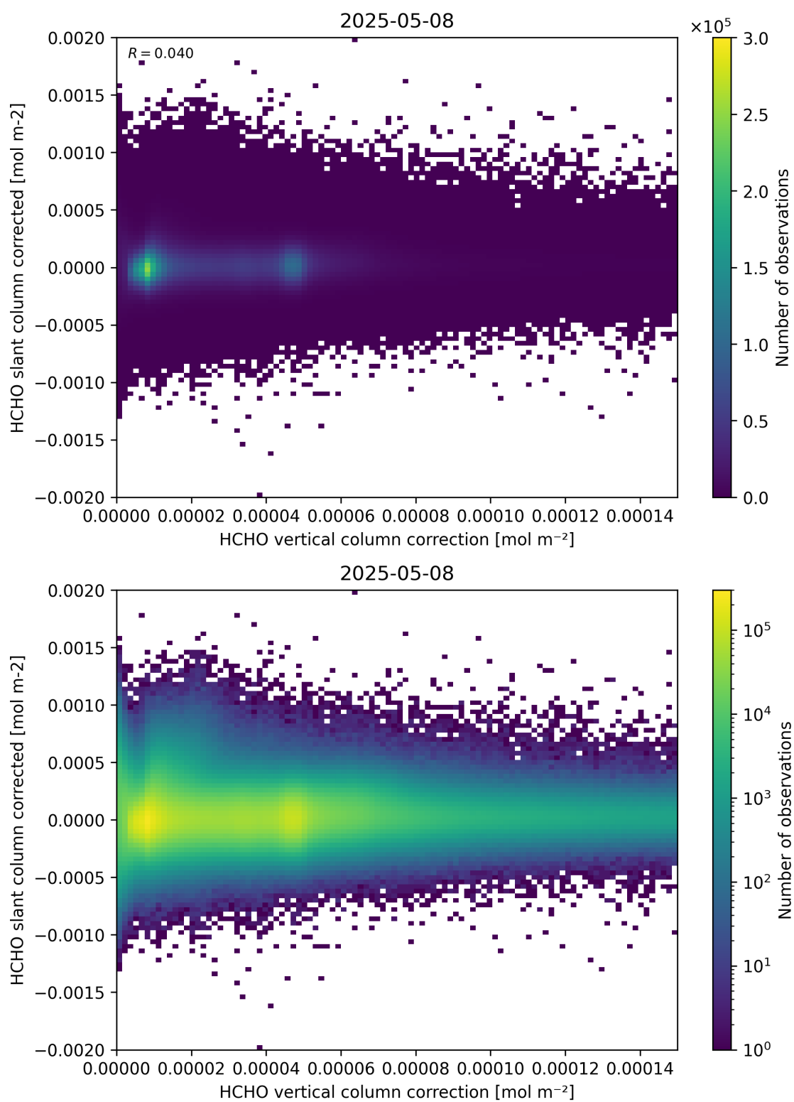
Figure 116: Scatter density plot of “HCHO vertical column correction” against “HCHO slant column corrected” for 2025-05-07 to 2025-05-09.
