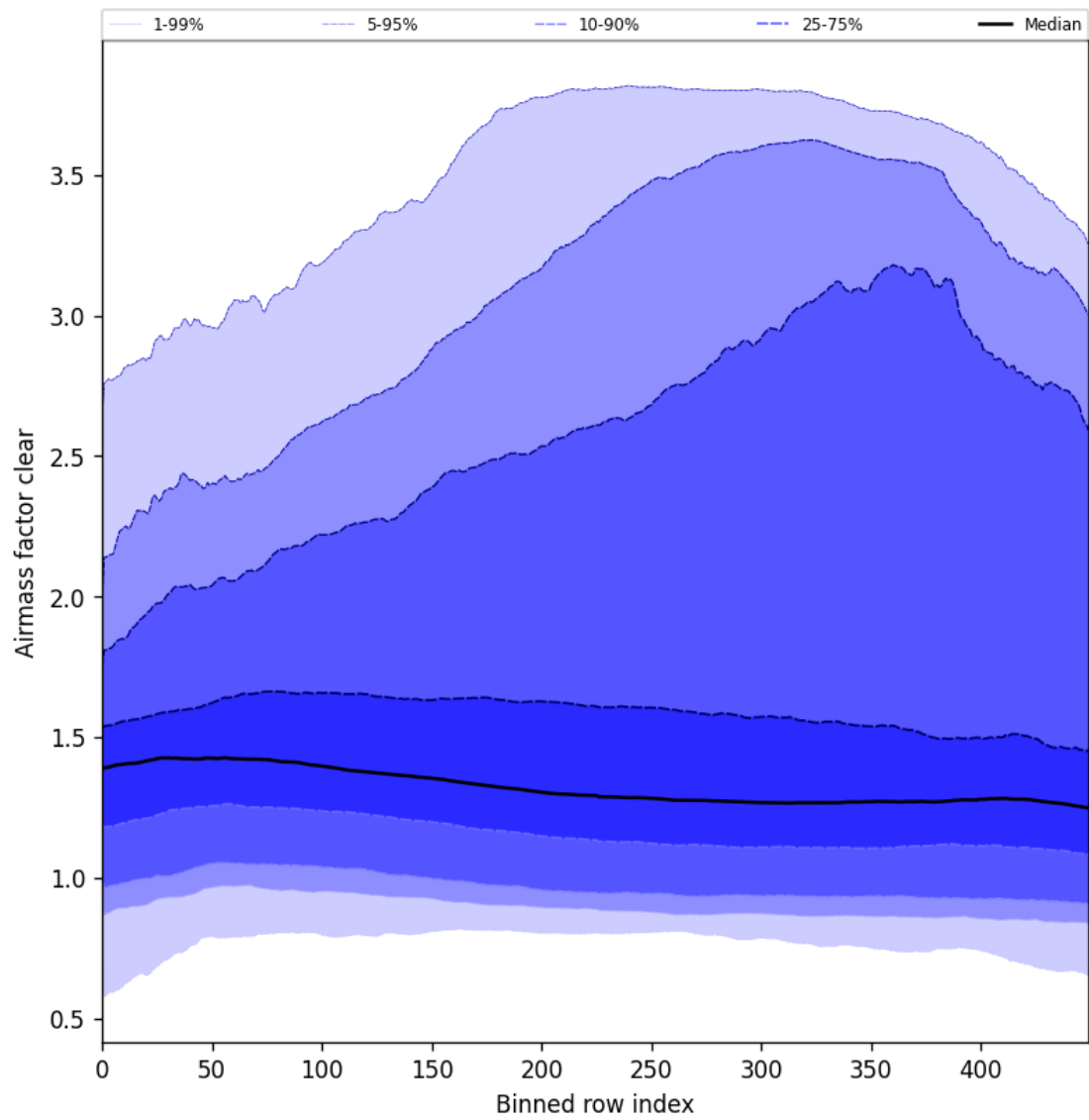
Figure 56: Along track statistics of “Airmass factor clear” for 2025-05-07 to 2025-05-09
