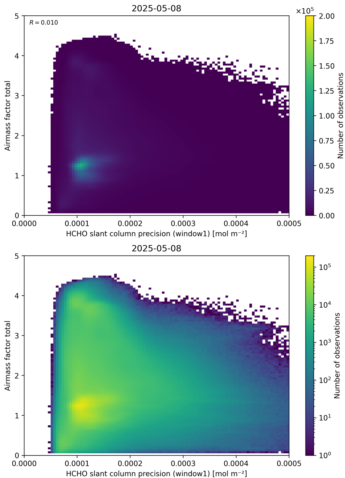
Figure 94: Scatter density plot of “HCHO slant column precision (window1)” against “Airmass factor total” for 2025-05-07 to 2025-05-09.
