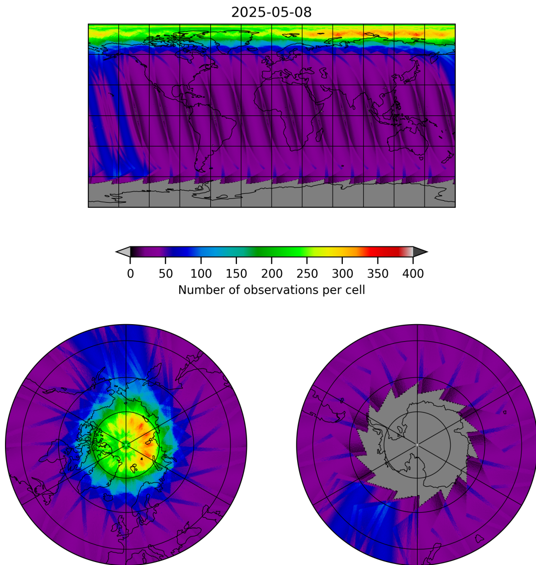
Figure 19: Map of the number of observations for 2025-05-07 to 2025-05-09
