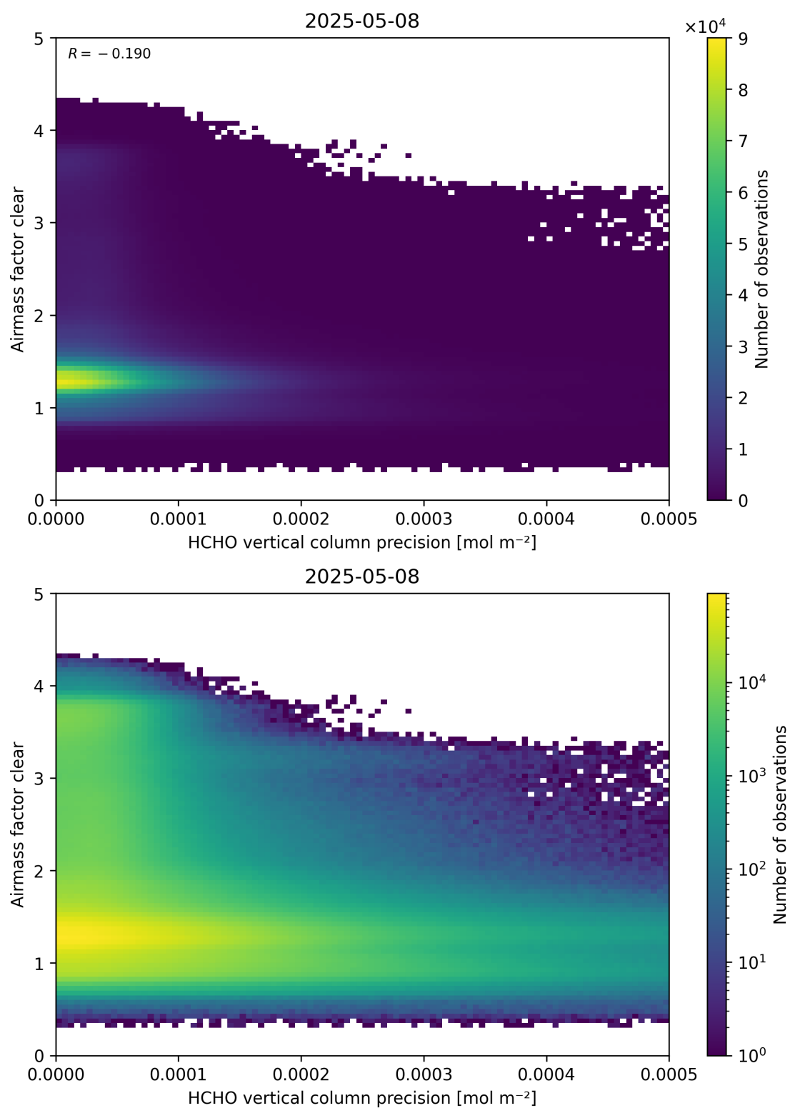
Figure 139: Scatter density plot of “HCHO vertical column precision” against “Airmass factor clear” for 2025-05-07 to 2025-05-09.
