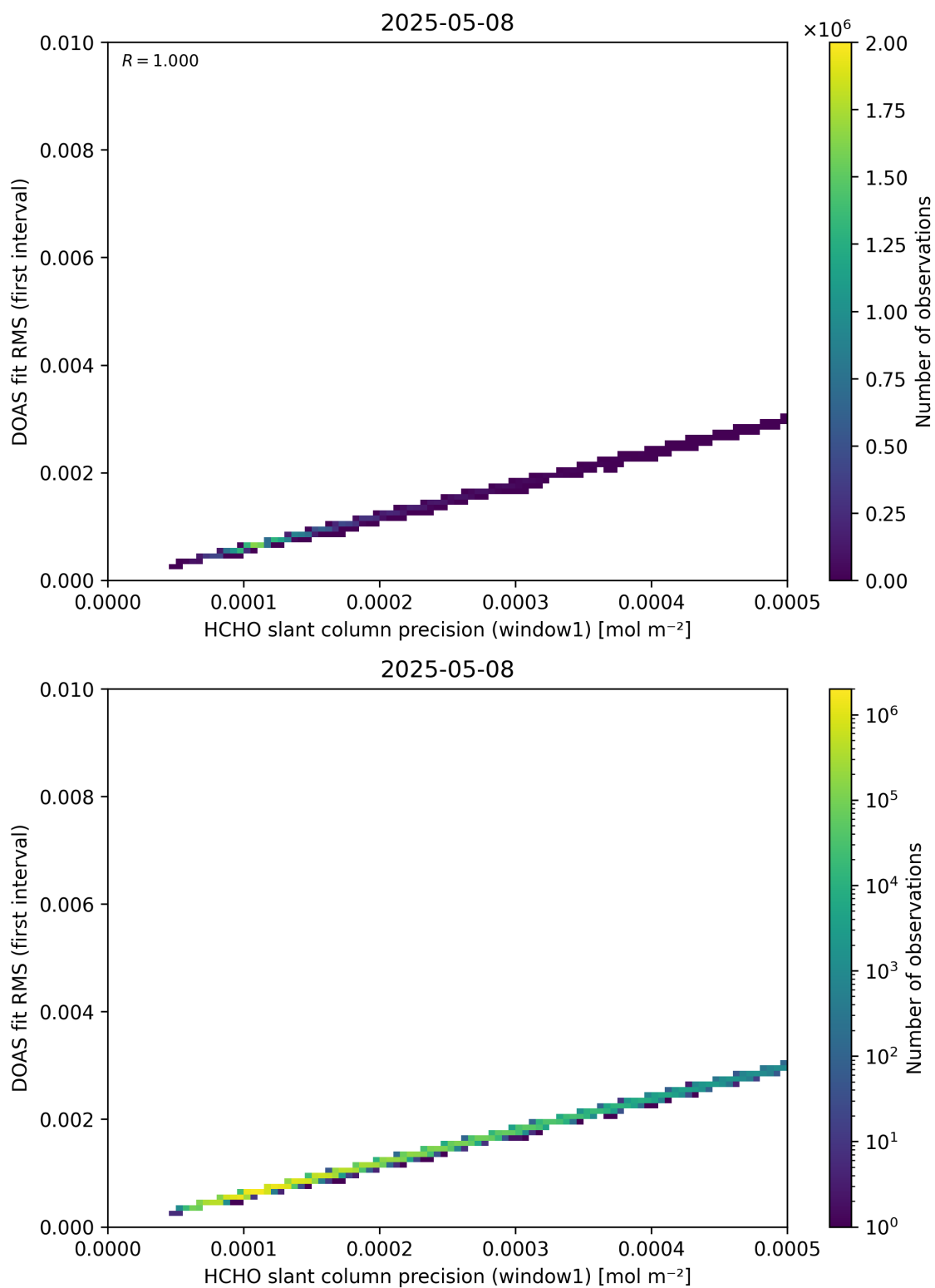
Figure 88: Scatter density plot of “HCHO slant column precision (window1)” against “DOAS fit RMS (first interval)” for 2025-05-07 to 2025-05-09.
