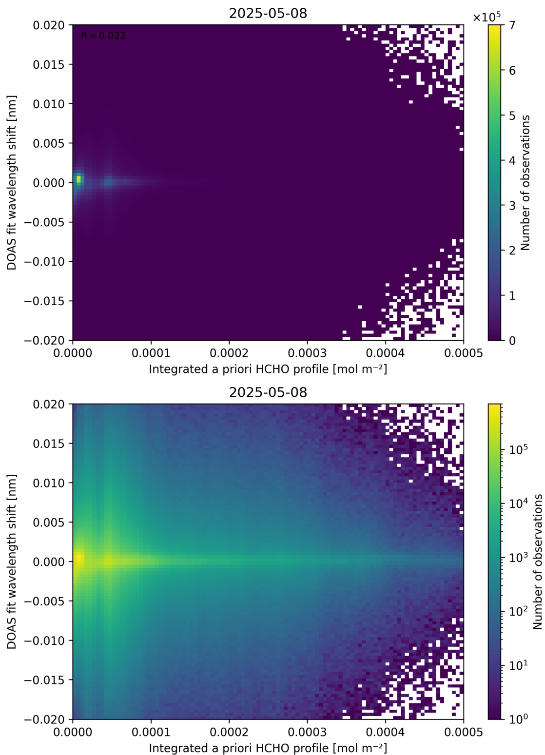
Figure 149: Scatter density plot of “Integrated a priori HCHO profile” against “DOAS fit wavelength shift” for 2025-05-07 to 2025-05-09.
