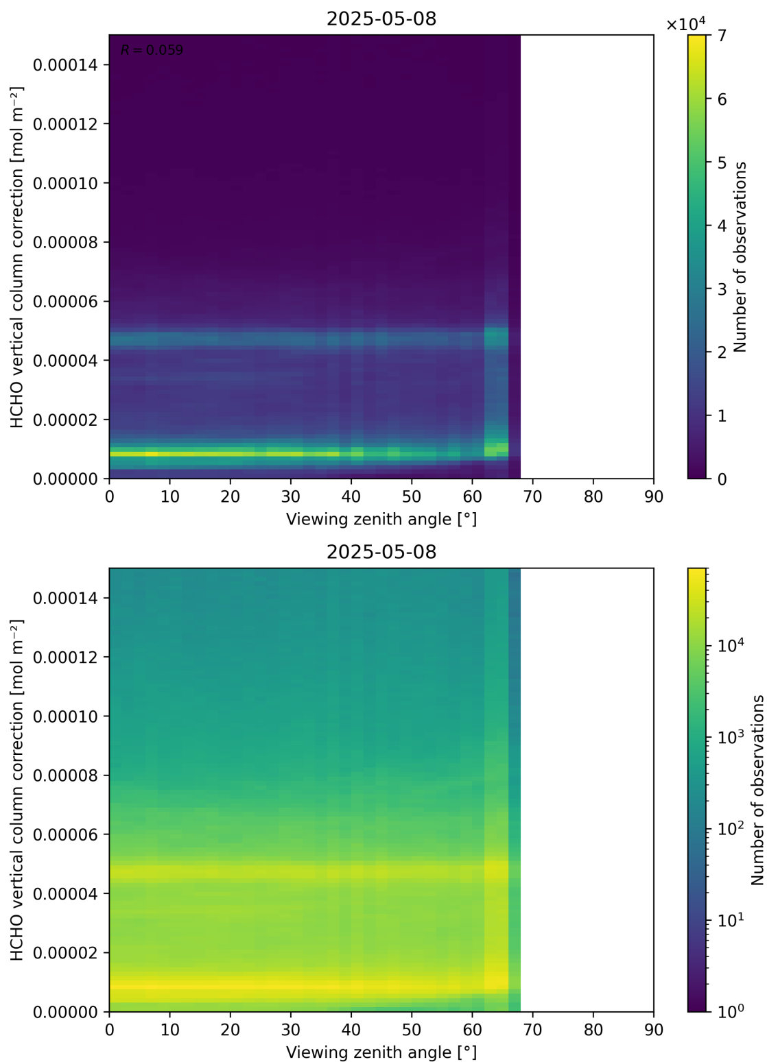
Figure 193: Scatter density plot of “Viewing zenith angle” against “HCHO vertical column correction” for 2025-05-07 to 2025-05-09.
