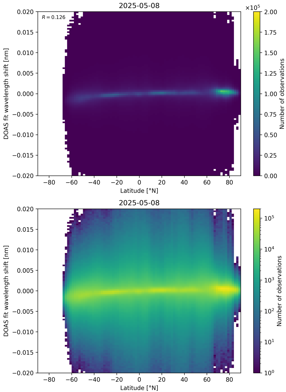
Figure 154: Scatter density plot of “Latitude” against “DOAS fit wavelength shift” for 2025-05-07 to 2025-05-09.
