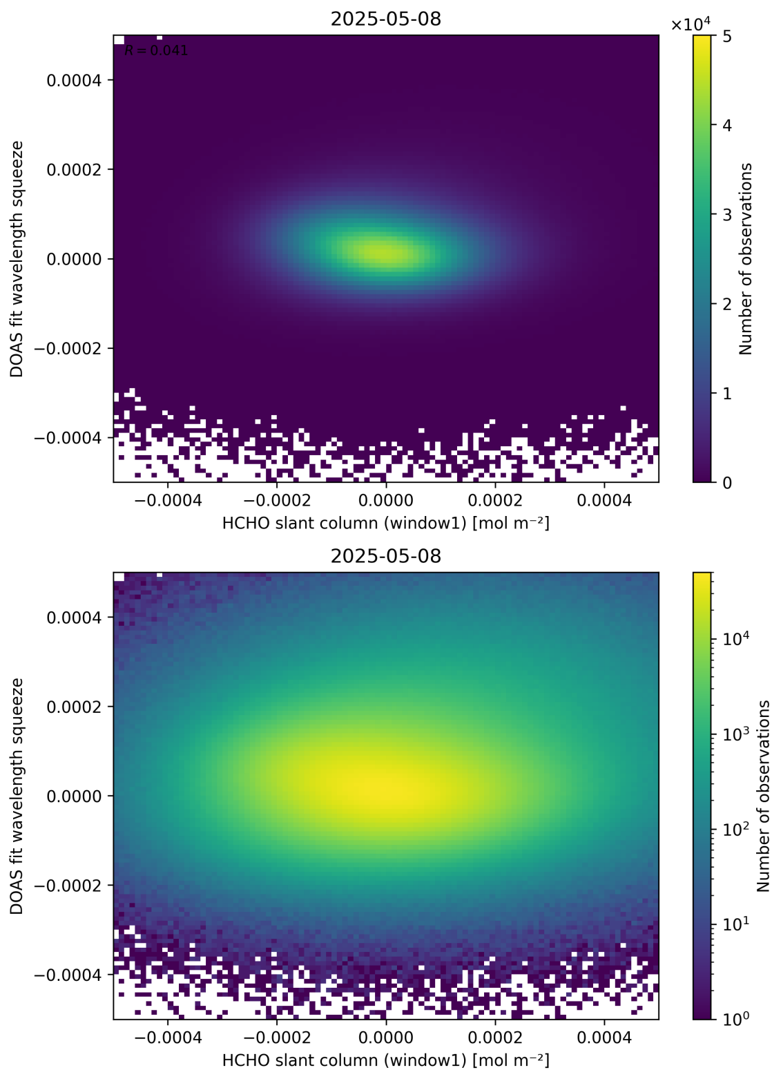
Figure 80: Scatter density plot of “HCHO slant column (window1)” against “DOAS fit wavelength squeeze” for 2025-05-07 to 2025-05-09.
