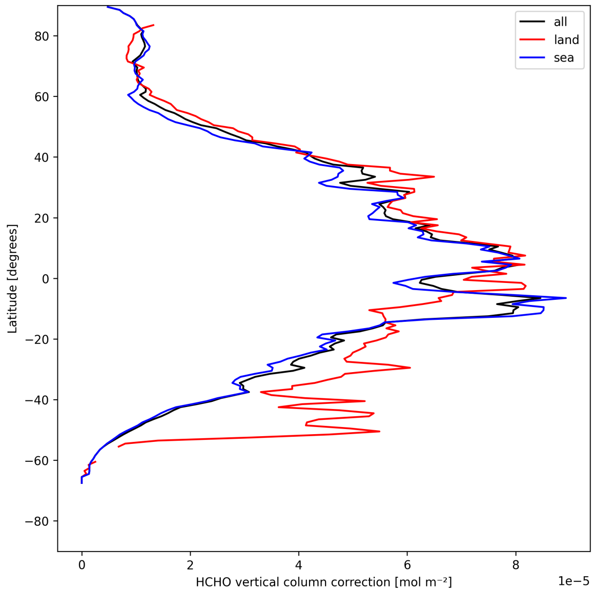
Figure 23: Zonal average of “HCHO vertical column correction” for 2025-05-07 to 2025-05-09.
