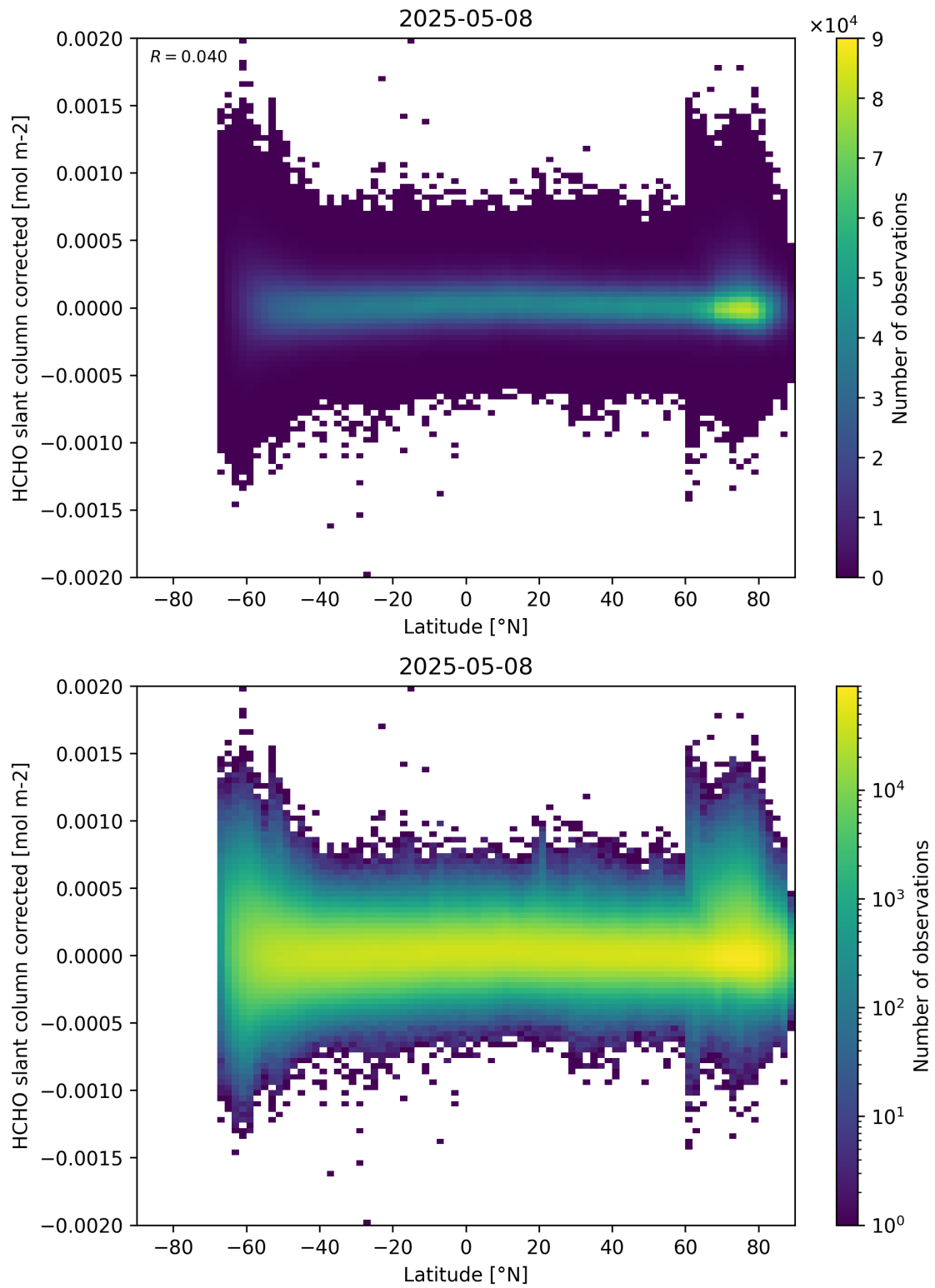
Figure 157: Scatter density plot of “Latitude” against “HCHO slant column corrected” for 2025-05-07 to 2025-05-09.
