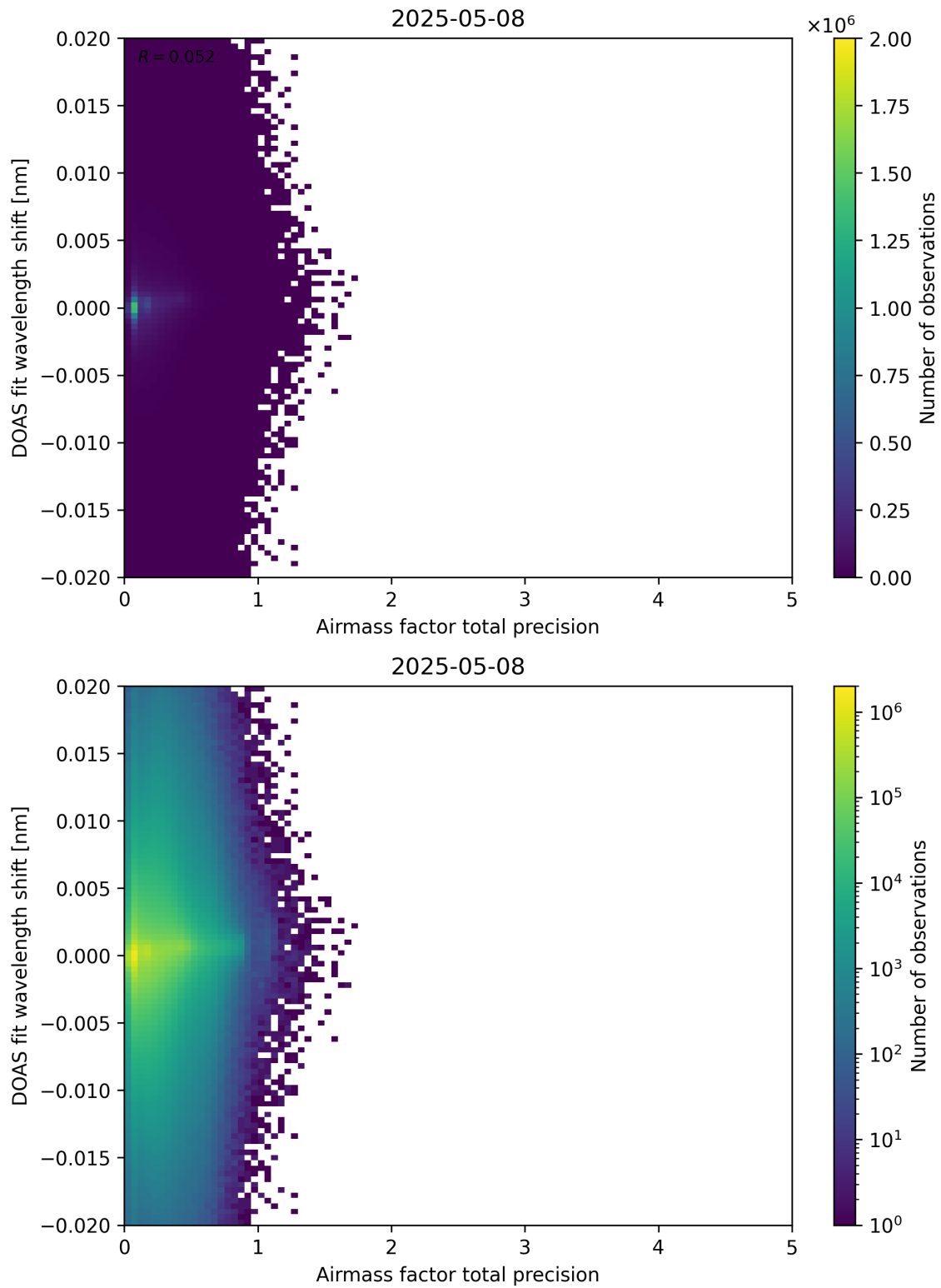
Figure 106: Scatter density plot of “Airmass factor total precision” against “DOAS fit wavelength shift” for 2025-05-07 to 2025-05-09.
