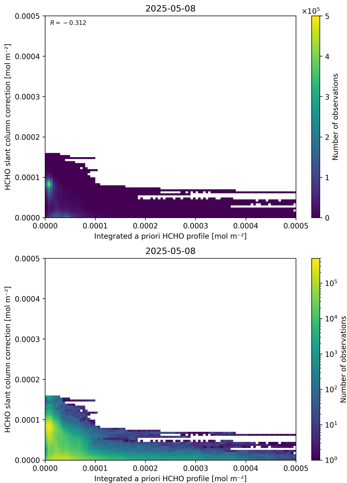
Figure 152: Scatter density plot of “Integrated a priori HCHO profile” against “HCHO slant column correction” for 2025-05-07 to 2025-05-09.
