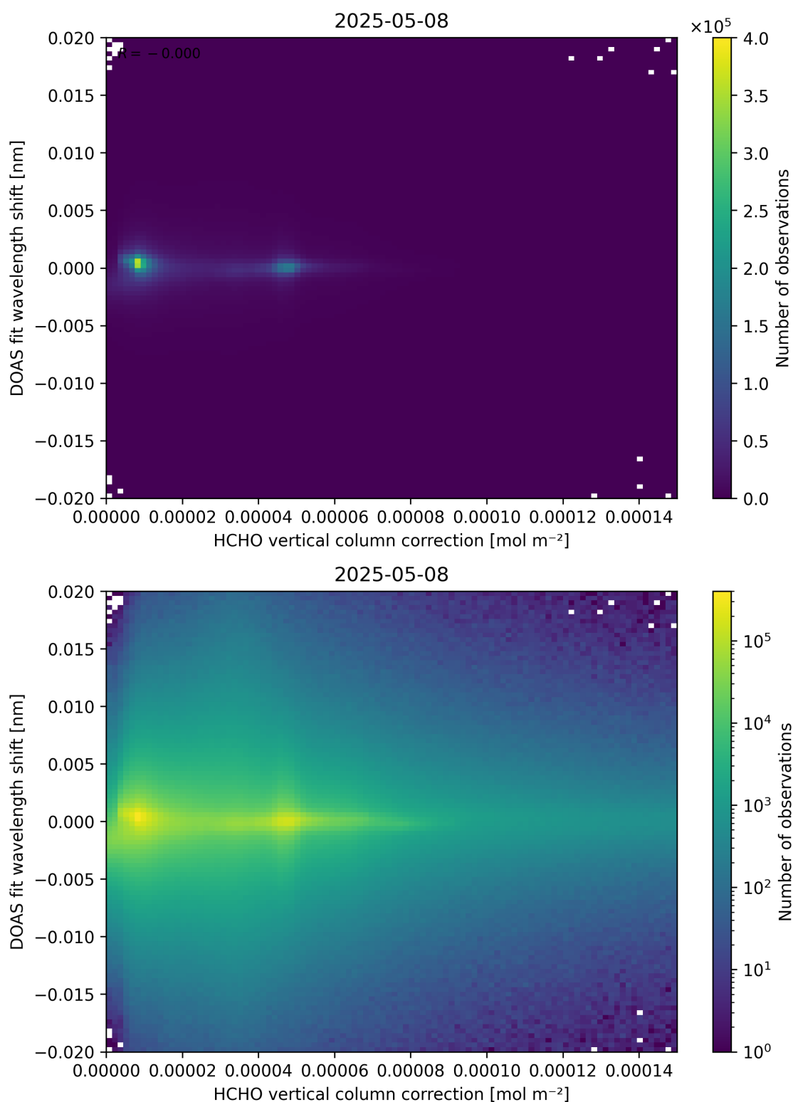
Figure 113: Scatter density plot of “HCHO vertical column correction” against “DOAS fit wavelength shift” for 2025-05-07 to 2025-05-09.
