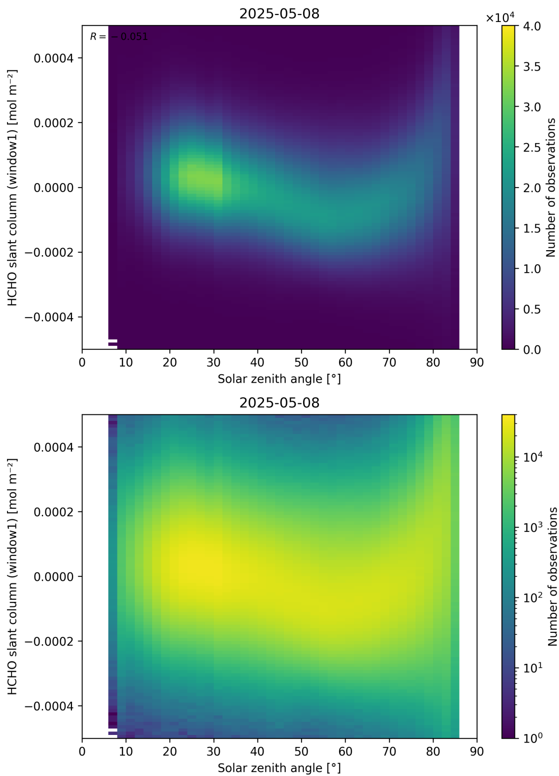
Figure 173: Scatter density plot of “Solar zenith angle” against “HCHO slant column (window1)” for 2025-05-07 to 2025-05-09.
