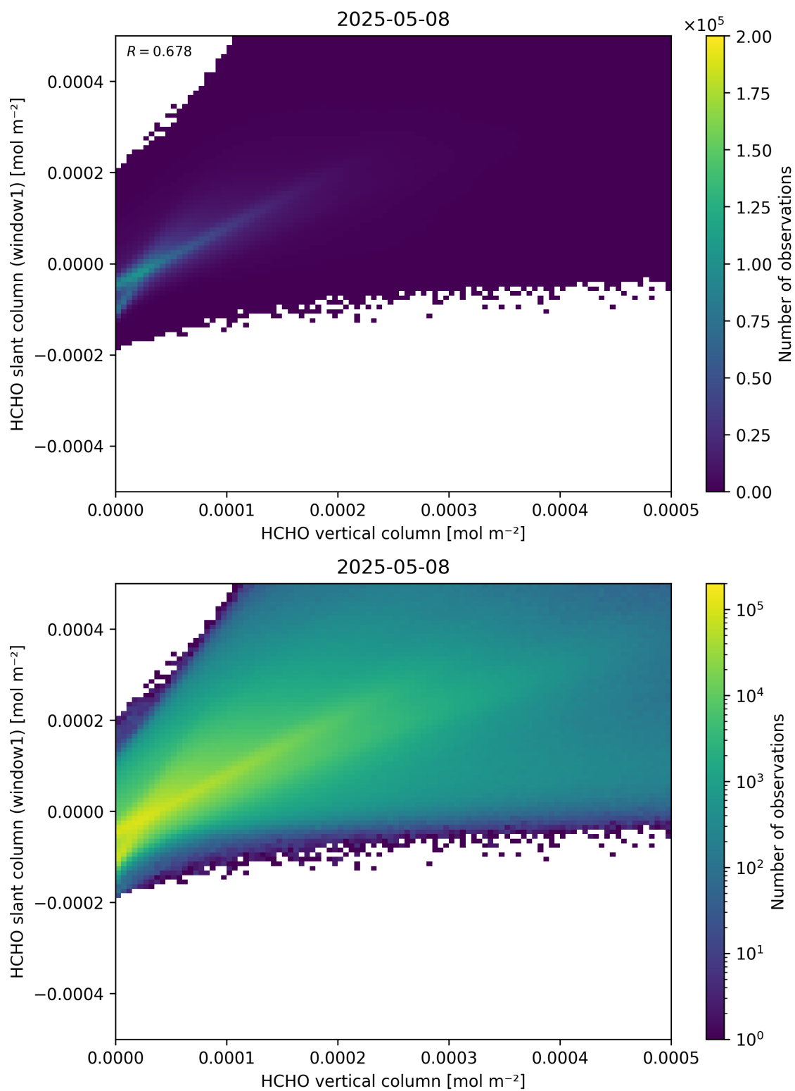
Figure 129: Scatter density plot of “HCHO vertical column” against “HCHO slant column (window1)” for 2025-05-07 to 2025-05-09.
