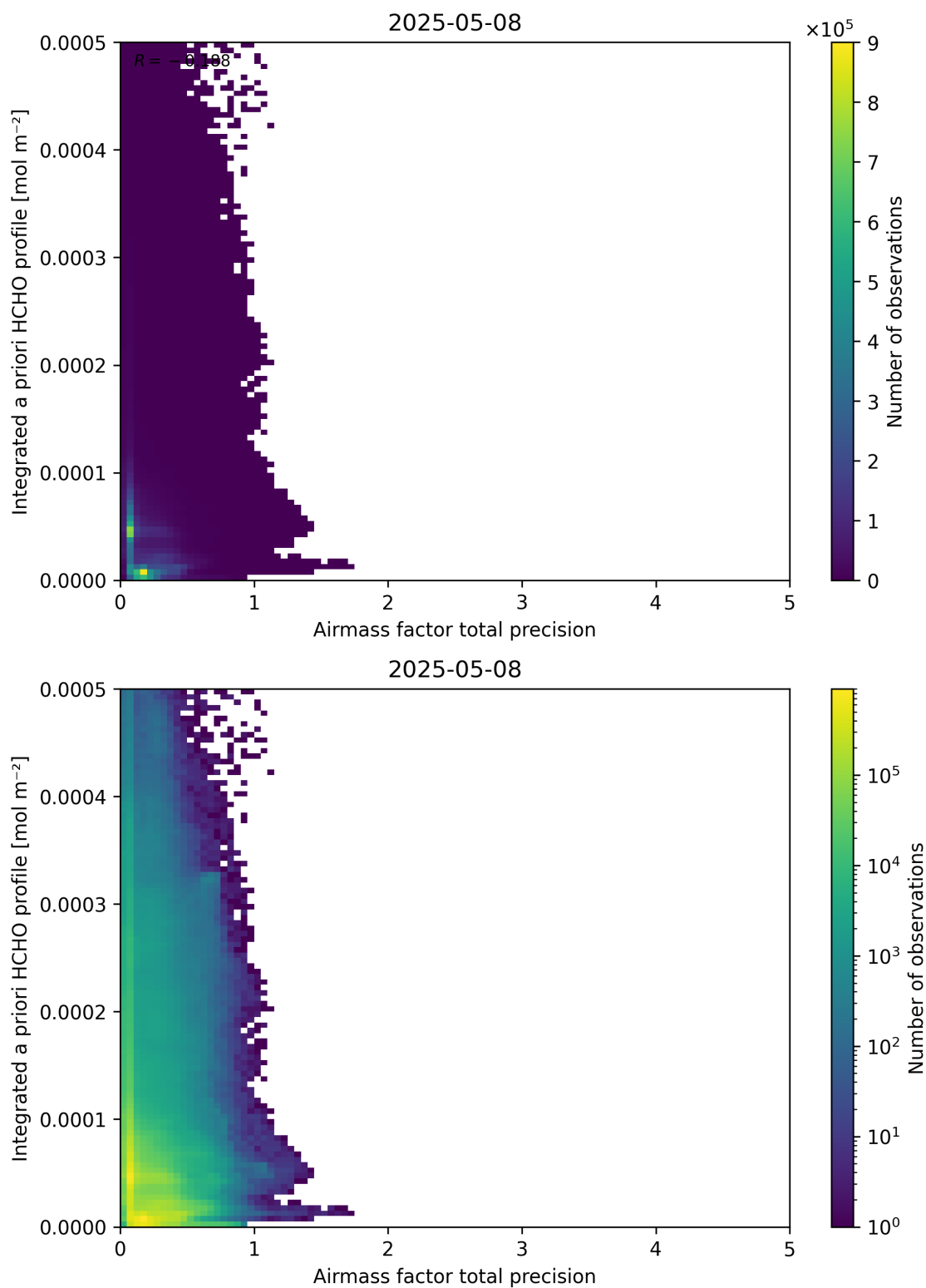
Figure 111: Scatter density plot of “Airmass factor total precision” against “Integrated a priori HCHO profile” for 2025-05-07 to 2025-05-09.
