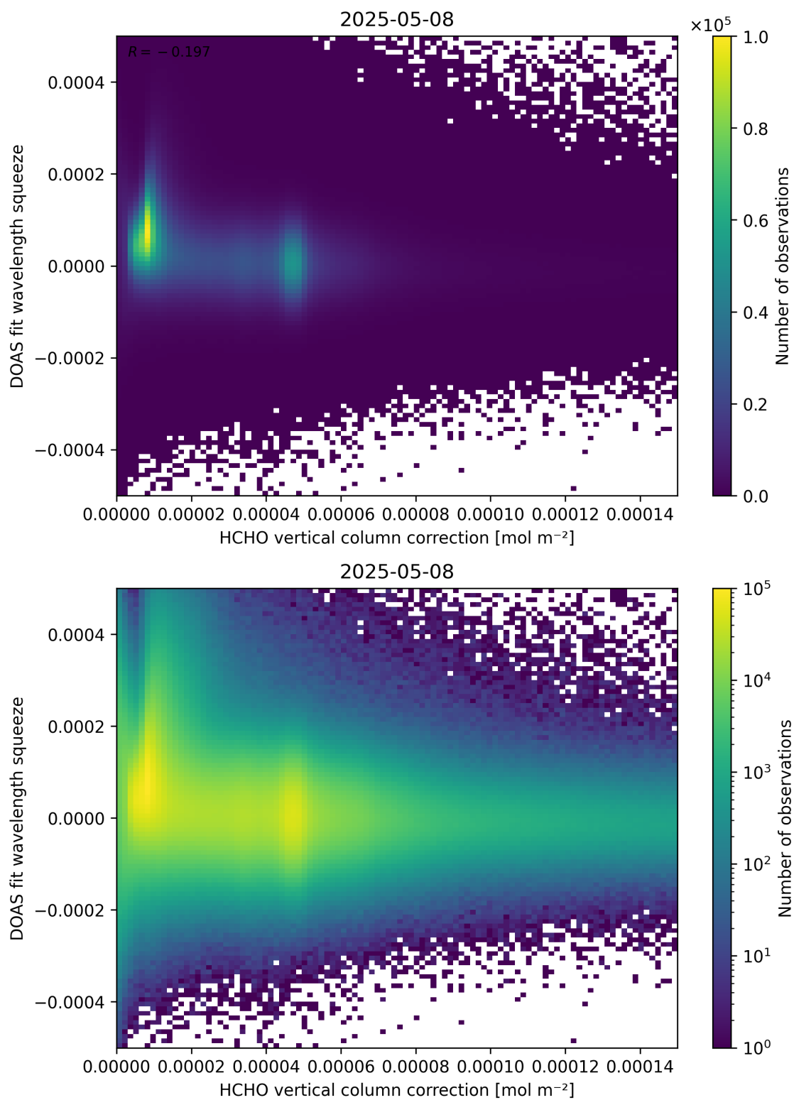
Figure 114: Scatter density plot of “HCHO vertical column correction” against “DOAS fit wavelength squeeze” for 2025-05-07 to 2025-05-09.
