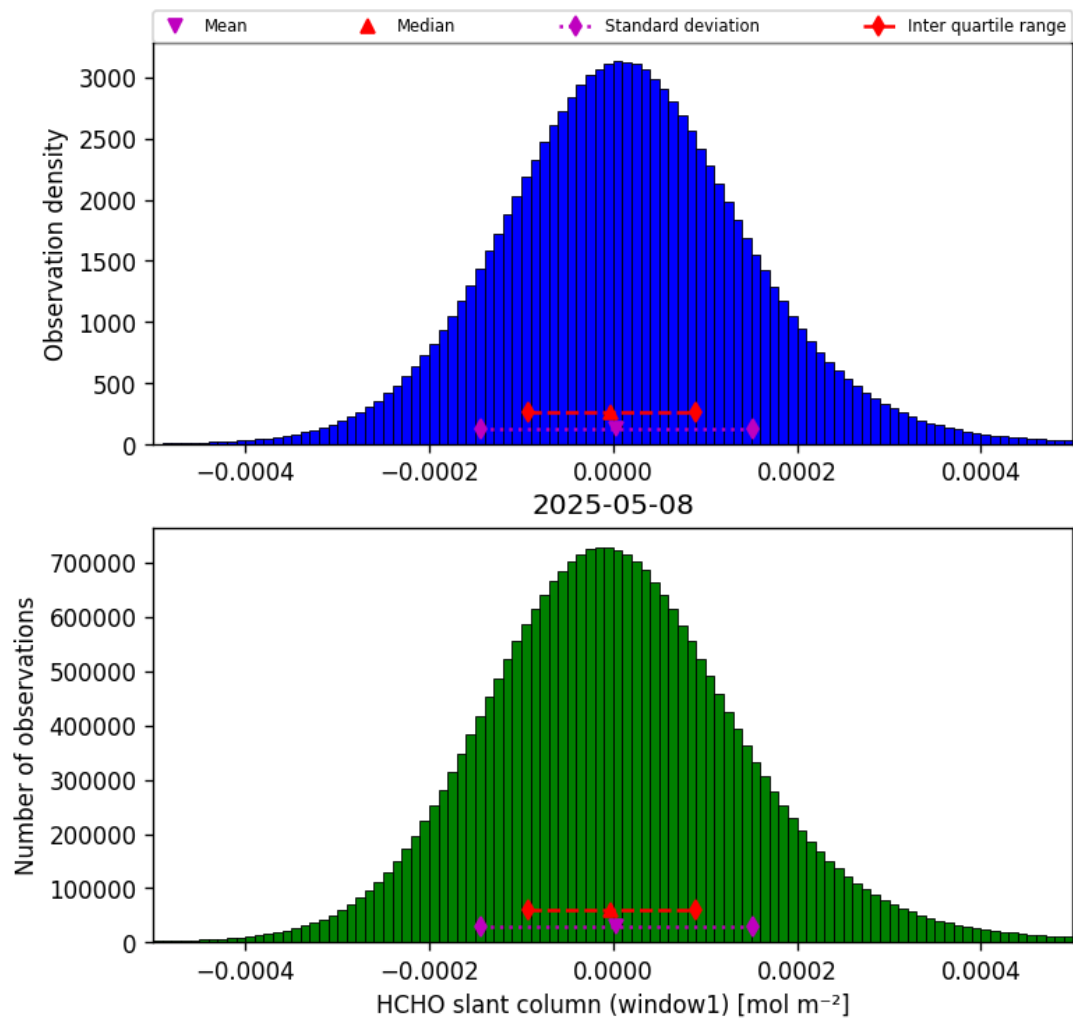
Figure 38: Histogram of “HCHO slant column (window1)” for 2025-05-07 to 2025-05-09
