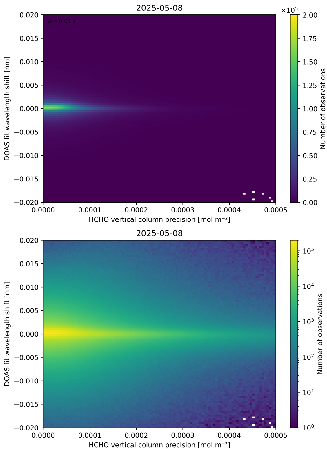
Figure 137: Scatter density plot of “HCHO vertical column precision” against “DOAS fit wavelength shift” for 2025-05-07 to 2025-05-09.
