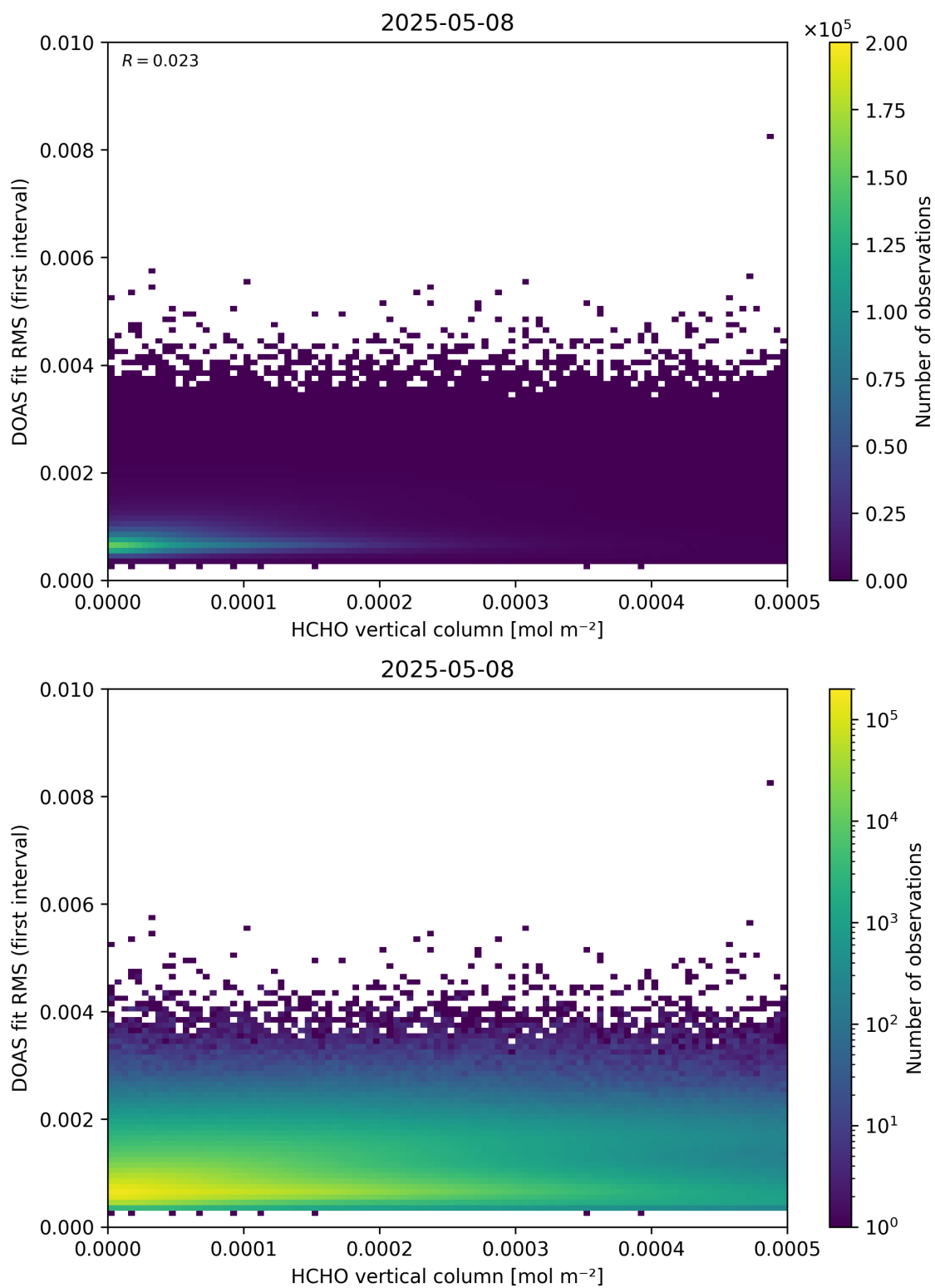
Figure 123: Scatter density plot of “HCHO vertical column” against “DOAS fit RMS (first interval)” for 2025-05-07 to 2025-05-09.
