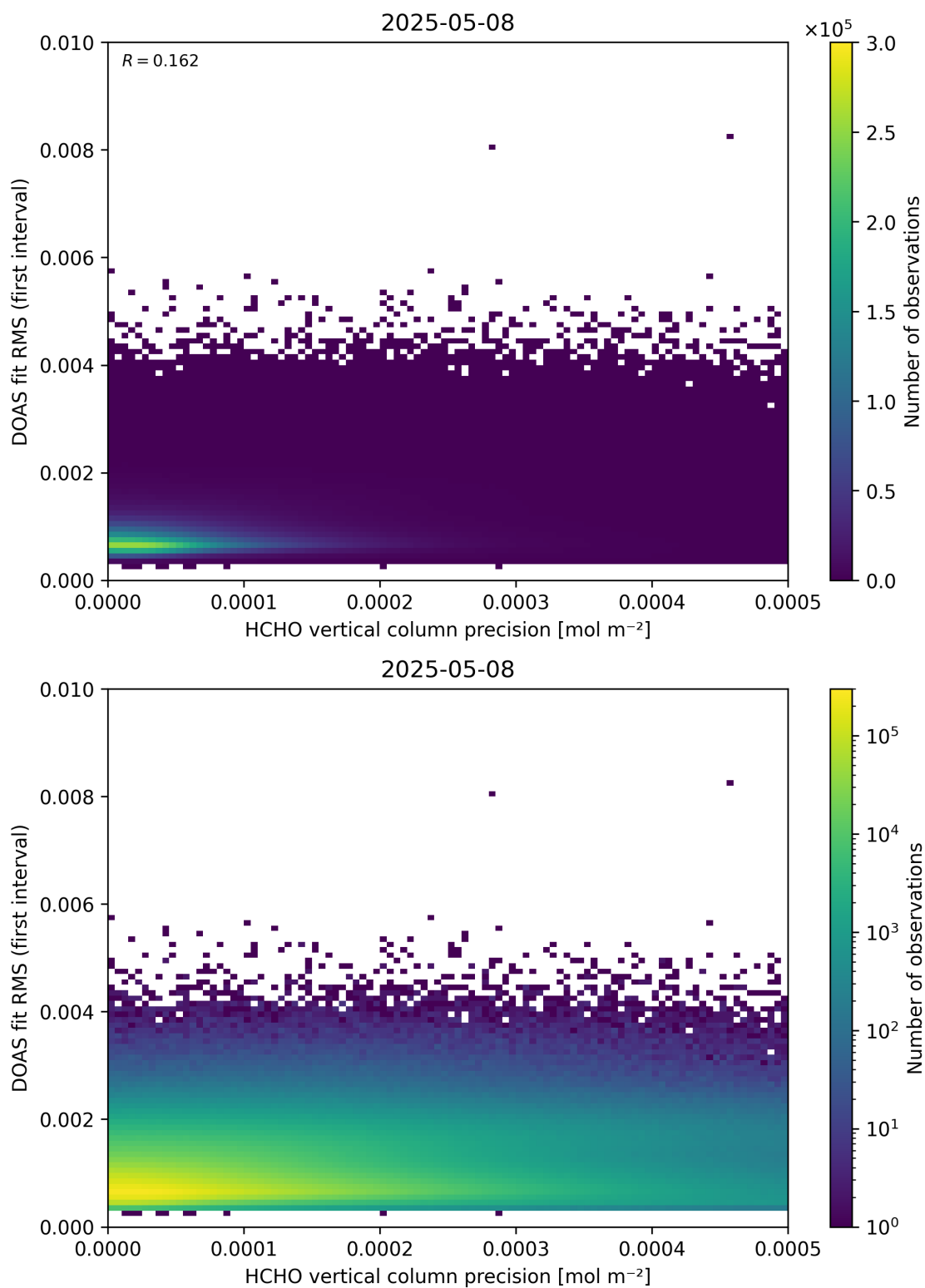
Figure 136: Scatter density plot of “HCHO vertical column precision” against “DOAS fit RMS (first interval)” for 2025-05-07 to 2025-05-09.
