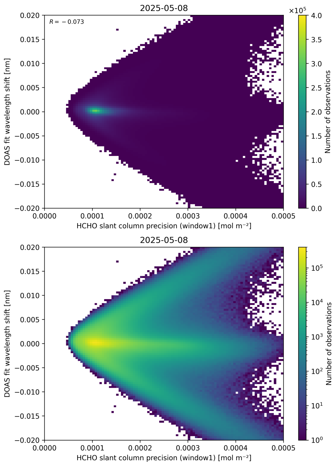
Figure 89: Scatter density plot of “HCHO slant column precision (window1)” against “DOAS fit wavelength shift” for 2025-05-07 to 2025-05-09.
