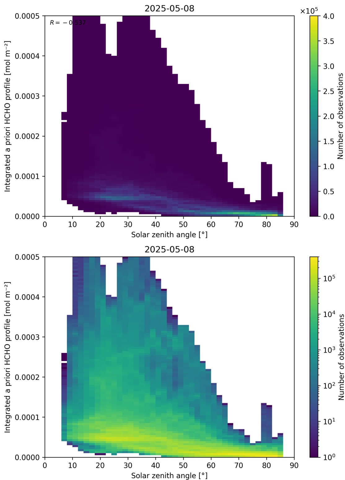
Figure 180: Scatter density plot of “Solar zenith angle” against “Integrated a priori HCHO profile” for 2025-05-07 to 2025-05-09.
