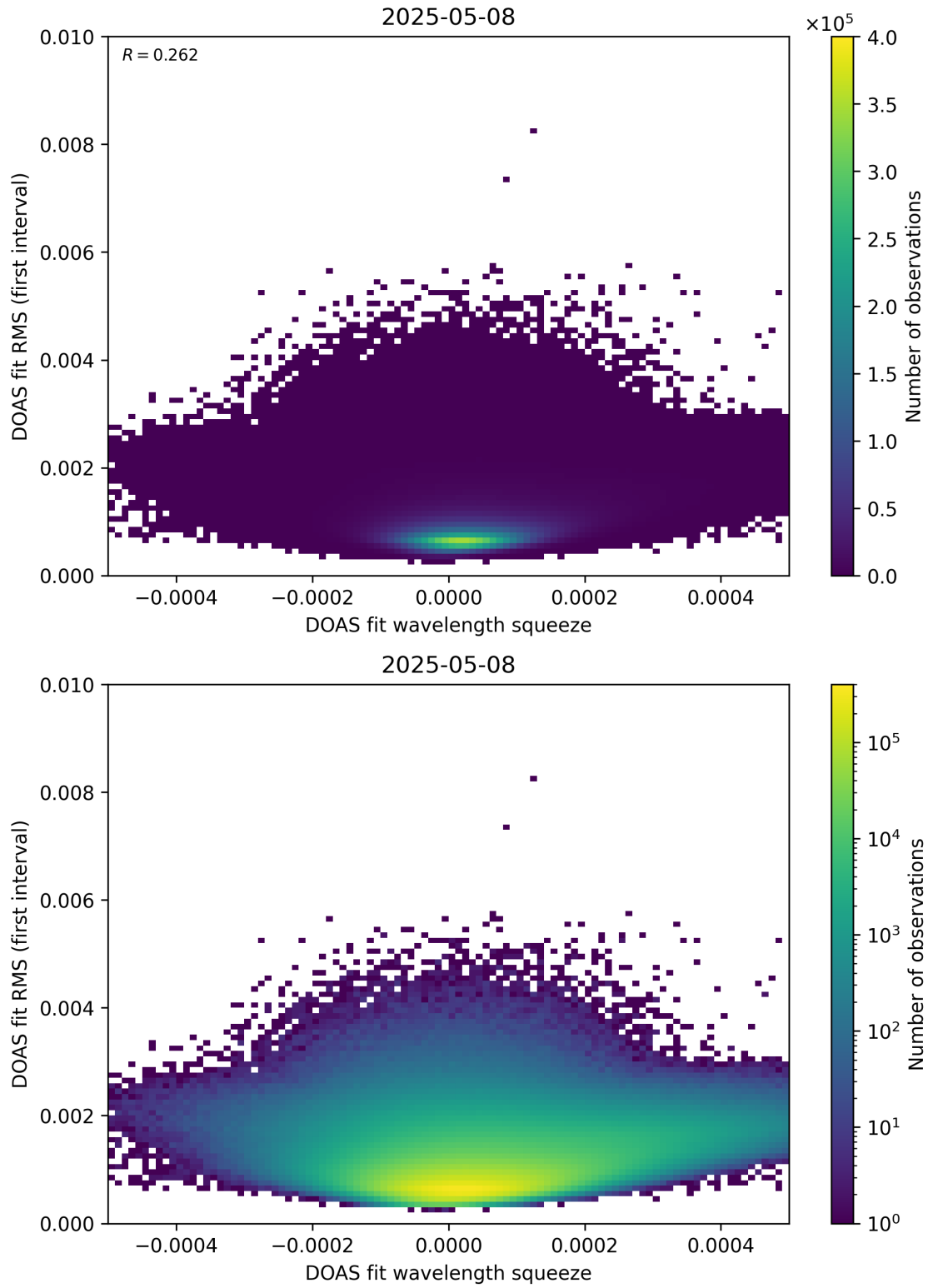
Figure 68: Scatter density plot of “DOAS fit wavelength squeeze” against “DOAS fit RMS (first interval)” for 2025-05-07 to 2025-05-09.
