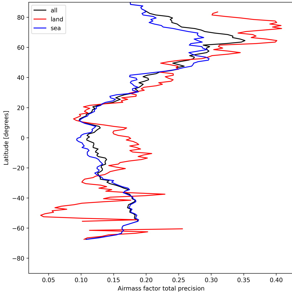
Figure 27: Zonal average of “Airmass factor total precision” for 2025-05-07 to 2025-05-09.
