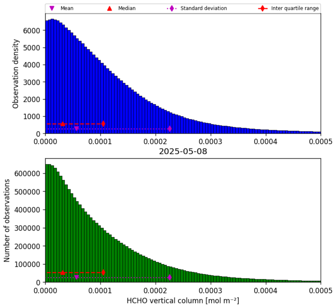
Figure 35: Histogram of “HCHO vertical column” for 2025-05-07 to 2025-05-09
