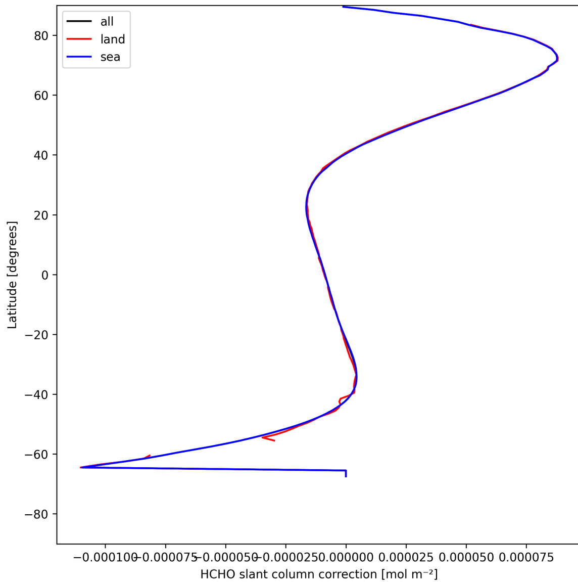
Figure 33: Zonal average of “HCHO slant column correction” for 2025-05-07 to 2025-05-09.
