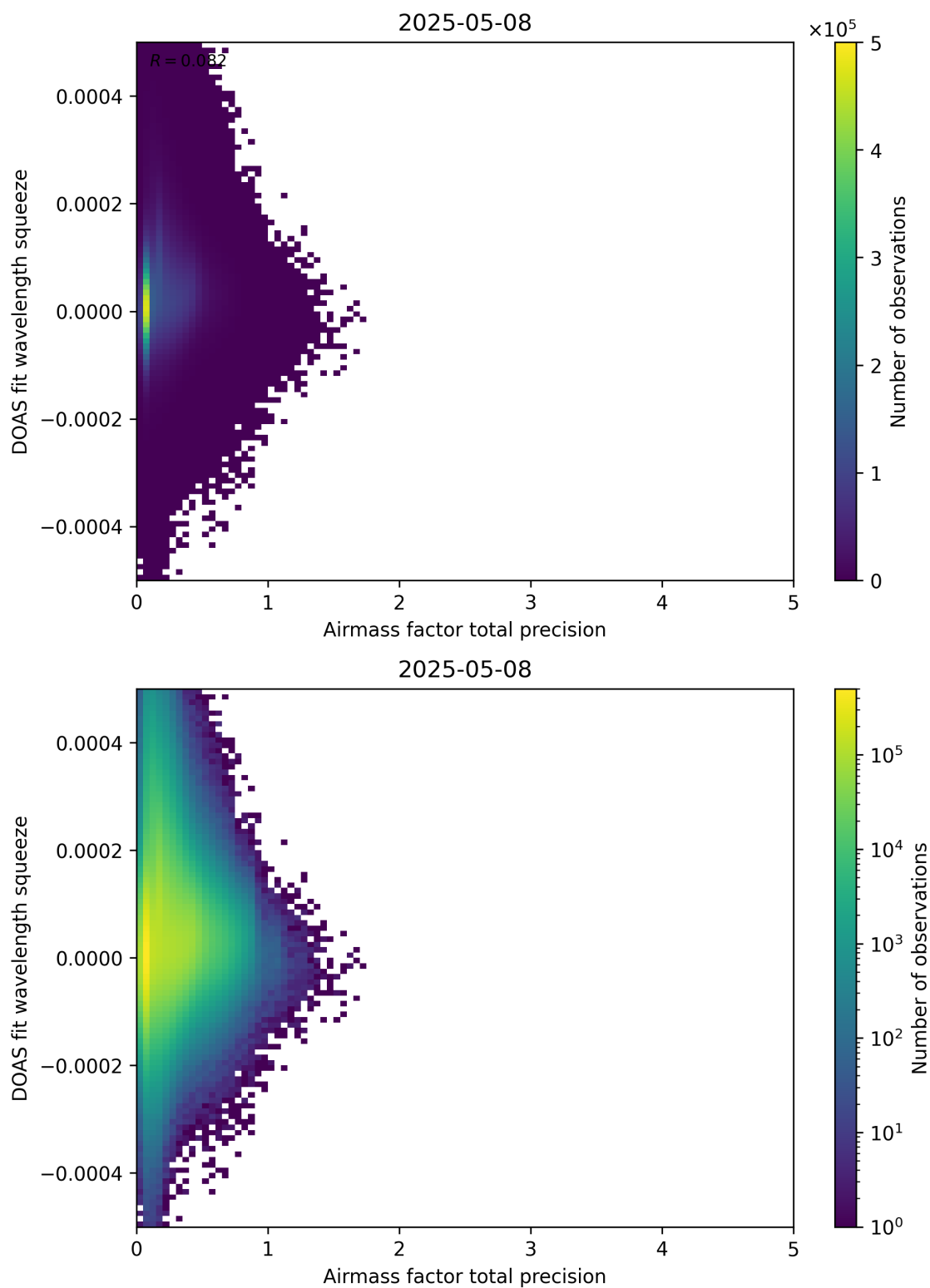
Figure 107: Scatter density plot of “Airmass factor total precision” against “DOAS fit wavelength squeeze” for 2025-05-07 to 2025-05-09.
