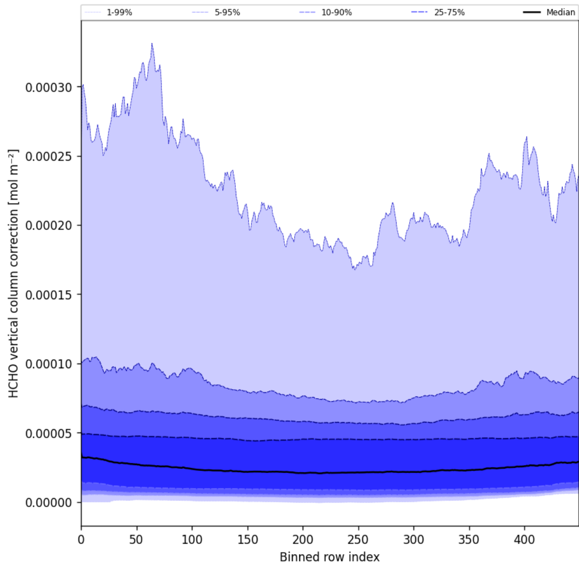
Figure 51: Along track statistics of “HCHO vertical column correction” for 2025-05-07 to 2025-05-09
