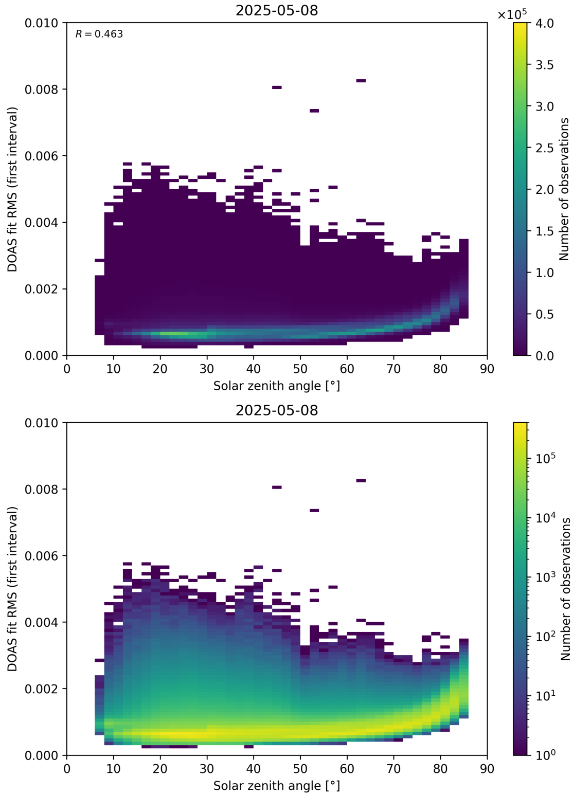
Figure 167: Scatter density plot of “Solar zenith angle” against “DOAS fit RMS (first interval)” for 2025-05-07 to 2025-05-09.
