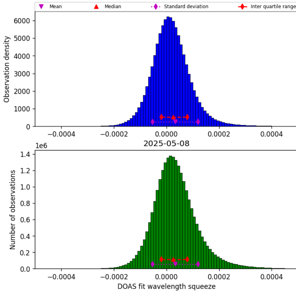
Figure 45: Histogram of “DOAS fit wavelength squeeze” for 2025-05-07 to 2025-05-09
