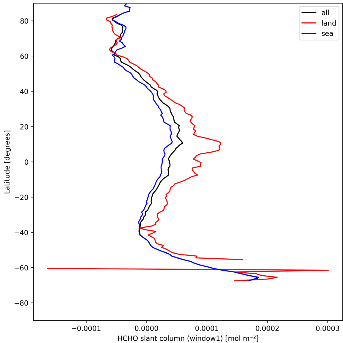
Figure 24: Zonal average of “HCHO slant column (window1)” for 2025-05-07 to 2025-05-09.
