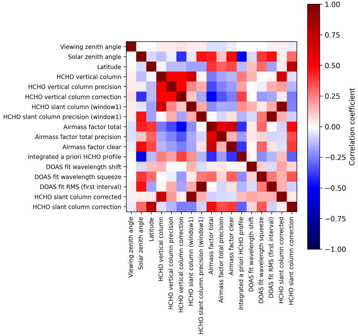
Figure 2: Map of correlation matrix for 2025-05-07 to 2025-05-09.
