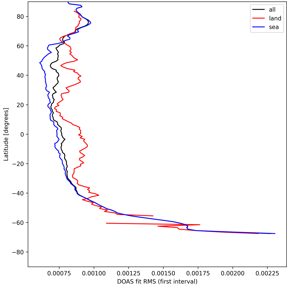
Figure 32: Zonal average of "DOAS fit RMS (first interval)" for 2025-05-07 to 2025-05-09.
