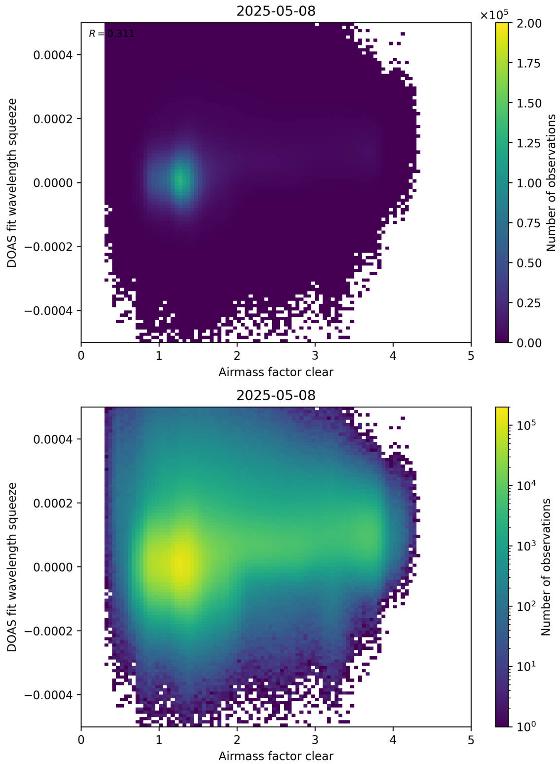
Figure 73: Scatter density plot of “Airmass factor clear” against “DOAS fit wavelength squeeze” for 2025-05-07 to 2025-05-09.
