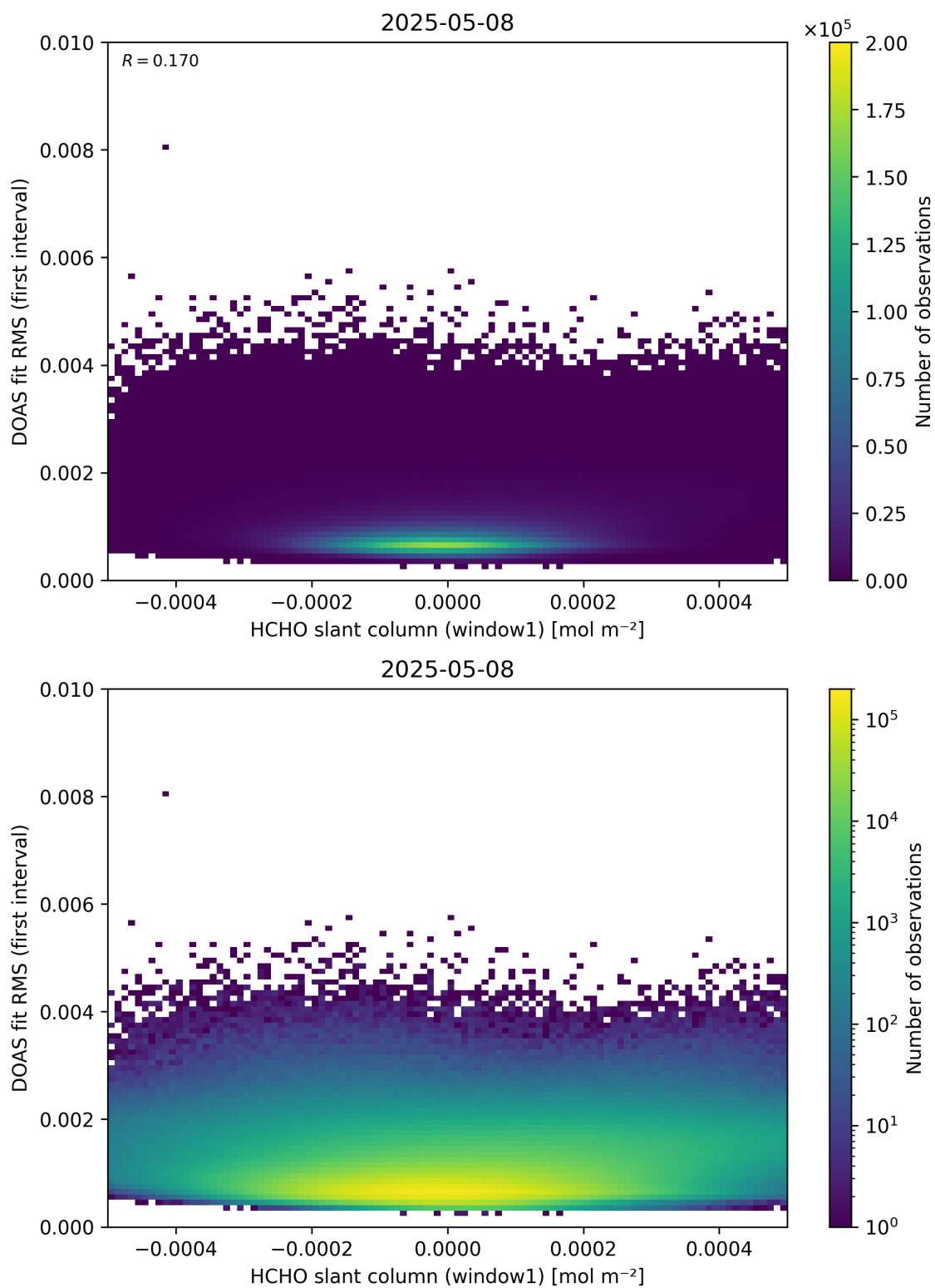
Figure 78: Scatter density plot of “HCHO slant column (window1)” against “DOAS fit RMS (first interval)” for 2025-05-07 to 2025-05-09.
