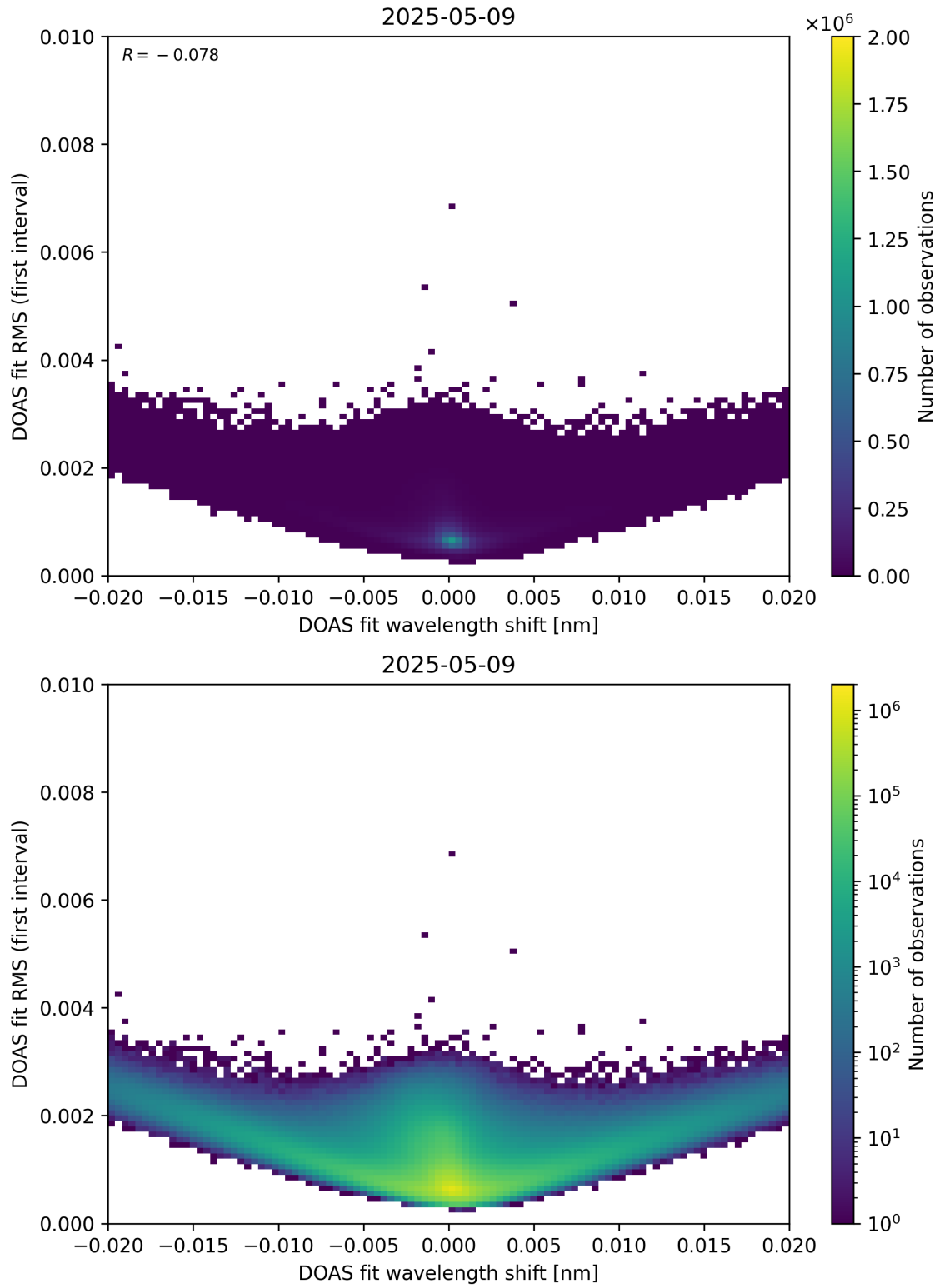
Figure 64: Scatter density plot of “DOAS fit wavelength shift” against “DOAS fit RMS (first interval)” for 2025-05-08 to 2025-05-10.
