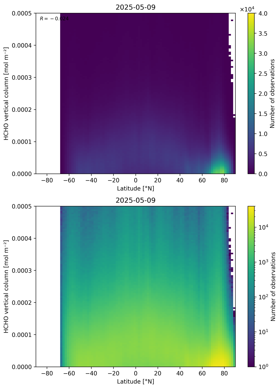
Figure 163: Scatter density plot of “Latitude” against “HCHO vertical column” for 2025-05-08 to 2025-05-10.
