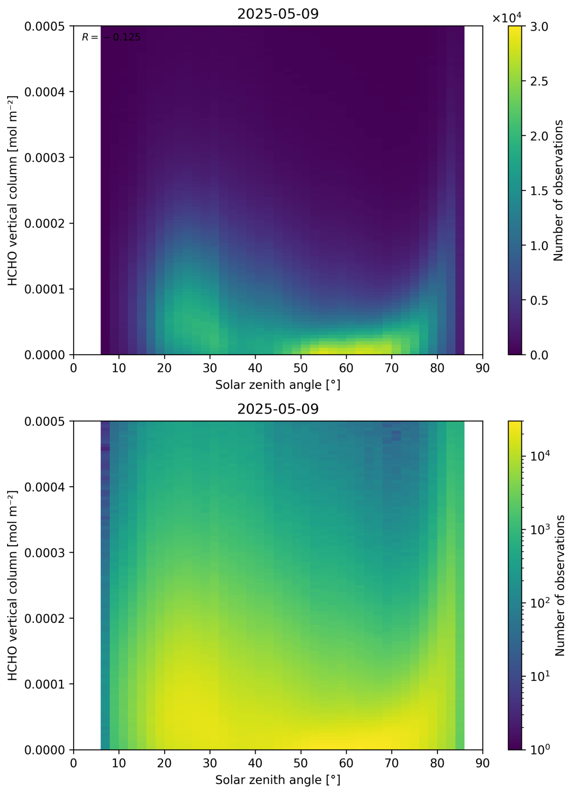
Figure 177: Scatter density plot of “Solar zenith angle” against “HCHO vertical column” for 2025-05-08 to 2025-05-10.
