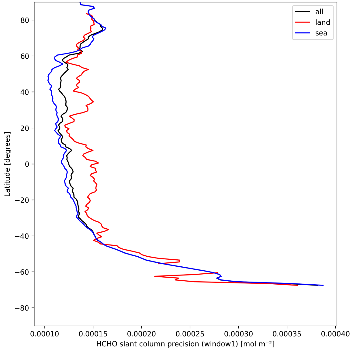
Figure 25: Zonal average of “HCHO slant column precision (window1)” for 2025-05-08 to 2025-05-10.
