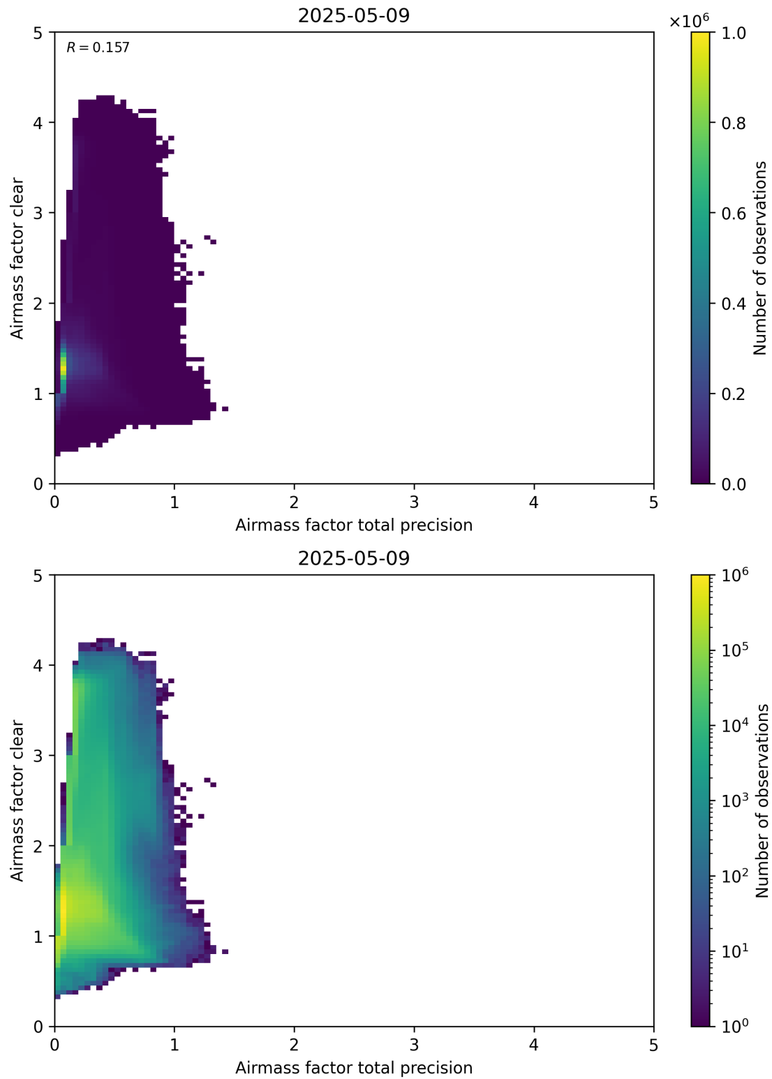
Figure 108: Scatter density plot of “Airmass factor total precision” against “Airmass factor clear” for 2025-05-08 to 2025-05-10.
