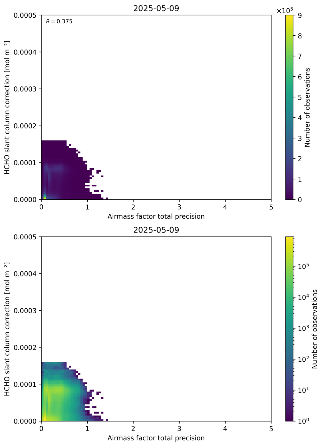
Figure 110: Scatter density plot of “Airmass factor total precision” against “HCHO slant column correction” for 2025-05-08 to 2025-05-10.
