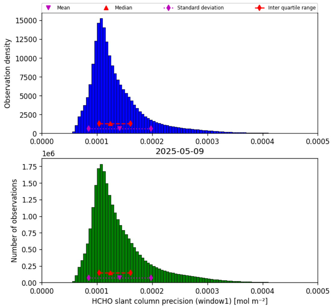
Figure 39: Histogram of “HCHO slant column precision (window1)” for 2025-05-08 to 2025-05-10
