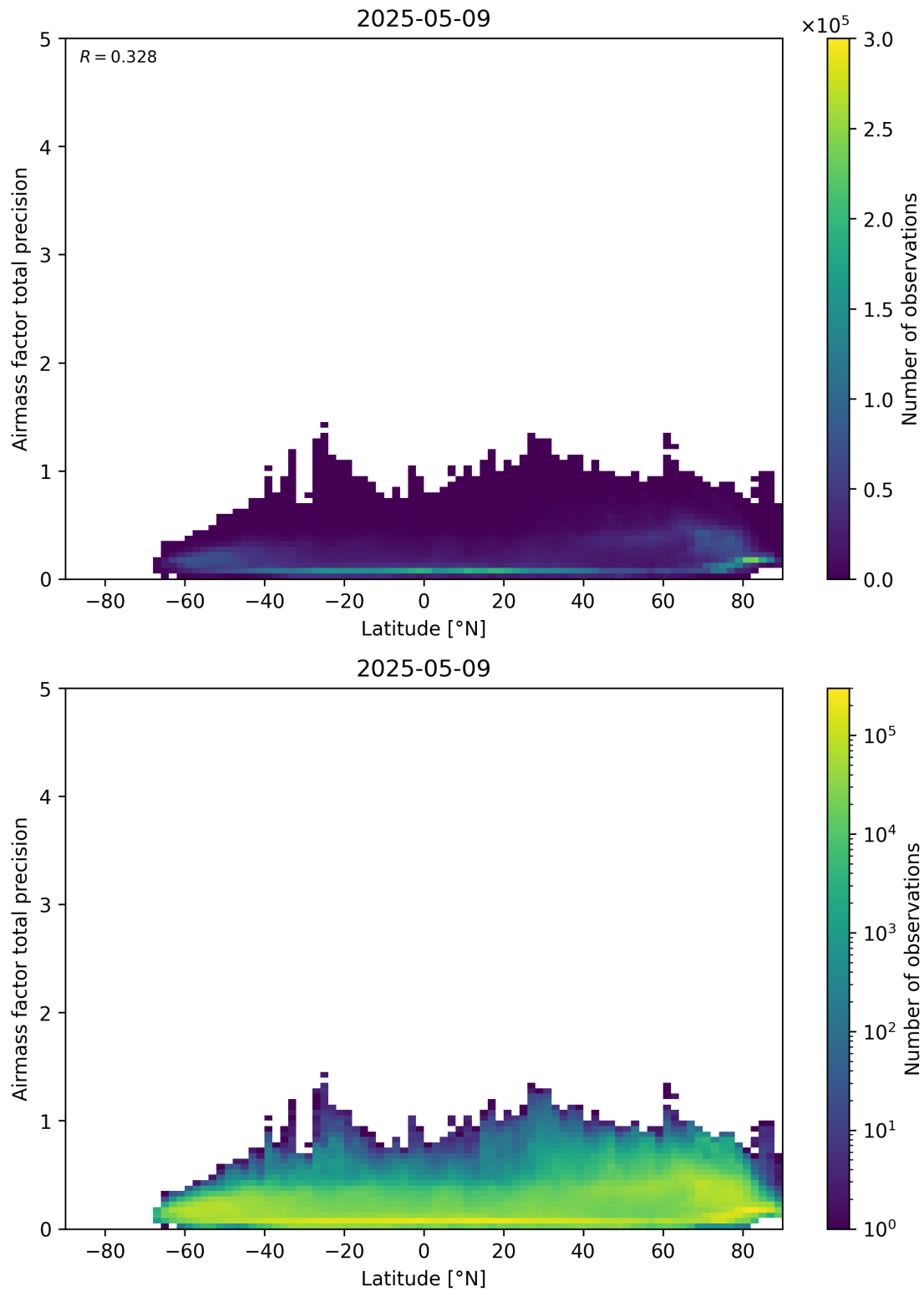
Figure 162: Scatter density plot of “Latitude” against “Airmass factor total precision” for 2025-05-08 to 2025-05-10.
