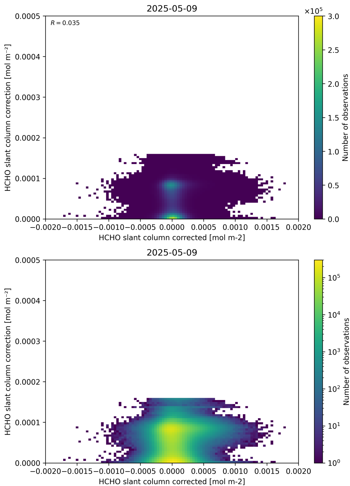
Figure 77: Scatter density plot of “HCHO slant column corrected” against “HCHO slant column correction” for 2025-05-08 to 2025-05-10.
