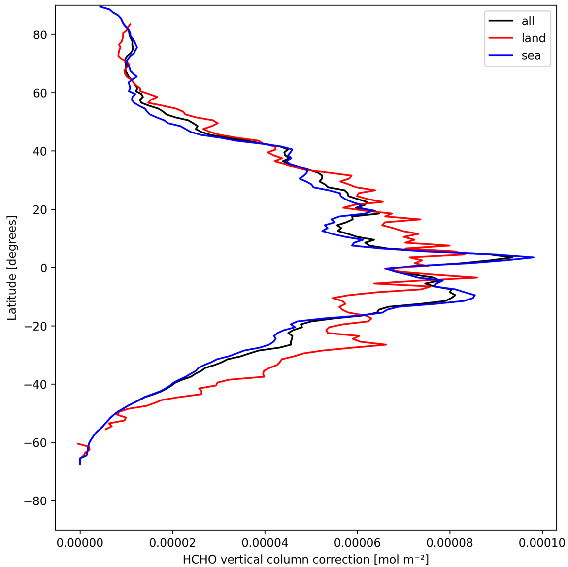
Figure 23: Zonal average of “HCHO vertical column correction” for 2025-05-08 to 2025-05-10.
