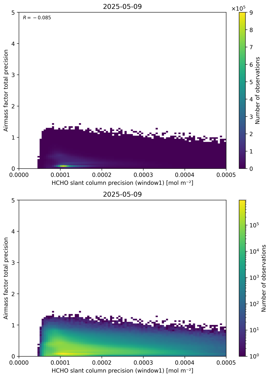
Figure 95: Scatter density plot of “HCHO slant column precision (window1)” against “Airmass factor total precision” for 2025-05-08 to 2025-05-10.
