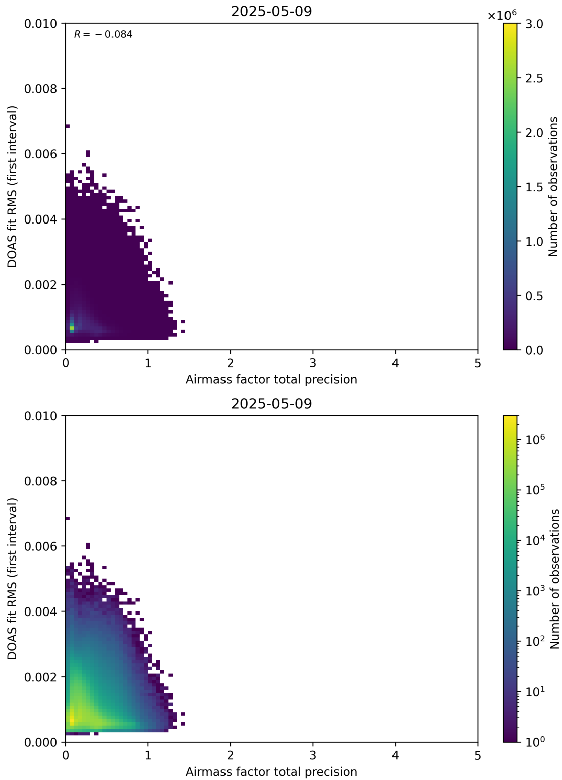
Figure 105: Scatter density plot of “Airmass factor total precision” against “DOAS fit RMS (first interval)” for 2025-05-08 to 2025-05-10.
