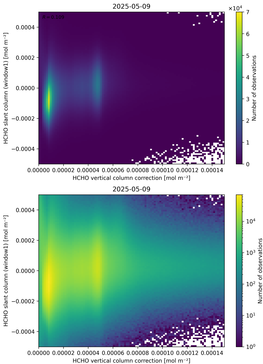
Figure 118: Scatter density plot of “HCHO vertical column correction” against “HCHO slant column (window1)” for 2025-05-08 to 2025-05-10.
