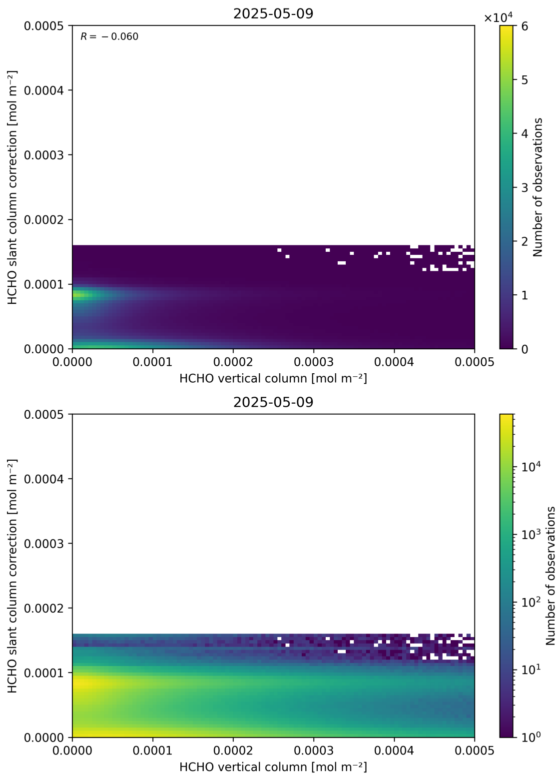
Figure 128: Scatter density plot of “HCHO vertical column” against “HCHO slant column correction” for 2025-05-08 to 2025-05-10.
