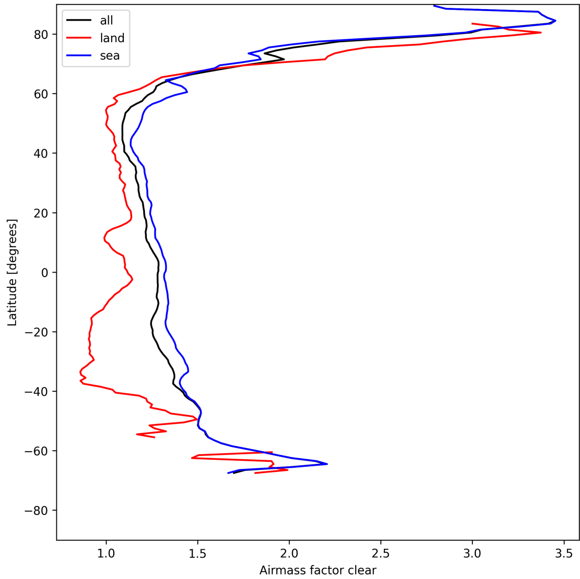
Figure 28: Zonal average of “Airmass factor clear” for 2025-05-08 to 2025-05-10.
