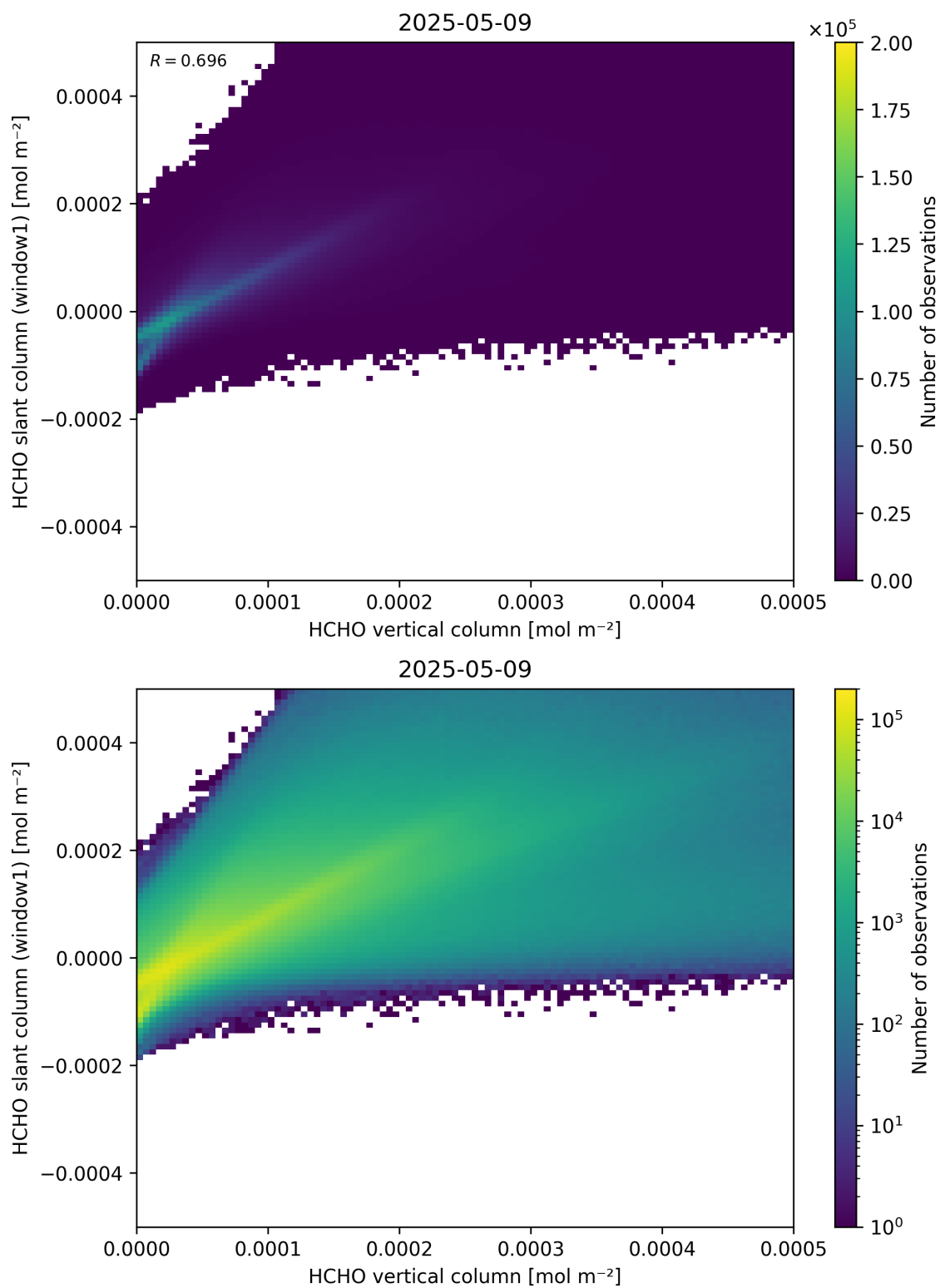
Figure 129: Scatter density plot of “HCHO vertical column” against “HCHO slant column (window1)” for 2025-05-08 to 2025-05-10.
