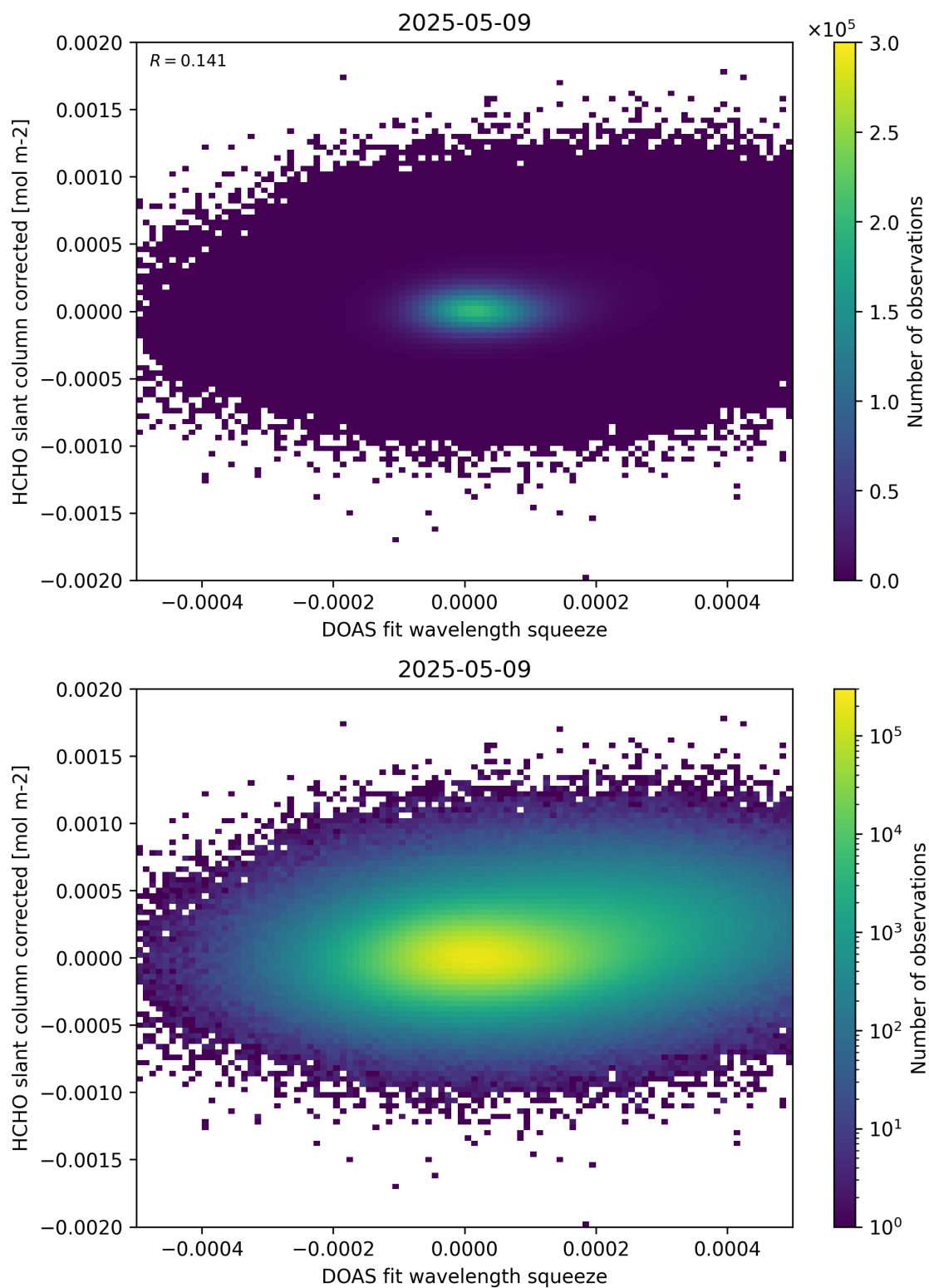
Figure 69: Scatter density plot of “DOAS fit wavelength squeeze” against “HCHO slant column corrected” for 2025-05-08 to 2025-05-10.
