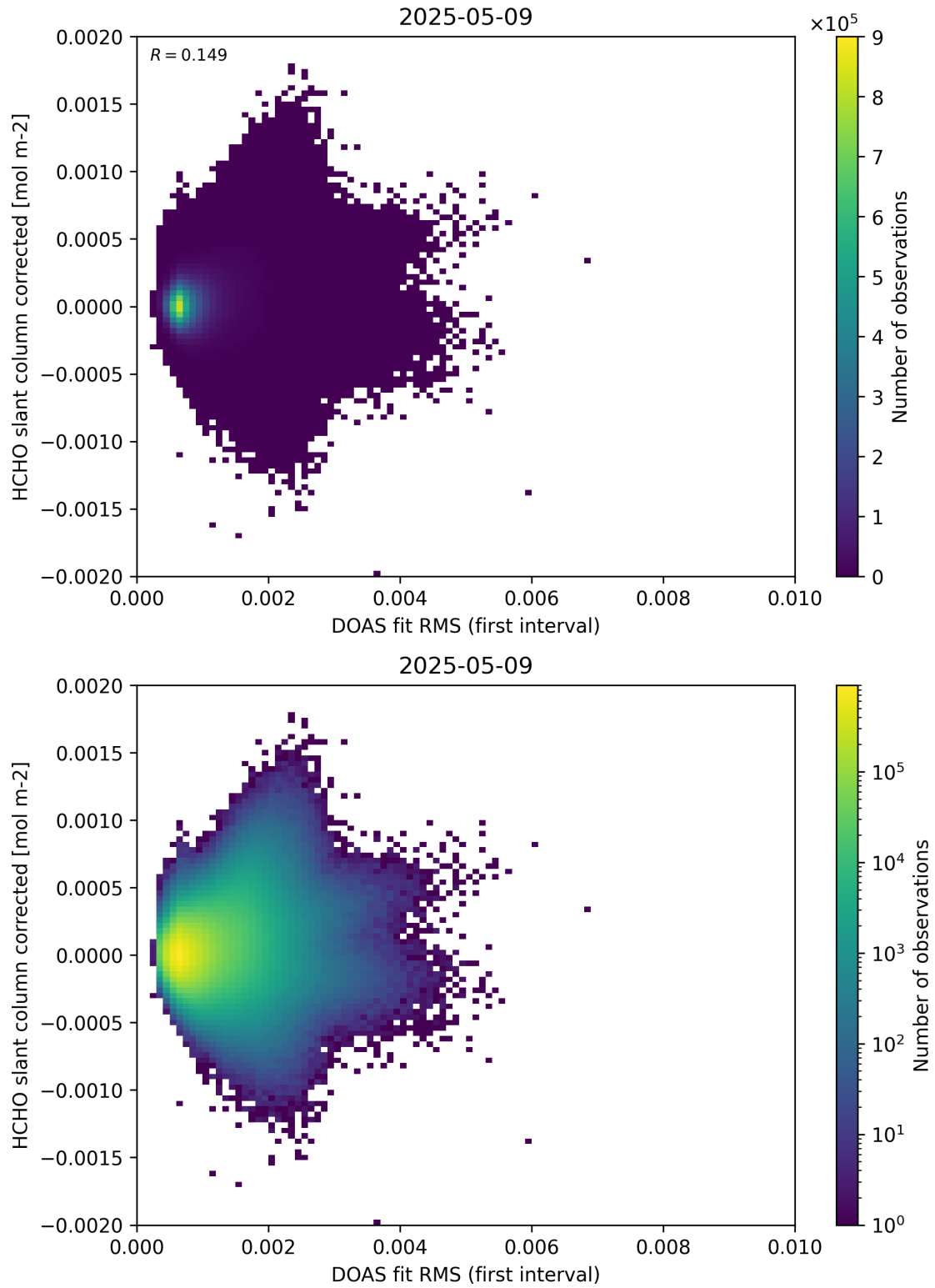
Figure 62: Scatter density plot of “DOAS fit RMS (first interval)” against “HCHO slant column corrected” for 2025-05-08 to 2025-05-10.
