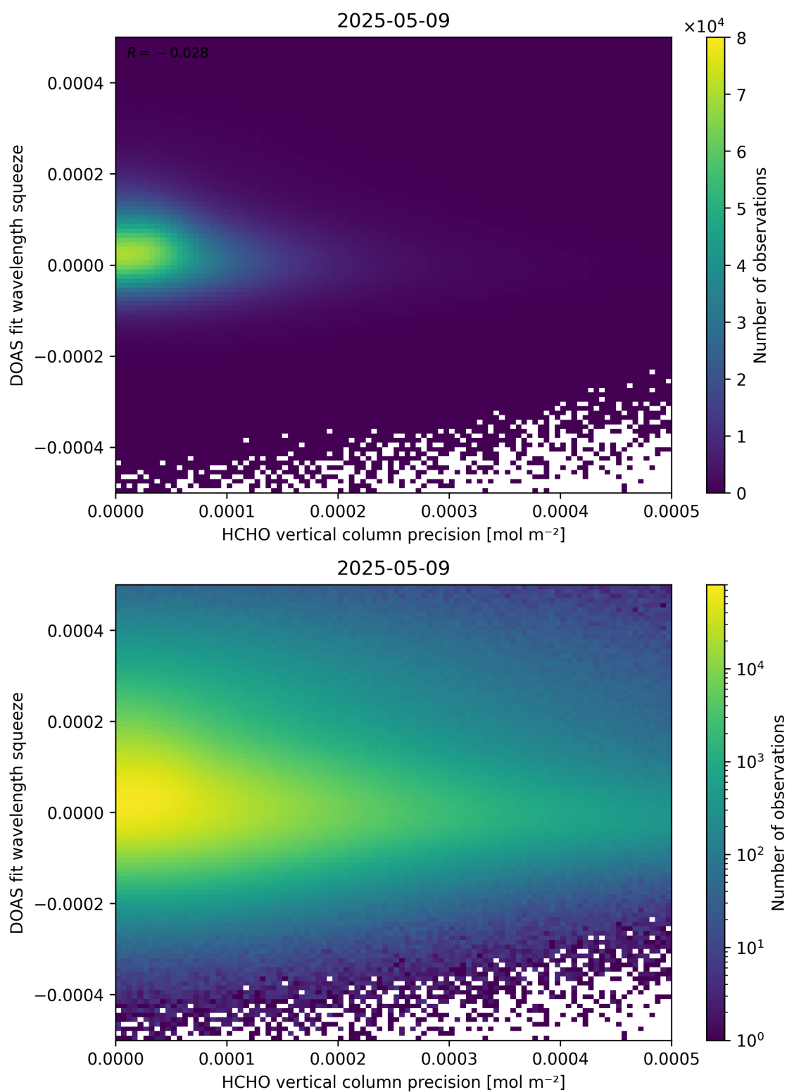
Figure 138: Scatter density plot of “HCHO vertical column precision” against “DOAS fit wavelength squeeze” for 2025-05-08 to 2025-05-10.
