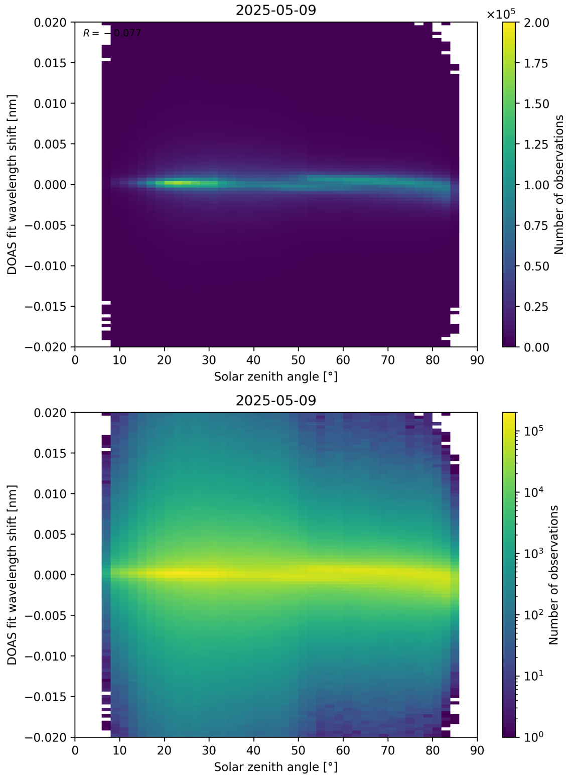
Figure 168: Scatter density plot of “Solar zenith angle” against “DOAS fit wavelength shift” for 2025-05-08 to 2025-05-10.
