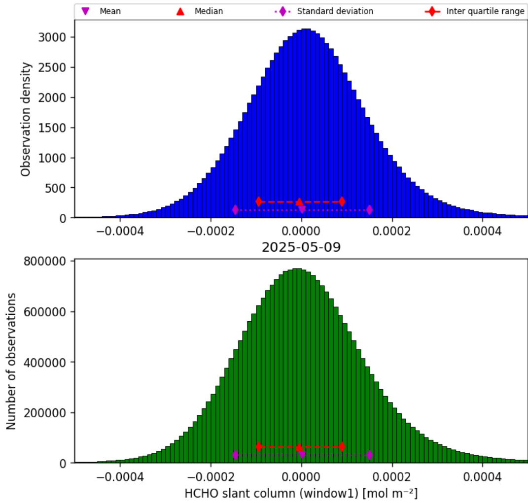
Figure 38: Histogram of “HCHO slant column (window1)” for 2025-05-08 to 2025-05-10
