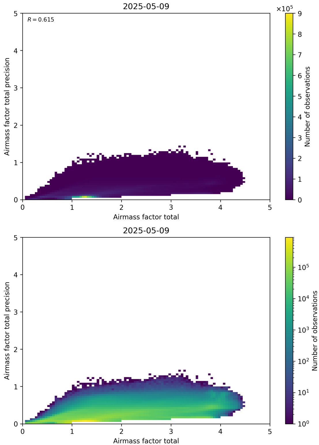
Figure 103: Scatter density plot of “Airmass factor total” against “Airmass factor total precision” for 2025-05-08 to 2025-05-10.
