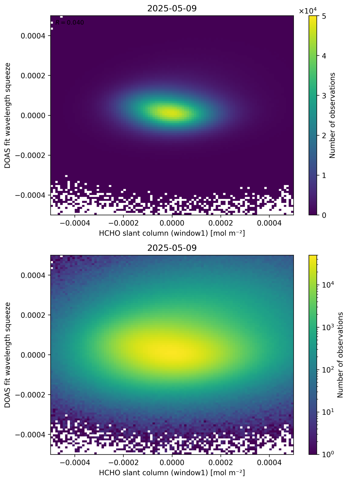
Figure 80: Scatter density plot of “HCHO slant column (window1)” against “DOAS fit wavelength squeeze” for 2025-05-08 to 2025-05-10.
