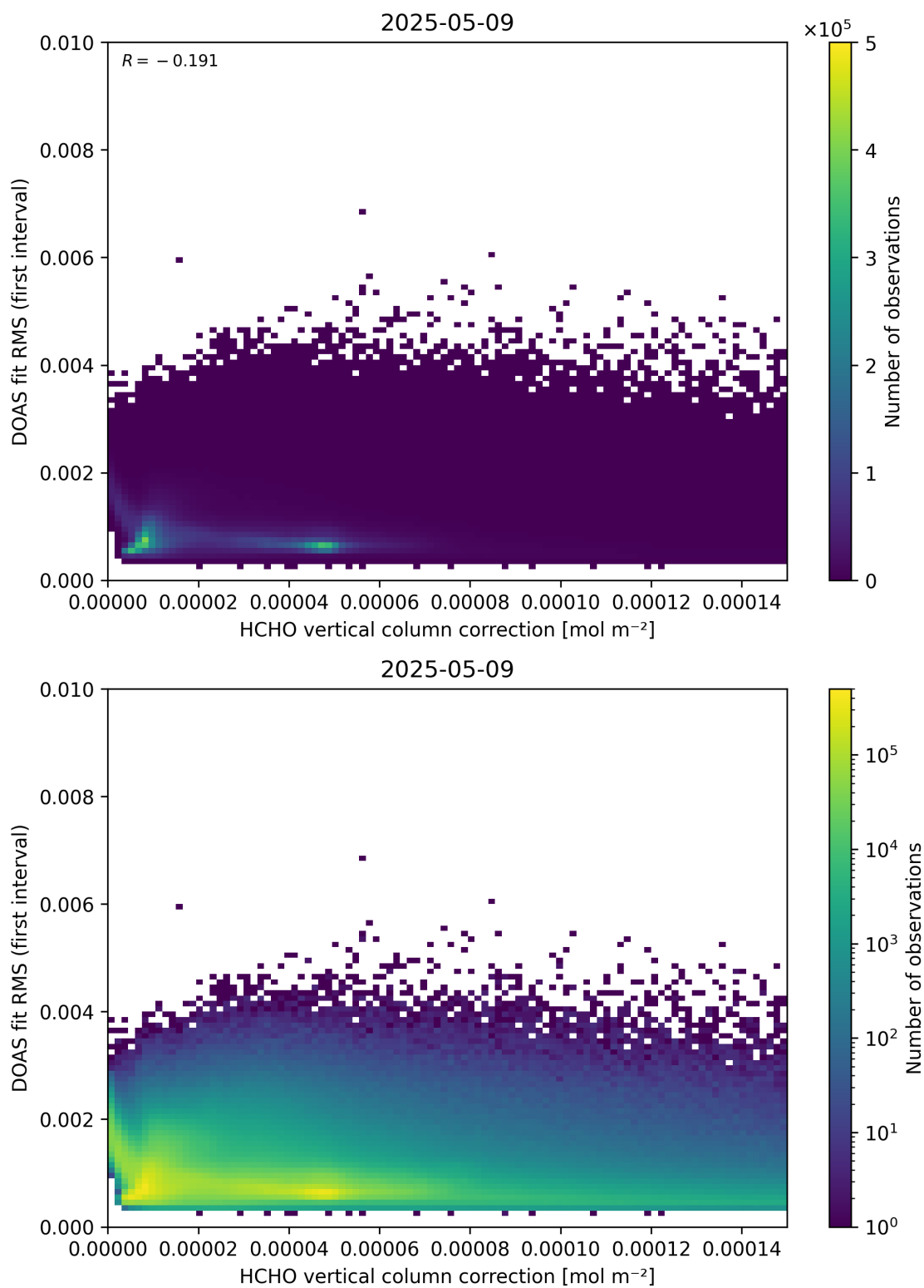
Figure 112: Scatter density plot of “HCHO vertical column correction” against “DOAS fit RMS (first interval)” for 2025-05-08 to 2025-05-10.
