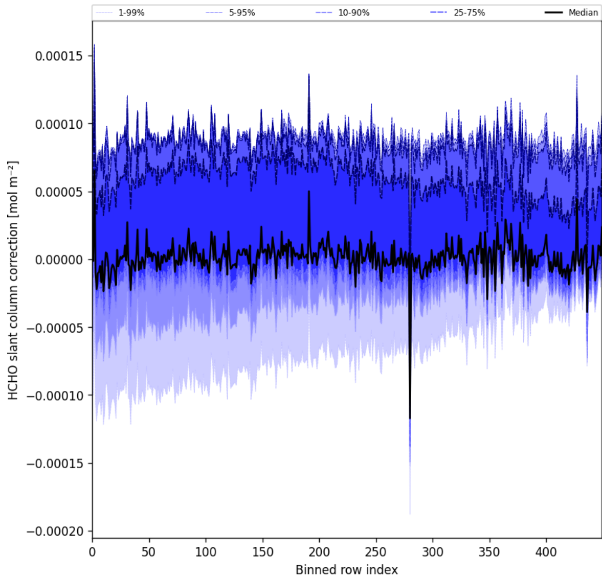
Figure 61: Along track statistics of “HCHO slant column correction” for 2025-05-08 to 2025-05-10
