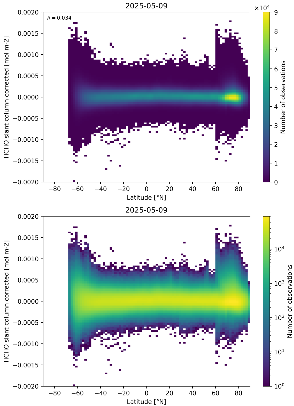
Figure 157: Scatter density plot of “Latitude” against “HCHO slant column corrected” for 2025-05-08 to 2025-05-10.
