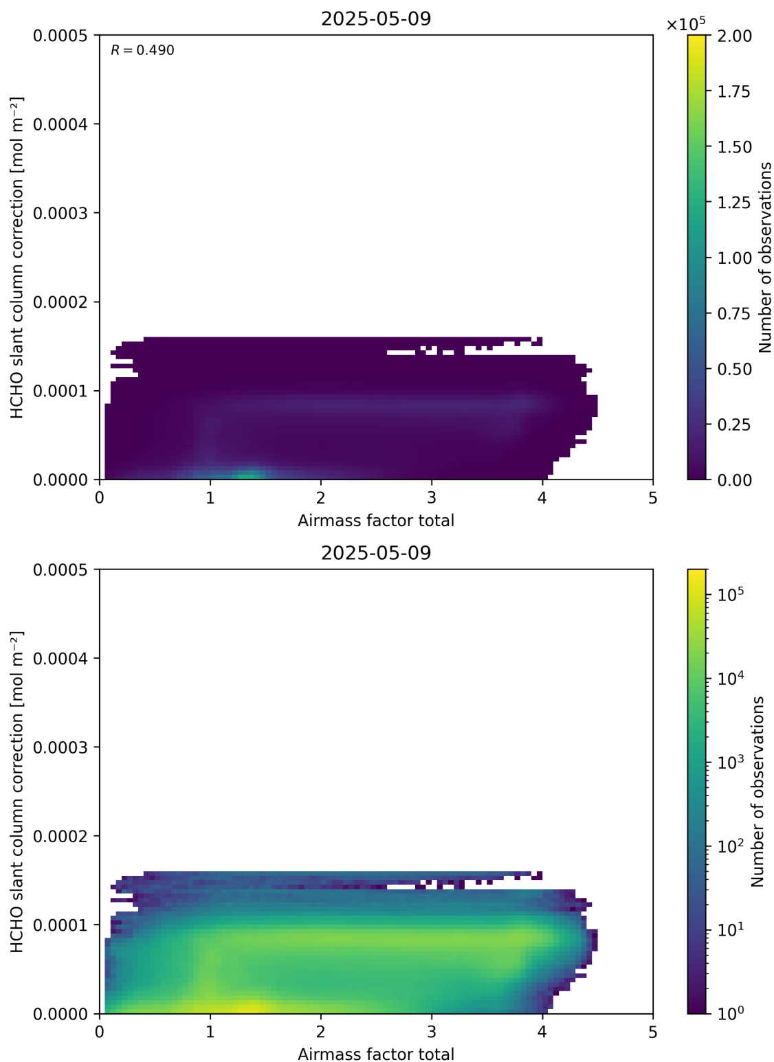
Figure 102: Scatter density plot of “Airmass factor total” against “HCHO slant column correction” for 2025-05-08 to 2025-05-10.
