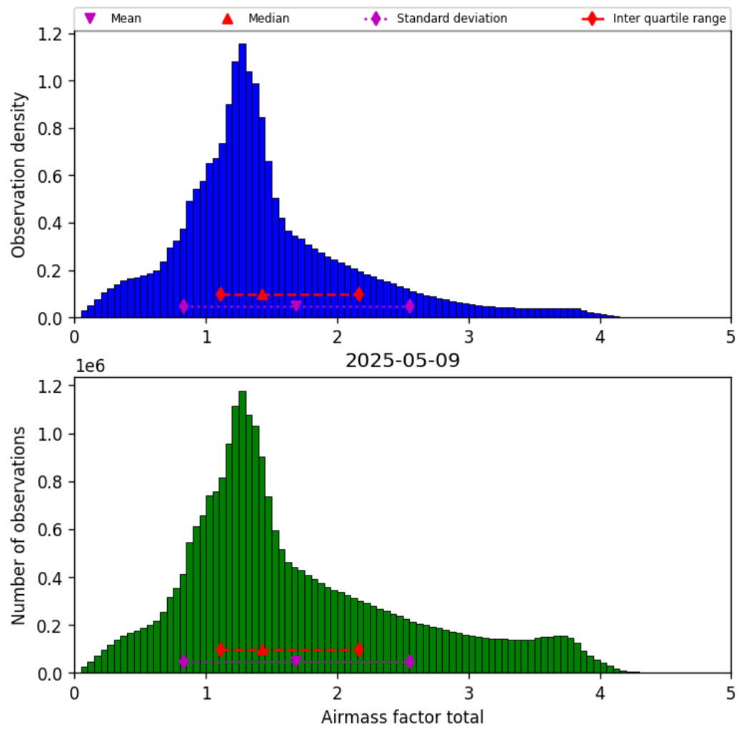
Figure 40: Histogram of “Airmass factor total” for 2025-05-08 to 2025-05-10
