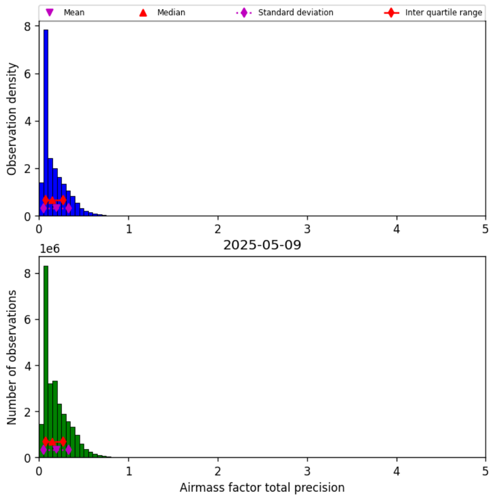
Figure 41: Histogram of “Airmass factor total precision” for 2025-05-08 to 2025-05-10
