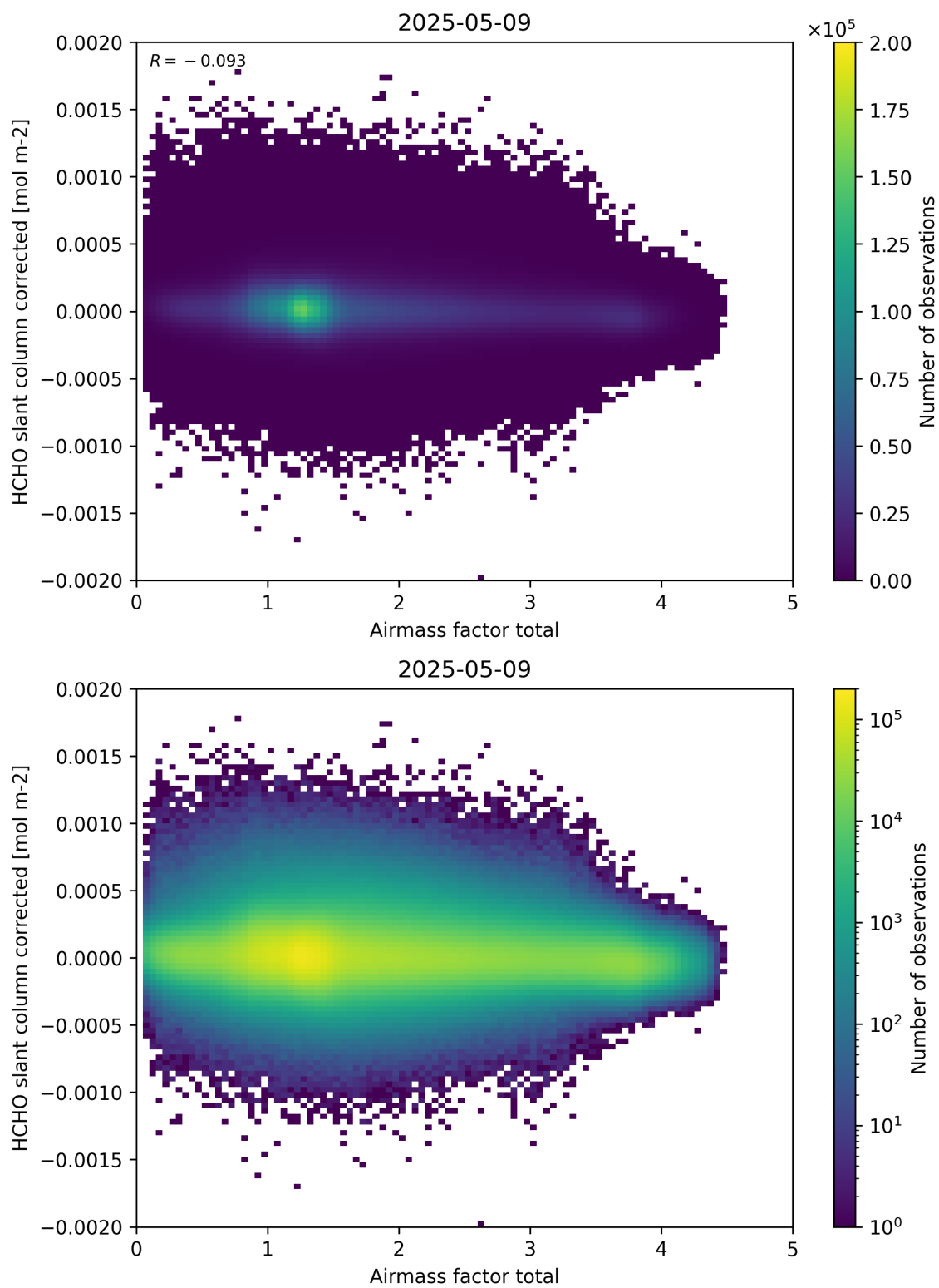
Figure 101: Scatter density plot of “Airmass factor total” against “HCHO slant column corrected” for 2025-05-08 to 2025-05-10.
