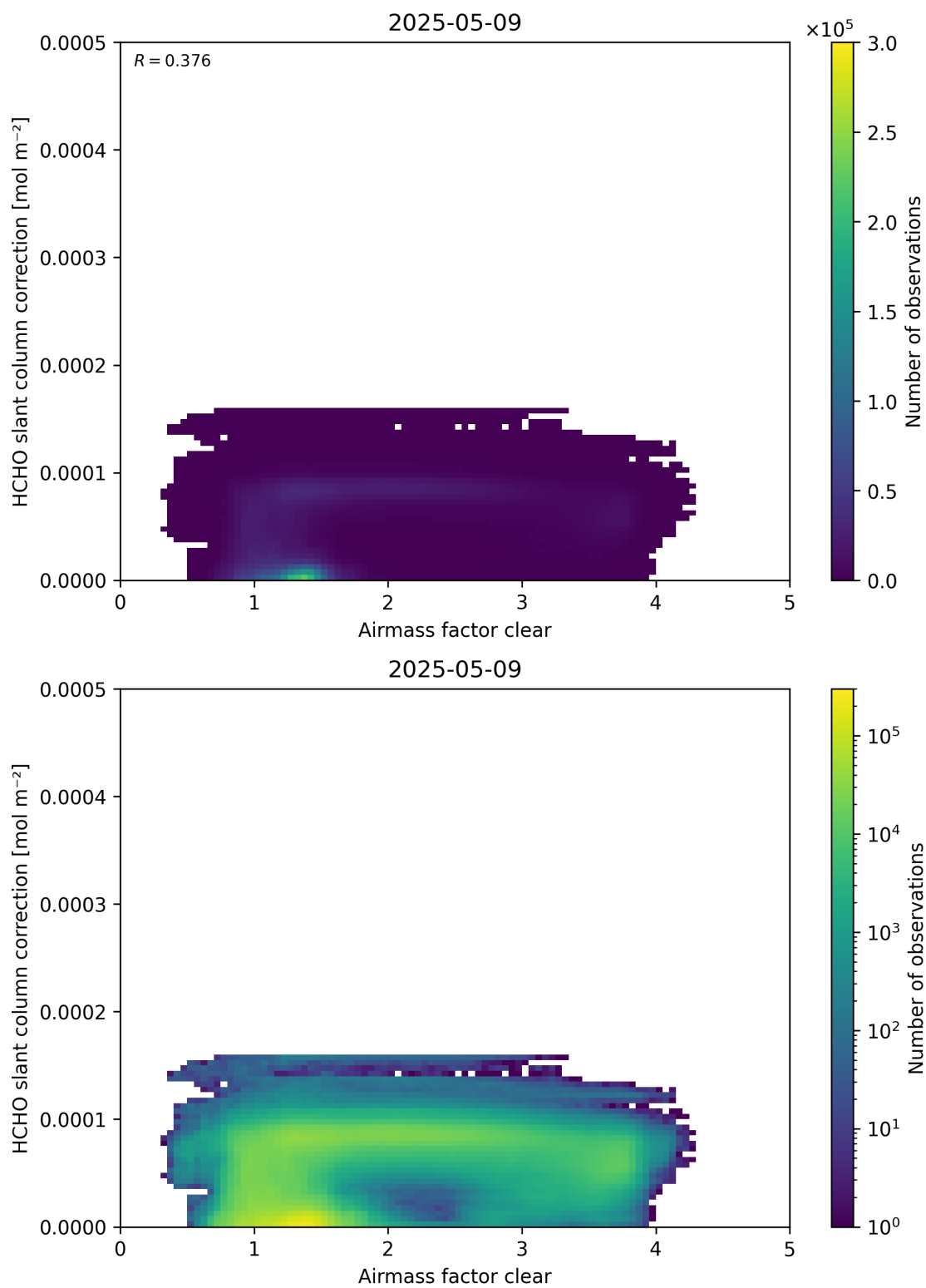
Figure 75: Scatter density plot of “Airmass factor clear” against “HCHO slant column correction” for 2025-05-08 to 2025-05-10.
