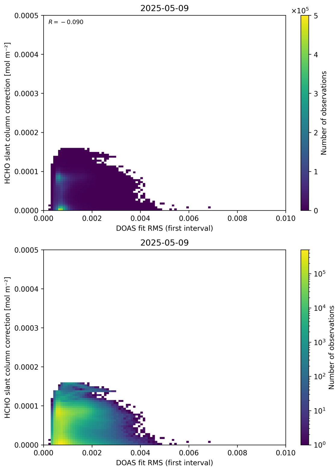
Figure 63: Scatter density plot of “DOAS fit RMS (first interval)” against “HCHO slant column correction” for 2025-05-08 to 2025-05-10.
