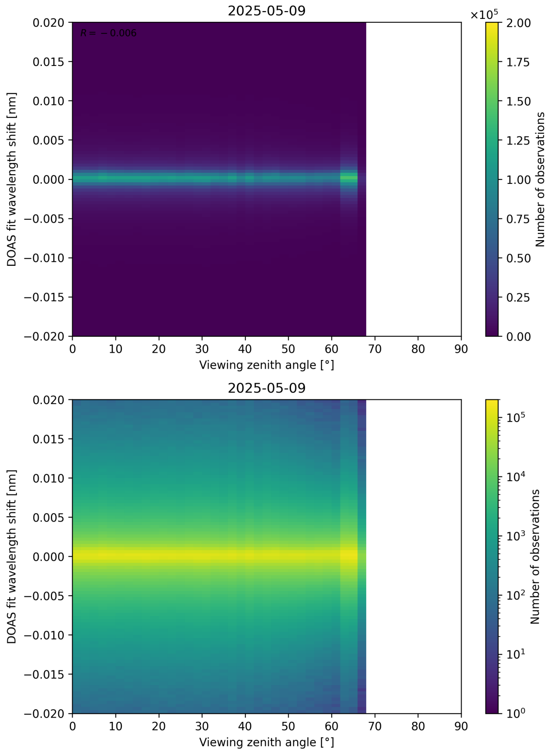
Figure 183: Scatter density plot of “Viewing zenith angle” against “DOAS fit wavelength shift” for 2025-05-08 to 2025-05-10.
