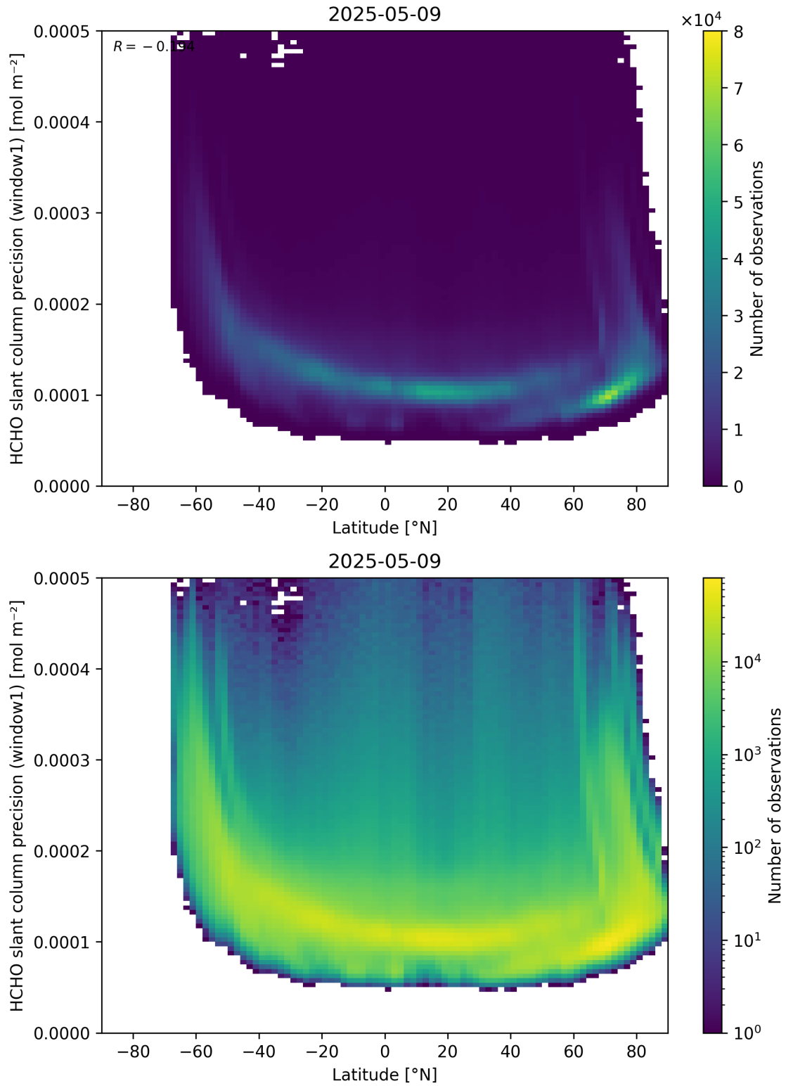
Figure 160: Scatter density plot of “Latitude” against “HCHO slant column precision (window1)” for 2025-05-08 to 2025-05-10.
