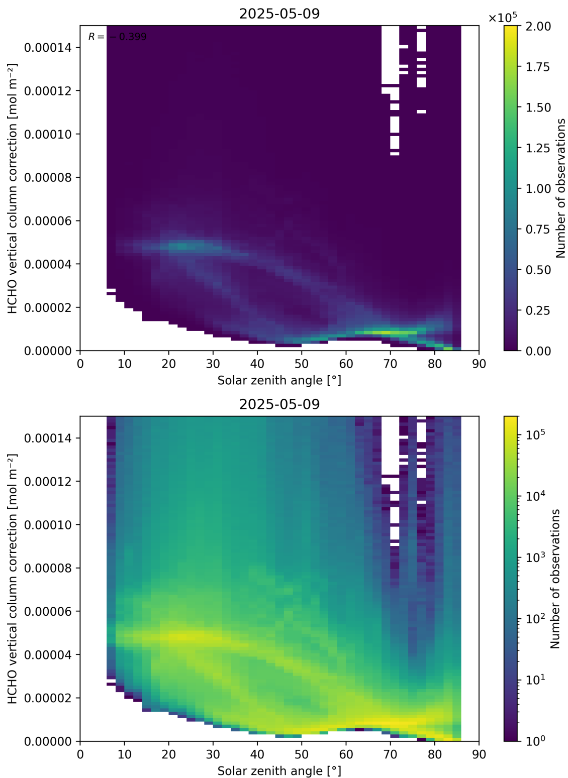
Figure 178: Scatter density plot of “Solar zenith angle” against “HCHO vertical column correction” for 2025-05-08 to 2025-05-10.
