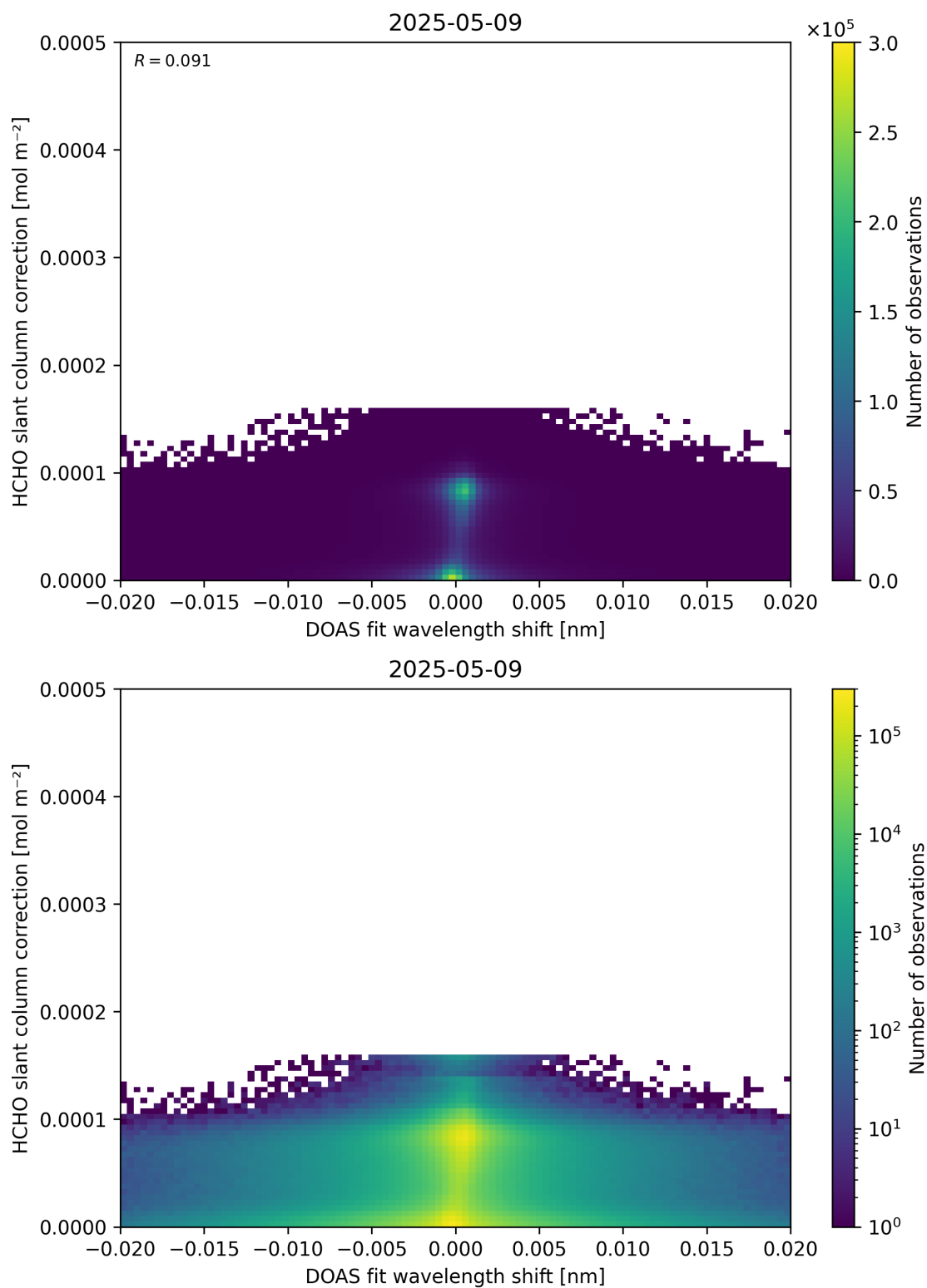
Figure 67: Scatter density plot of “DOAS fit wavelength shift” against “HCHO slant column correction” for 2025-05-08 to 2025-05-10.
