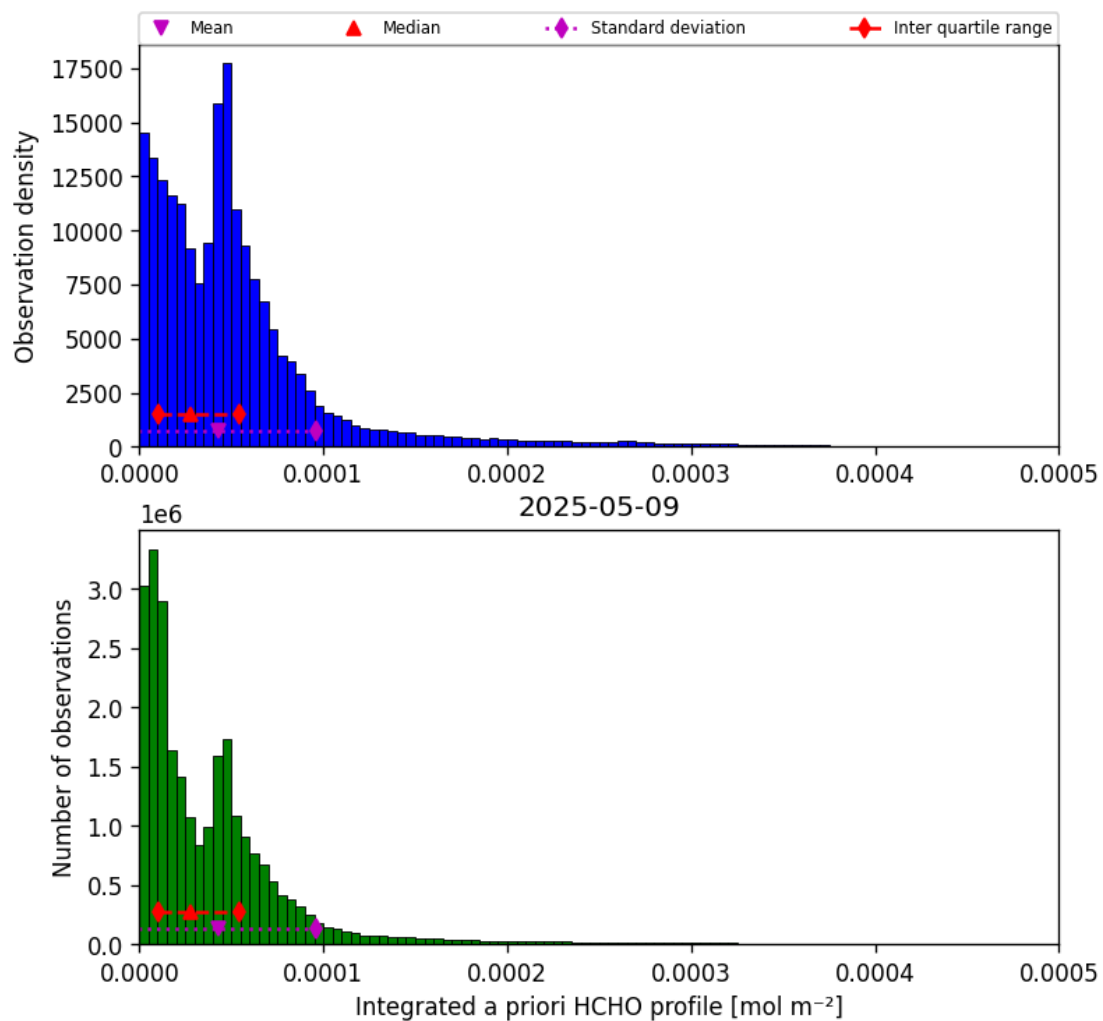
Figure 43: Histogram of “Integrated a priori HCHO profile” for 2025-05-08 to 2025-05-10
