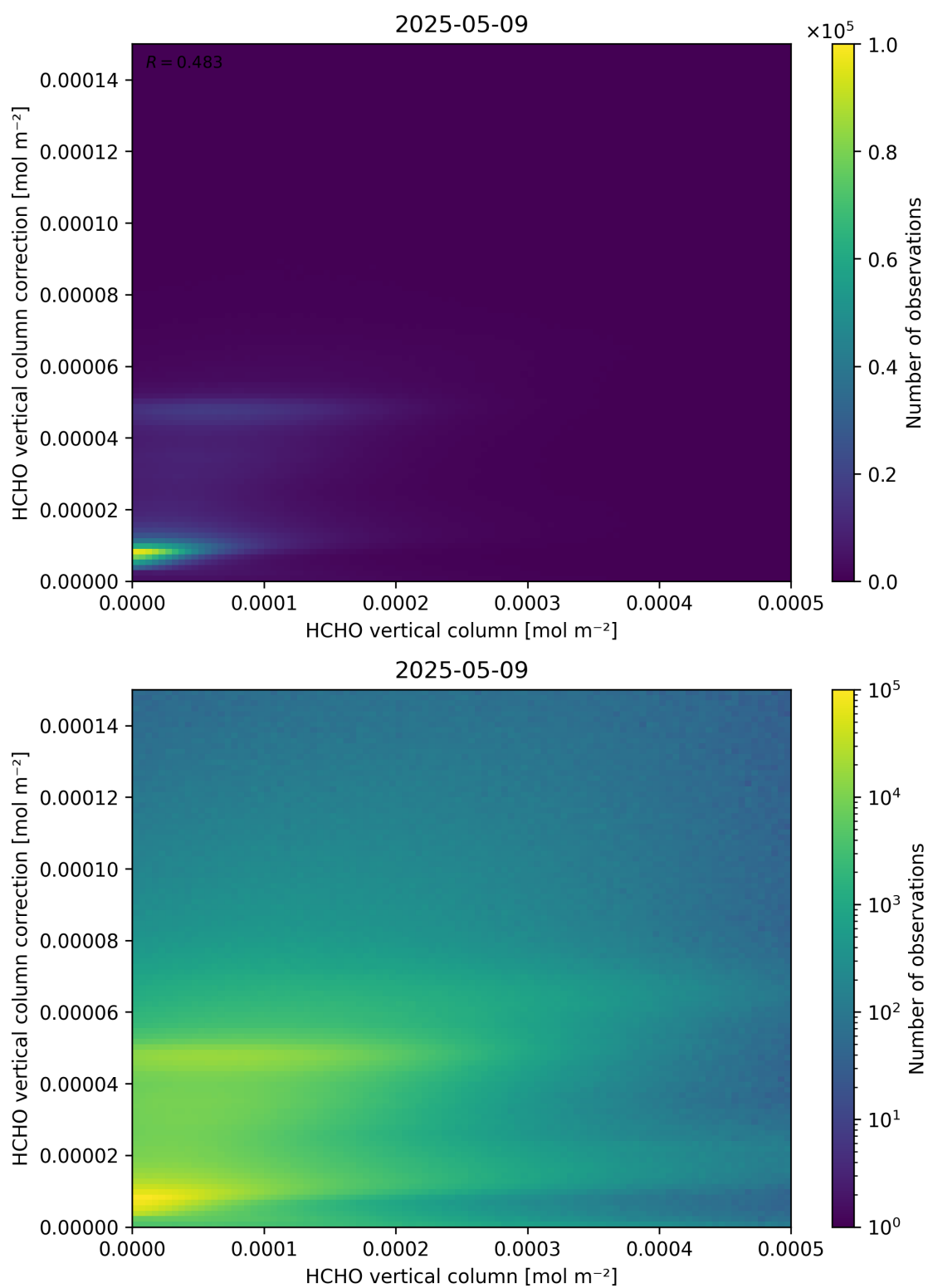
Figure 133: Scatter density plot of “HCHO vertical column” against “HCHO vertical column correction” for 2025-05-08 to 2025-05-10.
