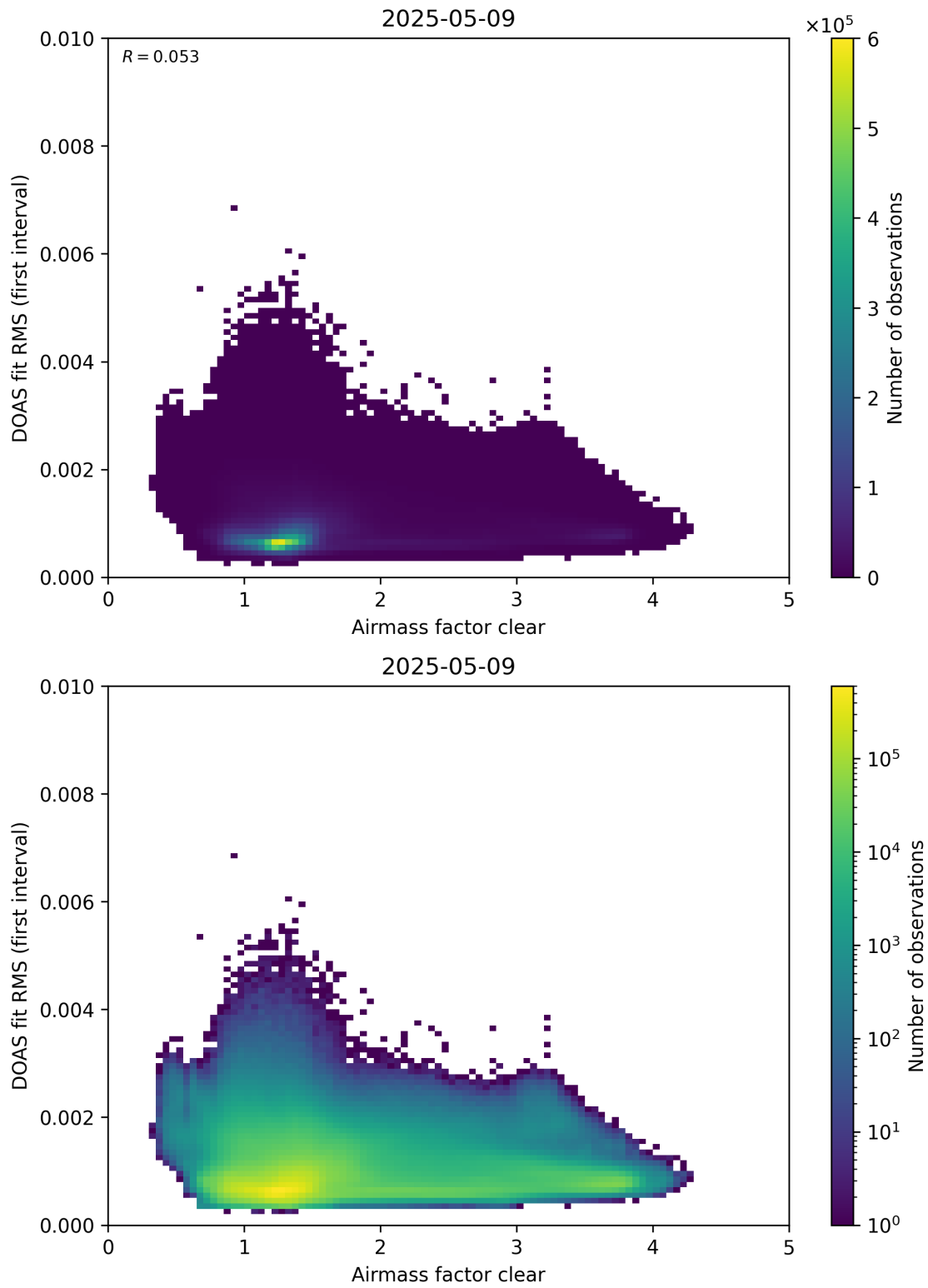
Figure 71: Scatter density plot of “Airmass factor clear” against “DOAS fit RMS (first interval)” for 2025-05-08 to 2025-05-10.
