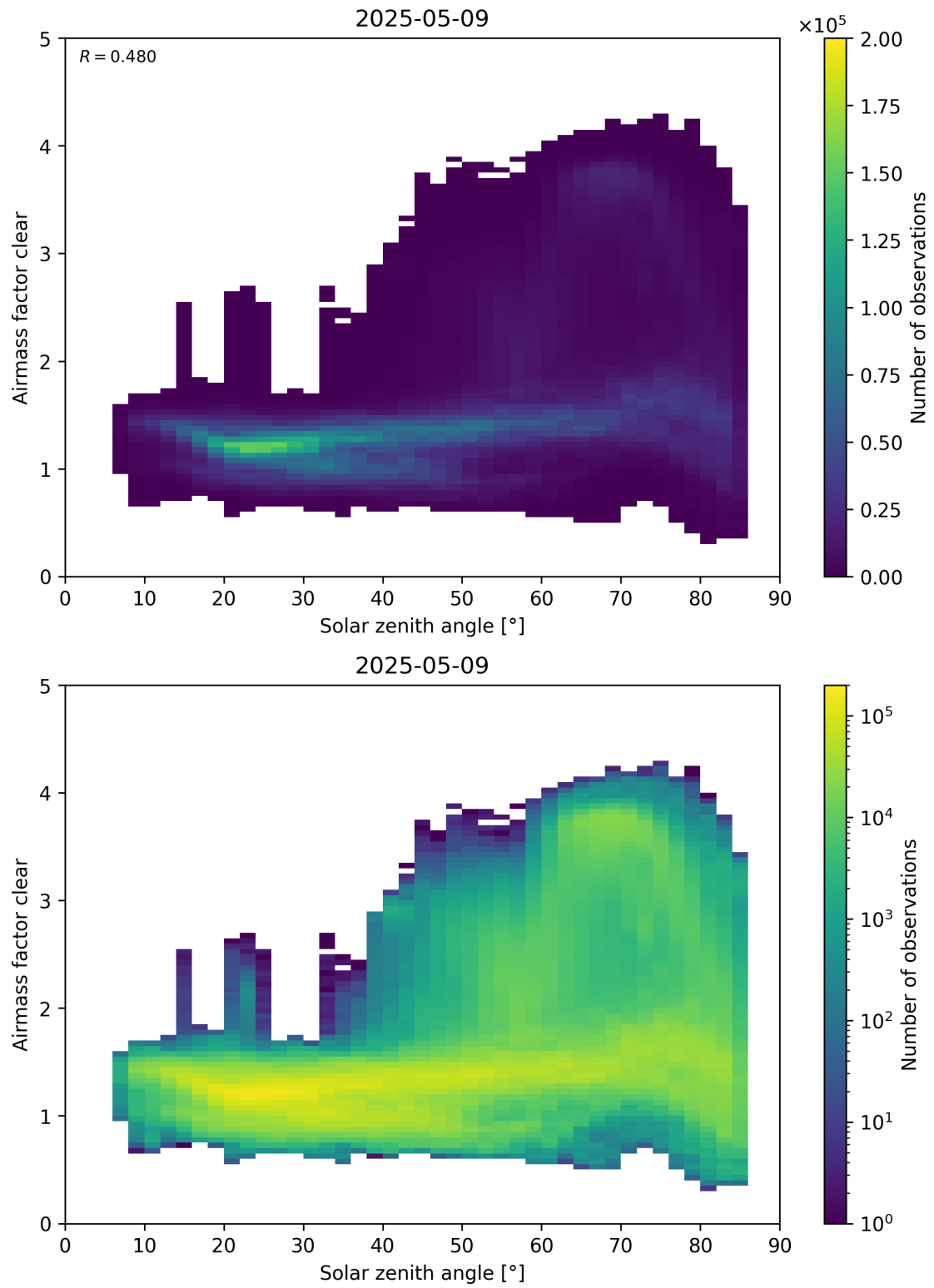
Figure 170: Scatter density plot of “Solar zenith angle” against “Airmass factor clear” for 2025-05-08 to 2025-05-10.
