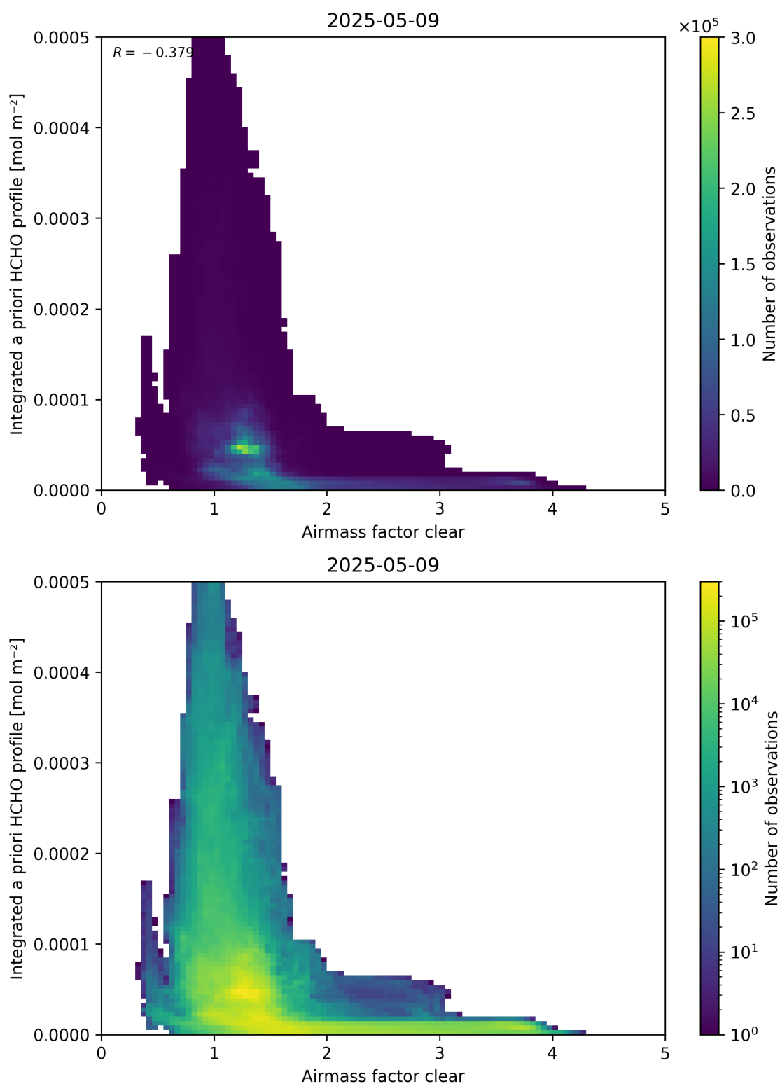
Figure 76: Scatter density plot of “Airmass factor clear” against “Integrated a priori HCHO profile” for 2025-05-08 to 2025-05-10.
