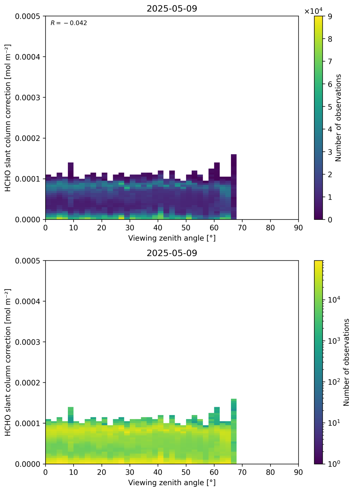
Figure 187: Scatter density plot of “Viewing zenith angle” against “HCHO slant column correction” for 2025-05-08 to 2025-05-10.
