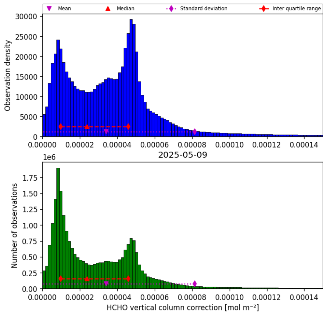
Figure 37: Histogram of “HCHO vertical column correction” for 2025-05-08 to 2025-05-10
