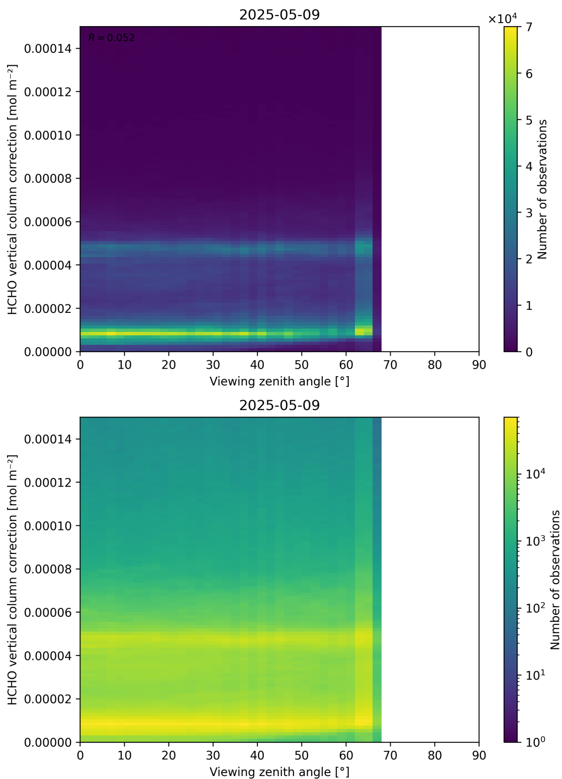
Figure 193: Scatter density plot of “Viewing zenith angle” against “HCHO vertical column correction” for 2025-05-08 to 2025-05-10.
