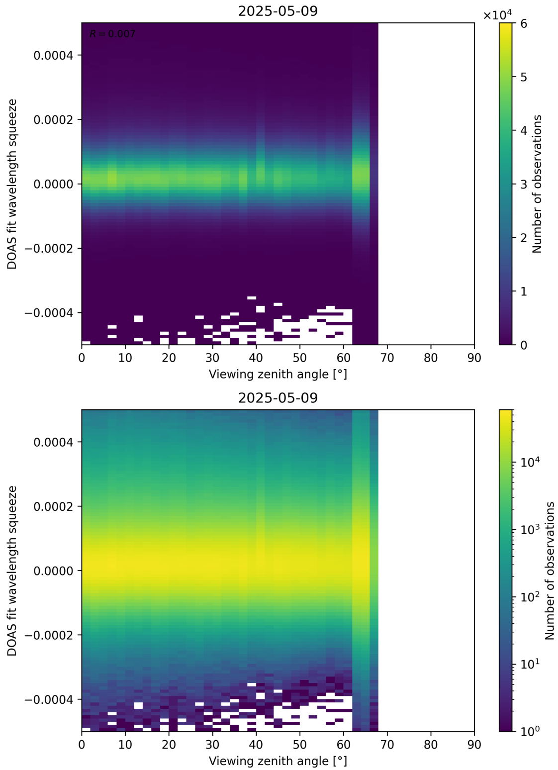
Figure 184: Scatter density plot of “Viewing zenith angle” against “DOAS fit wavelength squeeze” for 2025-05-08 to 2025-05-10.
