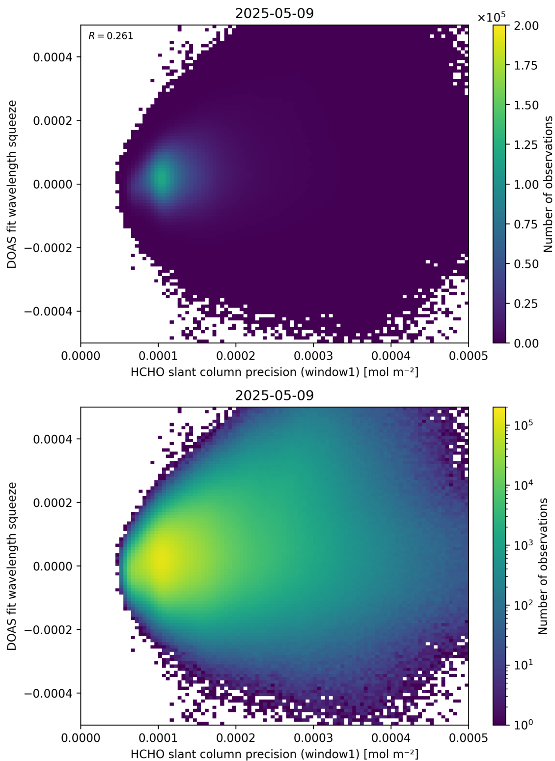
Figure 90: Scatter density plot of “HCHO slant column precision (window1)” against “DOAS fit wavelength squeeze” for 2025-05-08 to 2025-05-10.
