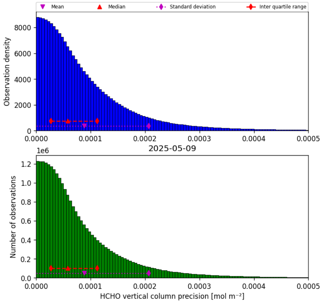
Figure 36: Histogram of “HCHO vertical column precision” for 2025-05-08 to 2025-05-10
