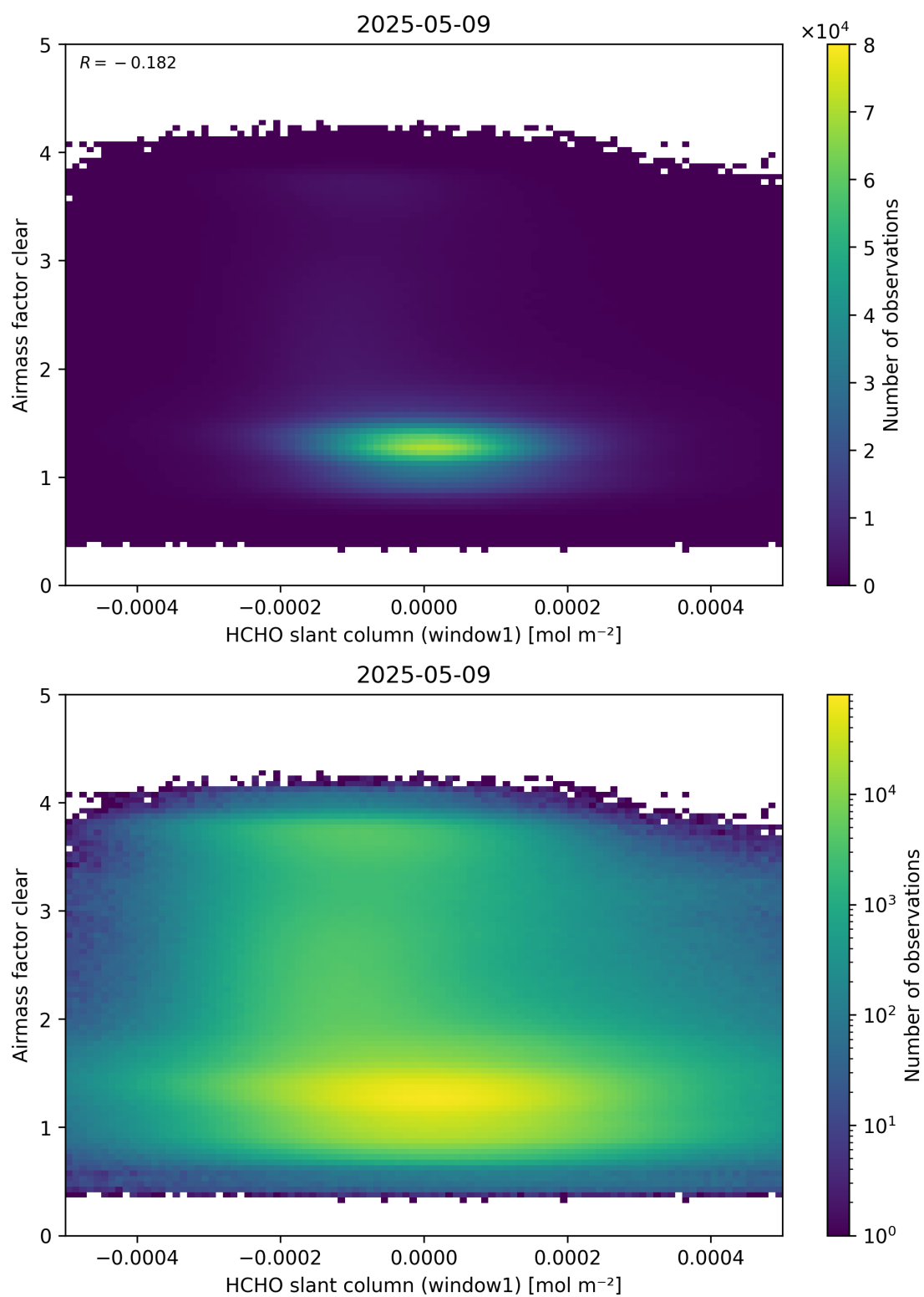
Figure 81: Scatter density plot of “HCHO slant column (window1)” against “Airmass factor clear” for 2025-05-08 to 2025-05-10.
