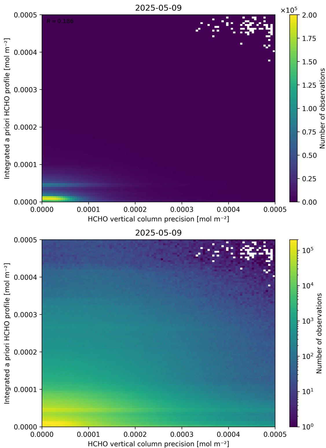
Figure 147: Scatter density plot of “HCHO vertical column precision” against “Integrated a priori HCHO profile” for 2025-05-08 to 2025-05-10.
