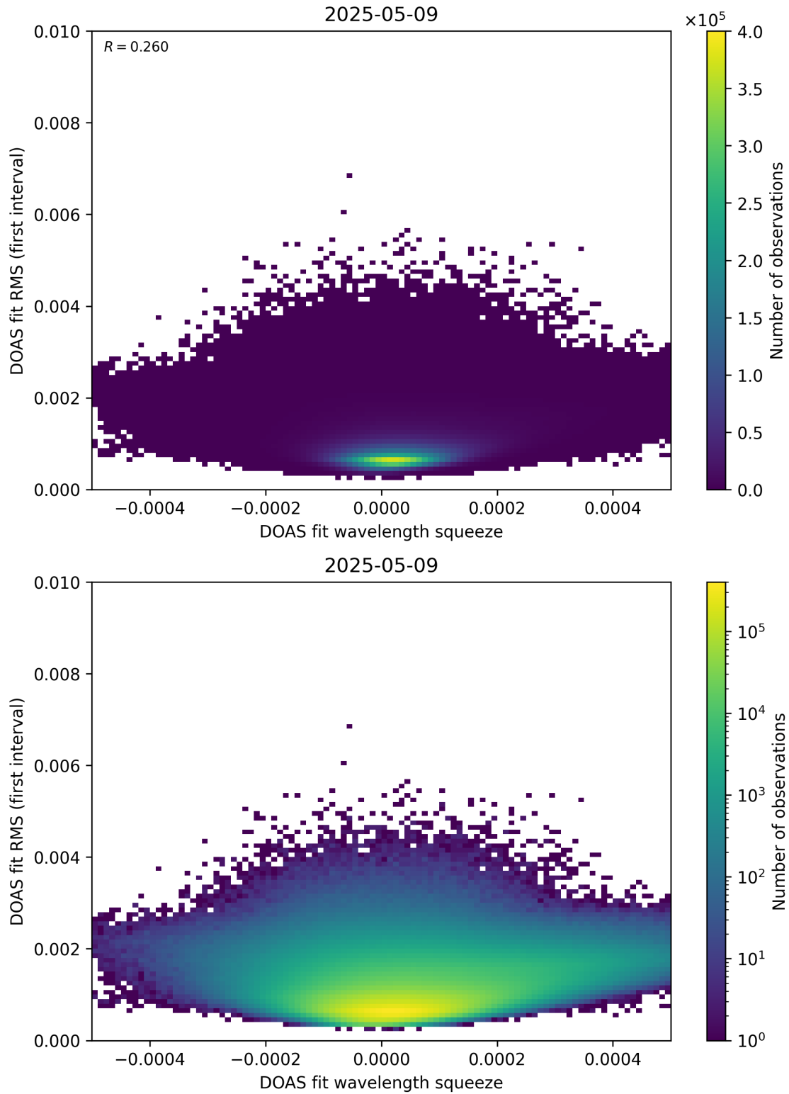
Figure 68: Scatter density plot of “DOAS fit wavelength squeeze” against “DOAS fit RMS (first interval)” for 2025-05-08 to 2025-05-10.
