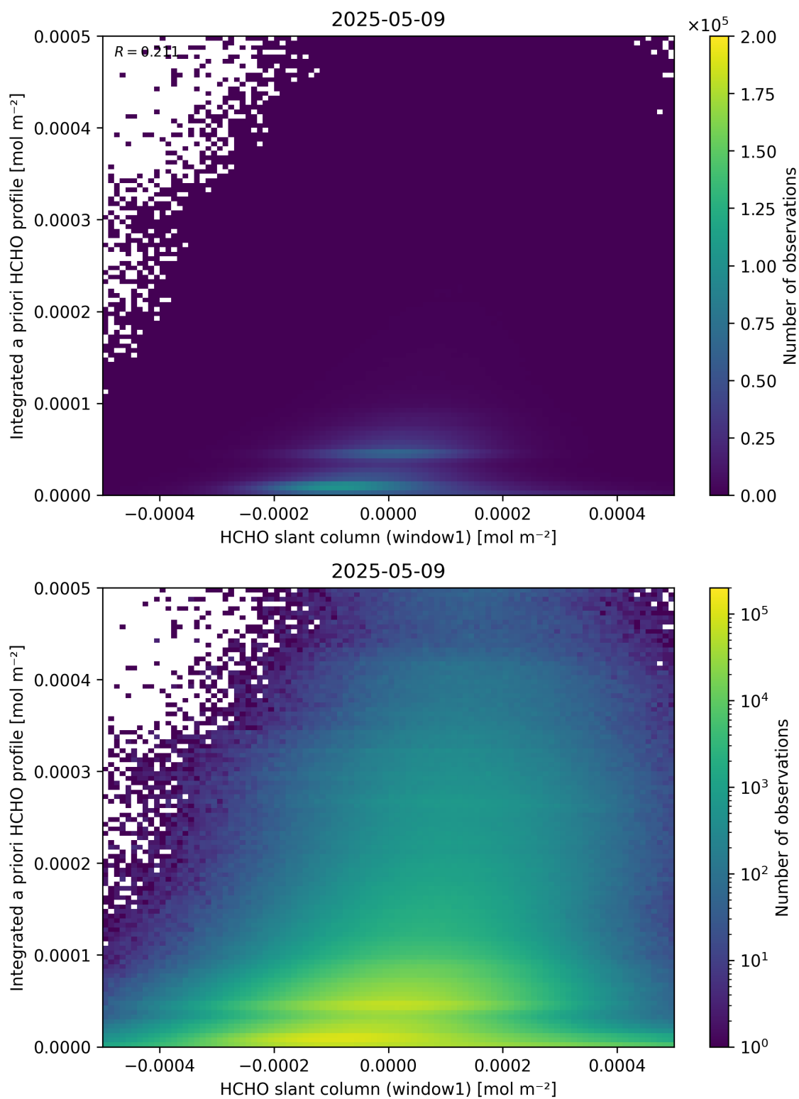
Figure 87: Scatter density plot of “HCHO slant column (window1)” against “Integrated a priori HCHO profile” for 2025-05-08 to 2025-05-10.
