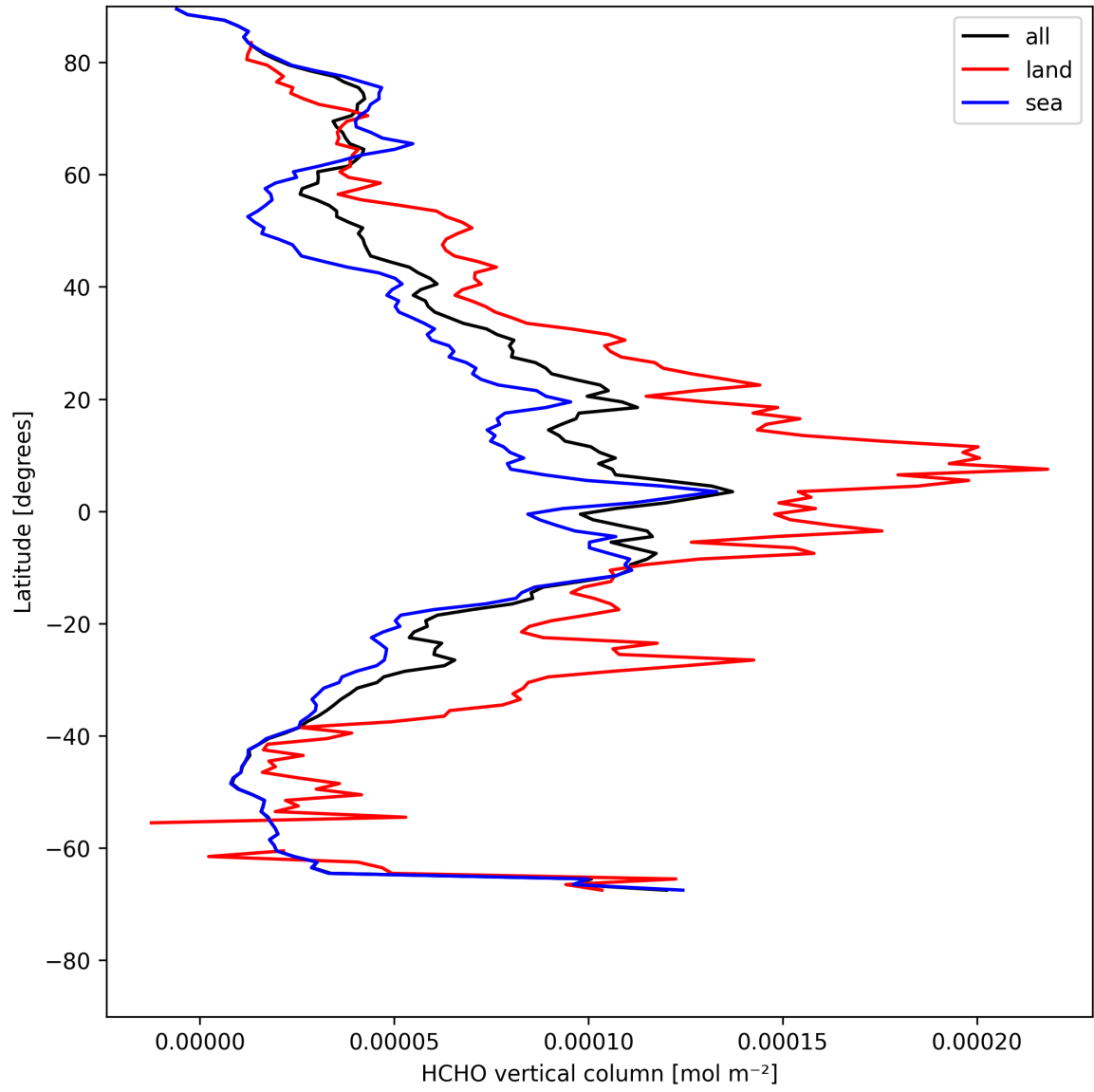
Figure 21: Zonal average of “HCHO vertical column” for 2025-05-08 to 2025-05-10.
