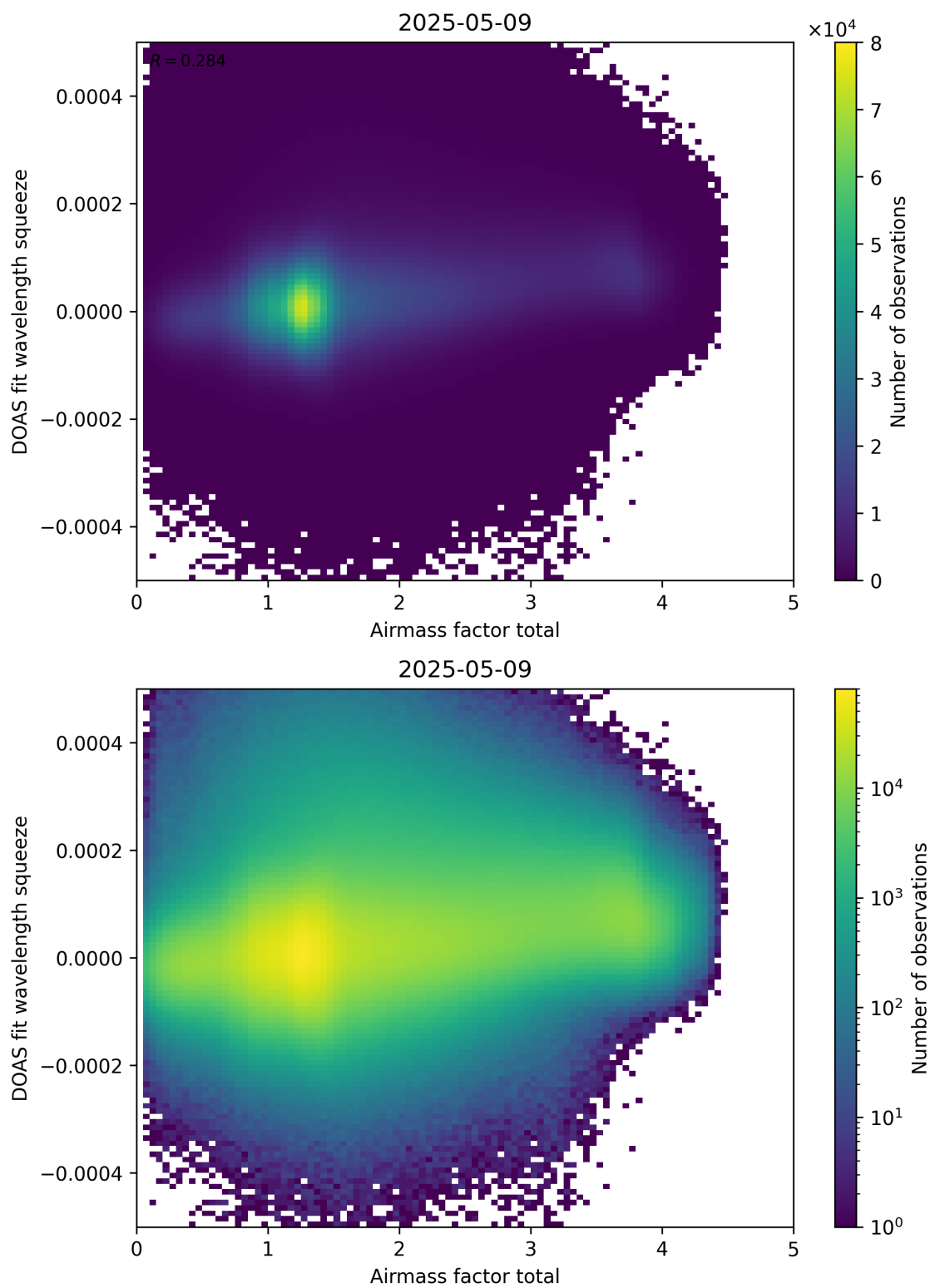
Figure 99: Scatter density plot of “Airmass factor total” against “DOAS fit wavelength squeeze” for 2025-05-08 to 2025-05-10.
