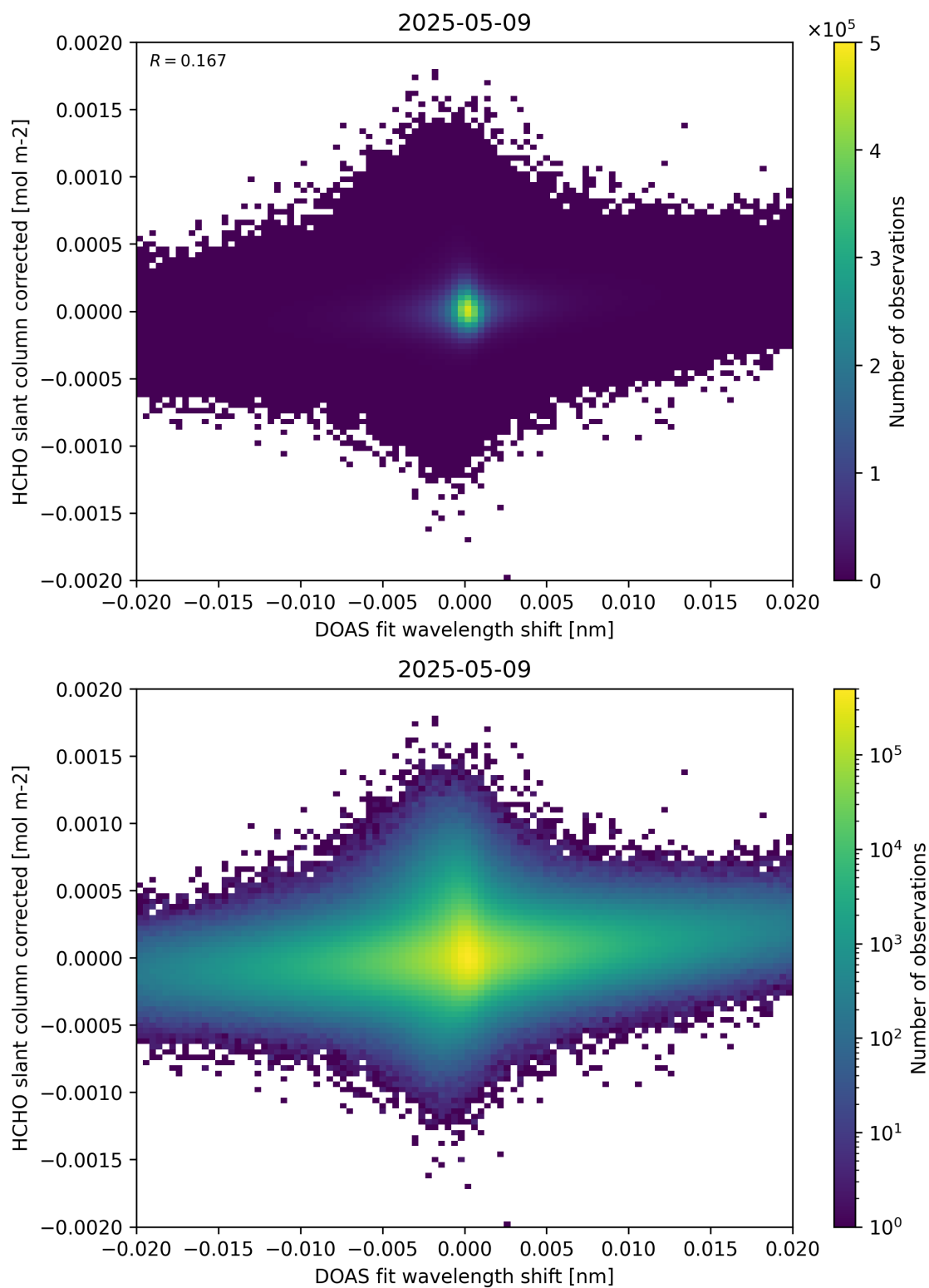
Figure 66: Scatter density plot of “DOAS fit wavelength shift” against “HCHO slant column corrected” for 2025-05-08 to 2025-05-10.
