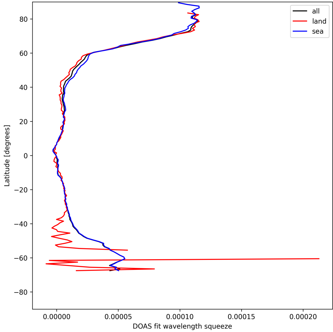
Figure 31: Zonal average of “DOAS fit wavelength squeeze” for 2025-05-08 to 2025-05-10.
