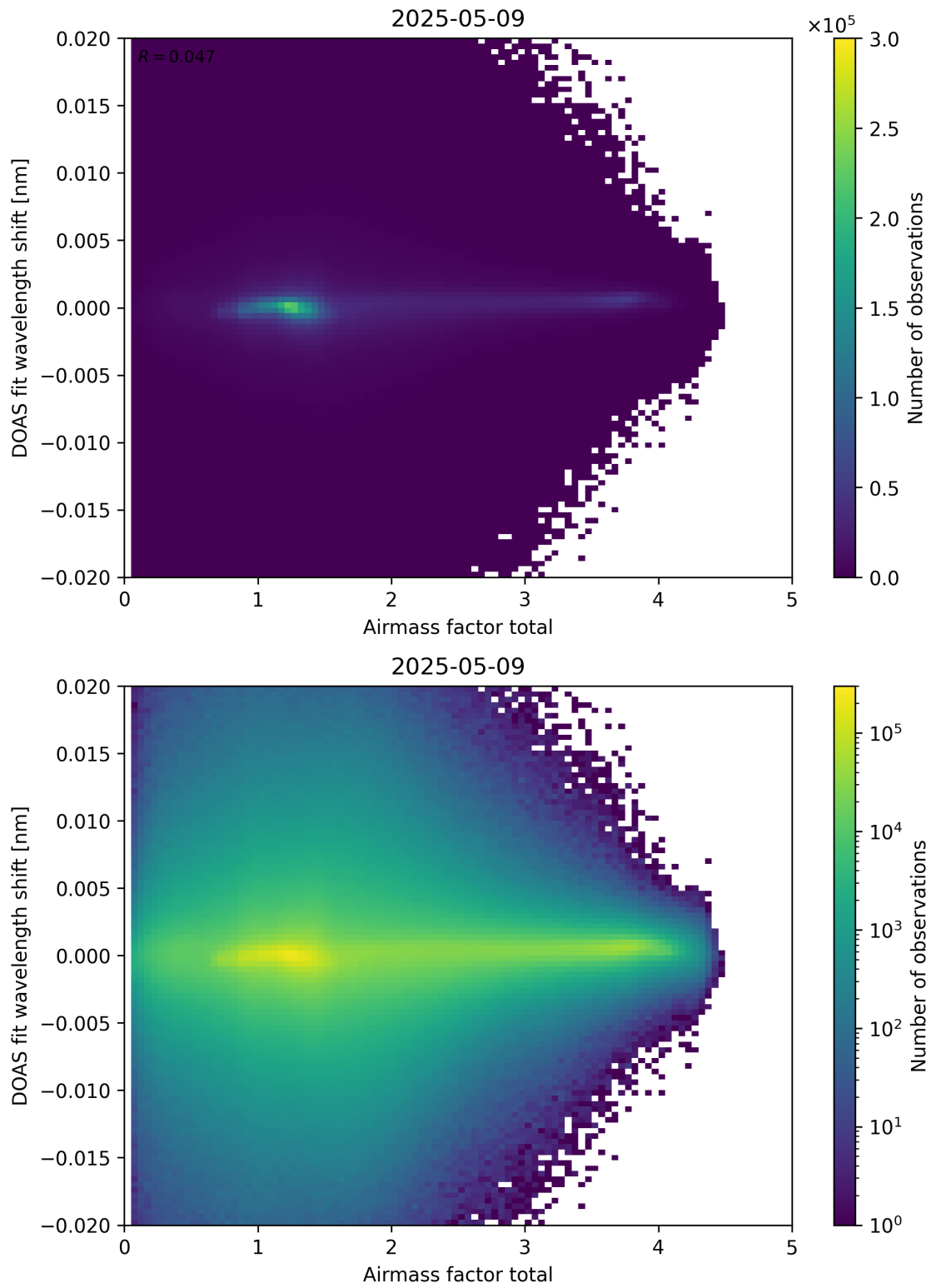
Figure 98: Scatter density plot of “Airmass factor total” against “DOAS fit wavelength shift” for 2025-05-08 to 2025-05-10.
