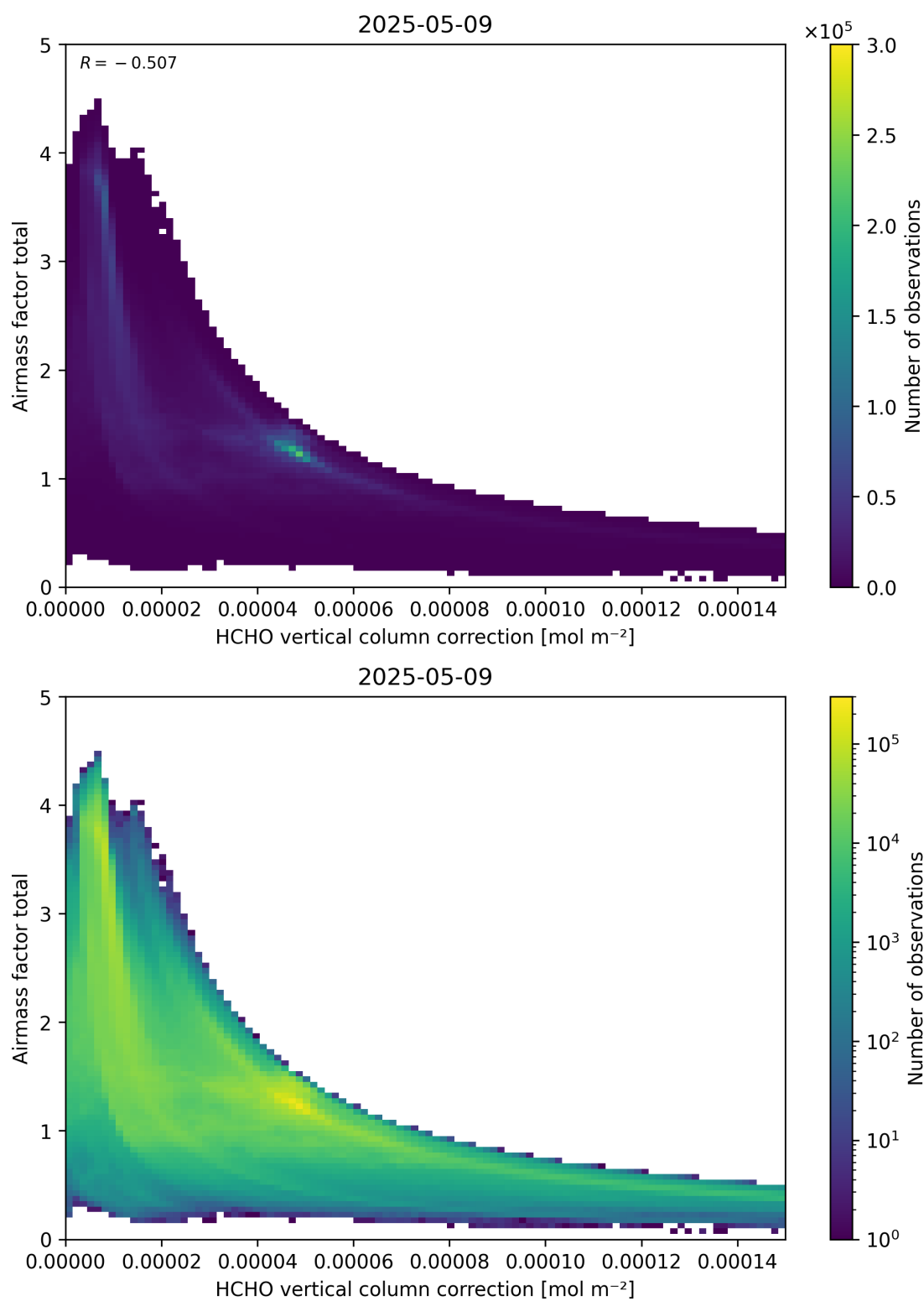
Figure 120: Scatter density plot of “HCHO vertical column correction” against “Airmass factor total” for 2025-05-08 to 2025-05-10.
