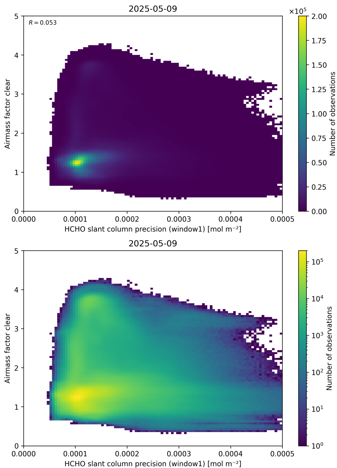
Figure 91: Scatter density plot of “HCHO slant column precision (window1)” against “Airmass factor clear” for 2025-05-08 to 2025-05-10.
