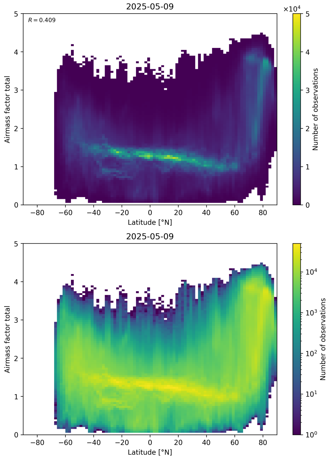
Figure 161: Scatter density plot of “Latitude” against “Airmass factor total” for 2025-05-08 to 2025-05-10.
