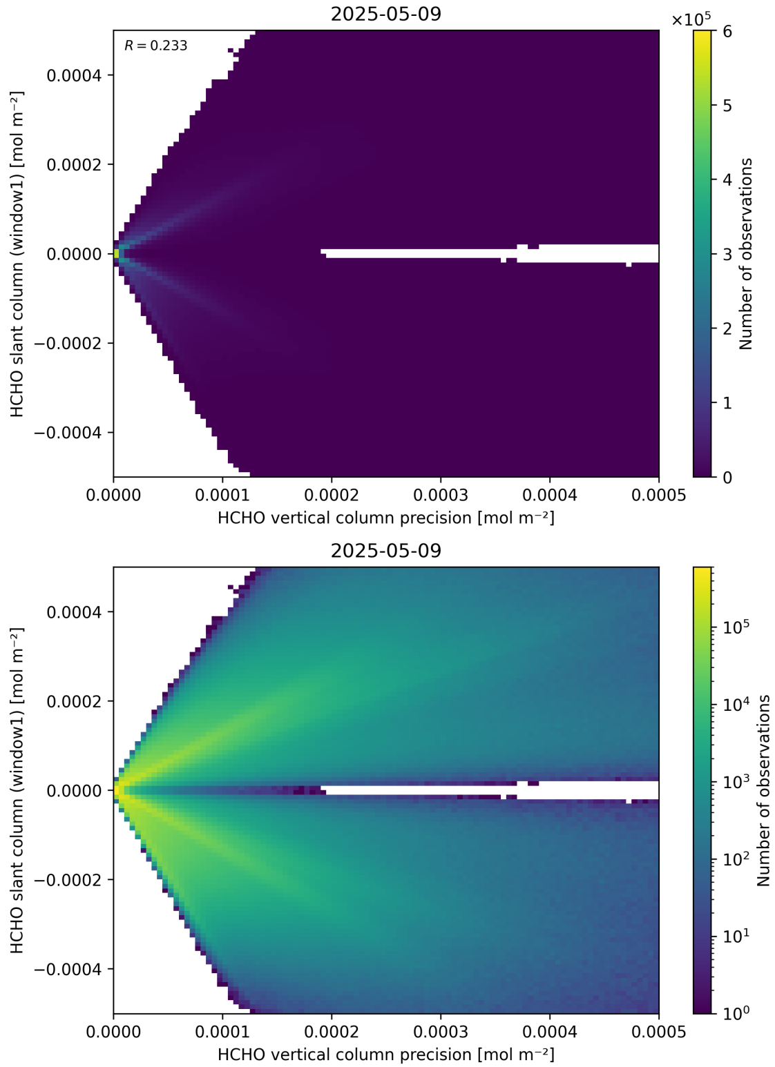
Figure 142: Scatter density plot of “HCHO vertical column precision” against “HCHO slant column (window1)” for 2025-05-08 to 2025-05-10.
