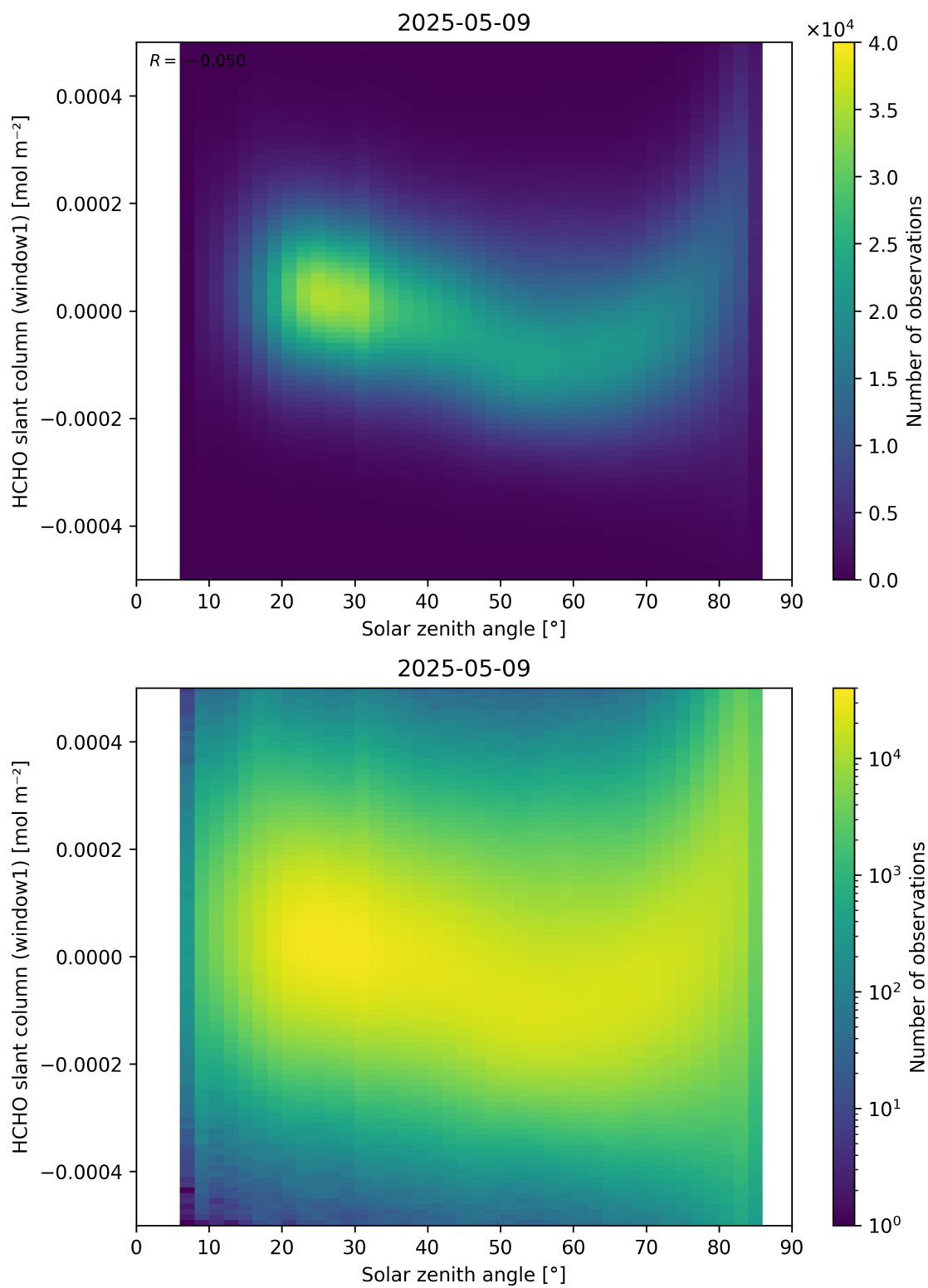
Figure 173: Scatter density plot of “Solar zenith angle” against “HCHO slant column (window1)” for 2025-05-08 to 2025-05-10.
