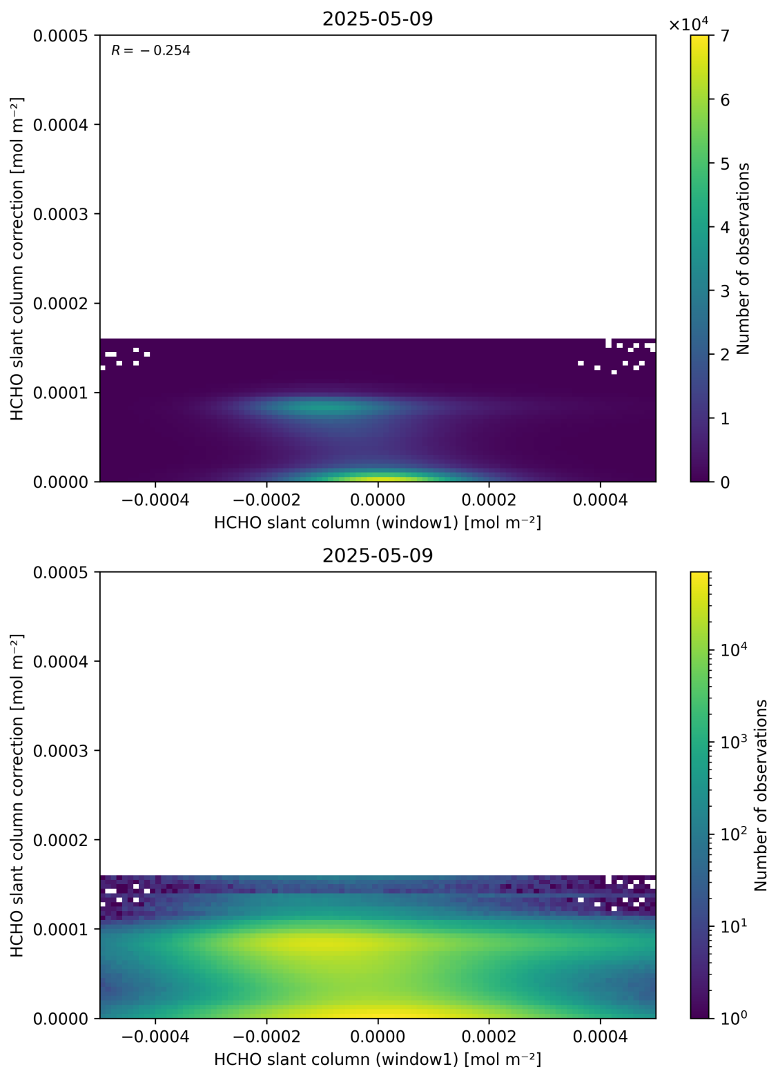
Figure 83: Scatter density plot of “HCHO slant column (window1)” against “HCHO slant column correction” for 2025-05-08 to 2025-05-10.
