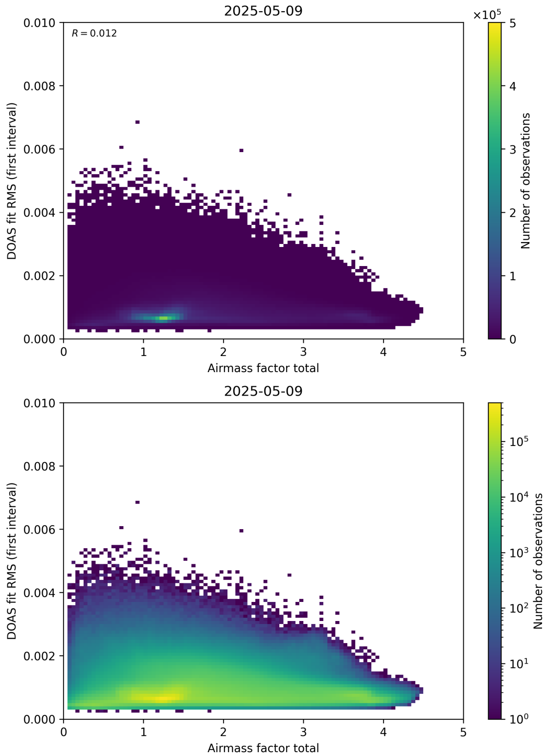
Figure 97: Scatter density plot of “Airmass factor total” against “DOAS fit RMS (first interval)” for 2025-05-08 to 2025-05-10.
