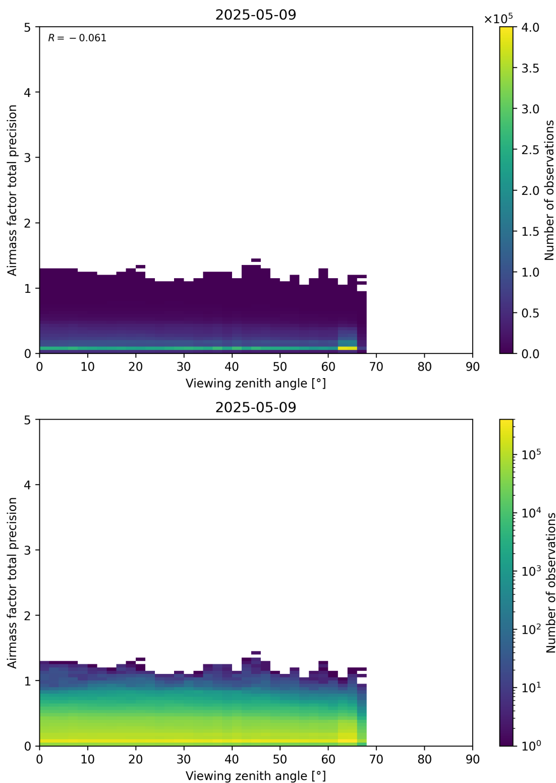
Figure 191: Scatter density plot of “Viewing zenith angle” against “Airmass factor total precision” for 2025-05-08 to 2025-05-10.
