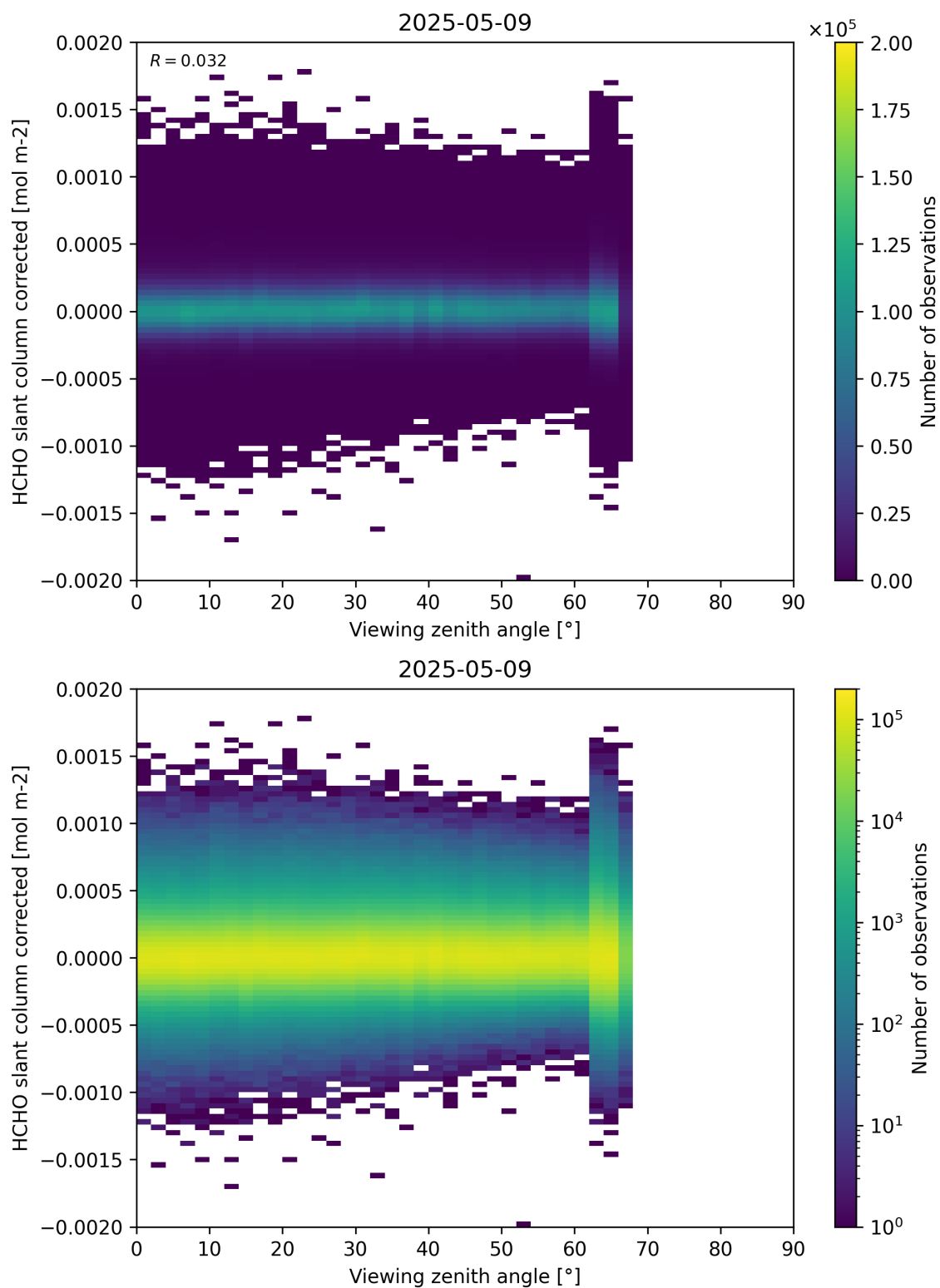
Figure 186: Scatter density plot of “Viewing zenith angle” against “HCHO slant column corrected” for 2025-05-08 to 2025-05-10.
