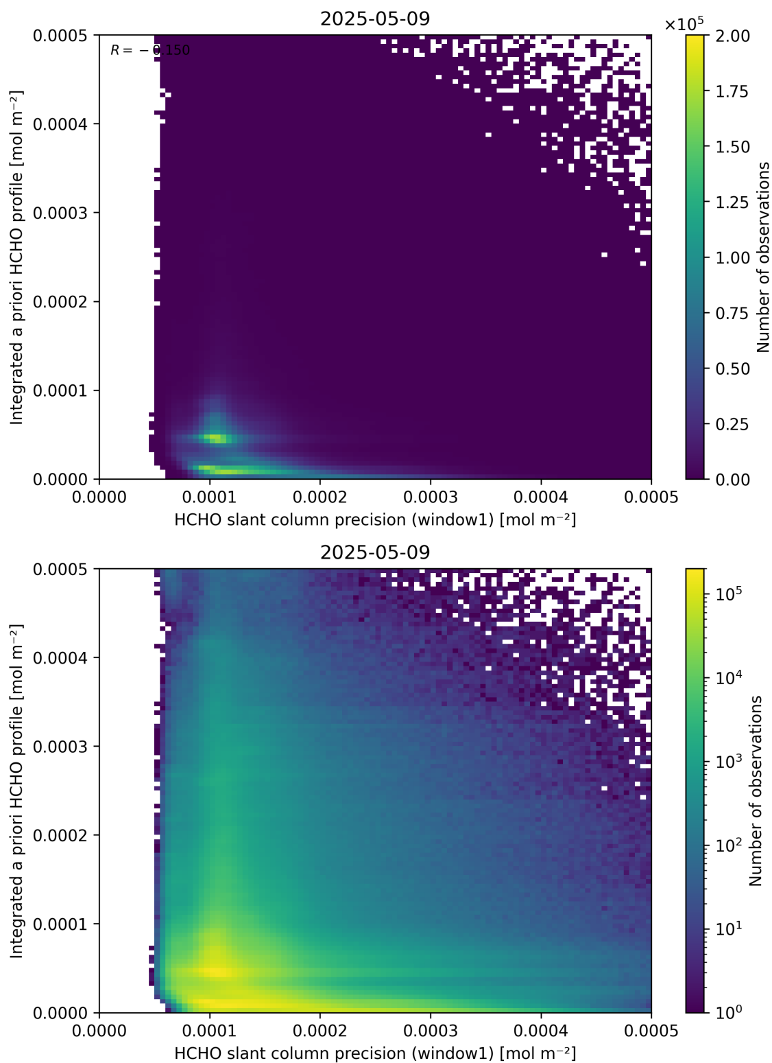
Figure 96: Scatter density plot of “HCHO slant column precision (window1)” against “Integrated a priori HCHO profile” for 2025-05-08 to 2025-05-10.
