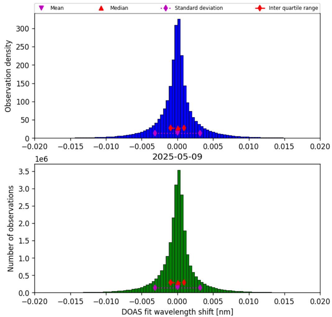
Figure 44: Histogram of “DOAS fit wavelength shift” for 2025-05-08 to 2025-05-10
