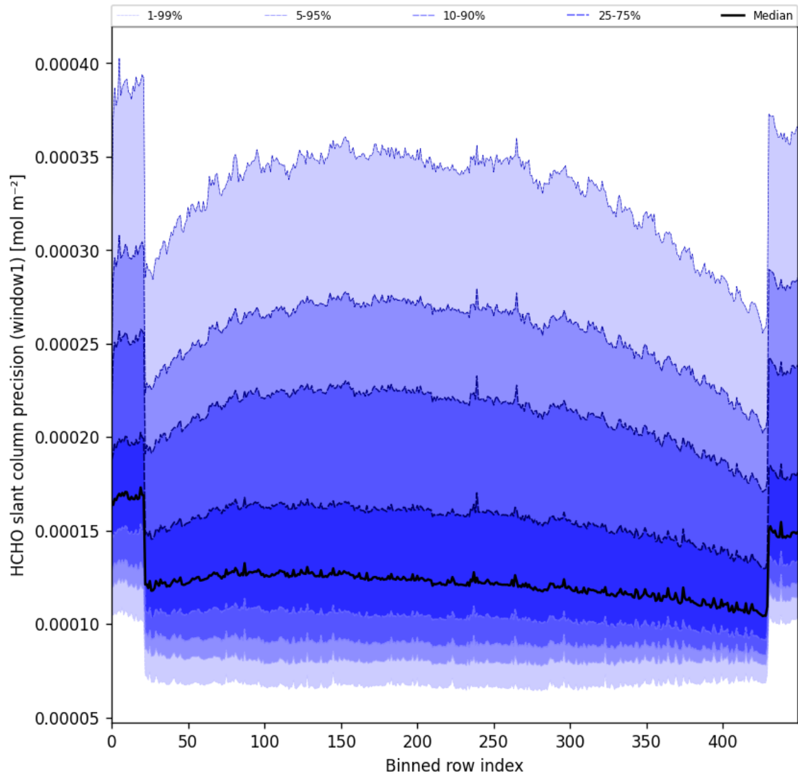
Figure 53: Along track statistics of “HCHO slant column precision (window1)” for 2025-05-08 to 2025-05-10
