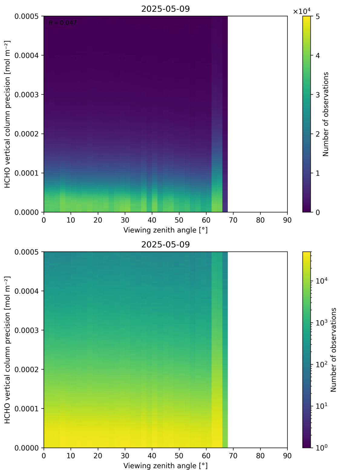
Figure 194: Scatter density plot of “Viewing zenith angle” against “HCHO vertical column precision” for 2025-05-08 to 2025-05-10.
