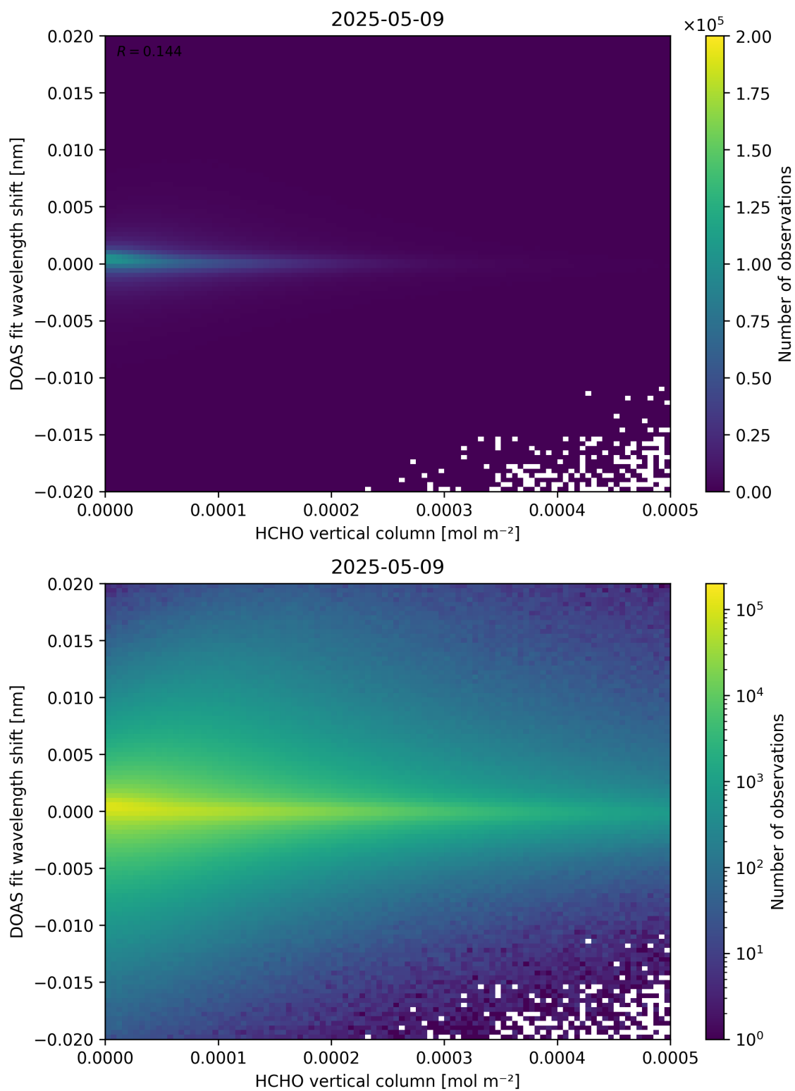
Figure 124: Scatter density plot of “HCHO vertical column” against “DOAS fit wavelength shift” for 2025-05-08 to 2025-05-10.
