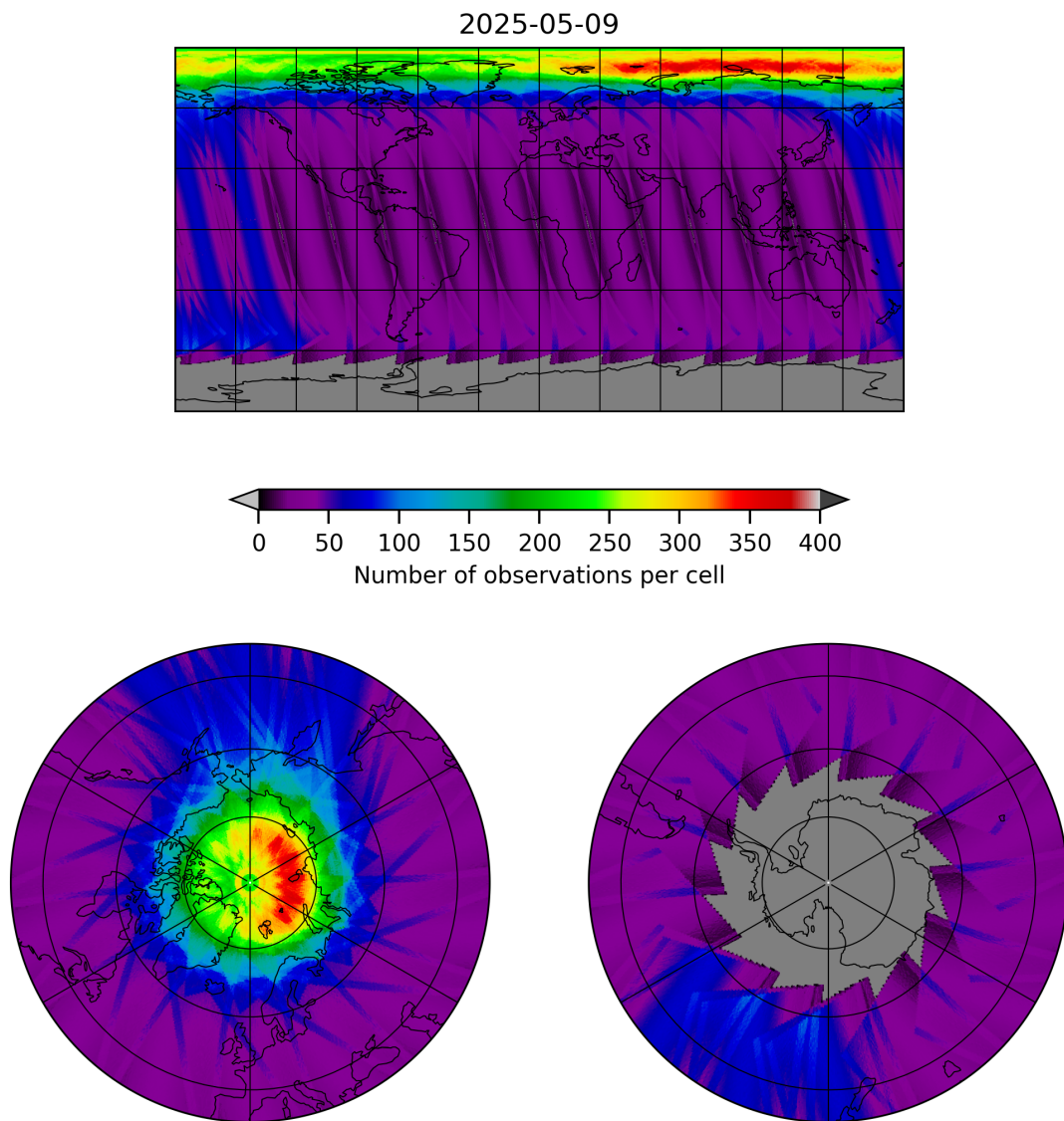
Figure 19: Map of the number of observations for 2025-05-08 to 2025-05-10
