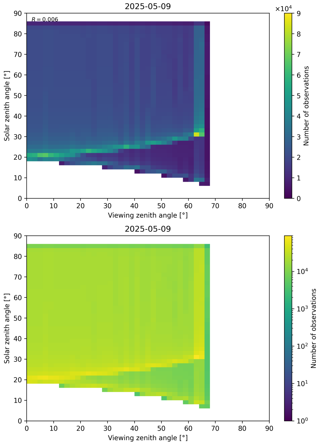
Figure 197: Scatter density plot of “Viewing zenith angle” against “Solar zenith angle” for 2025-05-08 to 2025-05-10.
