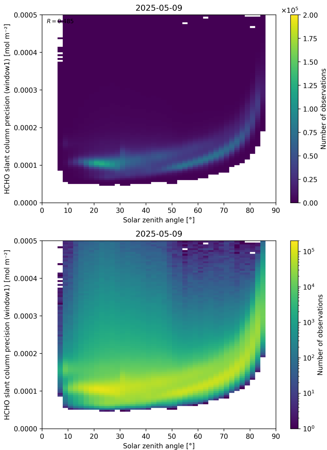
Figure 174: Scatter density plot of “Solar zenith angle” against “HCHO slant column precision (window1)” for 2025-05-08 to 2025-05-10.
