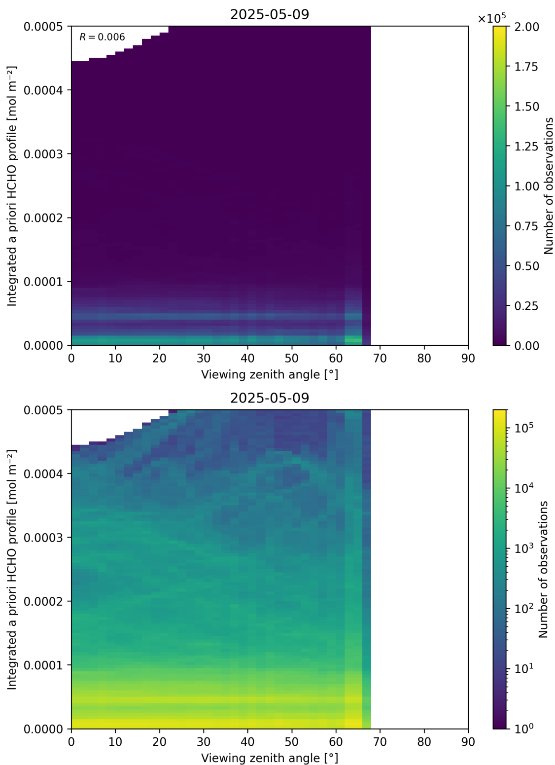
Figure 195: Scatter density plot of “Viewing zenith angle” against “Integrated a priori HCHO profile” for 2025-05-08 to 2025-05-10.
