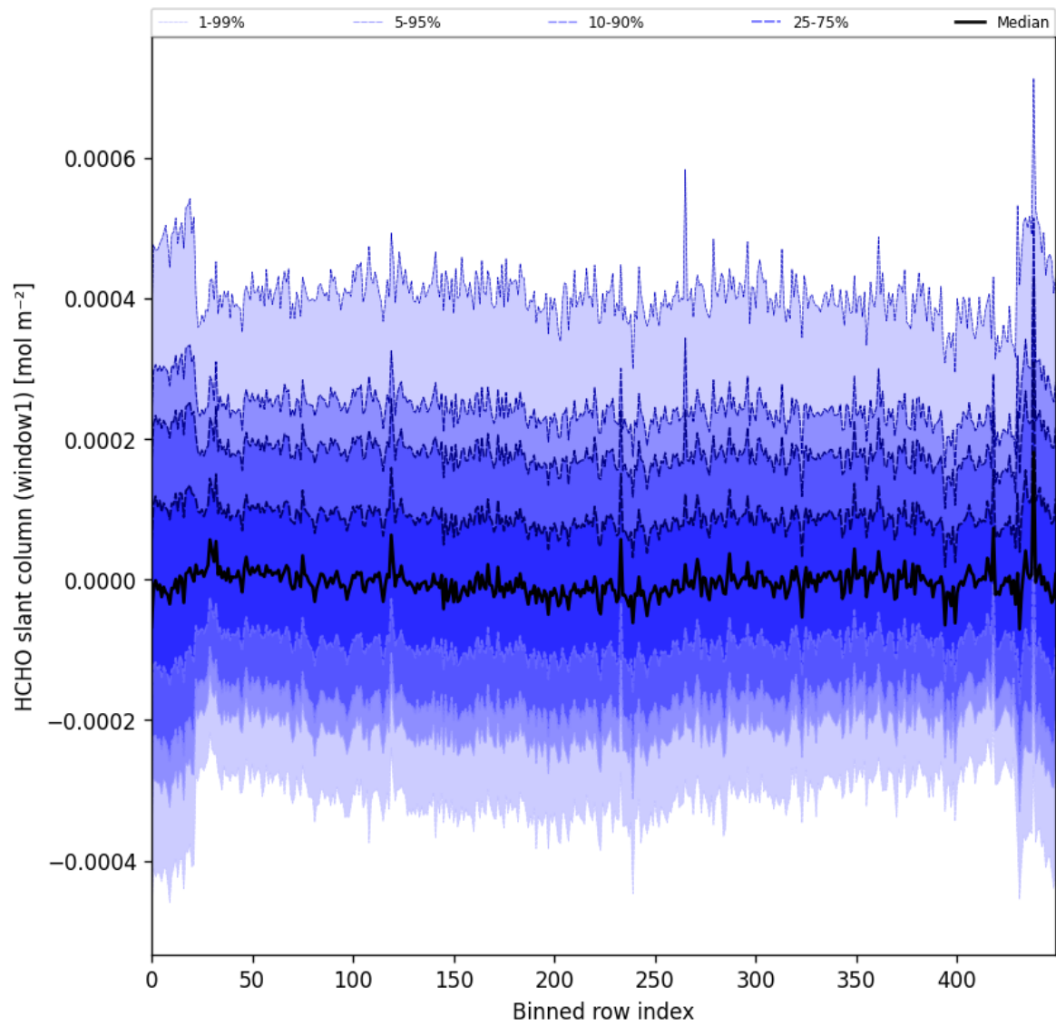
Figure 52: Along track statistics of “HCHO slant column (window1)” for 2025-05-08 to 2025-05-10
