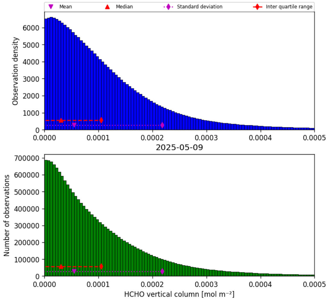
Figure 35: Histogram of “HCHO vertical column” for 2025-05-08 to 2025-05-10
