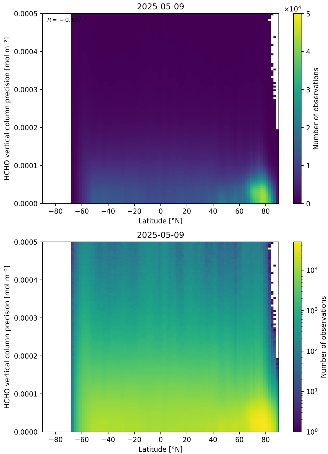
Figure 165: Scatter density plot of “Latitude” against “HCHO vertical column precision” for 2025-05-08 to 2025-05-10.
