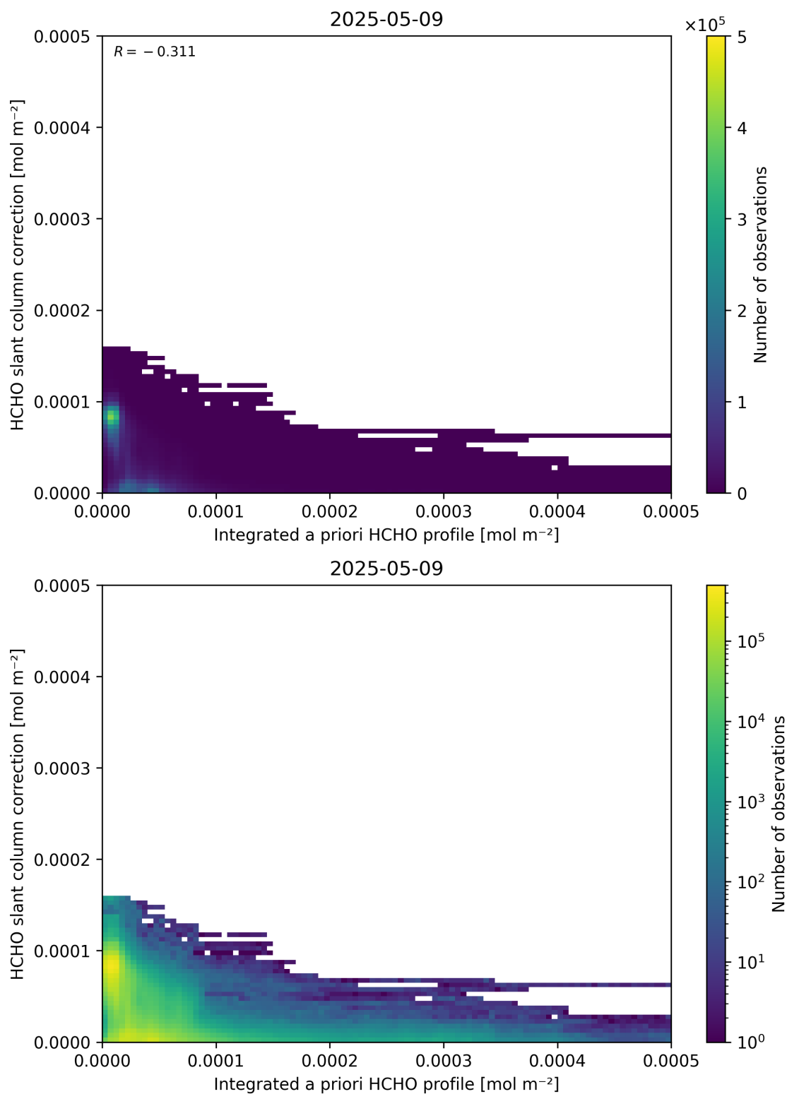
Figure 152: Scatter density plot of “Integrated a priori HCHO profile” against “HCHO slant column correction” for 2025-05-08 to 2025-05-10.
