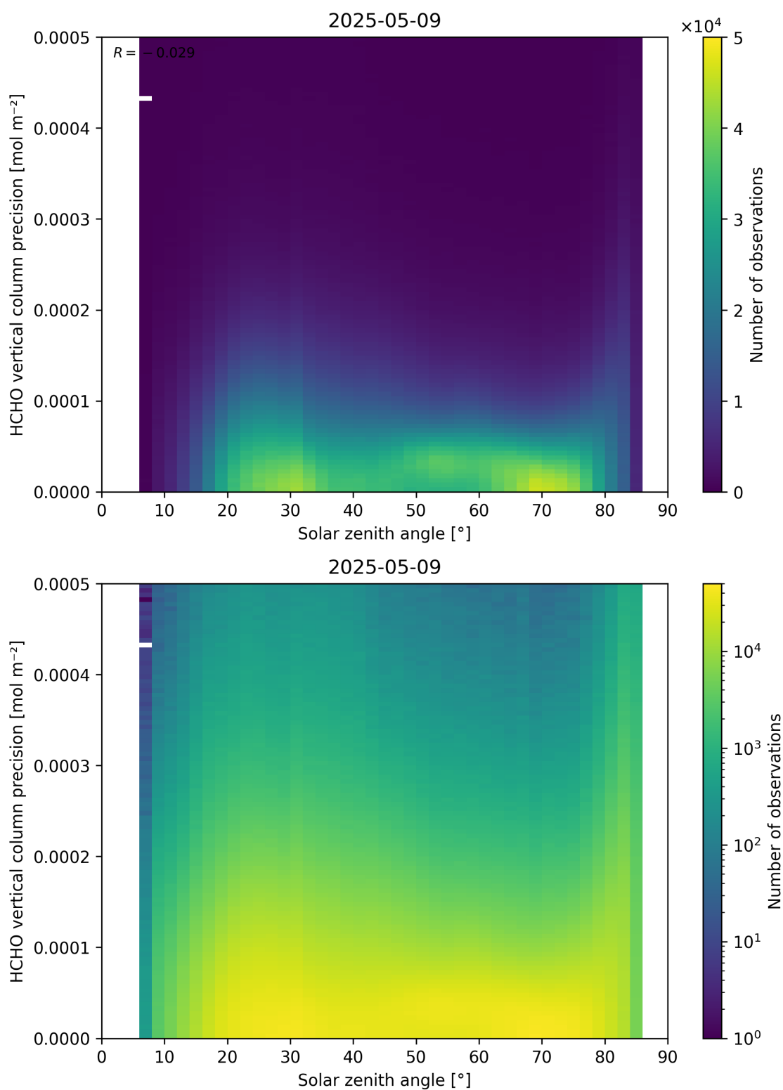
Figure 179: Scatter density plot of “Solar zenith angle” against “HCHO vertical column precision” for 2025-05-08 to 2025-05-10.
