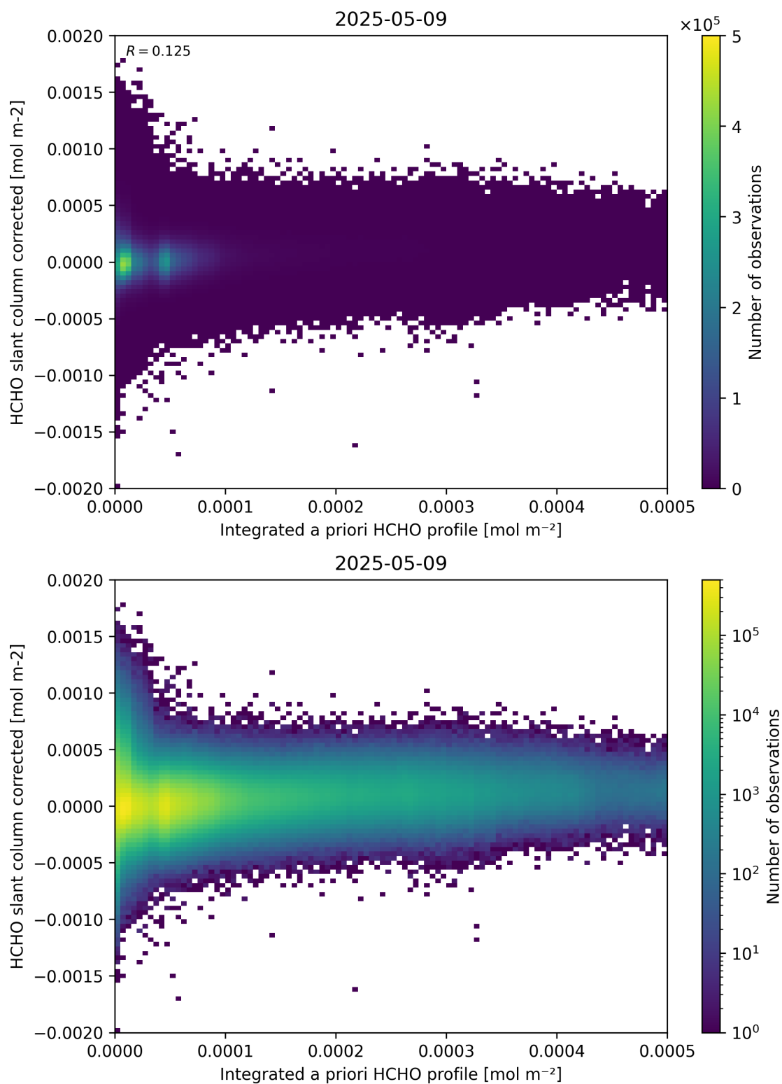
Figure 151: Scatter density plot of “Integrated a priori HCHO profile” against “HCHO slant column corrected” for 2025-05-08 to 2025-05-10.
