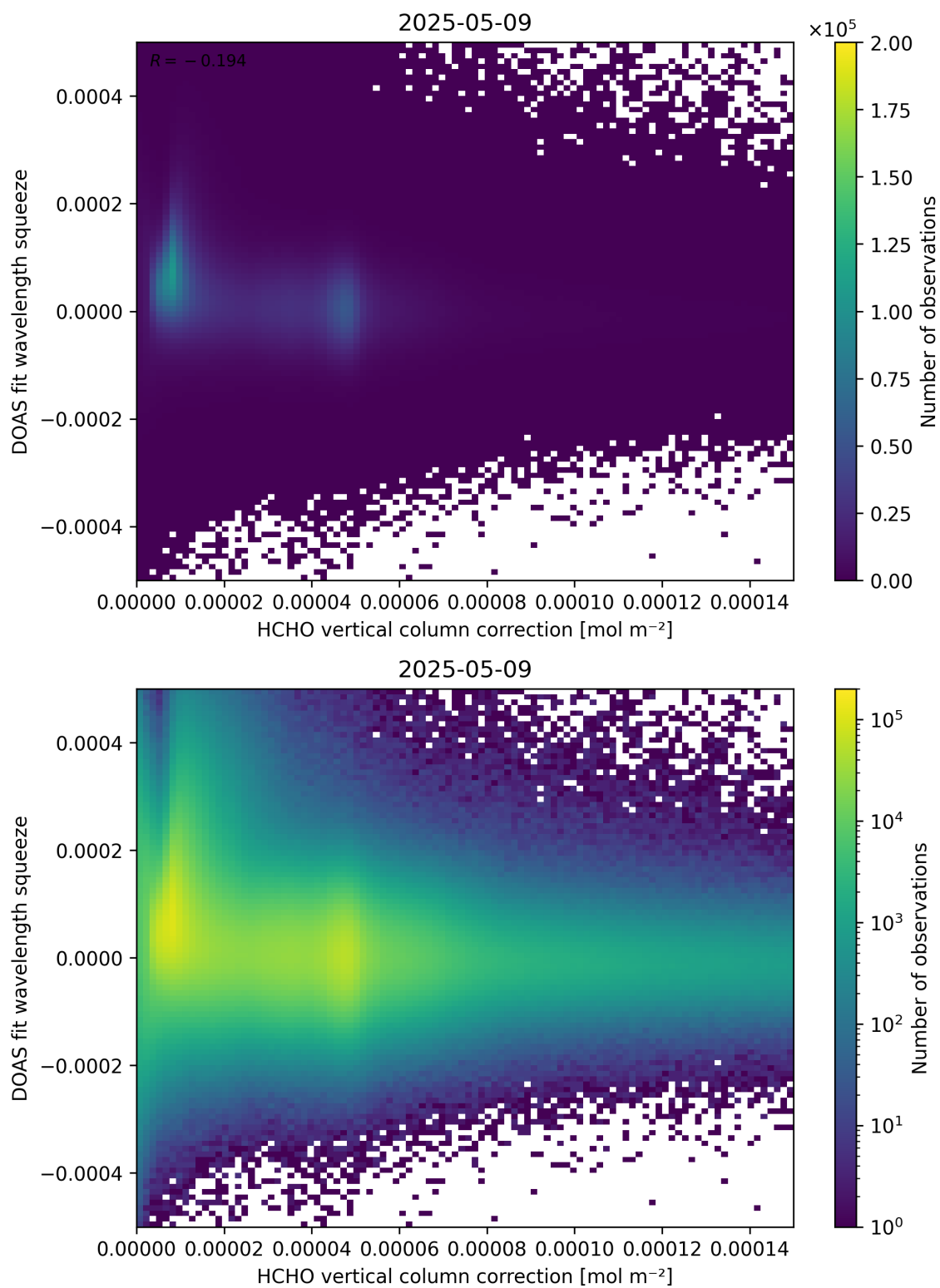
Figure 114: Scatter density plot of “HCHO vertical column correction” against “DOAS fit wavelength squeeze” for 2025-05-08 to 2025-05-10.
