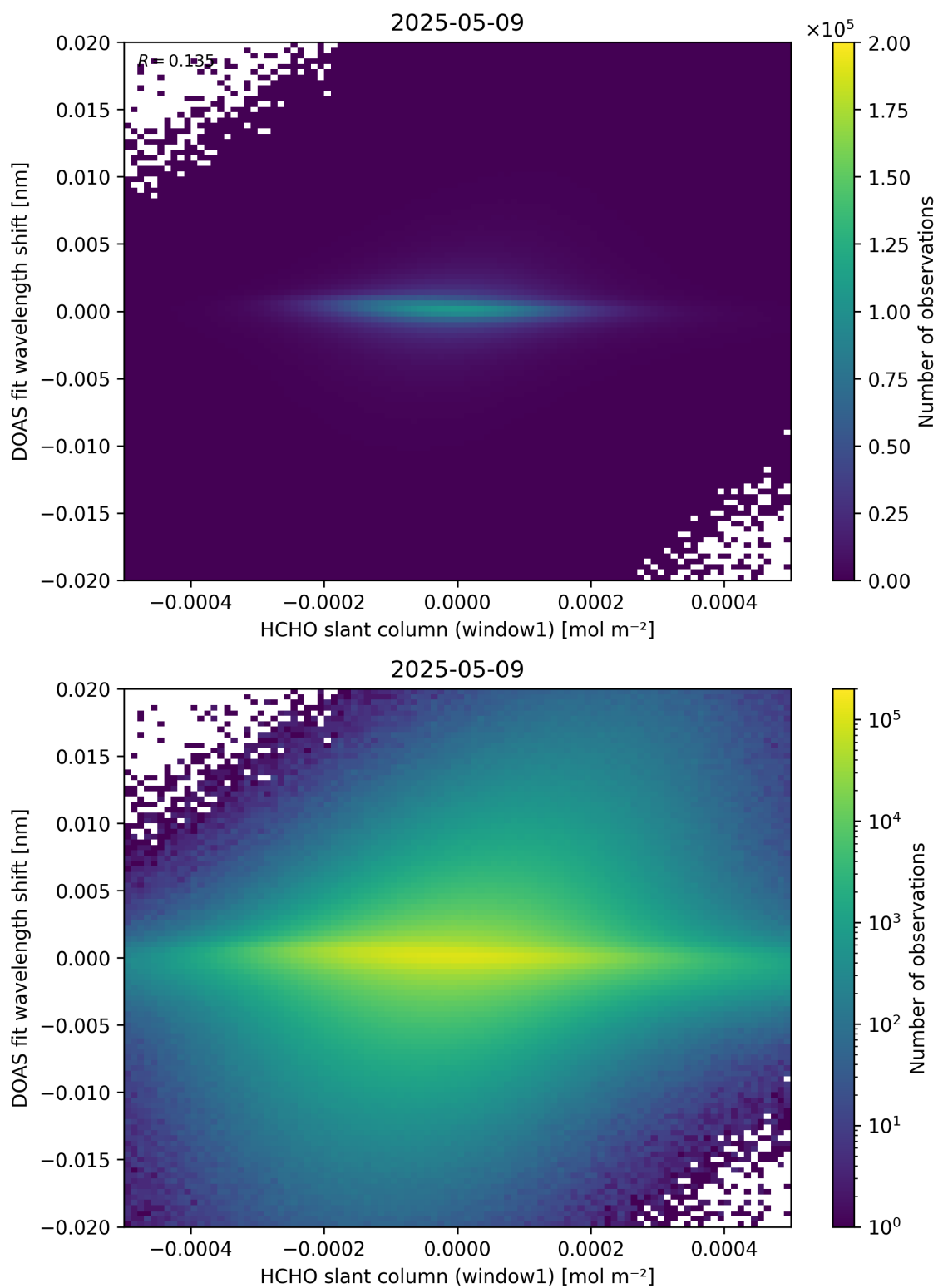
Figure 79: Scatter density plot of “HCHO slant column (window1)” against “DOAS fit wavelength shift” for 2025-05-08 to 2025-05-10.
