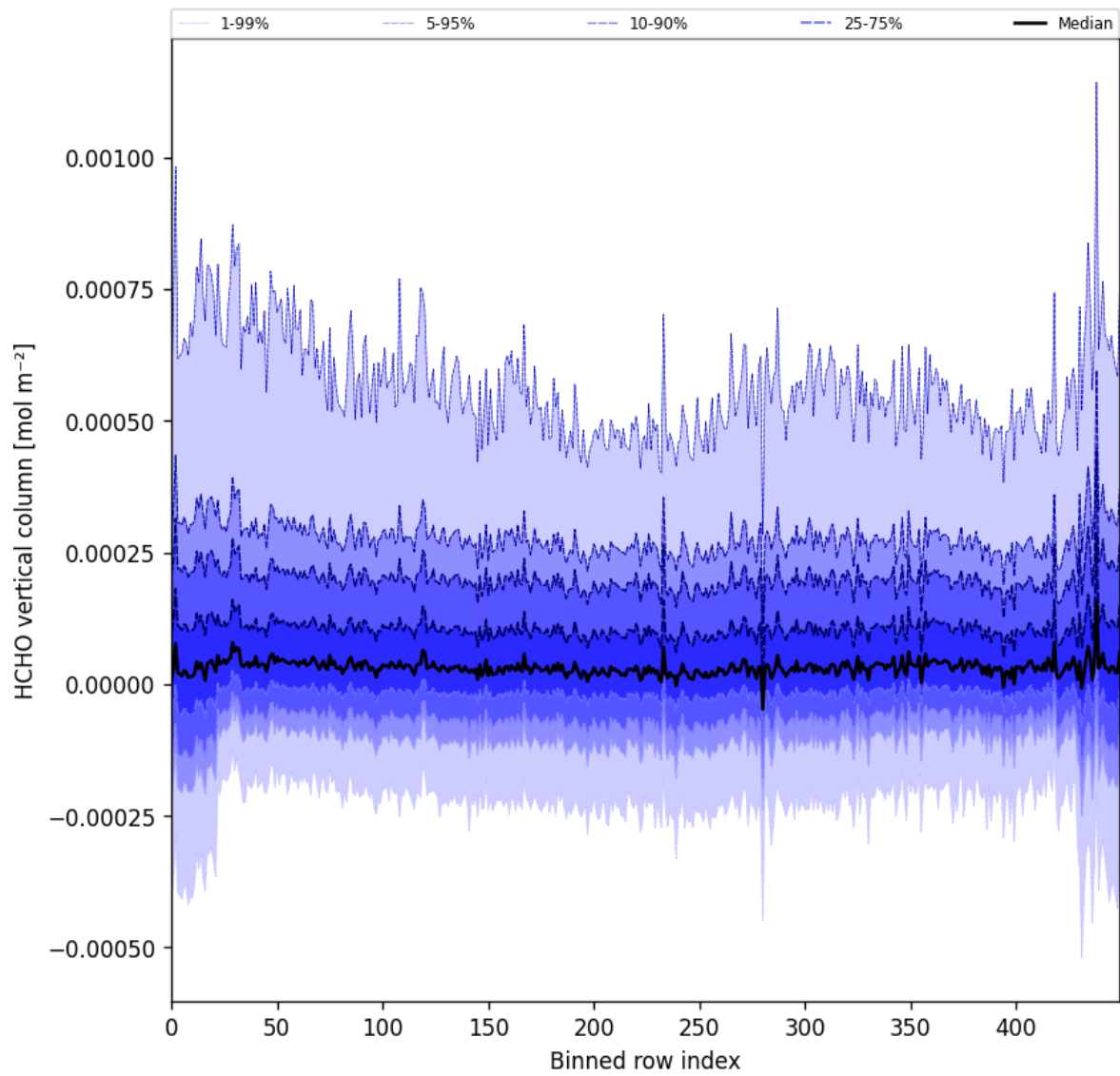
Figure 49: Along track statistics of “HCHO vertical column” for 2025-05-08 to 2025-05-10
