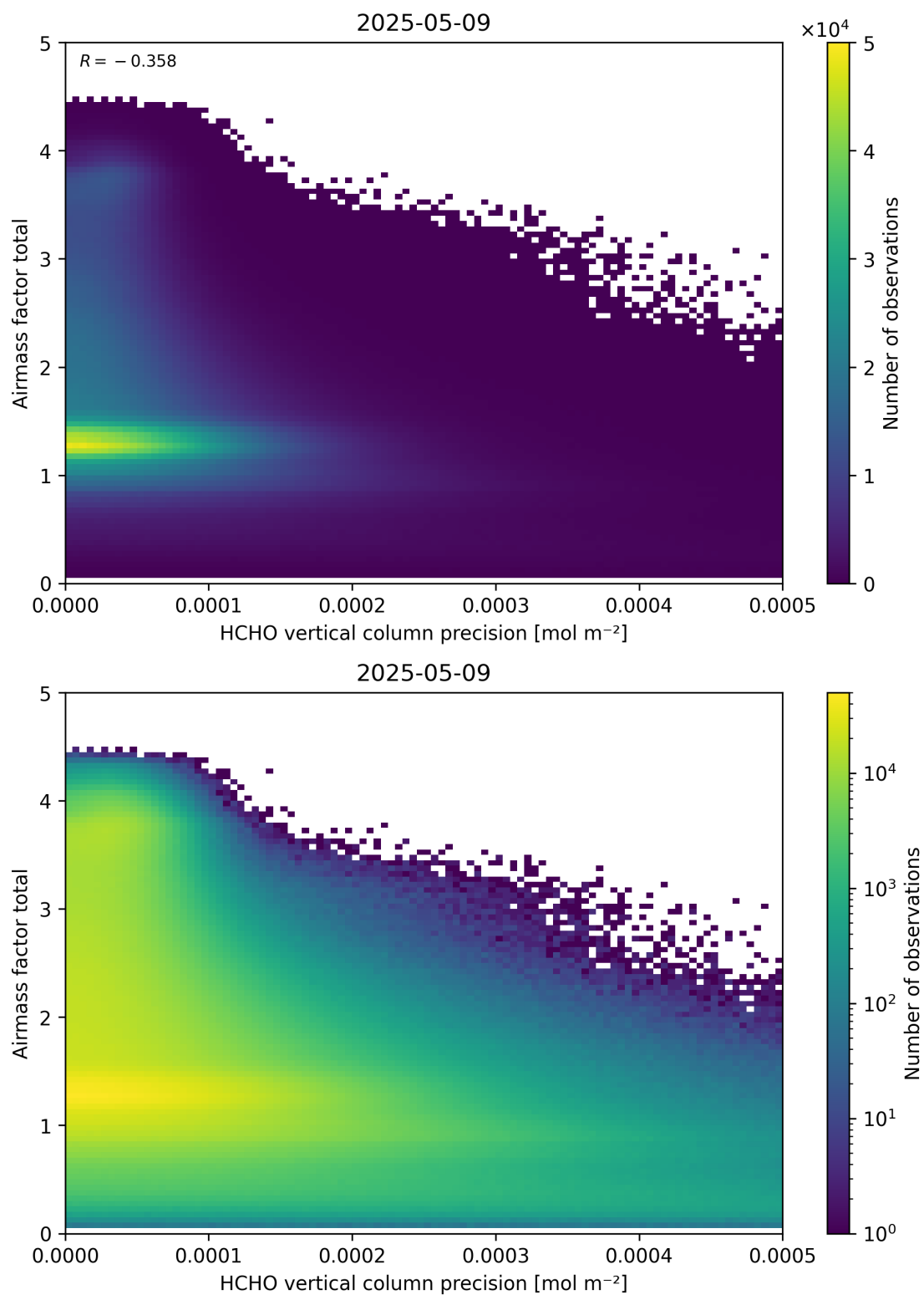
Figure 144: Scatter density plot of “HCHO vertical column precision” against “Airmass factor total” for 2025-05-08 to 2025-05-10.
