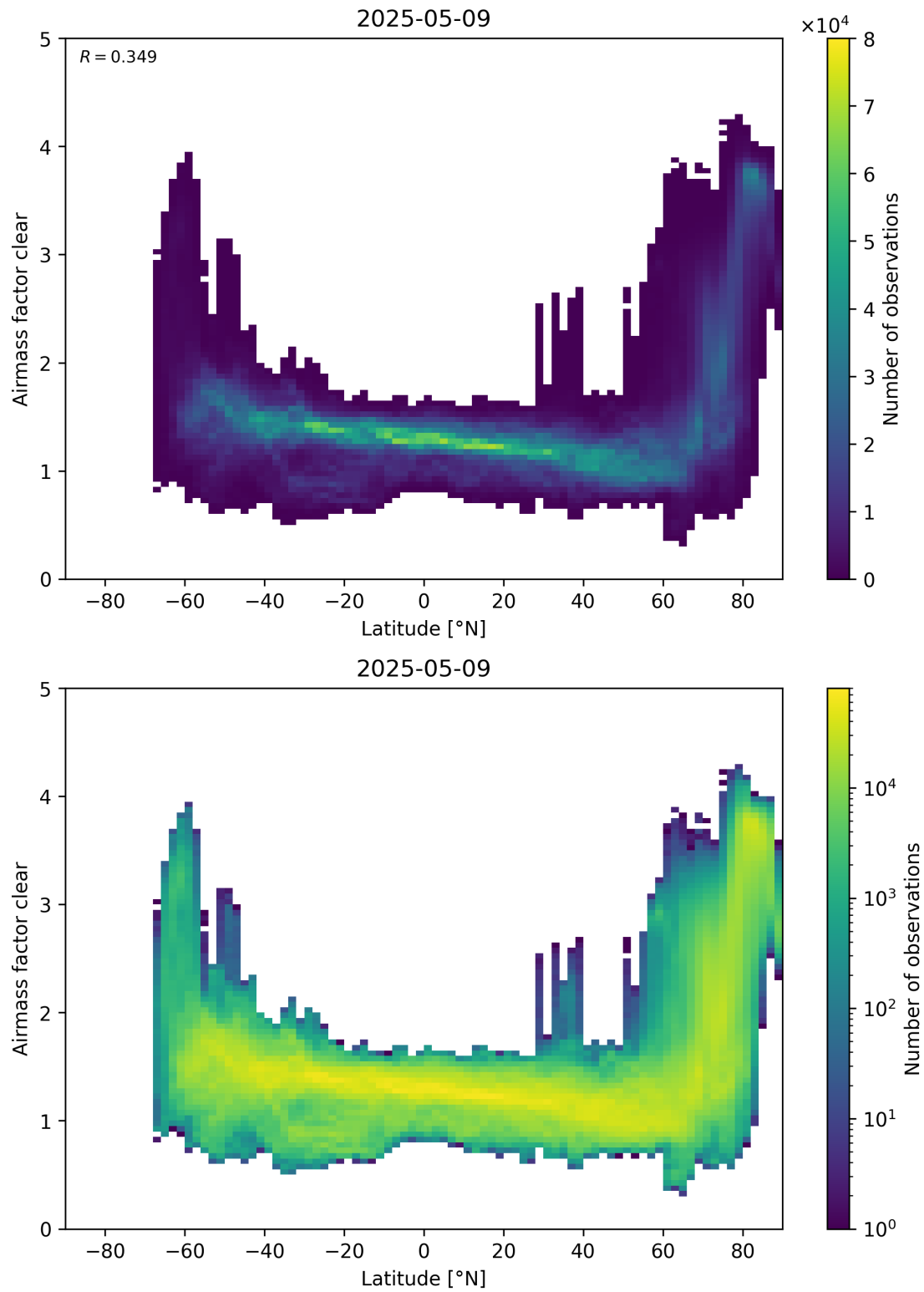
Figure 156: Scatter density plot of “Latitude” against “Airmass factor clear” for 2025-05-08 to 2025-05-10.
