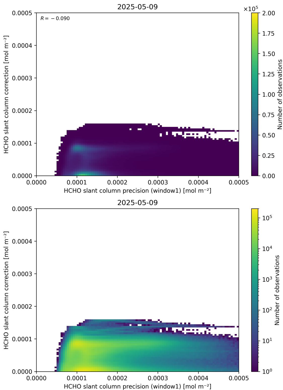
Figure 93: Scatter density plot of “HCHO slant column precision (window1)” against “HCHO slant column correction” for 2025-05-08 to 2025-05-10.
