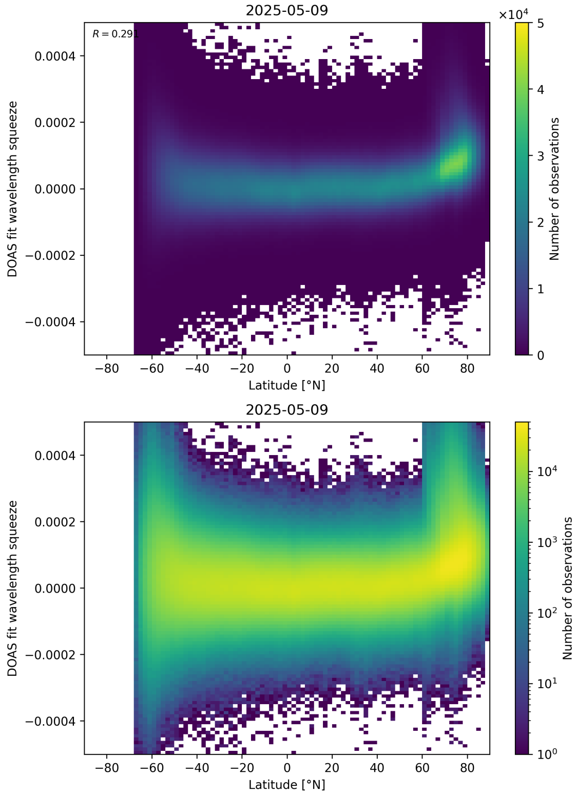
Figure 155: Scatter density plot of “Latitude” against “DOAS fit wavelength squeeze” for 2025-05-08 to 2025-05-10.
