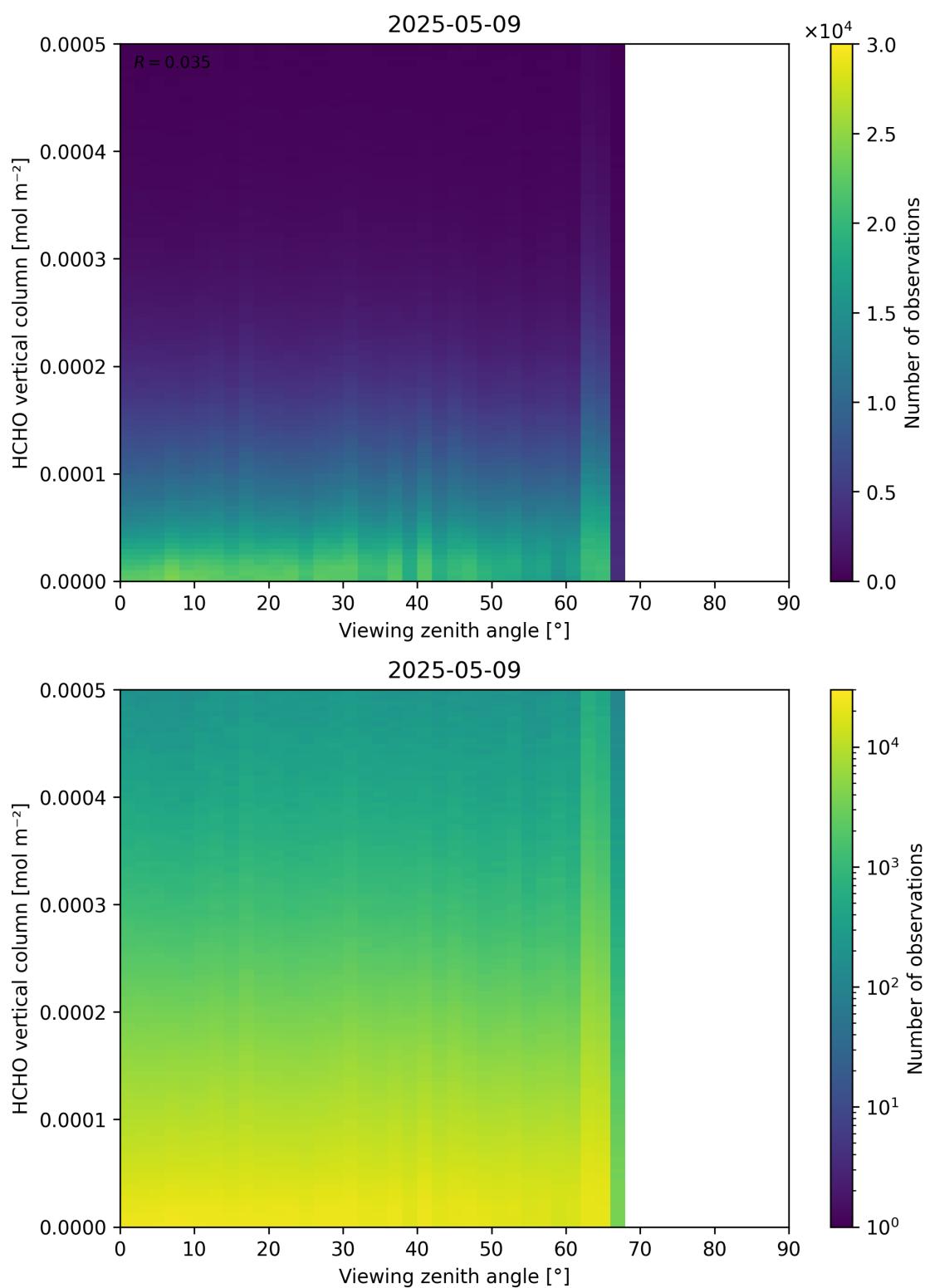
Figure 192: Scatter density plot of “Viewing zenith angle” against “HCHO vertical column” for 2025-05-08 to 2025-05-10.
