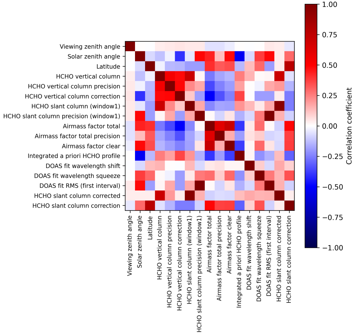
Figure 2: Map of correlation matrix for 2025-05-08 to 2025-05-10.
