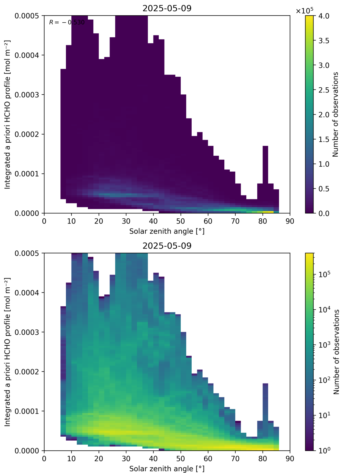
Figure 180: Scatter density plot of “Solar zenith angle” against “Integrated a priori HCHO profile” for 2025-05-08 to 2025-05-10.
