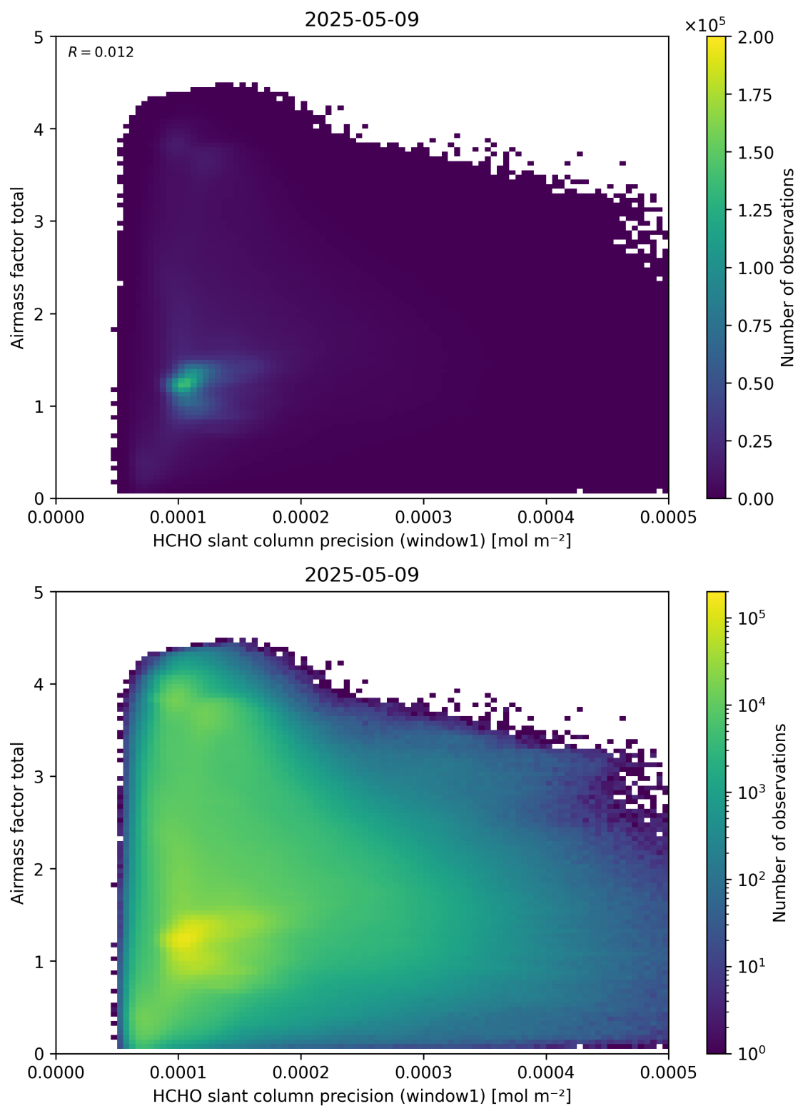
Figure 94: Scatter density plot of “HCHO slant column precision (window1)” against “Airmass factor total” for 2025-05-08 to 2025-05-10.
