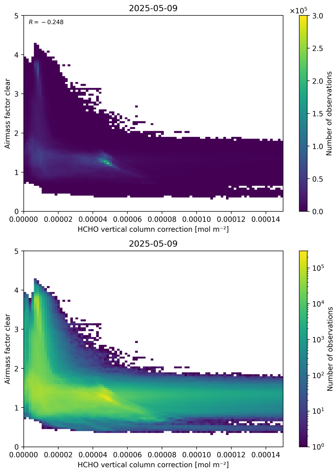
Figure 115: Scatter density plot of “HCHO vertical column correction” against “Airmass factor clear” for 2025-05-08 to 2025-05-10.
