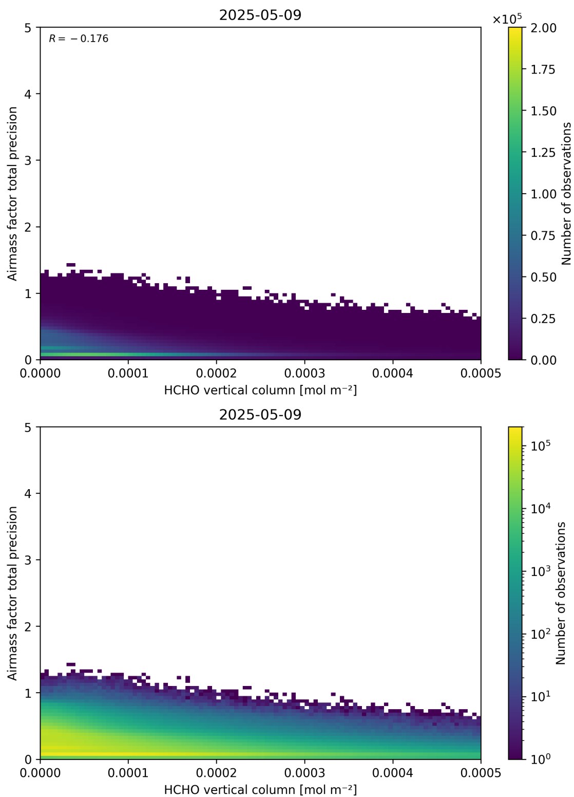
Figure 132: Scatter density plot of “HCHO vertical column” against “Airmass factor total precision” for 2025-05-08 to 2025-05-10.
