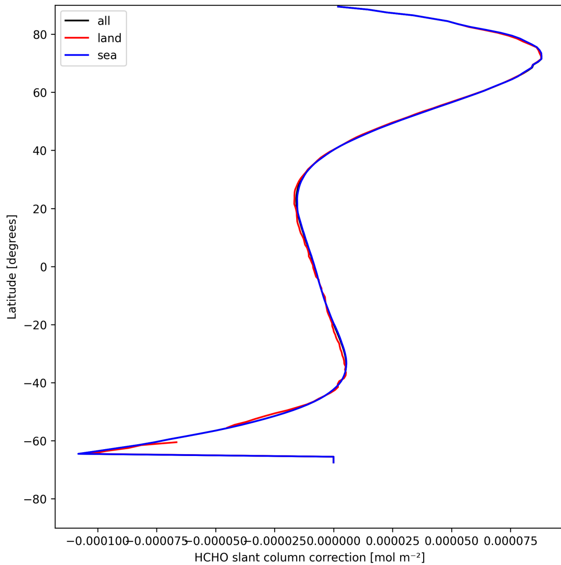
Figure 33: Zonal average of “HCHO slant column correction” for 2025-05-08 to 2025-05-10.
