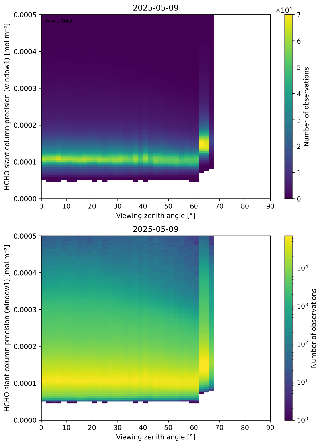
Figure 189: Scatter density plot of “Viewing zenith angle” against “HCHO slant column precision (window1)” for 2025-05-08 to 2025-05-10.
