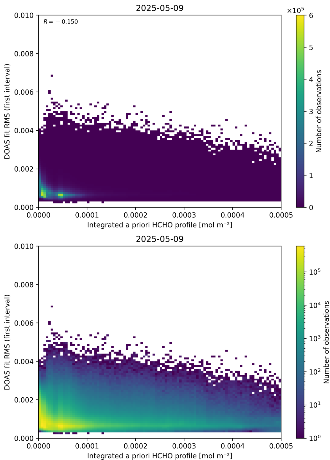
Figure 148: Scatter density plot of “Integrated a priori HCHO profile” against “DOAS fit RMS (first interval)” for 2025-05-08 to 2025-05-10.
