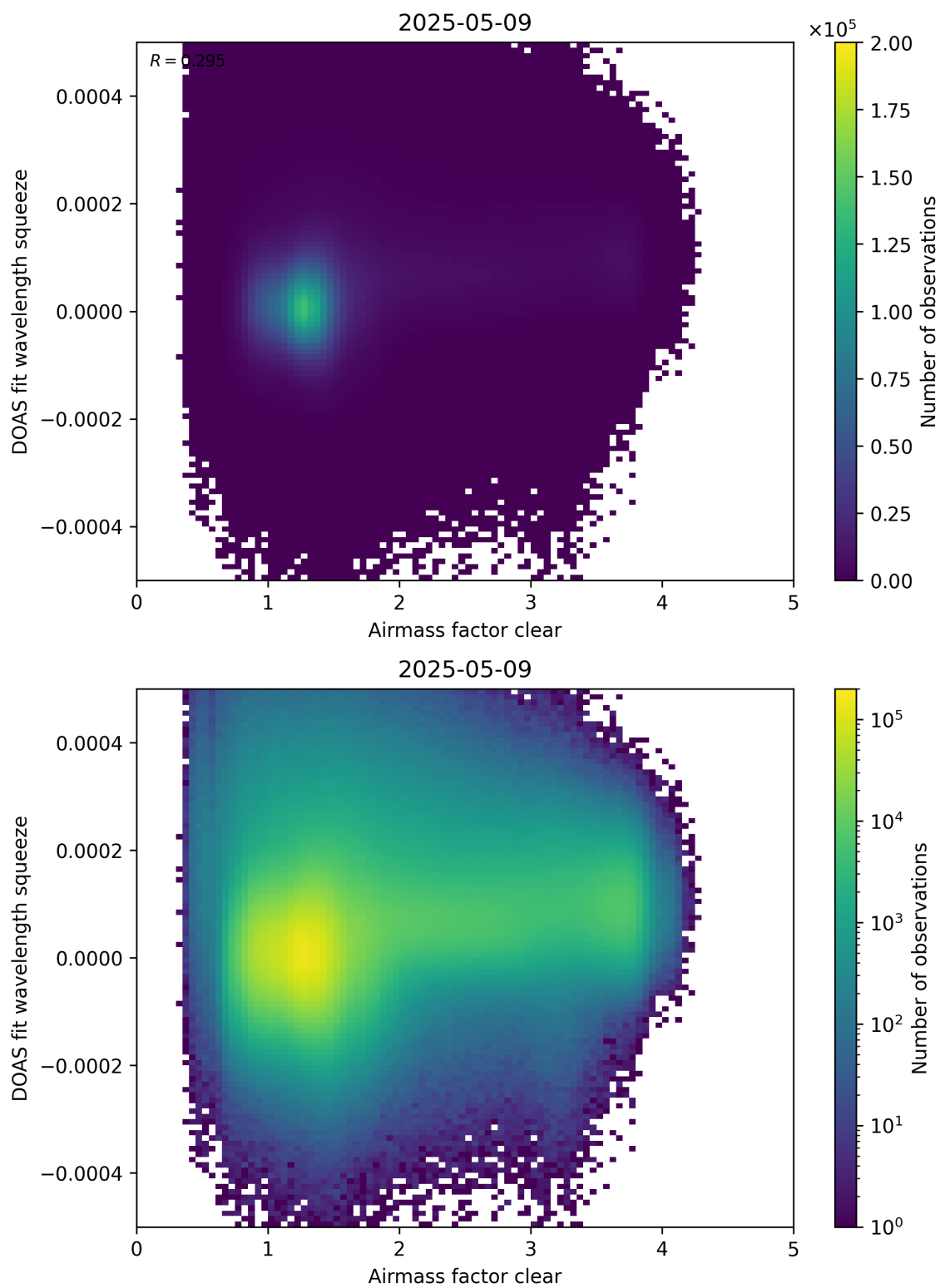
Figure 73: Scatter density plot of “Airmass factor clear” against “DOAS fit wavelength squeeze” for 2025-05-08 to 2025-05-10.
