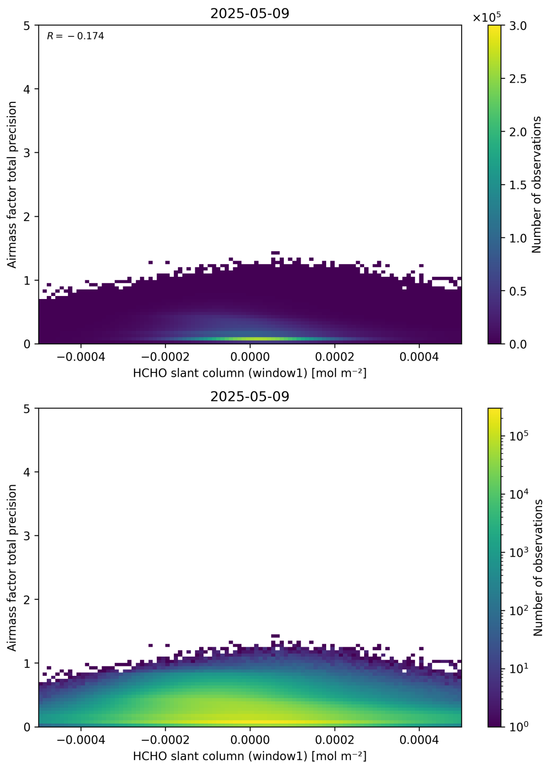
Figure 86: Scatter density plot of “HCHO slant column (window1)” against “Airmass factor total precision” for 2025-05-08 to 2025-05-10.
