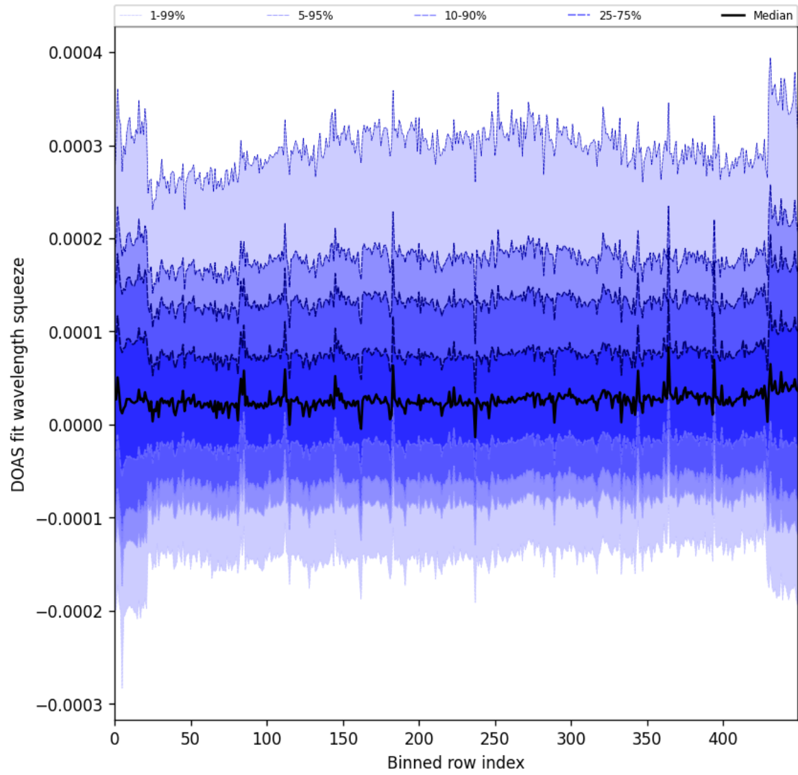
Figure 59: Along track statistics of “DOAS fit wavelength squeeze” for 2025-05-08 to 2025-05-10
