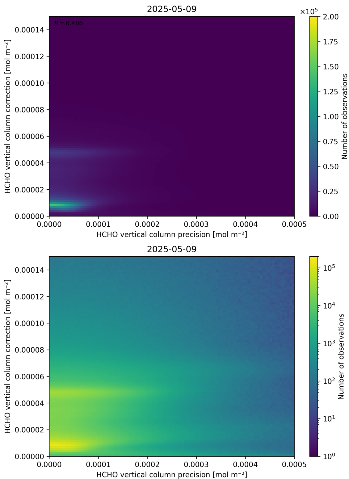
Figure 146: Scatter density plot of “HCHO vertical column precision” against “HCHO vertical column correction” for 2025-05-08 to 2025-05-10.
