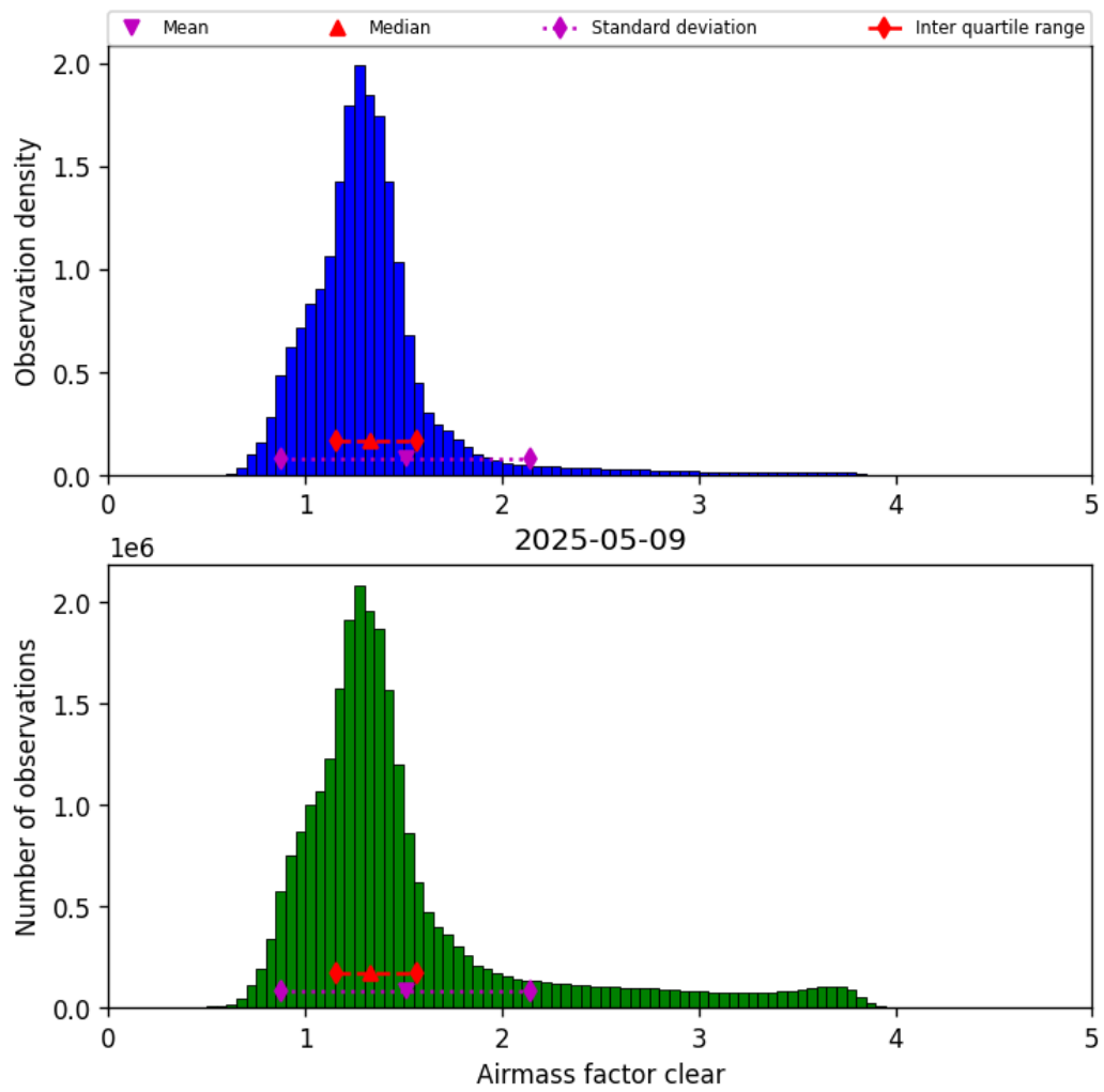
Figure 42: Histogram of “Airmass factor clear” for 2025-05-08 to 2025-05-10
