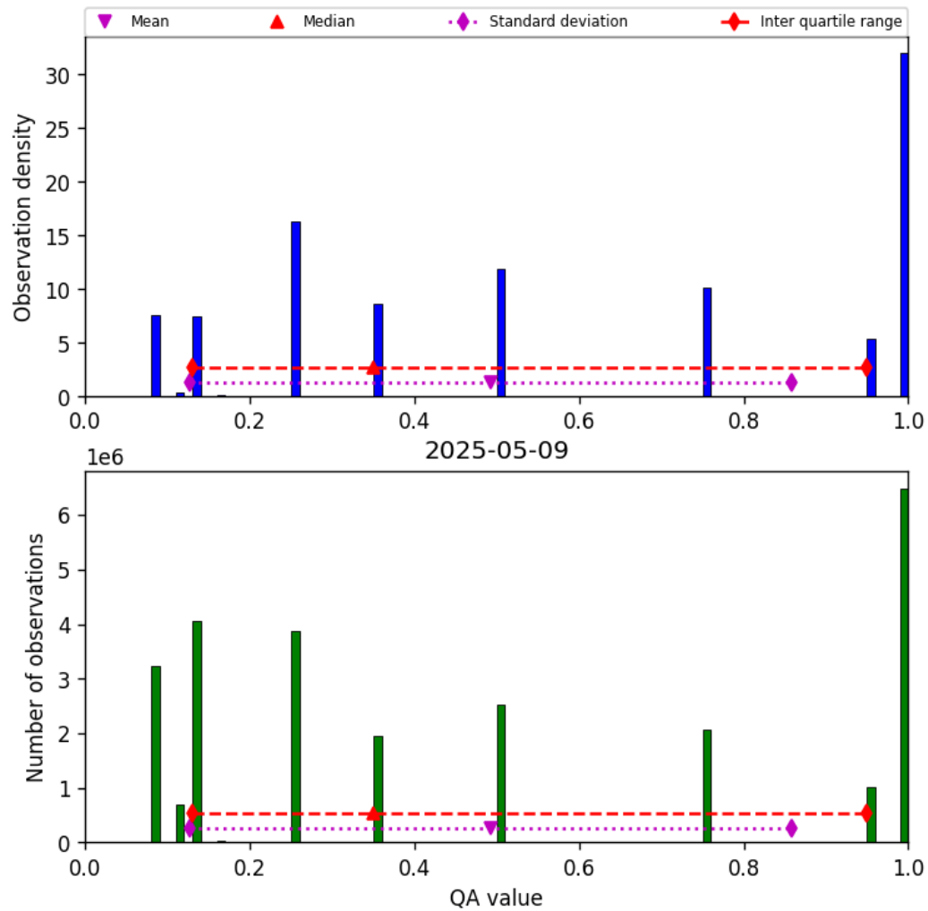
Figure 34: Histogram of “QA value” for 2025-05-08 to 2025-05-10
