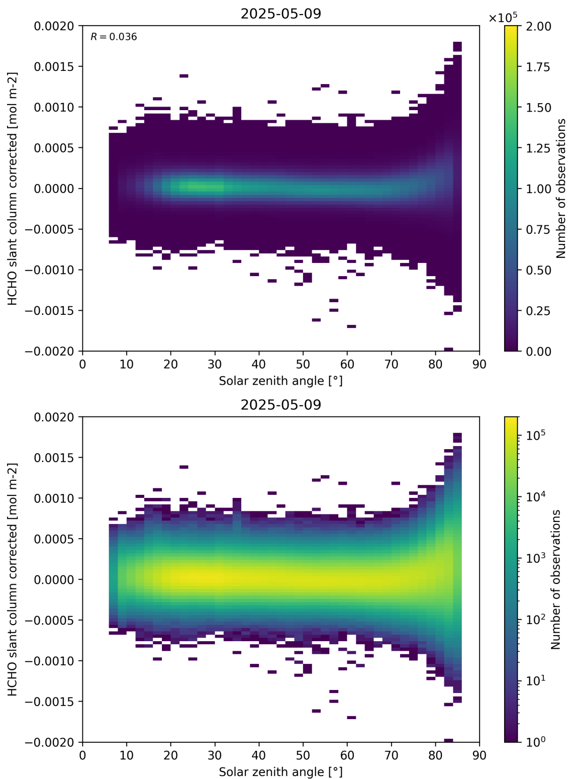
Figure 171: Scatter density plot of “Solar zenith angle” against “HCHO slant column corrected” for 2025-05-08 to 2025-05-10.
