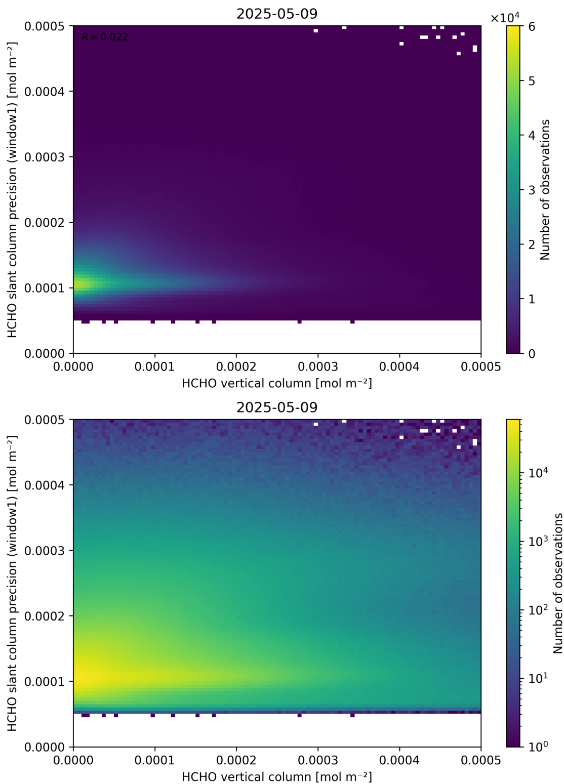
Figure 130: Scatter density plot of “HCHO vertical column” against “HCHO slant column precision (window1)” for 2025-05-08 to 2025-05-10.
