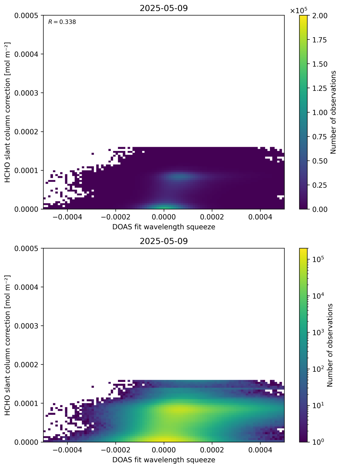
Figure 70: Scatter density plot of “DOAS fit wavelength squeeze” against “HCHO slant column correction” for 2025-05-08 to 2025-05-10.
