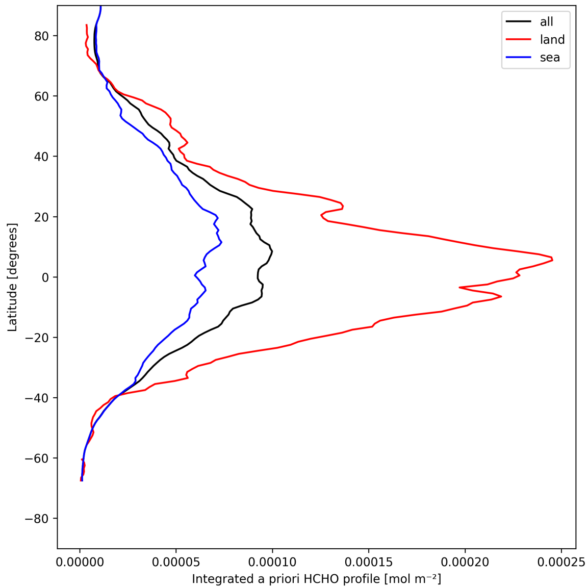
Figure 29: Zonal average of “Integrated a priori HCHO profile” for 2025-05-08 to 2025-05-10.
