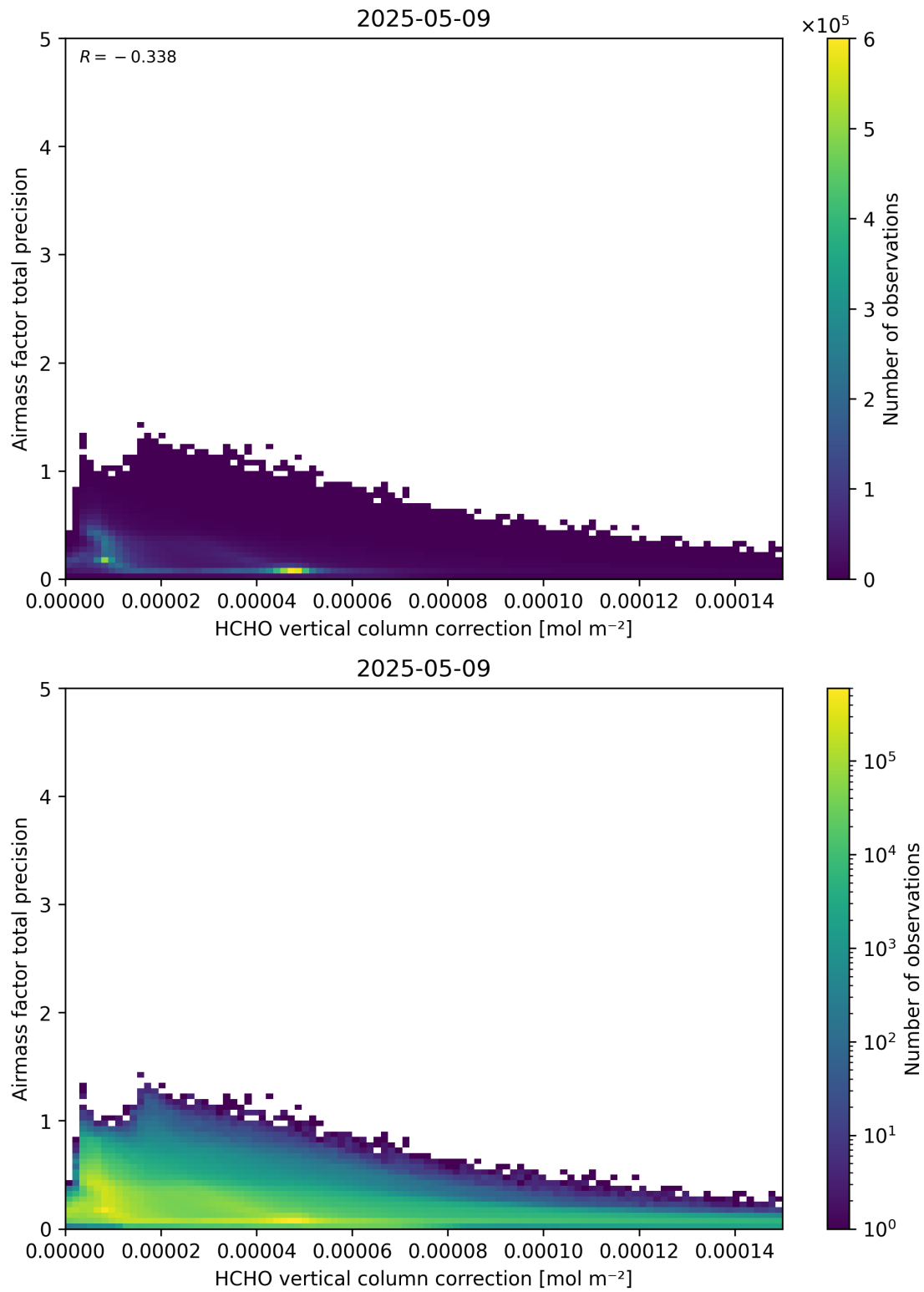
Figure 121: Scatter density plot of “HCHO vertical column correction” against “Airmass factor total precision” for 2025-05-08 to 2025-05-10.
