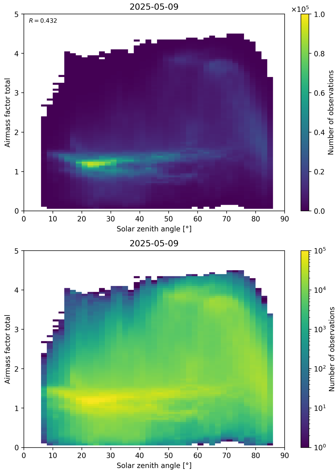
Figure 175: Scatter density plot of “Solar zenith angle” against “Airmass factor total” for 2025-05-08 to 2025-05-10.
