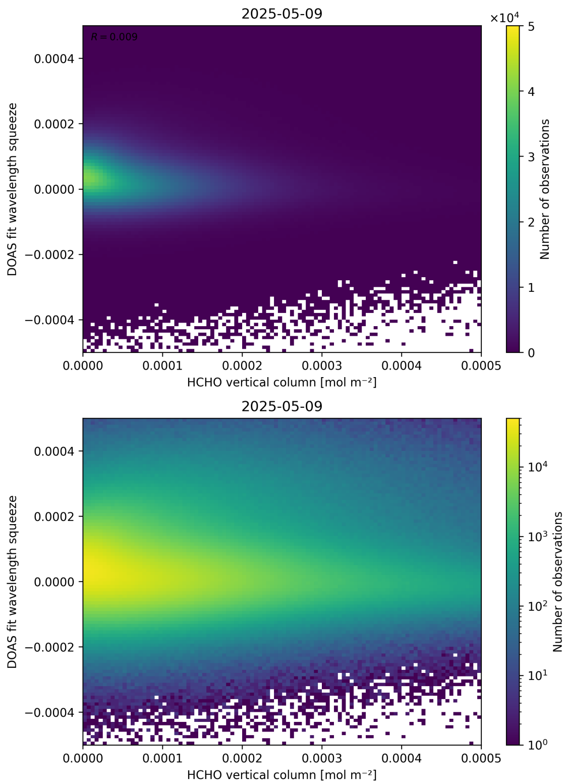
Figure 125: Scatter density plot of “HCHO vertical column” against “DOAS fit wavelength squeeze” for 2025-05-08 to 2025-05-10.
