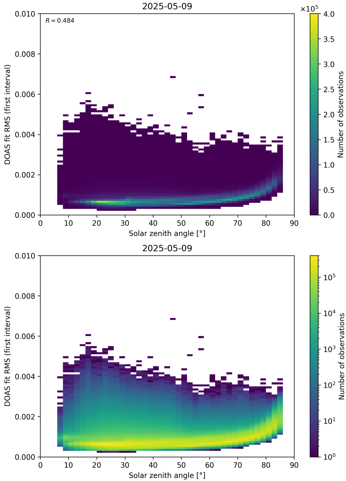
Figure 167: Scatter density plot of “Solar zenith angle” against “DOAS fit RMS (first interval)” for 2025-05-08 to 2025-05-10.
