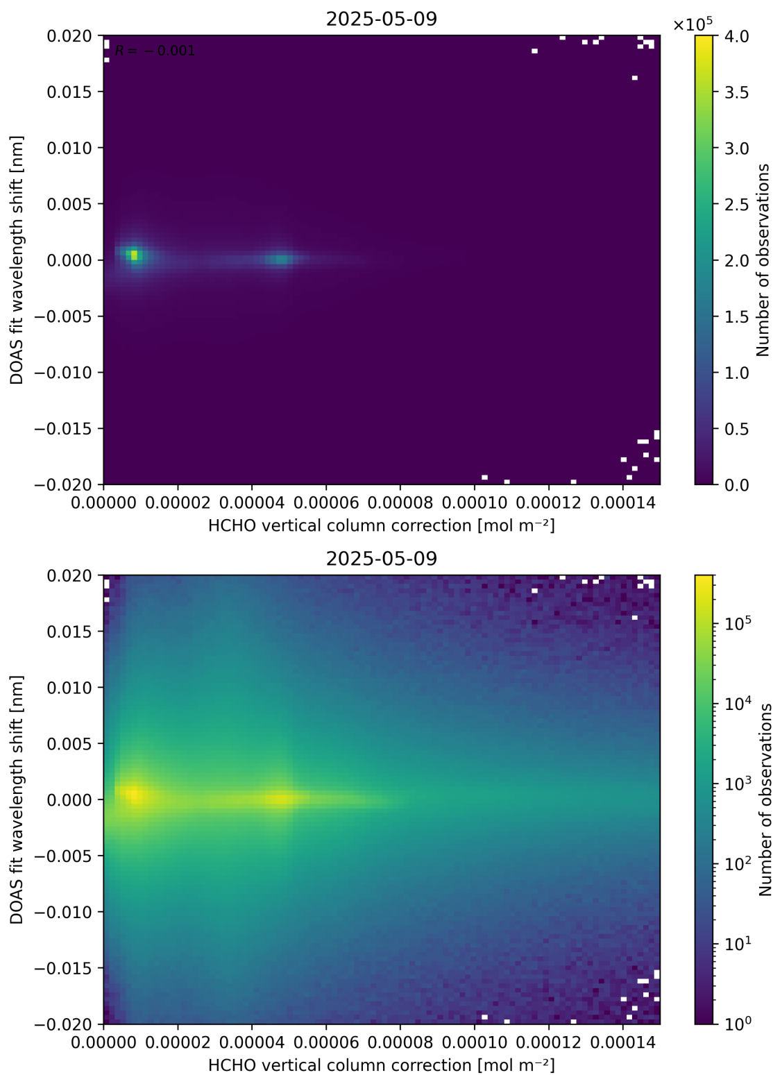
Figure 113: Scatter density plot of “HCHO vertical column correction” against “DOAS fit wavelength shift” for 2025-05-08 to 2025-05-10.
