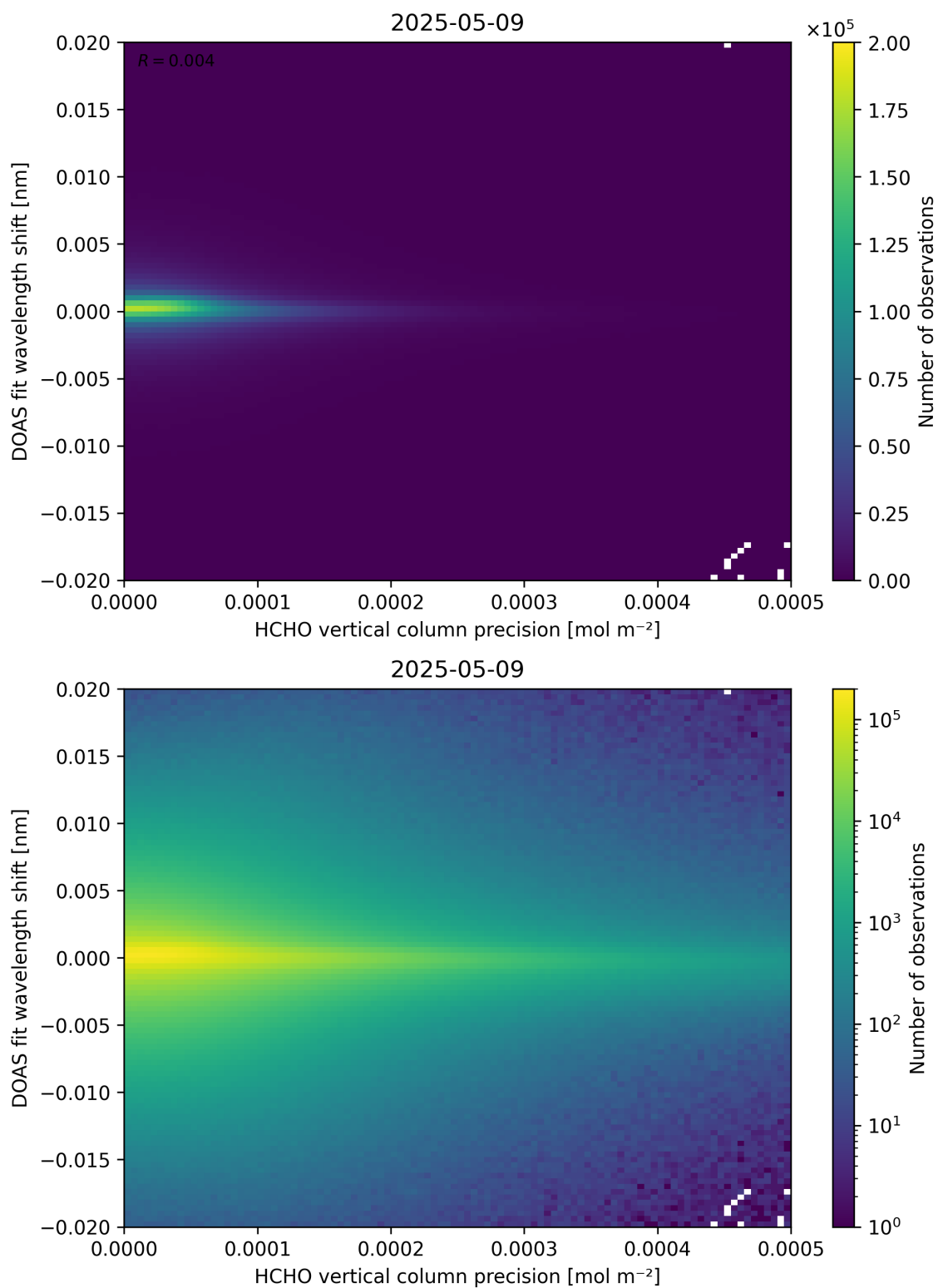
Figure 137: Scatter density plot of “HCHO vertical column precision” against “DOAS fit wavelength shift” for 2025-05-08 to 2025-05-10.
