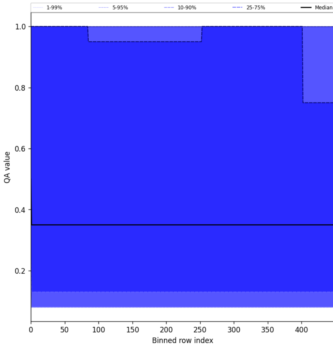
Figure 48: Along track statistics of “QA value” for 2025-05-08 to 2025-05-10
