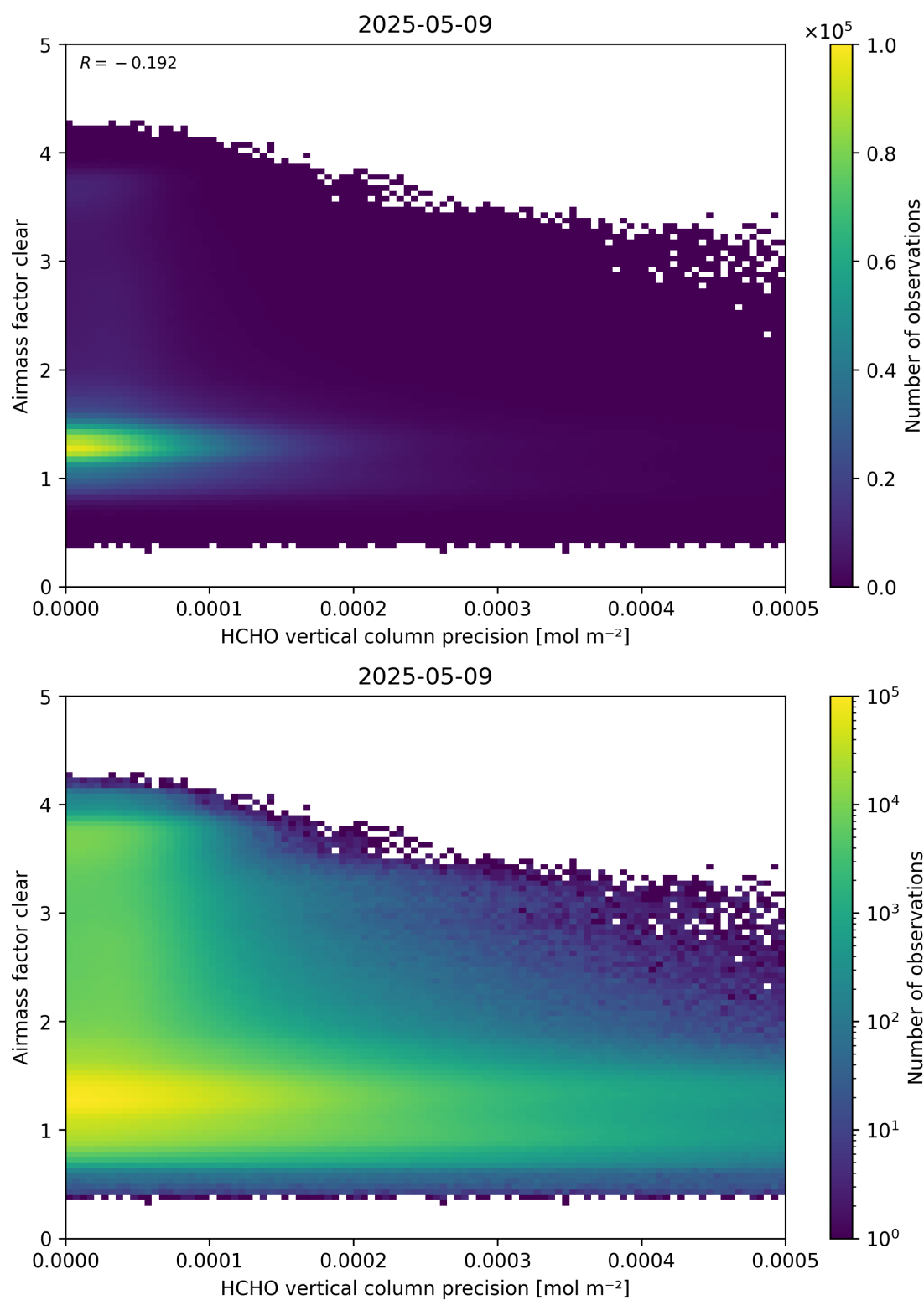
Figure 139: Scatter density plot of “HCHO vertical column precision” against “Airmass factor clear” for 2025-05-08 to 2025-05-10.
