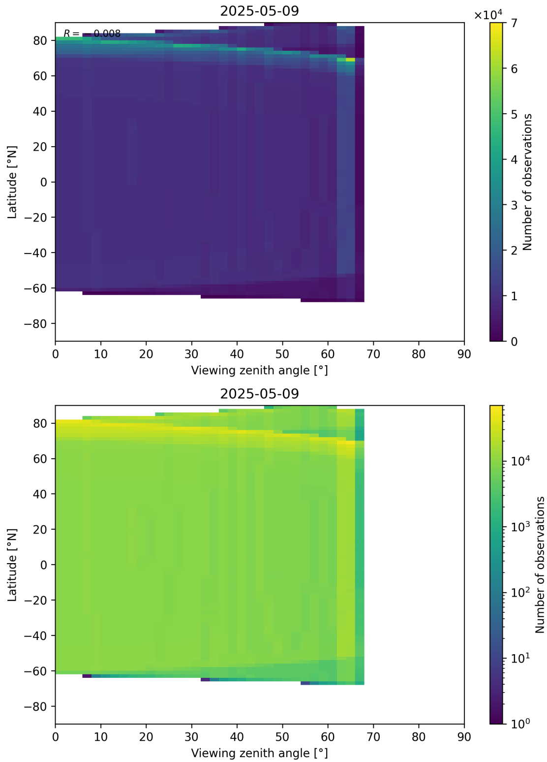
Figure 196: Scatter density plot of “Viewing zenith angle” against “Latitude” for 2025-05-08 to 2025-05-10.
