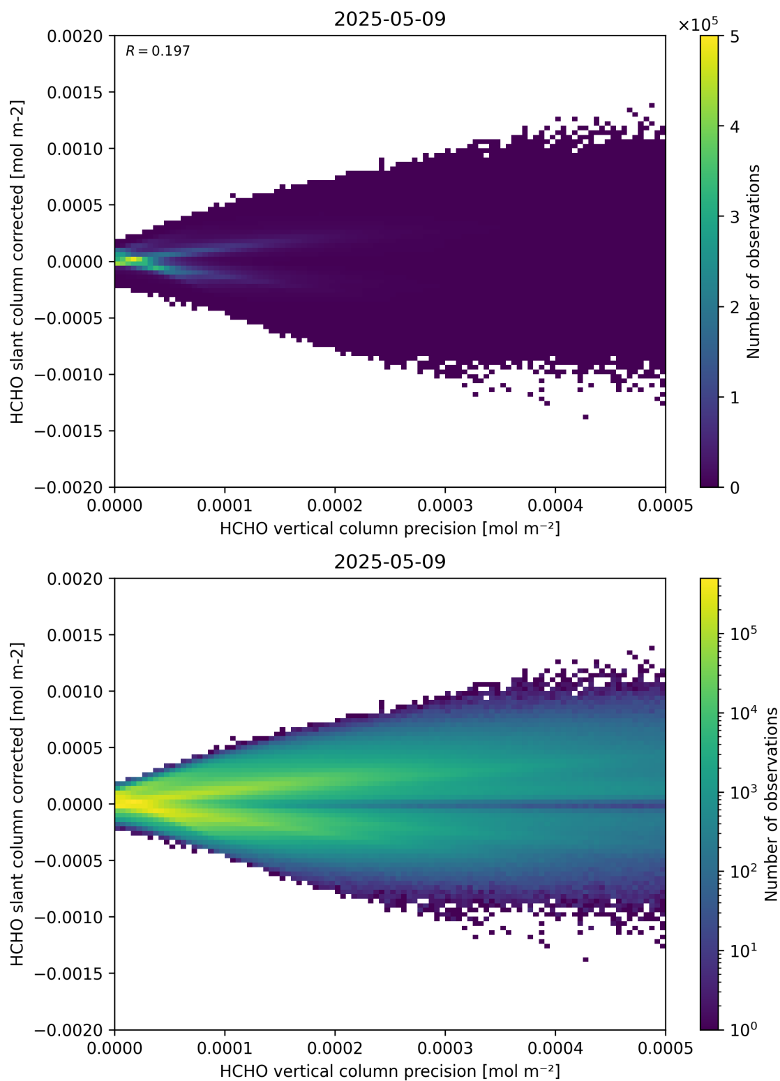
Figure 140: Scatter density plot of “HCHO vertical column precision” against “HCHO slant column corrected” for 2025-05-08 to 2025-05-10.
