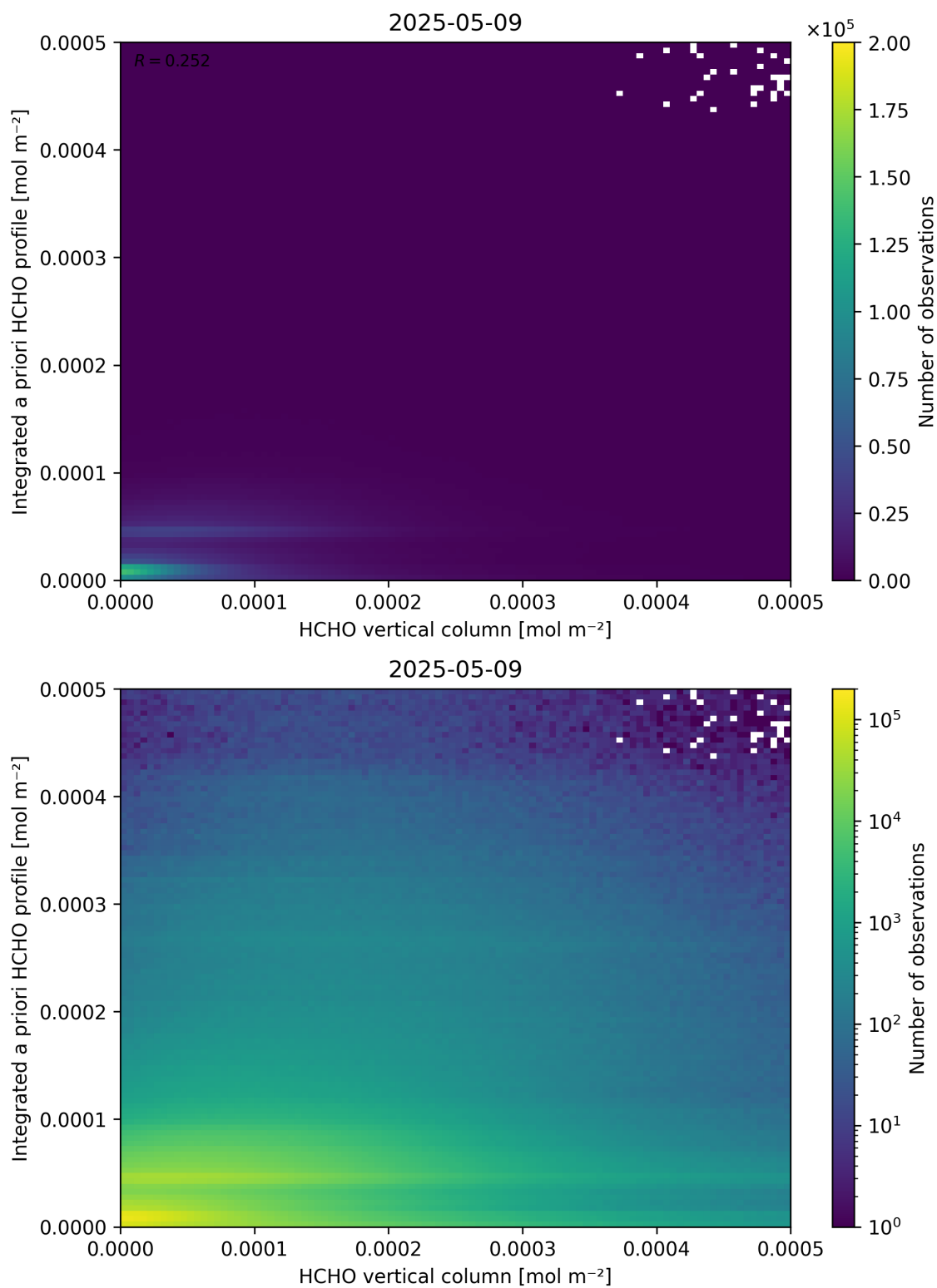
Figure 135: Scatter density plot of “HCHO vertical column” against “Integrated a priori HCHO profile” for 2025-05-08 to 2025-05-10.
