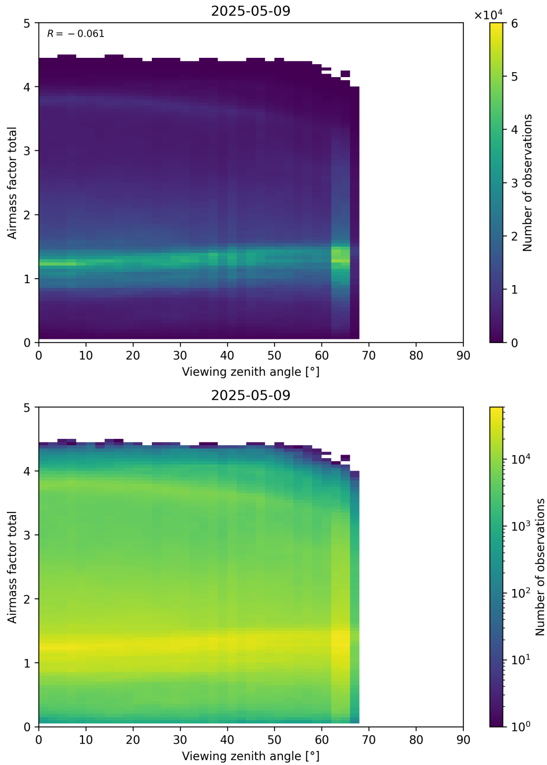
Figure 190: Scatter density plot of “Viewing zenith angle” against “Airmass factor total” for 2025-05-08 to 2025-05-10.
