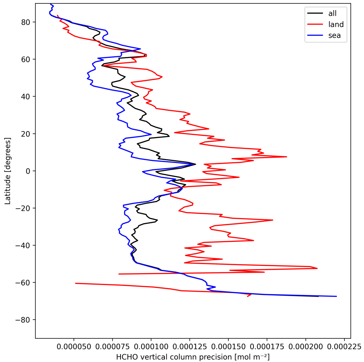
Figure 22: Zonal average of “HCHO vertical column precision” for 2025-05-08 to 2025-05-10.
