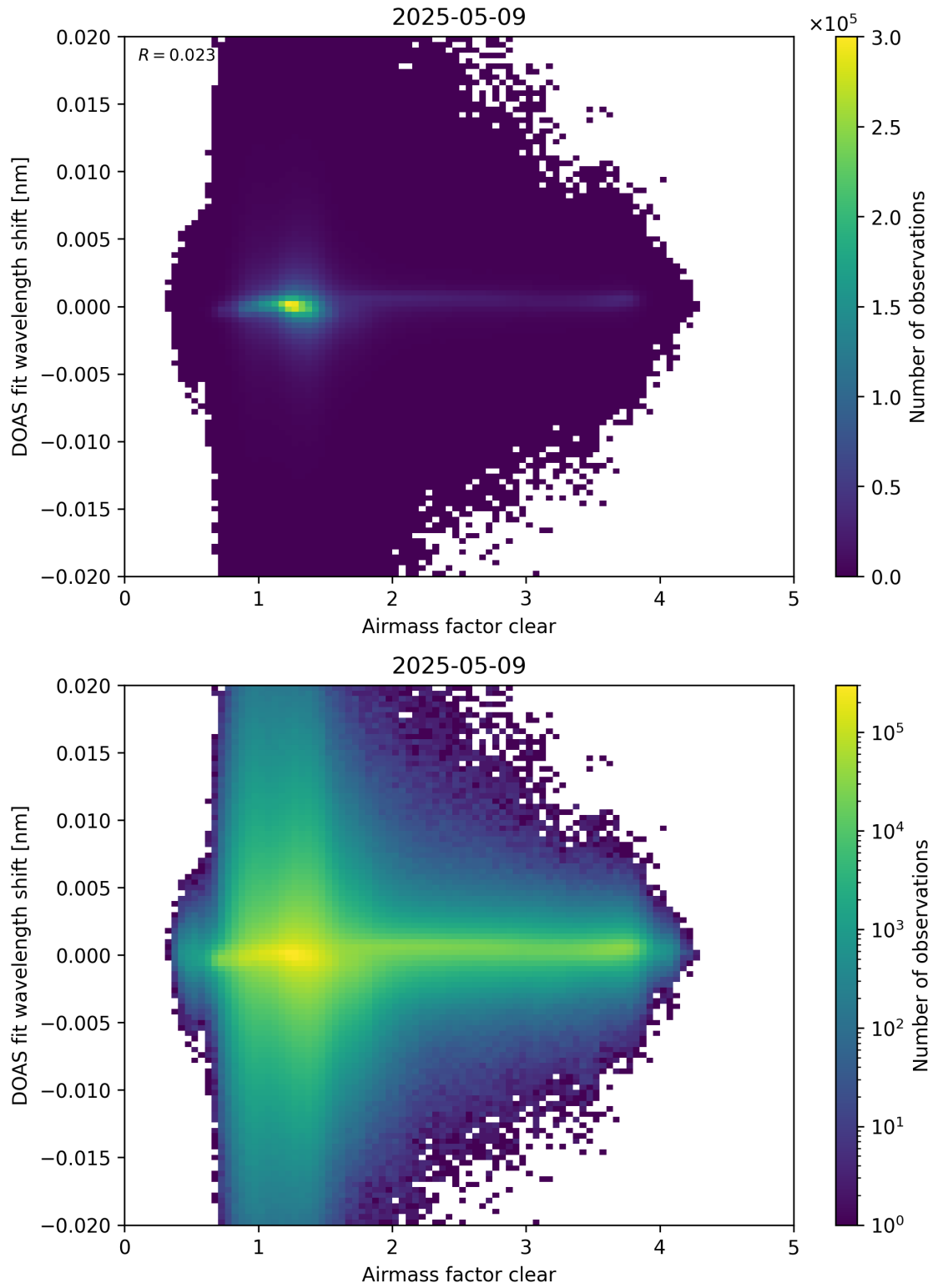
Figure 72: Scatter density plot of “Airmass factor clear” against “DOAS fit wavelength shift” for 2025-05-08 to 2025-05-10.
