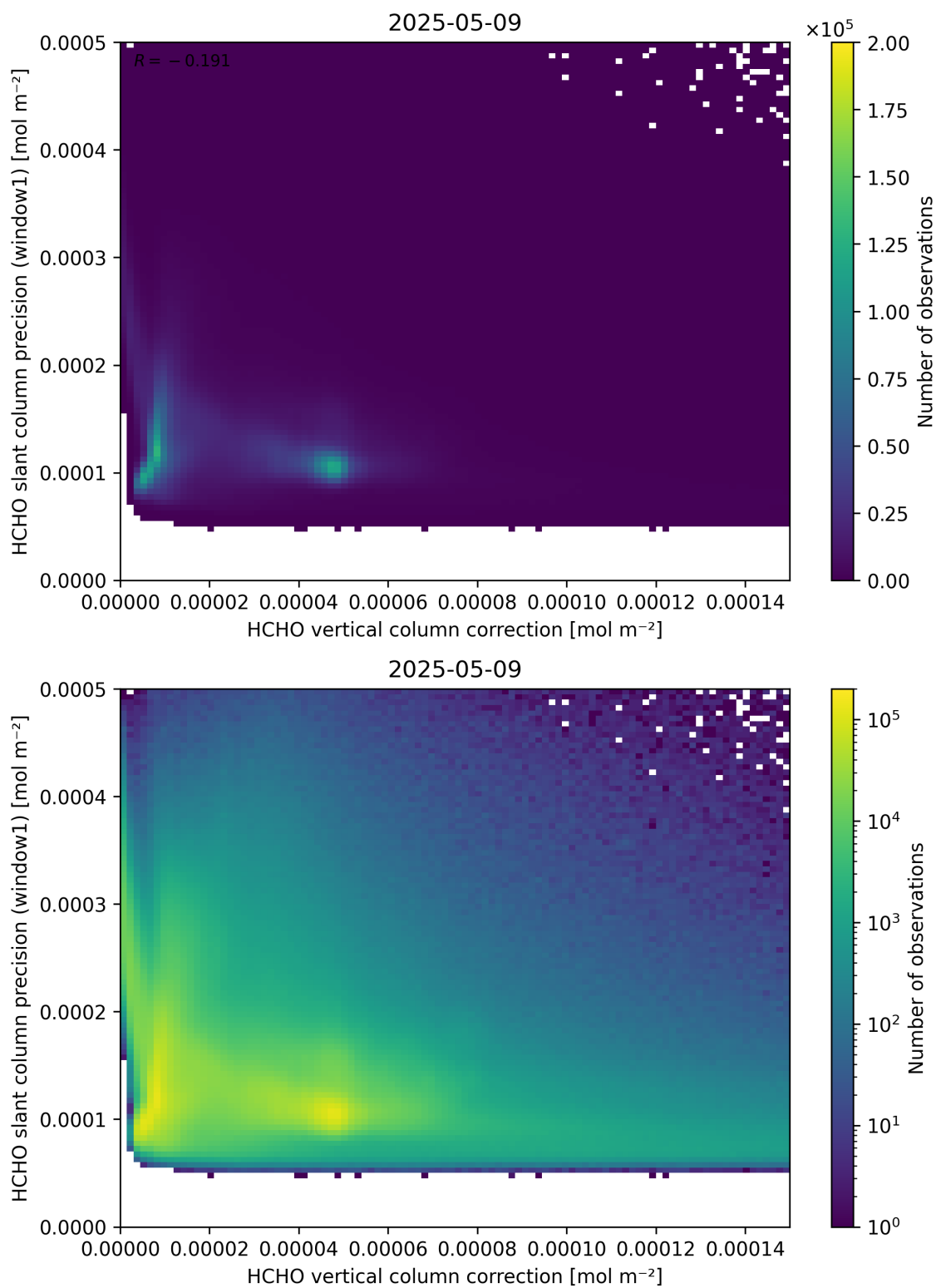
Figure 119: Scatter density plot of “HCHO vertical column correction” against “HCHO slant column precision (window1)” for 2025-05-08 to 2025-05-10.
