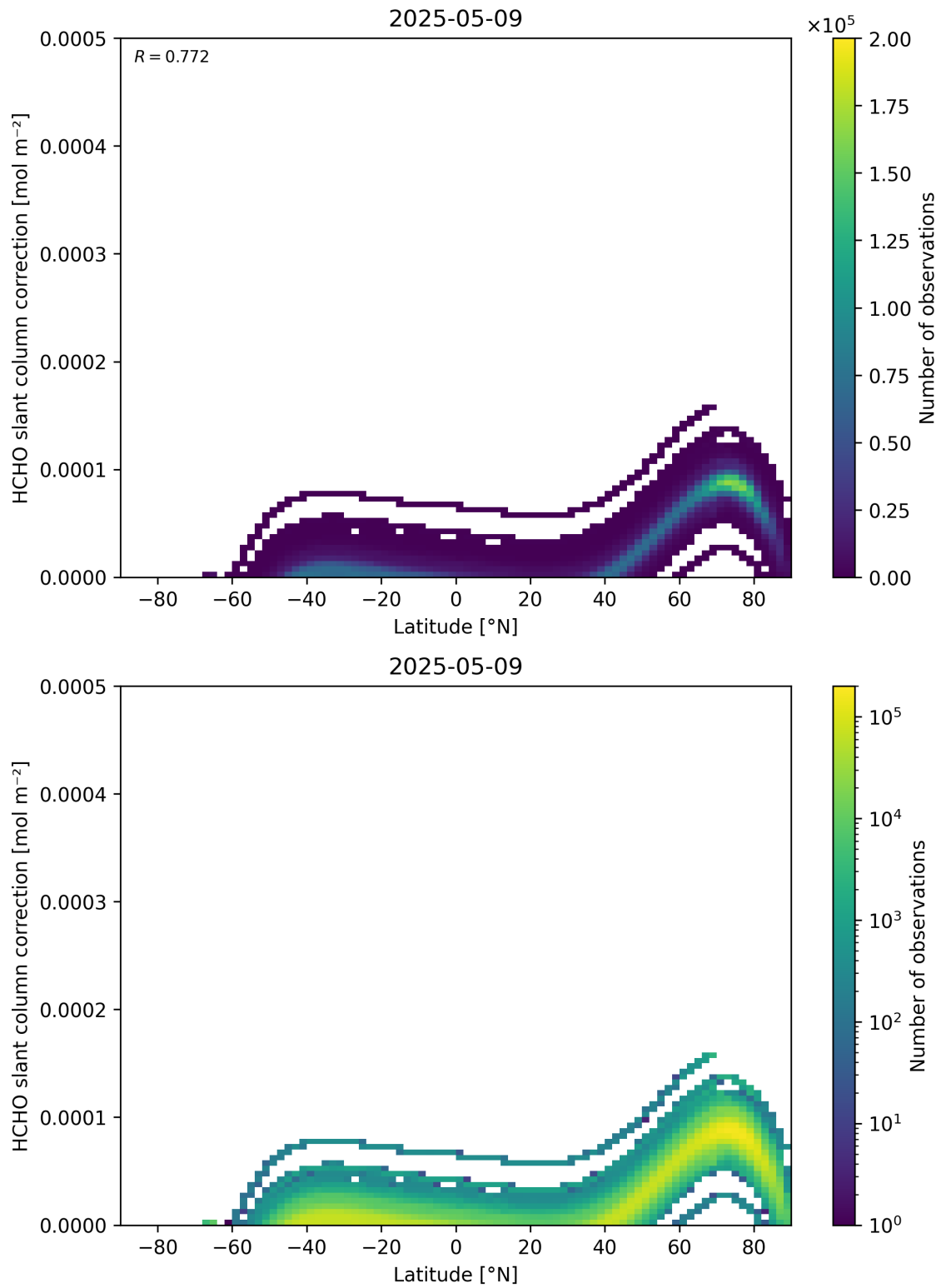
Figure 158: Scatter density plot of “Latitude” against “HCHO slant column correction” for 2025-05-08 to 2025-05-10.
