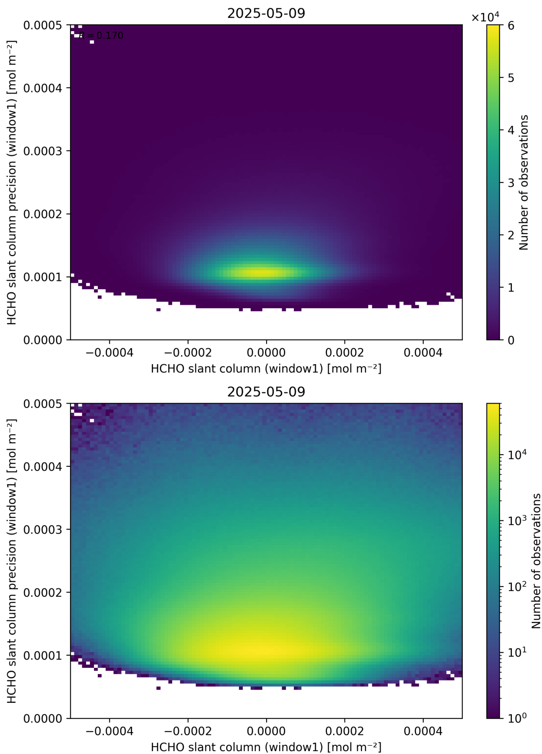
Figure 84: Scatter density plot of “HCHO slant column (window1)” against “HCHO slant column precision (window1)” for 2025-05-08 to 2025-05-10.
