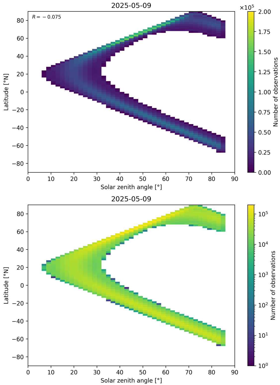
Figure 181: Scatter density plot of “Solar zenith angle” against “Latitude” for 2025-05-08 to 2025-05-10.
