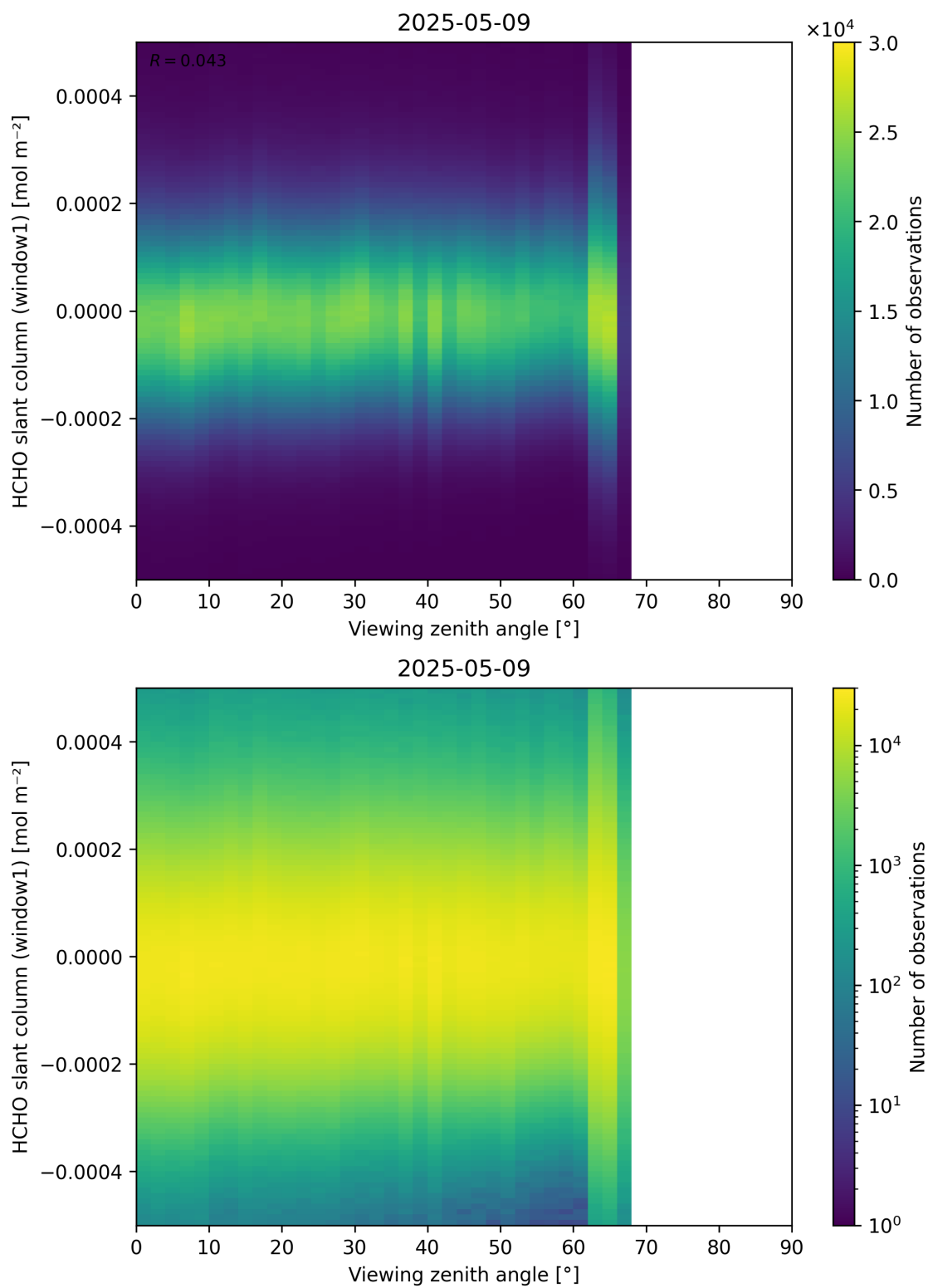
Figure 188: Scatter density plot of “Viewing zenith angle” against “HCHO slant column (window1)” for 2025-05-08 to 2025-05-10.
