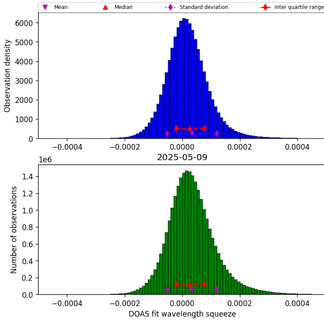
Figure 45: Histogram of “DOAS fit wavelength squeeze” for 2025-05-08 to 2025-05-10
