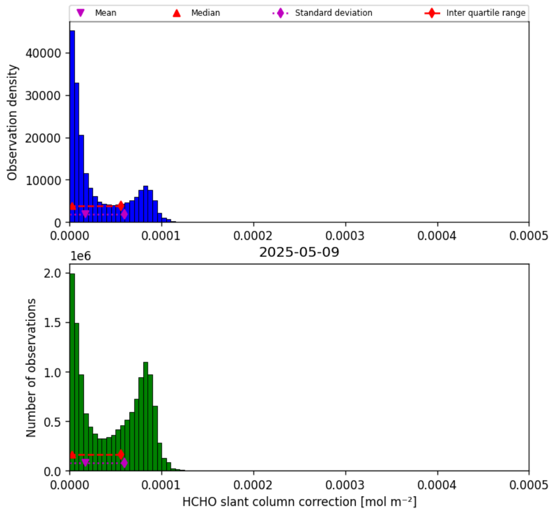
Figure 47: Histogram of “HCHO slant column correction” for 2025-05-08 to 2025-05-10
