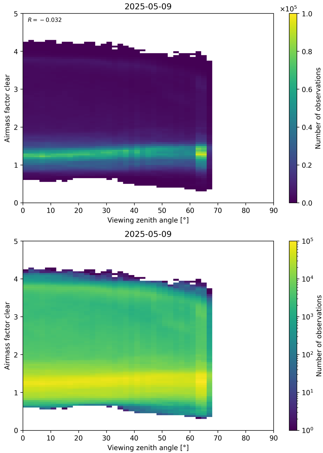
Figure 185: Scatter density plot of “Viewing zenith angle” against “Airmass factor clear” for 2025-05-08 to 2025-05-10.
