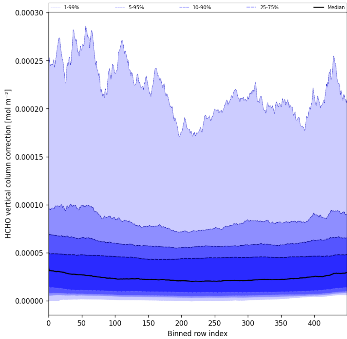
Figure 51: Along track statistics of “HCHO vertical column correction” for 2025-05-08 to 2025-05-10
