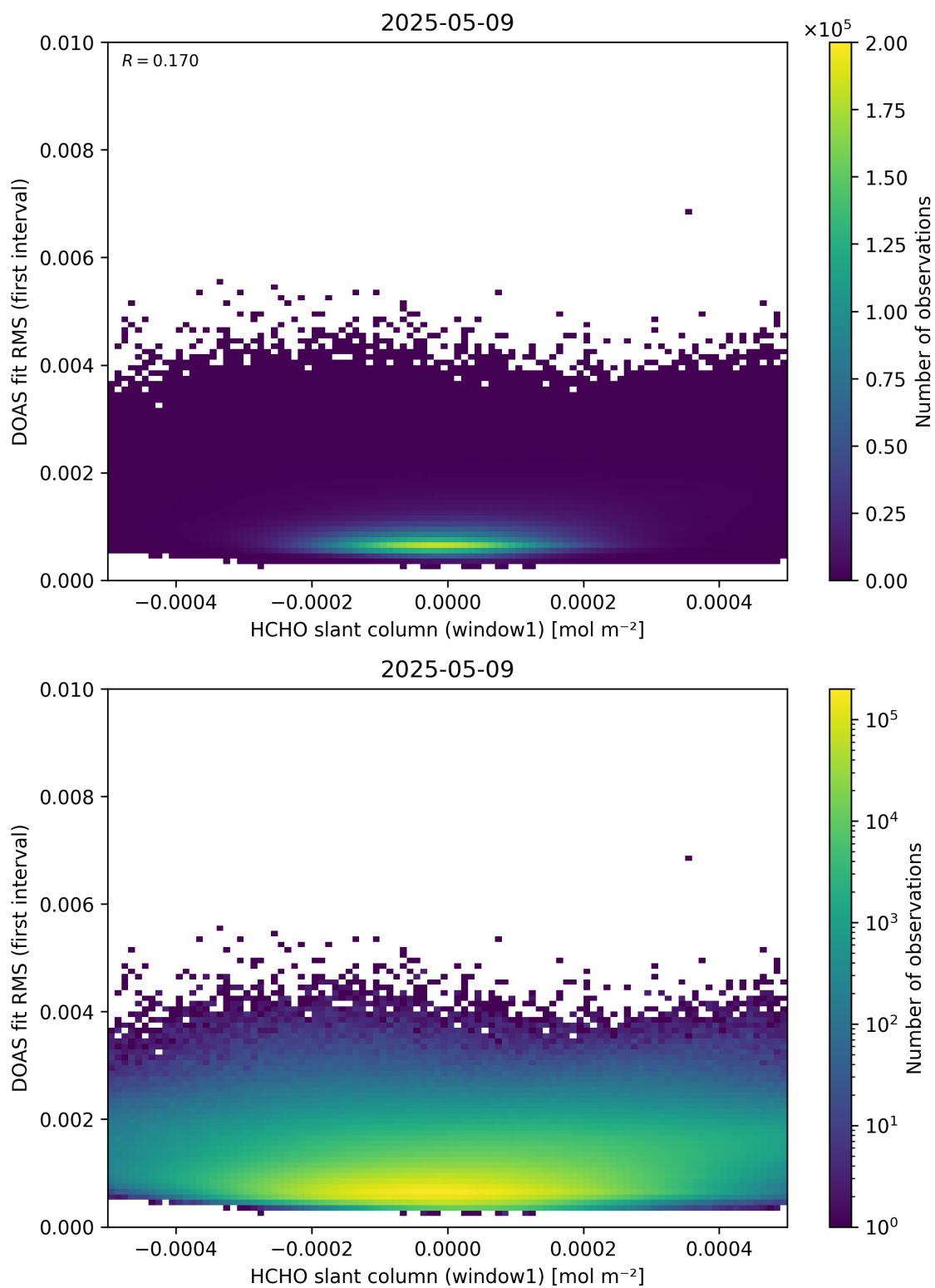
Figure 78: Scatter density plot of “HCHO slant column (window1)” against “DOAS fit RMS (first interval)” for 2025-05-08 to 2025-05-10.
