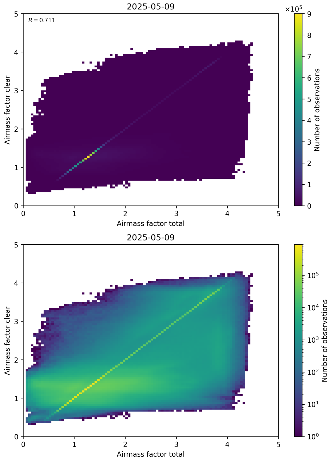
Figure 100: Scatter density plot of “Airmass factor total” against “Airmass factor clear” for 2025-05-08 to 2025-05-10.
