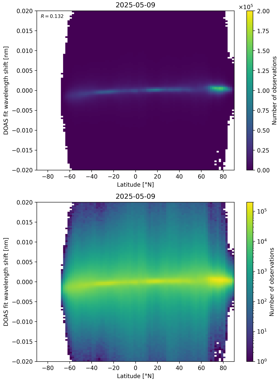
Figure 154: Scatter density plot of “Latitude” against “DOAS fit wavelength shift” for 2025-05-08 to 2025-05-10.
