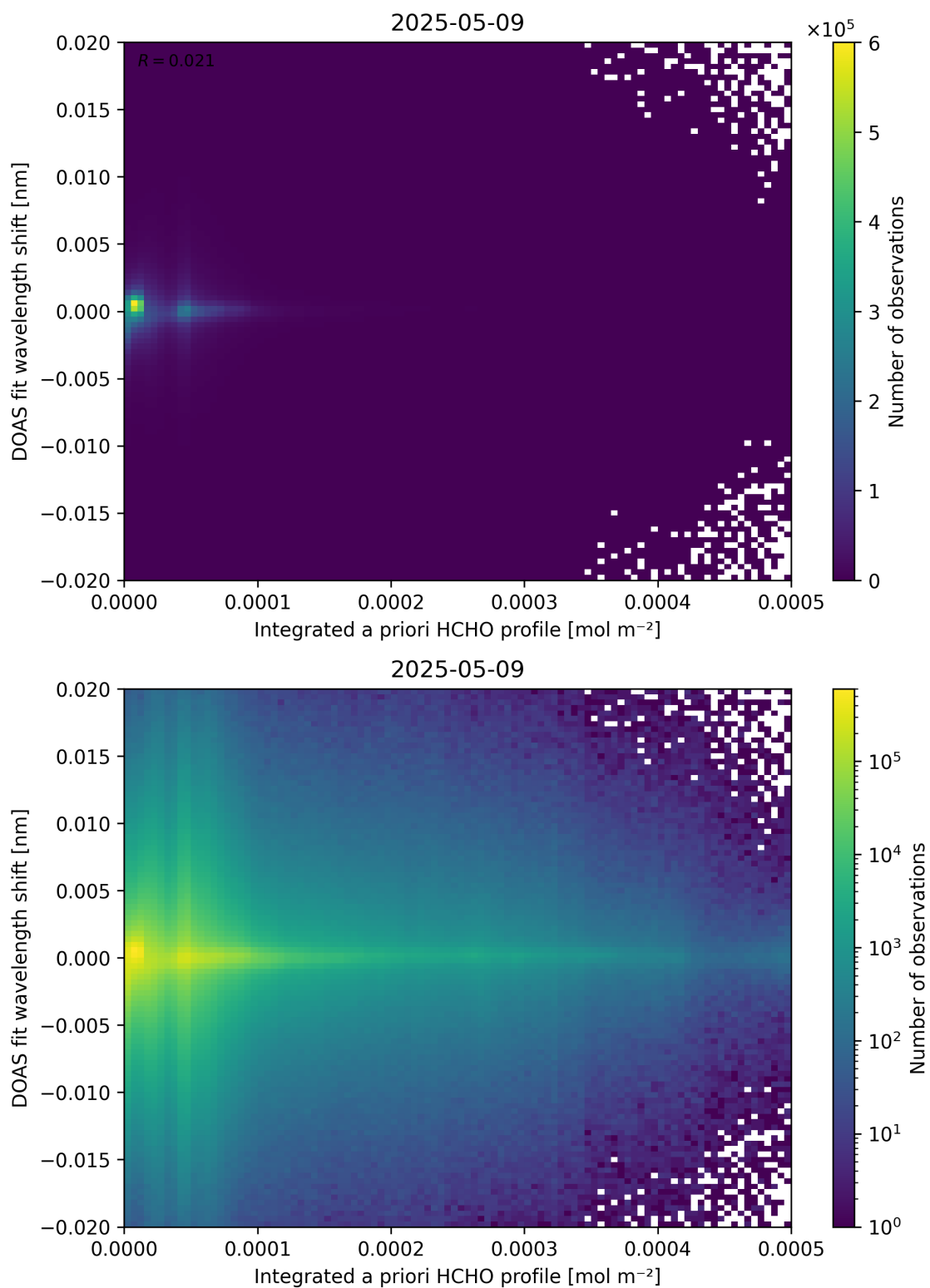
Figure 149: Scatter density plot of “Integrated a priori HCHO profile” against “DOAS fit wavelength shift” for 2025-05-08 to 2025-05-10.
