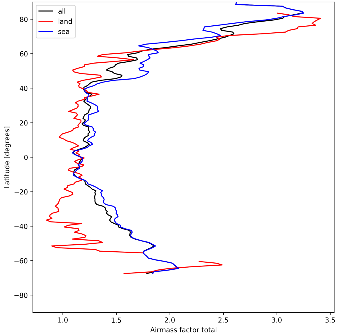
Figure 26: Zonal average of “Airmass factor total” for 2025-05-08 to 2025-05-10.
