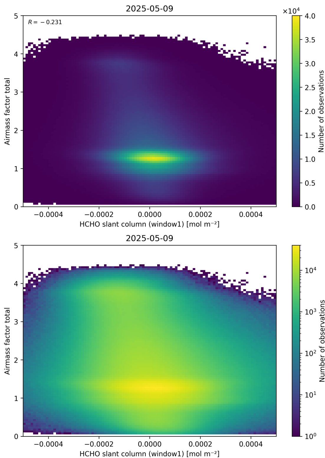
Figure 85: Scatter density plot of “HCHO slant column (window1)” against “Airmass factor total” for 2025-05-08 to 2025-05-10.
