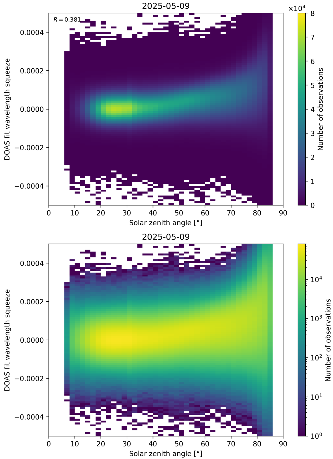
Figure 169: Scatter density plot of “Solar zenith angle” against “DOAS fit wavelength squeeze” for 2025-05-08 to 2025-05-10.
