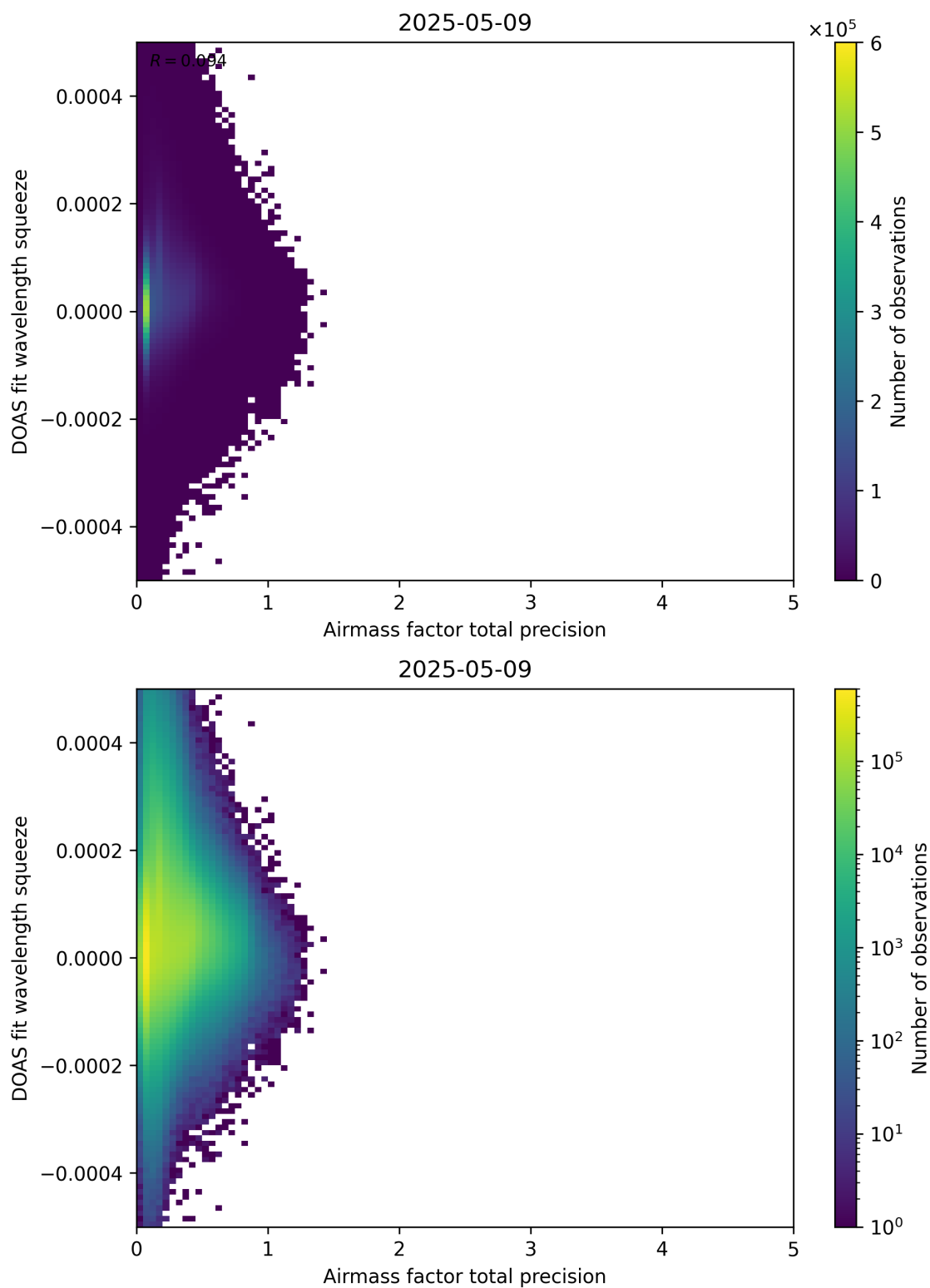
Figure 107: Scatter density plot of “Airmass factor total precision” against “DOAS fit wavelength squeeze” for 2025-05-08 to 2025-05-10.
