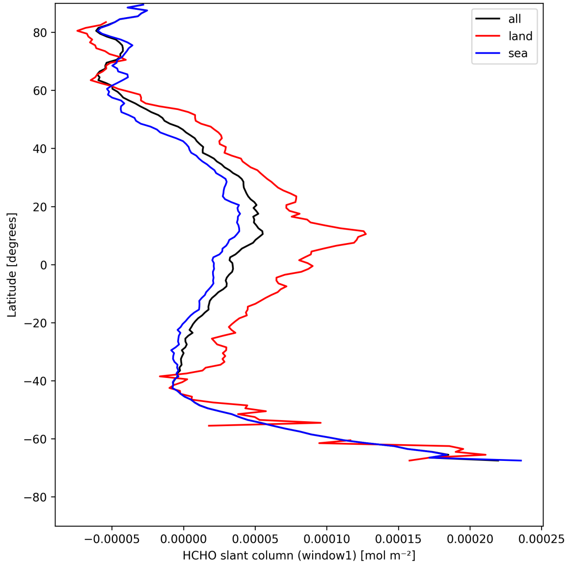
Figure 24: Zonal average of “HCHO slant column (window1)” for 2025-05-08 to 2025-05-10.
