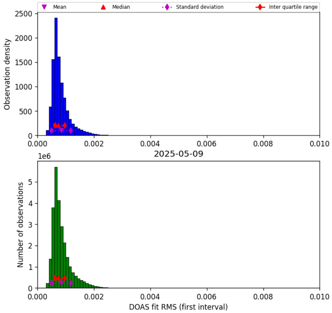
Figure 46: Histogram of “DOAS fit RMS (first interval)” for 2025-05-08 to 2025-05-10
