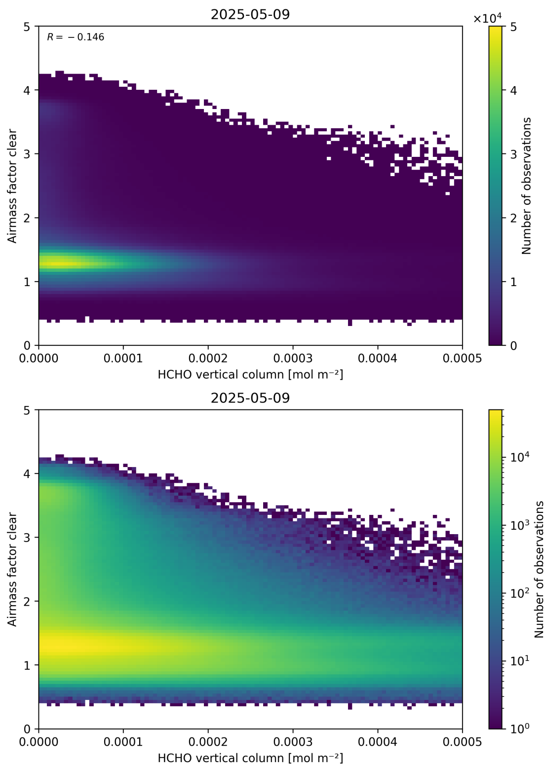
Figure 126: Scatter density plot of “HCHO vertical column” against “Airmass factor clear” for 2025-05-08 to 2025-05-10.
