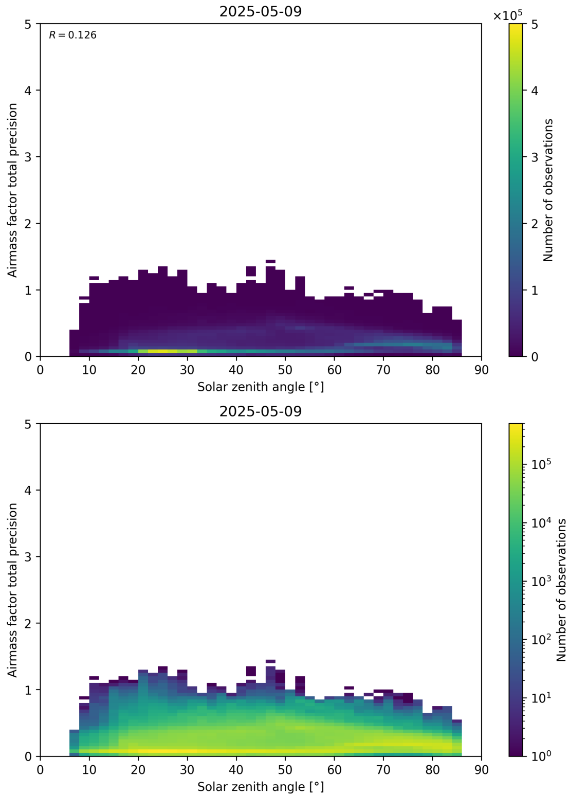
Figure 176: Scatter density plot of “Solar zenith angle” against “Airmass factor total precision” for 2025-05-08 to 2025-05-10.
