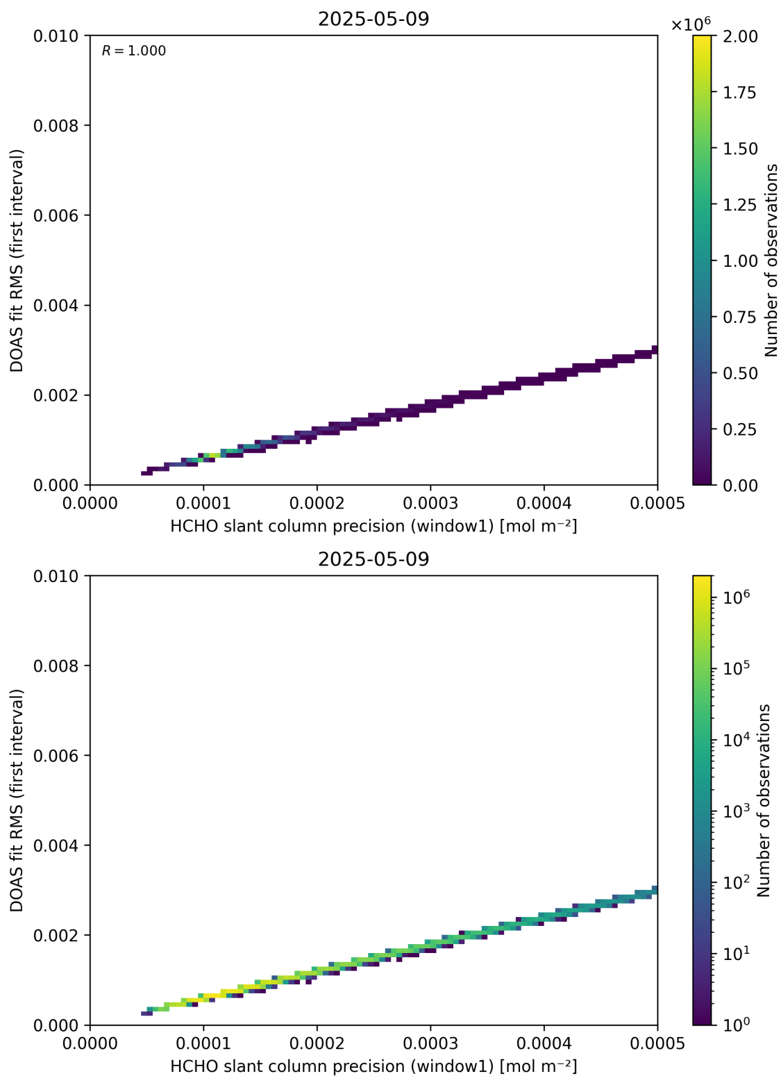
Figure 88: Scatter density plot of “HCHO slant column precision (window1)” against “DOAS fit RMS (first interval)” for 2025-05-08 to 2025-05-10.
