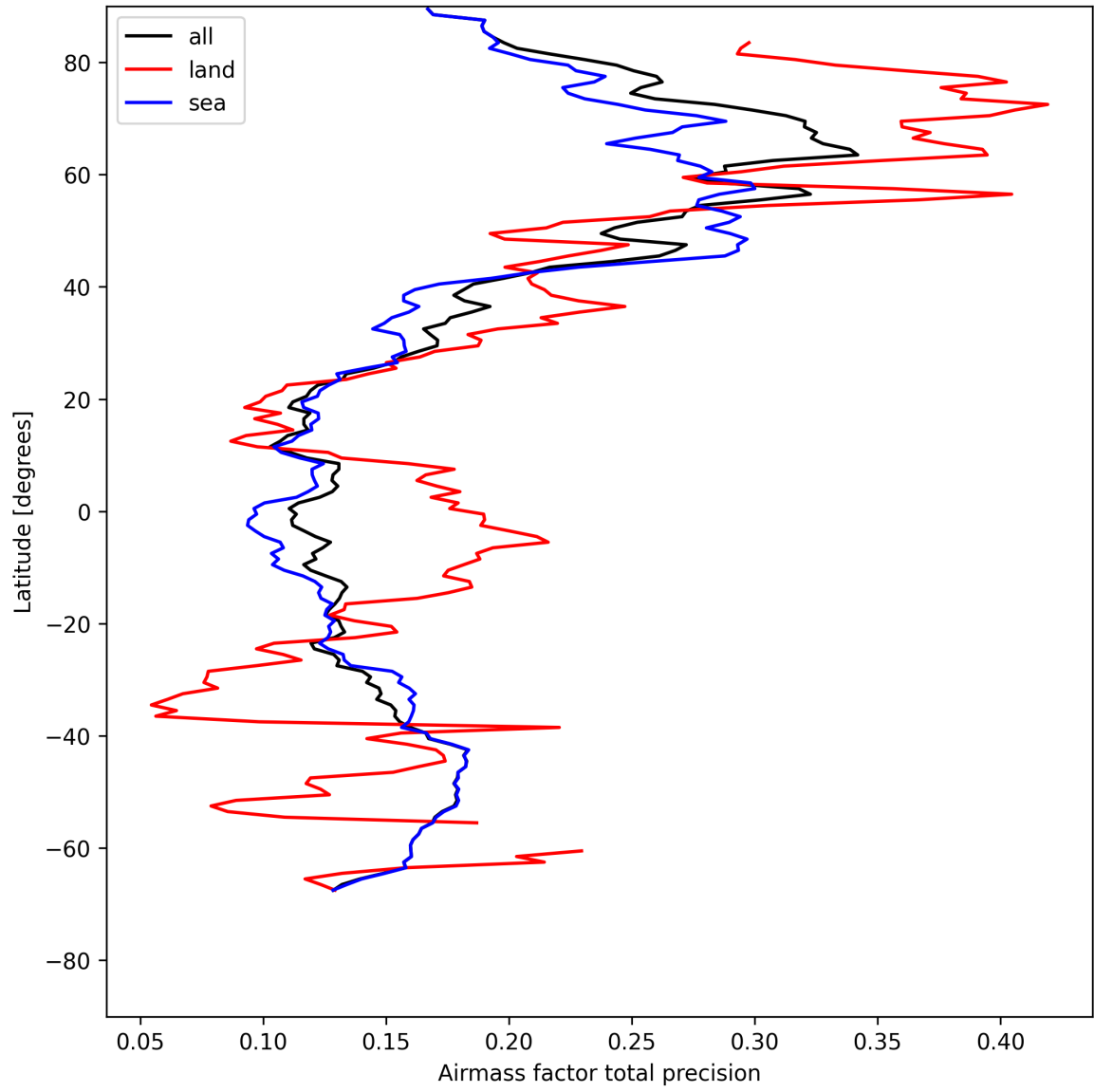
Figure 27: Zonal average of “Airmass factor total precision” for 2025-05-08 to 2025-05-10.
