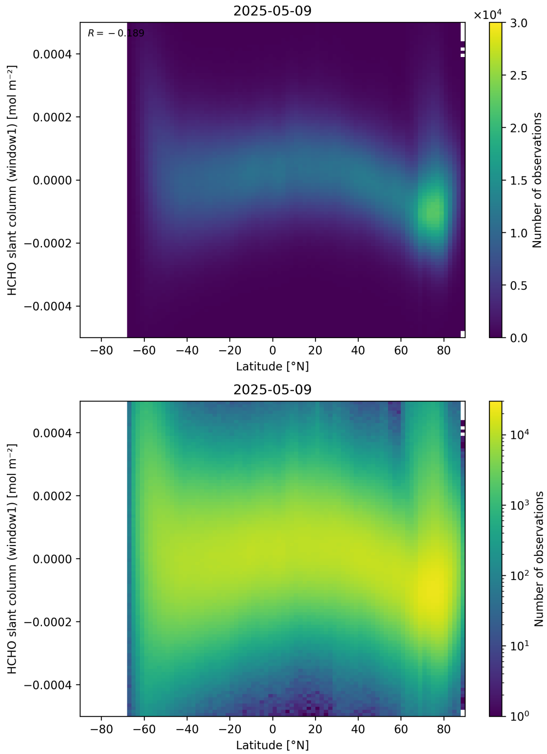
Figure 159: Scatter density plot of “Latitude” against “HCHO slant column (window1)” for 2025-05-08 to 2025-05-10.
