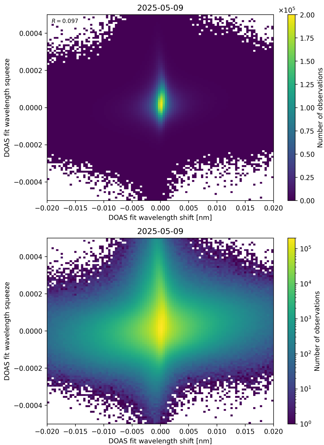
Figure 65: Scatter density plot of “DOAS fit wavelength shift” against “DOAS fit wavelength squeeze” for 2025-05-08 to 2025-05-10.
