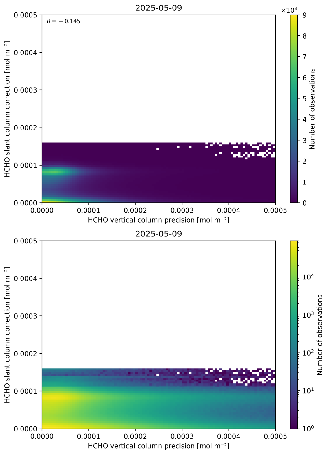
Figure 141: Scatter density plot of “HCHO vertical column precision” against “HCHO slant column correction” for 2025-05-08 to 2025-05-10.
