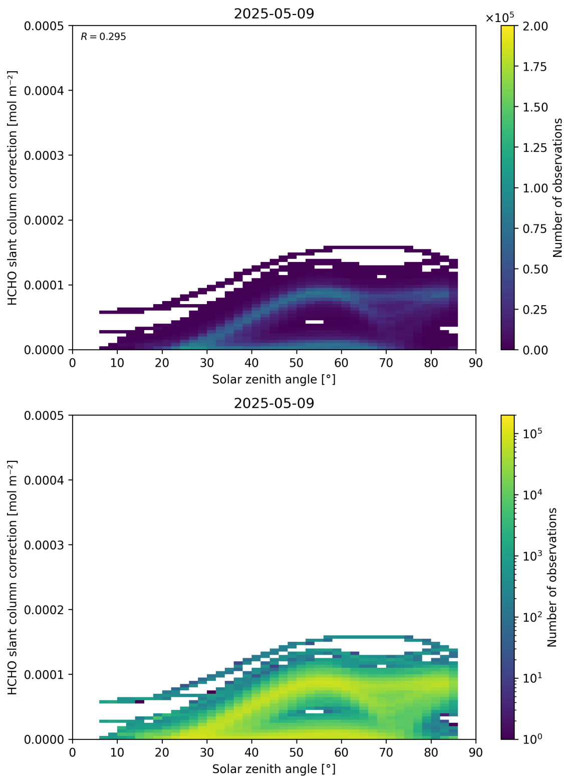
Figure 172: Scatter density plot of “Solar zenith angle” against “HCHO slant column correction” for 2025-05-08 to 2025-05-10.
