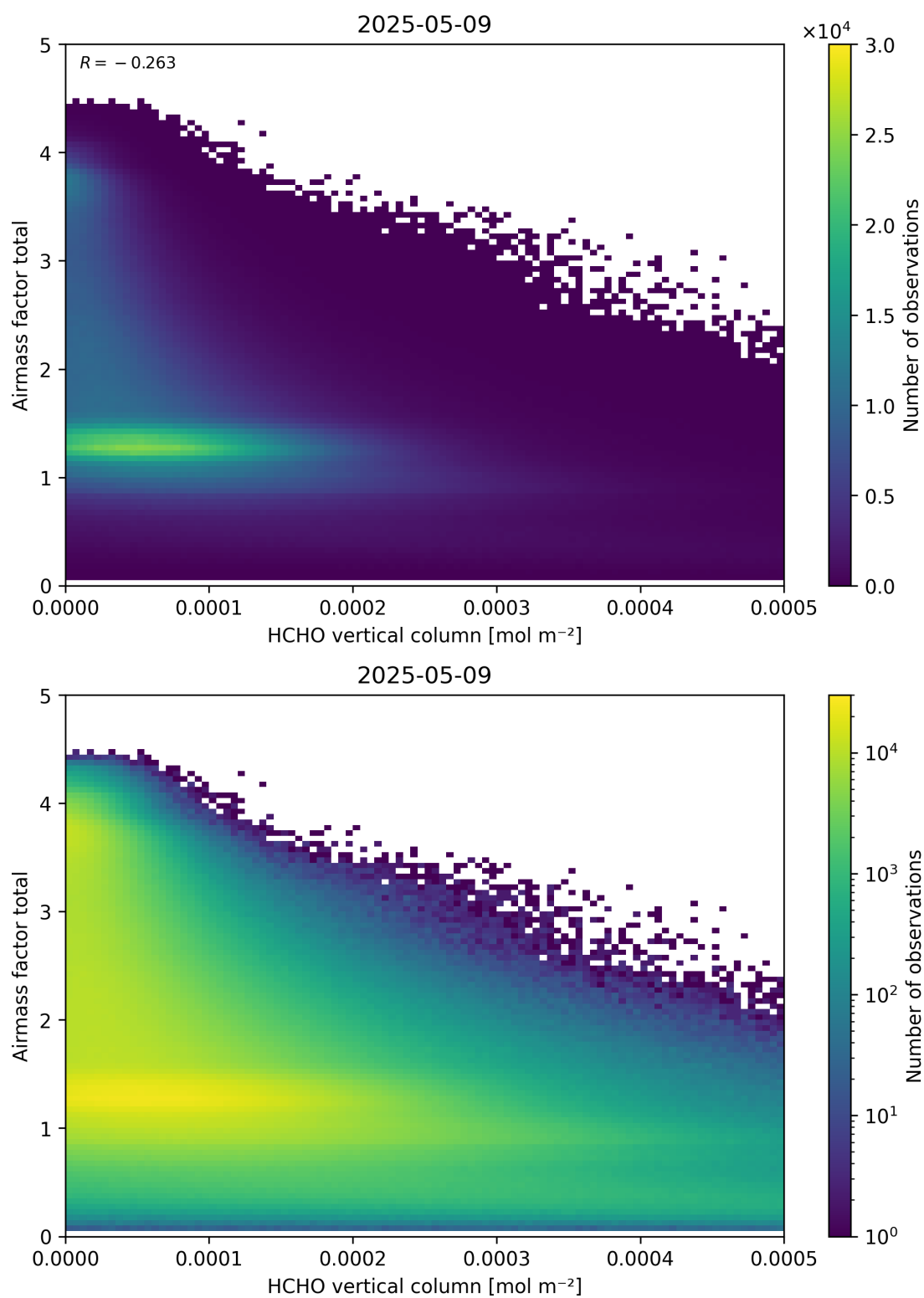
Figure 131: Scatter density plot of “HCHO vertical column” against “Airmass factor total” for 2025-05-08 to 2025-05-10.
