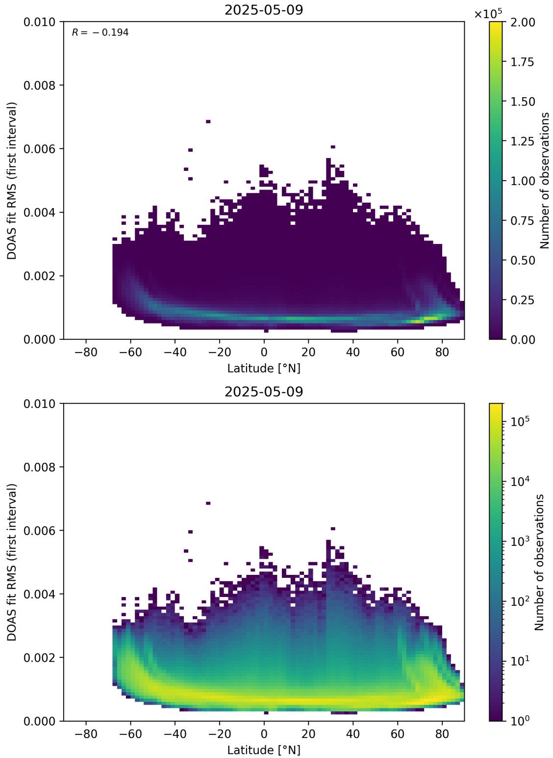
Figure 153: Scatter density plot of “Latitude” against “DOAS fit RMS (first interval)” for 2025-05-08 to 2025-05-10.
