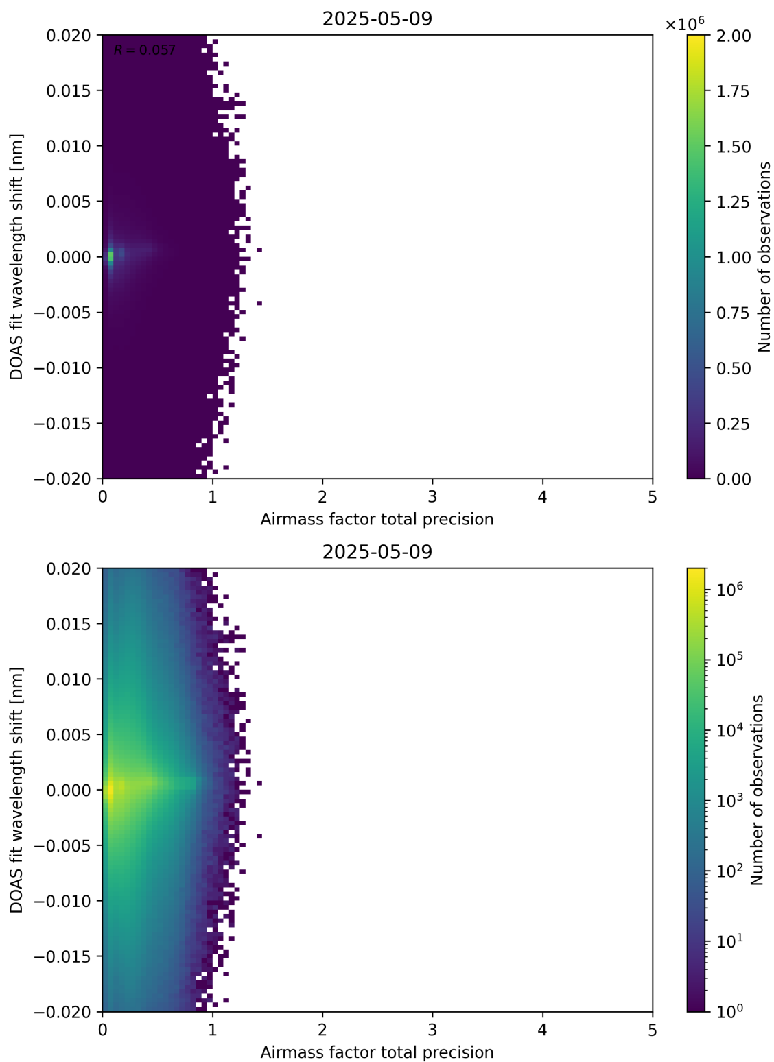
Figure 106: Scatter density plot of “Airmass factor total precision” against “DOAS fit wavelength shift” for 2025-05-08 to 2025-05-10.
