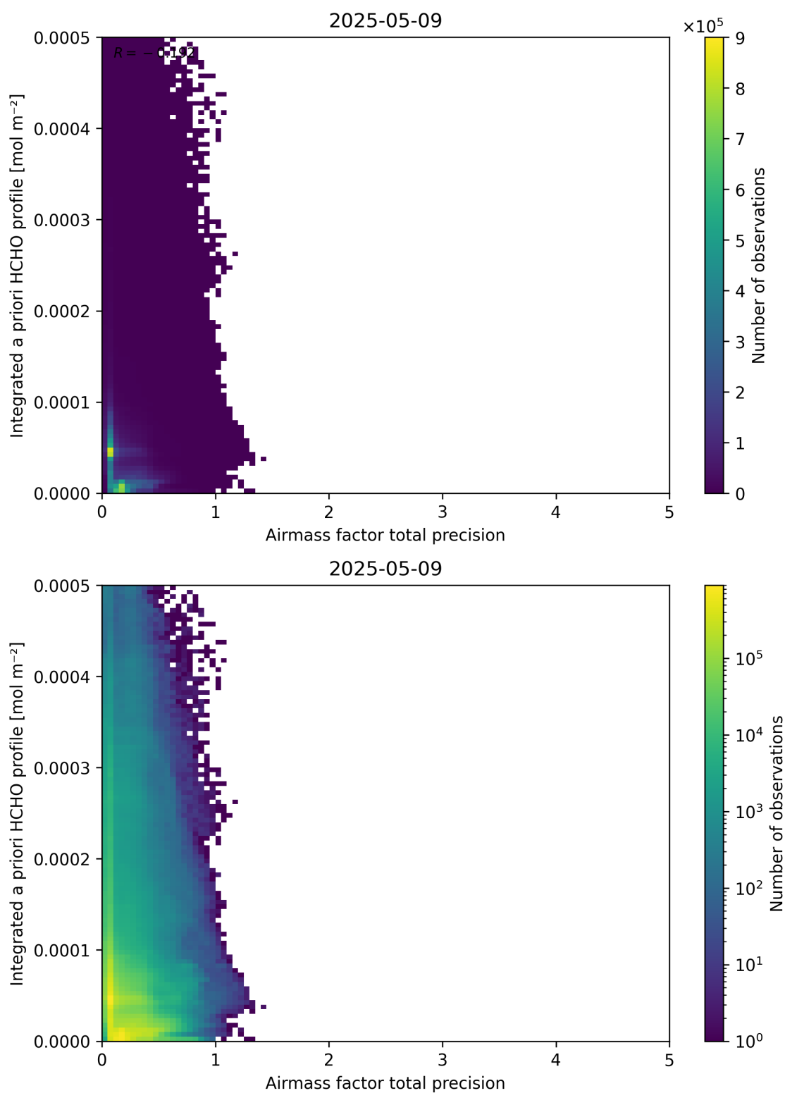
Figure 111: Scatter density plot of “Airmass factor total precision” against “Integrated a priori HCHO profile” for 2025-05-08 to 2025-05-10.
