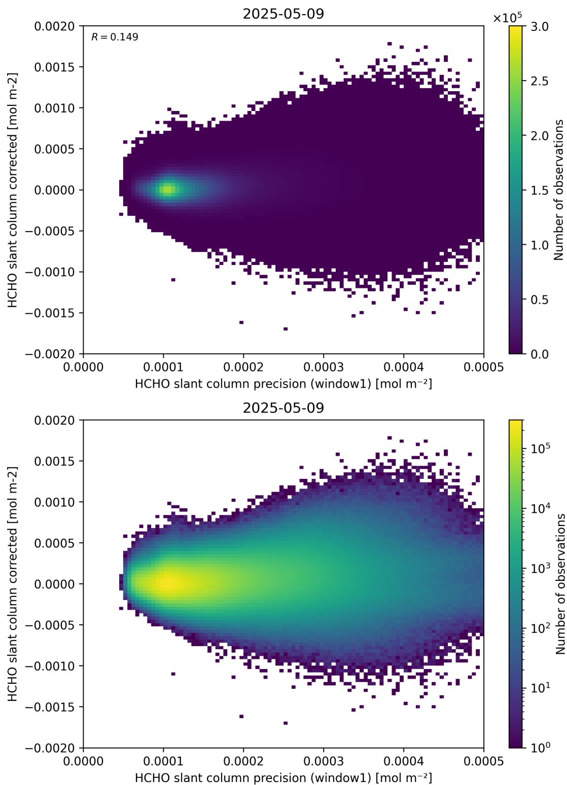
Figure 92: Scatter density plot of “HCHO slant column precision (window1)” against “HCHO slant column corrected” for 2025-05-08 to 2025-05-10.
