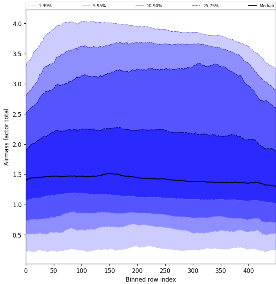
Figure 54: Along track statistics of “Airmass factor total” for 2025-05-08 to 2025-05-10
