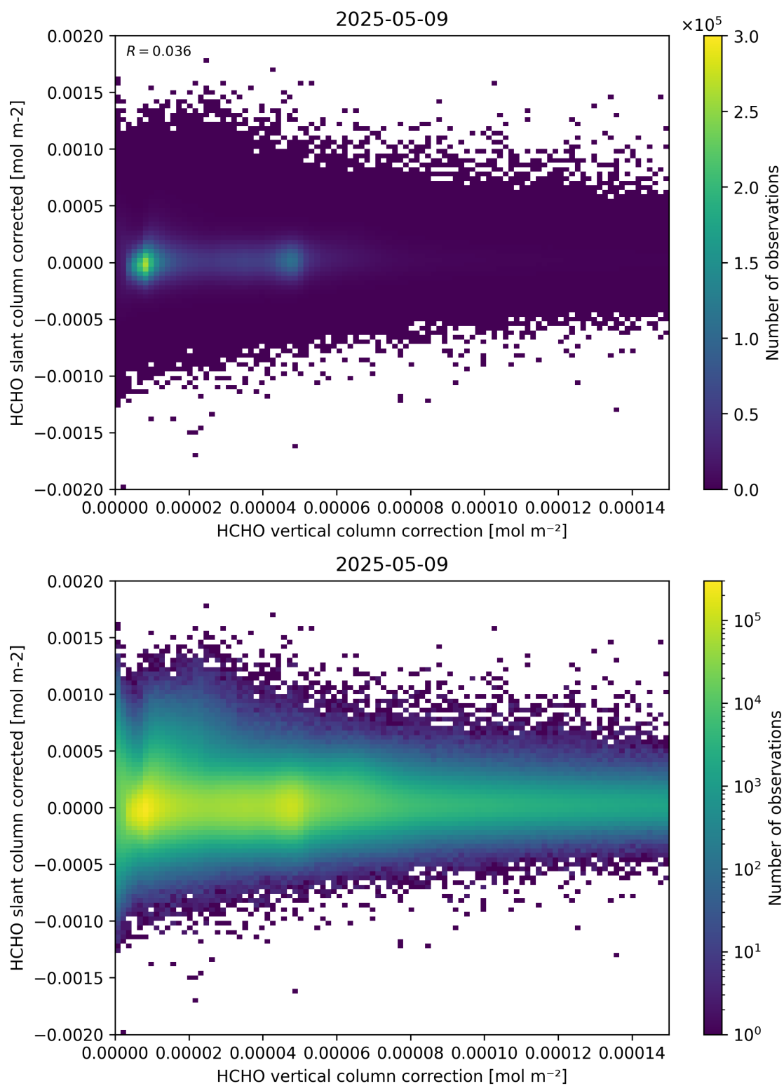
Figure 116: Scatter density plot of “HCHO vertical column correction” against “HCHO slant column corrected” for 2025-05-08 to 2025-05-10.
