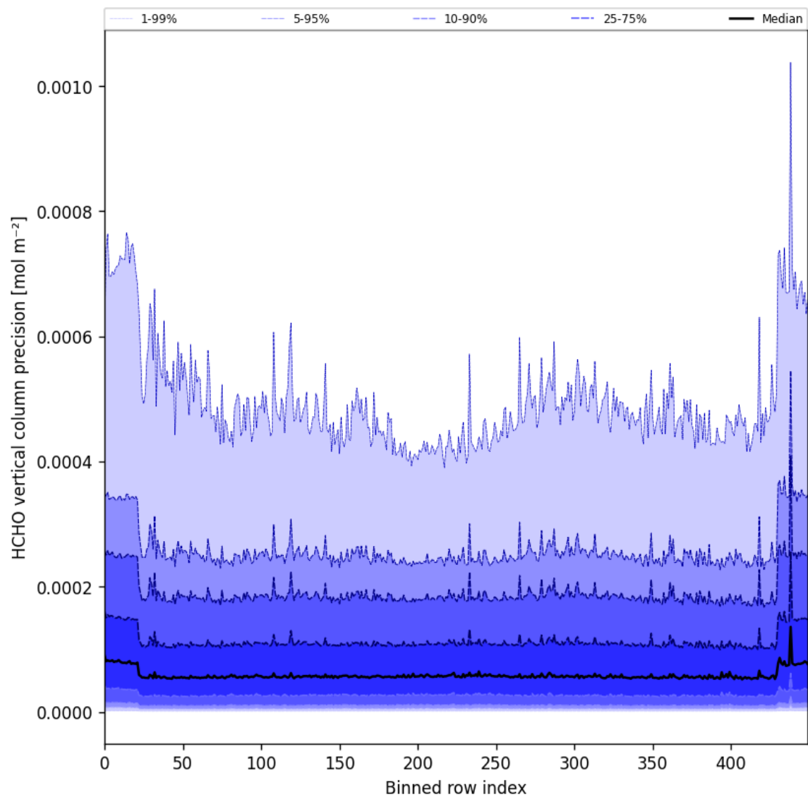
Figure 50: Along track statistics of “HCHO vertical column precision” for 2025-05-08 to 2025-05-10
