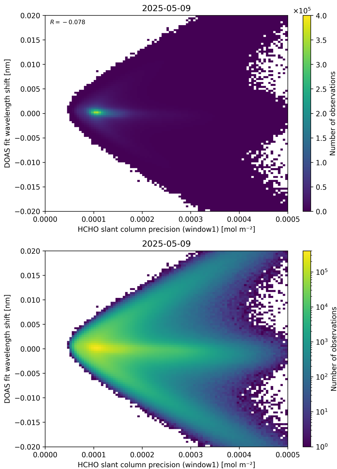
Figure 89: Scatter density plot of “HCHO slant column precision (window1)” against “DOAS fit wavelength shift” for 2025-05-08 to 2025-05-10.
