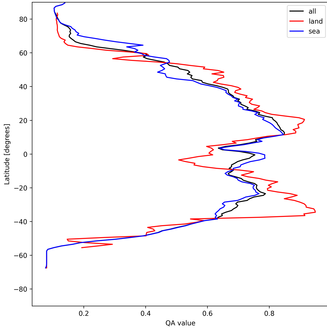
Figure 20: Zonal average of “QA value” for 2025-05-08 to 2025-05-10.
