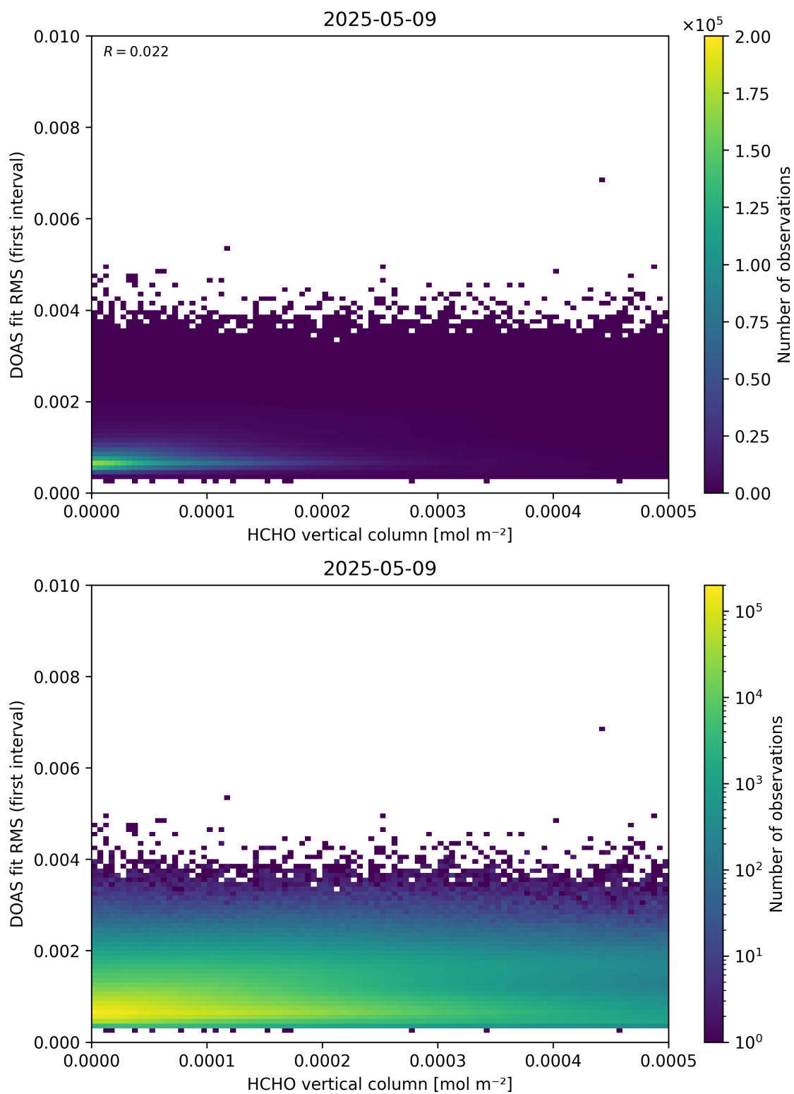
Figure 123: Scatter density plot of “HCHO vertical column” against “DOAS fit RMS (first interval)” for 2025-05-08 to 2025-05-10.
