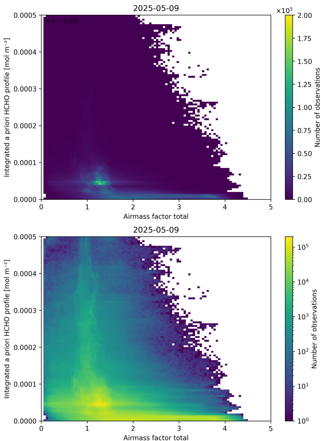
Figure 104: Scatter density plot of “Airmass factor total” against “Integrated a priori HCHO profile” for 2025-05-08 to 2025-05-10.
