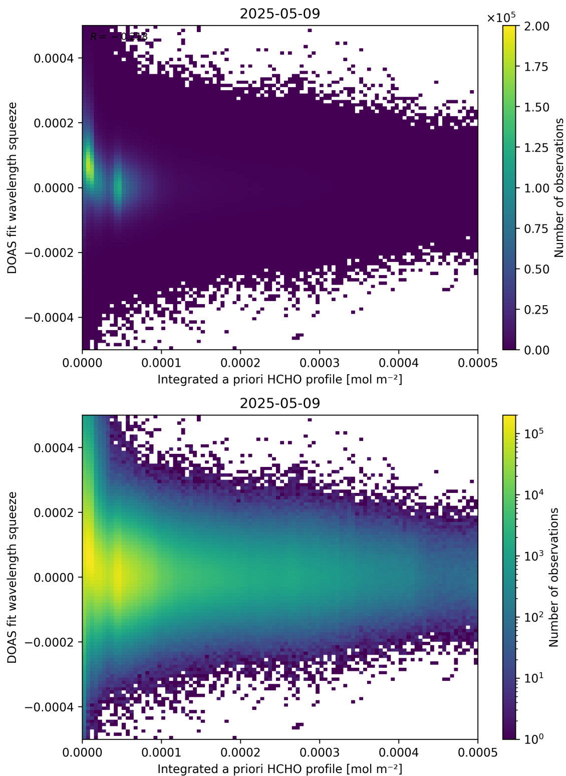
Figure 150: Scatter density plot of “Integrated a priori HCHO profile” against “DOAS fit wavelength squeeze” for 2025-05-08 to 2025-05-10.
