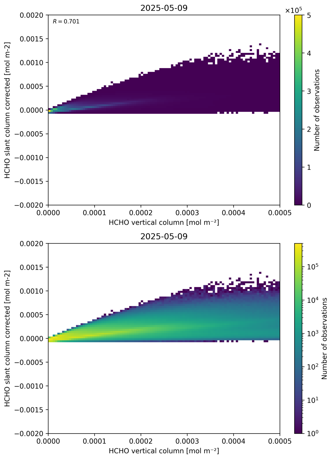
Figure 127: Scatter density plot of “HCHO vertical column” against “HCHO slant column corrected” for 2025-05-08 to 2025-05-10.
