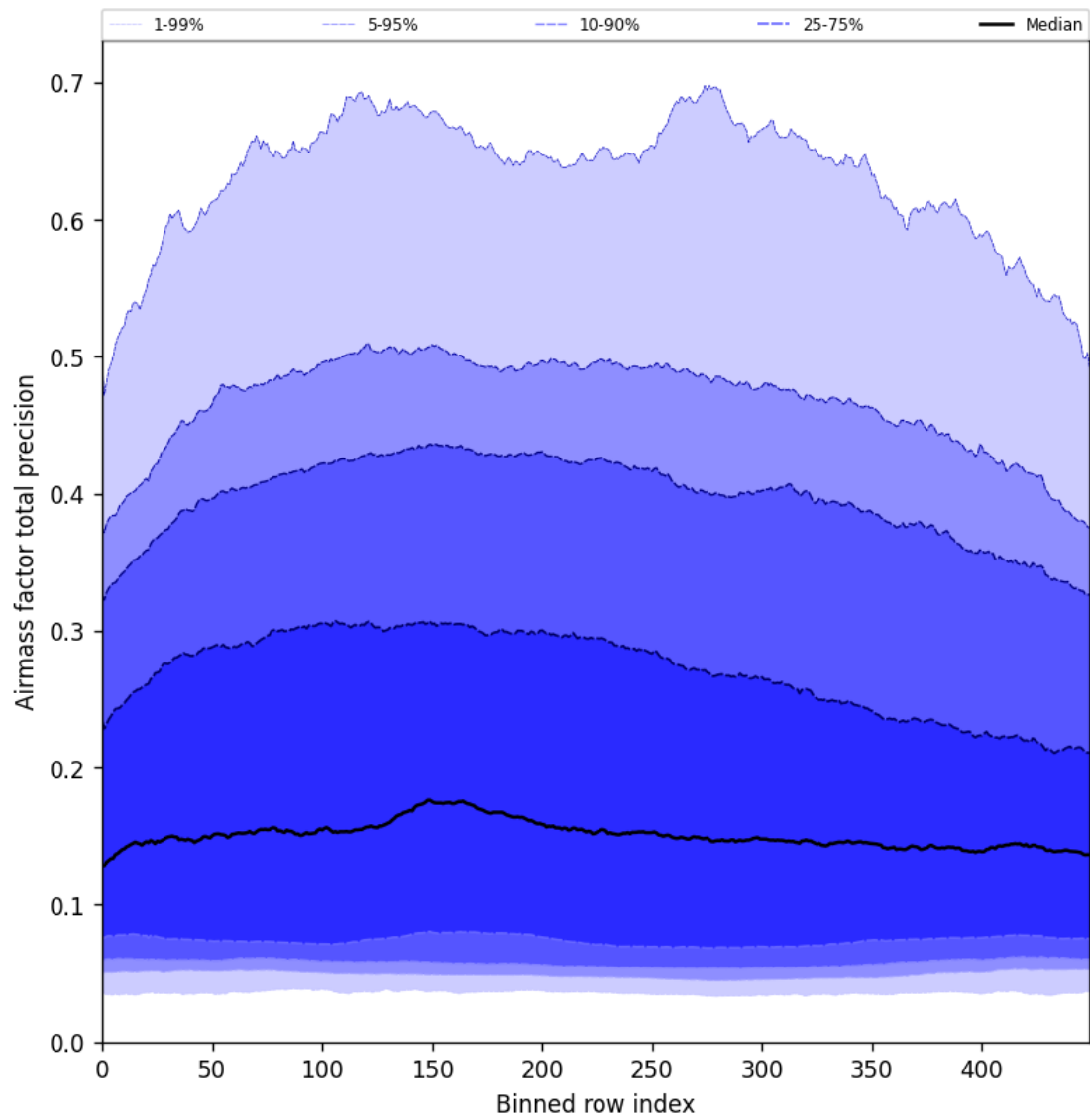
Figure 55: Along track statistics of “Airmass factor total precision” for 2025-05-08 to 2025-05-10
