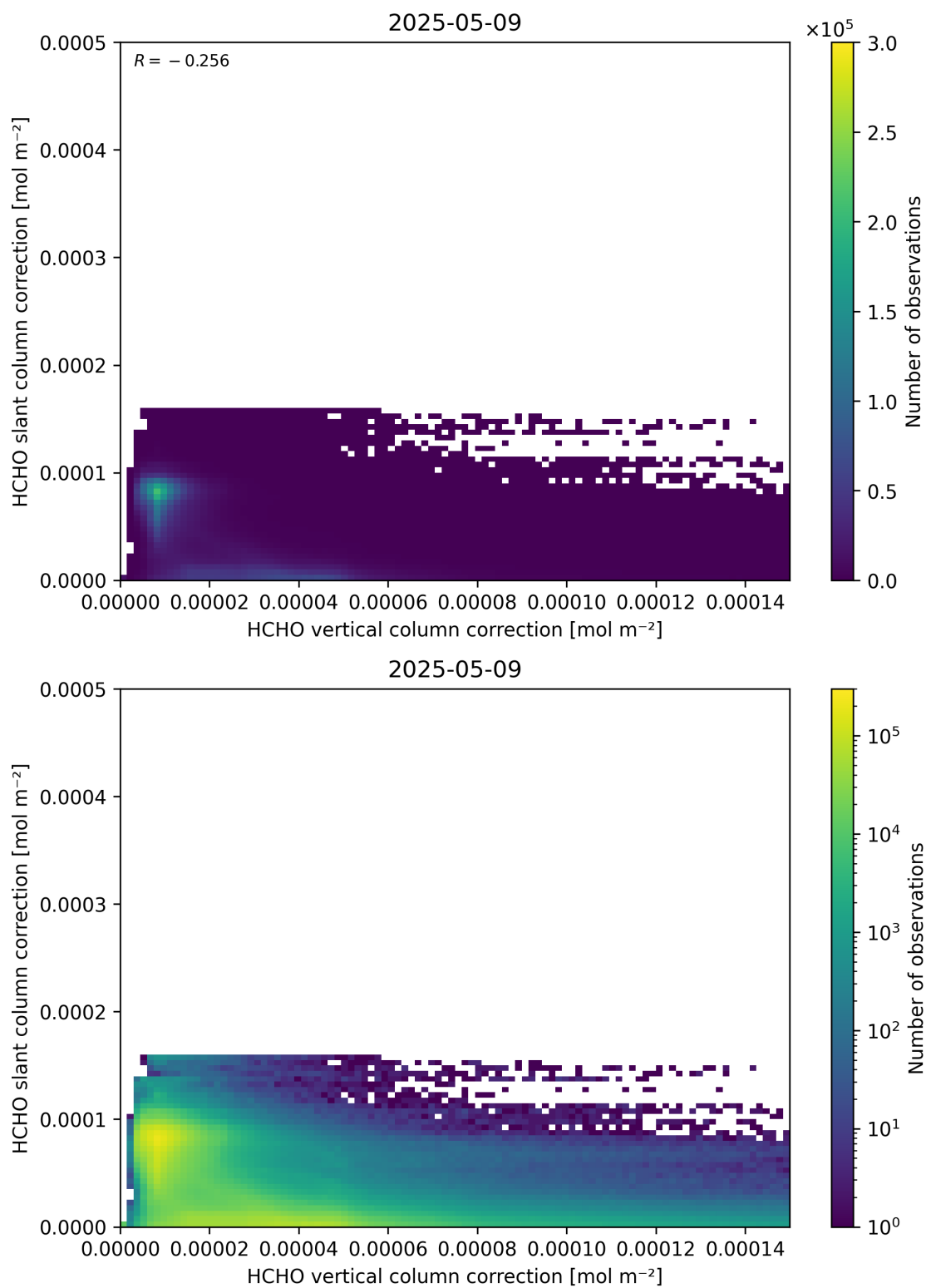
Figure 117: Scatter density plot of “HCHO vertical column correction” against “HCHO slant column correction” for 2025-05-08 to 2025-05-10.
