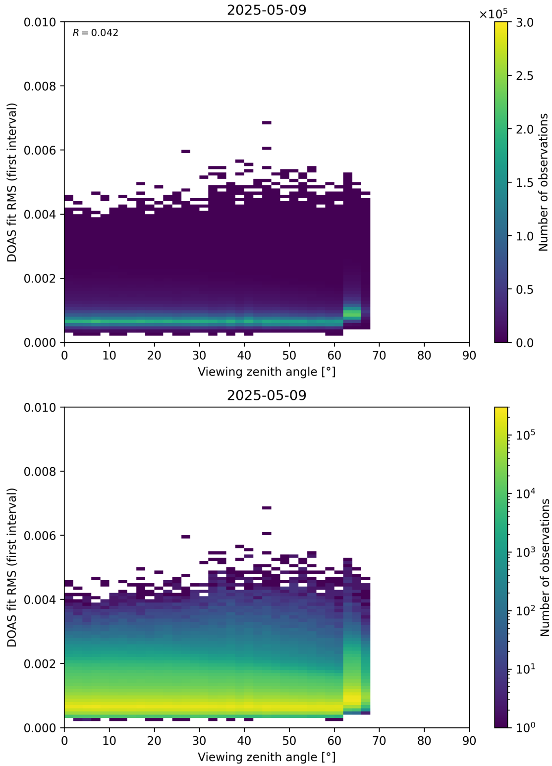
Figure 182: Scatter density plot of “Viewing zenith angle” against “DOAS fit RMS (first interval)” for 2025-05-08 to 2025-05-10.
