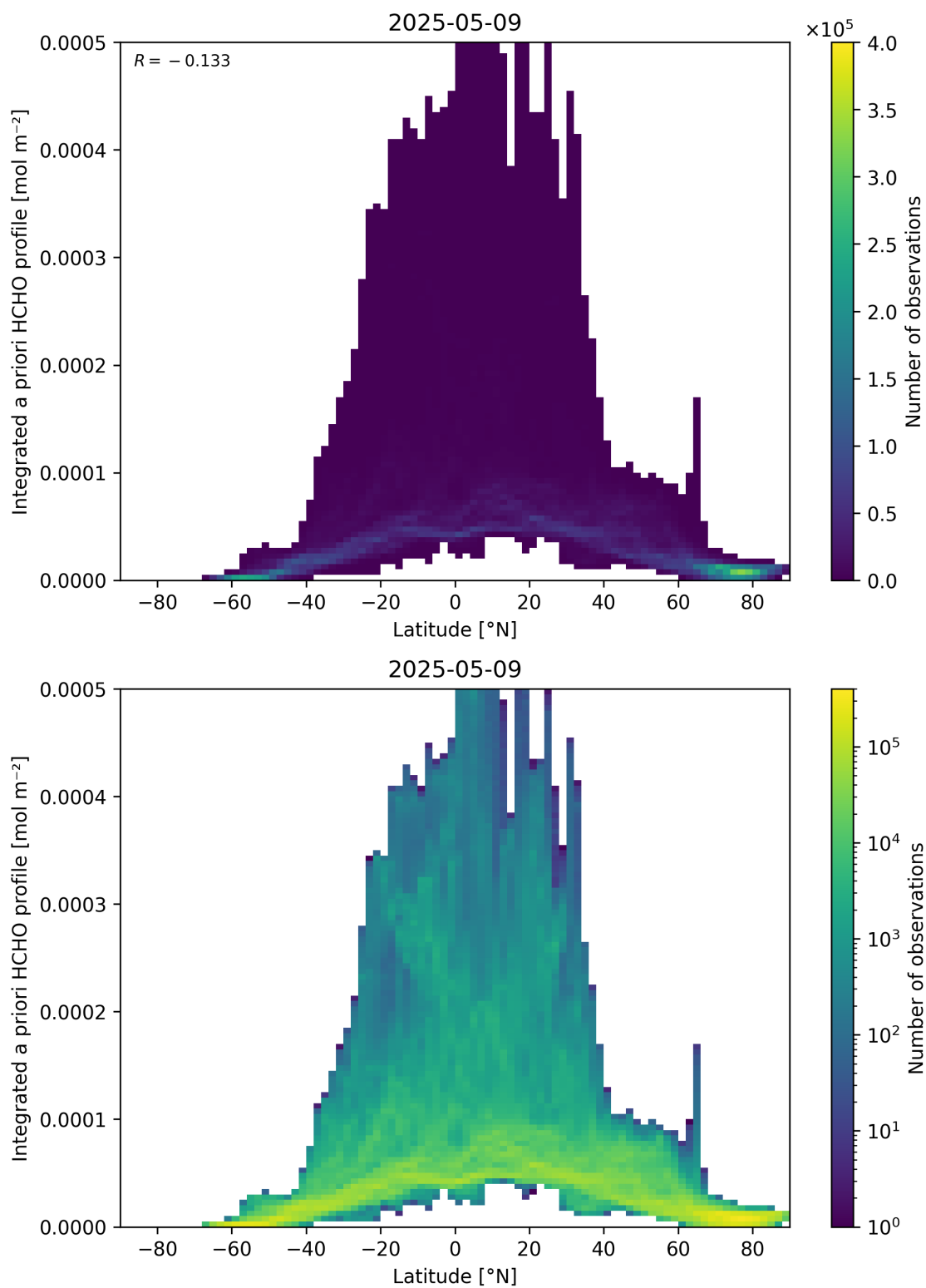
Figure 166: Scatter density plot of “Latitude” against “Integrated a priori HCHO profile” for 2025-05-08 to 2025-05-10.
