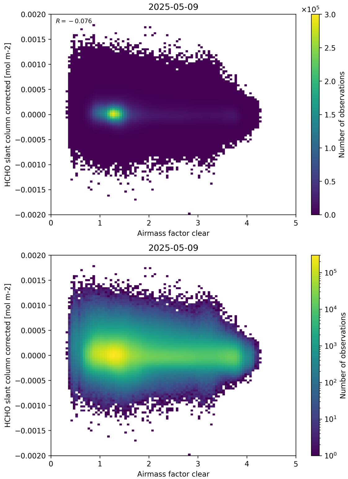
Figure 74: Scatter density plot of “Airmass factor clear” against “HCHO slant column corrected” for 2025-05-08 to 2025-05-10.
