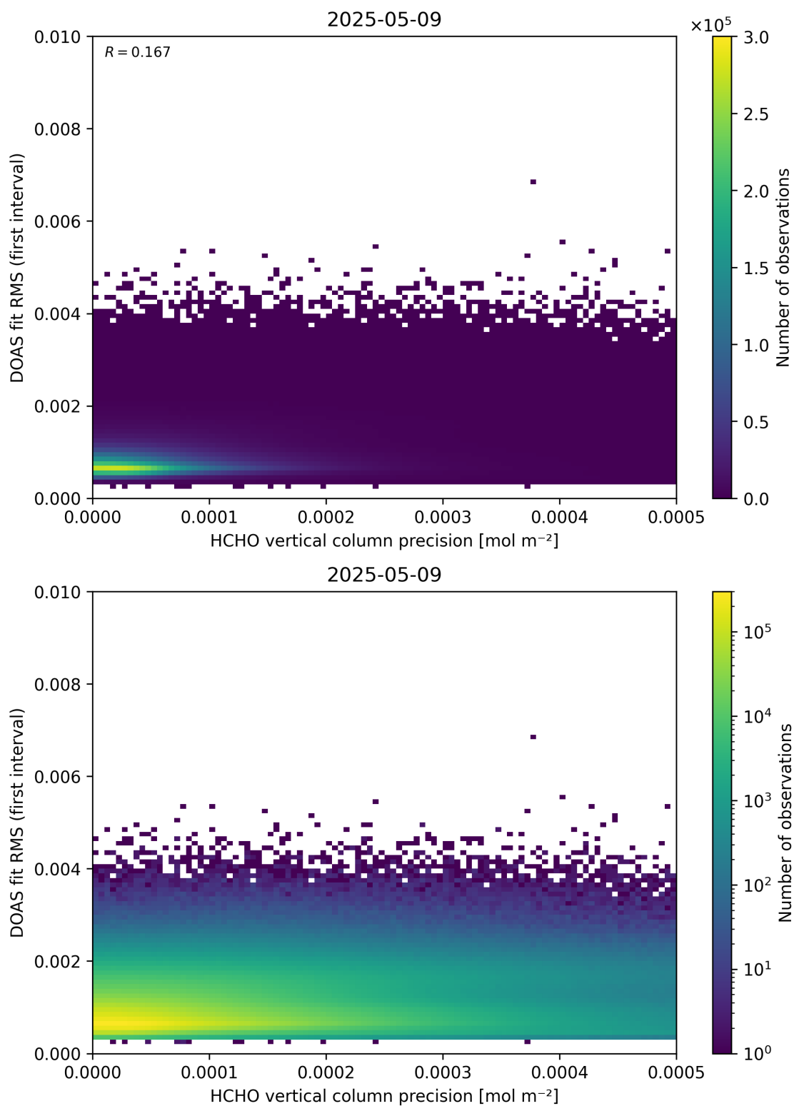
Figure 136: Scatter density plot of “HCHO vertical column precision” against “DOAS fit RMS (first interval)” for 2025-05-08 to 2025-05-10.
