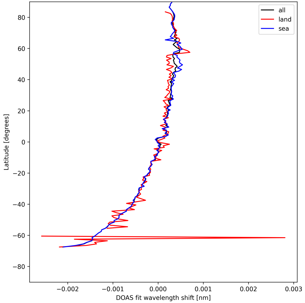
Figure 30: Zonal average of “DOAS fit wavelength shift” for 2025-05-08 to 2025-05-10.
