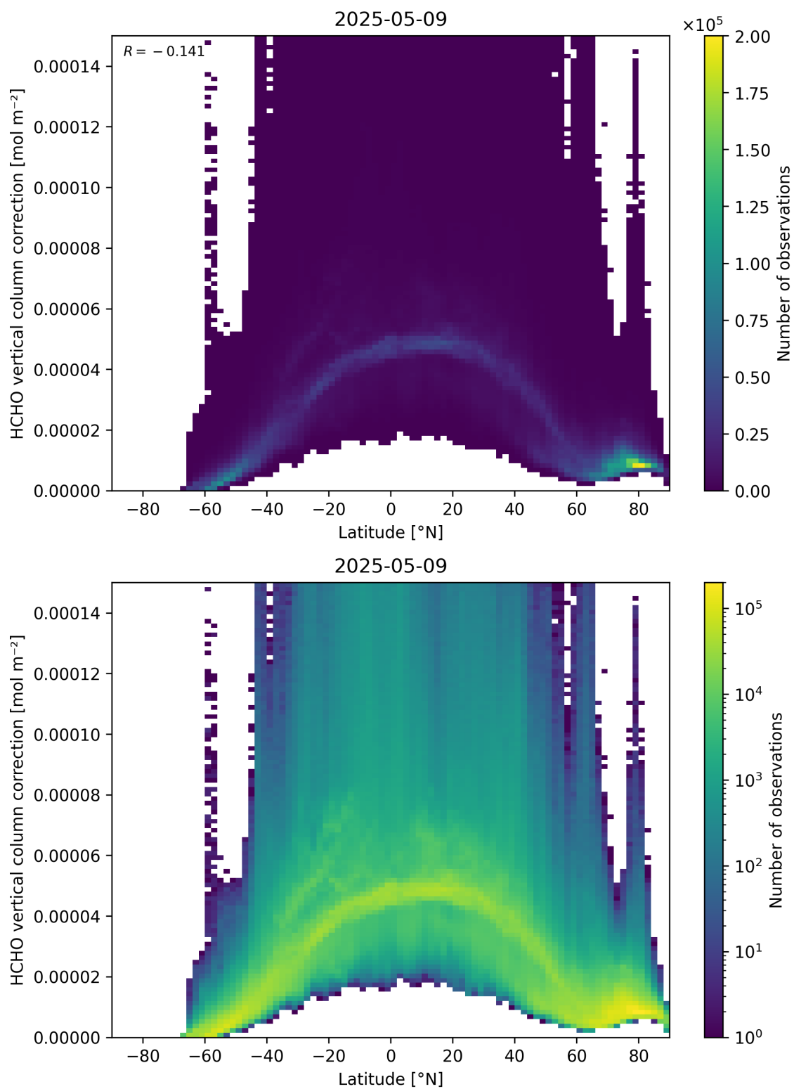
Figure 164: Scatter density plot of “Latitude” against “HCHO vertical column correction” for 2025-05-08 to 2025-05-10.
