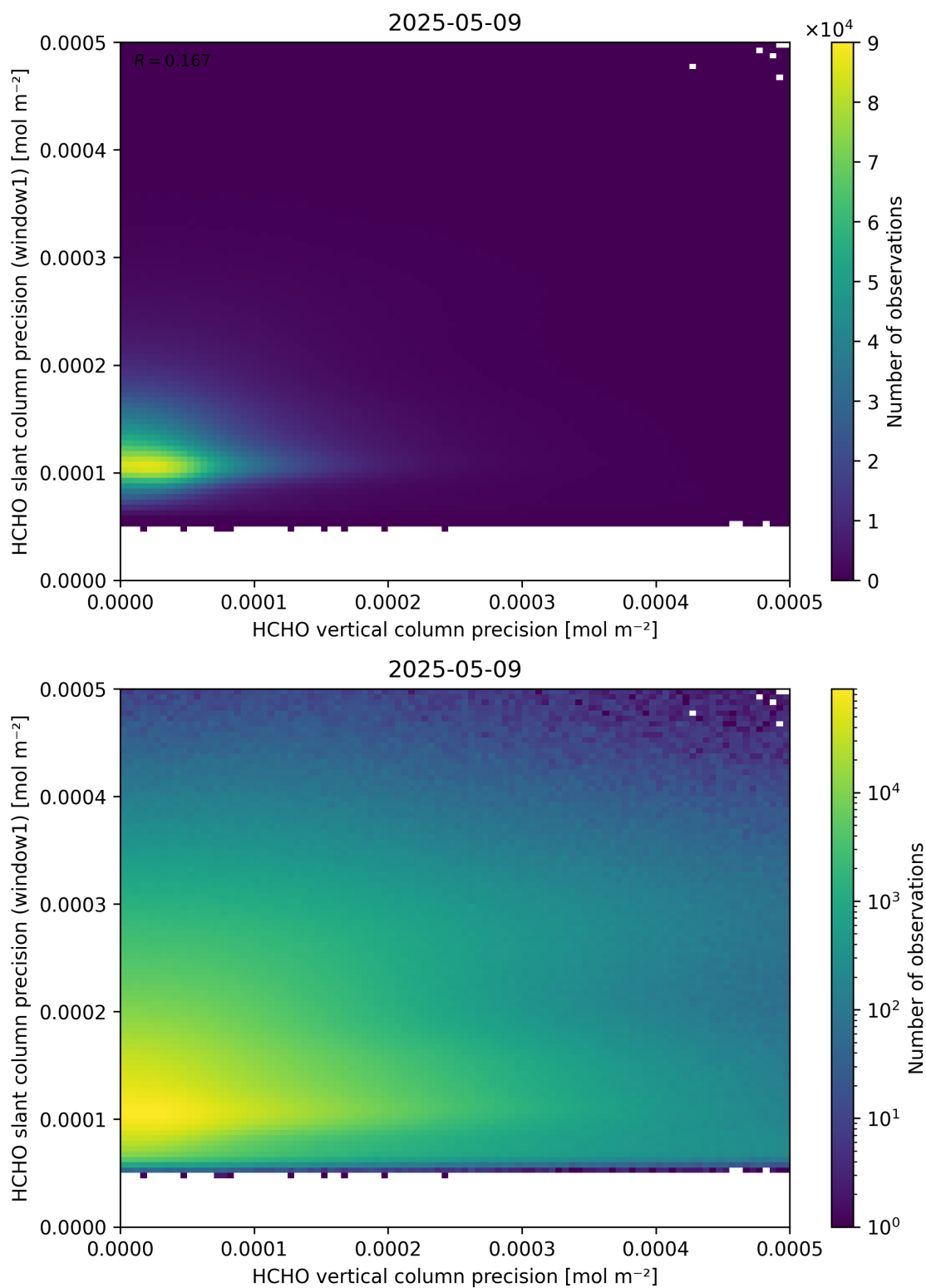
Figure 143: Scatter density plot of “HCHO vertical column precision” against “HCHO slant column precision (window1)” for 2025-05-08 to 2025-05-10.
