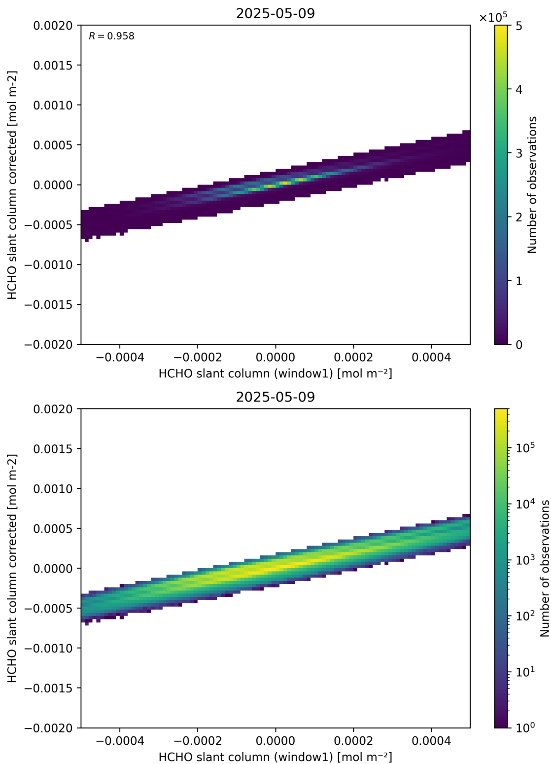
Figure 82: Scatter density plot of “HCHO slant column (window1)” against “HCHO slant column corrected” for 2025-05-08 to 2025-05-10.
