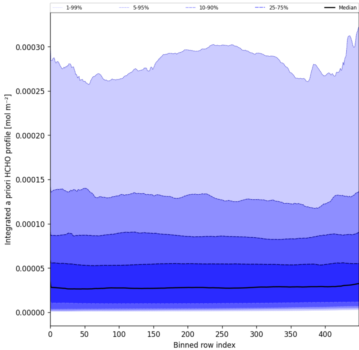
Figure 57: Along track statistics of “Integrated a priori HCHO profile” for 2025-05-08 to 2025-05-10
