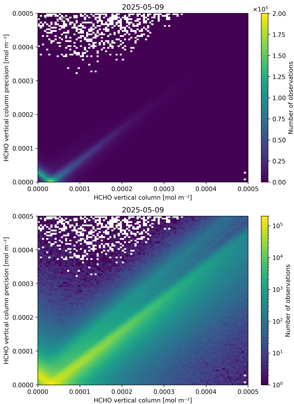
Figure 134: Scatter density plot of “HCHO vertical column” against “HCHO vertical column precision” for 2025-05-08 to 2025-05-10.
