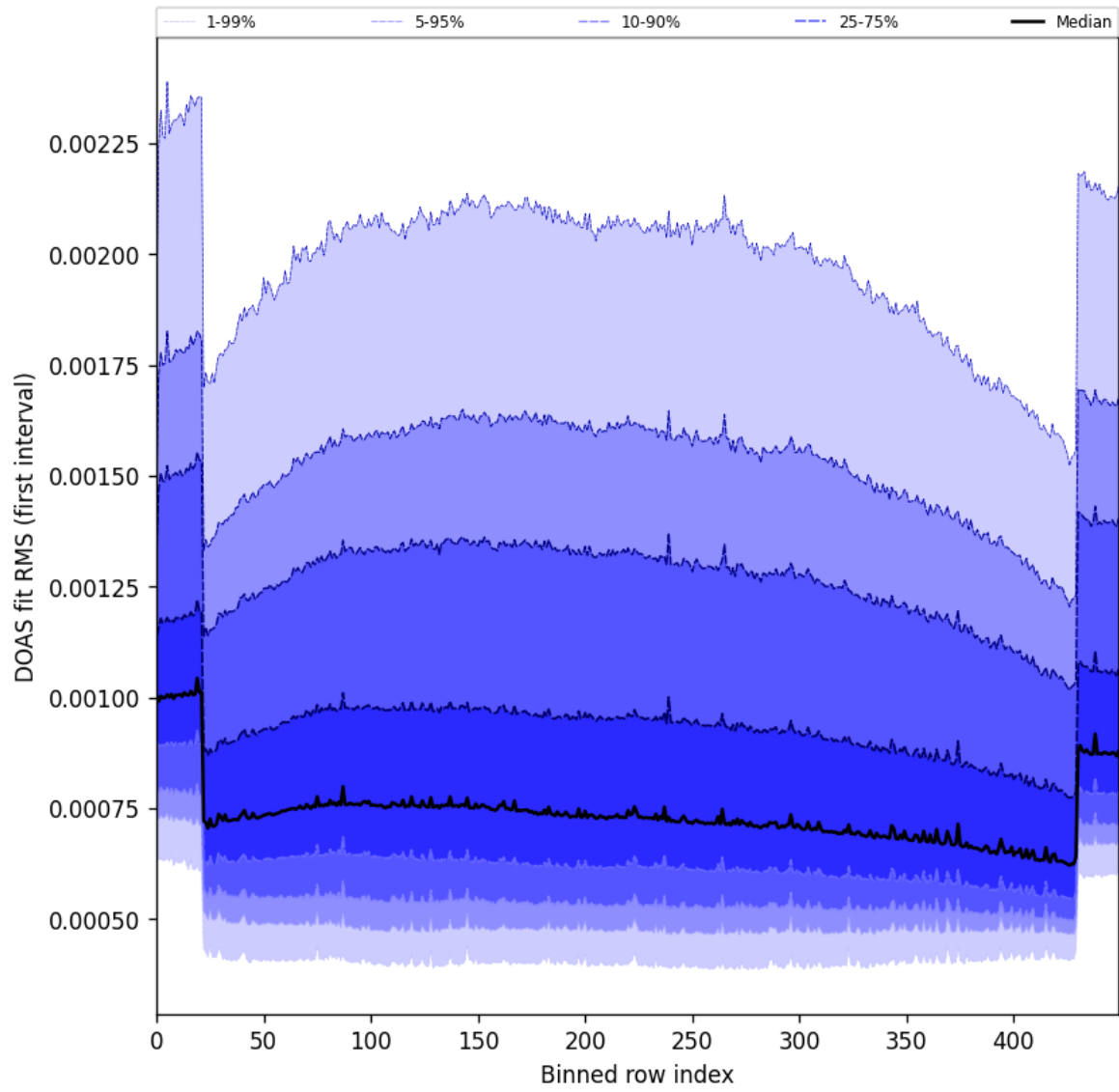
Figure 60: Along track statistics of “DOAS fit RMS (first interval)” for 2025-05-08 to 2025-05-10
