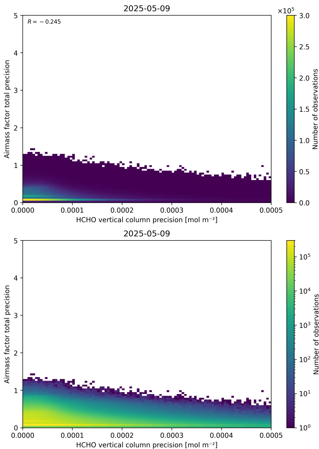
Figure 145: Scatter density plot of “HCHO vertical column precision” against “Airmass factor total precision” for 2025-05-08 to 2025-05-10.
