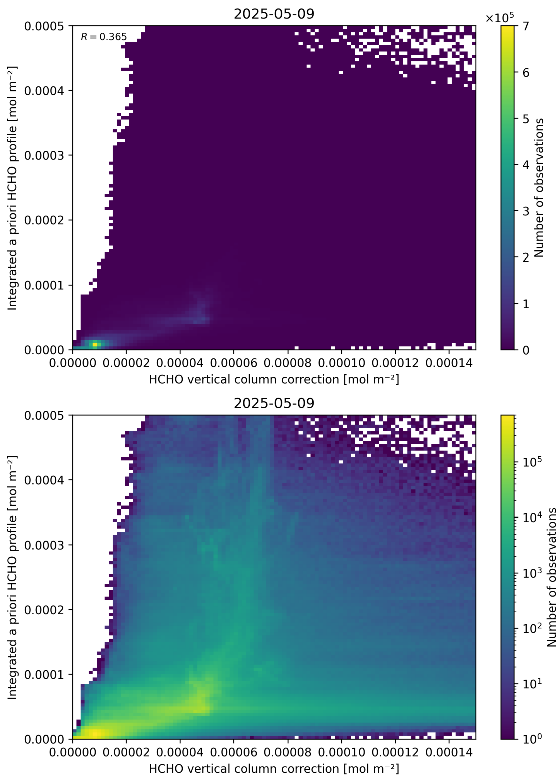
Figure 122: Scatter density plot of “HCHO vertical column correction” against “Integrated a priori HCHO profile” for 2025-05-08 to 2025-05-10.
