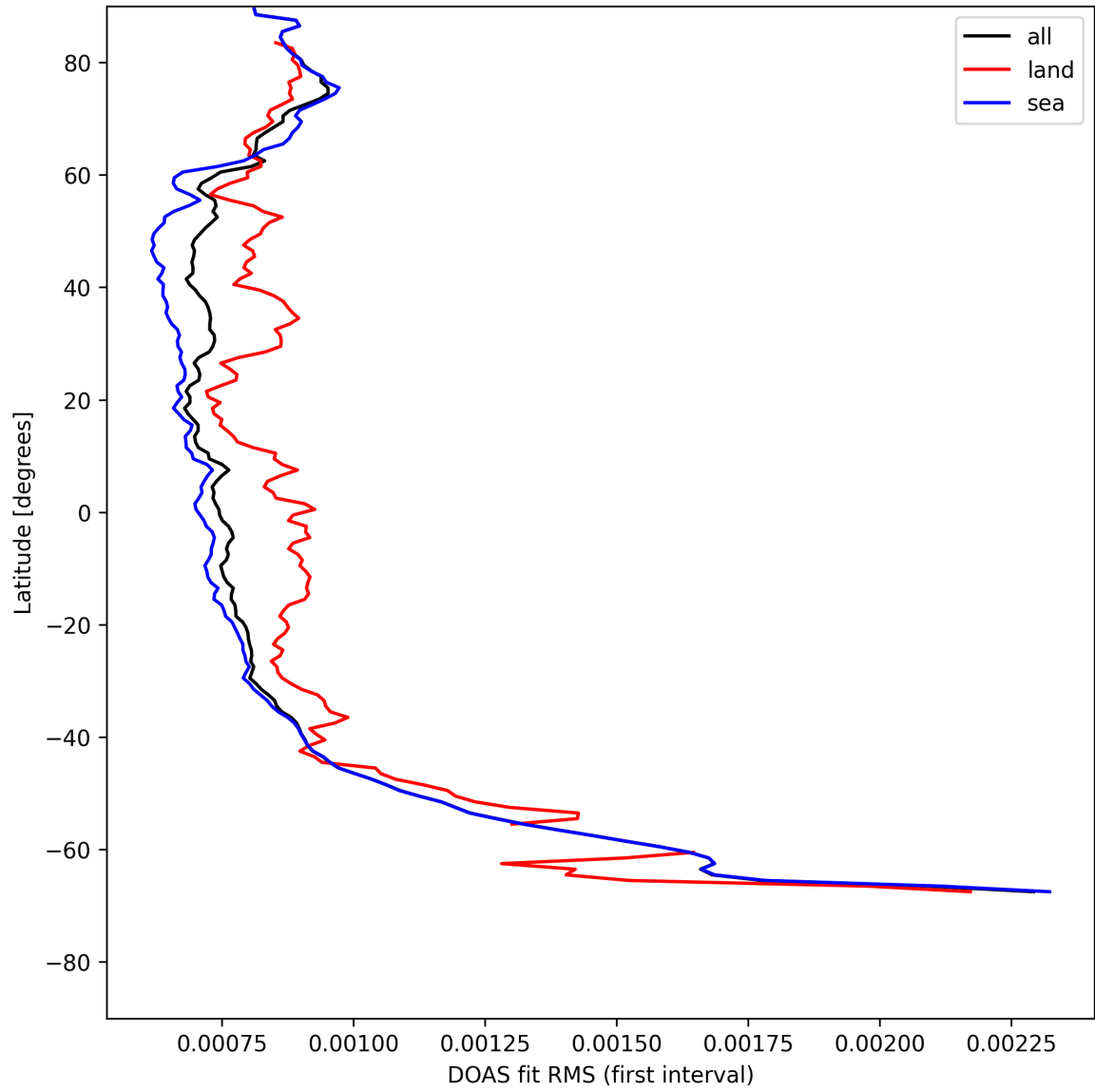
Figure 32: Zonal average of “DOAS fit RMS (first interval)” for 2025-05-08 to 2025-05-10.
