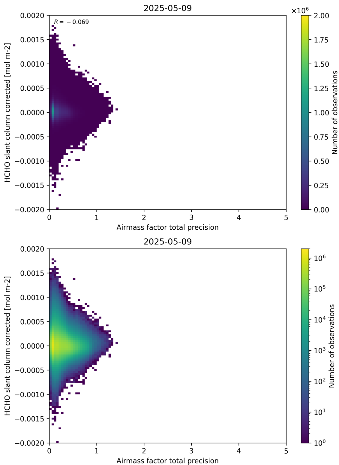
Figure 109: Scatter density plot of “Airmass factor total precision” against “HCHO slant column corrected” for 2025-05-08 to 2025-05-10.
