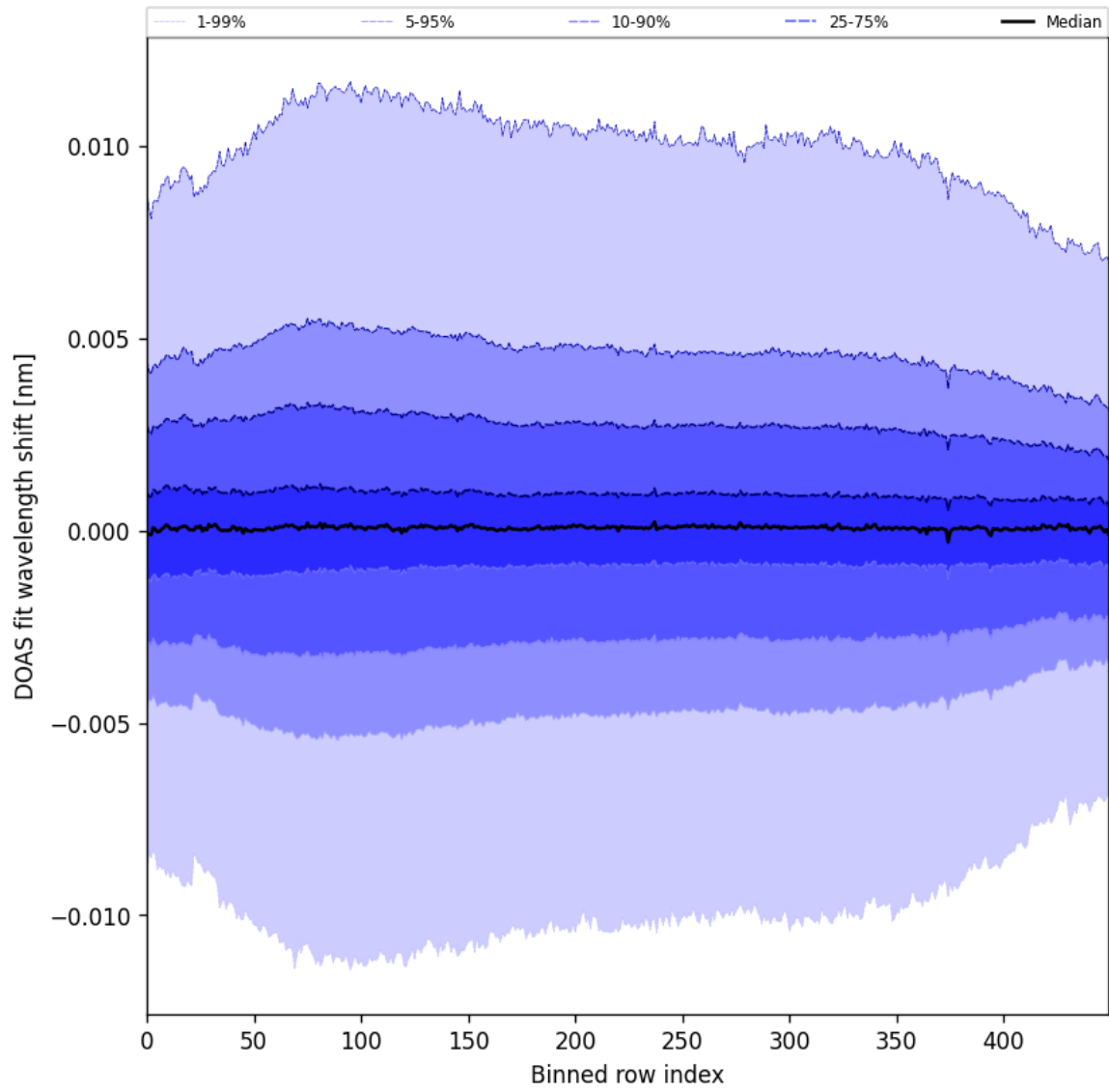
Figure 58: Along track statistics of “DOAS fit wavelength shift” for 2025-05-08 to 2025-05-10
