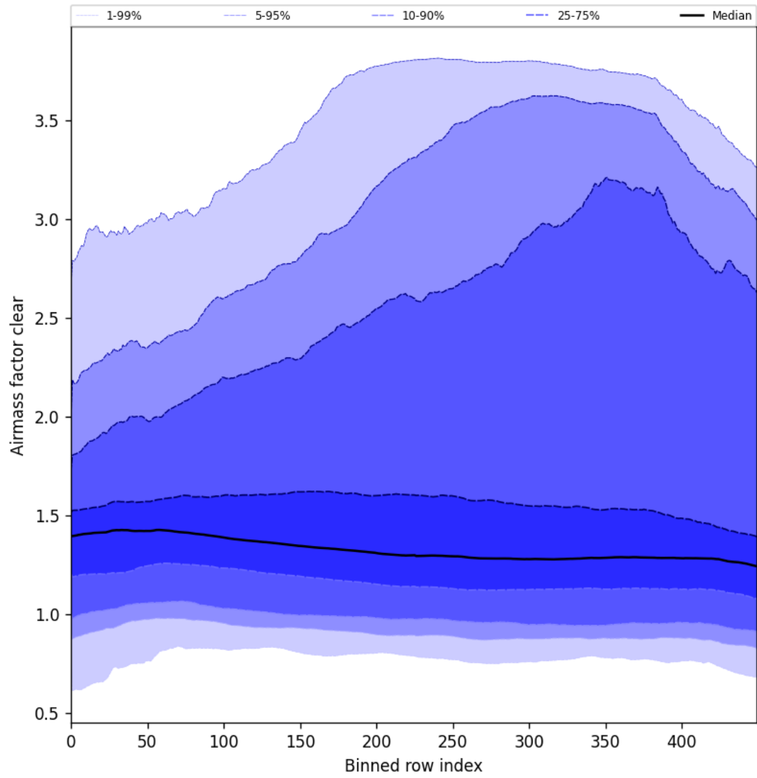
Figure 56: Along track statistics of “Airmass factor clear” for 2025-05-08 to 2025-05-10
