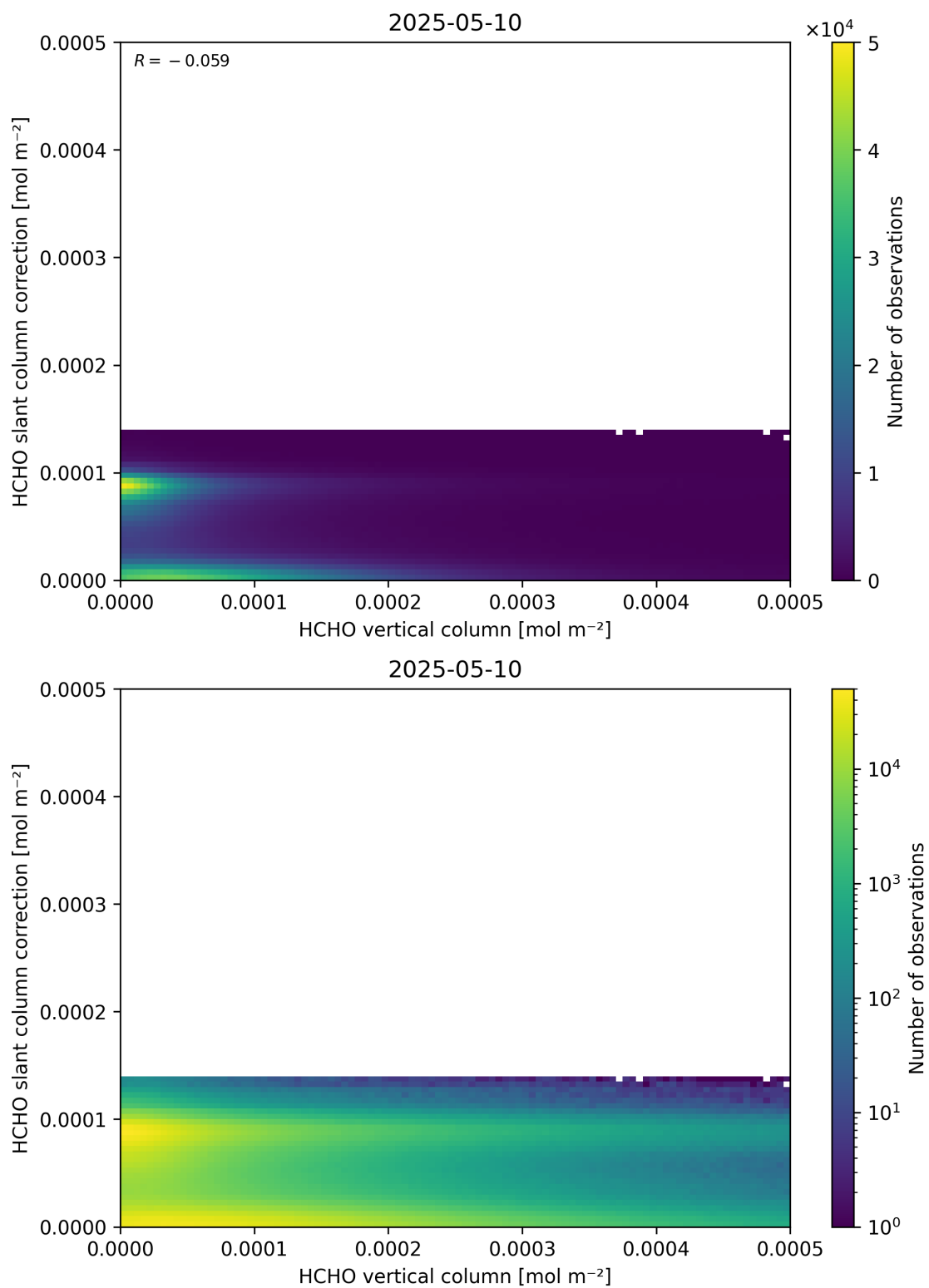
Figure 128: Scatter density plot of “HCHO vertical column” against “HCHO slant column correction” for 2025-05-10 to 2025-05-11.
