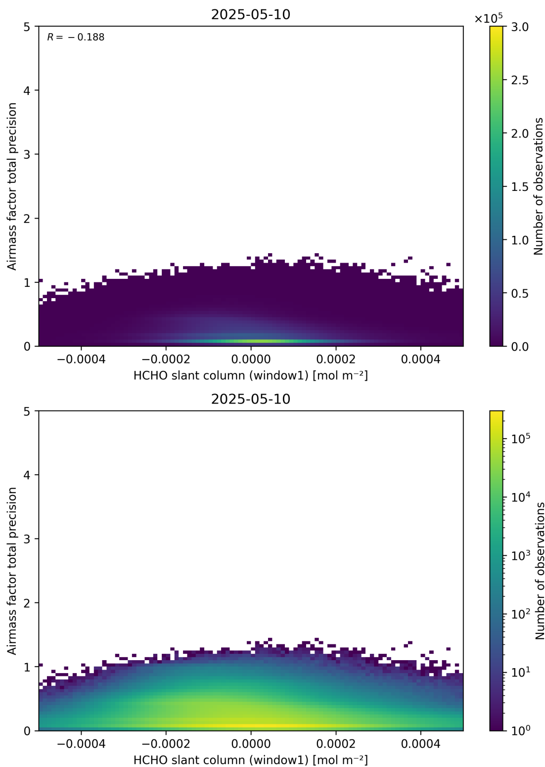
Figure 86: Scatter density plot of “HCHO slant column (window1)” against “Airmass factor total precision” for 2025-05-10 to 2025-05-11.
