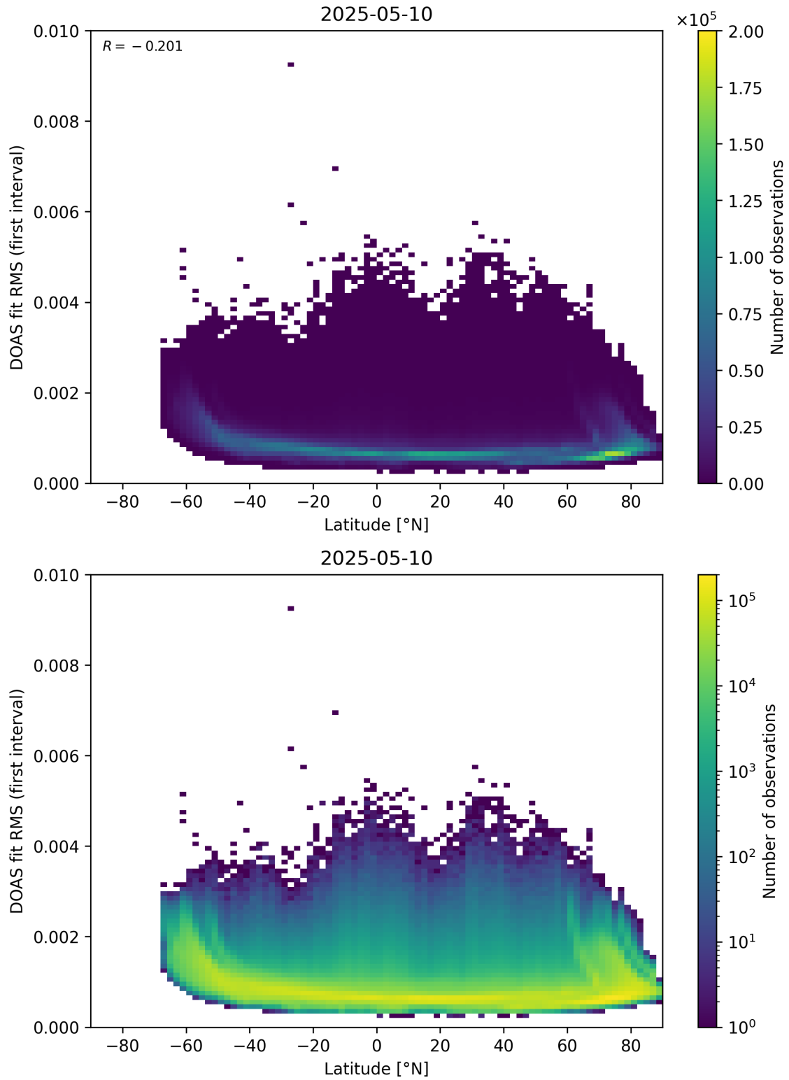
Figure 153: Scatter density plot of “Latitude” against “DOAS fit RMS (first interval)” for 2025-05-10 to 2025-05-11.
