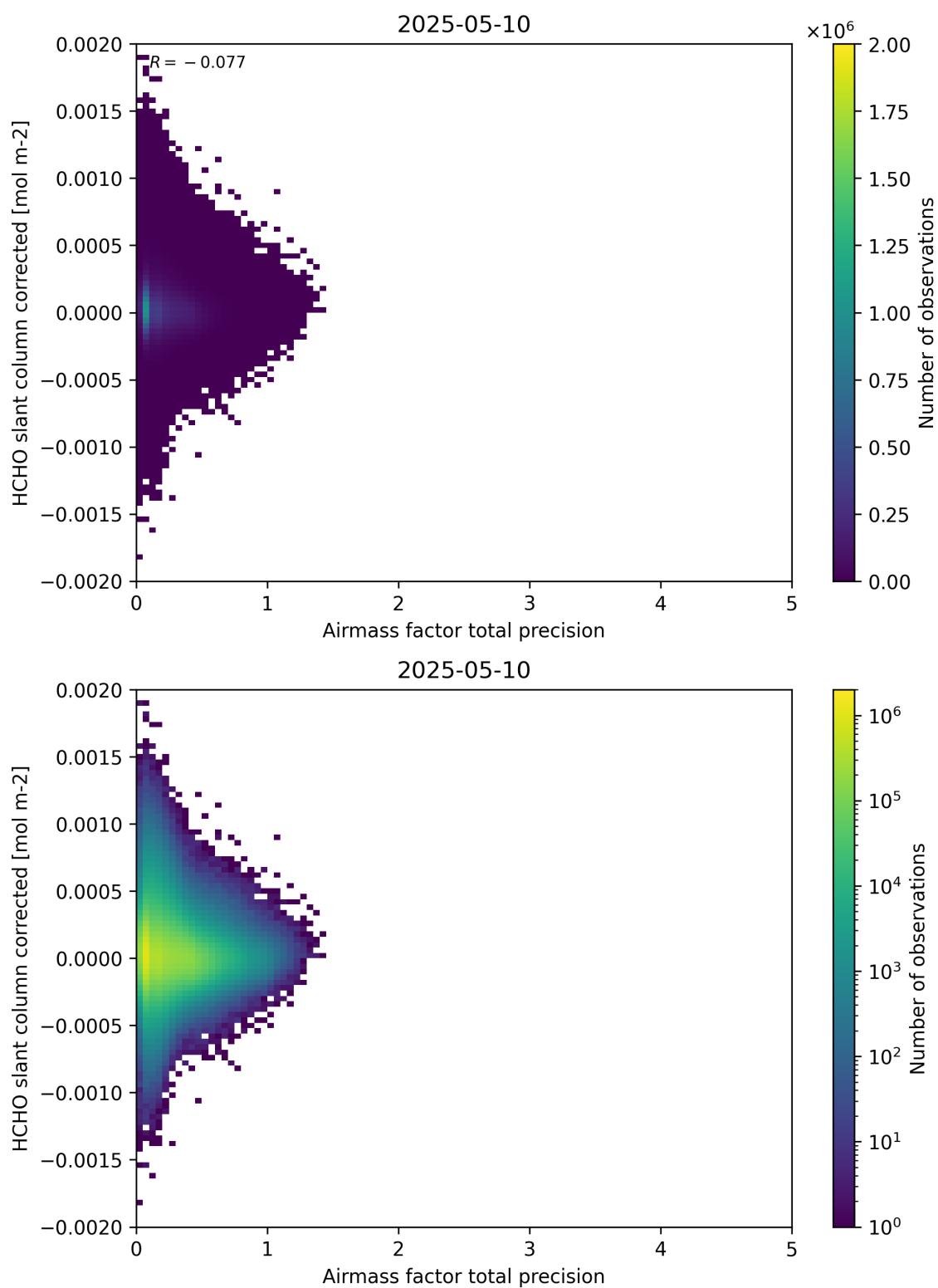
Figure 109: Scatter density plot of “Airmass factor total precision” against “HCHO slant column corrected” for 2025-05-10 to 2025-05-11.
