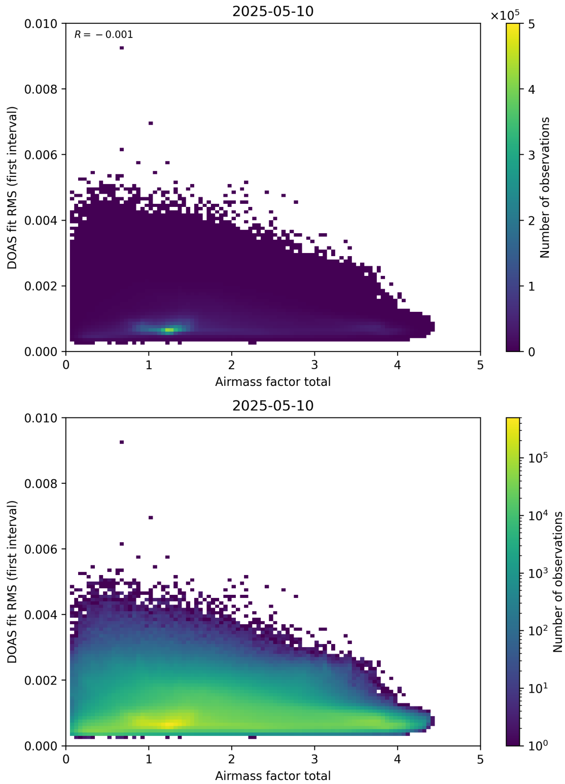
Figure 97: Scatter density plot of “Airmass factor total” against “DOAS fit RMS (first interval)” for 2025-05-10 to 2025-05-11.
