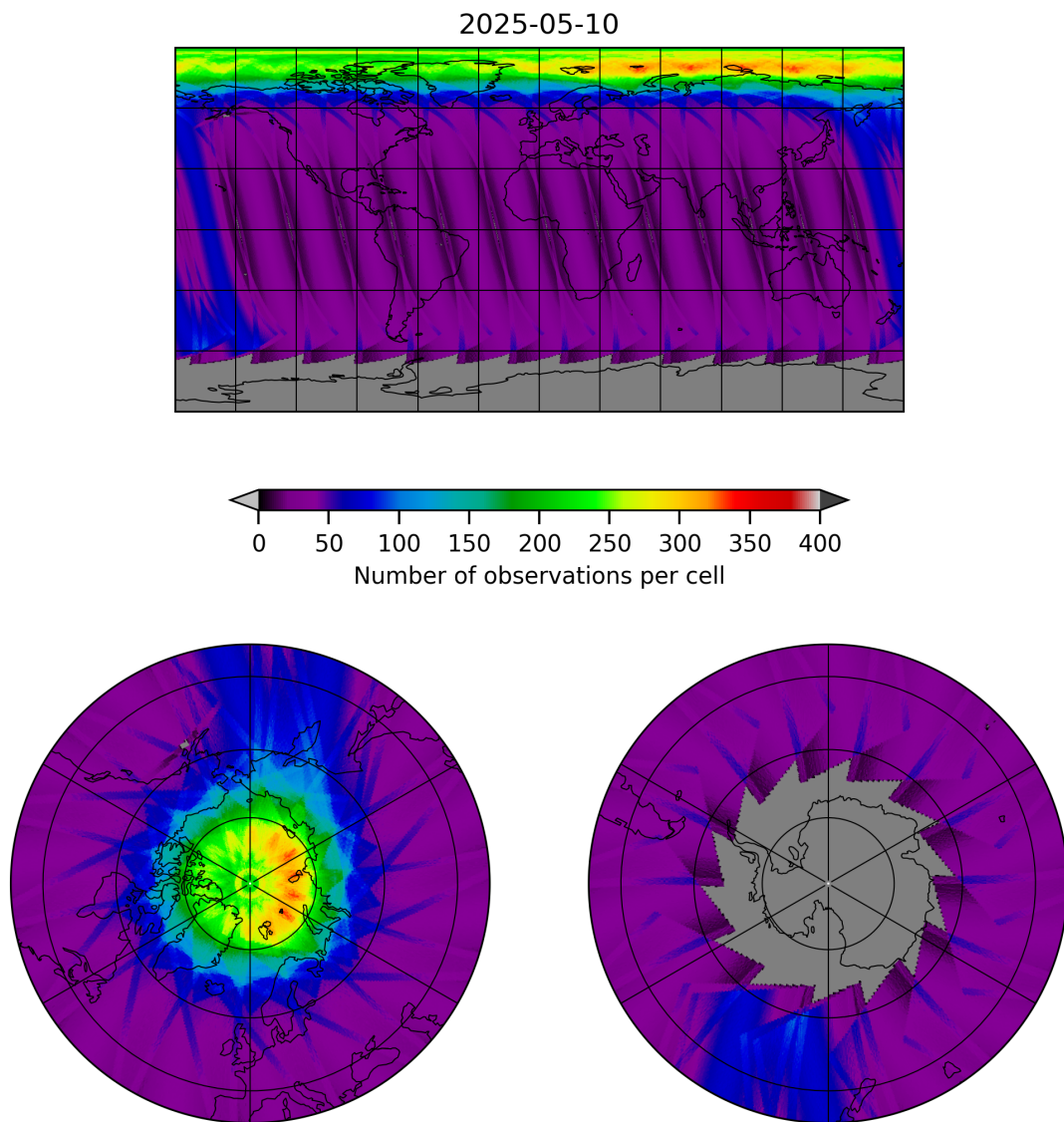
Figure 19: Map of the number of observations for 2025-05-10 to 2025-05-11
