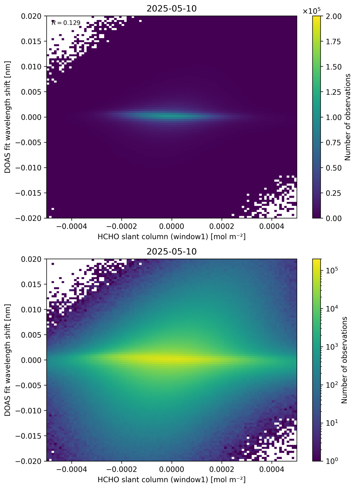
Figure 79: Scatter density plot of “HCHO slant column (window1)” against “DOAS fit wavelength shift” for 2025-05-10 to 2025-05-11.
