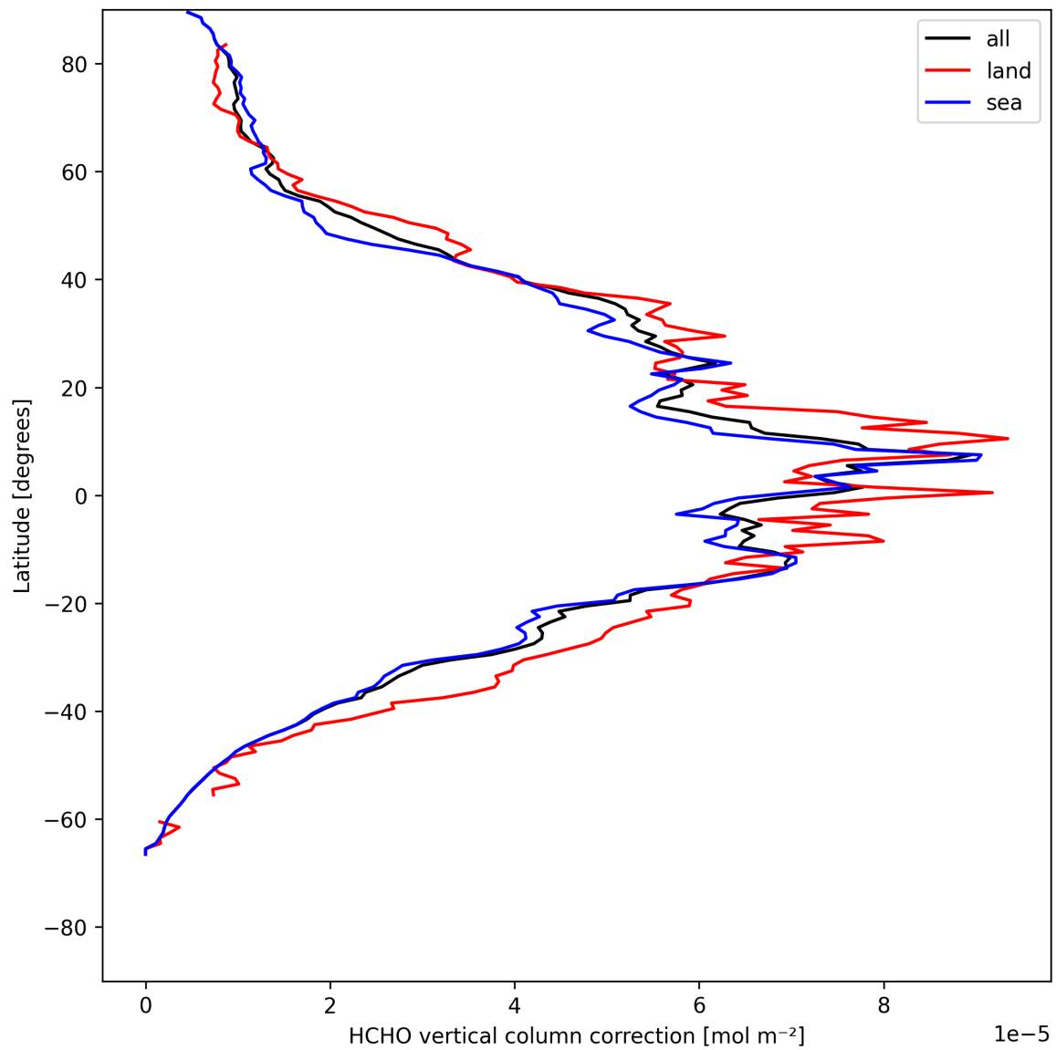
Figure 23: Zonal average of “HCHO vertical column correction” for 2025-05-10 to 2025-05-11.
