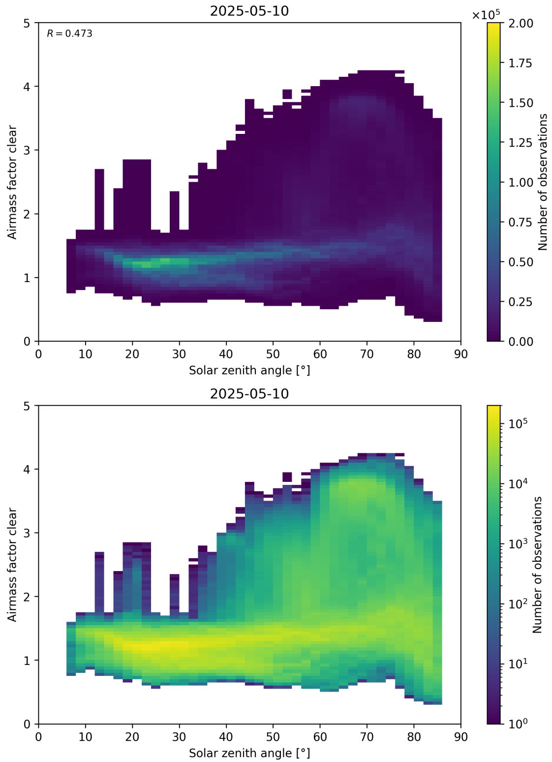
Figure 170: Scatter density plot of “Solar zenith angle” against “Airmass factor clear” for 2025-05-10 to 2025-05-11.
