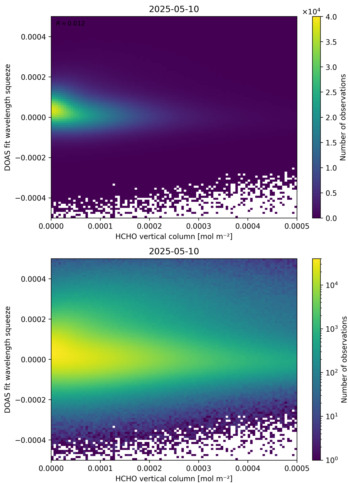
Figure 125: Scatter density plot of “HCHO vertical column” against “DOAS fit wavelength squeeze” for 2025-05-10 to 2025-05-11.
