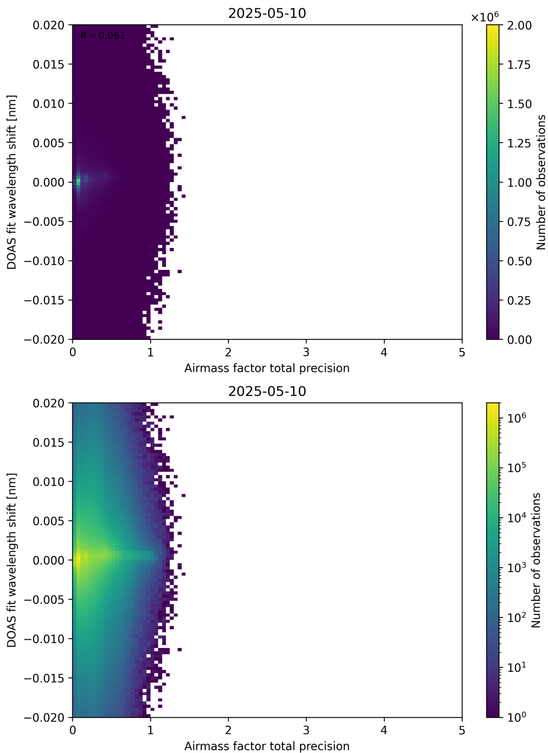
Figure 106: Scatter density plot of “Airmass factor total precision” against “DOAS fit wavelength shift” for 2025-05-10 to 2025-05-11.
