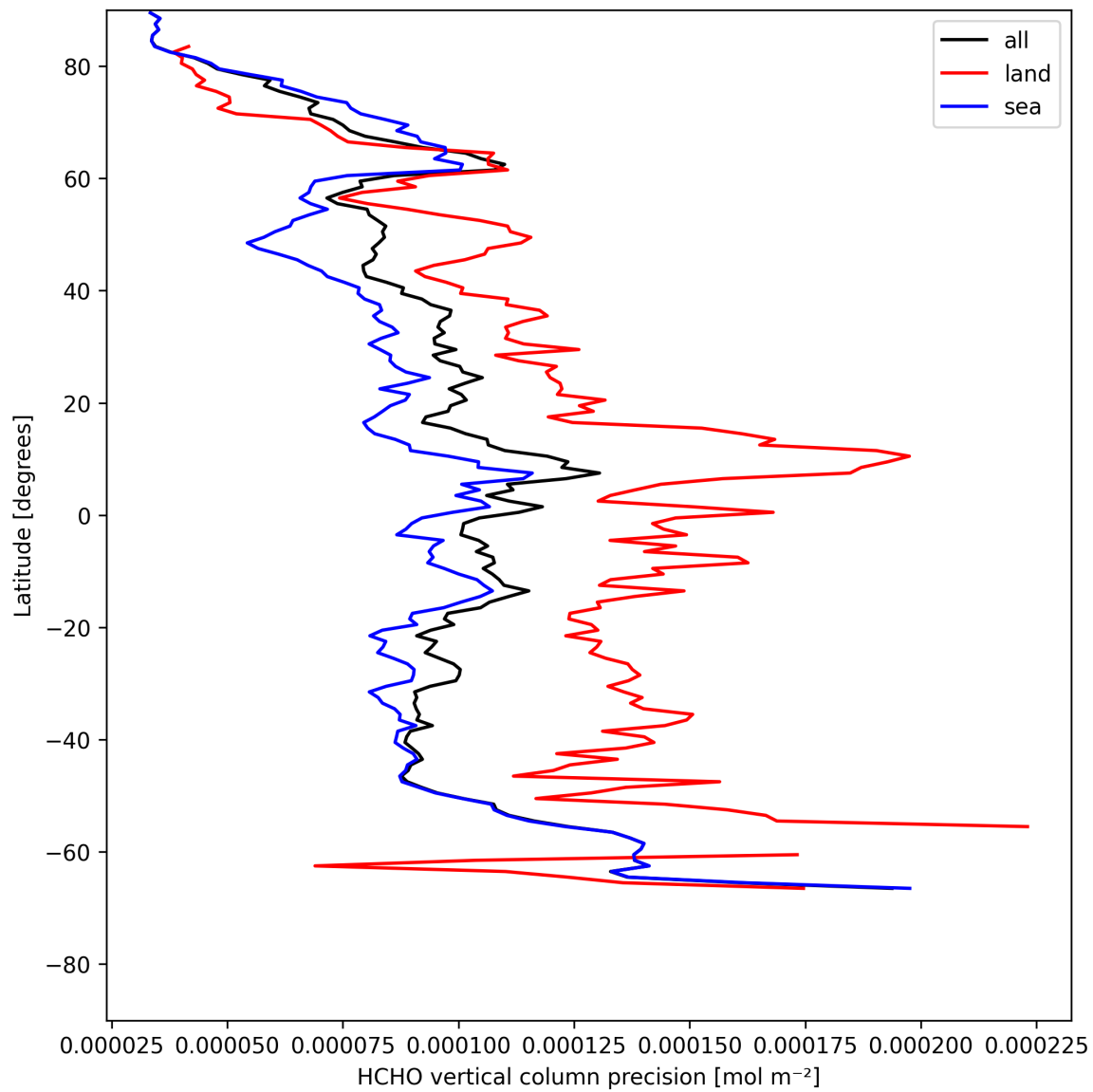
Figure 22: Zonal average of “HCHO vertical column precision” for 2025-05-10 to 2025-05-11.
