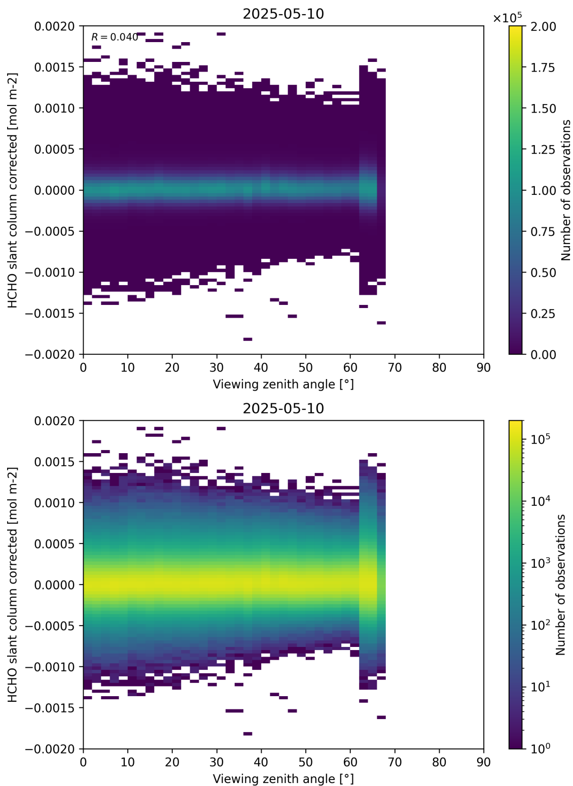
Figure 186: Scatter density plot of “Viewing zenith angle” against “HCHO slant column corrected” for 2025-05-10 to 2025-05-11.
