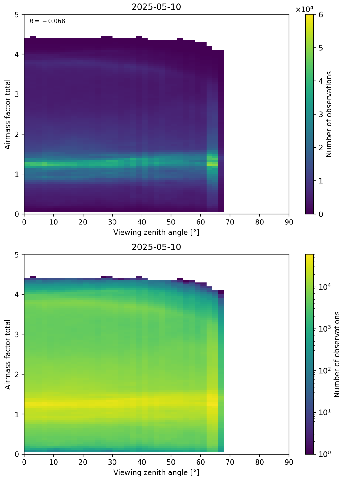
Figure 190: Scatter density plot of “Viewing zenith angle” against “Airmass factor total” for 2025-05-10 to 2025-05-11.
