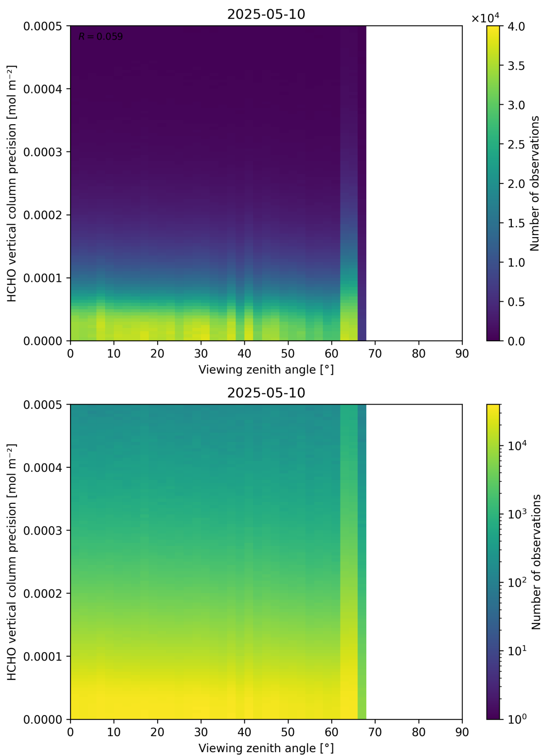
Figure 194: Scatter density plot of “Viewing zenith angle” against “HCHO vertical column precision” for 2025-05-10 to 2025-05-11.
