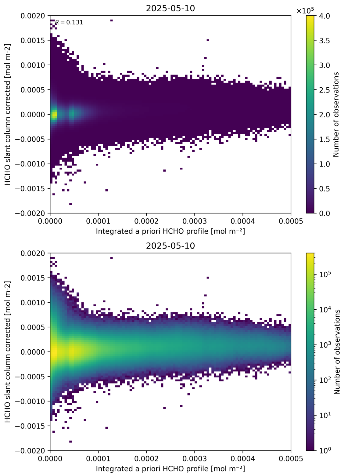
Figure 151: Scatter density plot of “Integrated a priori HCHO profile” against “HCHO slant column corrected” for 2025-05-10 to 2025-05-11.
