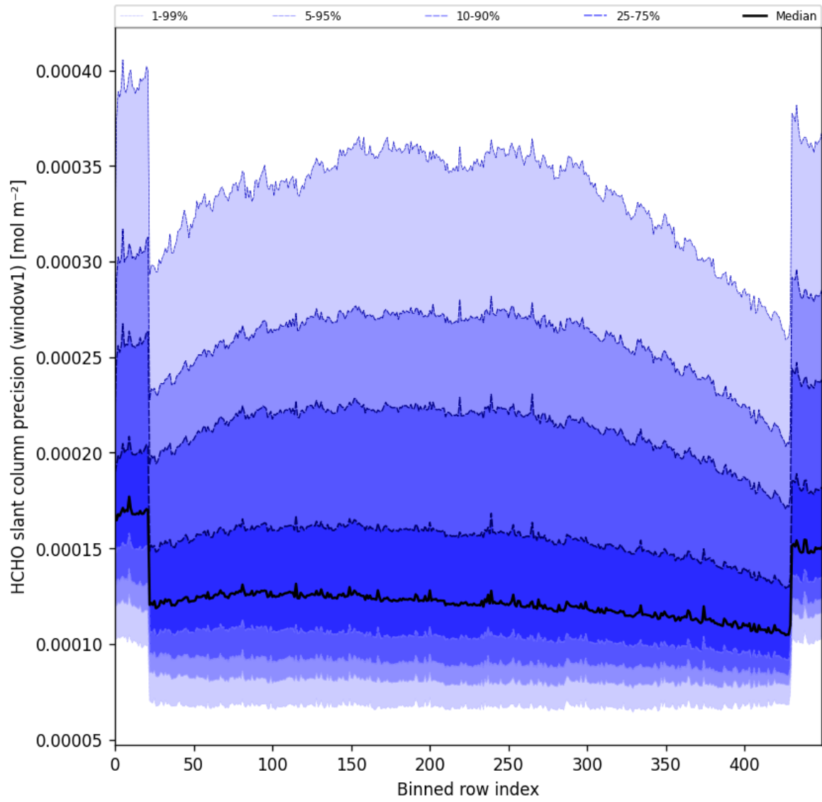
Figure 53: Along track statistics of “HCHO slant column precision (window1)” for 2025-05-10 to 2025-05-11
