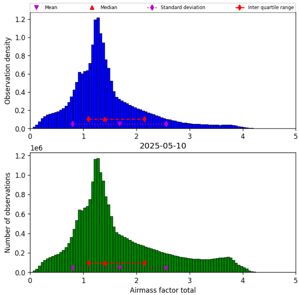
Figure 40: Histogram of “Airmass factor total” for 2025-05-10 to 2025-05-11
