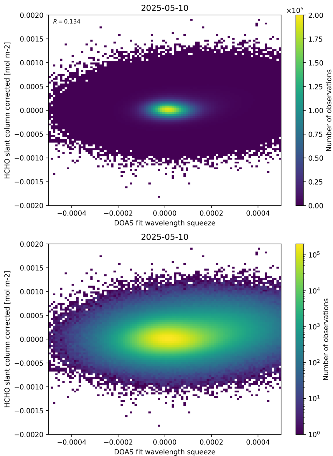
Figure 69: Scatter density plot of “DOAS fit wavelength squeeze” against “HCHO slant column corrected” for 2025-05-10 to 2025-05-11.
