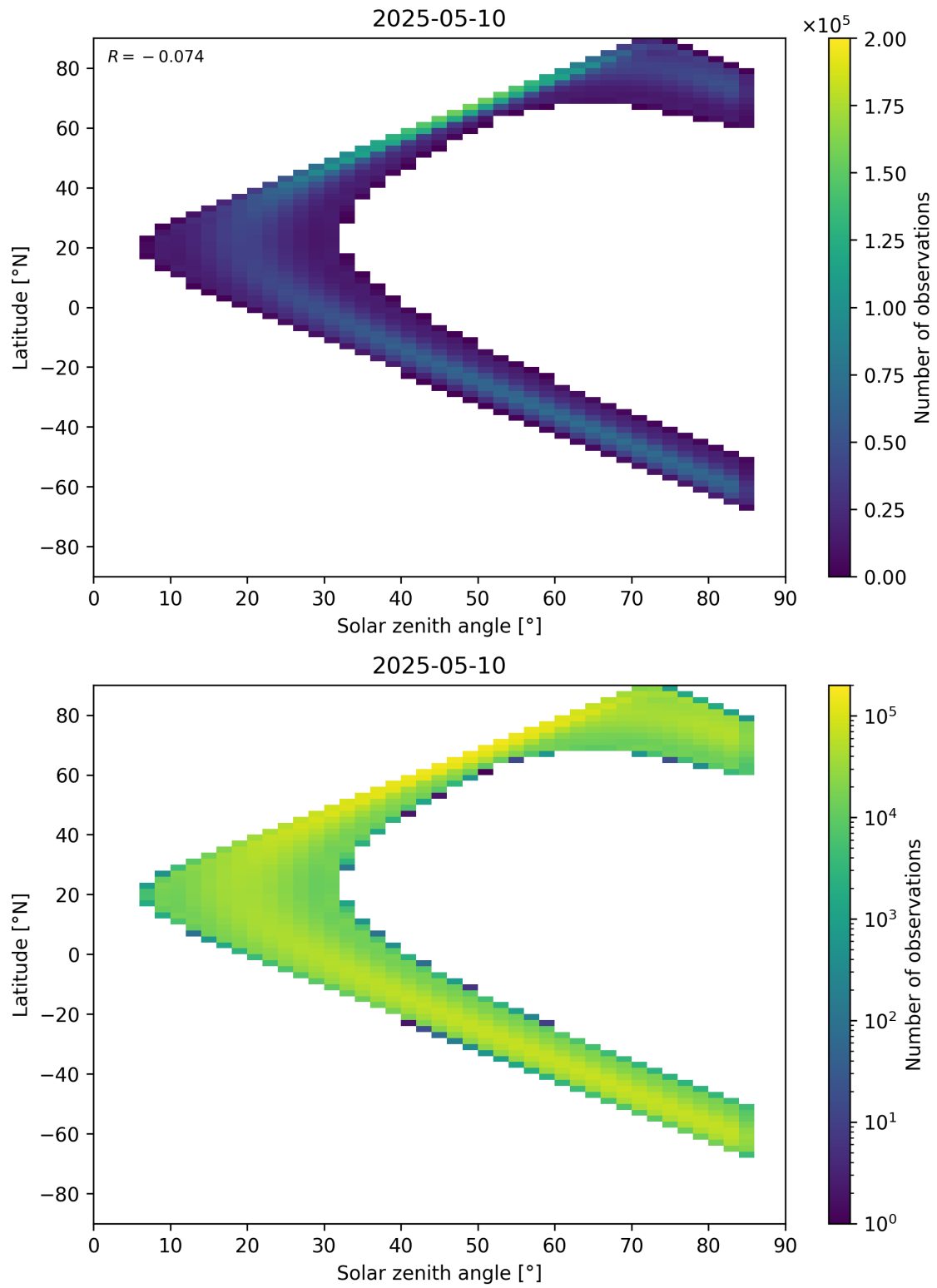
Figure 181: Scatter density plot of “Solar zenith angle” against “Latitude” for 2025-05-10 to 2025-05-11.
