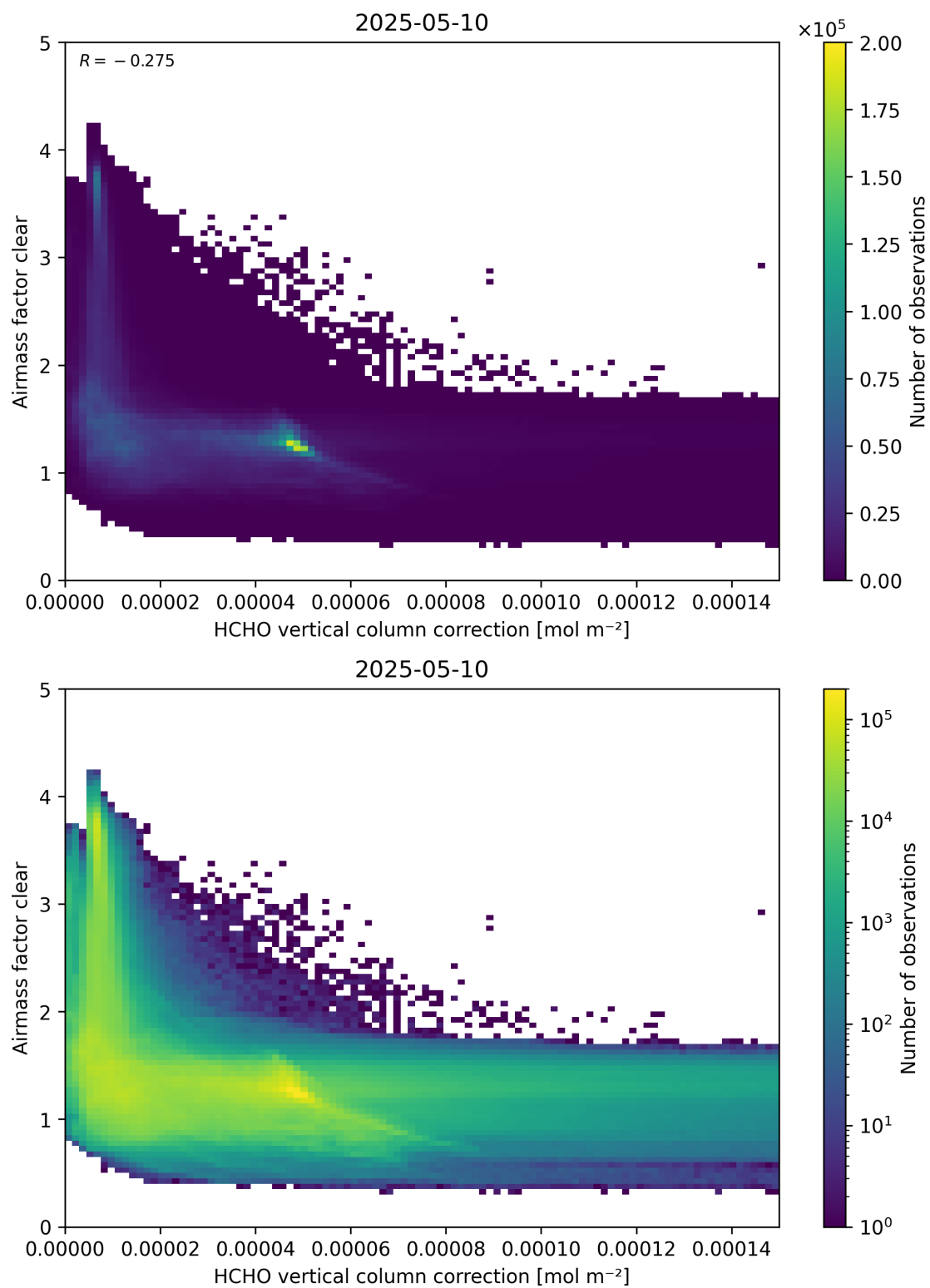
Figure 115: Scatter density plot of “HCHO vertical column correction” against “Airmass factor clear” for 2025-05-10 to 2025-05-11.
