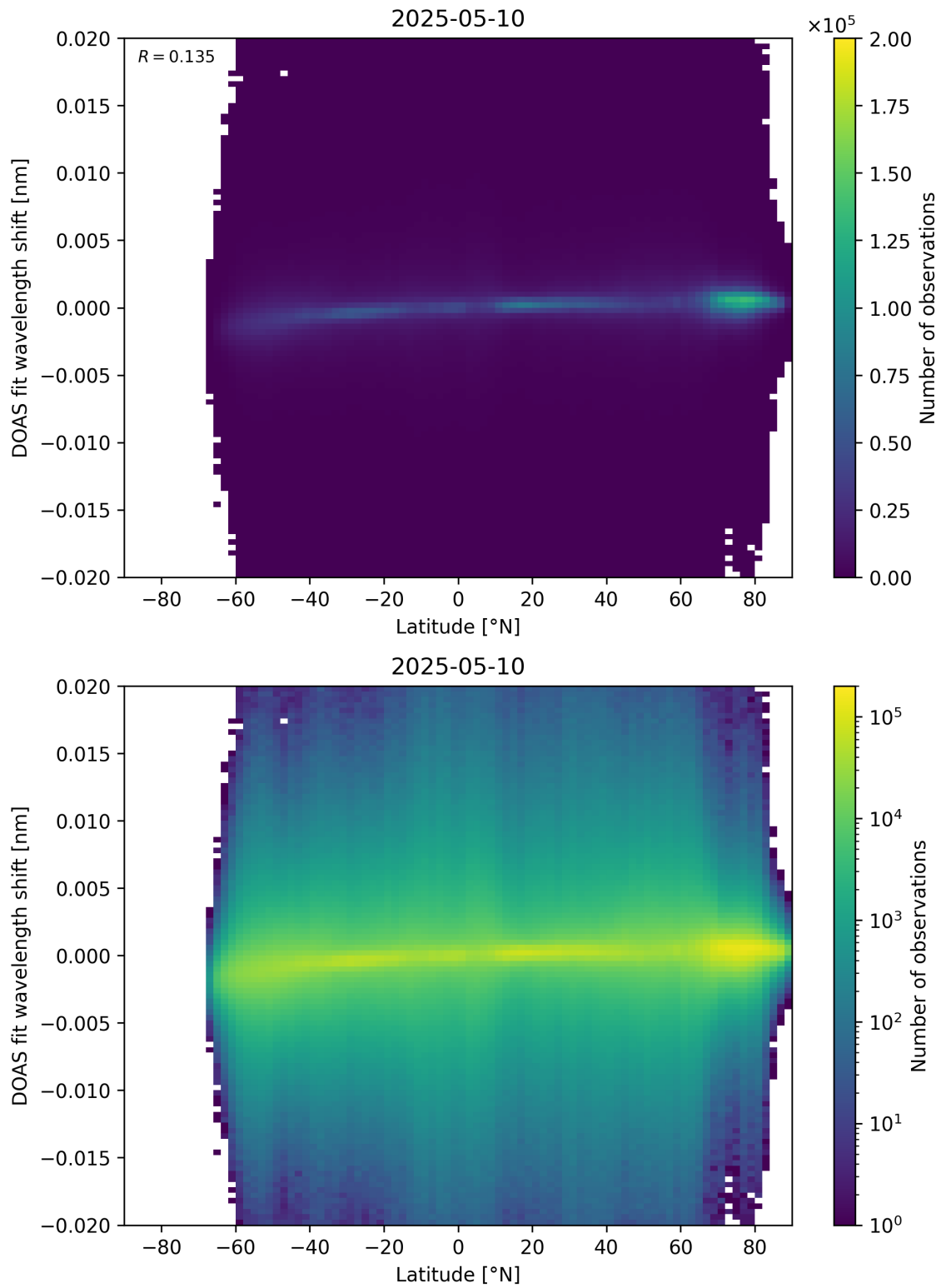
Figure 154: Scatter density plot of “Latitude” against “DOAS fit wavelength shift” for 2025-05-10 to 2025-05-11.
