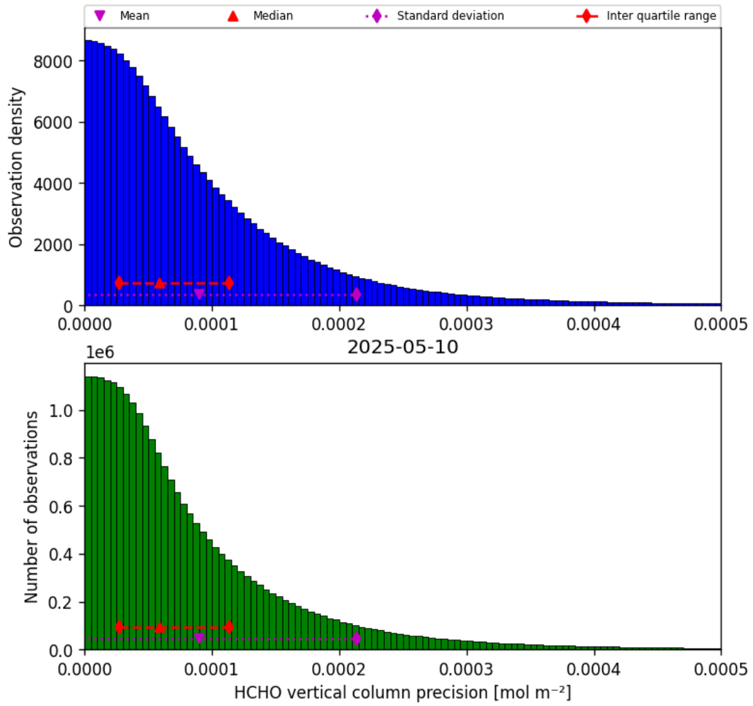
Figure 36: Histogram of “HCHO vertical column precision” for 2025-05-10 to 2025-05-11
