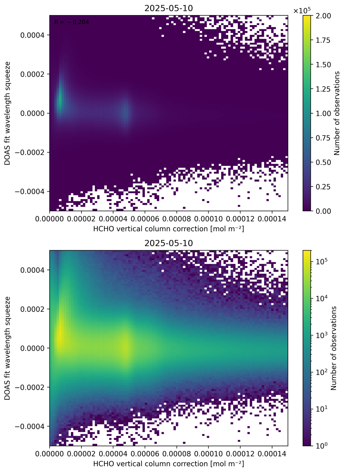
Figure 114: Scatter density plot of “HCHO vertical column correction” against “DOAS fit wavelength squeeze” for 2025-05-10 to 2025-05-11.
