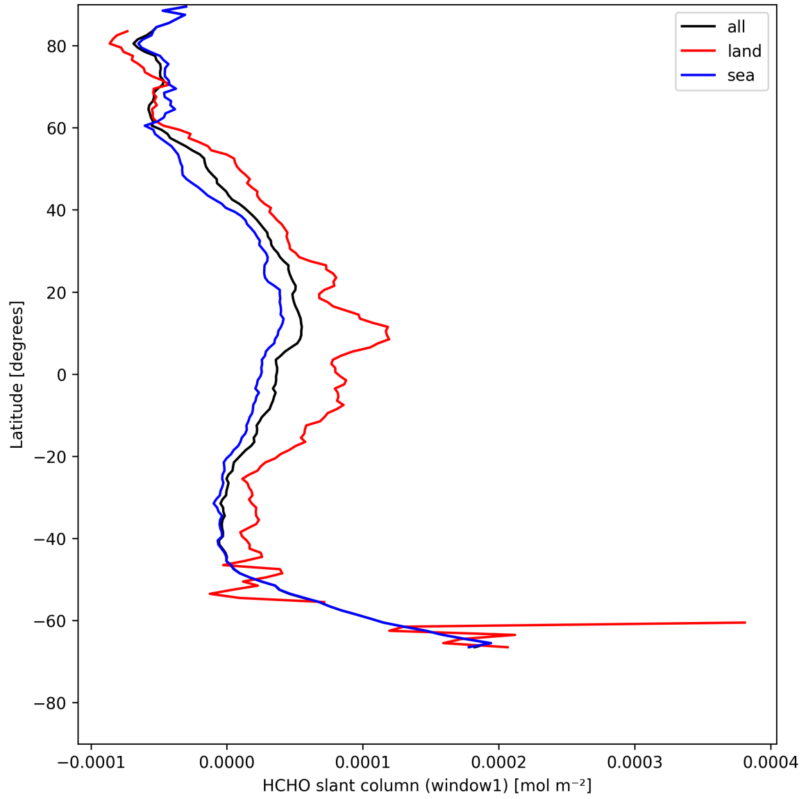
Figure 24: Zonal average of “HCHO slant column (window1)” for 2025-05-10 to 2025-05-11.
