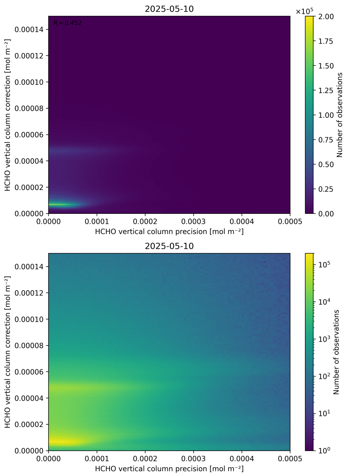
Figure 146: Scatter density plot of “HCHO vertical column precision” against “HCHO vertical column correction” for 2025-05-10 to 2025-05-11.
