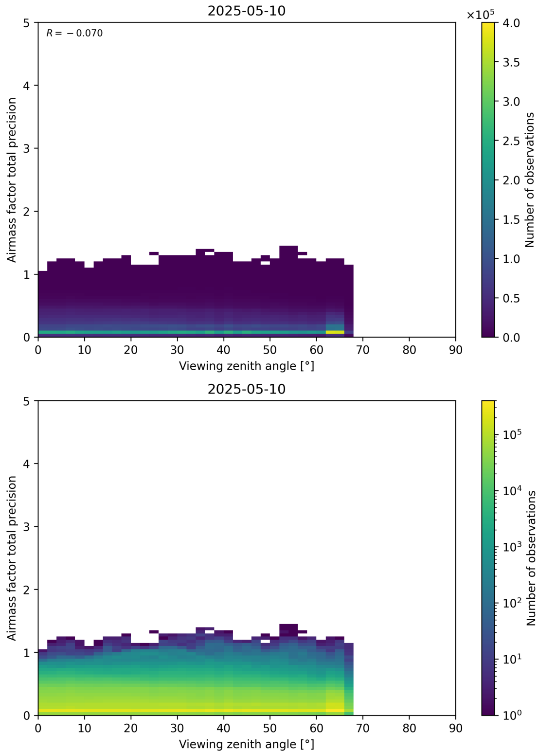
Figure 191: Scatter density plot of “Viewing zenith angle” against “Airmass factor total precision” for 2025-05-10 to 2025-05-11.
