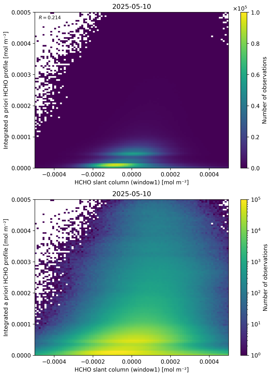
Figure 87: Scatter density plot of “HCHO slant column (window1)” against “Integrated a priori HCHO profile” for 2025-05-10 to 2025-05-11.
