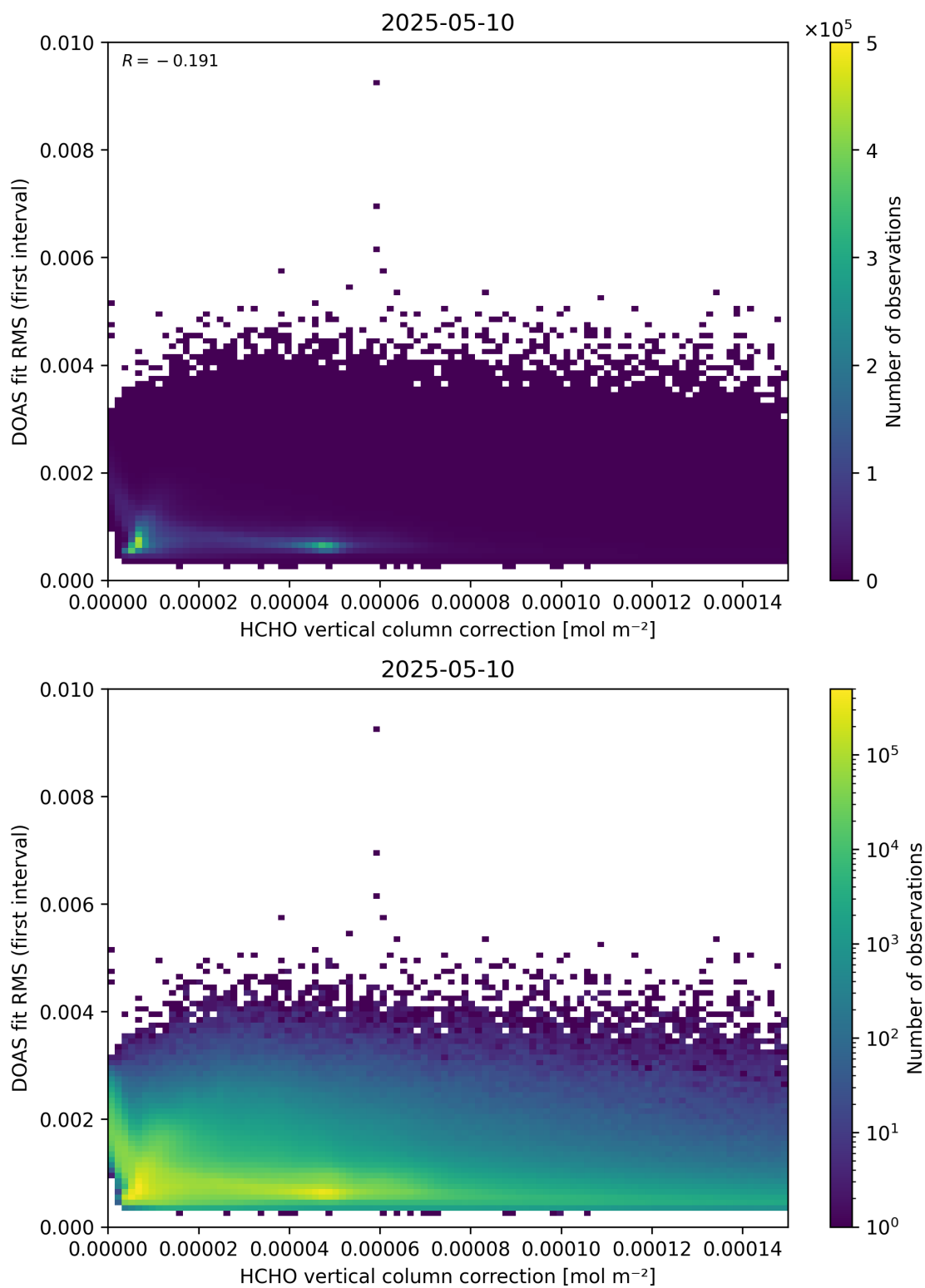
Figure 112: Scatter density plot of “HCHO vertical column correction” against “DOAS fit RMS (first interval)” for 2025-05-10 to 2025-05-11.
