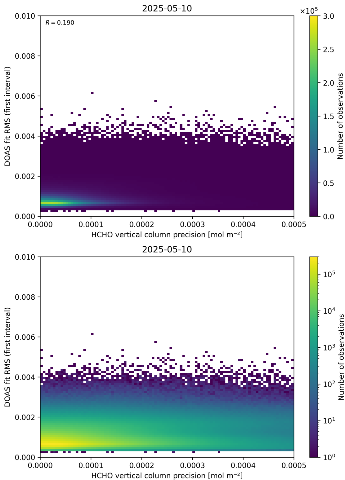
Figure 136: Scatter density plot of “HCHO vertical column precision” against “DOAS fit RMS (first interval)” for 2025-05-10 to 2025-05-11.
