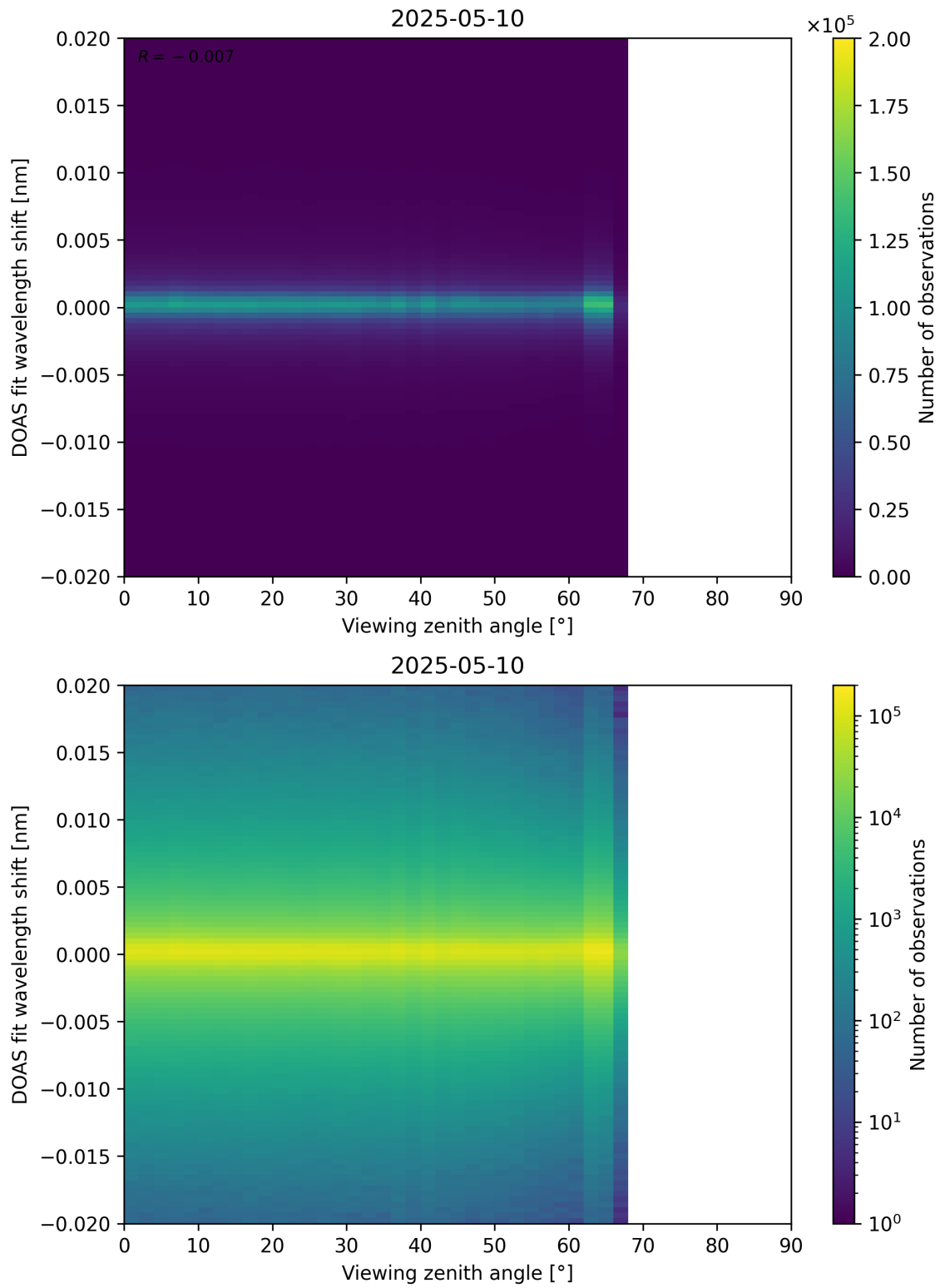
Figure 183: Scatter density plot of “Viewing zenith angle” against “DOAS fit wavelength shift” for 2025-05-10 to 2025-05-11.
