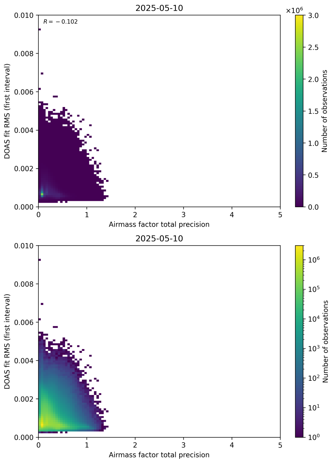
Figure 105: Scatter density plot of “Airmass factor total precision” against “DOAS fit RMS (first interval)” for 2025-05-10 to 2025-05-11.
