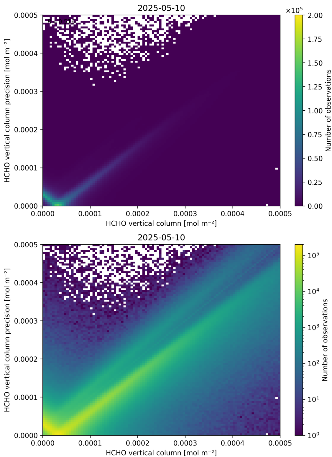
Figure 134: Scatter density plot of “HCHO vertical column” against “HCHO vertical column precision” for 2025-05-10 to 2025-05-11.
