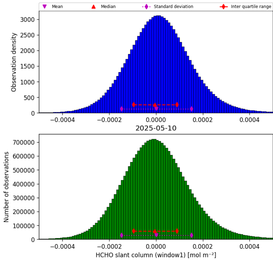
Figure 38: Histogram of “HCHO slant column (window1)” for 2025-05-10 to 2025-05-11
