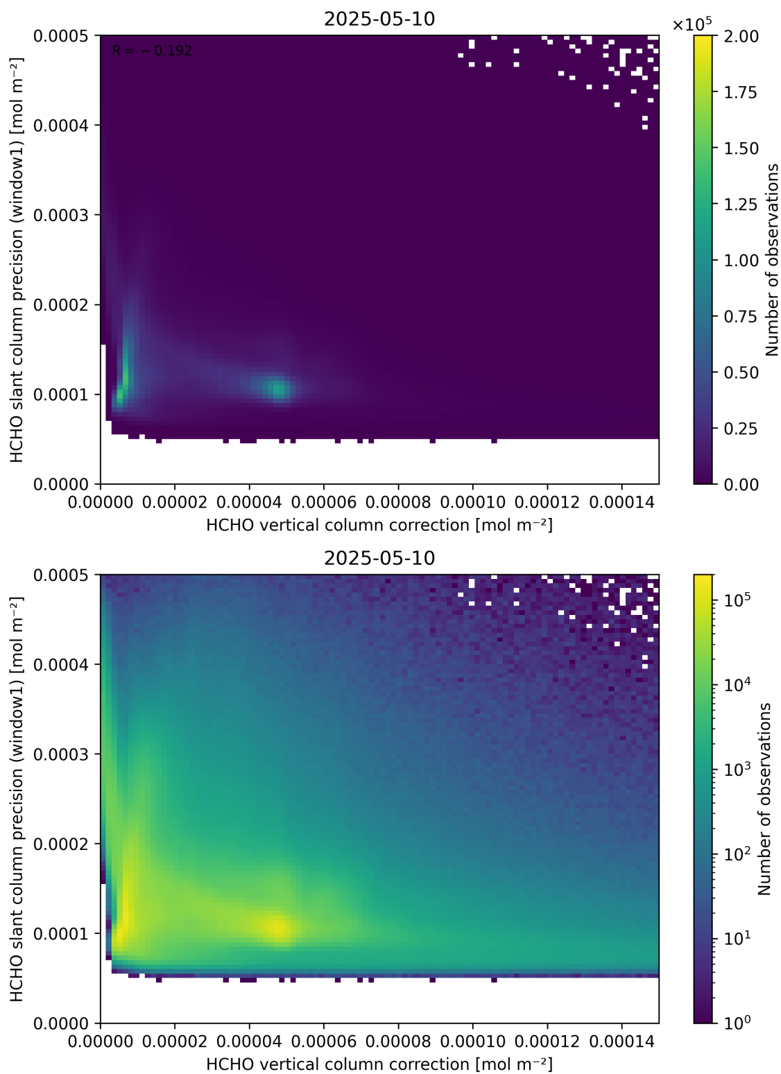
Figure 119: Scatter density plot of “HCHO vertical column correction” against “HCHO slant column precision (window1)” for 2025-05-10 to 2025-05-11.
