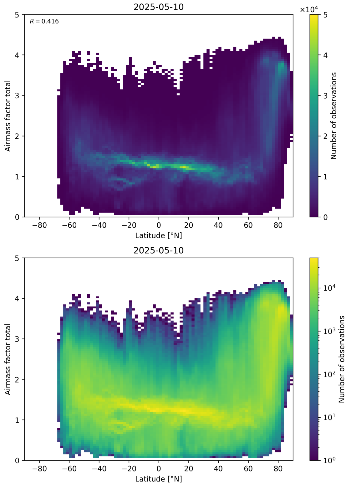
Figure 161: Scatter density plot of “Latitude” against “Airmass factor total” for 2025-05-10 to 2025-05-11.
