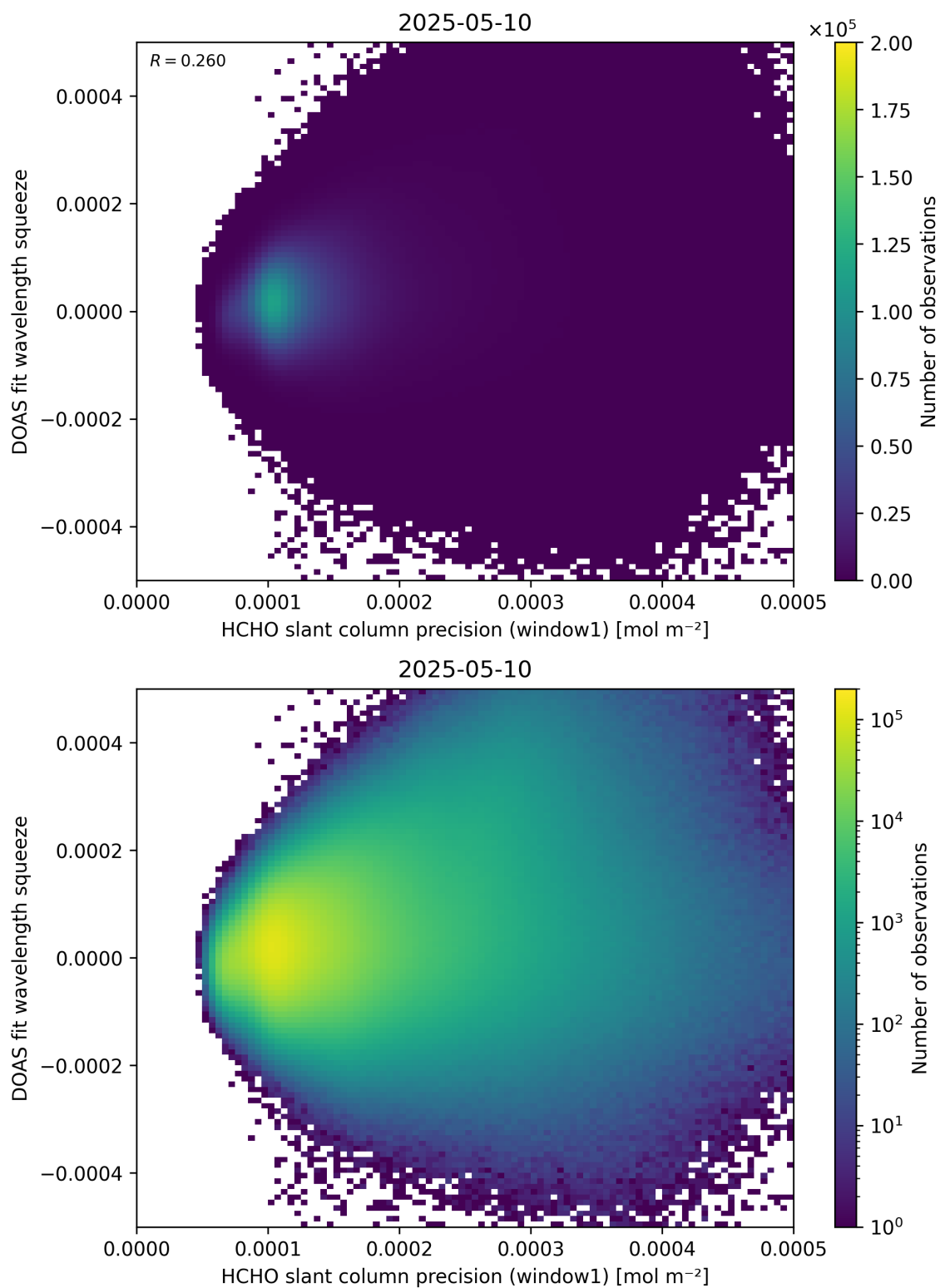
Figure 90: Scatter density plot of “HCHO slant column precision (window1)” against “DOAS fit wavelength squeeze” for 2025-05-10 to 2025-05-11.
