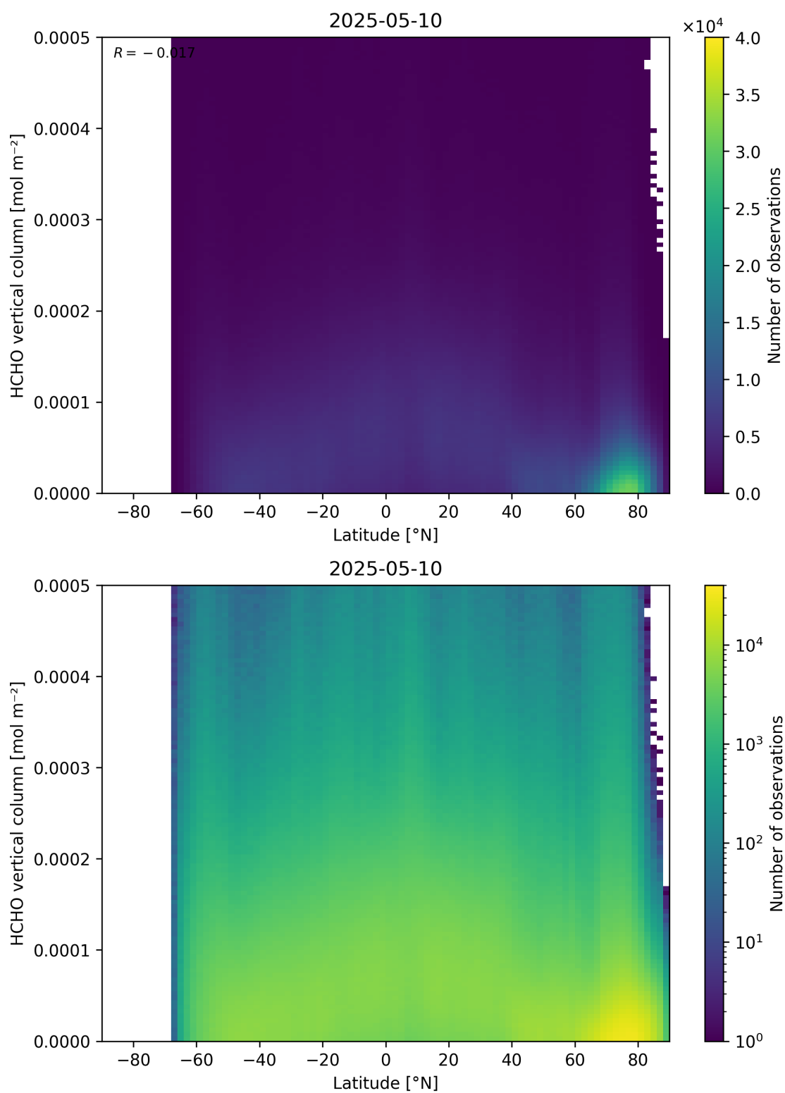
Figure 163: Scatter density plot of “Latitude” against “HCHO vertical column” for 2025-05-10 to 2025-05-11.
