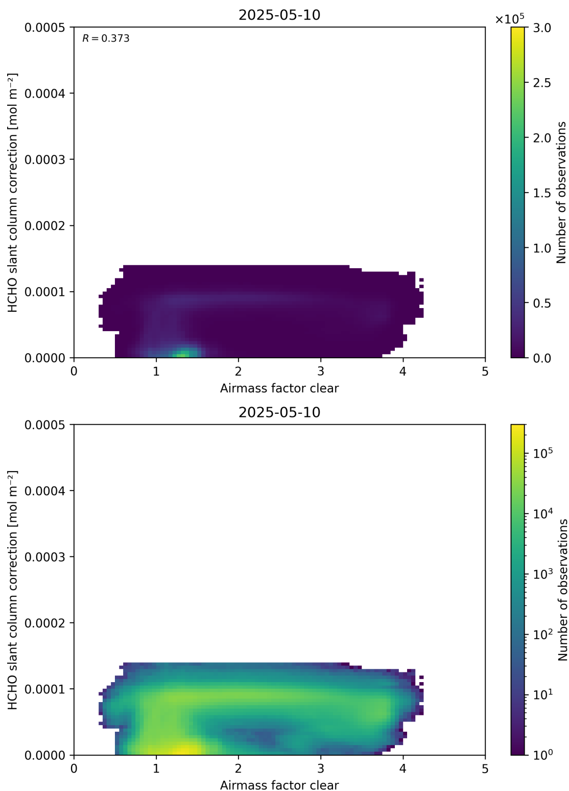
Figure 75: Scatter density plot of “Airmass factor clear” against “HCHO slant column correction” for 2025-05-10 to 2025-05-11.
