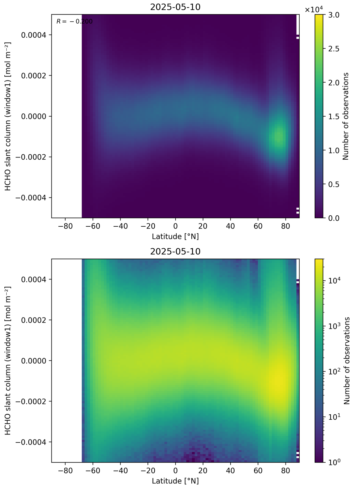
Figure 159: Scatter density plot of “Latitude” against “HCHO slant column (window1)” for 2025-05-10 to 2025-05-11.
