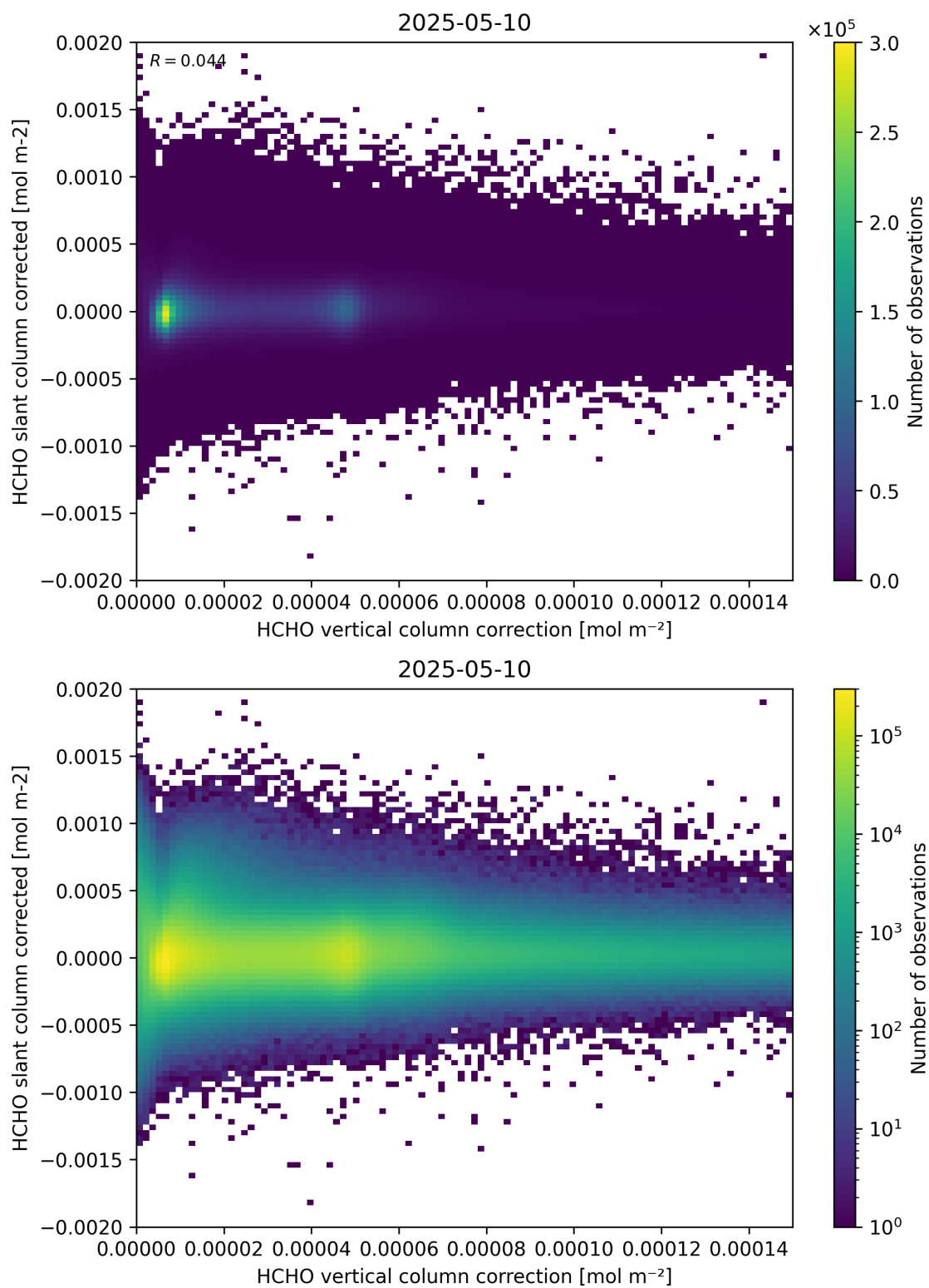
Figure 116: Scatter density plot of “HCHO vertical column correction” against “HCHO slant column corrected” for 2025-05-10 to 2025-05-11.
