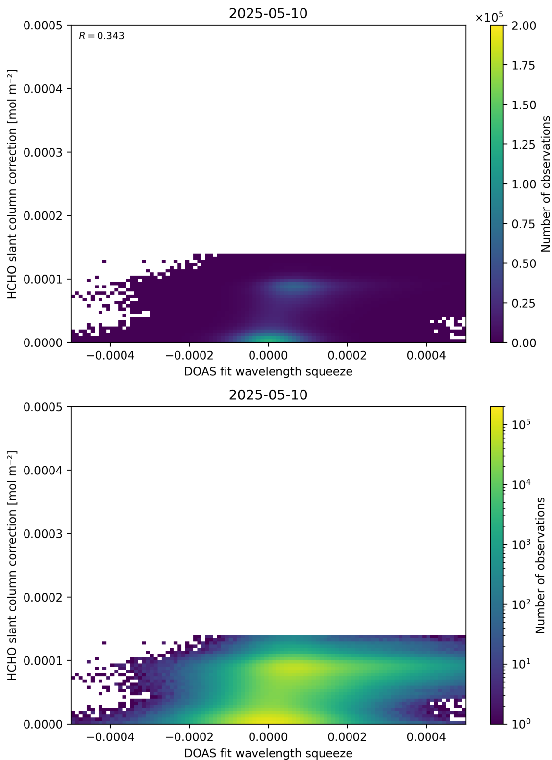
Figure 70: Scatter density plot of “DOAS fit wavelength squeeze” against “HCHO slant column correction” for 2025-05-10 to 2025-05-11.
