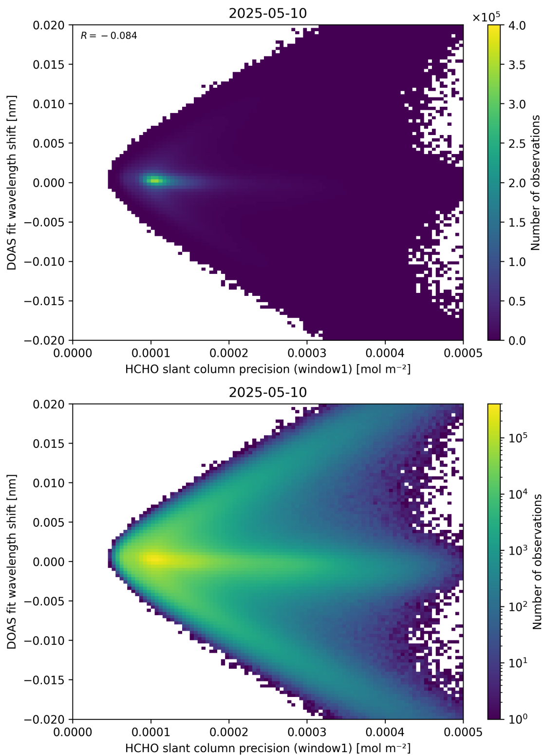
Figure 89: Scatter density plot of “HCHO slant column precision (window1)” against “DOAS fit wavelength shift” for 2025-05-10 to 2025-05-11.
