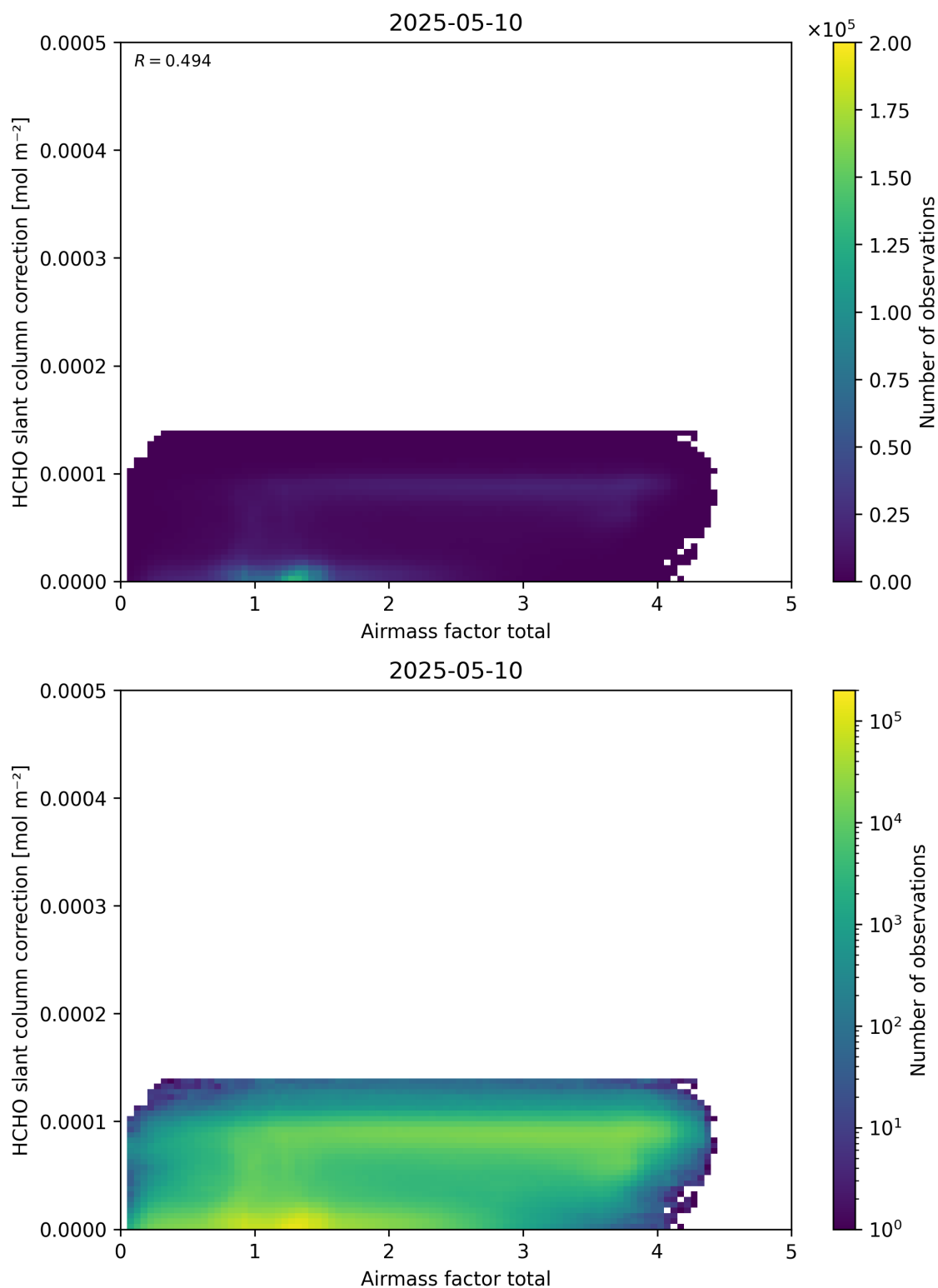
Figure 102: Scatter density plot of “Airmass factor total” against “HCHO slant column correction” for 2025-05-10 to 2025-05-11.
