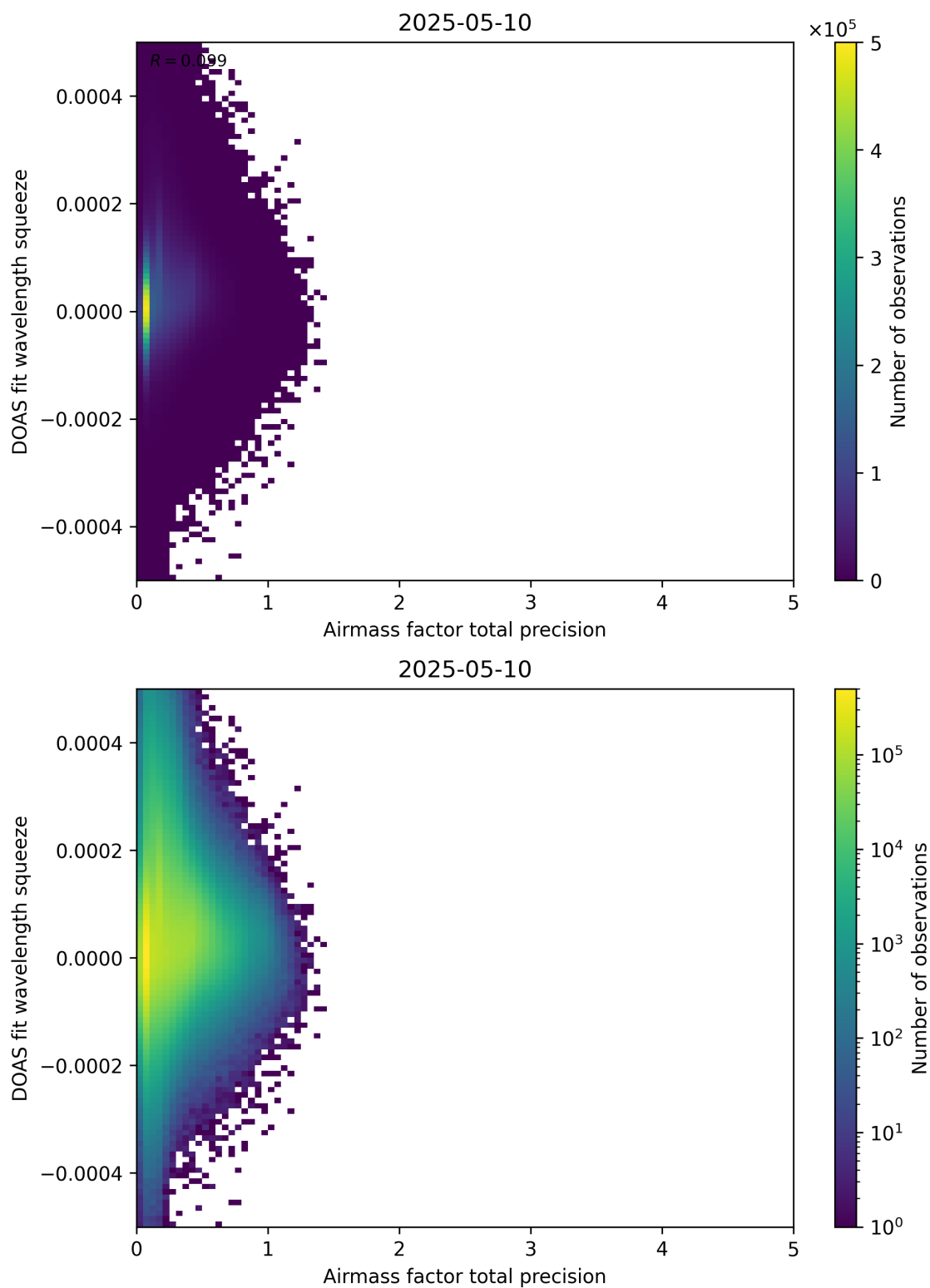
Figure 107: Scatter density plot of “Airmass factor total precision” against “DOAS fit wavelength squeeze” for 2025-05-10 to 2025-05-11.
