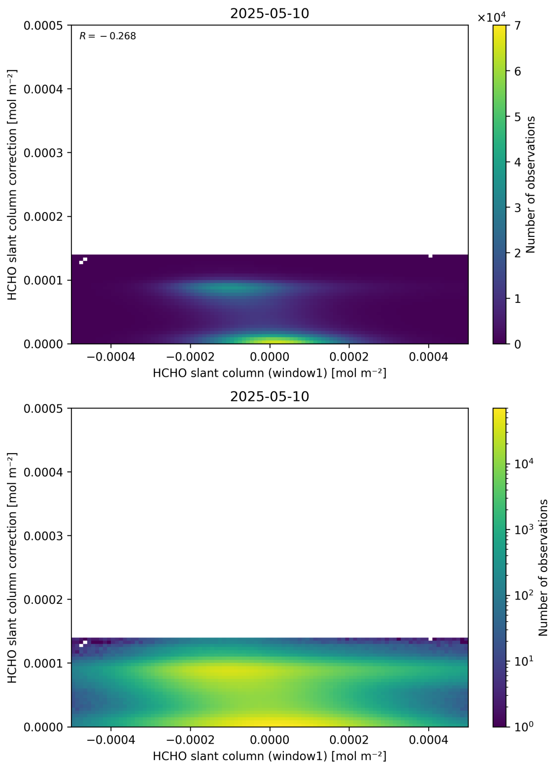
Figure 83: Scatter density plot of “HCHO slant column (window1)” against “HCHO slant column correction” for 2025-05-10 to 2025-05-11.
