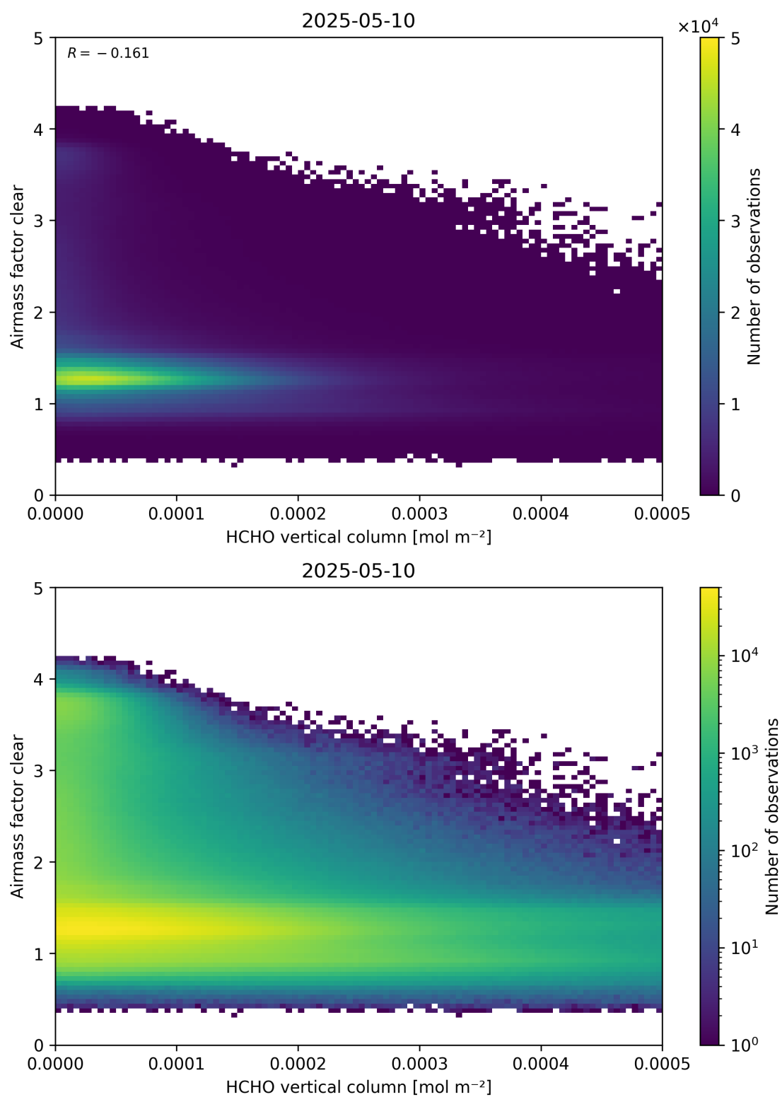
Figure 126: Scatter density plot of “HCHO vertical column” against “Airmass factor clear” for 2025-05-10 to 2025-05-11.
