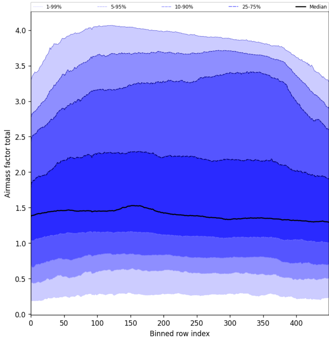
Figure 54: Along track statistics of “Airmass factor total” for 2025-05-10 to 2025-05-11
