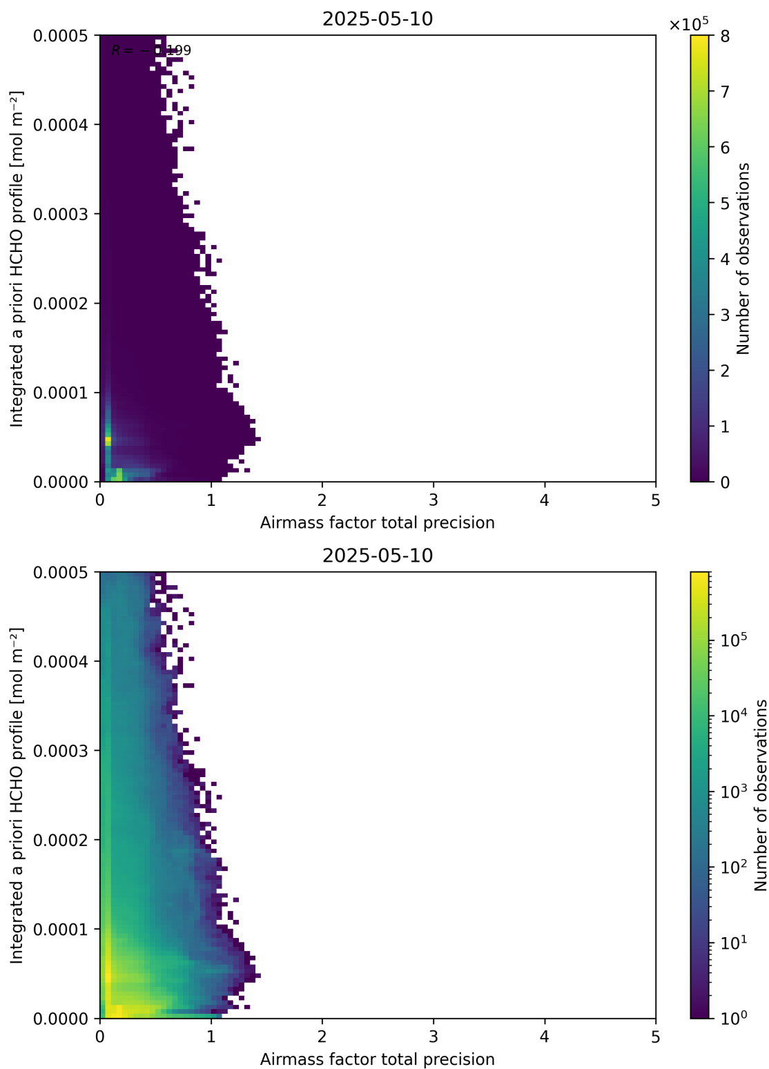
Figure 111: Scatter density plot of “Airmass factor total precision” against “Integrated a priori HCHO profile” for 2025-05-10 to 2025-05-11.
