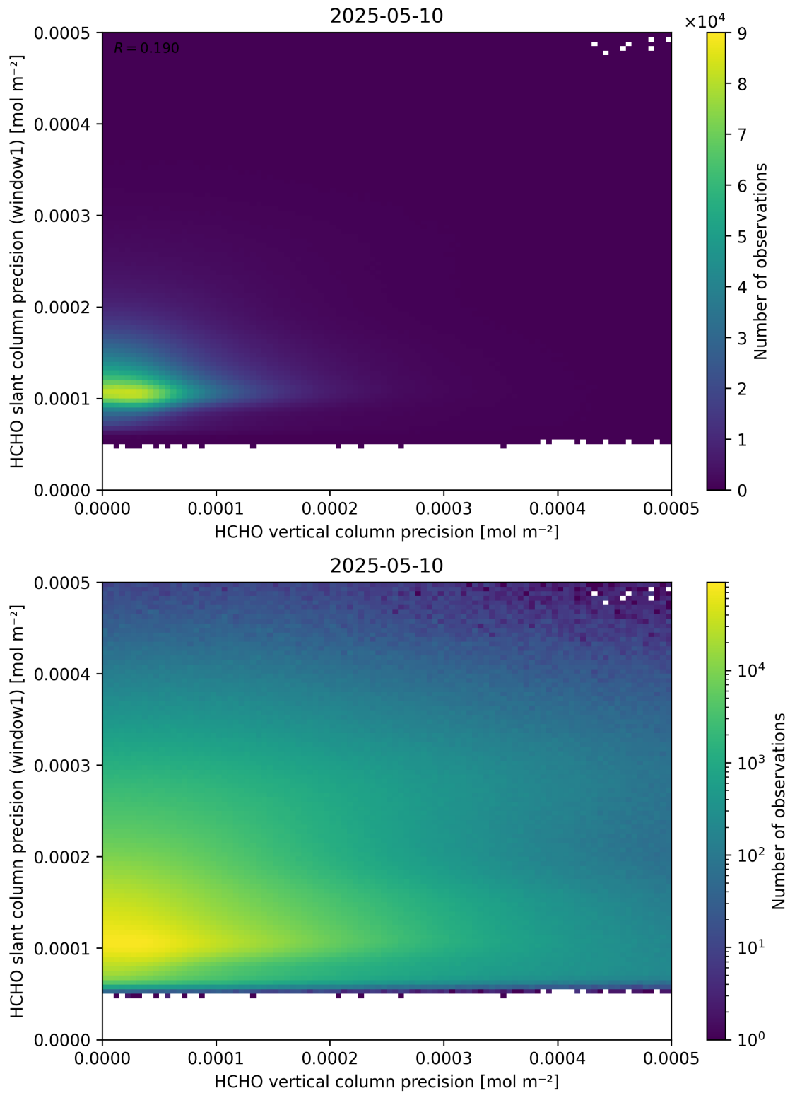
Figure 143: Scatter density plot of “HCHO vertical column precision” against “HCHO slant column precision (window1)” for 2025-05-10 to 2025-05-11.
