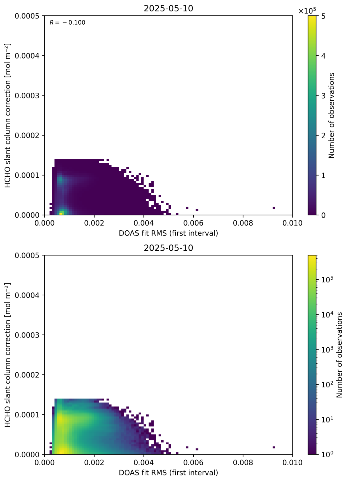
Figure 63: Scatter density plot of “DOAS fit RMS (first interval)” against “HCHO slant column correction” for 2025-05-10 to 2025-05-11.
