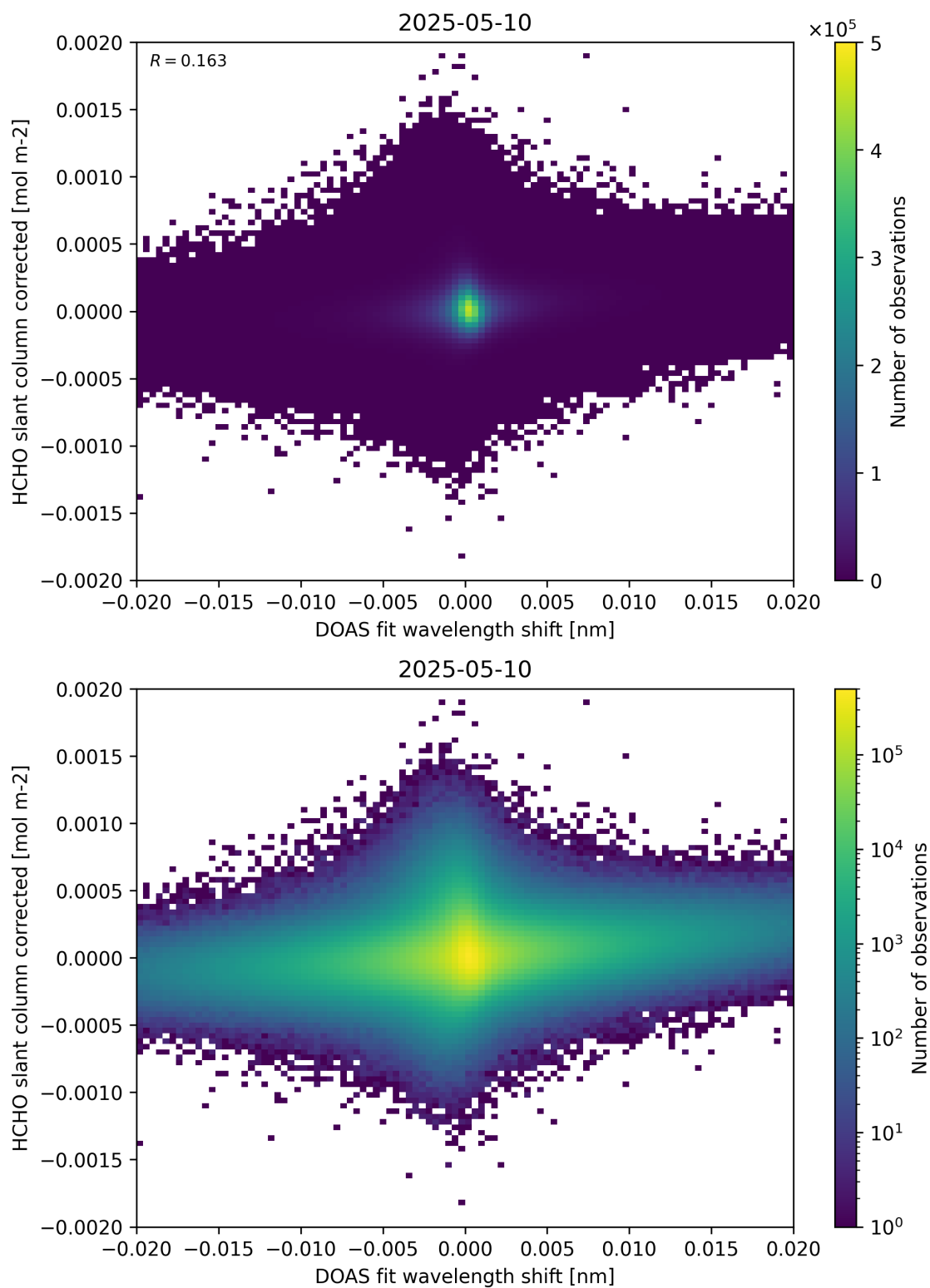
Figure 66: Scatter density plot of “DOAS fit wavelength shift” against “HCHO slant column corrected” for 2025-05-10 to 2025-05-11.
