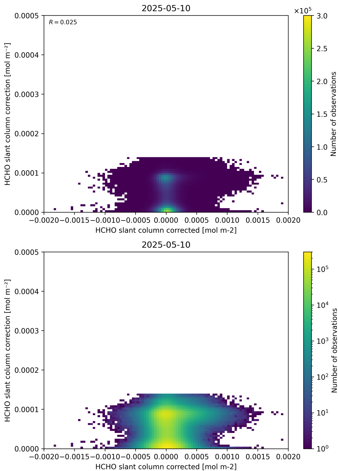
Figure 77: Scatter density plot of “HCHO slant column corrected” against “HCHO slant column correction” for 2025-05-10 to 2025-05-11.
