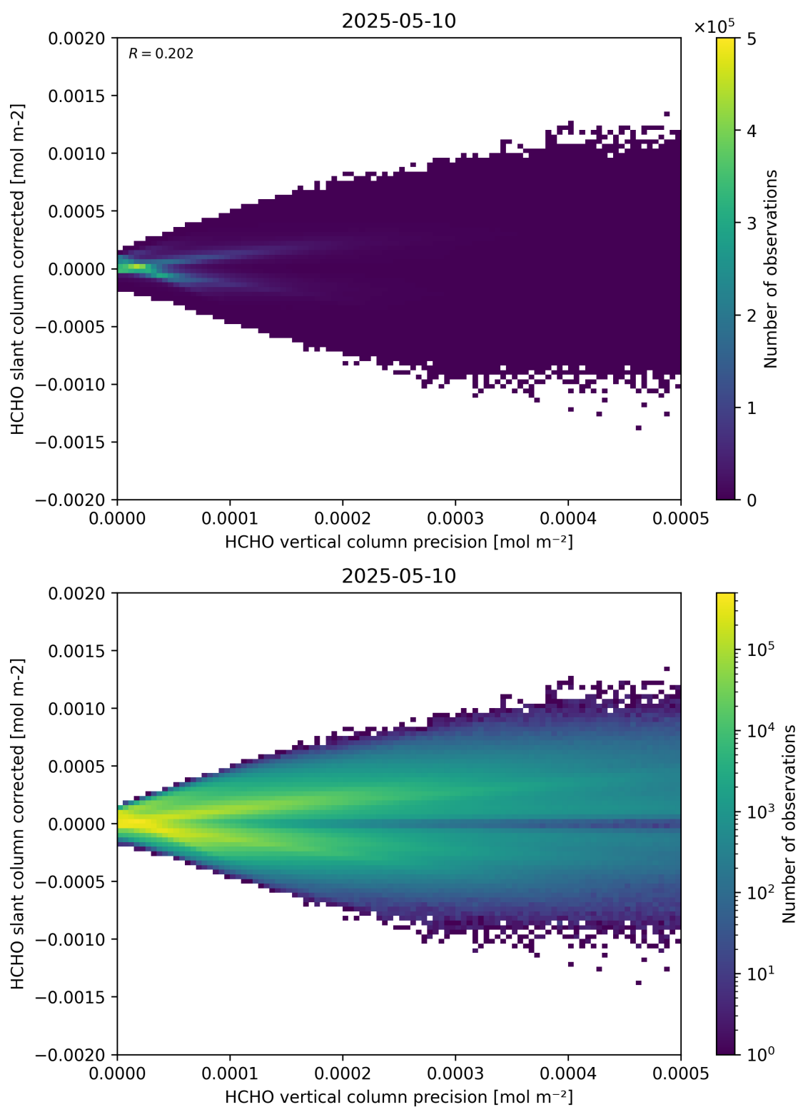
Figure 140: Scatter density plot of “HCHO vertical column precision” against “HCHO slant column corrected” for 2025-05-10 to 2025-05-11.
