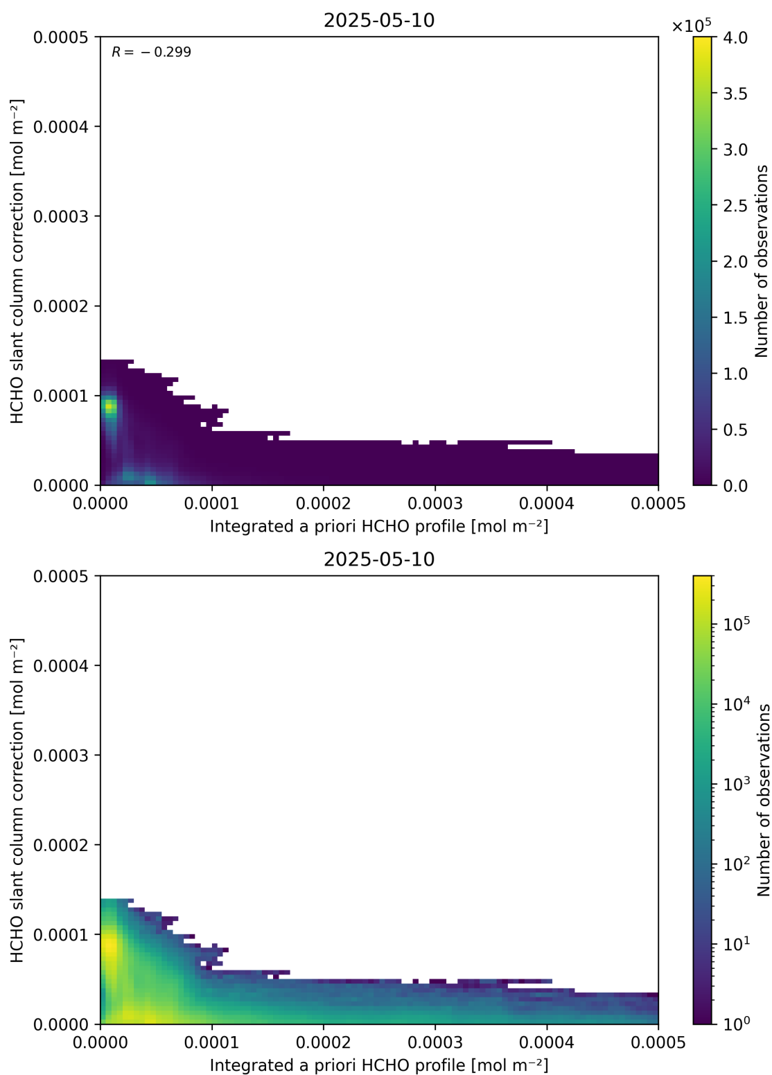
Figure 152: Scatter density plot of “Integrated a priori HCHO profile” against “HCHO slant column correction” for 2025-05-10 to 2025-05-11.
