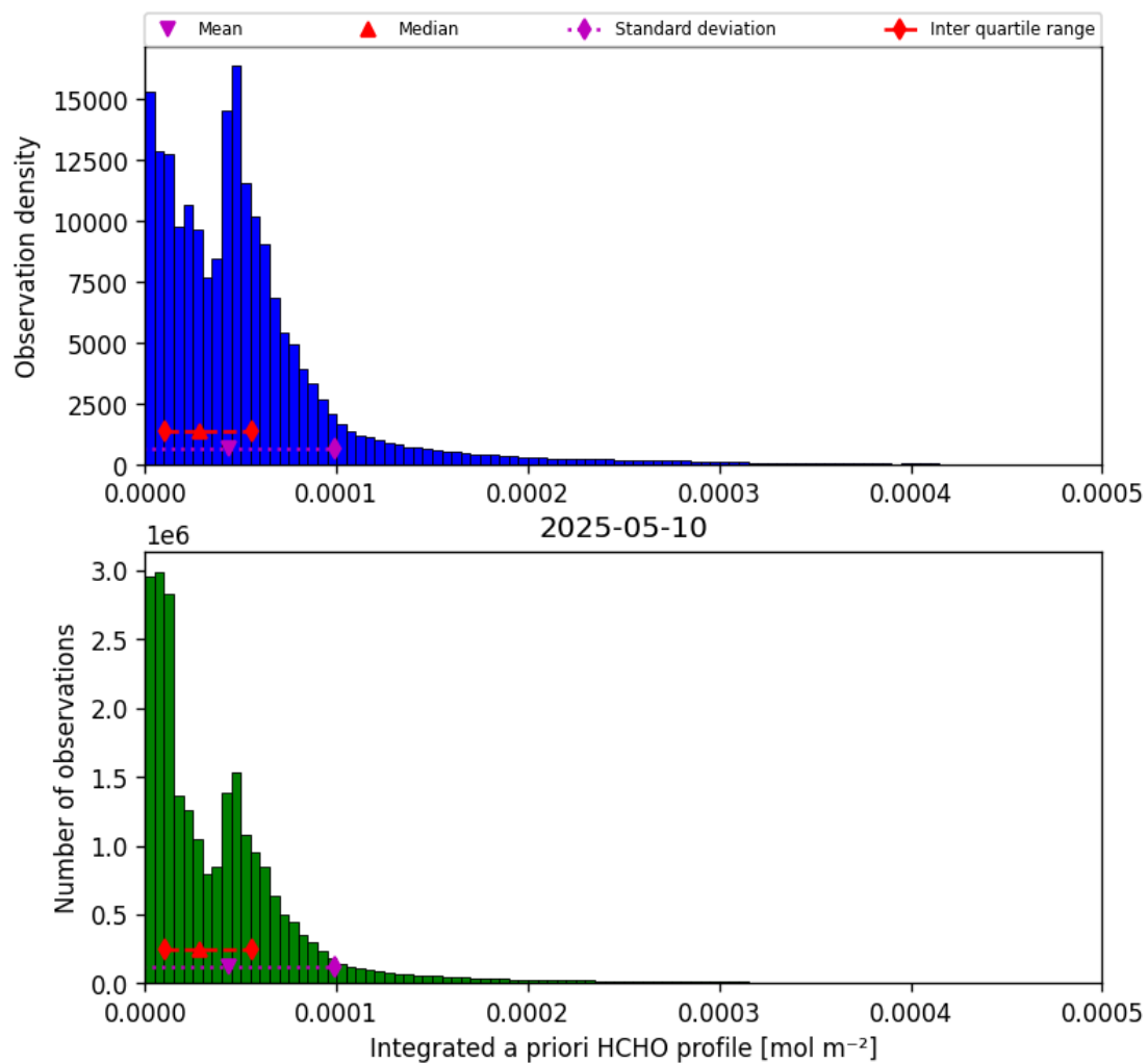
Figure 43: Histogram of “Integrated a priori HCHO profile” for 2025-05-10 to 2025-05-11
