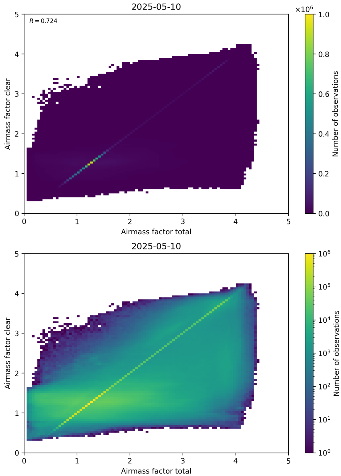
Figure 100: Scatter density plot of “Airmass factor total” against “Airmass factor clear” for 2025-05-10 to 2025-05-11.
