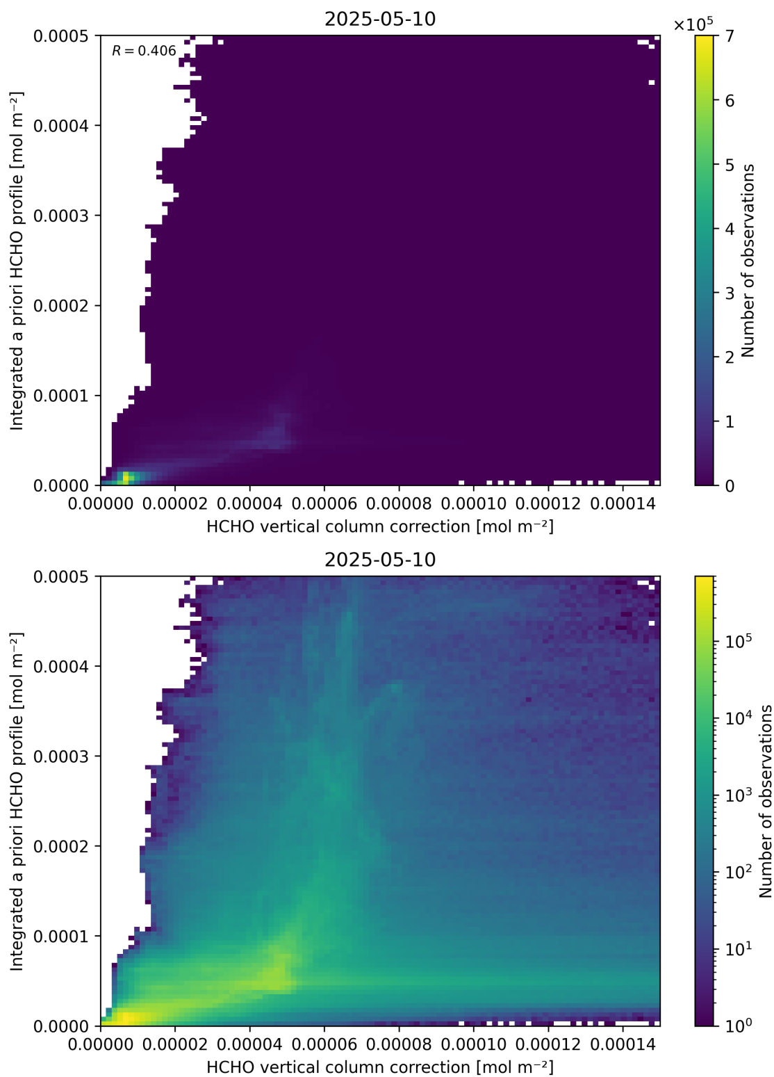
Figure 122: Scatter density plot of “HCHO vertical column correction” against “Integrated a priori HCHO profile” for 2025-05-10 to 2025-05-11.
