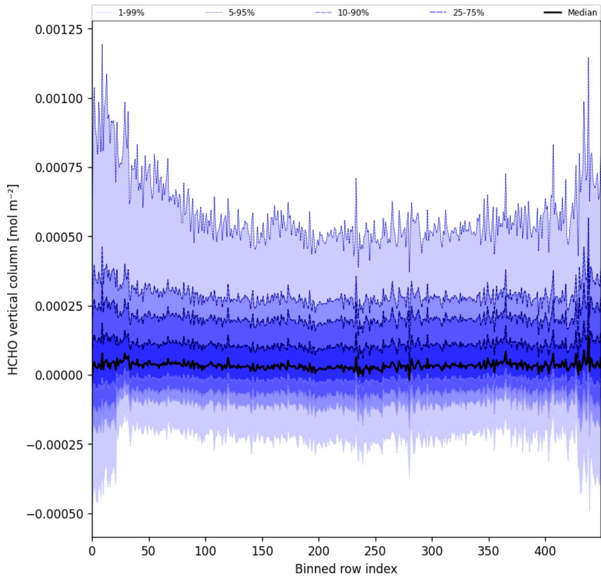
Figure 49: Along track statistics of “HCHO vertical column” for 2025-05-10 to 2025-05-11
