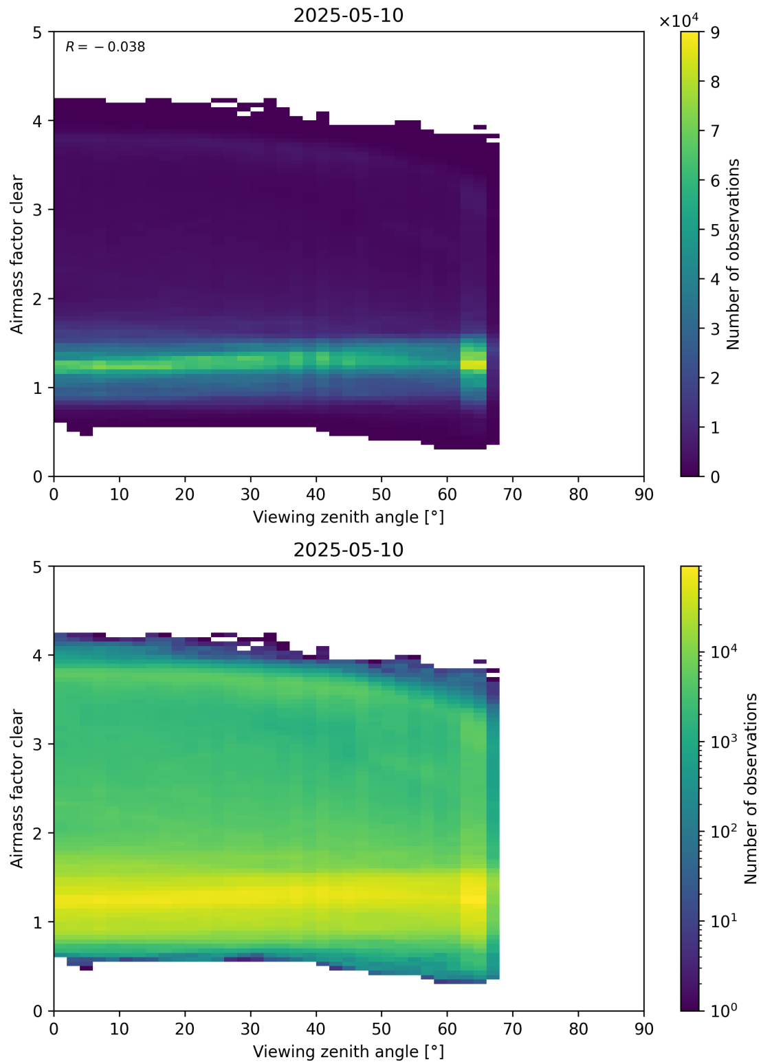
Figure 185: Scatter density plot of “Viewing zenith angle” against “Airmass factor clear” for 2025-05-10 to 2025-05-11.
