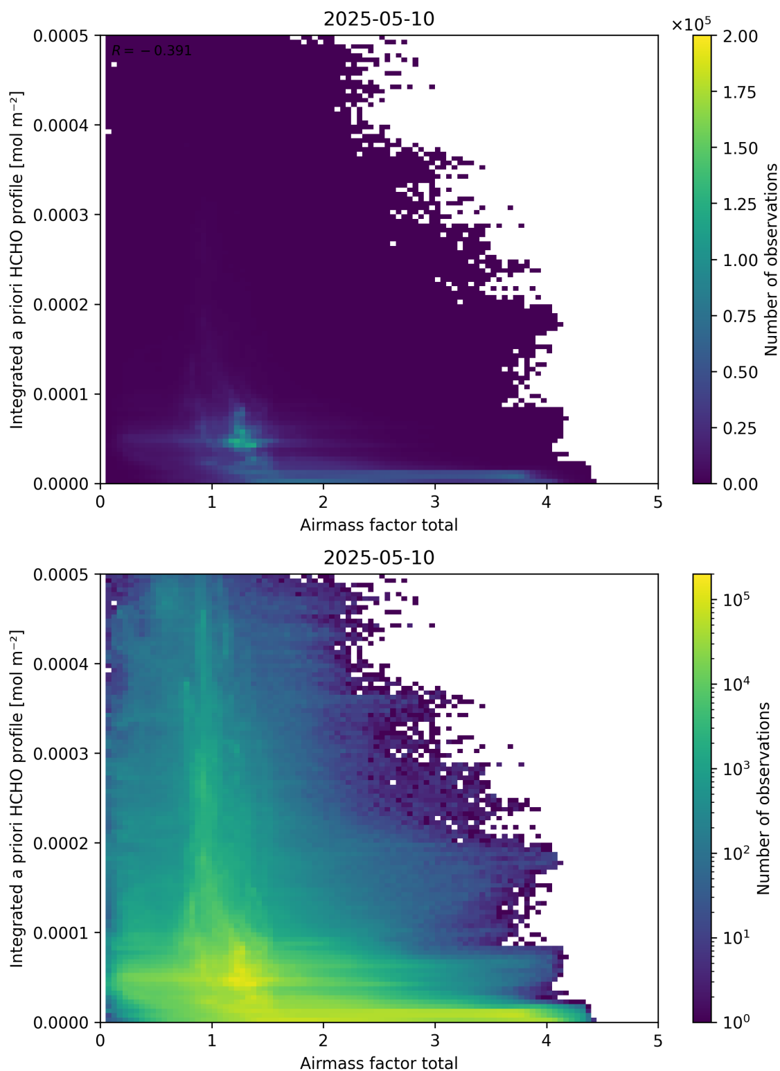
Figure 104: Scatter density plot of “Airmass factor total” against “Integrated a priori HCHO profile” for 2025-05-10 to 2025-05-11.
