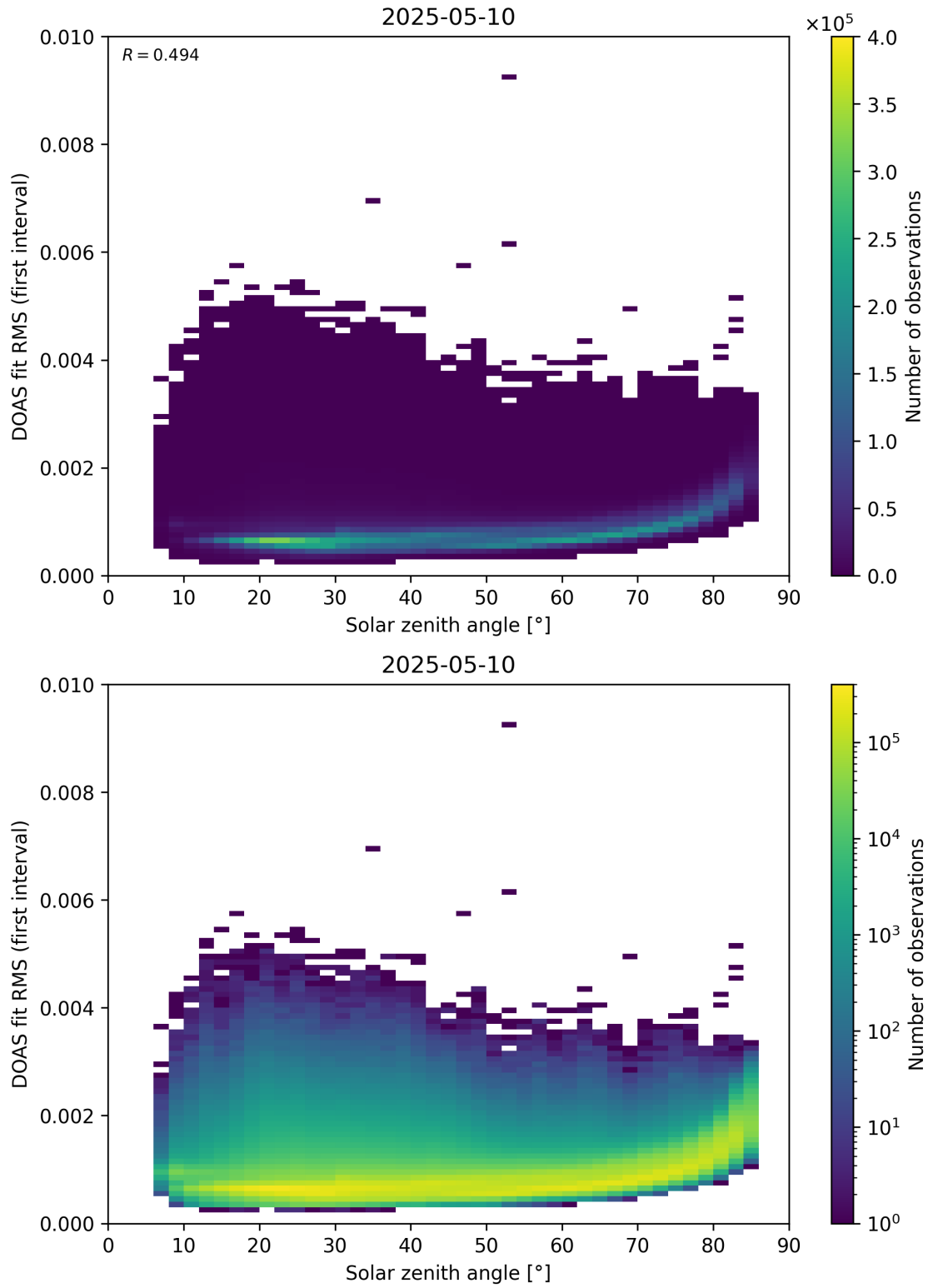
Figure 167: Scatter density plot of “Solar zenith angle” against “DOAS fit RMS (first interval)” for 2025-05-10 to 2025-05-11.
