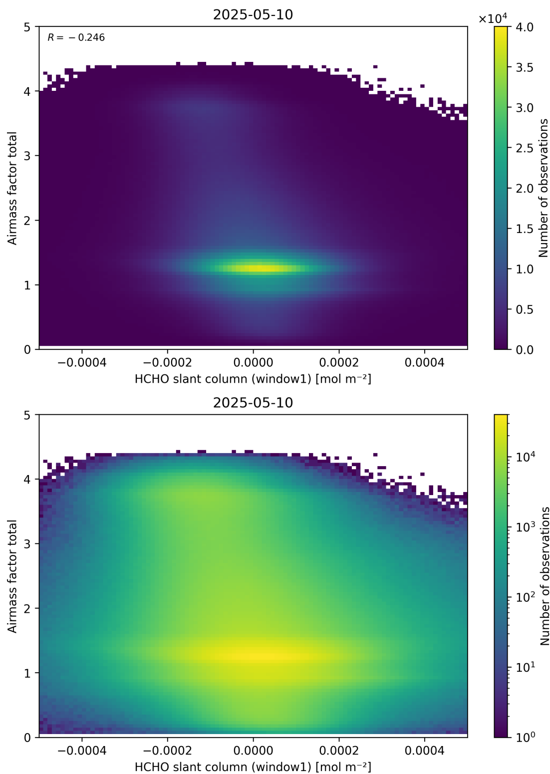
Figure 85: Scatter density plot of “HCHO slant column (window1)” against “Airmass factor total” for 2025-05-10 to 2025-05-11.
