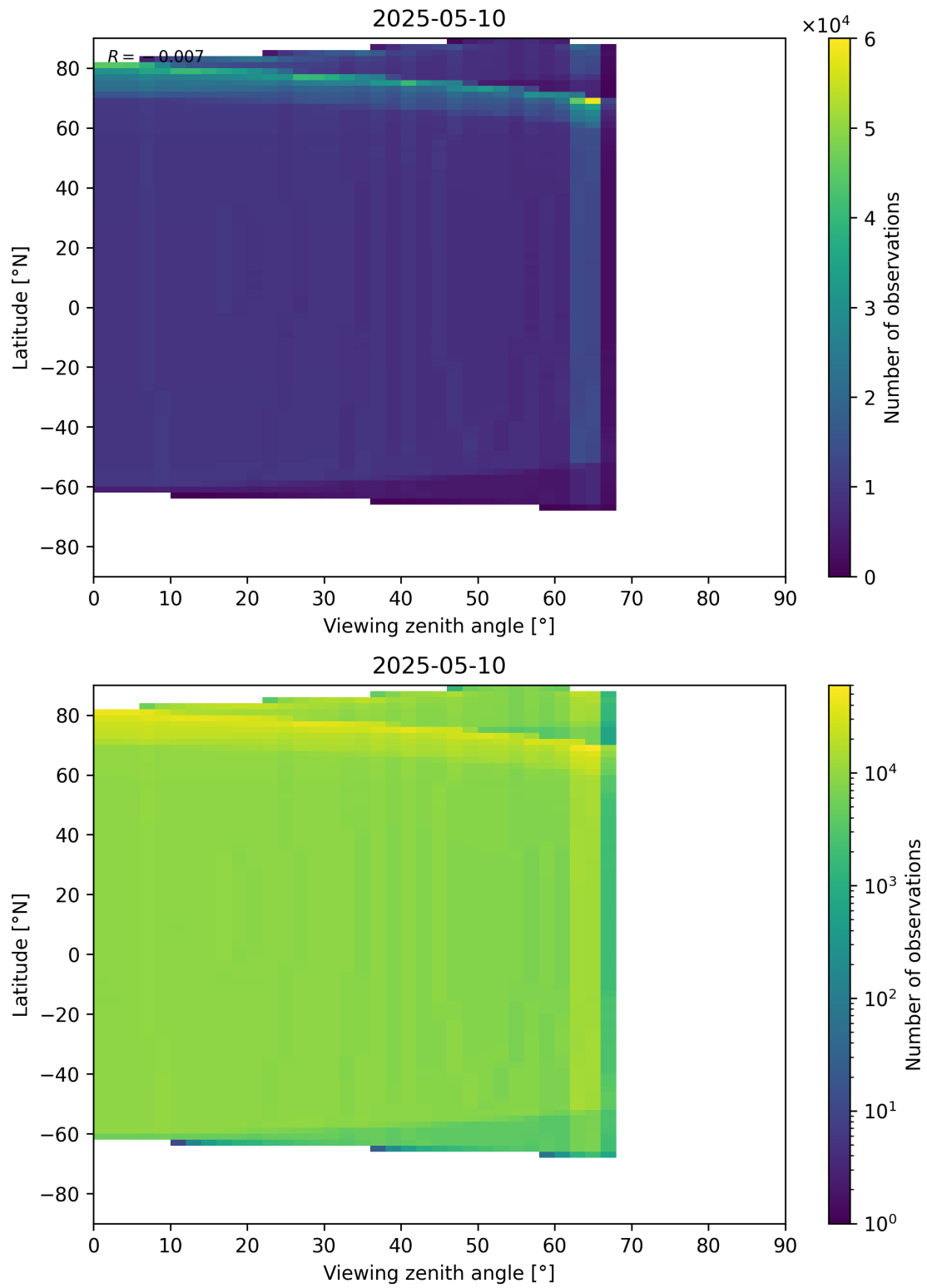
Figure 196: Scatter density plot of “Viewing zenith angle” against “Latitude” for 2025-05-10 to 2025-05-11.
