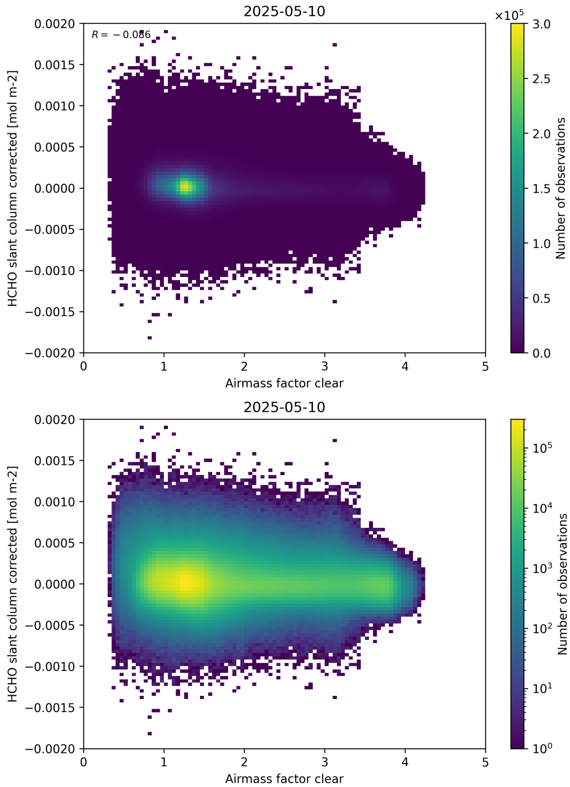
Figure 74: Scatter density plot of “Airmass factor clear” against “HCHO slant column corrected” for 2025-05-10 to 2025-05-11.
