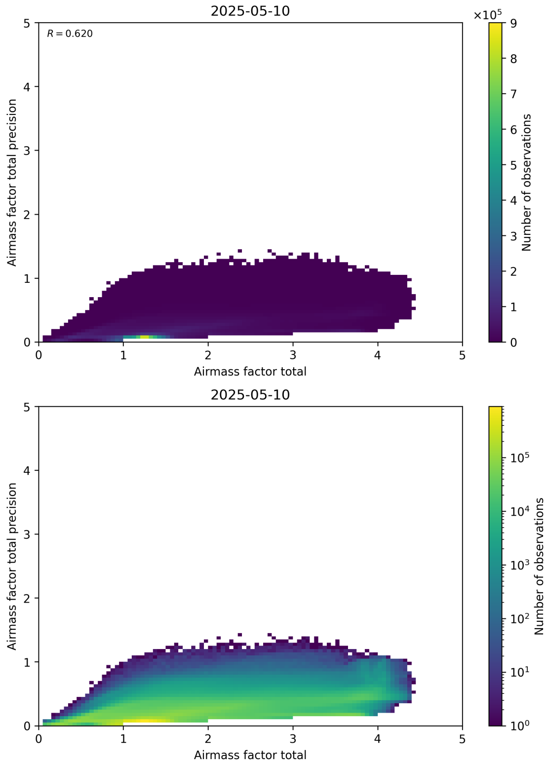
Figure 103: Scatter density plot of “Airmass factor total” against “Airmass factor total precision” for 2025-05-10 to 2025-05-11.
