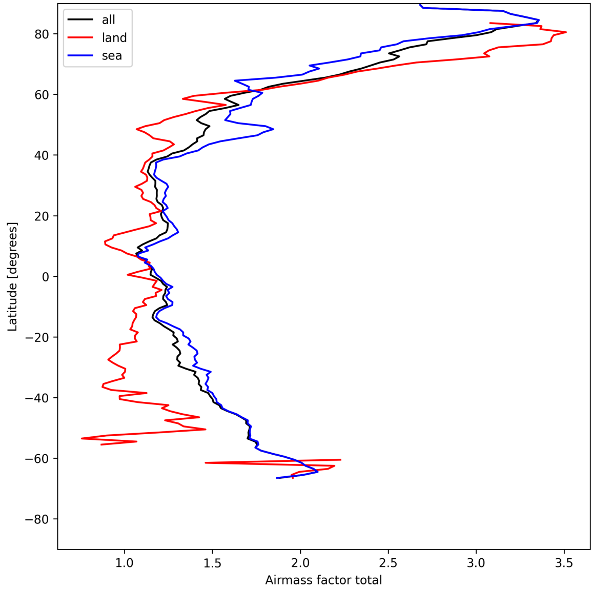
Figure 26: Zonal average of “Airmass factor total” for 2025-05-10 to 2025-05-11.
