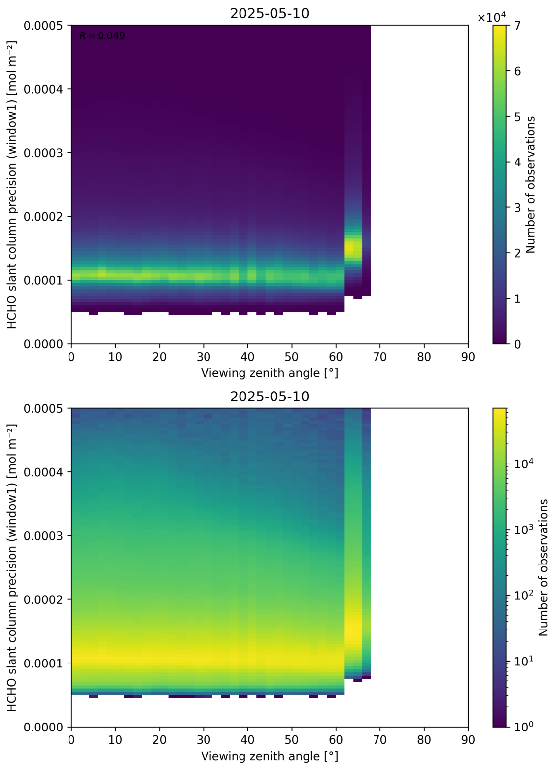
Figure 189: Scatter density plot of “Viewing zenith angle” against “HCHO slant column precision (window1)” for 2025-05-10 to 2025-05-11.
