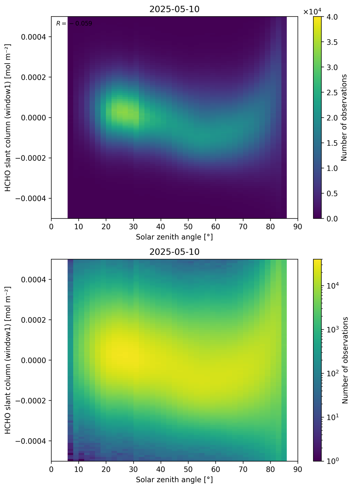
Figure 173: Scatter density plot of “Solar zenith angle” against “HCHO slant column (window1)” for 2025-05-10 to 2025-05-11.
