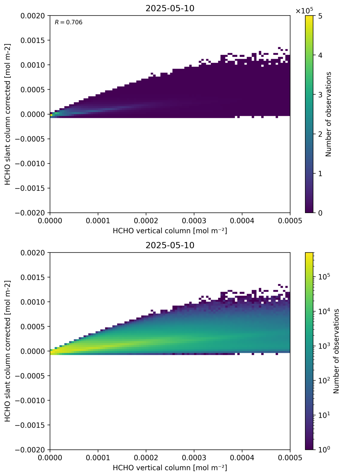
Figure 127: Scatter density plot of “HCHO vertical column” against “HCHO slant column corrected” for 2025-05-10 to 2025-05-11.
