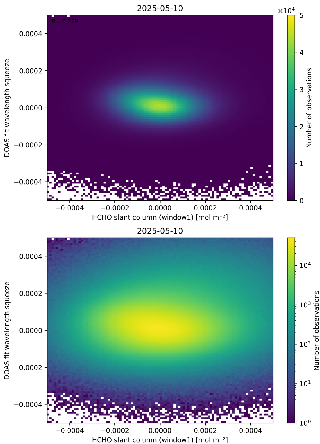
Figure 80: Scatter density plot of “HCHO slant column (window1)” against “DOAS fit wavelength squeeze” for 2025-05-10 to 2025-05-11.
