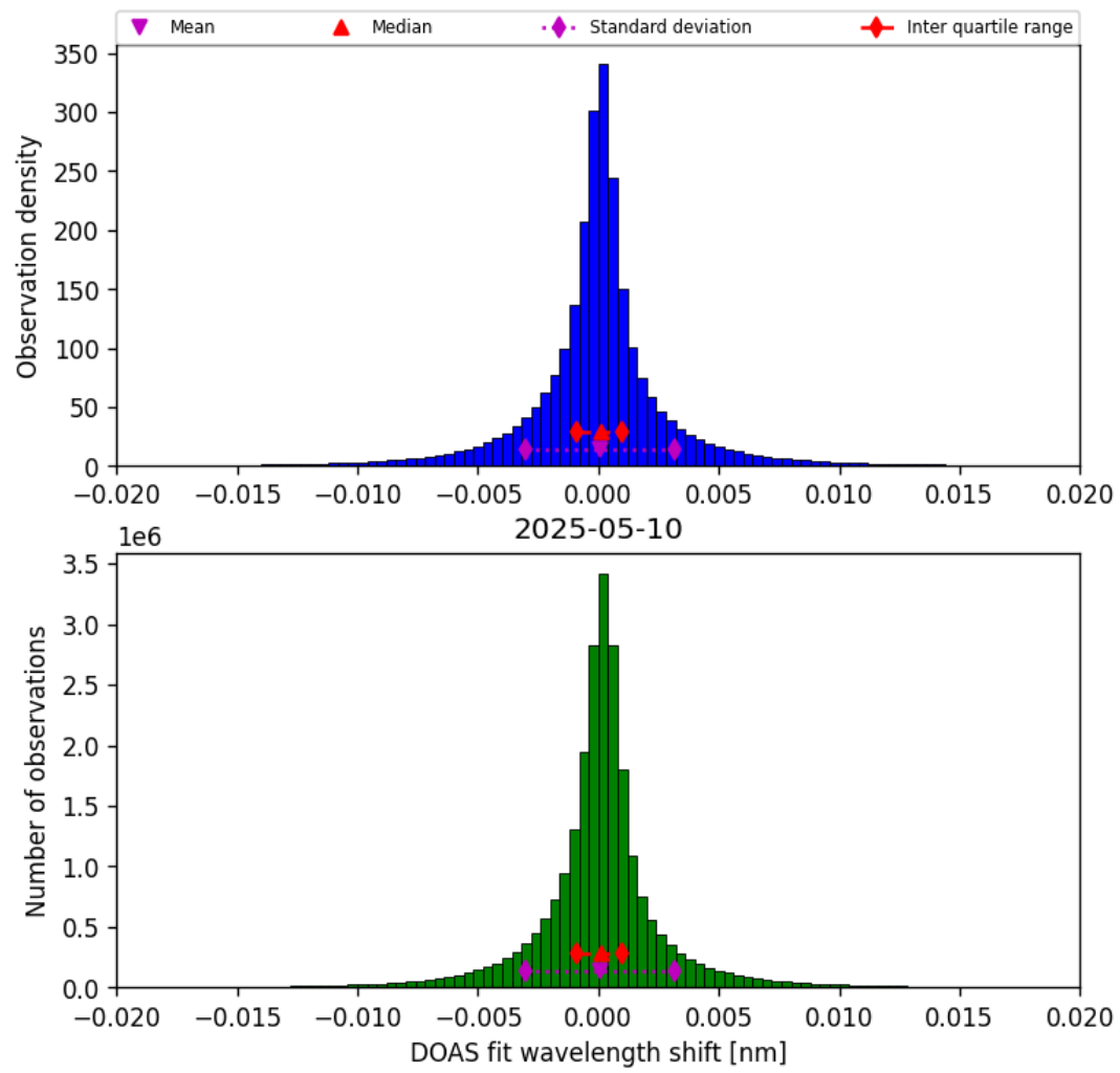
Figure 44: Histogram of “DOAS fit wavelength shift” for 2025-05-10 to 2025-05-11
