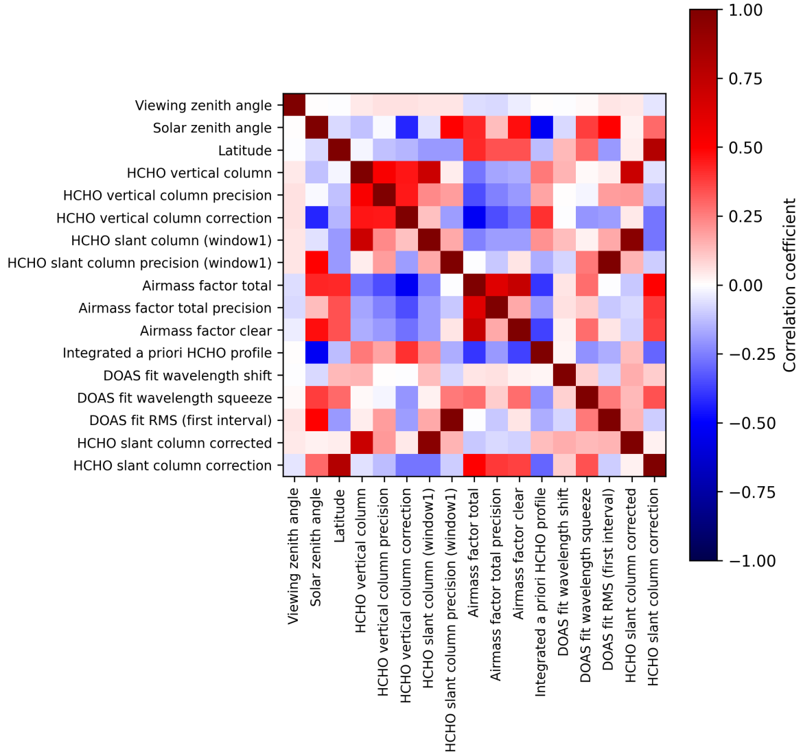
Figure 2: Map of correlation matrix for 2025-05-10 to 2025-05-11.
