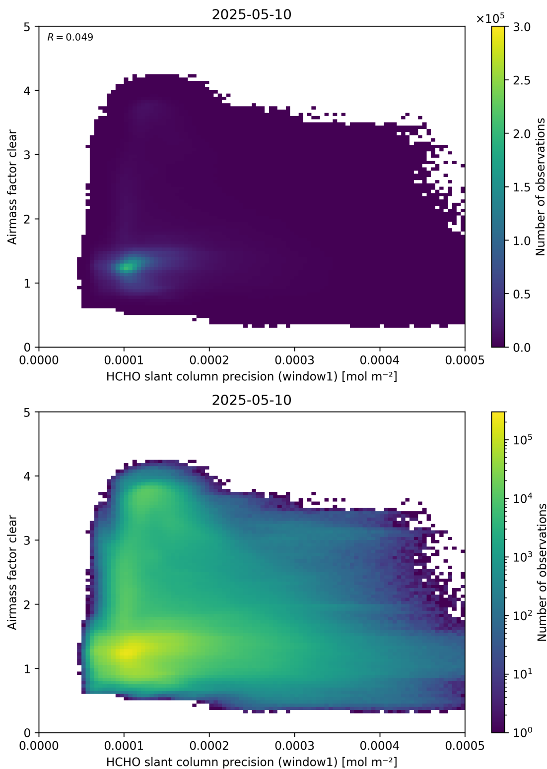
Figure 91: Scatter density plot of “HCHO slant column precision (window1)” against “Airmass factor clear” for 2025-05-10 to 2025-05-11.
