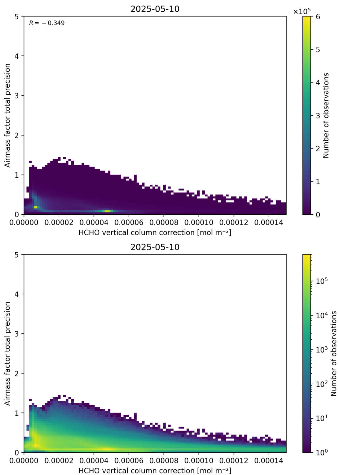
Figure 121: Scatter density plot of “HCHO vertical column correction” against “Airmass factor total precision” for 2025-05-10 to 2025-05-11.
