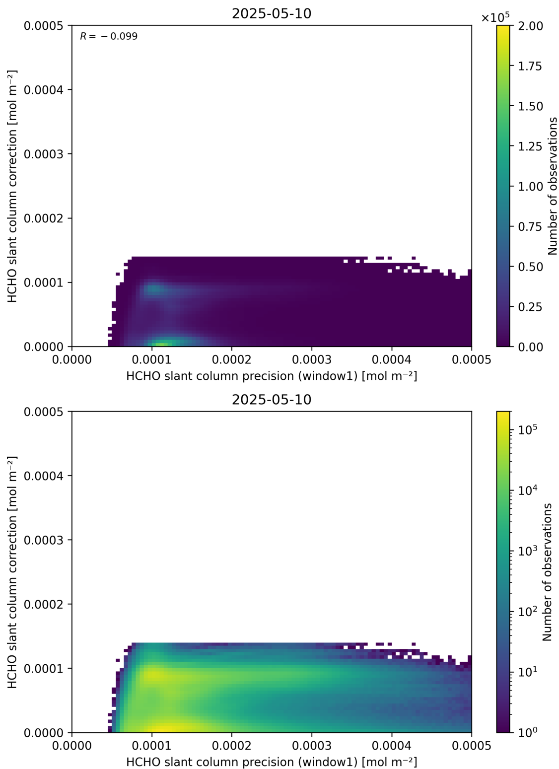
Figure 93: Scatter density plot of “HCHO slant column precision (window1)” against “HCHO slant column correction” for 2025-05-10 to 2025-05-11.
