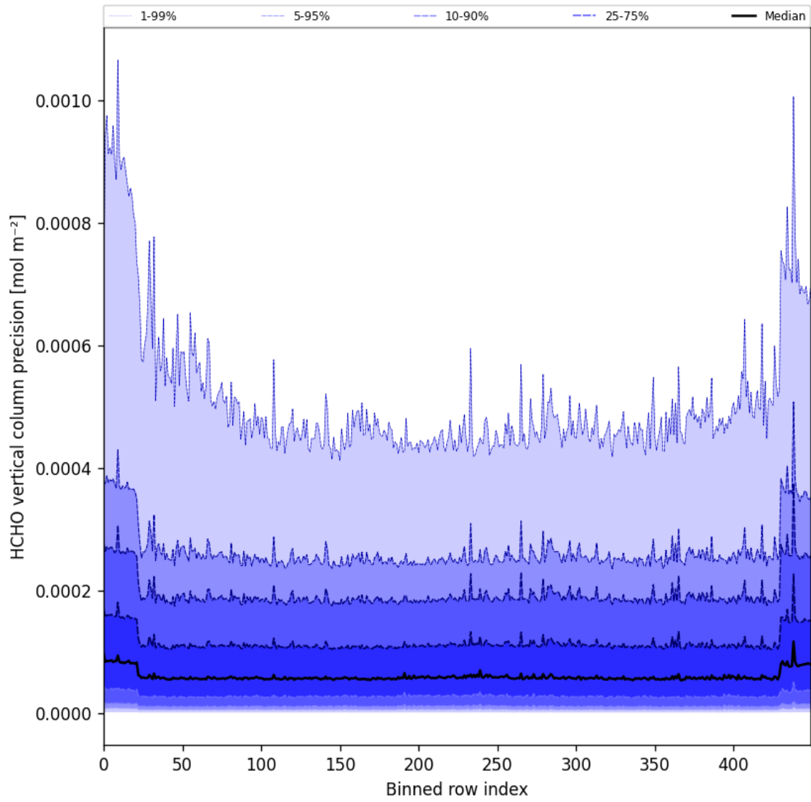
Figure 50: Along track statistics of “HCHO vertical column precision” for 2025-05-10 to 2025-05-11
