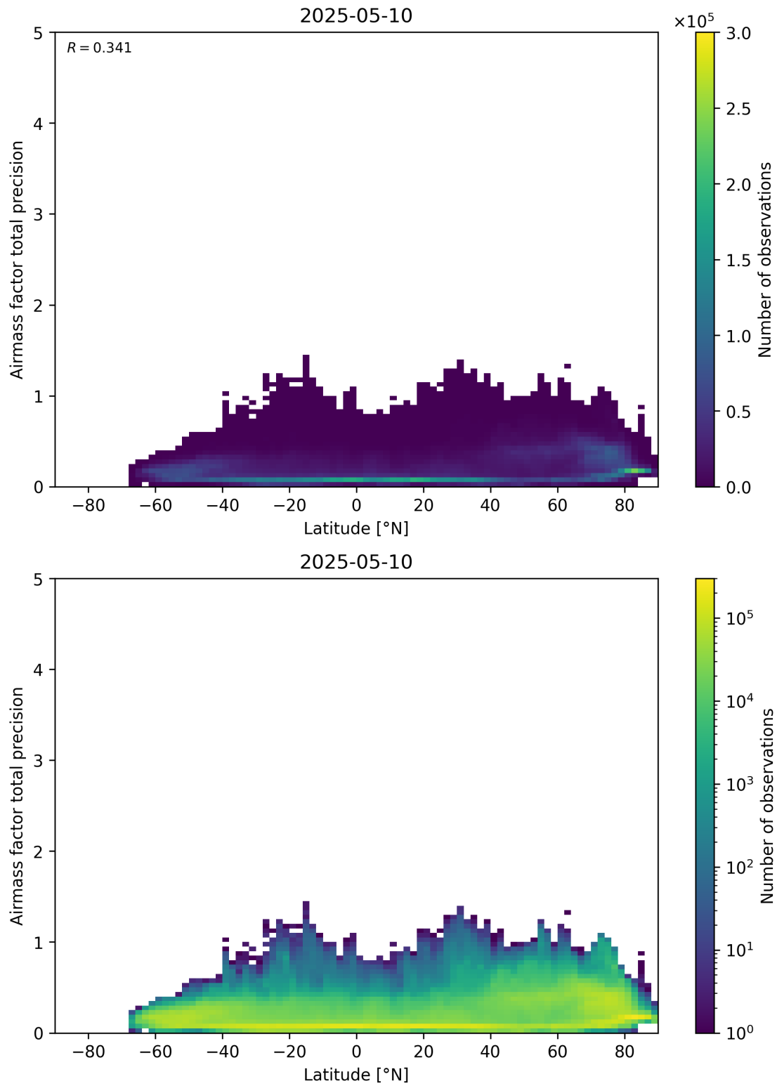
Figure 162: Scatter density plot of “Latitude” against “Airmass factor total precision” for 2025-05-10 to 2025-05-11.
