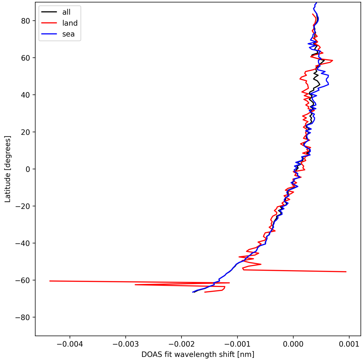
Figure 30: Zonal average of “DOAS fit wavelength shift” for 2025-05-10 to 2025-05-11.
