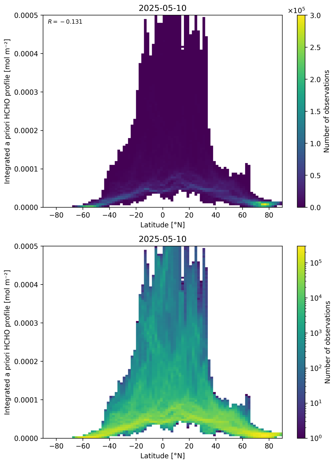
Figure 166: Scatter density plot of “Latitude” against “Integrated a priori HCHO profile” for 2025-05-10 to 2025-05-11.
