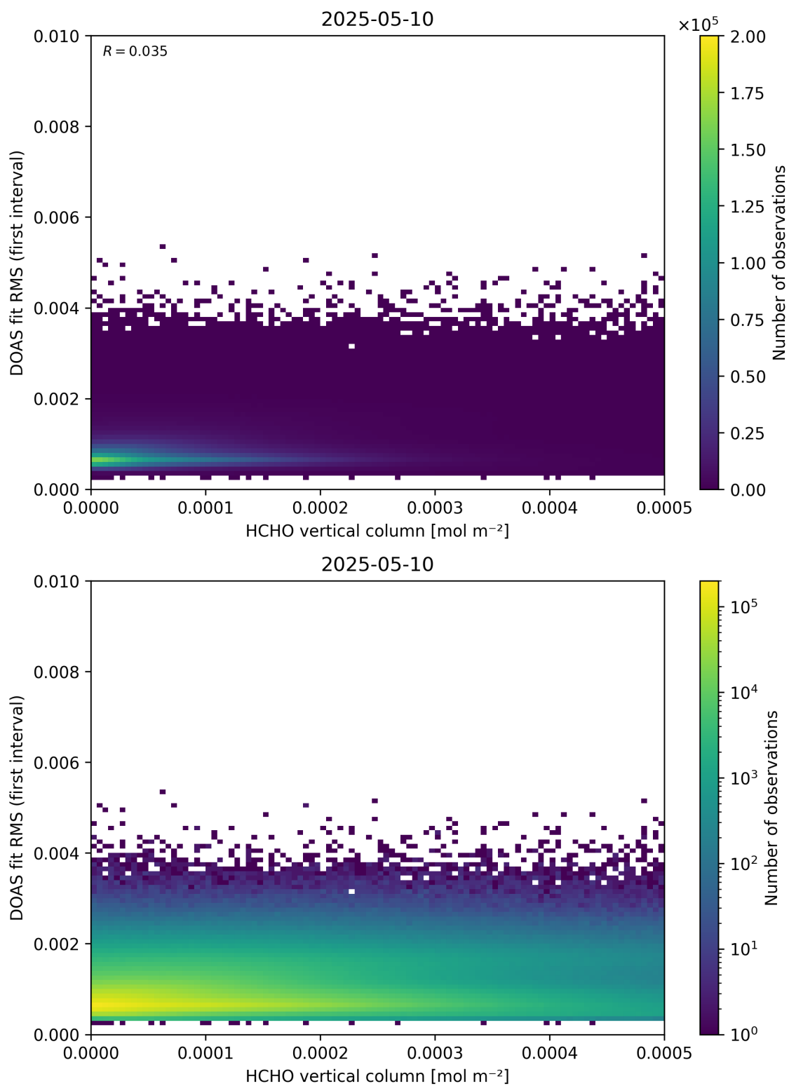
Figure 123: Scatter density plot of “HCHO vertical column” against “DOAS fit RMS (first interval)” for 2025-05-10 to 2025-05-11.
