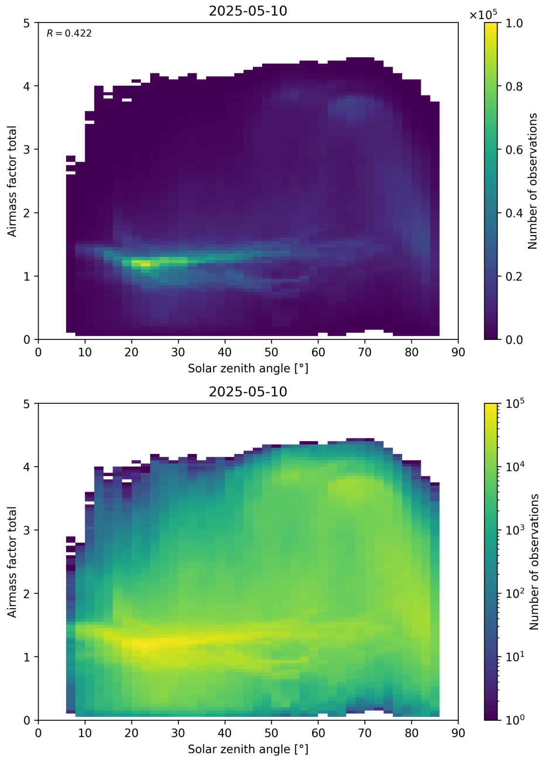
Figure 175: Scatter density plot of “Solar zenith angle” against “Airmass factor total” for 2025-05-10 to 2025-05-11.
