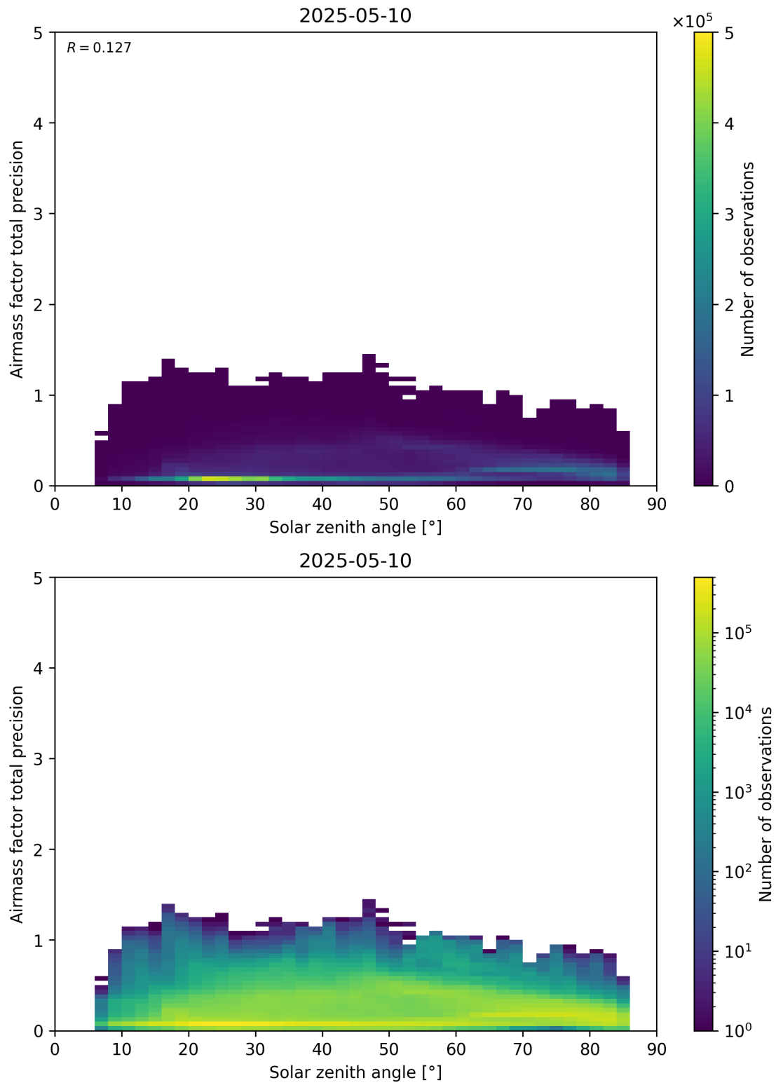
Figure 176: Scatter density plot of “Solar zenith angle” against “Airmass factor total precision” for 2025-05-10 to 2025-05-11.
