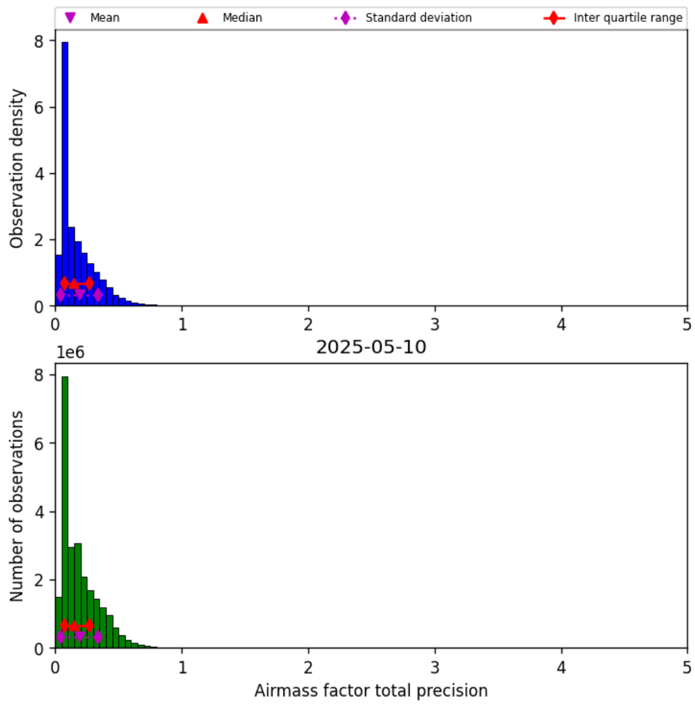
Figure 41: Histogram of “Airmass factor total precision” for 2025-05-10 to 2025-05-11
