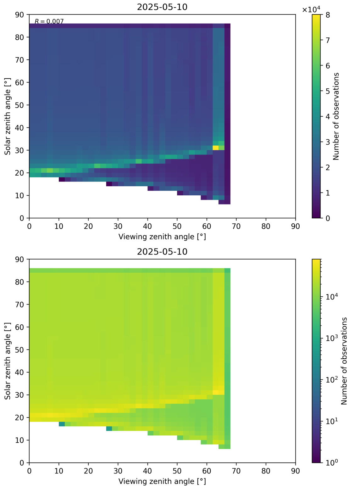
Figure 197: Scatter density plot of “Viewing zenith angle” against “Solar zenith angle” for 2025-05-10 to 2025-05-11.
