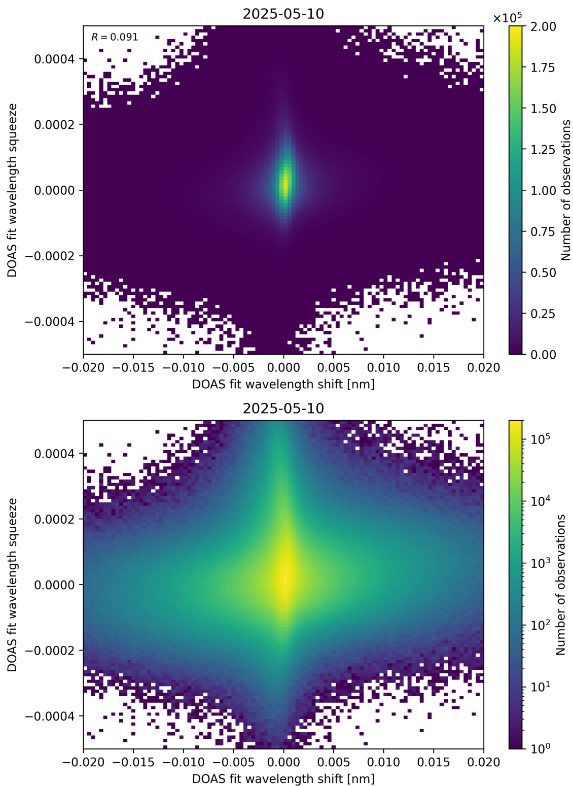
Figure 65: Scatter density plot of “DOAS fit wavelength shift” against “DOAS fit wavelength squeeze” for 2025-05-10 to 2025-05-11.
