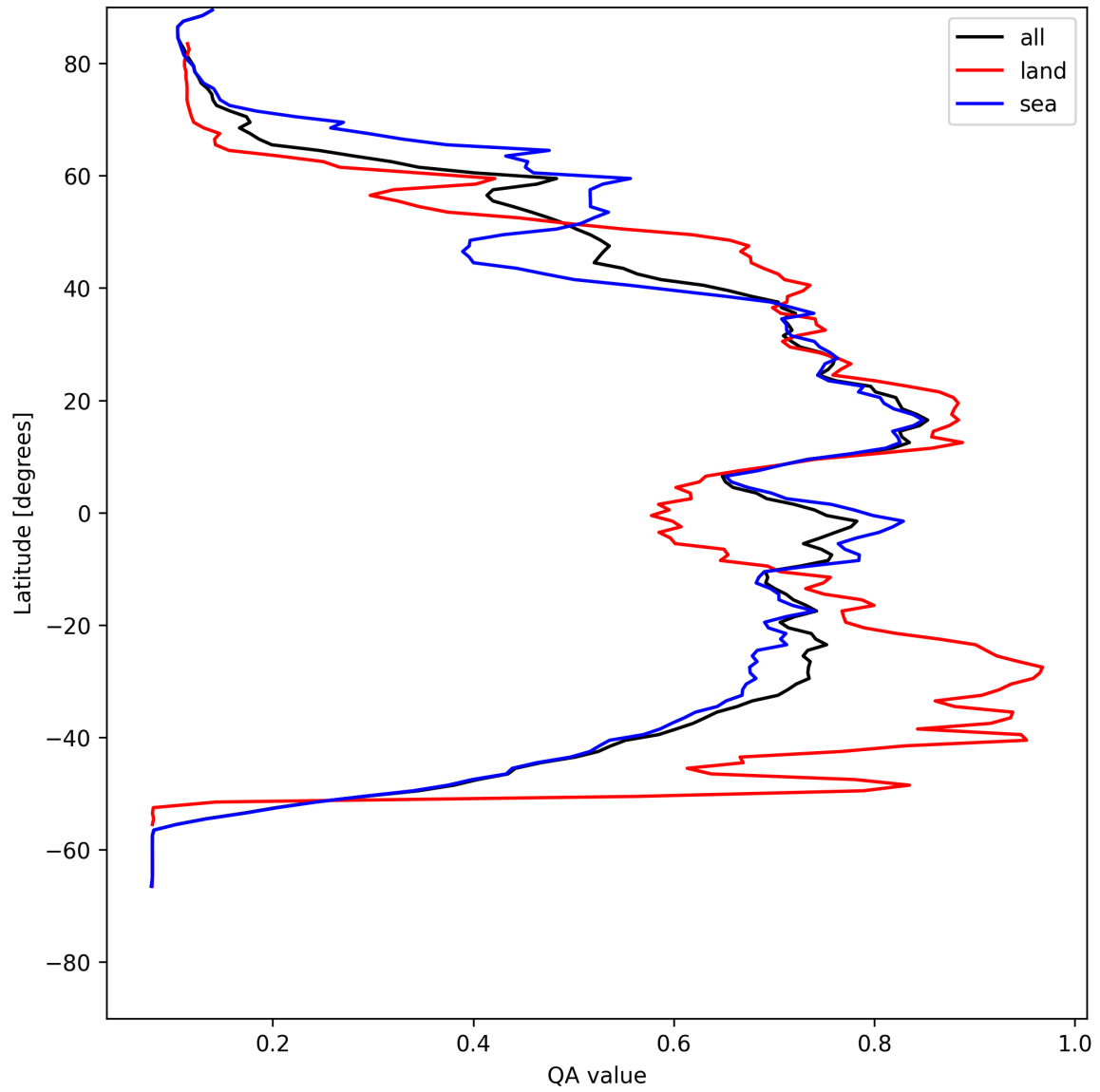
Figure 20: Zonal average of “QA value” for 2025-05-10 to 2025-05-11.
