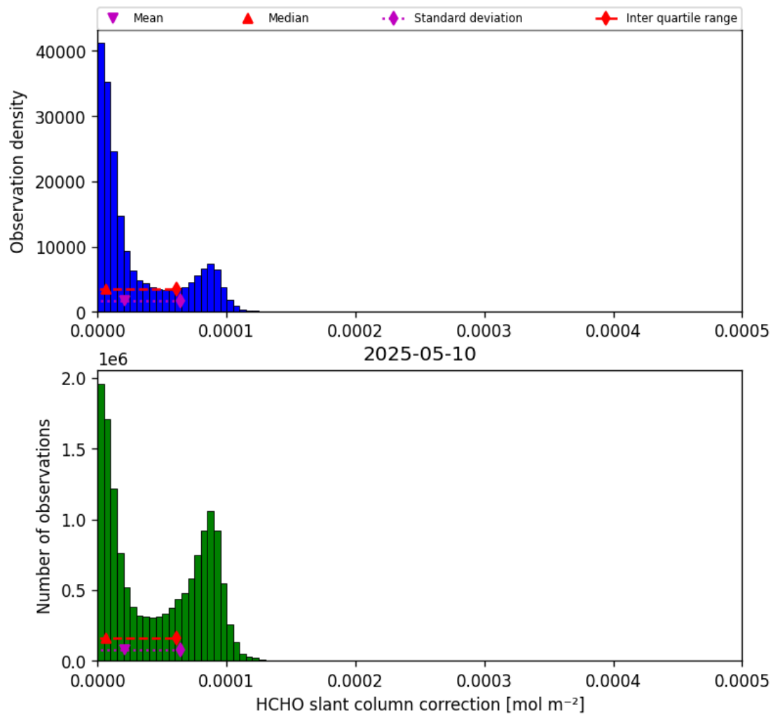
Figure 47: Histogram of “HCHO slant column correction” for 2025-05-10 to 2025-05-11
