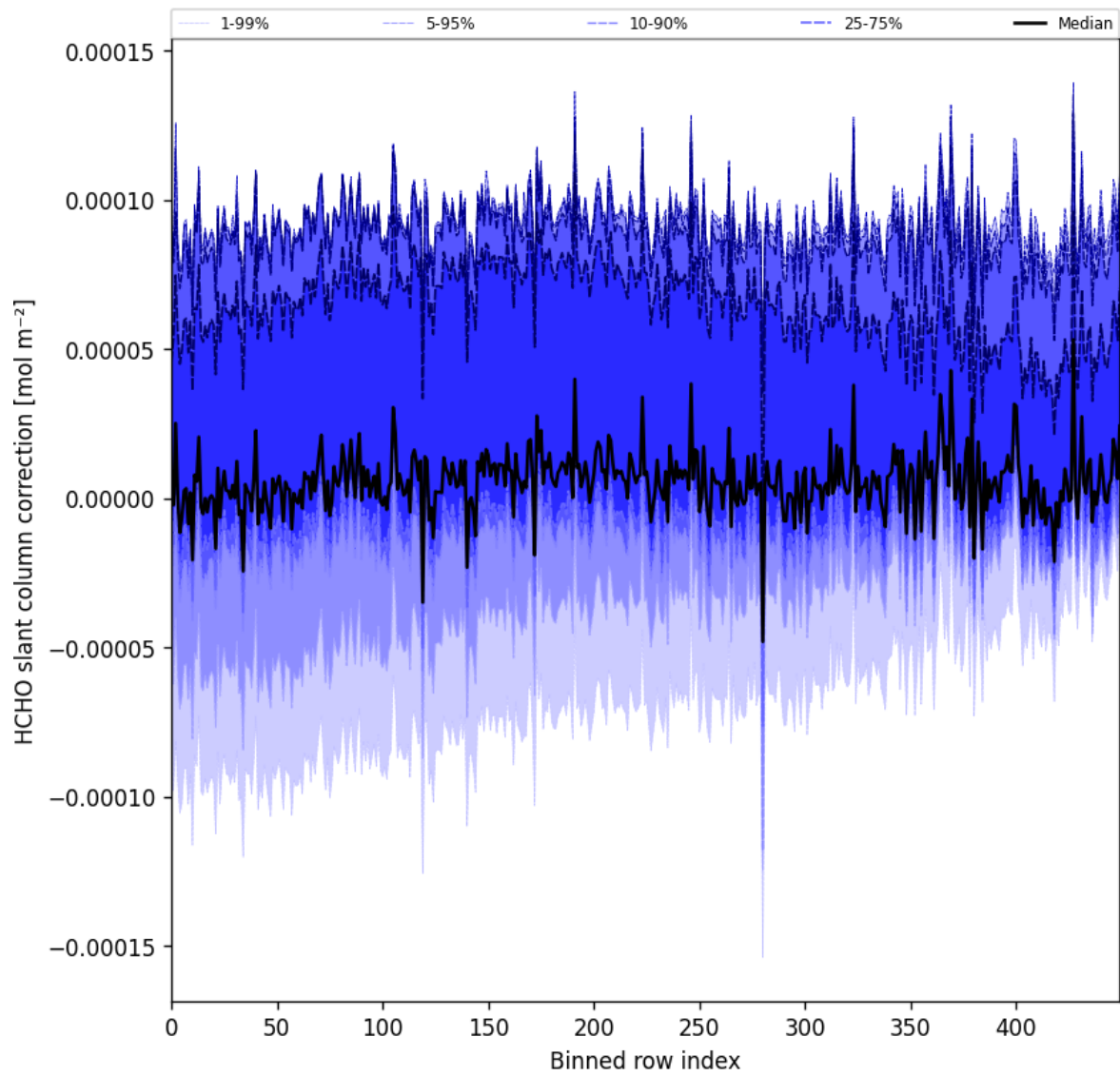
Figure 61: Along track statistics of “HCHO slant column correction” for 2025-05-10 to 2025-05-11
