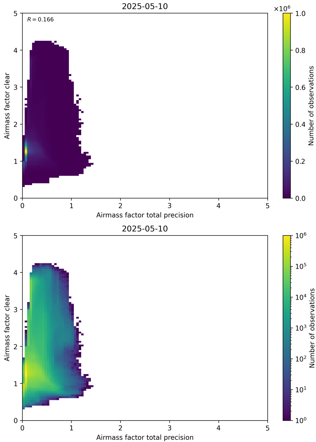
Figure 108: Scatter density plot of “Airmass factor total precision” against “Airmass factor clear” for 2025-05-10 to 2025-05-11.
