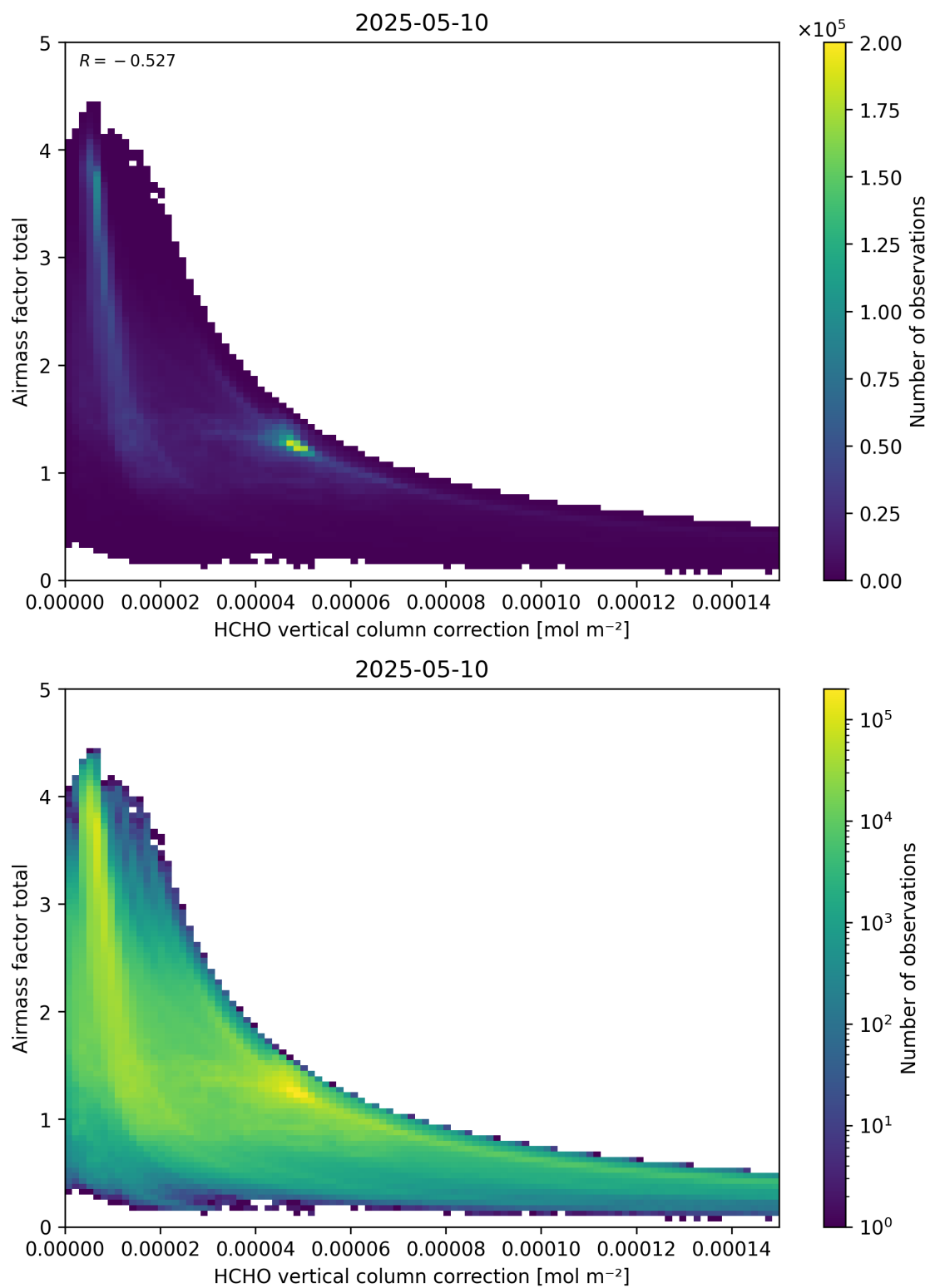
Figure 120: Scatter density plot of “HCHO vertical column correction” against “Airmass factor total” for 2025-05-10 to 2025-05-11.
