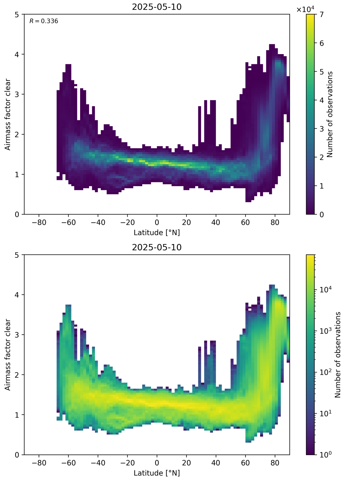
Figure 156: Scatter density plot of “Latitude” against “Airmass factor clear” for 2025-05-10 to 2025-05-11.
