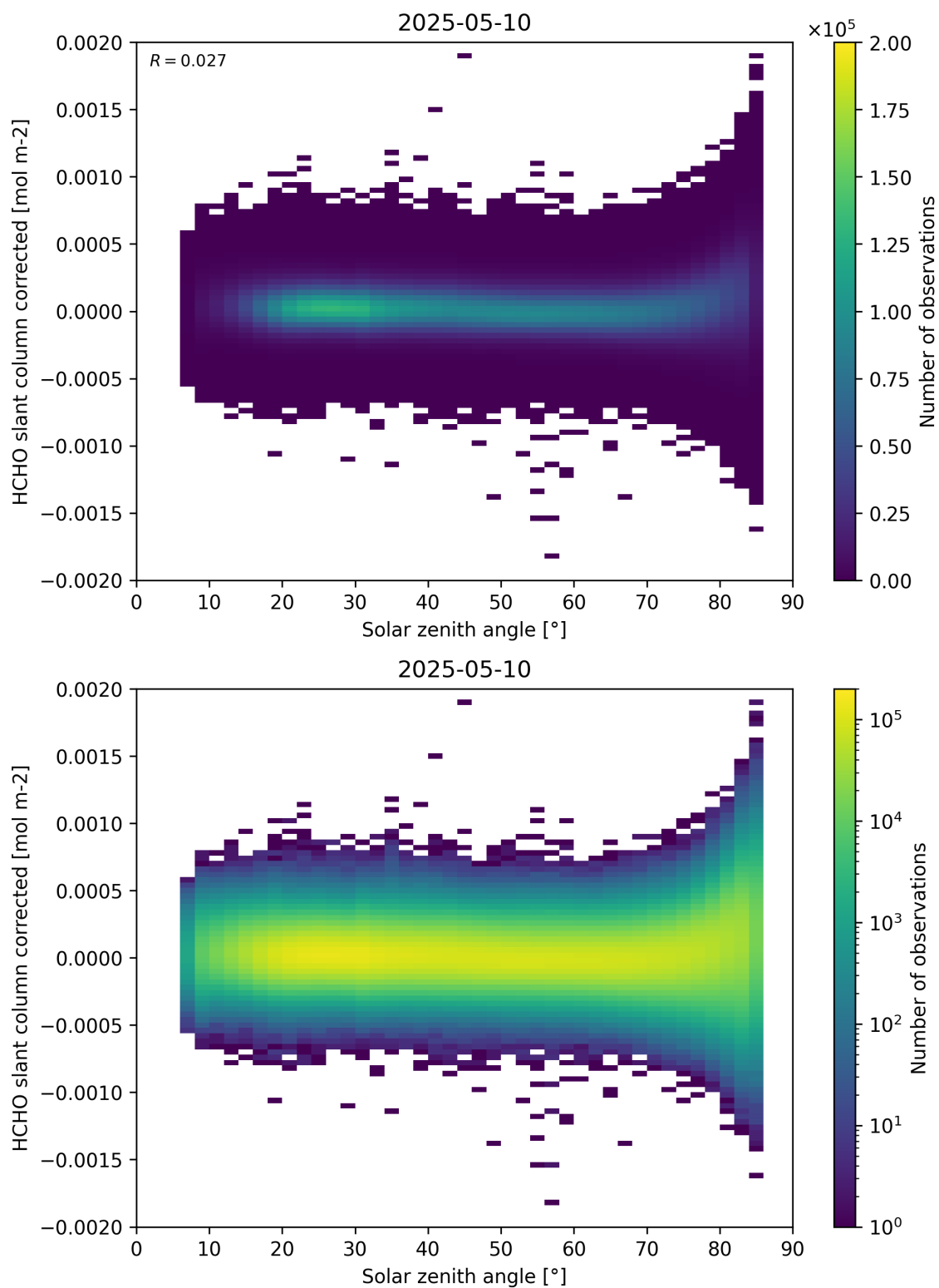
Figure 171: Scatter density plot of “Solar zenith angle” against “HCHO slant column corrected” for 2025-05-10 to 2025-05-11.
