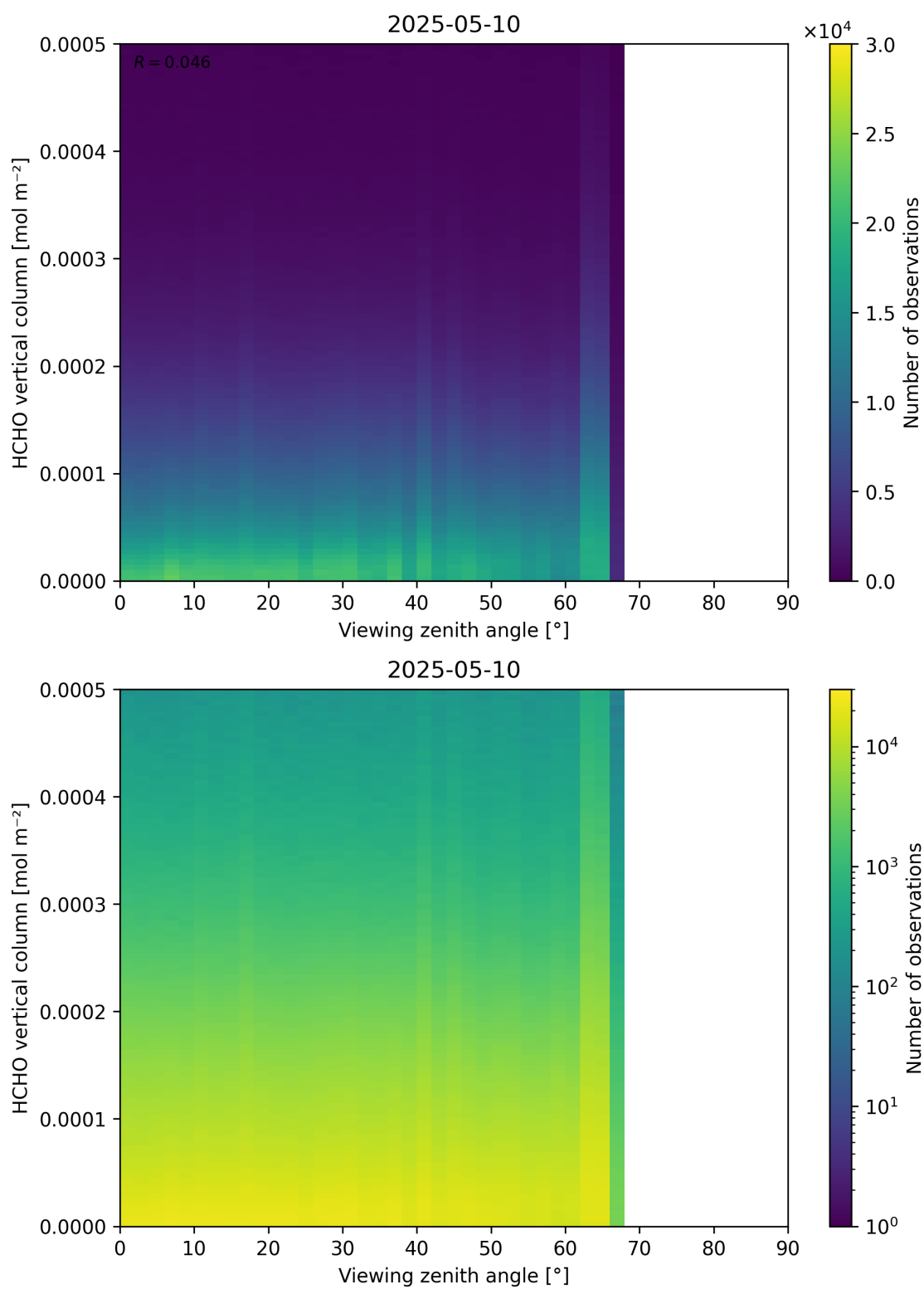
Figure 192: Scatter density plot of “Viewing zenith angle” against “HCHO vertical column” for 2025-05-10 to 2025-05-11.
