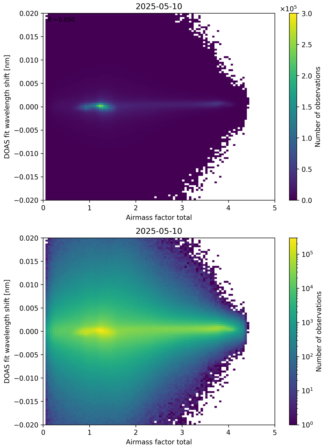
Figure 98: Scatter density plot of “Airmass factor total” against “DOAS fit wavelength shift” for 2025-05-10 to 2025-05-11.
