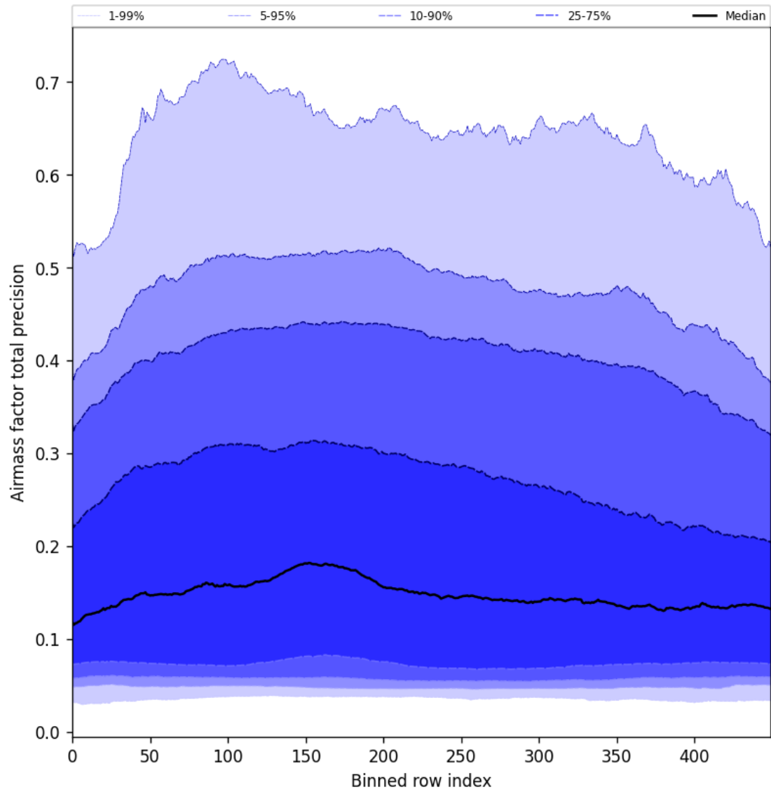
Figure 55: Along track statistics of “Airmass factor total precision” for 2025-05-10 to 2025-05-11
