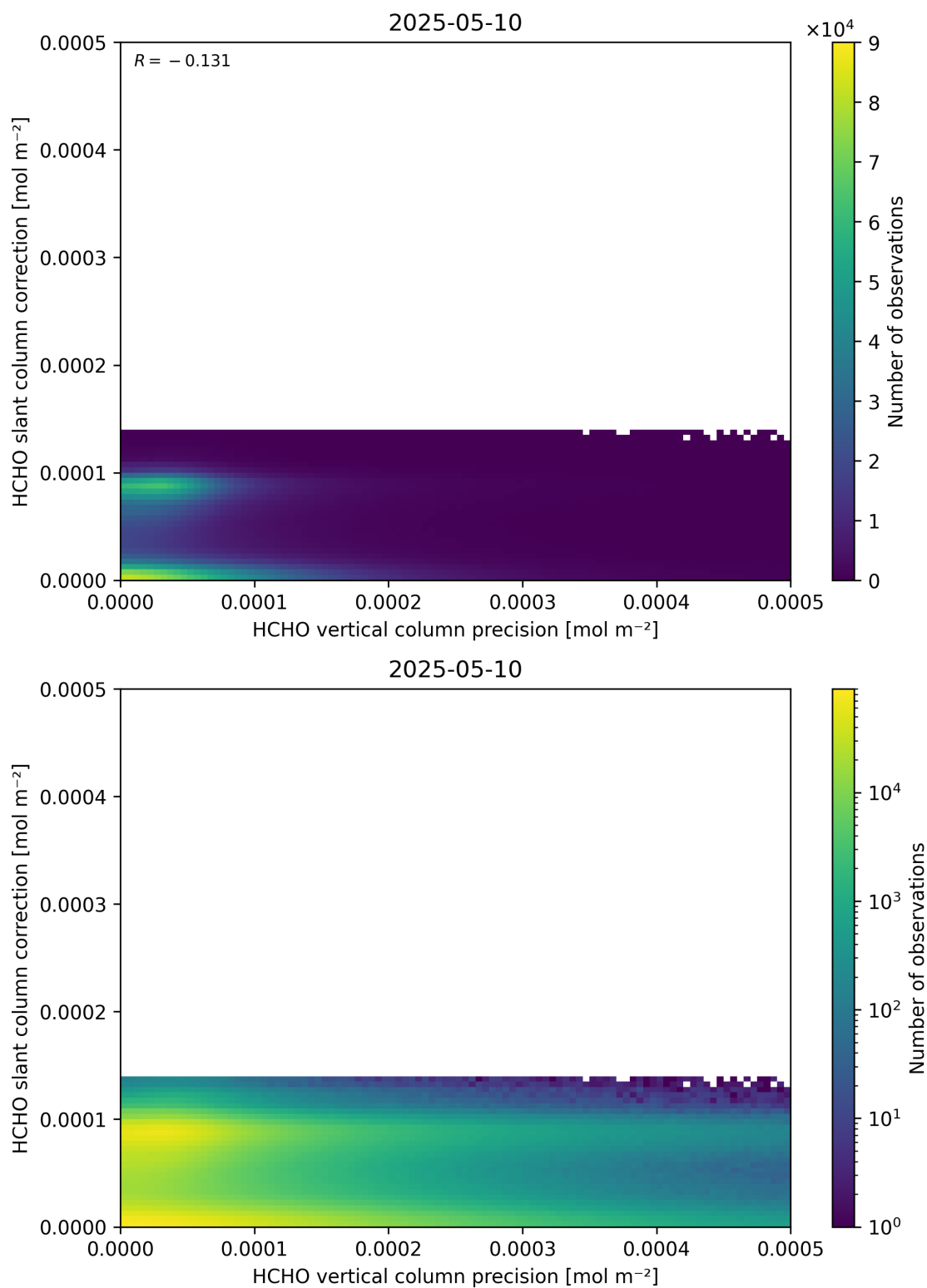
Figure 141: Scatter density plot of “HCHO vertical column precision” against “HCHO slant column correction” for 2025-05-10 to 2025-05-11.
