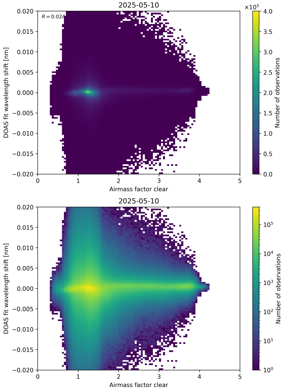
Figure 72: Scatter density plot of “Airmass factor clear” against “DOAS fit wavelength shift” for 2025-05-10 to 2025-05-11.
