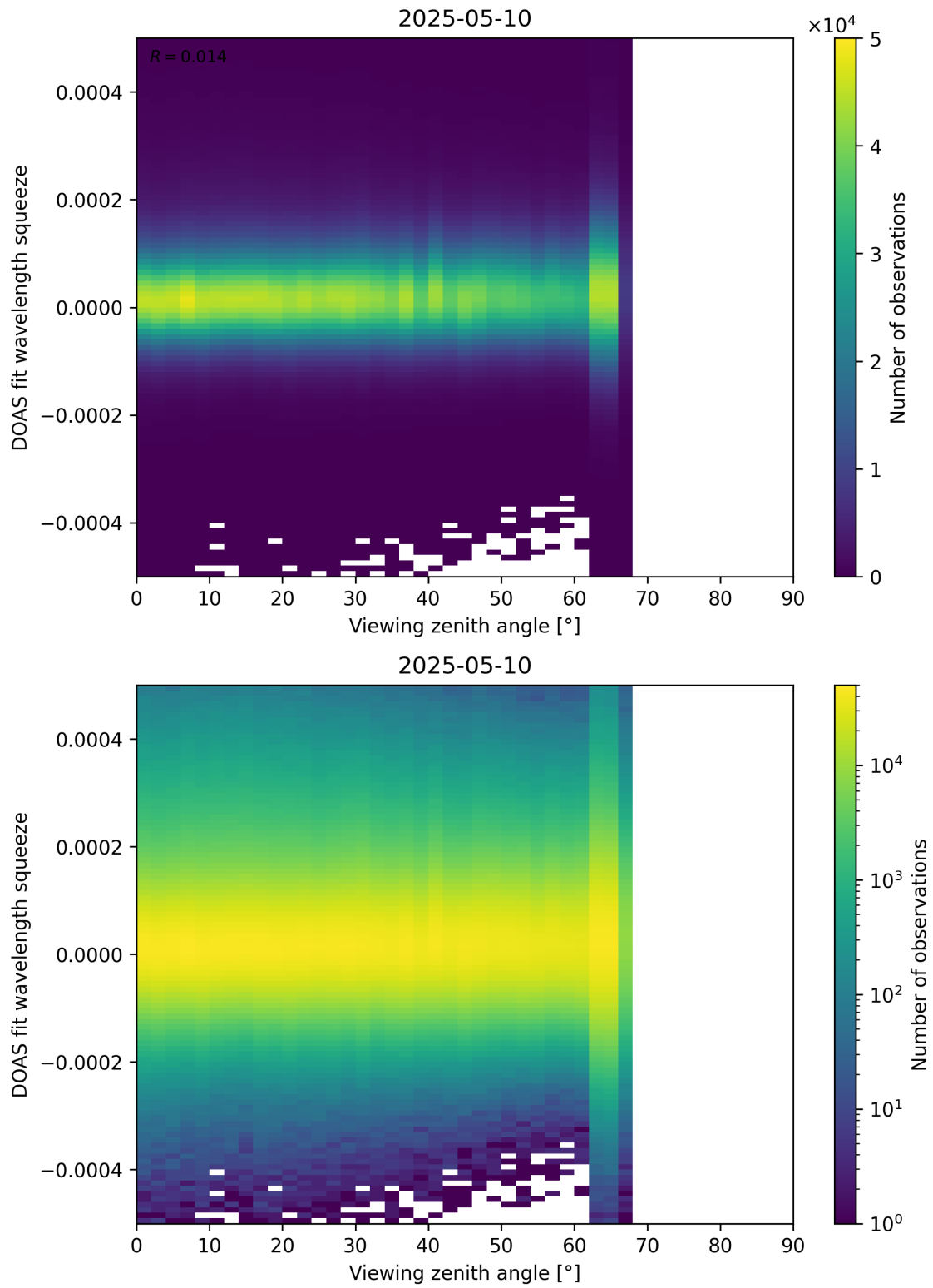
Figure 184: Scatter density plot of “Viewing zenith angle” against “DOAS fit wavelength squeeze” for 2025-05-10 to 2025-05-11.
