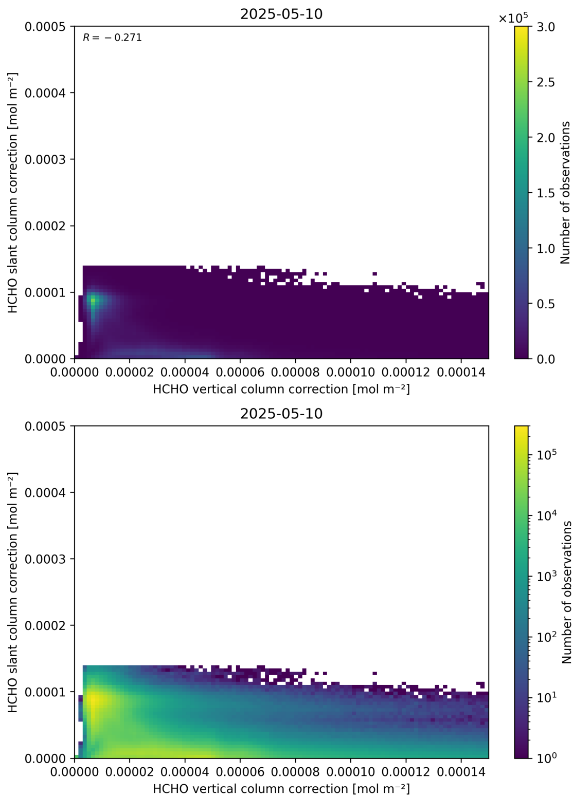
Figure 117: Scatter density plot of “HCHO vertical column correction” against “HCHO slant column correction” for 2025-05-10 to 2025-05-11.
