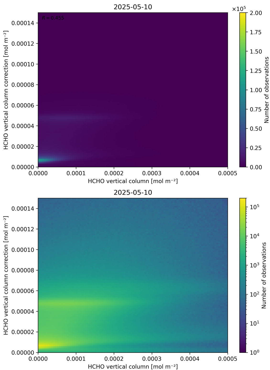
Figure 133: Scatter density plot of “HCHO vertical column” against “HCHO vertical column correction” for 2025-05-10 to 2025-05-11.
