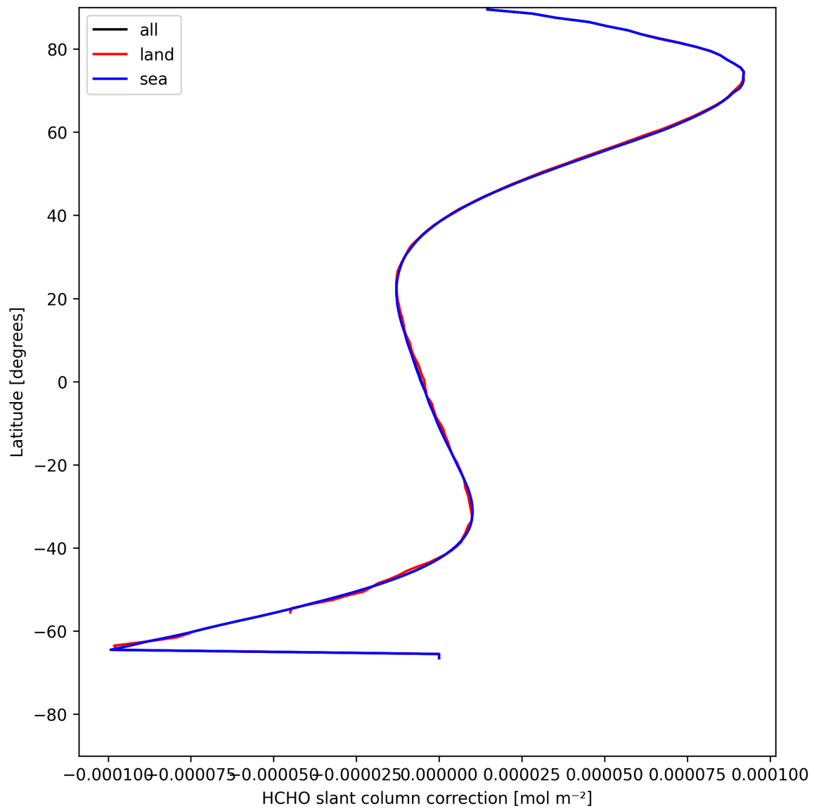
Figure 33: Zonal average of “HCHO slant column correction” for 2025-05-10 to 2025-05-11.
