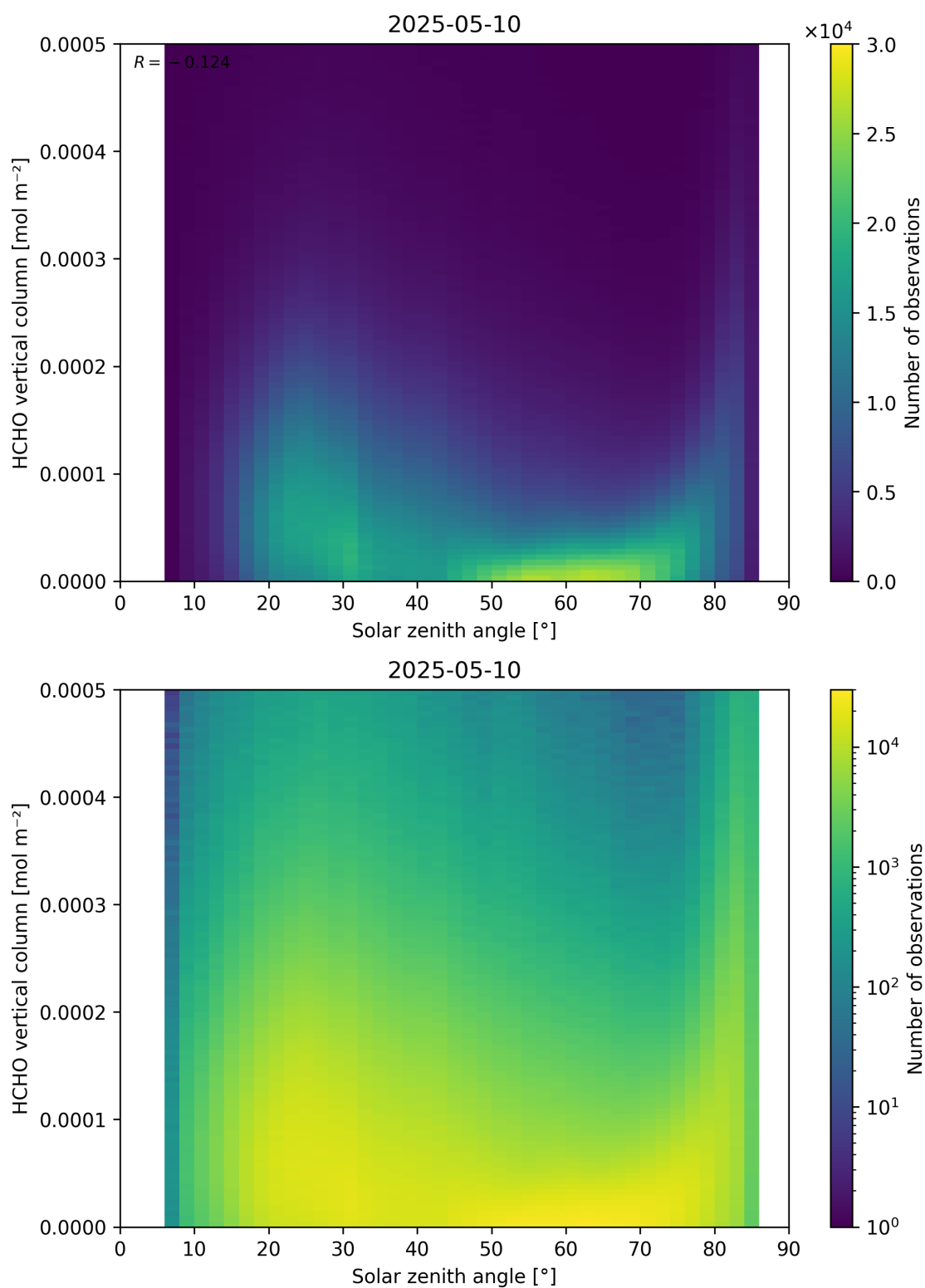
Figure 177: Scatter density plot of “Solar zenith angle” against “HCHO vertical column” for 2025-05-10 to 2025-05-11.
