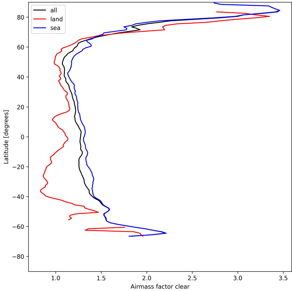
Figure 28: Zonal average of “Airmass factor clear” for 2025-05-10 to 2025-05-11.
