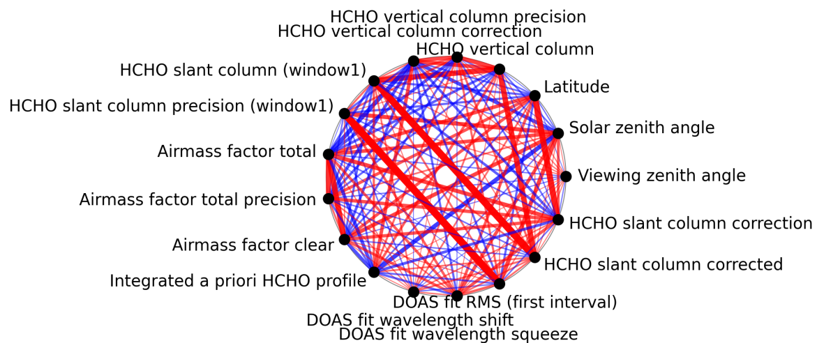
Figure 1: Map of correlation graph for 2025-05-10 to 2025-05-11.
