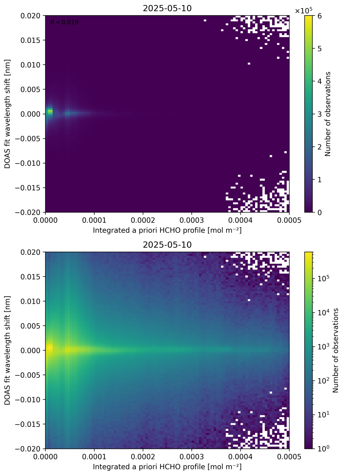
Figure 149: Scatter density plot of “Integrated a priori HCHO profile” against “DOAS fit wavelength shift” for 2025-05-10 to 2025-05-11.
