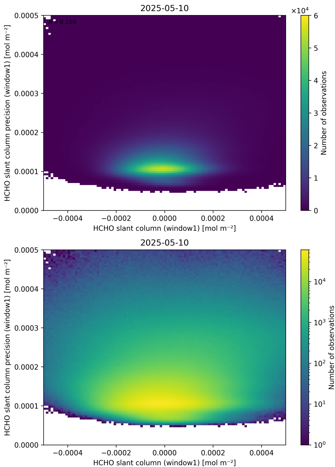
Figure 84: Scatter density plot of “HCHO slant column (window1)” against “HCHO slant column precision (window1)” for 2025-05-10 to 2025-05-11.
