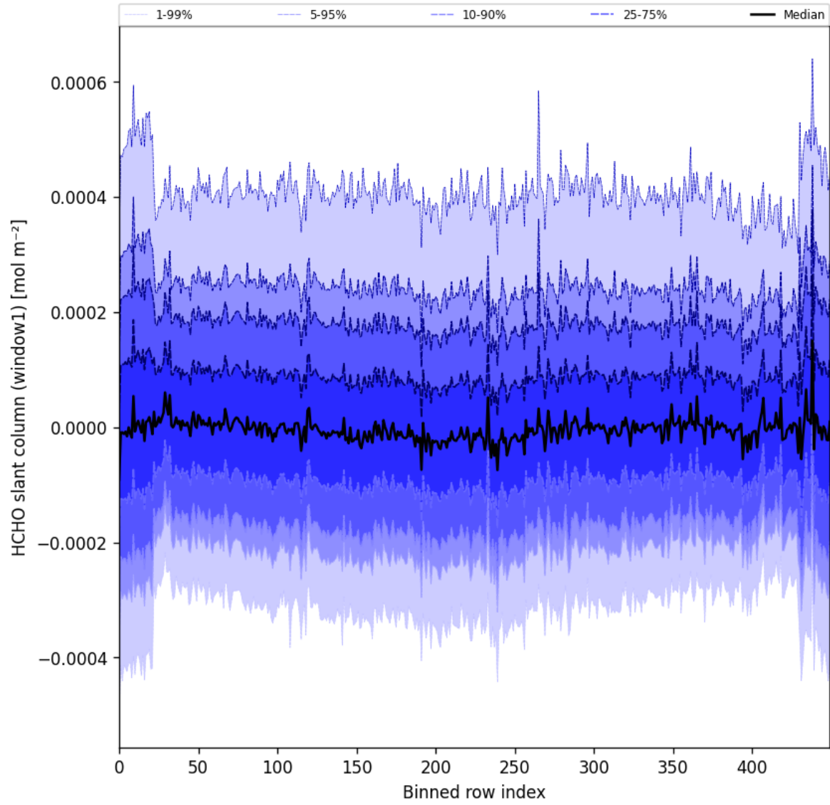
Figure 52: Along track statistics of “HCHO slant column (window1)” for 2025-05-10 to 2025-05-11
