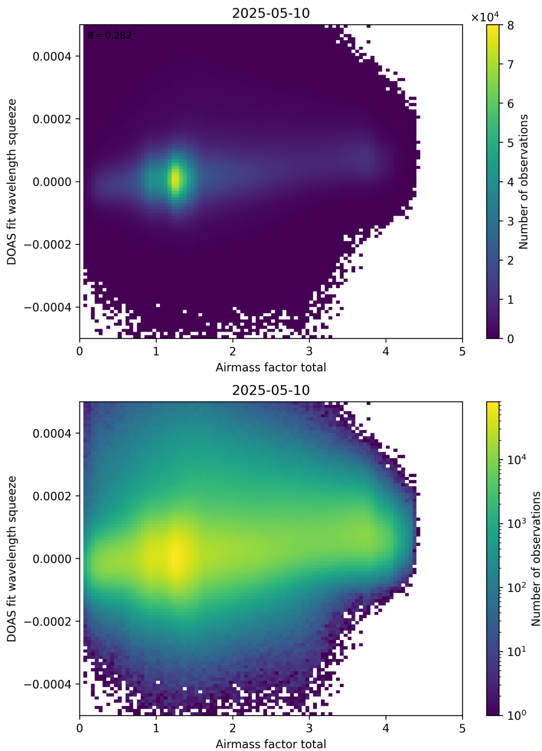
Figure 99: Scatter density plot of “Airmass factor total” against “DOAS fit wavelength squeeze” for 2025-05-10 to 2025-05-11.
