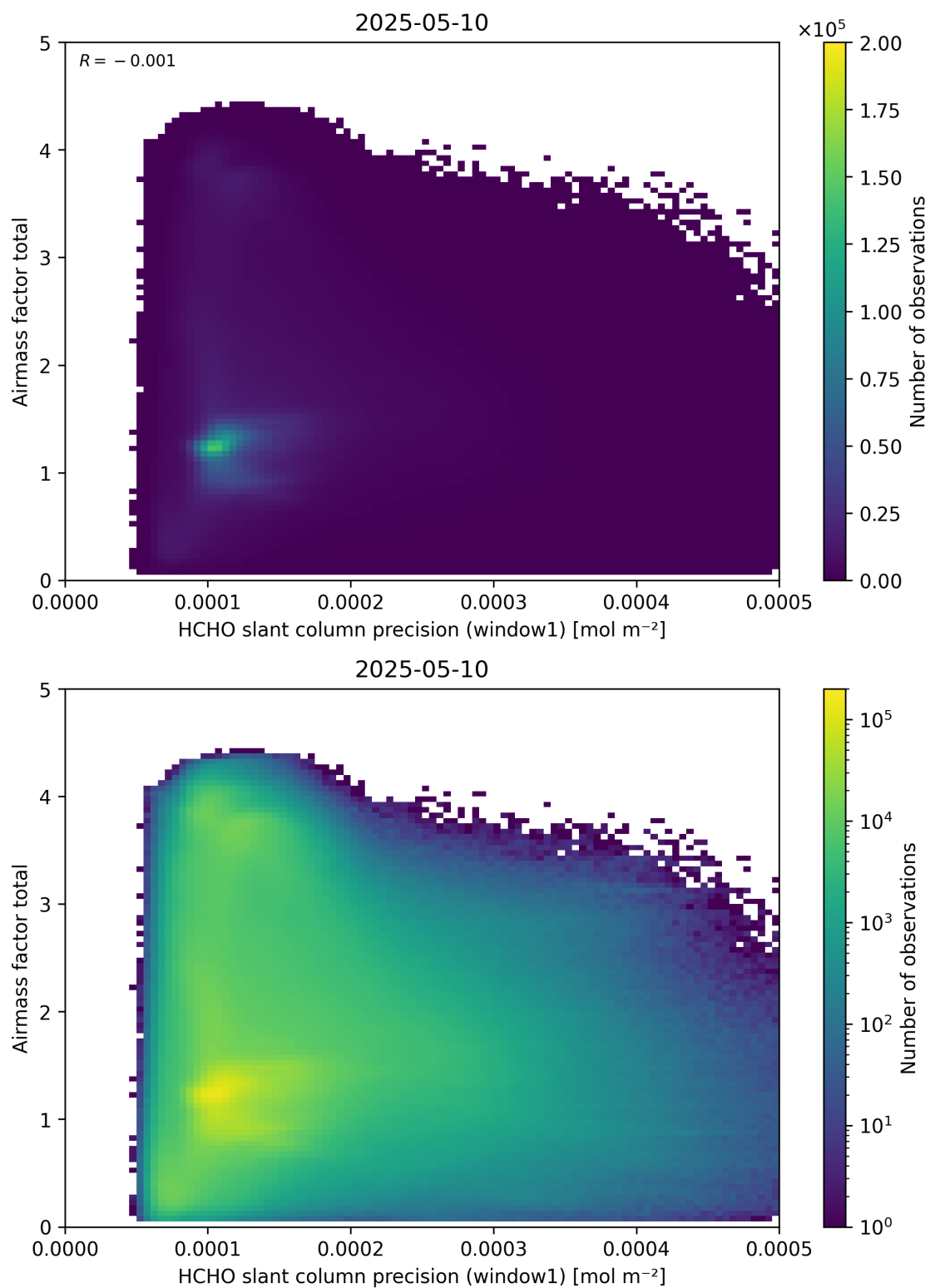
Figure 94: Scatter density plot of “HCHO slant column precision (window1)” against “Airmass factor total” for 2025-05-10 to 2025-05-11.
