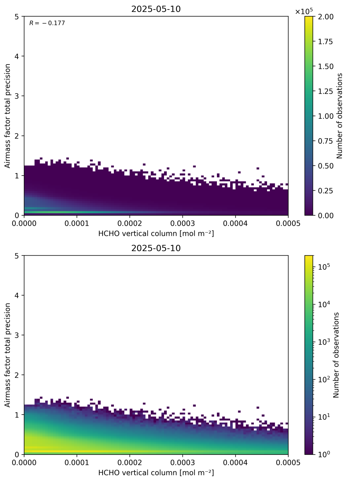
Figure 132: Scatter density plot of “HCHO vertical column” against “Airmass factor total precision” for 2025-05-10 to 2025-05-11.
