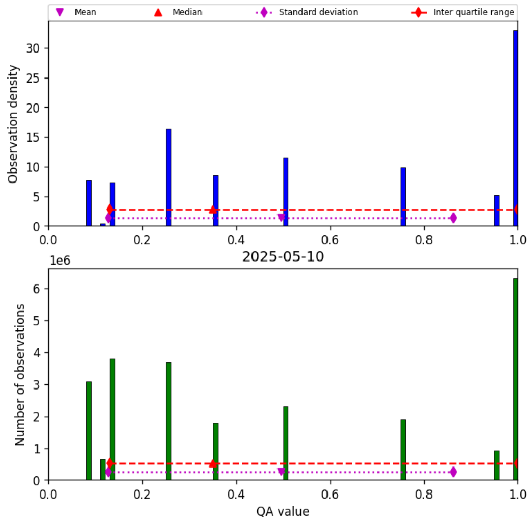
Figure 34: Histogram of “QA value” for 2025-05-10 to 2025-05-11
