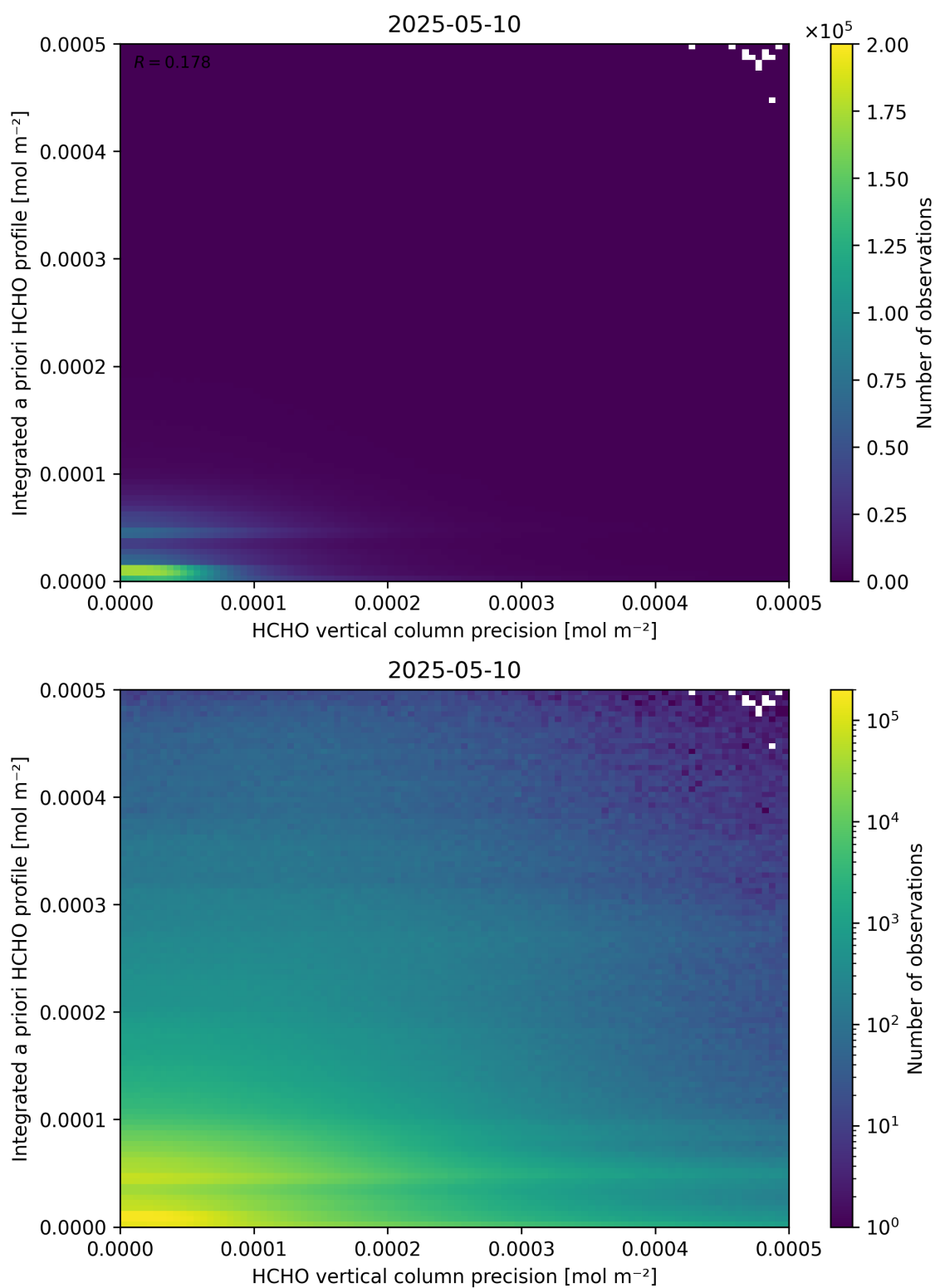
Figure 147: Scatter density plot of “HCHO vertical column precision” against “Integrated a priori HCHO profile” for 2025-05-10 to 2025-05-11.
