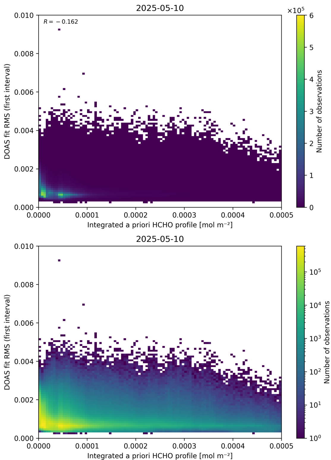
Figure 148: Scatter density plot of “Integrated a priori HCHO profile” against “DOAS fit RMS (first interval)” for 2025-05-10 to 2025-05-11.
