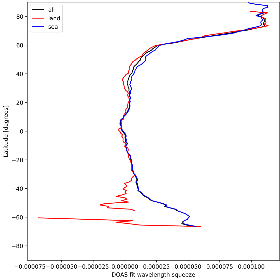
Figure 31: Zonal average of “DOAS fit wavelength squeeze” for 2025-05-10 to 2025-05-11.
