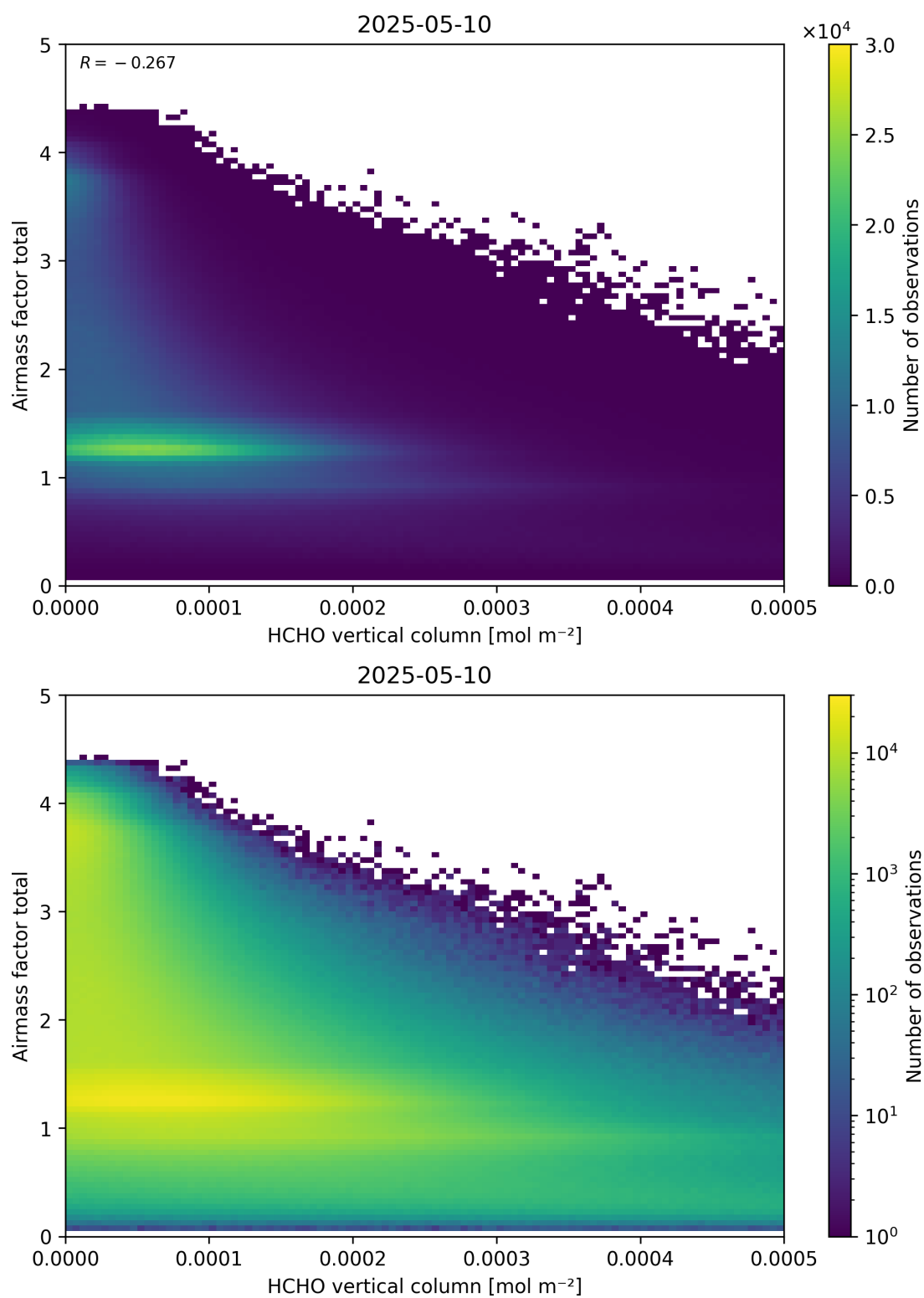
Figure 131: Scatter density plot of “HCHO vertical column” against “Airmass factor total” for 2025-05-10 to 2025-05-11.
