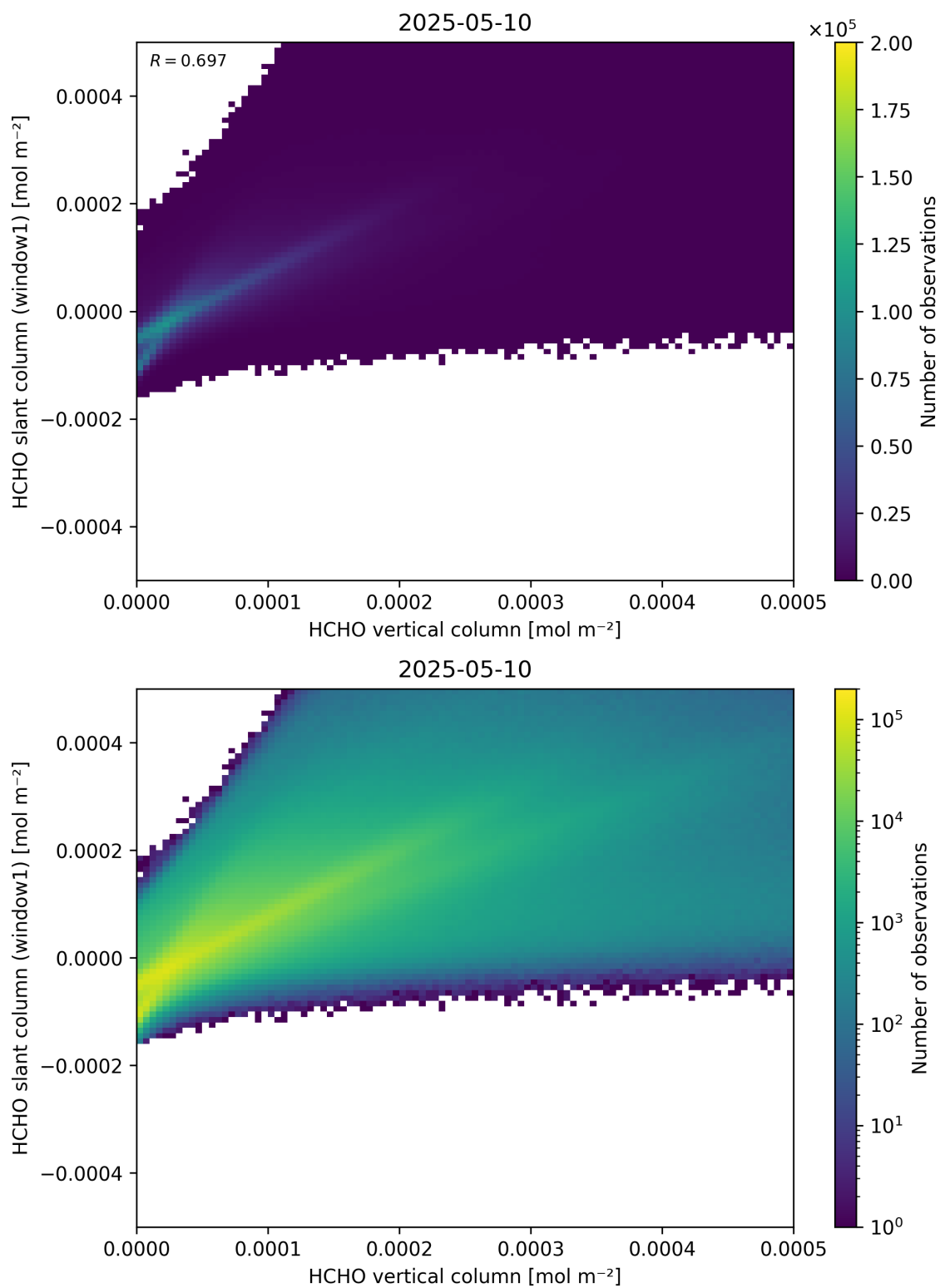
Figure 129: Scatter density plot of “HCHO vertical column” against “HCHO slant column (window1)” for 2025-05-10 to 2025-05-11.
