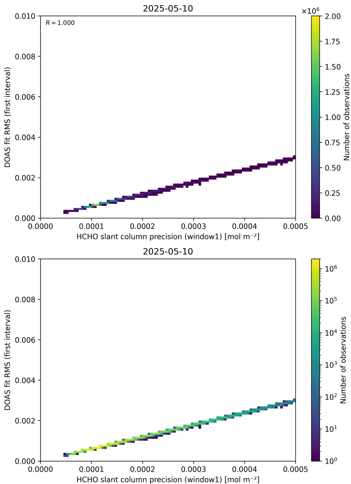
Figure 88: Scatter density plot of “HCHO slant column precision (window1)” against “DOAS fit RMS (first interval)” for 2025-05-10 to 2025-05-11.
