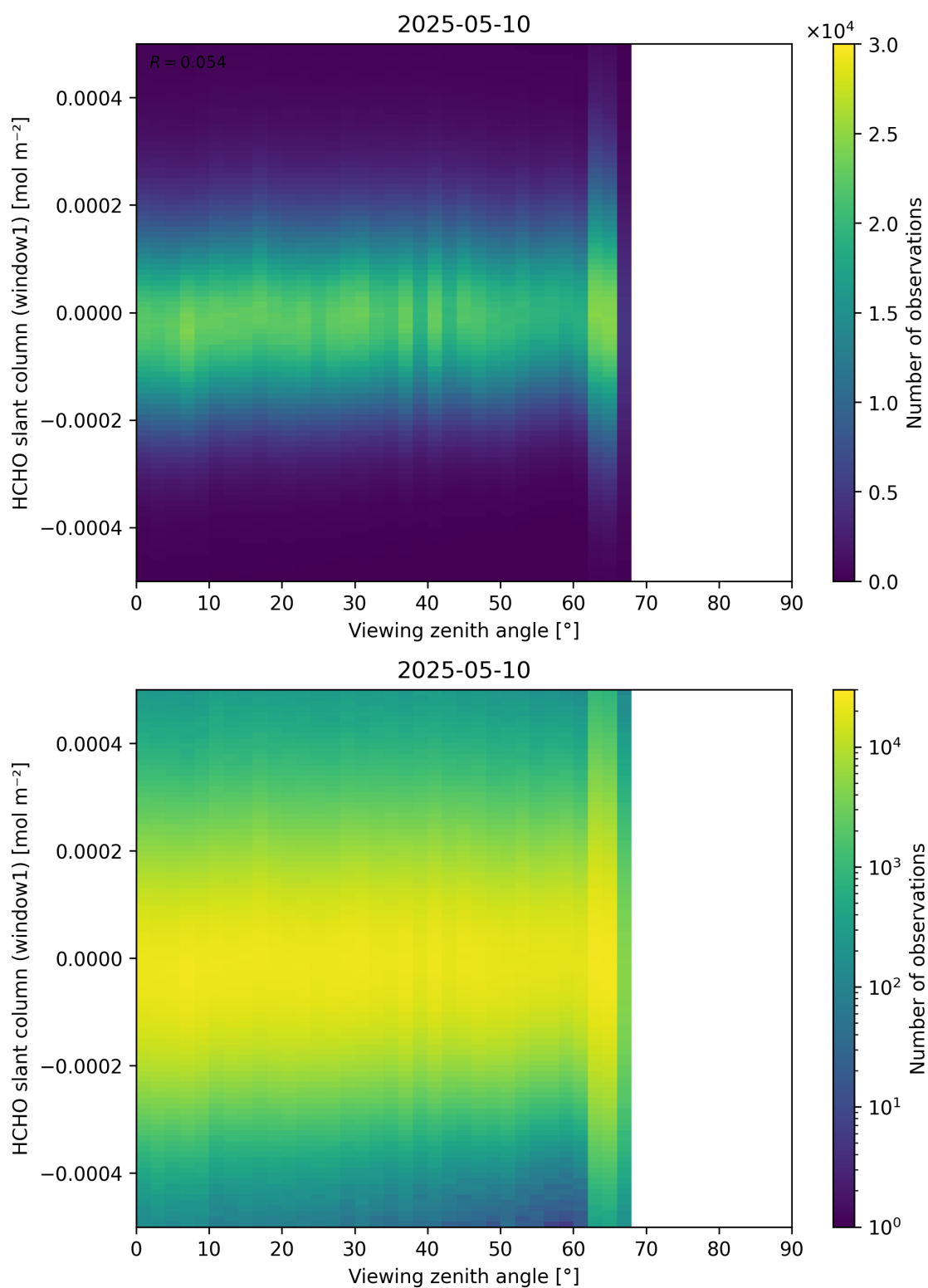
Figure 188: Scatter density plot of “Viewing zenith angle” against “HCHO slant column (window1)” for 2025-05-10 to 2025-05-11.
