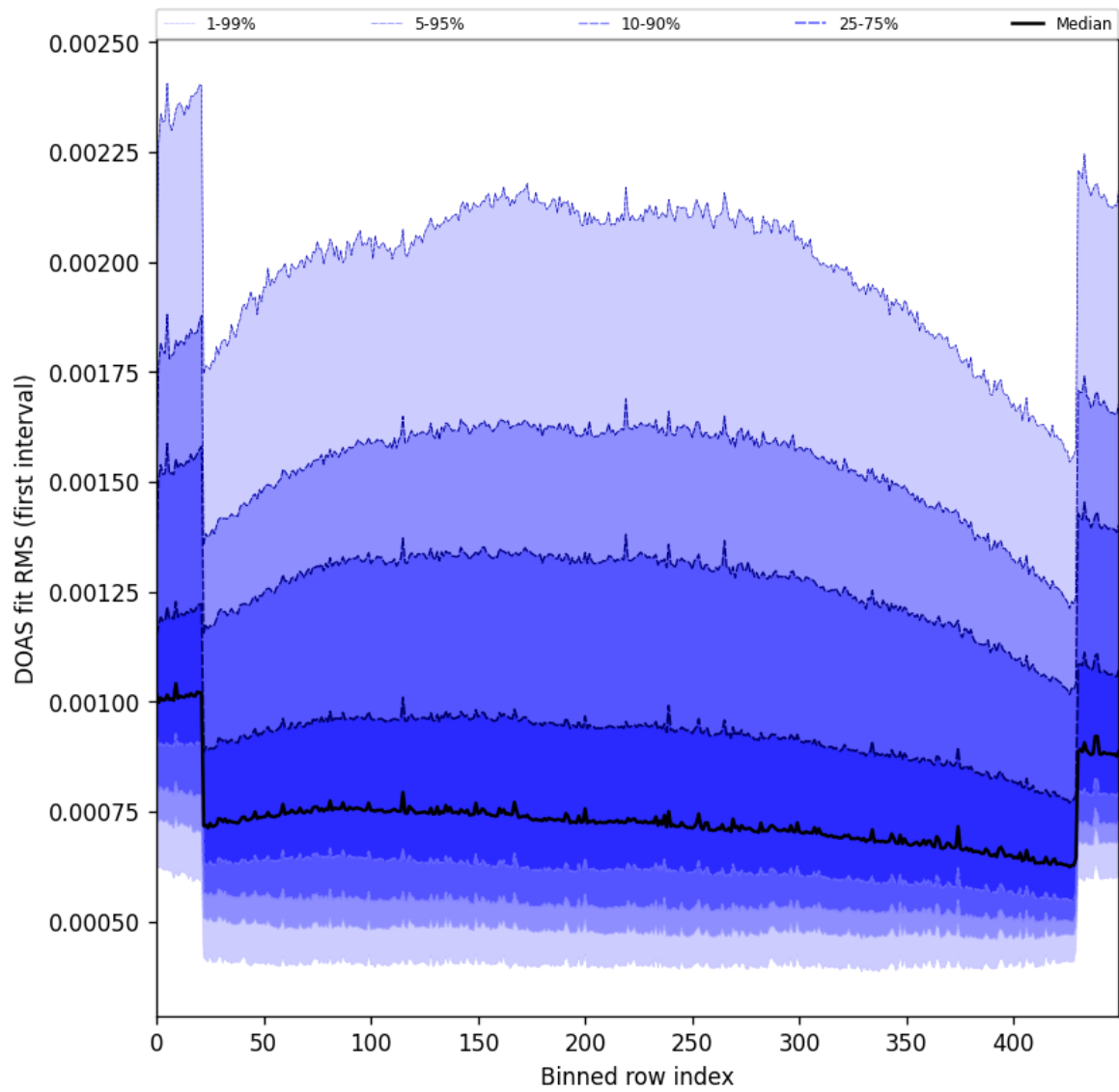
Figure 60: Along track statistics of “DOAS fit RMS (first interval)” for 2025-05-10 to 2025-05-11
