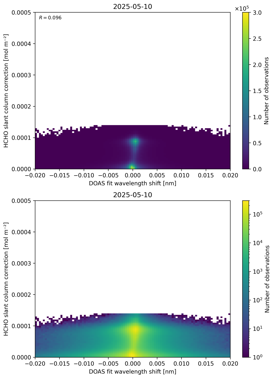
Figure 67: Scatter density plot of “DOAS fit wavelength shift” against “HCHO slant column correction” for 2025-05-10 to 2025-05-11.
