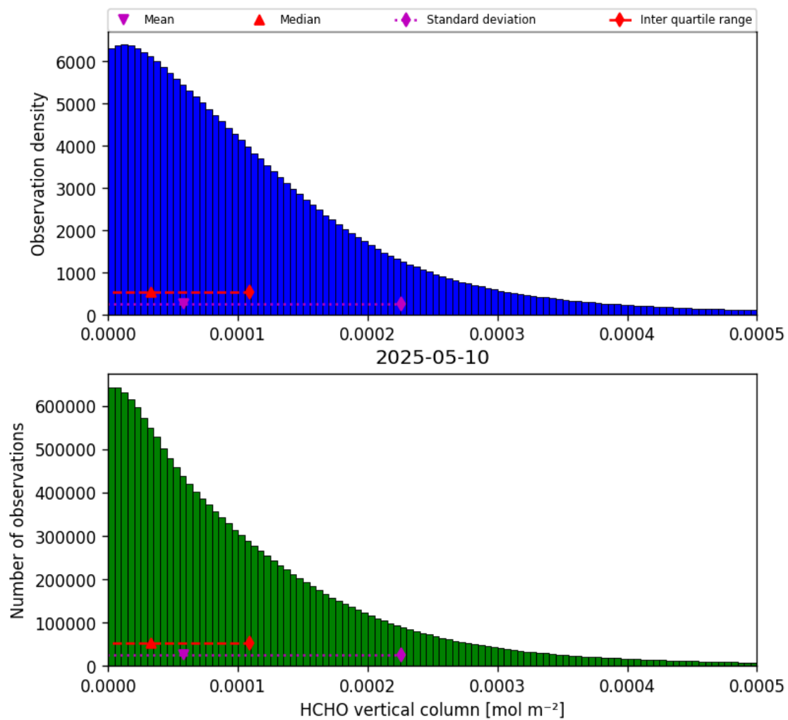
Figure 35: Histogram of “HCHO vertical column” for 2025-05-10 to 2025-05-11
