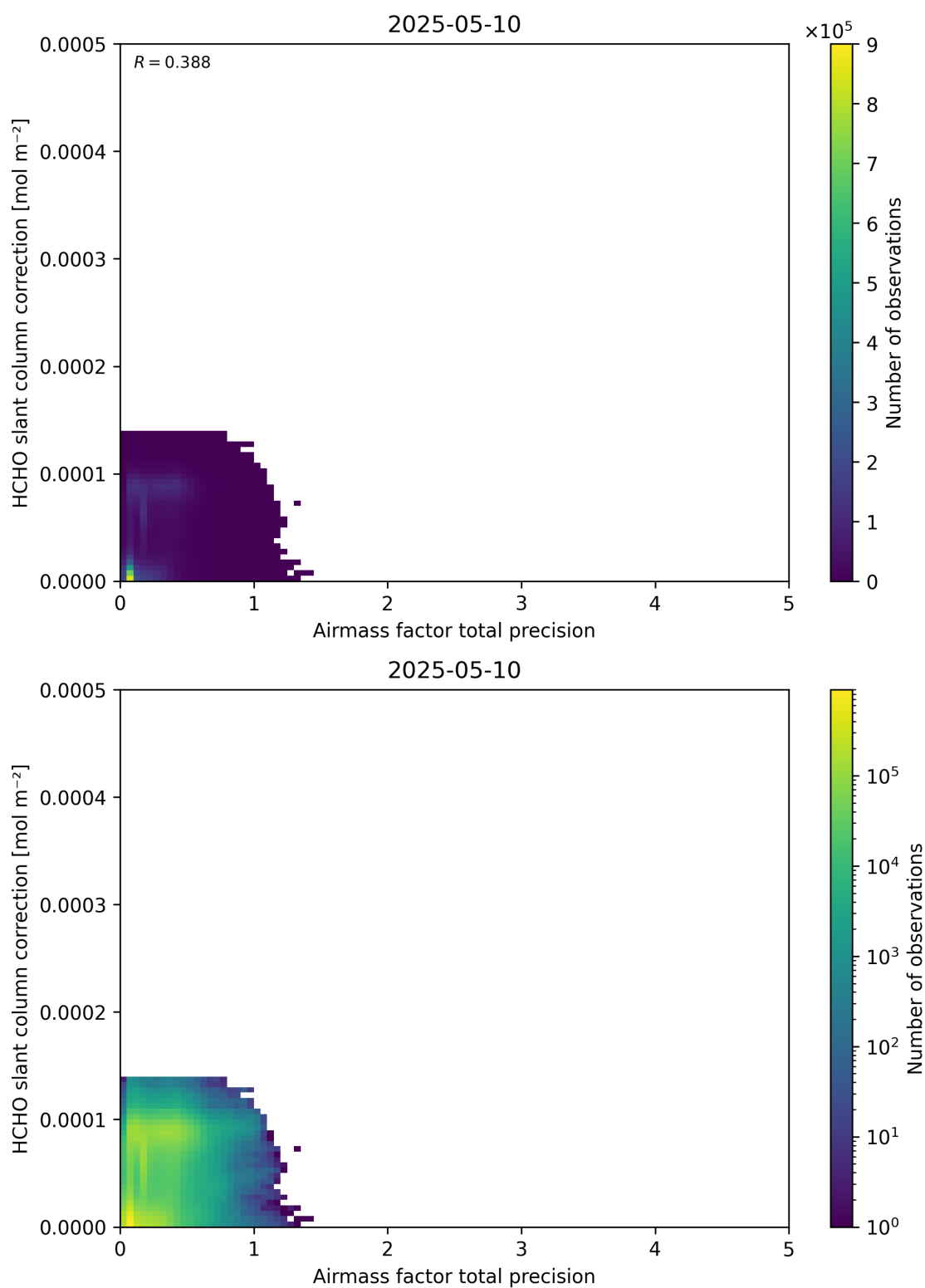
Figure 110: Scatter density plot of “Airmass factor total precision” against “HCHO slant column correction” for 2025-05-10 to 2025-05-11.
