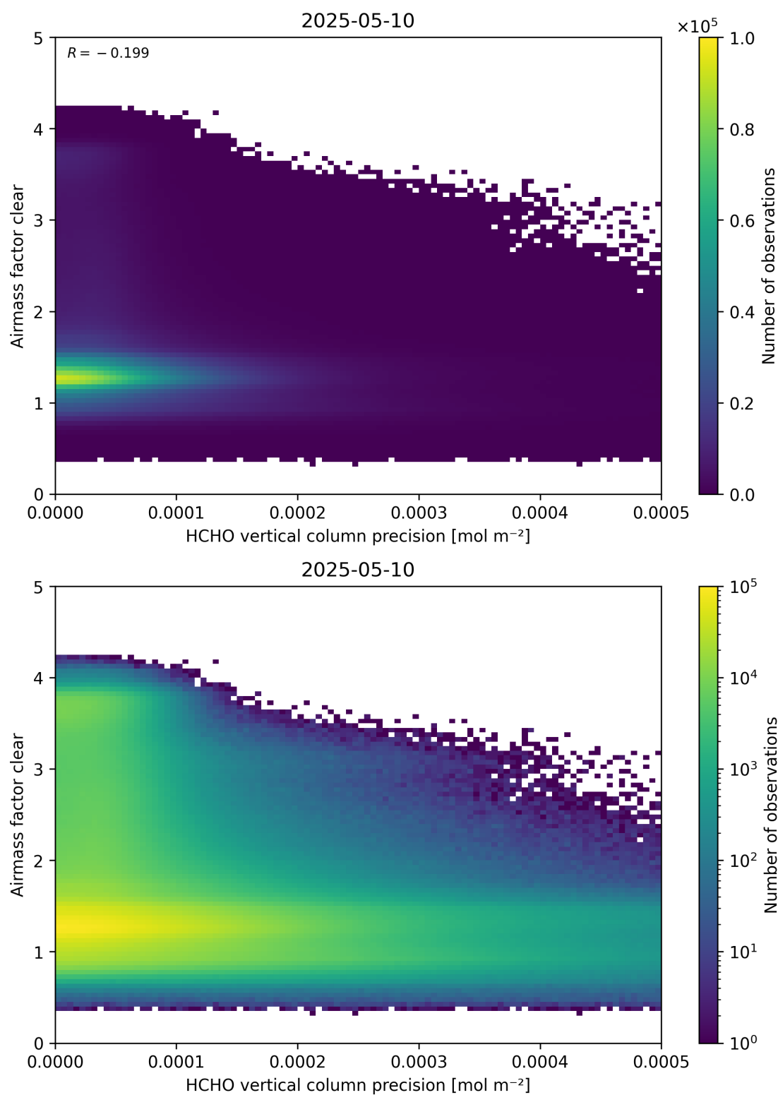
Figure 139: Scatter density plot of “HCHO vertical column precision” against “Airmass factor clear” for 2025-05-10 to 2025-05-11.
