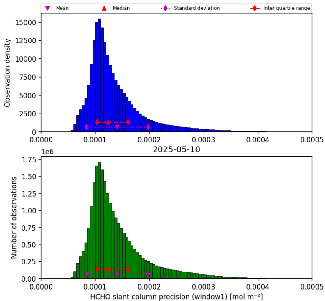
Figure 39: Histogram of “HCHO slant column precision (window1)” for 2025-05-10 to 2025-05-11
