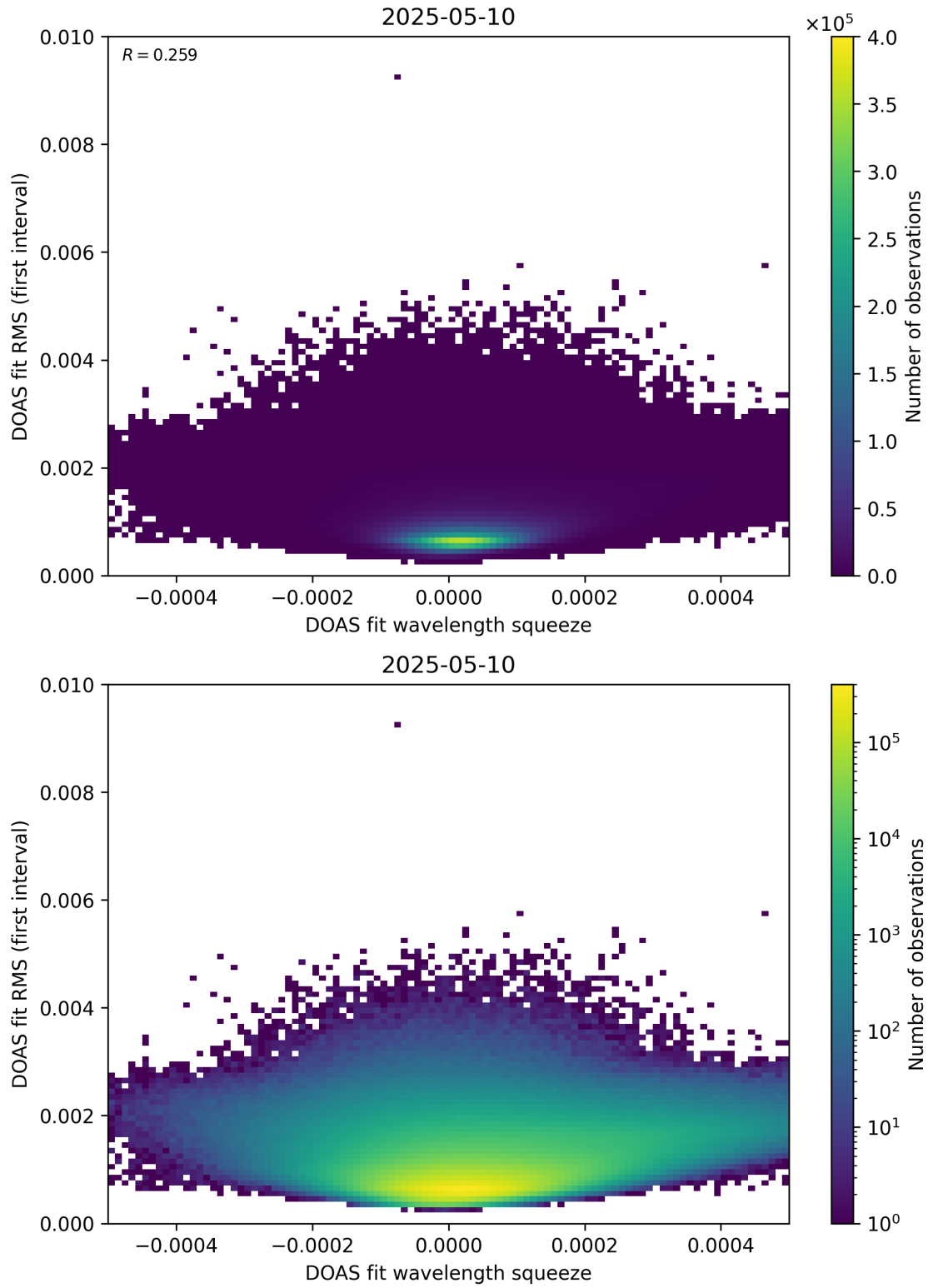
Figure 68: Scatter density plot of “DOAS fit wavelength squeeze” against “DOAS fit RMS (first interval)” for 2025-05-10 to 2025-05-11.
