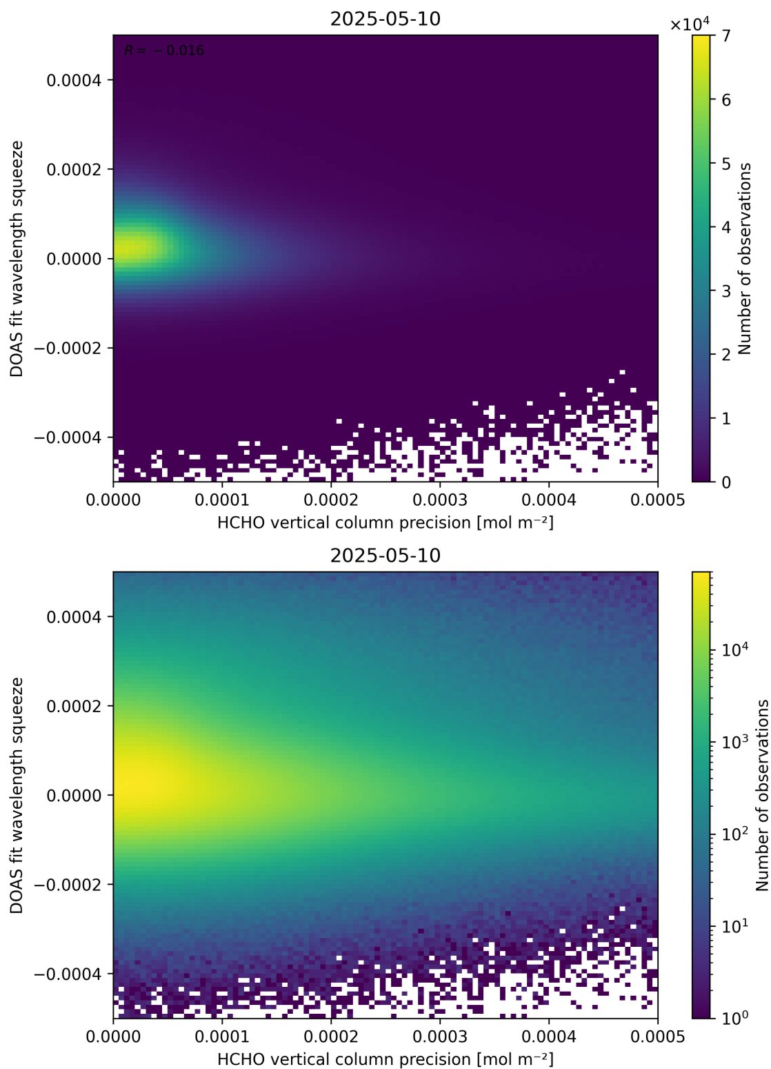
Figure 138: Scatter density plot of “HCHO vertical column precision” against “DOAS fit wavelength squeeze” for 2025-05-10 to 2025-05-11.
