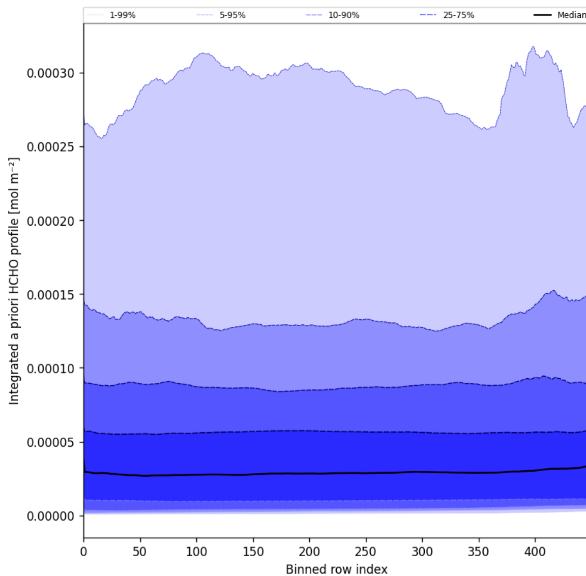
Figure 57: Along track statistics of "Integrated a priori HCHO profile" for 2025-05-10 to 2025-05-11
