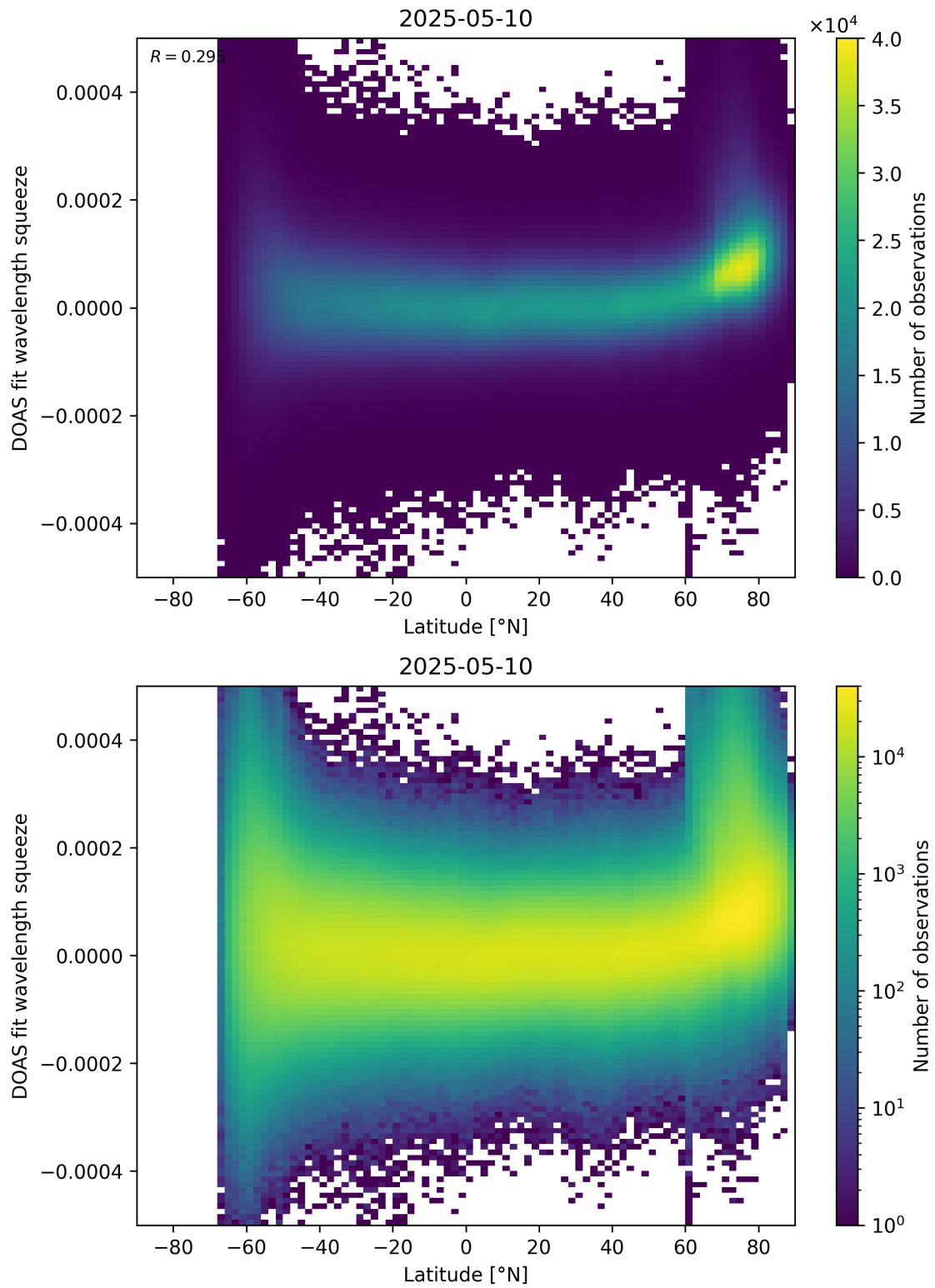
Figure 155: Scatter density plot of “Latitude” against “DOAS fit wavelength squeeze” for 2025-05-10 to 2025-05-11.
