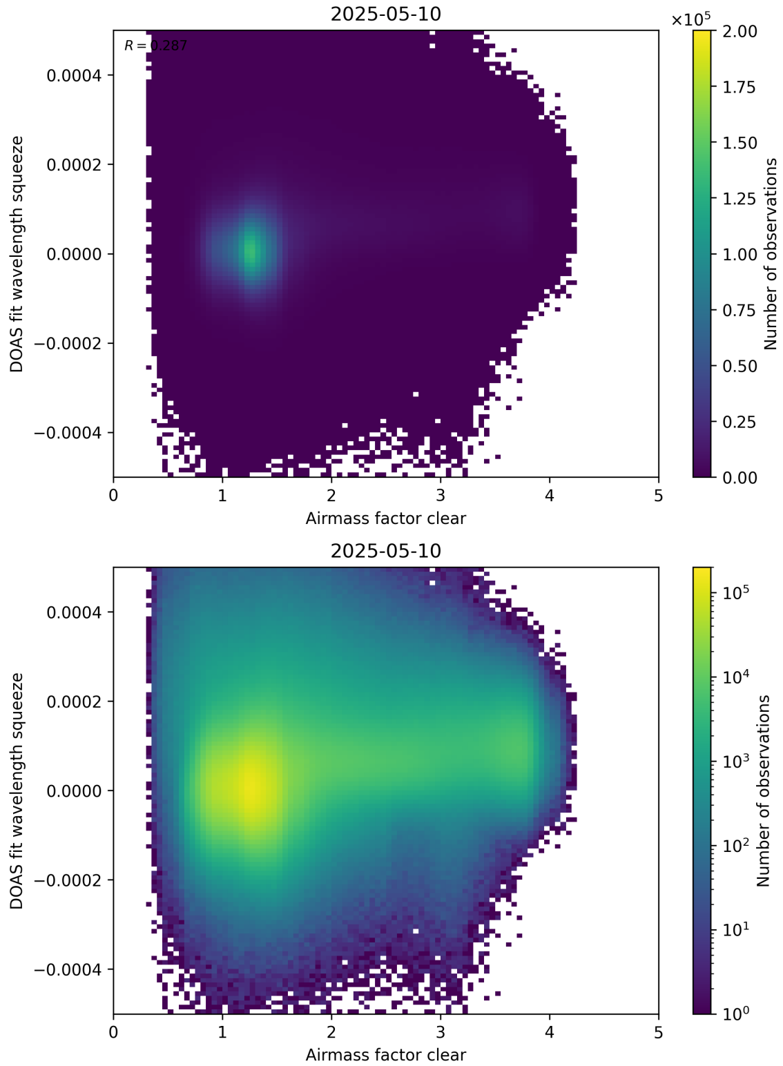
Figure 73: Scatter density plot of “Airmass factor clear” against “DOAS fit wavelength squeeze” for 2025-05-10 to 2025-05-11.
