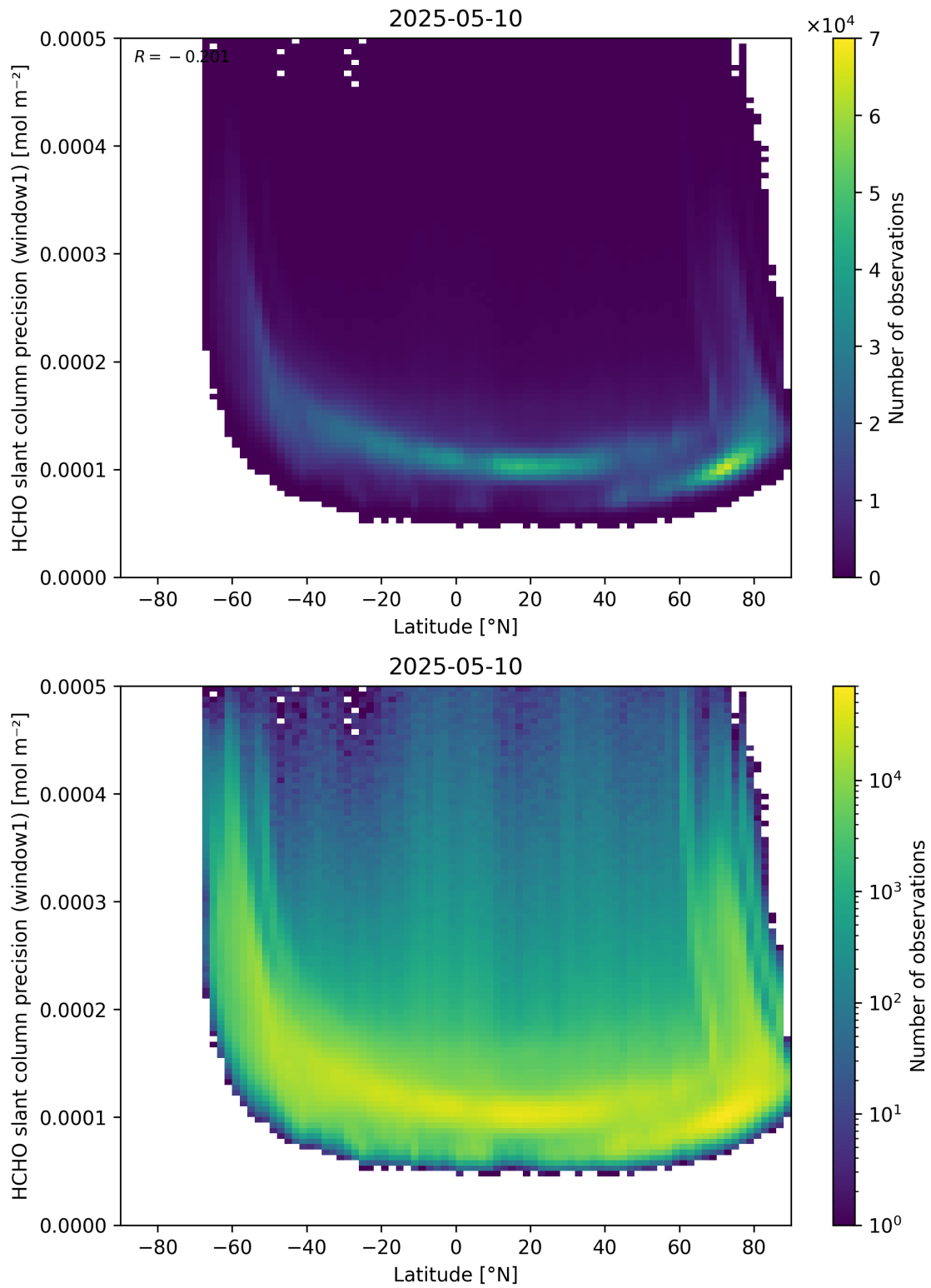
Figure 160: Scatter density plot of “Latitude” against “HCHO slant column precision (window1)” for 2025-05-10 to 2025-05-11.
