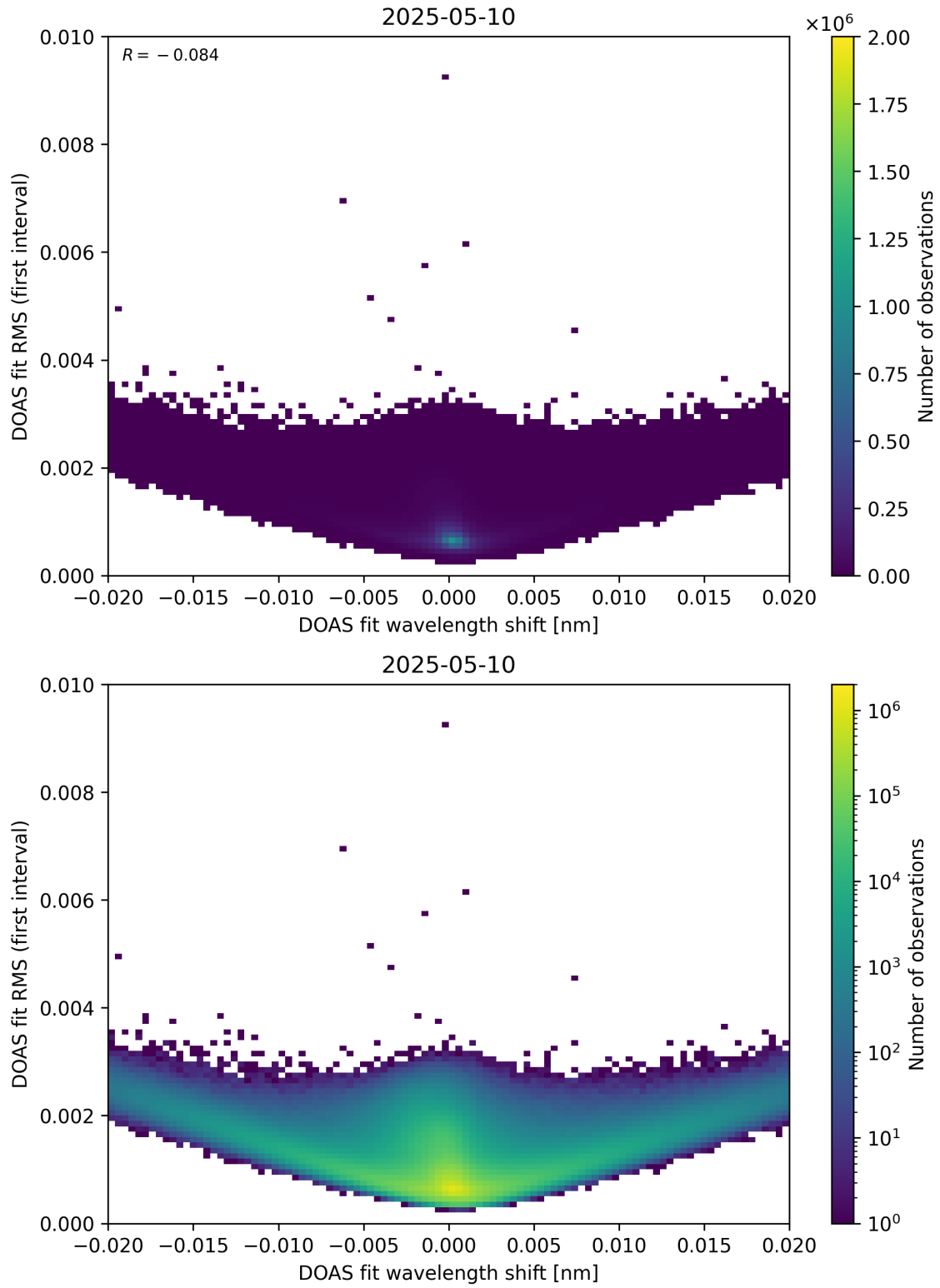
Figure 64: Scatter density plot of “DOAS fit wavelength shift” against “DOAS fit RMS (first interval)” for 2025-05-10 to 2025-05-11.
