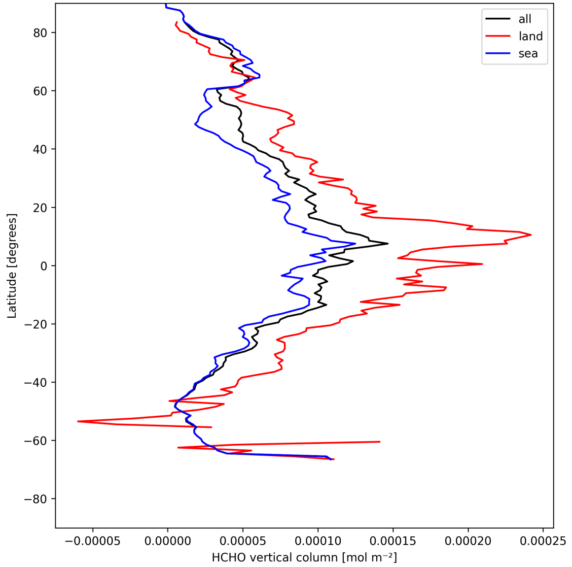
Figure 21: Zonal average of “HCHO vertical column” for 2025-05-10 to 2025-05-11.
