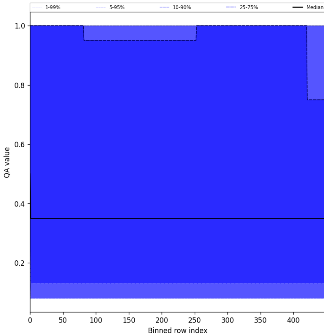
Figure 48: Along track statistics of “QA value” for 2025-05-10 to 2025-05-11
