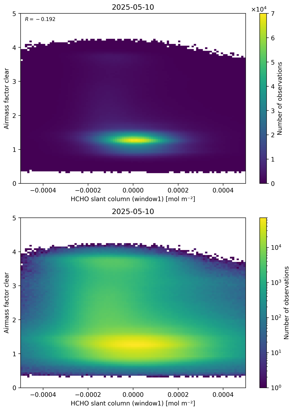
Figure 81: Scatter density plot of “HCHO slant column (window1)” against “Airmass factor clear” for 2025-05-10 to 2025-05-11.
