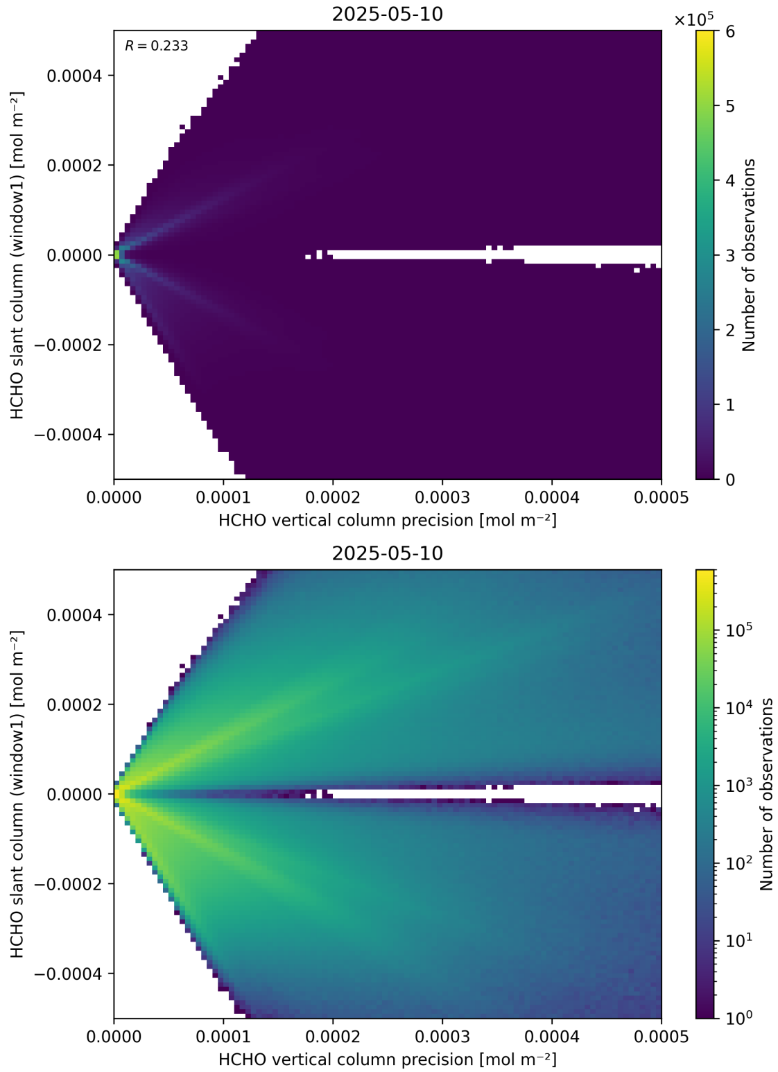
Figure 142: Scatter density plot of “HCHO vertical column precision” against “HCHO slant column (window1)” for 2025-05-10 to 2025-05-11.
