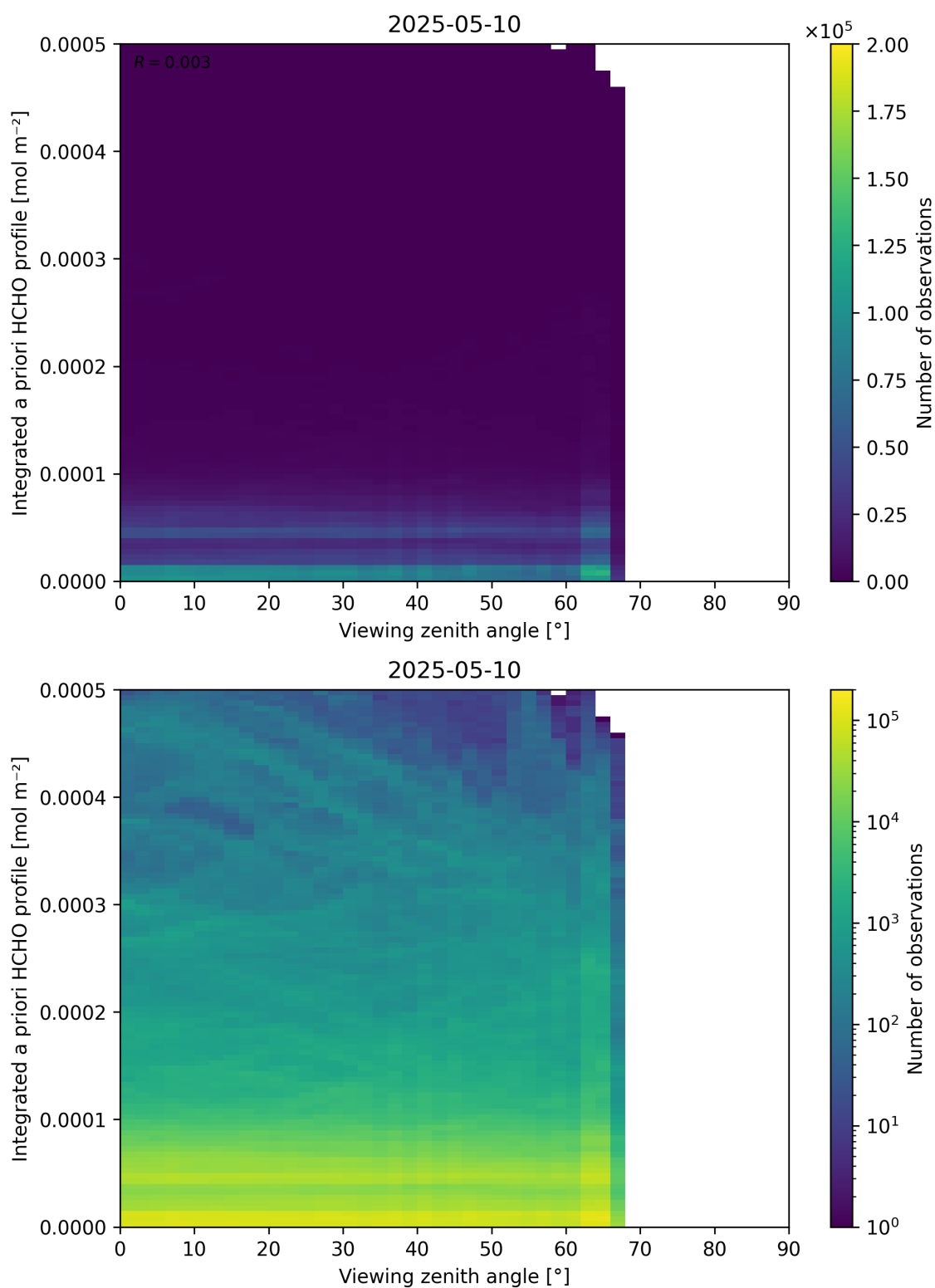
Figure 195: Scatter density plot of “Viewing zenith angle” against “Integrated a priori HCHO profile” for 2025-05-10 to 2025-05-11.
