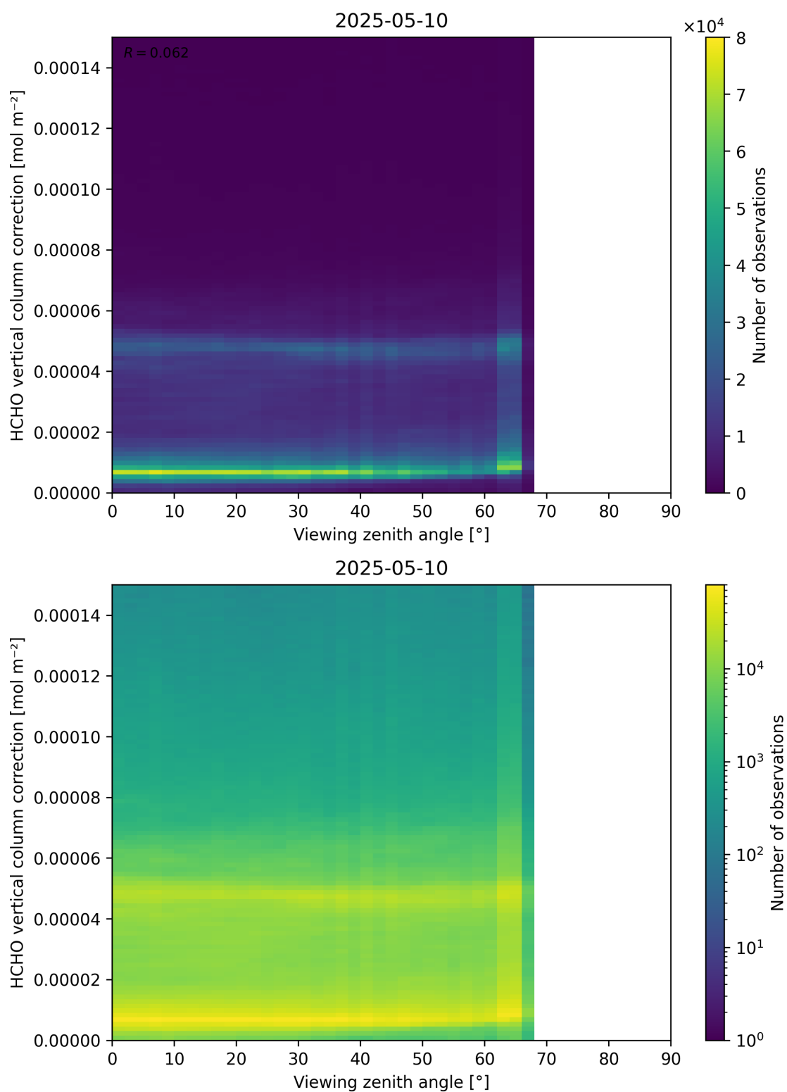
Figure 193: Scatter density plot of “Viewing zenith angle” against “HCHO vertical column correction” for 2025-05-10 to 2025-05-11.
