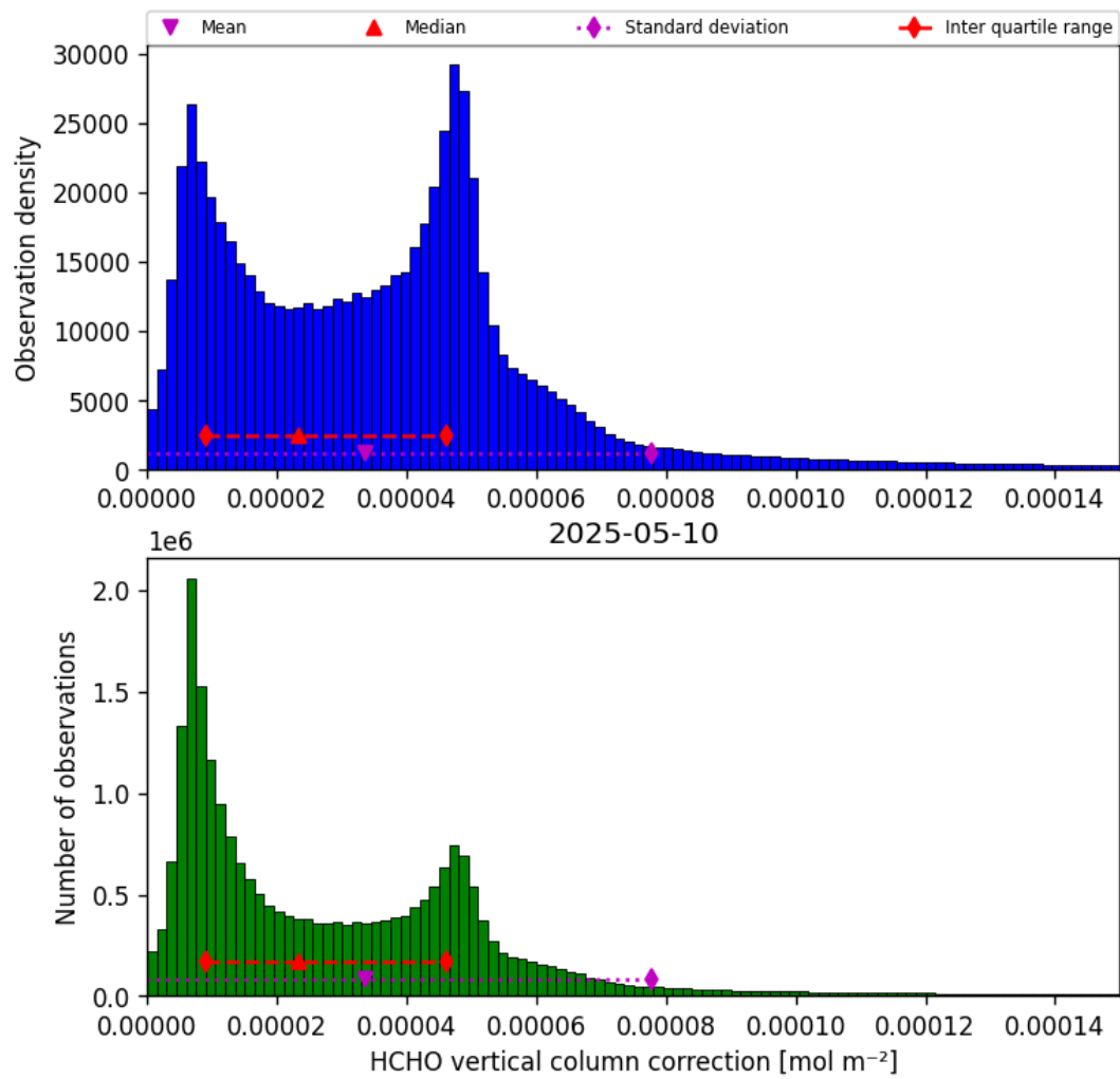
Figure 37: Histogram of “HCHO vertical column correction” for 2025-05-10 to 2025-05-11
