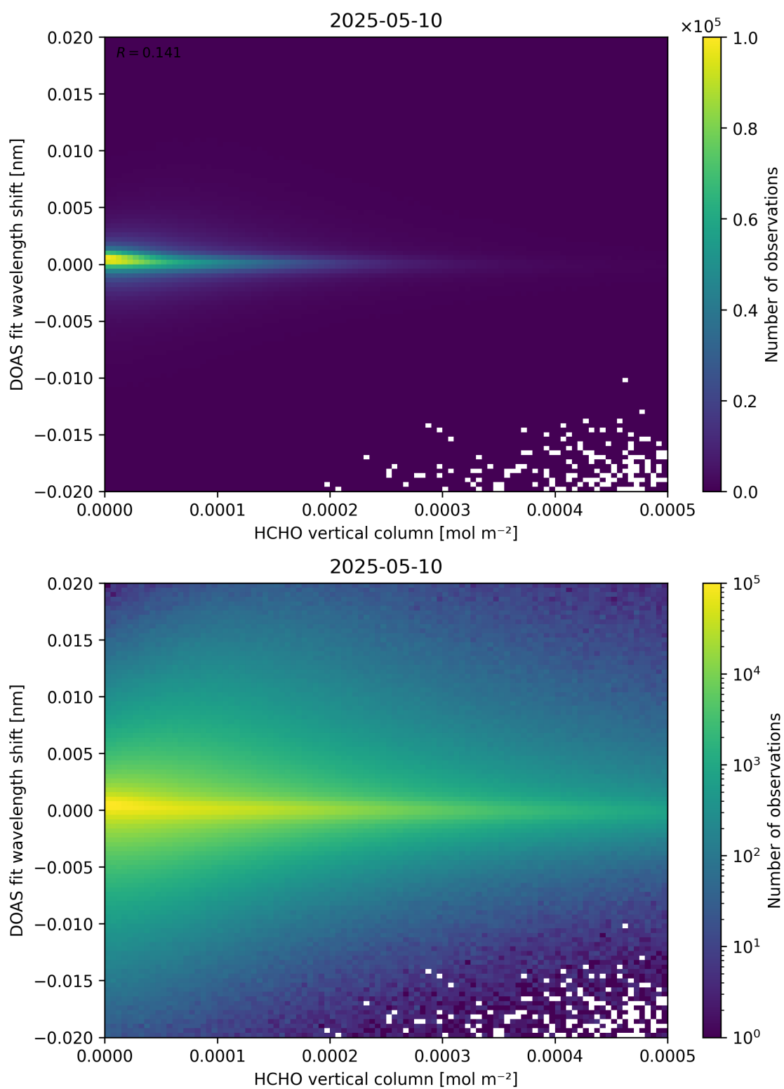
Figure 124: Scatter density plot of “HCHO vertical column” against “DOAS fit wavelength shift” for 2025-05-10 to 2025-05-11.
