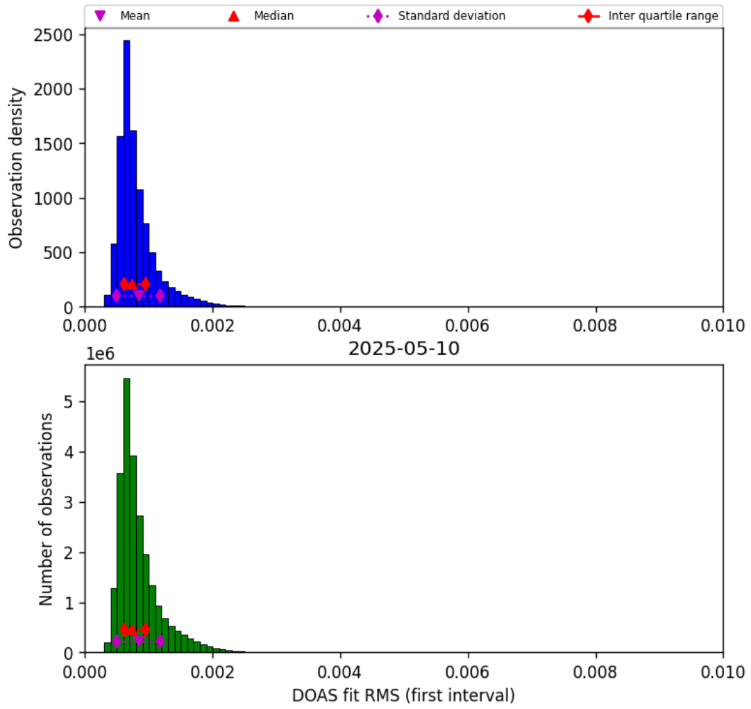
Figure 46: Histogram of “DOAS fit RMS (first interval)” for 2025-05-10 to 2025-05-11
