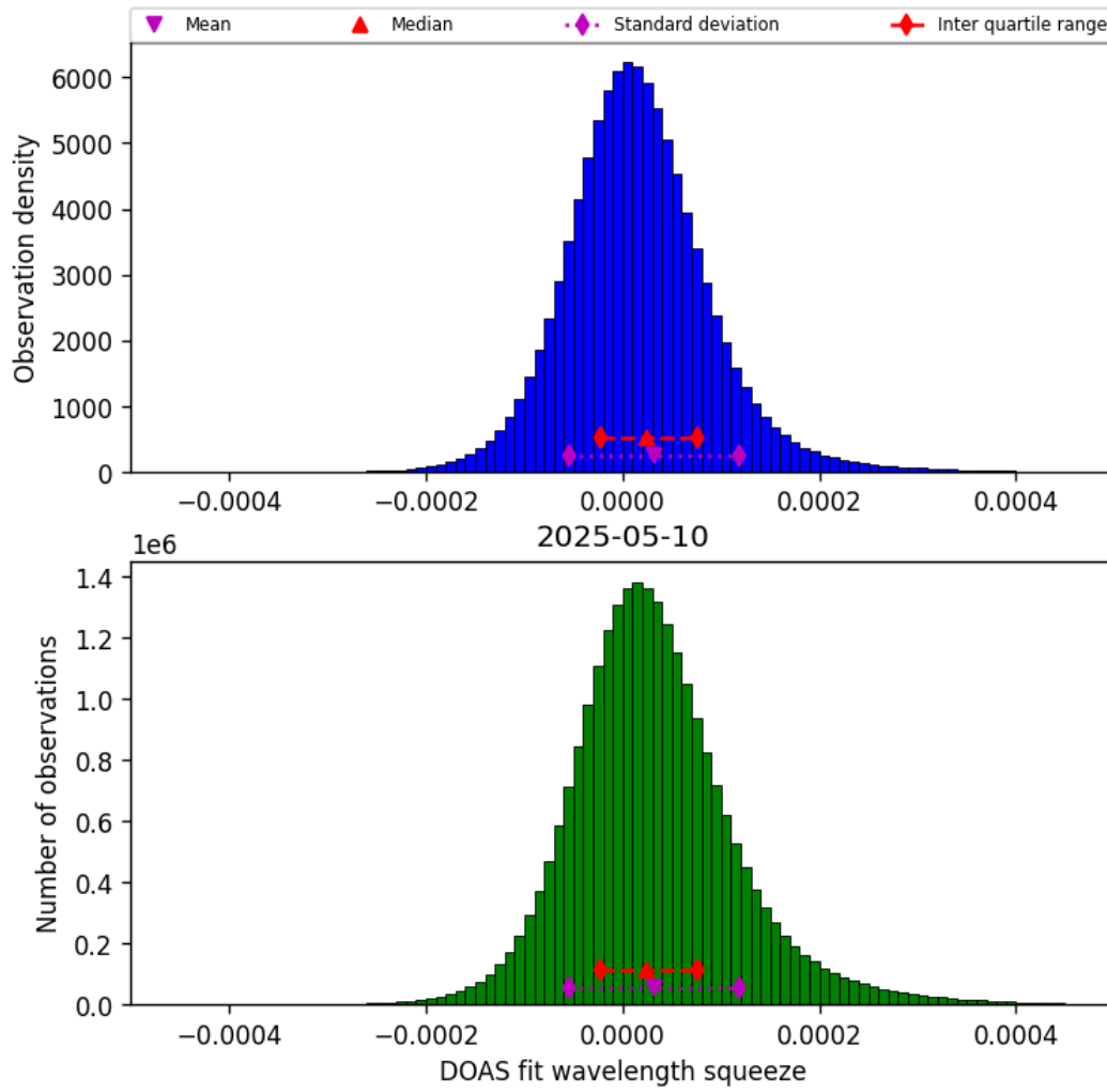
Figure 45: Histogram of “DOAS fit wavelength squeeze” for 2025-05-10 to 2025-05-11
