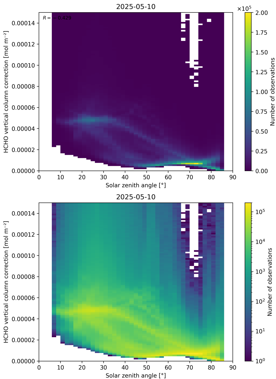
Figure 178: Scatter density plot of “Solar zenith angle” against “HCHO vertical column correction” for 2025-05-10 to 2025-05-11.
