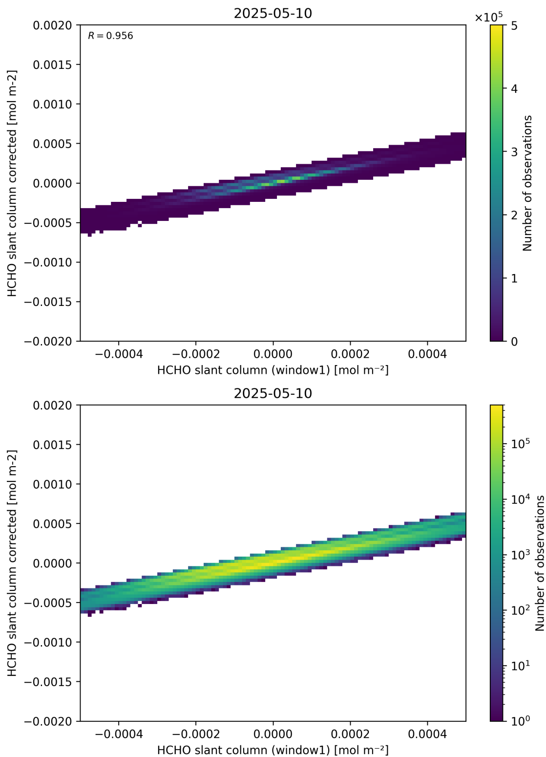
Figure 82: Scatter density plot of “HCHO slant column (window1)” against “HCHO slant column corrected” for 2025-05-10 to 2025-05-11.
