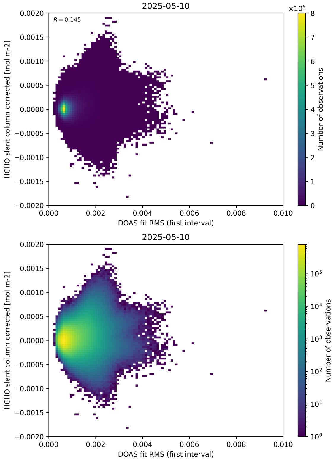
Figure 62: Scatter density plot of “DOAS fit RMS (first interval)” against “HCHO slant column corrected” for 2025-05-10 to 2025-05-11.
