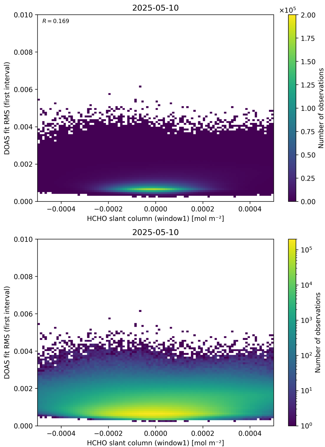
Figure 78: Scatter density plot of “HCHO slant column (window1)” against “DOAS fit RMS (first interval)” for 2025-05-10 to 2025-05-11.
