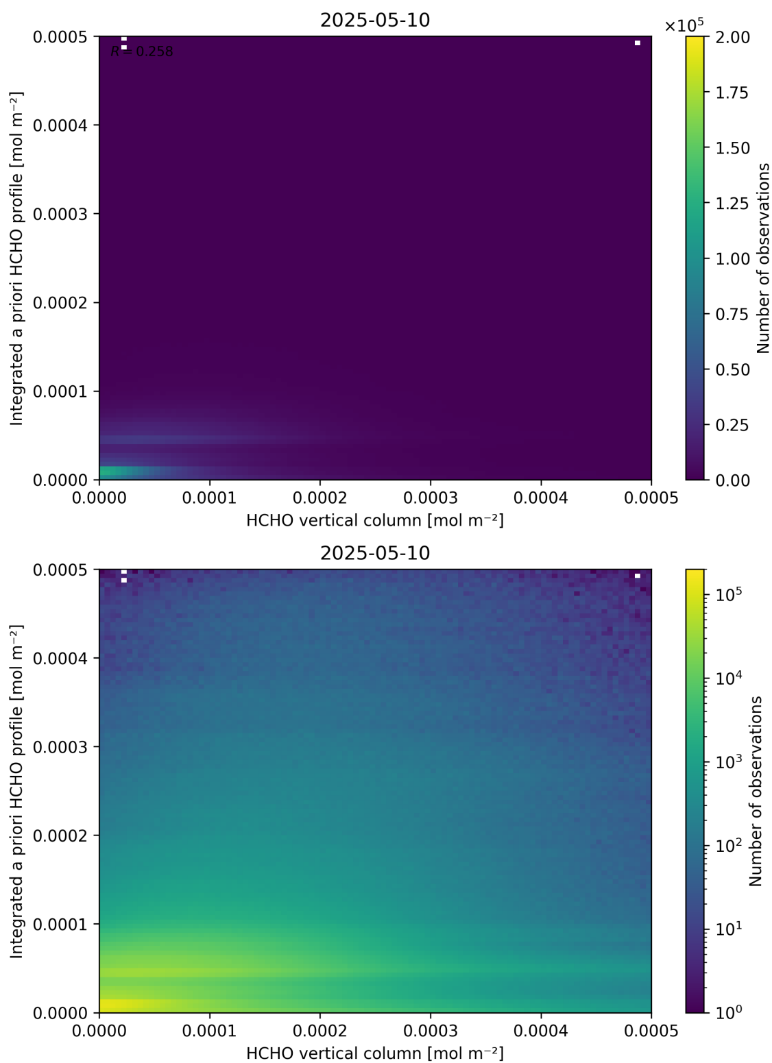
Figure 135: Scatter density plot of “HCHO vertical column” against “Integrated a priori HCHO profile” for 2025-05-10 to 2025-05-11.
