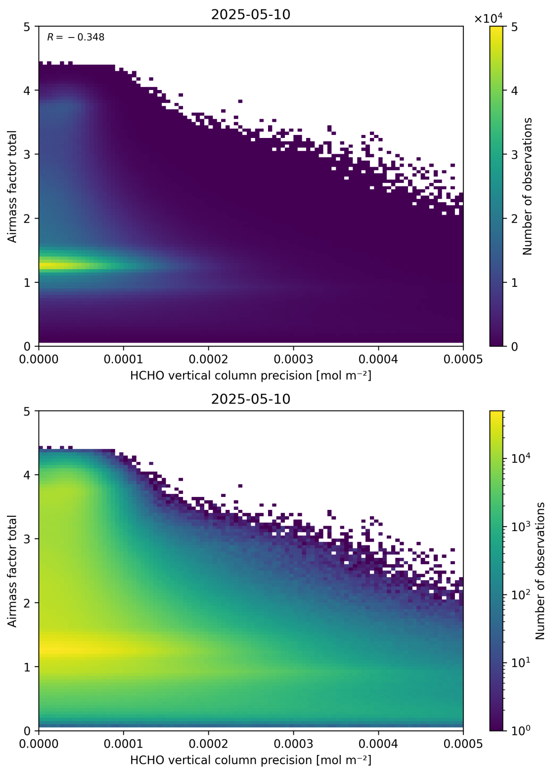
Figure 144: Scatter density plot of “HCHO vertical column precision” against “Airmass factor total” for 2025-05-10 to 2025-05-11.
