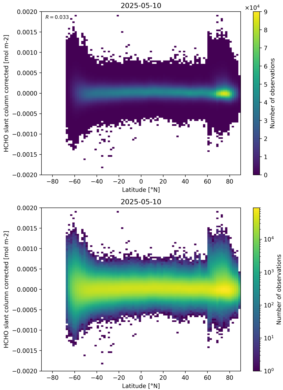
Figure 157: Scatter density plot of “Latitude” against “HCHO slant column corrected” for 2025-05-10 to 2025-05-11.
