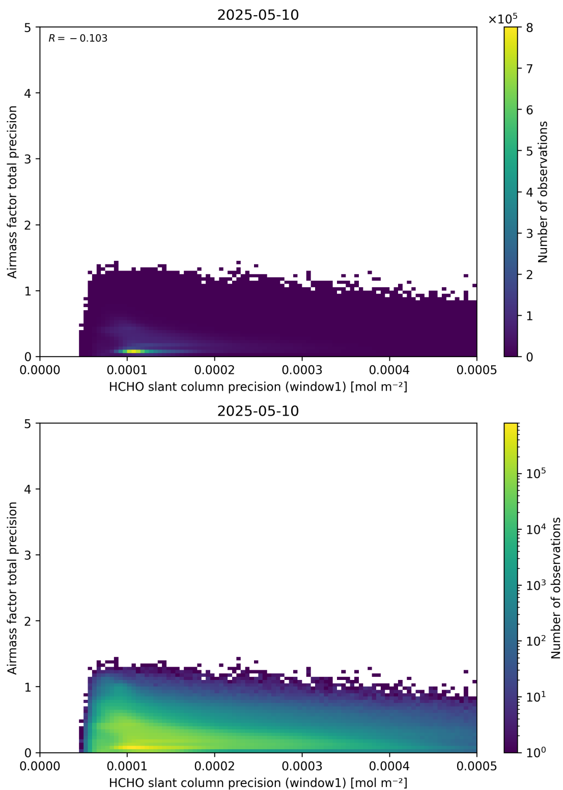
Figure 95: Scatter density plot of “HCHO slant column precision (window1)” against “Airmass factor total precision” for 2025-05-10 to 2025-05-11.
