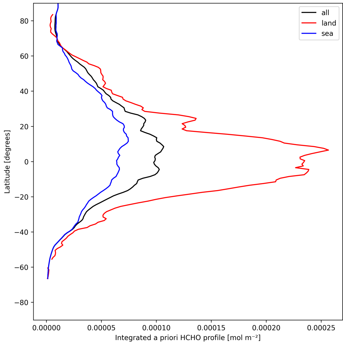
Figure 29: Zonal average of “Integrated a priori HCHO profile” for 2025-05-10 to 2025-05-11.
