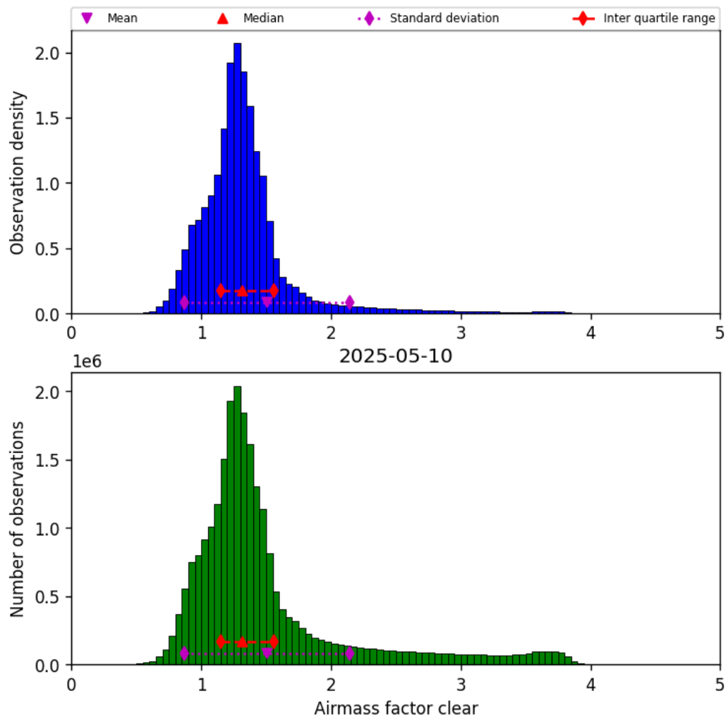
Figure 42: Histogram of “Airmass factor clear” for 2025-05-10 to 2025-05-11
