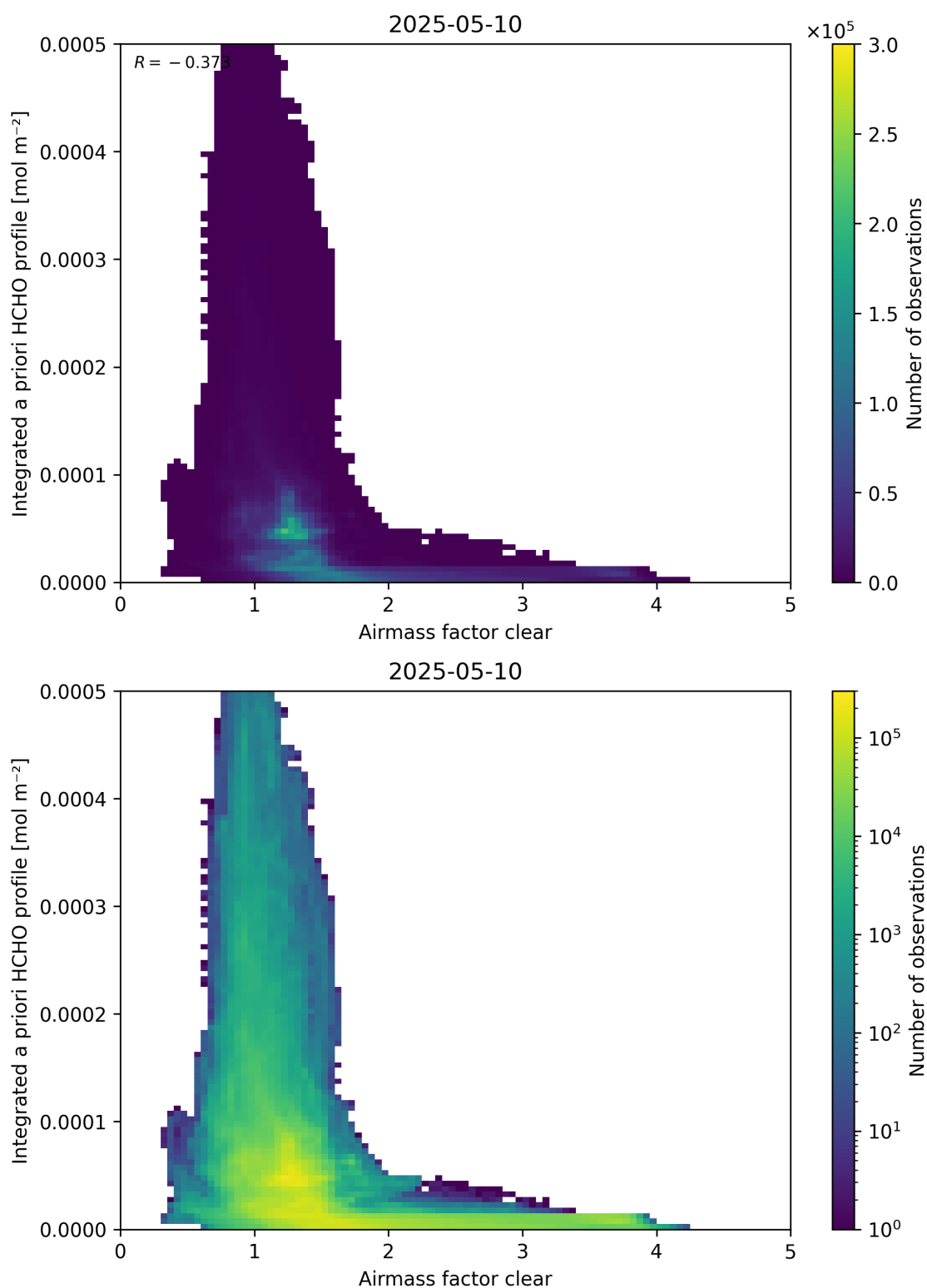
Figure 76: Scatter density plot of “Airmass factor clear” against “Integrated a priori HCHO profile” for 2025-05-10 to 2025-05-11.
