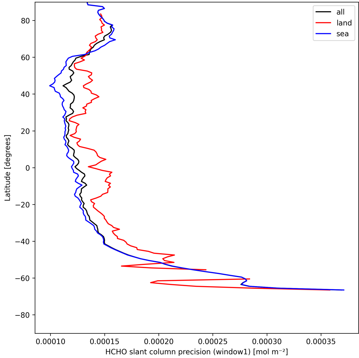
Figure 25: Zonal average of "HCHO slant column precision (window1)" for 2025-05-10 to 2025-05-11.
