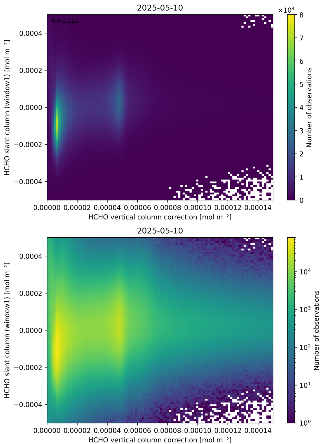
Figure 118: Scatter density plot of “HCHO vertical column correction” against “HCHO slant column (window1)” for 2025-05-10 to 2025-05-11.
