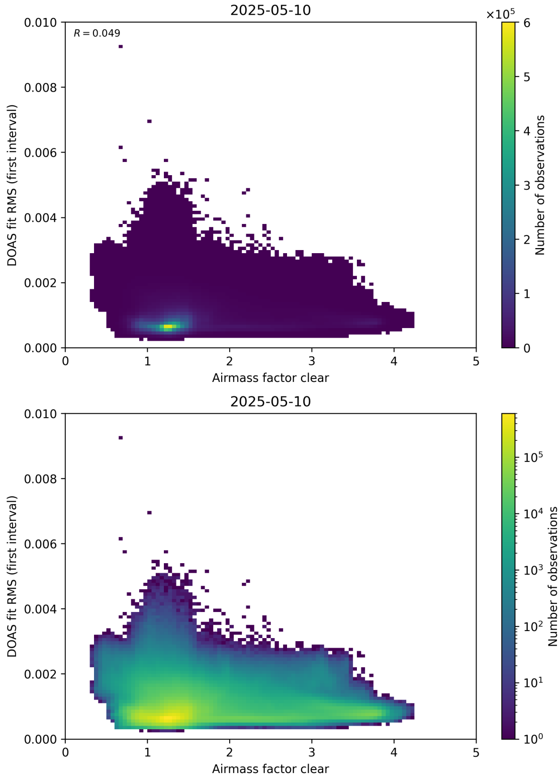
Figure 71: Scatter density plot of “Airmass factor clear” against “DOAS fit RMS (first interval)” for 2025-05-10 to 2025-05-11.
