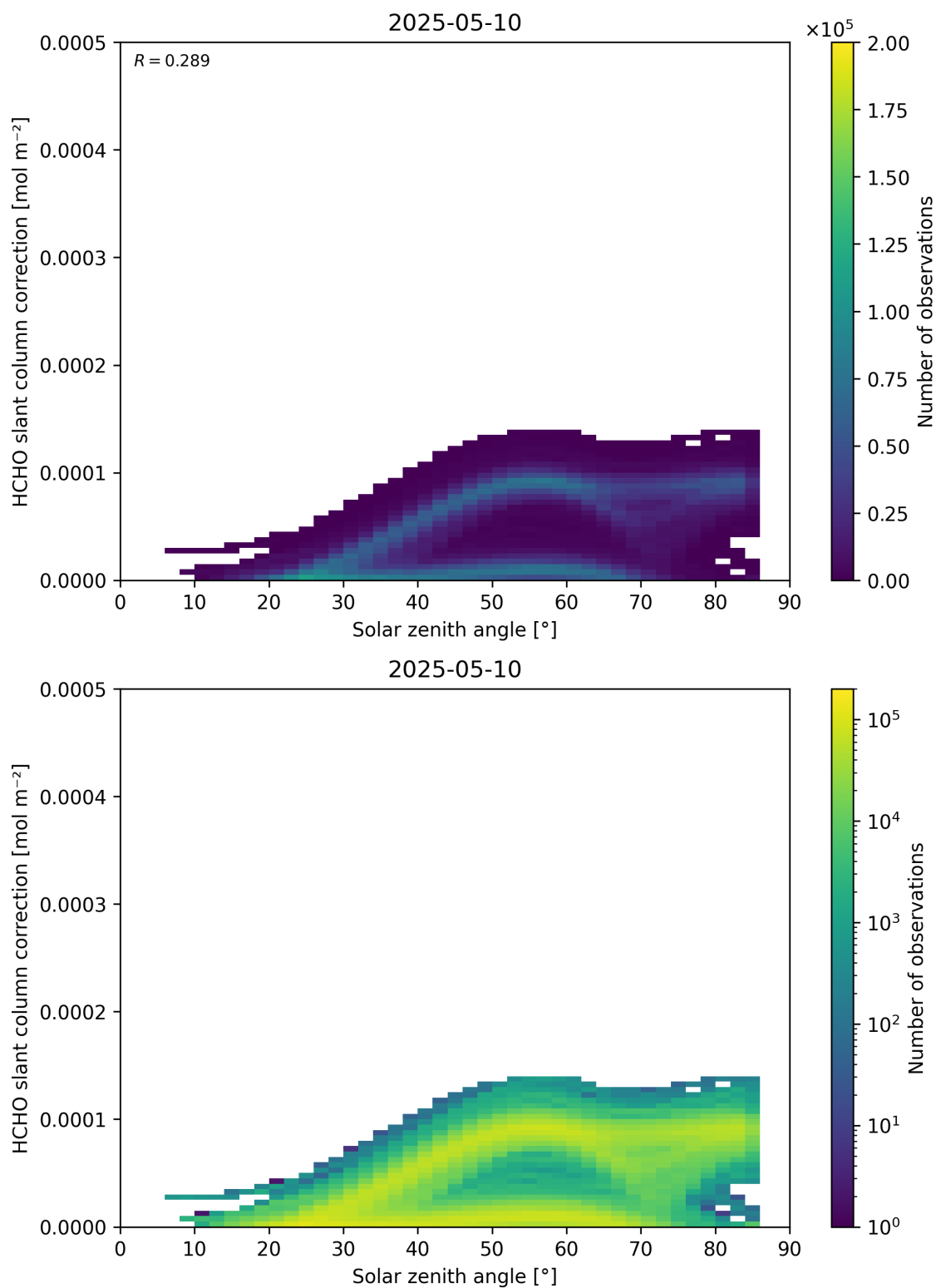
Figure 172: Scatter density plot of “Solar zenith angle” against “HCHO slant column correction” for 2025-05-10 to 2025-05-11.
