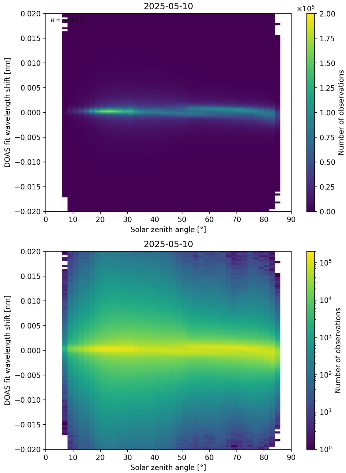
Figure 168: Scatter density plot of “Solar zenith angle” against “DOAS fit wavelength shift” for 2025-05-10 to 2025-05-11.
