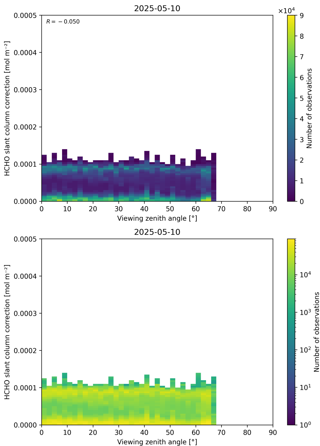
Figure 187: Scatter density plot of “Viewing zenith angle” against “HCHO slant column correction” for 2025-05-10 to 2025-05-11.
