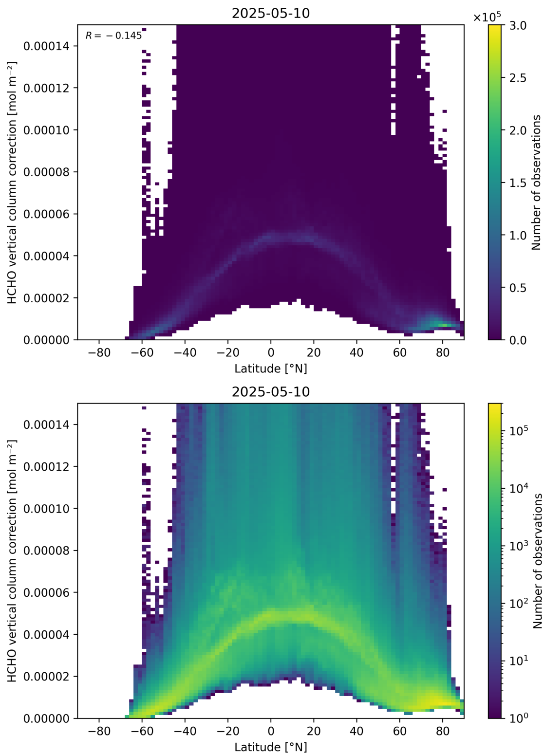
Figure 164: Scatter density plot of “Latitude” against “HCHO vertical column correction” for 2025-05-10 to 2025-05-11.
