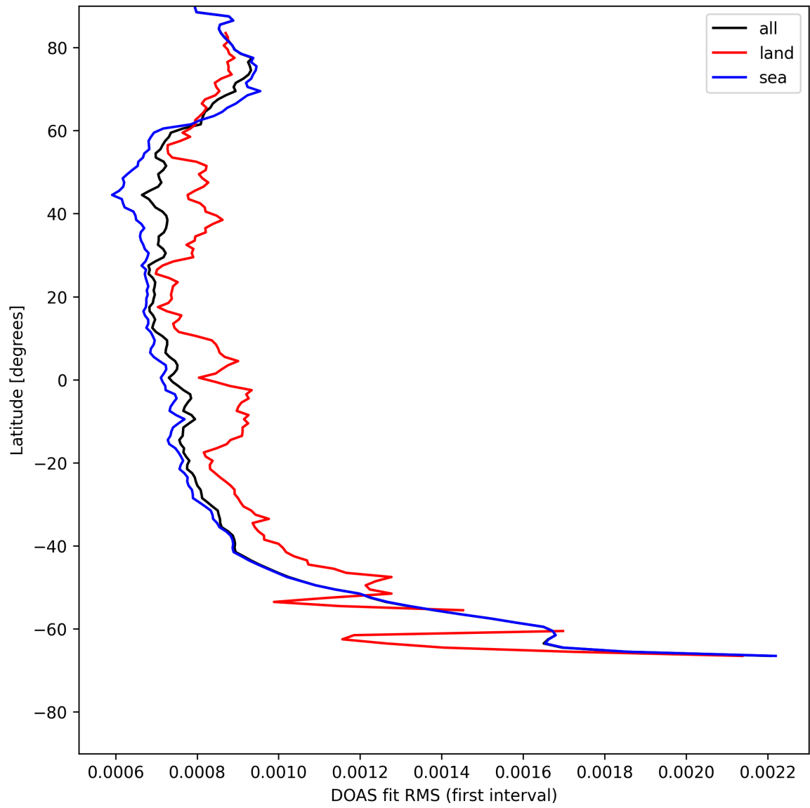
Figure 32: Zonal average of “DOAS fit RMS (first interval)” for 2025-05-10 to 2025-05-11.
