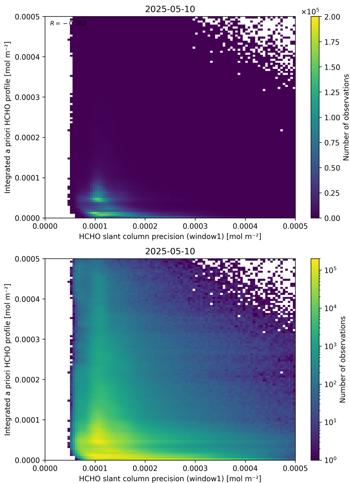
Figure 96: Scatter density plot of “HCHO slant column precision (window1)” against “Integrated a priori HCHO profile” for 2025-05-10 to 2025-05-11.
