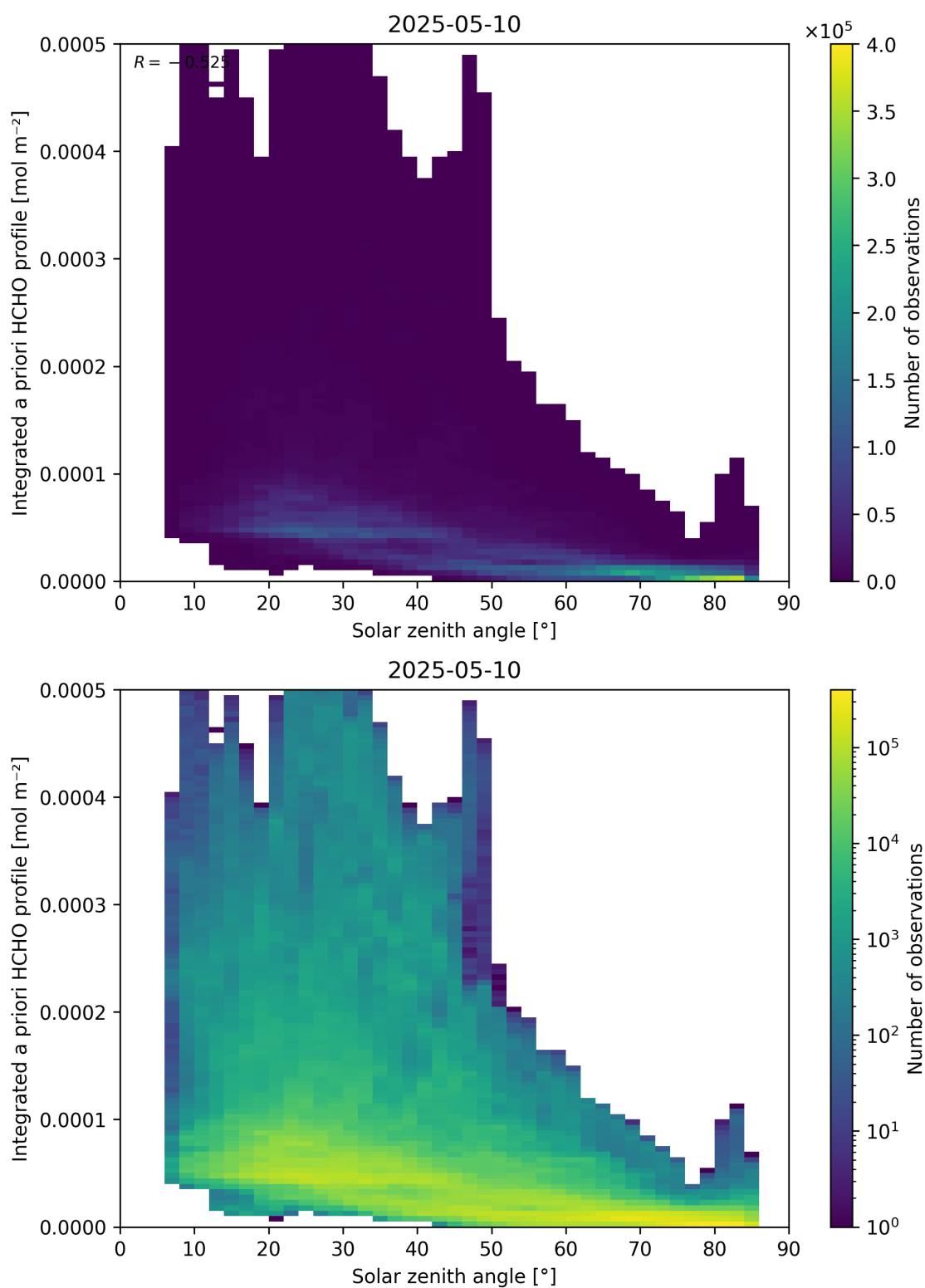
Figure 180: Scatter density plot of “Solar zenith angle” against “Integrated a priori HCHO profile” for 2025-05-10 to 2025-05-11.
