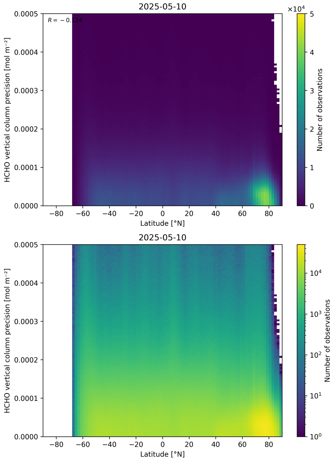
Figure 165: Scatter density plot of “Latitude” against “HCHO vertical column precision” for 2025-05-10 to 2025-05-11.
