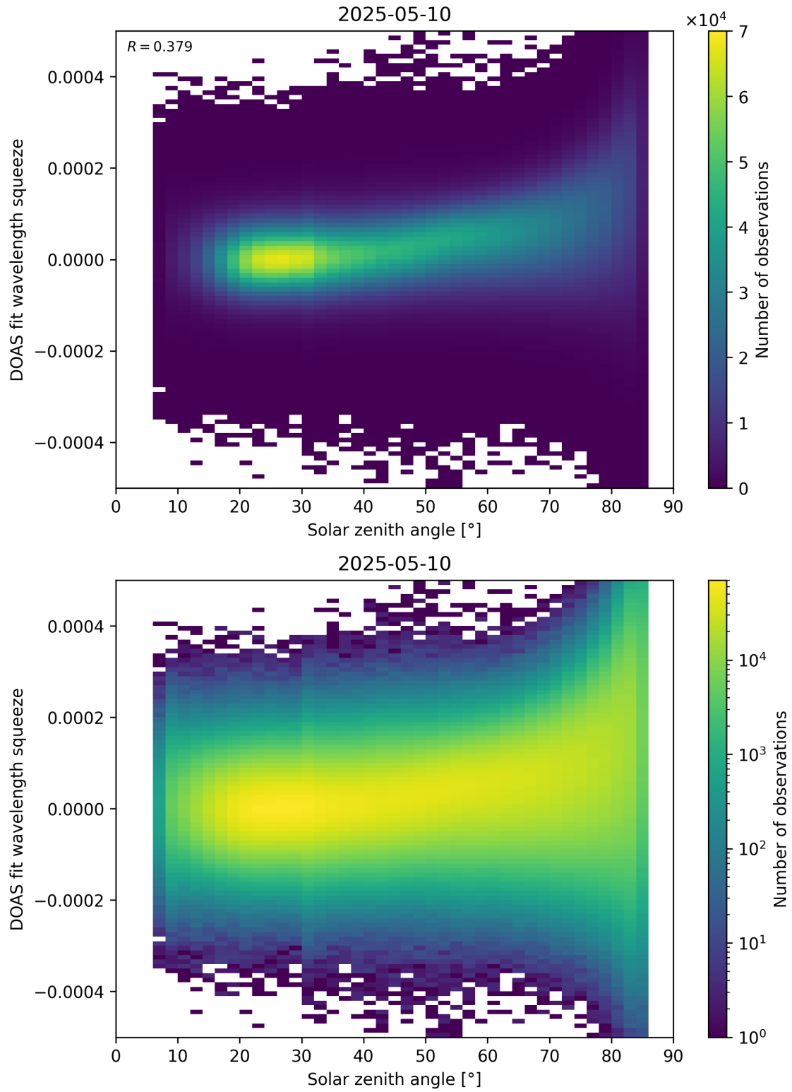
Figure 169: Scatter density plot of “Solar zenith angle” against “DOAS fit wavelength squeeze” for 2025-05-10 to 2025-05-11.
