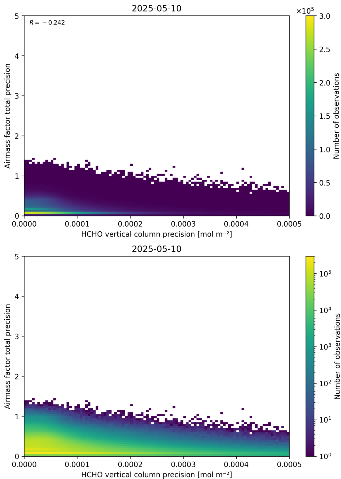
Figure 145: Scatter density plot of “HCHO vertical column precision” against “Airmass factor total precision” for 2025-05-10 to 2025-05-11.
