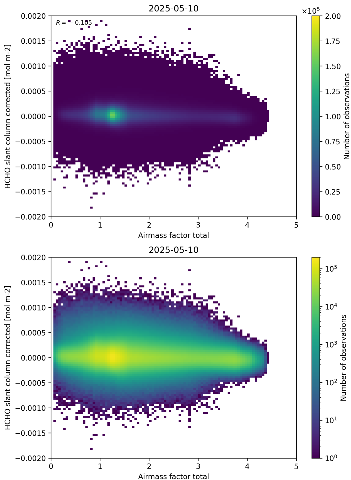
Figure 101: Scatter density plot of “Airmass factor total” against “HCHO slant column corrected” for 2025-05-10 to 2025-05-11.
