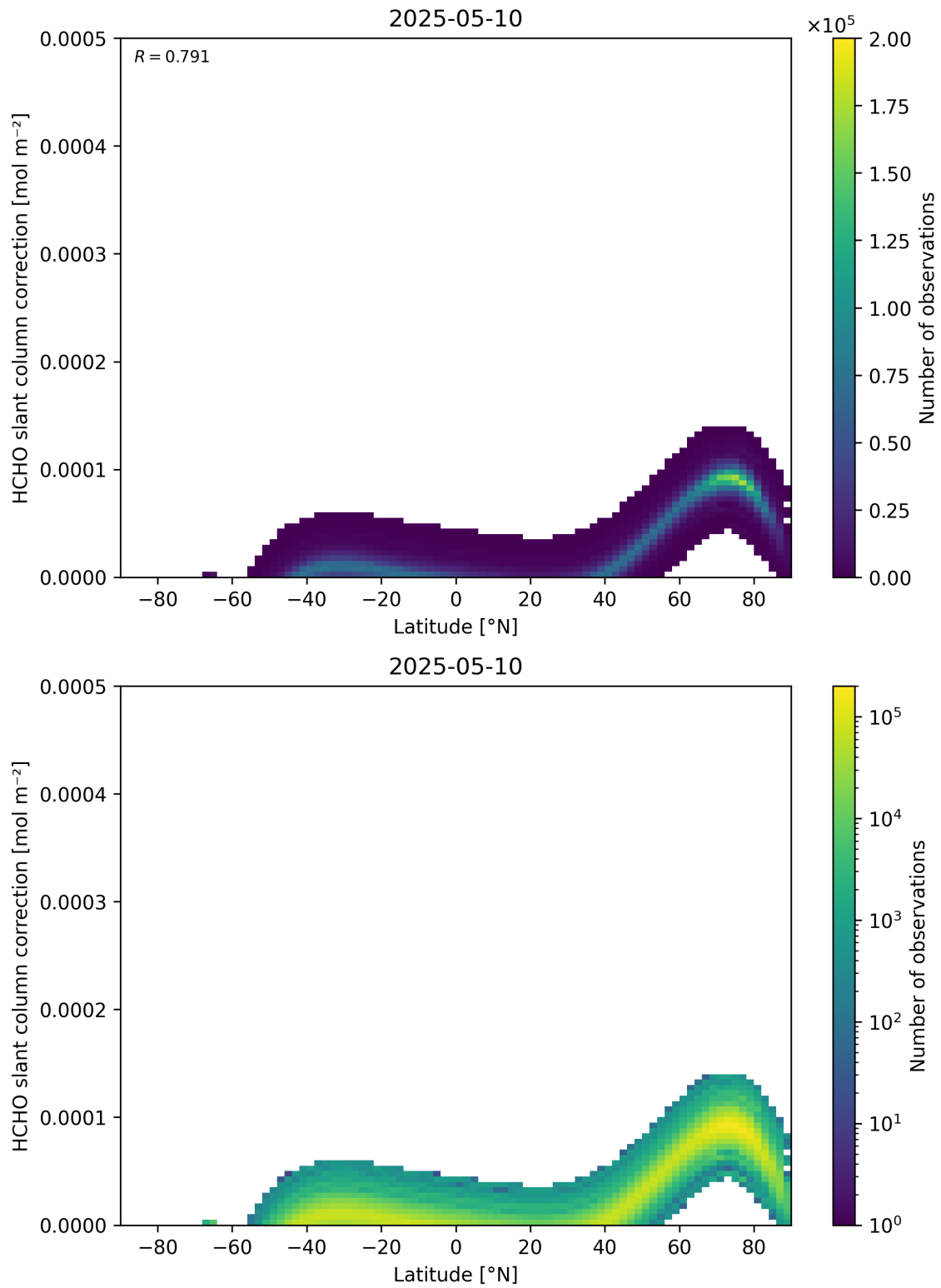
Figure 158: Scatter density plot of “Latitude” against “HCHO slant column correction” for 2025-05-10 to 2025-05-11.
