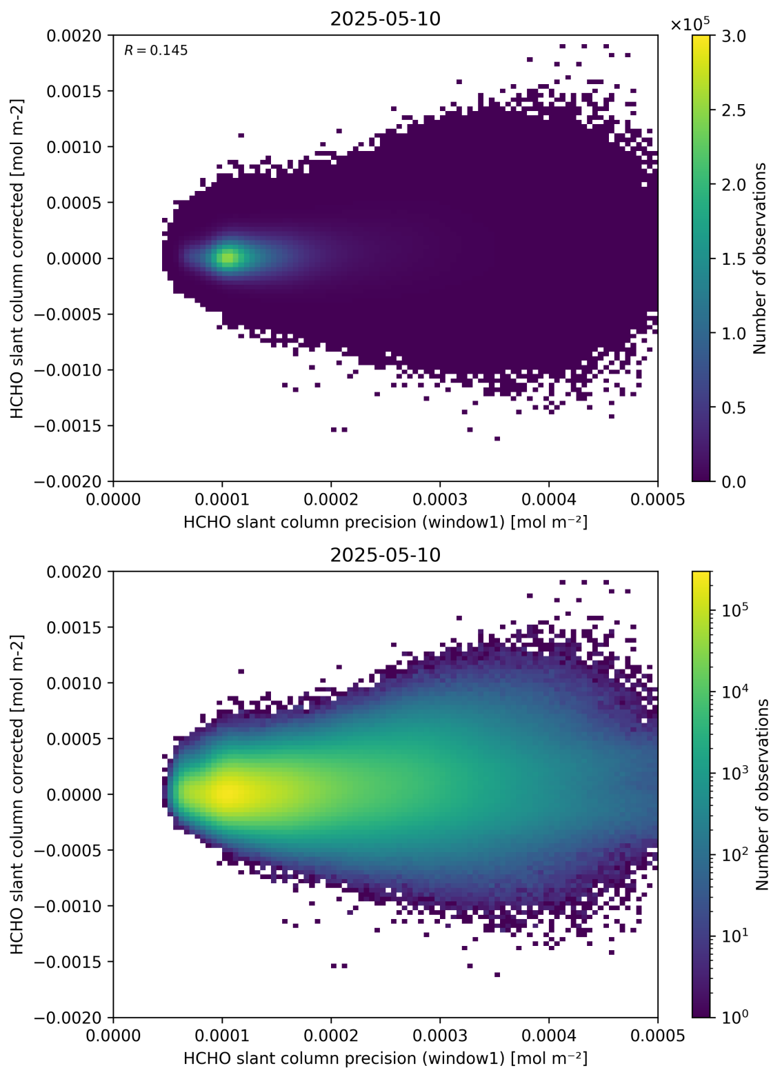
Figure 92: Scatter density plot of “HCHO slant column precision (window1)” against “HCHO slant column corrected” for 2025-05-10 to 2025-05-11.
