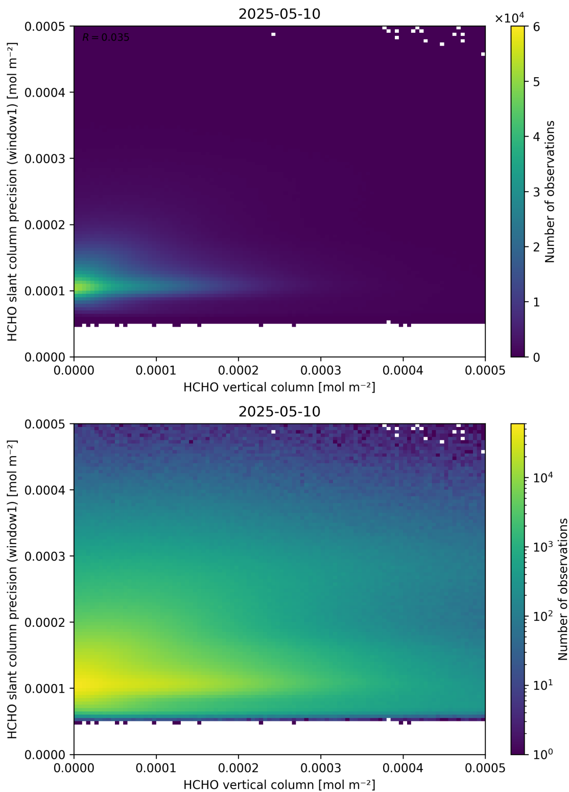
Figure 130: Scatter density plot of “HCHO vertical column” against “HCHO slant column precision (window1)” for 2025-05-10 to 2025-05-11.
