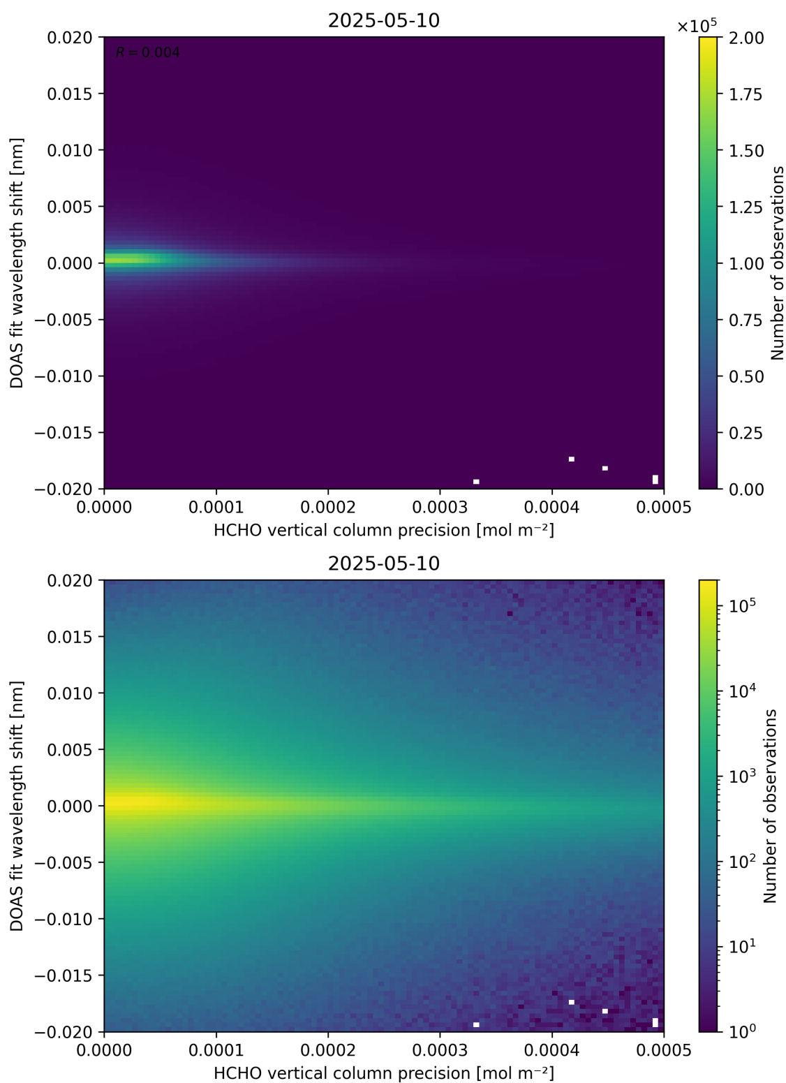
Figure 137: Scatter density plot of “HCHO vertical column precision” against “DOAS fit wavelength shift” for 2025-05-10 to 2025-05-11.
