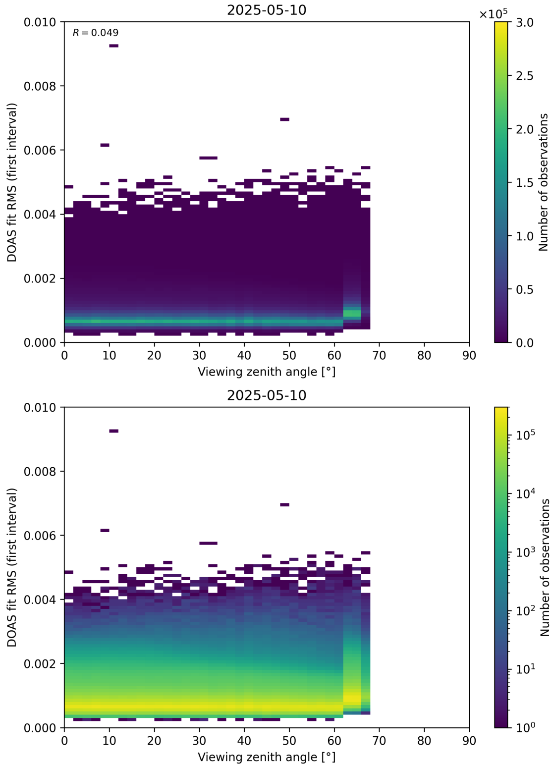
Figure 182: Scatter density plot of “Viewing zenith angle” against “DOAS fit RMS (first interval)” for 2025-05-10 to 2025-05-11.
