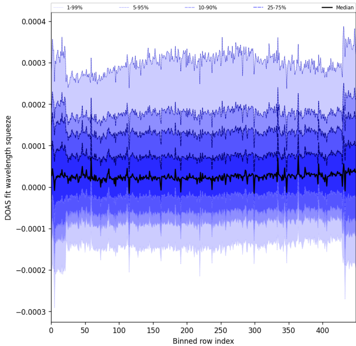
Figure 59: Along track statistics of “DOAS fit wavelength squeeze” for 2025-05-10 to 2025-05-11
