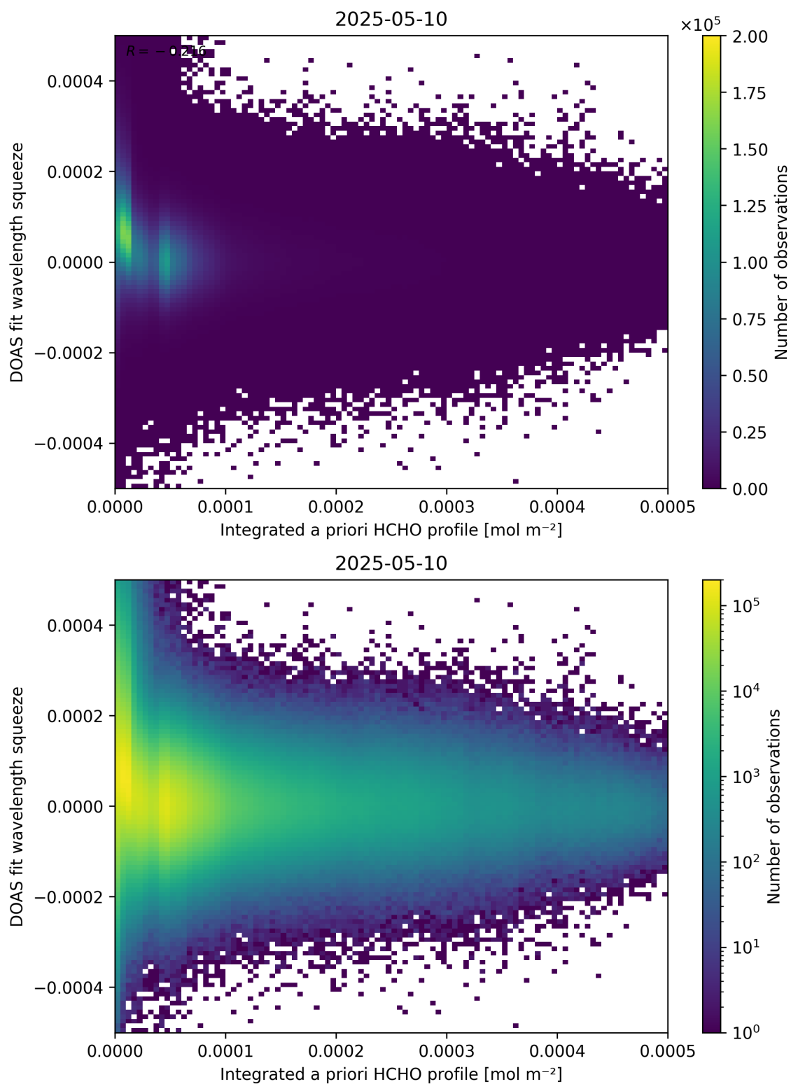
Figure 150: Scatter density plot of “Integrated a priori HCHO profile” against “DOAS fit wavelength squeeze” for 2025-05-10 to 2025-05-11.
