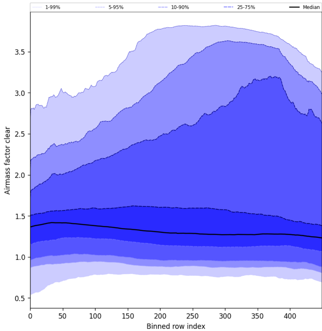
Figure 56: Along track statistics of “Airmass factor clear” for 2025-05-10 to 2025-05-11
