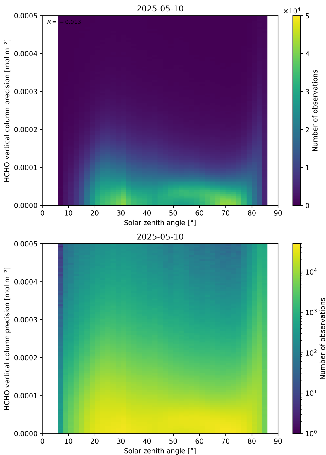
Figure 179: Scatter density plot of “Solar zenith angle” against “HCHO vertical column precision” for 2025-05-10 to 2025-05-11.
