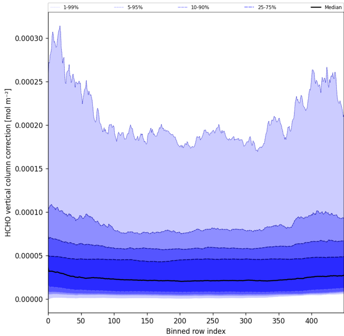
Figure 51: Along track statistics of “HCHO vertical column correction” for 2025-05-10 to 2025-05-11
