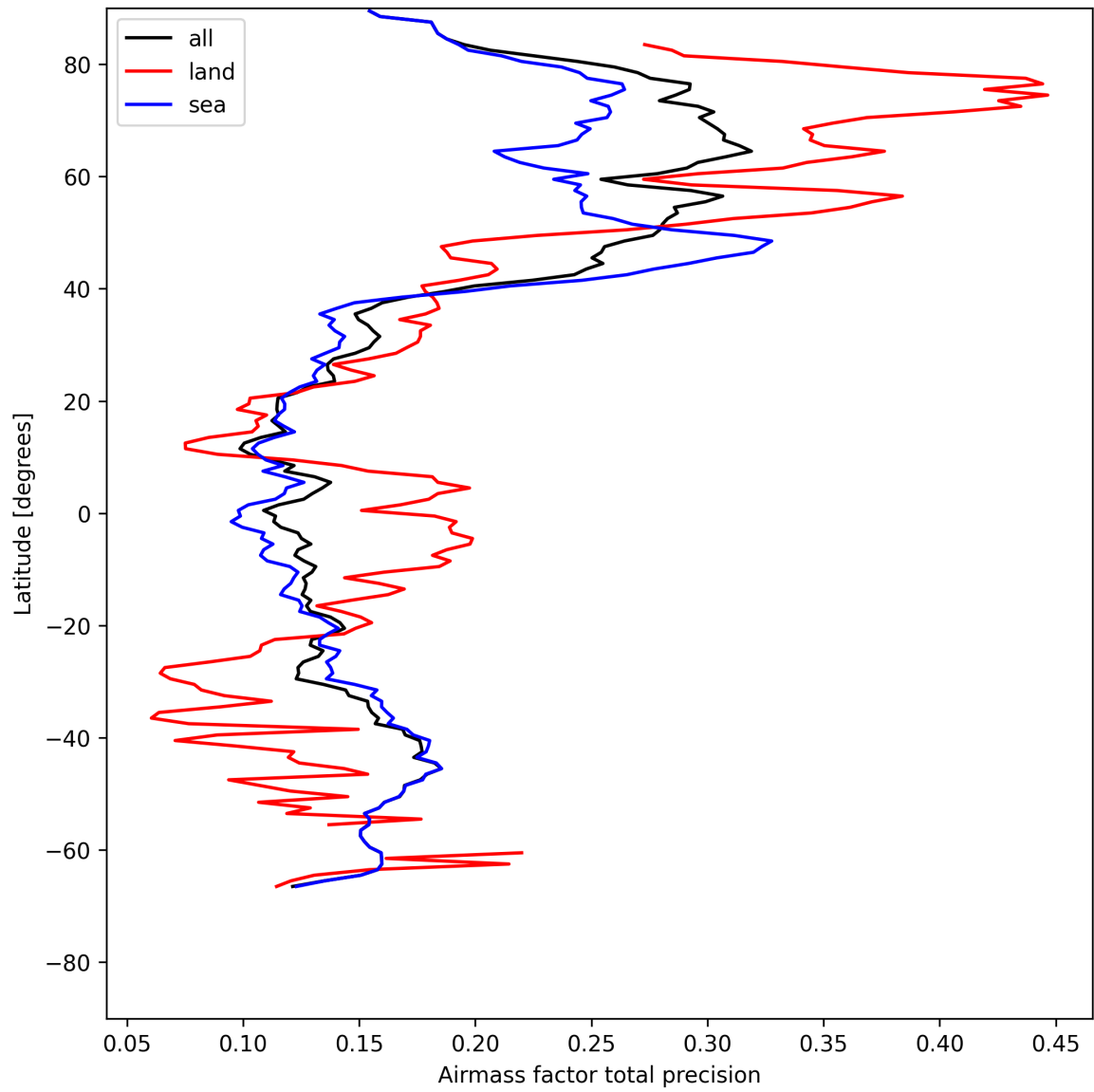
Figure 27: Zonal average of “Airmass factor total precision” for 2025-05-10 to 2025-05-11.
