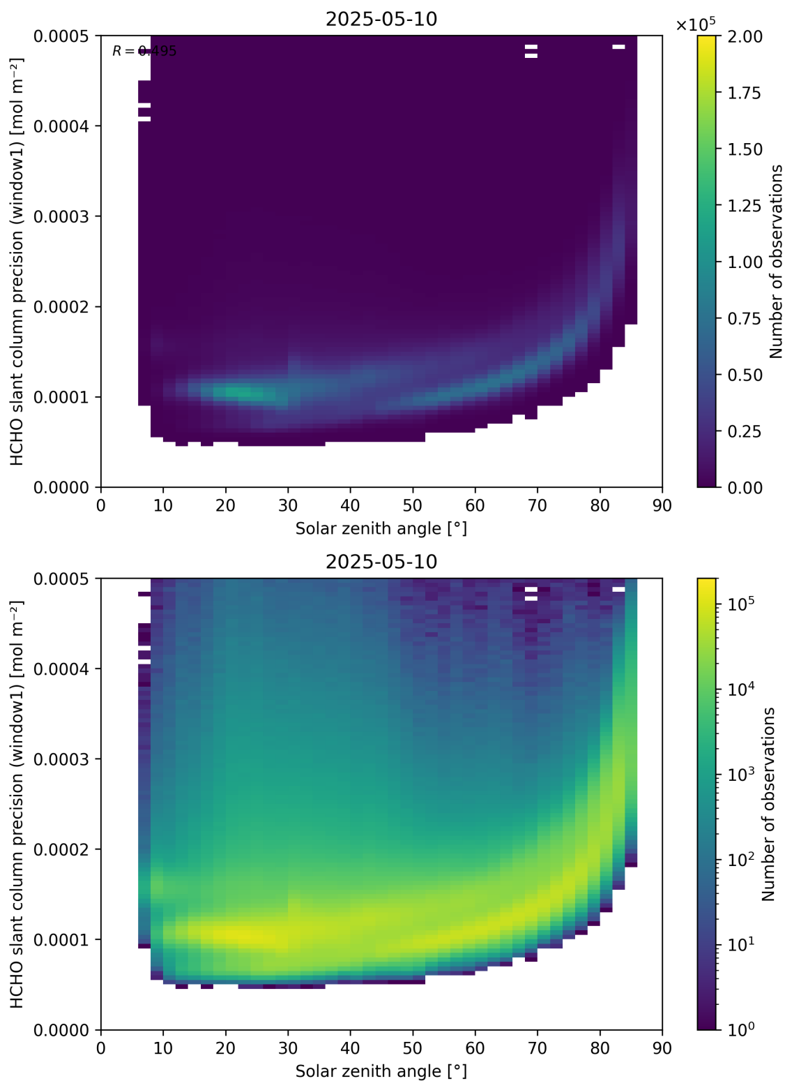
Figure 174: Scatter density plot of “Solar zenith angle” against “HCHO slant column precision (window1)” for 2025-05-10 to 2025-05-11.
