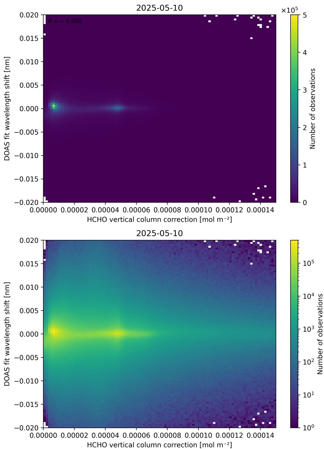
Figure 113: Scatter density plot of “HCHO vertical column correction” against “DOAS fit wavelength shift” for 2025-05-10 to 2025-05-11.
