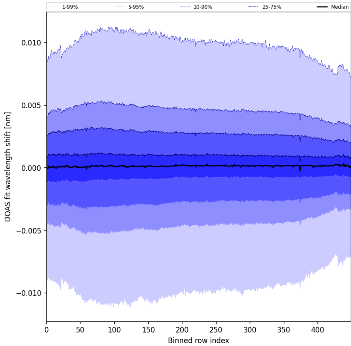
Figure 58: Along track statistics of “DOAS fit wavelength shift” for 2025-05-10 to 2025-05-11
