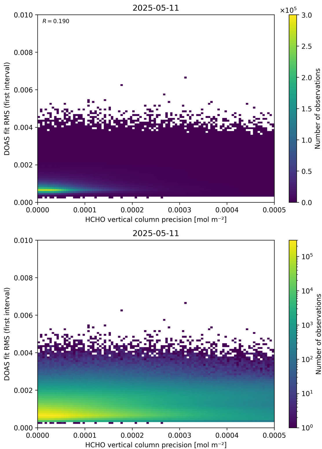
Figure 136: Scatter density plot of “HCHO vertical column precision” against “DOAS fit RMS (first interval)” for 2025-05-10 to 2025-05-12.
