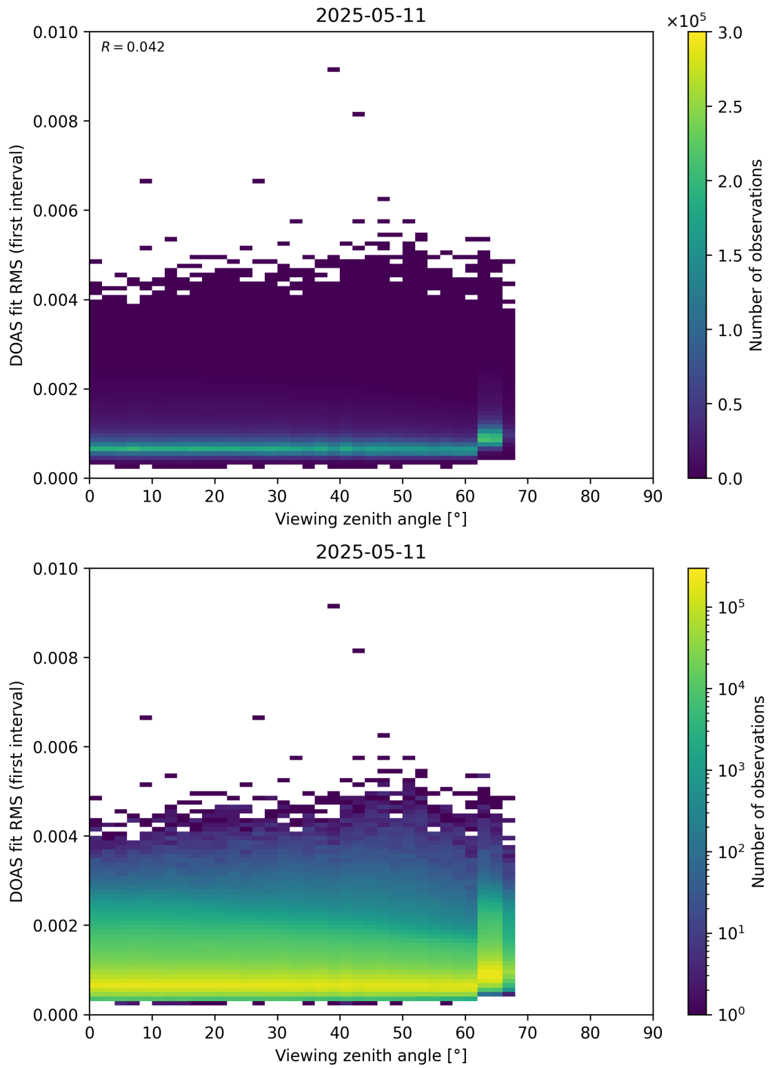
Figure 182: Scatter density plot of “Viewing zenith angle” against “DOAS fit RMS (first interval)” for 2025-05-10 to 2025-05-12.
