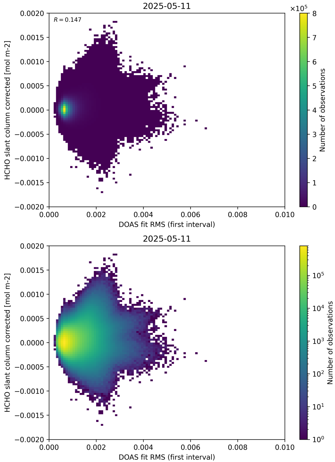
Figure 62: Scatter density plot of “DOAS fit RMS (first interval)” against “HCHO slant column corrected” for 2025-05-10 to 2025-05-12.
