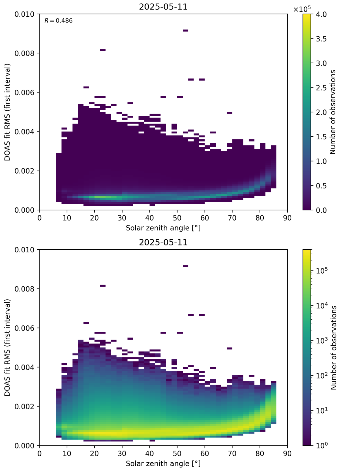
Figure 167: Scatter density plot of “Solar zenith angle” against “DOAS fit RMS (first interval)” for 2025-05-10 to 2025-05-12.
