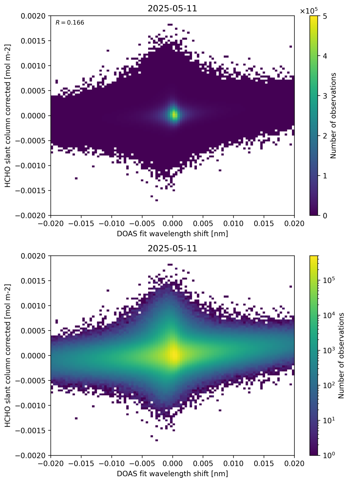
Figure 66: Scatter density plot of “DOAS fit wavelength shift” against “HCHO slant column corrected” for 2025-05-10 to 2025-05-12.
