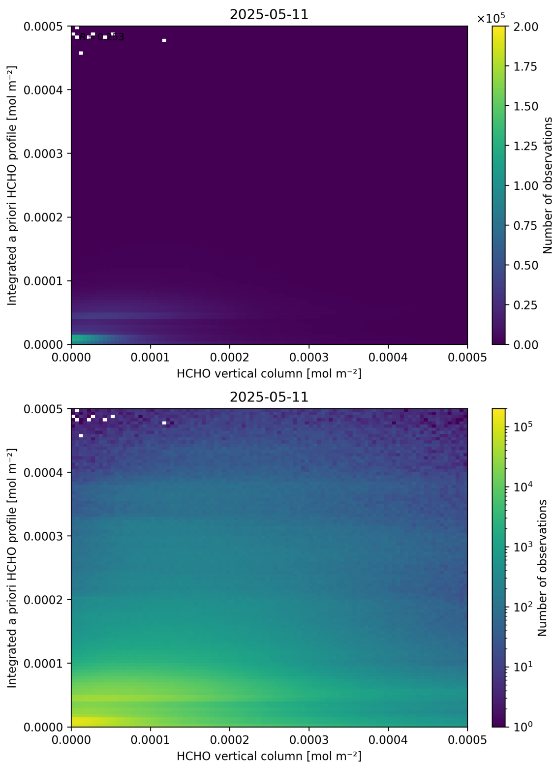
Figure 135: Scatter density plot of “HCHO vertical column” against “Integrated a priori HCHO profile” for 2025-05-10 to 2025-05-12.
