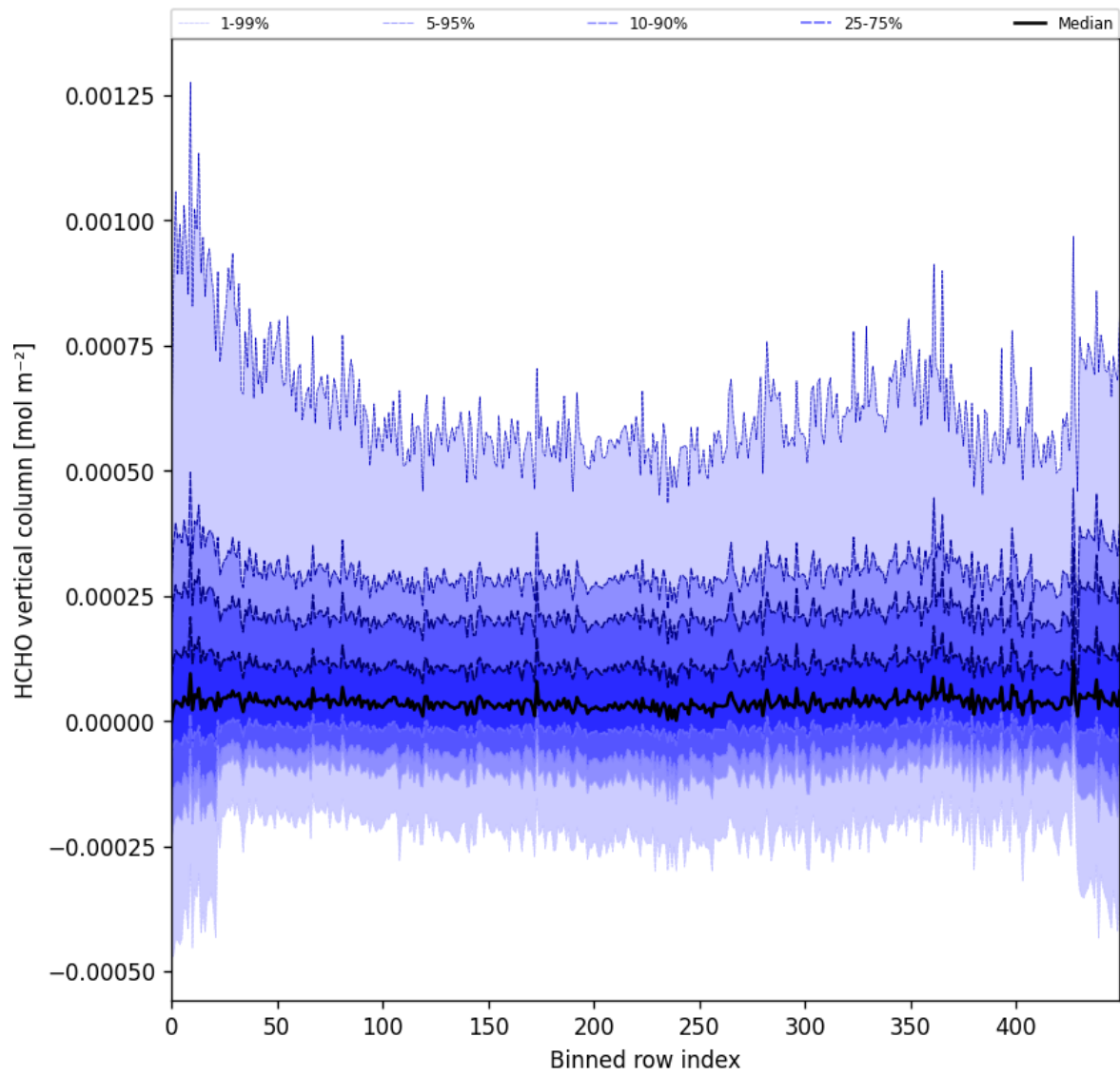
Figure 49: Along track statistics of “HCHO vertical column” for 2025-05-10 to 2025-05-12
