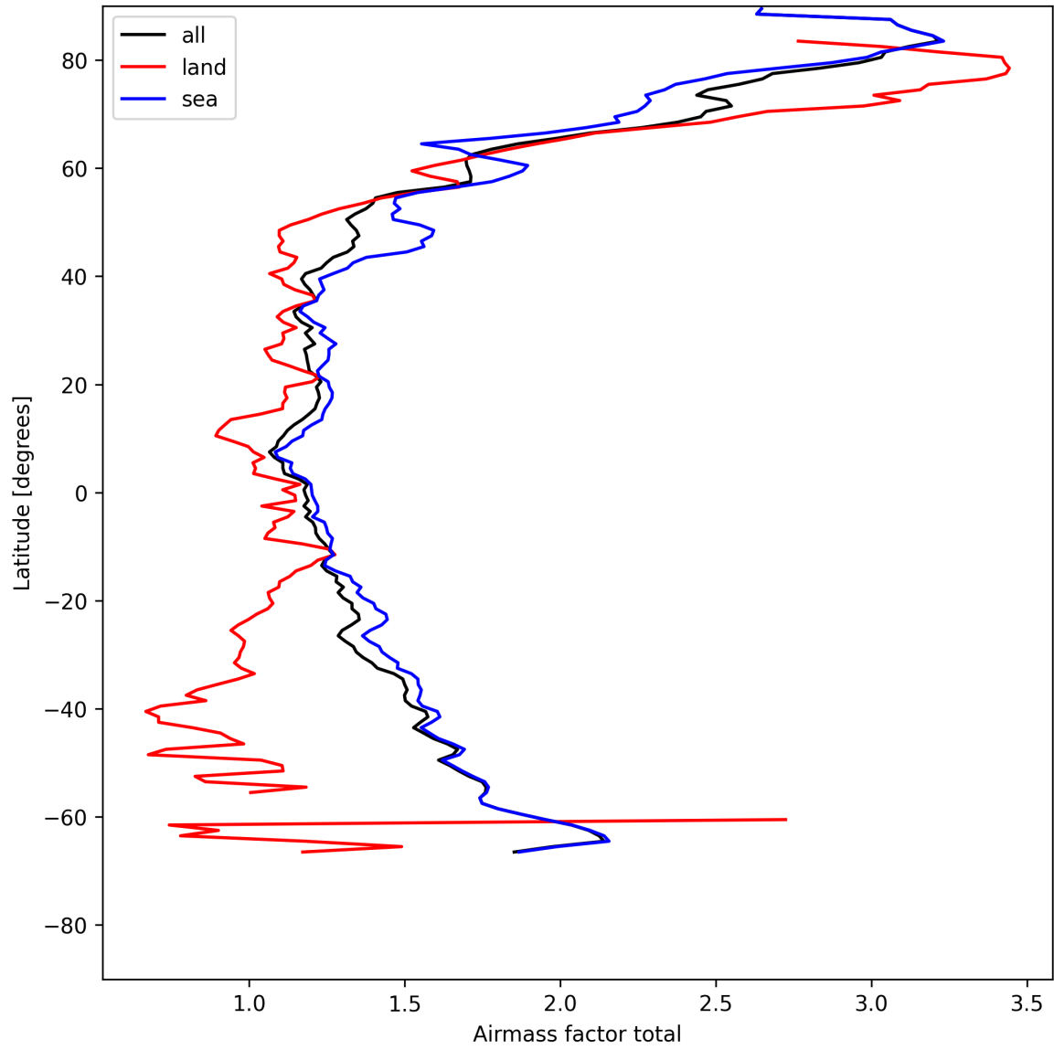
Figure 26: Zonal average of “Airmass factor total” for 2025-05-10 to 2025-05-12.
