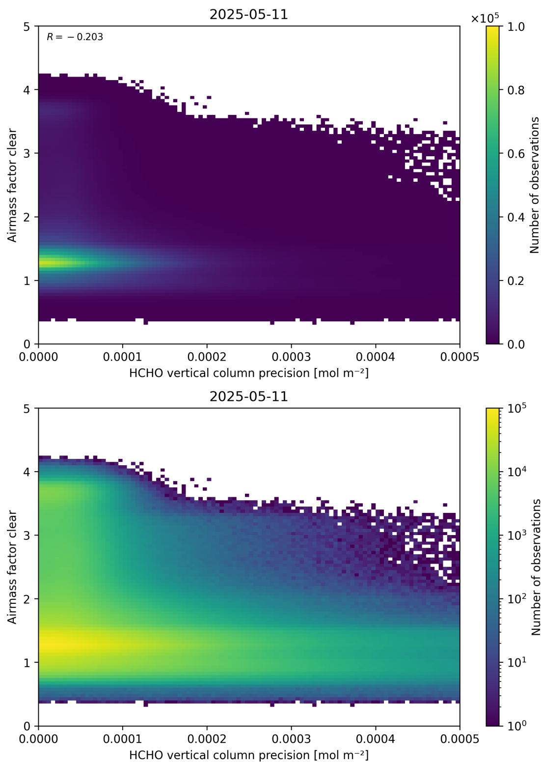
Figure 139: Scatter density plot of “HCHO vertical column precision” against “Airmass factor clear” for 2025-05-10 to 2025-05-12.
