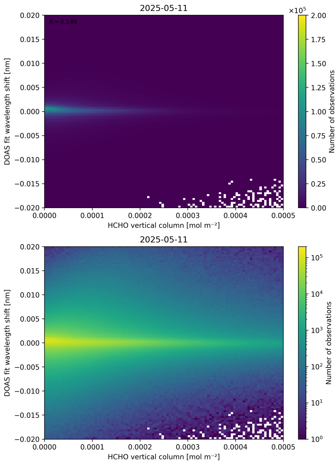
Figure 124: Scatter density plot of “HCHO vertical column” against “DOAS fit wavelength shift” for 2025-05-10 to 2025-05-12.
