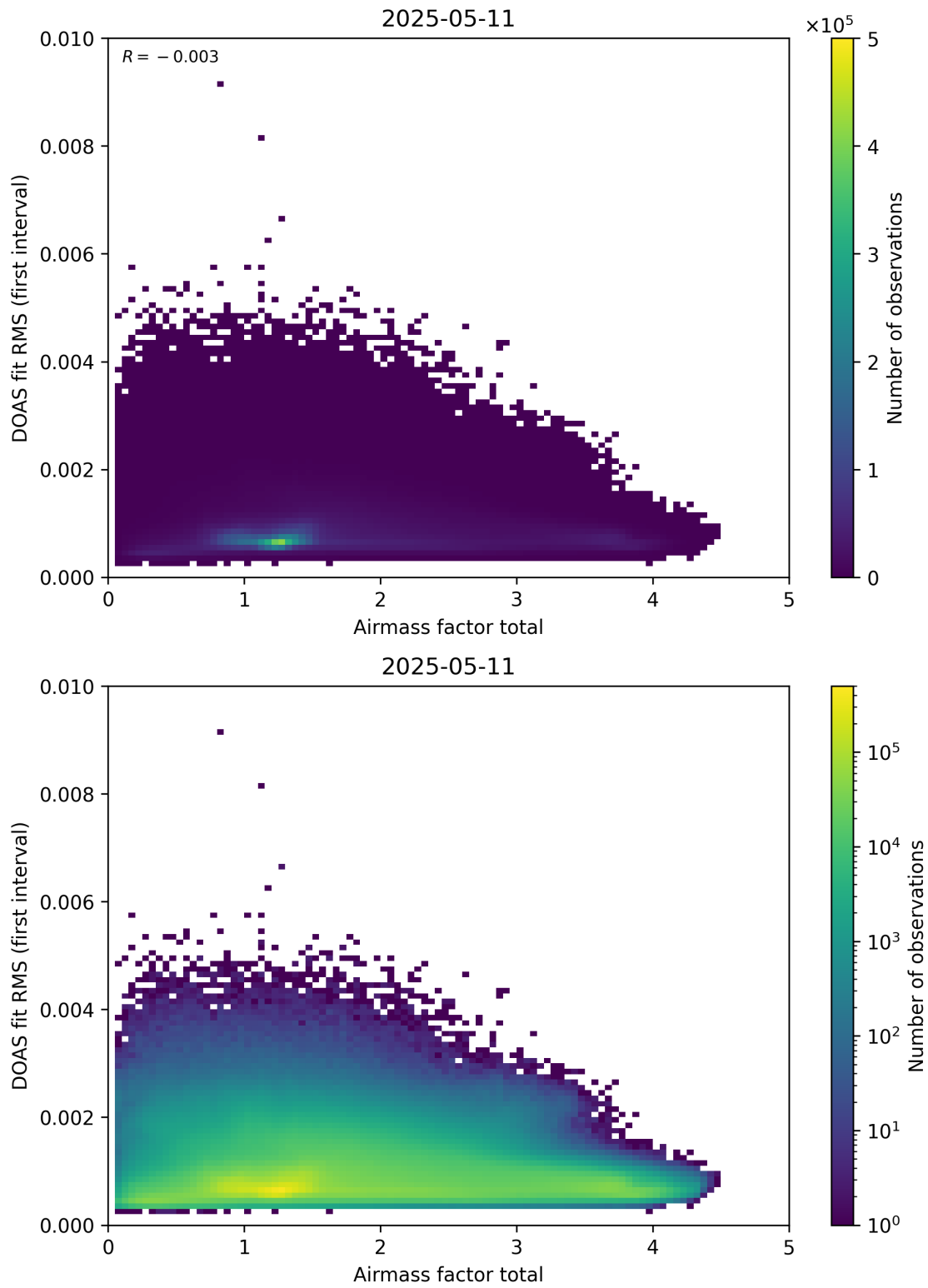
Figure 97: Scatter density plot of “Airmass factor total” against “DOAS fit RMS (first interval)” for 2025-05-10 to 2025-05-12.
