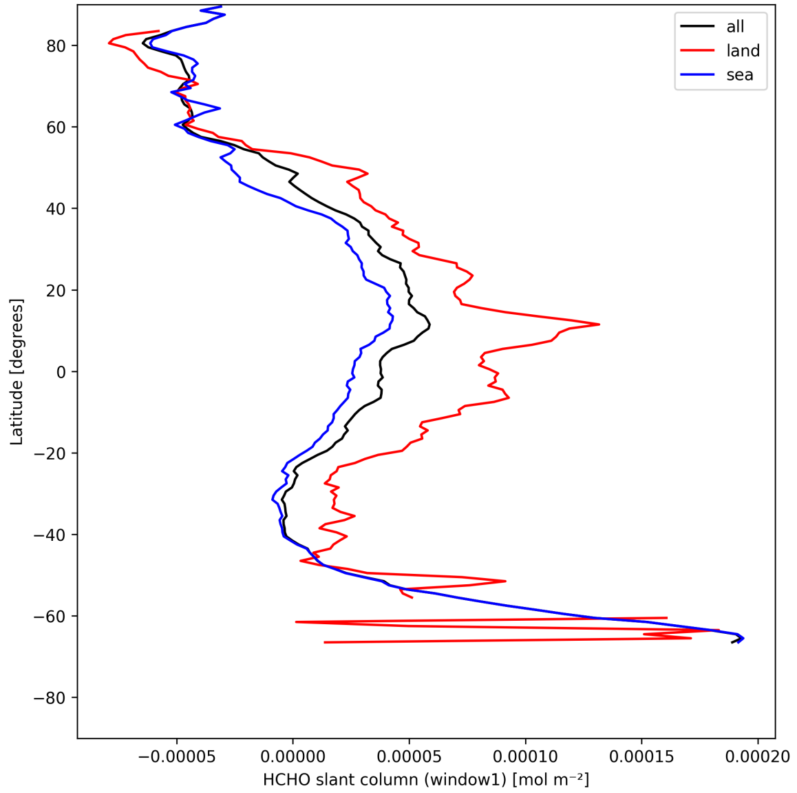
Figure 24: Zonal average of “HCHO slant column (window1)” for 2025-05-10 to 2025-05-12.
