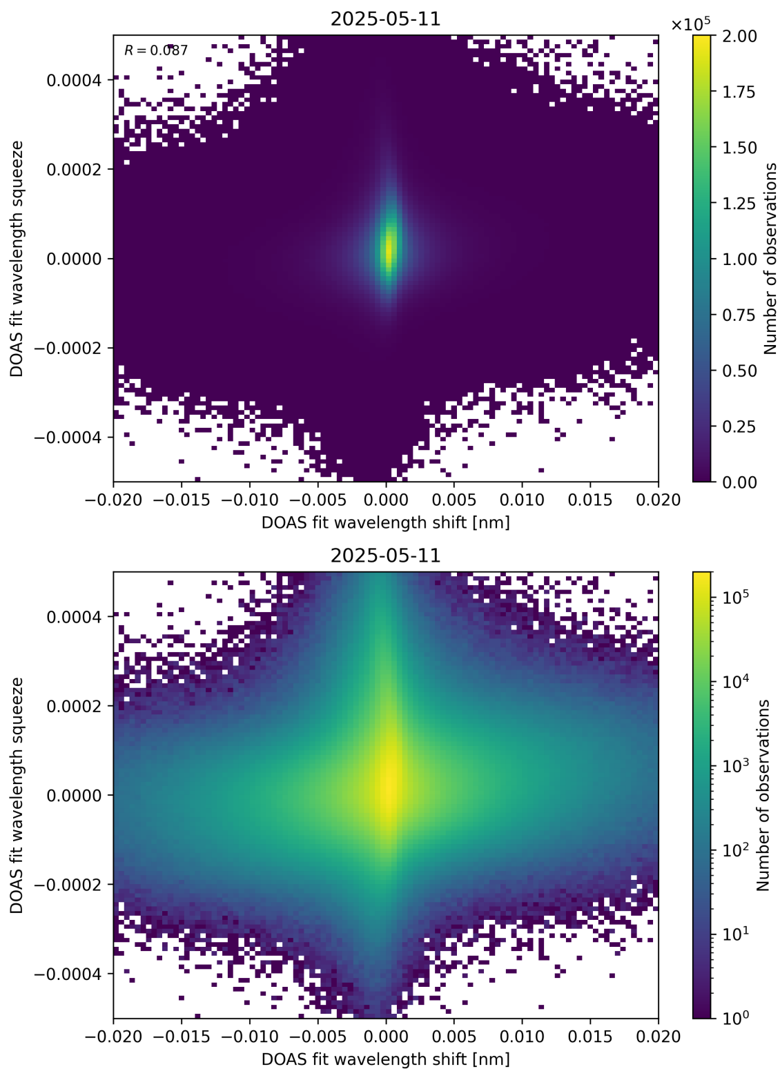
Figure 65: Scatter density plot of “DOAS fit wavelength shift” against “DOAS fit wavelength squeeze” for 2025-05-10 to 2025-05-12.
