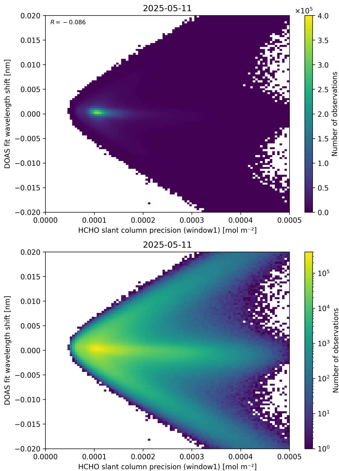
Figure 89: Scatter density plot of “HCHO slant column precision (window1)” against “DOAS fit wavelength shift” for 2025-05-10 to 2025-05-12.
