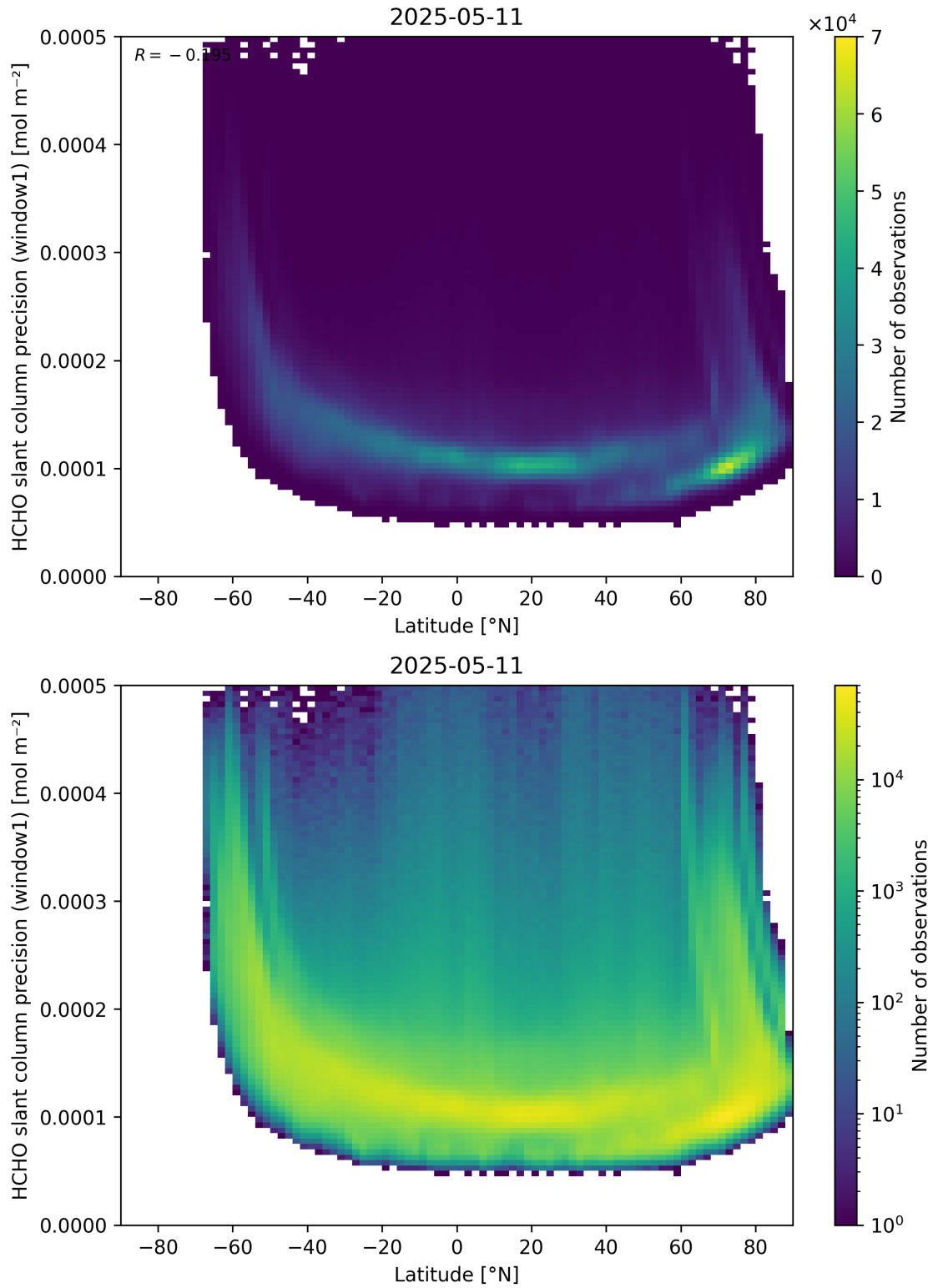
Figure 160: Scatter density plot of “Latitude” against “HCHO slant column precision (window1)” for 2025-05-10 to 2025-05-12.
