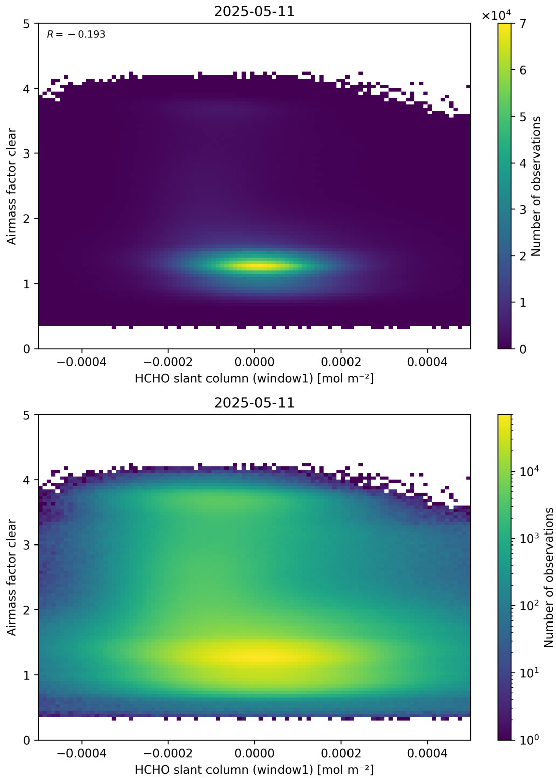
Figure 81: Scatter density plot of “HCHO slant column (window1)” against “Airmass factor clear” for 2025-05-10 to 2025-05-12.
