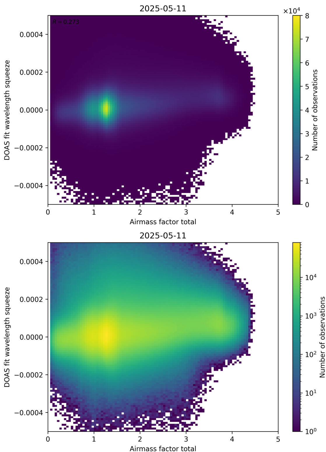
Figure 99: Scatter density plot of “Airmass factor total” against “DOAS fit wavelength squeeze” for 2025-05-10 to 2025-05-12.
