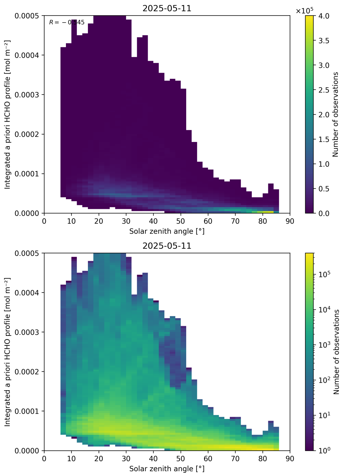
Figure 180: Scatter density plot of “Solar zenith angle” against “Integrated a priori HCHO profile” for 2025-05-10 to 2025-05-12.
