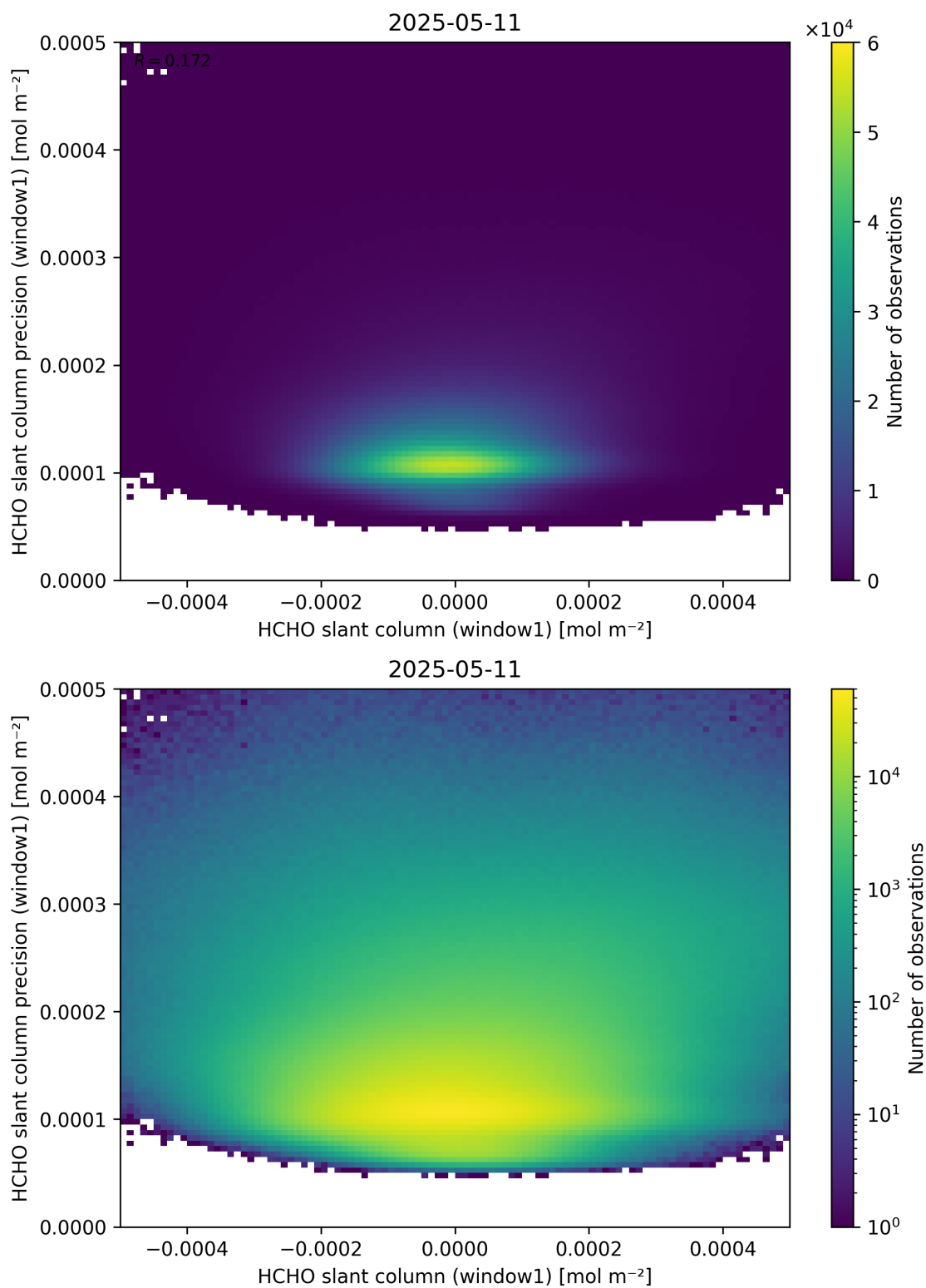
Figure 84: Scatter density plot of “HCHO slant column (window1)” against “HCHO slant column precision (window1)” for 2025-05-10 to 2025-05-12.
