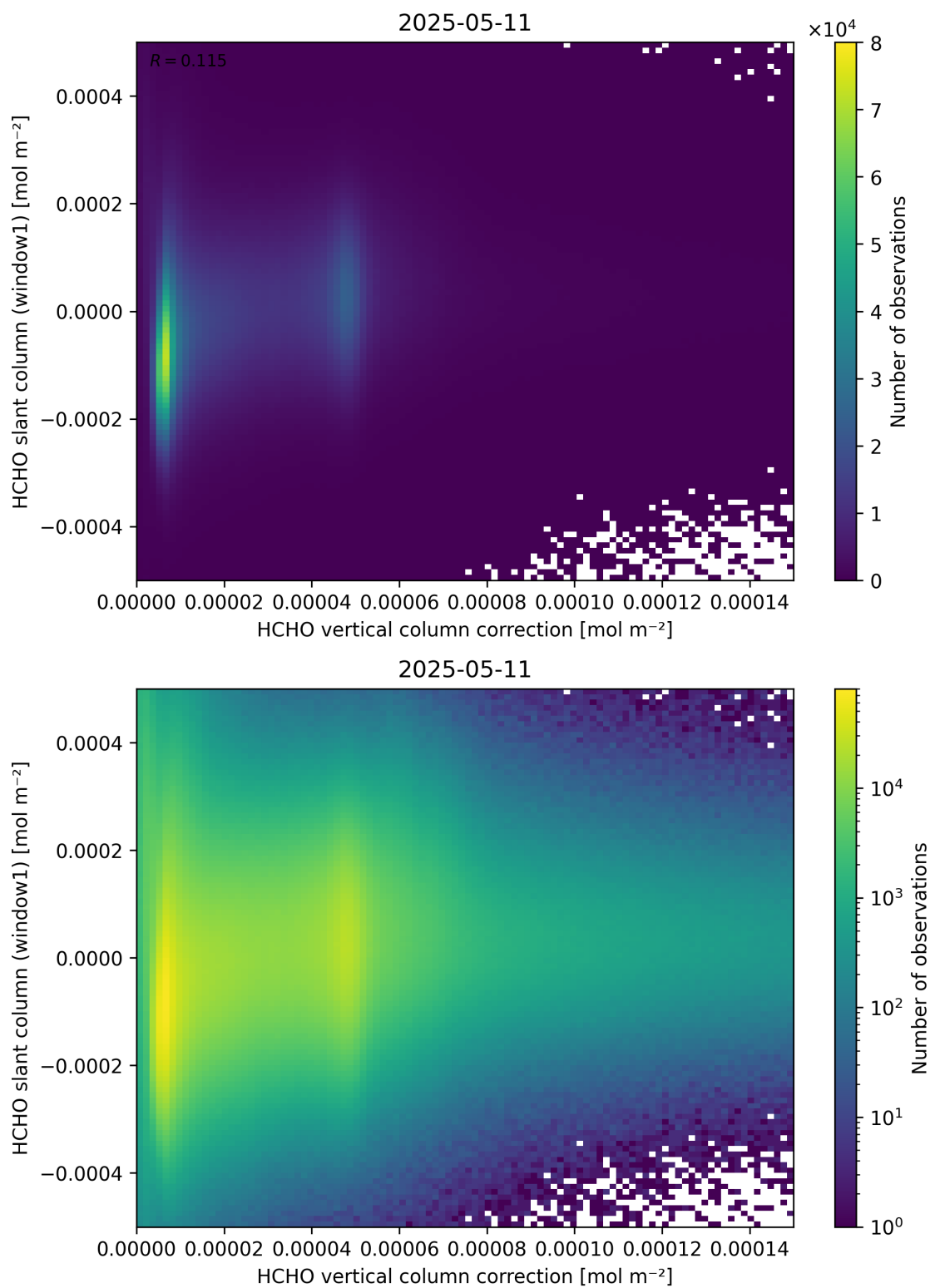
Figure 118: Scatter density plot of “HCHO vertical column correction” against “HCHO slant column (window1)” for 2025-05-10 to 2025-05-12.
