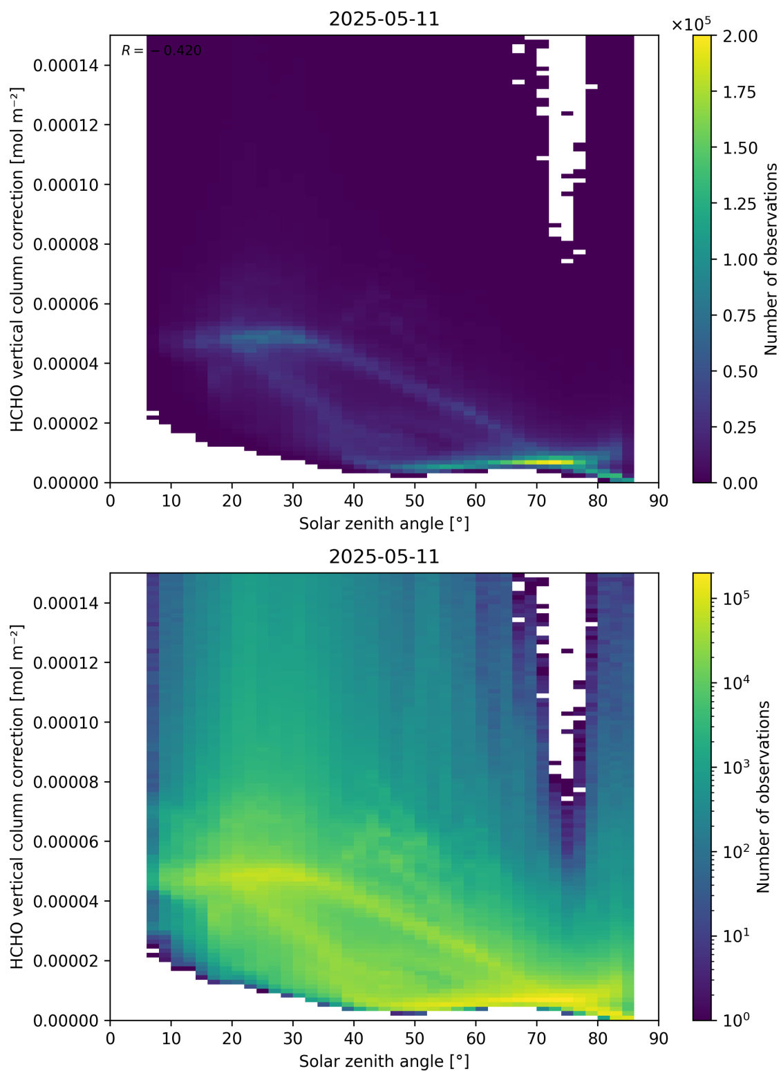
Figure 178: Scatter density plot of “Solar zenith angle” against “HCHO vertical column correction” for 2025-05-10 to 2025-05-12.
