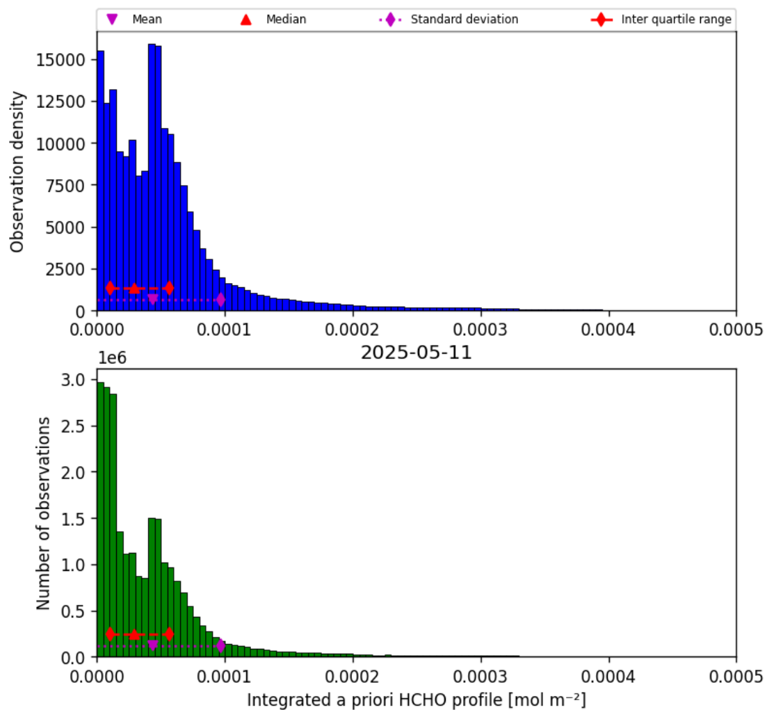
Figure 43: Histogram of “Integrated a priori HCHO profile” for 2025-05-10 to 2025-05-12
