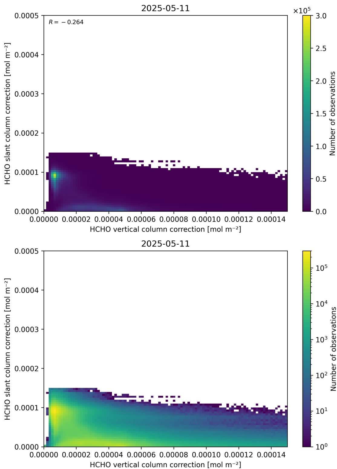
Figure 117: Scatter density plot of “HCHO vertical column correction” against “HCHO slant column correction” for 2025-05-10 to 2025-05-12.
