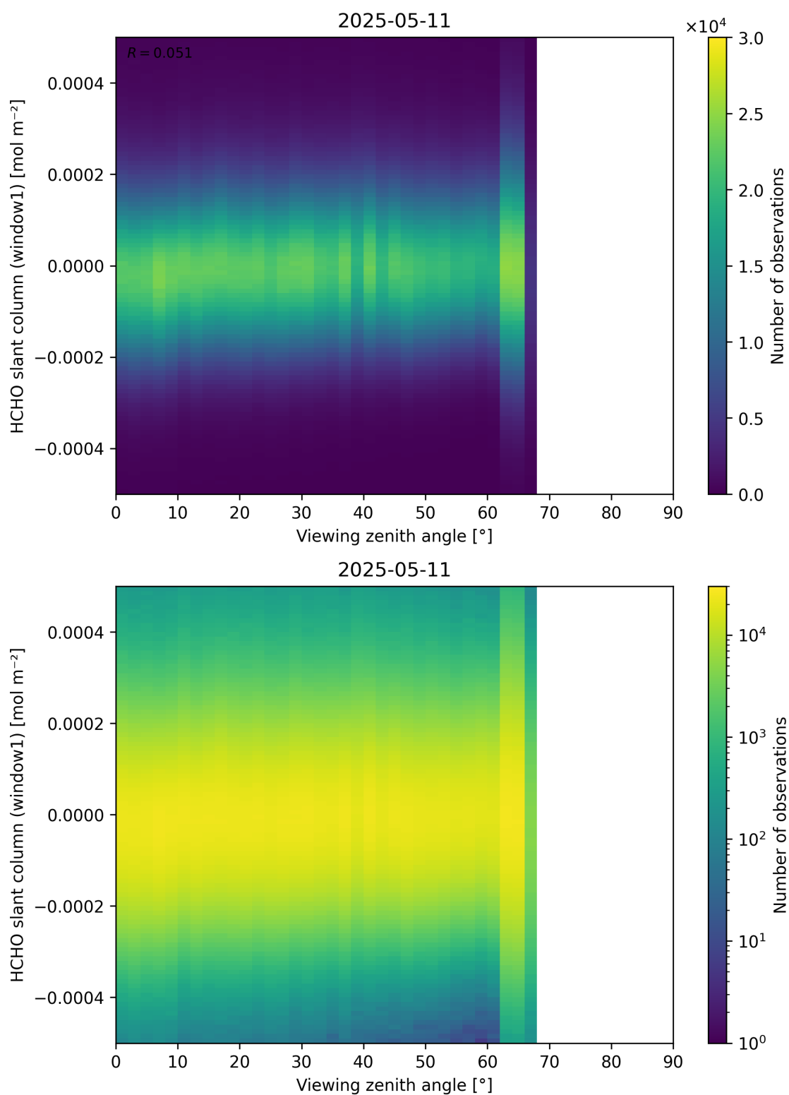
Figure 188: Scatter density plot of “Viewing zenith angle” against “HCHO slant column (window1)” for 2025-05-10 to 2025-05-12.
