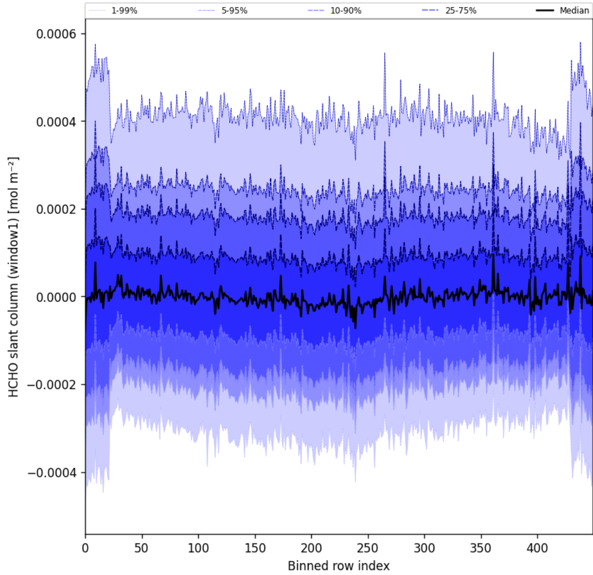
Figure 52: Along track statistics of “HCHO slant column (window1)” for 2025-05-10 to 2025-05-12
