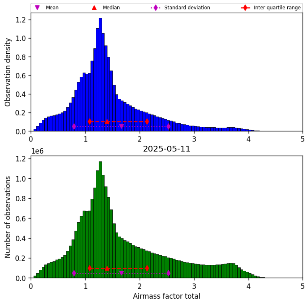
Figure 40: Histogram of “Airmass factor total” for 2025-05-10 to 2025-05-12
