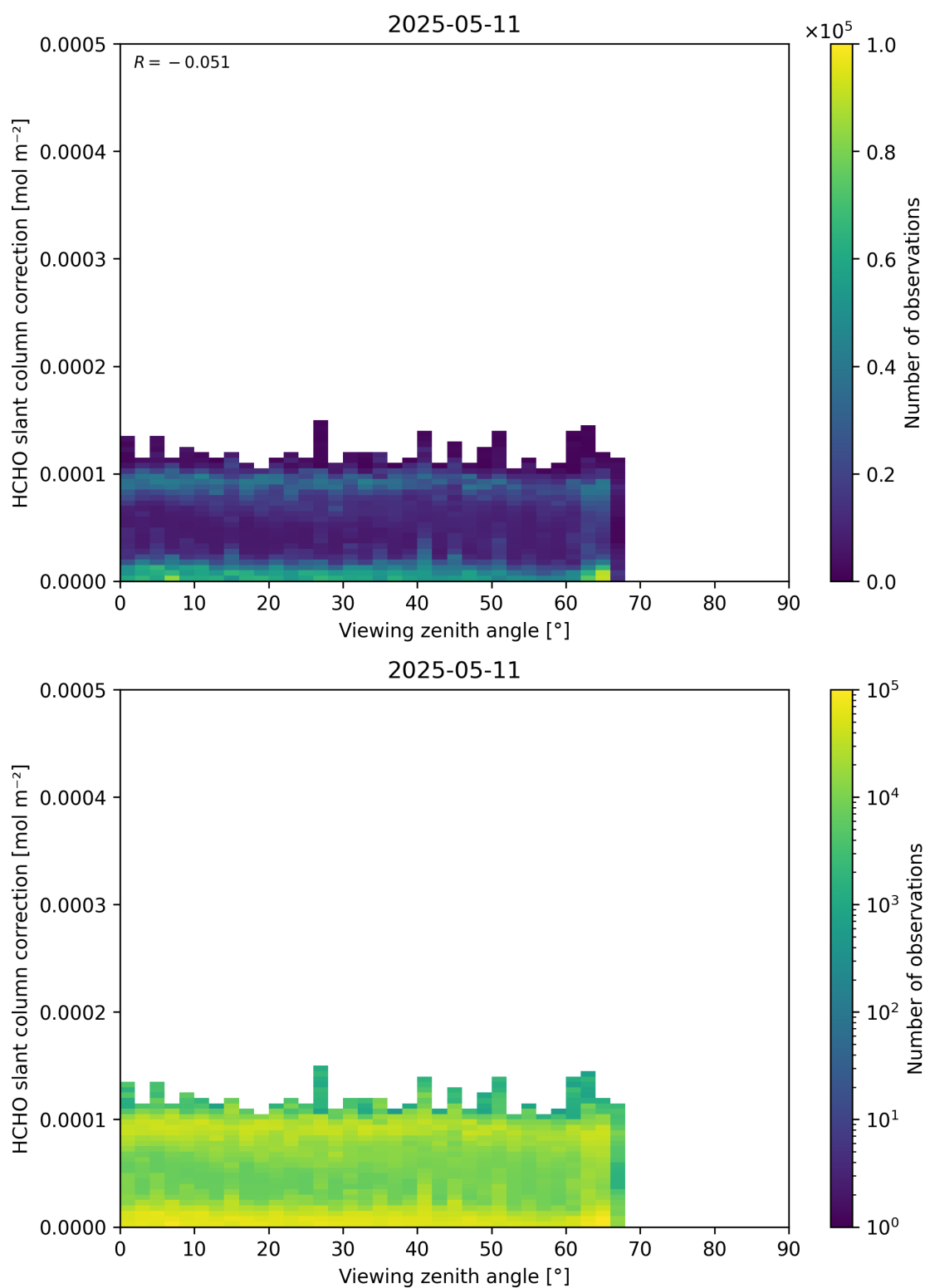
Figure 187: Scatter density plot of “Viewing zenith angle” against “HCHO slant column correction” for 2025-05-10 to 2025-05-12.
