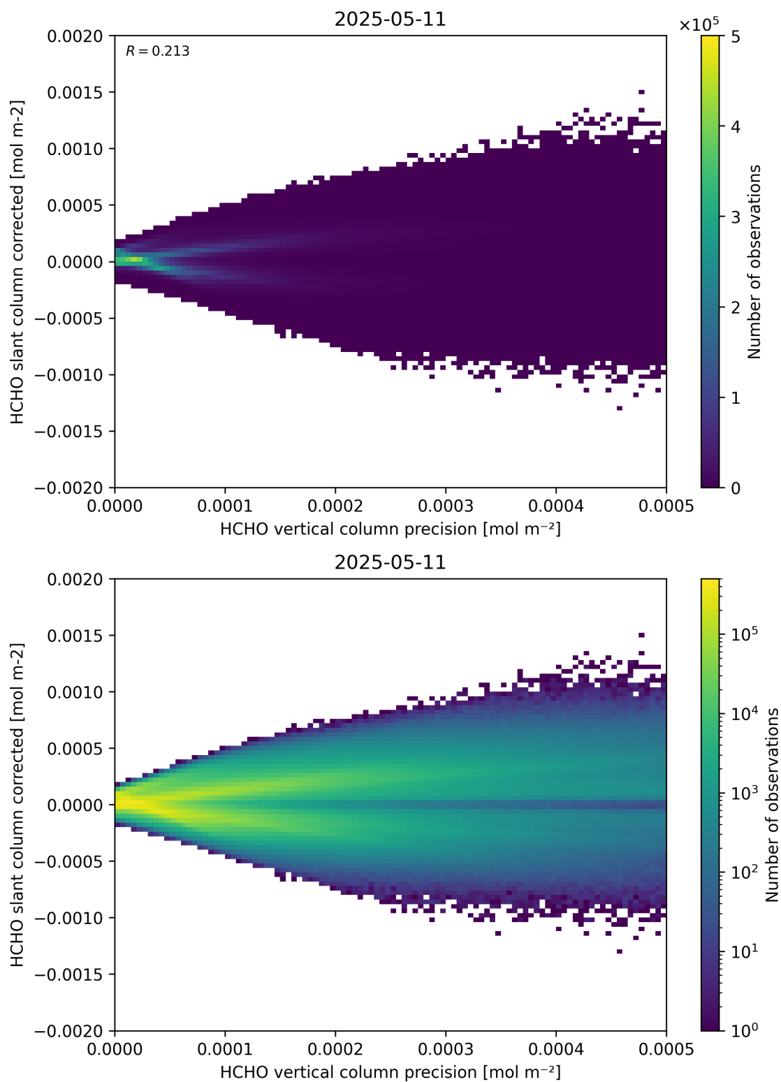
Figure 140: Scatter density plot of “HCHO vertical column precision” against “HCHO slant column corrected” for 2025-05-10 to 2025-05-12.
