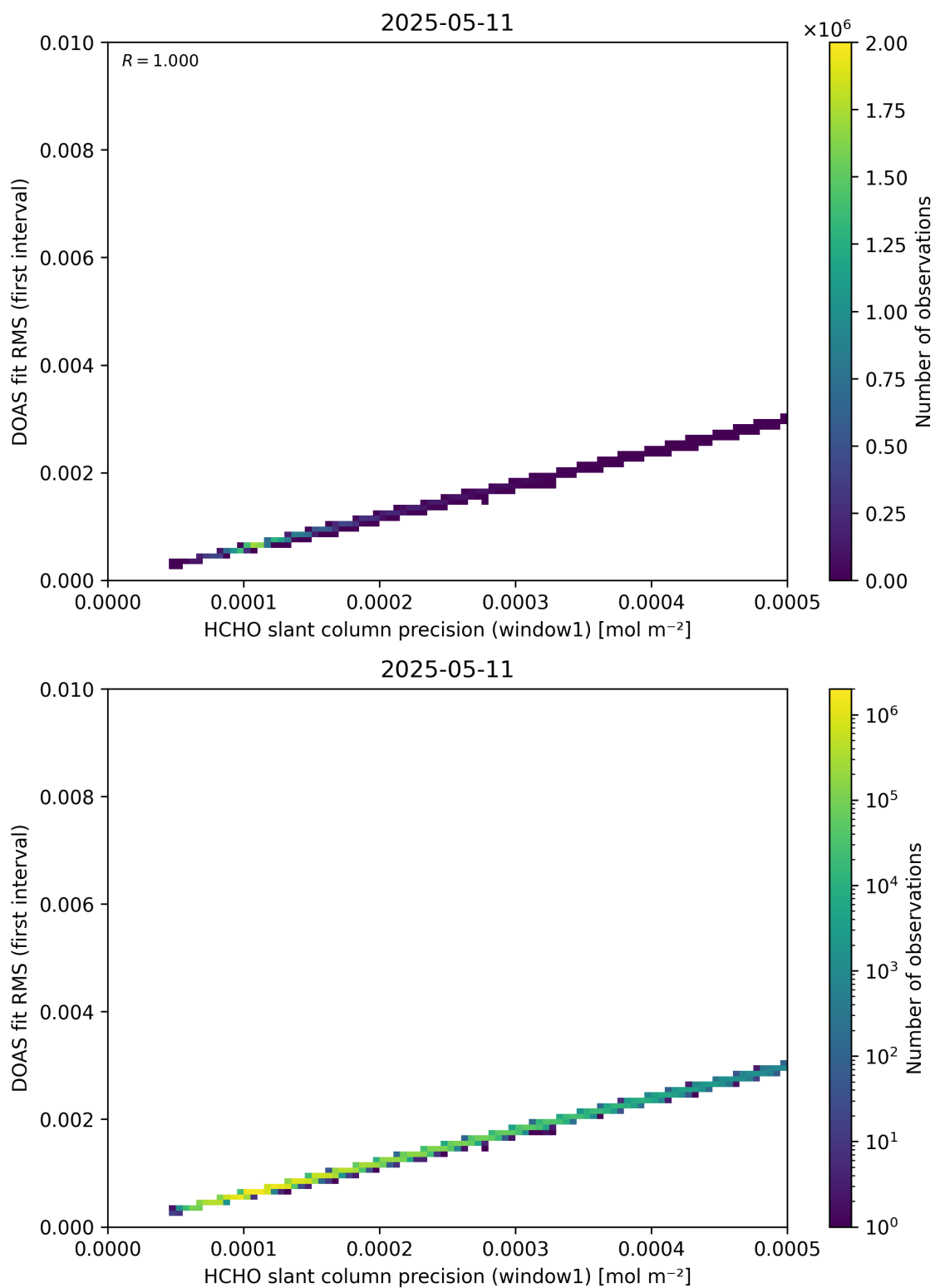
Figure 88: Scatter density plot of “HCHO slant column precision (window1)” against “DOAS fit RMS (first interval)” for 2025-05-10 to 2025-05-12.
