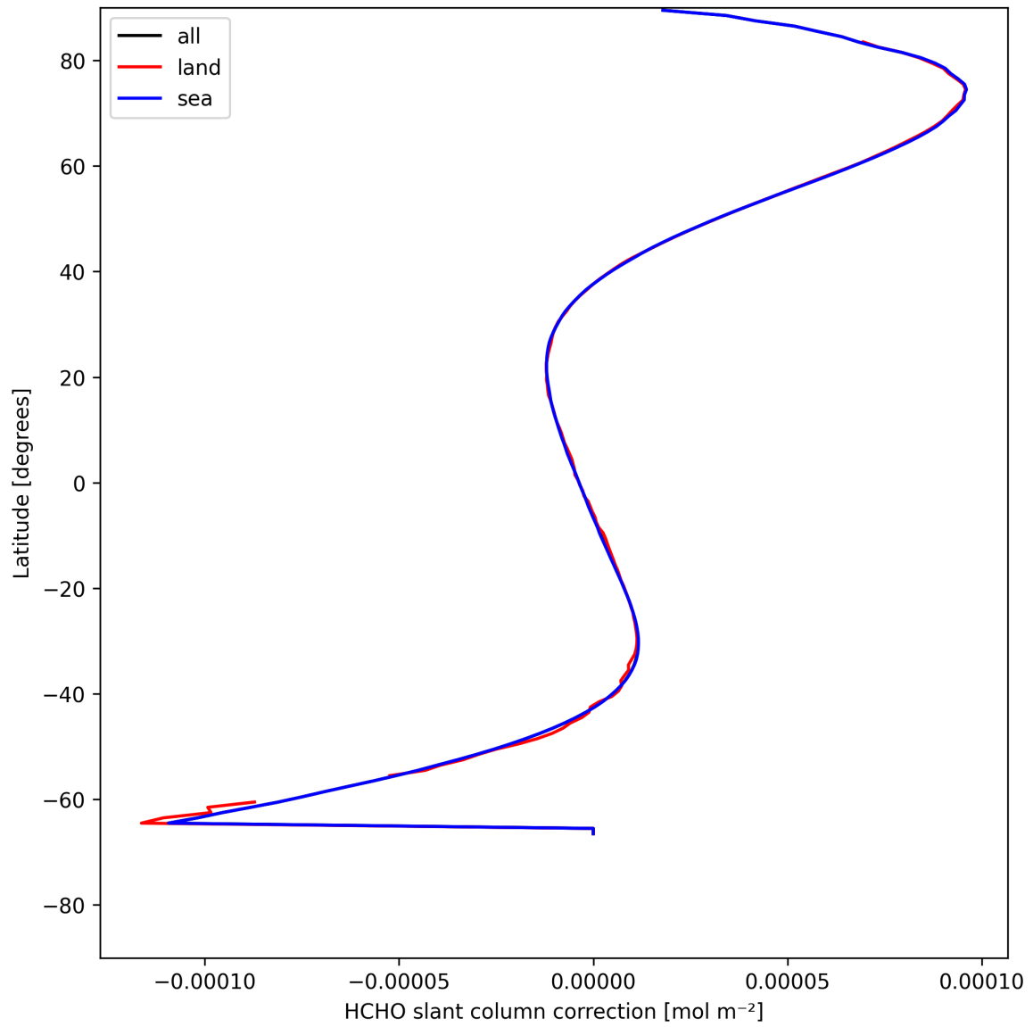
Figure 33: Zonal average of “HCHO slant column correction” for 2025-05-10 to 2025-05-12.
