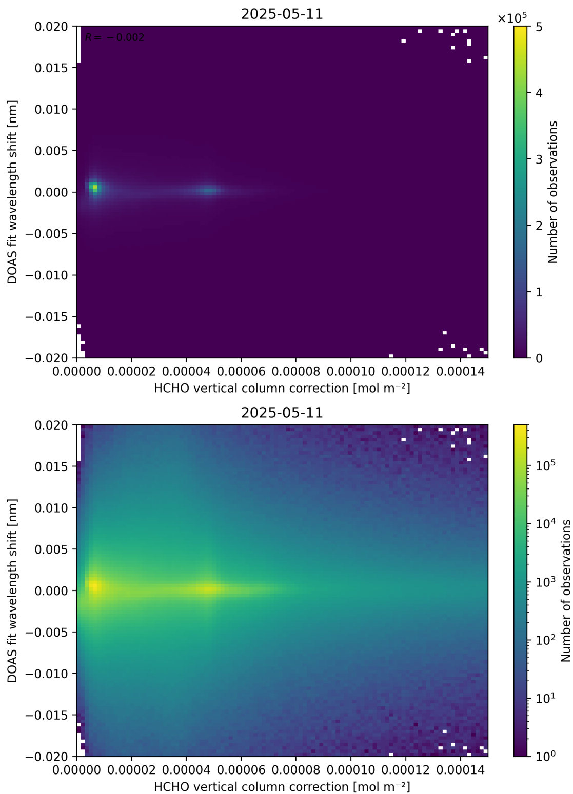
Figure 113: Scatter density plot of “HCHO vertical column correction” against “DOAS fit wavelength shift” for 2025-05-10 to 2025-05-12.
