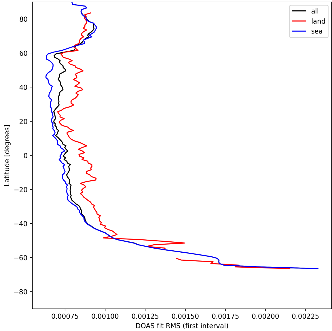
Figure 32: Zonal average of “DOAS fit RMS (first interval)” for 2025-05-10 to 2025-05-12.
