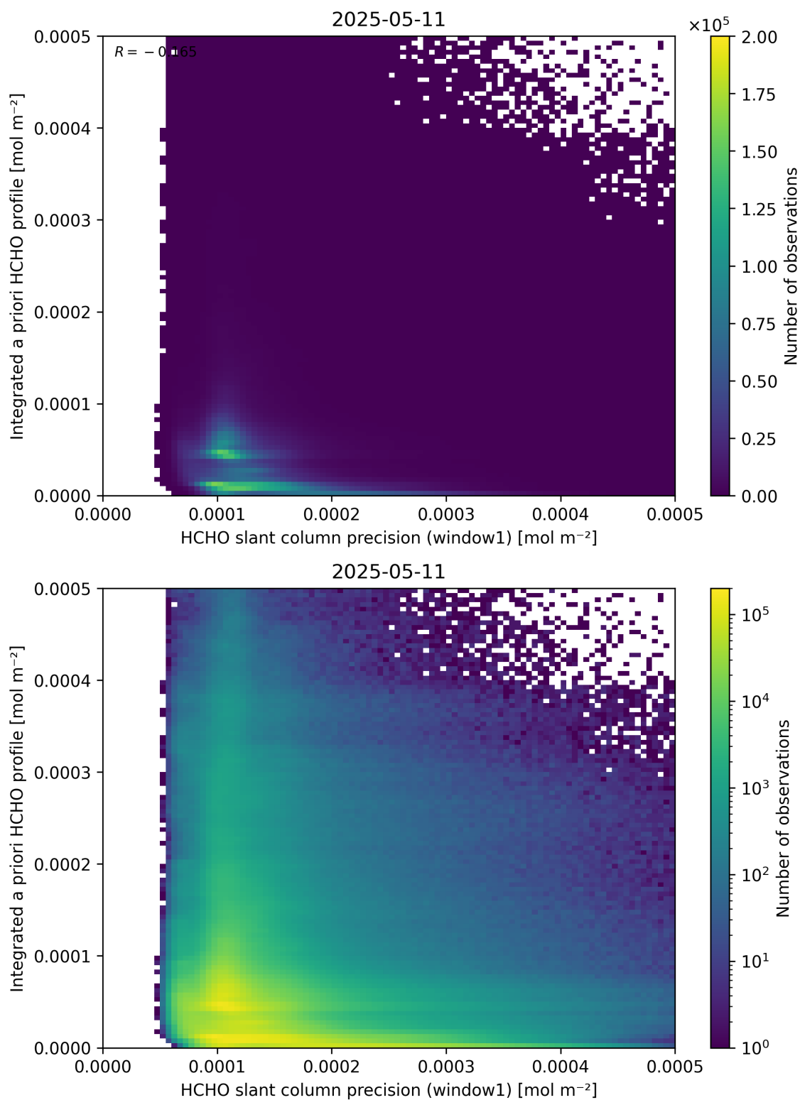
Figure 96: Scatter density plot of “HCHO slant column precision (window1)” against “Integrated a priori HCHO profile” for 2025-05-10 to 2025-05-12.
