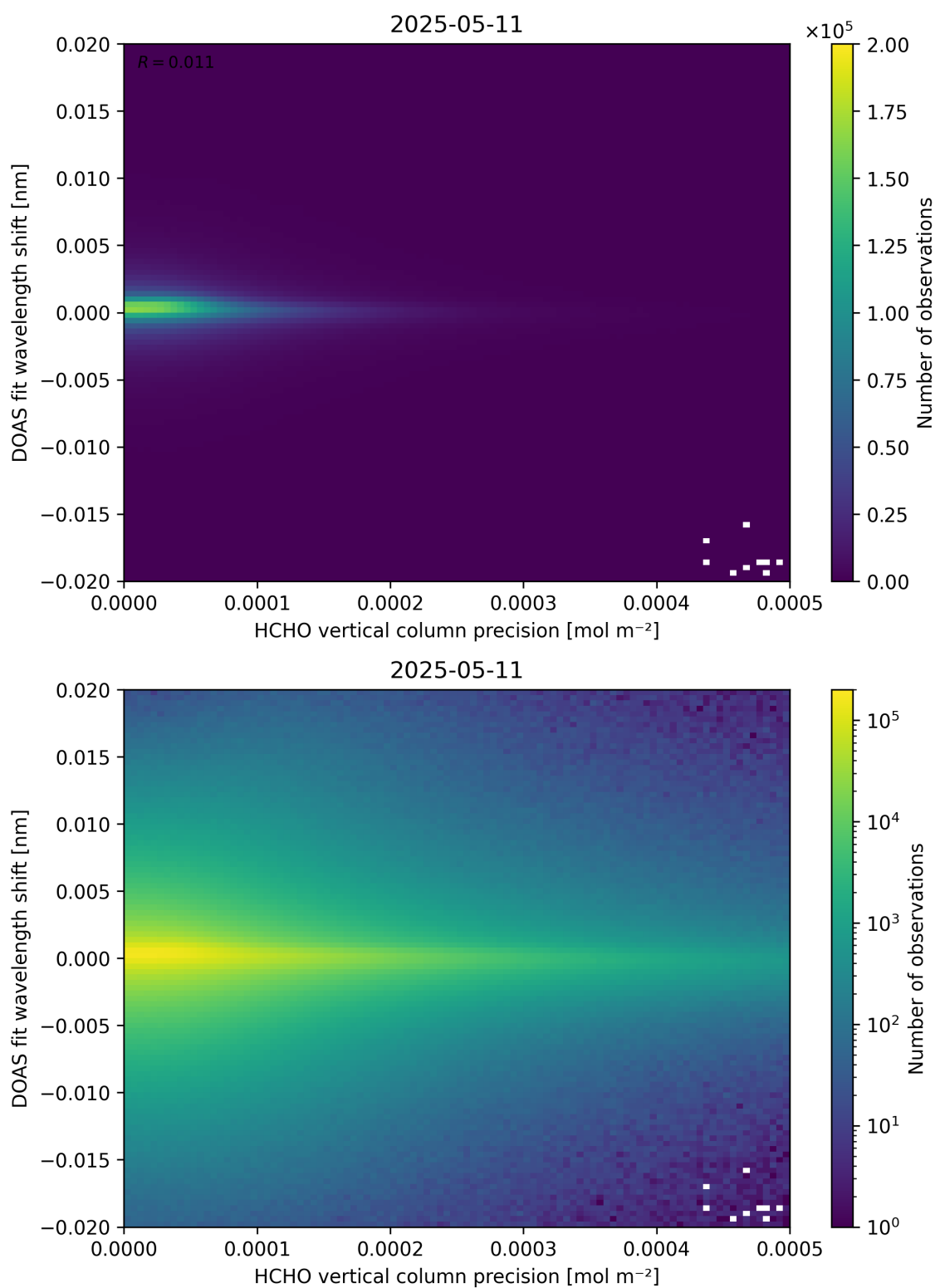
Figure 137: Scatter density plot of “HCHO vertical column precision” against “DOAS fit wavelength shift” for 2025-05-10 to 2025-05-12.
