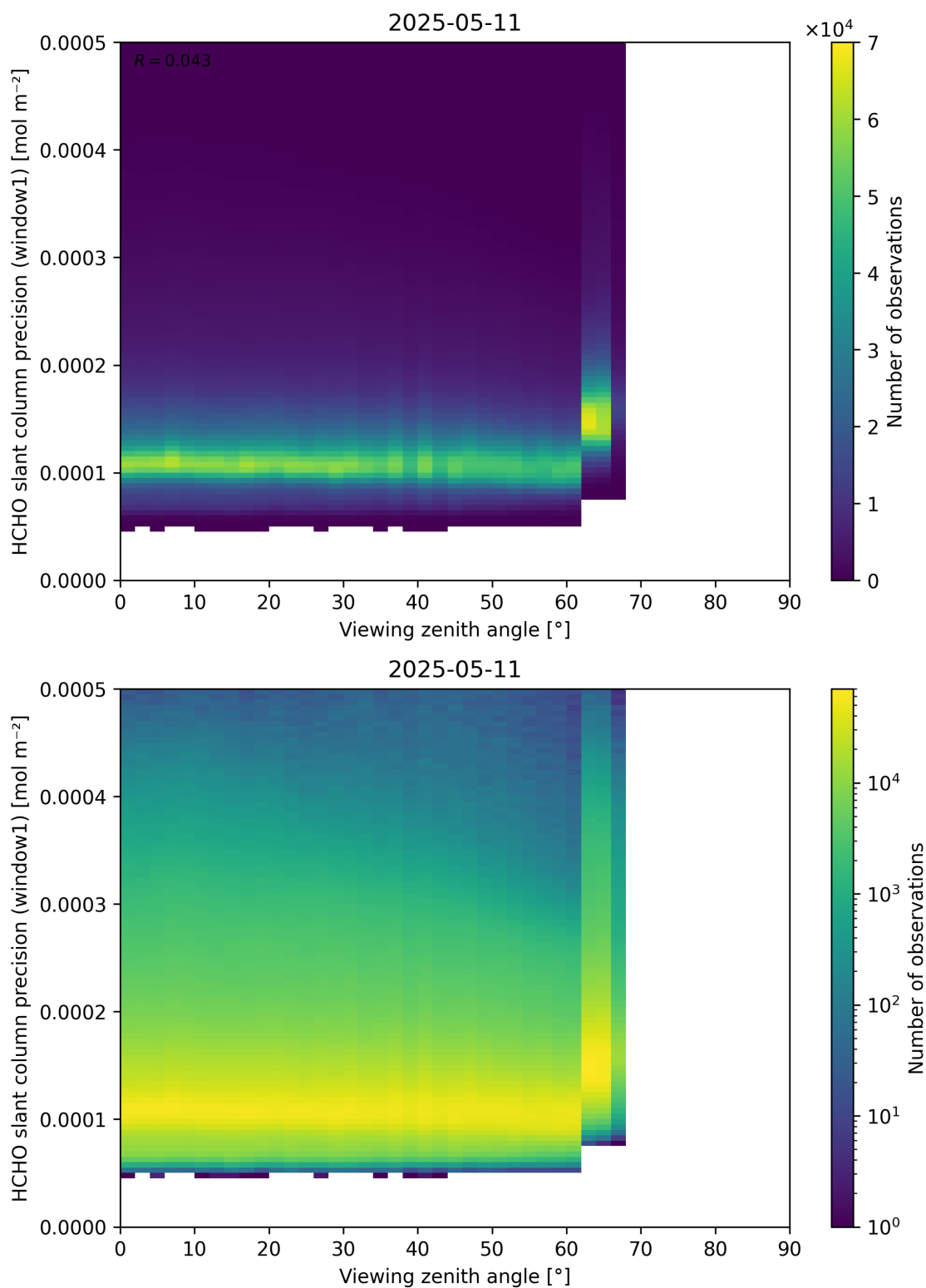
Figure 189: Scatter density plot of “Viewing zenith angle” against “HCHO slant column precision (window1)” for 2025-05-10 to 2025-05-12.
