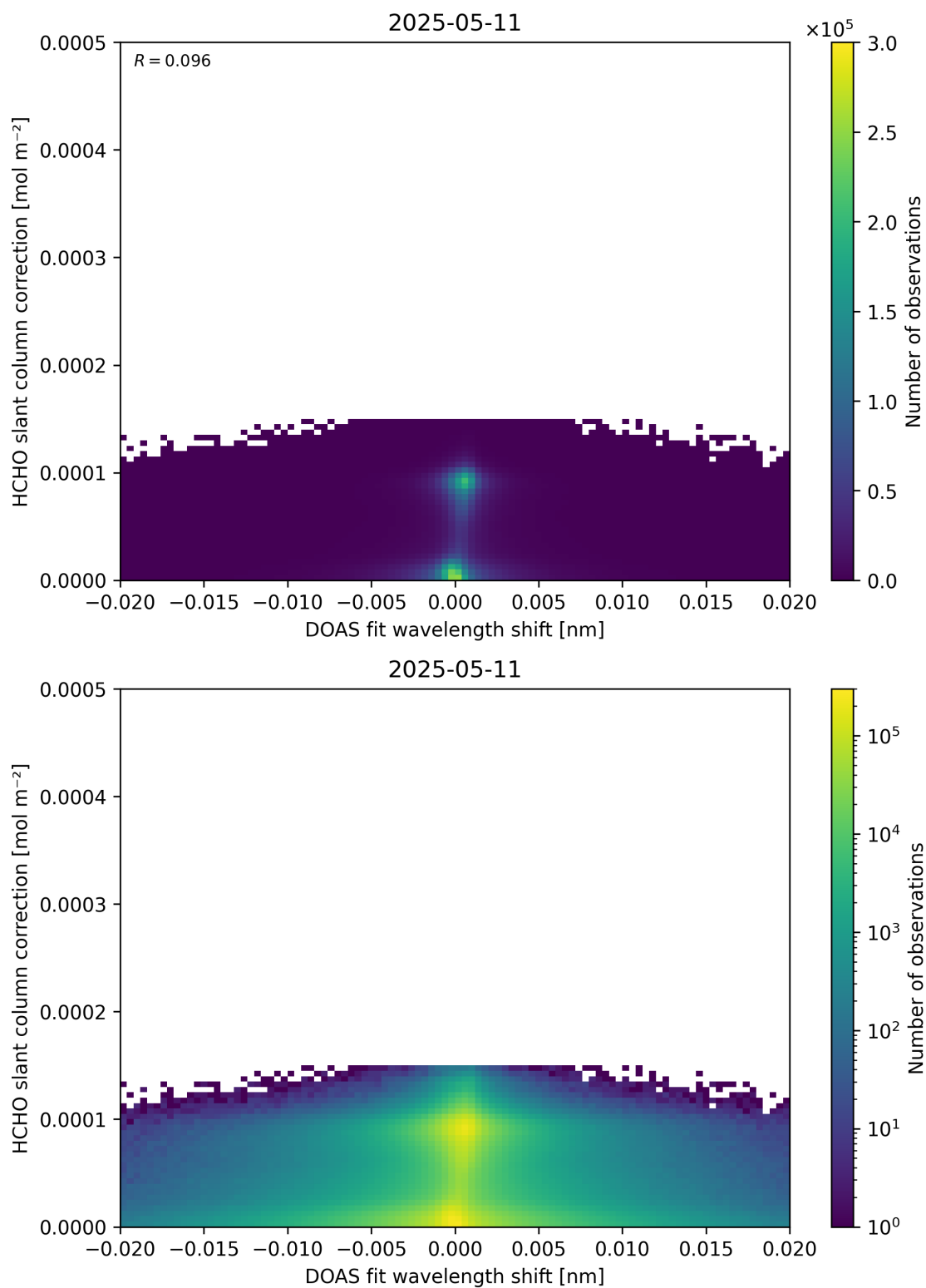
Figure 67: Scatter density plot of “DOAS fit wavelength shift” against “HCHO slant column correction” for 2025-05-10 to 2025-05-12.
