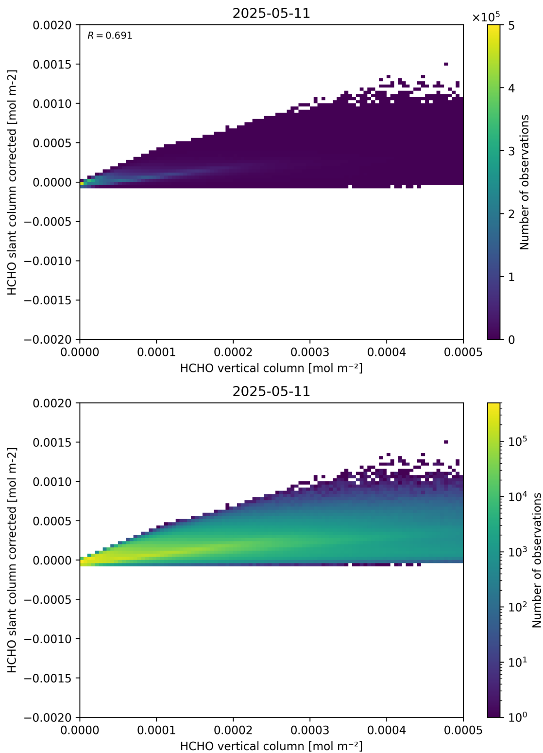
Figure 127: Scatter density plot of “HCHO vertical column” against “HCHO slant column corrected” for 2025-05-10 to 2025-05-12.
