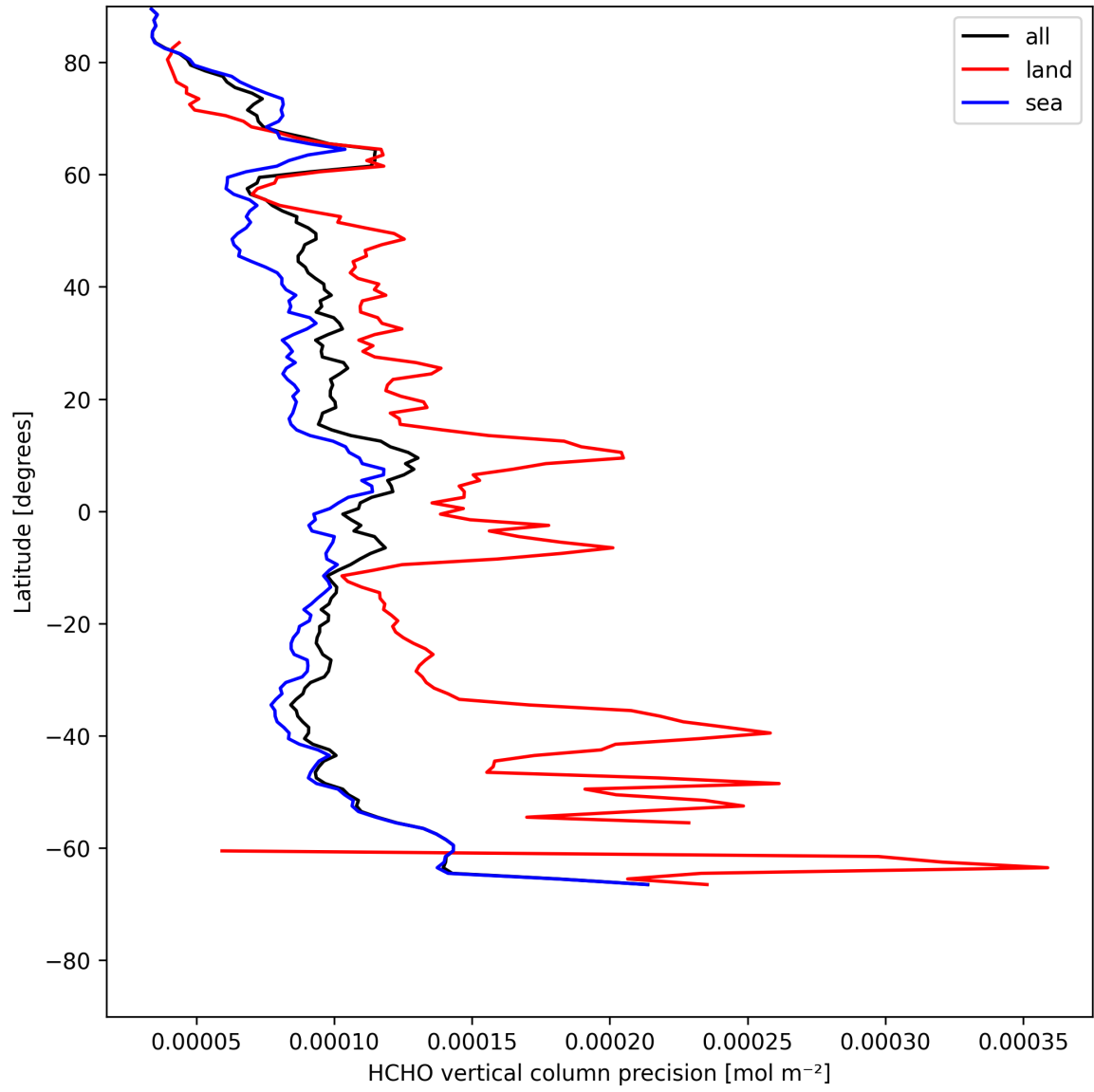
Figure 22: Zonal average of “HCHO vertical column precision” for 2025-05-10 to 2025-05-12.
