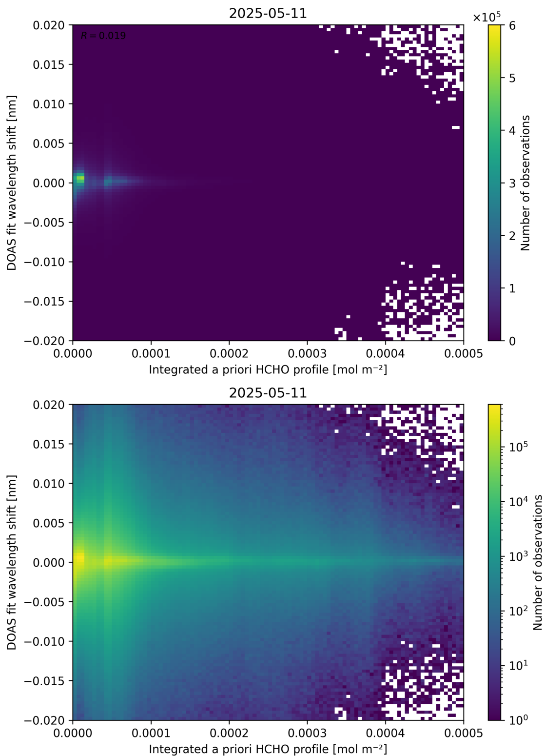
Figure 149: Scatter density plot of “Integrated a priori HCHO profile” against “DOAS fit wavelength shift” for 2025-05-10 to 2025-05-12.
