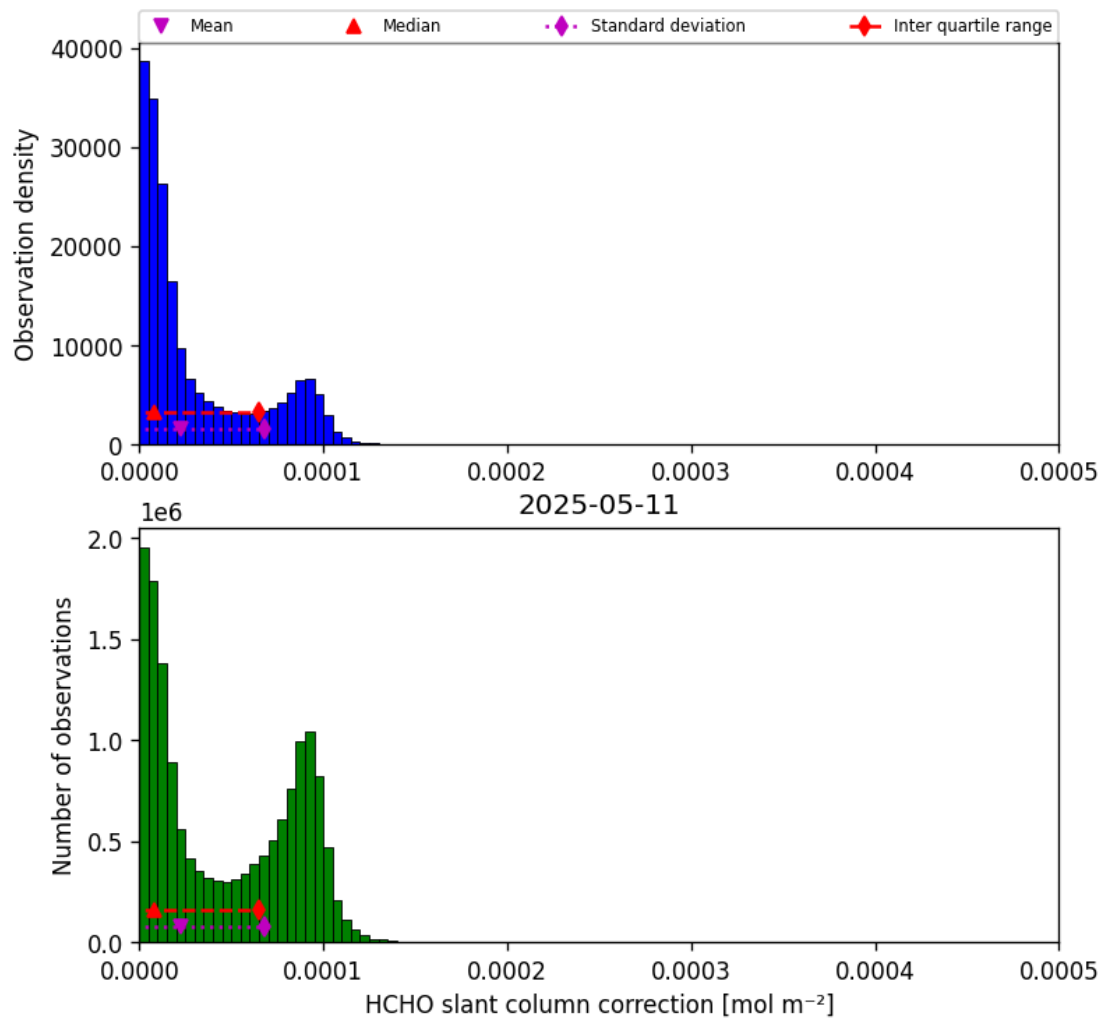
Figure 47: Histogram of “HCHO slant column correction” for 2025-05-10 to 2025-05-12
