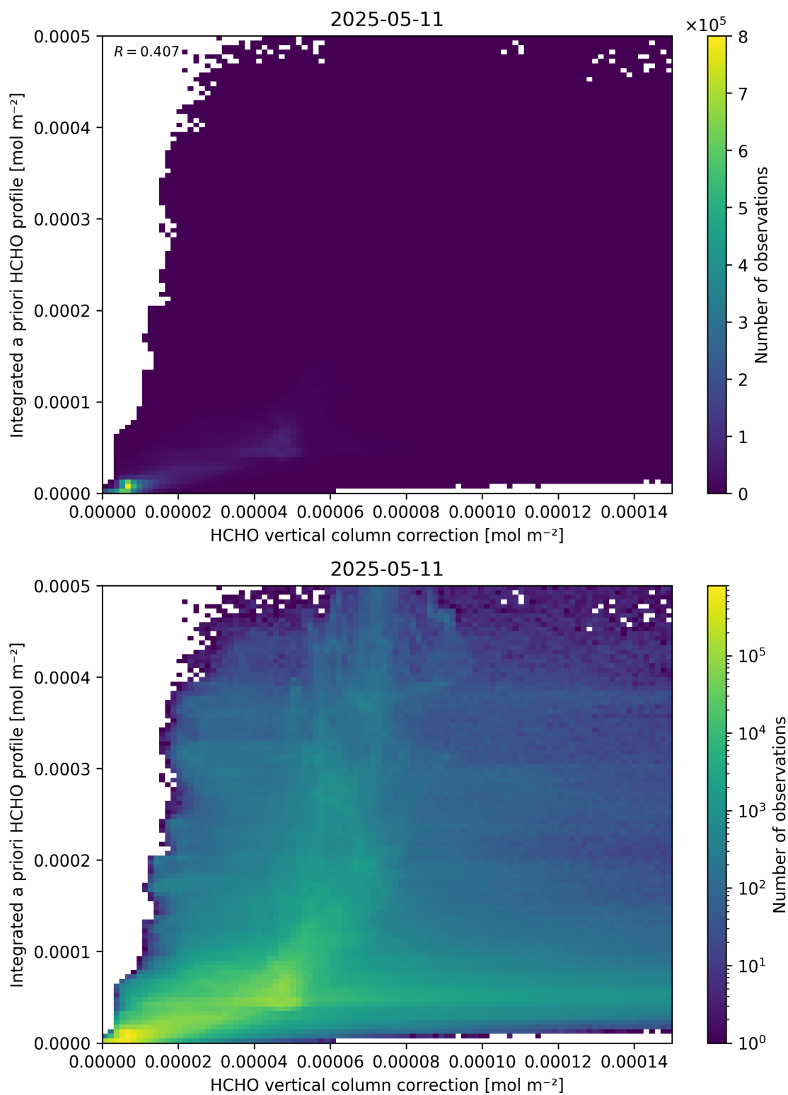
Figure 122: Scatter density plot of “HCHO vertical column correction” against “Integrated a priori HCHO profile” for 2025-05-10 to 2025-05-12.
