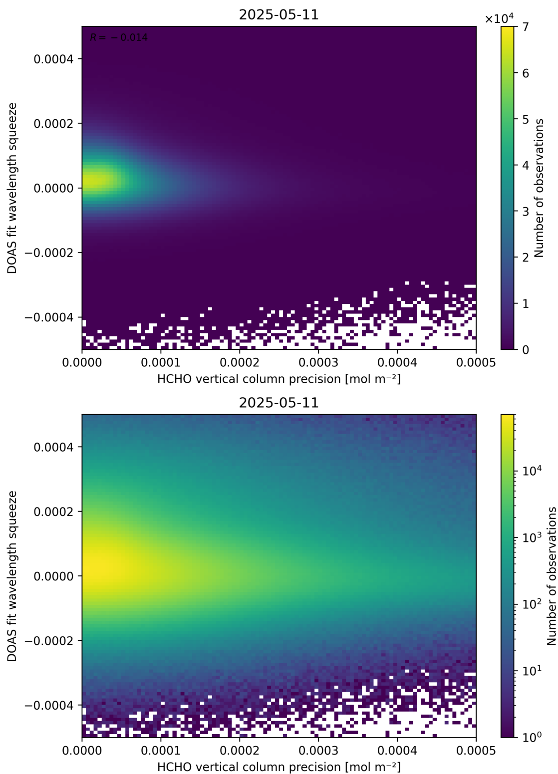
Figure 138: Scatter density plot of “HCHO vertical column precision” against “DOAS fit wavelength squeeze” for 2025-05-10 to 2025-05-12.
