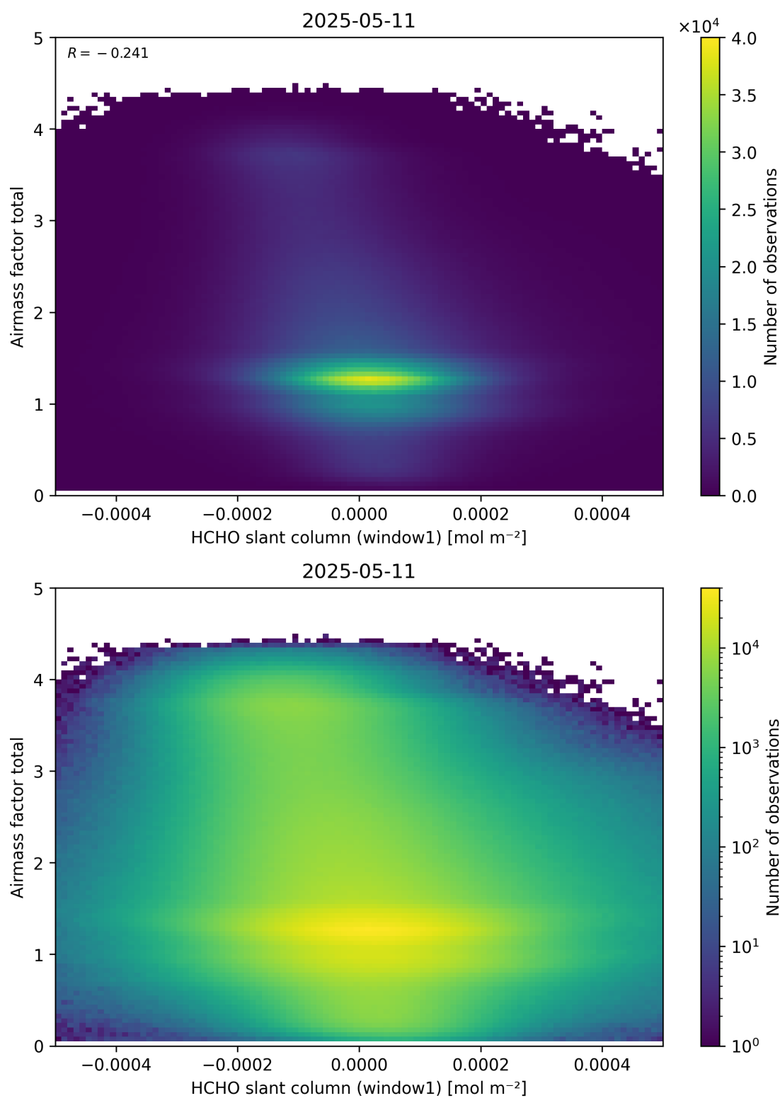
Figure 85: Scatter density plot of “HCHO slant column (window1)” against “Airmass factor total” for 2025-05-10 to 2025-05-12.
