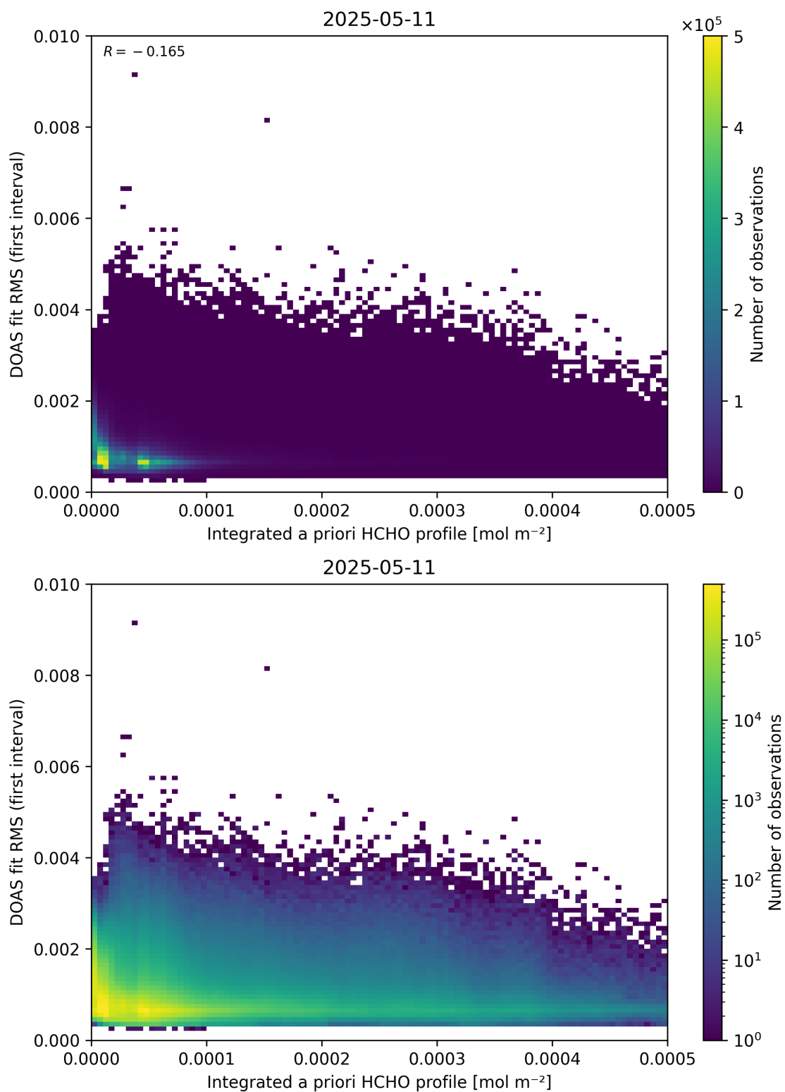
Figure 148: Scatter density plot of “Integrated a priori HCHO profile” against “DOAS fit RMS (first interval)” for 2025-05-10 to 2025-05-12.
