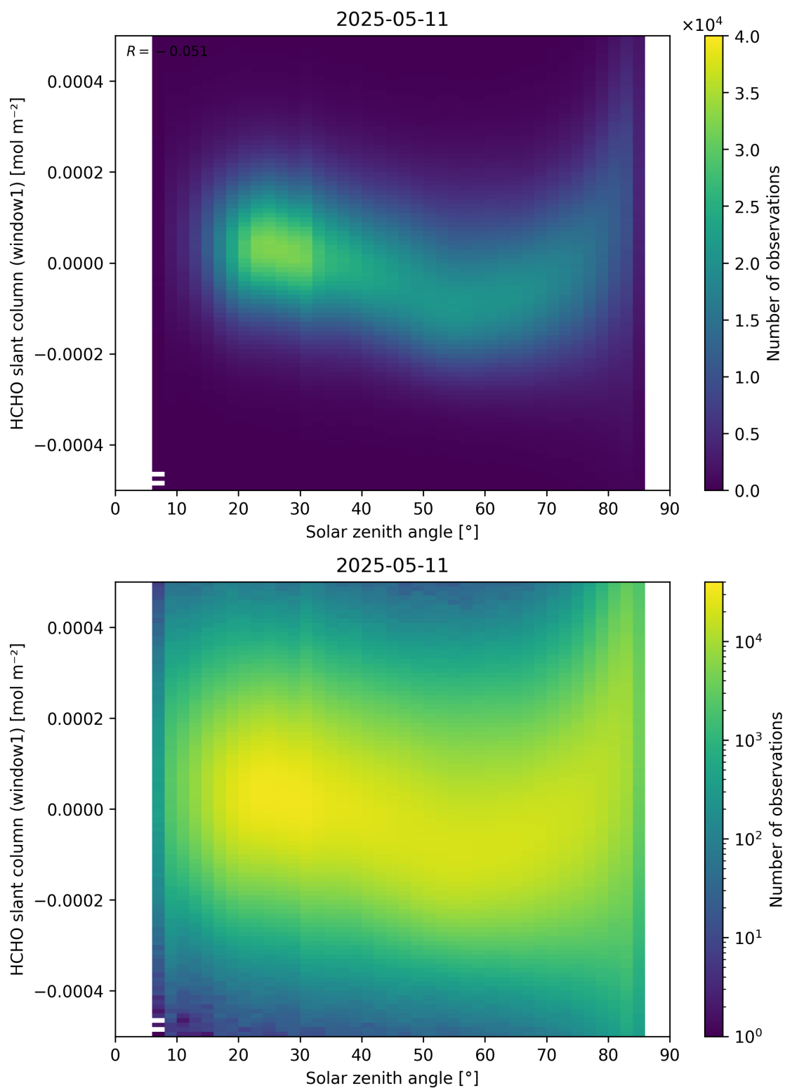
Figure 173: Scatter density plot of “Solar zenith angle” against “HCHO slant column (window1)” for 2025-05-10 to 2025-05-12.
