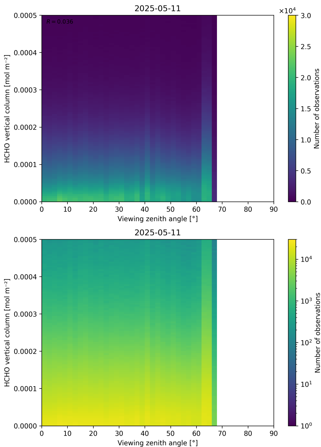
Figure 192: Scatter density plot of “Viewing zenith angle” against “HCHO vertical column” for 2025-05-10 to 2025-05-12.
