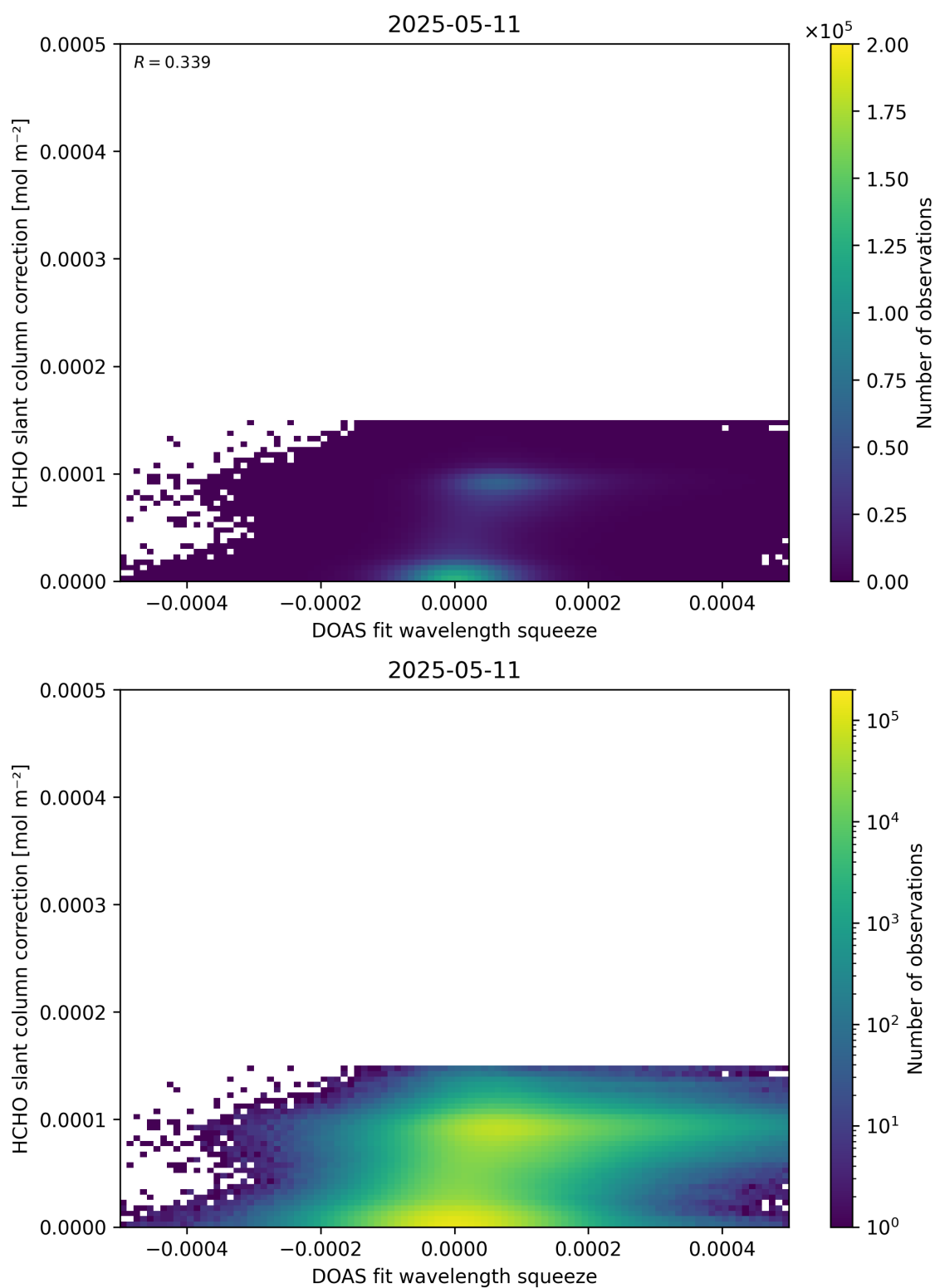
Figure 70: Scatter density plot of “DOAS fit wavelength squeeze” against “HCHO slant column correction” for 2025-05-10 to 2025-05-12.
