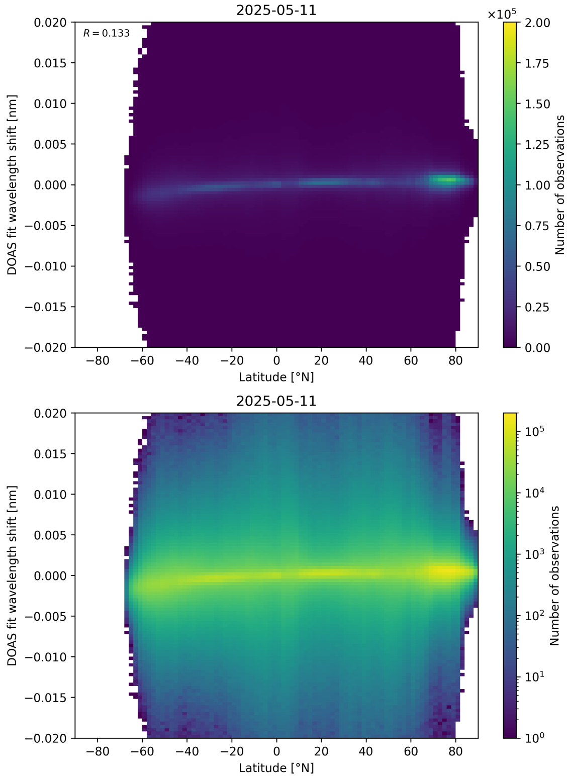
Figure 154: Scatter density plot of “Latitude” against “DOAS fit wavelength shift” for 2025-05-10 to 2025-05-12.
