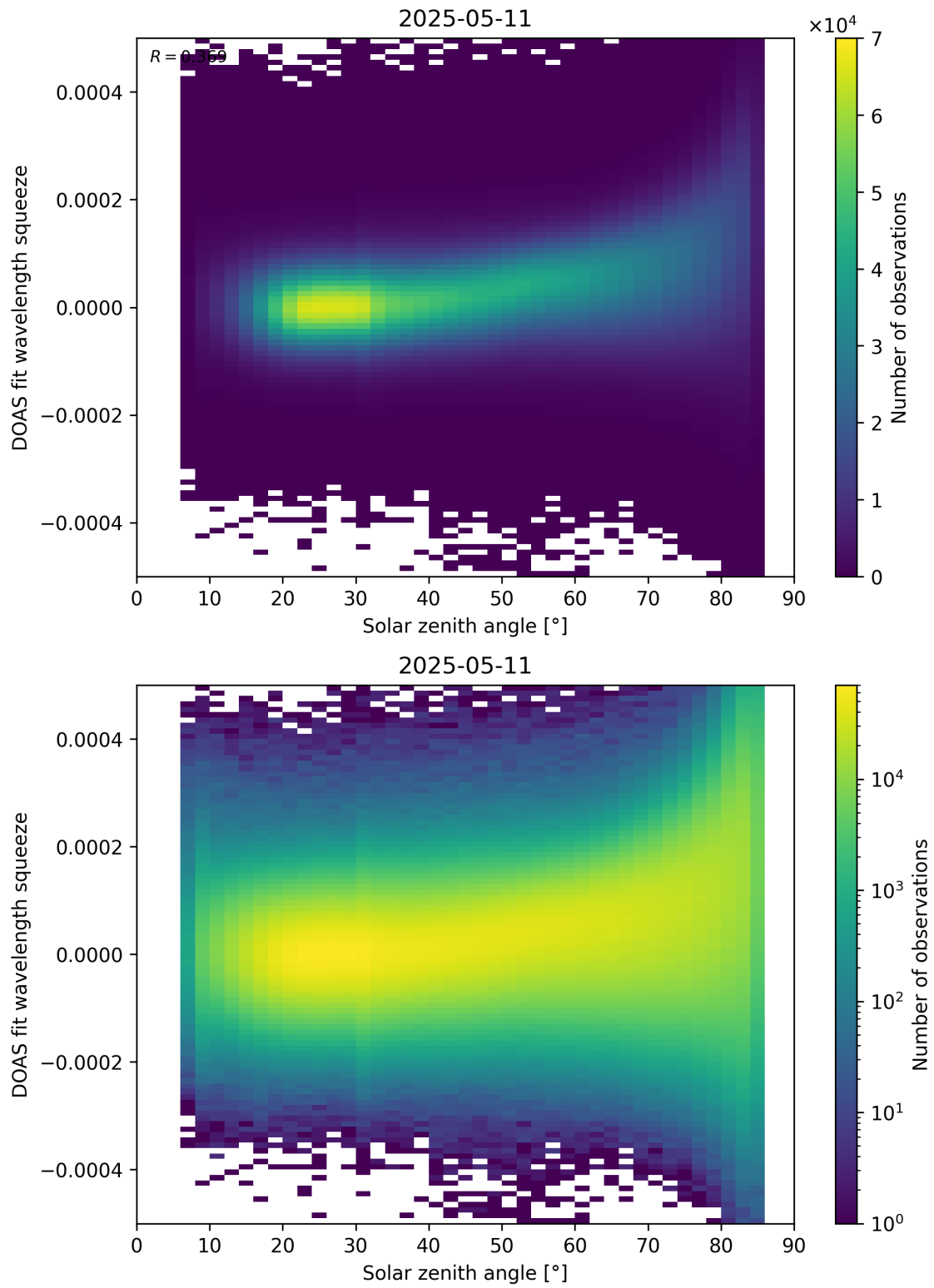
Figure 169: Scatter density plot of “Solar zenith angle” against “DOAS fit wavelength squeeze” for 2025-05-10 to 2025-05-12.
