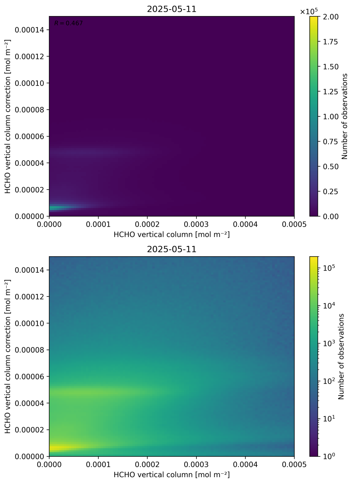
Figure 133: Scatter density plot of “HCHO vertical column” against “HCHO vertical column correction” for 2025-05-10 to 2025-05-12.
