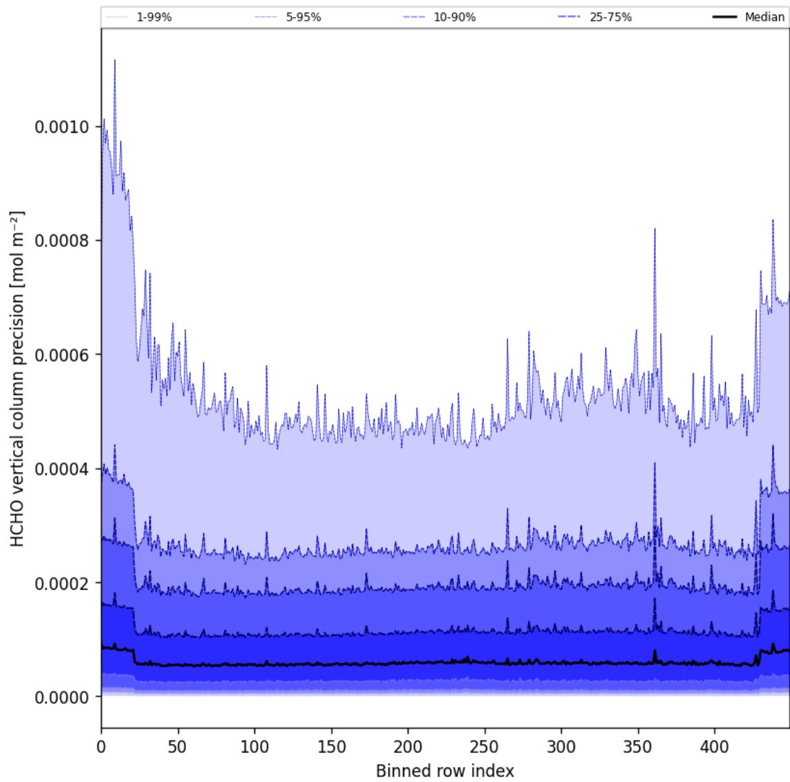
Figure 50: Along track statistics of “HCHO vertical column precision” for 2025-05-10 to 2025-05-12
