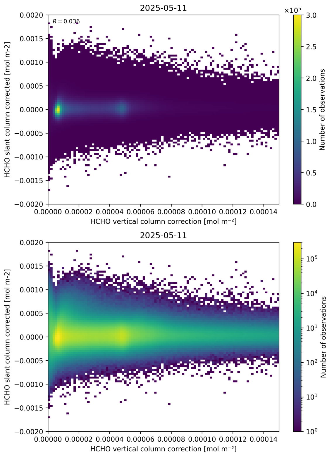
Figure 116: Scatter density plot of “HCHO vertical column correction” against “HCHO slant column corrected” for 2025-05-10 to 2025-05-12.
