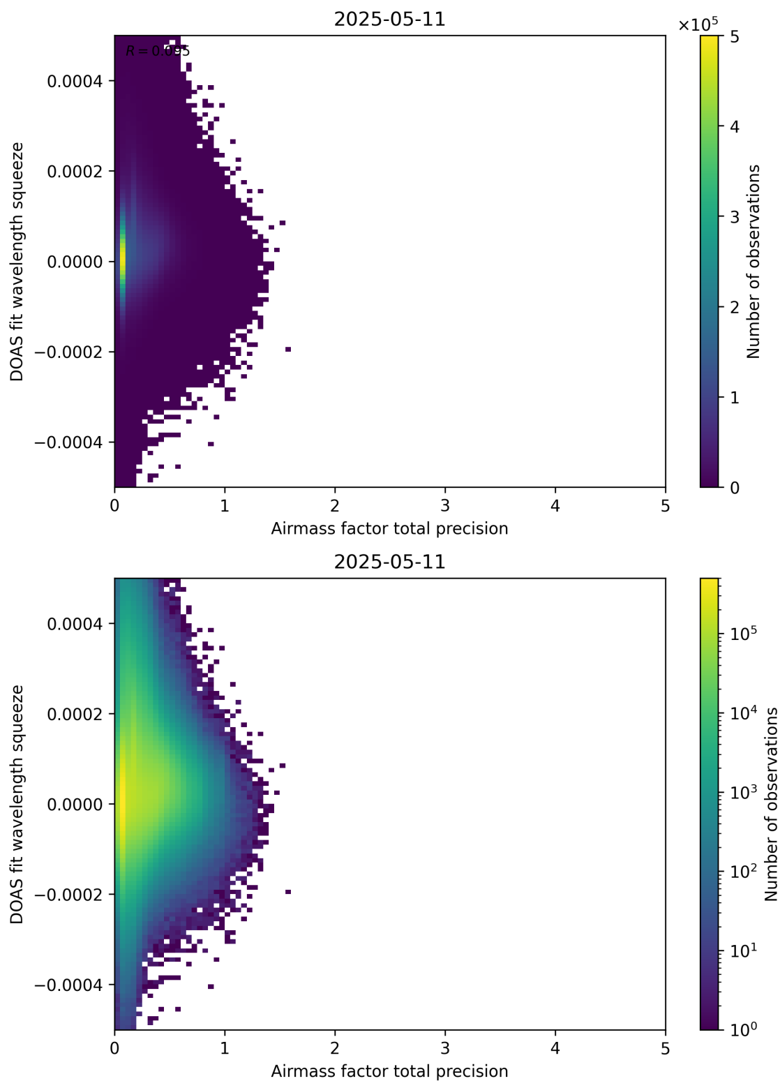
Figure 107: Scatter density plot of “Airmass factor total precision” against “DOAS fit wavelength squeeze” for 2025-05-10 to 2025-05-12.
