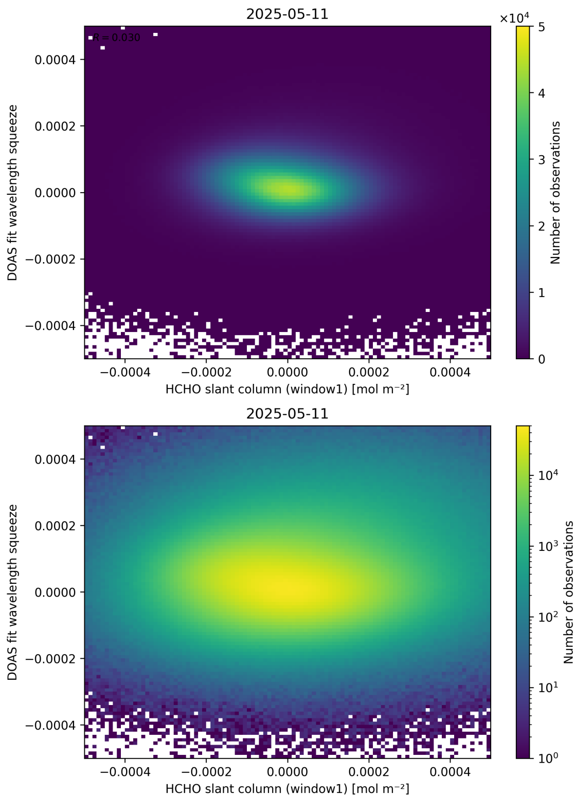
Figure 80: Scatter density plot of “HCHO slant column (window1)” against “DOAS fit wavelength squeeze” for 2025-05-10 to 2025-05-12.
