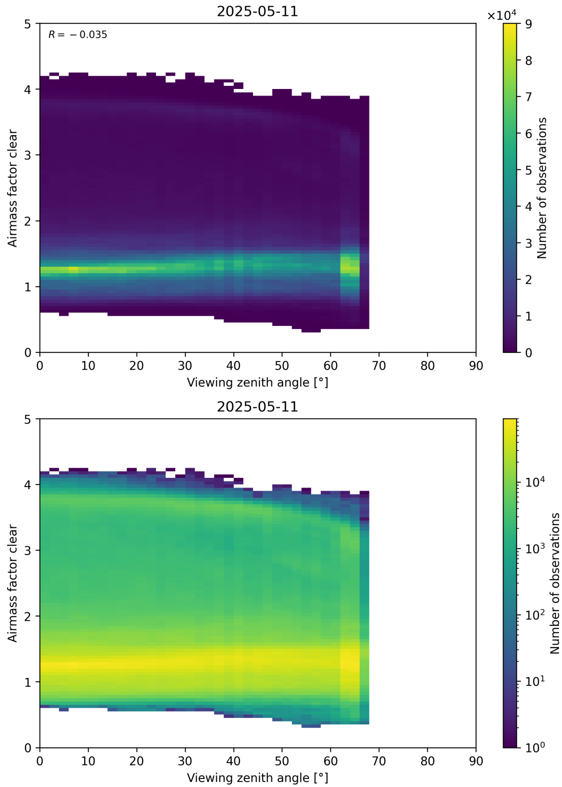
Figure 185: Scatter density plot of “Viewing zenith angle” against “Airmass factor clear” for 2025-05-10 to 2025-05-12.
