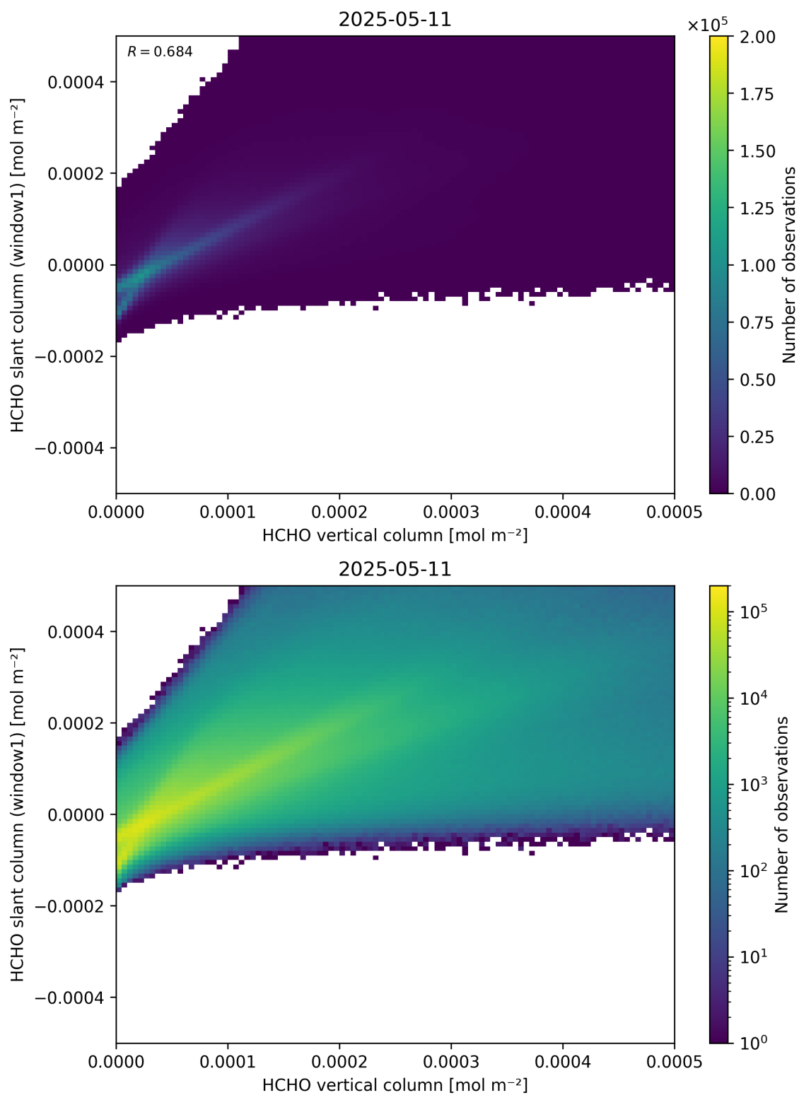
Figure 129: Scatter density plot of “HCHO vertical column” against “HCHO slant column (window1)” for 2025-05-10 to 2025-05-12.
