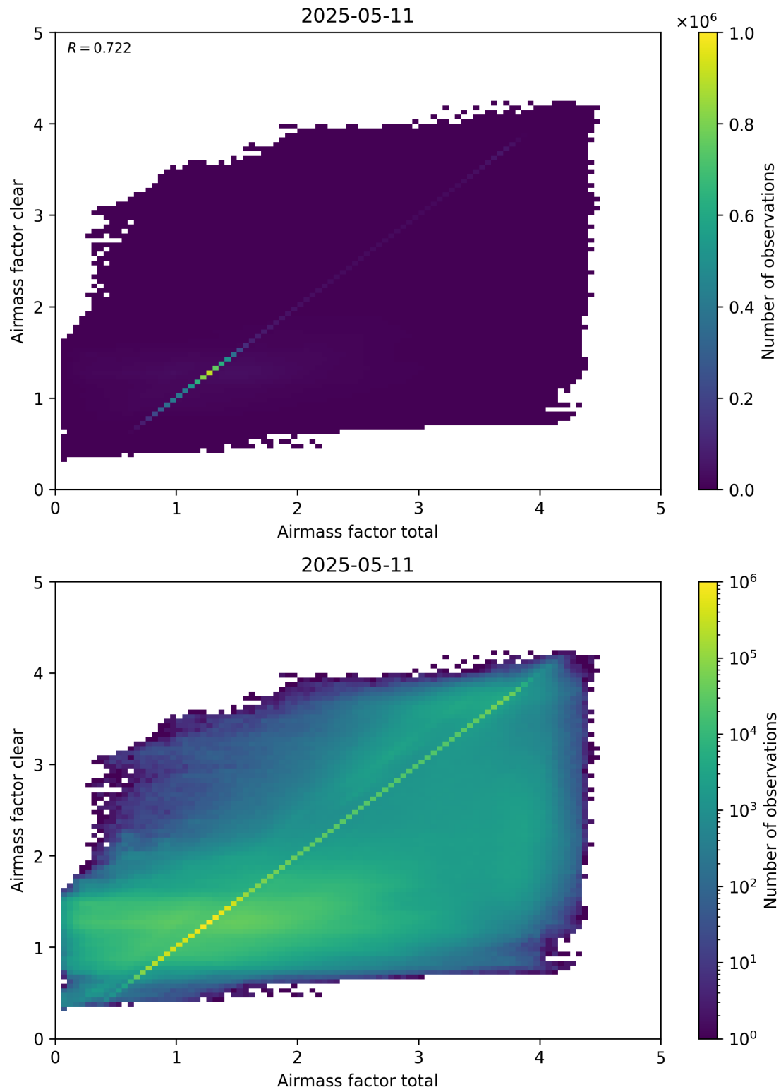
Figure 100: Scatter density plot of “Airmass factor total” against “Airmass factor clear” for 2025-05-10 to 2025-05-12.
