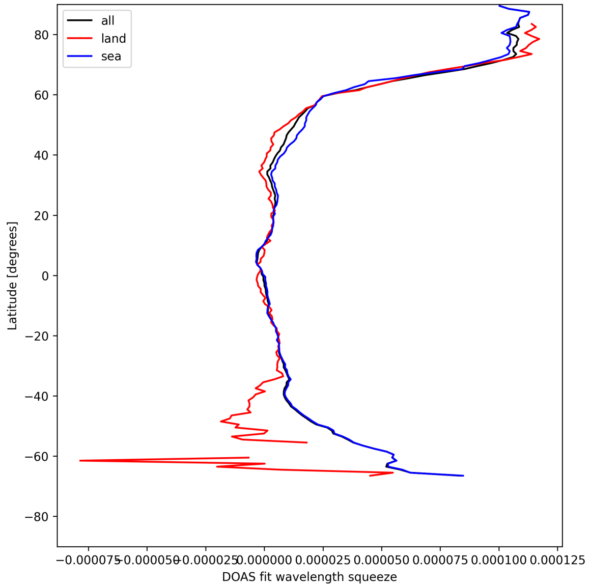
Figure 31: Zonal average of “DOAS fit wavelength squeeze” for 2025-05-10 to 2025-05-12.
