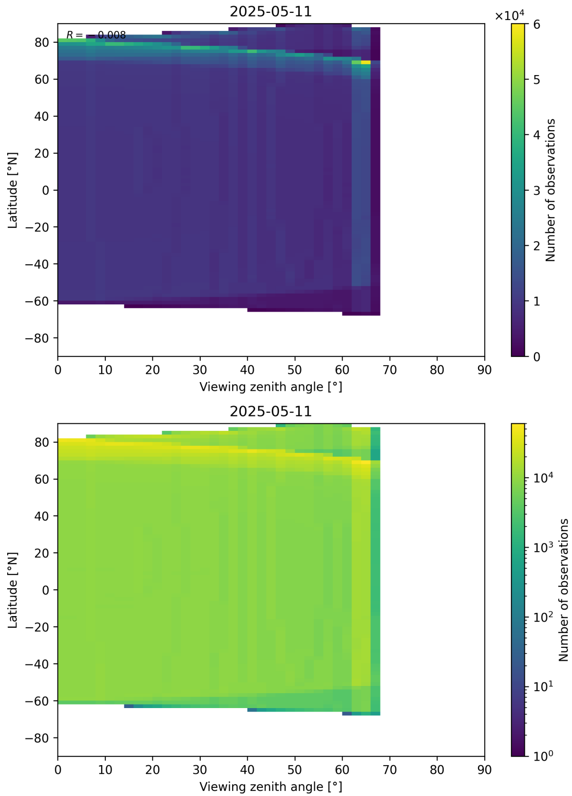
Figure 196: Scatter density plot of “Viewing zenith angle” against “Latitude” for 2025-05-10 to 2025-05-12.
