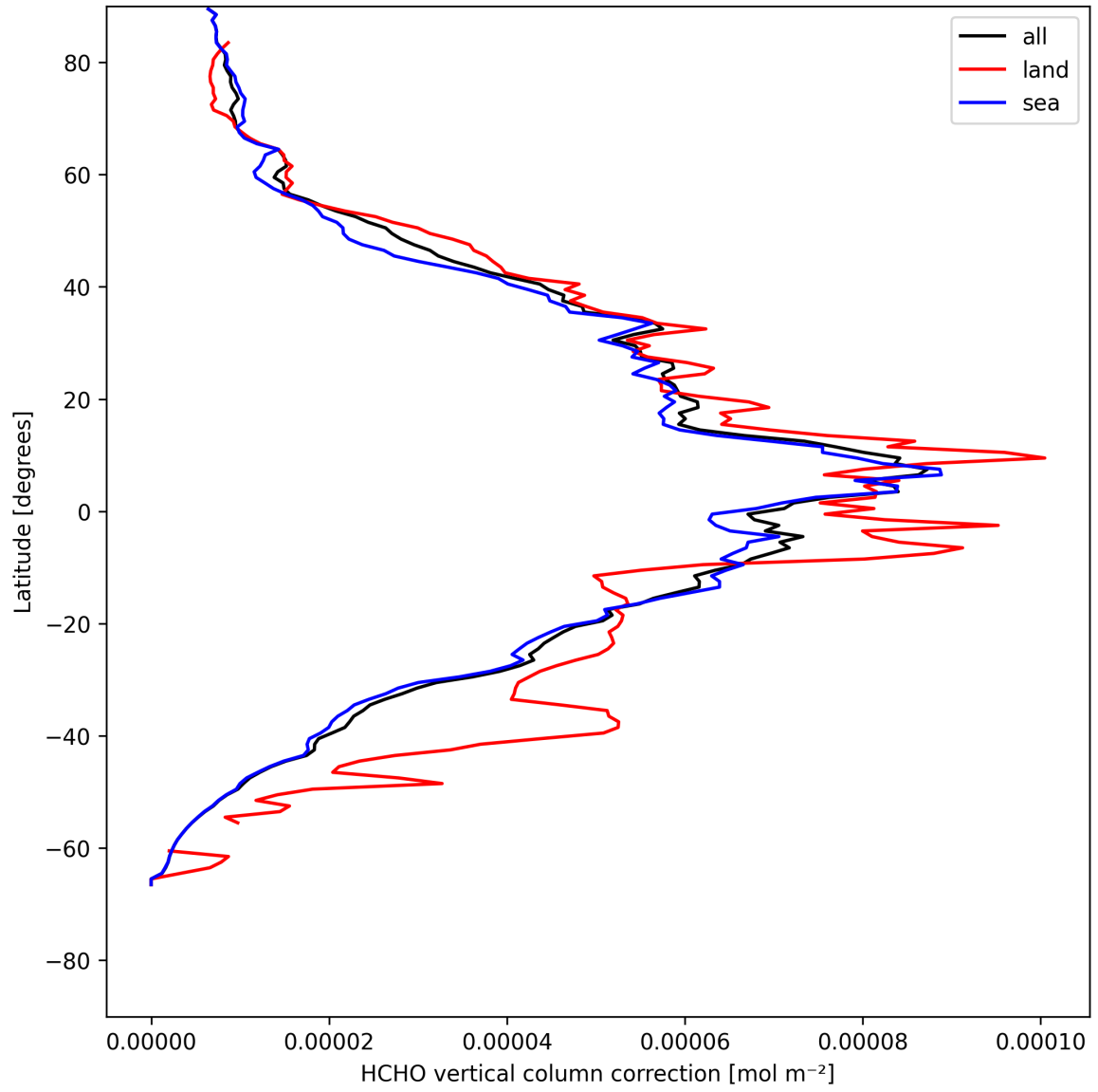
Figure 23: Zonal average of “HCHO vertical column correction” for 2025-05-10 to 2025-05-12.
