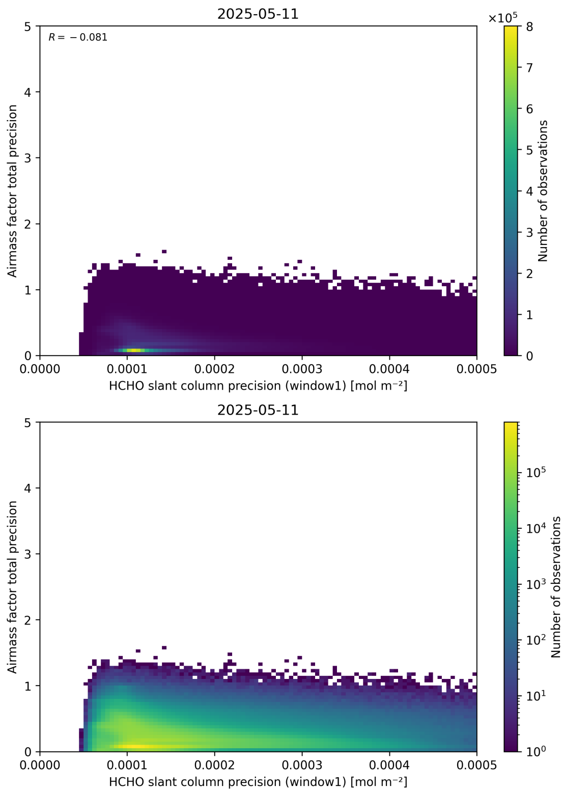
Figure 95: Scatter density plot of “HCHO slant column precision (window1)” against “Airmass factor total precision” for 2025-05-10 to 2025-05-12.
