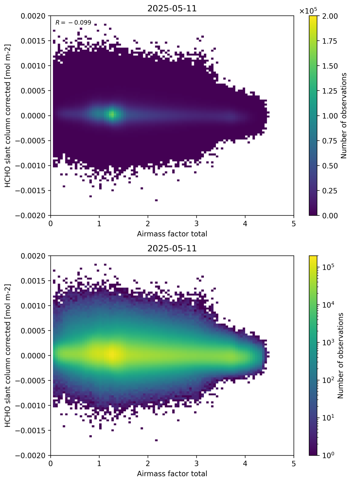
Figure 101: Scatter density plot of “Airmass factor total” against “HCHO slant column corrected” for 2025-05-10 to 2025-05-12.
