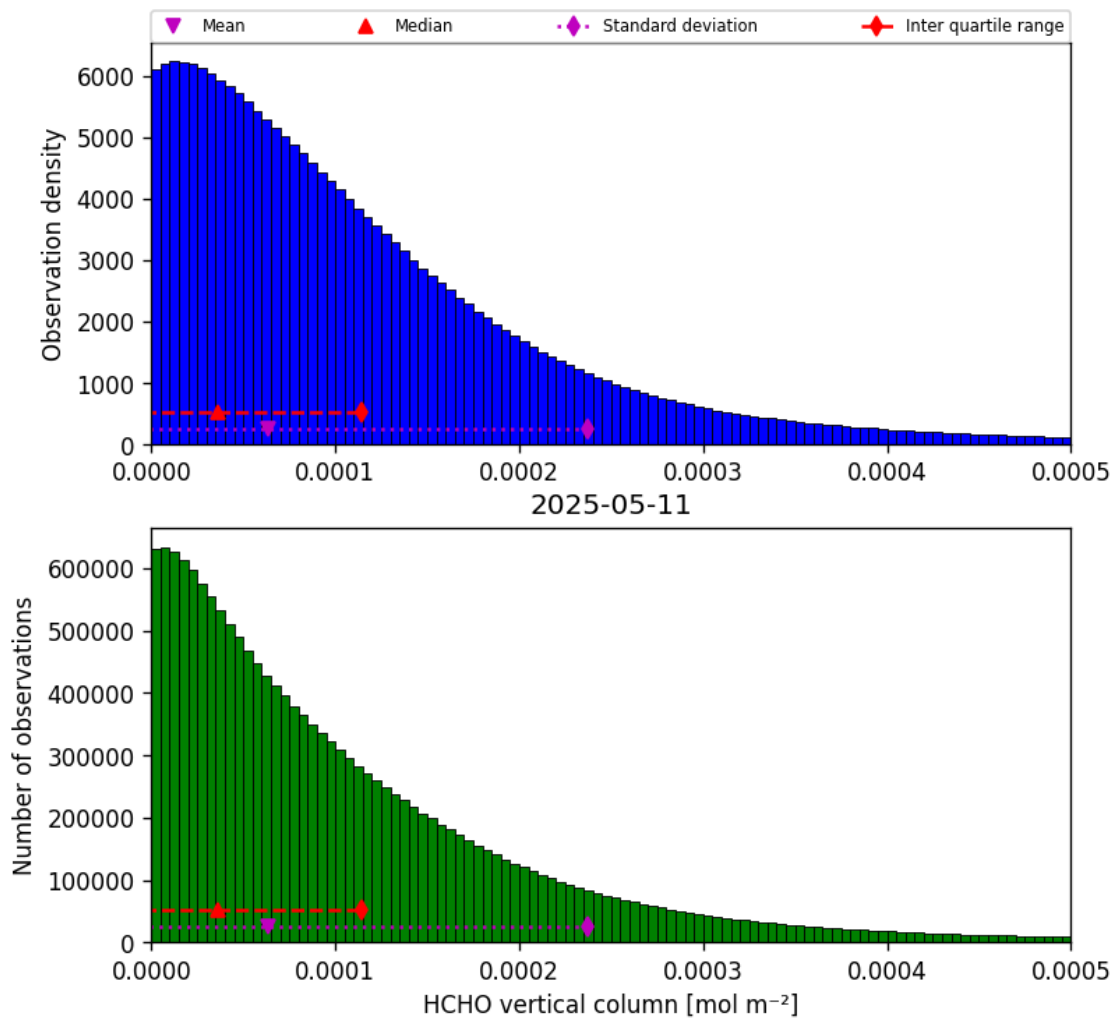
Figure 35: Histogram of “HCHO vertical column” for 2025-05-10 to 2025-05-12
