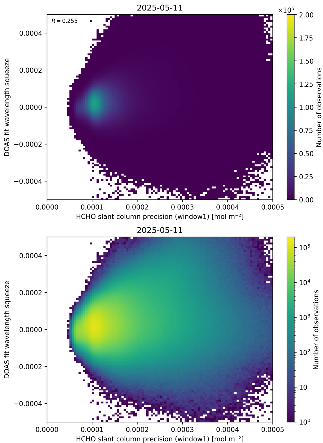
Figure 90: Scatter density plot of “HCHO slant column precision (window1)” against “DOAS fit wavelength squeeze” for 2025-05-10 to 2025-05-12.
