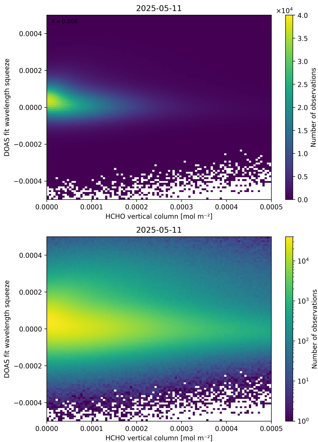
Figure 125: Scatter density plot of “HCHO vertical column” against “DOAS fit wavelength squeeze” for 2025-05-10 to 2025-05-12.
