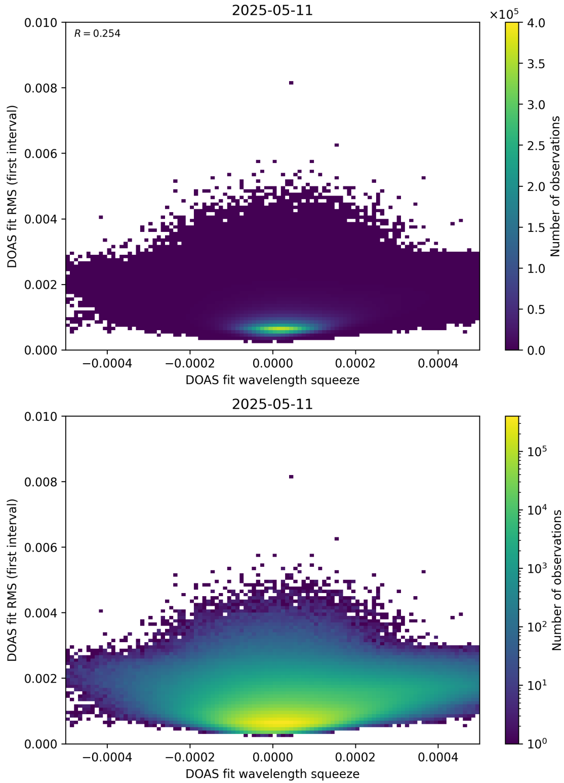
Figure 68: Scatter density plot of “DOAS fit wavelength squeeze” against “DOAS fit RMS (first interval)” for 2025-05-10 to 2025-05-12.
