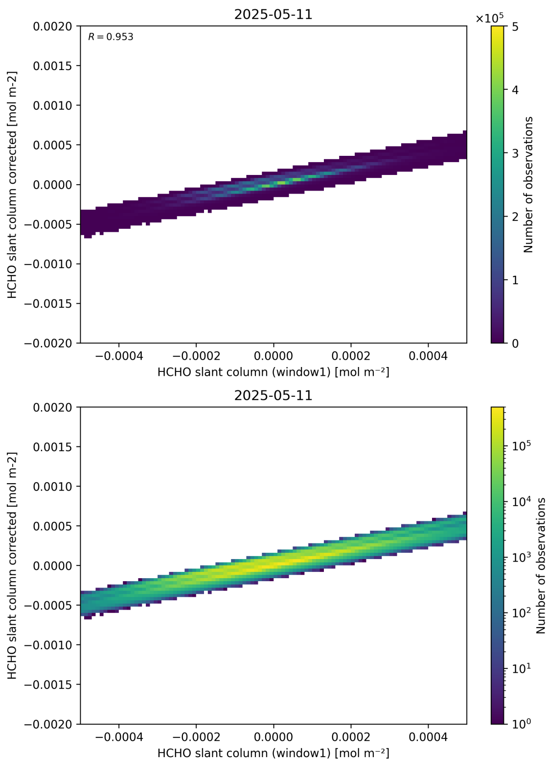
Figure 82: Scatter density plot of “HCHO slant column (window1)” against “HCHO slant column corrected” for 2025-05-10 to 2025-05-12.
