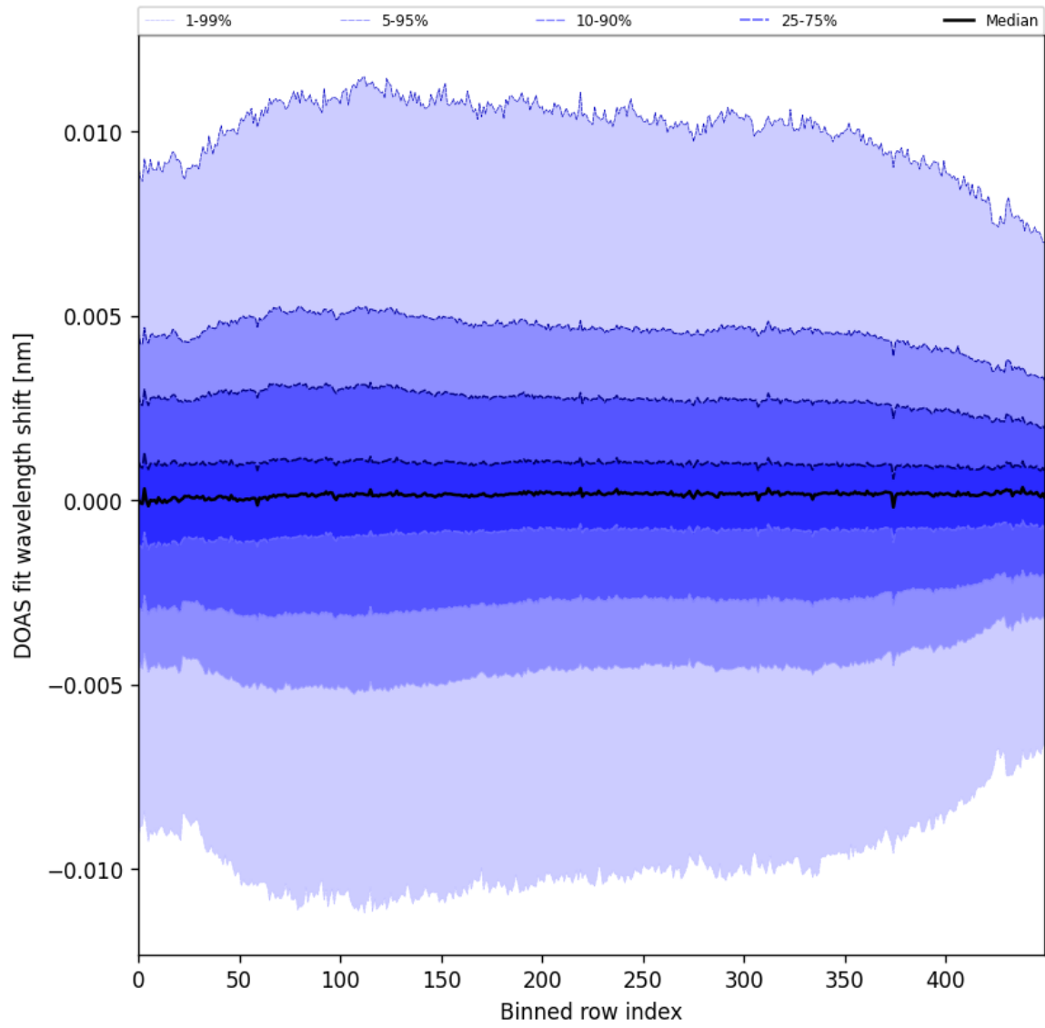
Figure 58: Along track statistics of “DOAS fit wavelength shift” for 2025-05-10 to 2025-05-12
