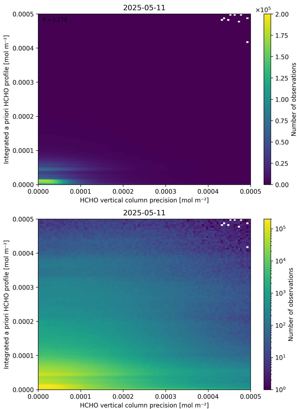
Figure 147: Scatter density plot of “HCHO vertical column precision” against “Integrated a priori HCHO profile” for 2025-05-10 to 2025-05-12.
