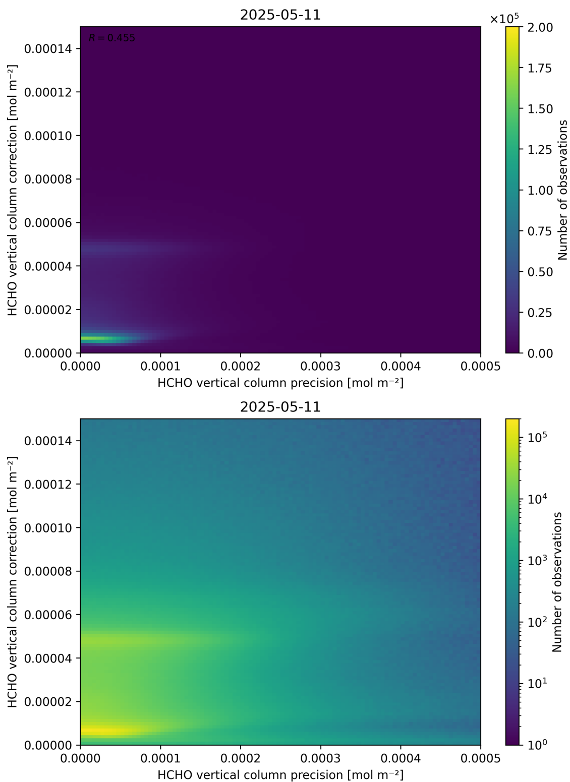
Figure 146: Scatter density plot of “HCHO vertical column precision” against “HCHO vertical column correction” for 2025-05-10 to 2025-05-12.
