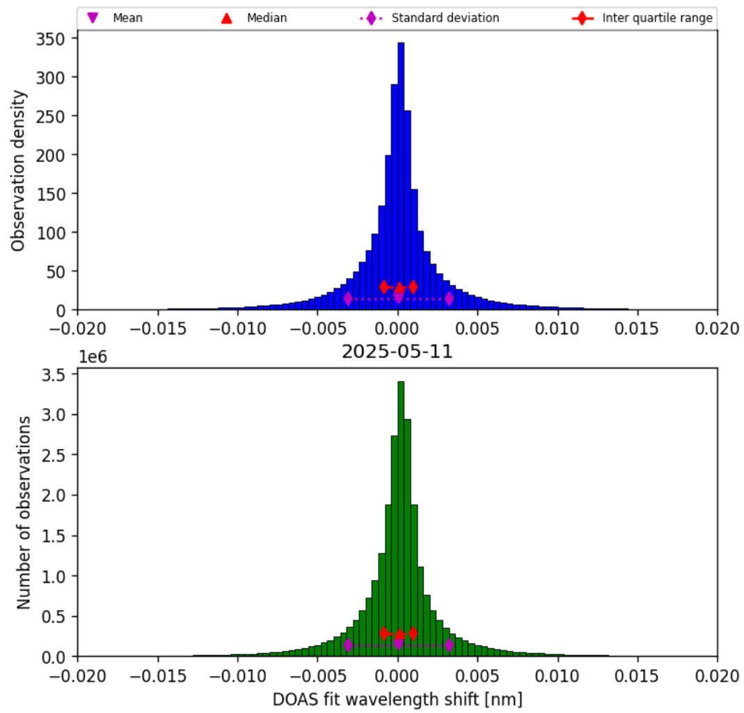
Figure 44: Histogram of “DOAS fit wavelength shift” for 2025-05-10 to 2025-05-12
