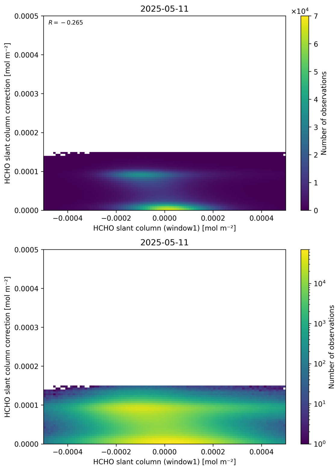
Figure 83: Scatter density plot of “HCHO slant column (window1)” against “HCHO slant column correction” for 2025-05-10 to 2025-05-12.
