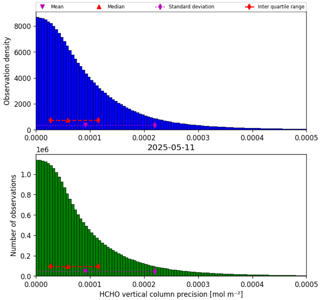
Figure 36: Histogram of “HCHO vertical column precision” for 2025-05-10 to 2025-05-12
