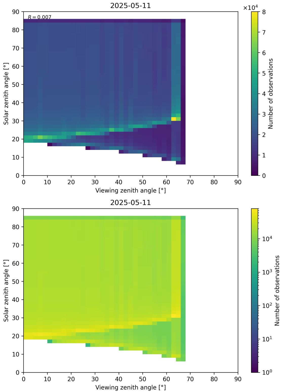
Figure 197: Scatter density plot of “Viewing zenith angle” against “Solar zenith angle” for 2025-05-10 to 2025-05-12.
