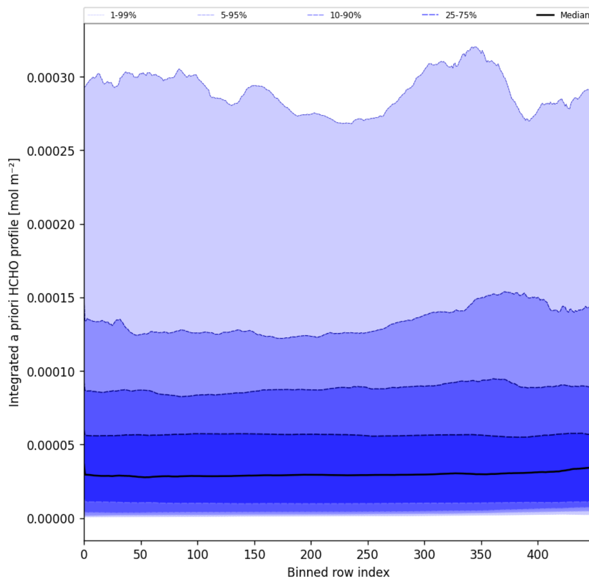
Figure 57: Along track statistics of “Integrated a priori HCHO profile” for 2025-05-10 to 2025-05-12
