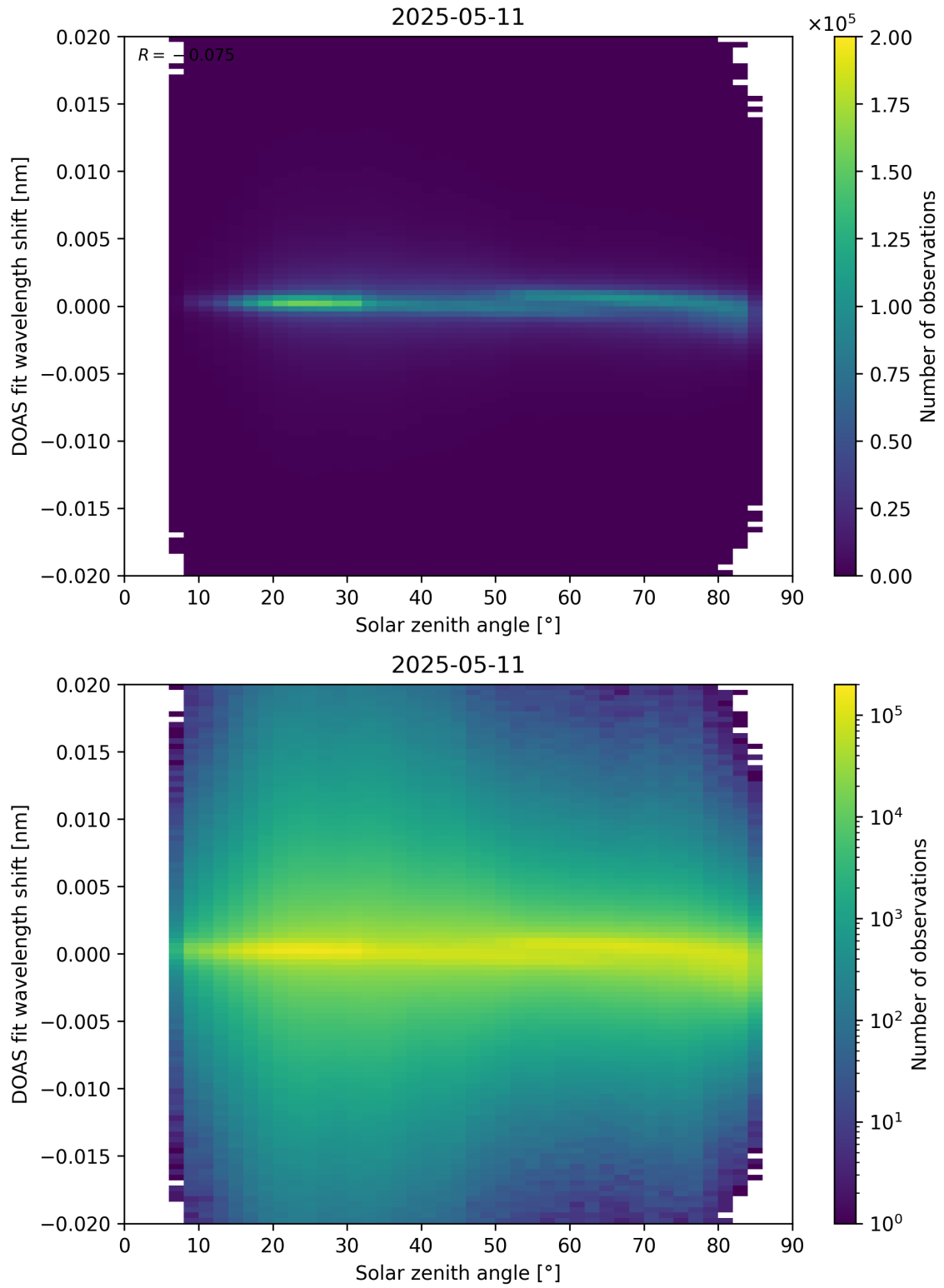
Figure 168: Scatter density plot of “Solar zenith angle” against “DOAS fit wavelength shift” for 2025-05-10 to 2025-05-12.
