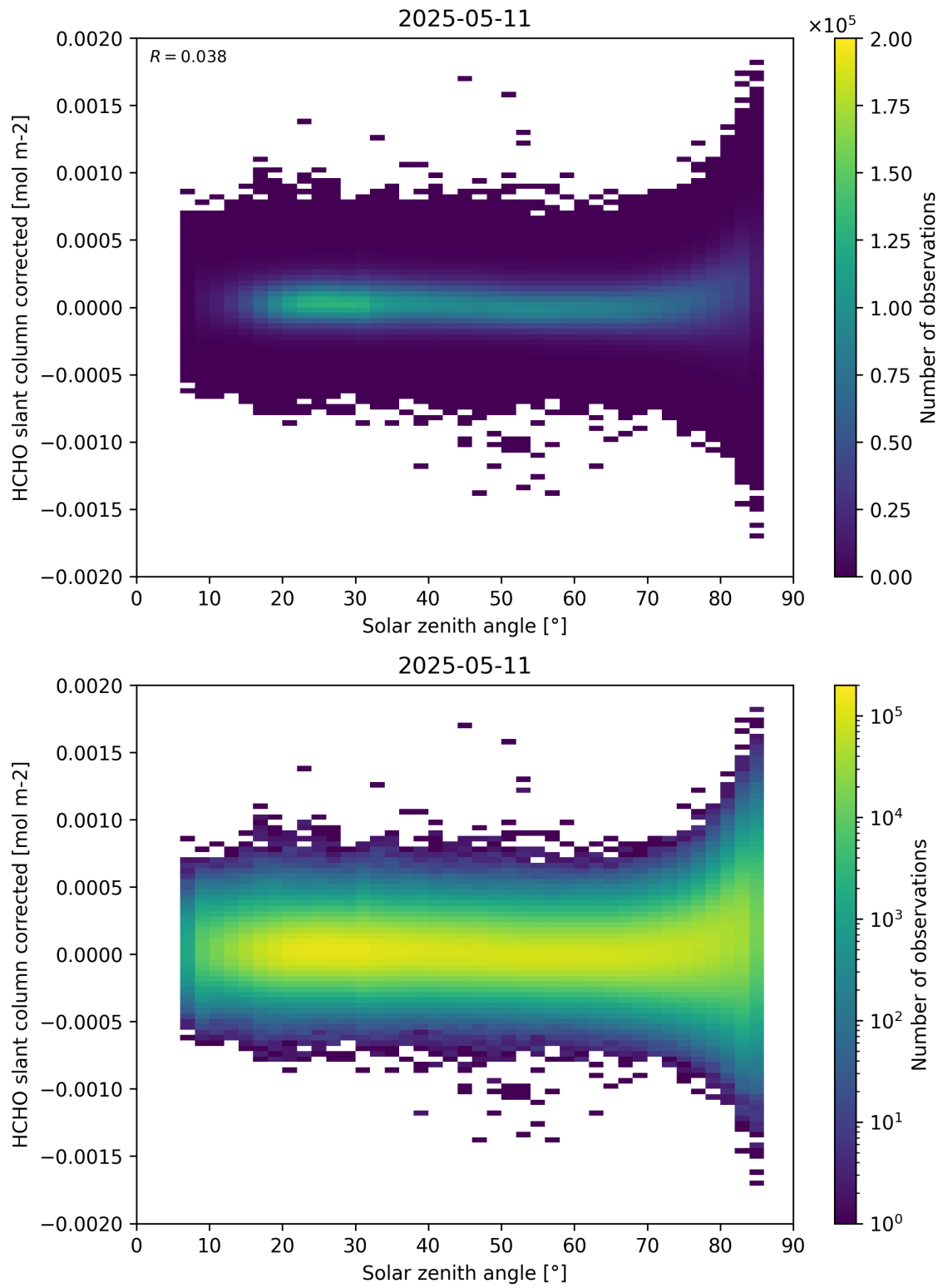
Figure 171: Scatter density plot of “Solar zenith angle” against “HCHO slant column corrected” for 2025-05-10 to 2025-05-12.
