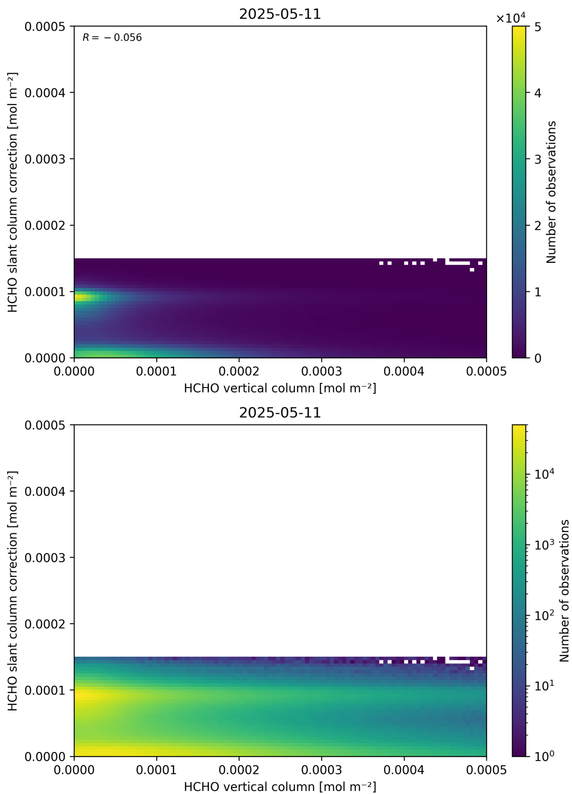
Figure 128: Scatter density plot of “HCHO vertical column” against “HCHO slant column correction” for 2025-05-10 to 2025-05-12.
