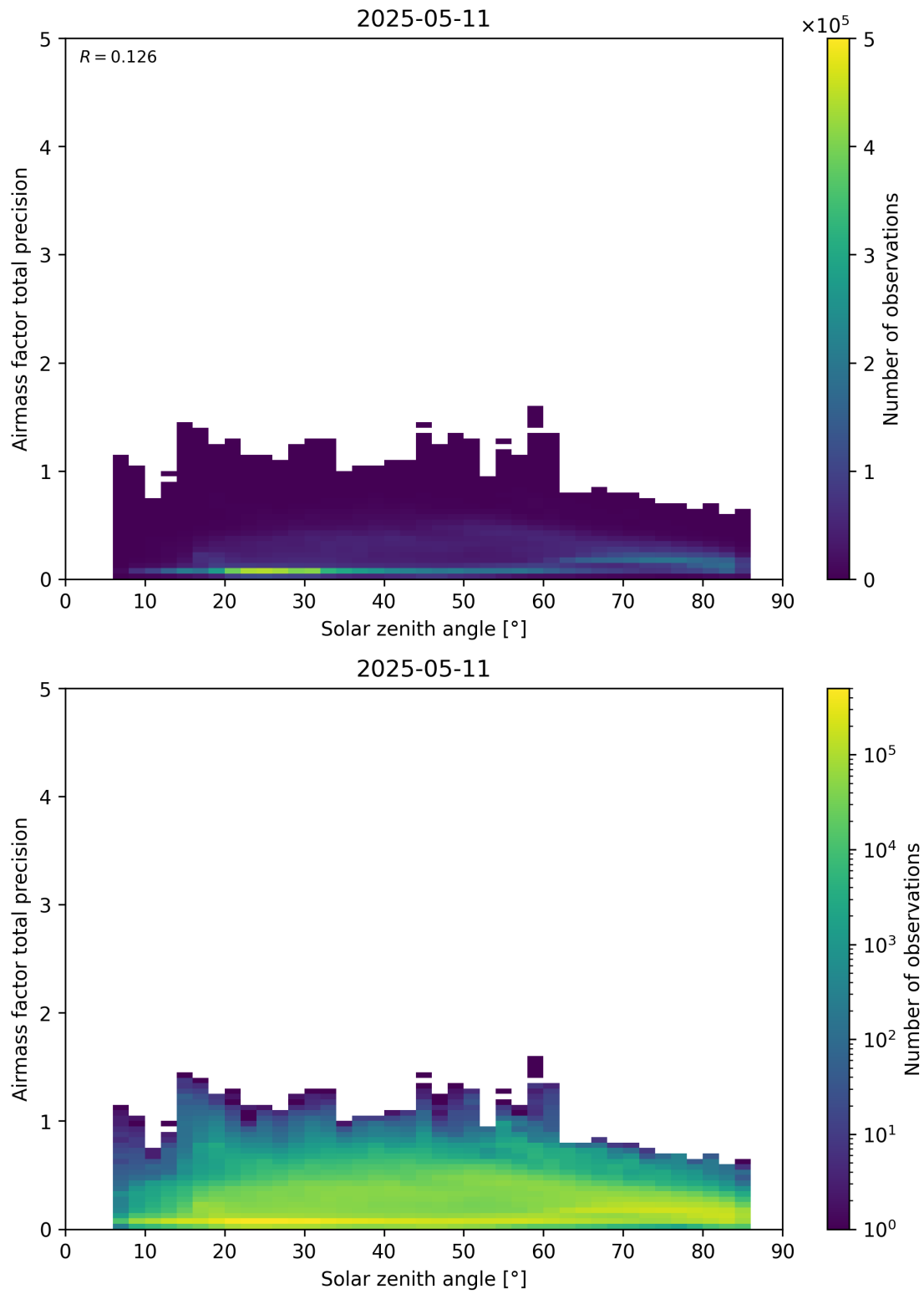
Figure 176: Scatter density plot of “Solar zenith angle” against “Airmass factor total precision” for 2025-05-10 to 2025-05-12.
