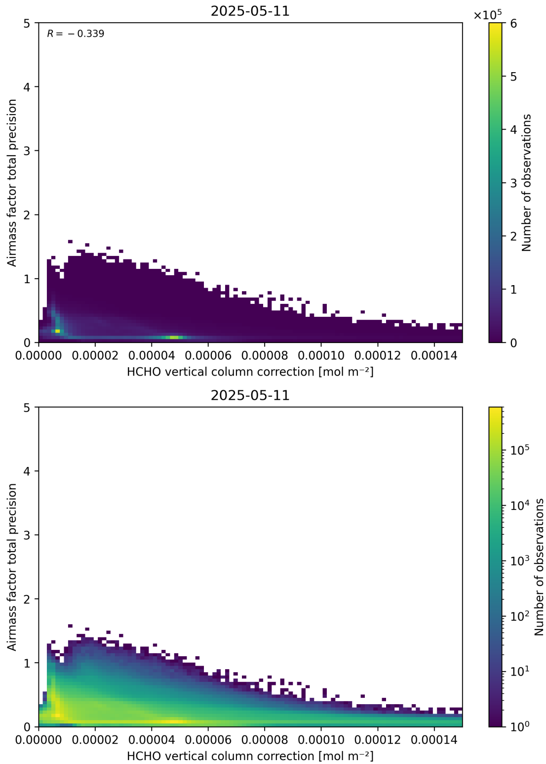
Figure 121: Scatter density plot of “HCHO vertical column correction” against “Airmass factor total precision” for 2025-05-10 to 2025-05-12.
