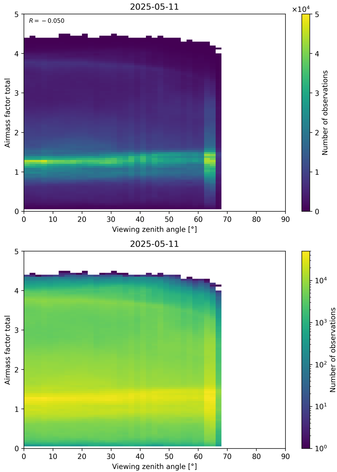
Figure 190: Scatter density plot of “Viewing zenith angle” against “Airmass factor total” for 2025-05-10 to 2025-05-12.
