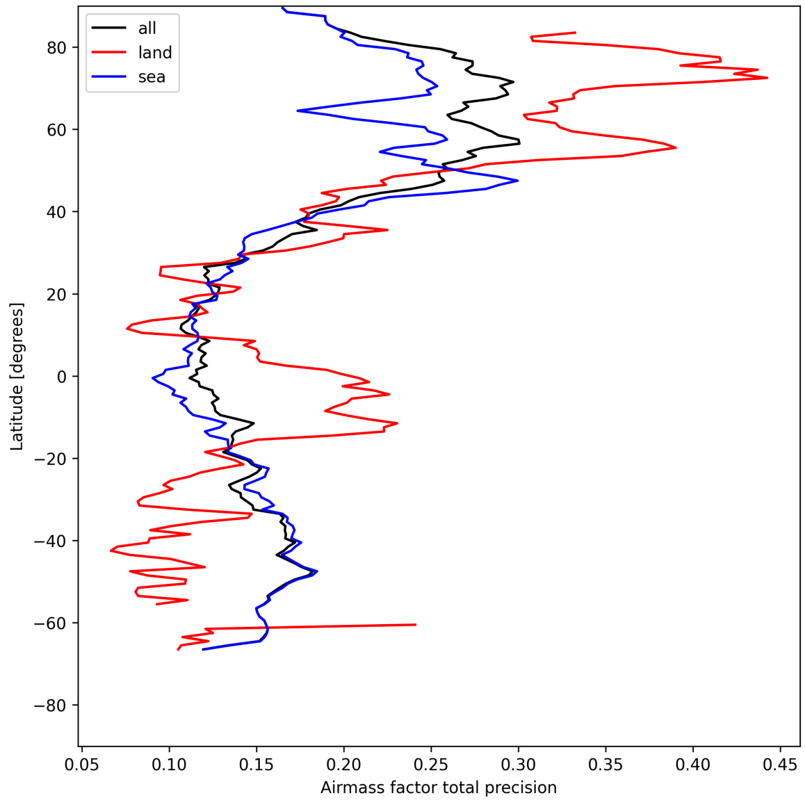
Figure 27: Zonal average of “Airmass factor total precision” for 2025-05-10 to 2025-05-12.
