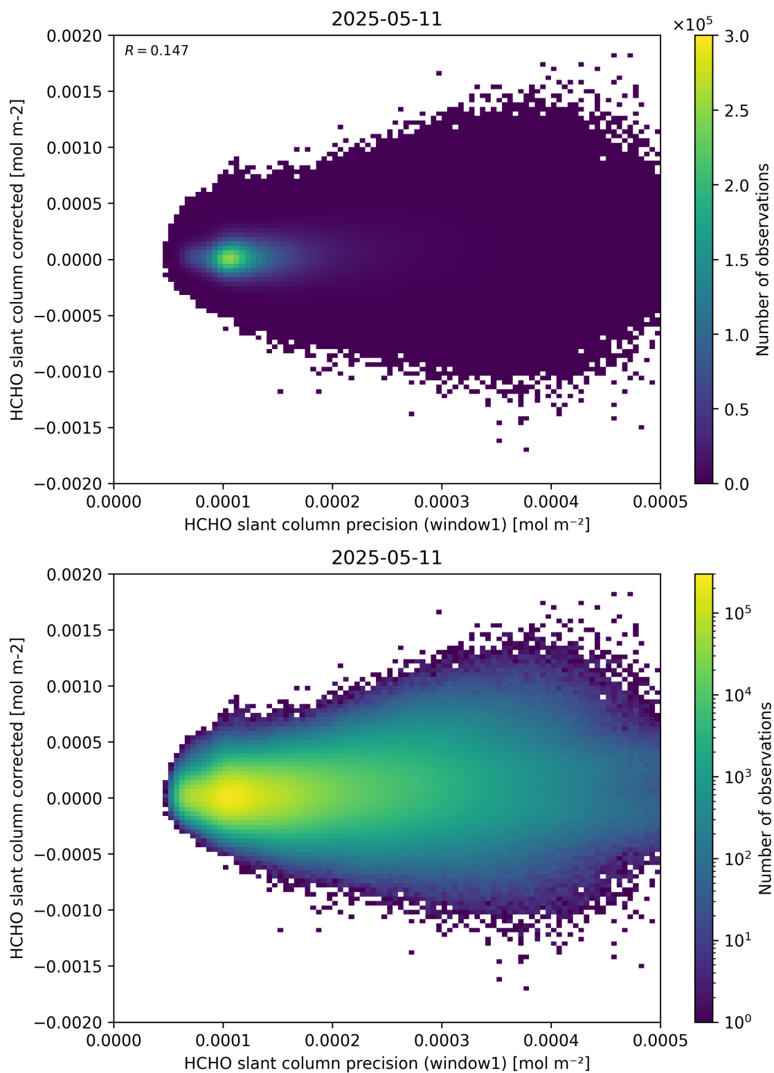
Figure 92: Scatter density plot of “HCHO slant column precision (window1)” against “HCHO slant column corrected” for 2025-05-10 to 2025-05-12.
