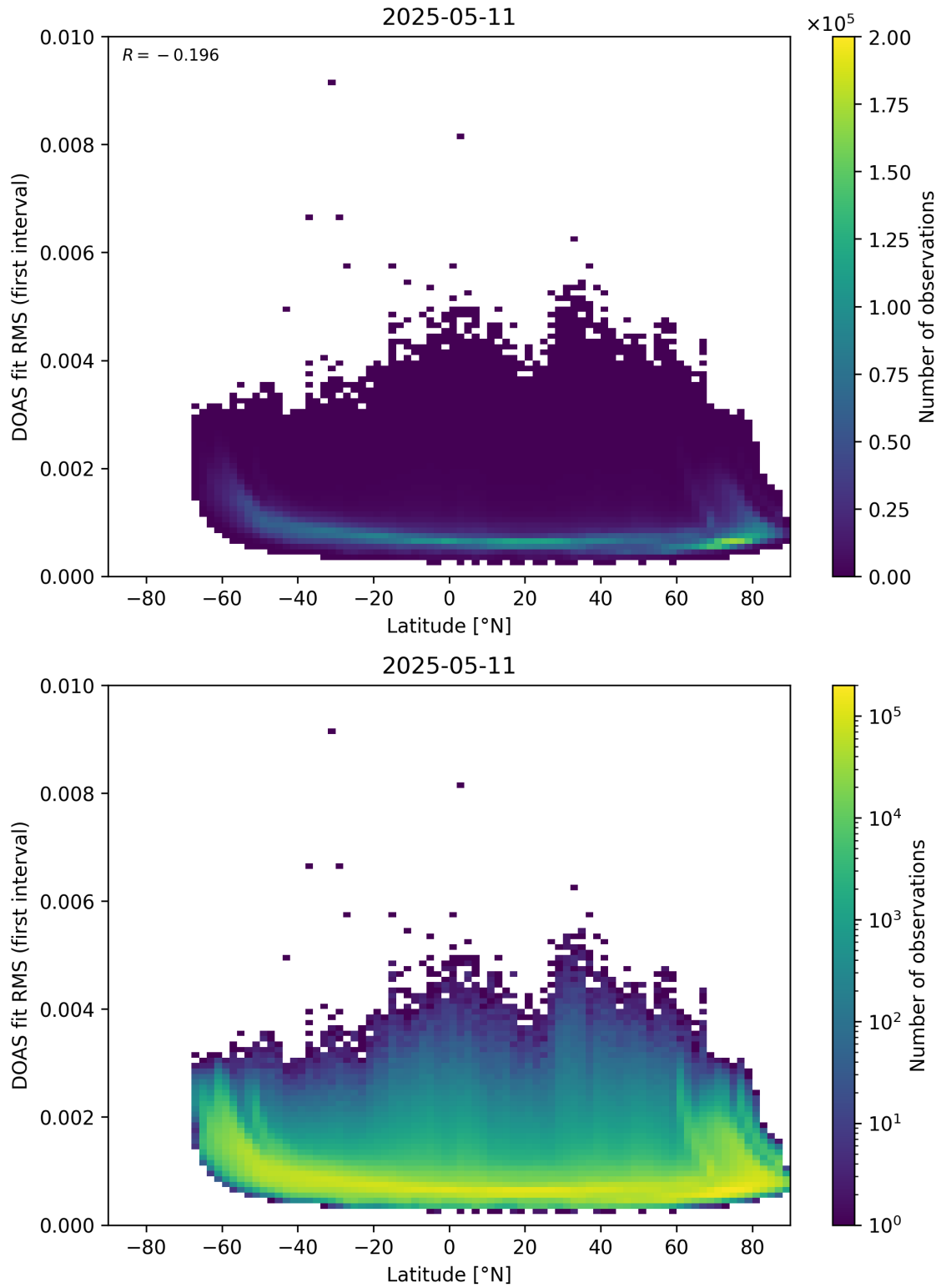
Figure 153: Scatter density plot of “Latitude” against “DOAS fit RMS (first interval)” for 2025-05-10 to 2025-05-12.
