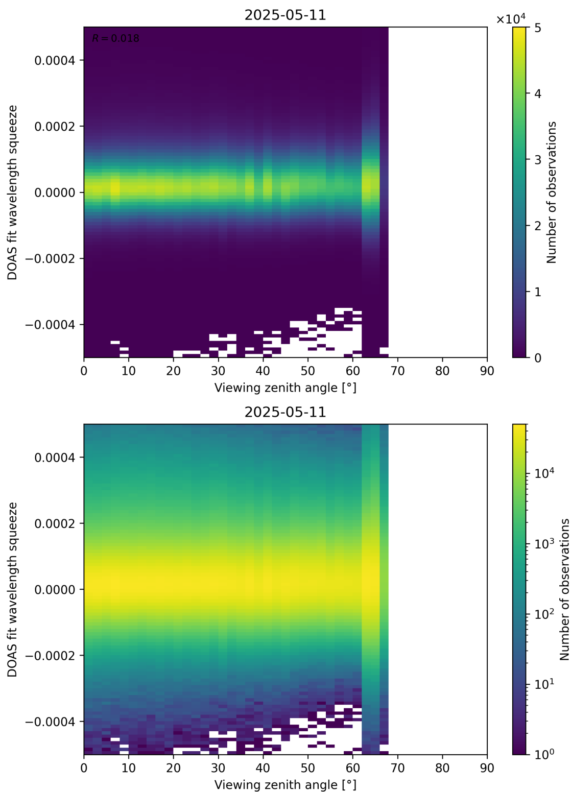
Figure 184: Scatter density plot of “Viewing zenith angle” against “DOAS fit wavelength squeeze” for 2025-05-10 to 2025-05-12.
