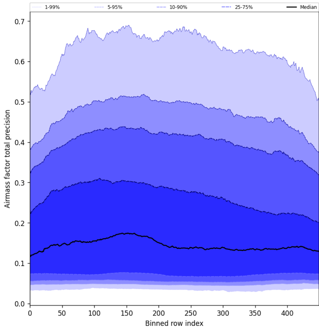
Figure 55: Along track statistics of “Airmass factor total precision” for 2025-05-10 to 2025-05-12
