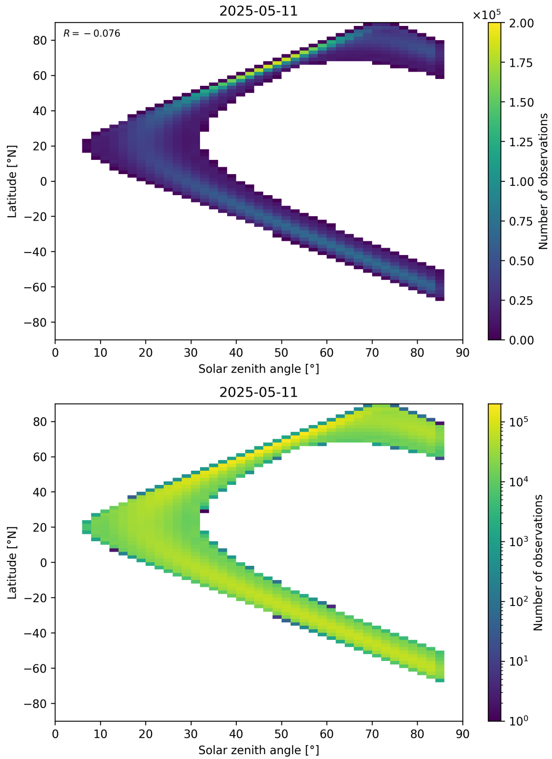
Figure 181: Scatter density plot of “Solar zenith angle” against “Latitude” for 2025-05-10 to 2025-05-12.
