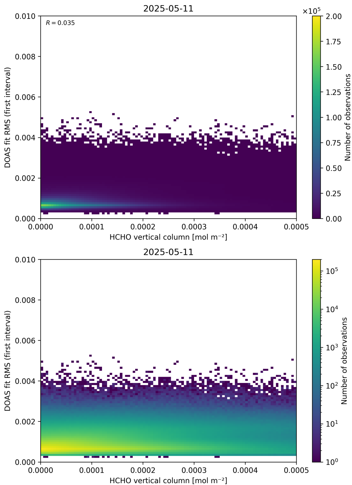
Figure 123: Scatter density plot of “HCHO vertical column” against “DOAS fit RMS (first interval)” for 2025-05-10 to 2025-05-12.
