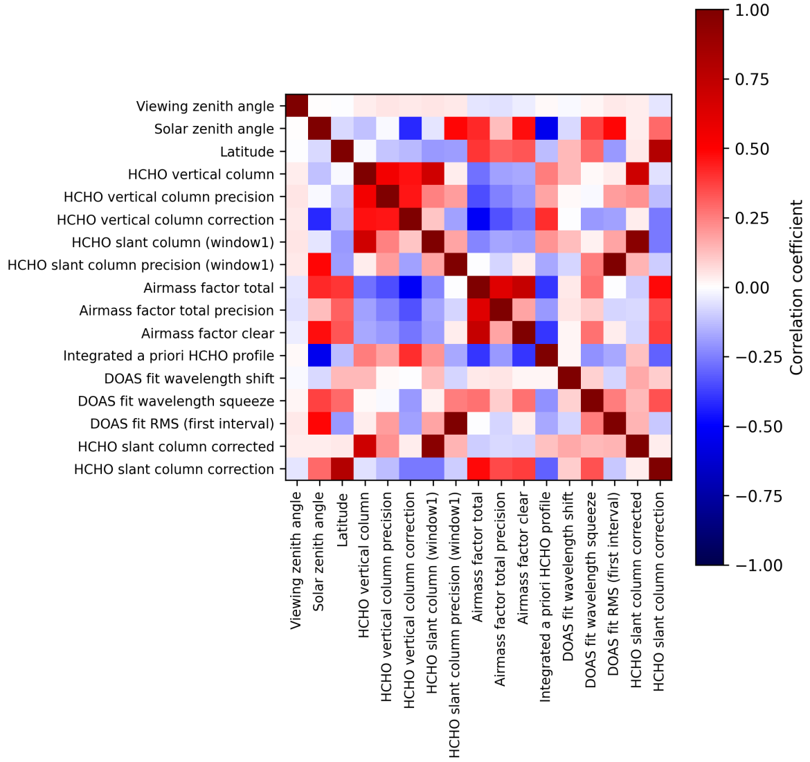
Figure 2: Map of correlation matrix for 2025-05-10 to 2025-05-12.
