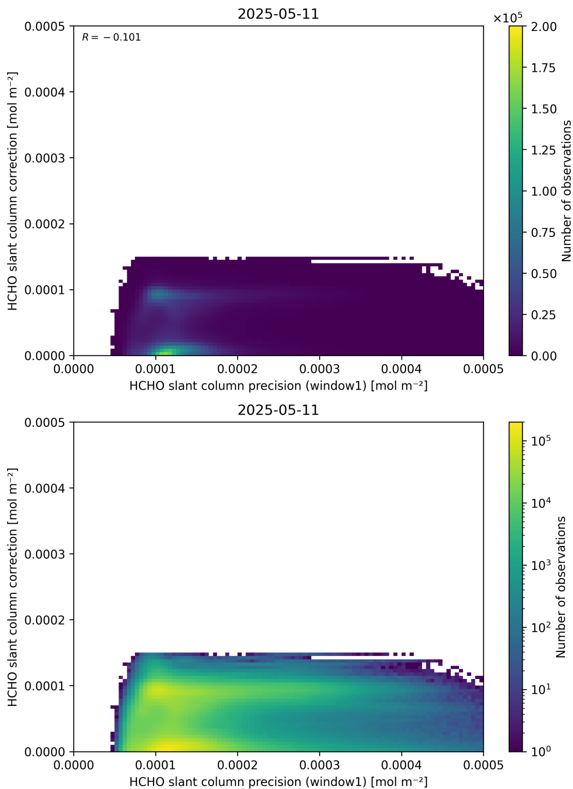
Figure 93: Scatter density plot of “HCHO slant column precision (window1)” against “HCHO slant column correction” for 2025-05-10 to 2025-05-12.
