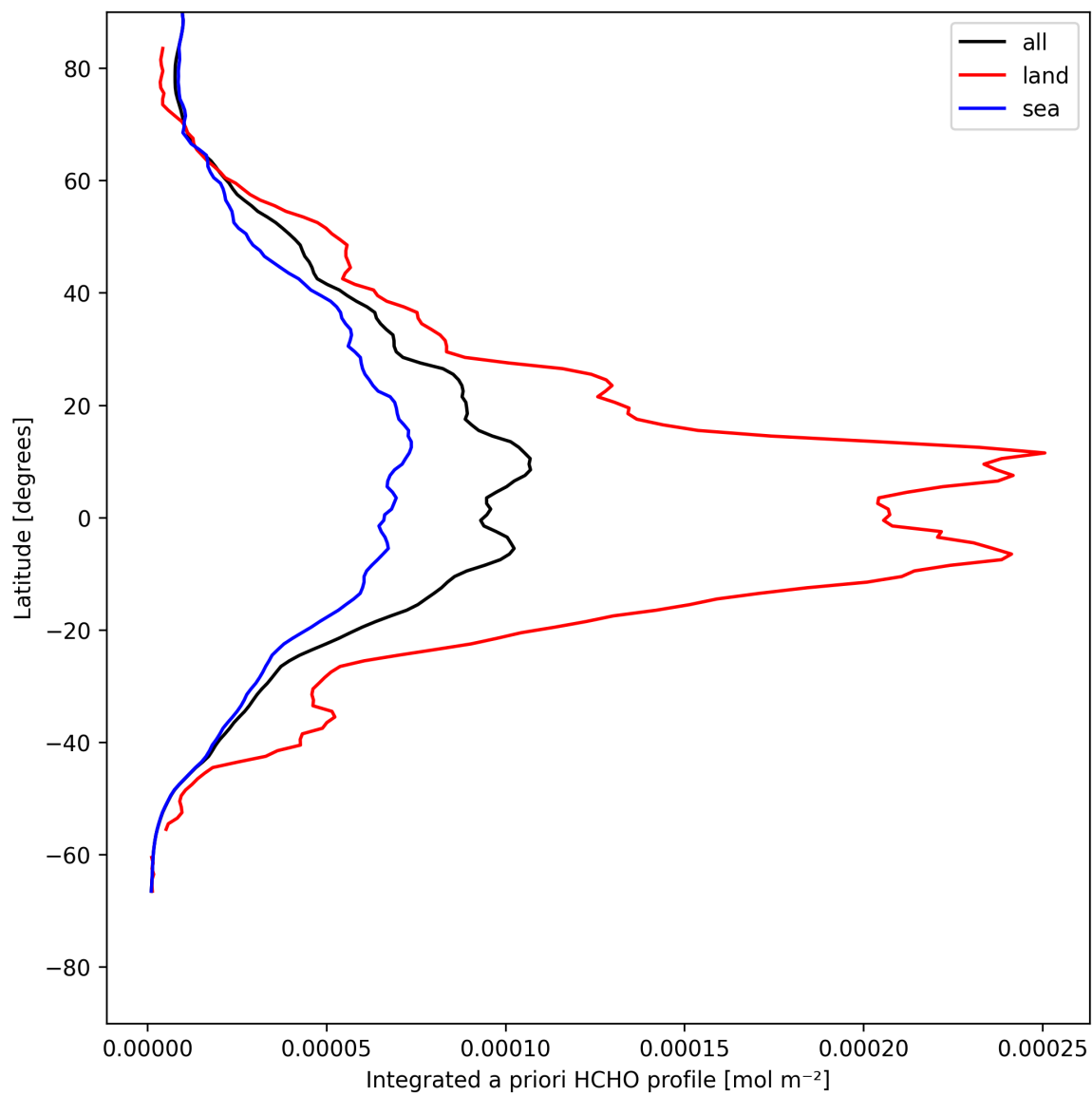
Figure 29: Zonal average of “Integrated a priori HCHO profile” for 2025-05-10 to 2025-05-12.
