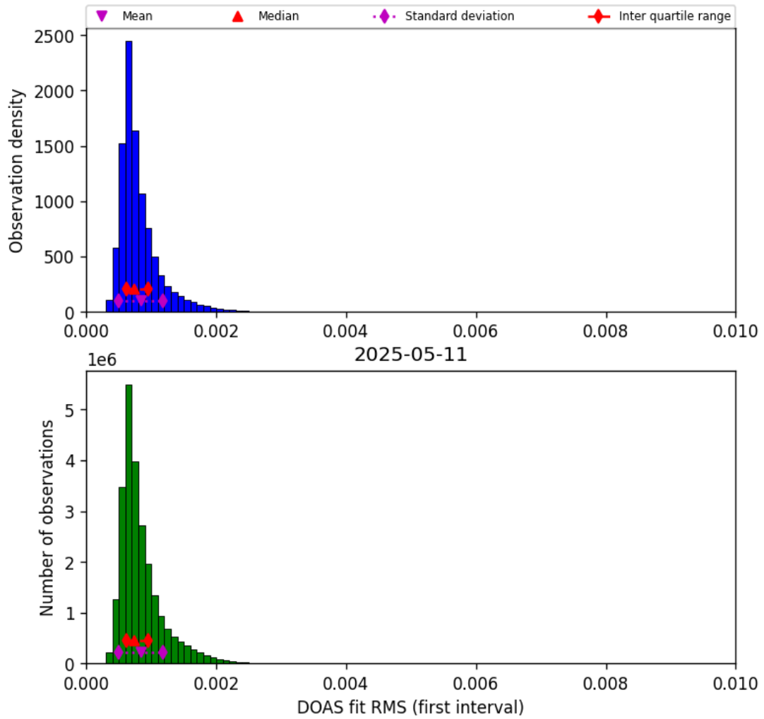
Figure 46: Histogram of “DOAS fit RMS (first interval)” for 2025-05-10 to 2025-05-12
