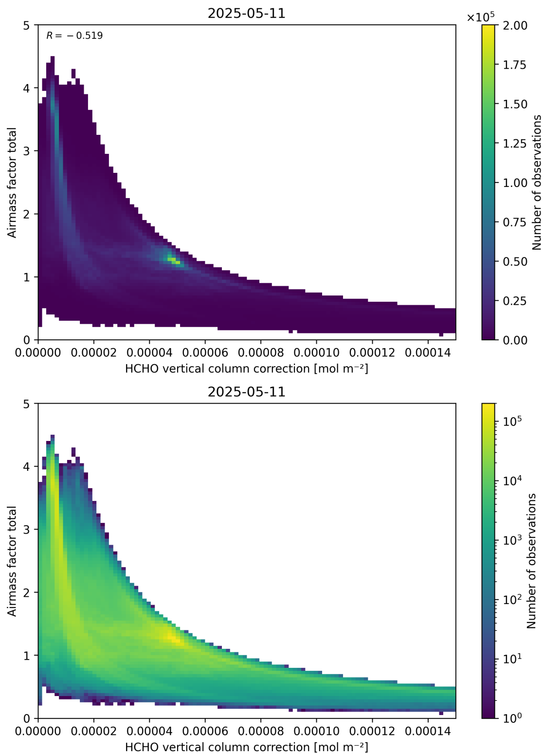
Figure 120: Scatter density plot of “HCHO vertical column correction” against “Airmass factor total” for 2025-05-10 to 2025-05-12.
