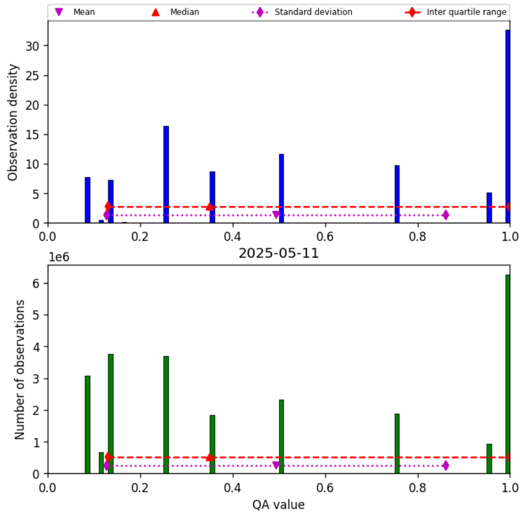
Figure 34: Histogram of “QA value” for 2025-05-10 to 2025-05-12
