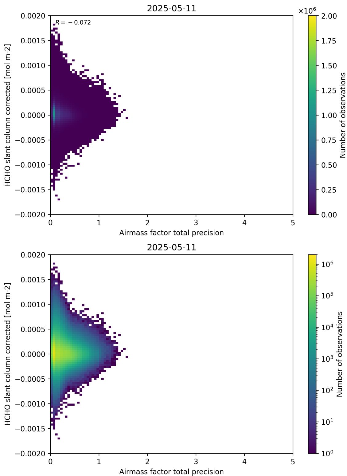
Figure 109: Scatter density plot of “Airmass factor total precision” against “HCHO slant column corrected” for 2025-05-10 to 2025-05-12.
