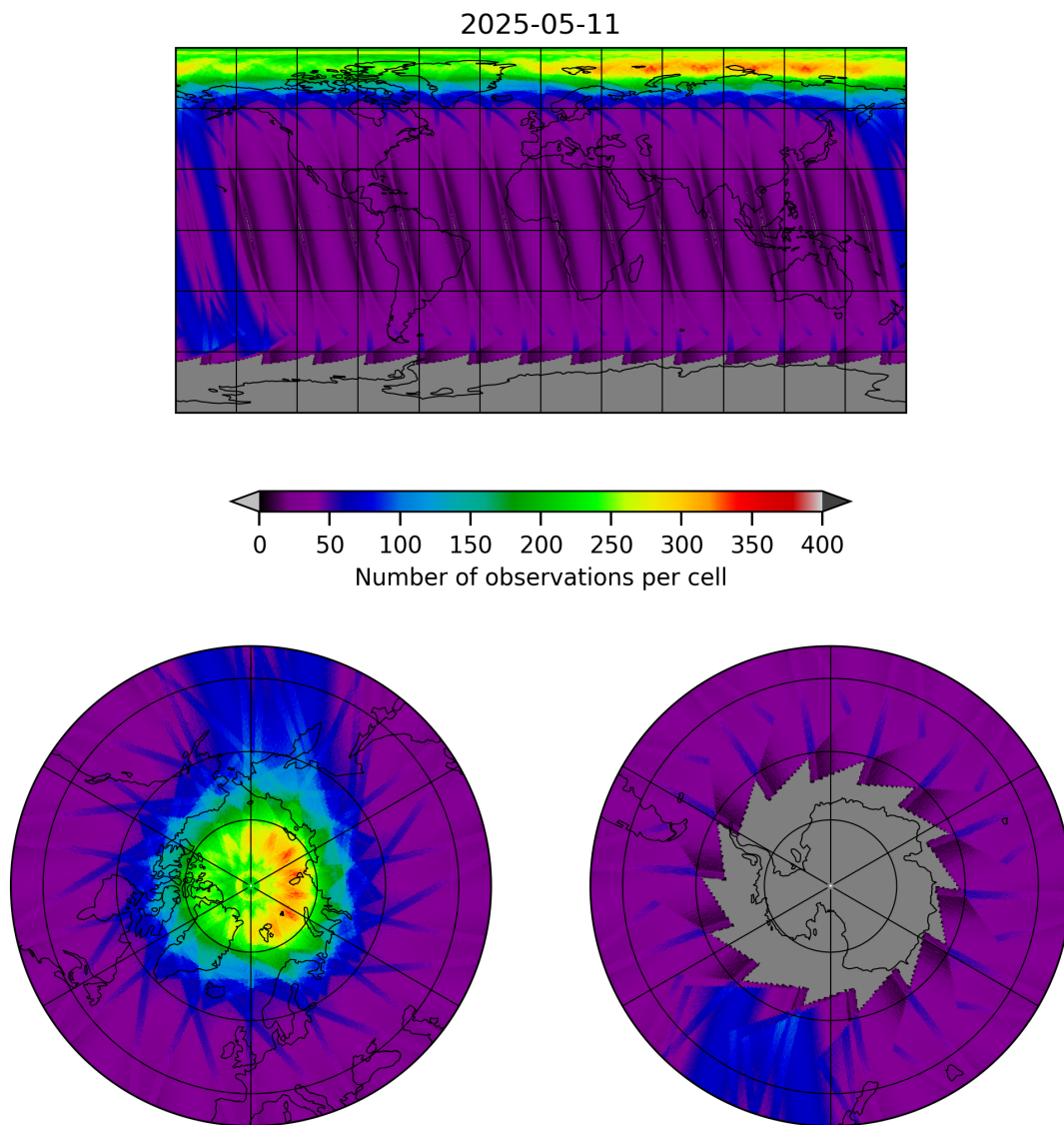
Figure 19: Map of the number of observations for 2025-05-10 to 2025-05-12
