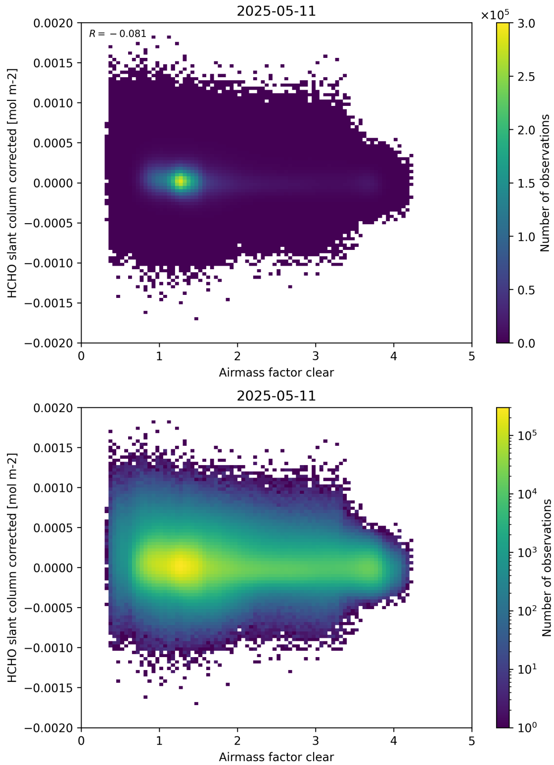
Figure 74: Scatter density plot of “Airmass factor clear” against “HCHO slant column corrected” for 2025-05-10 to 2025-05-12.
