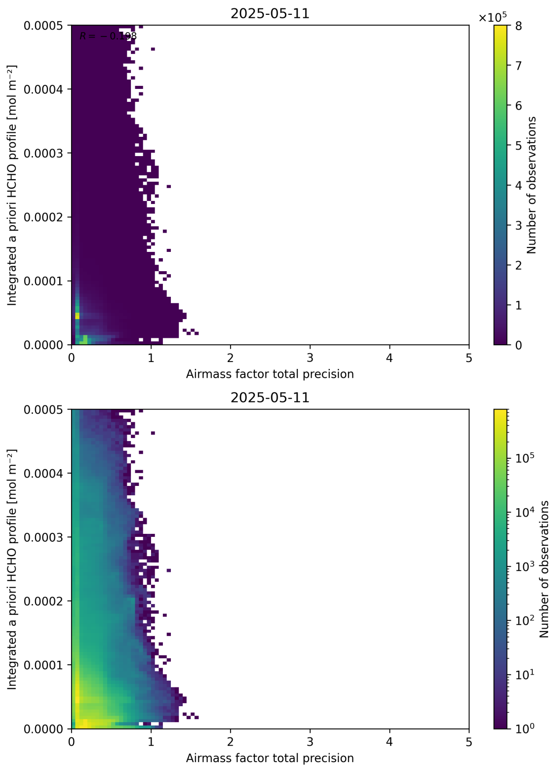
Figure 111: Scatter density plot of “Airmass factor total precision” against “Integrated a priori HCHO profile” for 2025-05-10 to 2025-05-12.
