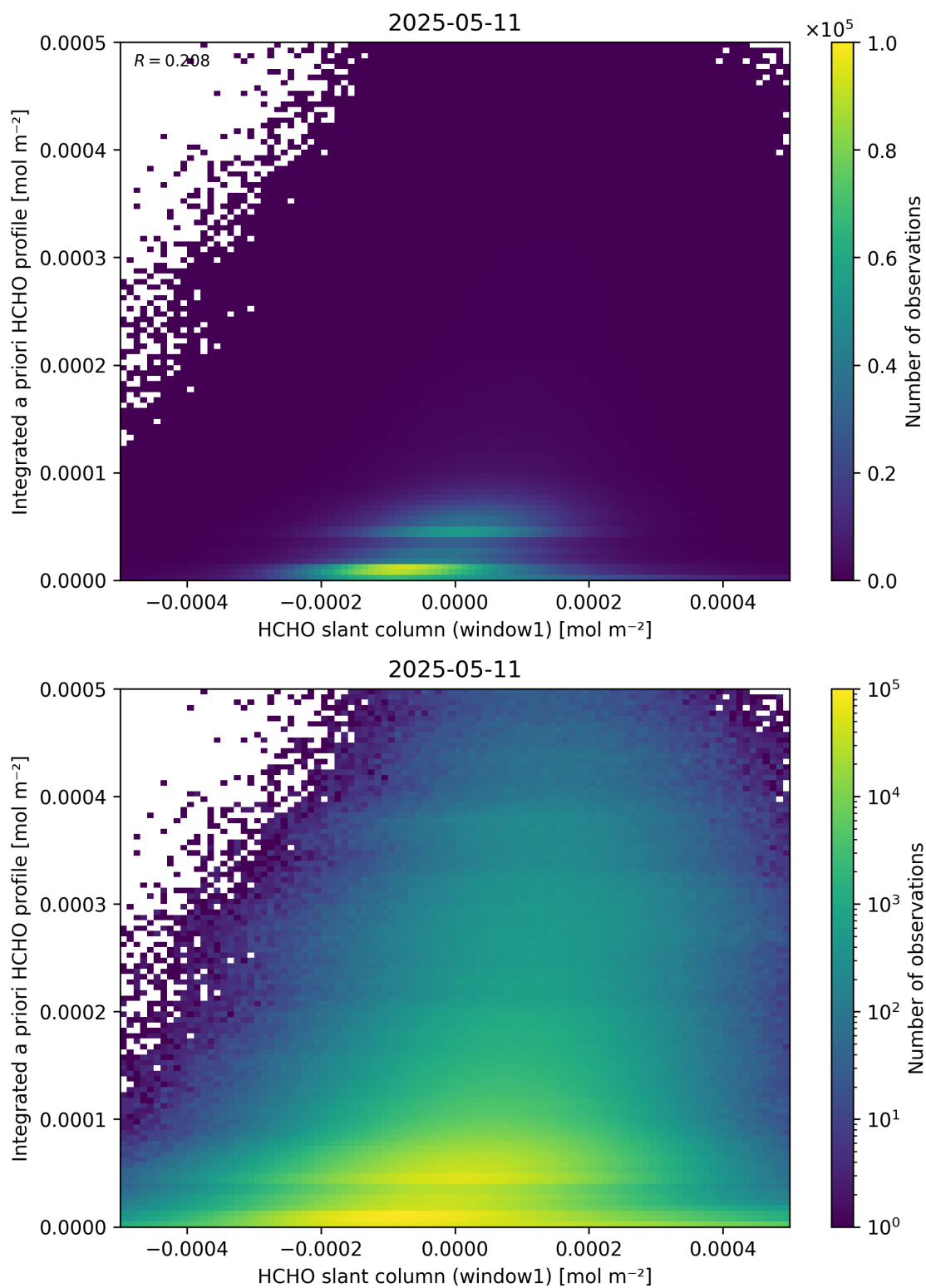
Figure 87: Scatter density plot of “HCHO slant column (window1)” against “Integrated a priori HCHO profile” for 2025-05-10 to 2025-05-12.
