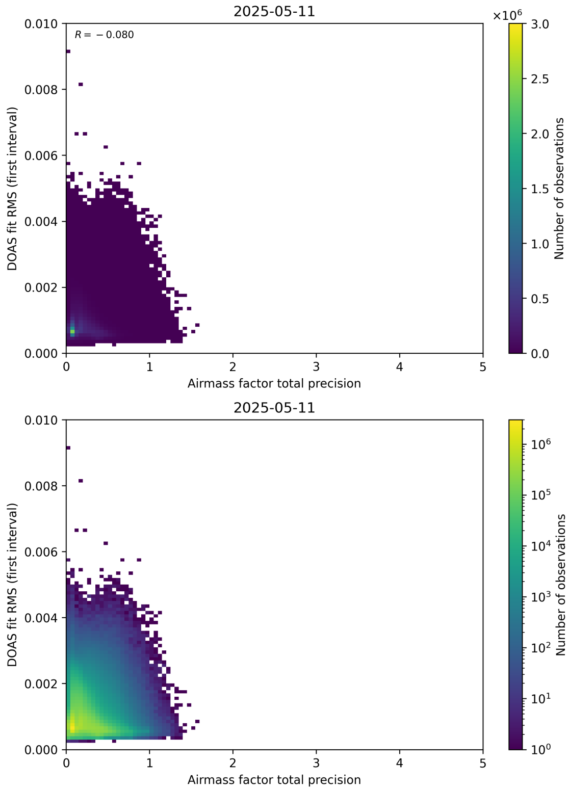
Figure 105: Scatter density plot of “Airmass factor total precision” against “DOAS fit RMS (first interval)” for 2025-05-10 to 2025-05-12.
