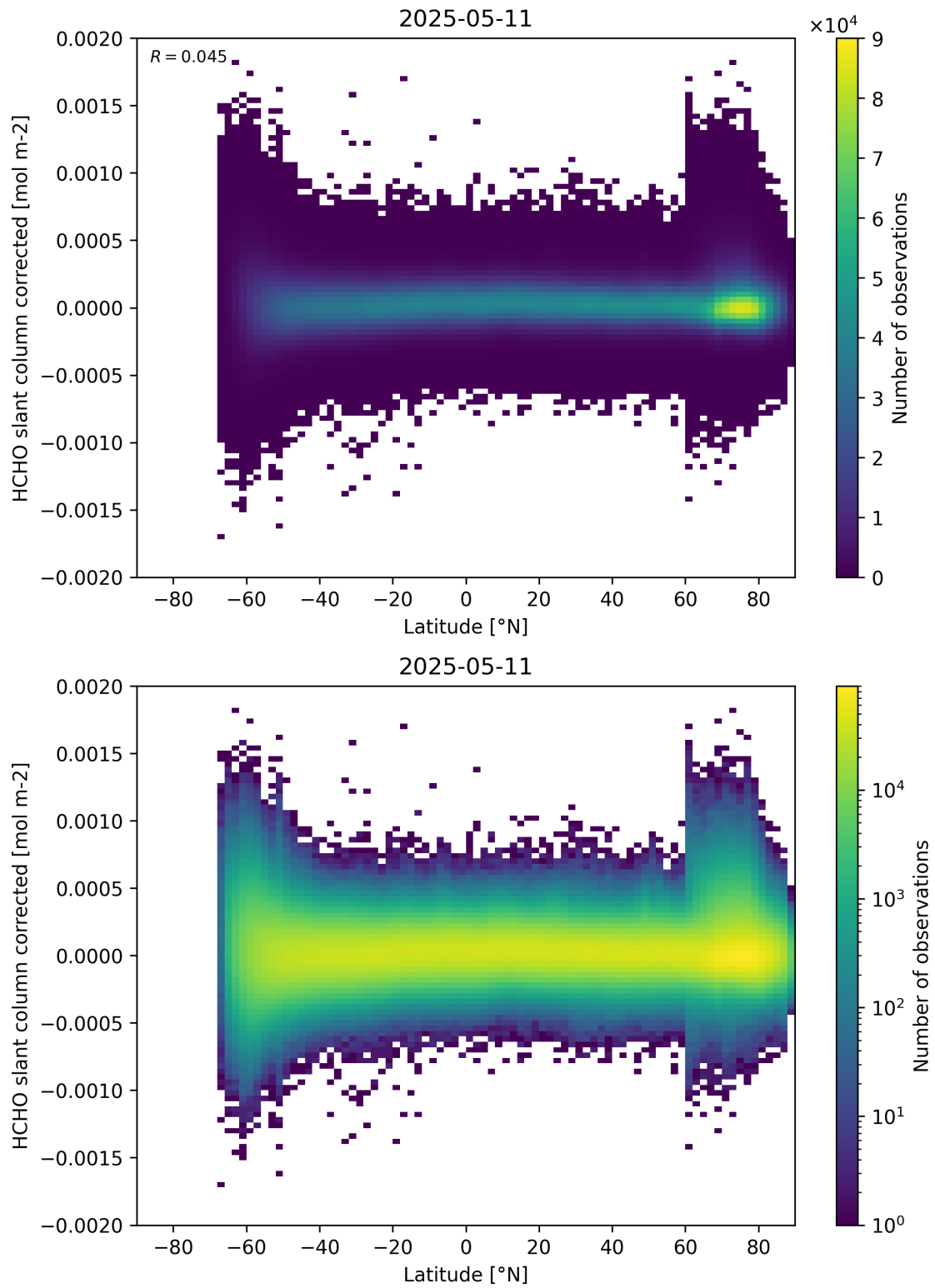
Figure 157: Scatter density plot of “Latitude” against “HCHO slant column corrected” for 2025-05-10 to 2025-05-12.
