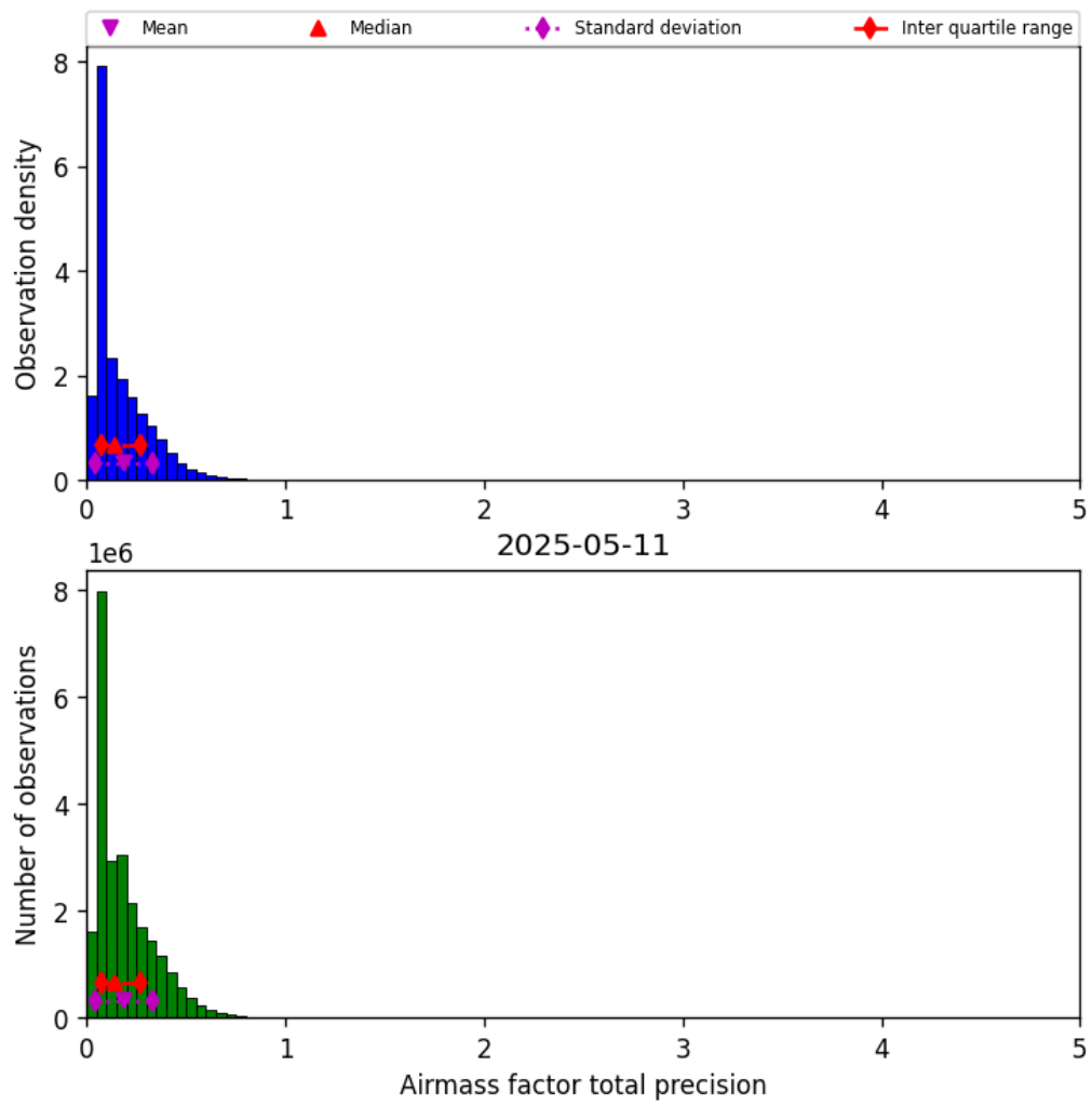
Figure 41: Histogram of “Airmass factor total precision” for 2025-05-10 to 2025-05-12
