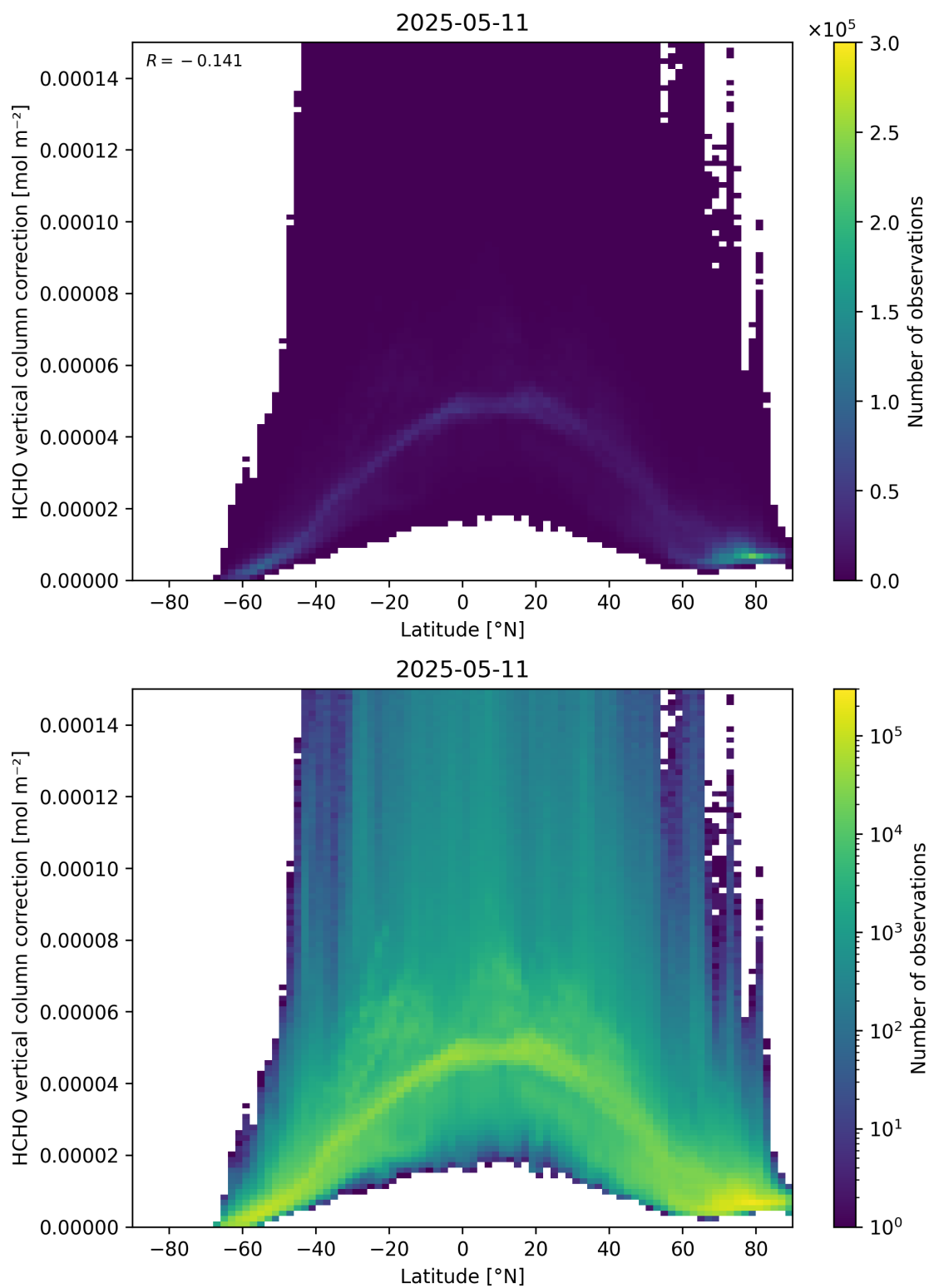
Figure 164: Scatter density plot of “Latitude” against “HCHO vertical column correction” for 2025-05-10 to 2025-05-12.
