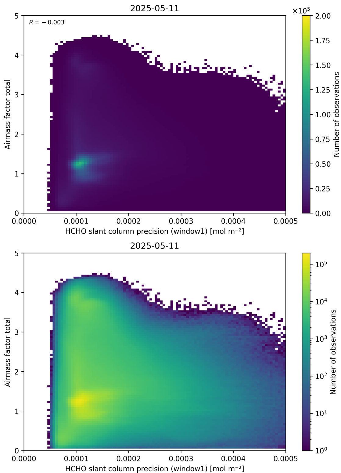
Figure 94: Scatter density plot of “HCHO slant column precision (window1)” against “Airmass factor total” for 2025-05-10 to 2025-05-12.
