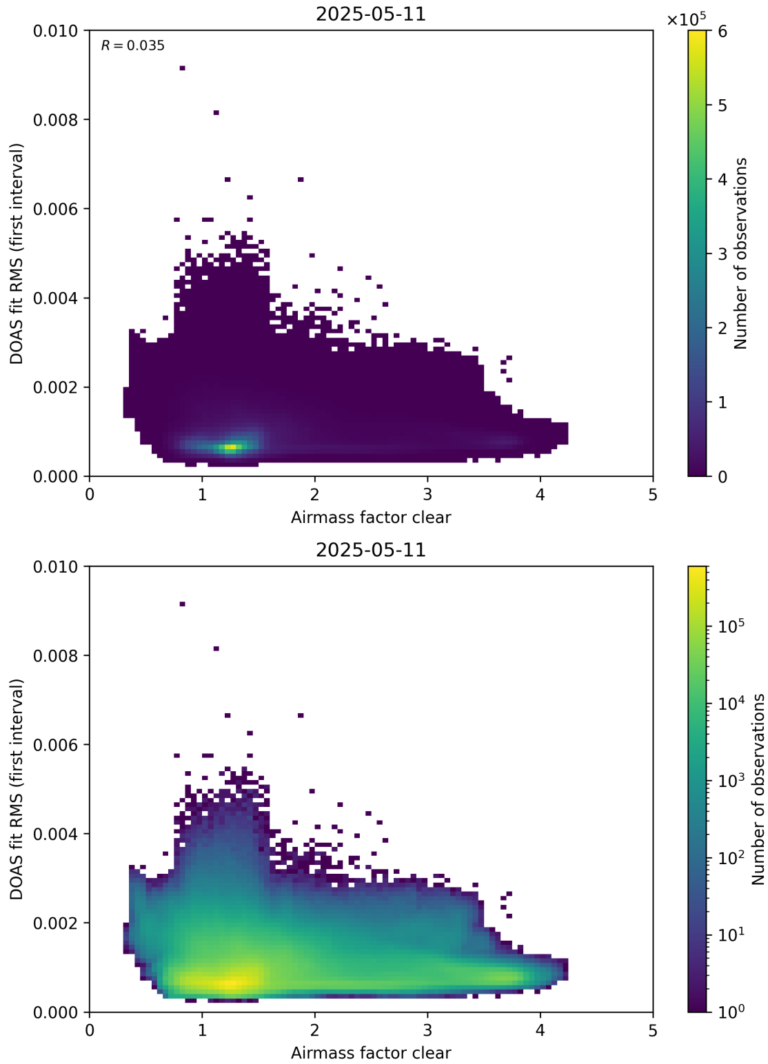
Figure 71: Scatter density plot of “Airmass factor clear” against “DOAS fit RMS (first interval)” for 2025-05-10 to 2025-05-12.
