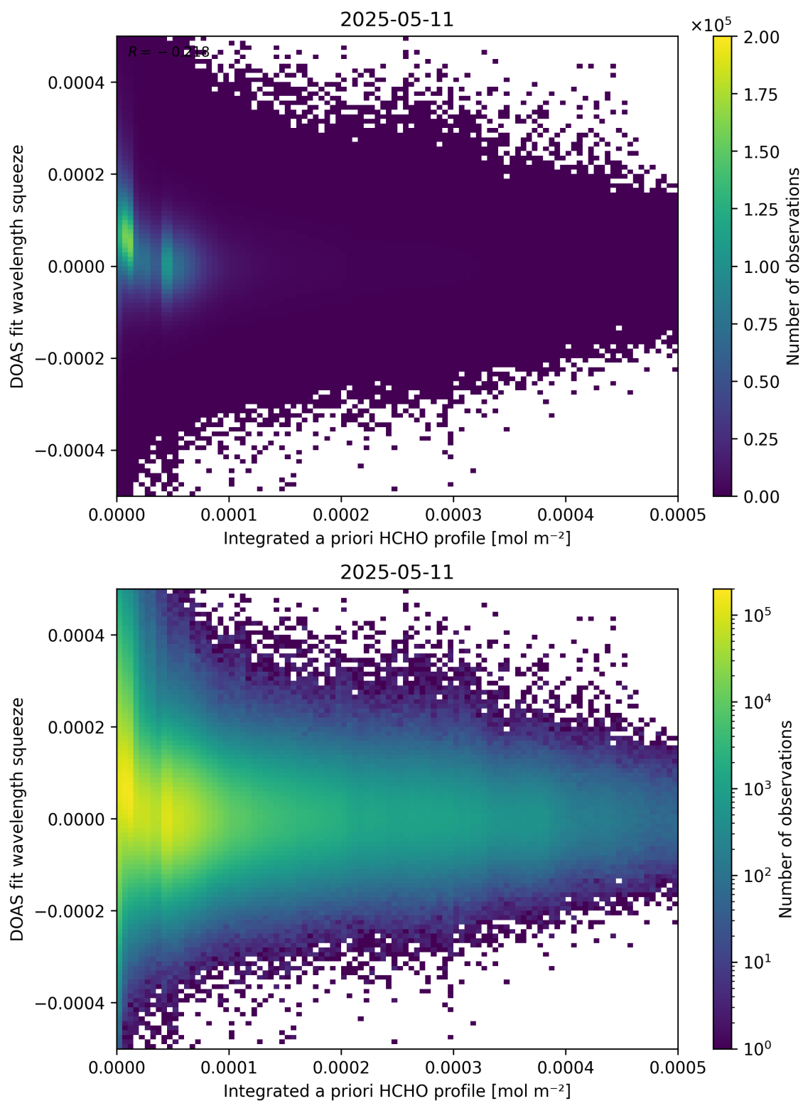
Figure 150: Scatter density plot of “Integrated a priori HCHO profile” against “DOAS fit wavelength squeeze” for 2025-05-10 to 2025-05-12.
