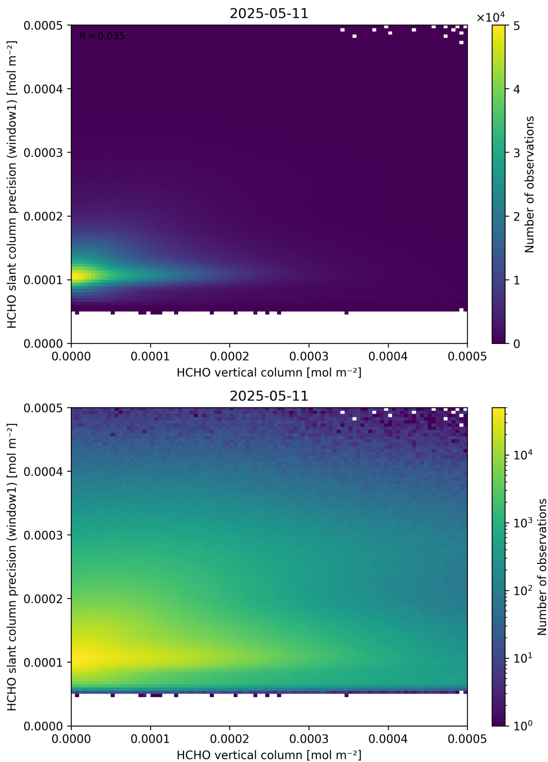
Figure 130: Scatter density plot of “HCHO vertical column” against “HCHO slant column precision (window1)” for 2025-05-10 to 2025-05-12.
