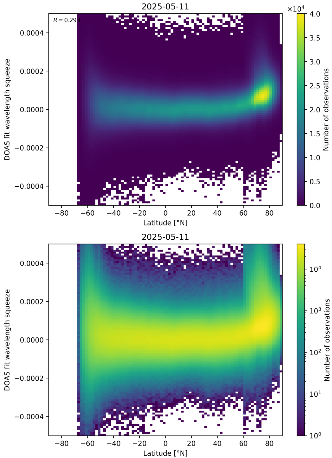
Figure 155: Scatter density plot of “Latitude” against “DOAS fit wavelength squeeze” for 2025-05-10 to 2025-05-12.
