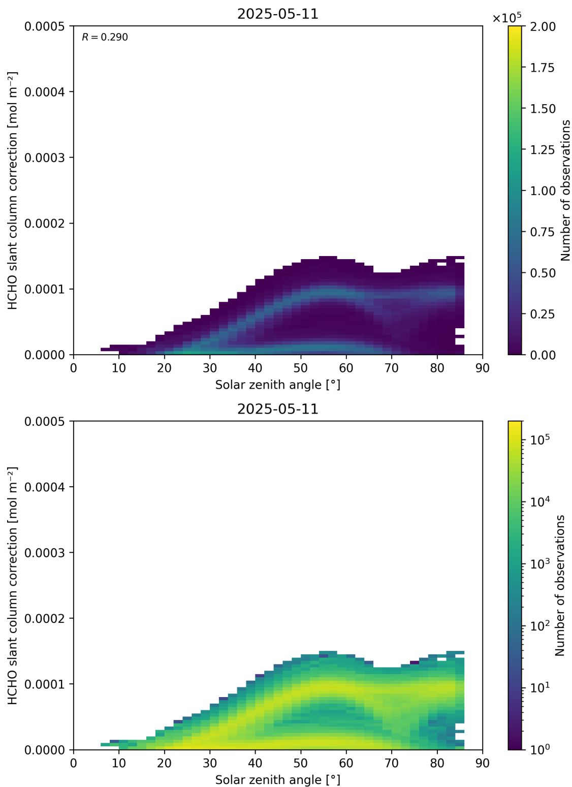
Figure 172: Scatter density plot of “Solar zenith angle” against “HCHO slant column correction” for 2025-05-10 to 2025-05-12.
