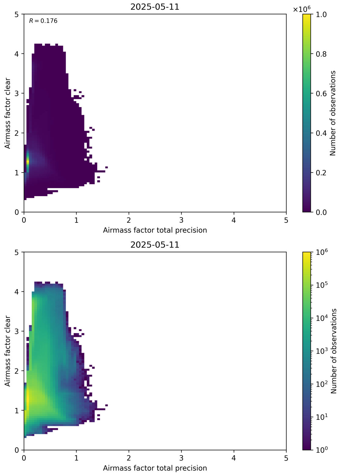
Figure 108: Scatter density plot of “Airmass factor total precision” against “Airmass factor clear” for 2025-05-10 to 2025-05-12.
