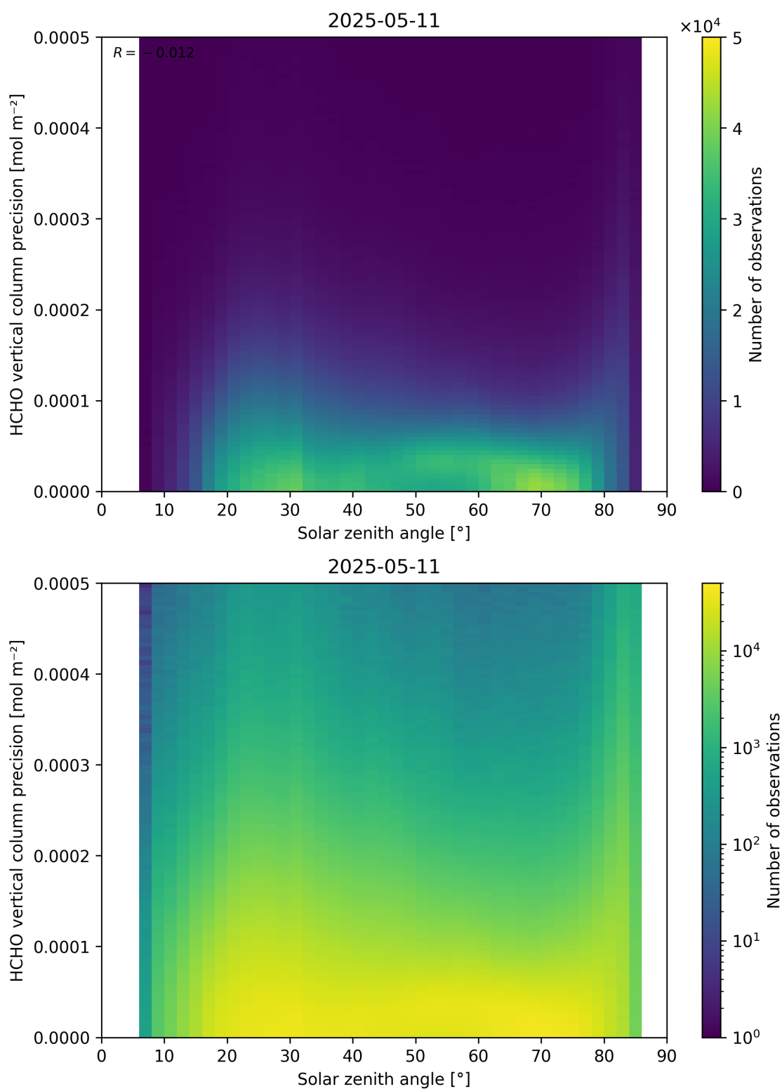
Figure 179: Scatter density plot of “Solar zenith angle” against “HCHO vertical column precision” for 2025-05-10 to 2025-05-12.
