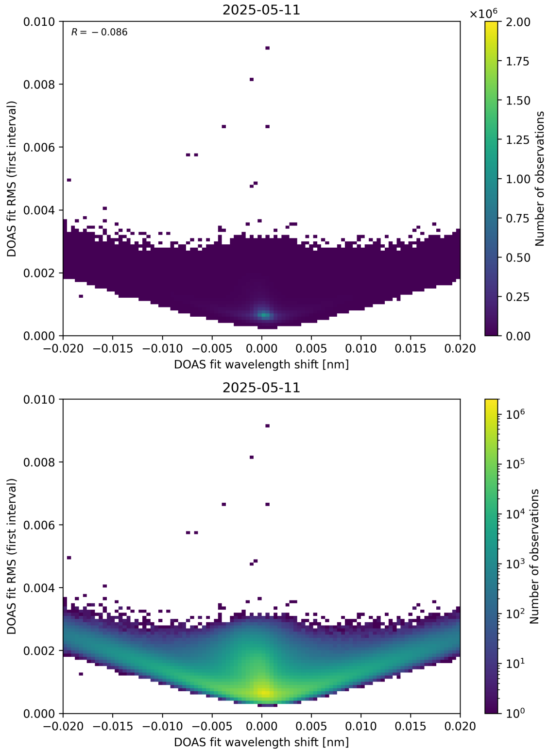
Figure 64: Scatter density plot of “DOAS fit wavelength shift” against “DOAS fit RMS (first interval)” for 2025-05-10 to 2025-05-12.
