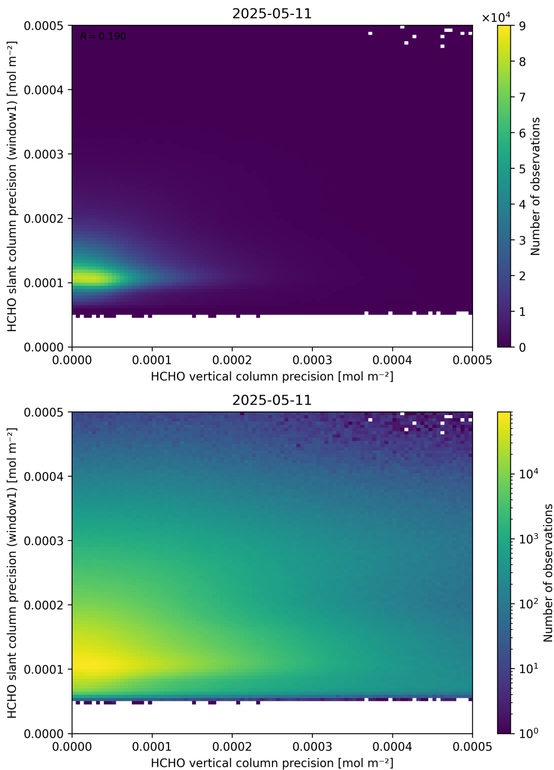
Figure 143: Scatter density plot of “HCHO vertical column precision” against “HCHO slant column precision (window1)” for 2025-05-10 to 2025-05-12.
