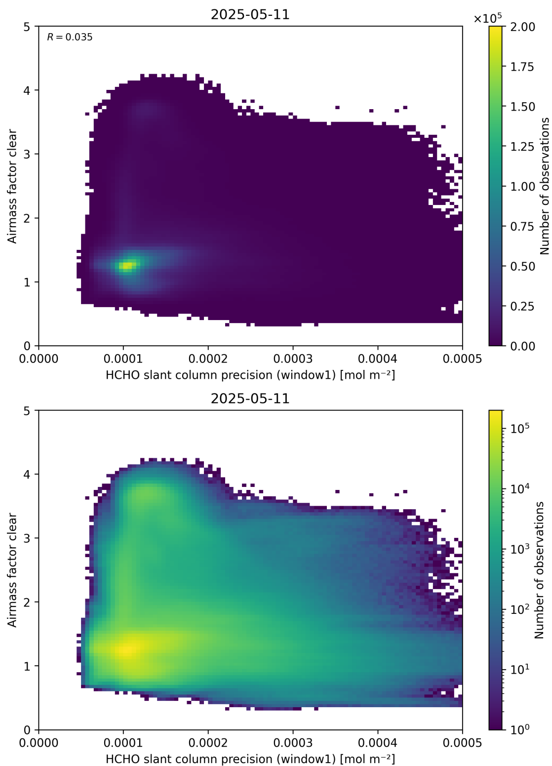
Figure 91: Scatter density plot of “HCHO slant column precision (window1)” against “Airmass factor clear” for 2025-05-10 to 2025-05-12.
