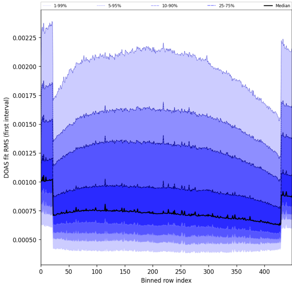
Figure 60: Along track statistics of “DOAS fit RMS (first interval)” for 2025-05-10 to 2025-05-12
