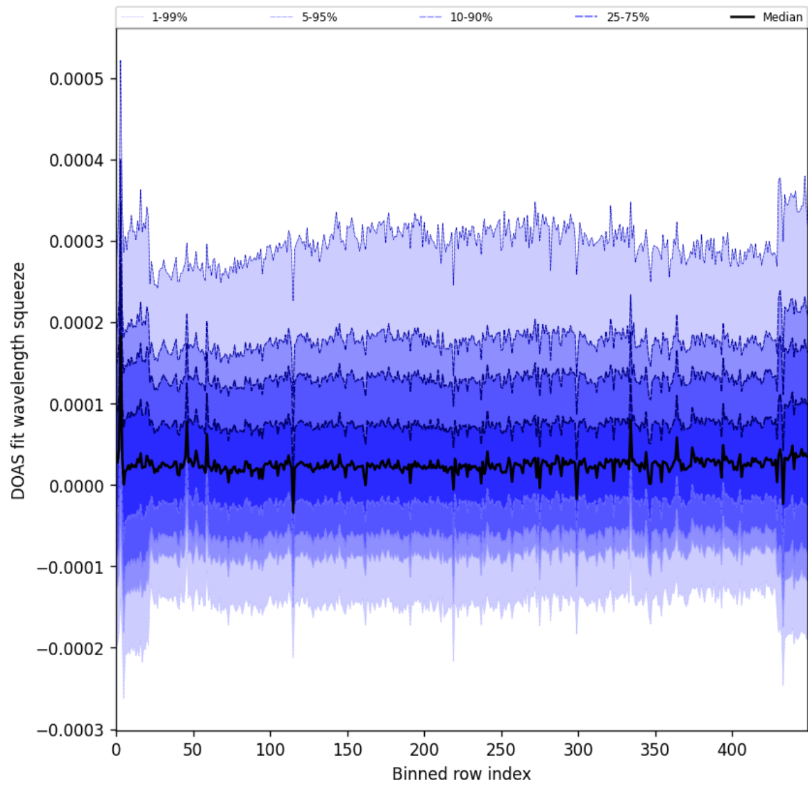
Figure 59: Along track statistics of “DOAS fit wavelength squeeze” for 2025-05-10 to 2025-05-12
