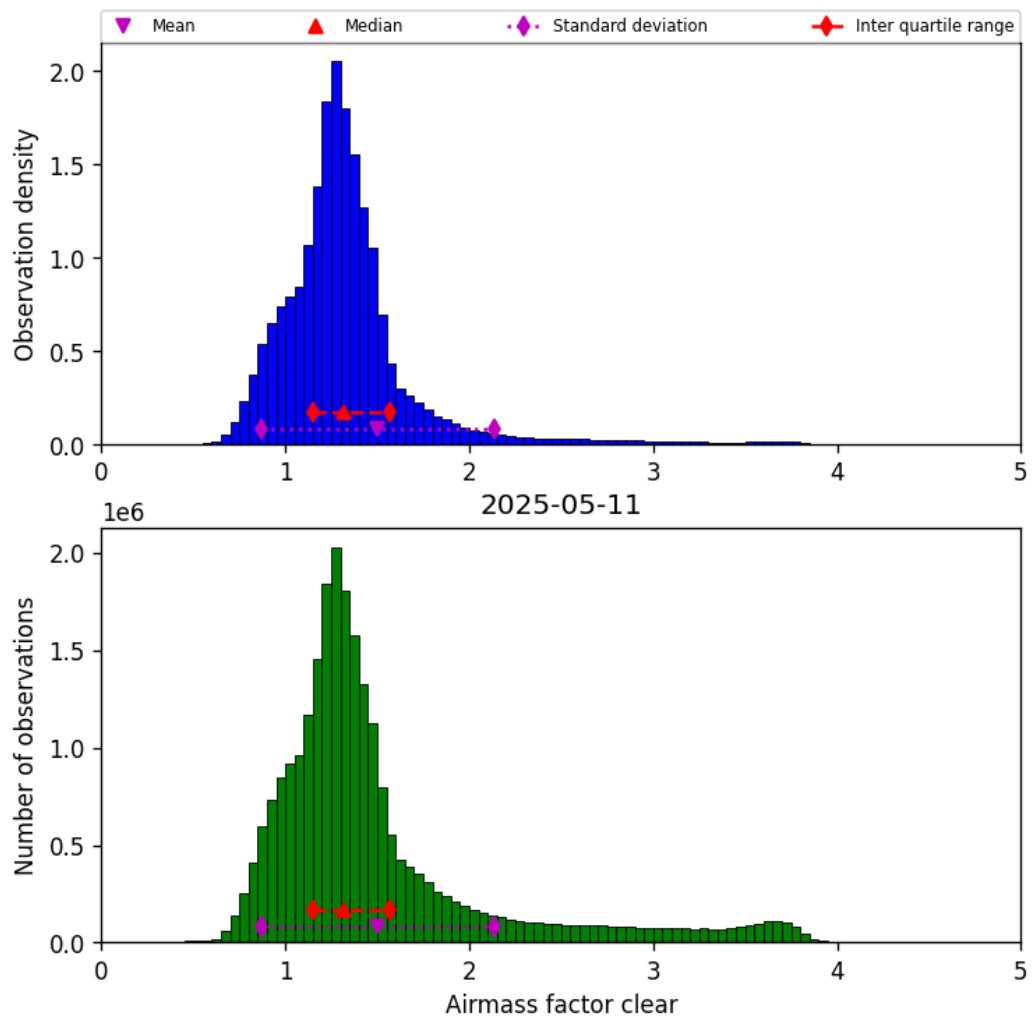
Figure 42: Histogram of “Airmass factor clear” for 2025-05-10 to 2025-05-12
