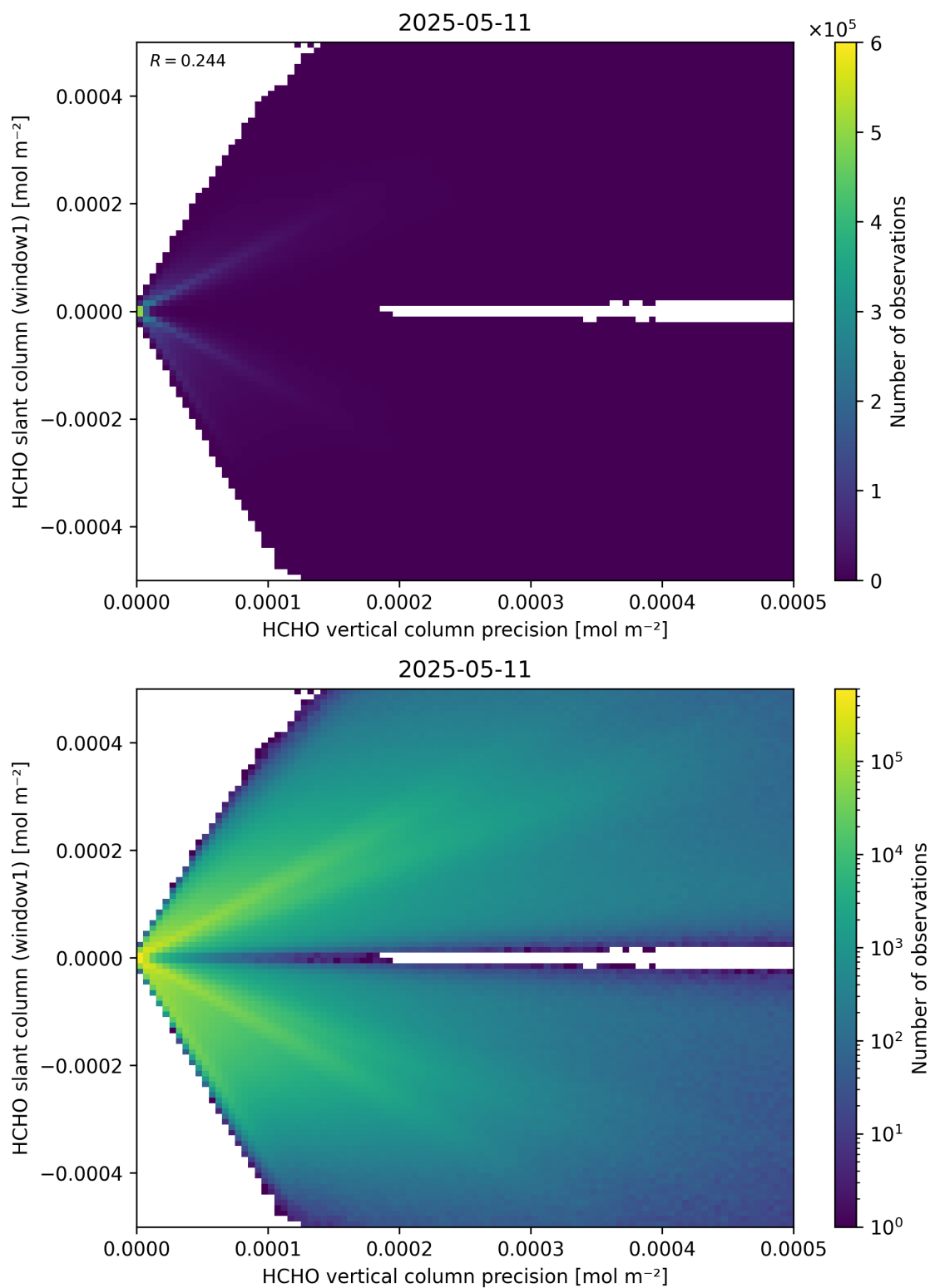
Figure 142: Scatter density plot of “HCHO vertical column precision” against “HCHO slant column (window1)” for 2025-05-10 to 2025-05-12.
