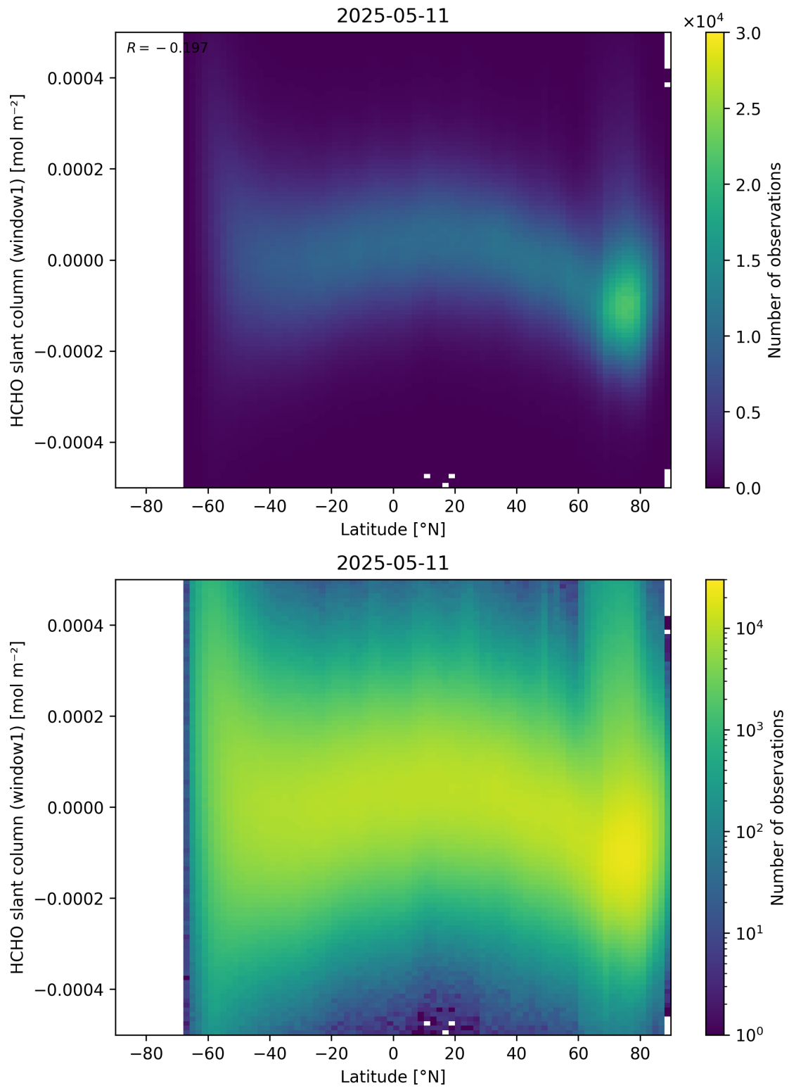
Figure 159: Scatter density plot of “Latitude” against “HCHO slant column (window1)” for 2025-05-10 to 2025-05-12.
