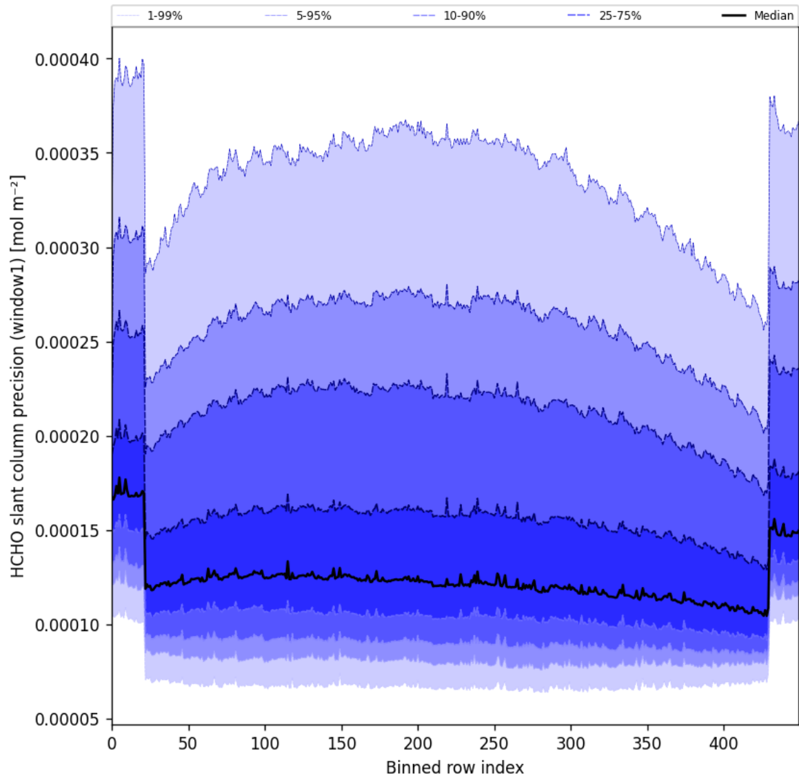
Figure 53: Along track statistics of “HCHO slant column precision (window1)” for 2025-05-10 to 2025-05-12
