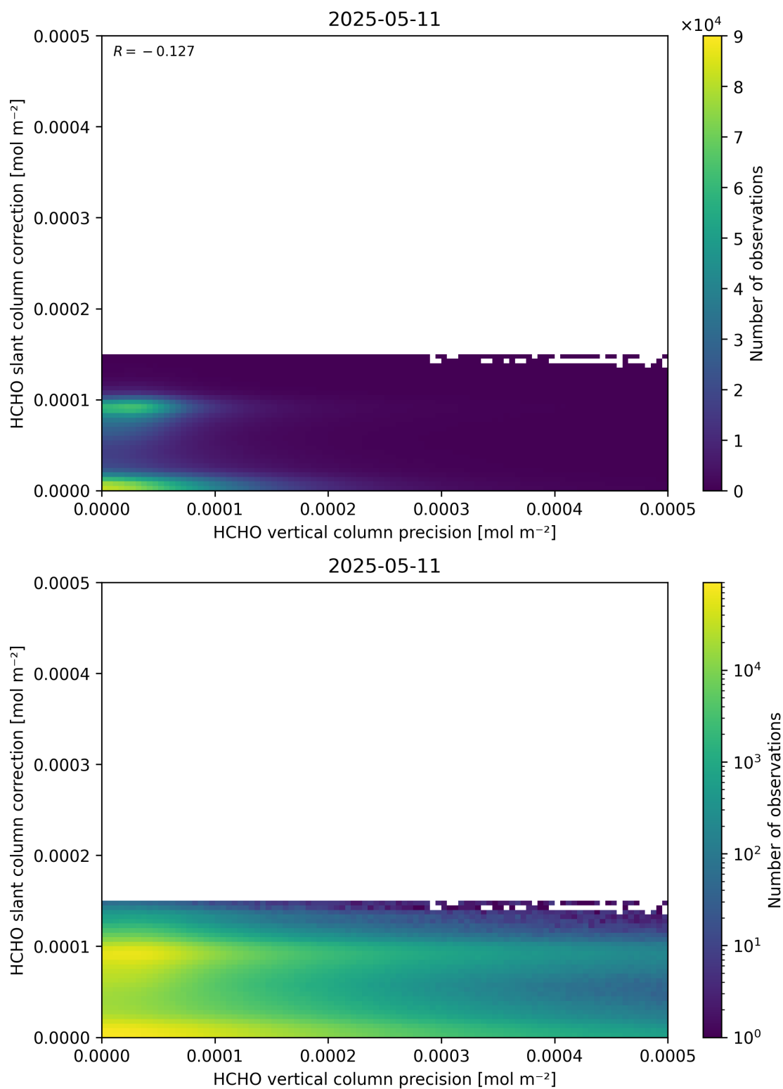
Figure 141: Scatter density plot of “HCHO vertical column precision” against “HCHO slant column correction” for 2025-05-10 to 2025-05-12.
