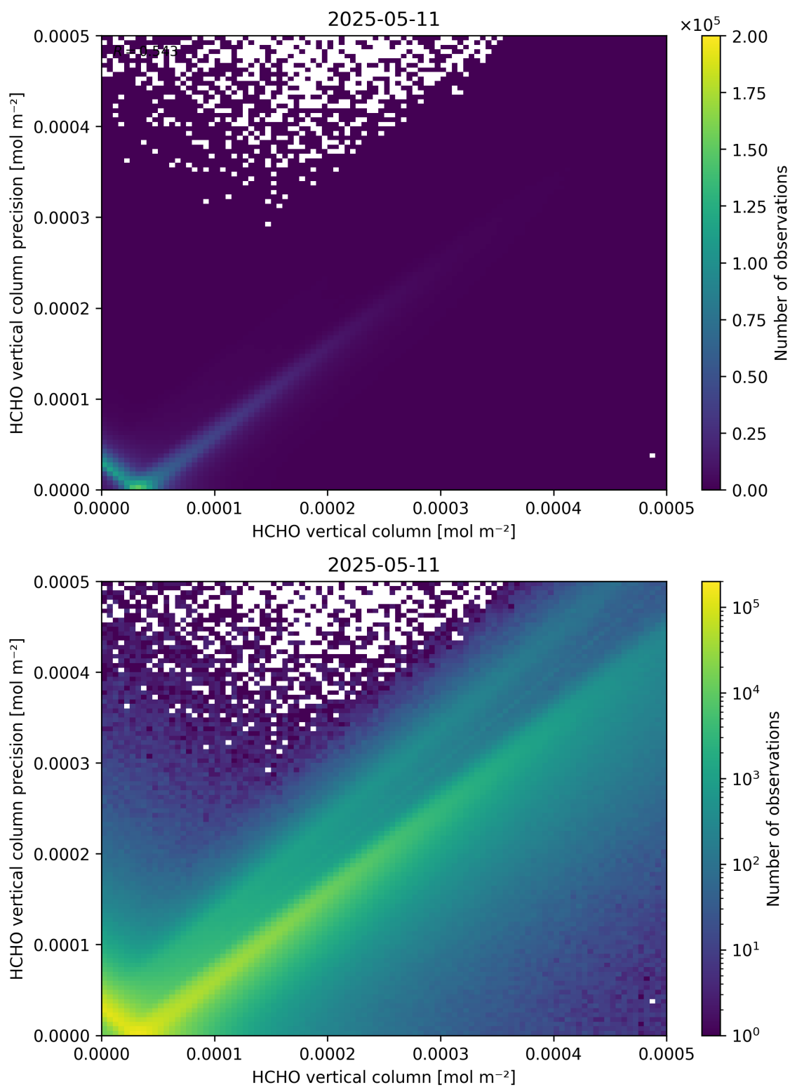
Figure 134: Scatter density plot of “HCHO vertical column” against “HCHO vertical column precision” for 2025-05-10 to 2025-05-12.
