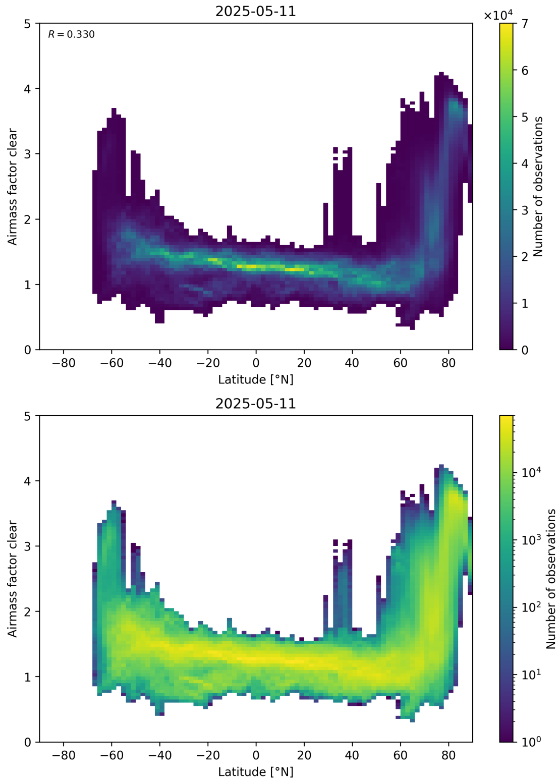
Figure 156: Scatter density plot of “Latitude” against “Airmass factor clear” for 2025-05-10 to 2025-05-12.
