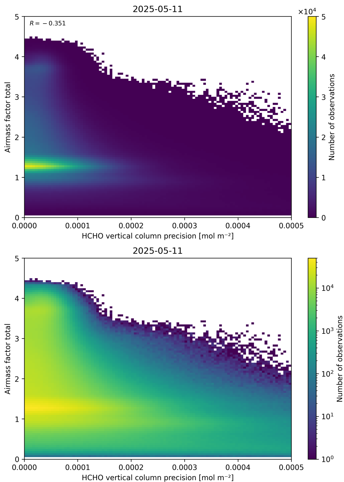
Figure 144: Scatter density plot of “HCHO vertical column precision” against “Airmass factor total” for 2025-05-10 to 2025-05-12.
