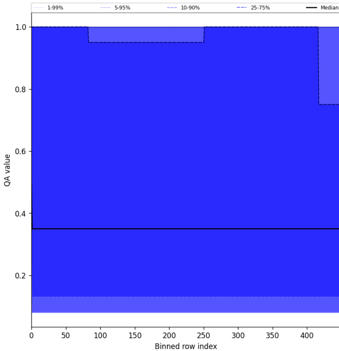
Figure 48: Along track statistics of “QA value” for 2025-05-10 to 2025-05-12
