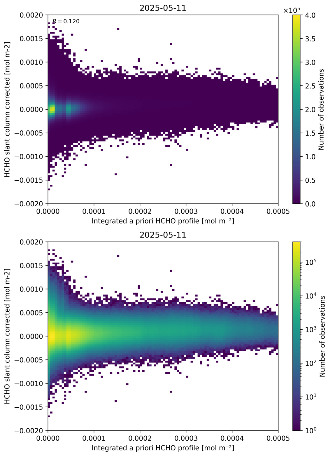
Figure 151: Scatter density plot of “Integrated a priori HCHO profile” against “HCHO slant column corrected” for 2025-05-10 to 2025-05-12.
