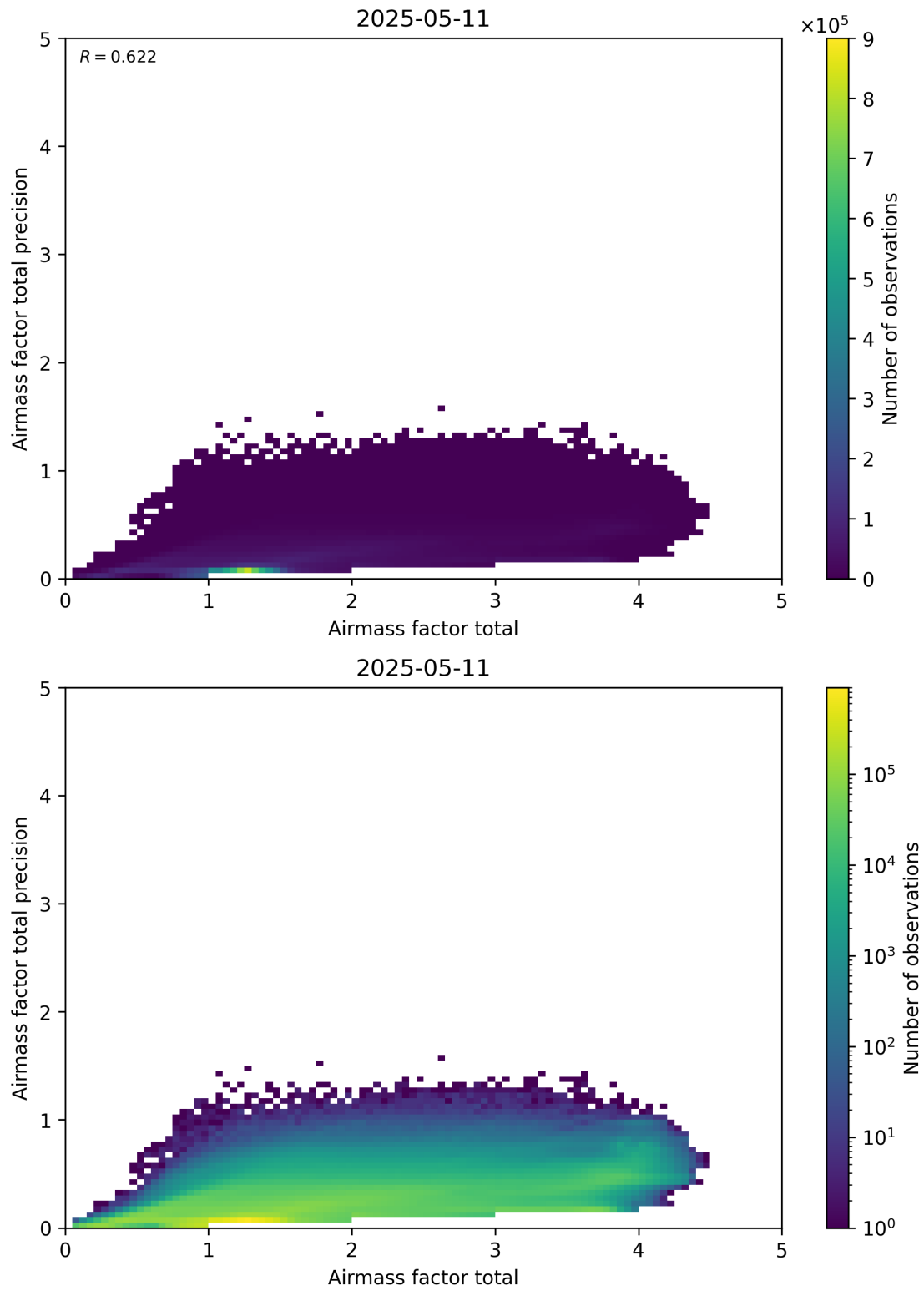
Figure 103: Scatter density plot of “Airmass factor total” against “Airmass factor total precision” for 2025-05-10 to 2025-05-12.
