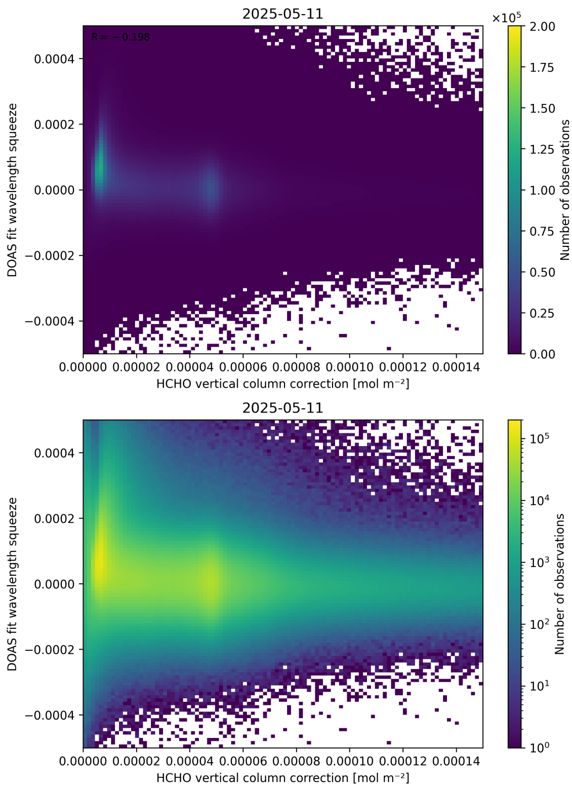
Figure 114: Scatter density plot of “HCHO vertical column correction” against “DOAS fit wavelength squeeze” for 2025-05-10 to 2025-05-12.
