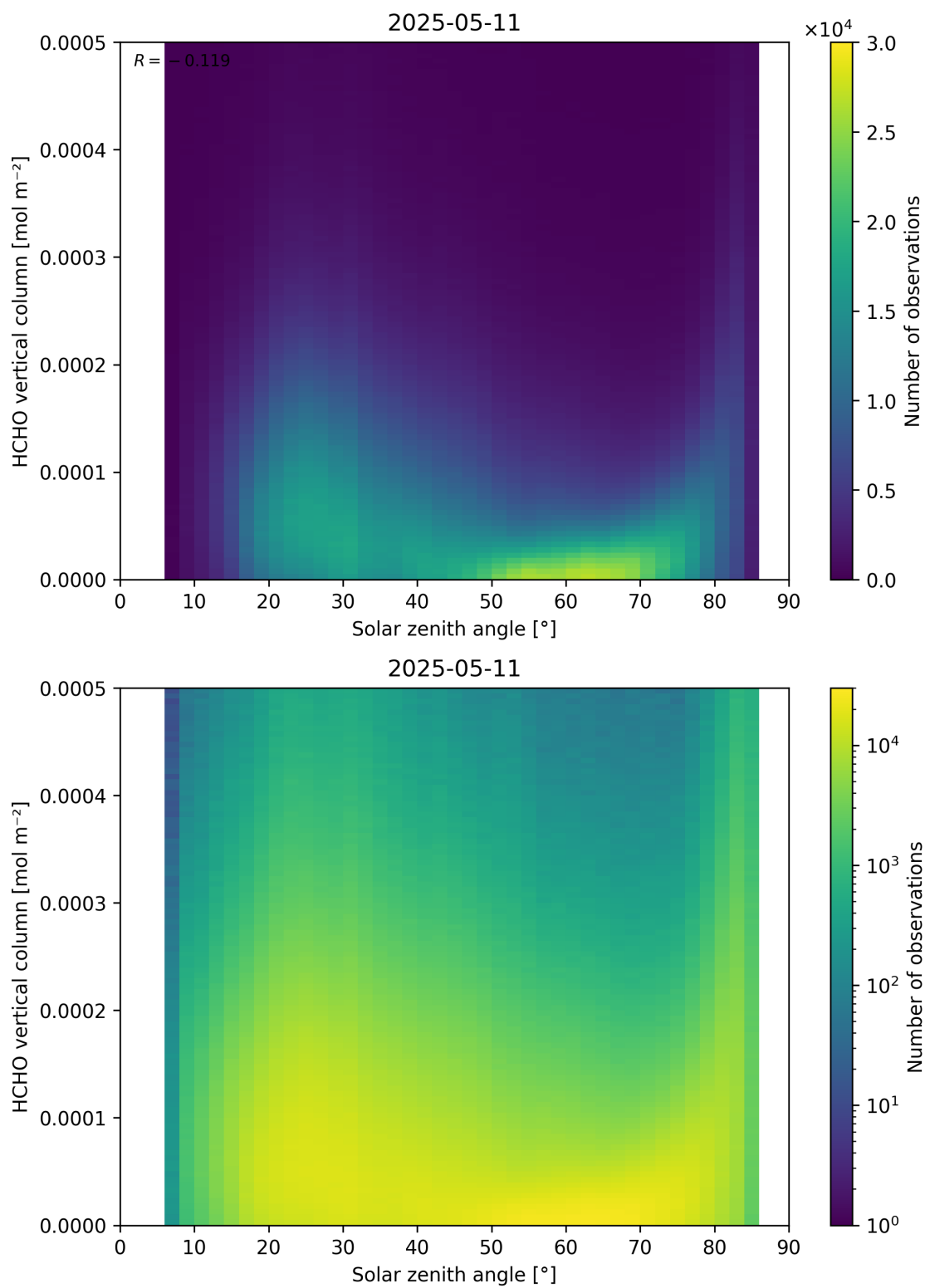
Figure 177: Scatter density plot of “Solar zenith angle” against “HCHO vertical column” for 2025-05-10 to 2025-05-12.
