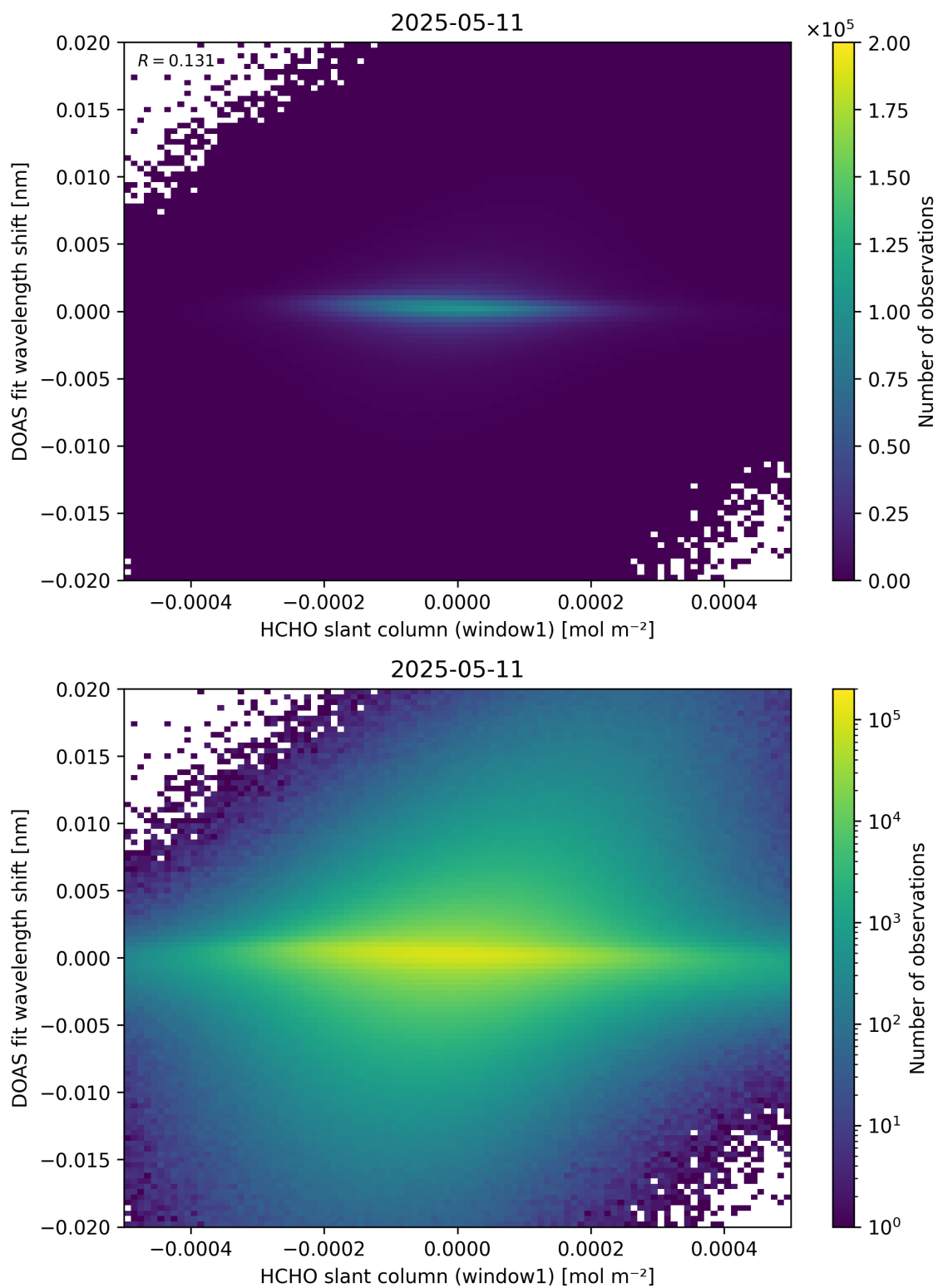
Figure 79: Scatter density plot of “HCHO slant column (window1)” against “DOAS fit wavelength shift” for 2025-05-10 to 2025-05-12.
