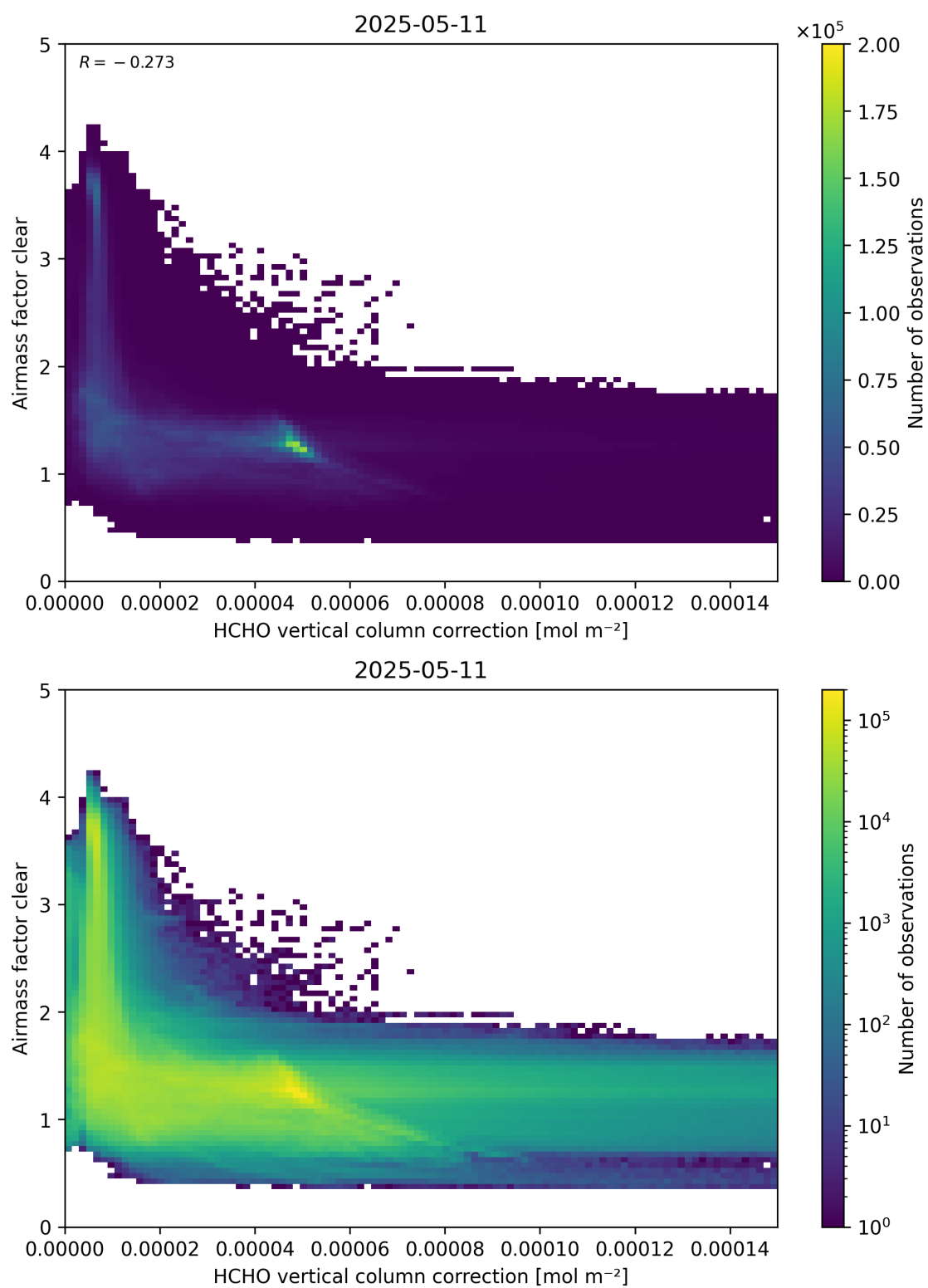
Figure 115: Scatter density plot of “HCHO vertical column correction” against “Airmass factor clear” for 2025-05-10 to 2025-05-12.
