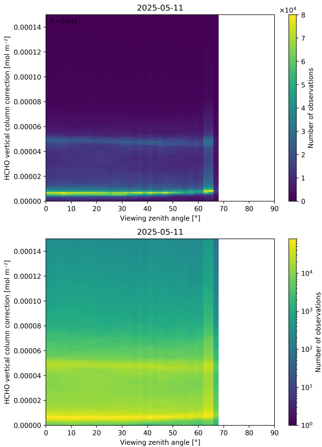
Figure 193: Scatter density plot of “Viewing zenith angle” against “HCHO vertical column correction” for 2025-05-10 to 2025-05-12.
