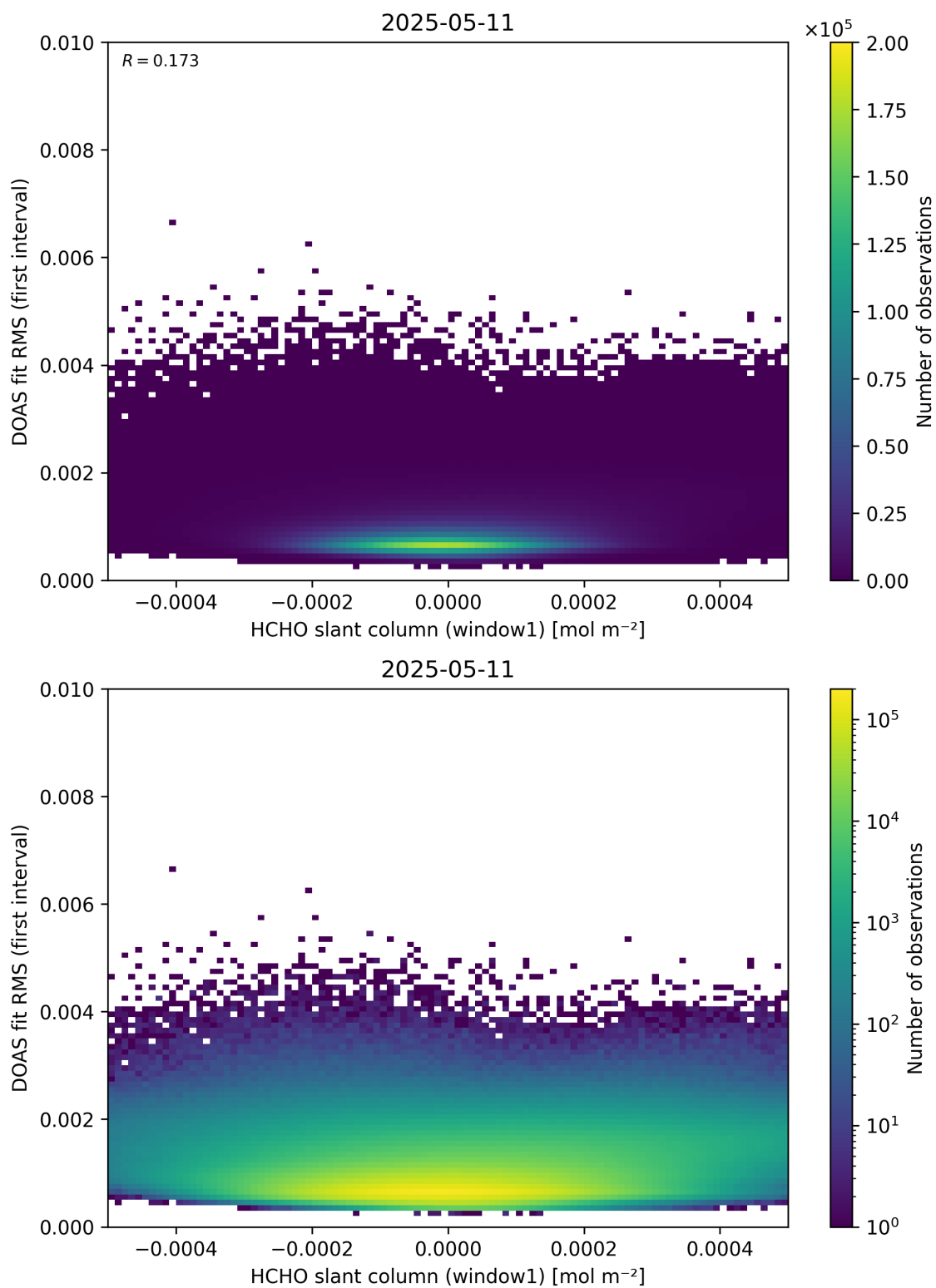
Figure 78: Scatter density plot of “HCHO slant column (window1)” against “DOAS fit RMS (first interval)” for 2025-05-10 to 2025-05-12.
