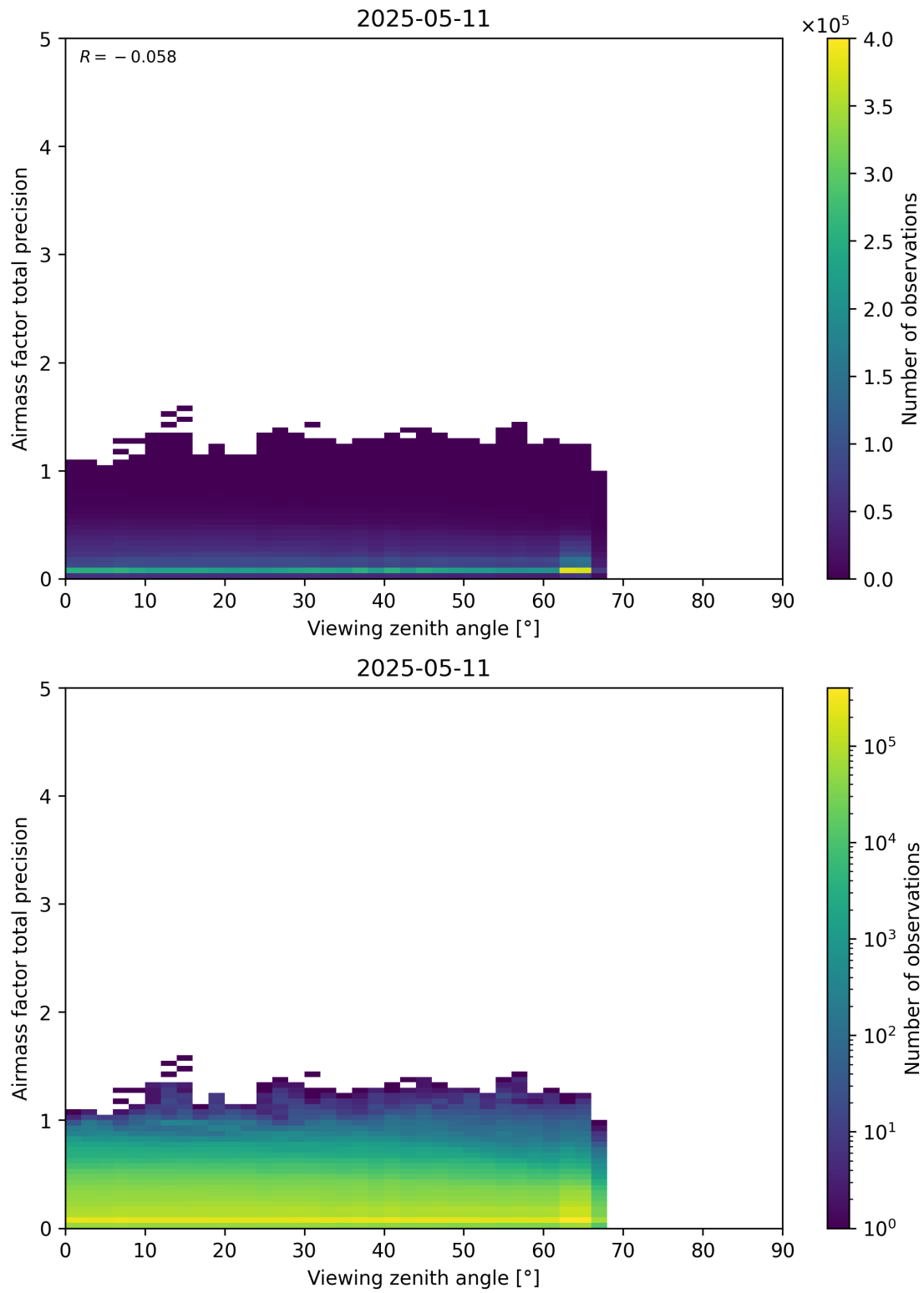
Figure 191: Scatter density plot of “Viewing zenith angle” against “Airmass factor total precision” for 2025-05-10 to 2025-05-12.
