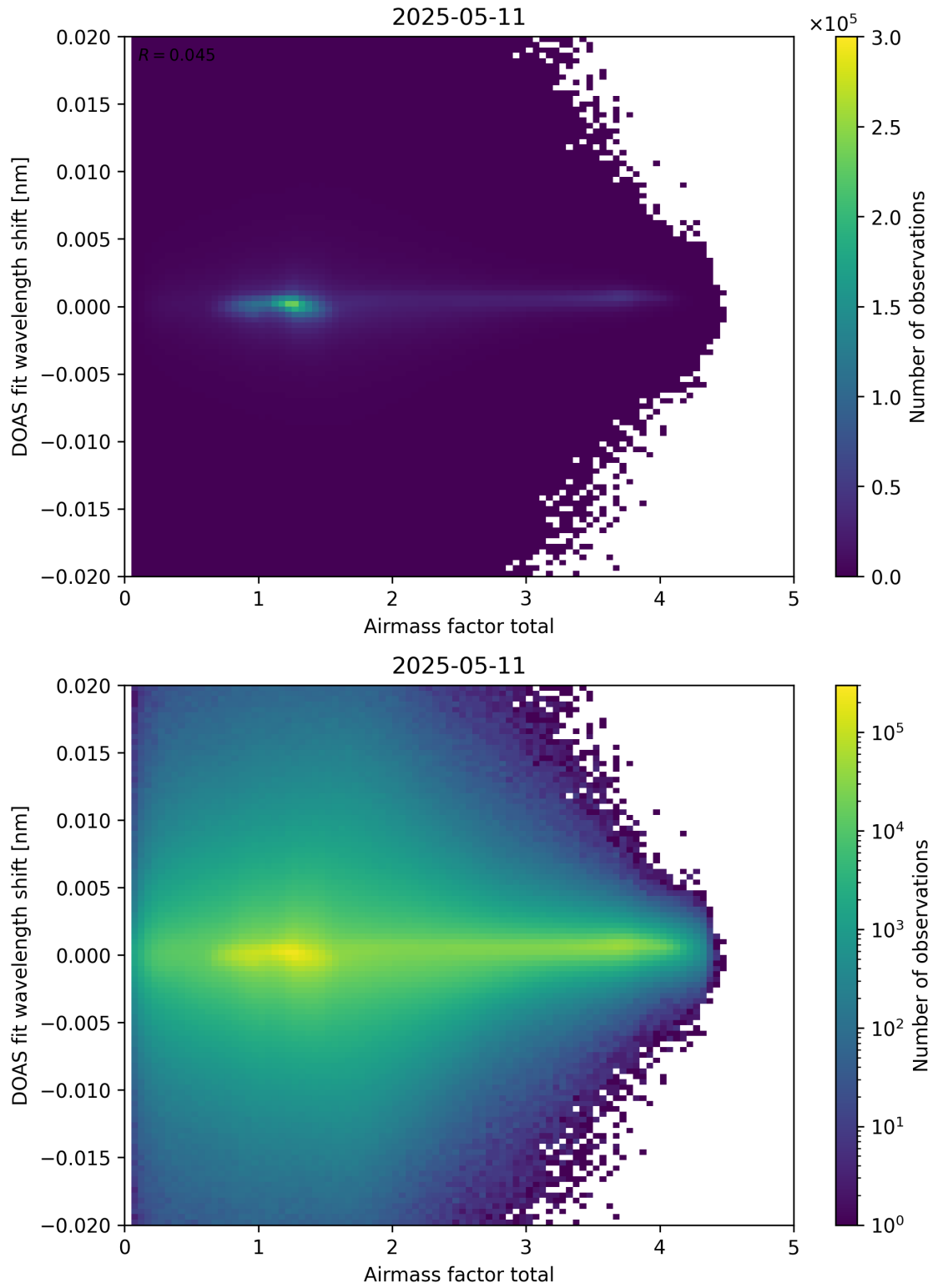
Figure 98: Scatter density plot of “Airmass factor total” against “DOAS fit wavelength shift” for 2025-05-10 to 2025-05-12.
