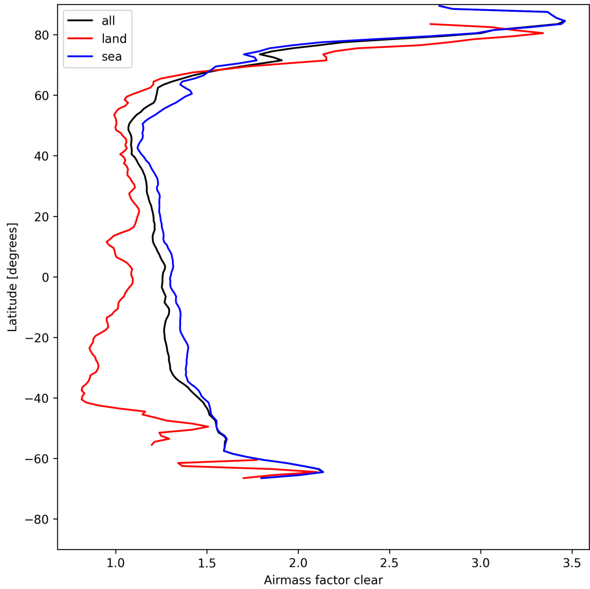
Figure 28: Zonal average of “Airmass factor clear” for 2025-05-10 to 2025-05-12.
