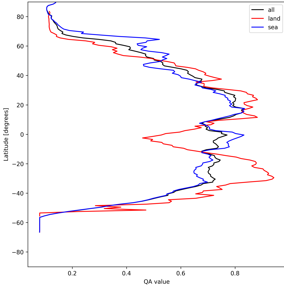
Figure 20: Zonal average of “QA value” for 2025-05-10 to 2025-05-12.
