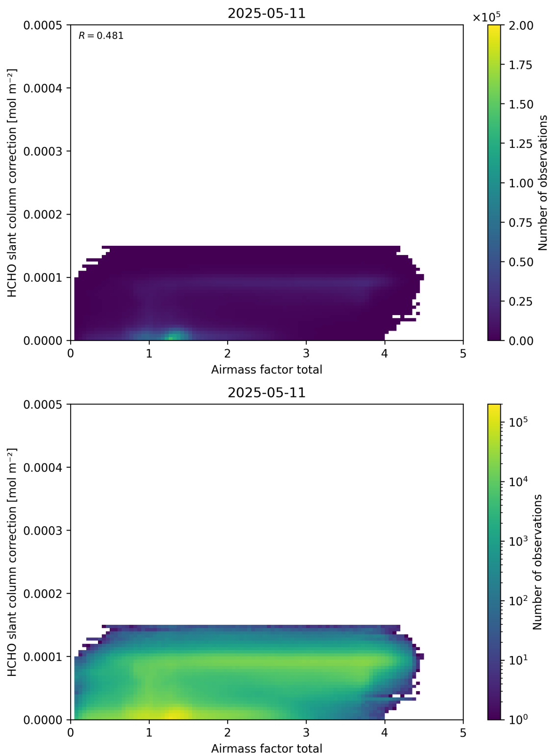
Figure 102: Scatter density plot of “Airmass factor total” against “HCHO slant column correction” for 2025-05-10 to 2025-05-12.
