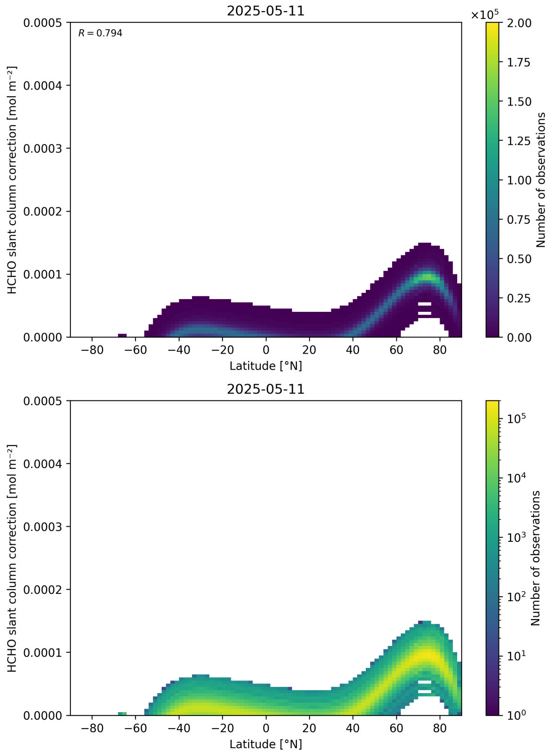
Figure 158: Scatter density plot of “Latitude” against “HCHO slant column correction” for 2025-05-10 to 2025-05-12.
