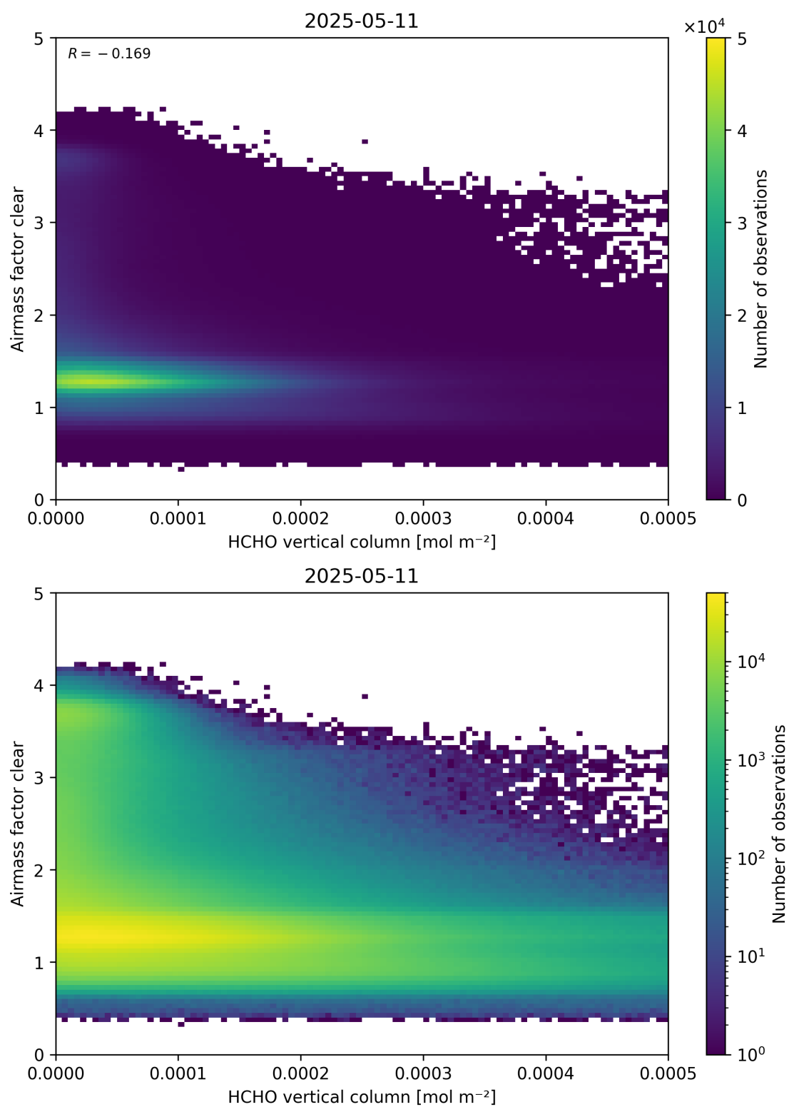
Figure 126: Scatter density plot of “HCHO vertical column” against “Airmass factor clear” for 2025-05-10 to 2025-05-12.
