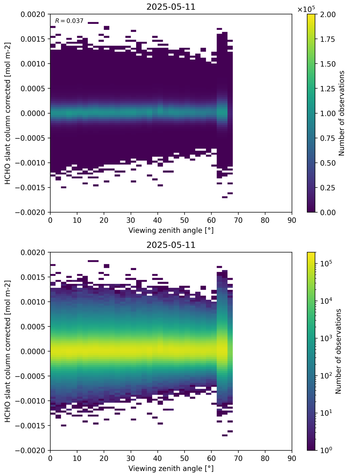
Figure 186: Scatter density plot of “Viewing zenith angle” against “HCHO slant column corrected” for 2025-05-10 to 2025-05-12.
