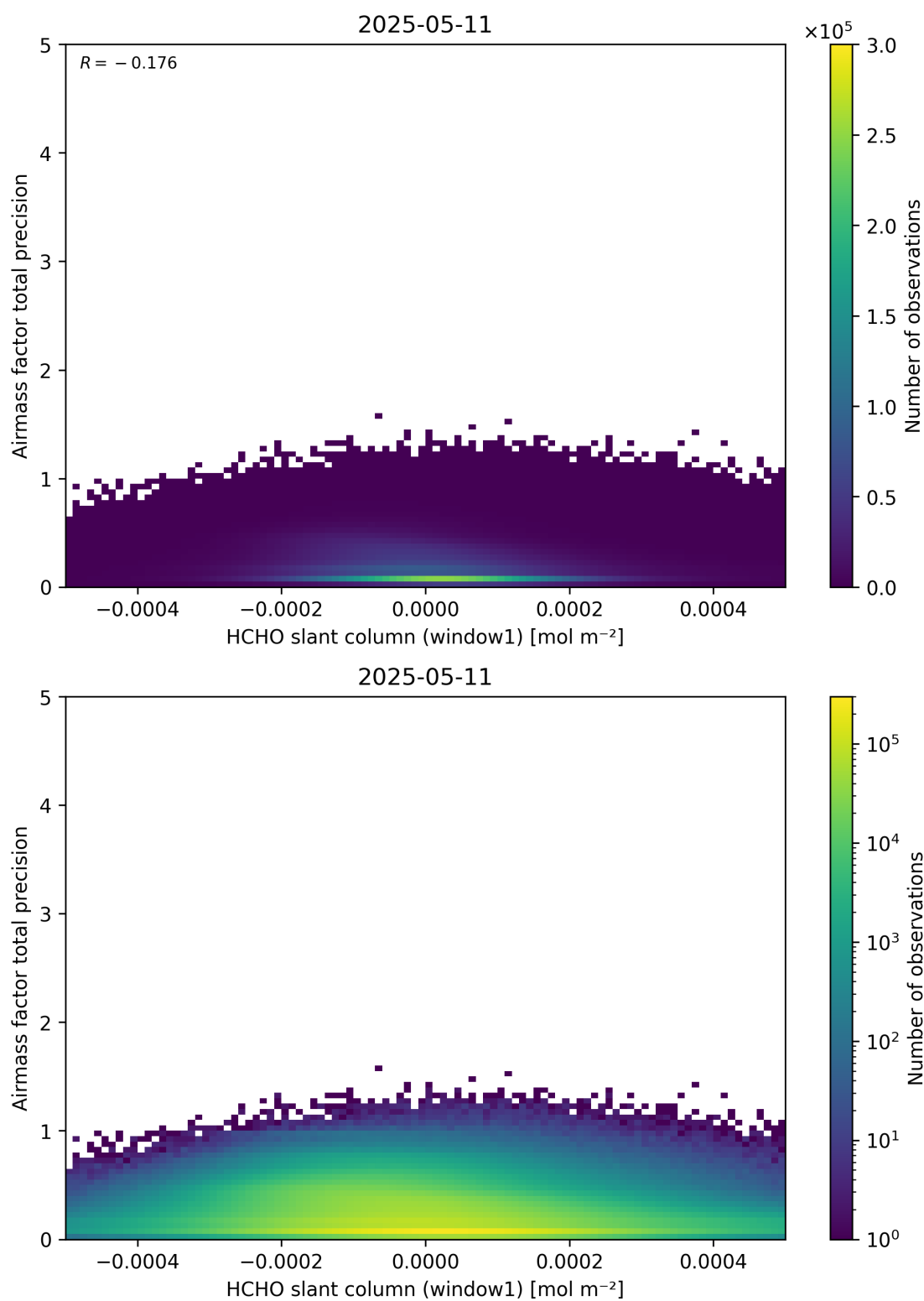
Figure 86: Scatter density plot of “HCHO slant column (window1)” against “Airmass factor total precision” for 2025-05-10 to 2025-05-12.
