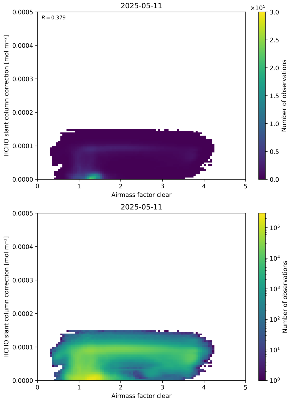
Figure 75: Scatter density plot of “Airmass factor clear” against “HCHO slant column correction” for 2025-05-10 to 2025-05-12.
