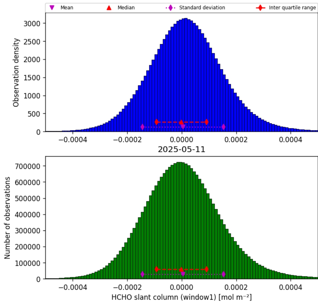
Figure 38: Histogram of “HCHO slant column (window1)” for 2025-05-10 to 2025-05-12
