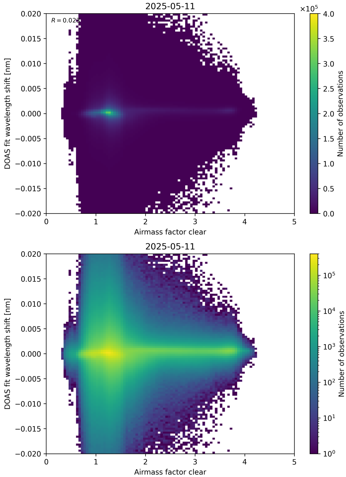
Figure 72: Scatter density plot of “Airmass factor clear” against “DOAS fit wavelength shift” for 2025-05-10 to 2025-05-12.
