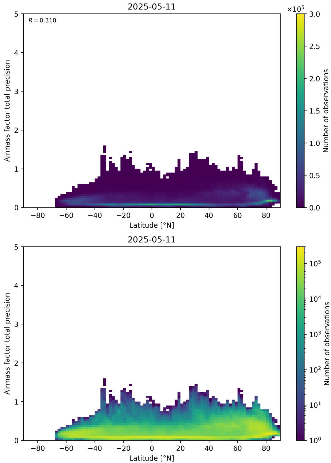
Figure 162: Scatter density plot of “Latitude” against “Airmass factor total precision” for 2025-05-10 to 2025-05-12.
