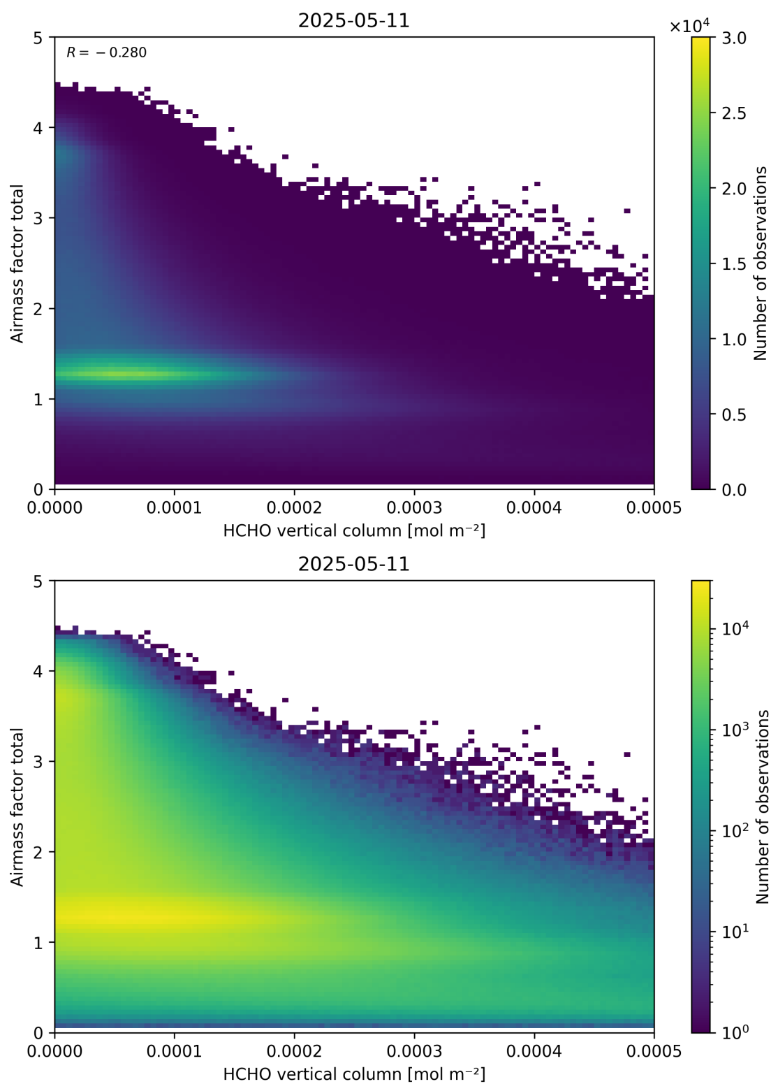
Figure 131: Scatter density plot of “HCHO vertical column” against “Airmass factor total” for 2025-05-10 to 2025-05-12.
