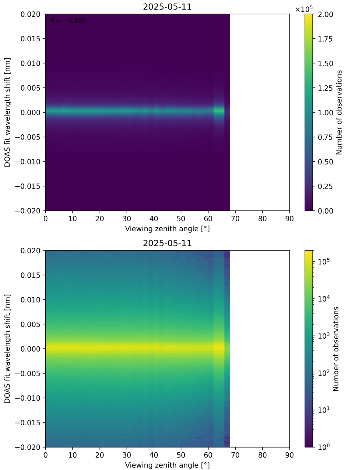
Figure 183: Scatter density plot of “Viewing zenith angle” against “DOAS fit wavelength shift” for 2025-05-10 to 2025-05-12.
