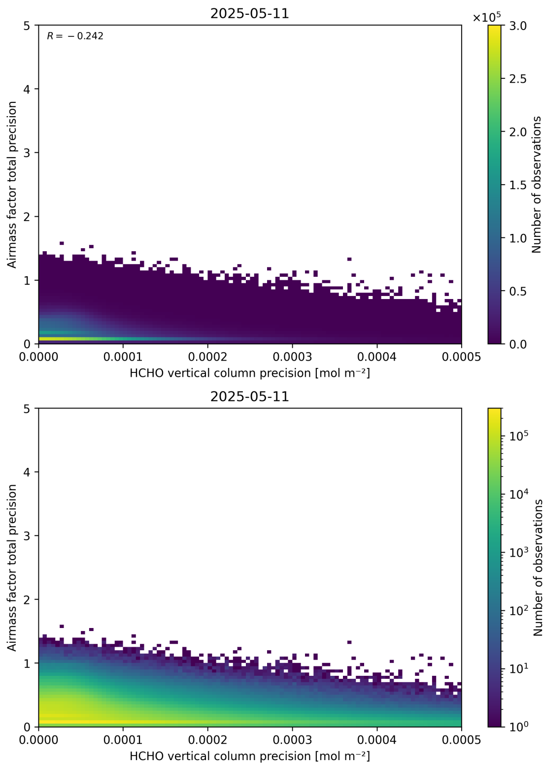
Figure 145: Scatter density plot of “HCHO vertical column precision” against “Airmass factor total precision” for 2025-05-10 to 2025-05-12.
