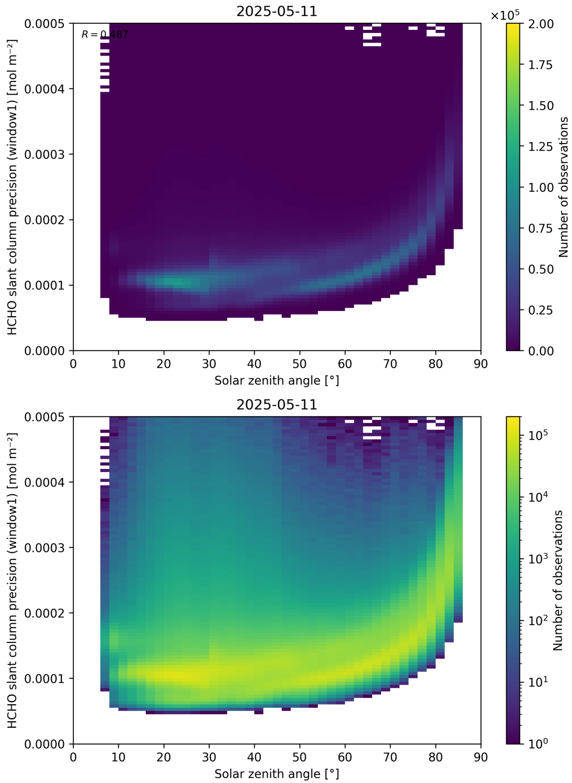
Figure 174: Scatter density plot of “Solar zenith angle” against “HCHO slant column precision (window1)” for 2025-05-10 to 2025-05-12.
