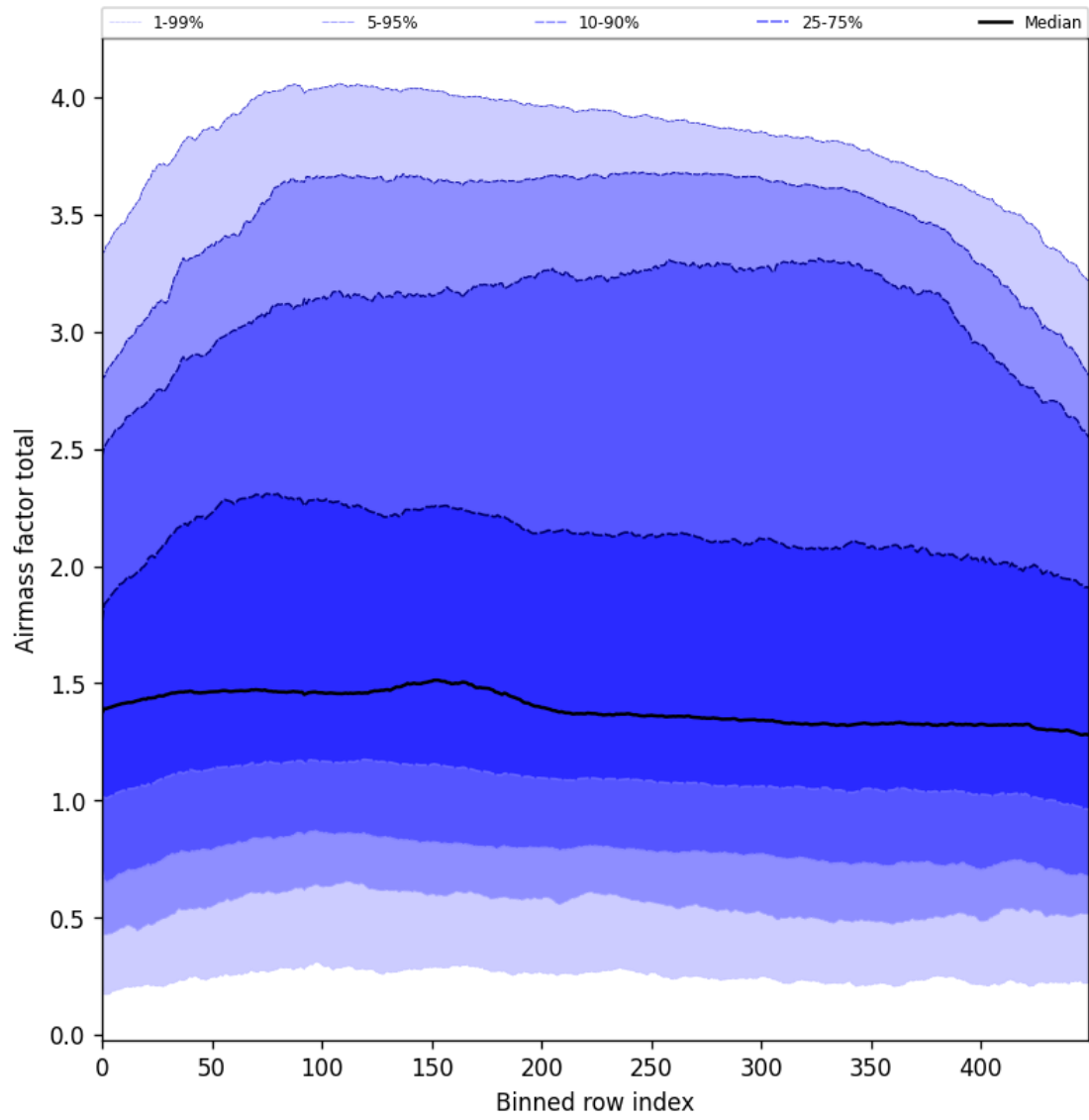
Figure 54: Along track statistics of “Airmass factor total” for 2025-05-10 to 2025-05-12
