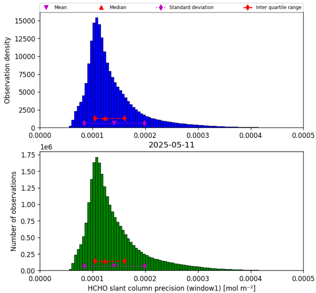
Figure 39: Histogram of “HCHO slant column precision (window1)” for 2025-05-10 to 2025-05-12
