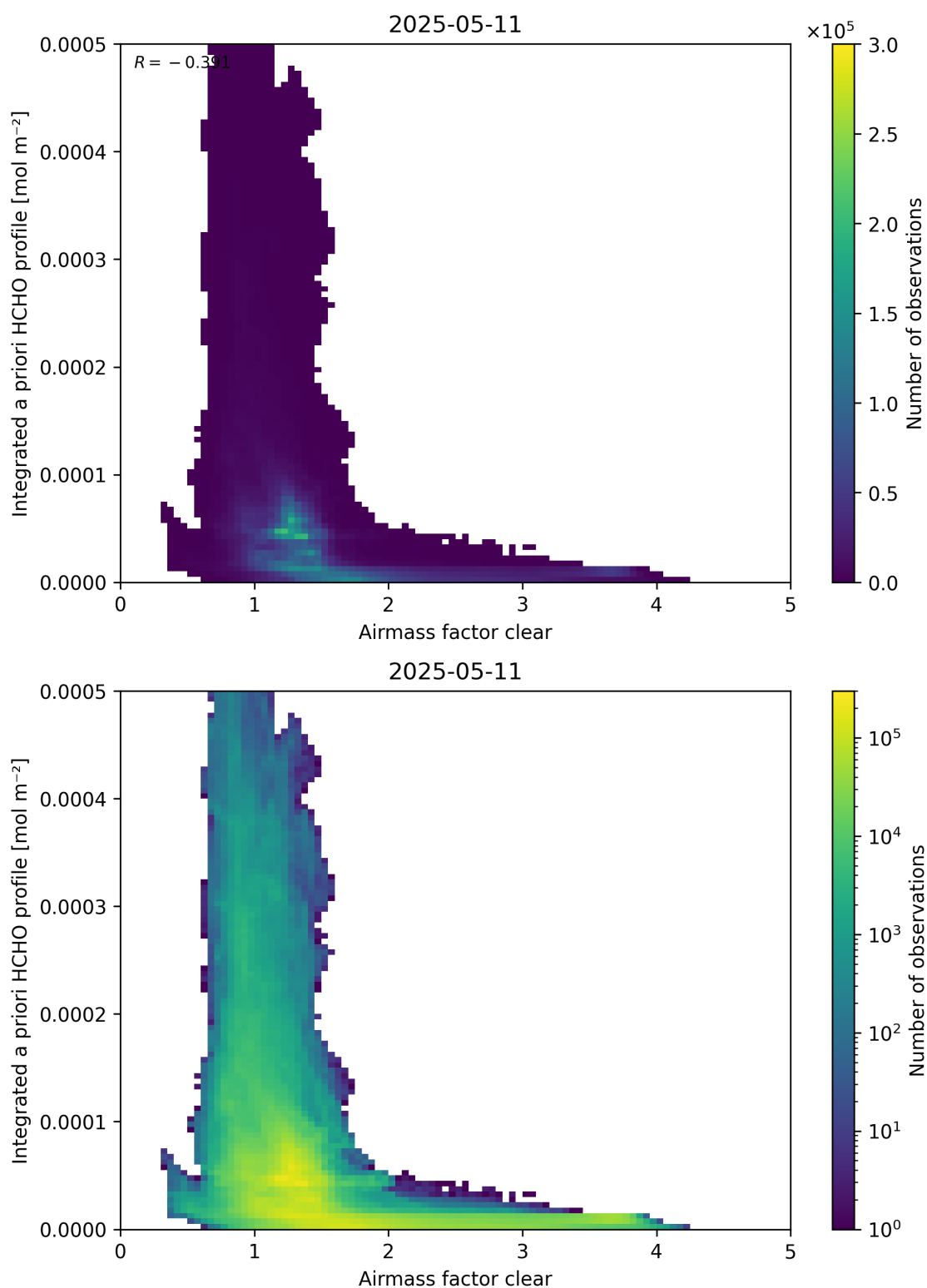
Figure 76: Scatter density plot of “Airmass factor clear” against “Integrated a priori HCHO profile” for 2025-05-10 to 2025-05-12.
