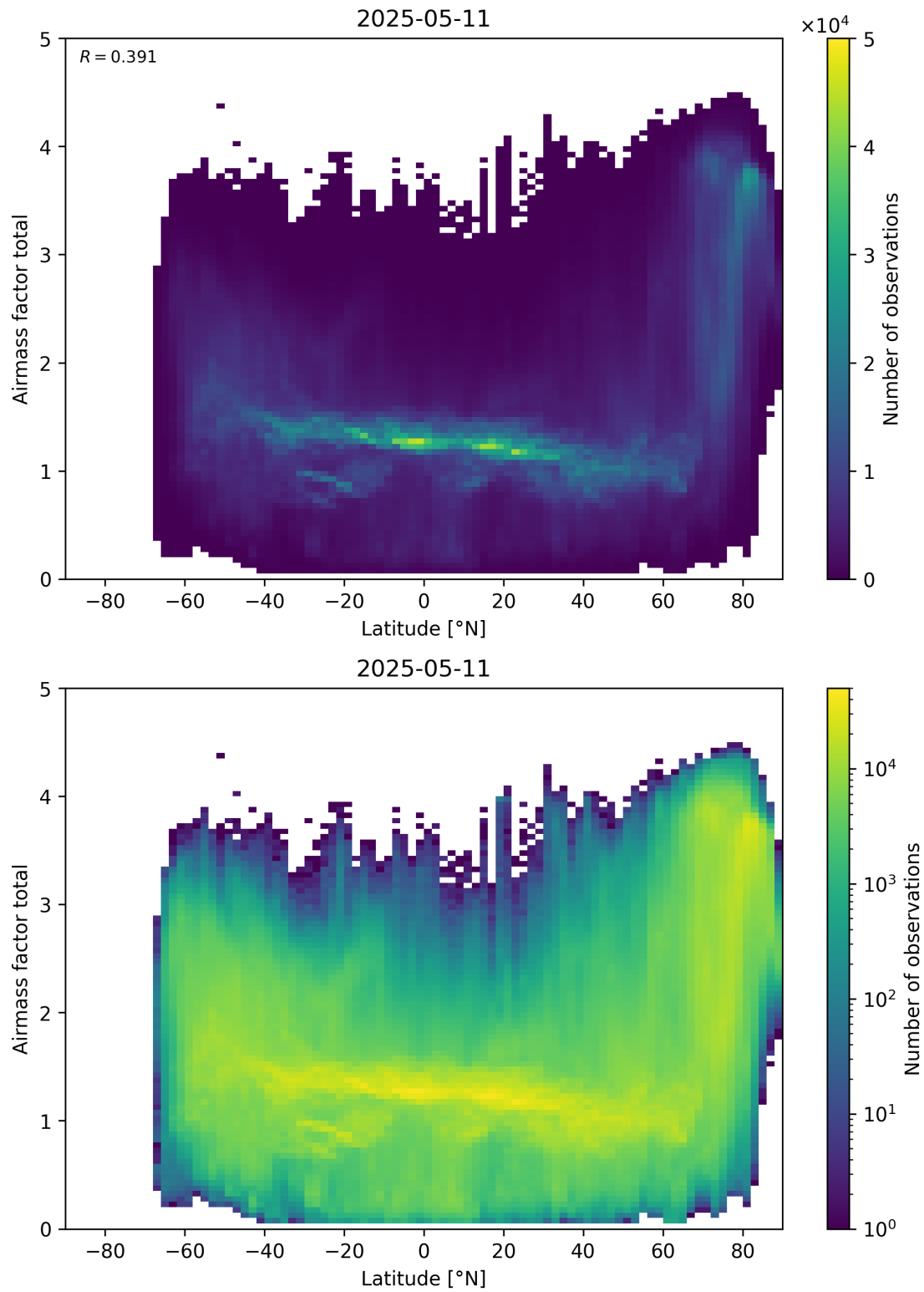
Figure 161: Scatter density plot of “Latitude” against “Airmass factor total” for 2025-05-10 to 2025-05-12.
