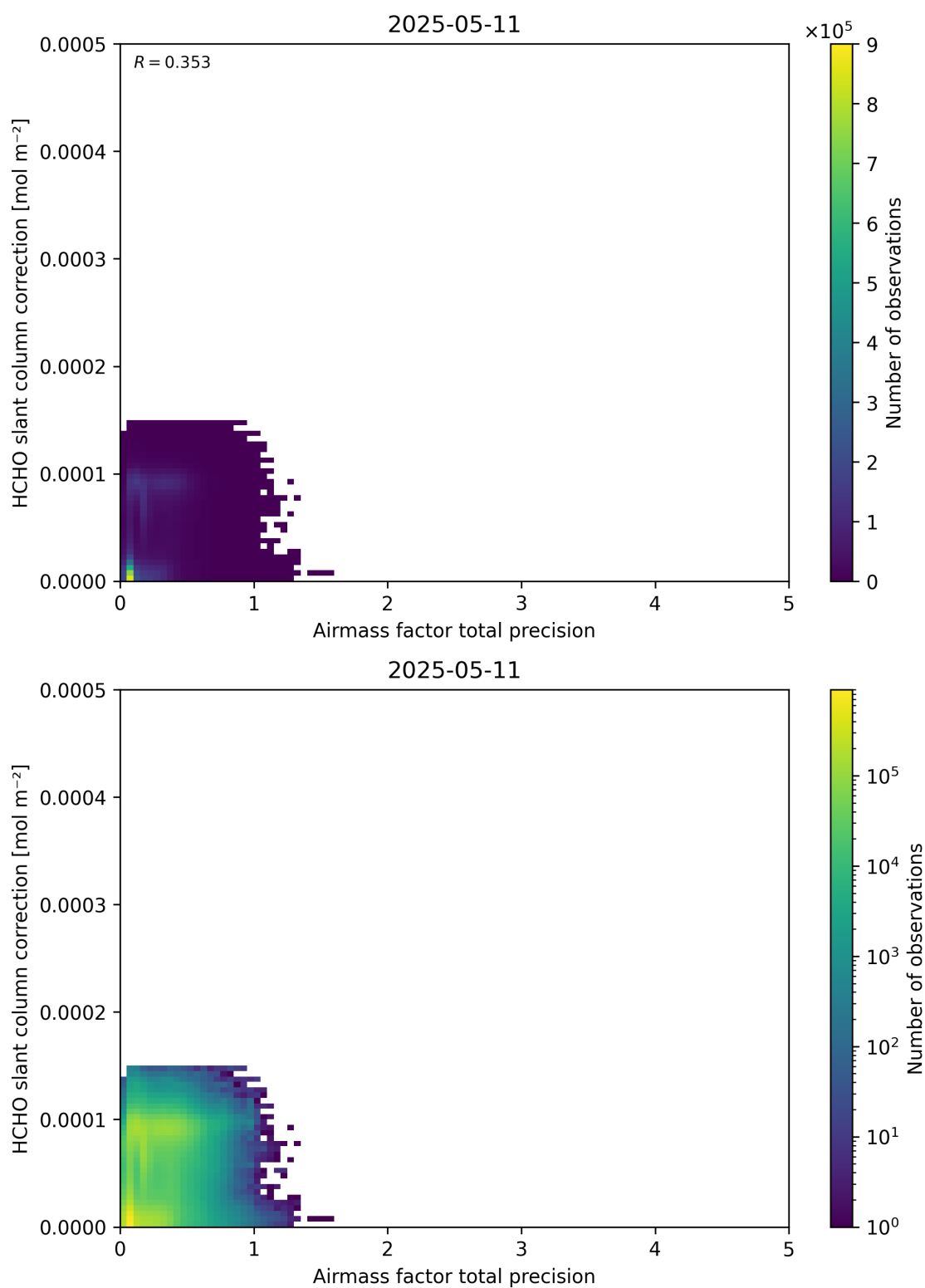
Figure 110: Scatter density plot of “Airmass factor total precision” against “HCHO slant column correction” for 2025-05-10 to 2025-05-12.
