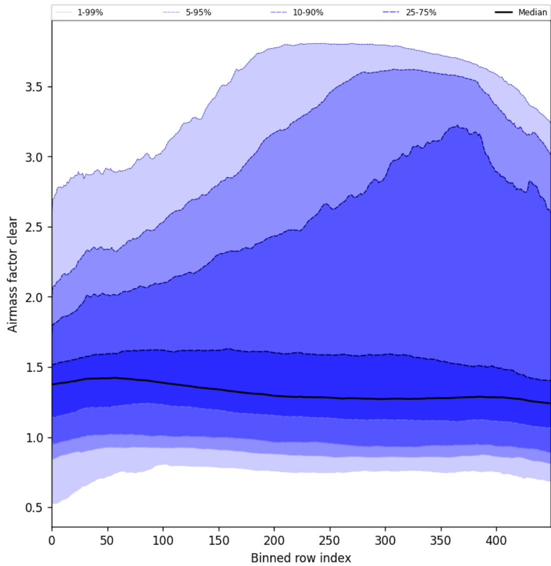
Figure 56: Along track statistics of “Airmass factor clear” for 2025-05-10 to 2025-05-12
