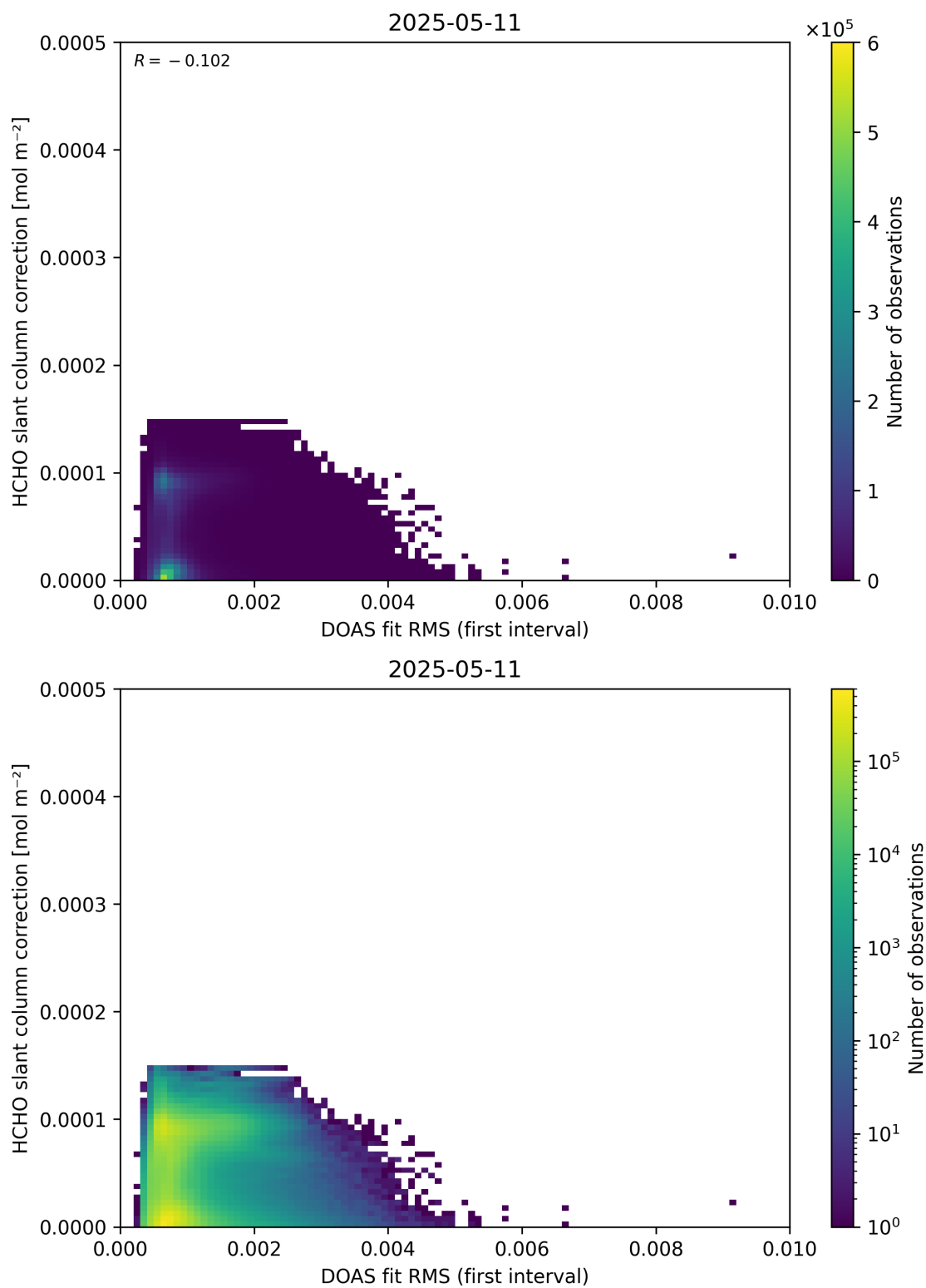
Figure 63: Scatter density plot of “DOAS fit RMS (first interval)” against “HCHO slant column correction” for 2025-05-10 to 2025-05-12.
