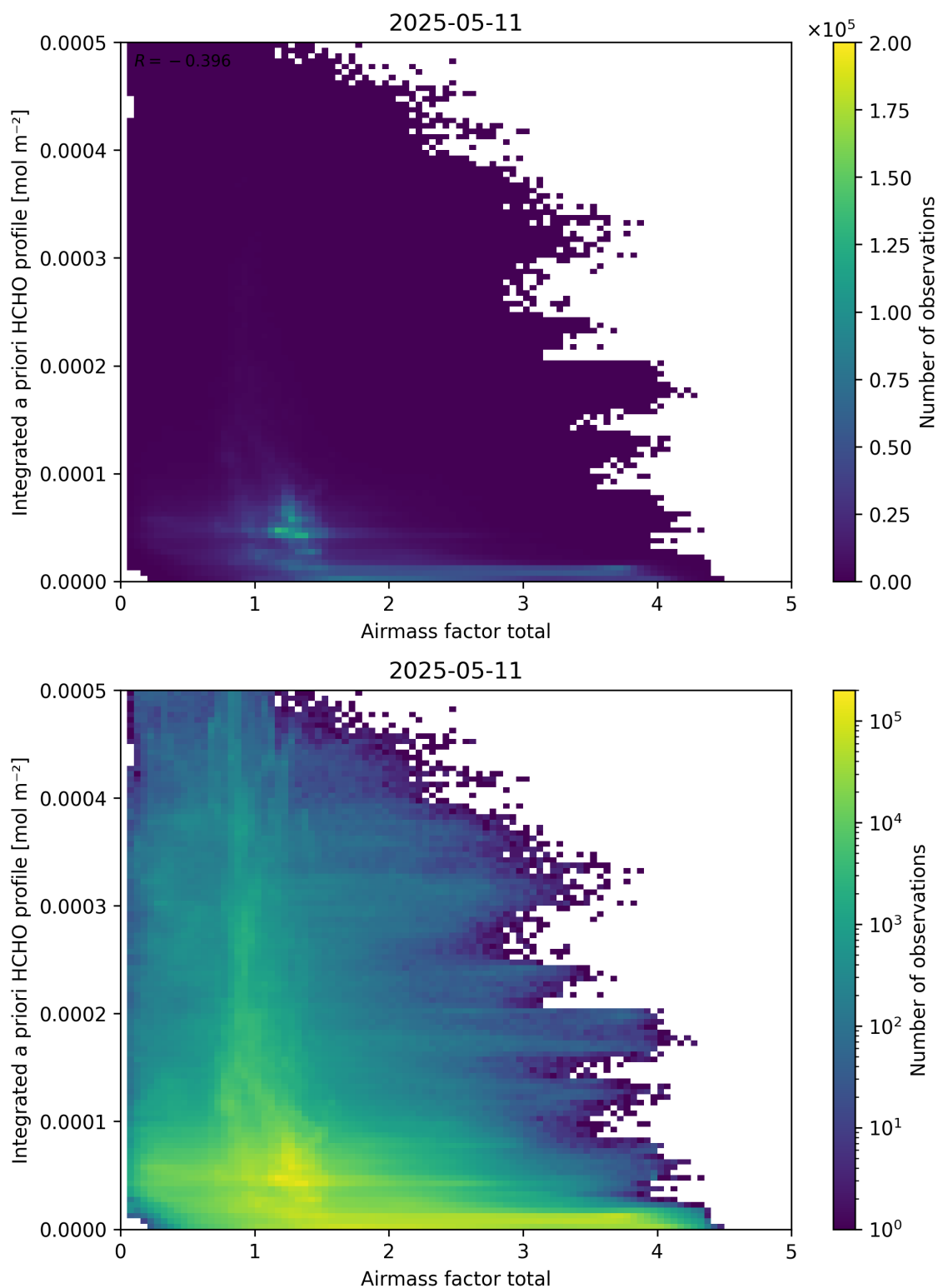
Figure 104: Scatter density plot of “Airmass factor total” against “Integrated a priori HCHO profile” for 2025-05-10 to 2025-05-12.
