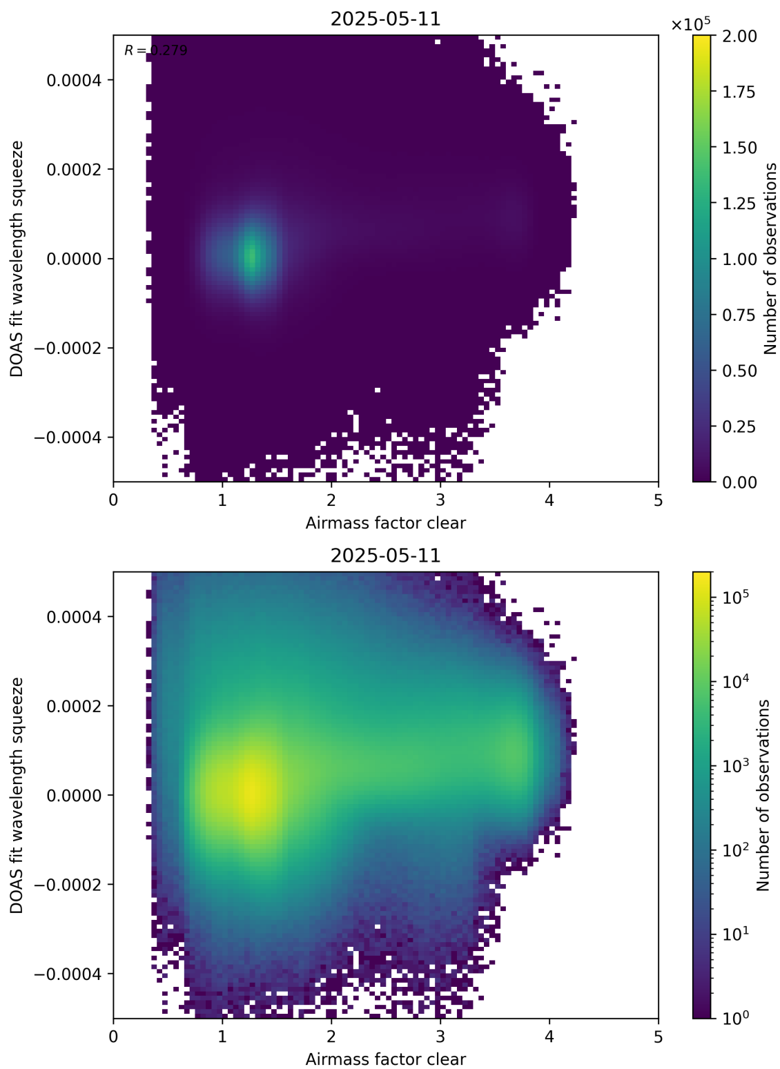
Figure 73: Scatter density plot of “Airmass factor clear” against “DOAS fit wavelength squeeze” for 2025-05-10 to 2025-05-12.
