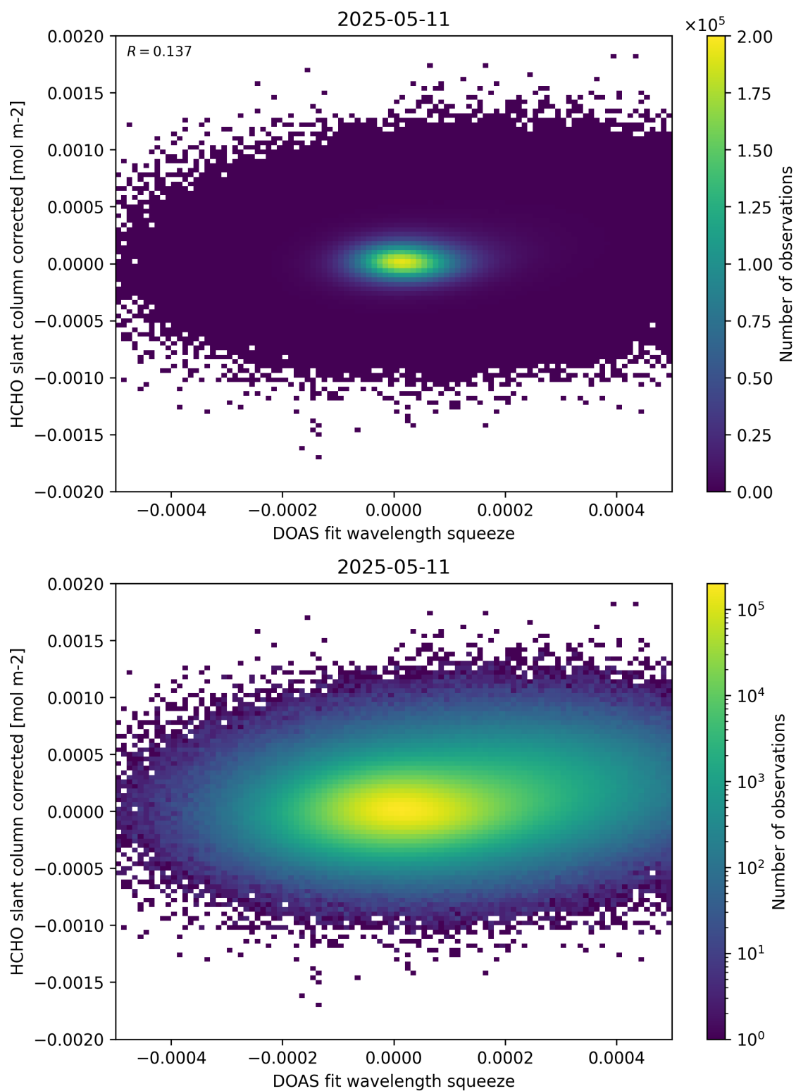
Figure 69: Scatter density plot of “DOAS fit wavelength squeeze” against “HCHO slant column corrected” for 2025-05-10 to 2025-05-12.
