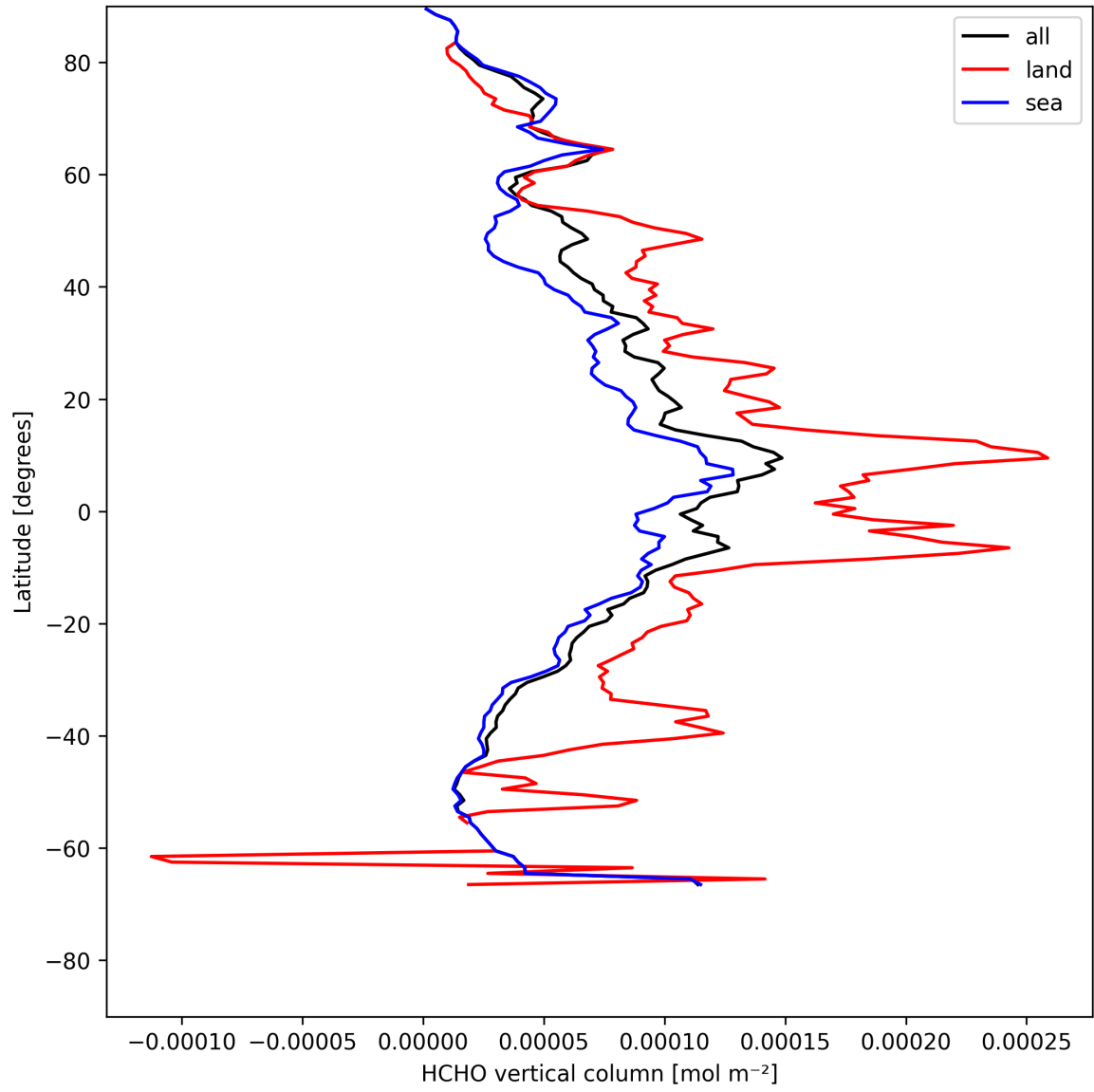
Figure 21: Zonal average of “HCHO vertical column” for 2025-05-10 to 2025-05-12.
