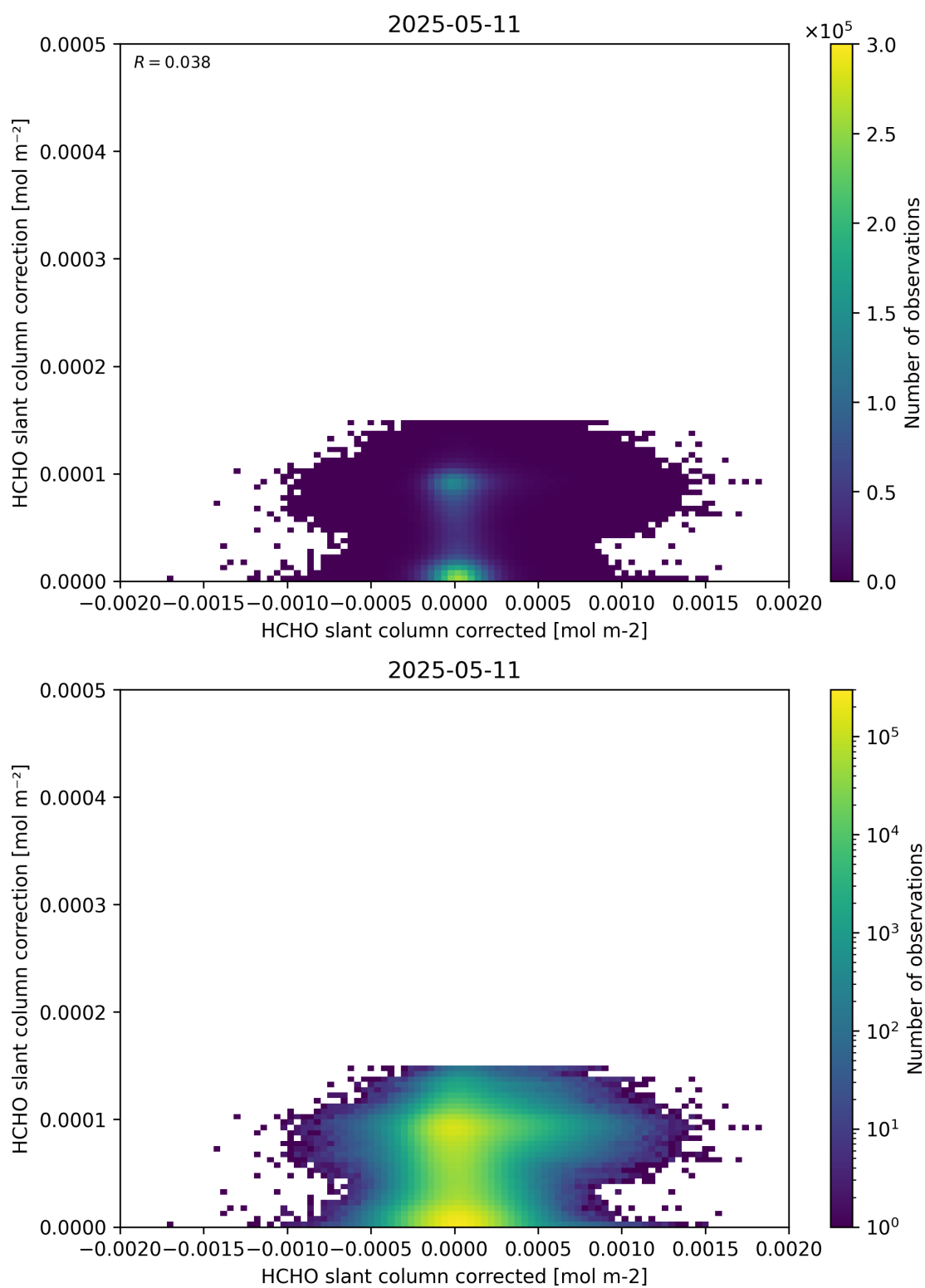
Figure 77: Scatter density plot of “HCHO slant column corrected” against “HCHO slant column correction” for 2025-05-10 to 2025-05-12.
