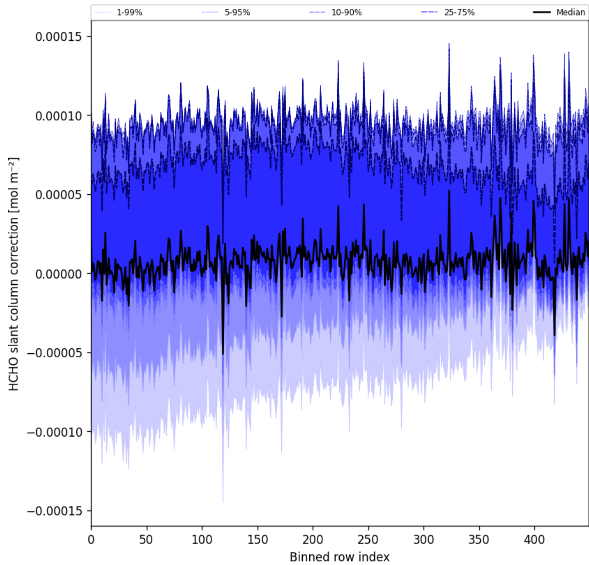
Figure 61: Along track statistics of “HCHO slant column correction” for 2025-05-10 to 2025-05-12
