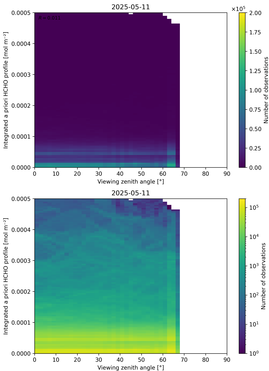
Figure 195: Scatter density plot of “Viewing zenith angle” against “Integrated a priori HCHO profile” for 2025-05-10 to 2025-05-12.
