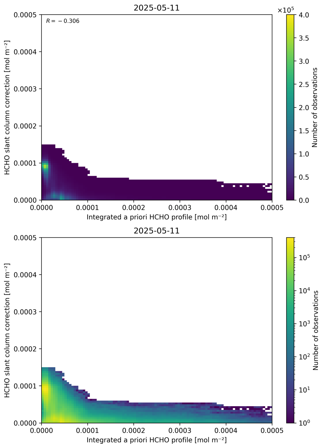
Figure 152: Scatter density plot of “Integrated a priori HCHO profile” against “HCHO slant column correction” for 2025-05-10 to 2025-05-12.
