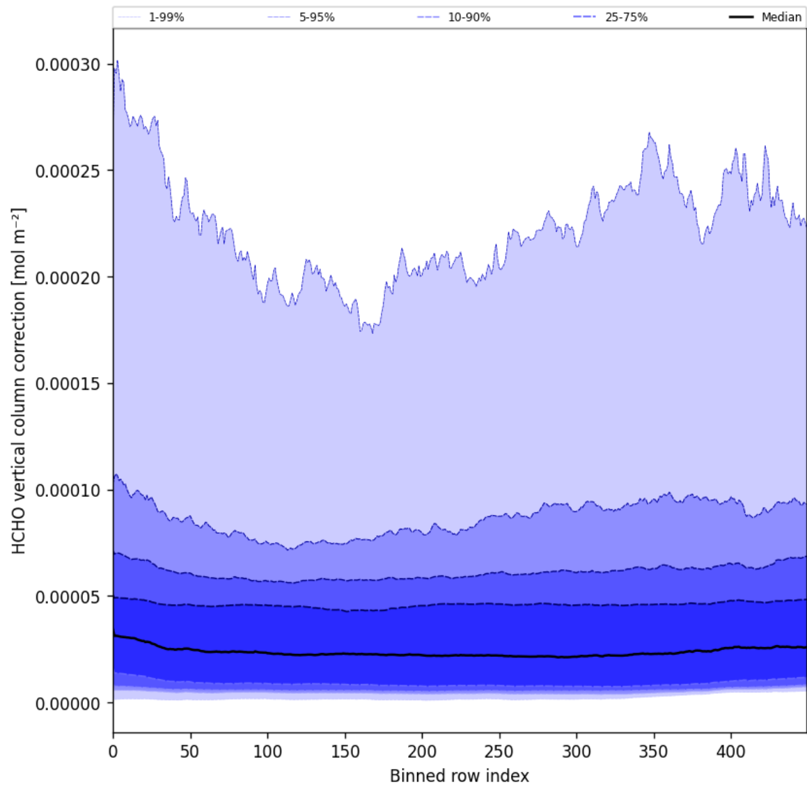
Figure 51: Along track statistics of “HCHO vertical column correction” for 2025-05-10 to 2025-05-12
