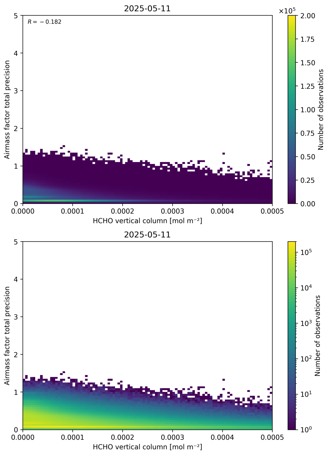
Figure 132: Scatter density plot of “HCHO vertical column” against “Airmass factor total precision” for 2025-05-10 to 2025-05-12.
