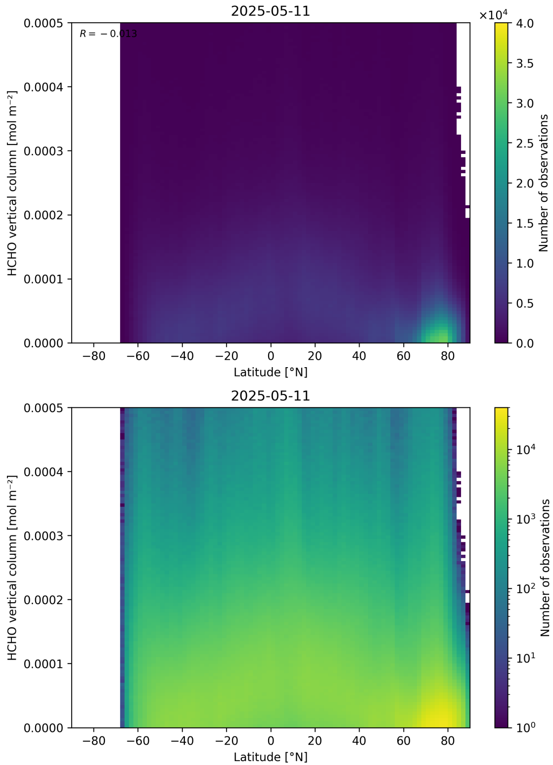
Figure 163: Scatter density plot of “Latitude” against “HCHO vertical column” for 2025-05-10 to 2025-05-12.
