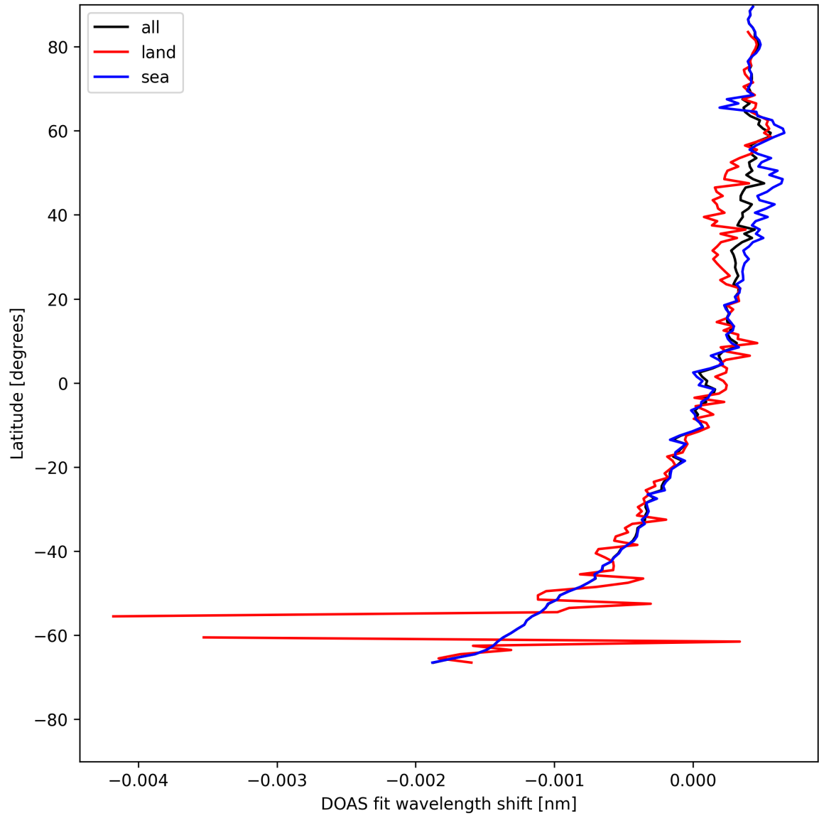
Figure 30: Zonal average of “DOAS fit wavelength shift” for 2025-05-10 to 2025-05-12.
