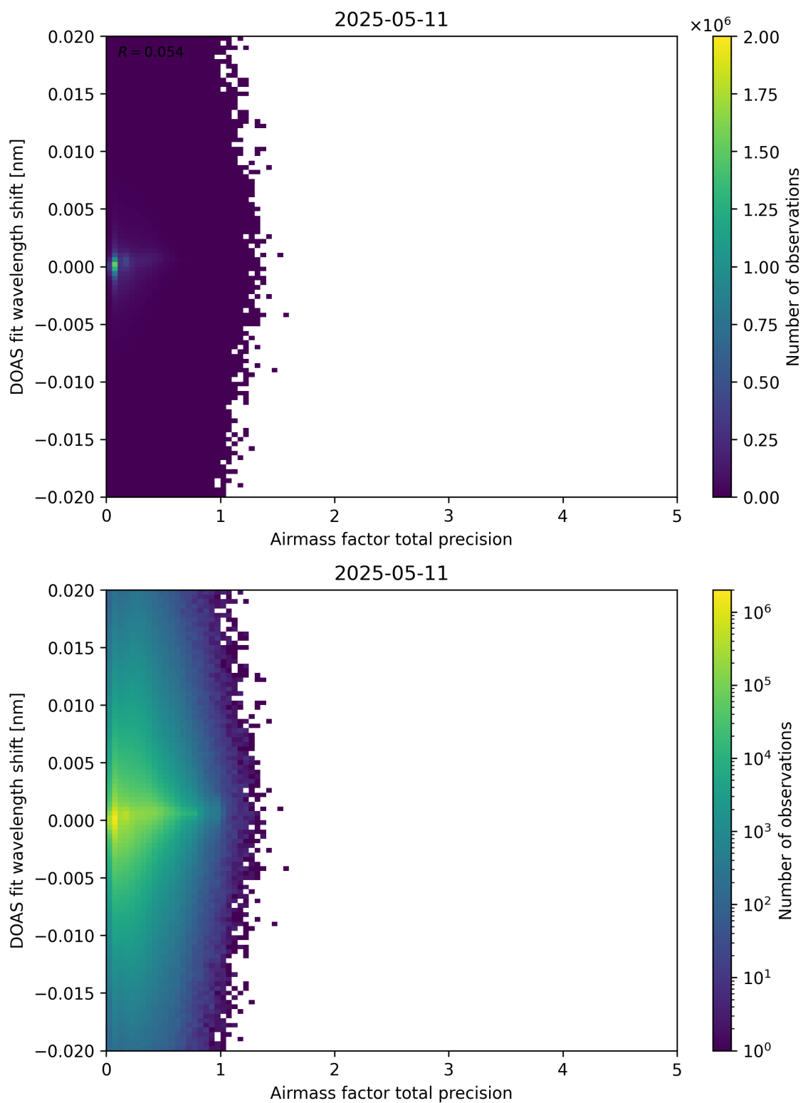
Figure 106: Scatter density plot of “Airmass factor total precision” against “DOAS fit wavelength shift” for 2025-05-10 to 2025-05-12.
