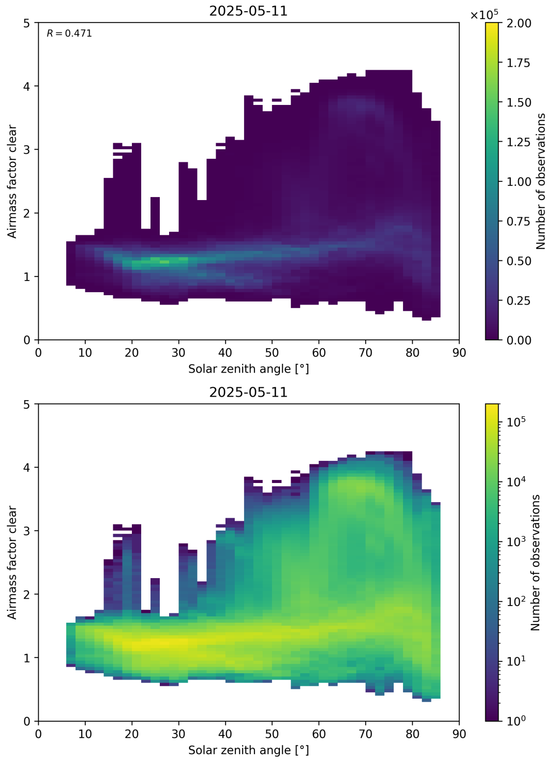
Figure 170: Scatter density plot of “Solar zenith angle” against “Airmass factor clear” for 2025-05-10 to 2025-05-12.
