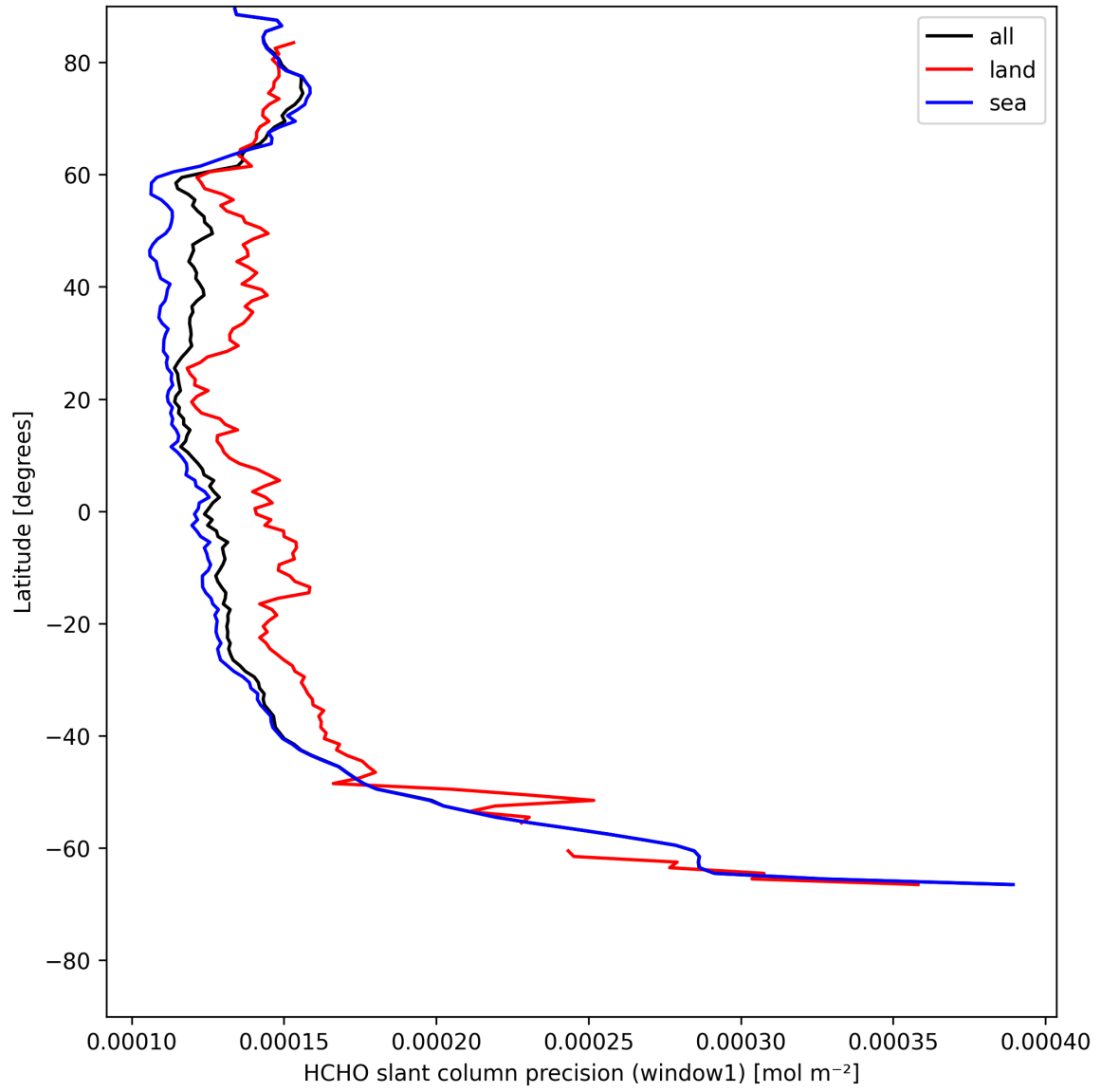
Figure 25: Zonal average of “HCHO slant column precision (window1)” for 2025-05-10 to 2025-05-12.
