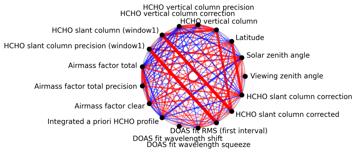
Figure 1: Map of correlation graph for 2025-05-10 to 2025-05-12.
