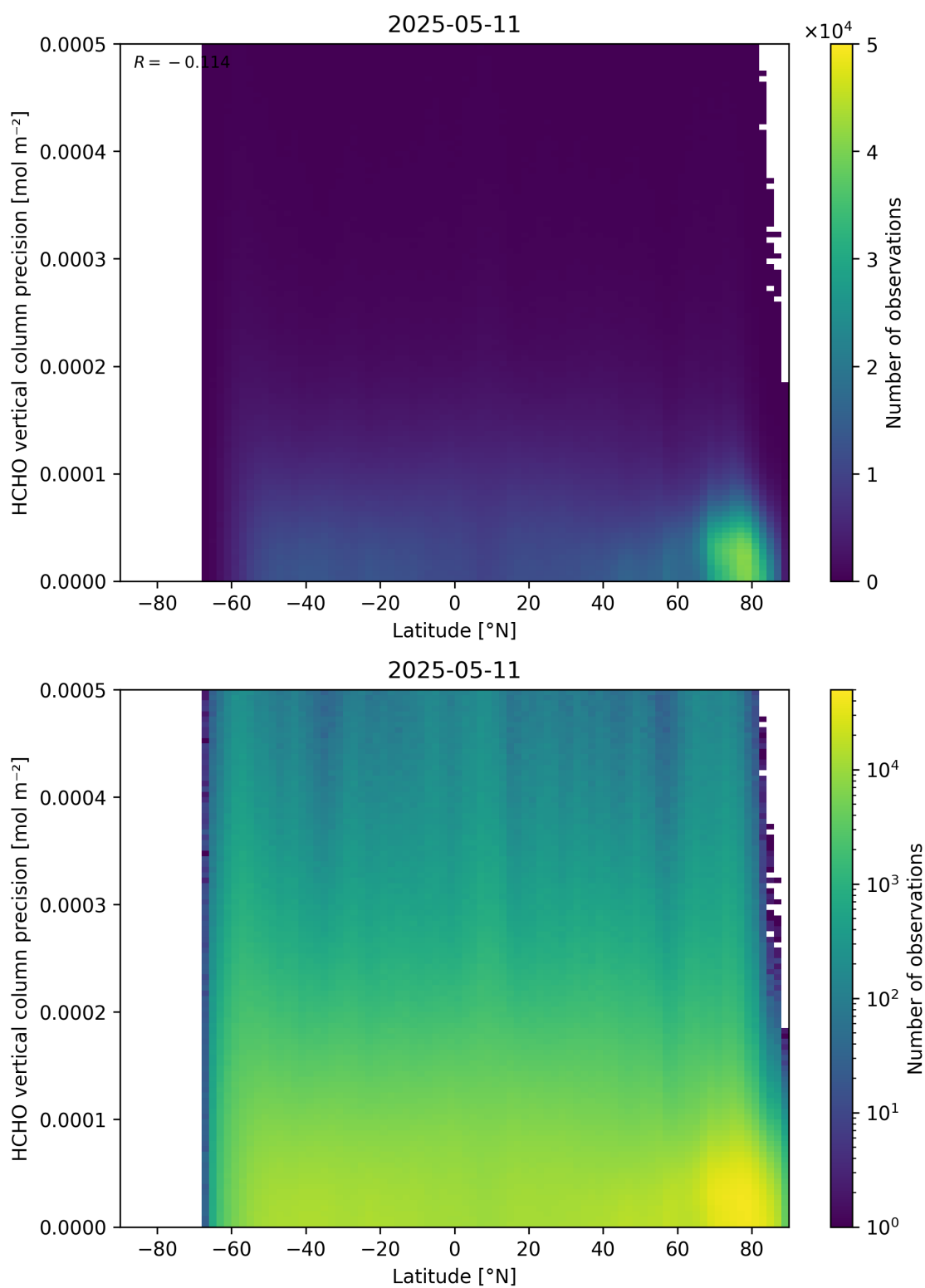
Figure 165: Scatter density plot of “Latitude” against “HCHO vertical column precision” for 2025-05-10 to 2025-05-12.
