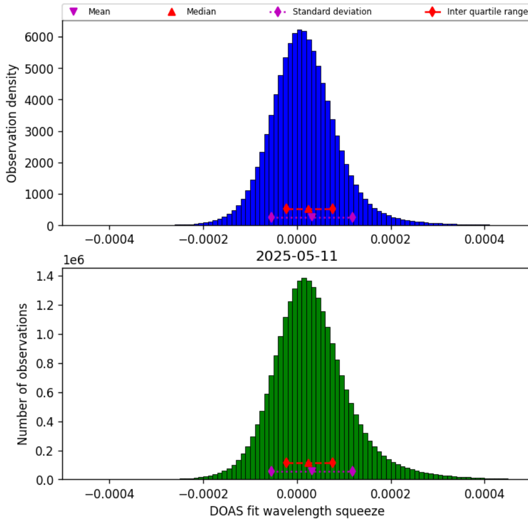
Figure 45: Histogram of “DOAS fit wavelength squeeze” for 2025-05-10 to 2025-05-12
