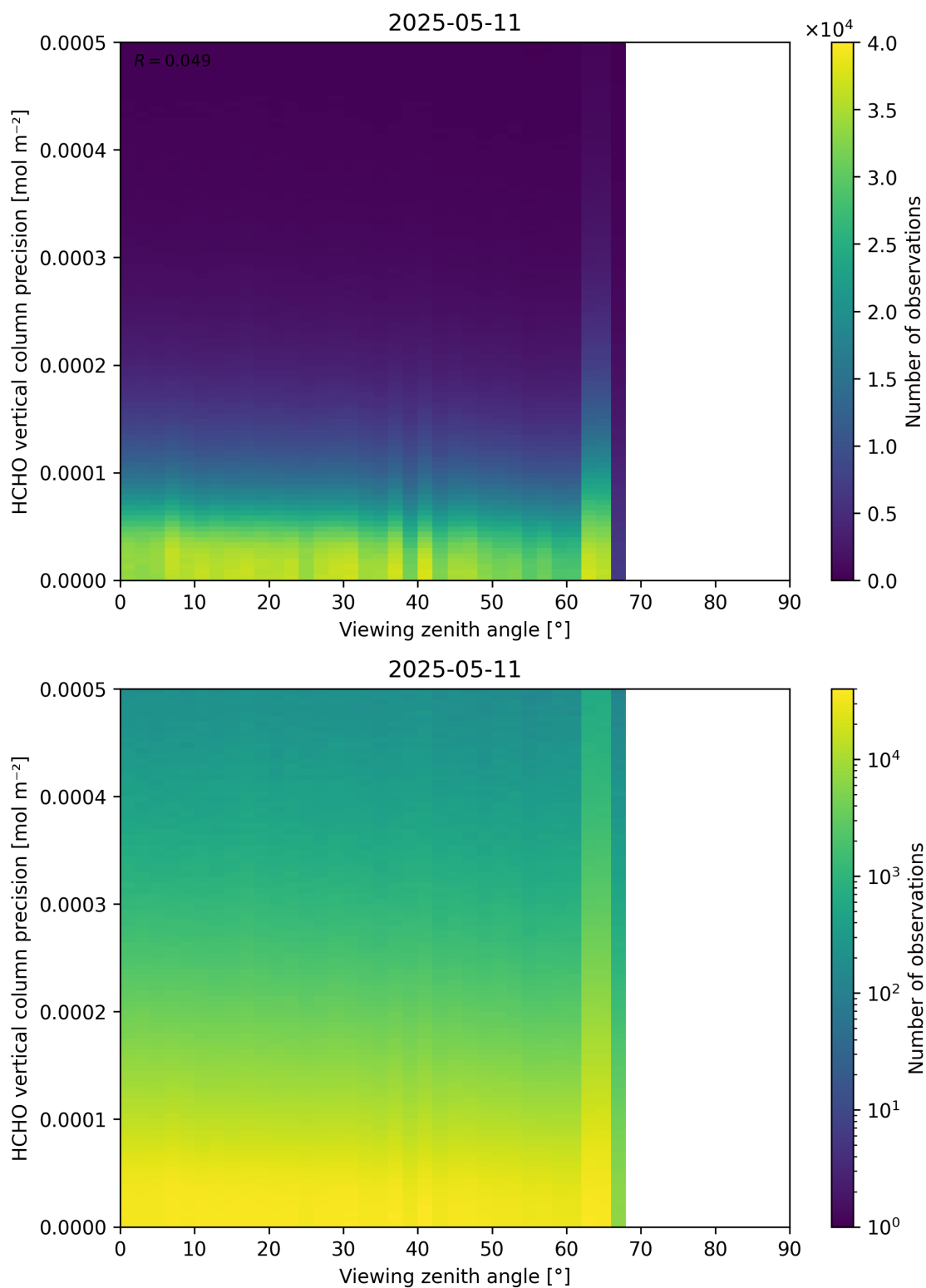
Figure 194: Scatter density plot of “Viewing zenith angle” against “HCHO vertical column precision” for 2025-05-10 to 2025-05-12.
