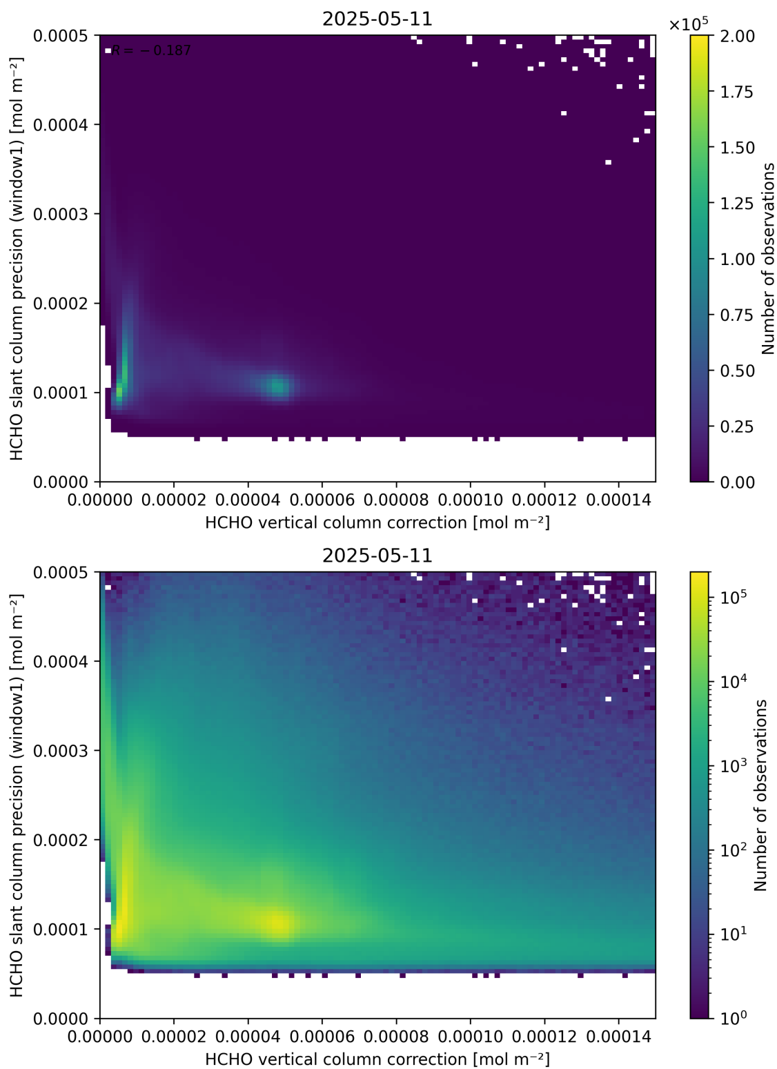
Figure 119: Scatter density plot of “HCHO vertical column correction” against “HCHO slant column precision (window1)” for 2025-05-10 to 2025-05-12.
