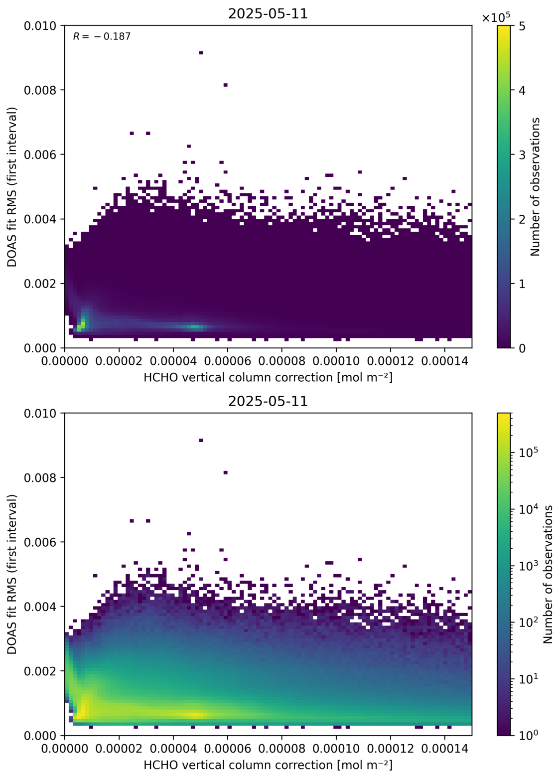
Figure 112: Scatter density plot of “HCHO vertical column correction” against “DOAS fit RMS (first interval)” for 2025-05-10 to 2025-05-12.
