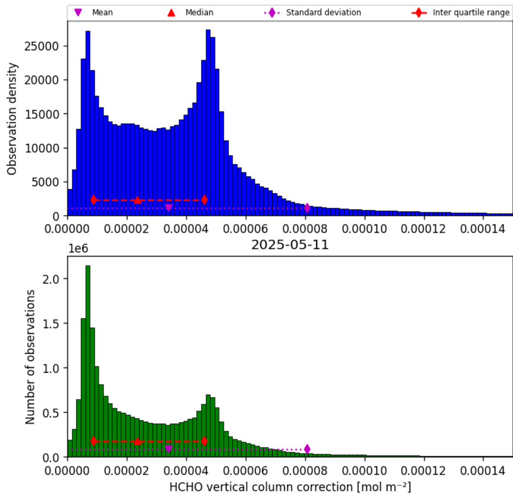
Figure 37: Histogram of “HCHO vertical column correction” for 2025-05-10 to 2025-05-12
