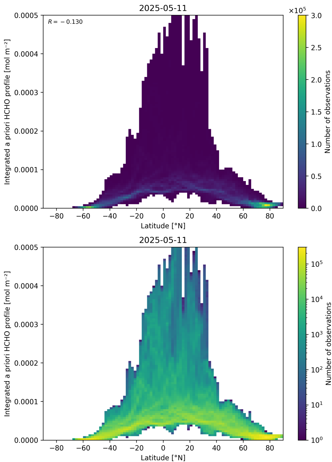
Figure 166: Scatter density plot of “Latitude” against “Integrated a priori HCHO profile” for 2025-05-10 to 2025-05-12.
