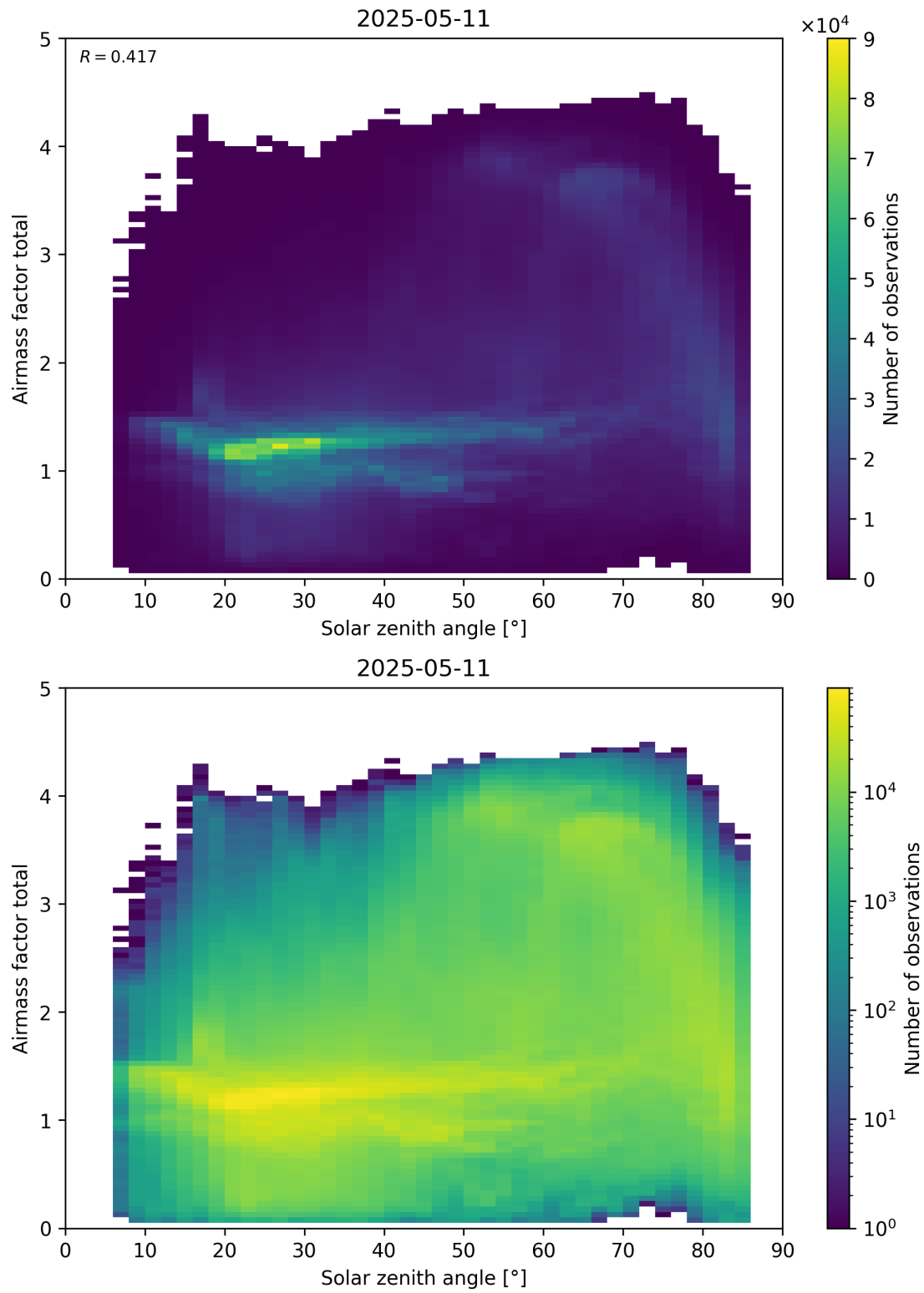
Figure 175: Scatter density plot of “Solar zenith angle” against “Airmass factor total” for 2025-05-10 to 2025-05-12.
