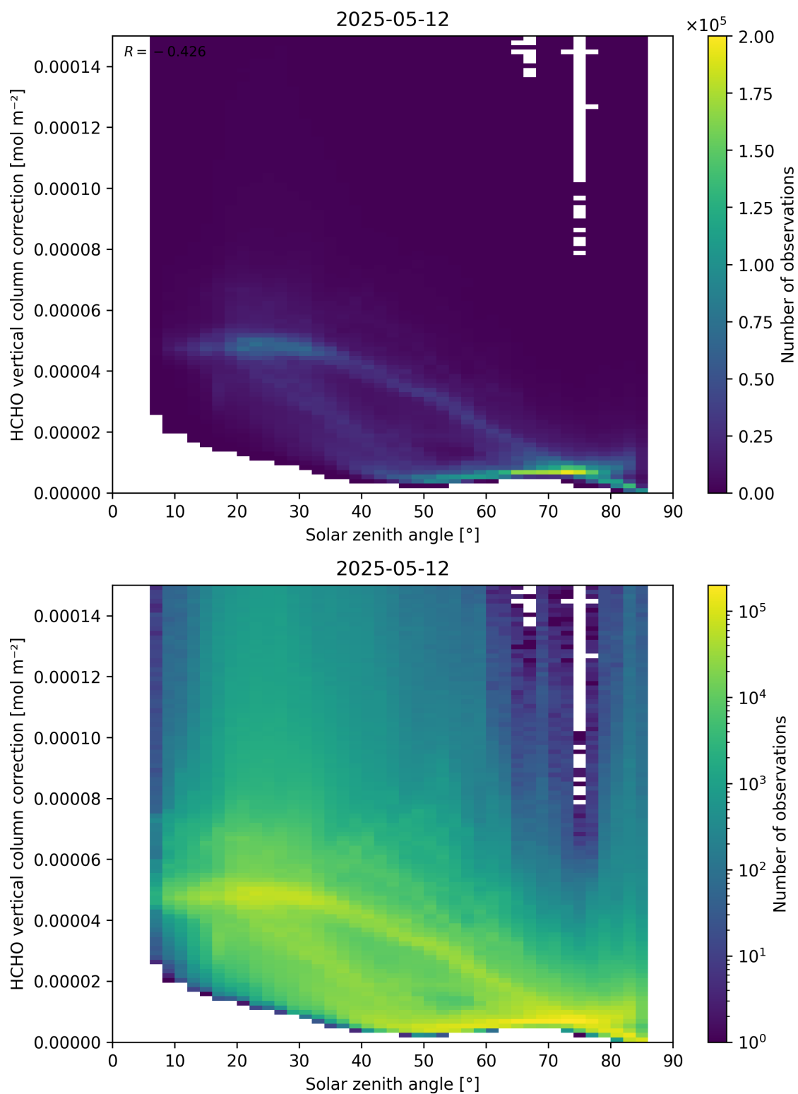
Figure 178: Scatter density plot of “Solar zenith angle” against “HCHO vertical column correction” for 2025-05-11 to 2025-05-13.
