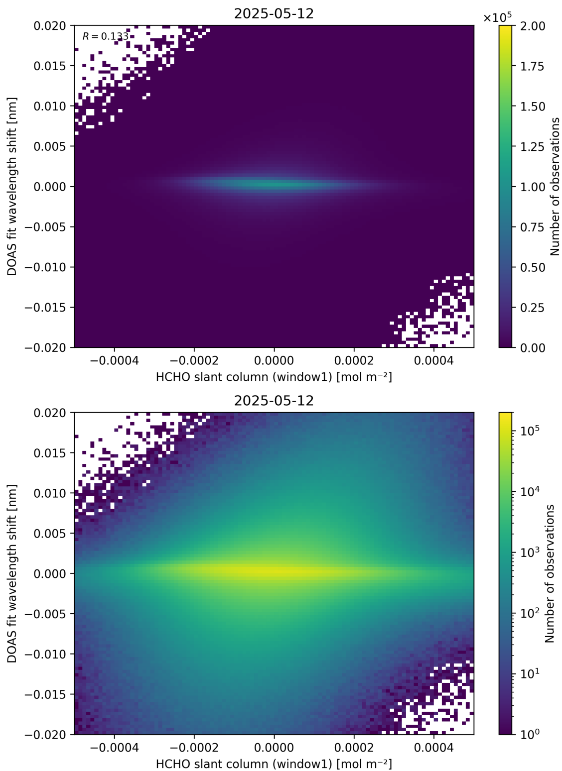
Figure 79: Scatter density plot of “HCHO slant column (window1)” against “DOAS fit wavelength shift” for 2025-05-11 to 2025-05-13.
