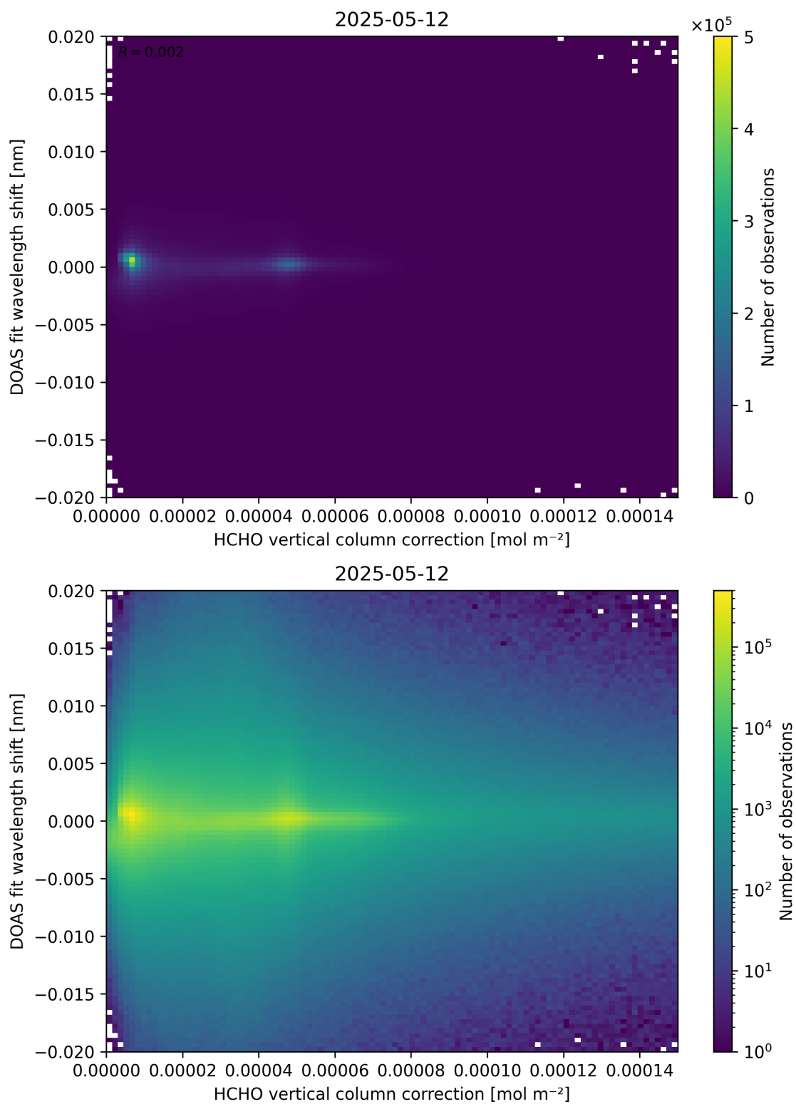
Figure 113: Scatter density plot of “HCHO vertical column correction” against “DOAS fit wavelength shift” for 2025-05-11 to 2025-05-13.
