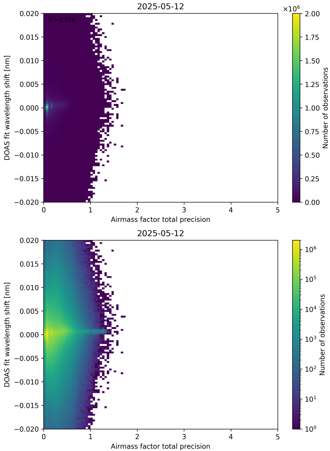
Figure 106: Scatter density plot of “Airmass factor total precision” against “DOAS fit wavelength shift” for 2025-05-11 to 2025-05-13.
