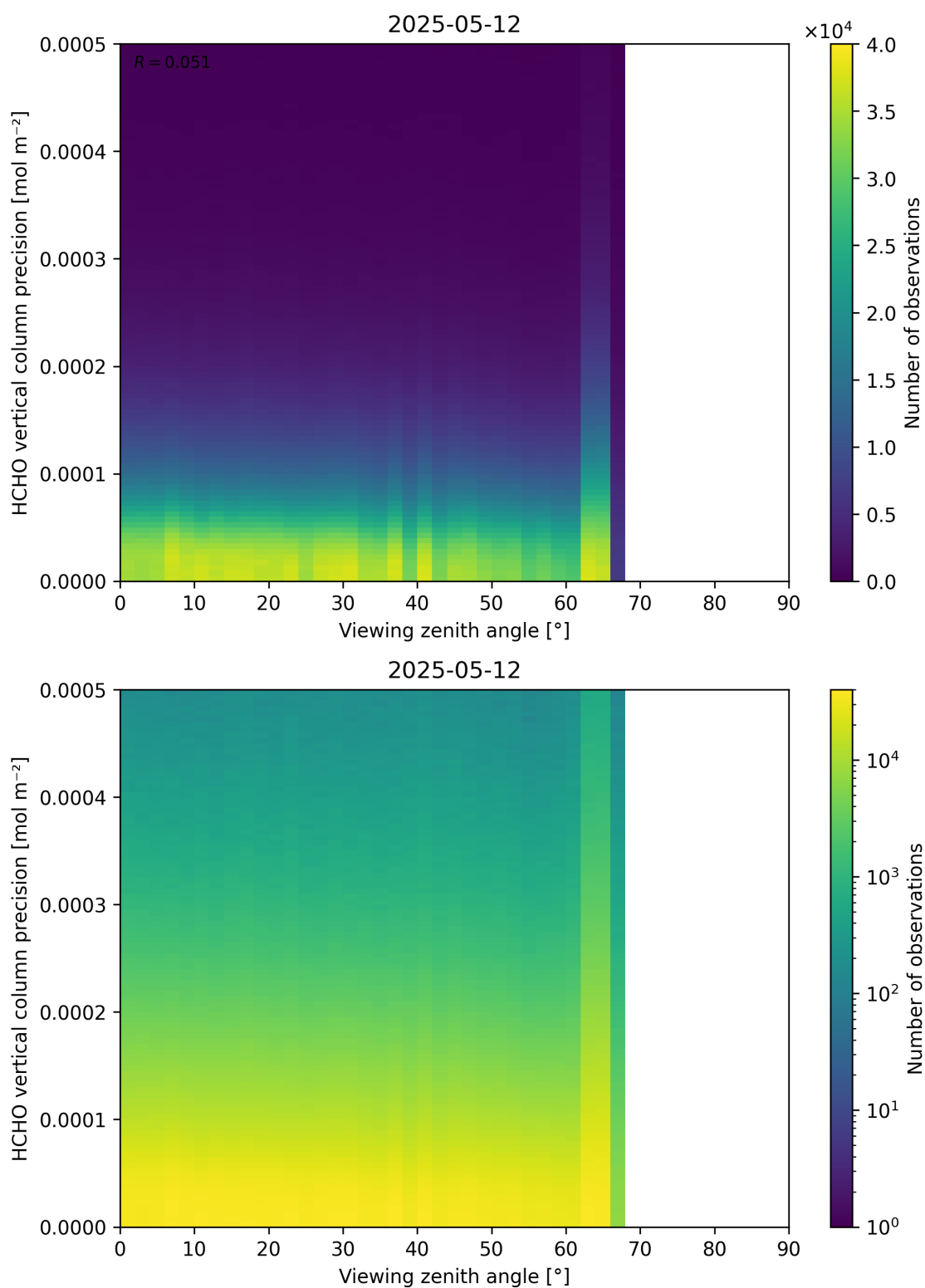
Figure 194: Scatter density plot of “Viewing zenith angle” against “HCHO vertical column precision” for 2025-05-11 to 2025-05-13.
