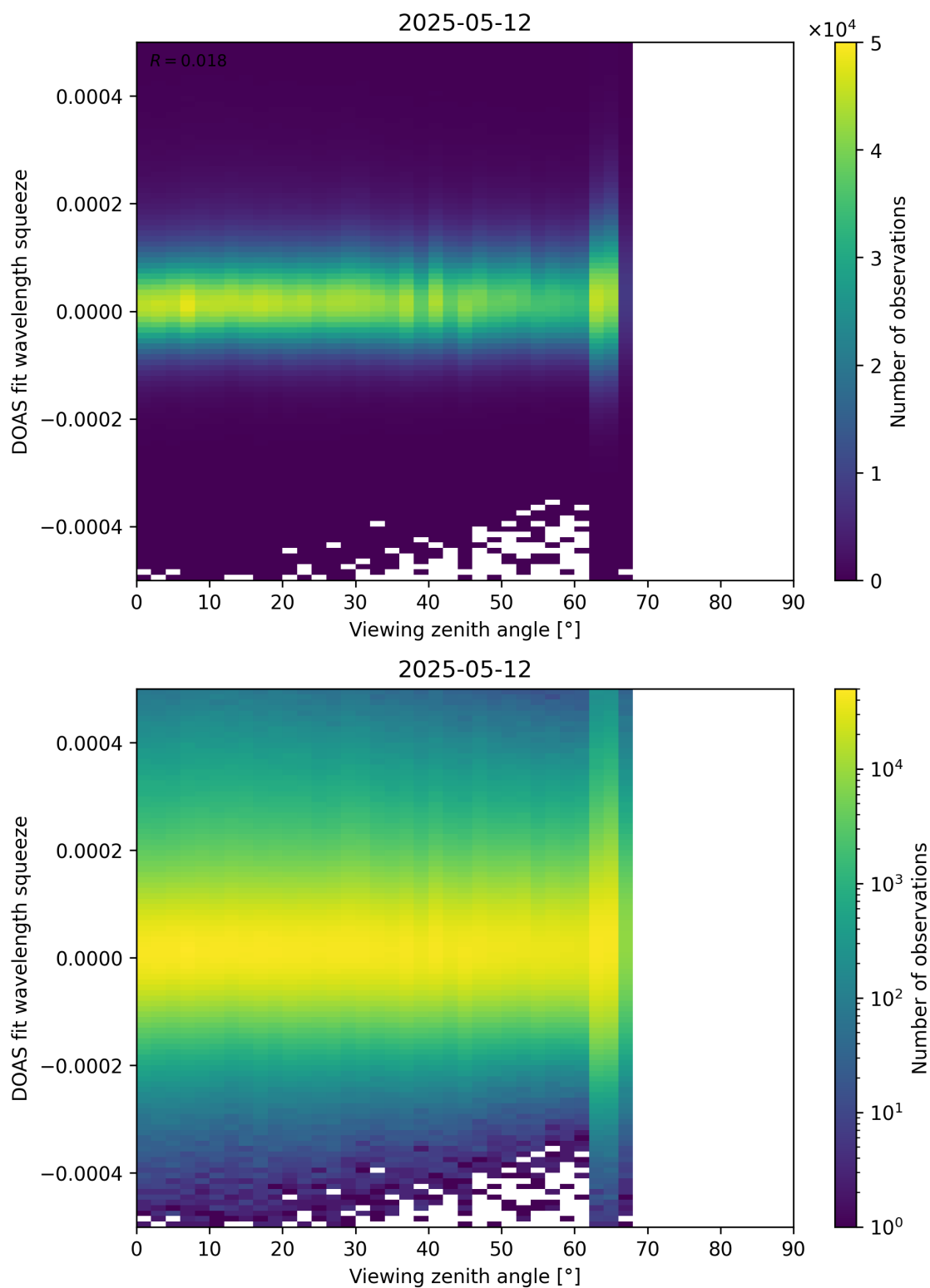
Figure 184: Scatter density plot of “Viewing zenith angle” against “DOAS fit wavelength squeeze” for 2025-05-11 to 2025-05-13.
