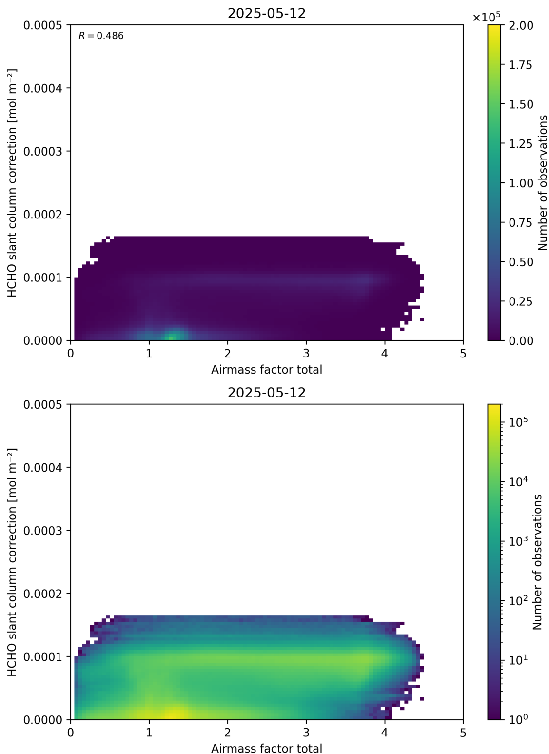
Figure 102: Scatter density plot of “Airmass factor total” against “HCHO slant column correction” for 2025-05-11 to 2025-05-13.
