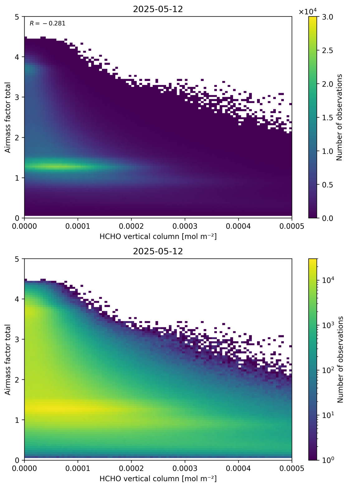
Figure 131: Scatter density plot of “HCHO vertical column” against “Airmass factor total” for 2025-05-11 to 2025-05-13.
