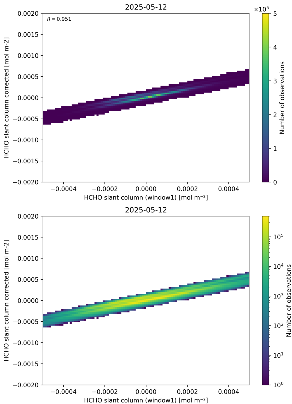
Figure 82: Scatter density plot of “HCHO slant column (window1)” against “HCHO slant column corrected” for 2025-05-11 to 2025-05-13.
