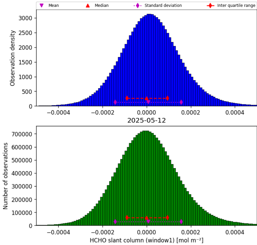
Figure 38: Histogram of “HCHO slant column (window1)” for 2025-05-11 to 2025-05-13
