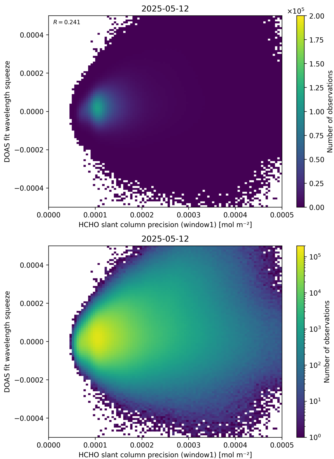
Figure 90: Scatter density plot of “HCHO slant column precision (window1)” against “DOAS fit wavelength squeeze” for 2025-05-11 to 2025-05-13.
