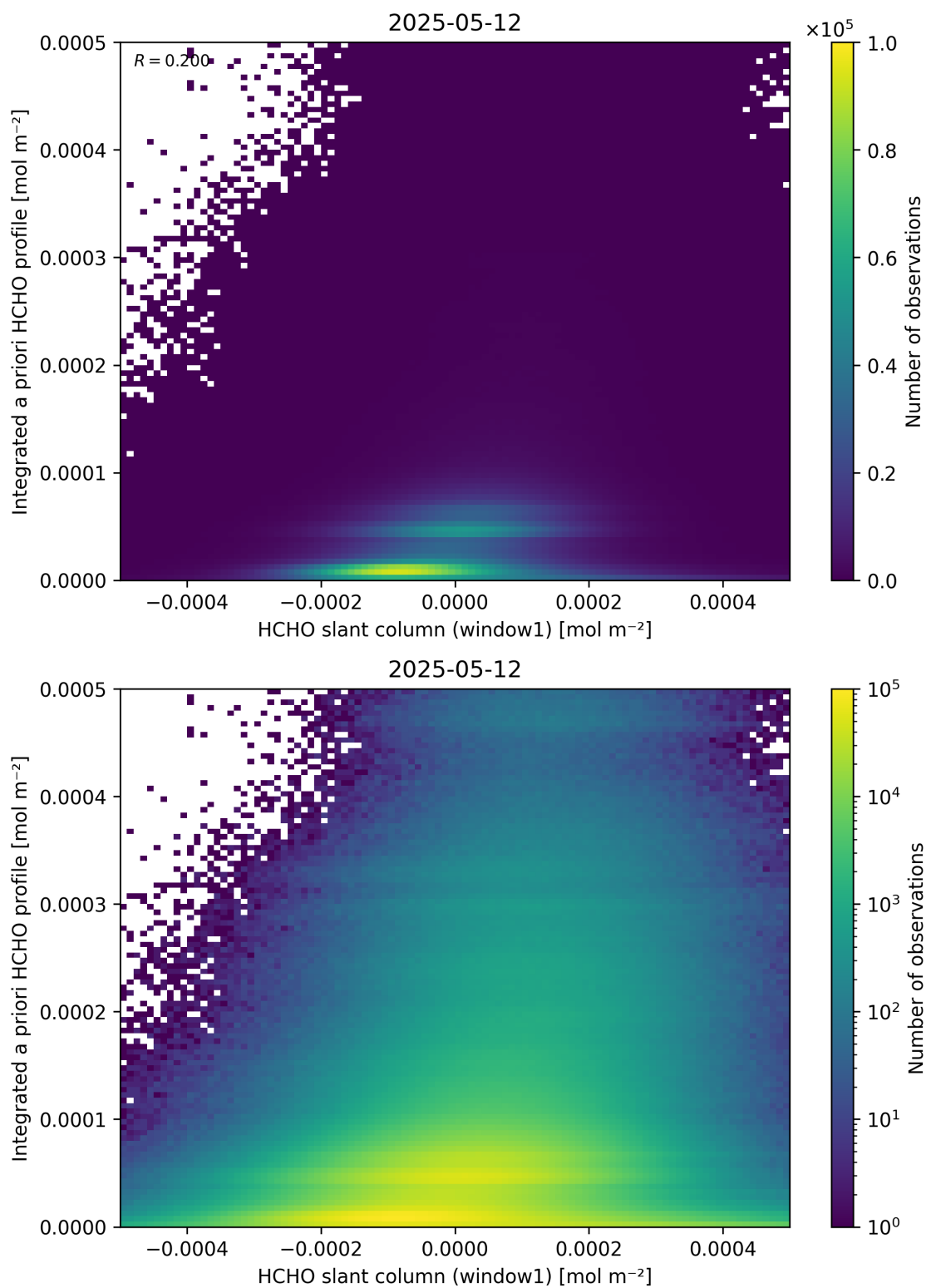
Figure 87: Scatter density plot of “HCHO slant column (window1)” against “Integrated a priori HCHO profile” for 2025-05-11 to 2025-05-13.
