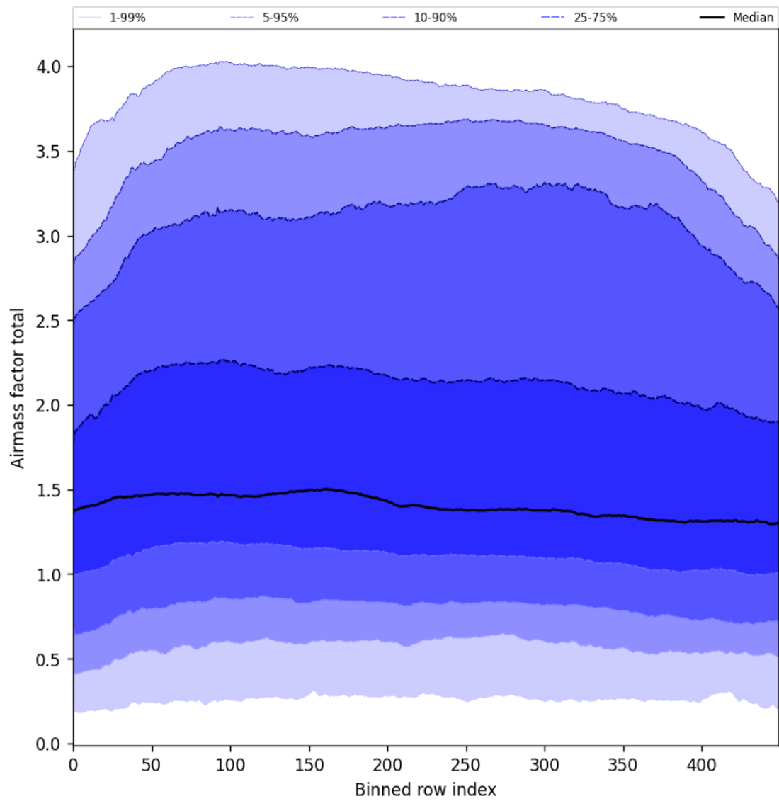
Figure 54: Along track statistics of “Airmass factor total” for 2025-05-11 to 2025-05-13
