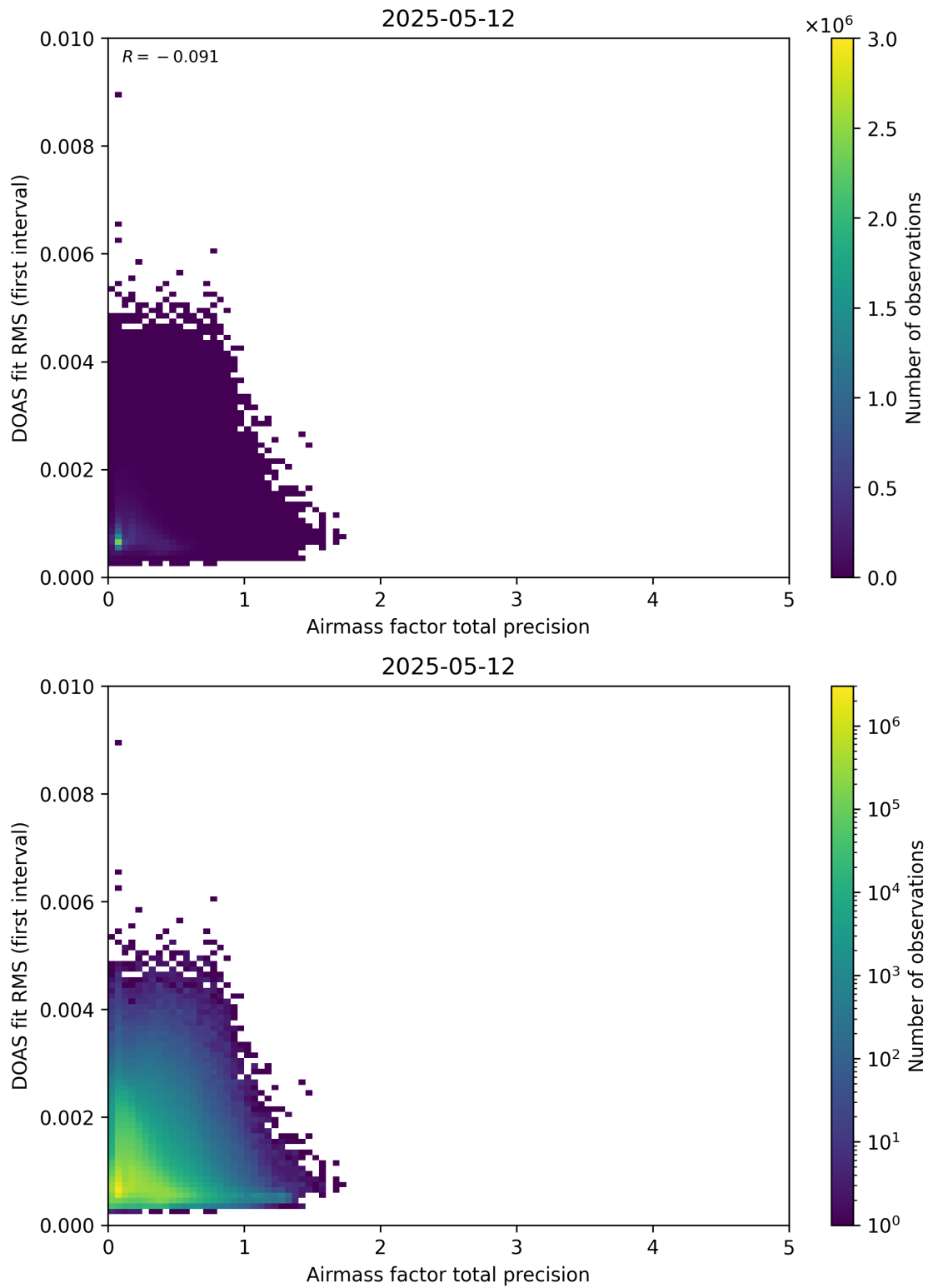
Figure 105: Scatter density plot of “Airmass factor total precision” against “DOAS fit RMS (first interval)” for 2025-05-11 to 2025-05-13.
