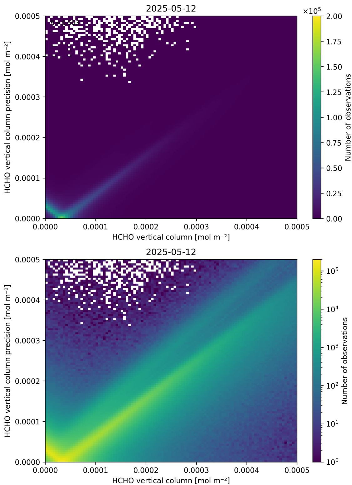
Figure 134: Scatter density plot of “HCHO vertical column” against “HCHO vertical column precision” for 2025-05-11 to 2025-05-13.
