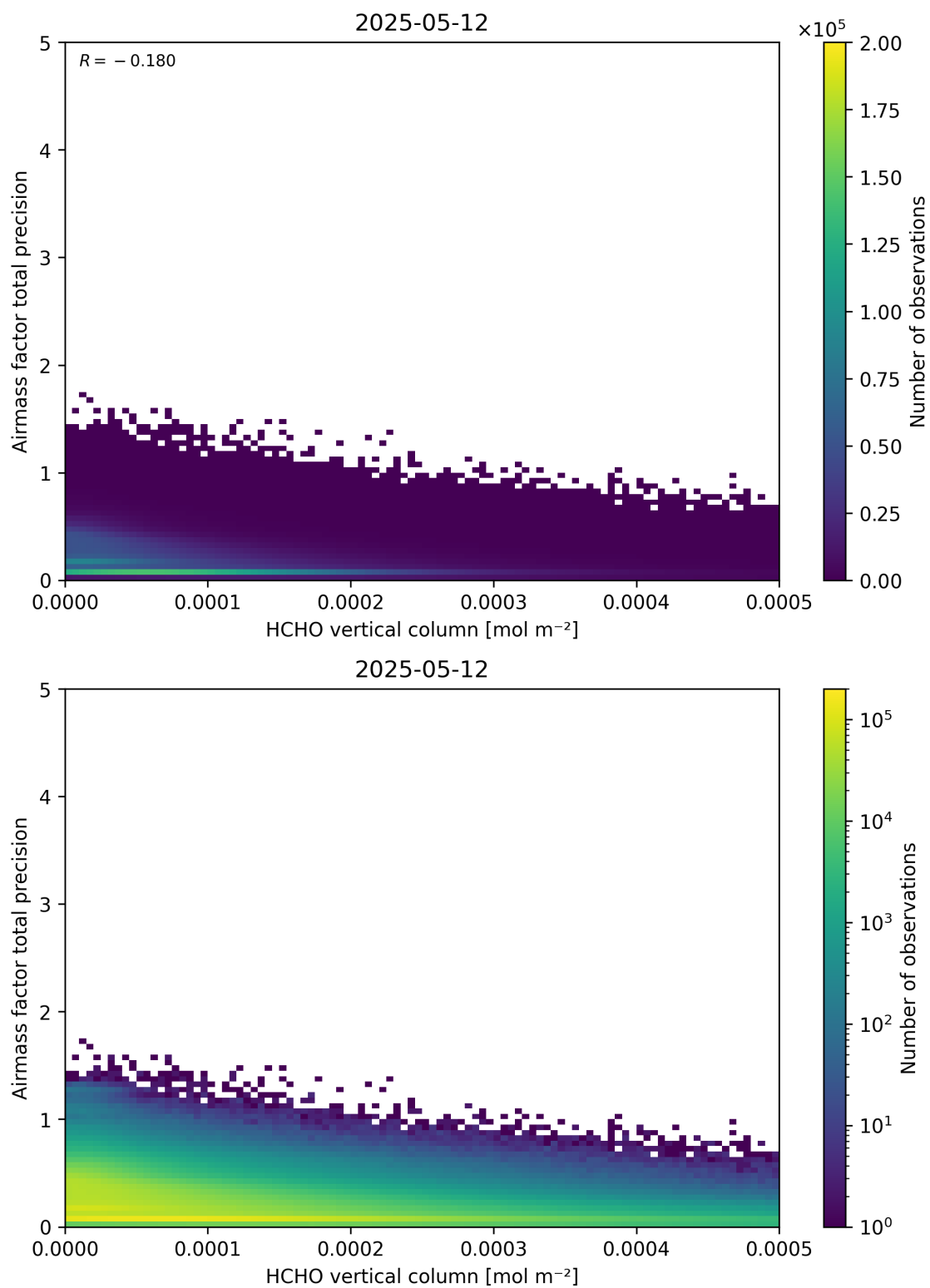
Figure 132: Scatter density plot of “HCHO vertical column” against “Airmass factor total precision” for 2025-05-11 to 2025-05-13.
