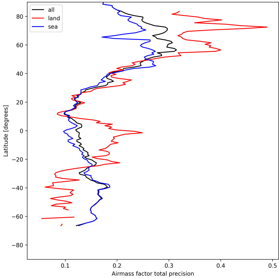
Figure 27: Zonal average of “Airmass factor total precision” for 2025-05-11 to 2025-05-13.
