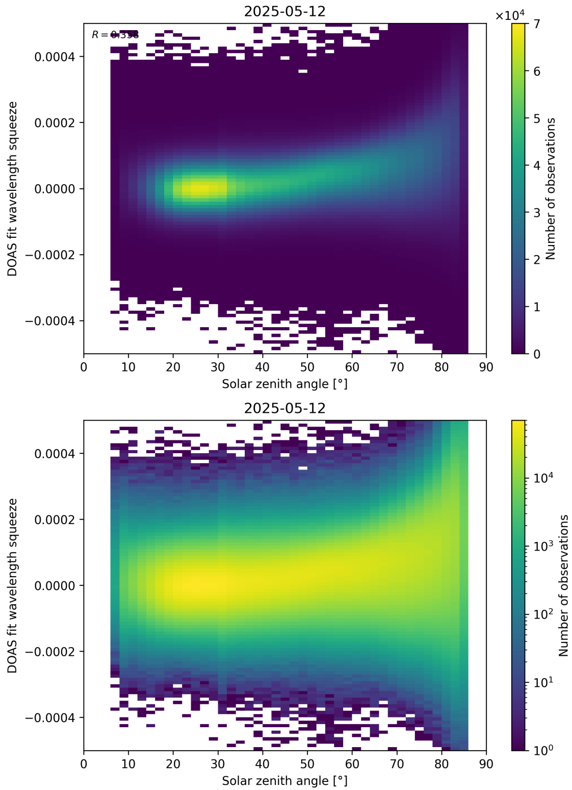
Figure 169: Scatter density plot of “Solar zenith angle” against “DOAS fit wavelength squeeze” for 2025-05-11 to 2025-05-13.
