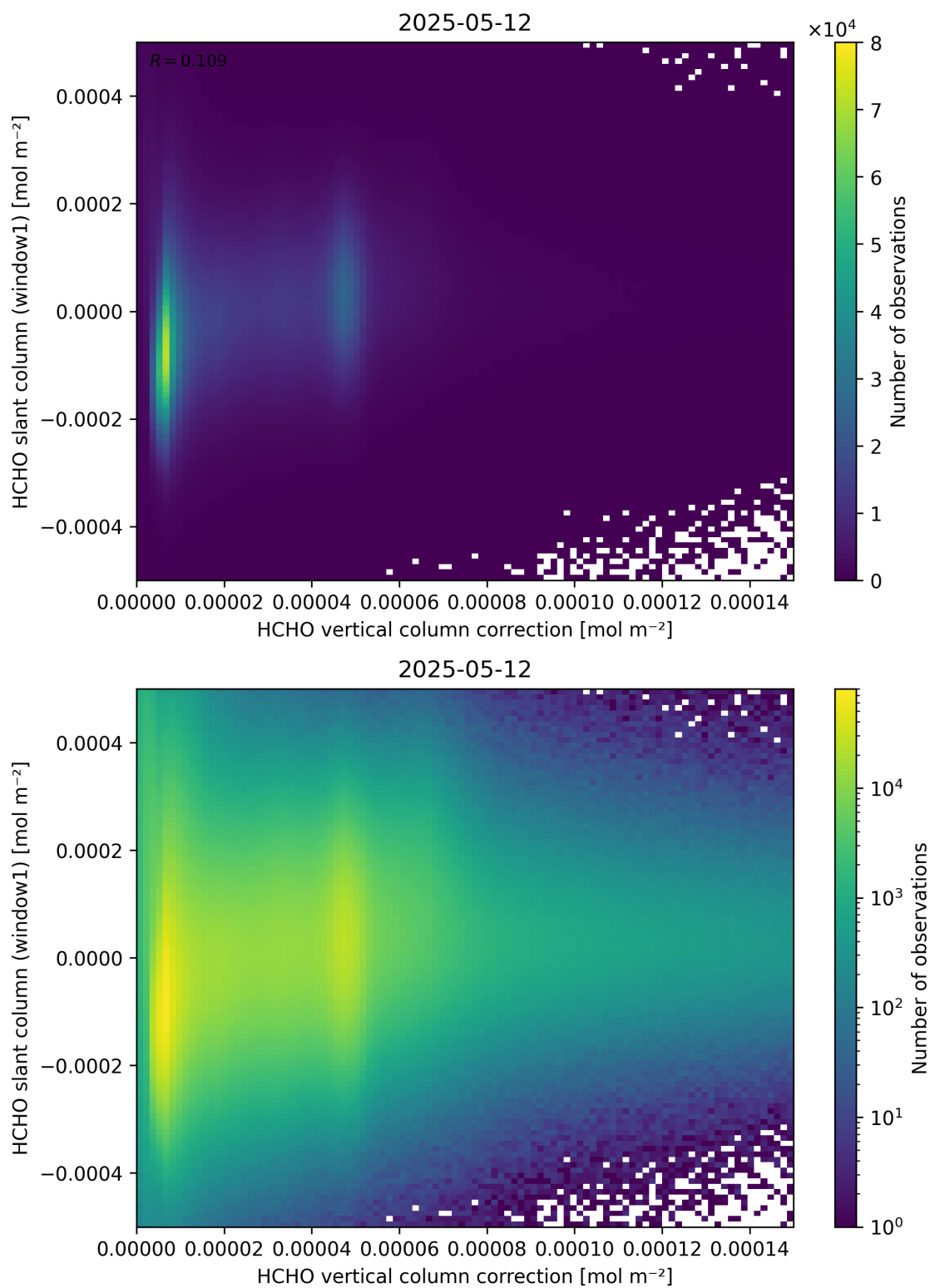
Figure 118: Scatter density plot of “HCHO vertical column correction” against “HCHO slant column (window1)” for 2025-05-11 to 2025-05-13.
