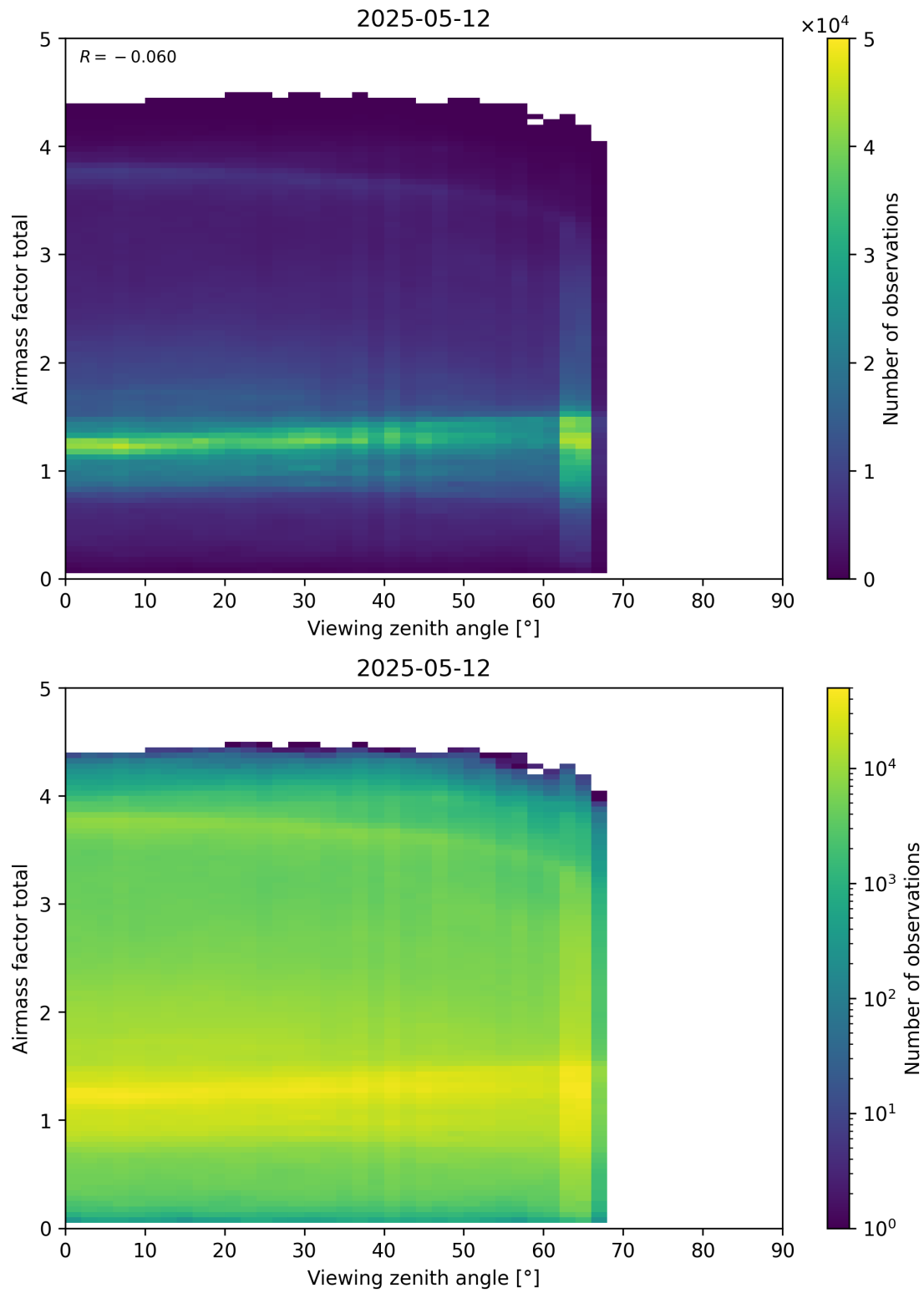
Figure 190: Scatter density plot of “Viewing zenith angle” against “Airmass factor total” for 2025-05-11 to 2025-05-13.
