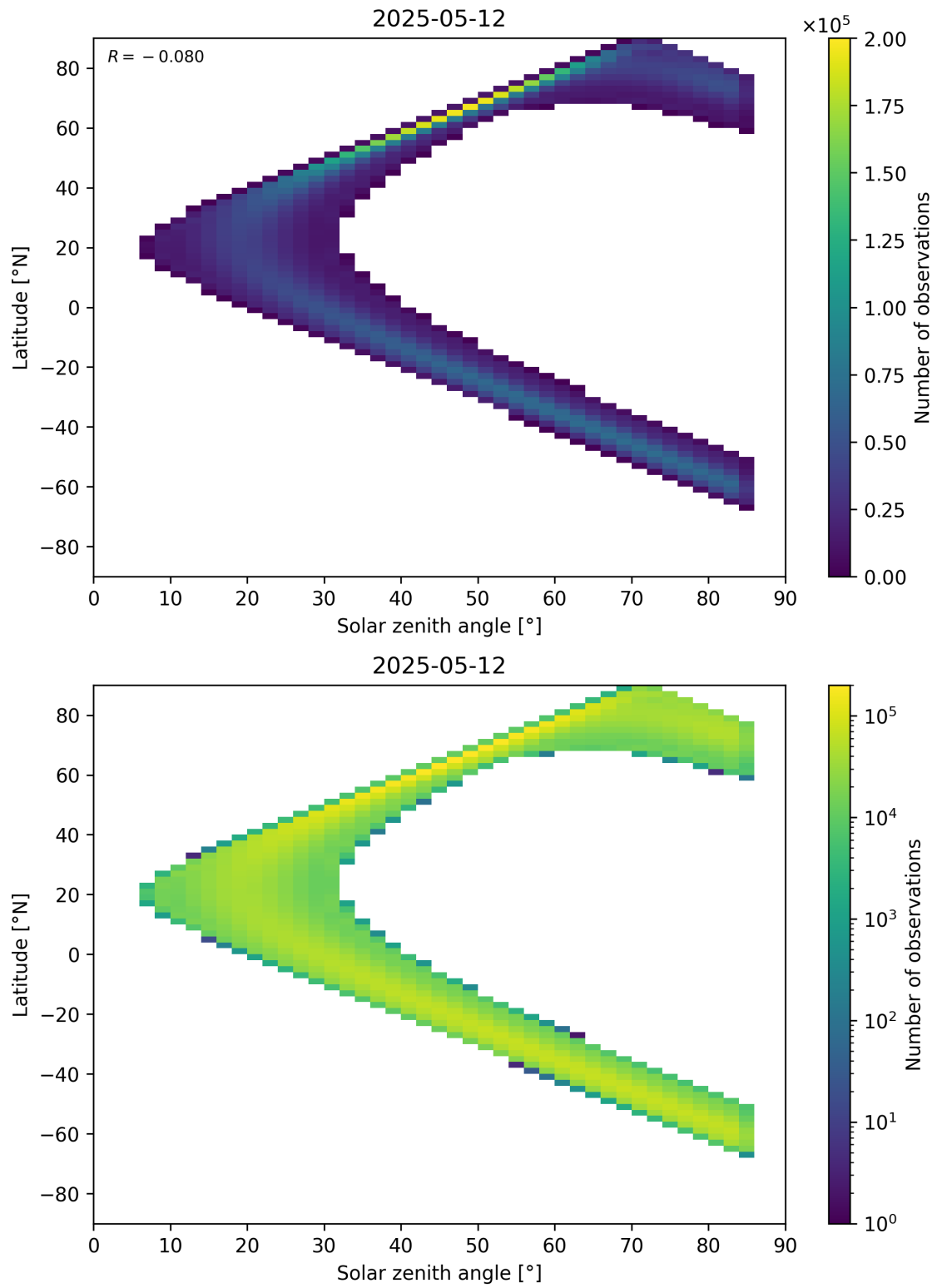
Figure 181: Scatter density plot of “Solar zenith angle” against “Latitude” for 2025-05-11 to 2025-05-13.
