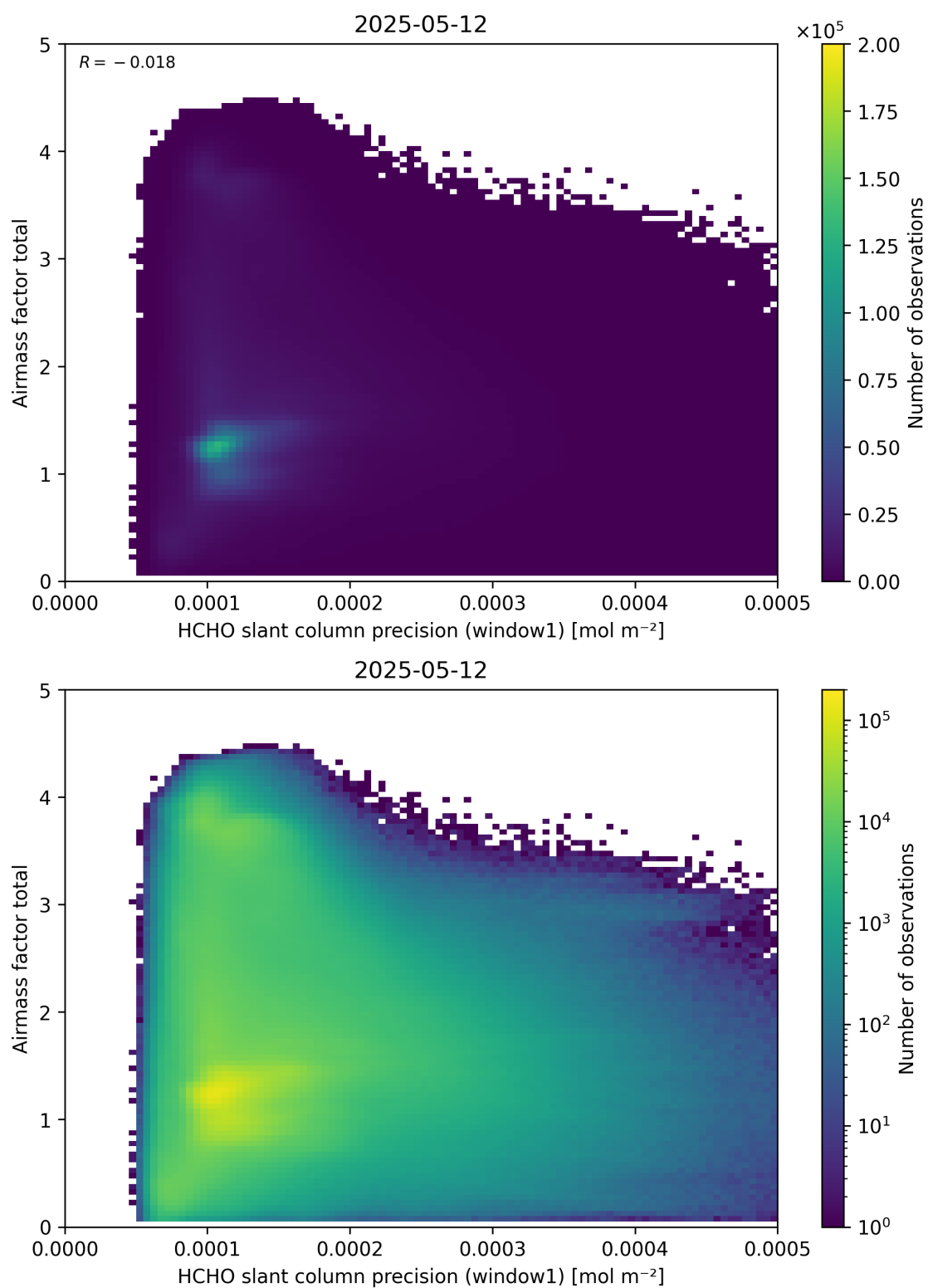
Figure 94: Scatter density plot of “HCHO slant column precision (window1)” against “Airmass factor total” for 2025-05-11 to 2025-05-13.
