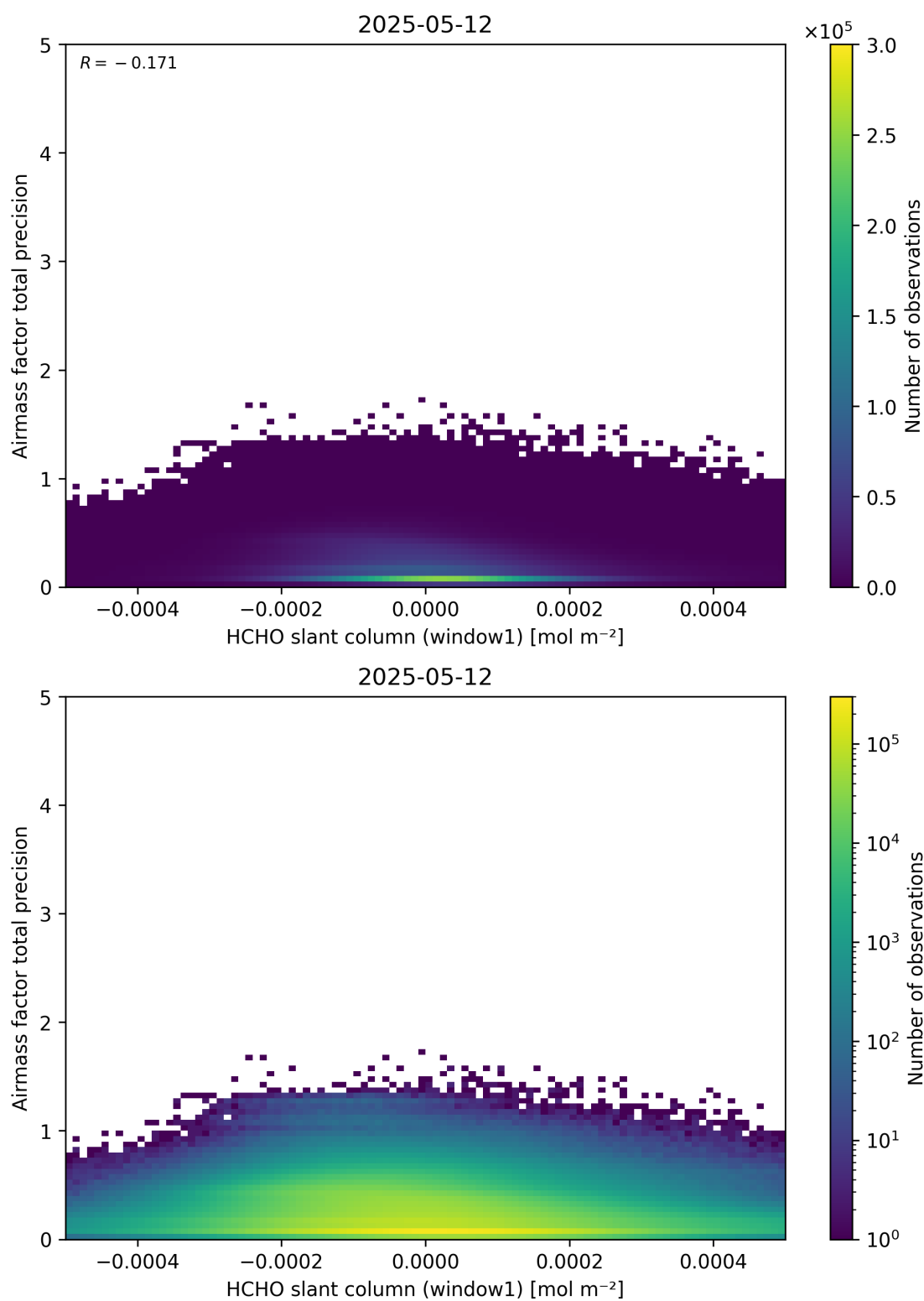
Figure 86: Scatter density plot of “HCHO slant column (window1)” against “Airmass factor total precision” for 2025-05-11 to 2025-05-13.
