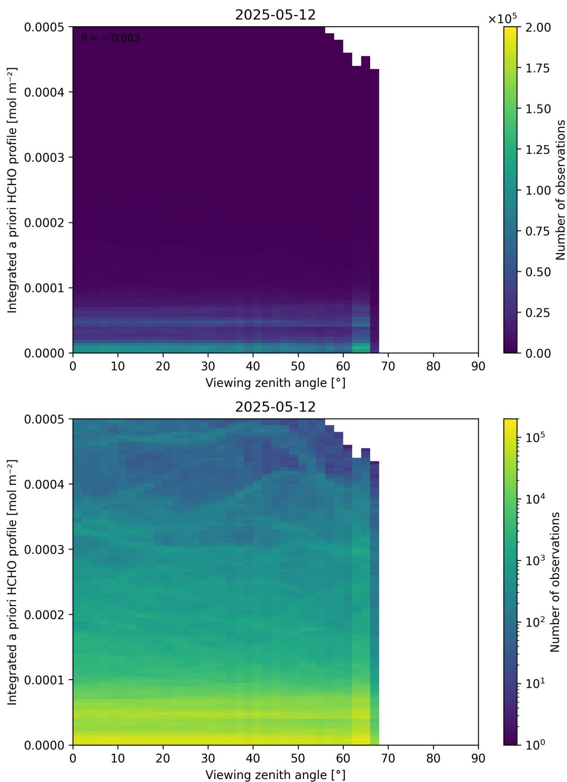
Figure 195: Scatter density plot of “Viewing zenith angle” against “Integrated a priori HCHO profile” for 2025-05-11 to 2025-05-13.
