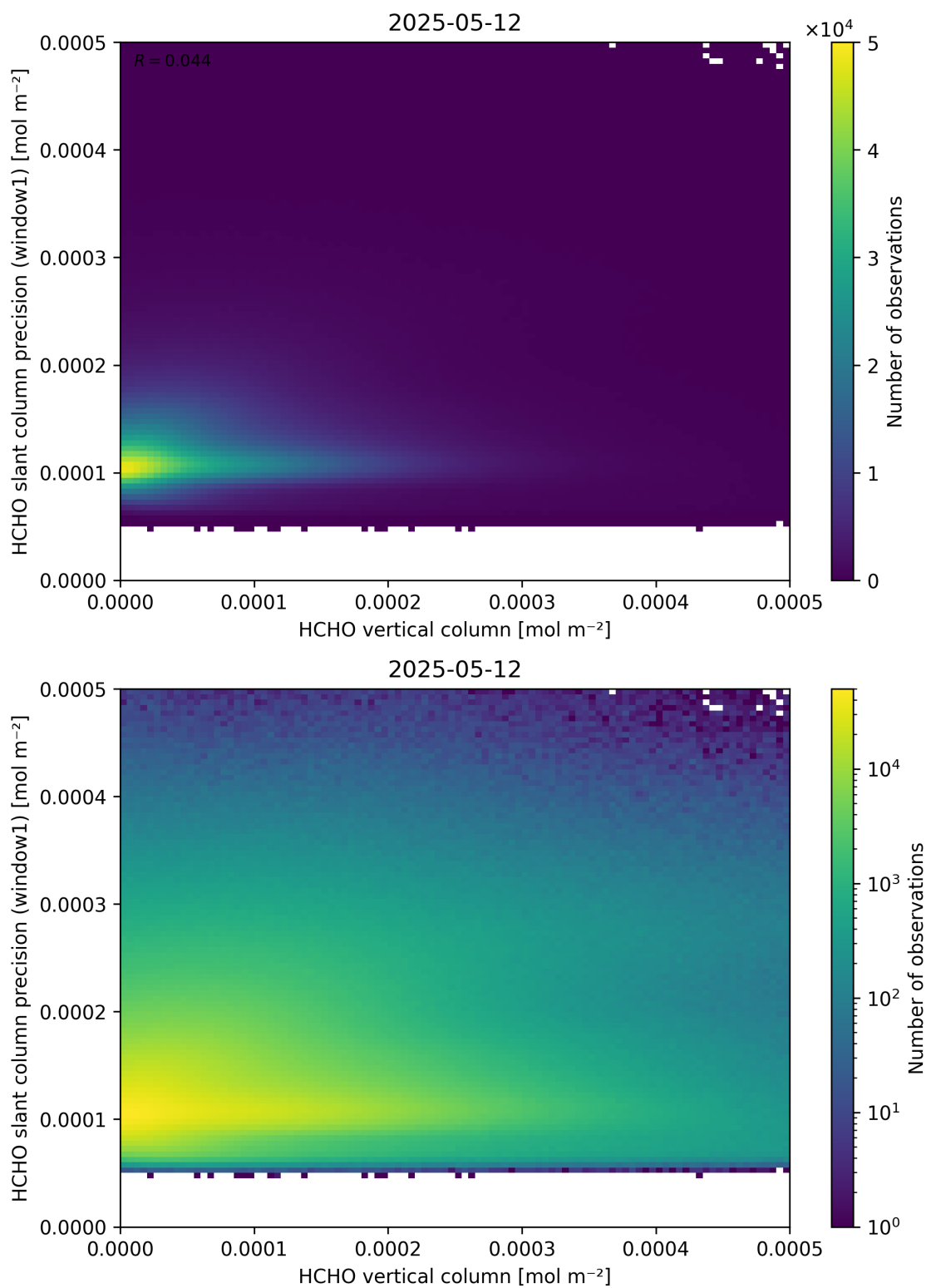
Figure 130: Scatter density plot of “HCHO vertical column” against “HCHO slant column precision (window1)” for 2025-05-11 to 2025-05-13.
