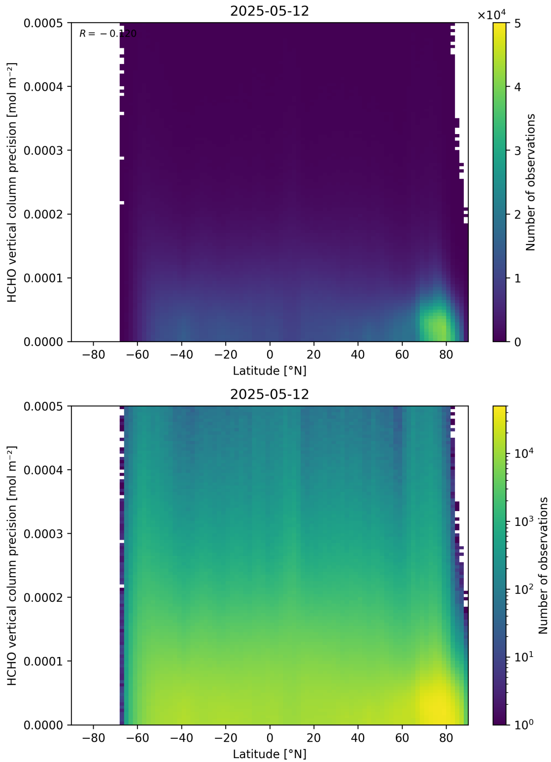
Figure 165: Scatter density plot of “Latitude” against “HCHO vertical column precision” for 2025-05-11 to 2025-05-13.
