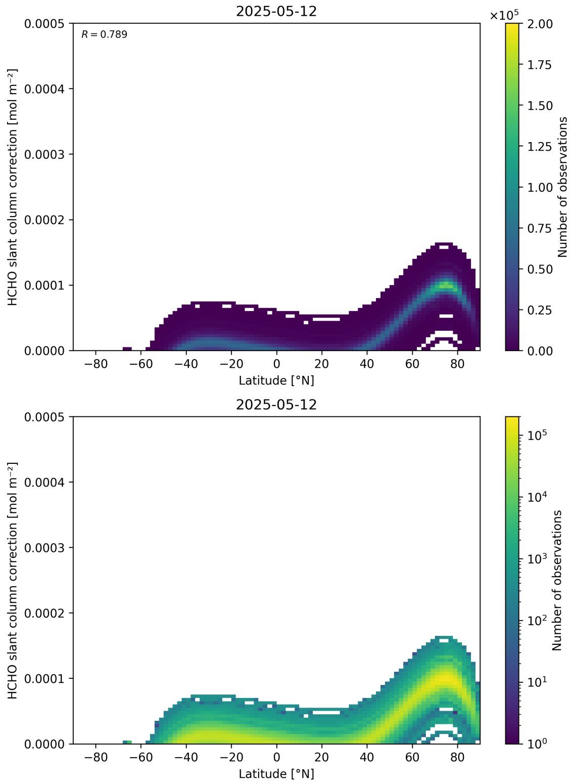
Figure 158: Scatter density plot of “Latitude” against “HCHO slant column correction” for 2025-05-11 to 2025-05-13.
