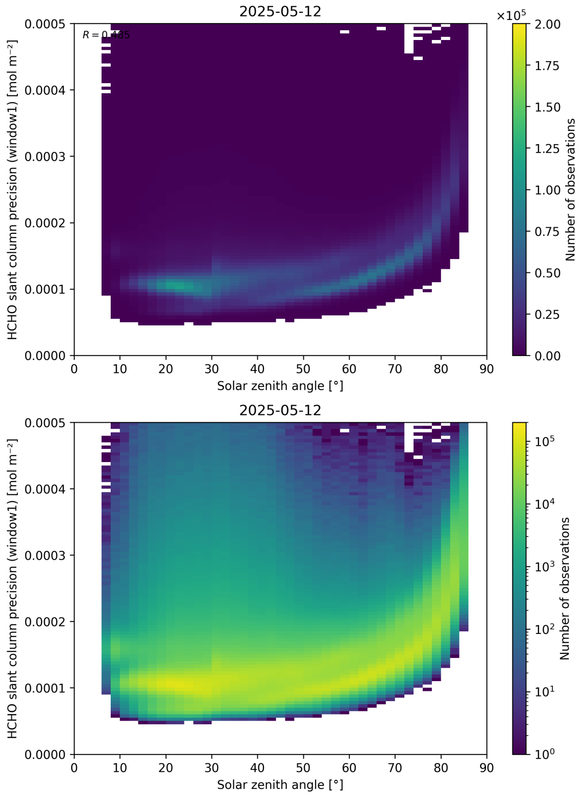
Figure 174: Scatter density plot of “Solar zenith angle” against “HCHO slant column precision (window1)” for 2025-05-11 to 2025-05-13.
