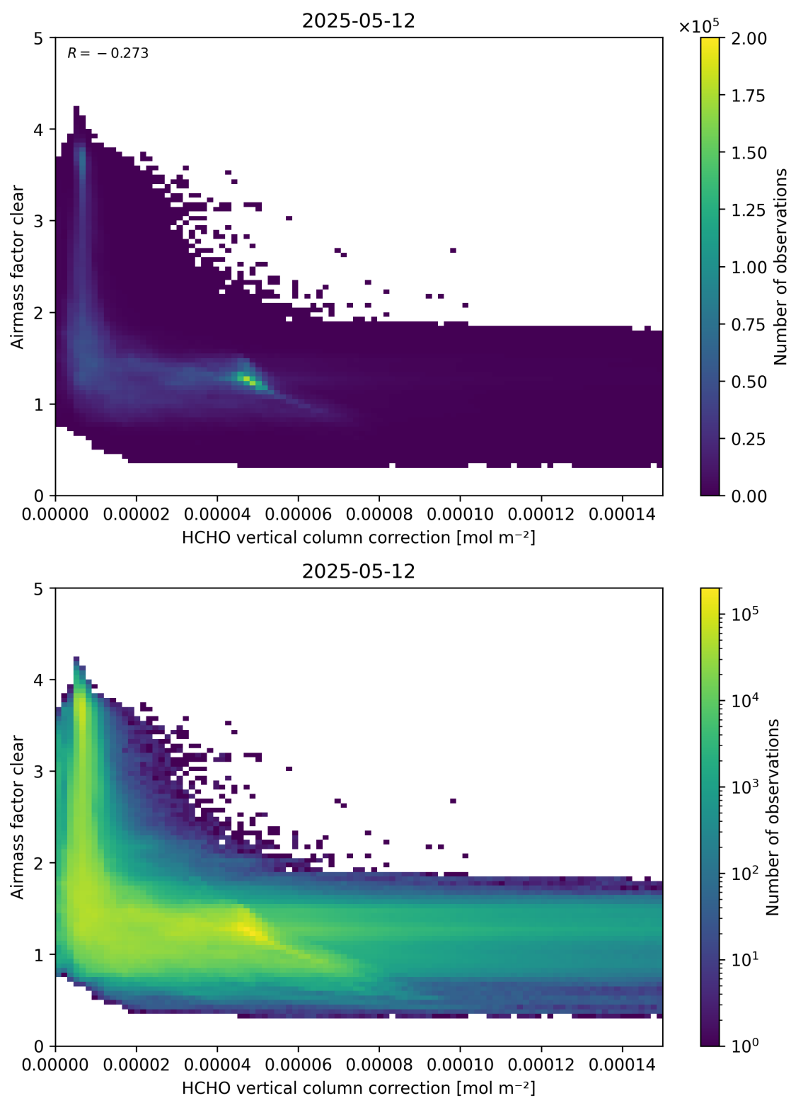
Figure 115: Scatter density plot of “HCHO vertical column correction” against “Airmass factor clear” for 2025-05-11 to 2025-05-13.
