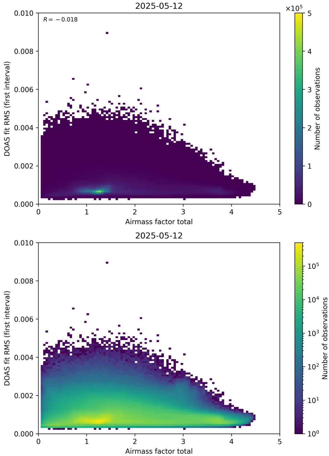
Figure 97: Scatter density plot of “Airmass factor total” against “DOAS fit RMS (first interval)” for 2025-05-11 to 2025-05-13.
