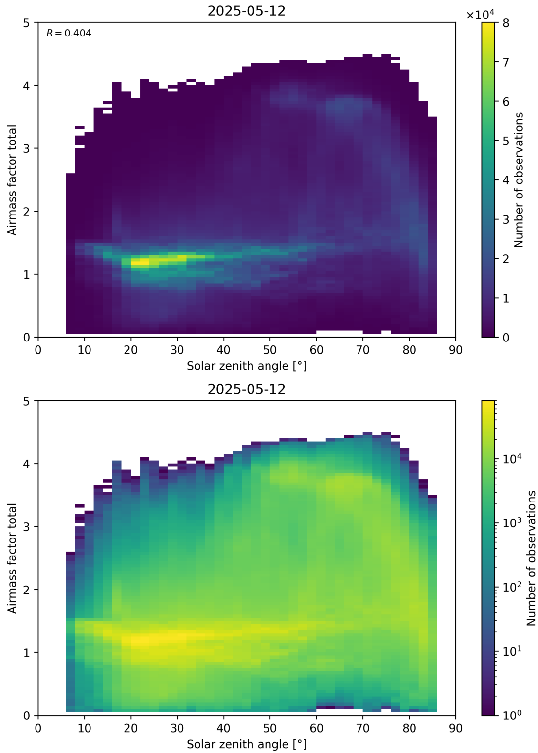
Figure 175: Scatter density plot of “Solar zenith angle” against “Airmass factor total” for 2025-05-11 to 2025-05-13.
