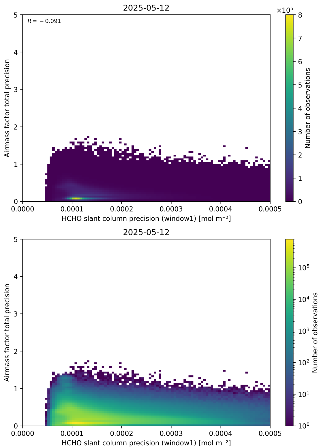
Figure 95: Scatter density plot of “HCHO slant column precision (window1)” against “Airmass factor total precision” for 2025-05-11 to 2025-05-13.
