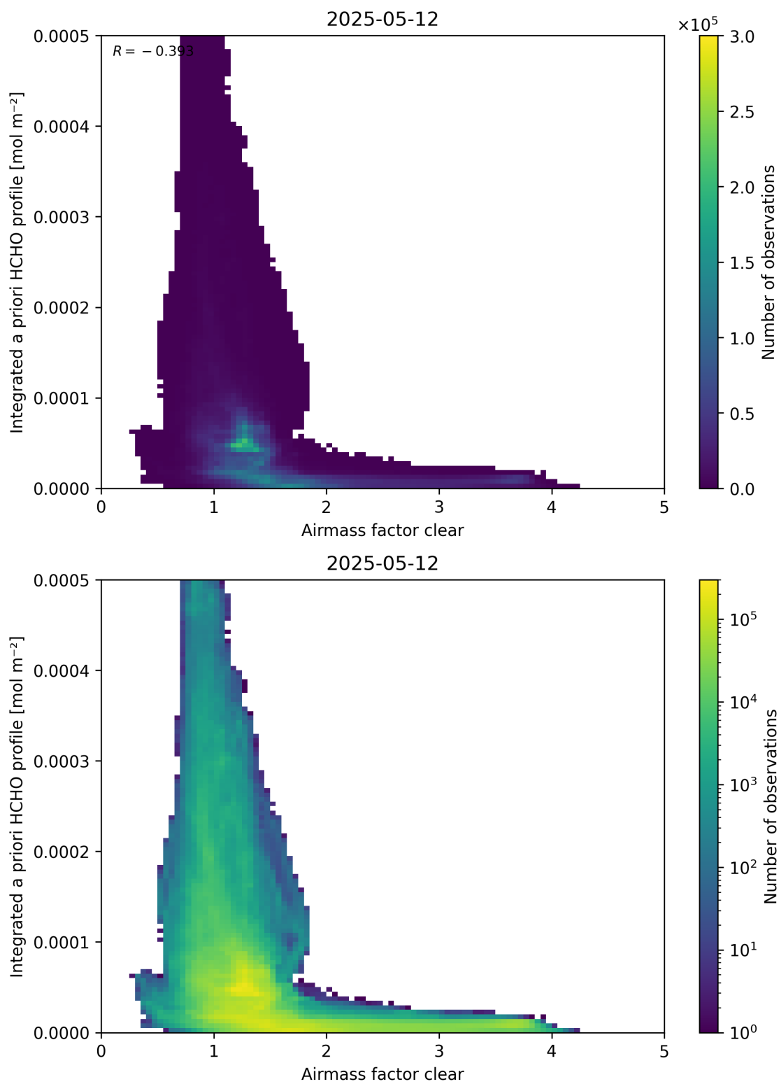
Figure 76: Scatter density plot of “Airmass factor clear” against “Integrated a priori HCHO profile” for 2025-05-11 to 2025-05-13.
