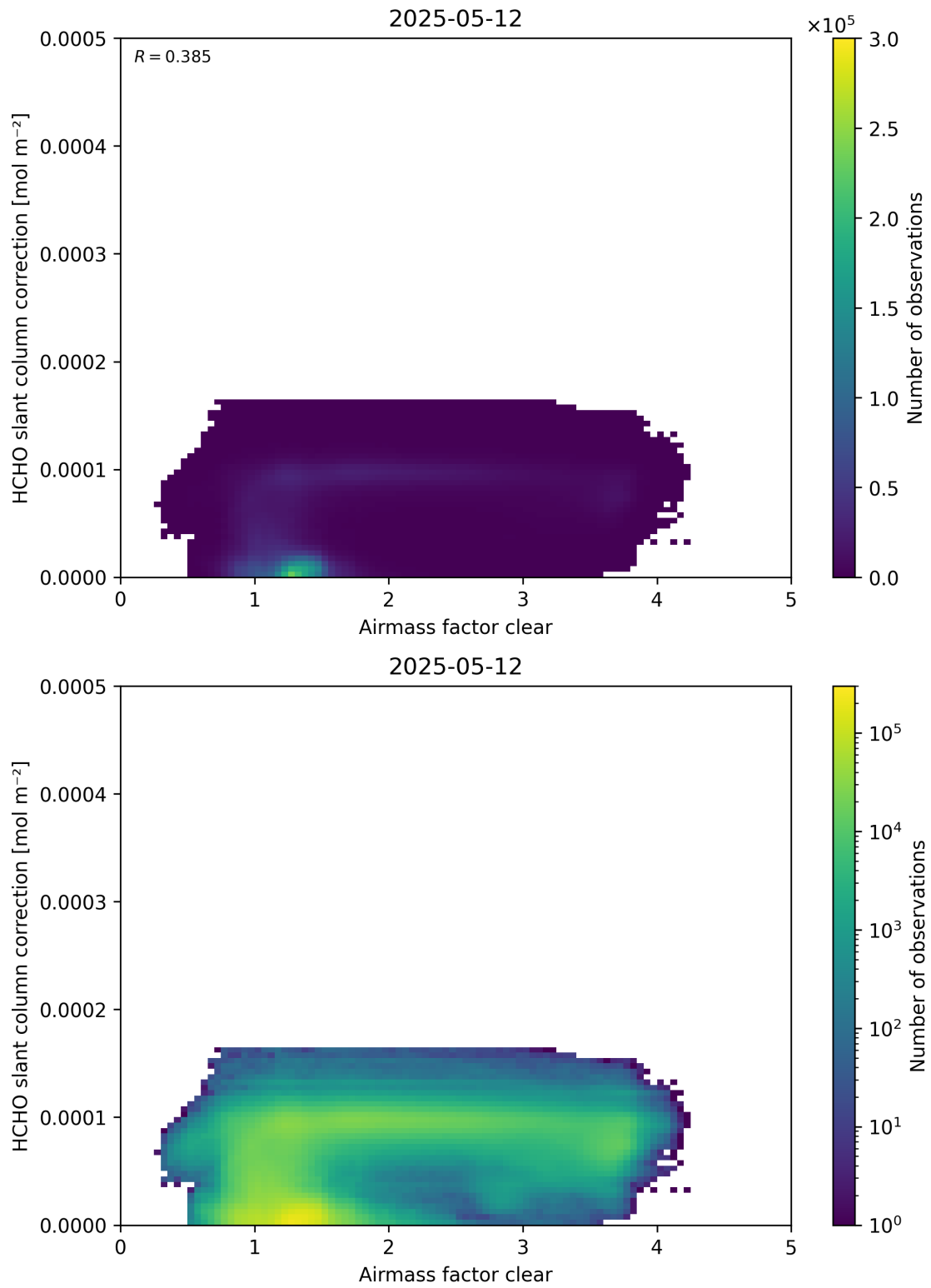
Figure 75: Scatter density plot of “Air mass factor clear” against “HCHO slant column correction” for 2025-05-11 to 2025-05-13.
