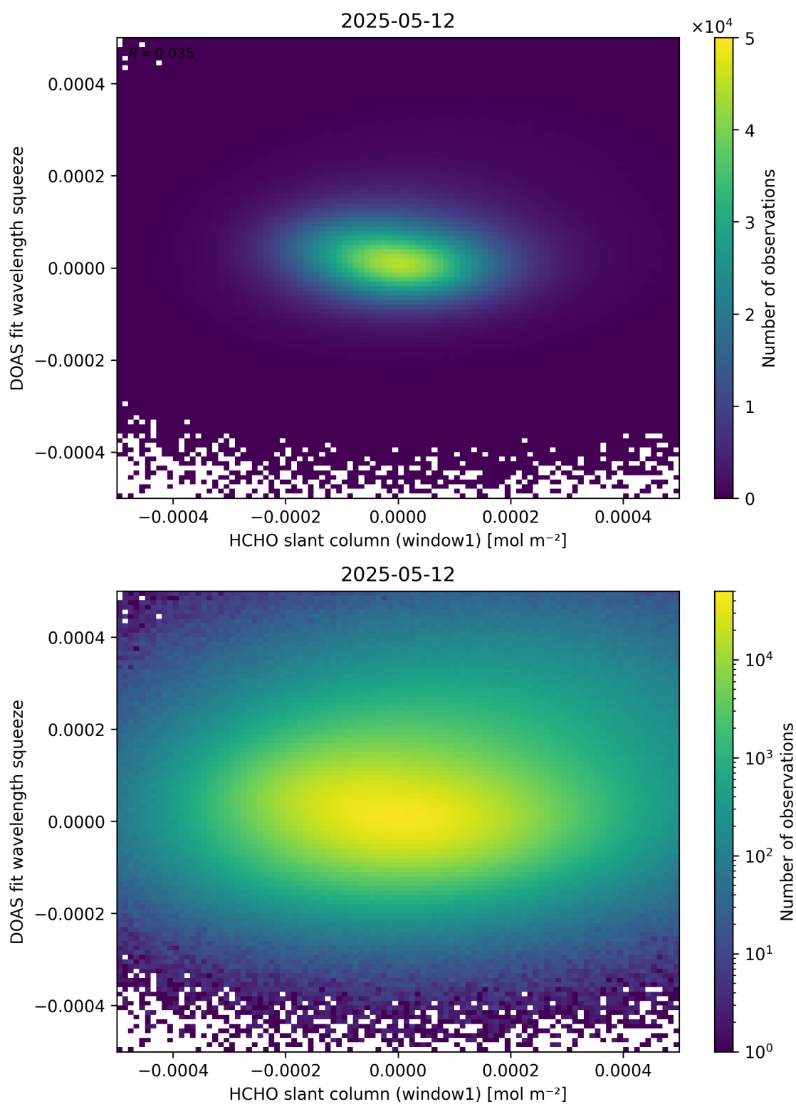
Figure 80: Scatter density plot of “HCHO slant column (window1)” against “DOAS fit wavelength squeeze” for 2025-05-11 to 2025-05-13.
