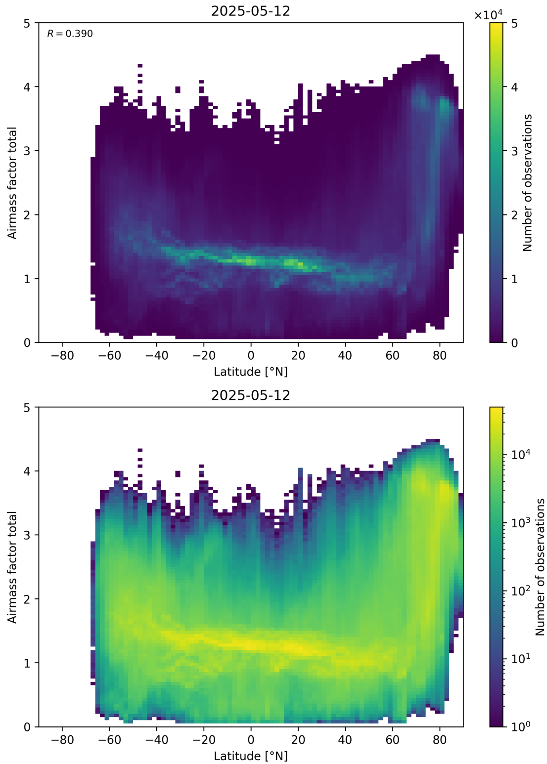
Figure 161: Scatter density plot of “Latitude” against “Airmass factor total” for 2025-05-11 to 2025-05-13.
