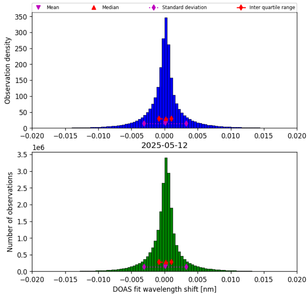
Figure 44: Histogram of “DOAS fit wavelength shift” for 2025-05-11 to 2025-05-13
