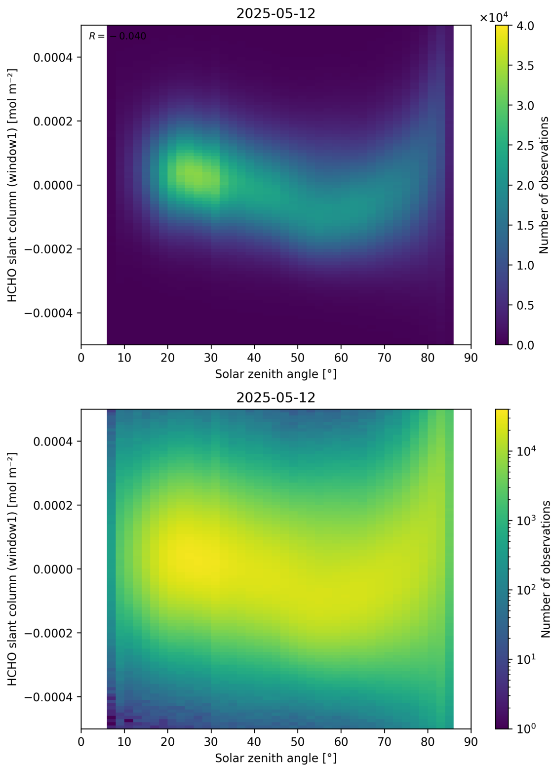
Figure 173: Scatter density plot of “Solar zenith angle” against “HCHO slant column (window1)” for 2025-05-11 to 2025-05-13.
