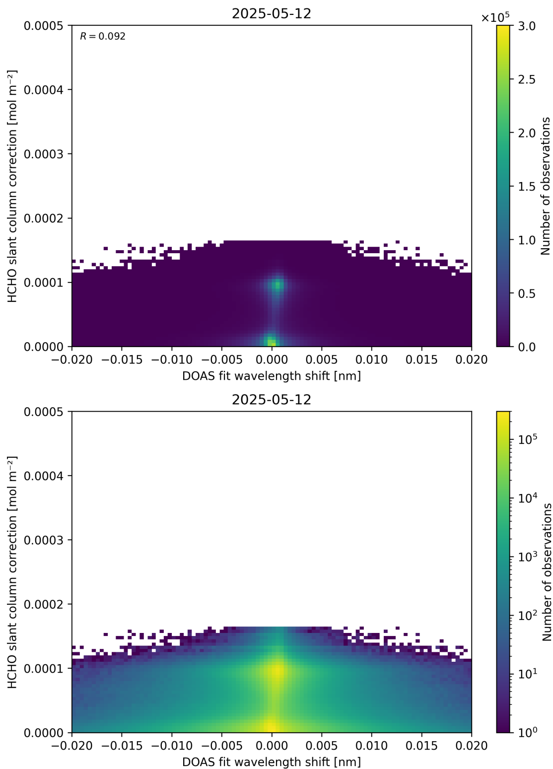
Figure 67: Scatter density plot of “DOAS fit wavelength shift” against “HCHO slant column correction” for 2025-05-11 to 2025-05-13.
