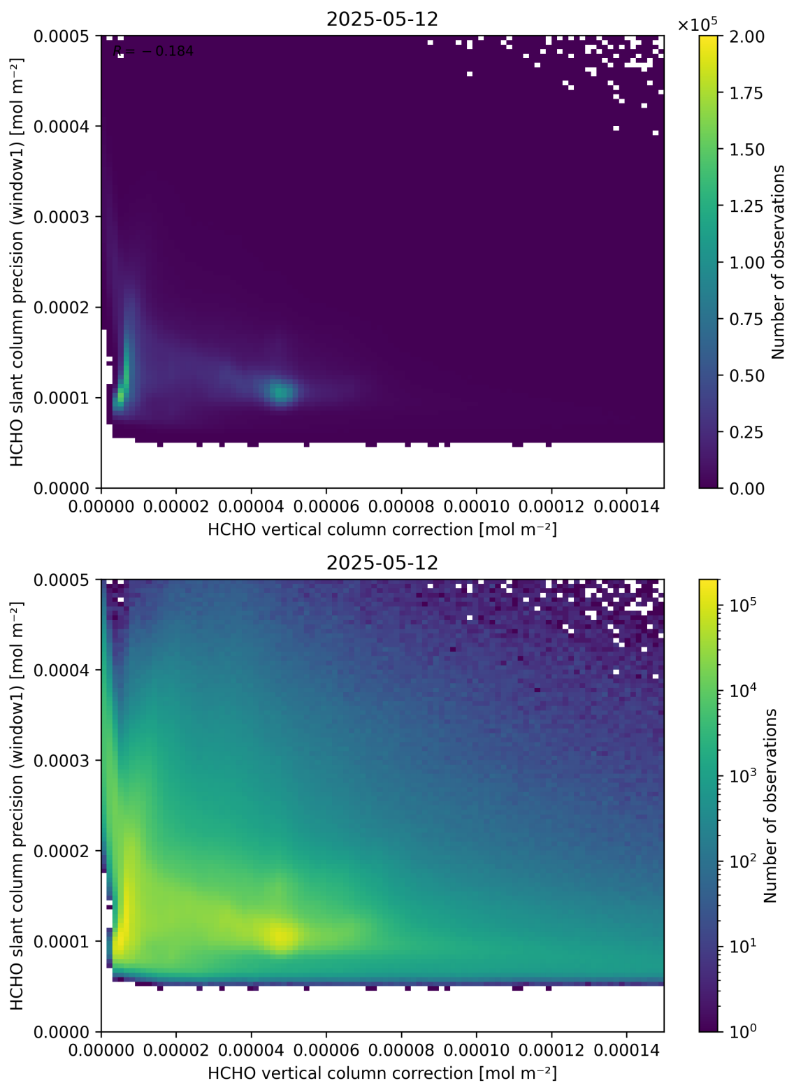
Figure 119: Scatter density plot of “HCHO vertical column correction” against “HCHO slant column precision (window1)” for 2025-05-11 to 2025-05-13.
