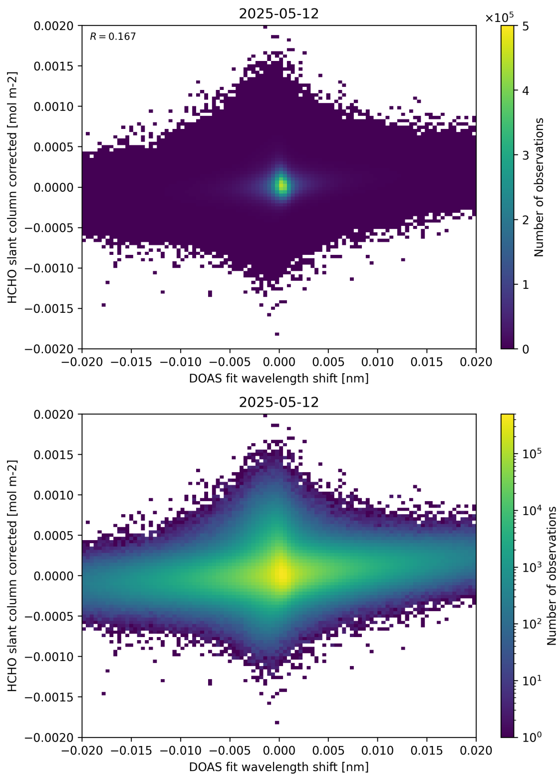
Figure 66: Scatter density plot of “DOAS fit wavelength shift” against “HCHO slant column corrected” for 2025-05-11 to 2025-05-13.
