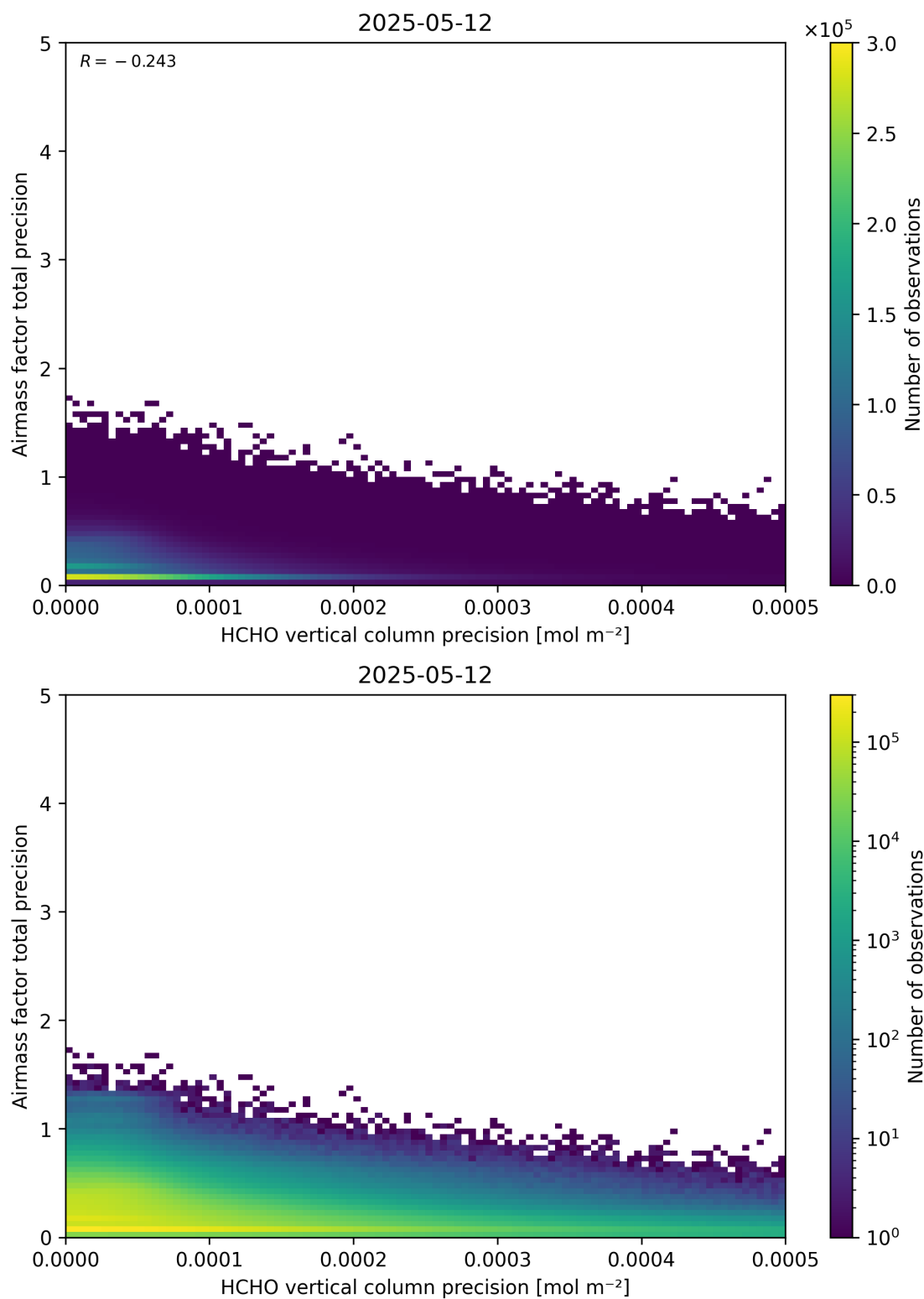
Figure 145: Scatter density plot of “HCHO vertical column precision” against “Airmass factor total precision” for 2025-05-11 to 2025-05-13.
