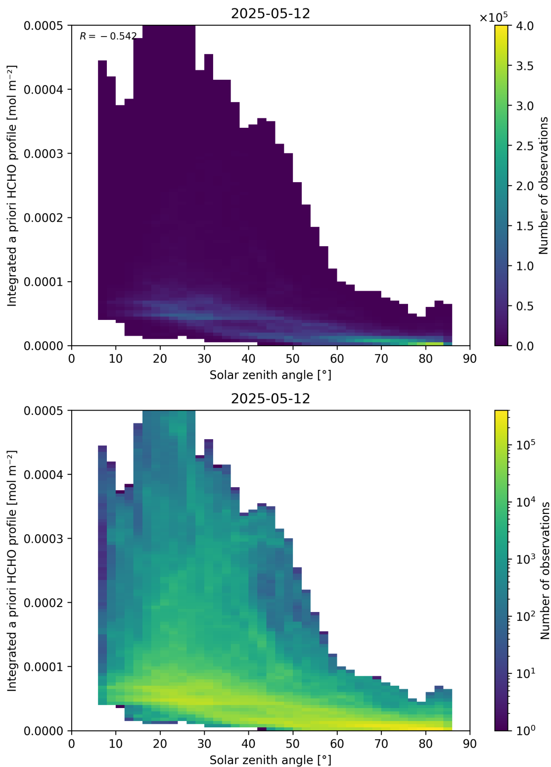
Figure 180: Scatter density plot of “Solar zenith angle” against “Integrated a priori HCHO profile” for 2025-05-11 to 2025-05-13.
