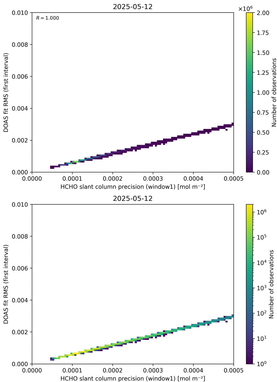
Figure 88: Scatter density plot of “HCHO slant column precision (window1)” against “DOAS fit RMS (first interval)” for 2025-05-11 to 2025-05-13.
