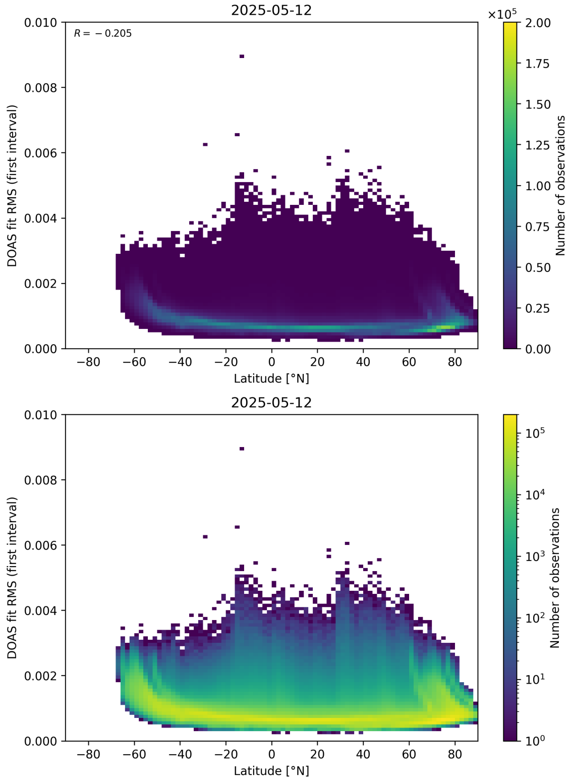
Figure 153: Scatter density plot of “Latitude” against “DOAS fit RMS (first interval)” for 2025-05-11 to 2025-05-13.
