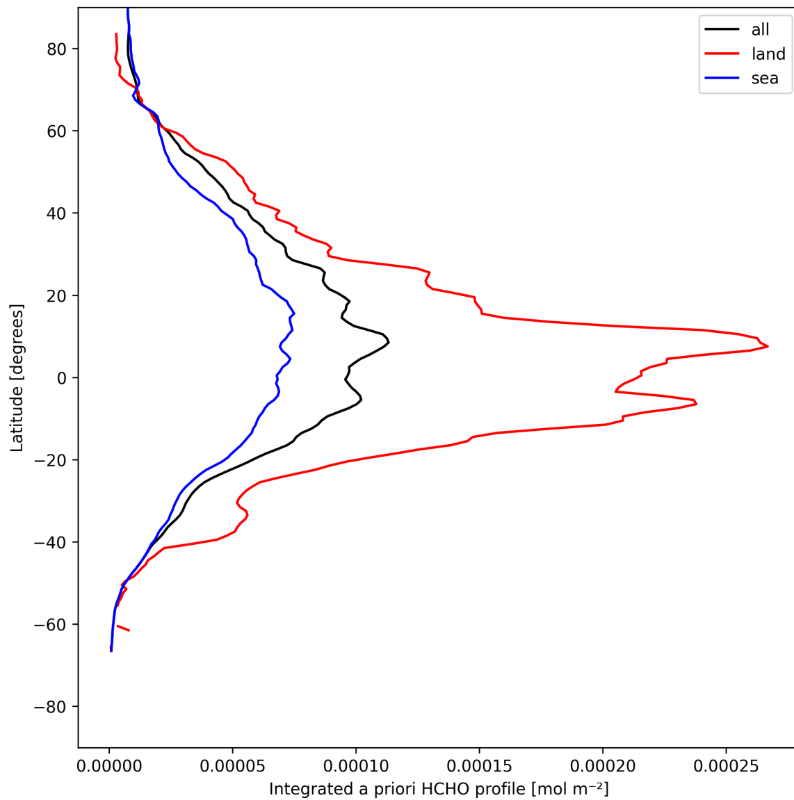
Figure 29: Zonal average of “Integrated a priori HCHO profile” for 2025-05-11 to 2025-05-13.
