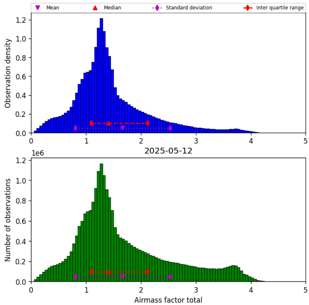
Figure 40: Histogram of “Airmass factor total” for 2025-05-11 to 2025-05-13
