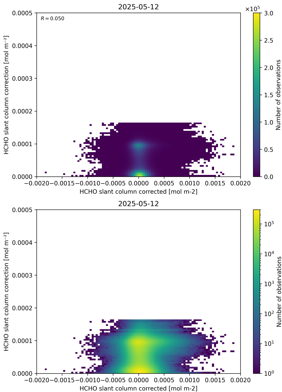
Figure 77: Scatter density plot of “HCHO slant column corrected” against “HCHO slant column correction” for 2025-05-11 to 2025-05-13.
