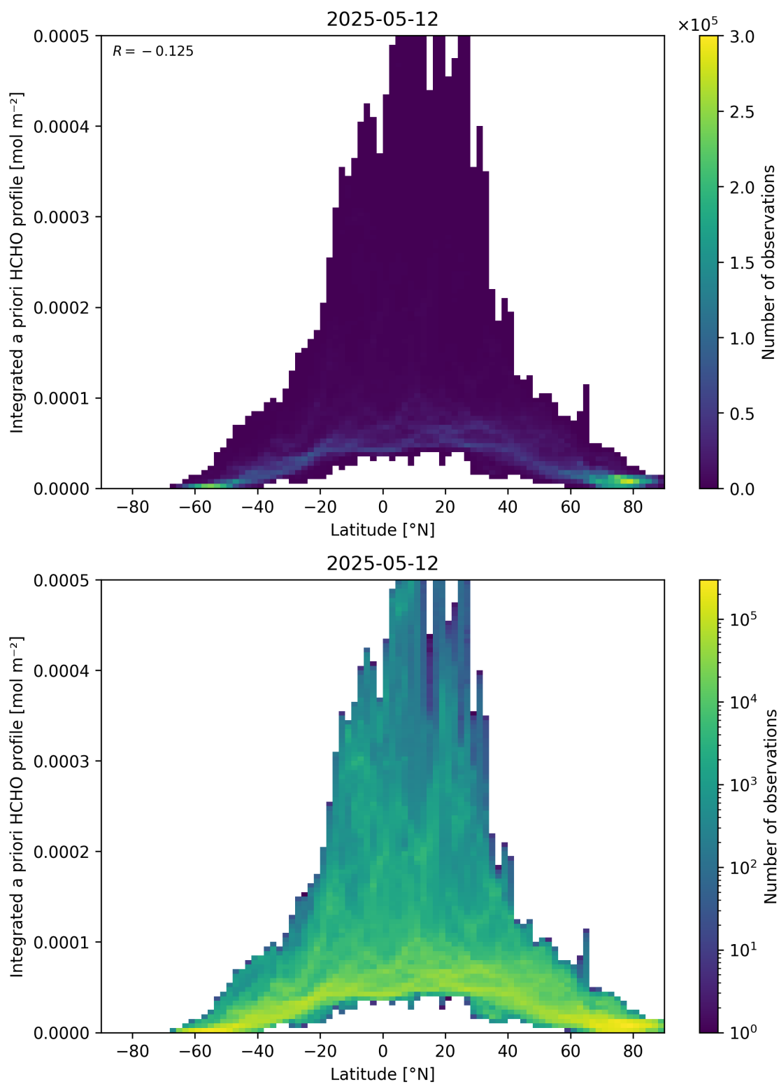
Figure 166: Scatter density plot of “Latitude” against “Integrated a priori HCHO profile” for 2025-05-11 to 2025-05-13.
