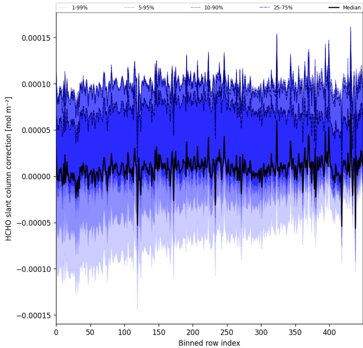
Figure 61: Along track statistics of “HCHO slant column correction” for 2025-05-11 to 2025-05-13
