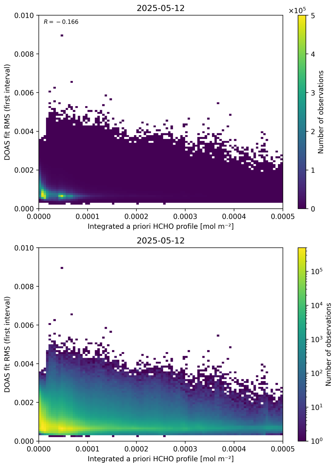
Figure 148: Scatter density plot of “Integrated a priori HCHO profile” against “DOAS fit RMS (first interval)” for 2025-05-11 to 2025-05-13.
