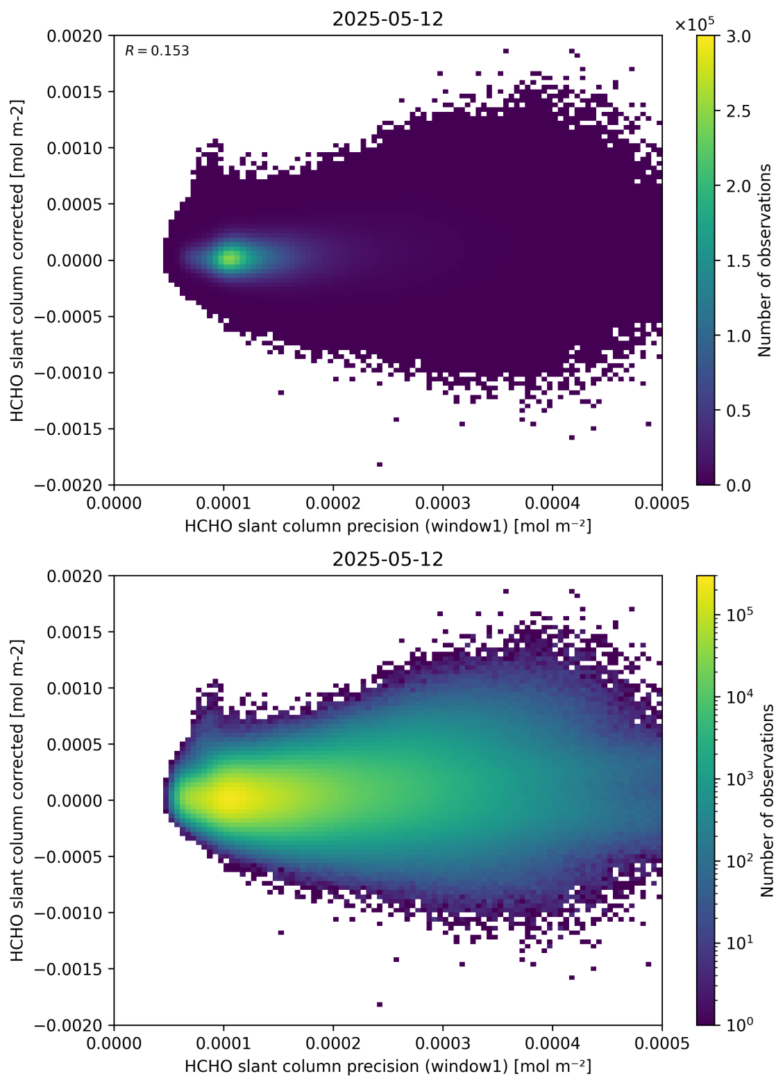
Figure 92: Scatter density plot of “HCHO slant column precision (window1)” against “HCHO slant column corrected” for 2025-05-11 to 2025-05-13.
