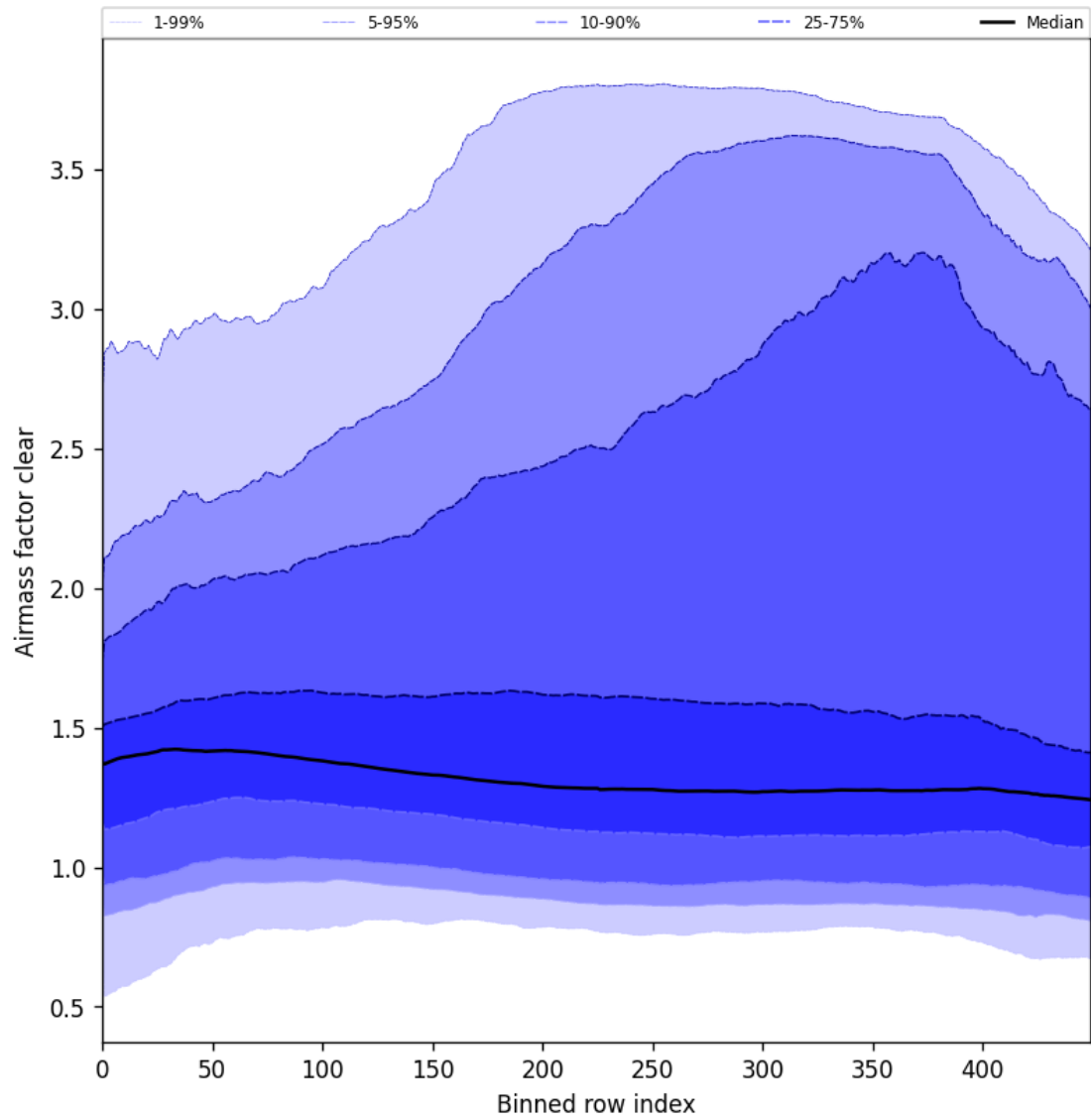
Figure 56: Along track statistics of “Airmass factor clear” for 2025-05-11 to 2025-05-13
