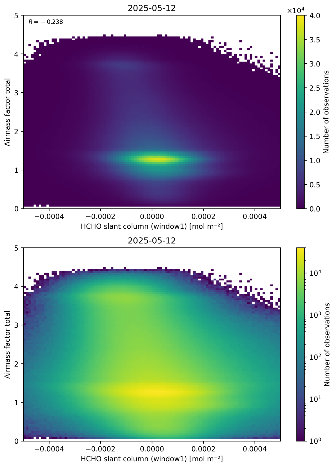
Figure 85: Scatter density plot of “HCHO slant column (window1)” against “Airmass factor total” for 2025-05-11 to 2025-05-13.
