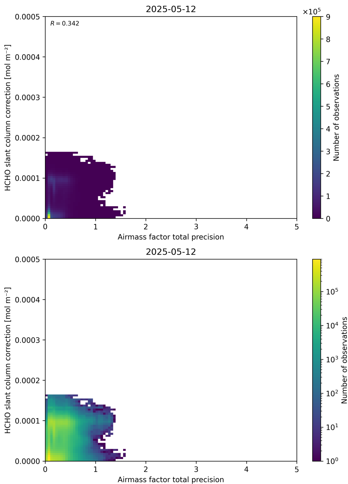
Figure 110: Scatter density plot of “Airmass factor total precision” against “HCHO slant column correction” for 2025-05-11 to 2025-05-13.
