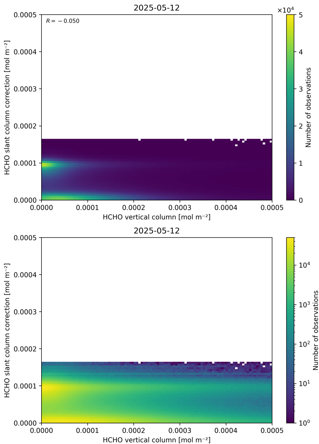
Figure 128: Scatter density plot of “HCHO vertical column” against “HCHO slant column correction” for 2025-05-11 to 2025-05-13.
