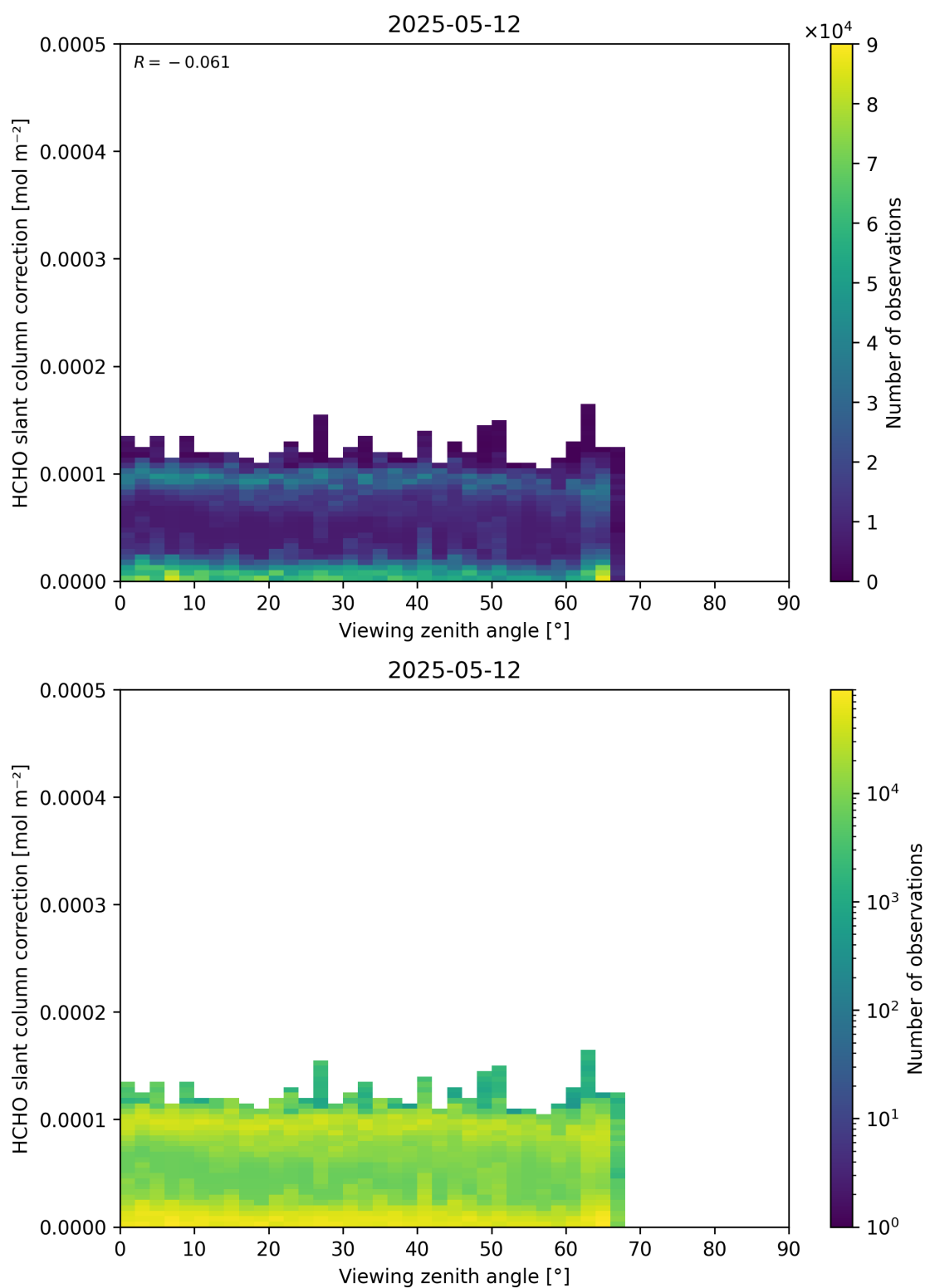
Figure 187: Scatter density plot of “Viewing zenith angle” against “HCHO slant column correction” for 2025-05-11 to 2025-05-13.
