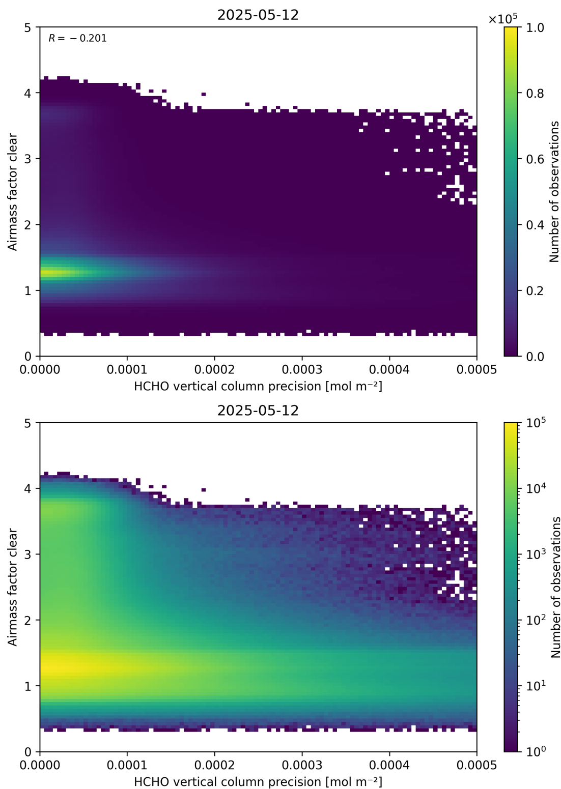
Figure 139: Scatter density plot of “HCHO vertical column precision” against “Airmass factor clear” for 2025-05-11 to 2025-05-13.
