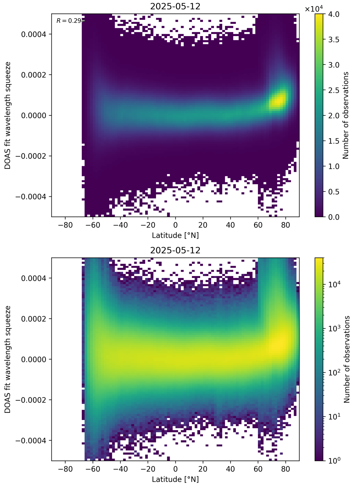
Figure 155: Scatter density plot of “Latitude” against “DOAS fit wavelength squeeze” for 2025-05-11 to 2025-05-13.
