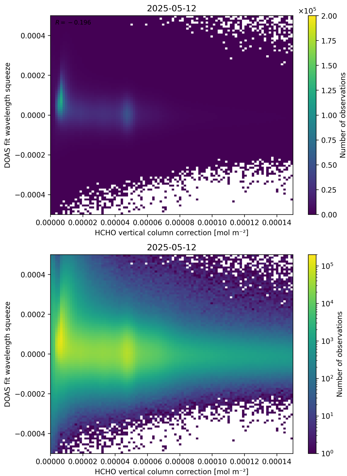
Figure 114: Scatter density plot of “HCHO vertical column correction” against “DOAS fit wavelength squeeze” for 2025-05-11 to 2025-05-13.
