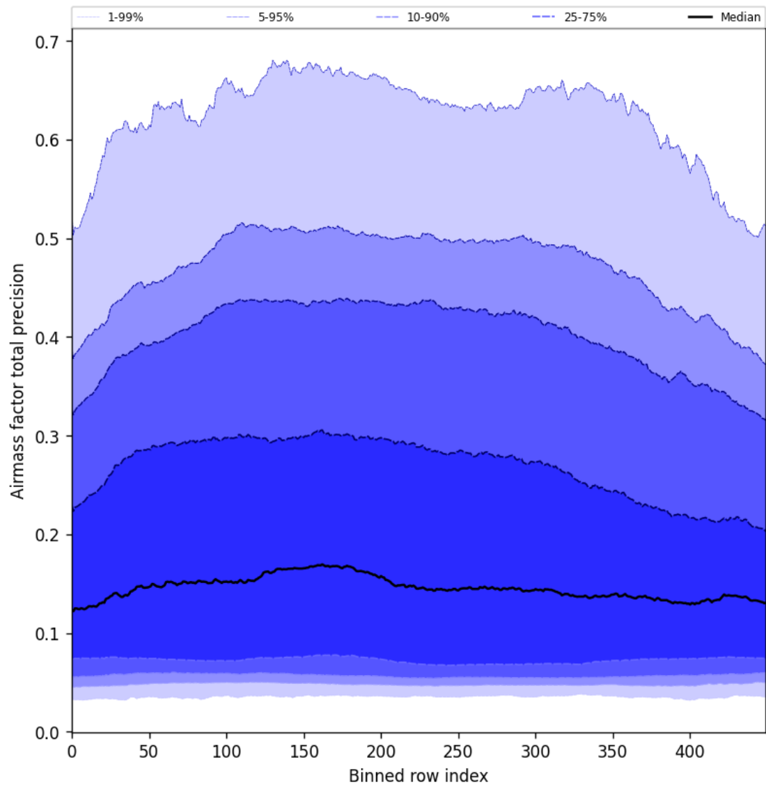
Figure 55: Along track statistics of “Airmass factor total precision” for 2025-05-11 to 2025-05-13
