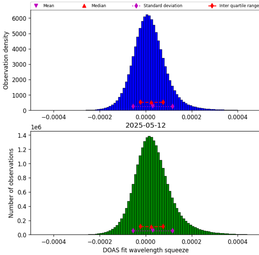
Figure 45: Histogram of “DOAS fit wavelength squeeze” for 2025-05-11 to 2025-05-13
