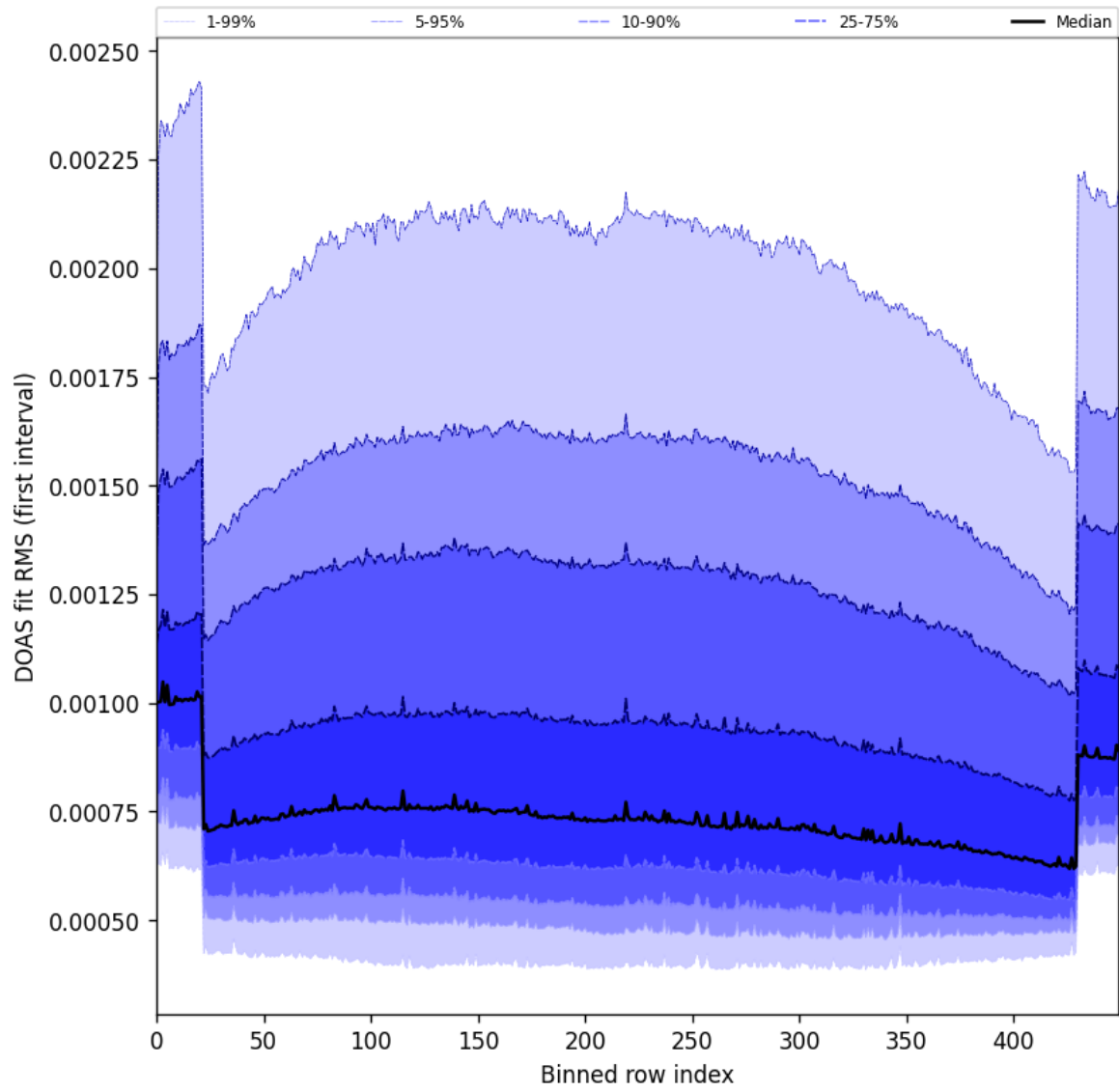
Figure 60: Along track statistics of “DOAS fit RMS (first interval)” for 2025-05-11 to 2025-05-13
