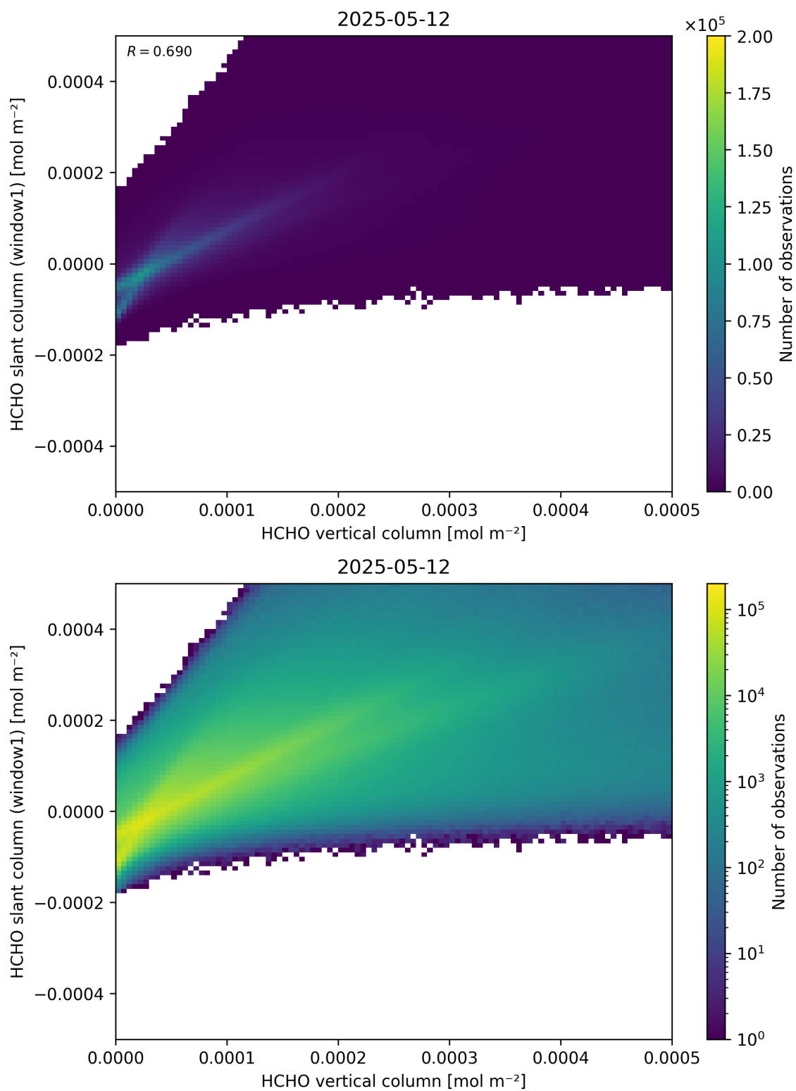
Figure 129: Scatter density plot of “HCHO vertical column” against “HCHO slant column (window1)” for 2025-05-11 to 2025-05-13.
