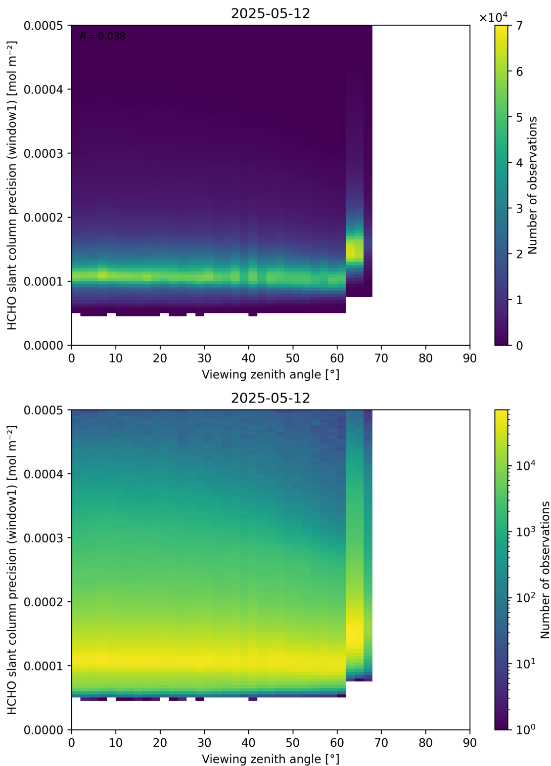
Figure 189: Scatter density plot of “Viewing zenith angle” against “HCHO slant column precision (window1)” for 2025-05-11 to 2025-05-13.
