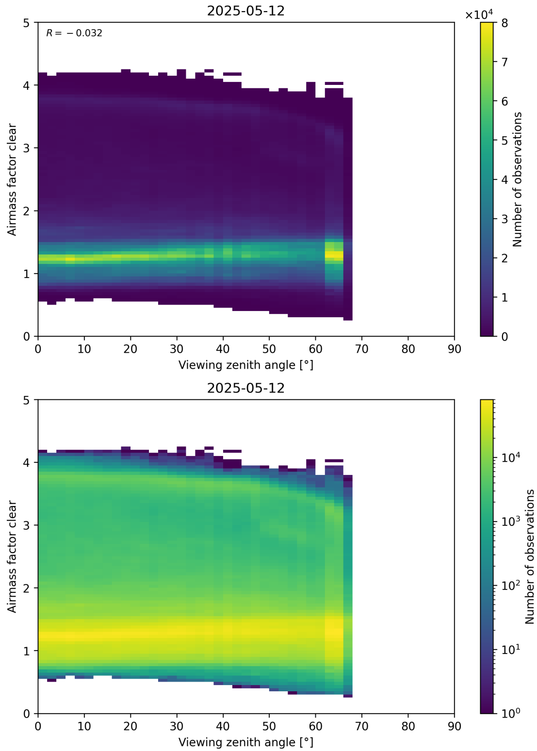
Figure 185: Scatter density plot of “Viewing zenith angle” against “Airmass factor clear” for 2025-05-11 to 2025-05-13.
