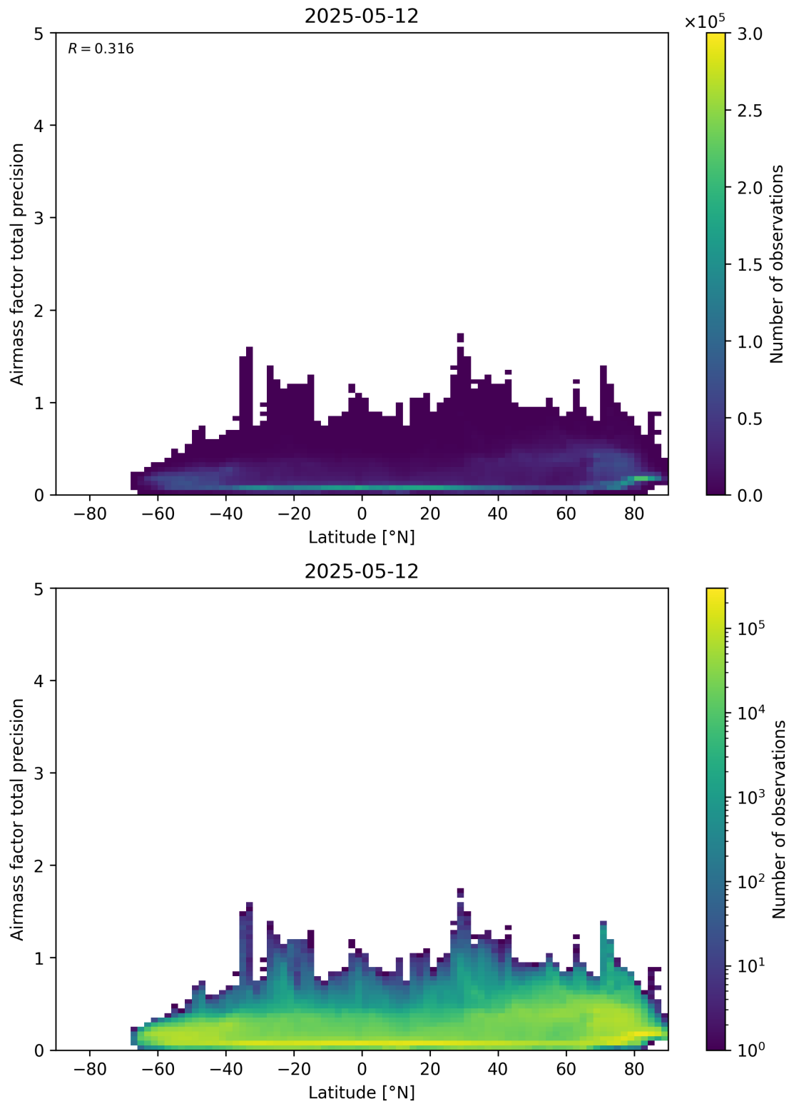
Figure 162: Scatter density plot of “Latitude” against “Airmass factor total precision” for 2025-05-11 to 2025-05-13.
