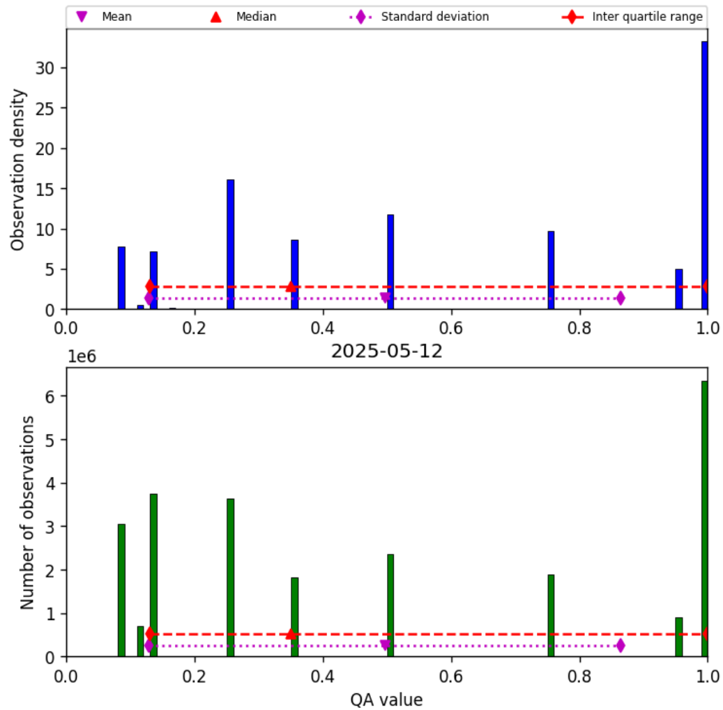
Figure 34: Histogram of “QA value” for 2025-05-11 to 2025-05-13
