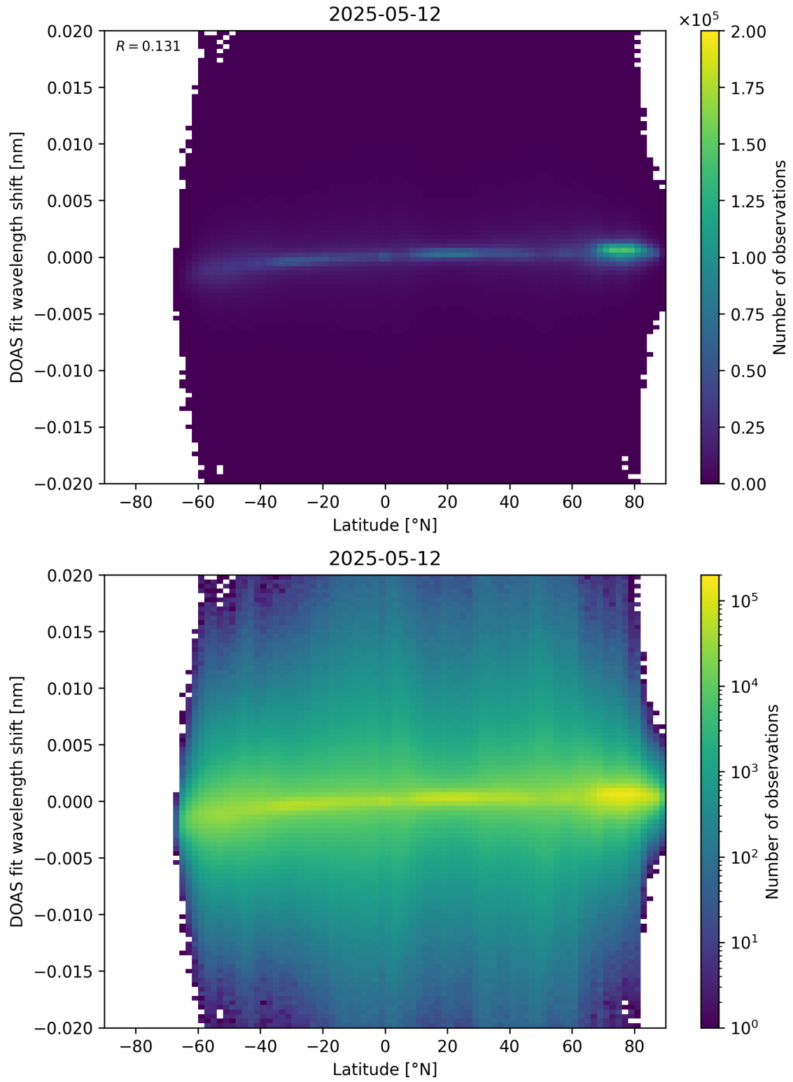
Figure 154: Scatter density plot of “Latitude” against “DOAS fit wavelength shift” for 2025-05-11 to 2025-05-13.
