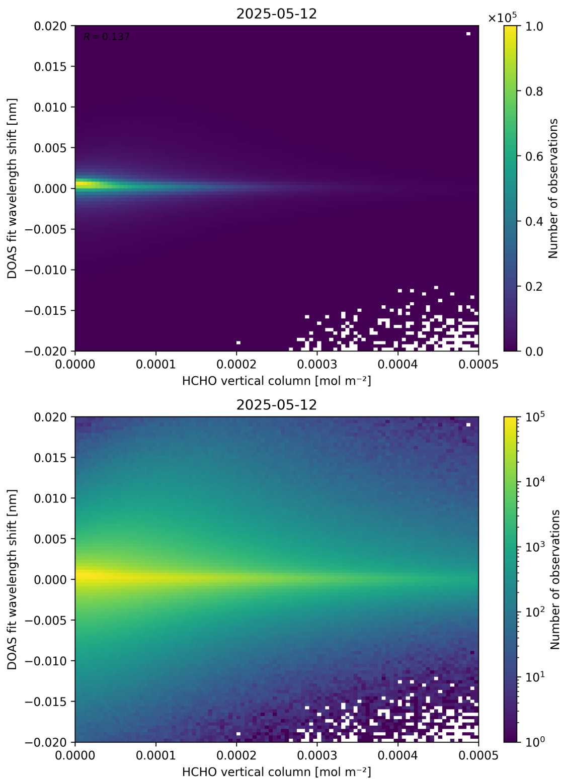
Figure 124: Scatter density plot of “HCHO vertical column” against “DOAS fit wavelength shift” for 2025-05-11 to 2025-05-13.
