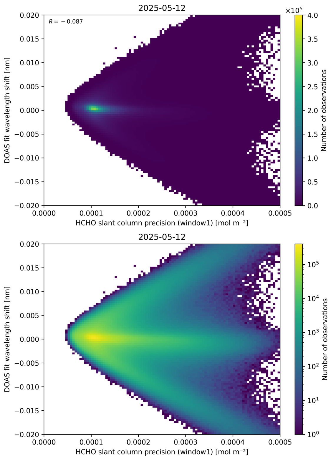
Figure 89: Scatter density plot of “HCHO slant column precision (window1)” against “DOAS fit wavelength shift” for 2025-05-11 to 2025-05-13.
