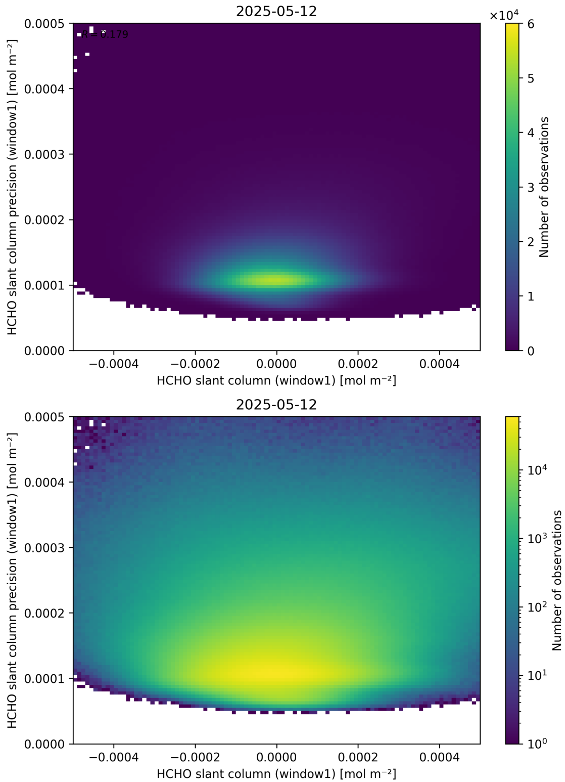
Figure 84: Scatter density plot of “HCHO slant column (window1)” against “HCHO slant column precision (window1)” for 2025-05-11 to 2025-05-13.
