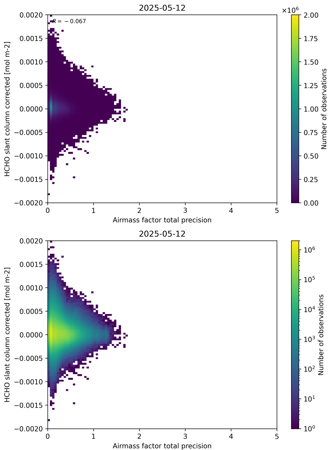
Figure 109: Scatter density plot of “Airmass factor total precision” against “HCHO slant column corrected” for 2025-05-11 to 2025-05-13.
