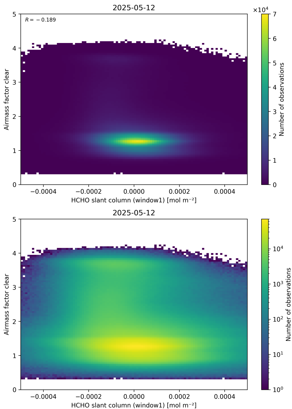
Figure 81: Scatter density plot of “HCHO slant column (window1)” against “Airmass factor clear” for 2025-05-11 to 2025-05-13.
