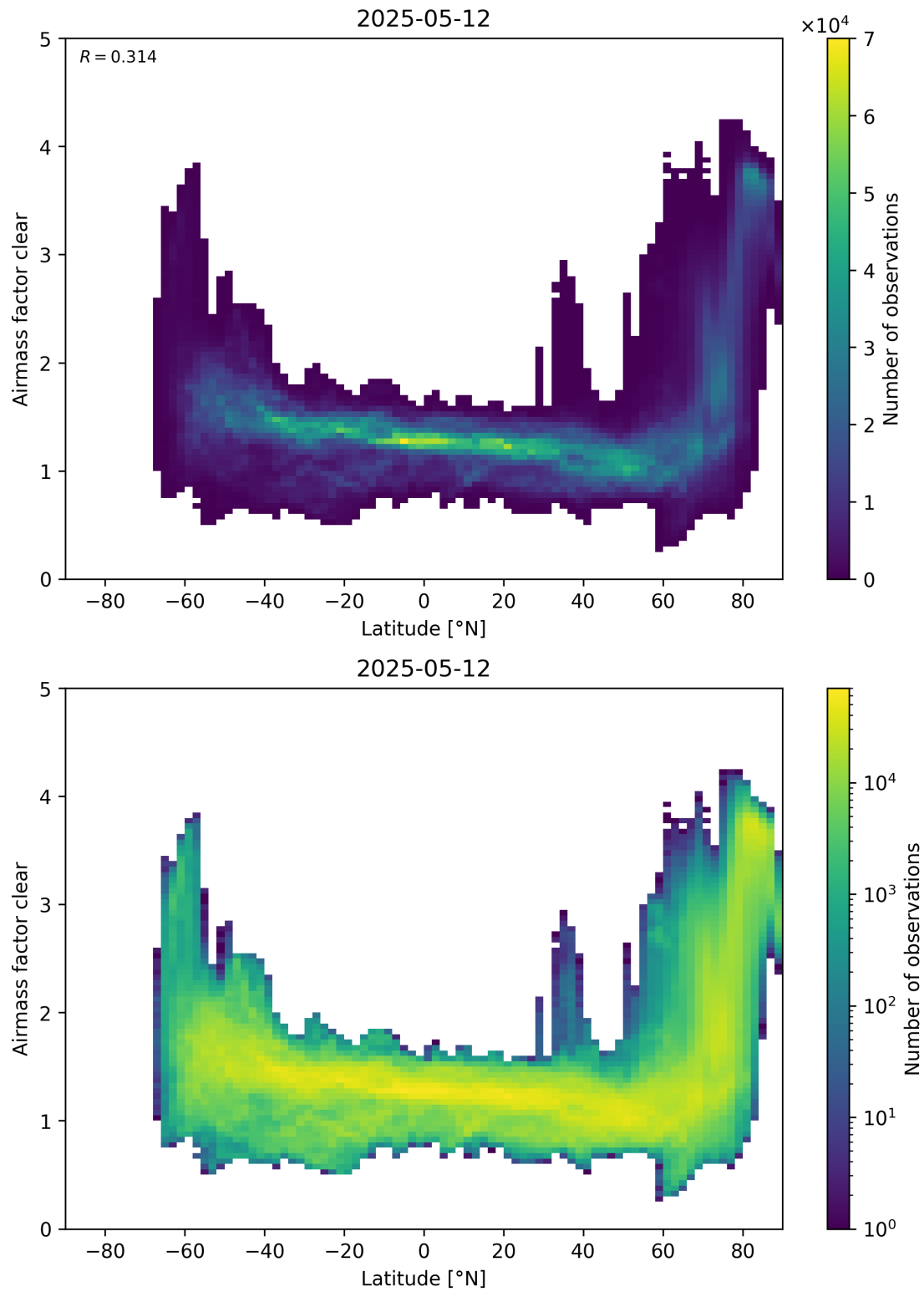
Figure 156: Scatter density plot of “Latitude” against “Airmass factor clear” for 2025-05-11 to 2025-05-13.
