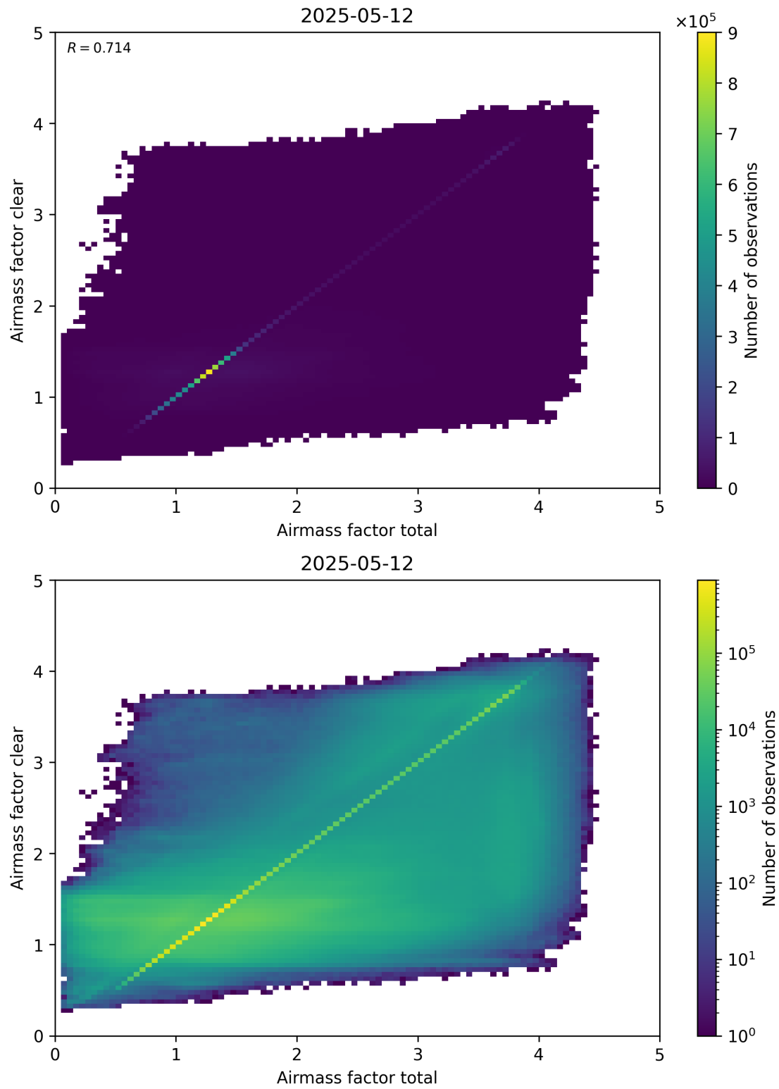
Figure 100: Scatter density plot of “Airmass factor total” against “Airmass factor clear” for 2025-05-11 to 2025-05-13.
