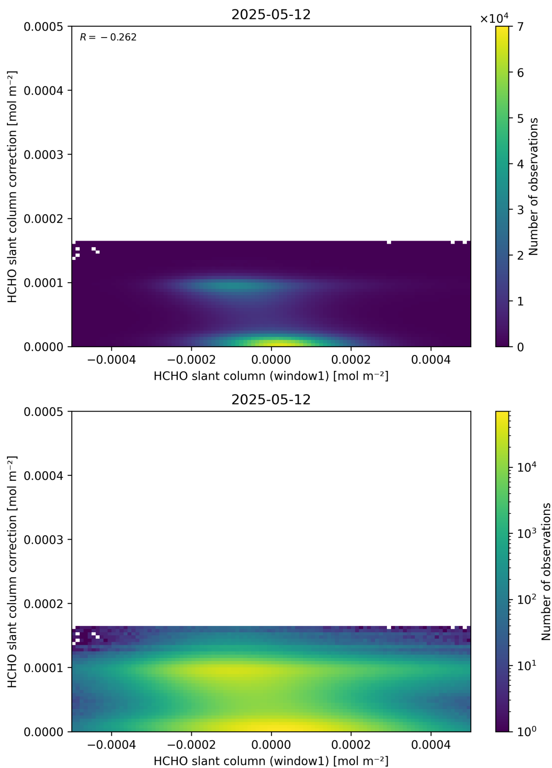
Figure 83: Scatter density plot of “HCHO slant column (window1)” against “HCHO slant column correction” for 2025-05-11 to 2025-05-13.
