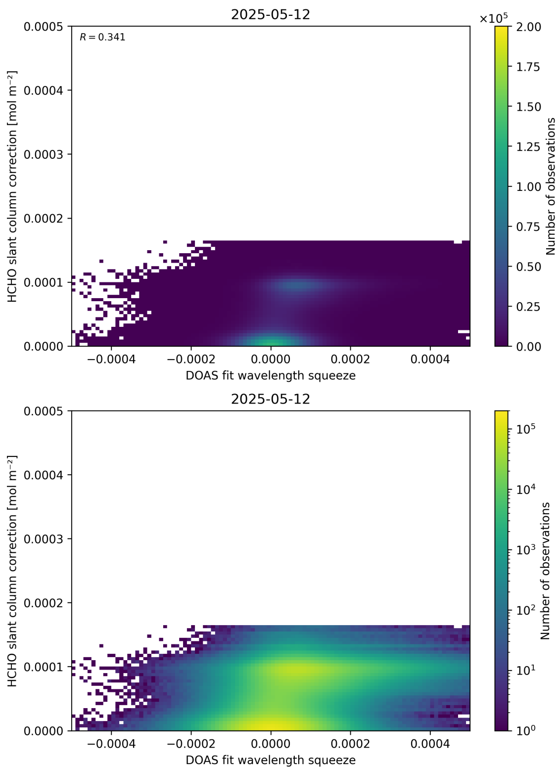
Figure 70: Scatter density plot of “DOAS fit wavelength squeeze” against “HCHO slant column correction” for 2025-05-11 to 2025-05-13.
