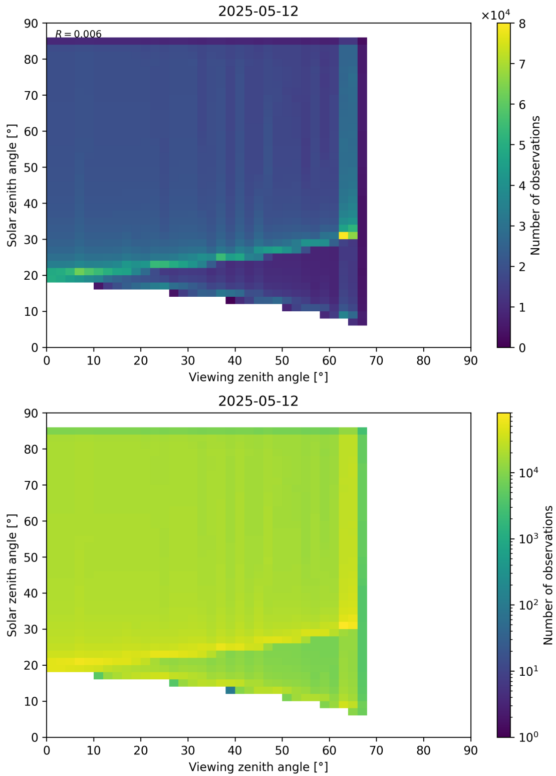
Figure 197: Scatter density plot of “Viewing zenith angle” against “Solar zenith angle” for 2025-05-11 to 2025-05-13.
