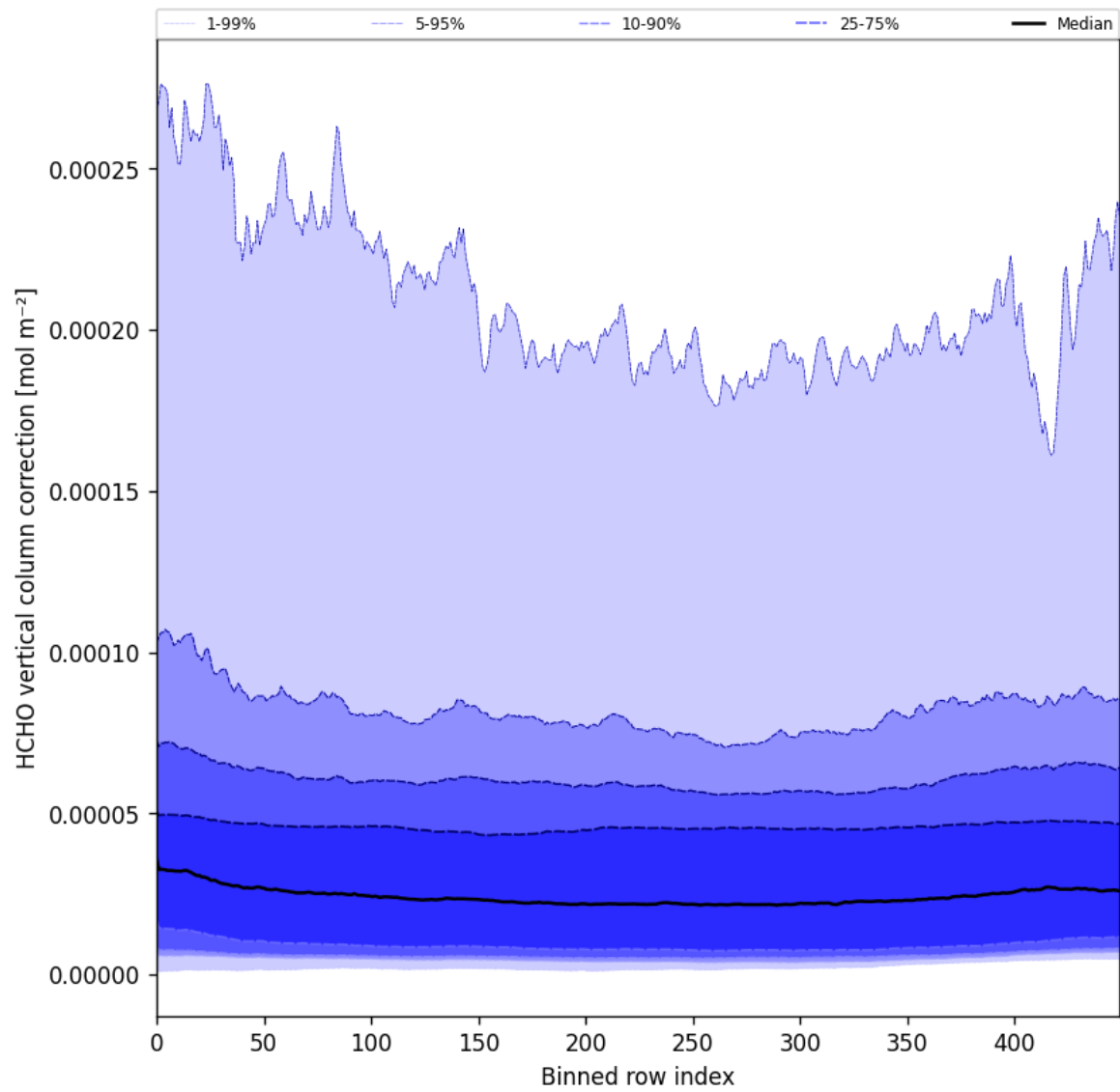
Figure 51: Along track statistics of “HCHO vertical column correction” for 2025-05-11 to 2025-05-13
