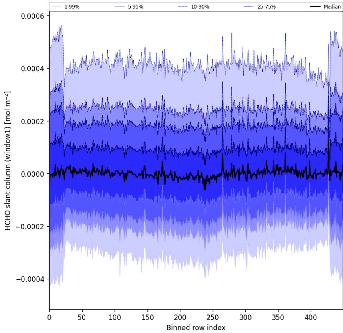
Figure 52: Along track statistics of “HCHO slant column (window1)” for 2025-05-11 to 2025-05-13
