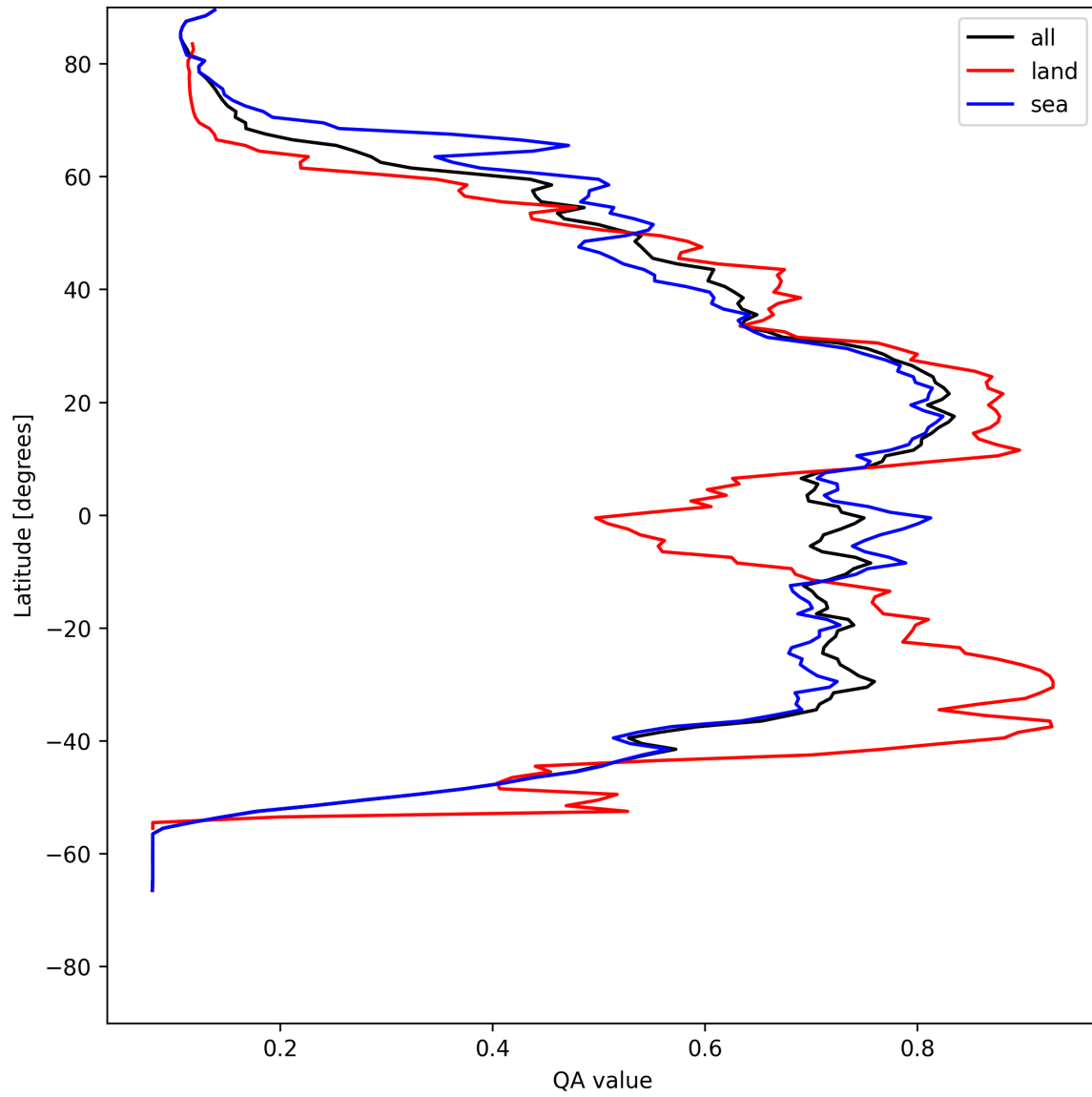
Figure 20: Zonal average of “QA value” for 2025-05-11 to 2025-05-13.
