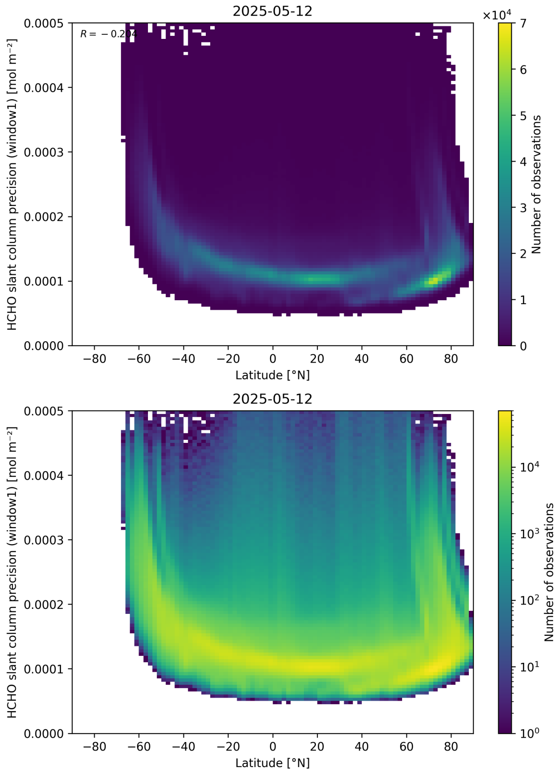
Figure 160: Scatter density plot of “Latitude” against “HCHO slant column precision (window1)” for 2025-05-11 to 2025-05-13.
