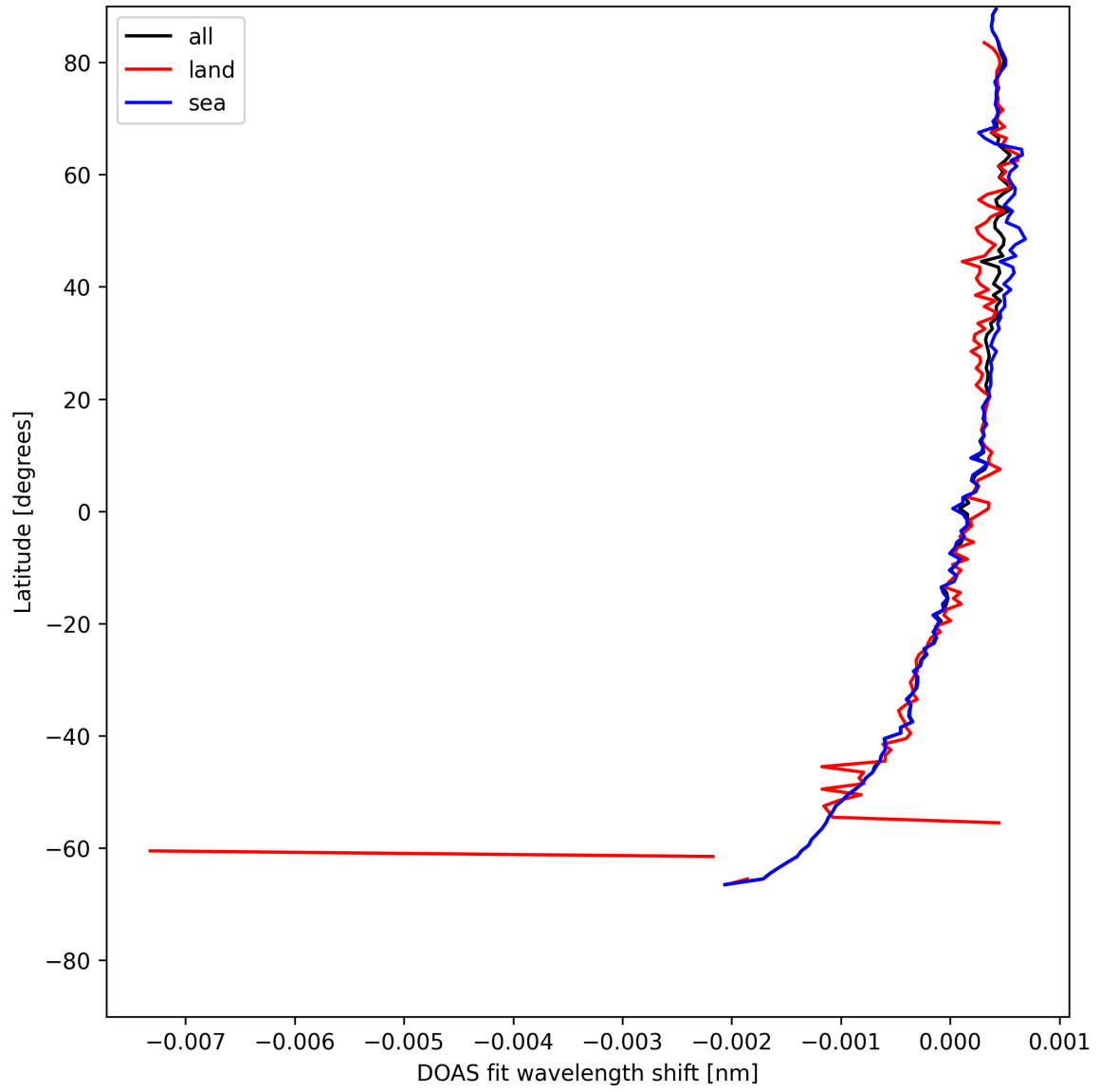
Figure 30: Zonal average of “DOAS fit wavelength shift” for 2025-05-11 to 2025-05-13.
