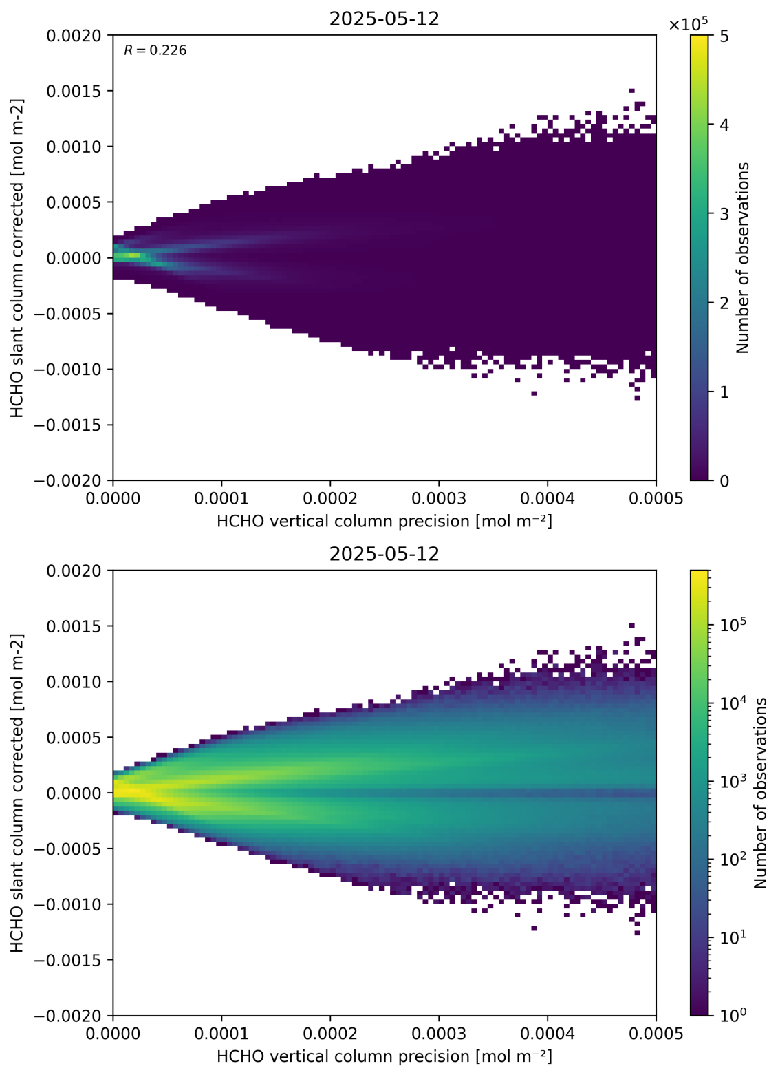
Figure 140: Scatter density plot of “HCHO vertical column precision” against “HCHO slant column corrected” for 2025-05-11 to 2025-05-13.
