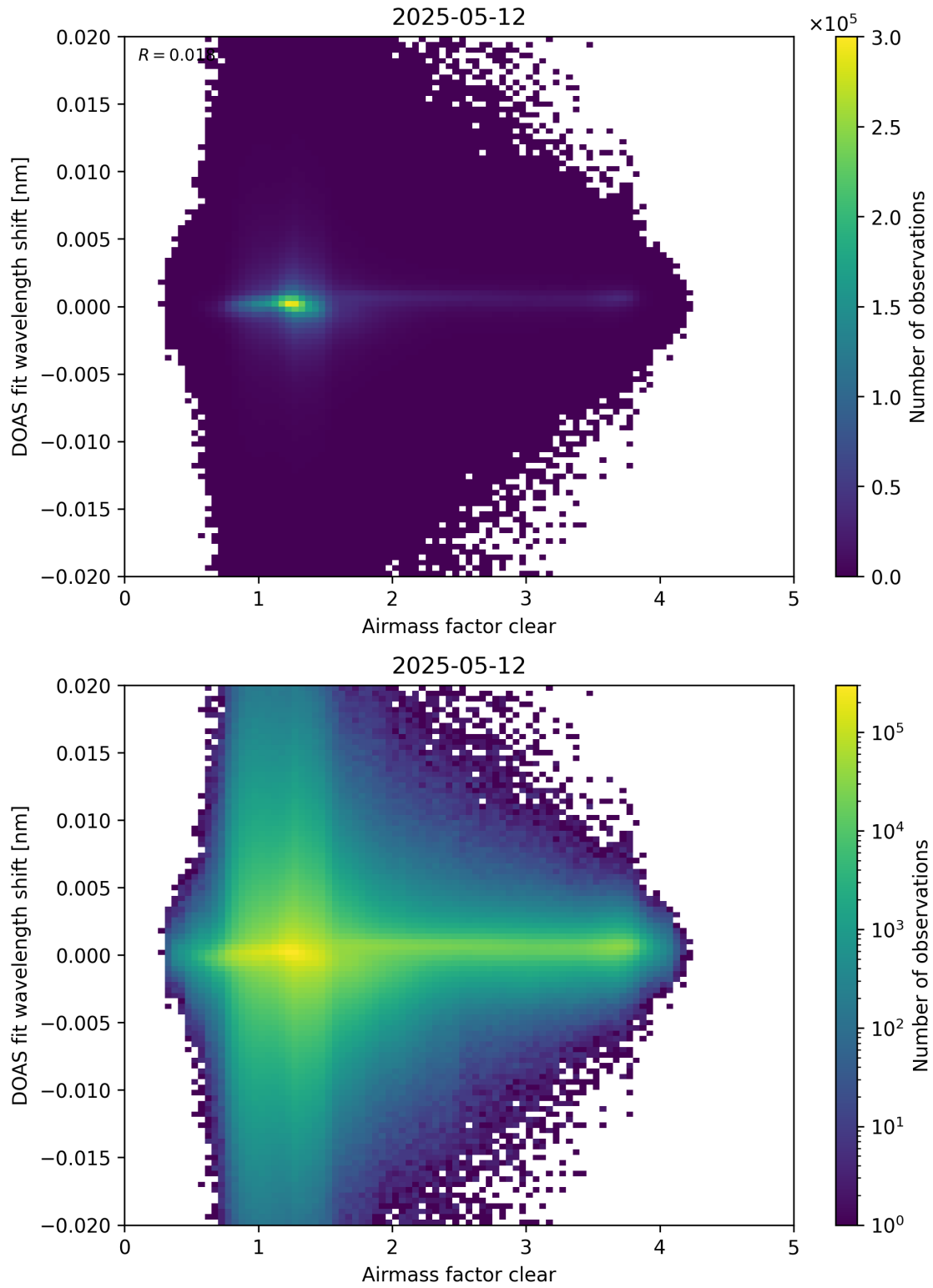
Figure 72: Scatter density plot of “Airmass factor clear” against “DOAS fit wavelength shift” for 2025-05-11 to 2025-05-13.
