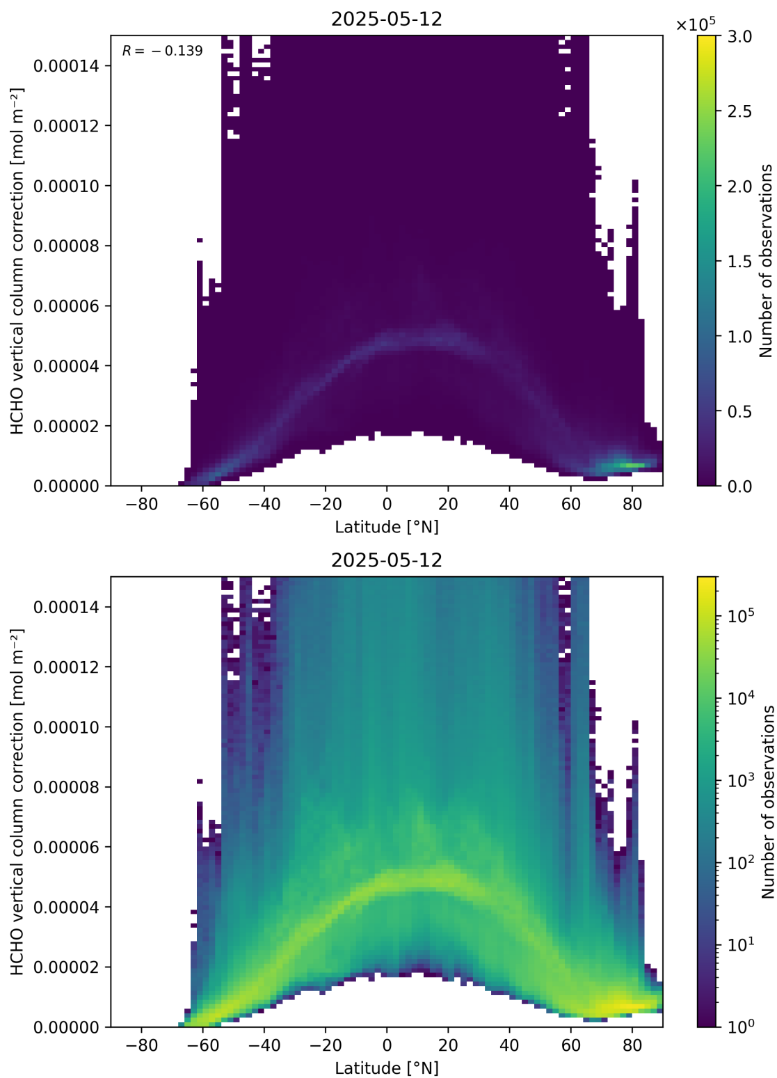
Figure 164: Scatter density plot of “Latitude” against “HCHO vertical column correction” for 2025-05-11 to 2025-05-13.
