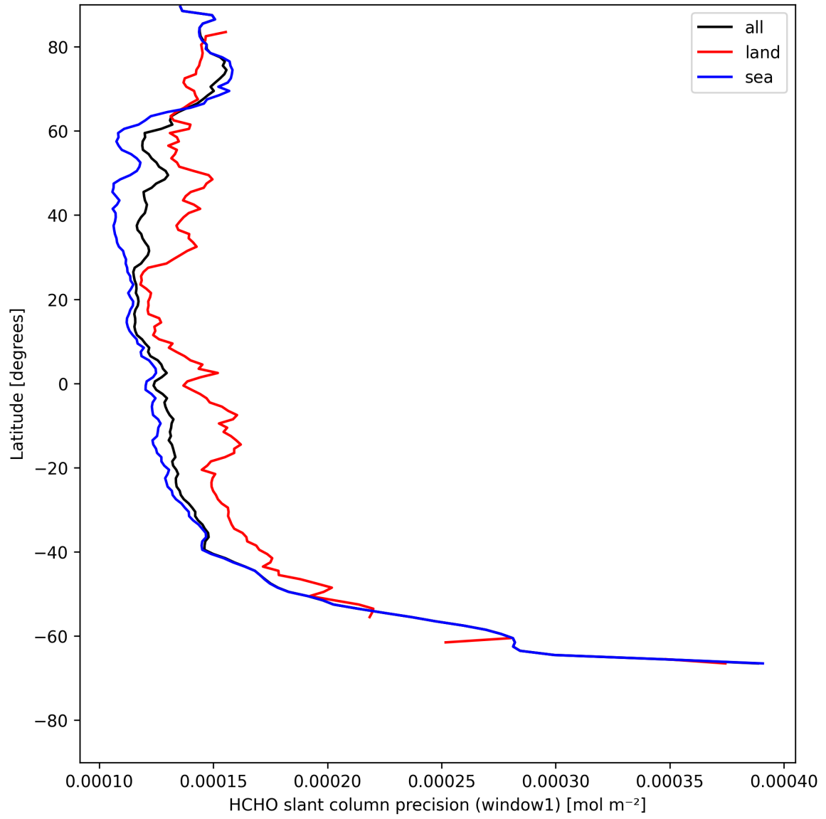
Figure 25: Zonal average of “HCHO slant column precision (window1)” for 2025-05-11 to 2025-05-13.
