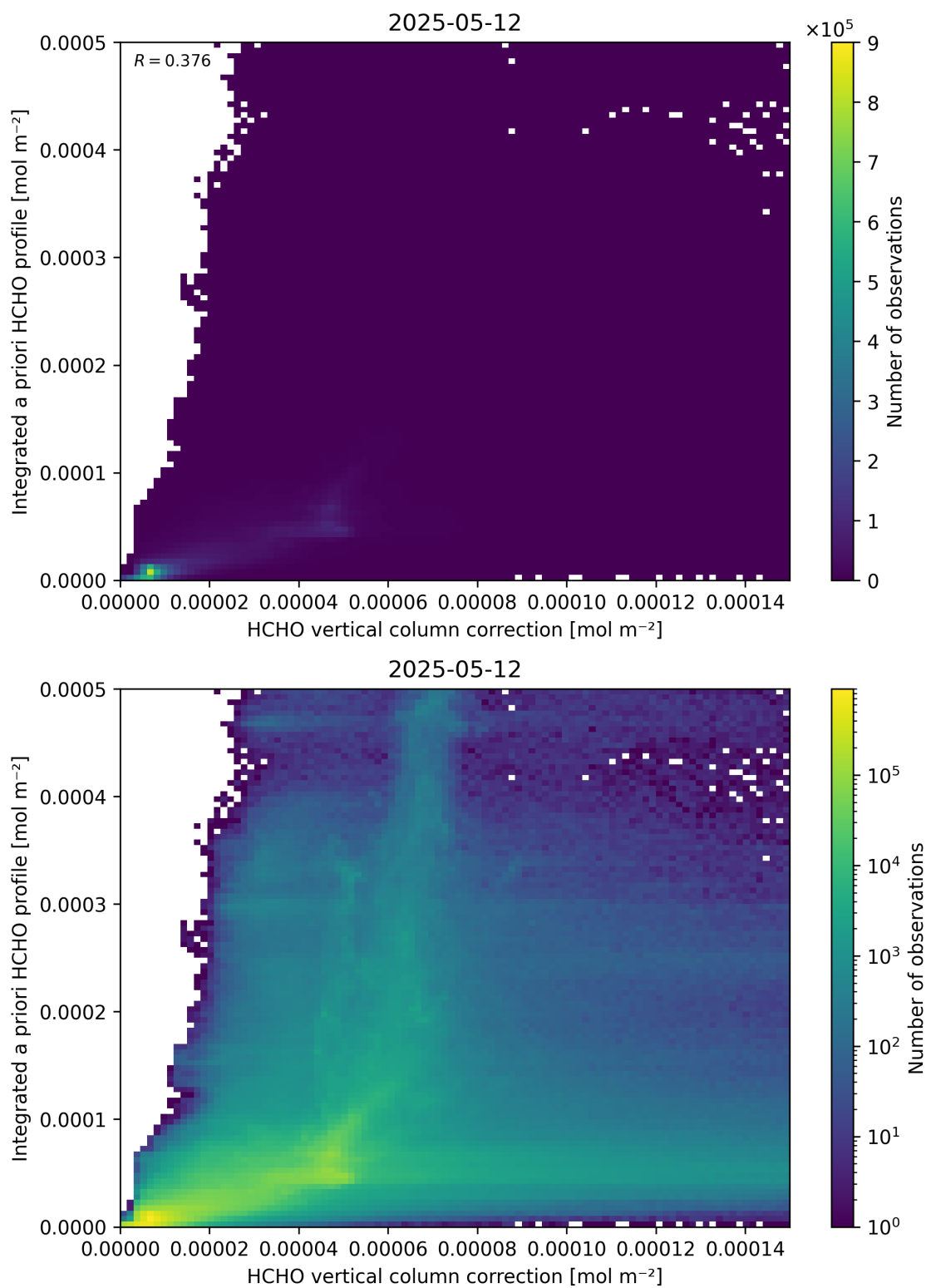
Figure 122: Scatter density plot of “HCHO vertical column correction” against “Integrated a priori HCHO profile” for 2025-05-11 to 2025-05-13.
