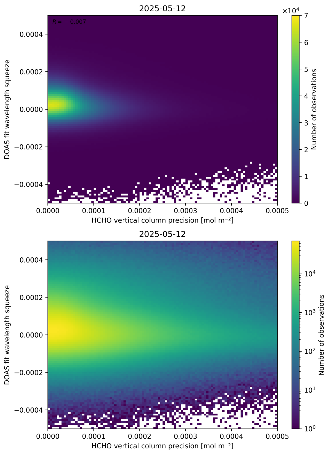
Figure 138: Scatter density plot of “HCHO vertical column precision” against “DOAS fit wavelength squeeze” for 2025-05-11 to 2025-05-13.
