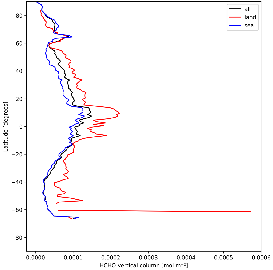
Figure 21: Zonal average of “HCHO vertical column” for 2025-05-11 to 2025-05-13.
