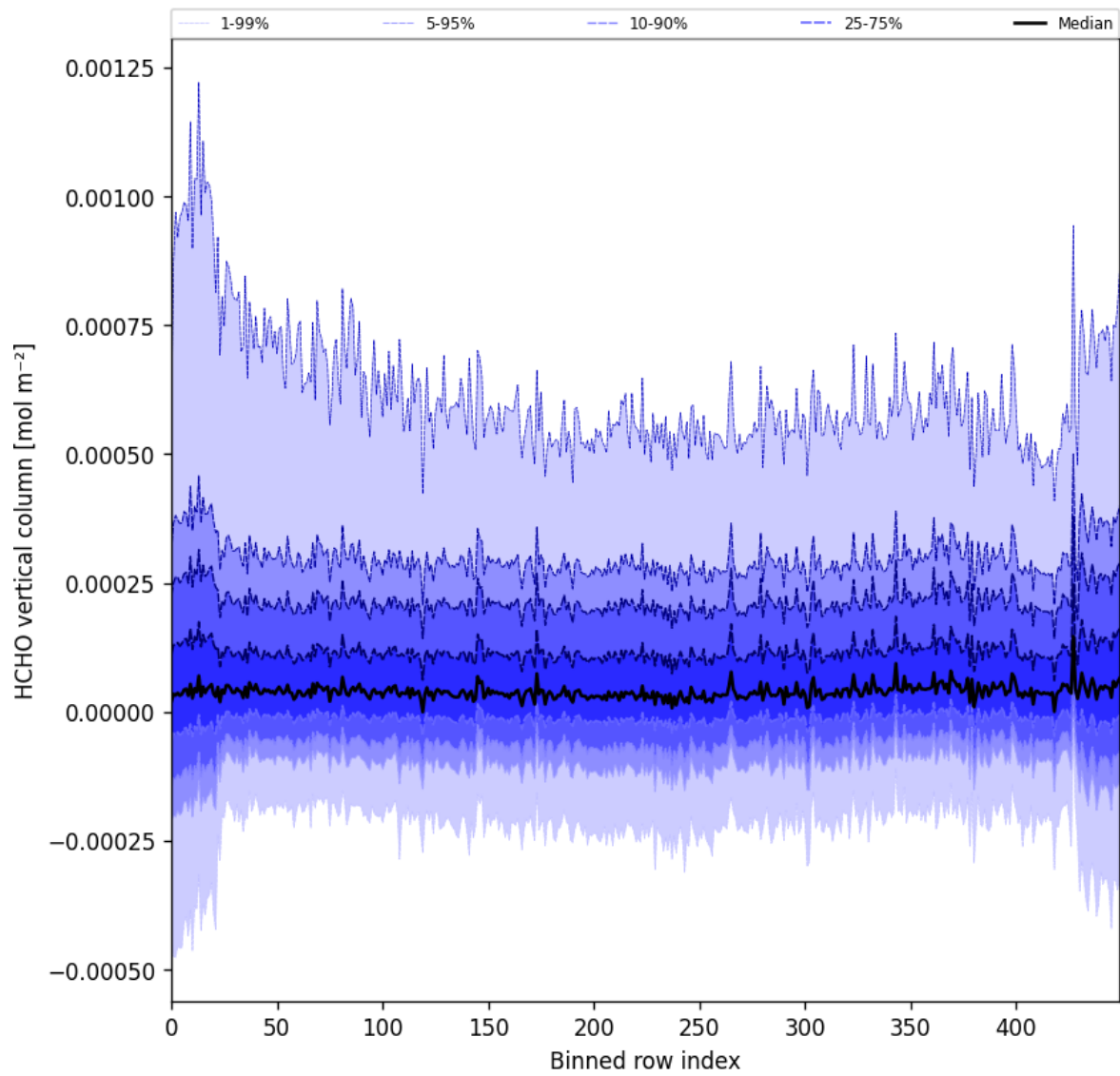
Figure 49: Along track statistics of “HCHO vertical column” for 2025-05-11 to 2025-05-13
