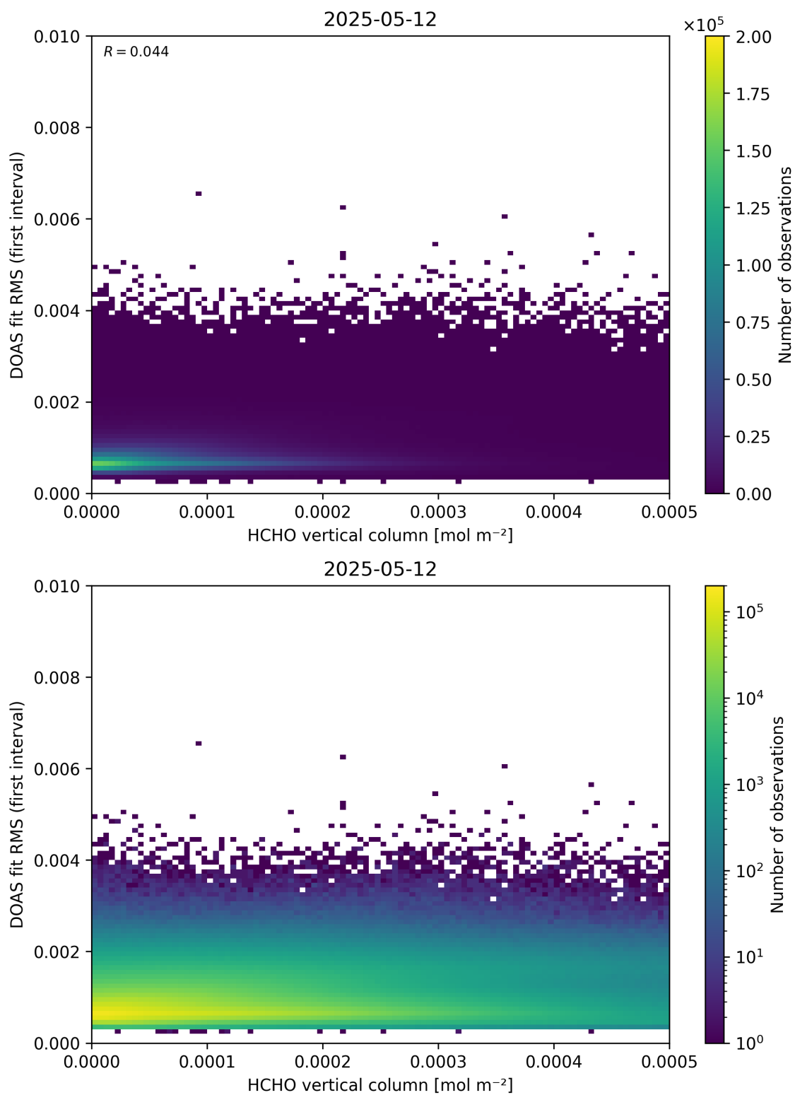
Figure 123: Scatter density plot of “HCHO vertical column” against “DOAS fit RMS (first interval)” for 2025-05-11 to 2025-05-13.
