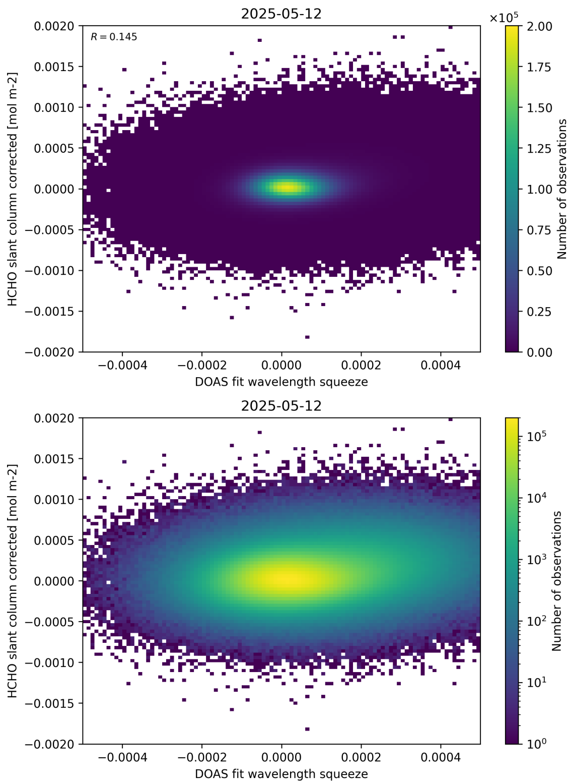
Figure 69: Scatter density plot of “DOAS fit wavelength squeeze” against “HCHO slant column corrected” for 2025-05-11 to 2025-05-13.
