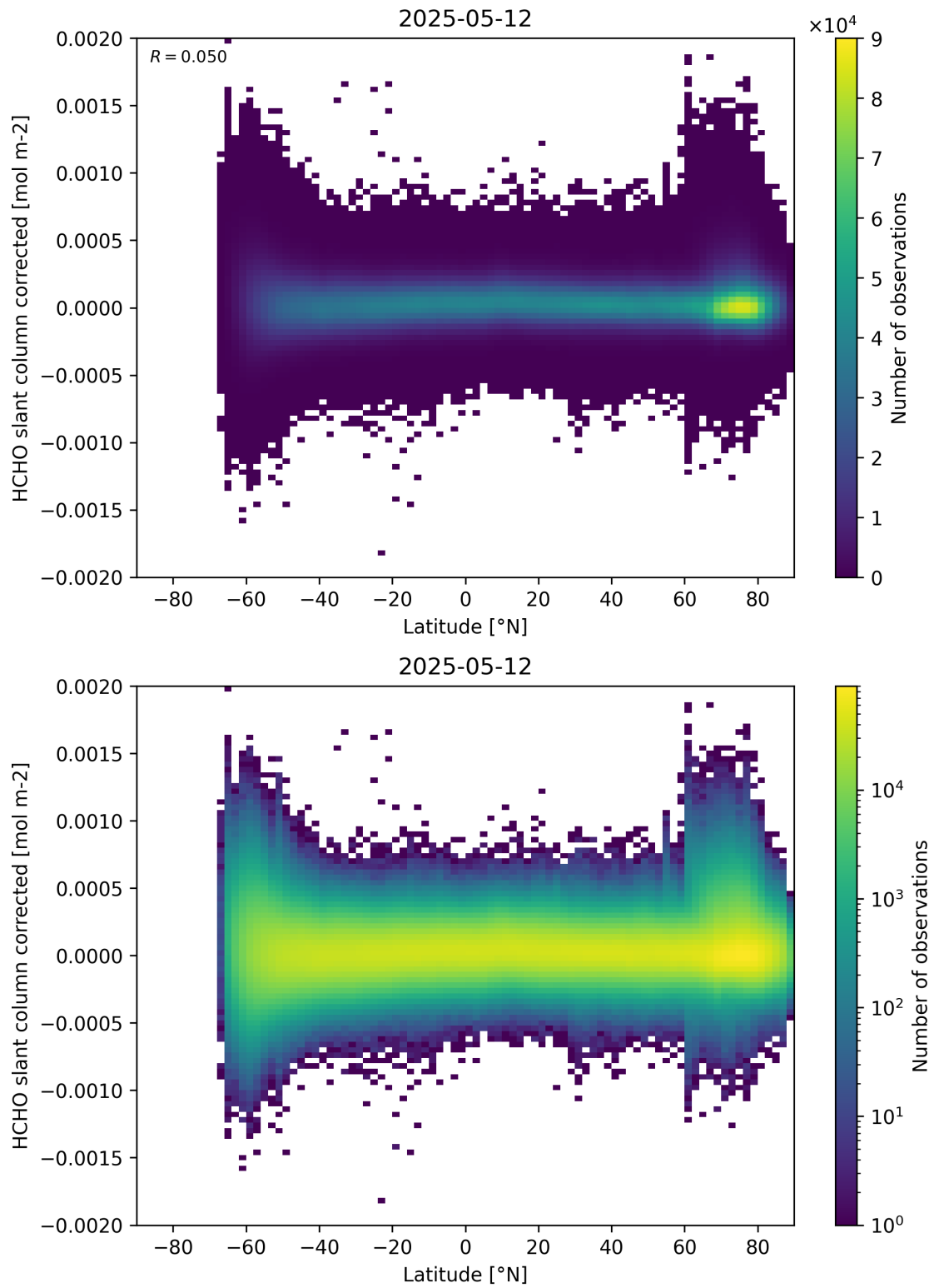
Figure 157: Scatter density plot of “Latitude” against “HCHO slant column corrected” for 2025-05-11 to 2025-05-13.
