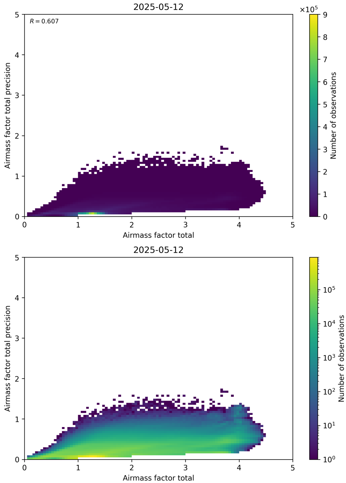
Figure 103: Scatter density plot of “Airmass factor total” against “Airmass factor total precision” for 2025-05-11 to 2025-05-13.
