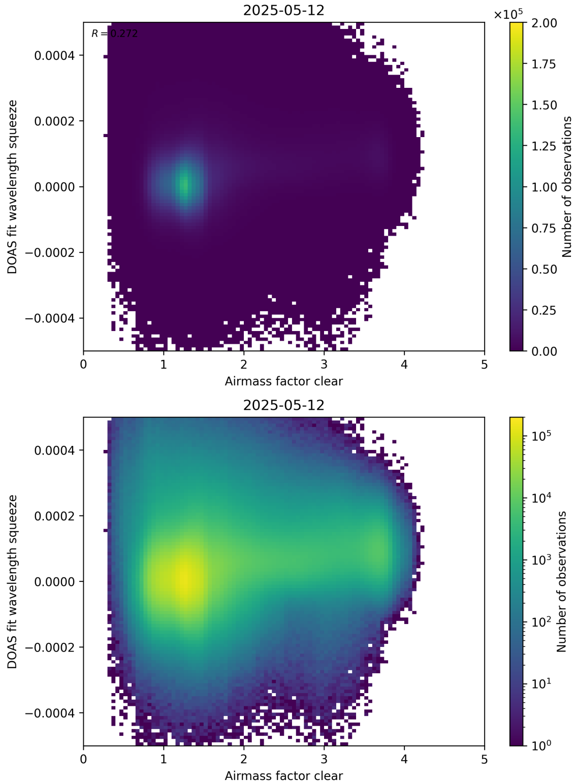
Figure 73: Scatter density plot of “Airmass factor clear” against “DOAS fit wavelength squeeze” for 2025-05-11 to 2025-05-13.
