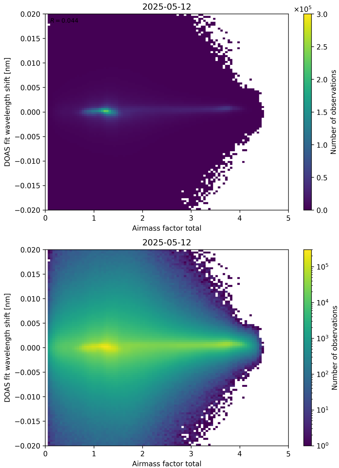
Figure 98: Scatter density plot of “Airmass factor total” against “DOAS fit wavelength shift” for 2025-05-11 to 2025-05-13.
