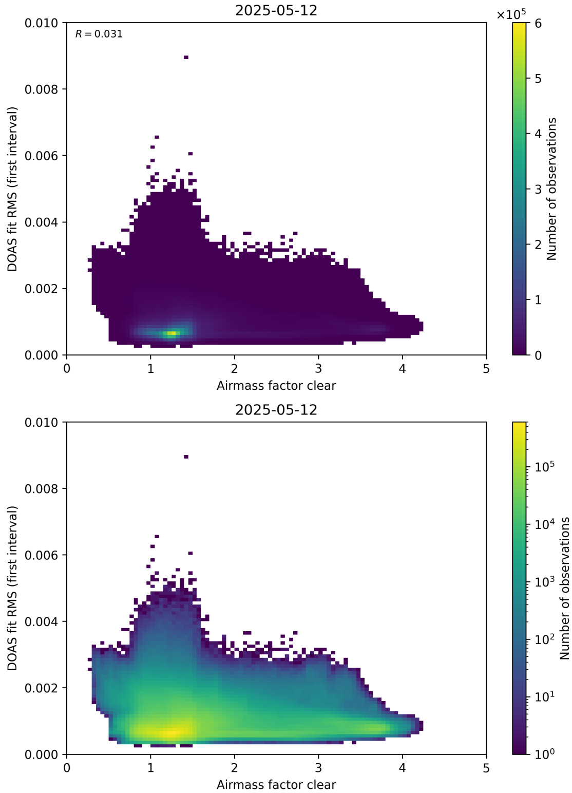
Figure 71: Scatter density plot of “Airmass factor clear” against “DOAS fit RMS (first interval)” for 2025-05-11 to 2025-05-13.
