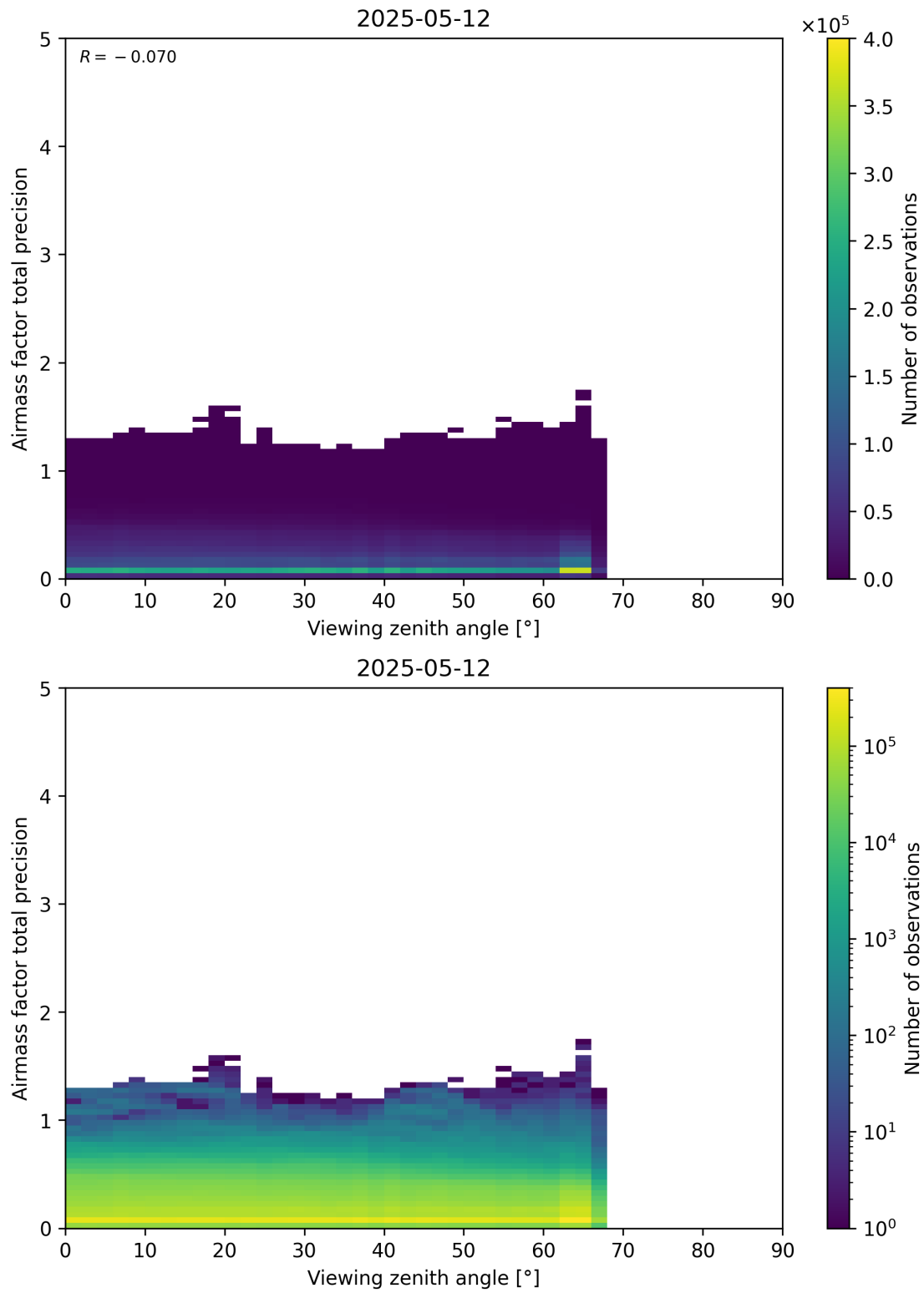
Figure 191: Scatter density plot of “Viewing zenith angle” against “Airmass factor total precision” for 2025-05-11 to 2025-05-13.
