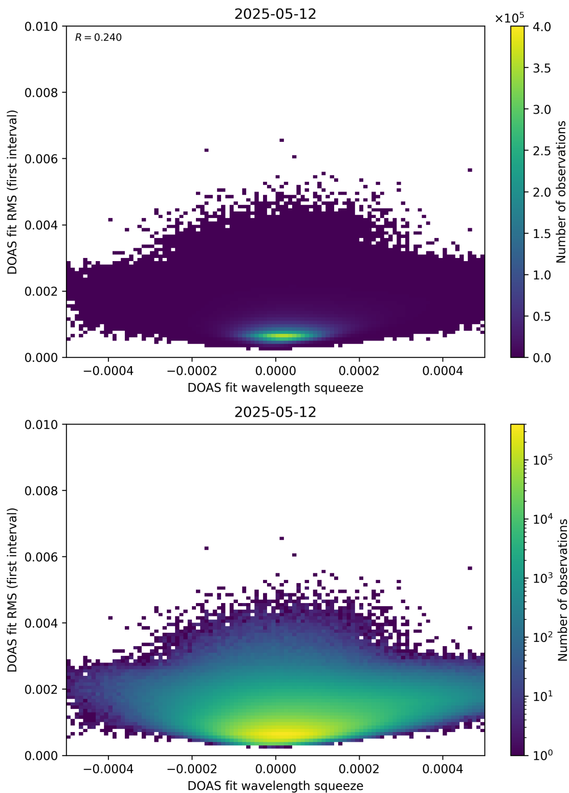
Figure 68: Scatter density plot of “DOAS fit wavelength squeeze” against “DOAS fit RMS (first interval)” for 2025-05-11 to 2025-05-13.
