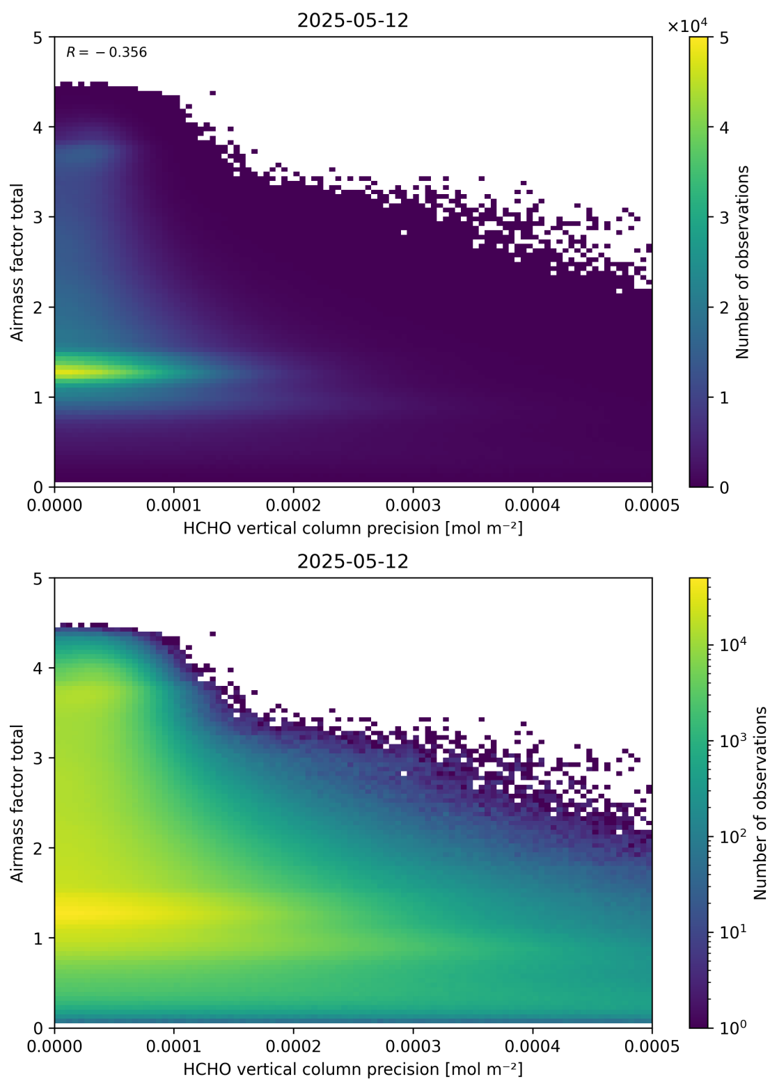
Figure 144: Scatter density plot of “HCHO vertical column precision” against “Airmass factor total” for 2025-05-11 to 2025-05-13.
