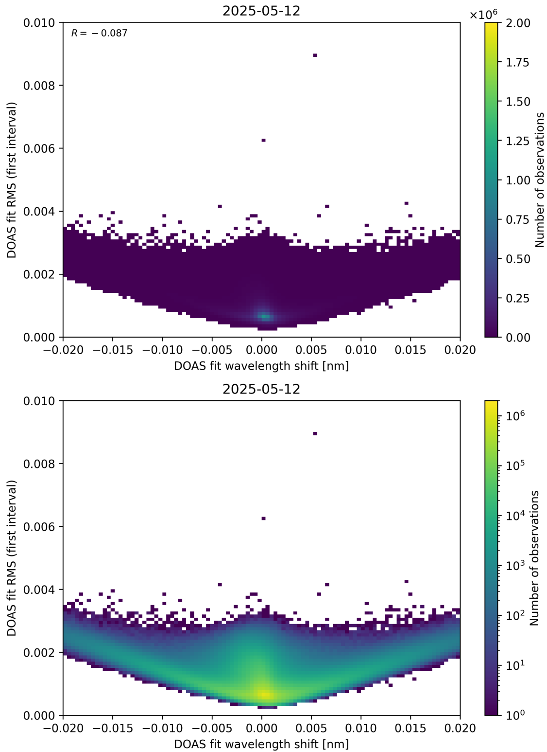
Figure 64: Scatter density plot of “DOAS fit wavelength shift” against “DOAS fit RMS (first interval)” for 2025-05-11 to 2025-05-13.
