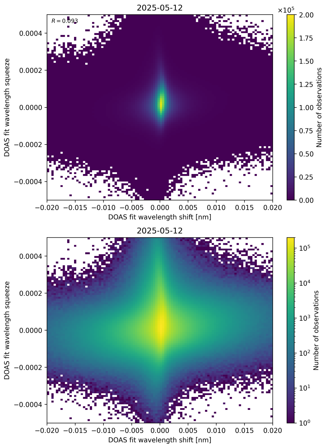
Figure 65: Scatter density plot of “DOAS fit wavelength shift” against “DOAS fit wavelength squeeze” for 2025-05-11 to 2025-05-13.
