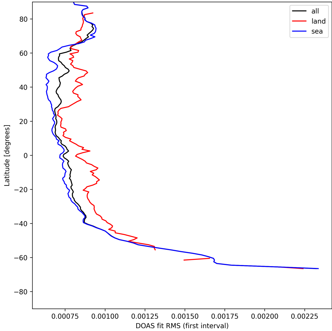
Figure 32: Zonal average of "DOAS fit RMS (first interval)" for 2025-05-11 to 2025-05-13.
