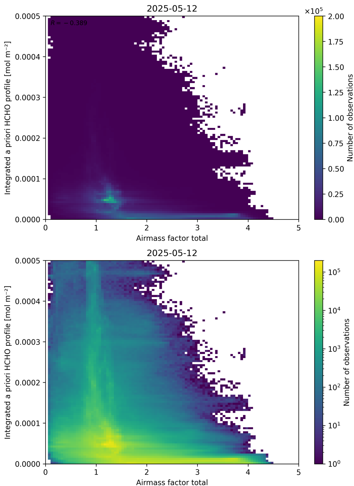
Figure 104: Scatter density plot of “Airmass factor total” against “Integrated a priori HCHO profile” for 2025-05-11 to 2025-05-13.
