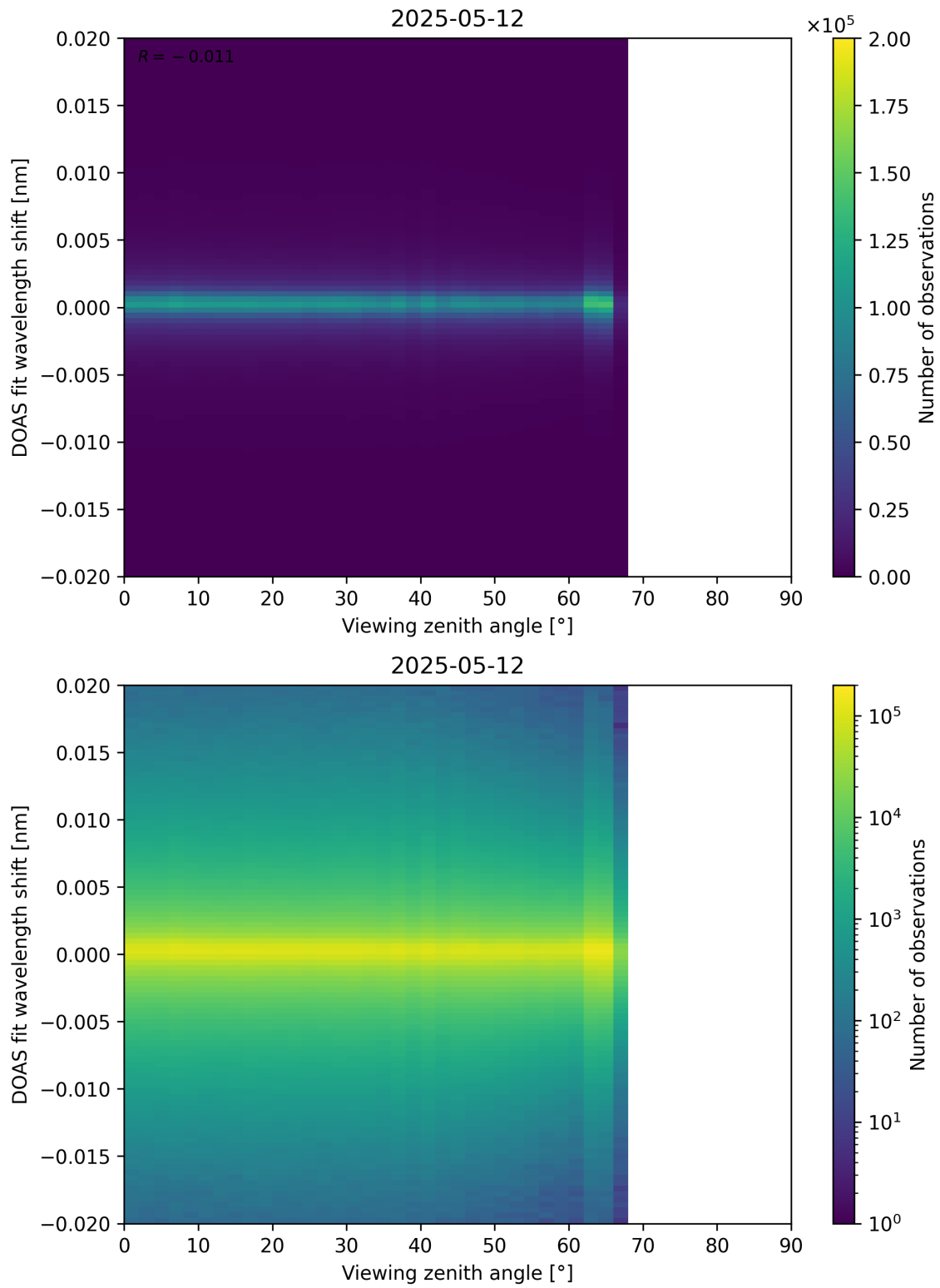
Figure 183: Scatter density plot of “Viewing zenith angle” against “DOAS fit wavelength shift” for 2025-05-11 to 2025-05-13.
