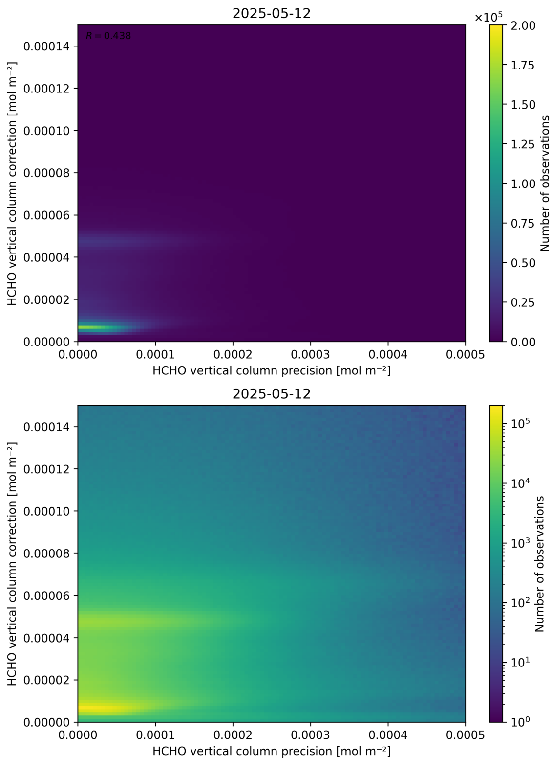
Figure 146: Scatter density plot of “HCHO vertical column precision” against “HCHO vertical column correction” for 2025-05-11 to 2025-05-13.
