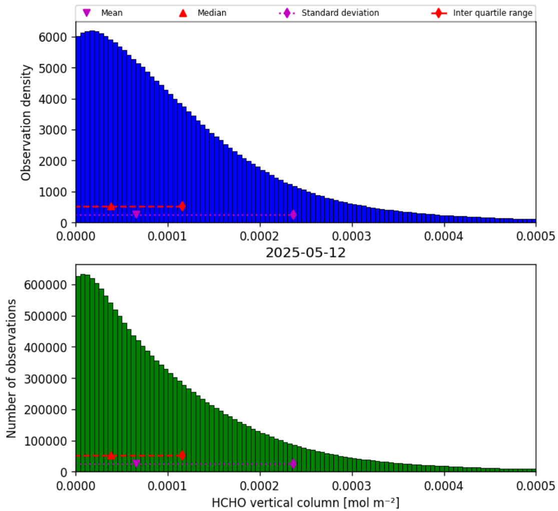
Figure 35: Histogram of “HCHO vertical column” for 2025-05-11 to 2025-05-13
