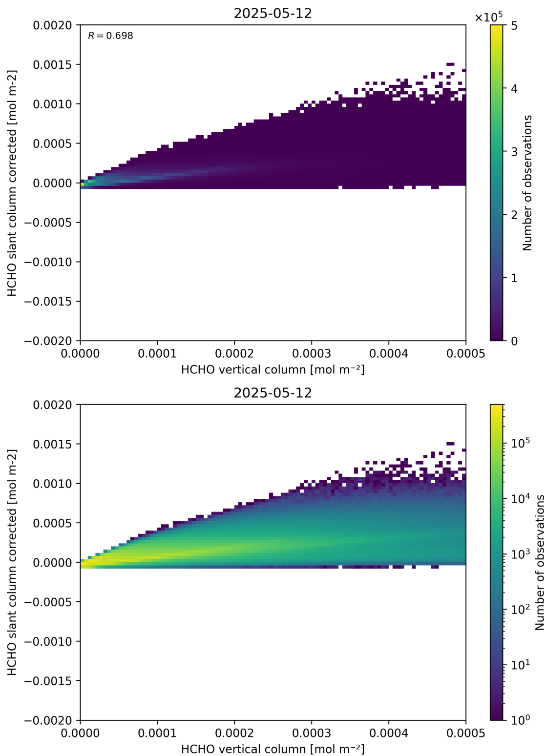
Figure 127: Scatter density plot of “HCHO vertical column” against “HCHO slant column corrected” for 2025-05-11 to 2025-05-13.
