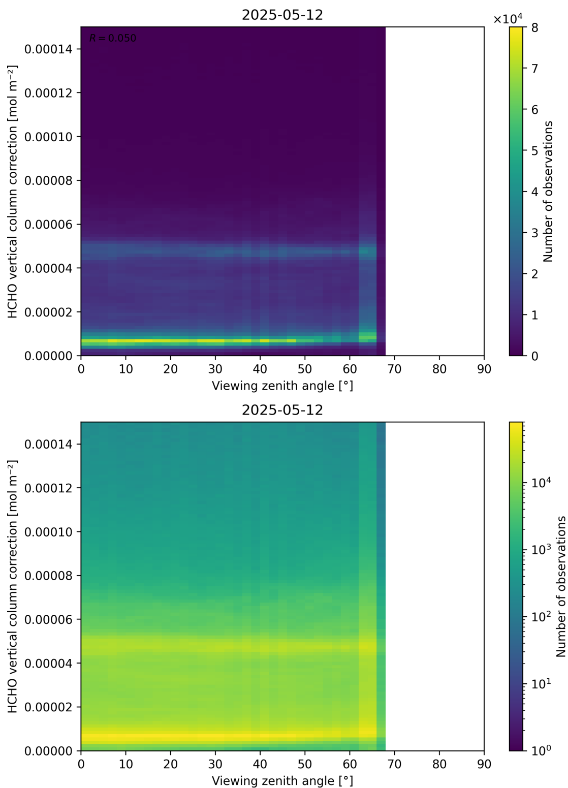
Figure 193: Scatter density plot of “Viewing zenith angle” against “HCHO vertical column correction” for 2025-05-11 to 2025-05-13.
