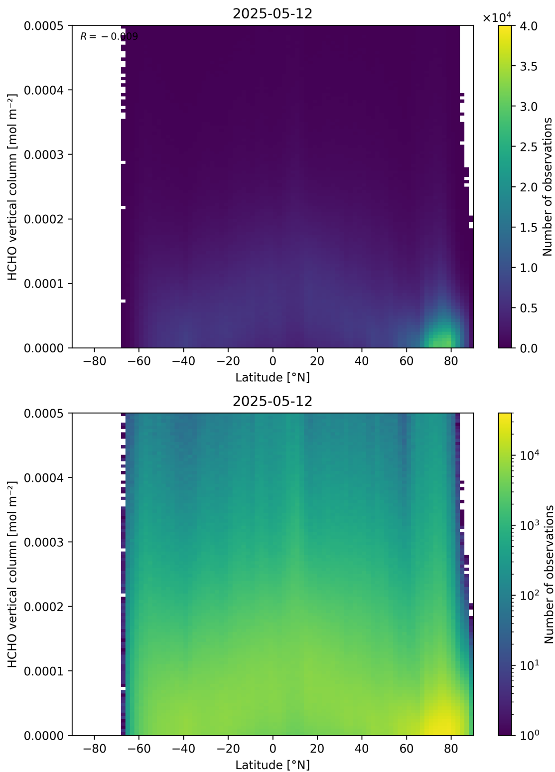
Figure 163: Scatter density plot of “Latitude” against “HCHO vertical column” for 2025-05-11 to 2025-05-13.
