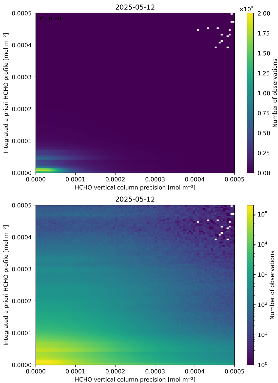
Figure 147: Scatter density plot of “HCHO vertical column precision” against “Integrated a priori HCHO profile” for 2025-05-11 to 2025-05-13.
