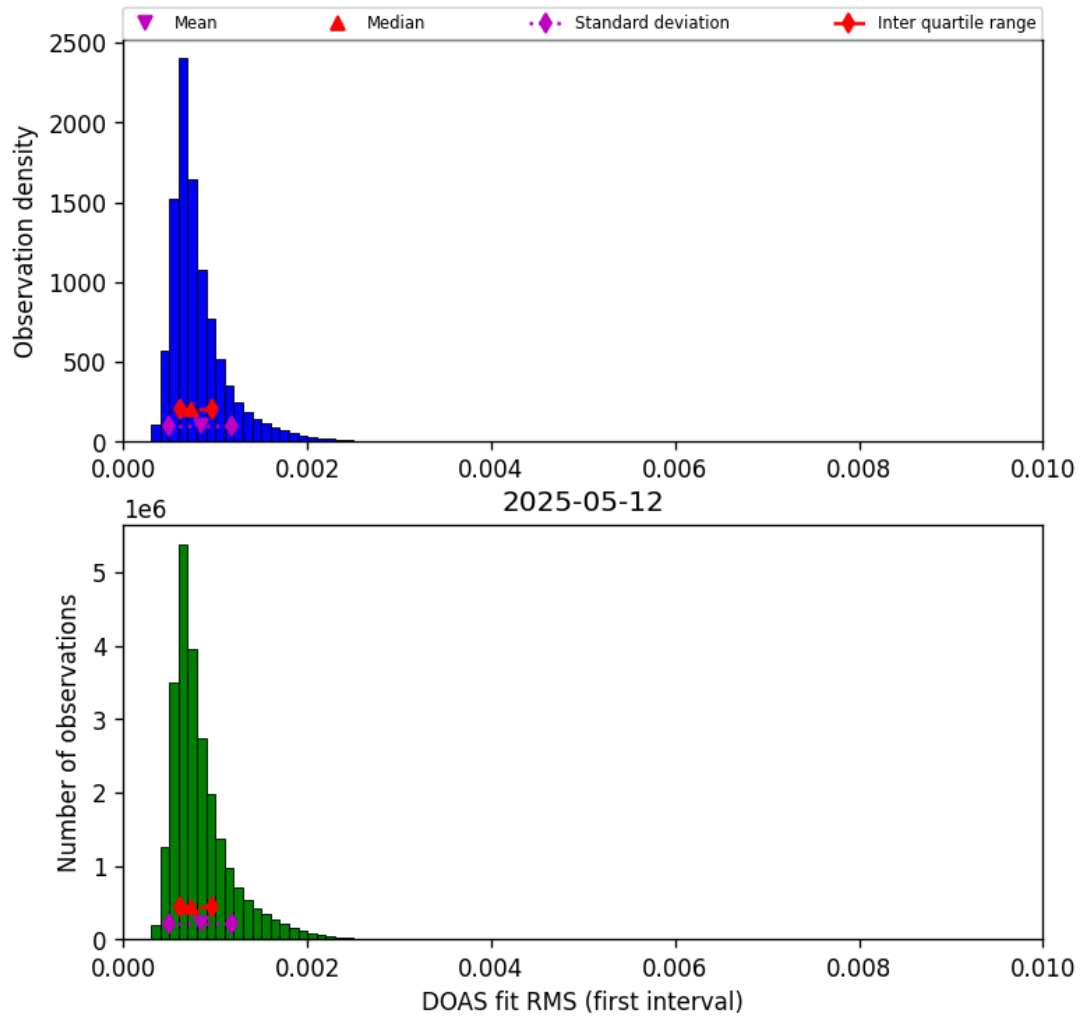
Figure 46: Histogram of “DOAS fit RMS (first interval)” for 2025-05-11 to 2025-05-13
