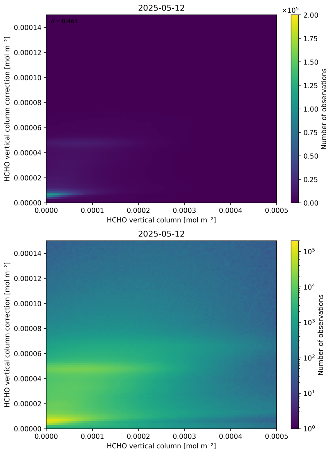
Figure 133: Scatter density plot of “HCHO vertical column” against “HCHO vertical column correction” for 2025-05-11 to 2025-05-13.
