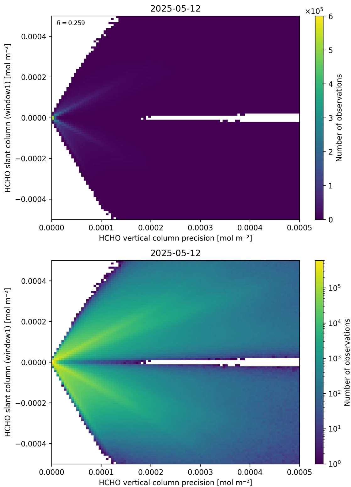
Figure 142: Scatter density plot of “HCHO vertical column precision” against “HCHO slant column (window1)” for 2025-05-11 to 2025-05-13.
