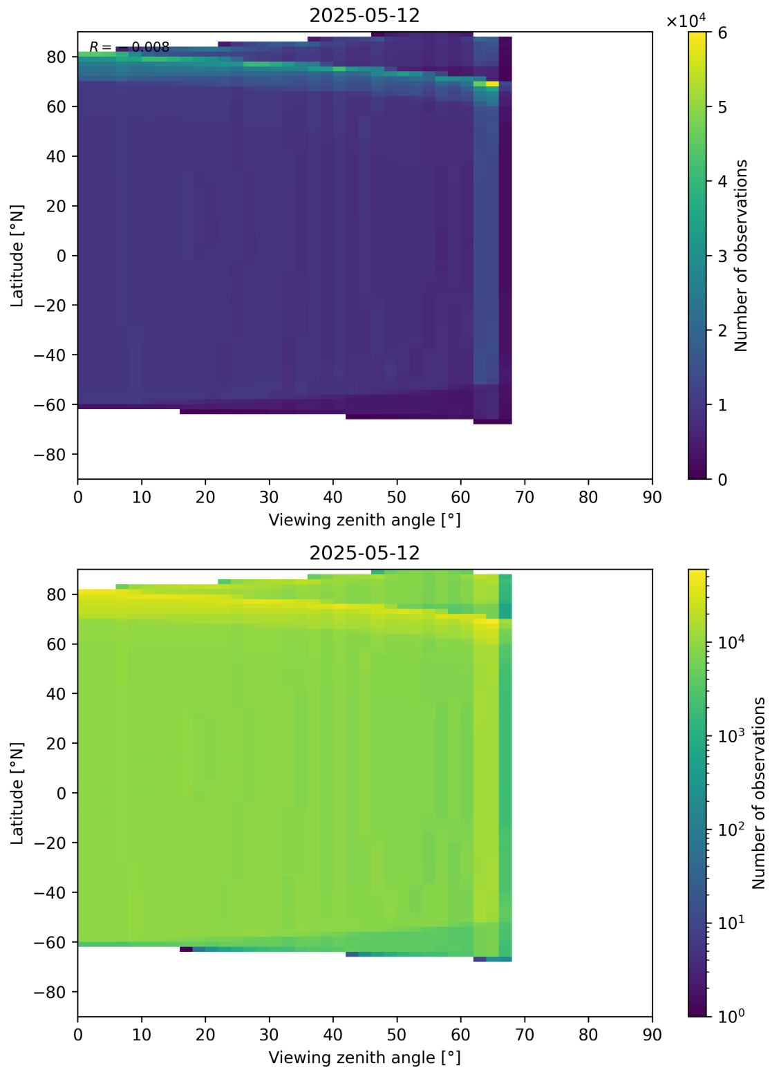
Figure 196: Scatter density plot of “Viewing zenith angle” against “Latitude” for 2025-05-11 to 2025-05-13.
