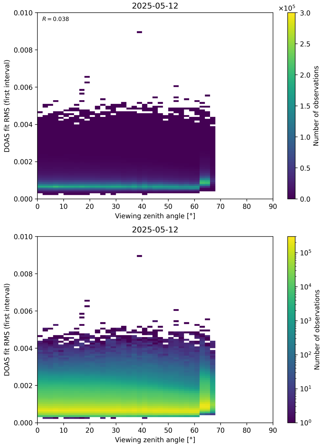
Figure 182: Scatter density plot of “Viewing zenith angle” against “DOAS fit RMS (first interval)” for 2025-05-11 to 2025-05-13.
