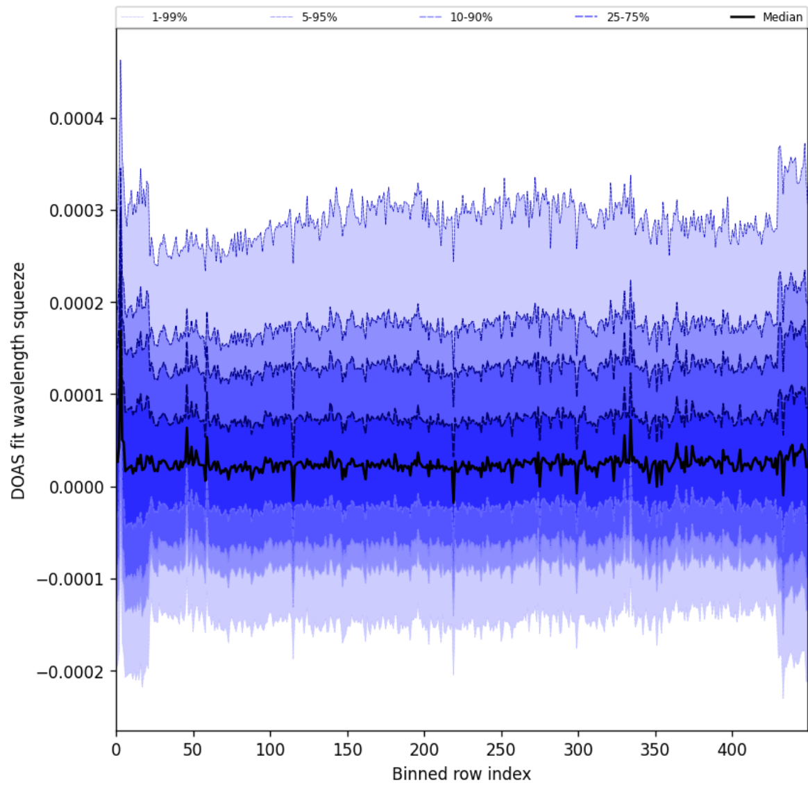
Figure 59: Along track statistics of “DOAS fit wavelength squeeze” for 2025-05-11 to 2025-05-13
