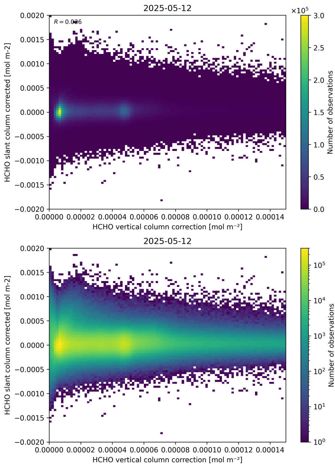
Figure 116: Scatter density plot of “HCHO vertical column correction” against “HCHO slant column corrected” for 2025-05-11 to 2025-05-13.
