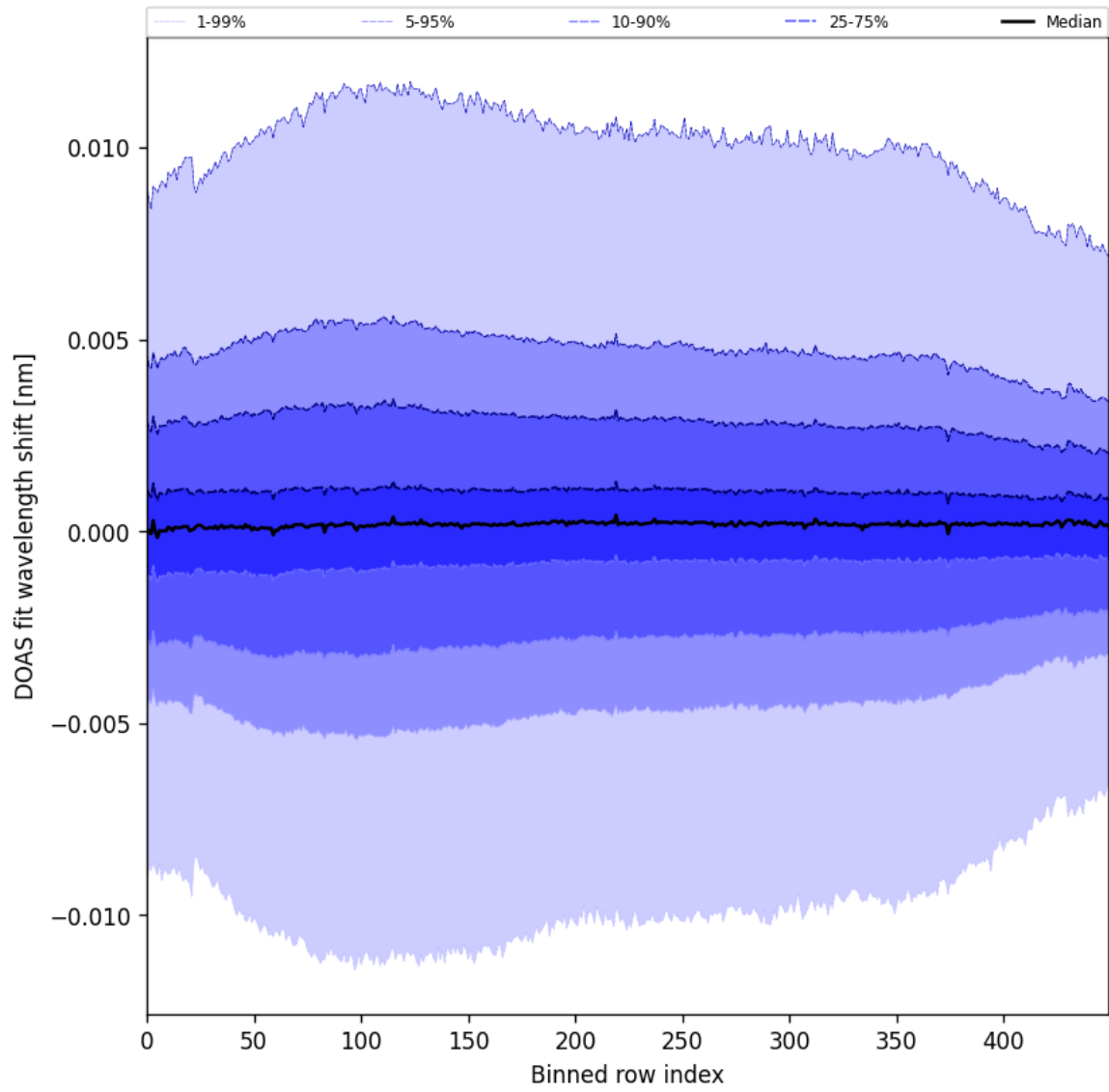
Figure 58: Along track statistics of “DOAS fit wavelength shift” for 2025-05-11 to 2025-05-13
