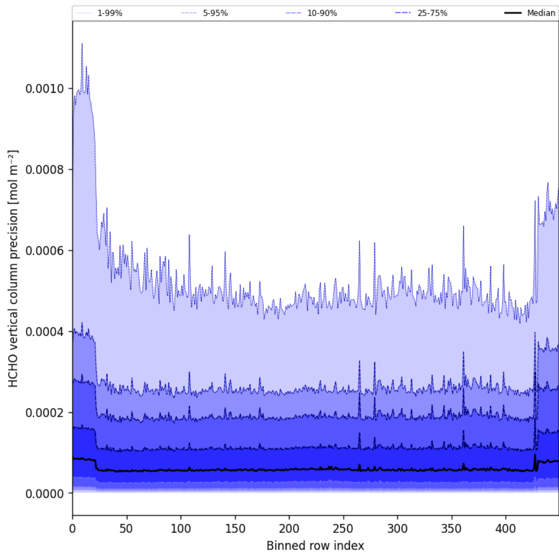
Figure 50: Along track statistics of “HCHO vertical column precision” for 2025-05-11 to 2025-05-13
