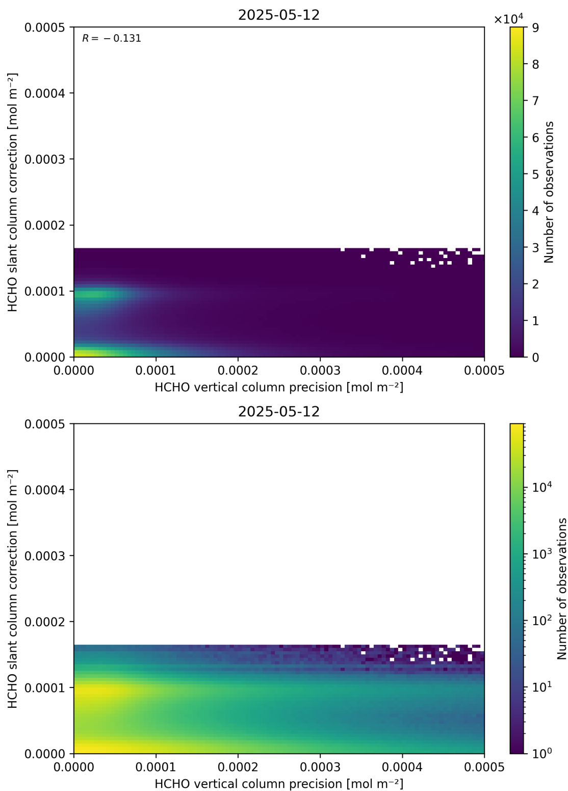
Figure 141: Scatter density plot of “HCHO vertical column precision” against “HCHO slant column correction” for 2025-05-11 to 2025-05-13.
