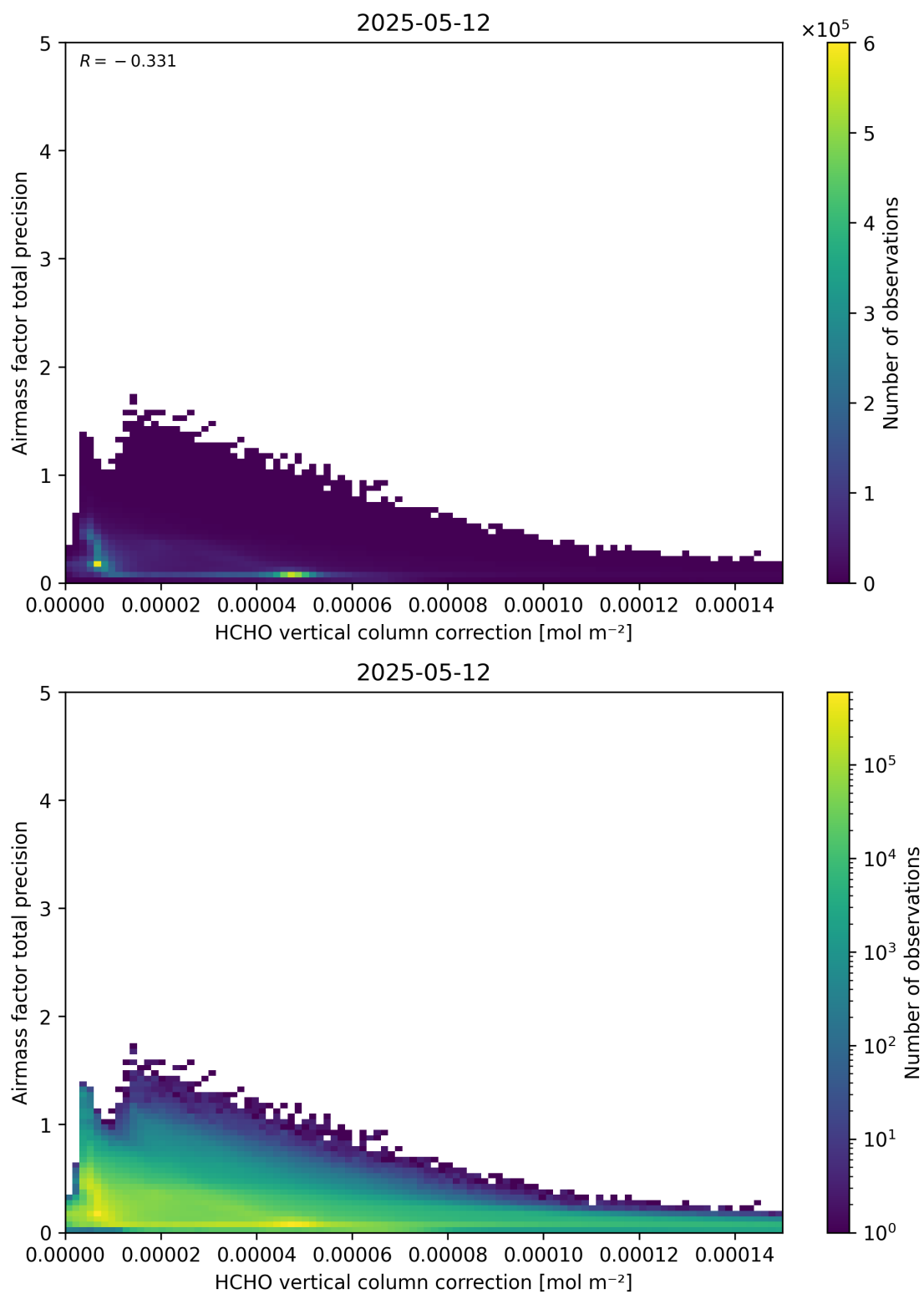
Figure 121: Scatter density plot of “HCHO vertical column correction” against “Airmass factor total precision” for 2025-05-11 to 2025-05-13.
