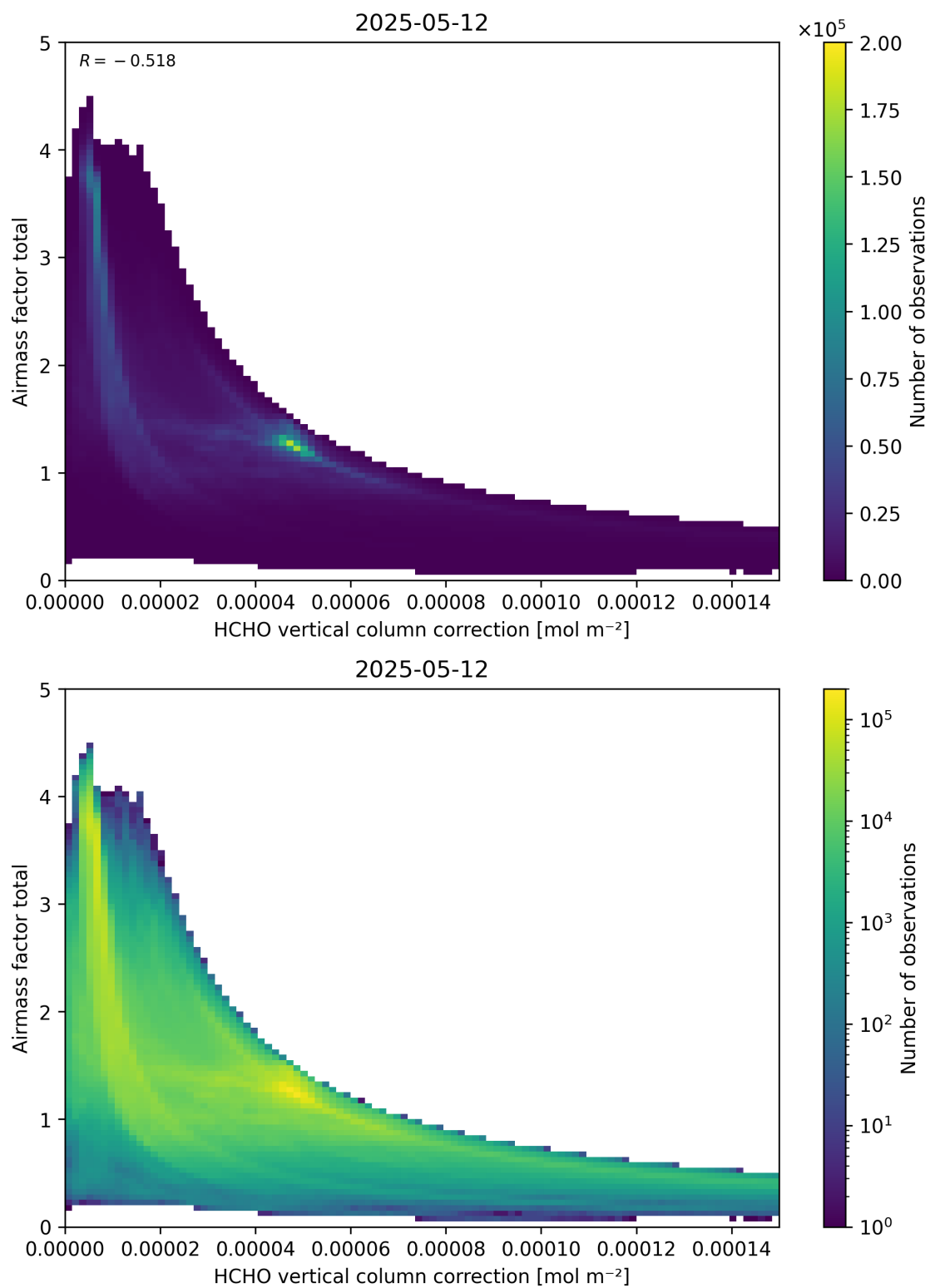
Figure 120: Scatter density plot of “HCHO vertical column correction” against “Airmass factor total” for 2025-05-11 to 2025-05-13.
