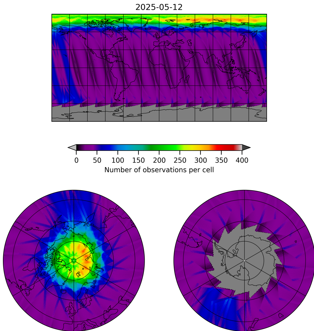
Figure 19: Map of the number of observations for 2025-05-11 to 2025-05-13
