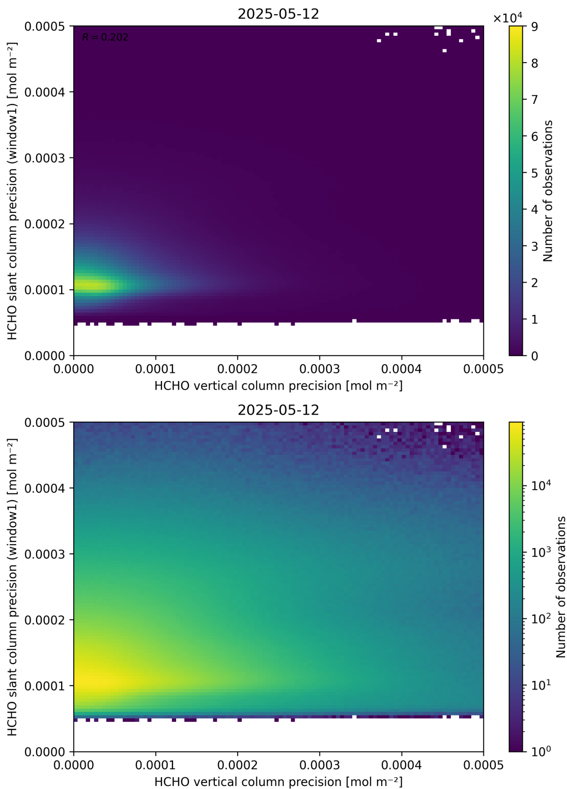
Figure 143: Scatter density plot of “HCHO vertical column precision” against “HCHO slant column precision (window1)” for 2025-05-11 to 2025-05-13.
