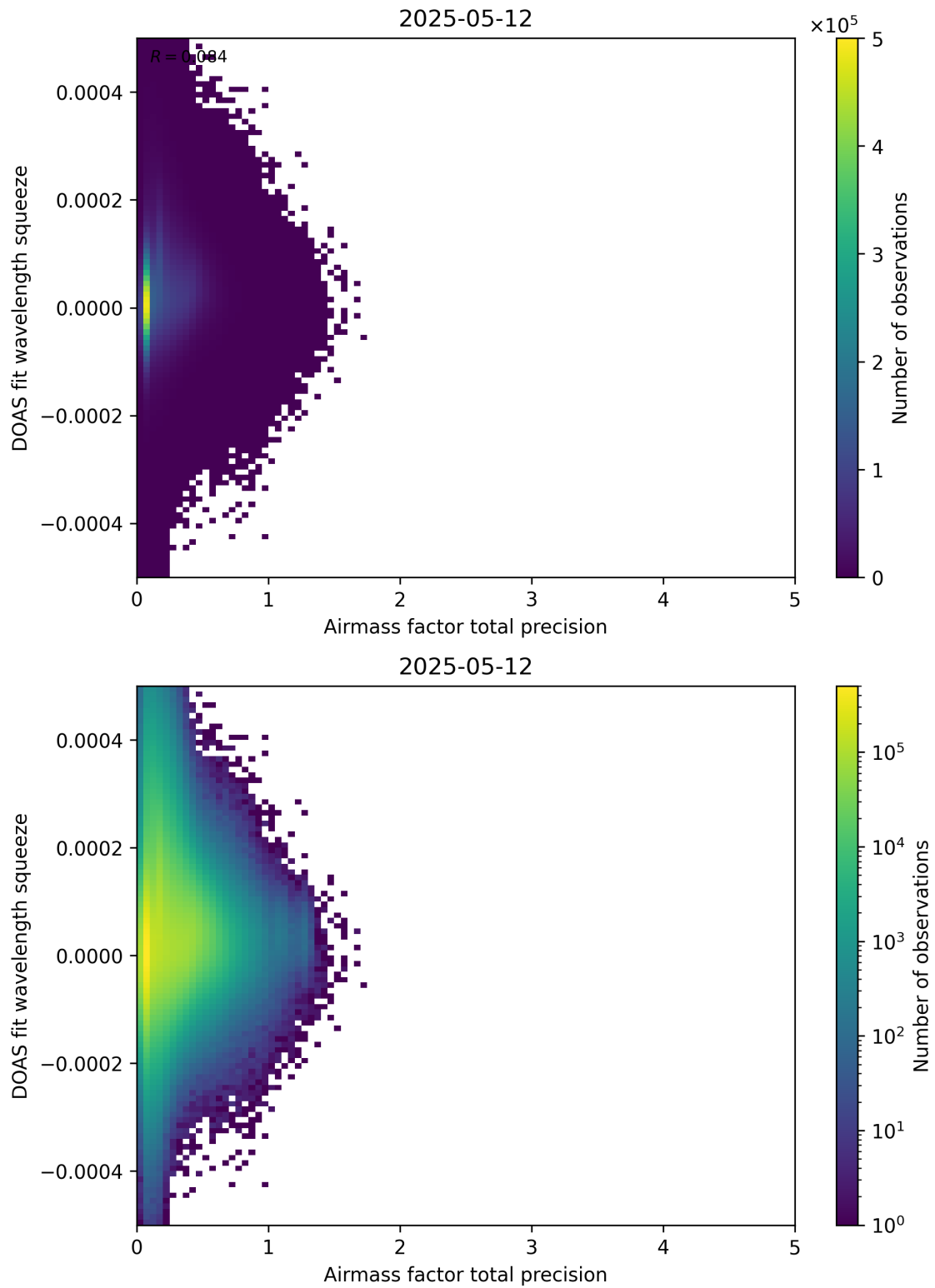
Figure 107: Scatter density plot of “Airmass factor total precision” against “DOAS fit wavelength squeeze” for 2025-05-11 to 2025-05-13.
