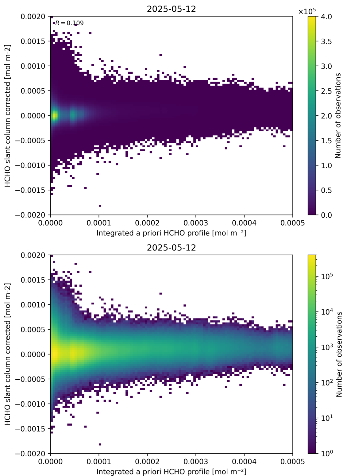
Figure 151: Scatter density plot of “Integrated a priori HCHO profile” against “HCHO slant column corrected” for 2025-05-11 to 2025-05-13.
