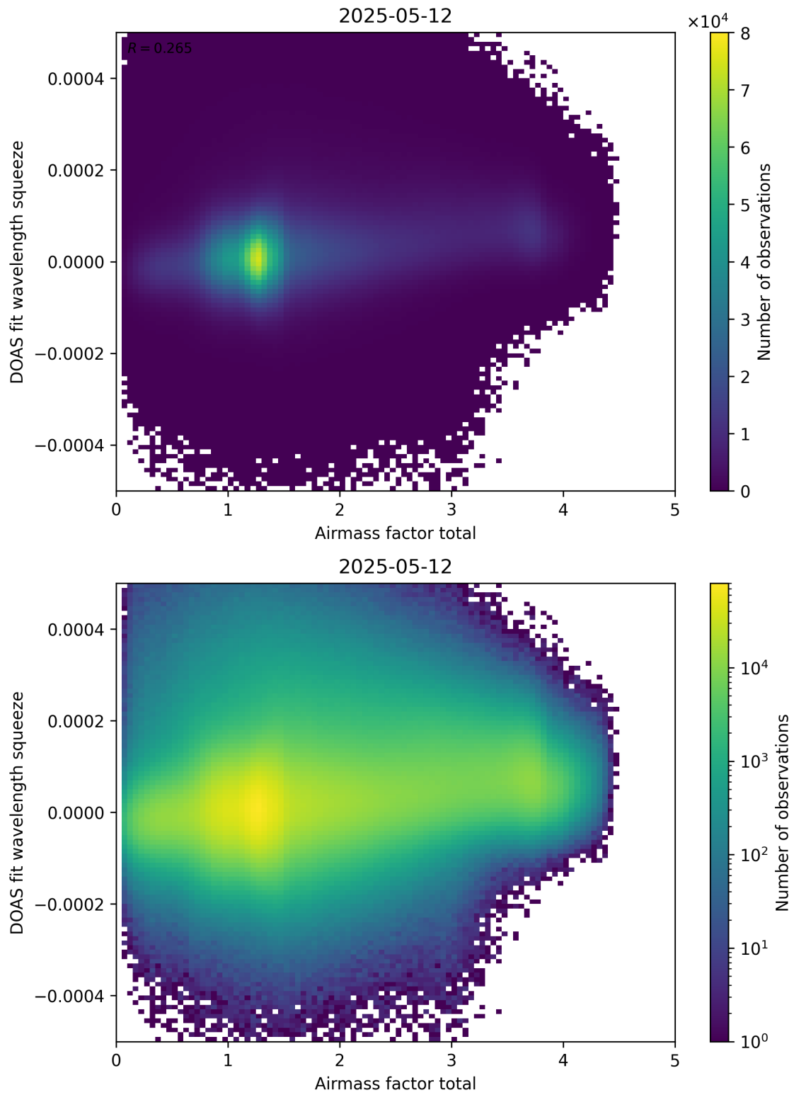
Figure 99: Scatter density plot of “Airmass factor total” against “DOAS fit wavelength squeeze” for 2025-05-11 to 2025-05-13.
