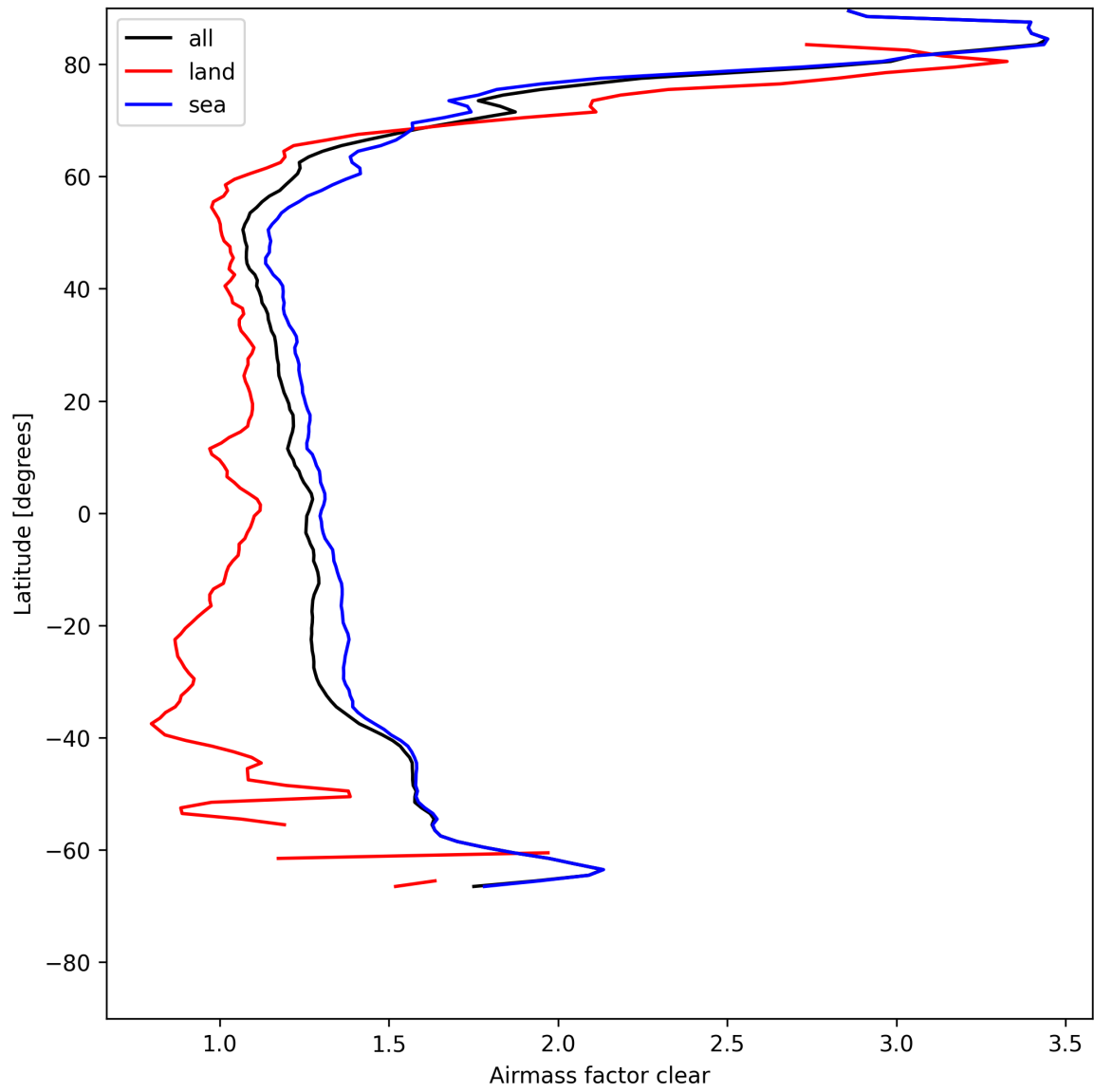
Figure 28: Zonal average of “Airmass factor clear” for 2025-05-11 to 2025-05-13.
