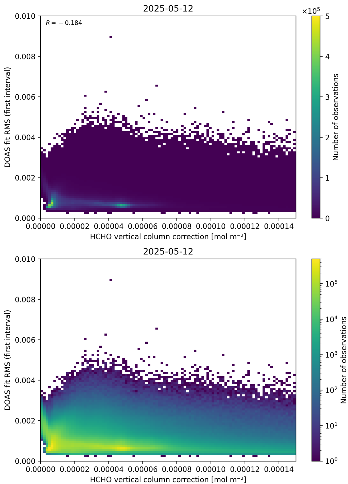
Figure 112: Scatter density plot of “HCHO vertical column correction” against “DOAS fit RMS (first interval)” for 2025-05-11 to 2025-05-13.
