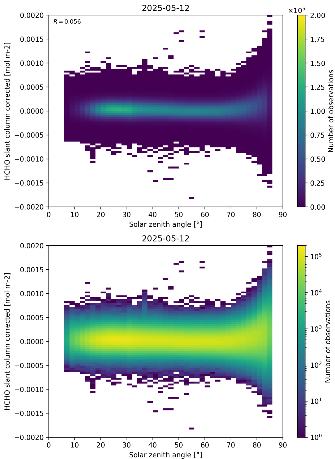
Figure 171: Scatter density plot of “Solar zenith angle” against “HCHO slant column corrected” for 2025-05-11 to 2025-05-13.
