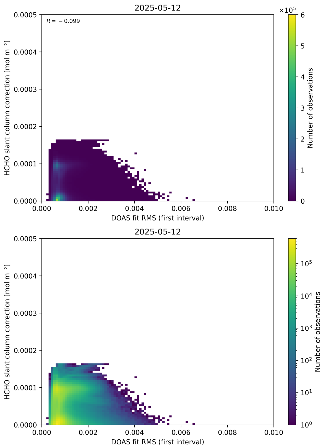
Figure 63: Scatter density plot of “DOAS fit RMS (first interval)” against “HCHO slant column correction” for 2025-05-11 to 2025-05-13.
