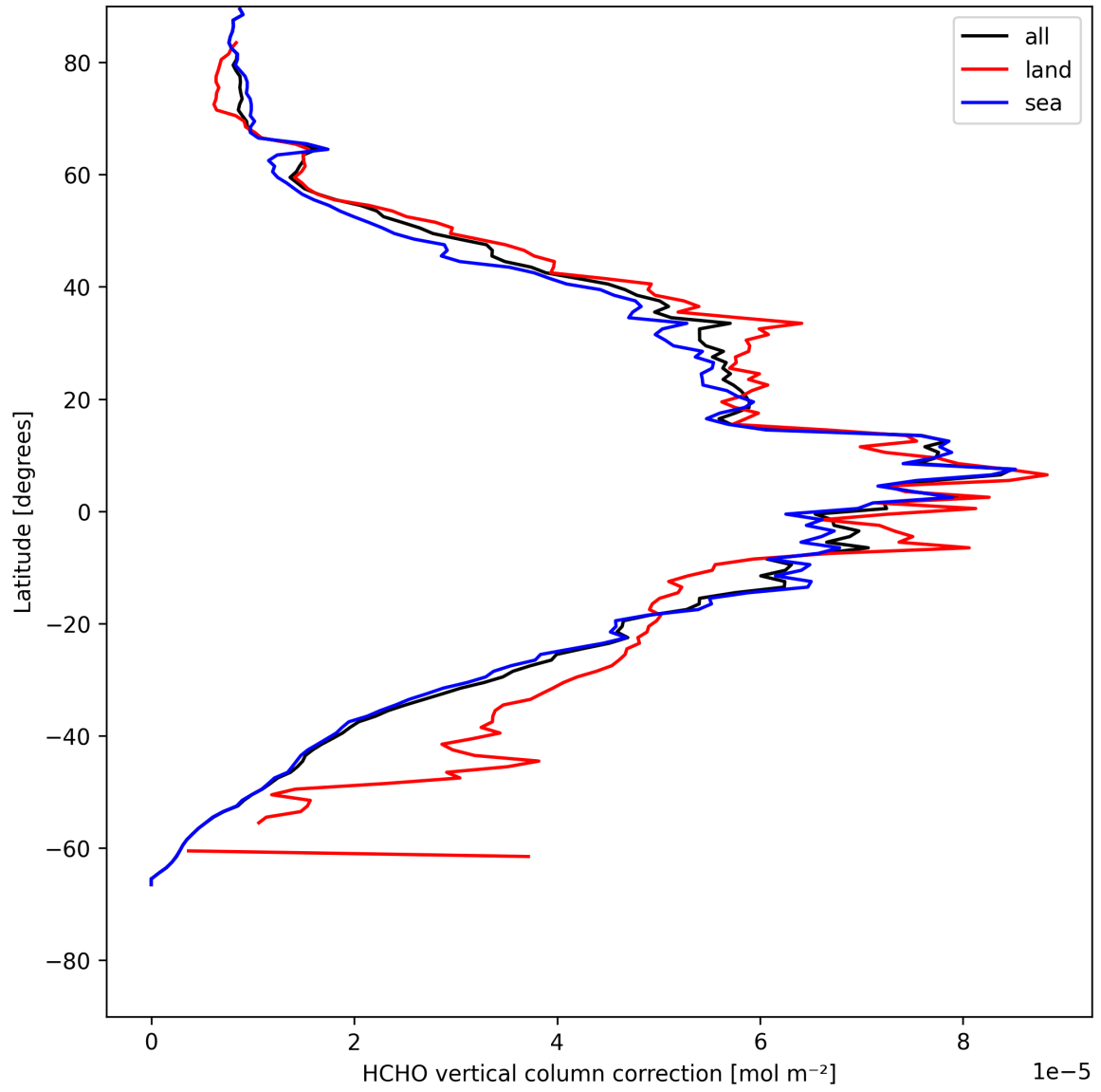
Figure 23: Zonal average of “HCHO vertical column correction” for 2025-05-11 to 2025-05-13.
