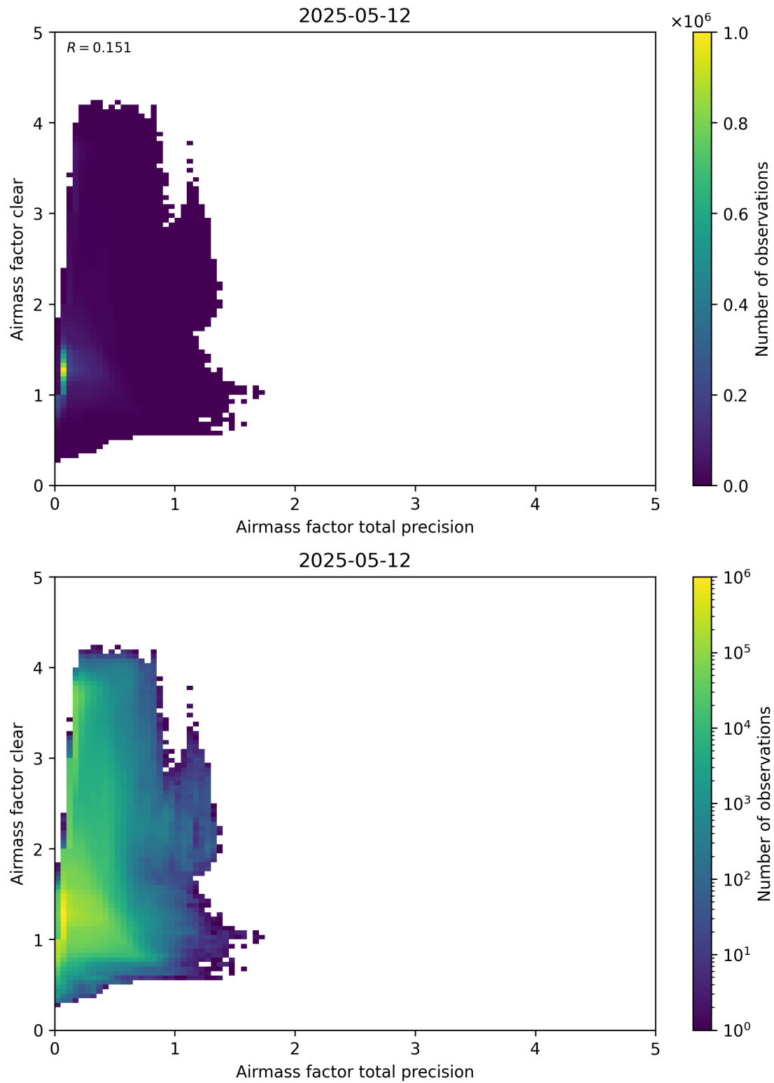
Figure 108: Scatter density plot of “Airmass factor total precision” against “Airmass factor clear” for 2025-05-11 to 2025-05-13.
