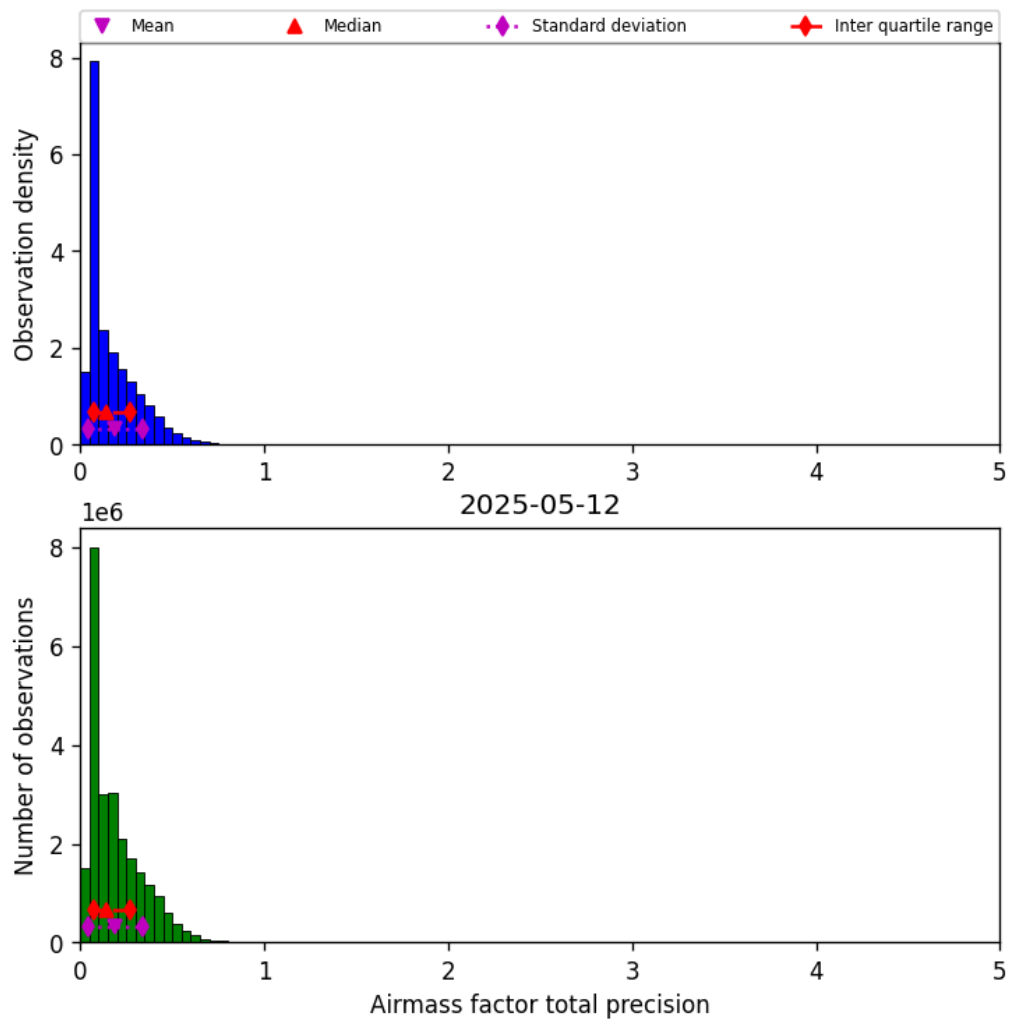
Figure 41: Histogram of “Airmass factor total precision” for 2025-05-11 to 2025-05-13
