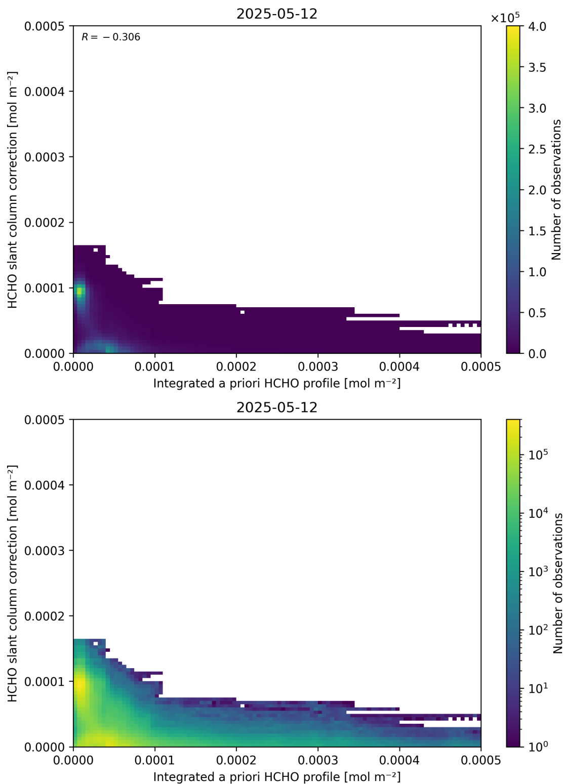
Figure 152: Scatter density plot of “Integrated a priori HCHO profile” against “HCHO slant column correction” for 2025-05-11 to 2025-05-13.
