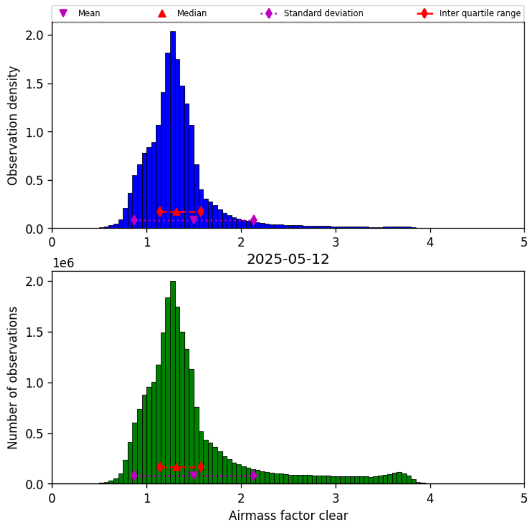
Figure 42: Histogram of “Airmass factor clear” for 2025-05-11 to 2025-05-13
