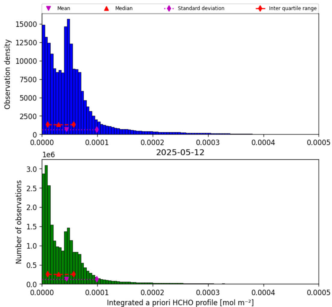
Figure 43: Histogram of “Integrated a priori HCHO profile” for 2025-05-11 to 2025-05-13
