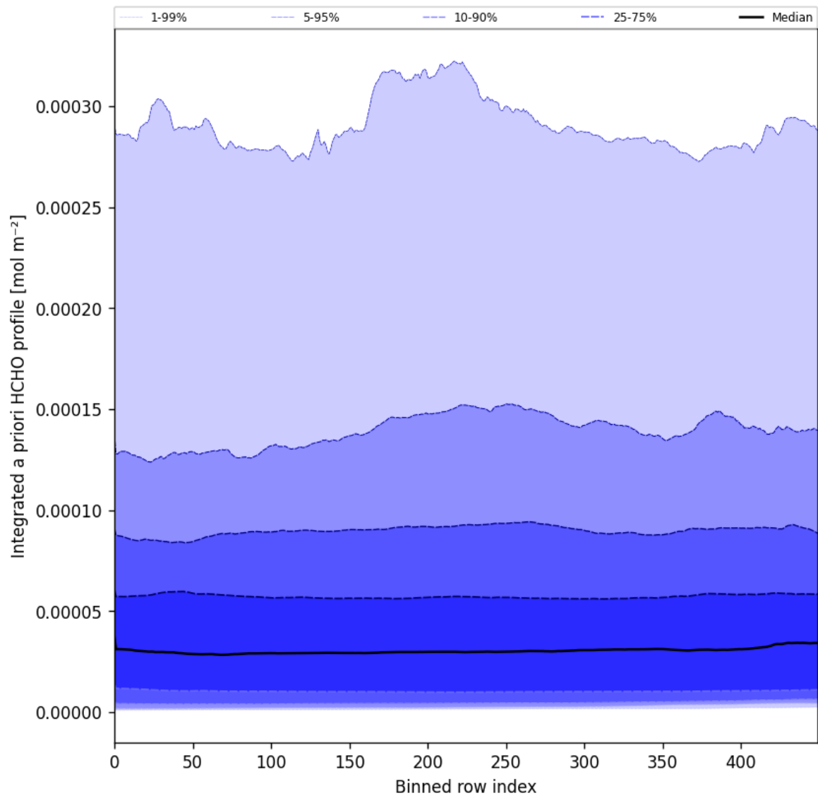
Figure 57: Along track statistics of "Integrated a priori HCHO profile" for 2025-05-11 to 2025-05-13
