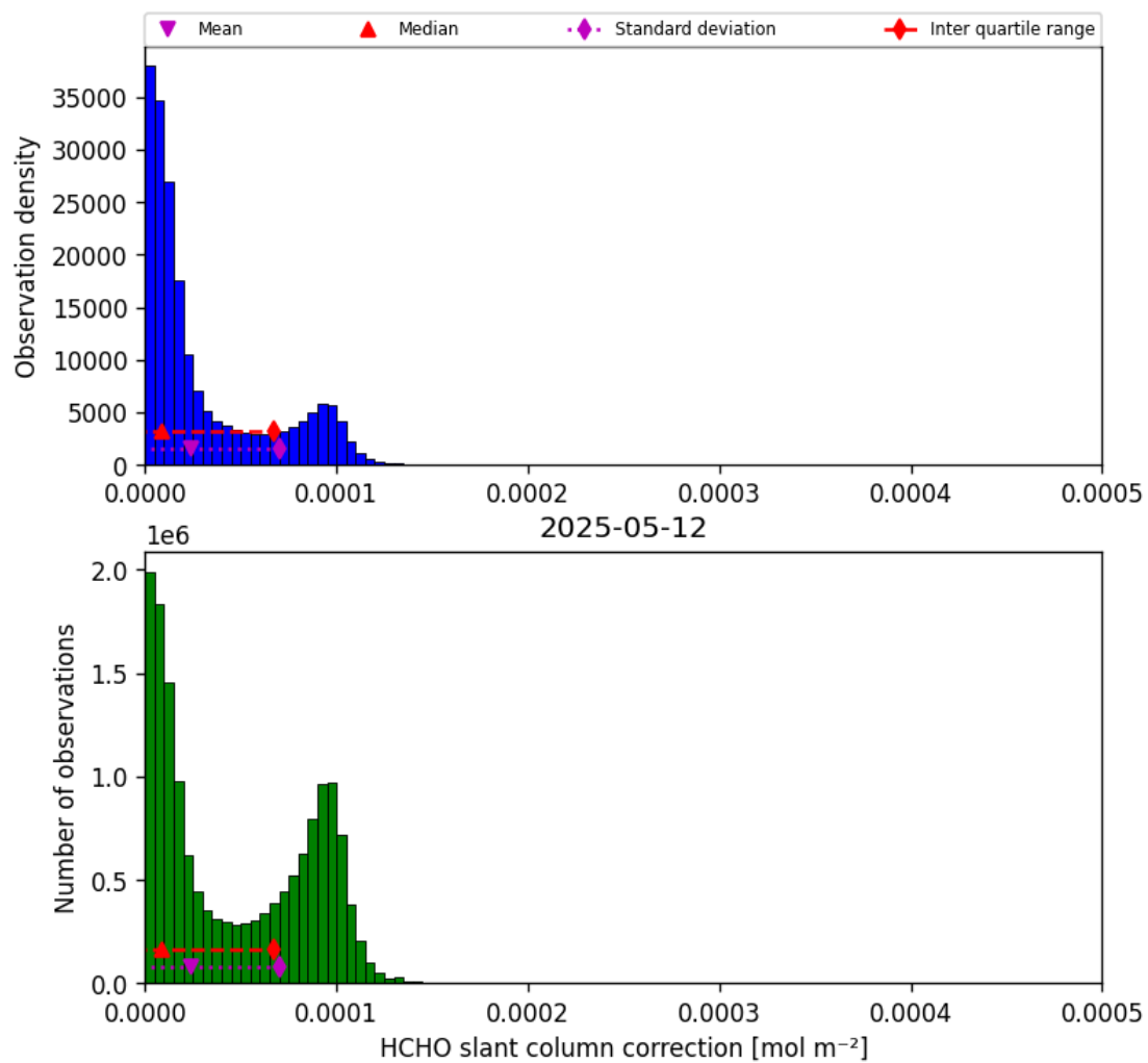
Figure 47: Histogram of “HCHO slant column correction” for 2025-05-11 to 2025-05-13
