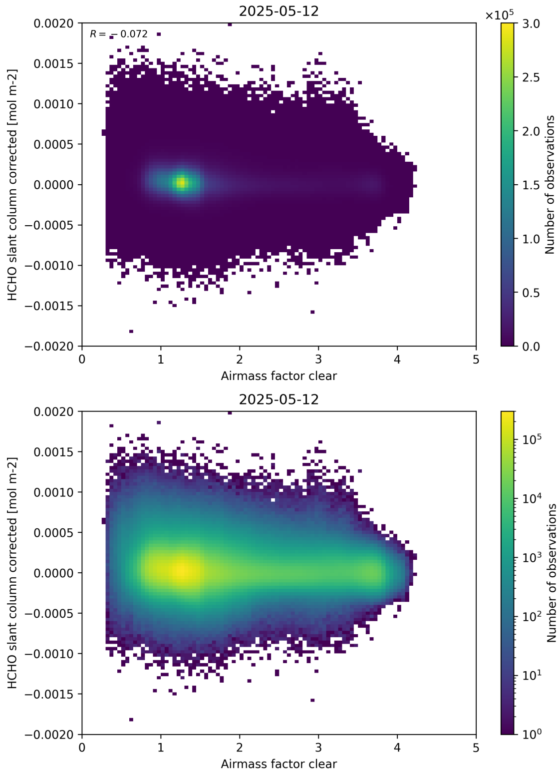
Figure 74: Scatter density plot of “Airmass factor clear” against “HCHO slant column corrected” for 2025-05-11 to 2025-05-13.
