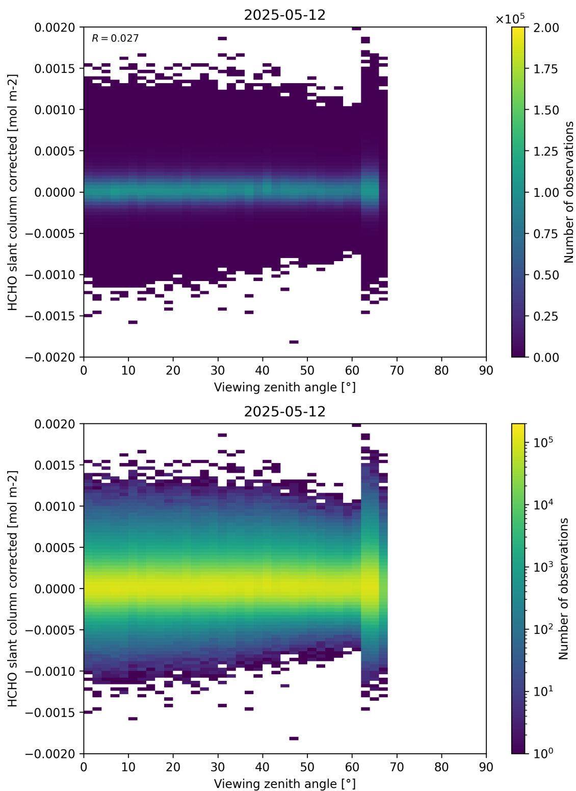
Figure 186: Scatter density plot of “Viewing zenith angle” against “HCHO slant column corrected” for 2025-05-11 to 2025-05-13.
