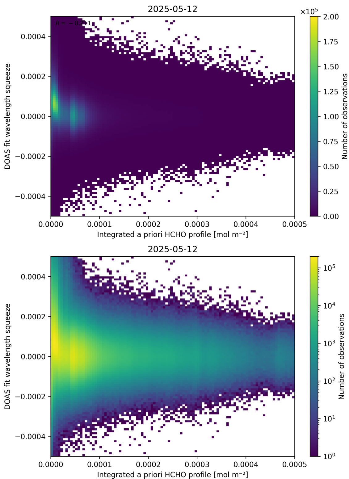
Figure 150: Scatter density plot of “Integrated a priori HCHO profile” against “DOAS fit wavelength squeeze” for 2025-05-11 to 2025-05-13.
