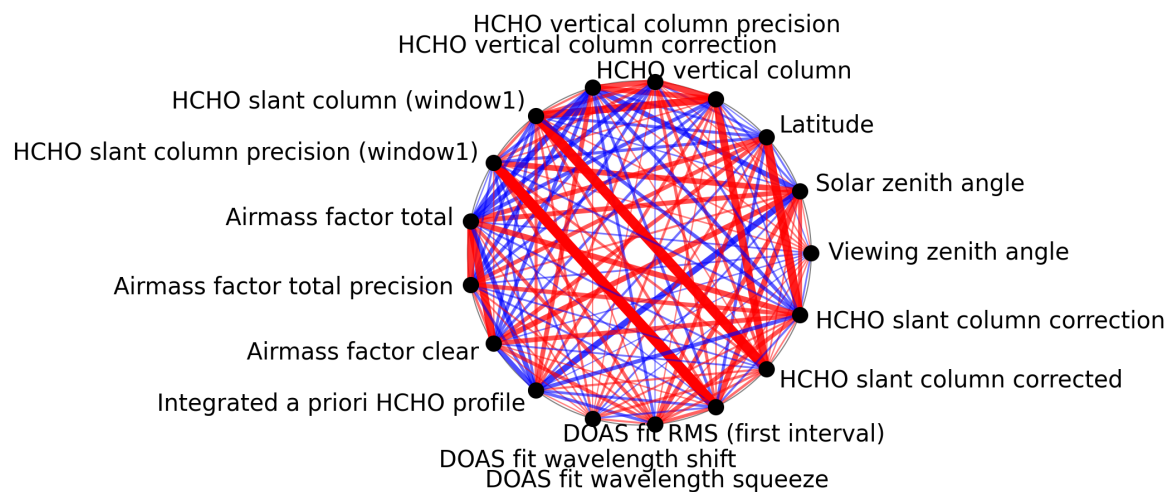
Figure 1: Map of correlation graph for 2025-05-11 to 2025-05-13.
