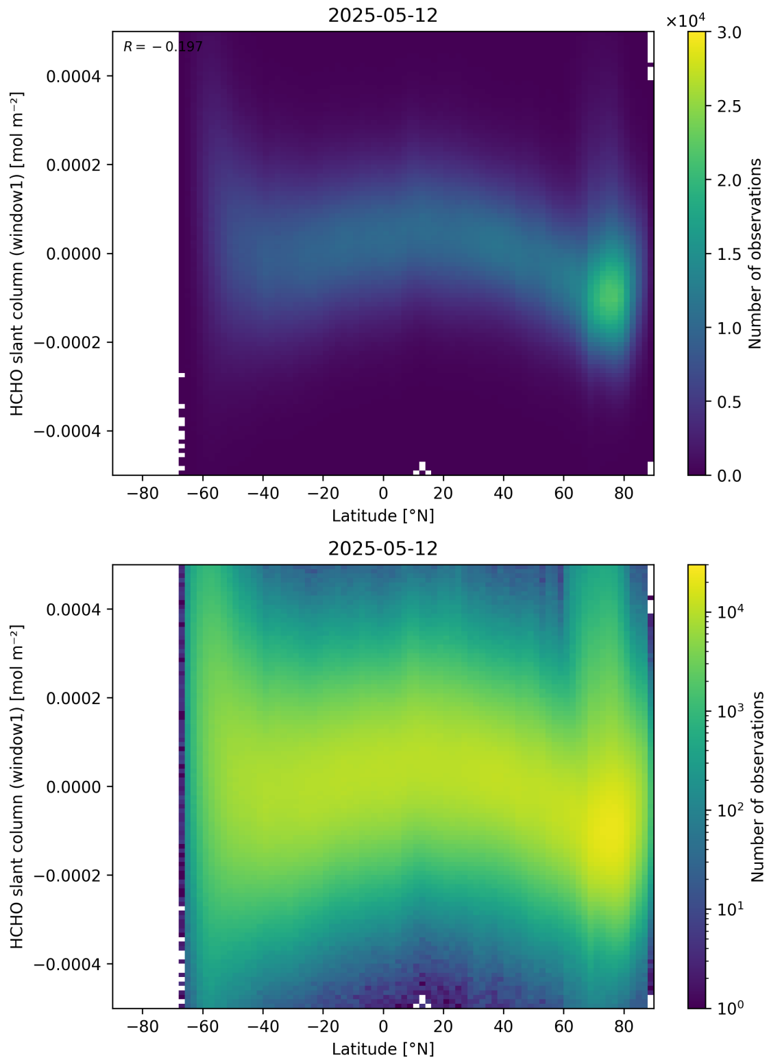
Figure 159: Scatter density plot of “Latitude” against “HCHO slant column (window1)” for 2025-05-11 to 2025-05-13.
