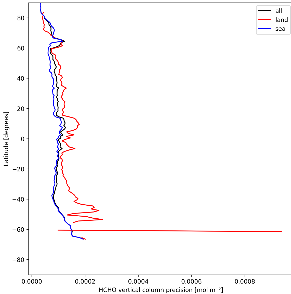
Figure 22: Zonal average of “HCHO vertical column precision” for 2025-05-11 to 2025-05-13.
