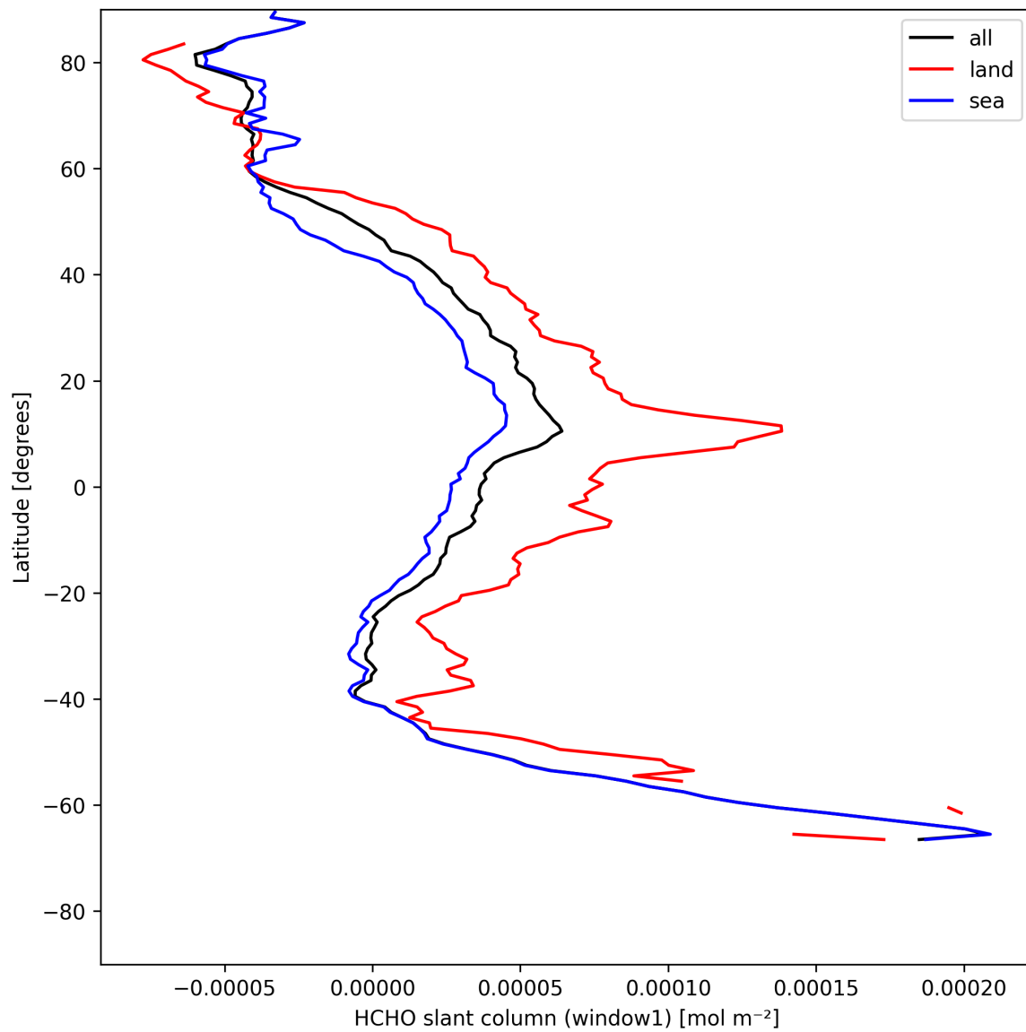
Figure 24: Zonal average of “HCHO slant column (window1)” for 2025-05-11 to 2025-05-13.
