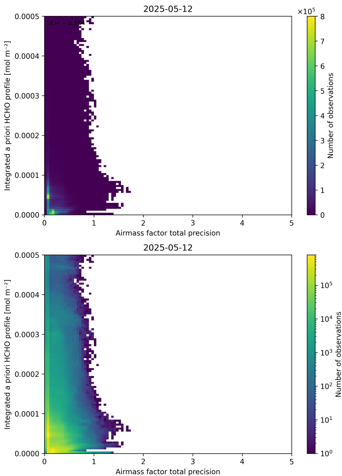
Figure 111: Scatter density plot of “Airmass factor total precision” against “Integrated a priori HCHO profile” for 2025-05-11 to 2025-05-13.
