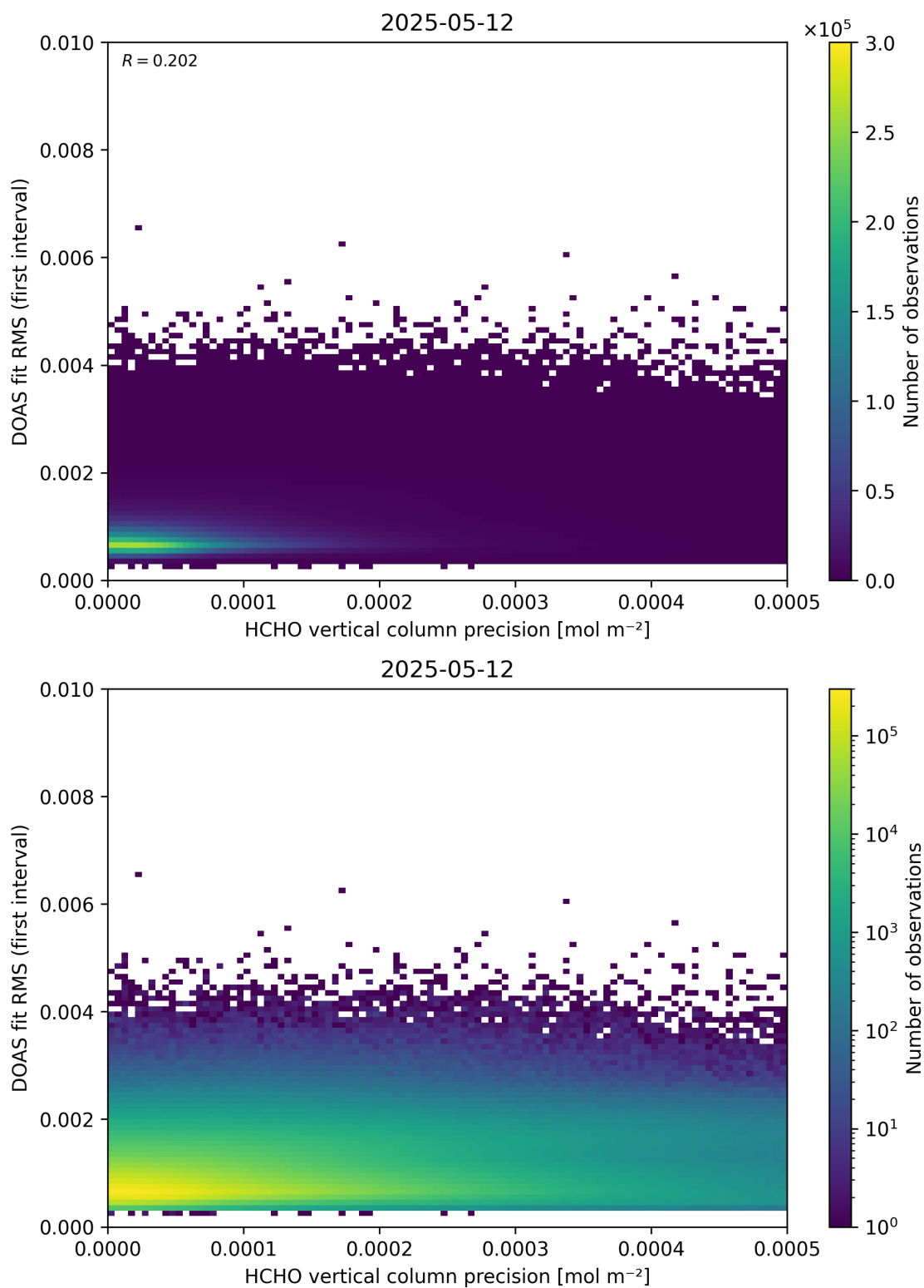
Figure 136: Scatter density plot of “HCHO vertical column precision” against “DOAS fit RMS (first interval)” for 2025-05-11 to 2025-05-13.
