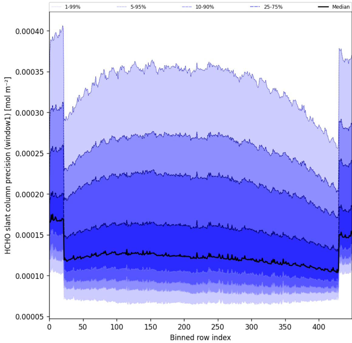
Figure 53: Along track statistics of "HCHO slant column precision (window1)" for 2025-05-11 to 2025-05-13
