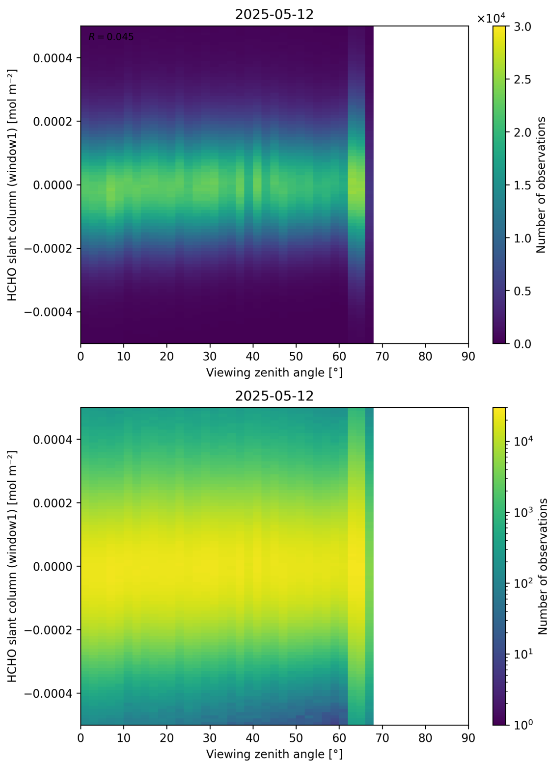
Figure 188: Scatter density plot of “Viewing zenith angle” against “HCHO slant column (window1)” for 2025-05-11 to 2025-05-13.
