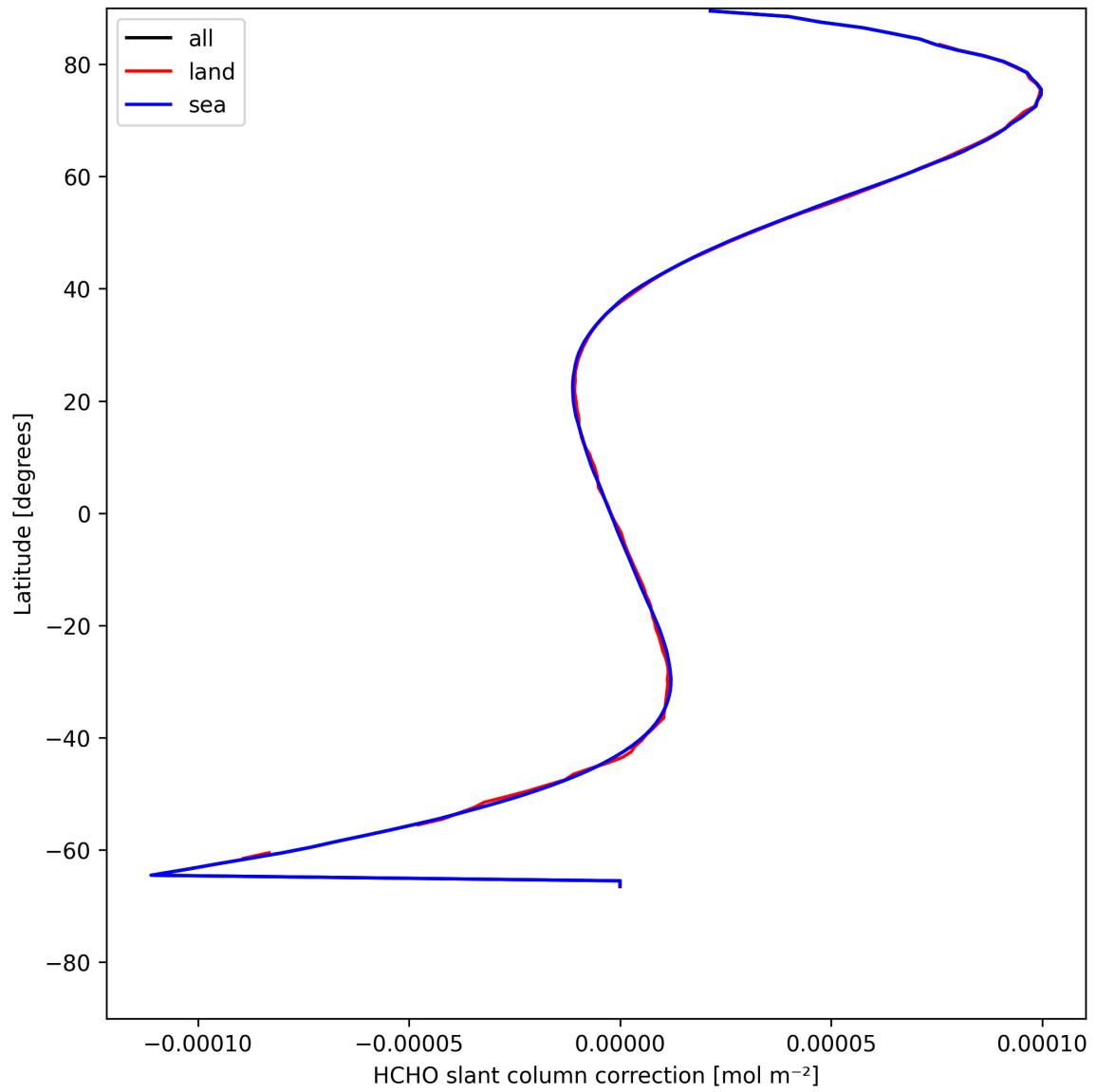
Figure 33: Zonal average of “HCHO slant column correction” for 2025-05-11 to 2025-05-13.
