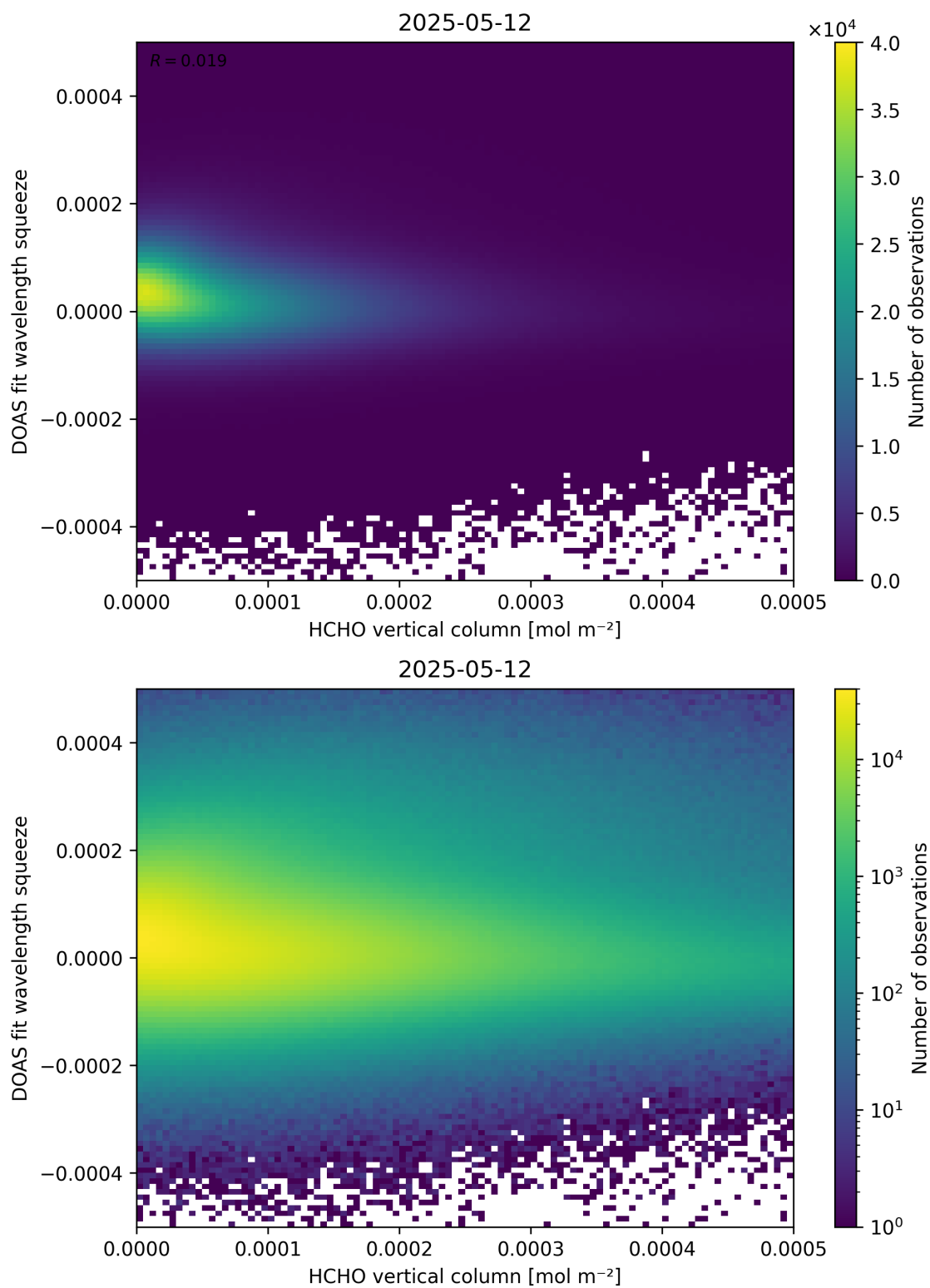
Figure 125: Scatter density plot of “HCHO vertical column” against “DOAS fit wavelength squeeze” for 2025-05-11 to 2025-05-13.
