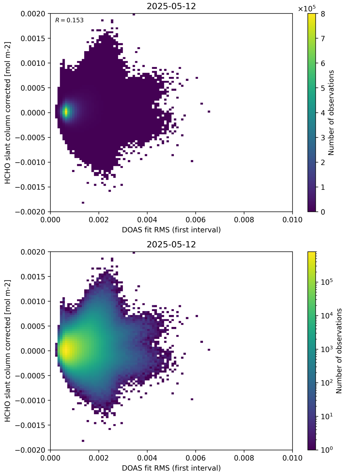
Figure 62: Scatter density plot of “DOAS fit RMS (first interval)” against “HCHO slant column corrected” for 2025-05-11 to 2025-05-13.
