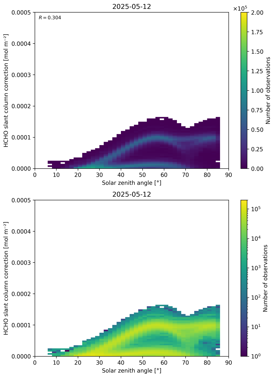
Figure 172: Scatter density plot of “Solar zenith angle” against “HCHO slant column correction” for 2025-05-11 to 2025-05-13.
