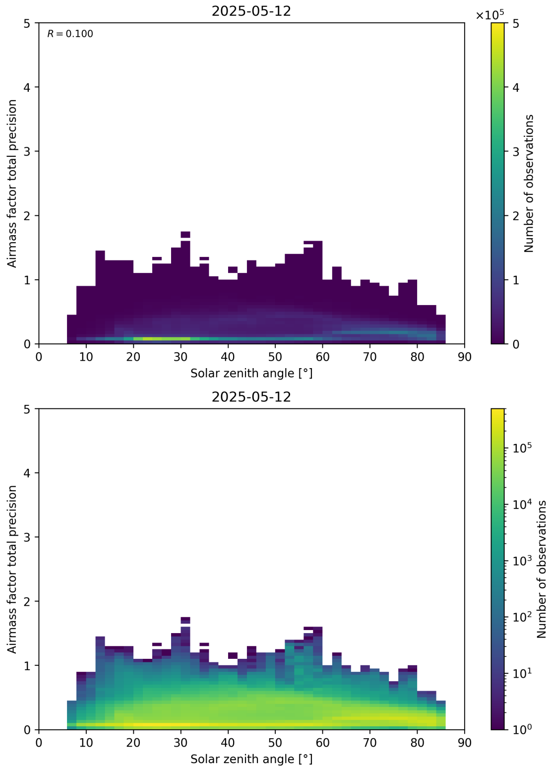
Figure 176: Scatter density plot of “Solar zenith angle” against “Airmass factor total precision” for 2025-05-11 to 2025-05-13.
