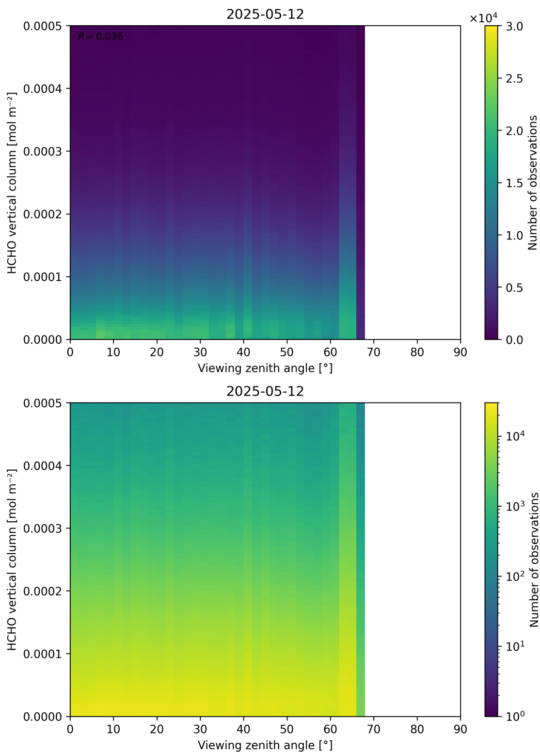
Figure 192: Scatter density plot of “Viewing zenith angle” against “HCHO vertical column” for 2025-05-11 to 2025-05-13.
