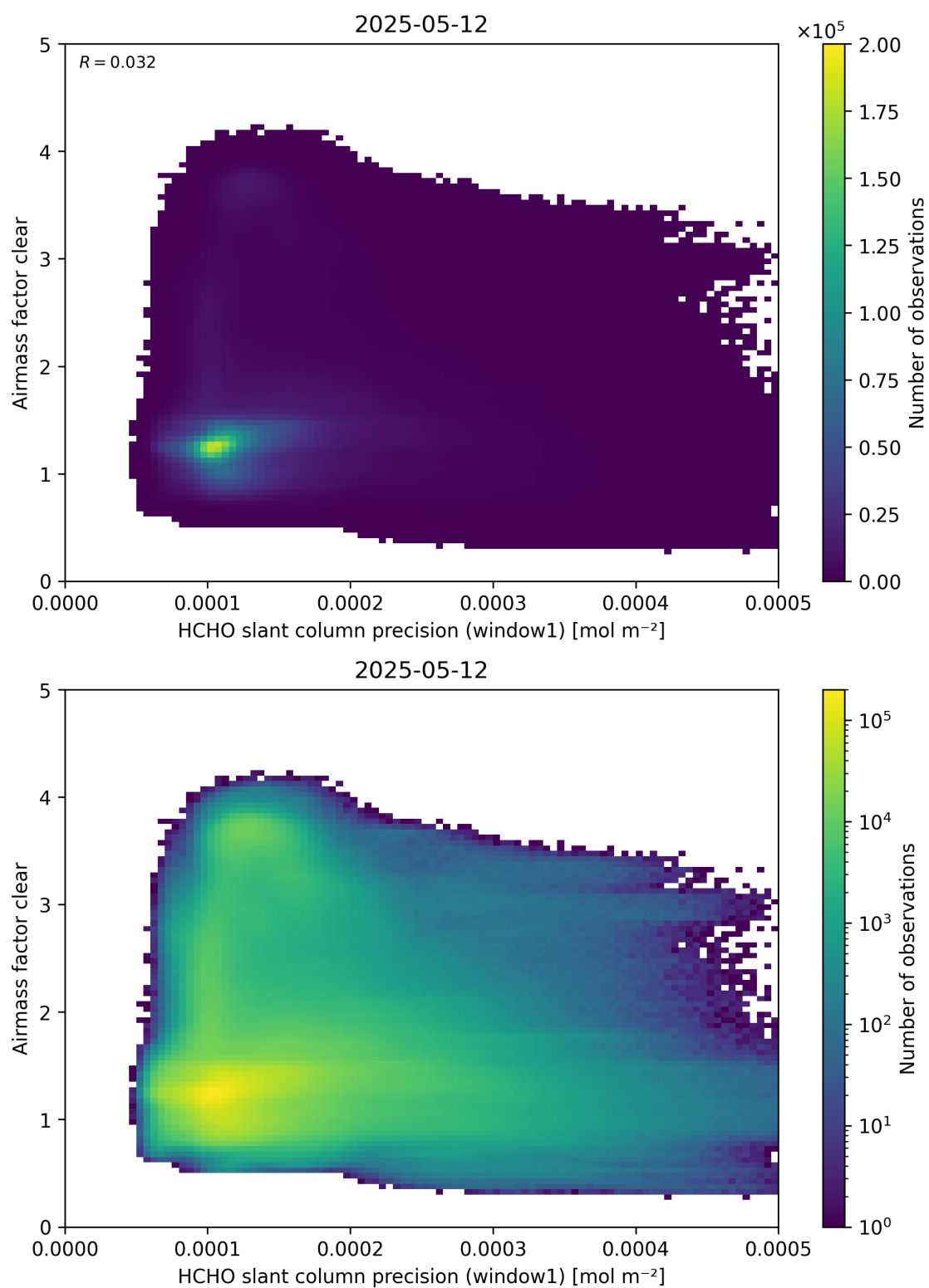
Figure 91: Scatter density plot of “HCHO slant column precision (window1)” against “Airmass factor clear” for 2025-05-11 to 2025-05-13.
