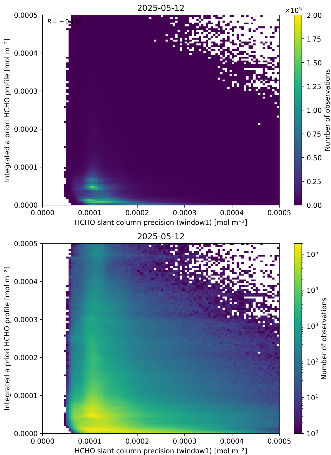
Figure 96: Scatter density plot of “HCHO slant column precision (window1)” against “Integrated a priori HCHO profile” for 2025-05-11 to 2025-05-13.
