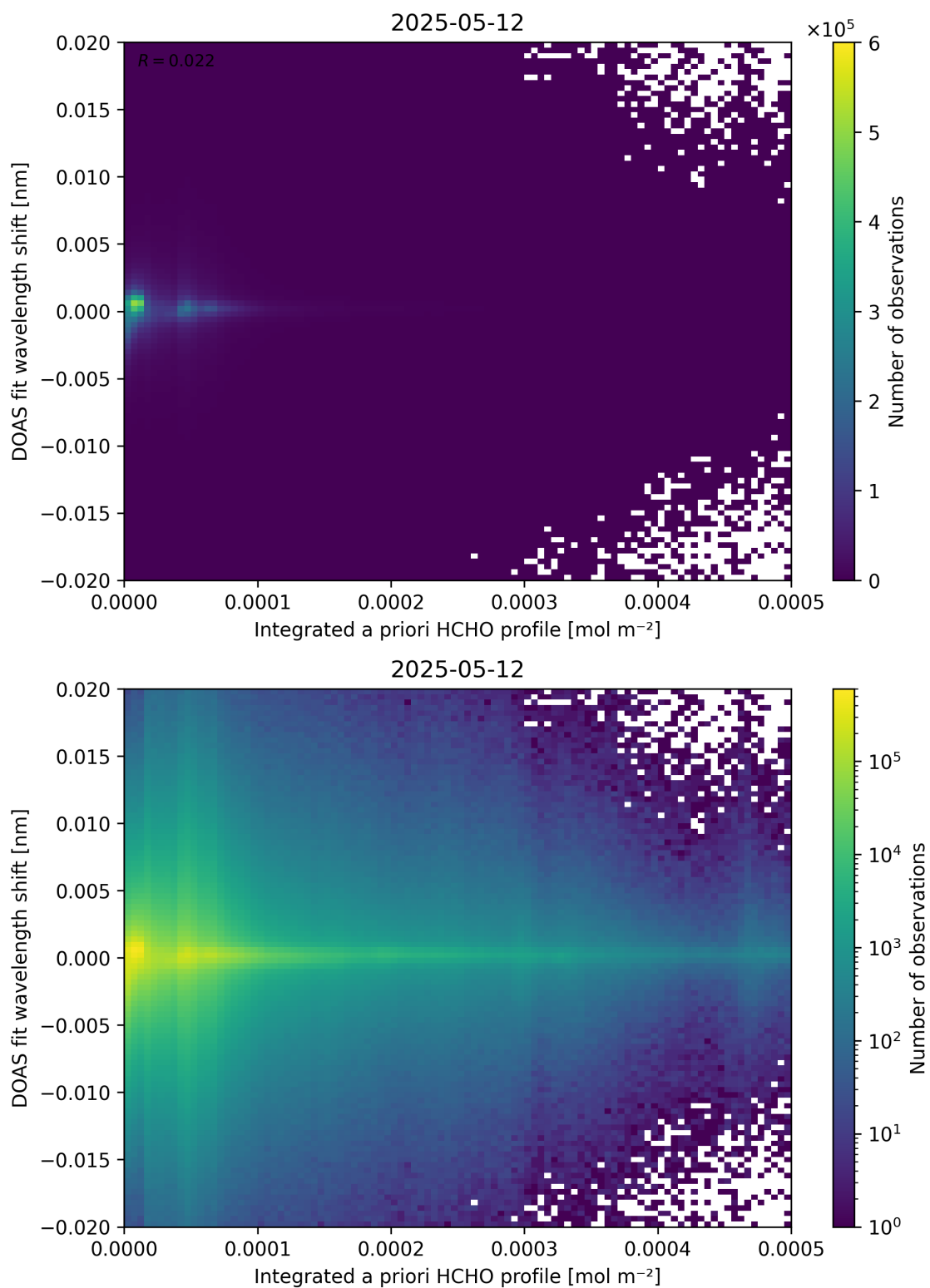
Figure 149: Scatter density plot of “Integrated a priori HCHO profile” against “DOAS fit wavelength shift” for 2025-05-11 to 2025-05-13.
