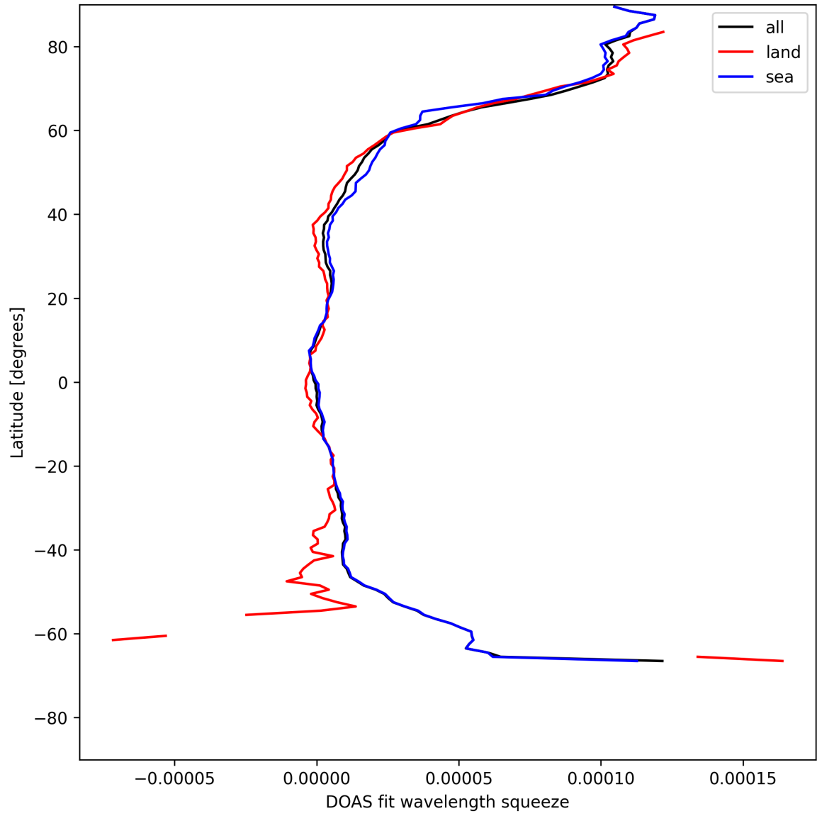
Figure 31: Zonal average of “DOAS fit wavelength squeeze” for 2025-05-11 to 2025-05-13.
