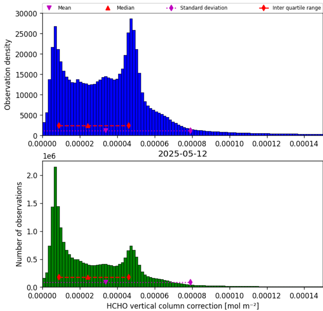
Figure 37: Histogram of “HCHO vertical column correction” for 2025-05-11 to 2025-05-13
