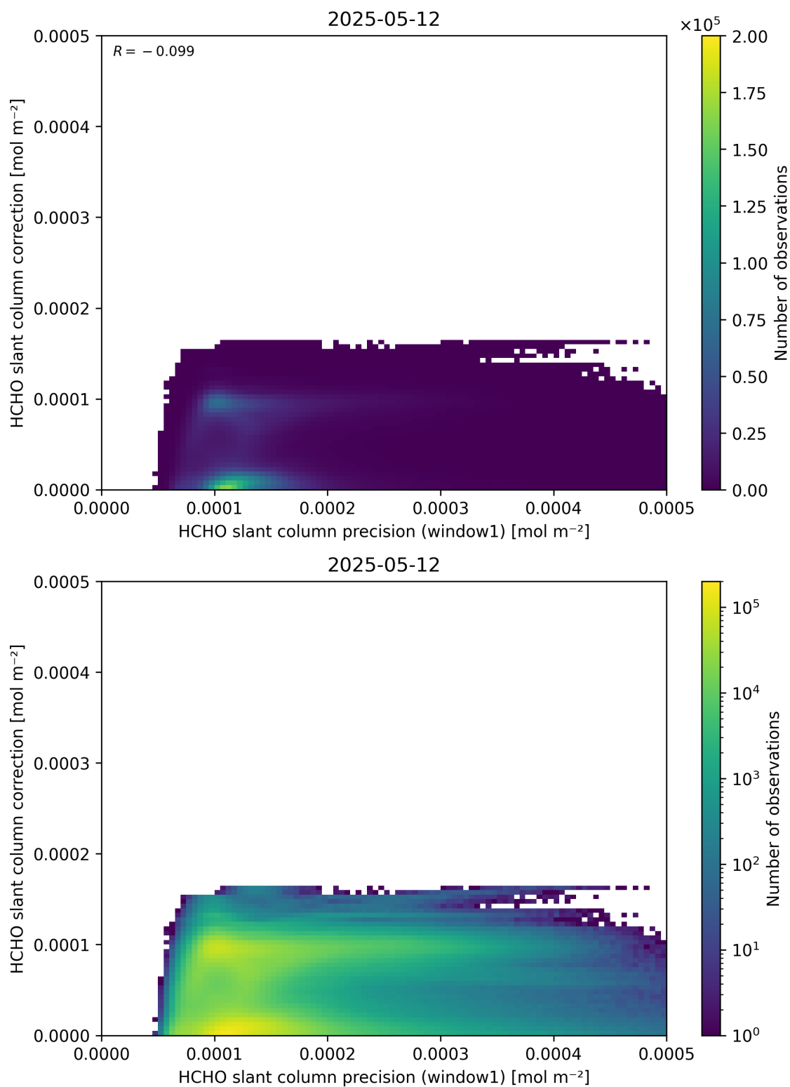
Figure 93: Scatter density plot of “HCHO slant column precision (window1)” against “HCHO slant column correction” for 2025-05-11 to 2025-05-13.
