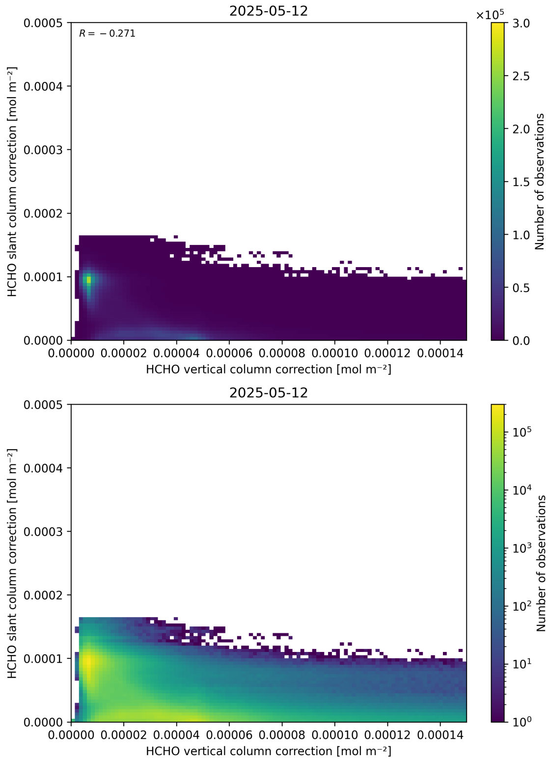
Figure 117: Scatter density plot of “HCHO vertical column correction” against “HCHO slant column correction” for 2025-05-11 to 2025-05-13.
