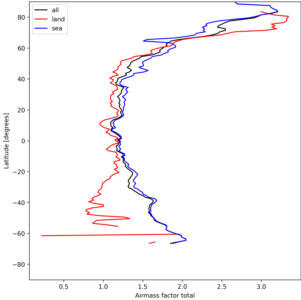
Figure 26: Zonal average of “Airmass factor total” for 2025-05-11 to 2025-05-13.
