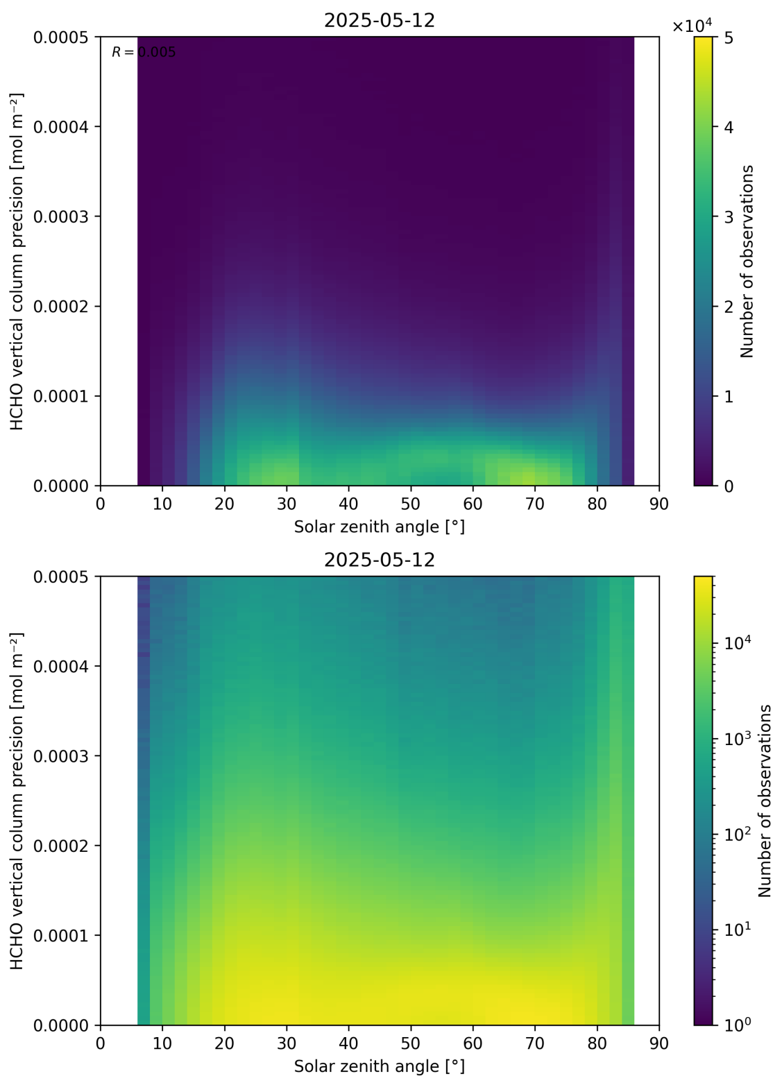
Figure 179: Scatter density plot of “Solar zenith angle” against “HCHO vertical column precision” for 2025-05-11 to 2025-05-13.
