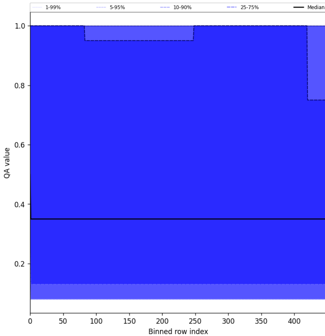
Figure 48: Along track statistics of “QA value” for 2025-05-11 to 2025-05-13
