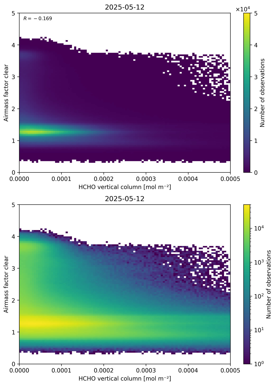
Figure 126: Scatter density plot of “HCHO vertical column” against “Airmass factor clear” for 2025-05-11 to 2025-05-13.
