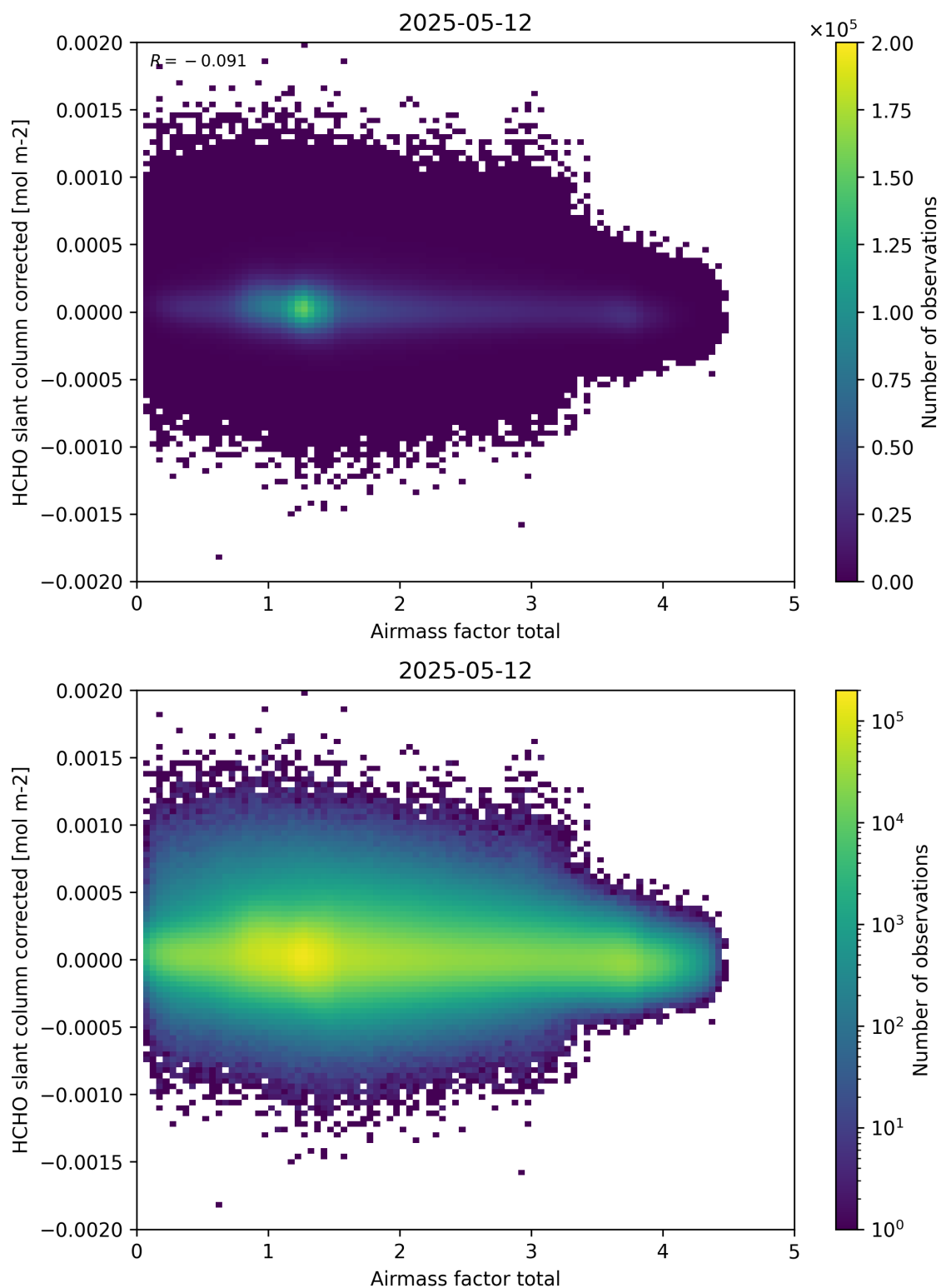
Figure 101: Scatter density plot of “Airmass factor total” against “HCHO slant column corrected” for 2025-05-11 to 2025-05-13.
