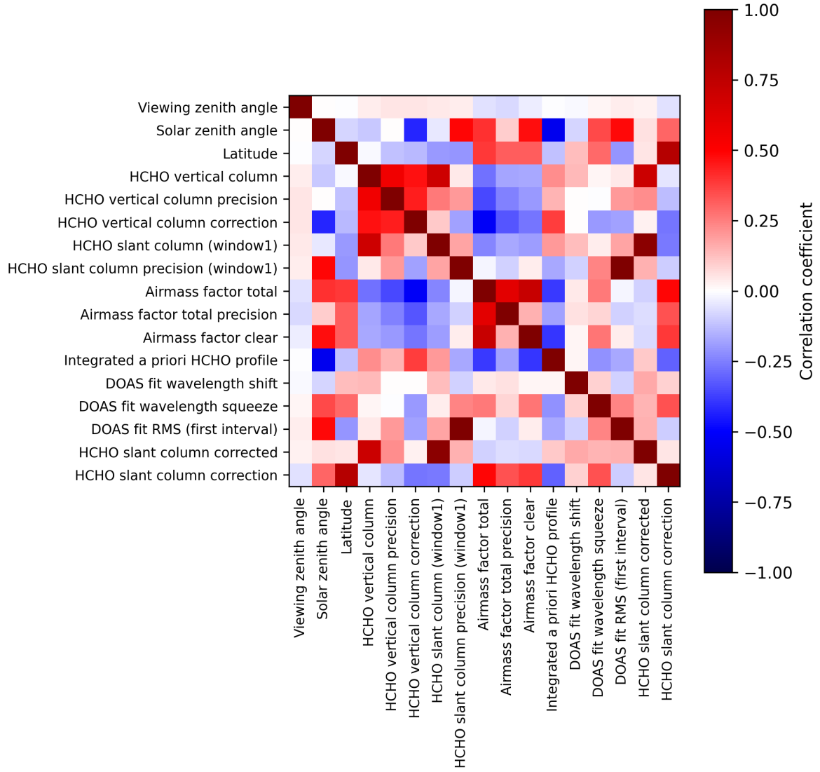
Figure 2: Map of correlation matrix for 2025-05-11 to 2025-05-13.
