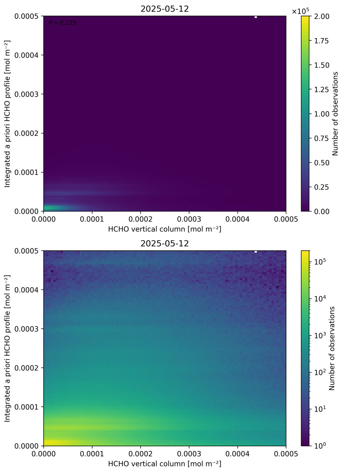
Figure 135: Scatter density plot of “HCHO vertical column” against “Integrated a priori HCHO profile” for 2025-05-11 to 2025-05-13.
