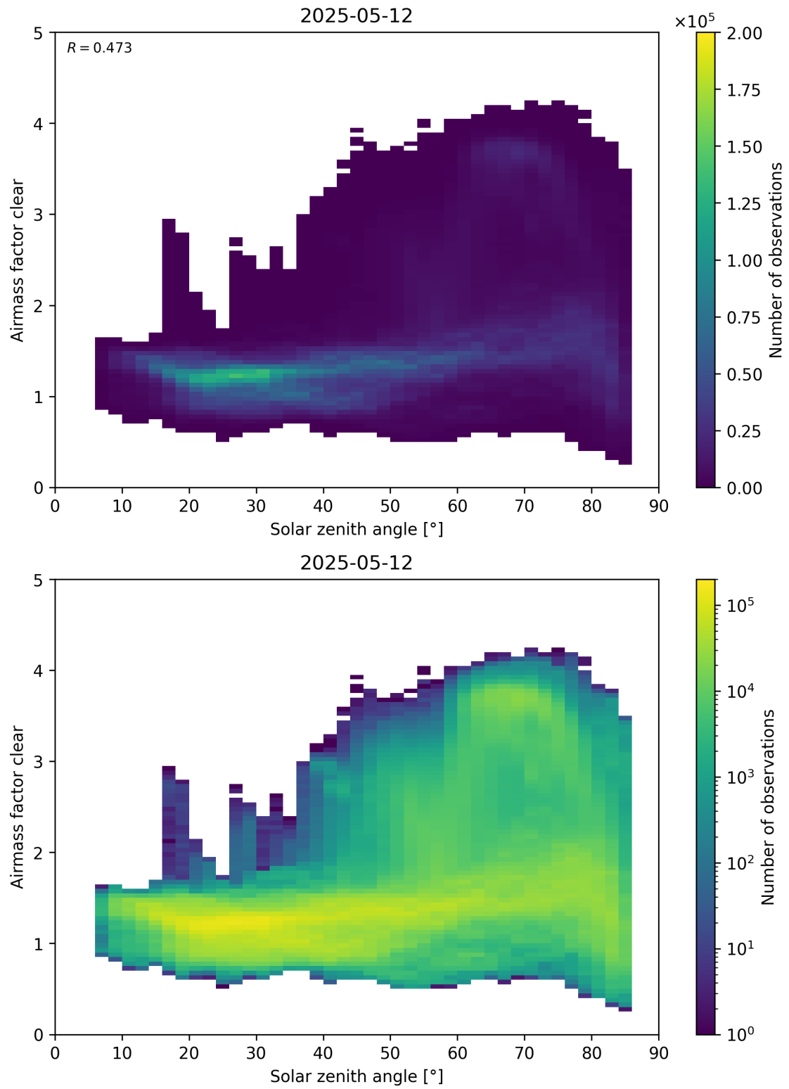
Figure 170: Scatter density plot of “Solar zenith angle” against “Airmass factor clear” for 2025-05-11 to 2025-05-13.
