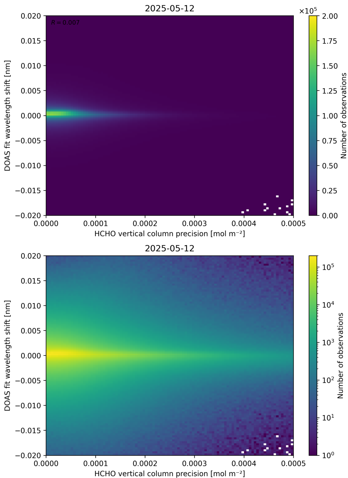
Figure 137: Scatter density plot of “HCHO vertical column precision” against “DOAS fit wavelength shift” for 2025-05-11 to 2025-05-13.
