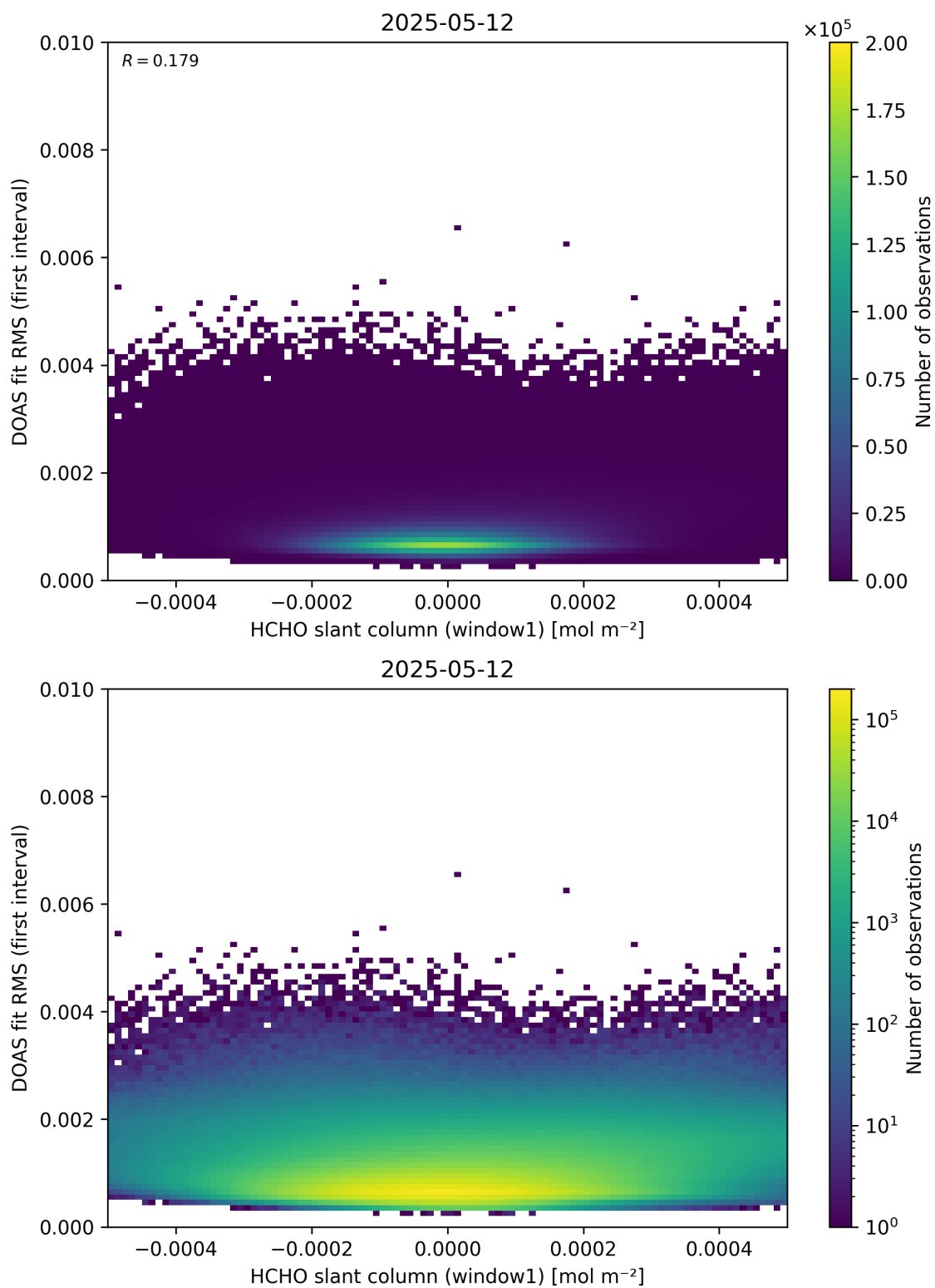
Figure 78: Scatter density plot of “HCHO slant column (window1)” against “DOAS fit RMS (first interval)” for 2025-05-11 to 2025-05-13.
