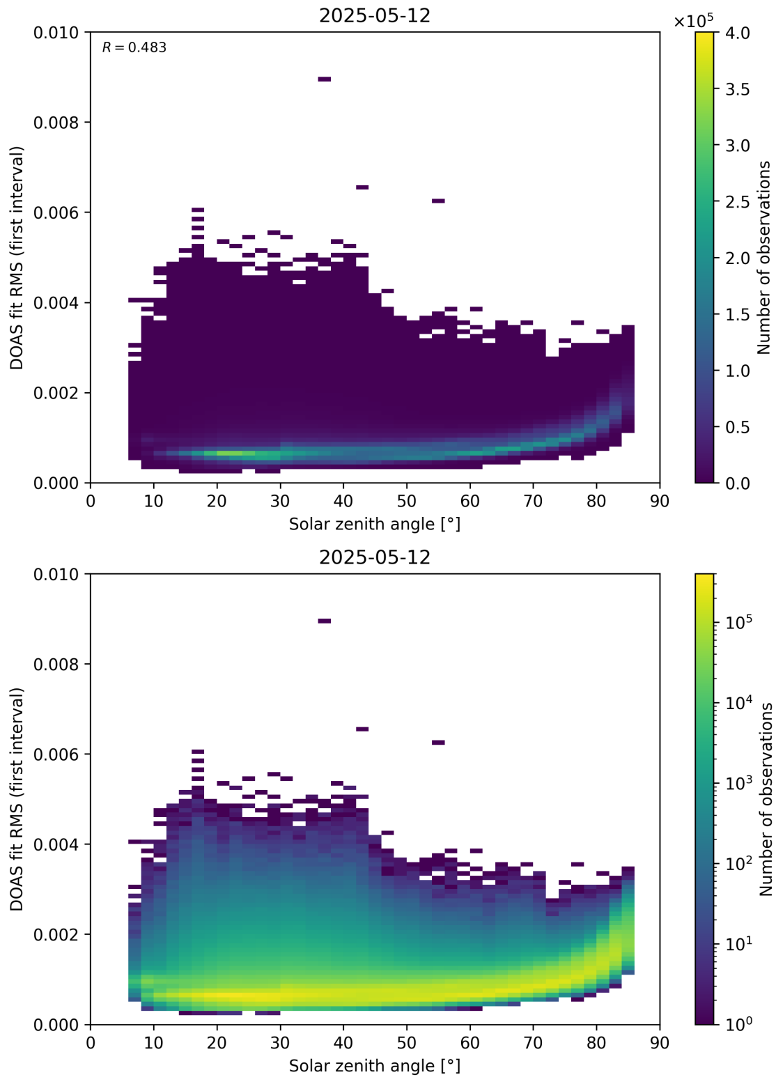
Figure 167: Scatter density plot of “Solar zenith angle” against “DOAS fit RMS (first interval)” for 2025-05-11 to 2025-05-13.
