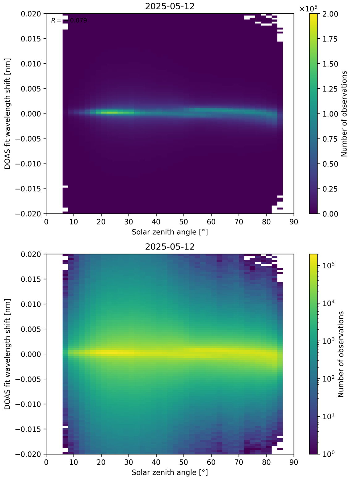
Figure 168: Scatter density plot of “Solar zenith angle” against “DOAS fit wavelength shift” for 2025-05-11 to 2025-05-13.
