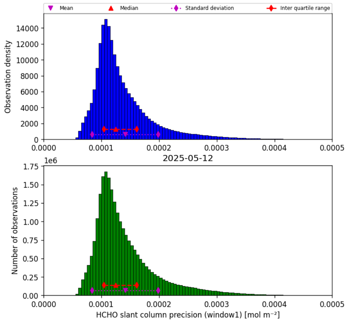
Figure 39: Histogram of “HCHO slant column precision (window1)” for 2025-05-11 to 2025-05-13
