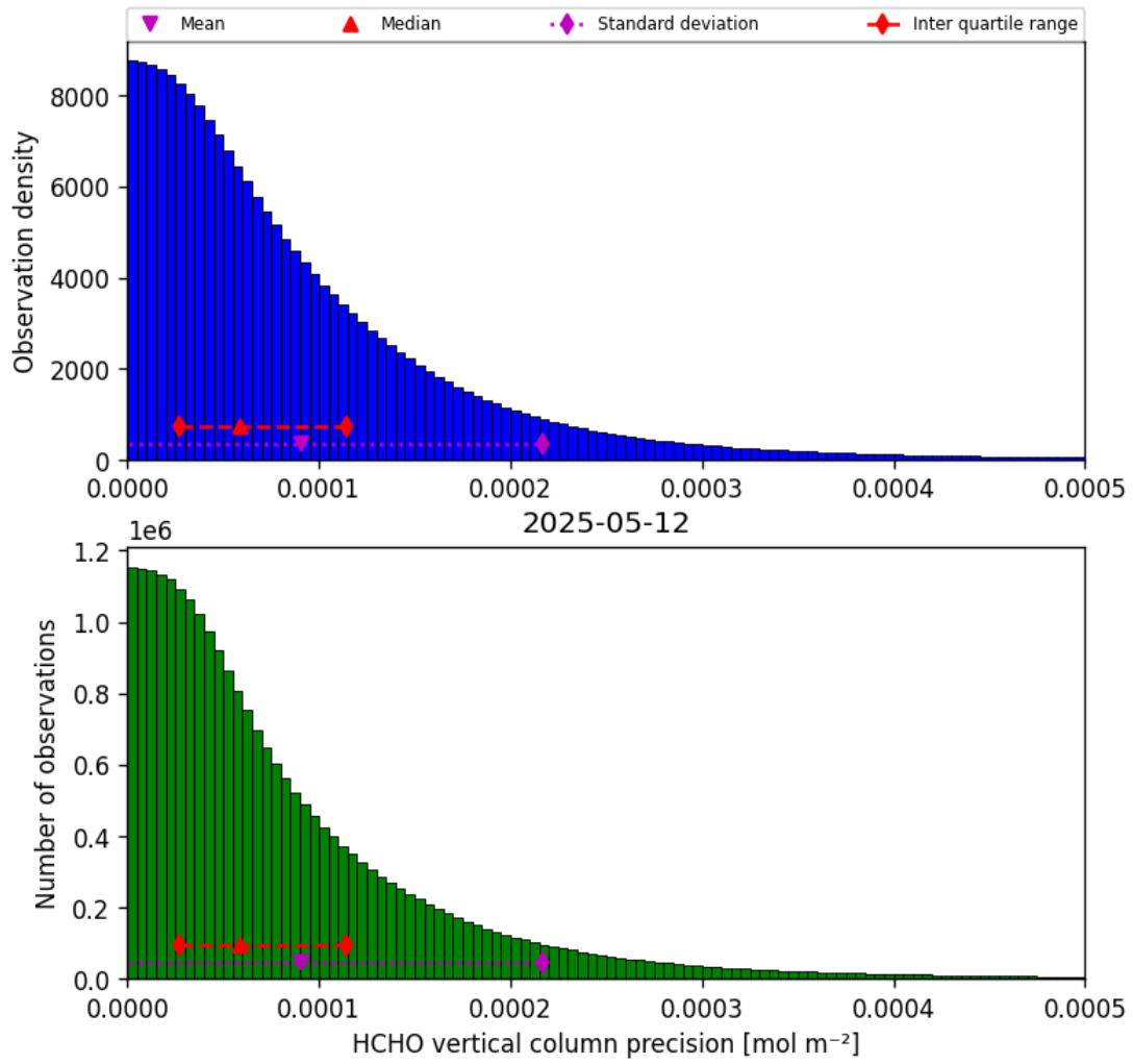
Figure 36: Histogram of “HCHO vertical column precision” for 2025-05-11 to 2025-05-13
