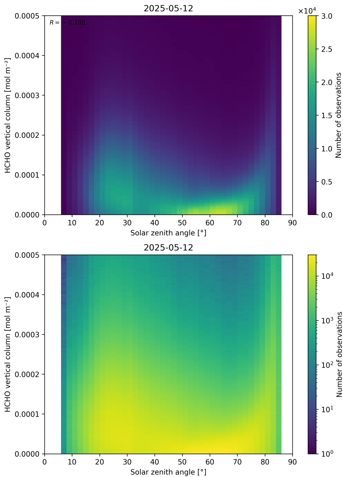
Figure 177: Scatter density plot of “Solar zenith angle” against “HCHO vertical column” for 2025-05-11 to 2025-05-13.
