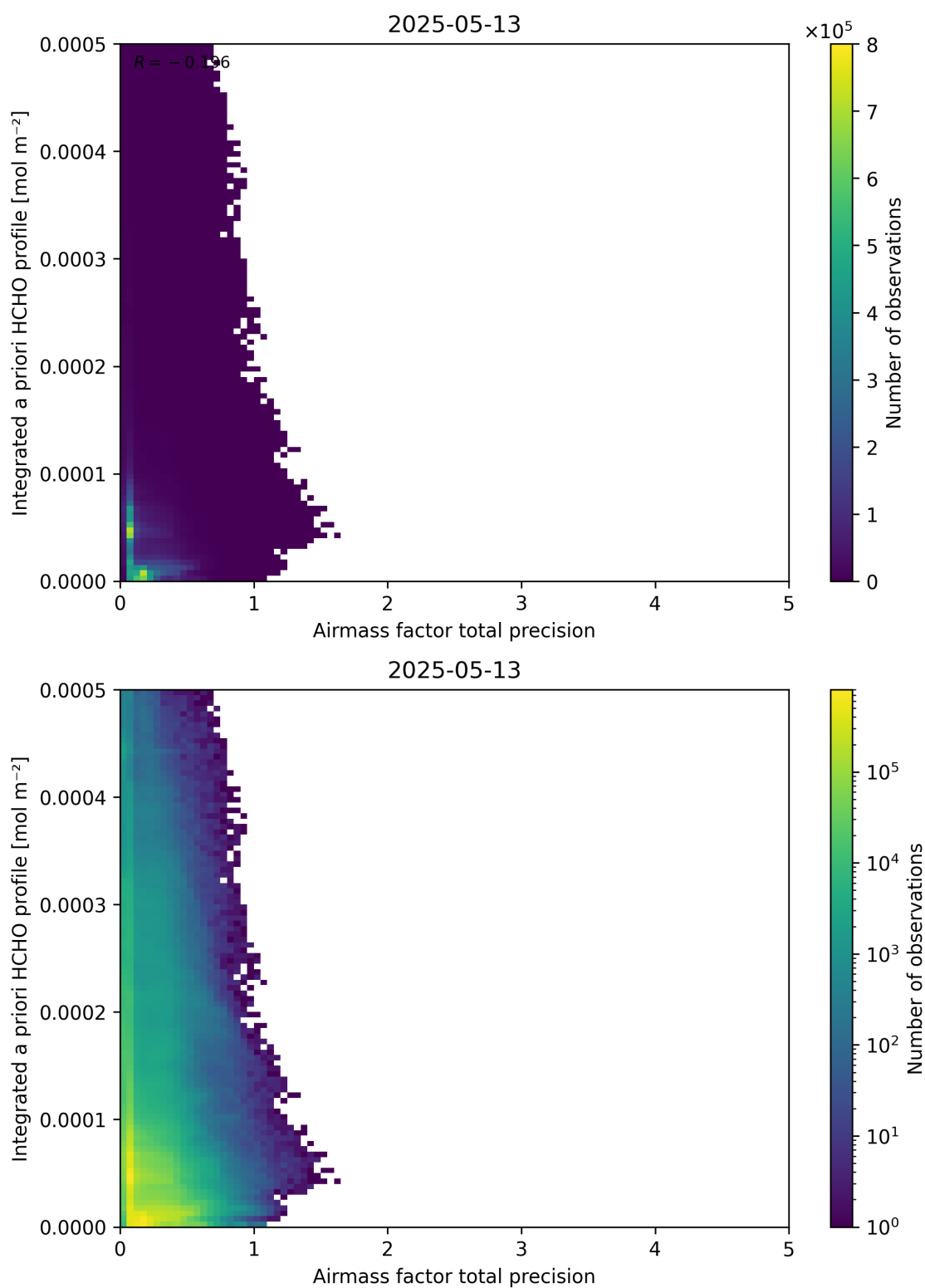
Figure 111: Scatter density plot of “Airmass factor total precision” against “Integrated a priori HCHO profile” for 2025-05-12 to 2025-05-14.
