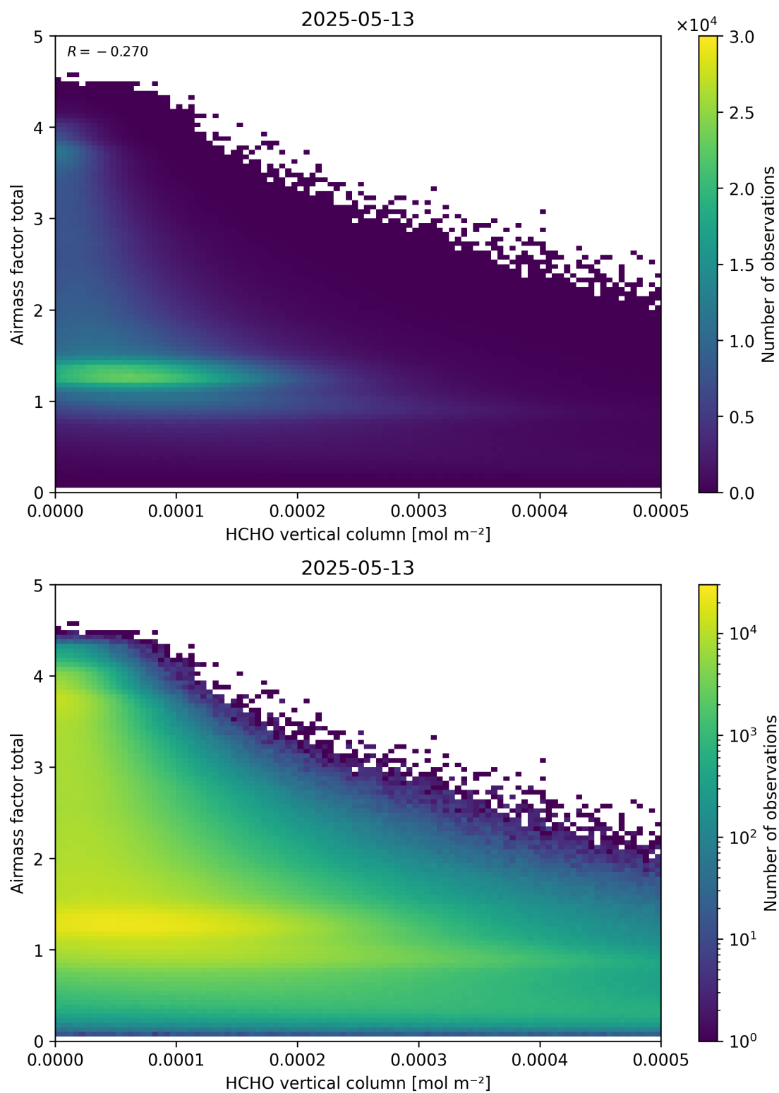
Figure 131: Scatter density plot of “HCHO vertical column” against “Airmass factor total” for 2025-05-12 to 2025-05-14.
