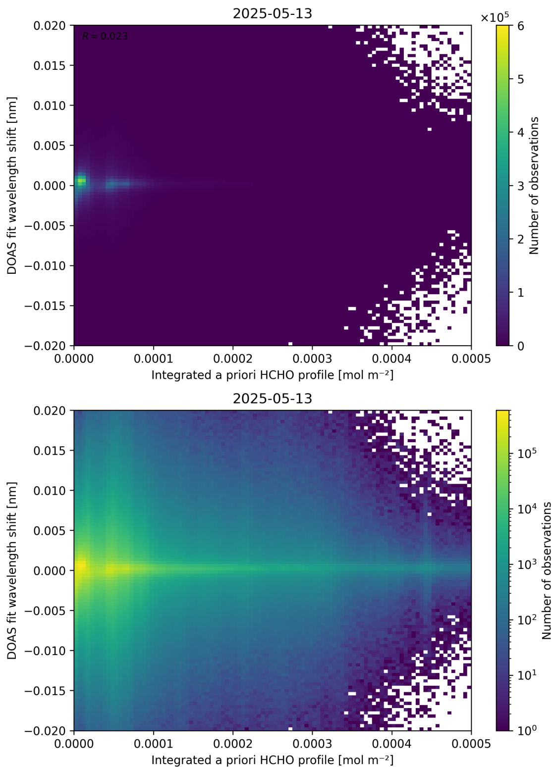
Figure 149: Scatter density plot of “Integrated a priori HCHO profile” against “DOAS fit wavelength shift” for 2025-05-12 to 2025-05-14.
