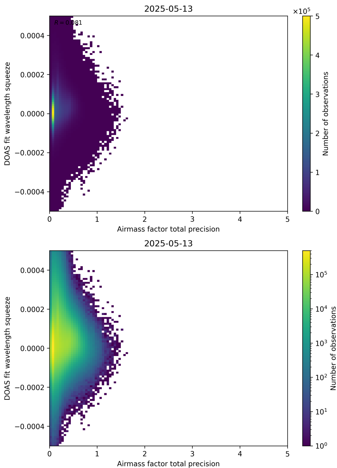
Figure 107: Scatter density plot of “Airmass factor total precision” against “DOAS fit wavelength squeeze” for 2025-05-12 to 2025-05-14.
