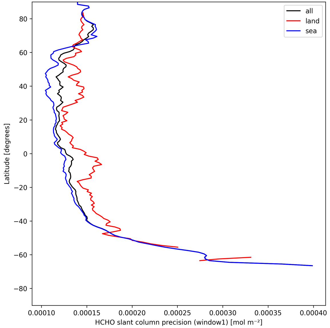
Figure 25: Zonal average of “HCHO slant column precision (window1)” for 2025-05-12 to 2025-05-14.
