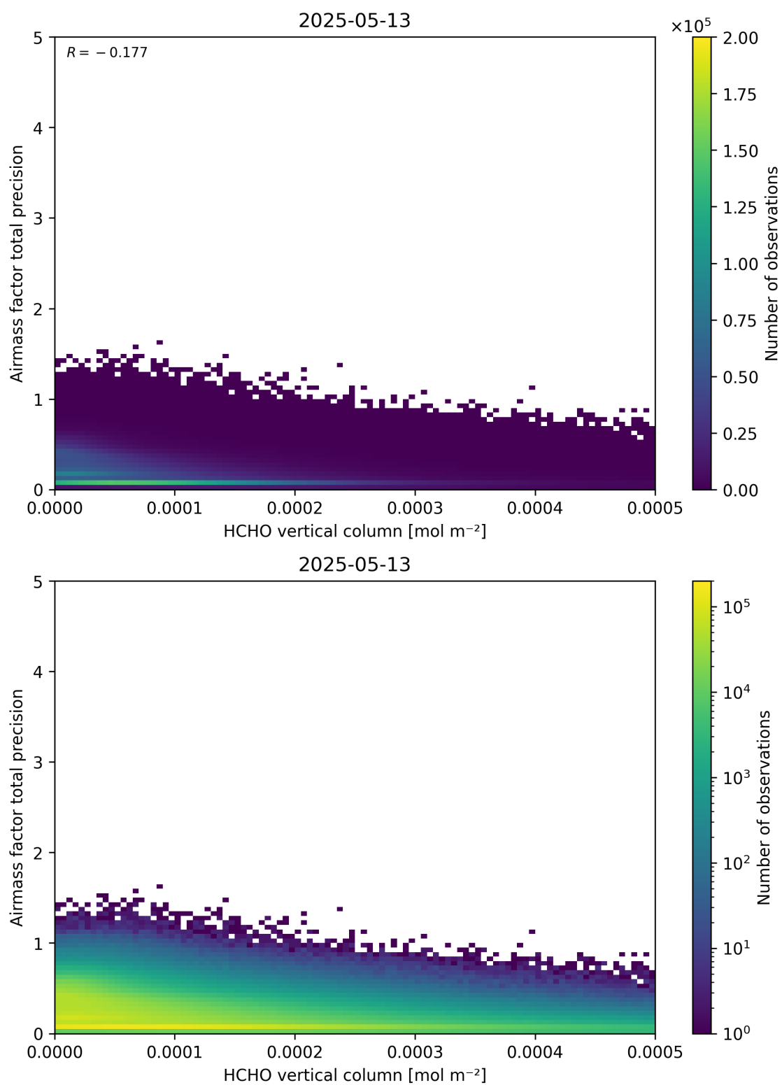
Figure 132: Scatter density plot of “HCHO vertical column” against “Airmass factor total precision” for 2025-05-12 to 2025-05-14.
