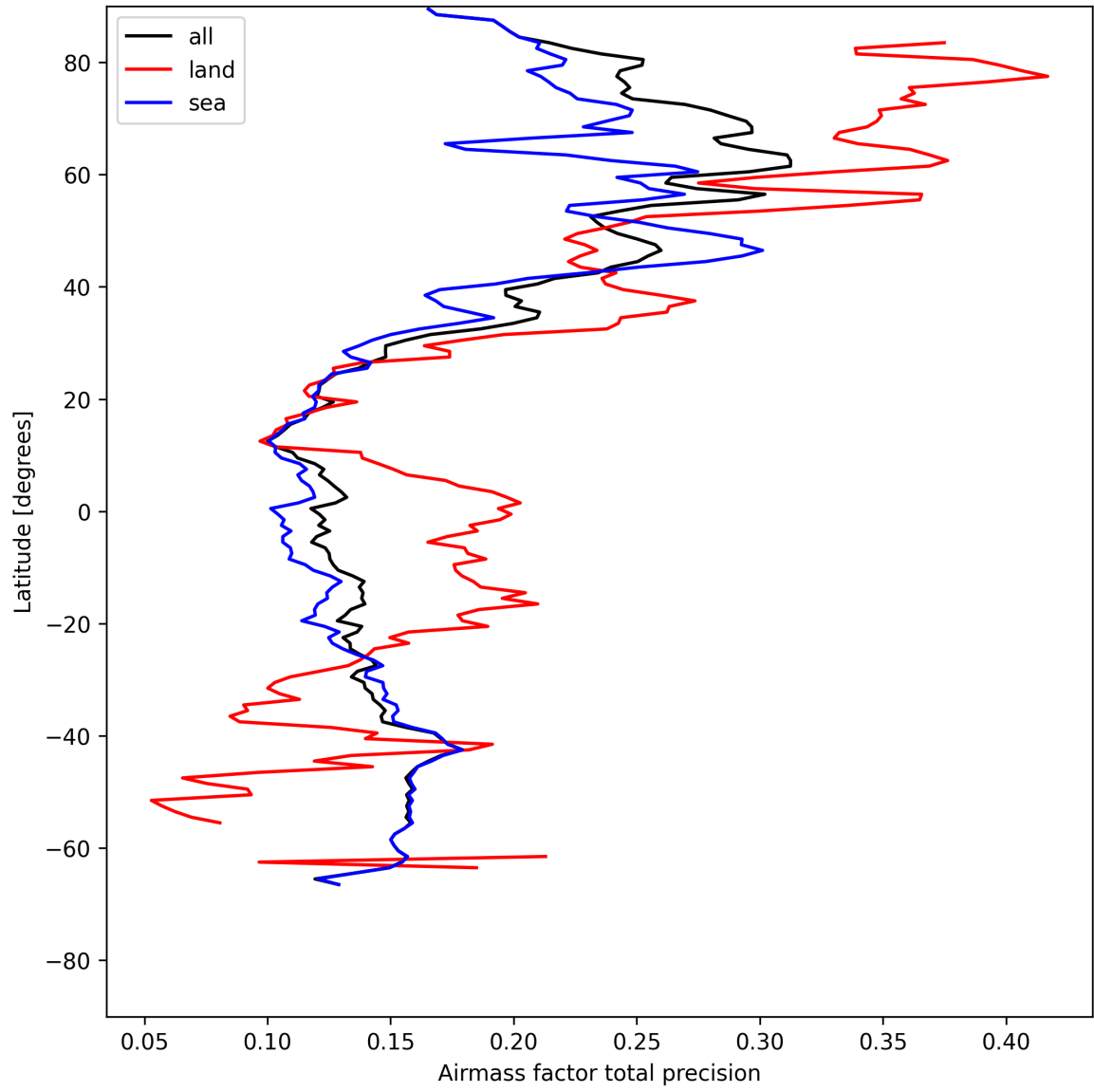
Figure 27: Zonal average of “Airmass factor total precision” for 2025-05-12 to 2025-05-14.
