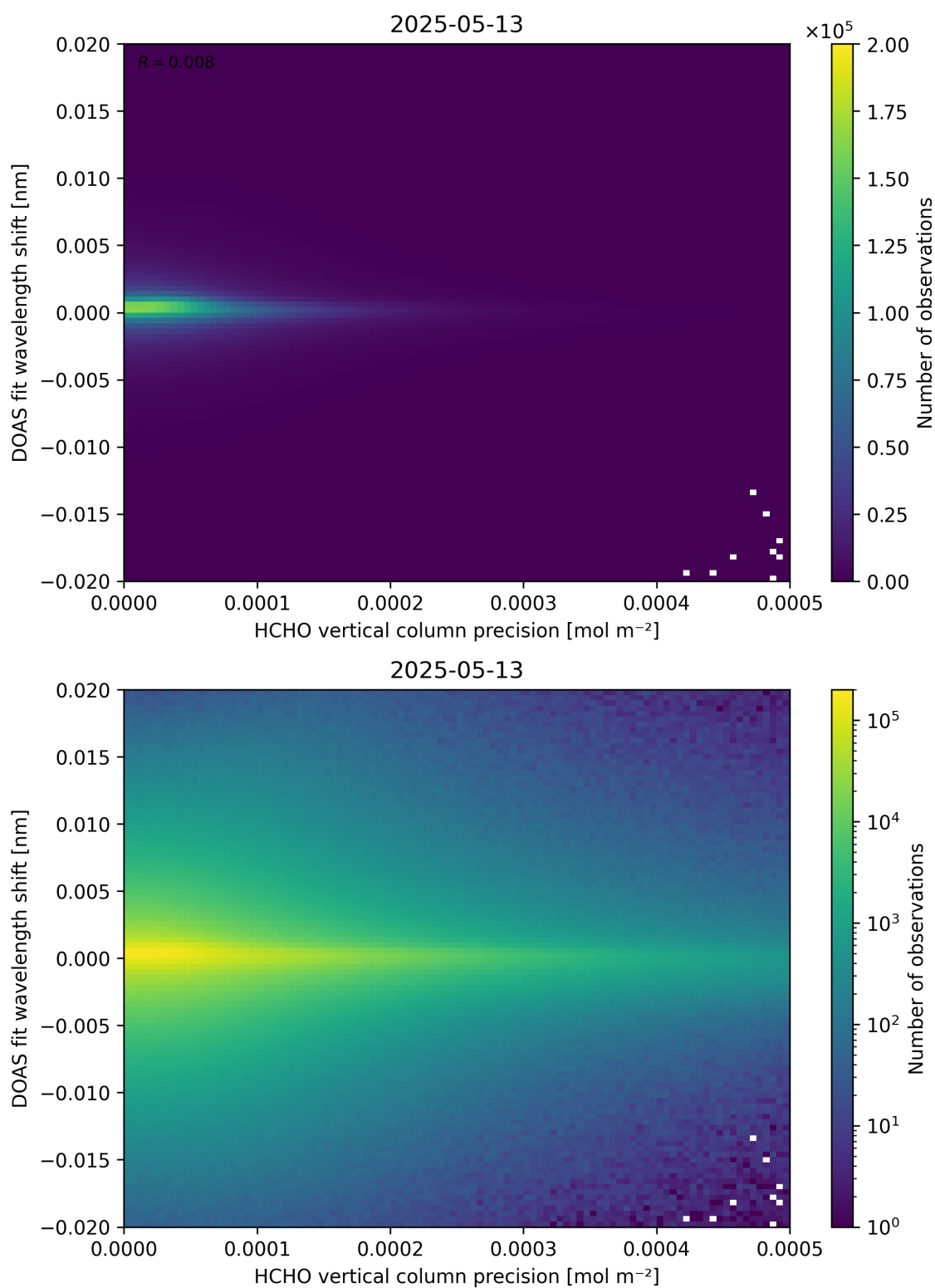
Figure 137: Scatter density plot of “HCHO vertical column precision” against “DOAS fit wavelength shift” for 2025-05-12 to 2025-05-14.
