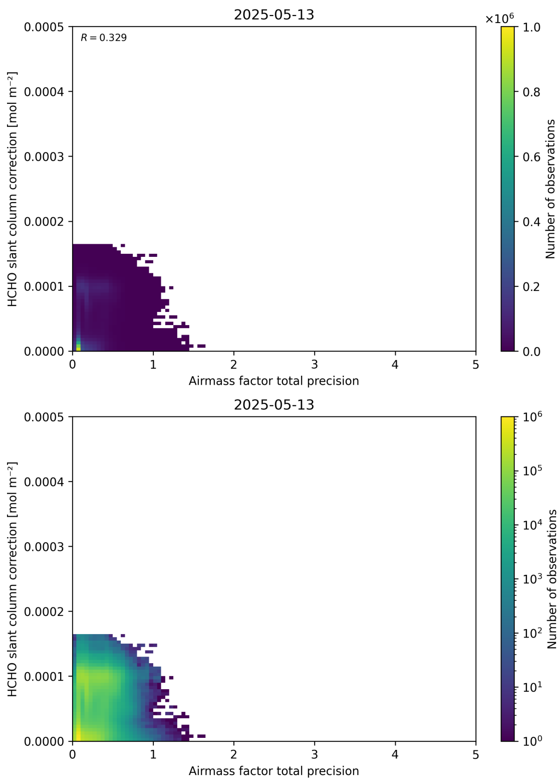
Figure 110: Scatter density plot of “Airmass factor total precision” against “HCHO slant column correction” for 2025-05-12 to 2025-05-14.
