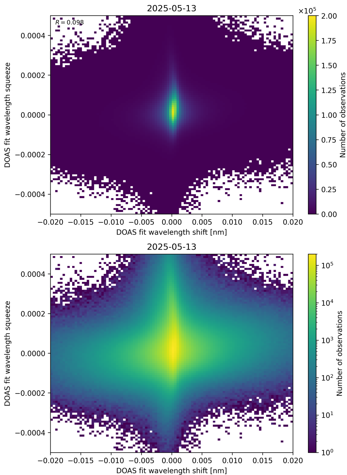
Figure 65: Scatter density plot of “DOAS fit wavelength shift” against “DOAS fit wavelength squeeze” for 2025-05-12 to 2025-05-14.
