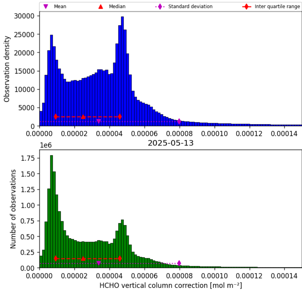
Figure 37: Histogram of “HCHO vertical column correction” for 2025-05-12 to 2025-05-14
