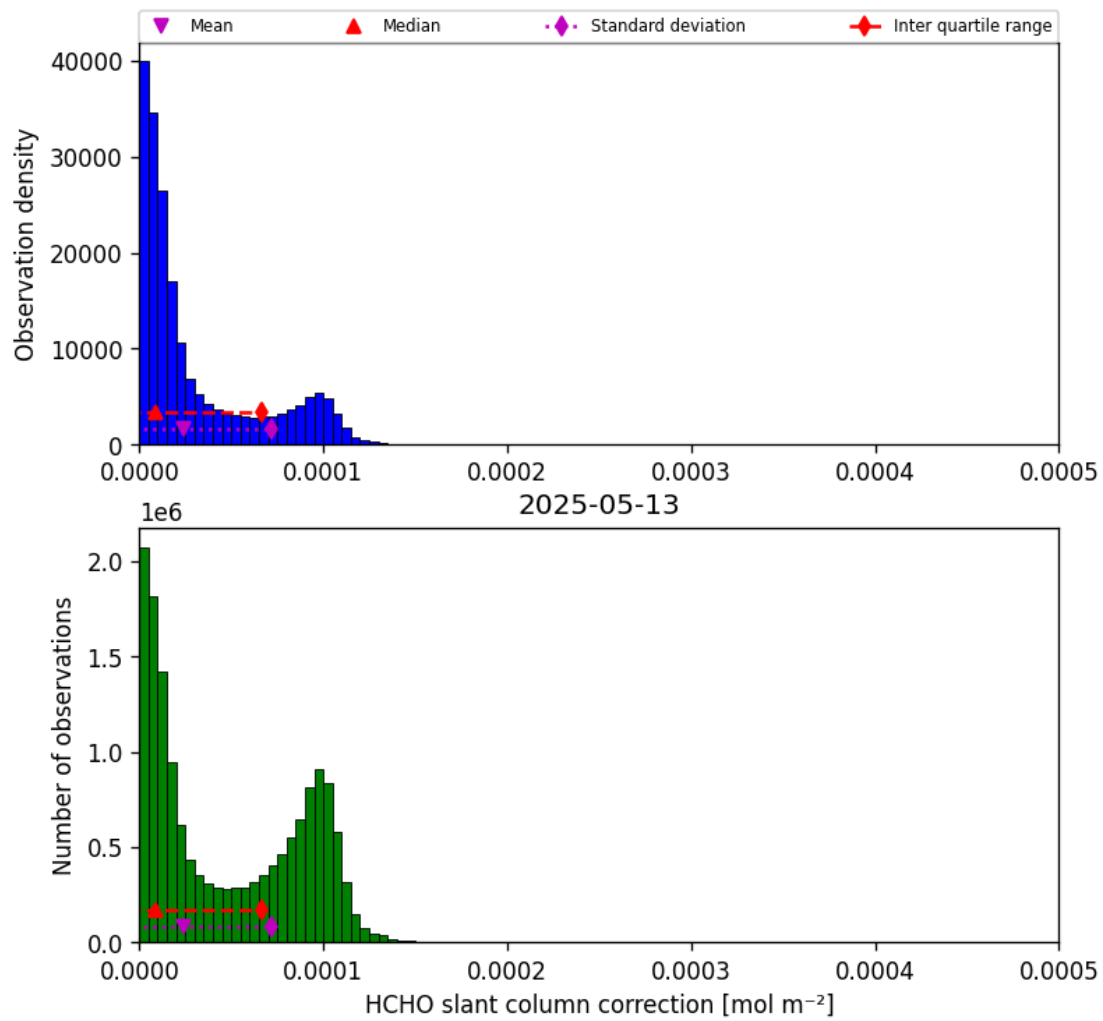
Figure 47: Histogram of “HCHO slant column correction” for 2025-05-12 to 2025-05-14
