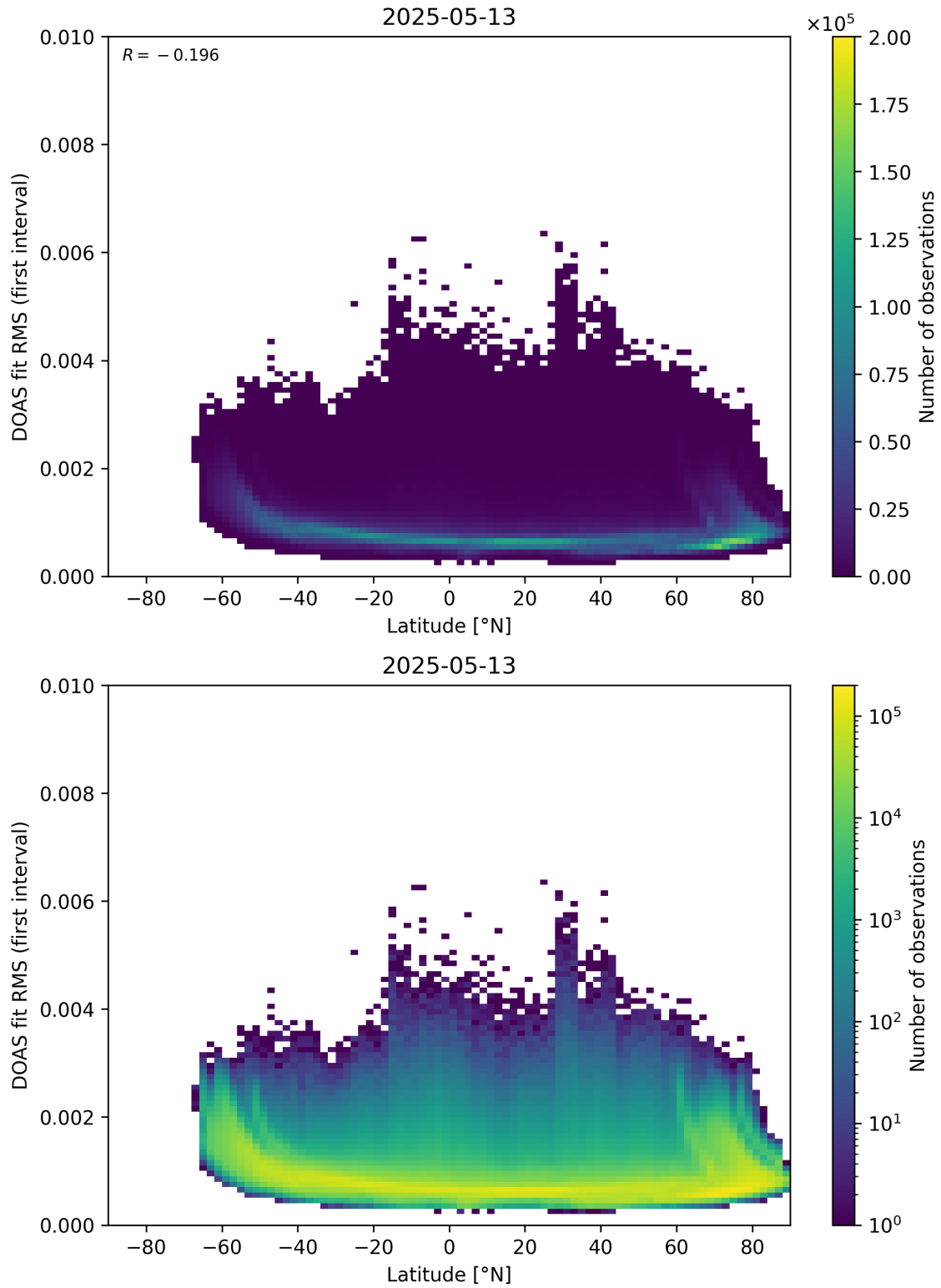
Figure 153: Scatter density plot of “Latitude” against “DOAS fit RMS (first interval)” for 2025-05-12 to 2025-05-14.
