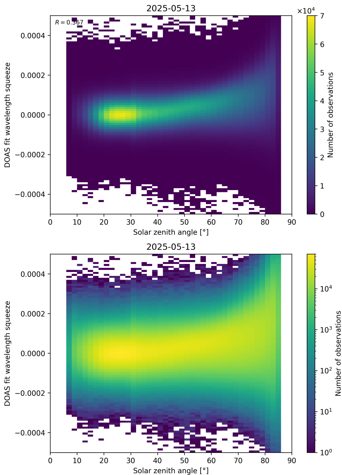
Figure 169: Scatter density plot of “Solar zenith angle” against “DOAS fit wavelength squeeze” for 2025-05-12 to 2025-05-14.
