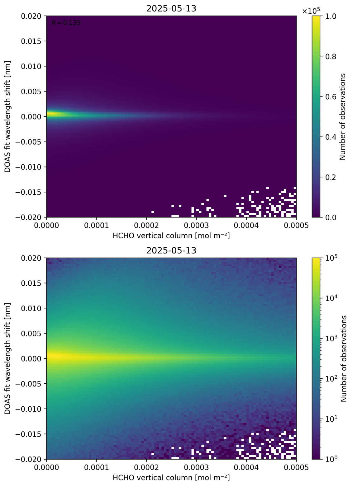
Figure 124: Scatter density plot of “HCHO vertical column” against “DOAS fit wavelength shift” for 2025-05-12 to 2025-05-14.
