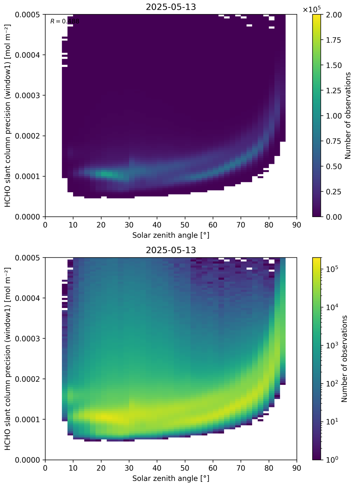
Figure 174: Scatter density plot of “Solar zenith angle” against “HCHO slant column precision (window1)” for 2025-05-12 to 2025-05-14.
