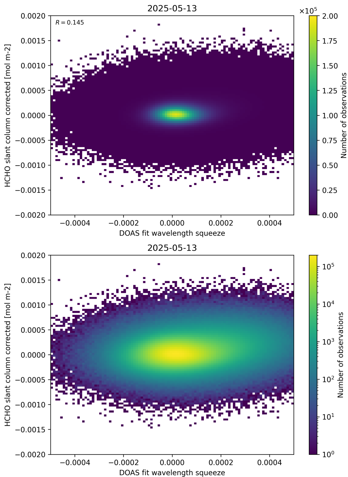
Figure 69: Scatter density plot of “DOAS fit wavelength squeeze” against “HCHO slant column corrected” for 2025-05-12 to 2025-05-14.
