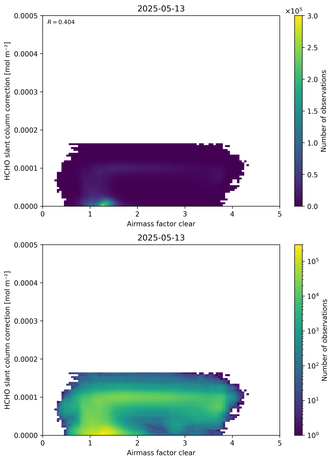
Figure 75: Scatter density plot of “Airmass factor clear” against “HCHO slant column correction” for 2025-05-12 to 2025-05-14.
