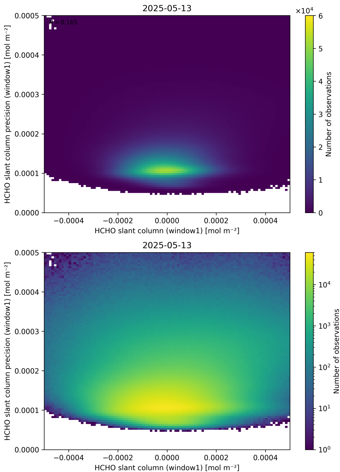
Figure 84: Scatter density plot of “HCHO slant column (window1)” against “HCHO slant column precision (window1)” for 2025-05-12 to 2025-05-14.
