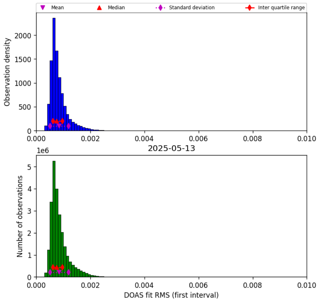
Figure 46: Histogram of “DOAS fit RMS (first interval)” for 2025-05-12 to 2025-05-14
