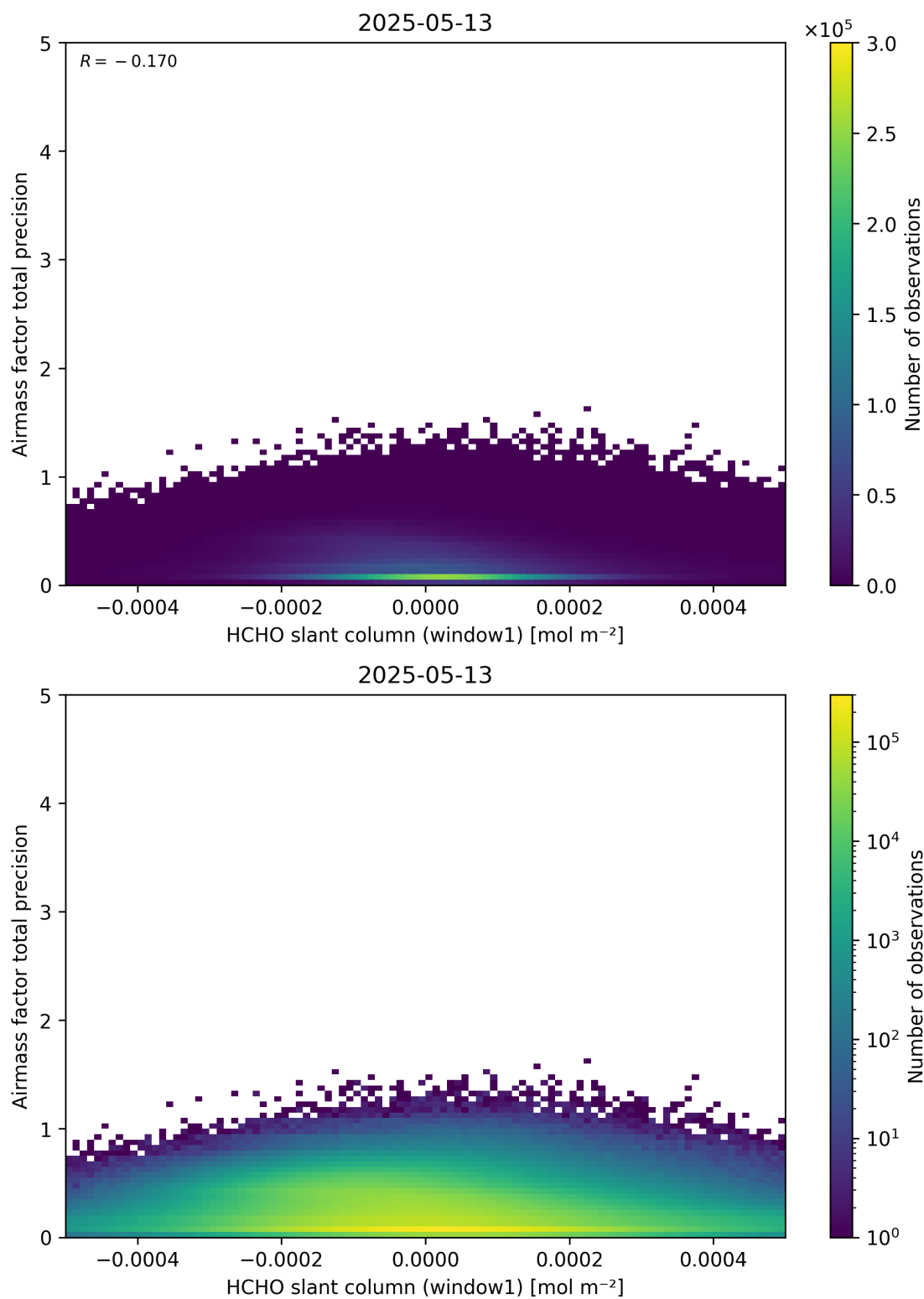
Figure 86: Scatter density plot of “HCHO slant column (window1)” against “Airmass factor total precision” for 2025-05-12 to 2025-05-14.
