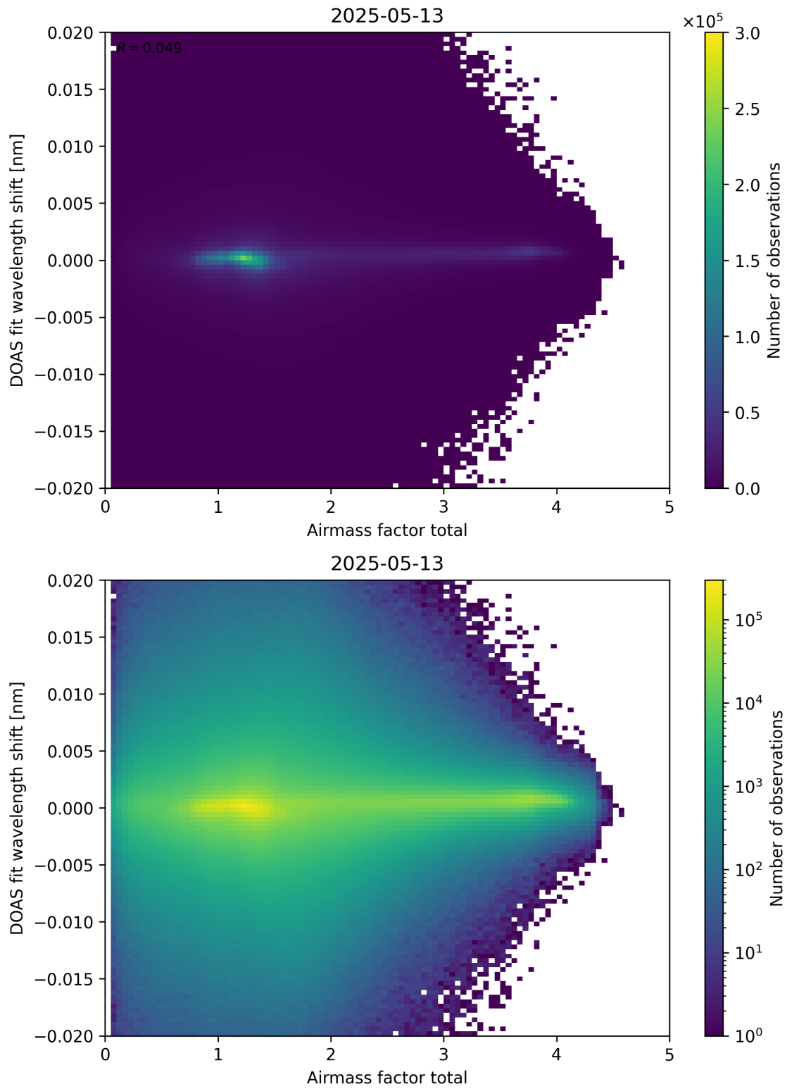
Figure 98: Scatter density plot of “Airmass factor total” against “DOAS fit wavelength shift” for 2025-05-12 to 2025-05-14.
