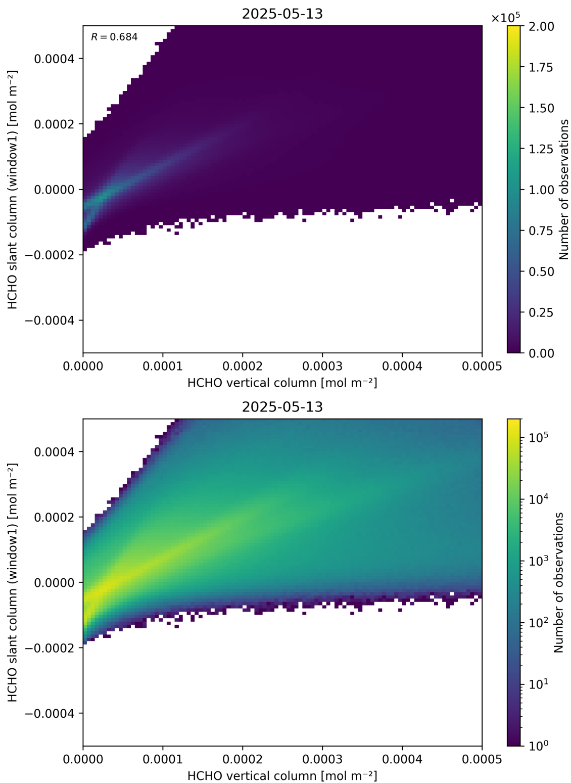
Figure 129: Scatter density plot of “HCHO vertical column” against “HCHO slant column (window1)” for 2025-05-12 to 2025-05-14.
