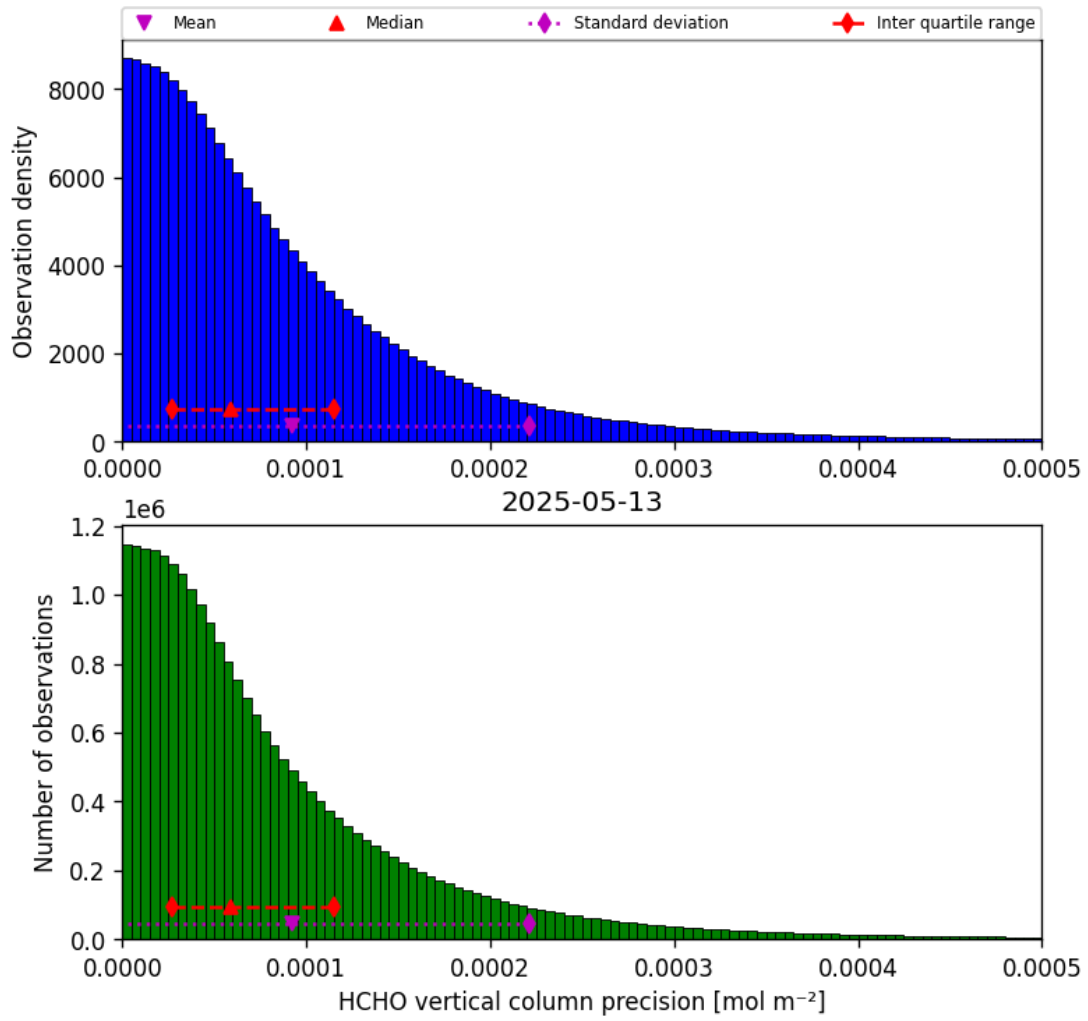
Figure 36: Histogram of “HCHO vertical column precision” for 2025-05-12 to 2025-05-14
