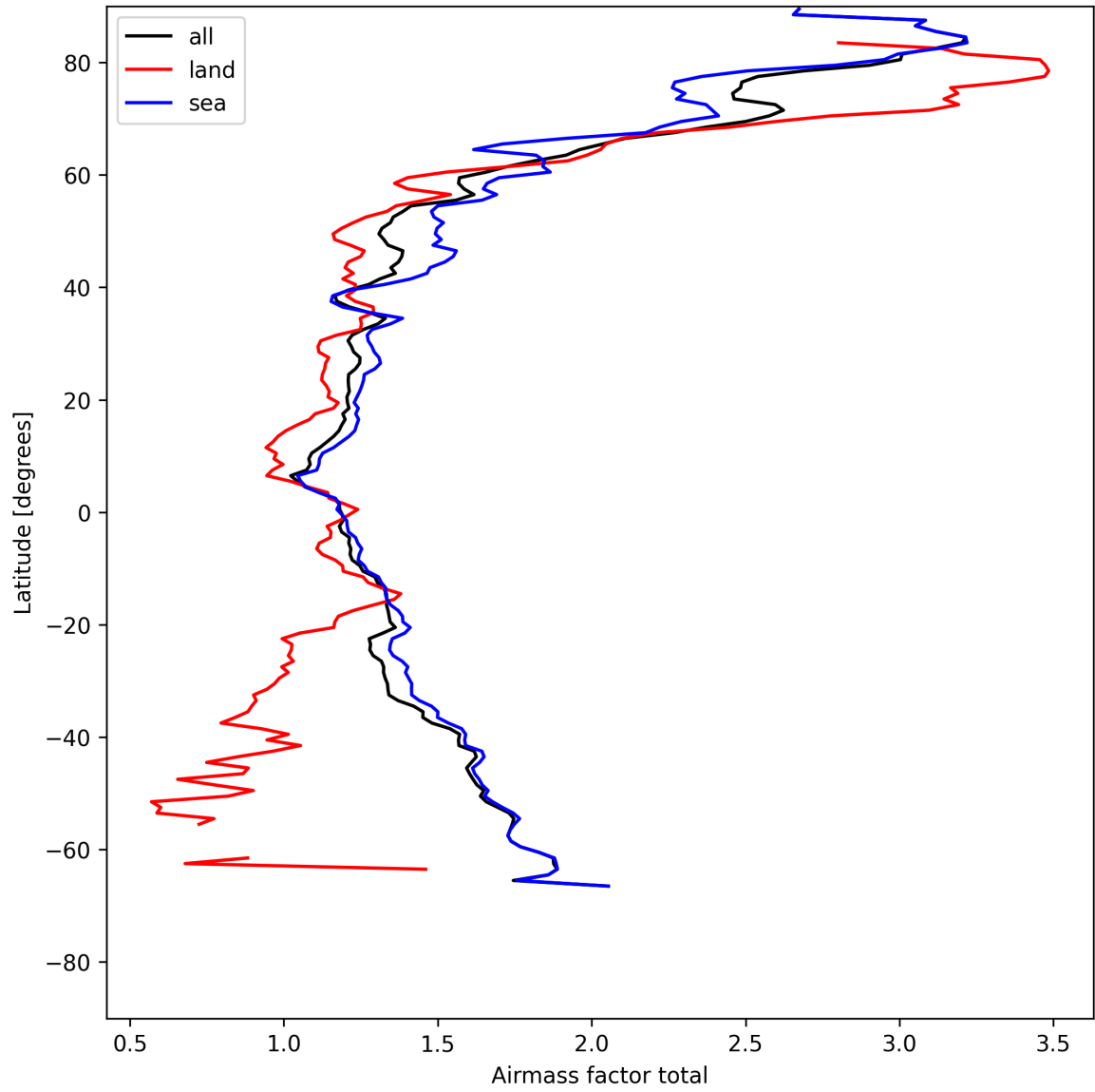
Figure 26: Zonal average of “Airmass factor total” for 2025-05-12 to 2025-05-14.
