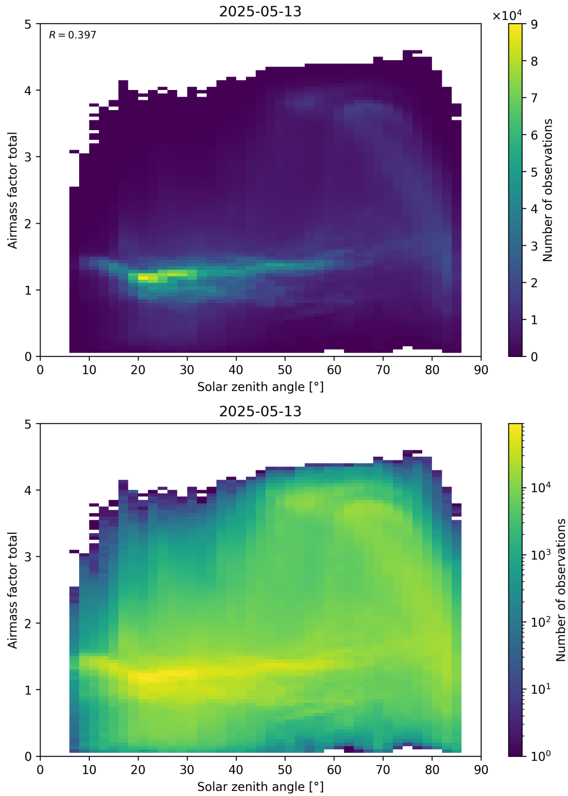
Figure 175: Scatter density plot of “Solar zenith angle” against “Airmass factor total” for 2025-05-12 to 2025-05-14.
