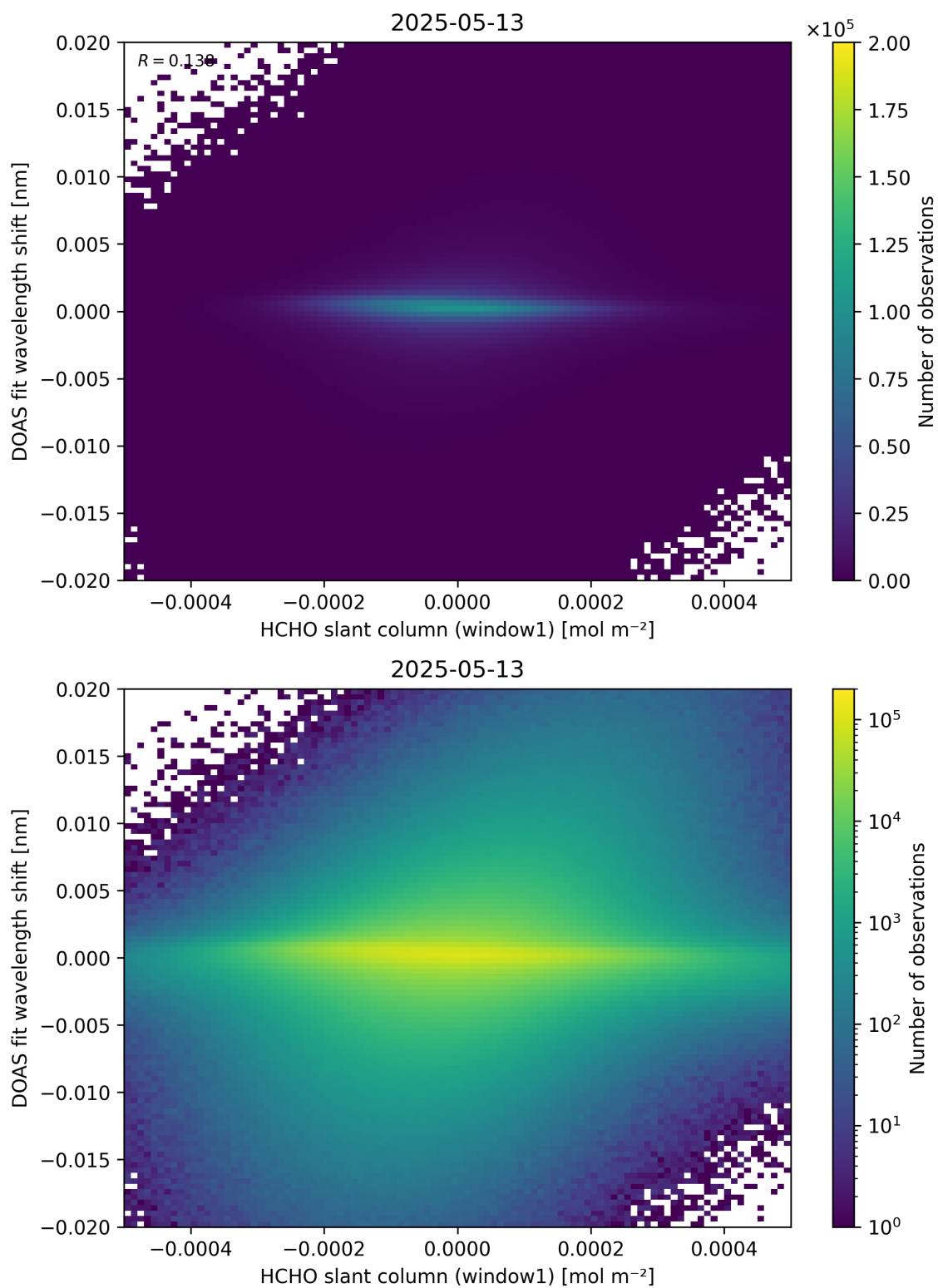
Figure 79: Scatter density plot of “HCHO slant column (window1)” against “DOAS fit wavelength shift” for 2025-05-12 to 2025-05-14.
