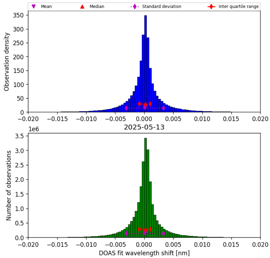
Figure 44: Histogram of “DOAS fit wavelength shift” for 2025-05-12 to 2025-05-14
