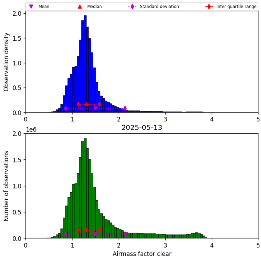
Figure 42: Histogram of “Airmass factor clear” for 2025-05-12 to 2025-05-14
