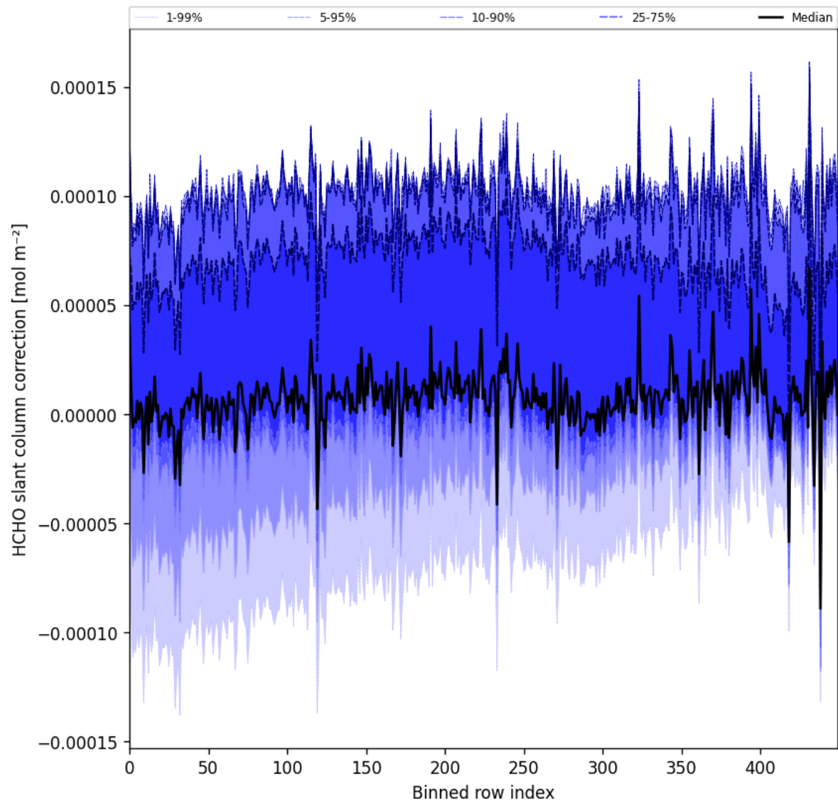
Figure 61: Along track statistics of "HCHO slant column correction" for 2025-05-12 to 2025-05-14
