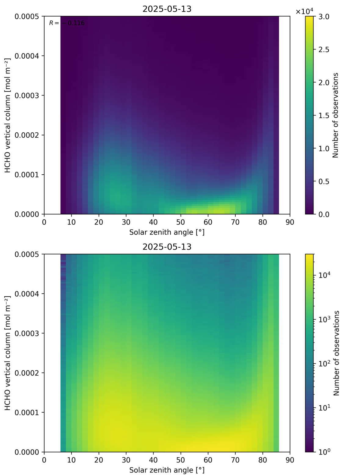
Figure 177: Scatter density plot of “Solar zenith angle” against “HCHO vertical column” for 2025-05-12 to 2025-05-14.
