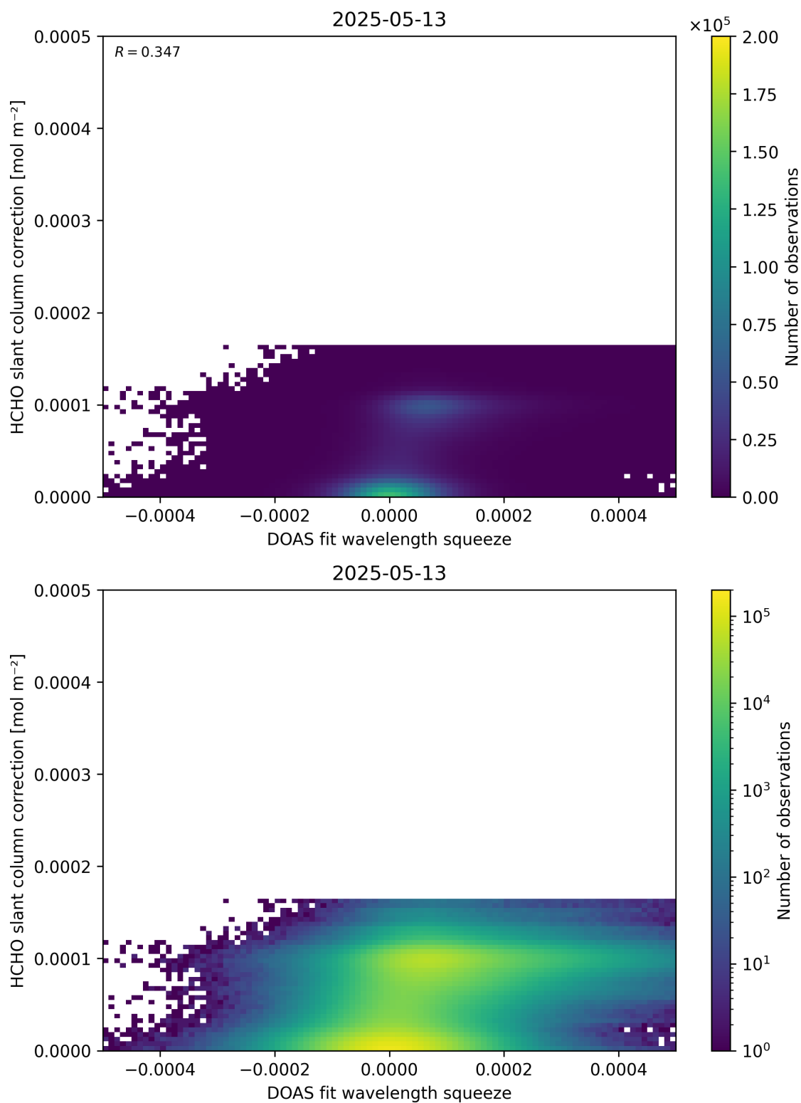
Figure 70: Scatter density plot of “DOAS fit wavelength squeeze” against “HCHO slant column correction” for 2025-05-12 to 2025-05-14.
