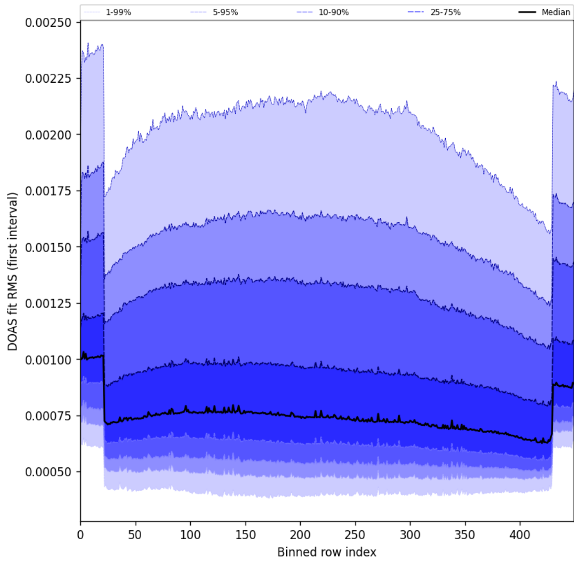
Figure 60: Along track statistics of “DOAS fit RMS (first interval)” for 2025-05-12 to 2025-05-14
