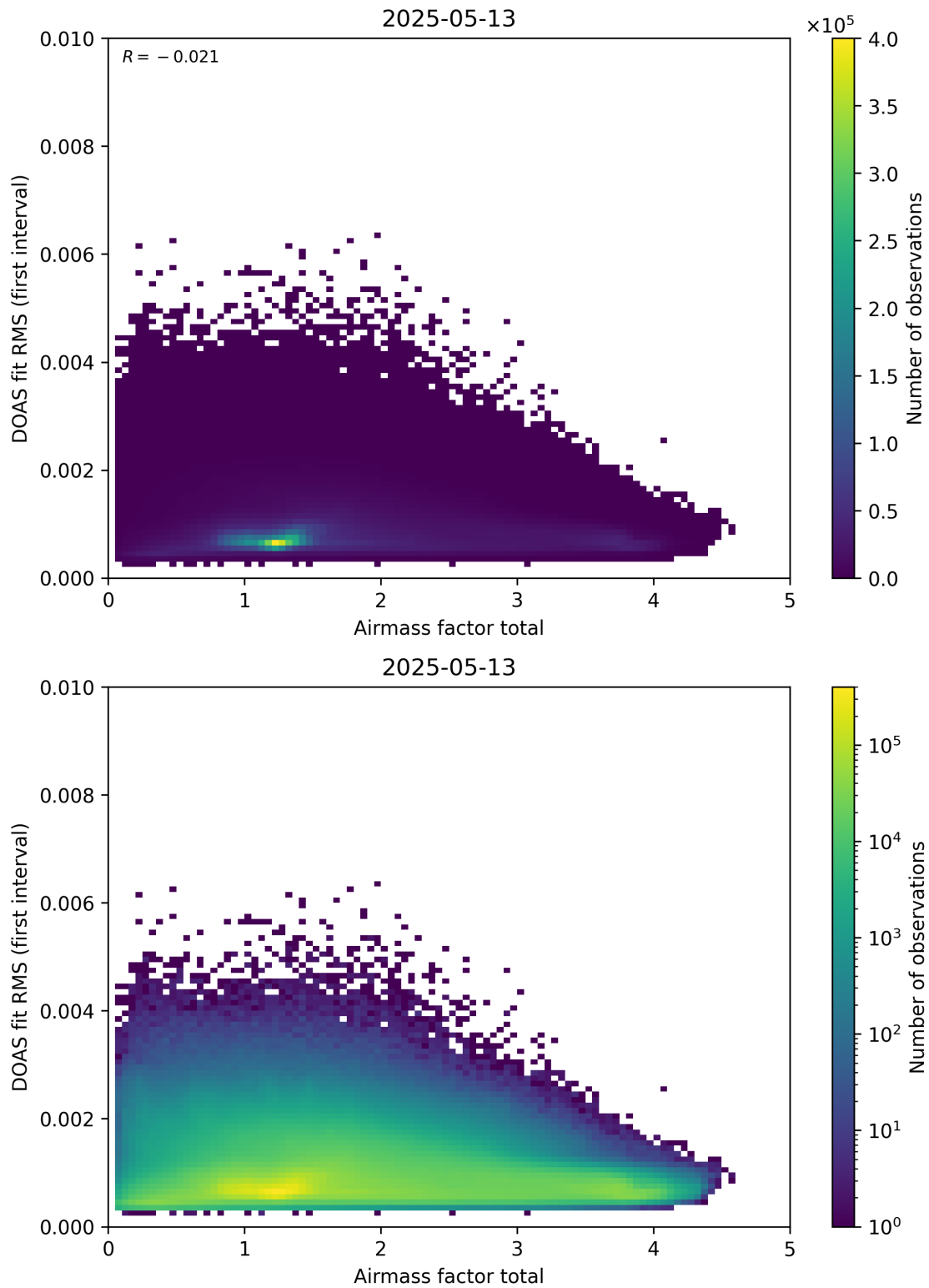
Figure 97: Scatter density plot of “Airmass factor total” against “DOAS fit RMS (first interval)” for 2025-05-12 to 2025-05-14.
