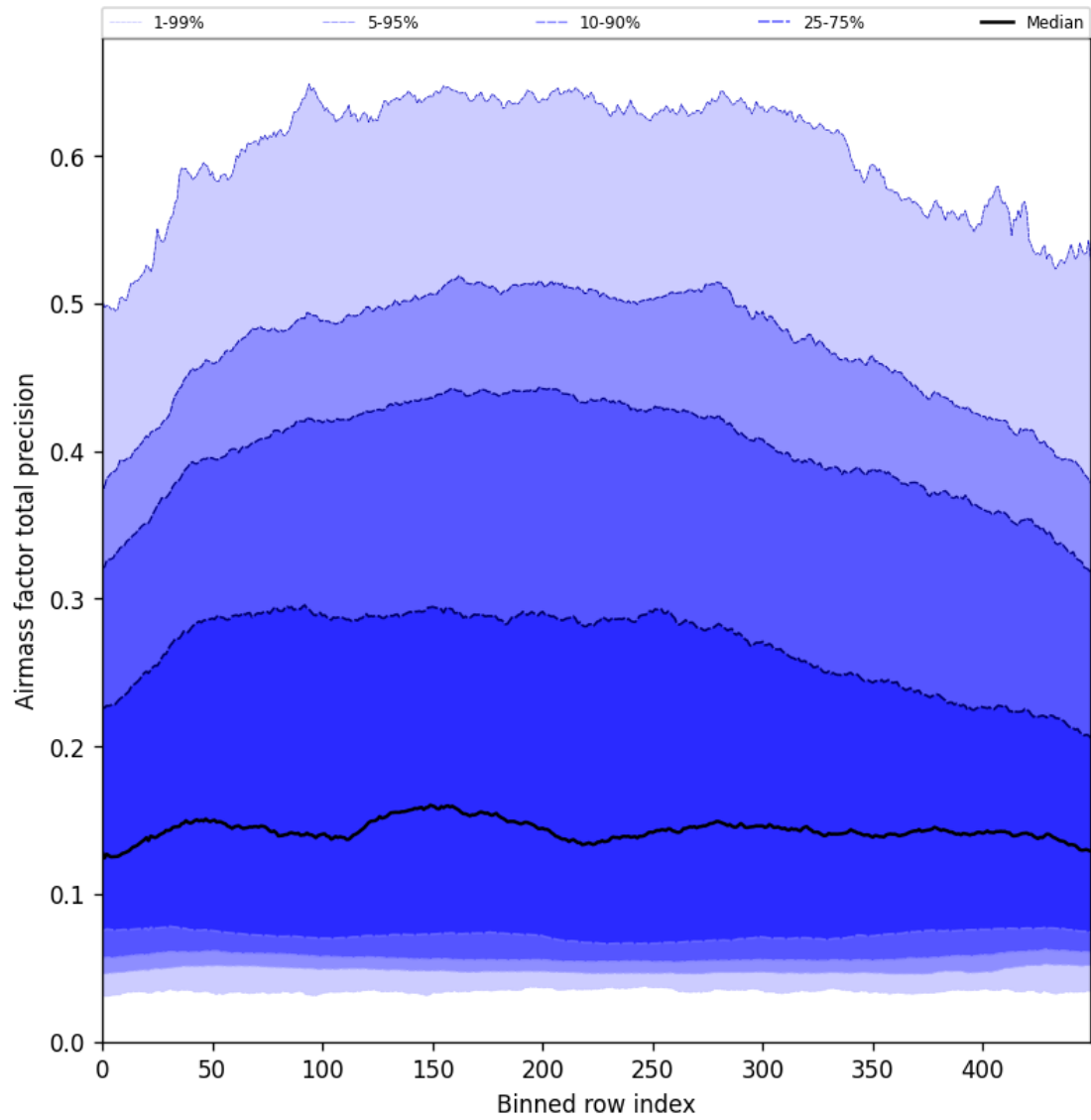
Figure 55: Along track statistics of “Airmass factor total precision” for 2025-05-12 to 2025-05-14
