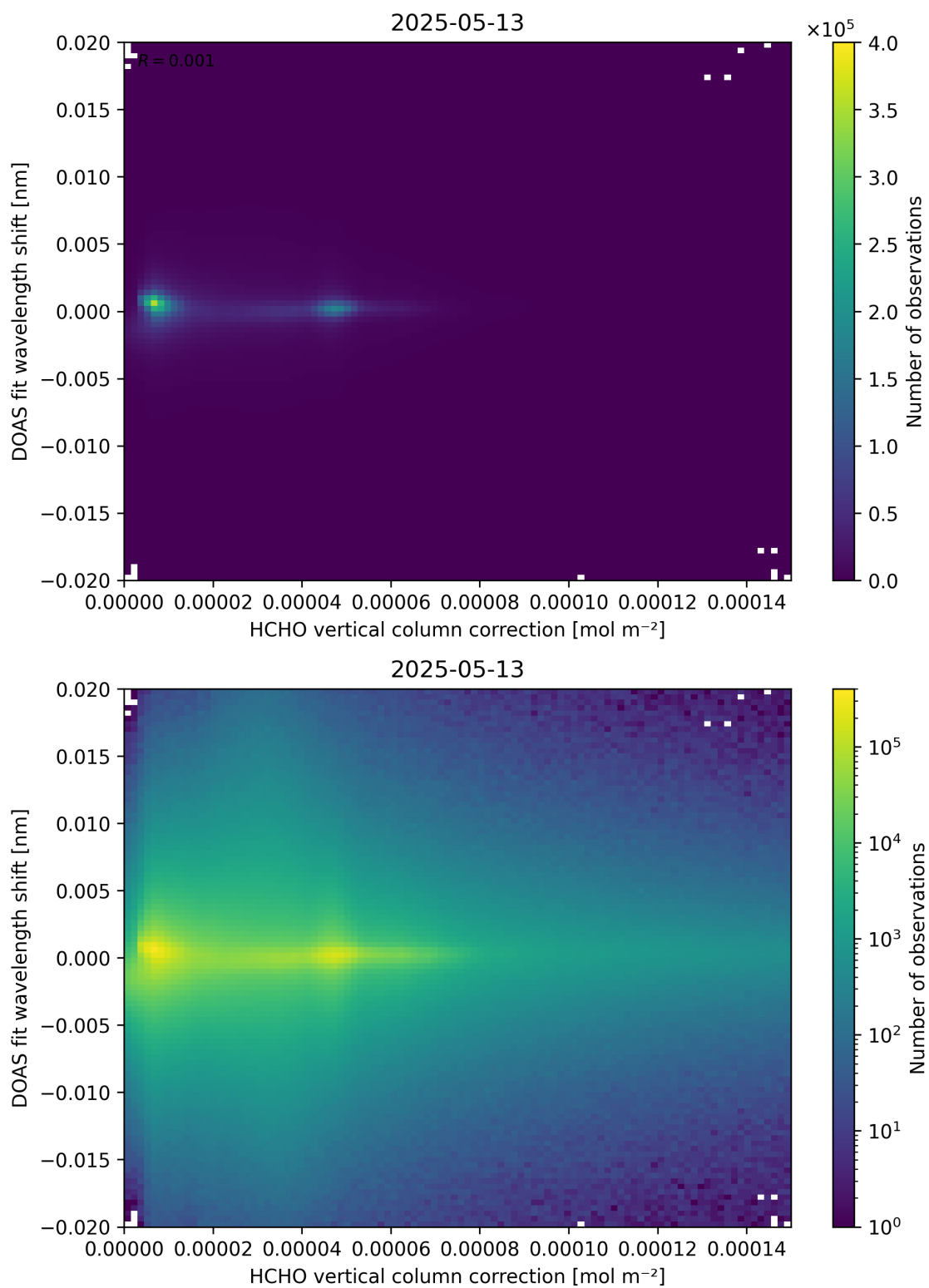
Figure 113: Scatter density plot of “HCHO vertical column correction” against “DOAS fit wavelength shift” for 2025-05-12 to 2025-05-14.
