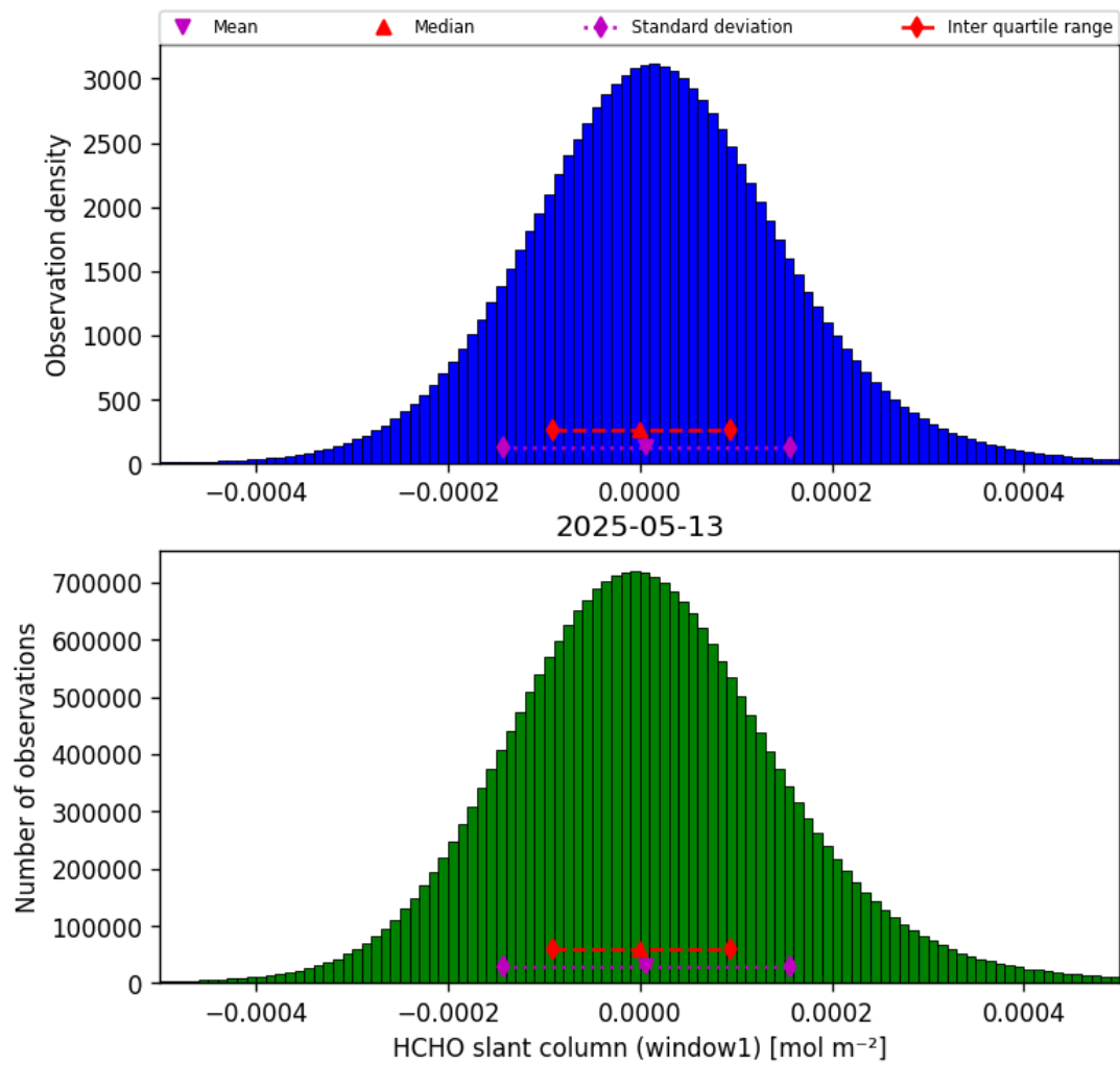
Figure 38: Histogram of “HCHO slant column (window1)” for 2025-05-12 to 2025-05-14
