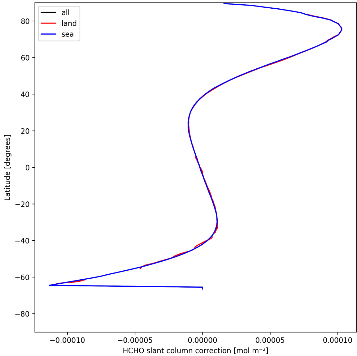
Figure 33: Zonal average of “HCHO slant column correction” for 2025-05-12 to 2025-05-14.
