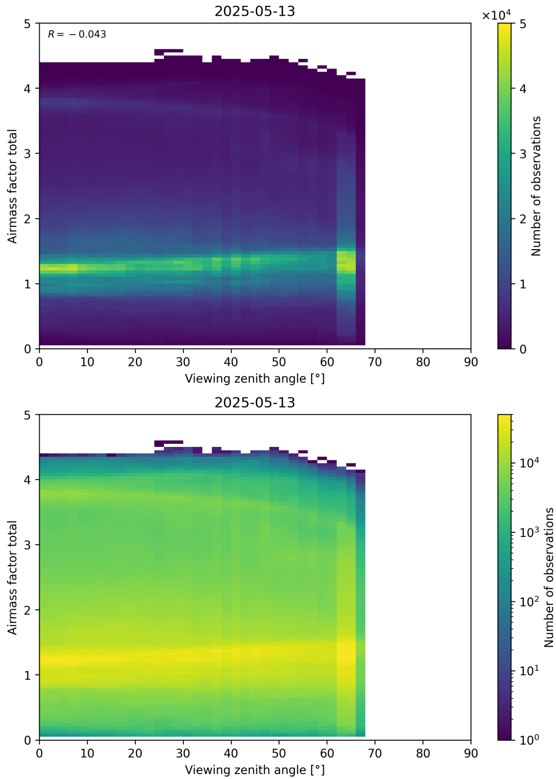
Figure 190: Scatter density plot of “Viewing zenith angle” against “Airmass factor total” for 2025-05-12 to 2025-05-14.
