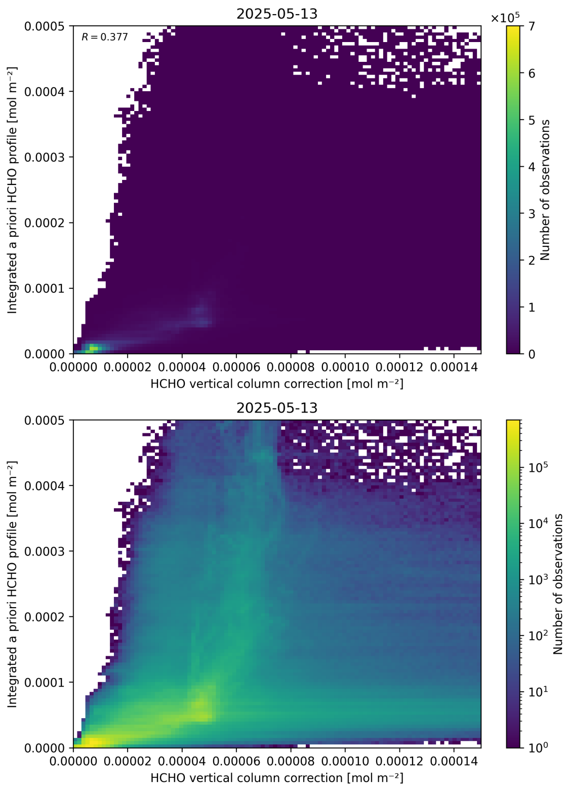
Figure 122: Scatter density plot of “HCHO vertical column correction” against “Integrated a priori HCHO profile” for 2025-05-12 to 2025-05-14.
