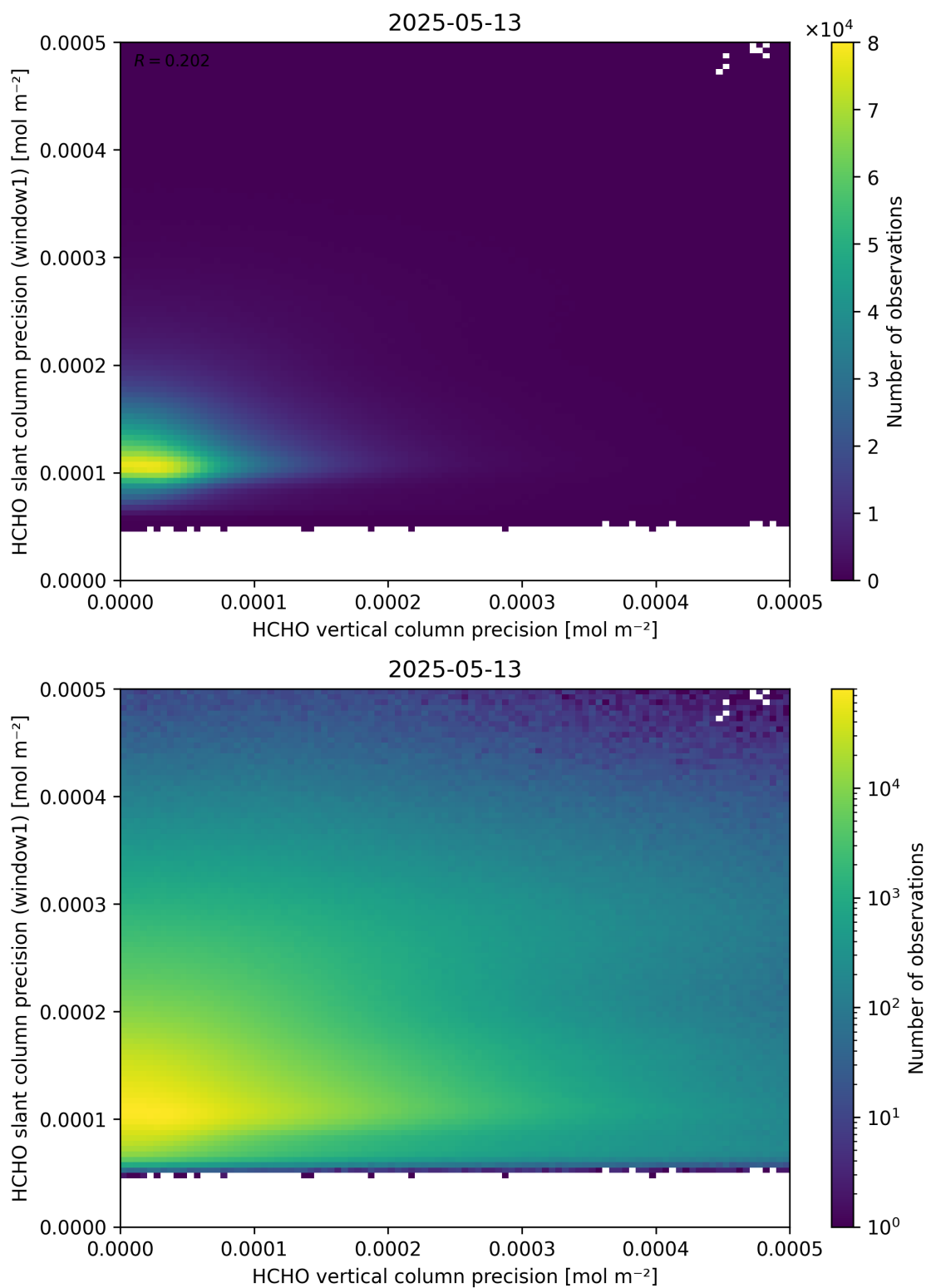
Figure 143: Scatter density plot of “HCHO vertical column precision” against “HCHO slant column precision (window1)” for 2025-05-12 to 2025-05-14.
