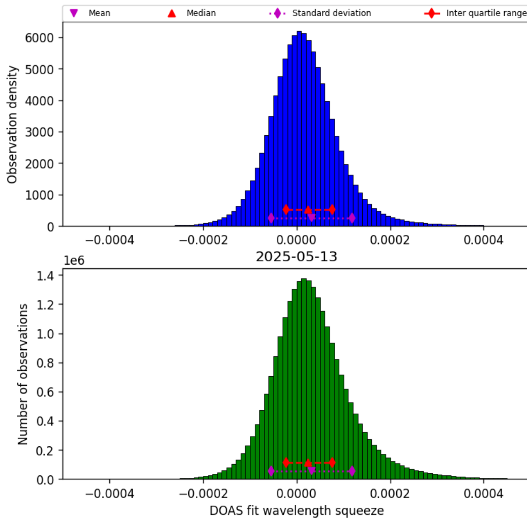
Figure 45: Histogram of “DOAS fit wavelength squeeze” for 2025-05-12 to 2025-05-14
