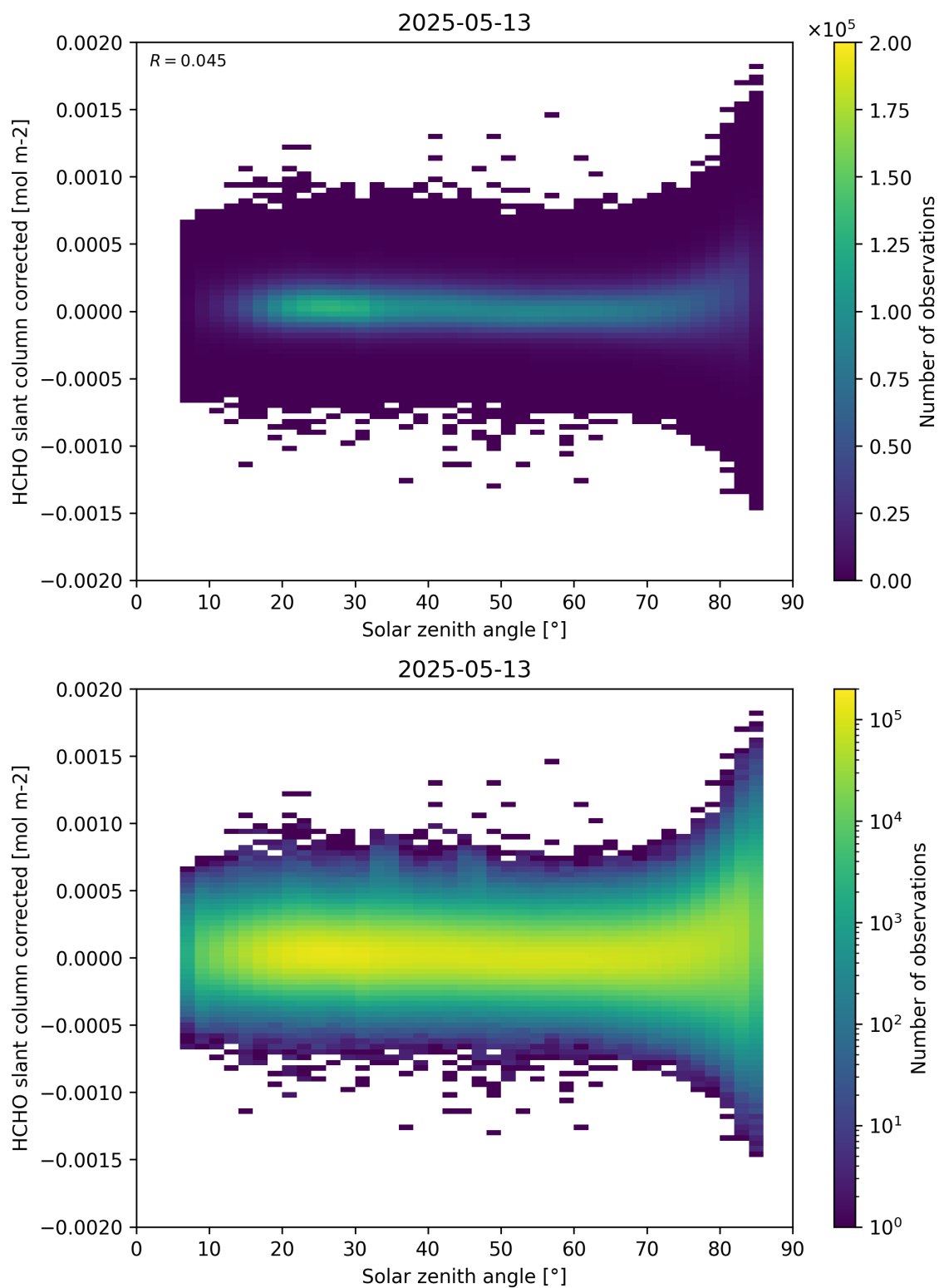
Figure 171: Scatter density plot of “Solar zenith angle” against “HCHO slant column corrected” for 2025-05-12 to 2025-05-14.
