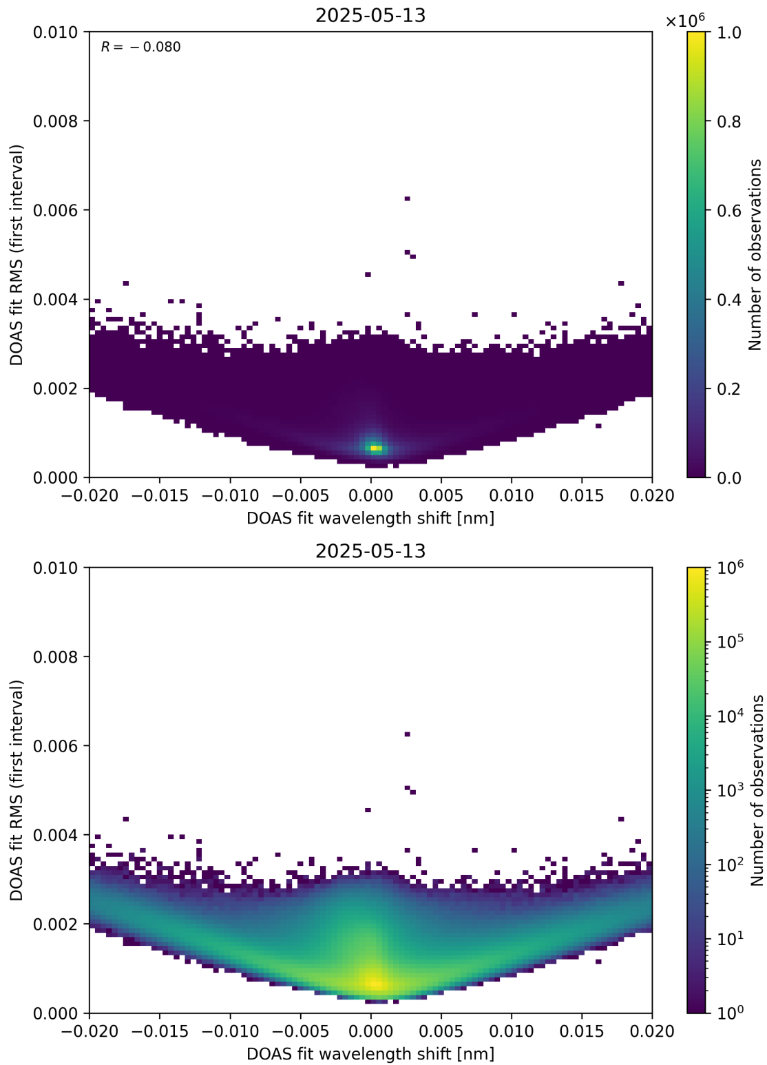
Figure 64: Scatter density plot of “DOAS fit wavelength shift” against “DOAS fit RMS (first interval)” for 2025-05-12 to 2025-05-14.
