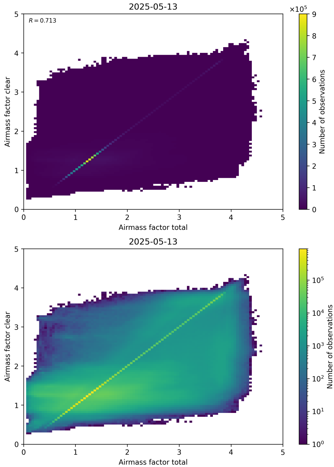
Figure 100: Scatter density plot of “Airmass factor total” against “Airmass factor clear” for 2025-05-12 to 2025-05-14.
