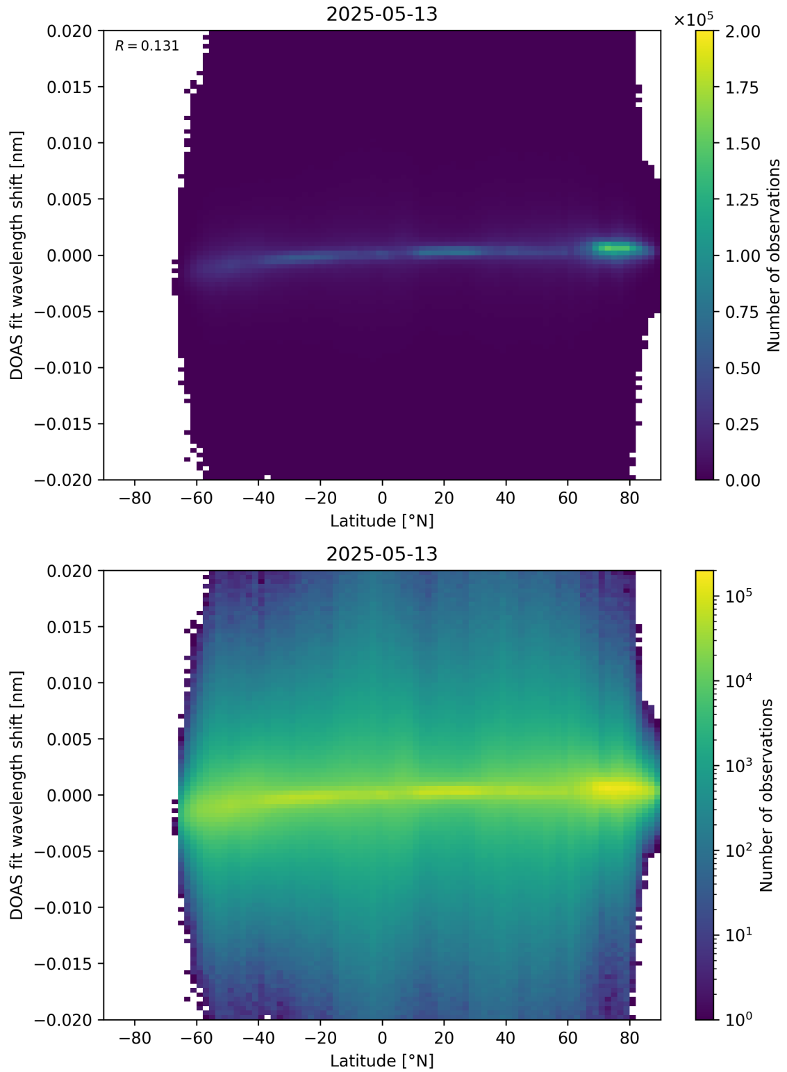
Figure 154: Scatter density plot of “Latitude” against “DOAS fit wavelength shift” for 2025-05-12 to 2025-05-14.
