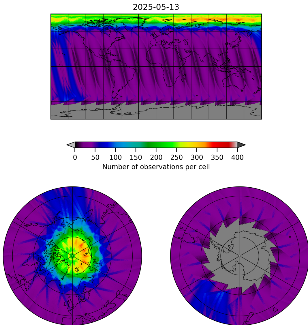
Figure 19: Map of the number of observations for 2025-05-12 to 2025-05-14
