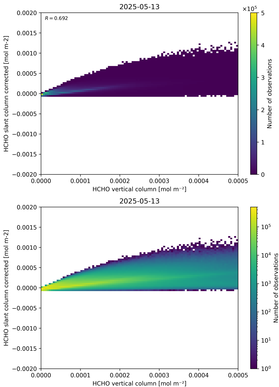
Figure 127: Scatter density plot of “HCHO vertical column” against “HCHO slant column corrected” for 2025-05-12 to 2025-05-14.
