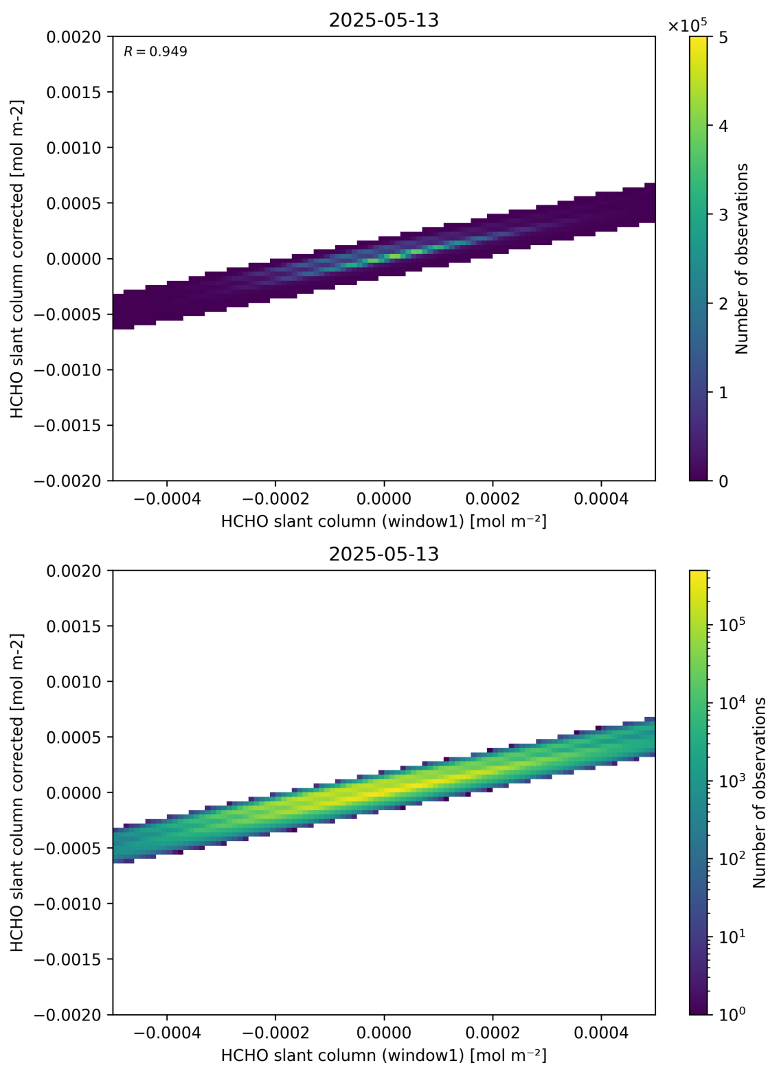
Figure 82: Scatter density plot of “HCHO slant column (window1)” against “HCHO slant column corrected” for 2025-05-12 to 2025-05-14.
