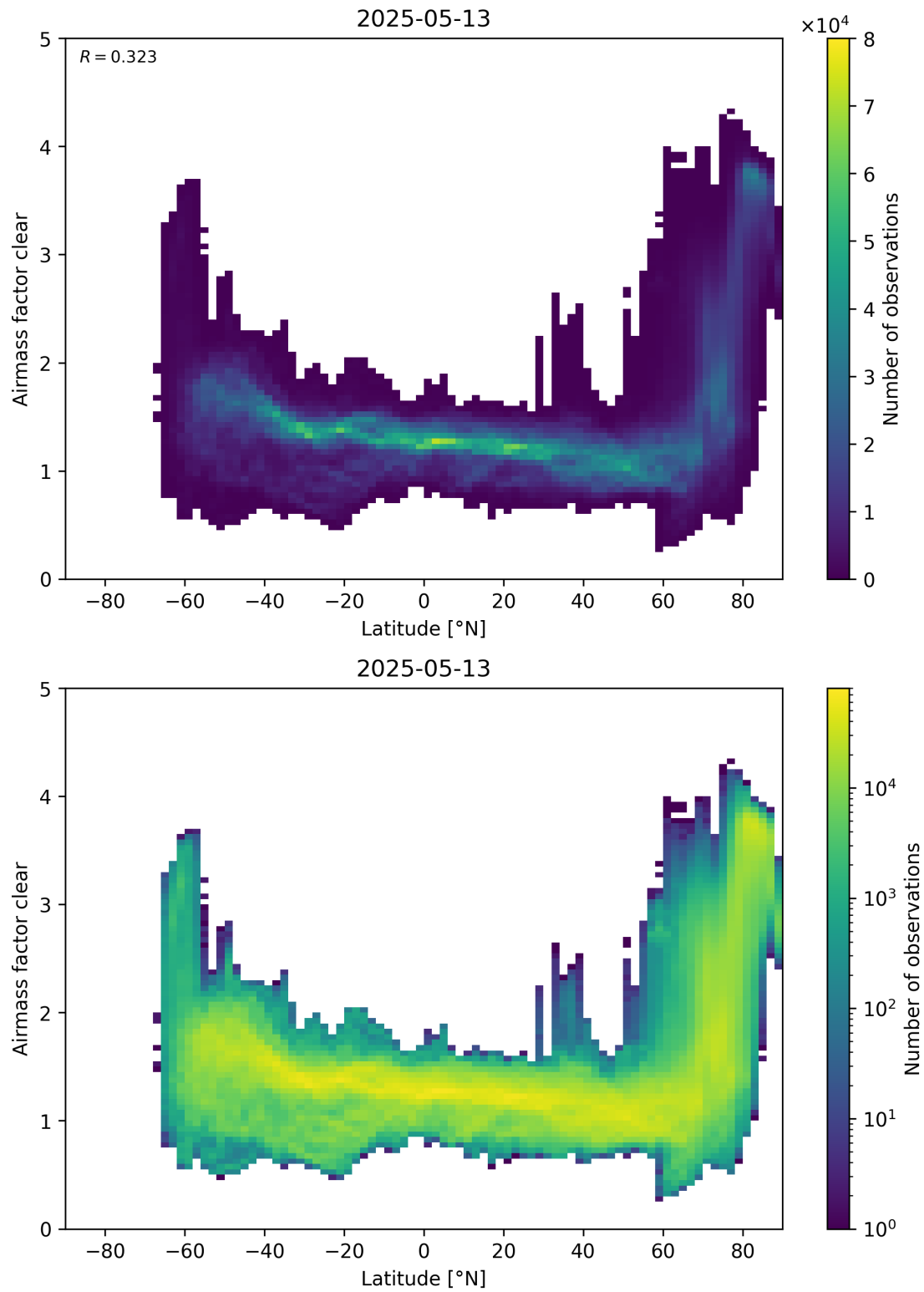
Figure 156: Scatter density plot of “Latitude” against “Airmass factor clear” for 2025-05-12 to 2025-05-14.
