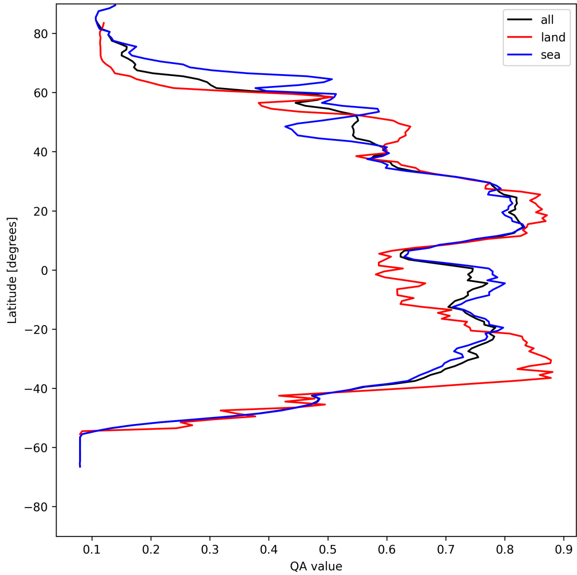
Figure 20: Zonal average of “QA value” for 2025-05-12 to 2025-05-14.
