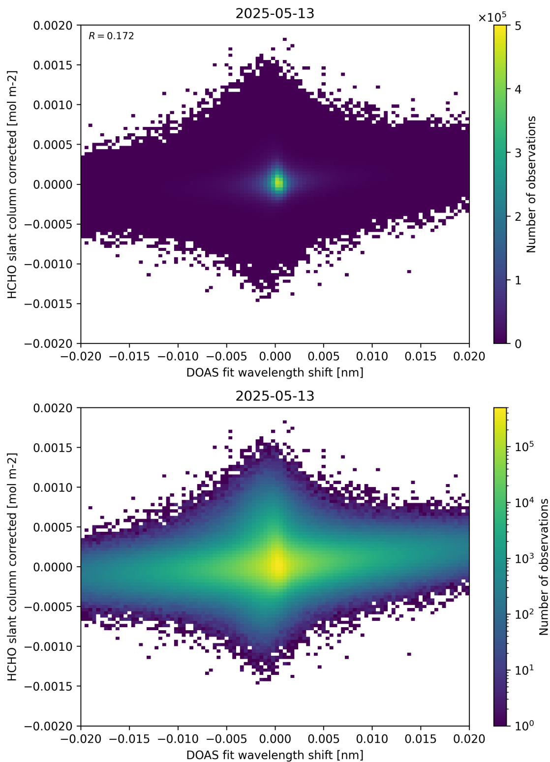
Figure 66: Scatter density plot of “DOAS fit wavelength shift” against “HCHO slant column corrected” for 2025-05-12 to 2025-05-14.
