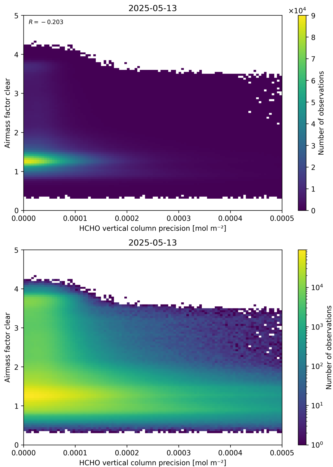
Figure 139: Scatter density plot of “HCHO vertical column precision” against “Airmass factor clear” for 2025-05-12 to 2025-05-14.
