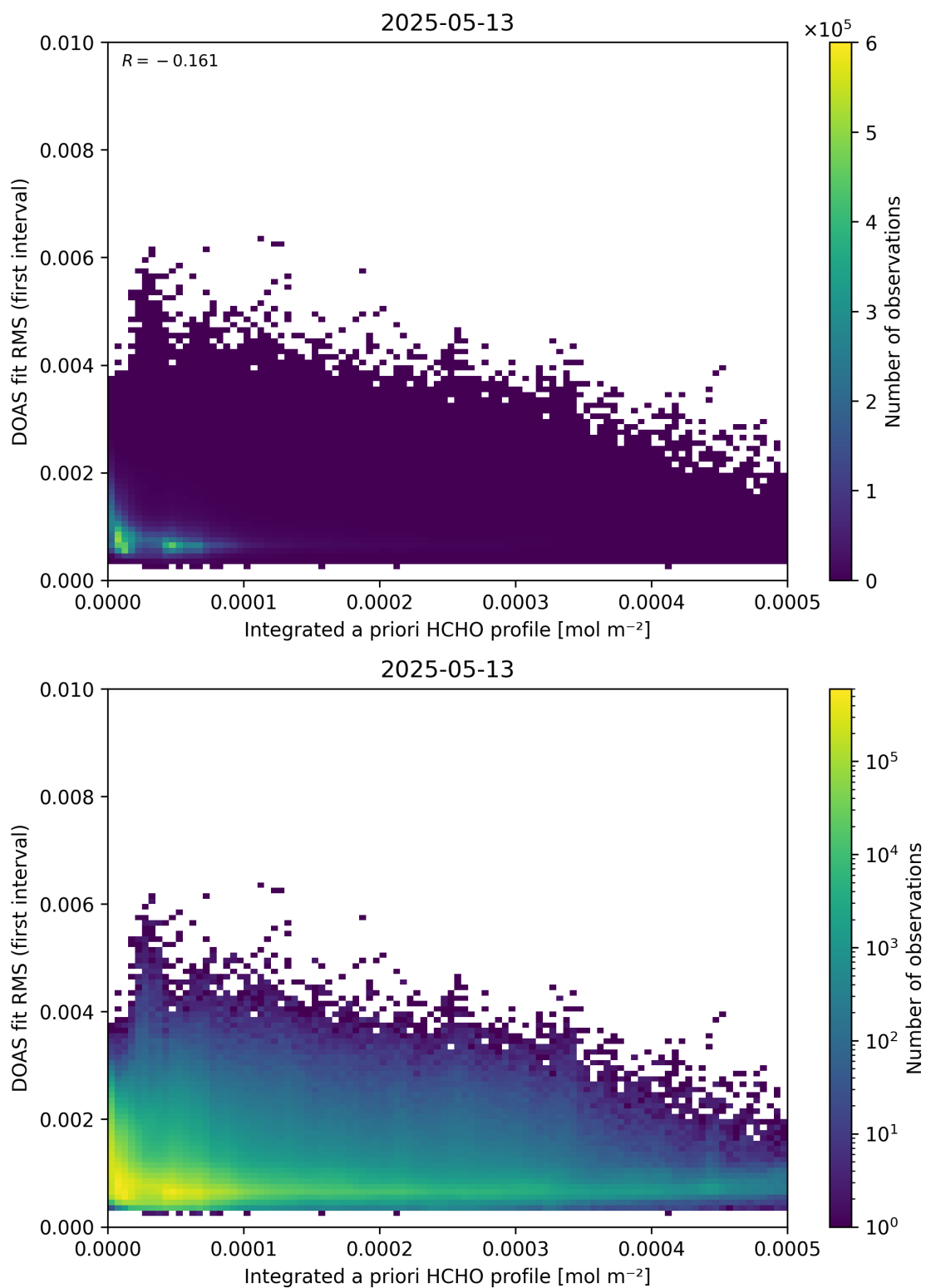
Figure 148: Scatter density plot of “Integrated a priori HCHO profile” against “DOAS fit RMS (first interval)” for 2025-05-12 to 2025-05-14.
