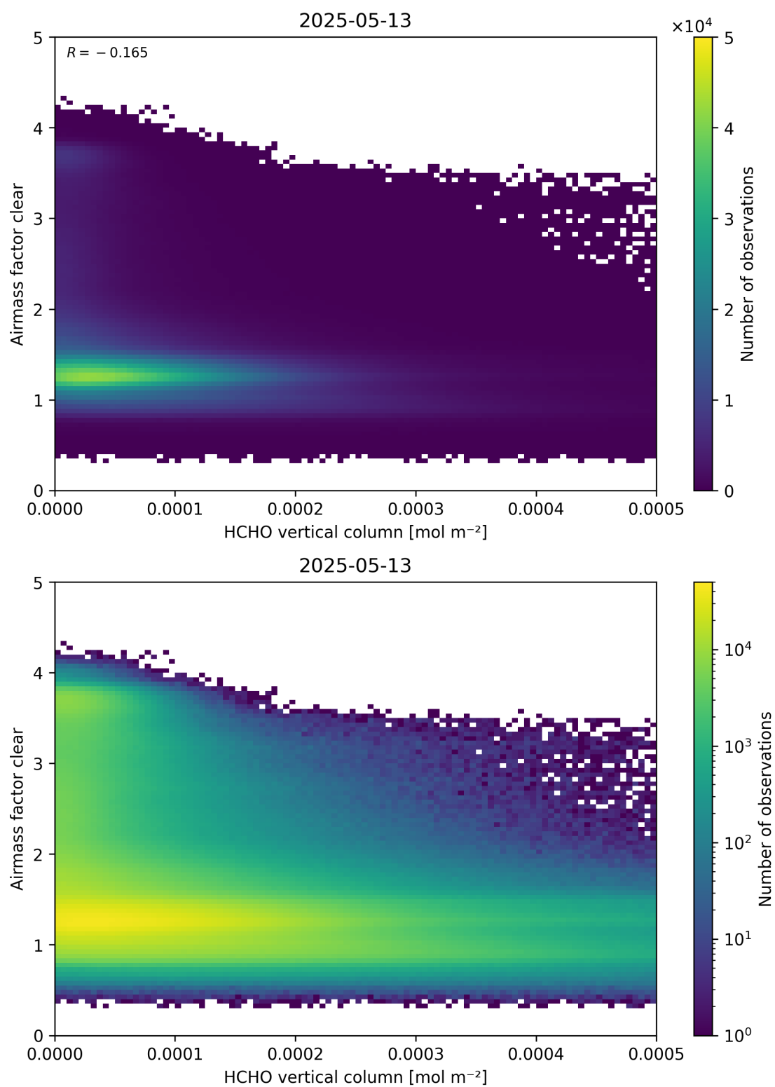
Figure 126: Scatter density plot of “HCHO vertical column” against “Airmass factor clear” for 2025-05-12 to 2025-05-14.
