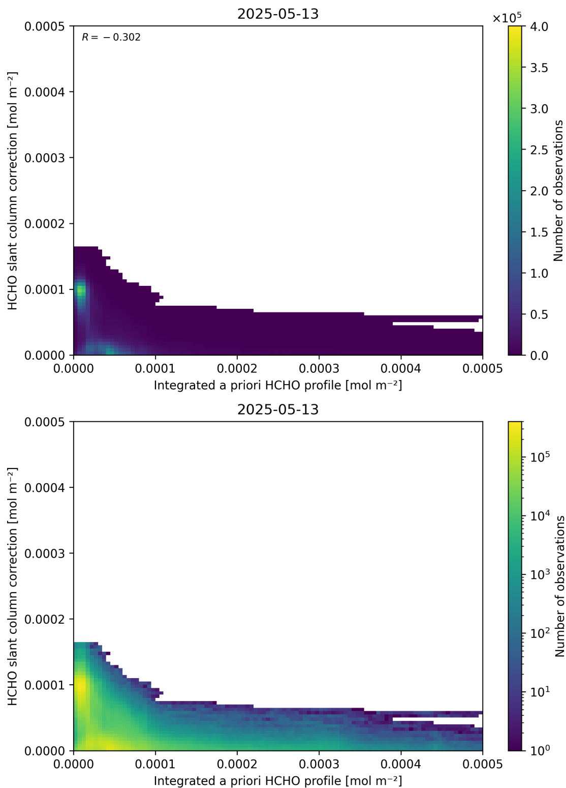
Figure 152: Scatter density plot of “Integrated a priori HCHO profile” against “HCHO slant column correction” for 2025-05-12 to 2025-05-14.
