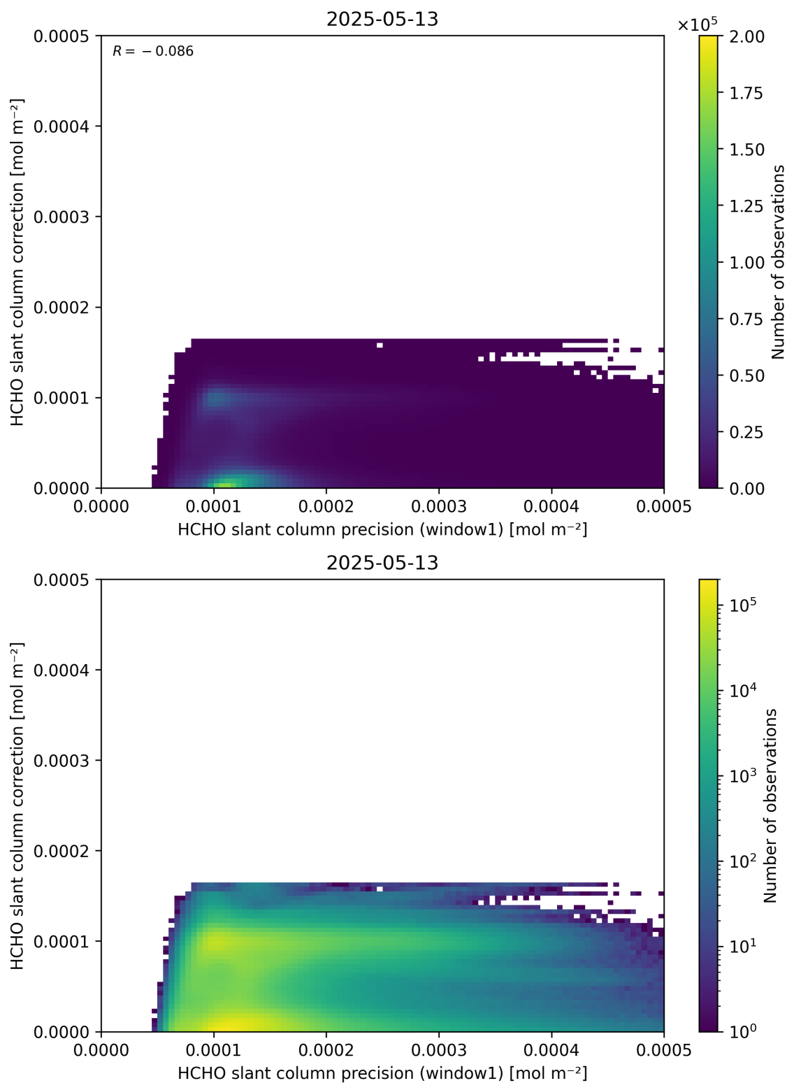
Figure 93: Scatter density plot of “HCHO slant column precision (window1)” against “HCHO slant column correction” for 2025-05-12 to 2025-05-14.
