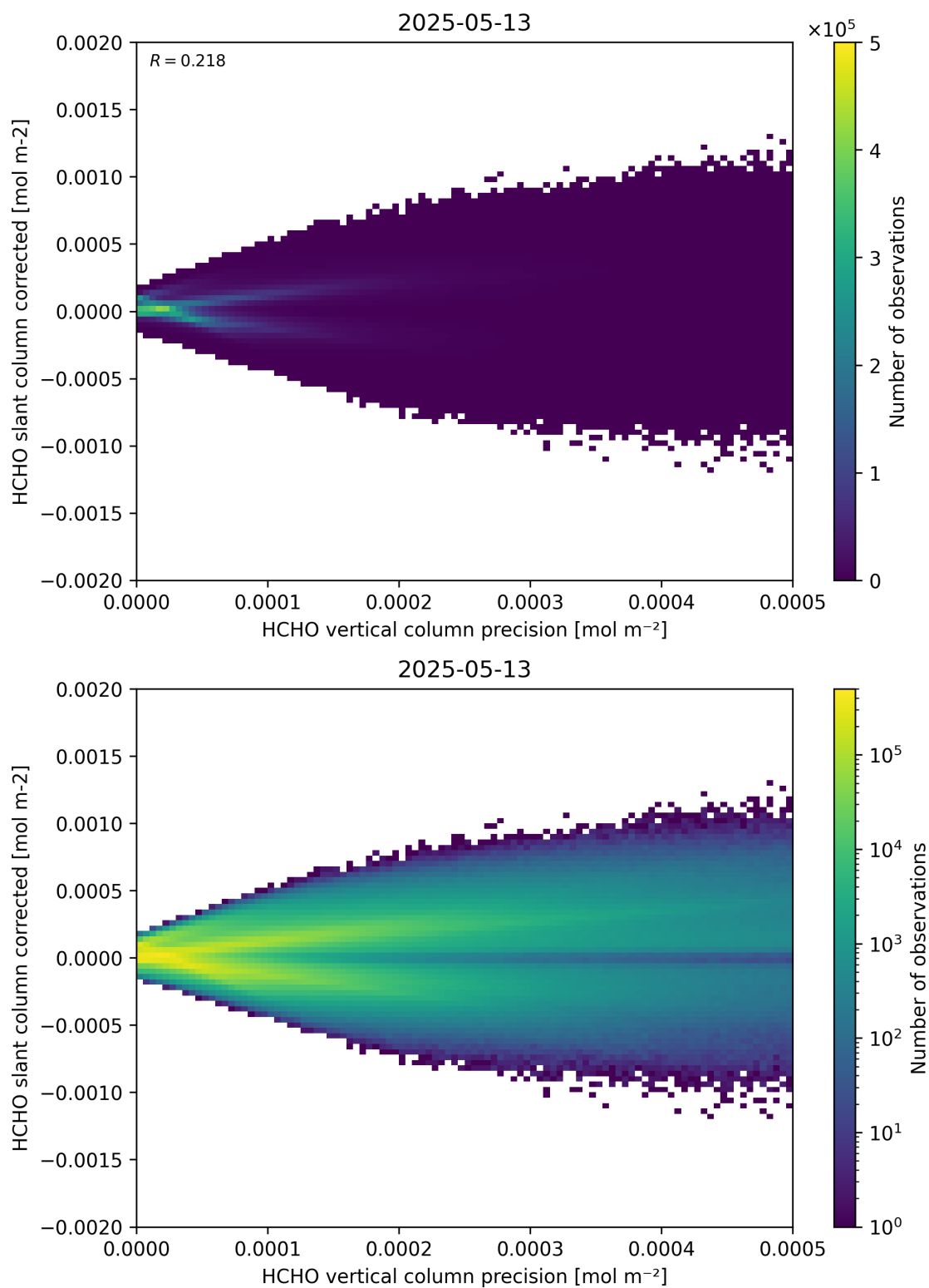
Figure 140: Scatter density plot of “HCHO vertical column precision” against “HCHO slant column corrected” for 2025-05-12 to 2025-05-14.
