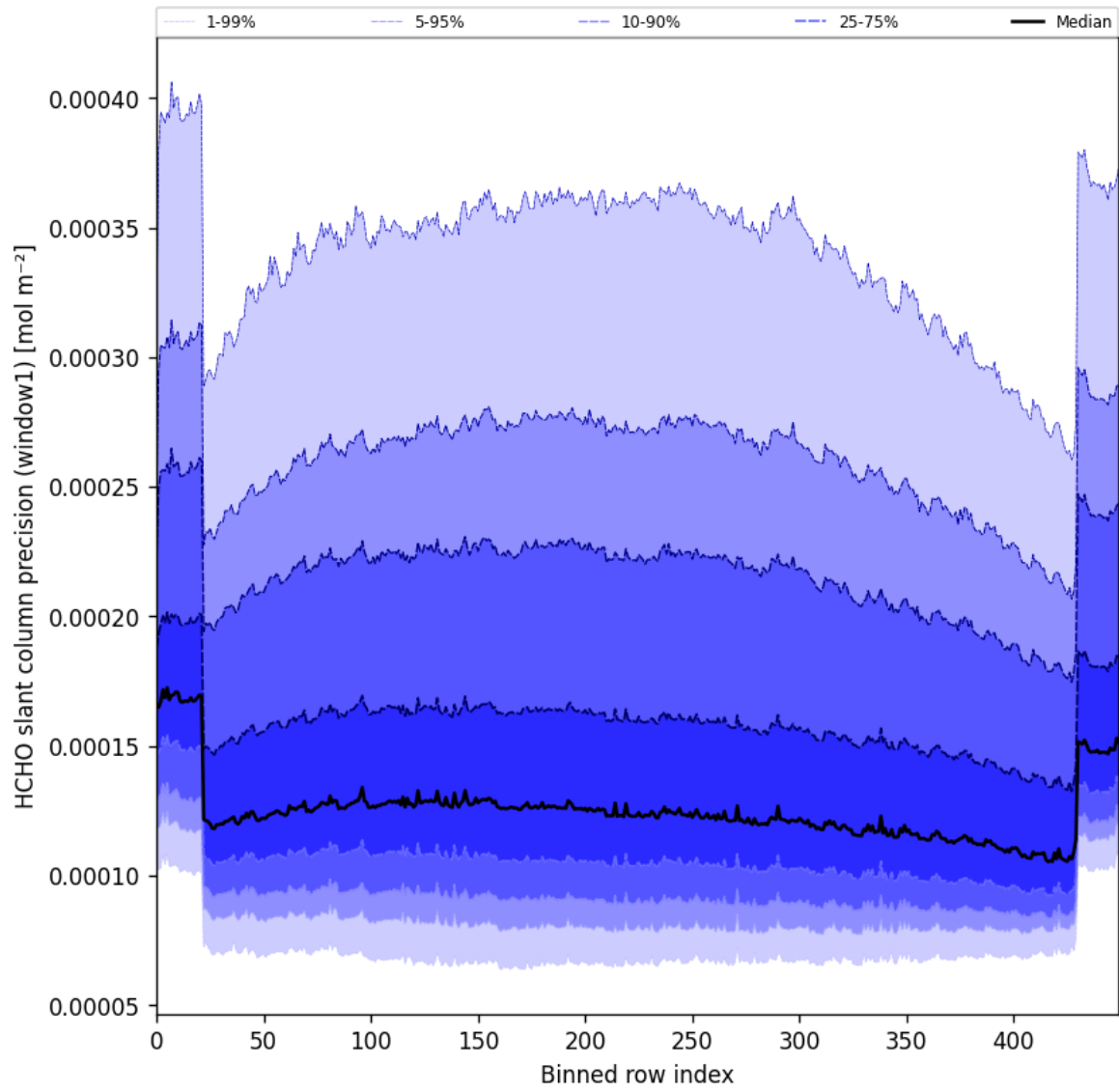
Figure 53: Along track statistics of “HCHO slant column precision (window1)” for 2025-05-12 to 2025-05-14
