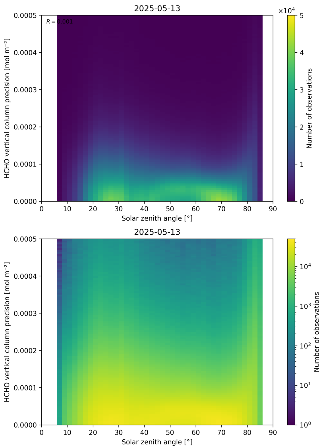
Figure 179: Scatter density plot of “Solar zenith angle” against “HCHO vertical column precision” for 2025-05-12 to 2025-05-14.
