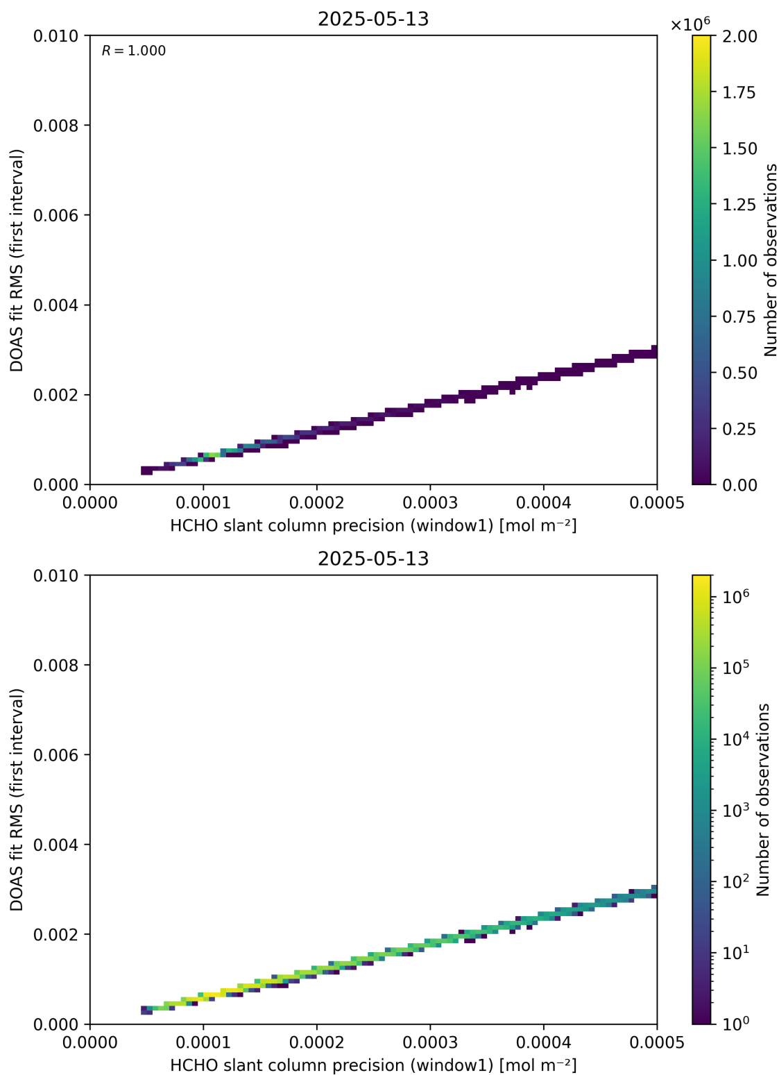
Figure 88: Scatter density plot of “HCHO slant column precision (window1)” against “DOAS fit RMS (first interval)” for 2025-05-12 to 2025-05-14.
