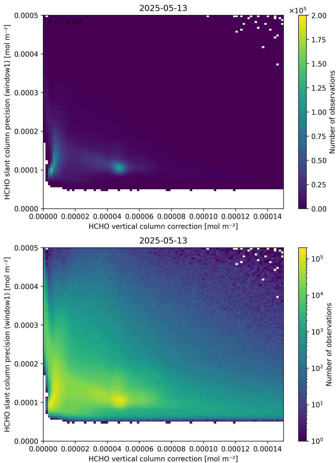
Figure 119: Scatter density plot of “HCHO vertical column correction” against “HCHO slant column precision (window1)” for 2025-05-12 to 2025-05-14.
