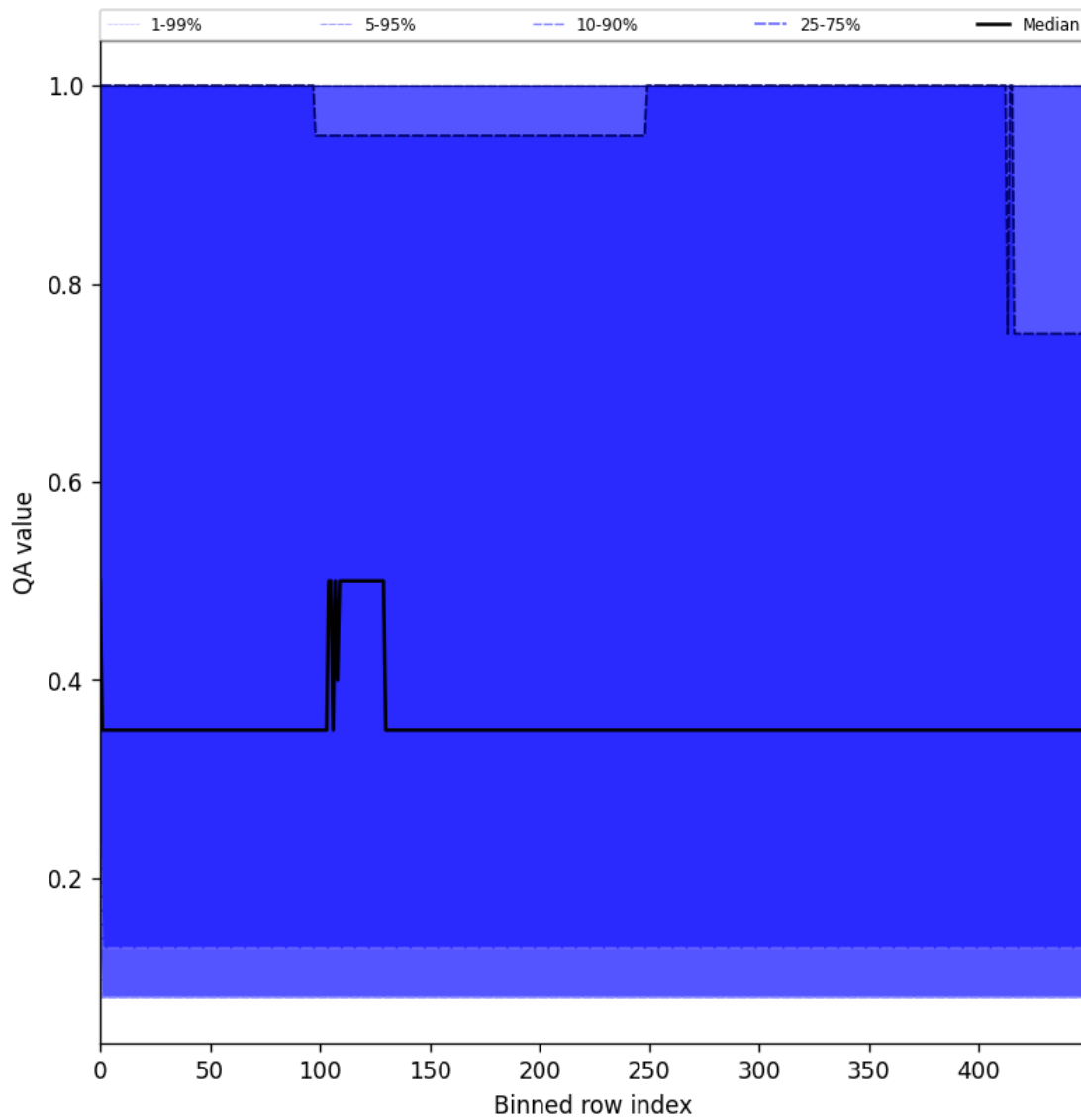
Figure 48: Along track statistics of “QA value” for 2025-05-12 to 2025-05-14
