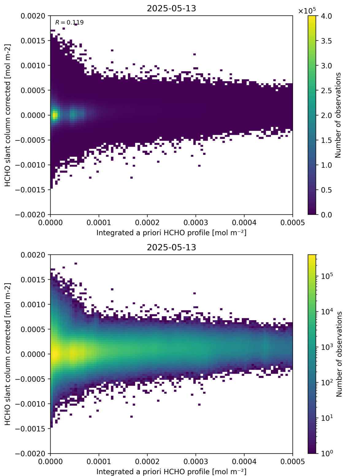
Figure 151: Scatter density plot of “Integrated a priori HCHO profile” against “HCHO slant column corrected” for 2025-05-12 to 2025-05-14.
