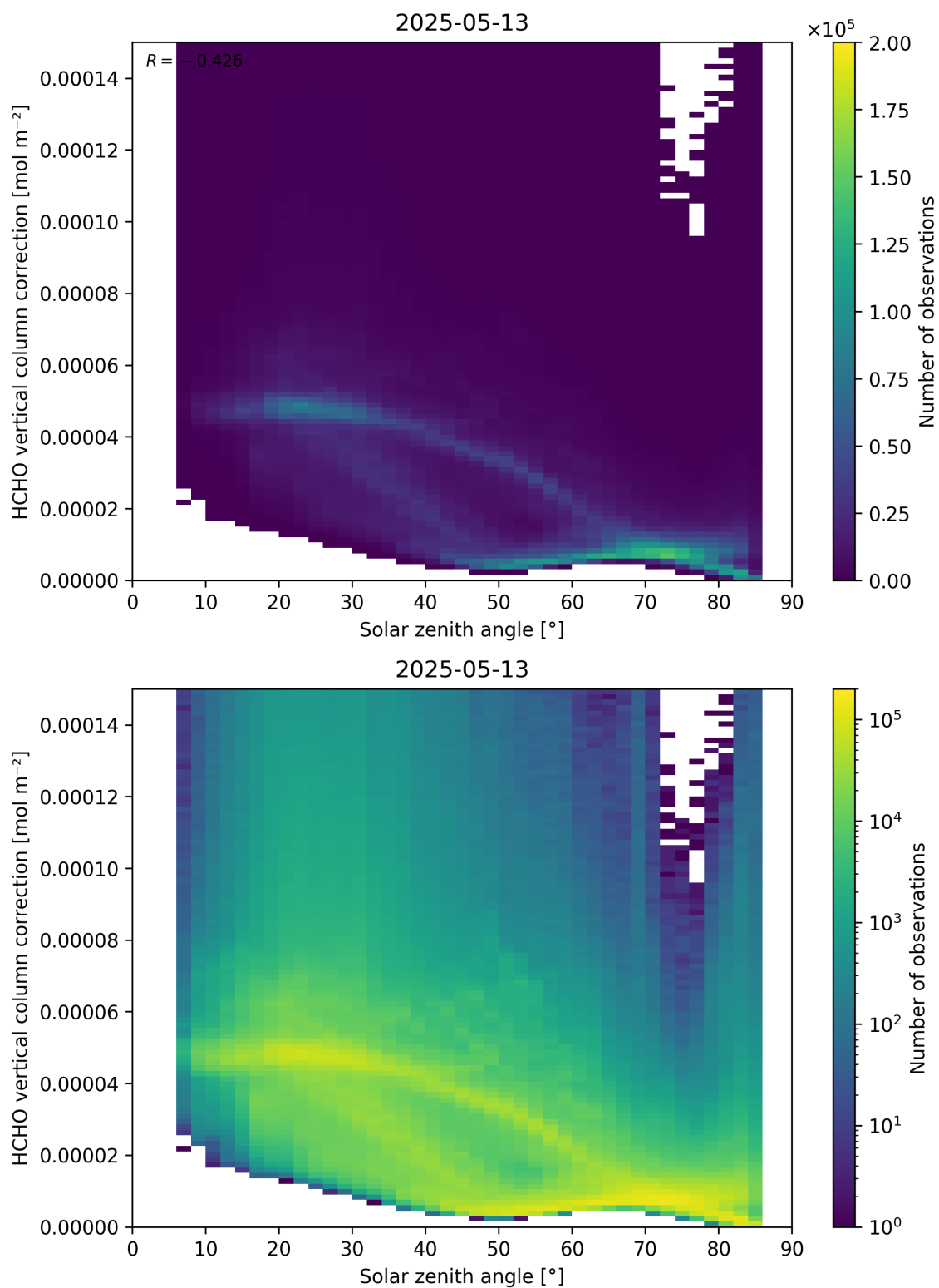
Figure 178: Scatter density plot of “Solar zenith angle” against “HCHO vertical column correction” for 2025-05-12 to 2025-05-14.
