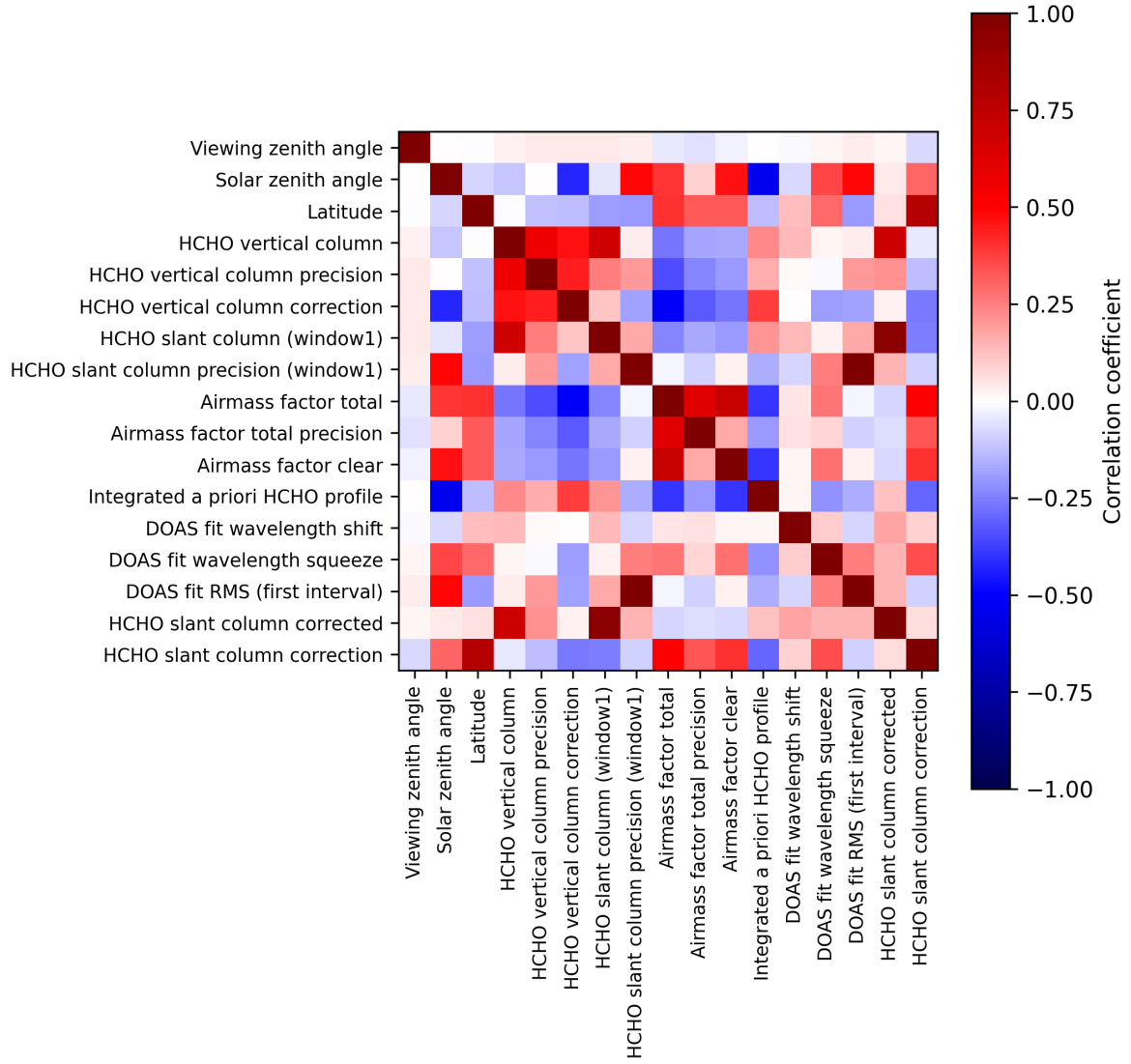
Figure 2: Map of correlation matrix for 2025-05-12 to 2025-05-14.
