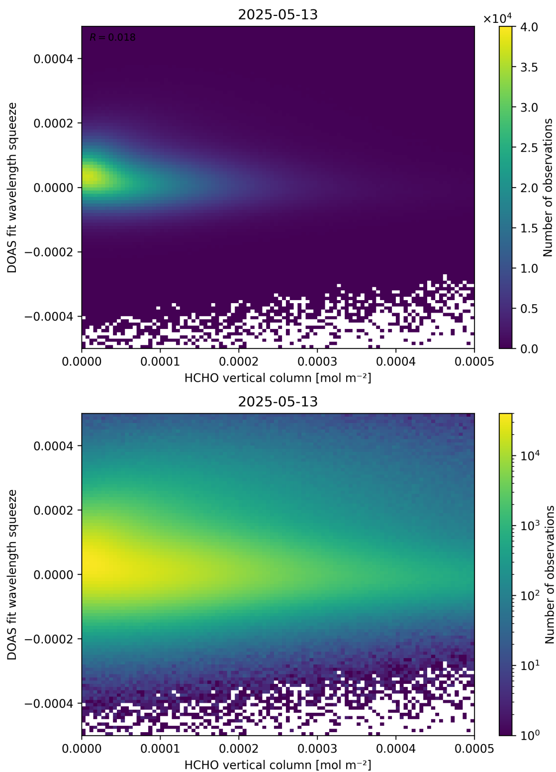
Figure 125: Scatter density plot of “HCHO vertical column” against “DOAS fit wavelength squeeze” for 2025-05-12 to 2025-05-14.
