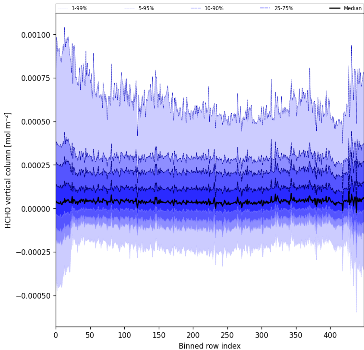
Figure 49: Along track statistics of “HCHO vertical column” for 2025-05-12 to 2025-05-14
