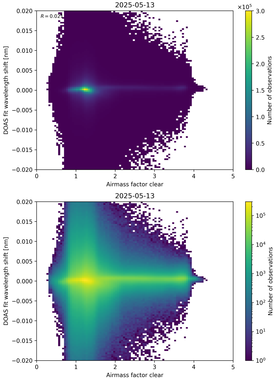
Figure 72: Scatter density plot of “Airmass factor clear” against “DOAS fit wavelength shift” for 2025-05-12 to 2025-05-14.
