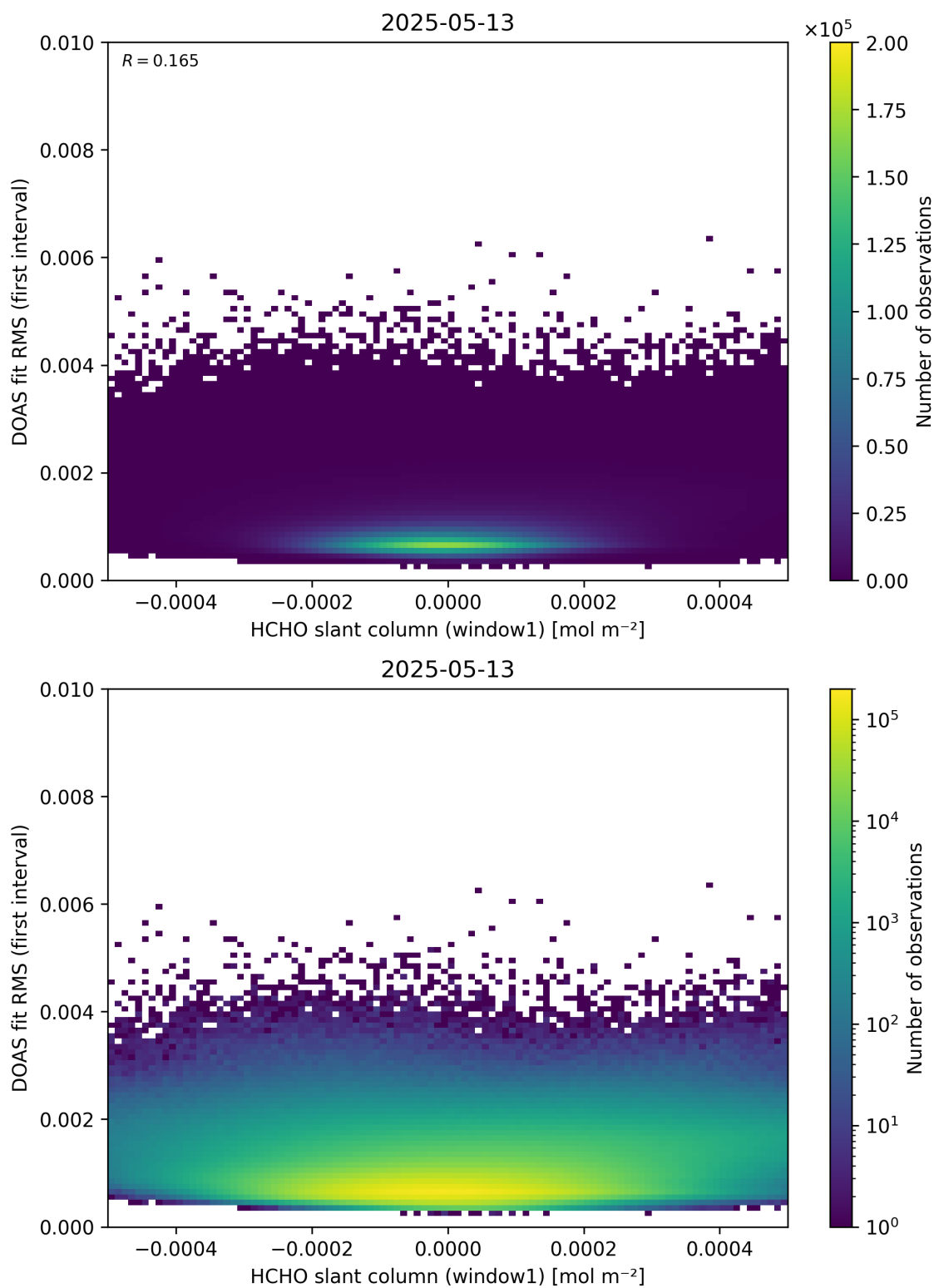
Figure 78: Scatter density plot of “HCHO slant column (window1)” against “DOAS fit RMS (first interval)” for 2025-05-12 to 2025-05-14.
