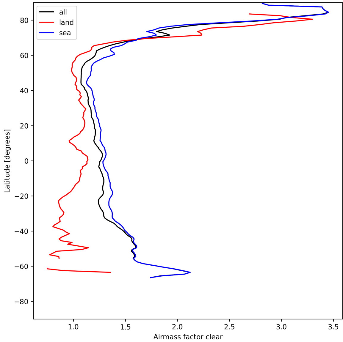
Figure 28: Zonal average of “Airmass factor clear” for 2025-05-12 to 2025-05-14.
