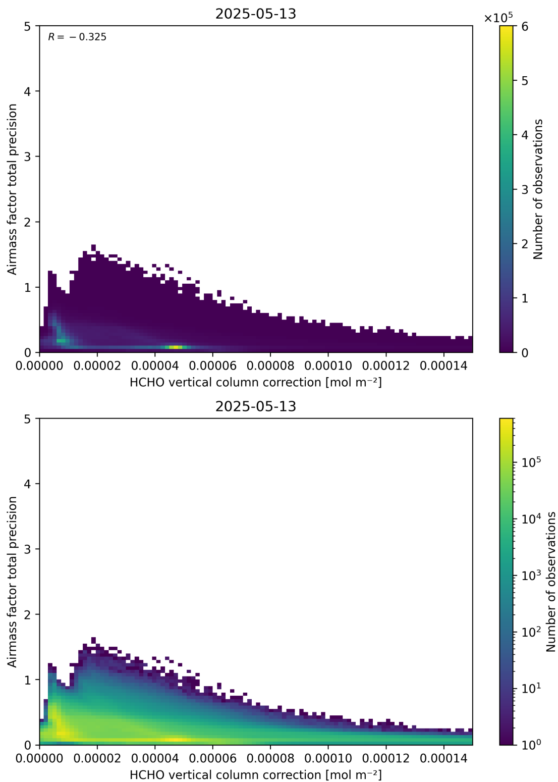
Figure 121: Scatter density plot of “HCHO vertical column correction” against “Airmass factor total precision” for 2025-05-12 to 2025-05-14.
