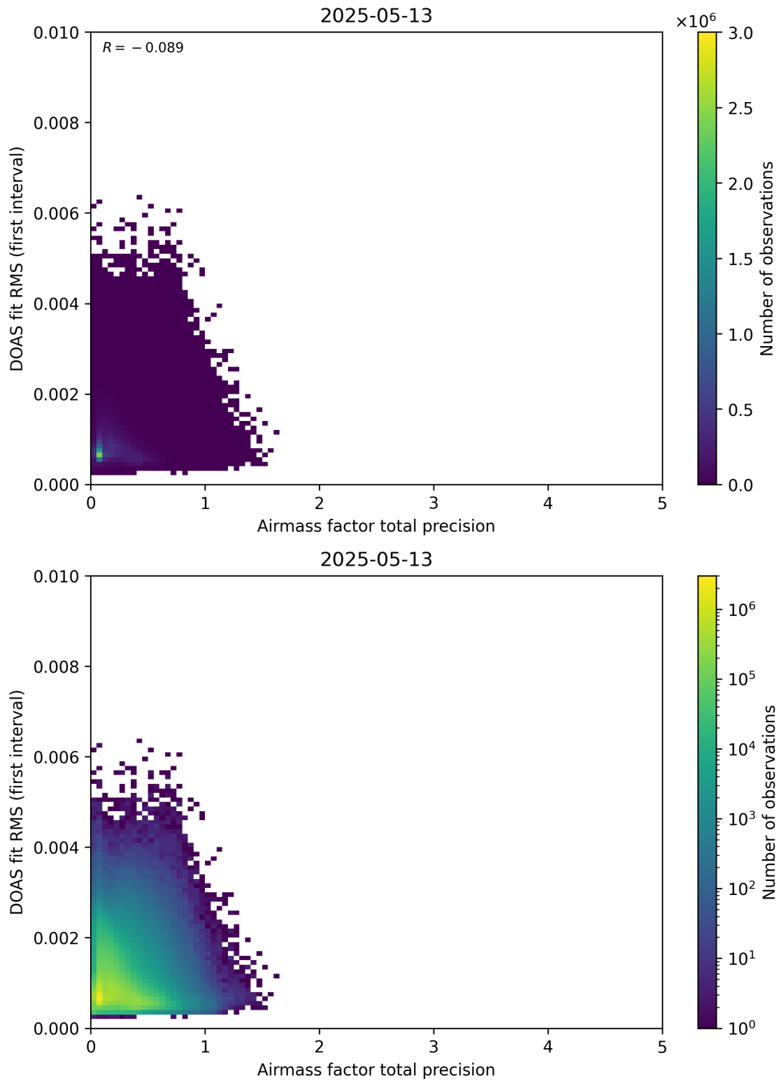
Figure 105: Scatter density plot of “Airmass factor total precision” against “DOAS fit RMS (first interval)” for 2025-05-12 to 2025-05-14.
