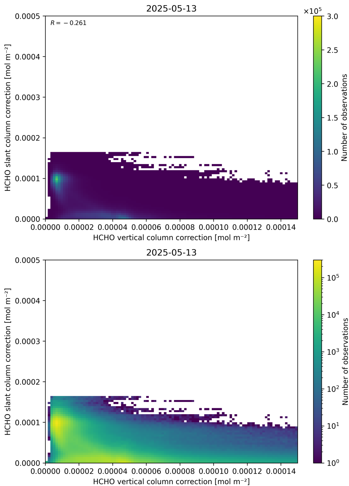
Figure 117: Scatter density plot of “HCHO vertical column correction” against “HCHO slant column correction” for 2025-05-12 to 2025-05-14.
