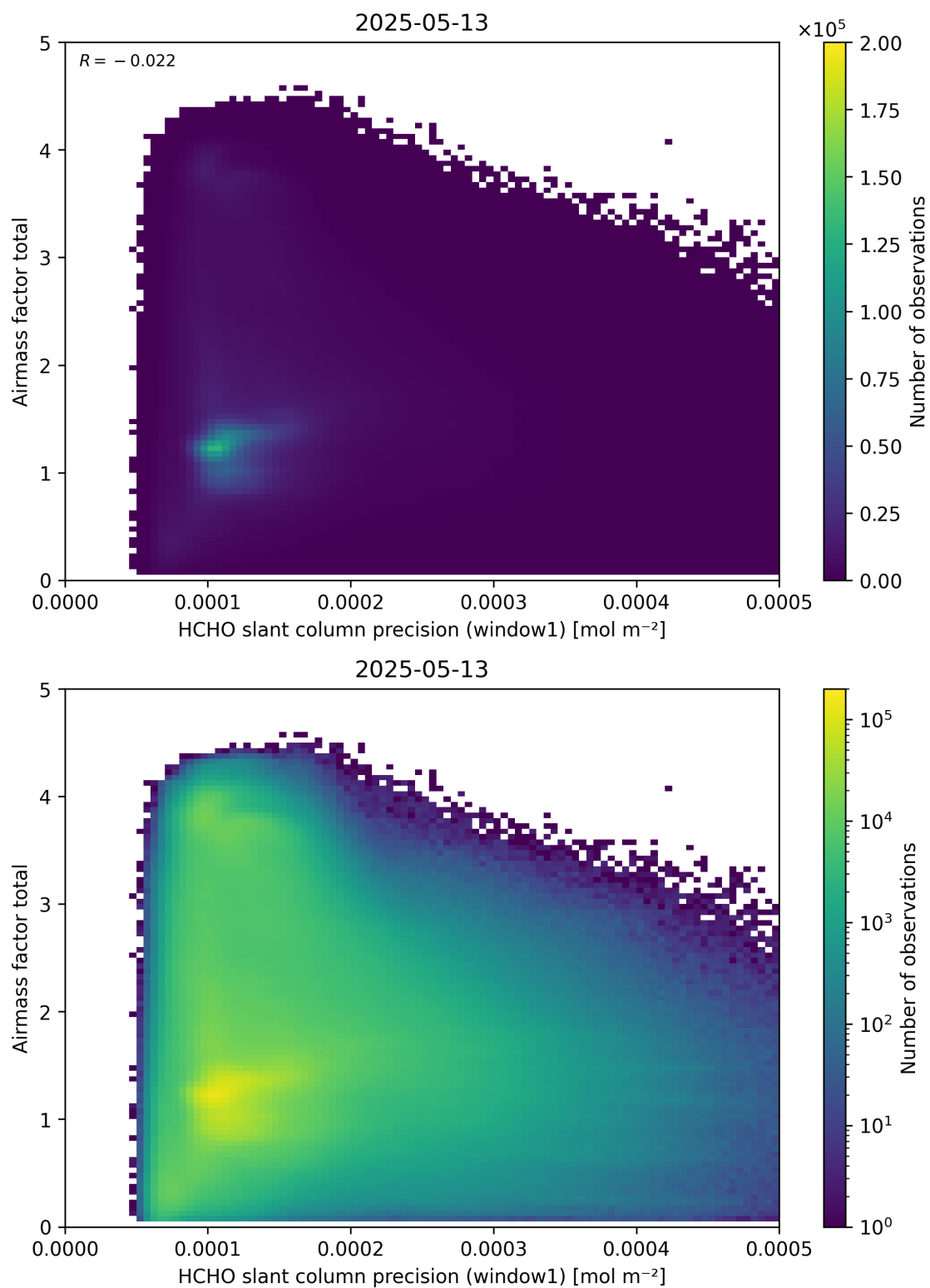
Figure 94: Scatter density plot of “HCHO slant column precision (window1)” against “Airmass factor total” for 2025-05-12 to 2025-05-14.
