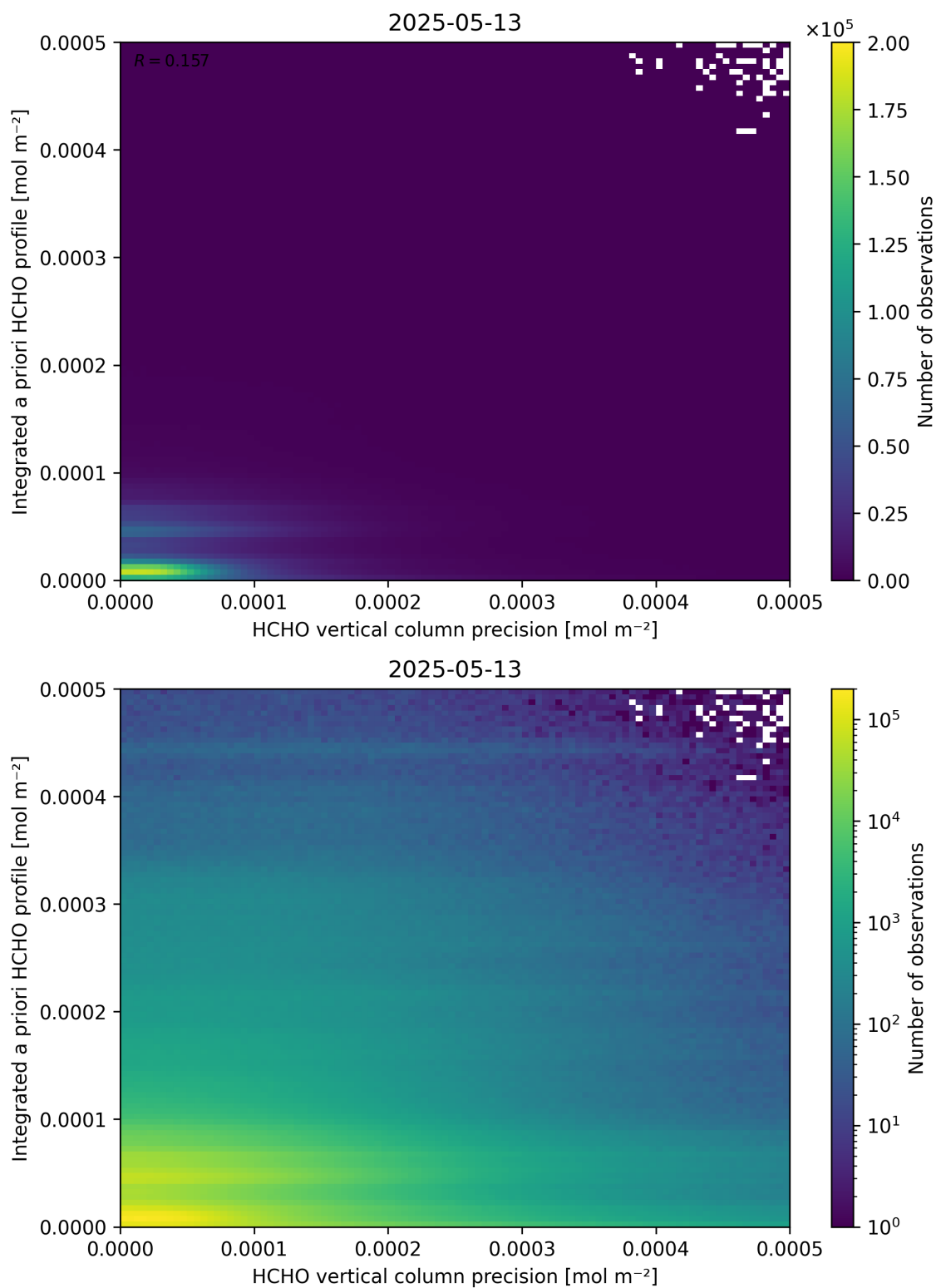
Figure 147: Scatter density plot of “HCHO vertical column precision” against “Integrated a priori HCHO profile” for 2025-05-12 to 2025-05-14.
