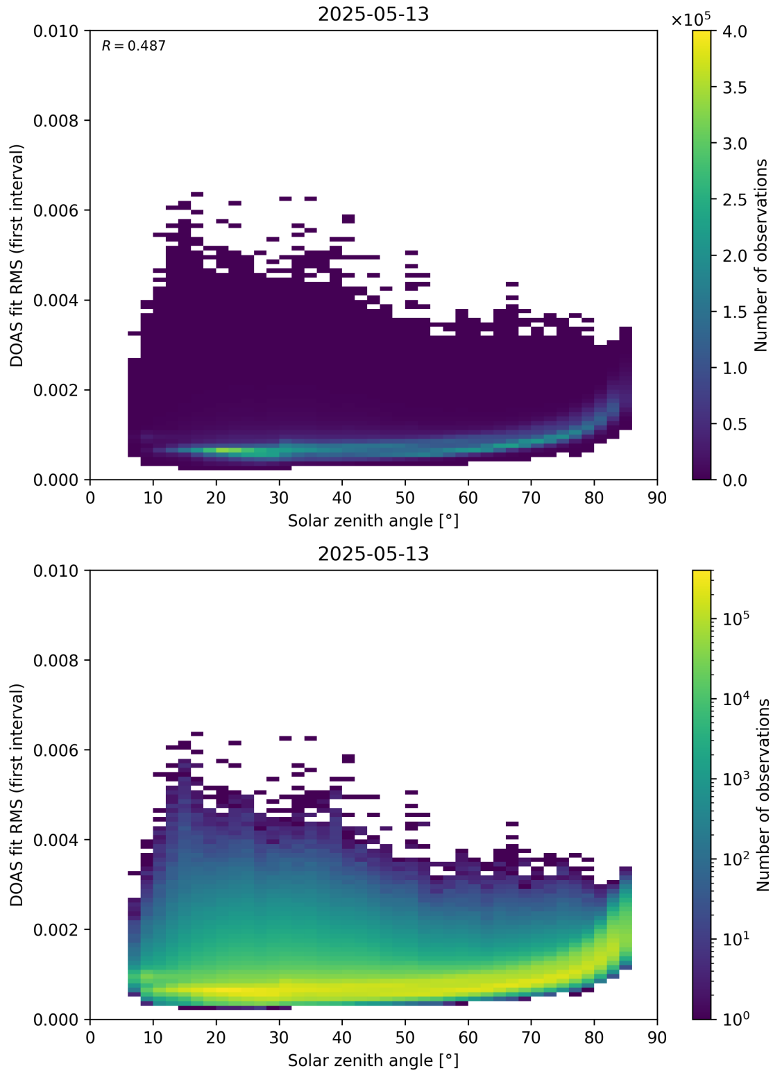
Figure 167: Scatter density plot of “Solar zenith angle” against “DOAS fit RMS (first interval)” for 2025-05-12 to 2025-05-14.
