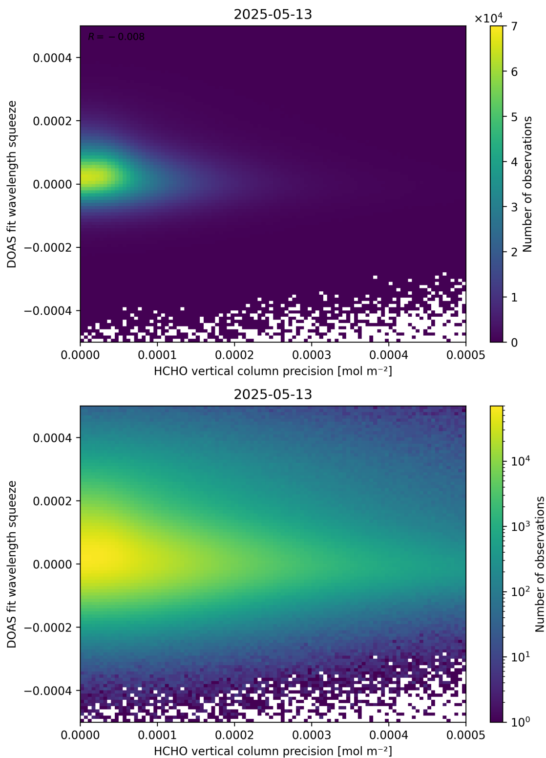
Figure 138: Scatter density plot of “HCHO vertical column precision” against “DOAS fit wavelength squeeze” for 2025-05-12 to 2025-05-14.
