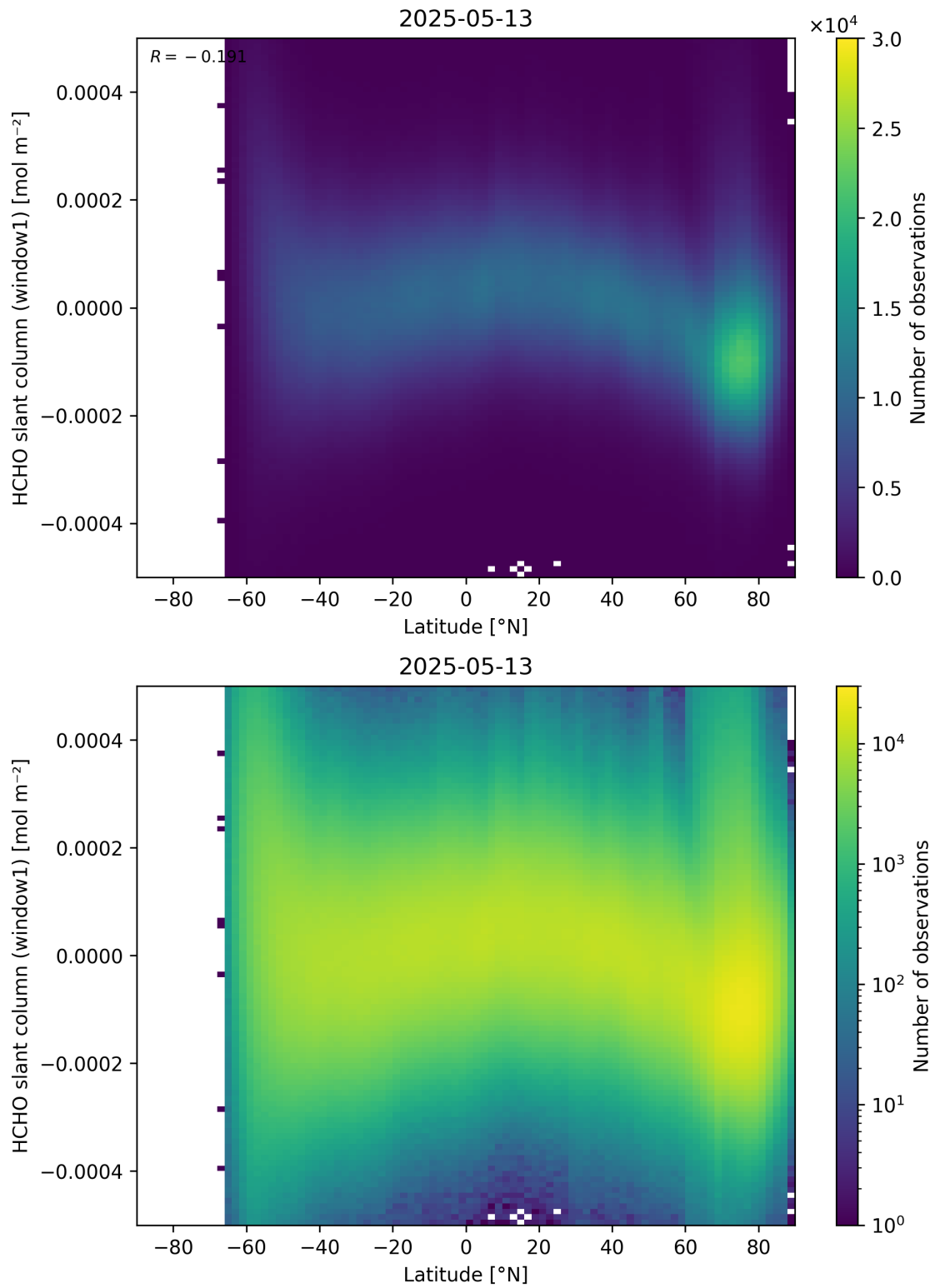
Figure 159: Scatter density plot of “Latitude” against “HCHO slant column (window1)” for 2025-05-12 to 2025-05-14.
