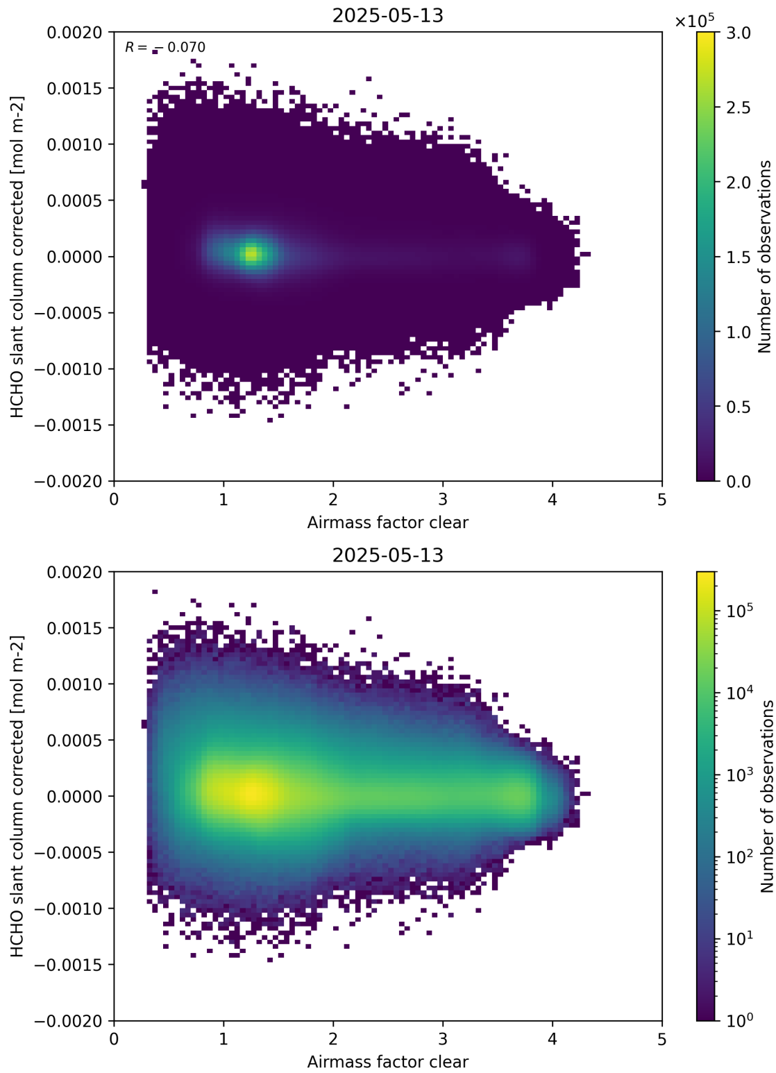
Figure 74: Scatter density plot of “Airmass factor clear” against “HCHO slant column corrected” for 2025-05-12 to 2025-05-14.
