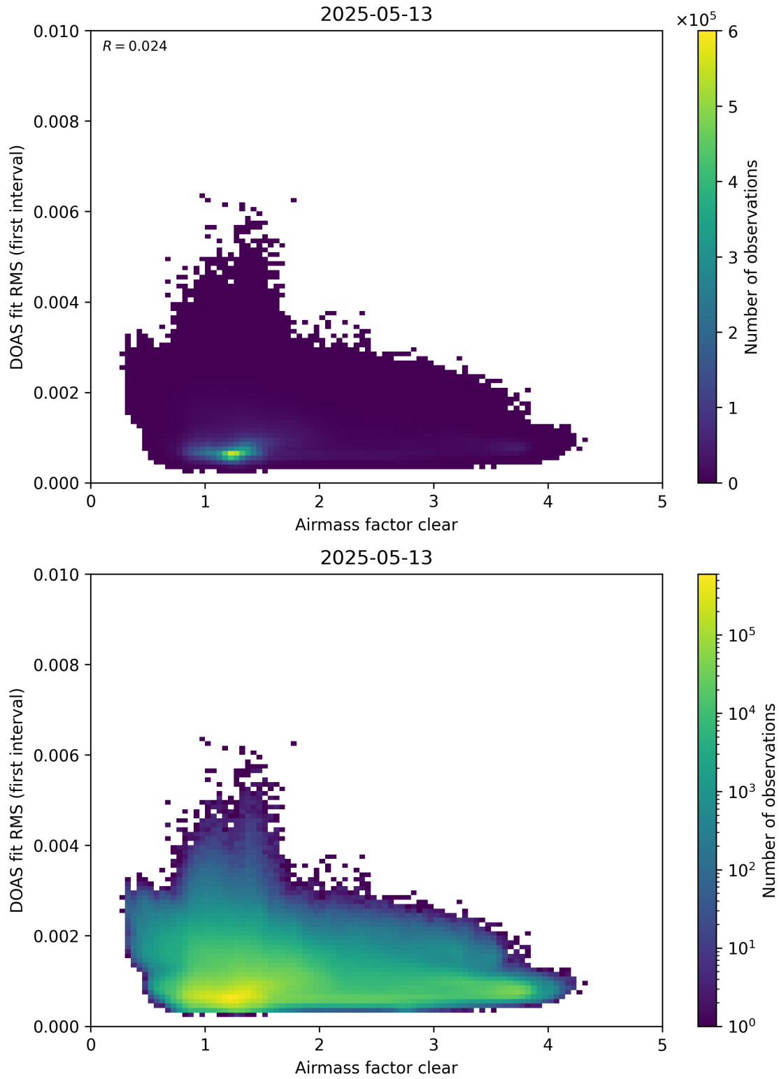
Figure 71: Scatter density plot of “Airmass factor clear” against “DOAS fit RMS (first interval)” for 2025-05-12 to 2025-05-14.
