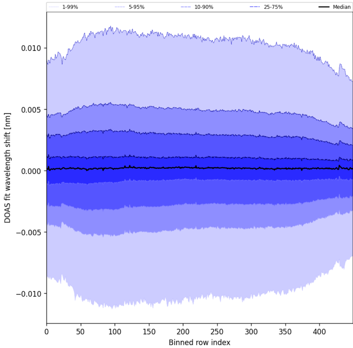
Figure 58: Along track statistics of “DOAS fit wavelength shift” for 2025-05-12 to 2025-05-14
