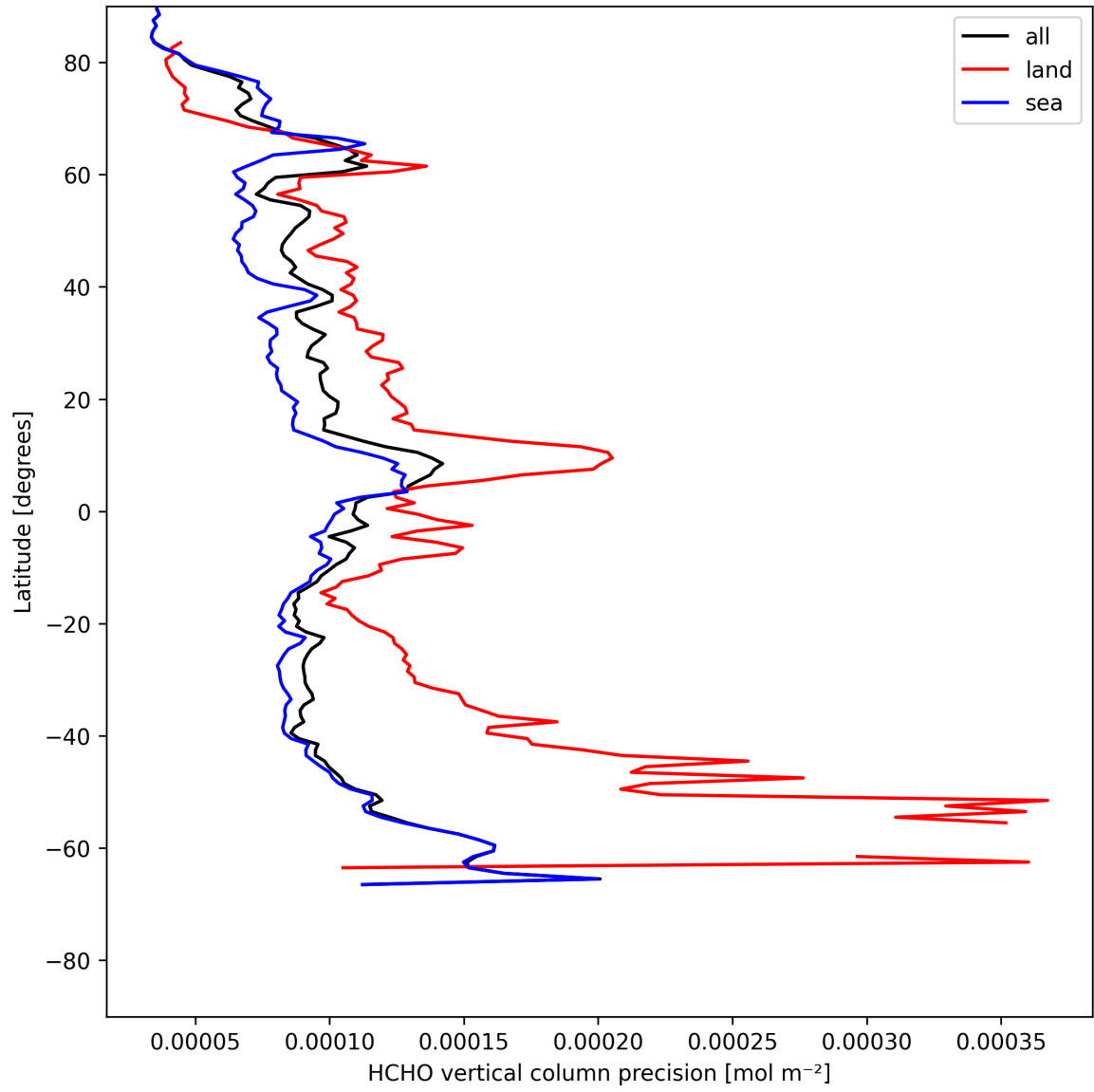
Figure 22: Zonal average of “HCHO vertical column precision” for 2025-05-12 to 2025-05-14.
