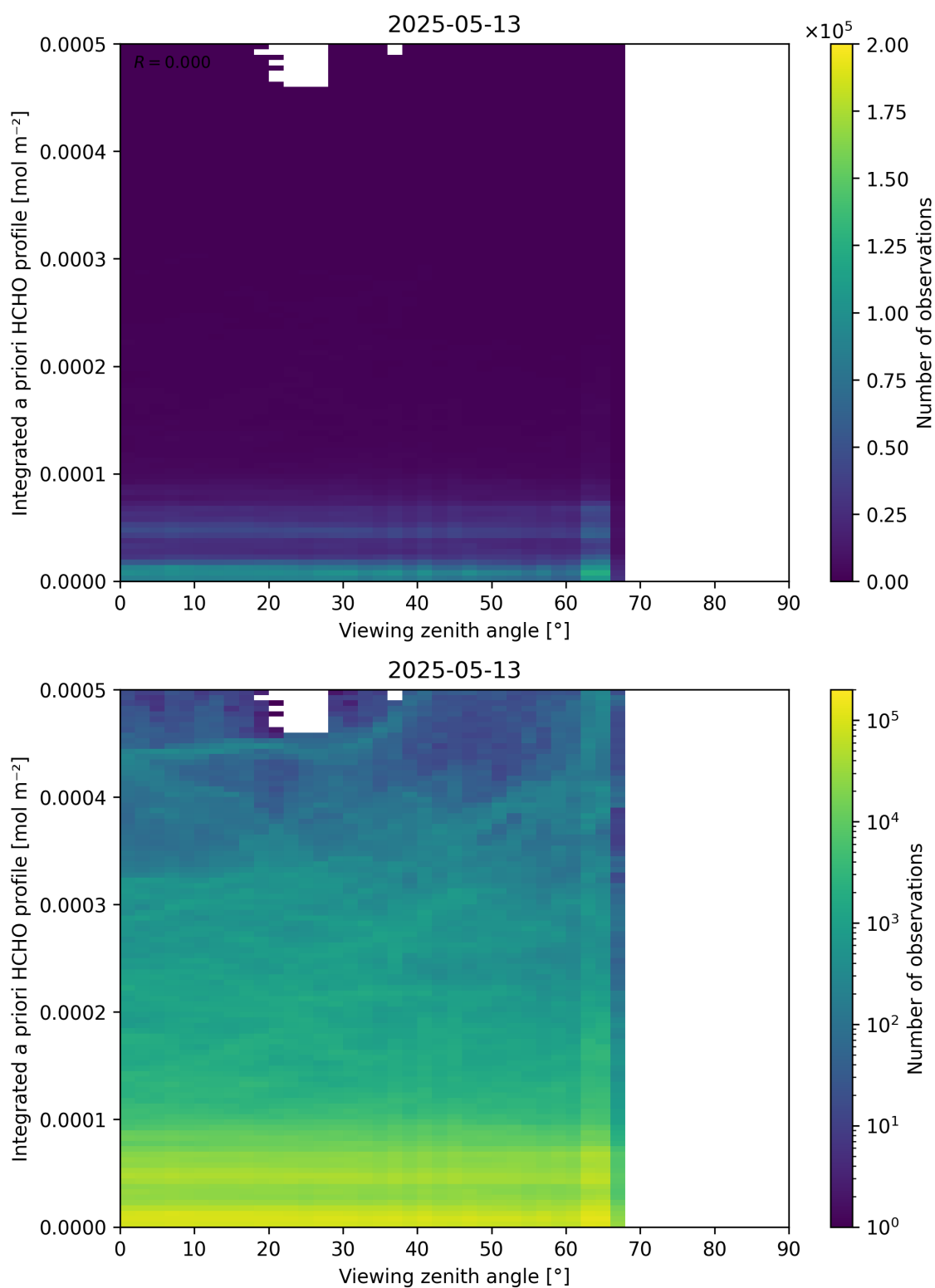
Figure 195: Scatter density plot of “Viewing zenith angle” against “Integrated a priori HCHO profile” for 2025-05-12 to 2025-05-14.
