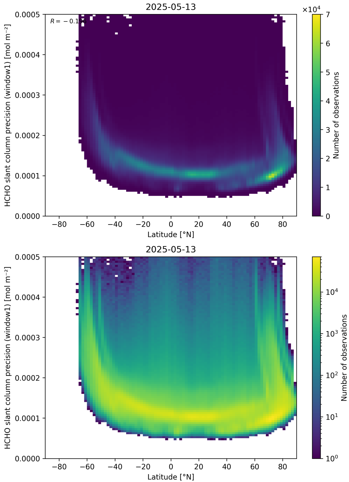
Figure 160: Scatter density plot of “Latitude” against “HCHO slant column precision (window1)” for 2025-05-12 to 2025-05-14.
