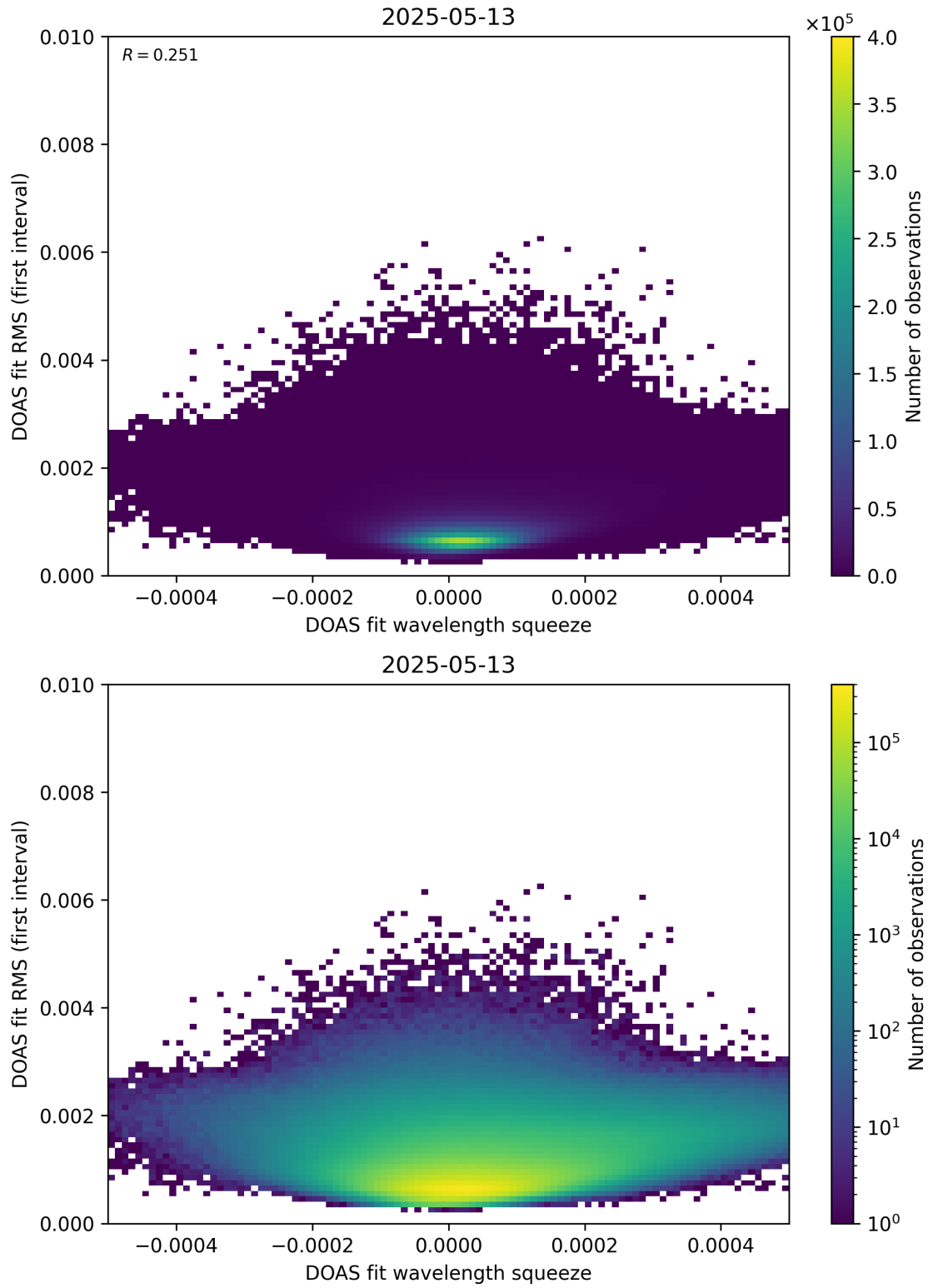
Figure 68: Scatter density plot of “DOAS fit wavelength squeeze” against “DOAS fit RMS (first interval)” for 2025-05-12 to 2025-05-14.
