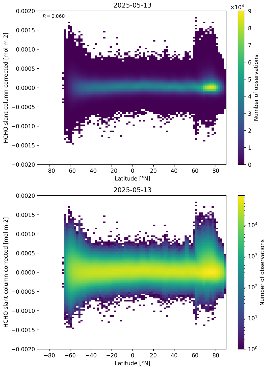
Figure 157: Scatter density plot of “Latitude” against “HCHO slant column corrected” for 2025-05-12 to 2025-05-14.
