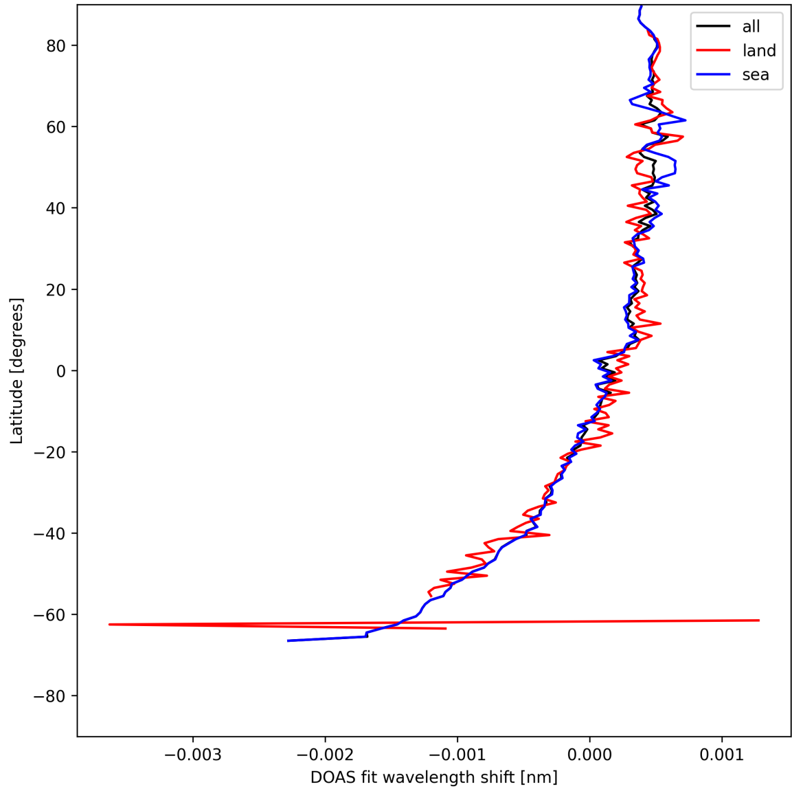
Figure 30: Zonal average of “DOAS fit wavelength shift” for 2025-05-12 to 2025-05-14.
