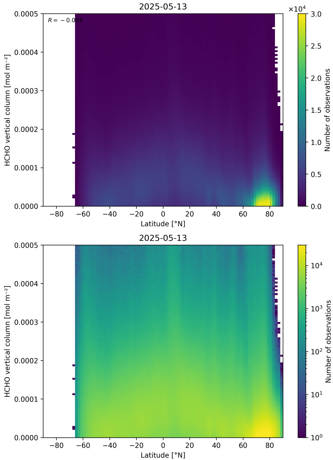
Figure 163: Scatter density plot of “Latitude” against “HCHO vertical column” for 2025-05-12 to 2025-05-14.
