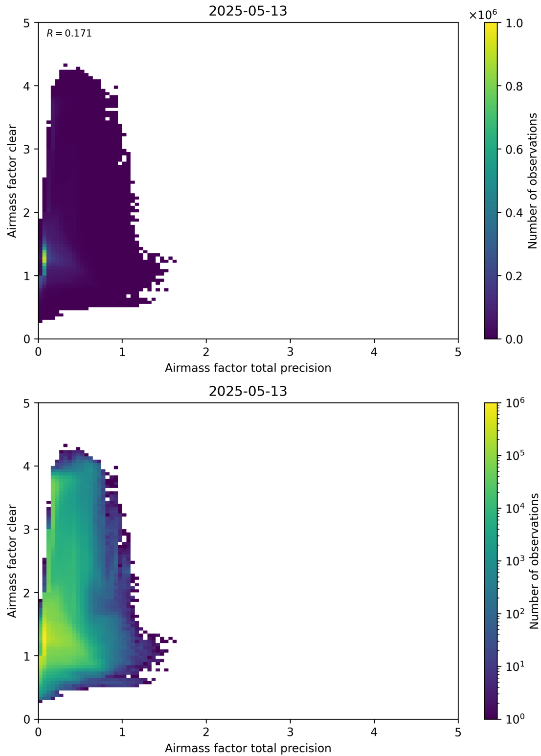
Figure 108: Scatter density plot of “Airmass factor total precision” against “Airmass factor clear” for 2025-05-12 to 2025-05-14.
