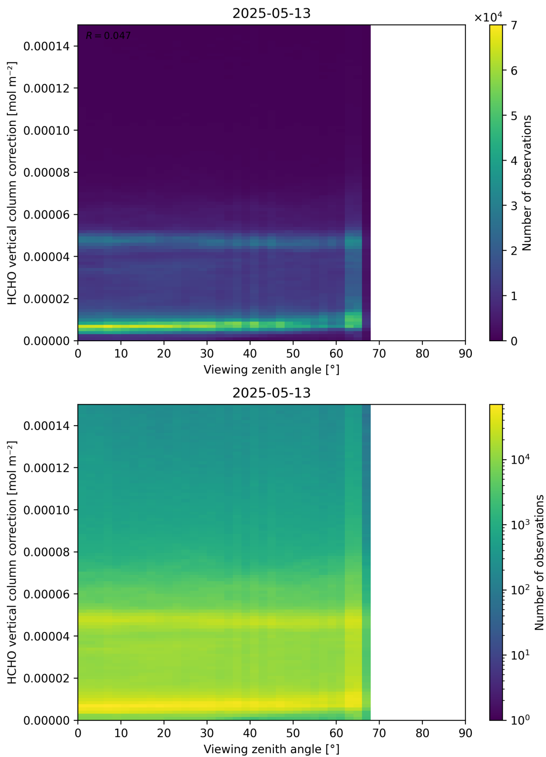
Figure 193: Scatter density plot of “Viewing zenith angle” against “HCHO vertical column correction” for 2025-05-12 to 2025-05-14.
