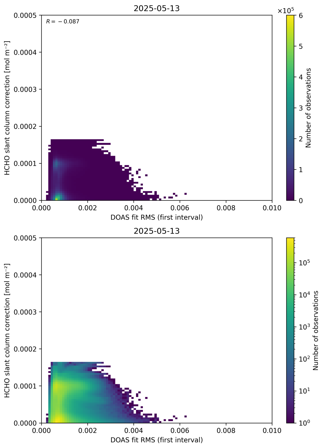
Figure 63: Scatter density plot of “DOAS fit RMS (first interval)” against “HCHO slant column correction” for 2025-05-12 to 2025-05-14.
