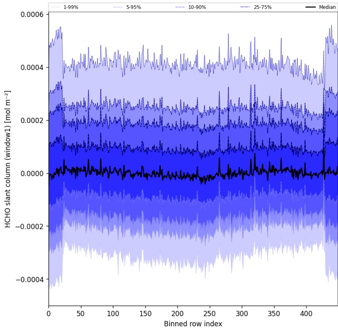
Figure 52: Along track statistics of “HCHO slant column (window1)” for 2025-05-12 to 2025-05-14
