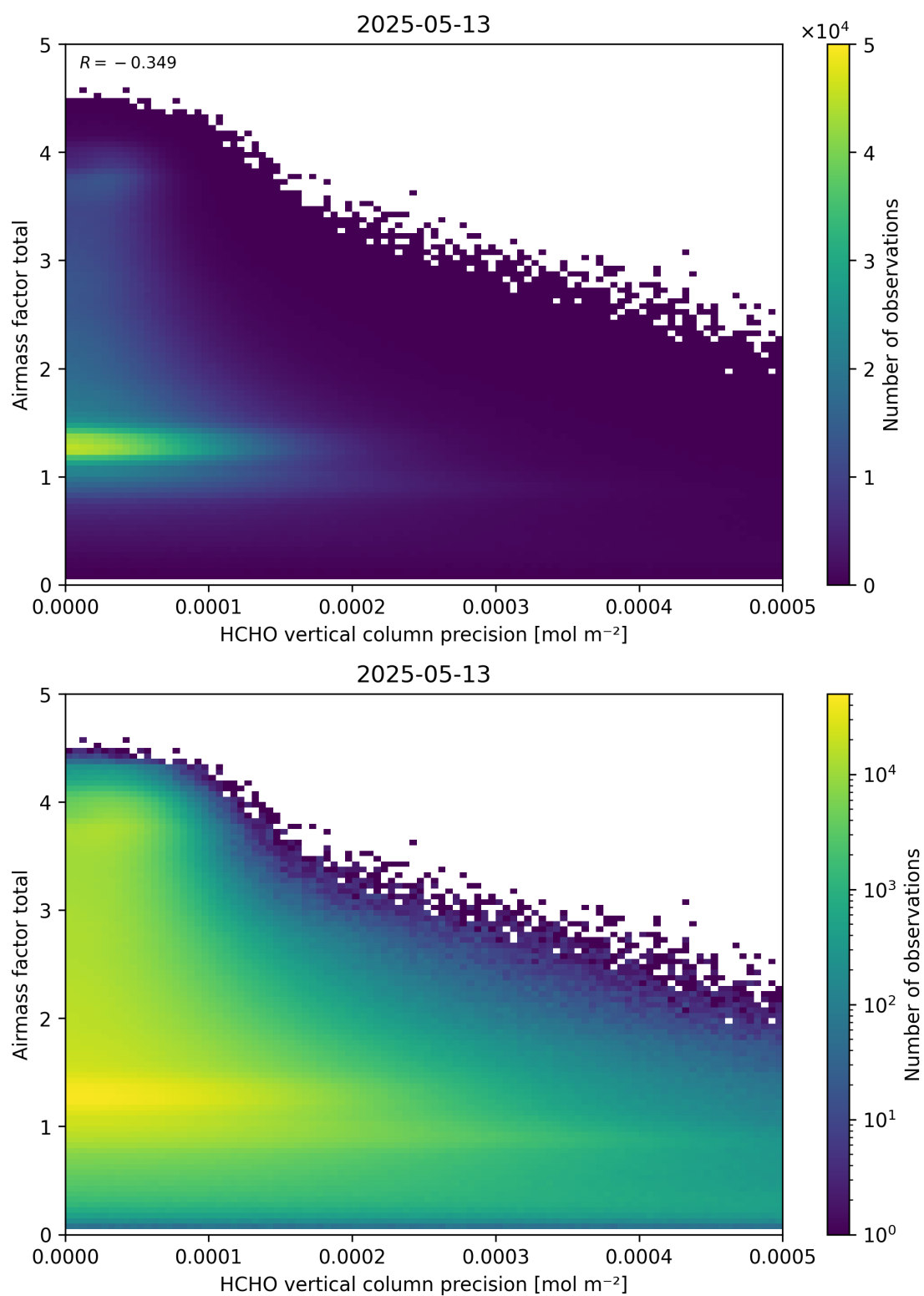
Figure 144: Scatter density plot of “HCHO vertical column precision” against “Airmass factor total” for 2025-05-12 to 2025-05-14.
