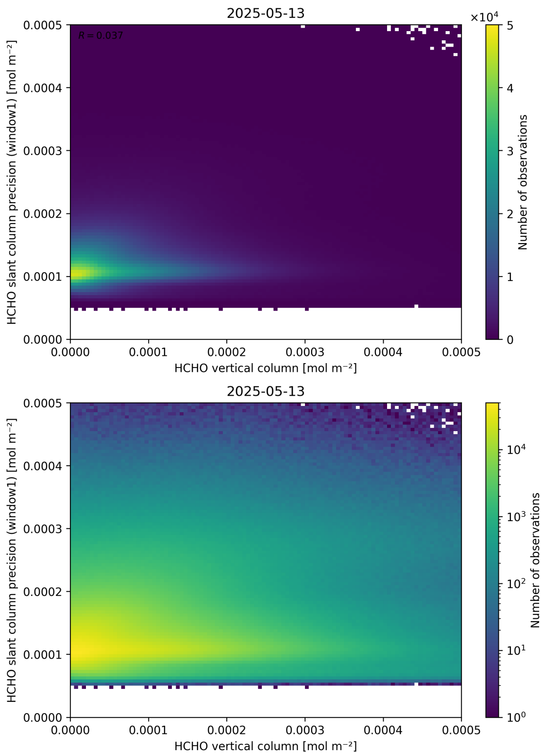
Figure 130: Scatter density plot of “HCHO vertical column” against “HCHO slant column precision (window1)” for 2025-05-12 to 2025-05-14.
