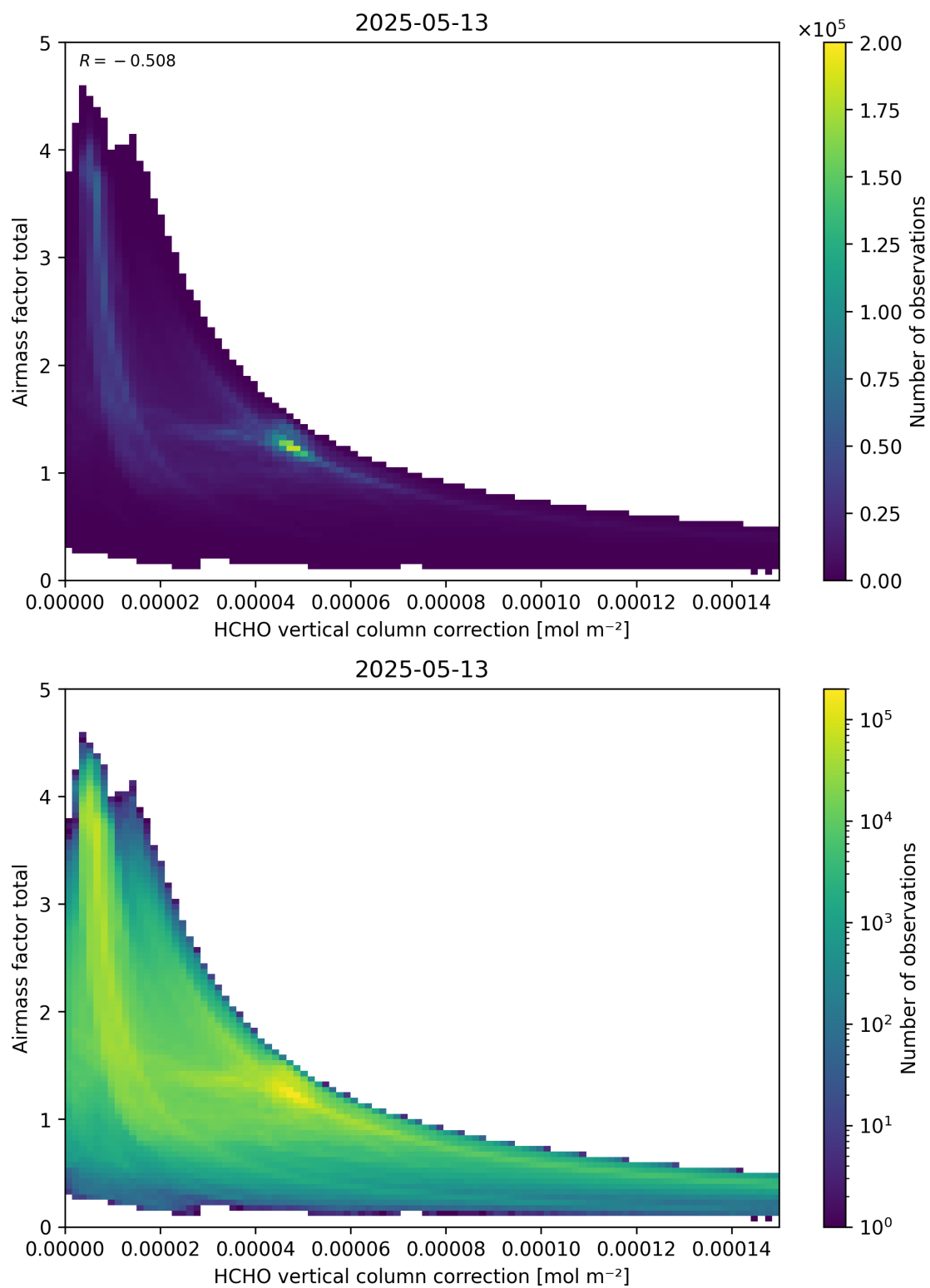
Figure 120: Scatter density plot of “HCHO vertical column correction” against “Airmass factor total” for 2025-05-12 to 2025-05-14.
