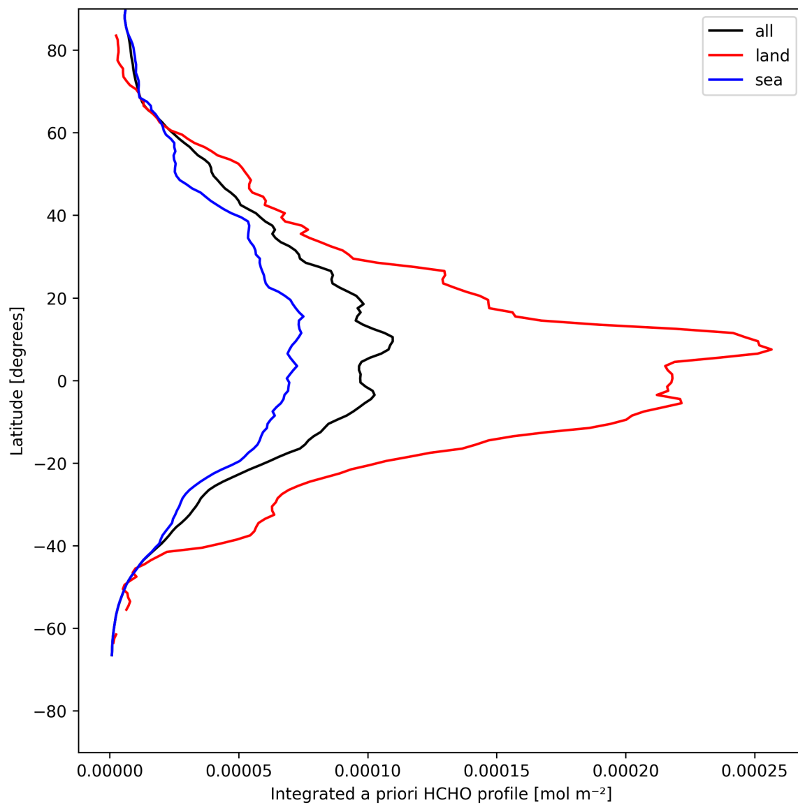
Figure 29: Zonal average of “Integrated a priori HCHO profile” for 2025-05-12 to 2025-05-14.
