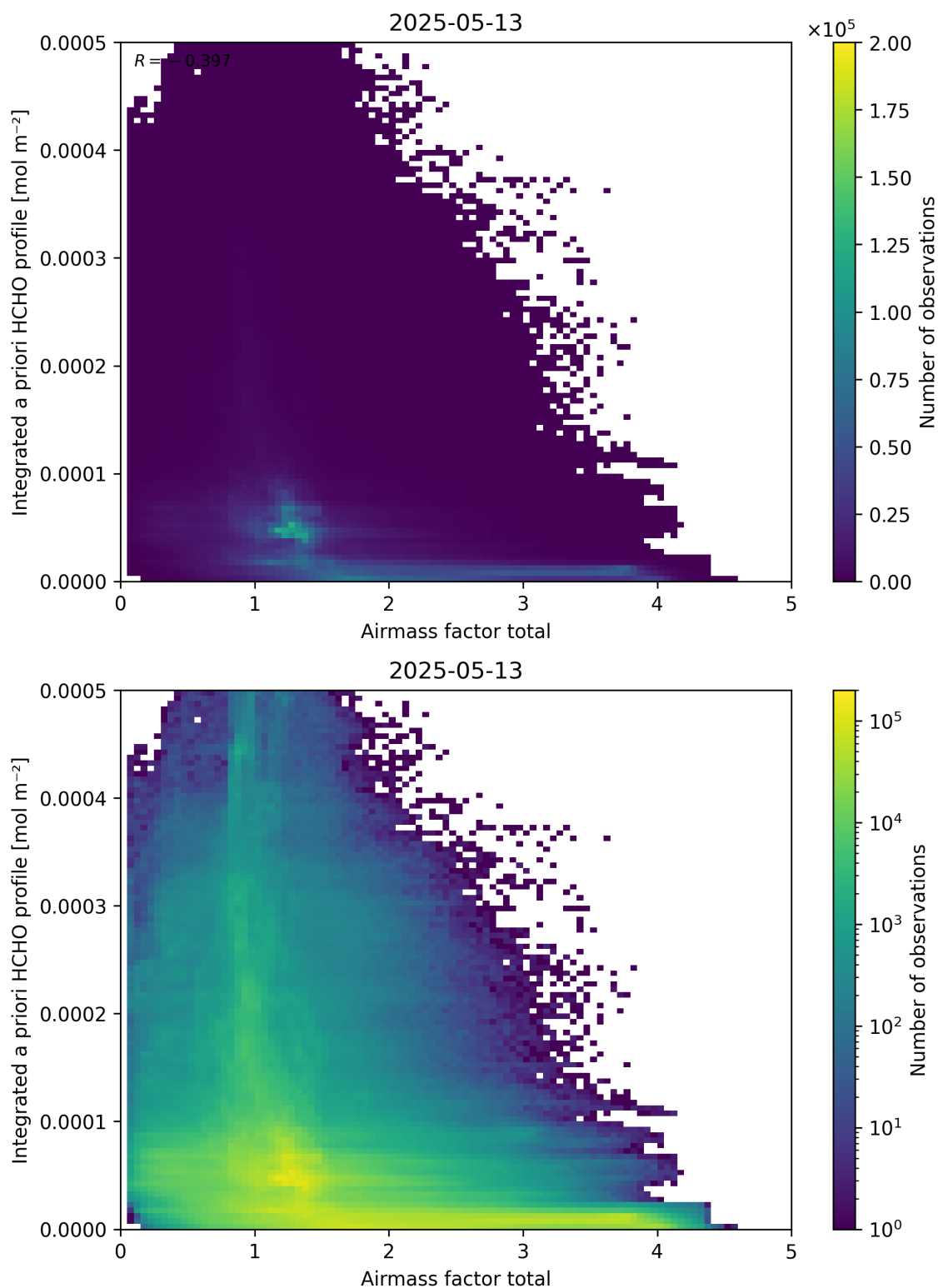
Figure 104: Scatter density plot of “Airmass factor total” against “Integrated a priori HCHO profile” for 2025-05-12 to 2025-05-14.
