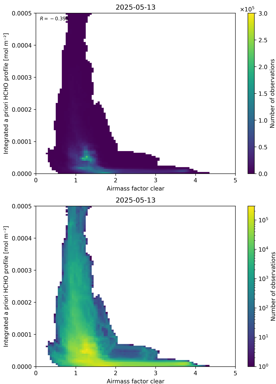
Figure 76: Scatter density plot of “Airmass factor clear” against “Integrated a priori HCHO profile” for 2025-05-12 to 2025-05-14.
