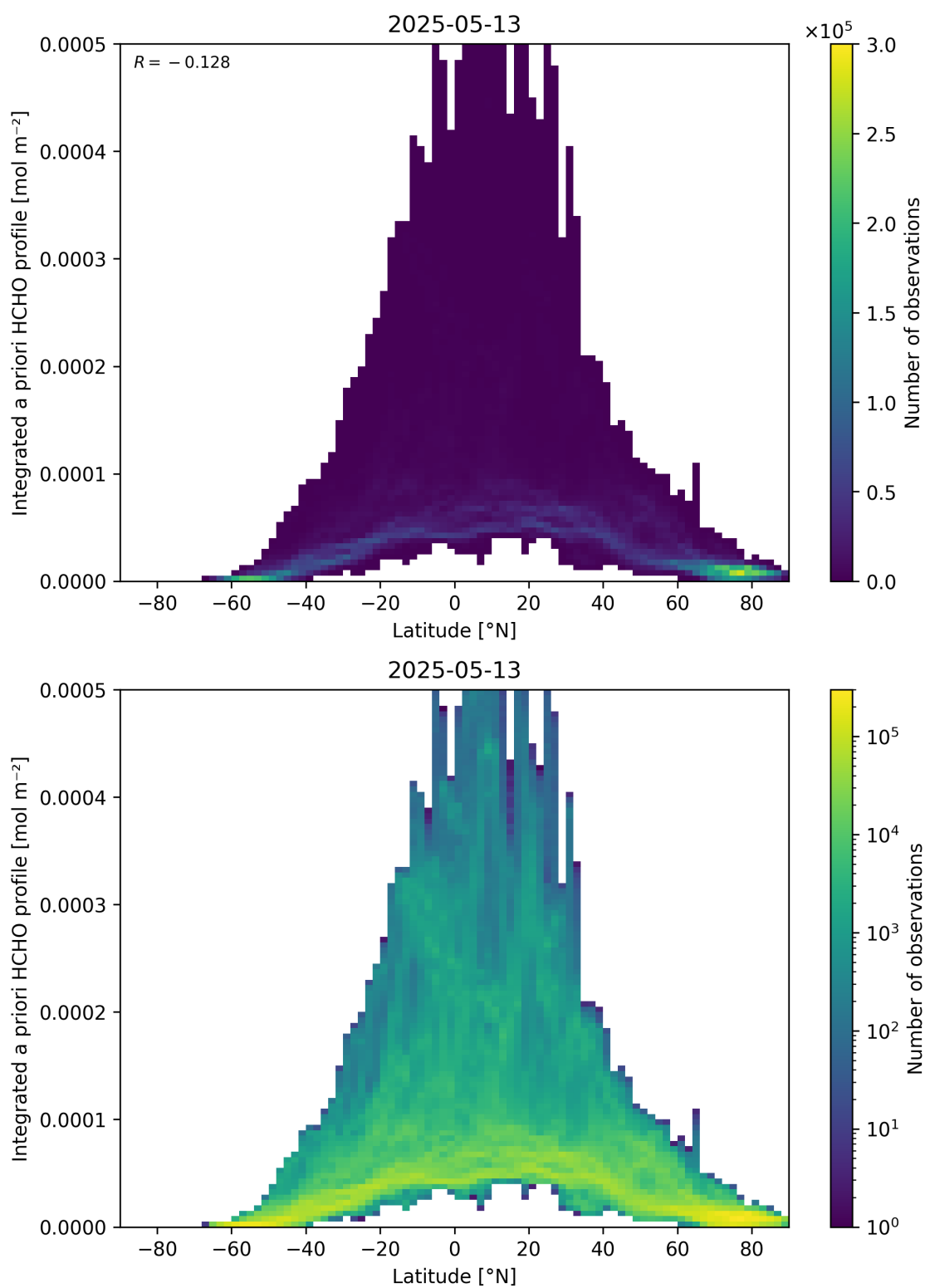
Figure 166: Scatter density plot of “Latitude” against “Integrated a priori HCHO profile” for 2025-05-12 to 2025-05-14.
