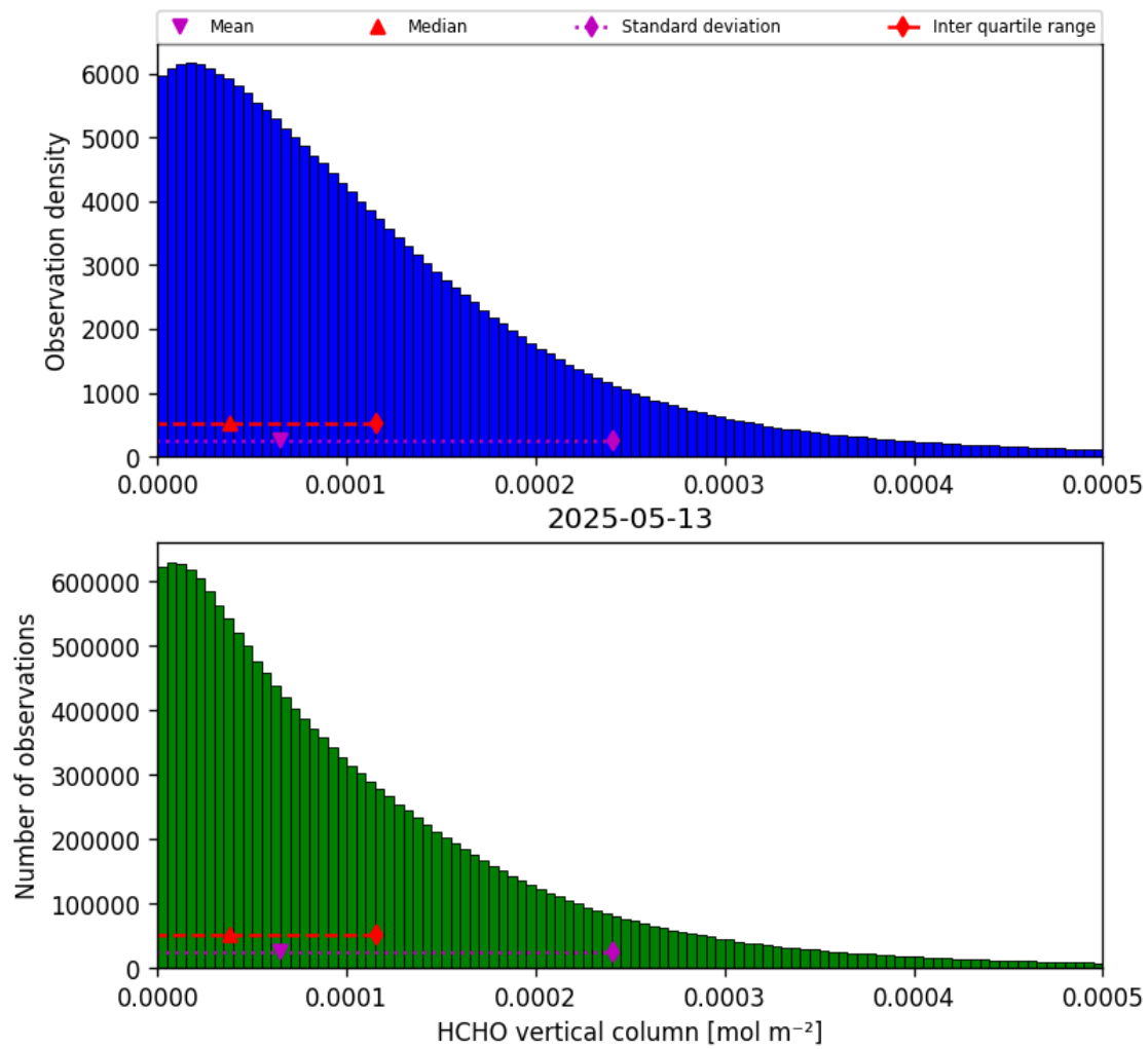
Figure 35: Histogram of “HCHO vertical column” for 2025-05-12 to 2025-05-14
