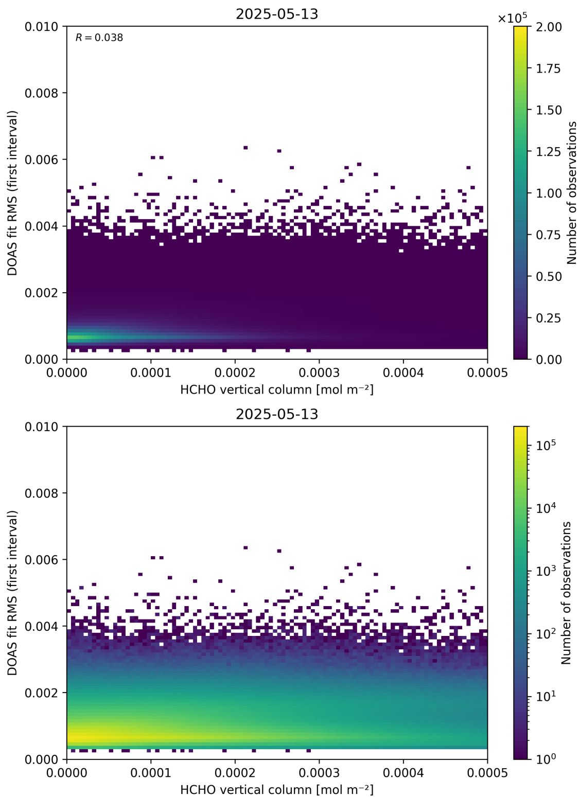
Figure 123: Scatter density plot of “HCHO vertical column” against “DOAS fit RMS (first interval)” for 2025-05-12 to 2025-05-14.
