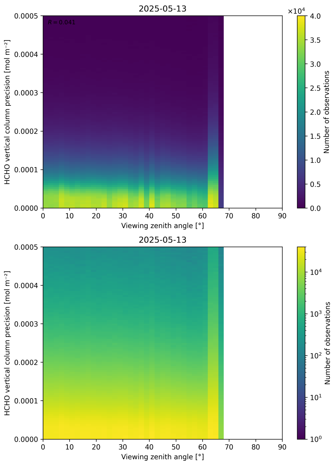
Figure 194: Scatter density plot of “Viewing zenith angle” against “HCHO vertical column precision” for 2025-05-12 to 2025-05-14.
