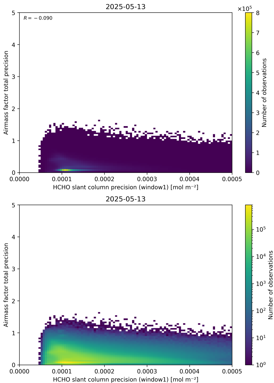
Figure 95: Scatter density plot of “HCHO slant column precision (window1)” against “Airmass factor total precision” for 2025-05-12 to 2025-05-14.
