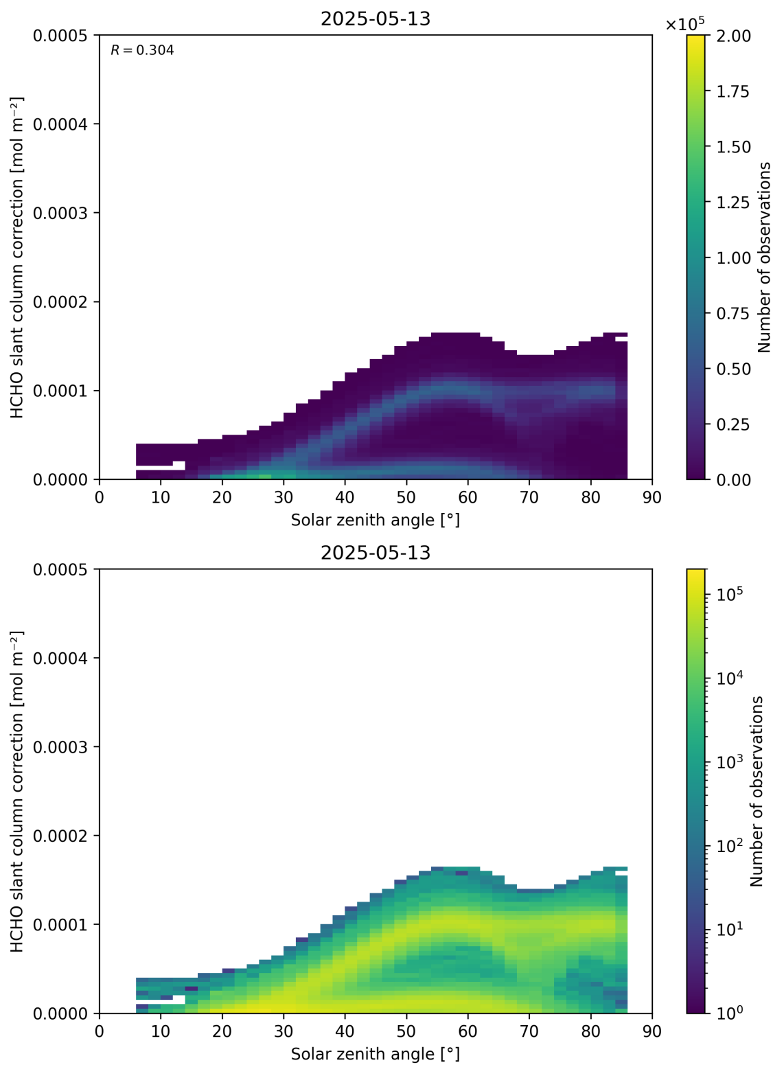
Figure 172: Scatter density plot of “Solar zenith angle” against “HCHO slant column correction” for 2025-05-12 to 2025-05-14.
