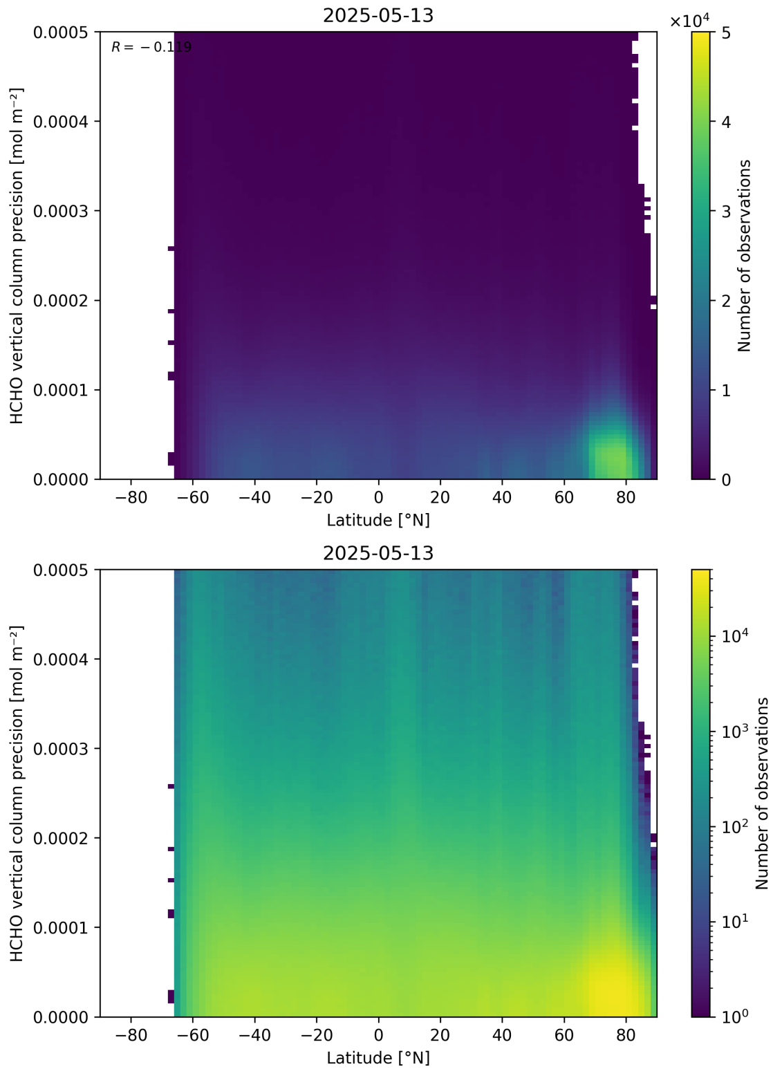
Figure 165: Scatter density plot of “Latitude” against “HCHO vertical column precision” for 2025-05-12 to 2025-05-14.
