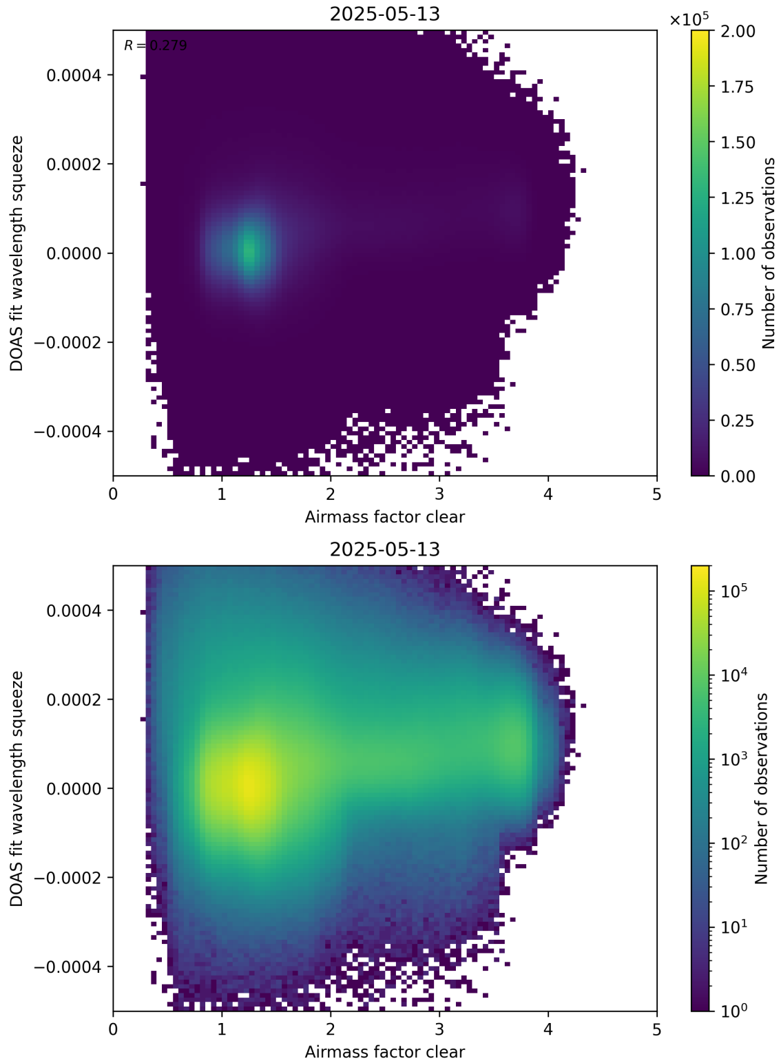
Figure 73: Scatter density plot of “Airmass factor clear” against “DOAS fit wavelength squeeze” for 2025-05-12 to 2025-05-14.
