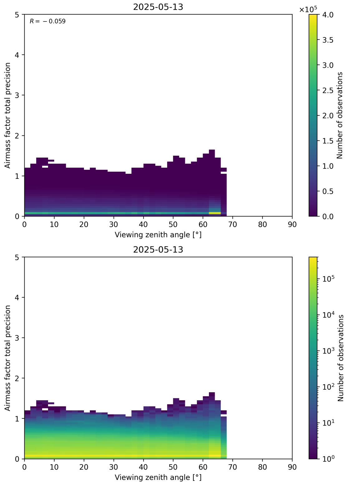
Figure 191: Scatter density plot of “Viewing zenith angle” against “Airmass factor total precision” for 2025-05-12 to 2025-05-14.
