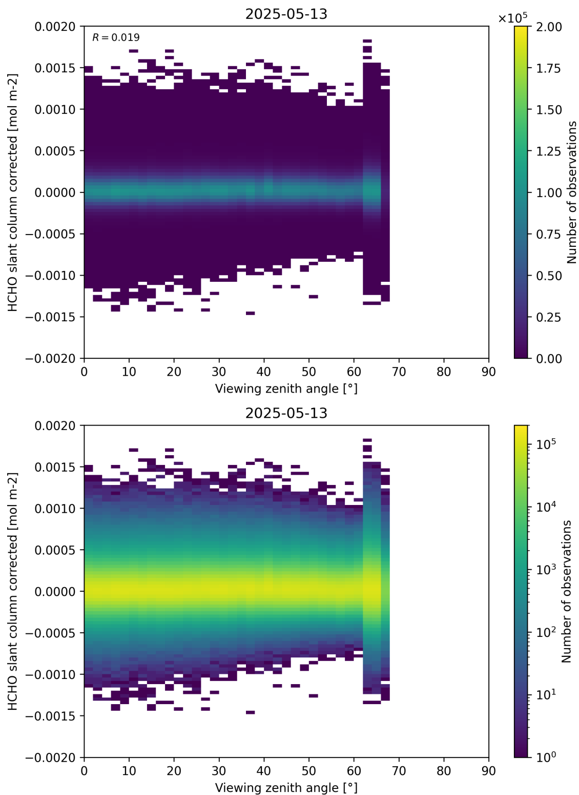
Figure 186: Scatter density plot of “Viewing zenith angle” against “HCHO slant column corrected” for 2025-05-12 to 2025-05-14.
