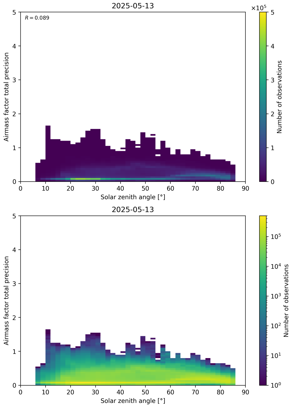
Figure 176: Scatter density plot of “Solar zenith angle” against “Airmass factor total precision” for 2025-05-12 to 2025-05-14.
