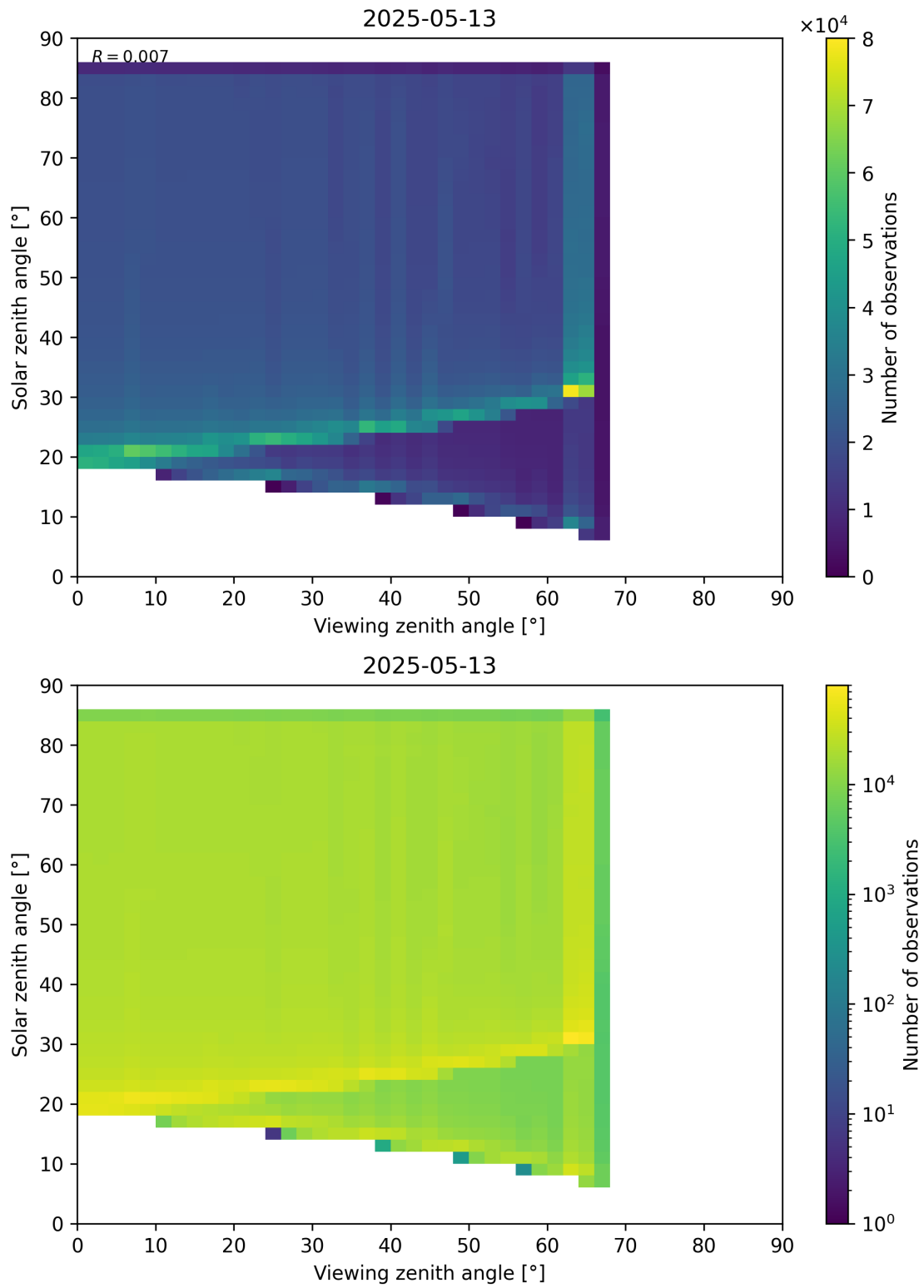
Figure 197: Scatter density plot of “Viewing zenith angle” against “Solar zenith angle” for 2025-05-12 to 2025-05-14.
