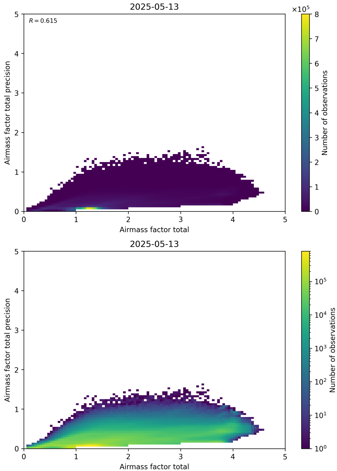
Figure 103: Scatter density plot of “Airmass factor total” against “Airmass factor total precision” for 2025-05-12 to 2025-05-14.
