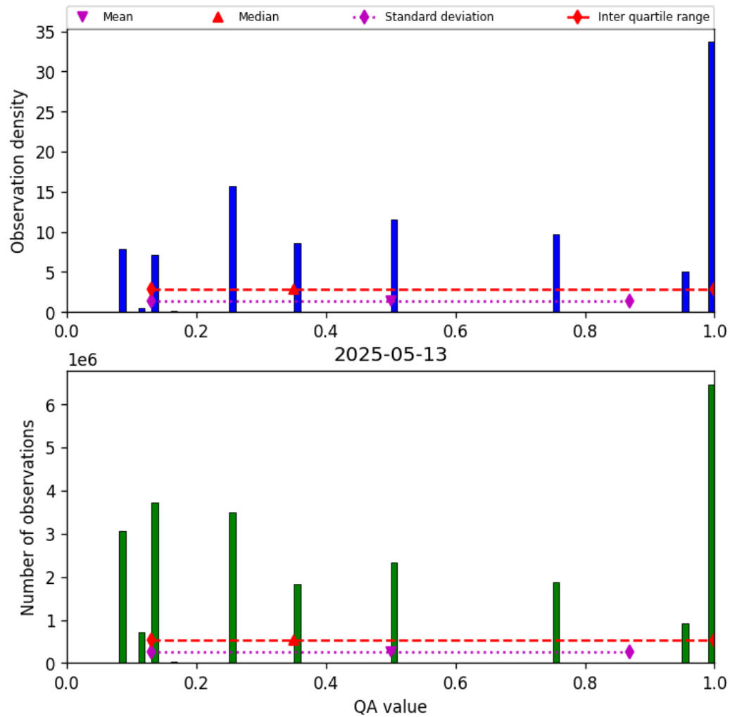
Figure 34: Histogram of “QA value” for 2025-05-12 to 2025-05-14
