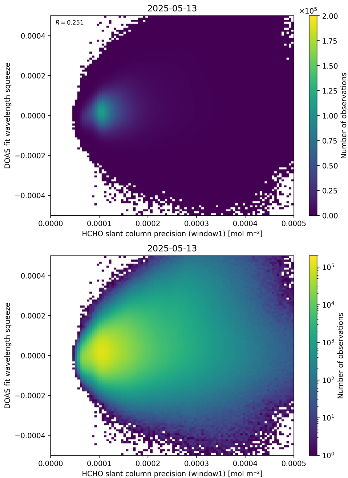
Figure 90: Scatter density plot of “HCHO slant column precision (window1)” against “DOAS fit wavelength squeeze” for 2025-05-12 to 2025-05-14.
