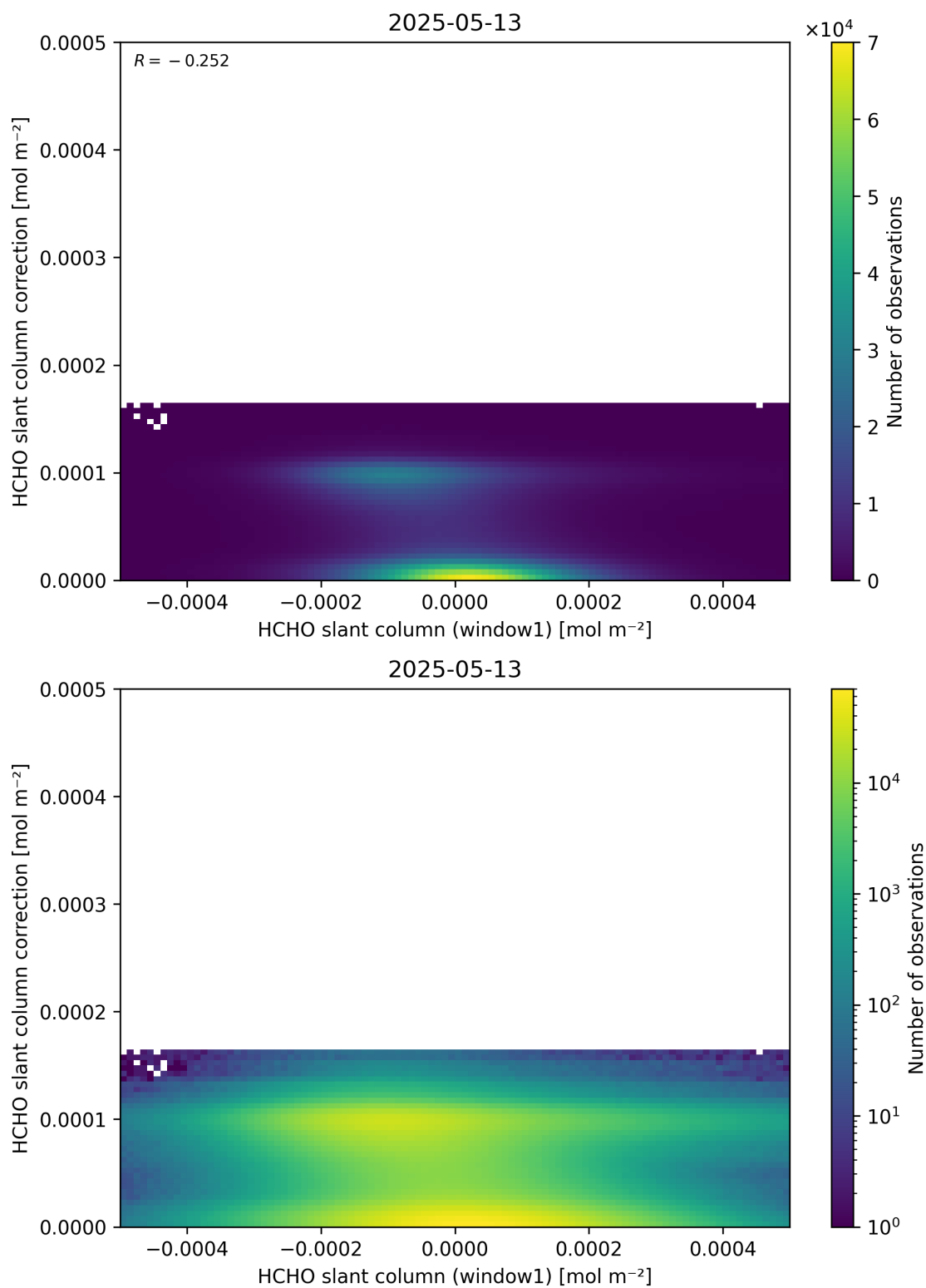
Figure 83: Scatter density plot of “HCHO slant column (window1)” against “HCHO slant column correction” for 2025-05-12 to 2025-05-14.
