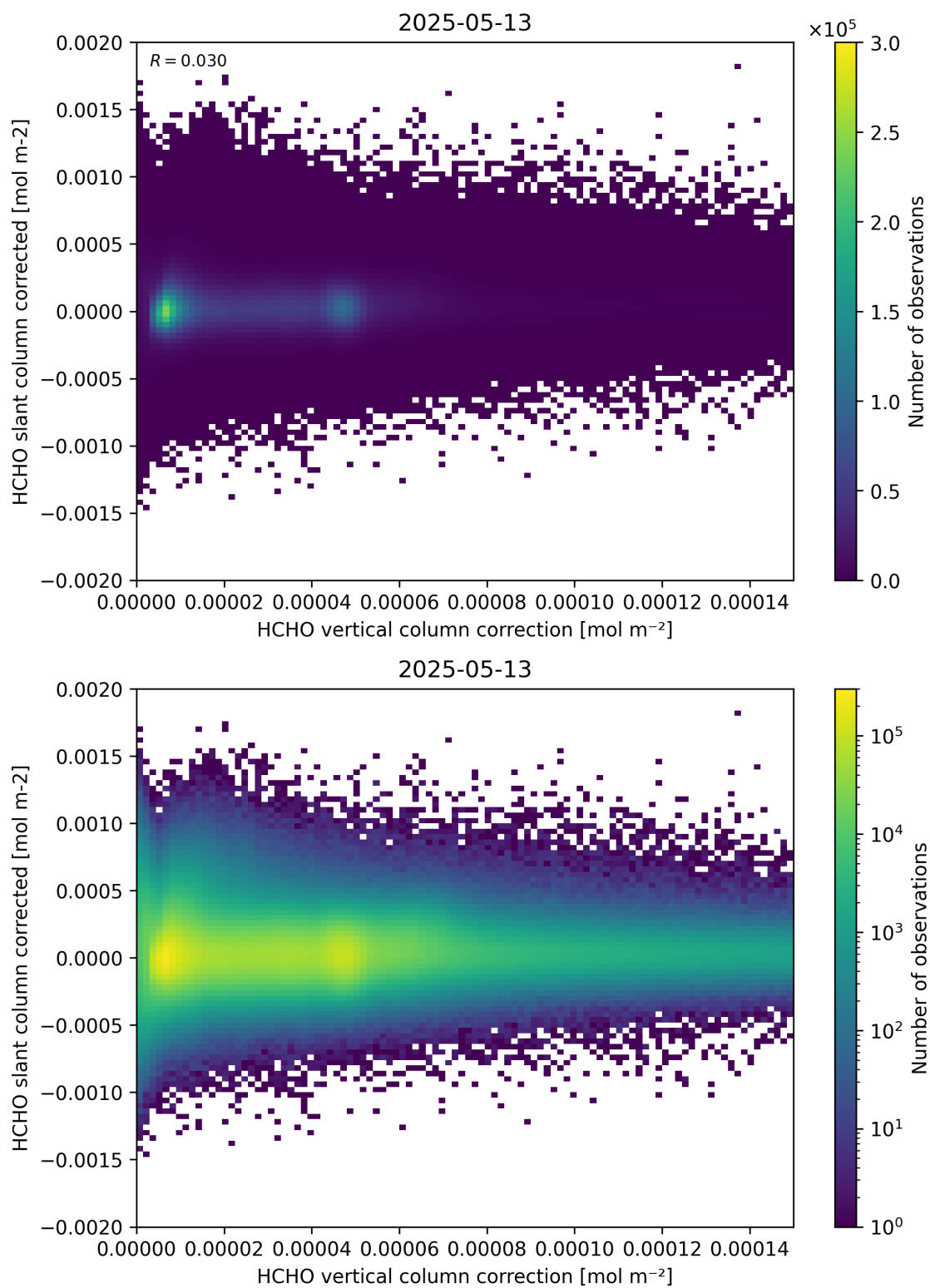
Figure 116: Scatter density plot of “HCHO vertical column correction” against “HCHO slant column corrected” for 2025-05-12 to 2025-05-14.
