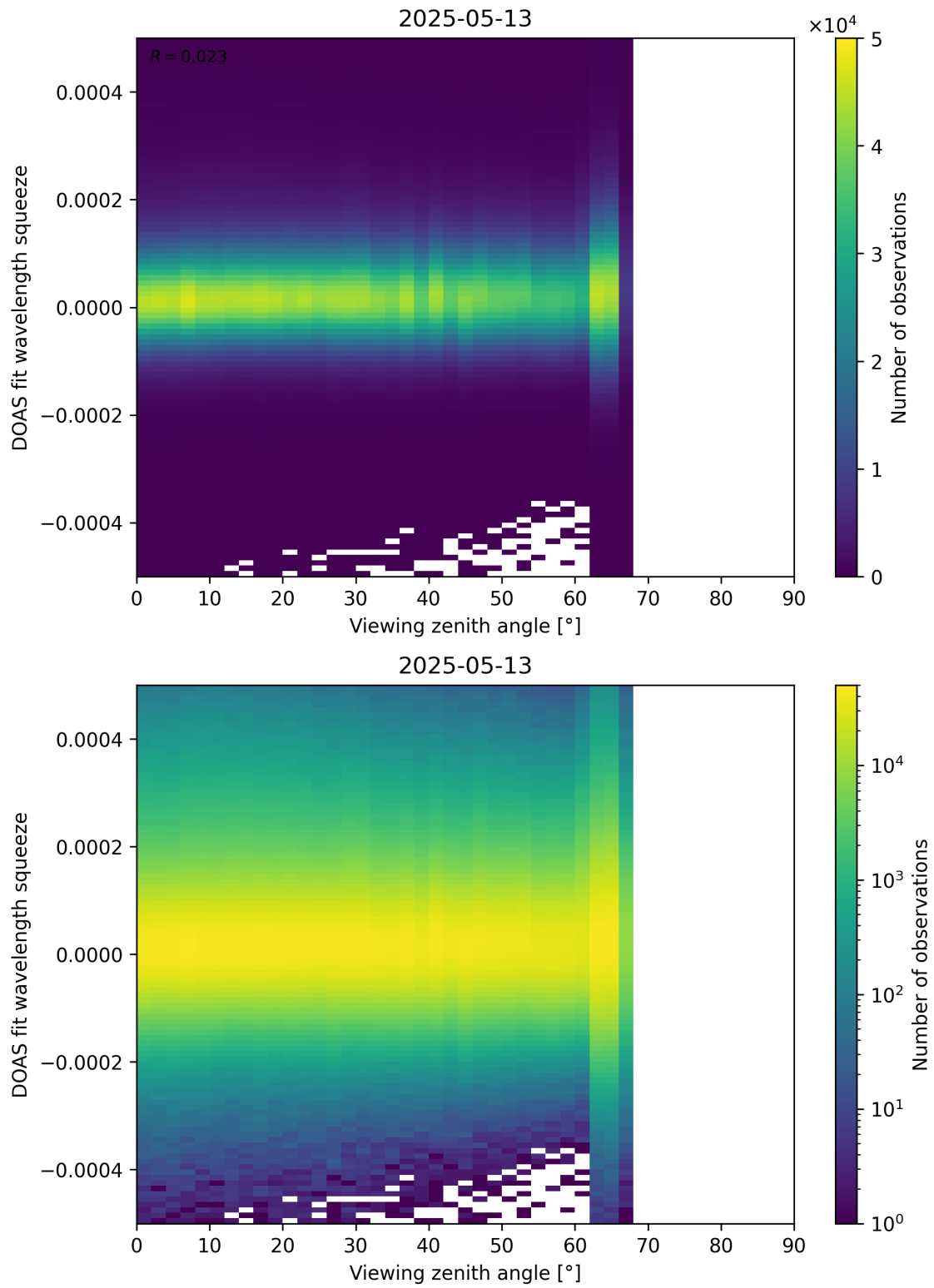
Figure 184: Scatter density plot of “Viewing zenith angle” against “DOAS fit wavelength squeeze” for 2025-05-12 to 2025-05-14.
