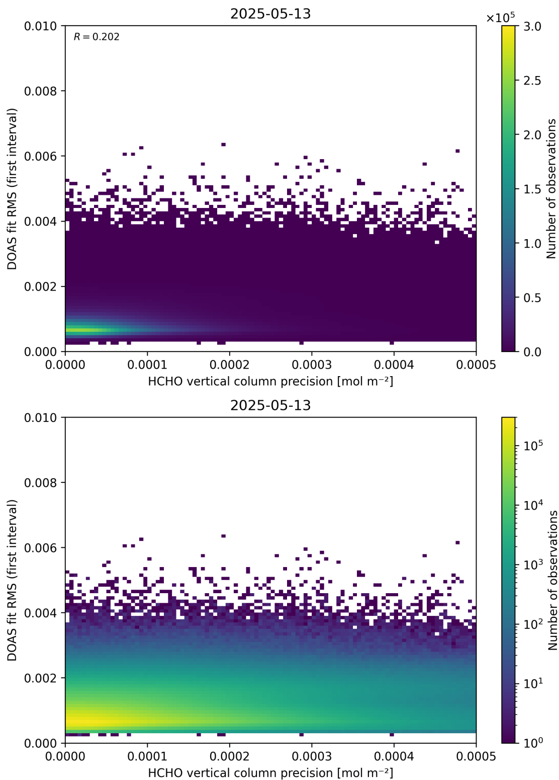
Figure 136: Scatter density plot of “HCHO vertical column precision” against “DOAS fit RMS (first interval)” for 2025-05-12 to 2025-05-14.
