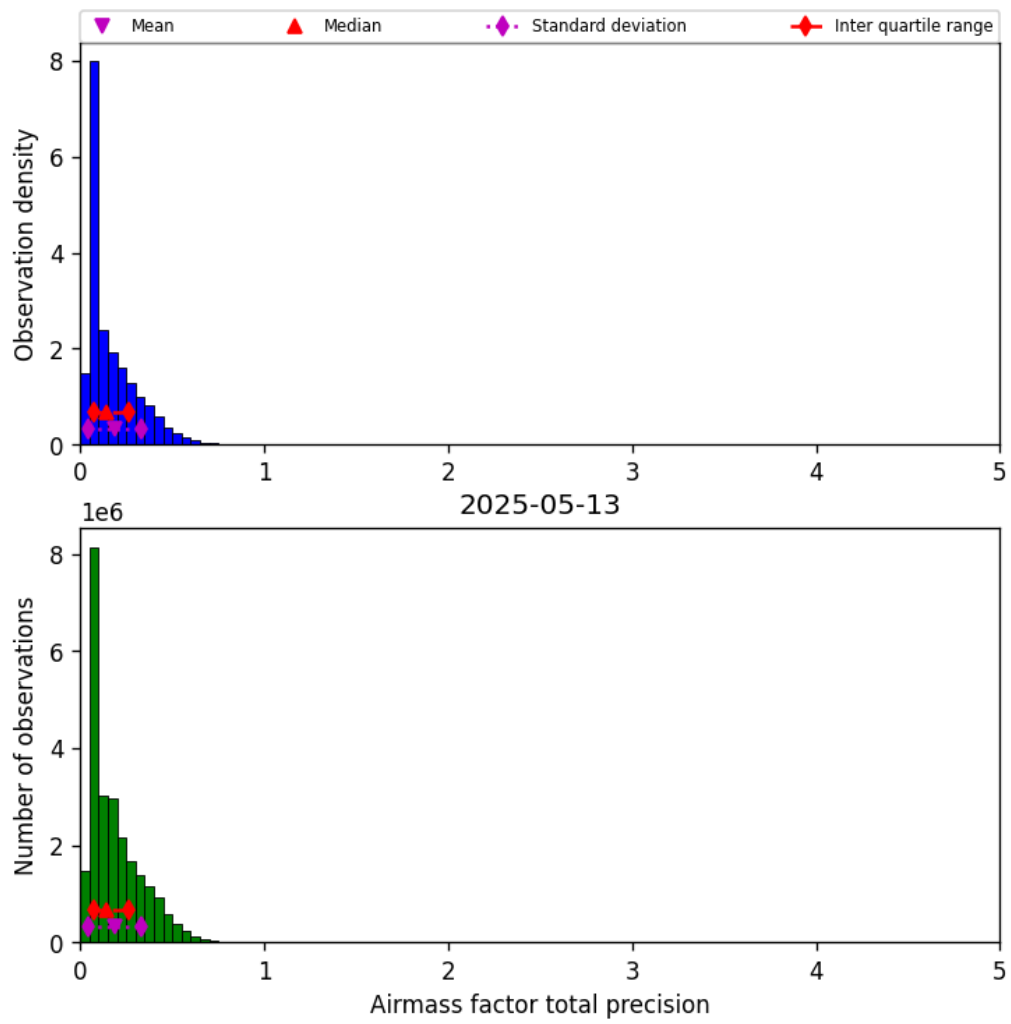
Figure 41: Histogram of “Airmass factor total precision” for 2025-05-12 to 2025-05-14
