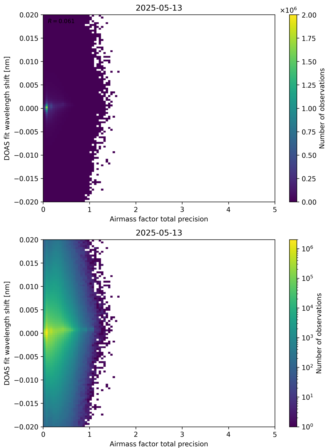
Figure 106: Scatter density plot of “Airmass factor total precision” against “DOAS fit wavelength shift” for 2025-05-12 to 2025-05-14.
