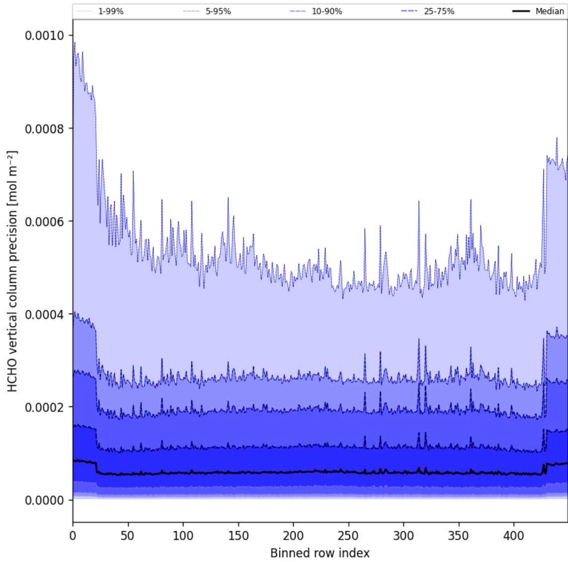
Figure 50: Along track statistics of “HCHO vertical column precision” for 2025-05-12 to 2025-05-14
