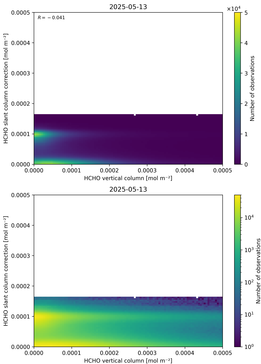
Figure 128: Scatter density plot of “HCHO vertical column” against “HCHO slant column correction” for 2025-05-12 to 2025-05-14.
