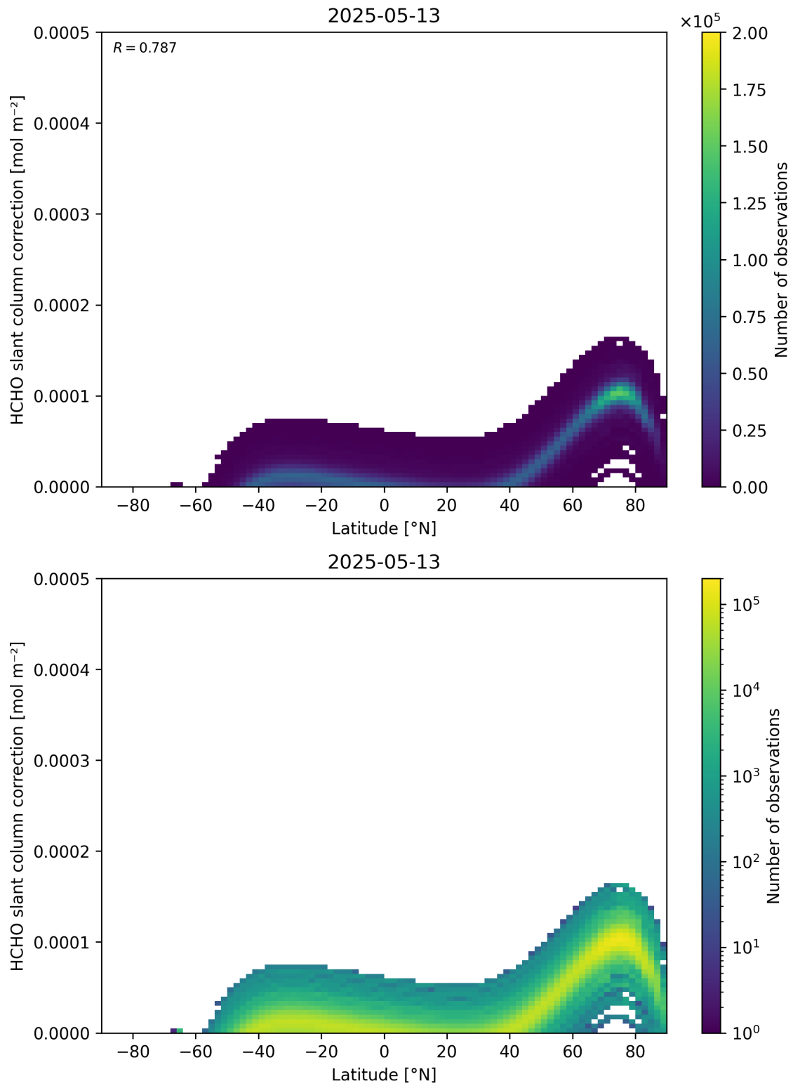
Figure 158: Scatter density plot of “Latitude” against “HCHO slant column correction” for 2025-05-12 to 2025-05-14.
