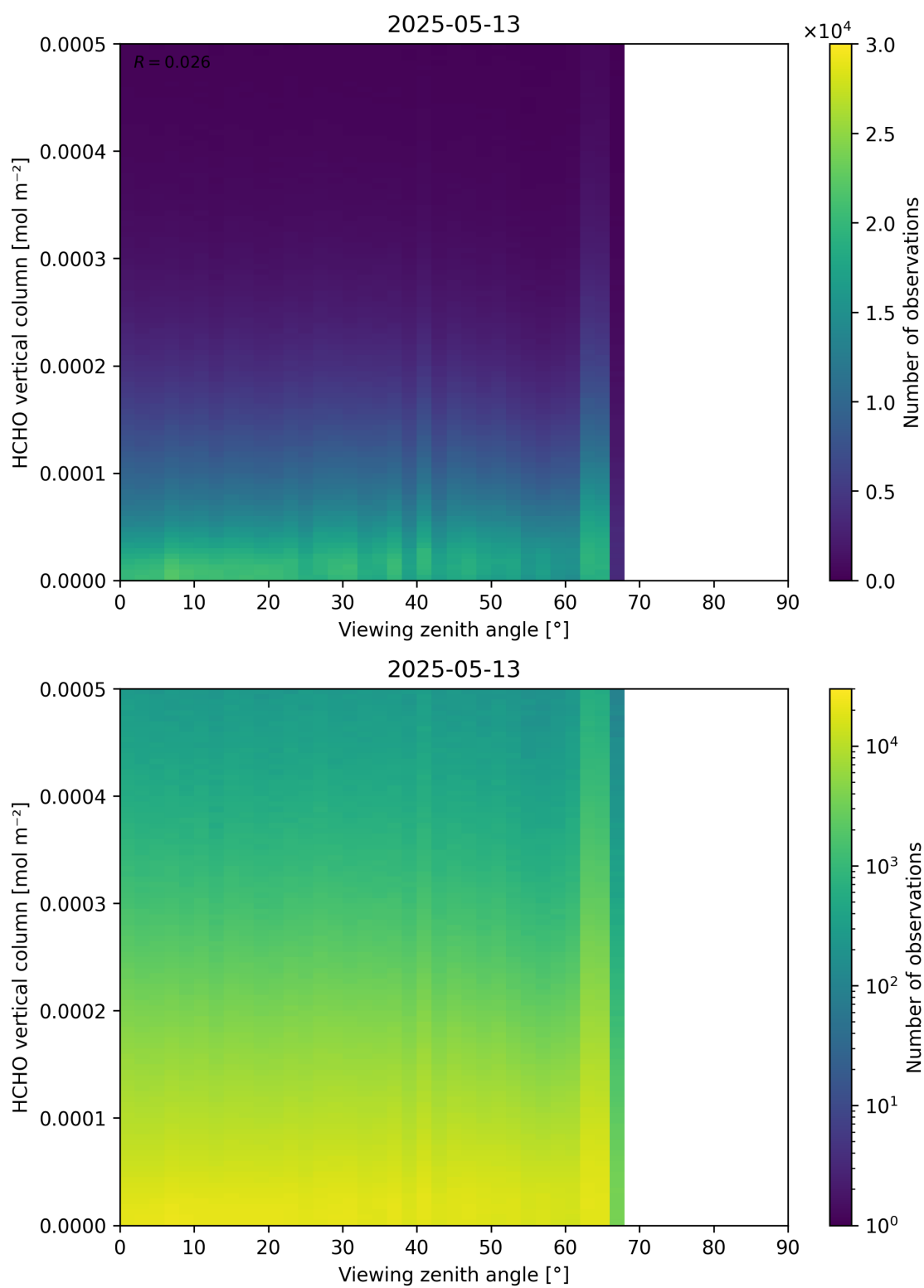
Figure 192: Scatter density plot of “Viewing zenith angle” against “HCHO vertical column” for 2025-05-12 to 2025-05-14.
