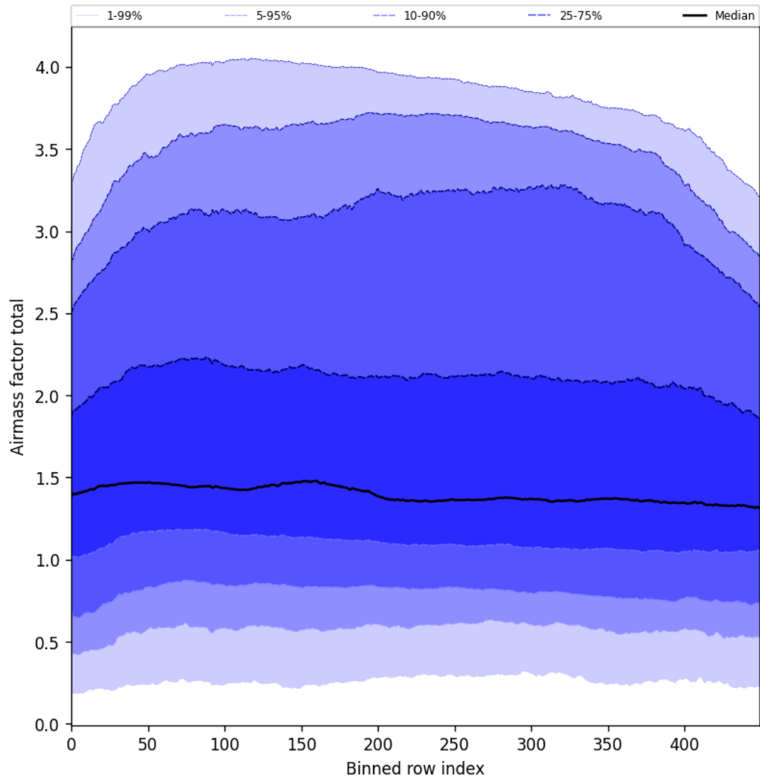
Figure 54: Along track statistics of “Airmass factor total” for 2025-05-12 to 2025-05-14
