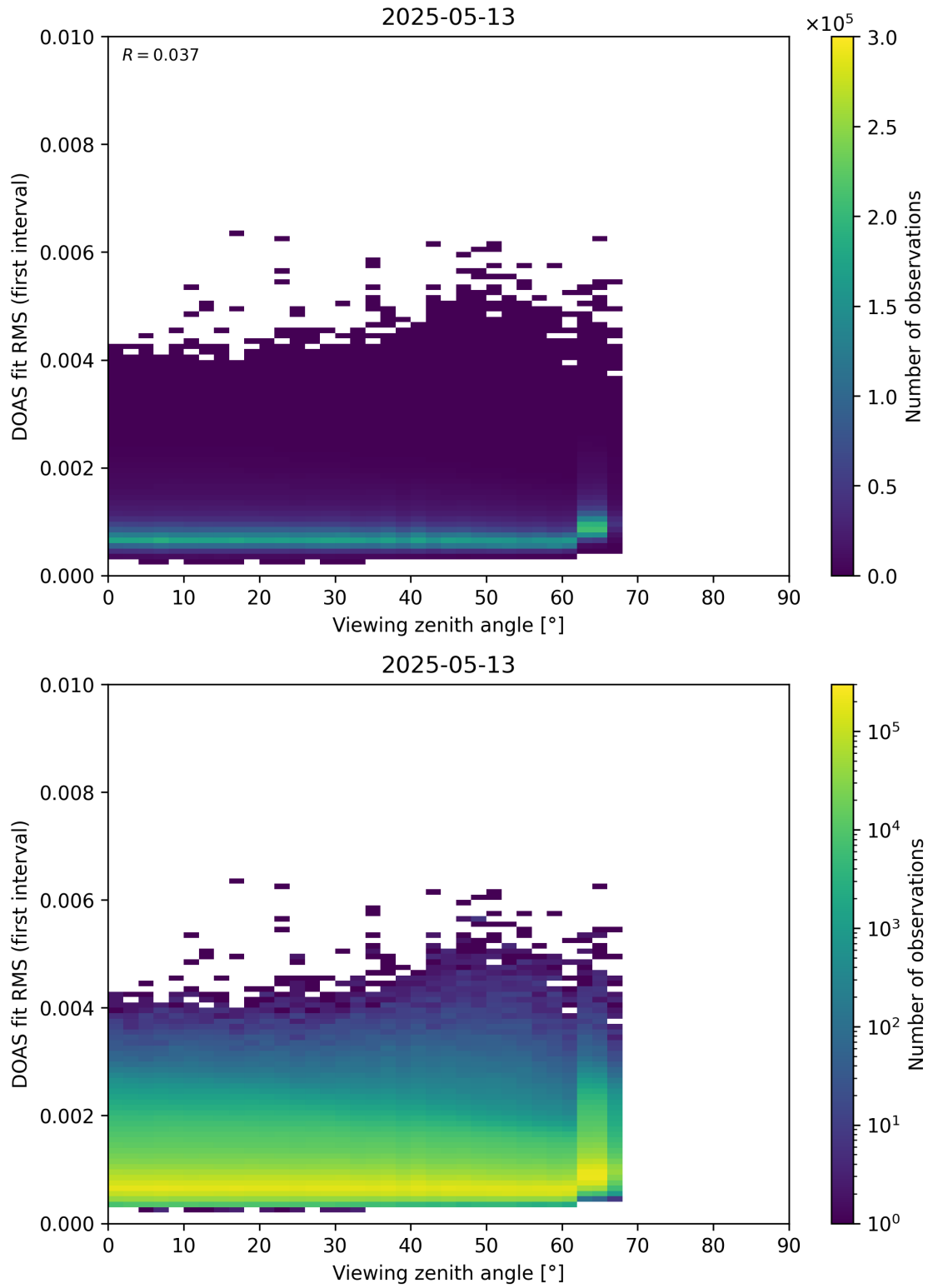
Figure 182: Scatter density plot of “Viewing zenith angle” against “DOAS fit RMS (first interval)” for 2025-05-12 to 2025-05-14.
