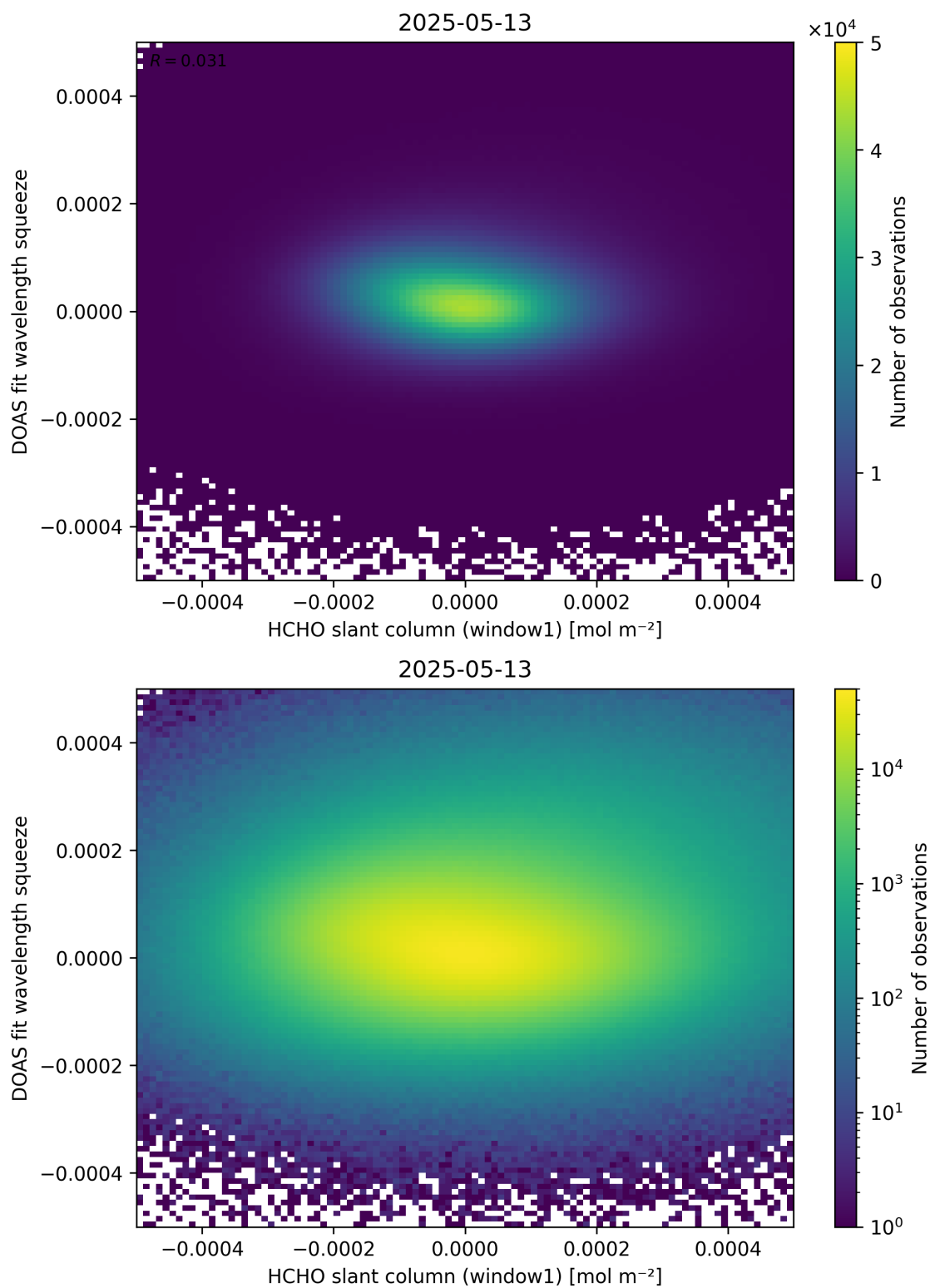
Figure 80: Scatter density plot of “HCHO slant column (window1)” against “DOAS fit wavelength squeeze” for 2025-05-12 to 2025-05-14.
