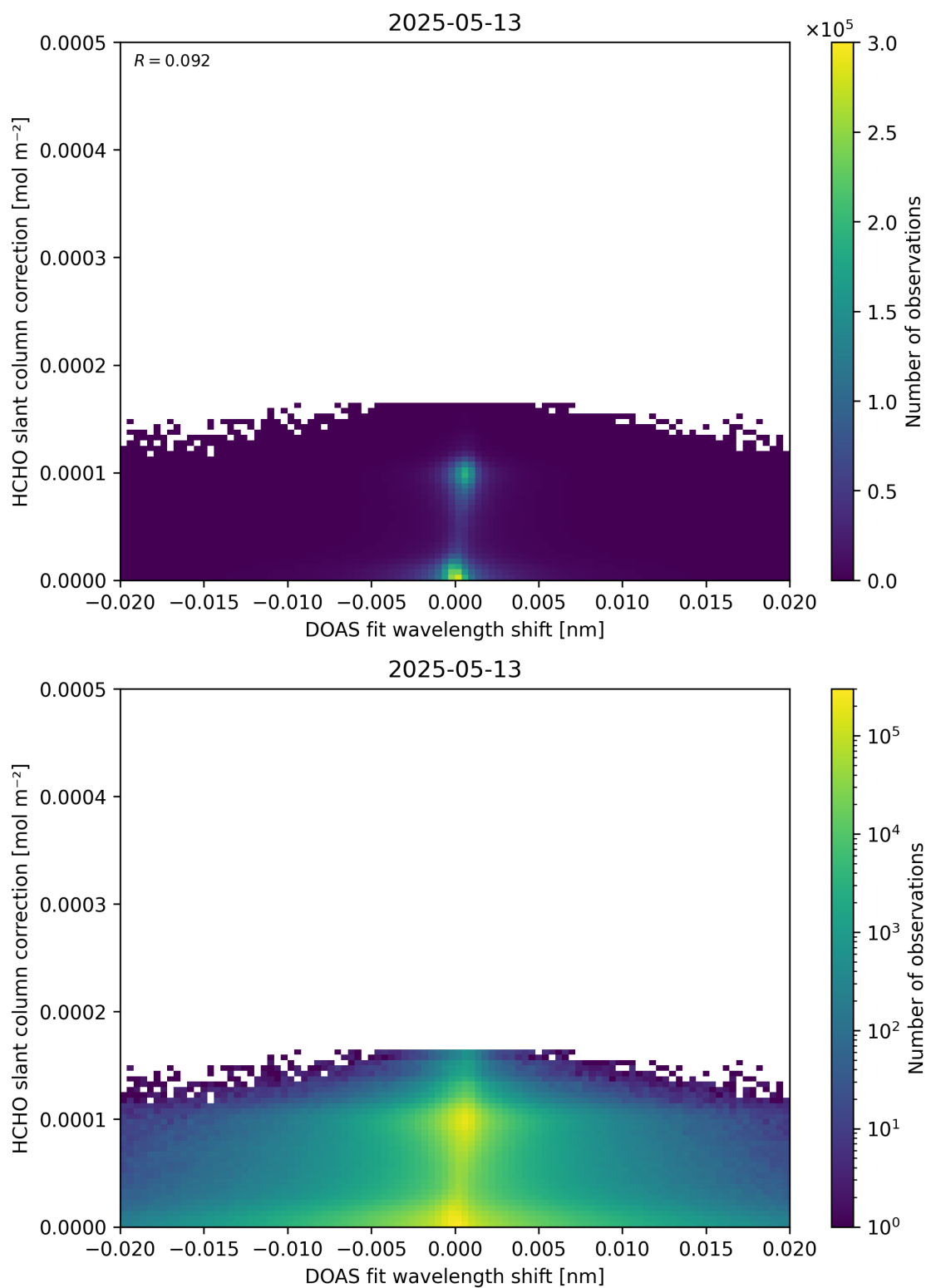
Figure 67: Scatter density plot of “DOAS fit wavelength shift” against “HCHO slant column correction” for 2025-05-12 to 2025-05-14.
