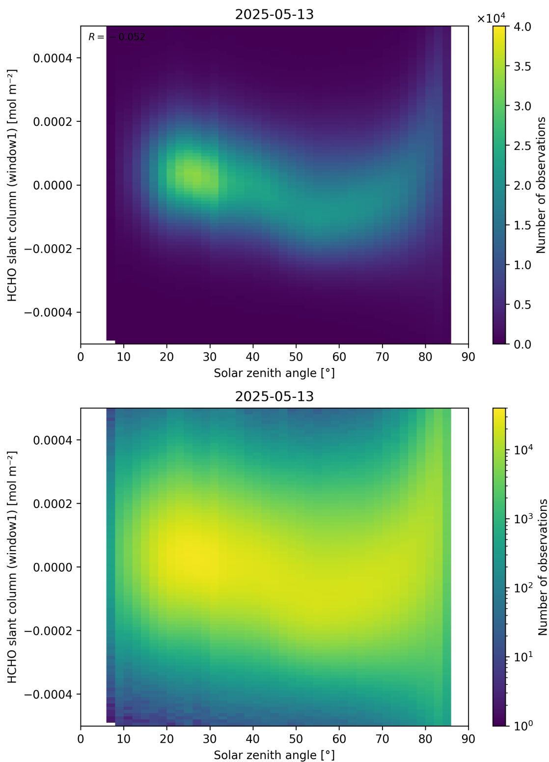
Figure 173: Scatter density plot of “Solar zenith angle” against “HCHO slant column (window1)” for 2025-05-12 to 2025-05-14.
