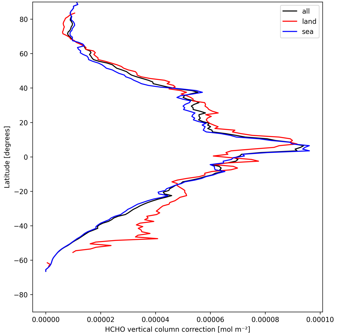
Figure 23: Zonal average of “HCHO vertical column correction” for 2025-05-12 to 2025-05-14.
