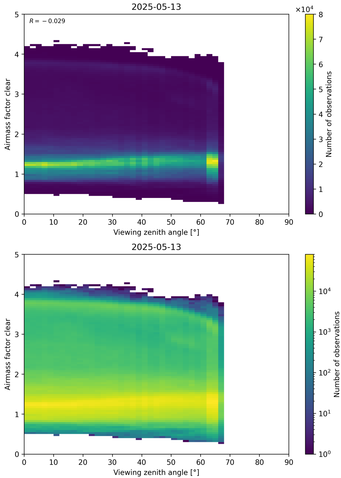
Figure 185: Scatter density plot of “Viewing zenith angle” against “Airmass factor clear” for 2025-05-12 to 2025-05-14.
