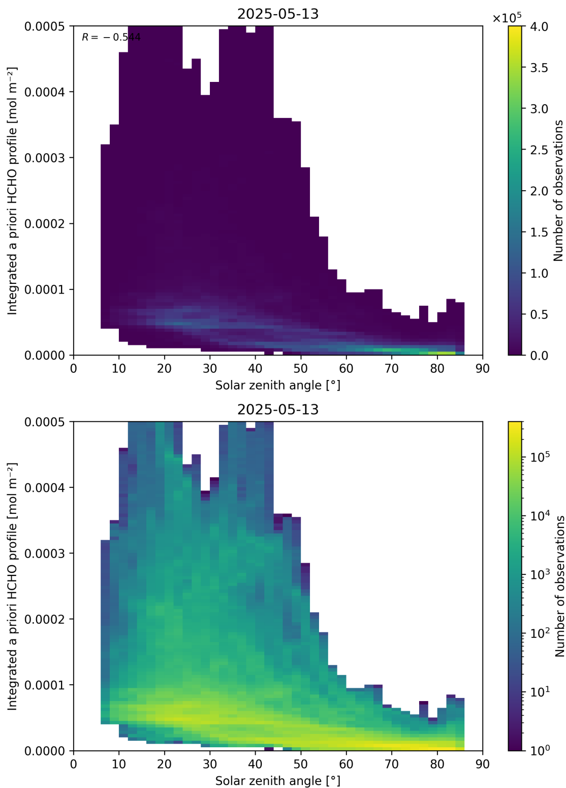
Figure 180: Scatter density plot of “Solar zenith angle” against “Integrated a priori HCHO profile” for 2025-05-12 to 2025-05-14.
