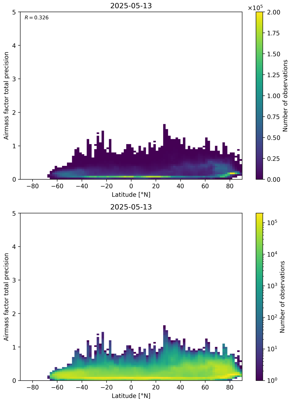
Figure 162: Scatter density plot of “Latitude” against “Airmass factor total precision” for 2025-05-12 to 2025-05-14.
