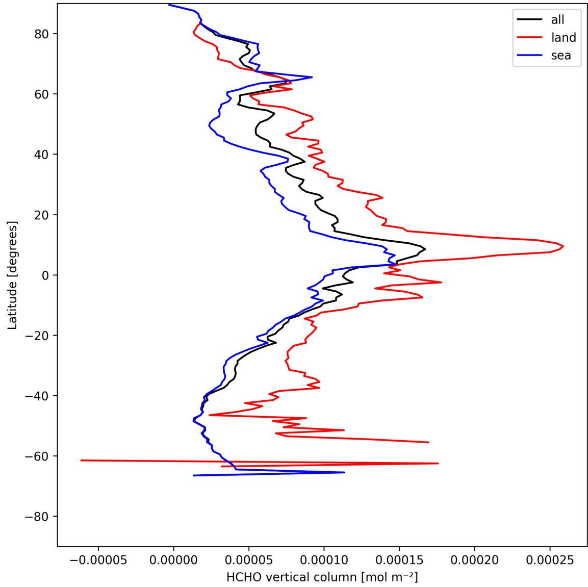
Figure 21: Zonal average of “HCHO vertical column” for 2025-05-12 to 2025-05-14.
