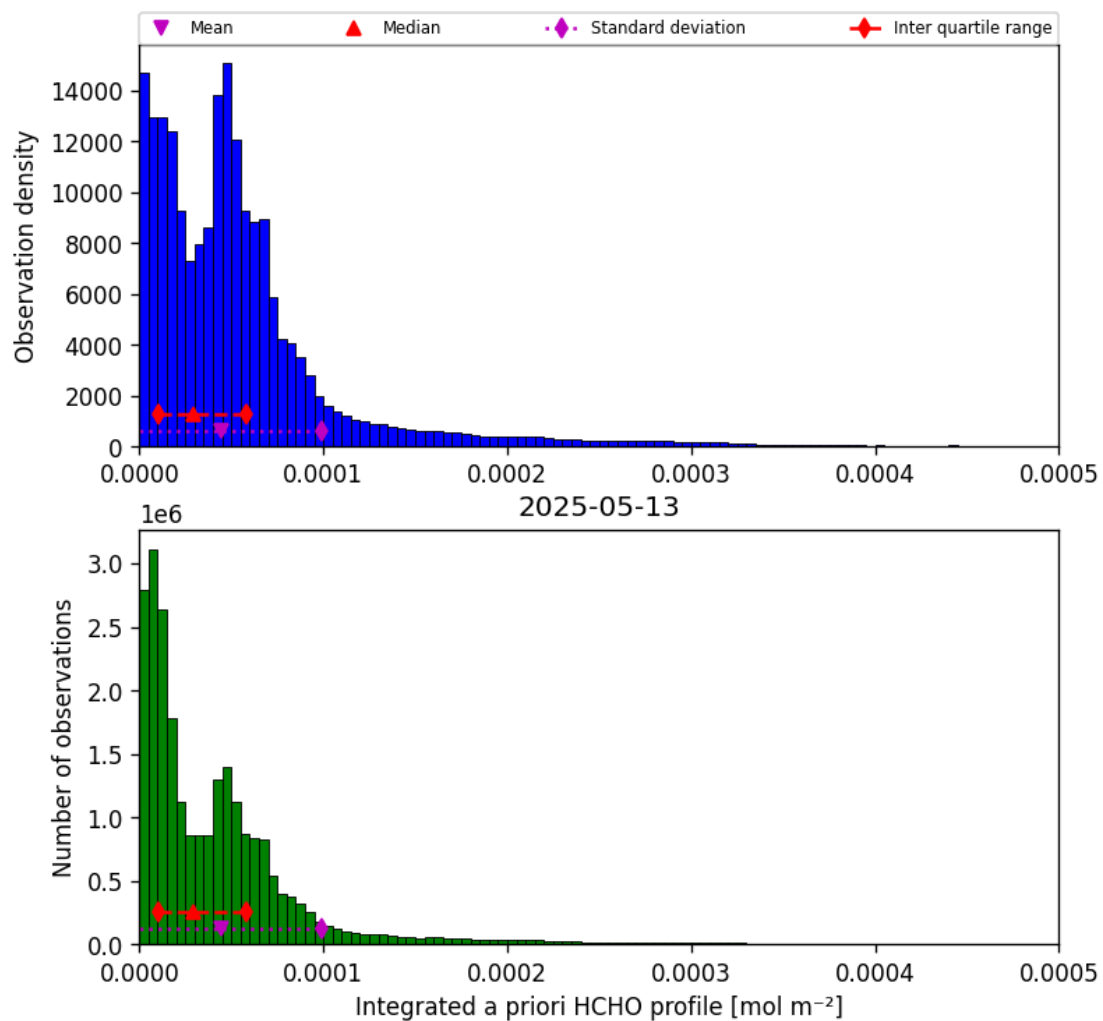
Figure 43: Histogram of “Integrated a priori HCHO profile” for 2025-05-12 to 2025-05-14
