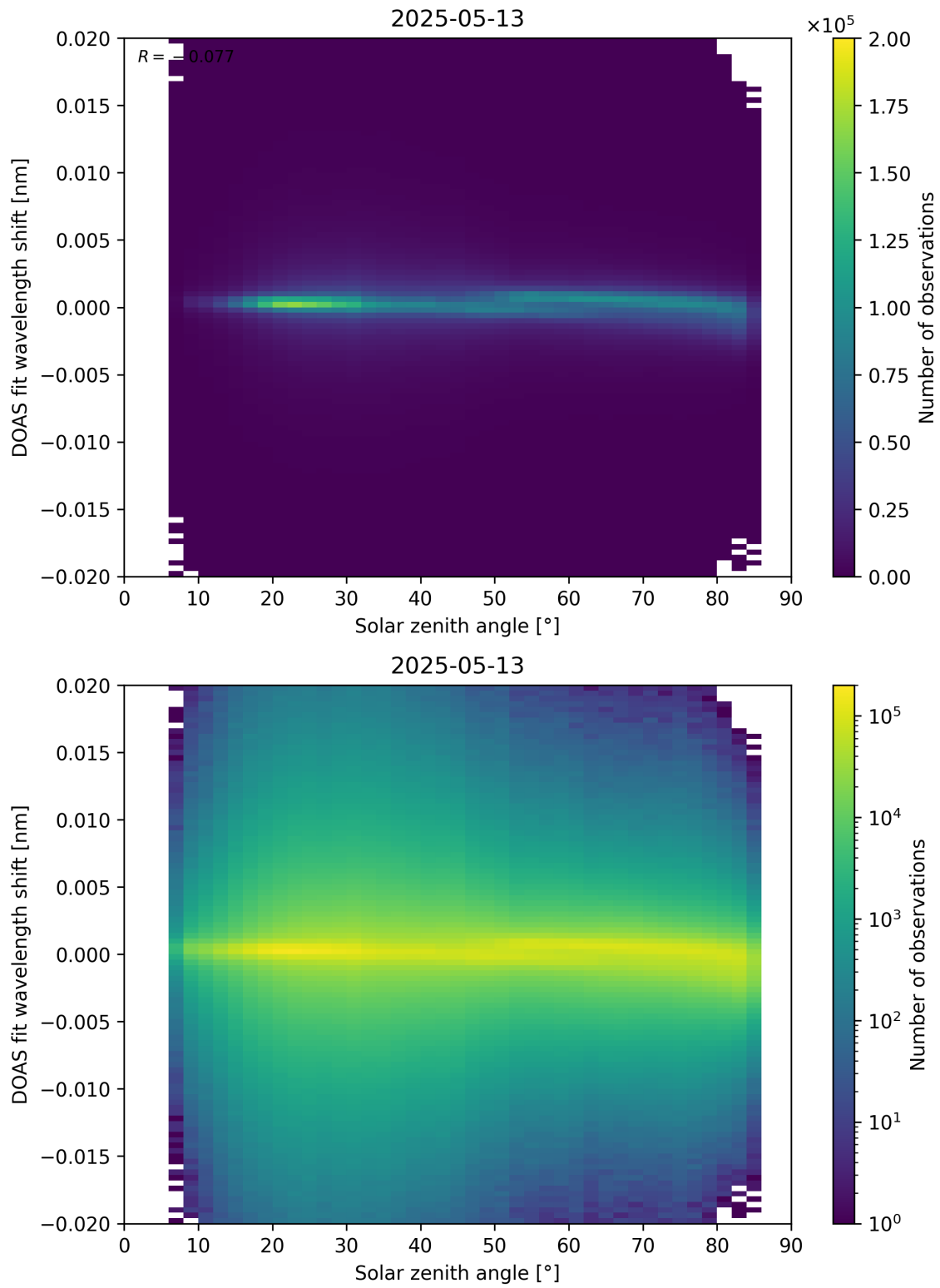
Figure 168: Scatter density plot of “Solar zenith angle” against “DOAS fit wavelength shift” for 2025-05-12 to 2025-05-14.
