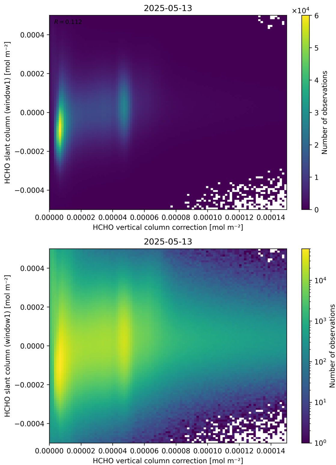
Figure 118: Scatter density plot of “HCHO vertical column correction” against “HCHO slant column (window1)” for 2025-05-12 to 2025-05-14.
