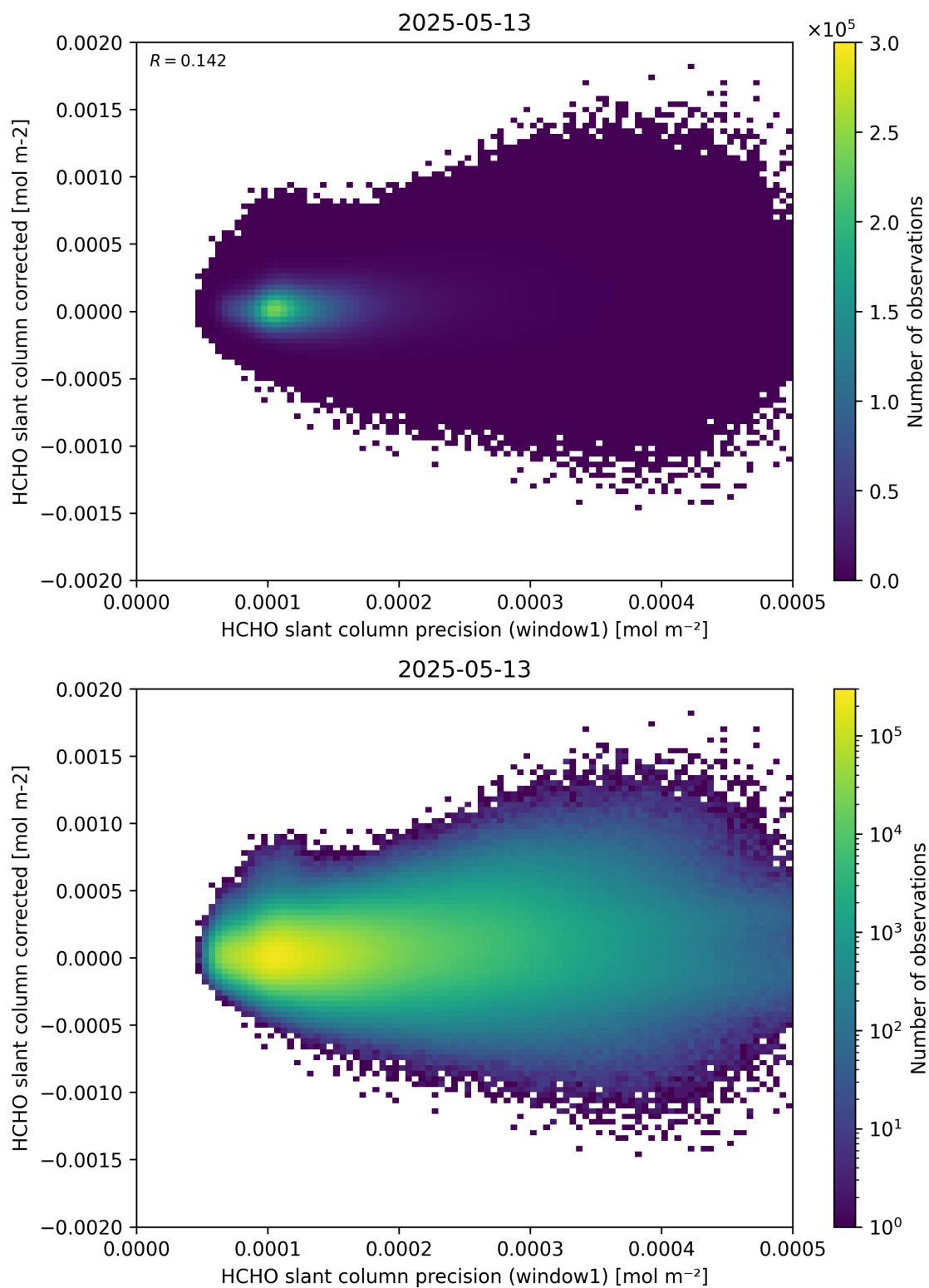
Figure 92: Scatter density plot of “HCHO slant column precision (window1)” against “HCHO slant column corrected” for 2025-05-12 to 2025-05-14.
