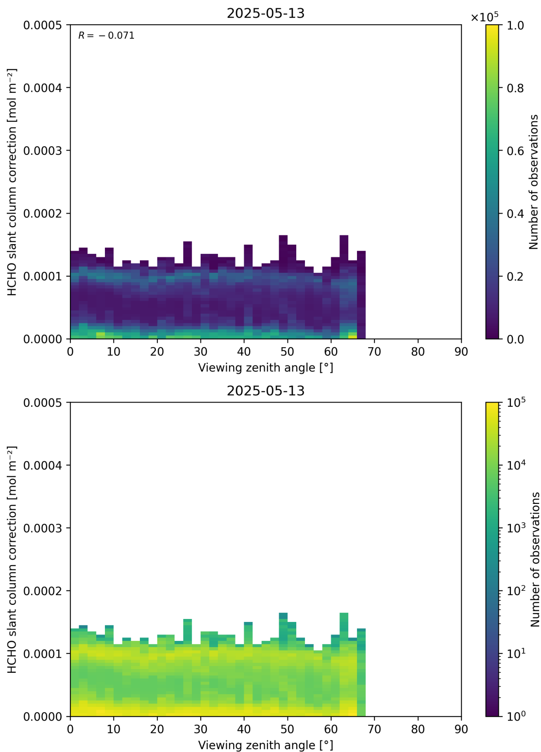
Figure 187: Scatter density plot of “Viewing zenith angle” against “HCHO slant column correction” for 2025-05-12 to 2025-05-14.
