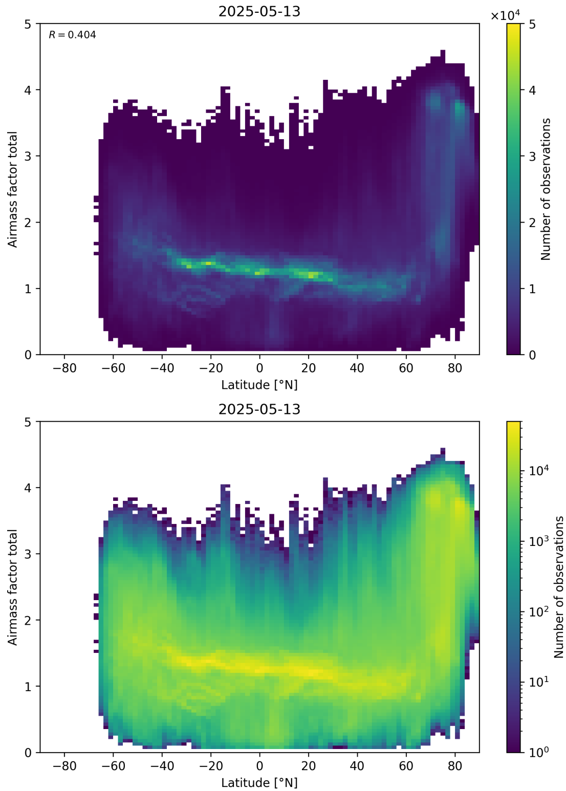
Figure 161: Scatter density plot of “Latitude” against “Airmass factor total” for 2025-05-12 to 2025-05-14.
