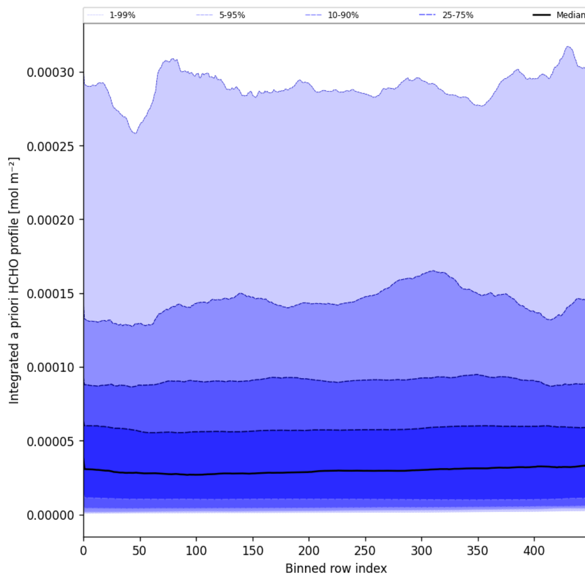
Figure 57: Along track statistics of “Integrated a priori HCHO profile” for 2025-05-12 to 2025-05-14
