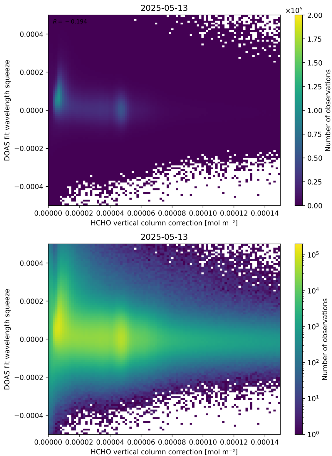
Figure 114: Scatter density plot of “HCHO vertical column correction” against “DOAS fit wavelength squeeze” for 2025-05-12 to 2025-05-14.
