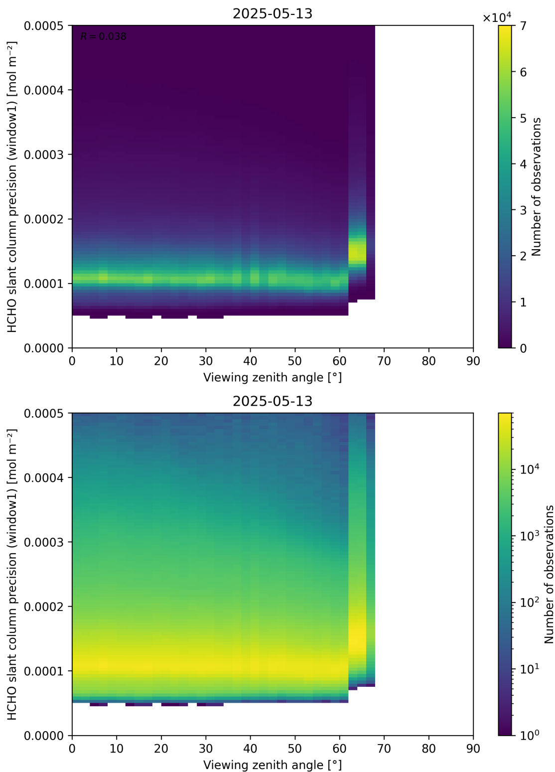
Figure 189: Scatter density plot of “Viewing zenith angle” against “HCHO slant column precision (window1)” for 2025-05-12 to 2025-05-14.
