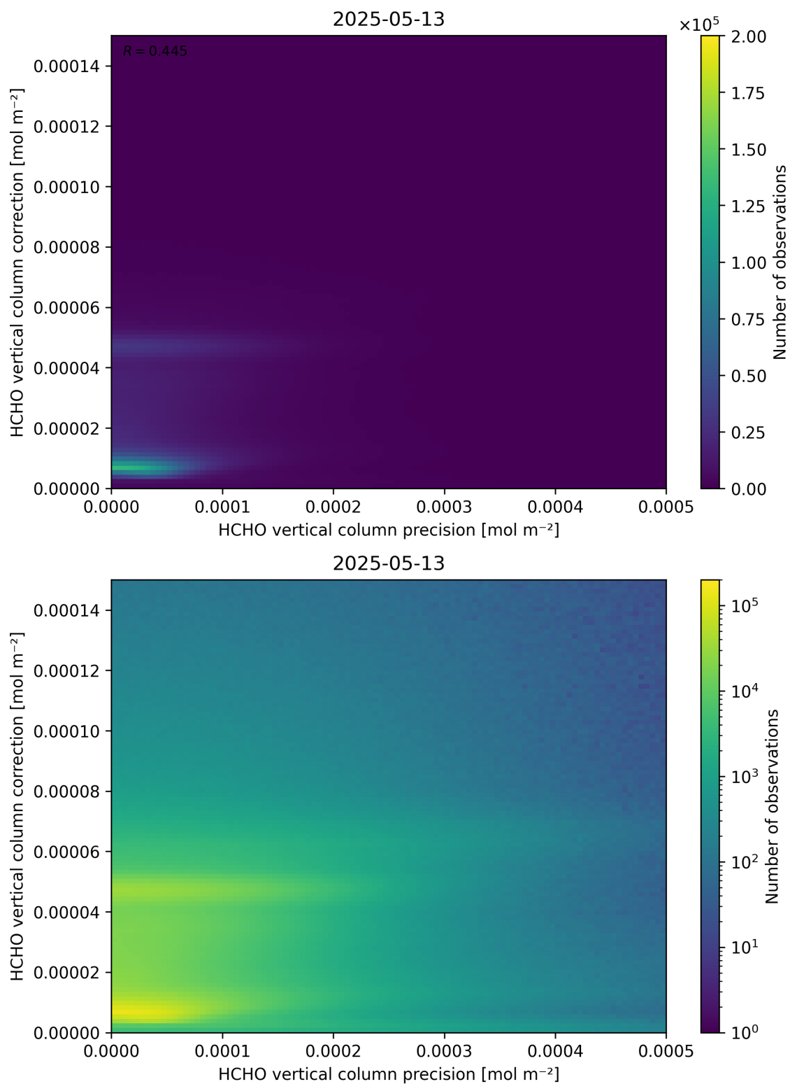
Figure 146: Scatter density plot of “HCHO vertical column precision” against “HCHO vertical column correction” for 2025-05-12 to 2025-05-14.
