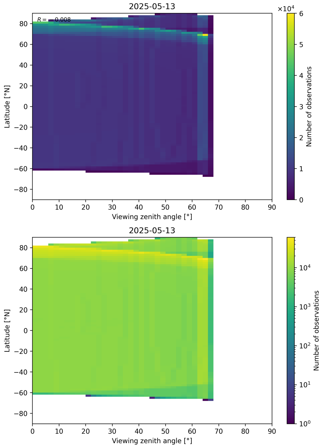
Figure 196: Scatter density plot of “Viewing zenith angle” against “Latitude” for 2025-05-12 to 2025-05-14.
