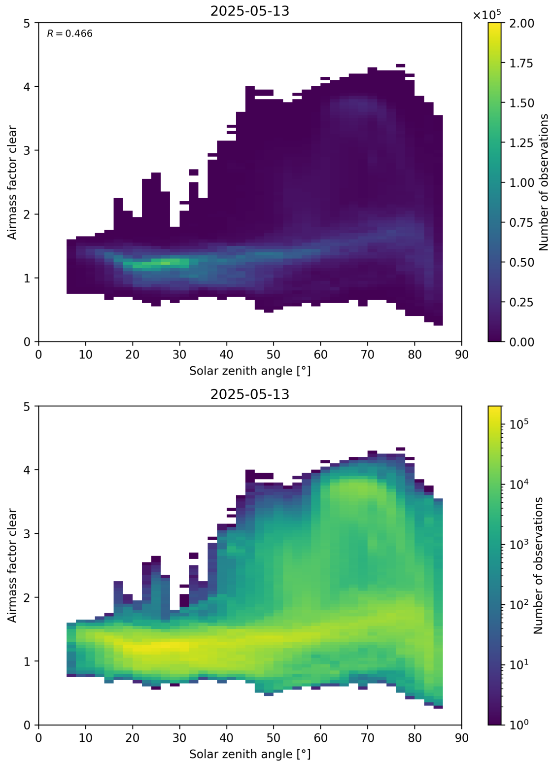
Figure 170: Scatter density plot of “Solar zenith angle” against “Airmass factor clear” for 2025-05-12 to 2025-05-14.
