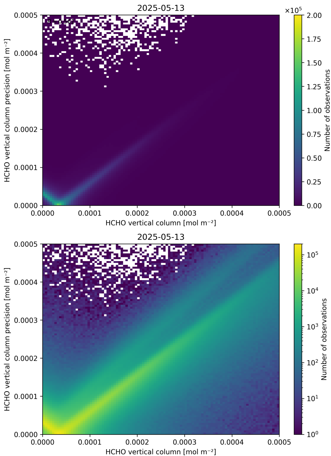
Figure 134: Scatter density plot of “HCHO vertical column” against “HCHO vertical column precision” for 2025-05-12 to 2025-05-14.
