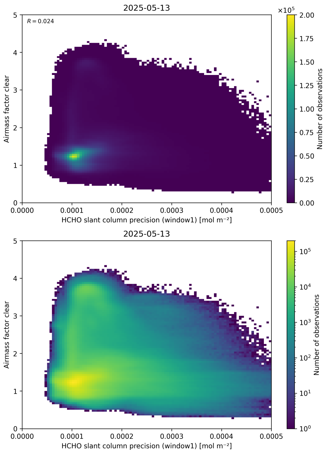
Figure 91: Scatter density plot of “HCHO slant column precision (window1)” against “Airmass factor clear” for 2025-05-12 to 2025-05-14.
