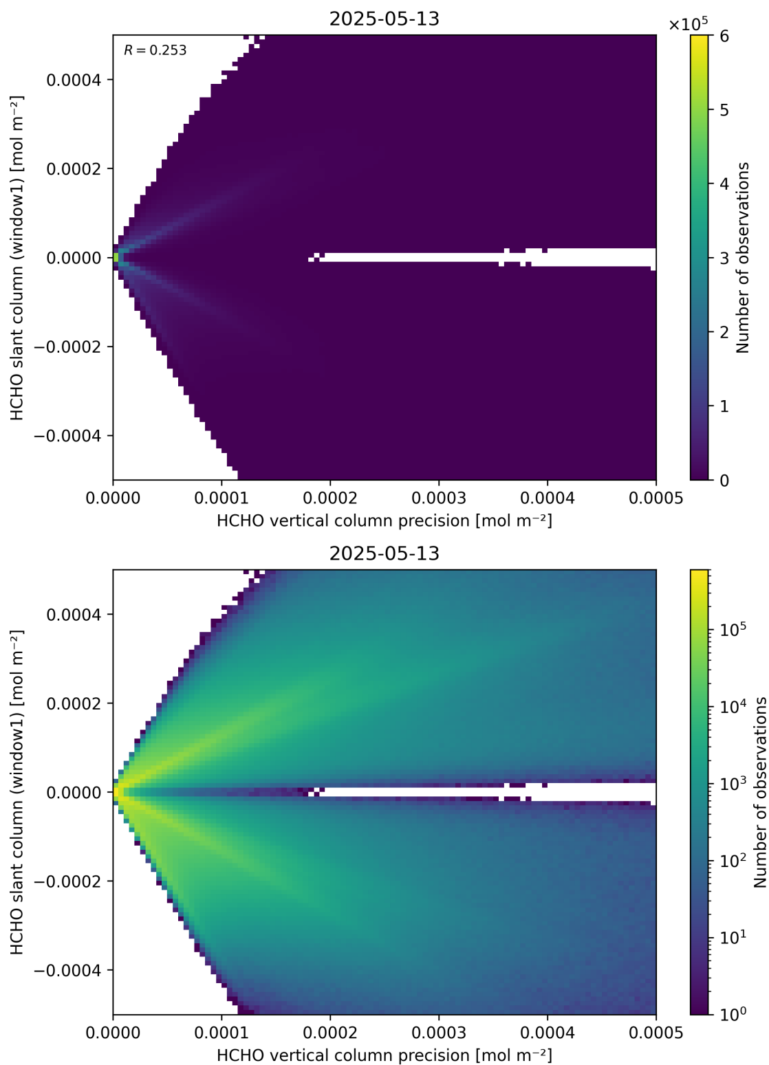
Figure 142: Scatter density plot of “HCHO vertical column precision” against “HCHO slant column (window1)” for 2025-05-12 to 2025-05-14.
