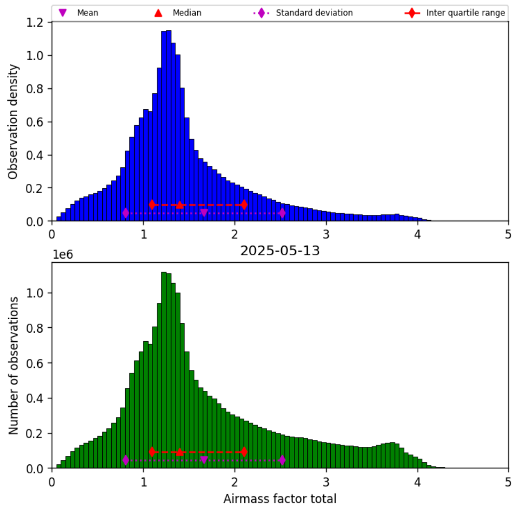
Figure 40: Histogram of “Airmass factor total” for 2025-05-12 to 2025-05-14
