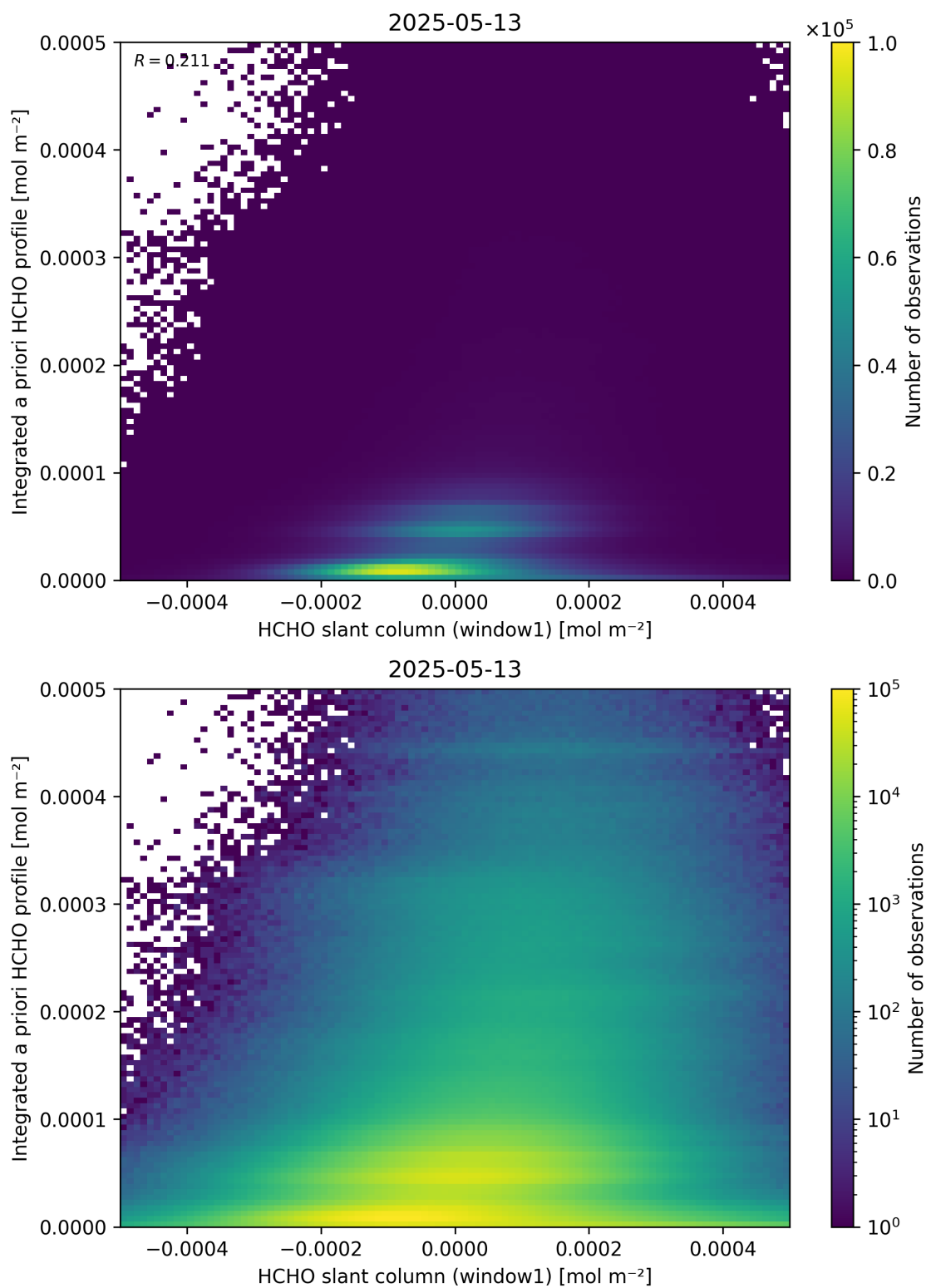
Figure 87: Scatter density plot of “HCHO slant column (window1)” against “Integrated a priori HCHO profile” for 2025-05-12 to 2025-05-14.
