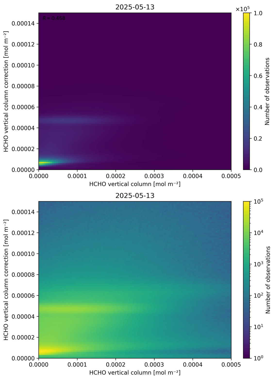
Figure 133: Scatter density plot of “HCHO vertical column” against “HCHO vertical column correction” for 2025-05-12 to 2025-05-14.
