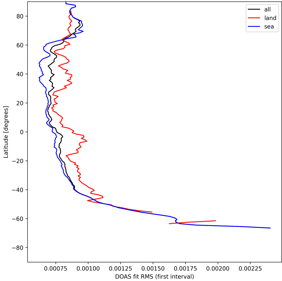
Figure 32: Zonal average of "DOAS fit RMS (first interval)" for 2025-05-12 to 2025-05-14.
