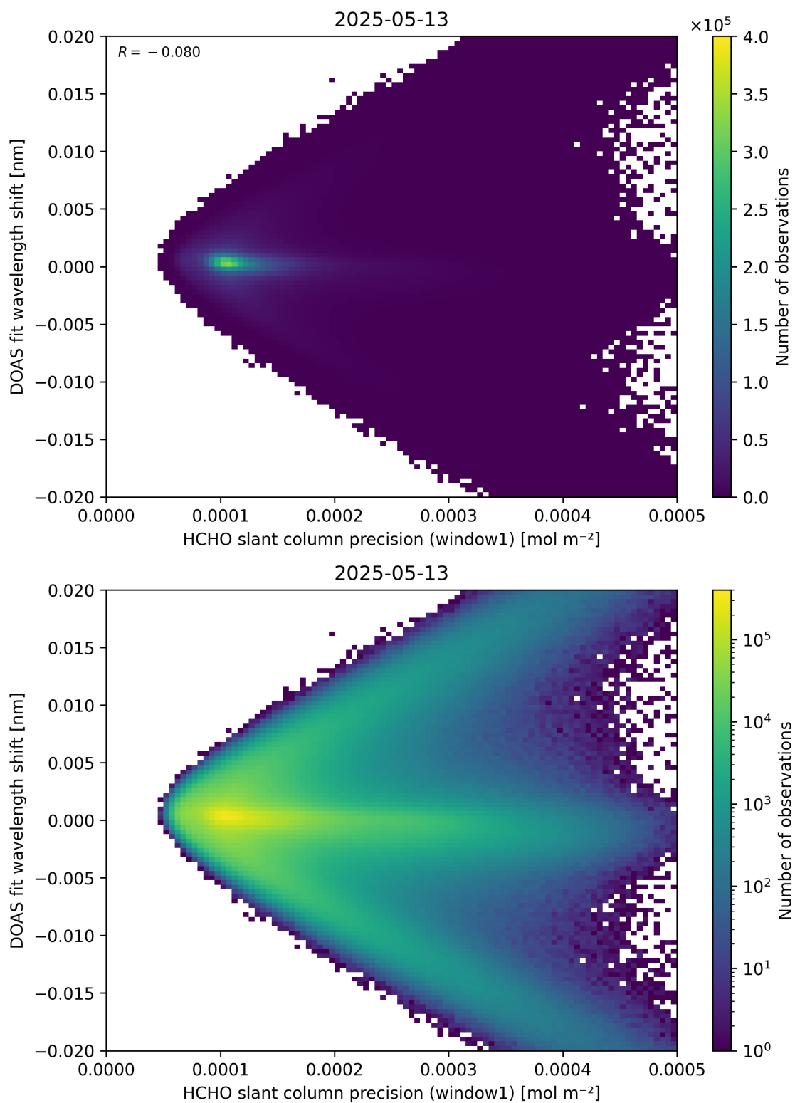
Figure 89: Scatter density plot of “HCHO slant column precision (window1)” against “DOAS fit wavelength shift” for 2025-05-12 to 2025-05-14.
