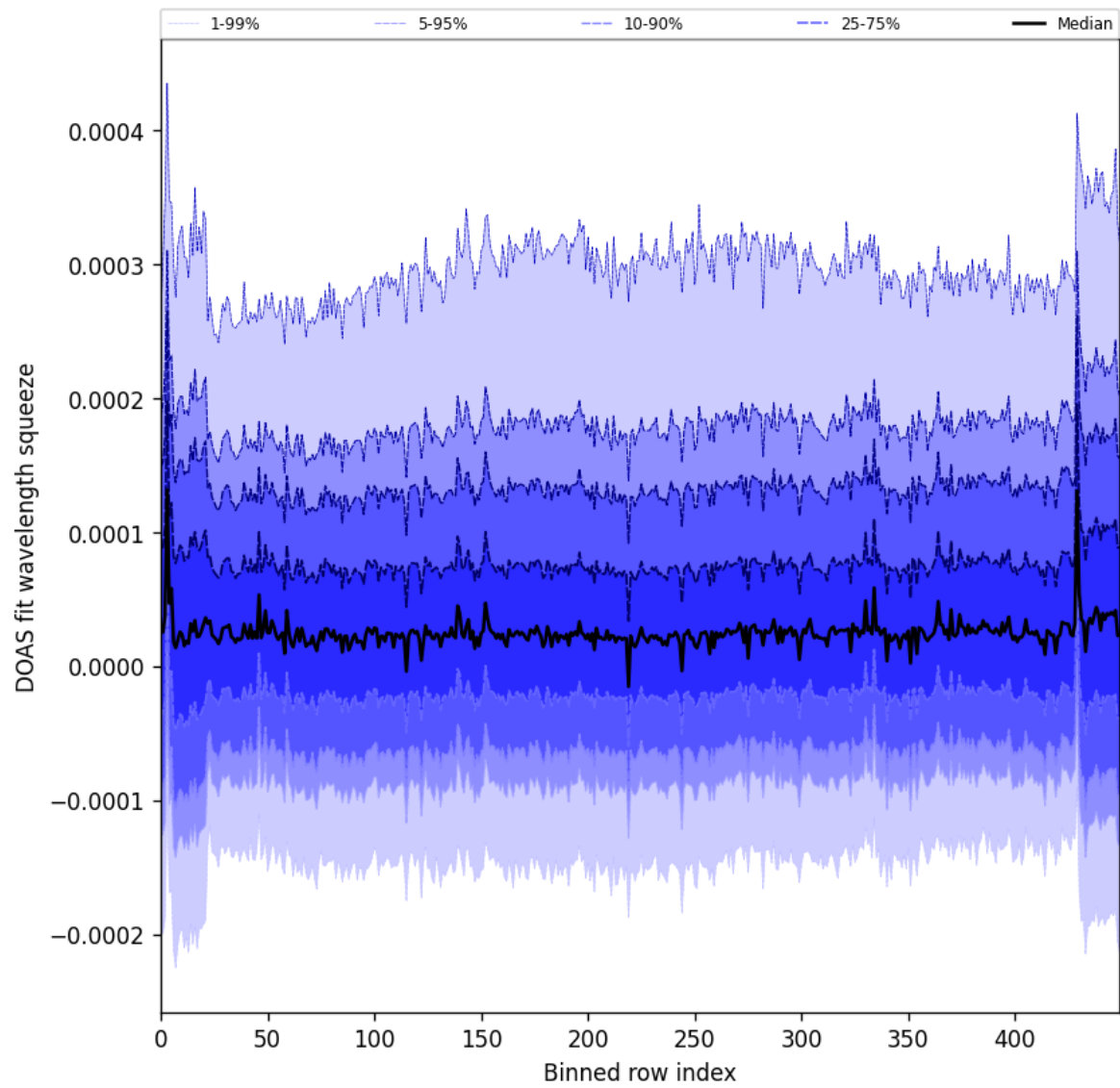
Figure 59: Along track statistics of “DOAS fit wavelength squeeze” for 2025-05-12 to 2025-05-14
