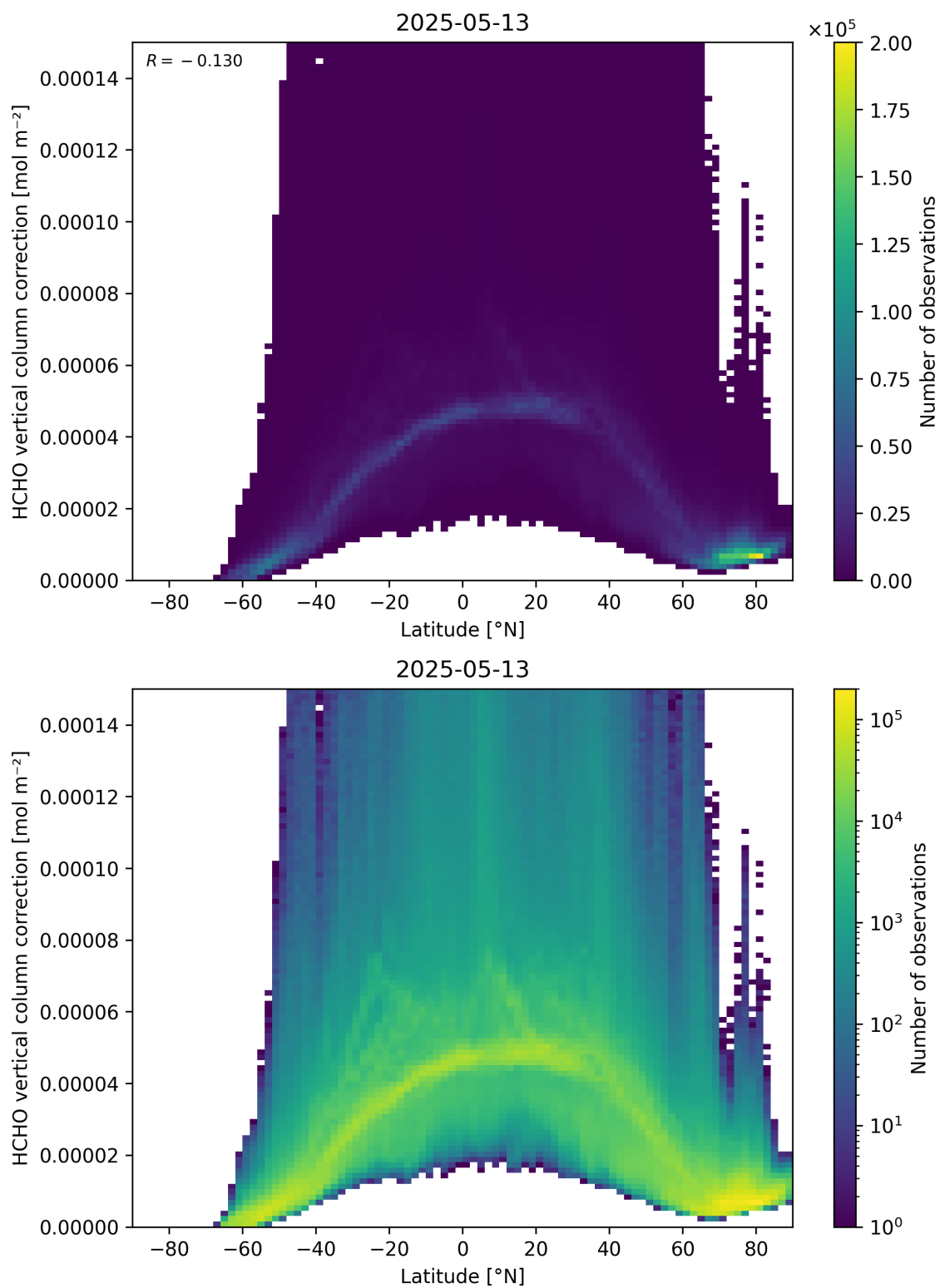
Figure 164: Scatter density plot of “Latitude” against “HCHO vertical column correction” for 2025-05-12 to 2025-05-14.
