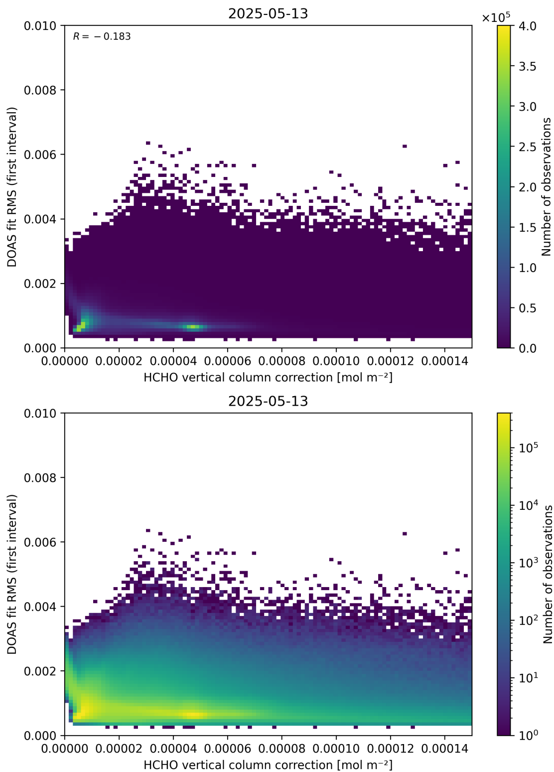
Figure 112: Scatter density plot of “HCHO vertical column correction” against “DOAS fit RMS (first interval)” for 2025-05-12 to 2025-05-14.
