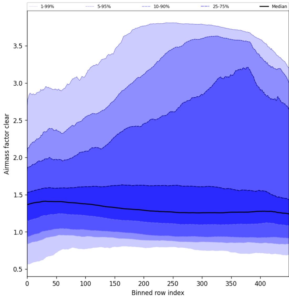
Figure 56: Along track statistics of “Airmass factor clear” for 2025-05-12 to 2025-05-14
