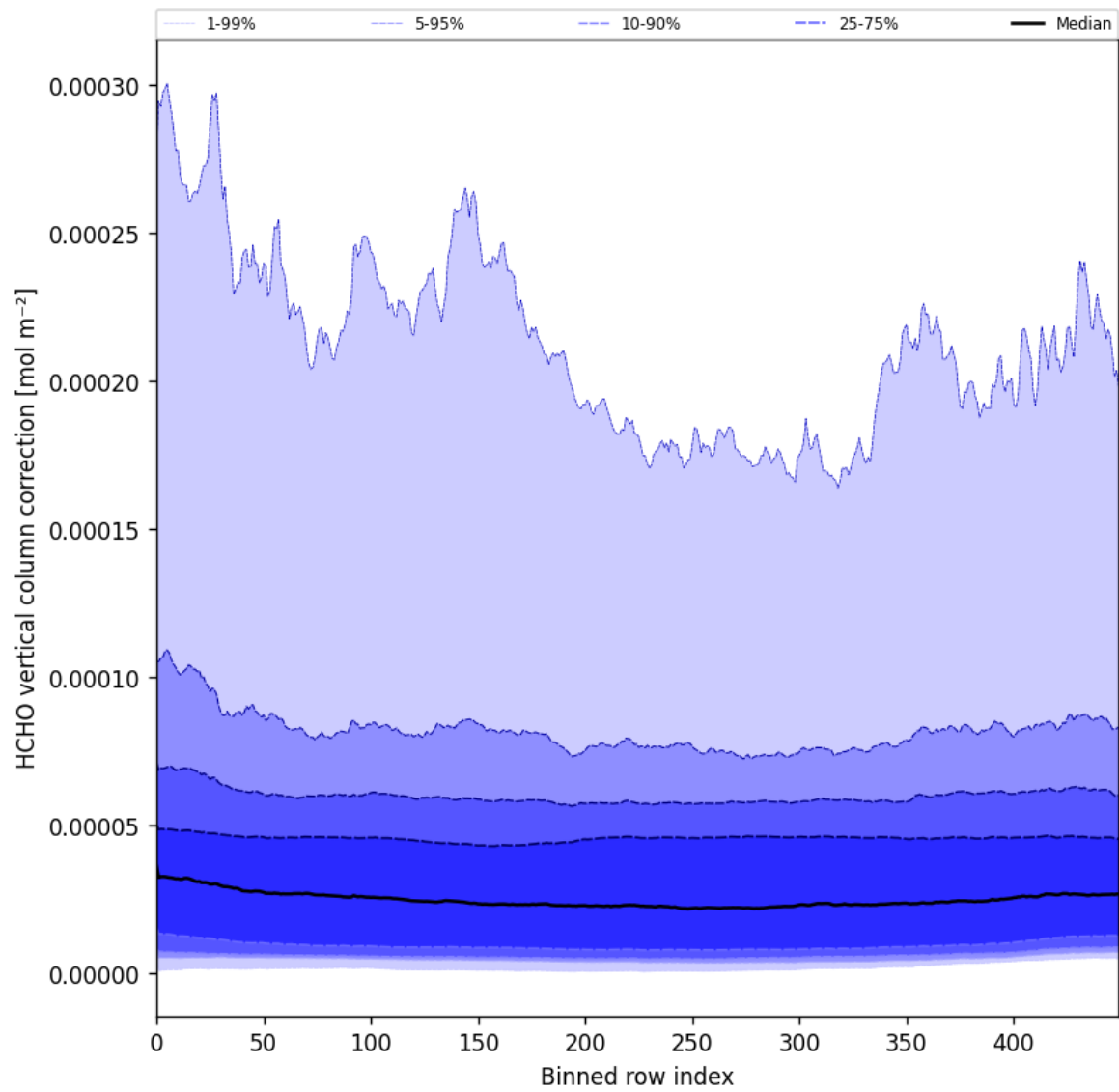
Figure 51: Along track statistics of “HCHO vertical column correction” for 2025-05-12 to 2025-05-14
