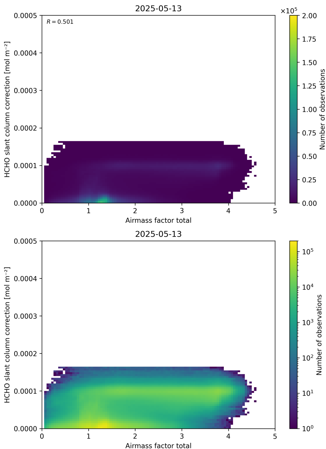
Figure 102: Scatter density plot of “Airmass factor total” against “HCHO slant column correction” for 2025-05-12 to 2025-05-14.
