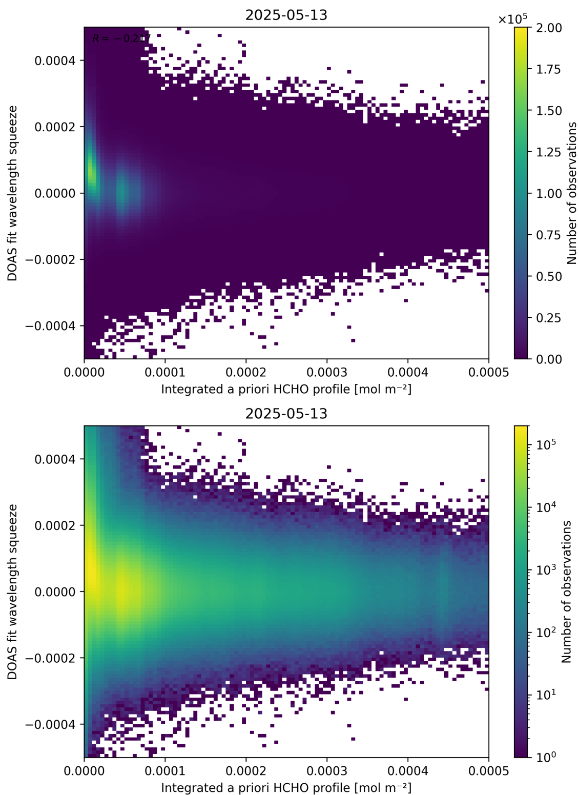
Figure 150: Scatter density plot of “Integrated a priori HCHO profile” against “DOAS fit wavelength squeeze” for 2025-05-12 to 2025-05-14.
