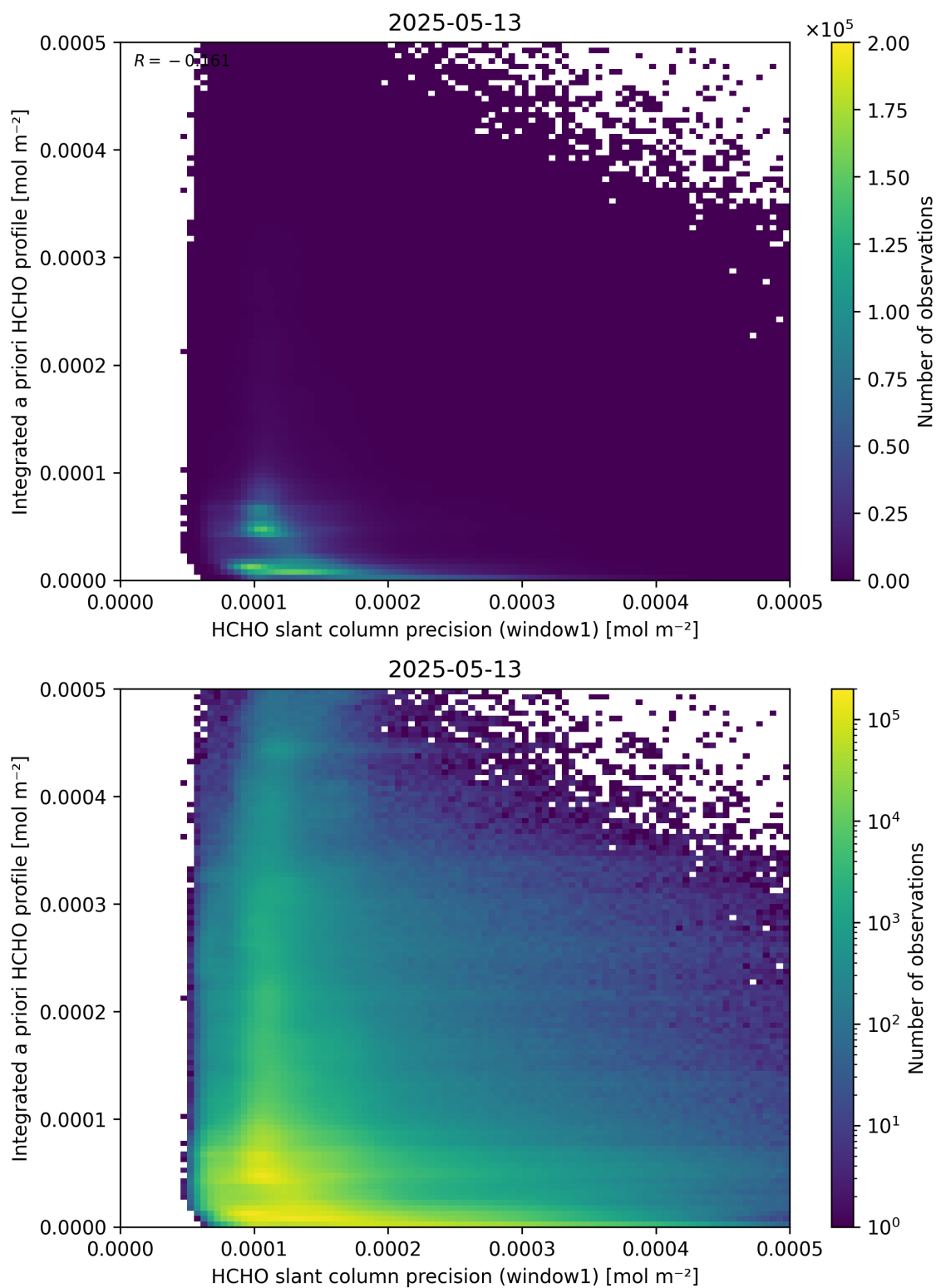
Figure 96: Scatter density plot of “HCHO slant column precision (window1)” against “Integrated a priori HCHO profile” for 2025-05-12 to 2025-05-14.
