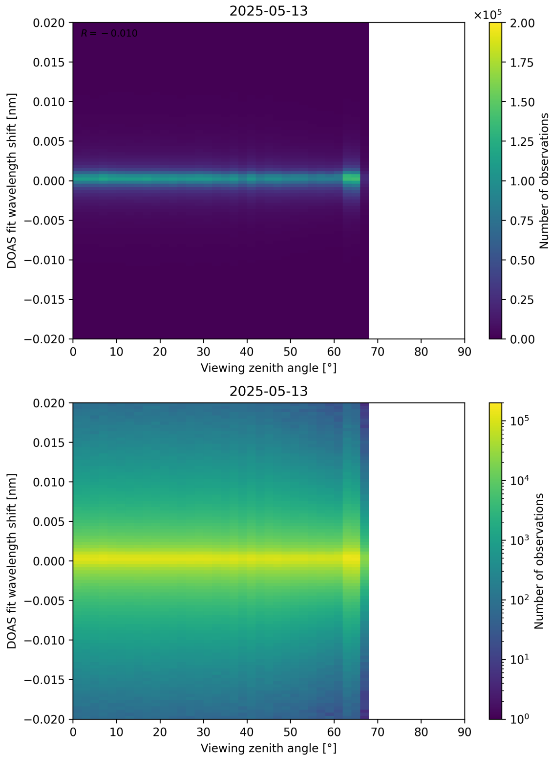
Figure 183: Scatter density plot of “Viewing zenith angle” against “DOAS fit wavelength shift” for 2025-05-12 to 2025-05-14.
