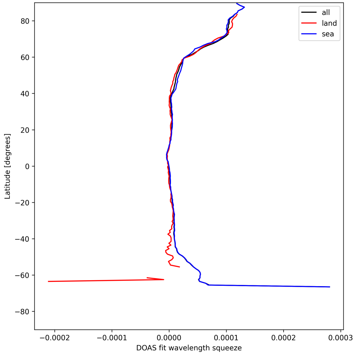
Figure 31: Zonal average of “DOAS fit wavelength squeeze” for 2025-05-12 to 2025-05-14.
