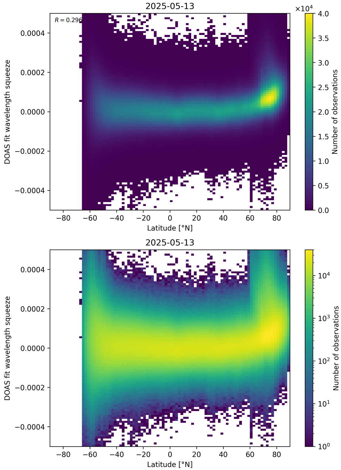
Figure 155: Scatter density plot of “Latitude” against “DOAS fit wavelength squeeze” for 2025-05-12 to 2025-05-14.
