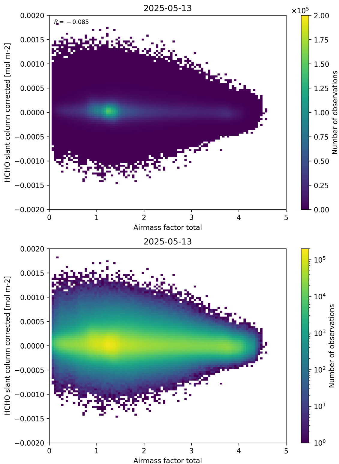
Figure 101: Scatter density plot of “Airmass factor total” against “HCHO slant column corrected” for 2025-05-12 to 2025-05-14.
