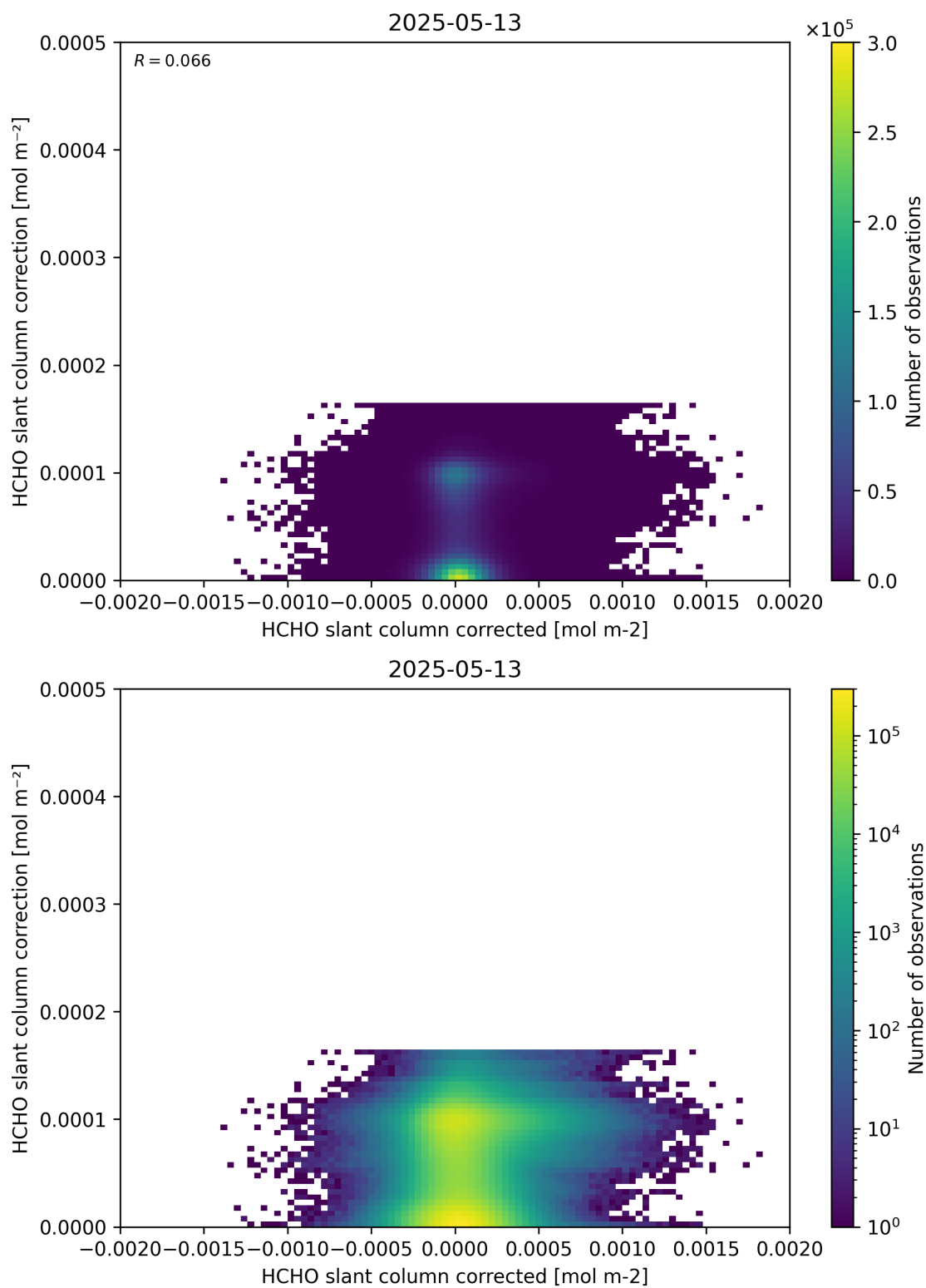
Figure 77: Scatter density plot of “HCHO slant column corrected” against “HCHO slant column correction” for 2025-05-12 to 2025-05-14.
