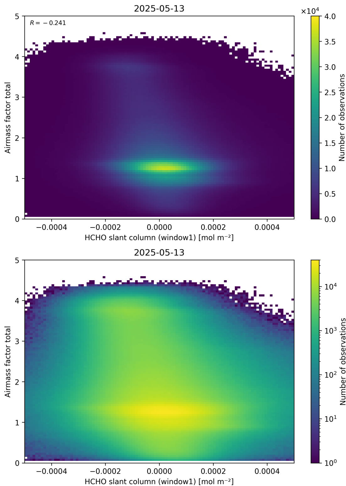
Figure 85: Scatter density plot of “HCHO slant column (window1)” against “Airmass factor total” for 2025-05-12 to 2025-05-14.
