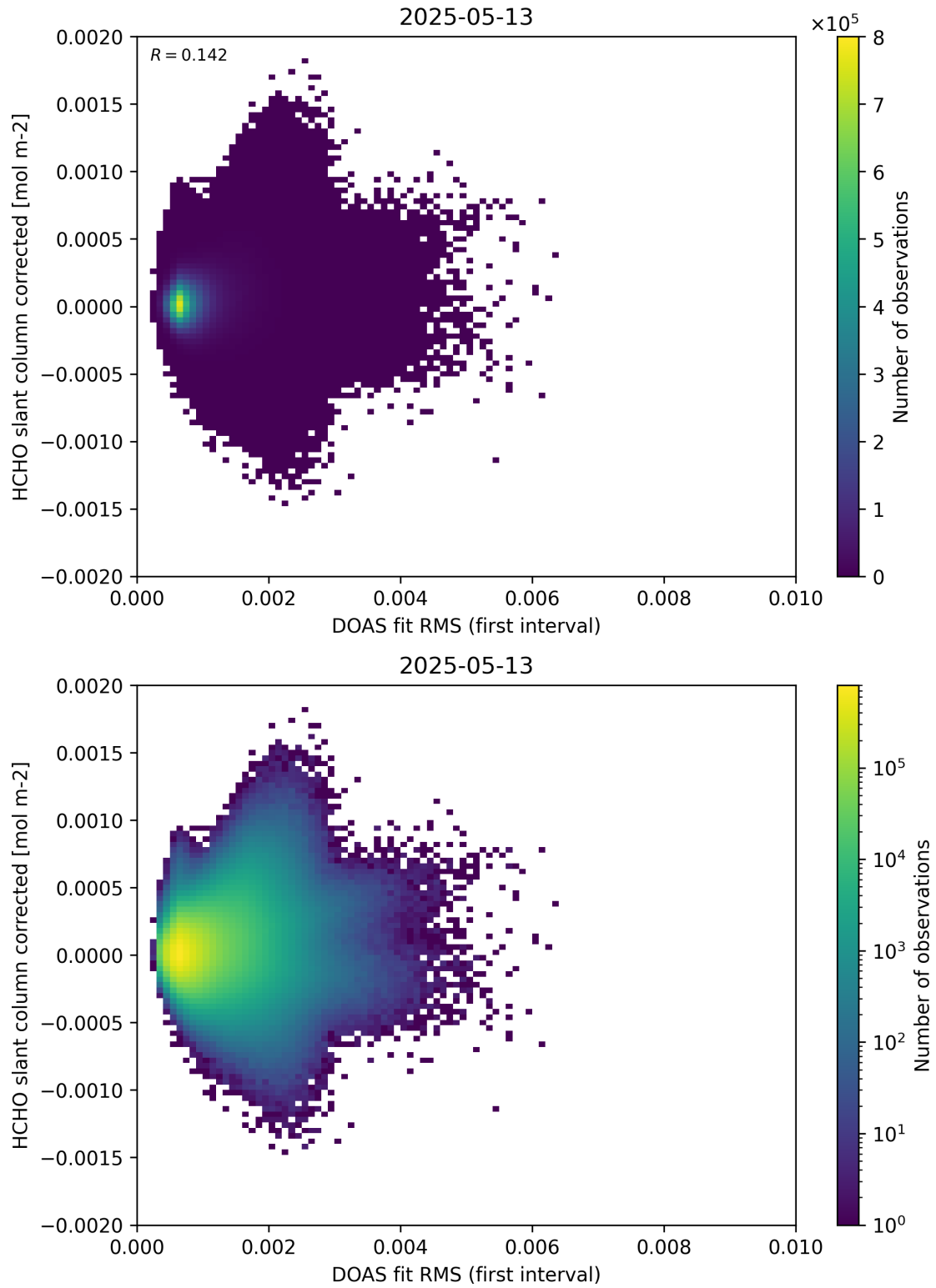
Figure 62: Scatter density plot of “DOAS fit RMS (first interval)” against “HCHO slant column corrected” for 2025-05-12 to 2025-05-14.
