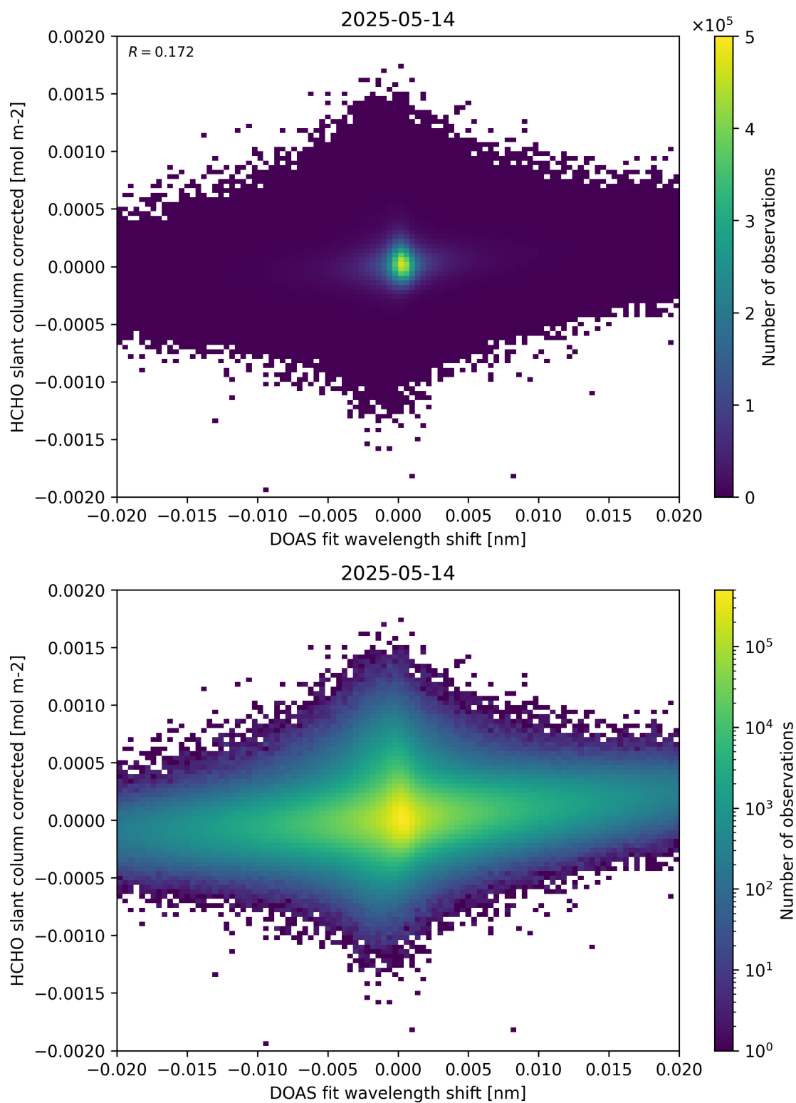
Figure 66: Scatter density plot of “DOAS fit wavelength shift” against “HCHO slant column corrected” for 2025-05-13 to 2025-05-15.
