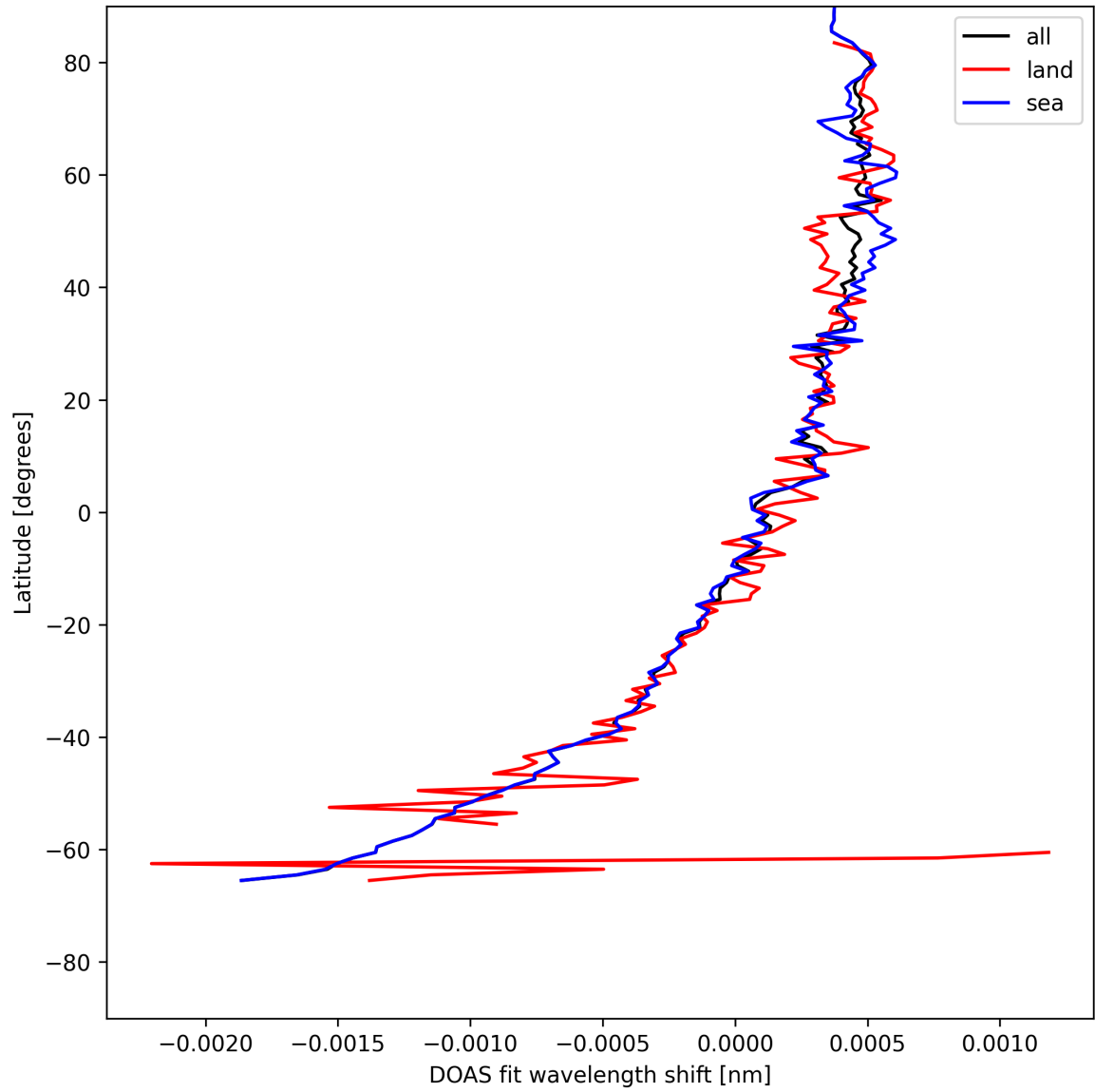
Figure 30: Zonal average of “DOAS fit wavelength shift” for 2025-05-13 to 2025-05-15.
