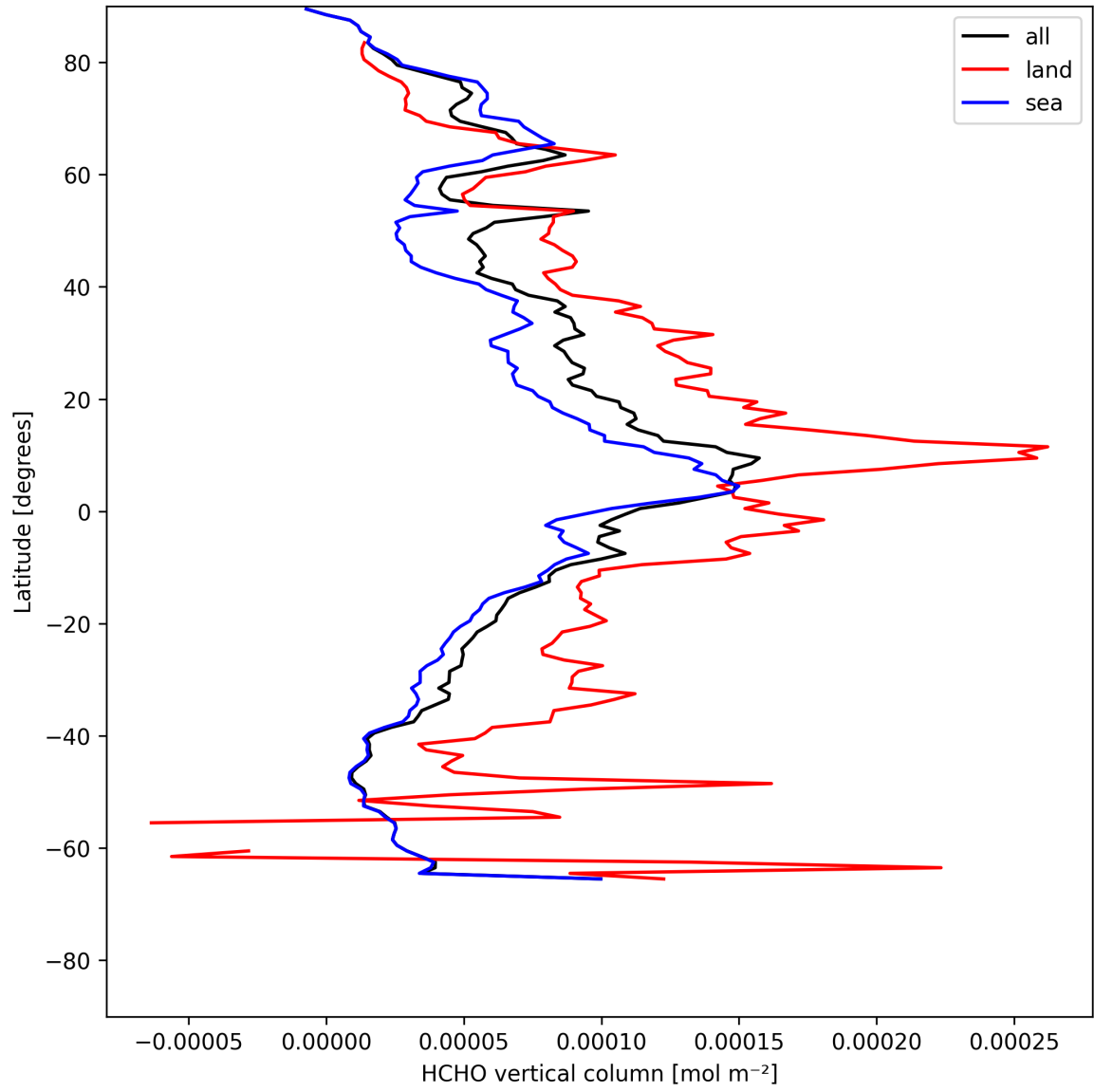
Figure 21: Zonal average of “HCHO vertical column” for 2025-05-13 to 2025-05-15.
