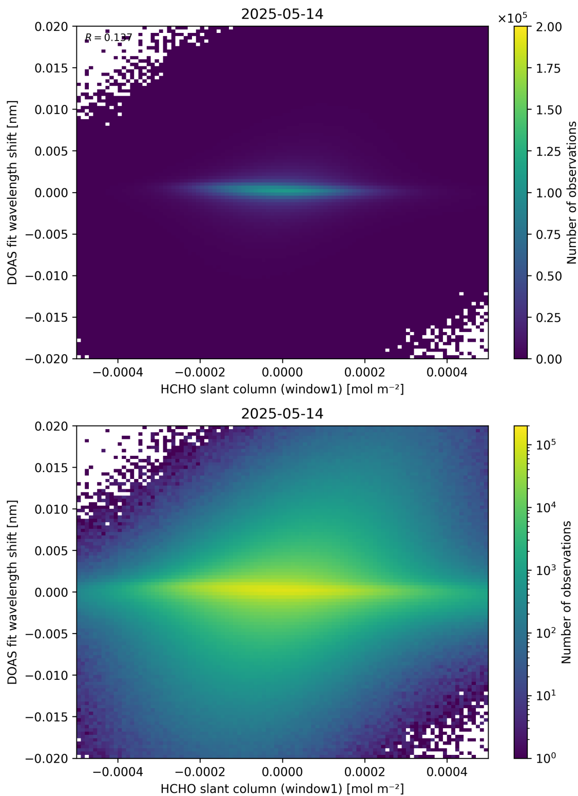
Figure 79: Scatter density plot of “HCHO slant column (window1)” against “DOAS fit wavelength shift” for 2025-05-13 to 2025-05-15.
