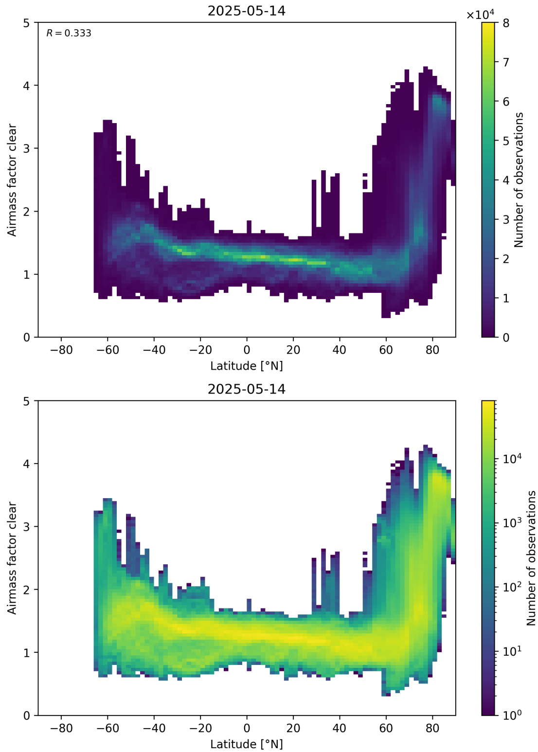
Figure 156: Scatter density plot of “Latitude” against “Airmass factor clear” for 2025-05-13 to 2025-05-15.
