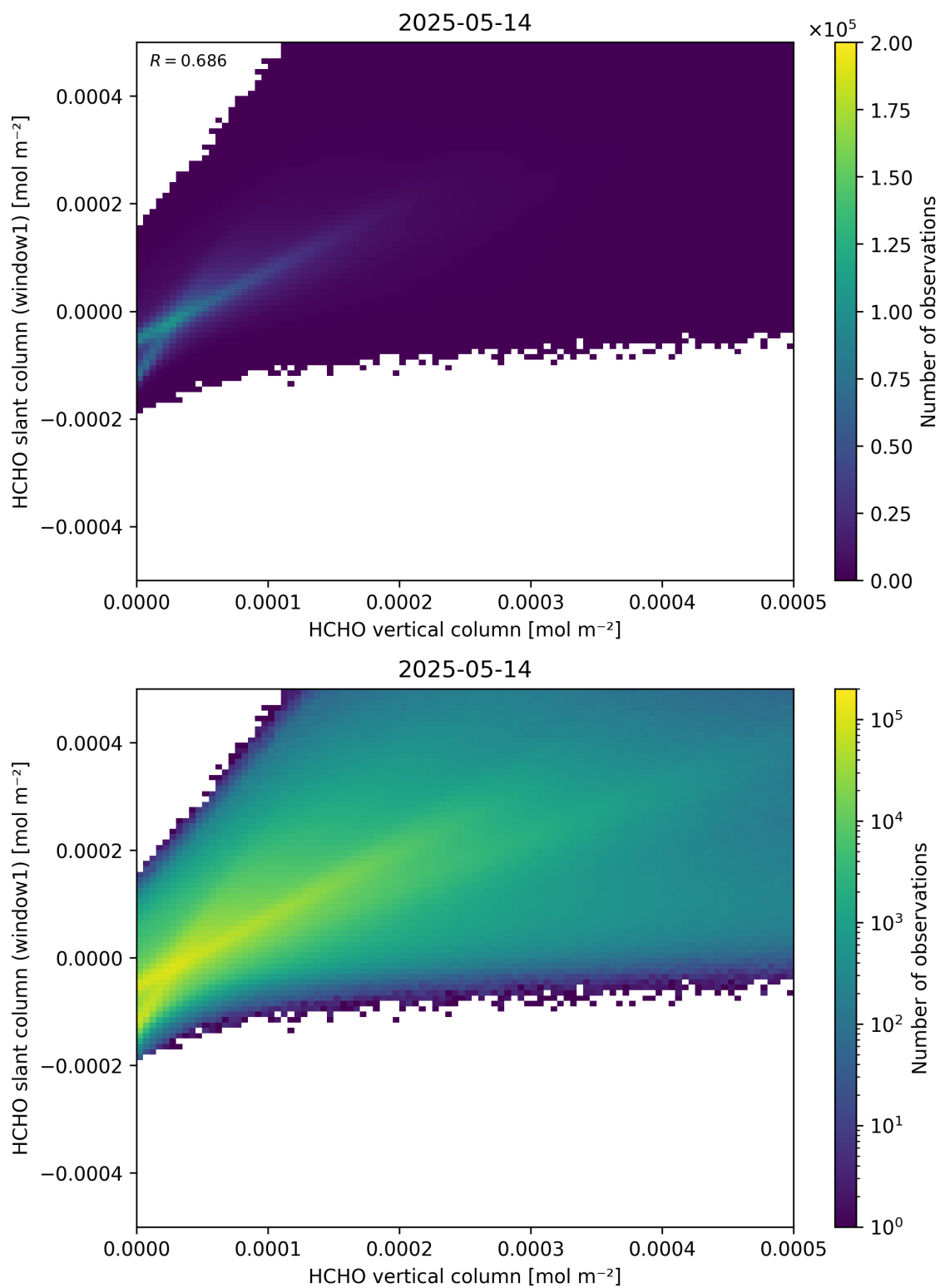
Figure 129: Scatter density plot of “HCHO vertical column” against “HCHO slant column (window1)” for 2025-05-13 to 2025-05-15.
