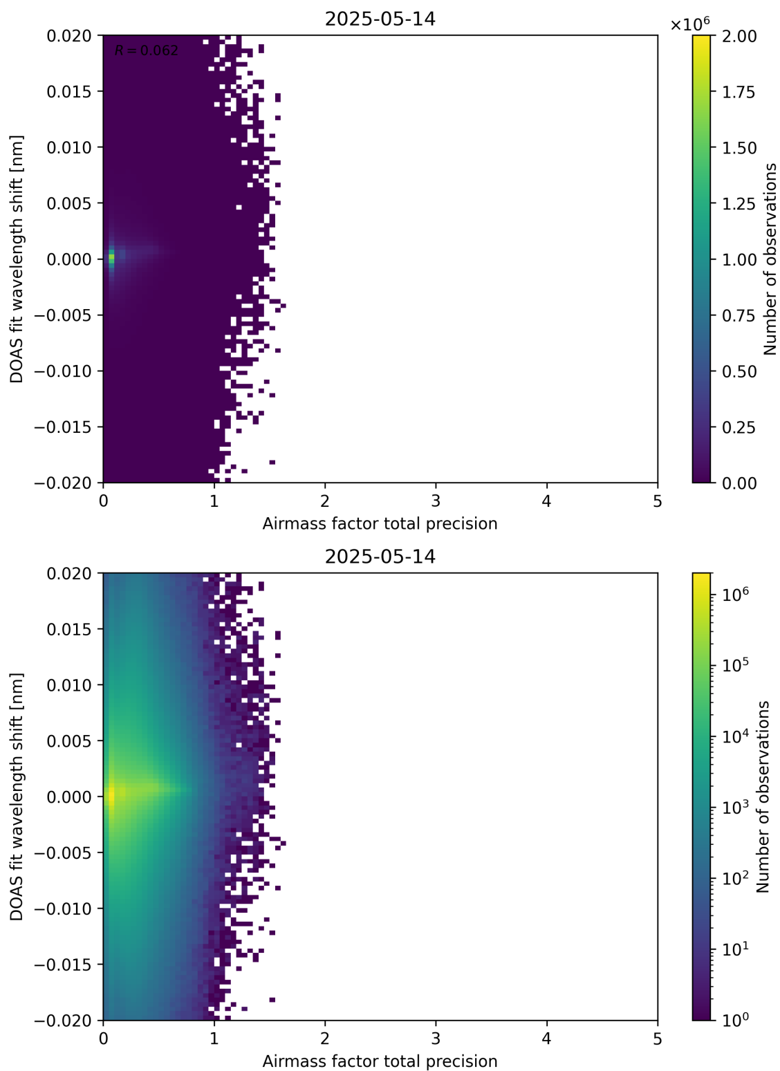
Figure 106: Scatter density plot of “Airmass factor total precision” against “DOAS fit wavelength shift” for 2025-05-13 to 2025-05-15.
