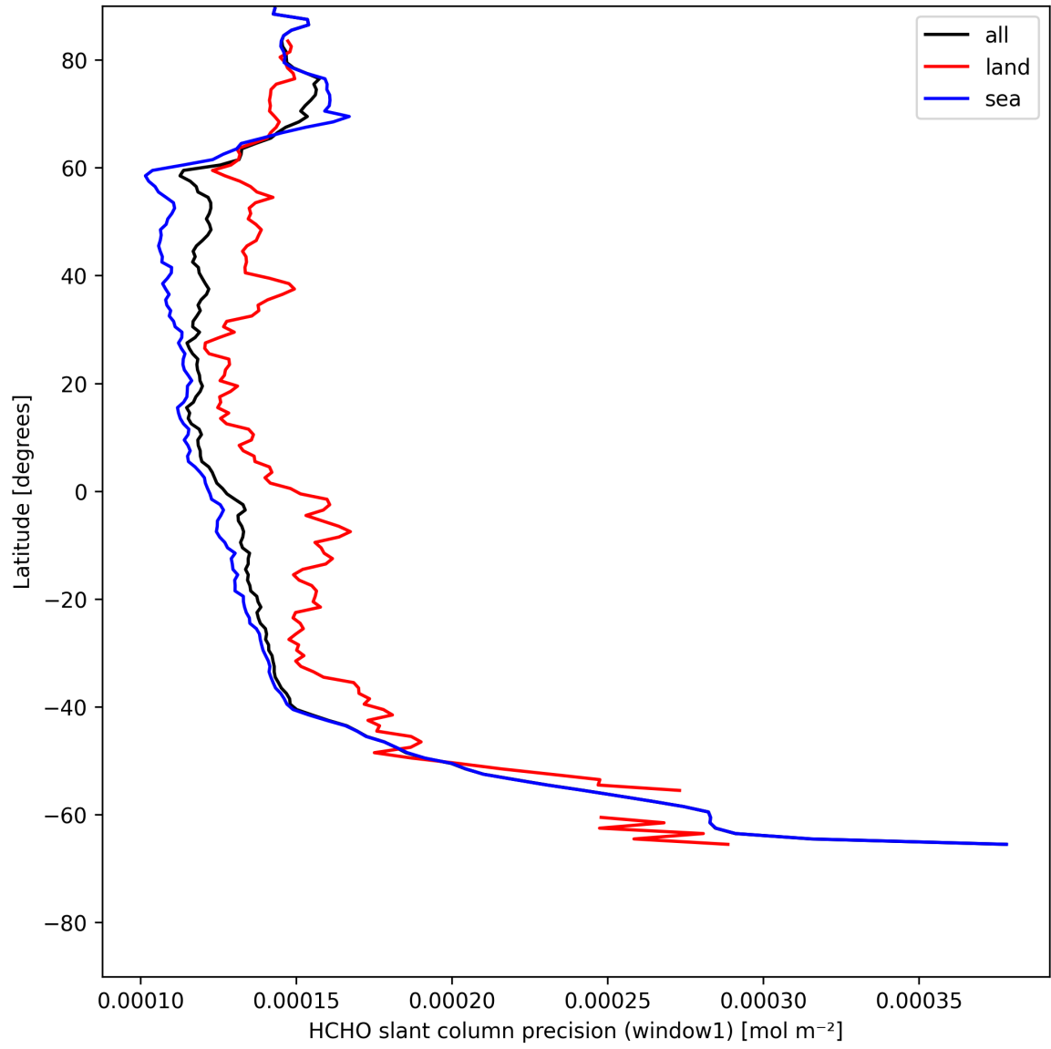
Figure 25: Zonal average of "HCHO slant column precision (window1)" for 2025-05-13 to 2025-05-15.
