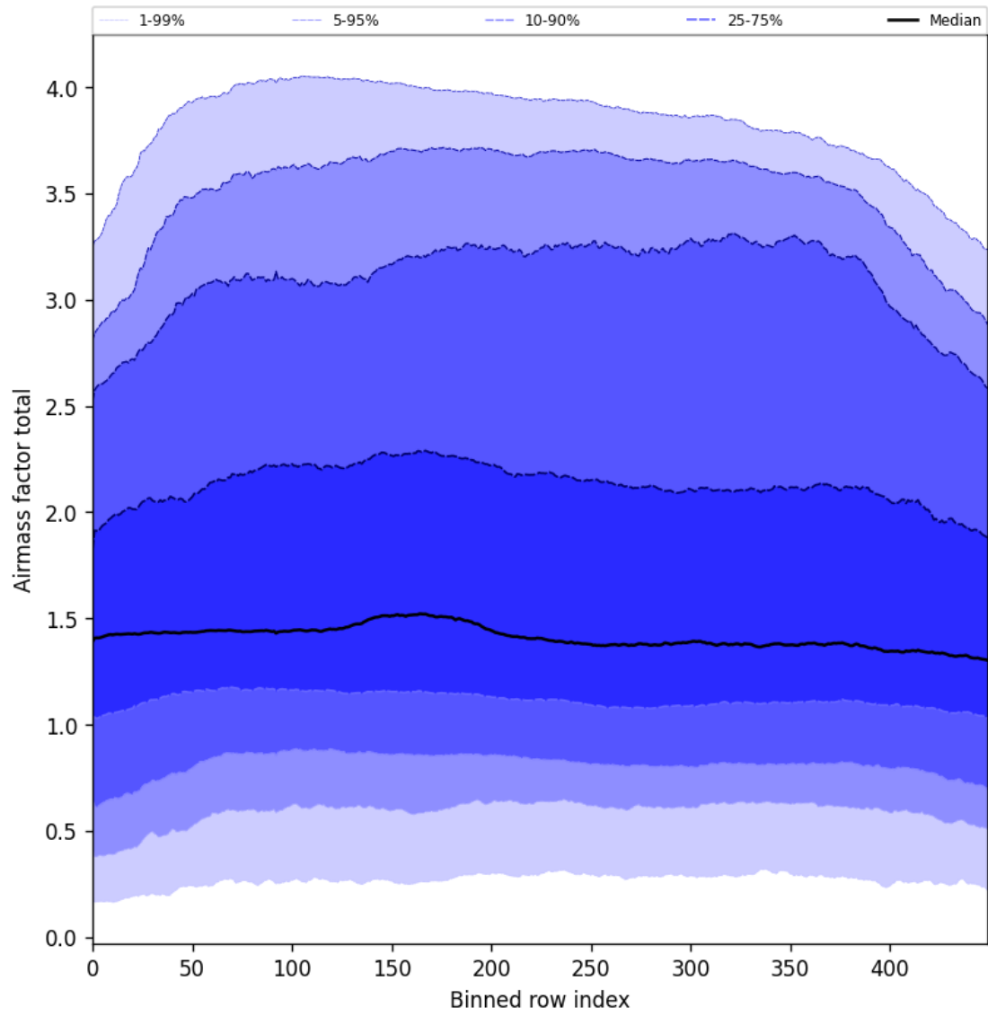
Figure 54: Along track statistics of “Airmass factor total” for 2025-05-13 to 2025-05-15
