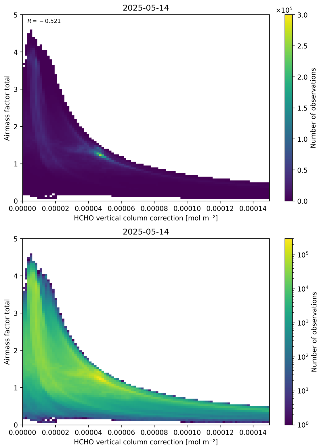
Figure 120: Scatter density plot of “HCHO vertical column correction” against “Airmass factor total” for 2025-05-13 to 2025-05-15.
