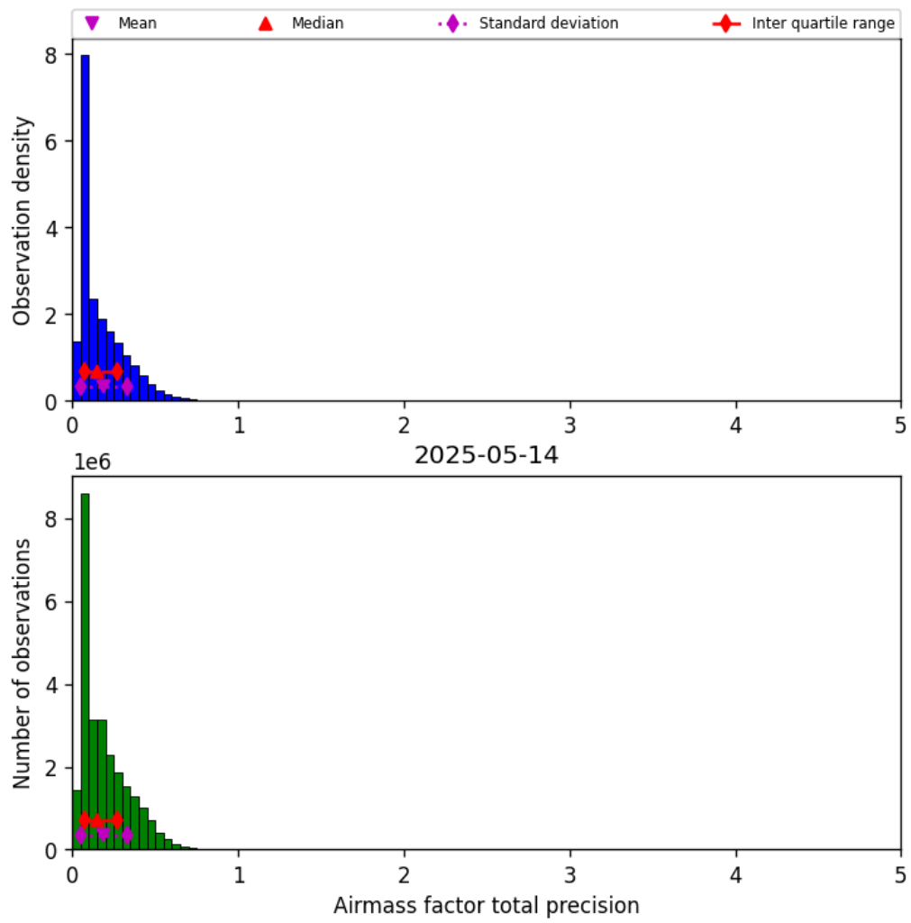
Figure 41: Histogram of “Airmass factor total precision” for 2025-05-13 to 2025-05-15
