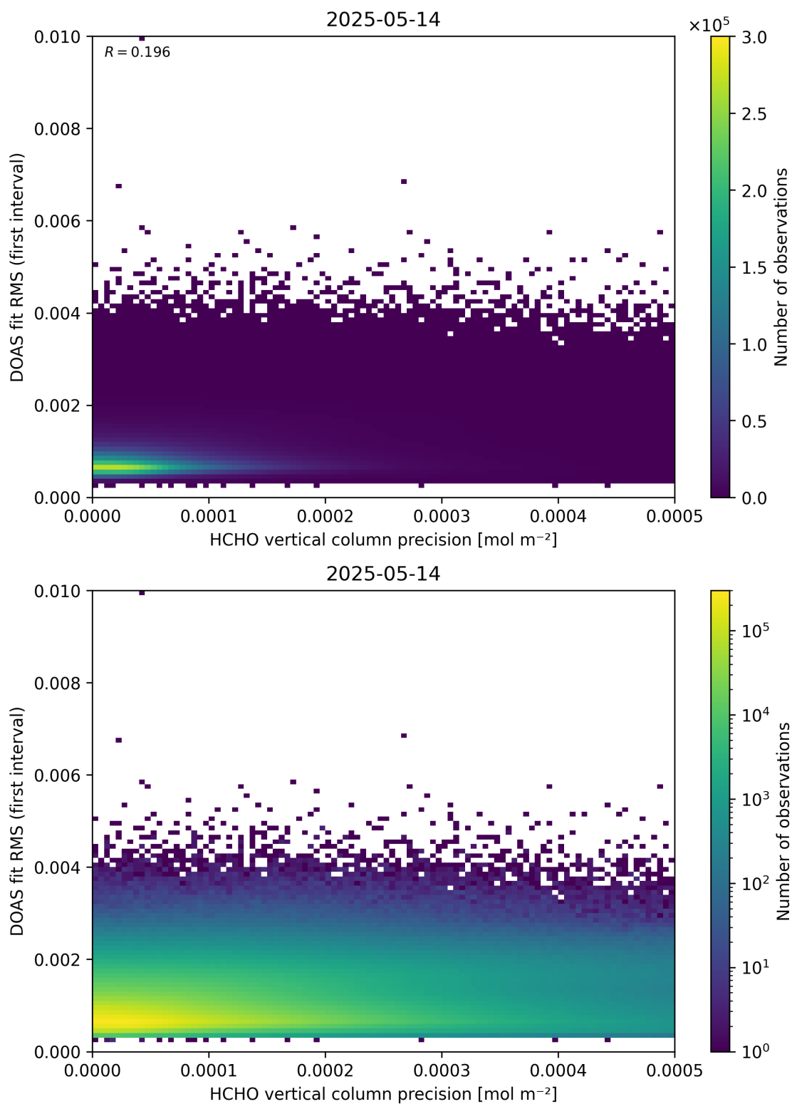
Figure 136: Scatter density plot of “HCHO vertical column precision” against “DOAS fit RMS (first interval)” for 2025-05-13 to 2025-05-15.
