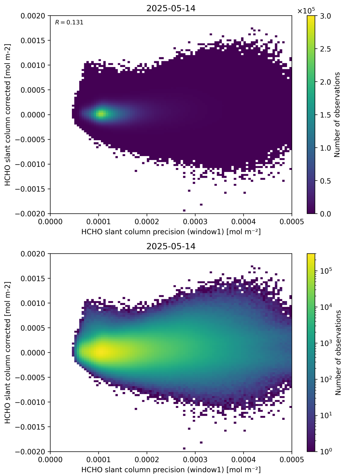
Figure 92: Scatter density plot of “HCHO slant column precision (window1)” against “HCHO slant column corrected” for 2025-05-13 to 2025-05-15.
