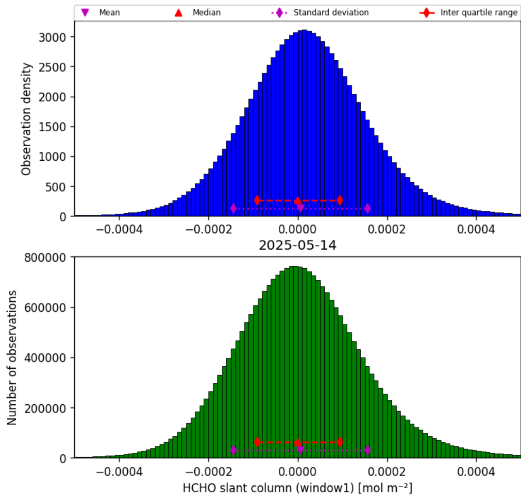
Figure 38: Histogram of “HCHO slant column (window1)” for 2025-05-13 to 2025-05-15
