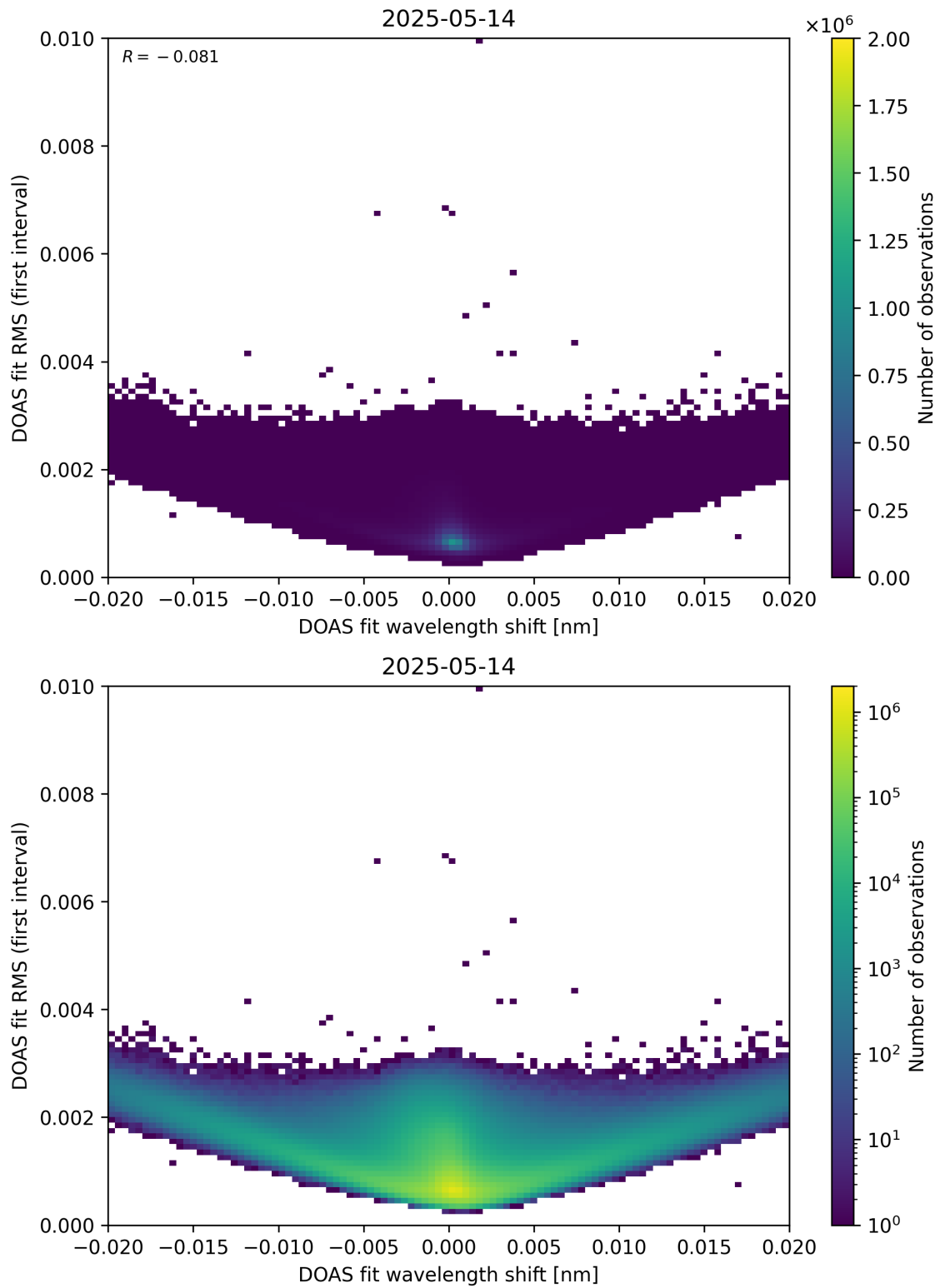
Figure 64: Scatter density plot of “DOAS fit wavelength shift” against “DOAS fit RMS (first interval)” for 2025-05-13 to 2025-05-15.
