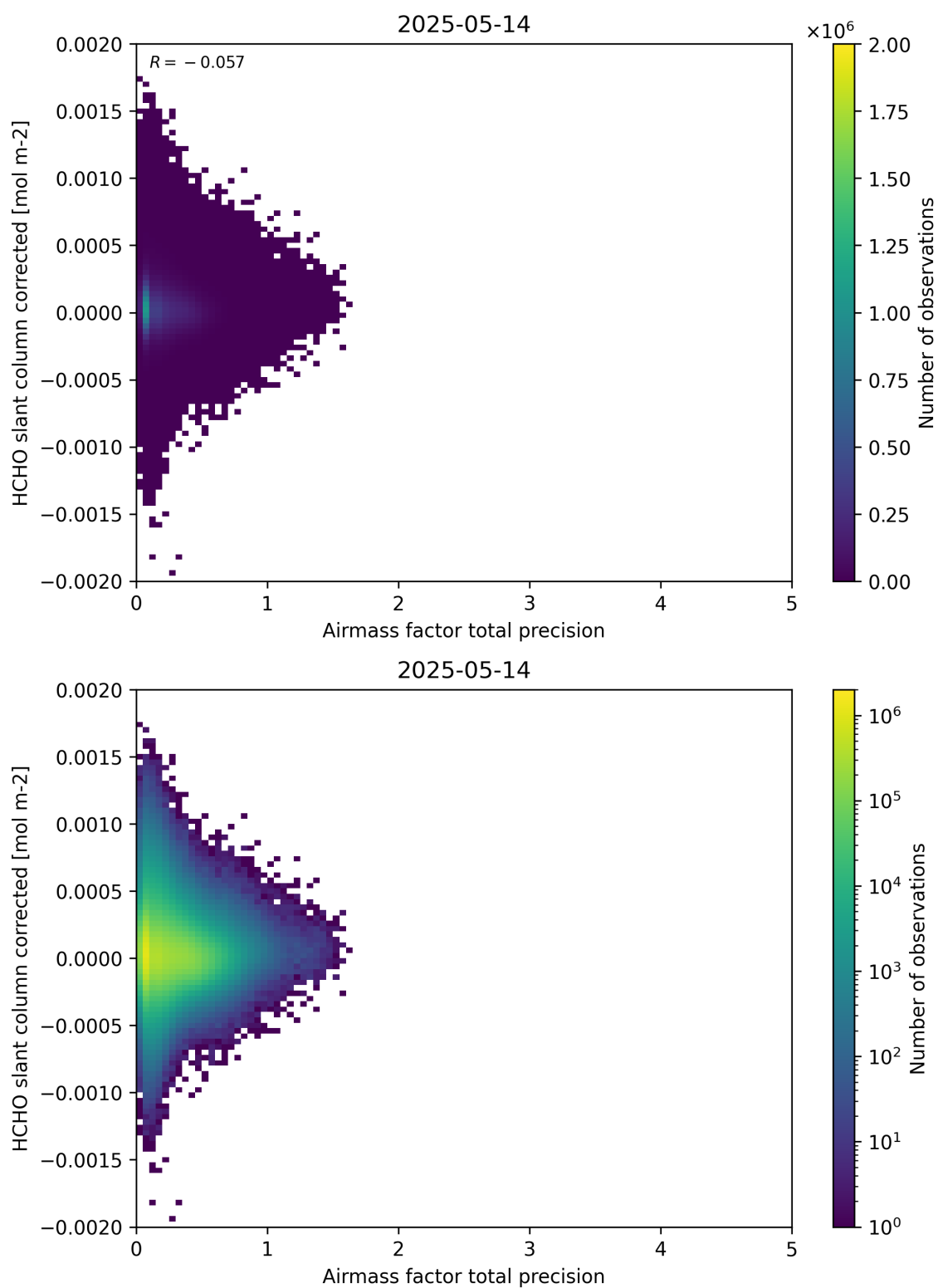
Figure 109: Scatter density plot of “Airmass factor total precision” against “HCHO slant column corrected” for 2025-05-13 to 2025-05-15.
