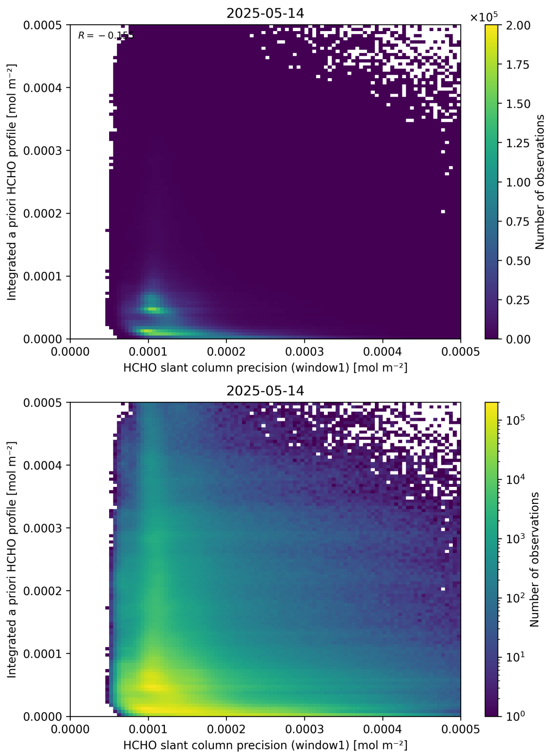
Figure 96: Scatter density plot of “HCHO slant column precision (window1)” against “Integrated a priori HCHO profile” for 2025-05-13 to 2025-05-15.
