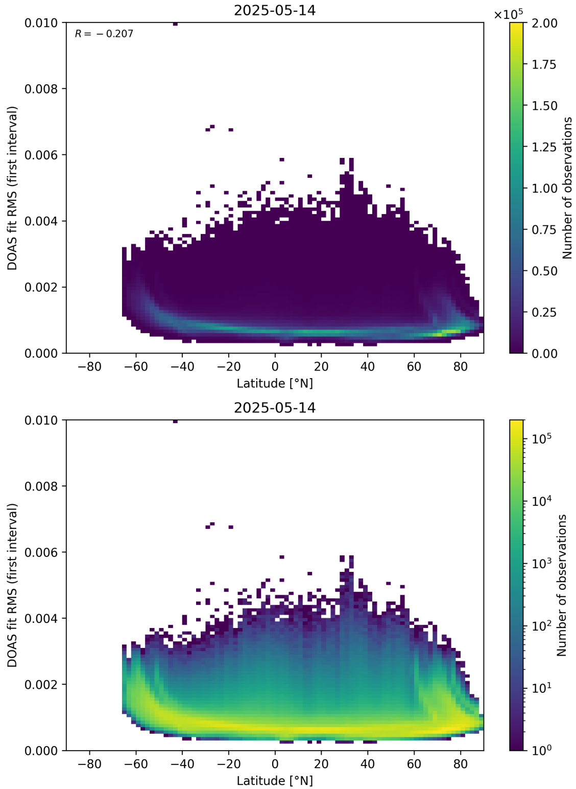
Figure 153: Scatter density plot of “Latitude” against “DOAS fit RMS (first interval)” for 2025-05-13 to 2025-05-15.
