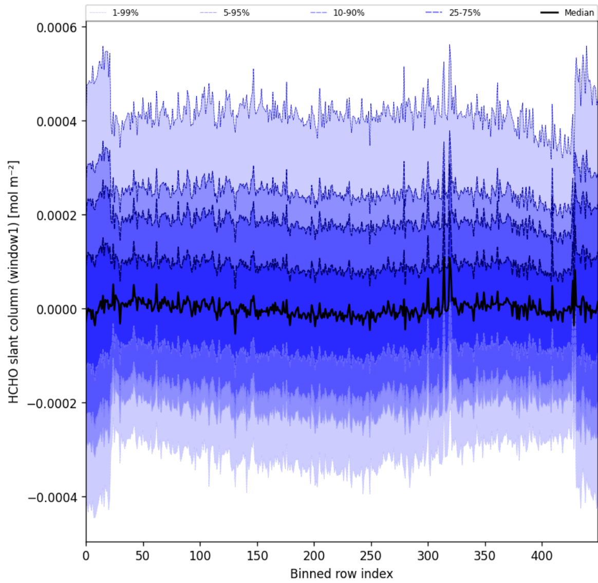
Figure 52: Along track statistics of “HCHO slant column (window1)” for 2025-05-13 to 2025-05-15
