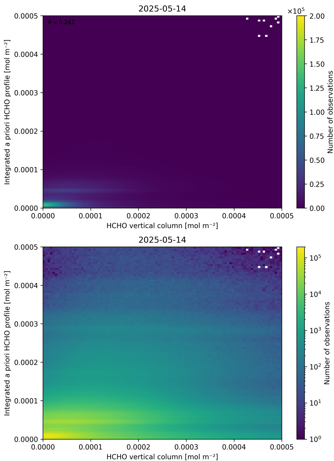
Figure 135: Scatter density plot of “HCHO vertical column” against “Integrated a priori HCHO profile” for 2025-05-13 to 2025-05-15.
