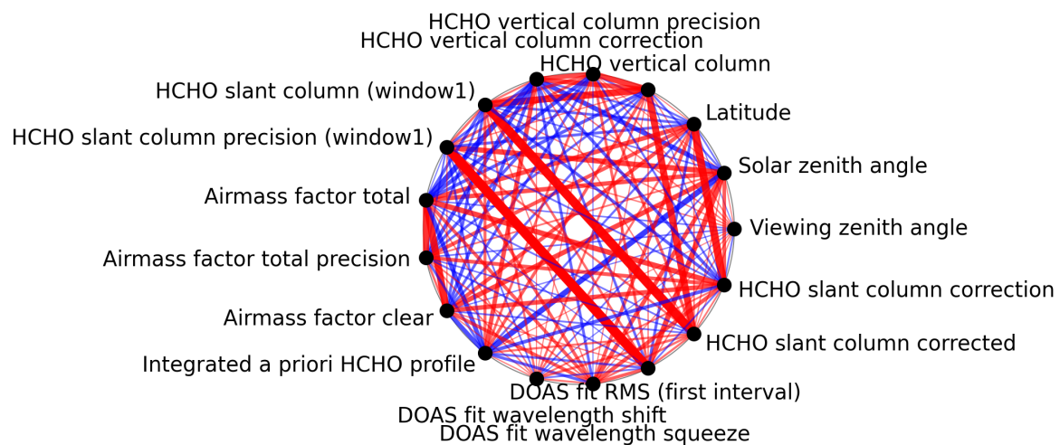
Figure 1: Map of correlation graph for 2025-05-13 to 2025-05-15.
