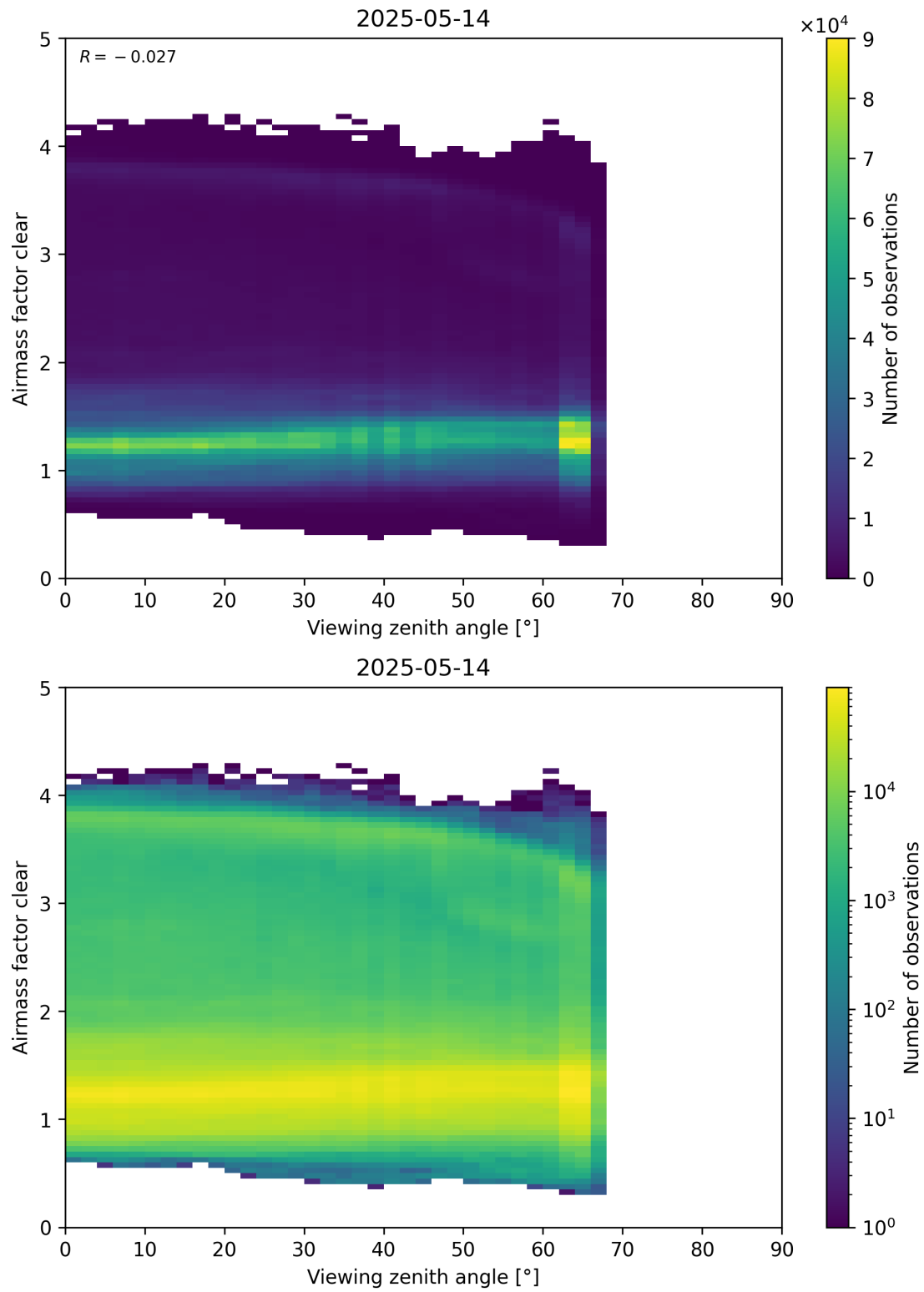
Figure 185: Scatter density plot of “Viewing zenith angle” against “Airmass factor clear” for 2025-05-13 to 2025-05-15.
