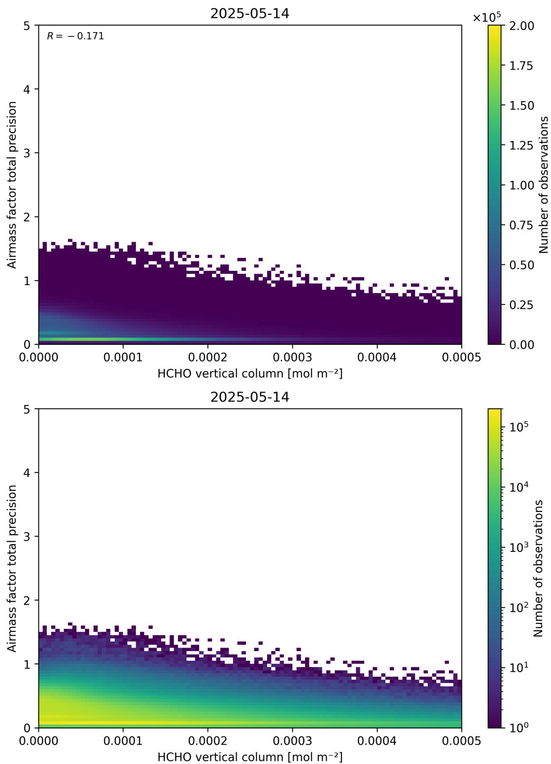
Figure 132: Scatter density plot of “HCHO vertical column” against “Airmass factor total precision” for 2025-05-13 to 2025-05-15.
