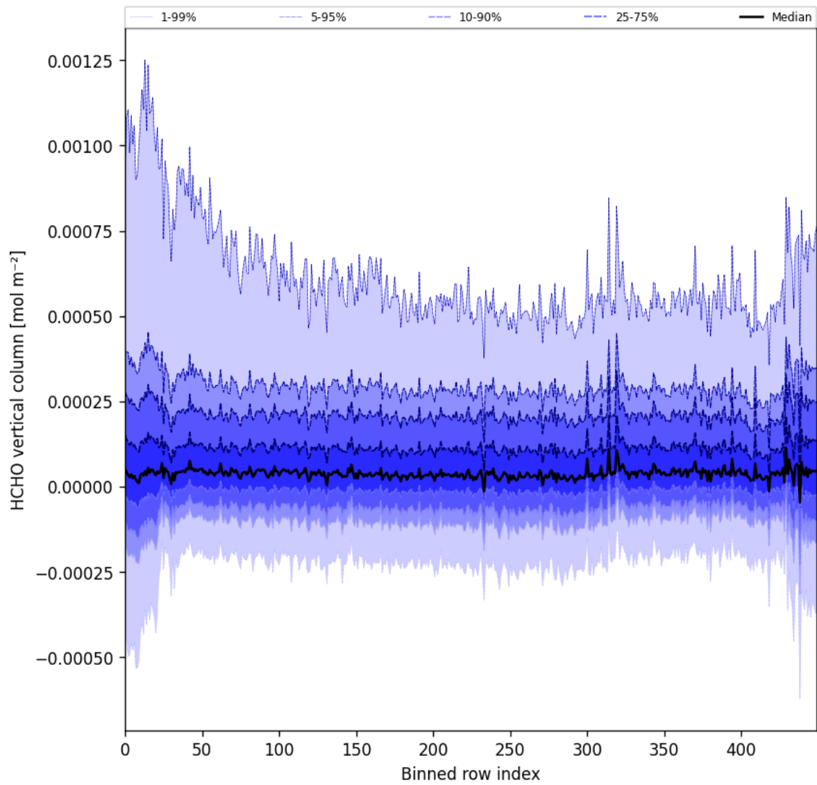
Figure 49: Along track statistics of “HCHO vertical column” for 2025-05-13 to 2025-05-15
