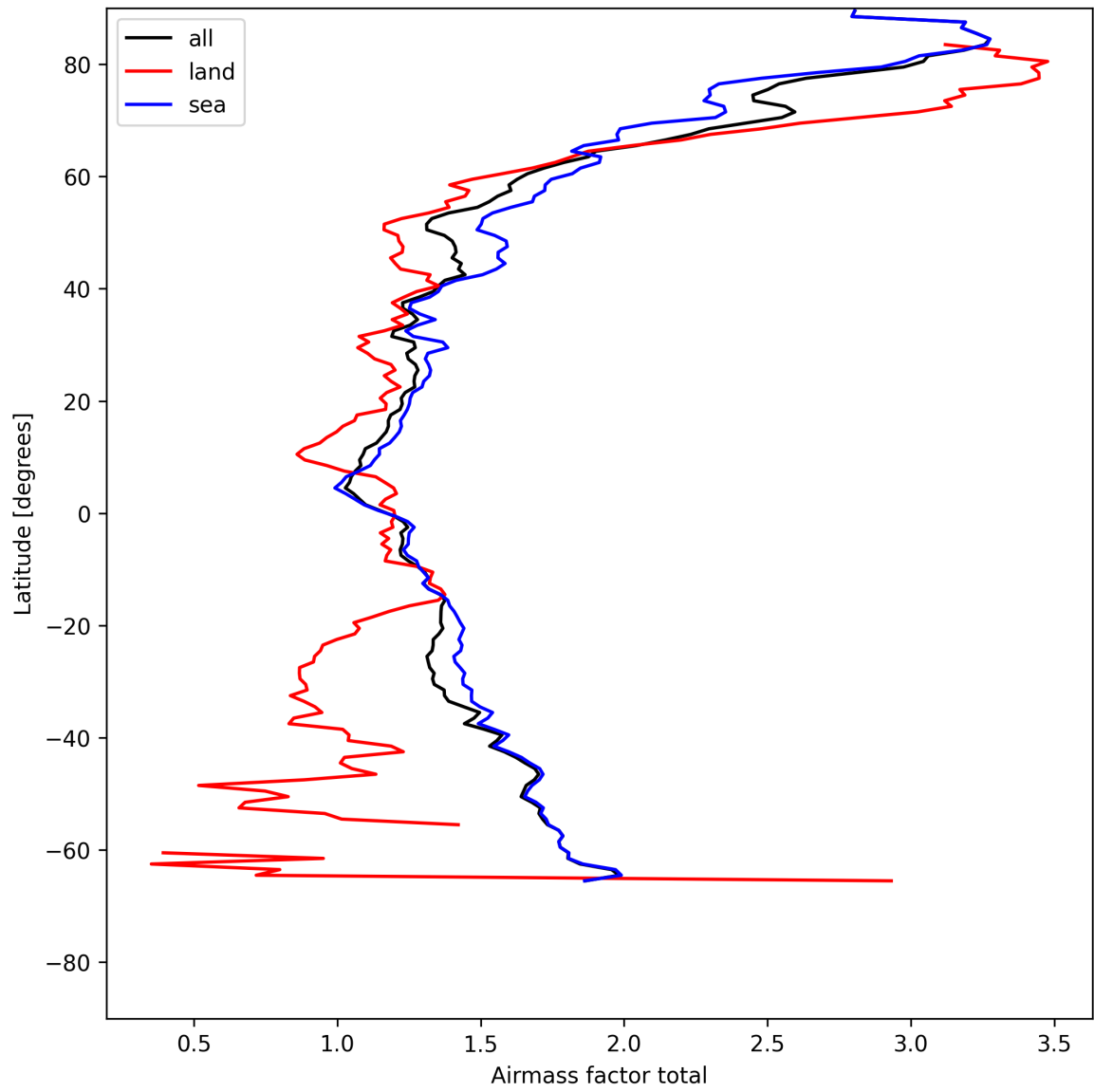
Figure 26: Zonal average of “Airmass factor total” for 2025-05-13 to 2025-05-15.
