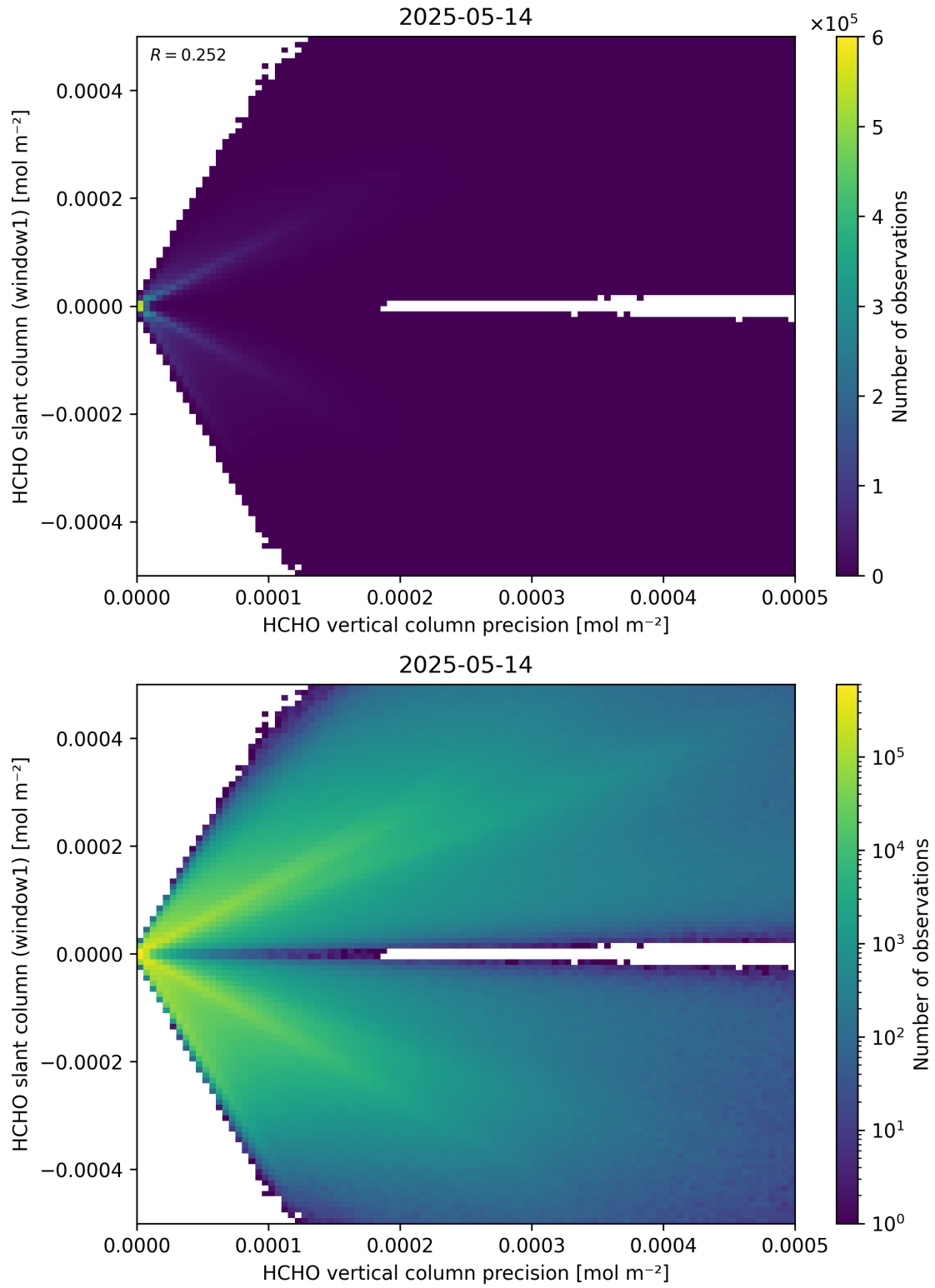
Figure 142: Scatter density plot of “HCHO vertical column precision” against “HCHO slant column (window1)” for 2025-05-13 to 2025-05-15.
