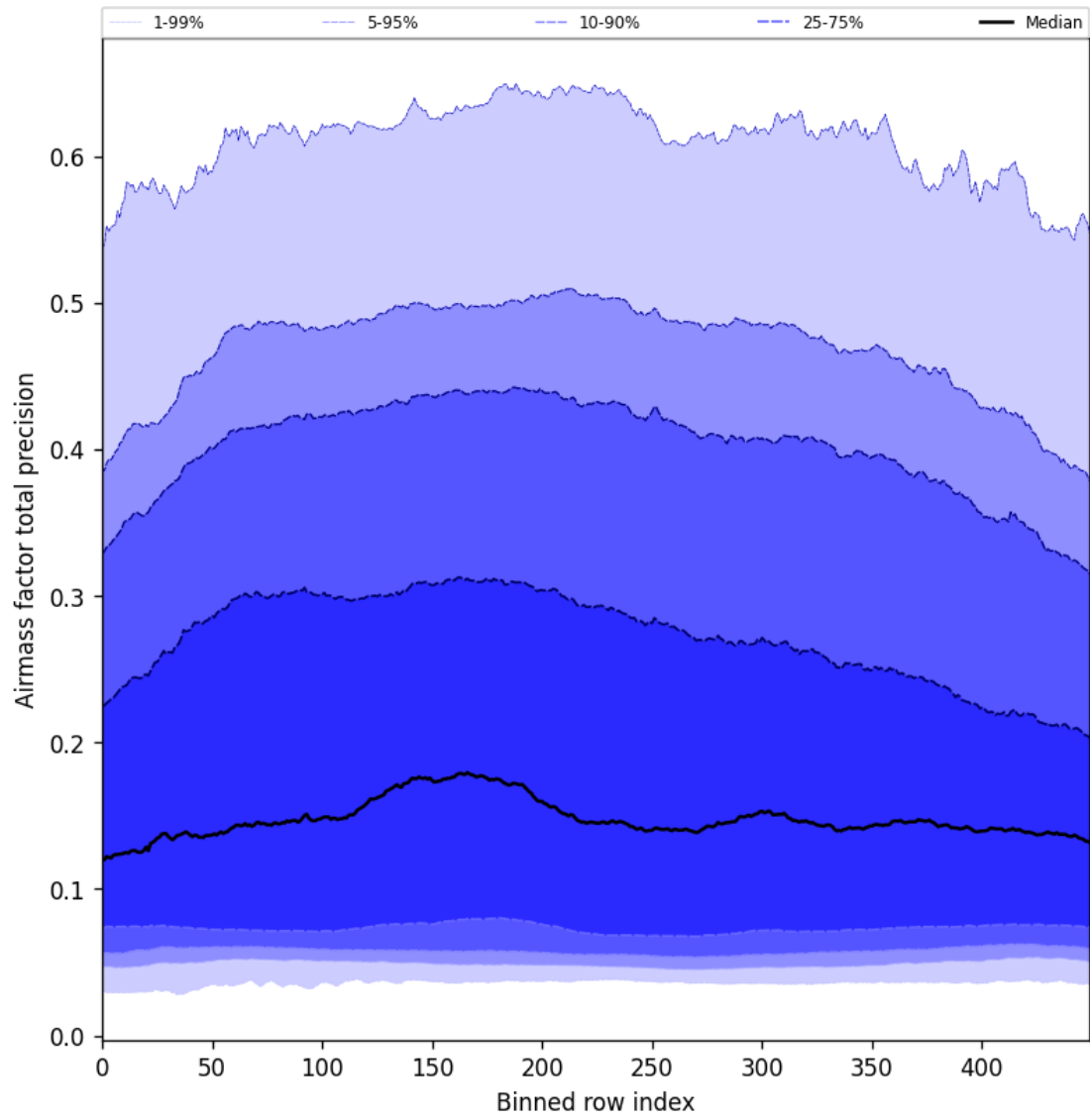
Figure 55: Along track statistics of “Airmass factor total precision” for 2025-05-13 to 2025-05-15
