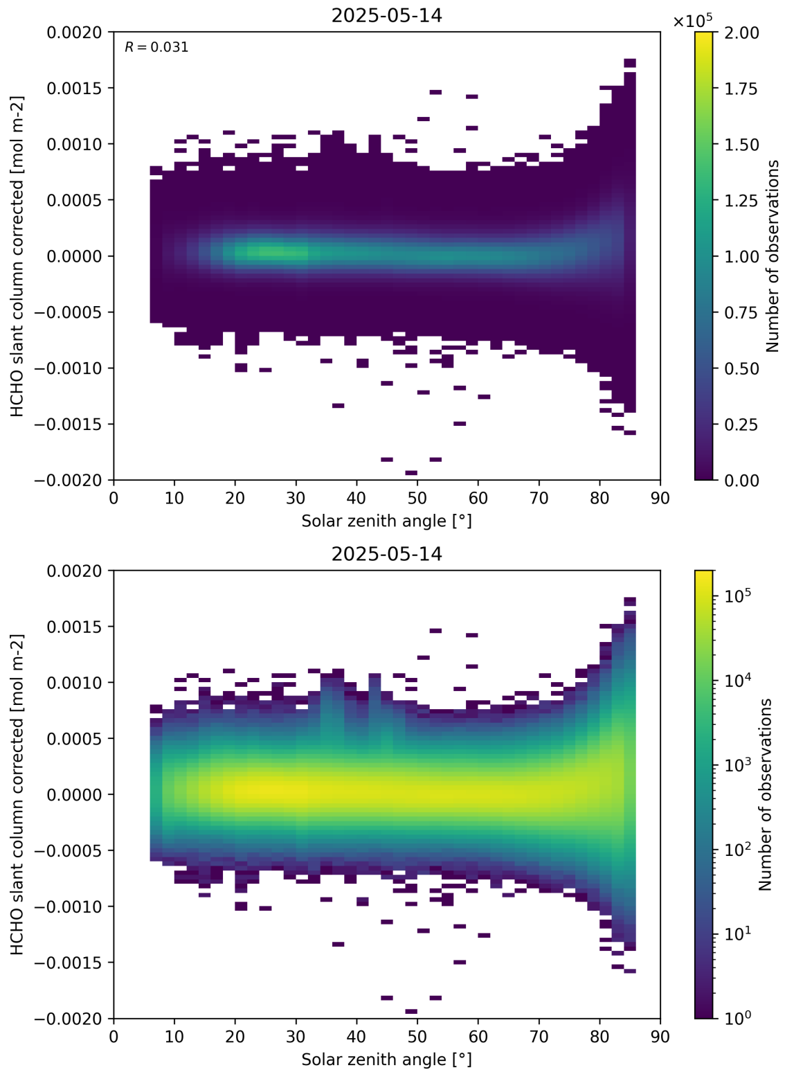
Figure 171: Scatter density plot of “Solar zenith angle” against “HCHO slant column corrected” for 2025-05-13 to 2025-05-15.
