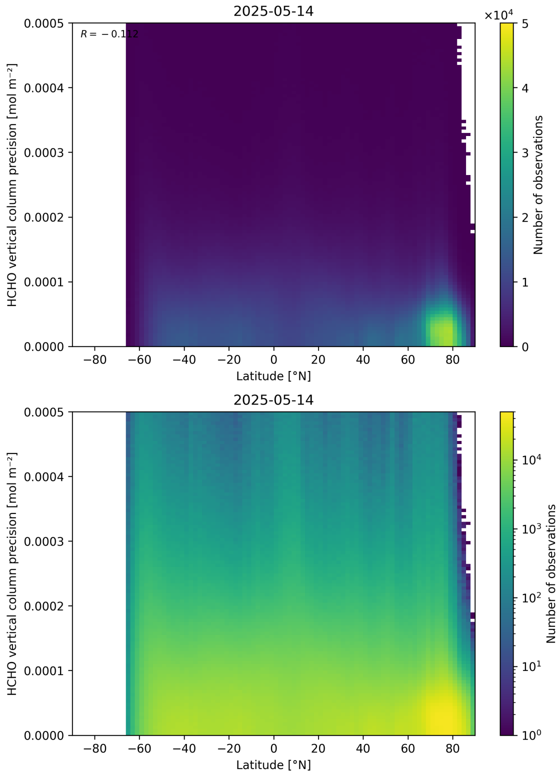
Figure 165: Scatter density plot of “Latitude” against “HCHO vertical column precision” for 2025-05-13 to 2025-05-15.
