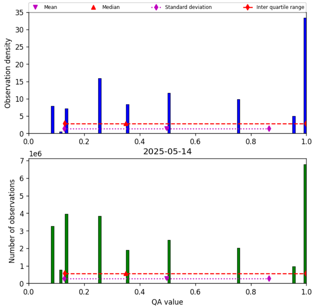
Figure 34: Histogram of “QA value” for 2025-05-13 to 2025-05-15
