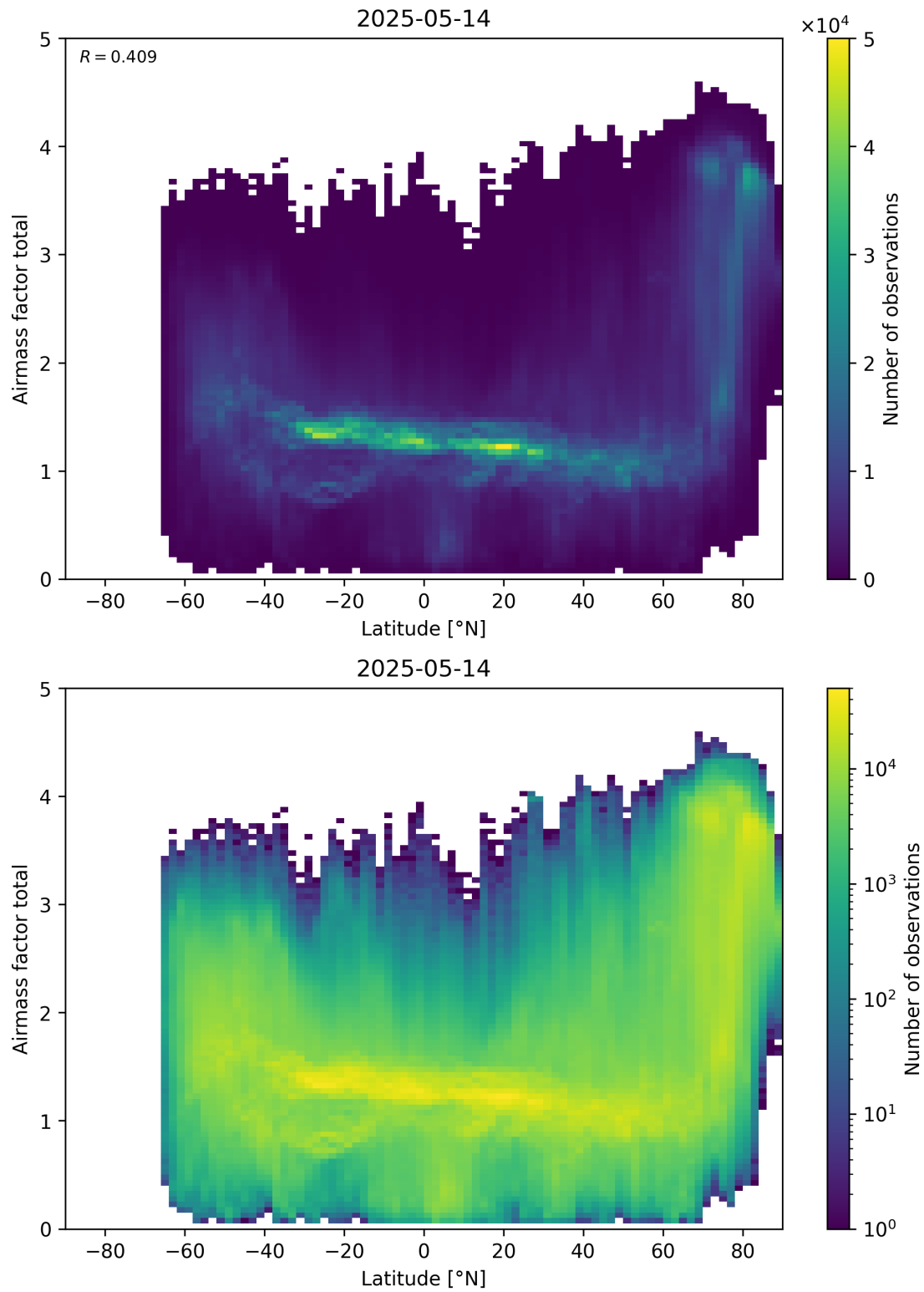
Figure 161: Scatter density plot of “Latitude” against “Airmass factor total” for 2025-05-13 to 2025-05-15.
