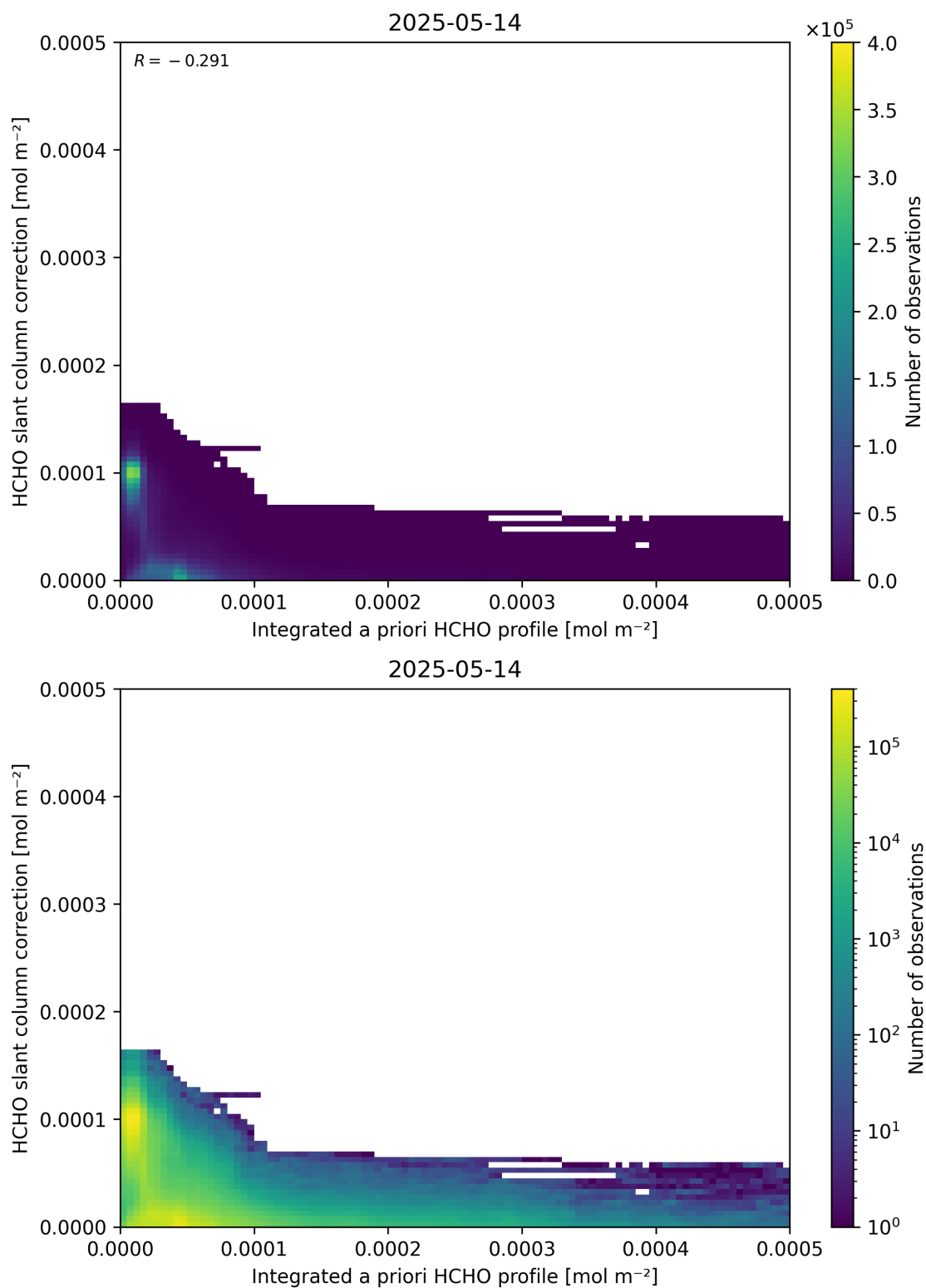
Figure 152: Scatter density plot of “Integrated a priori HCHO profile” against “HCHO slant column correction” for 2025-05-13 to 2025-05-15.
