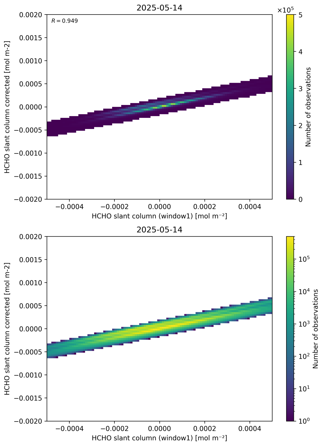
Figure 82: Scatter density plot of “HCHO slant column (window1)” against “HCHO slant column corrected” for 2025-05-13 to 2025-05-15.
