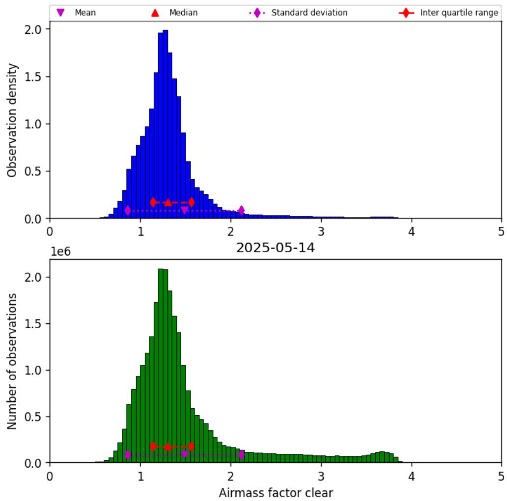
Figure 42: Histogram of “Airmass factor clear” for 2025-05-13 to 2025-05-15
