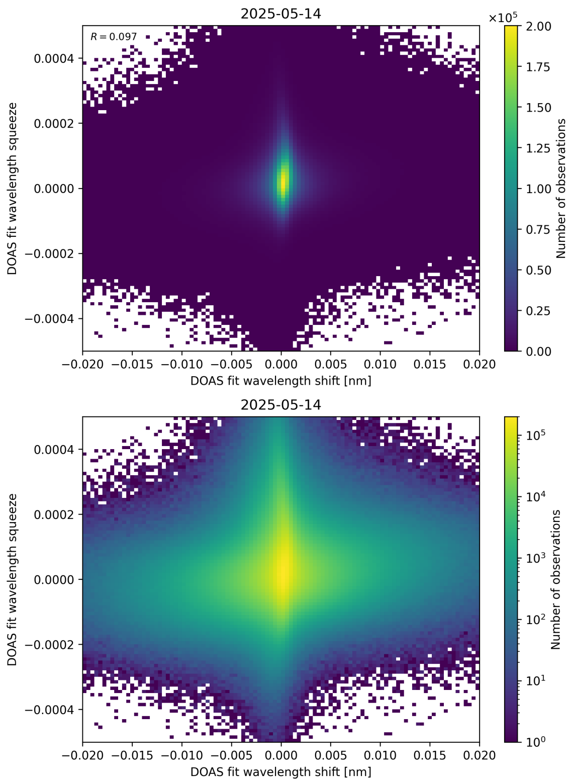
Figure 65: Scatter density plot of “DOAS fit wavelength shift” against “DOAS fit wavelength squeeze” for 2025-05-13 to 2025-05-15.
