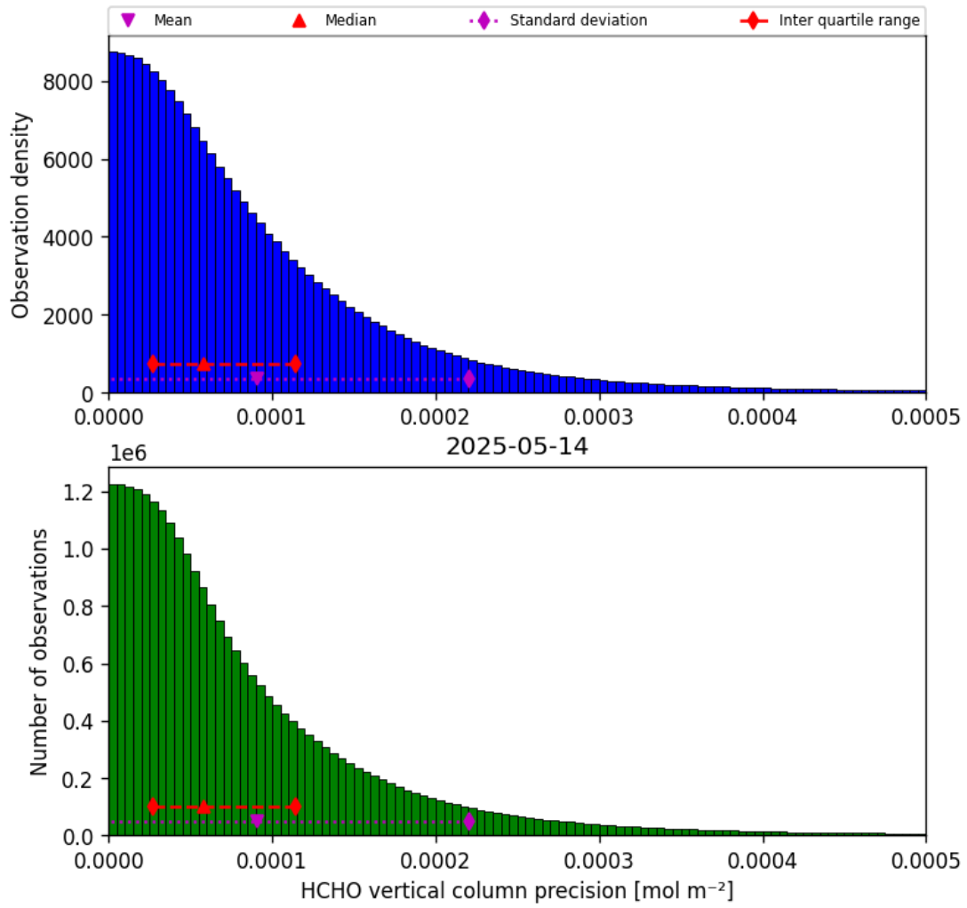
Figure 36: Histogram of “HCHO vertical column precision” for 2025-05-13 to 2025-05-15
