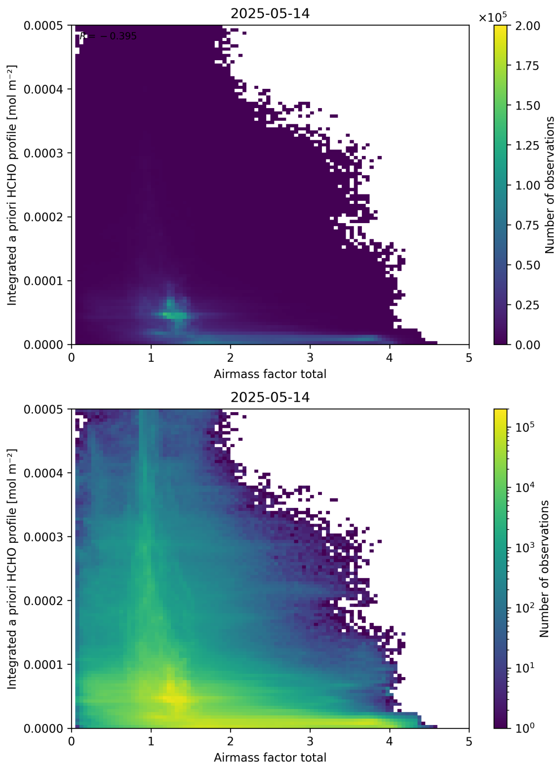
Figure 104: Scatter density plot of “Airmass factor total” against “Integrated a priori HCHO profile” for 2025-05-13 to 2025-05-15.
