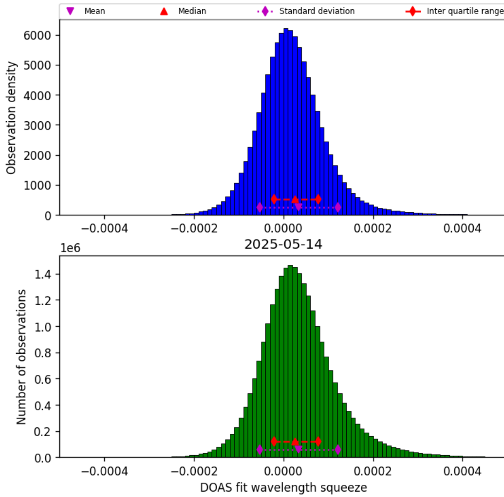
Figure 45: Histogram of “DOAS fit wavelength squeeze” for 2025-05-13 to 2025-05-15
