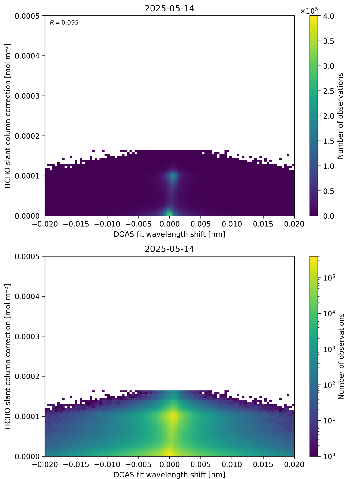
Figure 67: Scatter density plot of “DOAS fit wavelength shift” against “HCHO slant column correction” for 2025-05-13 to 2025-05-15.
