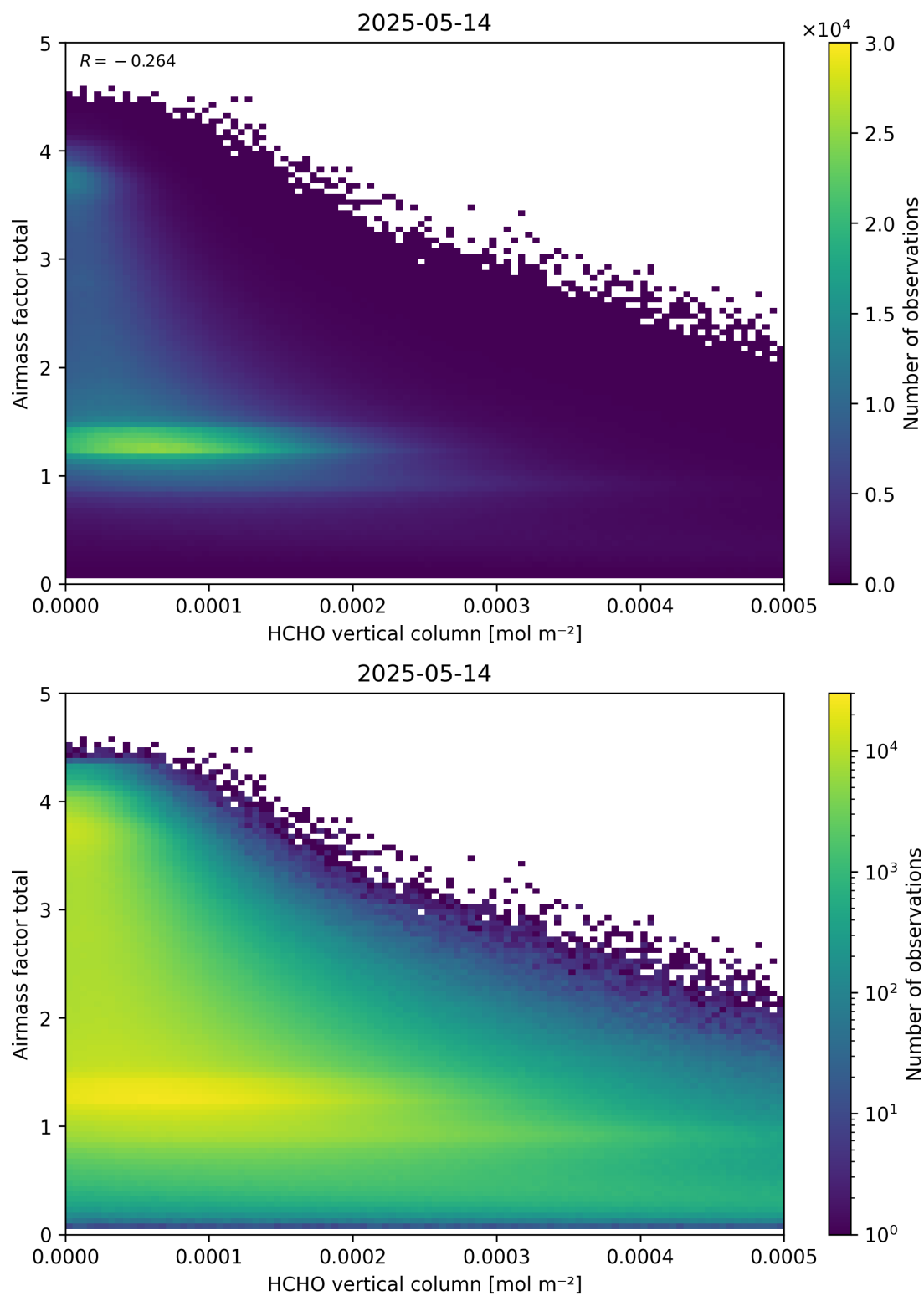
Figure 131: Scatter density plot of “HCHO vertical column” against “Airmass factor total” for 2025-05-13 to 2025-05-15.
