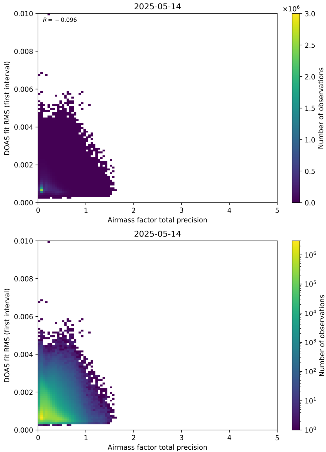
Figure 105: Scatter density plot of “Airmass factor total precision” against “DOAS fit RMS (first interval)” for 2025-05-13 to 2025-05-15.
