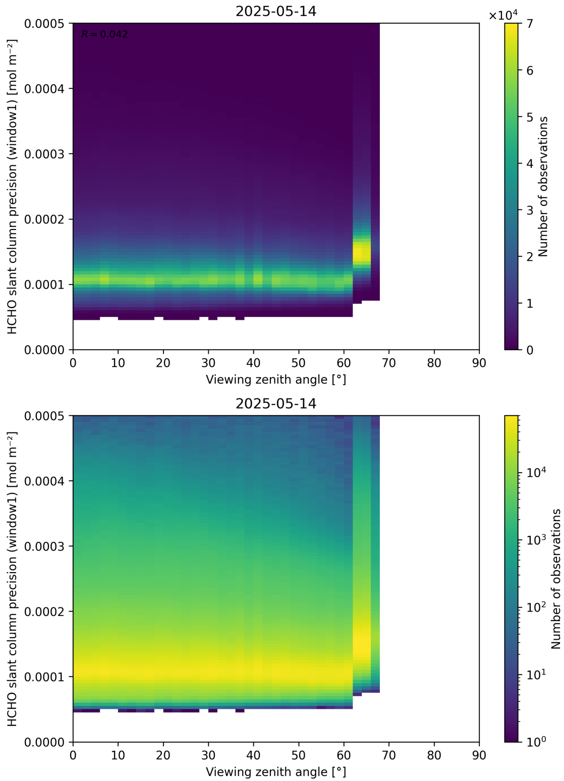
Figure 189: Scatter density plot of “Viewing zenith angle” against “HCHO slant column precision (window1)” for 2025-05-13 to 2025-05-15.
