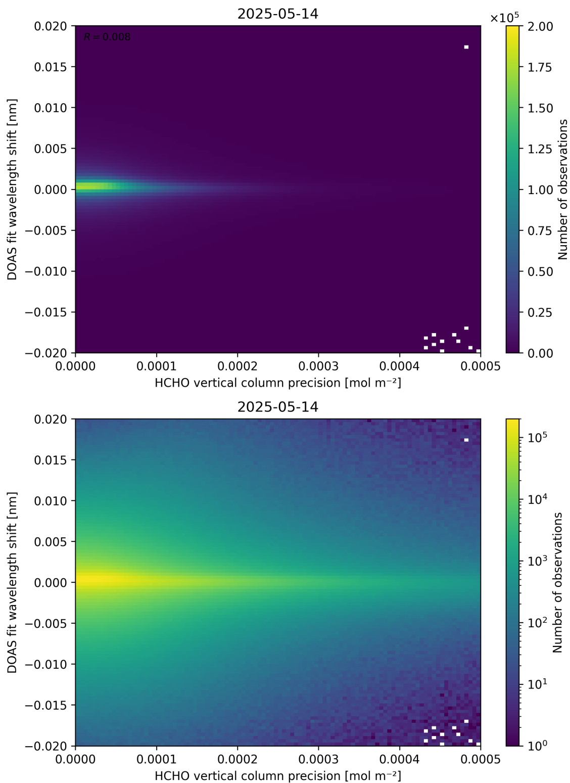
Figure 137: Scatter density plot of “HCHO vertical column precision” against “DOAS fit wavelength shift” for 2025-05-13 to 2025-05-15.
