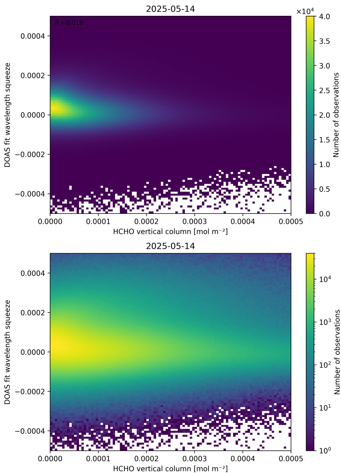
Figure 125: Scatter density plot of “HCHO vertical column” against “DOAS fit wavelength squeeze” for 2025-05-13 to 2025-05-15.
