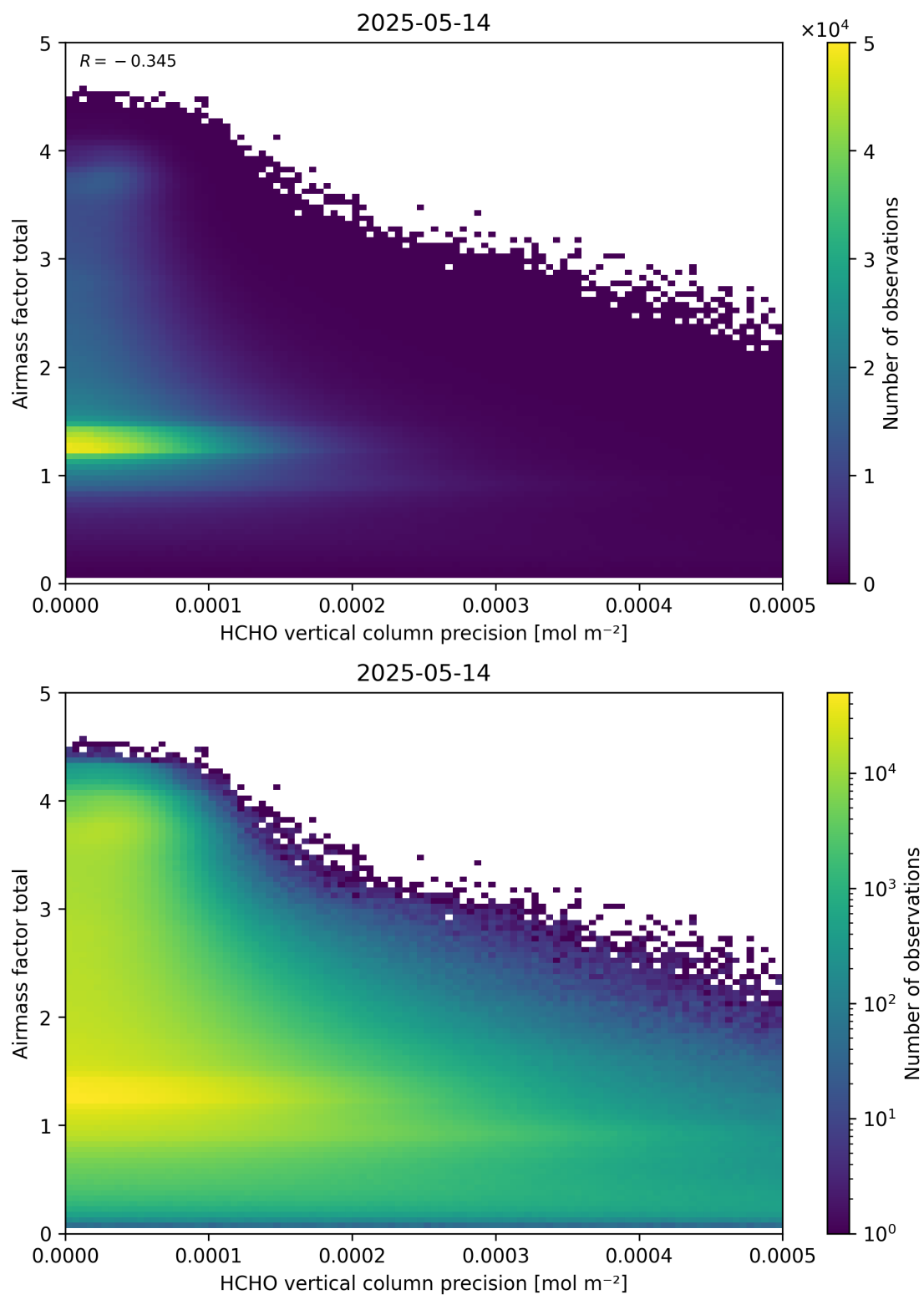
Figure 144: Scatter density plot of “HCHO vertical column precision” against “Airmass factor total” for 2025-05-13 to 2025-05-15.
