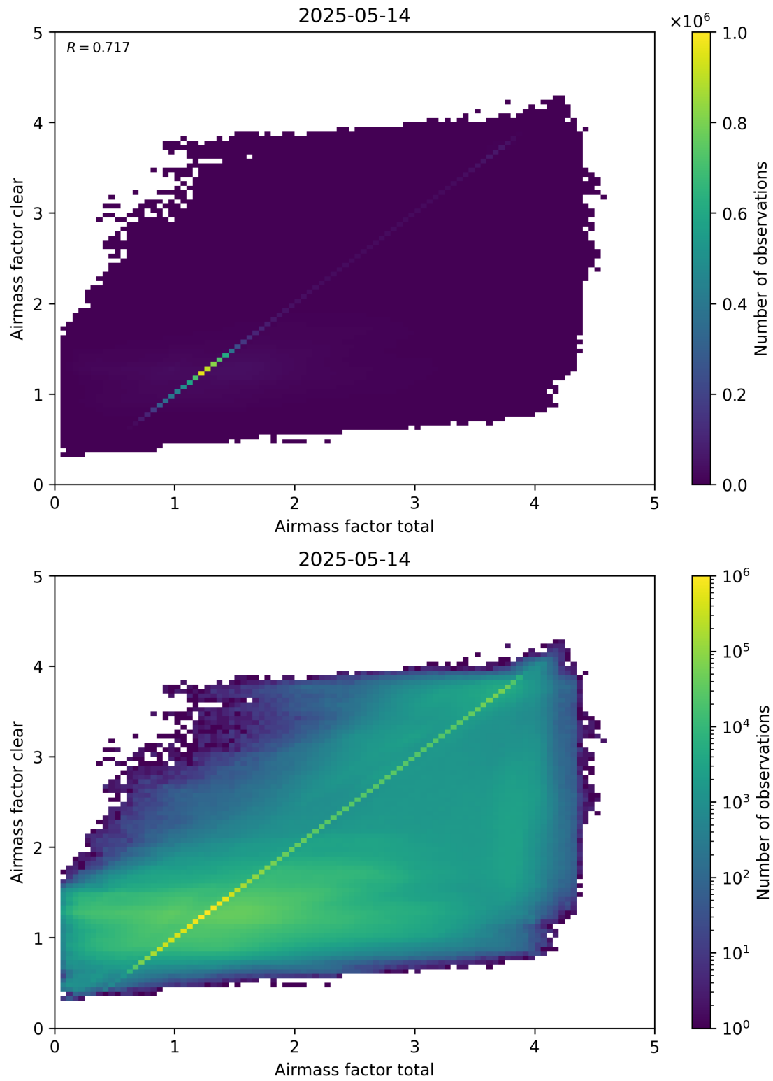
Figure 100: Scatter density plot of “Airmass factor total” against “Airmass factor clear” for 2025-05-13 to 2025-05-15.
