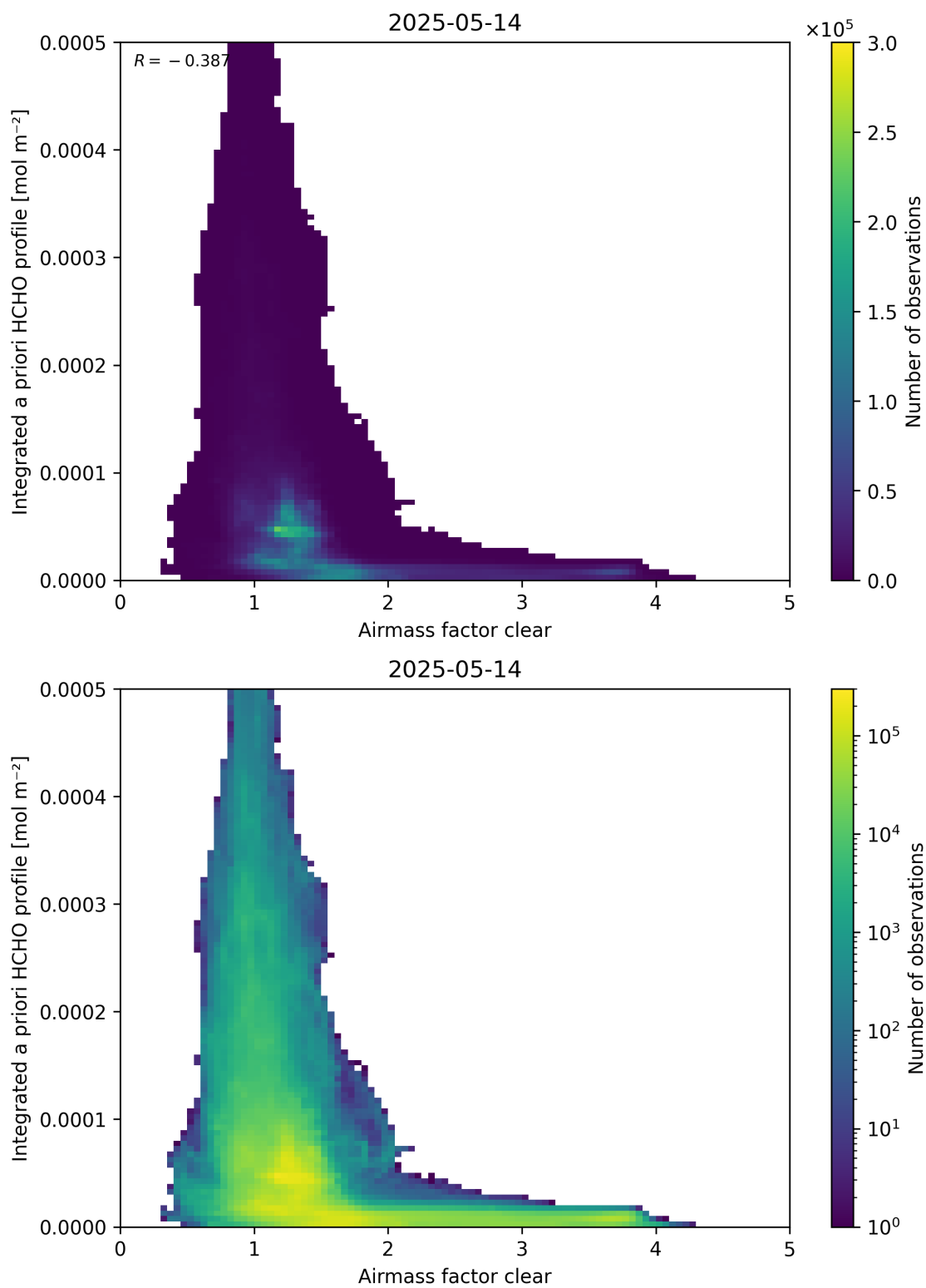
Figure 76: Scatter density plot of “Airmass factor clear” against “Integrated a priori HCHO profile” for 2025-05-13 to 2025-05-15.
