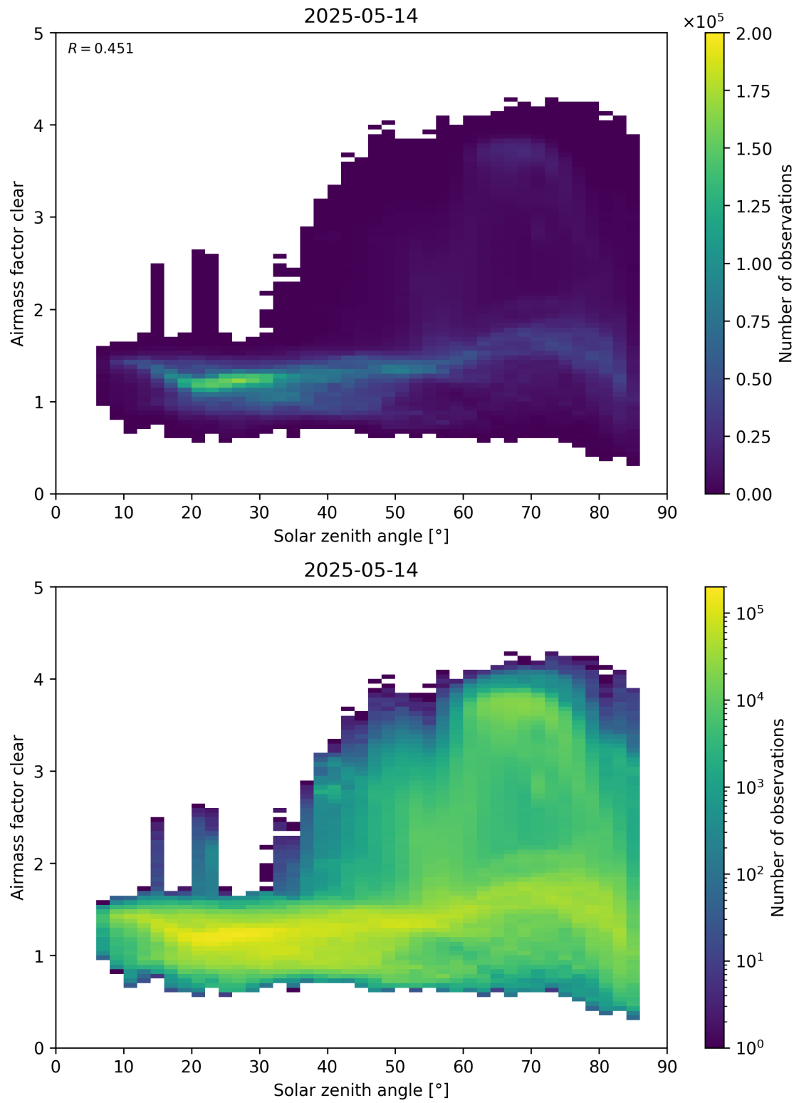
Figure 170: Scatter density plot of “Solar zenith angle” against “Airmass factor clear” for 2025-05-13 to 2025-05-15.
