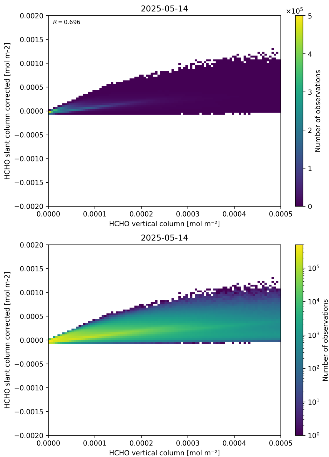
Figure 127: Scatter density plot of “HCHO vertical column” against “HCHO slant column corrected” for 2025-05-13 to 2025-05-15.
