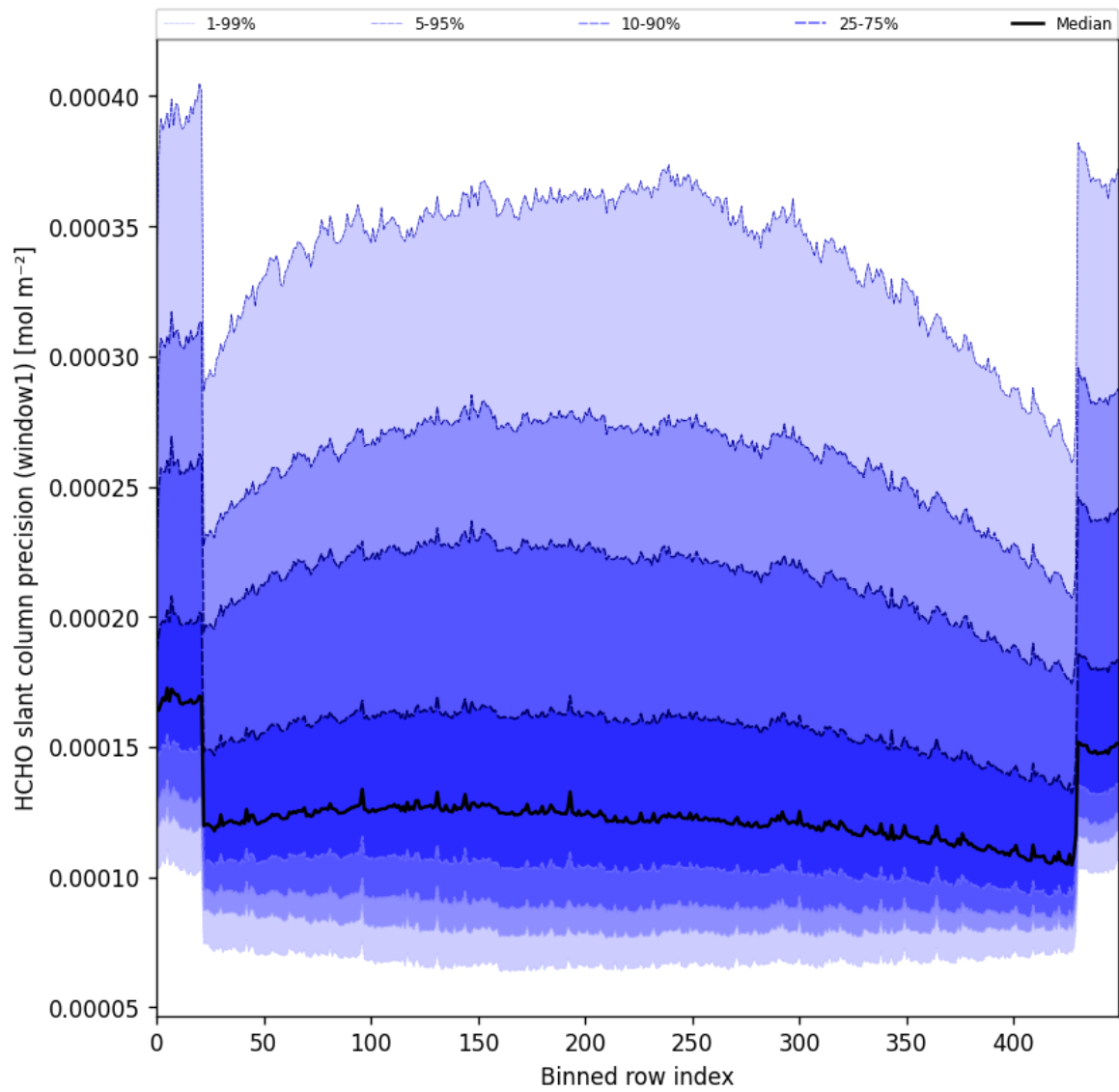
Figure 53: Along track statistics of “HCHO slant column precision (window1)” for 2025-05-13 to 2025-05-15
