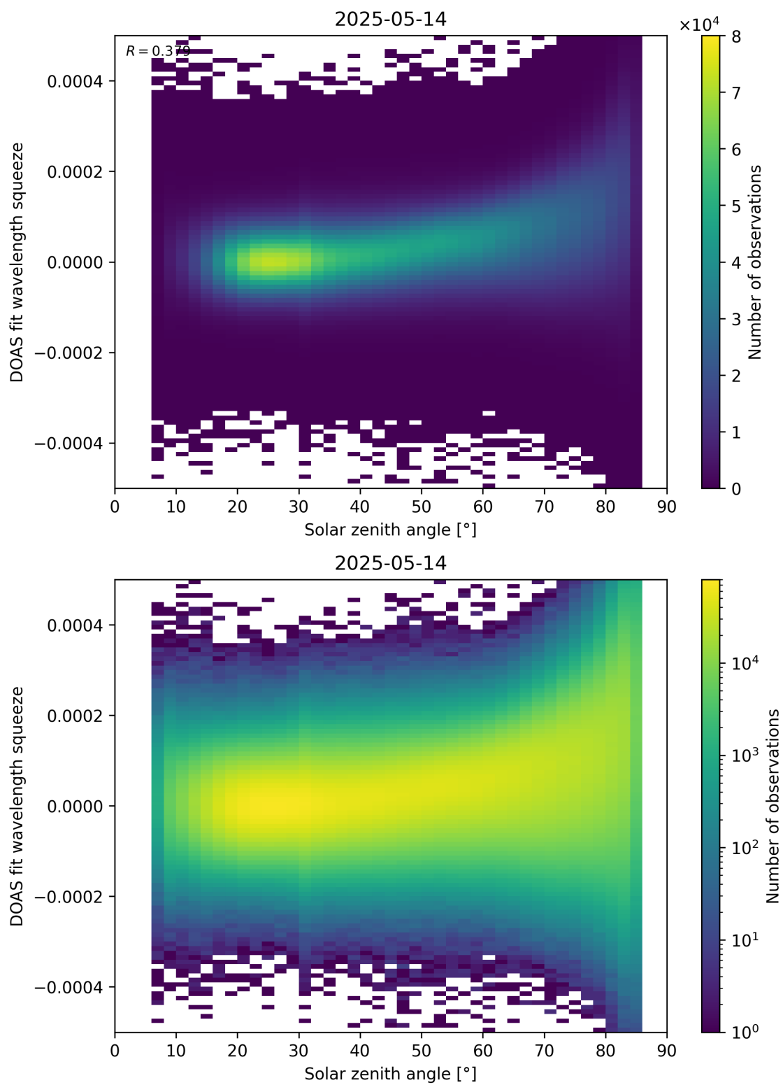
Figure 169: Scatter density plot of “Solar zenith angle” against “DOAS fit wavelength squeeze” for 2025-05-13 to 2025-05-15.
