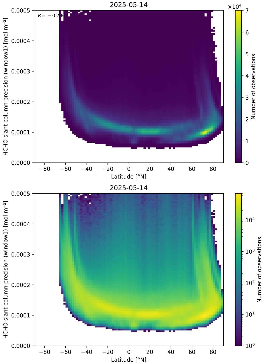
Figure 160: Scatter density plot of “Latitude” against “HCHO slant column precision (window1)” for 2025-05-13 to 2025-05-15.
