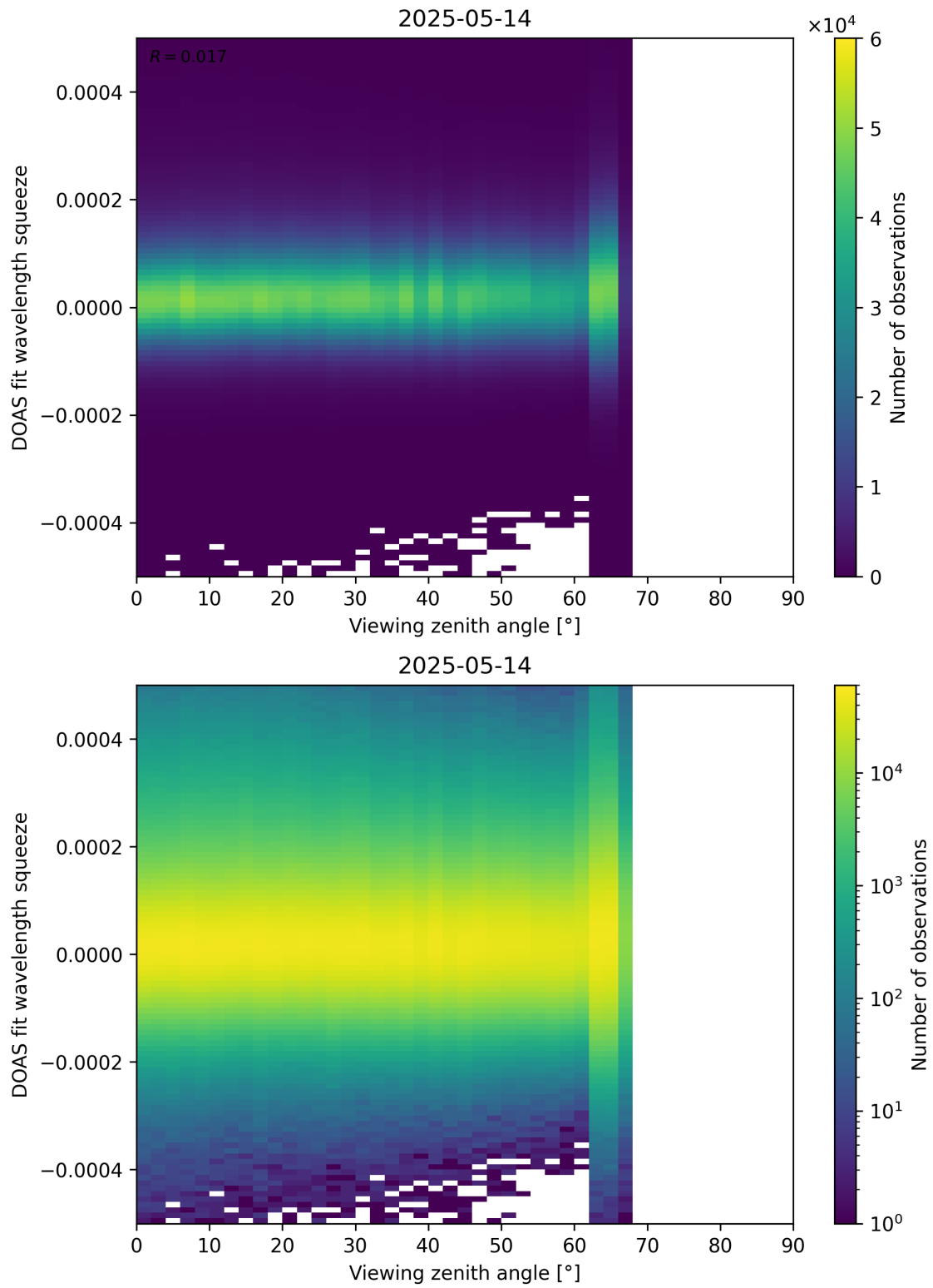
Figure 184: Scatter density plot of “Viewing zenith angle” against “DOAS fit wavelength squeeze” for 2025-05-13 to 2025-05-15.
