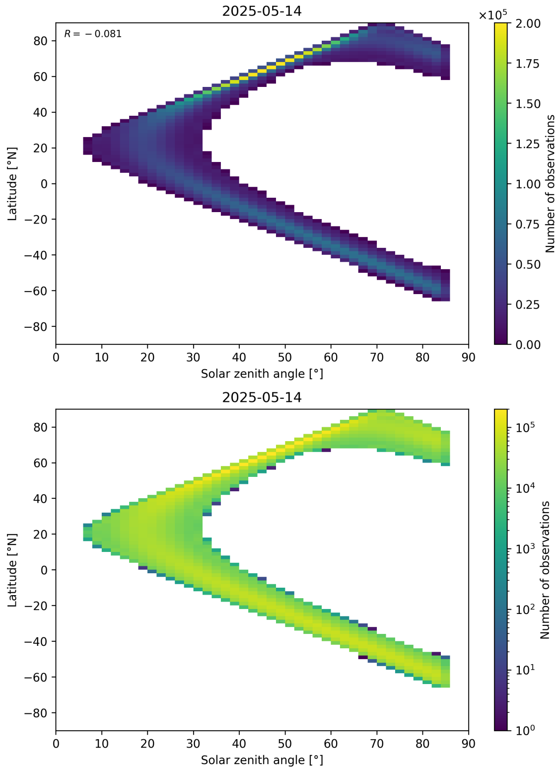
Figure 181: Scatter density plot of “Solar zenith angle” against “Latitude” for 2025-05-13 to 2025-05-15.
