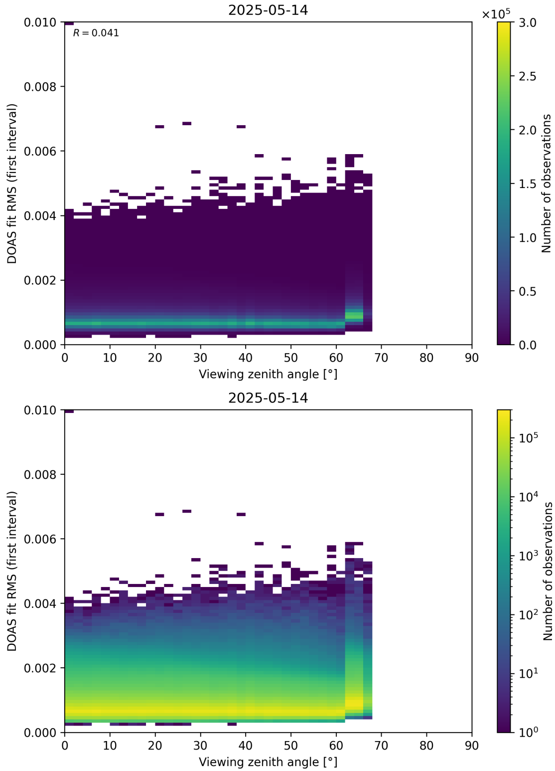
Figure 182: Scatter density plot of “Viewing zenith angle” against “DOAS fit RMS (first interval)” for 2025-05-13 to 2025-05-15.
