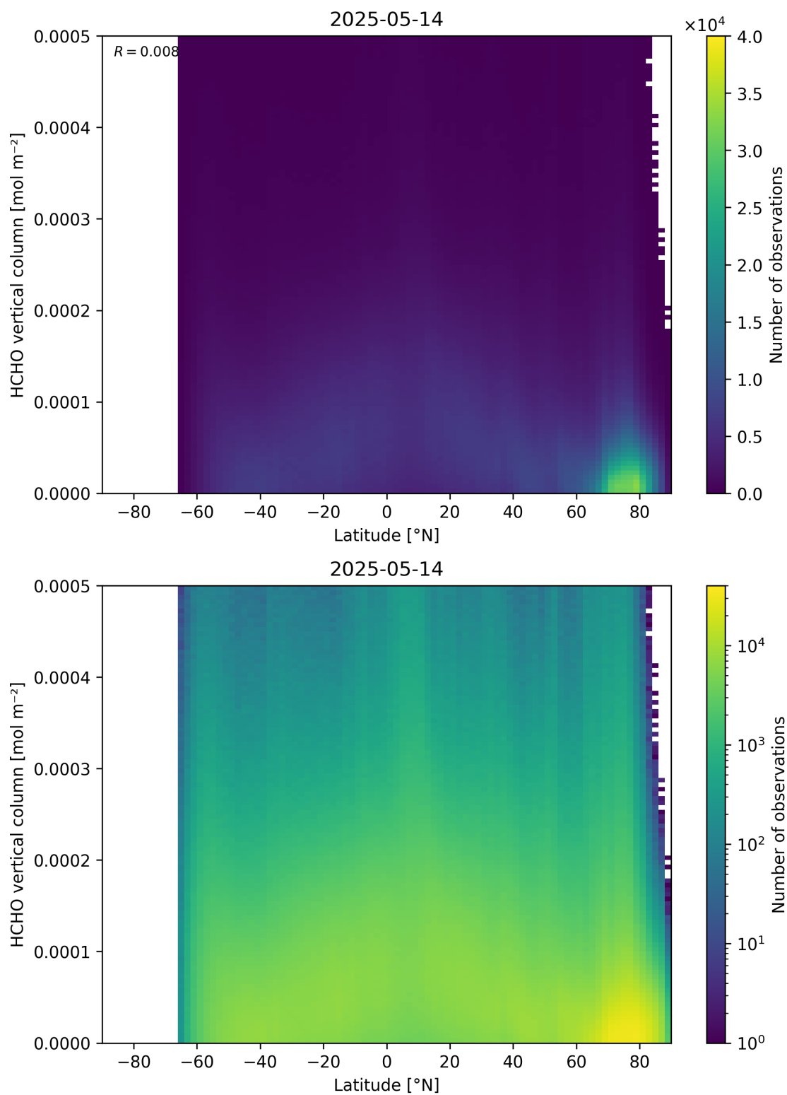
Figure 163: Scatter density plot of “Latitude” against “HCHO vertical column” for 2025-05-13 to 2025-05-15.
