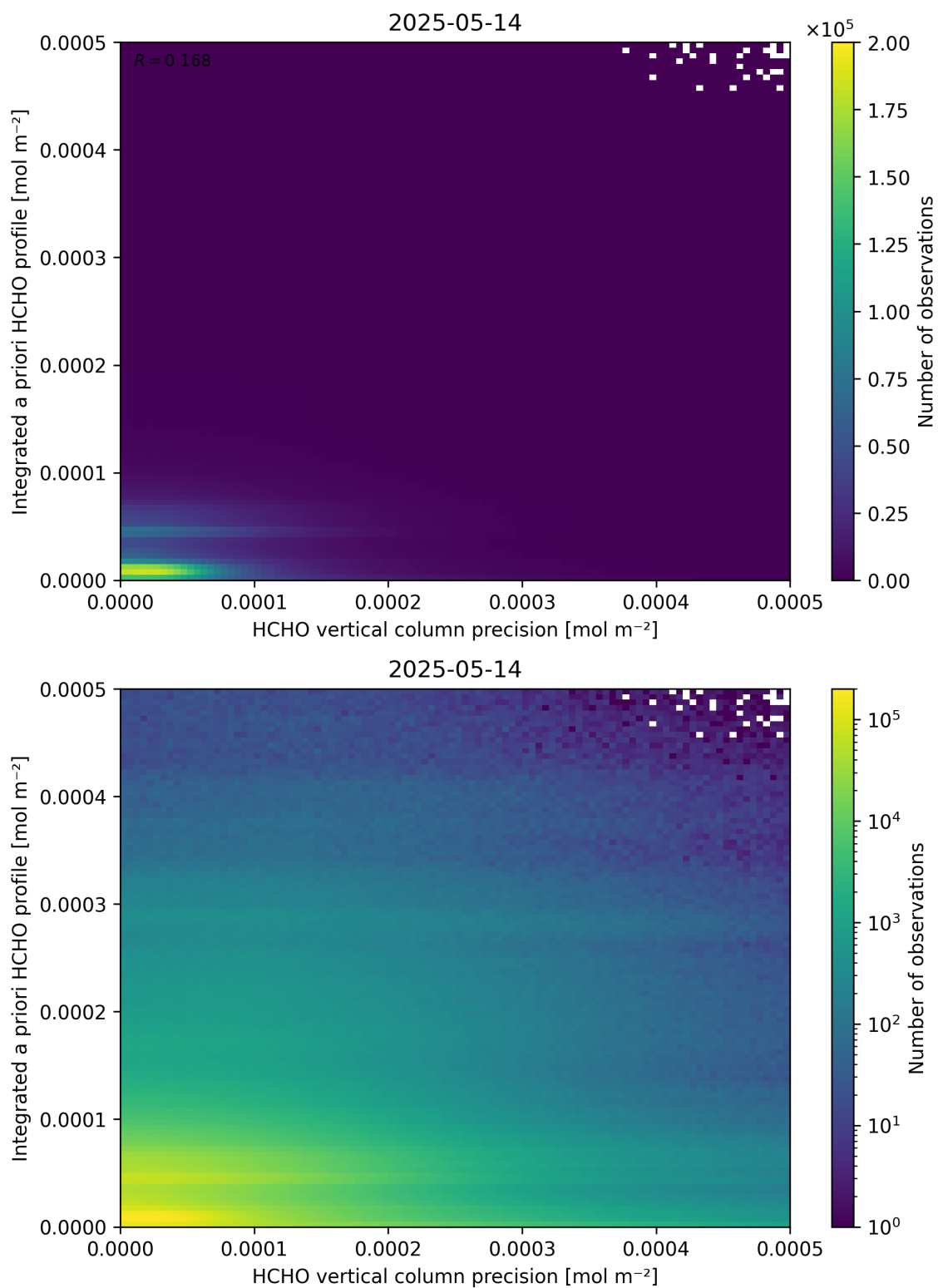
Figure 147: Scatter density plot of “HCHO vertical column precision” against “Integrated a priori HCHO profile” for 2025-05-13 to 2025-05-15.
