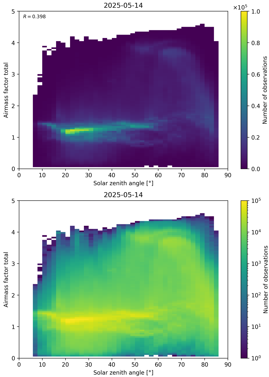
Figure 175: Scatter density plot of “Solar zenith angle” against “Airmass factor total” for 2025-05-13 to 2025-05-15.
