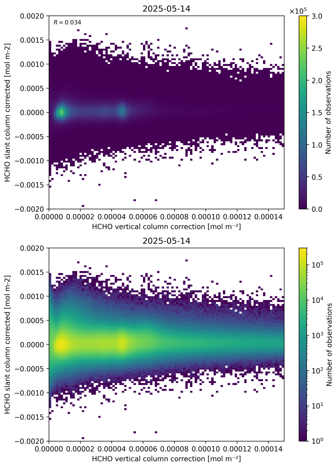
Figure 116: Scatter density plot of “HCHO vertical column correction” against “HCHO slant column corrected” for 2025-05-13 to 2025-05-15.
