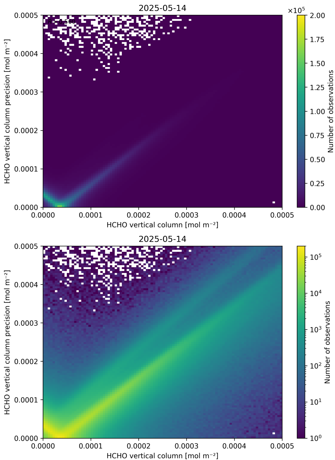
Figure 134: Scatter density plot of “HCHO vertical column” against “HCHO vertical column precision” for 2025-05-13 to 2025-05-15.
