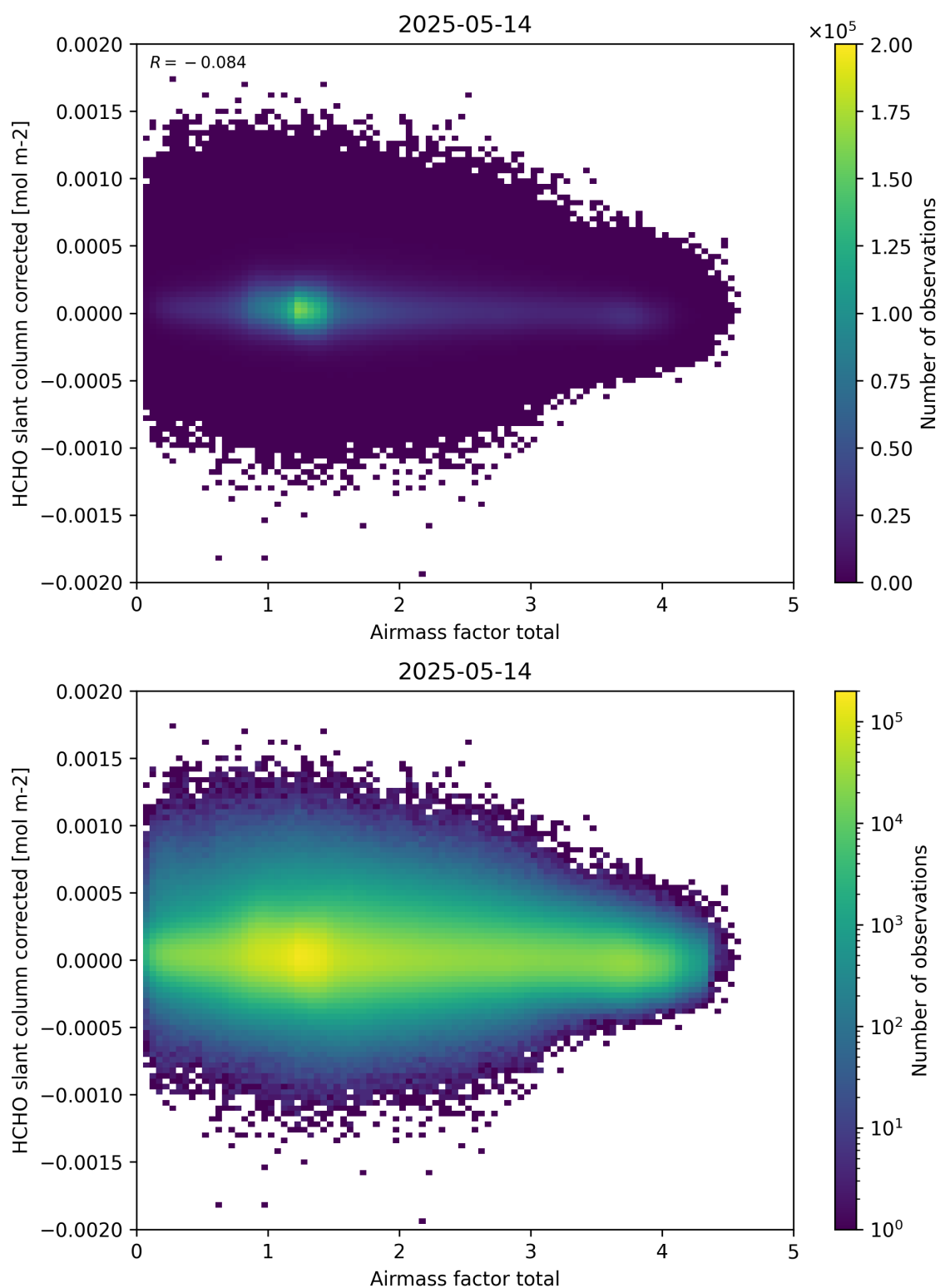
Figure 101: Scatter density plot of “Airmass factor total” against “HCHO slant column corrected” for 2025-05-13 to 2025-05-15.
