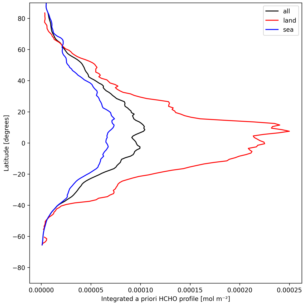
Figure 29: Zonal average of “Integrated a priori HCHO profile” for 2025-05-13 to 2025-05-15.
