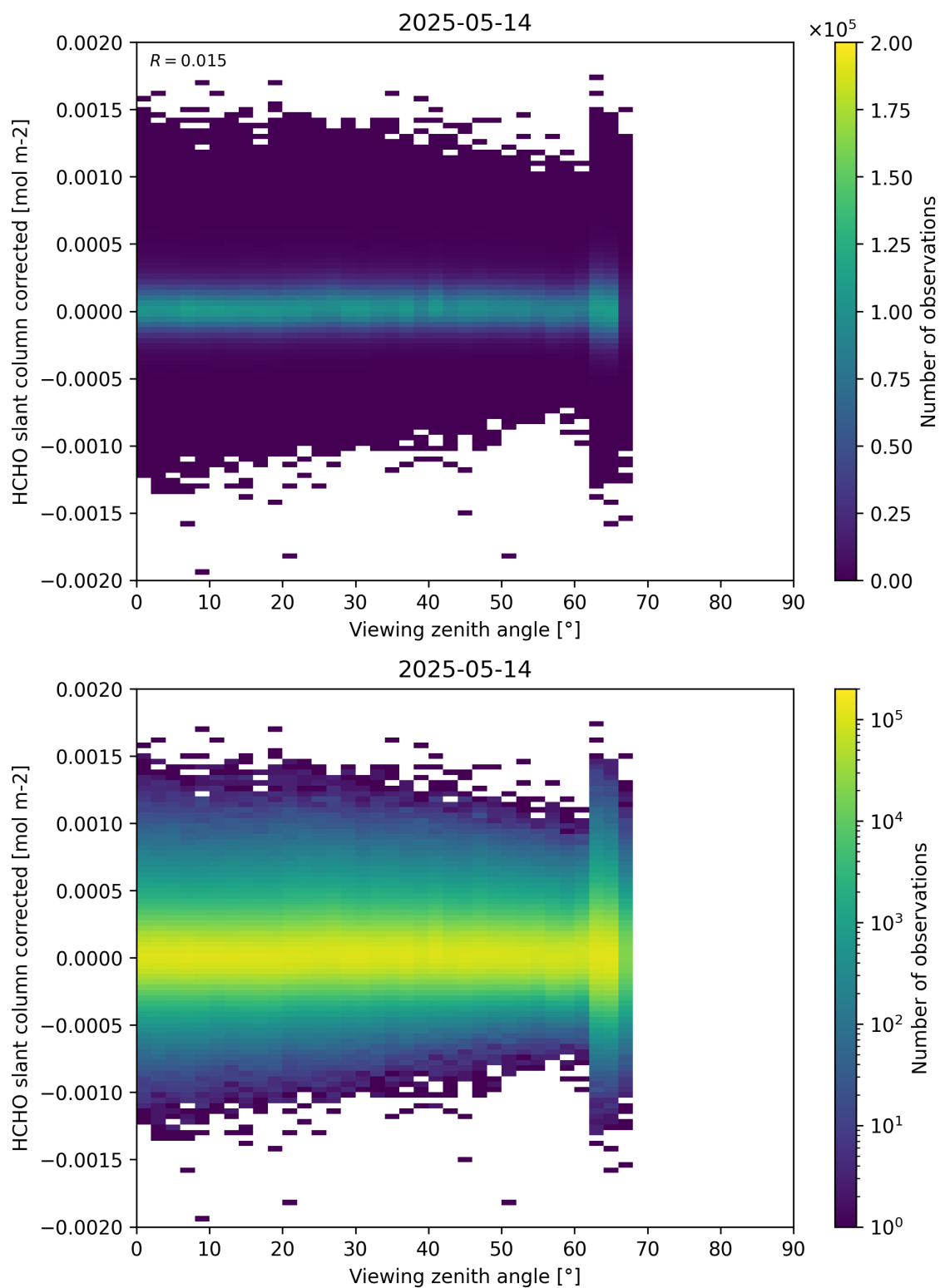
Figure 186: Scatter density plot of “Viewing zenith angle” against “HCHO slant column corrected” for 2025-05-13 to 2025-05-15.
