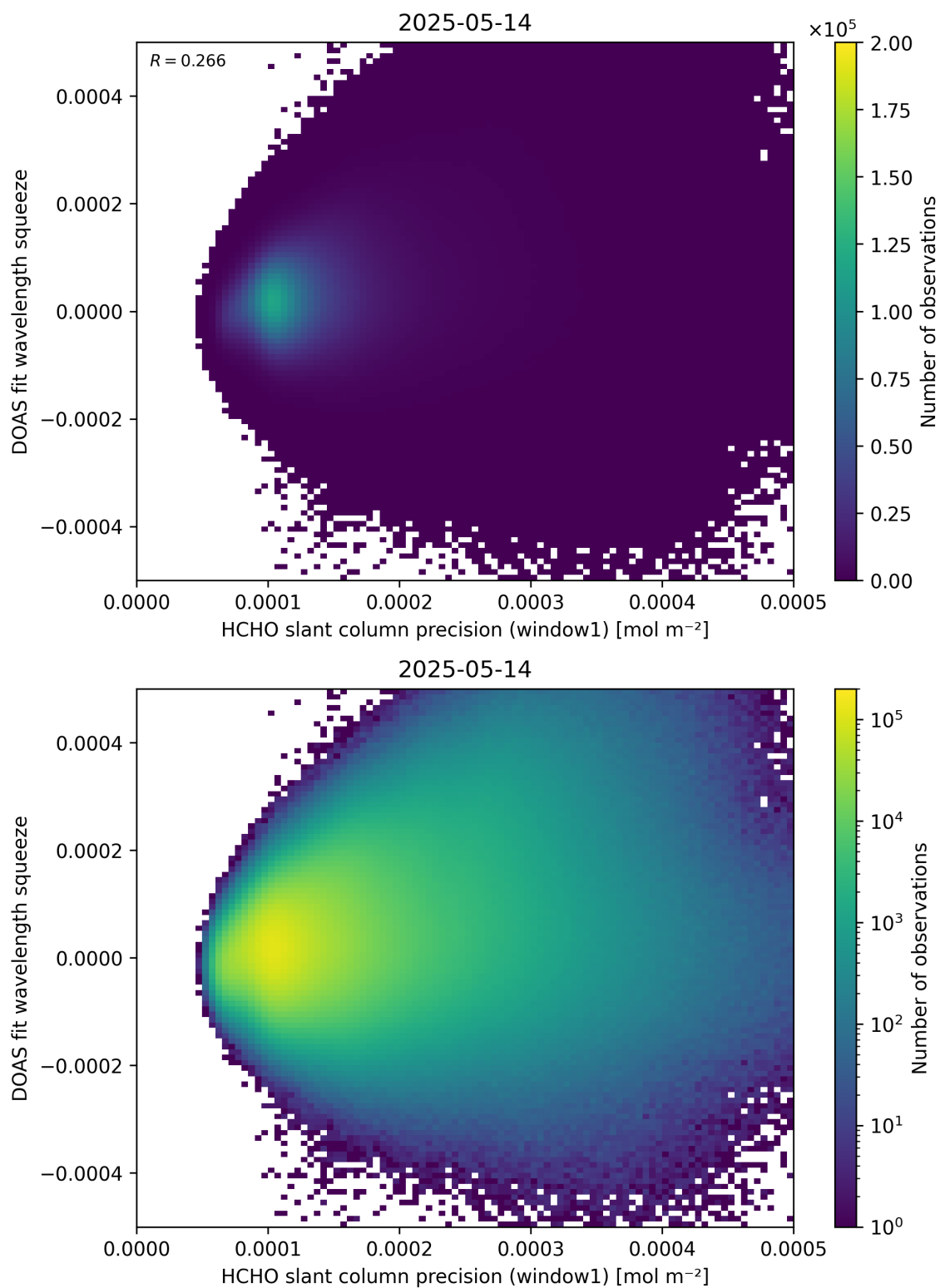
Figure 90: Scatter density plot of “HCHO slant column precision (window1)” against “DOAS fit wavelength squeeze” for 2025-05-13 to 2025-05-15.
