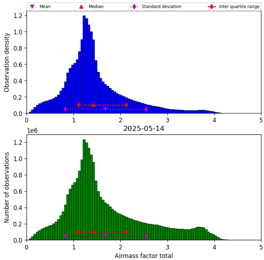
Figure 40: Histogram of “Airmass factor total” for 2025-05-13 to 2025-05-15
