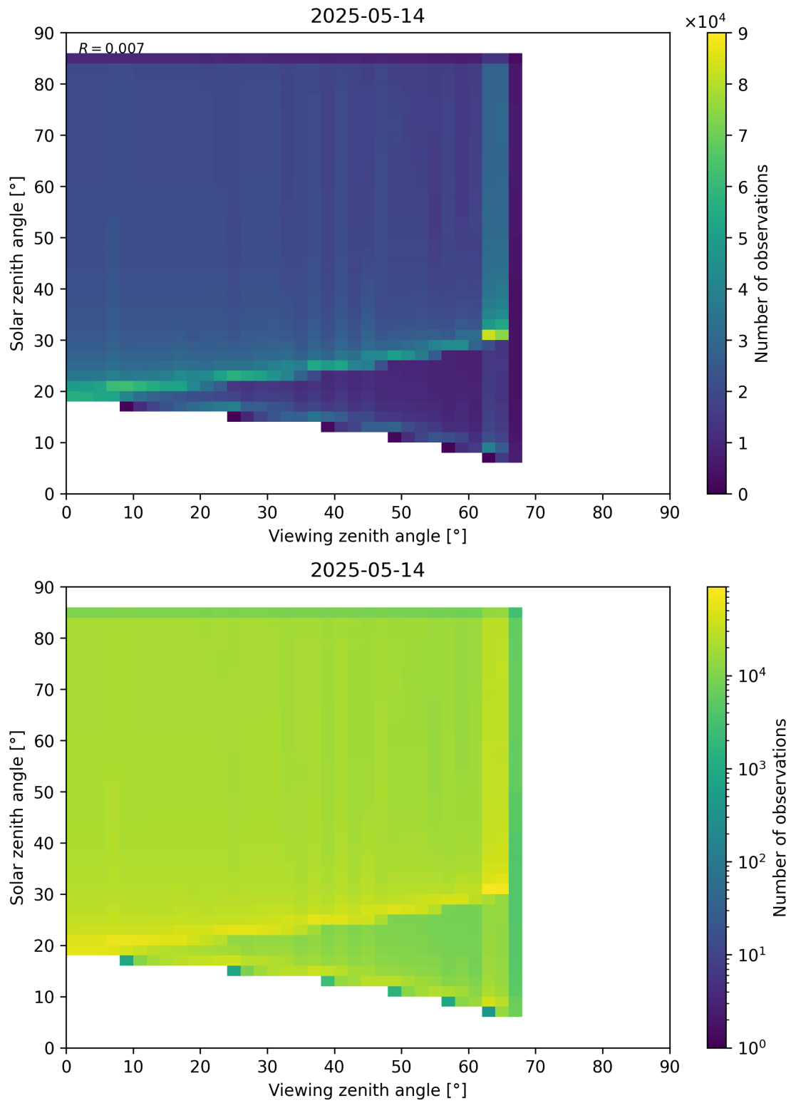
Figure 197: Scatter density plot of “Viewing zenith angle” against “Solar zenith angle” for 2025-05-13 to 2025-05-15.
