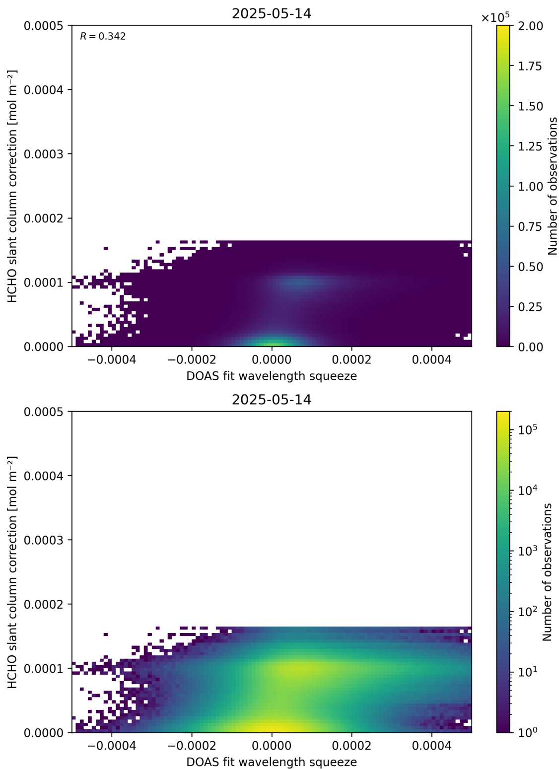
Figure 70: Scatter density plot of “DOAS fit wavelength squeeze” against “HCHO slant column correction” for 2025-05-13 to 2025-05-15.
