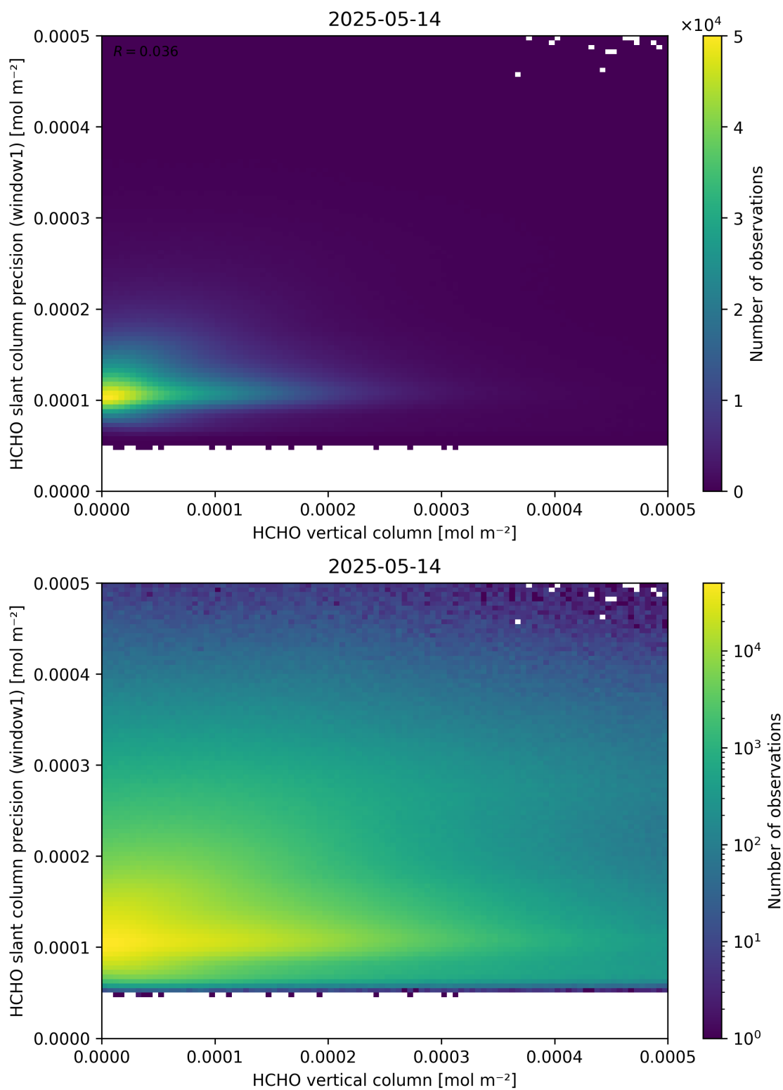
Figure 130: Scatter density plot of “HCHO vertical column” against “HCHO slant column precision (window1)” for 2025-05-13 to 2025-05-15.
