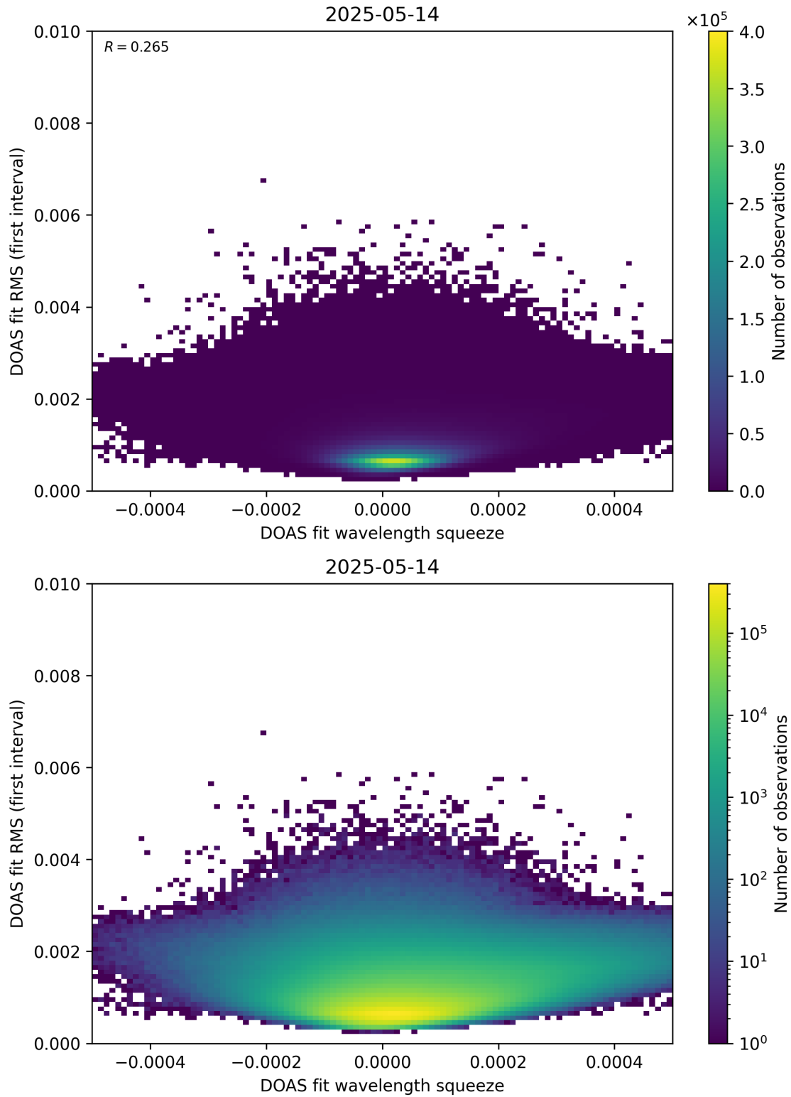
Figure 68: Scatter density plot of “DOAS fit wavelength squeeze” against “DOAS fit RMS (first interval)” for 2025-05-13 to 2025-05-15.
