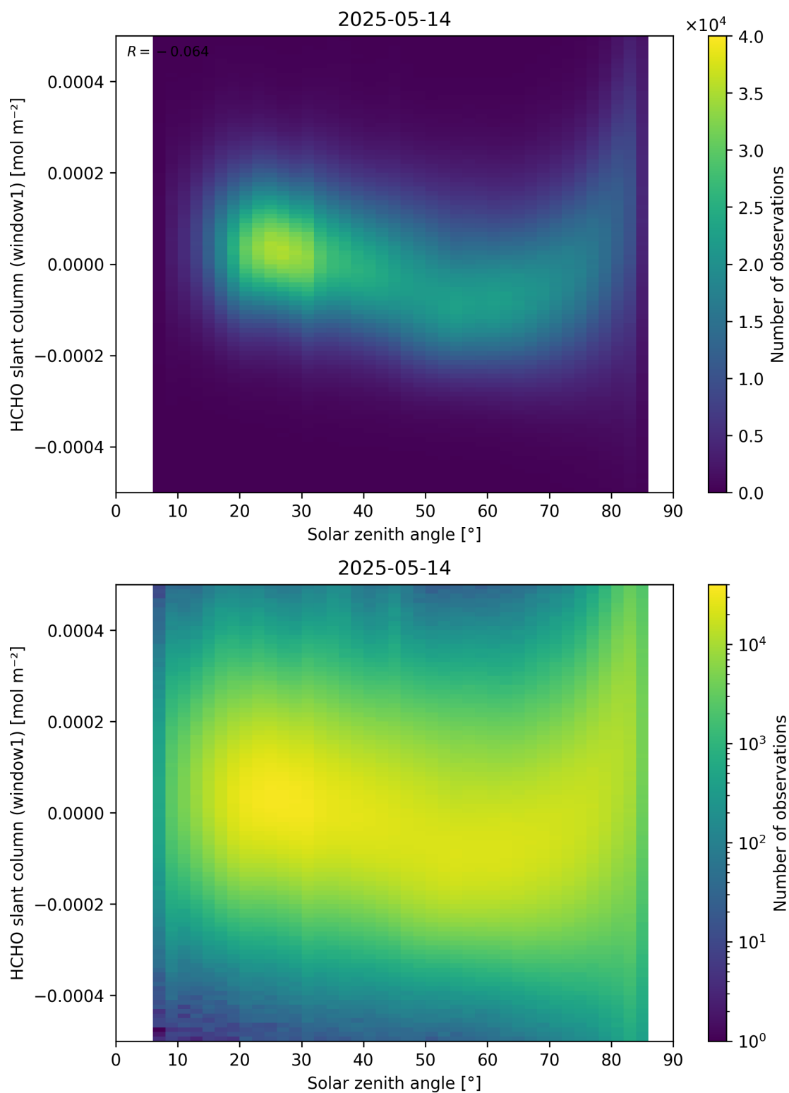
Figure 173: Scatter density plot of “Solar zenith angle” against “HCHO slant column (window1)” for 2025-05-13 to 2025-05-15.
