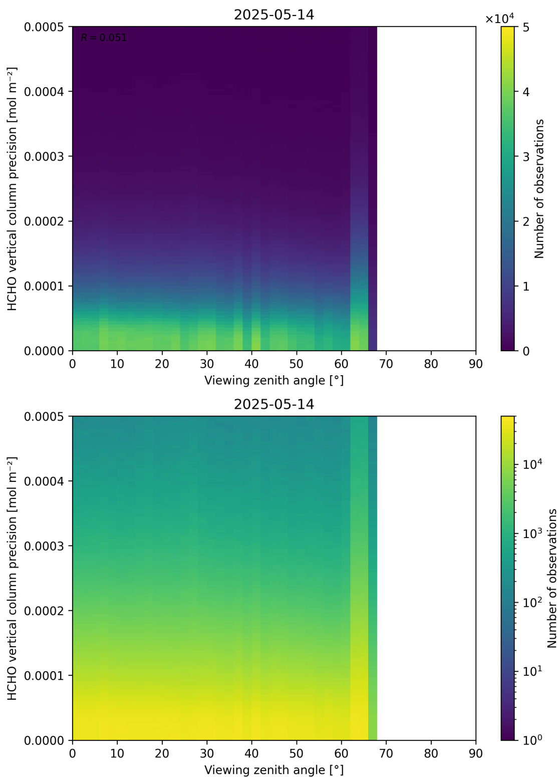
Figure 194: Scatter density plot of “Viewing zenith angle” against “HCHO vertical column precision” for 2025-05-13 to 2025-05-15.
