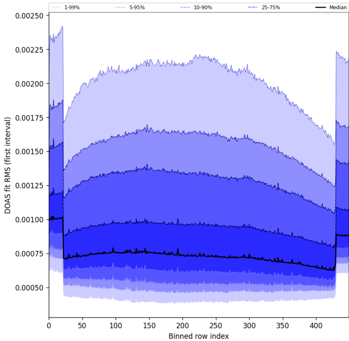
Figure 60: Along track statistics of “DOAS fit RMS (first interval)” for 2025-05-13 to 2025-05-15
