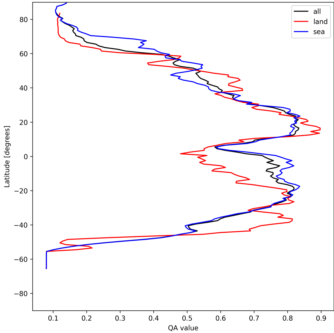
Figure 20: Zonal average of “QA value” for 2025-05-13 to 2025-05-15.
