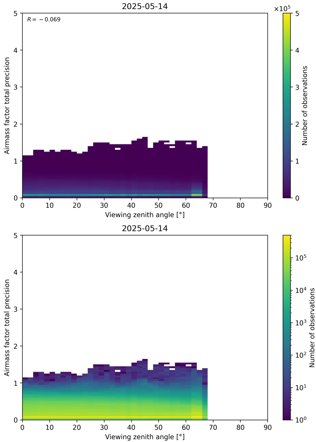
Figure 191: Scatter density plot of “Viewing zenith angle” against “Airmass factor total precision” for 2025-05-13 to 2025-05-15.
