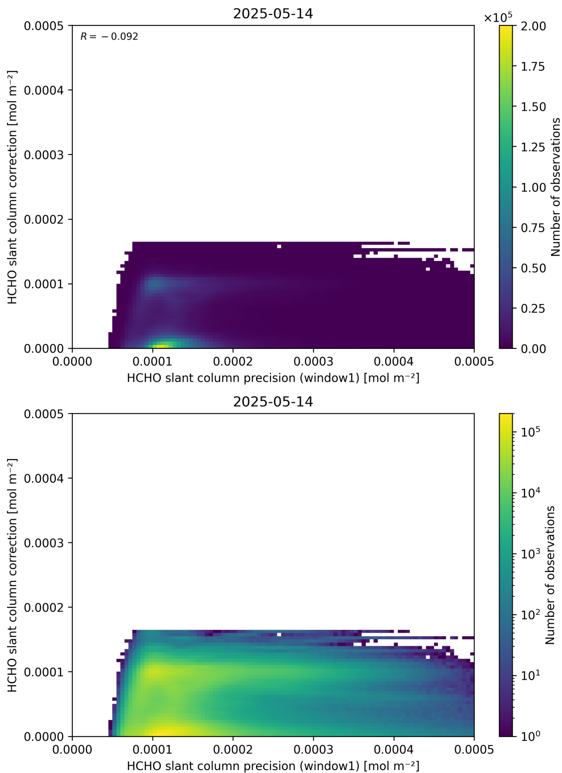
Figure 93: Scatter density plot of “HCHO slant column precision (window1)” against “HCHO slant column correction” for 2025-05-13 to 2025-05-15.
