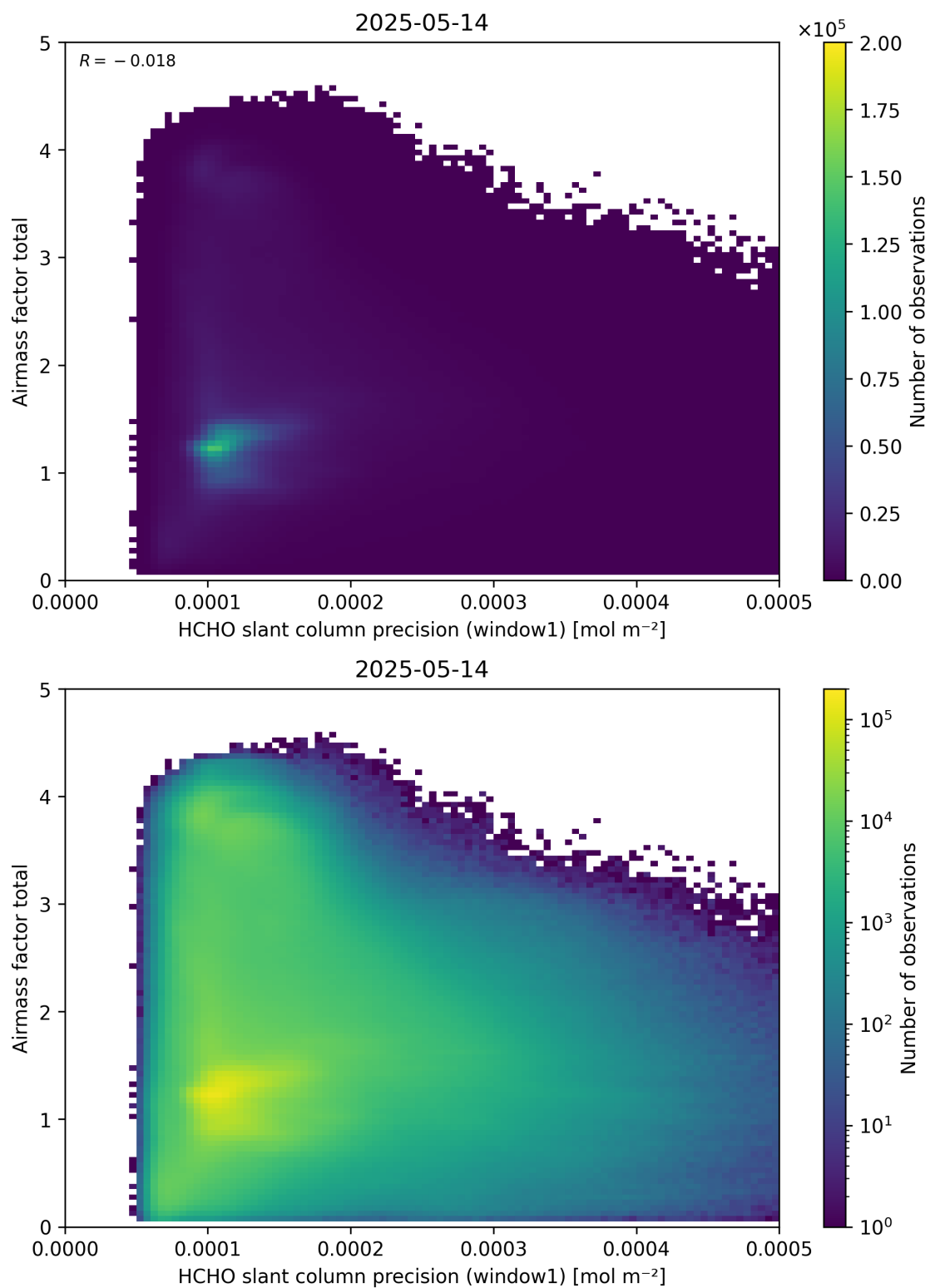
Figure 94: Scatter density plot of “HCHO slant column precision (window1)” against “Airmass factor total” for 2025-05-13 to 2025-05-15.
