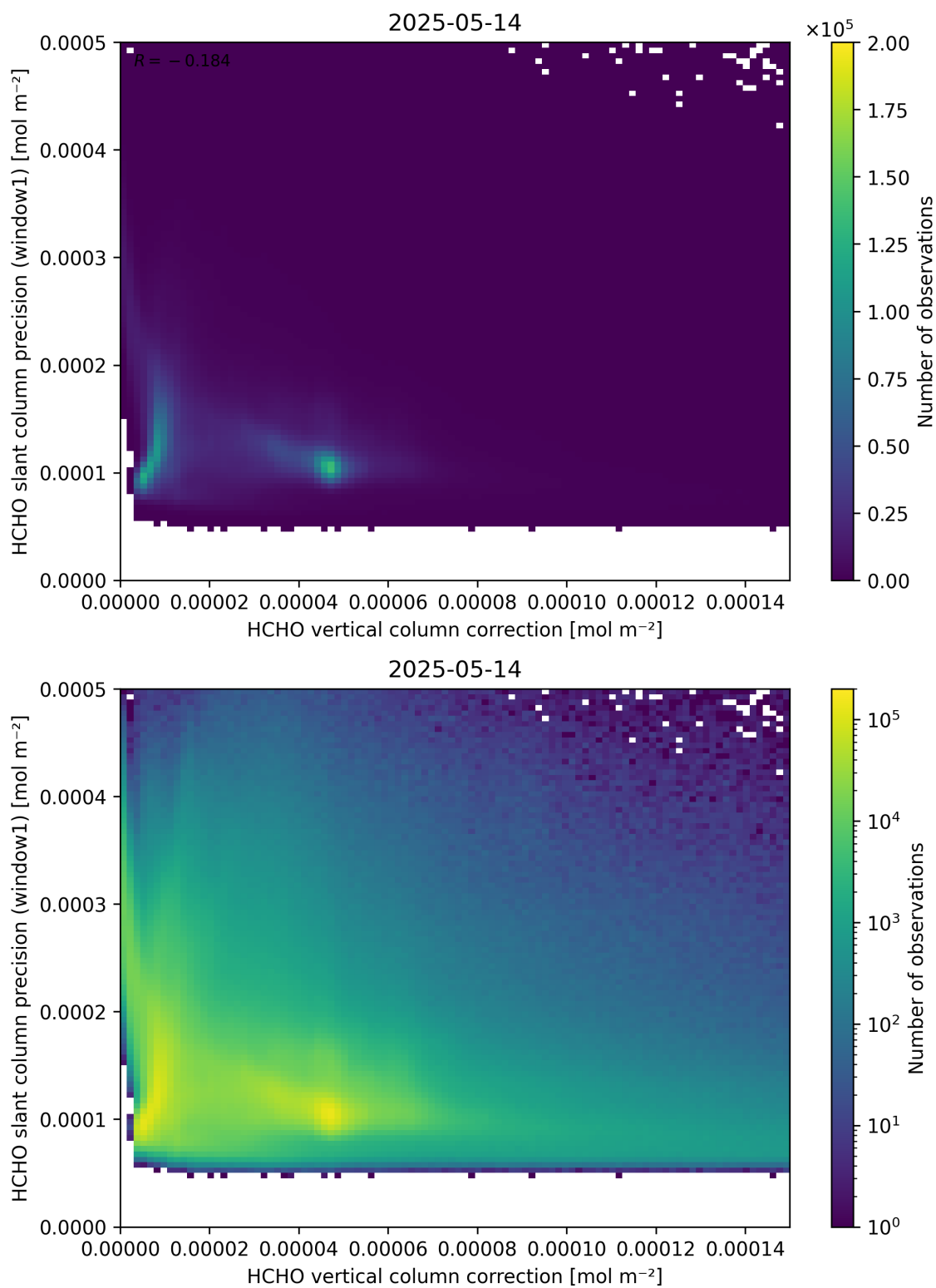
Figure 119: Scatter density plot of “HCHO vertical column correction” against “HCHO slant column precision (window1)” for 2025-05-13 to 2025-05-15.
