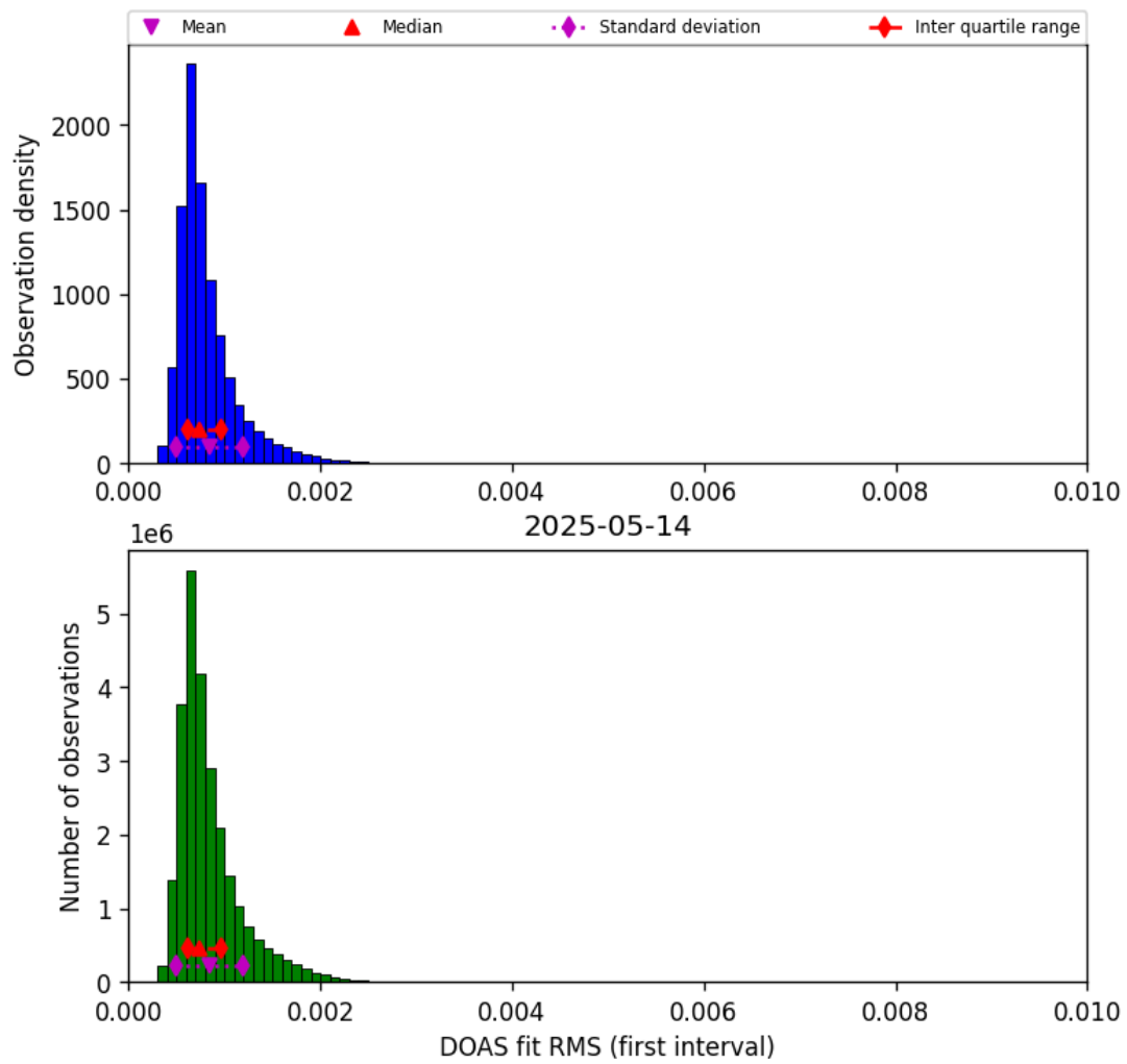
Figure 46: Histogram of “DOAS fit RMS (first interval)” for 2025-05-13 to 2025-05-15
