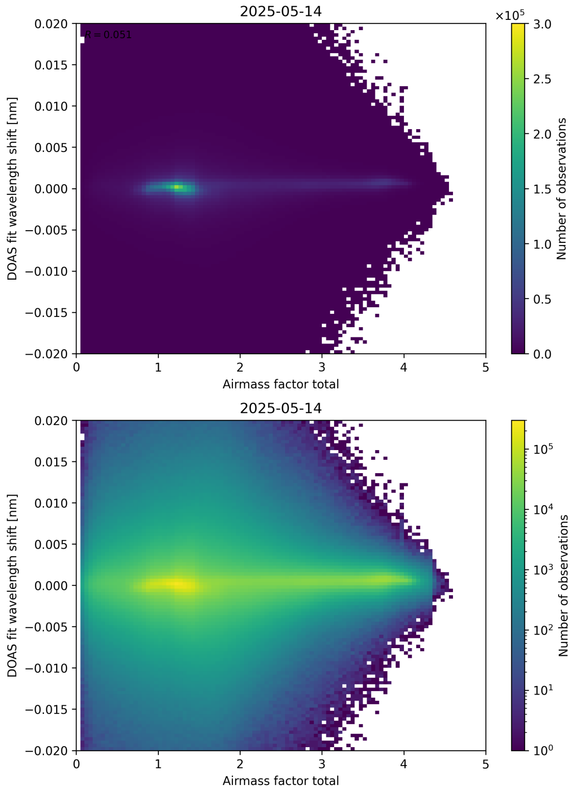
Figure 98: Scatter density plot of “Airmass factor total” against “DOAS fit wavelength shift” for 2025-05-13 to 2025-05-15.
