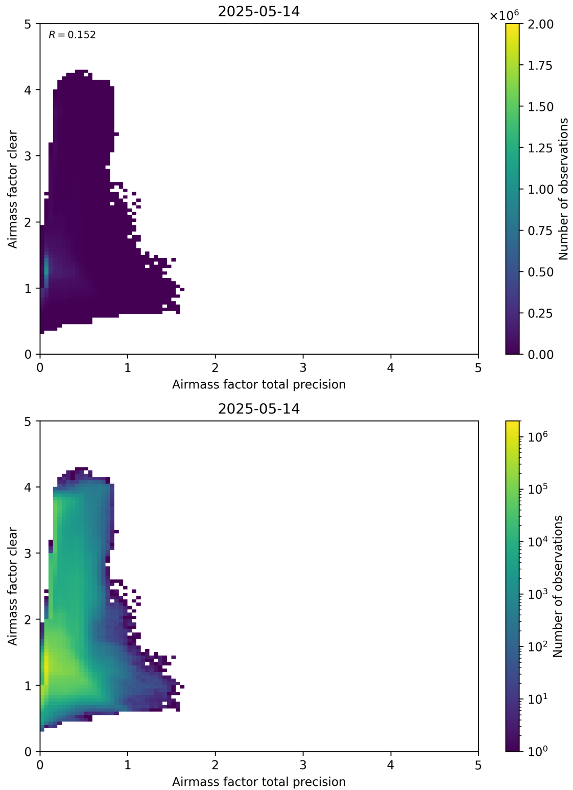
Figure 108: Scatter density plot of “Airmass factor total precision” against “Airmass factor clear” for 2025-05-13 to 2025-05-15.
