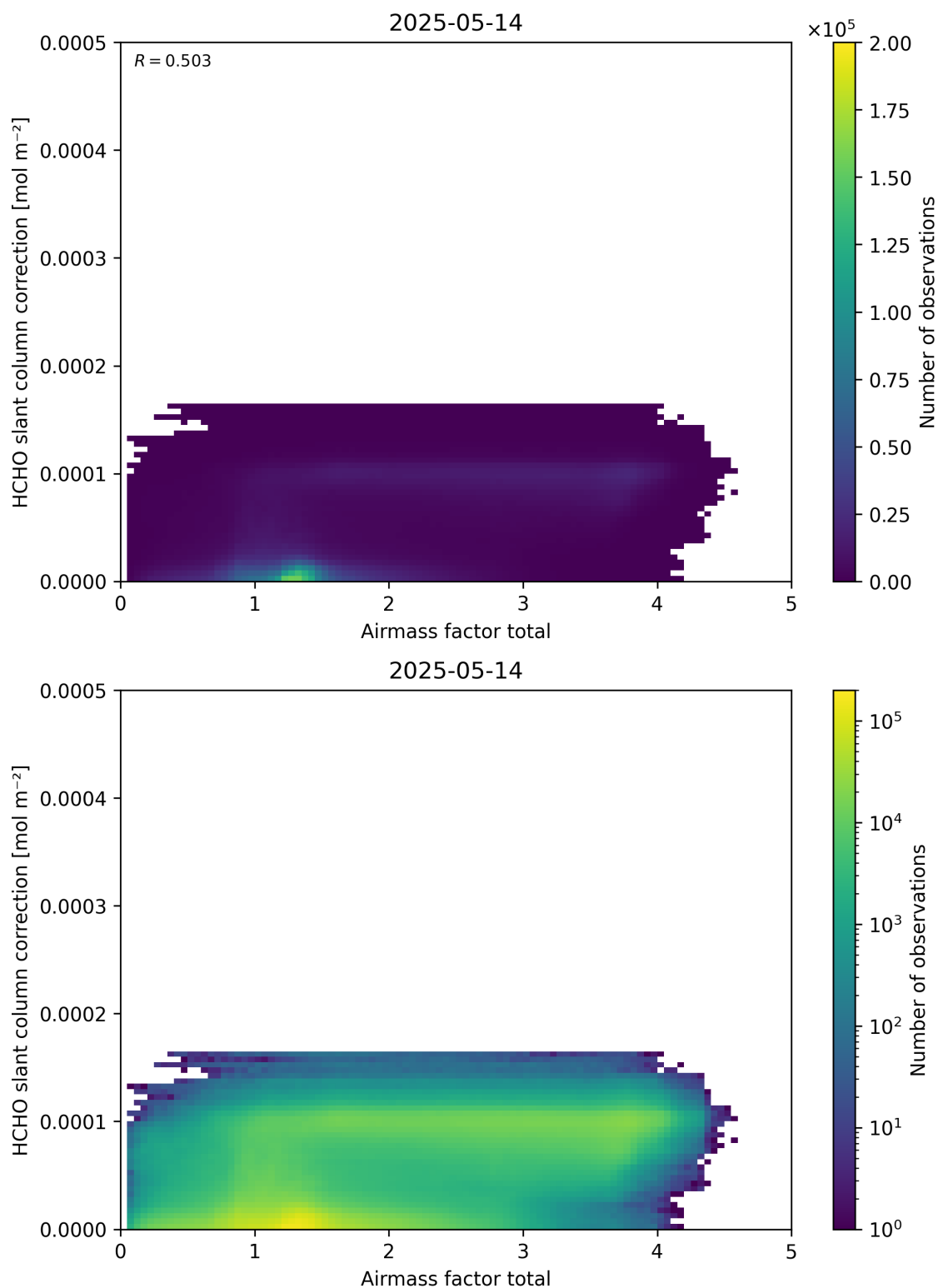
Figure 102: Scatter density plot of “Airmass factor total” against “HCHO slant column correction” for 2025-05-13 to 2025-05-15.
