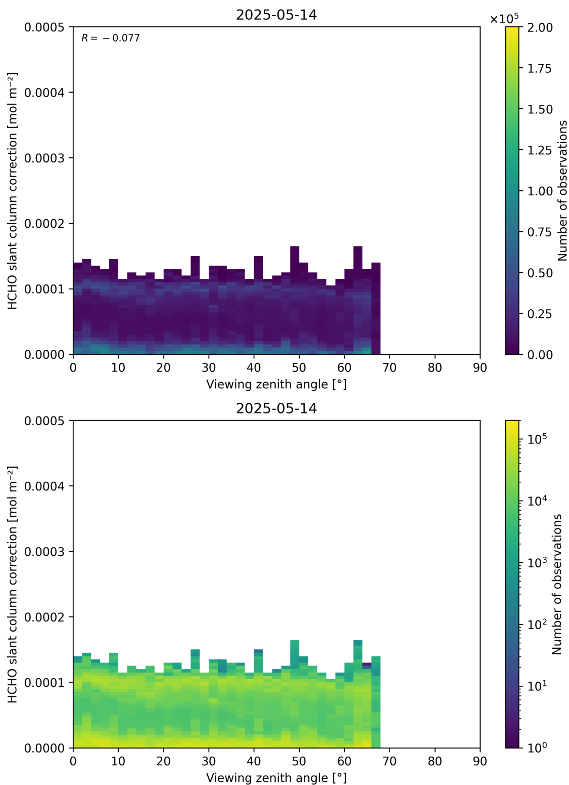
Figure 187: Scatter density plot of “Viewing zenith angle” against “HCHO slant column correction” for 2025-05-13 to 2025-05-15.
