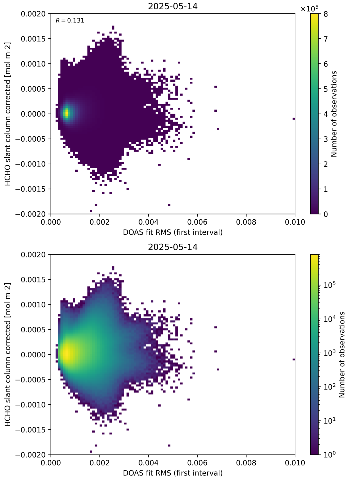
Figure 62: Scatter density plot of “DOAS fit RMS (first interval)” against “HCHO slant column corrected” for 2025-05-13 to 2025-05-15.
