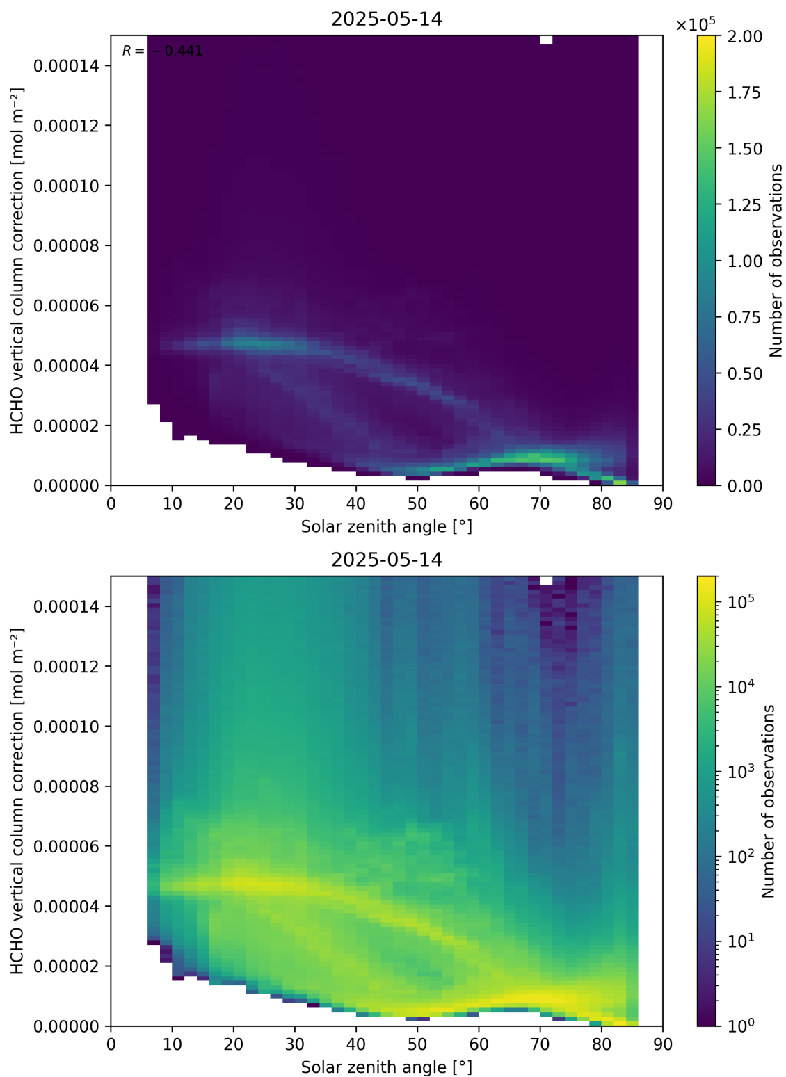
Figure 178: Scatter density plot of “Solar zenith angle” against “HCHO vertical column correction” for 2025-05-13 to 2025-05-15.
