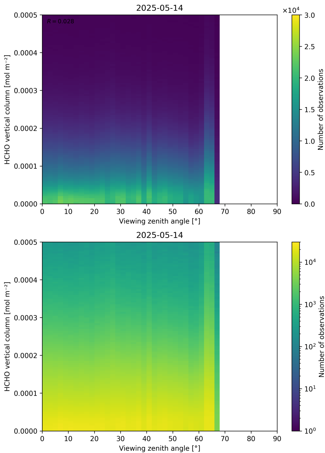
Figure 192: Scatter density plot of “Viewing zenith angle” against “HCHO vertical column” for 2025-05-13 to 2025-05-15.
