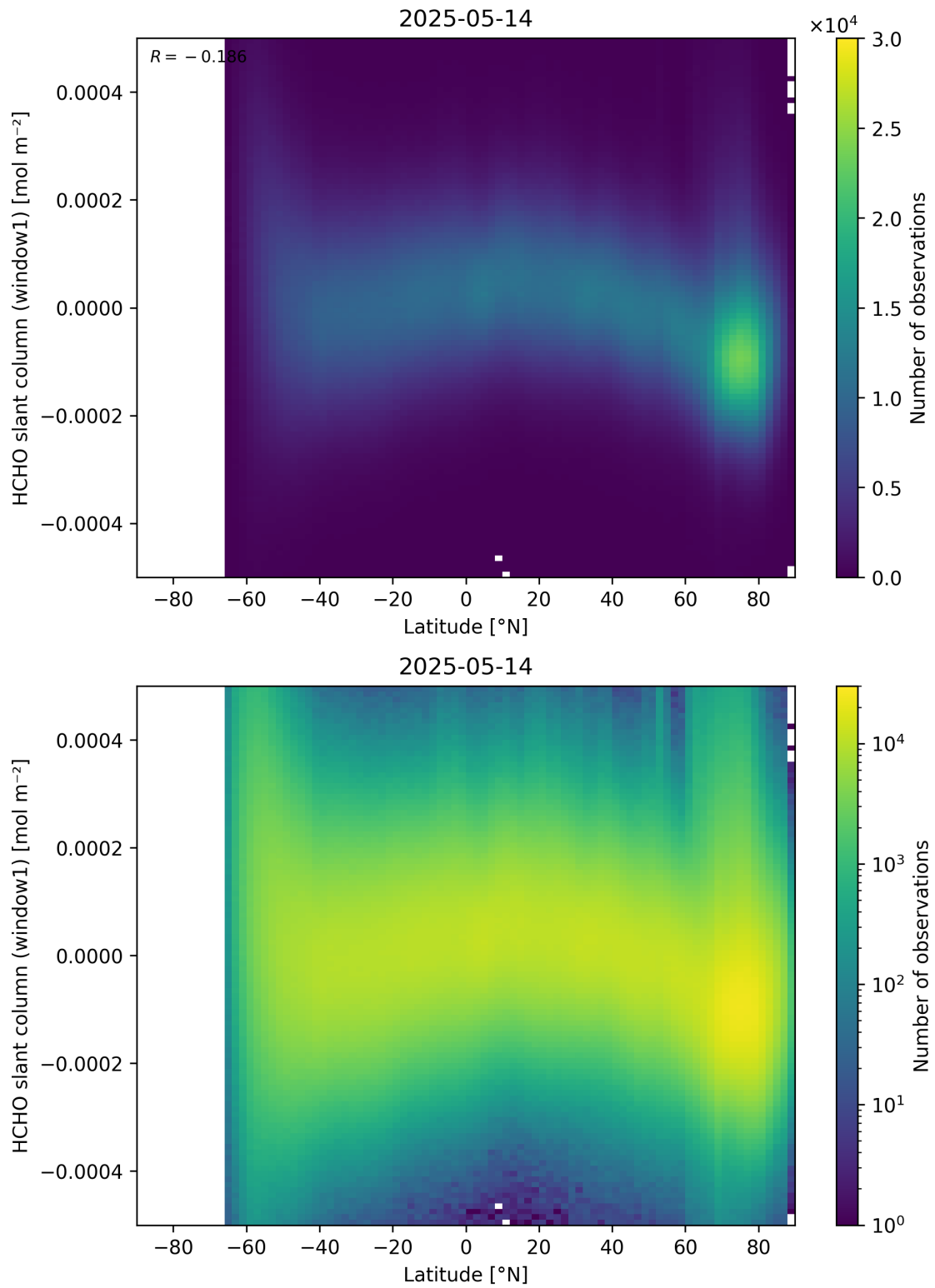
Figure 159: Scatter density plot of “Latitude” against “HCHO slant column (window1)” for 2025-05-13 to 2025-05-15.
