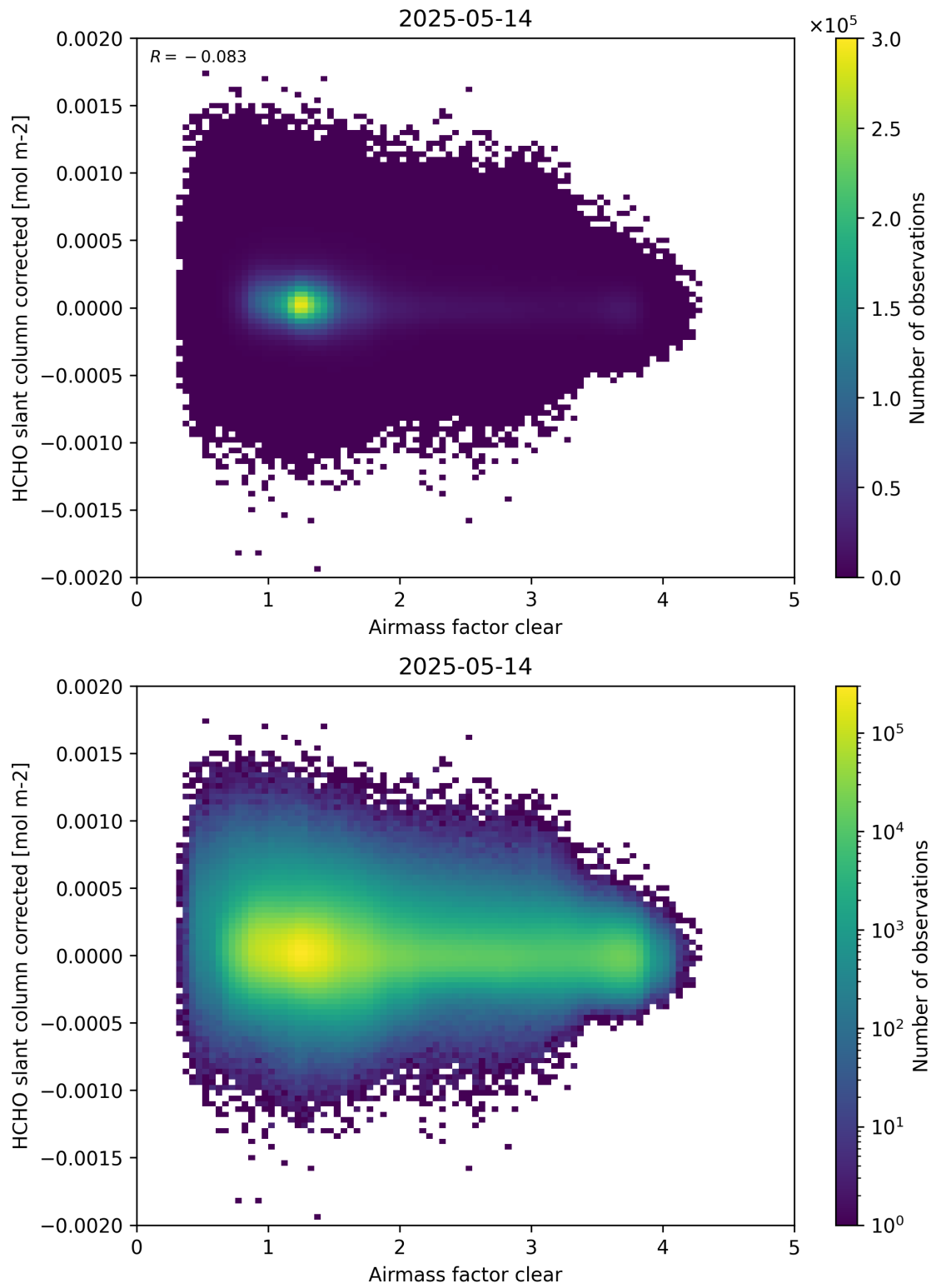
Figure 74: Scatter density plot of “Airmass factor clear” against “HCHO slant column corrected” for 2025-05-13 to 2025-05-15.
