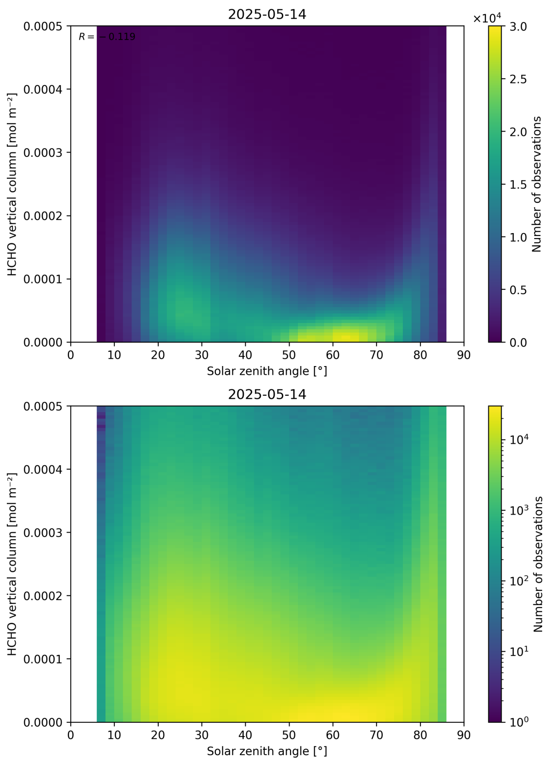
Figure 177: Scatter density plot of “Solar zenith angle” against “HCHO vertical column” for 2025-05-13 to 2025-05-15.
