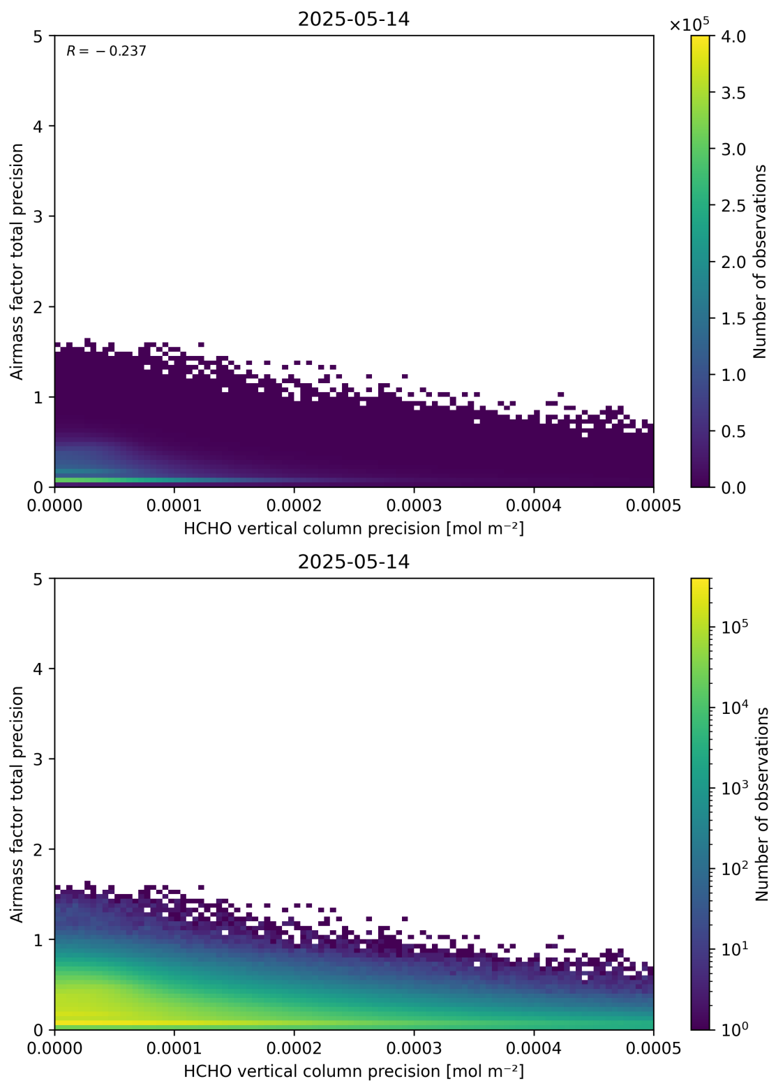
Figure 145: Scatter density plot of “HCHO vertical column precision” against “Airmass factor total precision” for 2025-05-13 to 2025-05-15.
