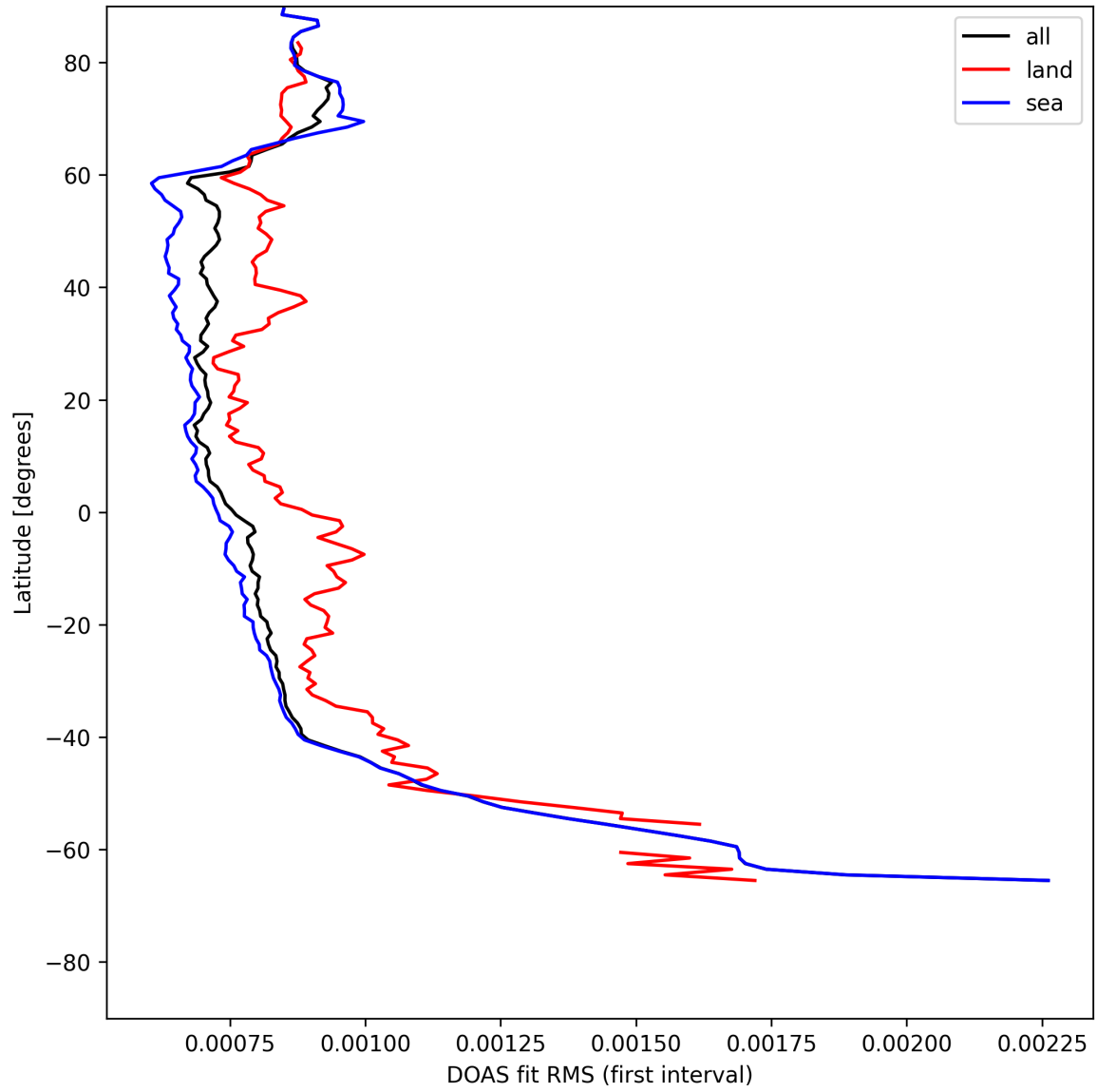
Figure 32: Zonal average of "DOAS fit RMS (first interval)" for 2025-05-13 to 2025-05-15.
