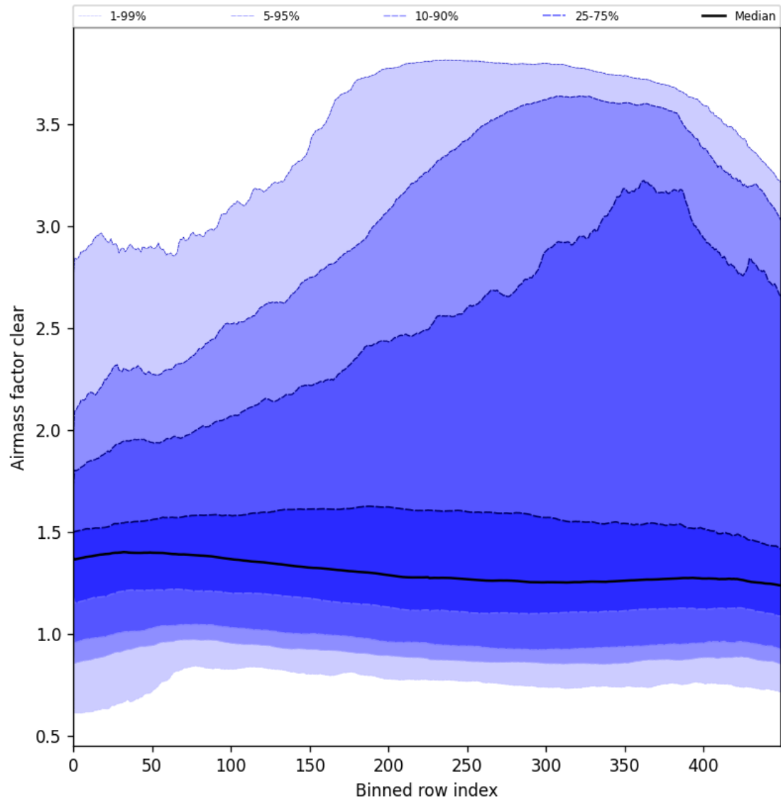
Figure 56: Along track statistics of “Airmass factor clear” for 2025-05-13 to 2025-05-15
