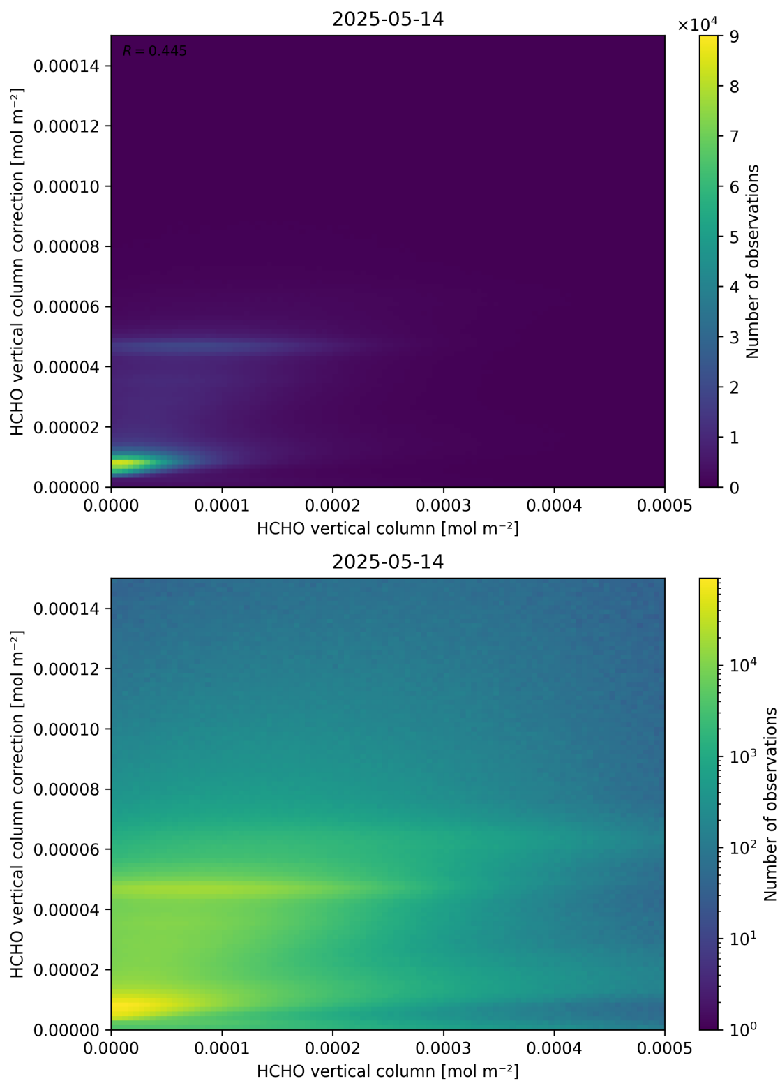
Figure 133: Scatter density plot of “HCHO vertical column” against “HCHO vertical column correction” for 2025-05-13 to 2025-05-15.
