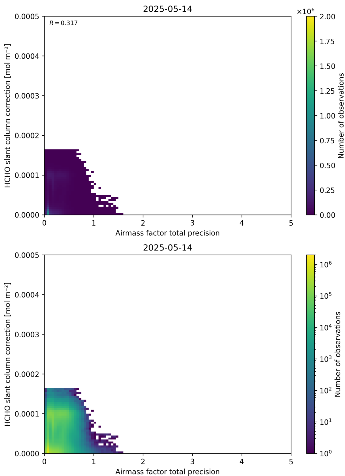
Figure 110: Scatter density plot of “Airmass factor total precision” against “HCHO slant column correction” for 2025-05-13 to 2025-05-15.
