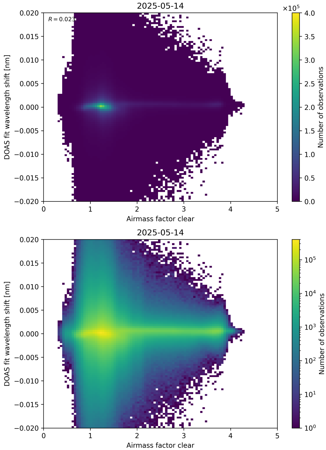
Figure 72: Scatter density plot of “Airmass factor clear” against “DOAS fit wavelength shift” for 2025-05-13 to 2025-05-15.
