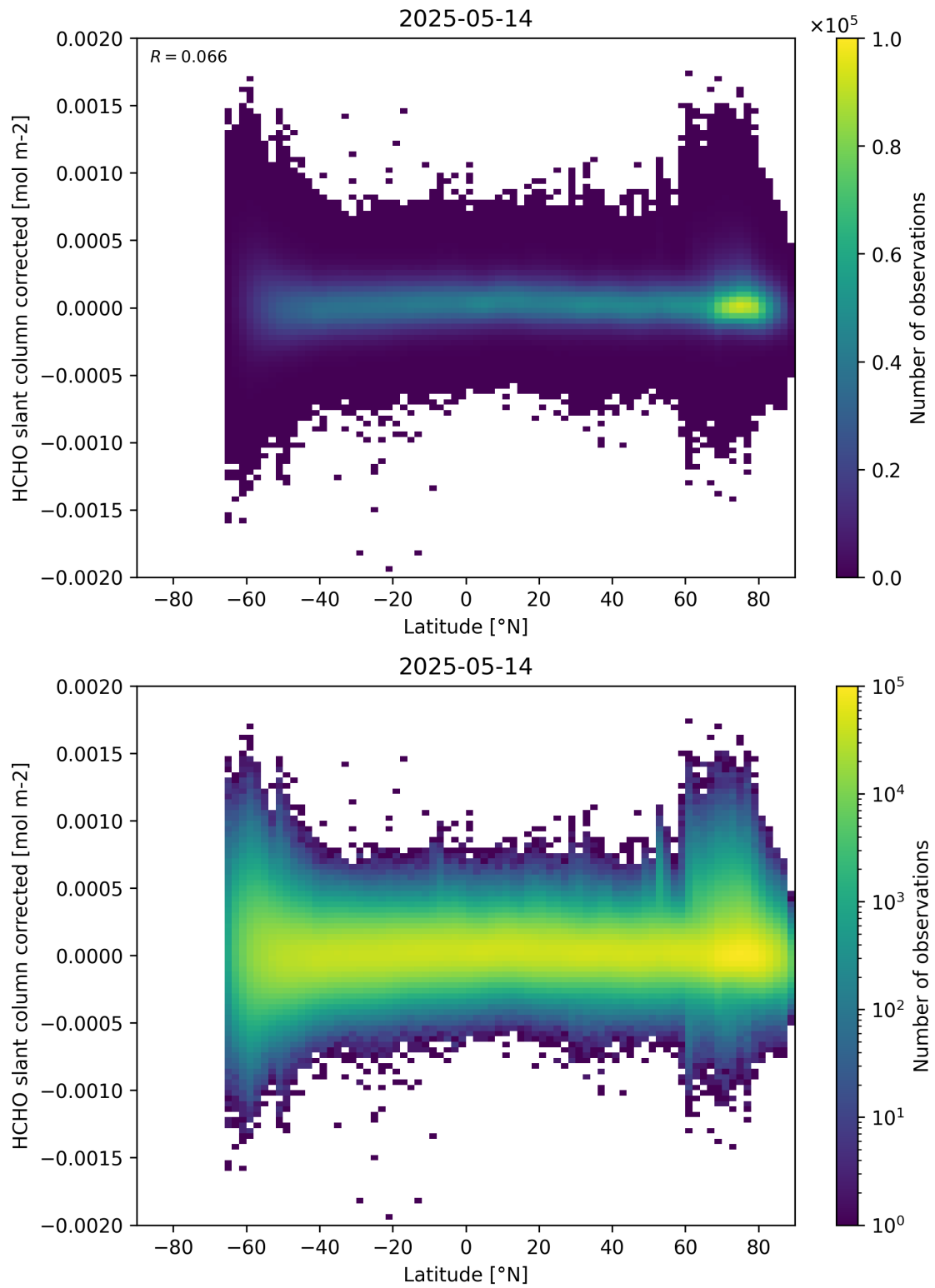
Figure 157: Scatter density plot of “Latitude” against “HCHO slant column corrected” for 2025-05-13 to 2025-05-15.
