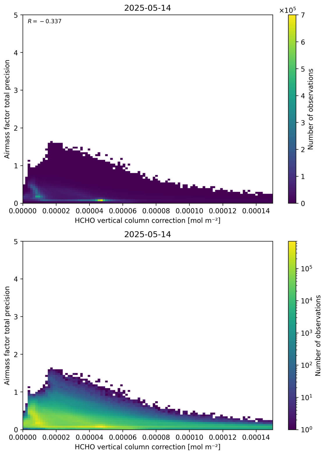
Figure 121: Scatter density plot of “HCHO vertical column correction” against “Airmass factor total precision” for 2025-05-13 to 2025-05-15.
