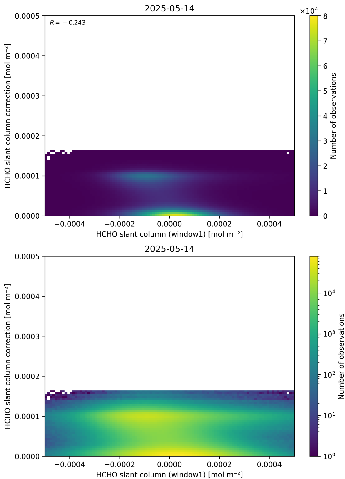
Figure 83: Scatter density plot of “HCHO slant column (window1)” against “HCHO slant column correction” for 2025-05-13 to 2025-05-15.
