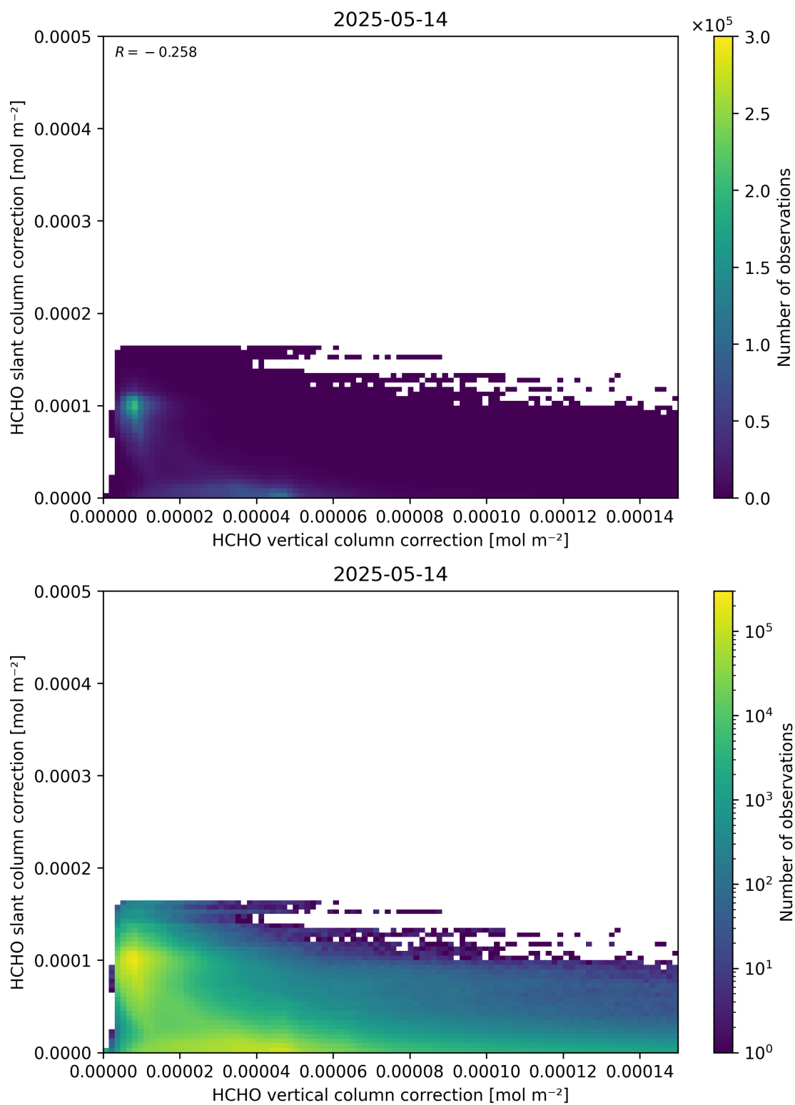
Figure 117: Scatter density plot of “HCHO vertical column correction” against “HCHO slant column correction” for 2025-05-13 to 2025-05-15.
