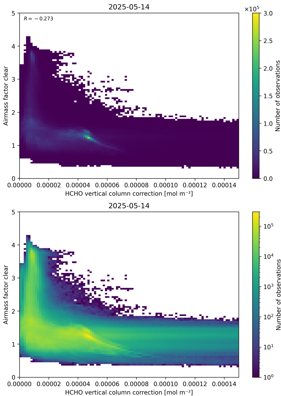
Figure 115: Scatter density plot of “HCHO vertical column correction” against “Airmass factor clear” for 2025-05-13 to 2025-05-15.
