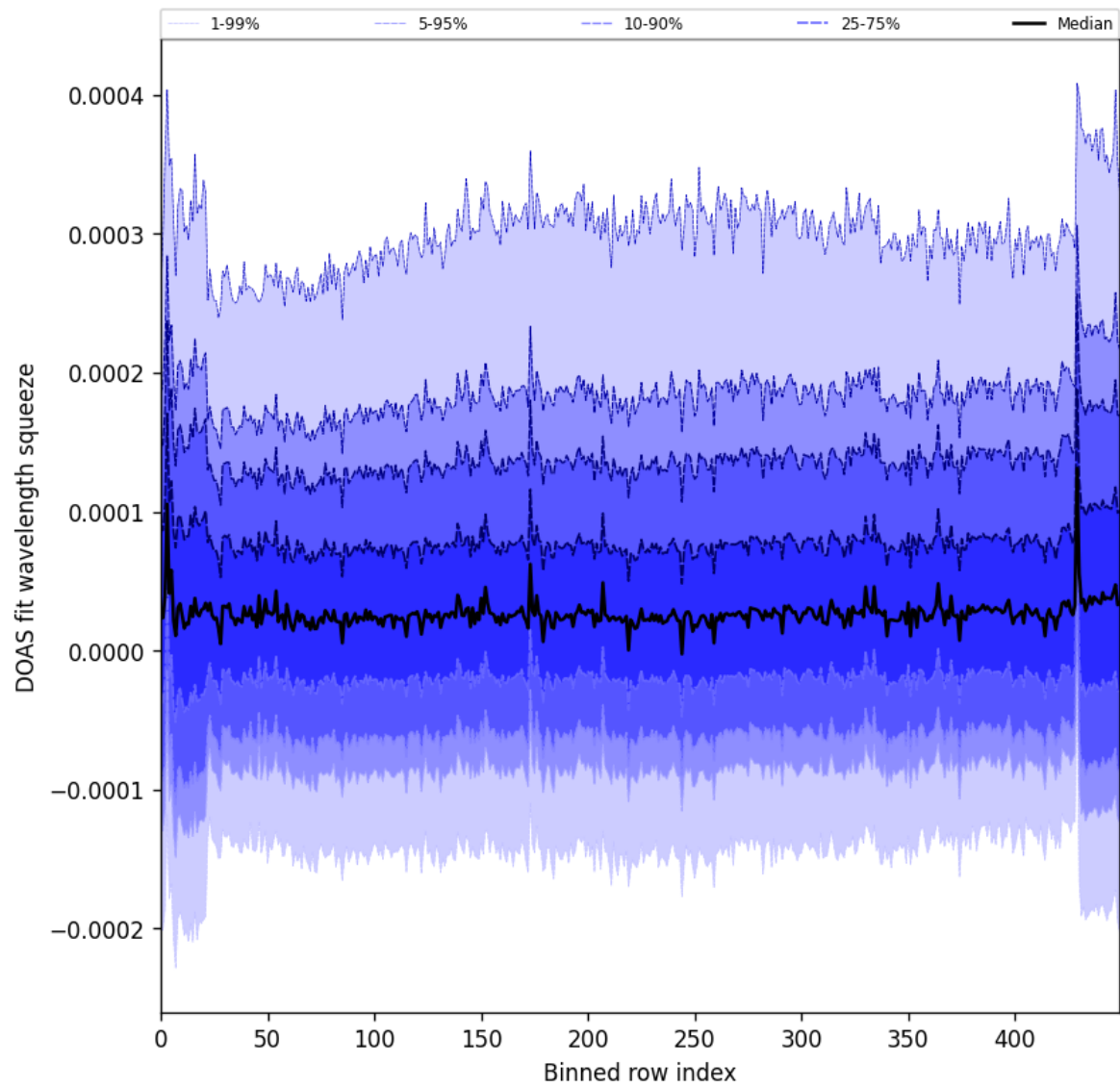
Figure 59: Along track statistics of “DOAS fit wavelength squeeze” for 2025-05-13 to 2025-05-15
