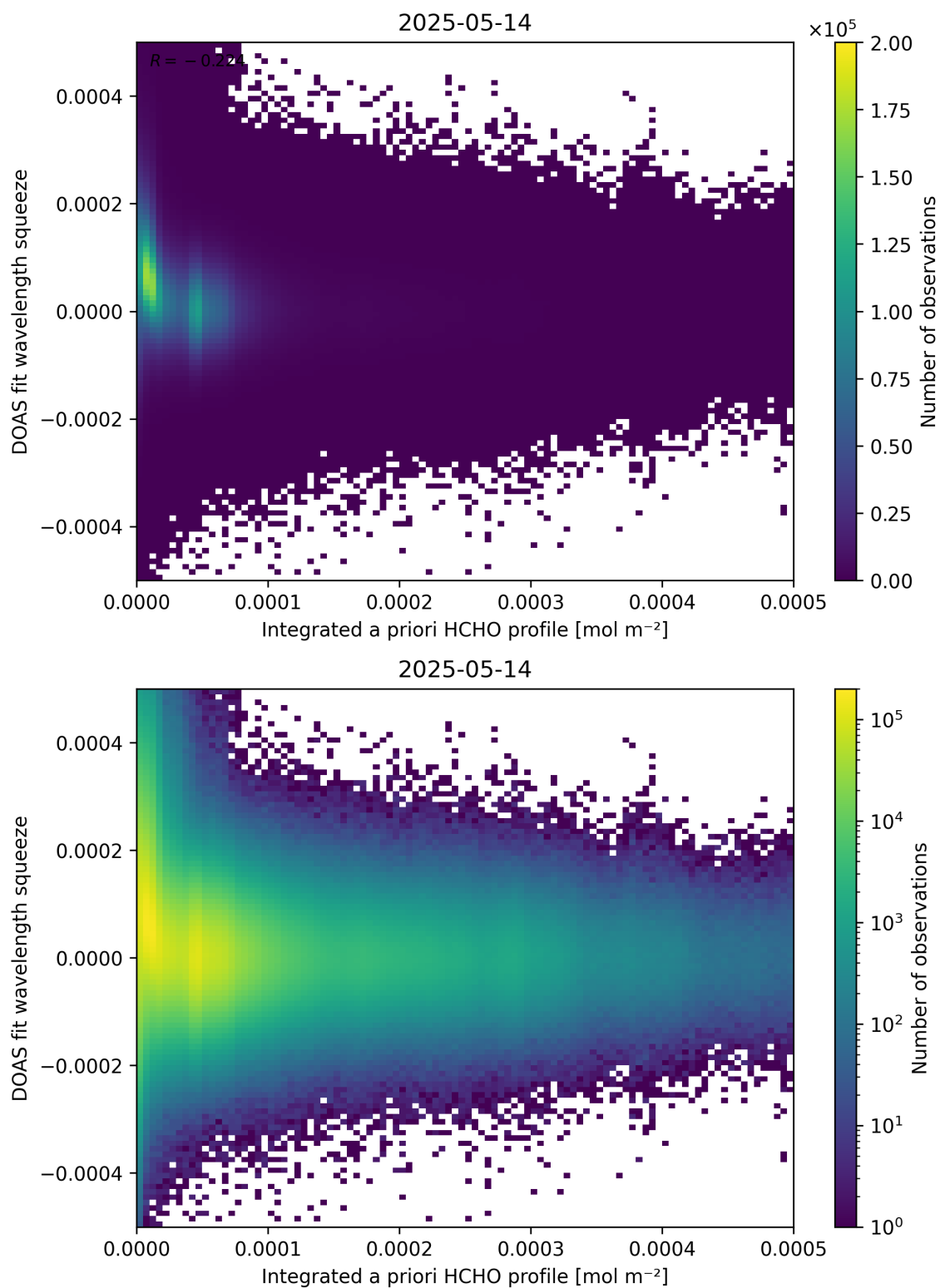
Figure 150: Scatter density plot of “Integrated a priori HCHO profile” against “DOAS fit wavelength squeeze” for 2025-05-13 to 2025-05-15.
