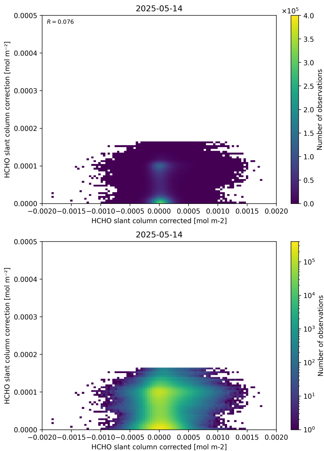
Figure 77: Scatter density plot of “HCHO slant column corrected” against “HCHO slant column correction” for 2025-05-13 to 2025-05-15.
