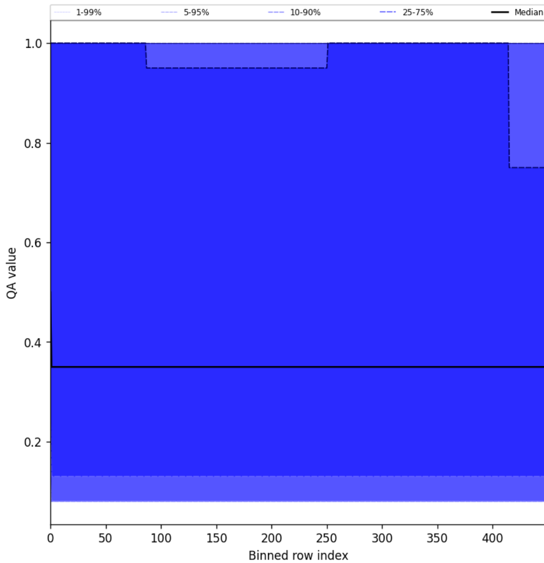
Figure 48: Along track statistics of “QA value” for 2025-05-13 to 2025-05-15
