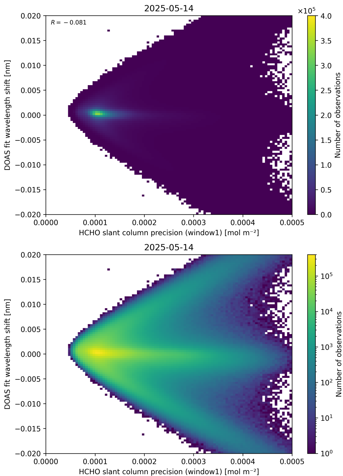
Figure 89: Scatter density plot of “HCHO slant column precision (window1)” against “DOAS fit wavelength shift” for 2025-05-13 to 2025-05-15.
