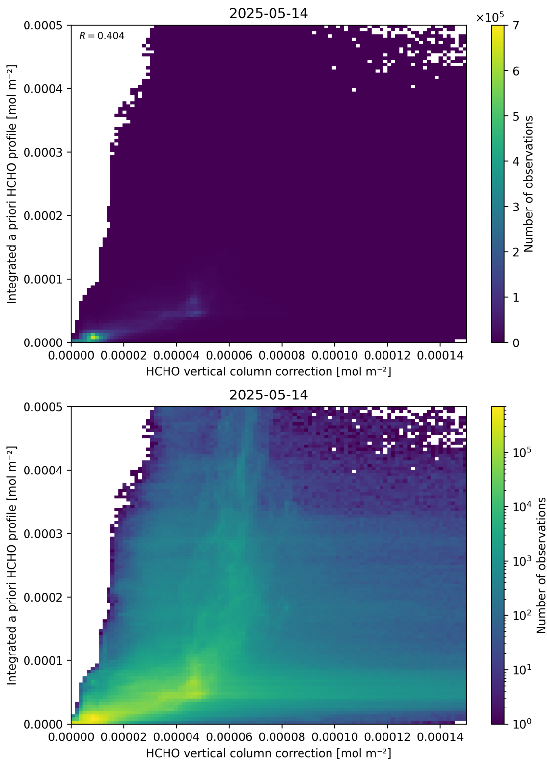
Figure 122: Scatter density plot of “HCHO vertical column correction” against “Integrated a priori HCHO profile” for 2025-05-13 to 2025-05-15.
