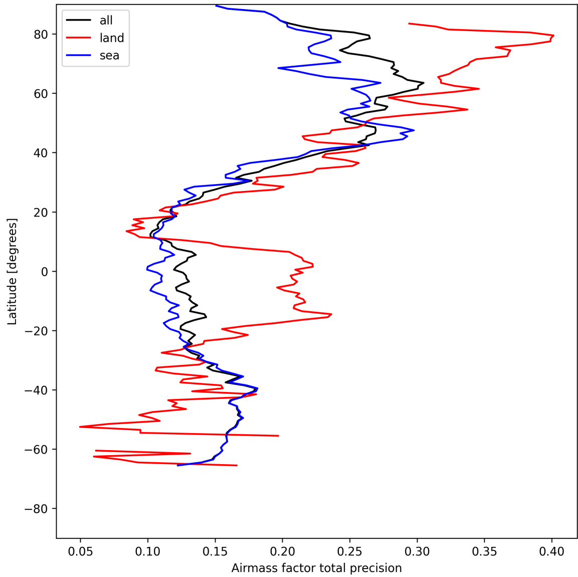
Figure 27: Zonal average of “Airmass factor total precision” for 2025-05-13 to 2025-05-15.
