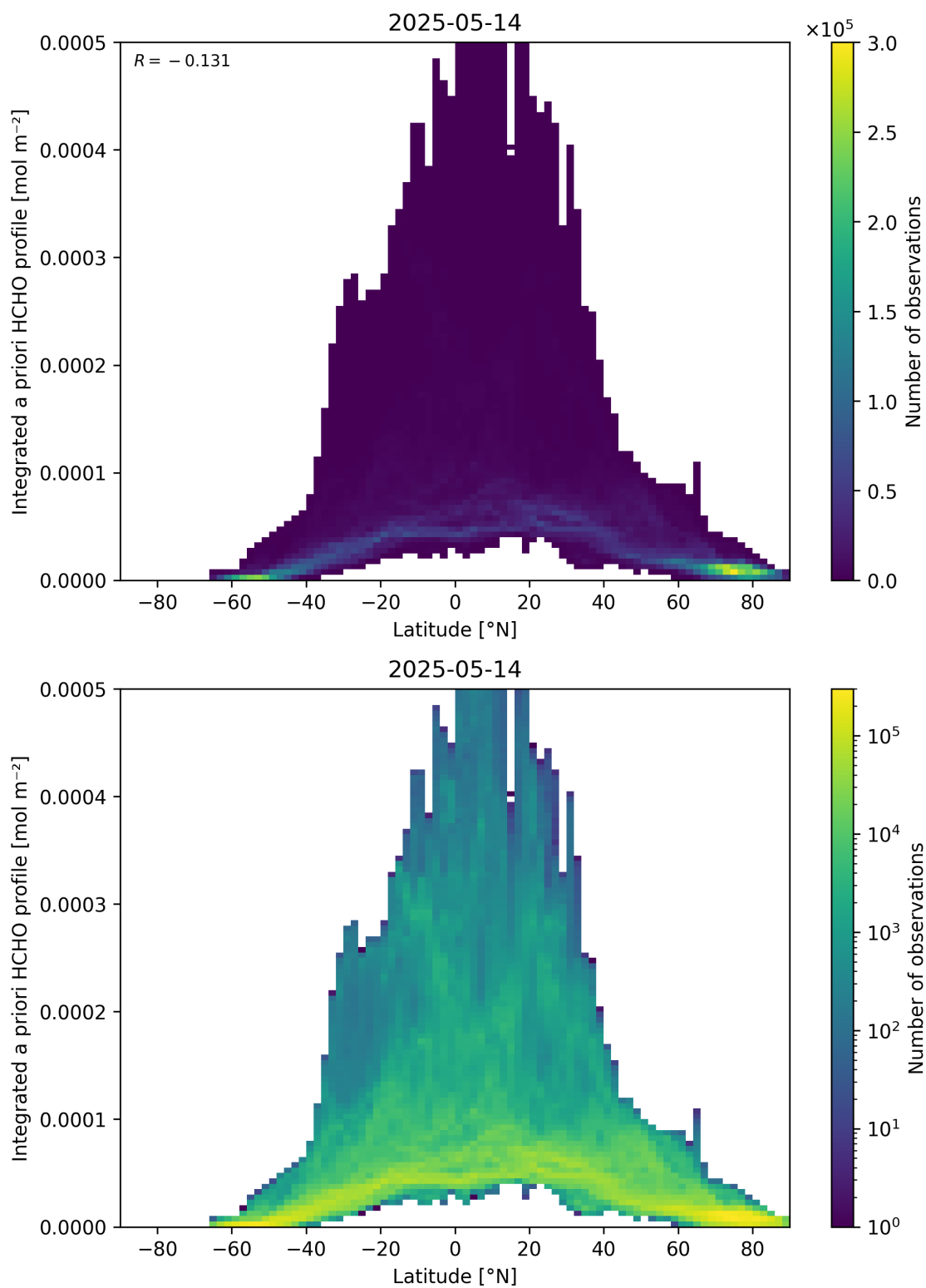
Figure 166: Scatter density plot of “Latitude” against “Integrated a priori HCHO profile” for 2025-05-13 to 2025-05-15.
