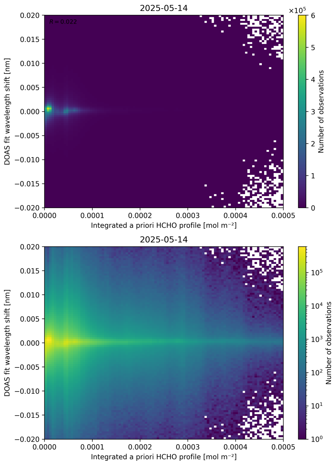
Figure 149: Scatter density plot of “Integrated a priori HCHO profile” against “DOAS fit wavelength shift” for 2025-05-13 to 2025-05-15.
