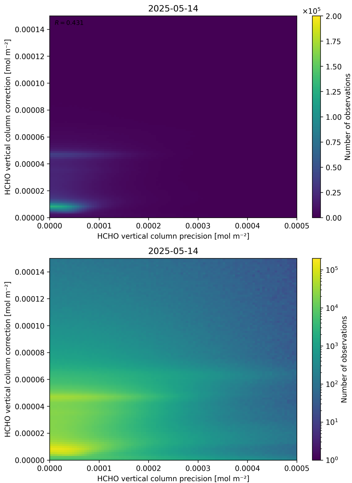
Figure 146: Scatter density plot of “HCHO vertical column precision” against “HCHO vertical column correction” for 2025-05-13 to 2025-05-15.
