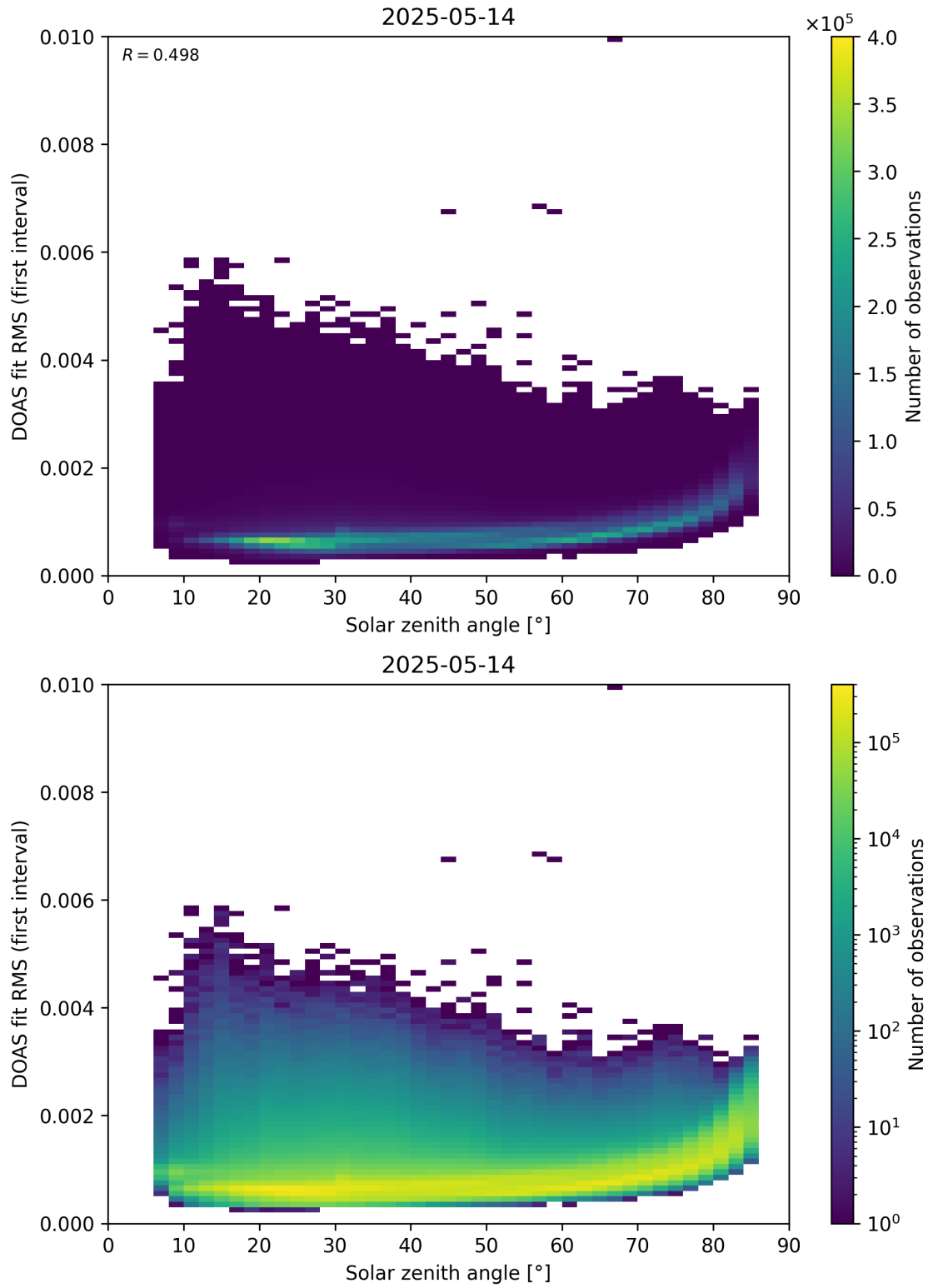
Figure 167: Scatter density plot of “Solar zenith angle” against “DOAS fit RMS (first interval)” for 2025-05-13 to 2025-05-15.
