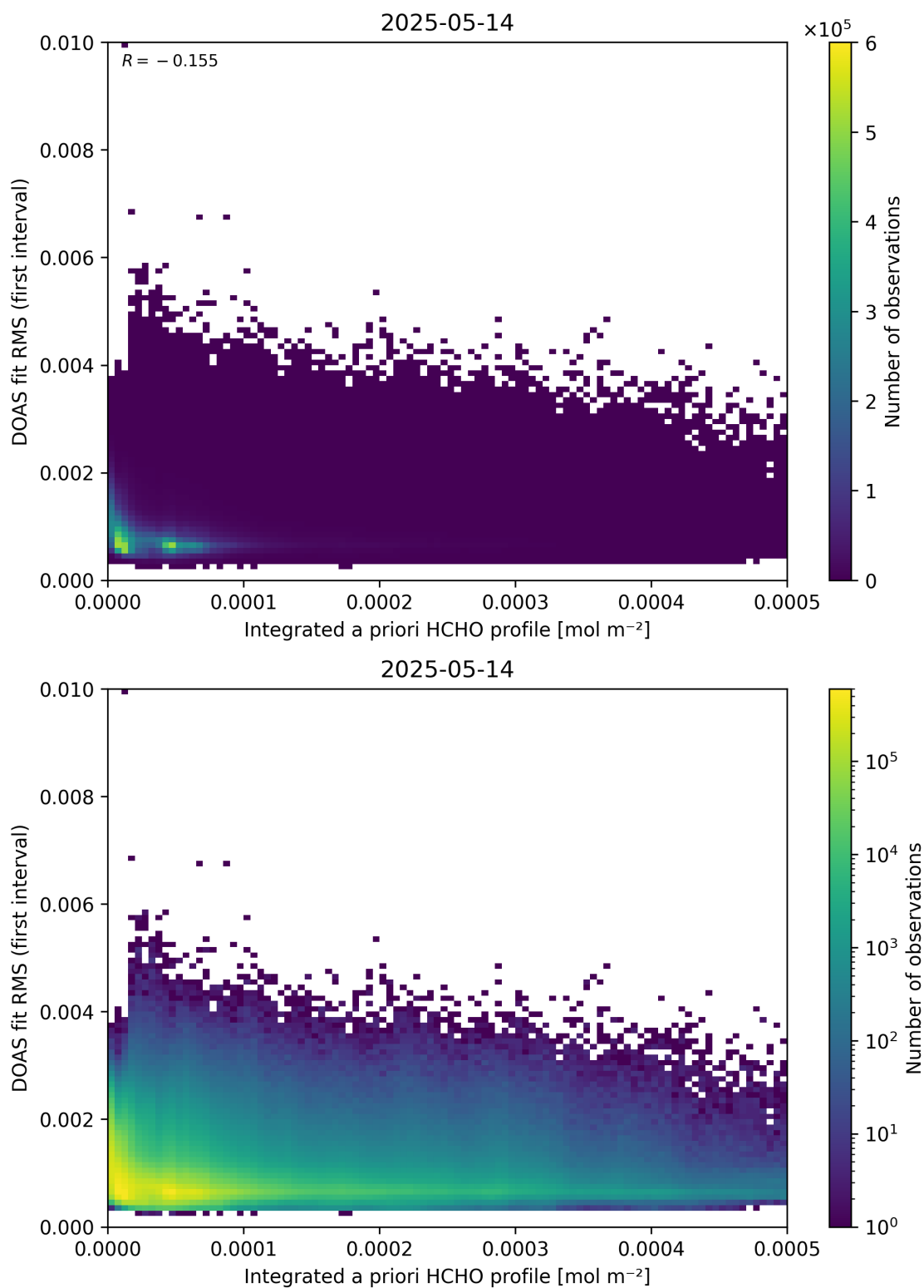
Figure 148: Scatter density plot of “Integrated a priori HCHO profile” against “DOAS fit RMS (first interval)” for 2025-05-13 to 2025-05-15.
