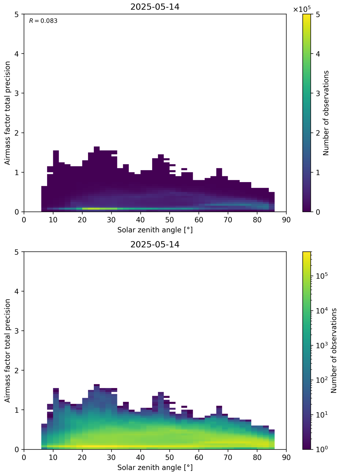
Figure 176: Scatter density plot of “Solar zenith angle” against “Airmass factor total precision” for 2025-05-13 to 2025-05-15.
