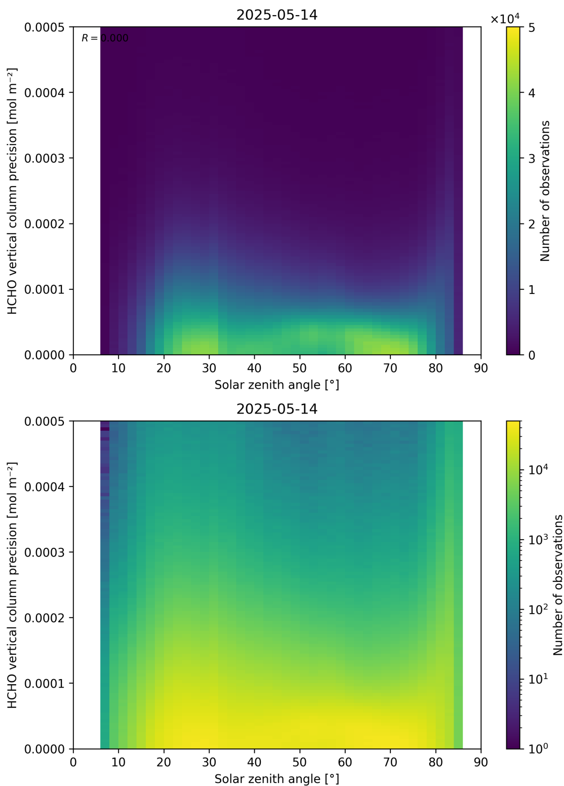
Figure 179: Scatter density plot of “Solar zenith angle” against “HCHO vertical column precision” for 2025-05-13 to 2025-05-15.
