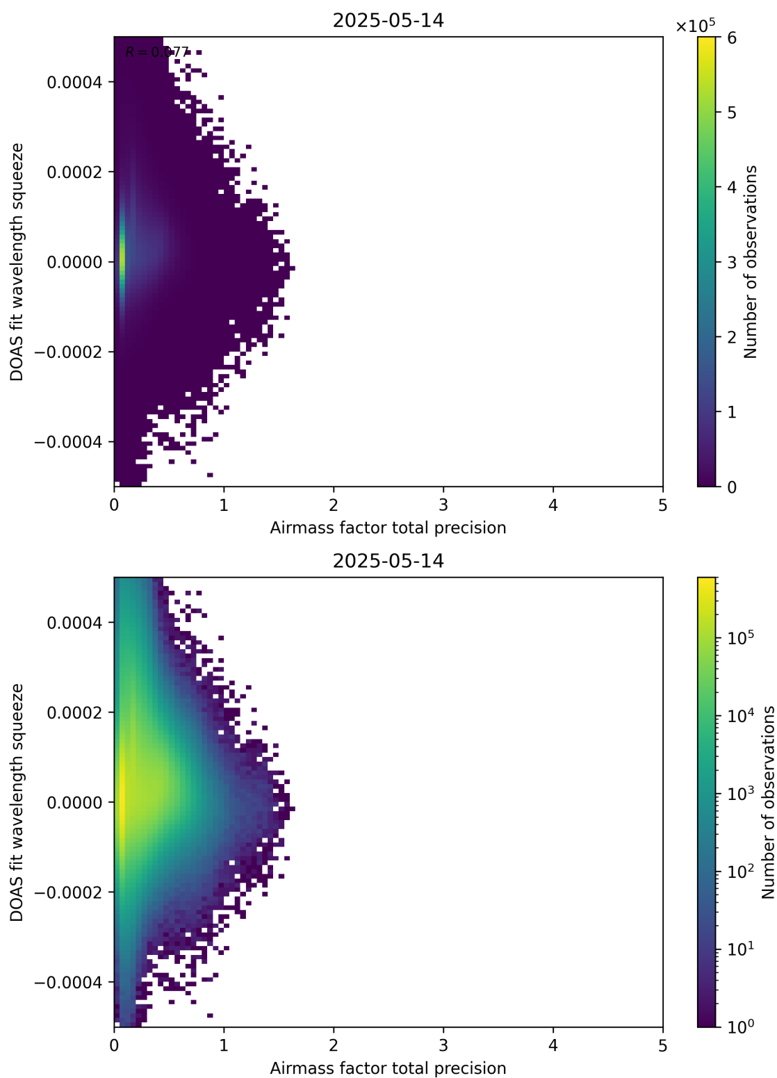
Figure 107: Scatter density plot of “Airmass factor total precision” against “DOAS fit wavelength squeeze” for 2025-05-13 to 2025-05-15.
