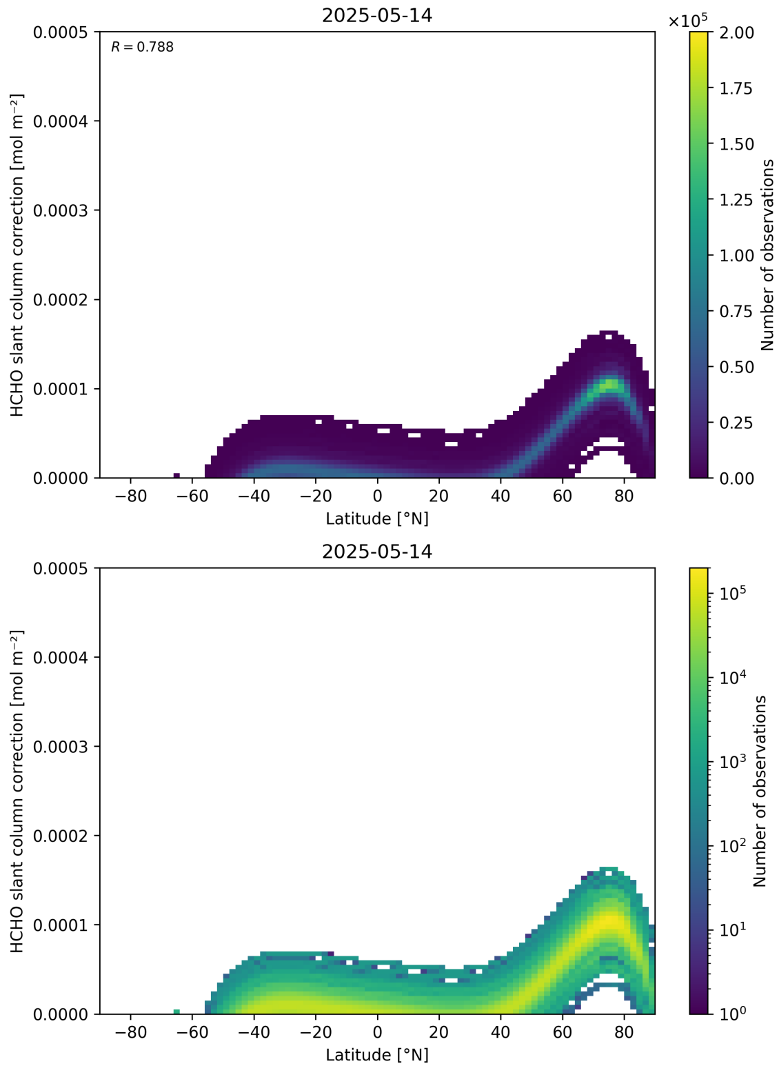
Figure 158: Scatter density plot of “Latitude” against “HCHO slant column correction” for 2025-05-13 to 2025-05-15.
