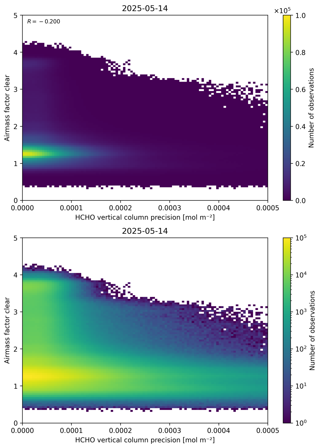
Figure 139: Scatter density plot of “HCHO vertical column precision” against “Airmass factor clear” for 2025-05-13 to 2025-05-15.
