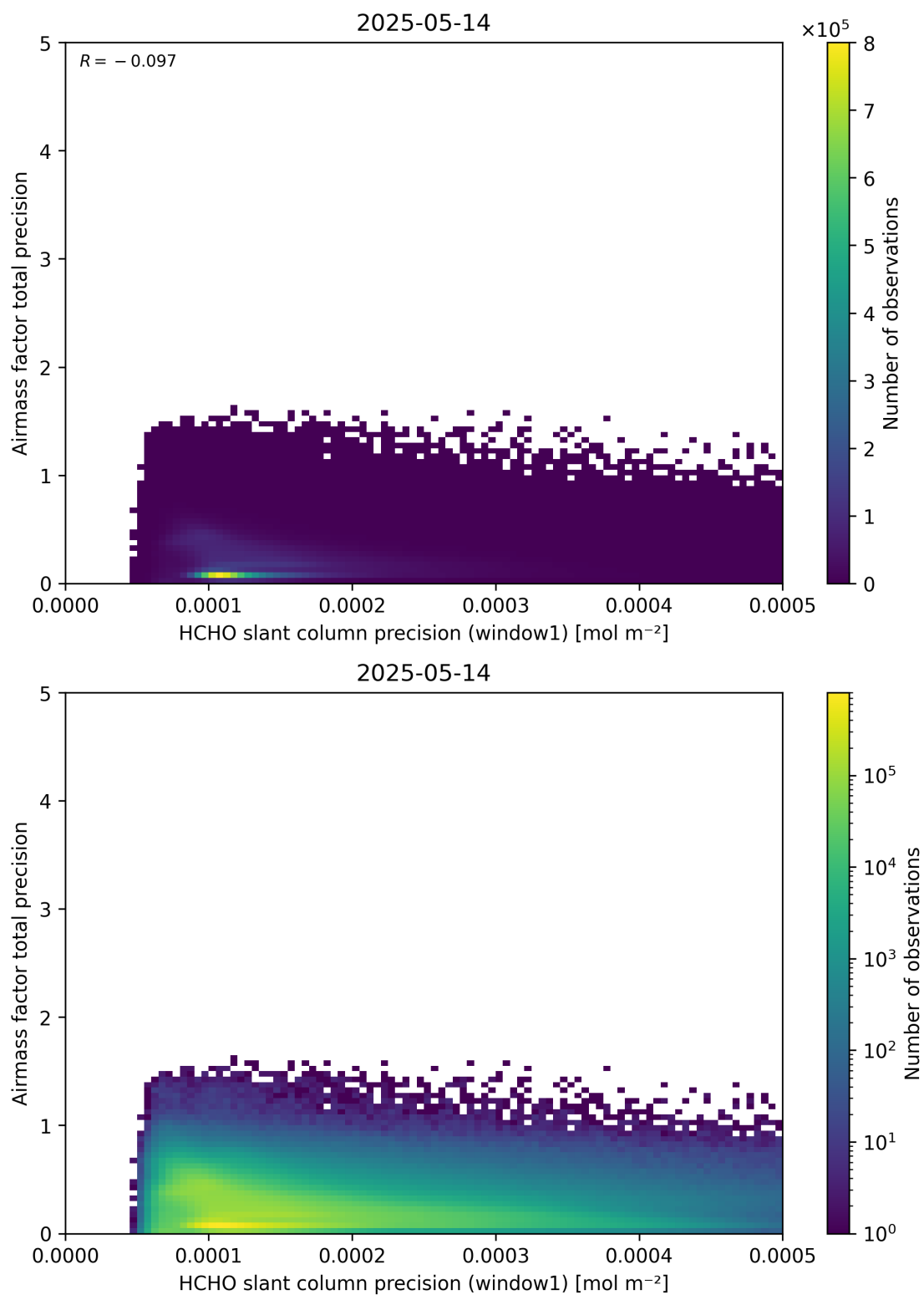
Figure 95: Scatter density plot of “HCHO slant column precision (window1)” against “Airmass factor total precision” for 2025-05-13 to 2025-05-15.
