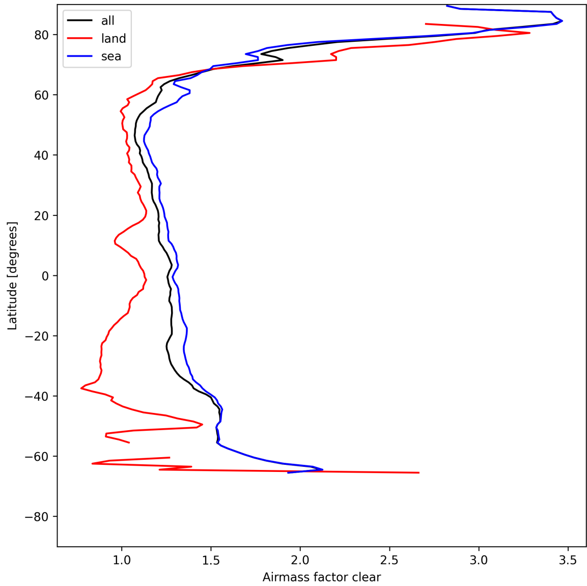
Figure 28: Zonal average of “Airmass factor clear” for 2025-05-13 to 2025-05-15.
