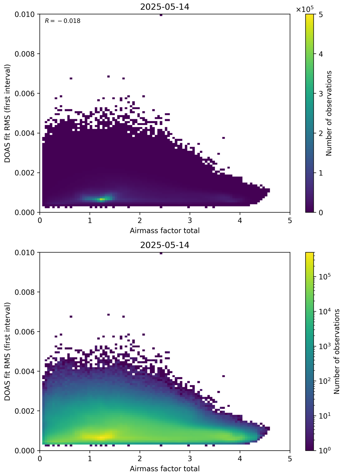
Figure 97: Scatter density plot of “Airmass factor total” against “DOAS fit RMS (first interval)” for 2025-05-13 to 2025-05-15.
