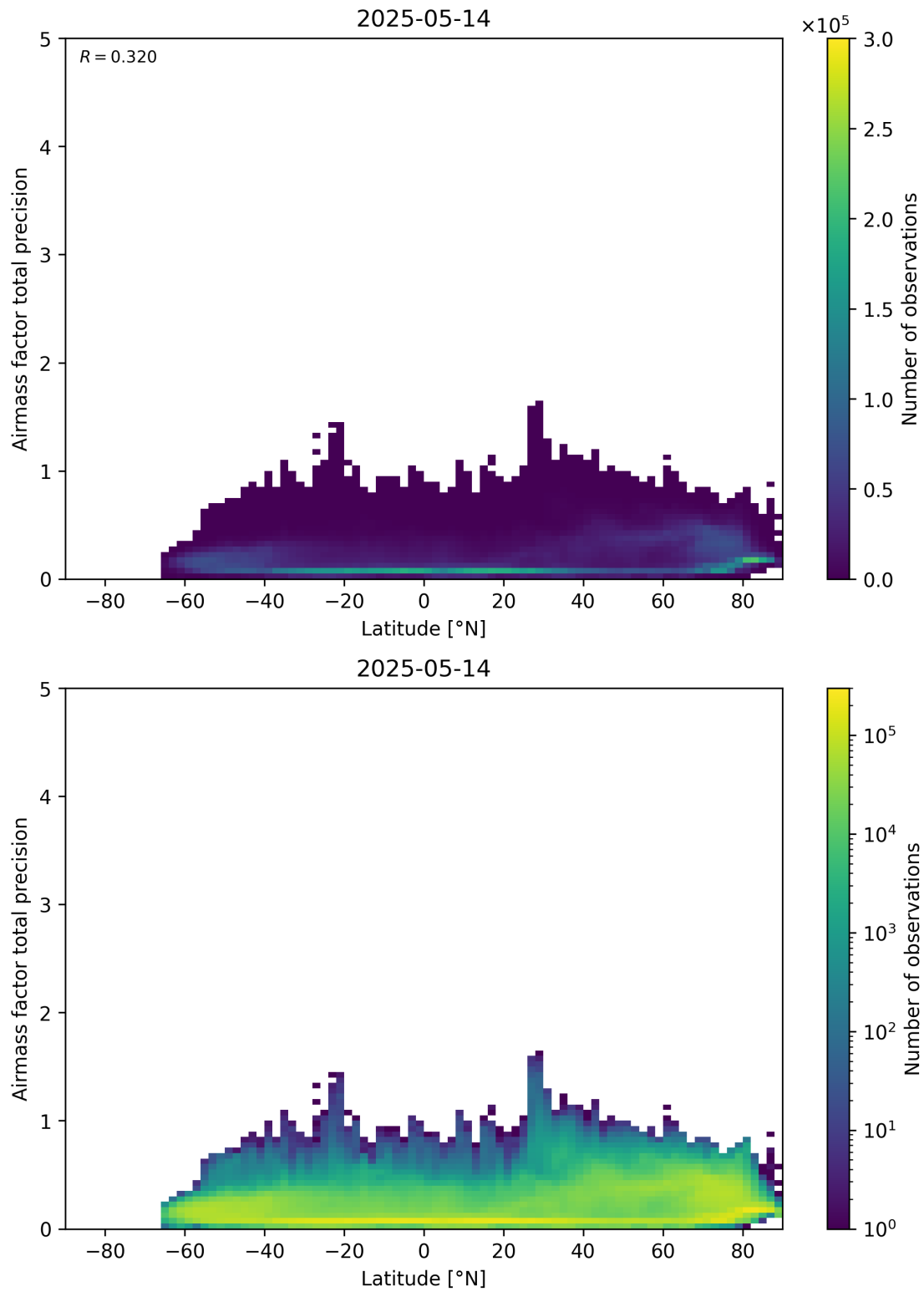
Figure 162: Scatter density plot of “Latitude” against “Airmass factor total precision” for 2025-05-13 to 2025-05-15.
