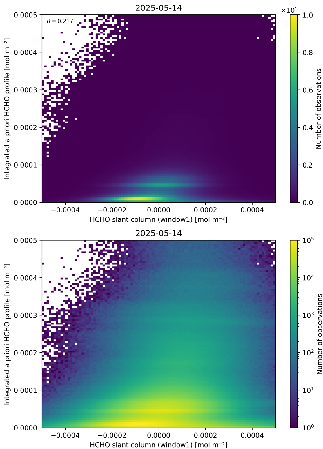
Figure 87: Scatter density plot of “HCHO slant column (window1)” against “Integrated a priori HCHO profile” for 2025-05-13 to 2025-05-15.
