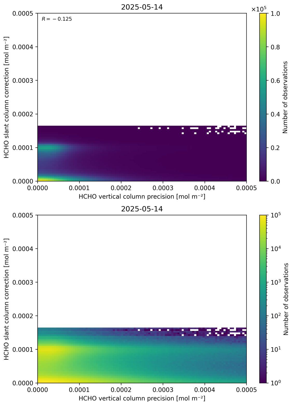
Figure 141: Scatter density plot of “HCHO vertical column precision” against “HCHO slant column correction” for 2025-05-13 to 2025-05-15.
