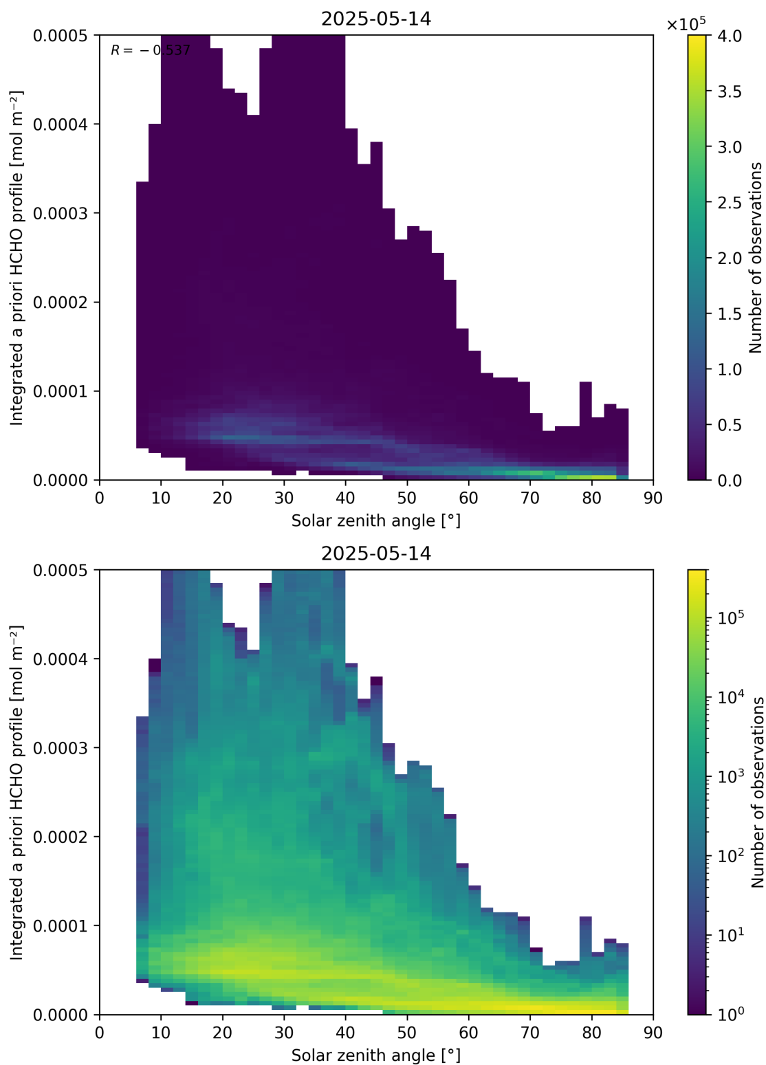
Figure 180: Scatter density plot of “Solar zenith angle” against “Integrated a priori HCHO profile” for 2025-05-13 to 2025-05-15.
