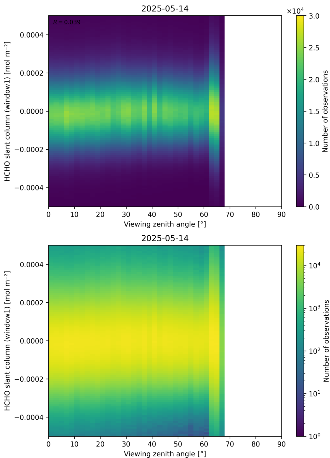
Figure 188: Scatter density plot of “Viewing zenith angle” against “HCHO slant column (window1)” for 2025-05-13 to 2025-05-15.
