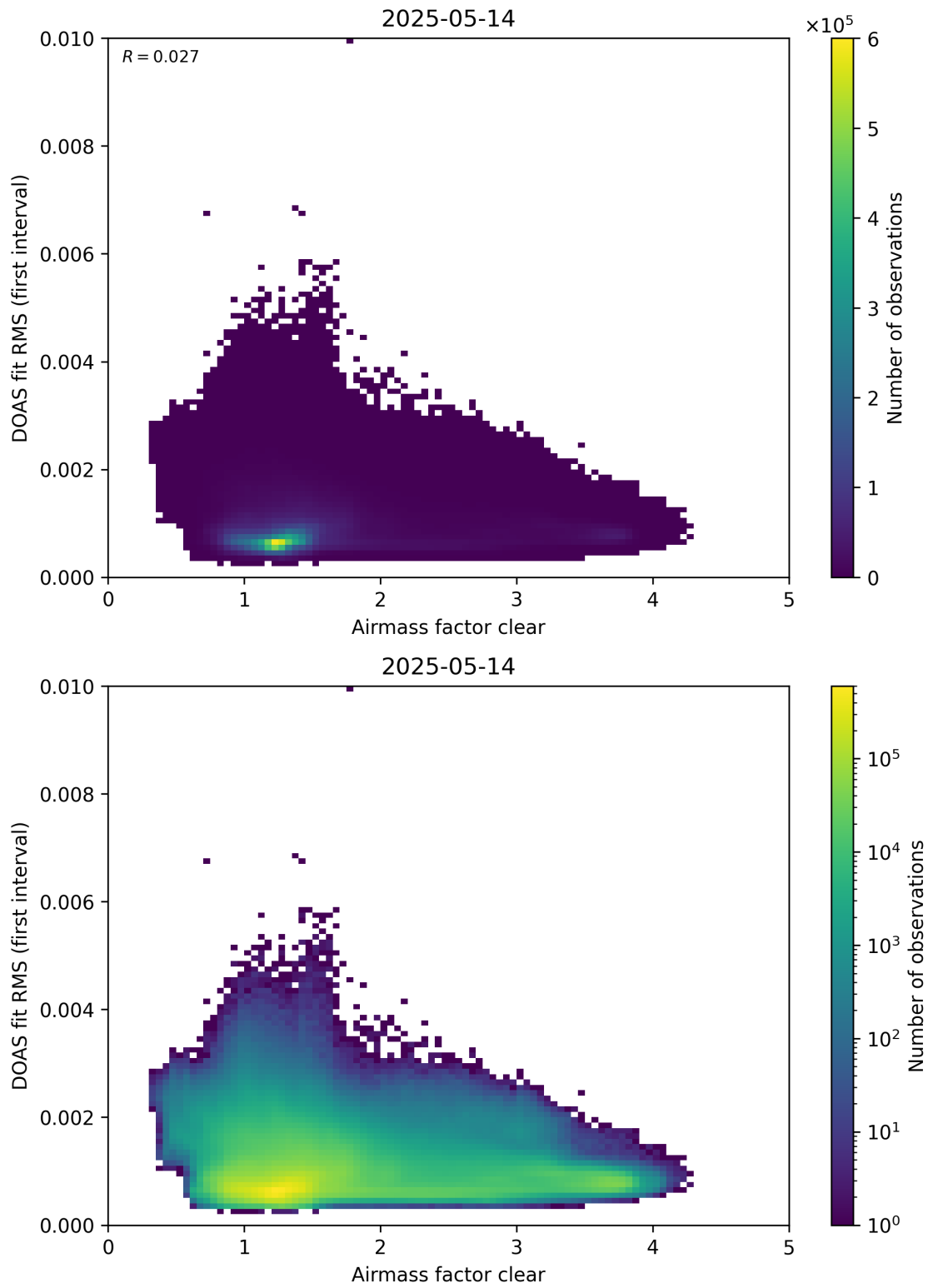
Figure 71: Scatter density plot of “Airmass factor clear” against “DOAS fit RMS (first interval)” for 2025-05-13 to 2025-05-15.
