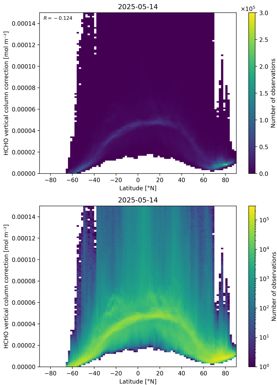
Figure 164: Scatter density plot of “Latitude” against “HCHO vertical column correction” for 2025-05-13 to 2025-05-15.
