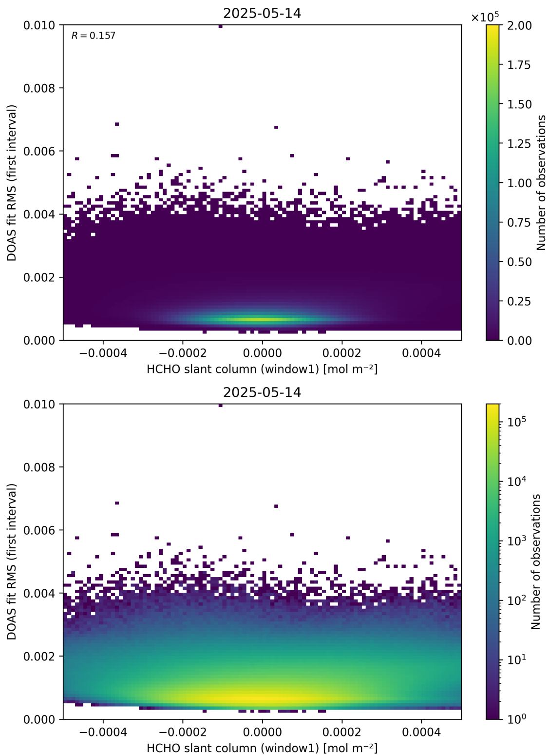
Figure 78: Scatter density plot of “HCHO slant column (window1)” against “DOAS fit RMS (first interval)” for 2025-05-13 to 2025-05-15.
