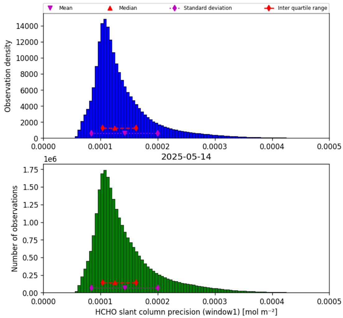
Figure 39: Histogram of “HCHO slant column precision (window1)” for 2025-05-13 to 2025-05-15
