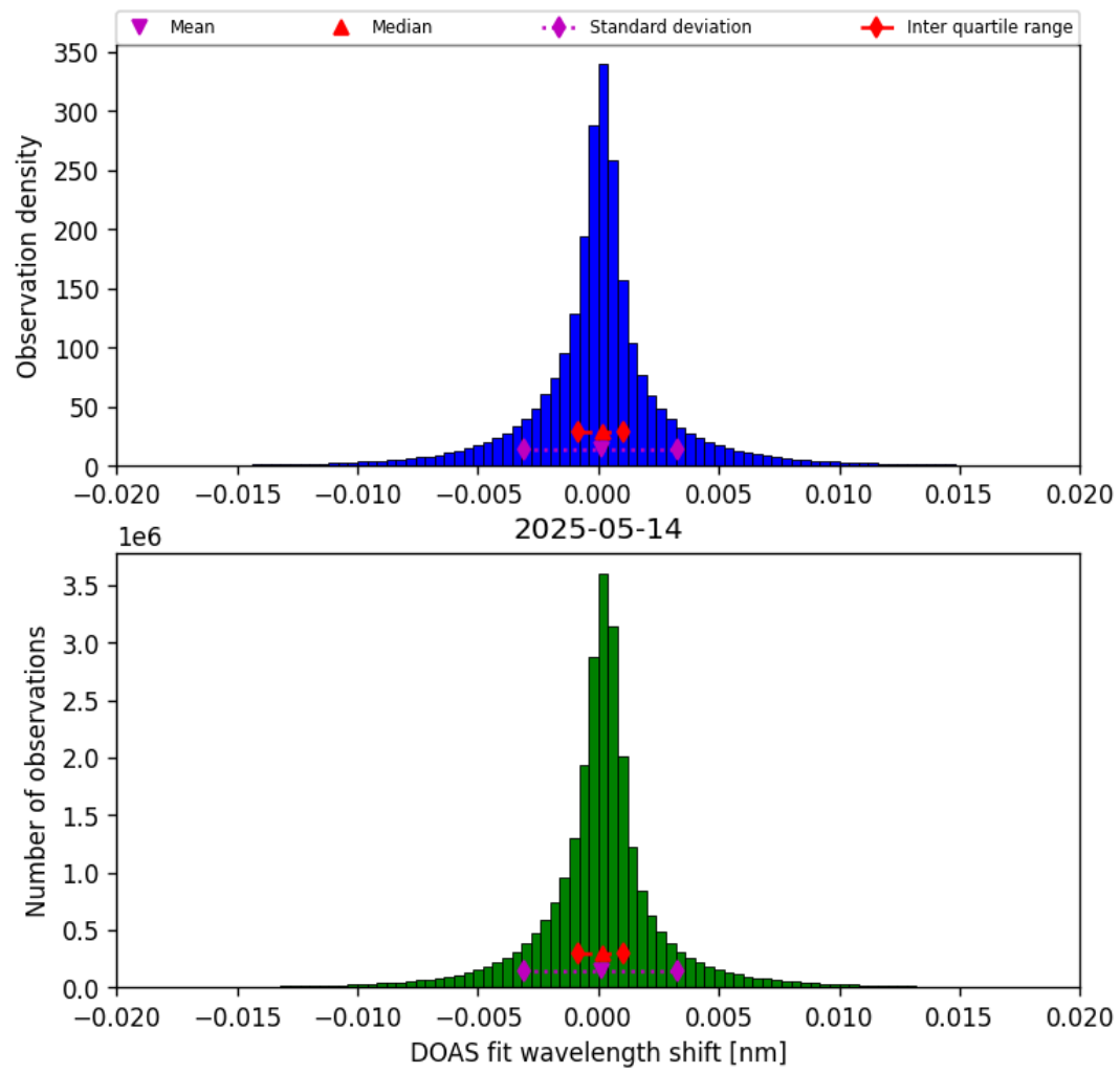
Figure 44: Histogram of “DOAS fit wavelength shift” for 2025-05-13 to 2025-05-15
