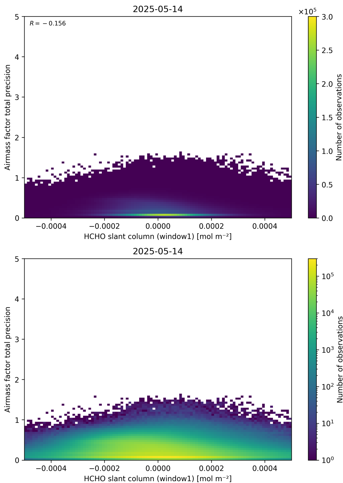
Figure 86: Scatter density plot of “HCHO slant column (window1)” against “Airmass factor total precision” for 2025-05-13 to 2025-05-15.
