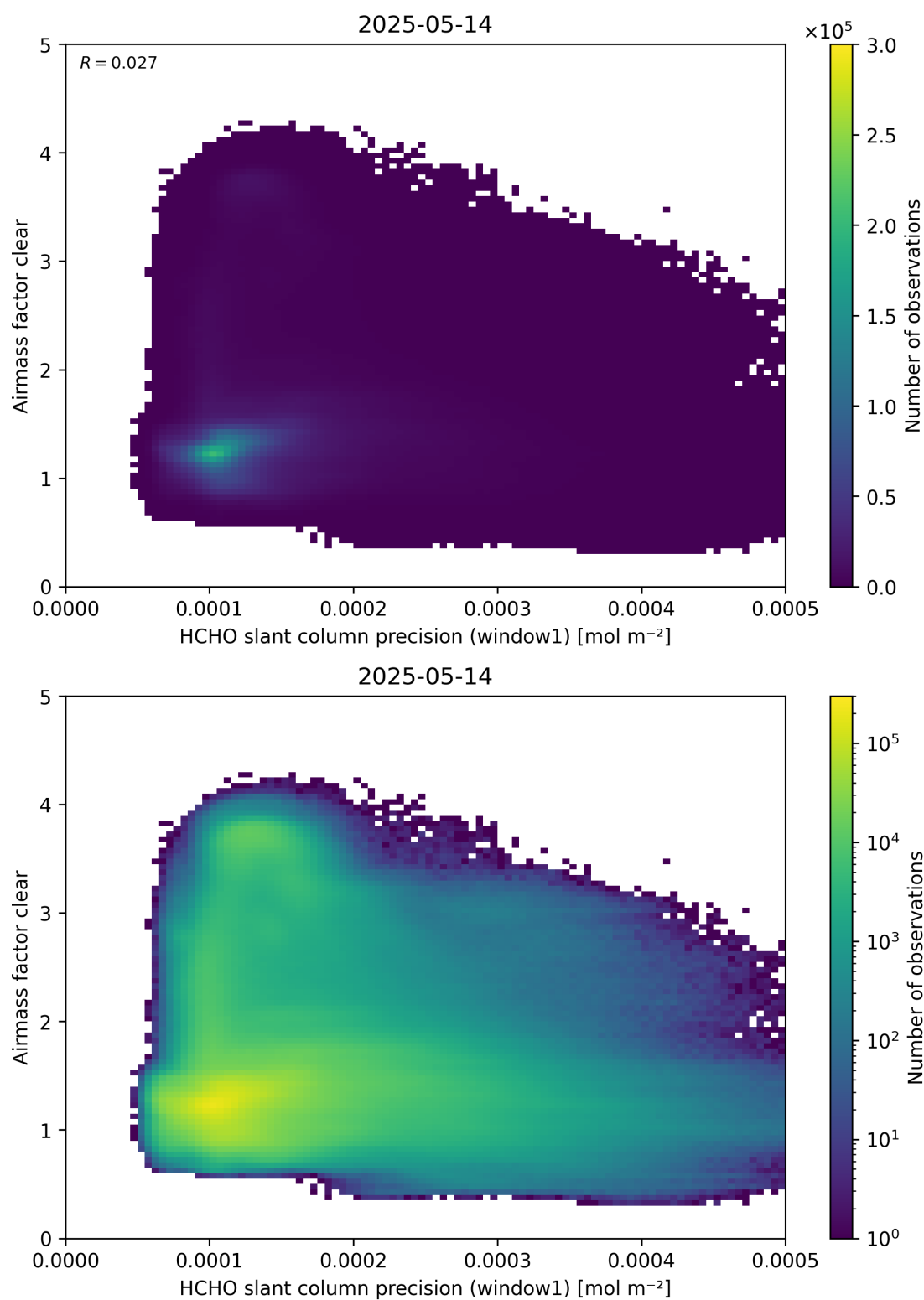
Figure 91: Scatter density plot of “HCHO slant column precision (window1)” against “Airmass factor clear” for 2025-05-13 to 2025-05-15.
