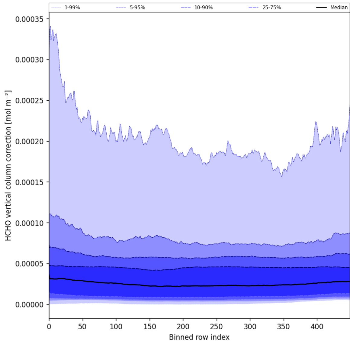
Figure 51: Along track statistics of “HCHO vertical column correction” for 2025-05-13 to 2025-05-15
