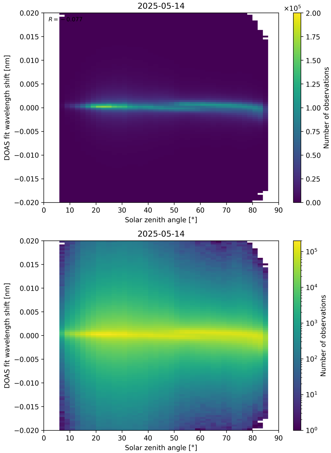
Figure 168: Scatter density plot of “Solar zenith angle” against “DOAS fit wavelength shift” for 2025-05-13 to 2025-05-15.
