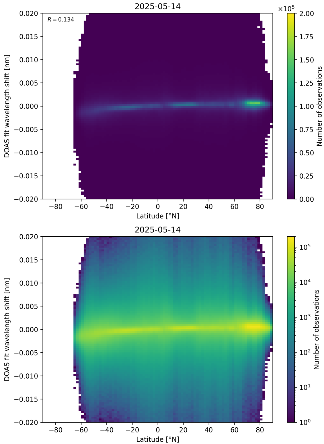
Figure 154: Scatter density plot of “Latitude” against “DOAS fit wavelength shift” for 2025-05-13 to 2025-05-15.
