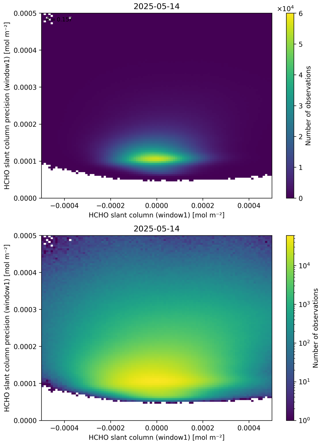
Figure 84: Scatter density plot of “HCHO slant column (window1)” against “HCHO slant column precision (window1)” for 2025-05-13 to 2025-05-15.
