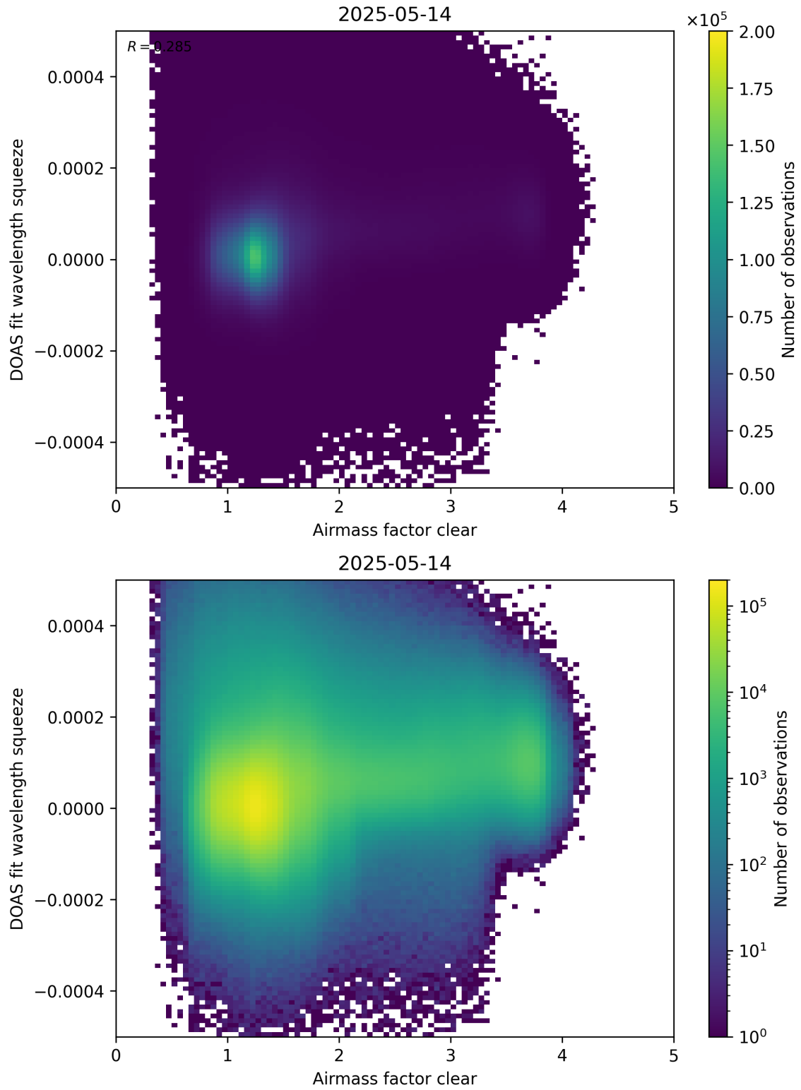
Figure 73: Scatter density plot of “Airmass factor clear” against “DOAS fit wavelength squeeze” for 2025-05-13 to 2025-05-15.
