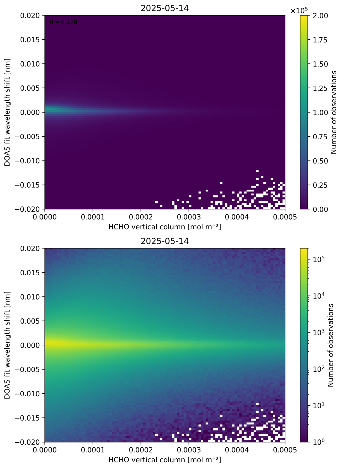
Figure 124: Scatter density plot of “HCHO vertical column” against “DOAS fit wavelength shift” for 2025-05-13 to 2025-05-15.
