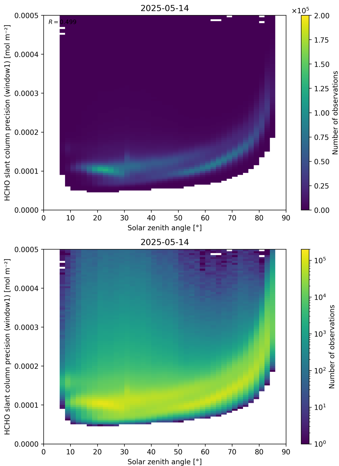
Figure 174: Scatter density plot of “Solar zenith angle” against “HCHO slant column precision (window1)” for 2025-05-13 to 2025-05-15.
