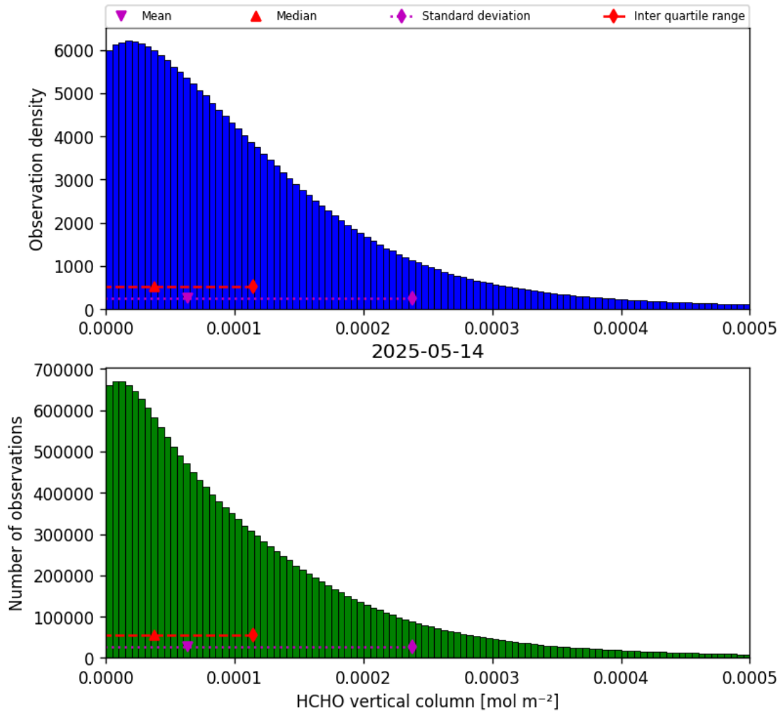
Figure 35: Histogram of “HCHO vertical column” for 2025-05-13 to 2025-05-15
