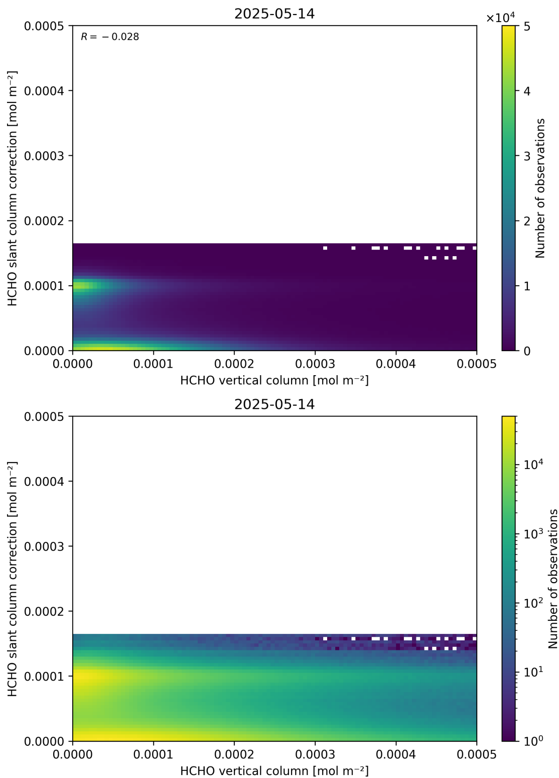
Figure 128: Scatter density plot of “HCHO vertical column” against “HCHO slant column correction” for 2025-05-13 to 2025-05-15.
