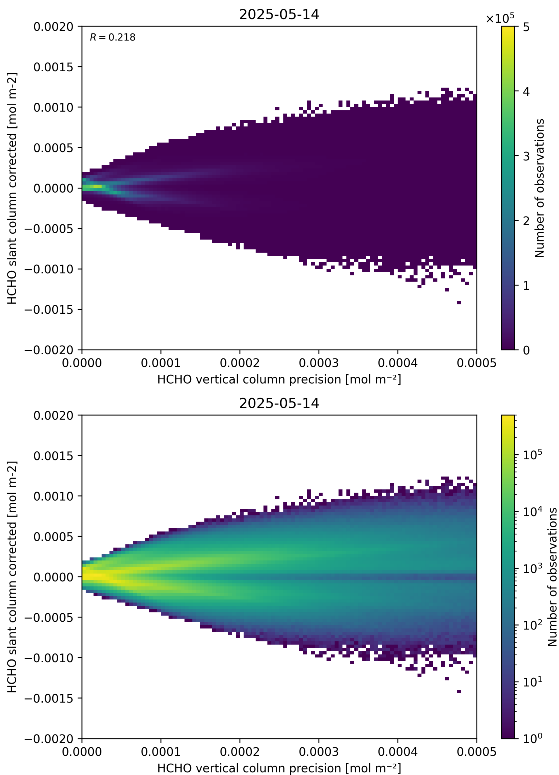
Figure 140: Scatter density plot of “HCHO vertical column precision” against “HCHO slant column corrected” for 2025-05-13 to 2025-05-15.
