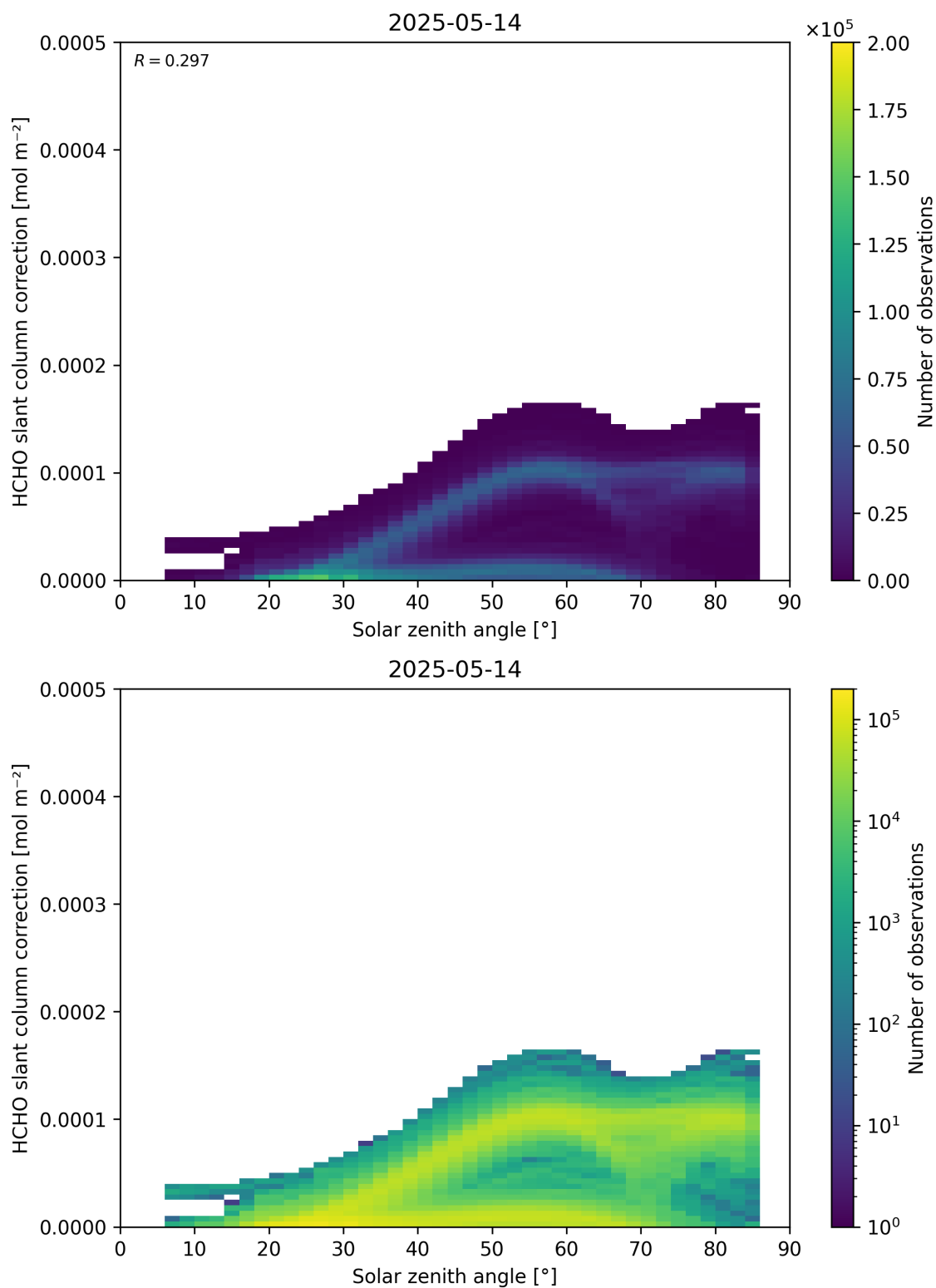
Figure 172: Scatter density plot of “Solar zenith angle” against “HCHO slant column correction” for 2025-05-13 to 2025-05-15.
