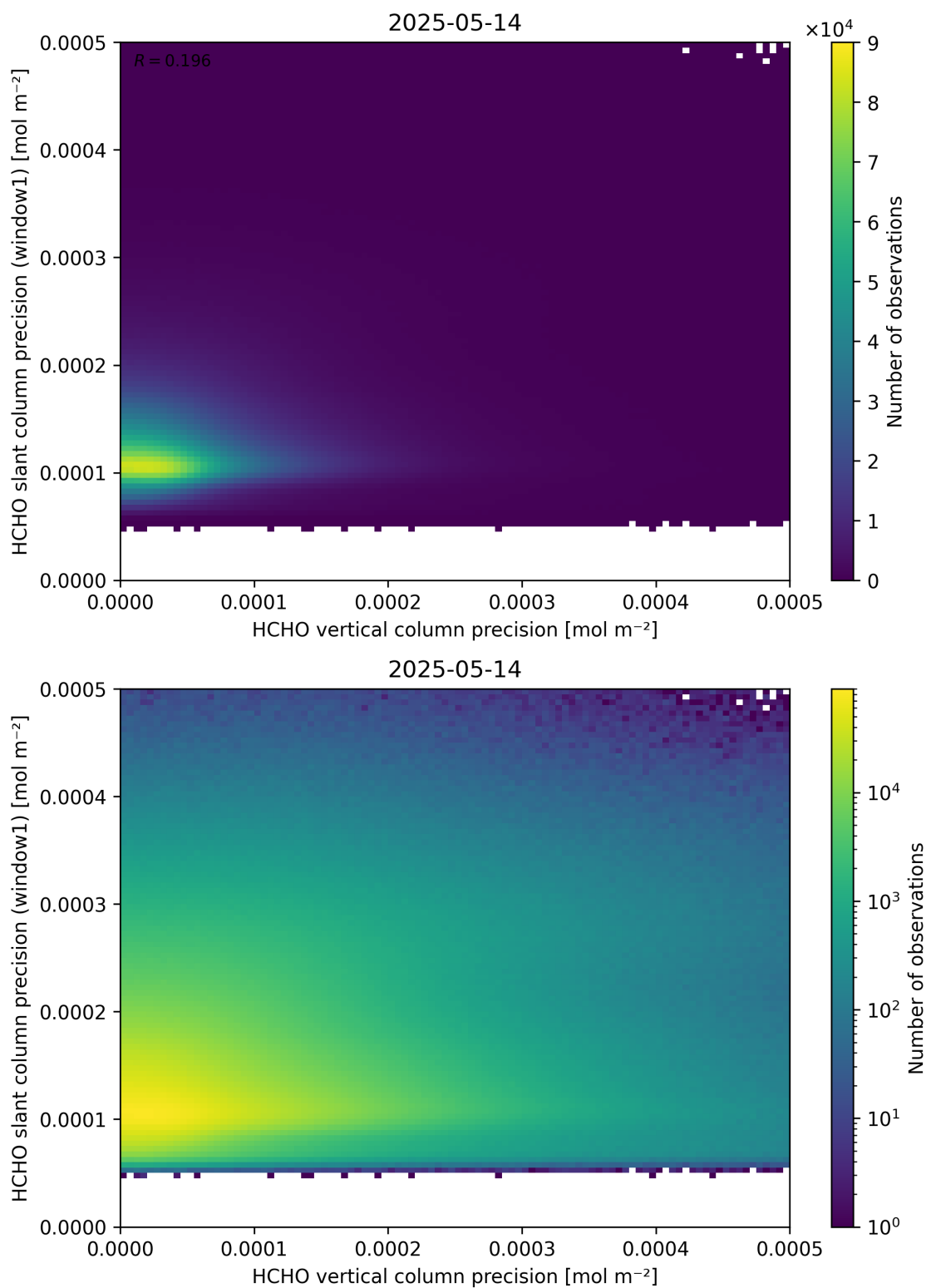
Figure 143: Scatter density plot of “HCHO vertical column precision” against “HCHO slant column precision (window1)” for 2025-05-13 to 2025-05-15.
