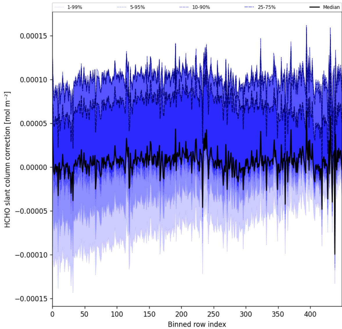
Figure 61: Along track statistics of “HCHO slant column correction” for 2025-05-13 to 2025-05-15
