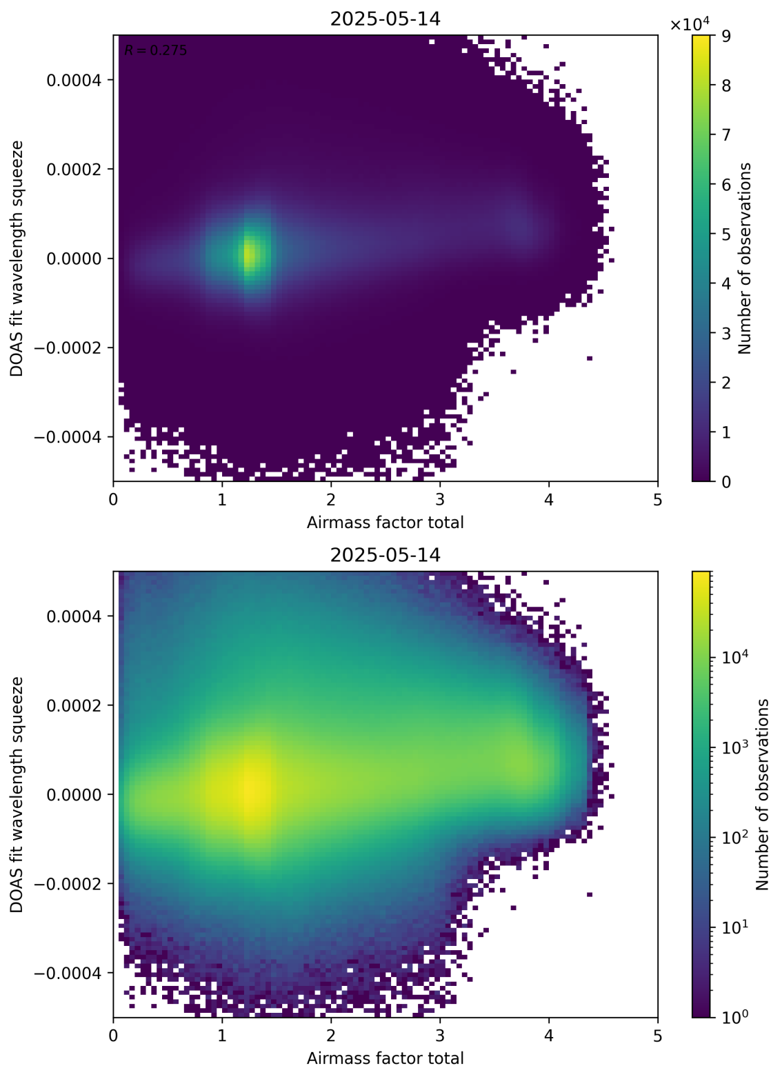
Figure 99: Scatter density plot of “Airmass factor total” against “DOAS fit wavelength squeeze” for 2025-05-13 to 2025-05-15.
