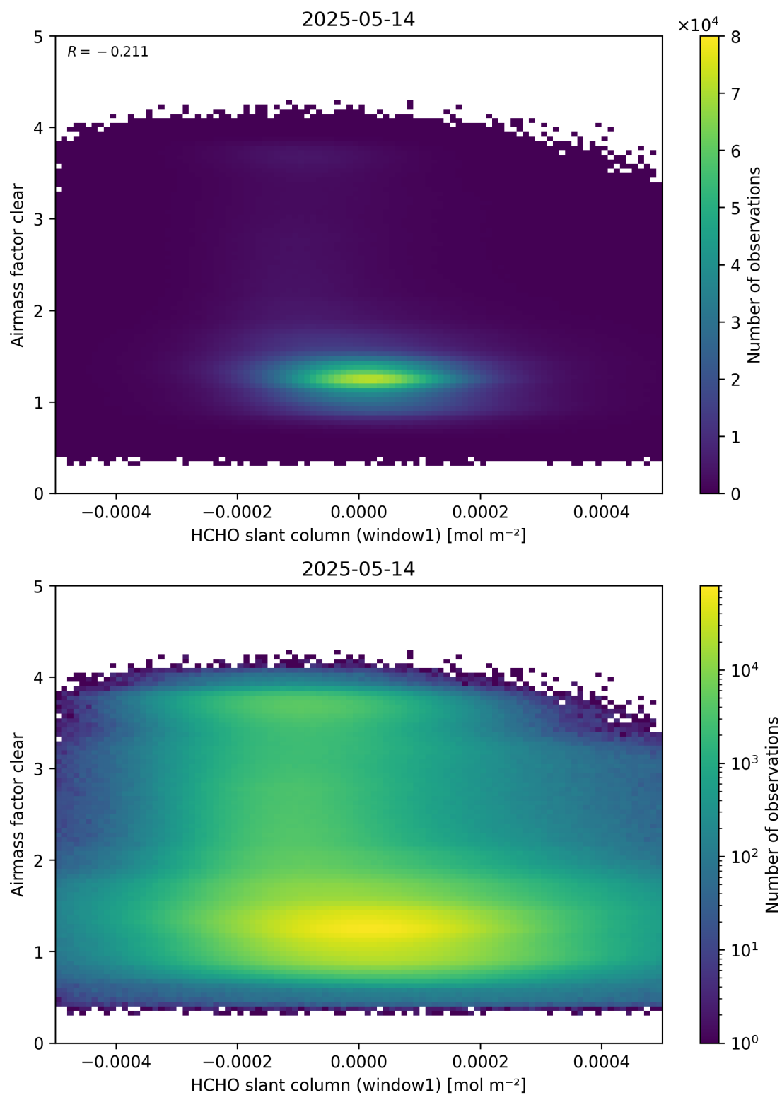
Figure 81: Scatter density plot of “HCHO slant column (window1)” against “Airmass factor clear” for 2025-05-13 to 2025-05-15.
