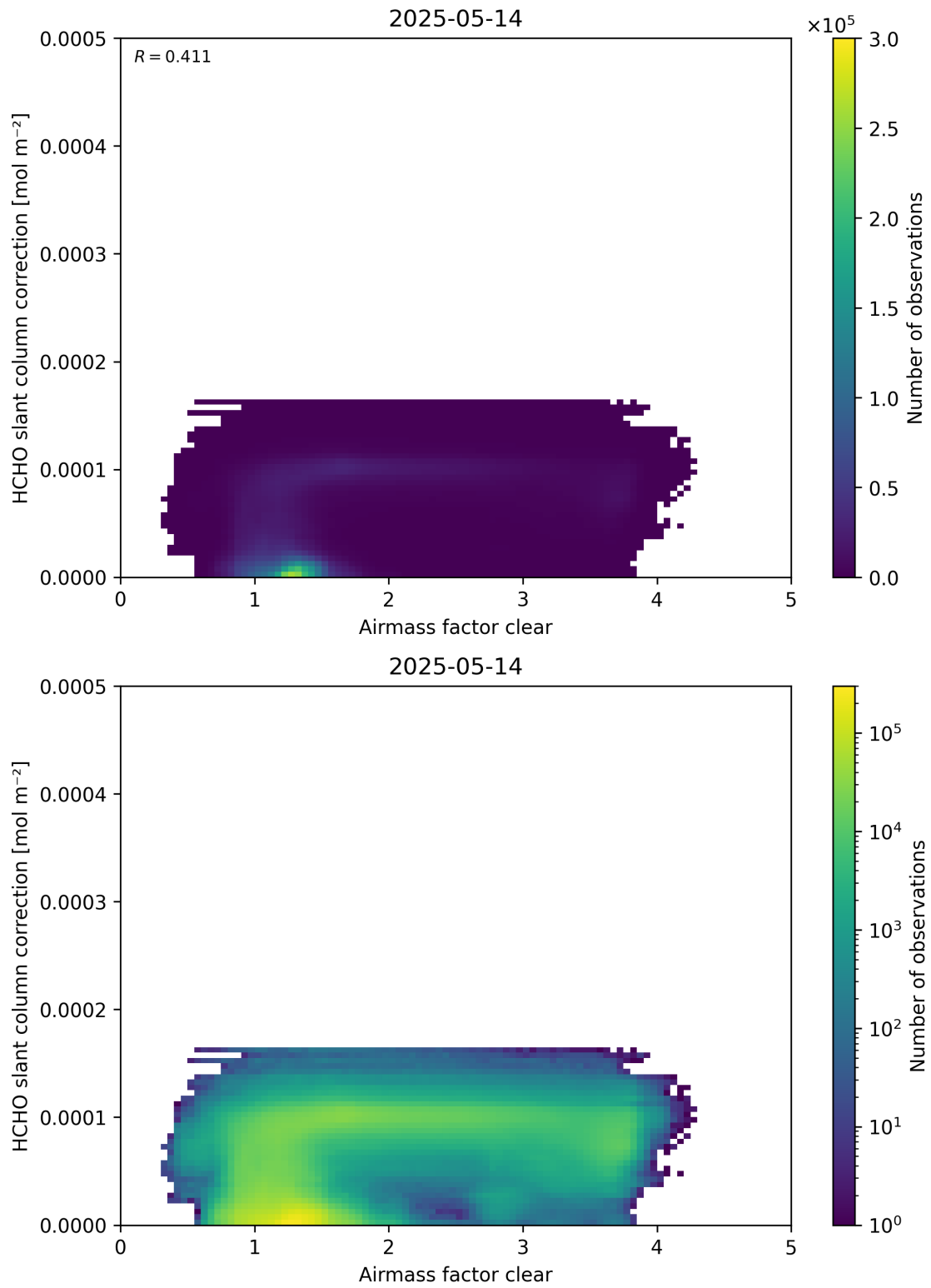
Figure 75: Scatter density plot of “Airmass factor clear” against “HCHO slant column correction” for 2025-05-13 to 2025-05-15.
