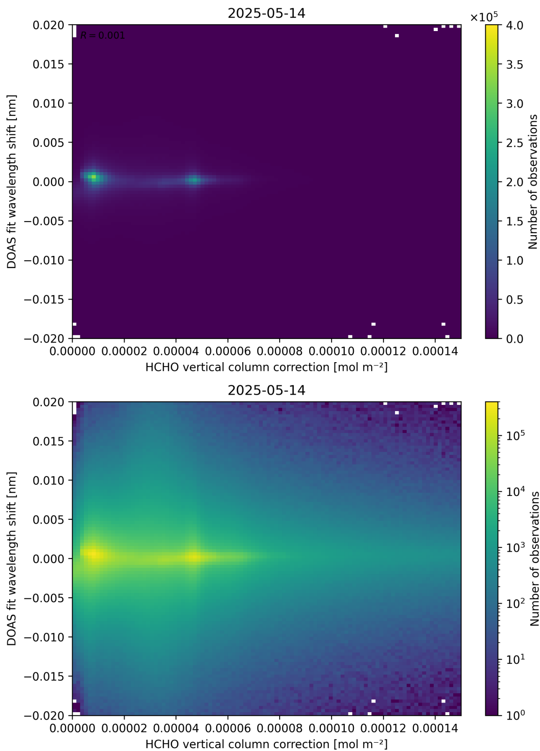
Figure 113: Scatter density plot of “HCHO vertical column correction” against “DOAS fit wavelength shift” for 2025-05-13 to 2025-05-15.
