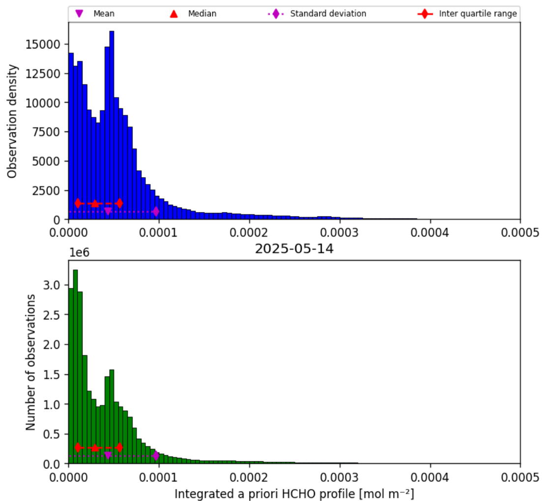
Figure 43: Histogram of “Integrated a priori HCHO profile” for 2025-05-13 to 2025-05-15
