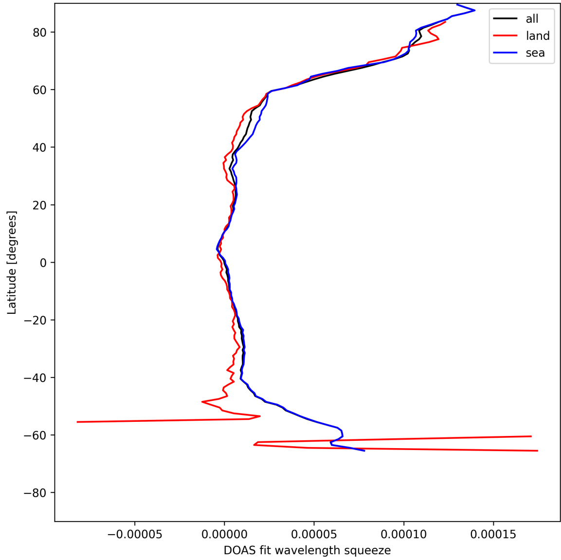
Figure 31: Zonal average of “DOAS fit wavelength squeeze” for 2025-05-13 to 2025-05-15.
