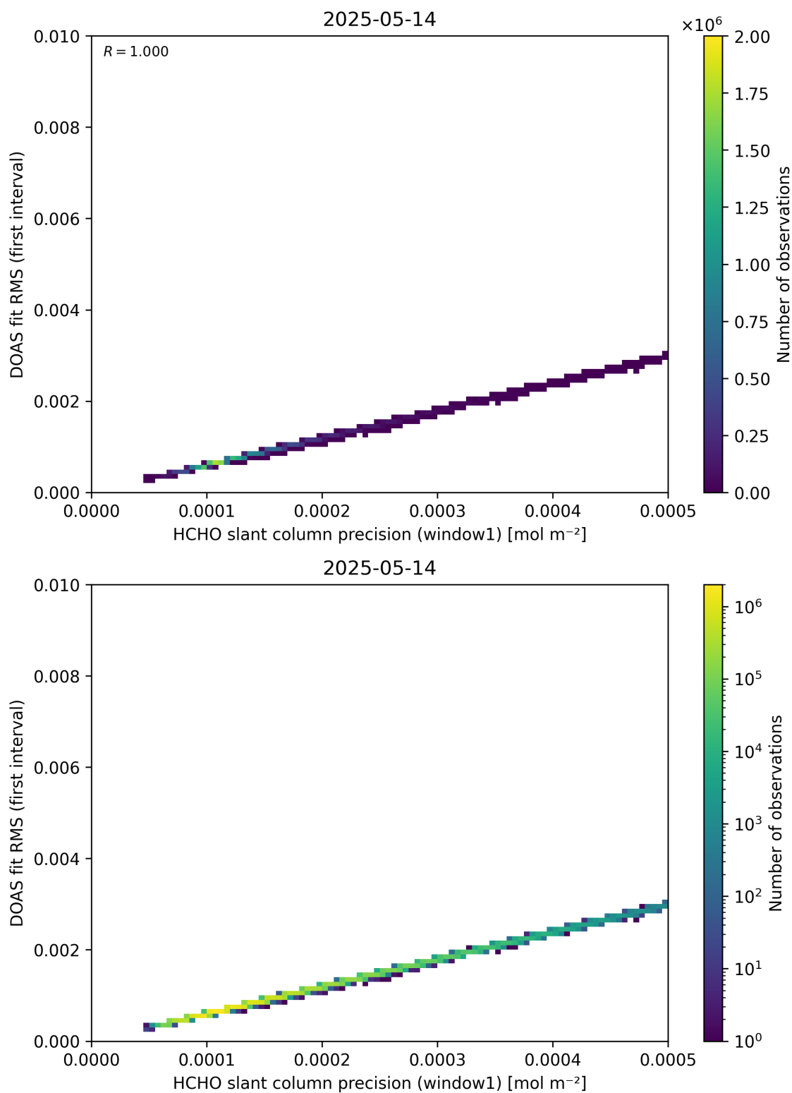
Figure 88: Scatter density plot of “HCHO slant column precision (window1)” against “DOAS fit RMS (first interval)” for 2025-05-13 to 2025-05-15.
