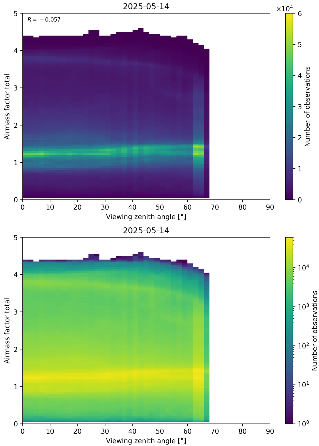
Figure 190: Scatter density plot of “Viewing zenith angle” against “Airmass factor total” for 2025-05-13 to 2025-05-15.
