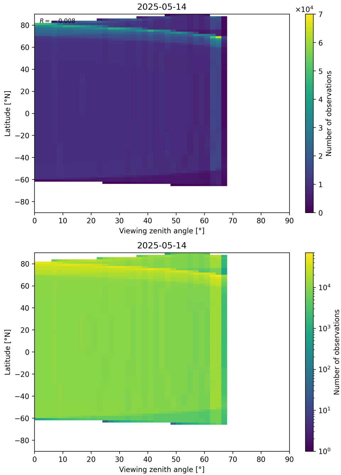
Figure 196: Scatter density plot of “Viewing zenith angle” against “Latitude” for 2025-05-13 to 2025-05-15.
