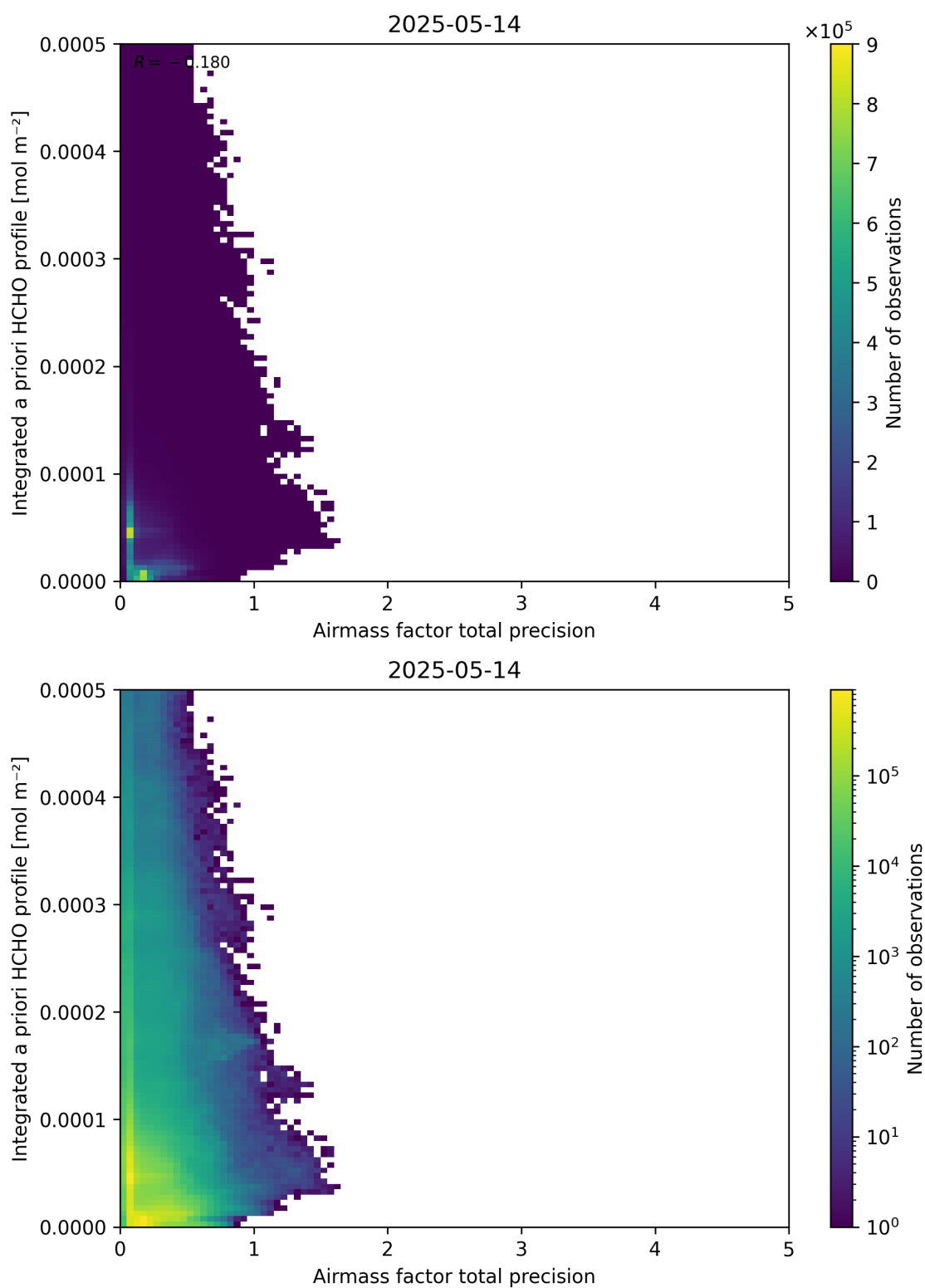
Figure 111: Scatter density plot of “Airmass factor total precision” against “Integrated a priori HCHO profile” for 2025-05-13 to 2025-05-15.
