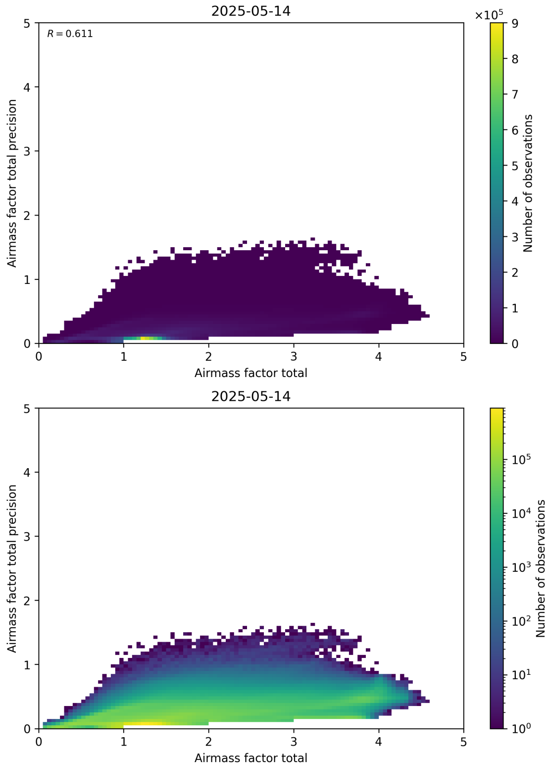
Figure 103: Scatter density plot of “Airmass factor total” against “Airmass factor total precision” for 2025-05-13 to 2025-05-15.
