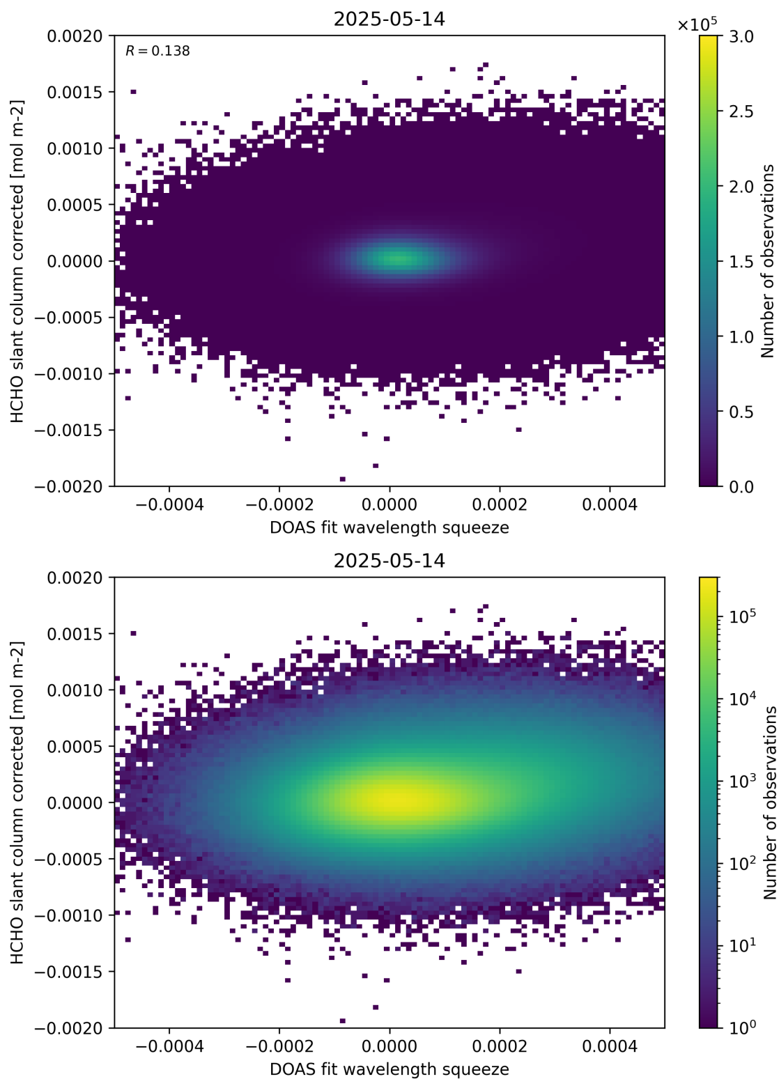
Figure 69: Scatter density plot of “DOAS fit wavelength squeeze” against “HCHO slant column corrected” for 2025-05-13 to 2025-05-15.
