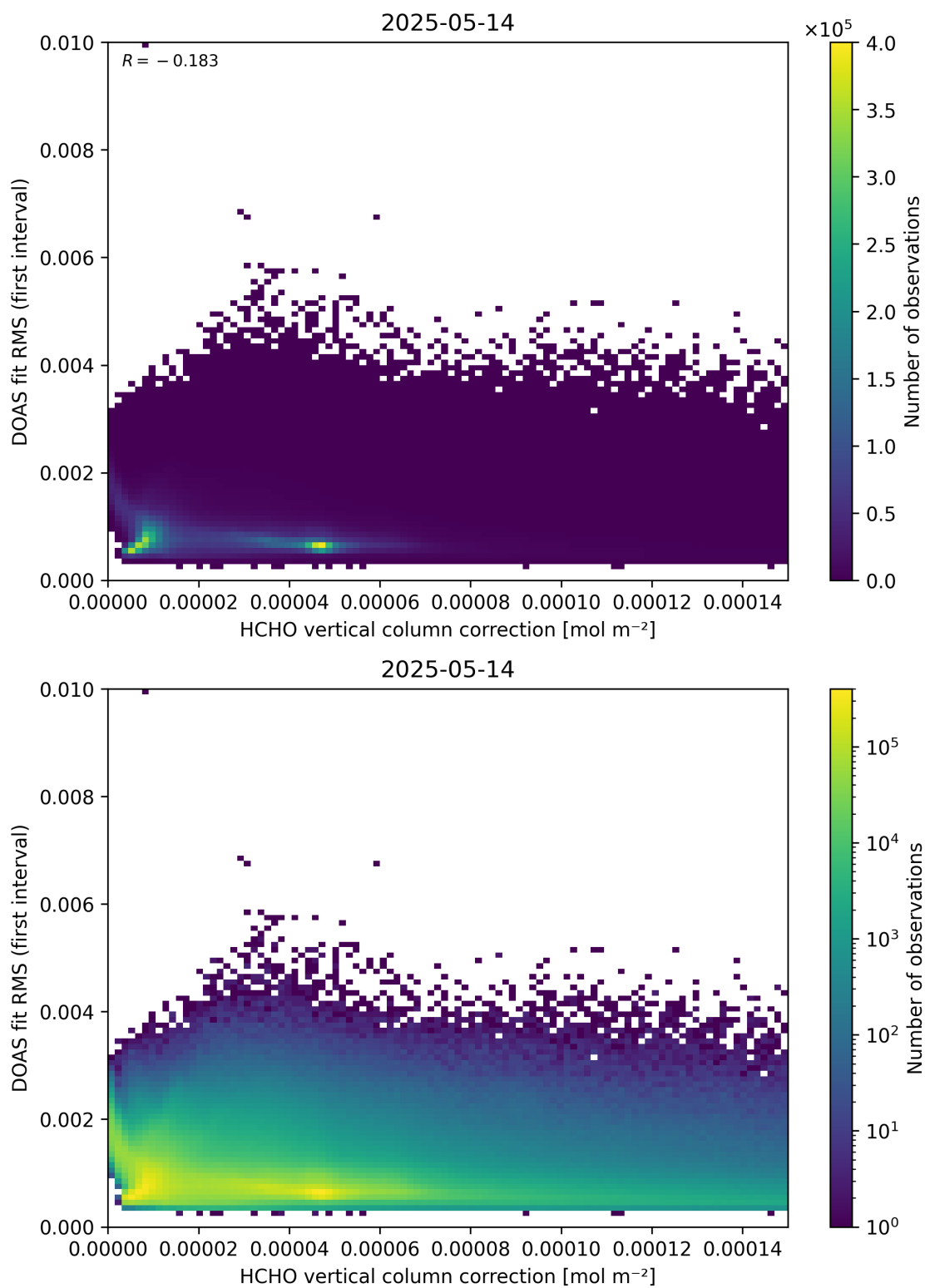
Figure 112: Scatter density plot of “HCHO vertical column correction” against “DOAS fit RMS (first interval)” for 2025-05-13 to 2025-05-15.
