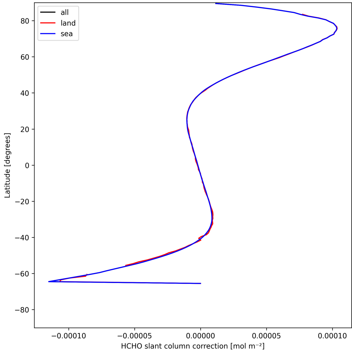
Figure 33: Zonal average of “HCHO slant column correction” for 2025-05-13 to 2025-05-15.
