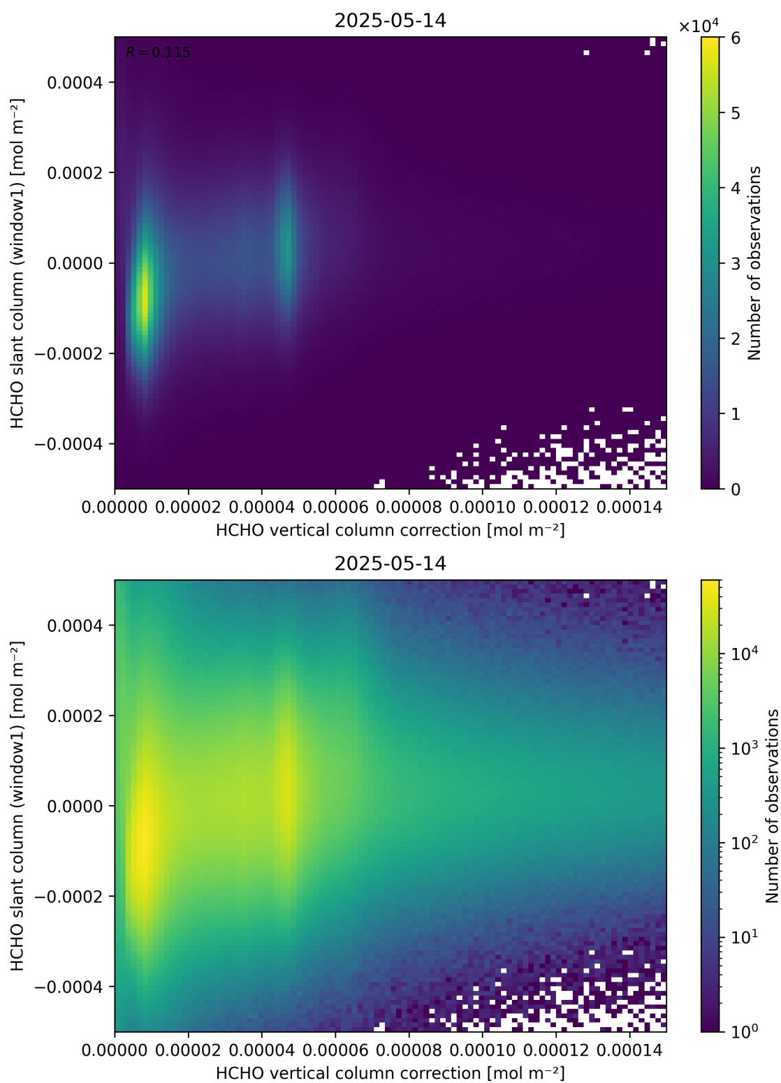
Figure 118: Scatter density plot of “HCHO vertical column correction” against “HCHO slant column (window1)” for 2025-05-13 to 2025-05-15.
