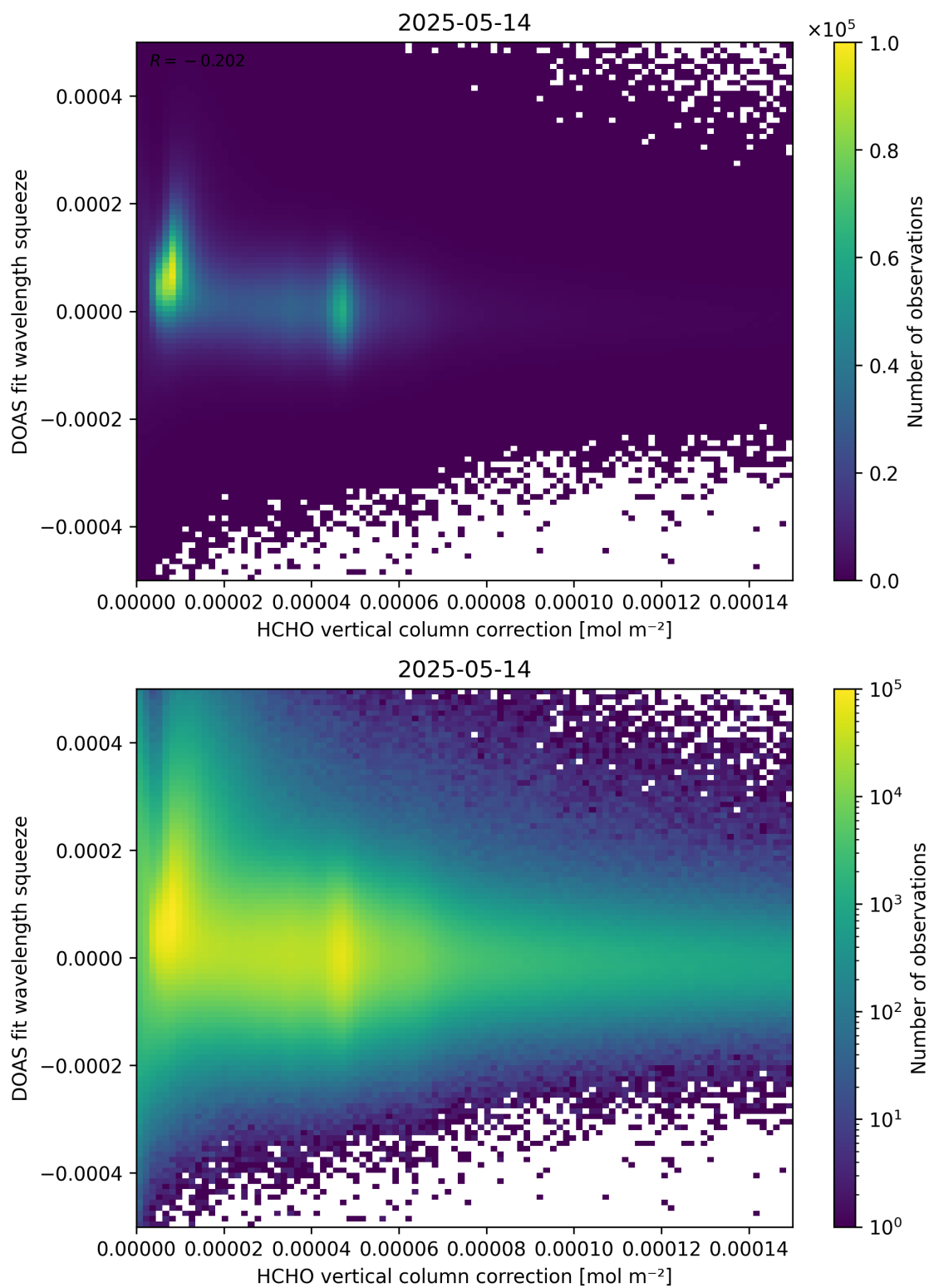
Figure 114: Scatter density plot of “HCHO vertical column correction” against “DOAS fit wavelength squeeze” for 2025-05-13 to 2025-05-15.
