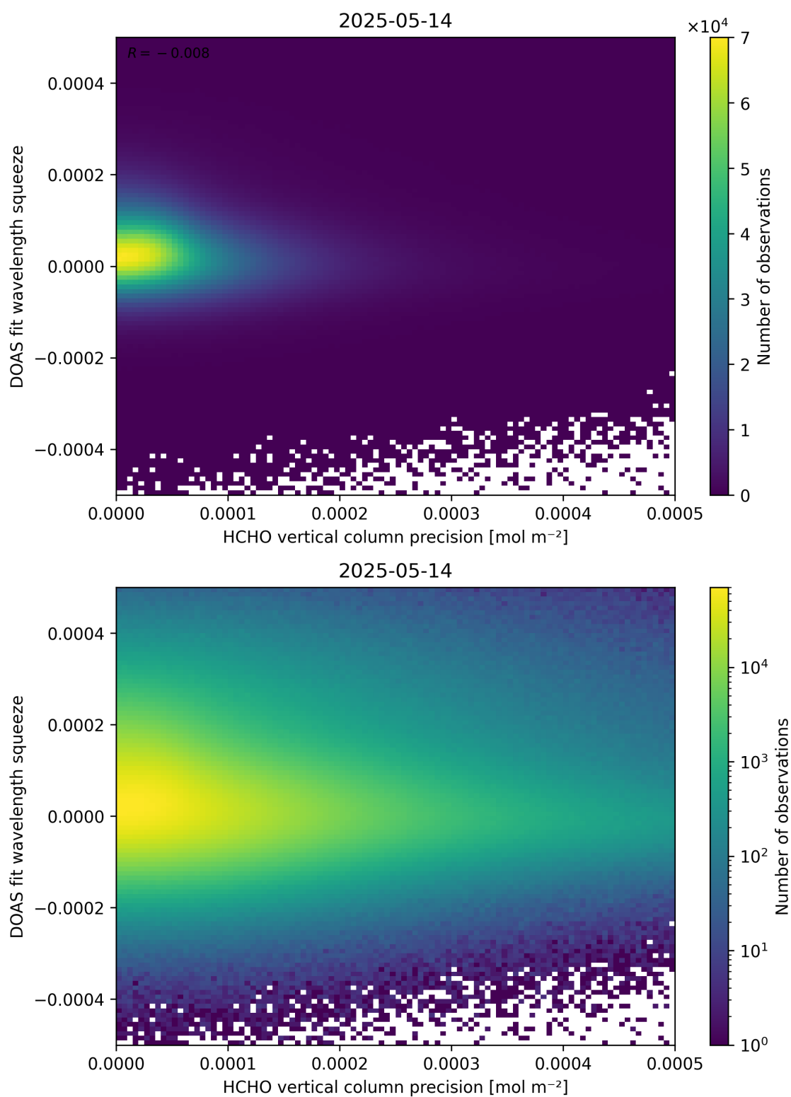
Figure 138: Scatter density plot of “HCHO vertical column precision” against “DOAS fit wavelength squeeze” for 2025-05-13 to 2025-05-15.
