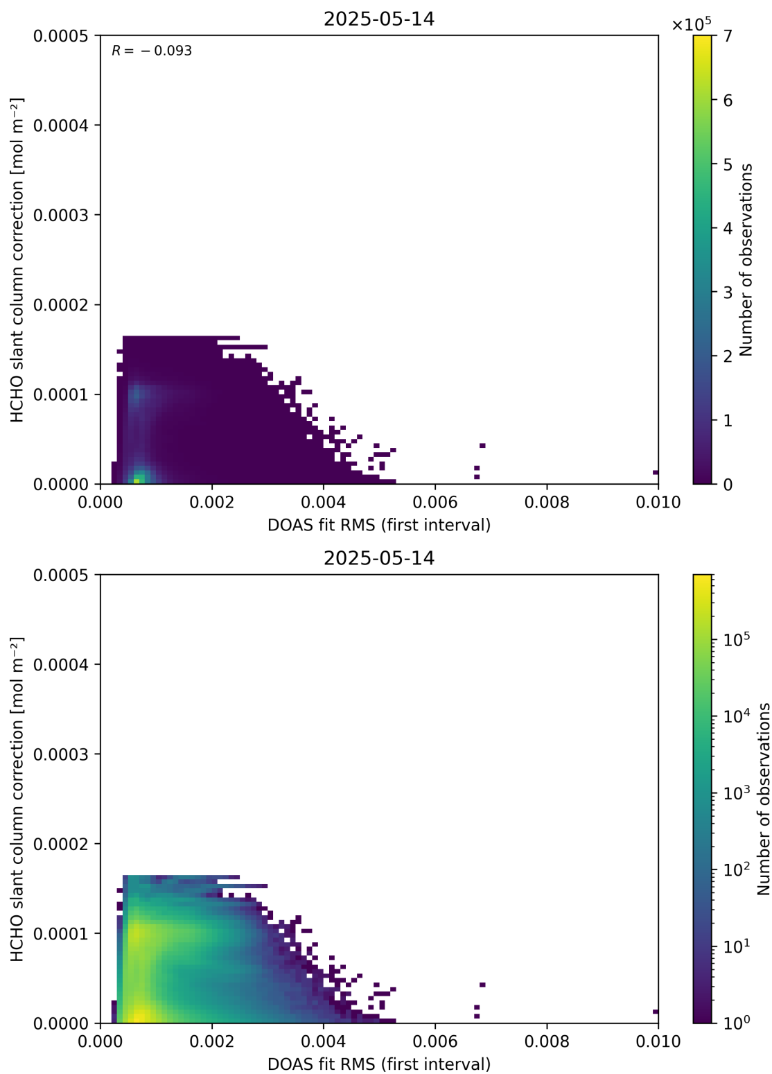
Figure 63: Scatter density plot of “DOAS fit RMS (first interval)” against “HCHO slant column correction” for 2025-05-13 to 2025-05-15.
