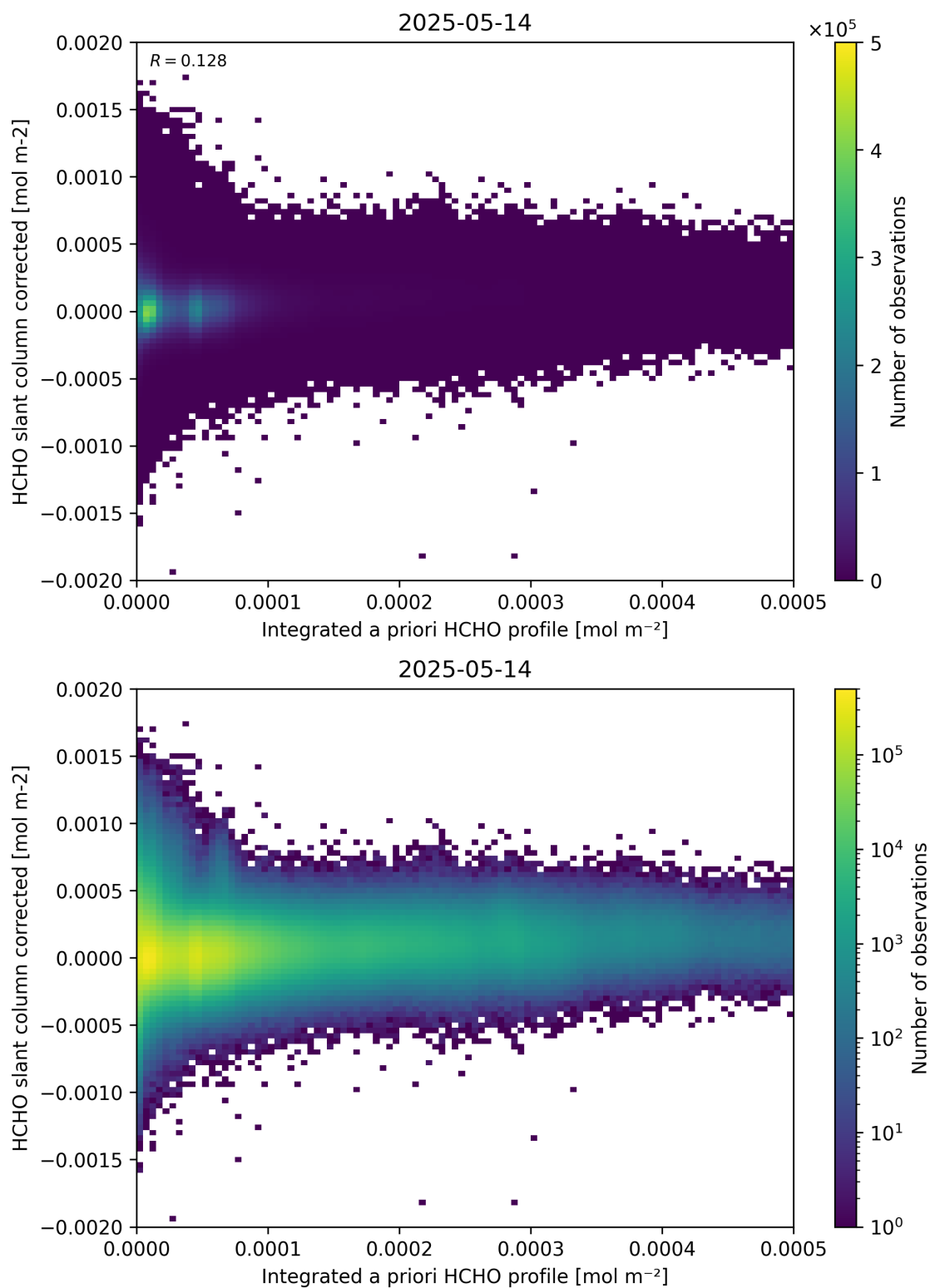
Figure 151: Scatter density plot of “Integrated a priori HCHO profile” against “HCHO slant column corrected” for 2025-05-13 to 2025-05-15.
