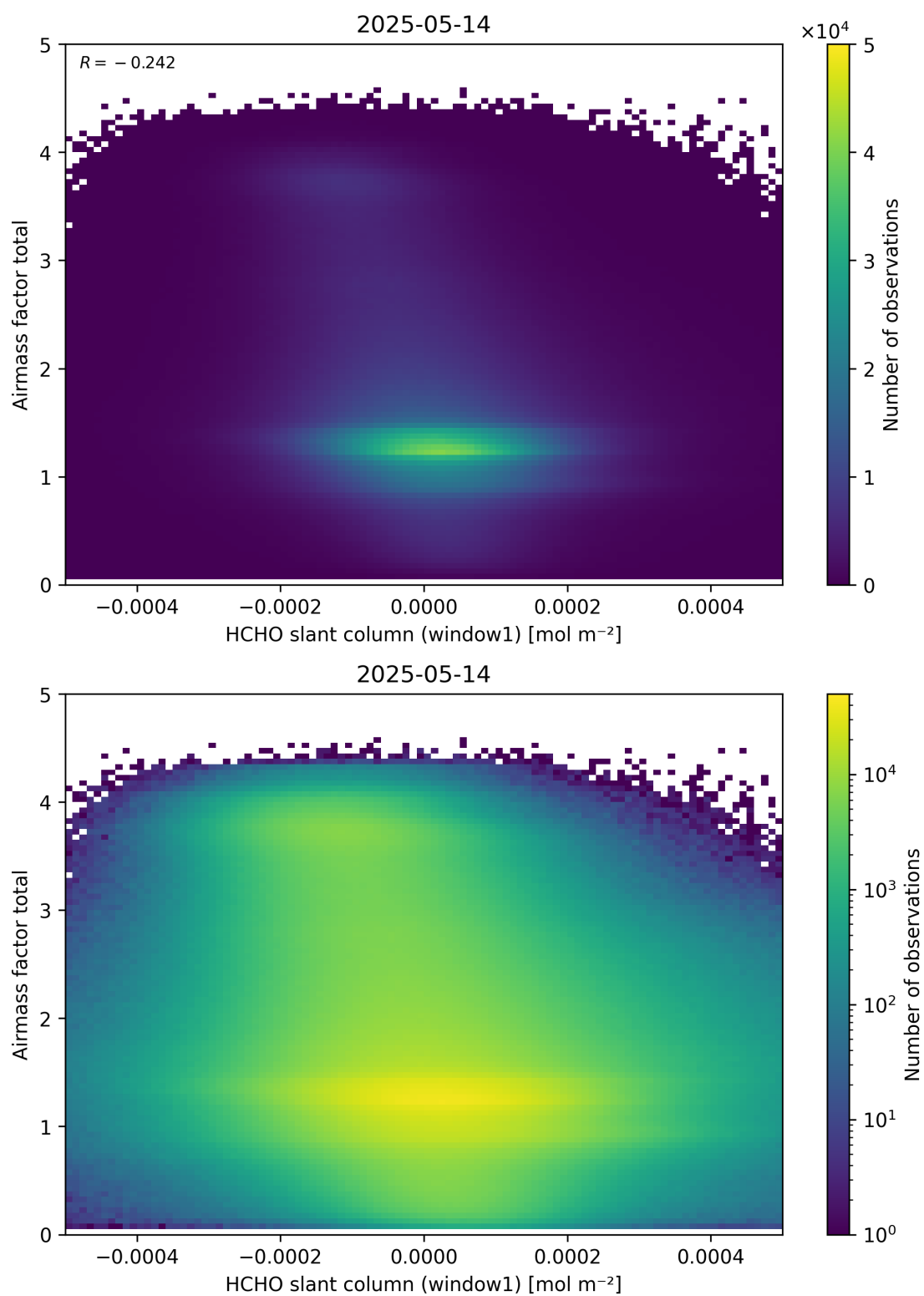
Figure 85: Scatter density plot of “HCHO slant column (window1)” against “Airmass factor total” for 2025-05-13 to 2025-05-15.
