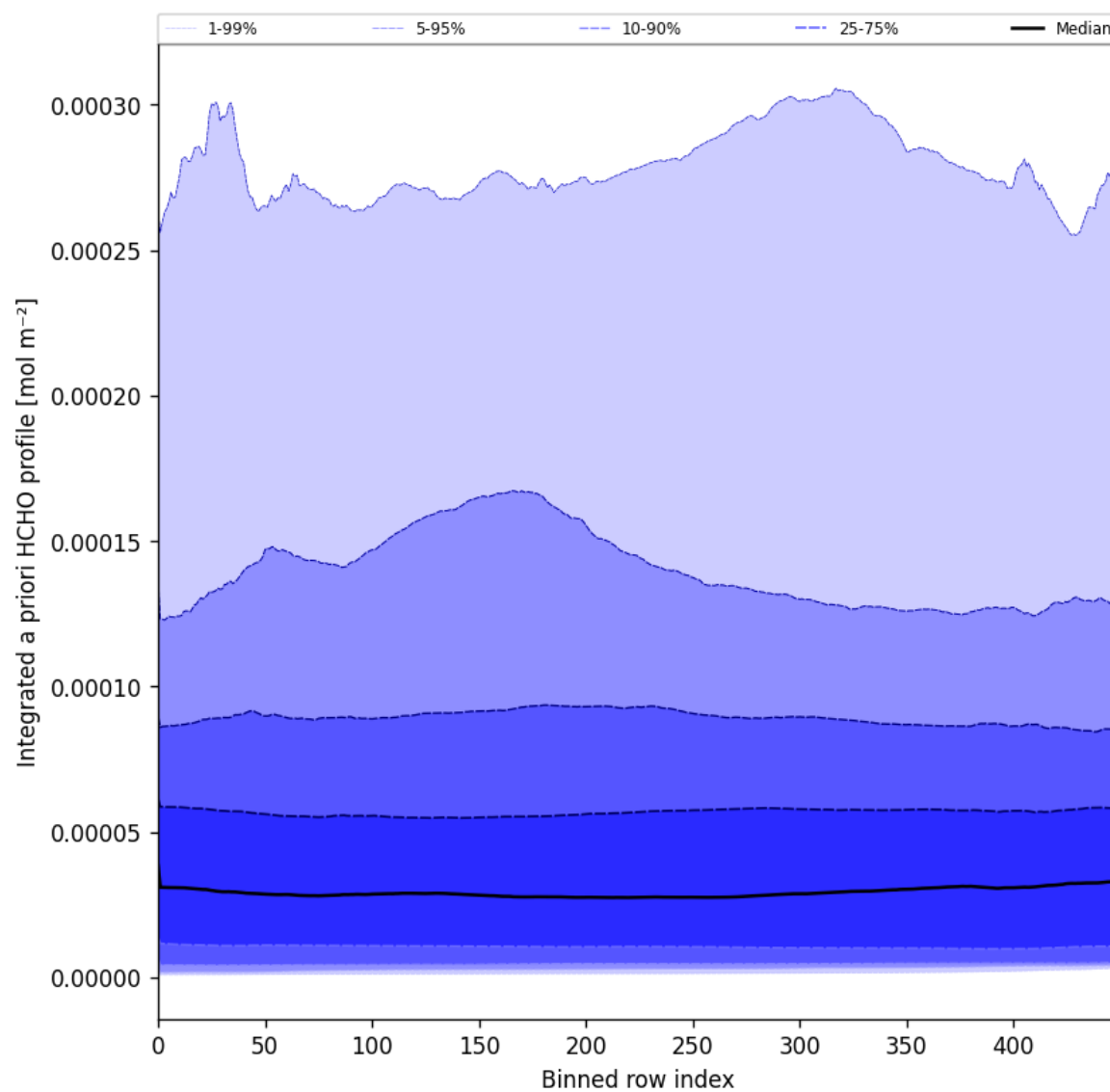
Figure 57: Along track statistics of “Integrated a priori HCHO profile” for 2025-05-13 to 2025-05-15
