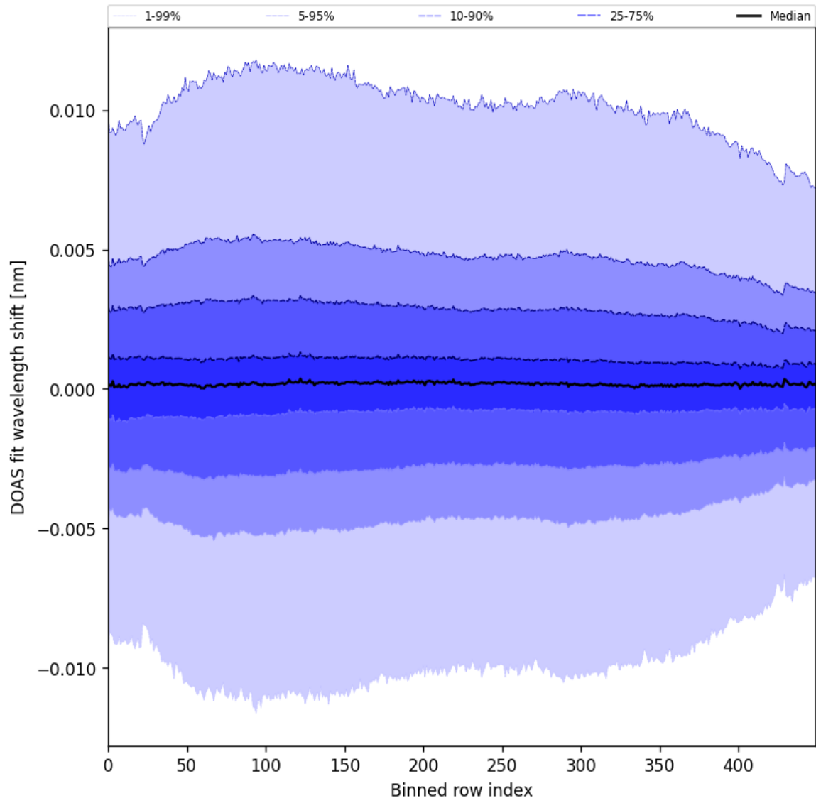
Figure 58: Along track statistics of “DOAS fit wavelength shift” for 2025-05-13 to 2025-05-15
