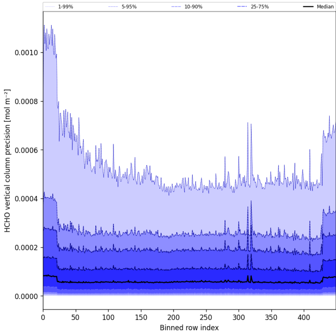
Figure 50: Along track statistics of “HCHO vertical column precision” for 2025-05-13 to 2025-05-15
