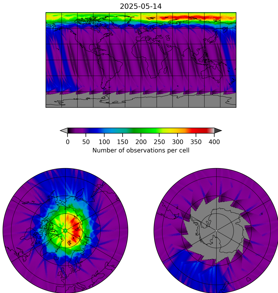
Figure 19: Map of the number of observations for 2025-05-13 to 2025-05-15
