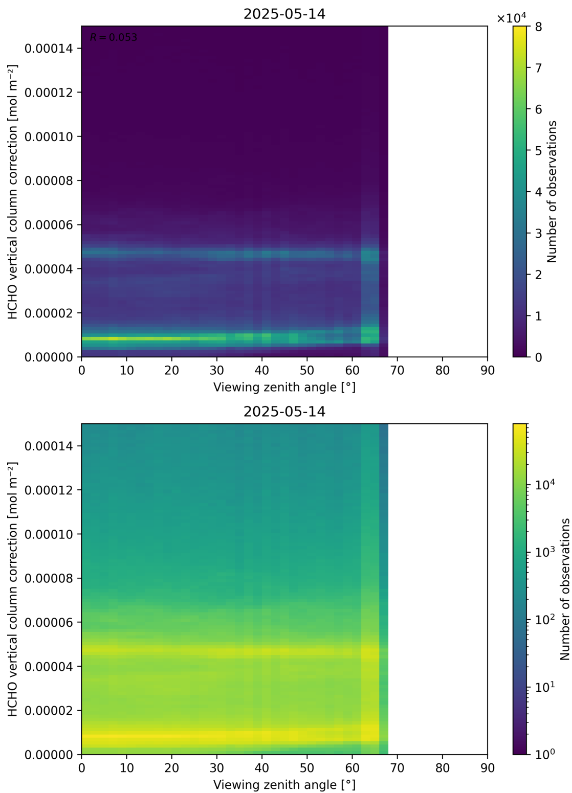
Figure 193: Scatter density plot of “Viewing zenith angle” against “HCHO vertical column correction” for 2025-05-13 to 2025-05-15.
