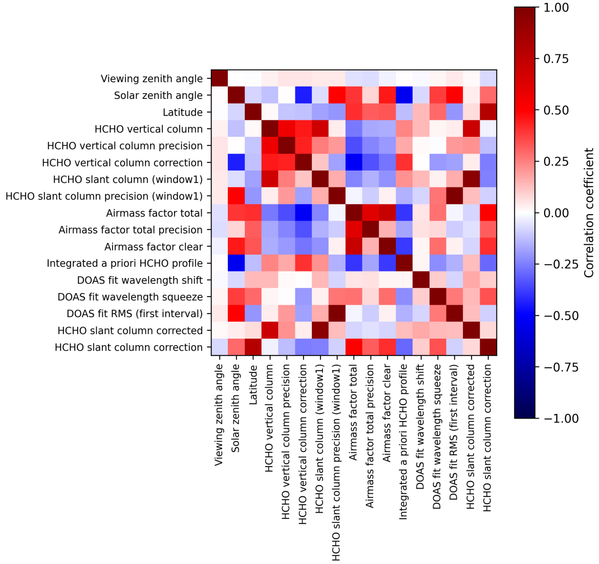
Figure 2: Map of correlation matrix for 2025-05-13 to 2025-05-15.
