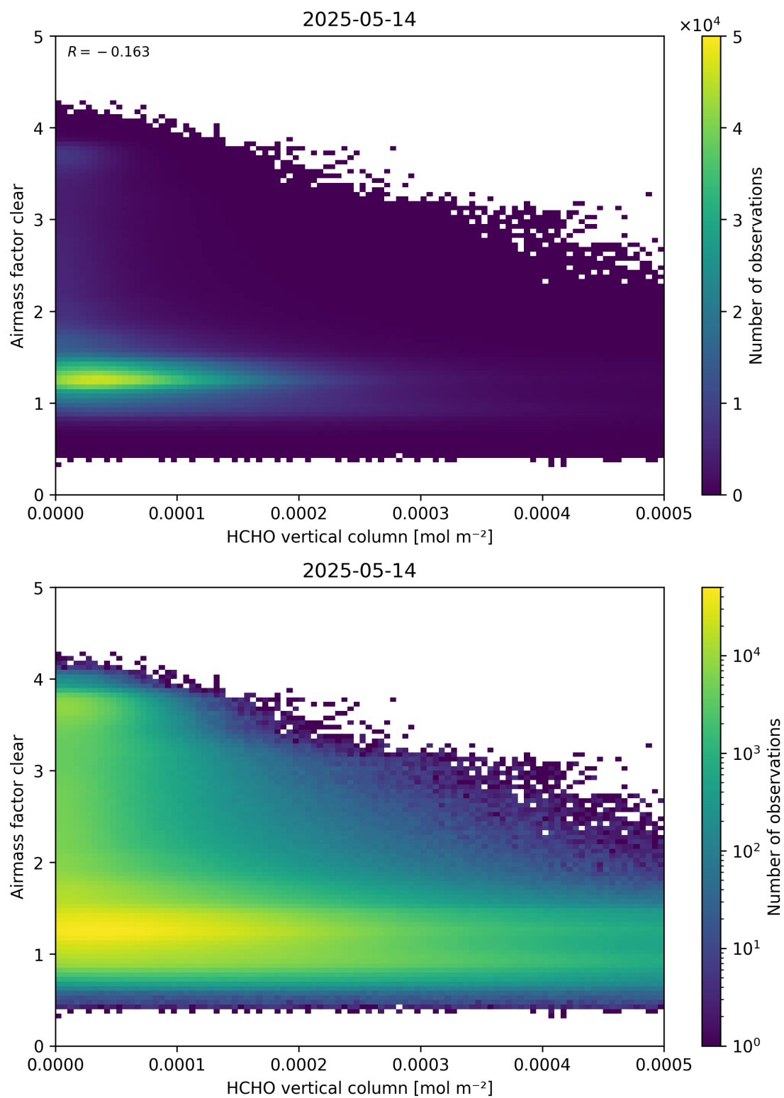
Figure 126: Scatter density plot of “HCHO vertical column” against “Airmass factor clear” for 2025-05-13 to 2025-05-15.
