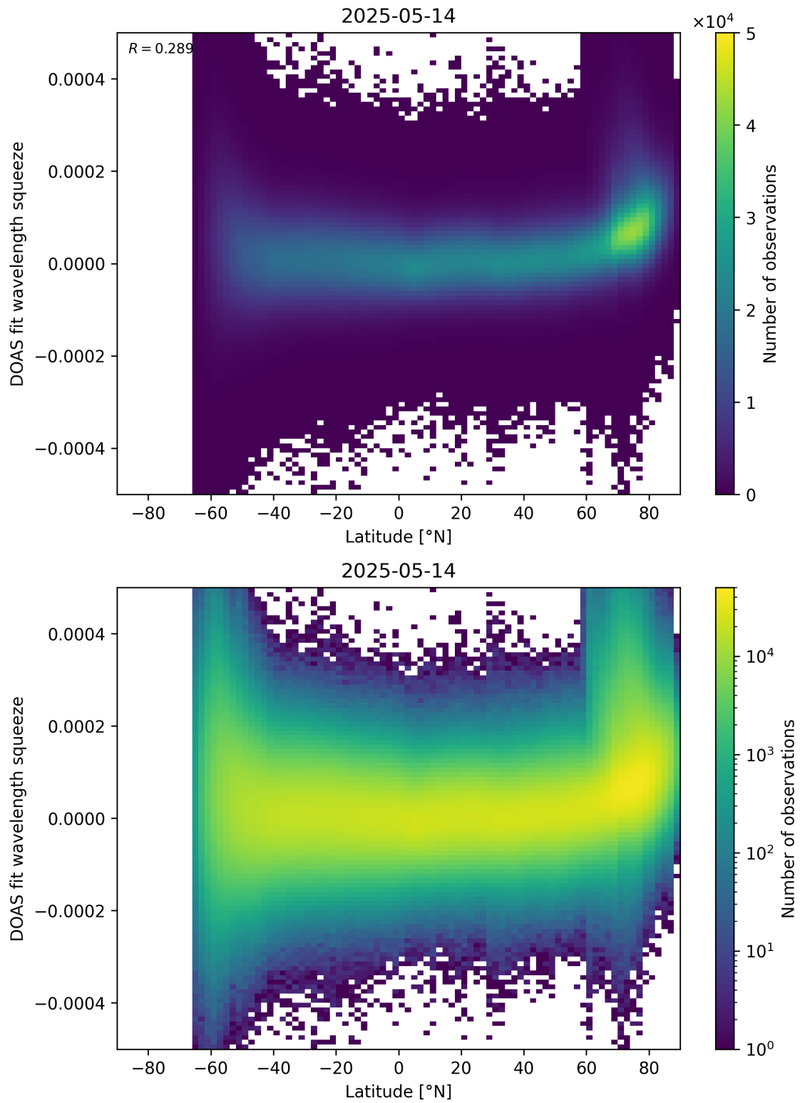
Figure 155: Scatter density plot of “Latitude” against “DOAS fit wavelength squeeze” for 2025-05-13 to 2025-05-15.
