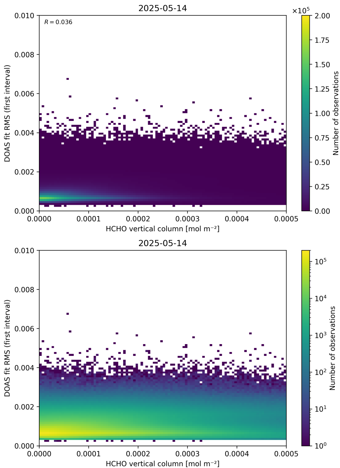
Figure 123: Scatter density plot of “HCHO vertical column” against “DOAS fit RMS (first interval)” for 2025-05-13 to 2025-05-15.
