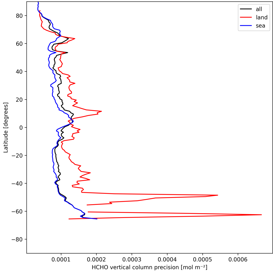
Figure 22: Zonal average of “HCHO vertical column precision” for 2025-05-13 to 2025-05-15.
