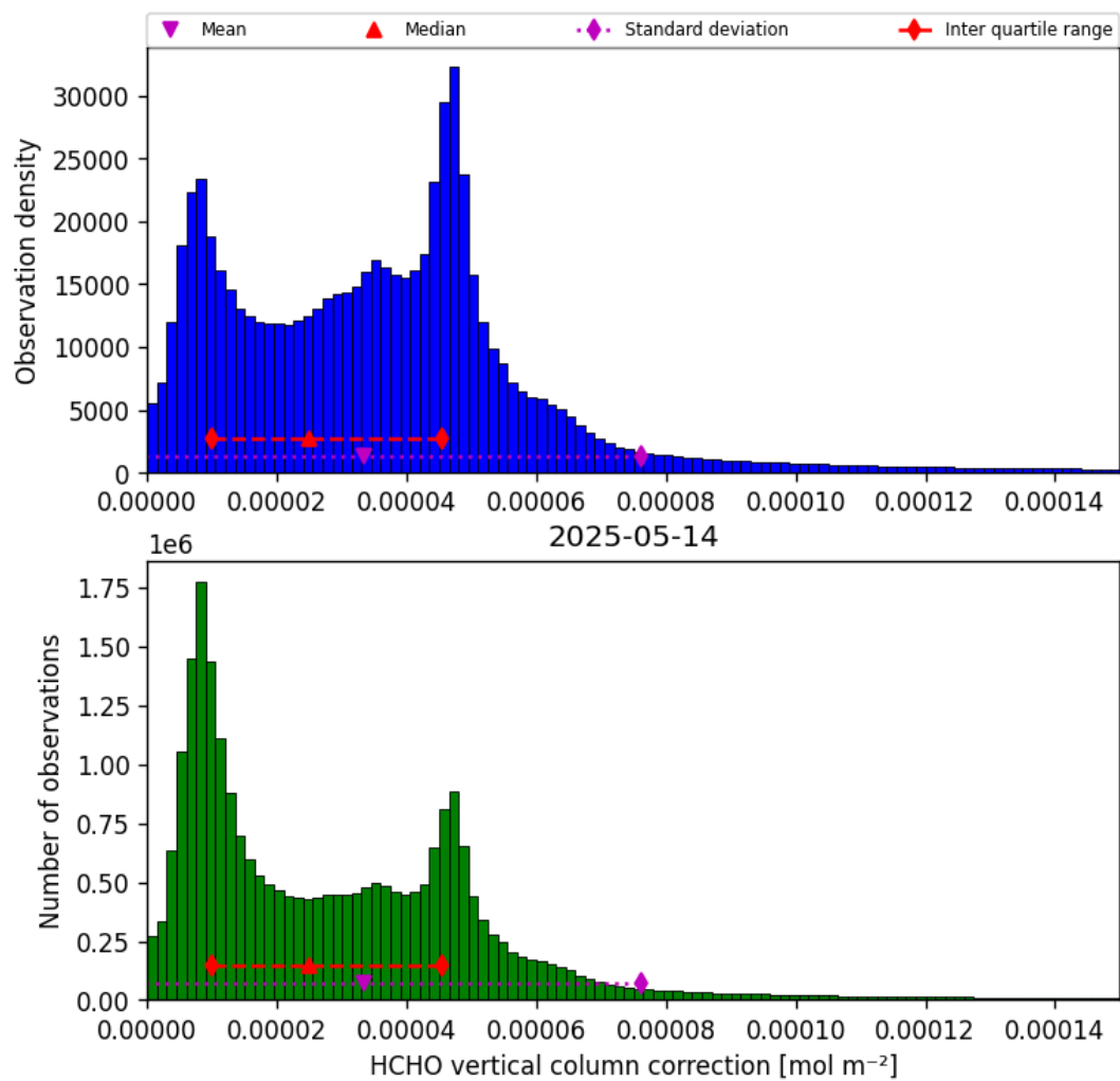
Figure 37: Histogram of “HCHO vertical column correction” for 2025-05-13 to 2025-05-15
