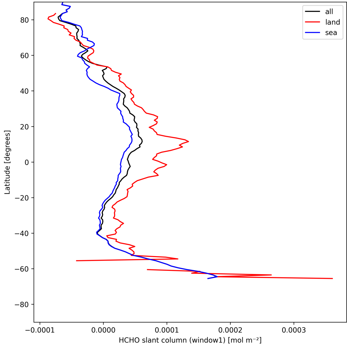
Figure 24: Zonal average of “HCHO slant column (window1)” for 2025-05-13 to 2025-05-15.
