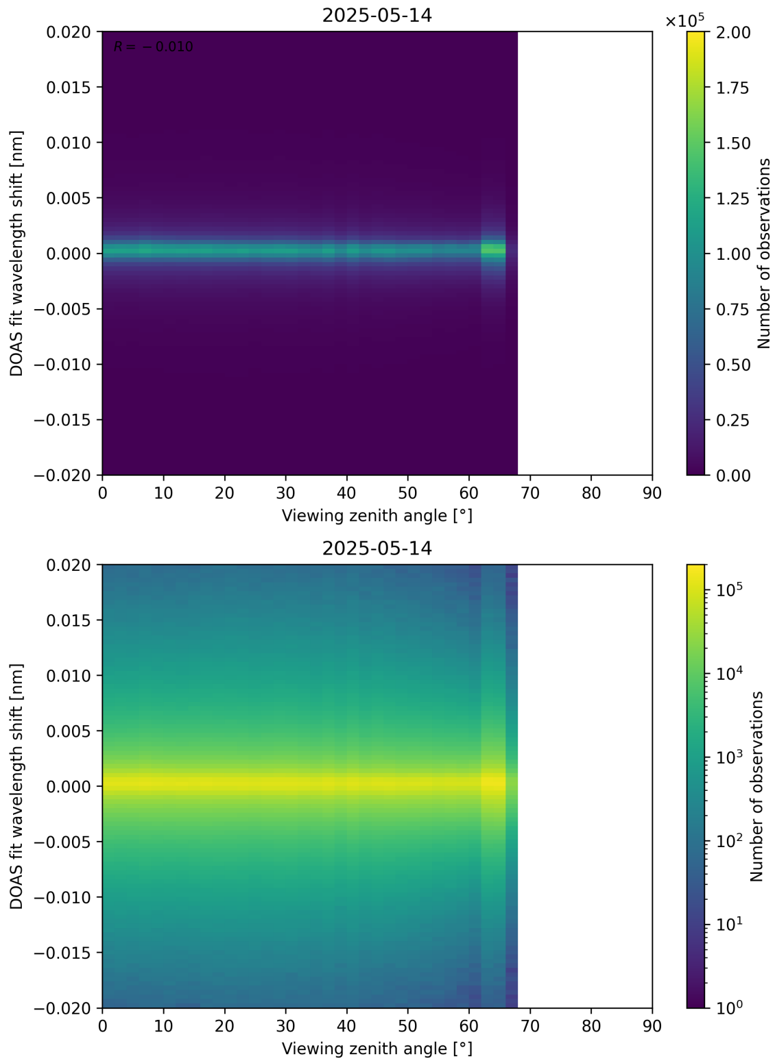
Figure 183: Scatter density plot of “Viewing zenith angle” against “DOAS fit wavelength shift” for 2025-05-13 to 2025-05-15.
