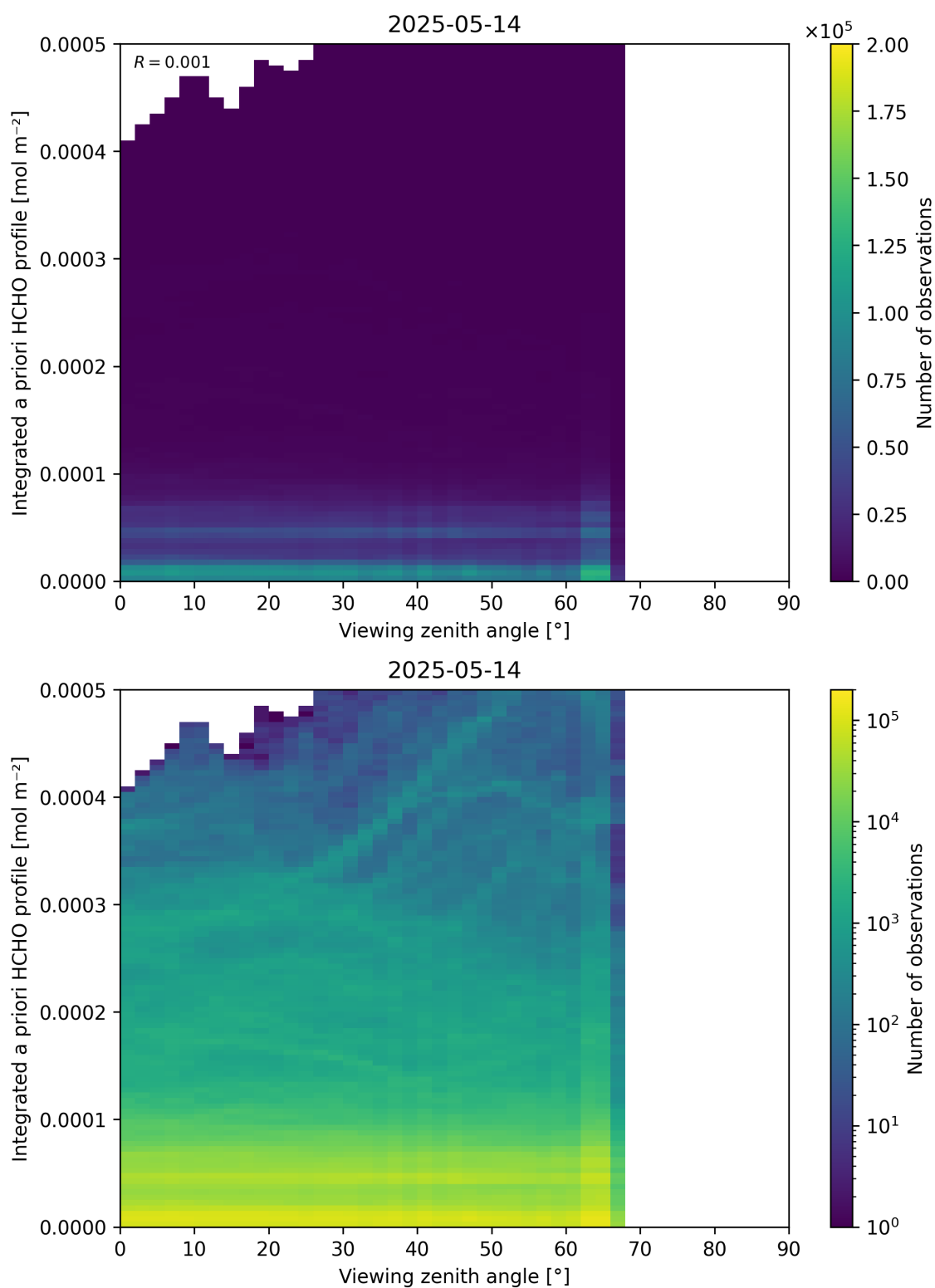
Figure 195: Scatter density plot of “Viewing zenith angle” against “Integrated a priori HCHO profile” for 2025-05-13 to 2025-05-15.
