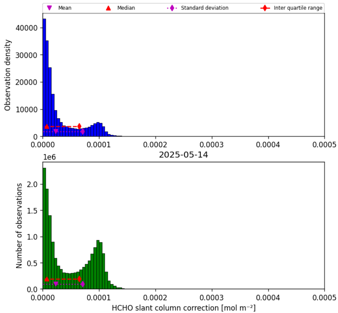
Figure 47: Histogram of “HCHO slant column correction” for 2025-05-13 to 2025-05-15
