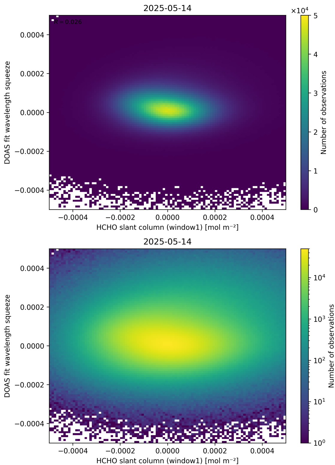
Figure 80: Scatter density plot of “HCHO slant column (window1)” against “DOAS fit wavelength squeeze” for 2025-05-13 to 2025-05-15.
