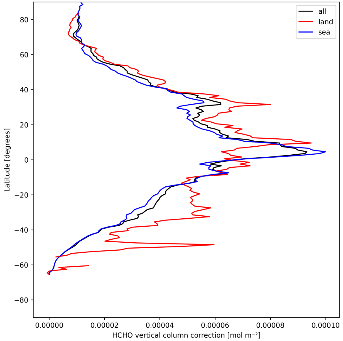
Figure 23: Zonal average of “HCHO vertical column correction” for 2025-05-13 to 2025-05-15.
