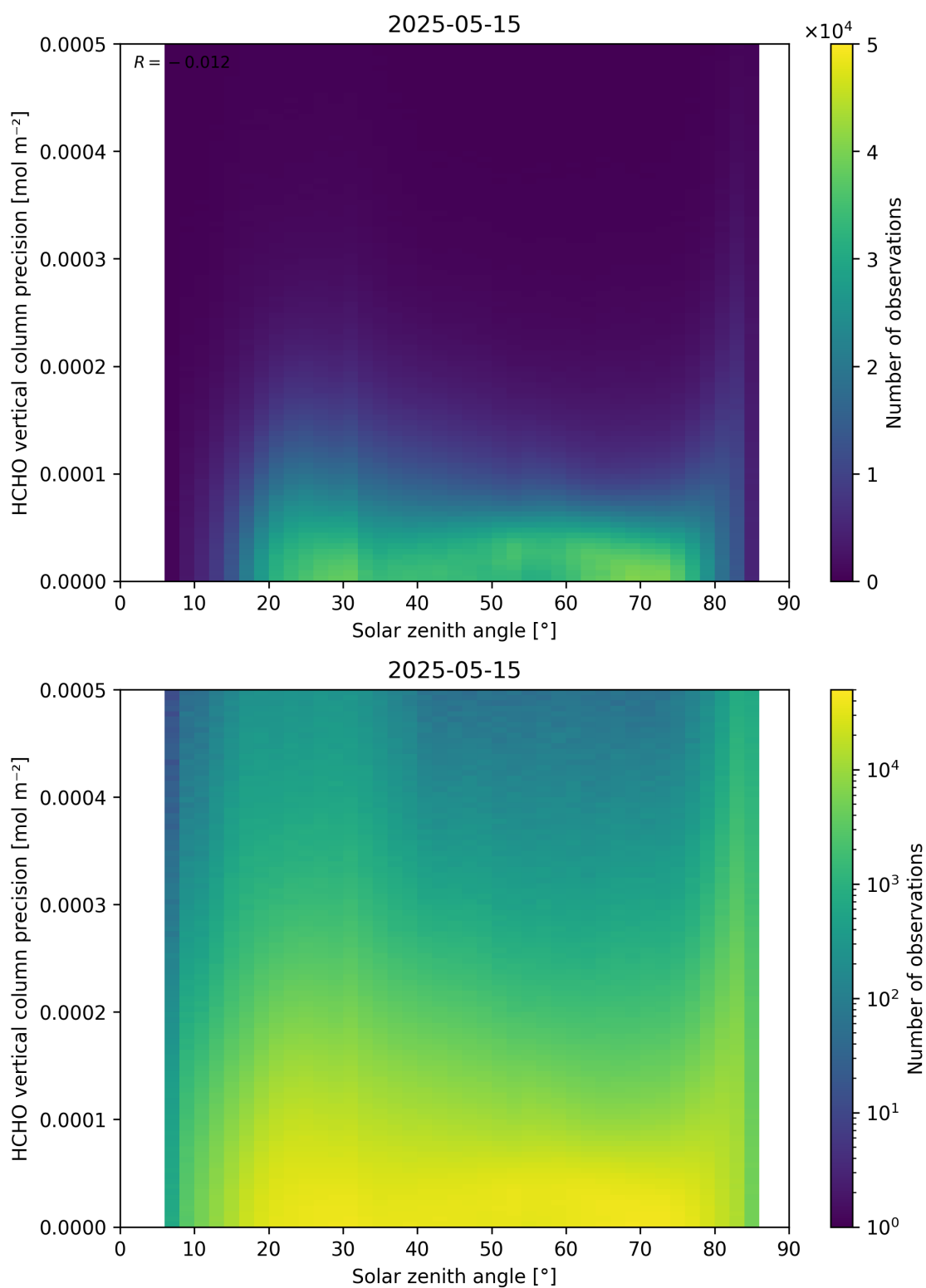
Figure 179: Scatter density plot of “Solar zenith angle” against “HCHO vertical column precision” for 2025-05-15 to 2025-05-16.
