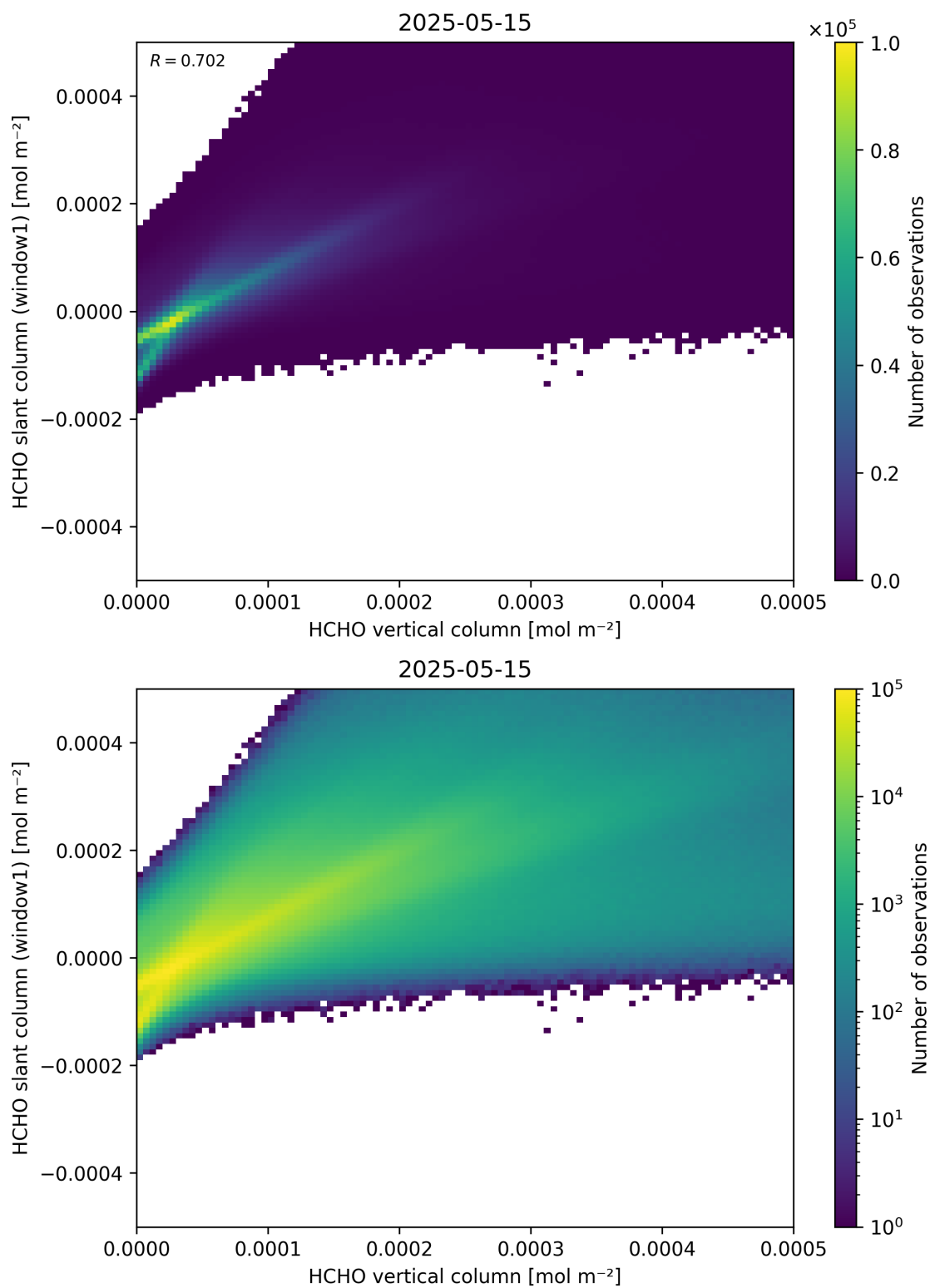
Figure 129: Scatter density plot of “HCHO vertical column” against “HCHO slant column (window1)” for 2025-05-15 to 2025-05-16.
