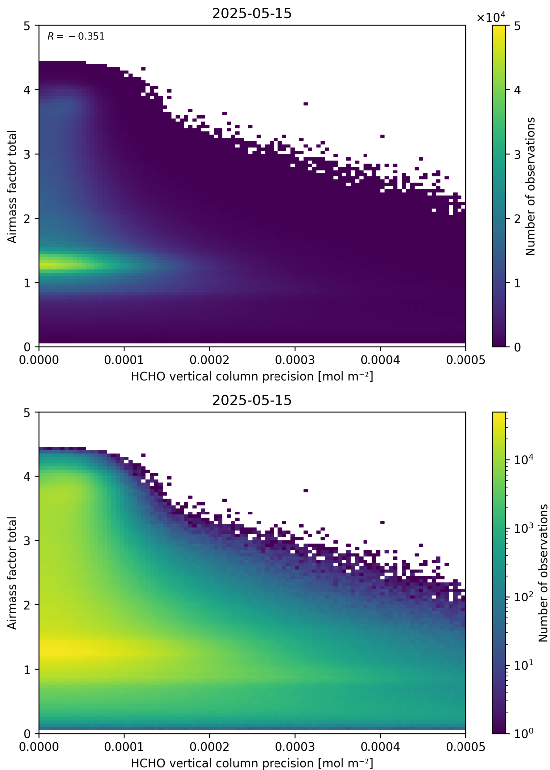
Figure 144: Scatter density plot of “HCHO vertical column precision” against “Airmass factor total” for 2025-05-15 to 2025-05-16.
