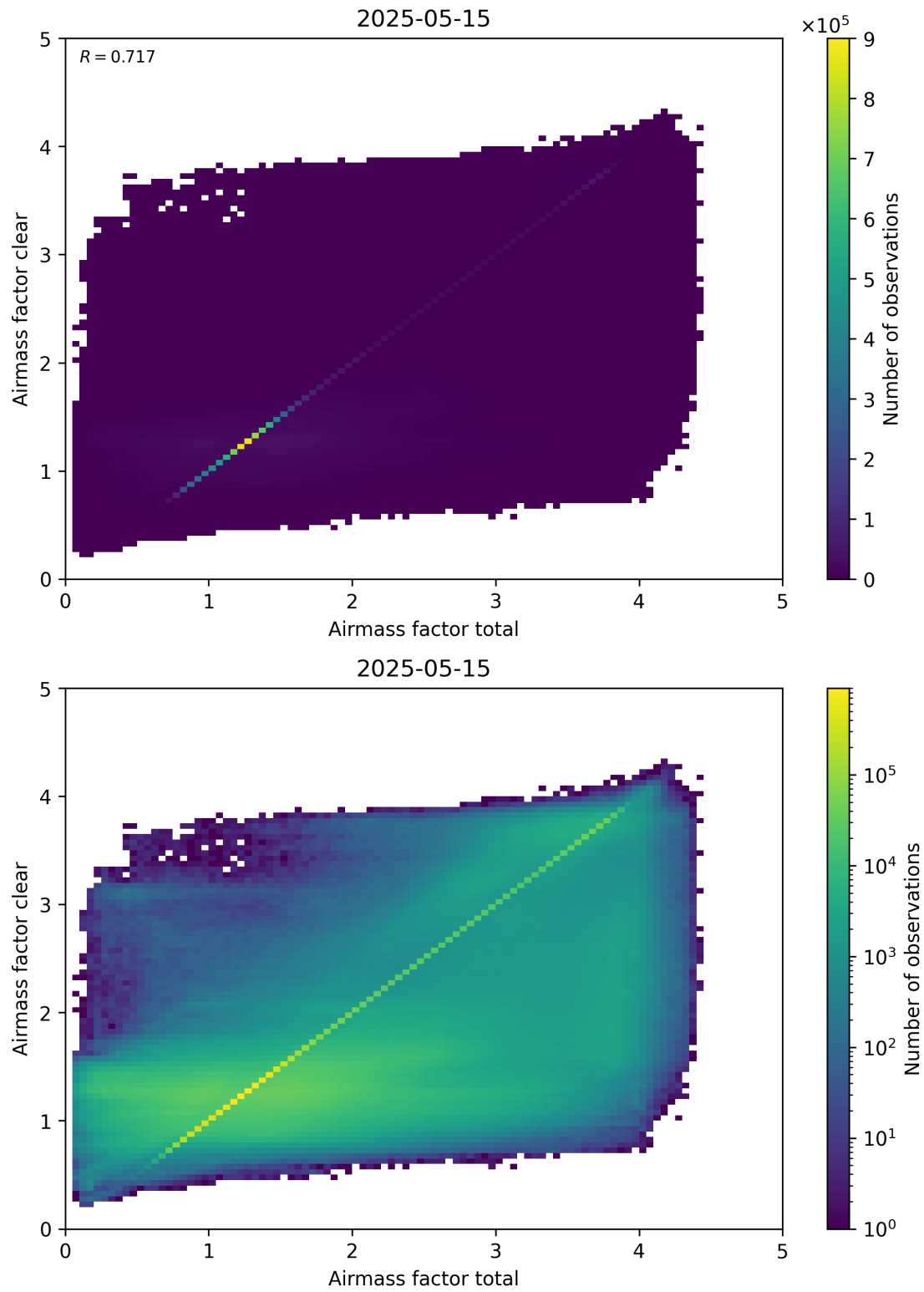
Figure 100: Scatter density plot of “Airmass factor total” against “Airmass factor clear” for 2025-05-15 to 2025-05-16.
