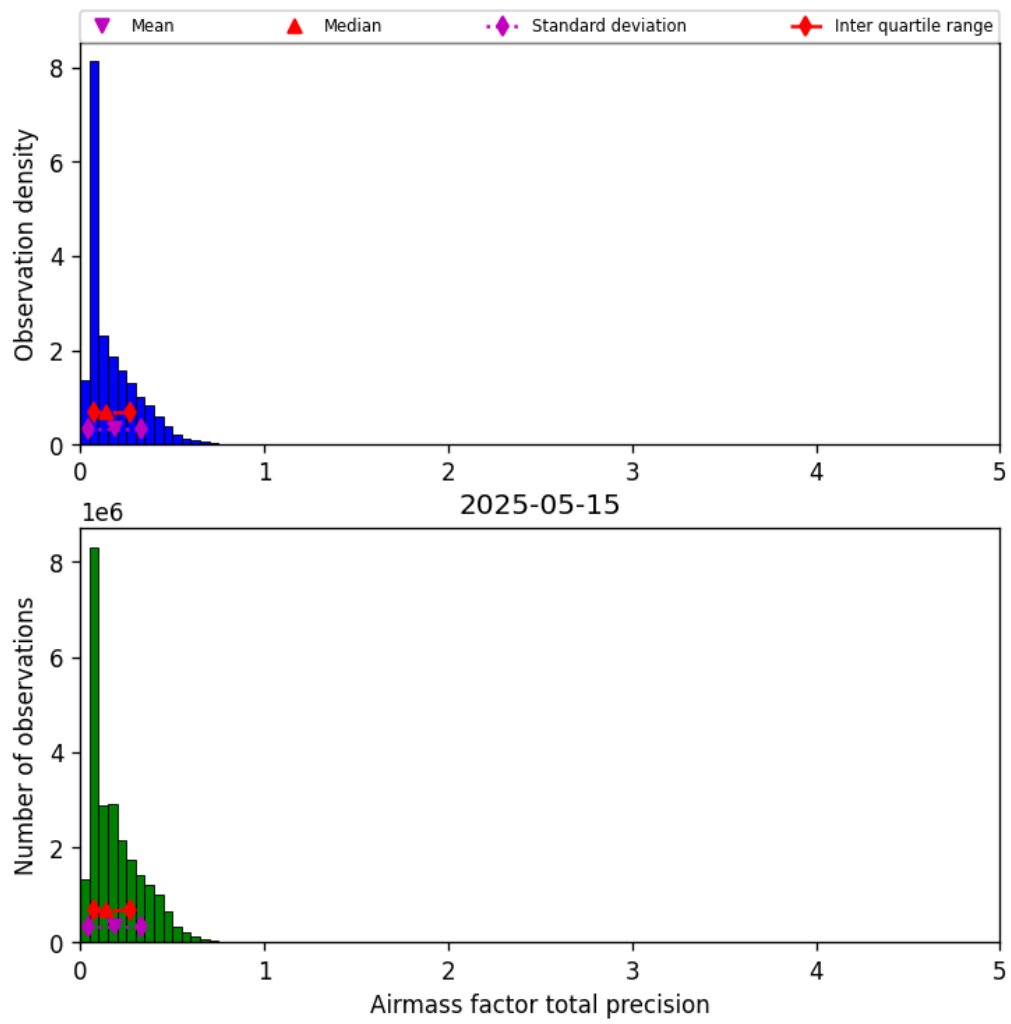
Figure 41: Histogram of “Airmass factor total precision” for 2025-05-15 to 2025-05-16
