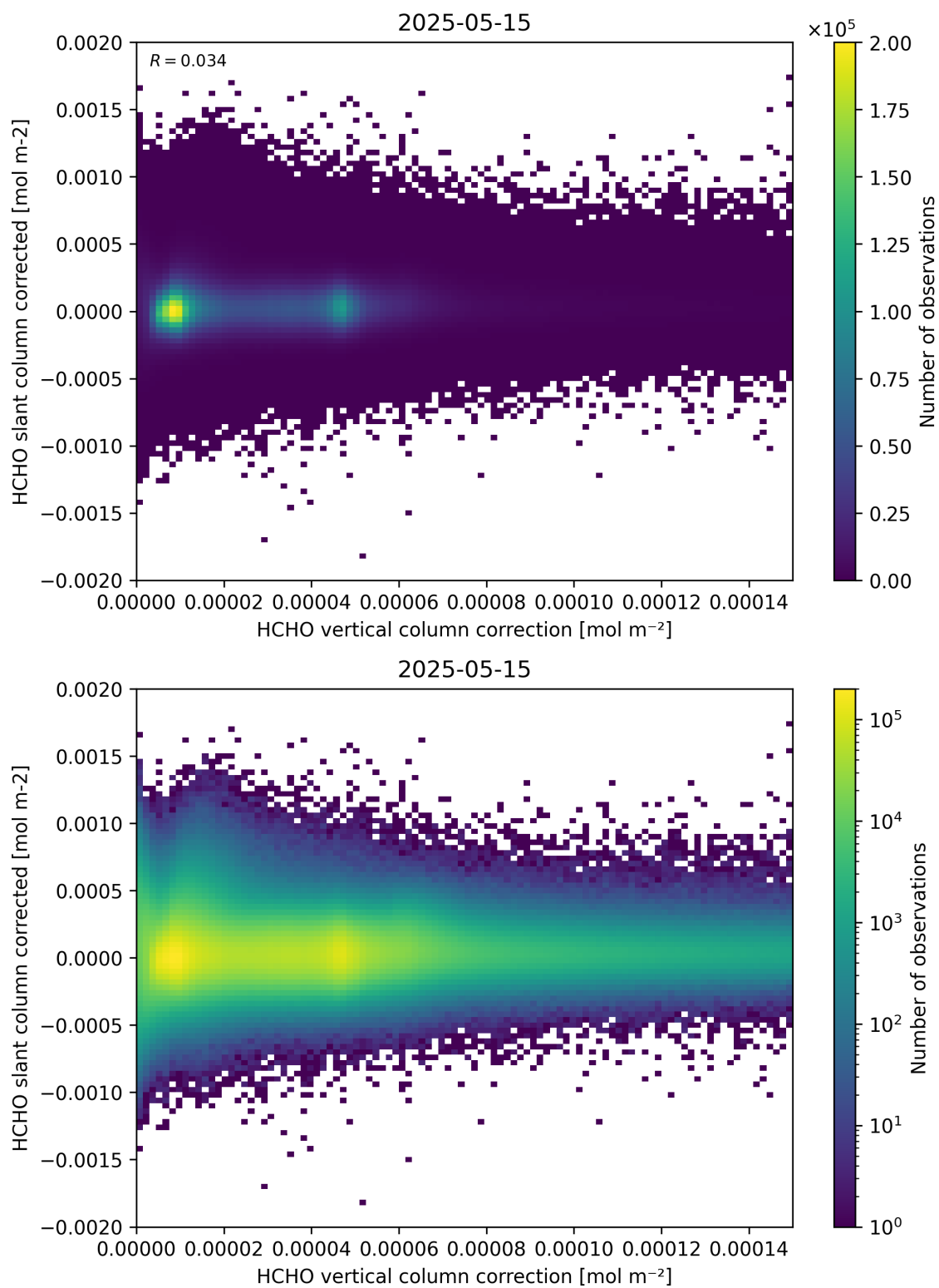
Figure 116: Scatter density plot of “HCHO vertical column correction” against “HCHO slant column corrected” for 2025-05-15 to 2025-05-16.
