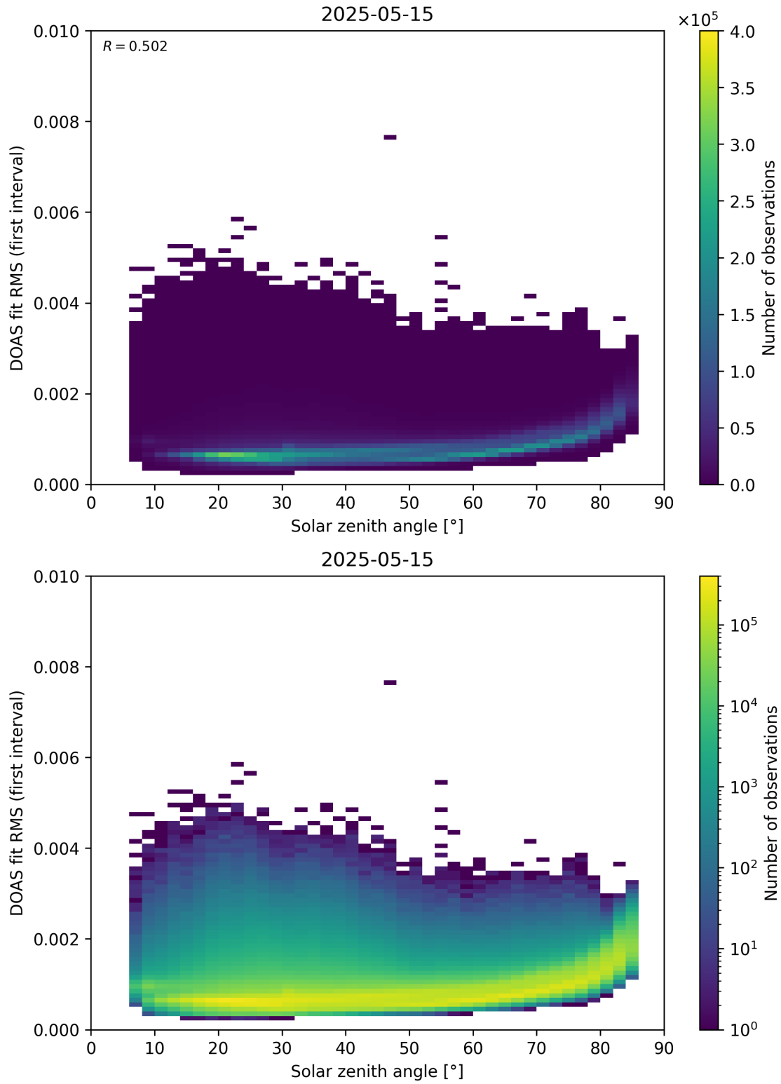
Figure 167: Scatter density plot of “Solar zenith angle” against “DOAS fit RMS (first interval)” for 2025-05-15 to 2025-05-16.
