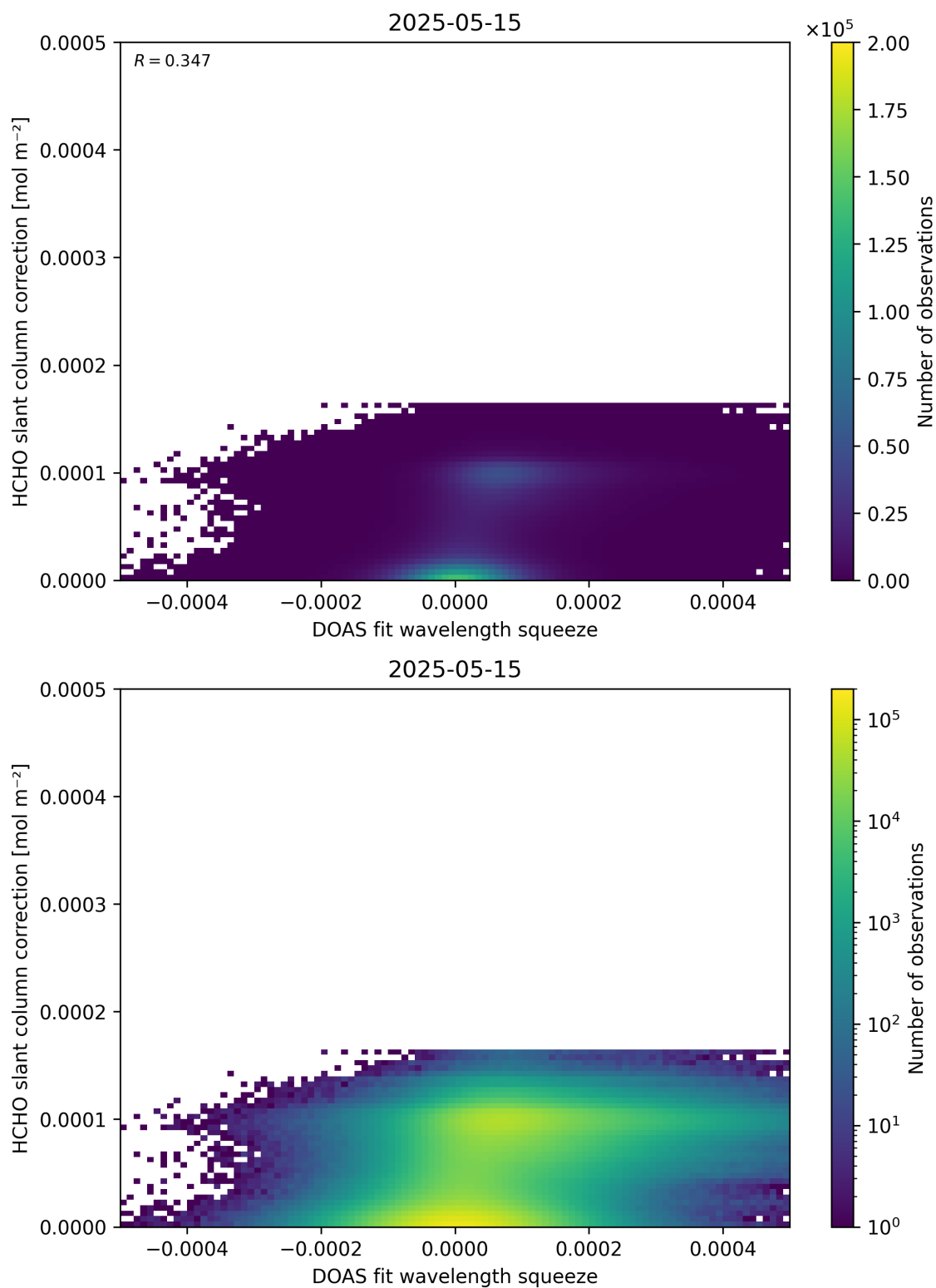
Figure 70: Scatter density plot of “DOAS fit wavelength squeeze” against “HCHO slant column correction” for 2025-05-15 to 2025-05-16.
