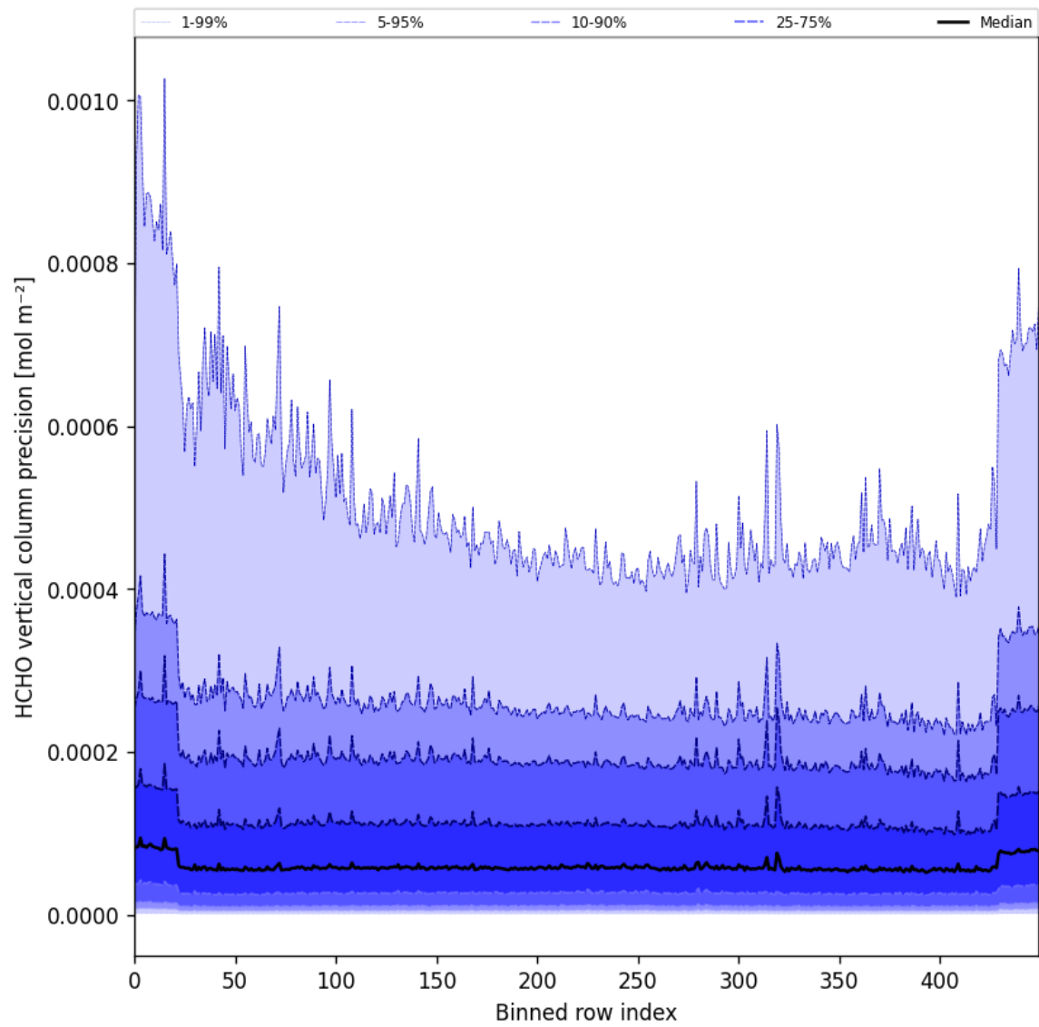
Figure 50: Along track statistics of “HCHO vertical column precision” for 2025-05-15 to 2025-05-16
