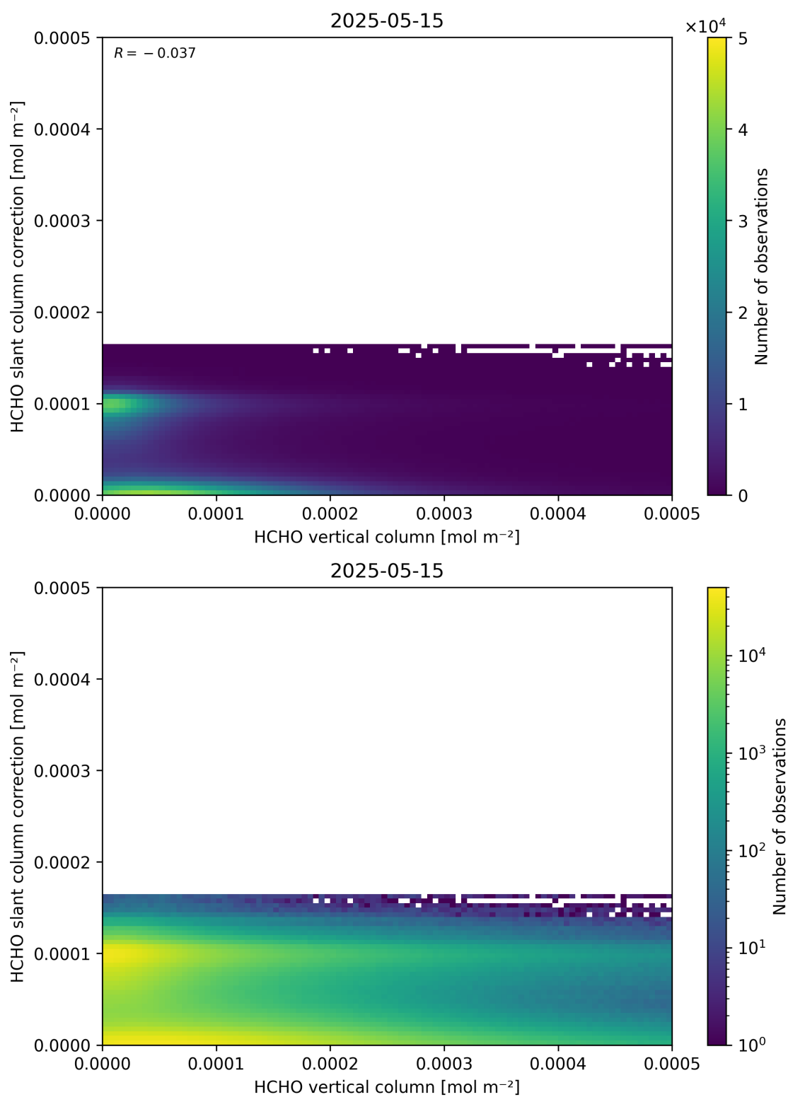
Figure 128: Scatter density plot of “HCHO vertical column” against “HCHO slant column correction” for 2025-05-15 to 2025-05-16.
