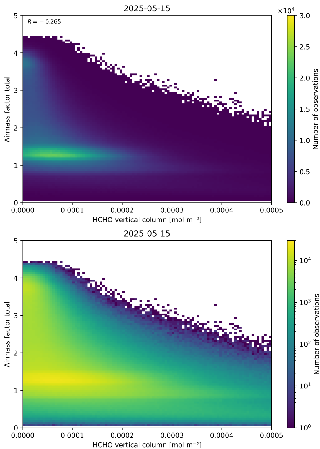
Figure 131: Scatter density plot of “HCHO vertical column” against “Airmass factor total” for 2025-05-15 to 2025-05-16.
