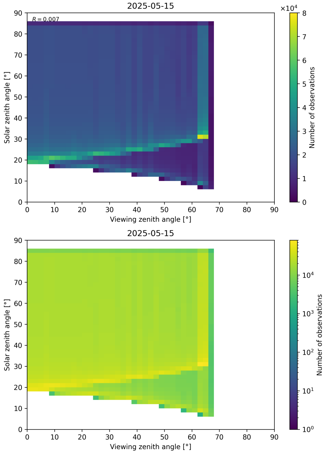
Figure 197: Scatter density plot of “Viewing zenith angle” against “Solar zenith angle” for 2025-05-15 to 2025-05-16.
