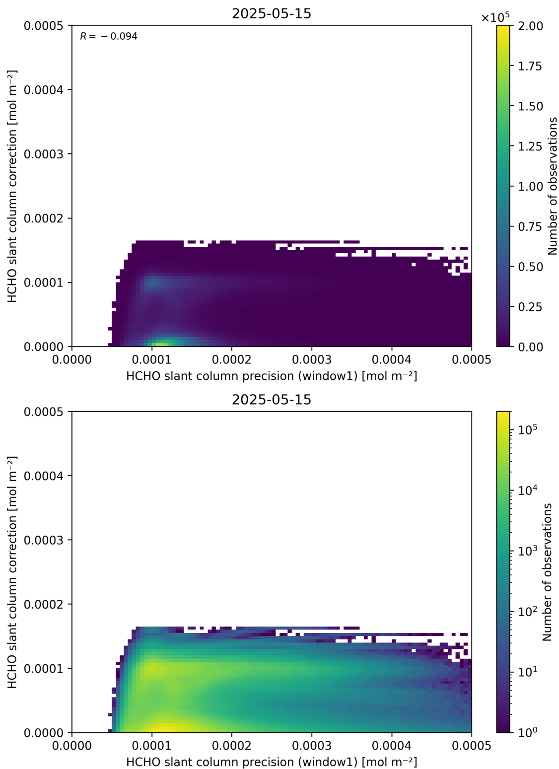
Figure 93: Scatter density plot of “HCHO slant column precision (window1)” against “HCHO slant column correction” for 2025-05-15 to 2025-05-16.
