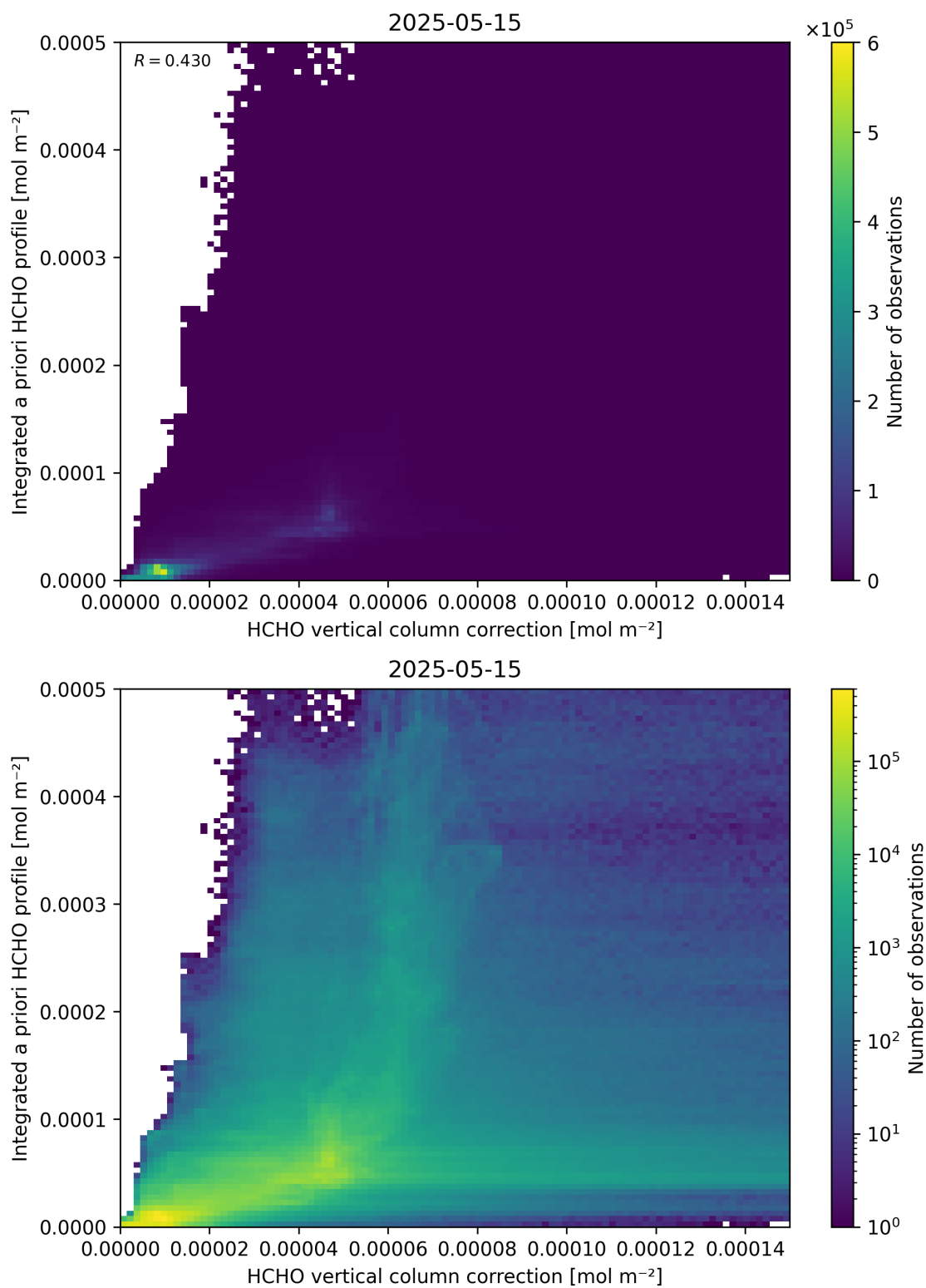
Figure 122: Scatter density plot of “HCHO vertical column correction” against “Integrated a priori HCHO profile” for 2025-05-15 to 2025-05-16.
