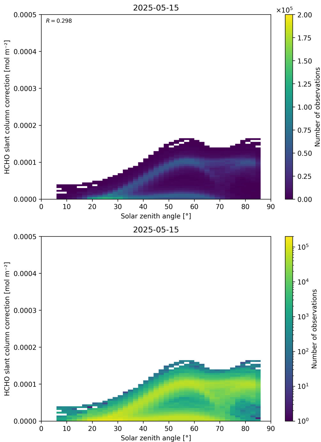
Figure 172: Scatter density plot of “Solar zenith angle” against “HCHO slant column correction” for 2025-05-15 to 2025-05-16.
