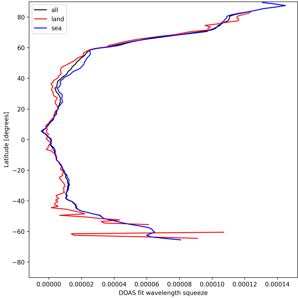
Figure 31: Zonal average of “DOAS fit wavelength squeeze” for 2025-05-15 to 2025-05-16.
