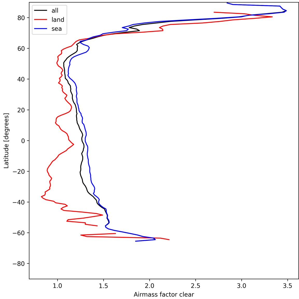
Figure 28: Zonal average of “Airmass factor clear” for 2025-05-15 to 2025-05-16.
