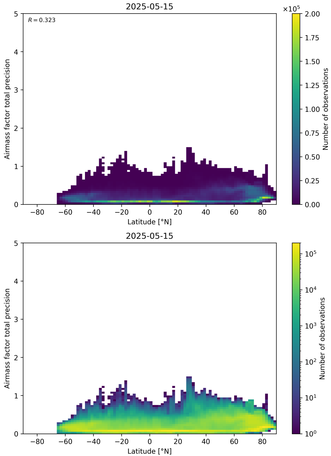
Figure 162: Scatter density plot of “Latitude” against “Airmass factor total precision” for 2025-05-15 to 2025-05-16.
