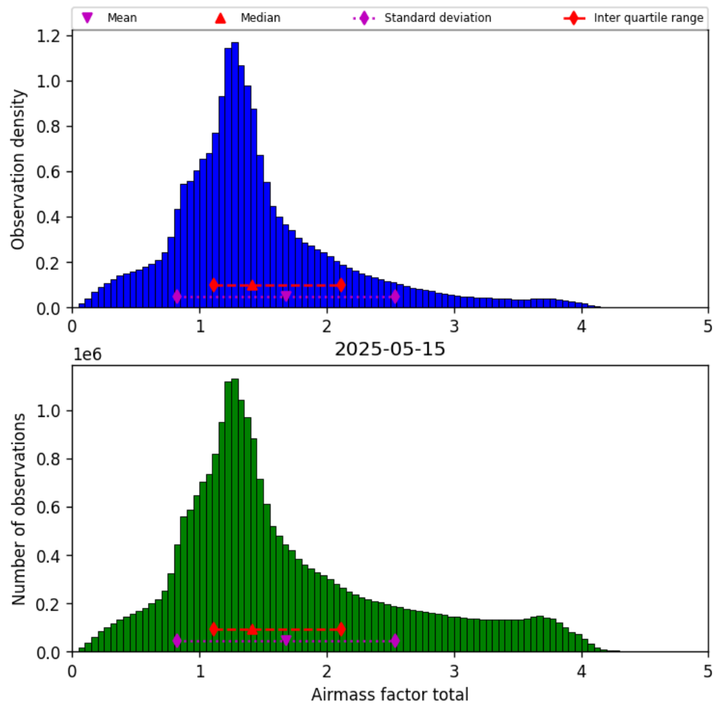
Figure 40: Histogram of “Airmass factor total” for 2025-05-15 to 2025-05-16
