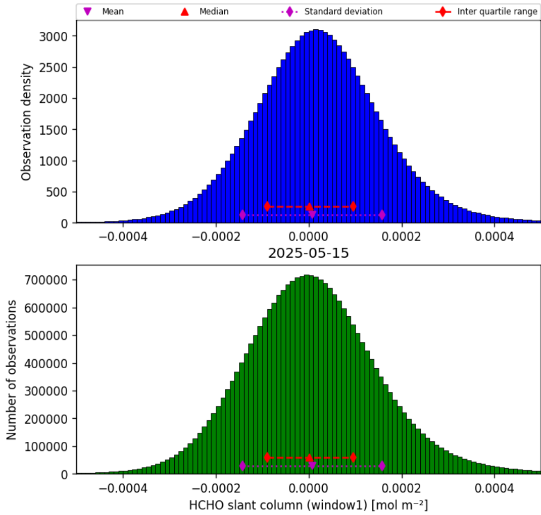
Figure 38: Histogram of “HCHO slant column (window1)” for 2025-05-15 to 2025-05-16
