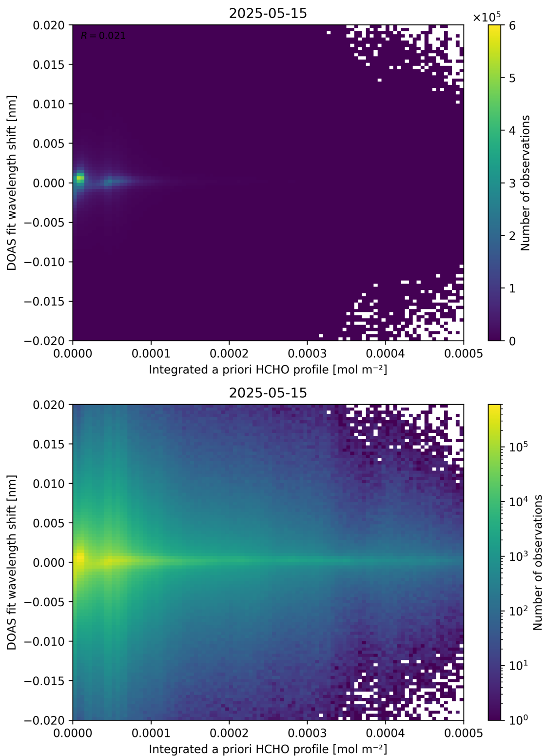
Figure 149: Scatter density plot of “Integrated a priori HCHO profile” against “DOAS fit wavelength shift” for 2025-05-15 to 2025-05-16.
