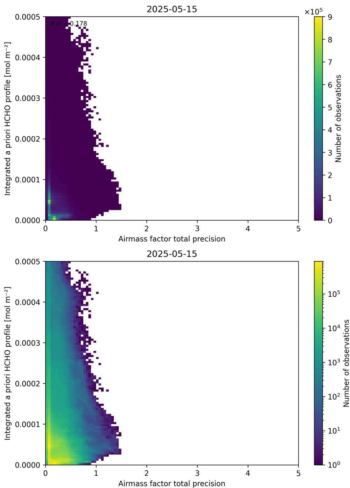
Figure 111: Scatter density plot of “Airmass factor total precision” against “Integrated a priori HCHO profile” for 2025-05-15 to 2025-05-16.
