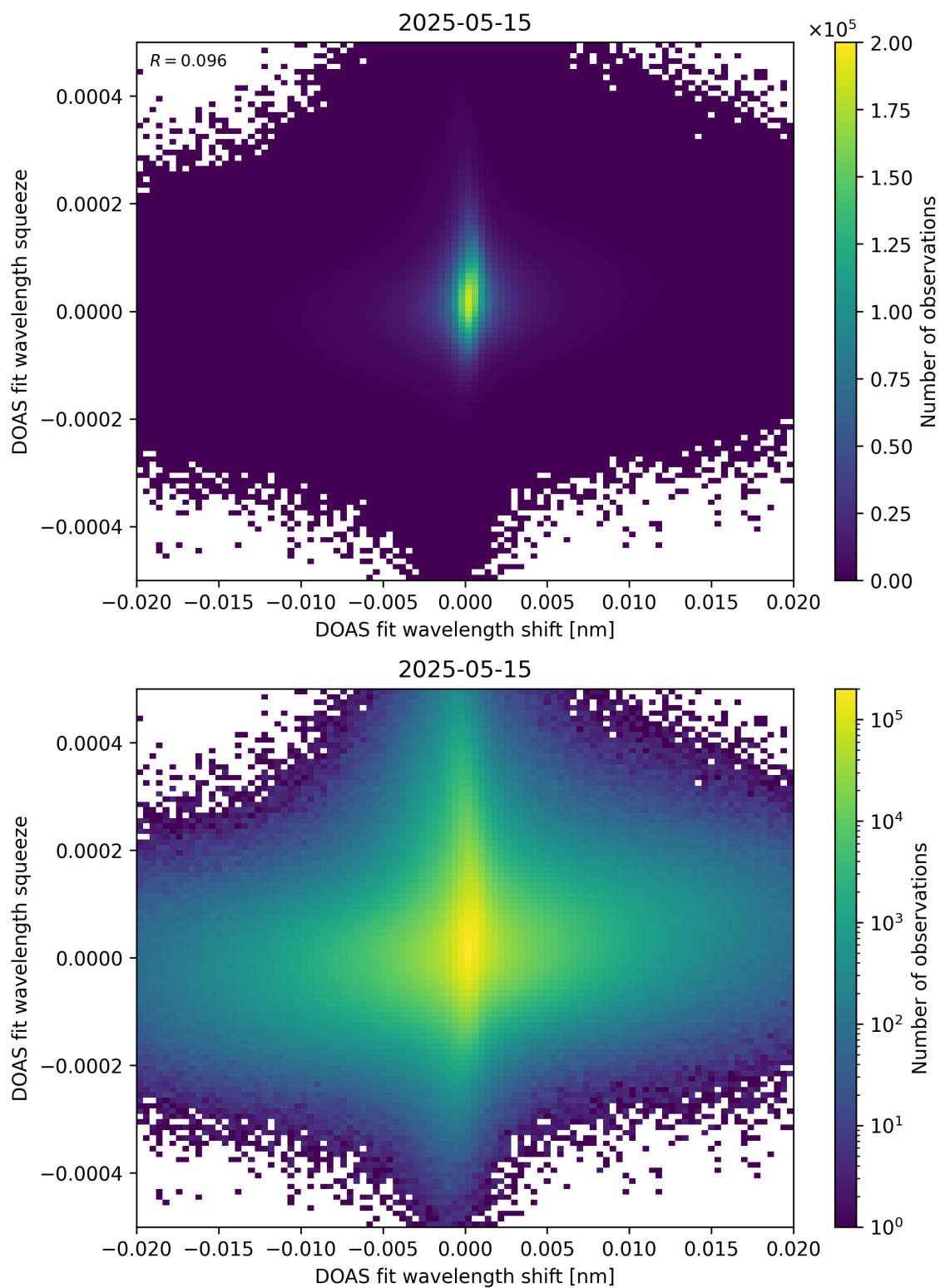
Figure 65: Scatter density plot of “DOAS fit wavelength shift” against “DOAS fit wavelength squeeze” for 2025-05-15 to 2025-05-16.
