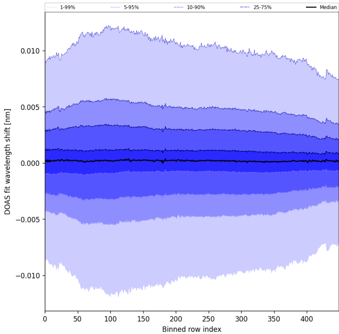
Figure 58: Along track statistics of “DOAS fit wavelength shift” for 2025-05-15 to 2025-05-16
