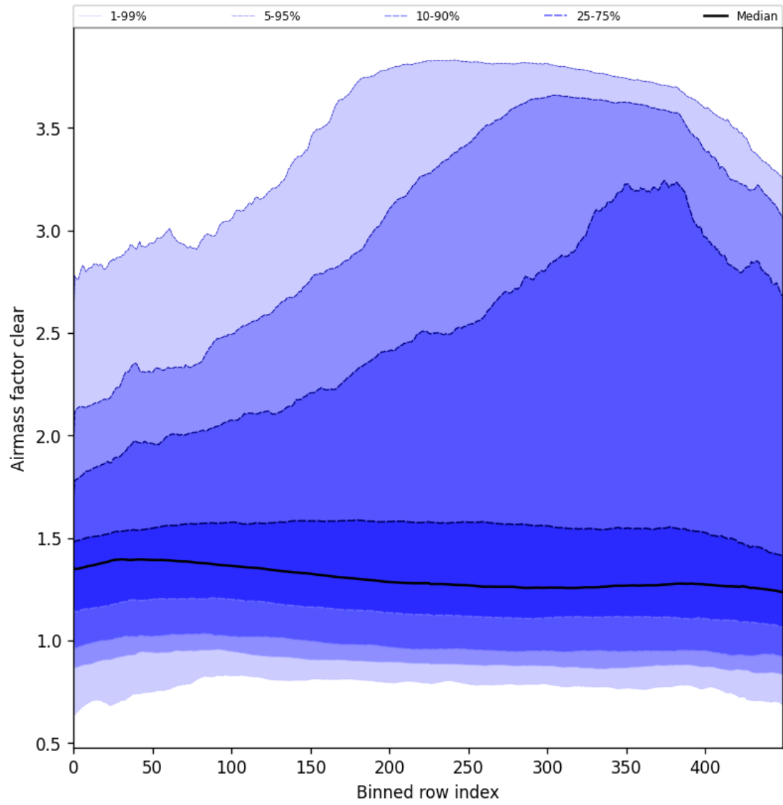
Figure 56: Along track statistics of “Airmass factor clear” for 2025-05-15 to 2025-05-16
