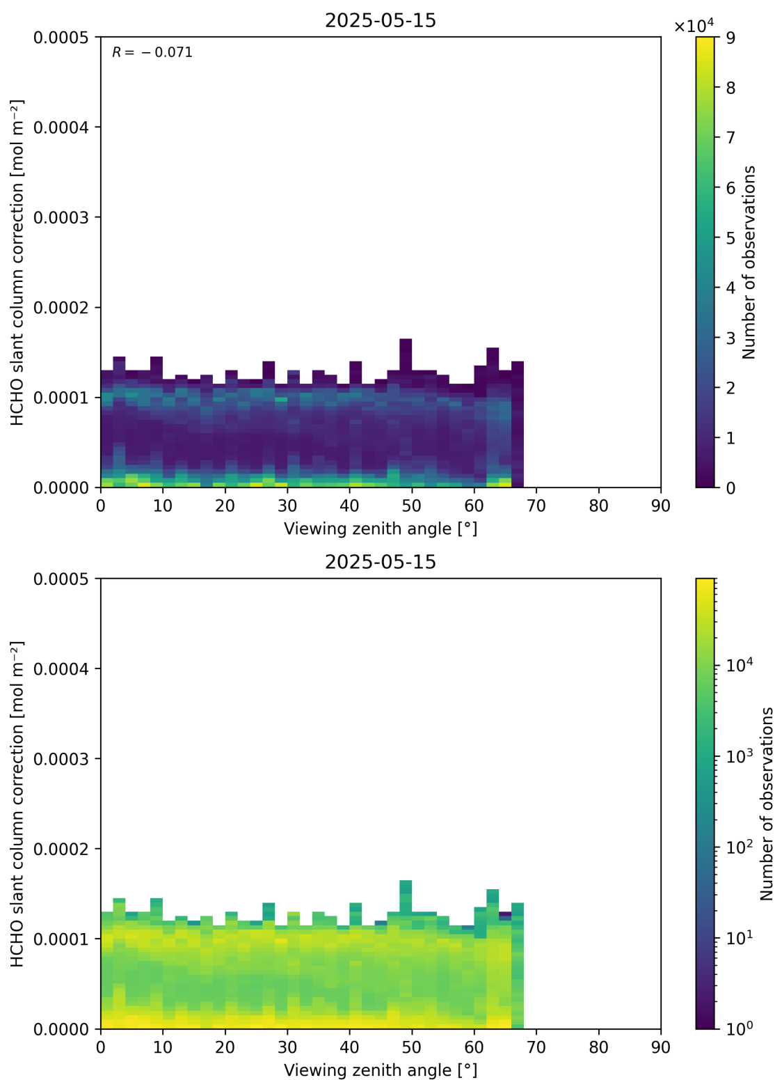
Figure 187: Scatter density plot of “Viewing zenith angle” against “HCHO slant column correction” for 2025-05-15 to 2025-05-16.
