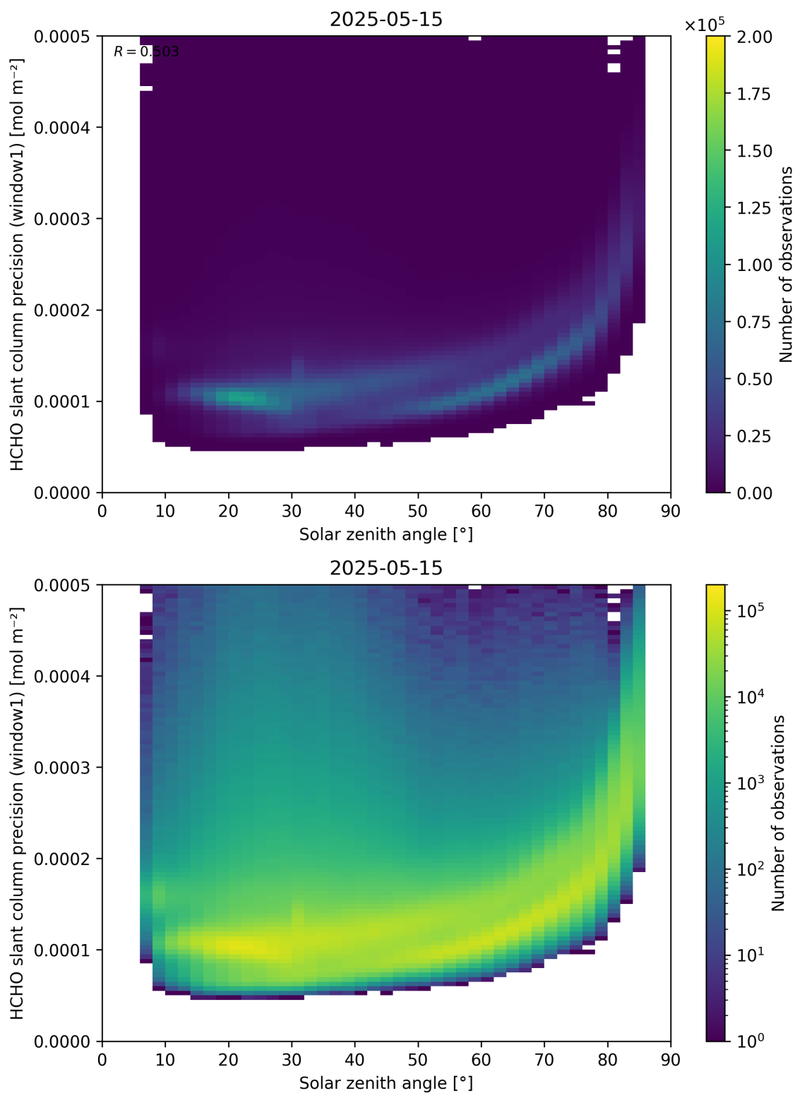
Figure 174: Scatter density plot of “Solar zenith angle” against “HCHO slant column precision (window1)” for 2025-05-15 to 2025-05-16.
