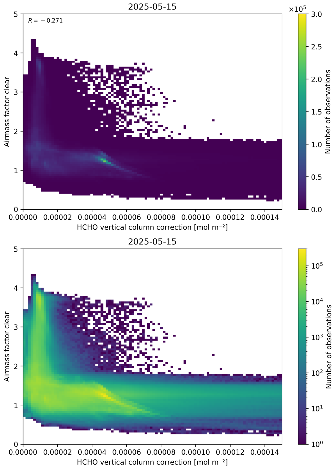
Figure 115: Scatter density plot of “HCHO vertical column correction” against “Airmass factor clear” for 2025-05-15 to 2025-05-16.
