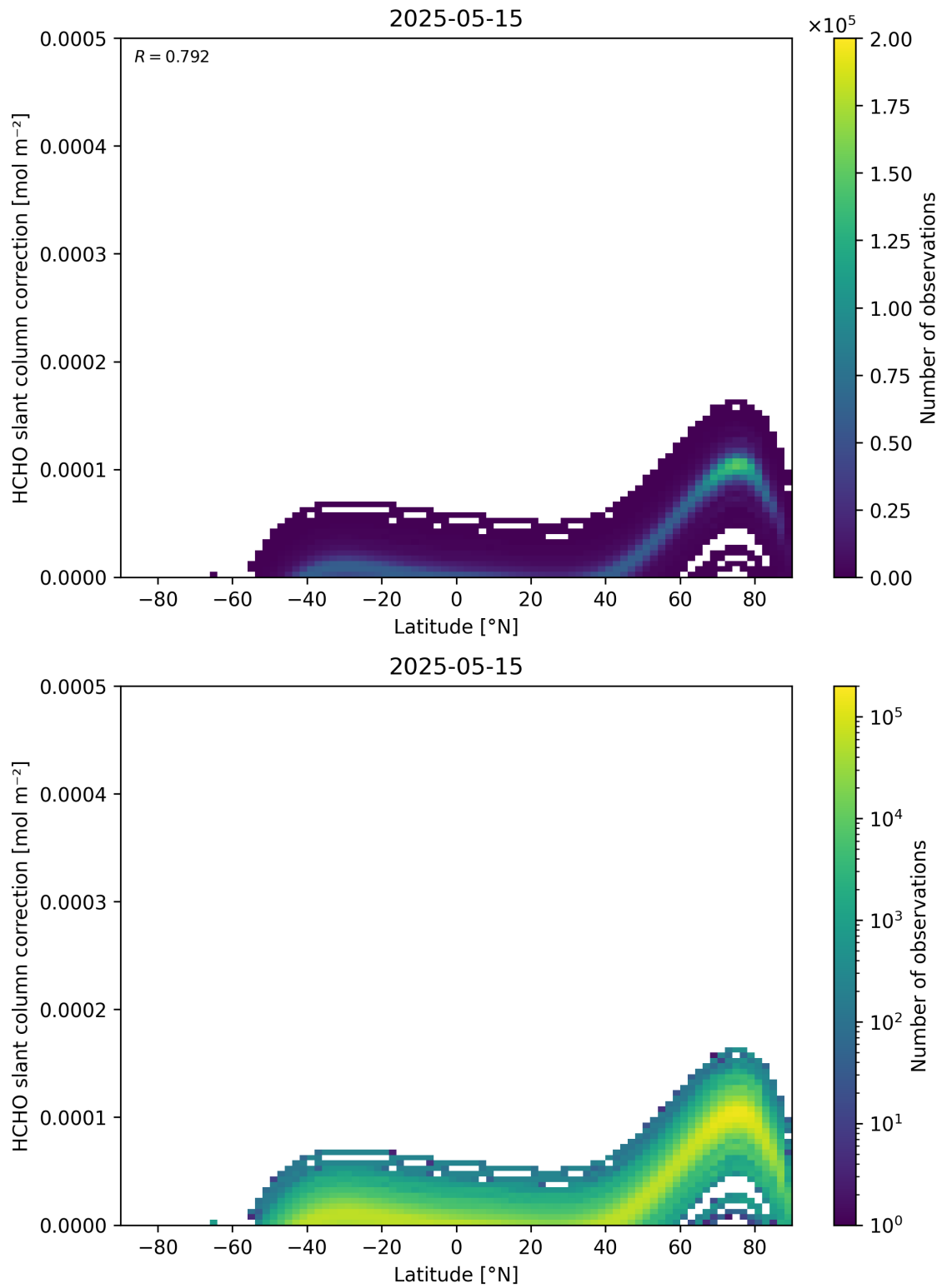
Figure 158: Scatter density plot of “Latitude” against “HCHO slant column correction” for 2025-05-15 to 2025-05-16.
