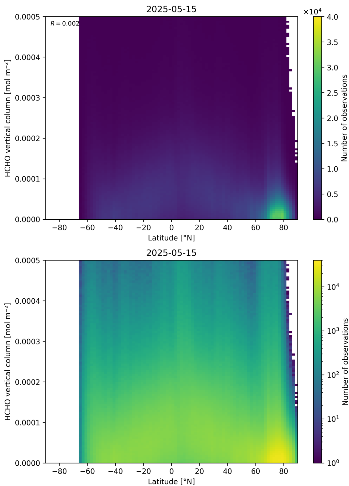
Figure 163: Scatter density plot of “Latitude” against “HCHO vertical column” for 2025-05-15 to 2025-05-16.
