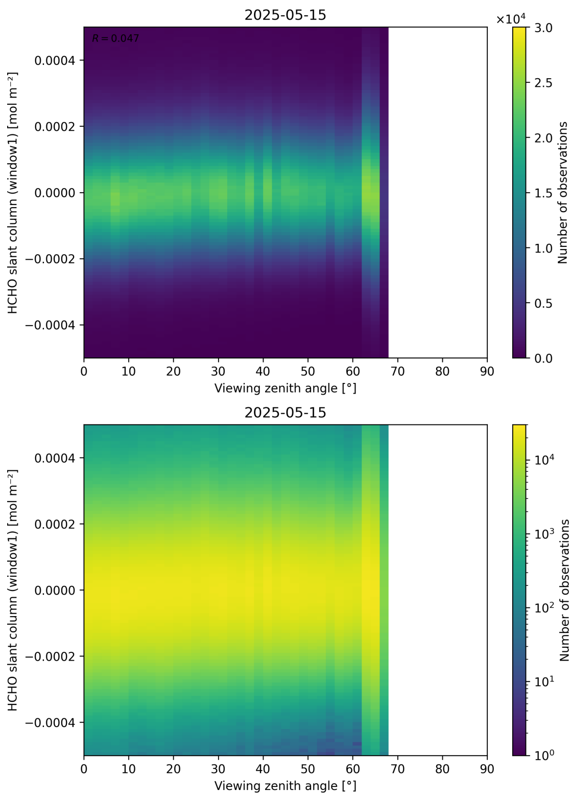
Figure 188: Scatter density plot of “Viewing zenith angle” against “HCHO slant column (window1)” for 2025-05-15 to 2025-05-16.
