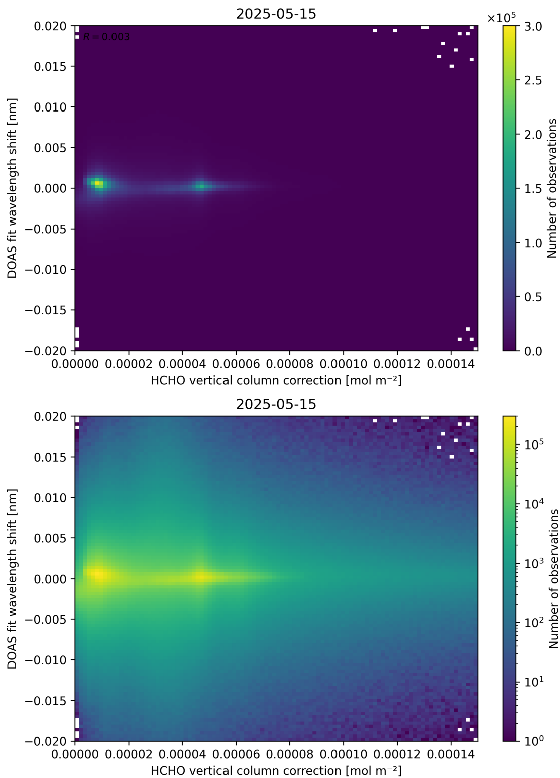
Figure 113: Scatter density plot of “HCHO vertical column correction” against “DOAS fit wavelength shift” for 2025-05-15 to 2025-05-16.
