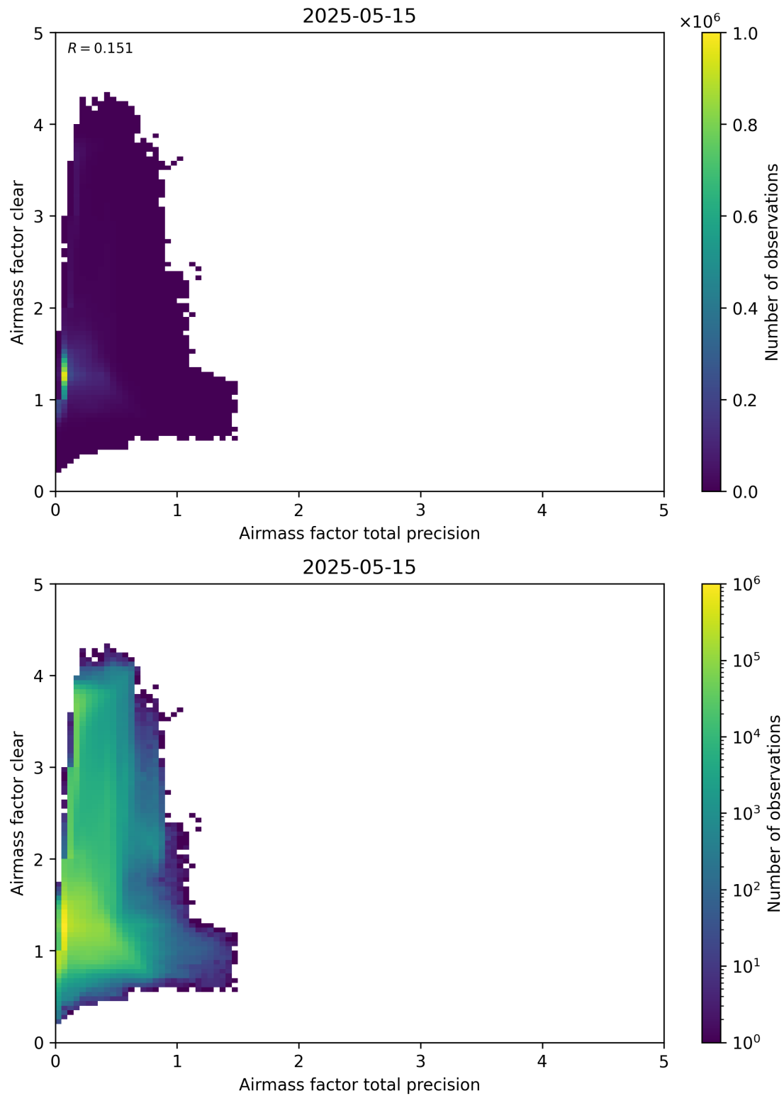
Figure 108: Scatter density plot of “Airmass factor total precision” against “Airmass factor clear” for 2025-05-15 to 2025-05-16.
