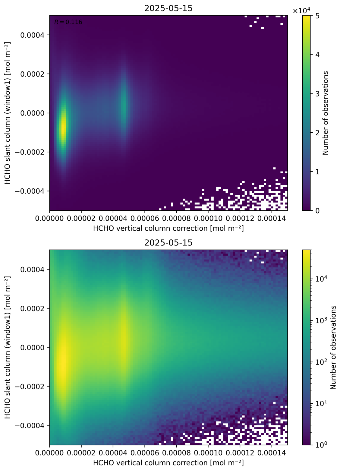
Figure 118: Scatter density plot of “HCHO vertical column correction” against “HCHO slant column (window1)” for 2025-05-15 to 2025-05-16.
