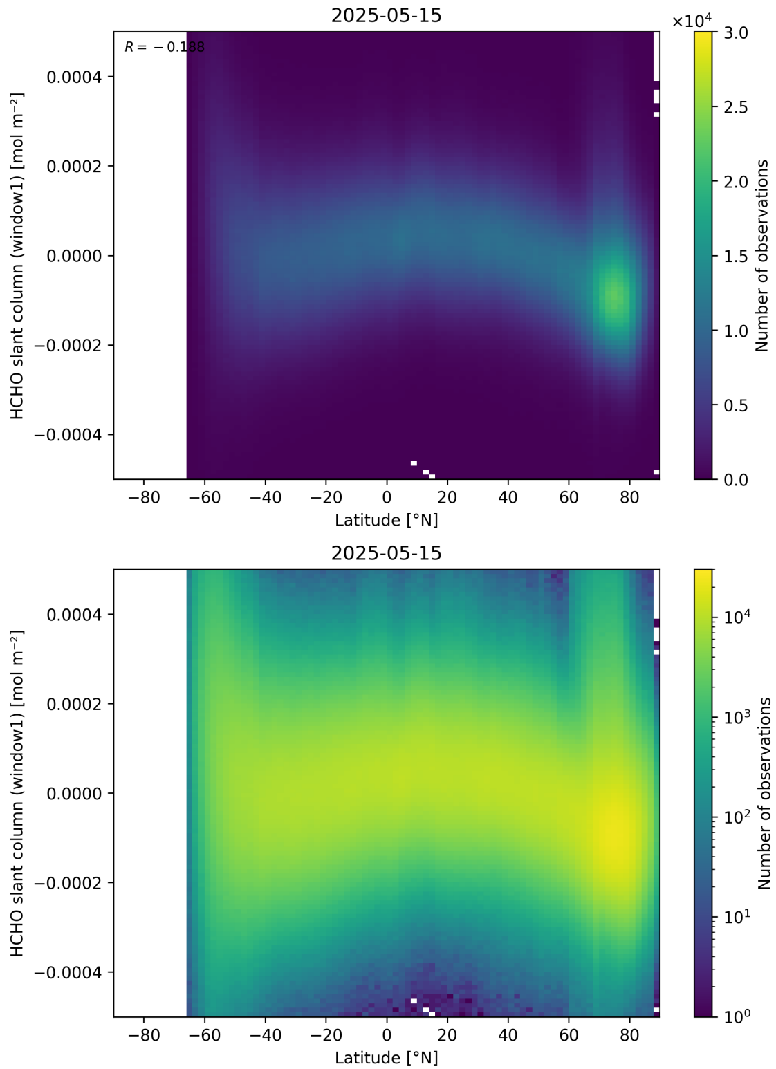
Figure 159: Scatter density plot of “Latitude” against “HCHO slant column (window1)” for 2025-05-15 to 2025-05-16.
