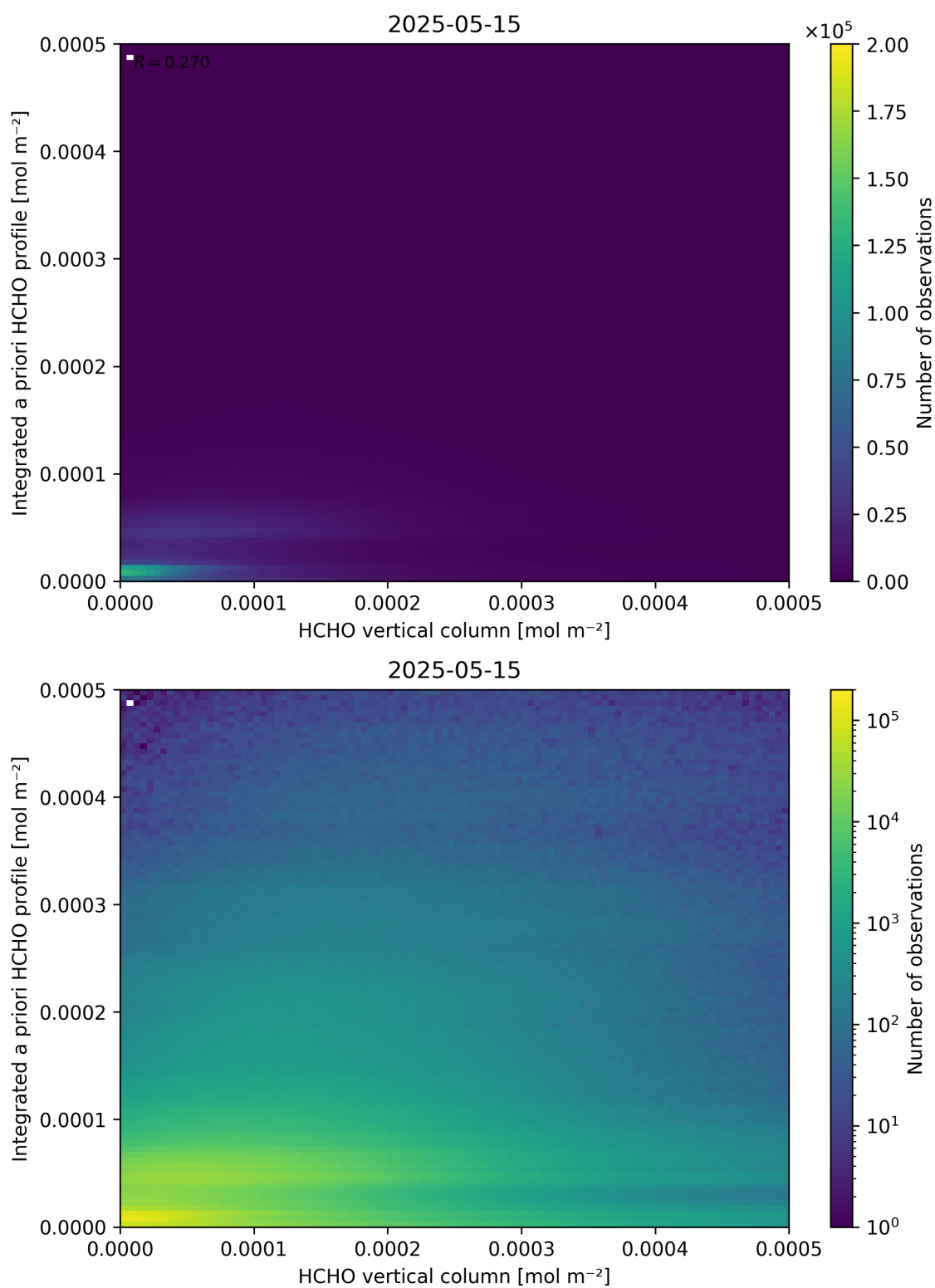
Figure 135: Scatter density plot of “HCHO vertical column” against “Integrated a priori HCHO profile” for 2025-05-15 to 2025-05-16.
