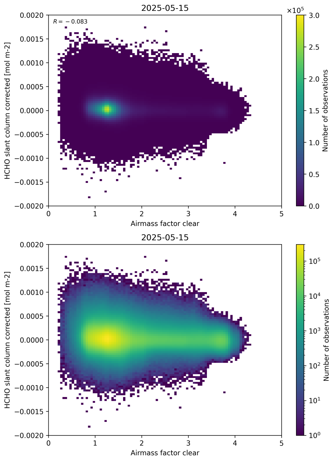
Figure 74: Scatter density plot of “Airmass factor clear” against “HCHO slant column corrected” for 2025-05-15 to 2025-05-16.
