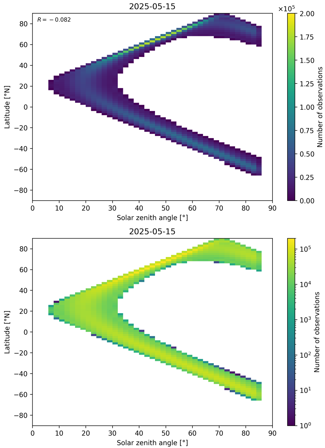
Figure 181: Scatter density plot of “Solar zenith angle” against “Latitude” for 2025-05-15 to 2025-05-16.
