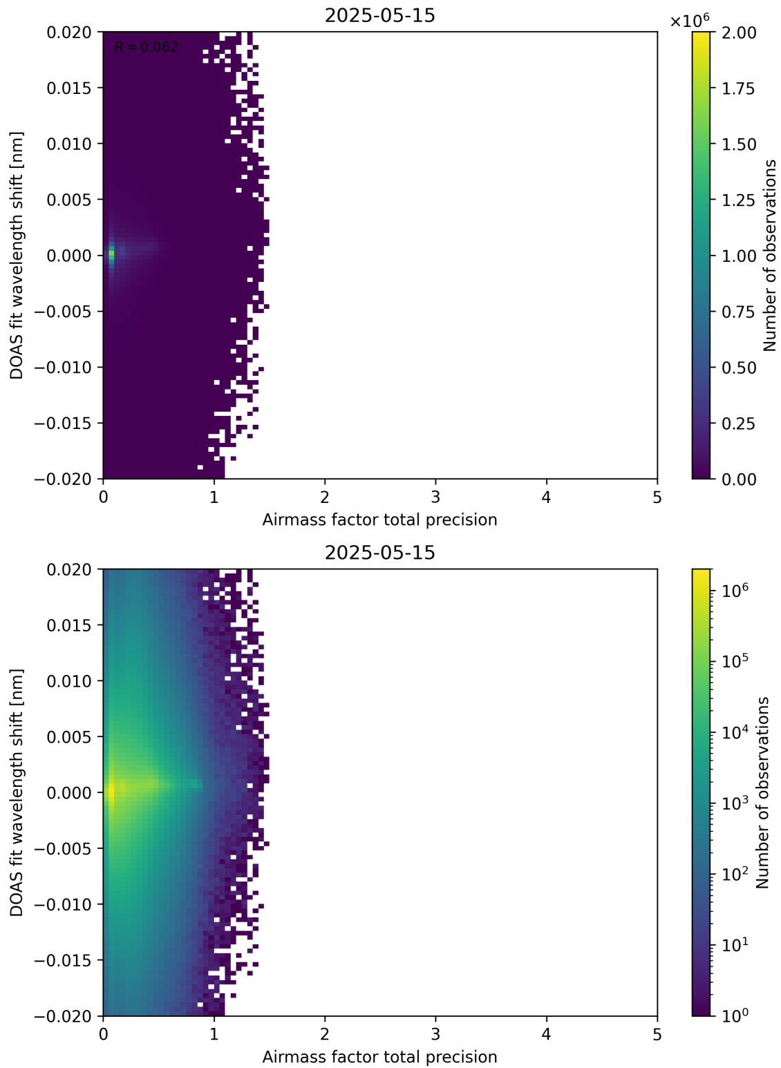
Figure 106: Scatter density plot of “Airmass factor total precision” against “DOAS fit wavelength shift” for 2025-05-15 to 2025-05-16.
