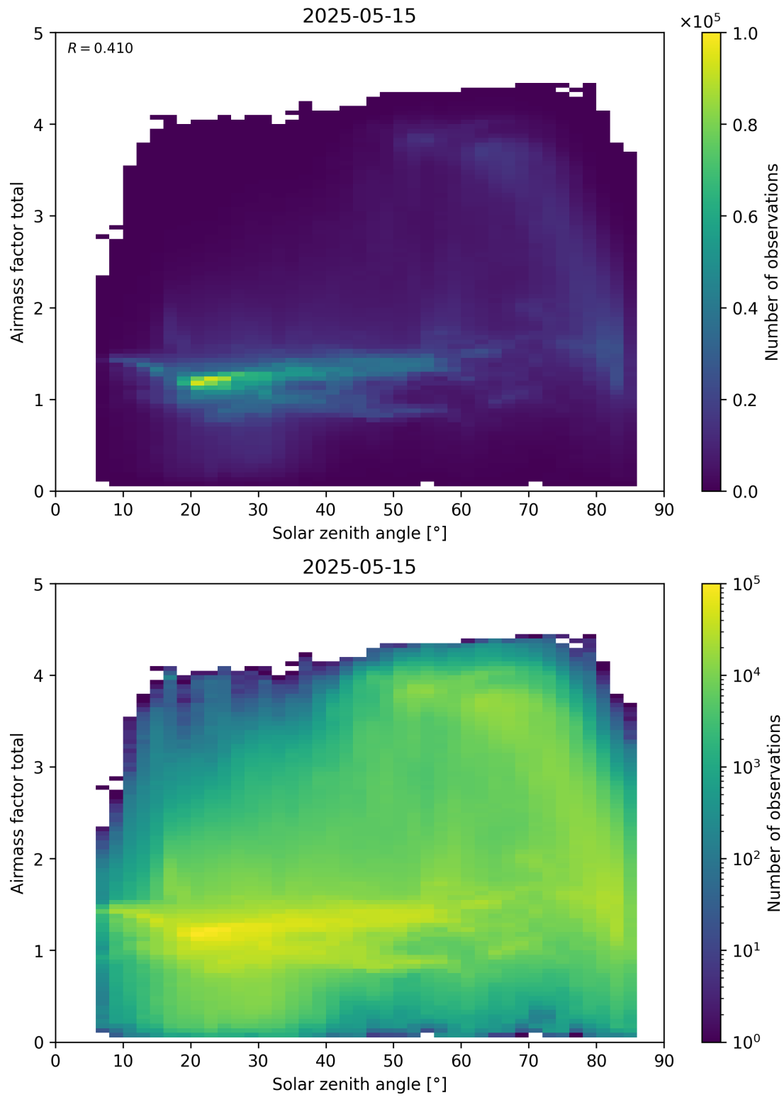
Figure 175: Scatter density plot of “Solar zenith angle” against “Airmass factor total” for 2025-05-15 to 2025-05-16.
