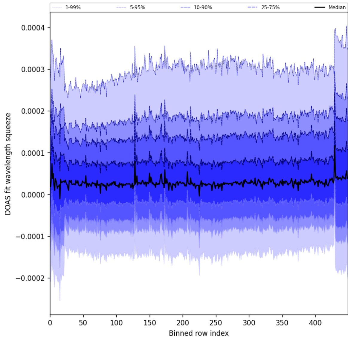
Figure 59: Along track statistics of “DOAS fit wavelength squeeze” for 2025-05-15 to 2025-05-16
