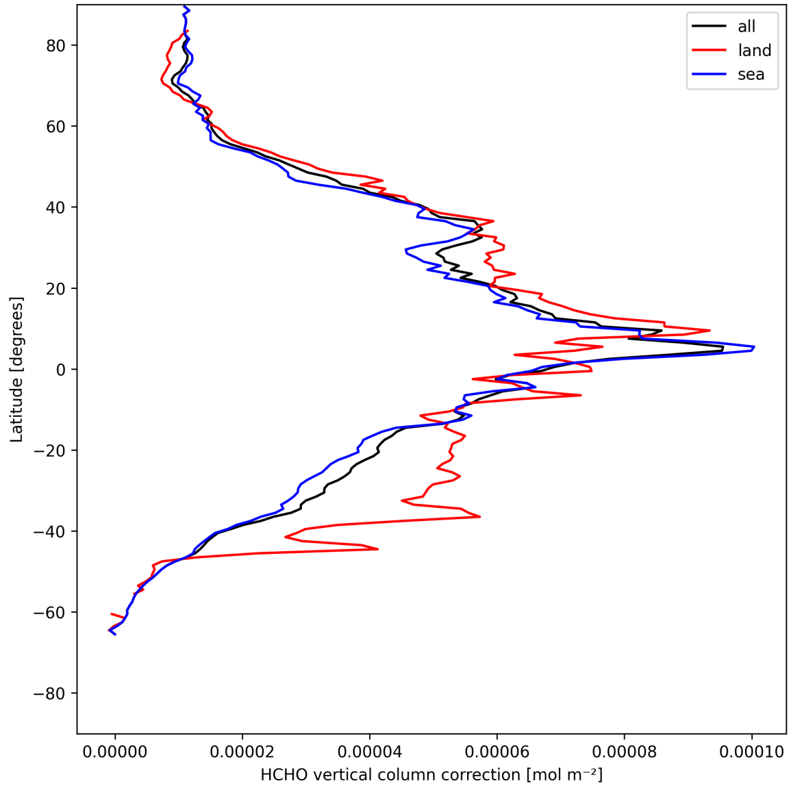
Figure 23: Zonal average of “HCHO vertical column correction” for 2025-05-15 to 2025-05-16.
