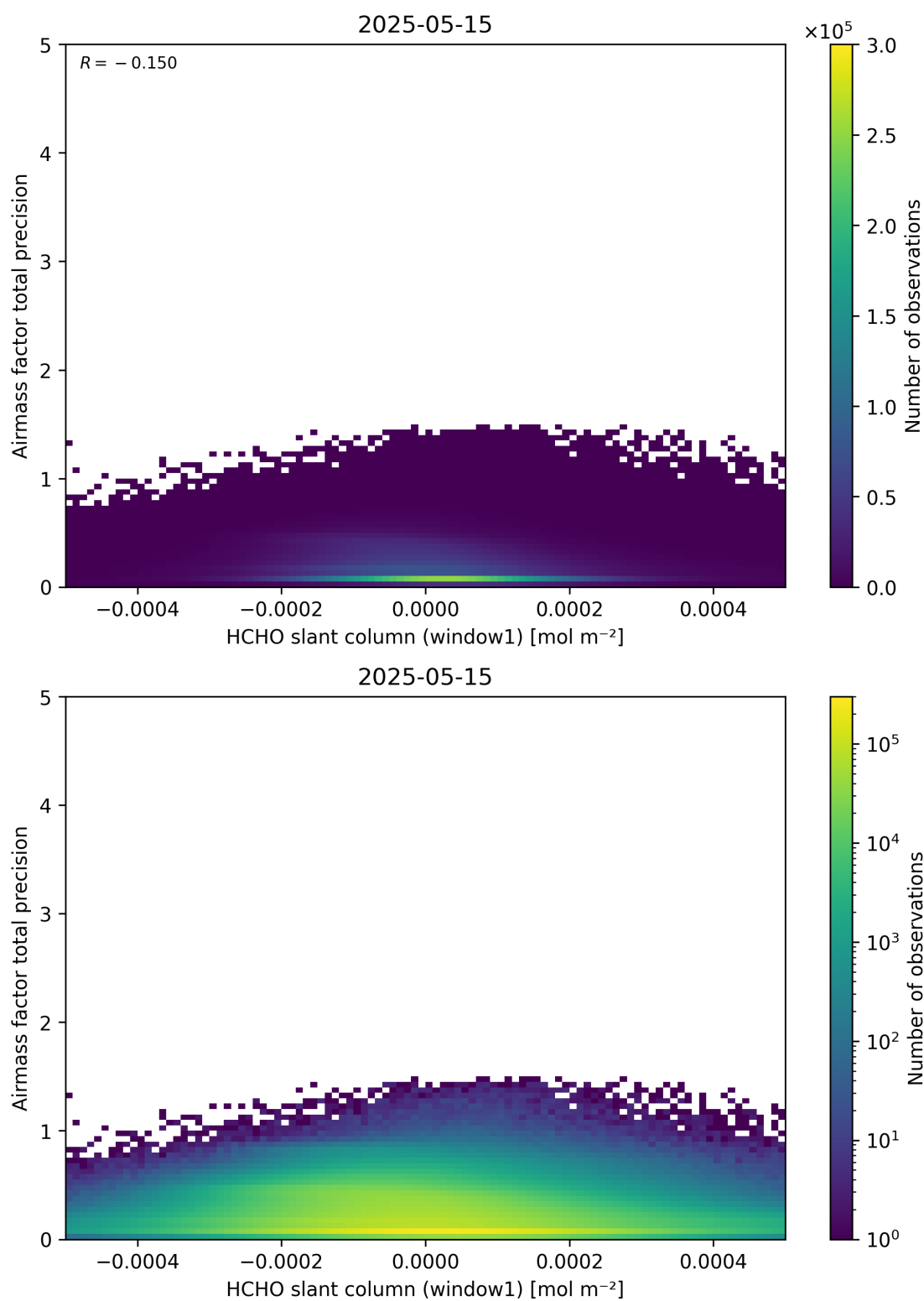
Figure 86: Scatter density plot of “HCHO slant column (window1)” against “Airmass factor total precision” for 2025-05-15 to 2025-05-16.
