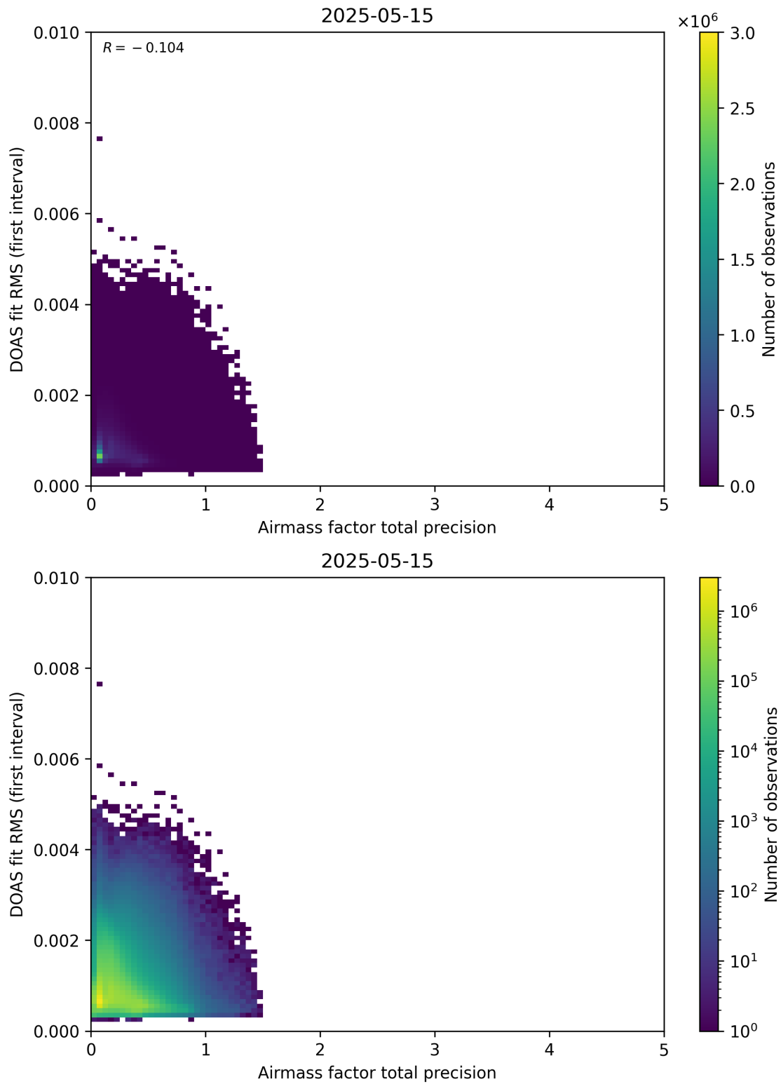
Figure 105: Scatter density plot of “Airmass factor total precision” against “DOAS fit RMS (first interval)” for 2025-05-15 to 2025-05-16.
