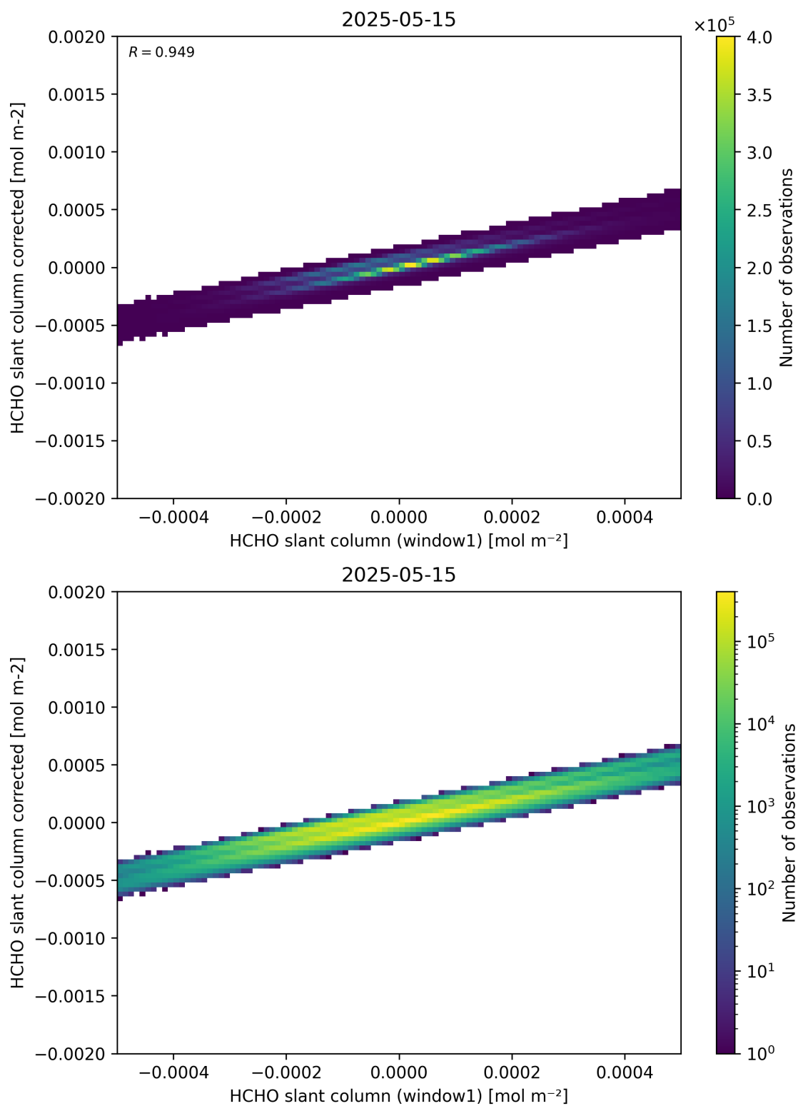
Figure 82: Scatter density plot of “HCHO slant column (window1)” against “HCHO slant column corrected” for 2025-05-15 to 2025-05-16.
