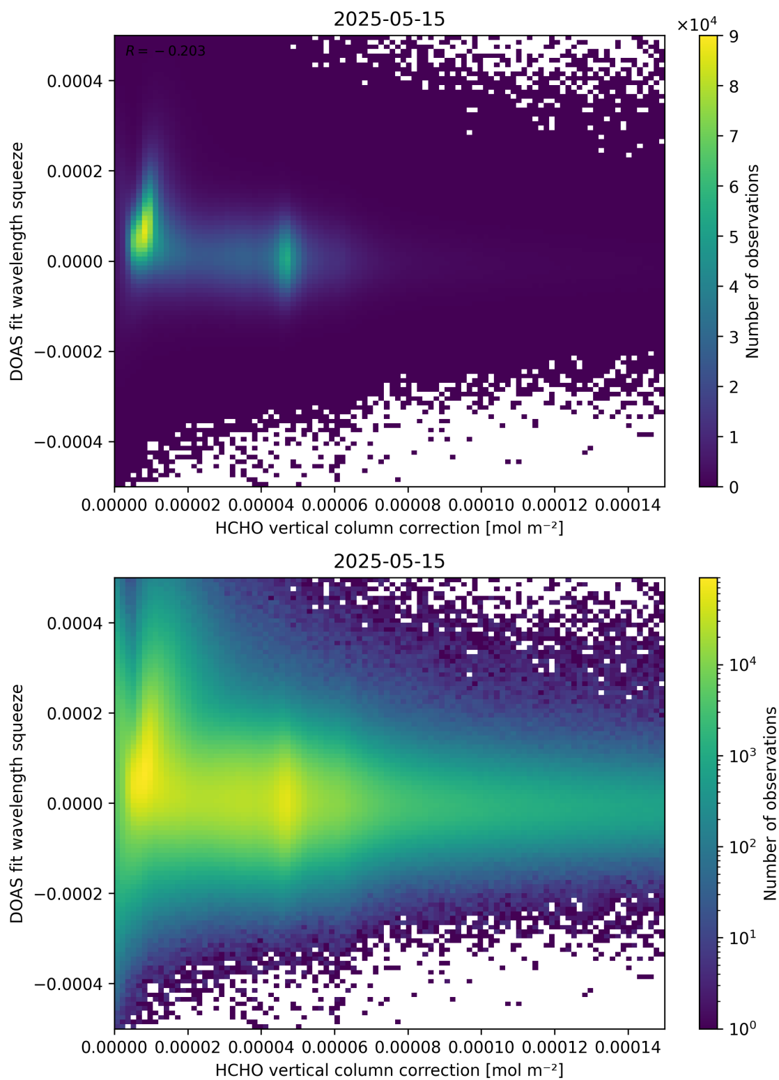
Figure 114: Scatter density plot of “HCHO vertical column correction” against “DOAS fit wavelength squeeze” for 2025-05-15 to 2025-05-16.
