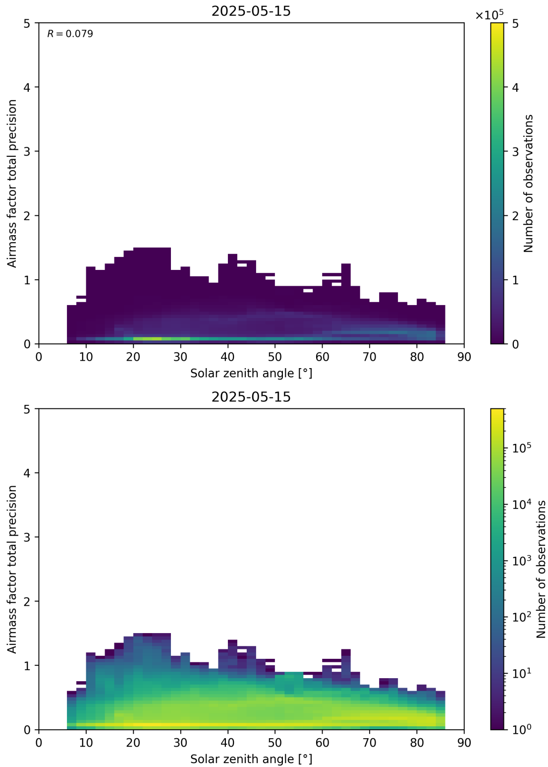
Figure 176: Scatter density plot of “Solar zenith angle” against “Airmass factor total precision” for 2025-05-15 to 2025-05-16.
