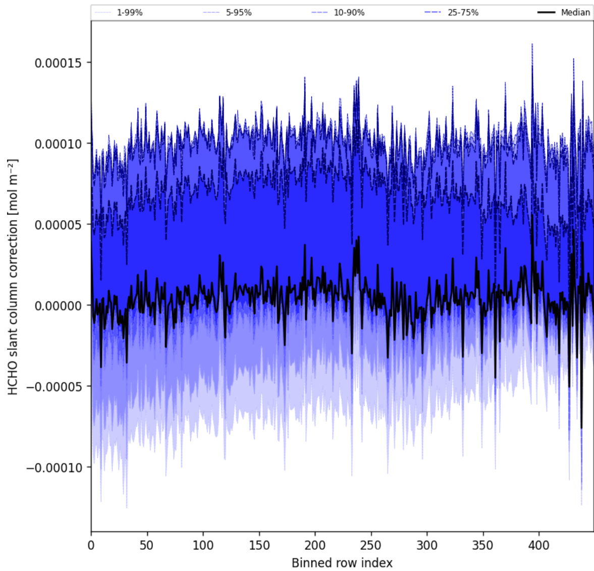
Figure 61: Along track statistics of “HCHO slant column correction” for 2025-05-15 to 2025-05-16
