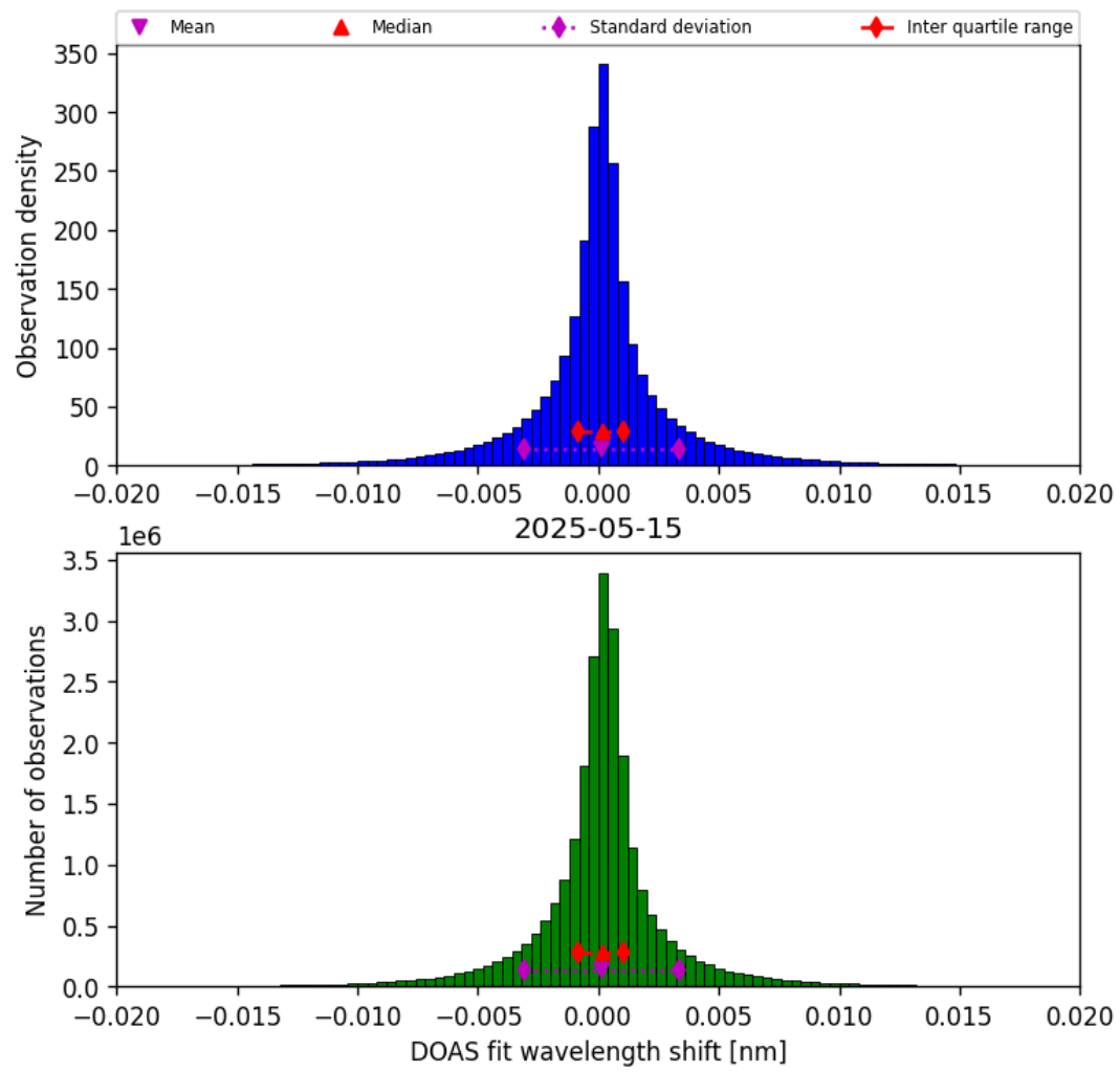
Figure 44: Histogram of “DOAS fit wavelength shift” for 2025-05-15 to 2025-05-16
