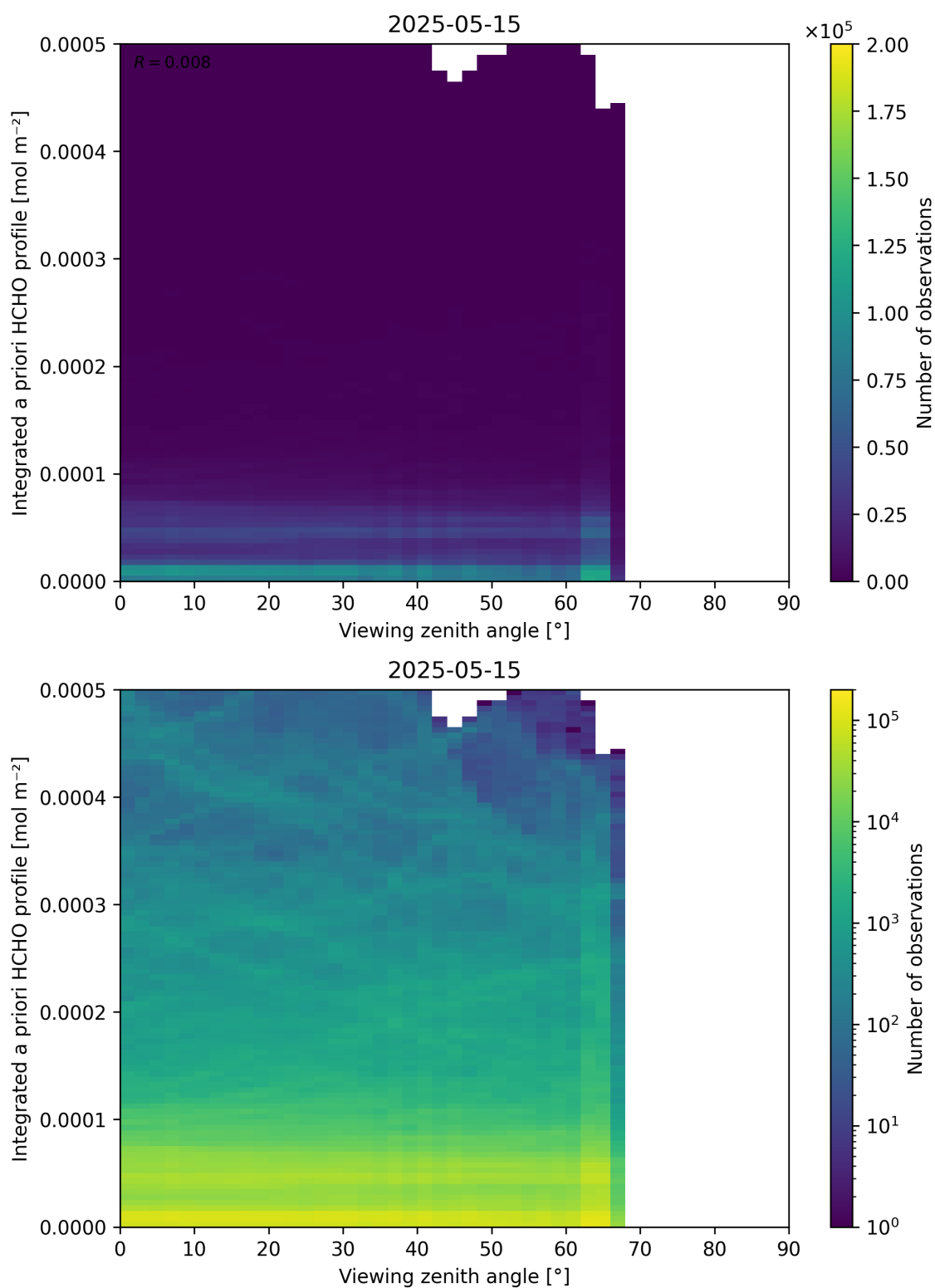
Figure 195: Scatter density plot of “Viewing zenith angle” against “Integrated a priori HCHO profile” for 2025-05-15 to 2025-05-16.
