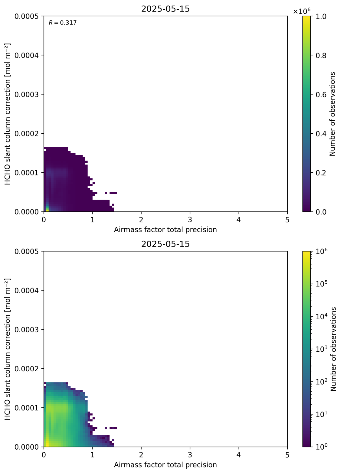
Figure 110: Scatter density plot of “Airmass factor total precision” against “HCHO slant column correction” for 2025-05-15 to 2025-05-16.
