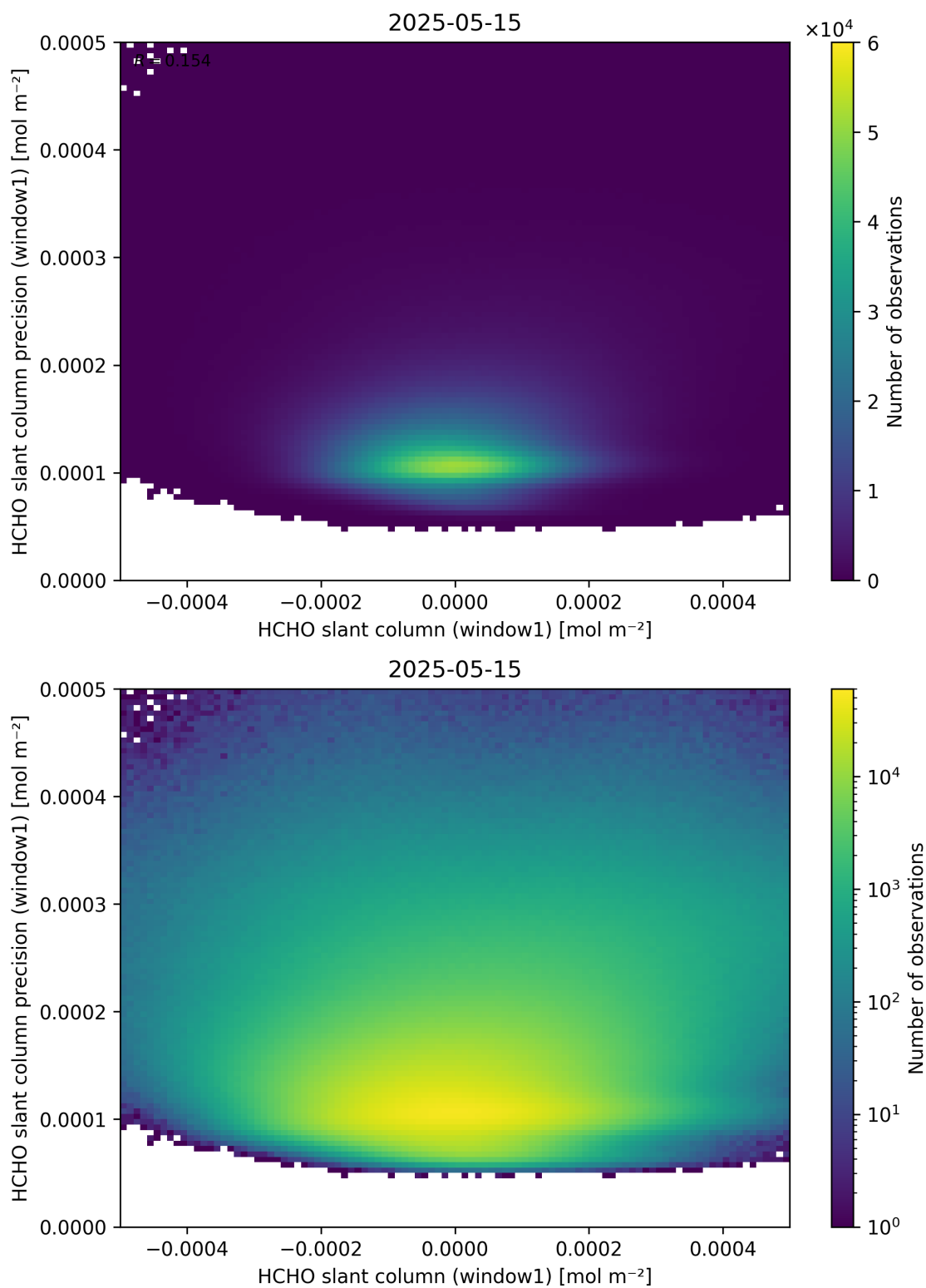
Figure 84: Scatter density plot of “HCHO slant column (window1)” against “HCHO slant column precision (window1)” for 2025-05-15 to 2025-05-16.
