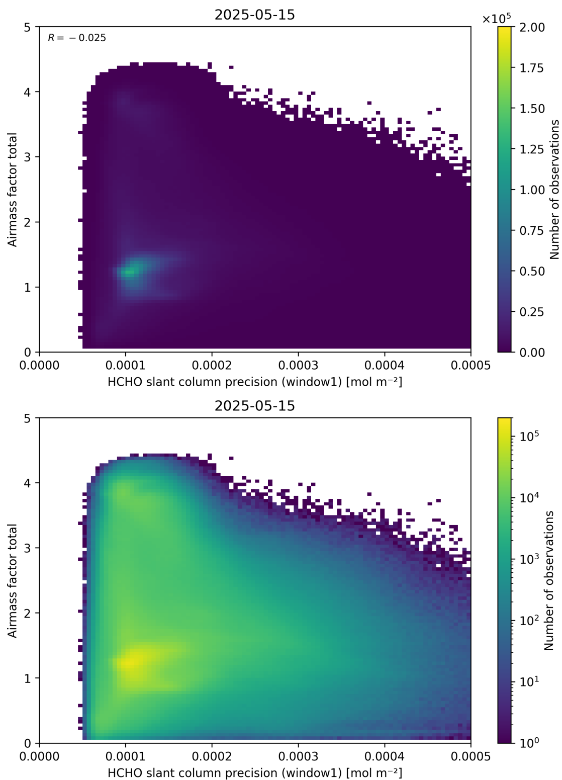
Figure 94: Scatter density plot of “HCHO slant column precision (window1)” against “Airmass factor total” for 2025-05-15 to 2025-05-16.
