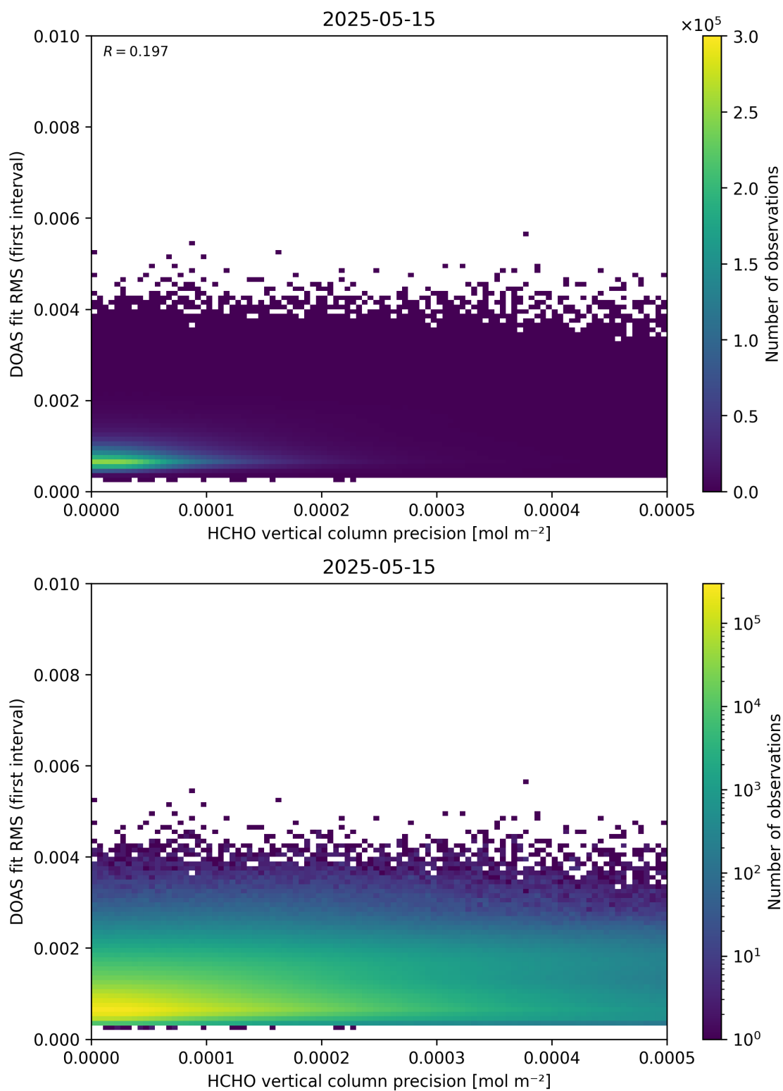
Figure 136: Scatter density plot of “HCHO vertical column precision” against “DOAS fit RMS (first interval)” for 2025-05-15 to 2025-05-16.
