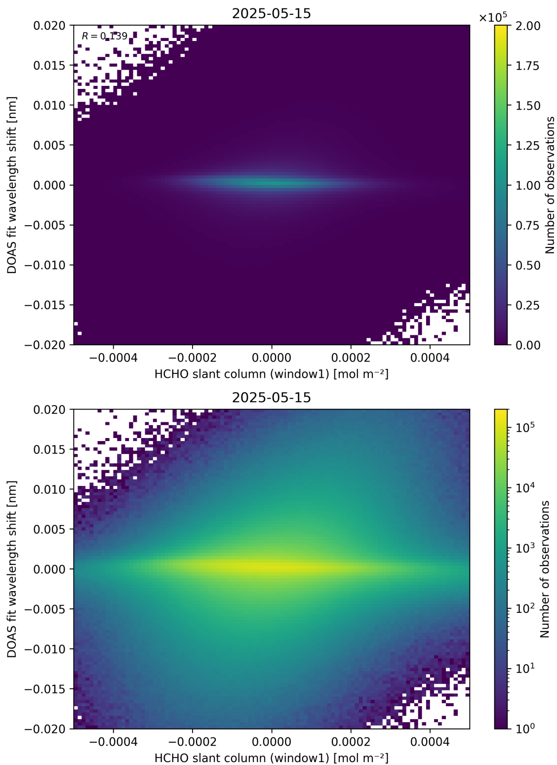
Figure 79: Scatter density plot of “HCHO slant column (window1)” against “DOAS fit wavelength shift” for 2025-05-15 to 2025-05-16.
