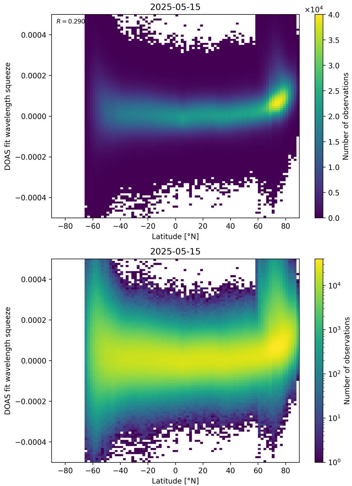
Figure 155: Scatter density plot of “Latitude” against “DOAS fit wavelength squeeze” for 2025-05-15 to 2025-05-16.
