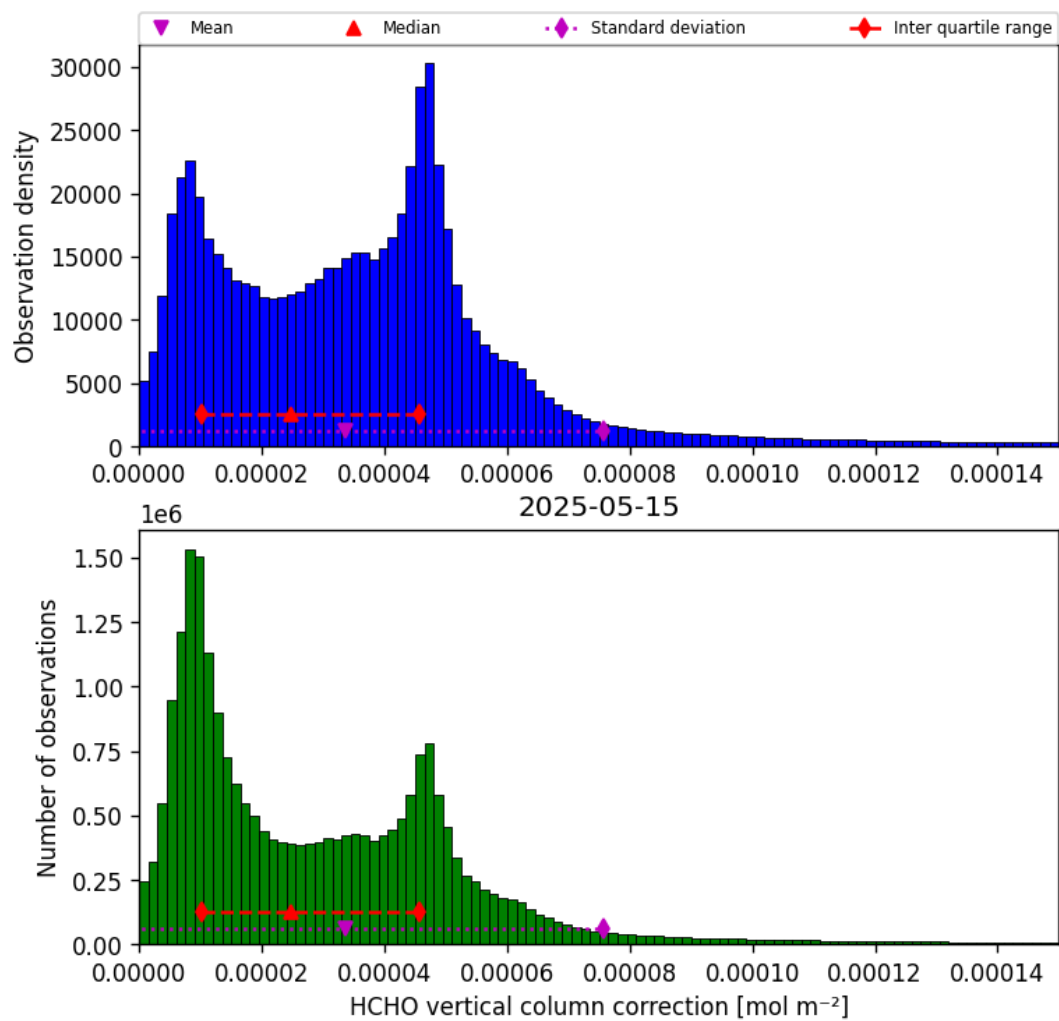
Figure 37: Histogram of “HCHO vertical column correction” for 2025-05-15 to 2025-05-16
