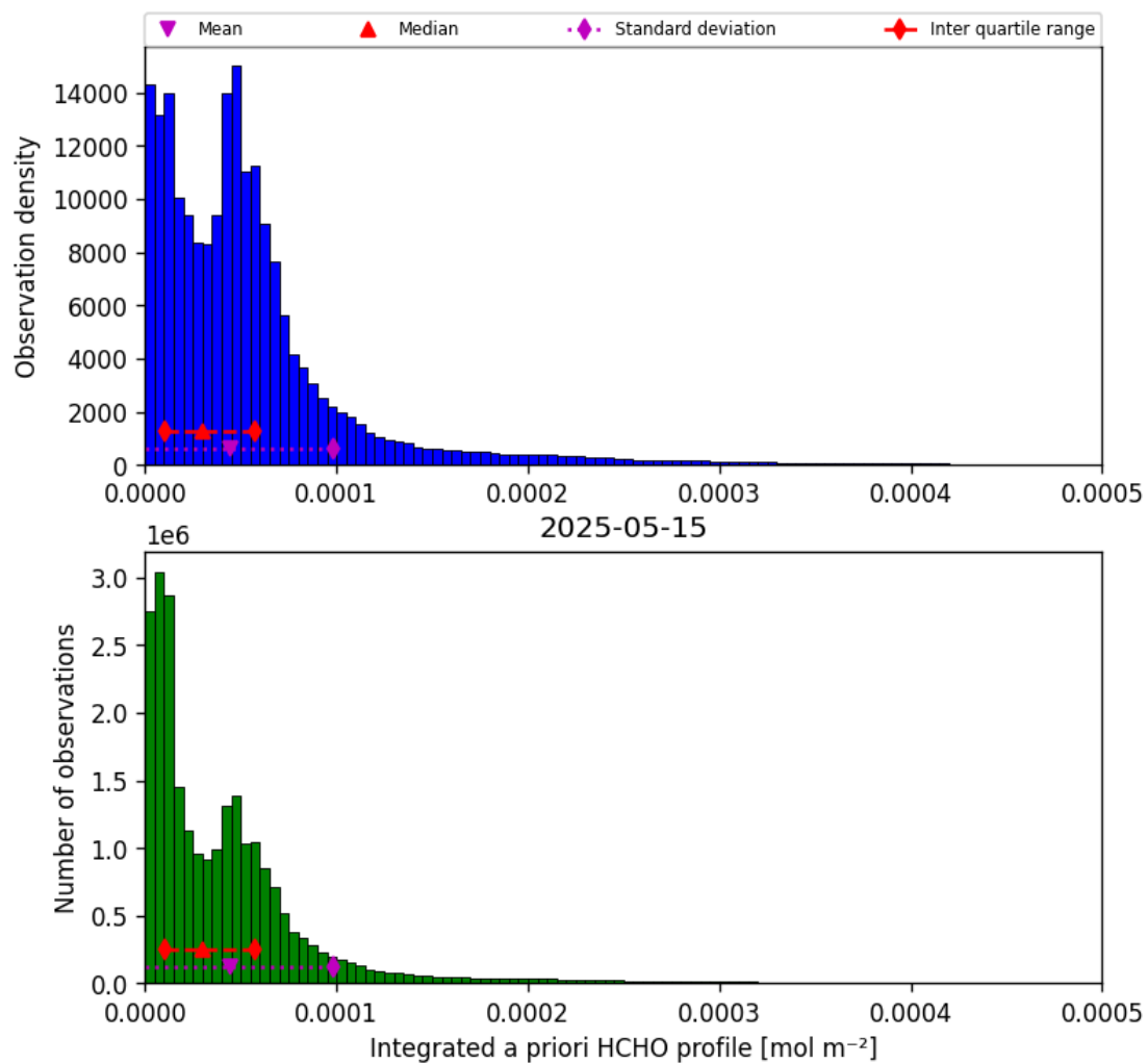
Figure 43: Histogram of “Integrated a priori HCHO profile” for 2025-05-15 to 2025-05-16
