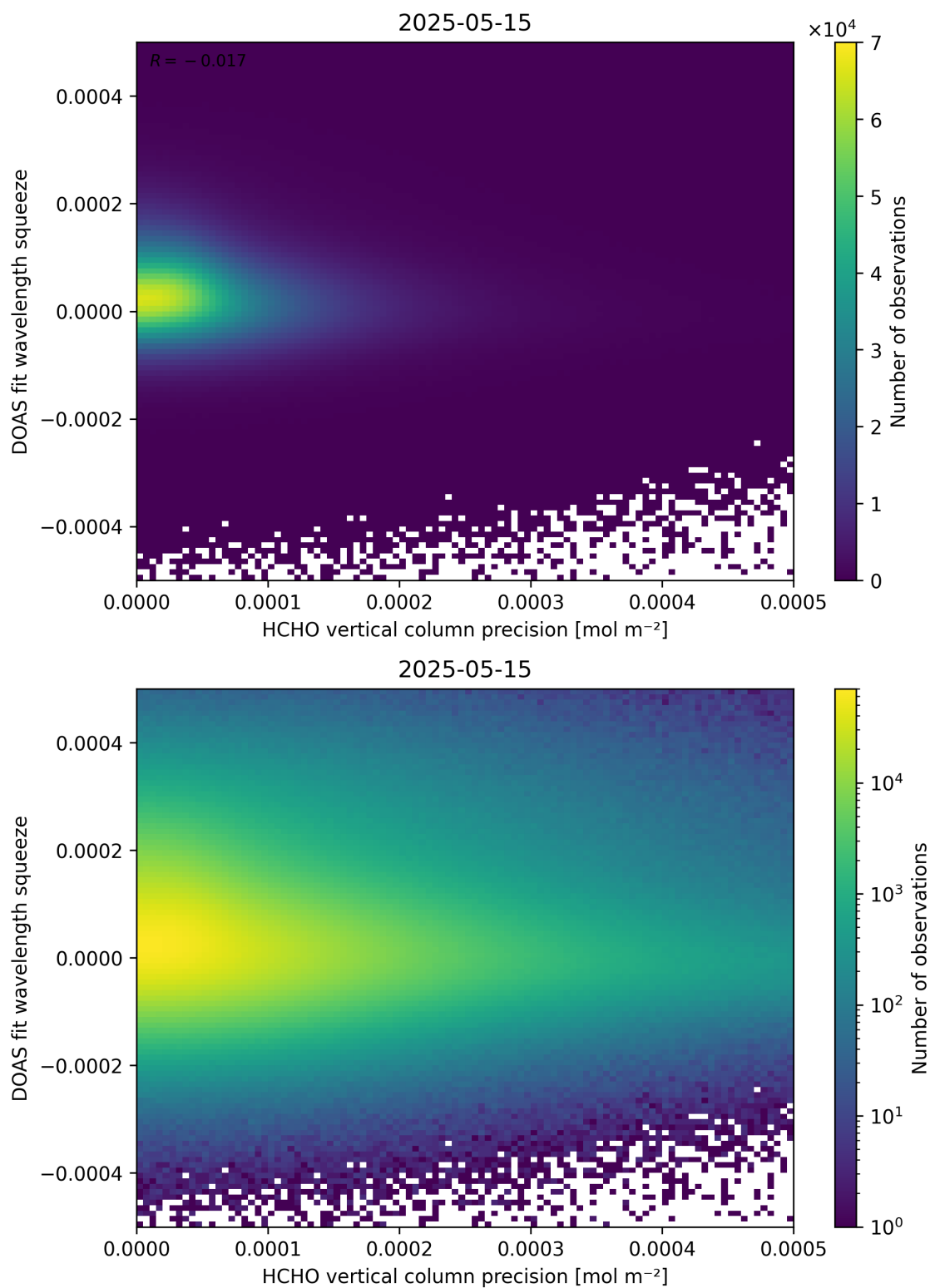
Figure 138: Scatter density plot of “HCHO vertical column precision” against “DOAS fit wavelength squeeze” for 2025-05-15 to 2025-05-16.
