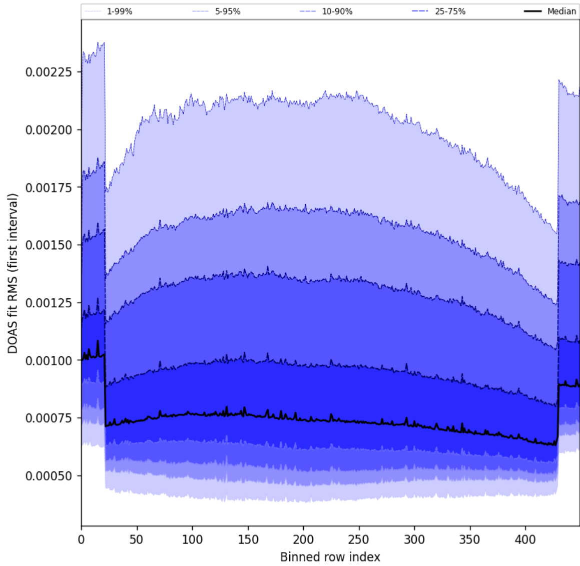
Figure 60: Along track statistics of “DOAS fit RMS (first interval)” for 2025-05-15 to 2025-05-16
