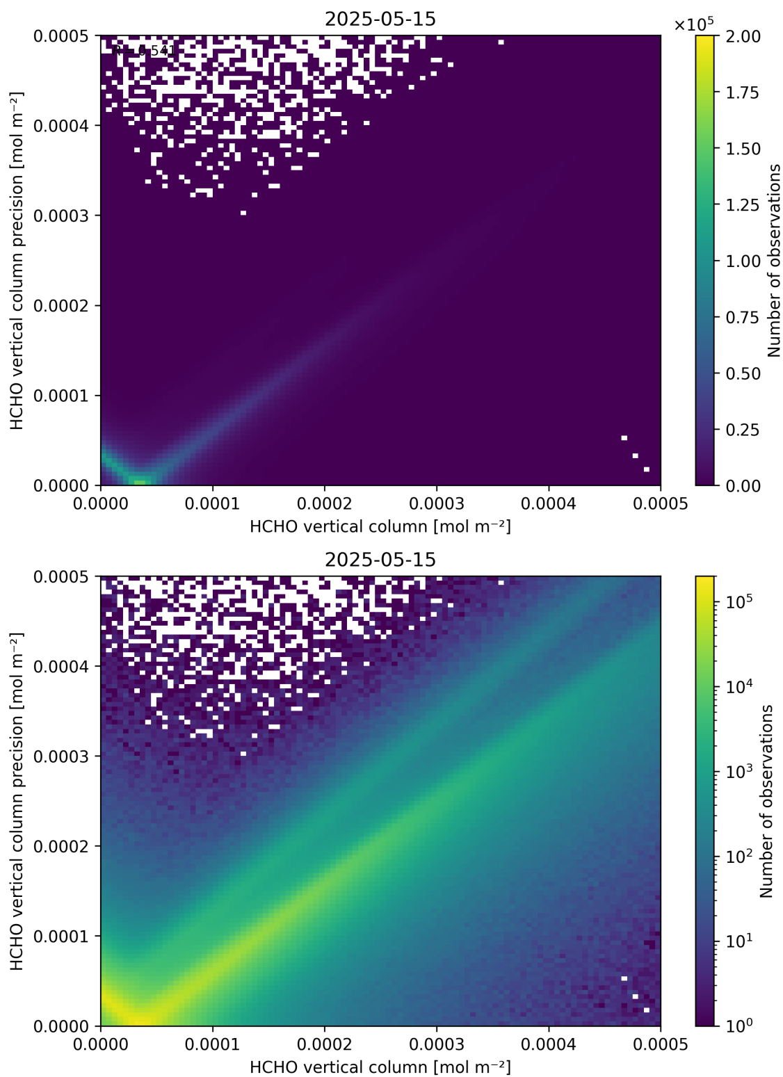
Figure 134: Scatter density plot of “HCHO vertical column” against “HCHO vertical column precision” for 2025-05-15 to 2025-05-16.
