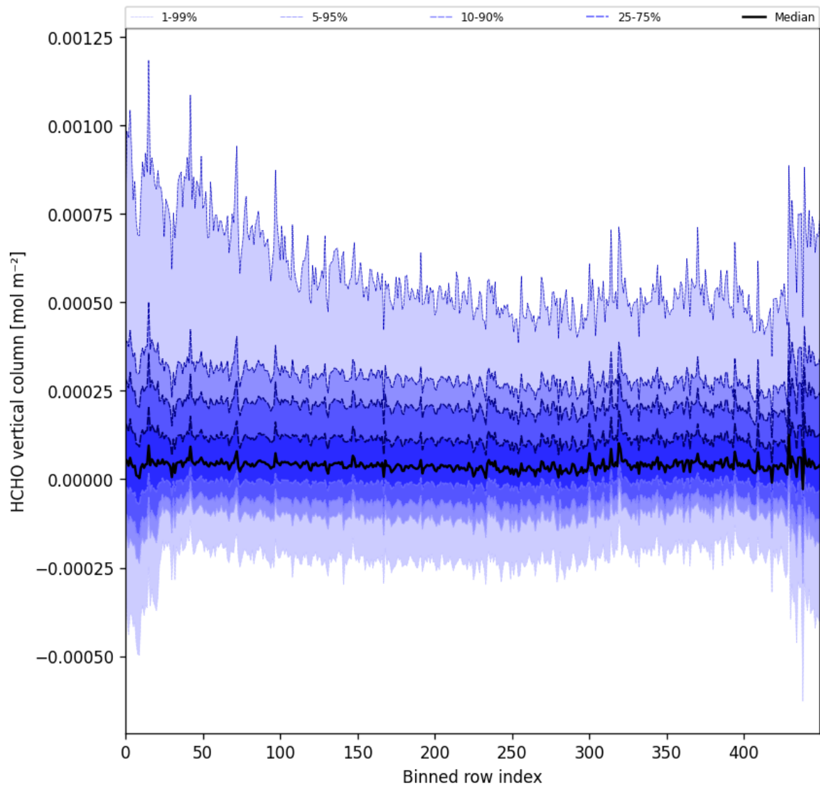
Figure 49: Along track statistics of “HCHO vertical column” for 2025-05-15 to 2025-05-16
