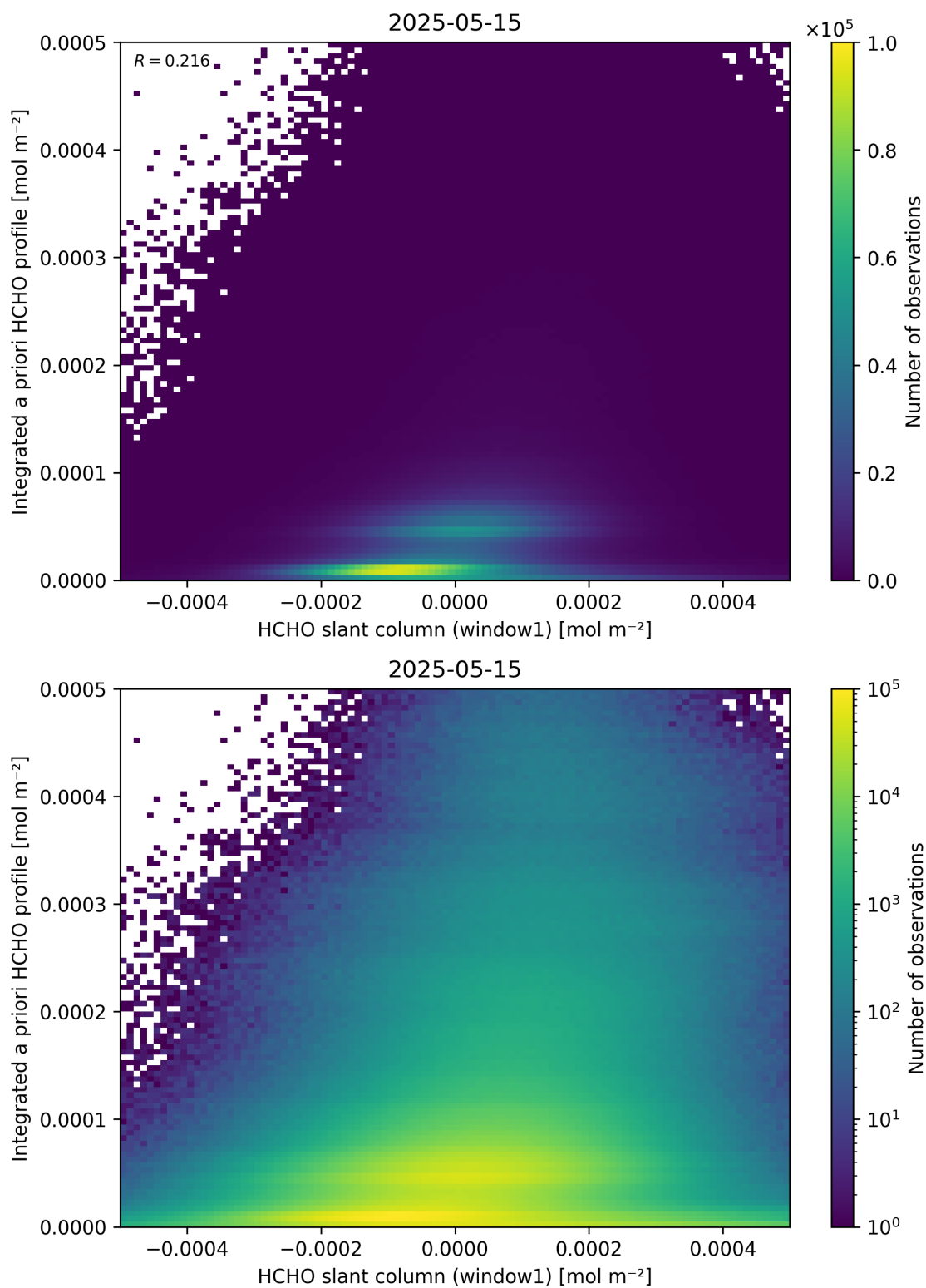
Figure 87: Scatter density plot of “HCHO slant column (window1)” against “Integrated a priori HCHO profile” for 2025-05-15 to 2025-05-16.
