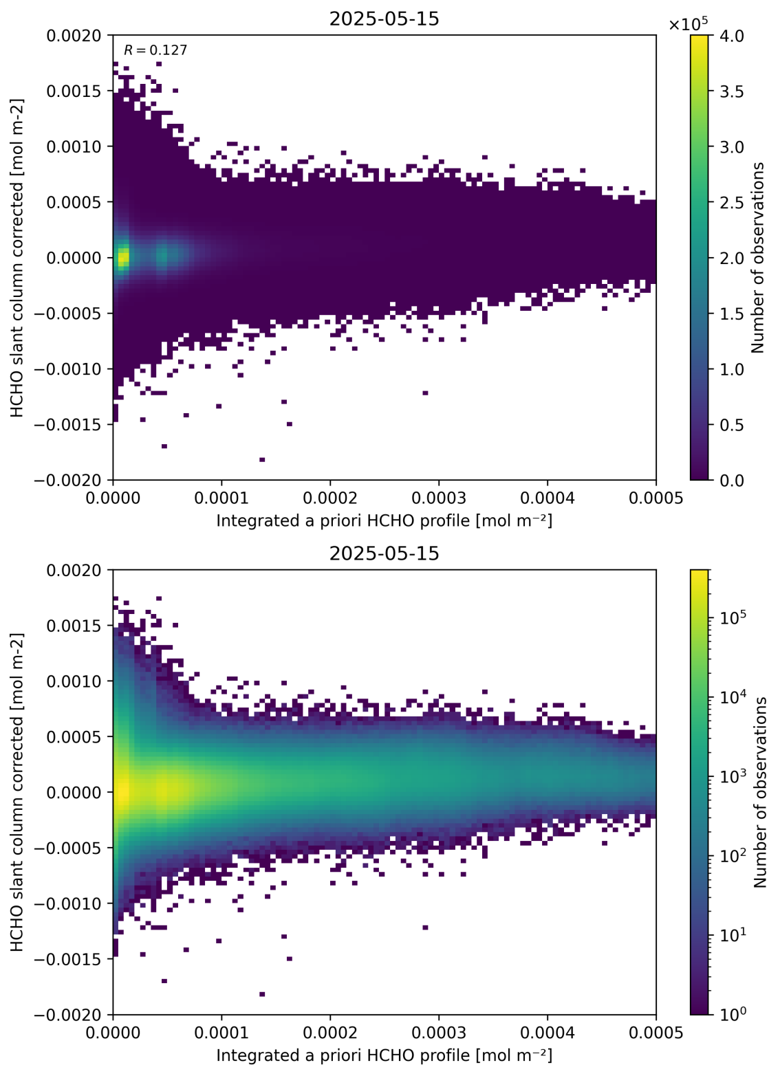
Figure 151: Scatter density plot of “Integrated a priori HCHO profile” against “HCHO slant column corrected” for 2025-05-15 to 2025-05-16.
