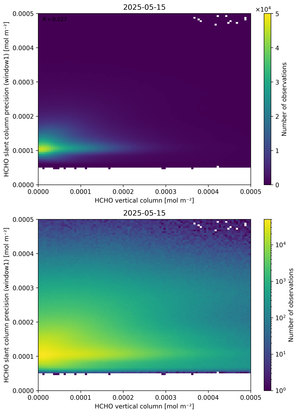
Figure 130: Scatter density plot of “HCHO vertical column” against “HCHO slant column precision (window1)” for 2025-05-15 to 2025-05-16.
