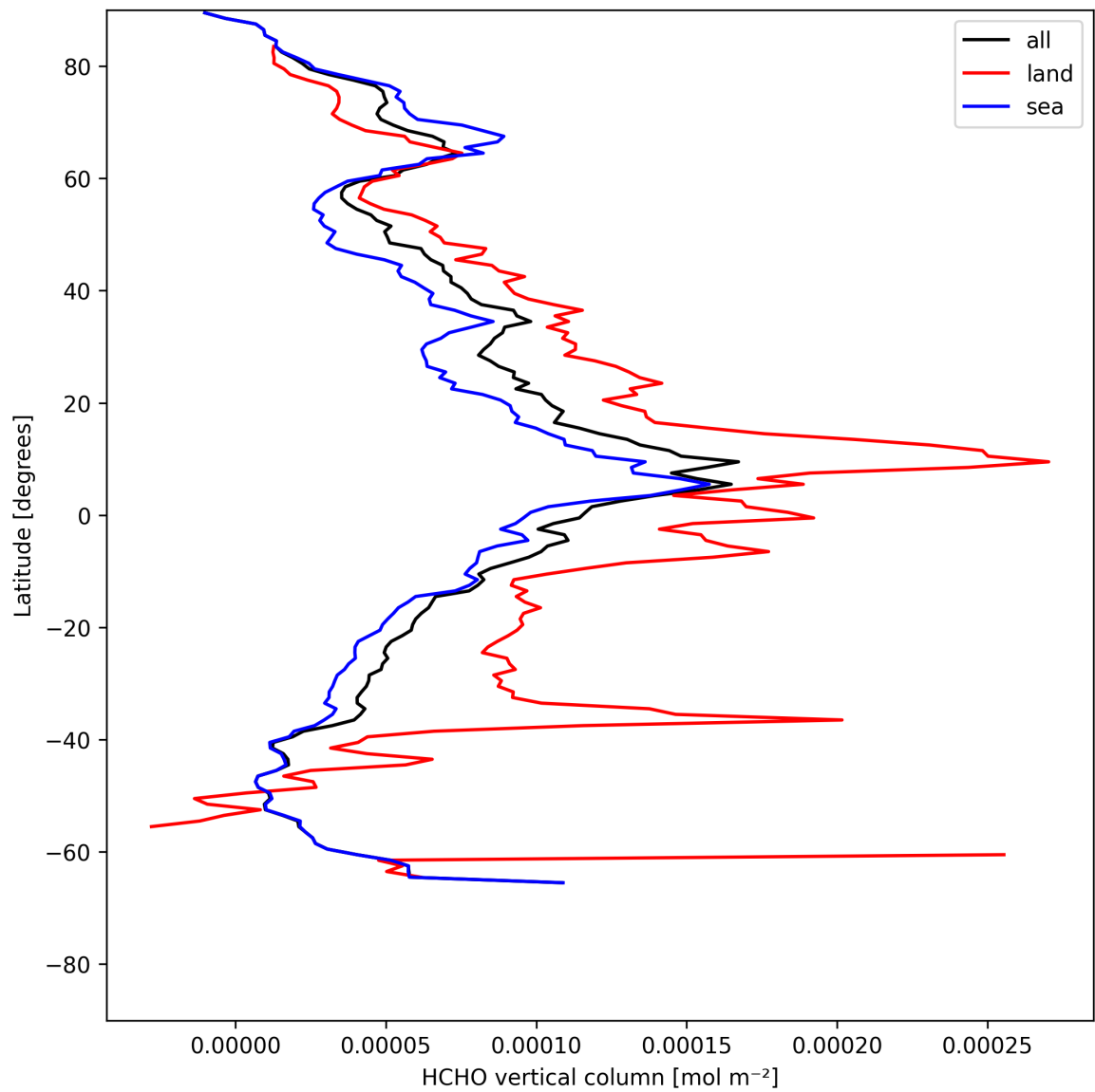
Figure 21: Zonal average of “HCHO vertical column” for 2025-05-15 to 2025-05-16.
