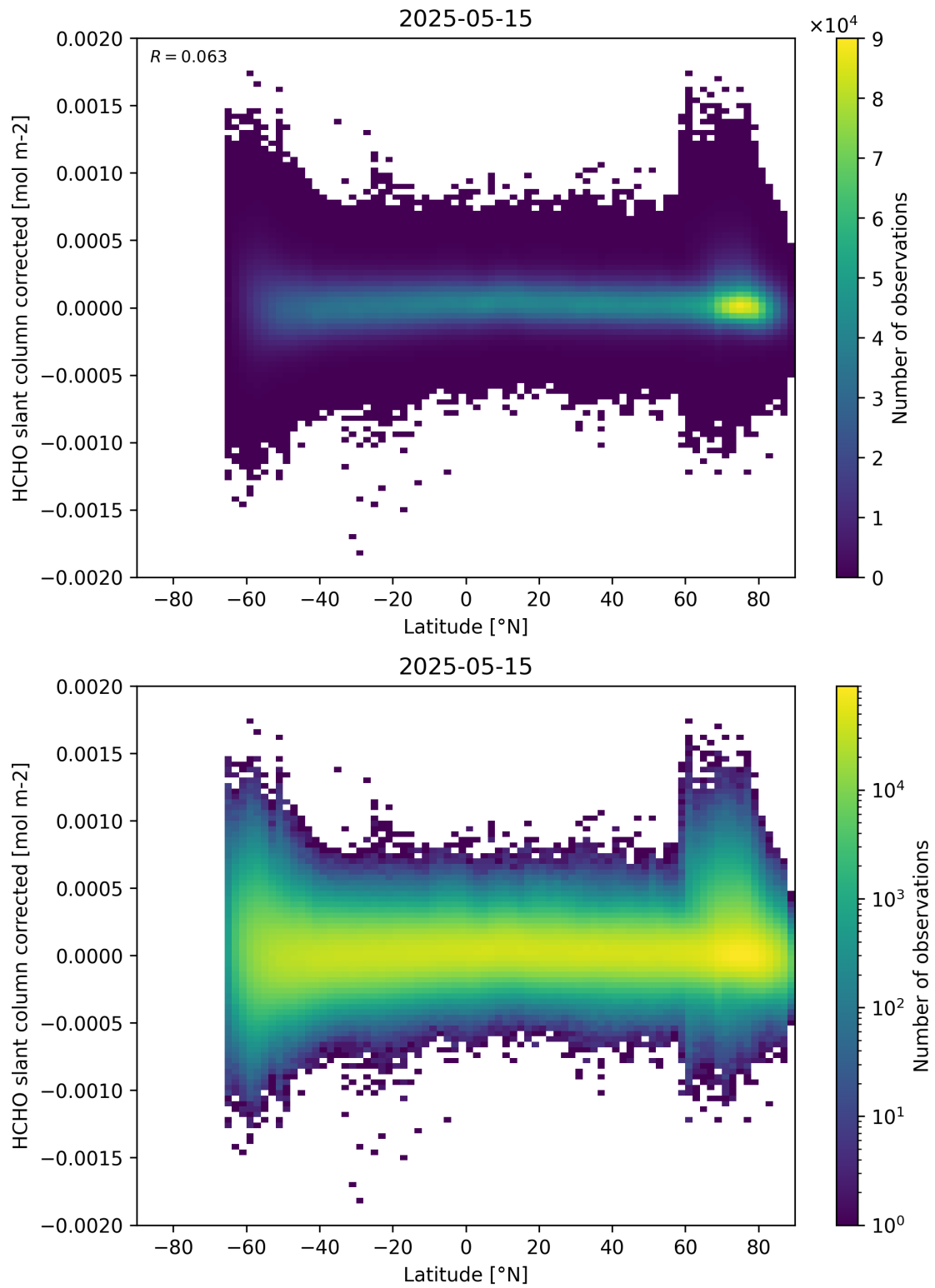
Figure 157: Scatter density plot of “Latitude” against “HCHO slant column corrected” for 2025-05-15 to 2025-05-16.
