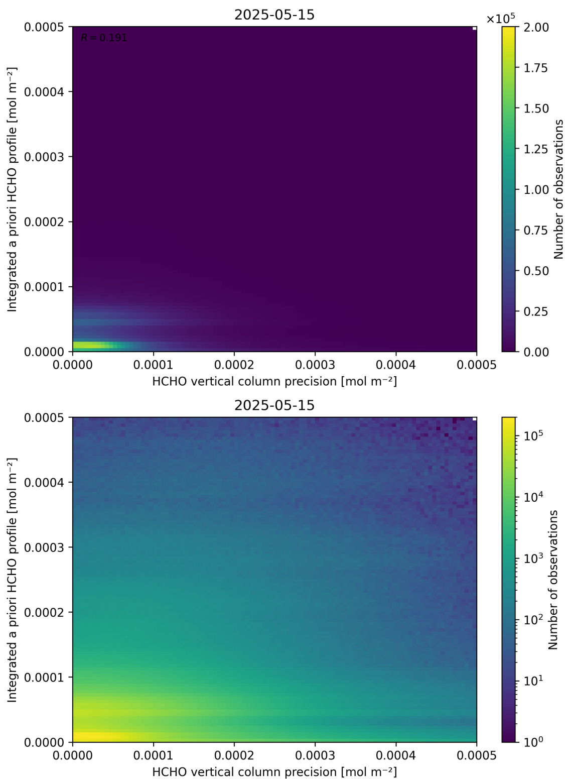
Figure 147: Scatter density plot of “HCHO vertical column precision” against “Integrated a priori HCHO profile” for 2025-05-15 to 2025-05-16.
