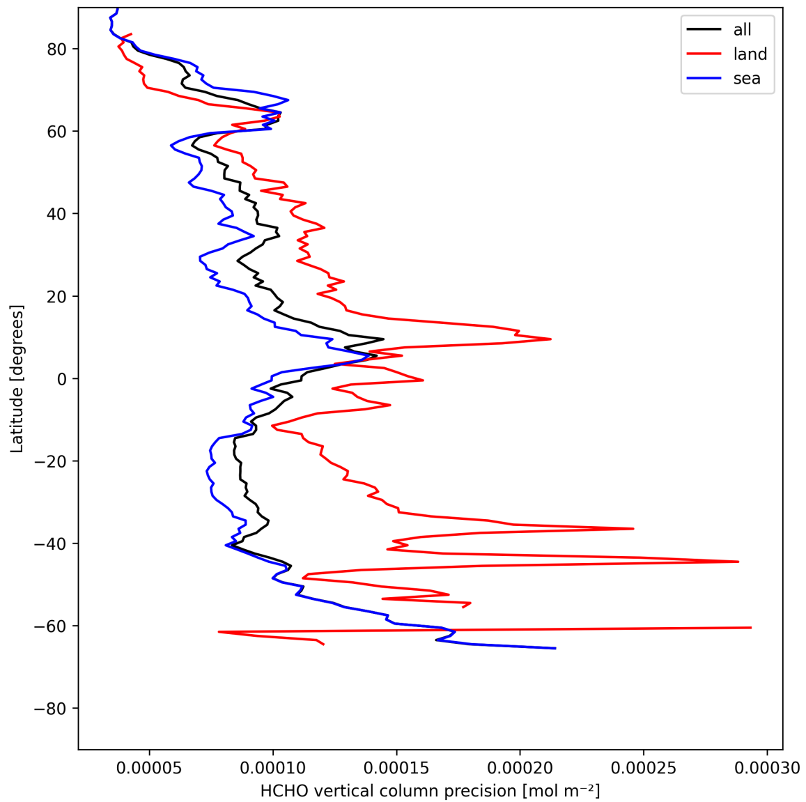
Figure 22: Zonal average of “HCHO vertical column precision” for 2025-05-15 to 2025-05-16.
