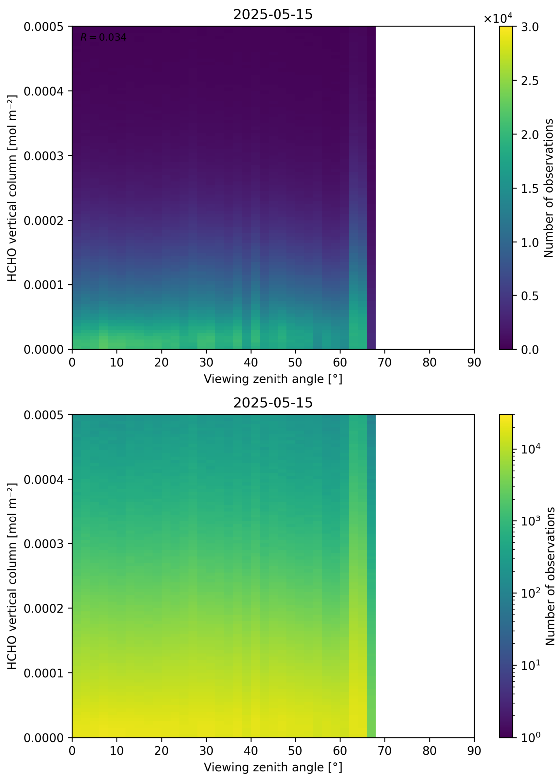
Figure 192: Scatter density plot of “Viewing zenith angle” against “HCHO vertical column” for 2025-05-15 to 2025-05-16.
