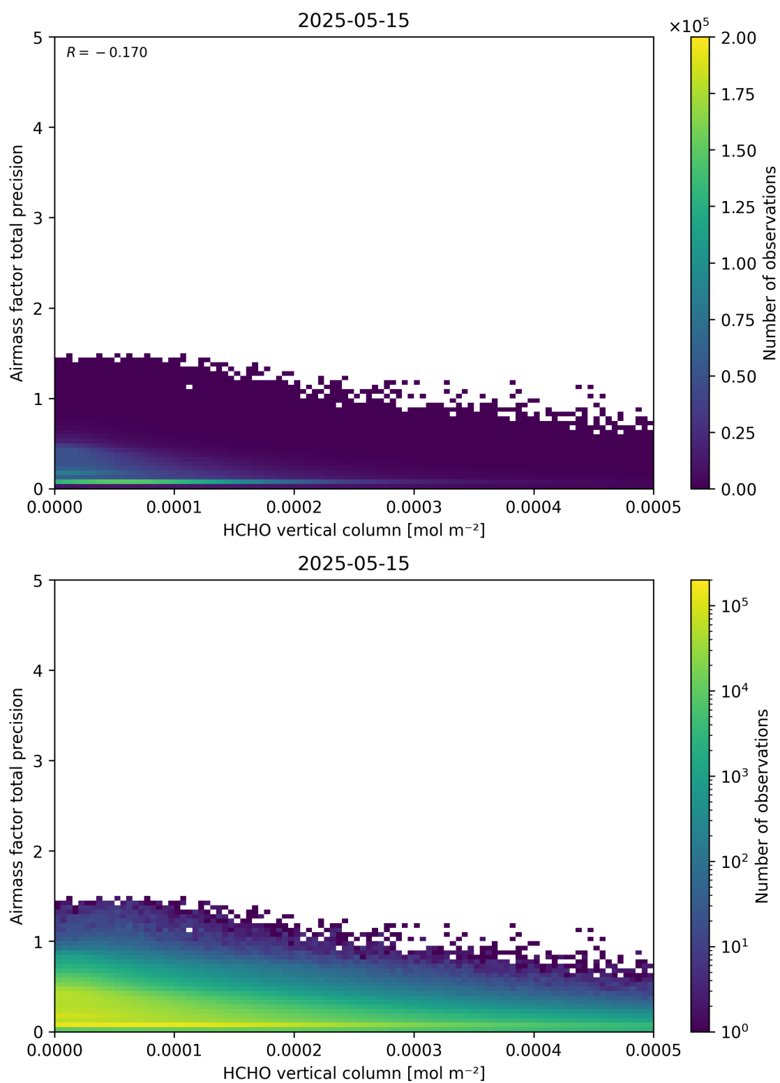
Figure 132: Scatter density plot of “HCHO vertical column” against “Airmass factor total precision” for 2025-05-15 to 2025-05-16.
