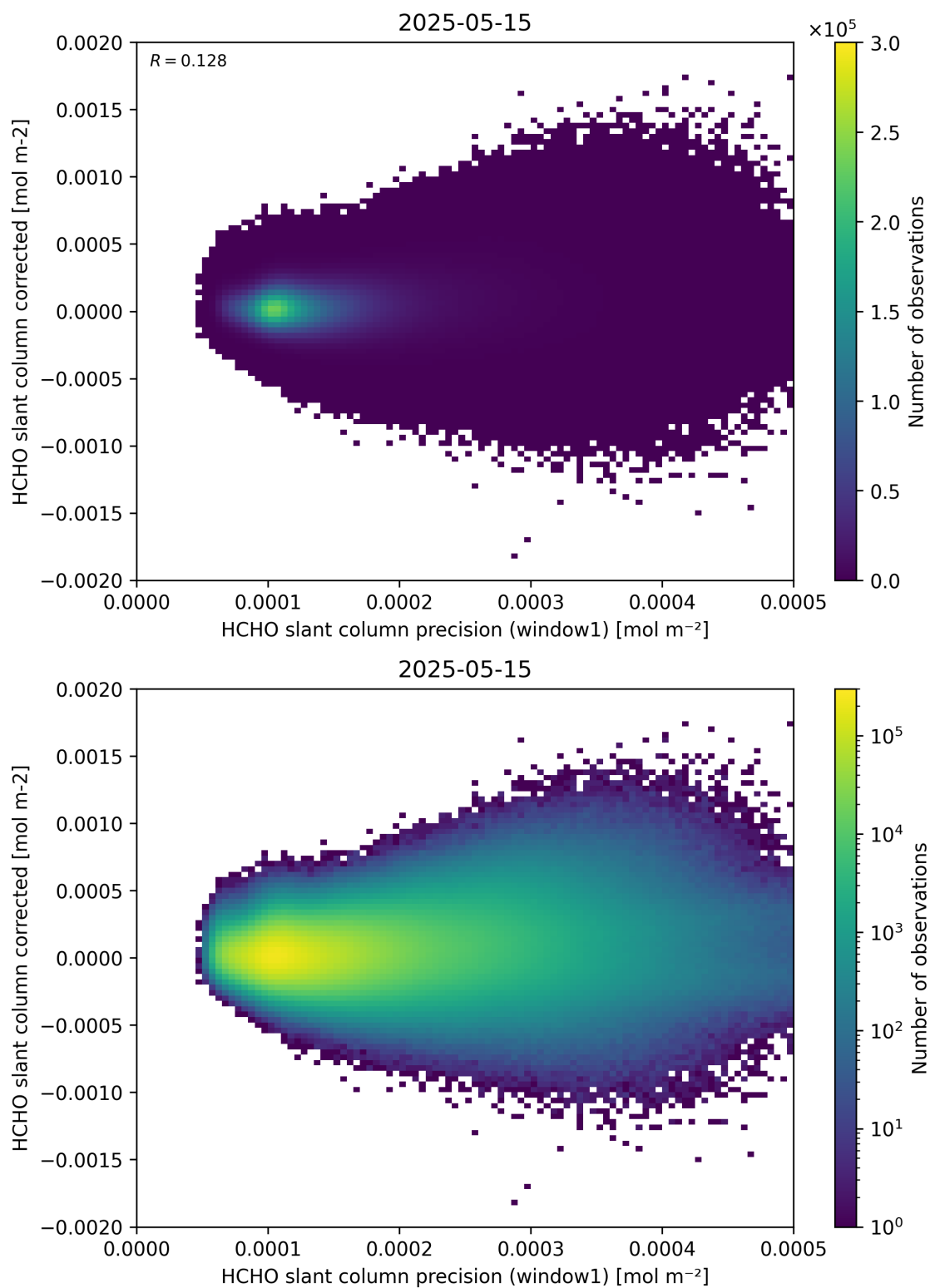
Figure 92: Scatter density plot of “HCHO slant column precision (window1)” against “HCHO slant column corrected” for 2025-05-15 to 2025-05-16.
