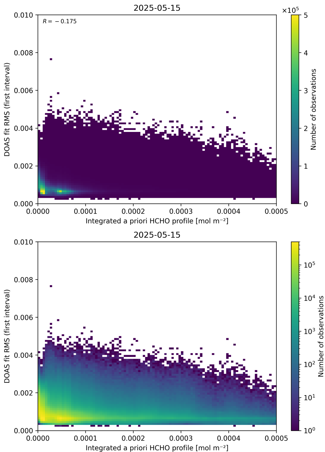
Figure 148: Scatter density plot of “Integrated a priori HCHO profile” against “DOAS fit RMS (first interval)” for 2025-05-15 to 2025-05-16.
