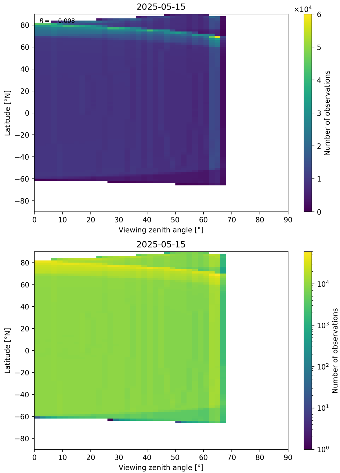
Figure 196: Scatter density plot of “Viewing zenith angle” against “Latitude” for 2025-05-15 to 2025-05-16.
