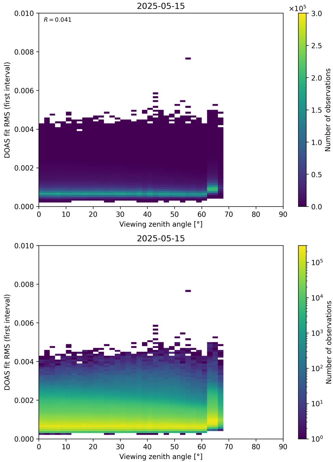
Figure 182: Scatter density plot of “Viewing zenith angle” against “DOAS fit RMS (first interval)” for 2025-05-15 to 2025-05-16.
