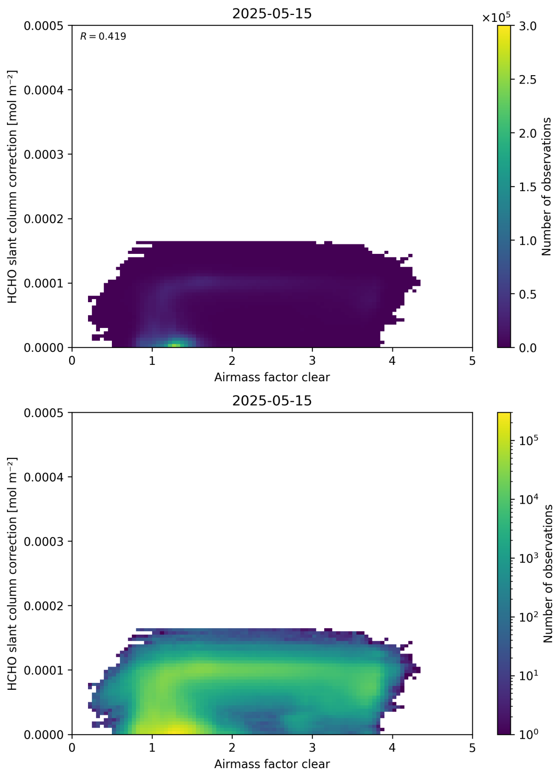
Figure 75: Scatter density plot of “Airmass factor clear” against “HCHO slant column correction” for 2025-05-15 to 2025-05-16.
