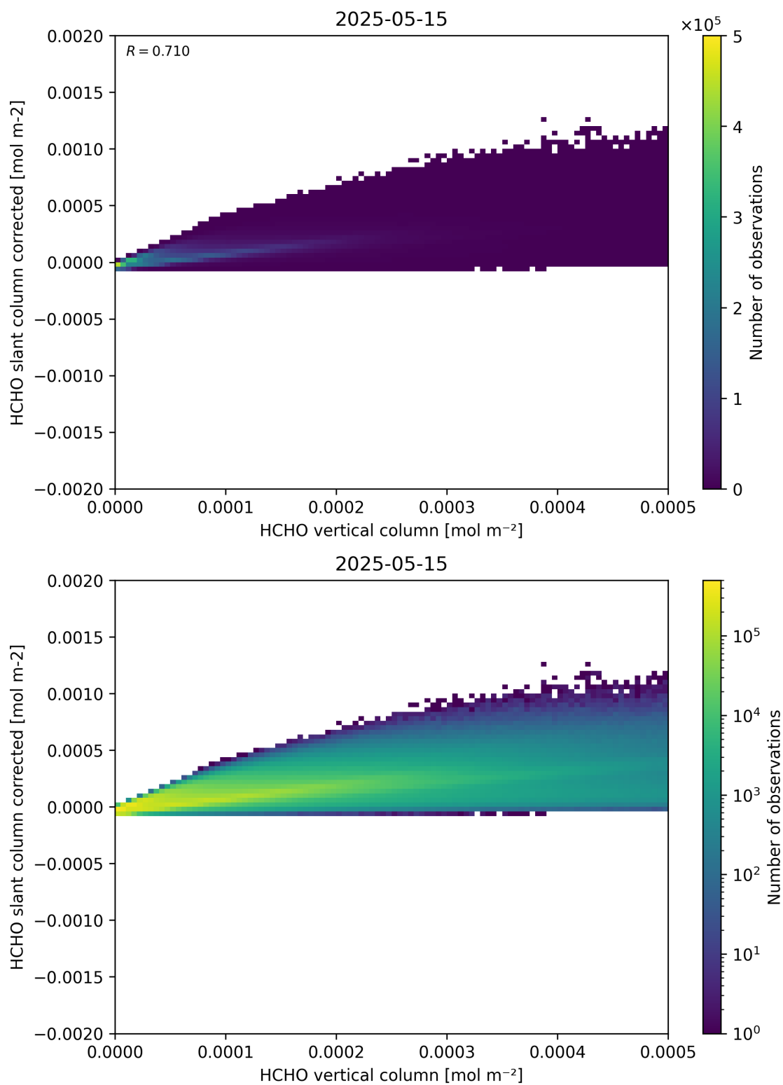
Figure 127: Scatter density plot of “HCHO vertical column” against “HCHO slant column corrected” for 2025-05-15 to 2025-05-16.
