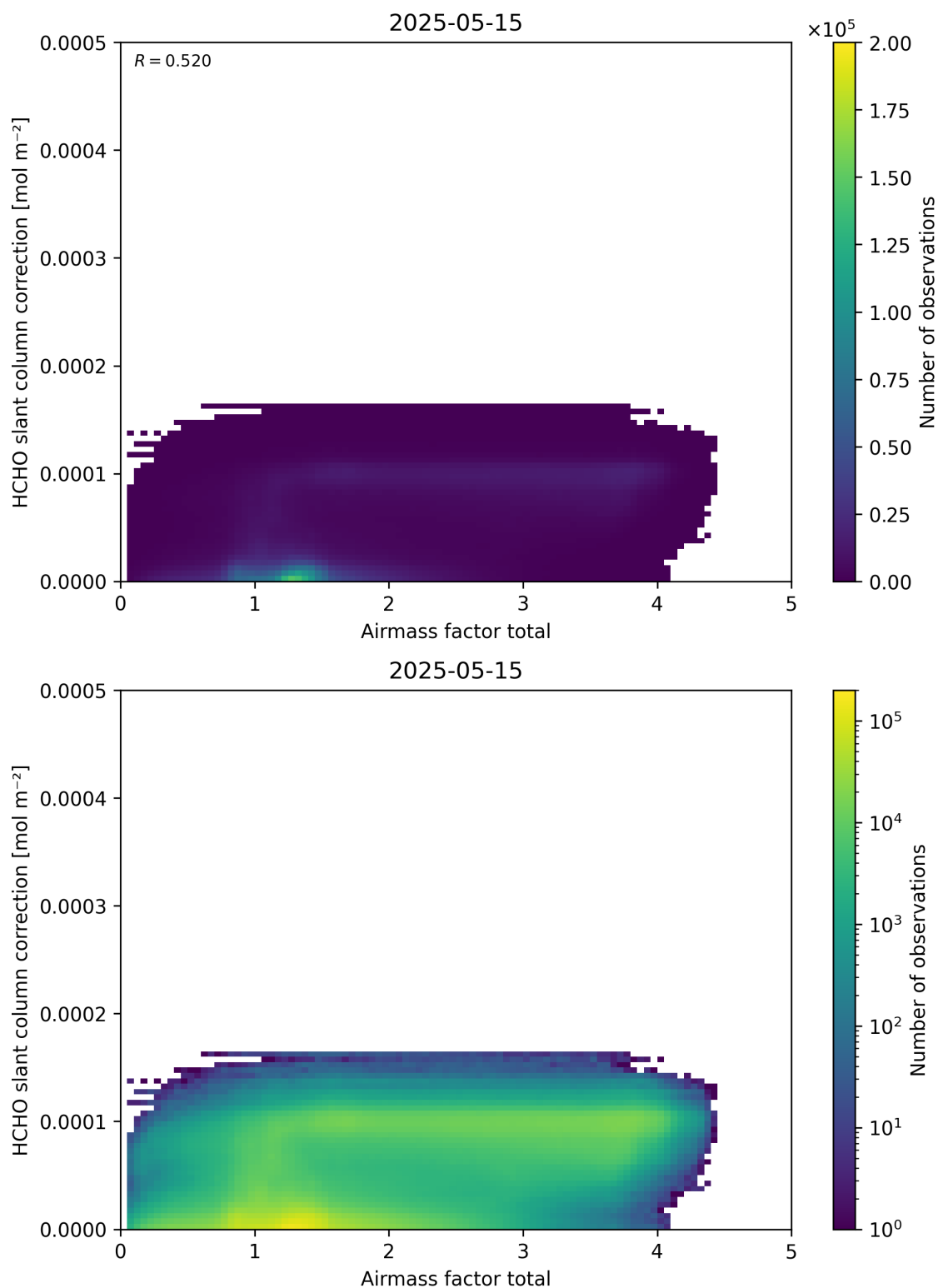
Figure 102: Scatter density plot of “Airmass factor total” against “HCHO slant column correction” for 2025-05-15 to 2025-05-16.
