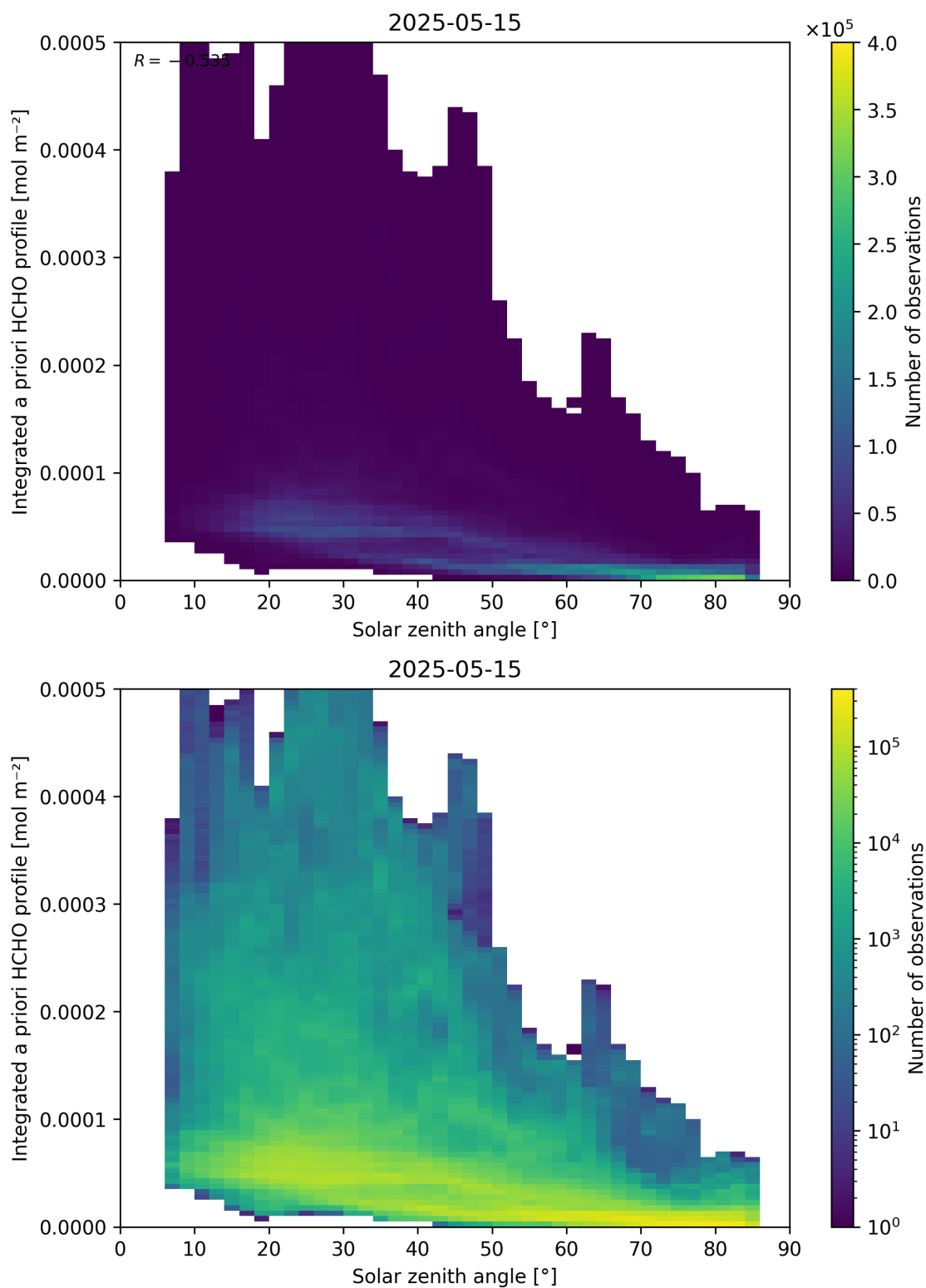
Figure 180: Scatter density plot of “Solar zenith angle” against “Integrated a priori HCHO profile” for 2025-05-15 to 2025-05-16.
