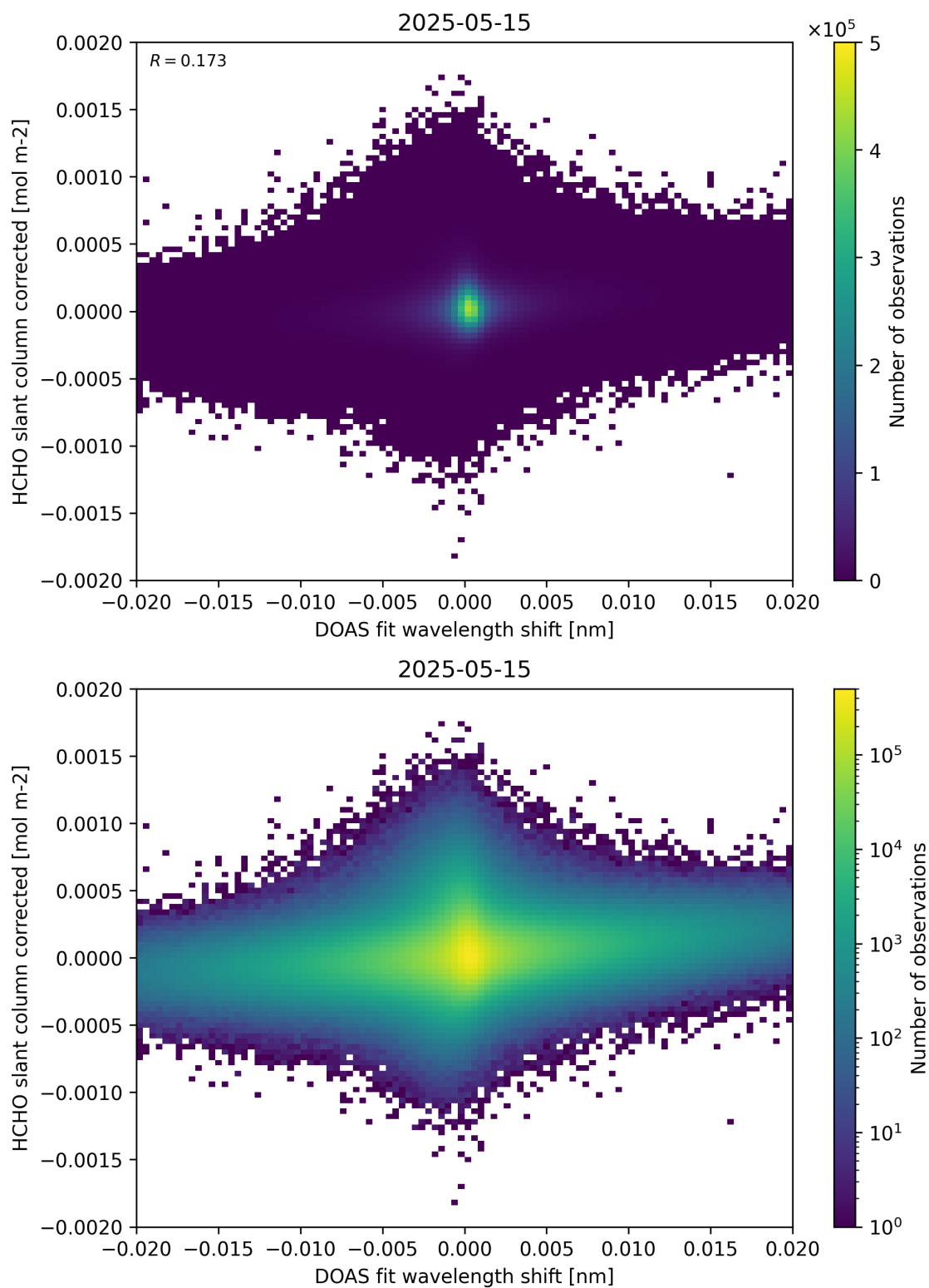
Figure 66: Scatter density plot of “DOAS fit wavelength shift” against “HCHO slant column corrected” for 2025-05-15 to 2025-05-16.
