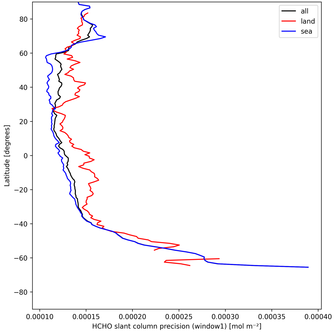
Figure 25: Zonal average of “HCHO slant column precision (window1)” for 2025-05-15 to 2025-05-16.
