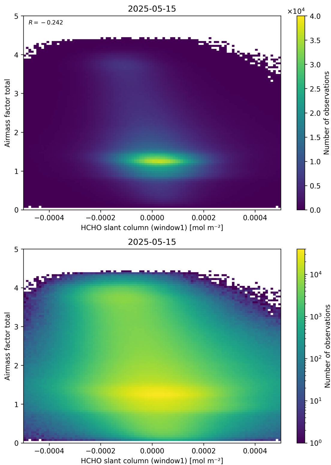
Figure 85: Scatter density plot of “HCHO slant column (window1)” against “Airmass factor total” for 2025-05-15 to 2025-05-16.
