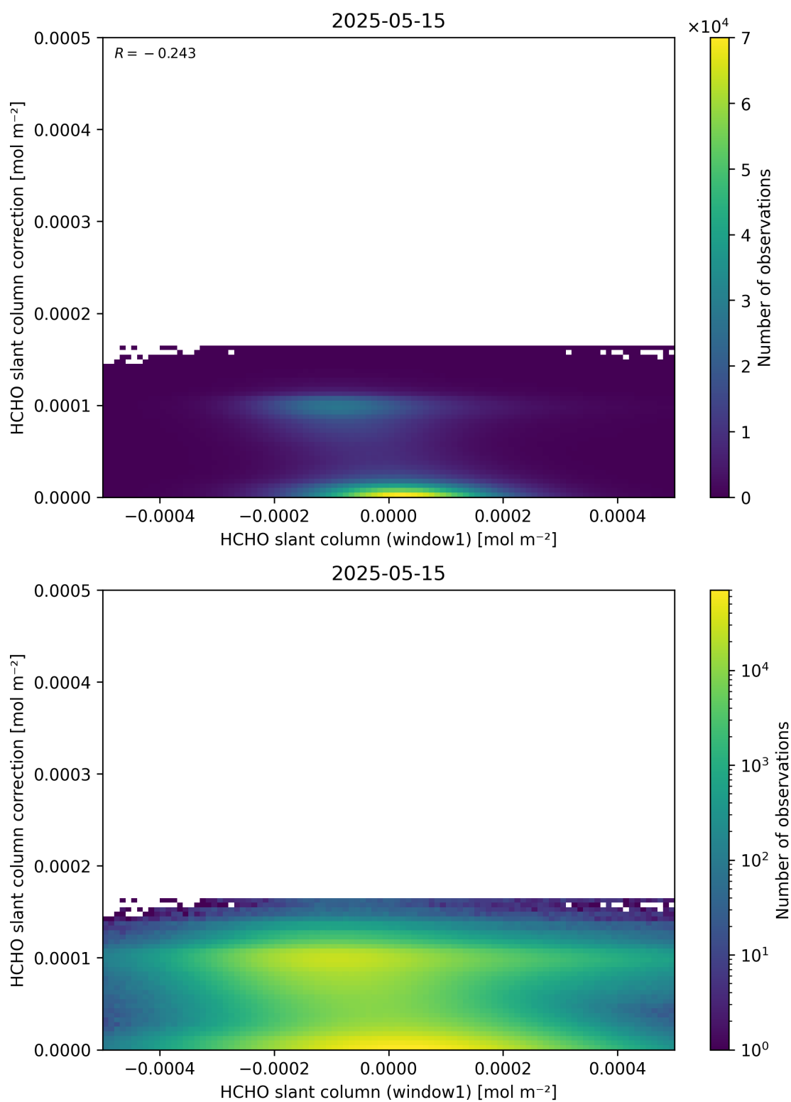
Figure 83: Scatter density plot of “HCHO slant column (window1)” against “HCHO slant column correction” for 2025-05-15 to 2025-05-16.
