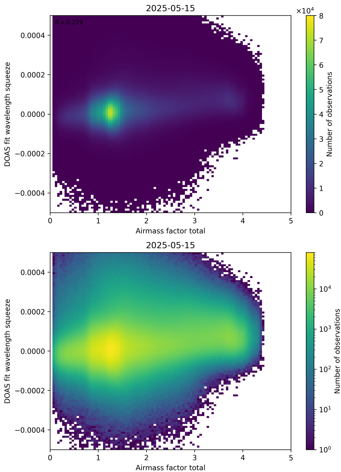
Figure 99: Scatter density plot of “Airmass factor total” against “DOAS fit wavelength squeeze” for 2025-05-15 to 2025-05-16.
