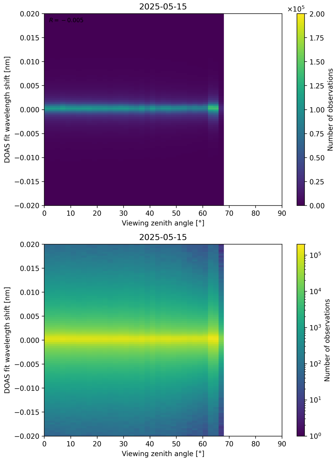
Figure 183: Scatter density plot of “Viewing zenith angle” against “DOAS fit wavelength shift” for 2025-05-15 to 2025-05-16.
