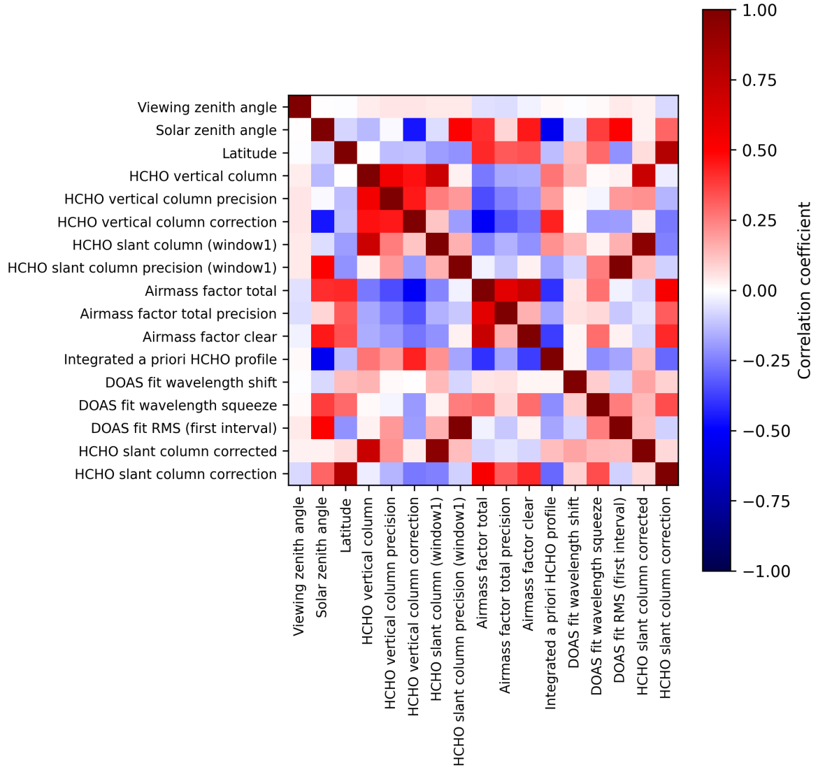
Figure 2: Map of correlation matrix for 2025-05-15 to 2025-05-16.
