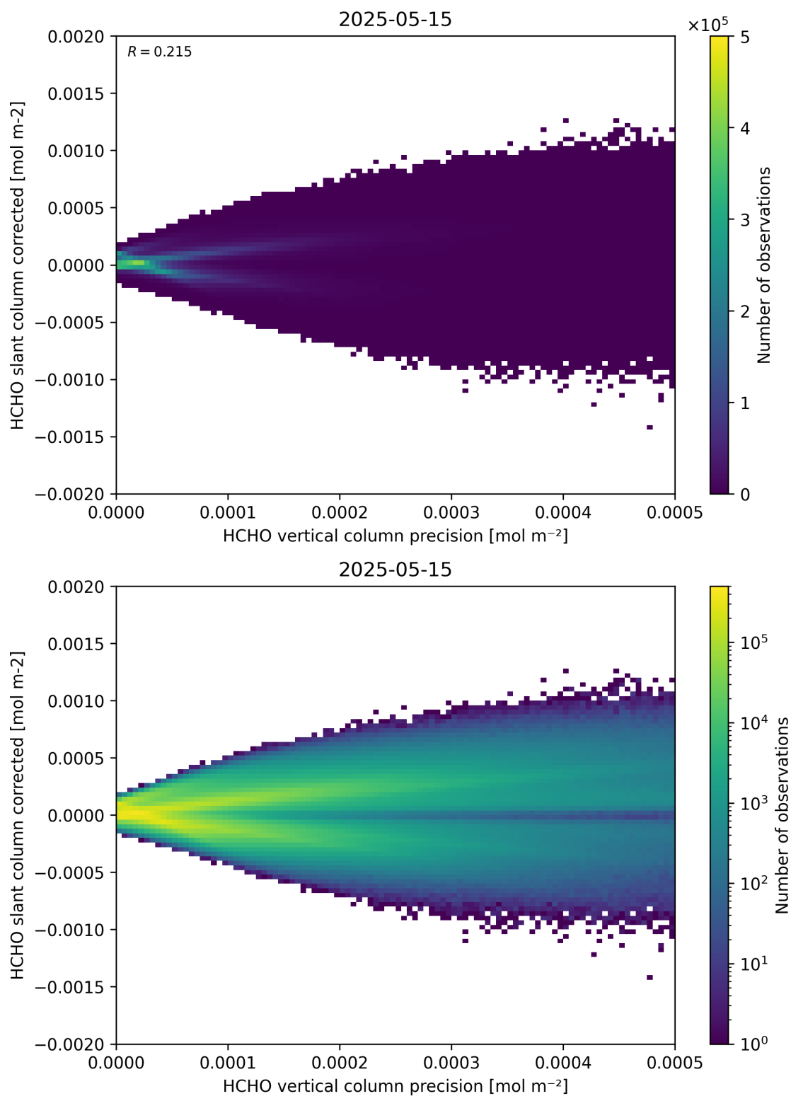
Figure 140: Scatter density plot of “HCHO vertical column precision” against “HCHO slant column corrected” for 2025-05-15 to 2025-05-16.
