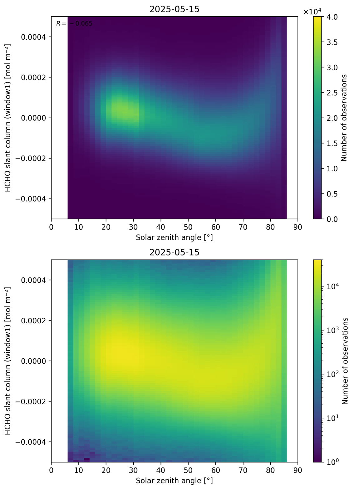
Figure 173: Scatter density plot of “Solar zenith angle” against “HCHO slant column (window1)” for 2025-05-15 to 2025-05-16.
