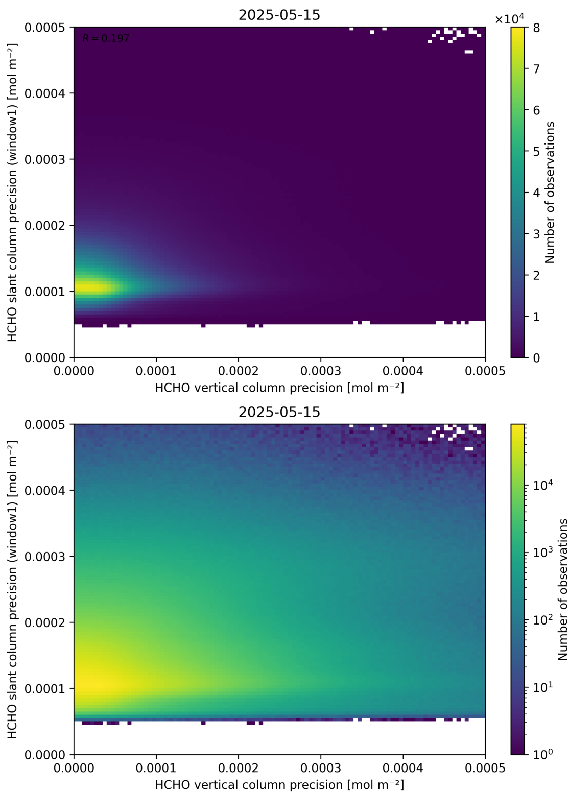
Figure 143: Scatter density plot of “HCHO vertical column precision” against “HCHO slant column precision (window1)” for 2025-05-15 to 2025-05-16.
