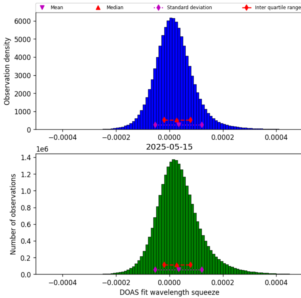
Figure 45: Histogram of "DOAS fit wavelength squeeze" for 2025-05-15 to 2025-05-16
