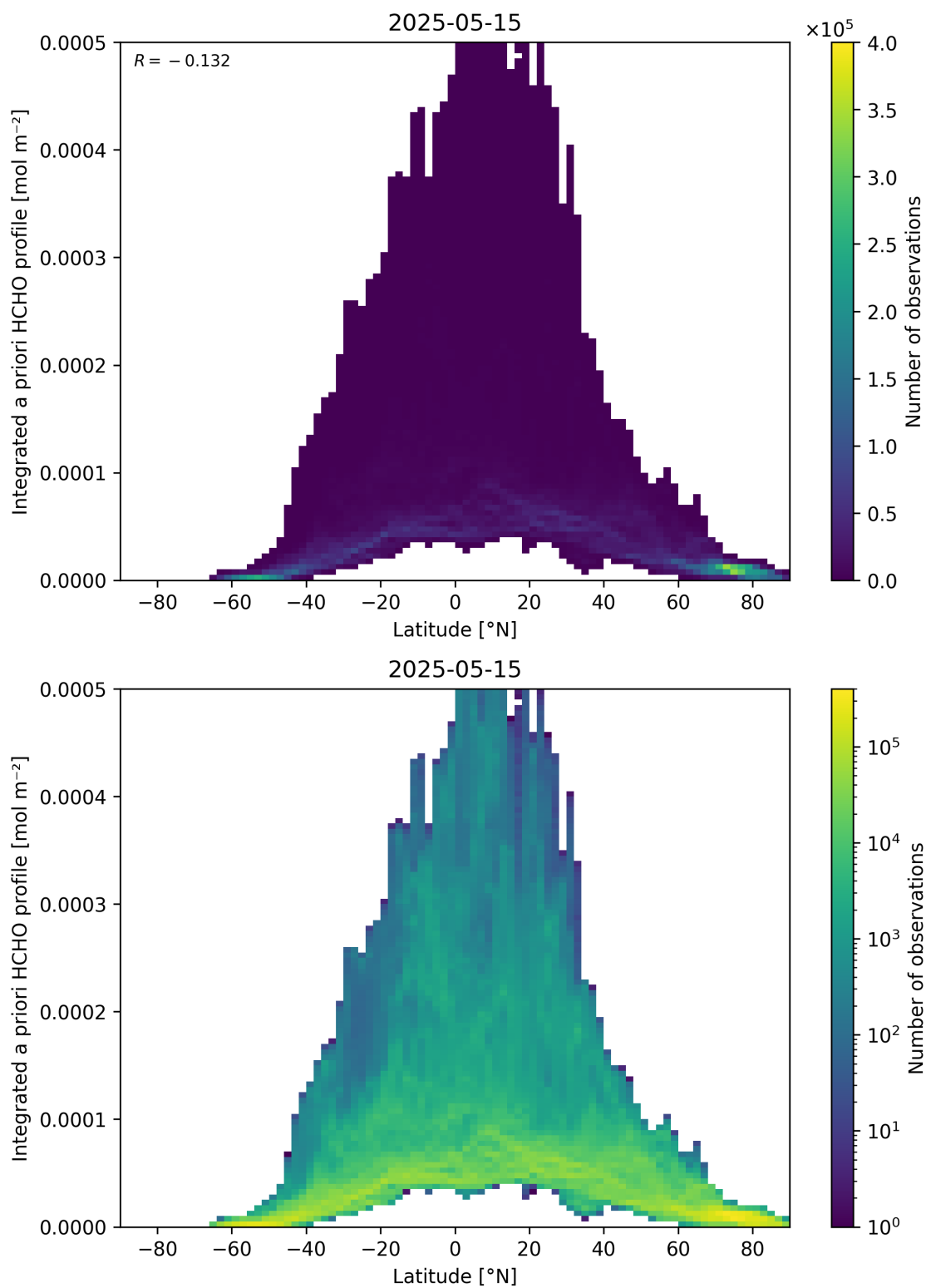
Figure 166: Scatter density plot of “Latitude” against “Integrated a priori HCHO profile” for 2025-05-15 to 2025-05-16.
