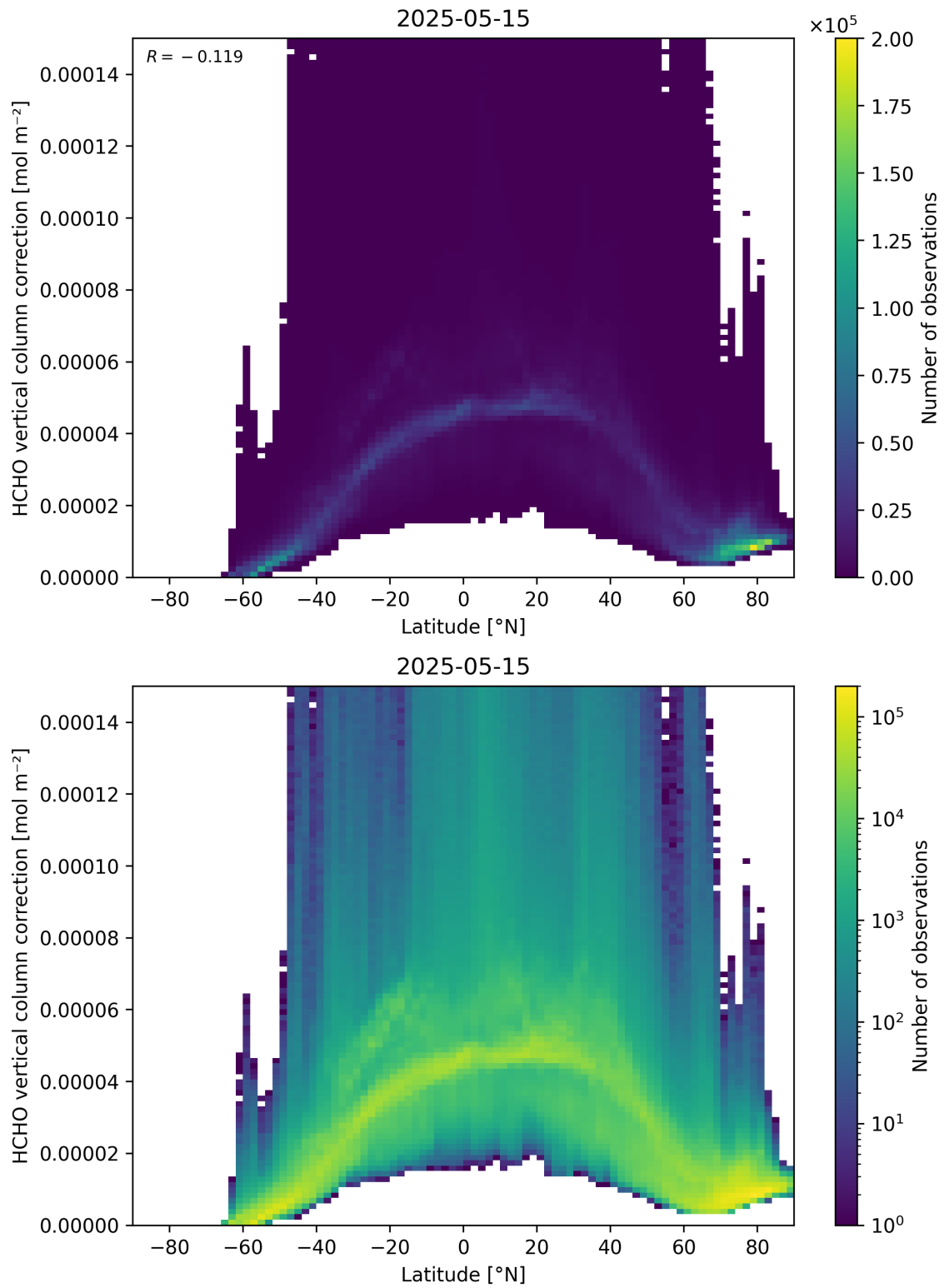
Figure 164: Scatter density plot of “Latitude” against “HCHO vertical column correction” for 2025-05-15 to 2025-05-16.
