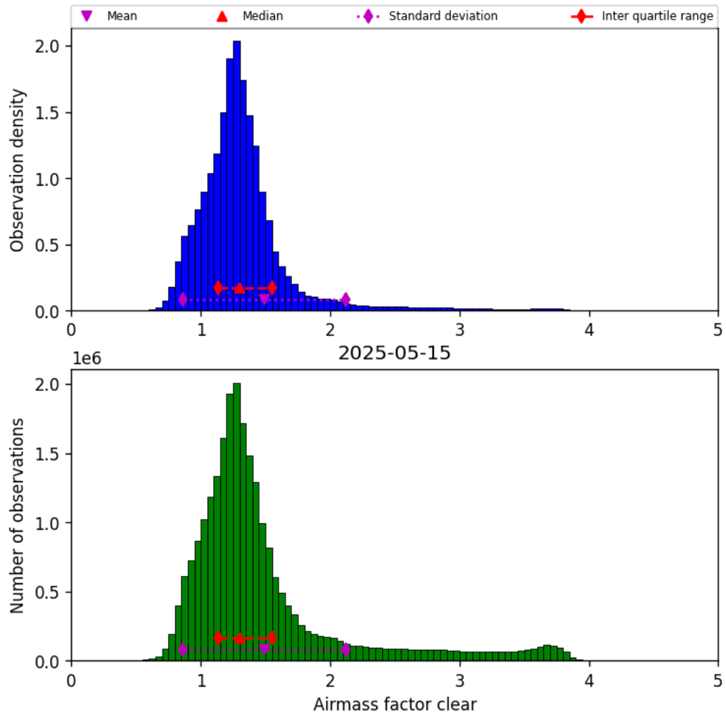
Figure 42: Histogram of “Airmass factor clear” for 2025-05-15 to 2025-05-16
