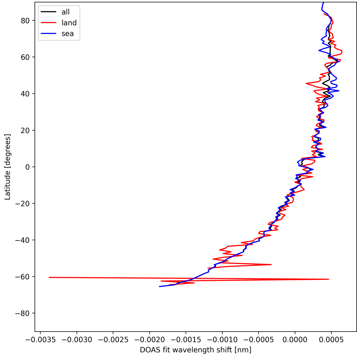
Figure 30: Zonal average of “DOAS fit wavelength shift” for 2025-05-15 to 2025-05-16.
