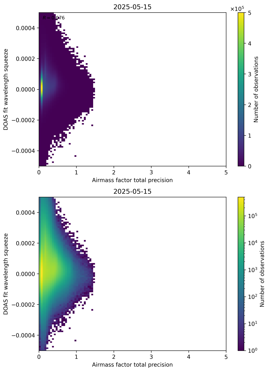
Figure 107: Scatter density plot of “Airmass factor total precision” against “DOAS fit wavelength squeeze” for 2025-05-15 to 2025-05-16.
