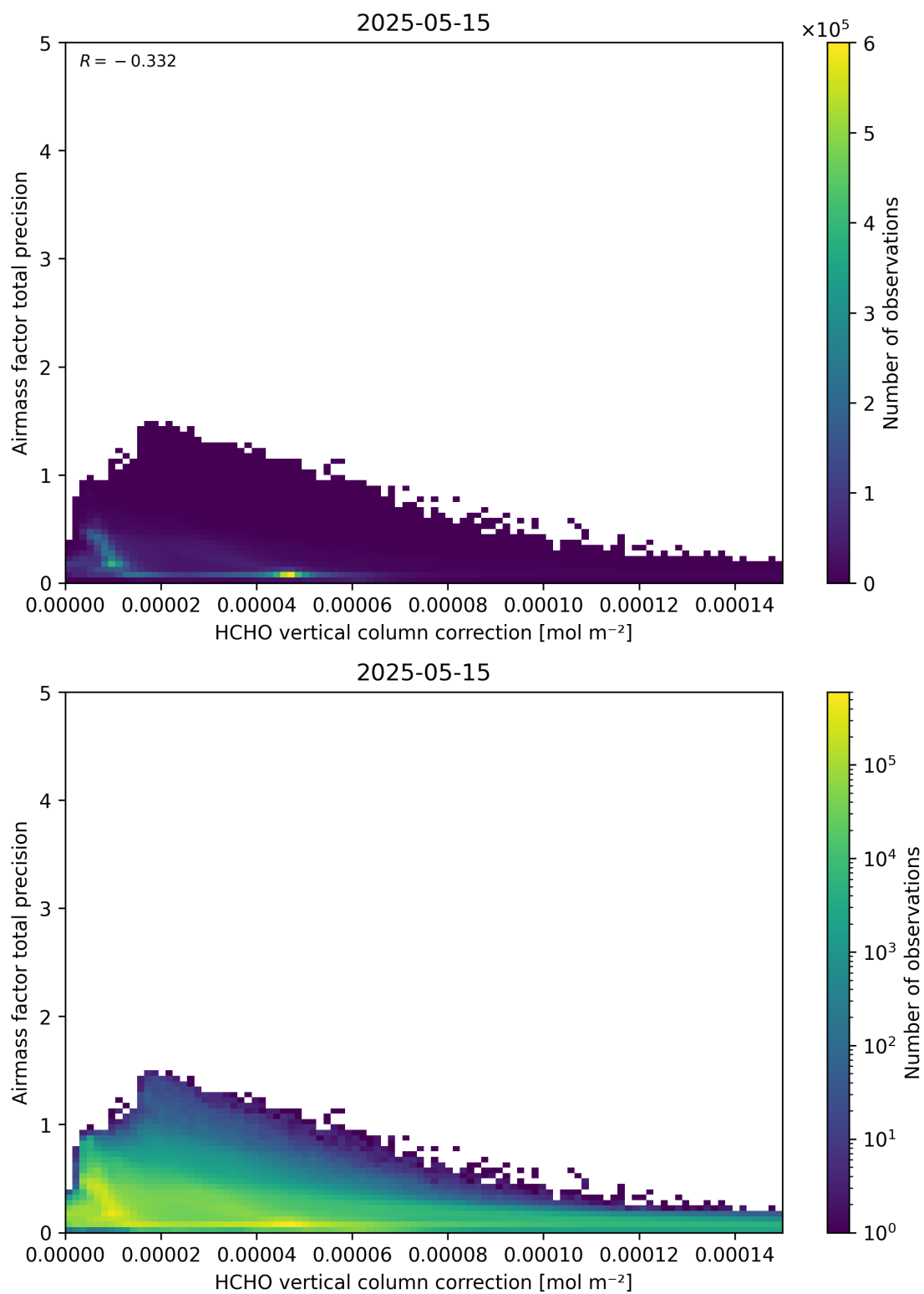
Figure 121: Scatter density plot of “HCHO vertical column correction” against “Airmass factor total precision” for 2025-05-15 to 2025-05-16.
