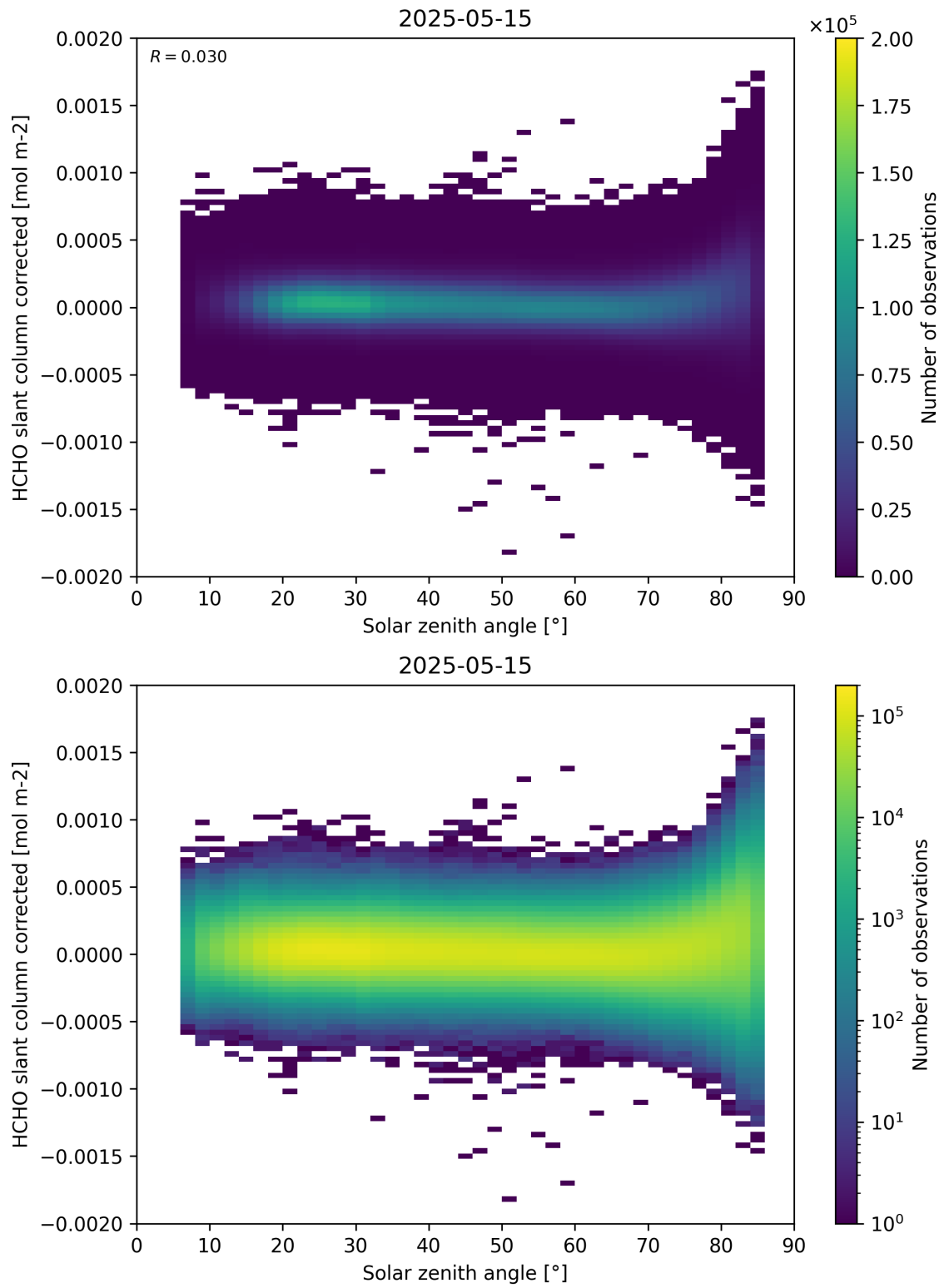
Figure 171: Scatter density plot of “Solar zenith angle” against “HCHO slant column corrected” for 2025-05-15 to 2025-05-16.
