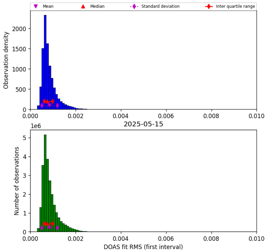
Figure 46: Histogram of “DOAS fit RMS (first interval)” for 2025-05-15 to 2025-05-16
