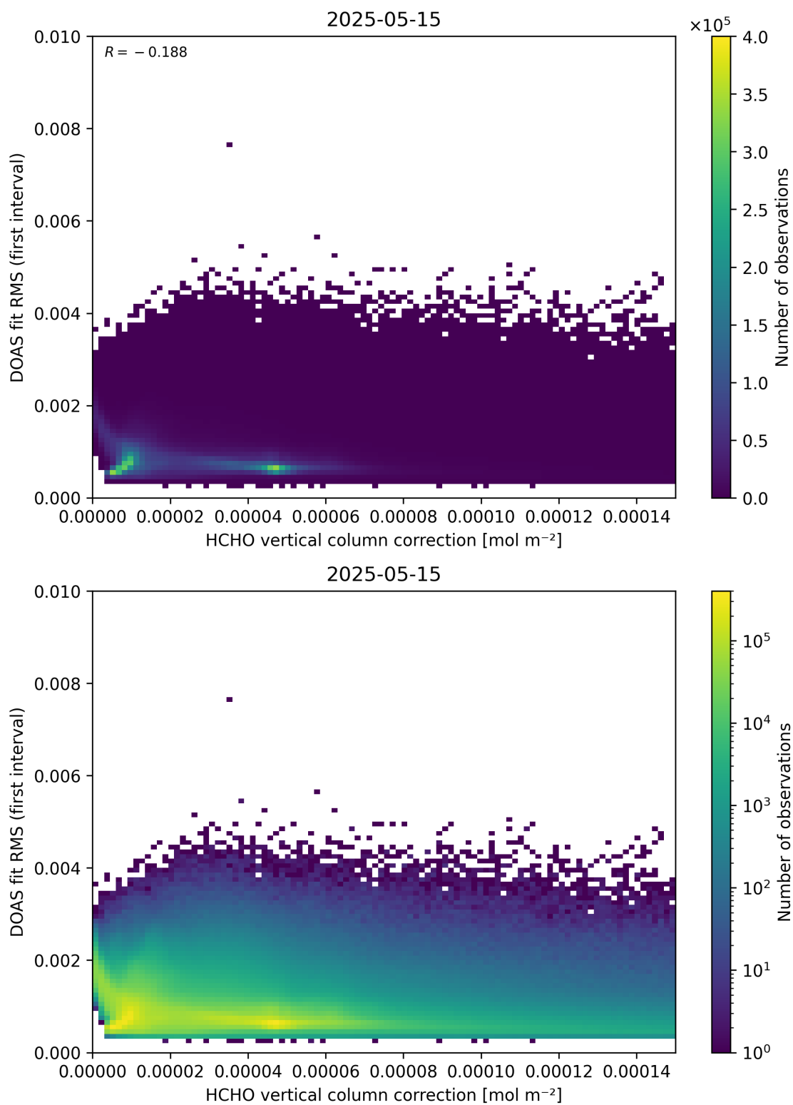
Figure 112: Scatter density plot of “HCHO vertical column correction” against “DOAS fit RMS (first interval)” for 2025-05-15 to 2025-05-16.
