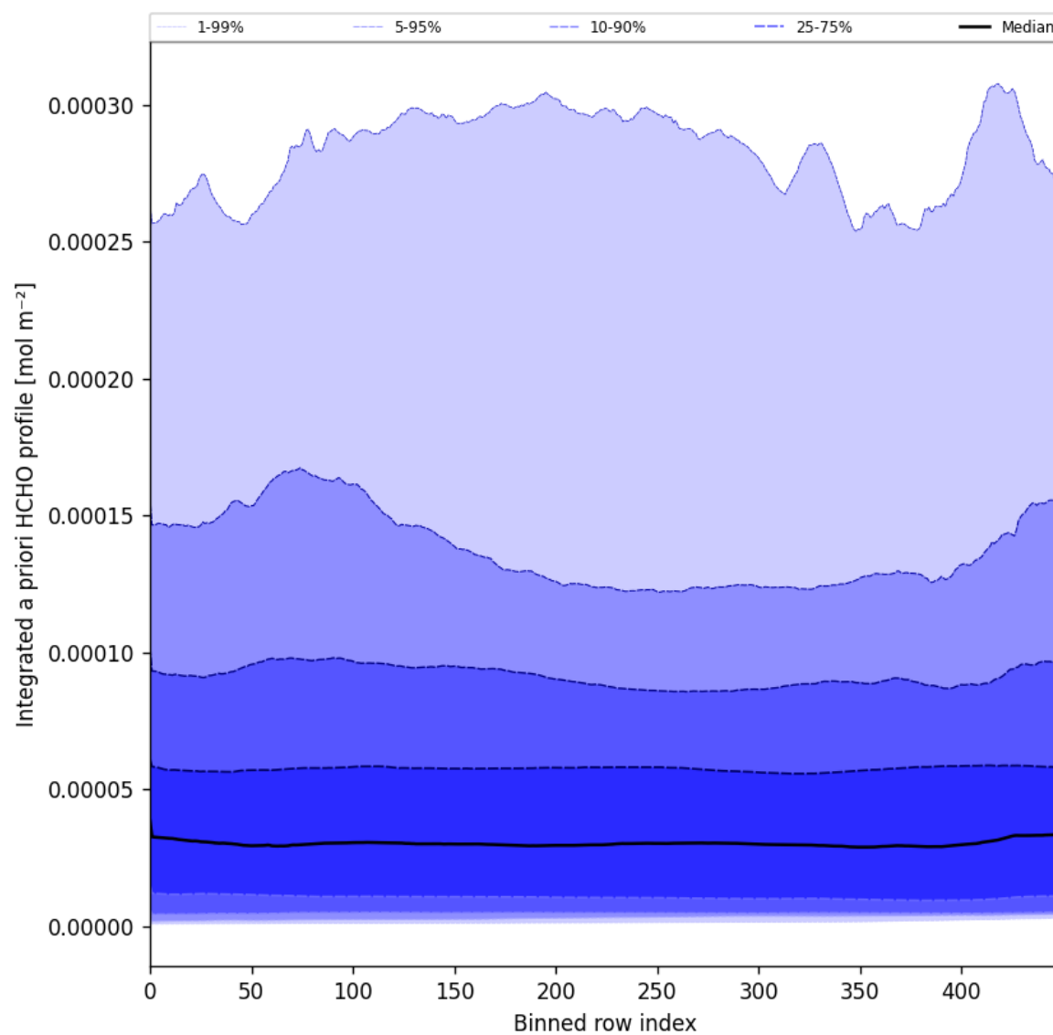
Figure 57: Along track statistics of “Integrated a priori HCHO profile” for 2025-05-15 to 2025-05-16
