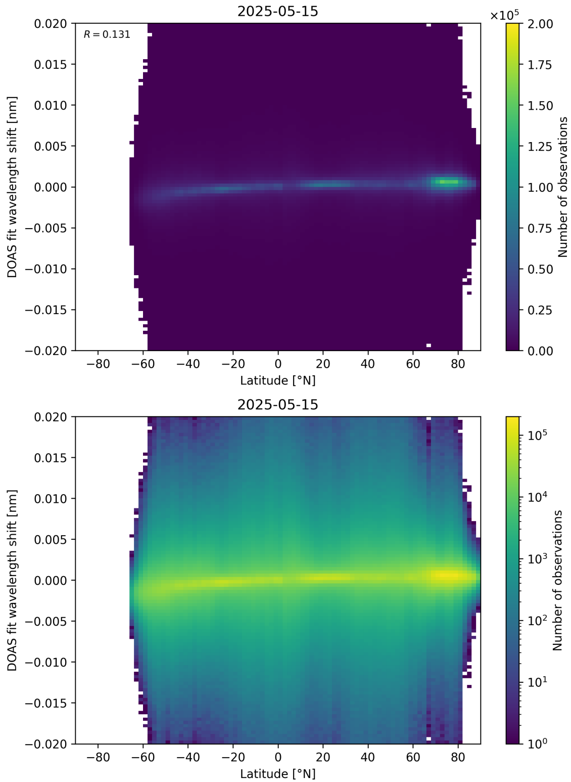
Figure 154: Scatter density plot of “Latitude” against “DOAS fit wavelength shift” for 2025-05-15 to 2025-05-16.
