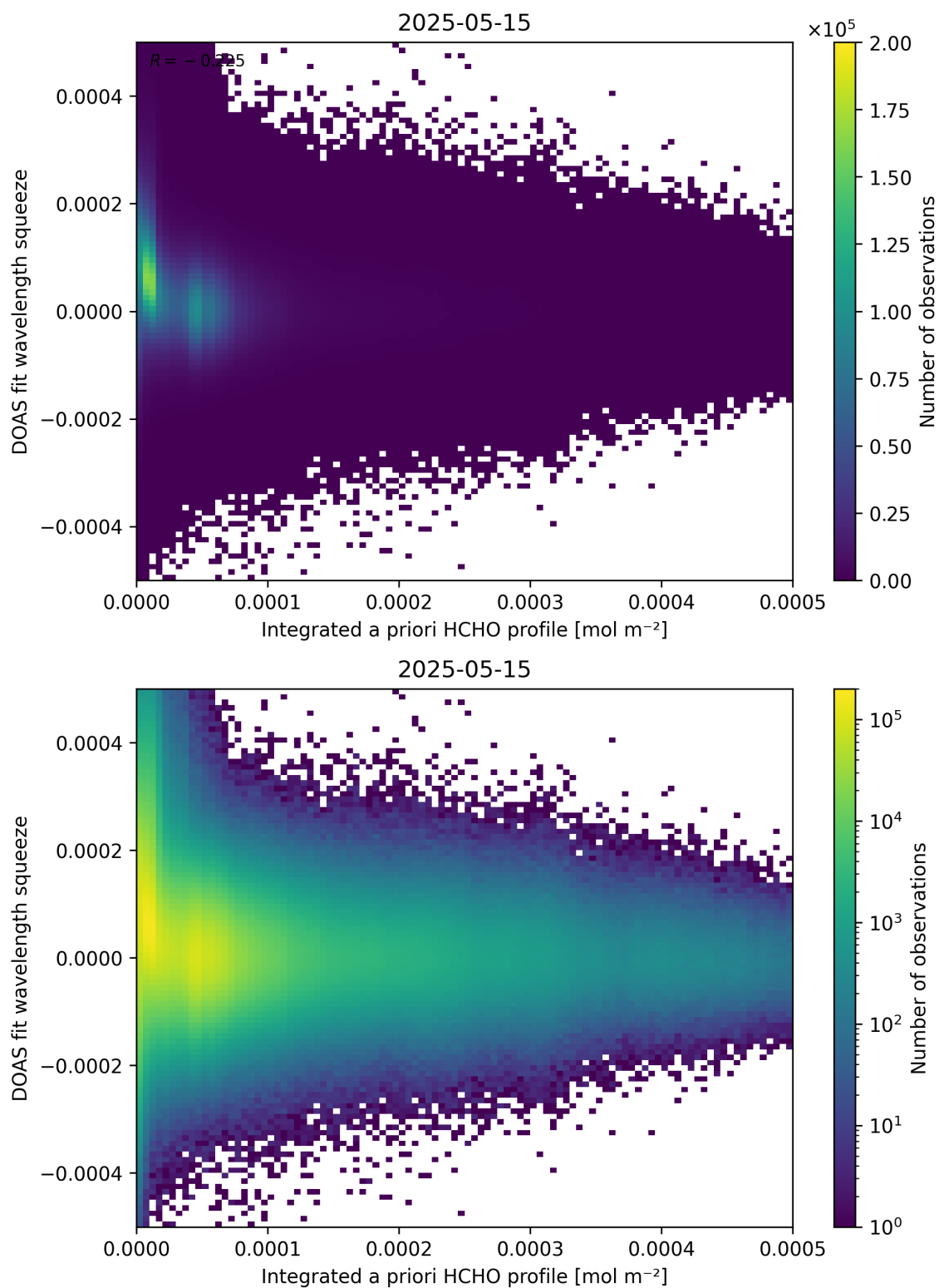
Figure 150: Scatter density plot of “Integrated a priori HCHO profile” against “DOAS fit wavelength squeeze” for 2025-05-15 to 2025-05-16.
