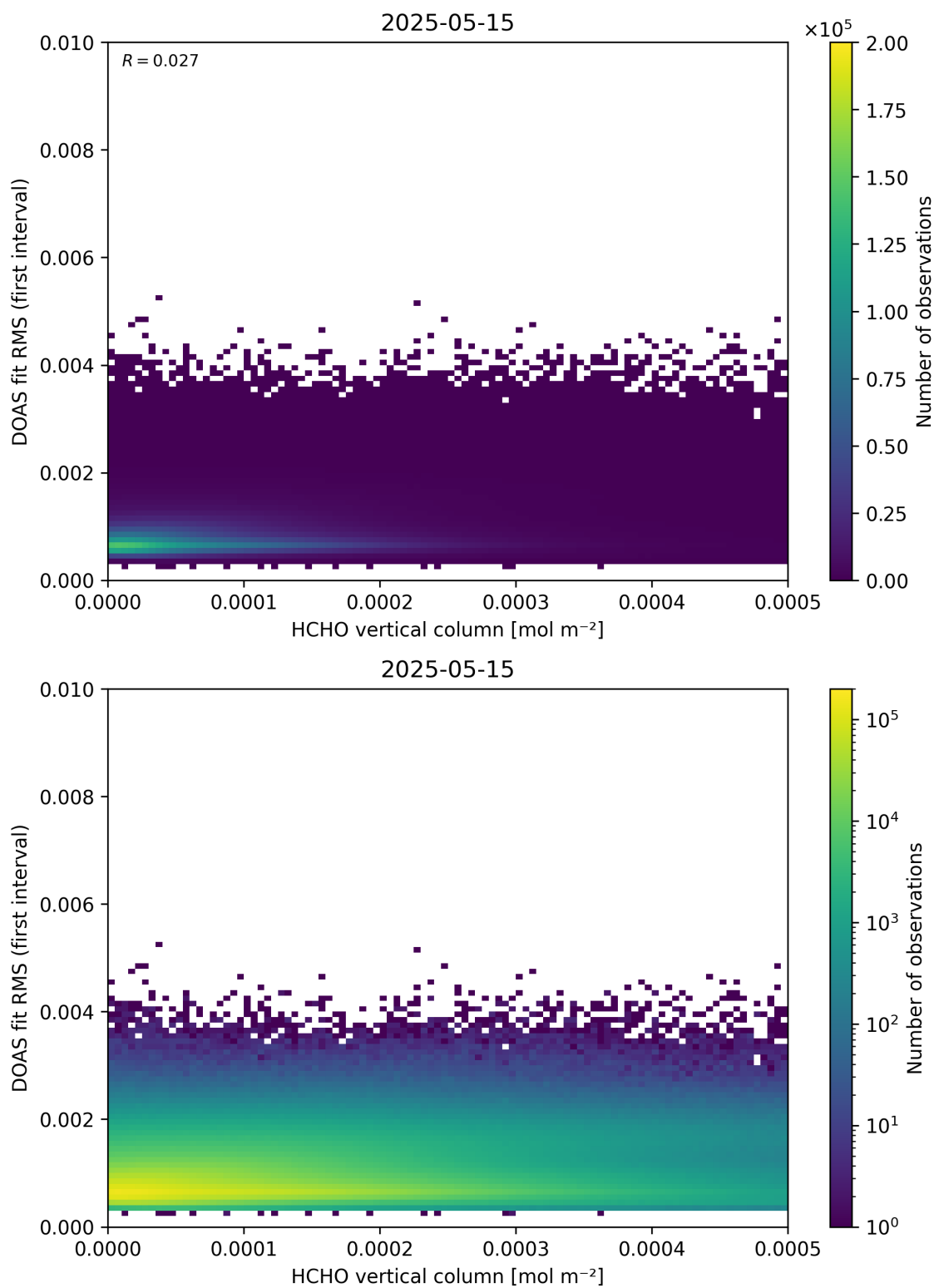
Figure 123: Scatter density plot of “HCHO vertical column” against “DOAS fit RMS (first interval)” for 2025-05-15 to 2025-05-16.
