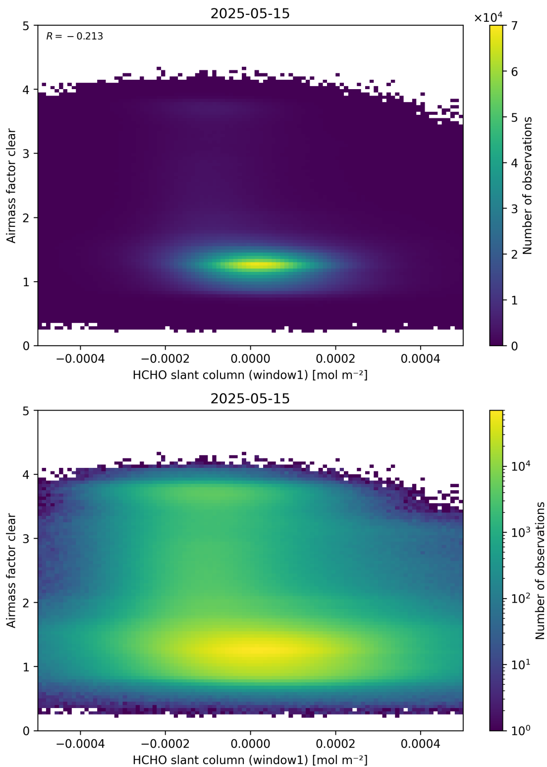
Figure 81: Scatter density plot of “HCHO slant column (window1)” against “Airmass factor clear” for 2025-05-15 to 2025-05-16.
