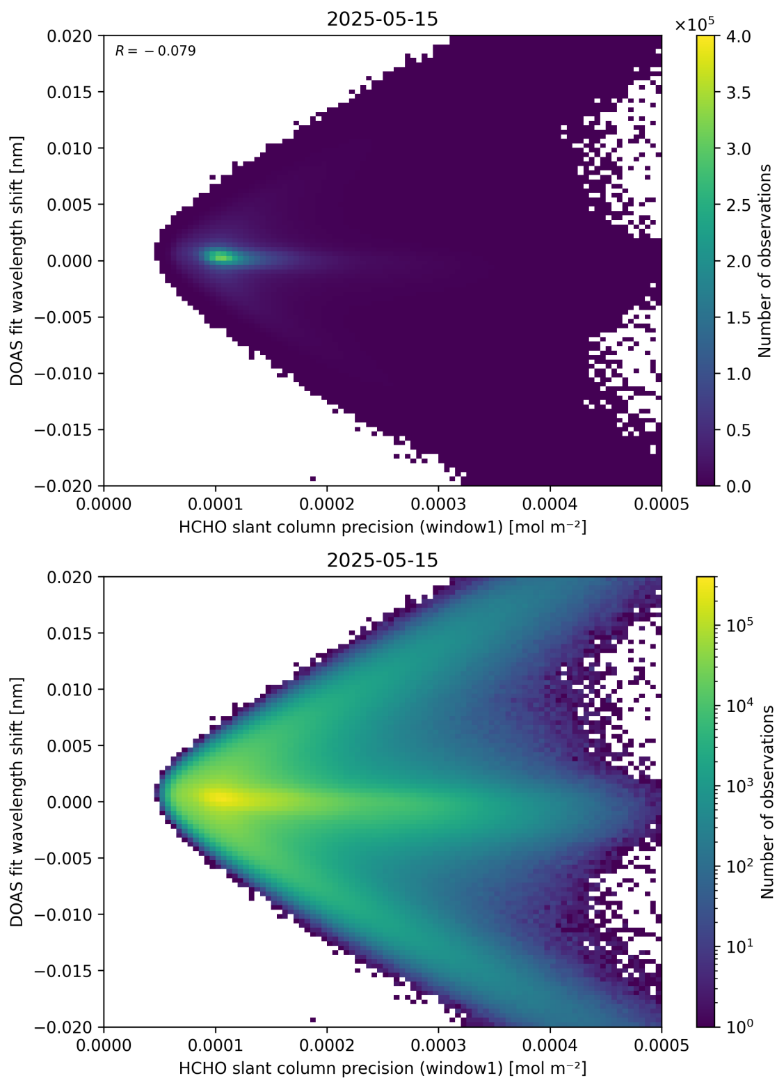
Figure 89: Scatter density plot of “HCHO slant column precision (window1)” against “DOAS fit wavelength shift” for 2025-05-15 to 2025-05-16.
