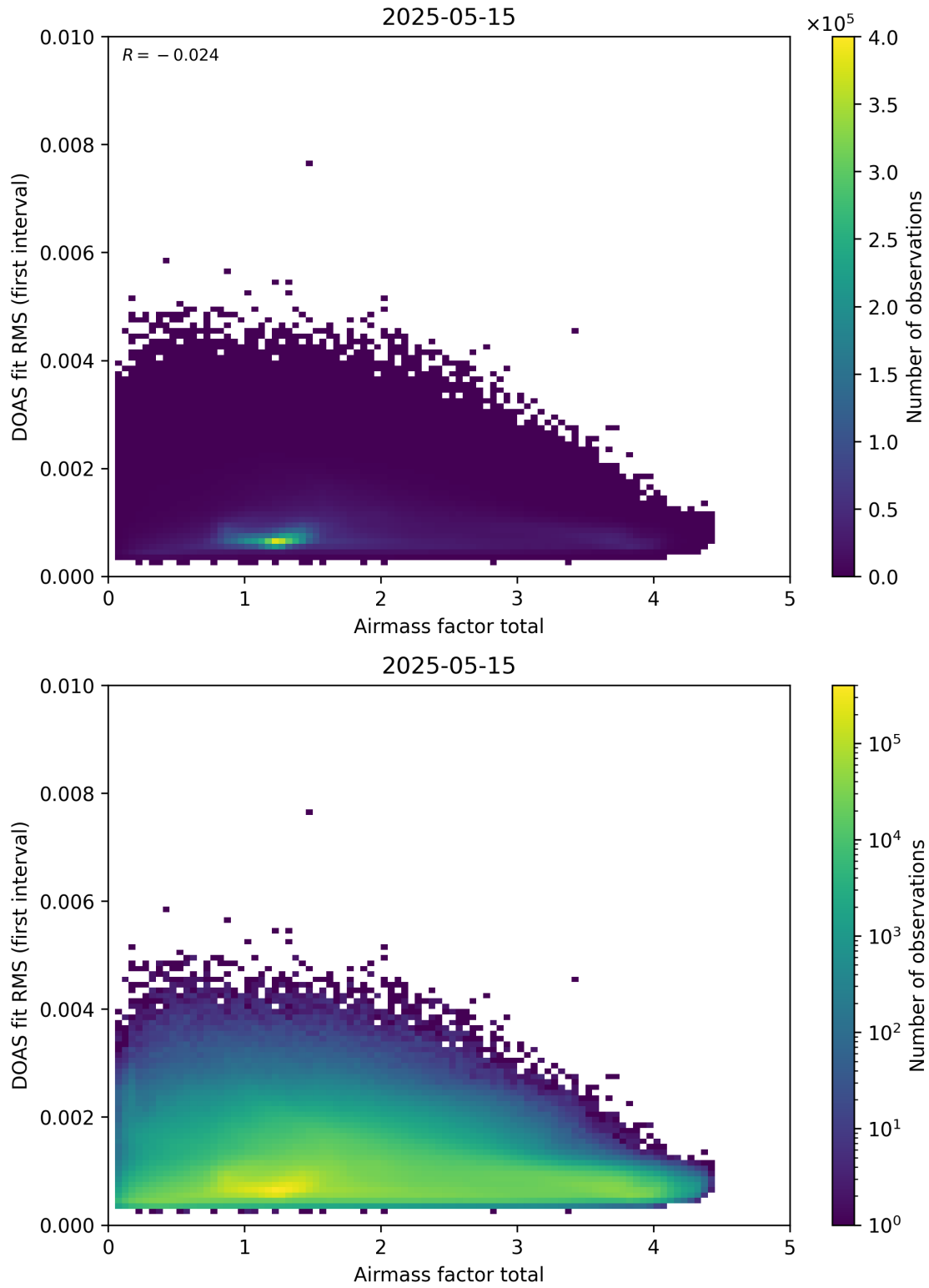
Figure 97: Scatter density plot of “Airmass factor total” against “DOAS fit RMS (first interval)” for 2025-05-15 to 2025-05-16.
