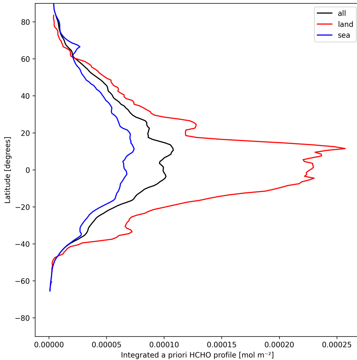
Figure 29: Zonal average of “Integrated a priori HCHO profile” for 2025-05-15 to 2025-05-16.
