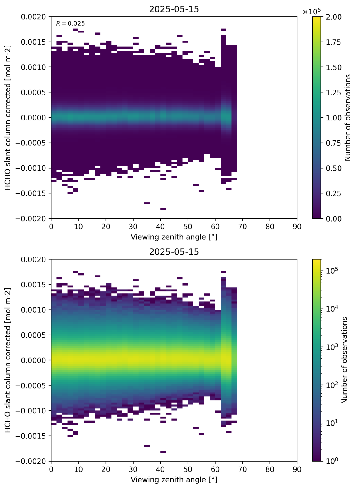
Figure 186: Scatter density plot of “Viewing zenith angle” against “HCHO slant column corrected” for 2025-05-15 to 2025-05-16.
