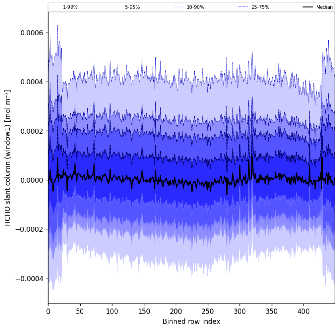
Figure 52: Along track statistics of “HCHO slant column (window1)” for 2025-05-15 to 2025-05-16
