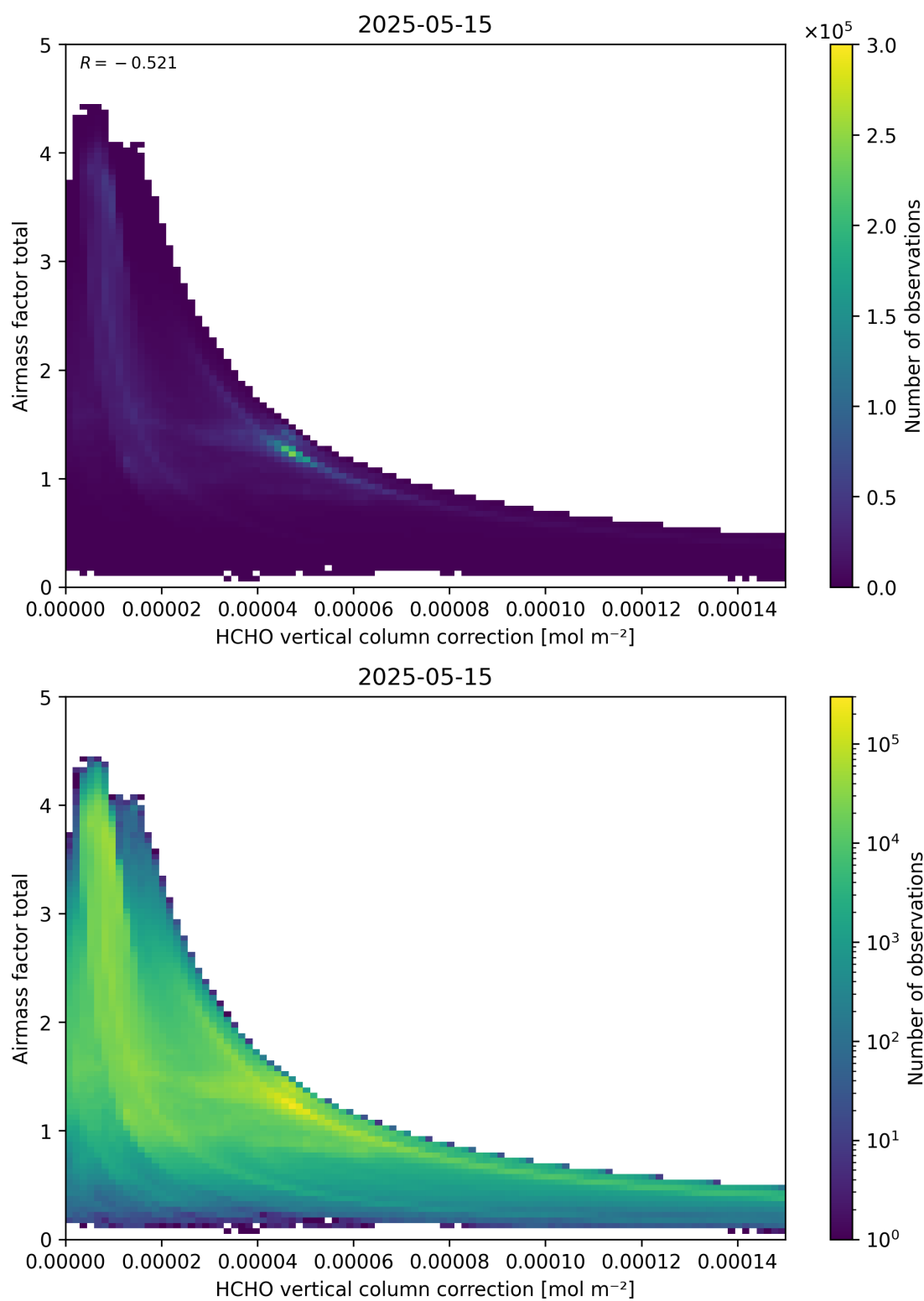
Figure 120: Scatter density plot of “HCHO vertical column correction” against “Airmass factor total” for 2025-05-15 to 2025-05-16.
