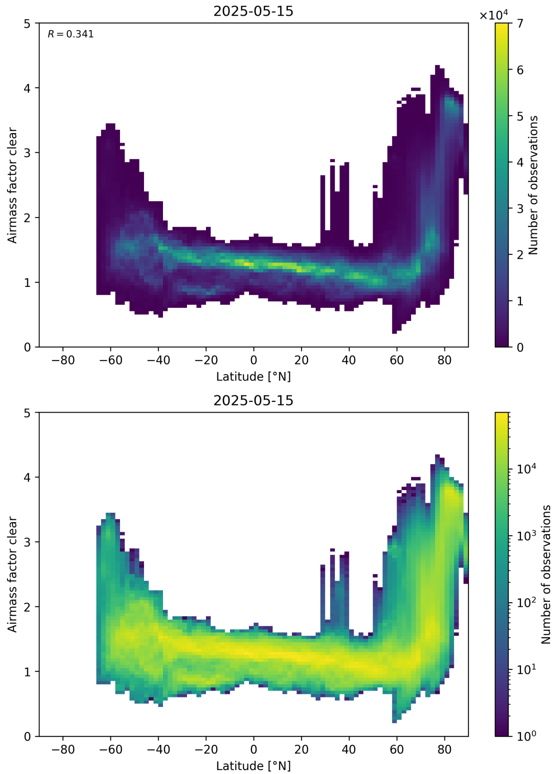
Figure 156: Scatter density plot of “Latitude” against “Airmass factor clear” for 2025-05-15 to 2025-05-16.
