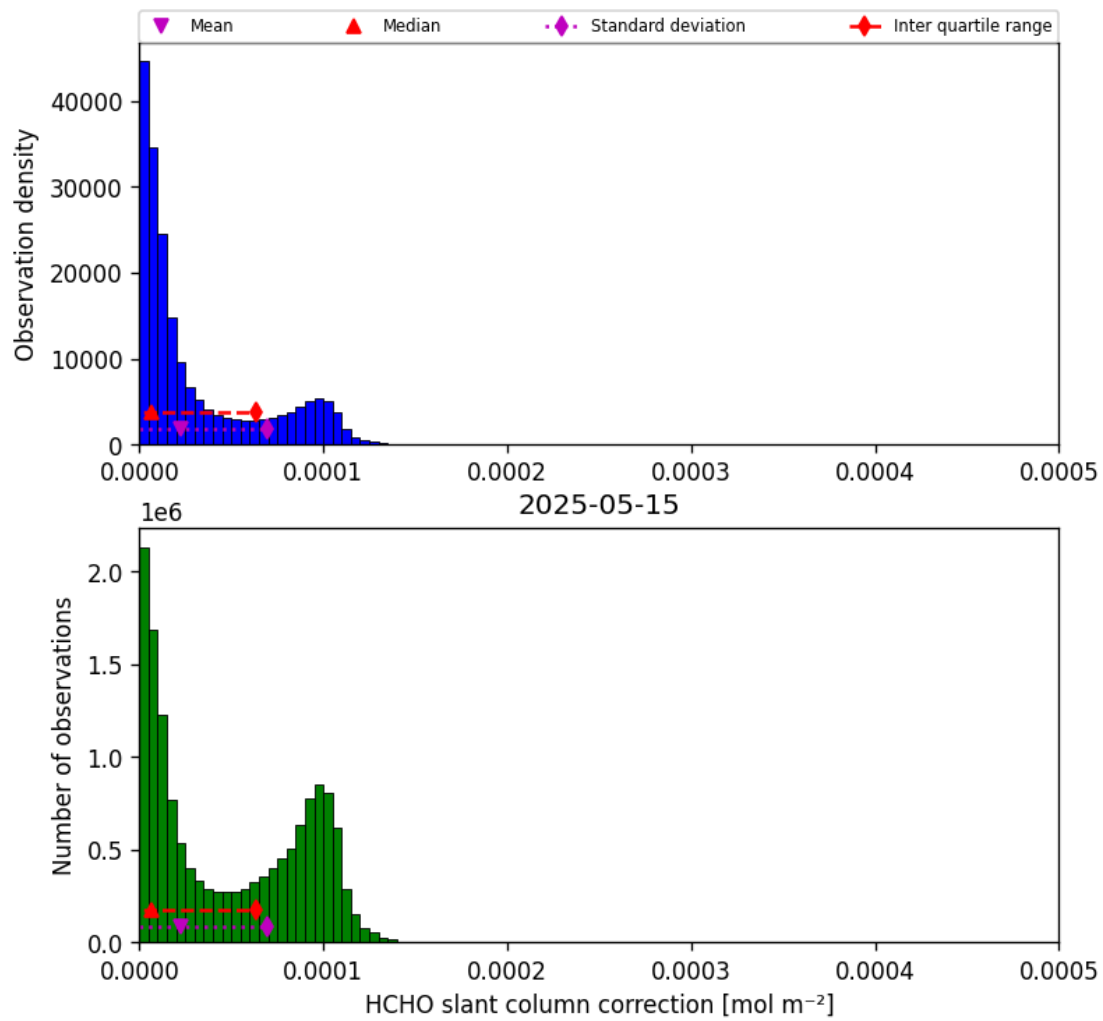
Figure 47: Histogram of “HCHO slant column correction” for 2025-05-15 to 2025-05-16
