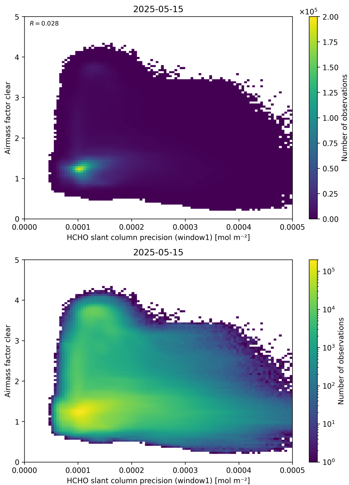
Figure 91: Scatter density plot of “HCHO slant column precision (window1)” against “Airmass factor clear” for 2025-05-15 to 2025-05-16.
