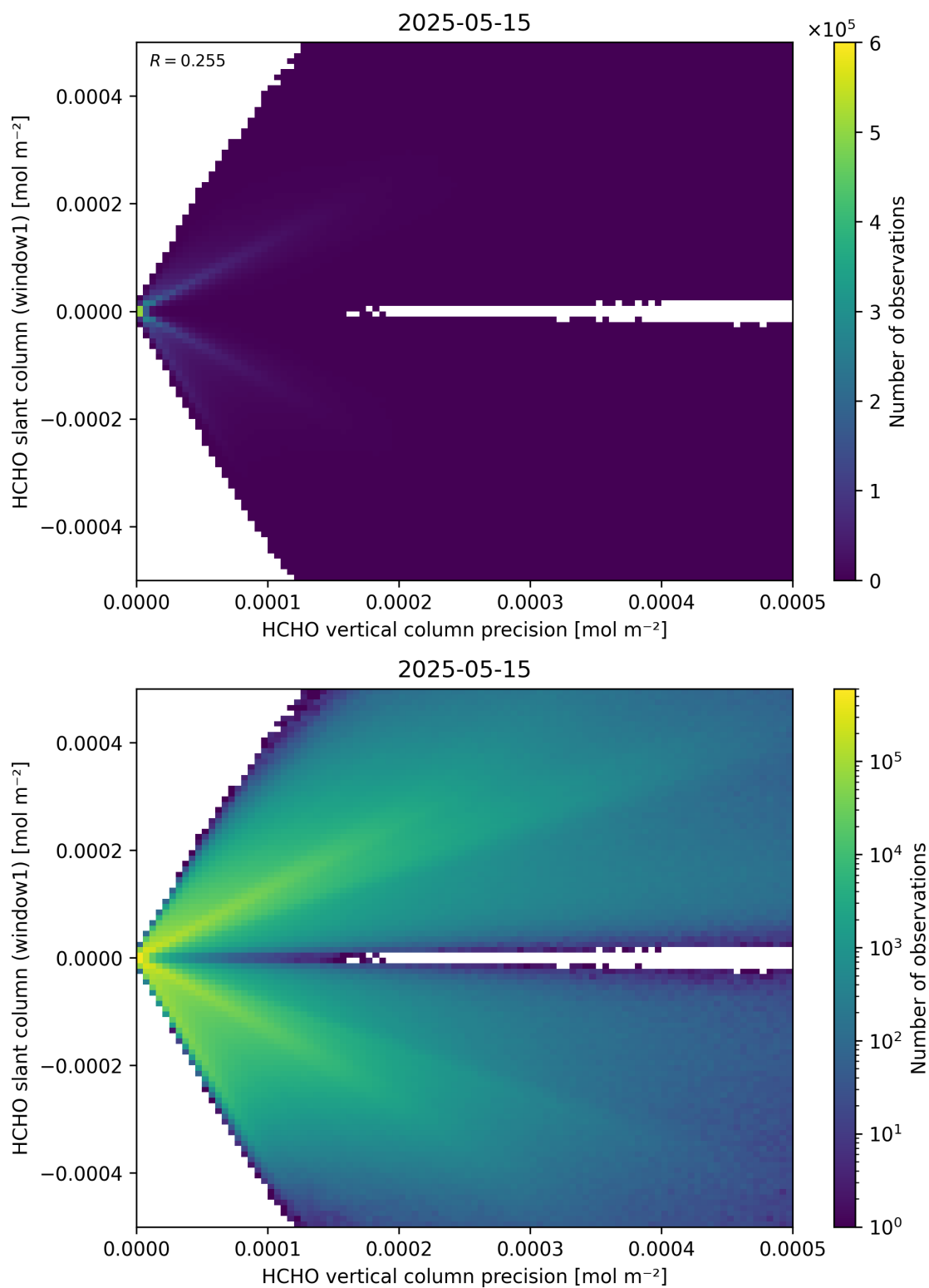
Figure 142: Scatter density plot of “HCHO vertical column precision” against “HCHO slant column (window1)” for 2025-05-15 to 2025-05-16.
