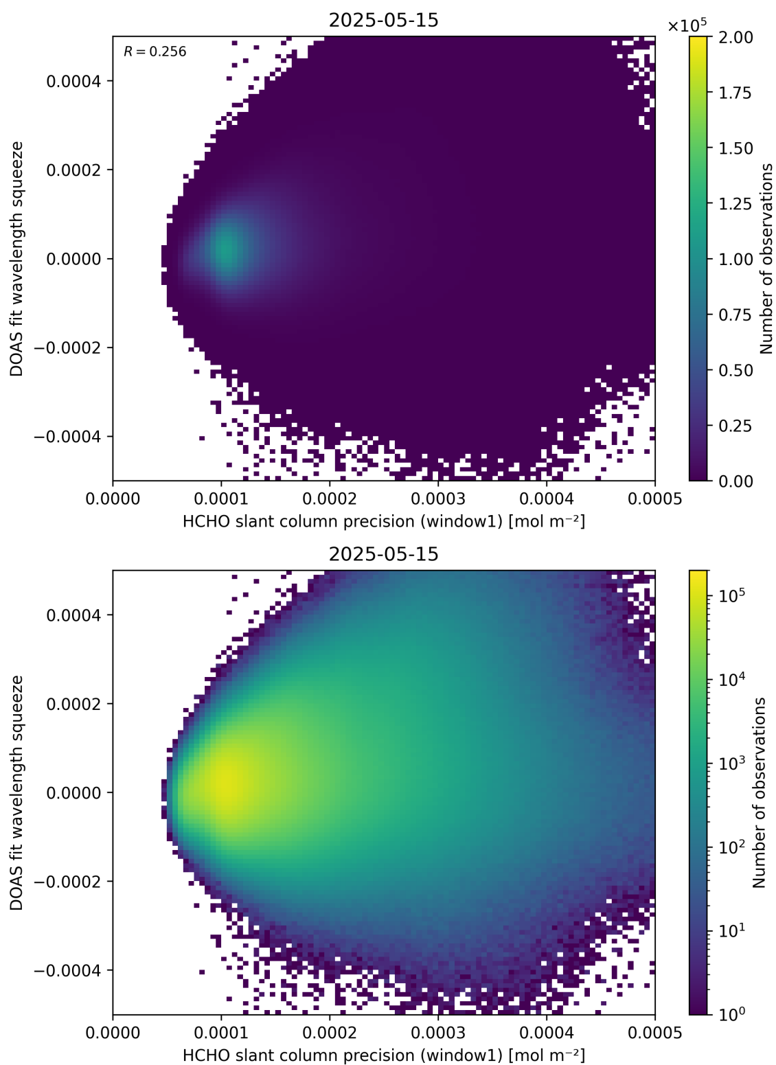
Figure 90: Scatter density plot of “HCHO slant column precision (window1)” against “DOAS fit wavelength squeeze” for 2025-05-15 to 2025-05-16.
