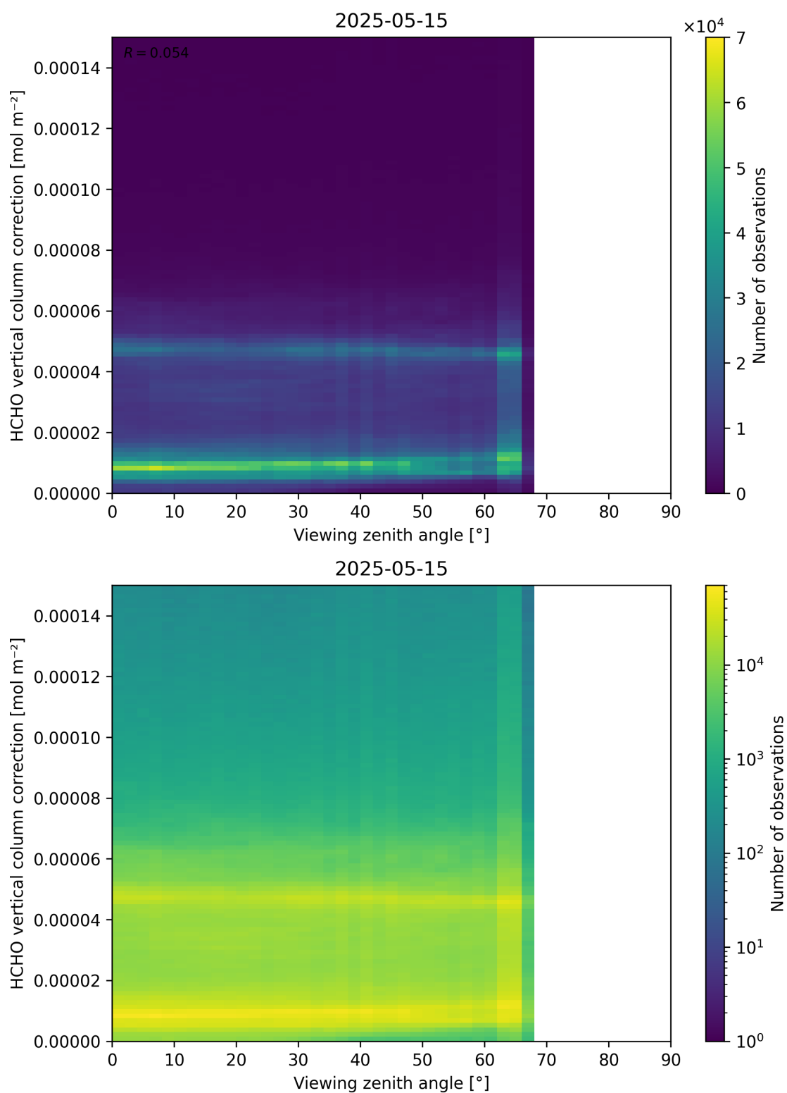
Figure 193: Scatter density plot of “Viewing zenith angle” against “HCHO vertical column correction” for 2025-05-15 to 2025-05-16.
