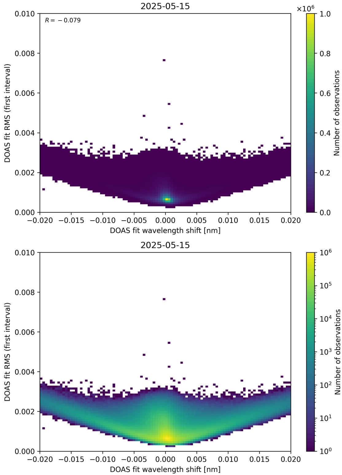
Figure 64: Scatter density plot of “DOAS fit wavelength shift” against “DOAS fit RMS (first interval)” for 2025-05-15 to 2025-05-16.
