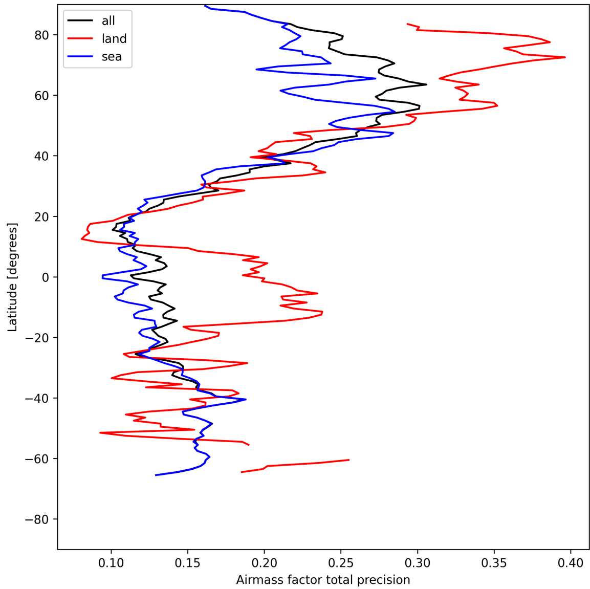
Figure 27: Zonal average of “Airmass factor total precision” for 2025-05-15 to 2025-05-16.
