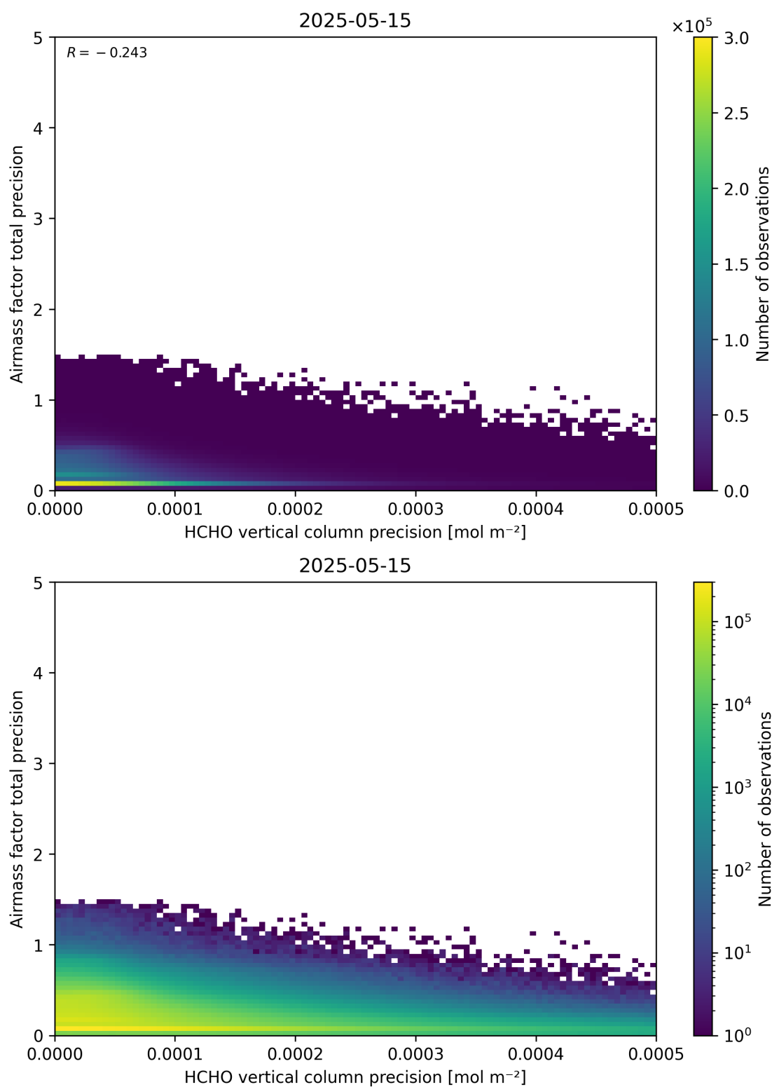
Figure 145: Scatter density plot of “HCHO vertical column precision” against “Airmass factor total precision” for 2025-05-15 to 2025-05-16.
