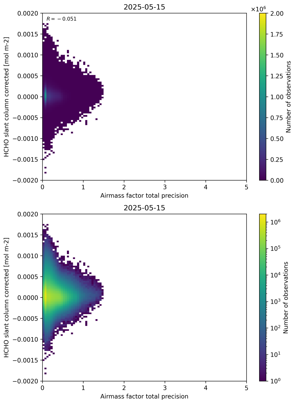
Figure 109: Scatter density plot of “Airmass factor total precision” against “HCHO slant column corrected” for 2025-05-15 to 2025-05-16.
