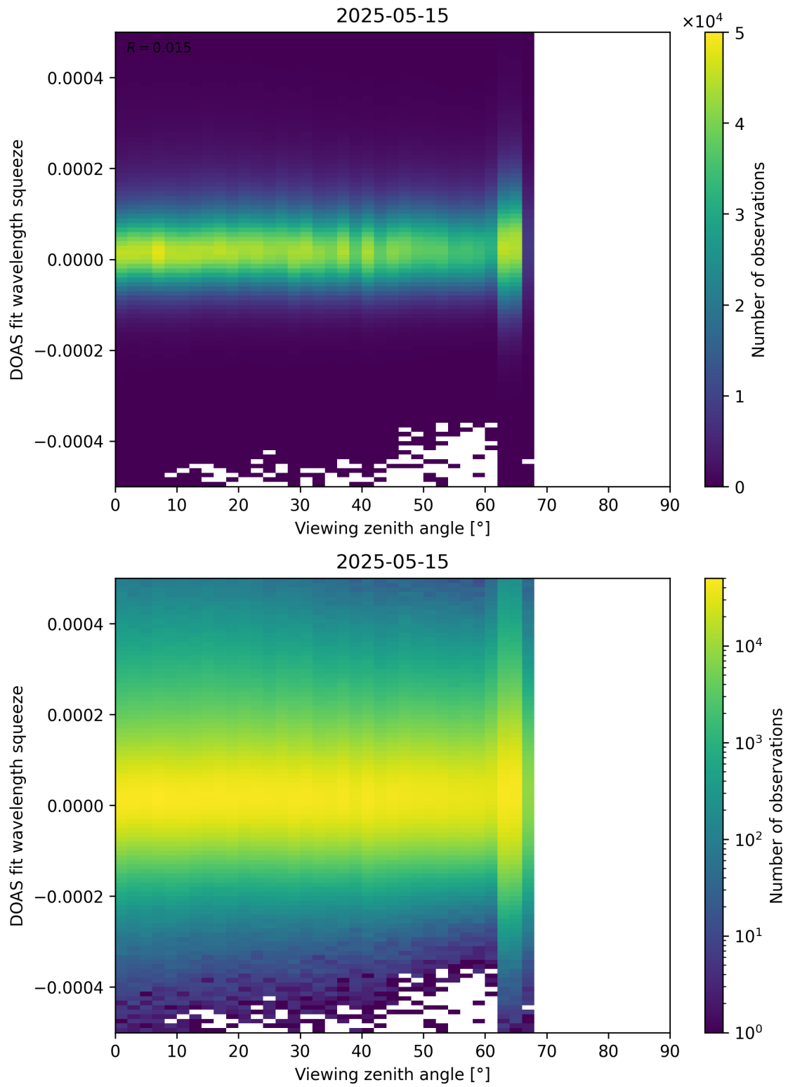
Figure 184: Scatter density plot of “Viewing zenith angle” against “DOAS fit wavelength squeeze” for 2025-05-15 to 2025-05-16.
