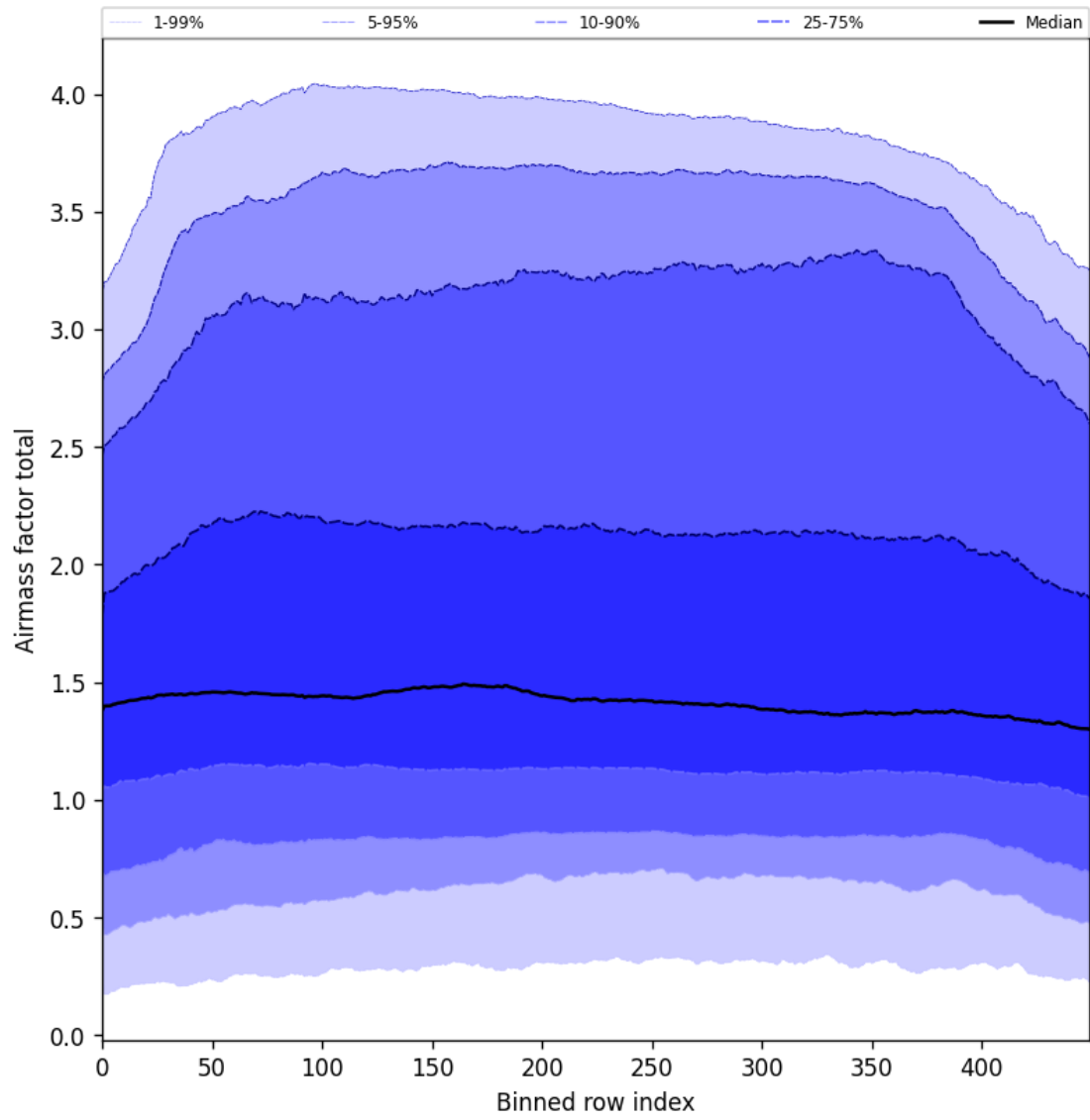
Figure 54: Along track statistics of “Airmass factor total” for 2025-05-15 to 2025-05-16
