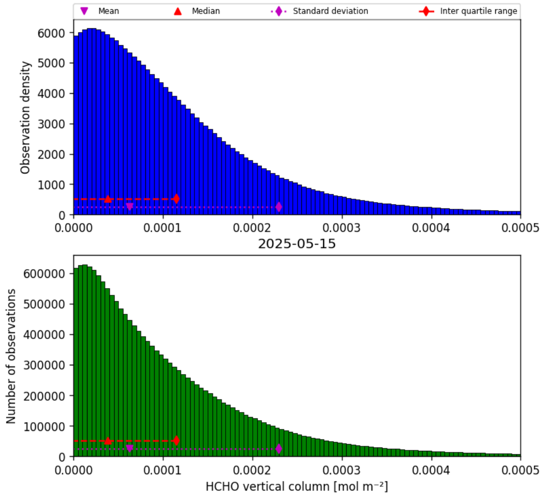
Figure 35: Histogram of “HCHO vertical column” for 2025-05-15 to 2025-05-16
