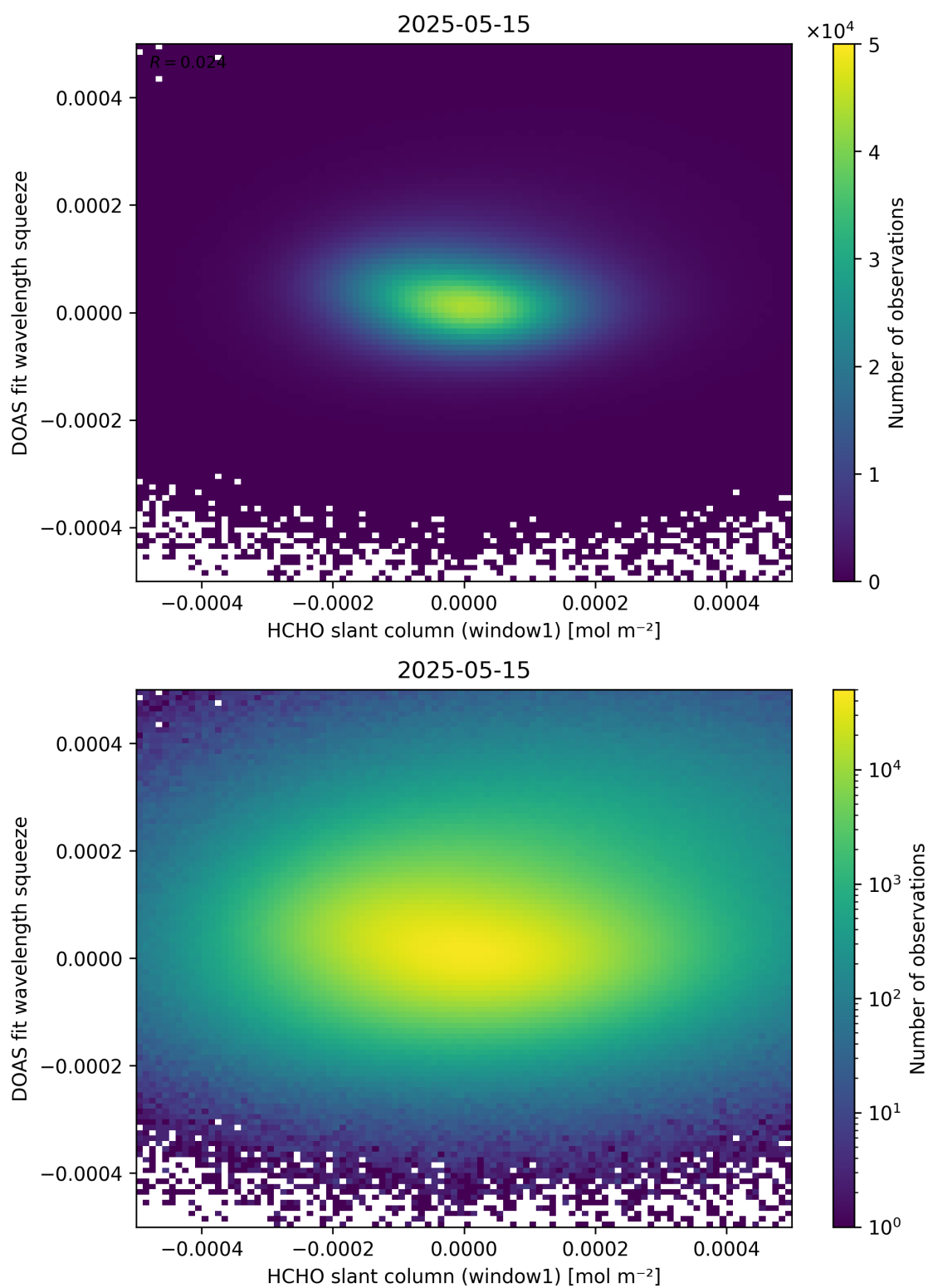
Figure 80: Scatter density plot of “HCHO slant column (window1)” against “DOAS fit wavelength squeeze” for 2025-05-15 to 2025-05-16.
