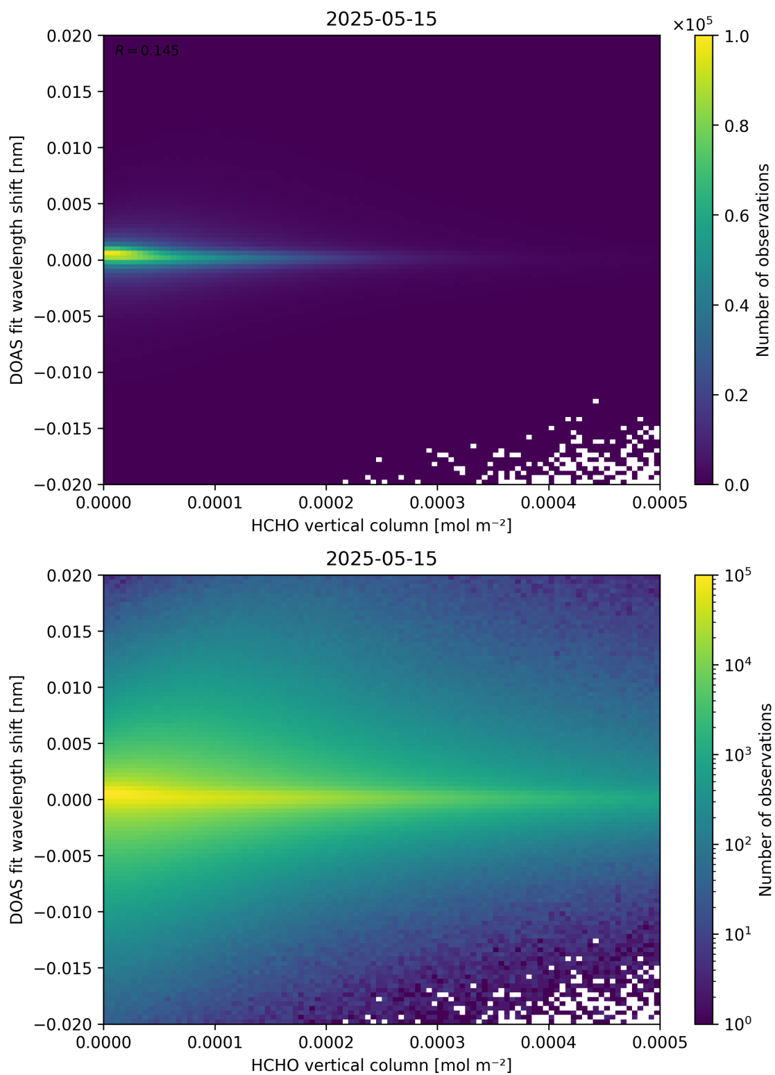
Figure 124: Scatter density plot of “HCHO vertical column” against “DOAS fit wavelength shift” for 2025-05-15 to 2025-05-16.
