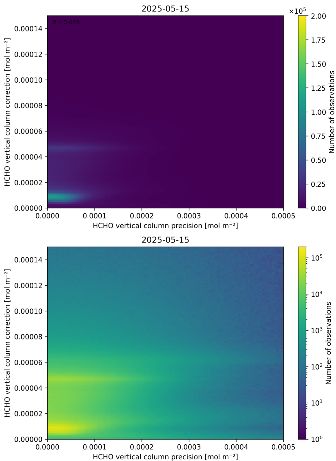
Figure 146: Scatter density plot of “HCHO vertical column precision” against “HCHO vertical column correction” for 2025-05-15 to 2025-05-16.
