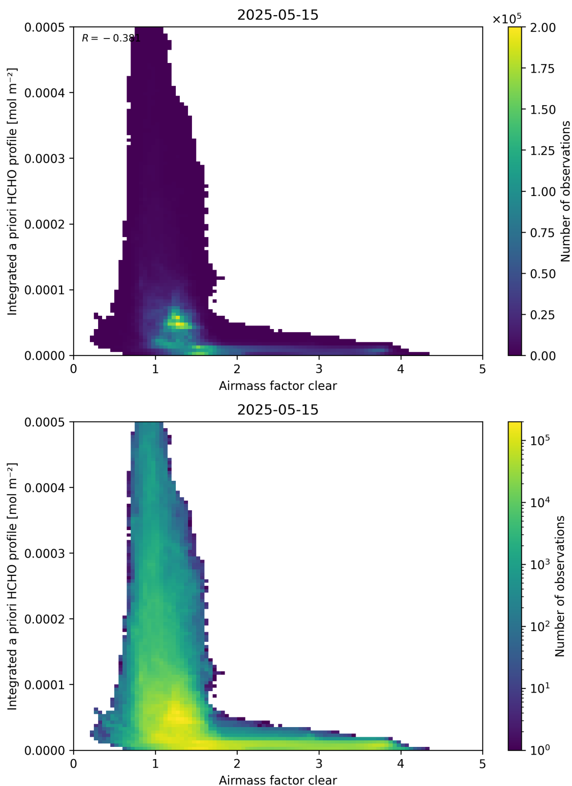
Figure 76: Scatter density plot of “Airmass factor clear” against “Integrated a priori HCHO profile” for 2025-05-15 to 2025-05-16.
