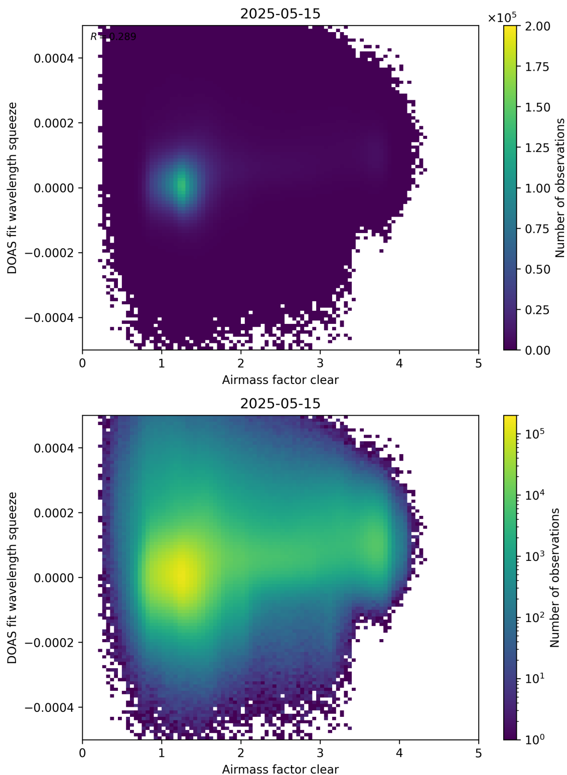
Figure 73: Scatter density plot of “Airmass factor clear” against “DOAS fit wavelength squeeze” for 2025-05-15 to 2025-05-16.
