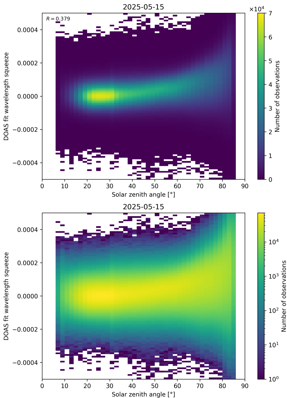
Figure 169: Scatter density plot of “Solar zenith angle” against “DOAS fit wavelength squeeze” for 2025-05-15 to 2025-05-16.
