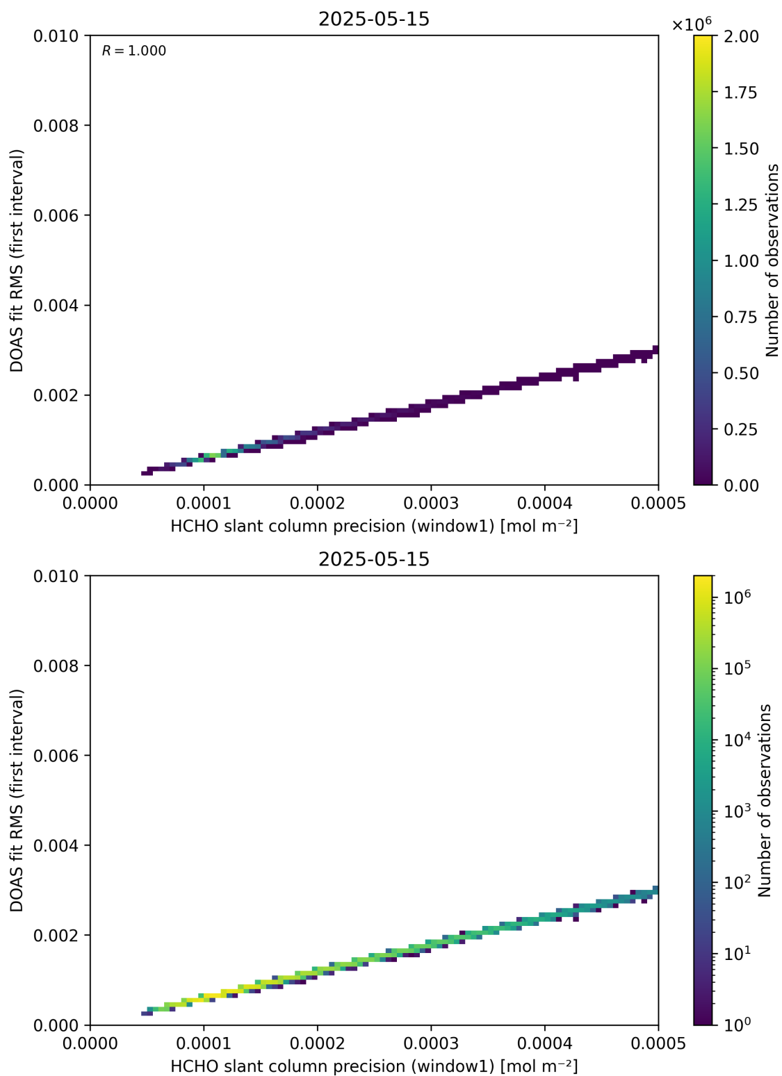
Figure 88: Scatter density plot of “HCHO slant column precision (window1)” against “DOAS fit RMS (first interval)” for 2025-05-15 to 2025-05-16.
