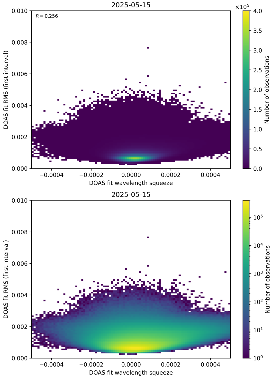
Figure 68: Scatter density plot of “DOAS fit wavelength squeeze” against “DOAS fit RMS (first interval)” for 2025-05-15 to 2025-05-16.
