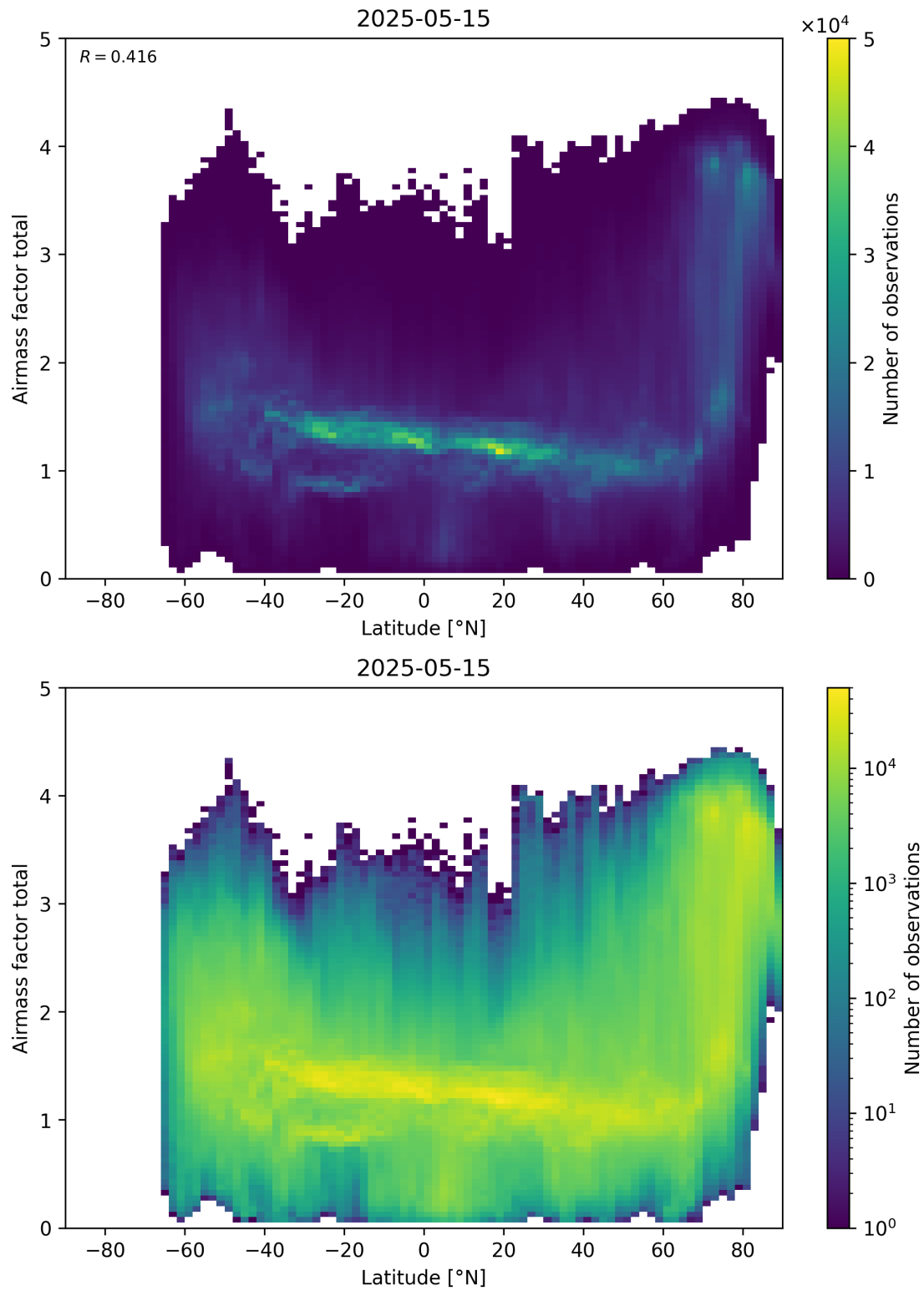
Figure 161: Scatter density plot of “Latitude” against “Airmass factor total” for 2025-05-15 to 2025-05-16.
