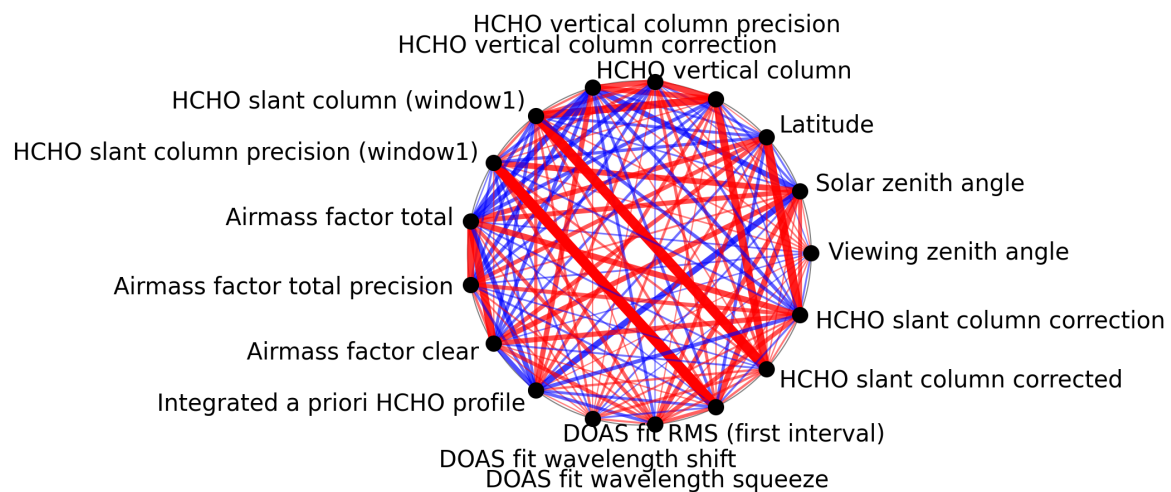
Figure 1: Map of correlation graph for 2025-05-15 to 2025-05-16.
