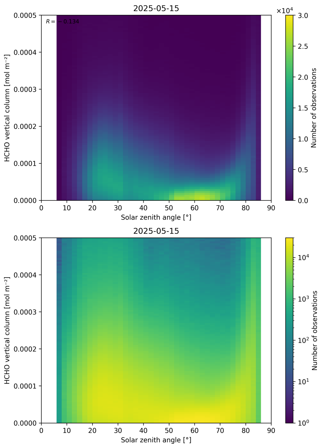
Figure 177: Scatter density plot of “Solar zenith angle” against “HCHO vertical column” for 2025-05-15 to 2025-05-16.
