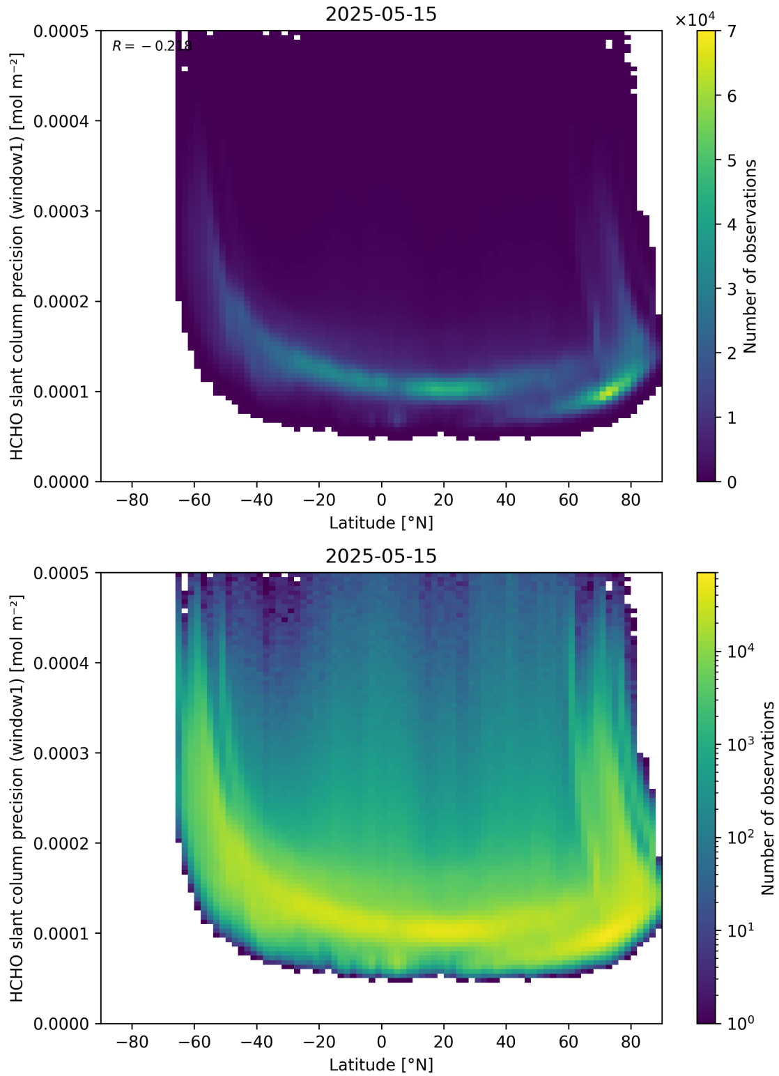
Figure 160: Scatter density plot of “Latitude” against “HCHO slant column precision (window1)” for 2025-05-15 to 2025-05-16.
