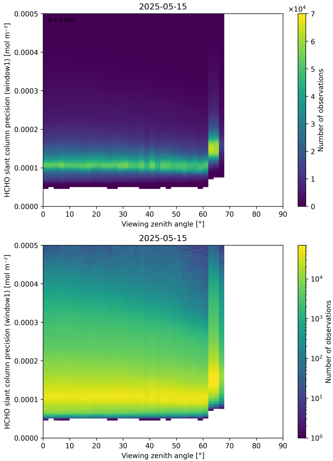
Figure 189: Scatter density plot of “Viewing zenith angle” against “HCHO slant column precision (window1)” for 2025-05-15 to 2025-05-16.
