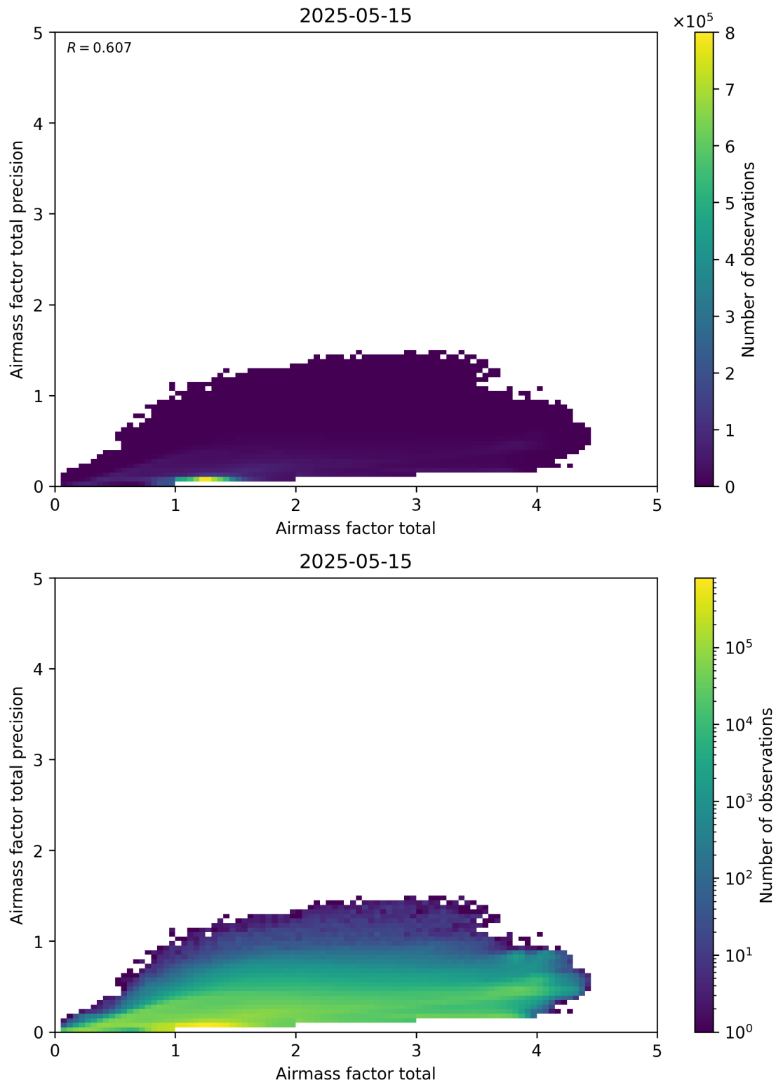
Figure 103: Scatter density plot of “Airmass factor total” against “Airmass factor total precision” for 2025-05-15 to 2025-05-16.
