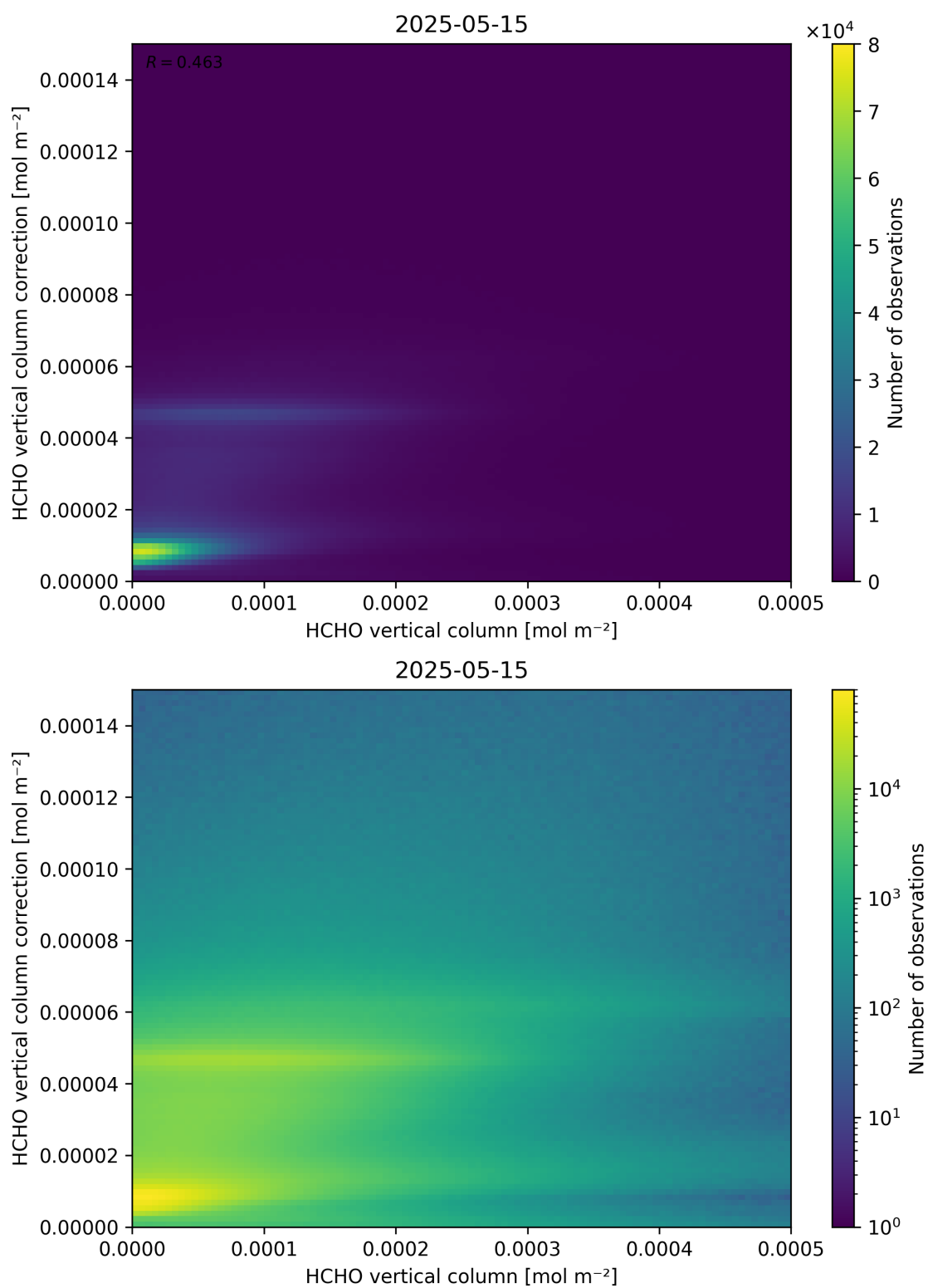
Figure 133: Scatter density plot of “HCHO vertical column” against “HCHO vertical column correction” for 2025-05-15 to 2025-05-16.
