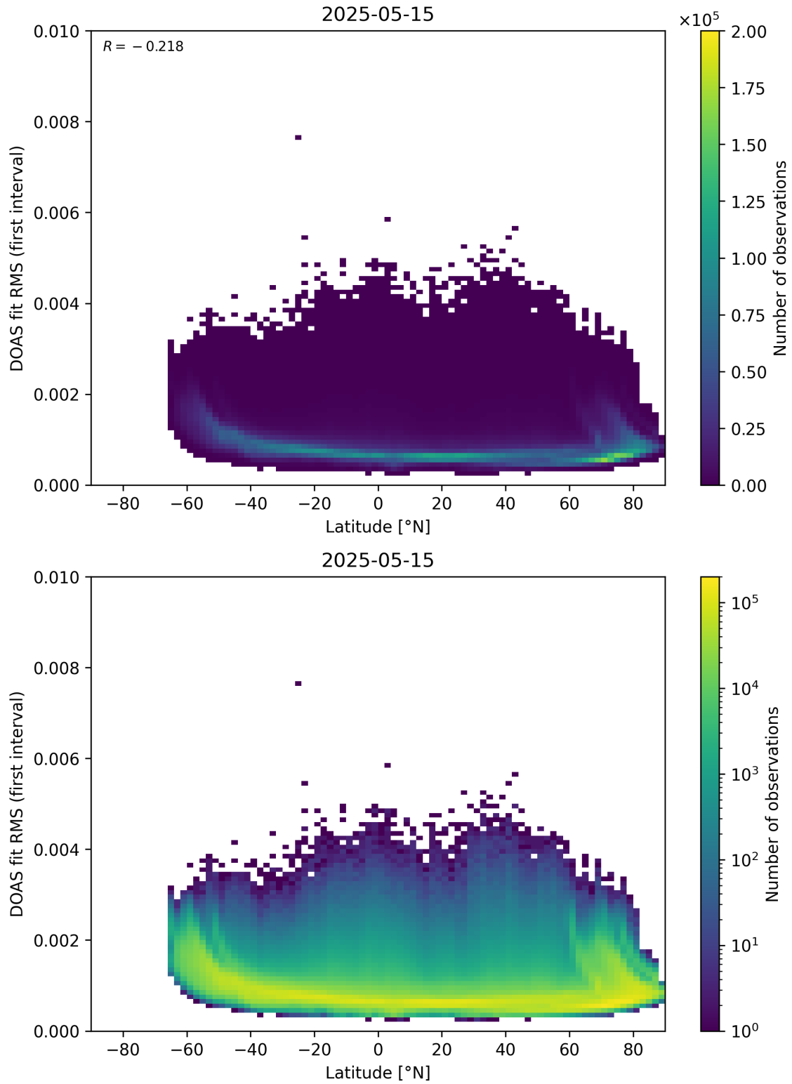
Figure 153: Scatter density plot of “Latitude” against “DOAS fit RMS (first interval)” for 2025-05-15 to 2025-05-16.
