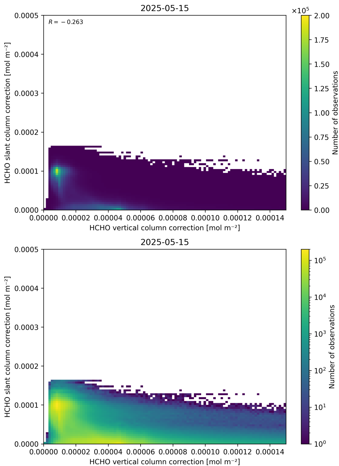
Figure 117: Scatter density plot of “HCHO vertical column correction” against “HCHO slant column correction” for 2025-05-15 to 2025-05-16.
