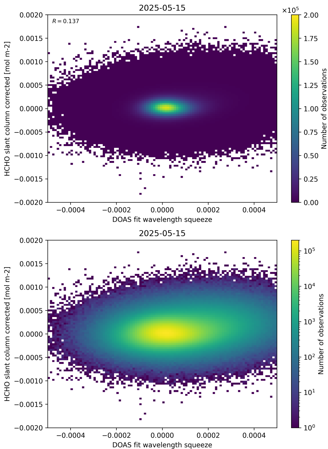
Figure 69: Scatter density plot of “DOAS fit wavelength squeeze” against “HCHO slant column corrected” for 2025-05-15 to 2025-05-16.
