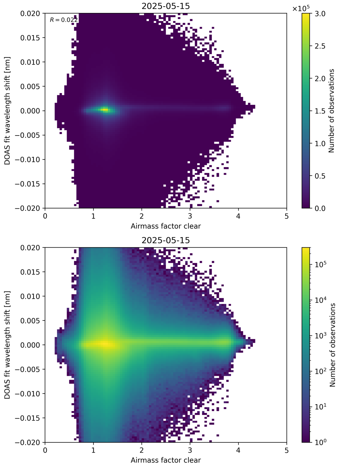
Figure 72: Scatter density plot of “Airmass factor clear” against “DOAS fit wavelength shift” for 2025-05-15 to 2025-05-16.
