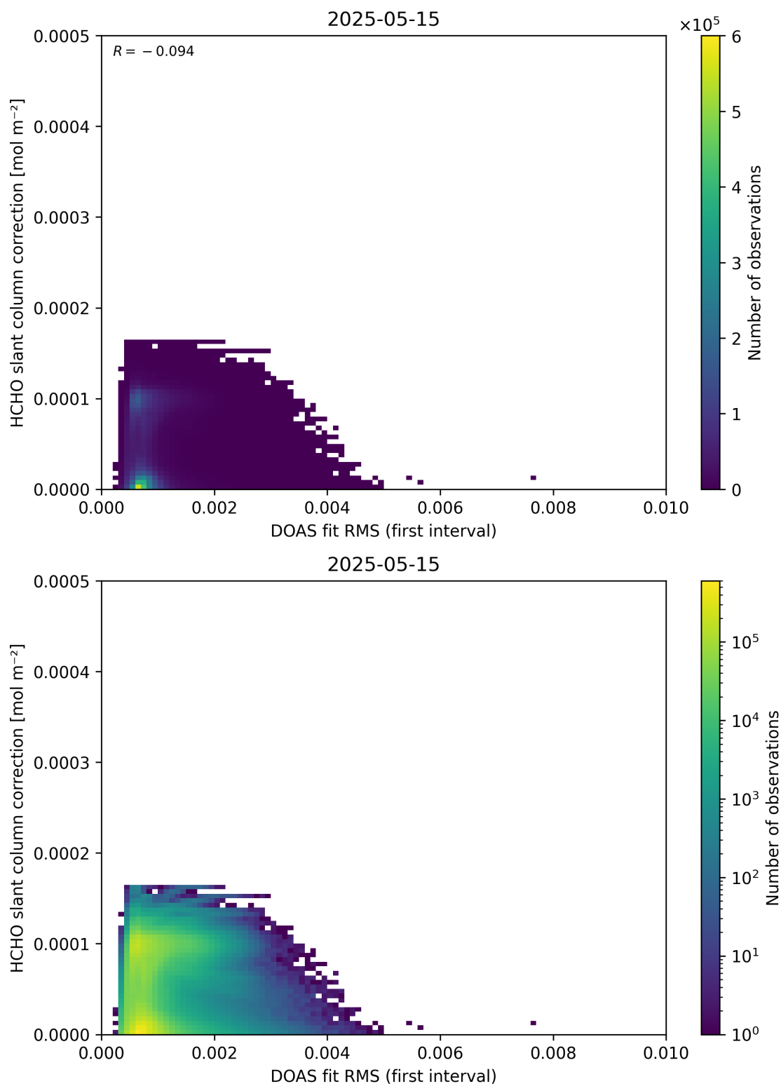
Figure 63: Scatter density plot of “DOAS fit RMS (first interval)” against “HCHO slant column correction” for 2025-05-15 to 2025-05-16.
