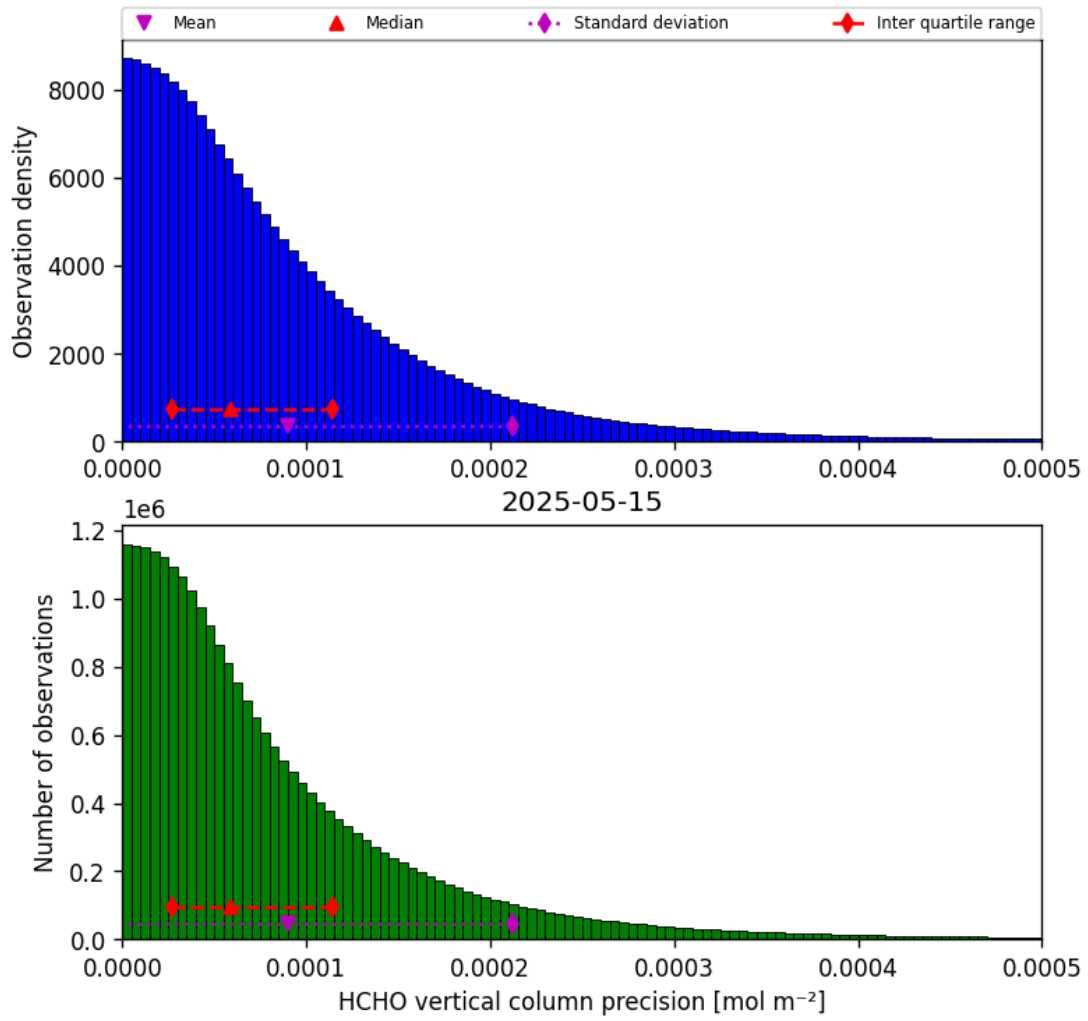
Figure 36: Histogram of “HCHO vertical column precision” for 2025-05-15 to 2025-05-16
