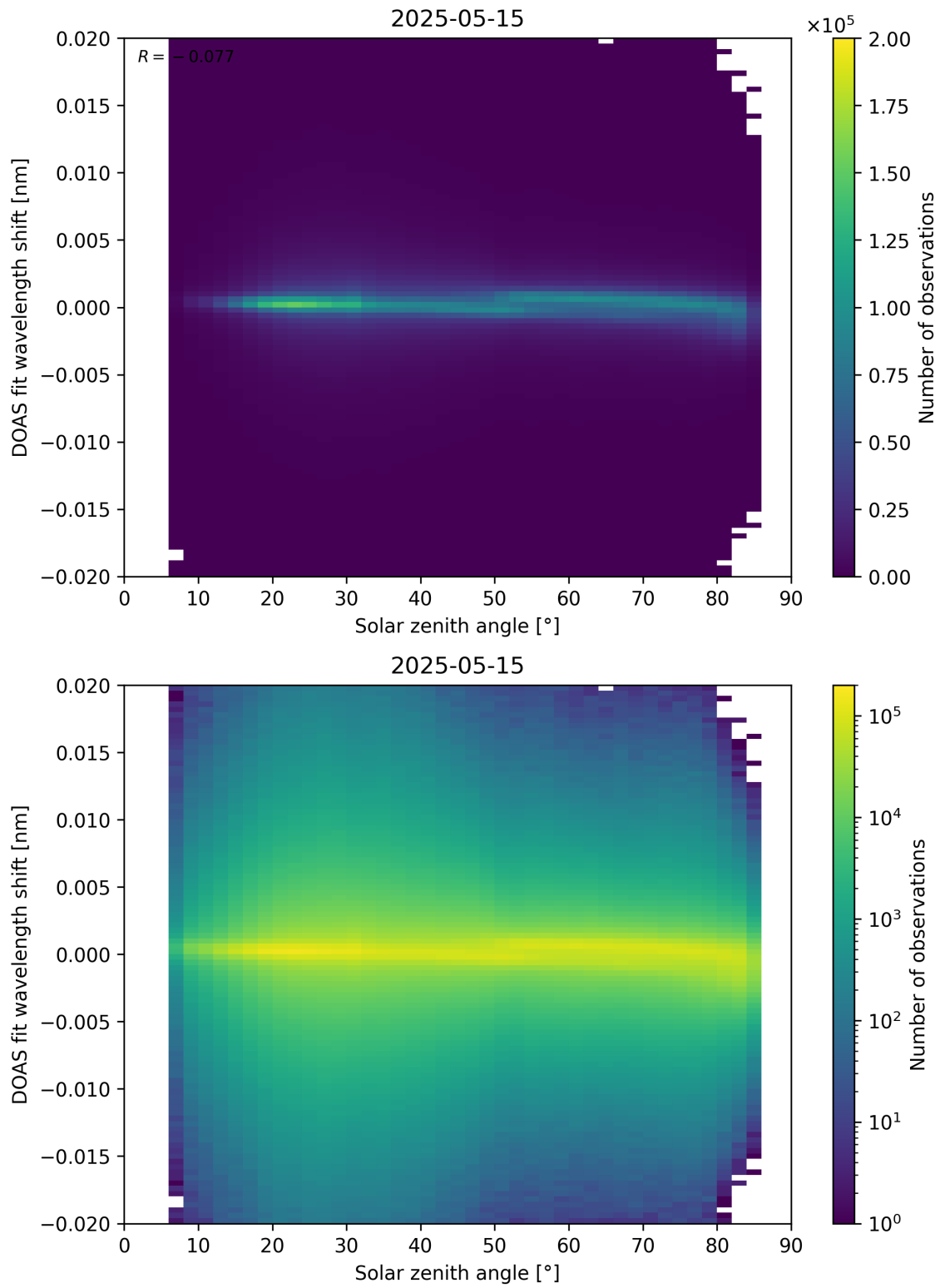
Figure 168: Scatter density plot of “Solar zenith angle” against “DOAS fit wavelength shift” for 2025-05-15 to 2025-05-16.
