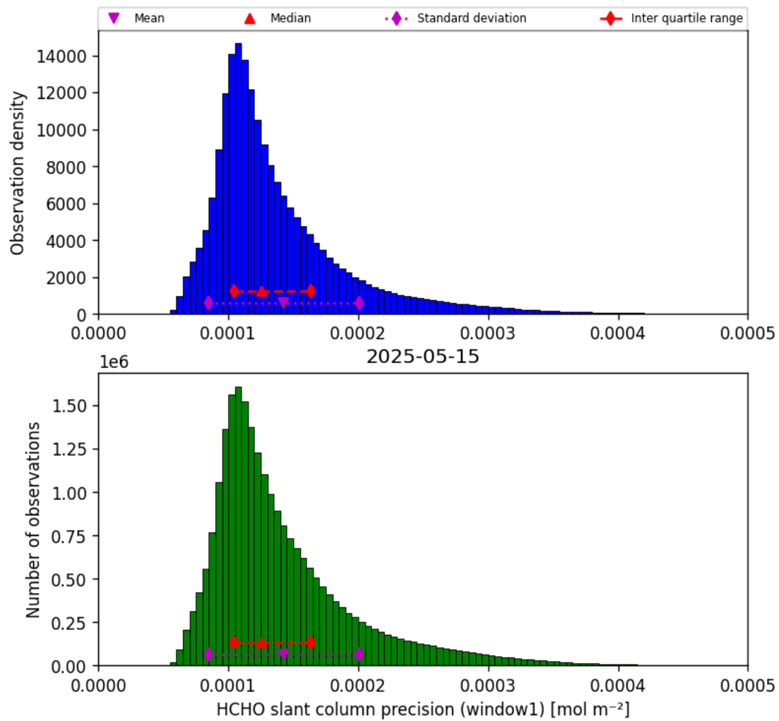
Figure 39: Histogram of “HCHO slant column precision (window1)” for 2025-05-15 to 2025-05-16
