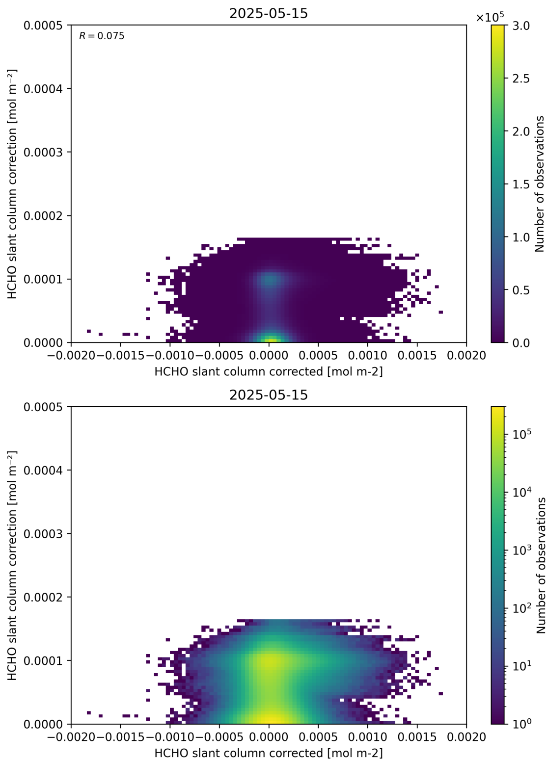
Figure 77: Scatter density plot of “HCHO slant column corrected” against “HCHO slant column correction” for 2025-05-15 to 2025-05-16.
