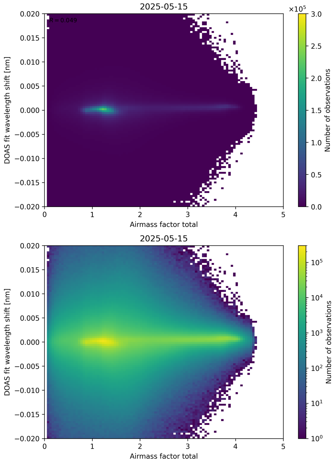
Figure 98: Scatter density plot of “Airmass factor total” against “DOAS fit wavelength shift” for 2025-05-15 to 2025-05-16.
