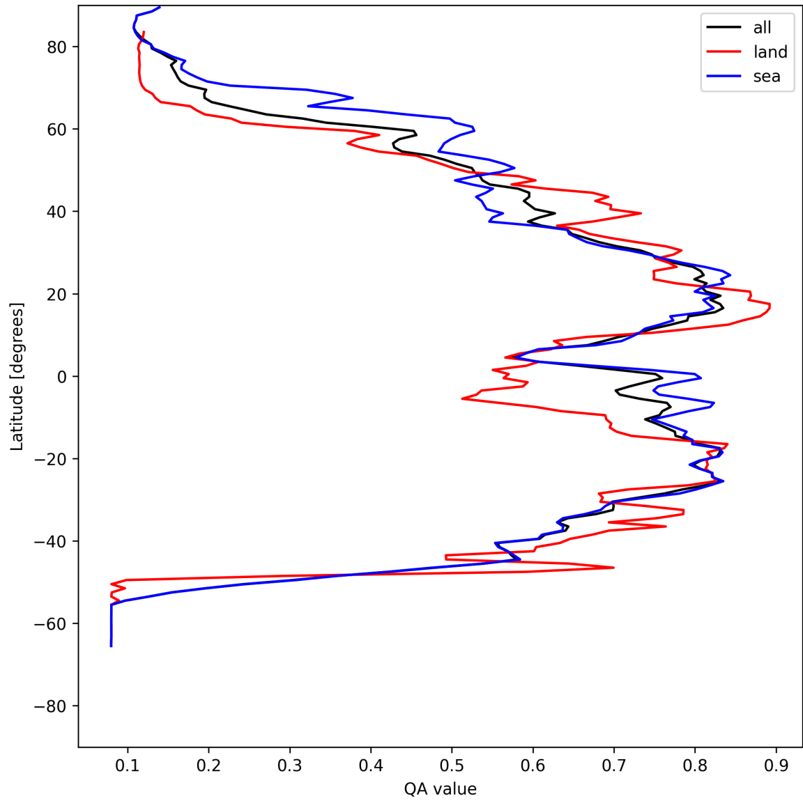
Figure 20: Zonal average of “QA value” for 2025-05-15 to 2025-05-16.
