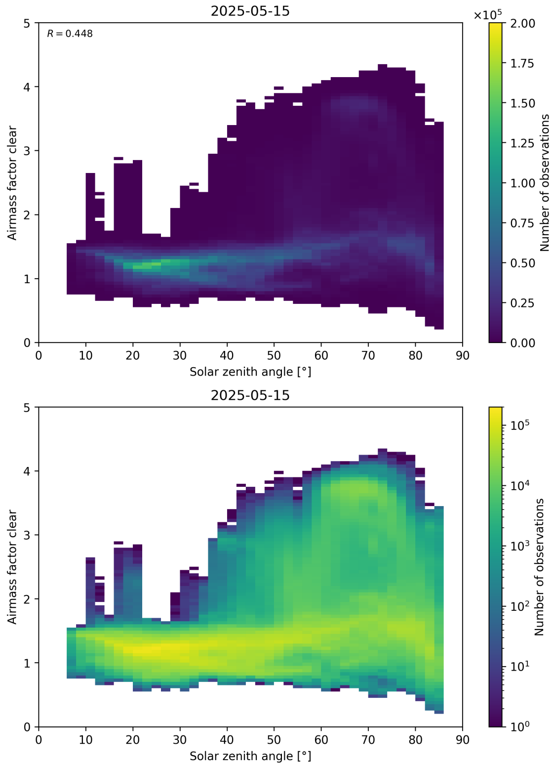
Figure 170: Scatter density plot of “Solar zenith angle” against “Airmass factor clear” for 2025-05-15 to 2025-05-16.
