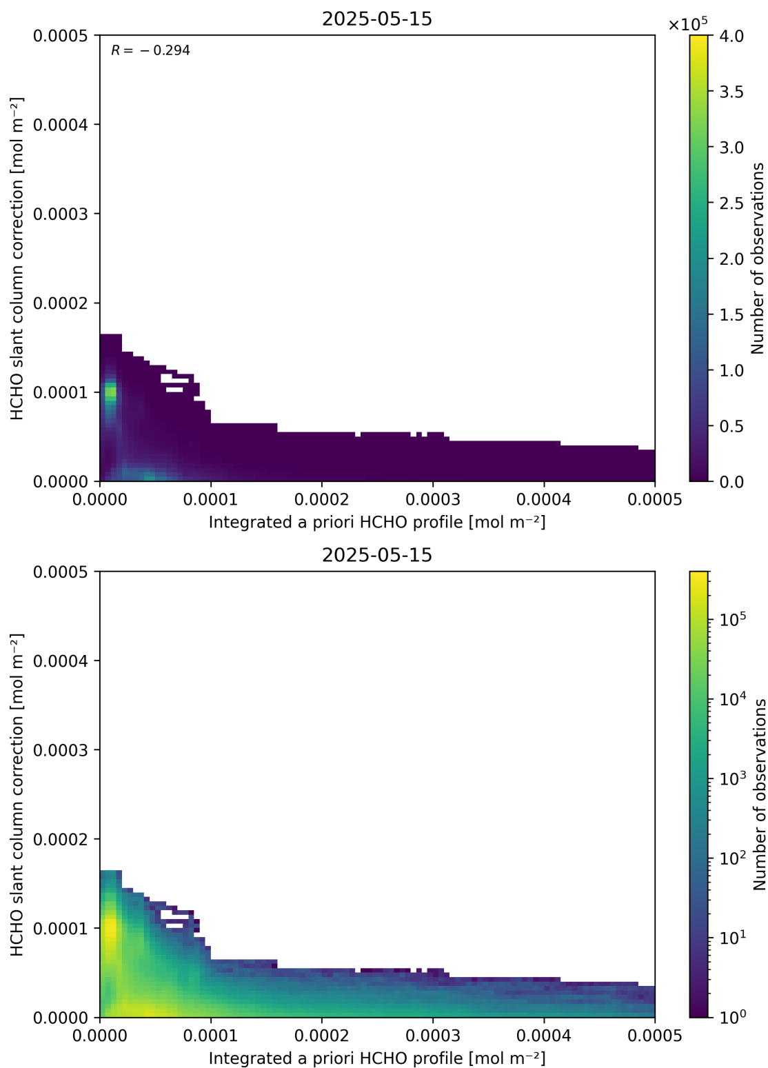
Figure 152: Scatter density plot of “Integrated a priori HCHO profile” against “HCHO slant column correction” for 2025-05-15 to 2025-05-16.
