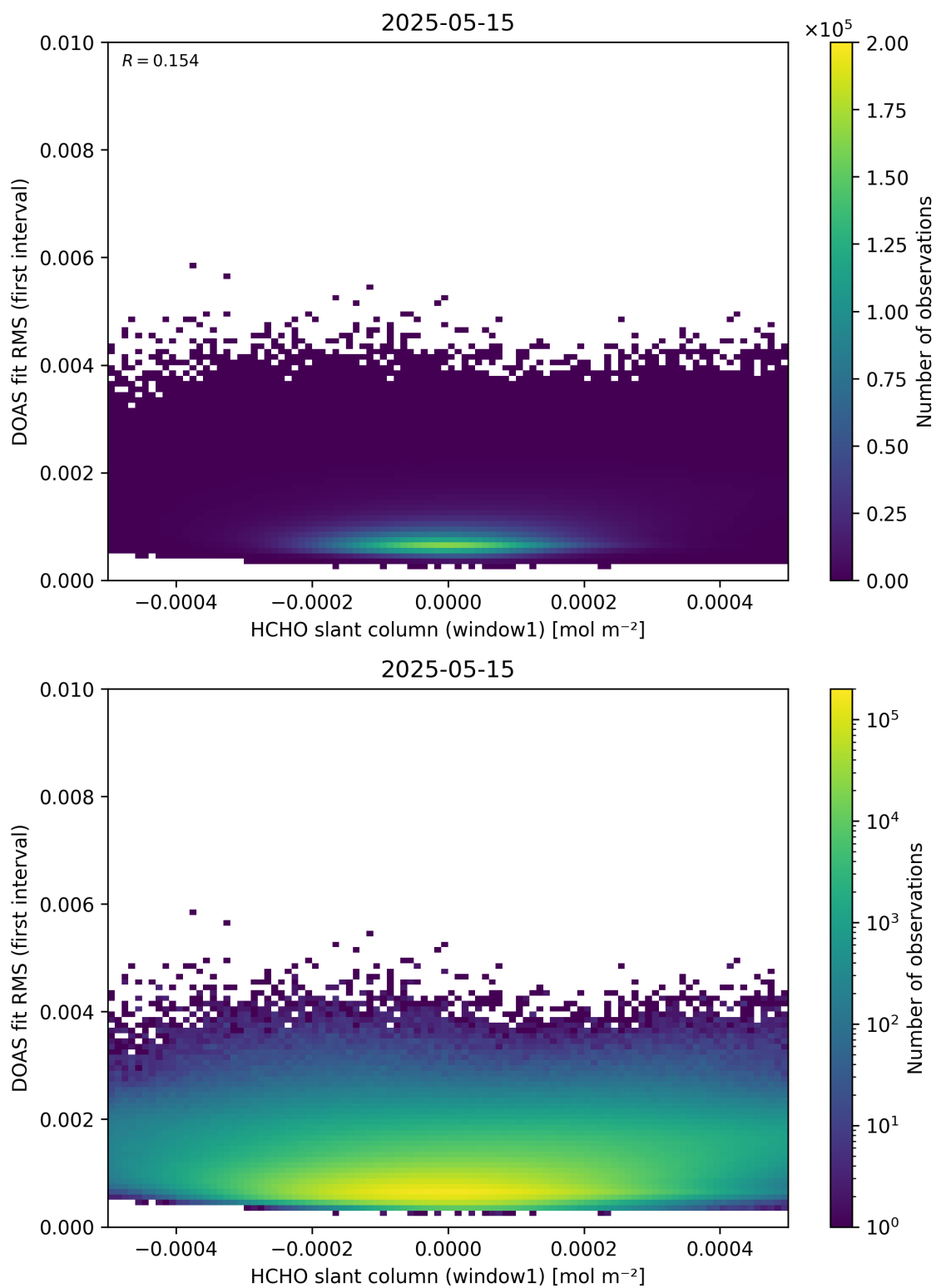
Figure 78: Scatter density plot of “HCHO slant column (window1)” against “DOAS fit RMS (first interval)” for 2025-05-15 to 2025-05-16.
