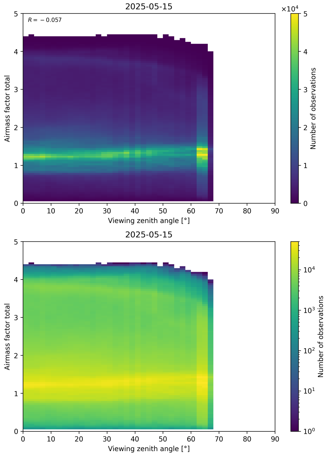
Figure 190: Scatter density plot of “Viewing zenith angle” against “Airmass factor total” for 2025-05-15 to 2025-05-16.
