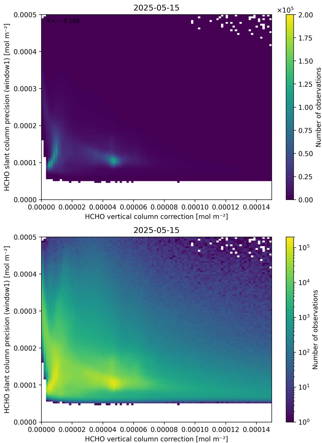
Figure 119: Scatter density plot of “HCHO vertical column correction” against “HCHO slant column precision (window1)” for 2025-05-15 to 2025-05-16.
