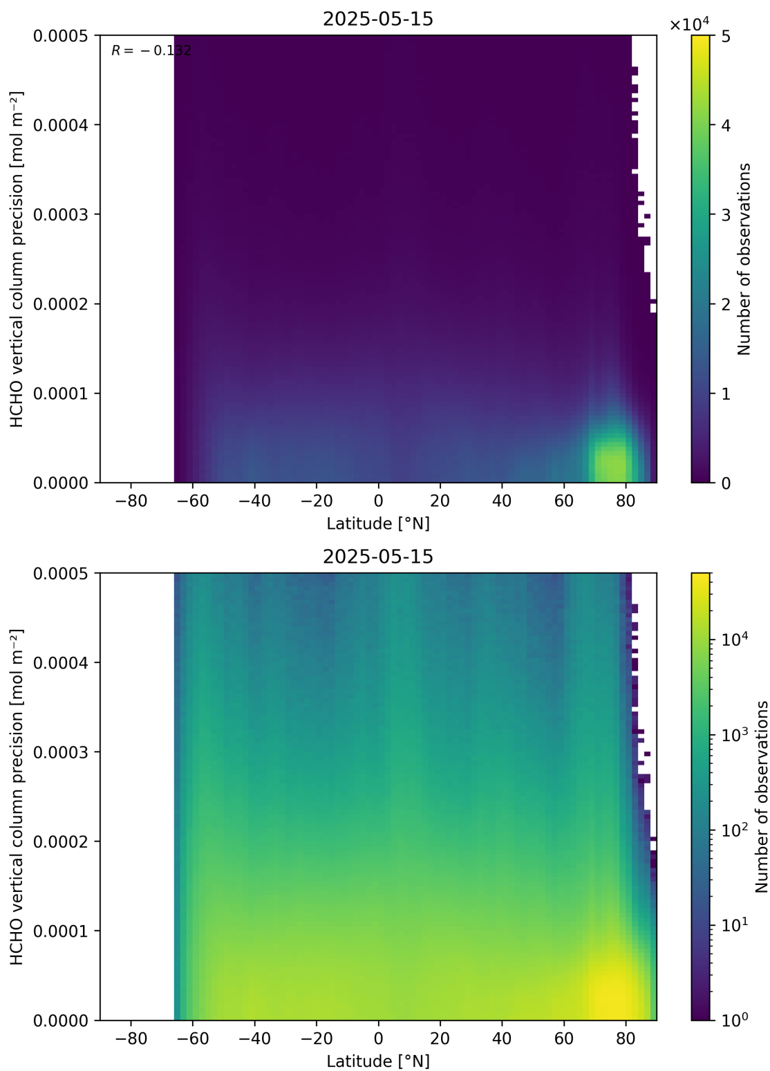
Figure 165: Scatter density plot of “Latitude” against “HCHO vertical column precision” for 2025-05-15 to 2025-05-16.
