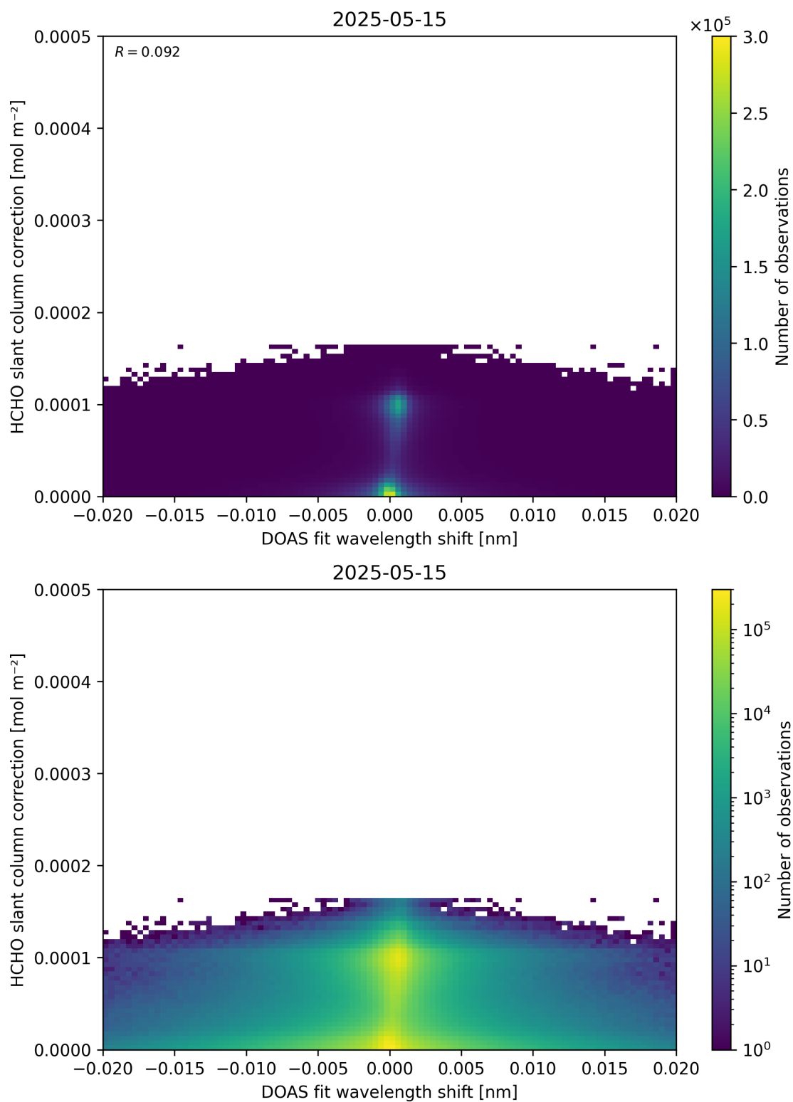
Figure 67: Scatter density plot of “DOAS fit wavelength shift” against “HCHO slant column correction” for 2025-05-15 to 2025-05-16.
