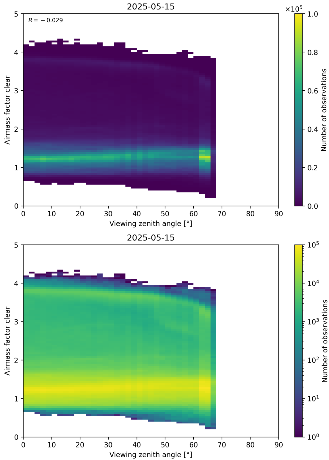
Figure 185: Scatter density plot of “Viewing zenith angle” against “Airmass factor clear” for 2025-05-15 to 2025-05-16.
