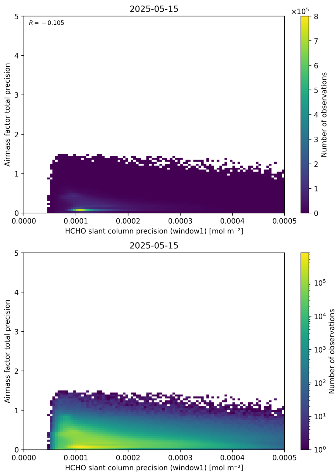
Figure 95: Scatter density plot of “HCHO slant column precision (window1)” against “Airmass factor total precision” for 2025-05-15 to 2025-05-16.
