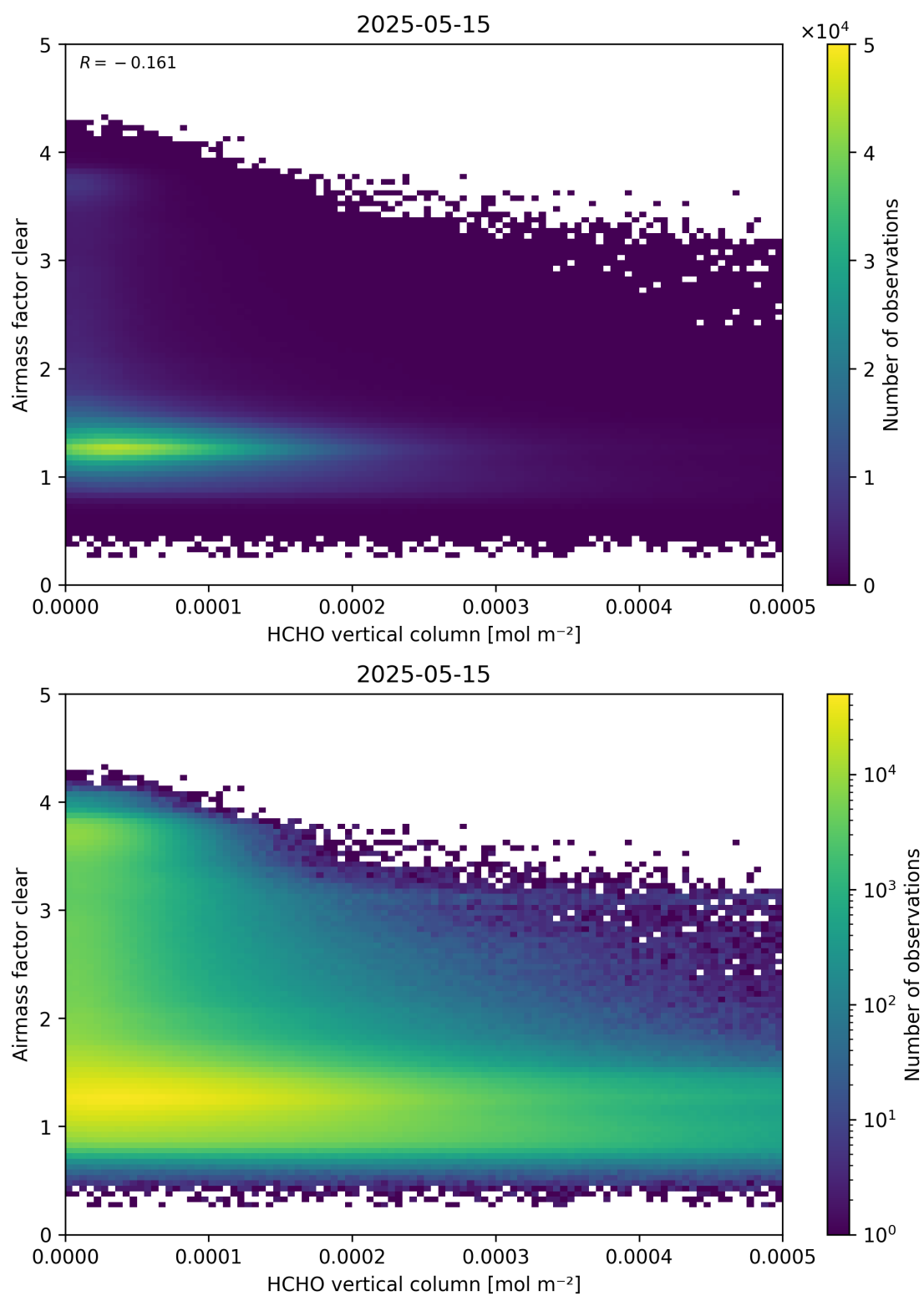
Figure 126: Scatter density plot of “HCHO vertical column” against “Airmass factor clear” for 2025-05-15 to 2025-05-16.
