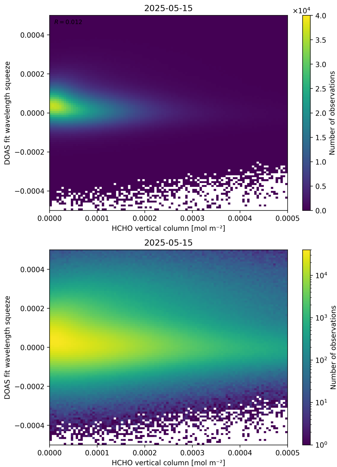
Figure 125: Scatter density plot of “HCHO vertical column” against “DOAS fit wavelength squeeze” for 2025-05-15 to 2025-05-16.
