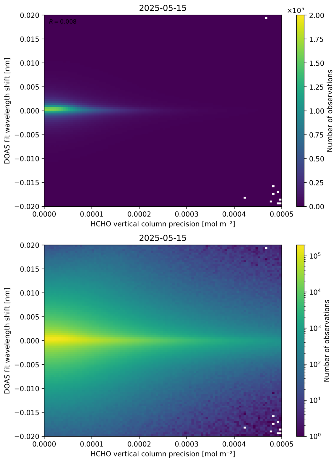
Figure 137: Scatter density plot of “HCHO vertical column precision” against “DOAS fit wavelength shift” for 2025-05-15 to 2025-05-16.
