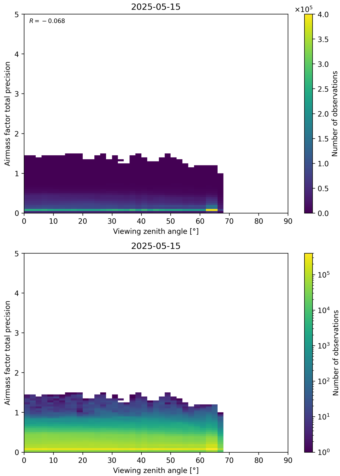
Figure 191: Scatter density plot of “Viewing zenith angle” against “Airmass factor total precision” for 2025-05-15 to 2025-05-16.
