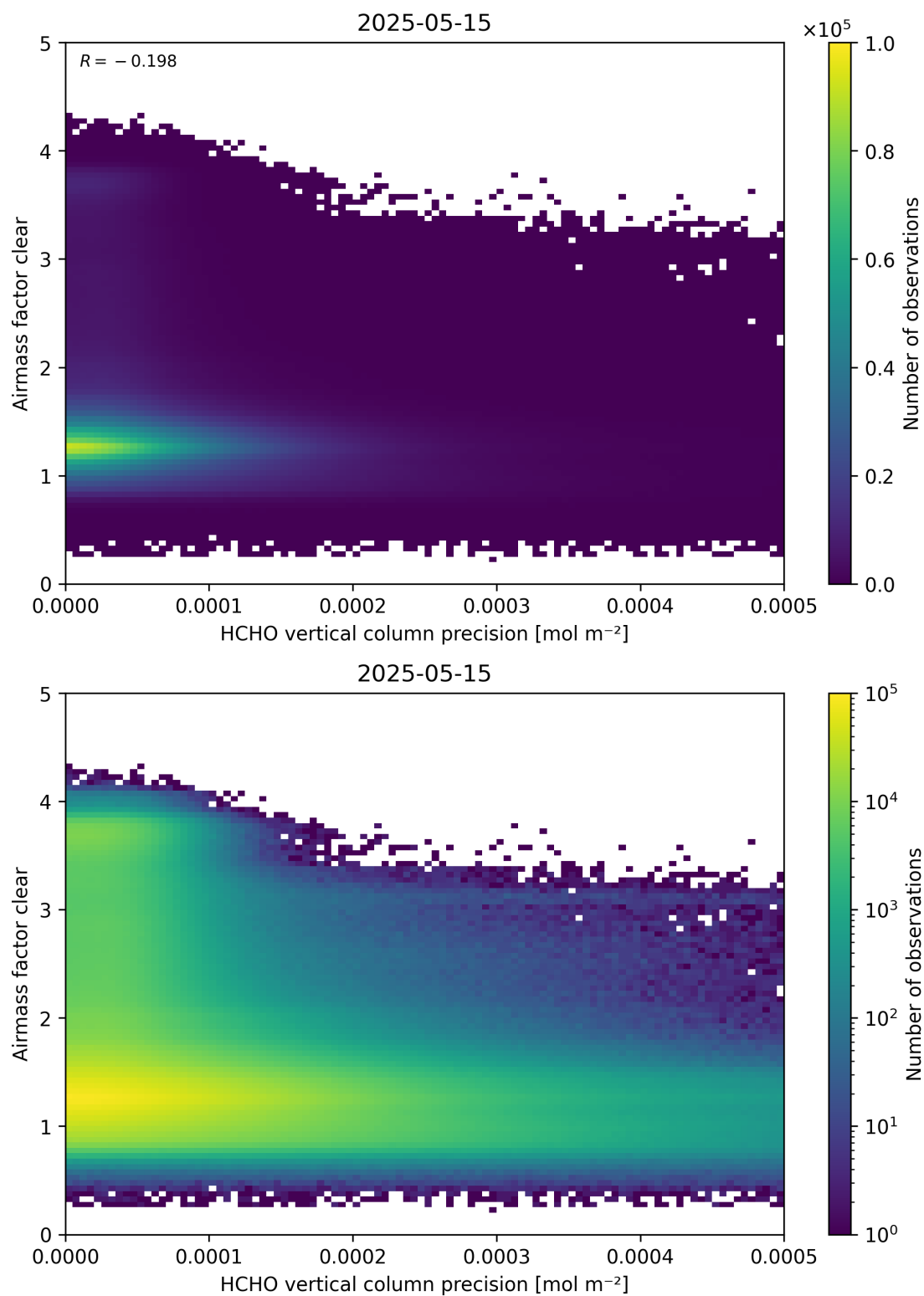
Figure 139: Scatter density plot of “HCHO vertical column precision” against “Airmass factor clear” for 2025-05-15 to 2025-05-16.
