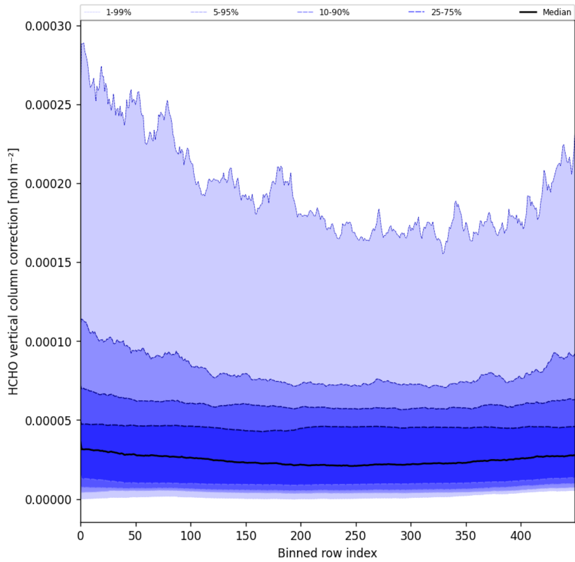
Figure 51: Along track statistics of “HCHO vertical column correction” for 2025-05-15 to 2025-05-16
