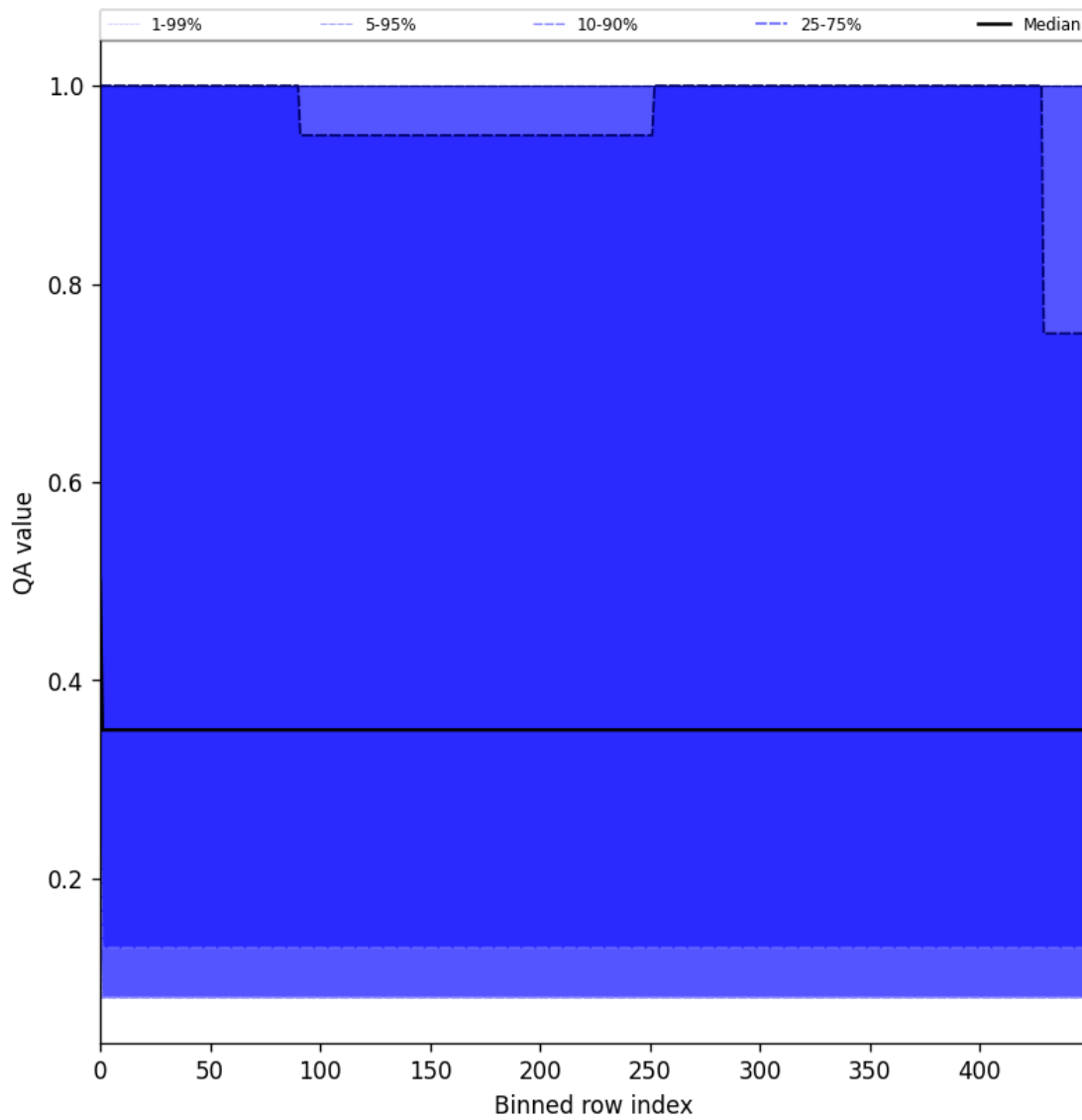
Figure 48: Along track statistics of “QA value” for 2025-05-15 to 2025-05-16
