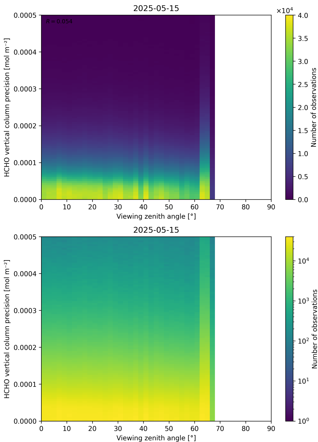
Figure 194: Scatter density plot of “Viewing zenith angle” against “HCHO vertical column precision” for 2025-05-15 to 2025-05-16.
