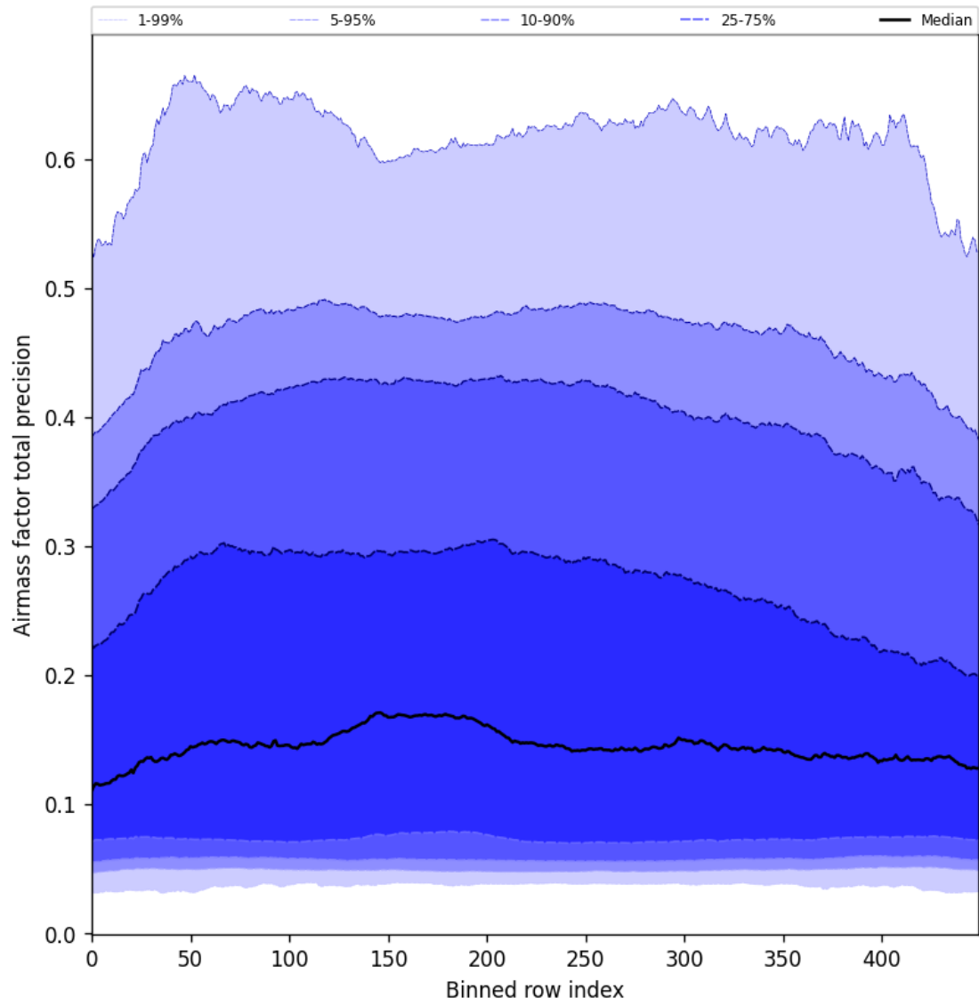
Figure 55: Along track statistics of “Airmass factor total precision” for 2025-05-15 to 2025-05-16
