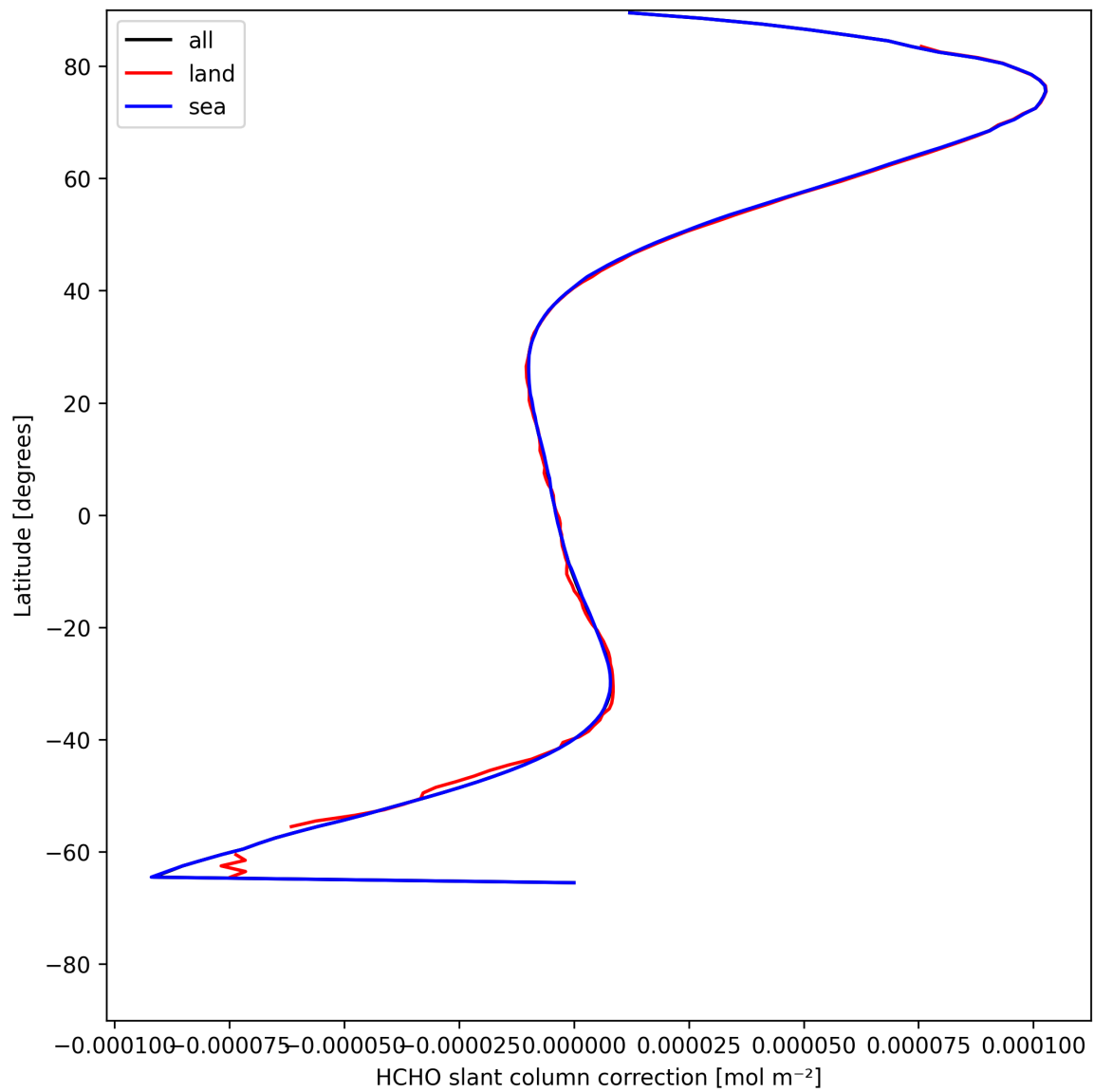
Figure 33: Zonal average of “HCHO slant column correction” for 2025-05-15 to 2025-05-16.
