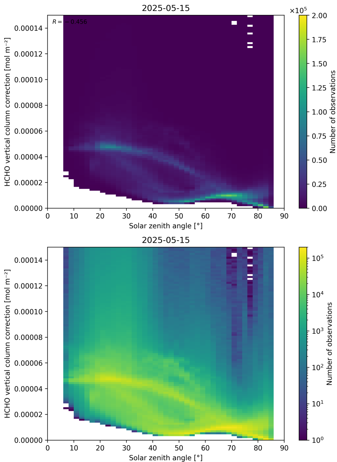
Figure 178: Scatter density plot of “Solar zenith angle” against “HCHO vertical column correction” for 2025-05-15 to 2025-05-16.
