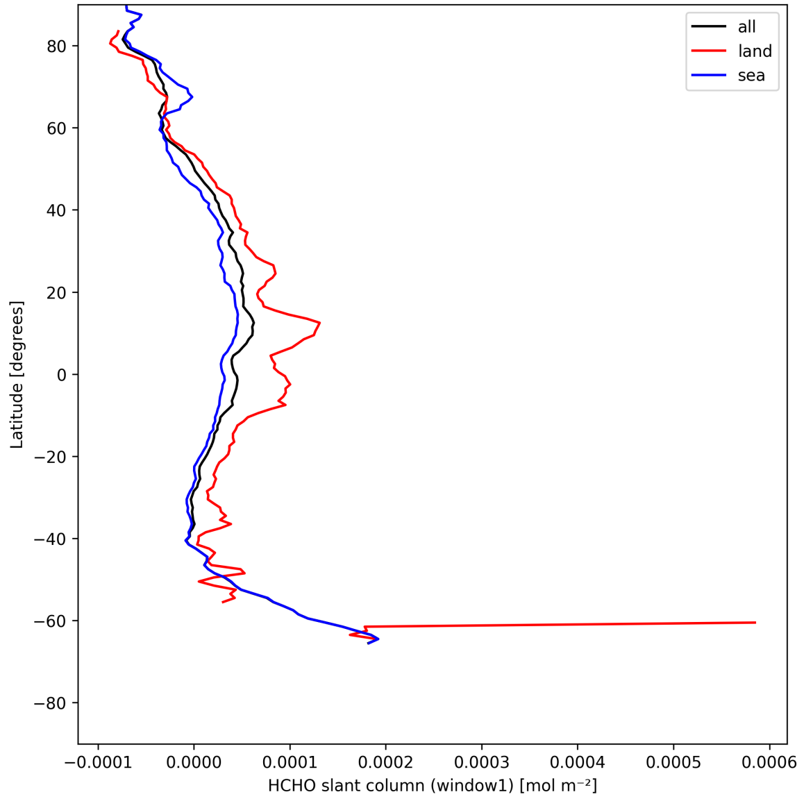
Figure 24: Zonal average of “HCHO slant column (window1)” for 2025-05-15 to 2025-05-16.
