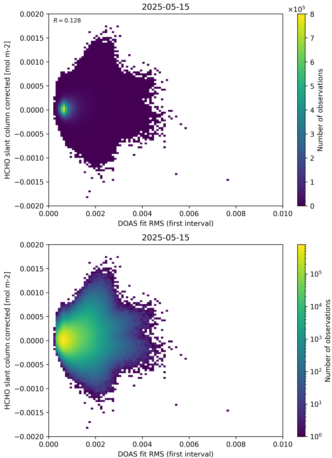
Figure 62: Scatter density plot of “DOAS fit RMS (first interval)” against “HCHO slant column corrected” for 2025-05-15 to 2025-05-16.
