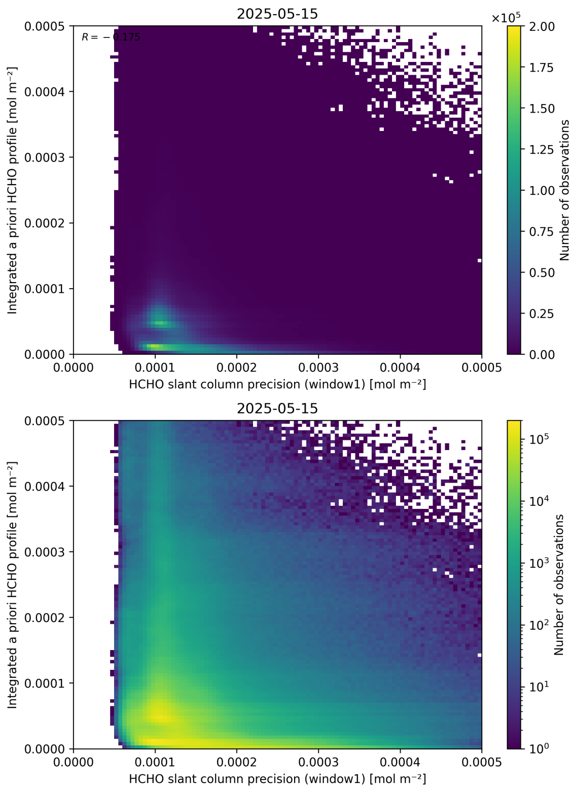
Figure 96: Scatter density plot of “HCHO slant column precision (window1)” against “Integrated a priori HCHO profile” for 2025-05-15 to 2025-05-16.
