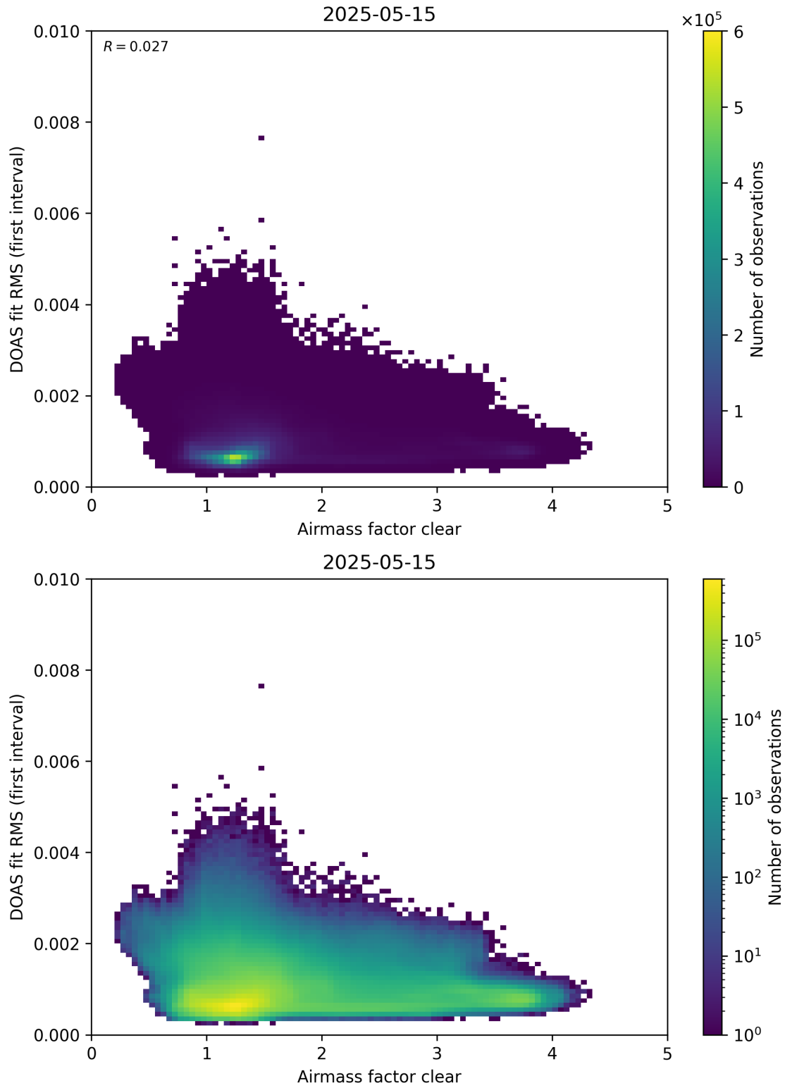
Figure 71: Scatter density plot of “Airmass factor clear” against “DOAS fit RMS (first interval)” for 2025-05-15 to 2025-05-16.
