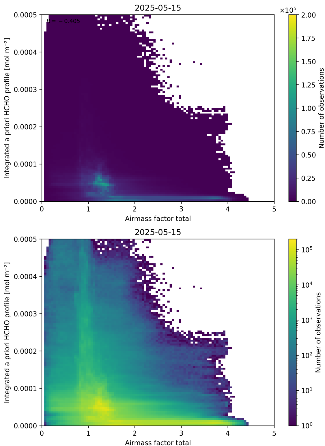
Figure 104: Scatter density plot of “Airmass factor total” against “Integrated a priori HCHO profile” for 2025-05-15 to 2025-05-16.
