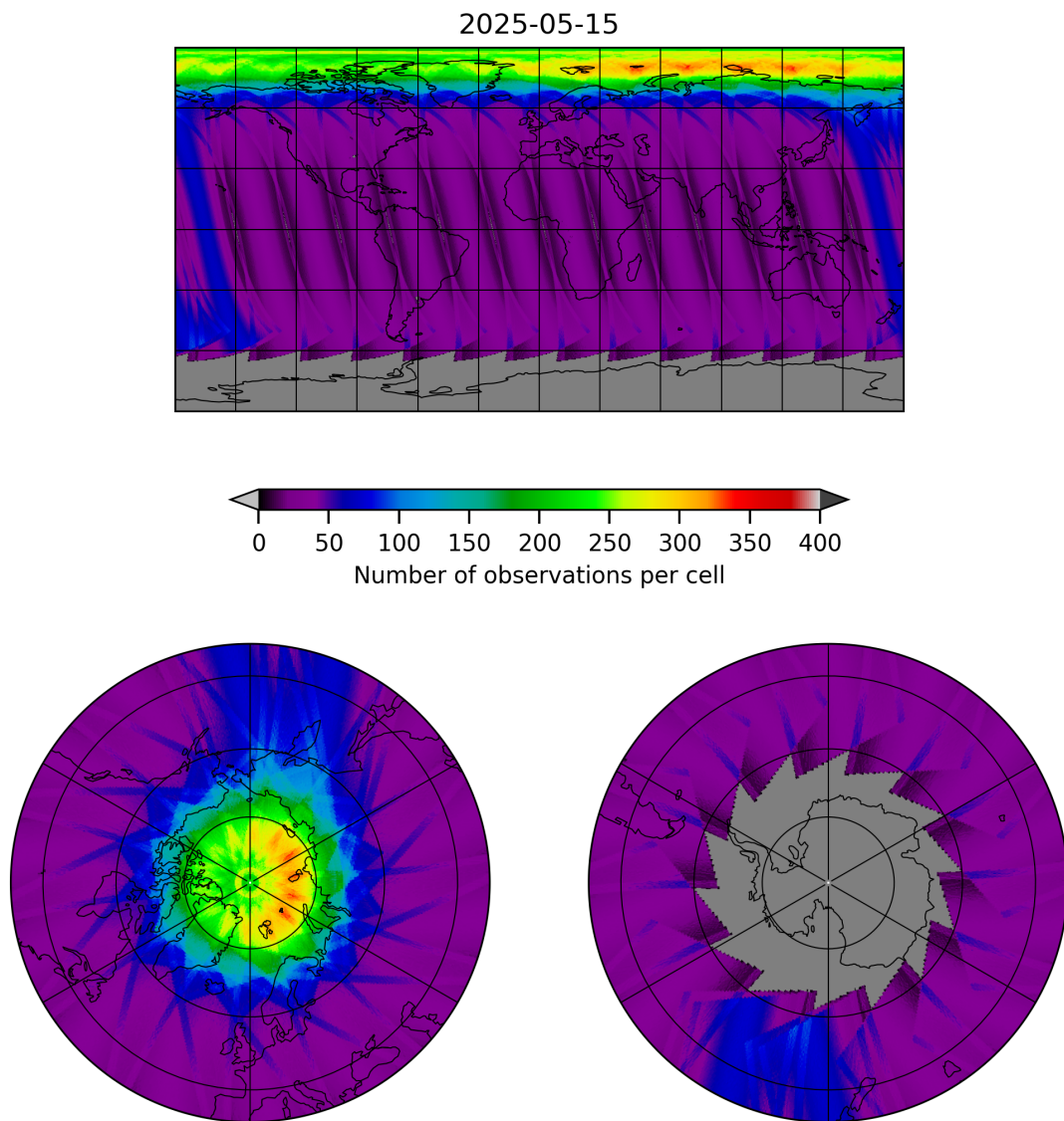
Figure 19: Map of the number of observations for 2025-05-15 to 2025-05-16
