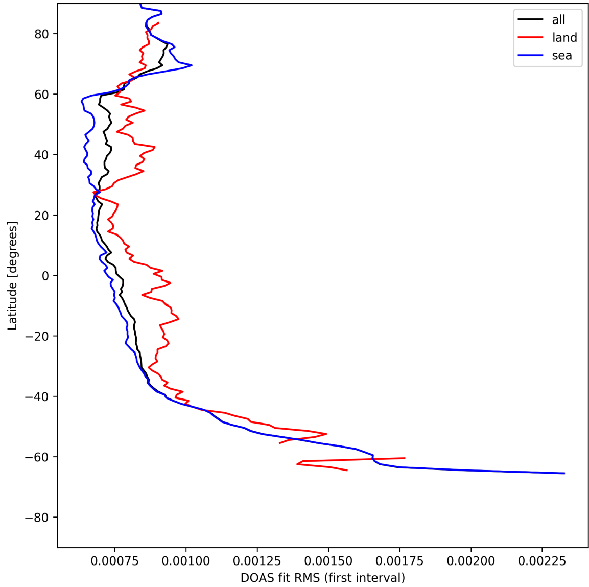
Figure 32: Zonal average of "DOAS fit RMS (first interval)" for 2025-05-15 to 2025-05-16.
