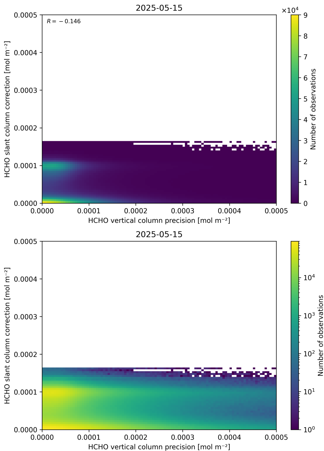
Figure 141: Scatter density plot of “HCHO vertical column precision” against “HCHO slant column correction” for 2025-05-15 to 2025-05-16.
