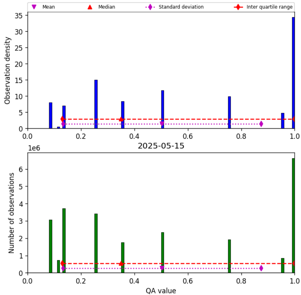
Figure 34: Histogram of “QA value” for 2025-05-15 to 2025-05-16
