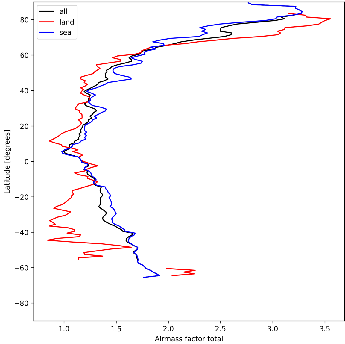
Figure 26: Zonal average of “Airmass factor total” for 2025-05-15 to 2025-05-16.
