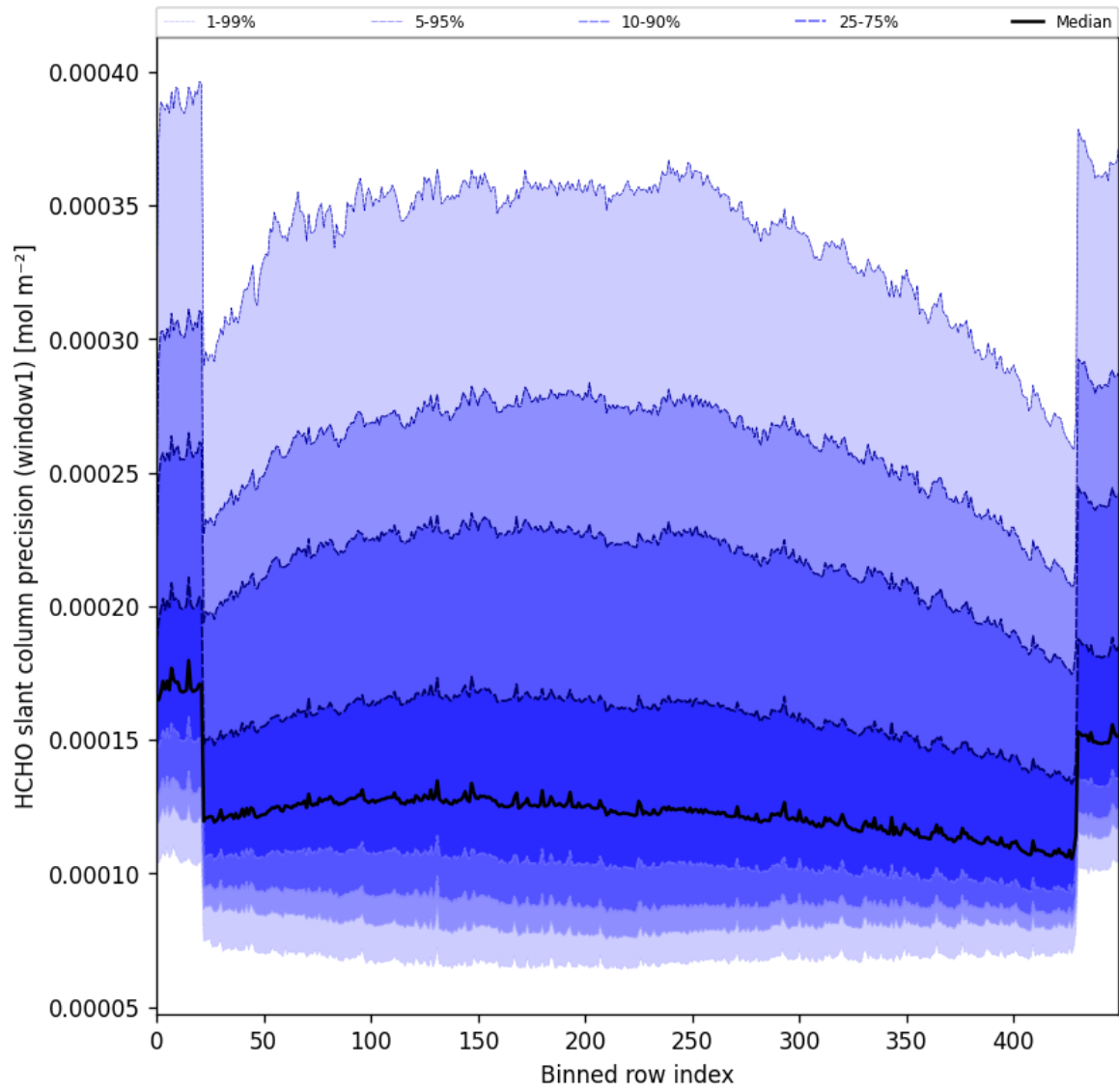
Figure 53: Along track statistics of “HCHO slant column precision (window1)” for 2025-05-15 to 2025-05-16
