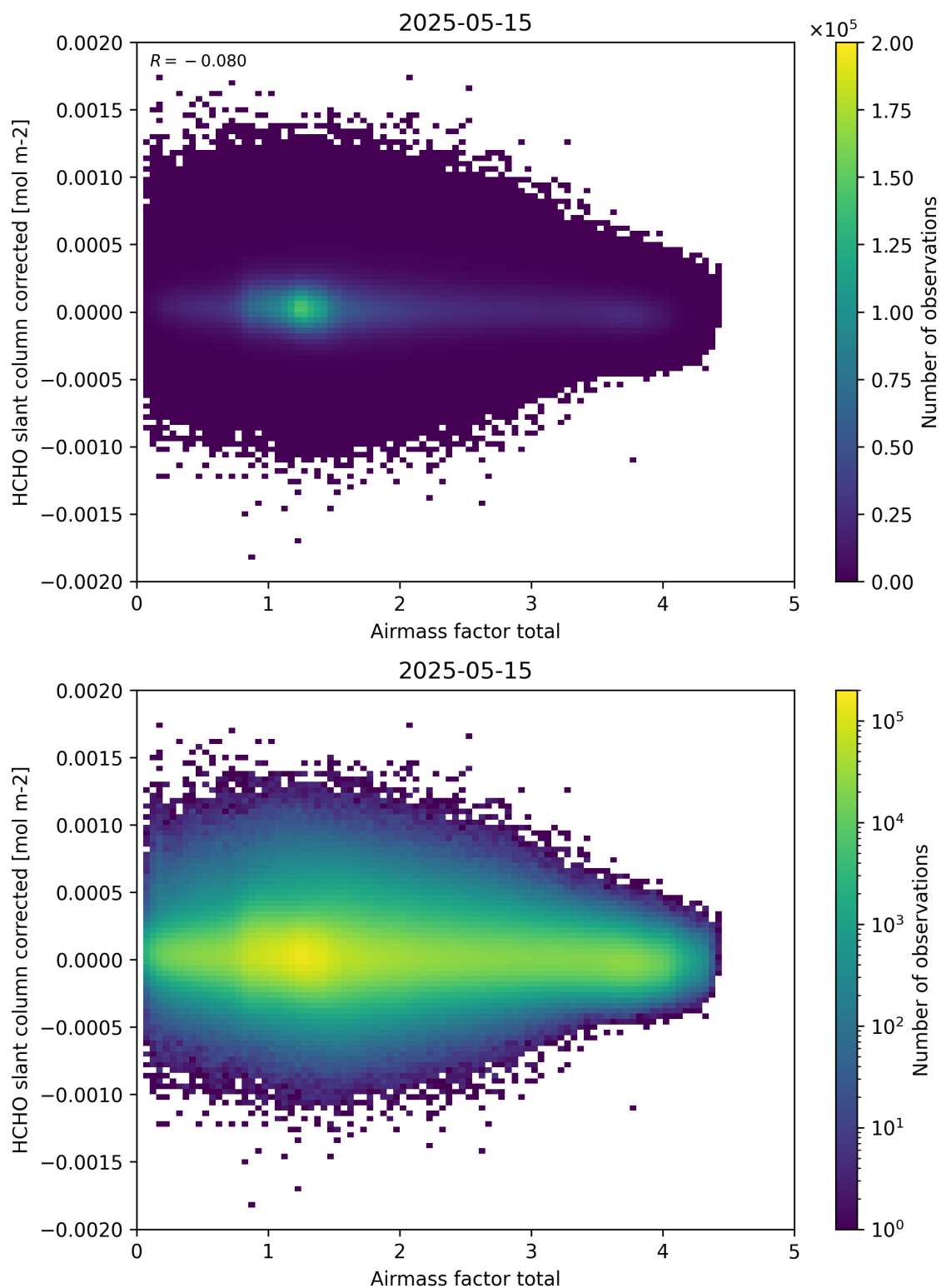
Figure 101: Scatter density plot of “Airmass factor total” against “HCHO slant column corrected” for 2025-05-15 to 2025-05-16.
