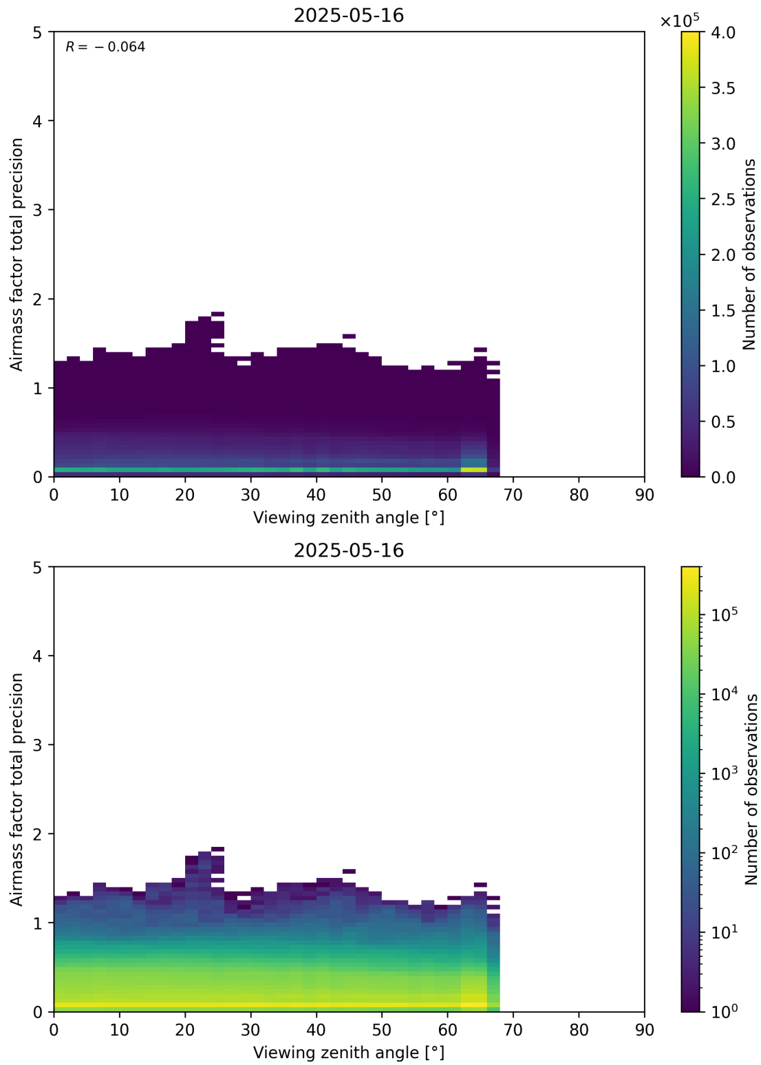
Figure 191: Scatter density plot of “Viewing zenith angle” against “Airmass factor total precision” for 2025-05-15 to 2025-05-17.
