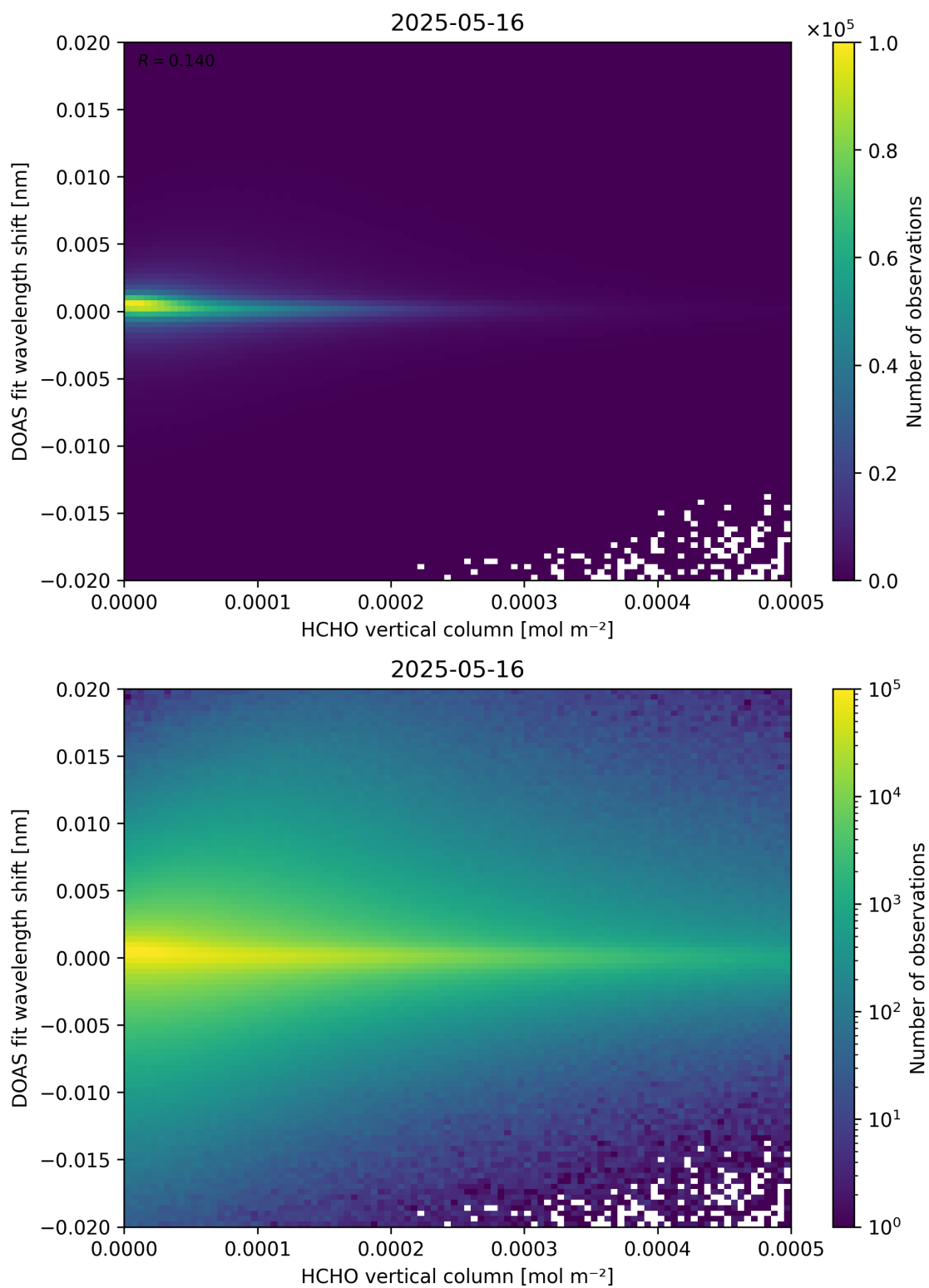
Figure 124: Scatter density plot of “HCHO vertical column” against “DOAS fit wavelength shift” for 2025-05-15 to 2025-05-17.
