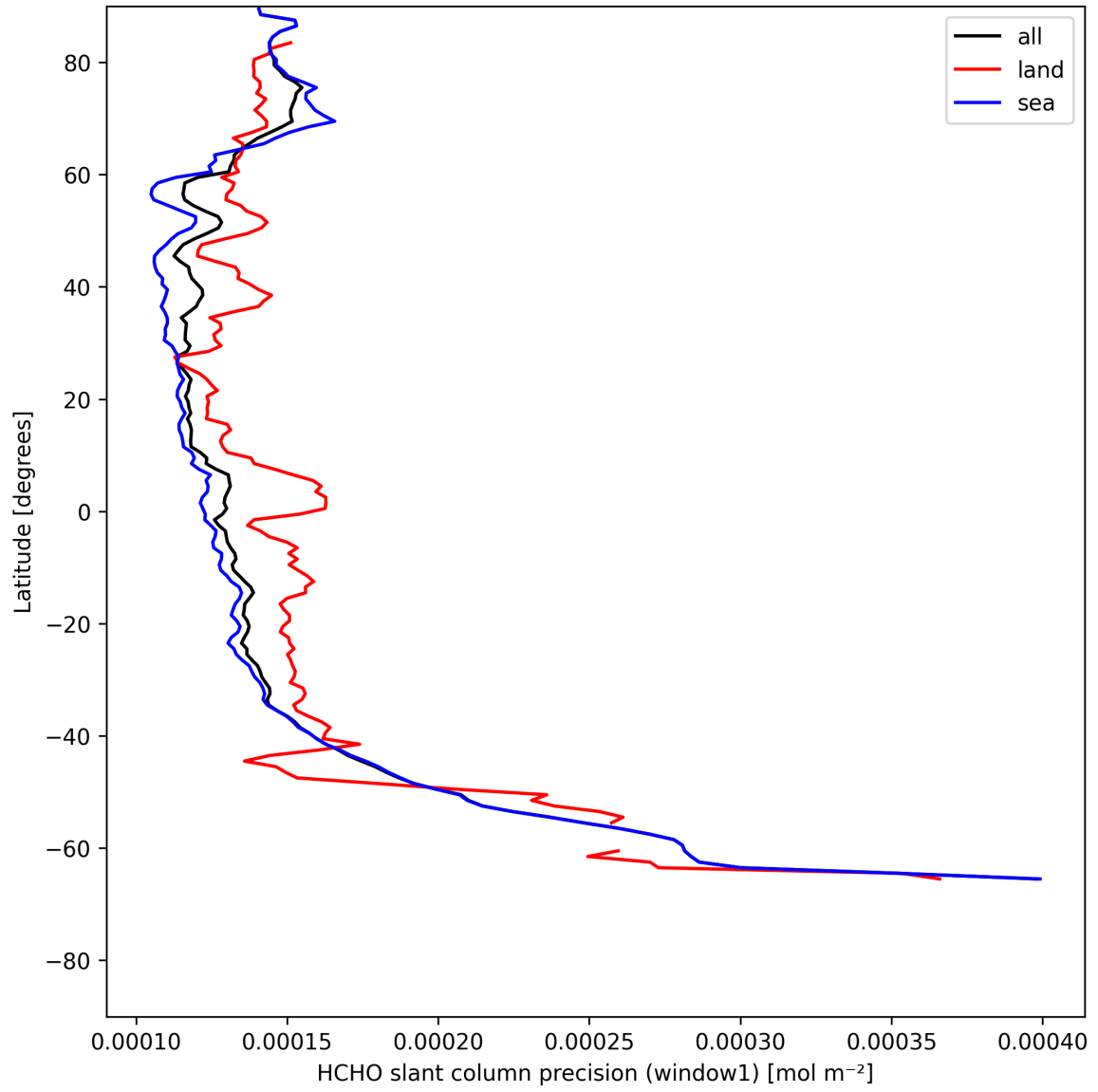
Figure 25: Zonal average of “HCHO slant column precision (window1)” for 2025-05-15 to 2025-05-17.
