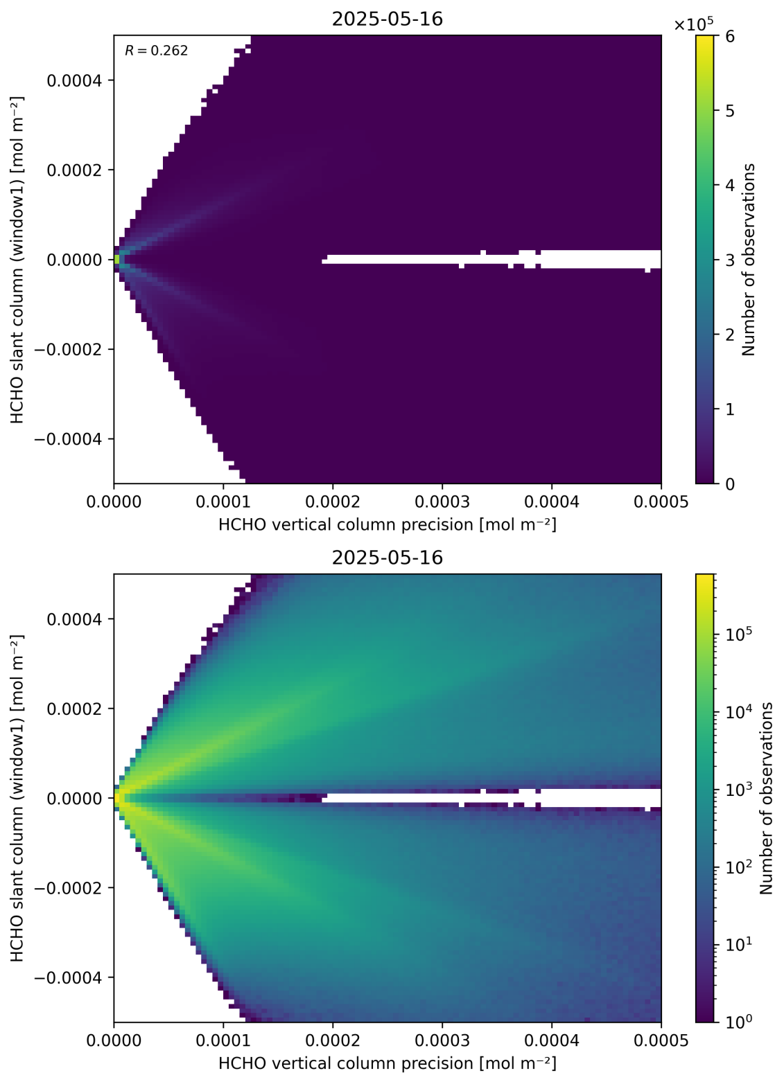
Figure 142: Scatter density plot of “HCHO vertical column precision” against “HCHO slant column (window1)” for 2025-05-15 to 2025-05-17.
