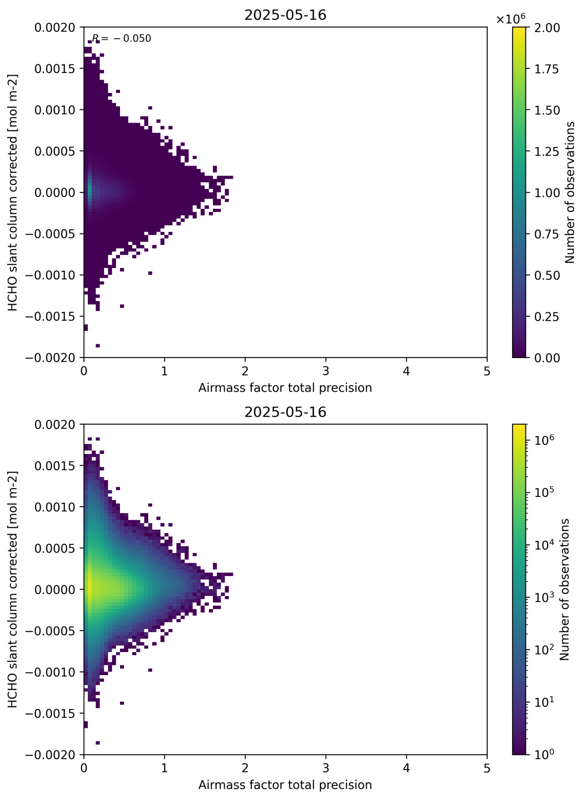
Figure 109: Scatter density plot of “Airmass factor total precision” against “HCHO slant column corrected” for 2025-05-15 to 2025-05-17.
