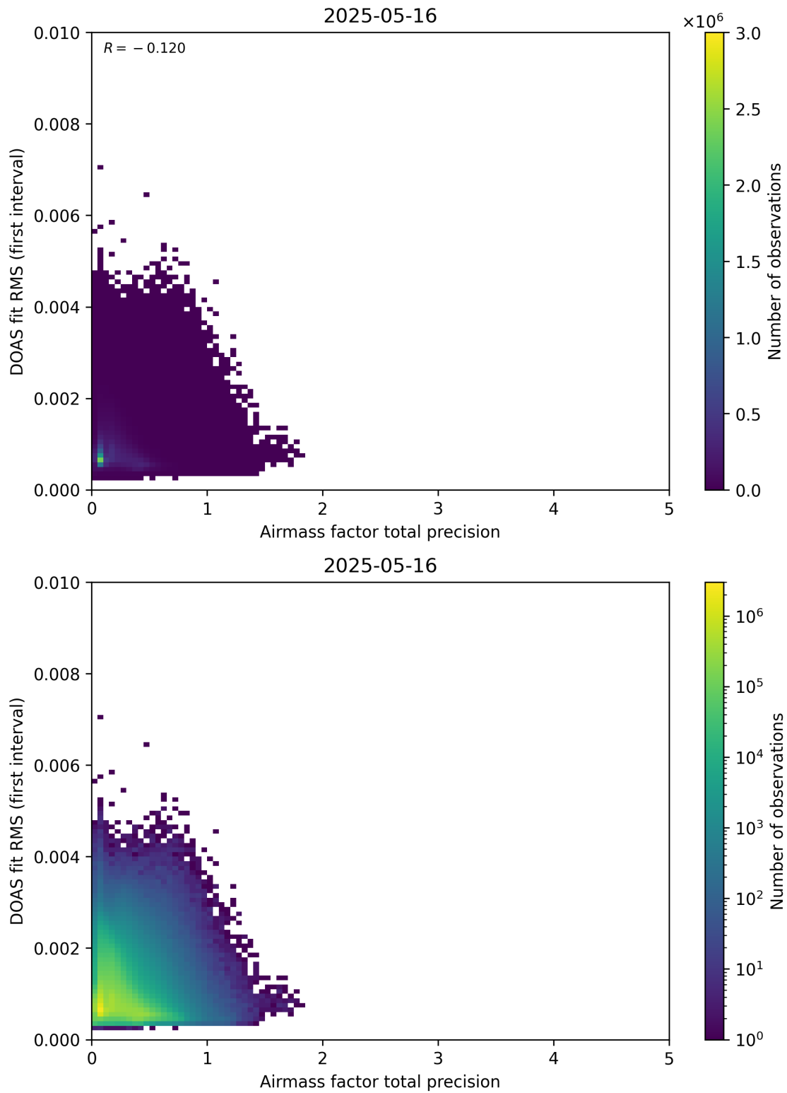
Figure 105: Scatter density plot of “Airmass factor total precision” against “DOAS fit RMS (first interval)” for 2025-05-15 to 2025-05-17.
