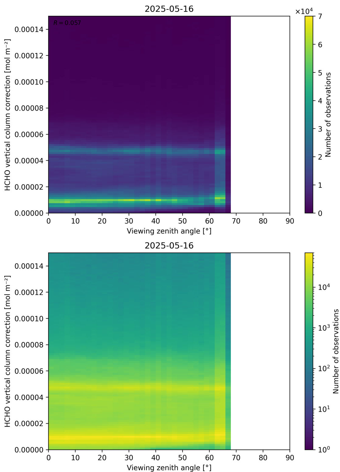
Figure 193: Scatter density plot of “Viewing zenith angle” against “HCHO vertical column correction” for 2025-05-15 to 2025-05-17.
