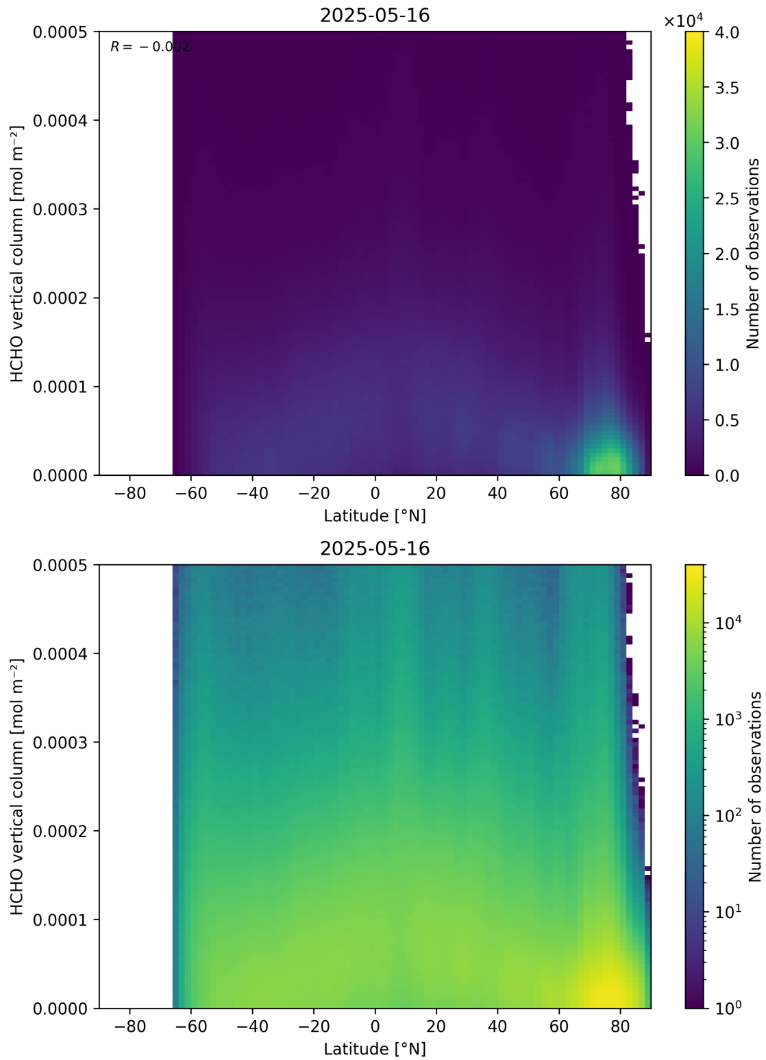
Figure 163: Scatter density plot of “Latitude” against “HCHO vertical column” for 2025-05-15 to 2025-05-17.
