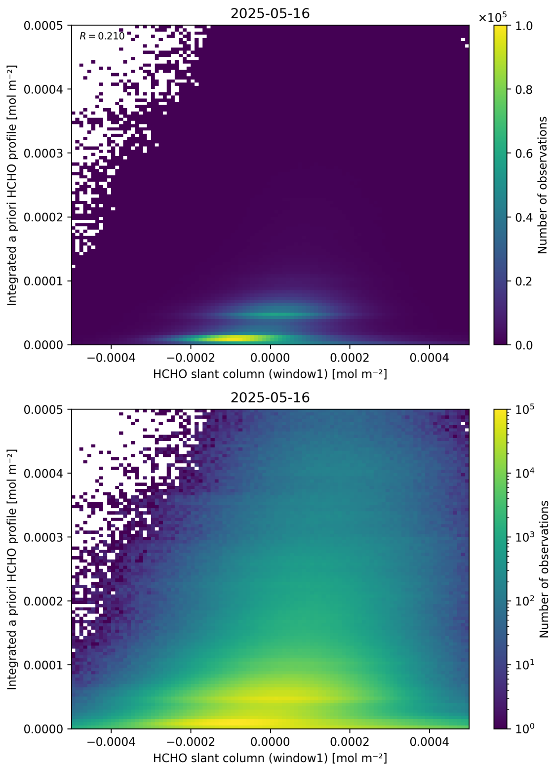
Figure 87: Scatter density plot of “HCHO slant column (window1)” against “Integrated a priori HCHO profile” for 2025-05-15 to 2025-05-17.
