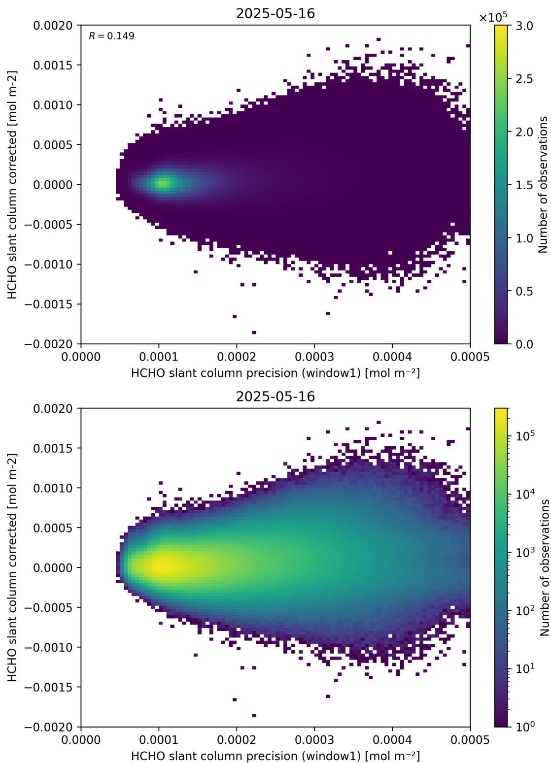
Figure 92: Scatter density plot of “HCHO slant column precision (window1)” against “HCHO slant column corrected” for 2025-05-15 to 2025-05-17.
