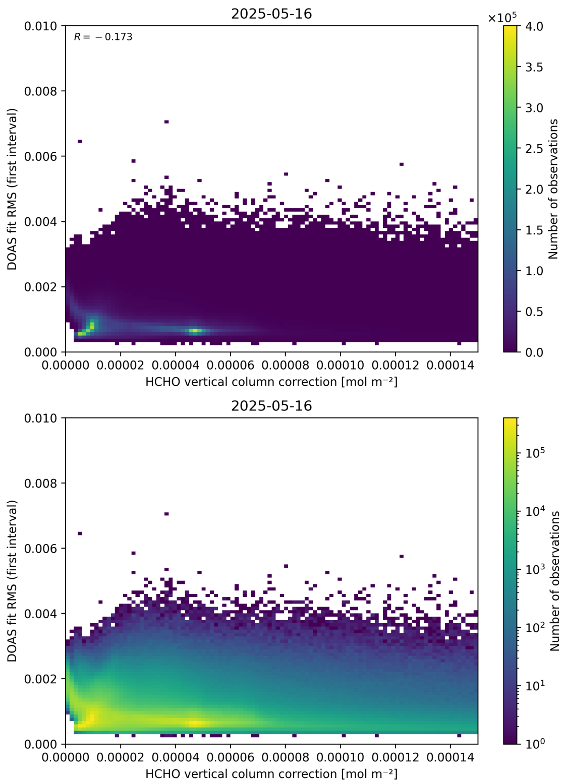
Figure 112: Scatter density plot of “HCHO vertical column correction” against “DOAS fit RMS (first interval)” for 2025-05-15 to 2025-05-17.
