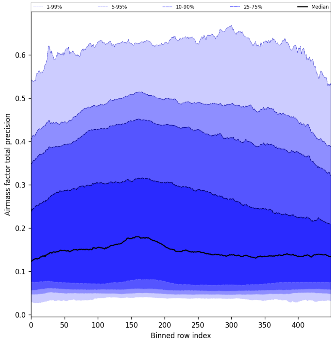
Figure 55: Along track statistics of “Airmass factor total precision” for 2025-05-15 to 2025-05-17
