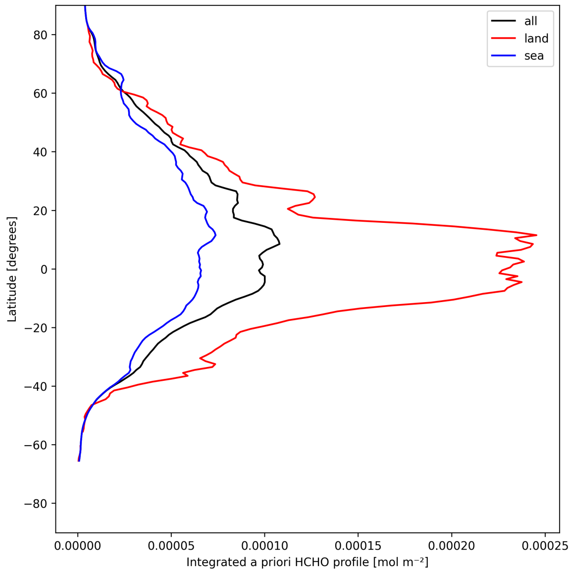
Figure 29: Zonal average of “Integrated a priori HCHO profile” for 2025-05-15 to 2025-05-17.
