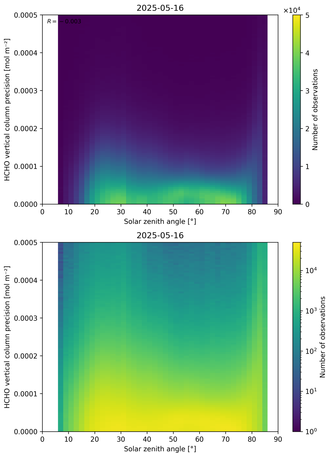
Figure 179: Scatter density plot of “Solar zenith angle” against “HCHO vertical column precision” for 2025-05-15 to 2025-05-17.
