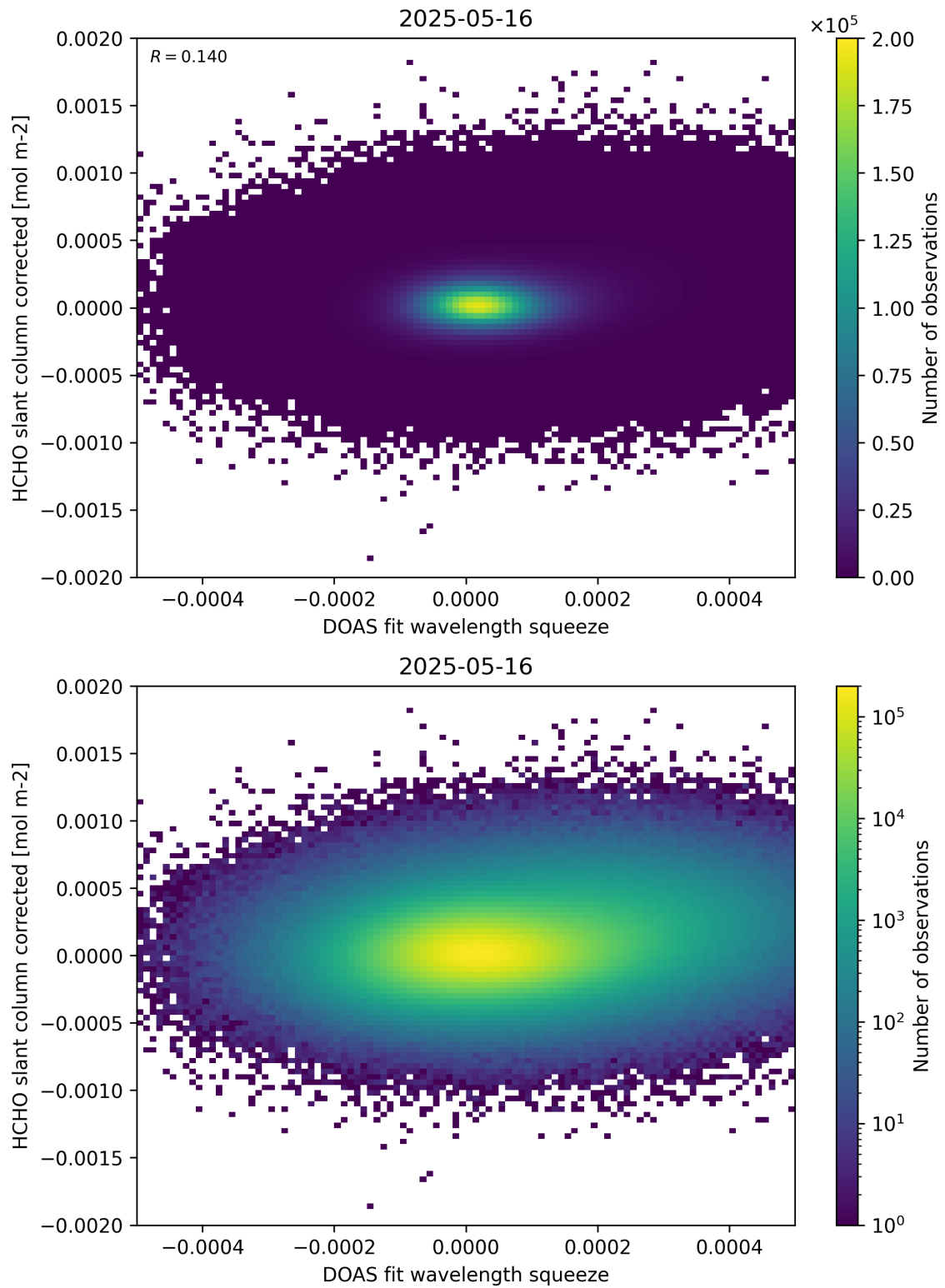
Figure 69: Scatter density plot of “DOAS fit wavelength squeeze” against “HCHO slant column corrected” for 2025-05-15 to 2025-05-17.
