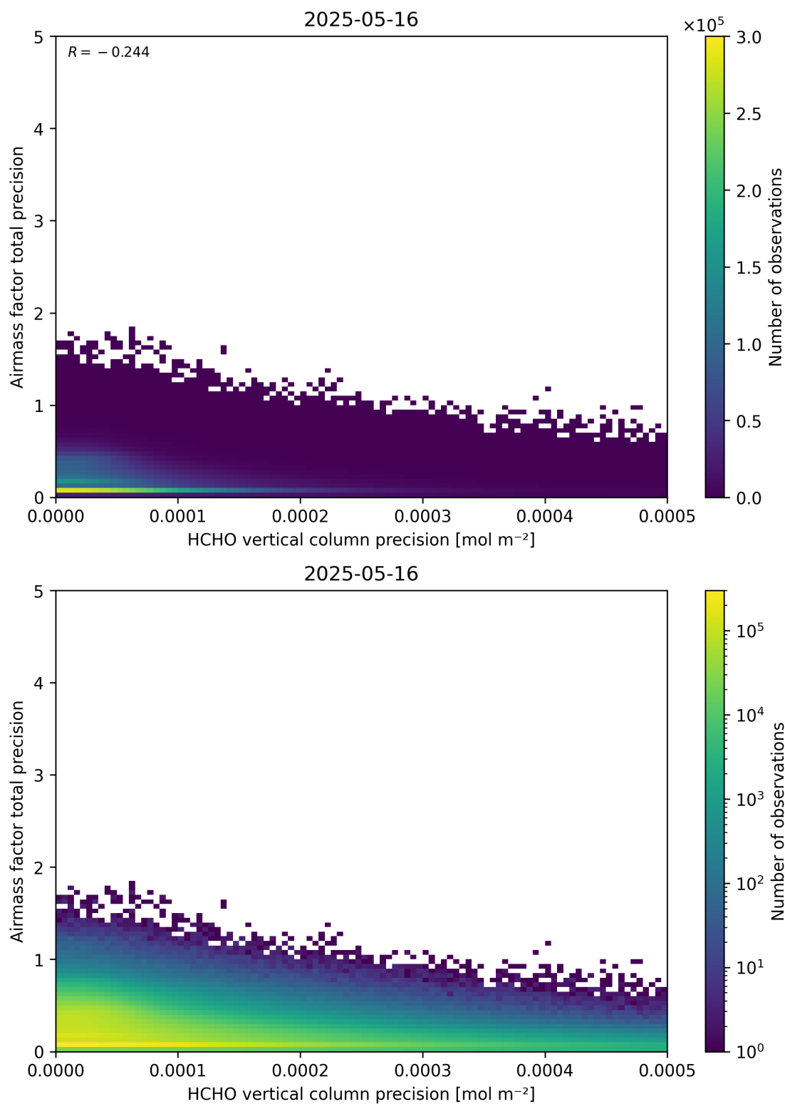
Figure 145: Scatter density plot of “HCHO vertical column precision” against “Airmass factor total precision” for 2025-05-15 to 2025-05-17.
