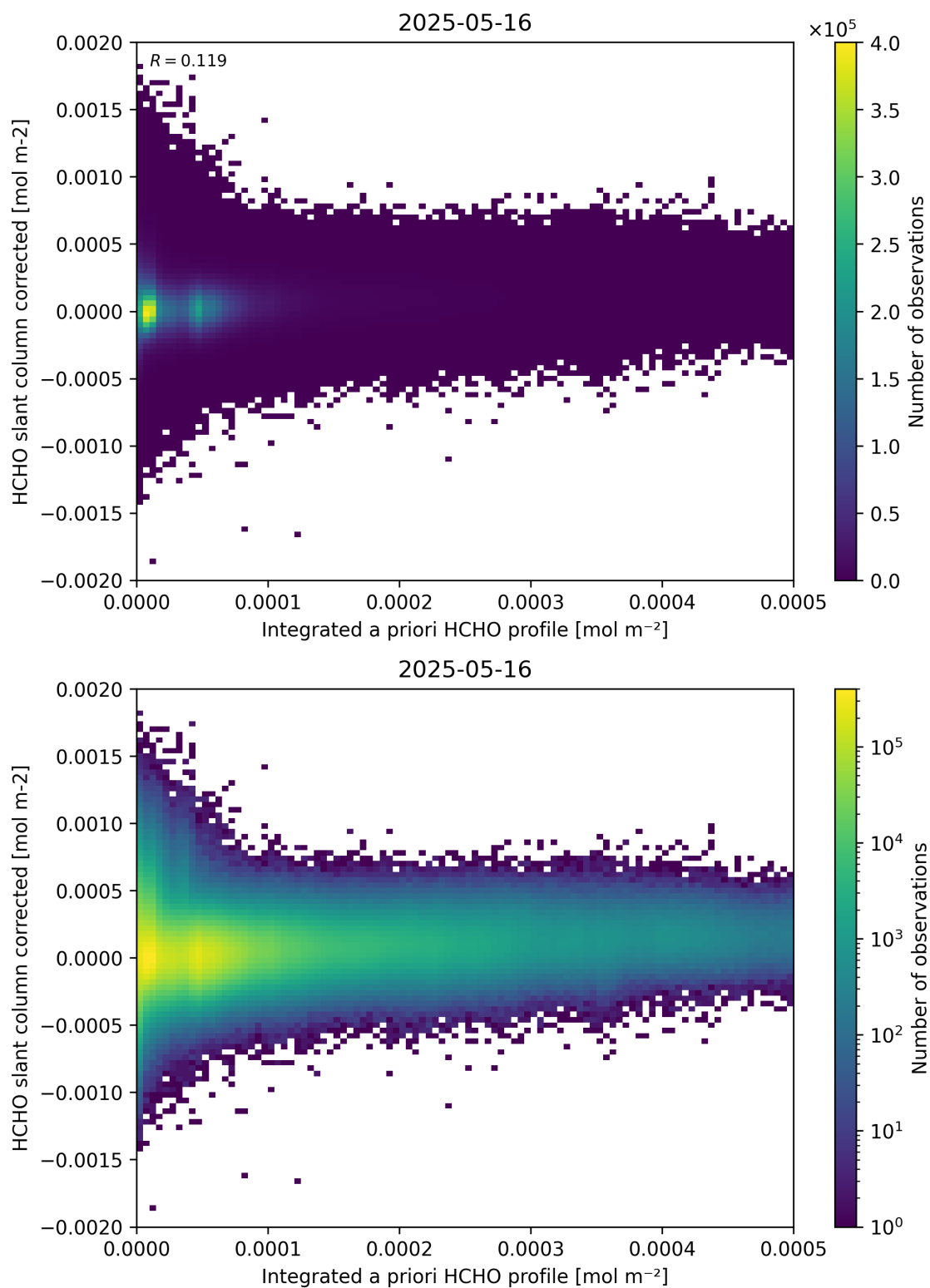
Figure 151: Scatter density plot of “Integrated a priori HCHO profile” against “HCHO slant column corrected” for 2025-05-15 to 2025-05-17.
