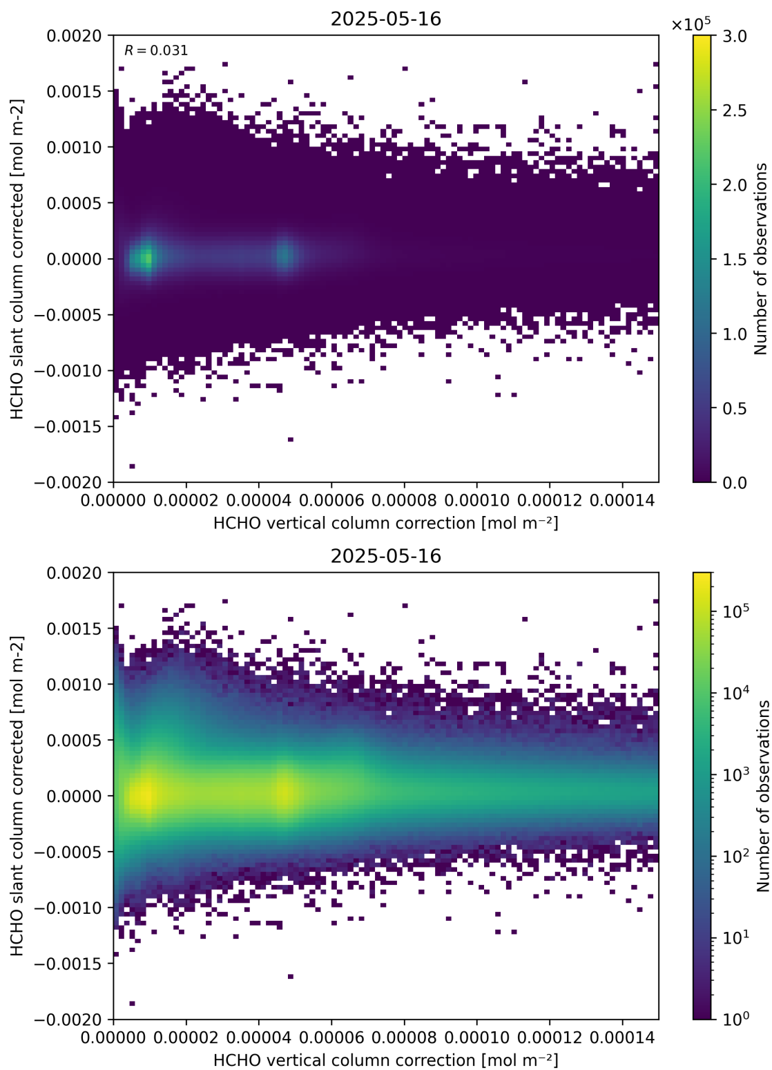
Figure 116: Scatter density plot of “HCHO vertical column correction” against “HCHO slant column corrected” for 2025-05-15 to 2025-05-17.
