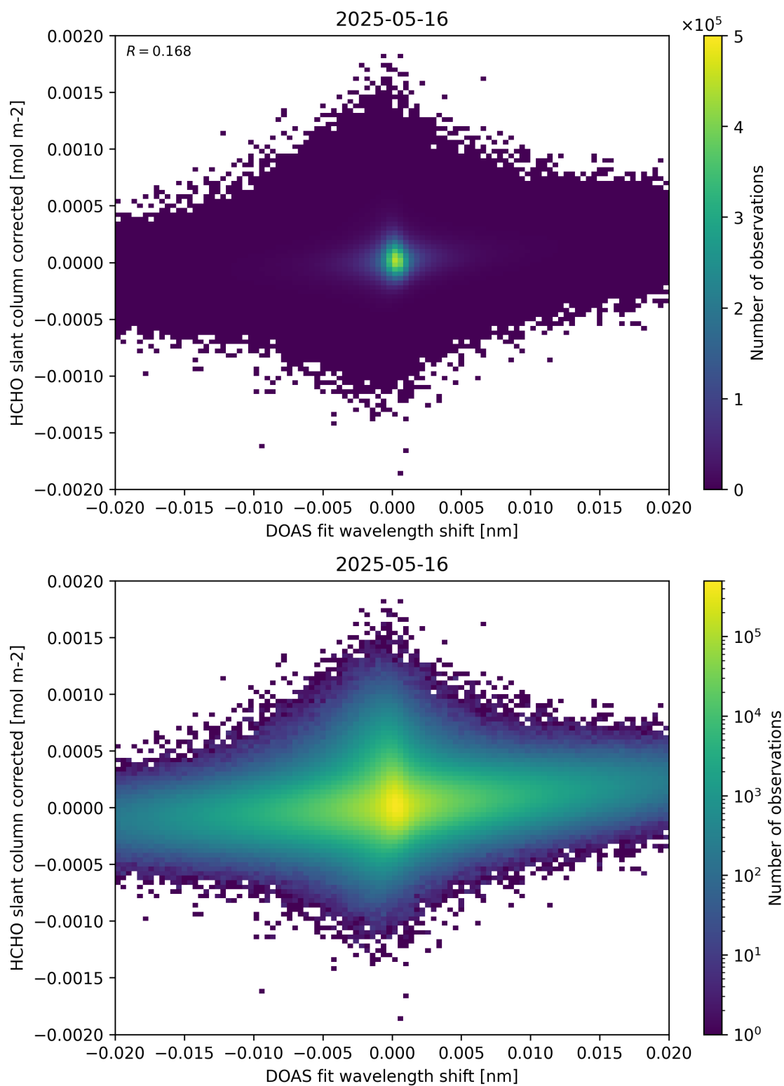
Figure 66: Scatter density plot of “DOAS fit wavelength shift” against “HCHO slant column corrected” for 2025-05-15 to 2025-05-17.
