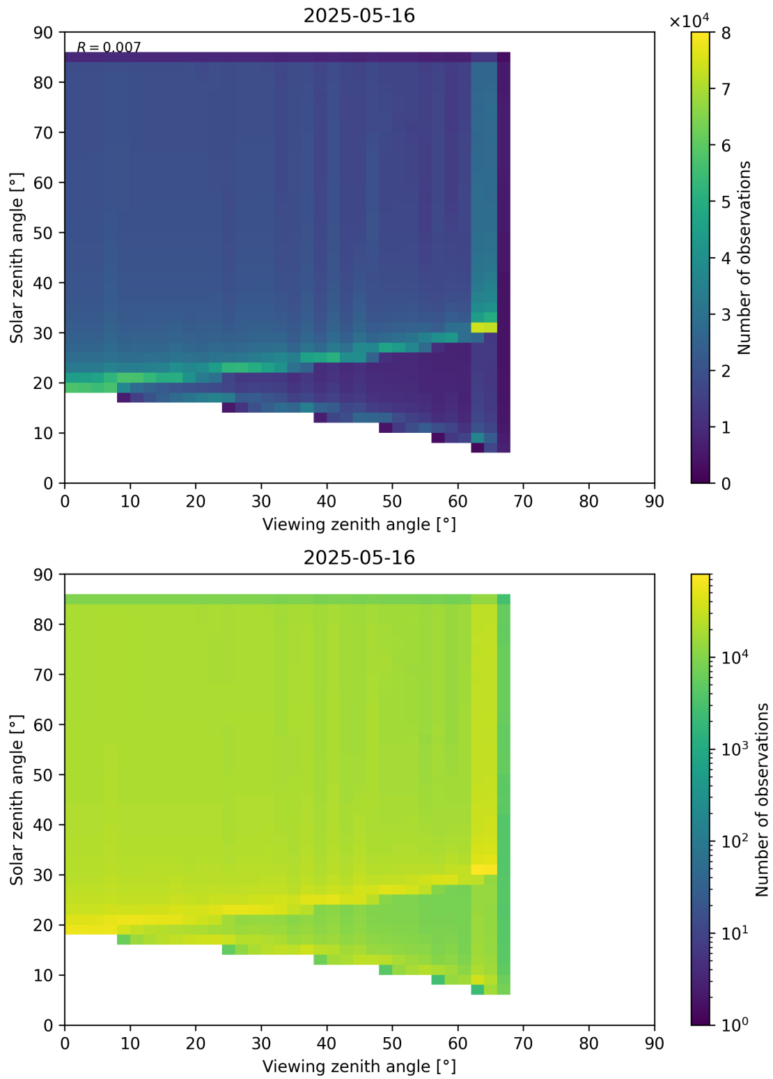
Figure 197: Scatter density plot of “Viewing zenith angle” against “Solar zenith angle” for 2025-05-15 to 2025-05-17.
