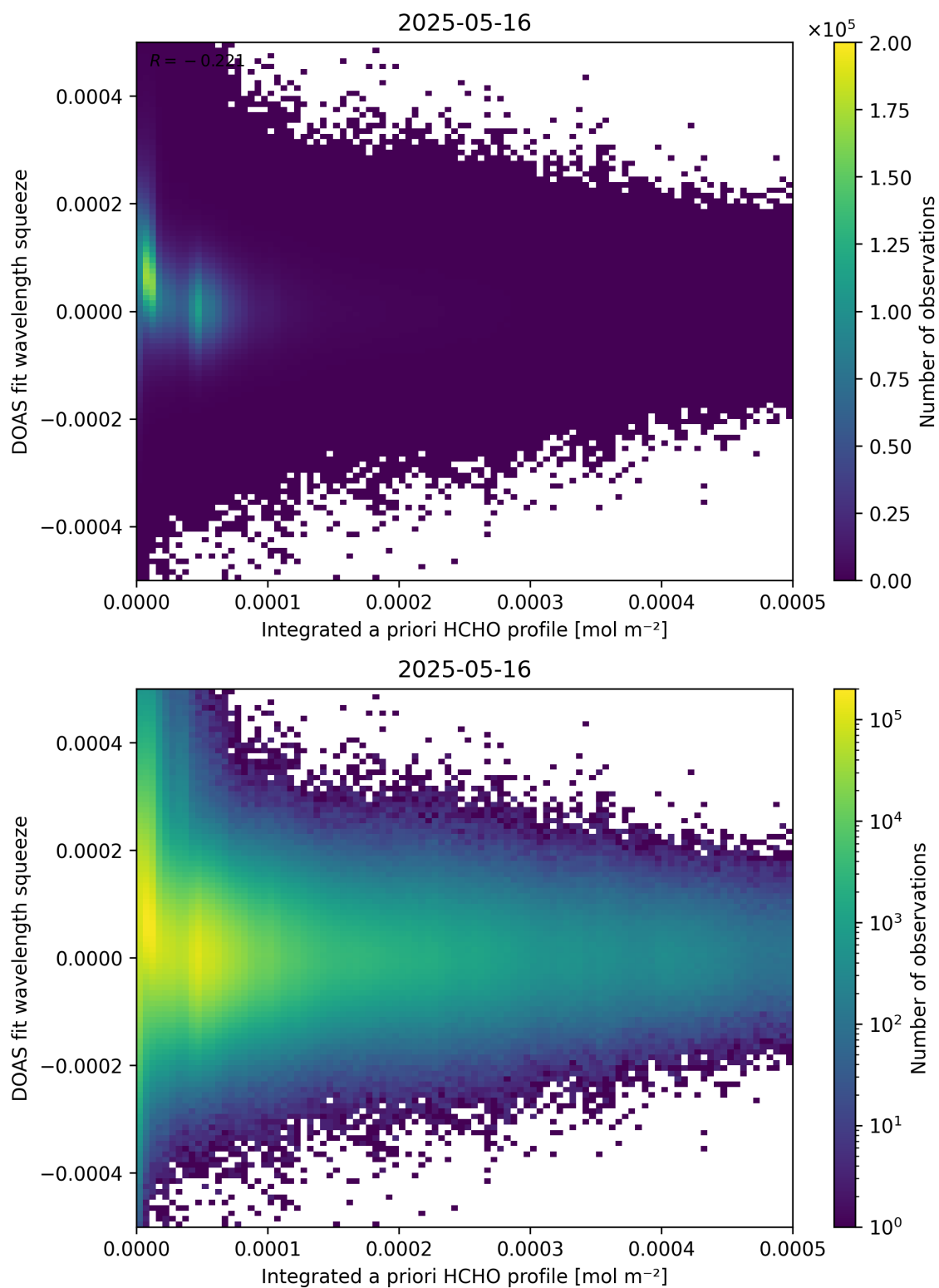
Figure 150: Scatter density plot of “Integrated a priori HCHO profile” against “DOAS fit wavelength squeeze” for 2025-05-15 to 2025-05-17.
