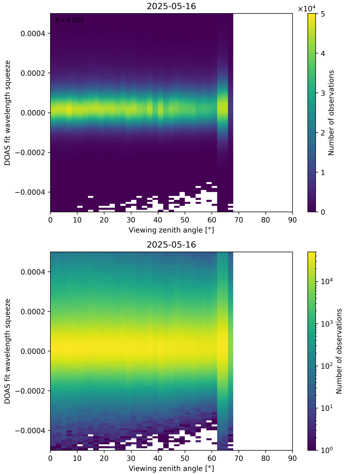
Figure 184: Scatter density plot of “Viewing zenith angle” against “DOAS fit wavelength squeeze” for 2025-05-15 to 2025-05-17.
