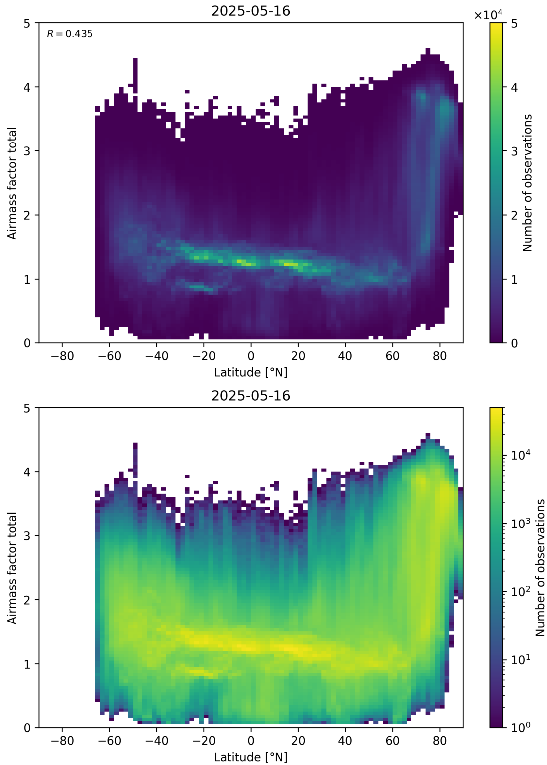
Figure 161: Scatter density plot of “Latitude” against “Airmass factor total” for 2025-05-15 to 2025-05-17.
