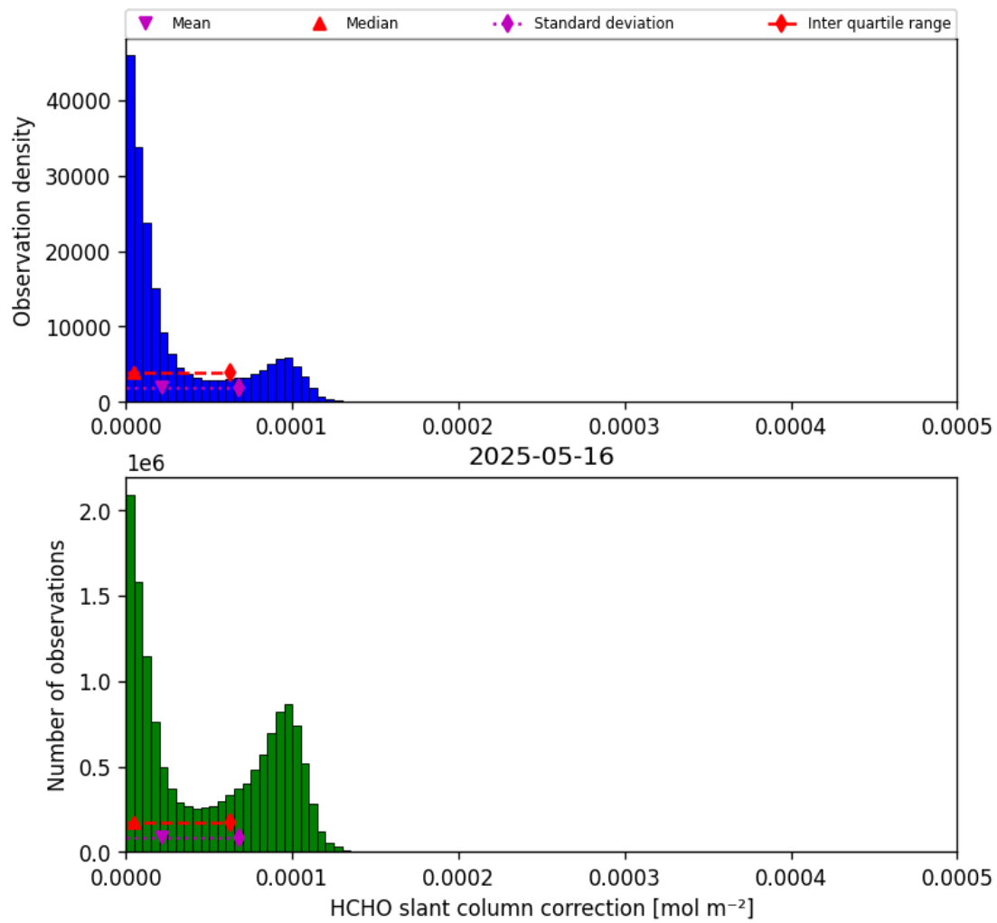
Figure 47: Histogram of "HCHO slant column correction" for 2025-05-15 to 2025-05-17
