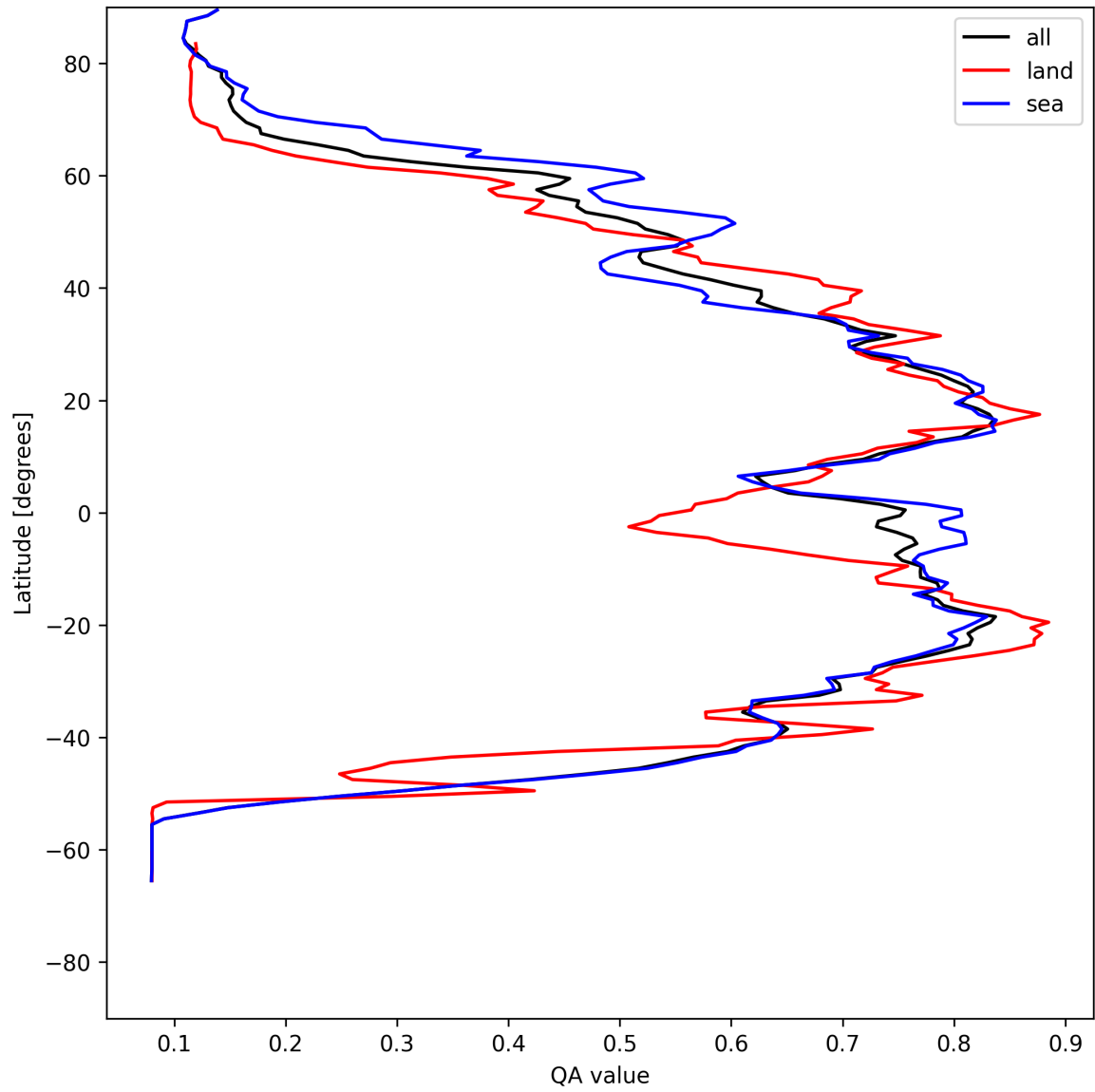
Figure 20: Zonal average of “QA value” for 2025-05-15 to 2025-05-17.
