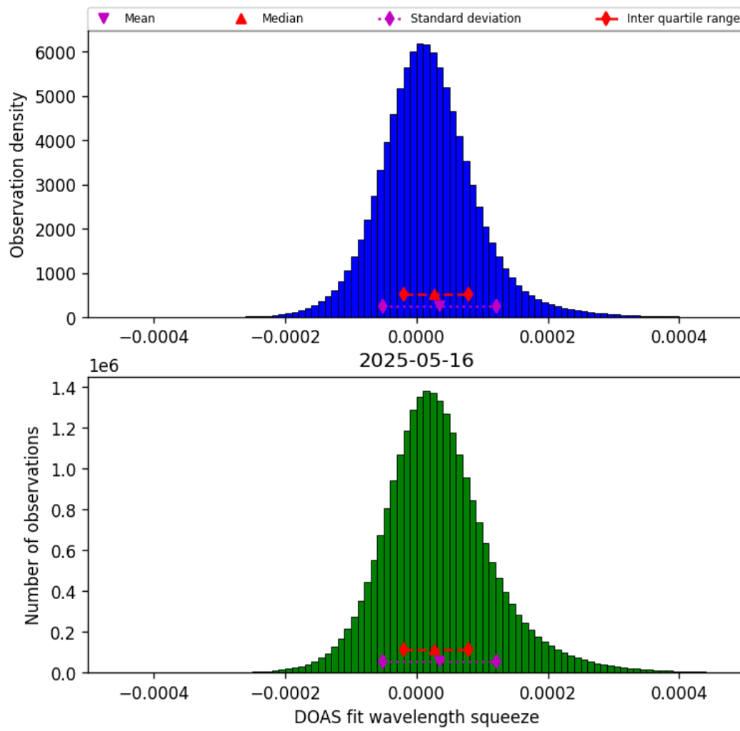
Figure 45: Histogram of “DOAS fit wavelength squeeze” for 2025-05-15 to 2025-05-17
