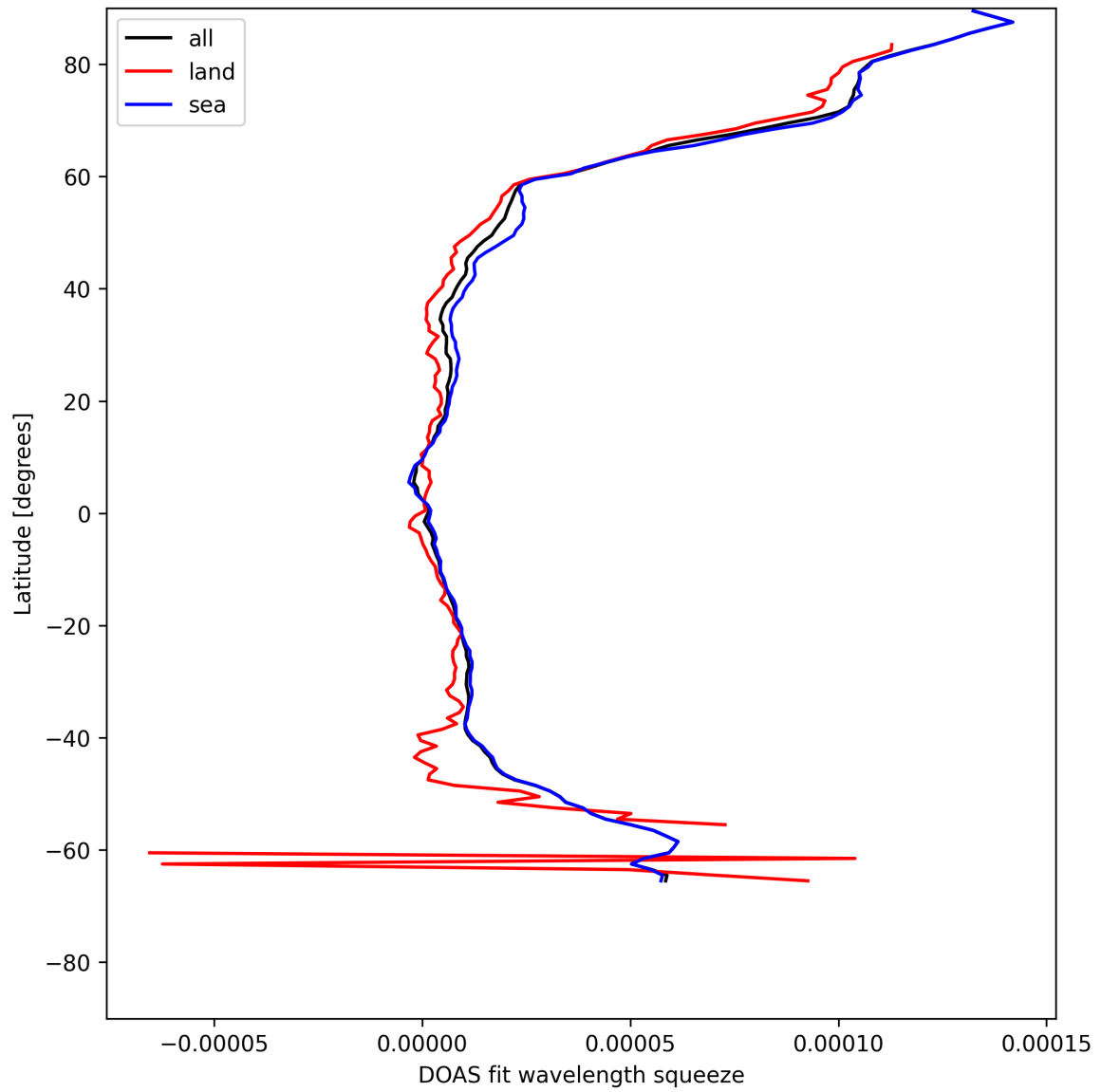
Figure 31: Zonal average of “DOAS fit wavelength squeeze” for 2025-05-15 to 2025-05-17.
