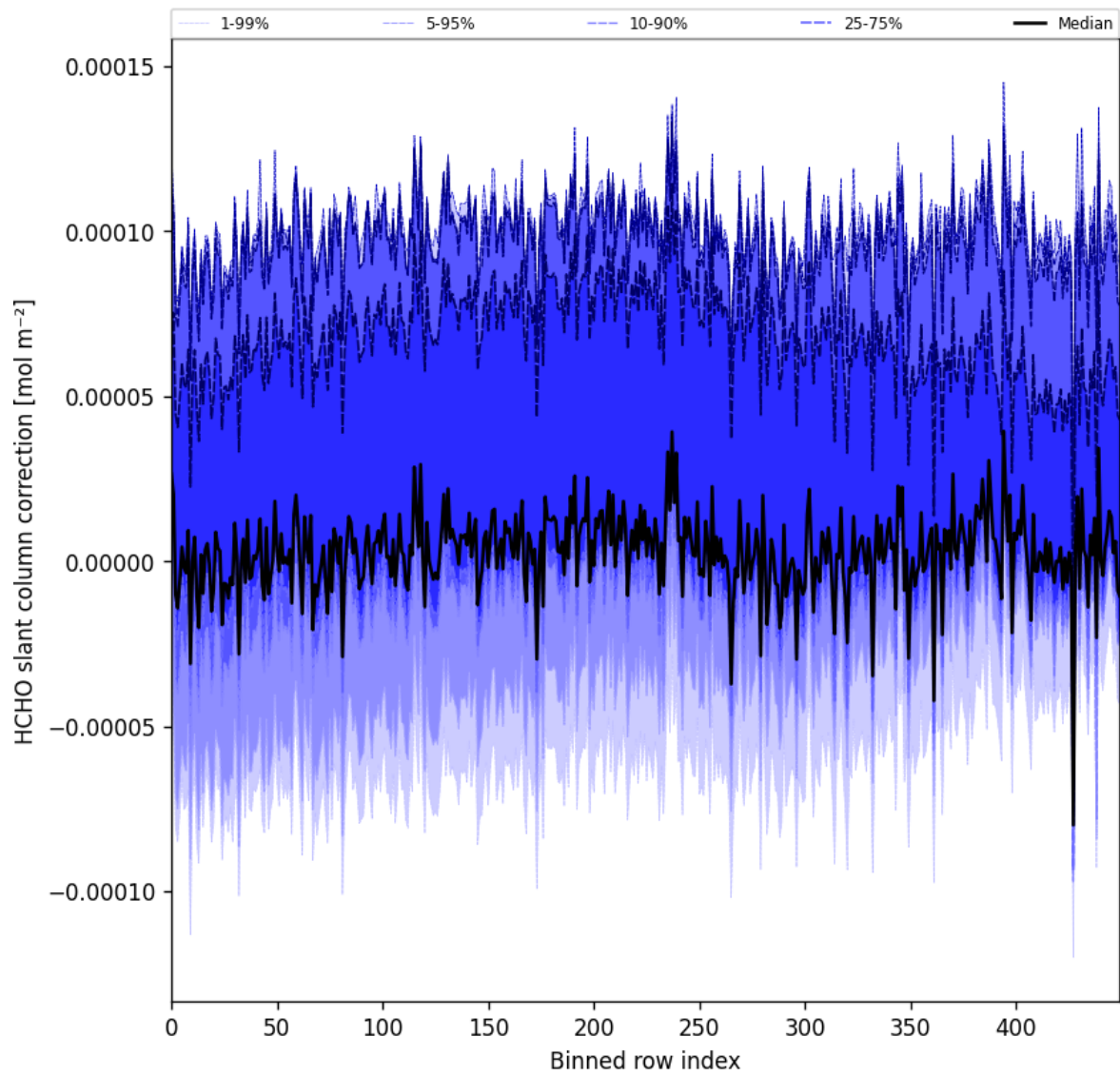
Figure 61: Along track statistics of "HCHO slant column correction" for 2025-05-15 to 2025-05-17
