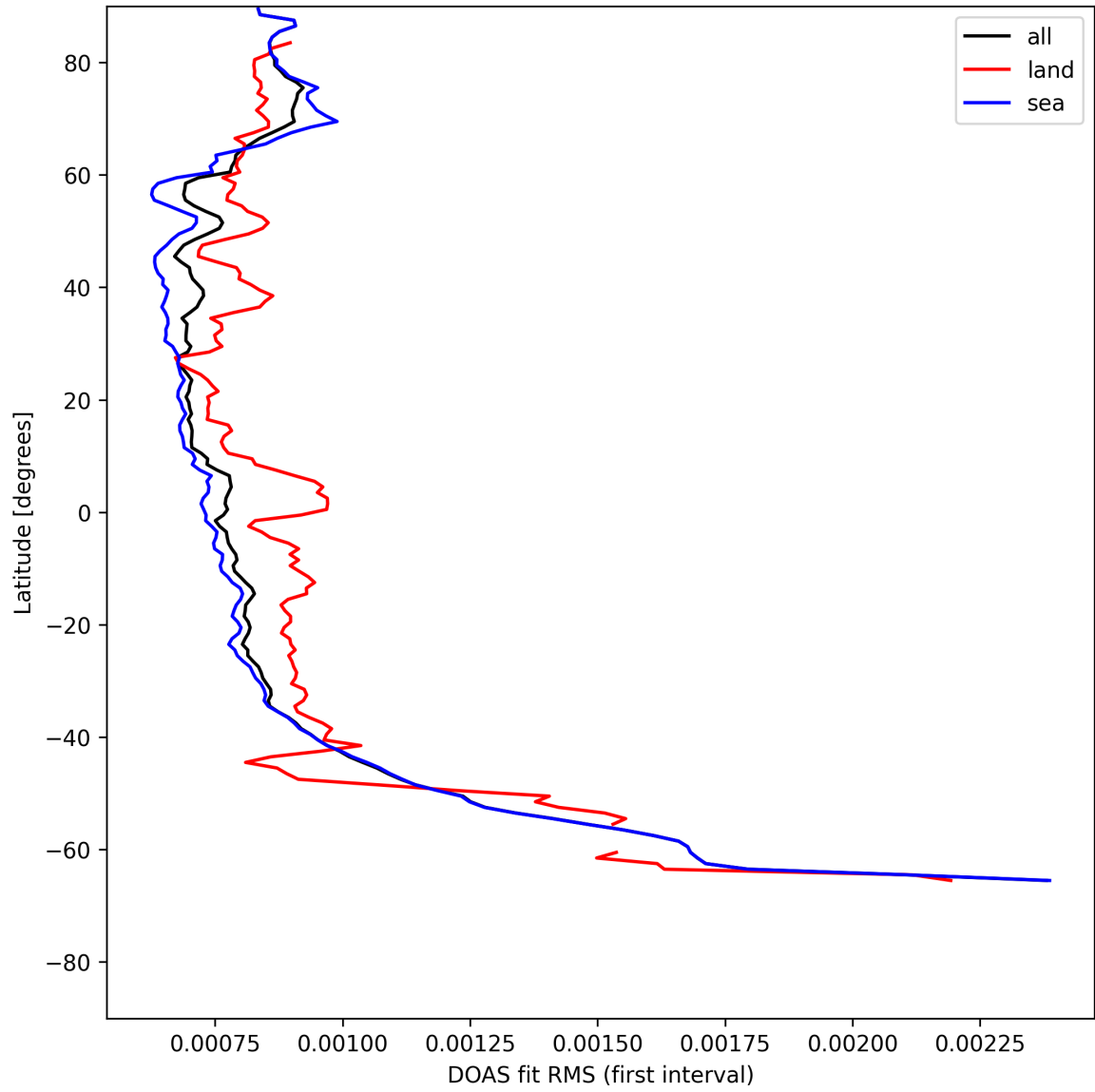
Figure 32: Zonal average of "DOAS fit RMS (first interval)" for 2025-05-15 to 2025-05-17.
