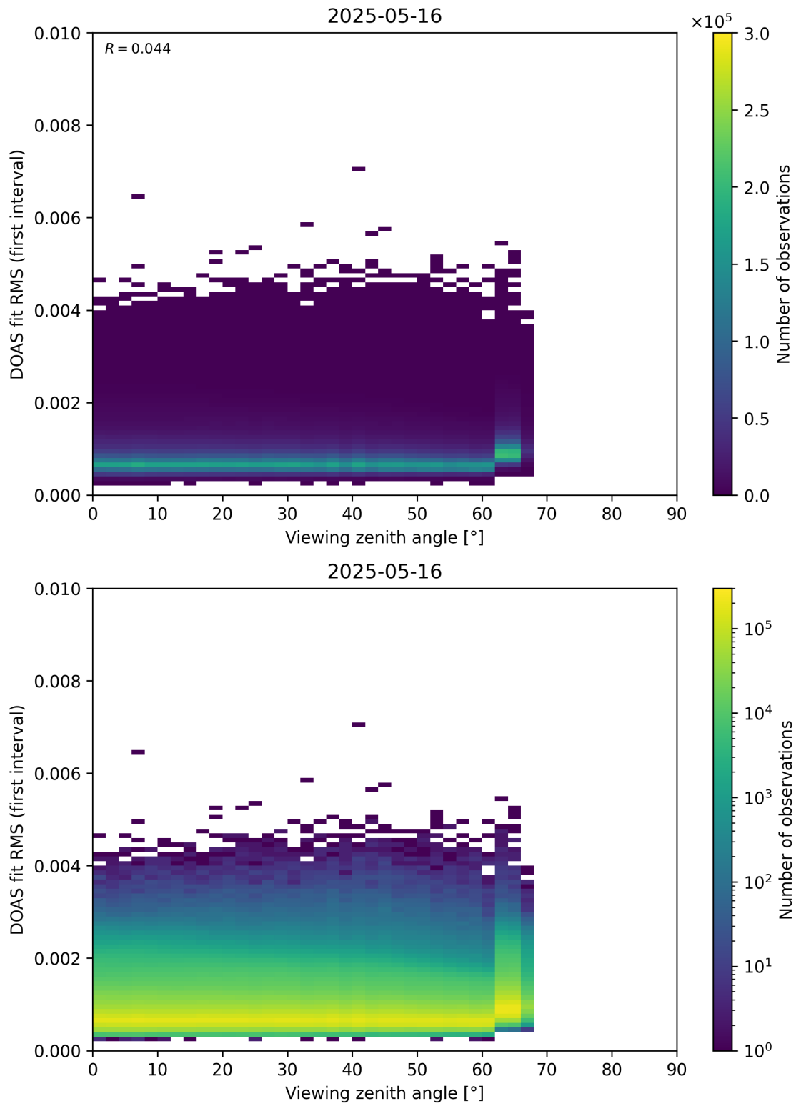
Figure 182: Scatter density plot of “Viewing zenith angle” against “DOAS fit RMS (first interval)” for 2025-05-15 to 2025-05-17.
