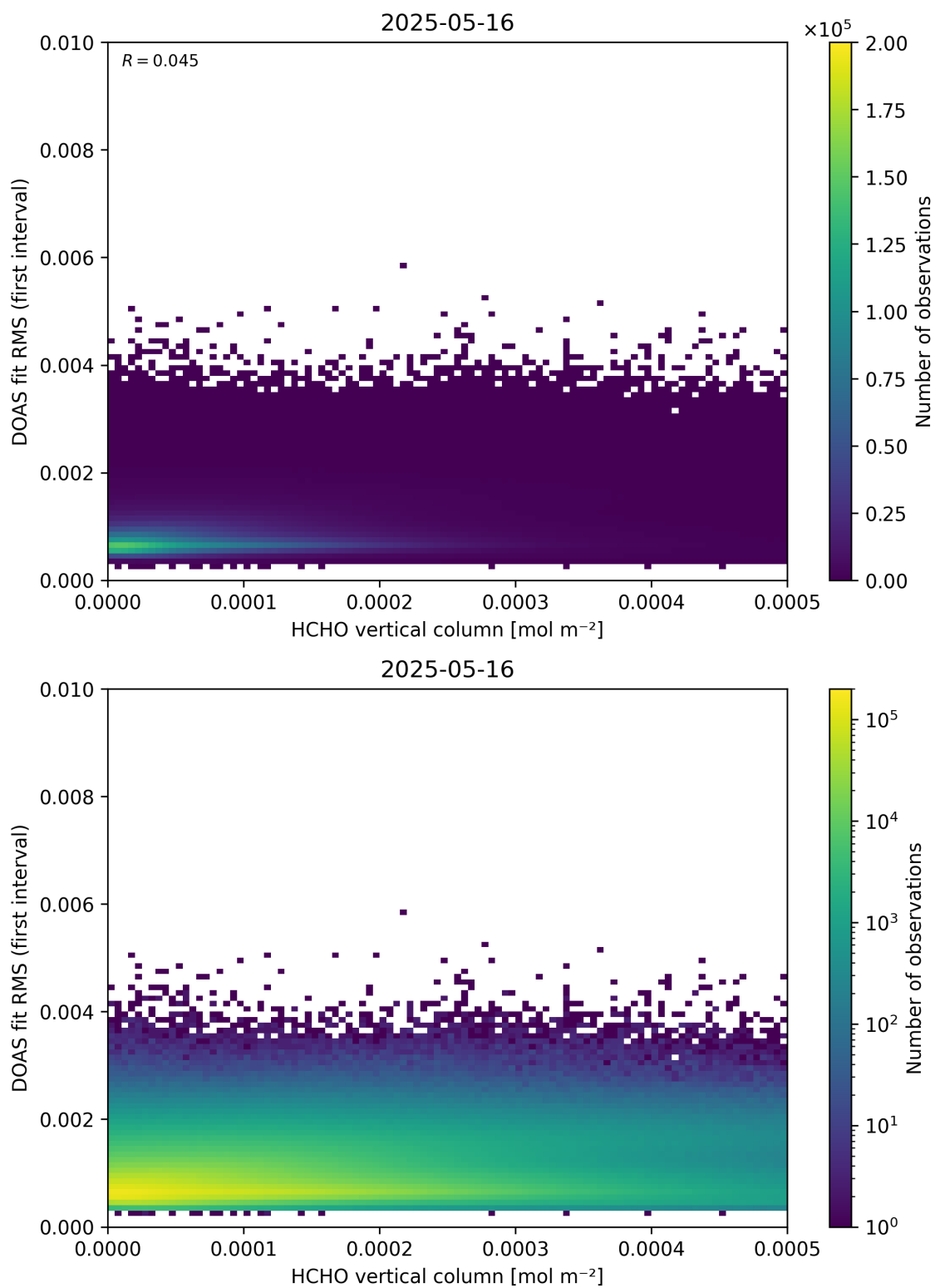
Figure 123: Scatter density plot of “HCHO vertical column” against “DOAS fit RMS (first interval)” for 2025-05-15 to 2025-05-17.
