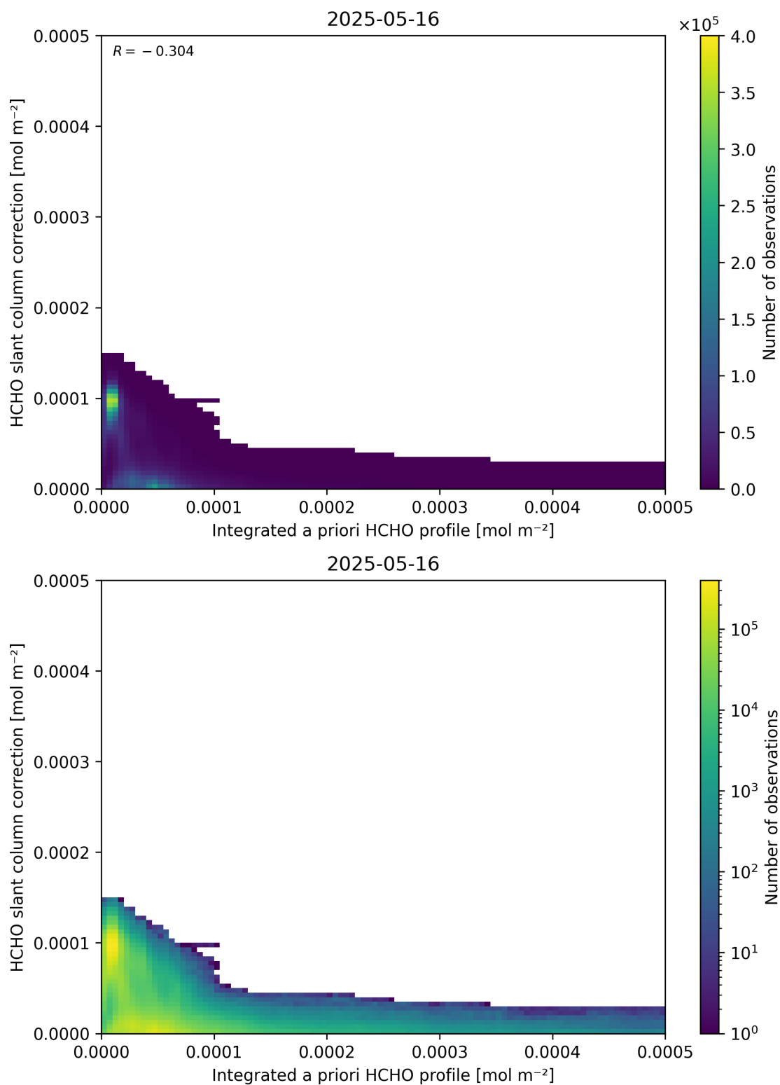
Figure 152: Scatter density plot of “Integrated a priori HCHO profile” against “HCHO slant column correction” for 2025-05-15 to 2025-05-17.
