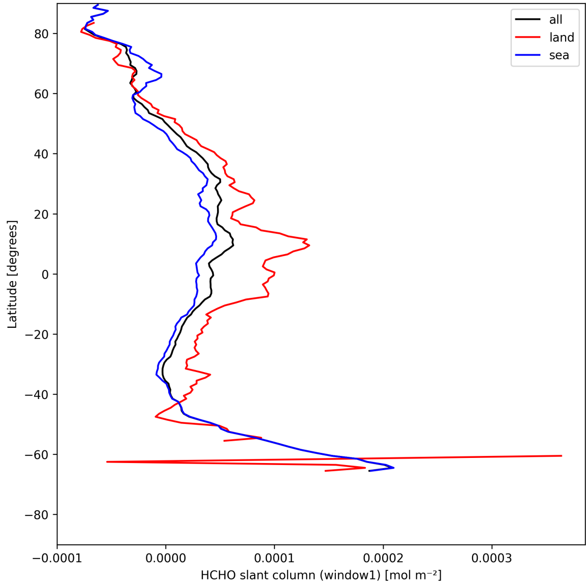
Figure 24: Zonal average of “HCHO slant column (window1)” for 2025-05-15 to 2025-05-17.
