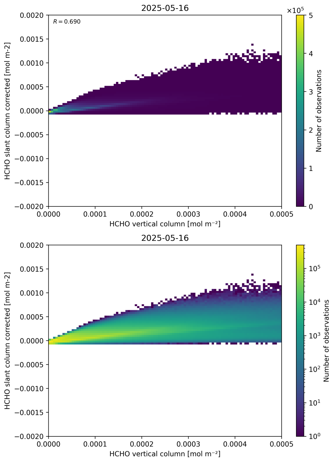
Figure 127: Scatter density plot of “HCHO vertical column” against “HCHO slant column corrected” for 2025-05-15 to 2025-05-17.
