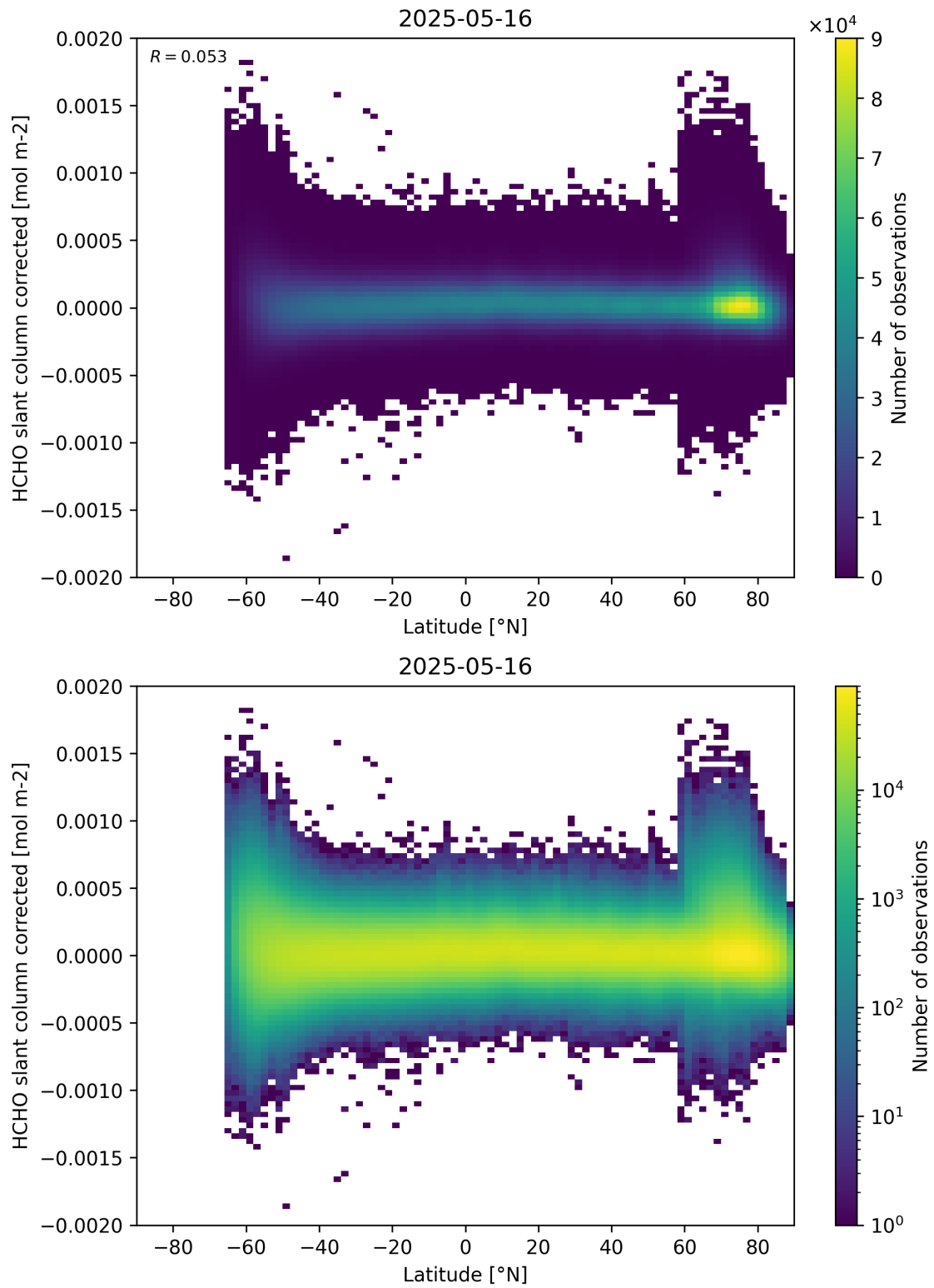
Figure 157: Scatter density plot of “Latitude” against “HCHO slant column corrected” for 2025-05-15 to 2025-05-17.
