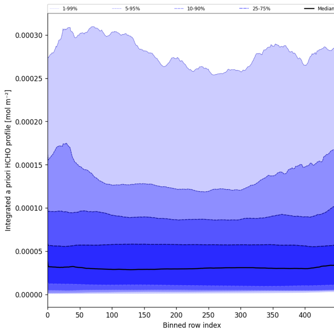
Figure 57: Along track statistics of "Integrated a priori HCHO profile" for 2025-05-15 to 2025-05-17
