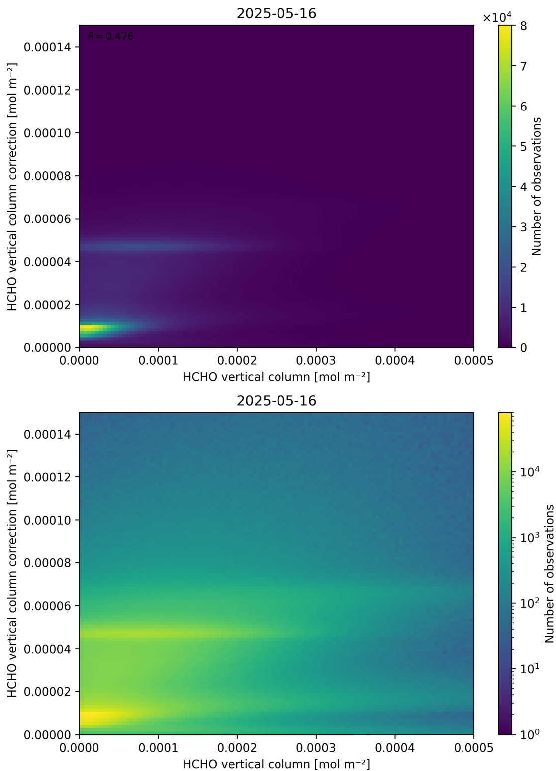
Figure 133: Scatter density plot of “HCHO vertical column” against “HCHO vertical column correction” for 2025-05-15 to 2025-05-17.
