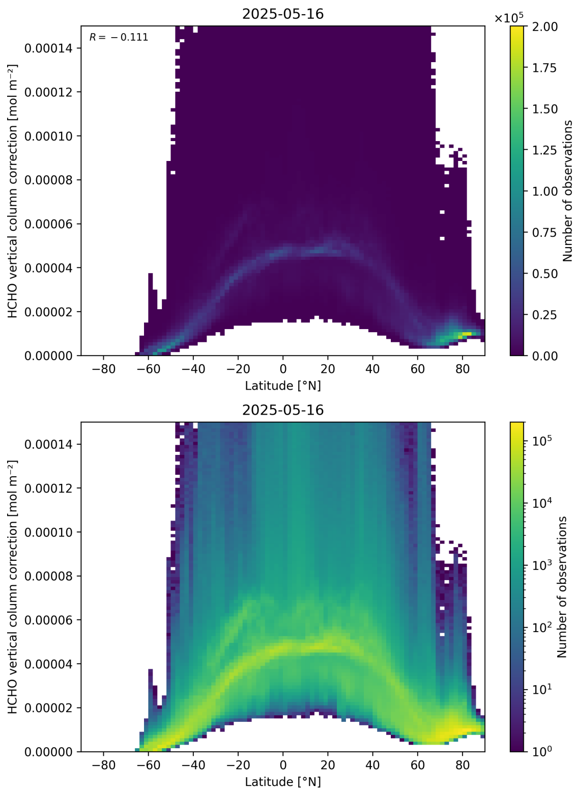
Figure 164: Scatter density plot of “Latitude” against “HCHO vertical column correction” for 2025-05-15 to 2025-05-17.
