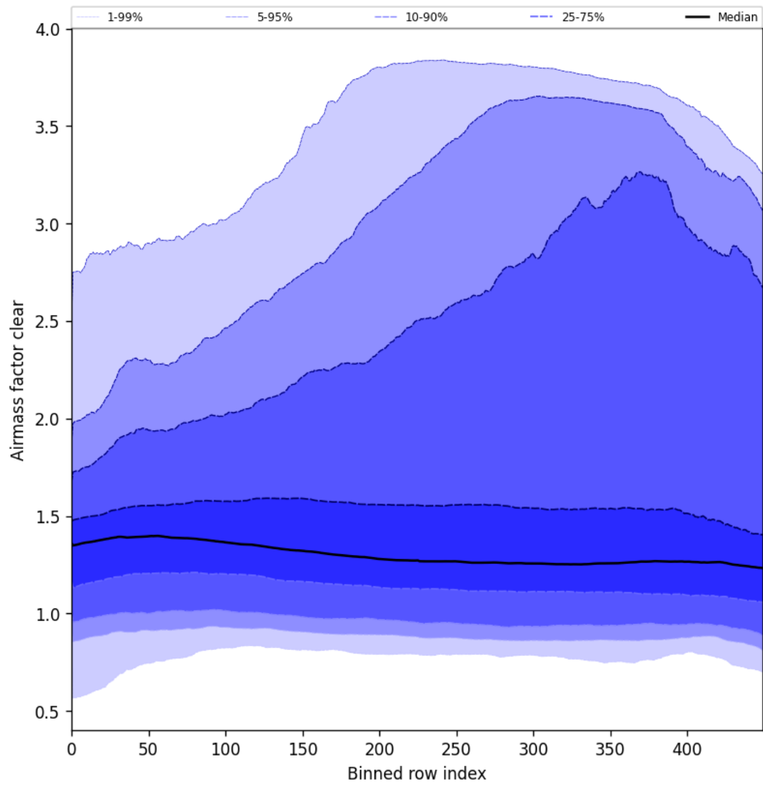
Figure 56: Along track statistics of “Airmass factor clear” for 2025-05-15 to 2025-05-17
