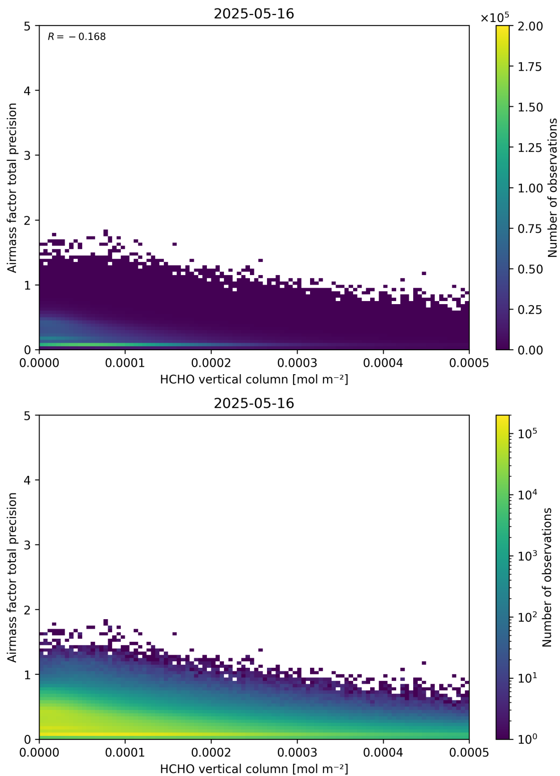
Figure 132: Scatter density plot of “HCHO vertical column” against “Airmass factor total precision” for 2025-05-15 to 2025-05-17.
