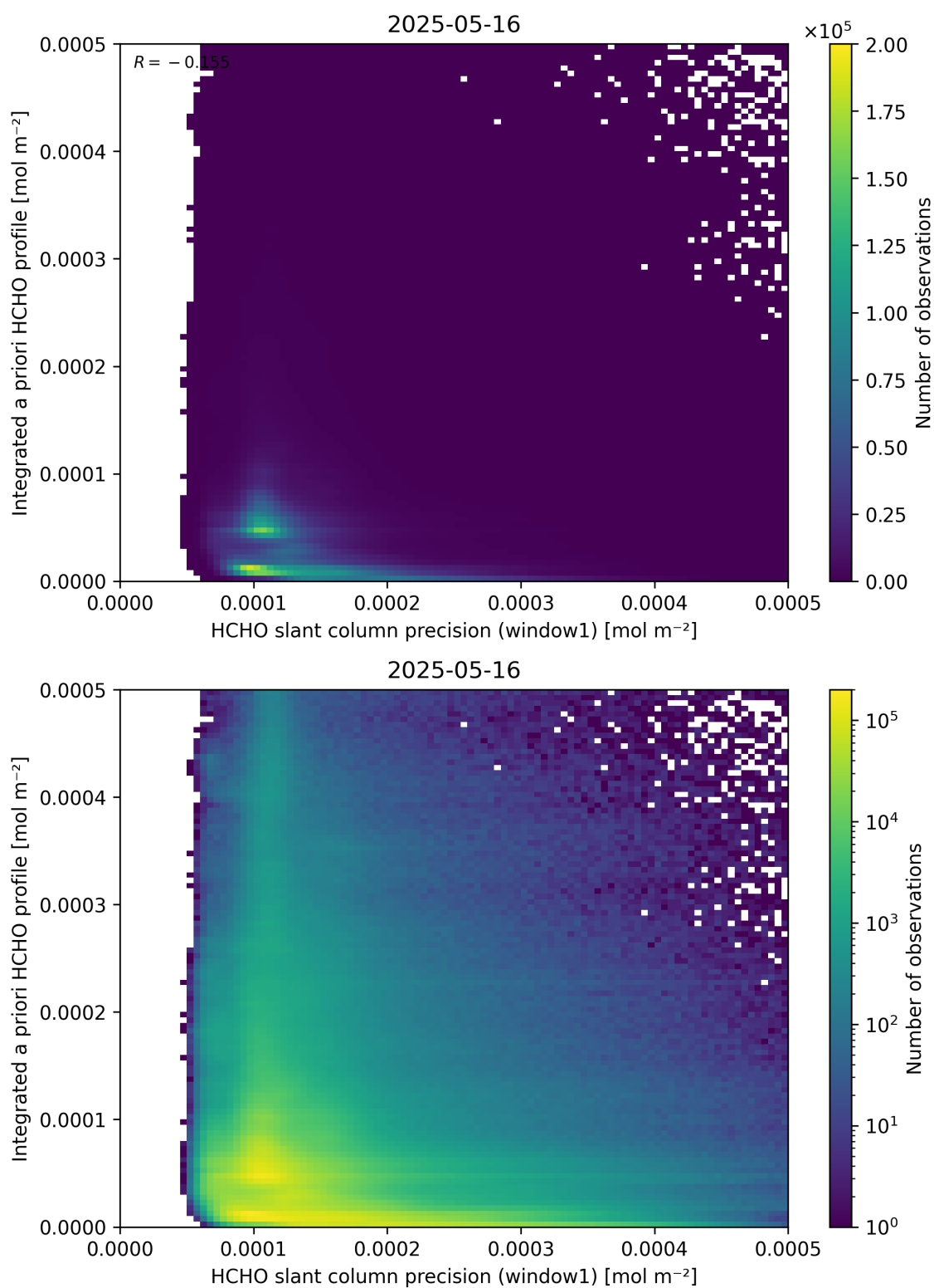
Figure 96: Scatter density plot of “HCHO slant column precision (window1)” against “Integrated a priori HCHO profile” for 2025-05-15 to 2025-05-17.
