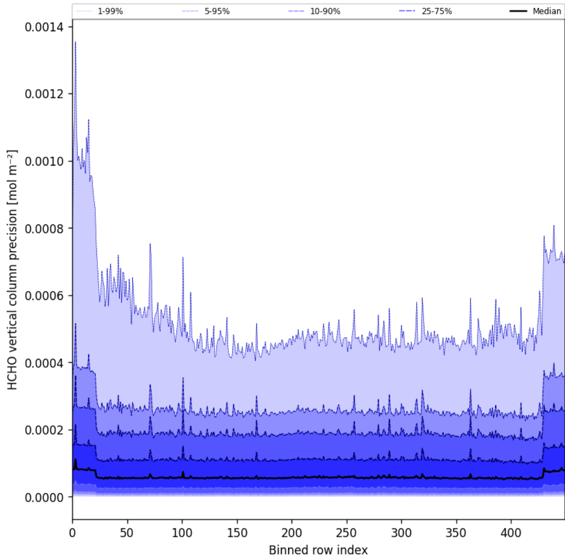
Figure 50: Along track statistics of “HCHO vertical column precision” for 2025-05-15 to 2025-05-17
