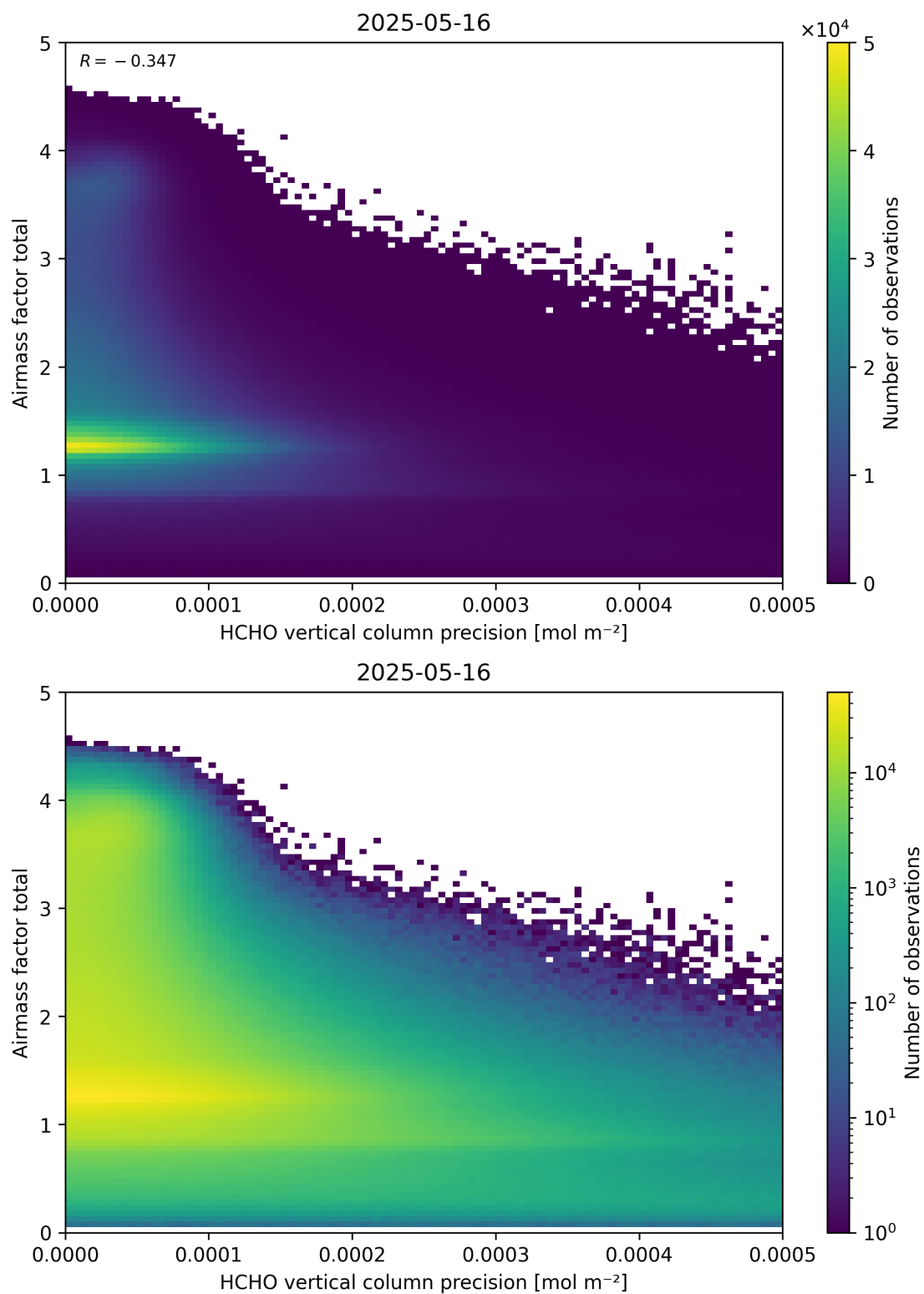
Figure 144: Scatter density plot of “HCHO vertical column precision” against “Airmass factor total” for 2025-05-15 to 2025-05-17.
