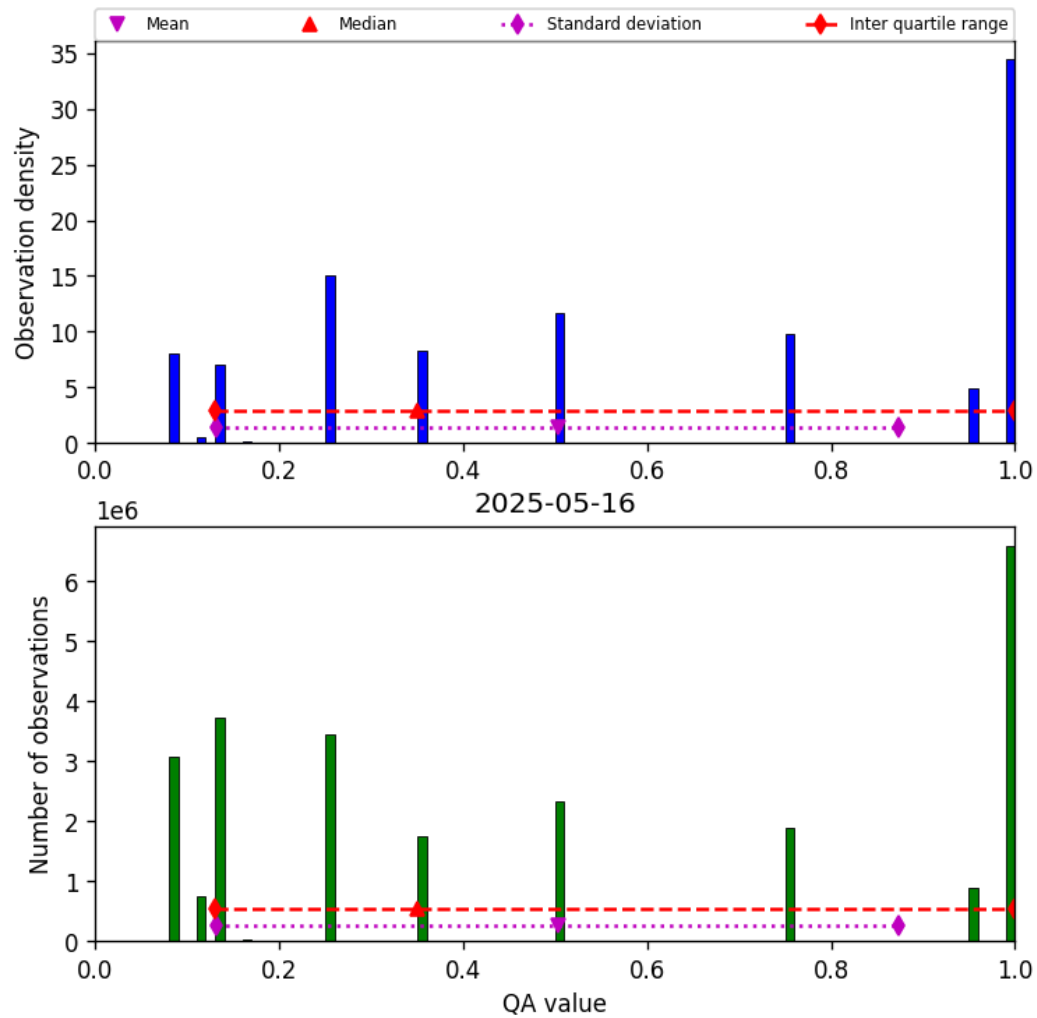
Figure 34: Histogram of “QA value” for 2025-05-15 to 2025-05-17
