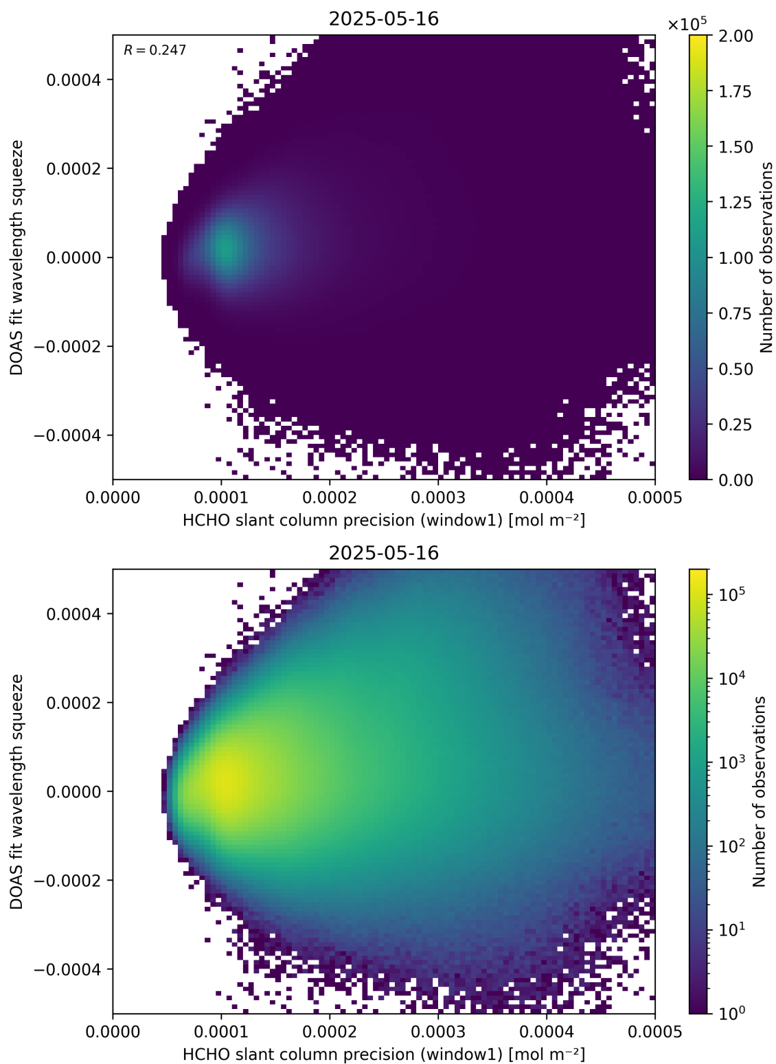
Figure 90: Scatter density plot of “HCHO slant column precision (window1)” against “DOAS fit wavelength squeeze” for 2025-05-15 to 2025-05-17.
