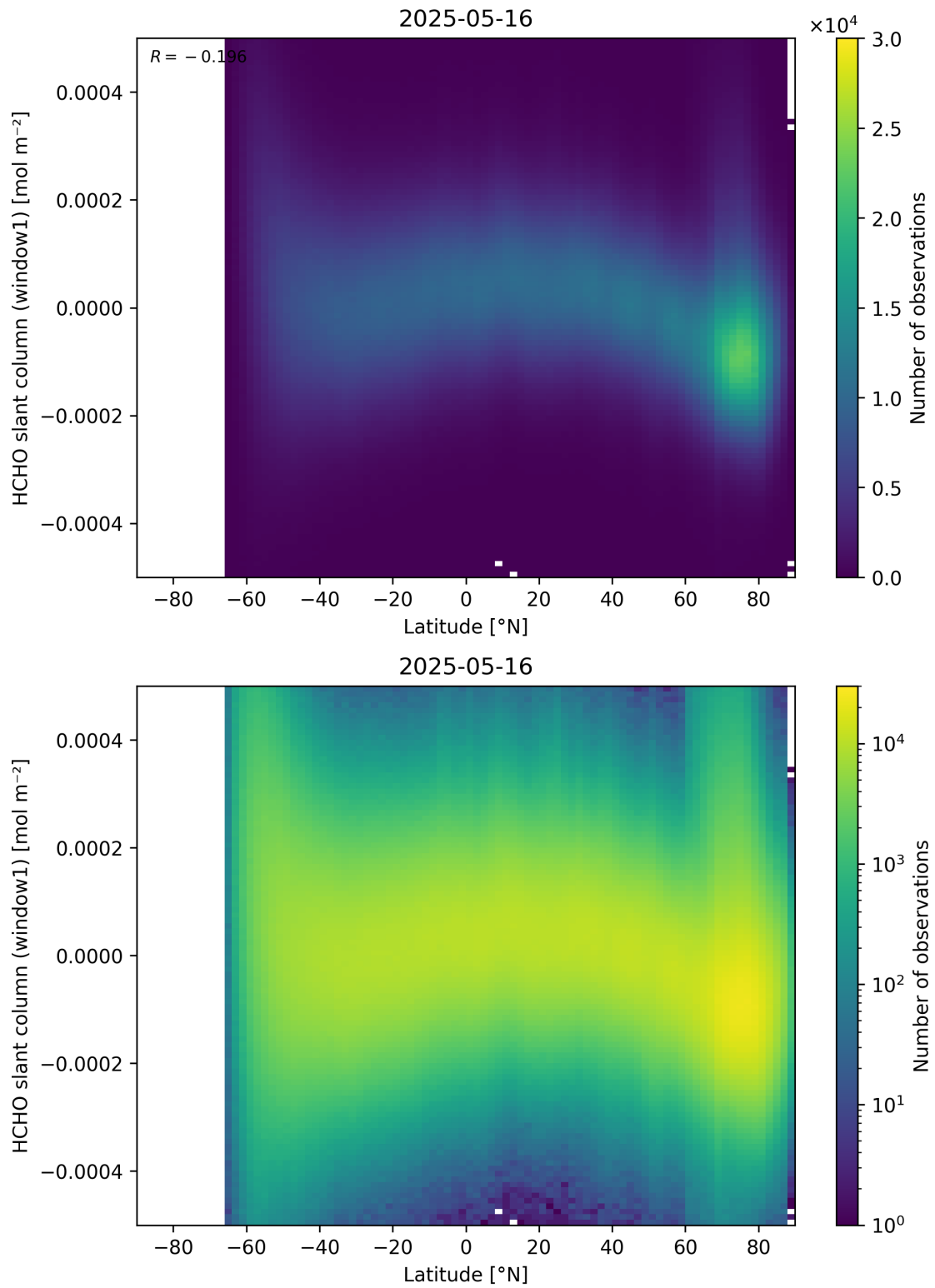
Figure 159: Scatter density plot of “Latitude” against “HCHO slant column (window1)” for 2025-05-15 to 2025-05-17.
