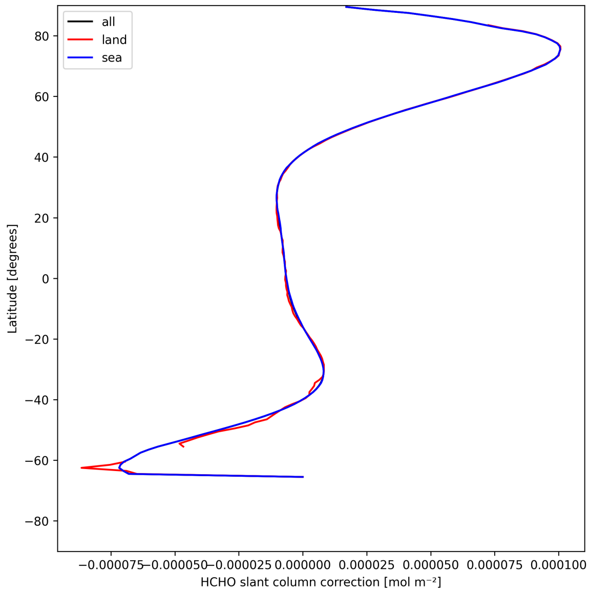
Figure 33: Zonal average of “HCHO slant column correction” for 2025-05-15 to 2025-05-17.
