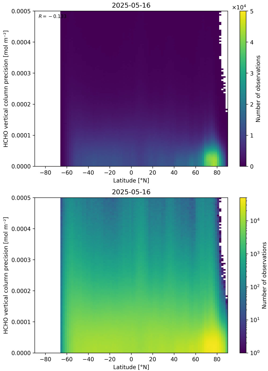
Figure 165: Scatter density plot of “Latitude” against “HCHO vertical column precision” for 2025-05-15 to 2025-05-17.
