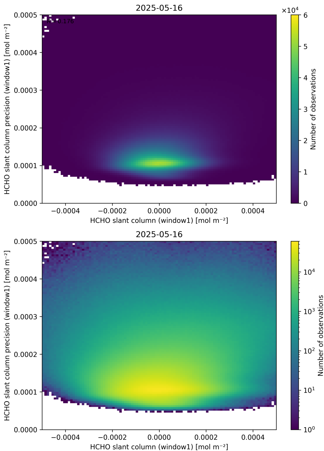
Figure 84: Scatter density plot of “HCHO slant column (window1)” against “HCHO slant column precision (window1)” for 2025-05-15 to 2025-05-17.
