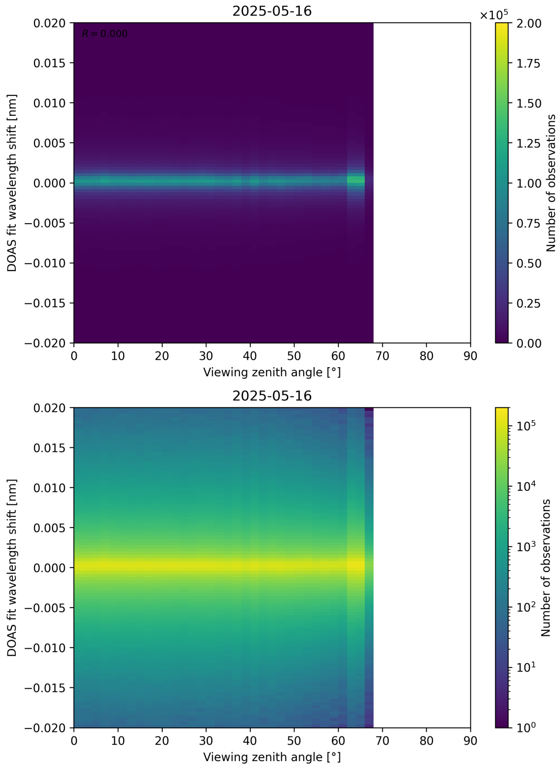
Figure 183: Scatter density plot of “Viewing zenith angle” against “DOAS fit wavelength shift” for 2025-05-15 to 2025-05-17.
