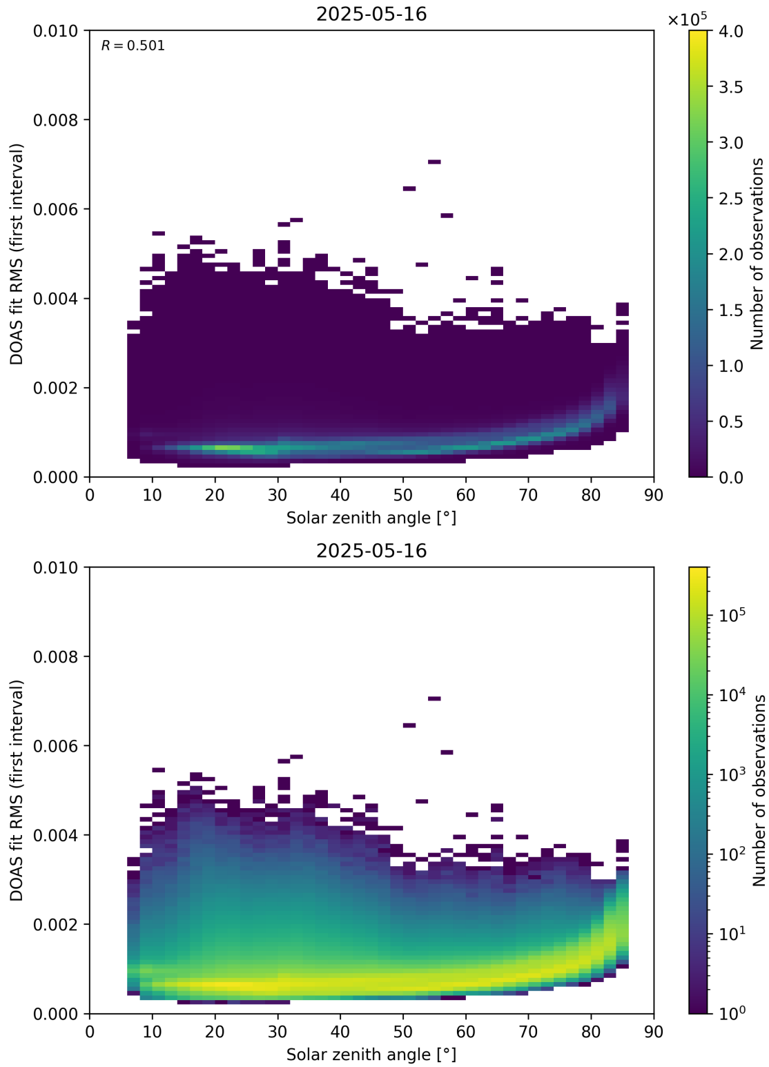
Figure 167: Scatter density plot of “Solar zenith angle” against “DOAS fit RMS (first interval)” for 2025-05-15 to 2025-05-17.
