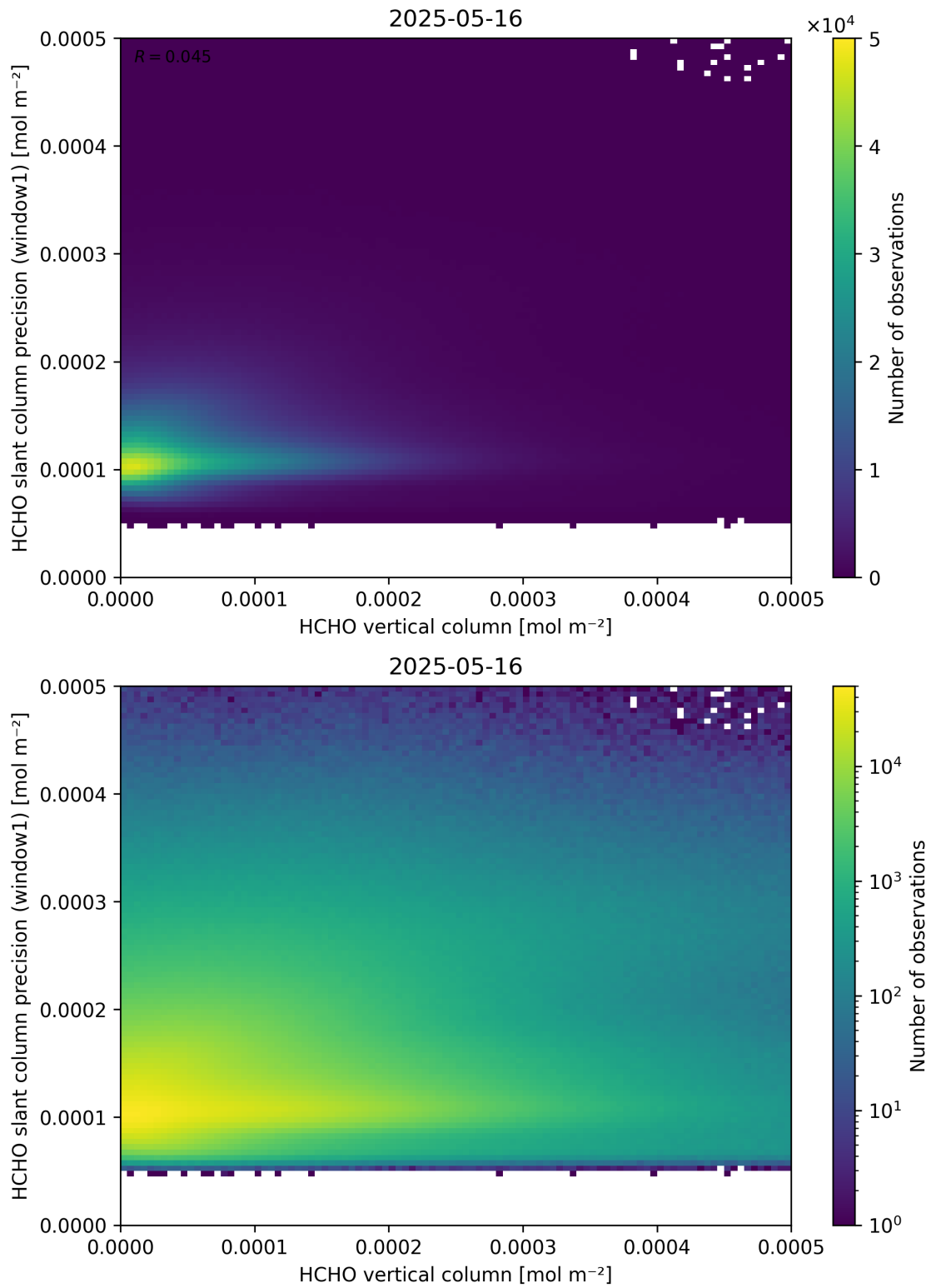
Figure 130: Scatter density plot of “HCHO vertical column” against “HCHO slant column precision (window1)” for 2025-05-15 to 2025-05-17.
