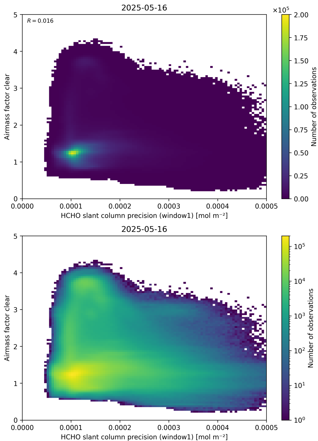
Figure 91: Scatter density plot of “HCHO slant column precision (window1)” against “Airmass factor clear” for 2025-05-15 to 2025-05-17.
