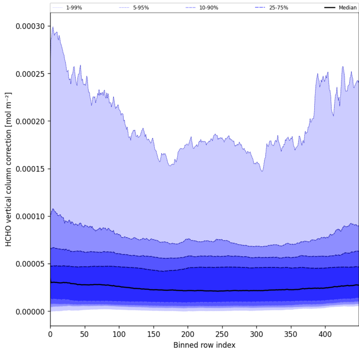
Figure 51: Along track statistics of "HCHO vertical column correction" for 2025-05-15 to 2025-05-17
