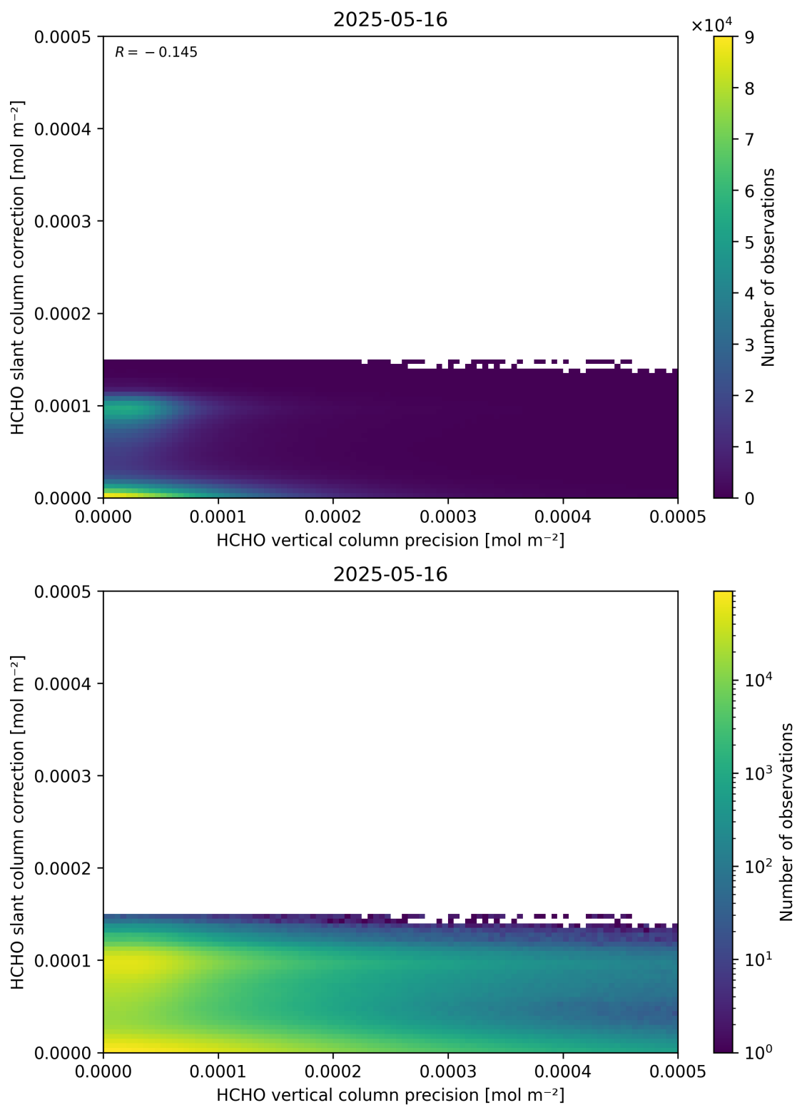
Figure 141: Scatter density plot of “HCHO vertical column precision” against “HCHO slant column correction” for 2025-05-15 to 2025-05-17.
