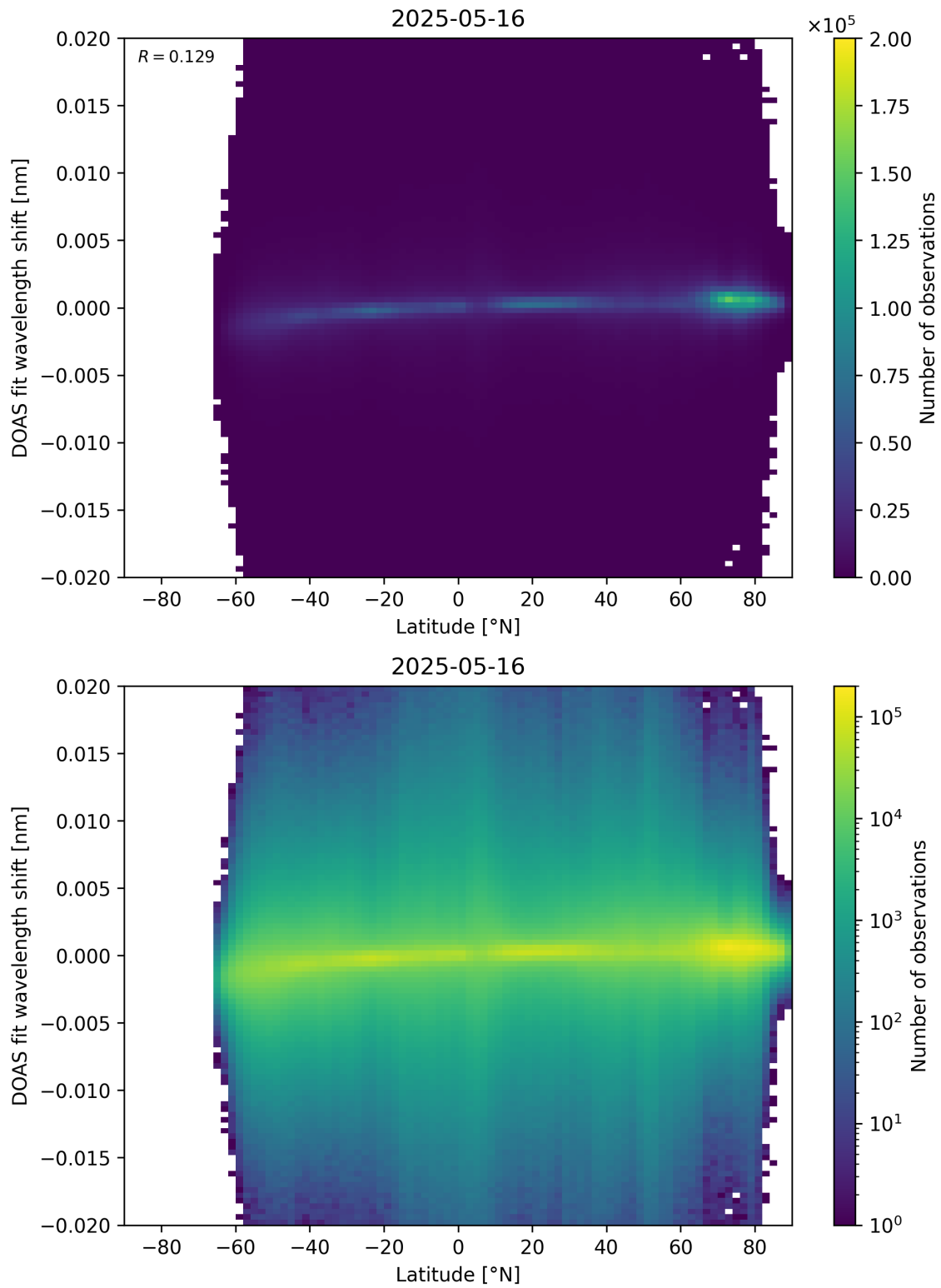
Figure 154: Scatter density plot of “Latitude” against “DOAS fit wavelength shift” for 2025-05-15 to 2025-05-17.
