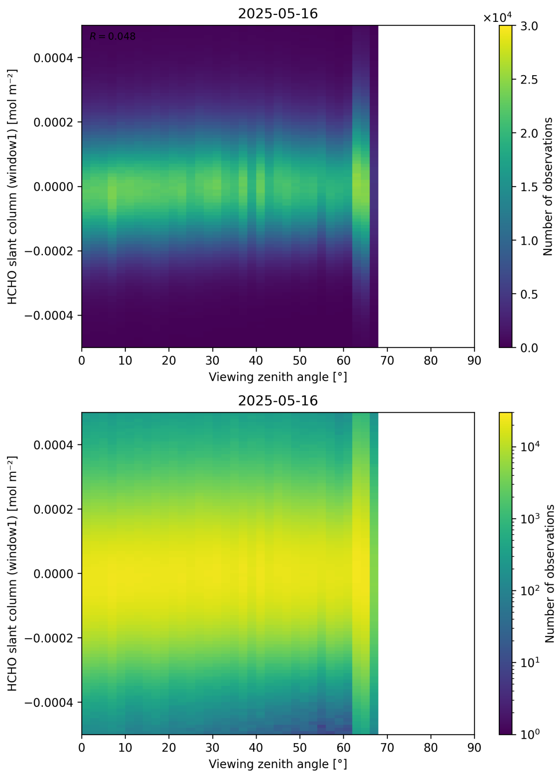
Figure 188: Scatter density plot of “Viewing zenith angle” against “HCHO slant column (window1)” for 2025-05-15 to 2025-05-17.
