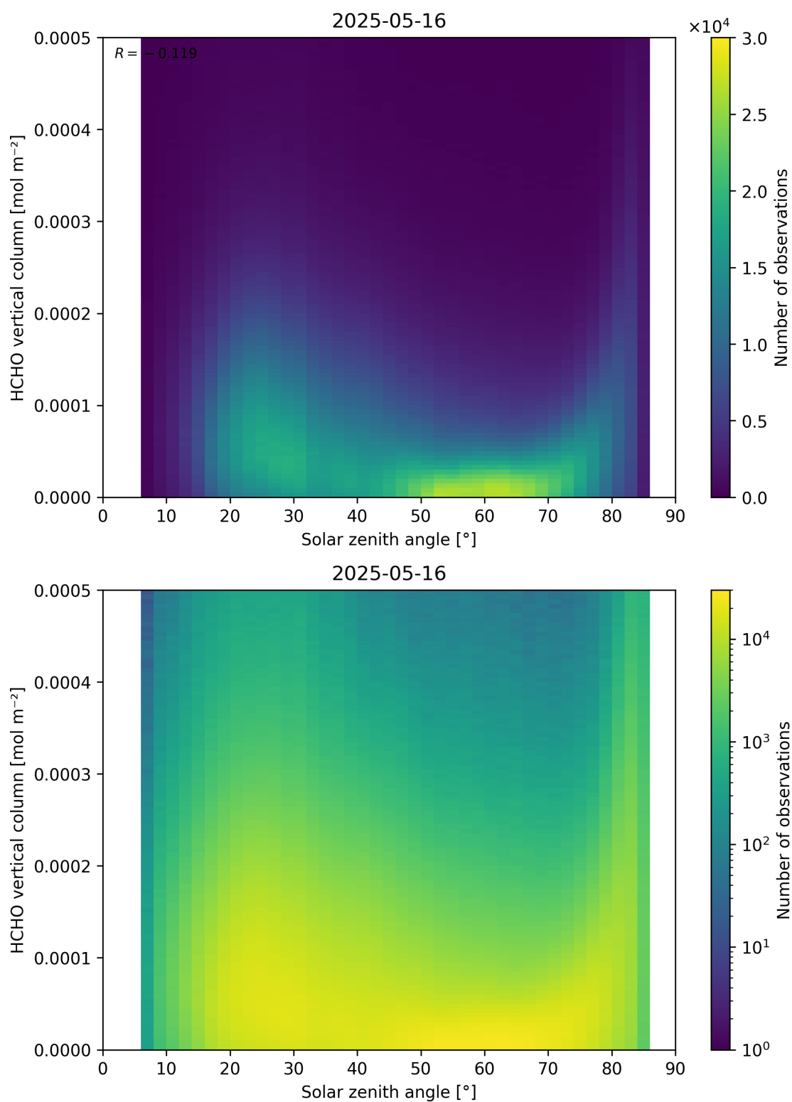
Figure 177: Scatter density plot of “Solar zenith angle” against “HCHO vertical column” for 2025-05-15 to 2025-05-17.
