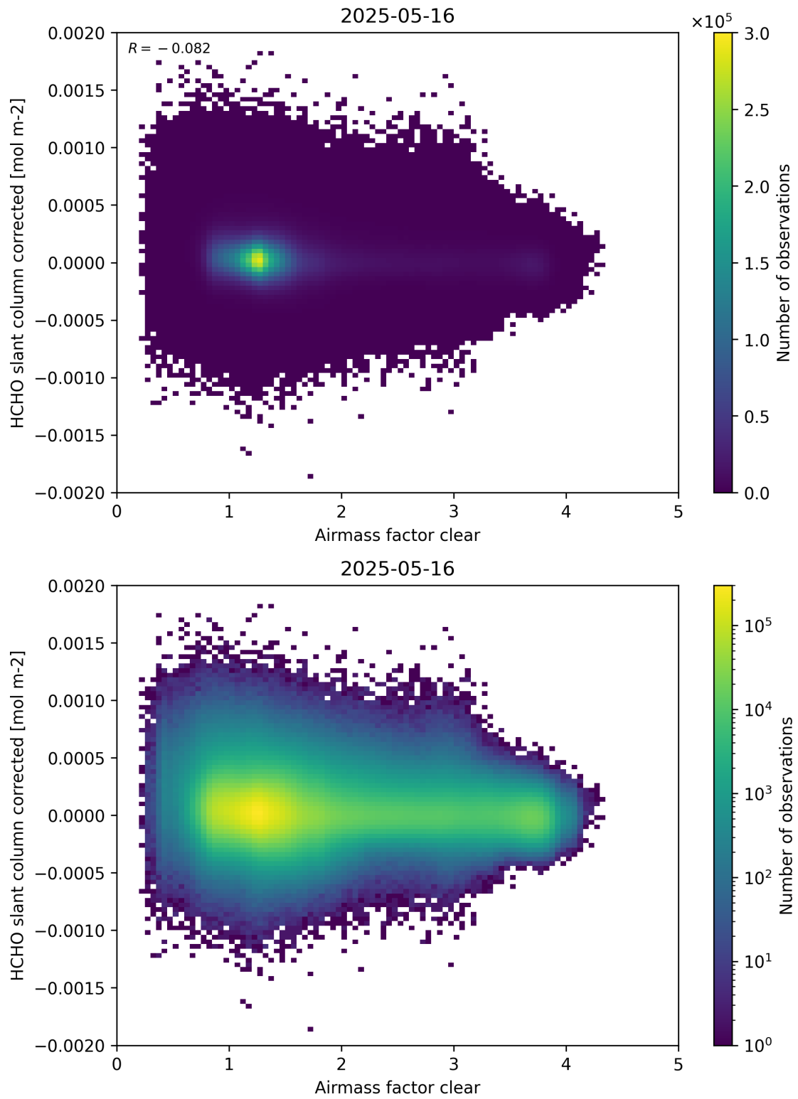
Figure 74: Scatter density plot of “Airmass factor clear” against “HCHO slant column corrected” for 2025-05-15 to 2025-05-17.
