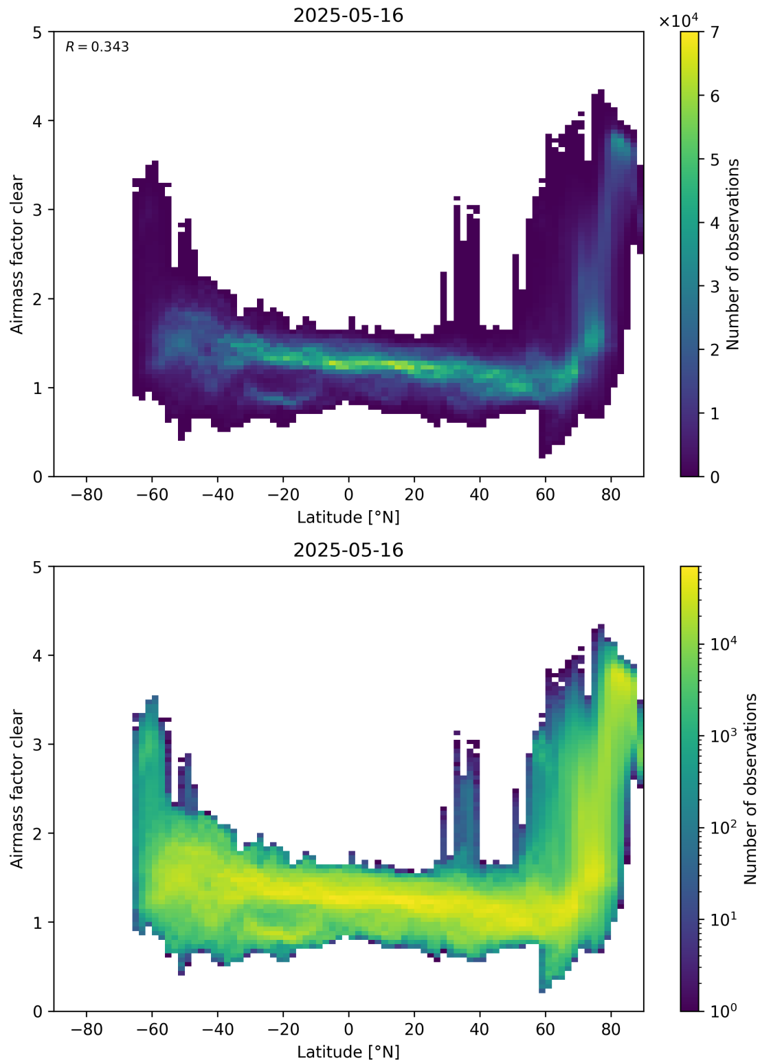
Figure 156: Scatter density plot of “Latitude” against “Airmass factor clear” for 2025-05-15 to 2025-05-17.
