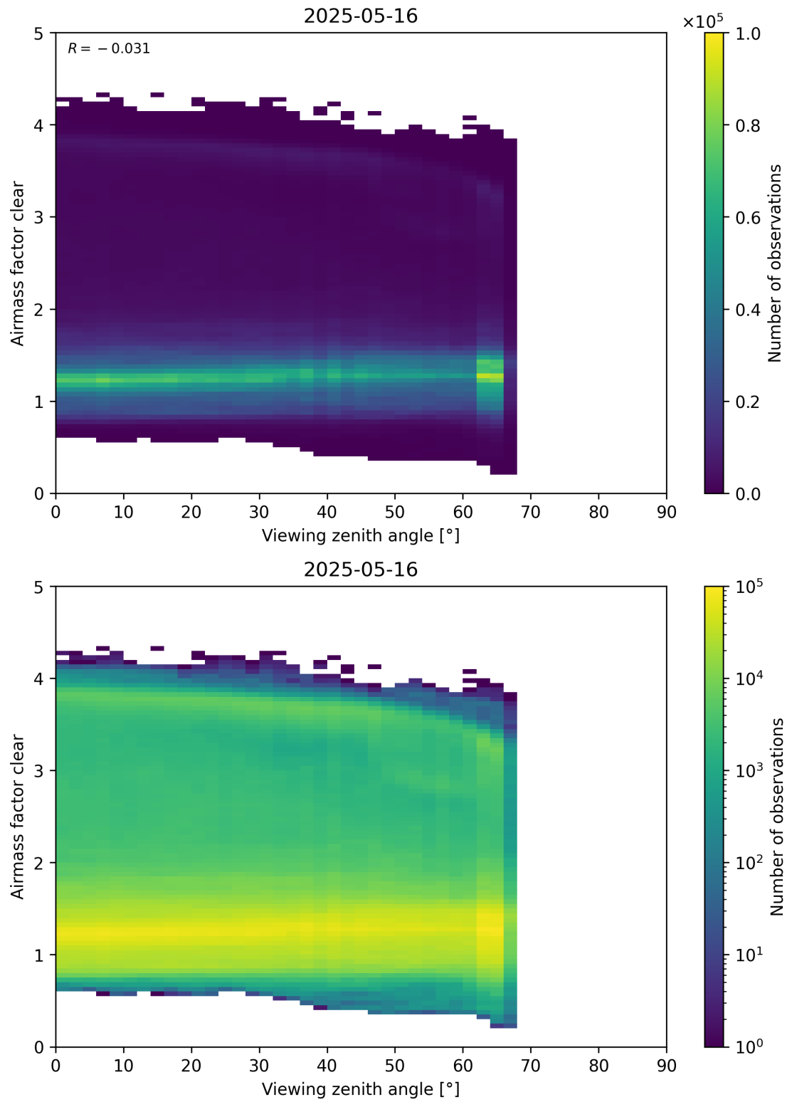
Figure 185: Scatter density plot of “Viewing zenith angle” against “Airmass factor clear” for 2025-05-15 to 2025-05-17.
