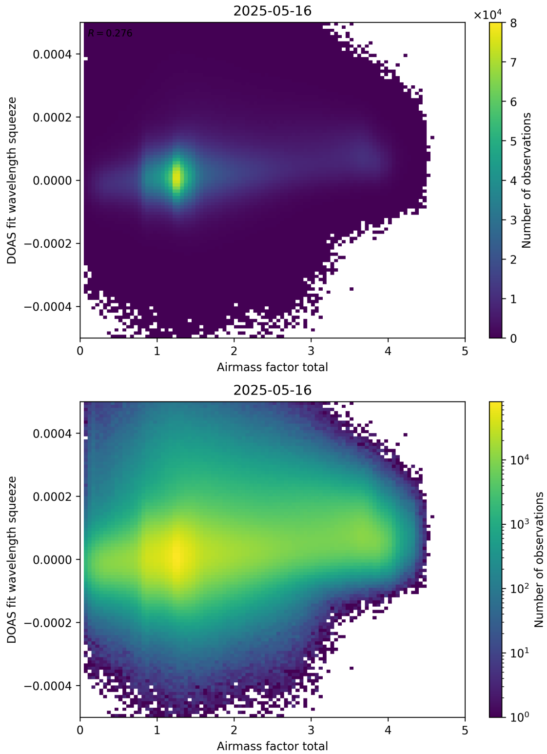
Figure 99: Scatter density plot of “Airmass factor total” against “DOAS fit wavelength squeeze” for 2025-05-15 to 2025-05-17.
