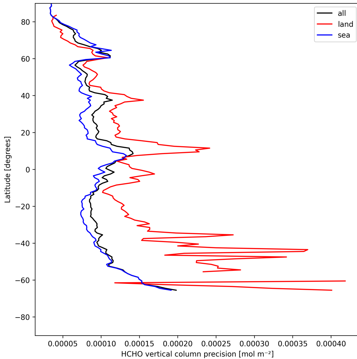
Figure 22: Zonal average of “HCHO vertical column precision” for 2025-05-15 to 2025-05-17.
