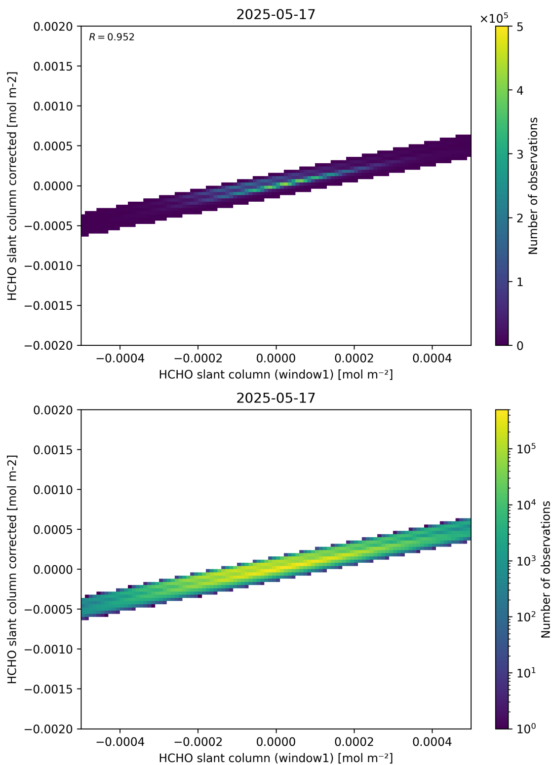
Figure 82: Scatter density plot of “HCHO slant column (window1)” against “HCHO slant column corrected” for 2025-05-16 to 2025-05-18.
