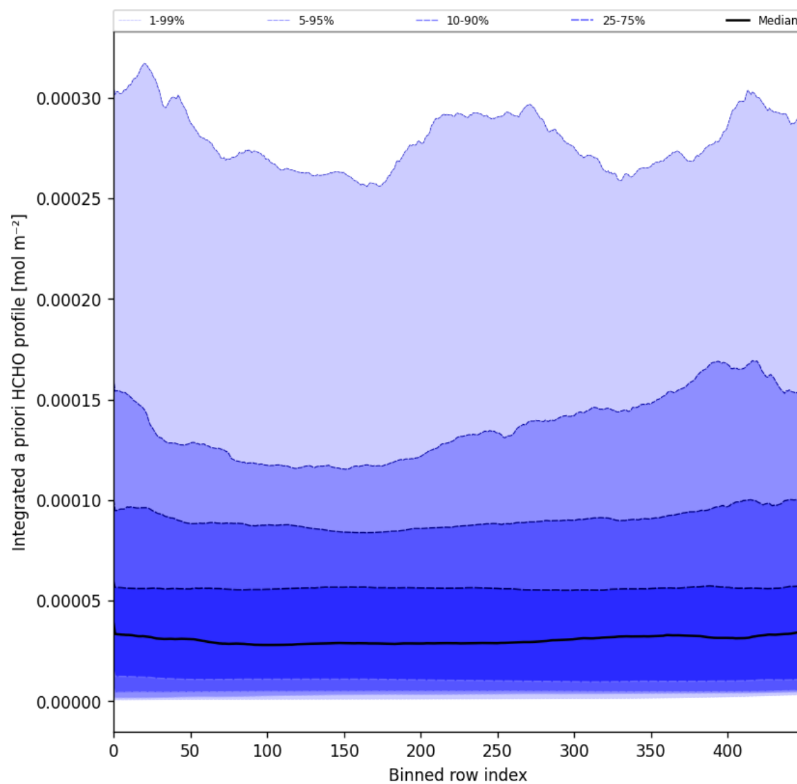
Figure 57: Along track statistics of “Integrated a priori HCHO profile” for 2025-05-16 to 2025-05-18
