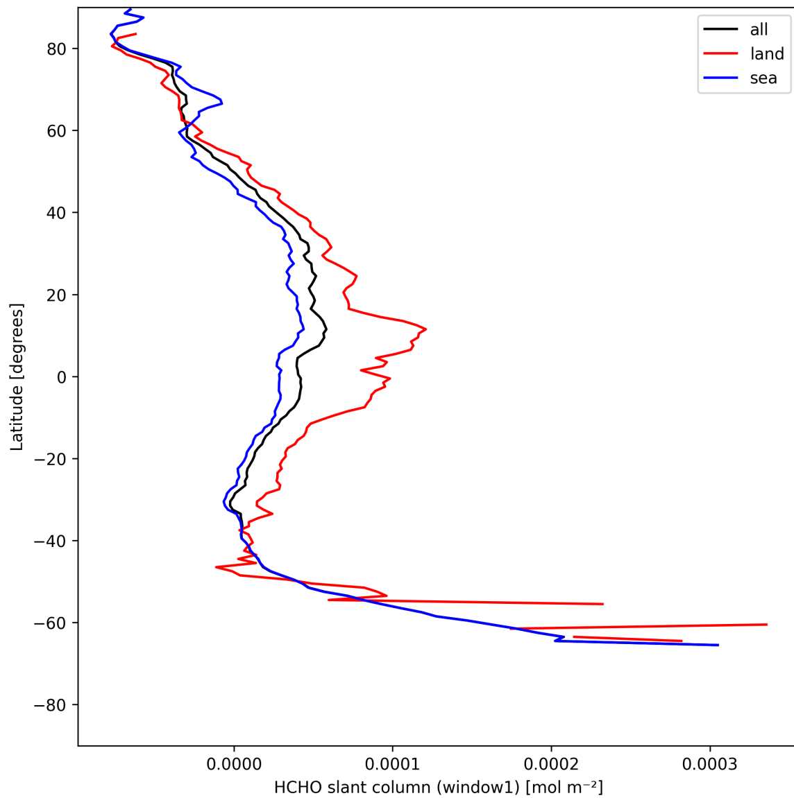
Figure 24: Zonal average of “HCHO slant column (window1)” for 2025-05-16 to 2025-05-18.
