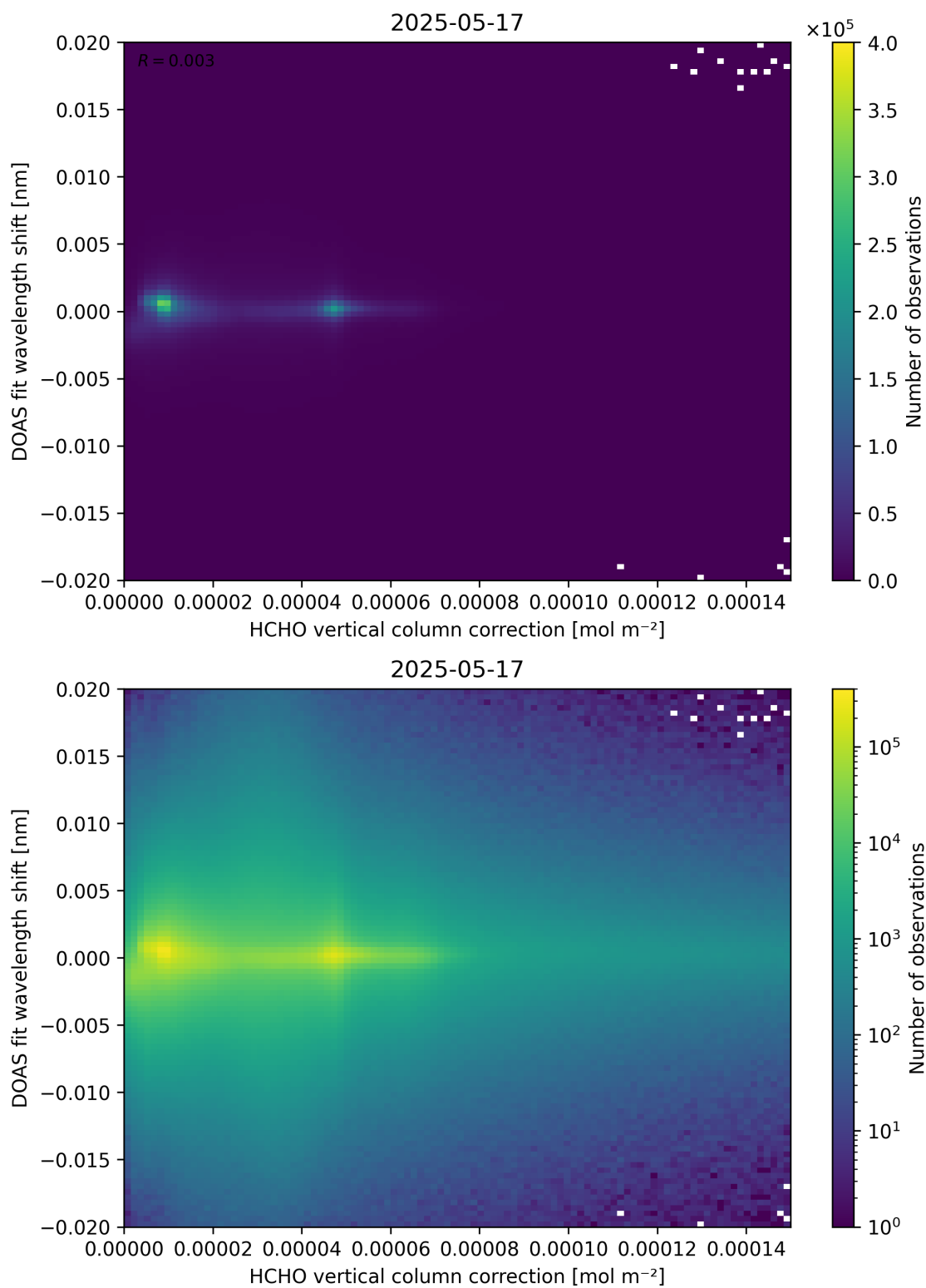
Figure 113: Scatter density plot of “HCHO vertical column correction” against “DOAS fit wavelength shift” for 2025-05-16 to 2025-05-18.
