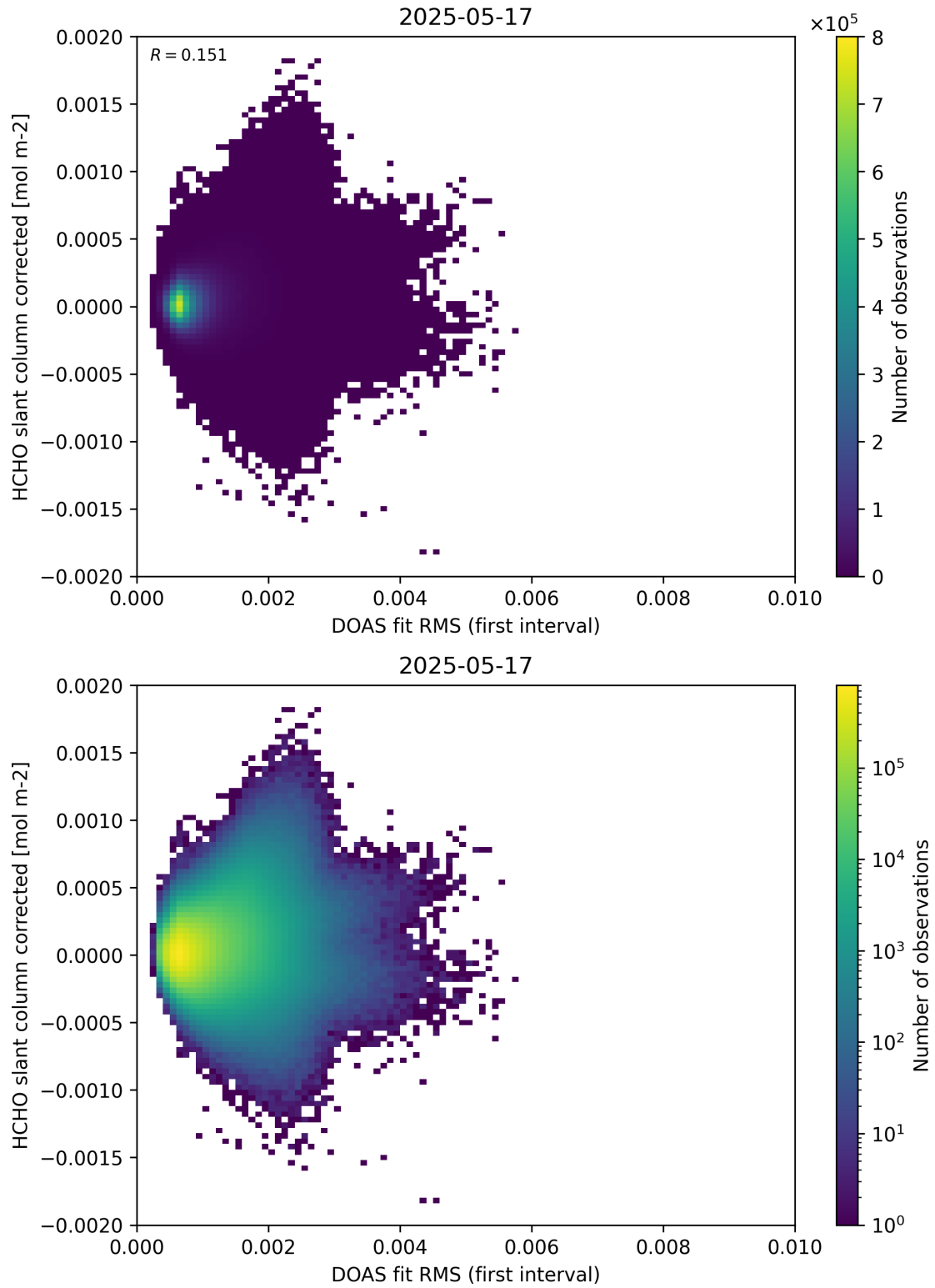
Figure 62: Scatter density plot of “DOAS fit RMS (first interval)” against “HCHO slant column corrected” for 2025-05-16 to 2025-05-18.
