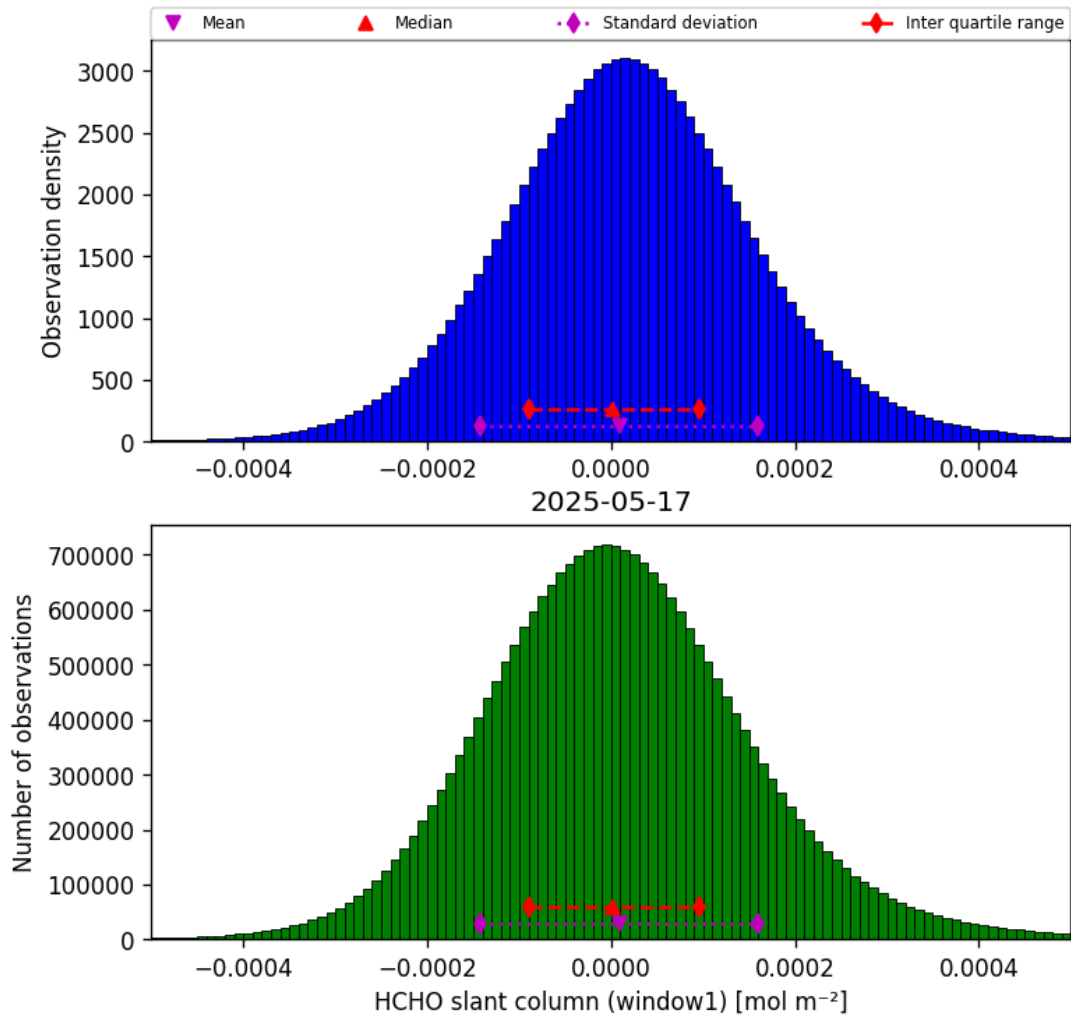
Figure 38: Histogram of “HCHO slant column (window1)” for 2025-05-16 to 2025-05-18
