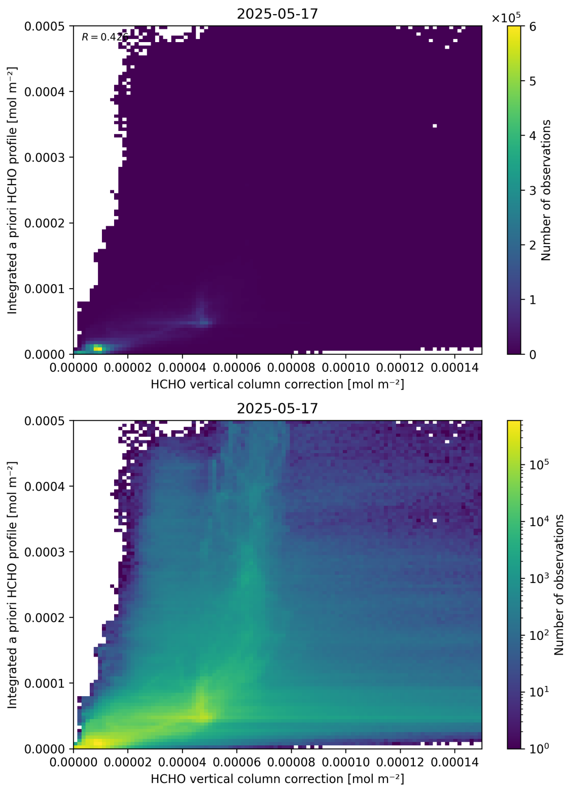
Figure 122: Scatter density plot of “HCHO vertical column correction” against “Integrated a priori HCHO profile” for 2025-05-16 to 2025-05-18.
