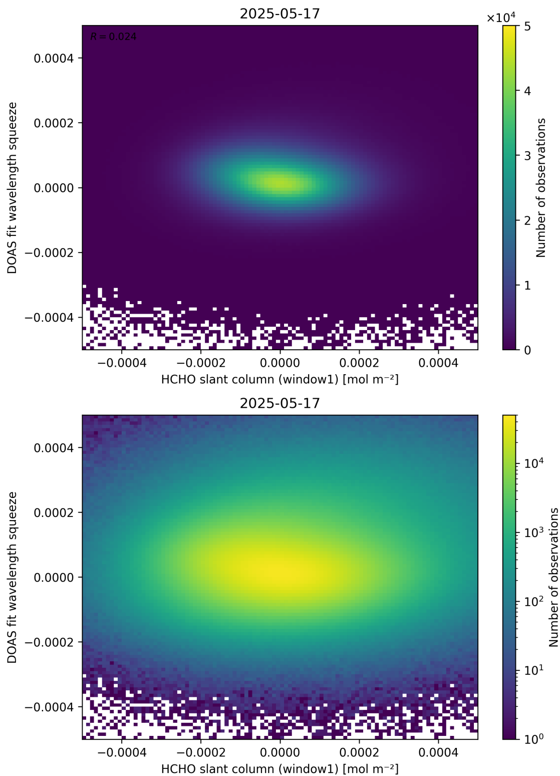
Figure 80: Scatter density plot of “HCHO slant column (window1)” against “DOAS fit wavelength squeeze” for 2025-05-16 to 2025-05-18.
