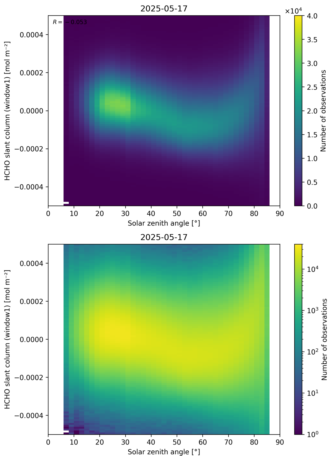
Figure 173: Scatter density plot of “Solar zenith angle” against “HCHO slant column (window1)” for 2025-05-16 to 2025-05-18.
