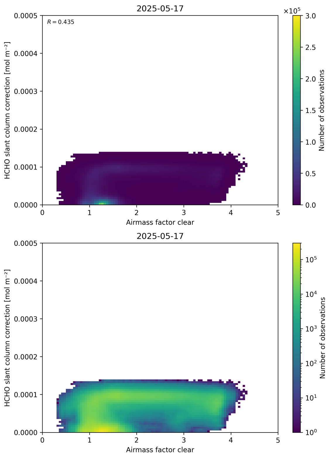
Figure 75: Scatter density plot of “Airmass factor clear” against “HCHO slant column correction” for 2025-05-16 to 2025-05-18.
