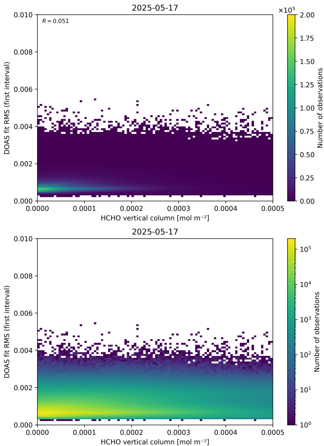
Figure 123: Scatter density plot of “HCHO vertical column” against “DOAS fit RMS (first interval)” for 2025-05-16 to 2025-05-18.
