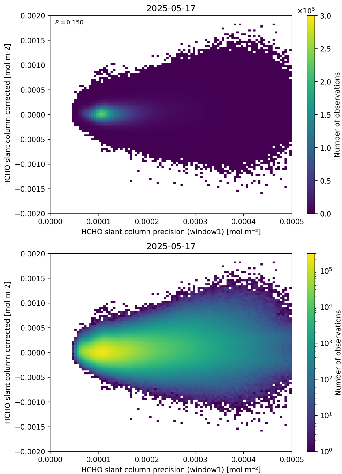
Figure 92: Scatter density plot of “HCHO slant column precision (window1)” against “HCHO slant column corrected” for 2025-05-16 to 2025-05-18.
