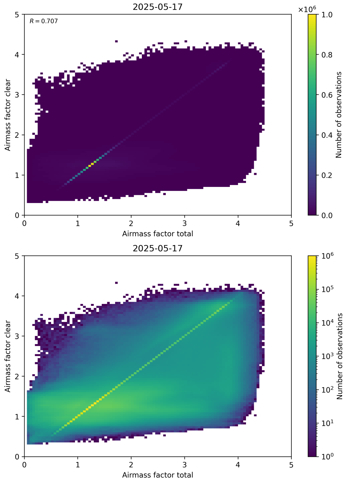
Figure 100: Scatter density plot of “Airmass factor total” against “Airmass factor clear” for 2025-05-16 to 2025-05-18.
