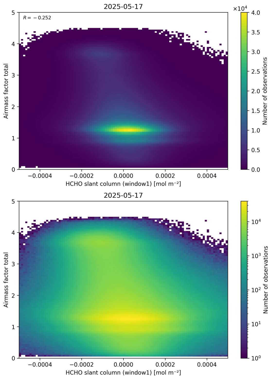
Figure 85: Scatter density plot of “HCHO slant column (window1)” against “Airmass factor total” for 2025-05-16 to 2025-05-18.
