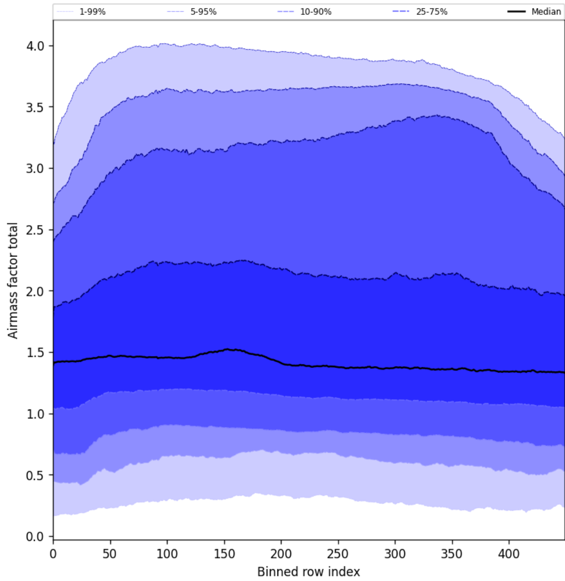
Figure 54: Along track statistics of “Airmass factor total” for 2025-05-16 to 2025-05-18
