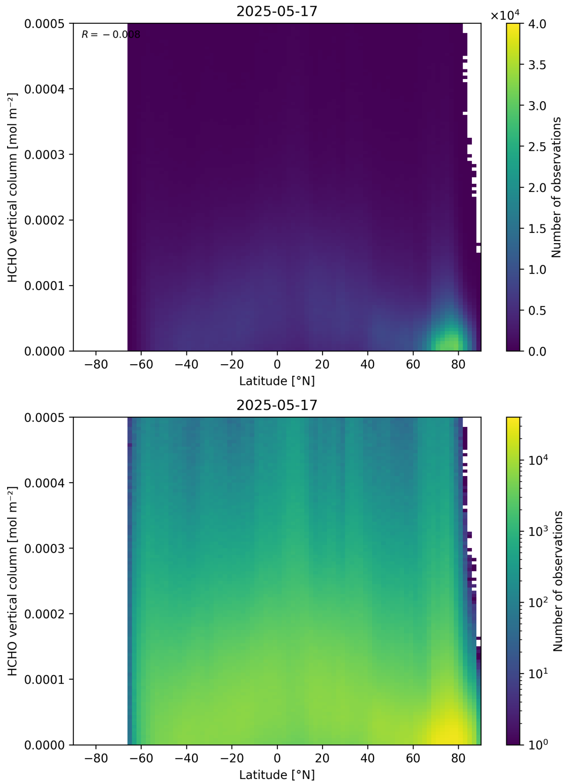
Figure 163: Scatter density plot of “Latitude” against “HCHO vertical column” for 2025-05-16 to 2025-05-18.
