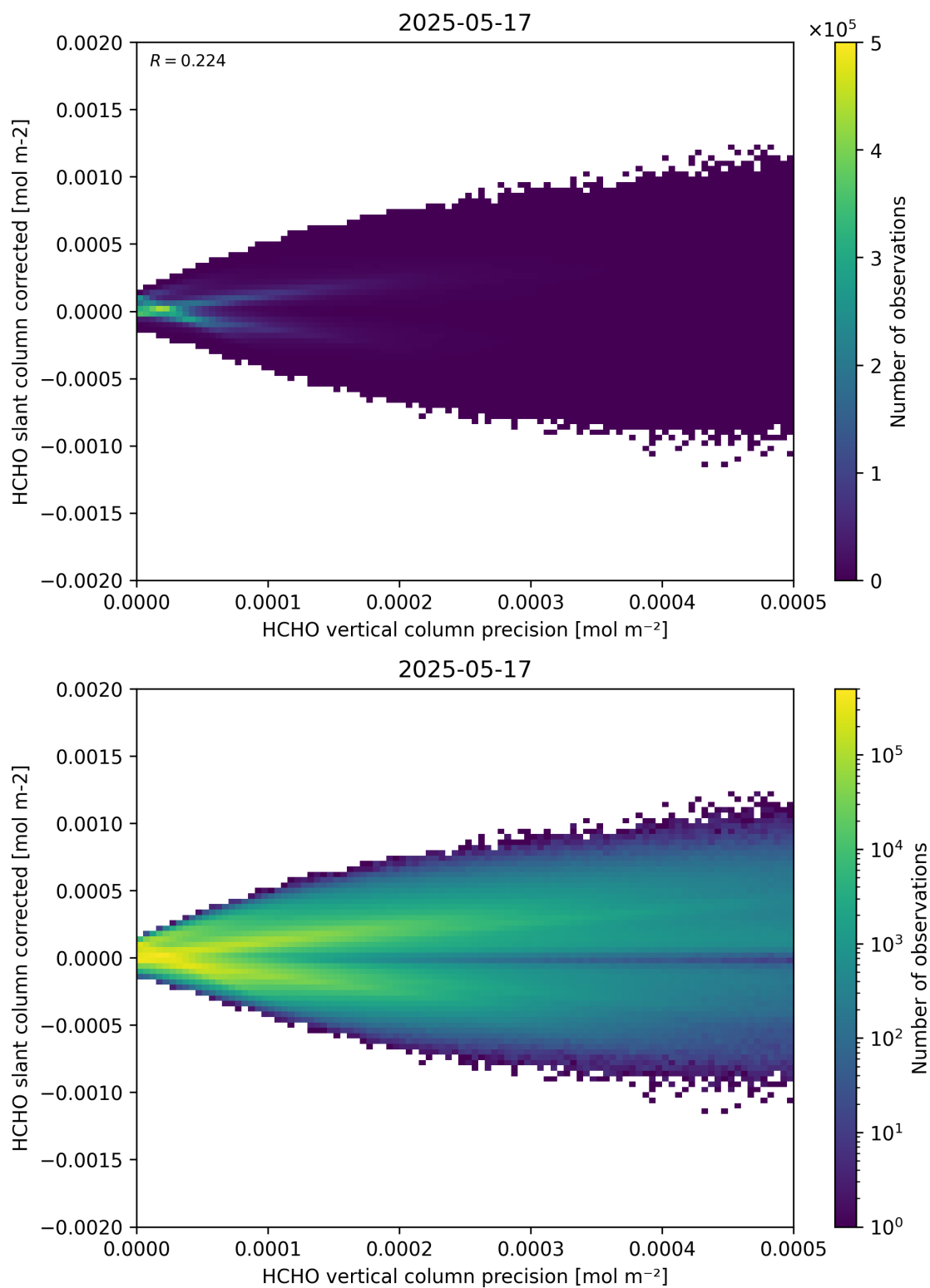
Figure 140: Scatter density plot of “HCHO vertical column precision” against “HCHO slant column corrected” for 2025-05-16 to 2025-05-18.
