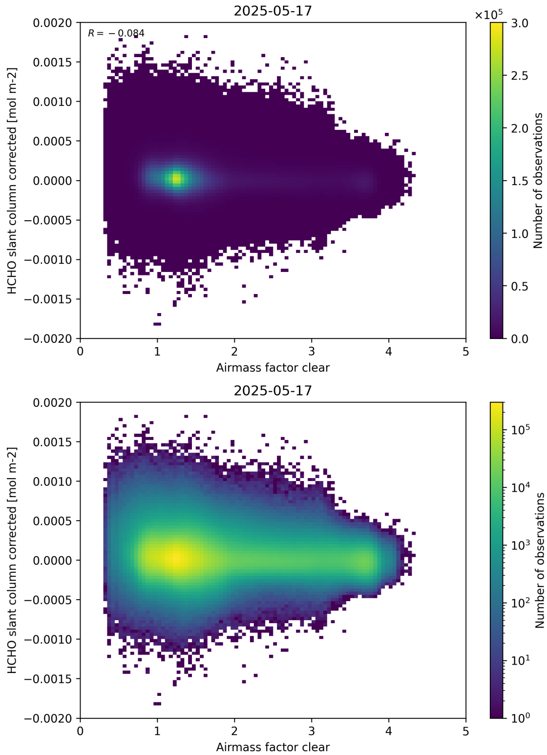
Figure 74: Scatter density plot of “Airmass factor clear” against “HCHO slant column corrected” for 2025-05-16 to 2025-05-18.
