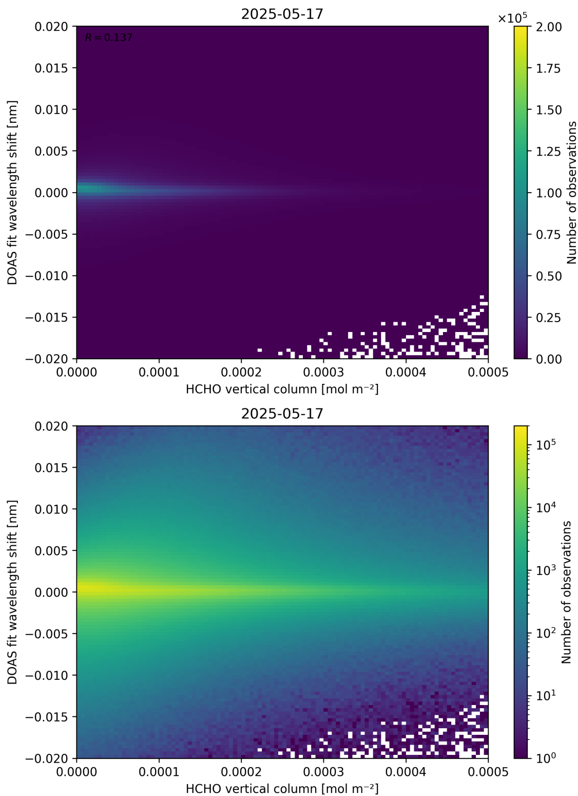
Figure 124: Scatter density plot of “HCHO vertical column” against “DOAS fit wavelength shift” for 2025-05-16 to 2025-05-18.
