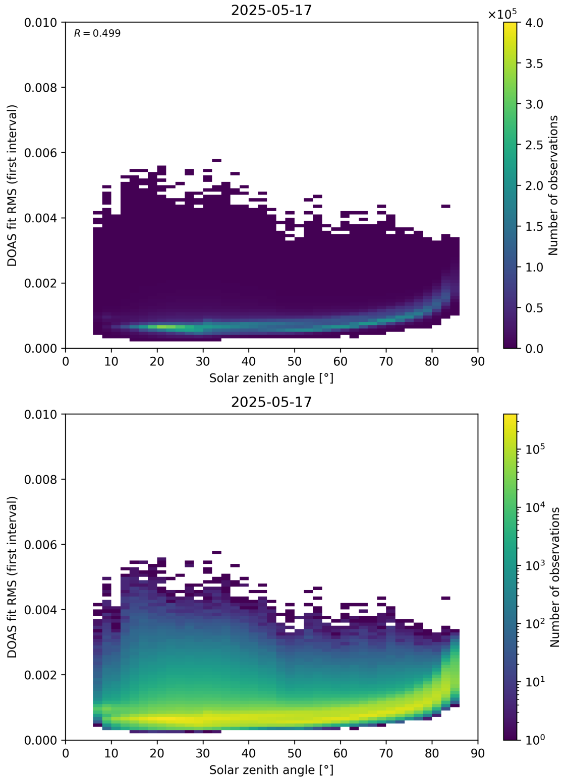
Figure 167: Scatter density plot of “Solar zenith angle” against “DOAS fit RMS (first interval)” for 2025-05-16 to 2025-05-18.
