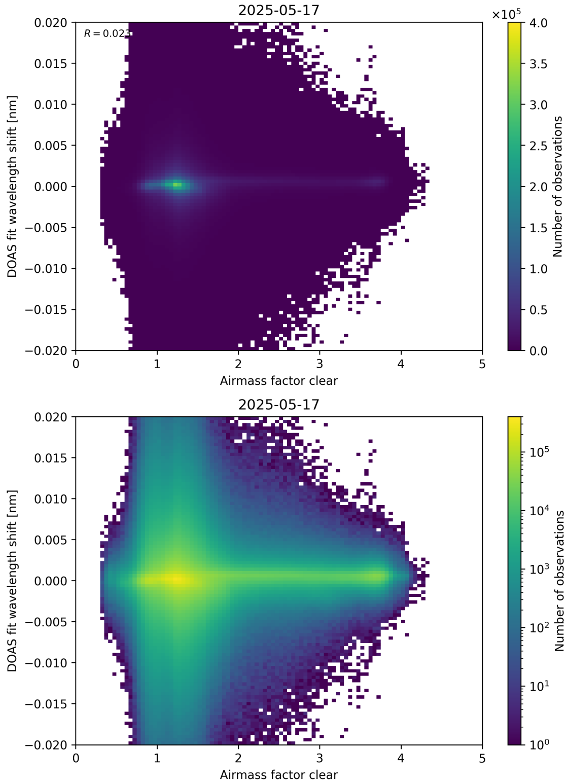
Figure 72: Scatter density plot of “Airmass factor clear” against “DOAS fit wavelength shift” for 2025-05-16 to 2025-05-18.
