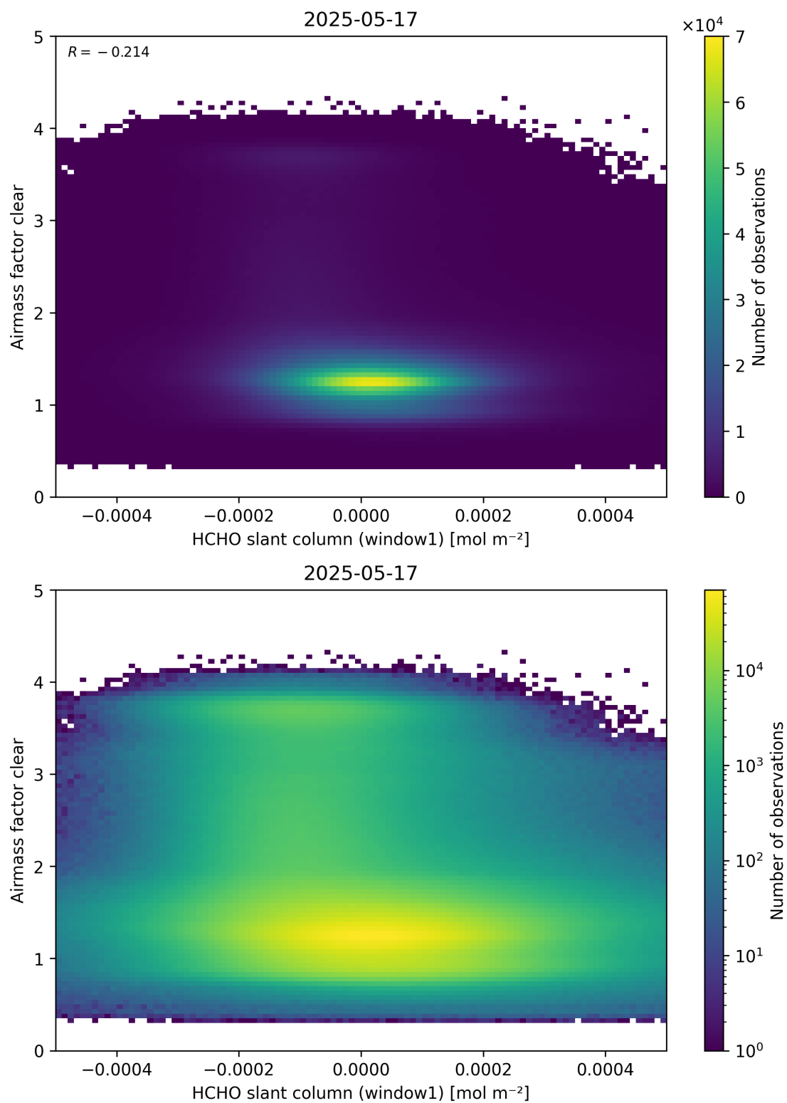
Figure 81: Scatter density plot of “HCHO slant column (window1)” against “Airmass factor clear” for 2025-05-16 to 2025-05-18.
