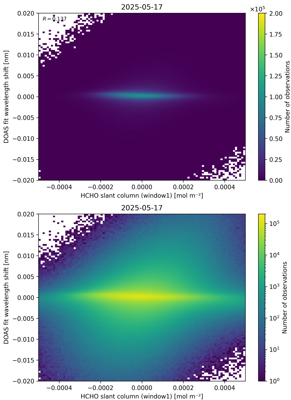
Figure 79: Scatter density plot of “HCHO slant column (window1)” against “DOAS fit wavelength shift” for 2025-05-16 to 2025-05-18.
