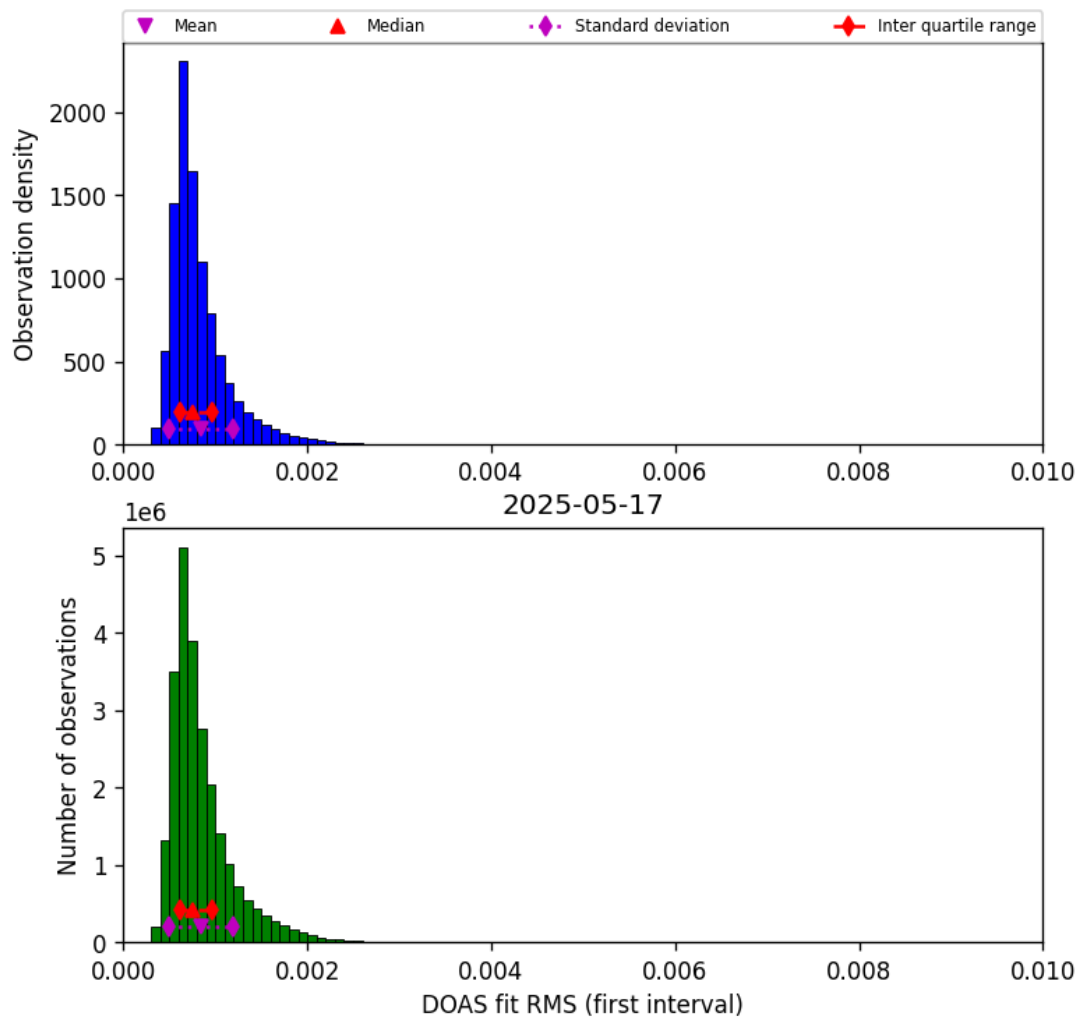
Figure 46: Histogram of “DOAS fit RMS (first interval)” for 2025-05-16 to 2025-05-18
