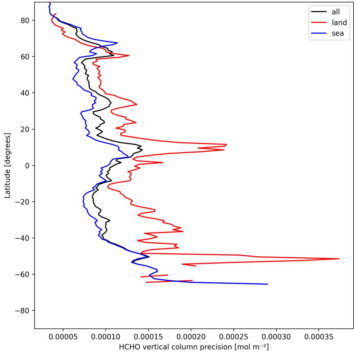
Figure 22: Zonal average of “HCHO vertical column precision” for 2025-05-16 to 2025-05-18.
