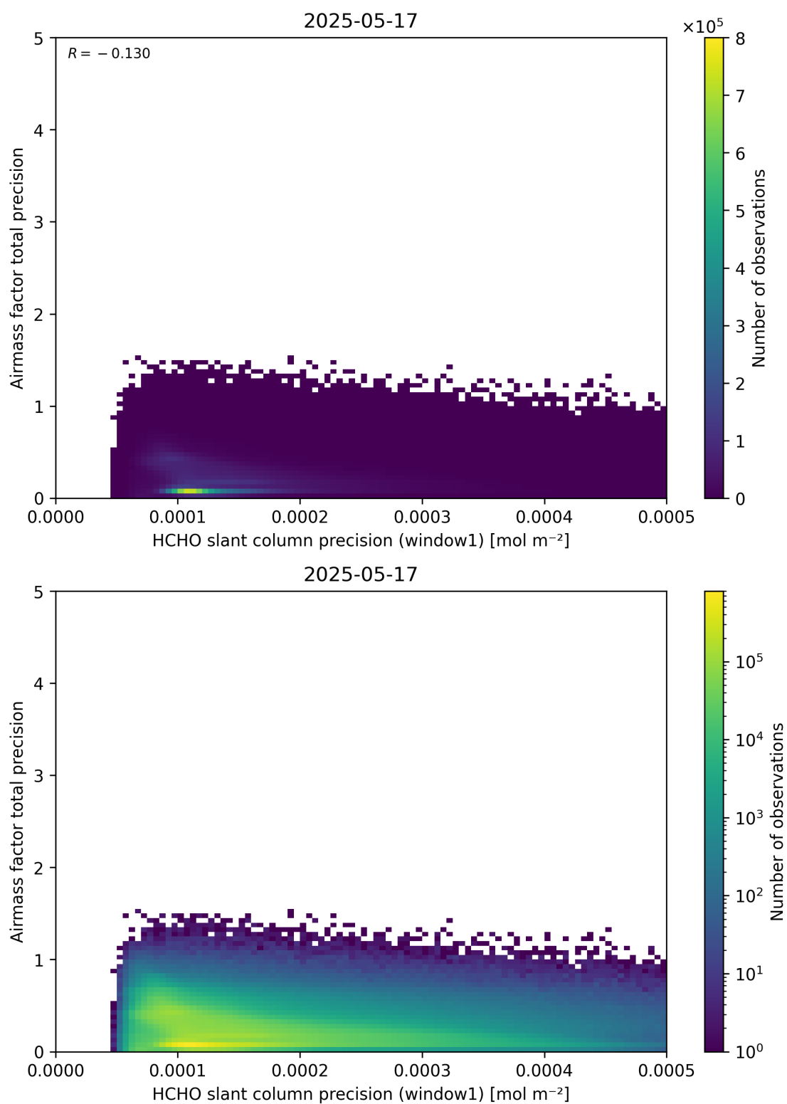
Figure 95: Scatter density plot of “HCHO slant column precision (window1)” against “Airmass factor total precision” for 2025-05-16 to 2025-05-18.
