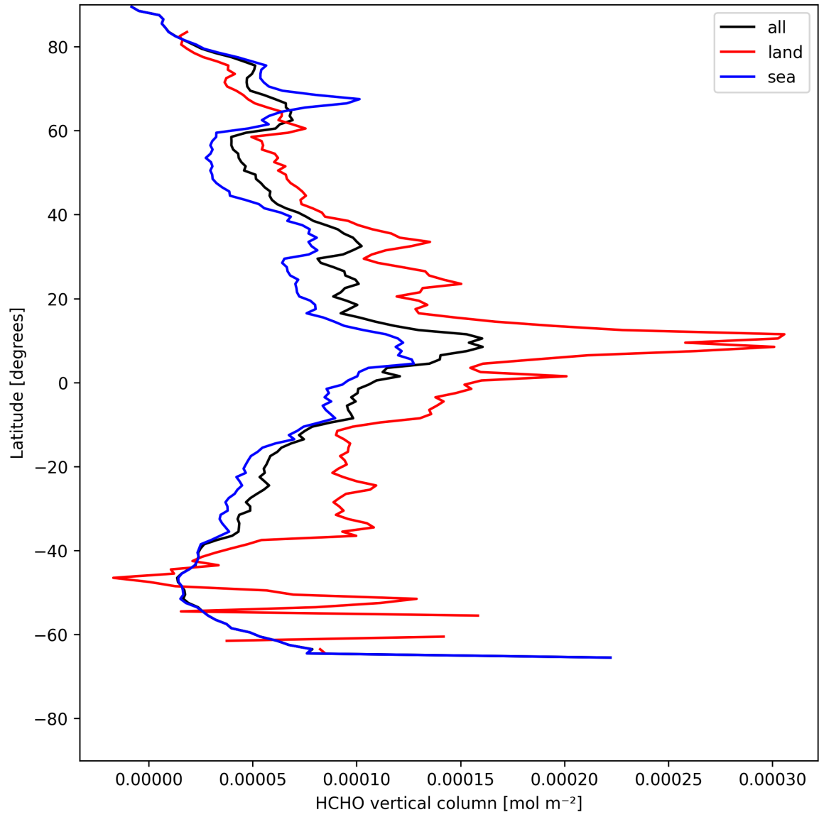
Figure 21: Zonal average of “HCHO vertical column” for 2025-05-16 to 2025-05-18.
