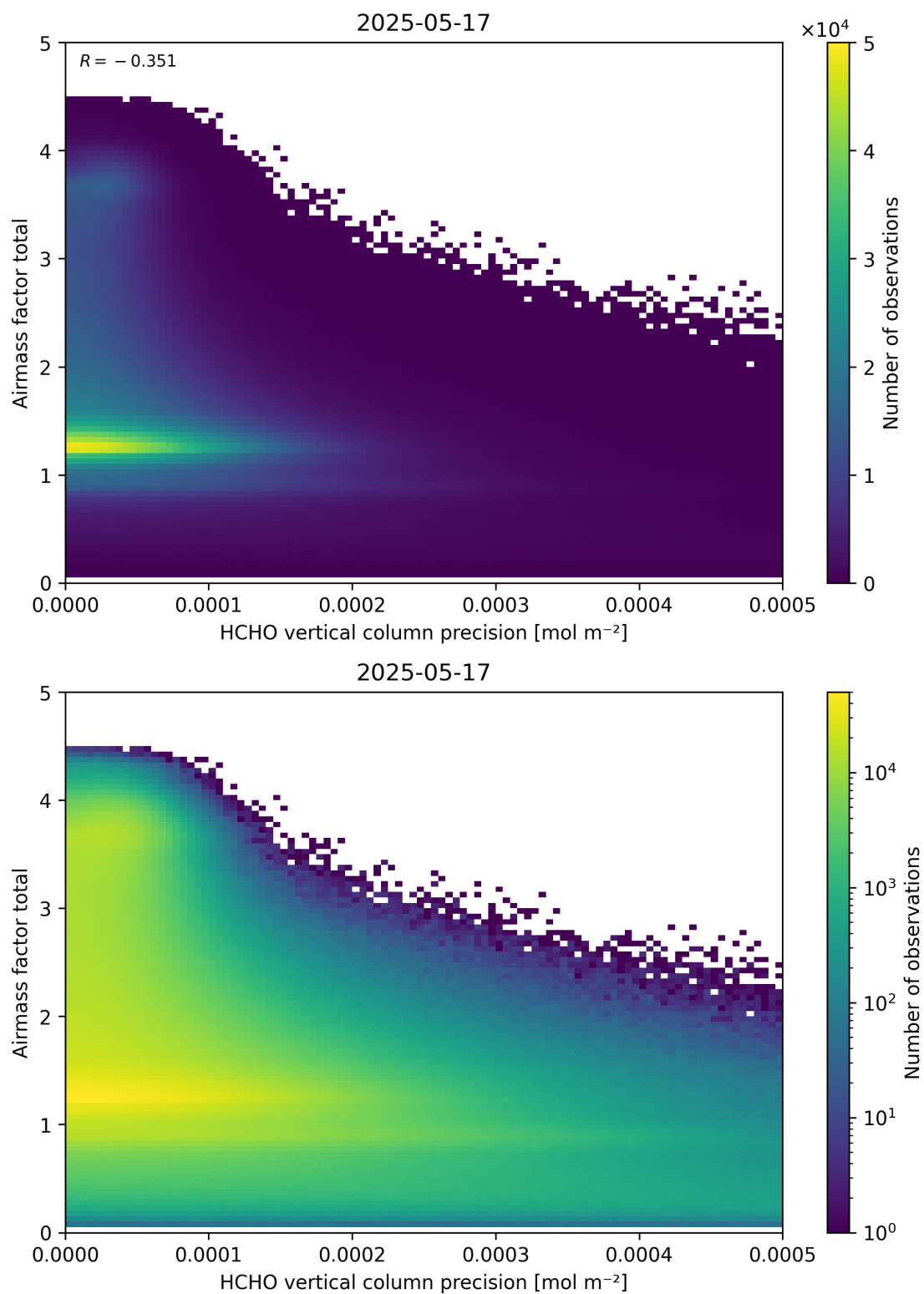
Figure 144: Scatter density plot of “HCHO vertical column precision” against “Airmass factor total” for 2025-05-16 to 2025-05-18.
