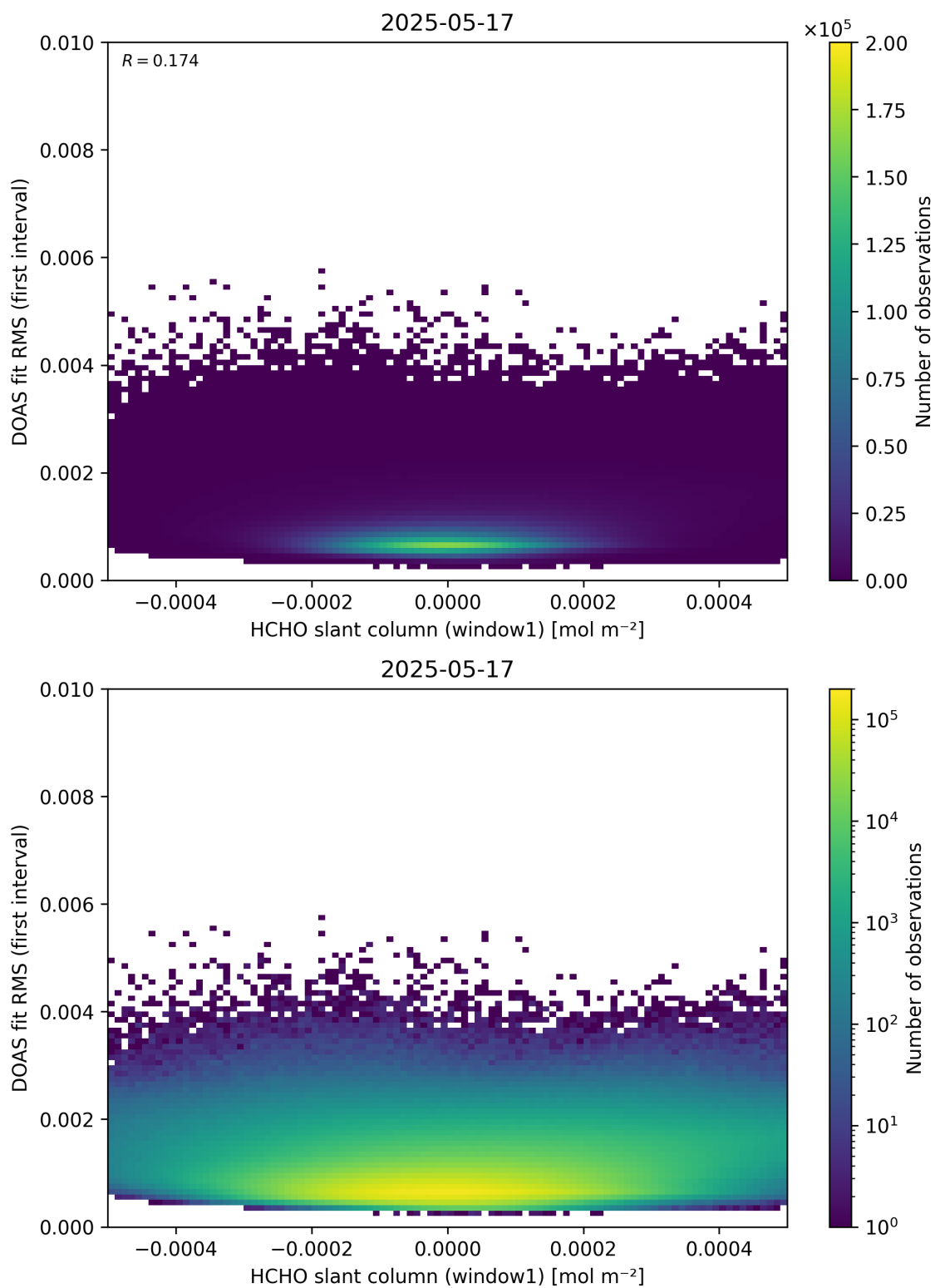
Figure 78: Scatter density plot of “HCHO slant column (window1)” against “DOAS fit RMS (first interval)” for 2025-05-16 to 2025-05-18.
