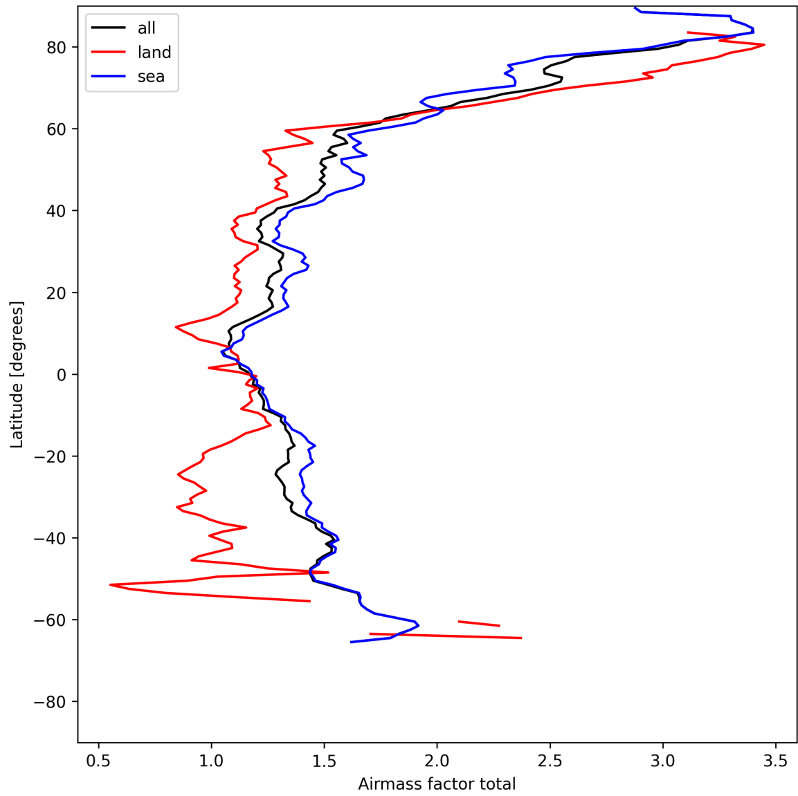
Figure 26: Zonal average of “Airmass factor total” for 2025-05-16 to 2025-05-18.
