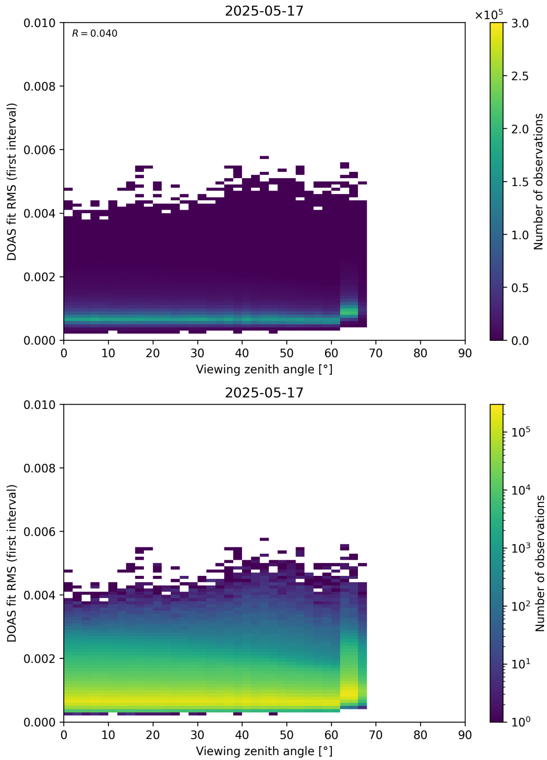
Figure 182: Scatter density plot of “Viewing zenith angle” against “DOAS fit RMS (first interval)” for 2025-05-16 to 2025-05-18.
