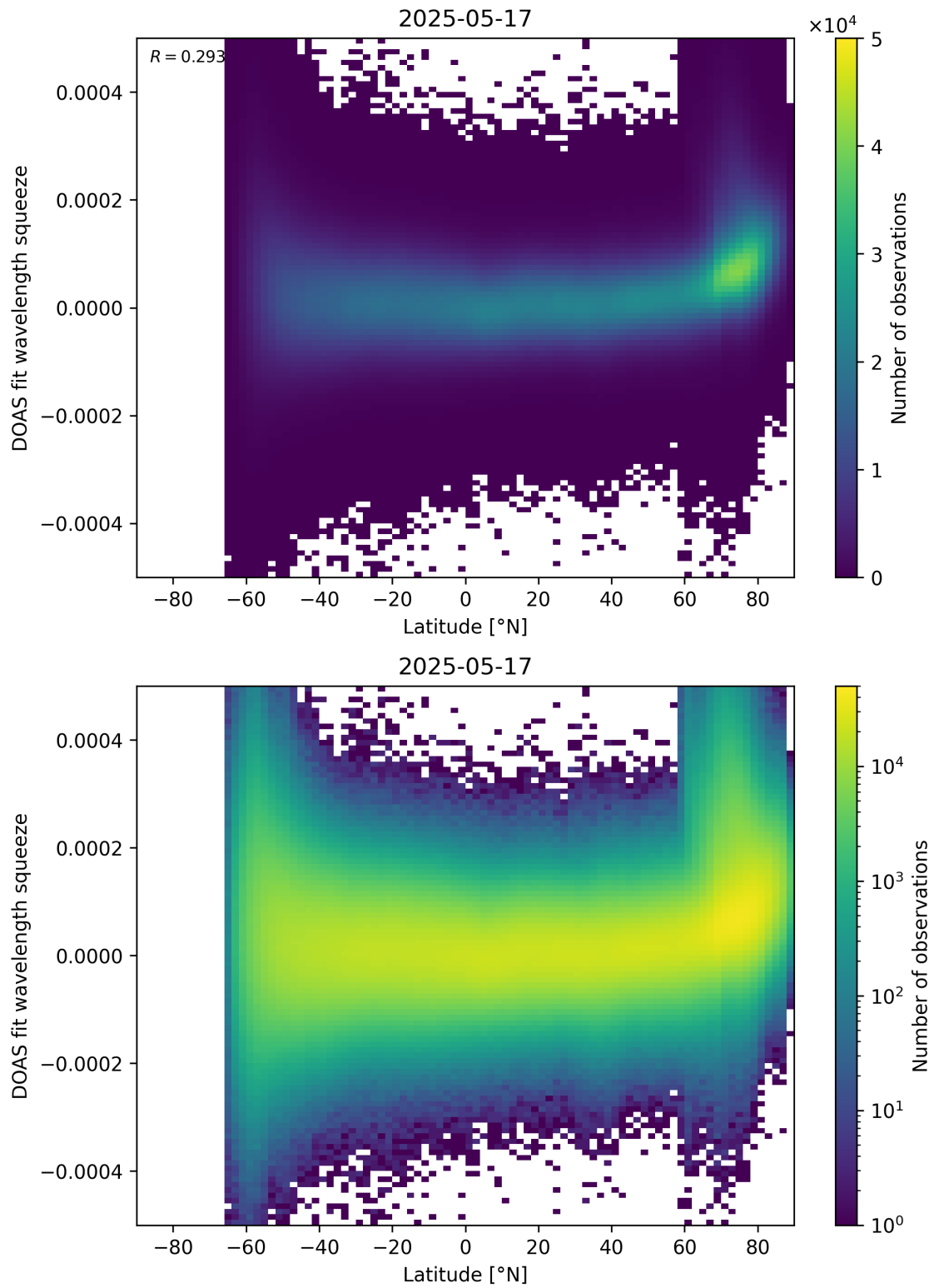
Figure 155: Scatter density plot of “Latitude” against “DOAS fit wavelength squeeze” for 2025-05-16 to 2025-05-18.
