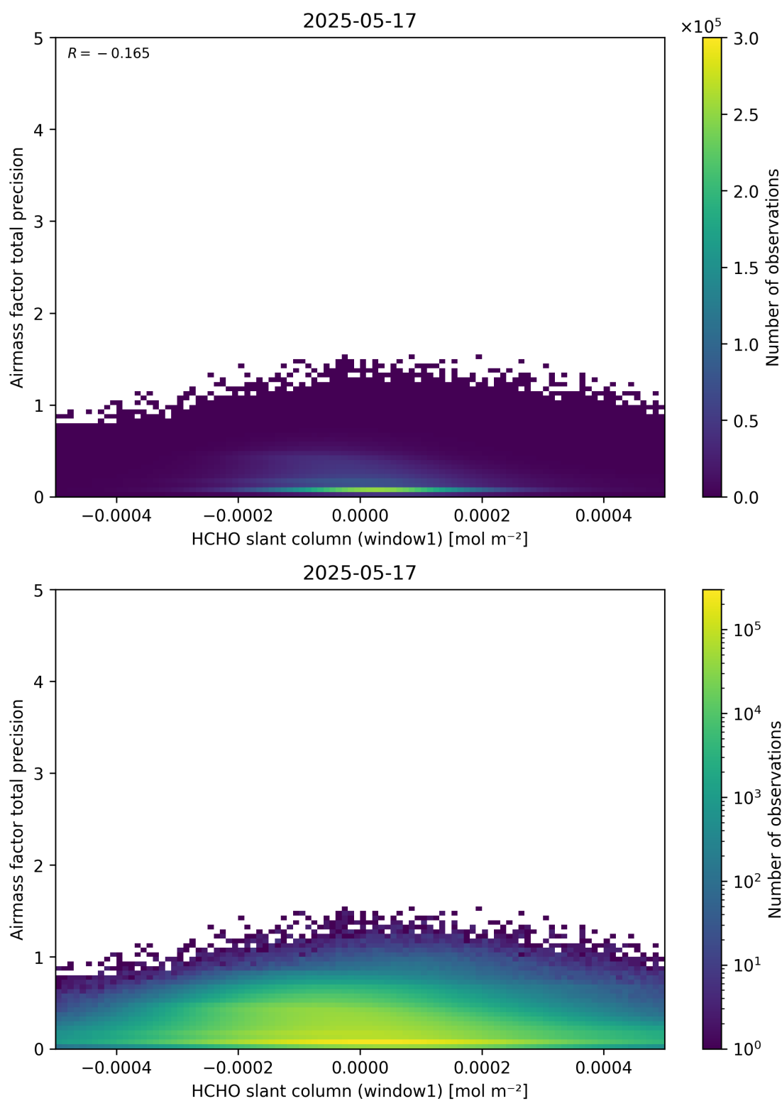
Figure 86: Scatter density plot of “HCHO slant column (window1)” against “Airmass factor total precision” for 2025-05-16 to 2025-05-18.
