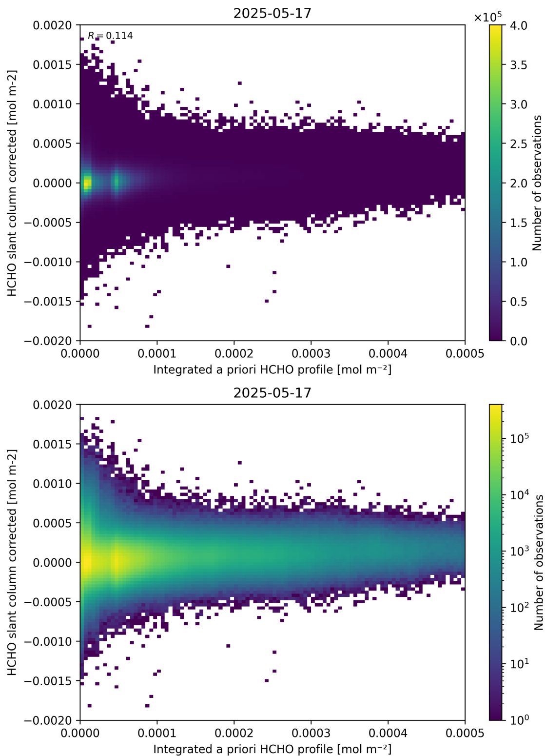
Figure 151: Scatter density plot of “Integrated a priori HCHO profile” against “HCHO slant column corrected” for 2025-05-16 to 2025-05-18.
