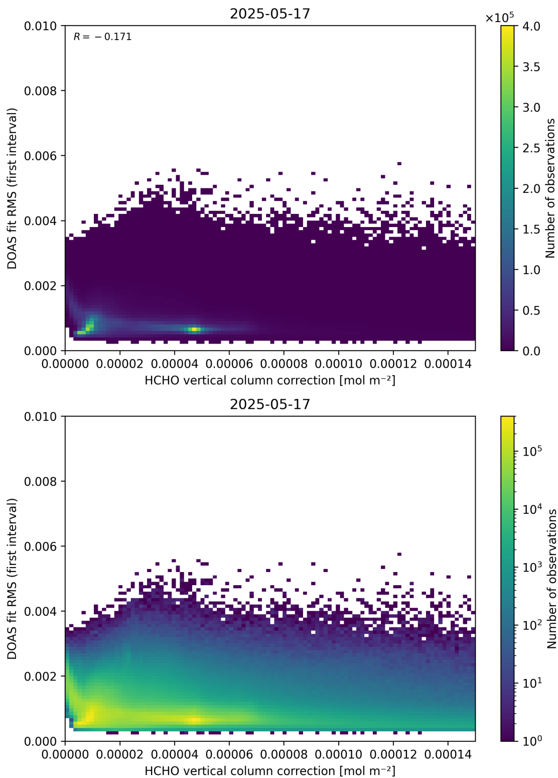
Figure 112: Scatter density plot of “HCHO vertical column correction” against “DOAS fit RMS (first interval)” for 2025-05-16 to 2025-05-18.
