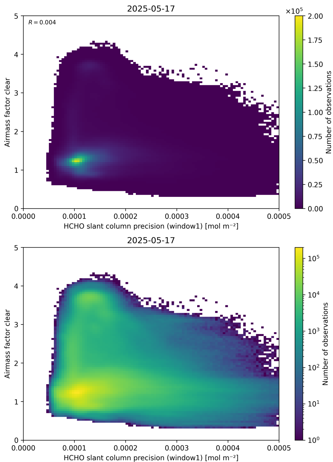
Figure 91: Scatter density plot of “HCHO slant column precision (window1)” against “Airmass factor clear” for 2025-05-16 to 2025-05-18.
