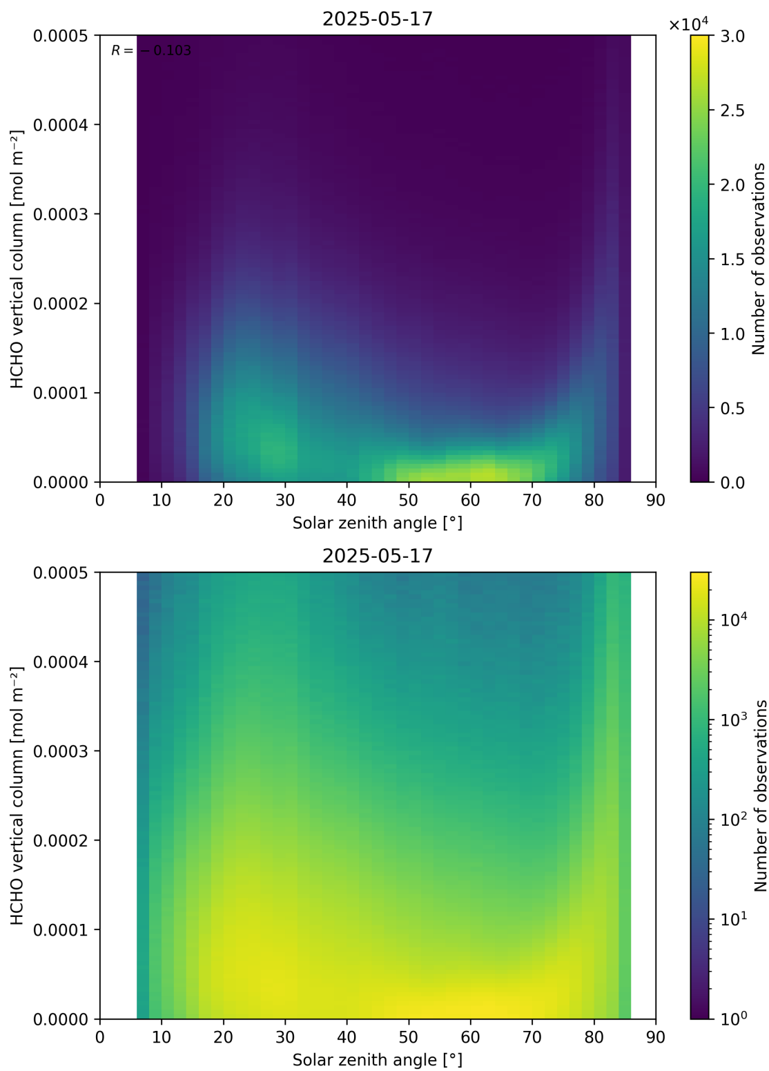
Figure 177: Scatter density plot of “Solar zenith angle” against “HCHO vertical column” for 2025-05-16 to 2025-05-18.
