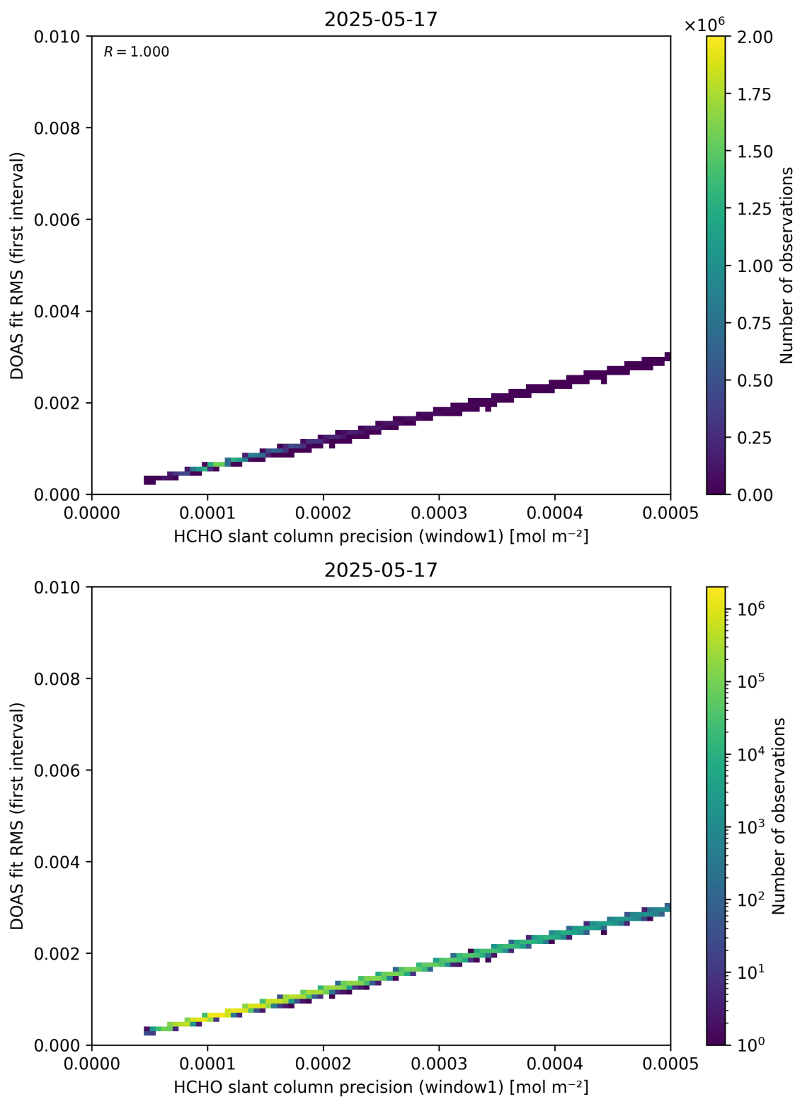
Figure 88: Scatter density plot of “HCHO slant column precision (window1)” against “DOAS fit RMS (first interval)” for 2025-05-16 to 2025-05-18.
