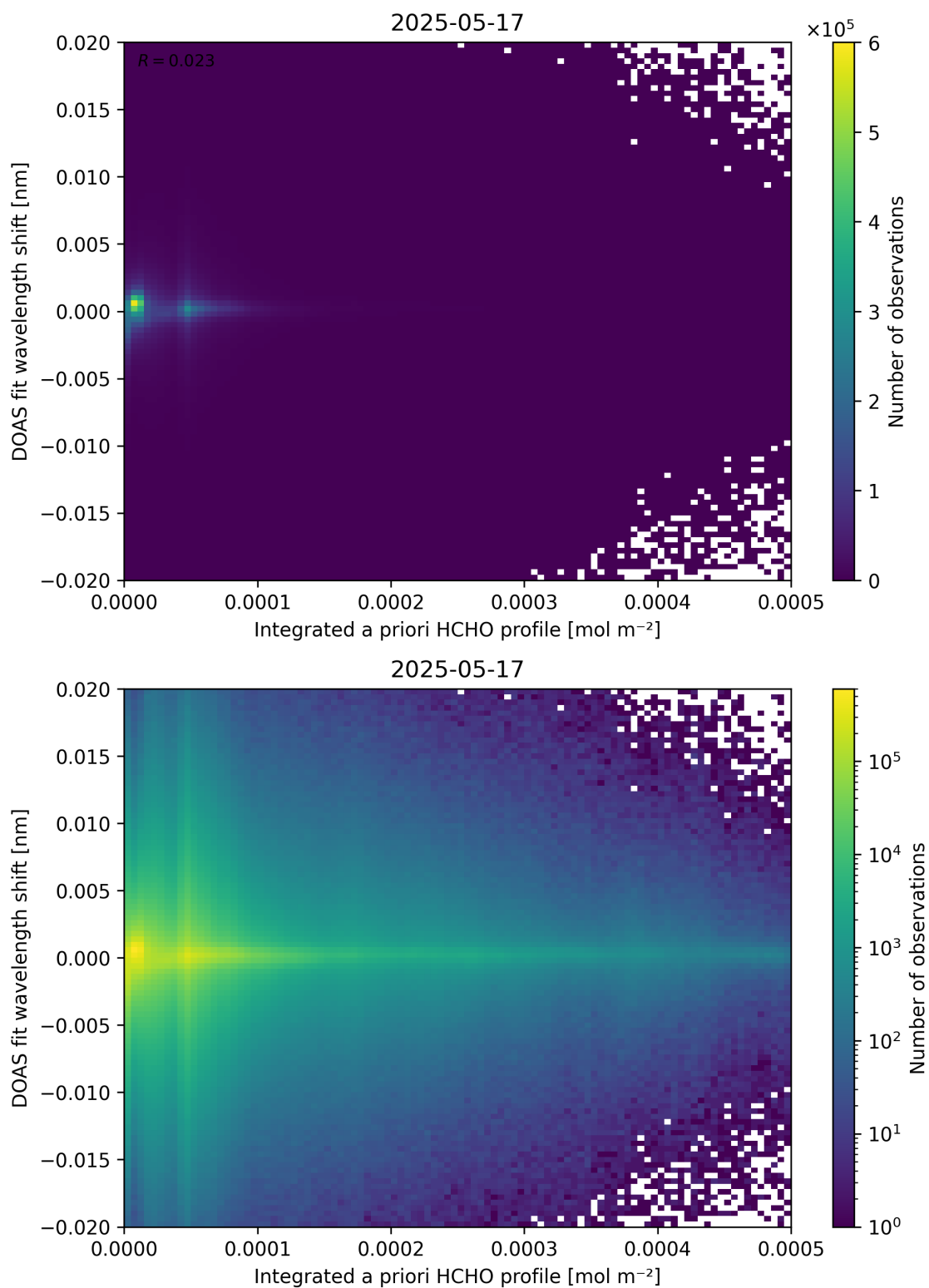
Figure 149: Scatter density plot of “Integrated a priori HCHO profile” against “DOAS fit wavelength shift” for 2025-05-16 to 2025-05-18.
