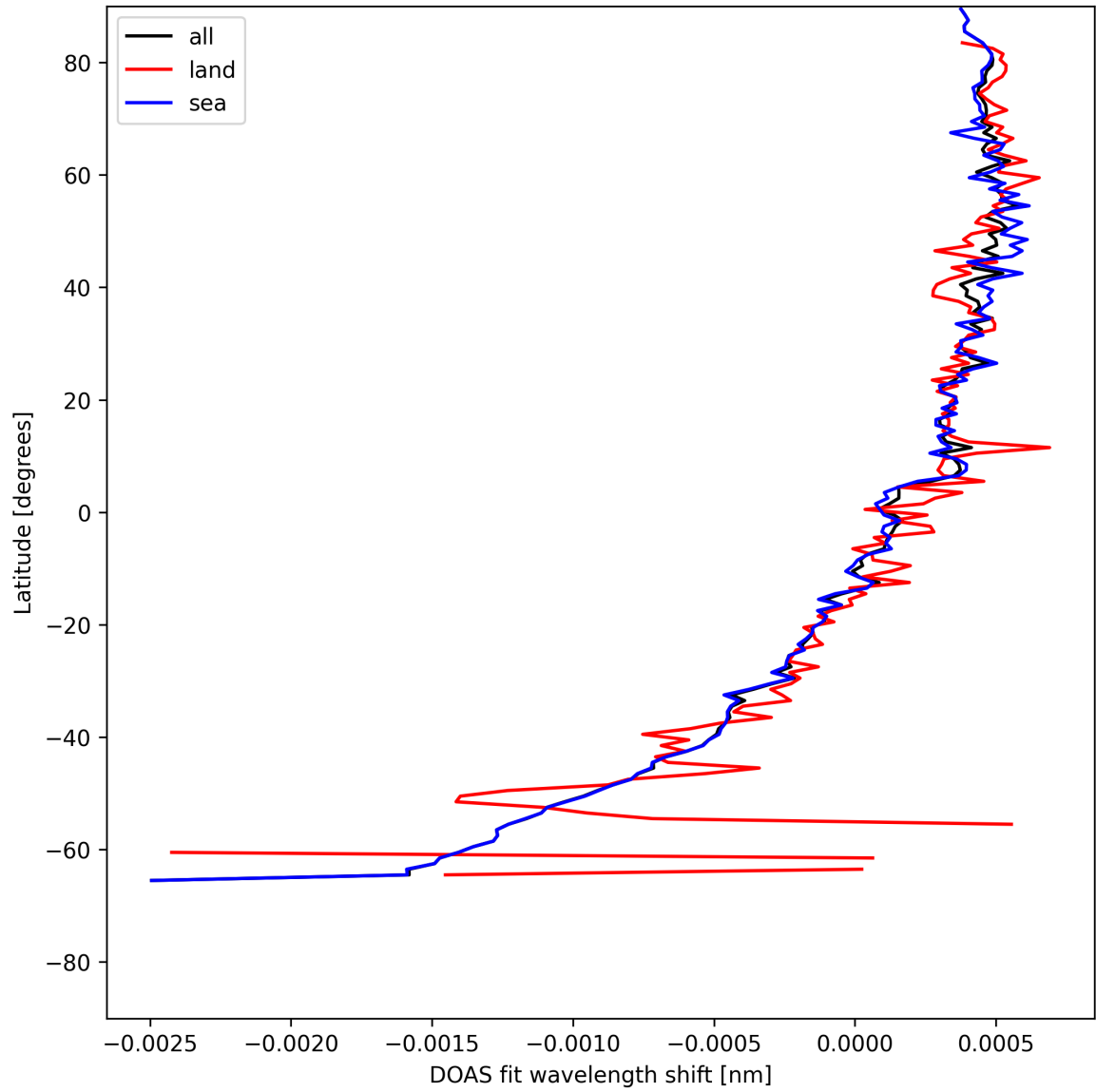
Figure 30: Zonal average of “DOAS fit wavelength shift” for 2025-05-16 to 2025-05-18.
