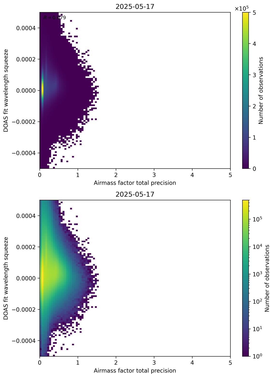
Figure 107: Scatter density plot of “Airmass factor total precision” against “DOAS fit wavelength squeeze” for 2025-05-16 to 2025-05-18.
