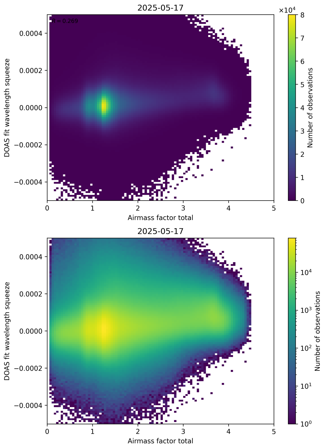
Figure 99: Scatter density plot of “Airmass factor total” against “DOAS fit wavelength squeeze” for 2025-05-16 to 2025-05-18.
