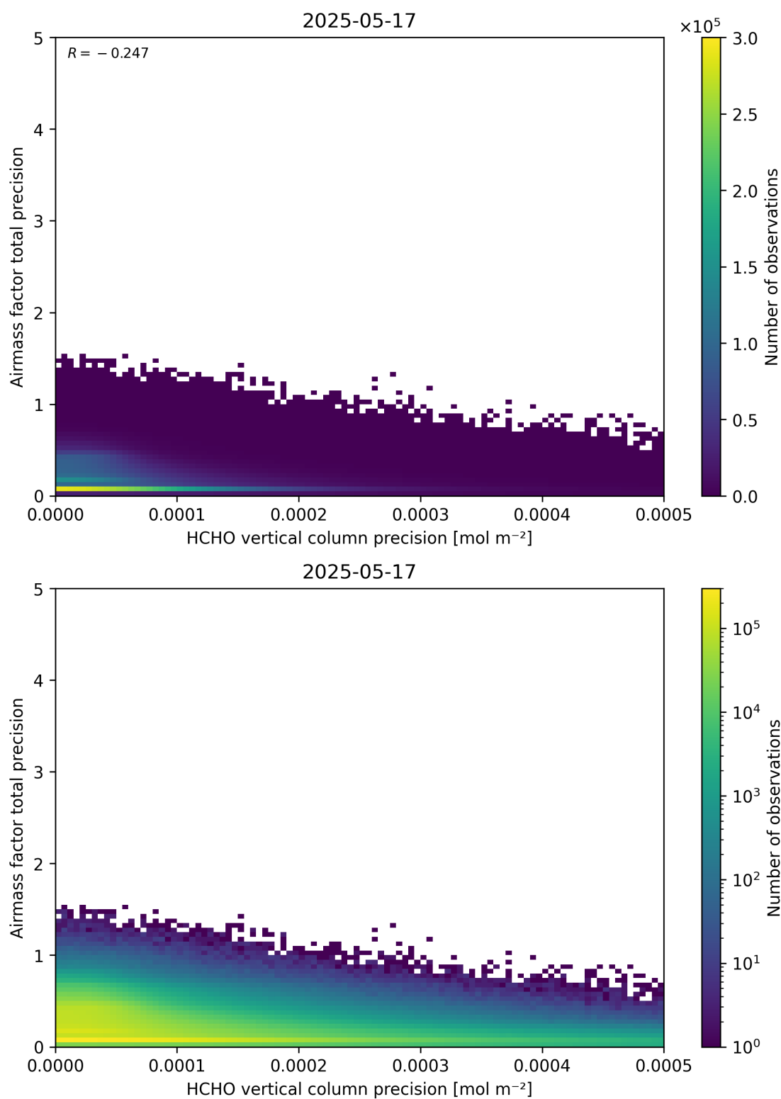
Figure 145: Scatter density plot of “HCHO vertical column precision” against “Airmass factor total precision” for 2025-05-16 to 2025-05-18.
