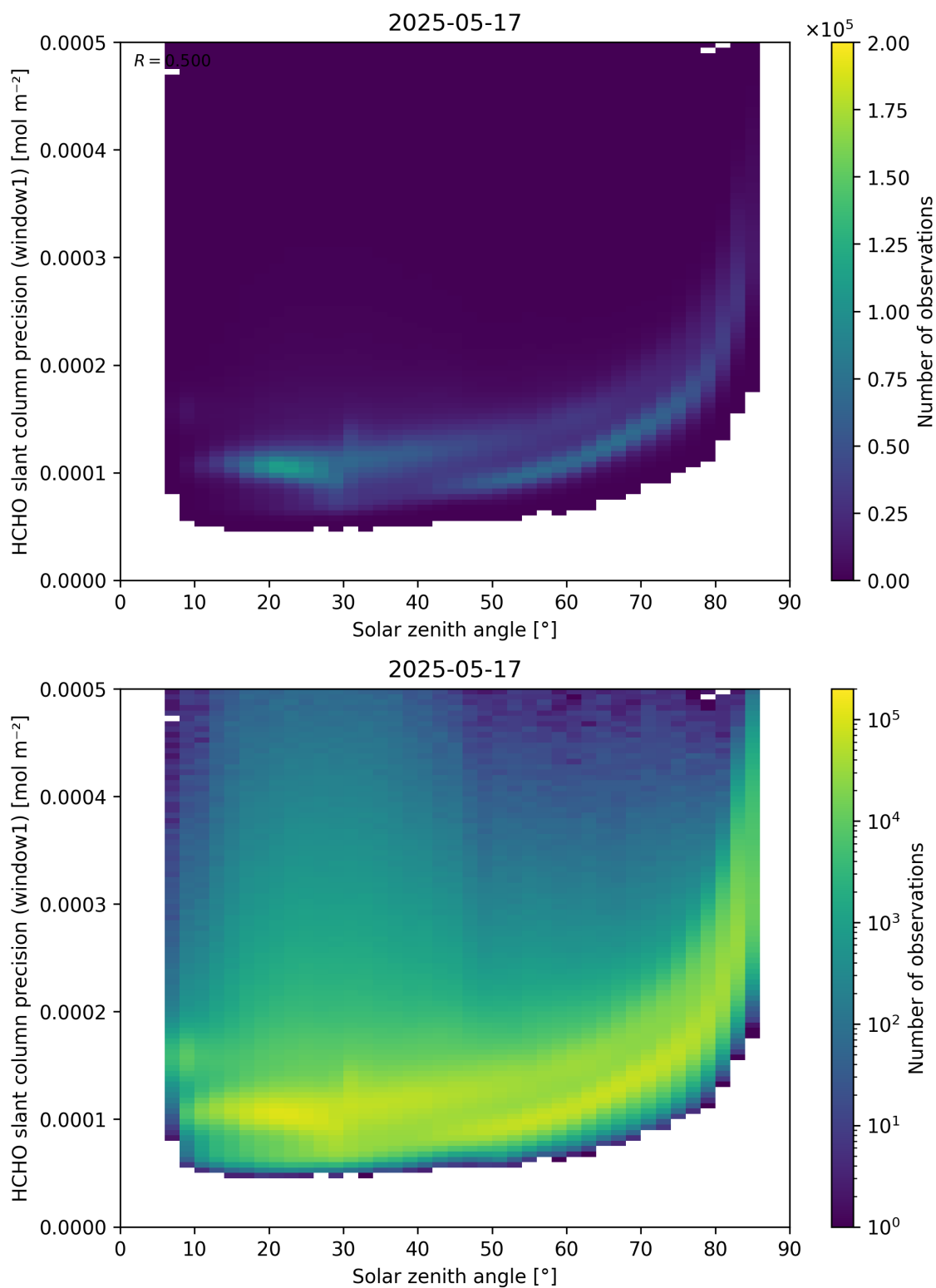
Figure 174: Scatter density plot of “Solar zenith angle” against “HCHO slant column precision (window1)” for 2025-05-16 to 2025-05-18.
