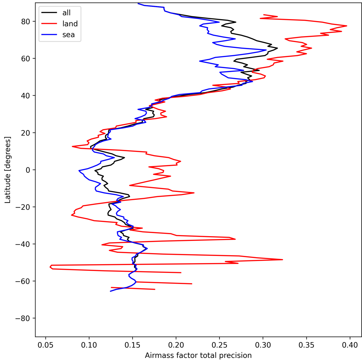
Figure 27: Zonal average of “Airmass factor total precision” for 2025-05-16 to 2025-05-18.
