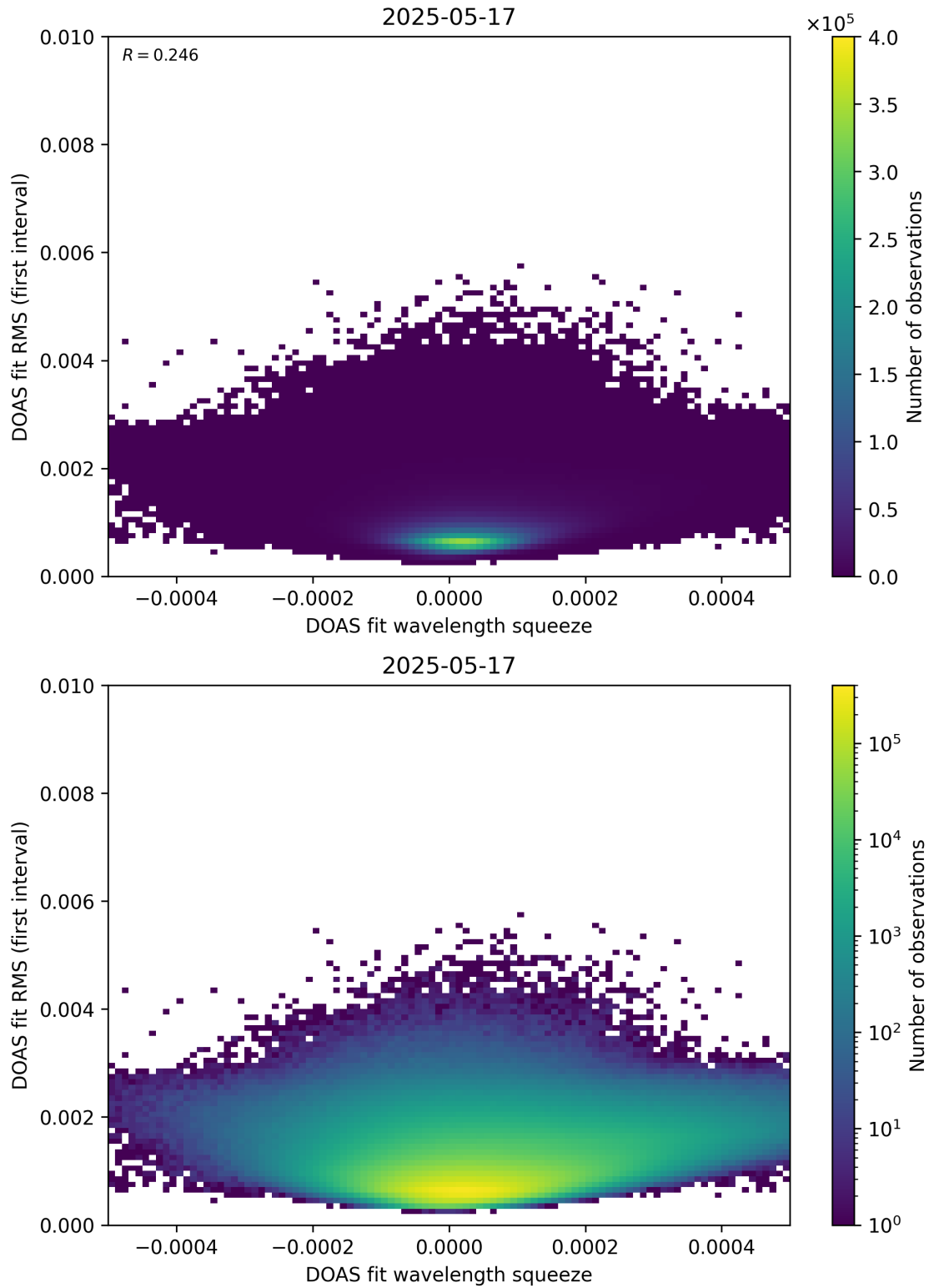
Figure 68: Scatter density plot of “DOAS fit wavelength squeeze” against “DOAS fit RMS (first interval)” for 2025-05-16 to 2025-05-18.
