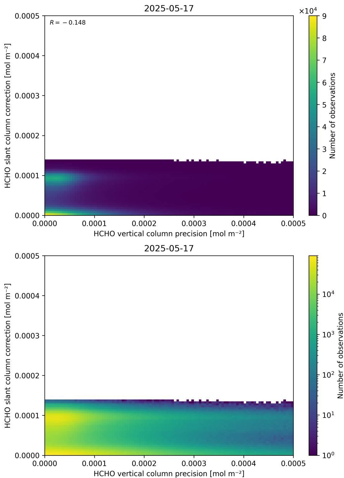
Figure 141: Scatter density plot of “HCHO vertical column precision” against “HCHO slant column correction” for 2025-05-16 to 2025-05-18.
