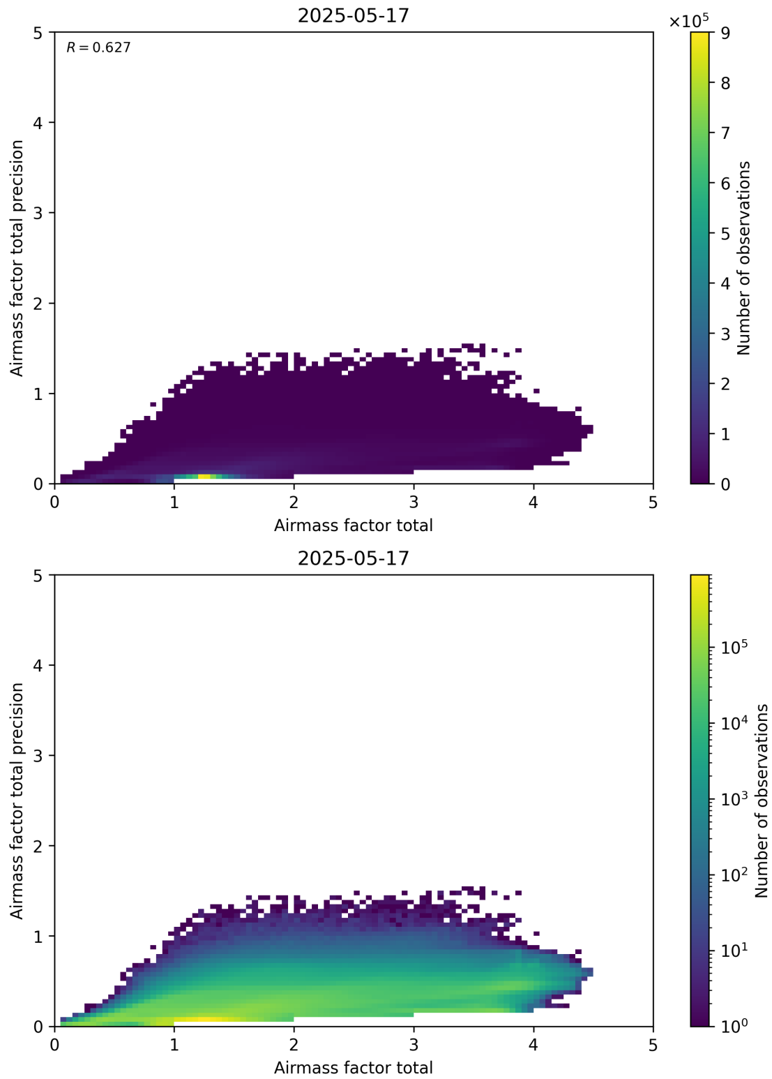
Figure 103: Scatter density plot of “Airmass factor total” against “Airmass factor total precision” for 2025-05-16 to 2025-05-18.
