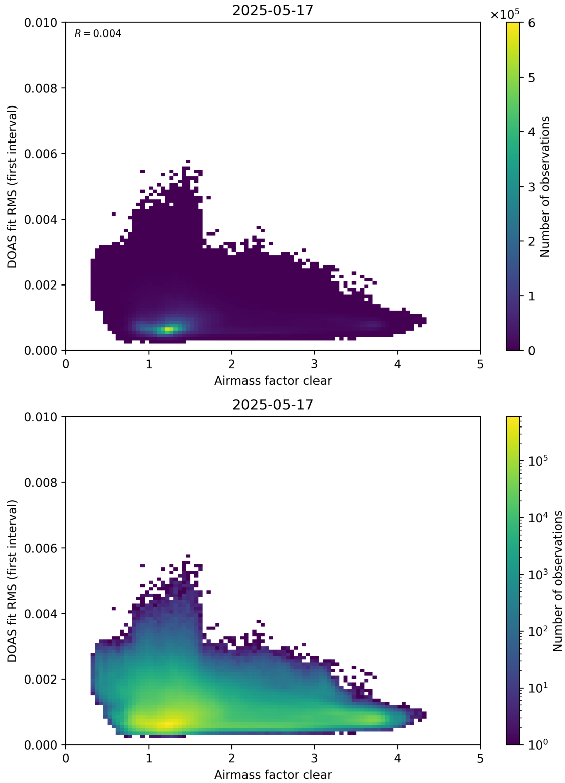
Figure 71: Scatter density plot of “Airmass factor clear” against “DOAS fit RMS (first interval)” for 2025-05-16 to 2025-05-18.
