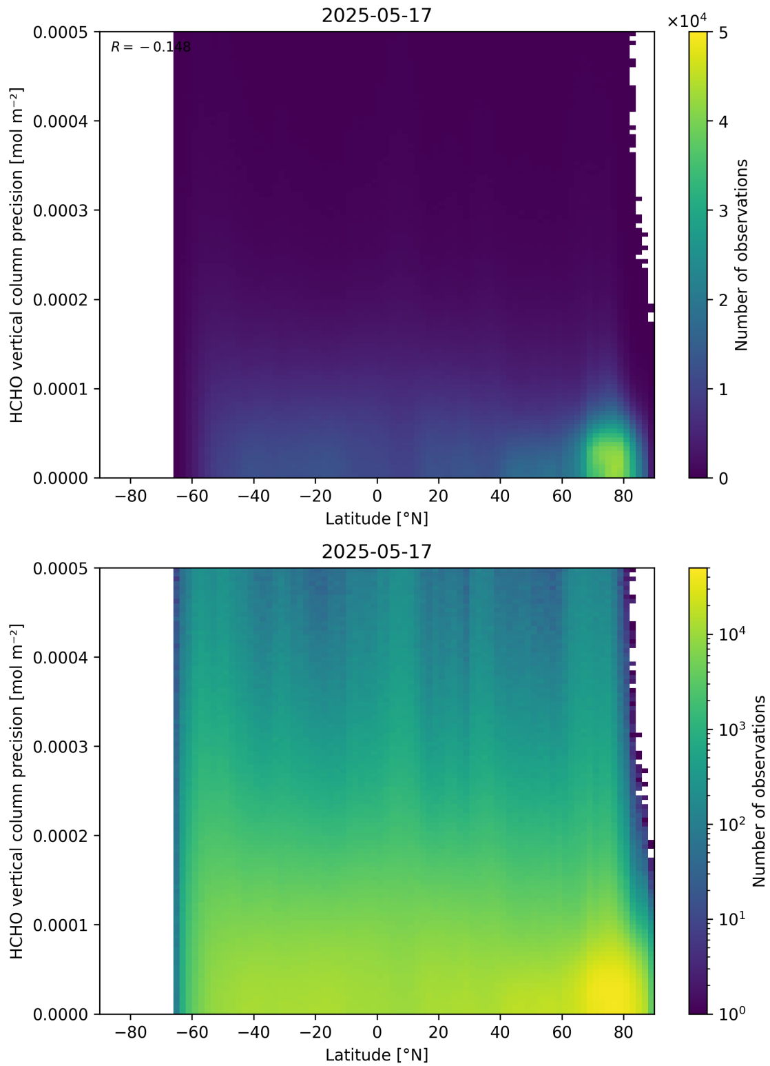
Figure 165: Scatter density plot of “Latitude” against “HCHO vertical column precision” for 2025-05-16 to 2025-05-18.
