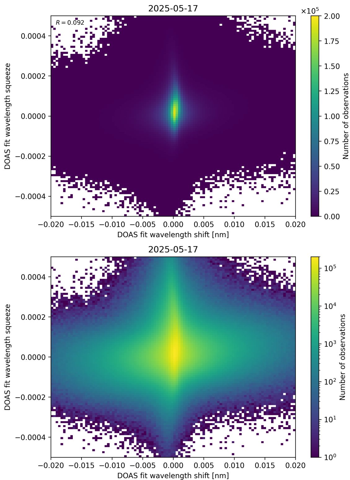
Figure 65: Scatter density plot of “DOAS fit wavelength shift” against “DOAS fit wavelength squeeze” for 2025-05-16 to 2025-05-18.
