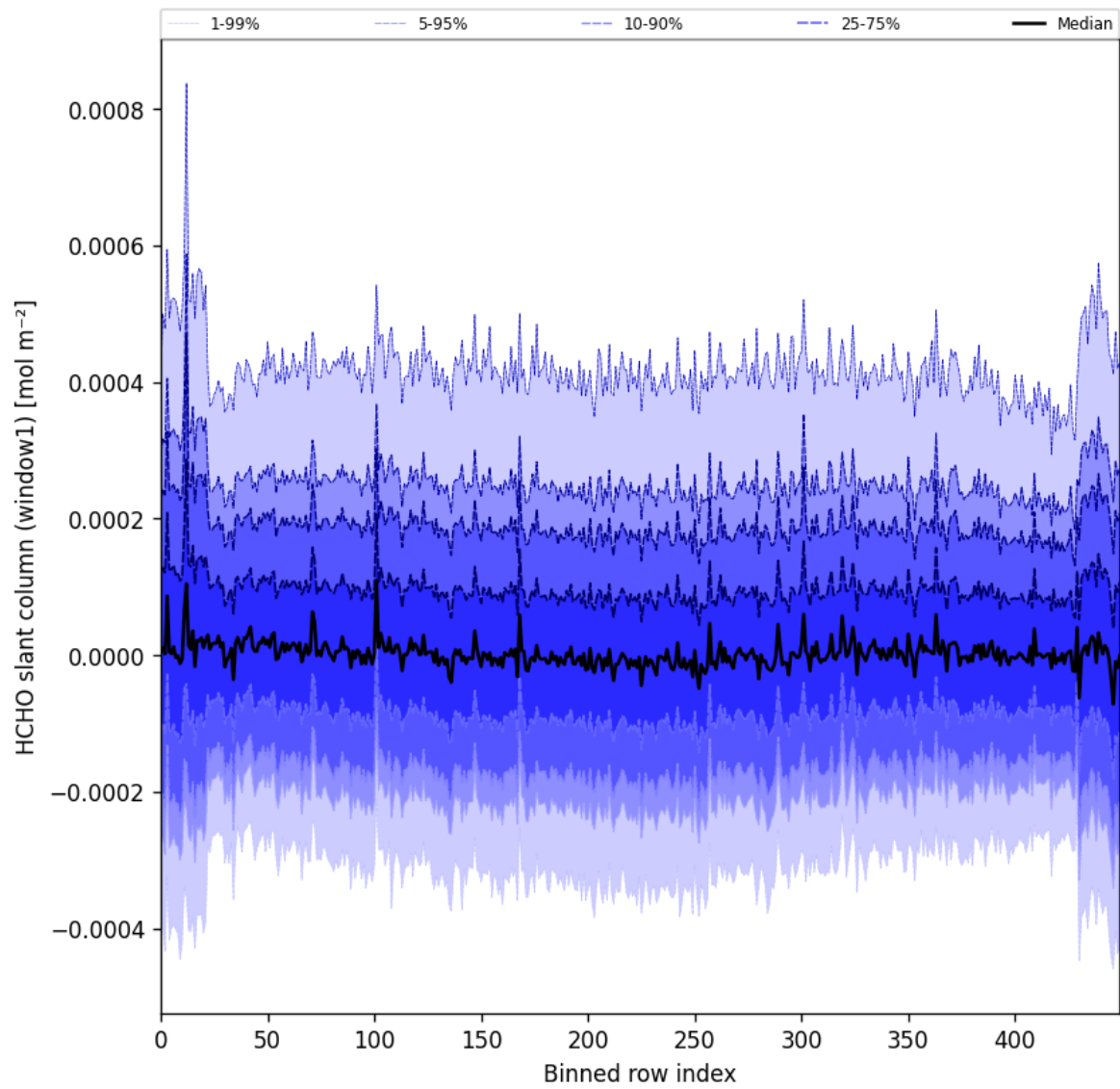
Figure 52: Along track statistics of "HCHO slant column (window1)" for 2025-05-16 to 2025-05-18
