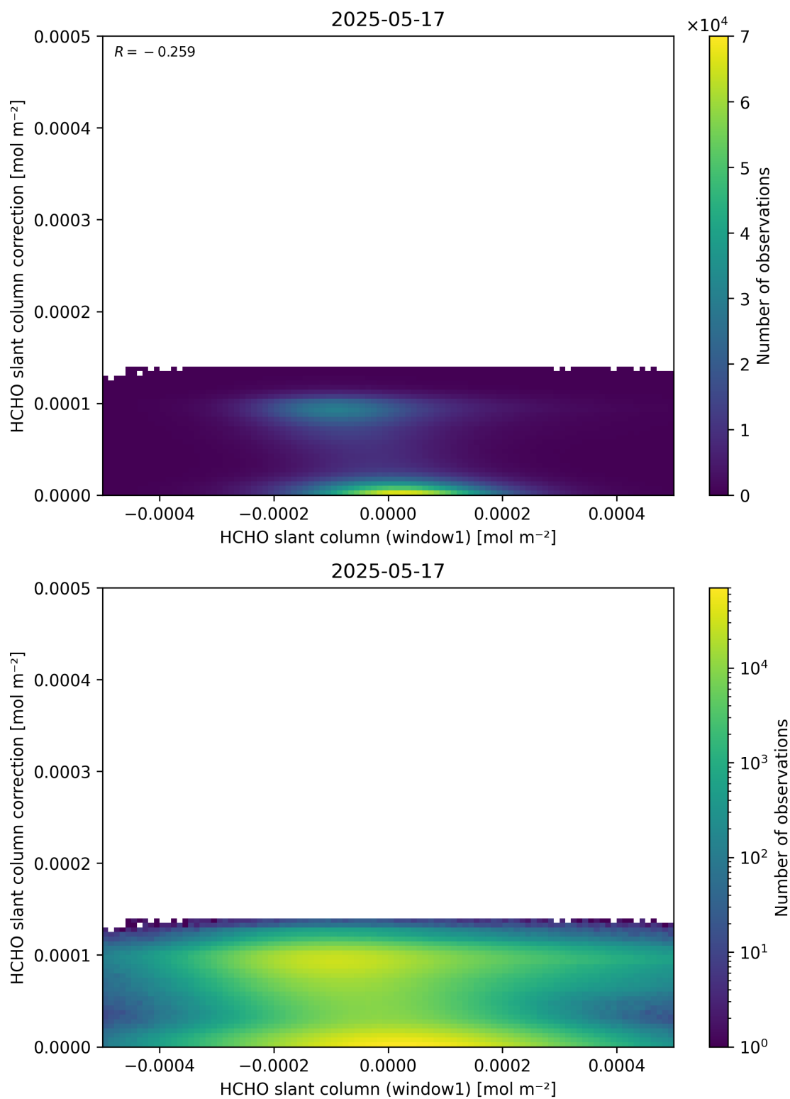
Figure 83: Scatter density plot of “HCHO slant column (window1)” against “HCHO slant column correction” for 2025-05-16 to 2025-05-18.
