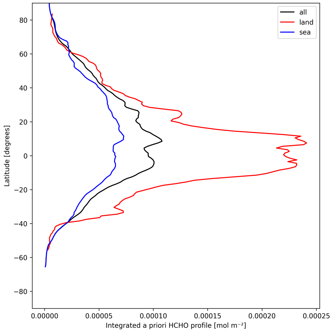
Figure 29: Zonal average of “Integrated a priori HCHO profile” for 2025-05-16 to 2025-05-18.
