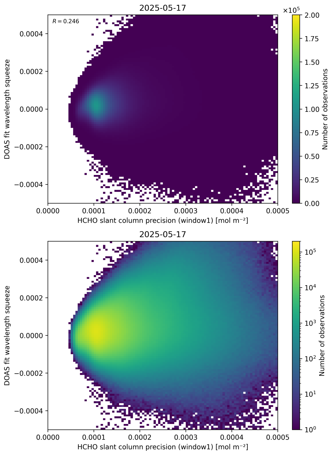
Figure 90: Scatter density plot of “HCHO slant column precision (window1)” against “DOAS fit wavelength squeeze” for 2025-05-16 to 2025-05-18.
