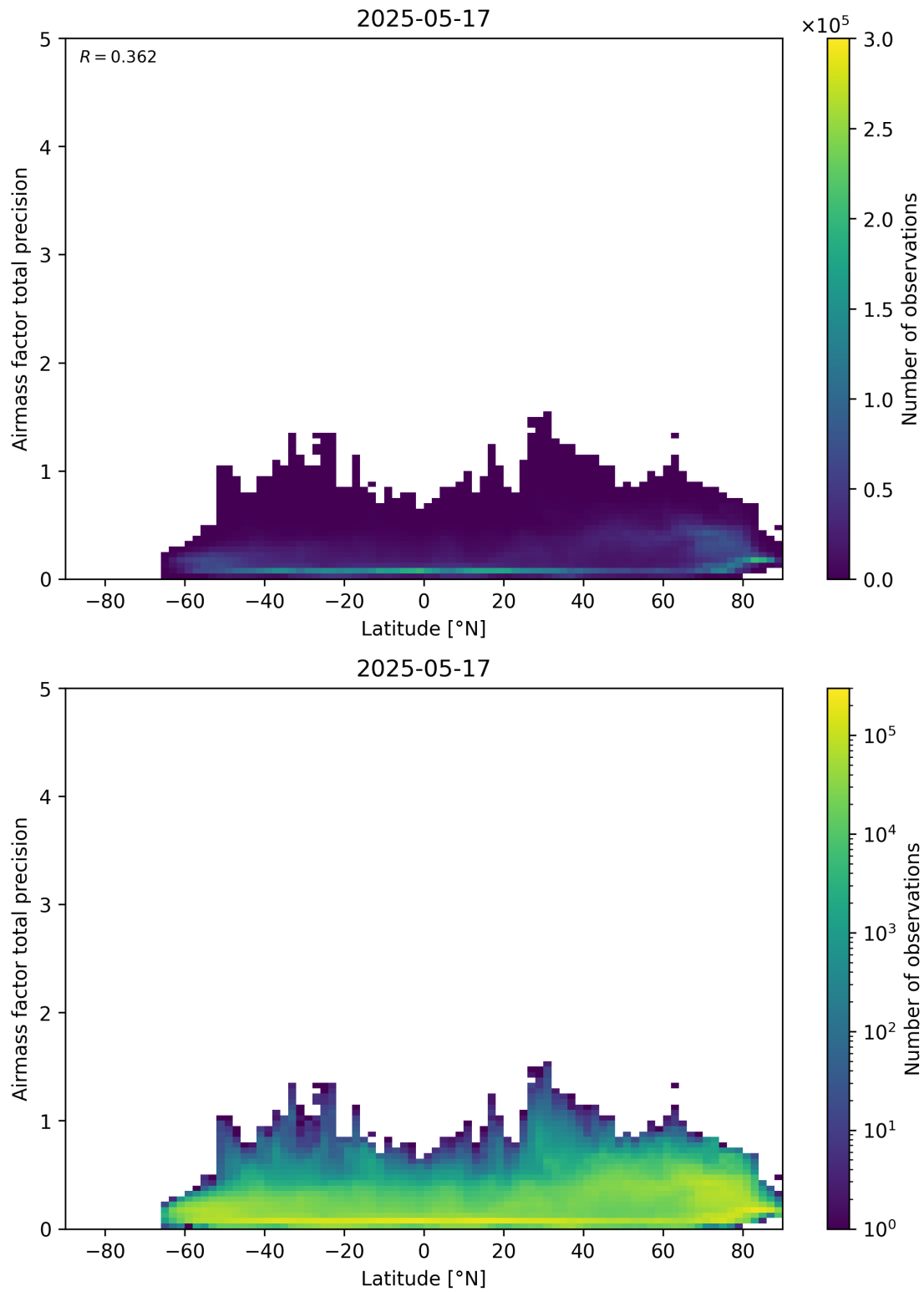
Figure 162: Scatter density plot of “Latitude” against “Airmass factor total precision” for 2025-05-16 to 2025-05-18.
