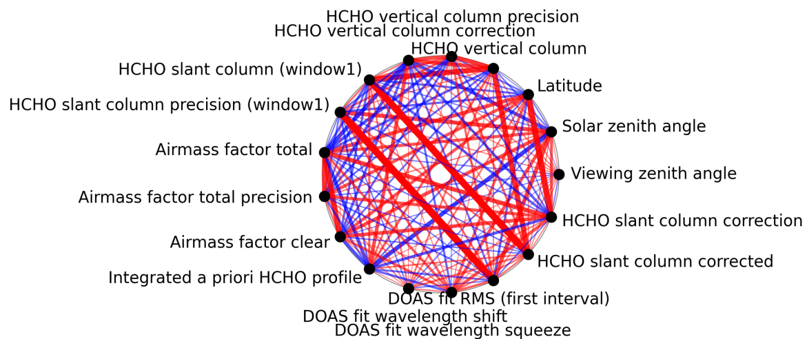
Figure 1: Map of correlation graph for 2025-05-16 to 2025-05-18.
