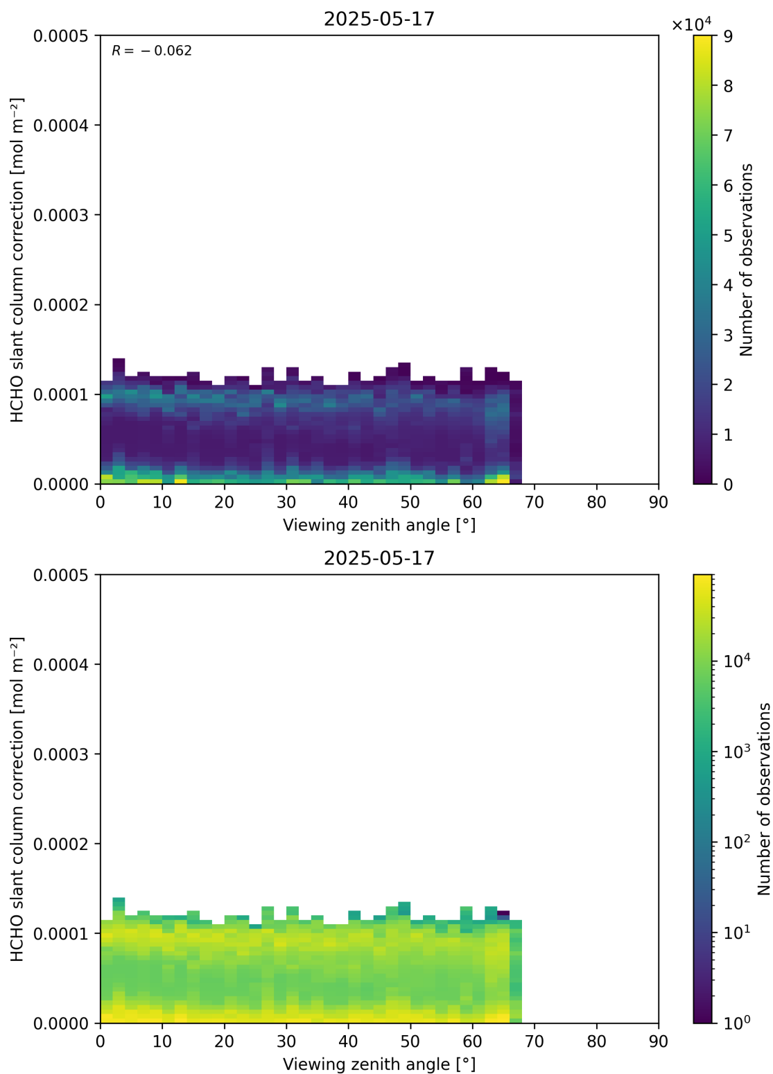
Figure 187: Scatter density plot of “Viewing zenith angle” against “HCHO slant column correction” for 2025-05-16 to 2025-05-18.
