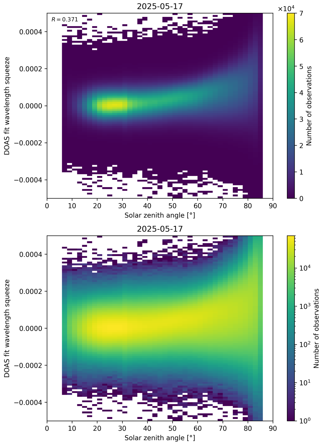
Figure 169: Scatter density plot of “Solar zenith angle” against “DOAS fit wavelength squeeze” for 2025-05-16 to 2025-05-18.
