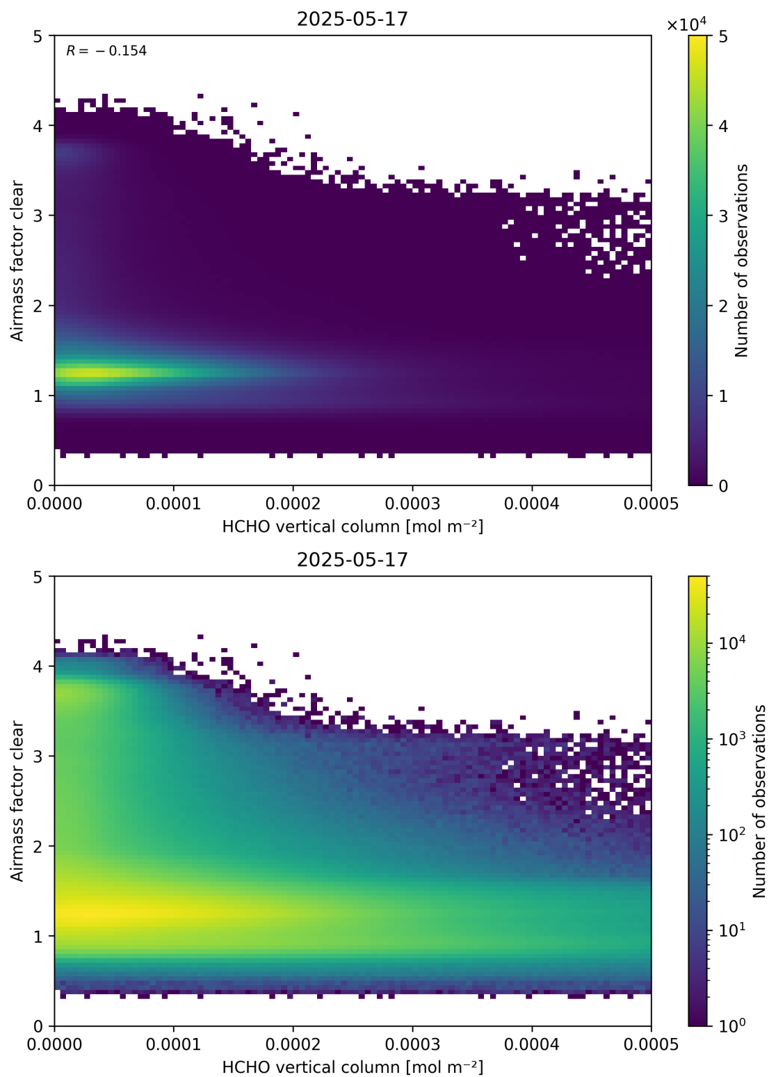
Figure 126: Scatter density plot of “HCHO vertical column” against “Airmass factor clear” for 2025-05-16 to 2025-05-18.
