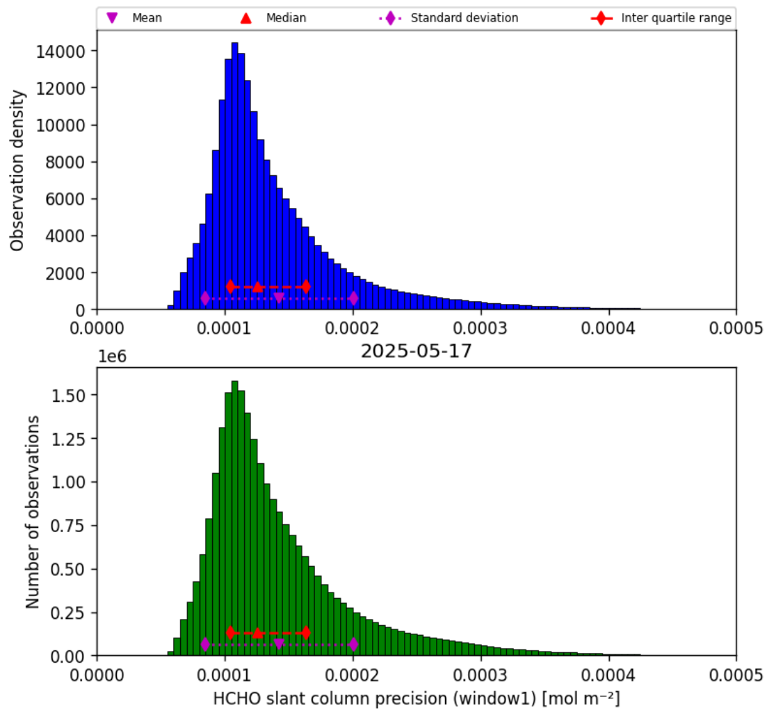
Figure 39: Histogram of “HCHO slant column precision (window1)” for 2025-05-16 to 2025-05-18
