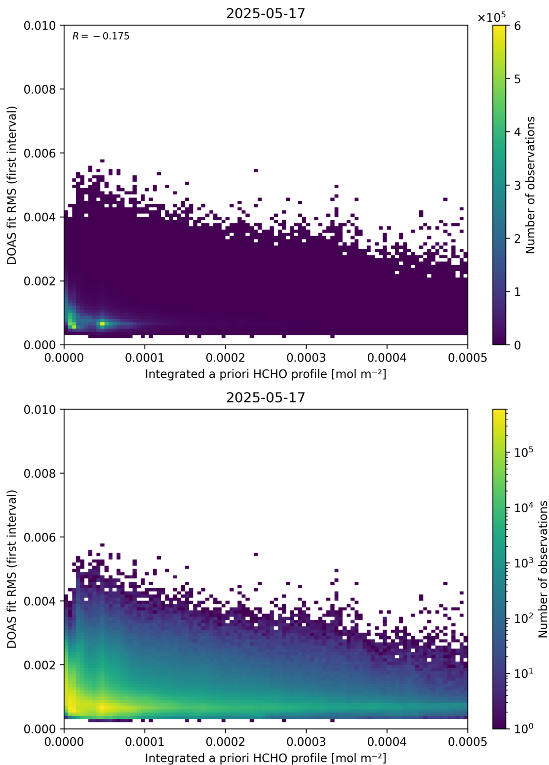
Figure 148: Scatter density plot of “Integrated a priori HCHO profile” against “DOAS fit RMS (first interval)” for 2025-05-16 to 2025-05-18.
