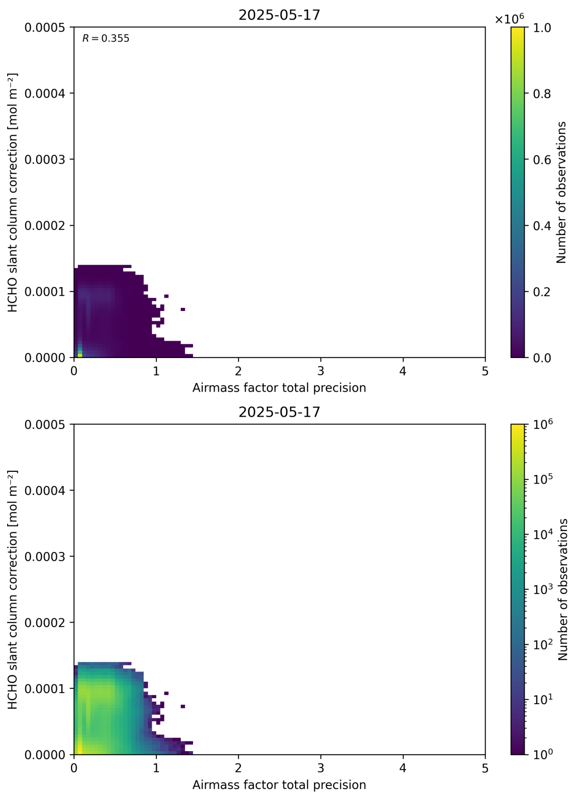
Figure 110: Scatter density plot of “Airmass factor total precision” against “HCHO slant column correction” for 2025-05-16 to 2025-05-18.
