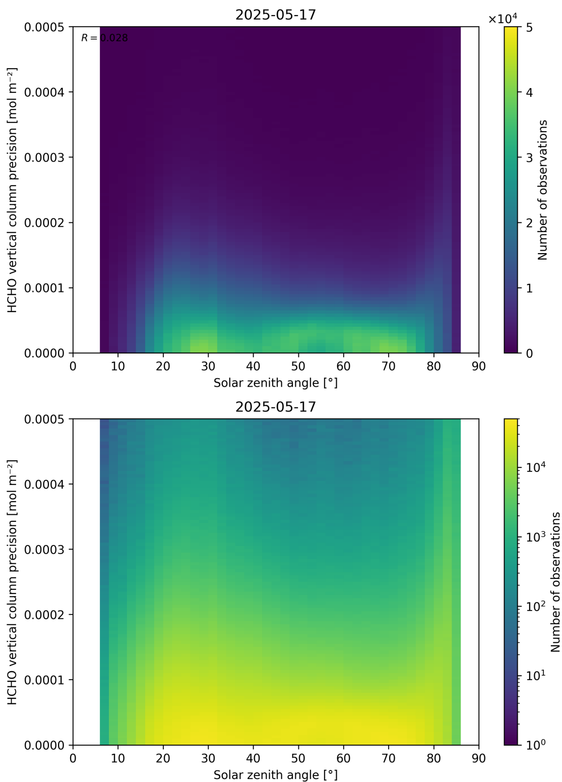
Figure 179: Scatter density plot of “Solar zenith angle” against “HCHO vertical column precision” for 2025-05-16 to 2025-05-18.
