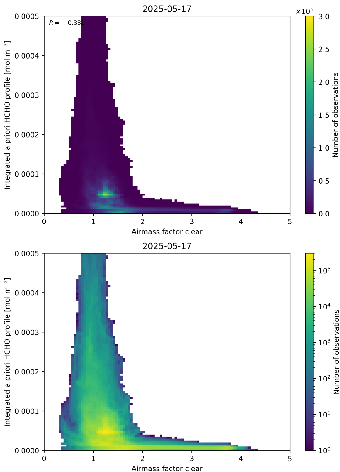
Figure 76: Scatter density plot of “Airmass factor clear” against “Integrated a priori HCHO profile” for 2025-05-16 to 2025-05-18.
