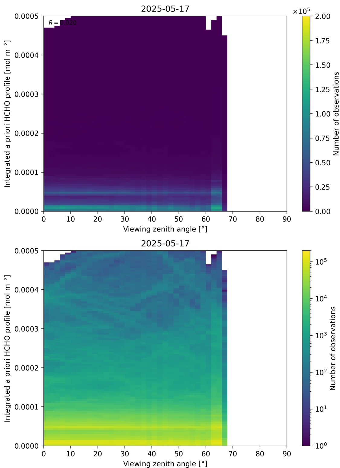
Figure 195: Scatter density plot of “Viewing zenith angle” against “Integrated a priori HCHO profile” for 2025-05-16 to 2025-05-18.
