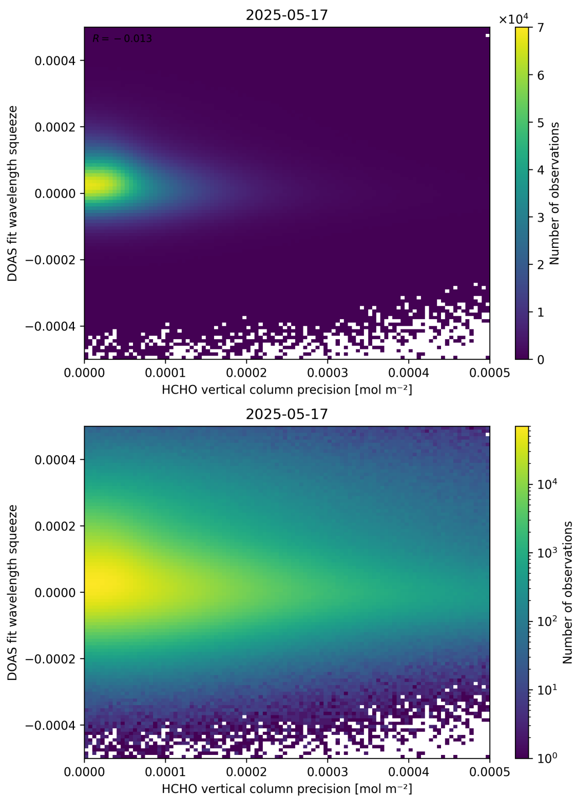
Figure 138: Scatter density plot of “HCHO vertical column precision” against “DOAS fit wavelength squeeze” for 2025-05-16 to 2025-05-18.
