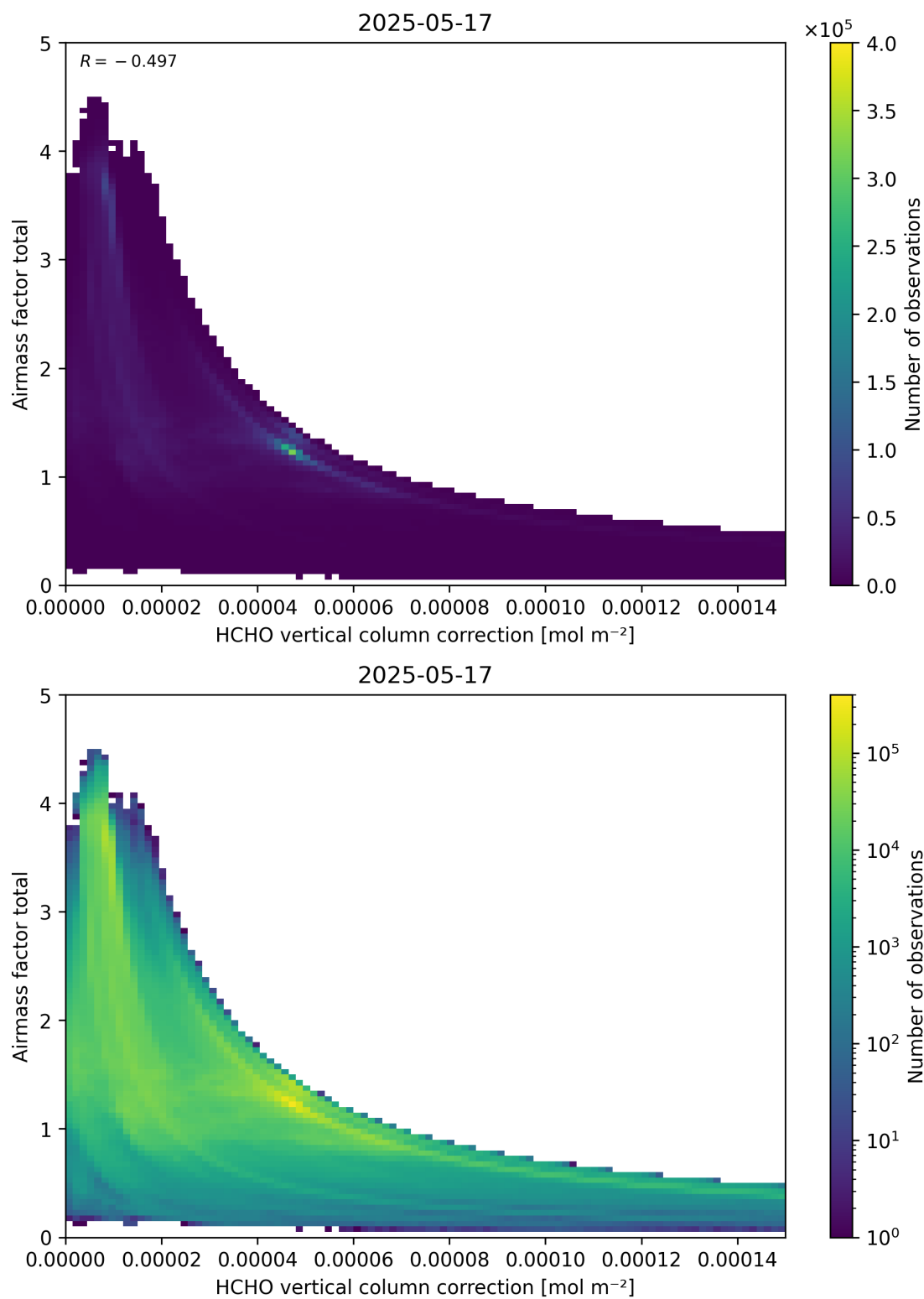
Figure 120: Scatter density plot of “HCHO vertical column correction” against “Airmass factor total” for 2025-05-16 to 2025-05-18.
