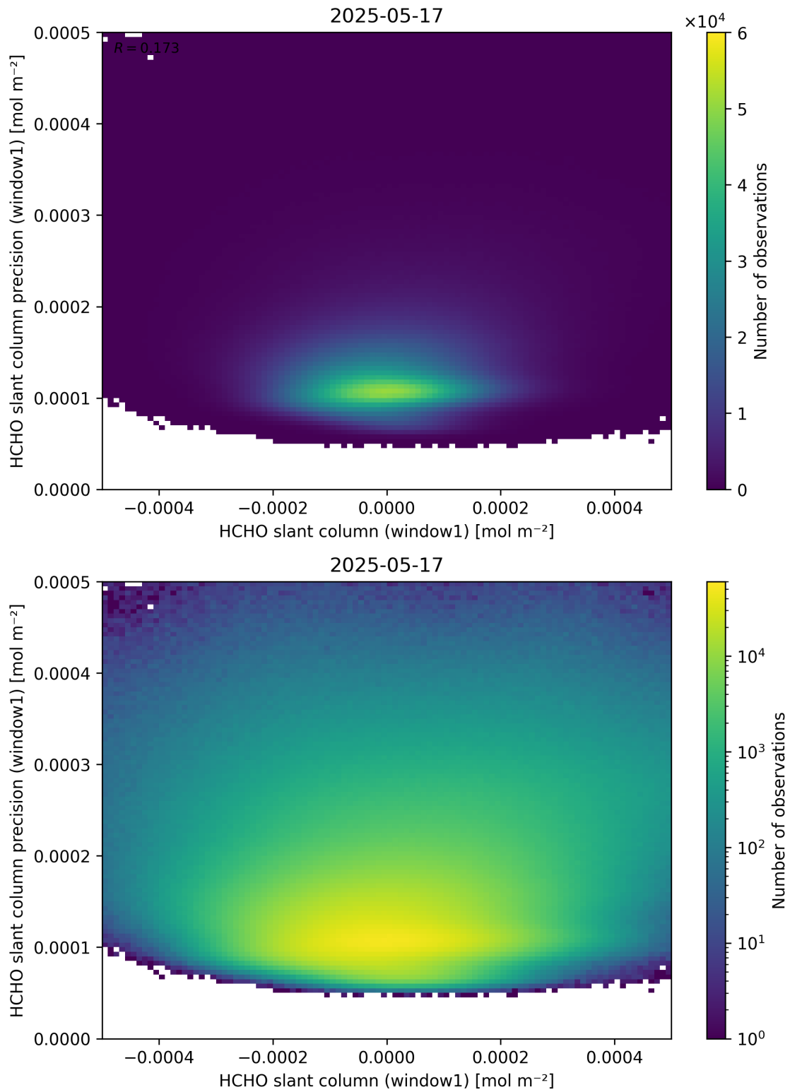
Figure 84: Scatter density plot of “HCHO slant column (window1)” against “HCHO slant column precision (window1)” for 2025-05-16 to 2025-05-18.
