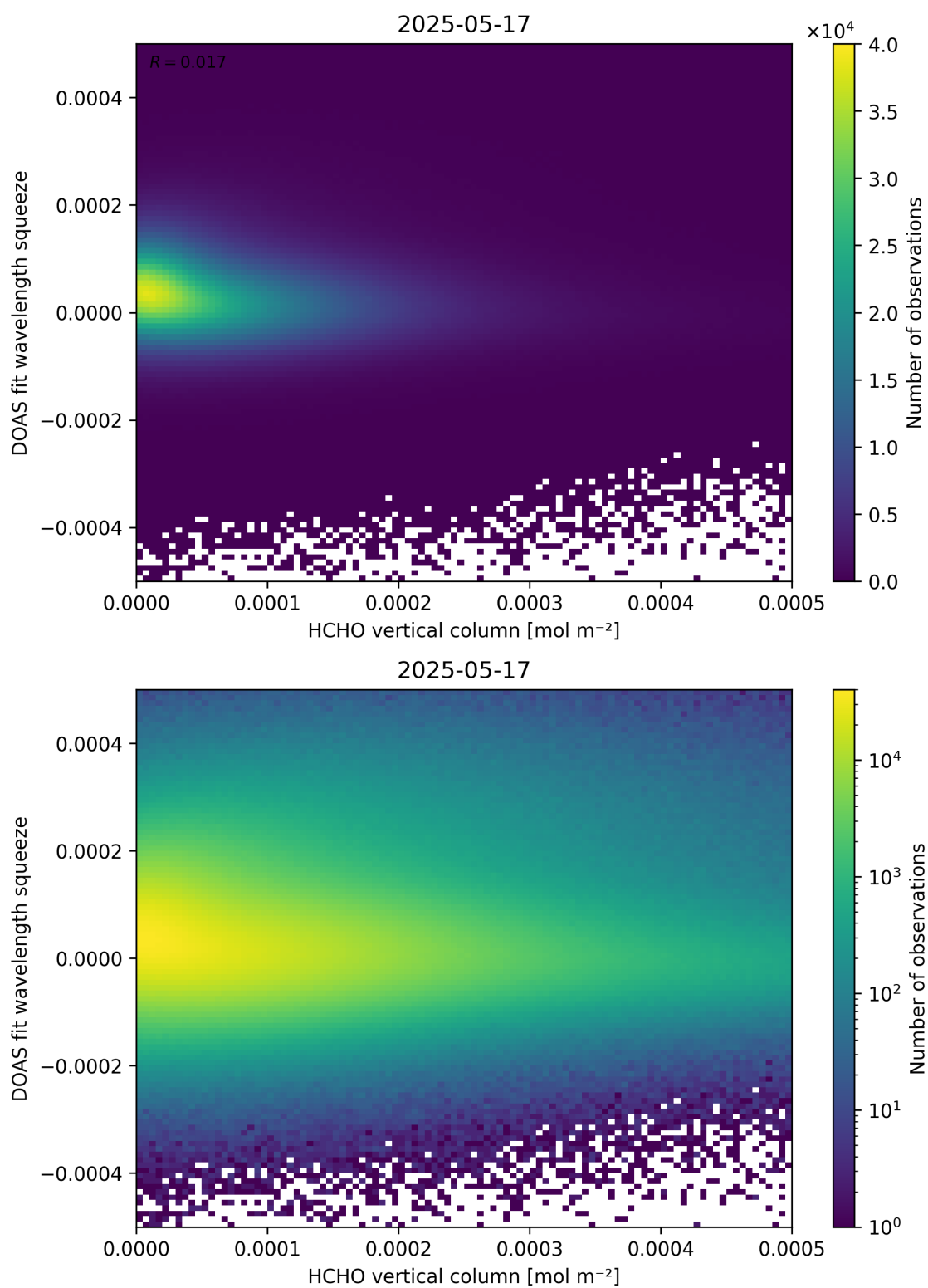
Figure 125: Scatter density plot of “HCHO vertical column” against “DOAS fit wavelength squeeze” for 2025-05-16 to 2025-05-18.
