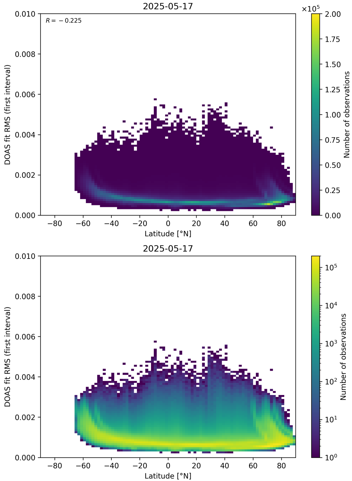
Figure 153: Scatter density plot of “Latitude” against “DOAS fit RMS (first interval)” for 2025-05-16 to 2025-05-18.
