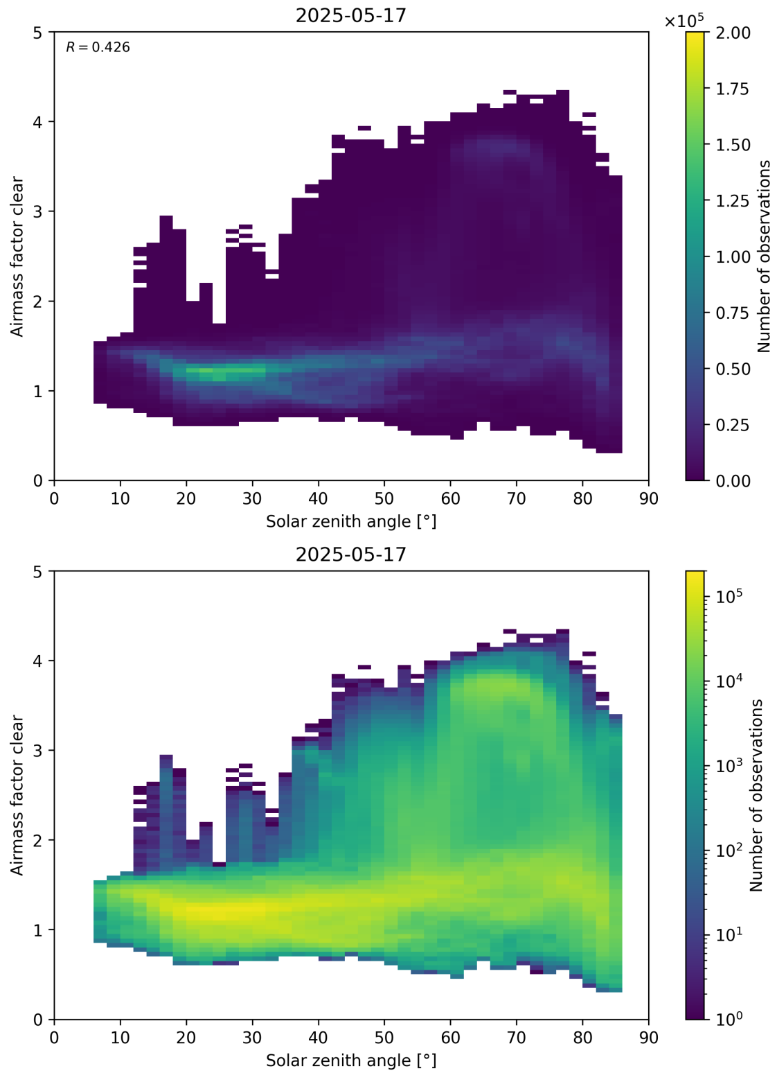
Figure 170: Scatter density plot of “Solar zenith angle” against “Airmass factor clear” for 2025-05-16 to 2025-05-18.
