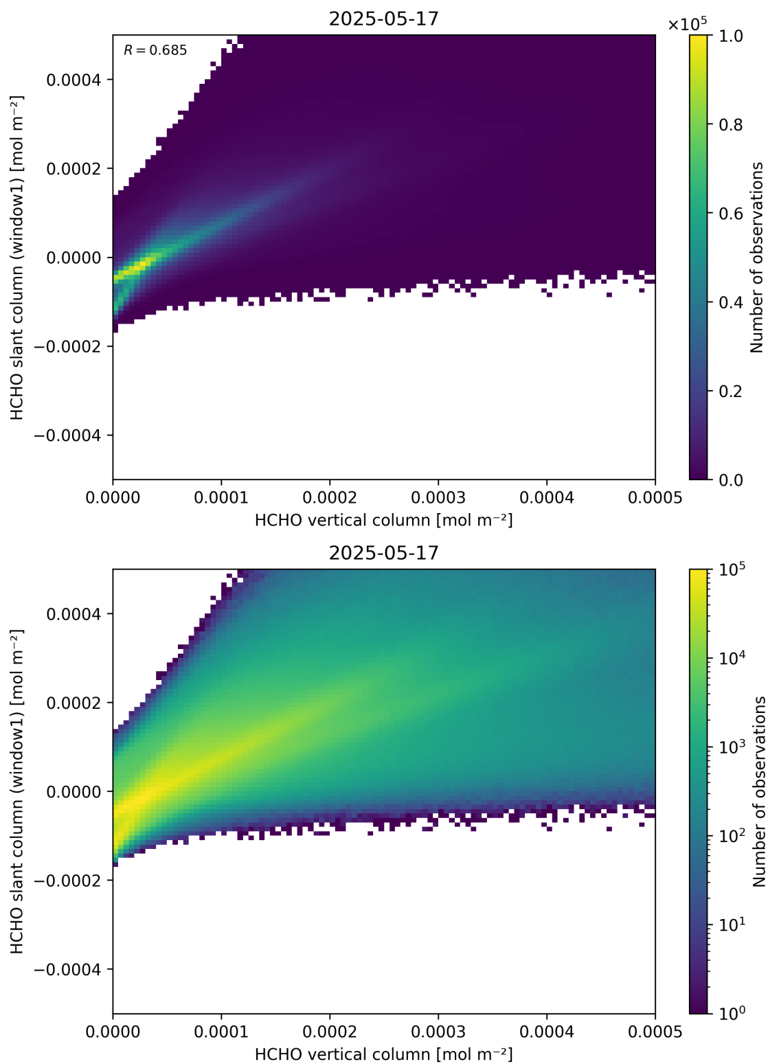
Figure 129: Scatter density plot of “HCHO vertical column” against “HCHO slant column (window1)” for 2025-05-16 to 2025-05-18.
