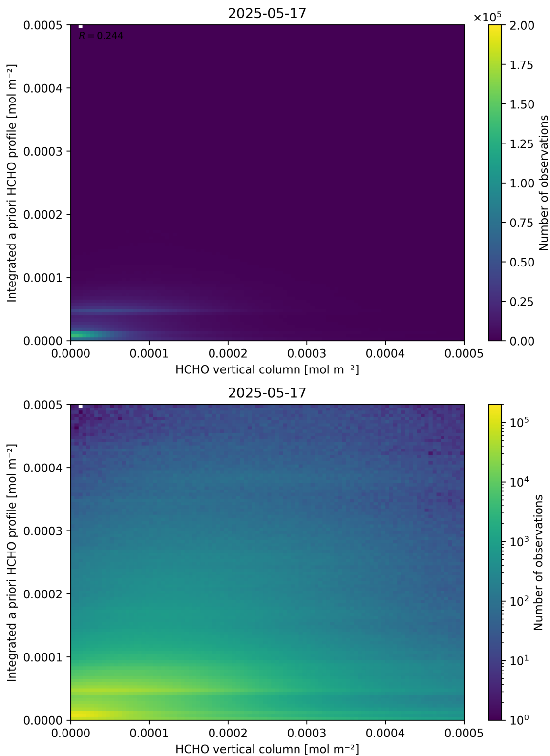
Figure 135: Scatter density plot of “HCHO vertical column” against “Integrated a priori HCHO profile” for 2025-05-16 to 2025-05-18.
