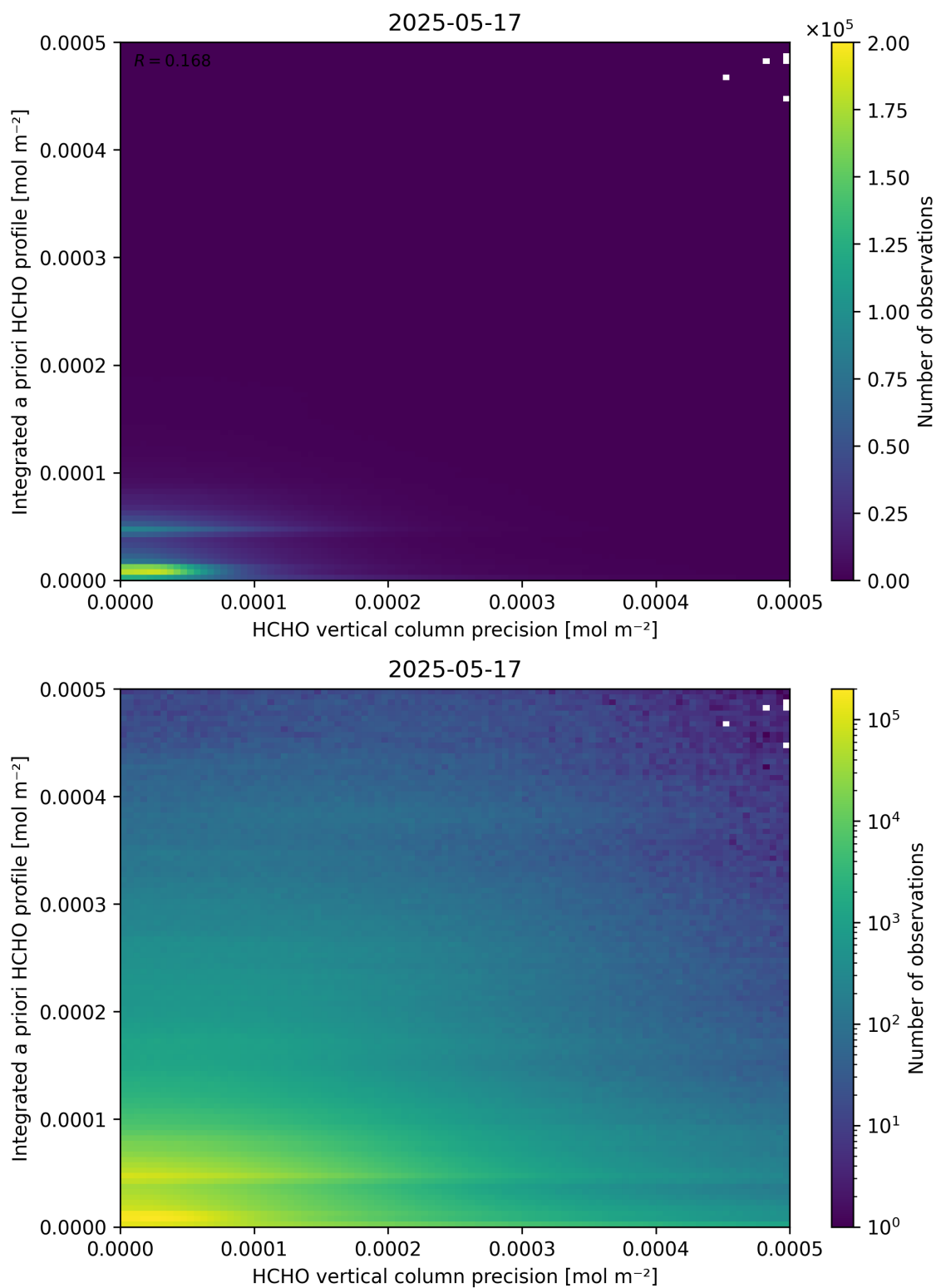
Figure 147: Scatter density plot of “HCHO vertical column precision” against “Integrated a priori HCHO profile” for 2025-05-16 to 2025-05-18.
