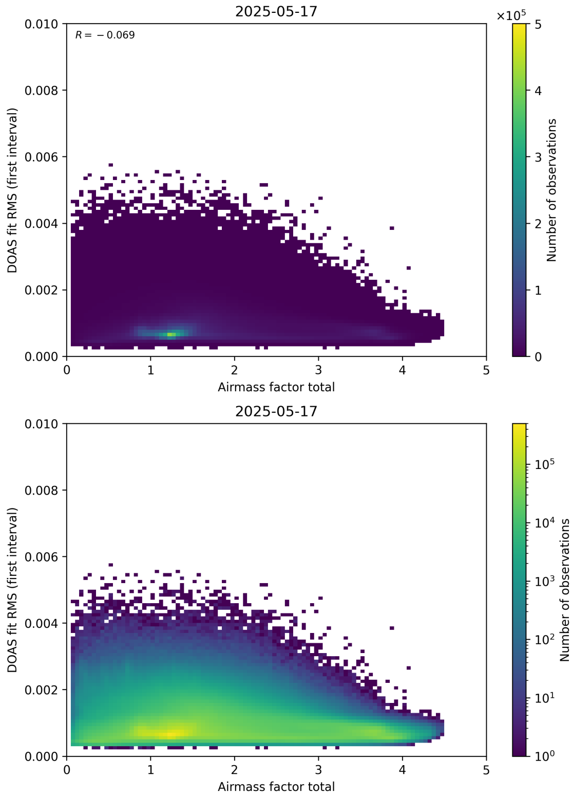
Figure 97: Scatter density plot of “Airmass factor total” against “DOAS fit RMS (first interval)” for 2025-05-16 to 2025-05-18.
