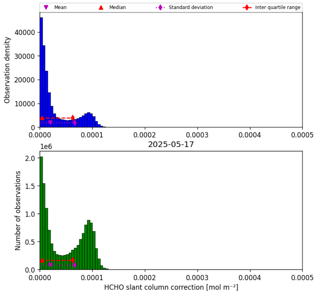
Figure 47: Histogram of “HCHO slant column correction” for 2025-05-16 to 2025-05-18
