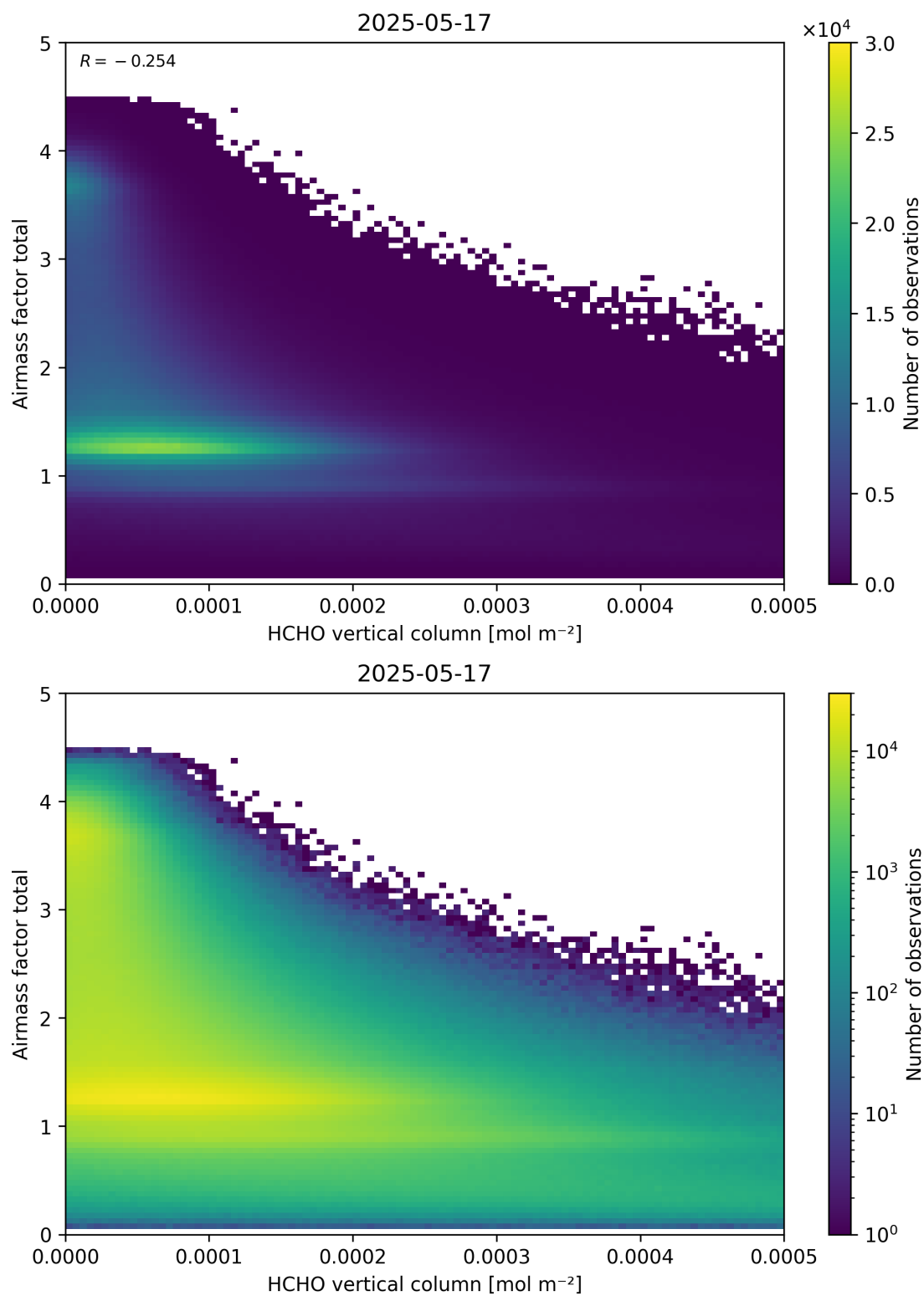
Figure 131: Scatter density plot of “HCHO vertical column” against “Airmass factor total” for 2025-05-16 to 2025-05-18.
