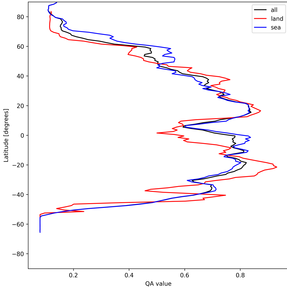
Figure 20: Zonal average of “QA value” for 2025-05-16 to 2025-05-18.
