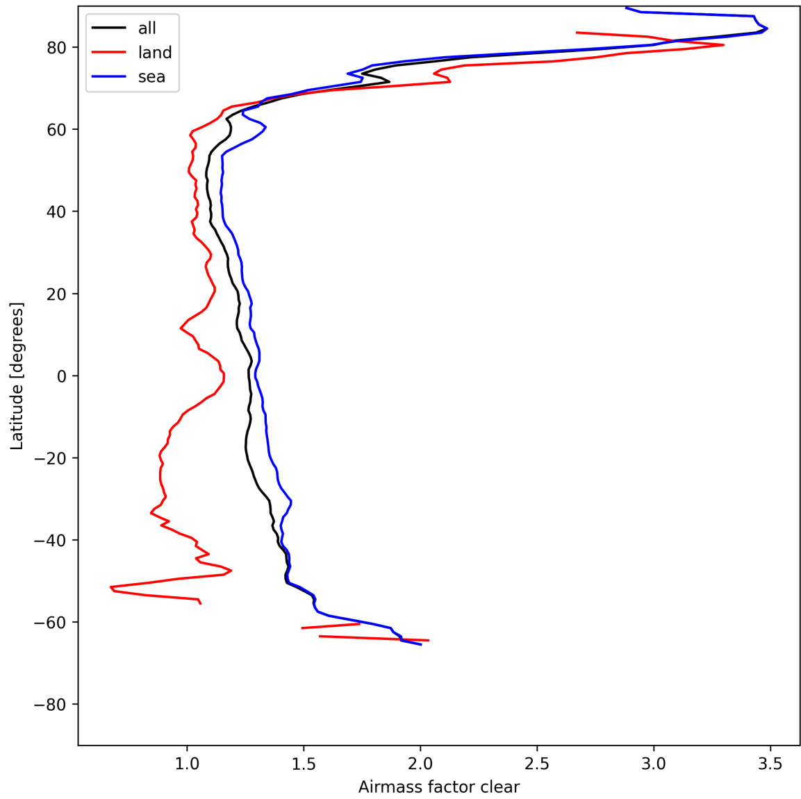
Figure 28: Zonal average of “Airmass factor clear” for 2025-05-16 to 2025-05-18.
