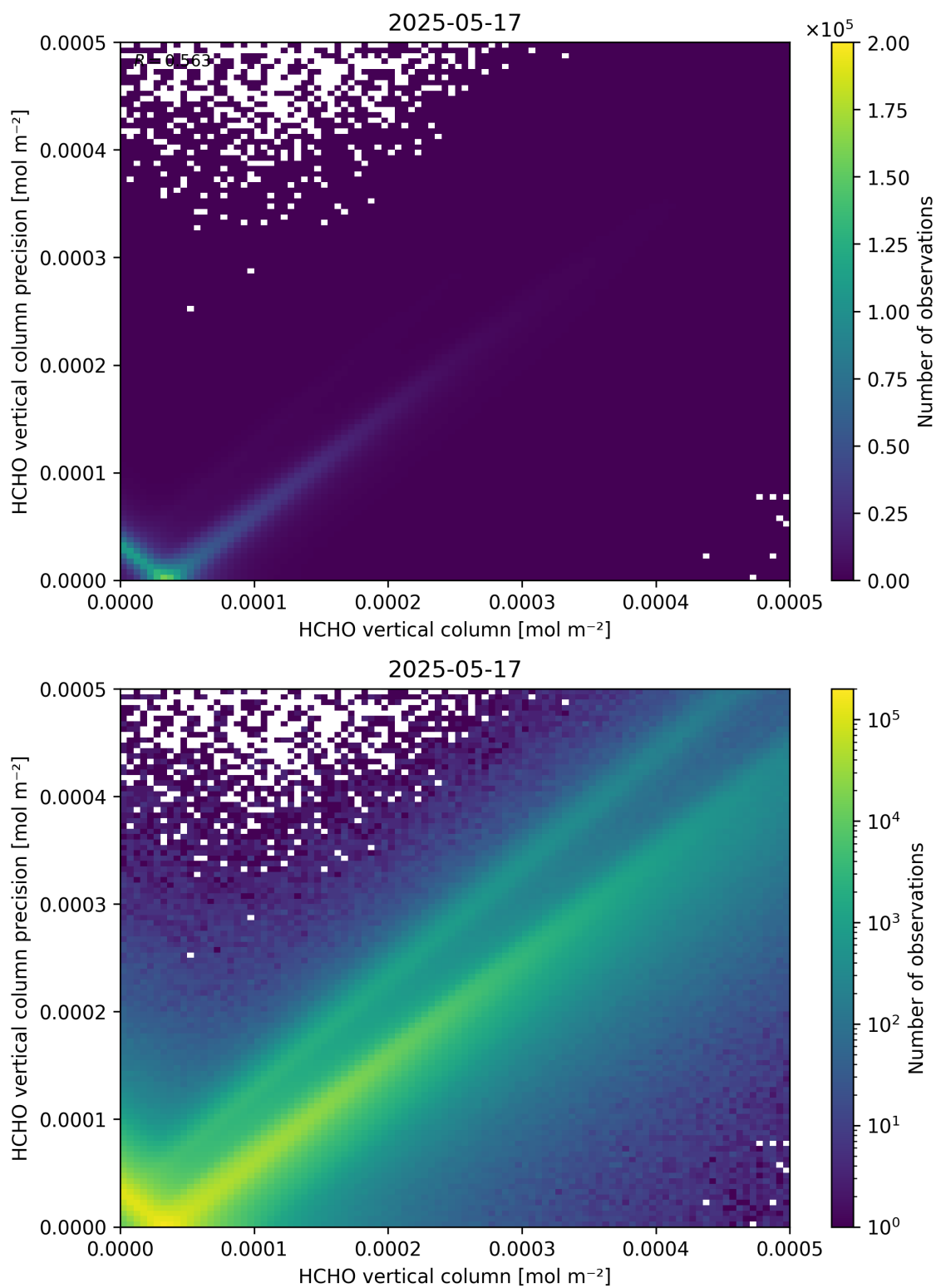
Figure 134: Scatter density plot of “HCHO vertical column” against “HCHO vertical column precision” for 2025-05-16 to 2025-05-18.
