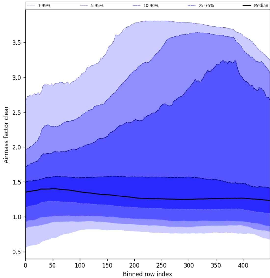
Figure 56: Along track statistics of “Airmass factor clear” for 2025-05-16 to 2025-05-18
