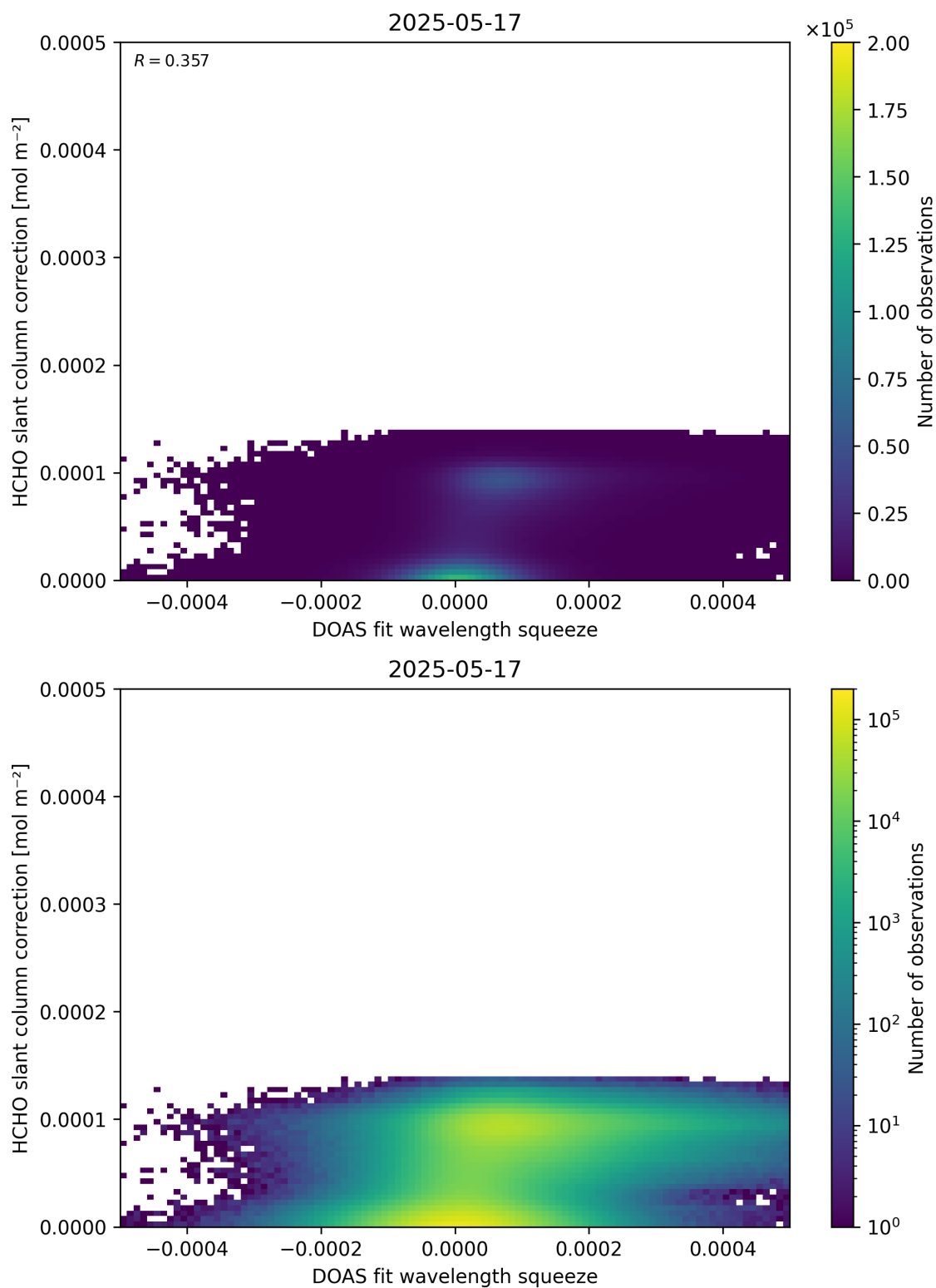
Figure 70: Scatter density plot of “DOAS fit wavelength squeeze” against “HCHO slant column correction” for 2025-05-16 to 2025-05-18.
