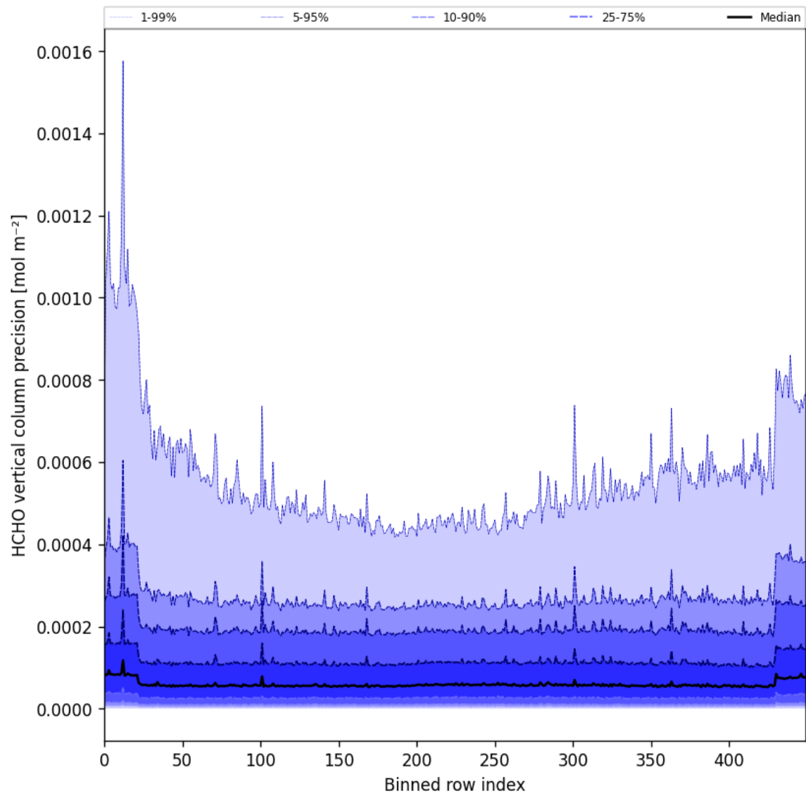
Figure 50: Along track statistics of “HCHO vertical column precision” for 2025-05-16 to 2025-05-18
