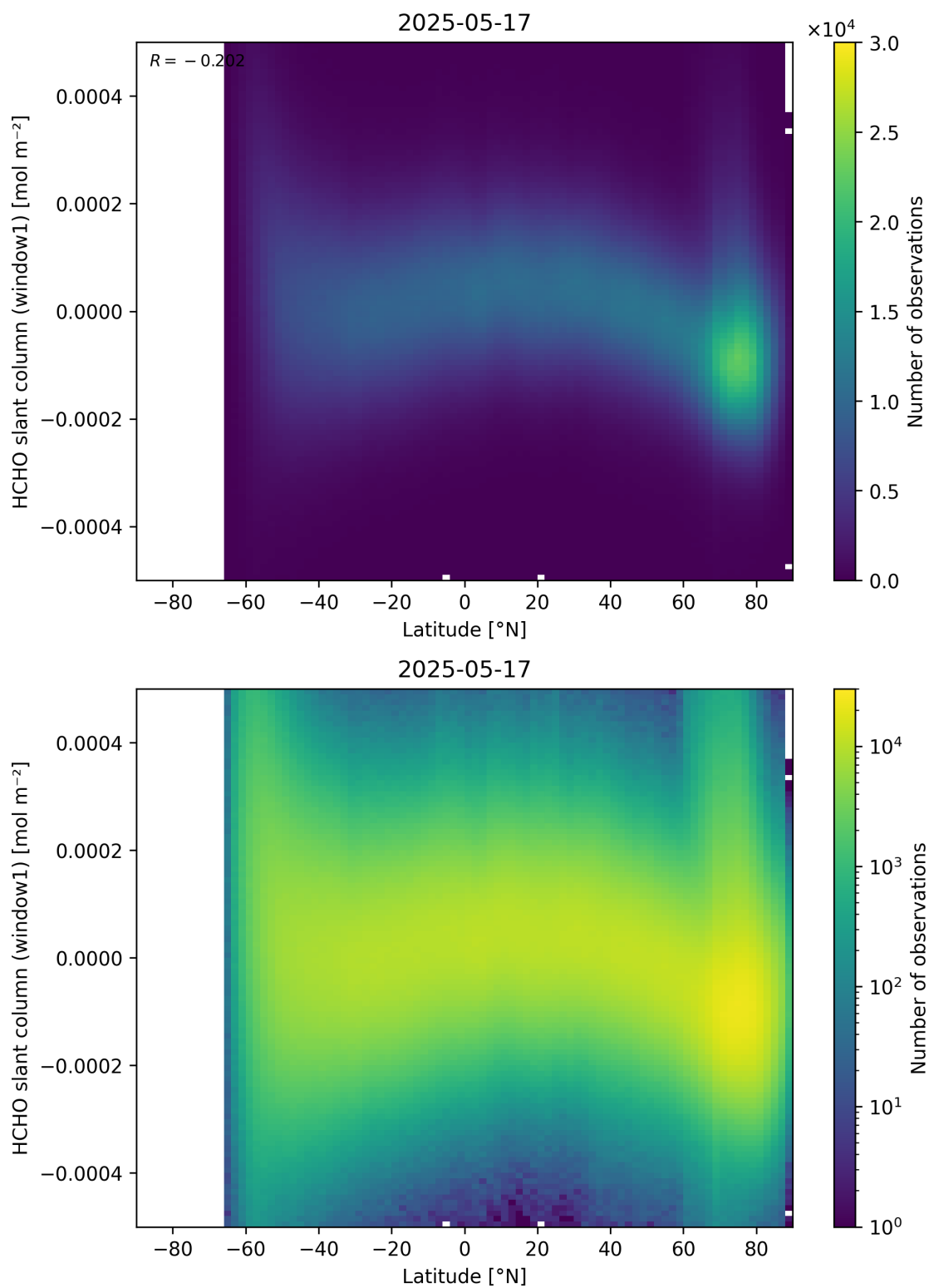
Figure 159: Scatter density plot of “Latitude” against “HCHO slant column (window1)” for 2025-05-16 to 2025-05-18.
