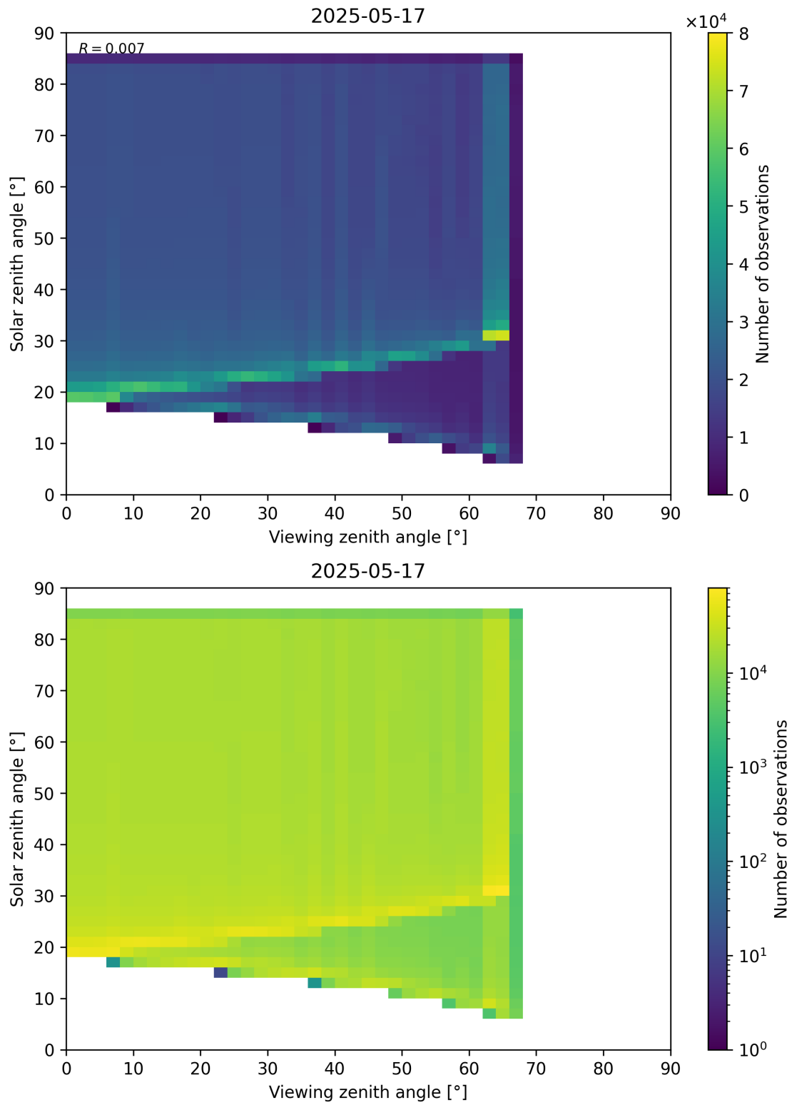
Figure 197: Scatter density plot of “Viewing zenith angle” against “Solar zenith angle” for 2025-05-16 to 2025-05-18.
