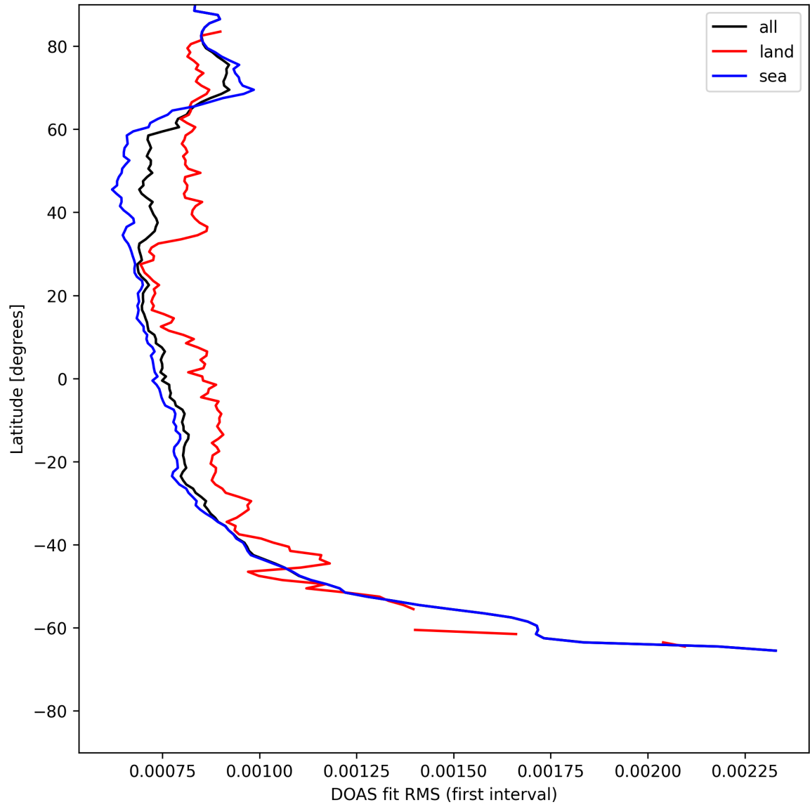
Figure 32: Zonal average of "DOAS fit RMS (first interval)" for 2025-05-16 to 2025-05-18.
