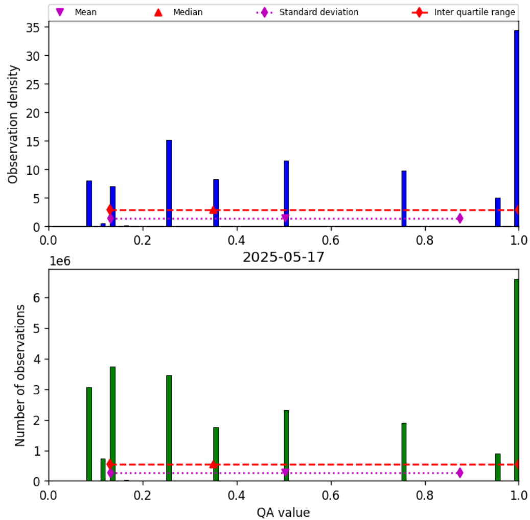
Figure 34: Histogram of “QA value” for 2025-05-16 to 2025-05-18
