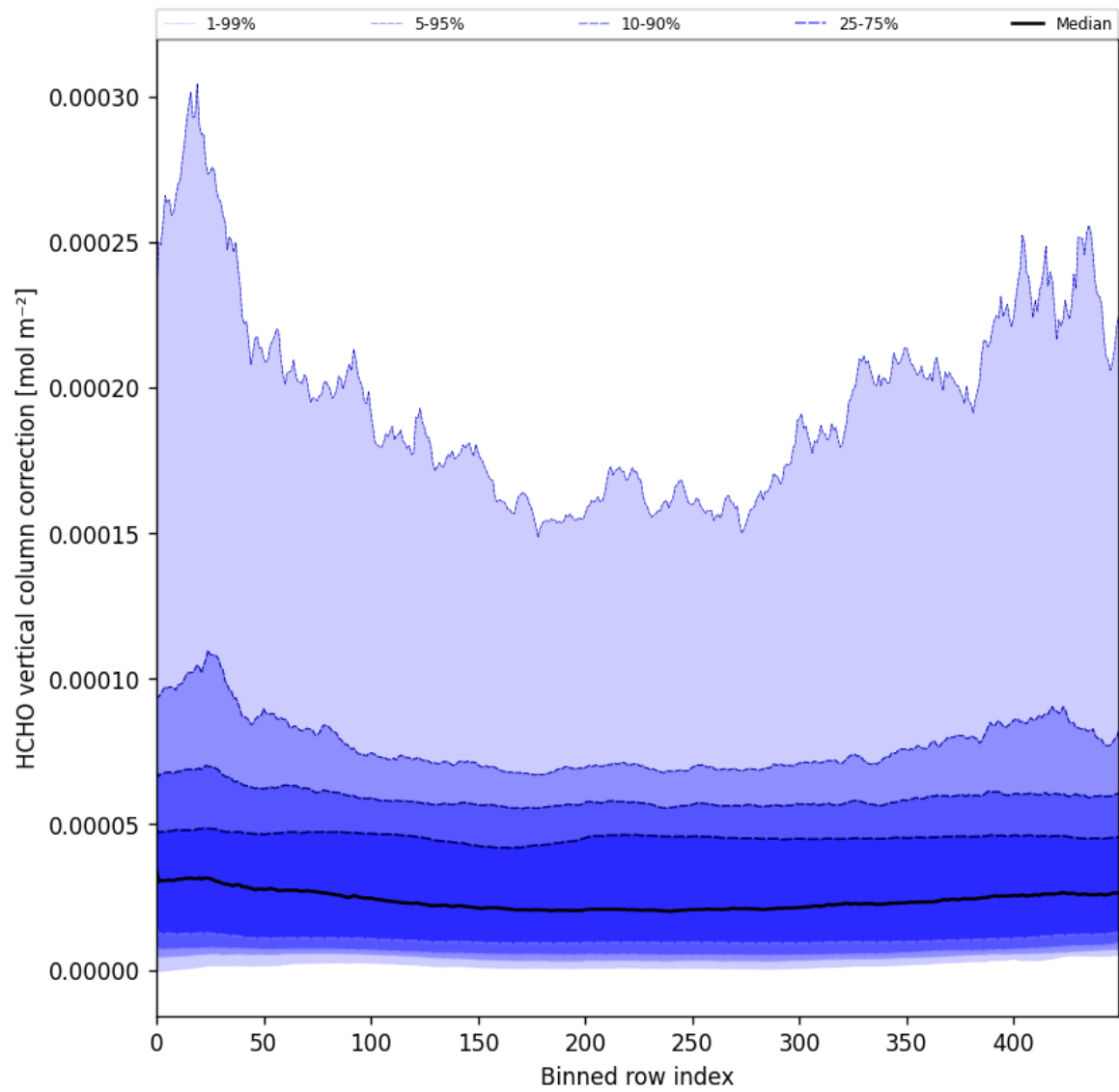
Figure 51: Along track statistics of “HCHO vertical column correction” for 2025-05-16 to 2025-05-18
