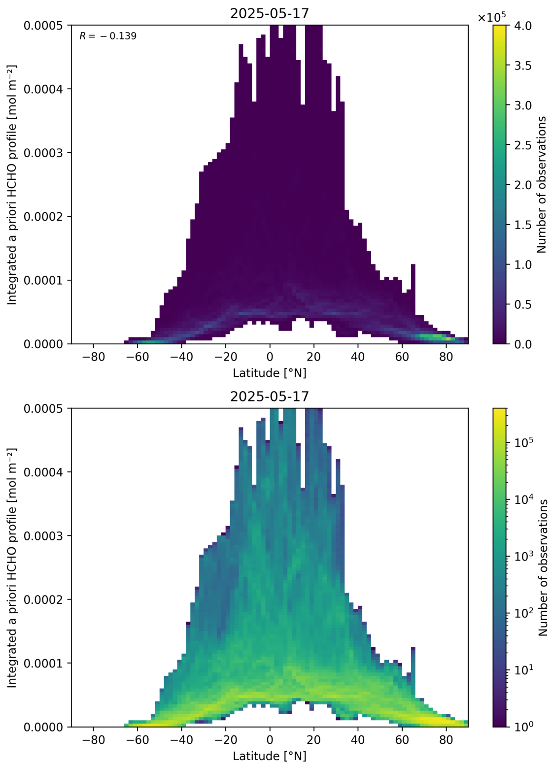
Figure 166: Scatter density plot of “Latitude” against “Integrated a priori HCHO profile” for 2025-05-16 to 2025-05-18.
