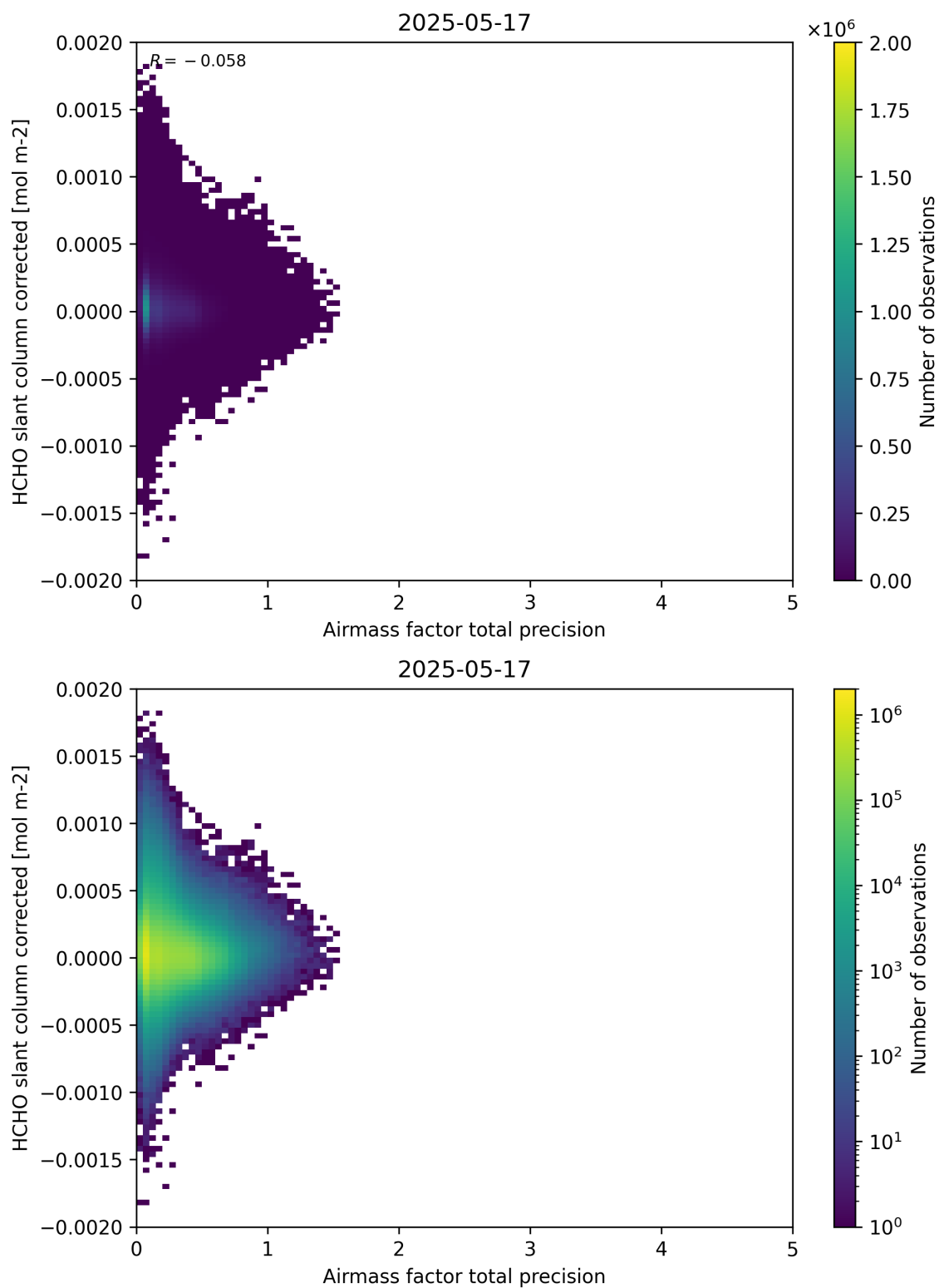
Figure 109: Scatter density plot of “Airmass factor total precision” against “HCHO slant column corrected” for 2025-05-16 to 2025-05-18.
