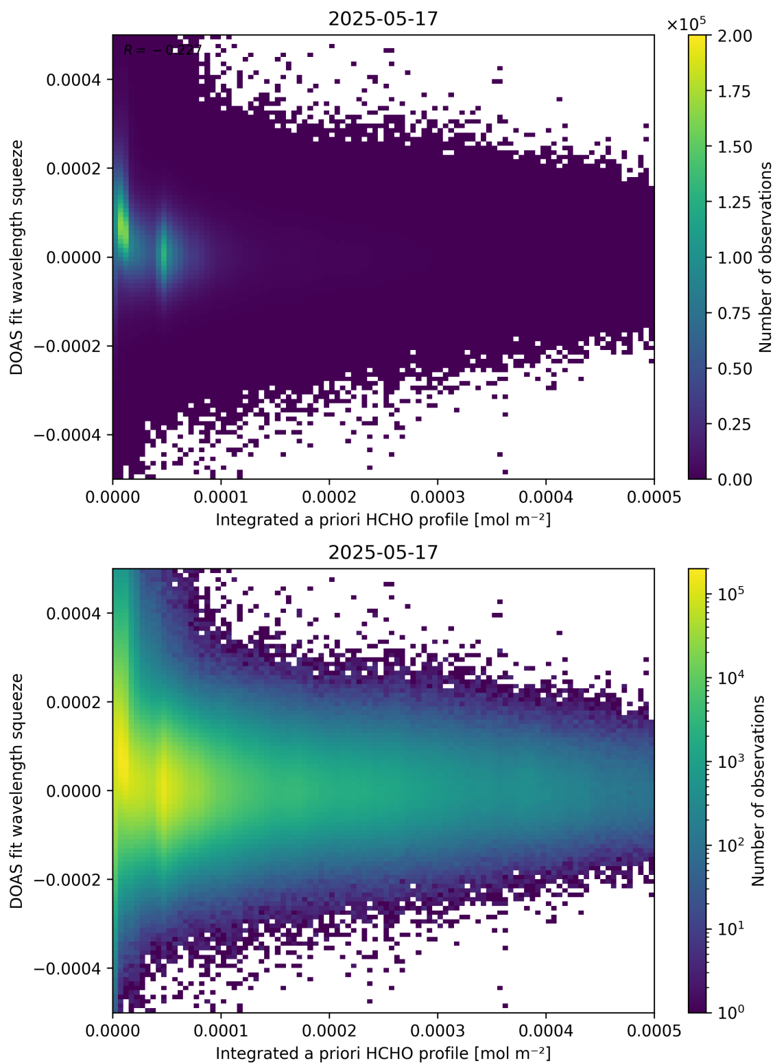
Figure 150: Scatter density plot of “Integrated a priori HCHO profile” against “DOAS fit wavelength squeeze” for 2025-05-16 to 2025-05-18.
