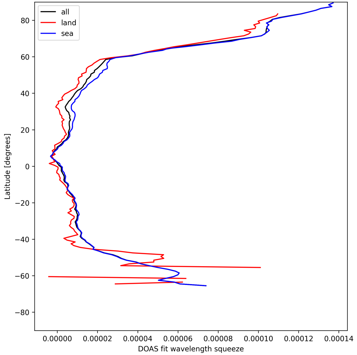
Figure 31: Zonal average of “DOAS fit wavelength squeeze” for 2025-05-16 to 2025-05-18.
