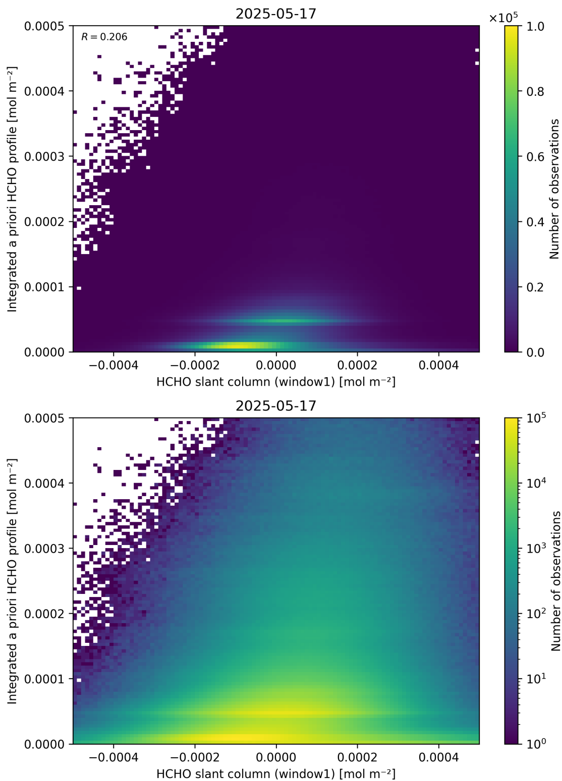
Figure 87: Scatter density plot of “HCHO slant column (window1)” against “Integrated a priori HCHO profile” for 2025-05-16 to 2025-05-18.
