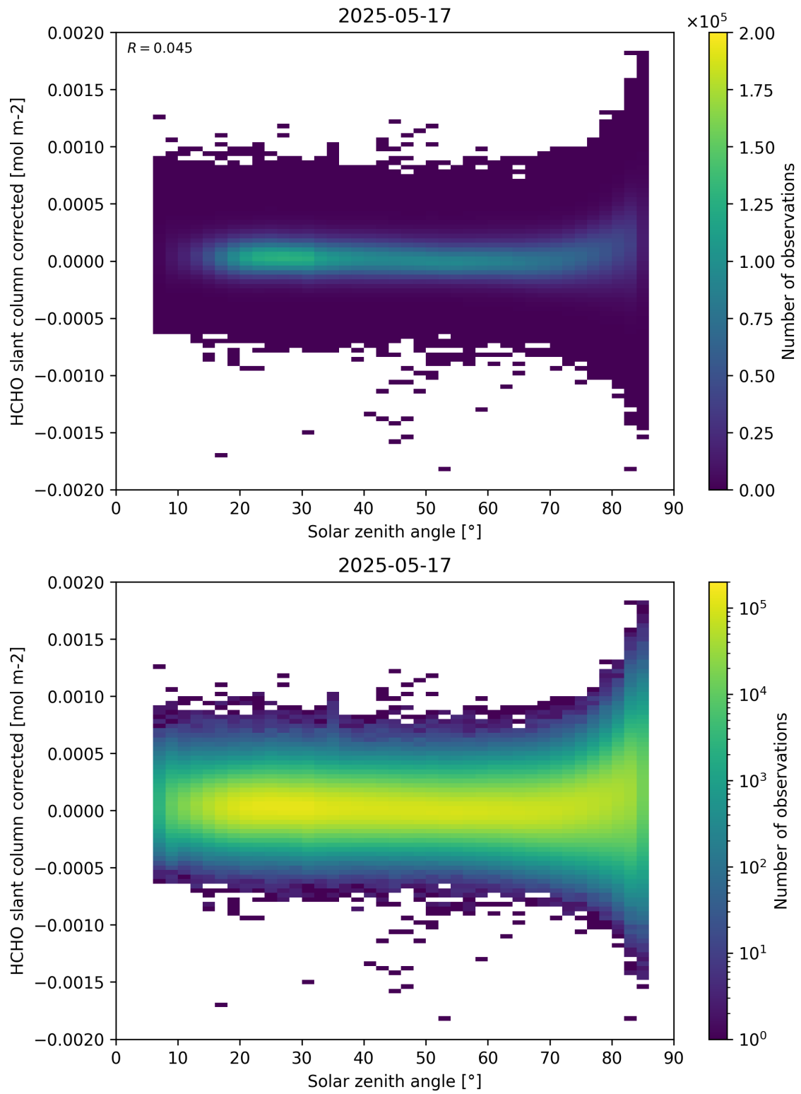
Figure 171: Scatter density plot of “Solar zenith angle” against “HCHO slant column corrected” for 2025-05-16 to 2025-05-18.
