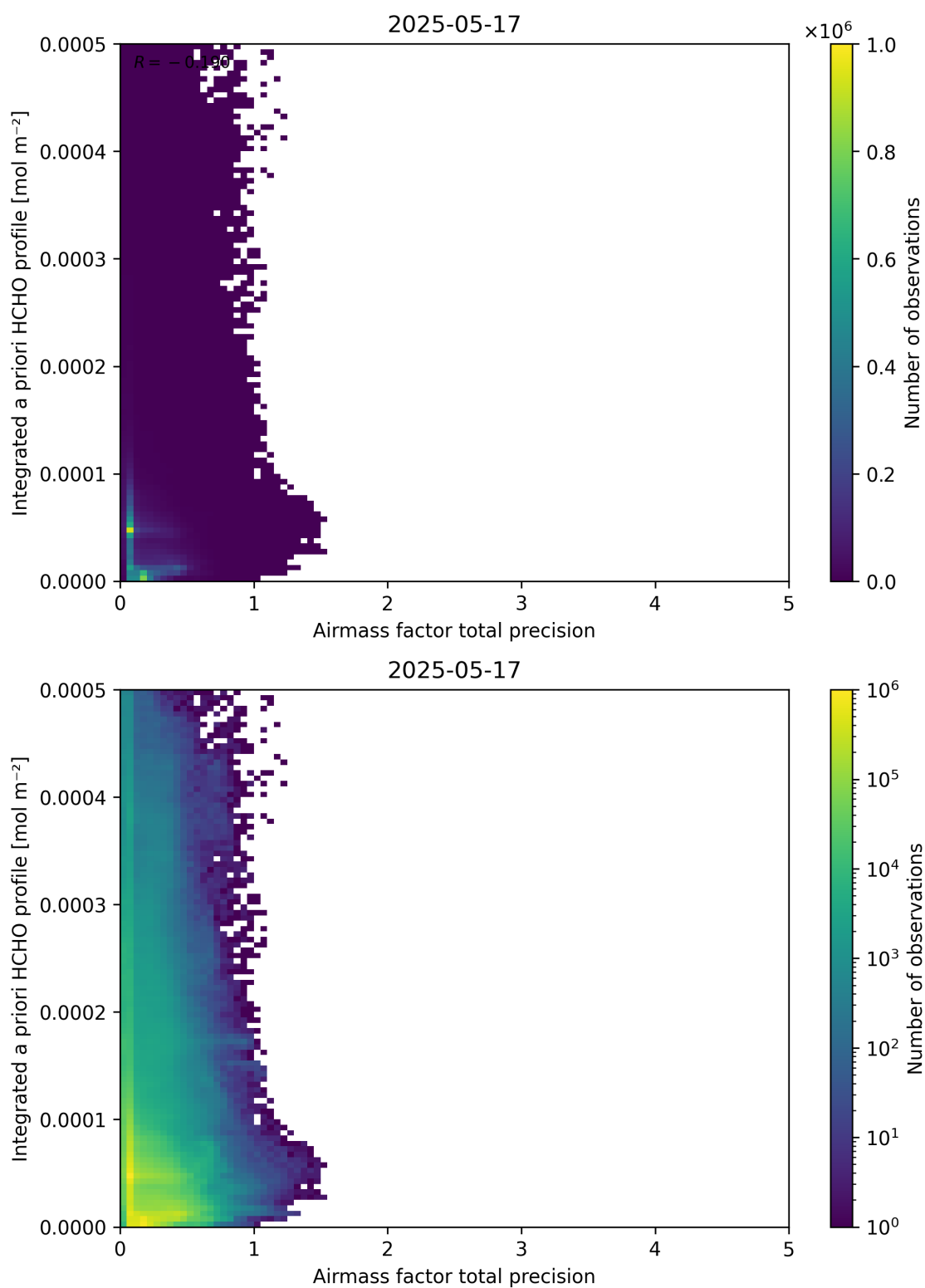
Figure 111: Scatter density plot of “Airmass factor total precision” against “Integrated a priori HCHO profile” for 2025-05-16 to 2025-05-18.
