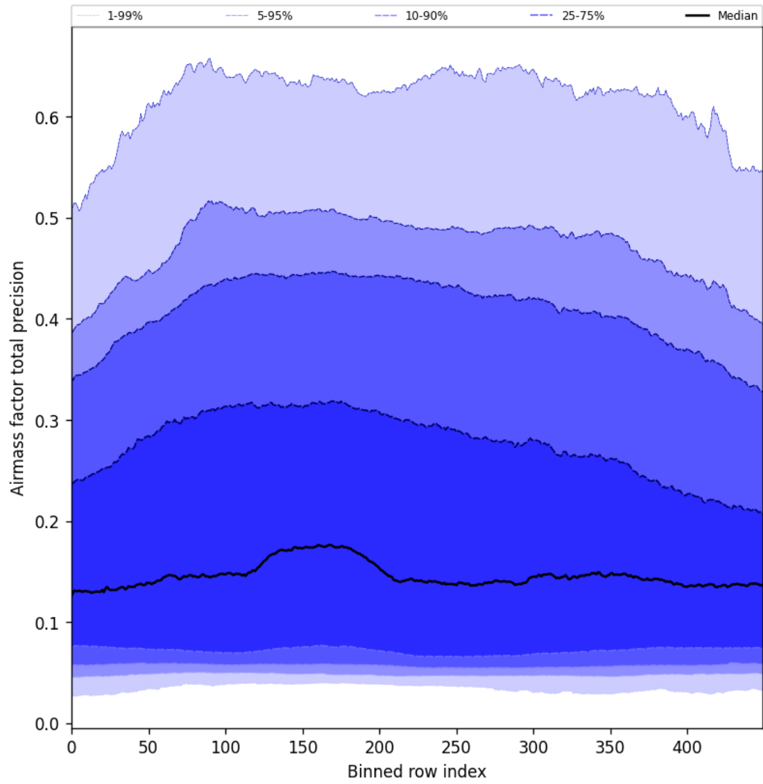
Figure 55: Along track statistics of “Airmass factor total precision” for 2025-05-16 to 2025-05-18
