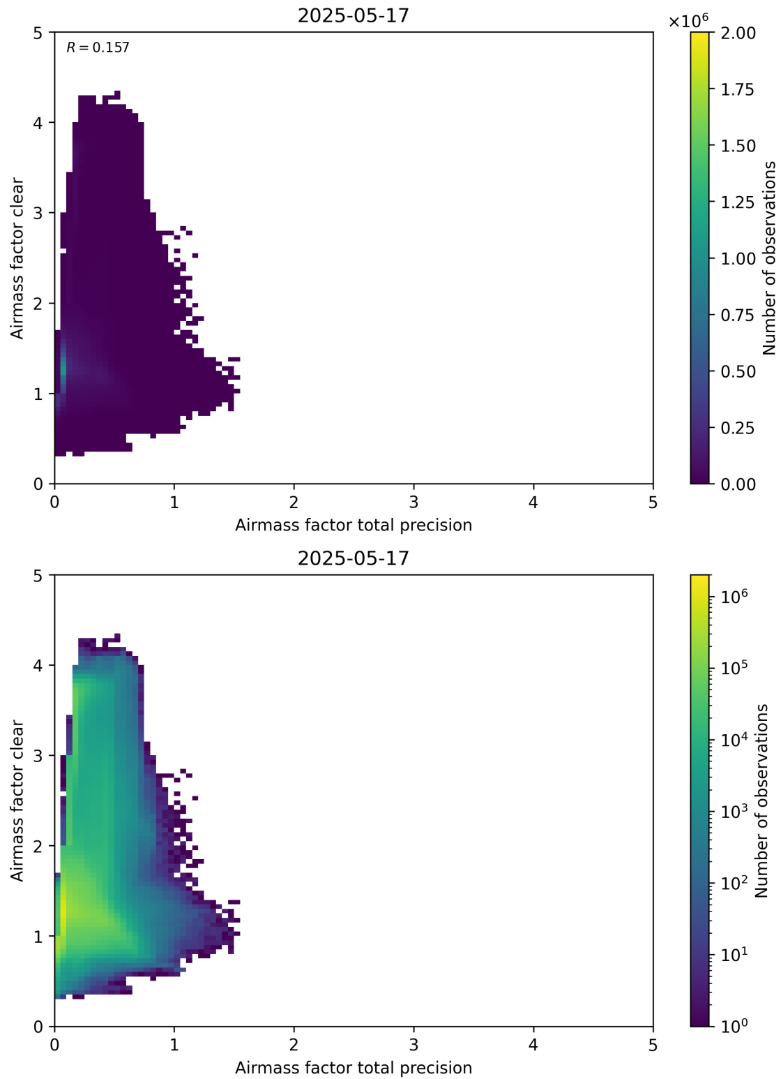
Figure 108: Scatter density plot of “Airmass factor total precision” against “Airmass factor clear” for 2025-05-16 to 2025-05-18.
