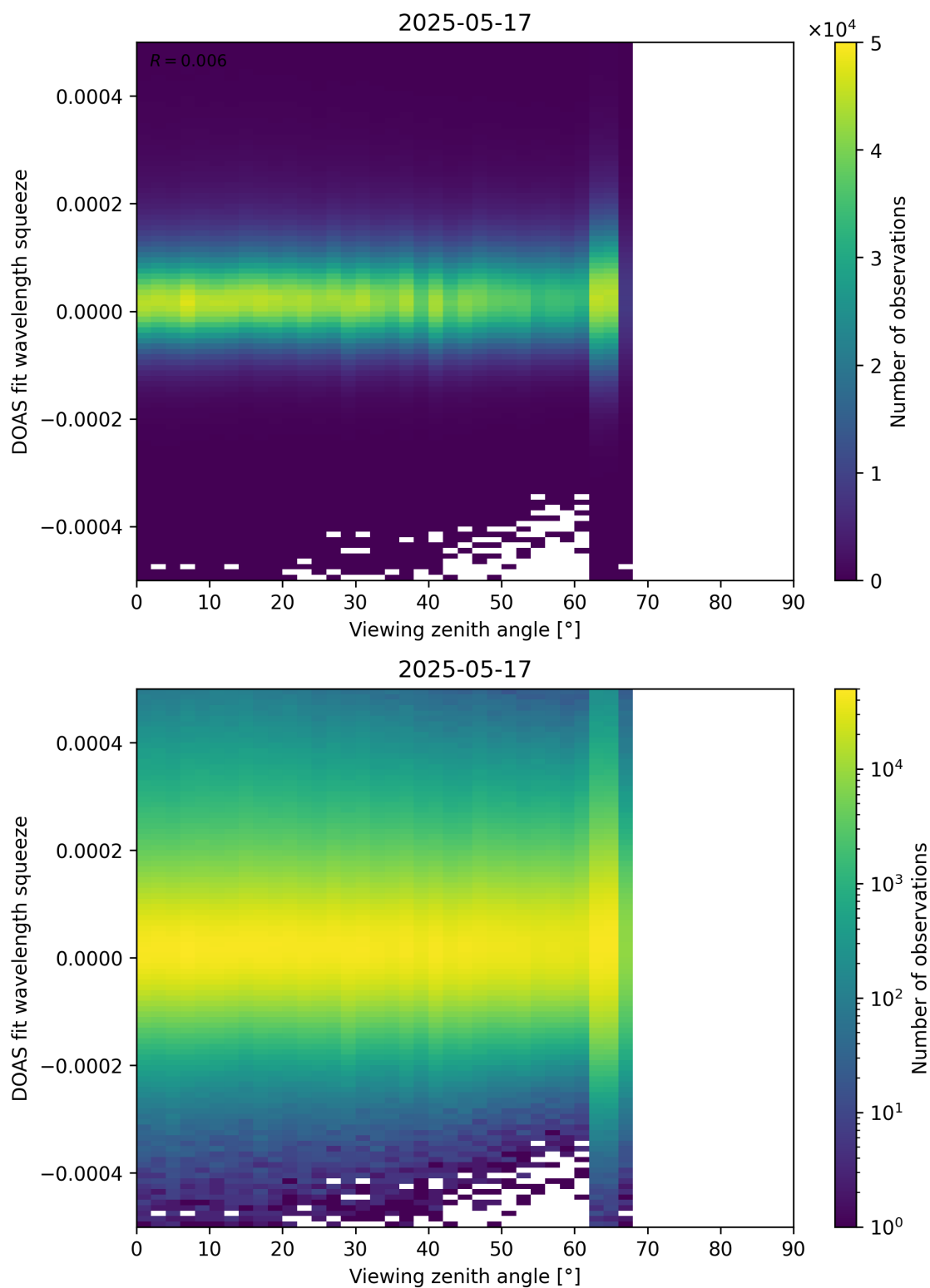
Figure 184: Scatter density plot of “Viewing zenith angle” against “DOAS fit wavelength squeeze” for 2025-05-16 to 2025-05-18.
