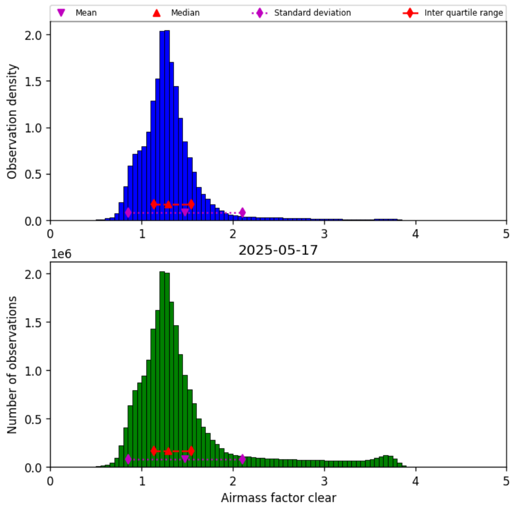
Figure 42: Histogram of “Airmass factor clear” for 2025-05-16 to 2025-05-18
