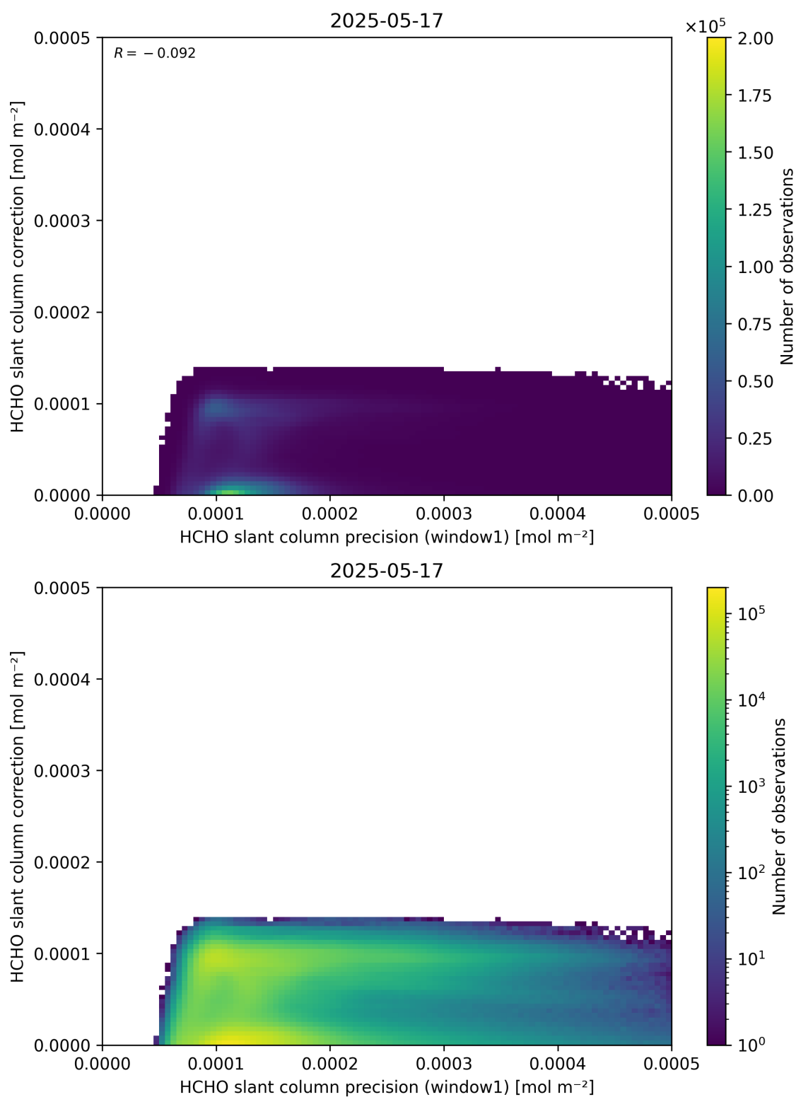
Figure 93: Scatter density plot of “HCHO slant column precision (window1)” against “HCHO slant column correction” for 2025-05-16 to 2025-05-18.
