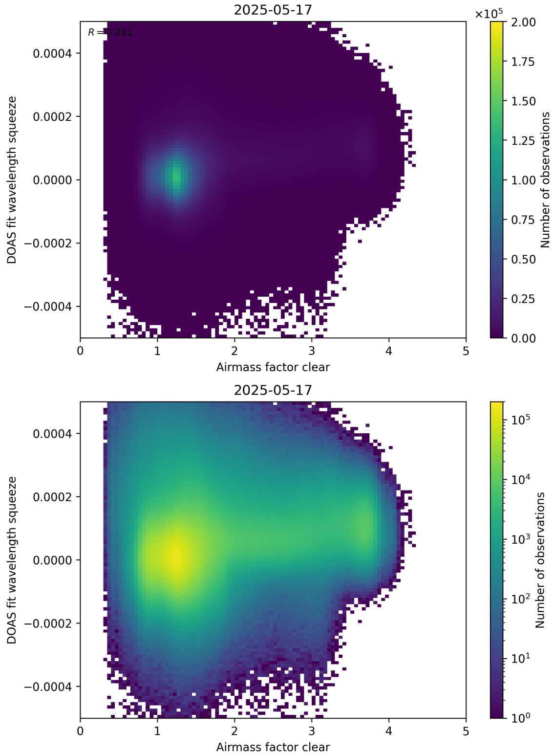
Figure 73: Scatter density plot of “Airmass factor clear” against “DOAS fit wavelength squeeze” for 2025-05-16 to 2025-05-18.
