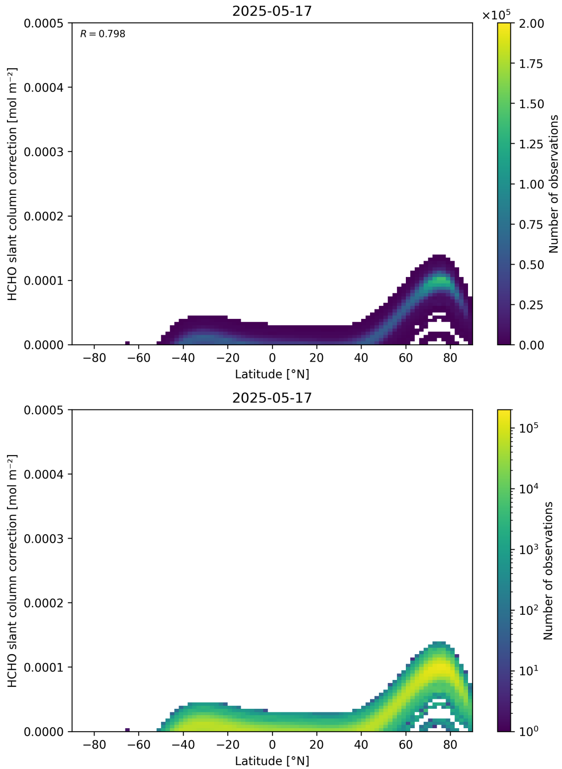
Figure 158: Scatter density plot of “Latitude” against “HCHO slant column correction” for 2025-05-16 to 2025-05-18.
