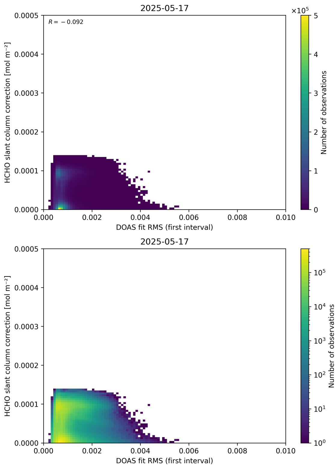
Figure 63: Scatter density plot of “DOAS fit RMS (first interval)” against “HCHO slant column correction” for 2025-05-16 to 2025-05-18.
