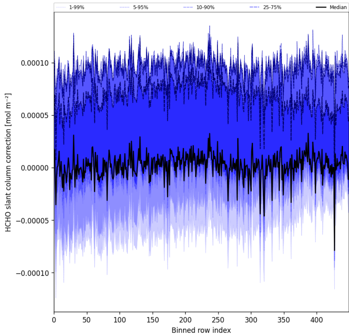
Figure 61: Along track statistics of “HCHO slant column correction” for 2025-05-16 to 2025-05-18
