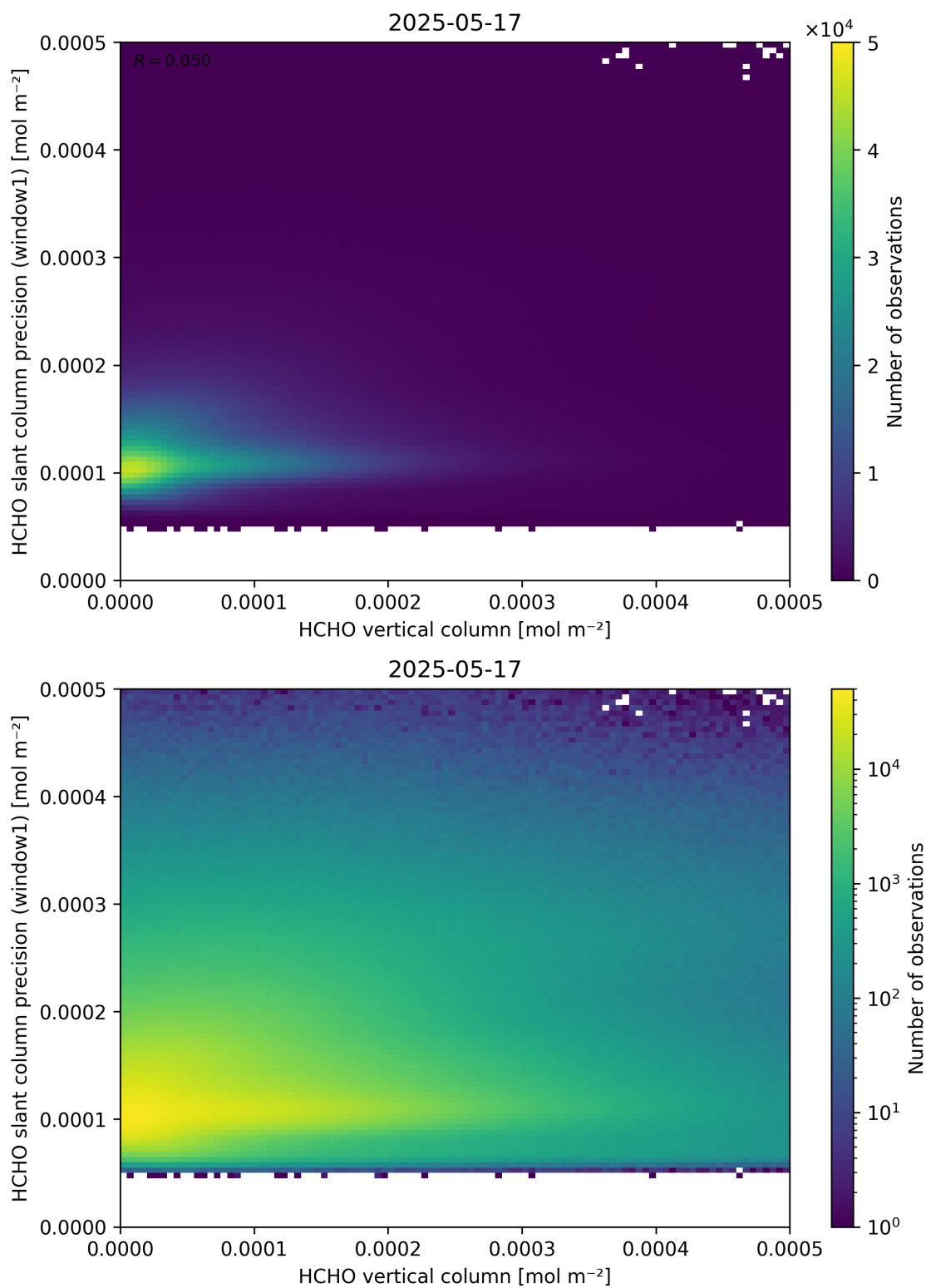
Figure 130: Scatter density plot of “HCHO vertical column” against “HCHO slant column precision (window1)” for 2025-05-16 to 2025-05-18.
