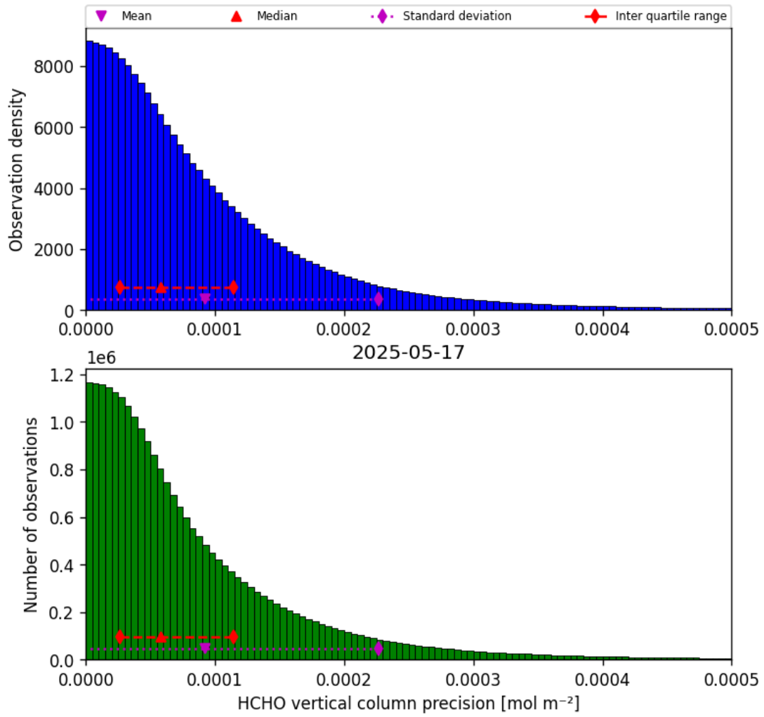
Figure 36: Histogram of “HCHO vertical column precision” for 2025-05-16 to 2025-05-18
