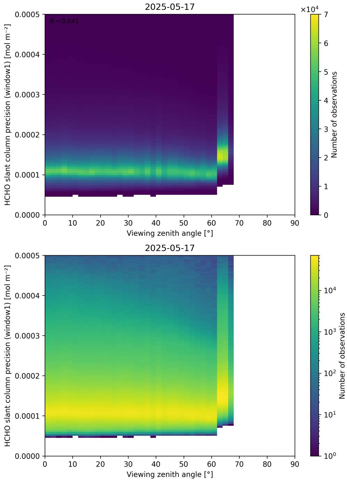
Figure 189: Scatter density plot of “Viewing zenith angle” against “HCHO slant column precision (window1)” for 2025-05-16 to 2025-05-18.
