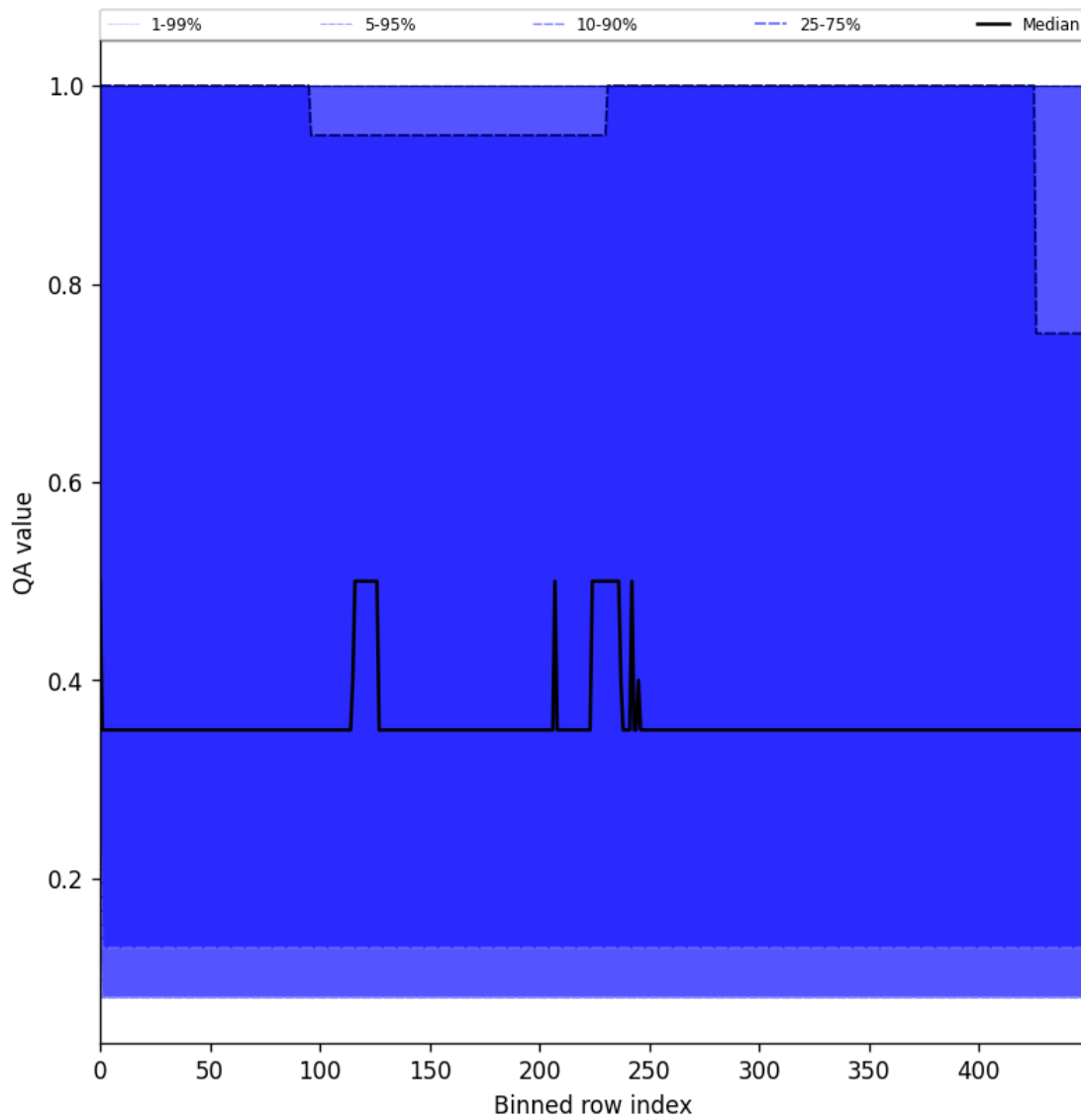
Figure 48: Along track statistics of “QA value” for 2025-05-16 to 2025-05-18
