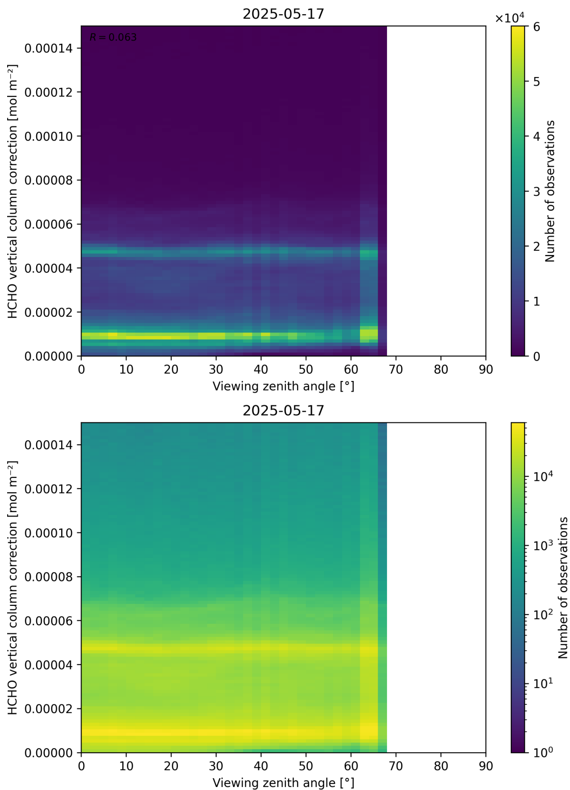
Figure 193: Scatter density plot of “Viewing zenith angle” against “HCHO vertical column correction” for 2025-05-16 to 2025-05-18.
