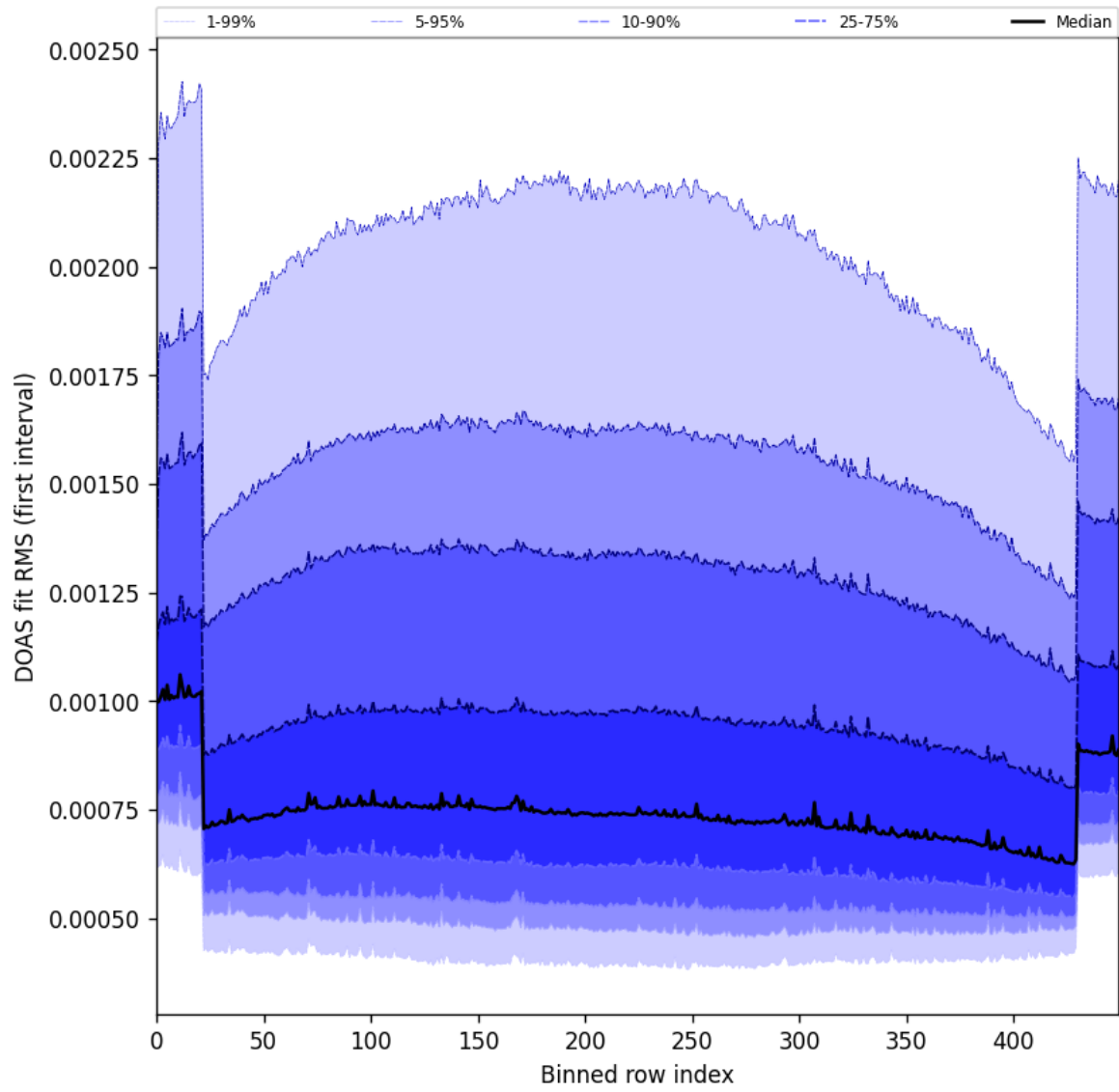
Figure 60: Along track statistics of “DOAS fit RMS (first interval)” for 2025-05-16 to 2025-05-18
