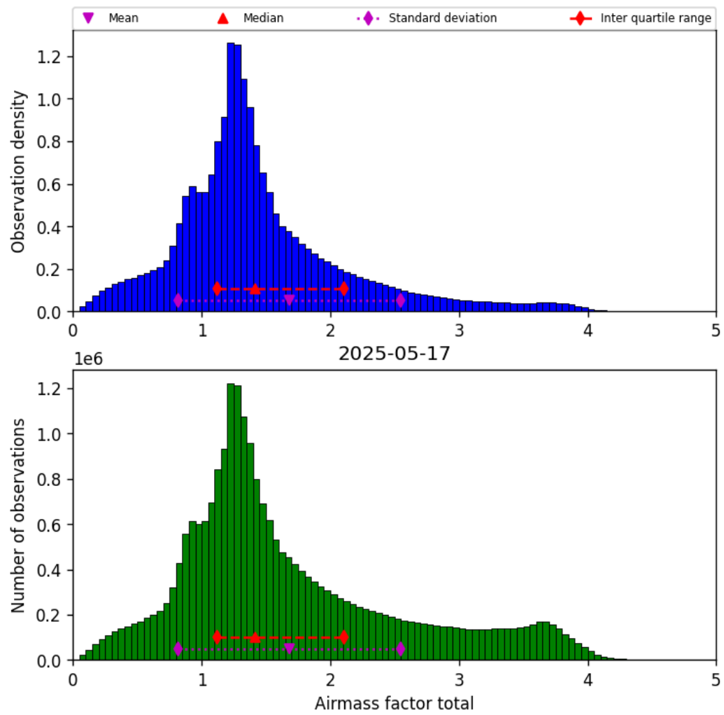
Figure 40: Histogram of “Airmass factor total” for 2025-05-16 to 2025-05-18
