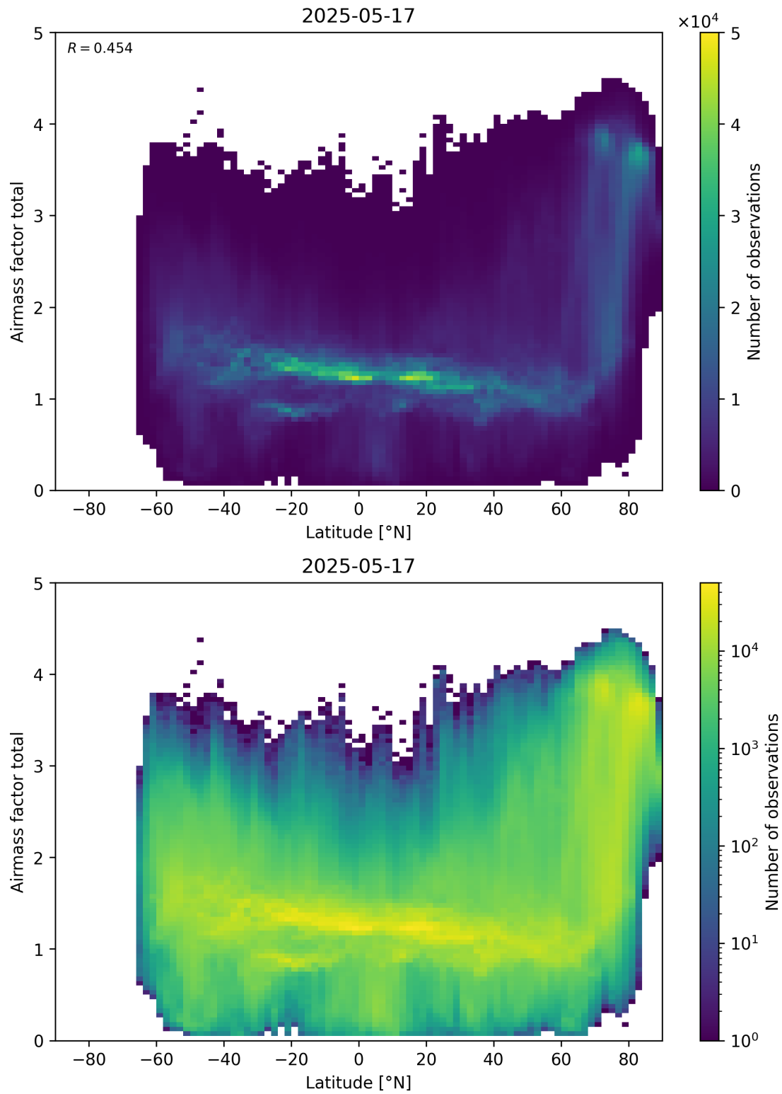
Figure 161: Scatter density plot of “Latitude” against “Airmass factor total” for 2025-05-16 to 2025-05-18.
