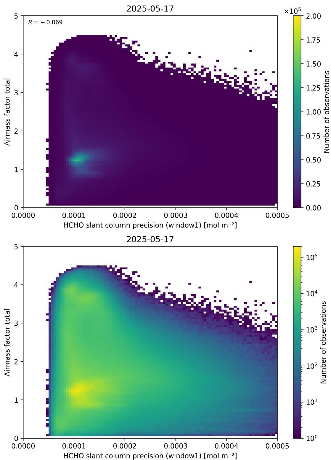
Figure 94: Scatter density plot of “HCHO slant column precision (window1)” against “Airmass factor total” for 2025-05-16 to 2025-05-18.
