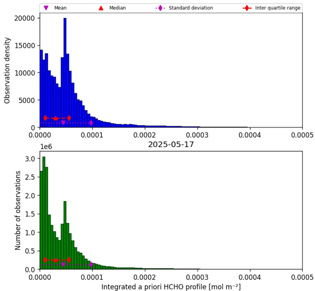
Figure 43: Histogram of “Integrated a priori HCHO profile” for 2025-05-16 to 2025-05-18
