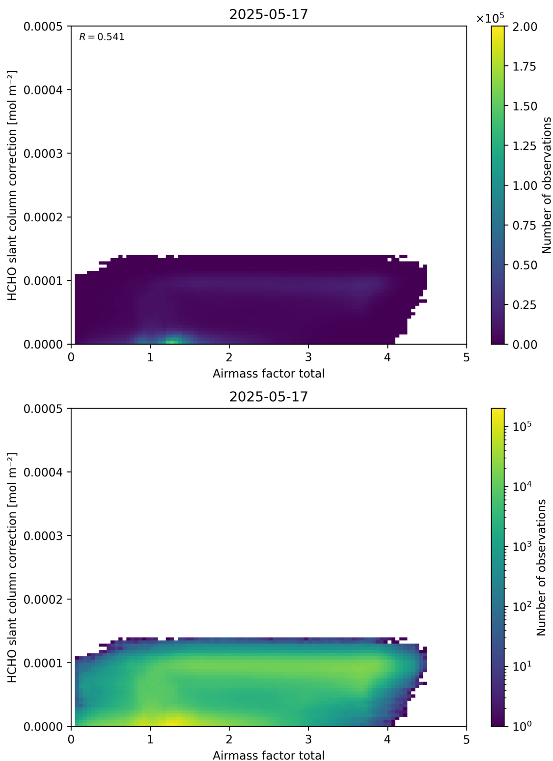
Figure 102: Scatter density plot of “Airmass factor total” against “HCHO slant column correction” for 2025-05-16 to 2025-05-18.
