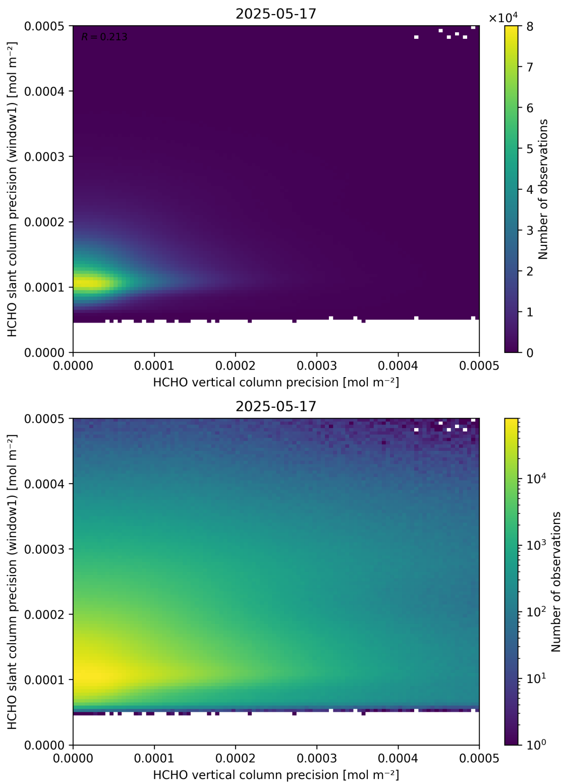
Figure 143: Scatter density plot of “HCHO vertical column precision” against “HCHO slant column precision (window1)” for 2025-05-16 to 2025-05-18.
