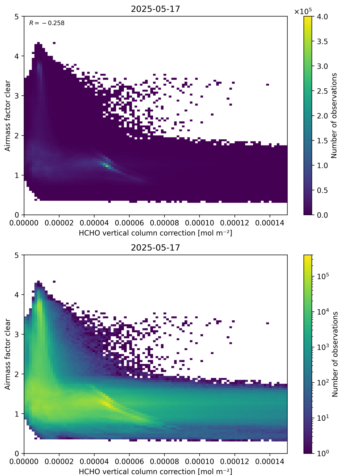
Figure 115: Scatter density plot of “HCHO vertical column correction” against “Airmass factor clear” for 2025-05-16 to 2025-05-18.
