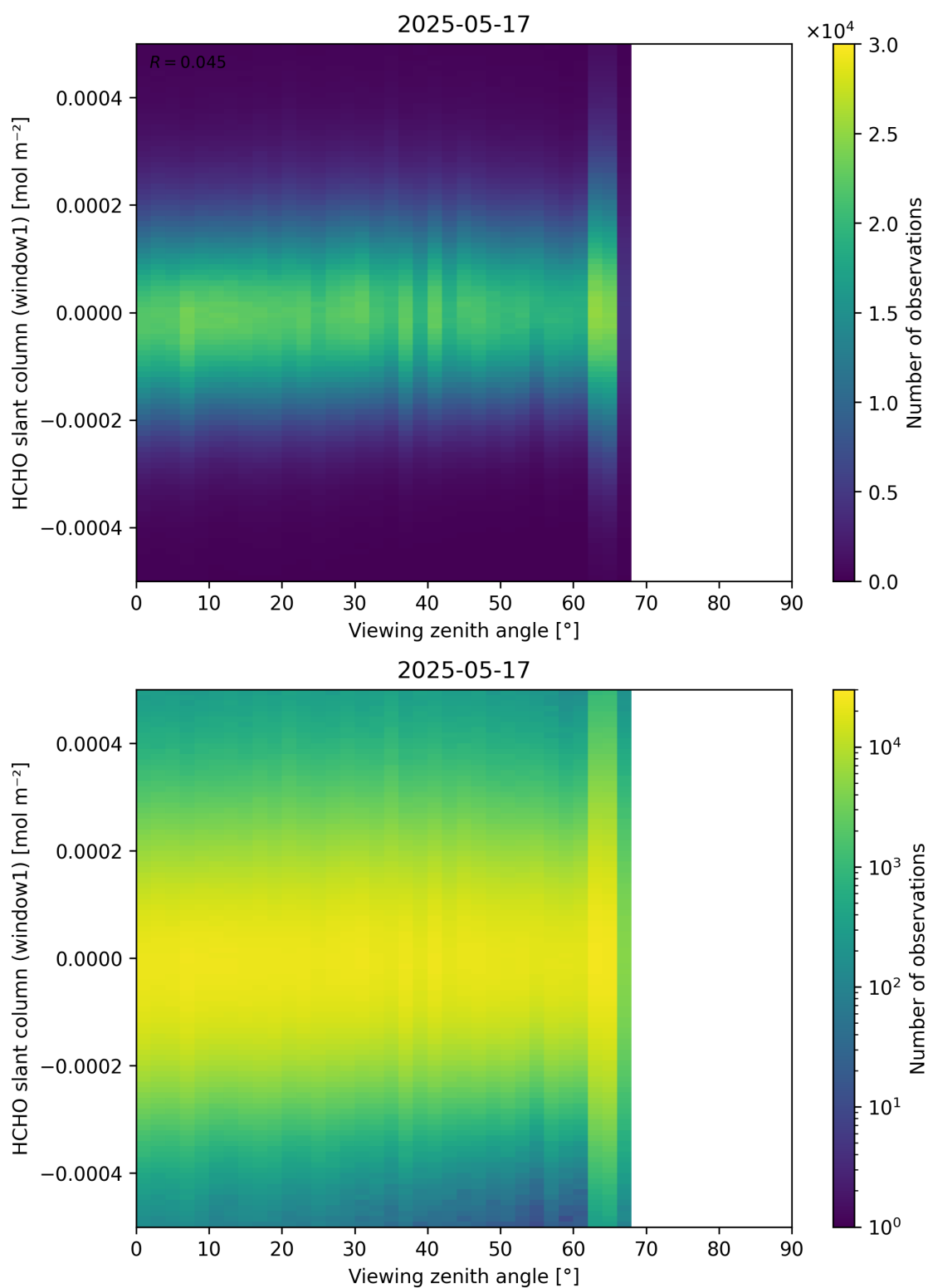
Figure 188: Scatter density plot of “Viewing zenith angle” against “HCHO slant column (window1)” for 2025-05-16 to 2025-05-18.
