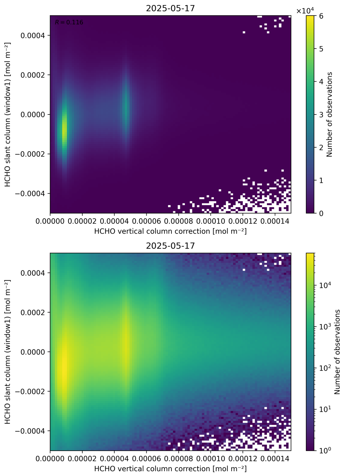
Figure 118: Scatter density plot of “HCHO vertical column correction” against “HCHO slant column (window1)” for 2025-05-16 to 2025-05-18.
