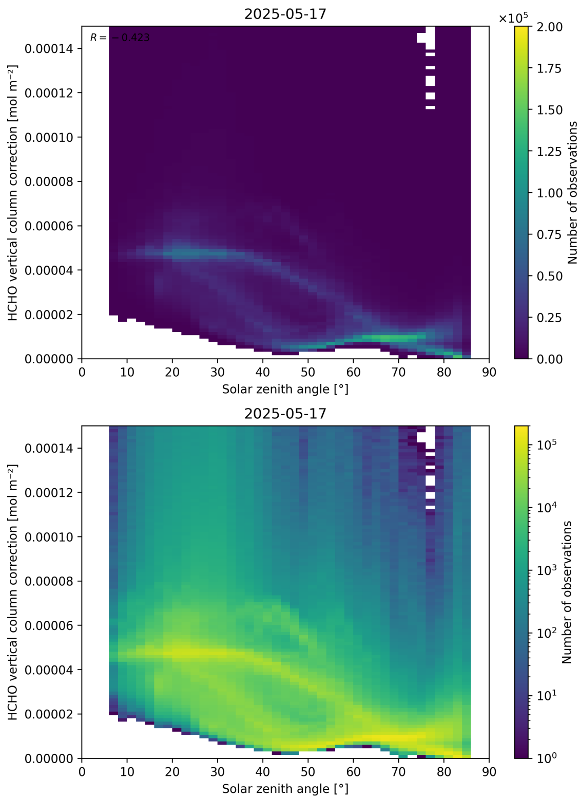
Figure 178: Scatter density plot of “Solar zenith angle” against “HCHO vertical column correction” for 2025-05-16 to 2025-05-18.
