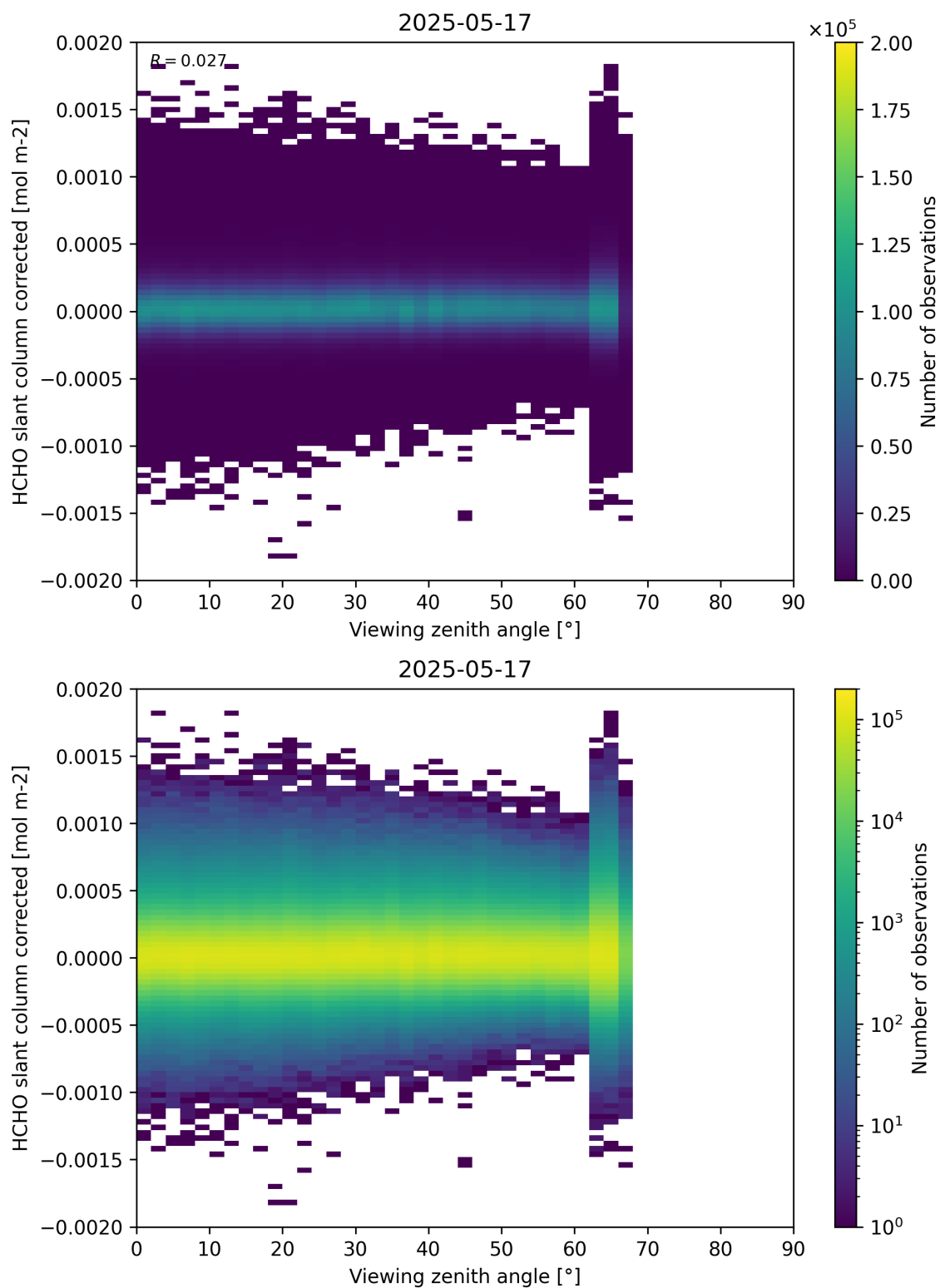
Figure 186: Scatter density plot of “Viewing zenith angle” against “HCHO slant column corrected” for 2025-05-16 to 2025-05-18.
