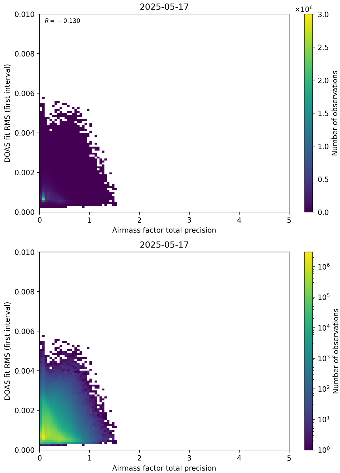
Figure 105: Scatter density plot of “Airmass factor total precision” against “DOAS fit RMS (first interval)” for 2025-05-16 to 2025-05-18.
