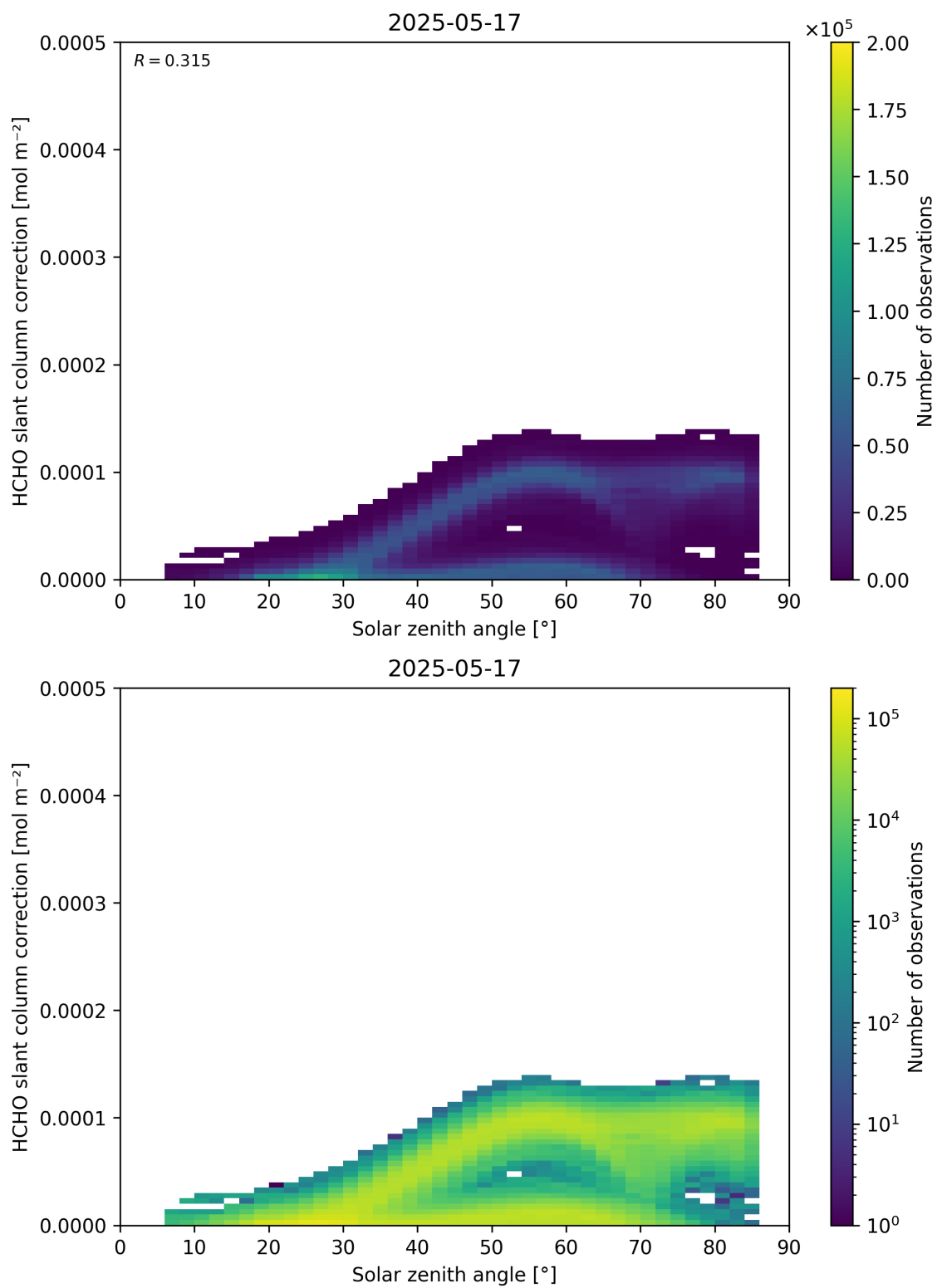
Figure 172: Scatter density plot of “Solar zenith angle” against “HCHO slant column correction” for 2025-05-16 to 2025-05-18.
