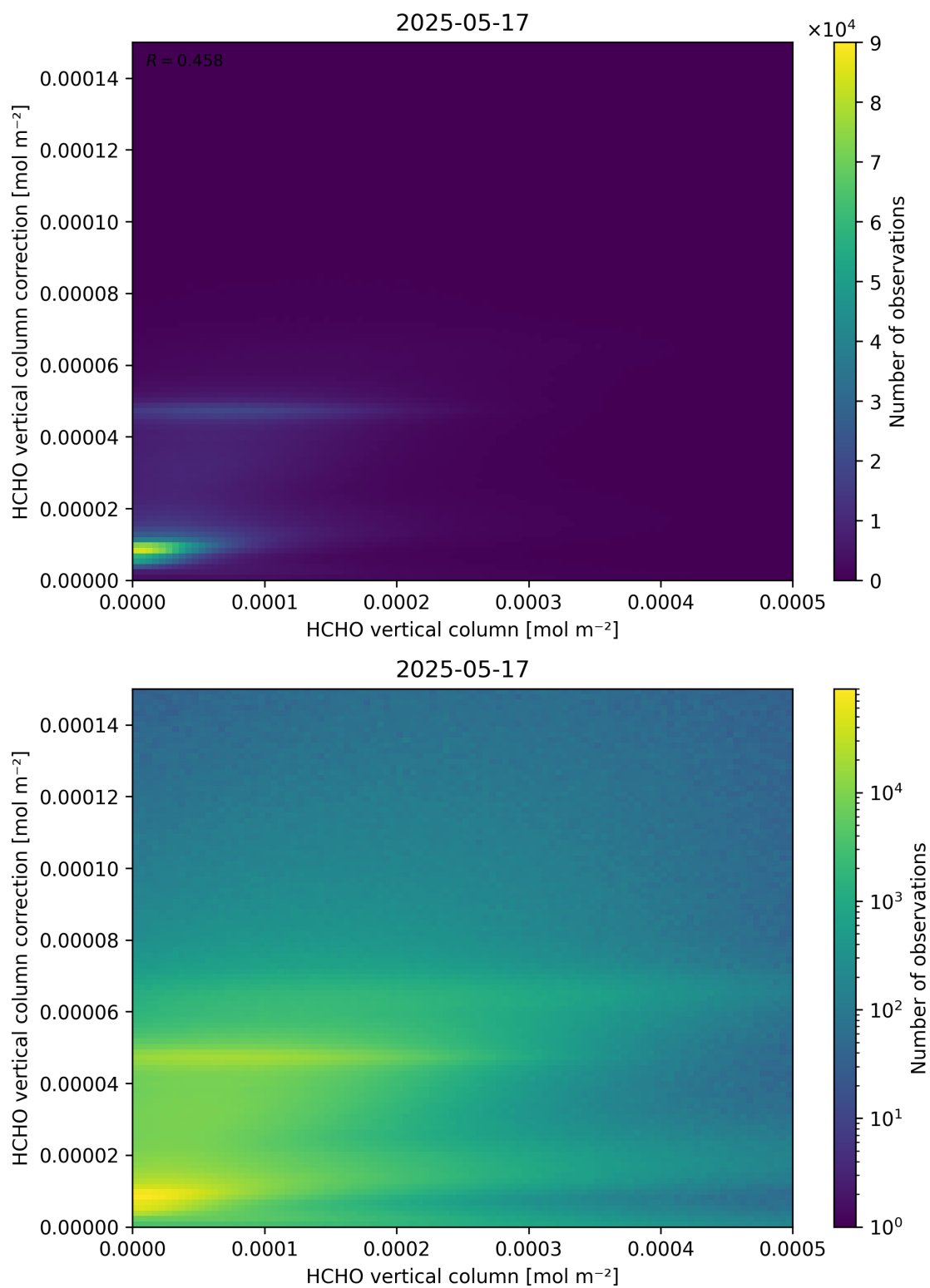
Figure 133: Scatter density plot of “HCHO vertical column” against “HCHO vertical column correction” for 2025-05-16 to 2025-05-18.
