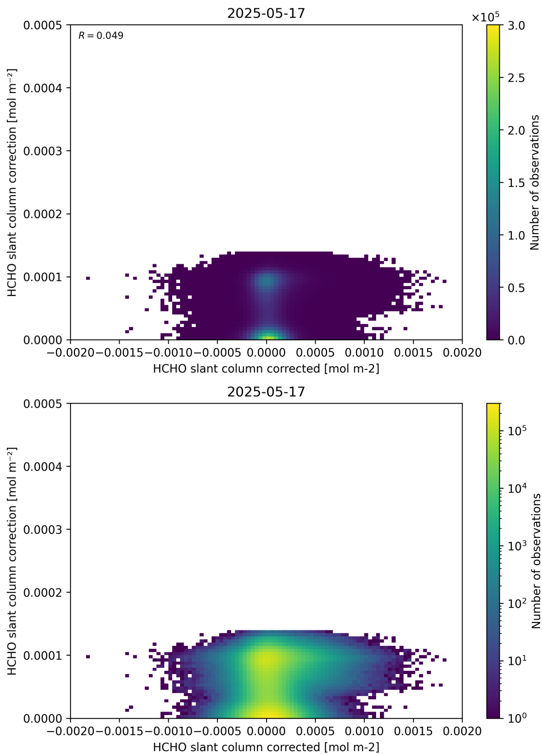
Figure 77: Scatter density plot of “HCHO slant column corrected” against “HCHO slant column correction” for 2025-05-16 to 2025-05-18.
