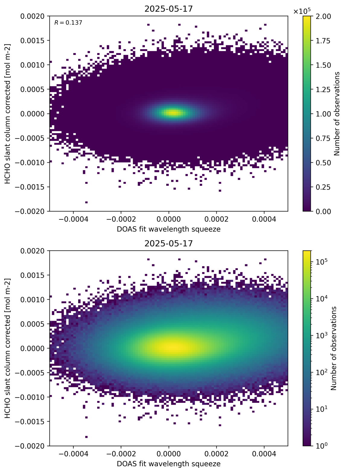
Figure 69: Scatter density plot of “DOAS fit wavelength squeeze” against “HCHO slant column corrected” for 2025-05-16 to 2025-05-18.
