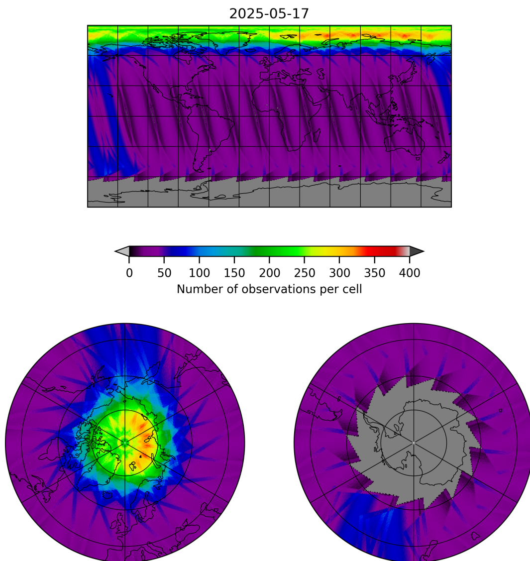
Figure 19: Map of the number of observations for 2025-05-16 to 2025-05-18
