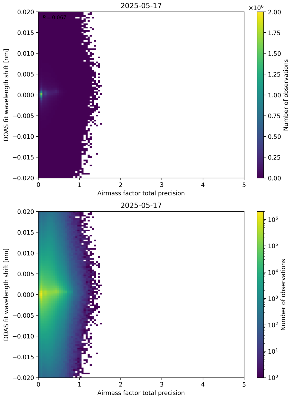
Figure 106: Scatter density plot of “Airmass factor total precision” against “DOAS fit wavelength shift” for 2025-05-16 to 2025-05-18.
