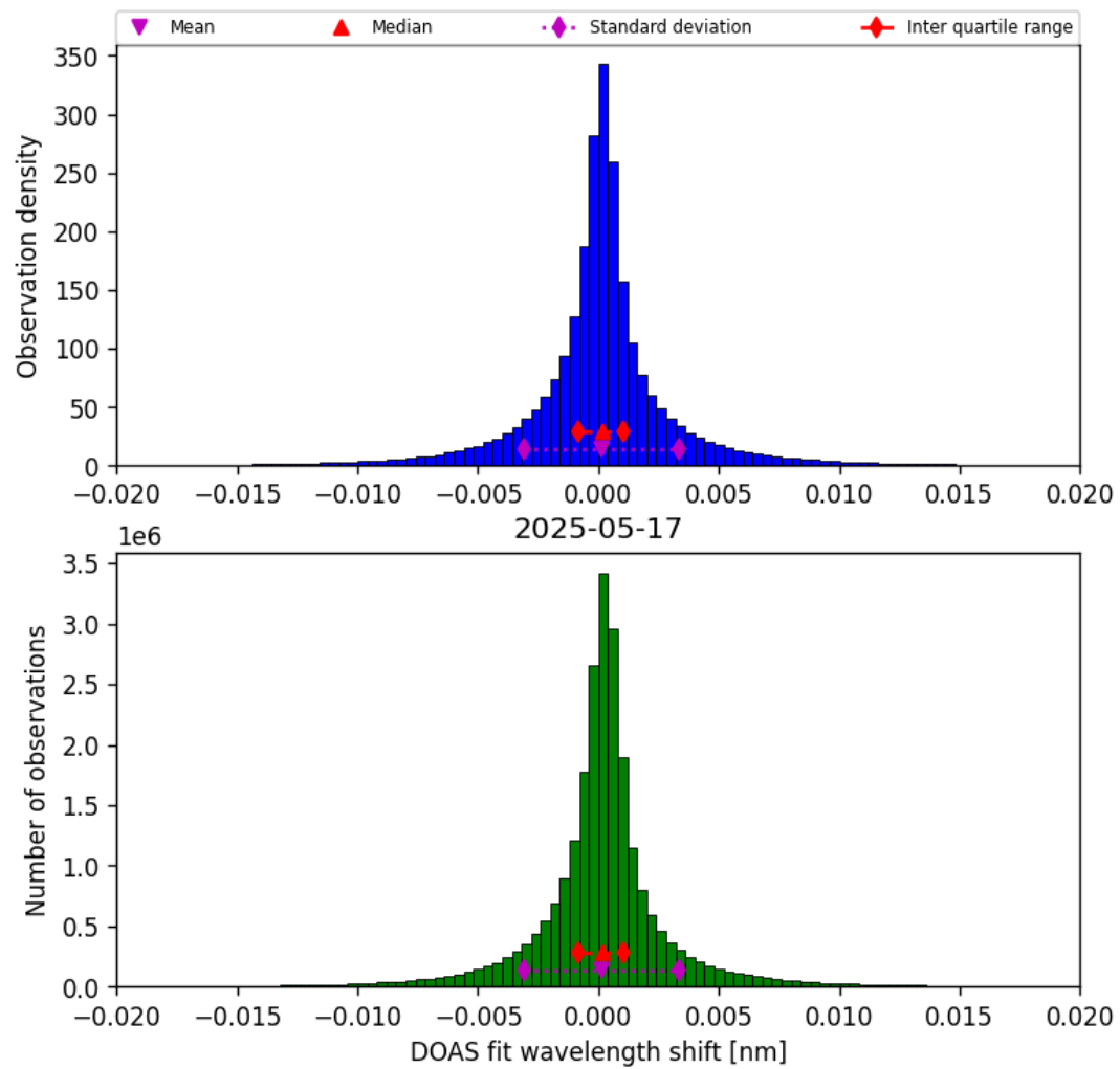
Figure 44: Histogram of “DOAS fit wavelength shift” for 2025-05-16 to 2025-05-18
