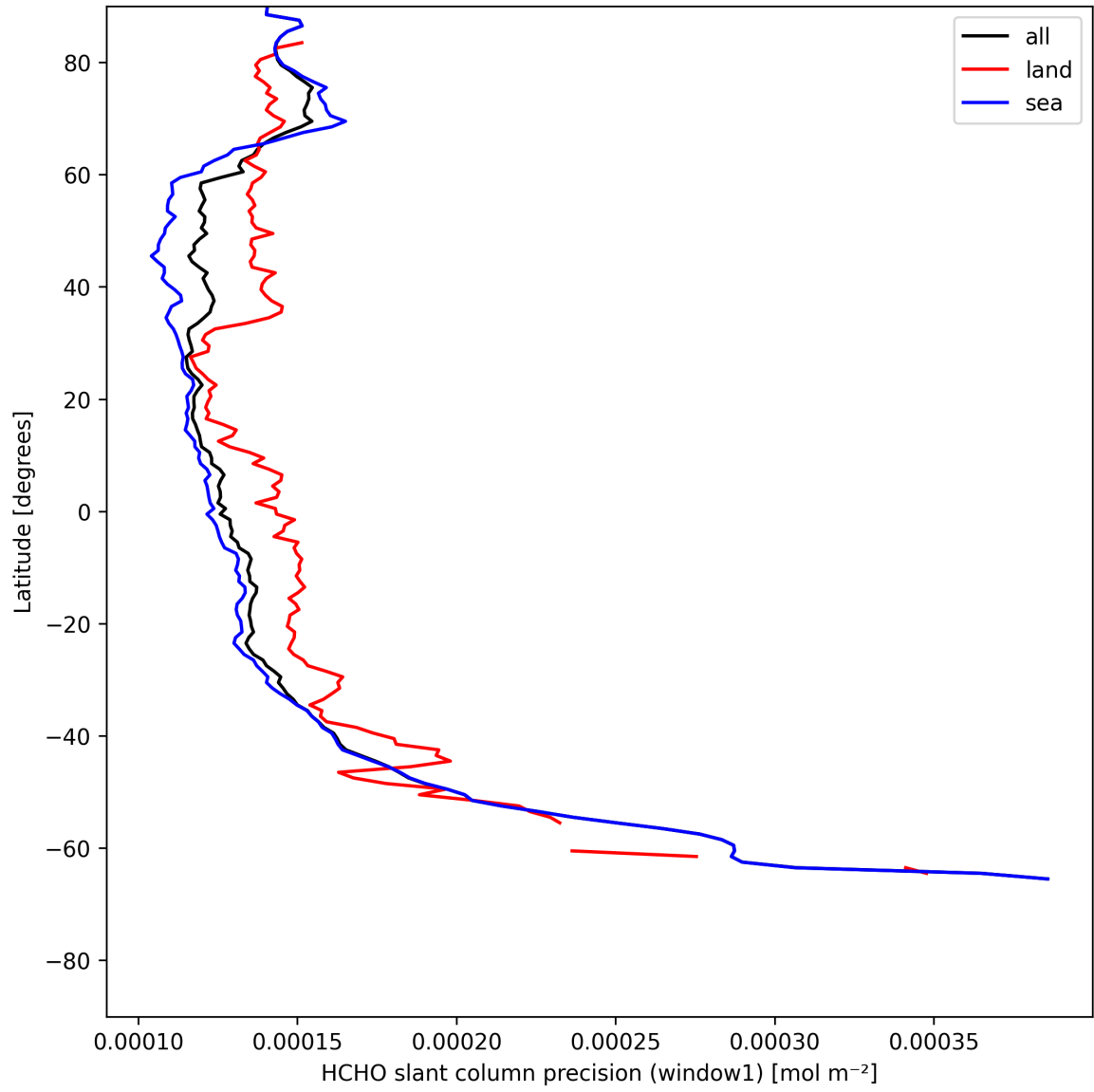
Figure 25: Zonal average of “HCHO slant column precision (window1)” for 2025-05-16 to 2025-05-18.
