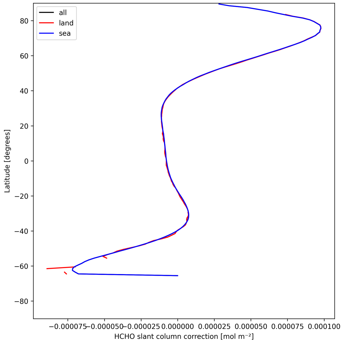
Figure 33: Zonal average of “HCHO slant column correction” for 2025-05-16 to 2025-05-18.
