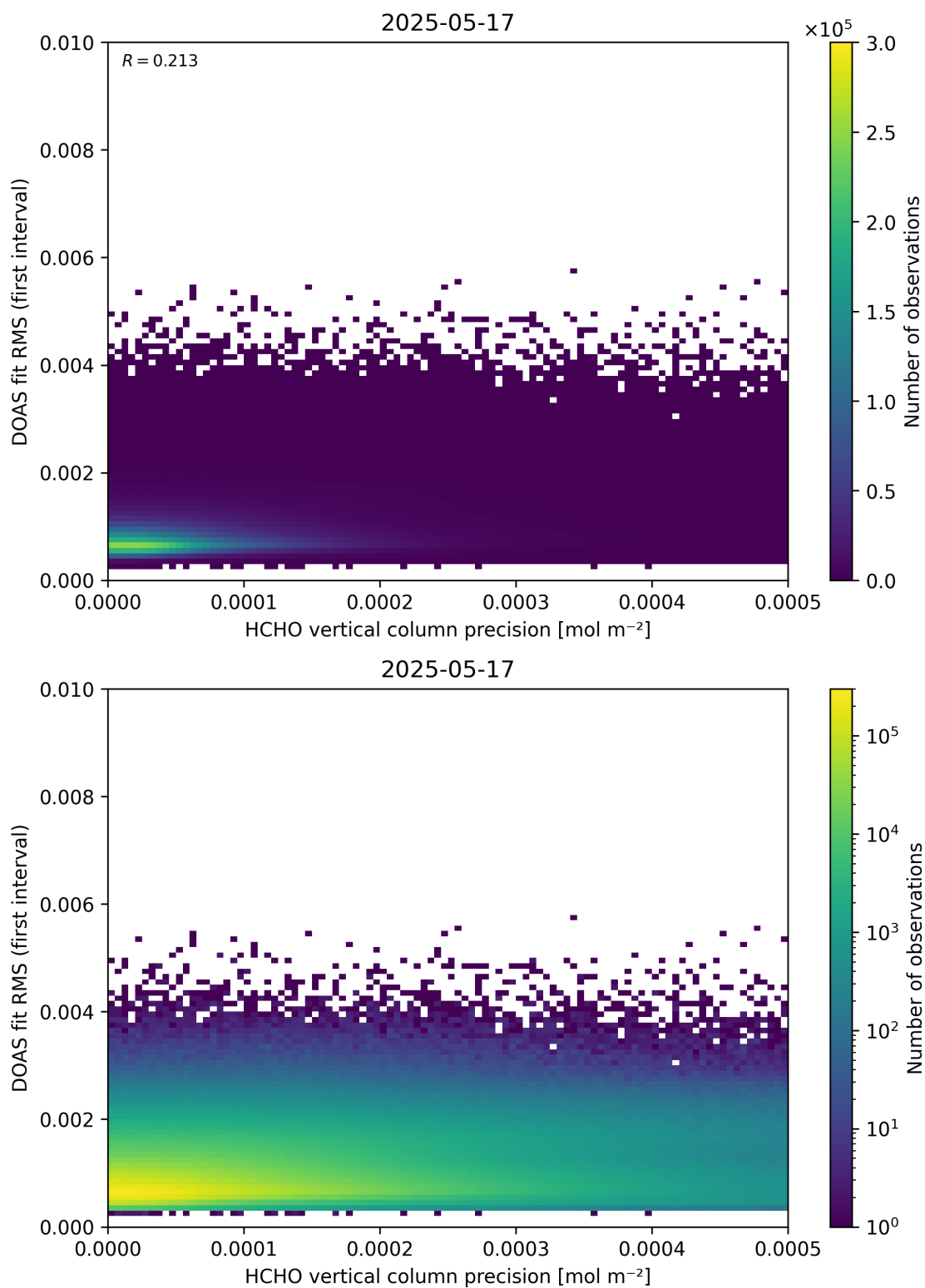
Figure 136: Scatter density plot of “HCHO vertical column precision” against “DOAS fit RMS (first interval)” for 2025-05-16 to 2025-05-18.
