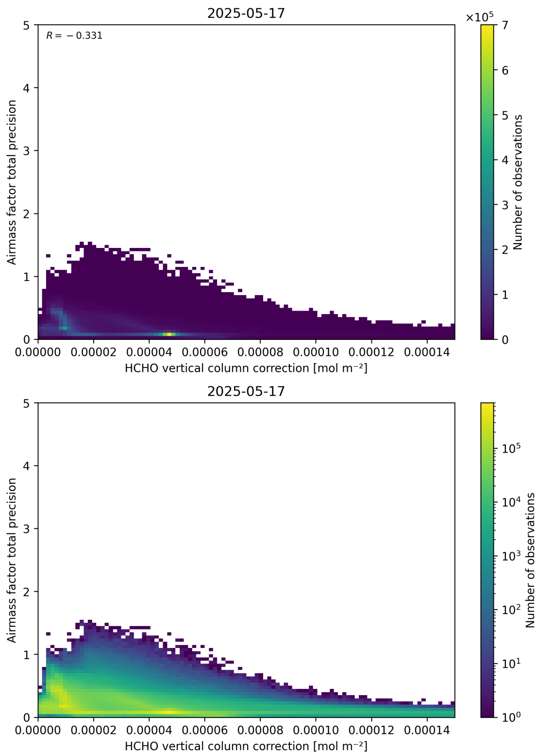
Figure 121: Scatter density plot of “HCHO vertical column correction” against “Airmass factor total precision” for 2025-05-16 to 2025-05-18.
