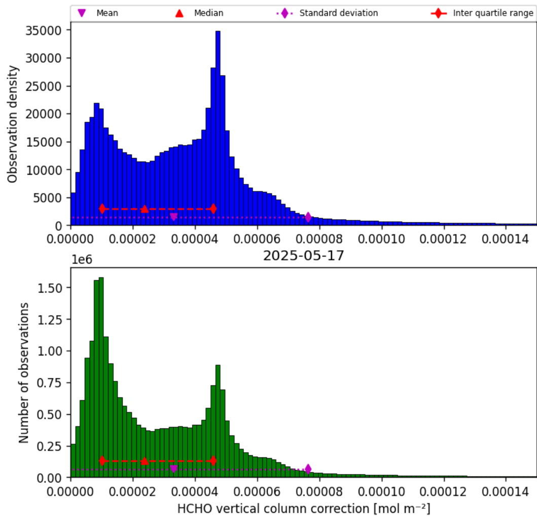
Figure 37: Histogram of “HCHO vertical column correction” for 2025-05-16 to 2025-05-18
