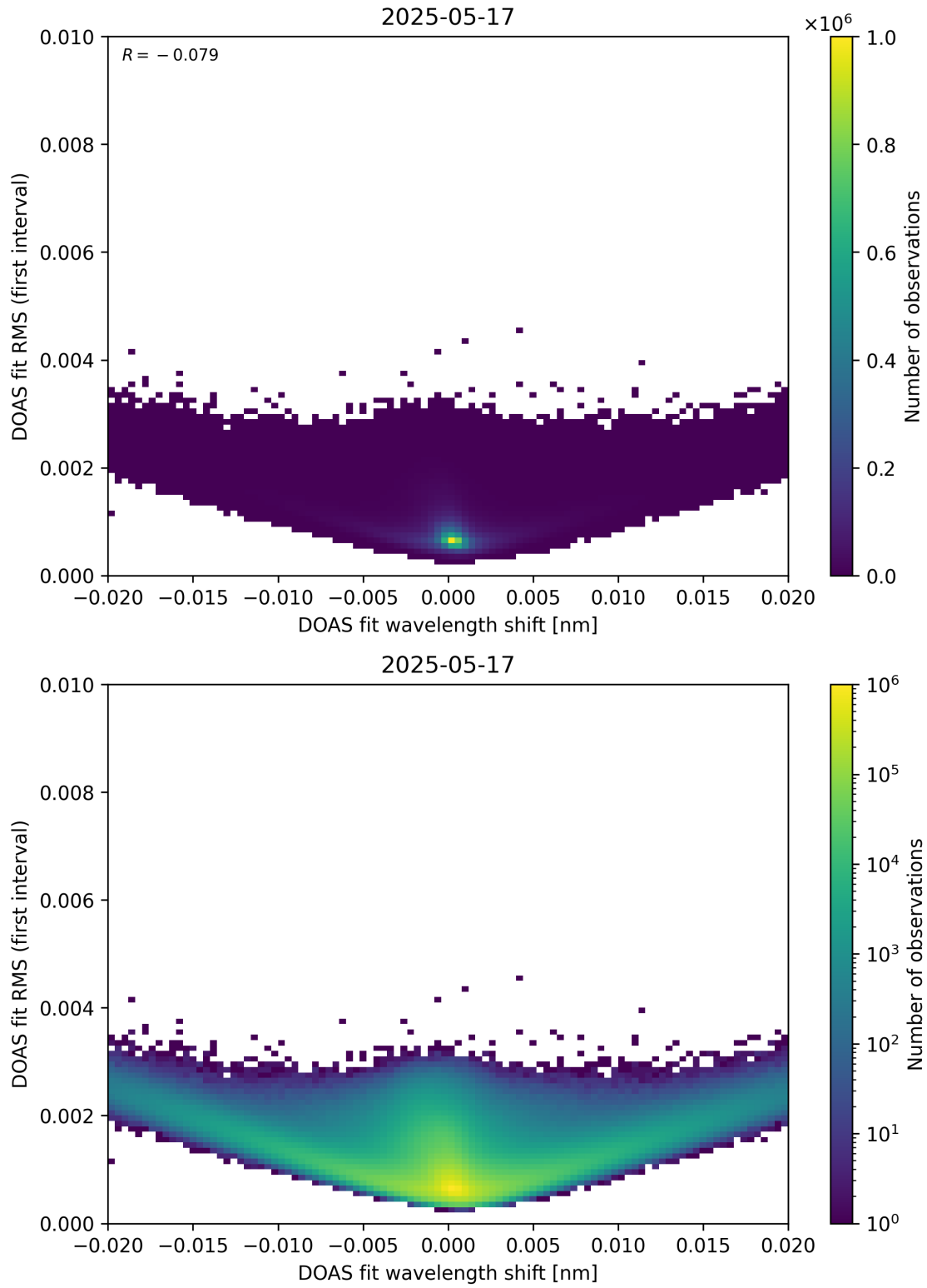
Figure 64: Scatter density plot of “DOAS fit wavelength shift” against “DOAS fit RMS (first interval)” for 2025-05-16 to 2025-05-18.
