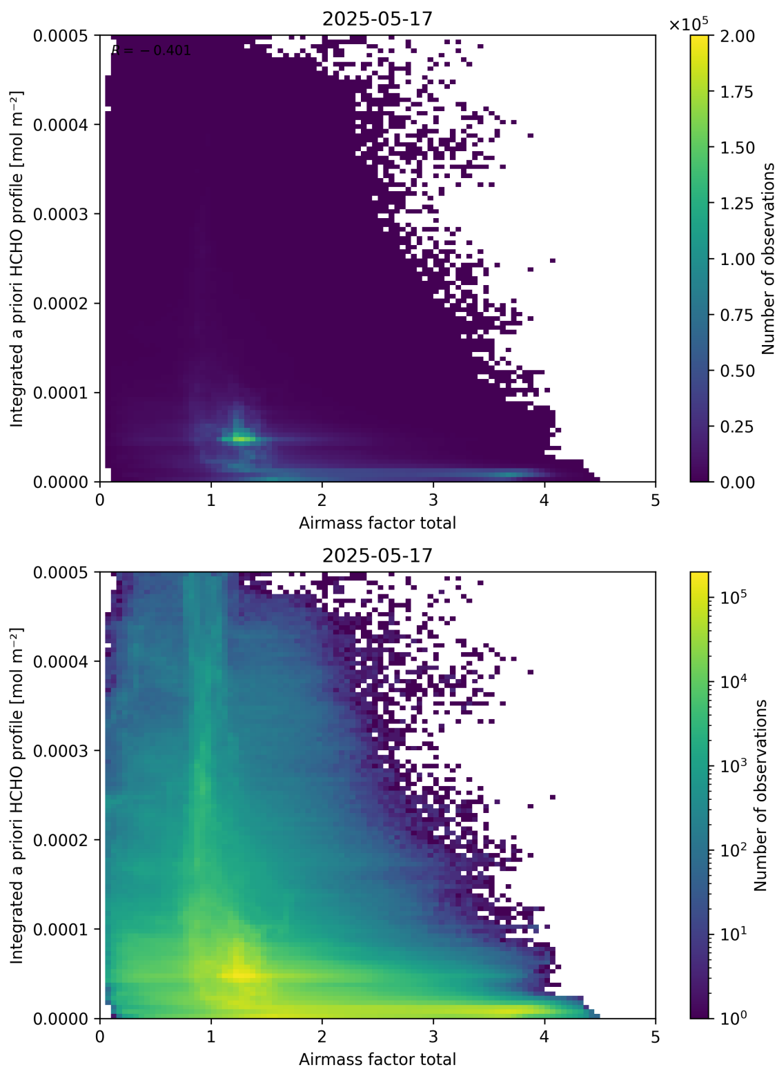
Figure 104: Scatter density plot of “Airmass factor total” against “Integrated a priori HCHO profile” for 2025-05-16 to 2025-05-18.
