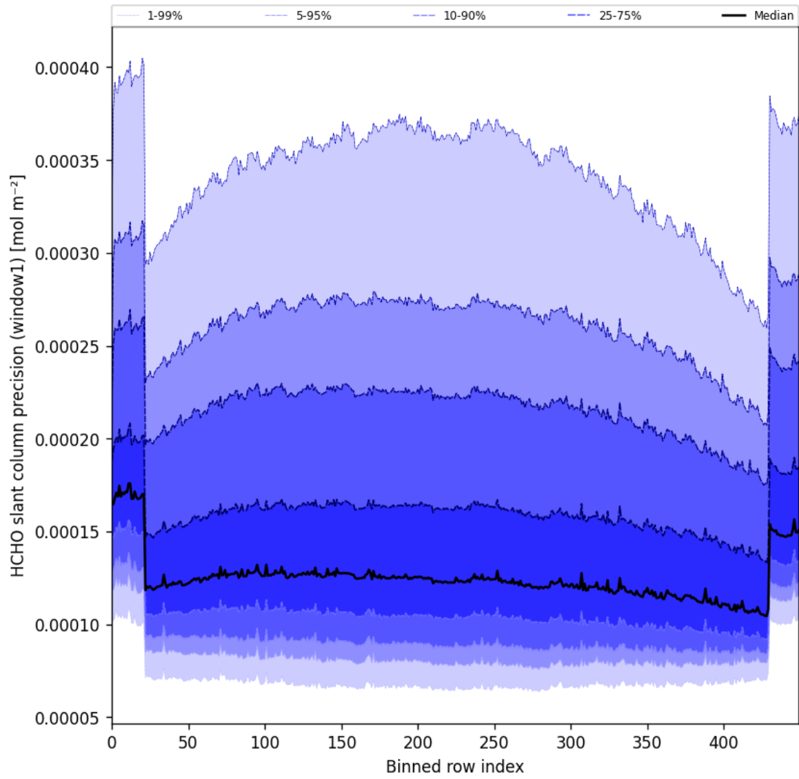
Figure 53: Along track statistics of “HCHO slant column precision (window1)” for 2025-05-16 to 2025-05-18
