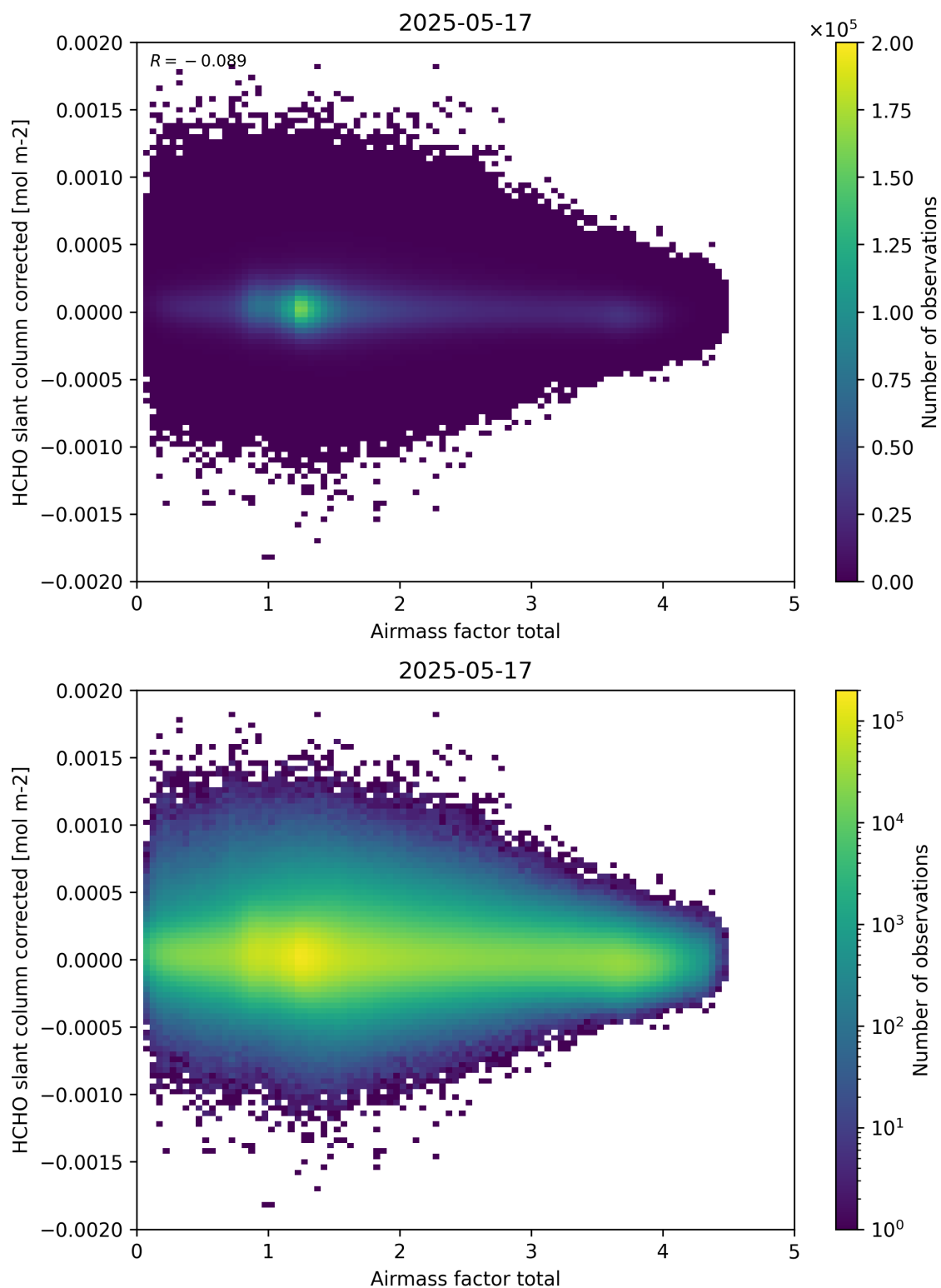
Figure 101: Scatter density plot of “Airmass factor total” against “HCHO slant column corrected” for 2025-05-16 to 2025-05-18.
