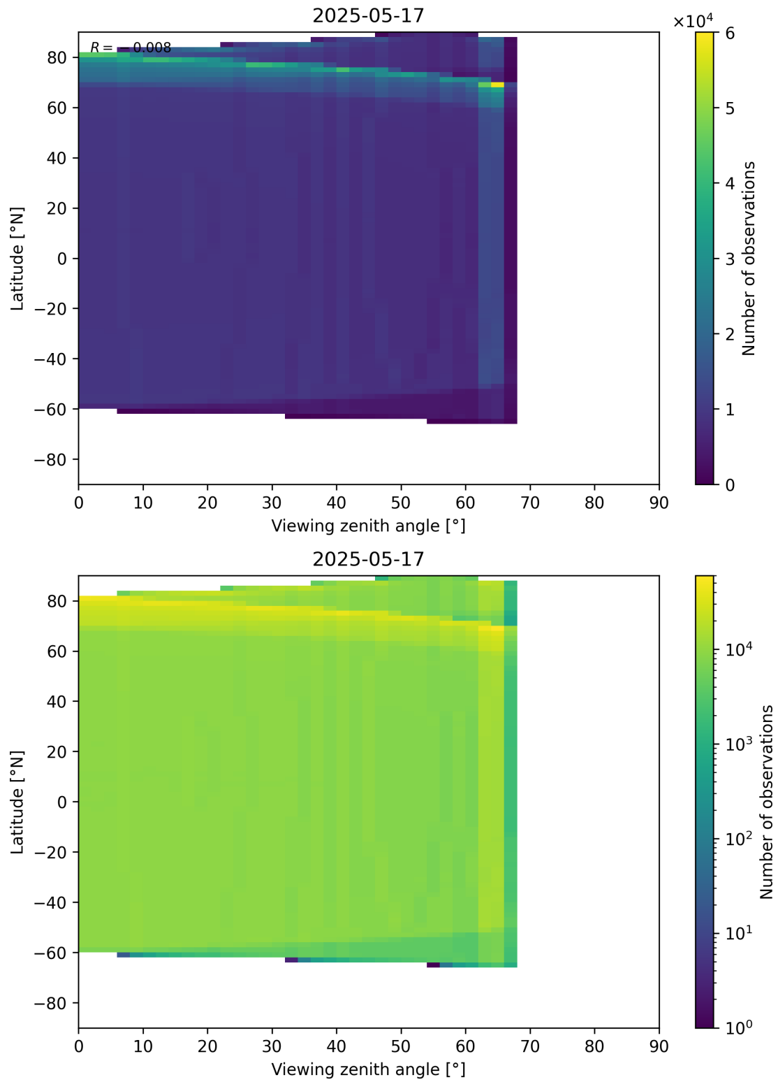
Figure 196: Scatter density plot of “Viewing zenith angle” against “Latitude” for 2025-05-16 to 2025-05-18.
