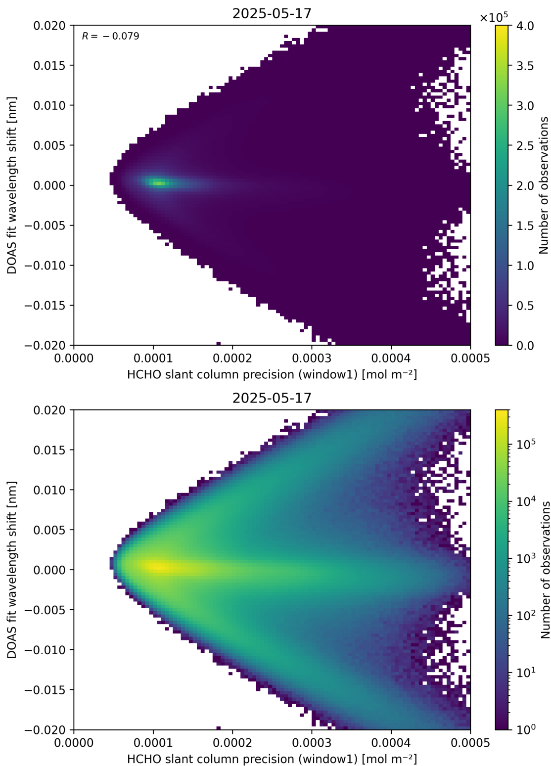
Figure 89: Scatter density plot of “HCHO slant column precision (window1)” against “DOAS fit wavelength shift” for 2025-05-16 to 2025-05-18.
