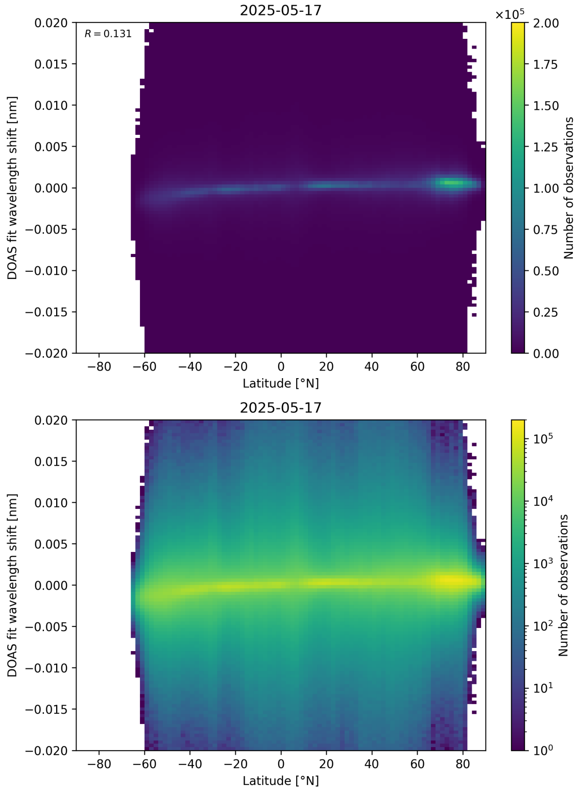
Figure 154: Scatter density plot of “Latitude” against “DOAS fit wavelength shift” for 2025-05-16 to 2025-05-18.
