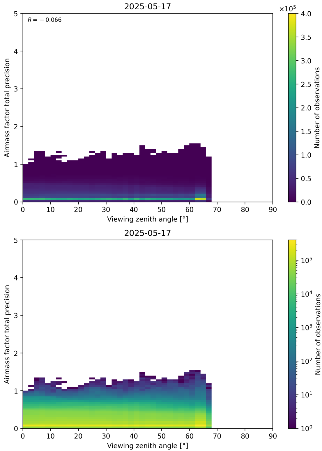
Figure 191: Scatter density plot of “Viewing zenith angle” against “Airmass factor total precision” for 2025-05-16 to 2025-05-18.
