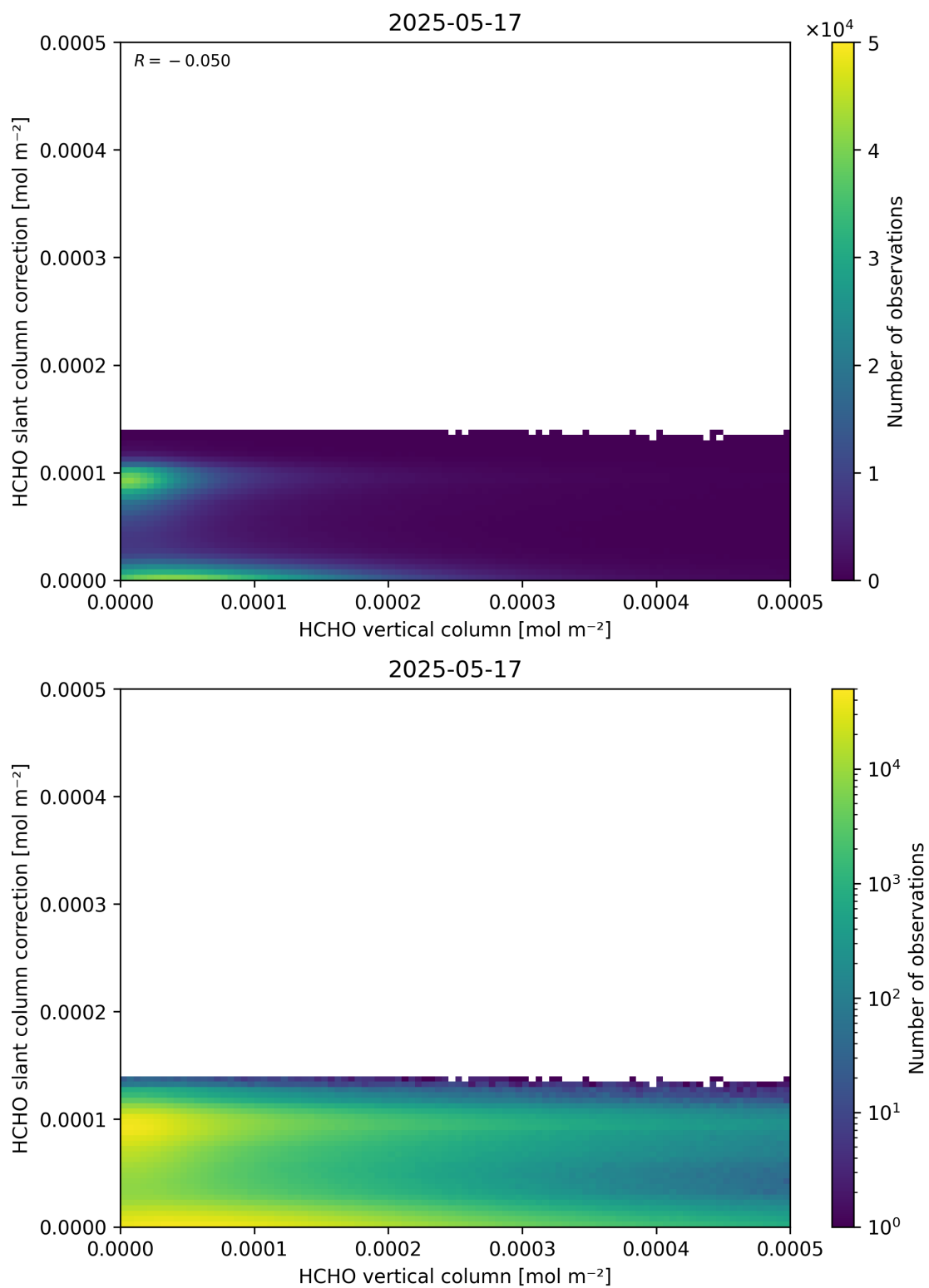
Figure 128: Scatter density plot of “HCHO vertical column” against “HCHO slant column correction” for 2025-05-16 to 2025-05-18.
