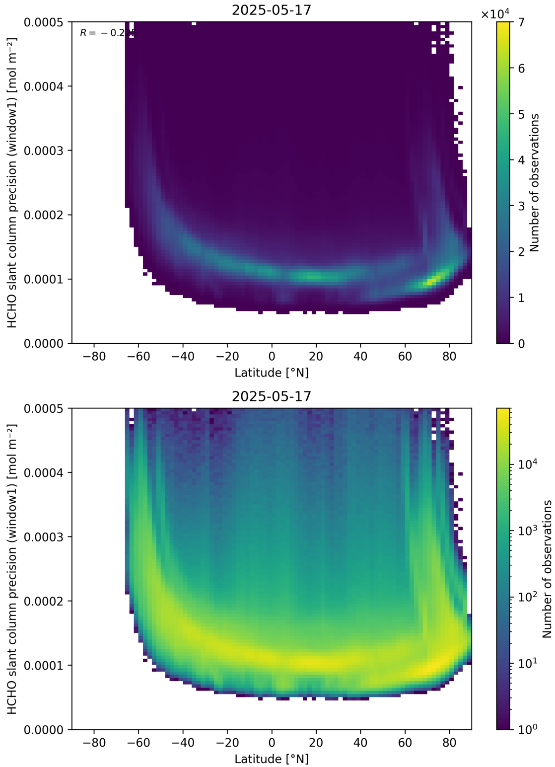
Figure 160: Scatter density plot of “Latitude” against “HCHO slant column precision (window1)” for 2025-05-16 to 2025-05-18.
