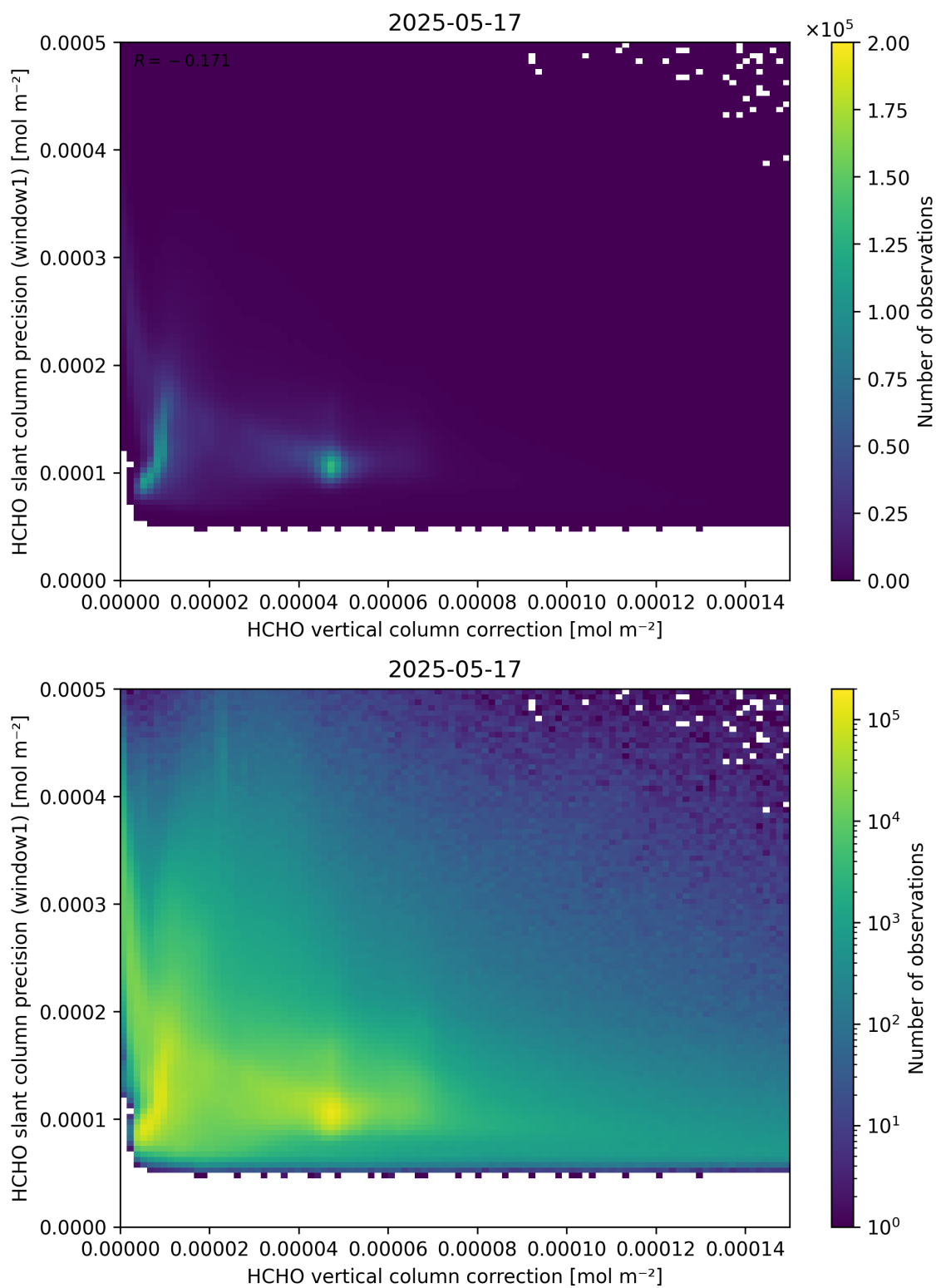
Figure 119: Scatter density plot of “HCHO vertical column correction” against “HCHO slant column precision (window1)” for 2025-05-16 to 2025-05-18.
