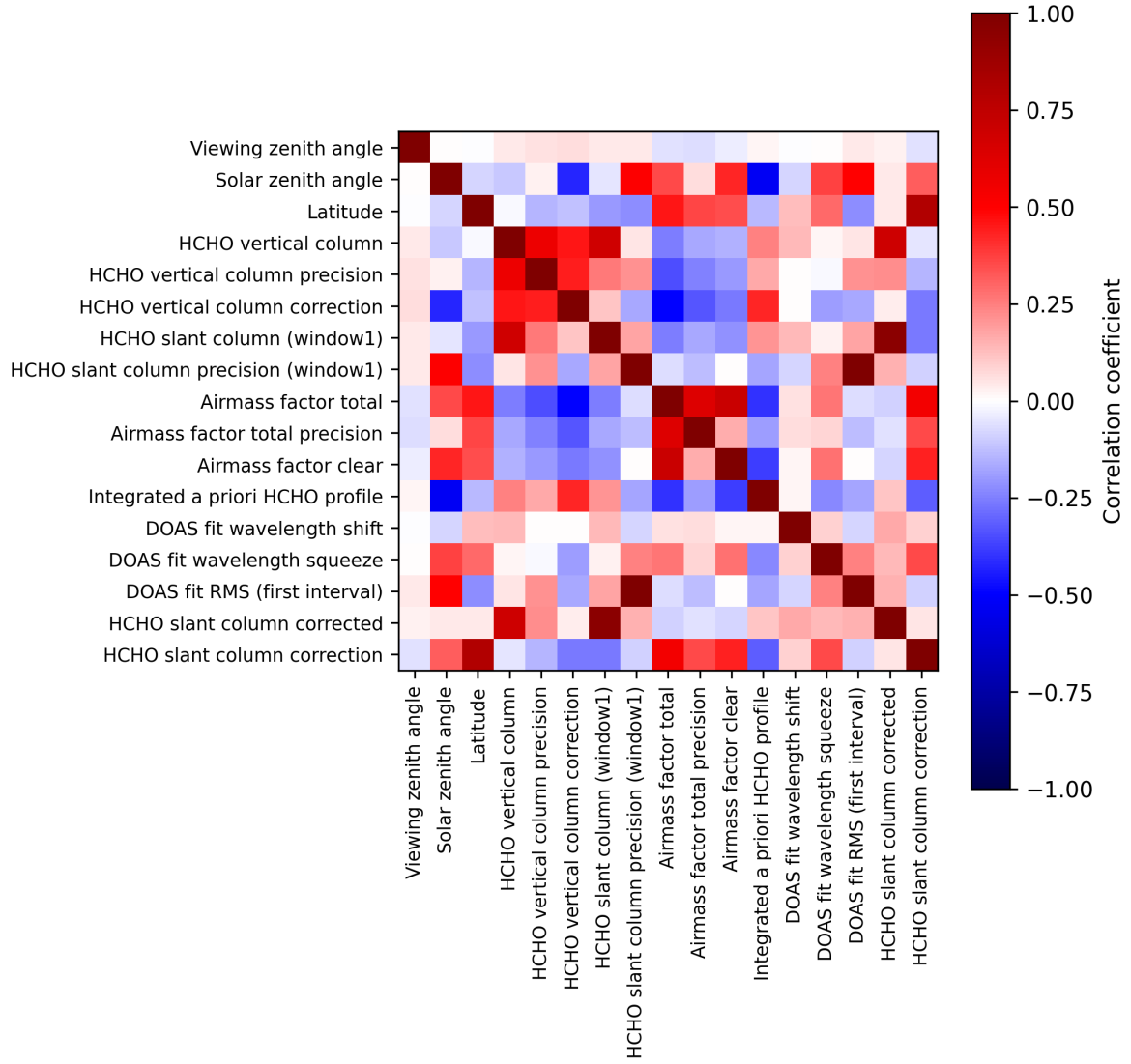
Figure 2: Map of correlation matrix for 2025-05-16 to 2025-05-18.
