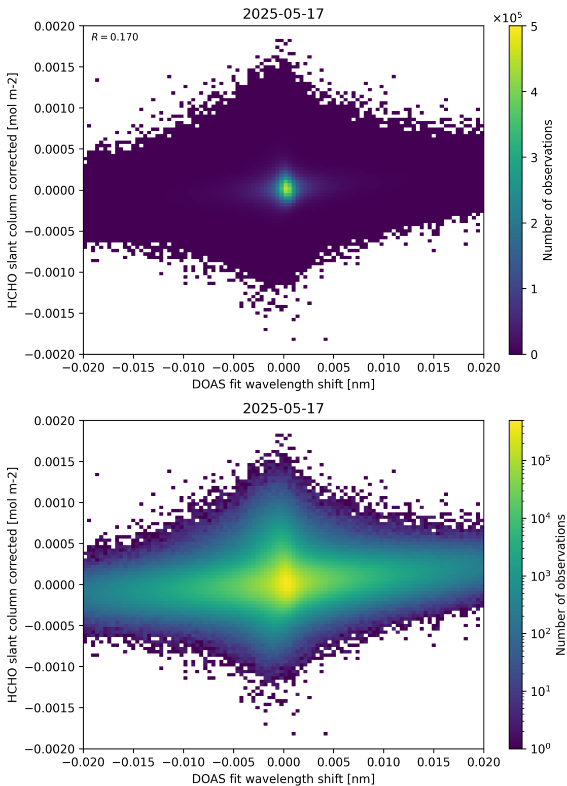
Figure 66: Scatter density plot of “DOAS fit wavelength shift” against “HCHO slant column corrected” for 2025-05-16 to 2025-05-18.
