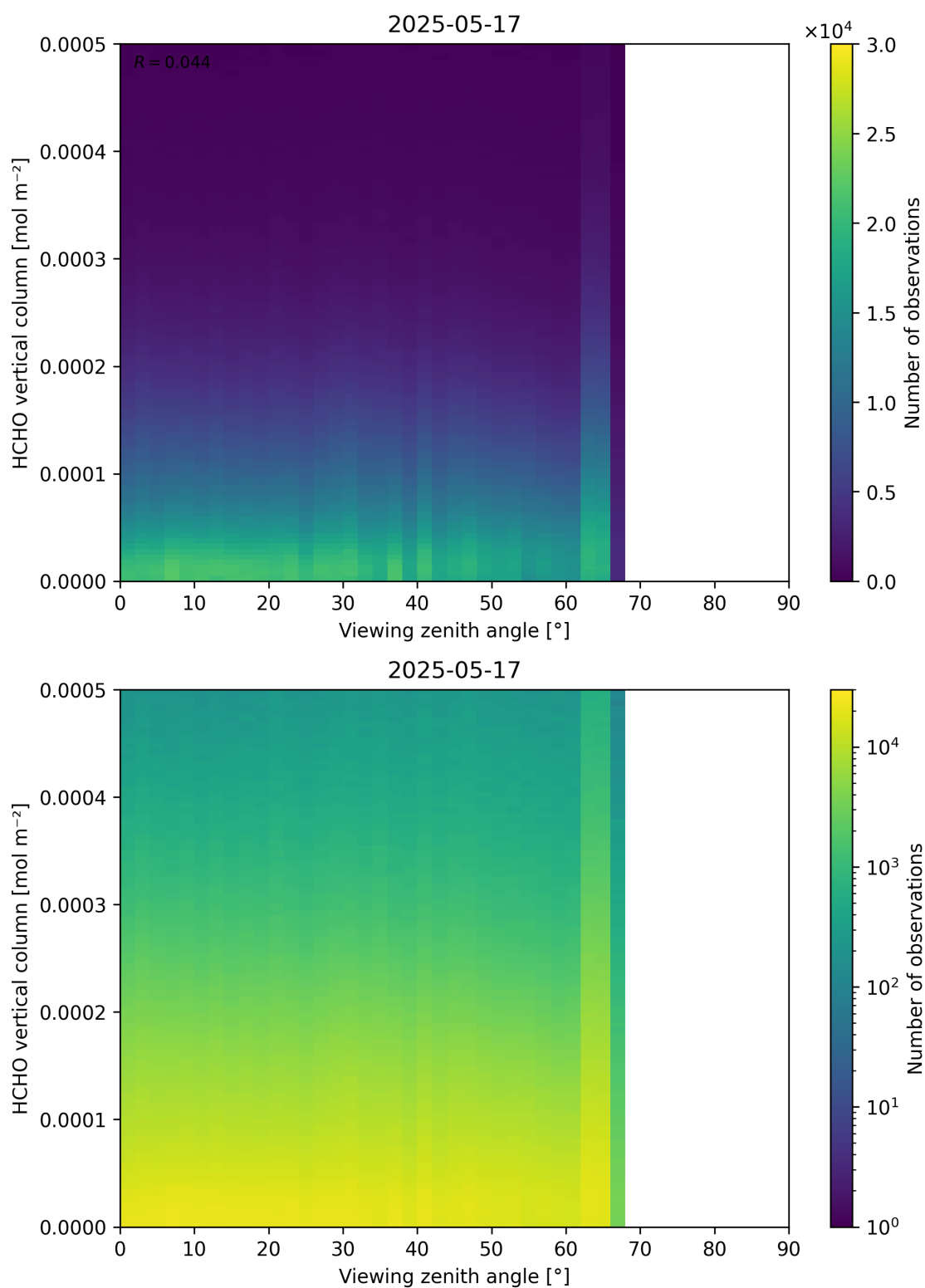
Figure 192: Scatter density plot of “Viewing zenith angle” against “HCHO vertical column” for 2025-05-16 to 2025-05-18.
