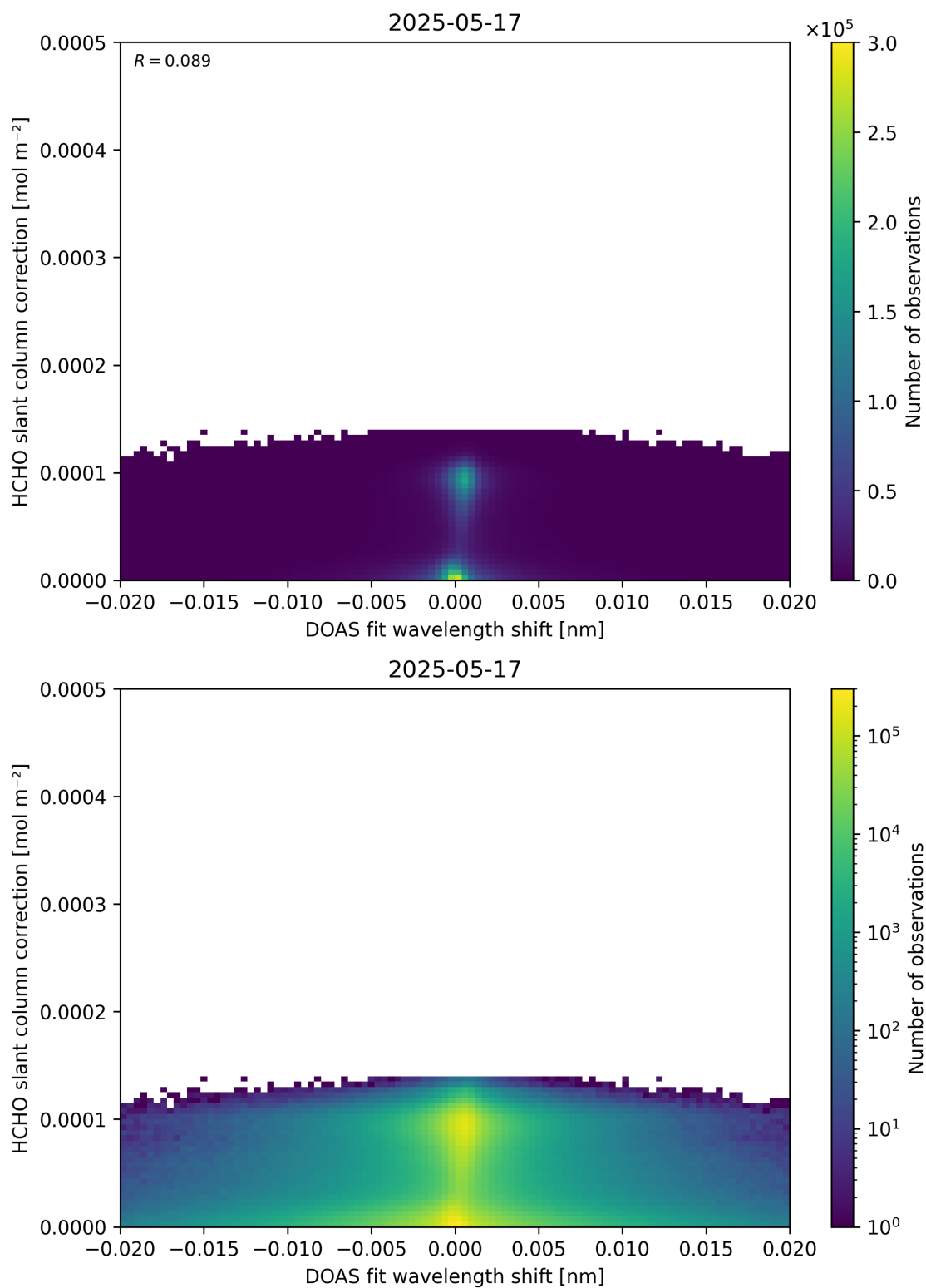
Figure 67: Scatter density plot of “DOAS fit wavelength shift” against “HCHO slant column correction” for 2025-05-16 to 2025-05-18.
