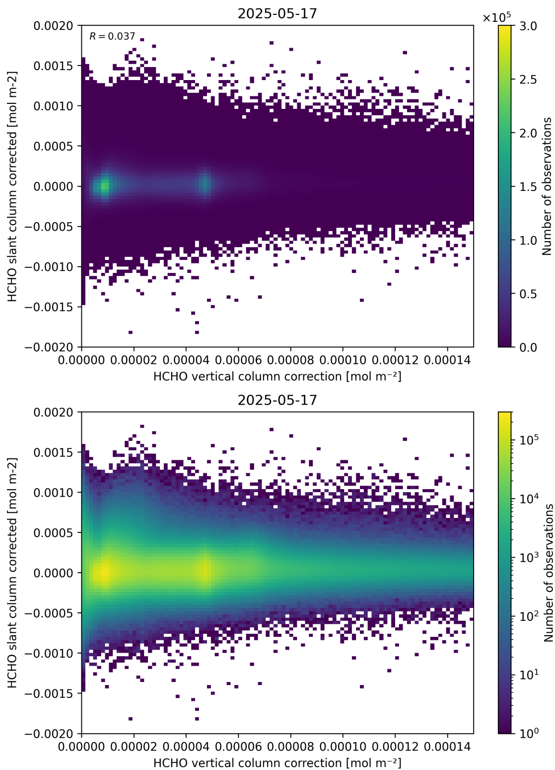
Figure 116: Scatter density plot of “HCHO vertical column correction” against “HCHO slant column corrected” for 2025-05-16 to 2025-05-18.
