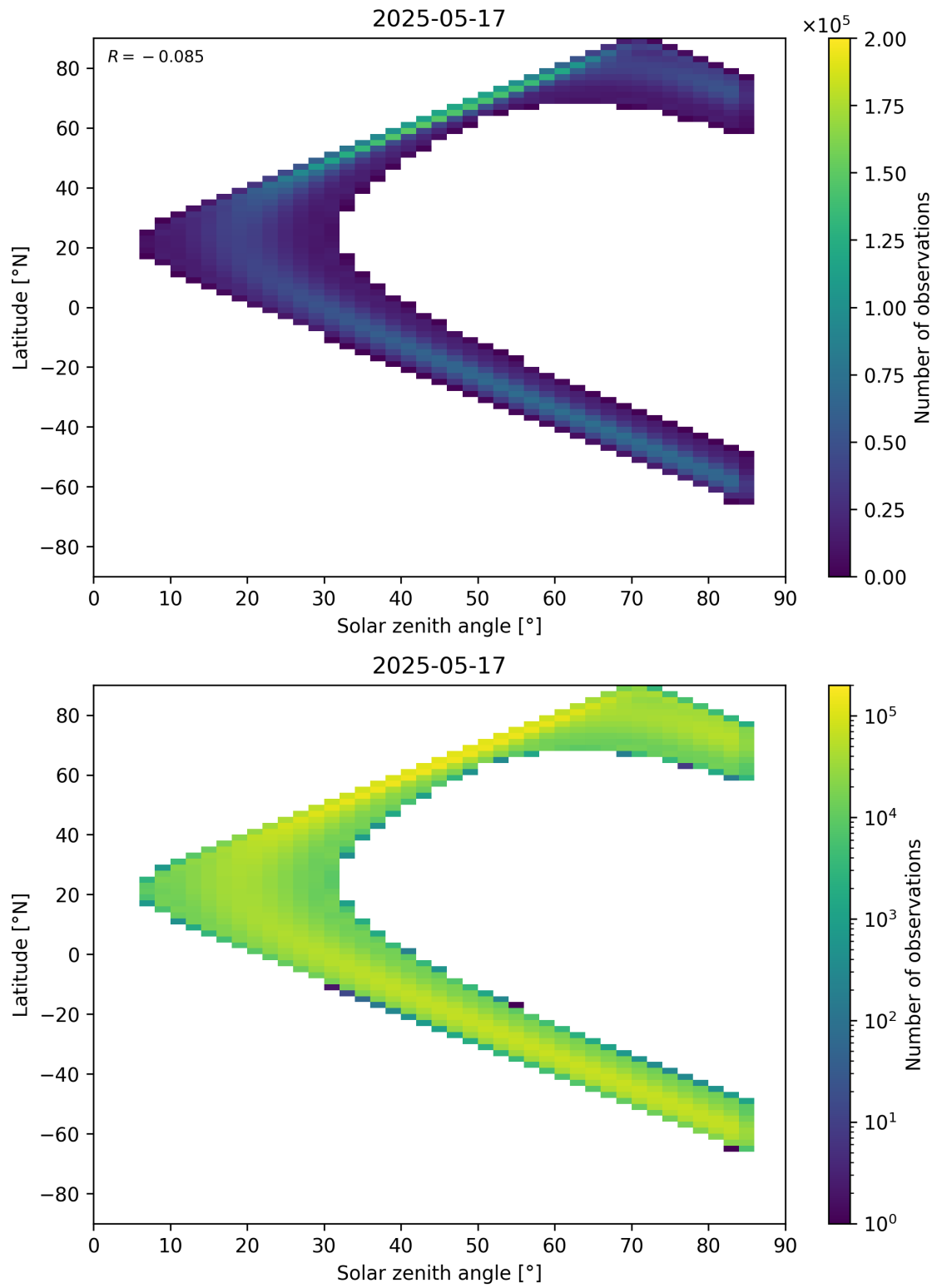
Figure 181: Scatter density plot of “Solar zenith angle” against “Latitude” for 2025-05-16 to 2025-05-18.
