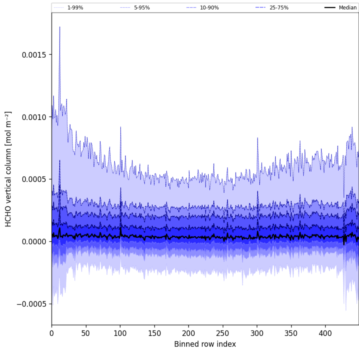
Figure 49: Along track statistics of “HCHO vertical column” for 2025-05-16 to 2025-05-18
