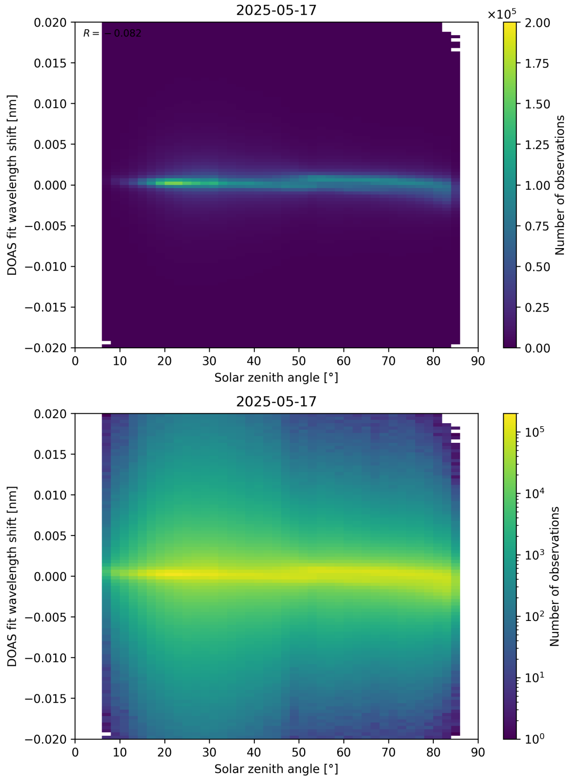
Figure 168: Scatter density plot of “Solar zenith angle” against “DOAS fit wavelength shift” for 2025-05-16 to 2025-05-18.
