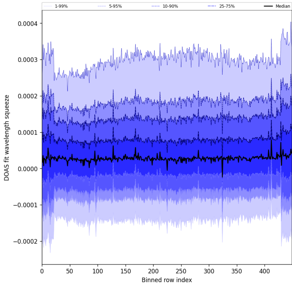
Figure 59: Along track statistics of “DOAS fit wavelength squeeze” for 2025-05-16 to 2025-05-18
