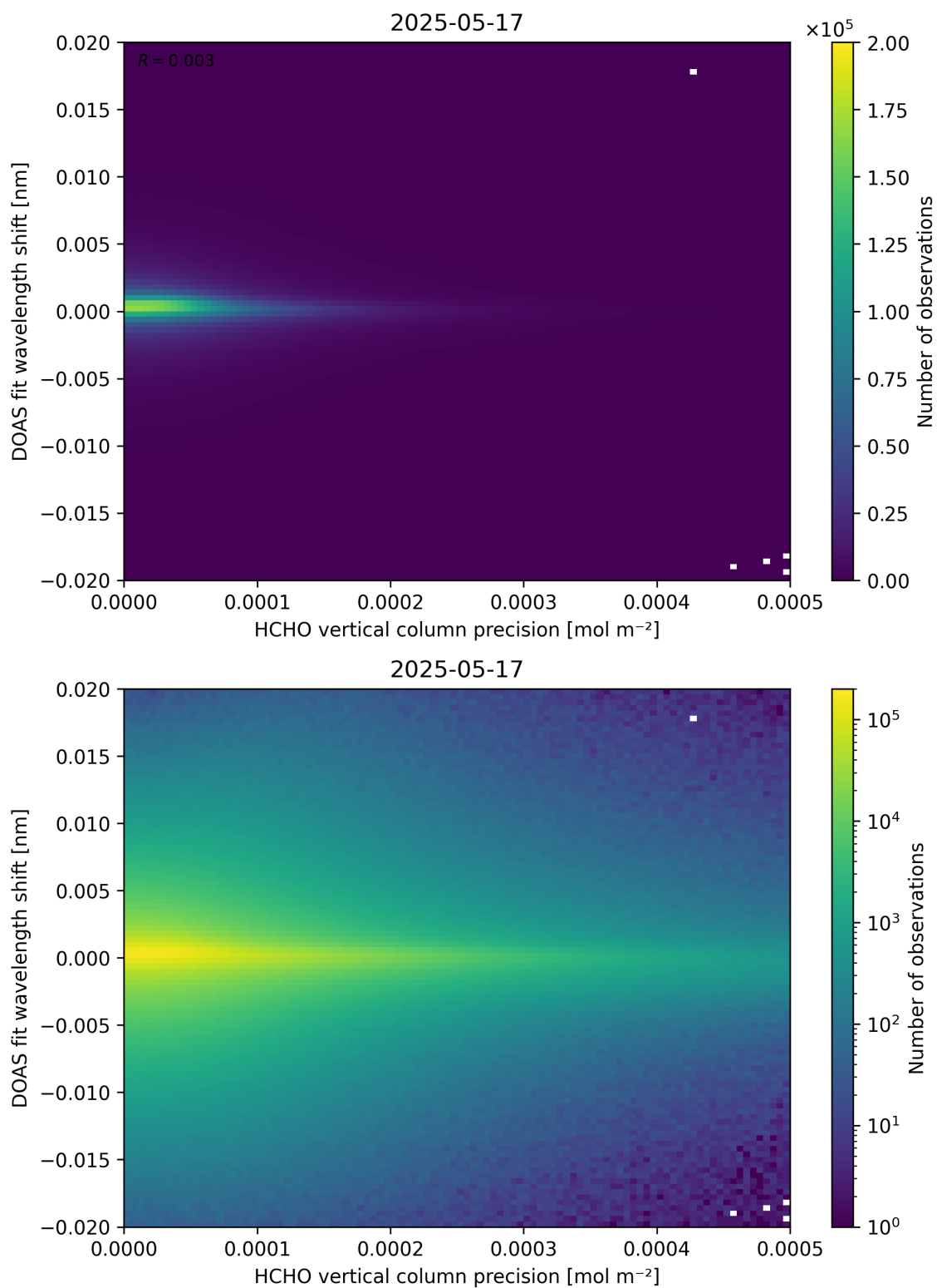
Figure 137: Scatter density plot of “HCHO vertical column precision” against “DOAS fit wavelength shift” for 2025-05-16 to 2025-05-18.
