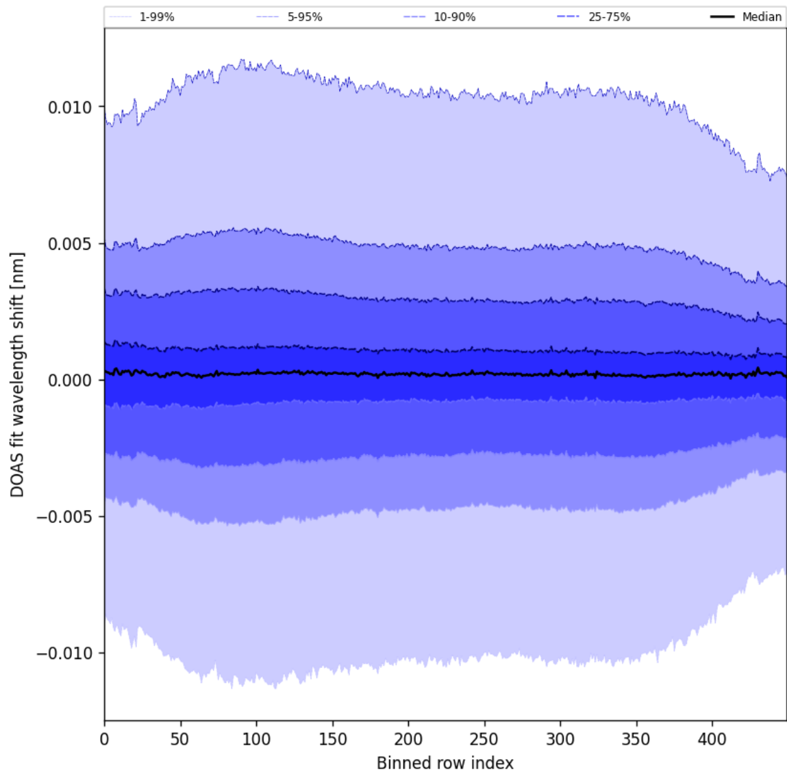
Figure 58: Along track statistics of “DOAS fit wavelength shift” for 2025-05-16 to 2025-05-18
