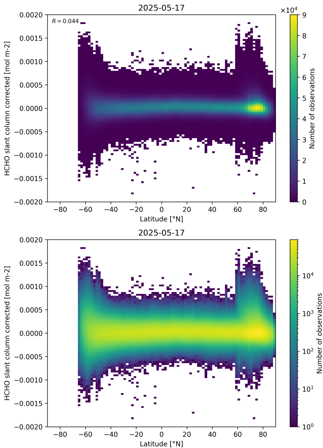
Figure 157: Scatter density plot of “Latitude” against “HCHO slant column corrected” for 2025-05-16 to 2025-05-18.
