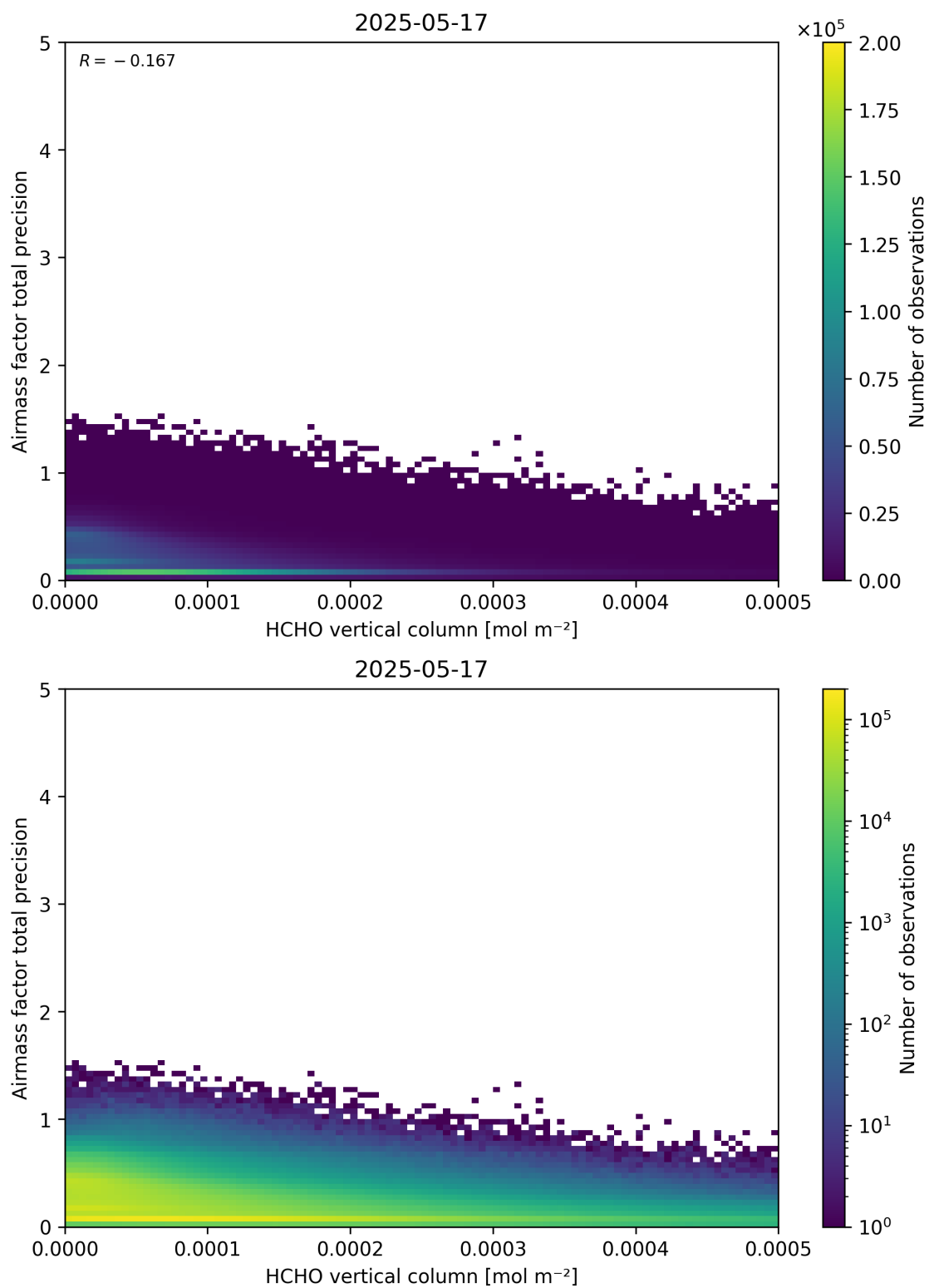
Figure 132: Scatter density plot of “HCHO vertical column” against “Airmass factor total precision” for 2025-05-16 to 2025-05-18.
