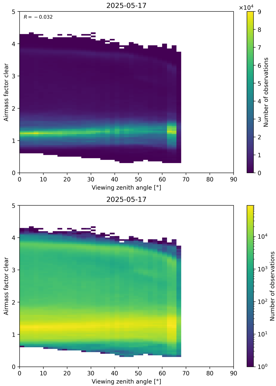
Figure 185: Scatter density plot of “Viewing zenith angle” against “Airmass factor clear” for 2025-05-16 to 2025-05-18.
