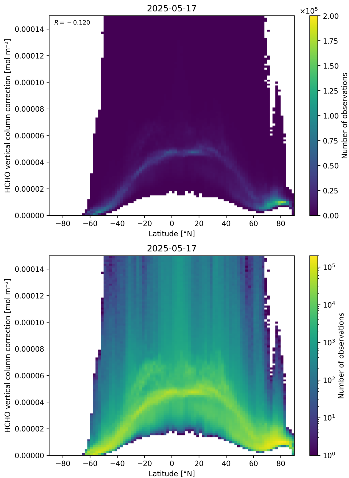
Figure 164: Scatter density plot of “Latitude” against “HCHO vertical column correction” for 2025-05-16 to 2025-05-18.
