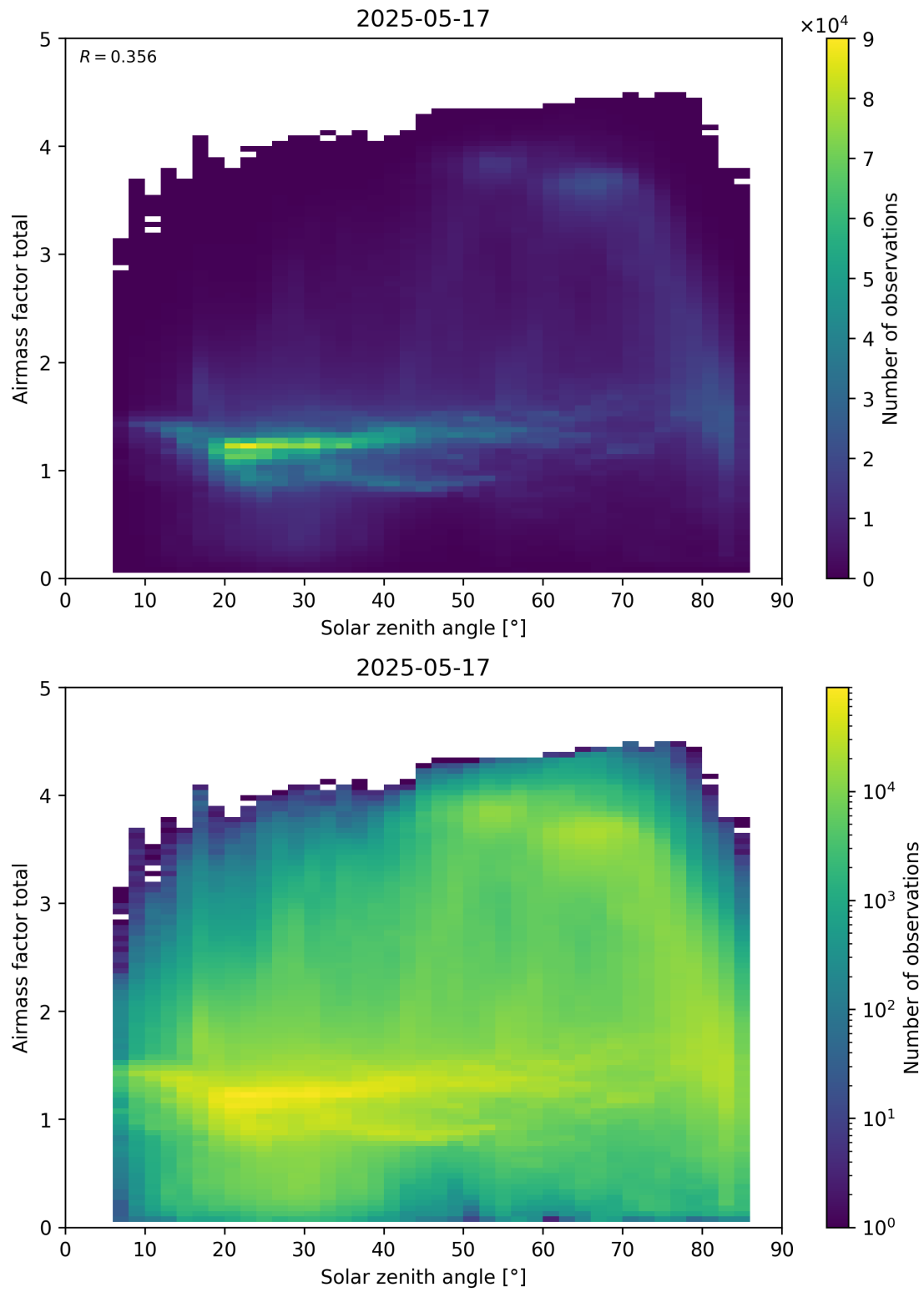
Figure 175: Scatter density plot of “Solar zenith angle” against “Airmass factor total” for 2025-05-16 to 2025-05-18.
