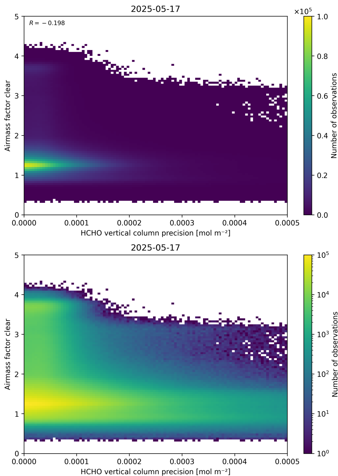
Figure 139: Scatter density plot of “HCHO vertical column precision” against “Airmass factor clear” for 2025-05-16 to 2025-05-18.
