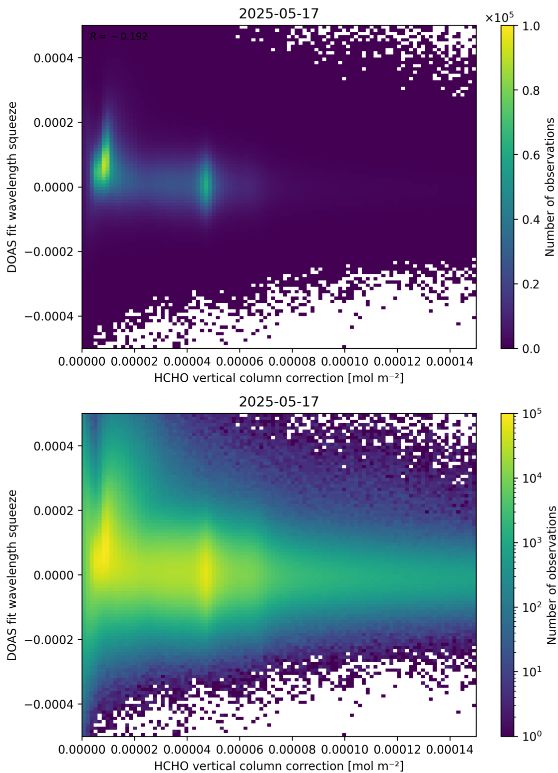
Figure 114: Scatter density plot of “HCHO vertical column correction” against “DOAS fit wavelength squeeze” for 2025-05-16 to 2025-05-18.
