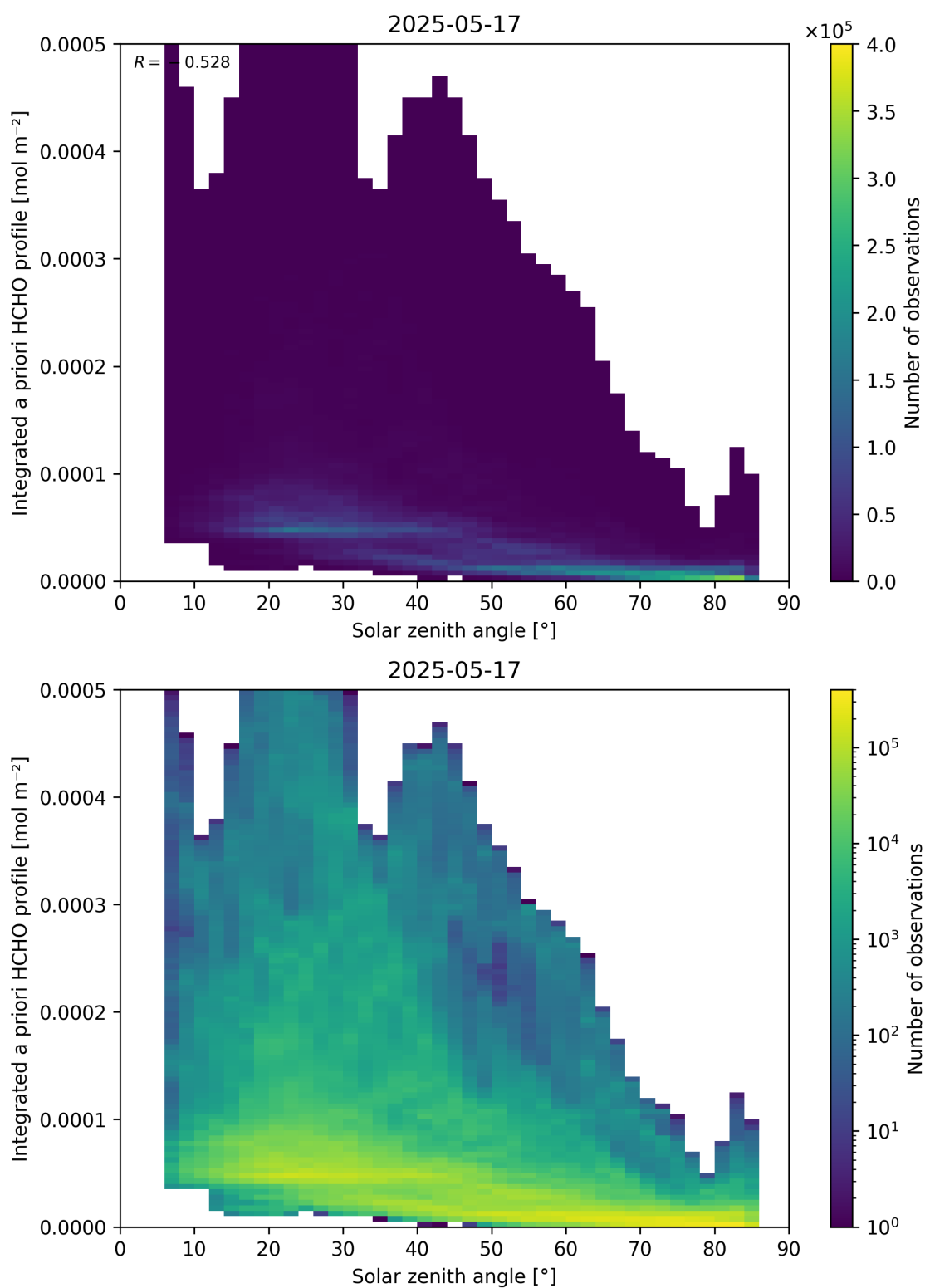
Figure 180: Scatter density plot of “Solar zenith angle” against “Integrated a priori HCHO profile” for 2025-05-16 to 2025-05-18.
