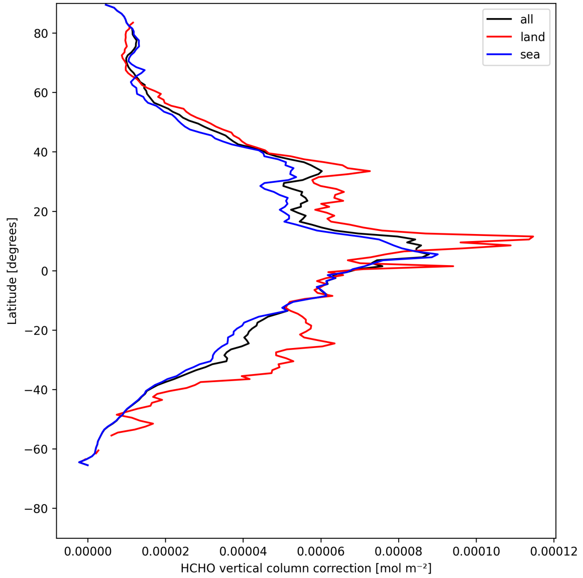
Figure 23: Zonal average of “HCHO vertical column correction” for 2025-05-16 to 2025-05-18.
