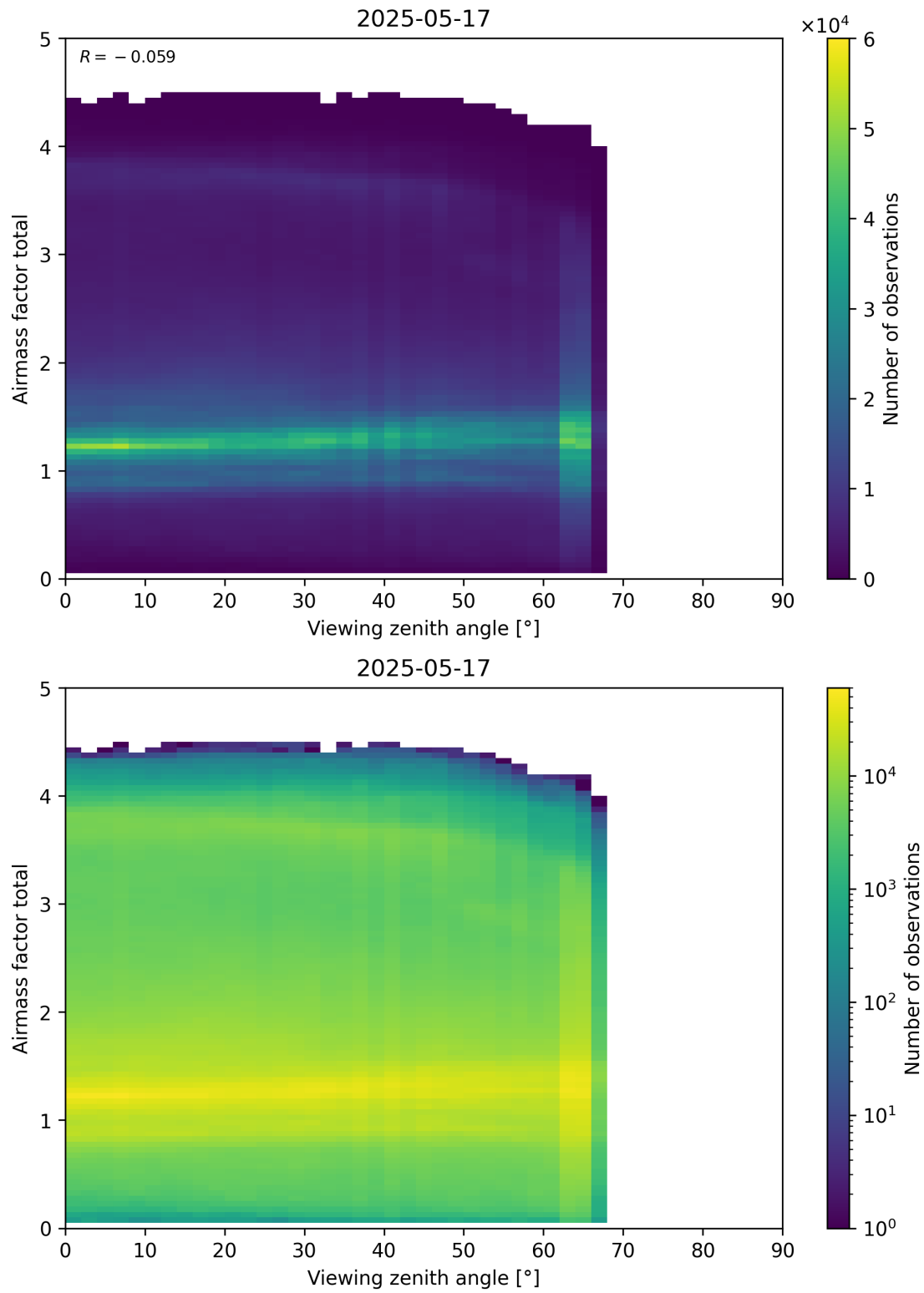
Figure 190: Scatter density plot of “Viewing zenith angle” against “Airmass factor total” for 2025-05-16 to 2025-05-18.
