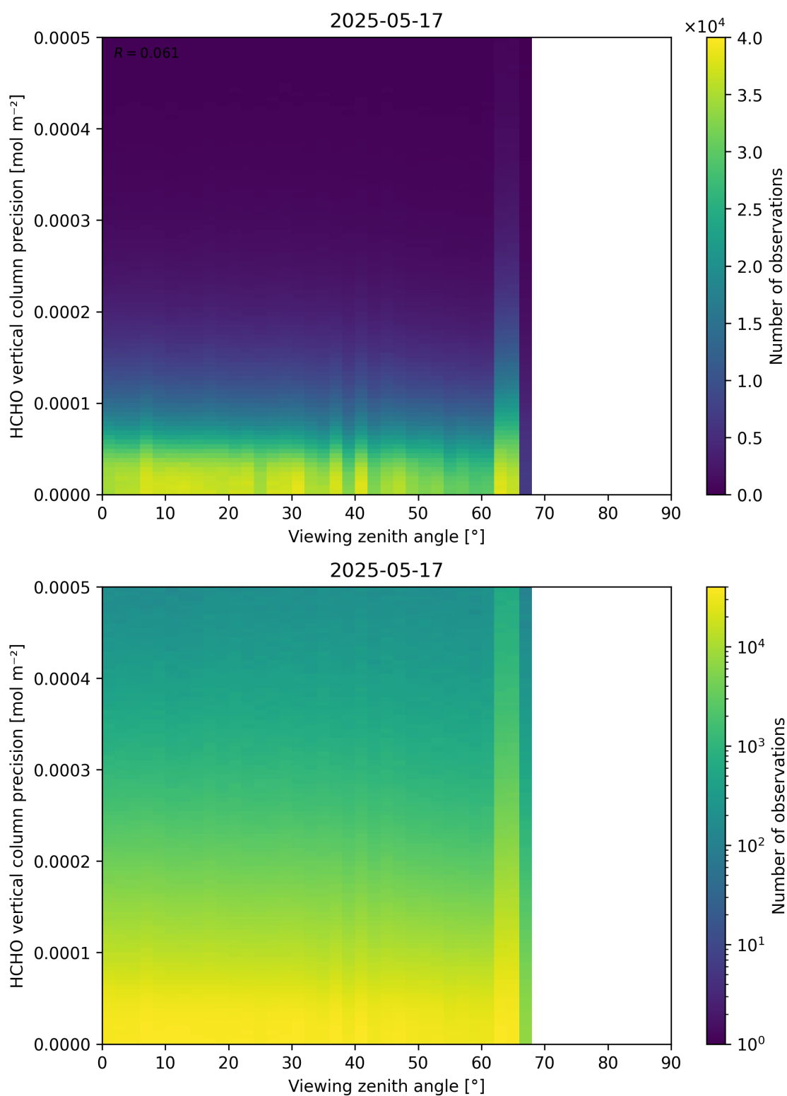
Figure 194: Scatter density plot of “Viewing zenith angle” against “HCHO vertical column precision” for 2025-05-16 to 2025-05-18.
