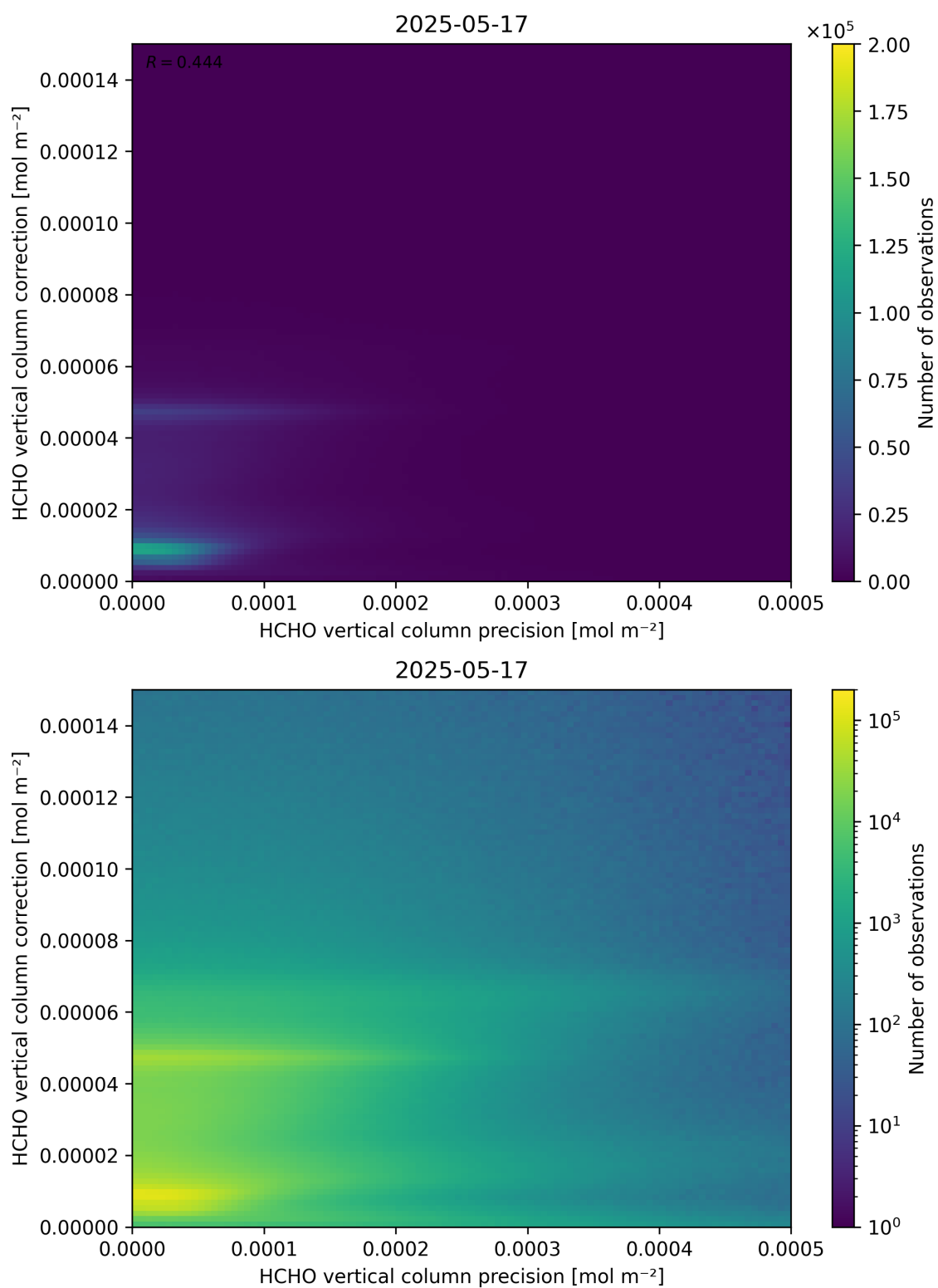
Figure 146: Scatter density plot of “HCHO vertical column precision” against “HCHO vertical column correction” for 2025-05-16 to 2025-05-18.
