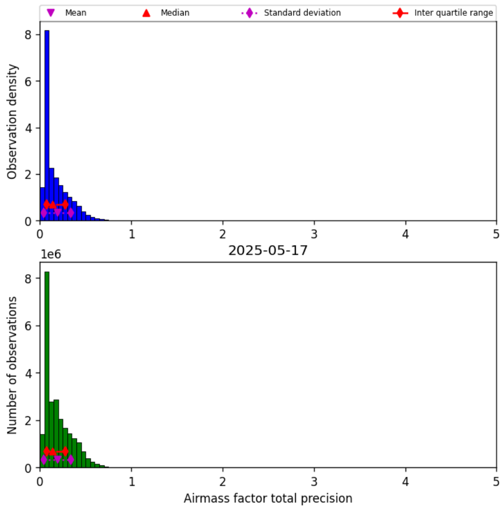
Figure 41: Histogram of “Airmass factor total precision” for 2025-05-16 to 2025-05-18
