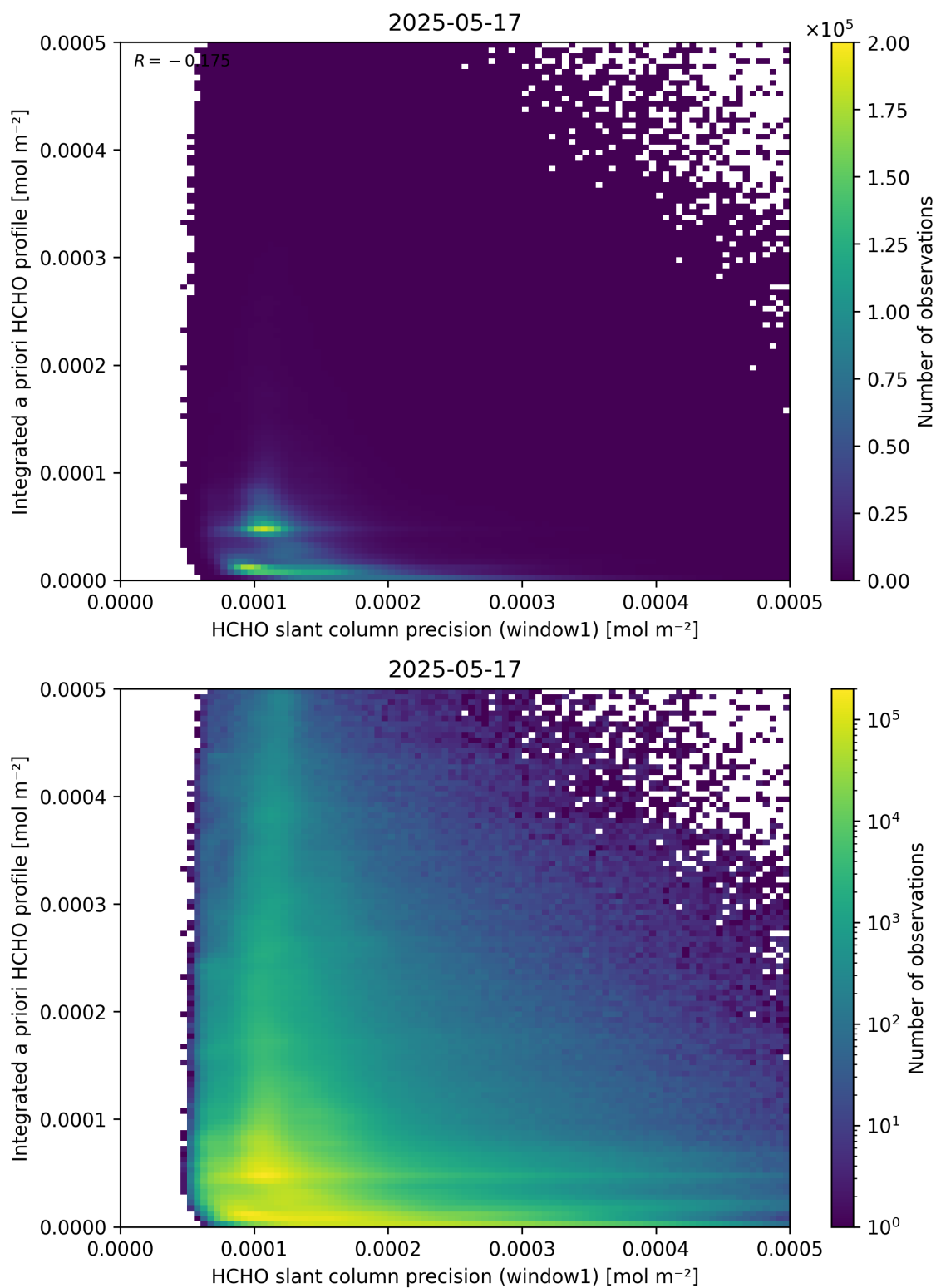
Figure 96: Scatter density plot of “HCHO slant column precision (window1)” against “Integrated a priori HCHO profile” for 2025-05-16 to 2025-05-18.
