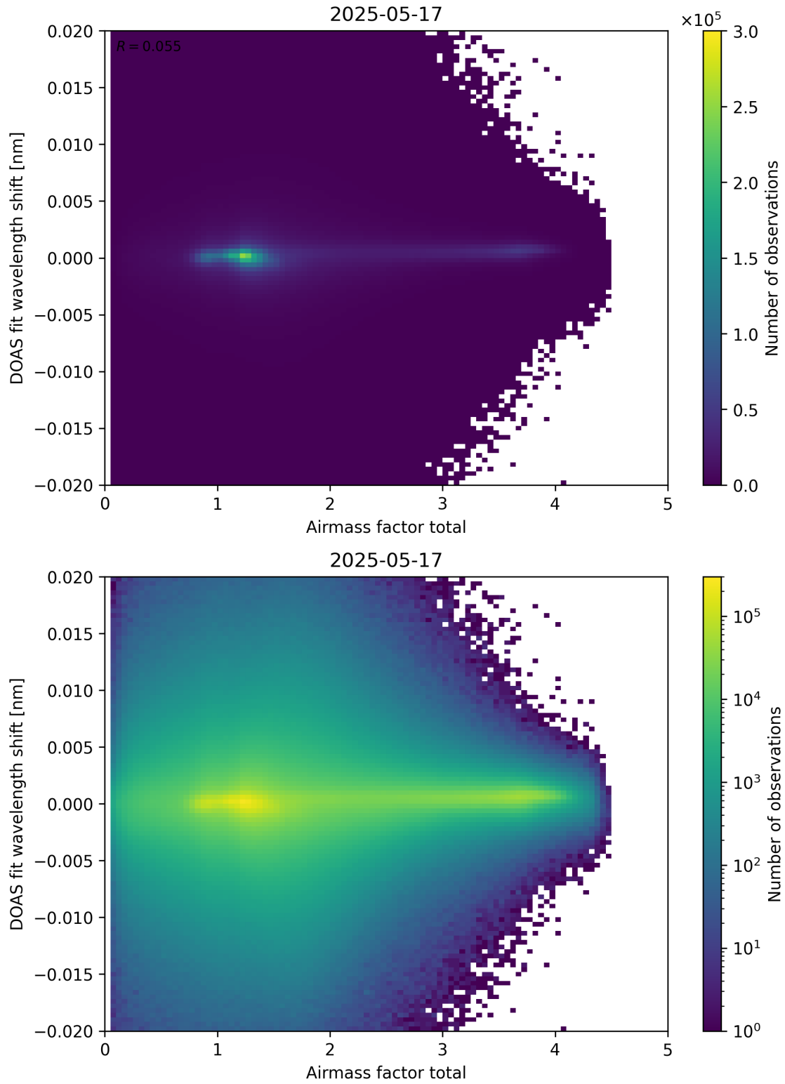
Figure 98: Scatter density plot of “Airmass factor total” against “DOAS fit wavelength shift” for 2025-05-16 to 2025-05-18.
