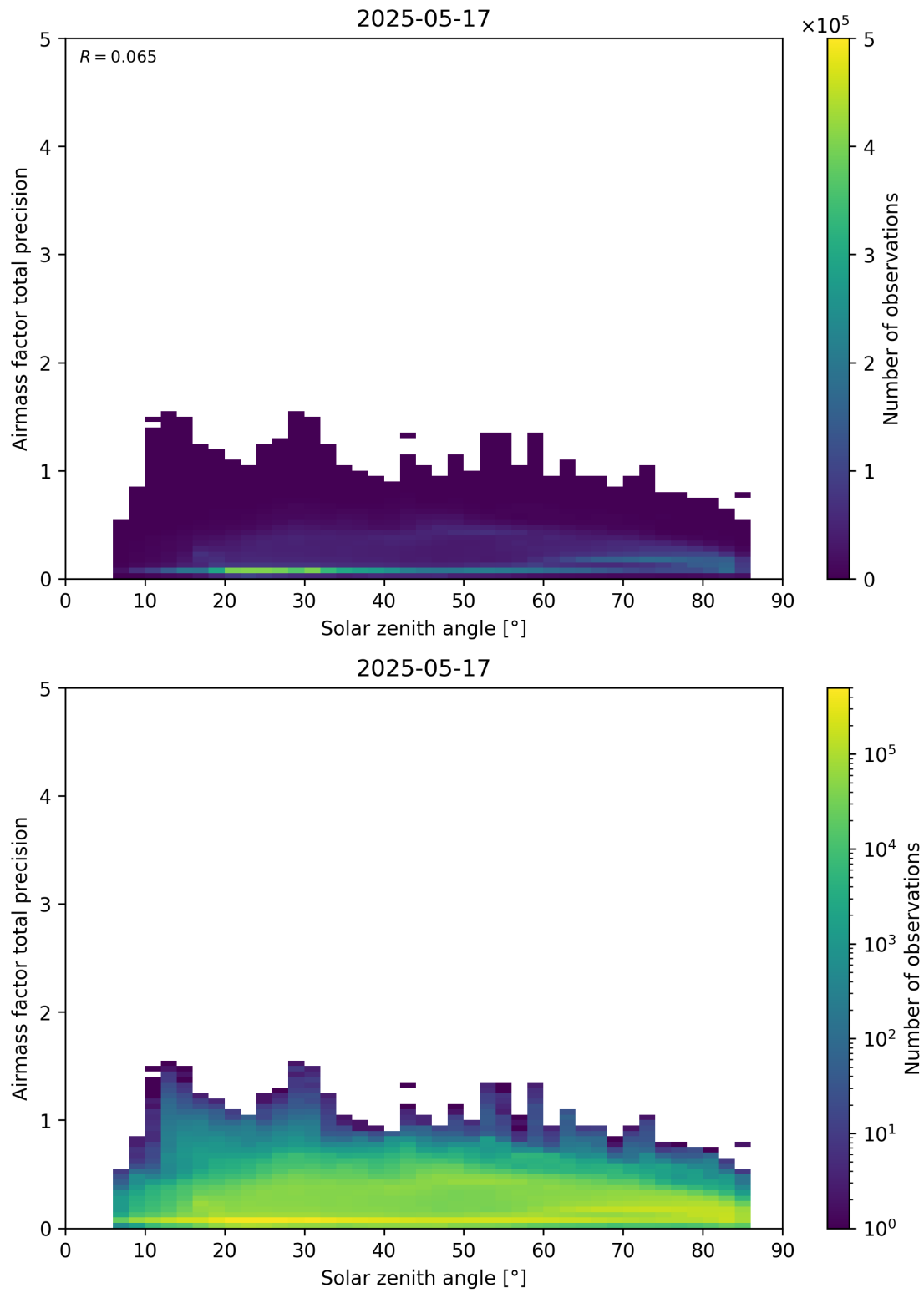
Figure 176: Scatter density plot of “Solar zenith angle” against “Airmass factor total precision” for 2025-05-16 to 2025-05-18.
