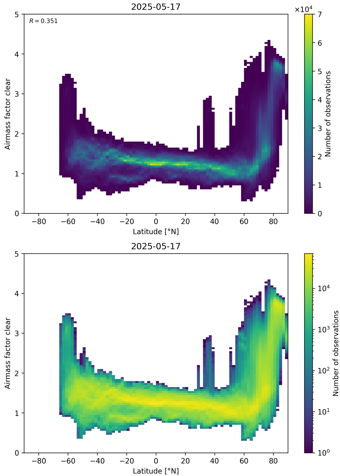
Figure 156: Scatter density plot of “Latitude” against “Airmass factor clear” for 2025-05-16 to 2025-05-18.
