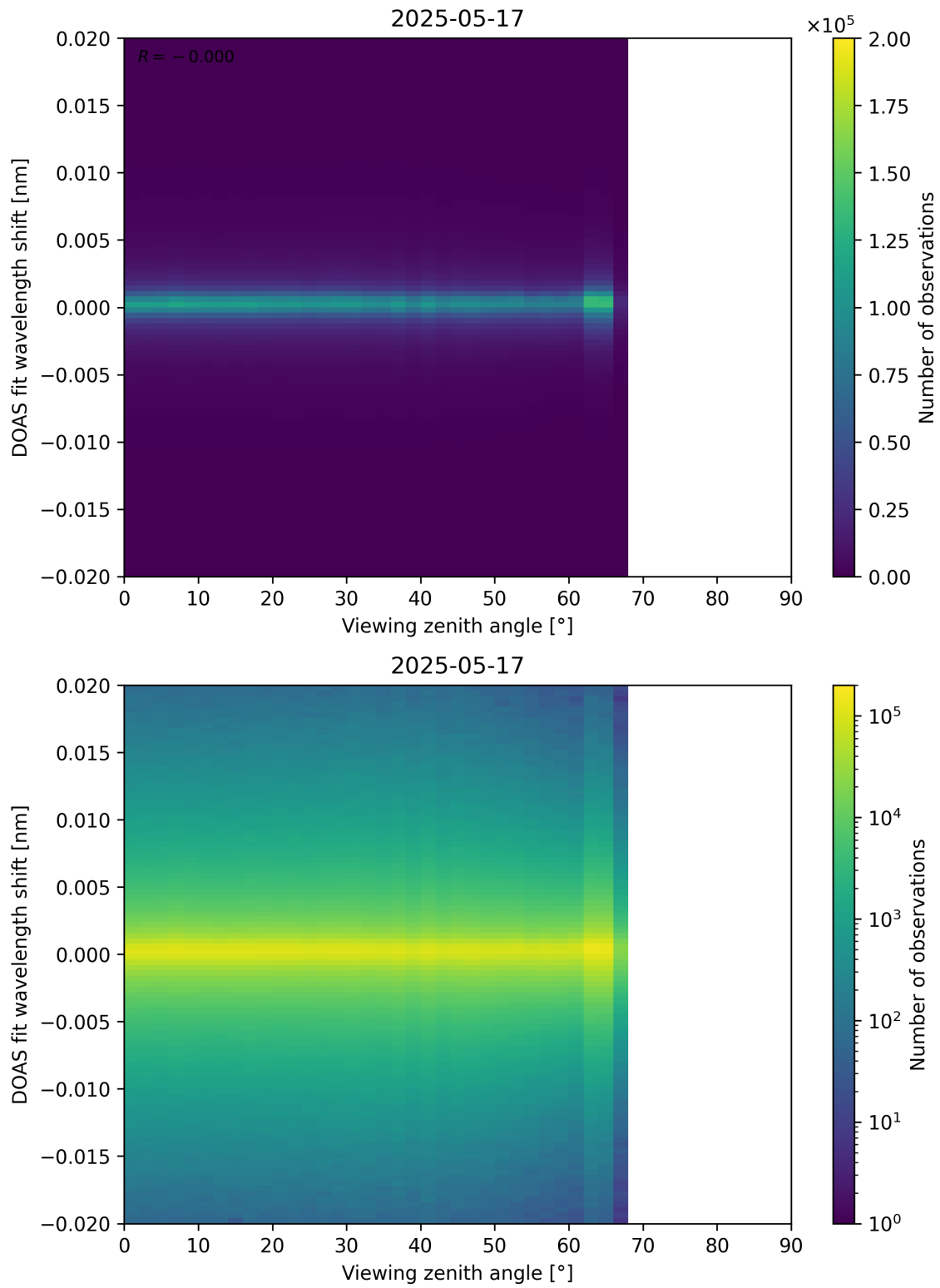
Figure 183: Scatter density plot of “Viewing zenith angle” against “DOAS fit wavelength shift” for 2025-05-16 to 2025-05-18.
