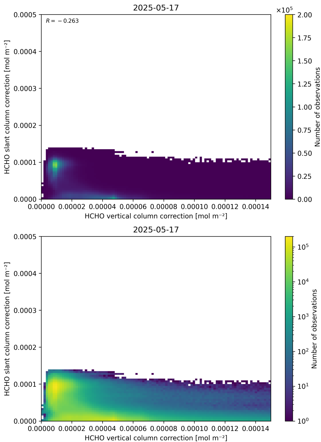
Figure 117: Scatter density plot of “HCHO vertical column correction” against “HCHO slant column correction” for 2025-05-16 to 2025-05-18.
