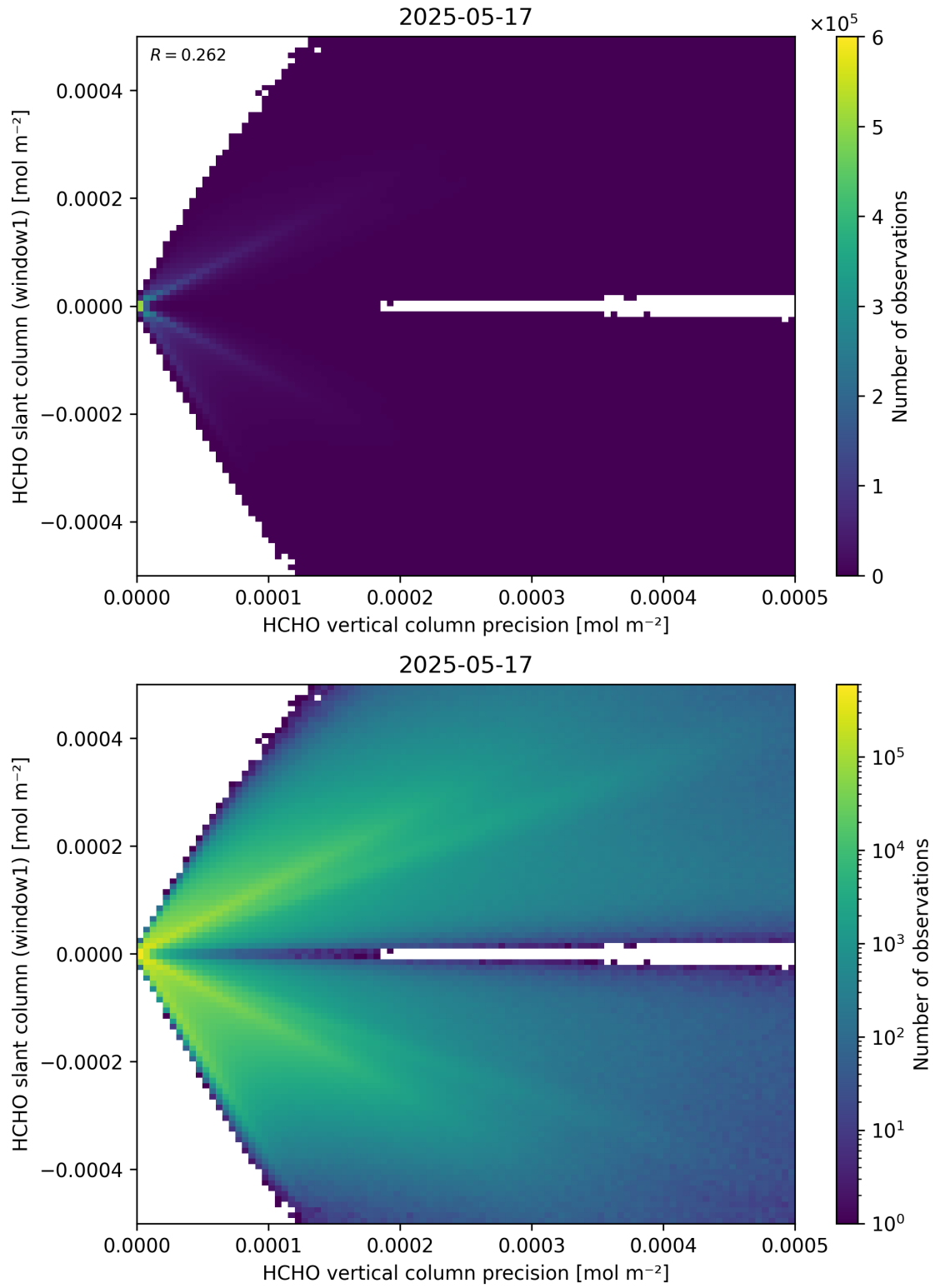
Figure 142: Scatter density plot of “HCHO vertical column precision” against “HCHO slant column (window1)” for 2025-05-16 to 2025-05-18.
