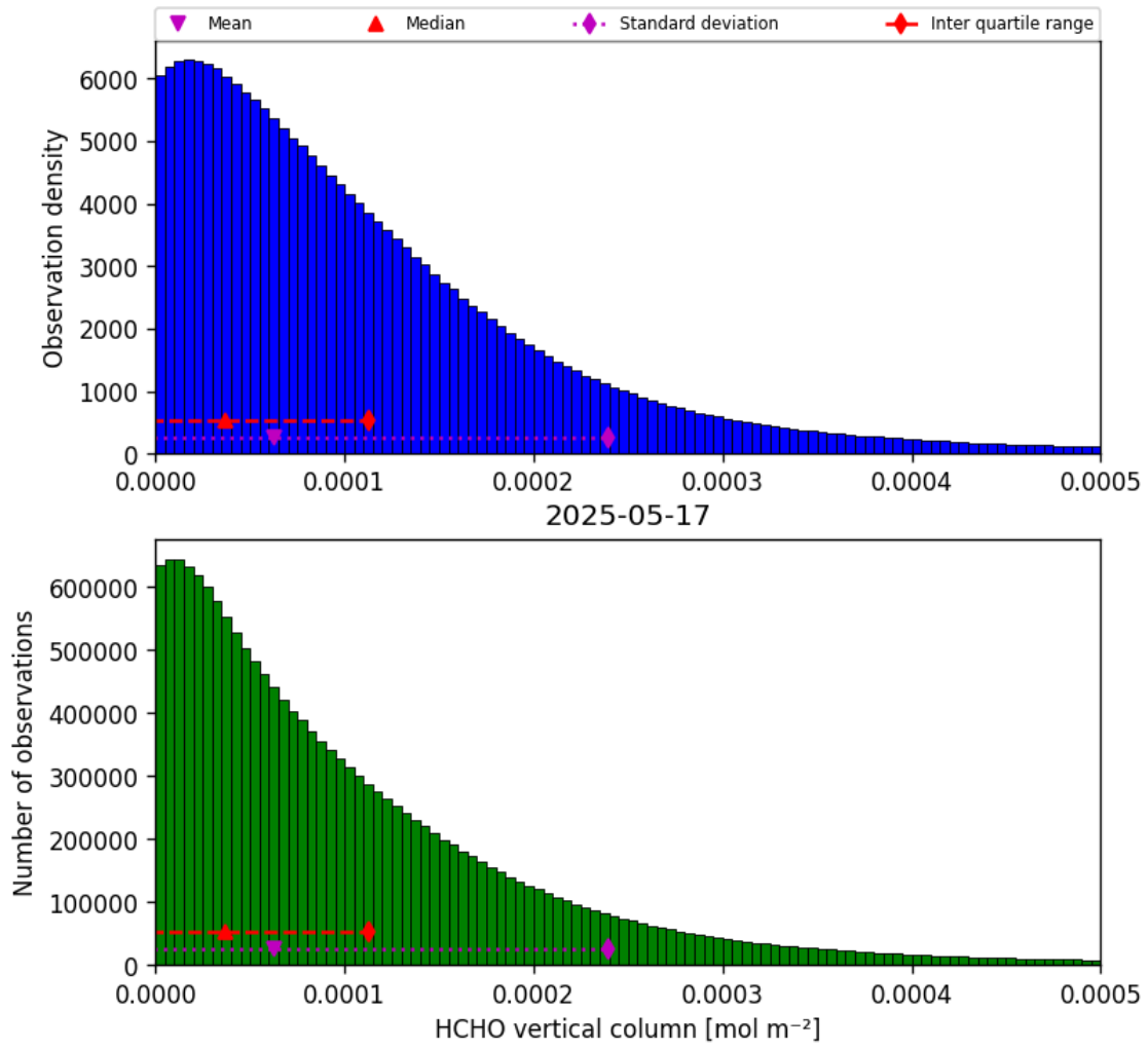
Figure 35: Histogram of “HCHO vertical column” for 2025-05-16 to 2025-05-18
