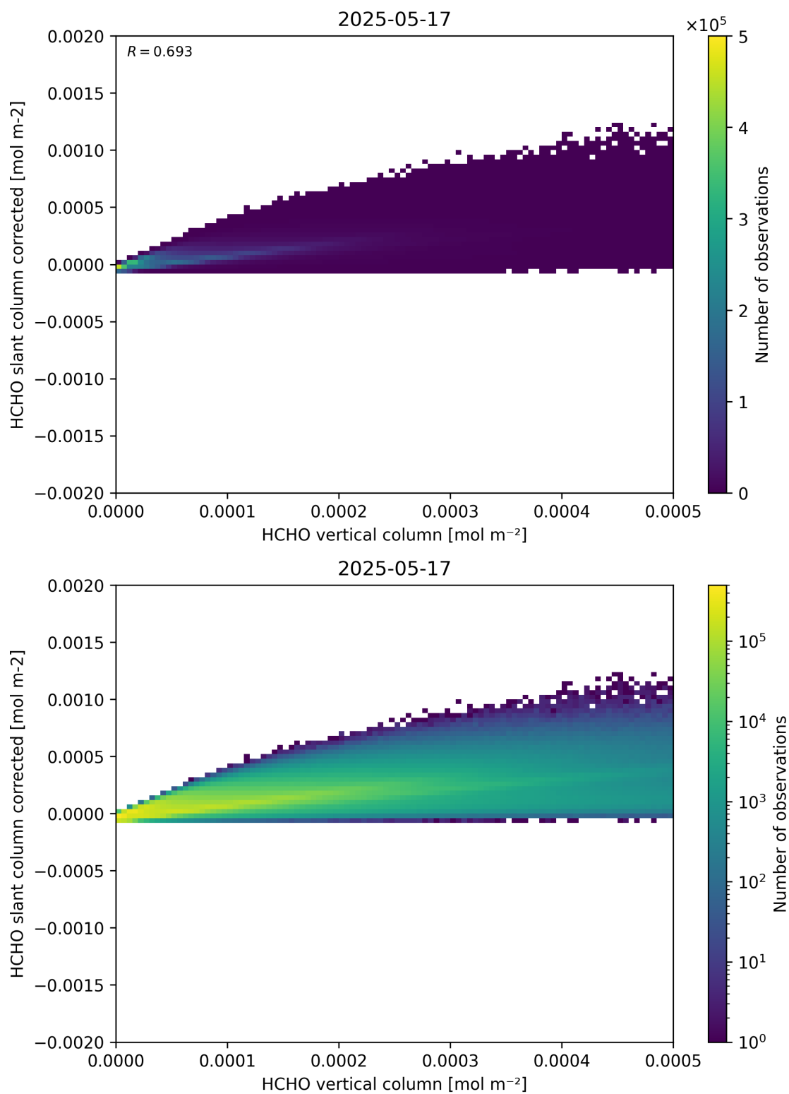
Figure 127: Scatter density plot of “HCHO vertical column” against “HCHO slant column corrected” for 2025-05-16 to 2025-05-18.
