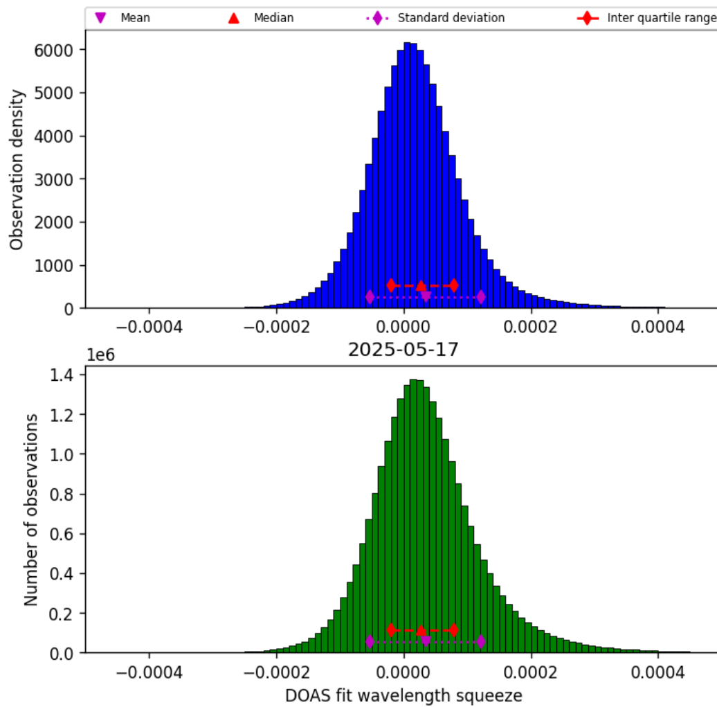
Figure 45: Histogram of “DOAS fit wavelength squeeze” for 2025-05-16 to 2025-05-18
