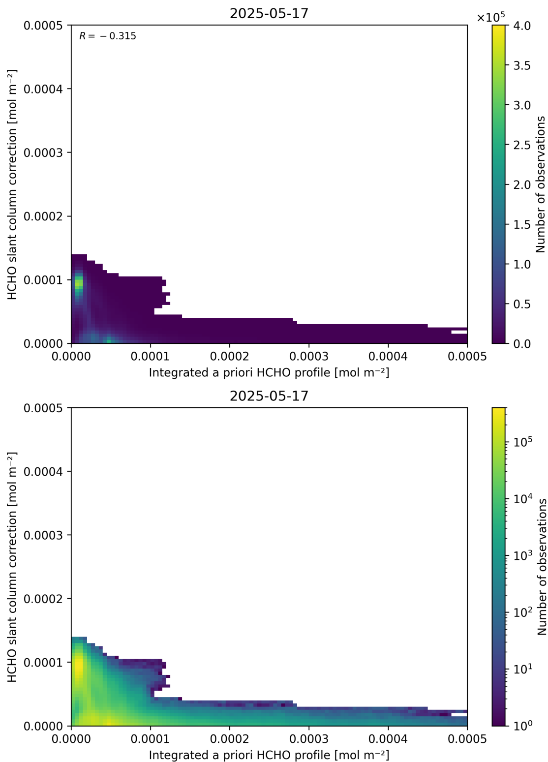
Figure 152: Scatter density plot of “Integrated a priori HCHO profile” against “HCHO slant column correction” for 2025-05-16 to 2025-05-18.
