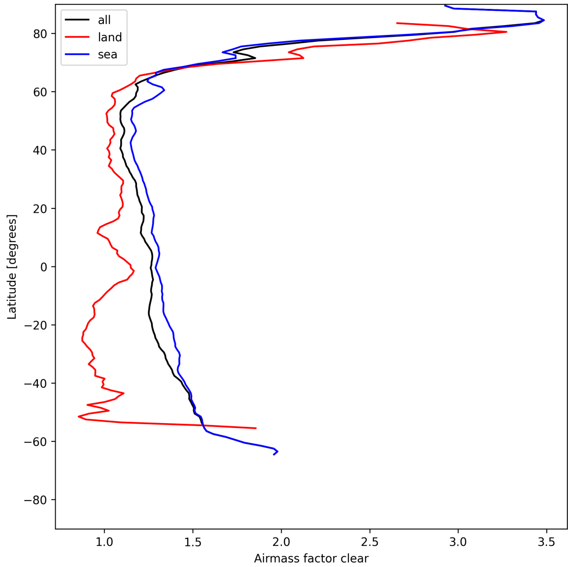
Figure 28: Zonal average of “Airmass factor clear” for 2025-05-17 to 2025-05-19.
