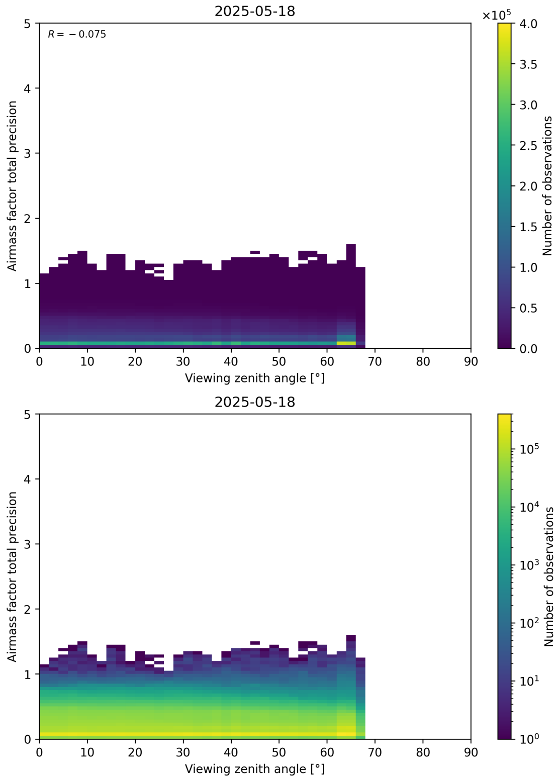
Figure 191: Scatter density plot of “Viewing zenith angle” against “Airmass factor total precision” for 2025-05-17 to 2025-05-19.
