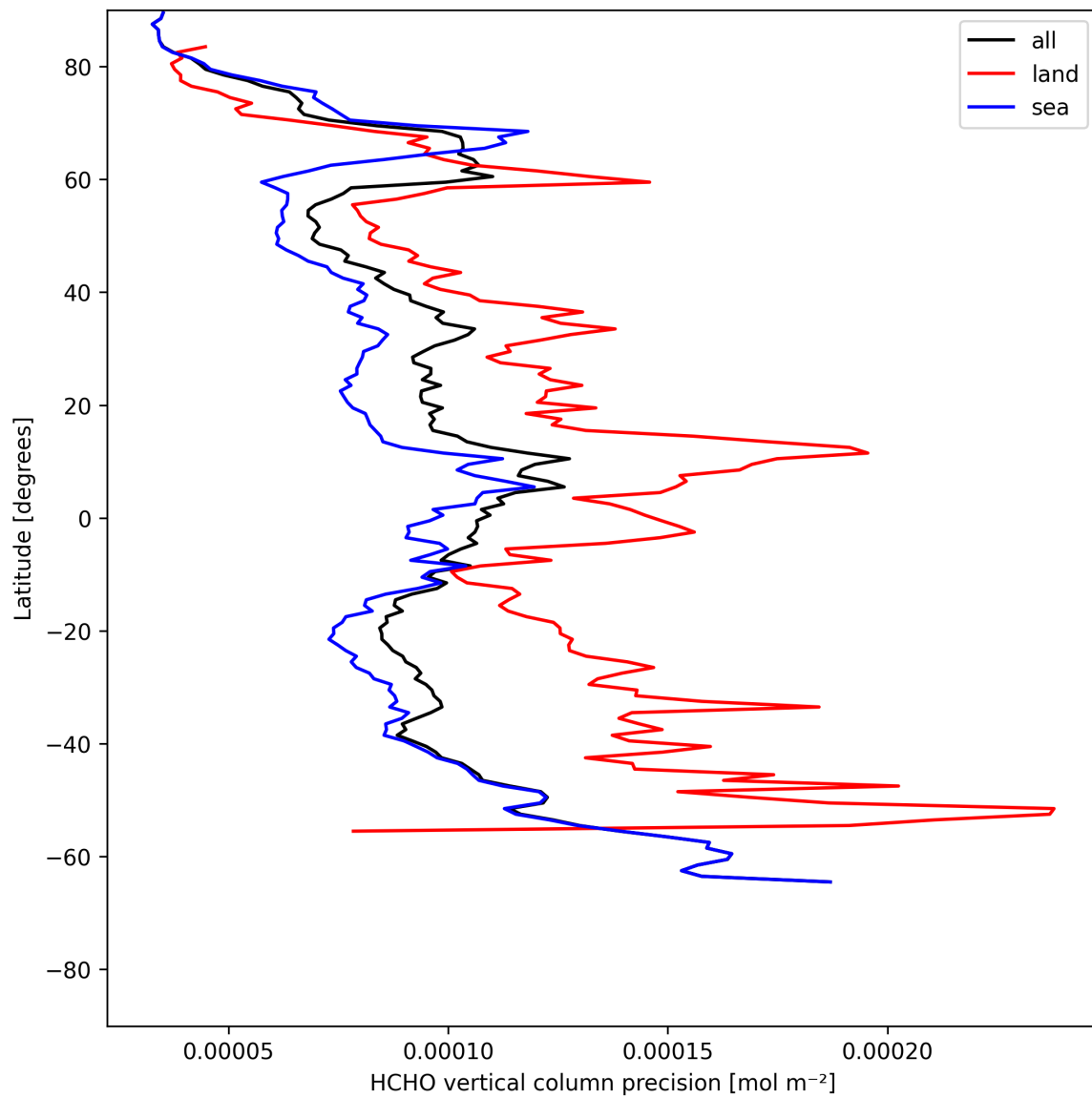
Figure 22: Zonal average of “HCHO vertical column precision” for 2025-05-17 to 2025-05-19.
