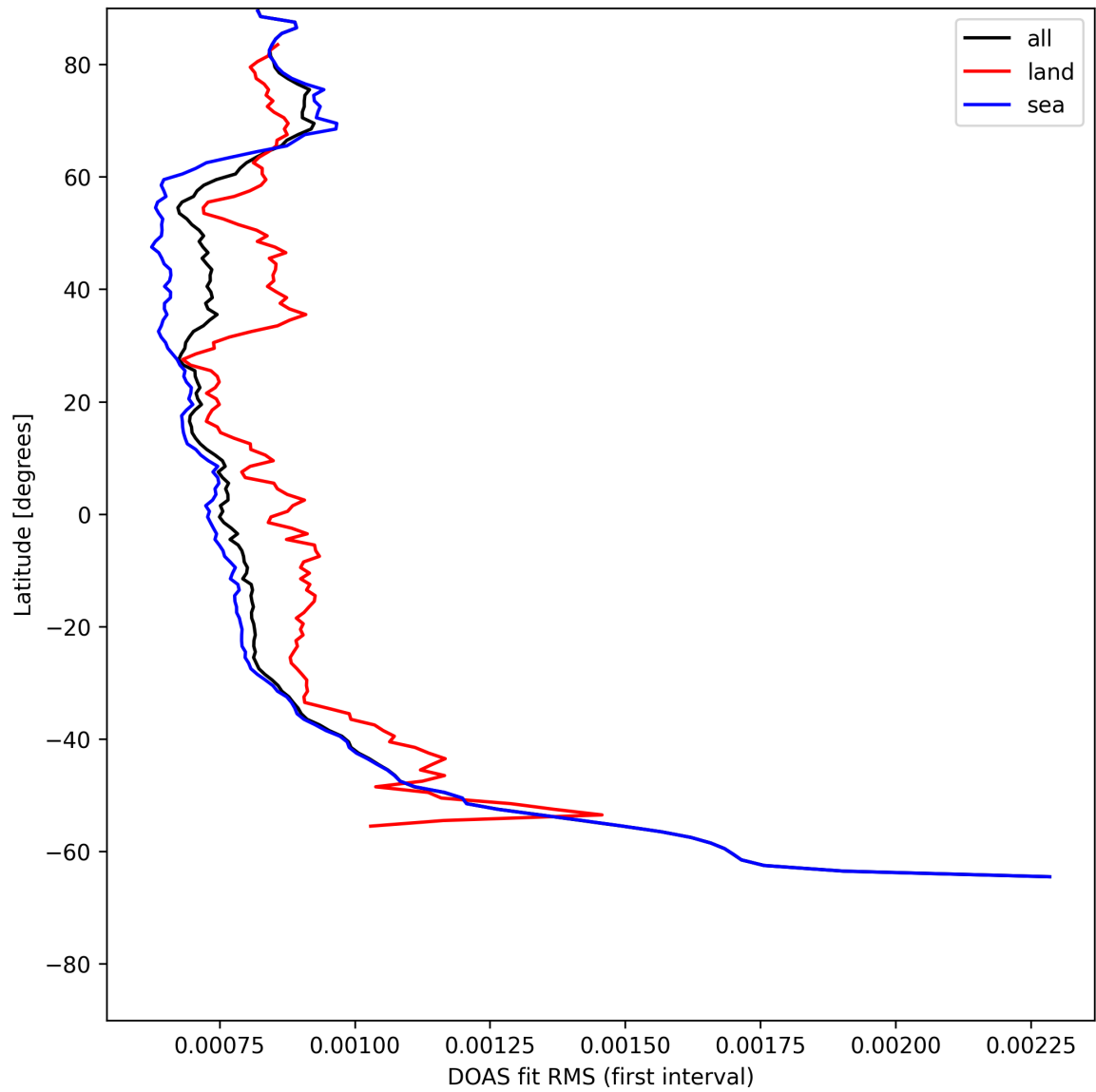
Figure 32: Zonal average of "DOAS fit RMS (first interval)" for 2025-05-17 to 2025-05-19.
