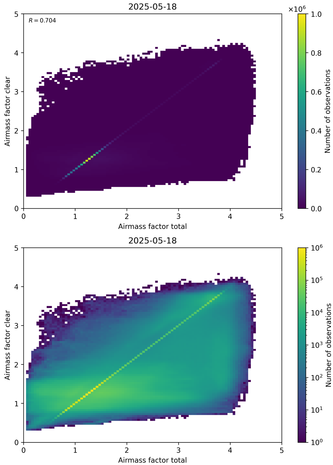
Figure 100: Scatter density plot of “Airmass factor total” against “Airmass factor clear” for 2025-05-17 to 2025-05-19.
