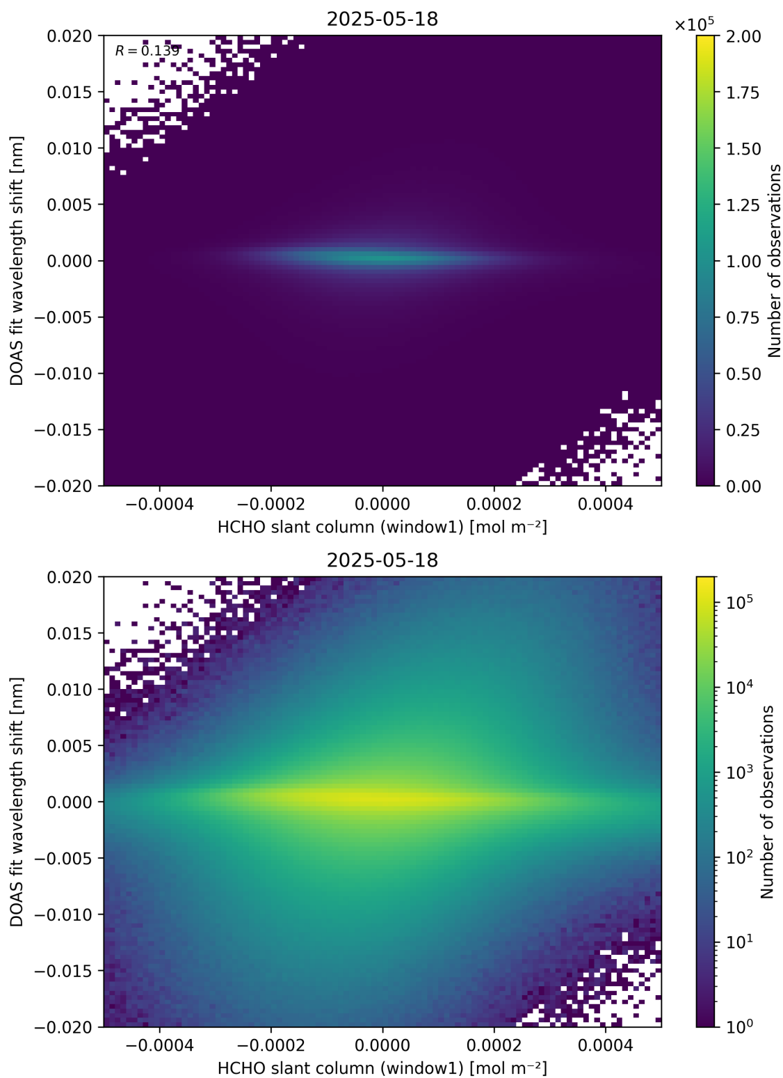
Figure 79: Scatter density plot of “HCHO slant column (window1)” against “DOAS fit wavelength shift” for 2025-05-17 to 2025-05-19.
