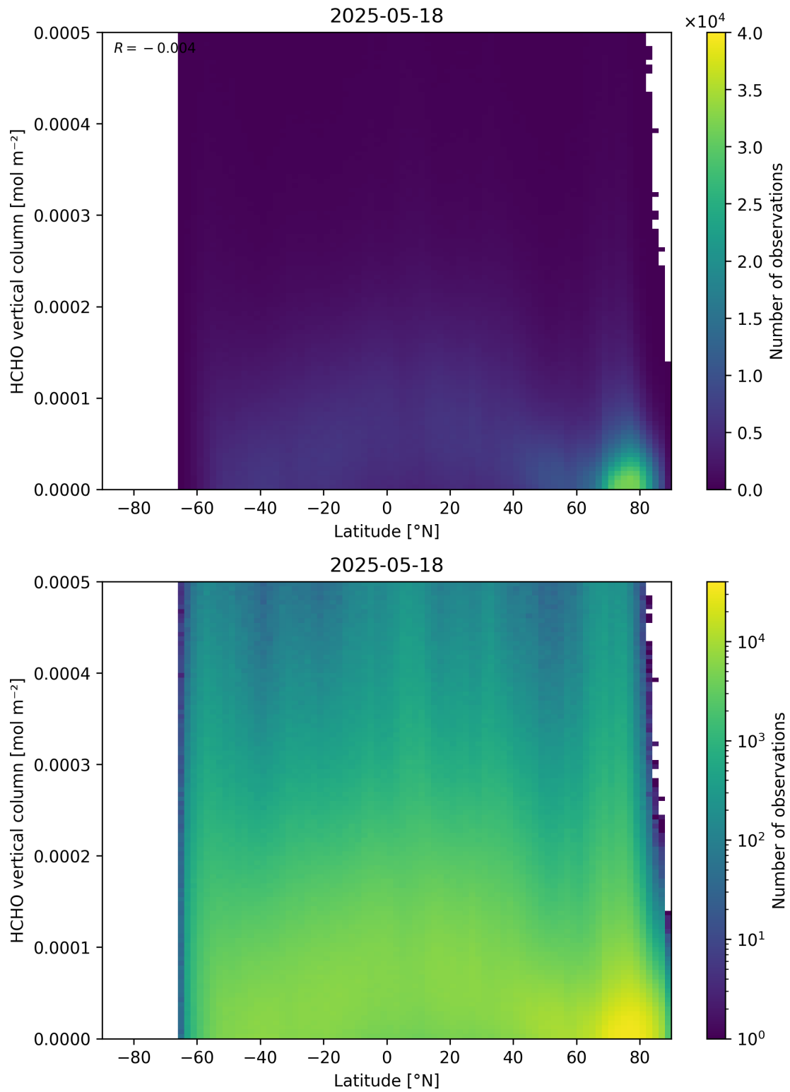
Figure 163: Scatter density plot of “Latitude” against “HCHO vertical column” for 2025-05-17 to 2025-05-19.
