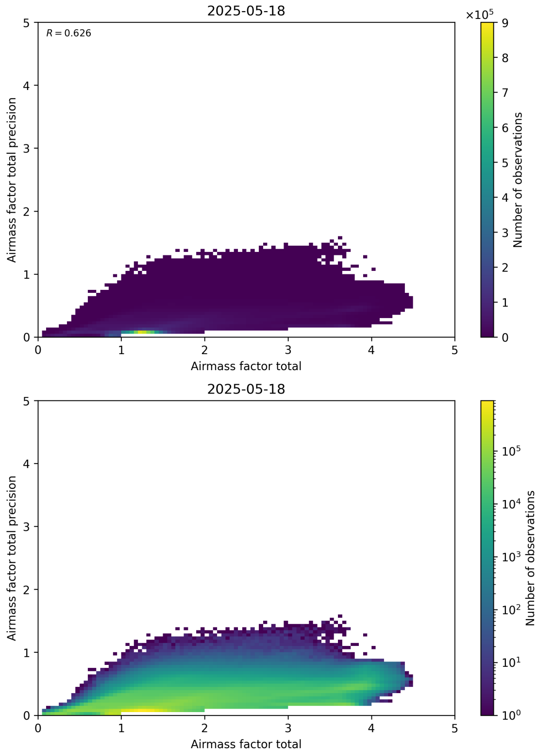
Figure 103: Scatter density plot of “Airmass factor total” against “Airmass factor total precision” for 2025-05-17 to 2025-05-19.
