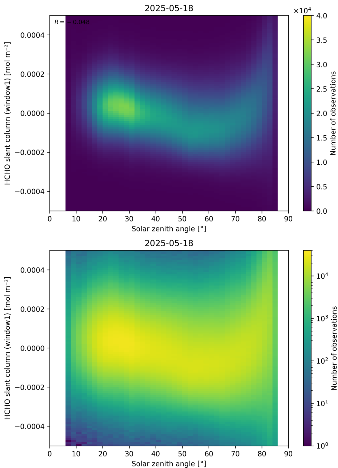
Figure 173: Scatter density plot of “Solar zenith angle” against “HCHO slant column (window1)” for 2025-05-17 to 2025-05-19.
