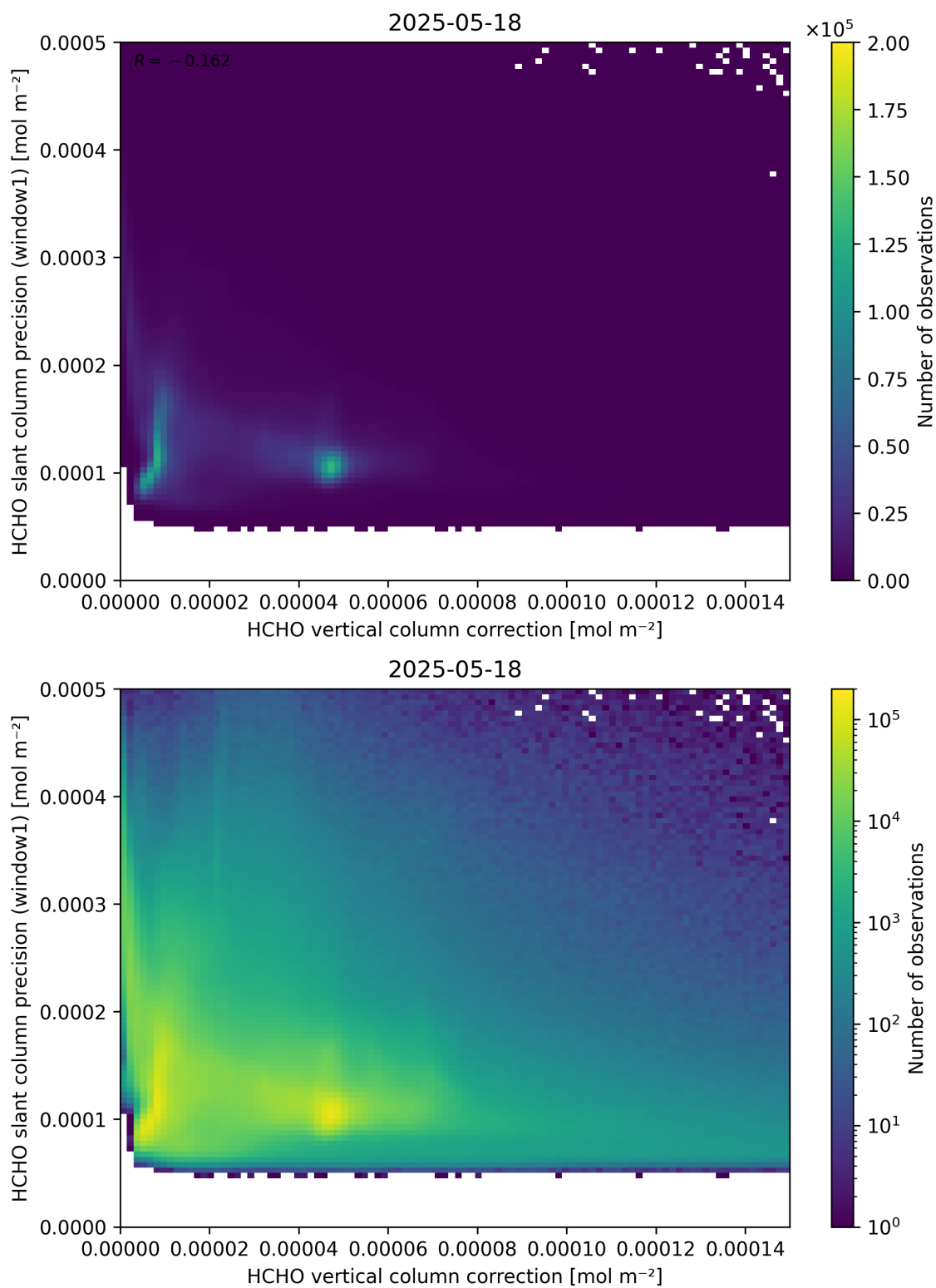
Figure 119: Scatter density plot of “HCHO vertical column correction” against “HCHO slant column precision (window1)” for 2025-05-17 to 2025-05-19.
