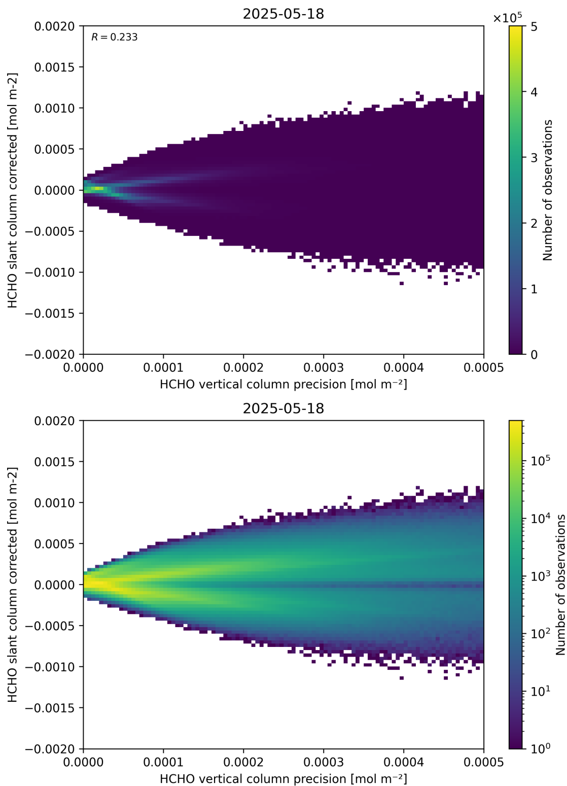
Figure 140: Scatter density plot of “HCHO vertical column precision” against “HCHO slant column corrected” for 2025-05-17 to 2025-05-19.
