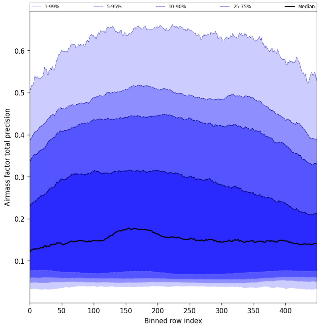
Figure 55: Along track statistics of “Airmass factor total precision” for 2025-05-17 to 2025-05-19
