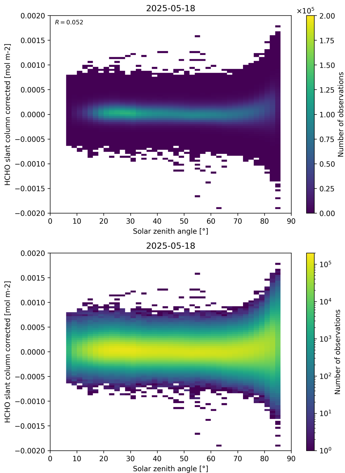
Figure 171: Scatter density plot of “Solar zenith angle” against “HCHO slant column corrected” for 2025-05-17 to 2025-05-19.
