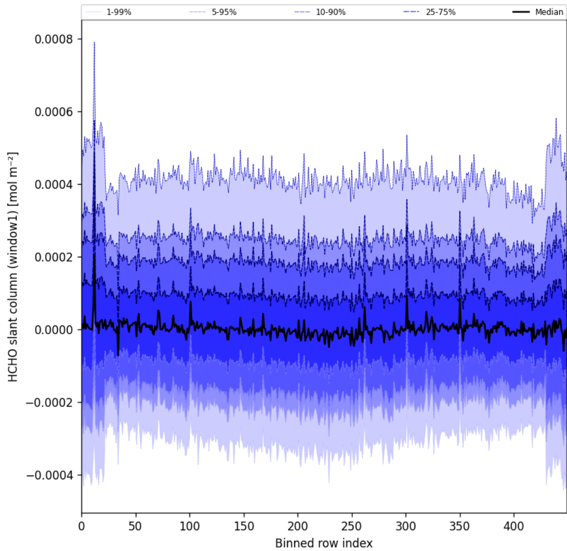
Figure 52: Along track statistics of “HCHO slant column (window1)” for 2025-05-17 to 2025-05-19
