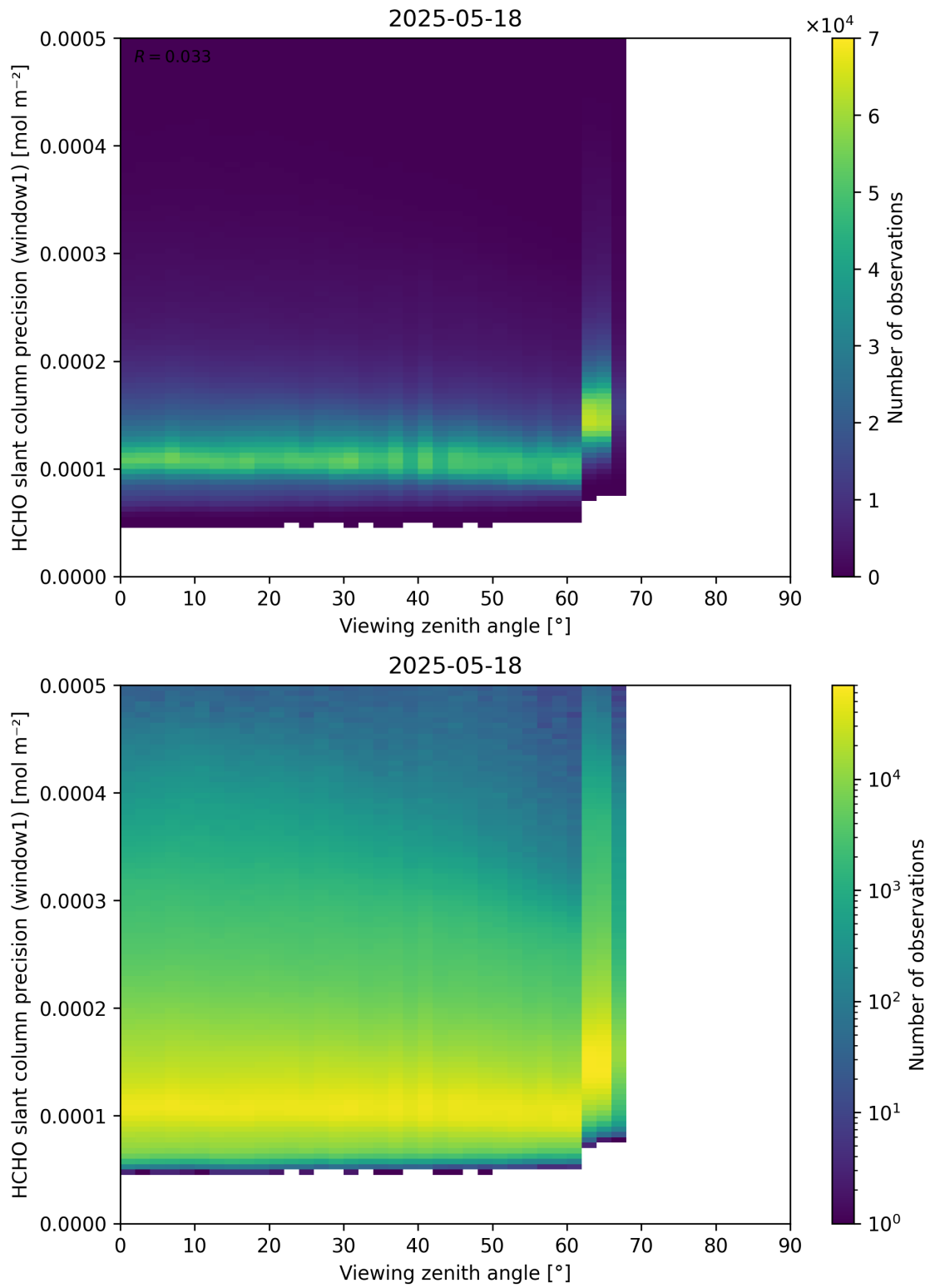
Figure 189: Scatter density plot of “Viewing zenith angle” against “HCHO slant column precision (window1)” for 2025-05-17 to 2025-05-19.
