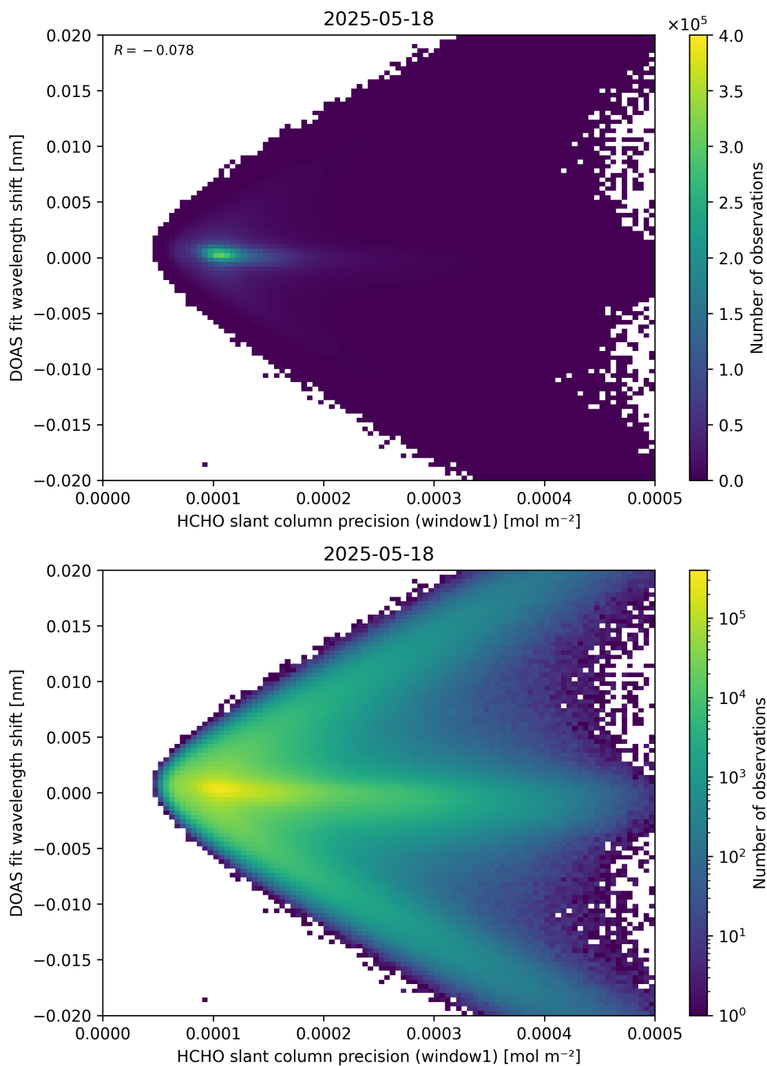
Figure 89: Scatter density plot of “HCHO slant column precision (window1)” against “DOAS fit wavelength shift” for 2025-05-17 to 2025-05-19.
