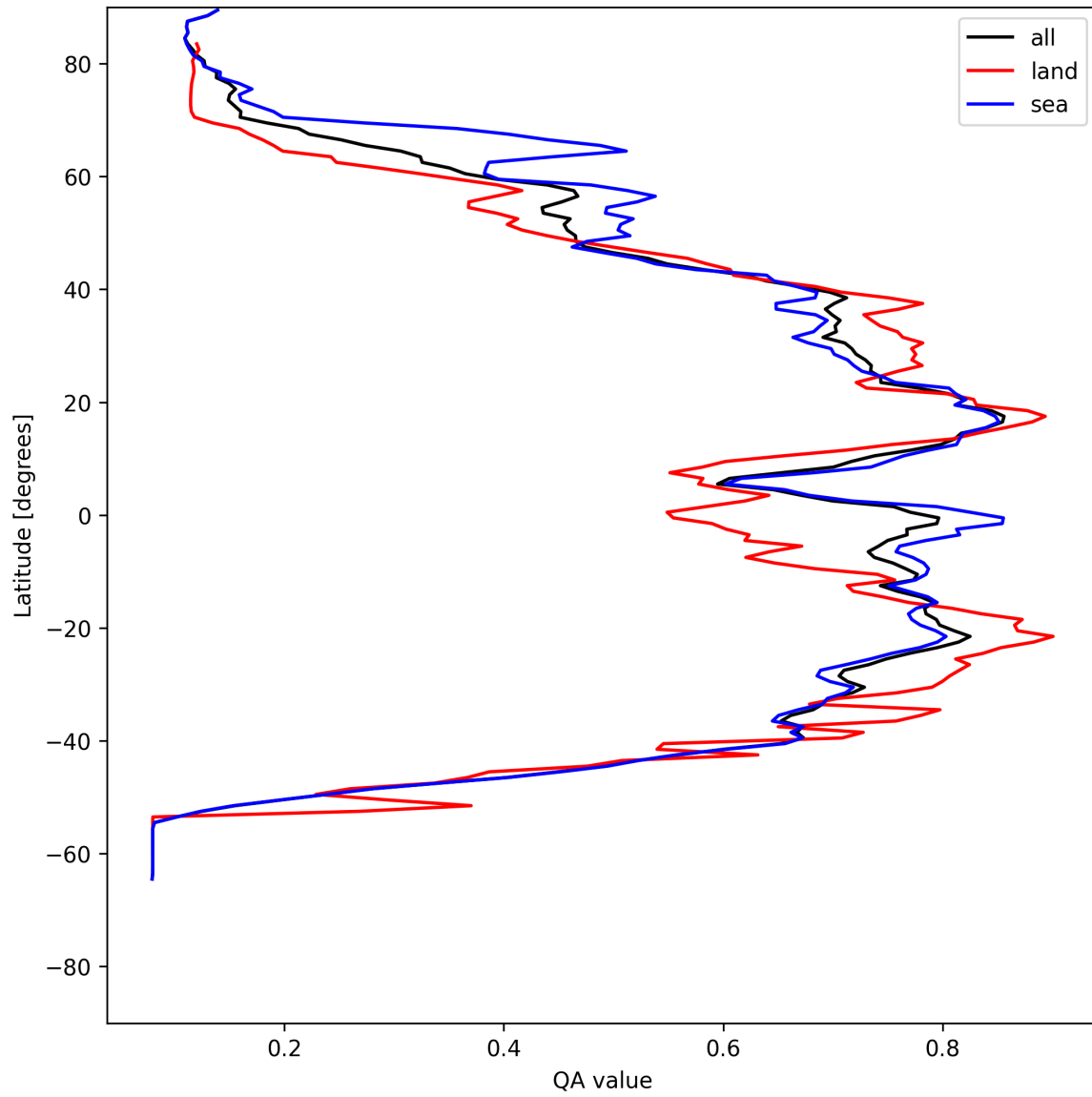
Figure 20: Zonal average of “QA value” for 2025-05-17 to 2025-05-19.
