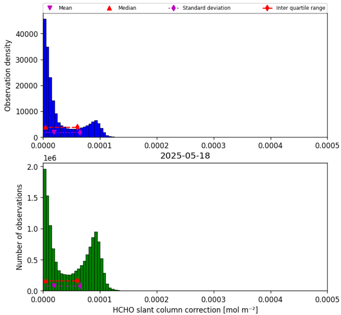
Figure 47: Histogram of “HCHO slant column correction” for 2025-05-17 to 2025-05-19
