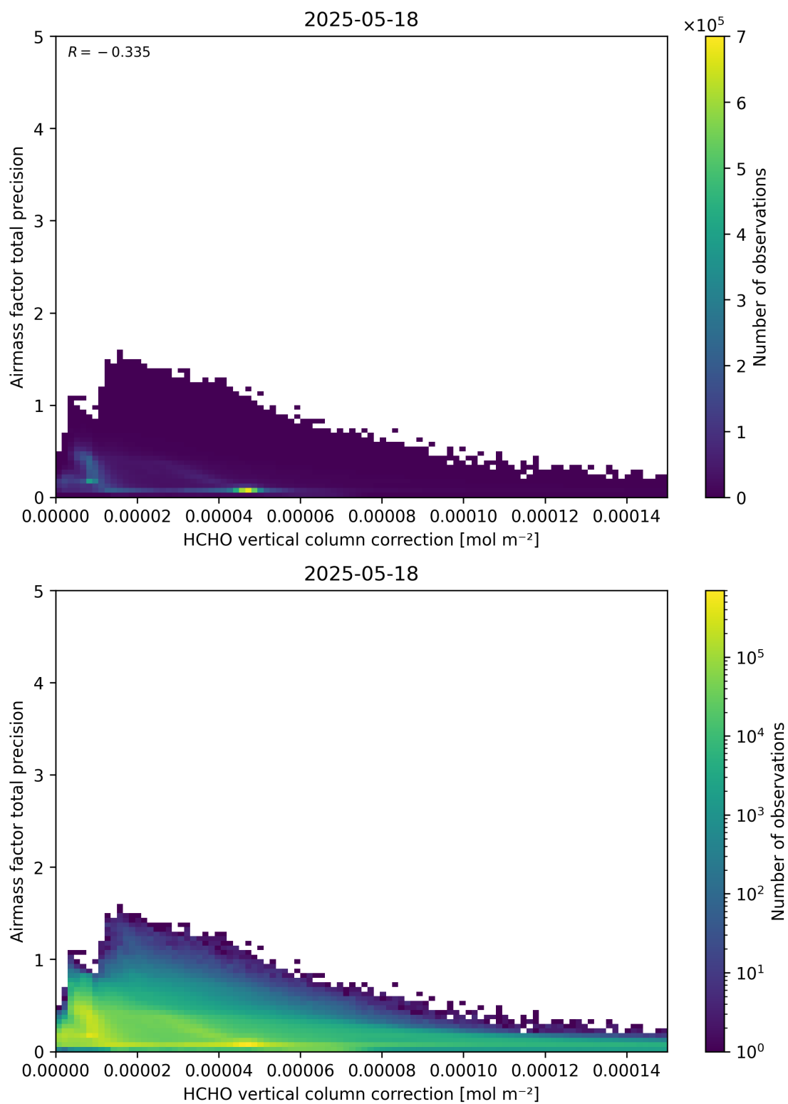
Figure 121: Scatter density plot of “HCHO vertical column correction” against “Airmass factor total precision” for 2025-05-17 to 2025-05-19.
