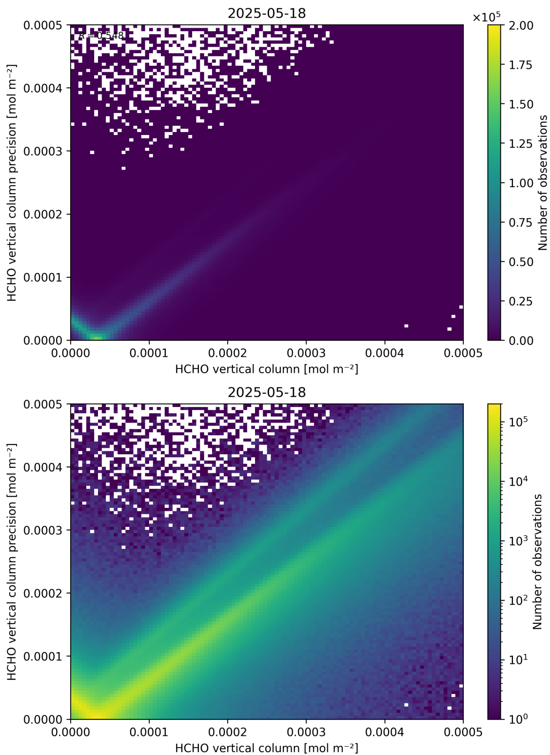
Figure 134: Scatter density plot of “HCHO vertical column” against “HCHO vertical column precision” for 2025-05-17 to 2025-05-19.
