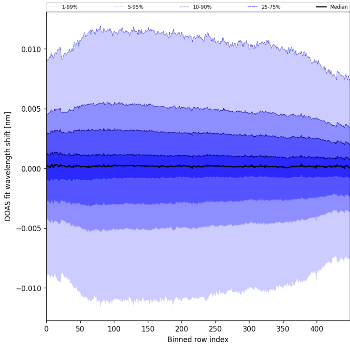
Figure 58: Along track statistics of “DOAS fit wavelength shift” for 2025-05-17 to 2025-05-19
