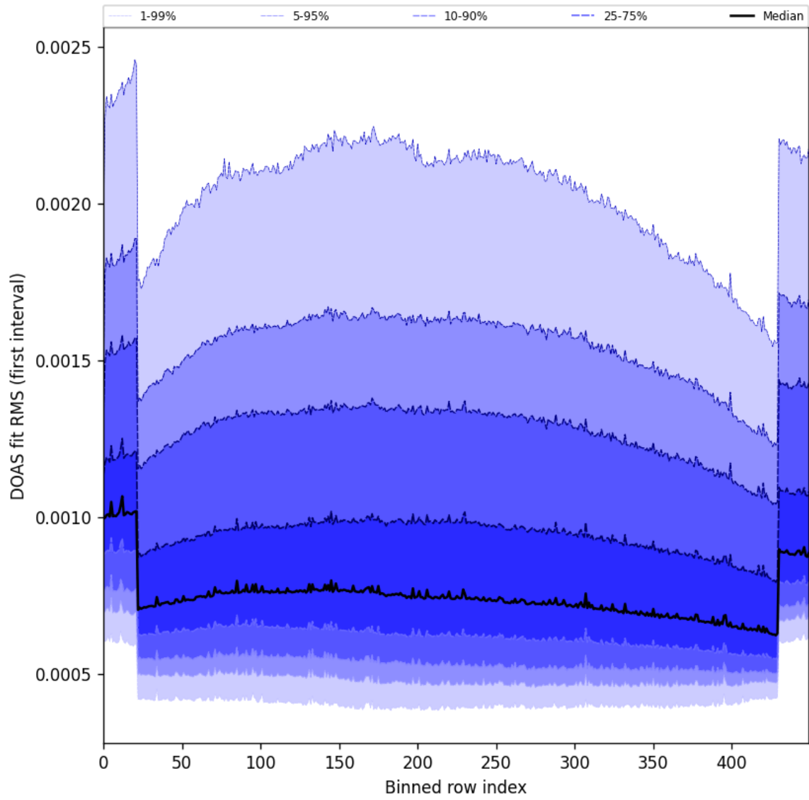
Figure 60: Along track statistics of “DOAS fit RMS (first interval)” for 2025-05-17 to 2025-05-19
