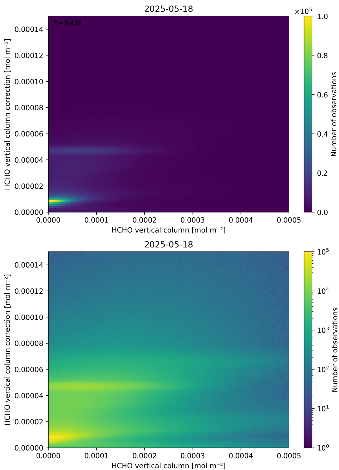
Figure 133: Scatter density plot of “HCHO vertical column” against “HCHO vertical column correction” for 2025-05-17 to 2025-05-19.
