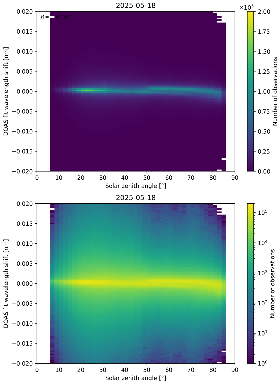
Figure 168: Scatter density plot of “Solar zenith angle” against “DOAS fit wavelength shift” for 2025-05-17 to 2025-05-19.
