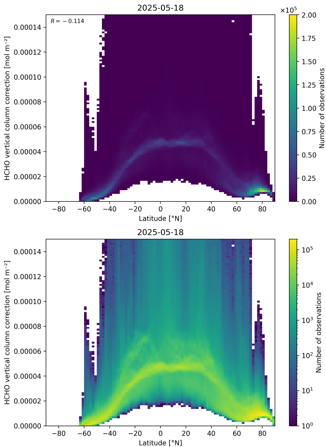
Figure 164: Scatter density plot of “Latitude” against “HCHO vertical column correction” for 2025-05-17 to 2025-05-19.
