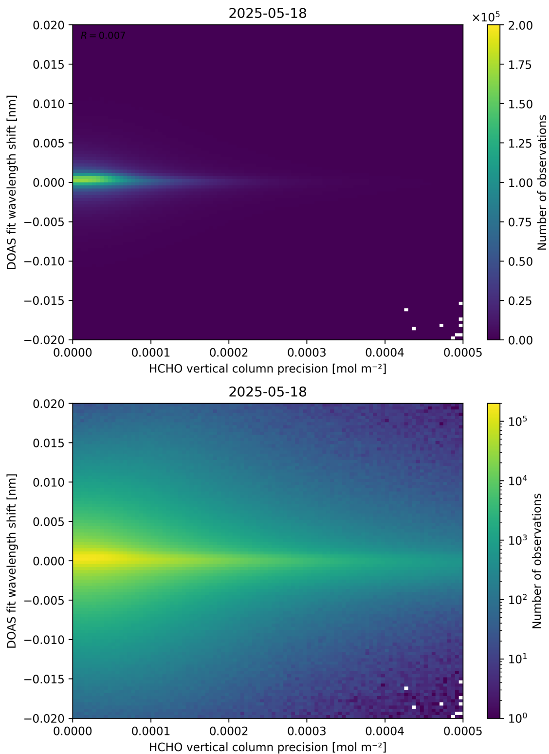
Figure 137: Scatter density plot of “HCHO vertical column precision” against “DOAS fit wavelength shift” for 2025-05-17 to 2025-05-19.
