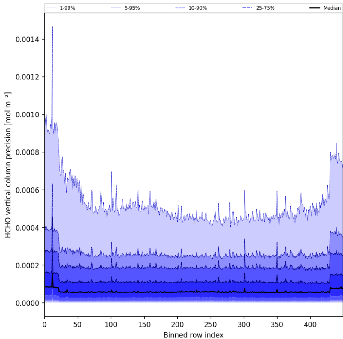
Figure 50: Along track statistics of “HCHO vertical column precision” for 2025-05-17 to 2025-05-19
