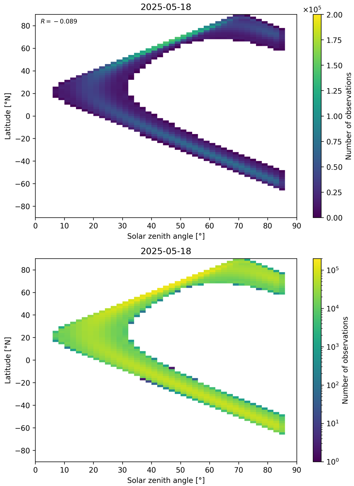
Figure 181: Scatter density plot of “Solar zenith angle” against “Latitude” for 2025-05-17 to 2025-05-19.
