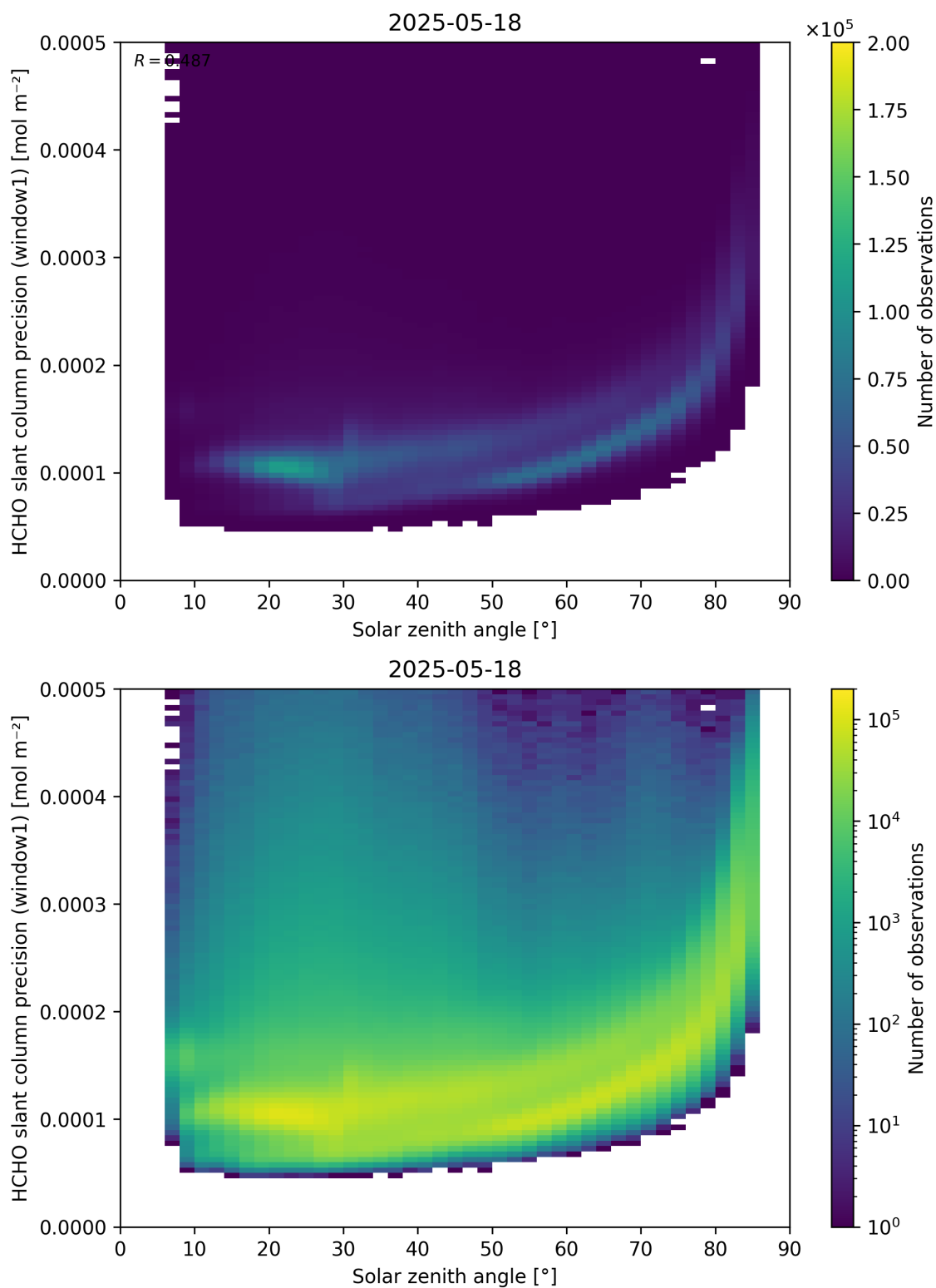
Figure 174: Scatter density plot of “Solar zenith angle” against “HCHO slant column precision (window1)” for 2025-05-17 to 2025-05-19.
