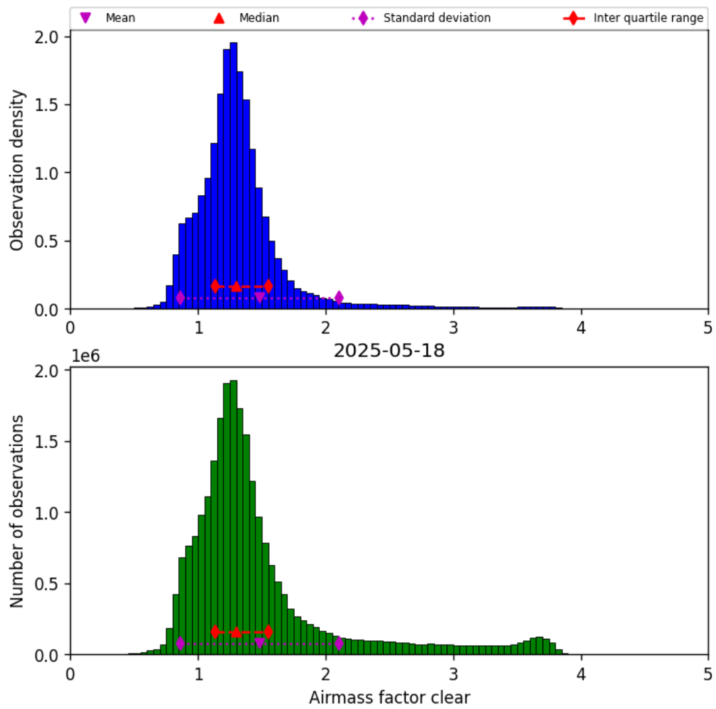
Figure 42: Histogram of “Airmass factor clear” for 2025-05-17 to 2025-05-19
