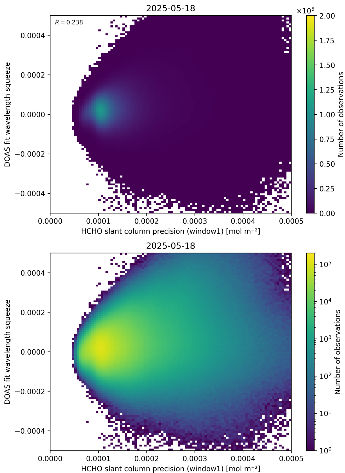
Figure 90: Scatter density plot of “HCHO slant column precision (window1)” against “DOAS fit wavelength squeeze” for 2025-05-17 to 2025-05-19.
