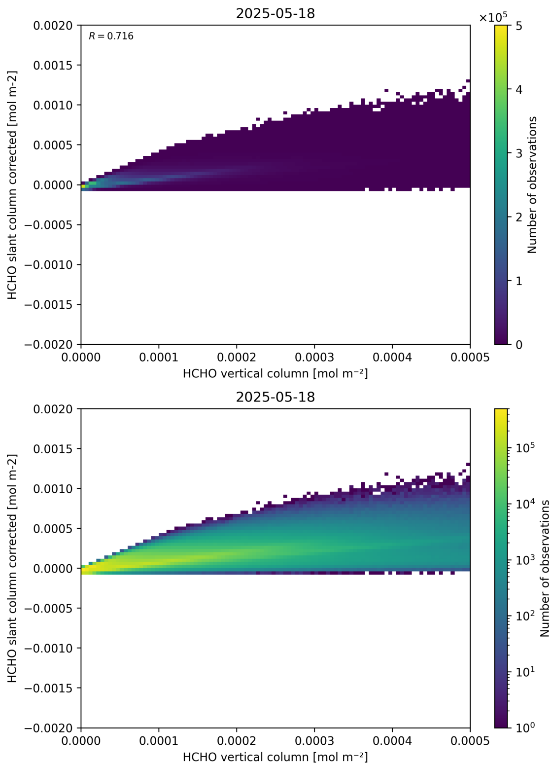
Figure 127: Scatter density plot of “HCHO vertical column” against “HCHO slant column corrected” for 2025-05-17 to 2025-05-19.
