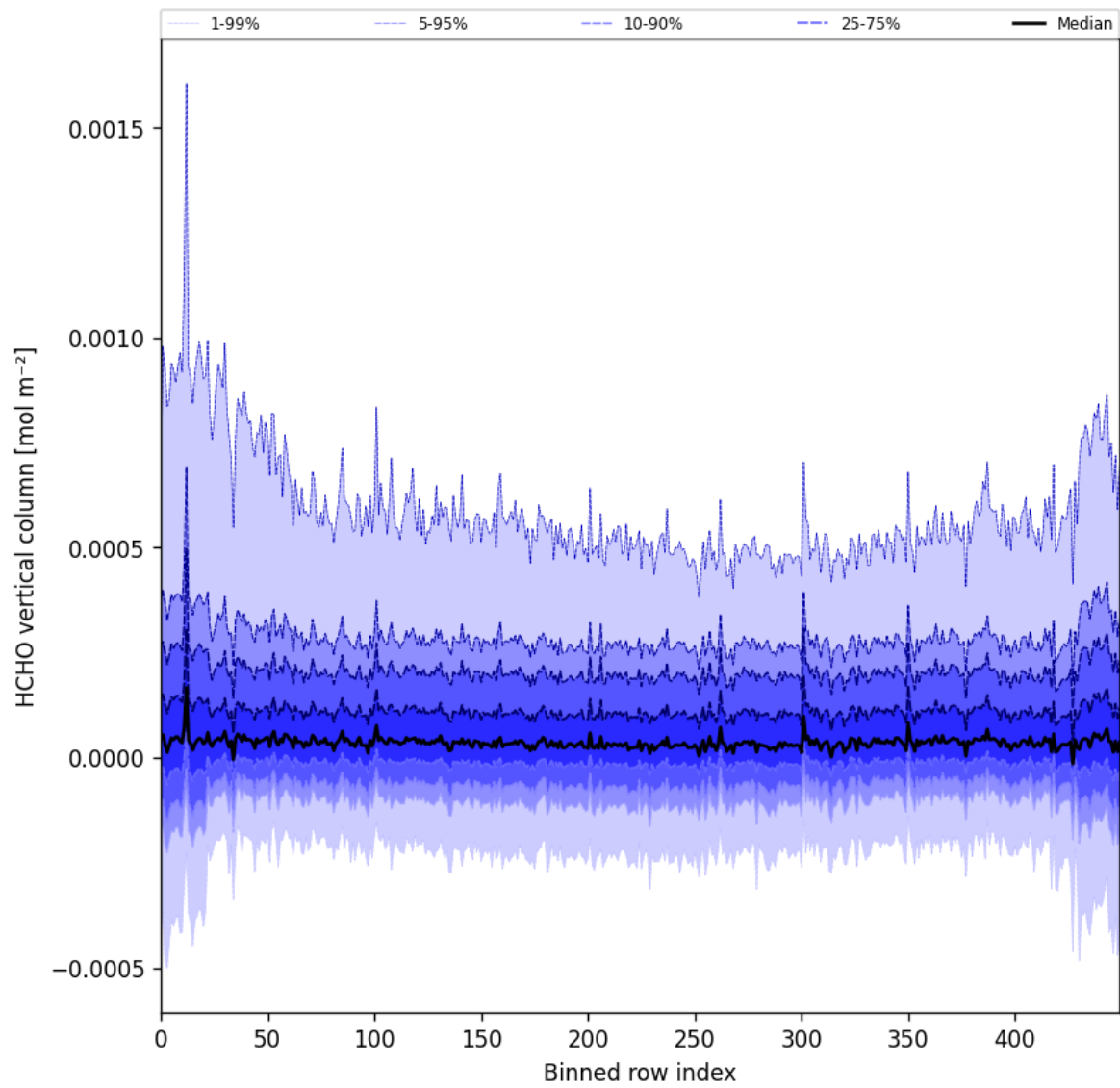
Figure 49: Along track statistics of “HCHO vertical column” for 2025-05-17 to 2025-05-19
