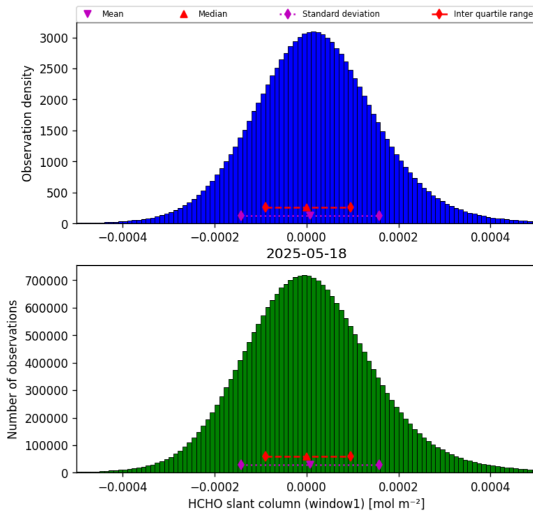
Figure 38: Histogram of “HCHO slant column (window1)” for 2025-05-17 to 2025-05-19
