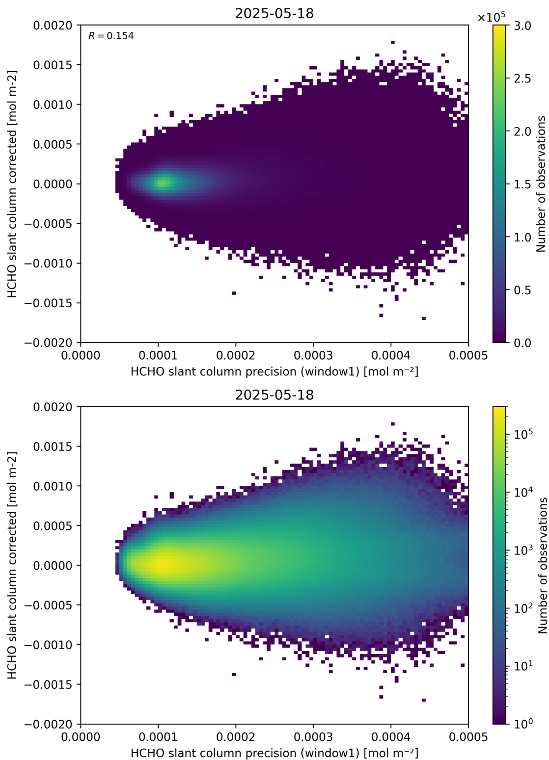
Figure 92: Scatter density plot of “HCHO slant column precision (window1)” against “HCHO slant column corrected” for 2025-05-17 to 2025-05-19.
