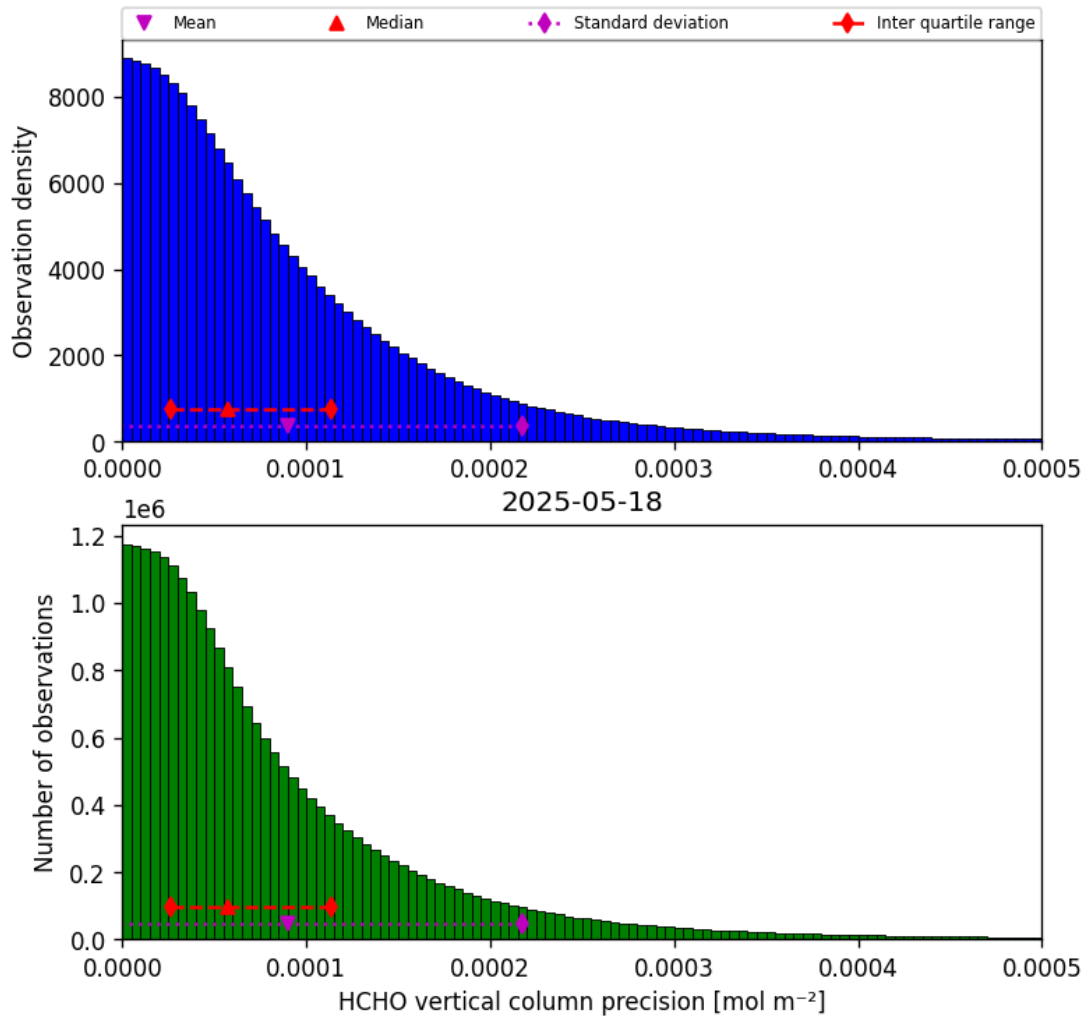
Figure 36: Histogram of “HCHO vertical column precision” for 2025-05-17 to 2025-05-19
