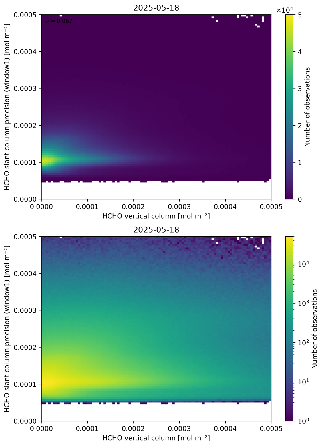
Figure 130: Scatter density plot of “HCHO vertical column” against “HCHO slant column precision (window1)” for 2025-05-17 to 2025-05-19.
