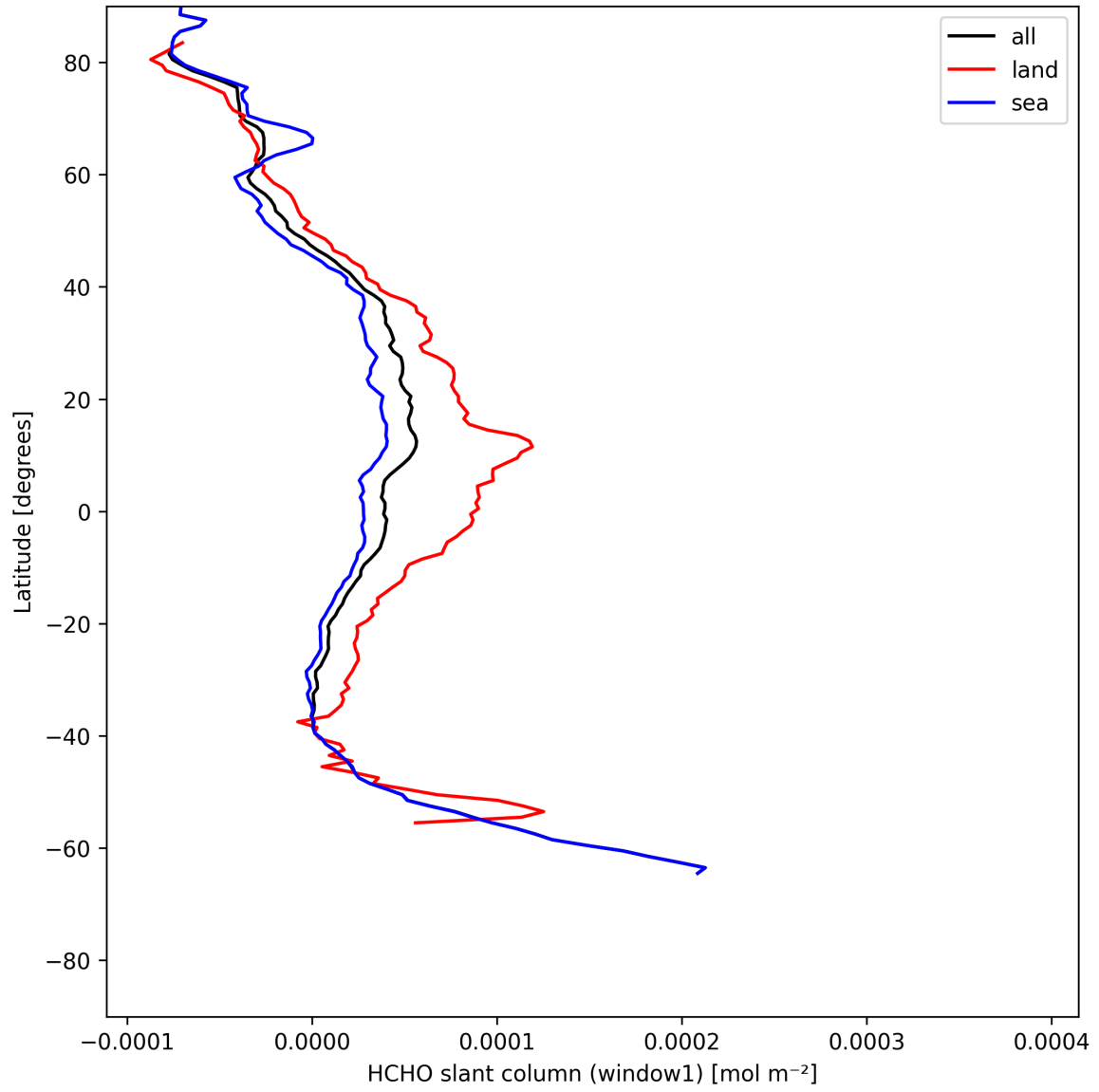
Figure 24: Zonal average of “HCHO slant column (window1)” for 2025-05-17 to 2025-05-19.
