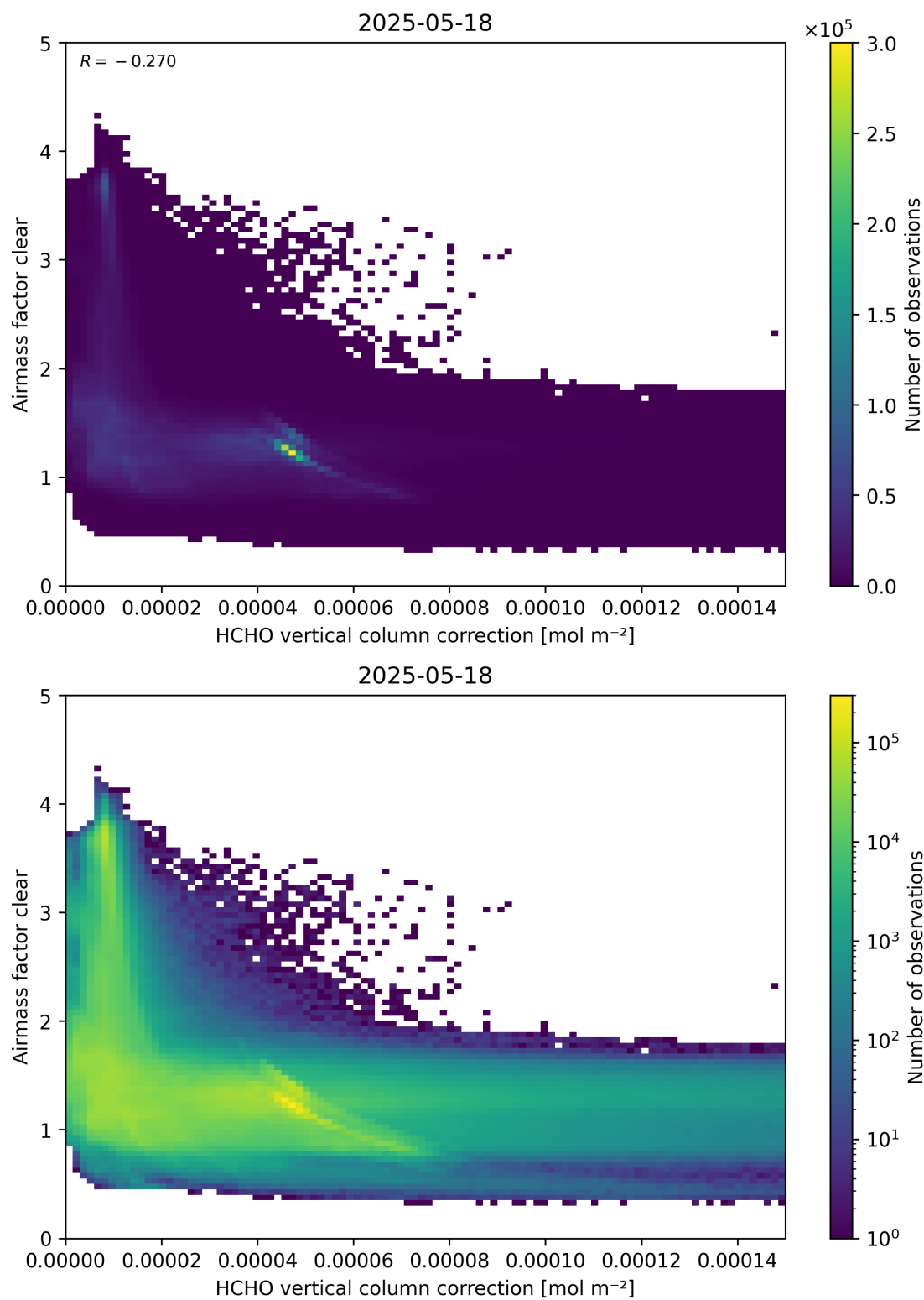
Figure 115: Scatter density plot of “HCHO vertical column correction” against “Airmass factor clear” for 2025-05-17 to 2025-05-19.
