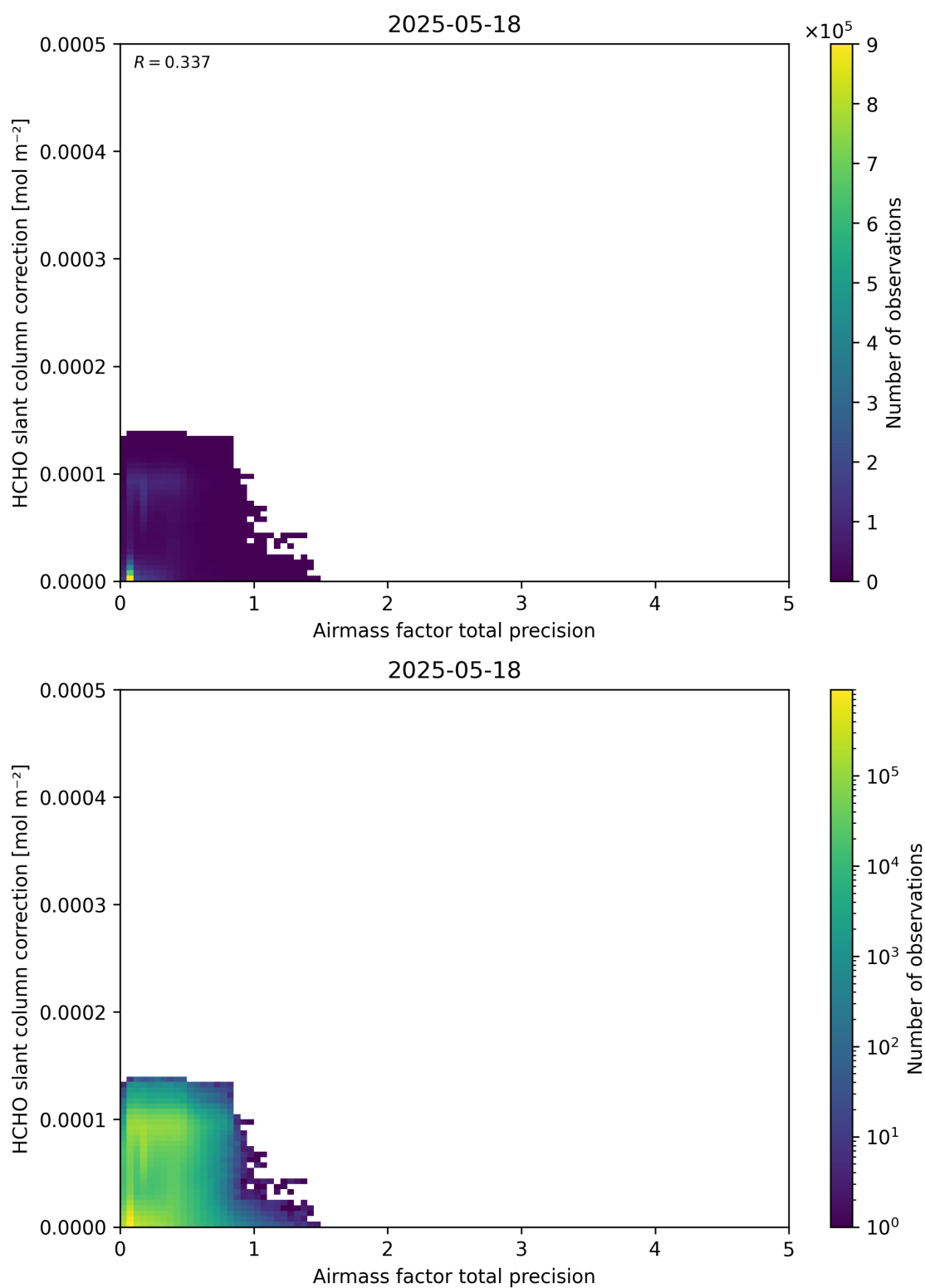
Figure 110: Scatter density plot of “Airmass factor total precision” against “HCHO slant column correction” for 2025-05-17 to 2025-05-19.
