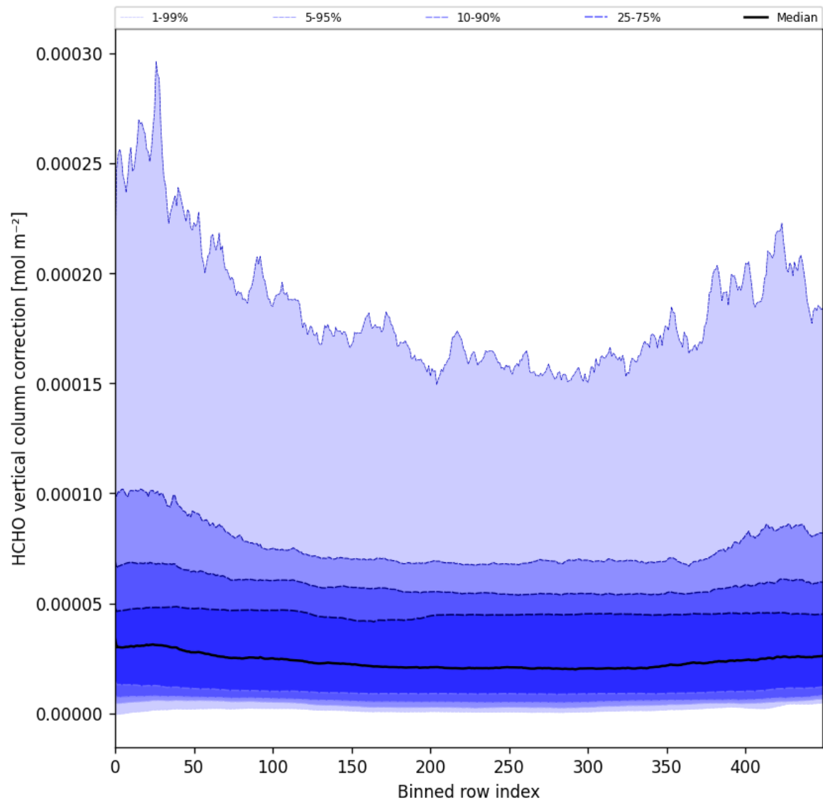
Figure 51: Along track statistics of “HCHO vertical column correction” for 2025-05-17 to 2025-05-19
