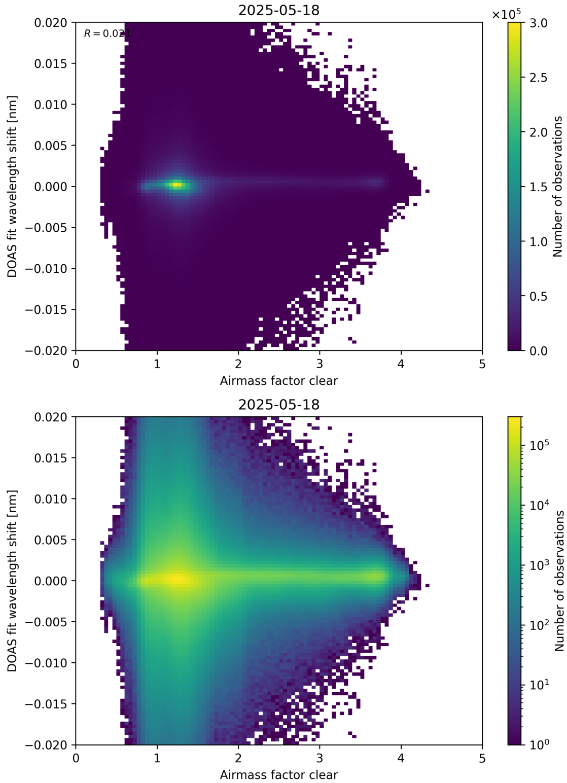
Figure 72: Scatter density plot of “Airmass factor clear” against “DOAS fit wavelength shift” for 2025-05-17 to 2025-05-19.
