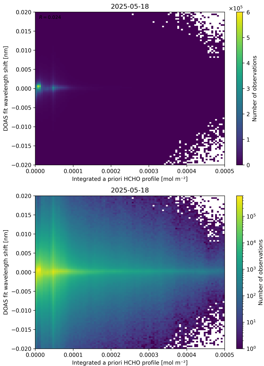
Figure 149: Scatter density plot of “Integrated a priori HCHO profile” against “DOAS fit wavelength shift” for 2025-05-17 to 2025-05-19.
