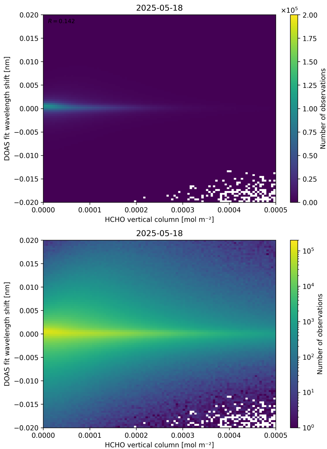
Figure 124: Scatter density plot of “HCHO vertical column” against “DOAS fit wavelength shift” for 2025-05-17 to 2025-05-19.
