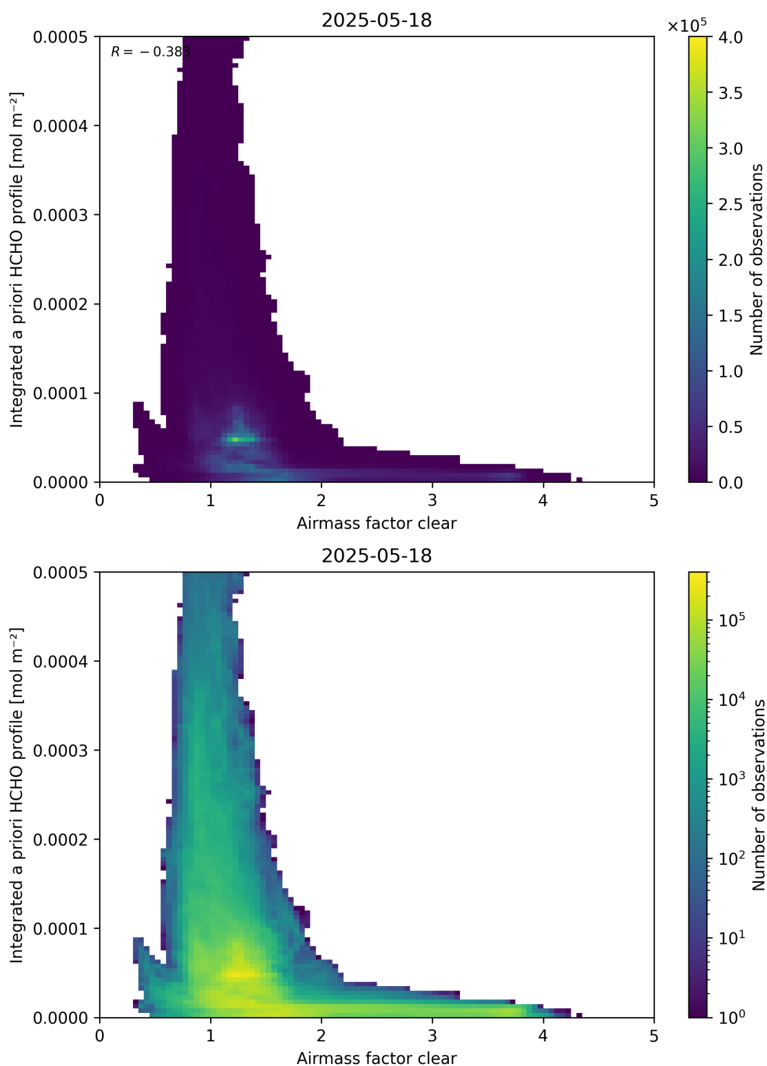
Figure 76: Scatter density plot of “Airmass factor clear” against “Integrated a priori HCHO profile” for 2025-05-17 to 2025-05-19.
