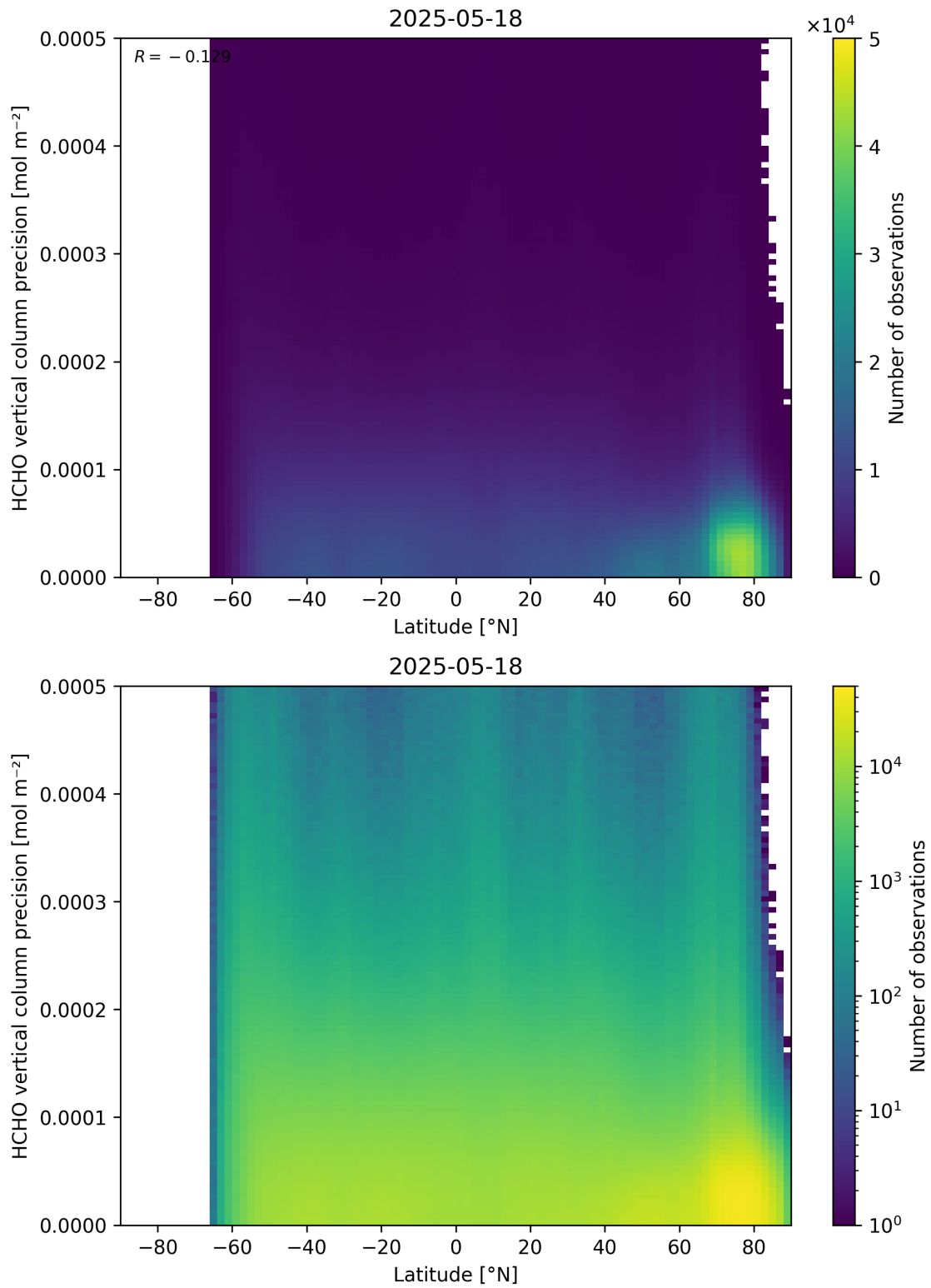
Figure 165: Scatter density plot of “Latitude” against “HCHO vertical column precision” for 2025-05-17 to 2025-05-19.
