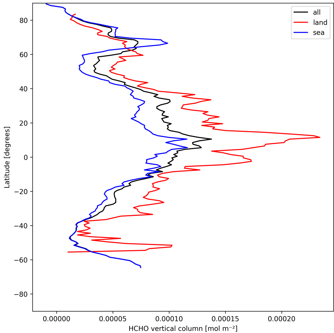
Figure 21: Zonal average of “HCHO vertical column” for 2025-05-17 to 2025-05-19.
