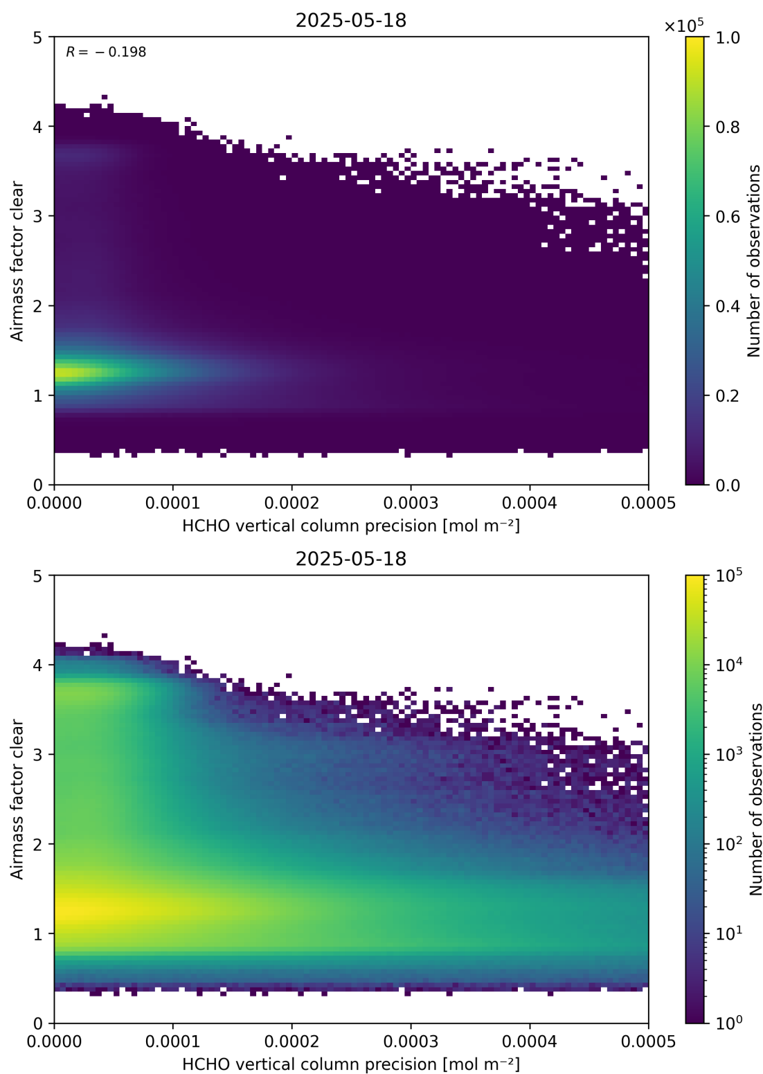
Figure 139: Scatter density plot of “HCHO vertical column precision” against “Airmass factor clear” for 2025-05-17 to 2025-05-19.
