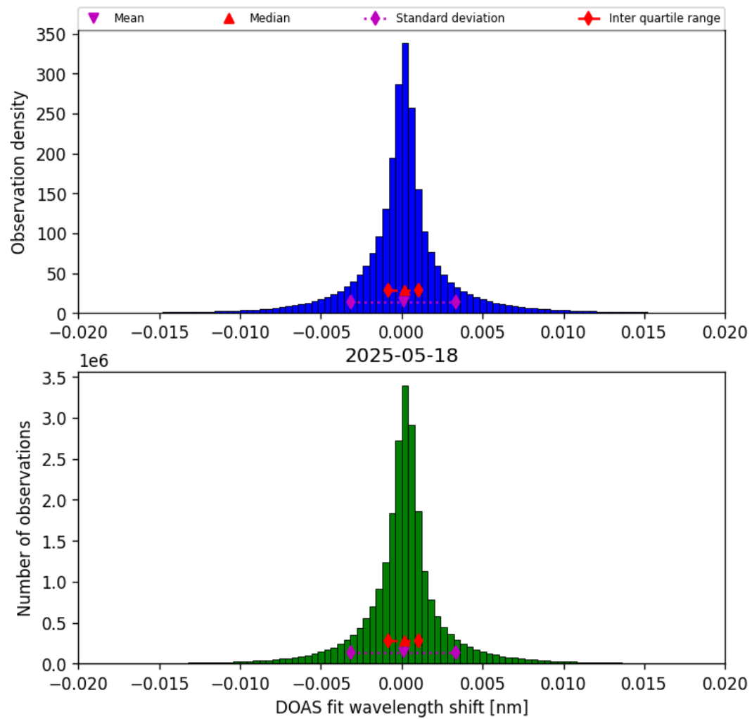
Figure 44: Histogram of “DOAS fit wavelength shift” for 2025-05-17 to 2025-05-19
