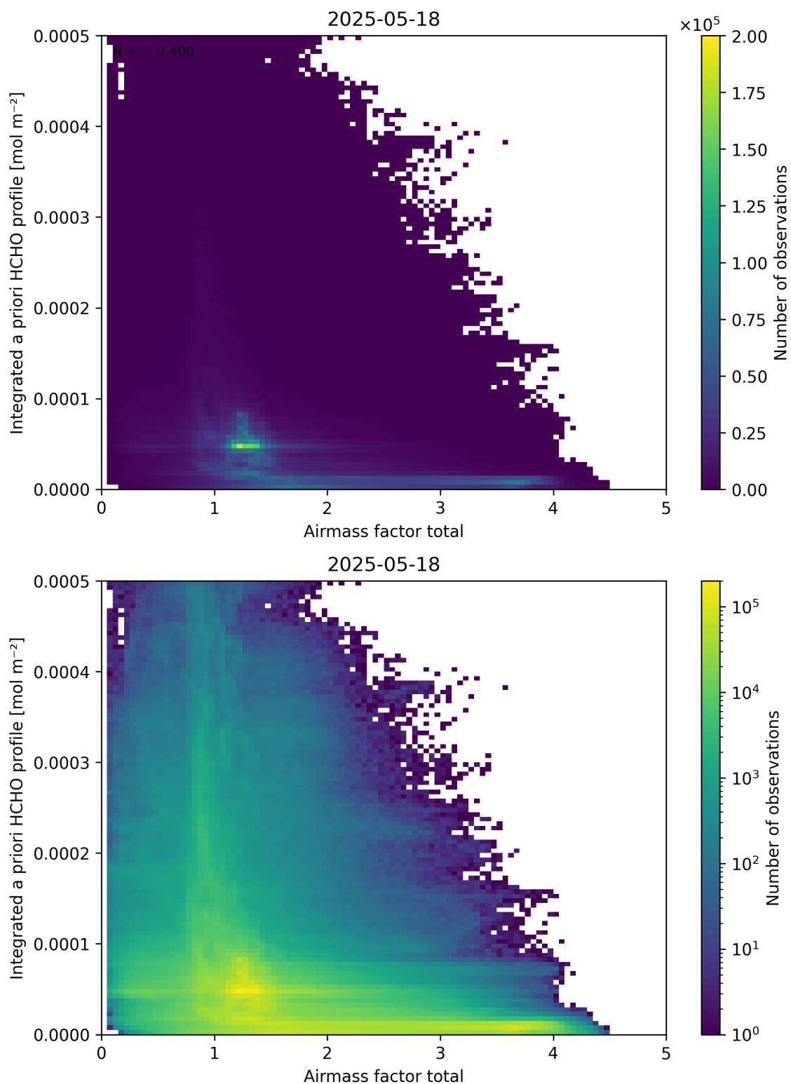
Figure 104: Scatter density plot of “Airmass factor total” against “Integrated a priori HCHO profile” for 2025-05-17 to 2025-05-19.
