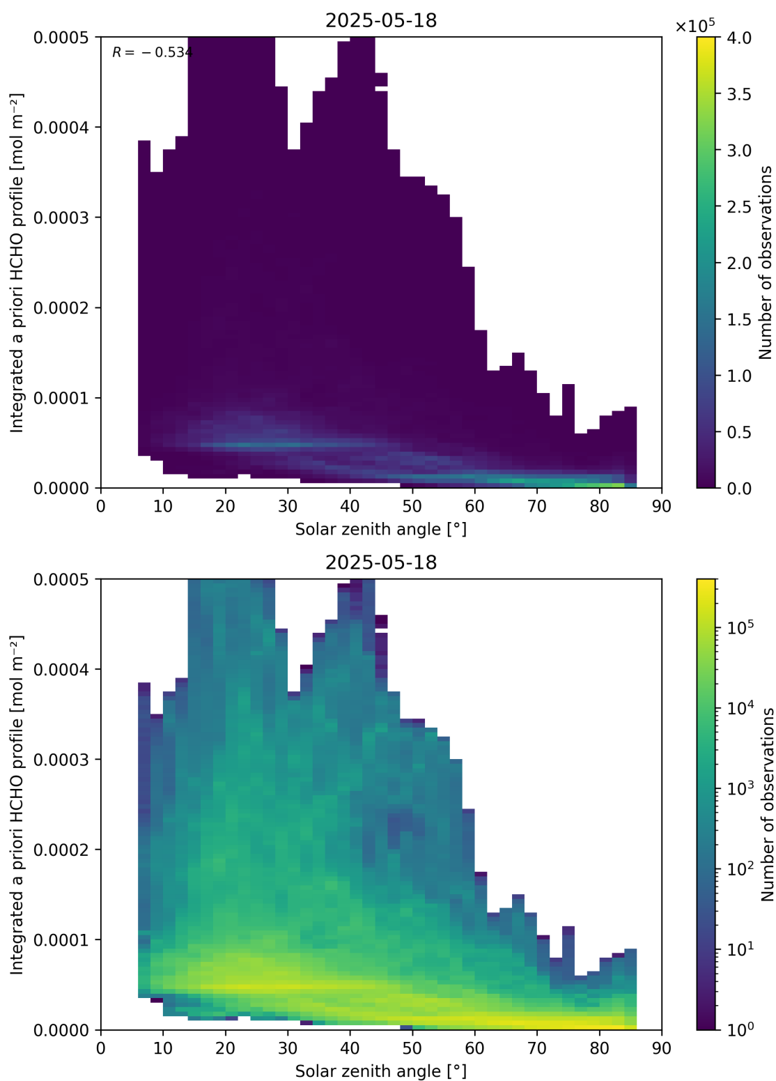
Figure 180: Scatter density plot of “Solar zenith angle” against “Integrated a priori HCHO profile” for 2025-05-17 to 2025-05-19.
