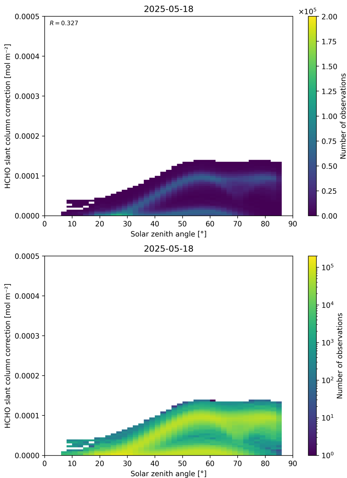
Figure 172: Scatter density plot of “Solar zenith angle” against “HCHO slant column correction” for 2025-05-17 to 2025-05-19.
