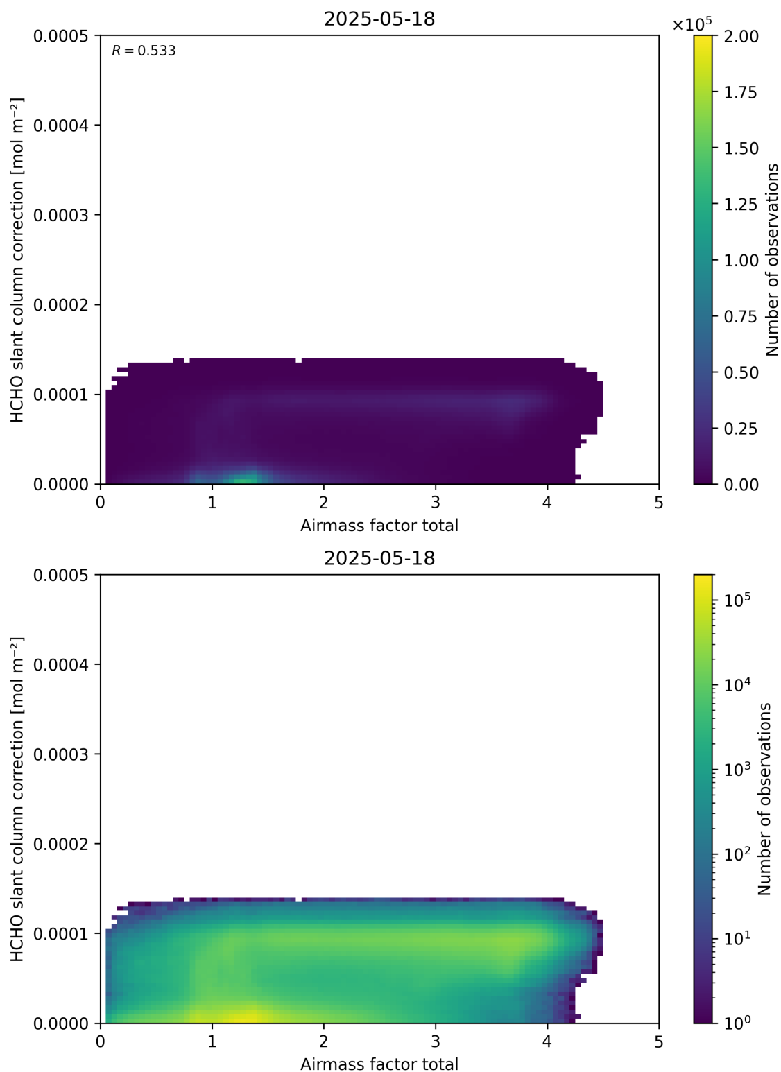
Figure 102: Scatter density plot of “Airmass factor total” against “HCHO slant column correction” for 2025-05-17 to 2025-05-19.
