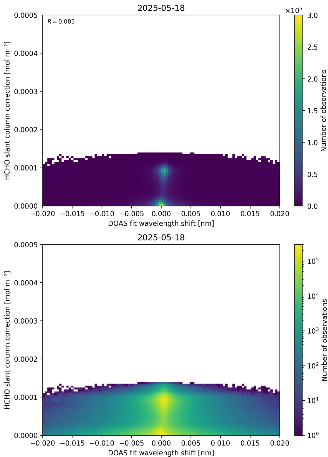
Figure 67: Scatter density plot of “DOAS fit wavelength shift” against “HCHO slant column correction” for 2025-05-17 to 2025-05-19.
