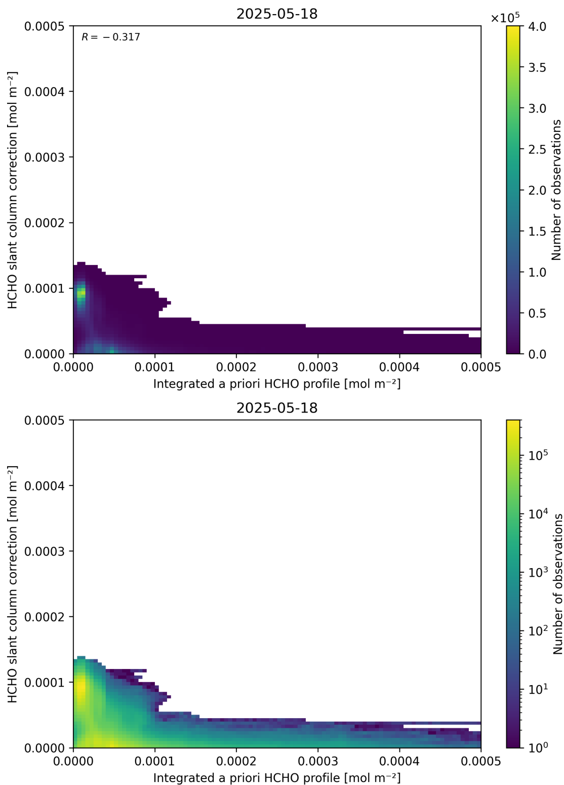
Figure 152: Scatter density plot of “Integrated a priori HCHO profile” against “HCHO slant column correction” for 2025-05-17 to 2025-05-19.
