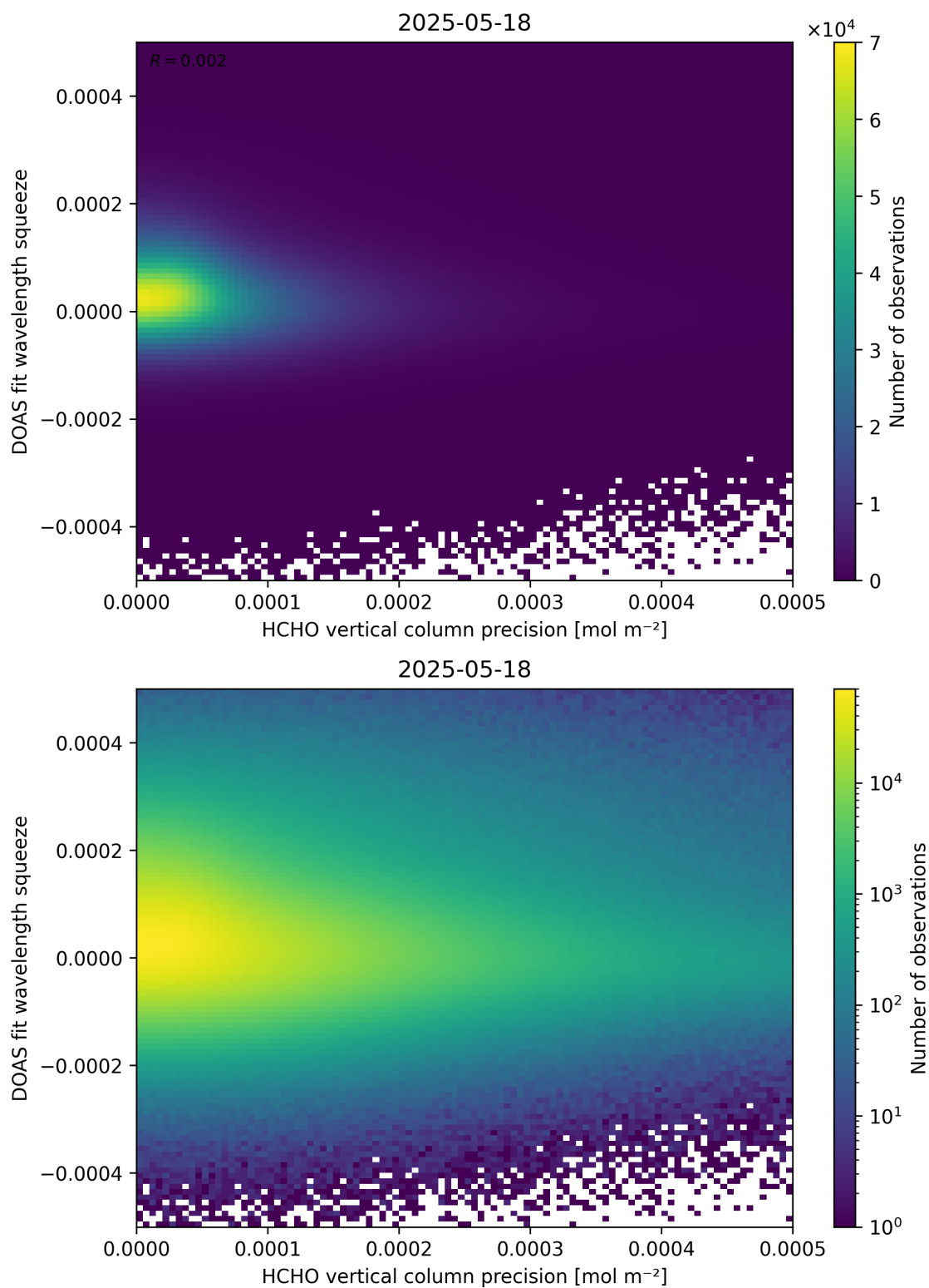
Figure 138: Scatter density plot of “HCHO vertical column precision” against “DOAS fit wavelength squeeze” for 2025-05-17 to 2025-05-19.
