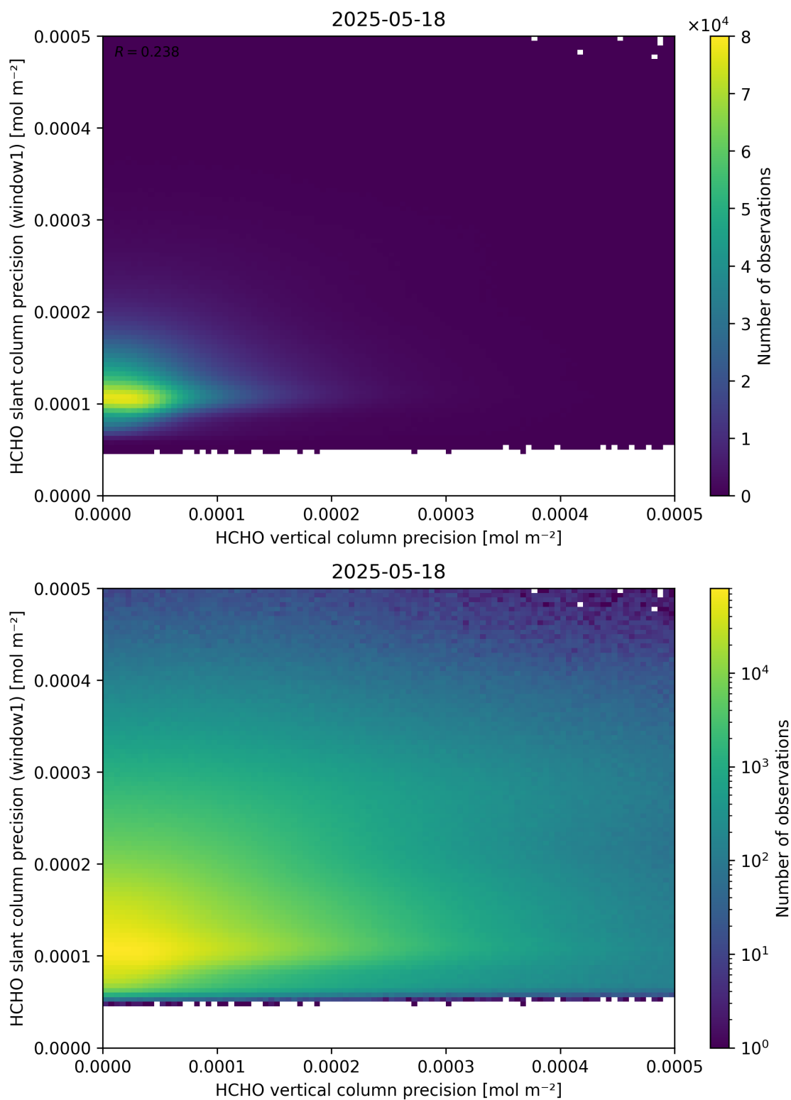
Figure 143: Scatter density plot of “HCHO vertical column precision” against “HCHO slant column precision (window1)” for 2025-05-17 to 2025-05-19.
