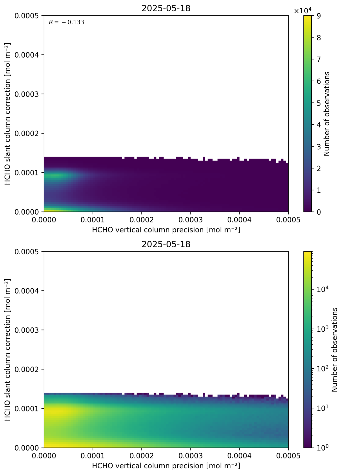
Figure 141: Scatter density plot of “HCHO vertical column precision” against “HCHO slant column correction” for 2025-05-17 to 2025-05-19.
