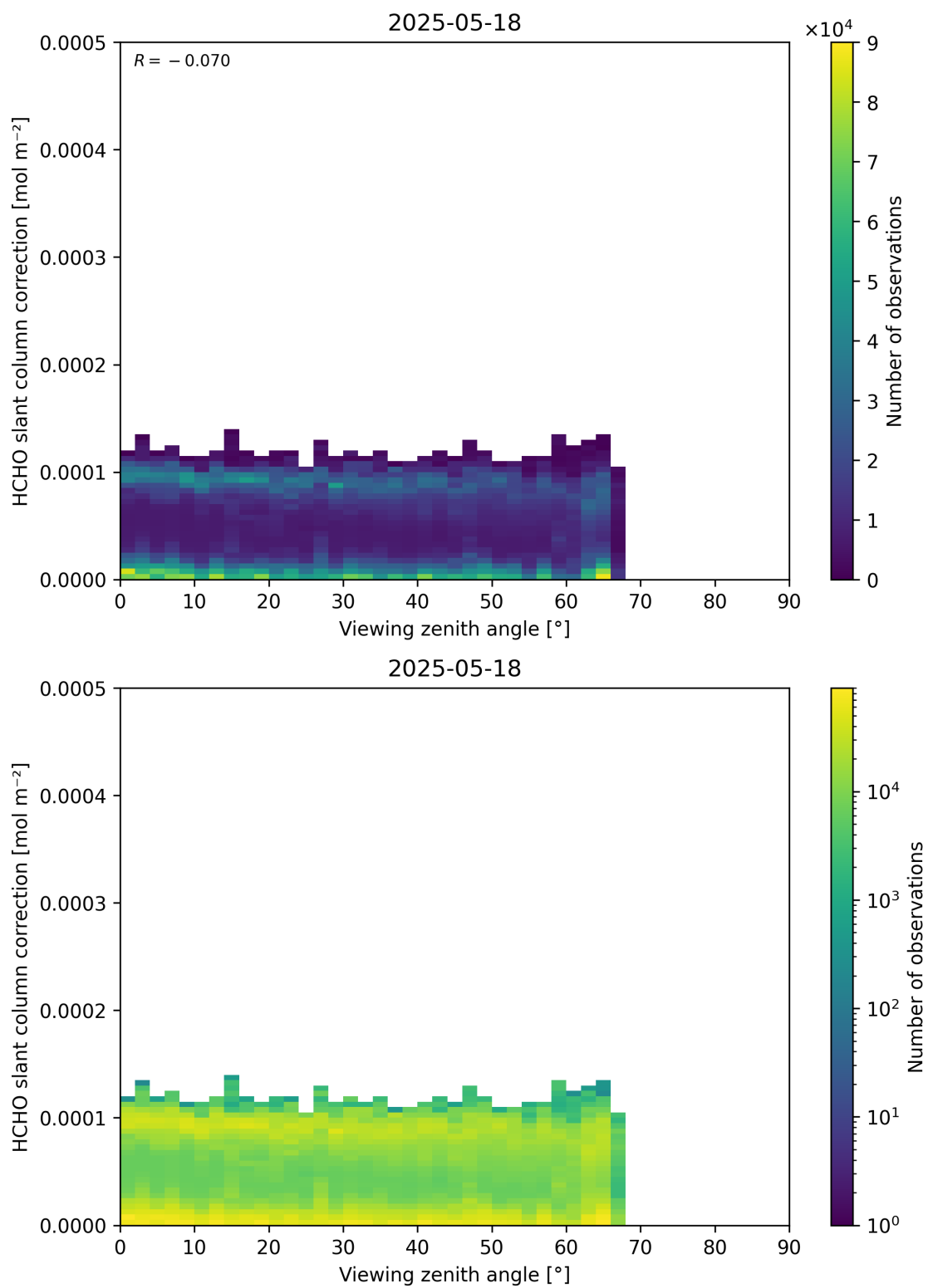
Figure 187: Scatter density plot of “Viewing zenith angle” against “HCHO slant column correction” for 2025-05-17 to 2025-05-19.
