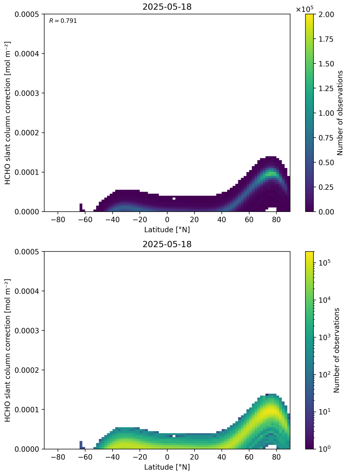
Figure 158: Scatter density plot of “Latitude” against “HCHO slant column correction” for 2025-05-17 to 2025-05-19.
