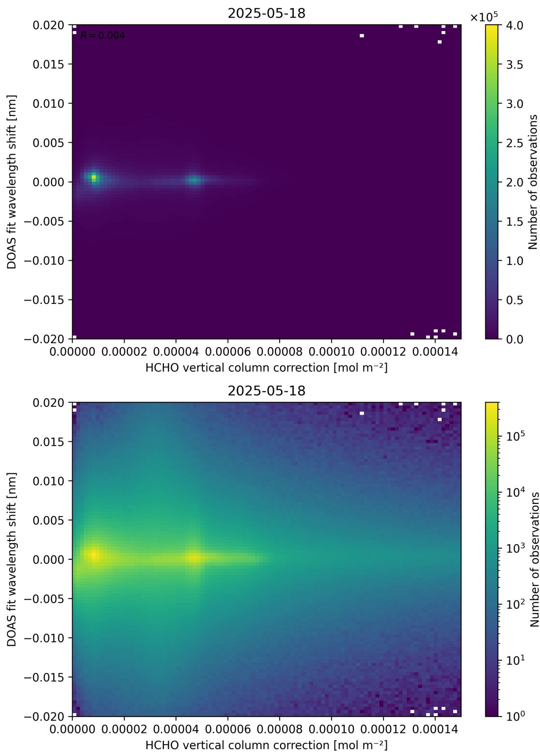
Figure 113: Scatter density plot of “HCHO vertical column correction” against “DOAS fit wavelength shift” for 2025-05-17 to 2025-05-19.
