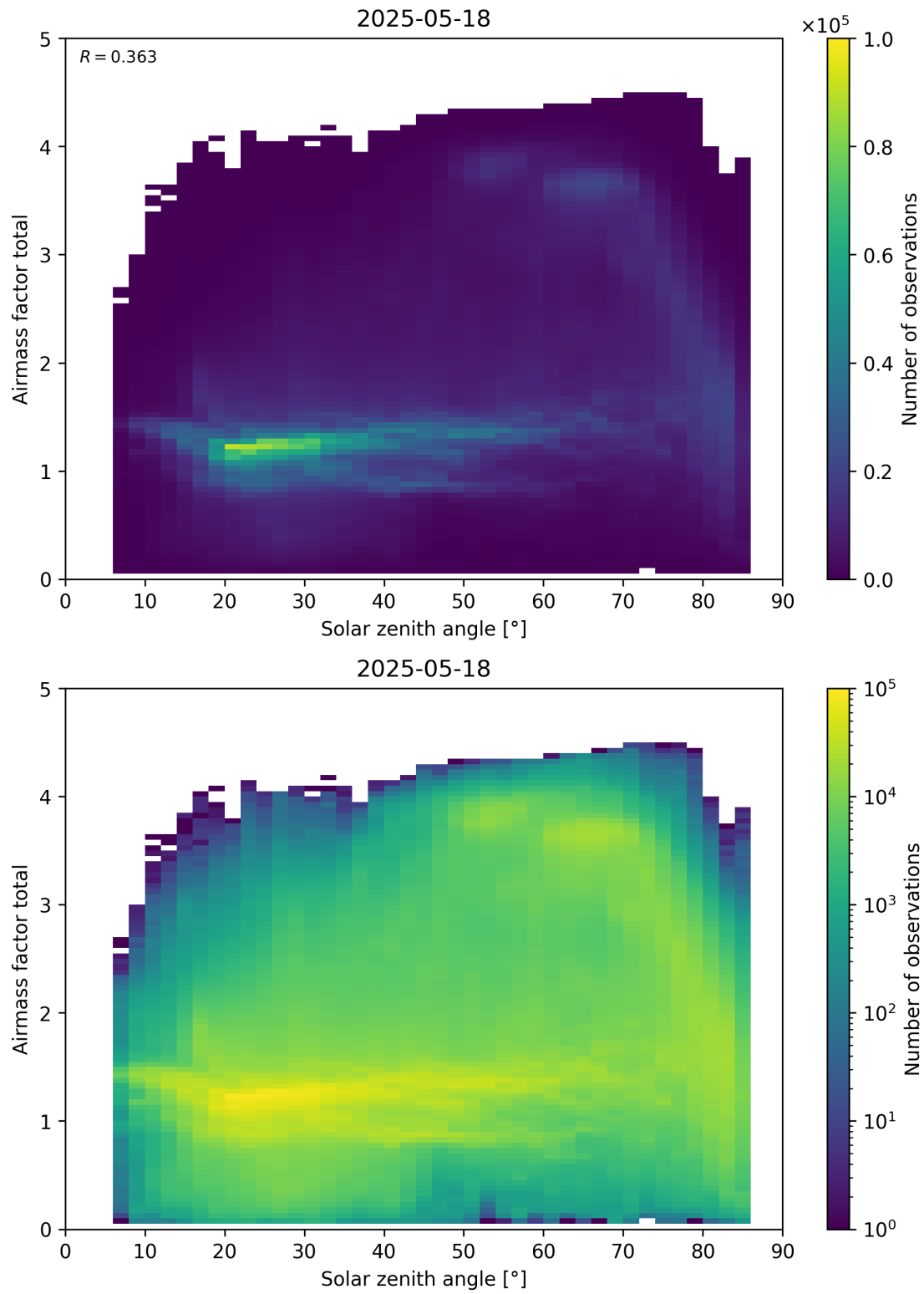
Figure 175: Scatter density plot of “Solar zenith angle” against “Airmass factor total” for 2025-05-17 to 2025-05-19.
