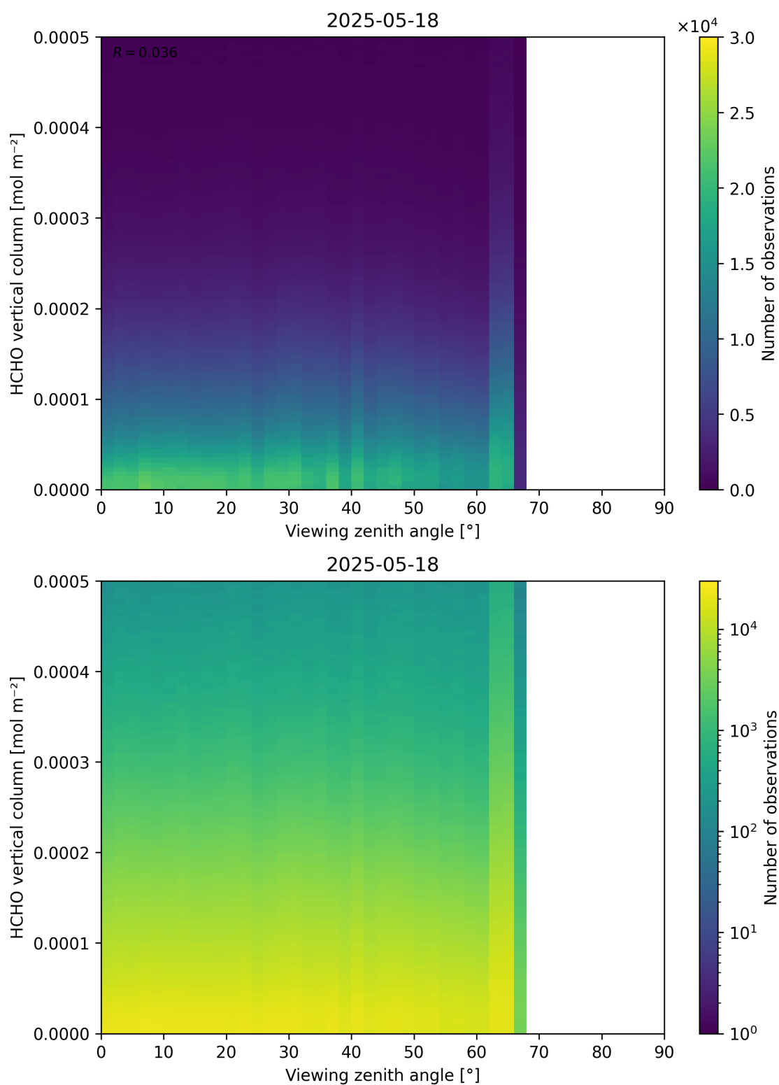
Figure 192: Scatter density plot of “Viewing zenith angle” against “HCHO vertical column” for 2025-05-17 to 2025-05-19.
