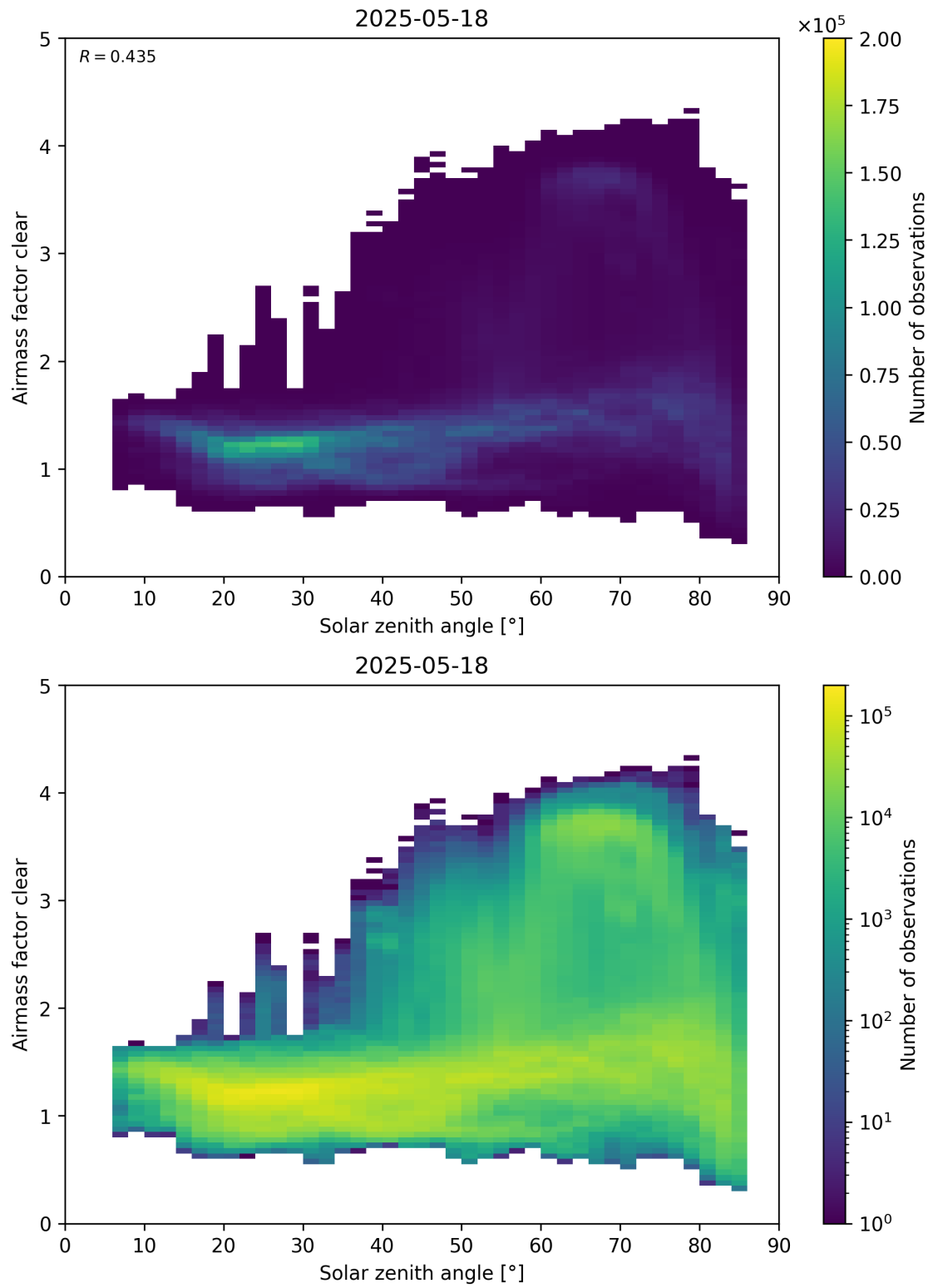
Figure 170: Scatter density plot of “Solar zenith angle” against “Airmass factor clear” for 2025-05-17 to 2025-05-19.
