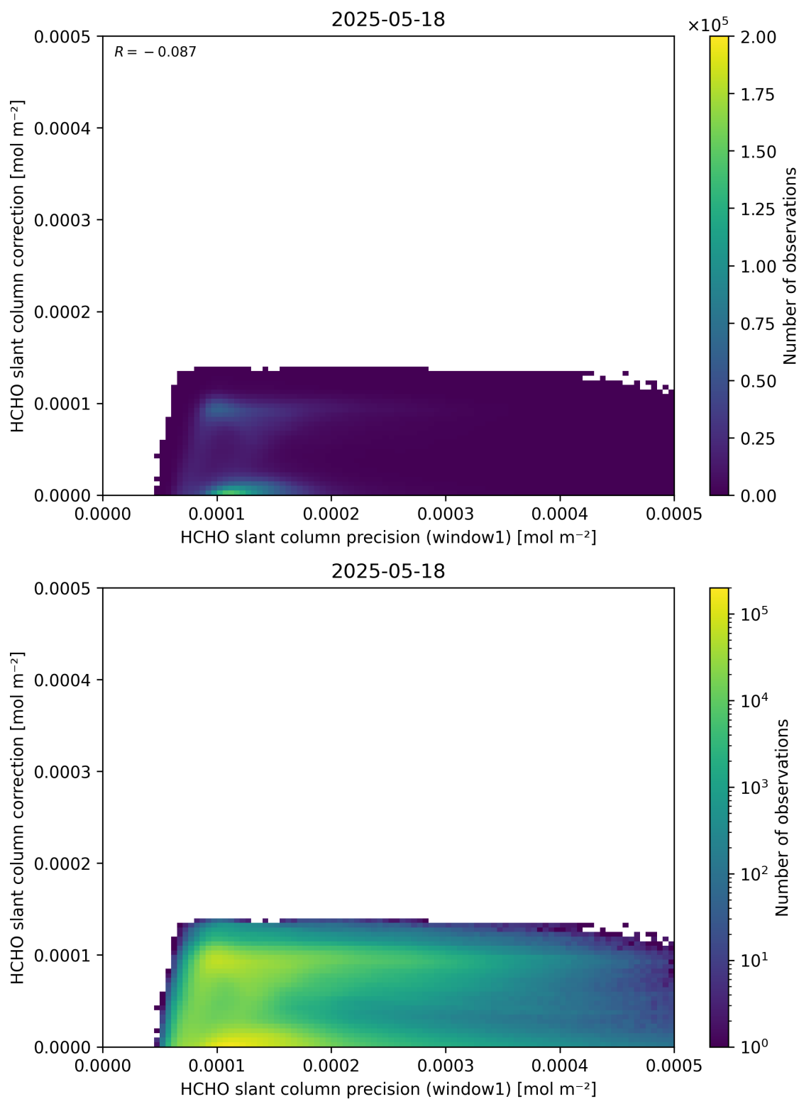
Figure 93: Scatter density plot of “HCHO slant column precision (window1)” against “HCHO slant column correction” for 2025-05-17 to 2025-05-19.
