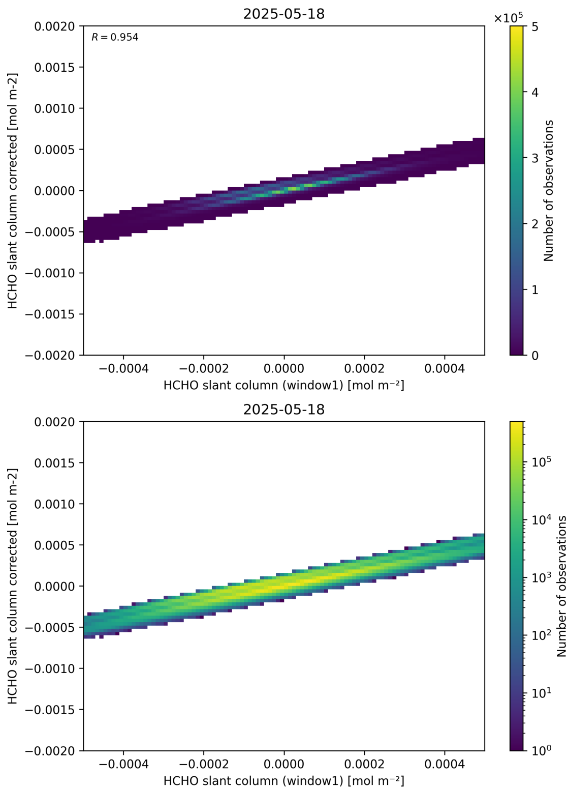
Figure 82: Scatter density plot of “HCHO slant column (window1)” against “HCHO slant column corrected” for 2025-05-17 to 2025-05-19.
