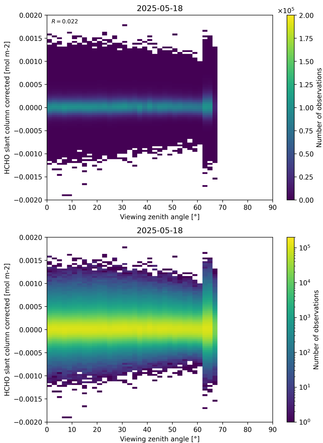
Figure 186: Scatter density plot of “Viewing zenith angle” against “HCHO slant column corrected” for 2025-05-17 to 2025-05-19.
