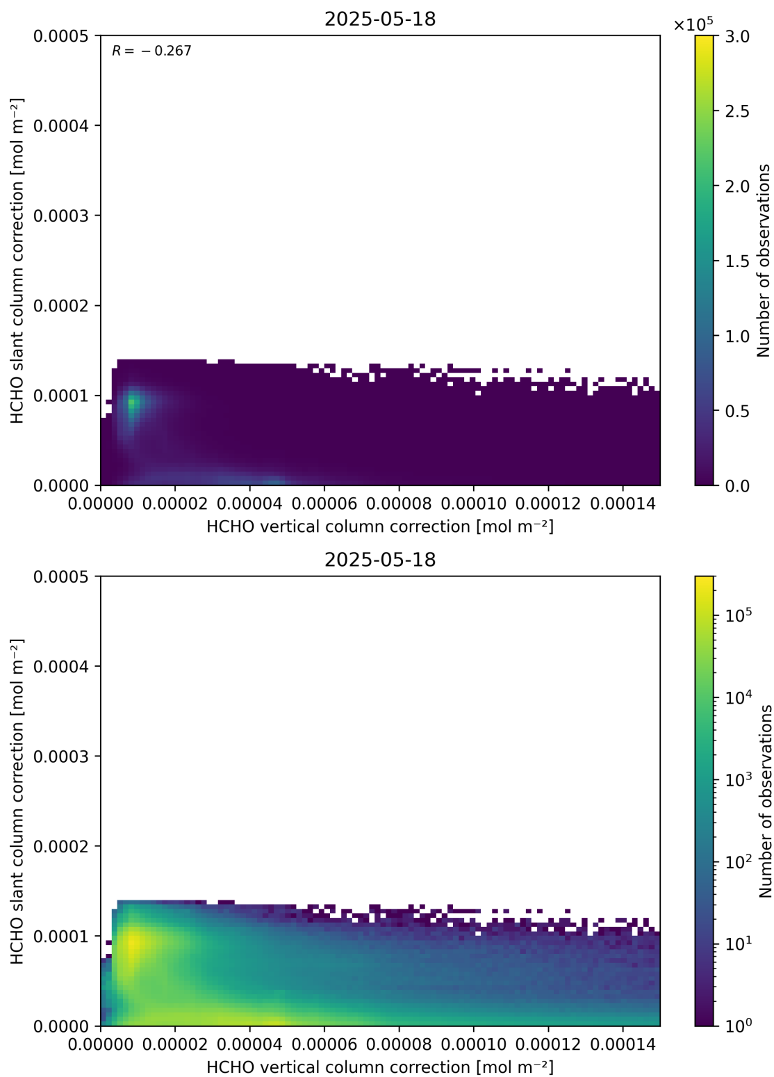
Figure 117: Scatter density plot of “HCHO vertical column correction” against “HCHO slant column correction” for 2025-05-17 to 2025-05-19.
