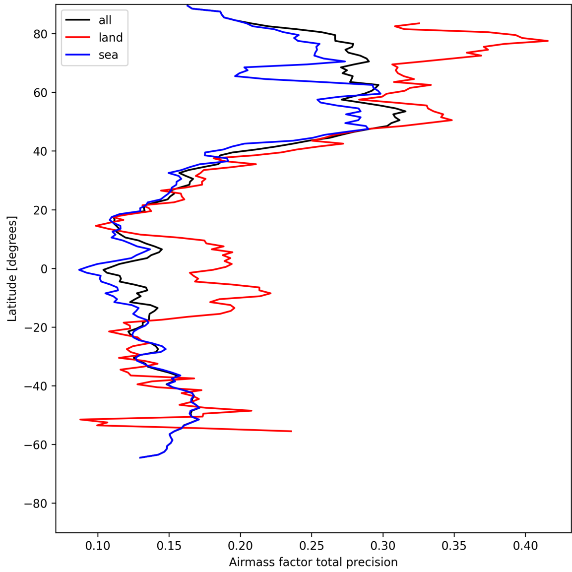
Figure 27: Zonal average of “Airmass factor total precision” for 2025-05-17 to 2025-05-19.
