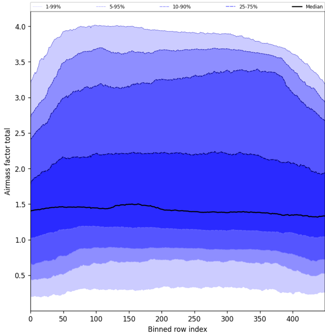
Figure 54: Along track statistics of “Airmass factor total” for 2025-05-17 to 2025-05-19
