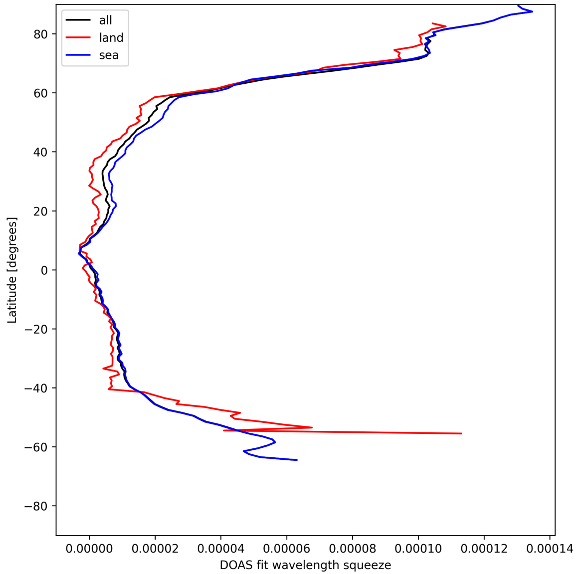
Figure 31: Zonal average of “DOAS fit wavelength squeeze” for 2025-05-17 to 2025-05-19.
