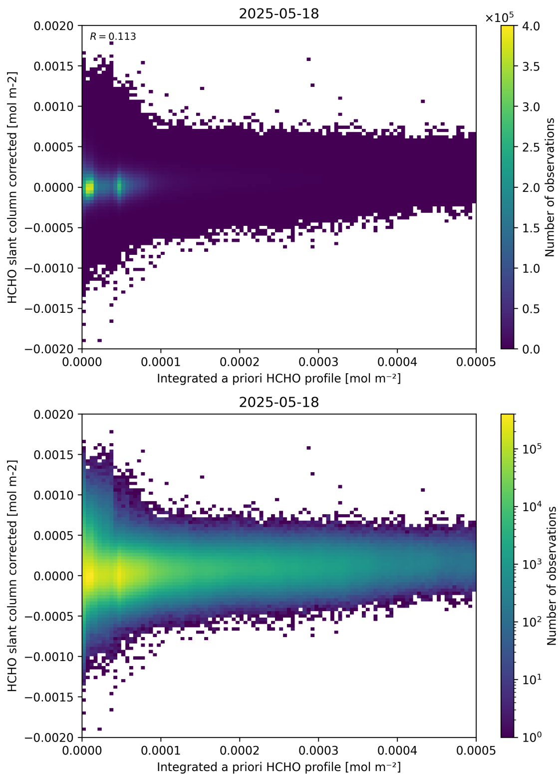
Figure 151: Scatter density plot of “Integrated a priori HCHO profile” against “HCHO slant column corrected” for 2025-05-17 to 2025-05-19.
