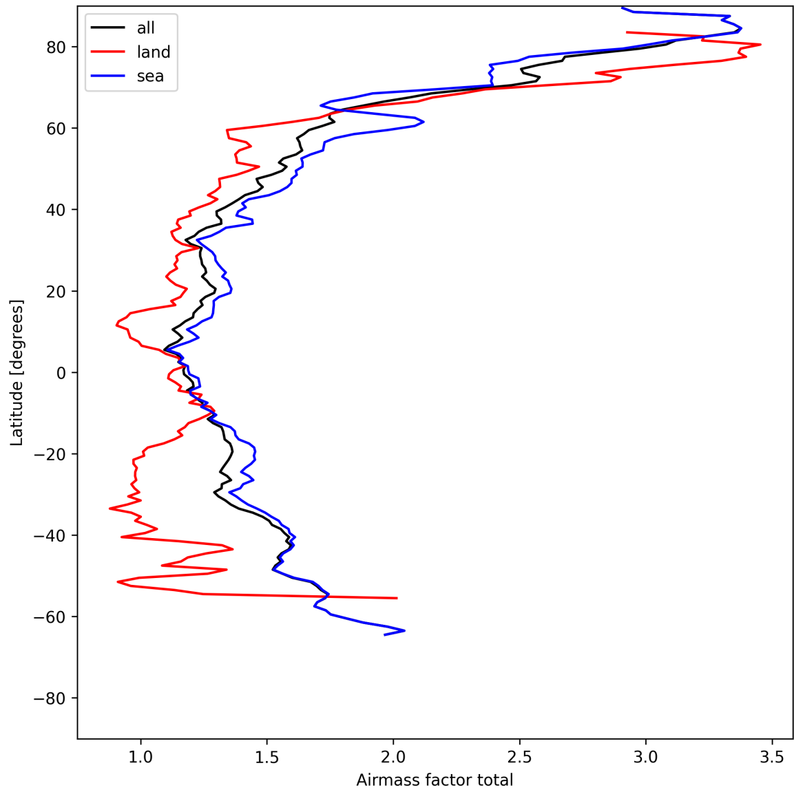
Figure 26: Zonal average of “Airmass factor total” for 2025-05-17 to 2025-05-19.
