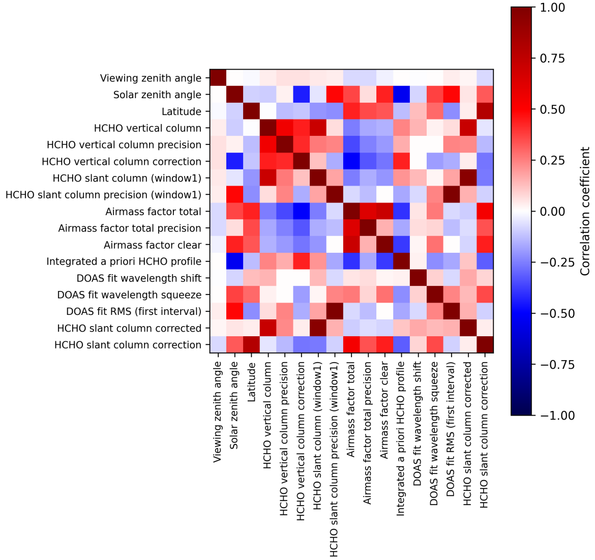
Figure 2: Map of correlation matrix for 2025-05-17 to 2025-05-19.
