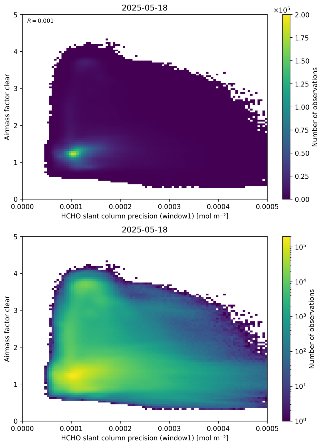
Figure 91: Scatter density plot of “HCHO slant column precision (window1)” against “Airmass factor clear” for 2025-05-17 to 2025-05-19.
