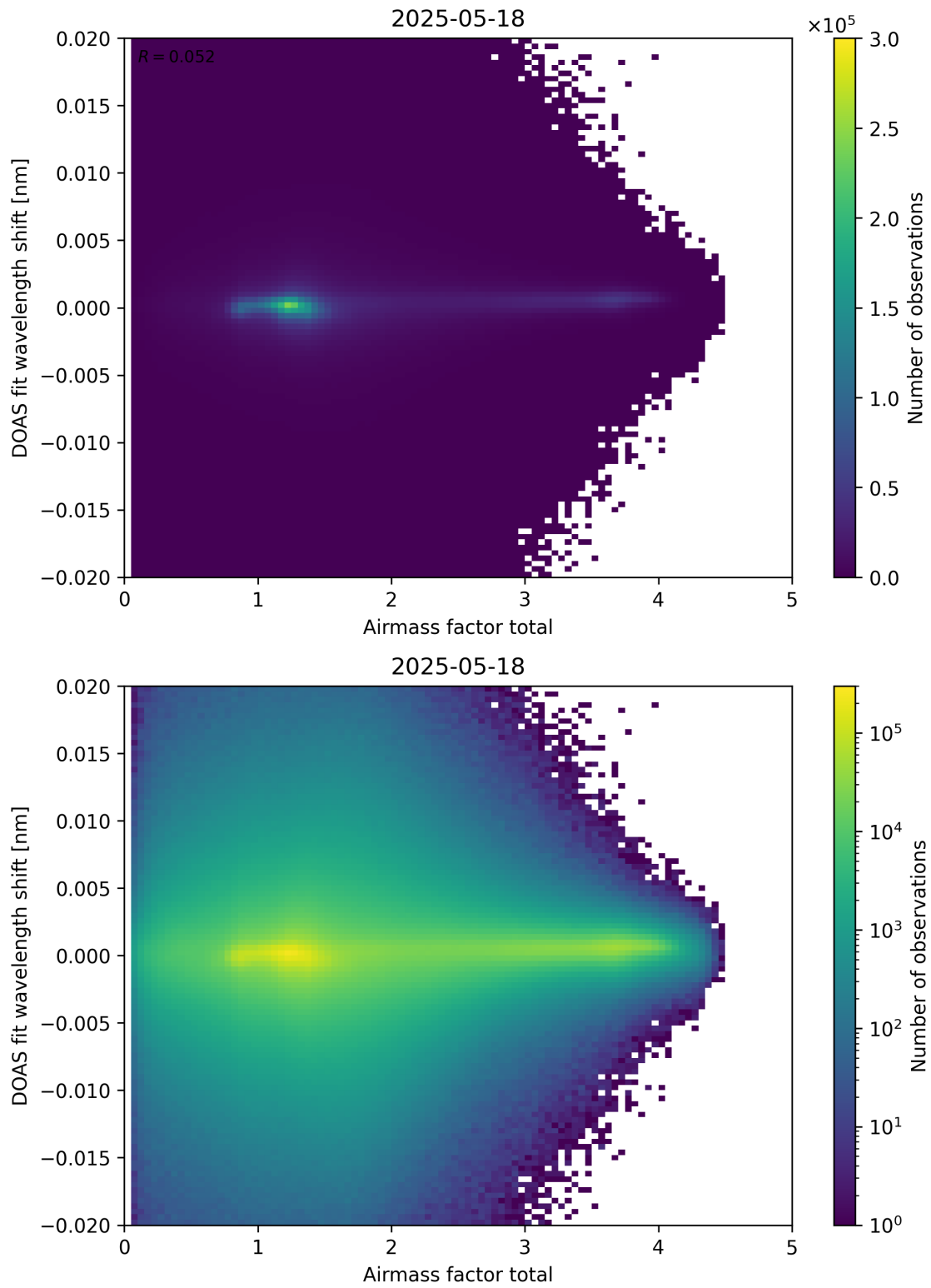
Figure 98: Scatter density plot of “Airmass factor total” against “DOAS fit wavelength shift” for 2025-05-17 to 2025-05-19.
