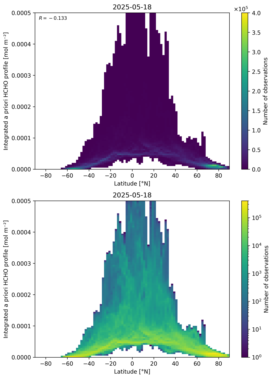
Figure 166: Scatter density plot of “Latitude” against “Integrated a priori HCHO profile” for 2025-05-17 to 2025-05-19.
