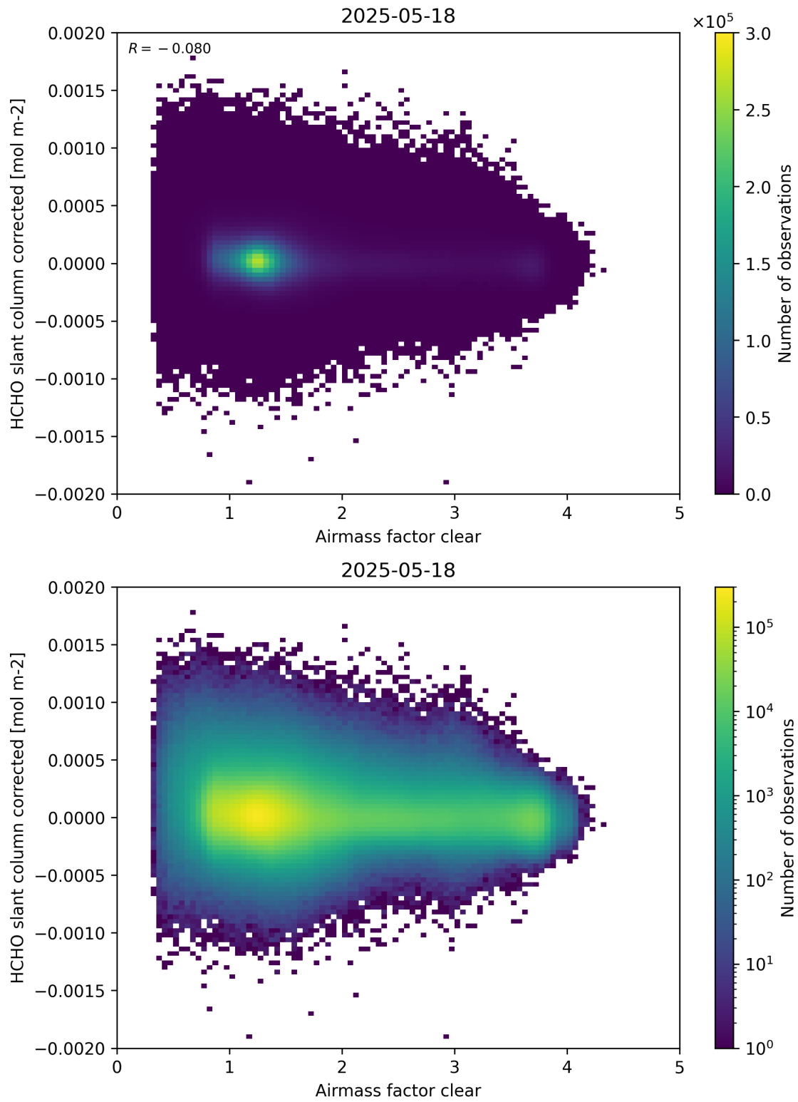
Figure 74: Scatter density plot of “Airmass factor clear” against “HCHO slant column corrected” for 2025-05-17 to 2025-05-19.
