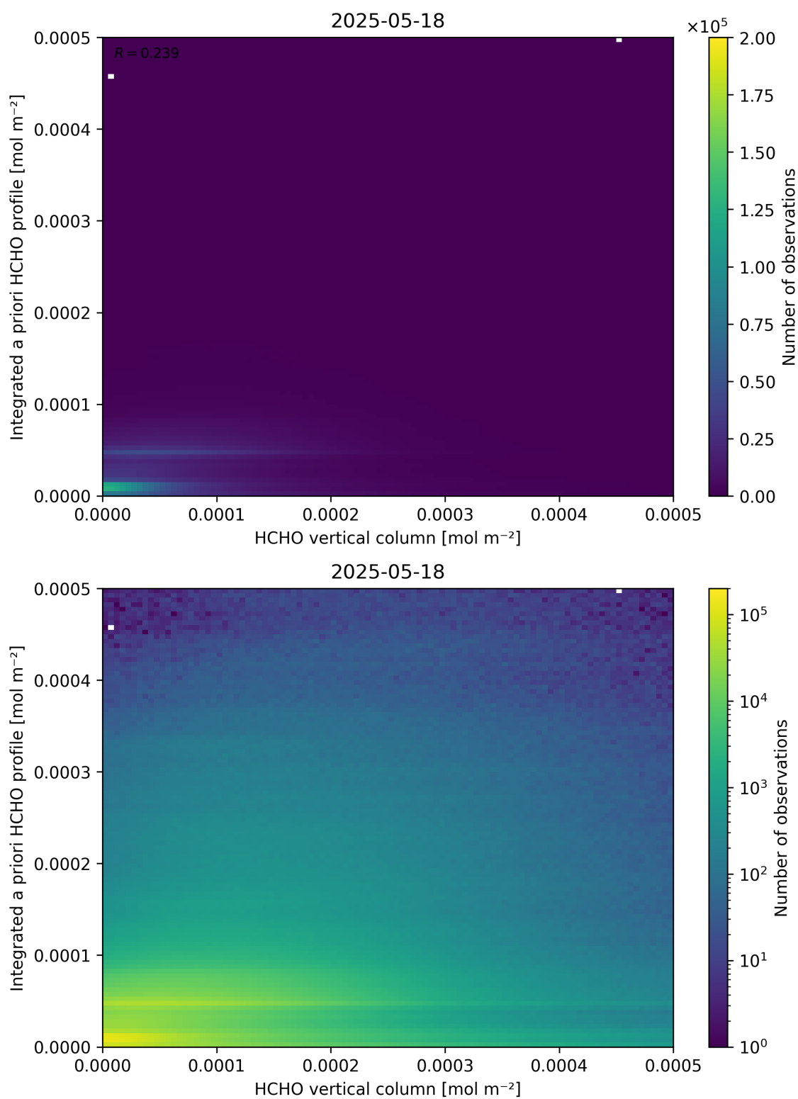
Figure 135: Scatter density plot of “HCHO vertical column” against “Integrated a priori HCHO profile” for 2025-05-17 to 2025-05-19.
