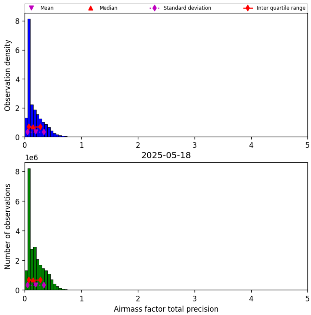
Figure 41: Histogram of “Airmass factor total precision” for 2025-05-17 to 2025-05-19
