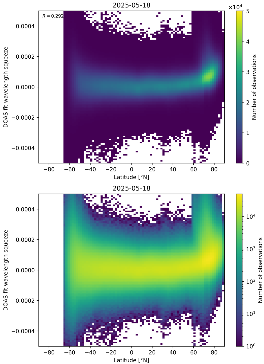
Figure 155: Scatter density plot of “Latitude” against “DOAS fit wavelength squeeze” for 2025-05-17 to 2025-05-19.
