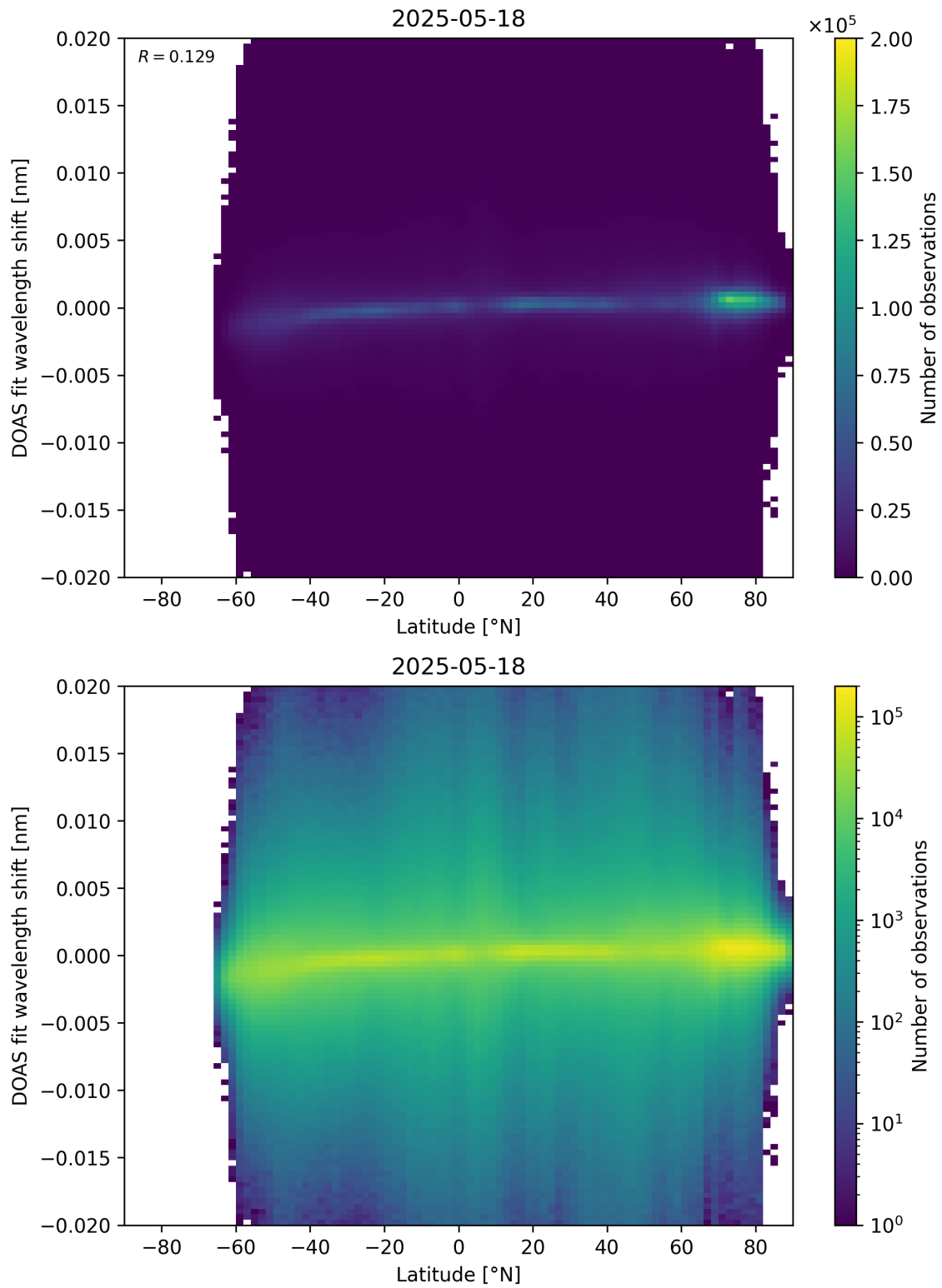
Figure 154: Scatter density plot of “Latitude” against “DOAS fit wavelength shift” for 2025-05-17 to 2025-05-19.
