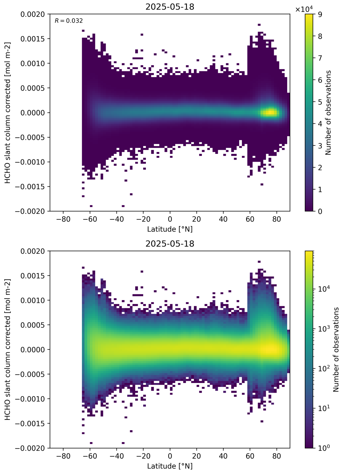
Figure 157: Scatter density plot of “Latitude” against “HCHO slant column corrected” for 2025-05-17 to 2025-05-19.
