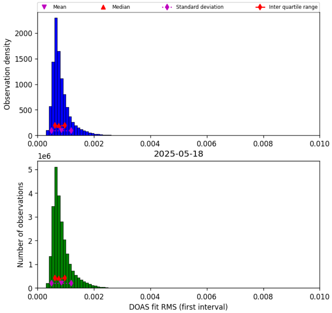
Figure 46: Histogram of “DOAS fit RMS (first interval)” for 2025-05-17 to 2025-05-19
