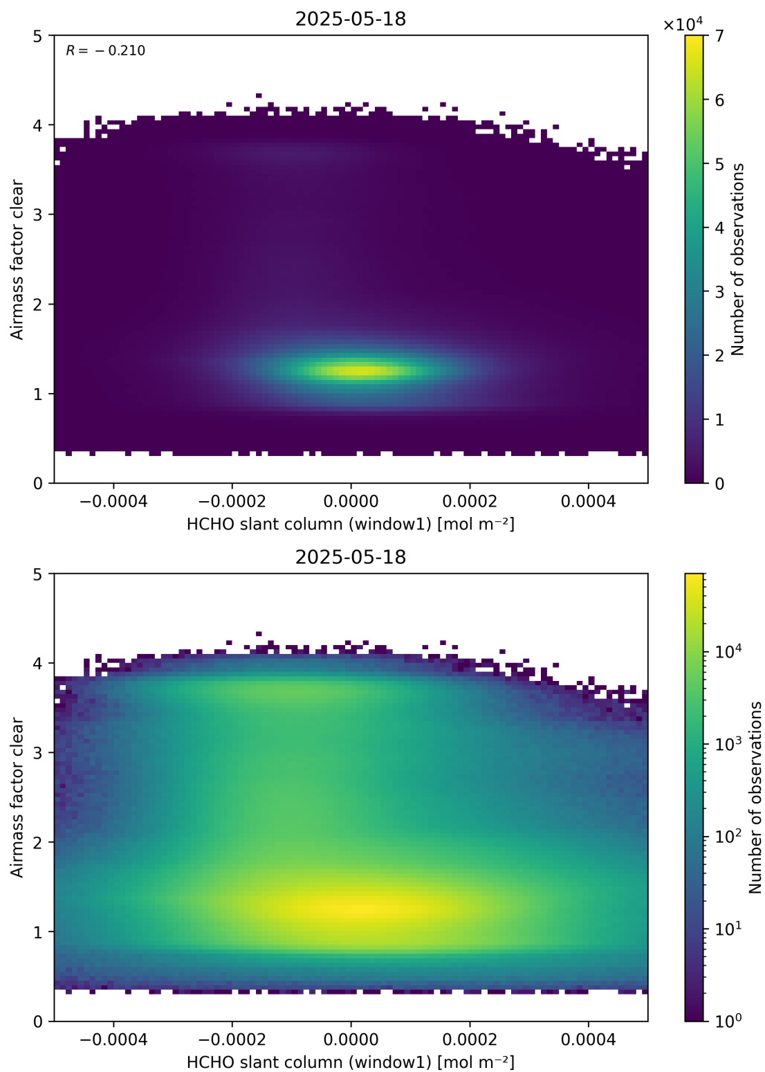
Figure 81: Scatter density plot of “HCHO slant column (window1)” against “Airmass factor clear” for 2025-05-17 to 2025-05-19.
