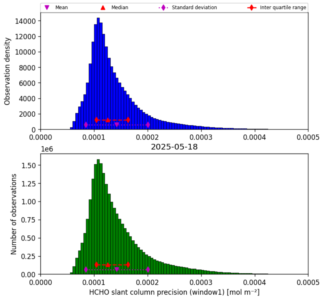
Figure 39: Histogram of “HCHO slant column precision (window1)” for 2025-05-17 to 2025-05-19
