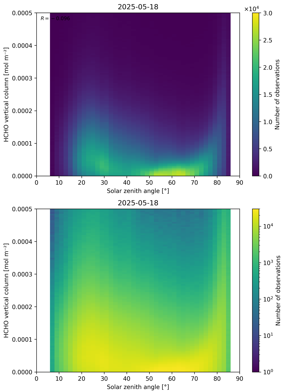
Figure 177: Scatter density plot of “Solar zenith angle” against “HCHO vertical column” for 2025-05-17 to 2025-05-19.
