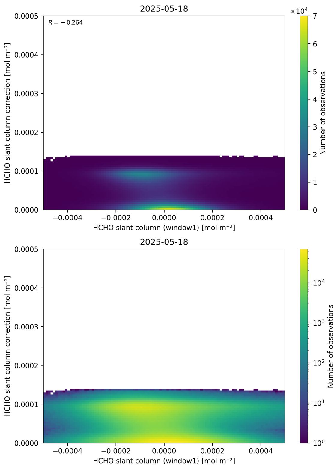
Figure 83: Scatter density plot of “HCHO slant column (window1)” against “HCHO slant column correction” for 2025-05-17 to 2025-05-19.
