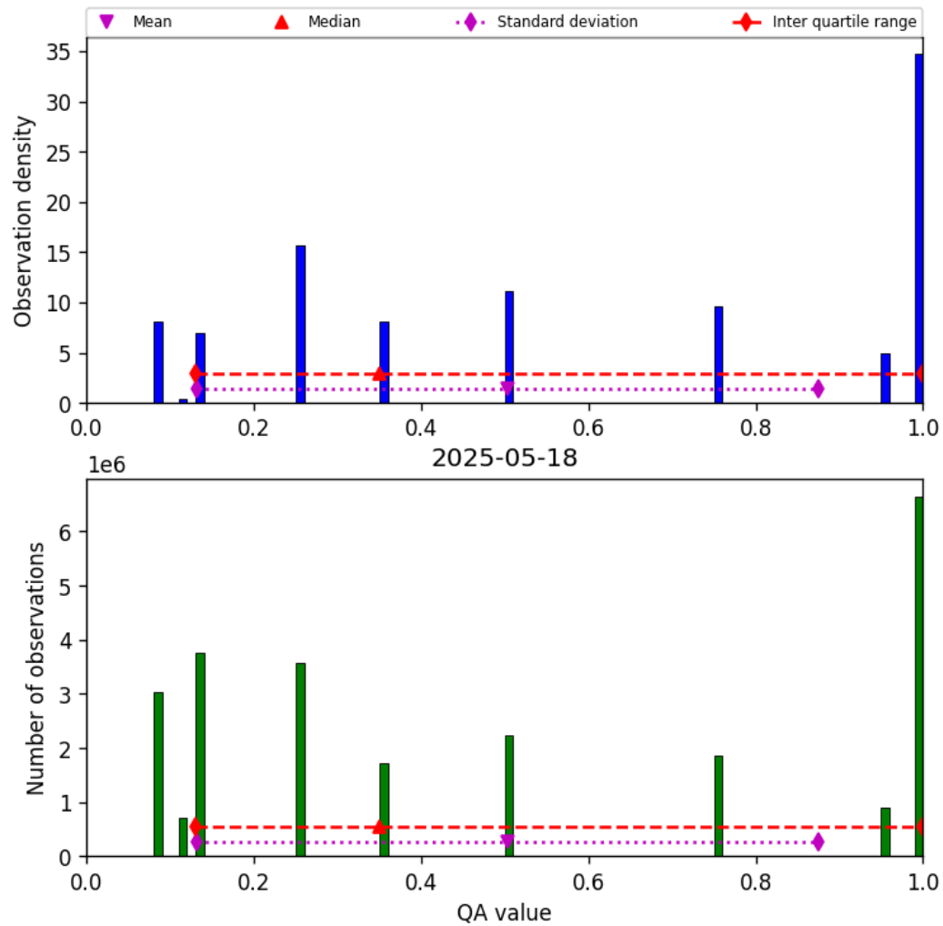
Figure 34: Histogram of “QA value” for 2025-05-17 to 2025-05-19
