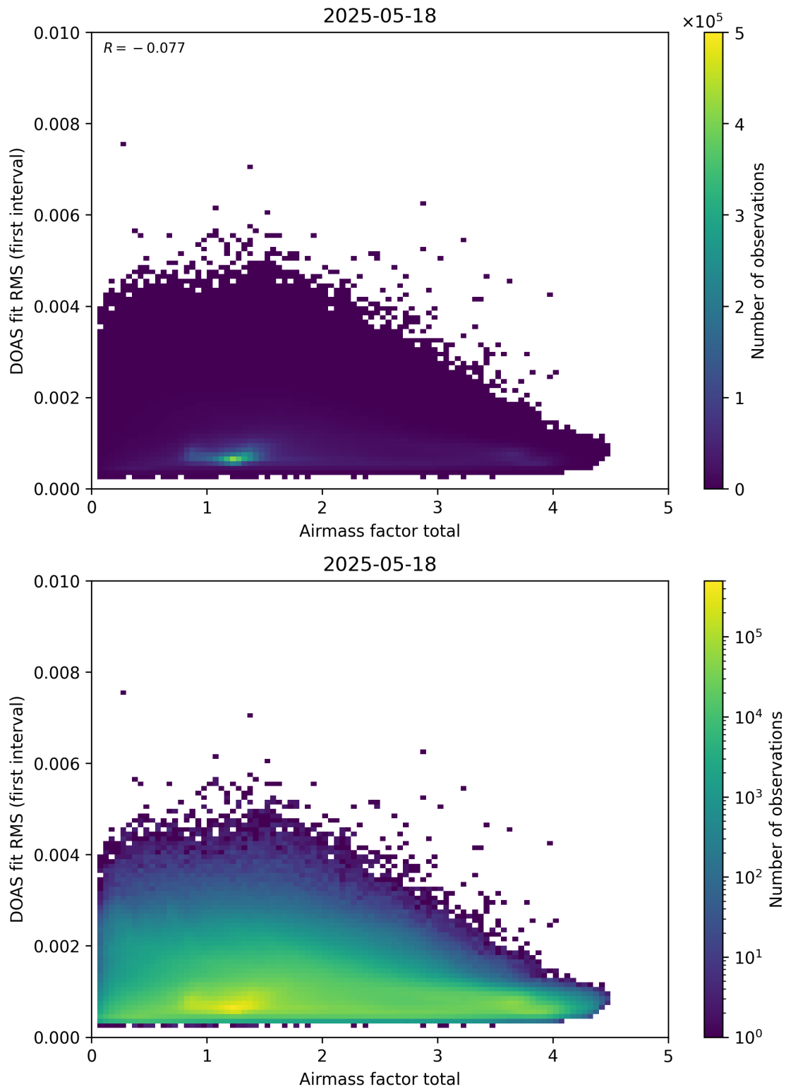
Figure 97: Scatter density plot of “Airmass factor total” against “DOAS fit RMS (first interval)” for 2025-05-17 to 2025-05-19.
