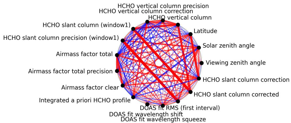
Figure 1: Map of correlation graph for 2025-05-17 to 2025-05-19.
