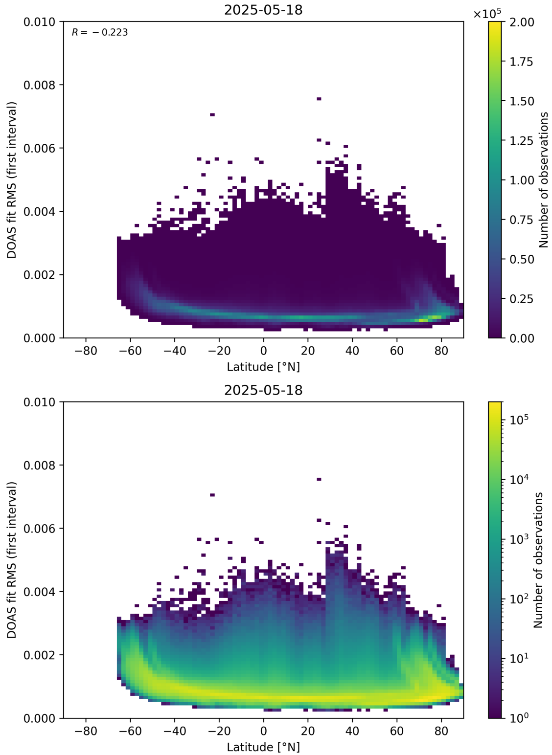
Figure 153: Scatter density plot of “Latitude” against “DOAS fit RMS (first interval)” for 2025-05-17 to 2025-05-19.
