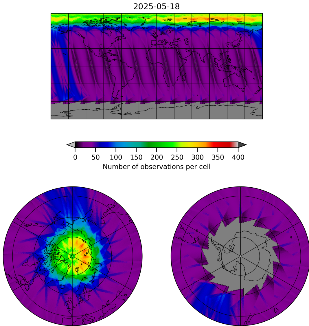
Figure 19: Map of the number of observations for 2025-05-17 to 2025-05-19
