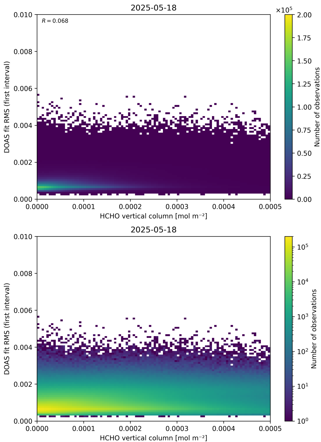
Figure 123: Scatter density plot of “HCHO vertical column” against “DOAS fit RMS (first interval)” for 2025-05-17 to 2025-05-19.
