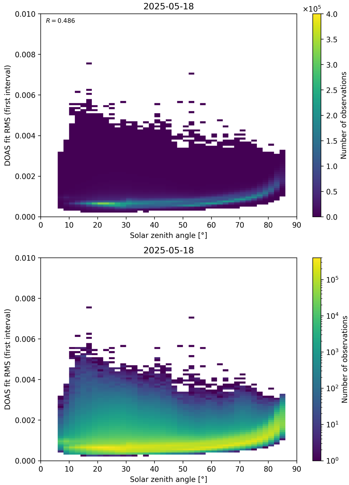
Figure 167: Scatter density plot of “Solar zenith angle” against “DOAS fit RMS (first interval)” for 2025-05-17 to 2025-05-19.
