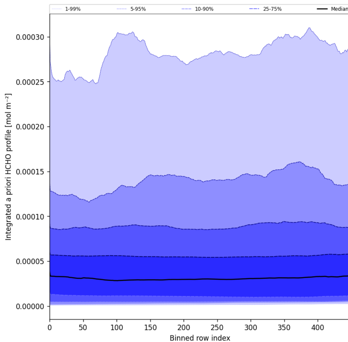
Figure 57: Along track statistics of “Integrated a priori HCHO profile” for 2025-05-17 to 2025-05-19
