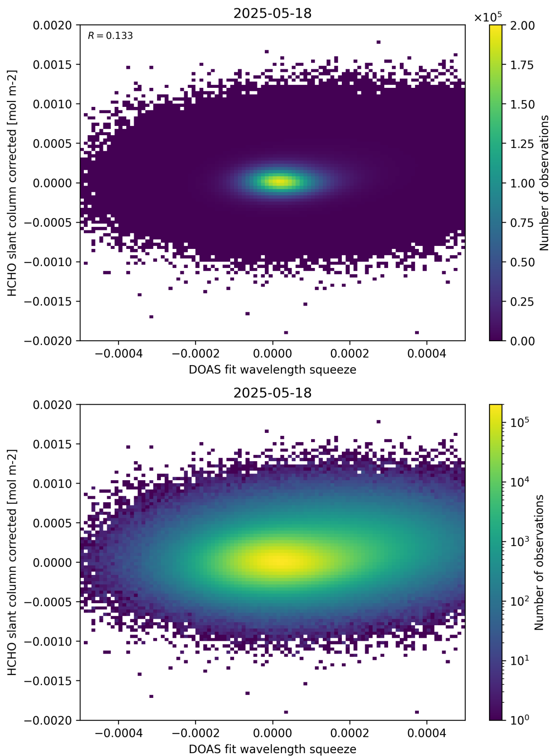
Figure 69: Scatter density plot of “DOAS fit wavelength squeeze” against “HCHO slant column corrected” for 2025-05-17 to 2025-05-19.
