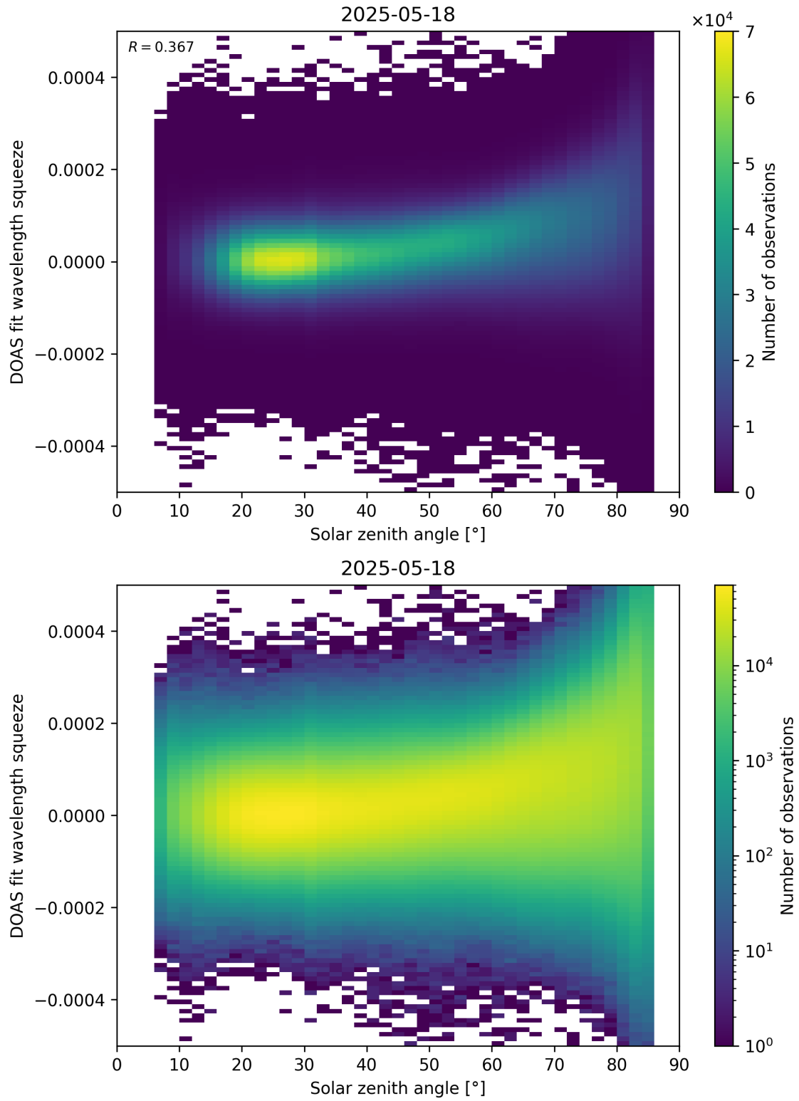
Figure 169: Scatter density plot of “Solar zenith angle” against “DOAS fit wavelength squeeze” for 2025-05-17 to 2025-05-19.
