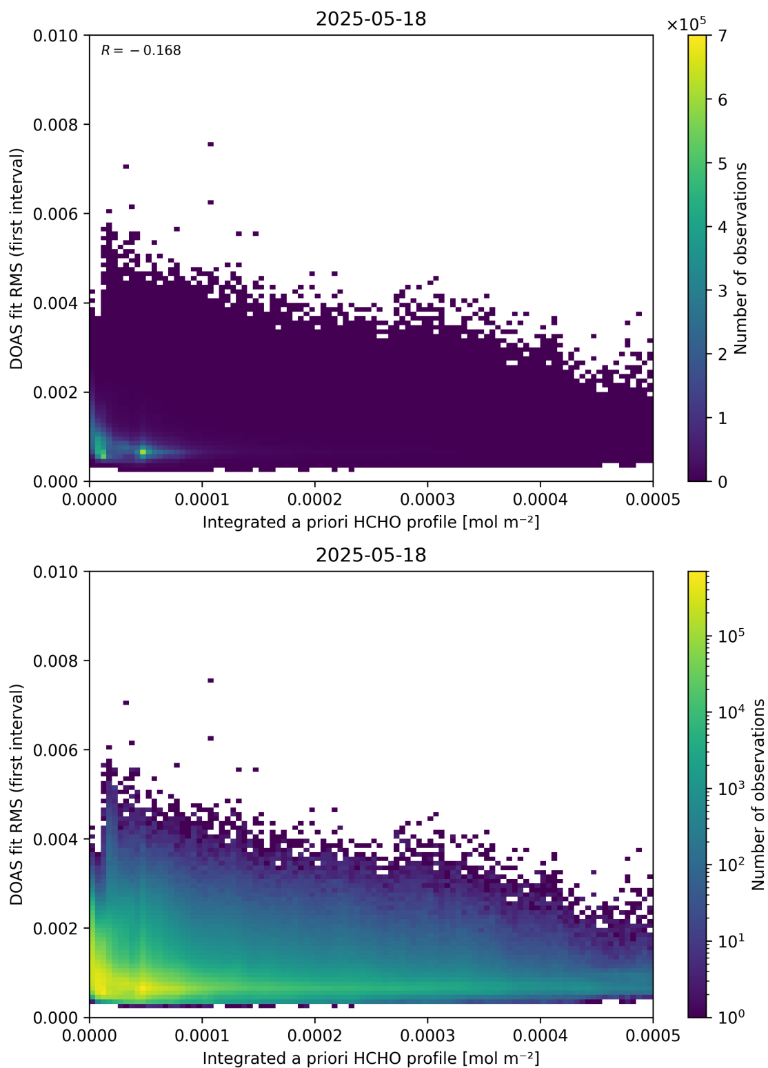
Figure 148: Scatter density plot of “Integrated a priori HCHO profile” against “DOAS fit RMS (first interval)” for 2025-05-17 to 2025-05-19.
