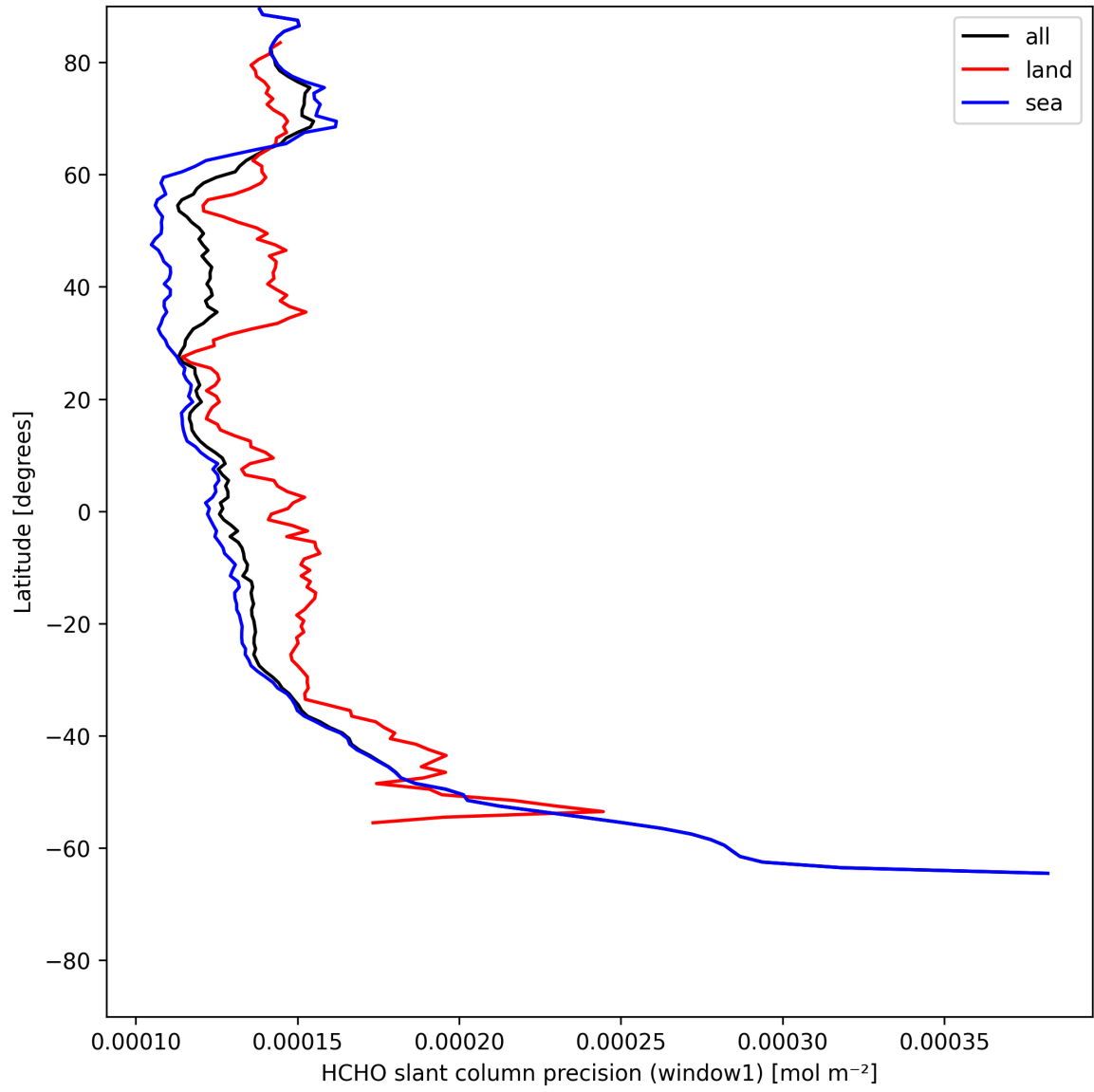
Figure 25: Zonal average of "HCHO slant column precision (window1)" for 2025-05-17 to 2025-05-19.
