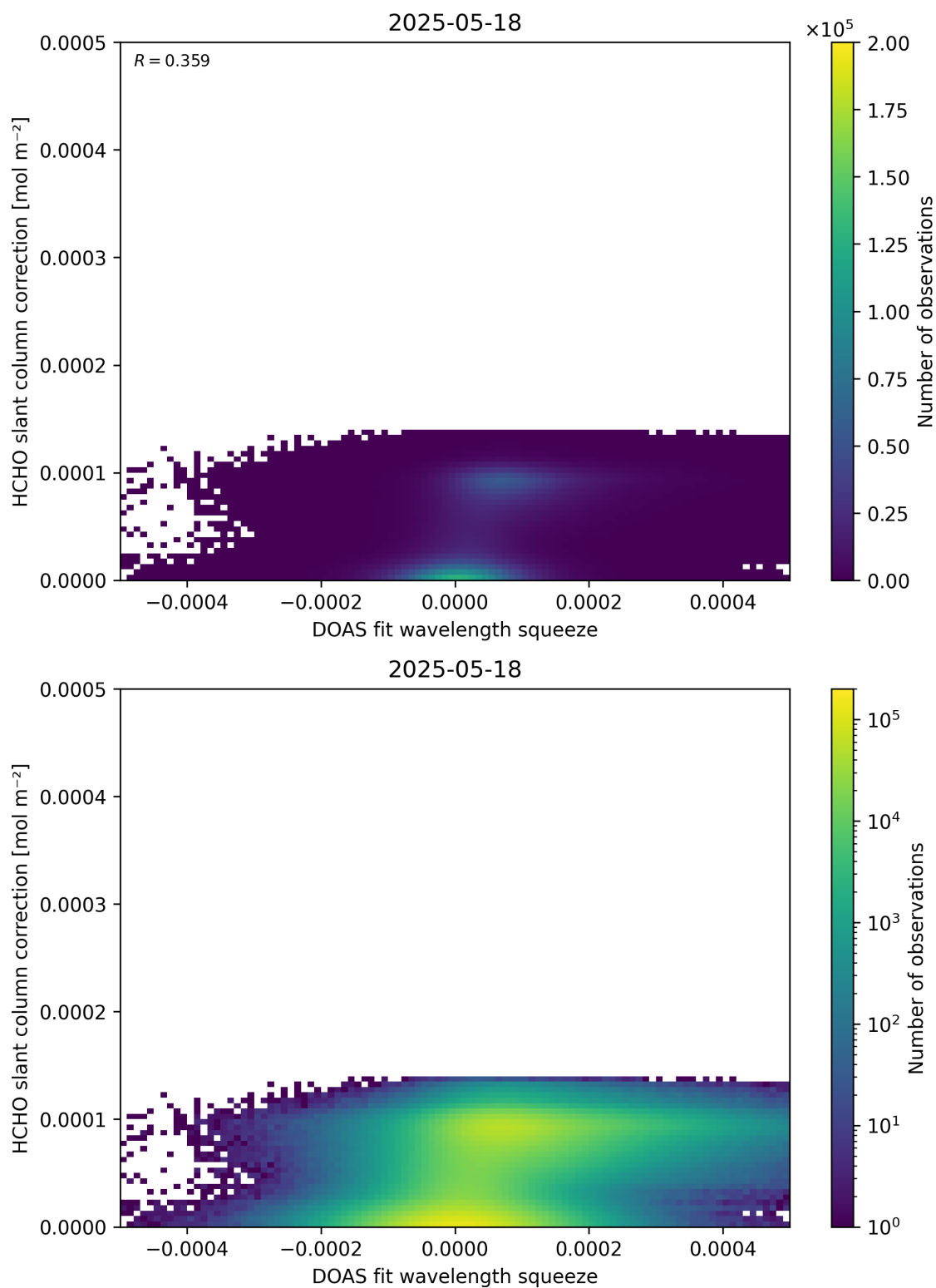
Figure 70: Scatter density plot of “DOAS fit wavelength squeeze” against “HCHO slant column correction” for 2025-05-17 to 2025-05-19.
