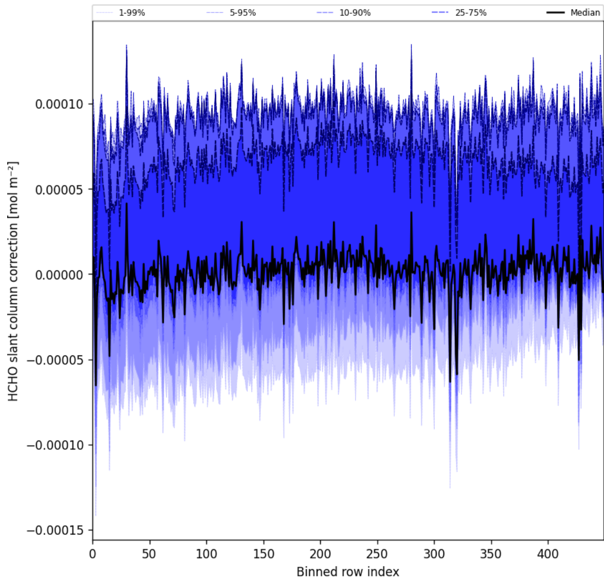
Figure 61: Along track statistics of “HCHO slant column correction” for 2025-05-17 to 2025-05-19
