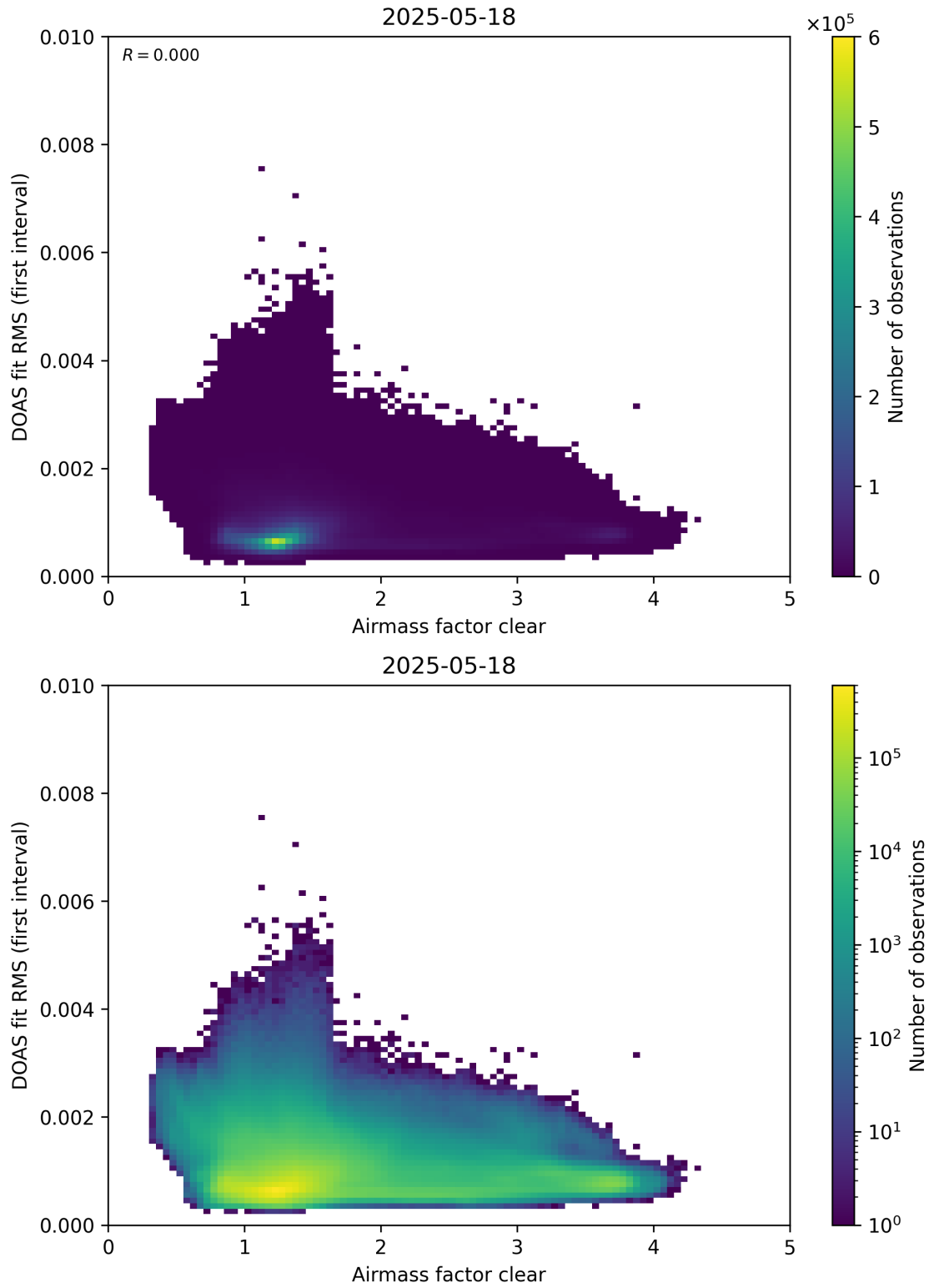
Figure 71: Scatter density plot of “Airmass factor clear” against “DOAS fit RMS (first interval)” for 2025-05-17 to 2025-05-19.
