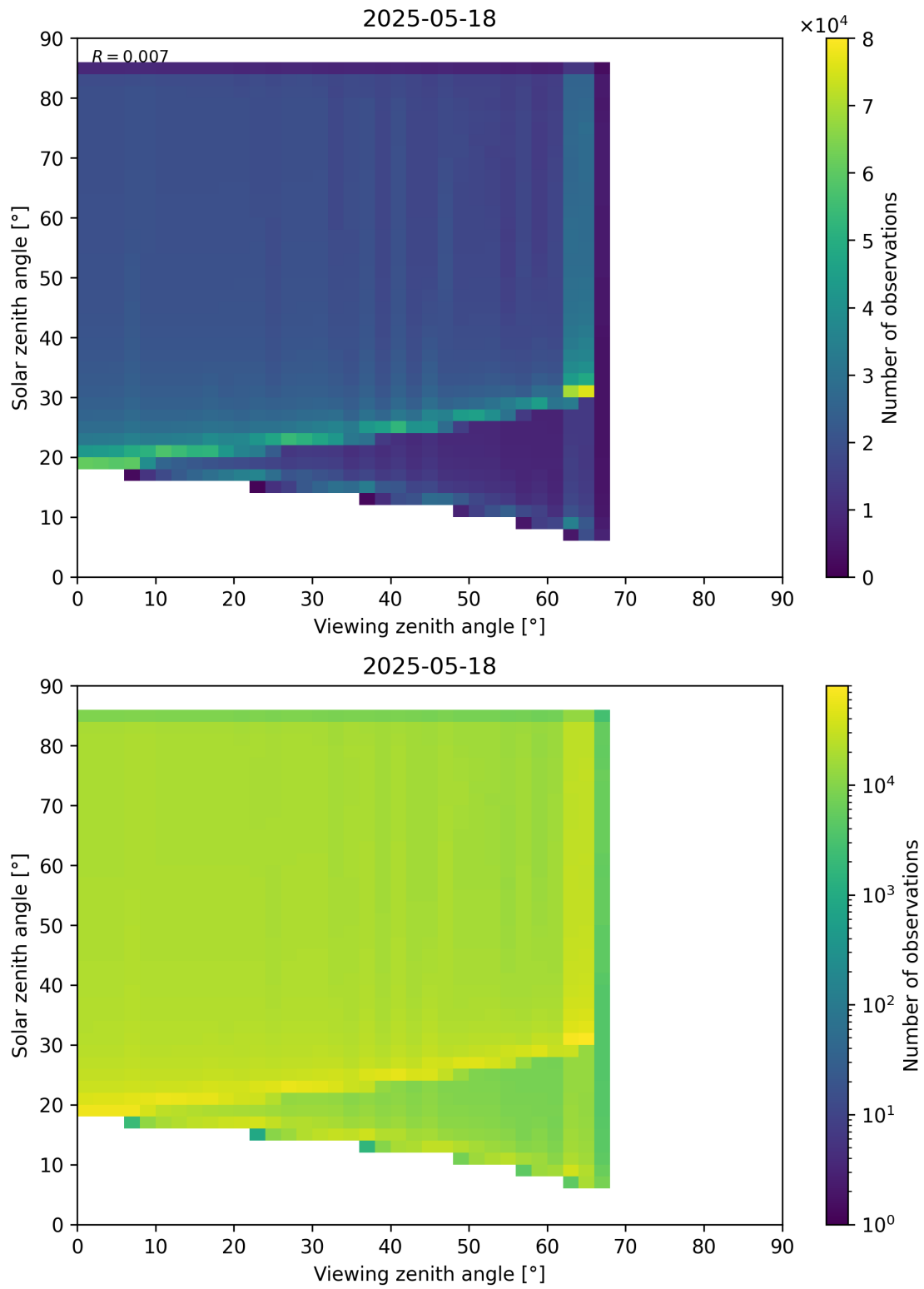
Figure 197: Scatter density plot of “Viewing zenith angle” against “Solar zenith angle” for 2025-05-17 to 2025-05-19.
