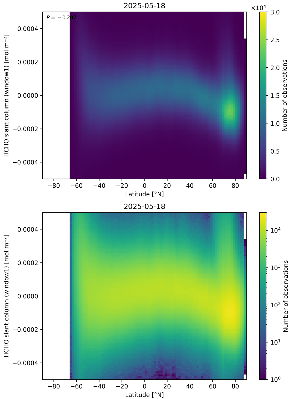
Figure 159: Scatter density plot of “Latitude” against “HCHO slant column (window1)” for 2025-05-17 to 2025-05-19.
