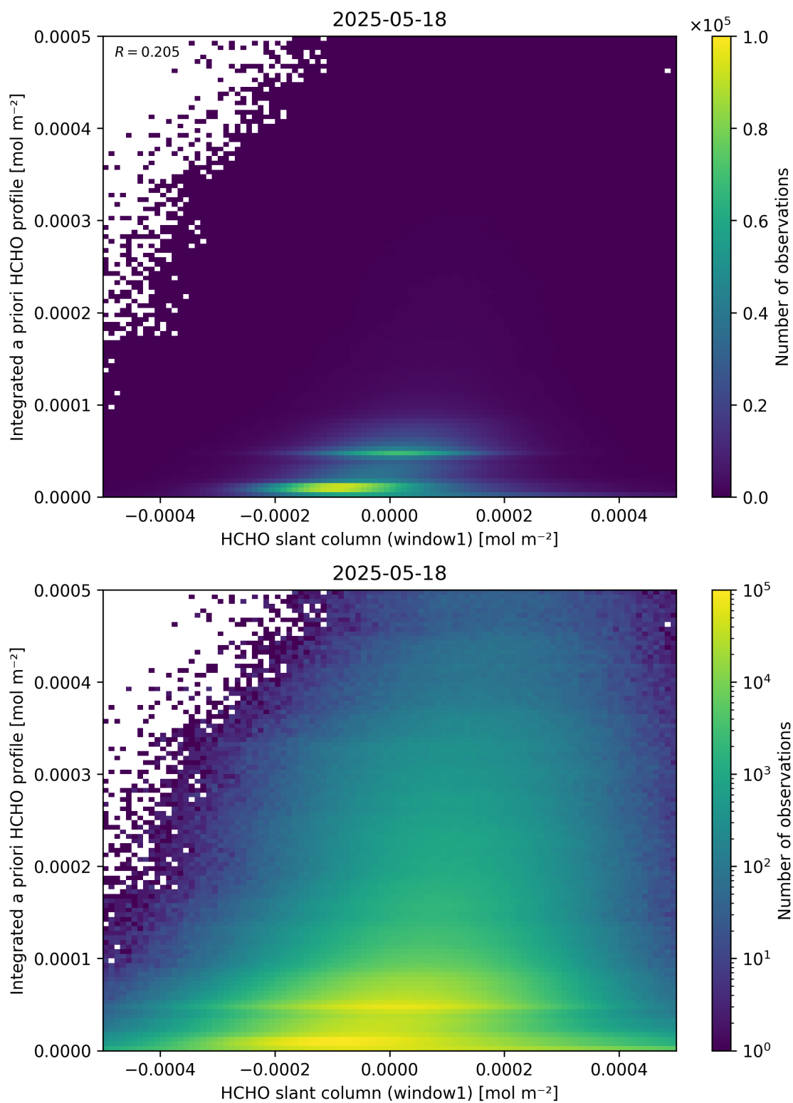
Figure 87: Scatter density plot of “HCHO slant column (window1)” against “Integrated a priori HCHO profile” for 2025-05-17 to 2025-05-19.
