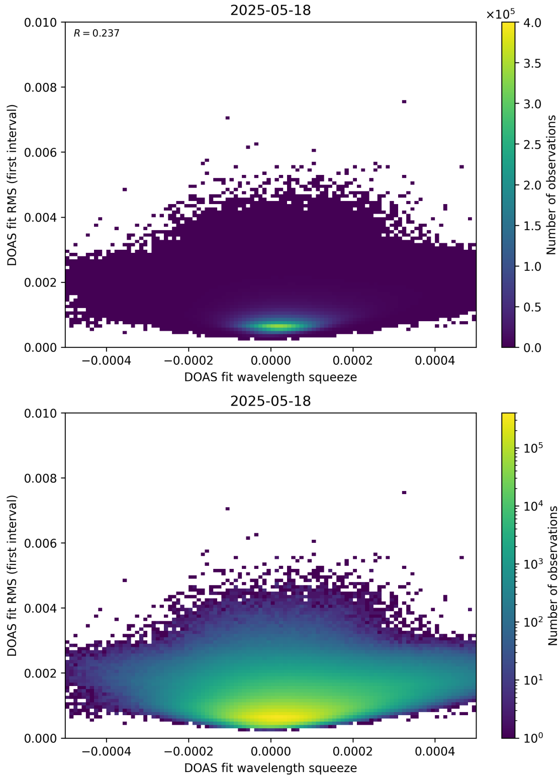
Figure 68: Scatter density plot of “DOAS fit wavelength squeeze” against “DOAS fit RMS (first interval)” for 2025-05-17 to 2025-05-19.
