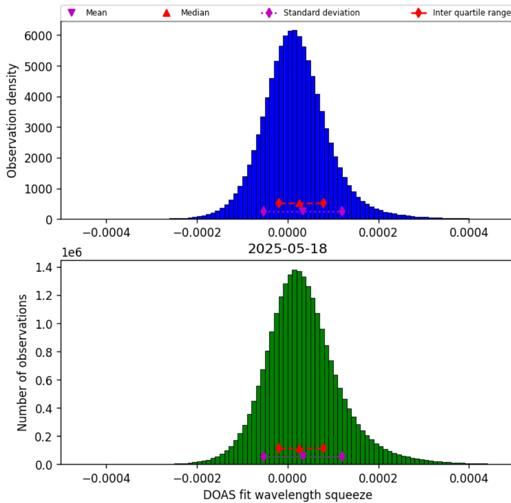
Figure 45: Histogram of “DOAS fit wavelength squeeze” for 2025-05-17 to 2025-05-19
