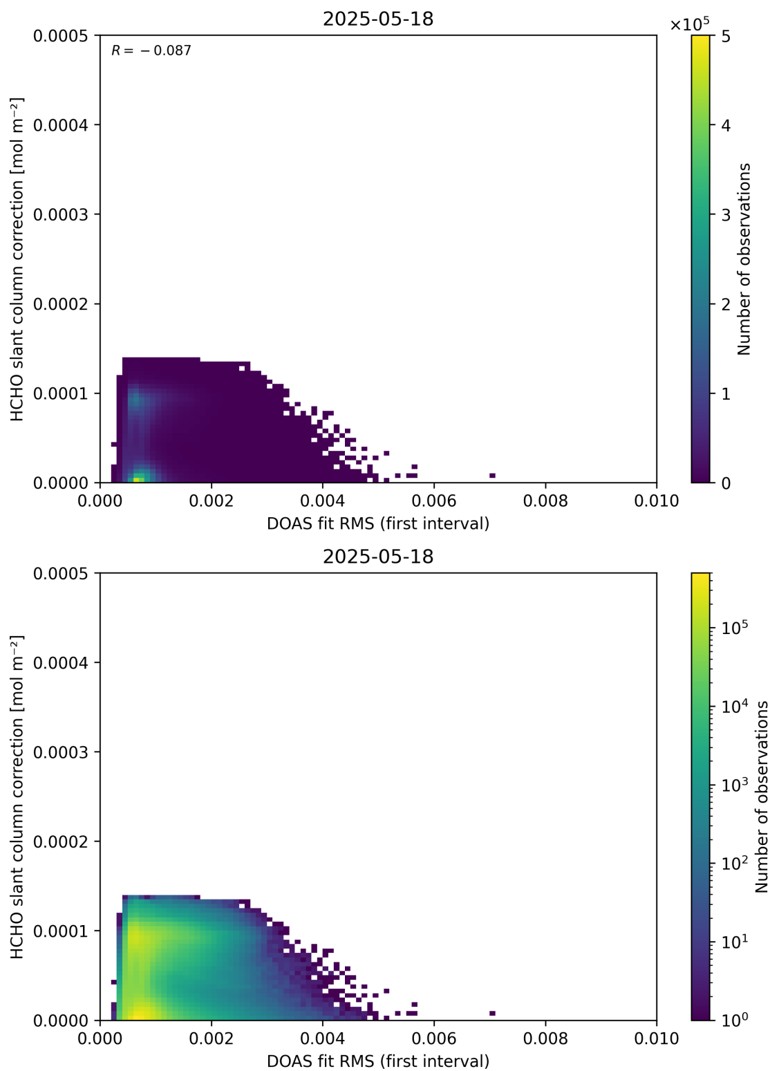
Figure 63: Scatter density plot of “DOAS fit RMS (first interval)” against “HCHO slant column correction” for 2025-05-17 to 2025-05-19.
