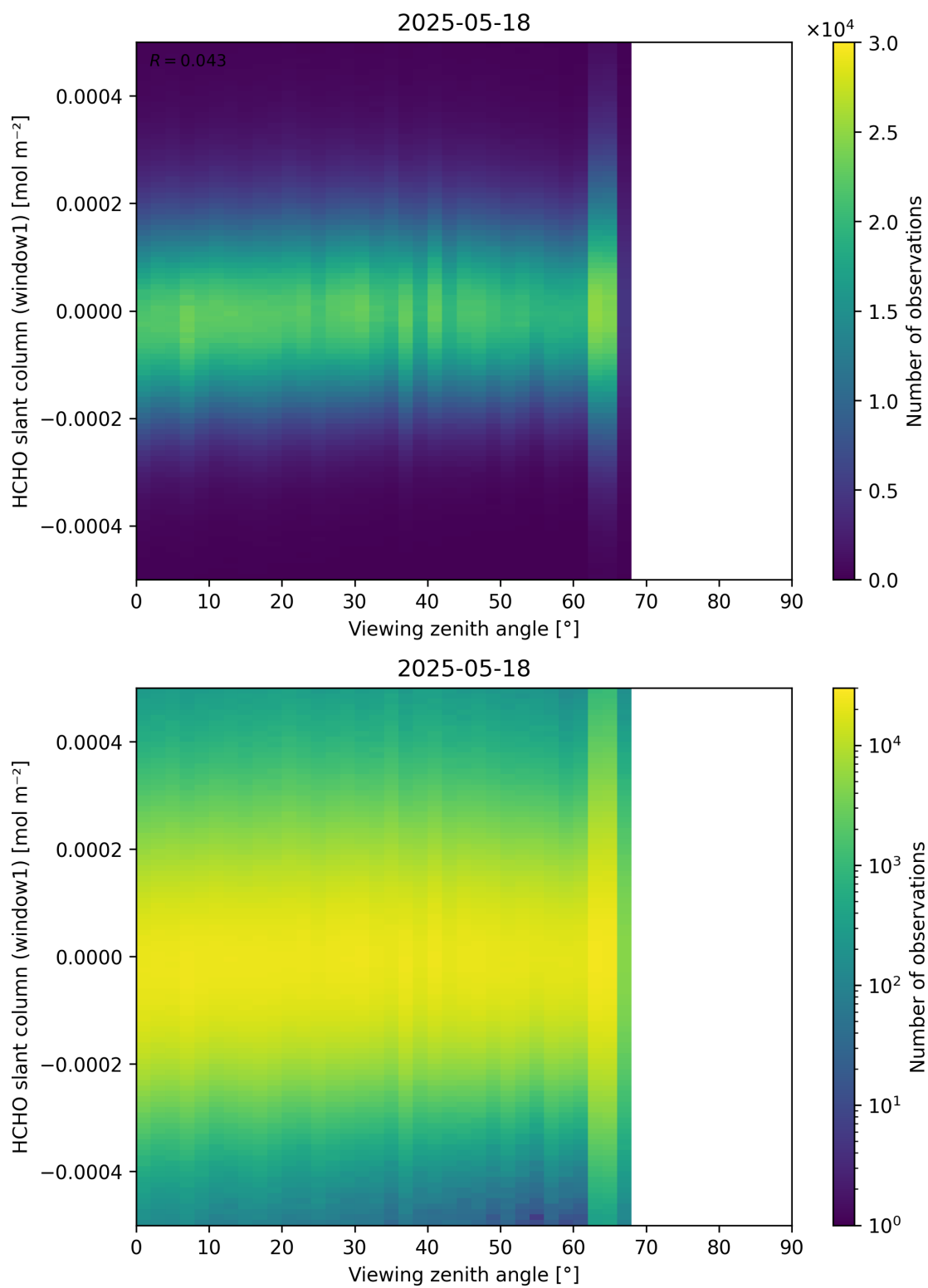
Figure 188: Scatter density plot of “Viewing zenith angle” against “HCHO slant column (window1)” for 2025-05-17 to 2025-05-19.
