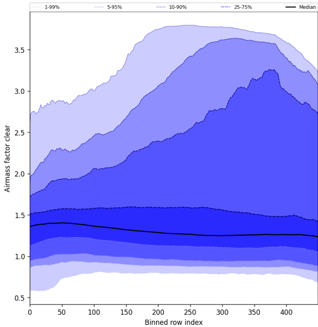
Figure 56: Along track statistics of “Airmass factor clear” for 2025-05-17 to 2025-05-19
