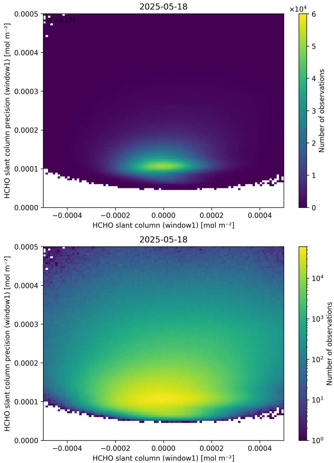
Figure 84: Scatter density plot of “HCHO slant column (window1)” against “HCHO slant column precision (window1)” for 2025-05-17 to 2025-05-19.
