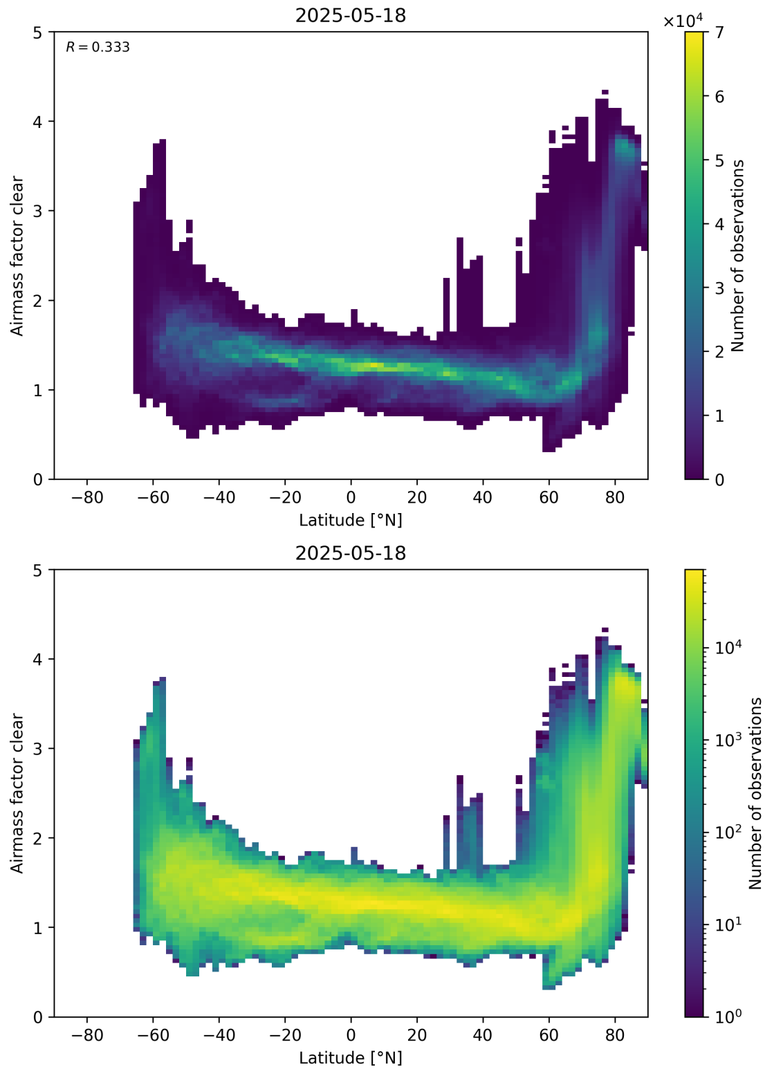
Figure 156: Scatter density plot of “Latitude” against “Airmass factor clear” for 2025-05-17 to 2025-05-19.
