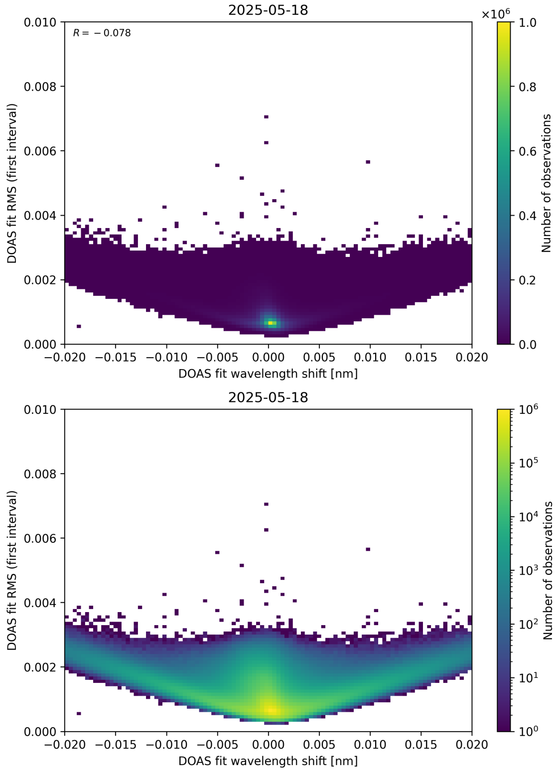
Figure 64: Scatter density plot of “DOAS fit wavelength shift” against “DOAS fit RMS (first interval)” for 2025-05-17 to 2025-05-19.
