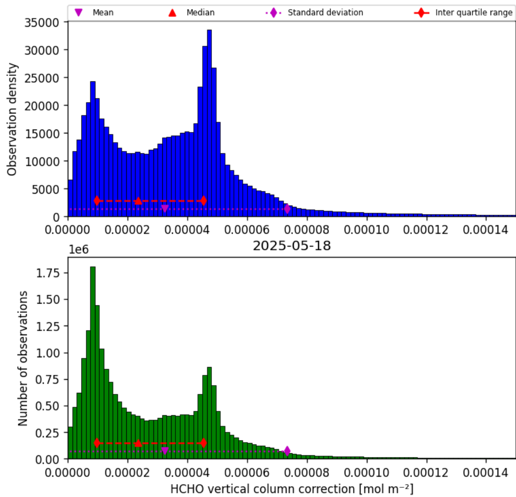
Figure 37: Histogram of “HCHO vertical column correction” for 2025-05-17 to 2025-05-19
