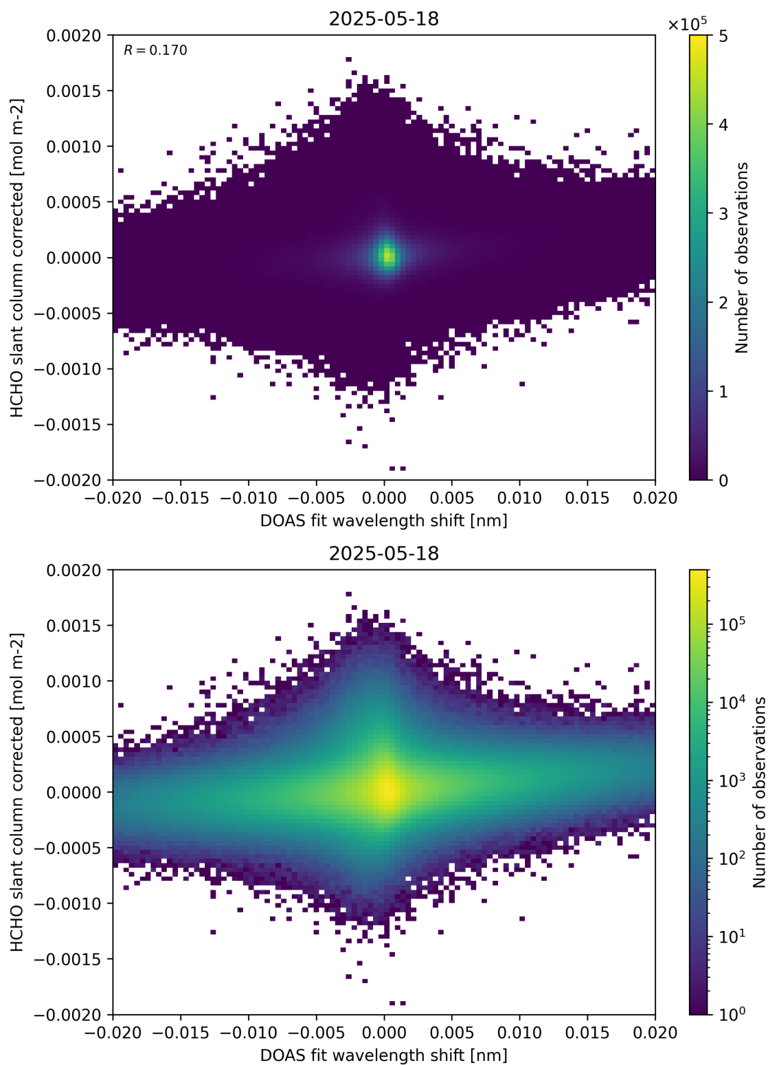
Figure 66: Scatter density plot of “DOAS fit wavelength shift” against “HCHO slant column corrected” for 2025-05-17 to 2025-05-19.
