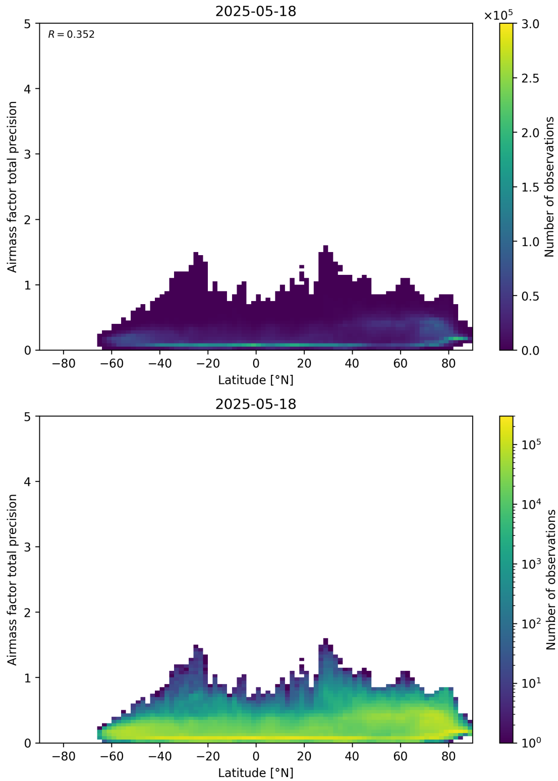
Figure 162: Scatter density plot of “Latitude” against “Airmass factor total precision” for 2025-05-17 to 2025-05-19.
