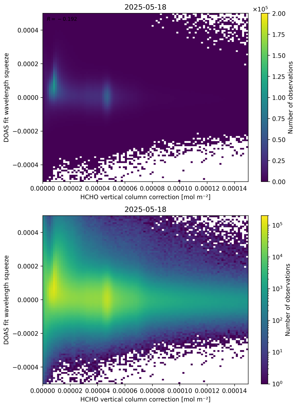
Figure 114: Scatter density plot of “HCHO vertical column correction” against “DOAS fit wavelength squeeze” for 2025-05-17 to 2025-05-19.
