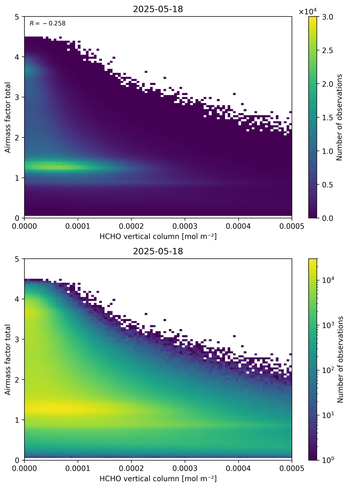
Figure 131: Scatter density plot of “HCHO vertical column” against “Airmass factor total” for 2025-05-17 to 2025-05-19.
