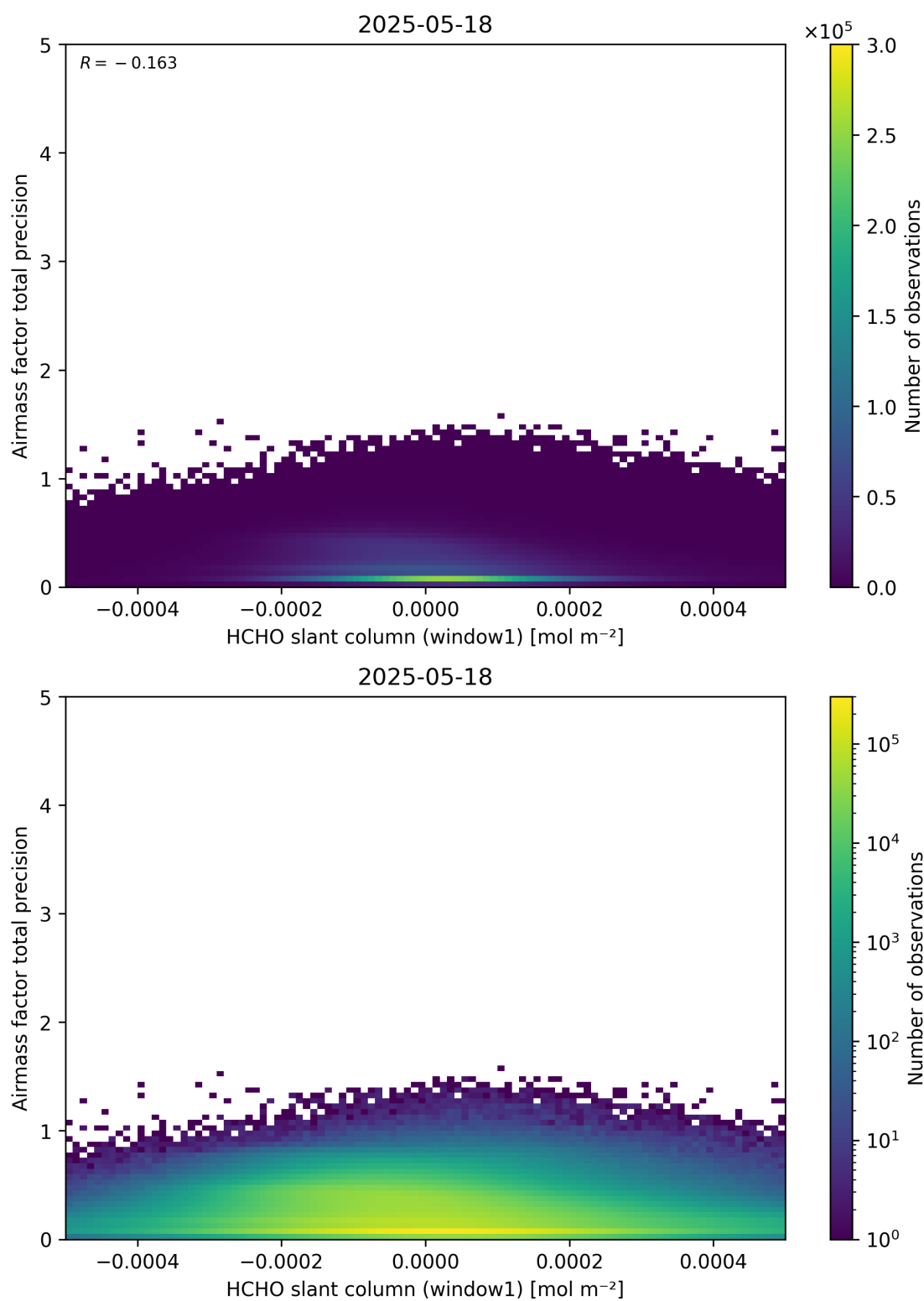
Figure 86: Scatter density plot of “HCHO slant column (window1)” against “Airmass factor total precision” for 2025-05-17 to 2025-05-19.
