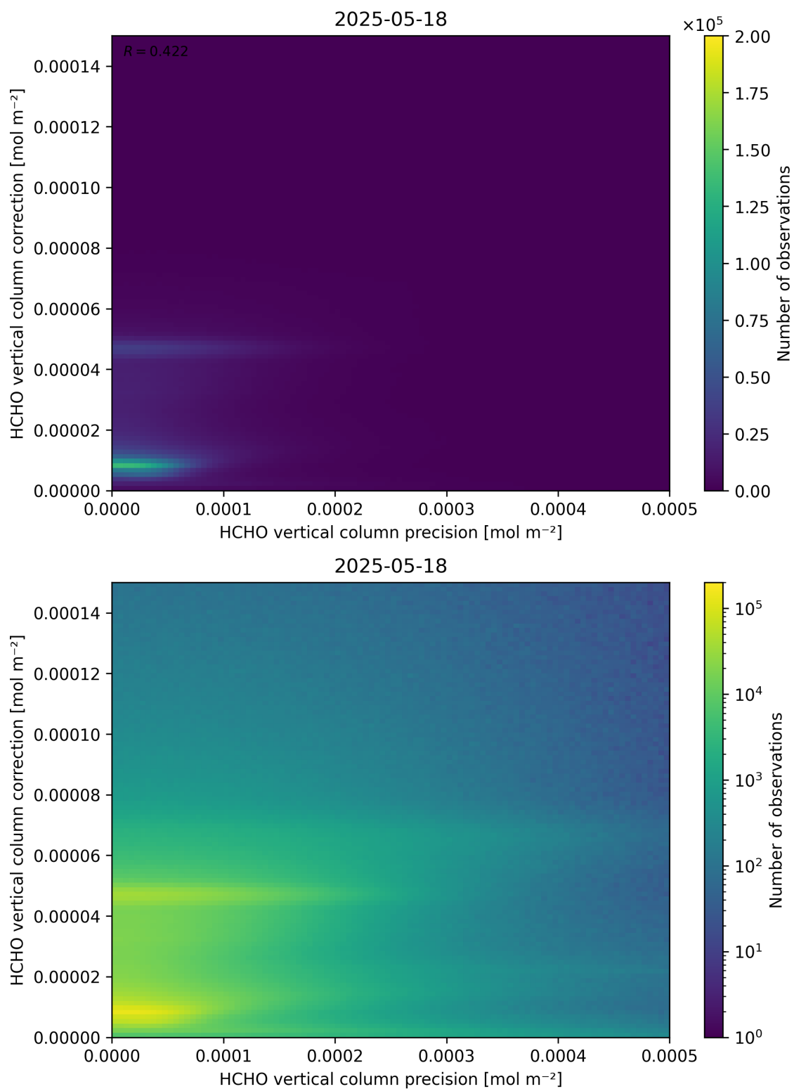
Figure 146: Scatter density plot of “HCHO vertical column precision” against “HCHO vertical column correction” for 2025-05-17 to 2025-05-19.
