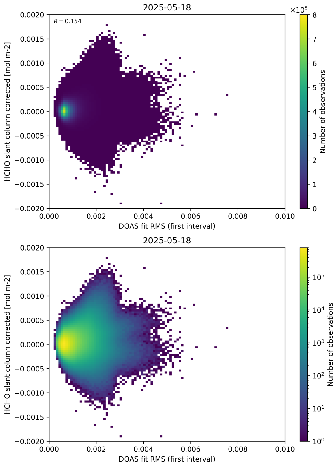
Figure 62: Scatter density plot of “DOAS fit RMS (first interval)” against “HCHO slant column corrected” for 2025-05-17 to 2025-05-19.
