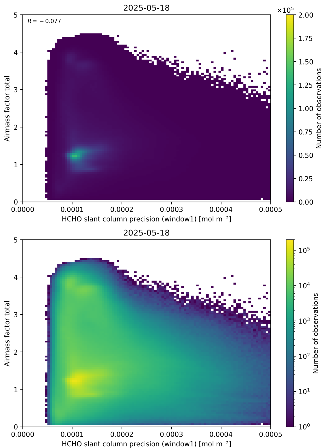
Figure 94: Scatter density plot of “HCHO slant column precision (window1)” against “Airmass factor total” for 2025-05-17 to 2025-05-19.
