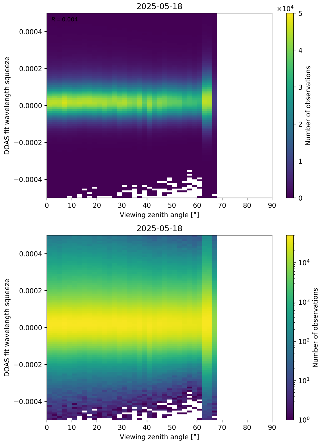
Figure 184: Scatter density plot of “Viewing zenith angle” against “DOAS fit wavelength squeeze” for 2025-05-17 to 2025-05-19.
