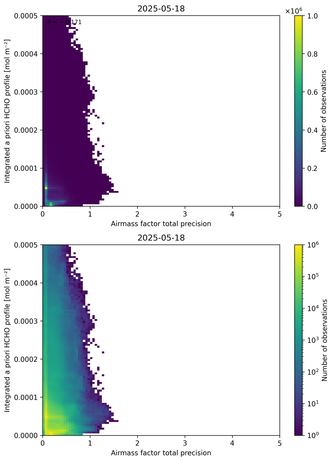
Figure 111: Scatter density plot of “Airmass factor total precision” against “Integrated a priori HCHO profile” for 2025-05-17 to 2025-05-19.
