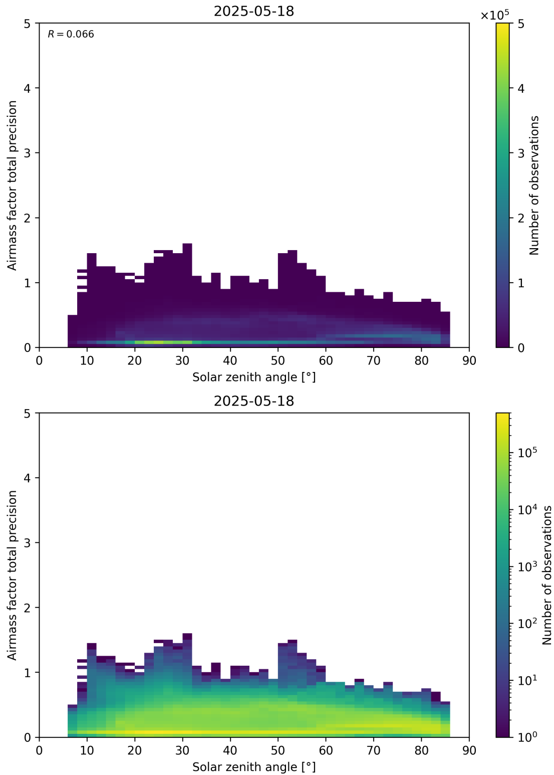
Figure 176: Scatter density plot of “Solar zenith angle” against “Airmass factor total precision” for 2025-05-17 to 2025-05-19.
