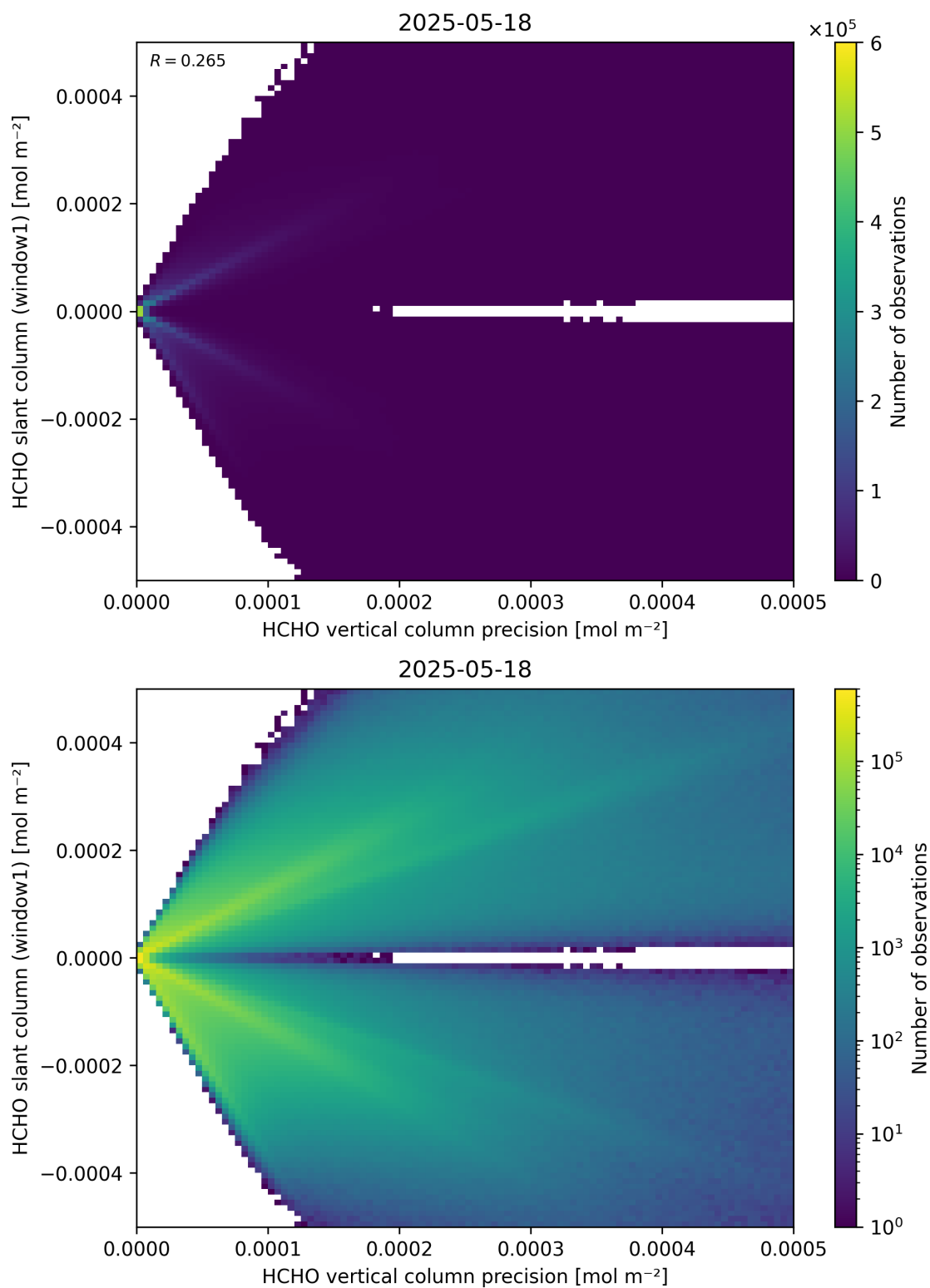
Figure 142: Scatter density plot of “HCHO vertical column precision” against “HCHO slant column (window1)” for 2025-05-17 to 2025-05-19.
