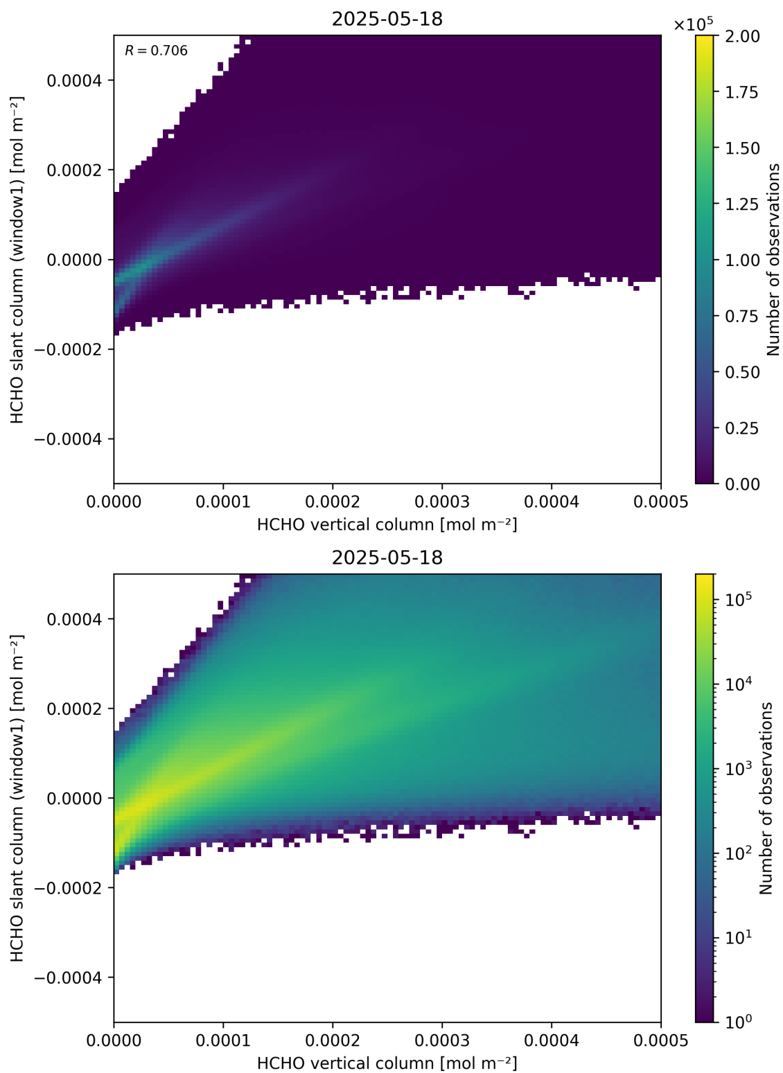
Figure 129: Scatter density plot of “HCHO vertical column” against “HCHO slant column (window1)” for 2025-05-17 to 2025-05-19.
