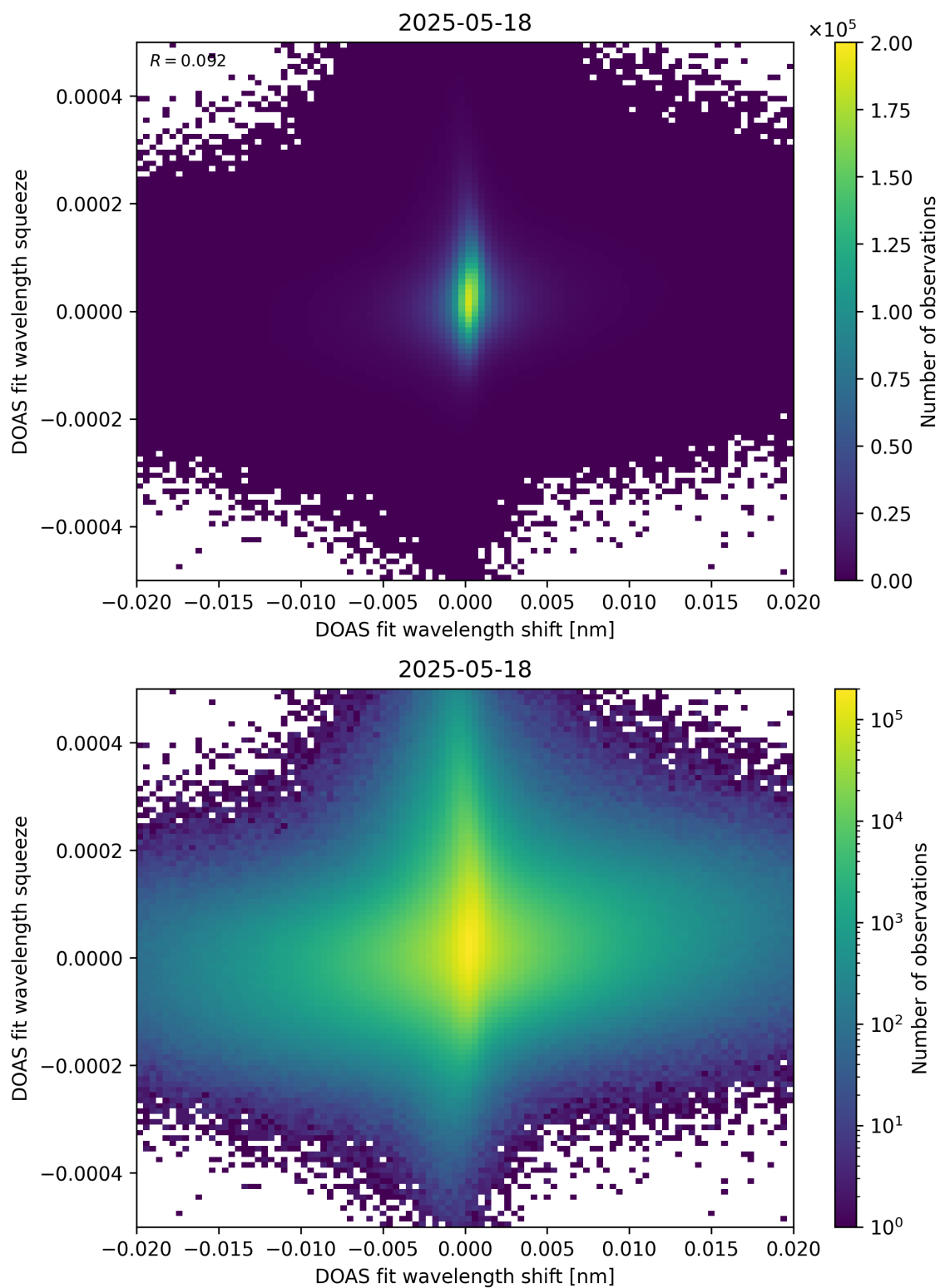
Figure 65: Scatter density plot of “DOAS fit wavelength shift” against “DOAS fit wavelength squeeze” for 2025-05-17 to 2025-05-19.
