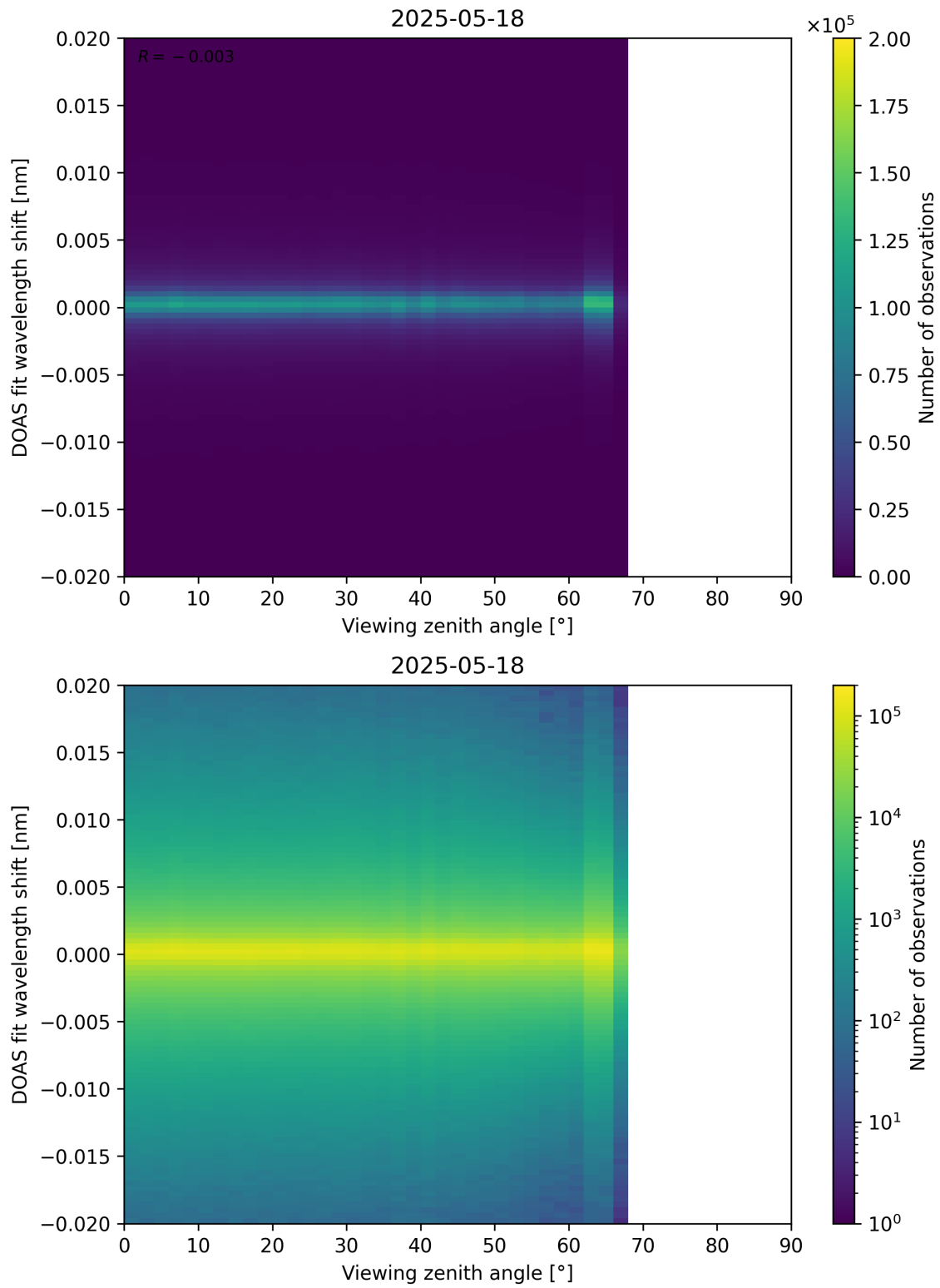
Figure 183: Scatter density plot of “Viewing zenith angle” against “DOAS fit wavelength shift” for 2025-05-17 to 2025-05-19.
