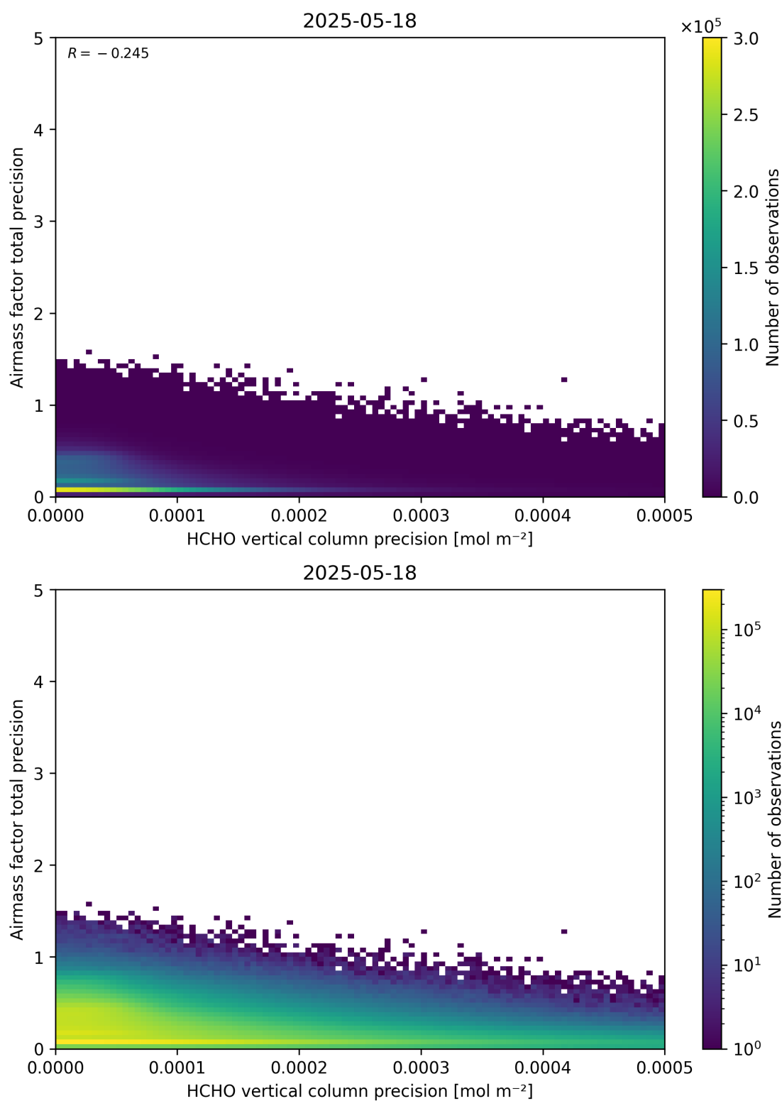
Figure 145: Scatter density plot of “HCHO vertical column precision” against “Airmass factor total precision” for 2025-05-17 to 2025-05-19.
