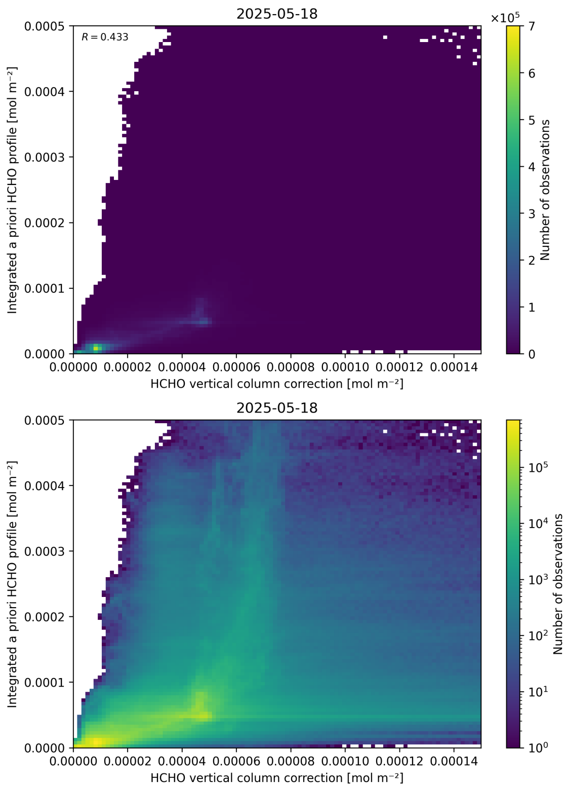
Figure 122: Scatter density plot of “HCHO vertical column correction” against “Integrated a priori HCHO profile” for 2025-05-17 to 2025-05-19.
