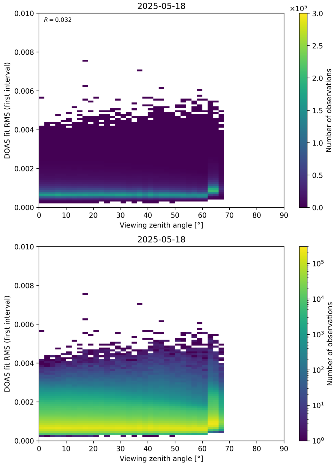
Figure 182: Scatter density plot of “Viewing zenith angle” against “DOAS fit RMS (first interval)” for 2025-05-17 to 2025-05-19.
