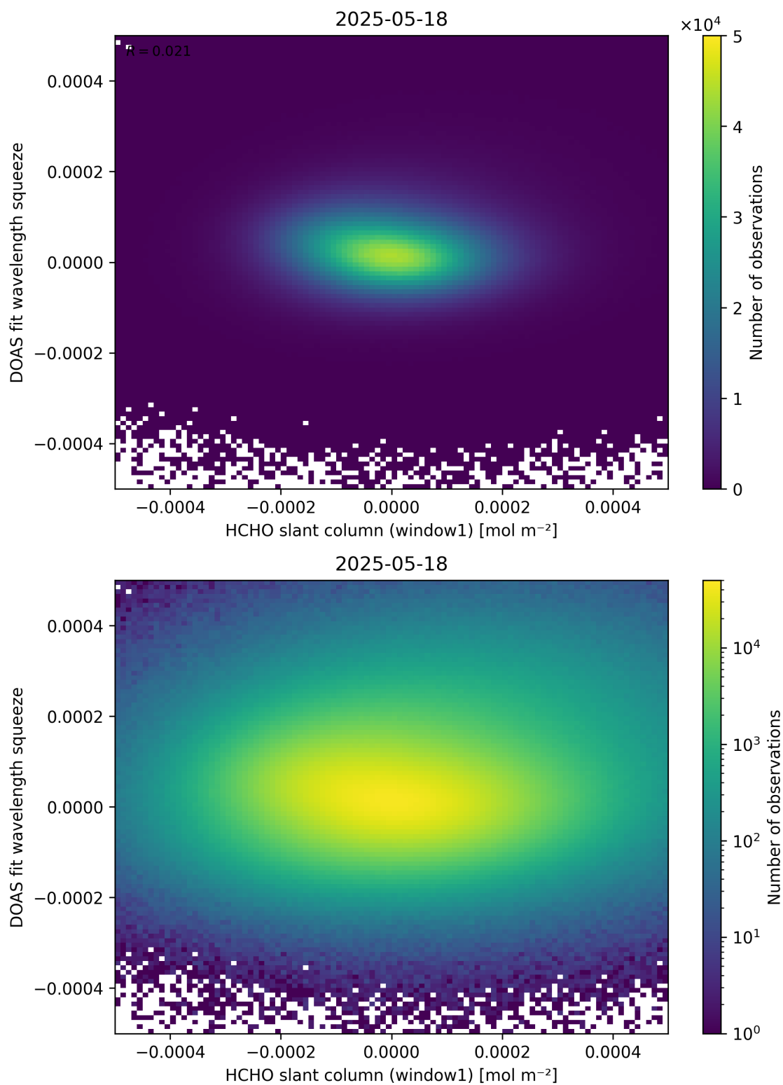
Figure 80: Scatter density plot of “HCHO slant column (window1)” against “DOAS fit wavelength squeeze” for 2025-05-17 to 2025-05-19.
