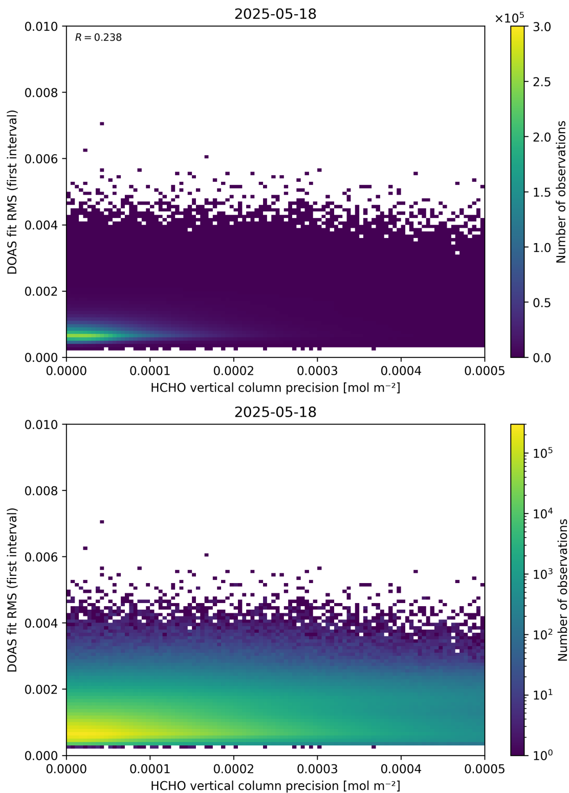
Figure 136: Scatter density plot of “HCHO vertical column precision” against “DOAS fit RMS (first interval)” for 2025-05-17 to 2025-05-19.
