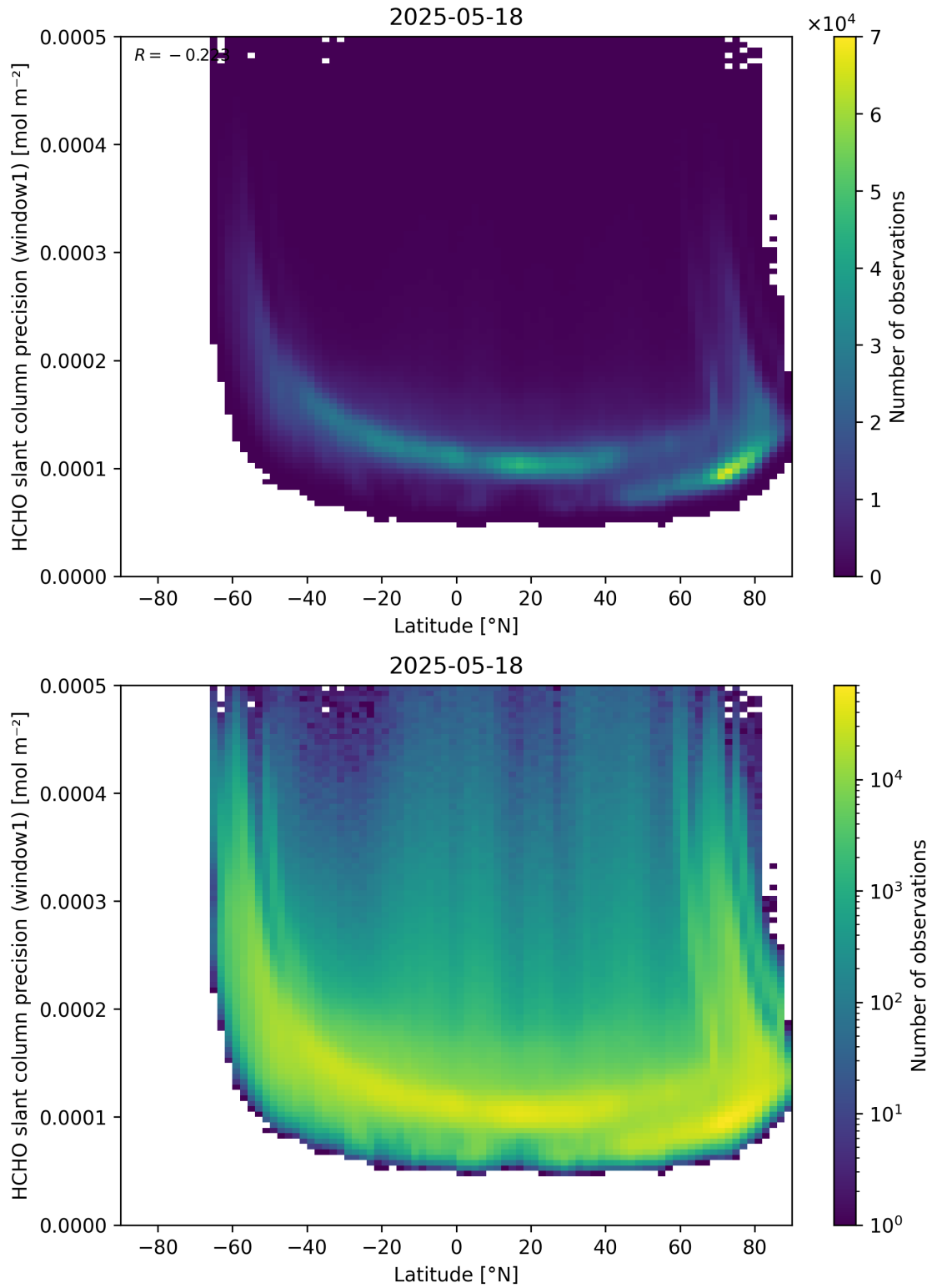
Figure 160: Scatter density plot of “Latitude” against “HCHO slant column precision (window1)” for 2025-05-17 to 2025-05-19.
