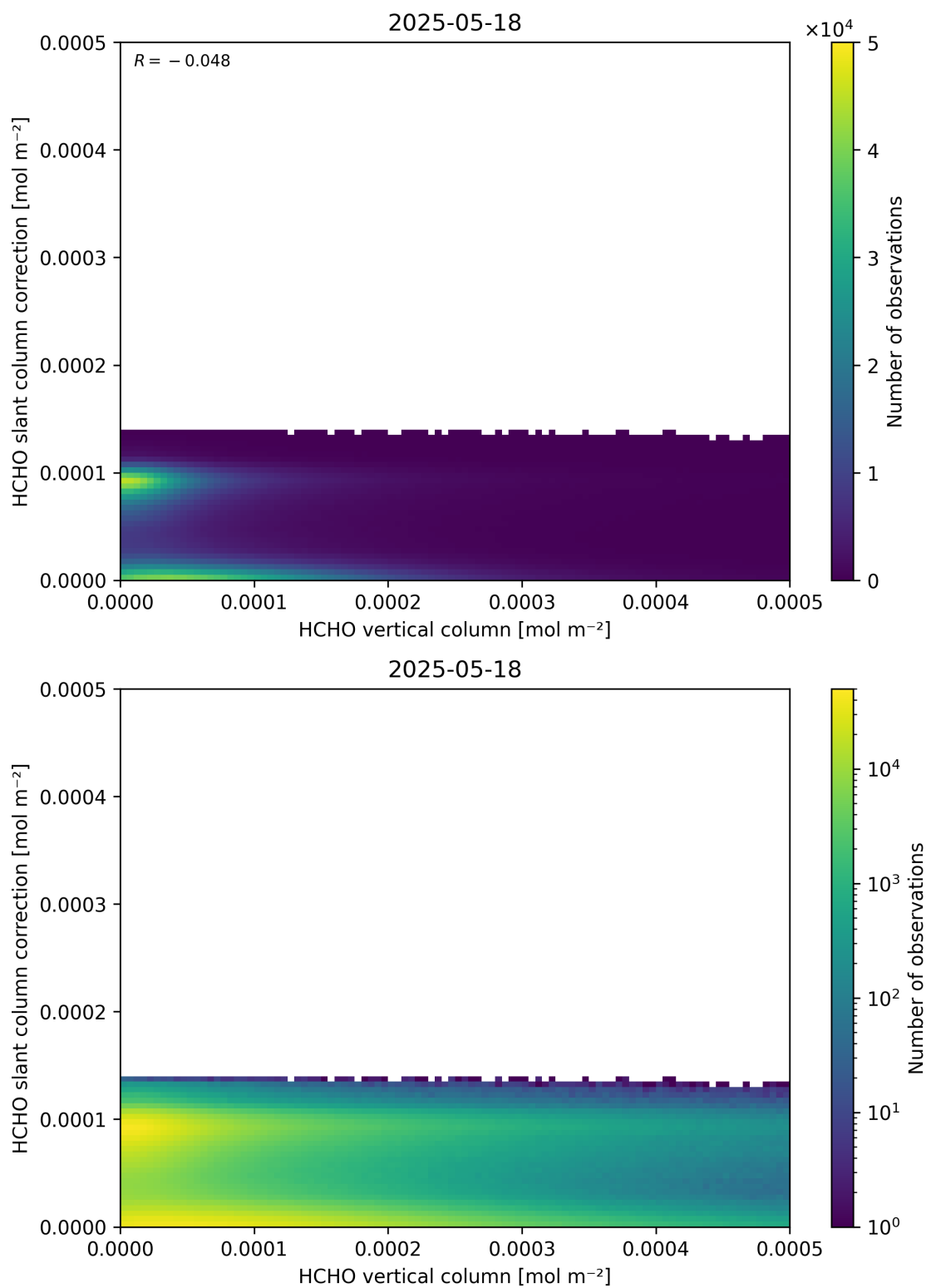
Figure 128: Scatter density plot of “HCHO vertical column” against “HCHO slant column correction” for 2025-05-17 to 2025-05-19.
