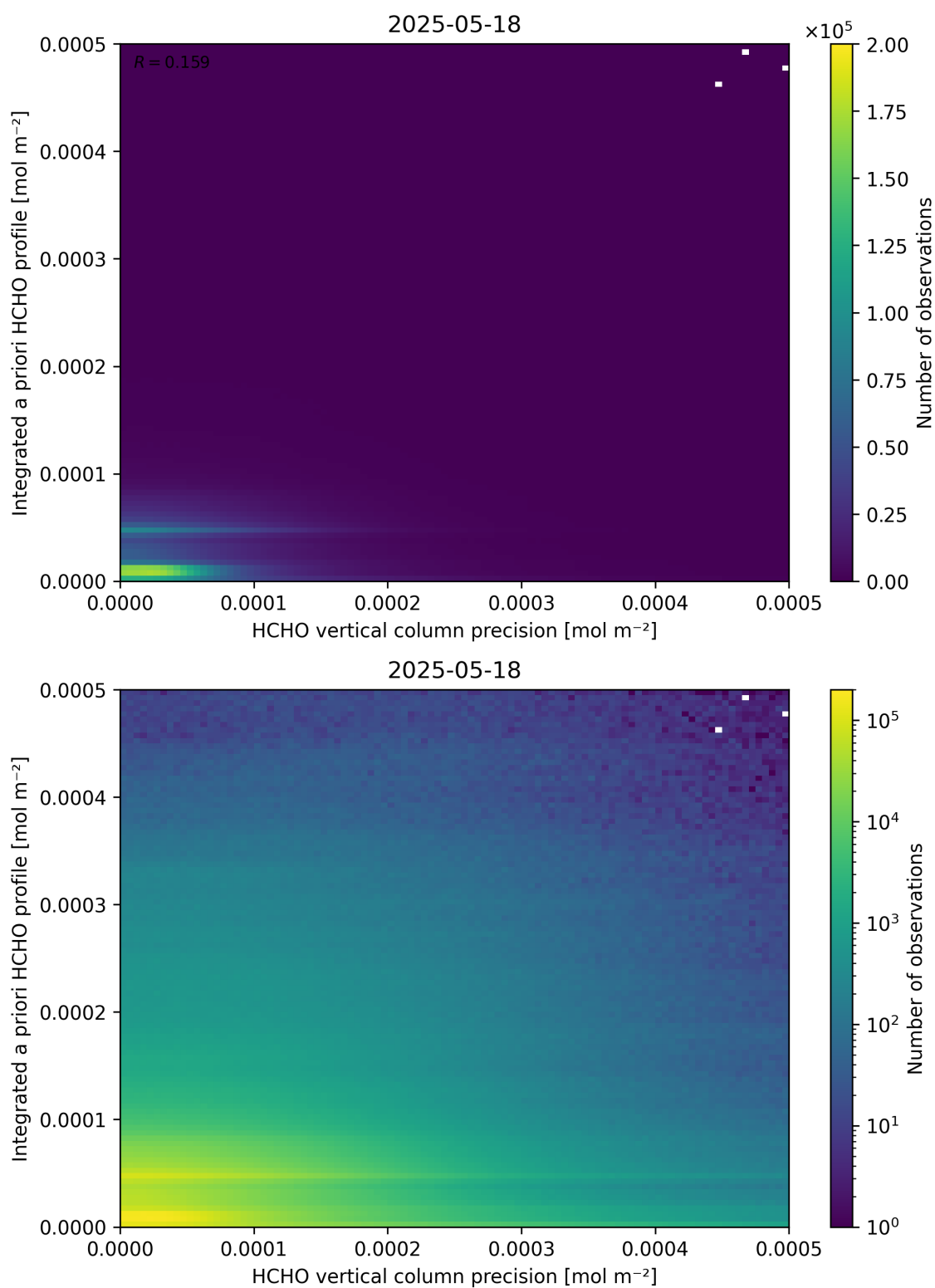
Figure 147: Scatter density plot of “HCHO vertical column precision” against “Integrated a priori HCHO profile” for 2025-05-17 to 2025-05-19.
