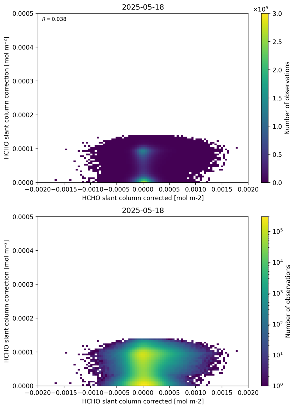
Figure 77: Scatter density plot of “HCHO slant column corrected” against “HCHO slant column correction” for 2025-05-17 to 2025-05-19.
