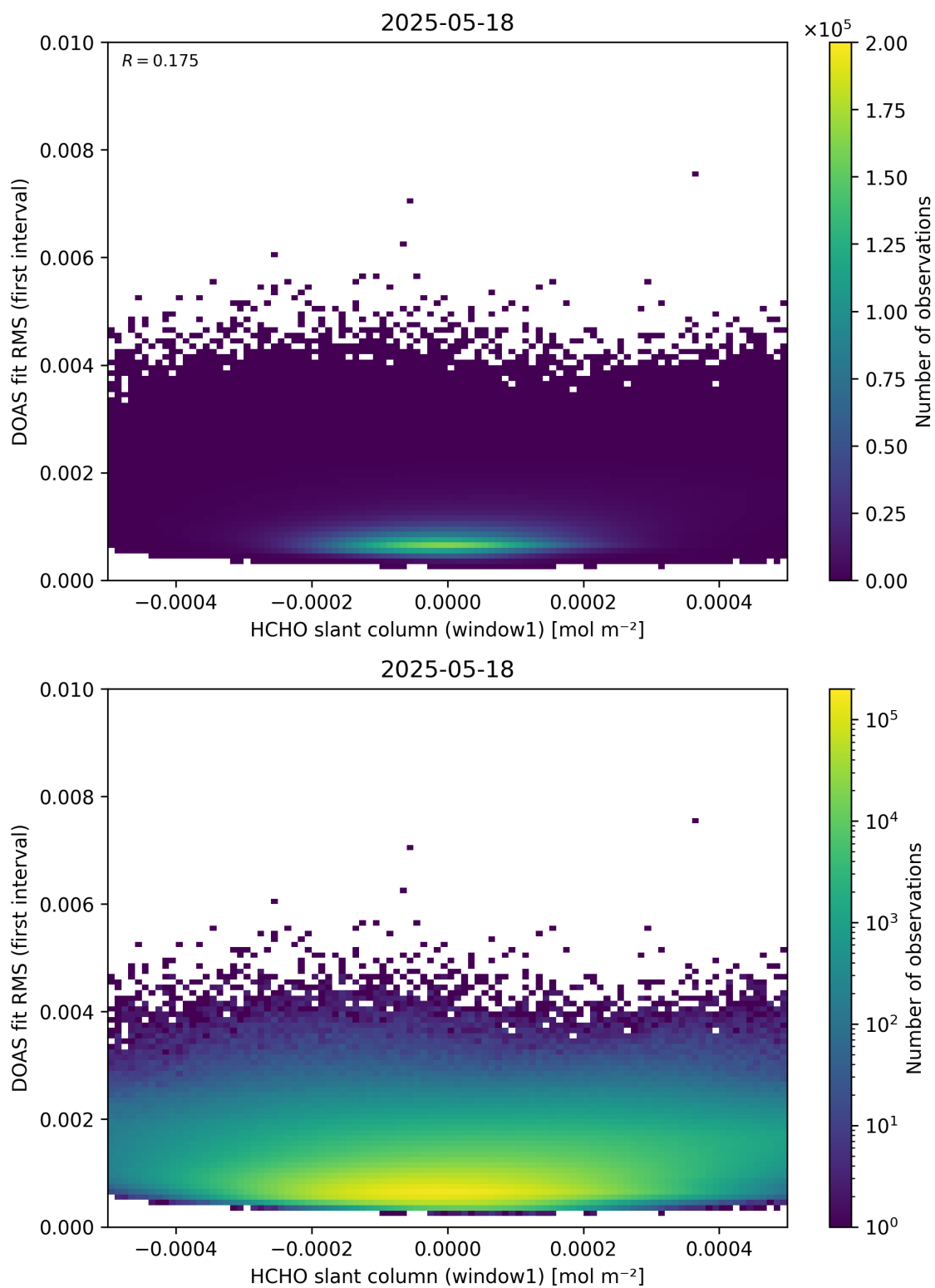
Figure 78: Scatter density plot of “HCHO slant column (window1)” against “DOAS fit RMS (first interval)” for 2025-05-17 to 2025-05-19.
