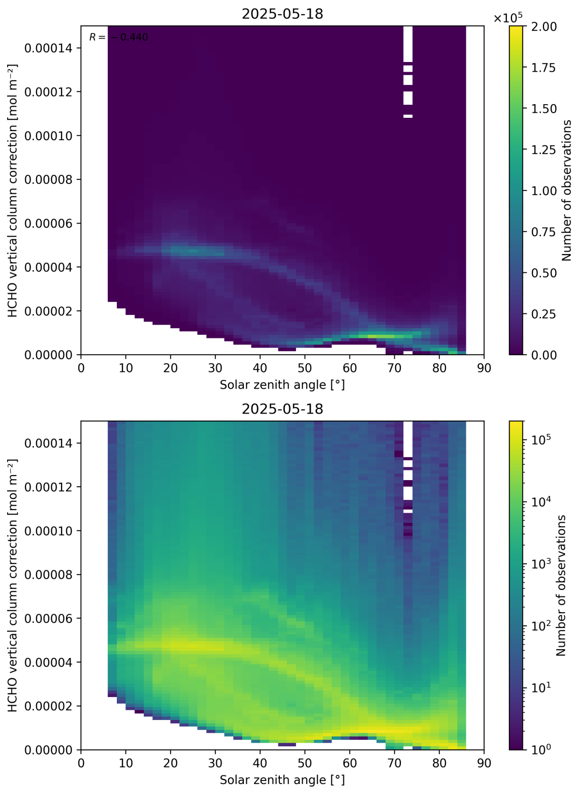
Figure 178: Scatter density plot of “Solar zenith angle” against “HCHO vertical column correction” for 2025-05-17 to 2025-05-19.
