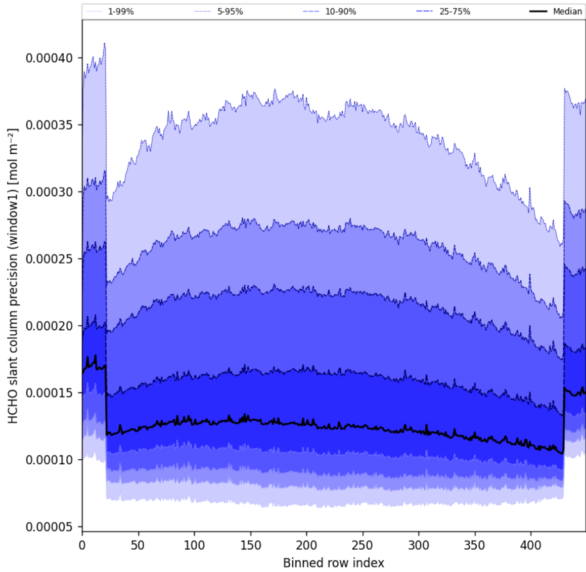
Figure 53: Along track statistics of “HCHO slant column precision (window1)” for 2025-05-17 to 2025-05-19
