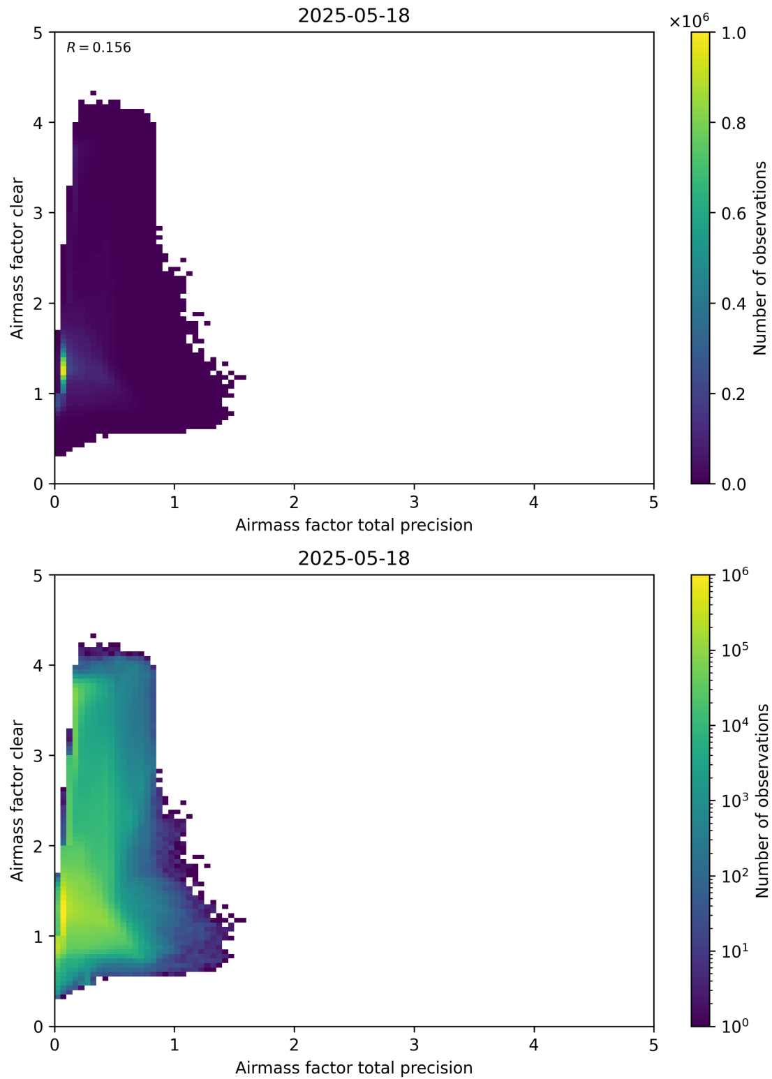
Figure 108: Scatter density plot of “Airmass factor total precision” against “Airmass factor clear” for 2025-05-17 to 2025-05-19.
