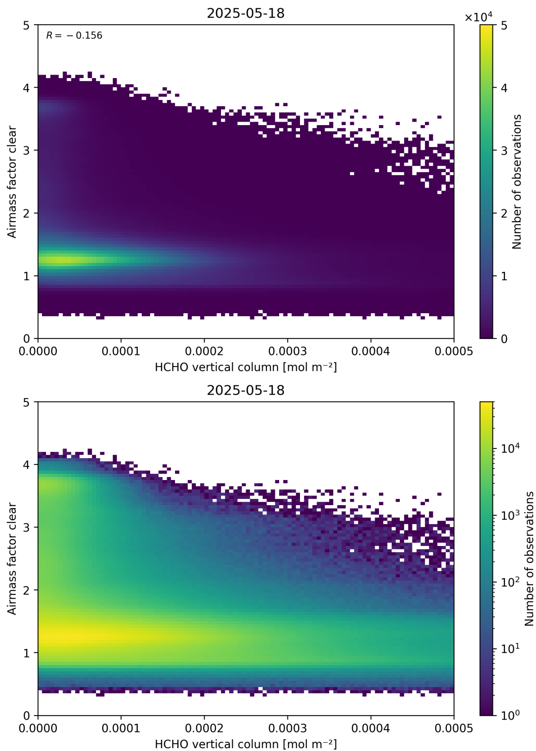
Figure 126: Scatter density plot of “HCHO vertical column” against “Airmass factor clear” for 2025-05-17 to 2025-05-19.
