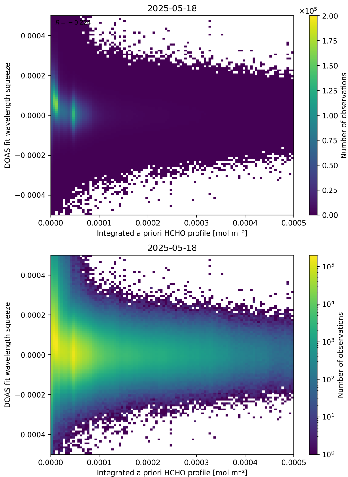
Figure 150: Scatter density plot of “Integrated a priori HCHO profile” against “DOAS fit wavelength squeeze” for 2025-05-17 to 2025-05-19.
