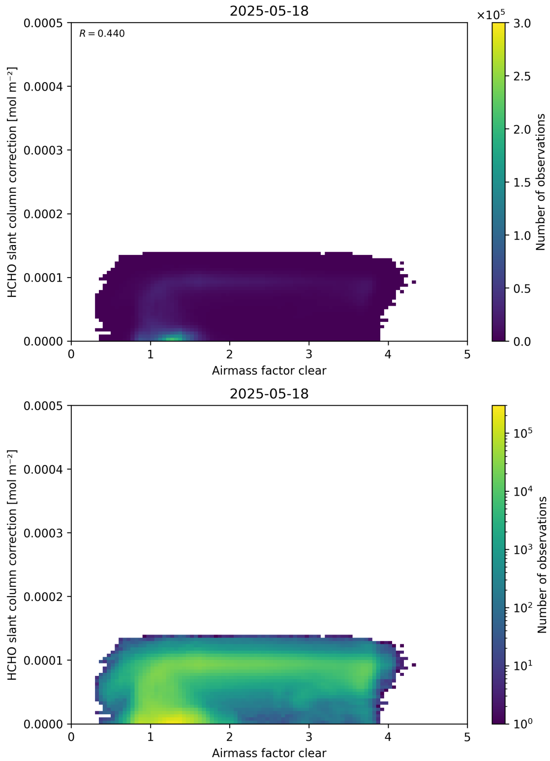
Figure 75: Scatter density plot of “Airmass factor clear” against “HCHO slant column correction” for 2025-05-17 to 2025-05-19.
