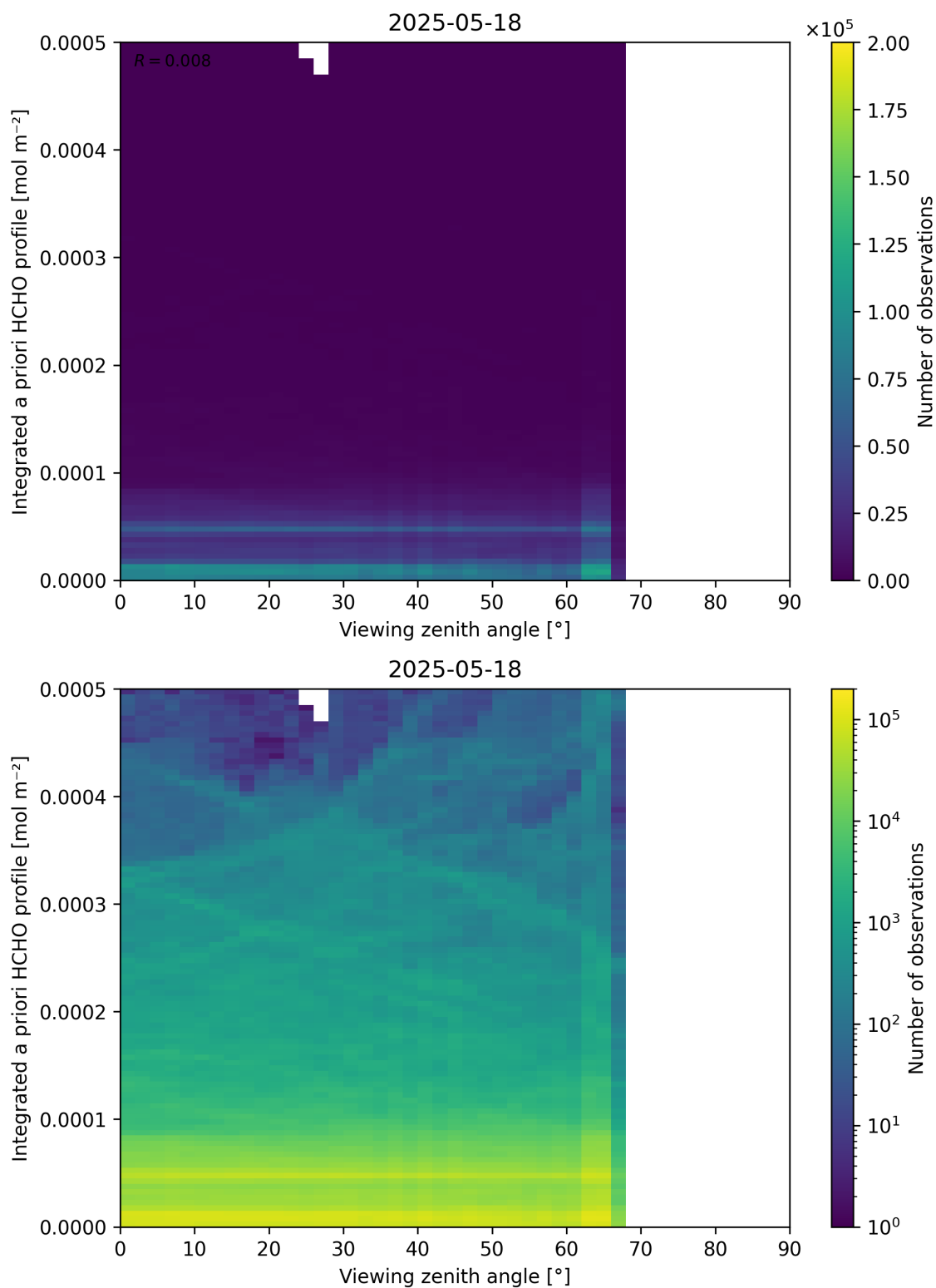
Figure 195: Scatter density plot of “Viewing zenith angle” against “Integrated a priori HCHO profile” for 2025-05-17 to 2025-05-19.
