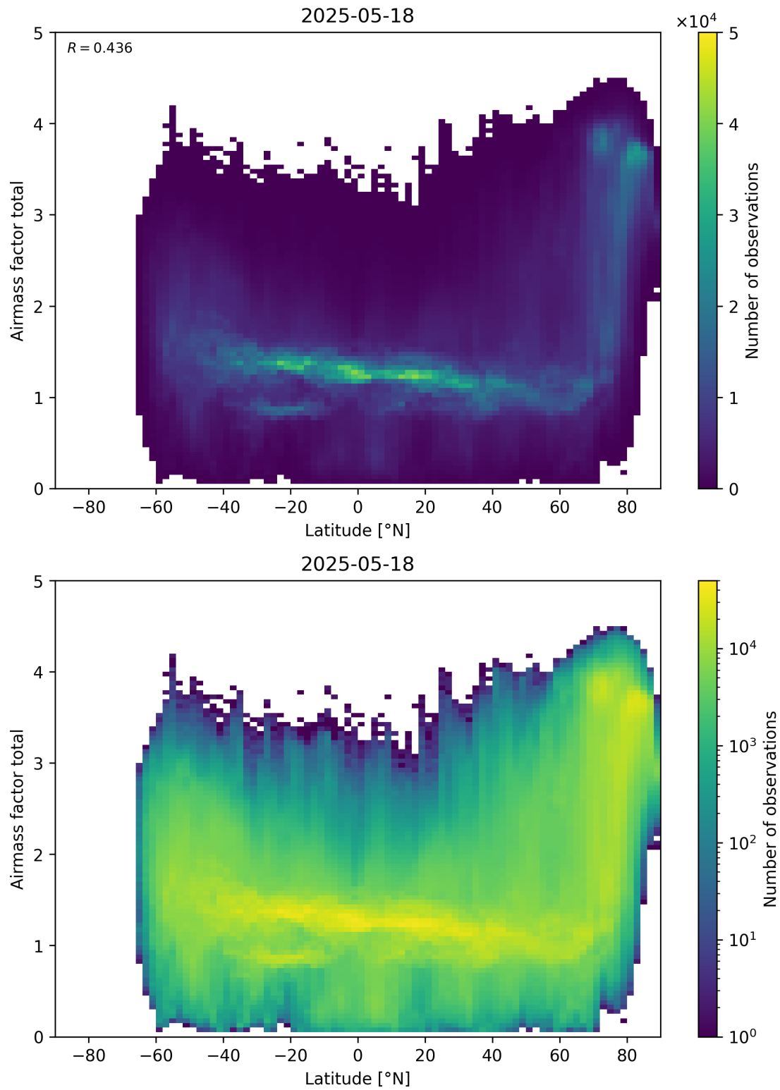
Figure 161: Scatter density plot of “Latitude” against “Airmass factor total” for 2025-05-17 to 2025-05-19.
