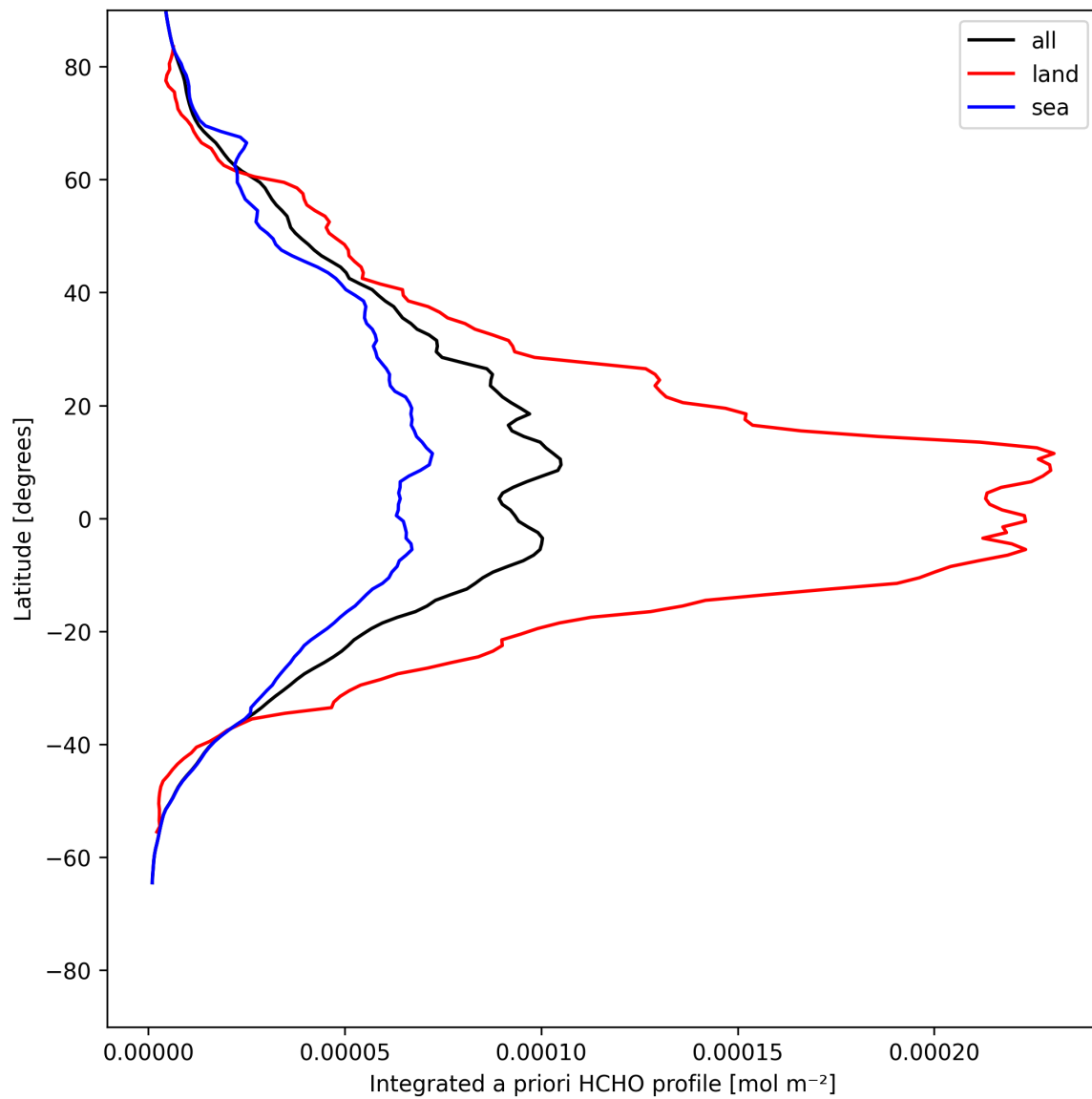
Figure 29: Zonal average of “Integrated a priori HCHO profile” for 2025-05-17 to 2025-05-19.
