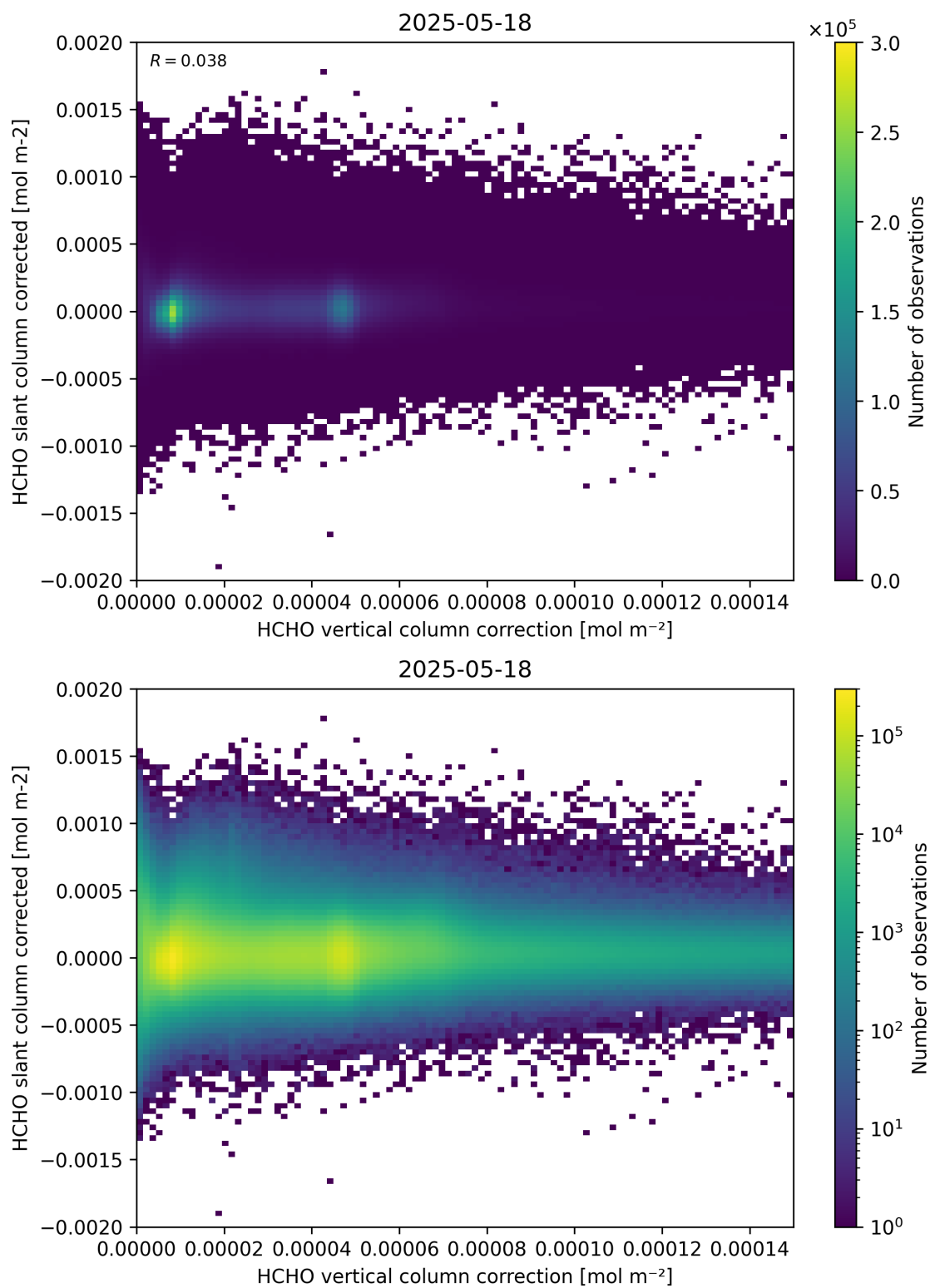
Figure 116: Scatter density plot of “HCHO vertical column correction” against “HCHO slant column corrected” for 2025-05-17 to 2025-05-19.
