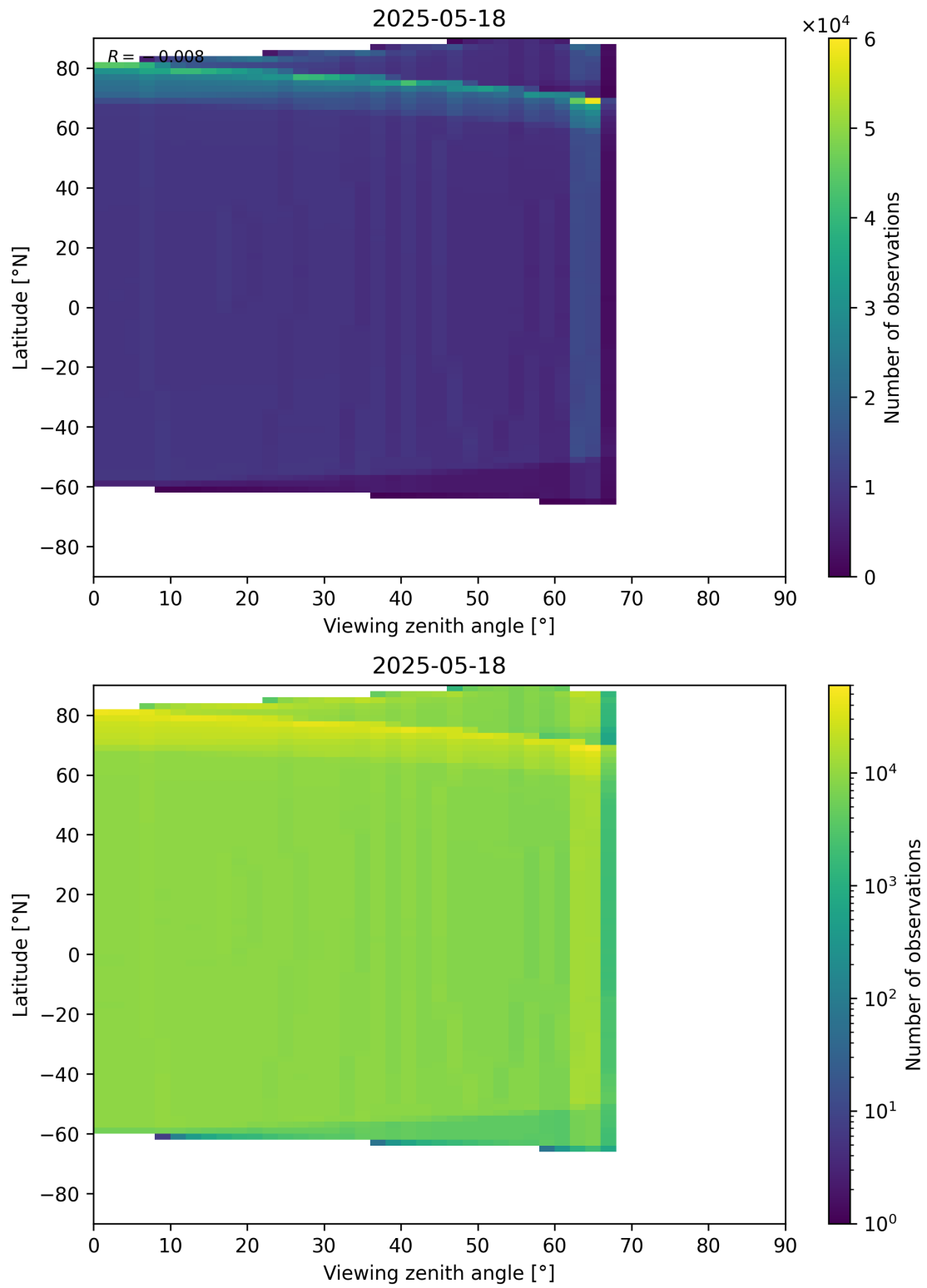
Figure 196: Scatter density plot of “Viewing zenith angle” against “Latitude” for 2025-05-17 to 2025-05-19.
