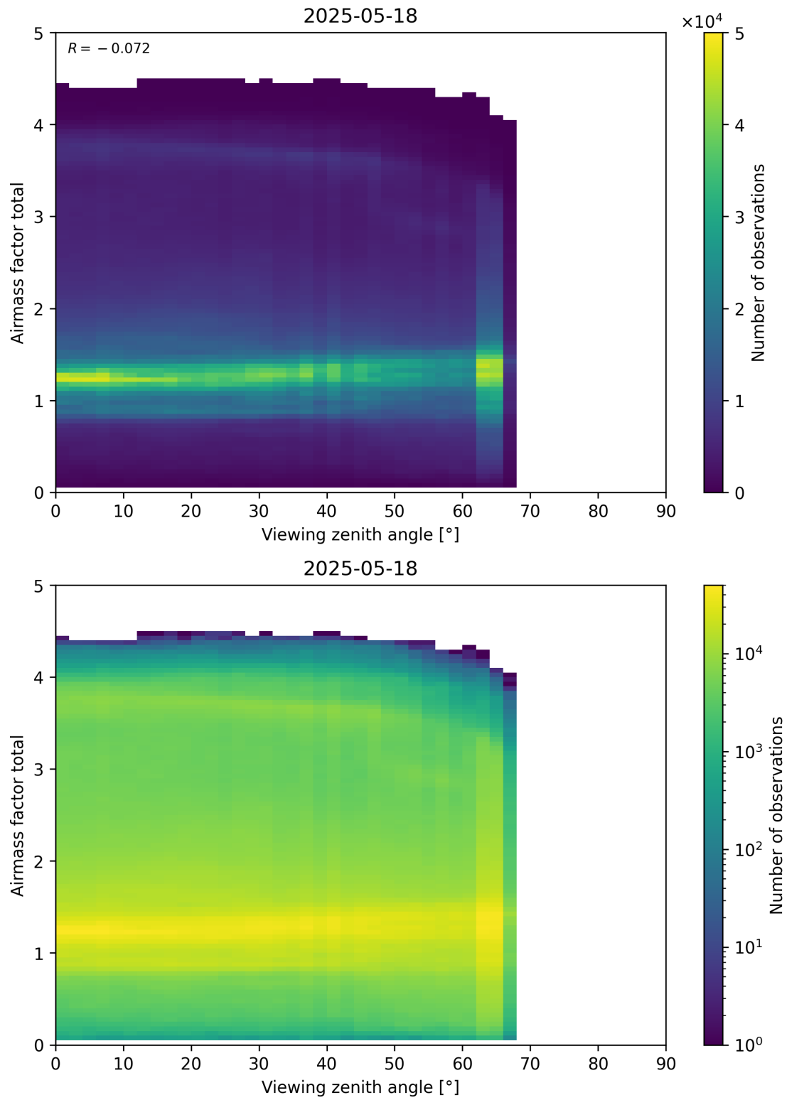
Figure 190: Scatter density plot of “Viewing zenith angle” against “Airmass factor total” for 2025-05-17 to 2025-05-19.
