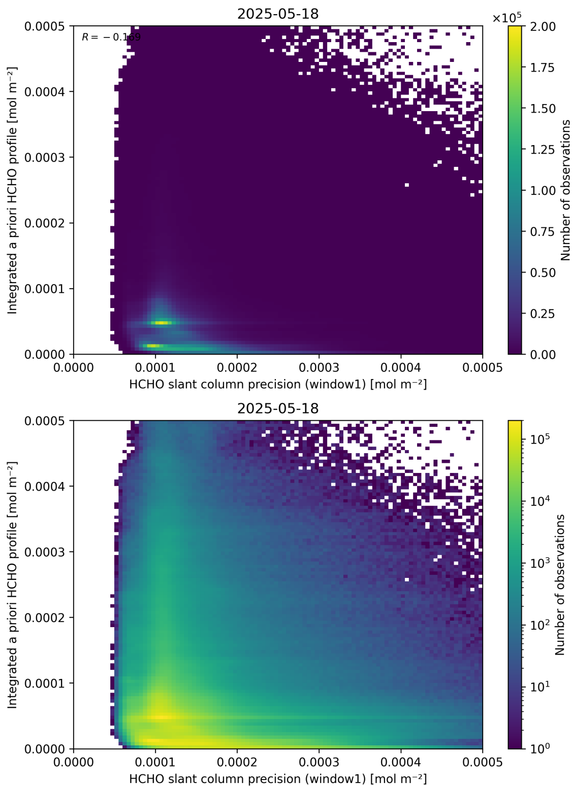
Figure 96: Scatter density plot of “HCHO slant column precision (window1)” against “Integrated a priori HCHO profile” for 2025-05-17 to 2025-05-19.
