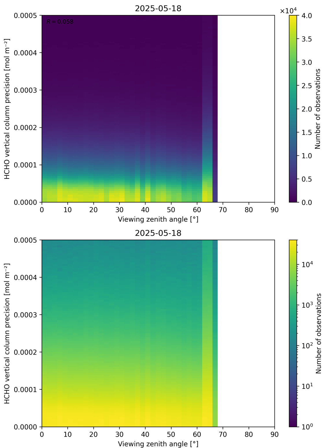
Figure 194: Scatter density plot of “Viewing zenith angle” against “HCHO vertical column precision” for 2025-05-17 to 2025-05-19.
