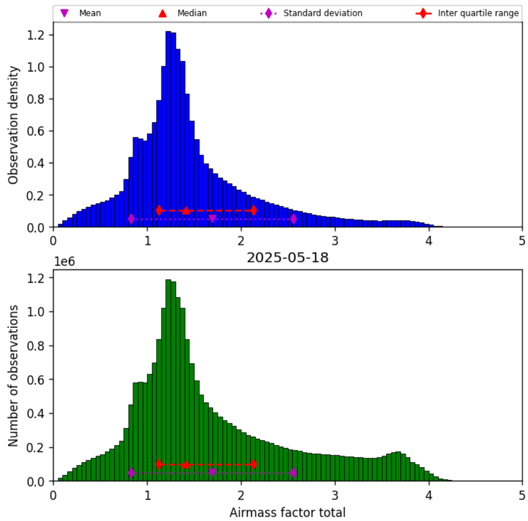
Figure 40: Histogram of “Airmass factor total” for 2025-05-17 to 2025-05-19
