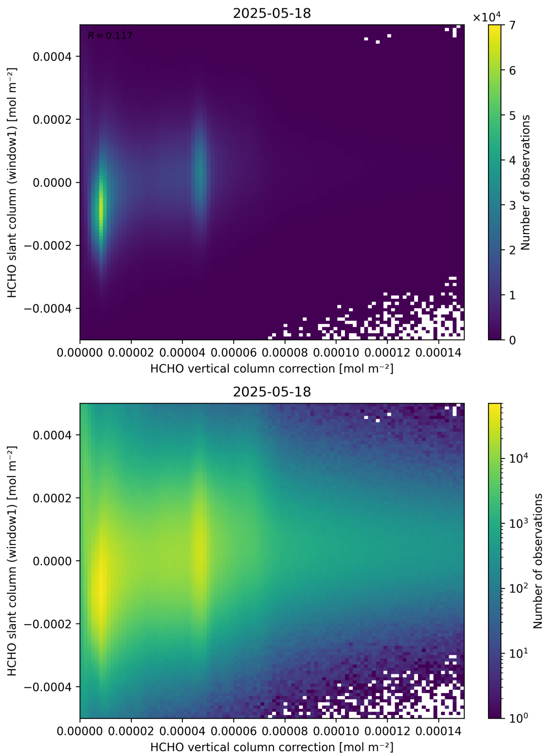
Figure 118: Scatter density plot of “HCHO vertical column correction” against “HCHO slant column (window1)” for 2025-05-17 to 2025-05-19.
