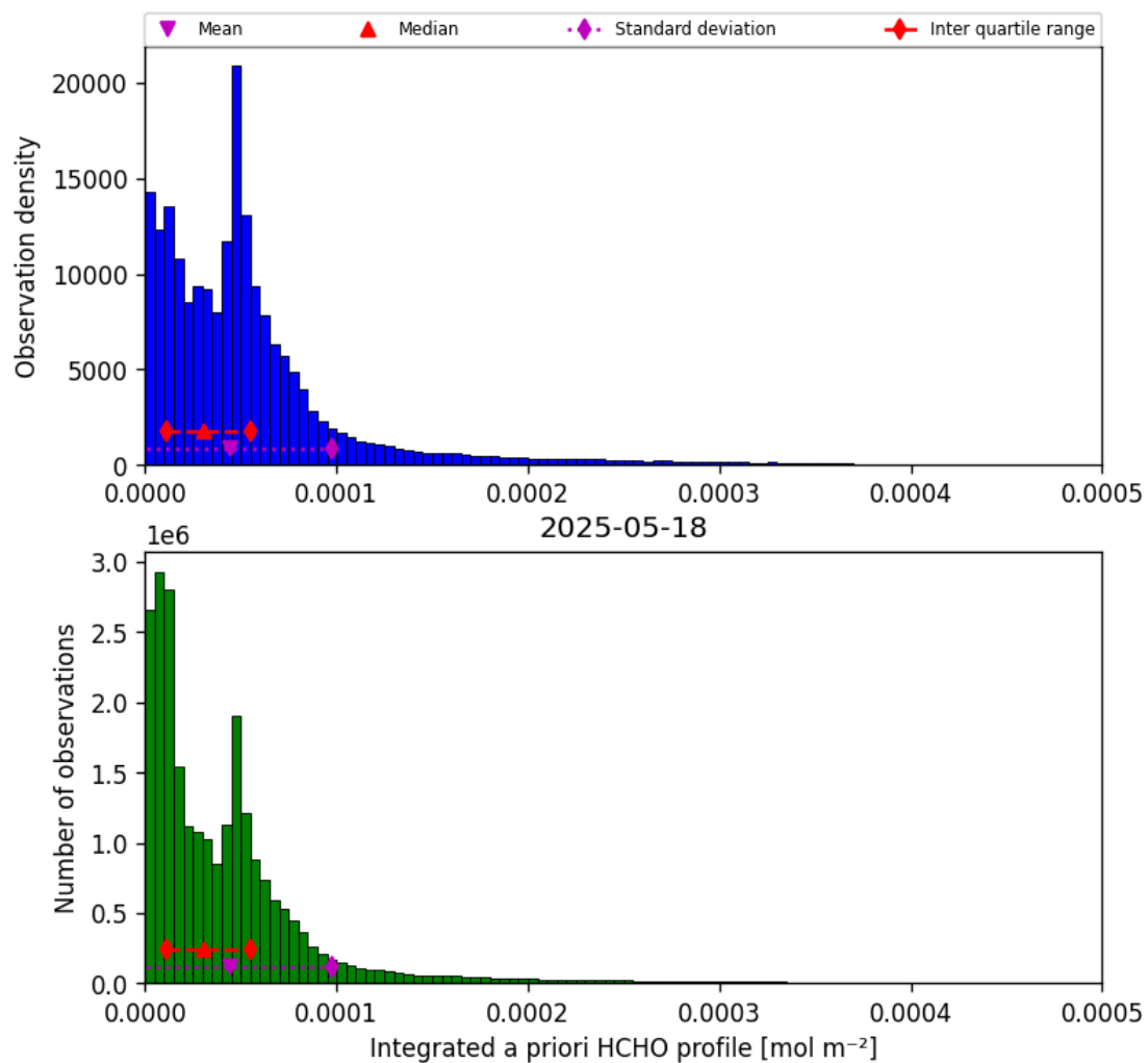
Figure 43: Histogram of “Integrated a priori HCHO profile” for 2025-05-17 to 2025-05-19
