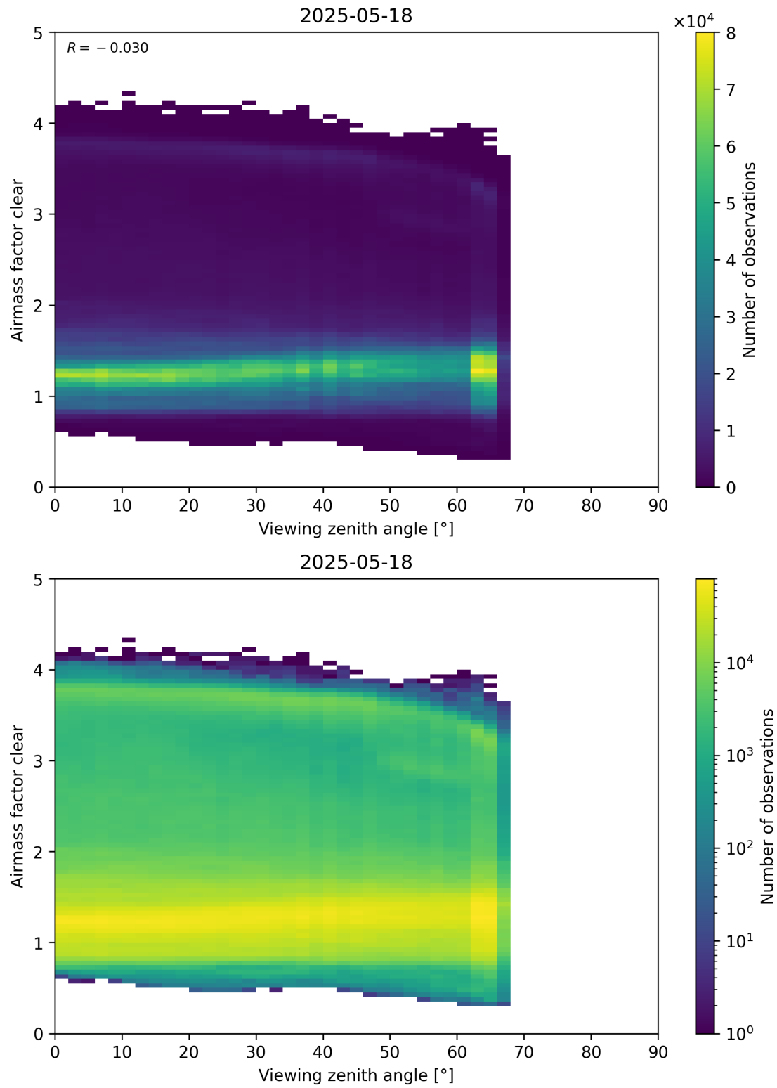
Figure 185: Scatter density plot of “Viewing zenith angle” against “Airmass factor clear” for 2025-05-17 to 2025-05-19.
