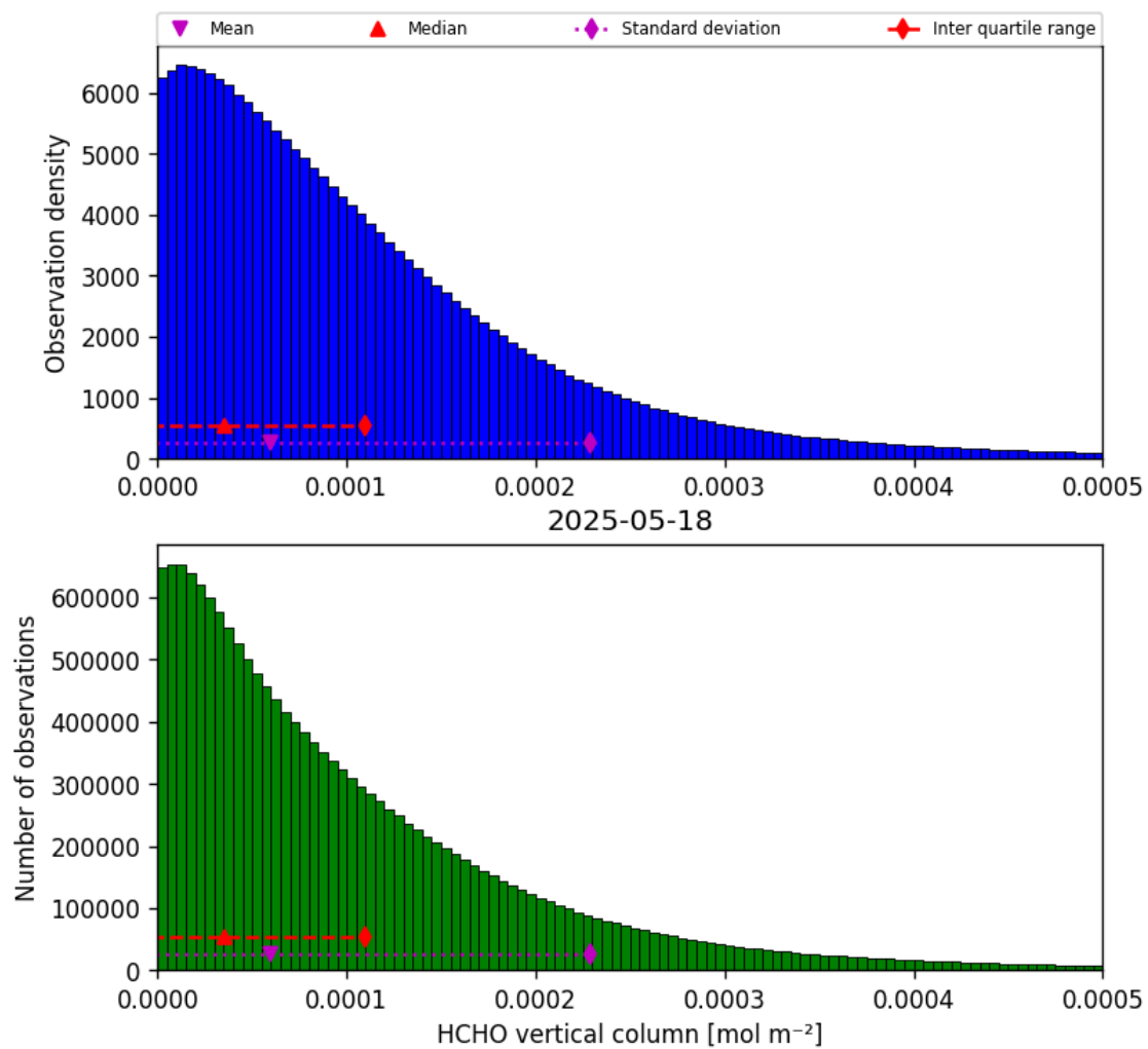
Figure 35: Histogram of “HCHO vertical column” for 2025-05-17 to 2025-05-19
