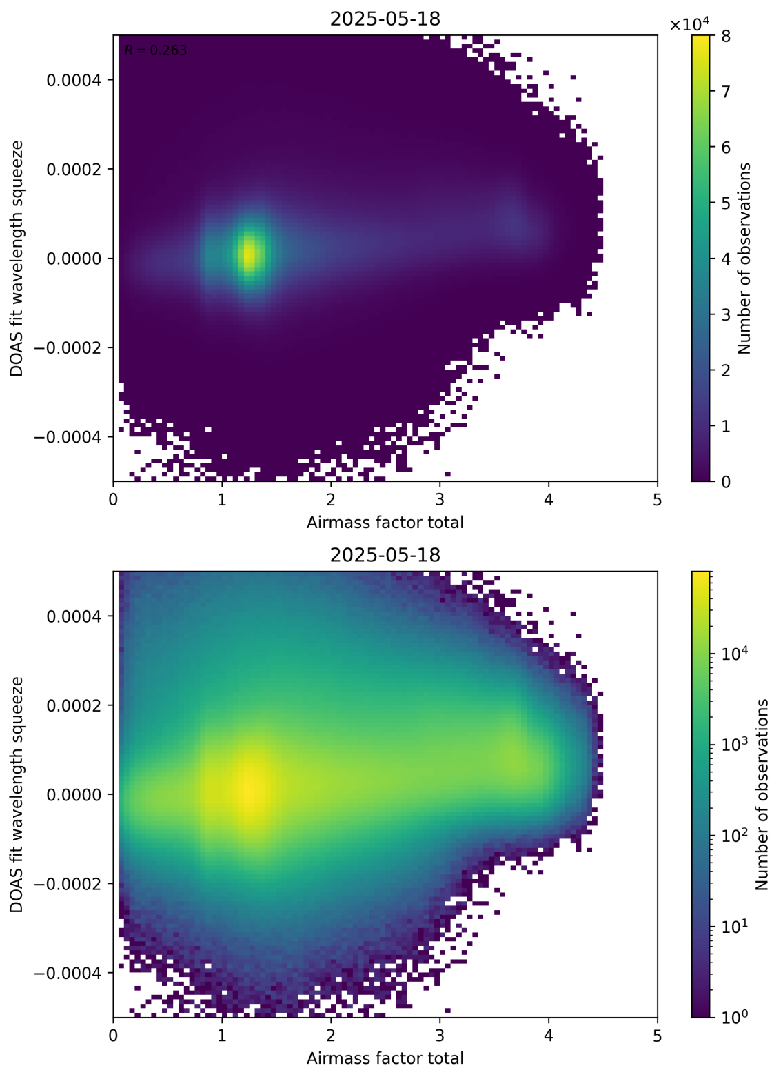
Figure 99: Scatter density plot of “Airmass factor total” against “DOAS fit wavelength squeeze” for 2025-05-17 to 2025-05-19.
