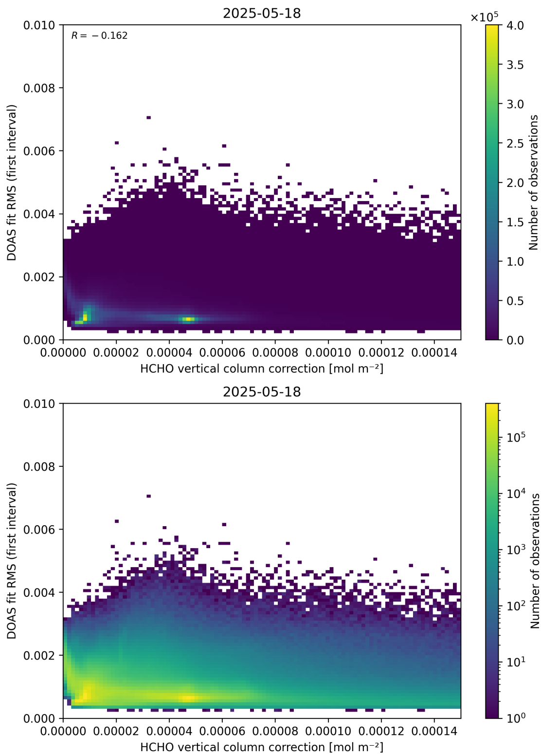
Figure 112: Scatter density plot of “HCHO vertical column correction” against “DOAS fit RMS (first interval)” for 2025-05-17 to 2025-05-19.
