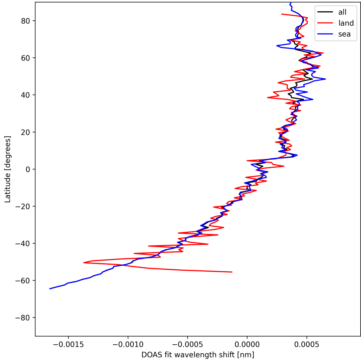
Figure 30: Zonal average of “DOAS fit wavelength shift” for 2025-05-17 to 2025-05-19.
