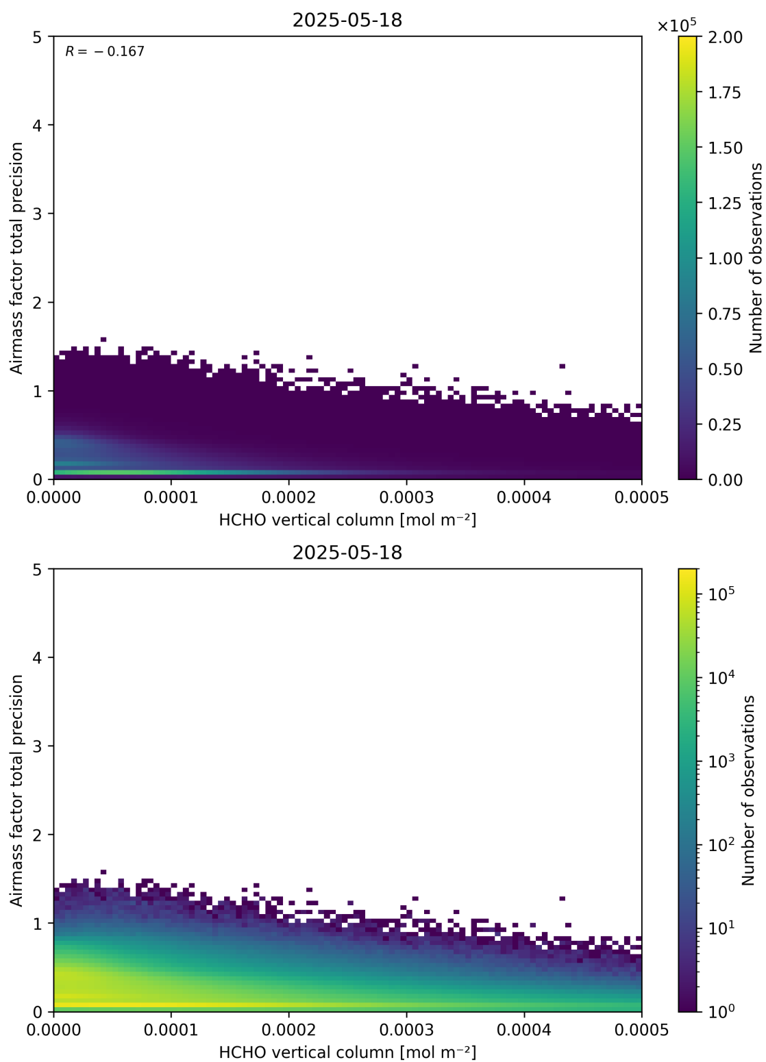
Figure 132: Scatter density plot of “HCHO vertical column” against “Airmass factor total precision” for 2025-05-17 to 2025-05-19.
