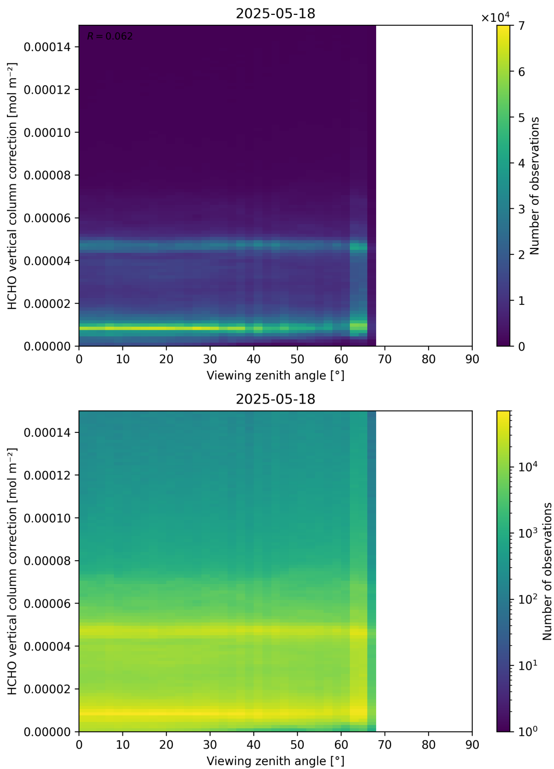
Figure 193: Scatter density plot of “Viewing zenith angle” against “HCHO vertical column correction” for 2025-05-17 to 2025-05-19.
