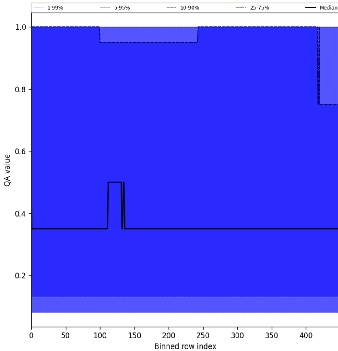
Figure 48: Along track statistics of “QA value” for 2025-05-17 to 2025-05-19
