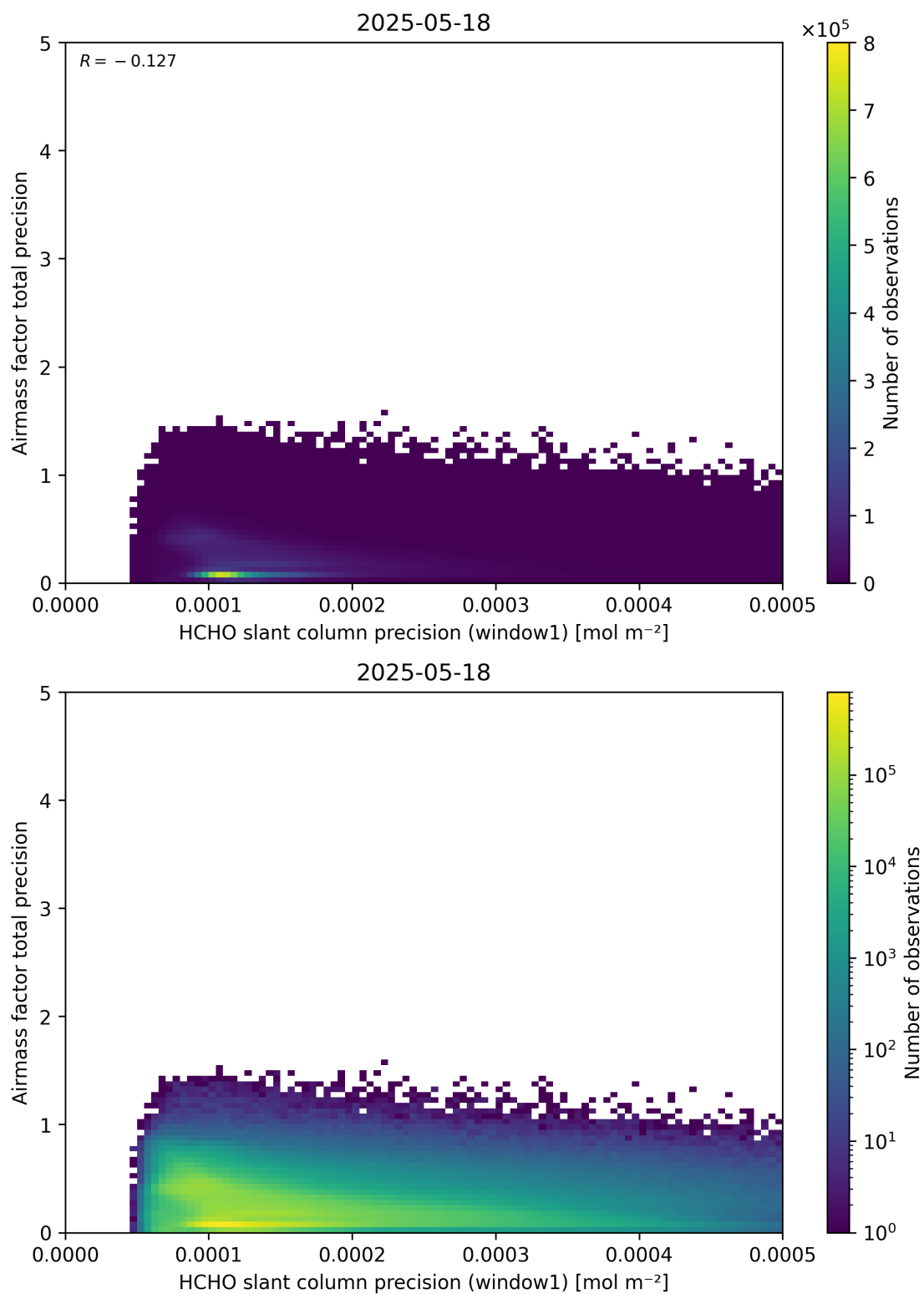
Figure 95: Scatter density plot of “HCHO slant column precision (window1)” against “Airmass factor total precision” for 2025-05-17 to 2025-05-19.
