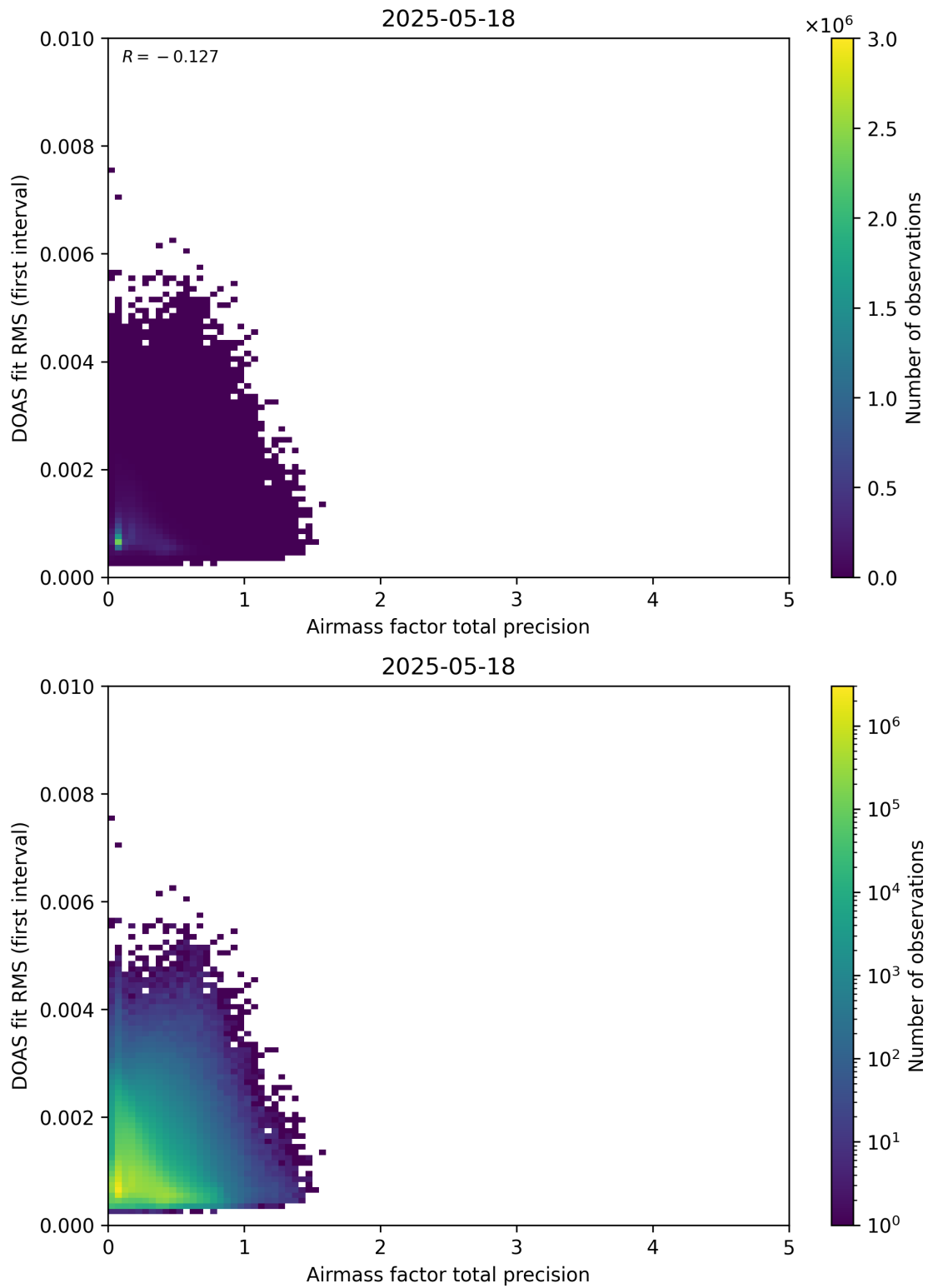
Figure 105: Scatter density plot of “Airmass factor total precision” against “DOAS fit RMS (first interval)” for 2025-05-17 to 2025-05-19.
