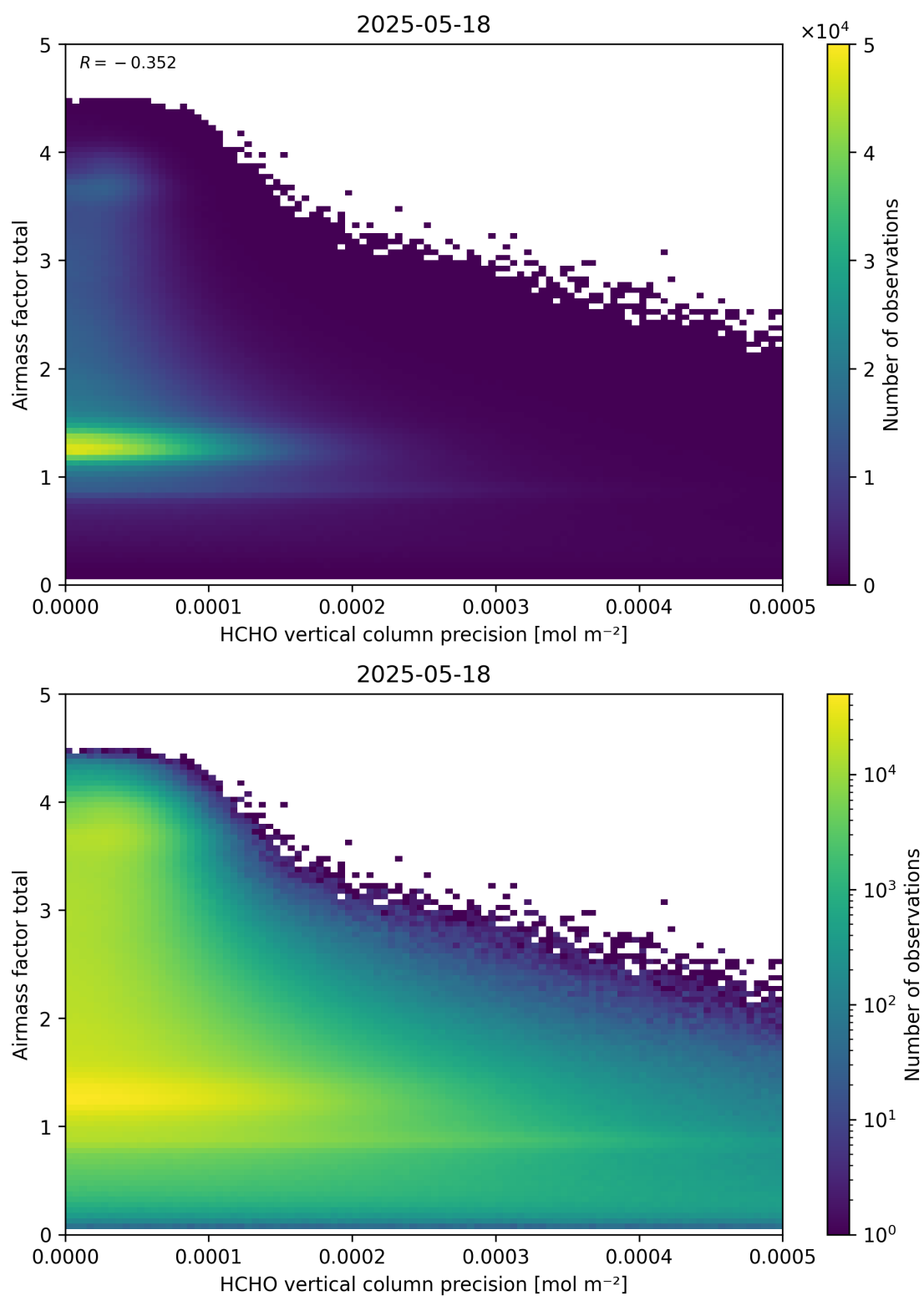
Figure 144: Scatter density plot of “HCHO vertical column precision” against “Airmass factor total” for 2025-05-17 to 2025-05-19.
