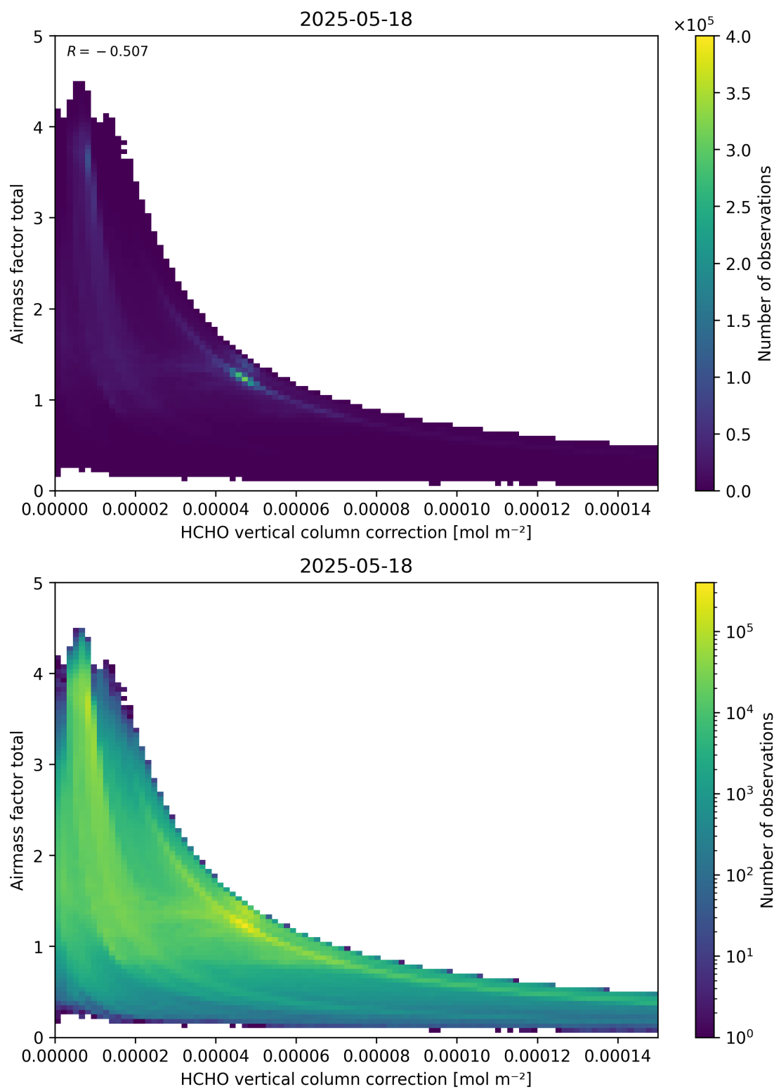
Figure 120: Scatter density plot of “HCHO vertical column correction” against “Airmass factor total” for 2025-05-17 to 2025-05-19.
