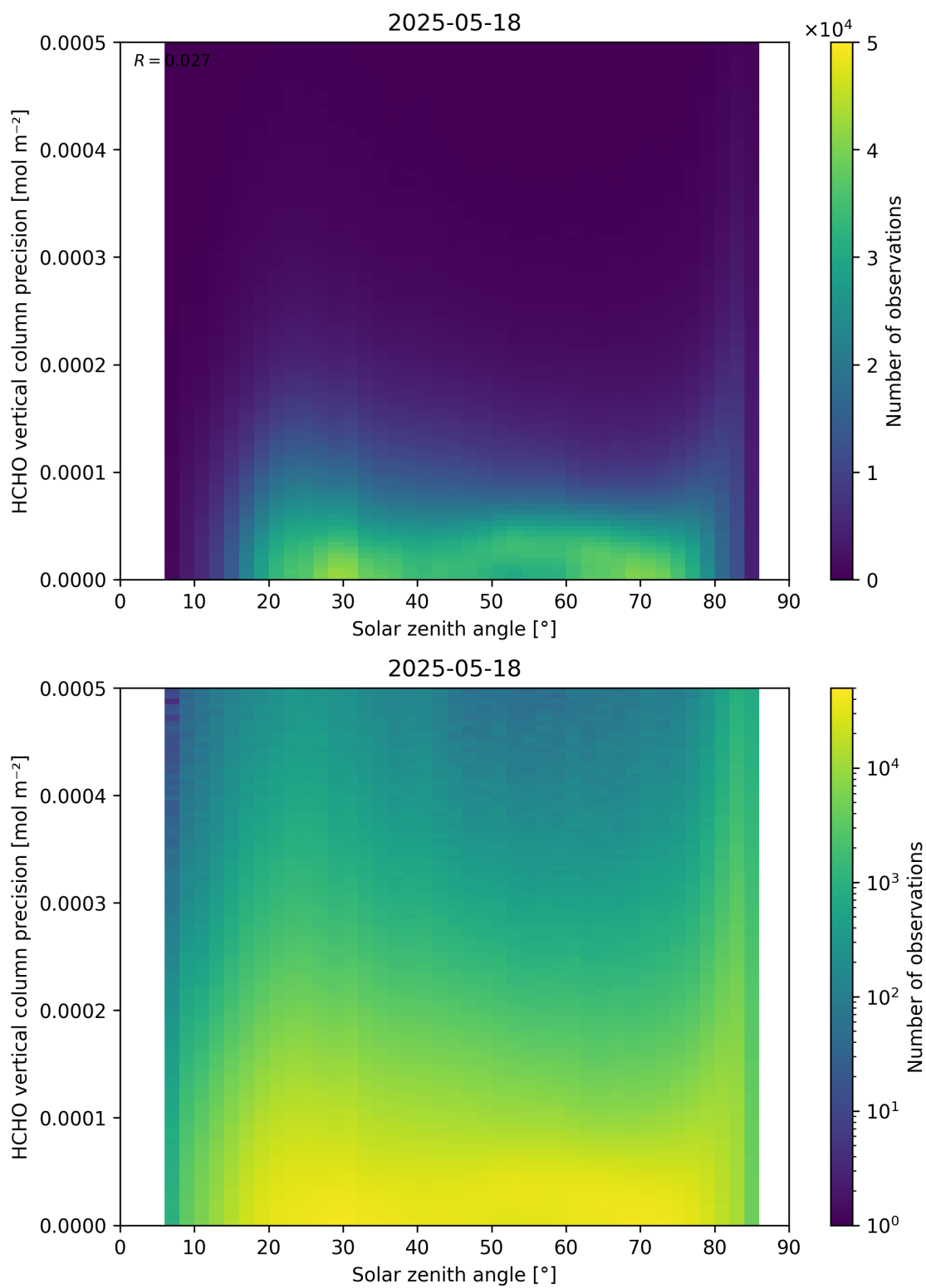
Figure 179: Scatter density plot of “Solar zenith angle” against “HCHO vertical column precision” for 2025-05-17 to 2025-05-19.
