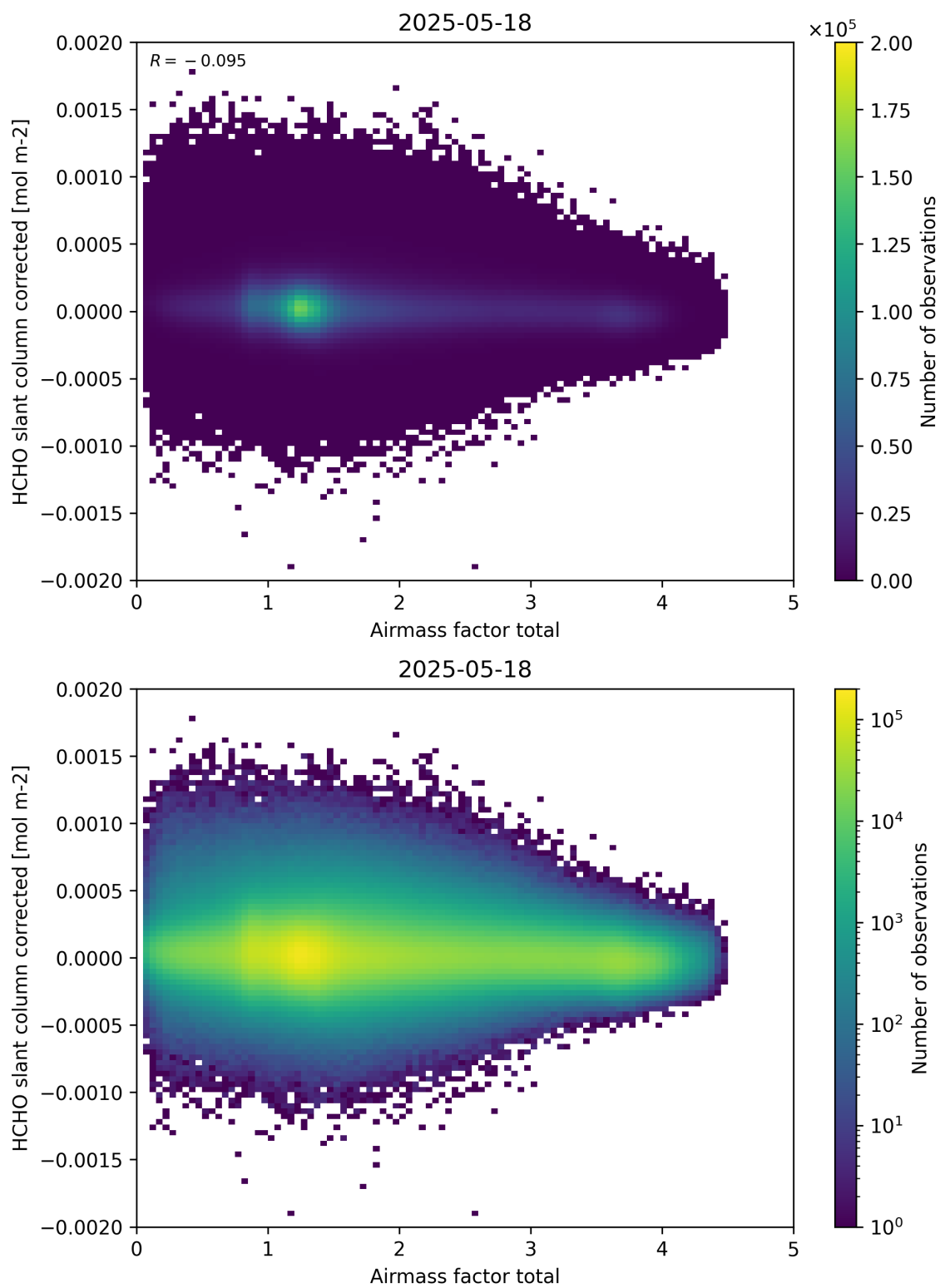
Figure 101: Scatter density plot of “Airmass factor total” against “HCHO slant column corrected” for 2025-05-17 to 2025-05-19.
