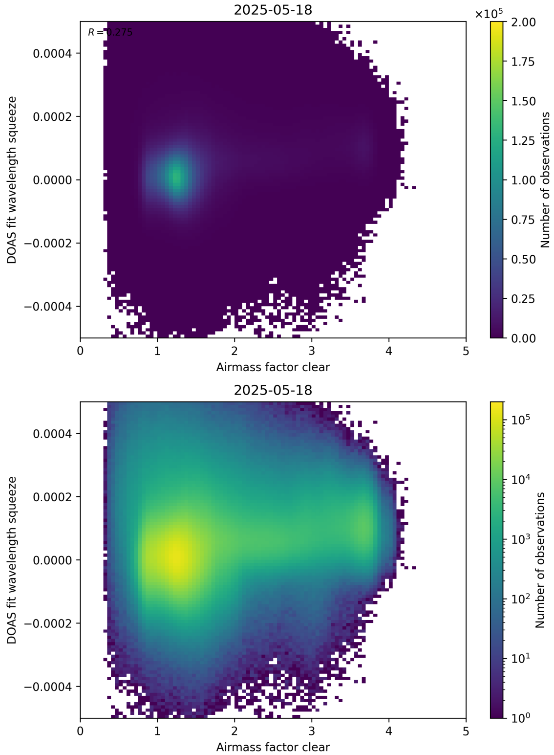
Figure 73: Scatter density plot of “Airmass factor clear” against “DOAS fit wavelength squeeze” for 2025-05-17 to 2025-05-19.
