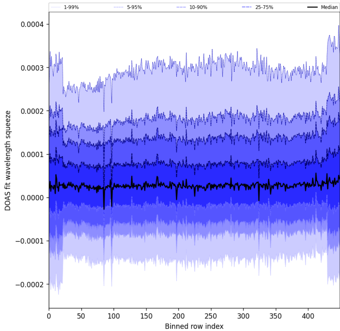
Figure 59: Along track statistics of “DOAS fit wavelength squeeze” for 2025-05-17 to 2025-05-19
