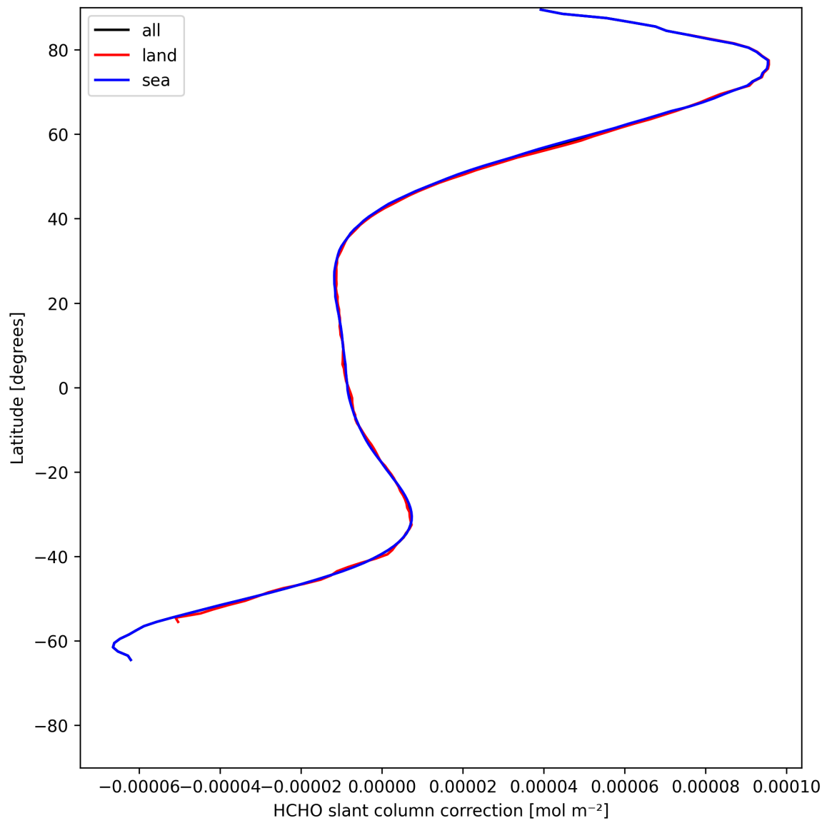
Figure 33: Zonal average of “HCHO slant column correction” for 2025-05-17 to 2025-05-19.
