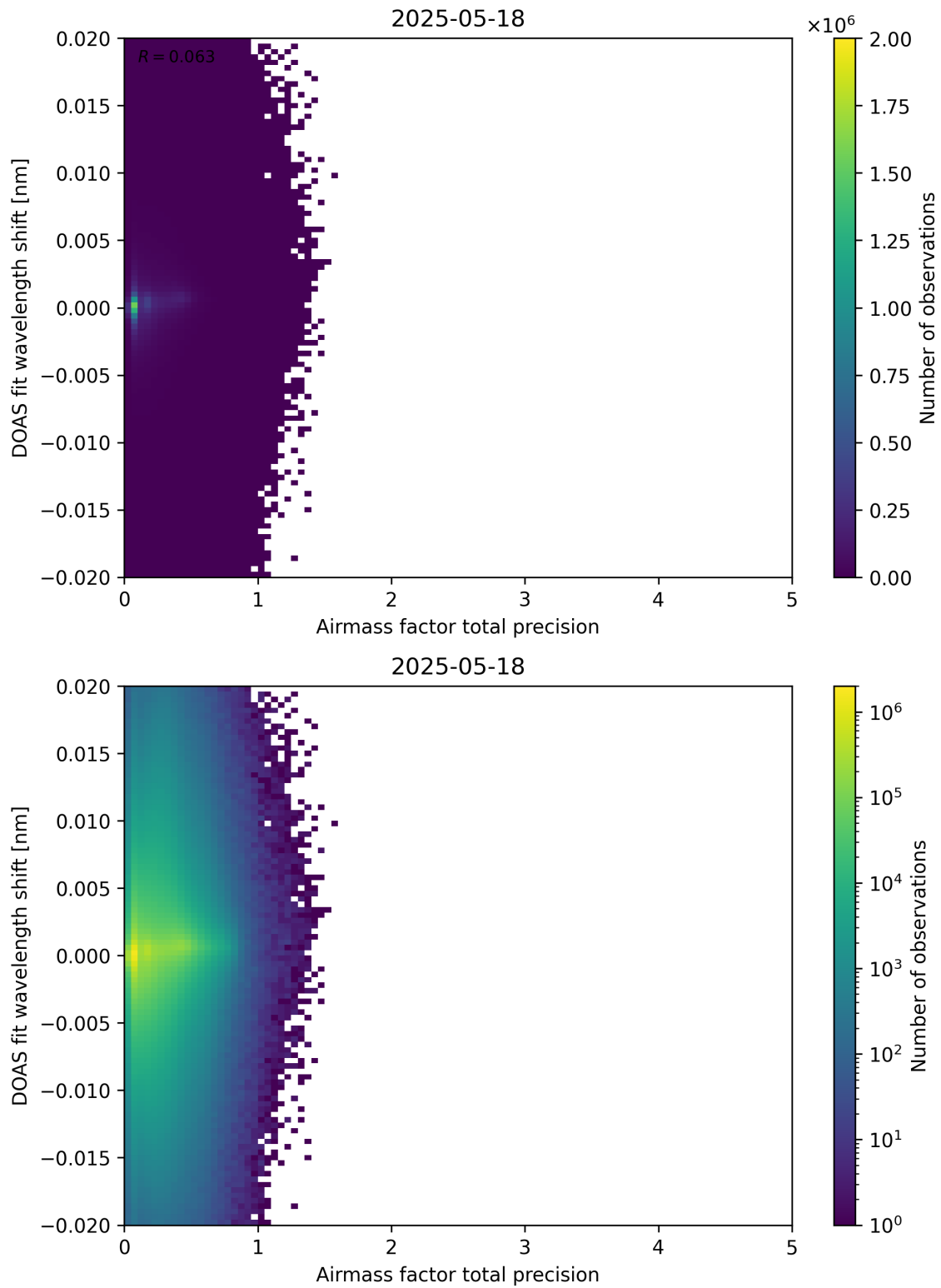
Figure 106: Scatter density plot of “Airmass factor total precision” against “DOAS fit wavelength shift” for 2025-05-17 to 2025-05-19.
