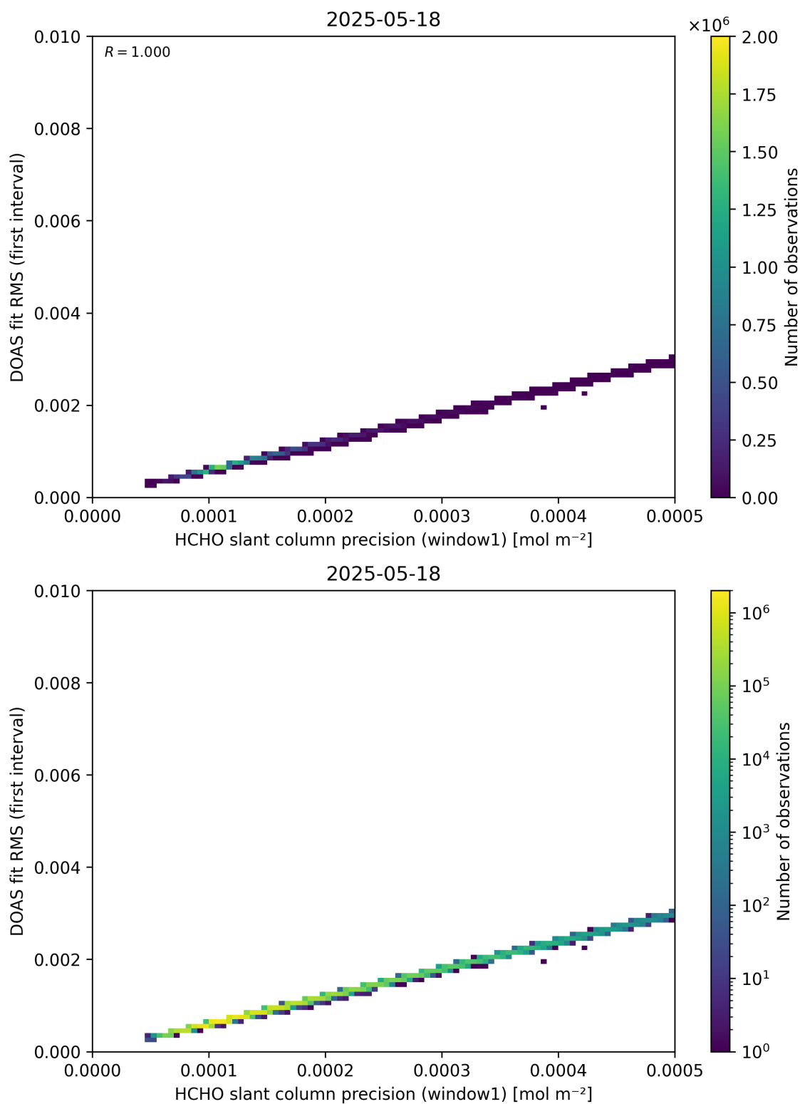
Figure 88: Scatter density plot of “HCHO slant column precision (window1)” against “DOAS fit RMS (first interval)” for 2025-05-17 to 2025-05-19.
