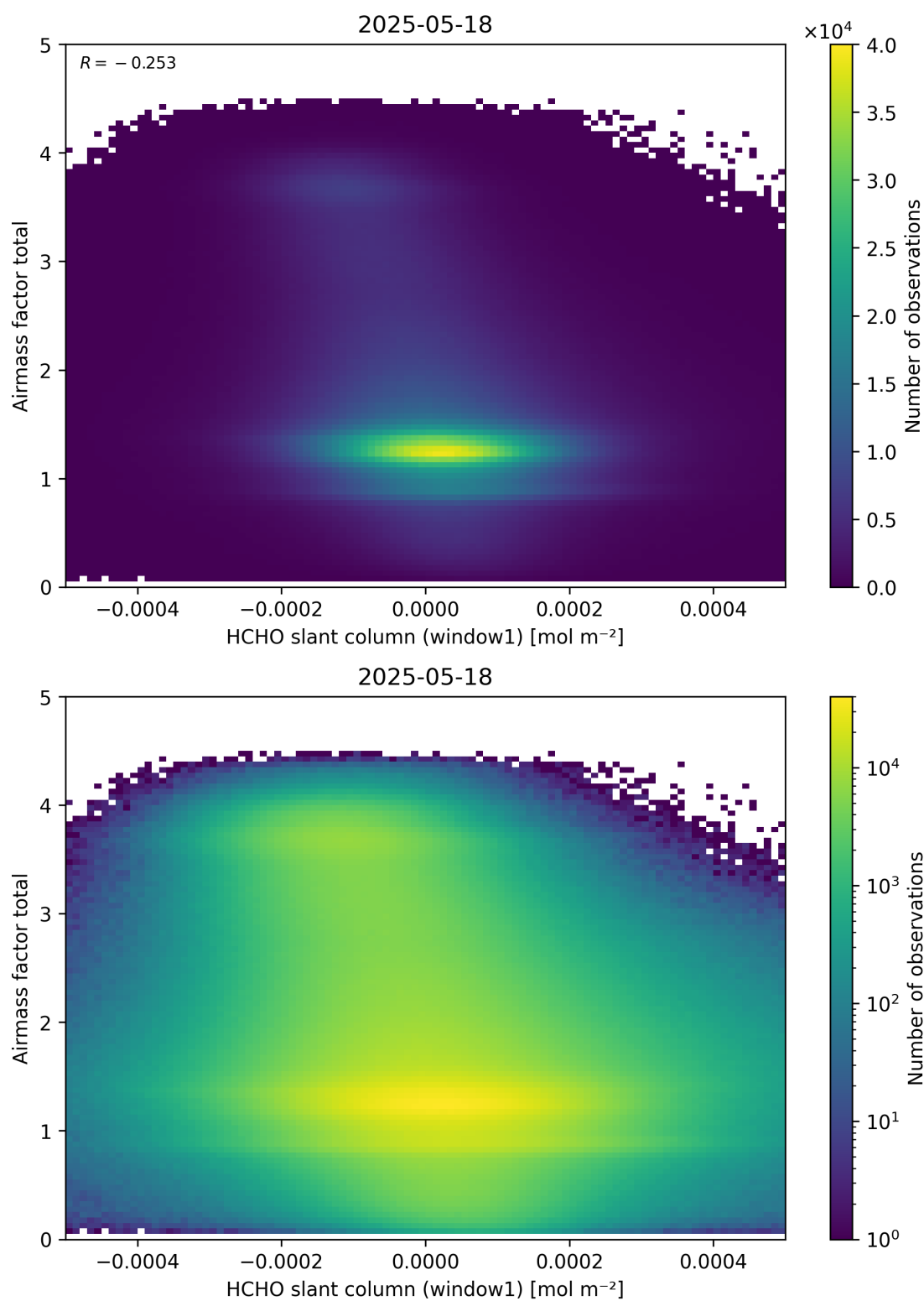
Figure 85: Scatter density plot of “HCHO slant column (window1)” against “Airmass factor total” for 2025-05-17 to 2025-05-19.
