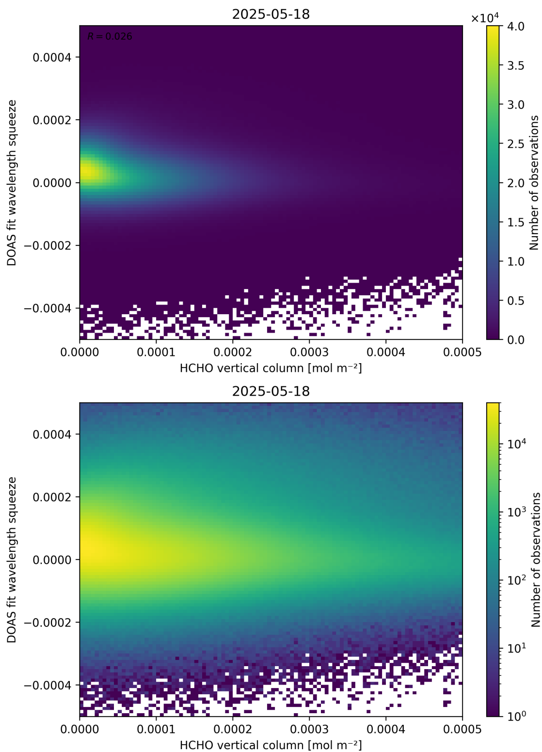
Figure 125: Scatter density plot of “HCHO vertical column” against “DOAS fit wavelength squeeze” for 2025-05-17 to 2025-05-19.
