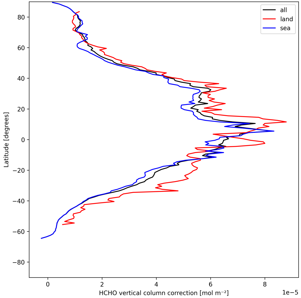
Figure 23: Zonal average of “HCHO vertical column correction” for 2025-05-17 to 2025-05-19.
