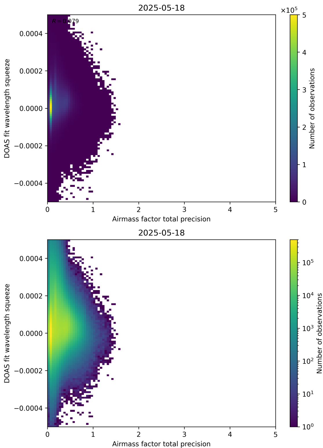
Figure 107: Scatter density plot of “Airmass factor total precision” against “DOAS fit wavelength squeeze” for 2025-05-17 to 2025-05-19.
