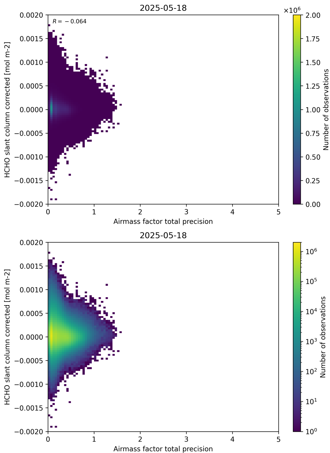
Figure 109: Scatter density plot of “Airmass factor total precision” against “HCHO slant column corrected” for 2025-05-17 to 2025-05-19.
