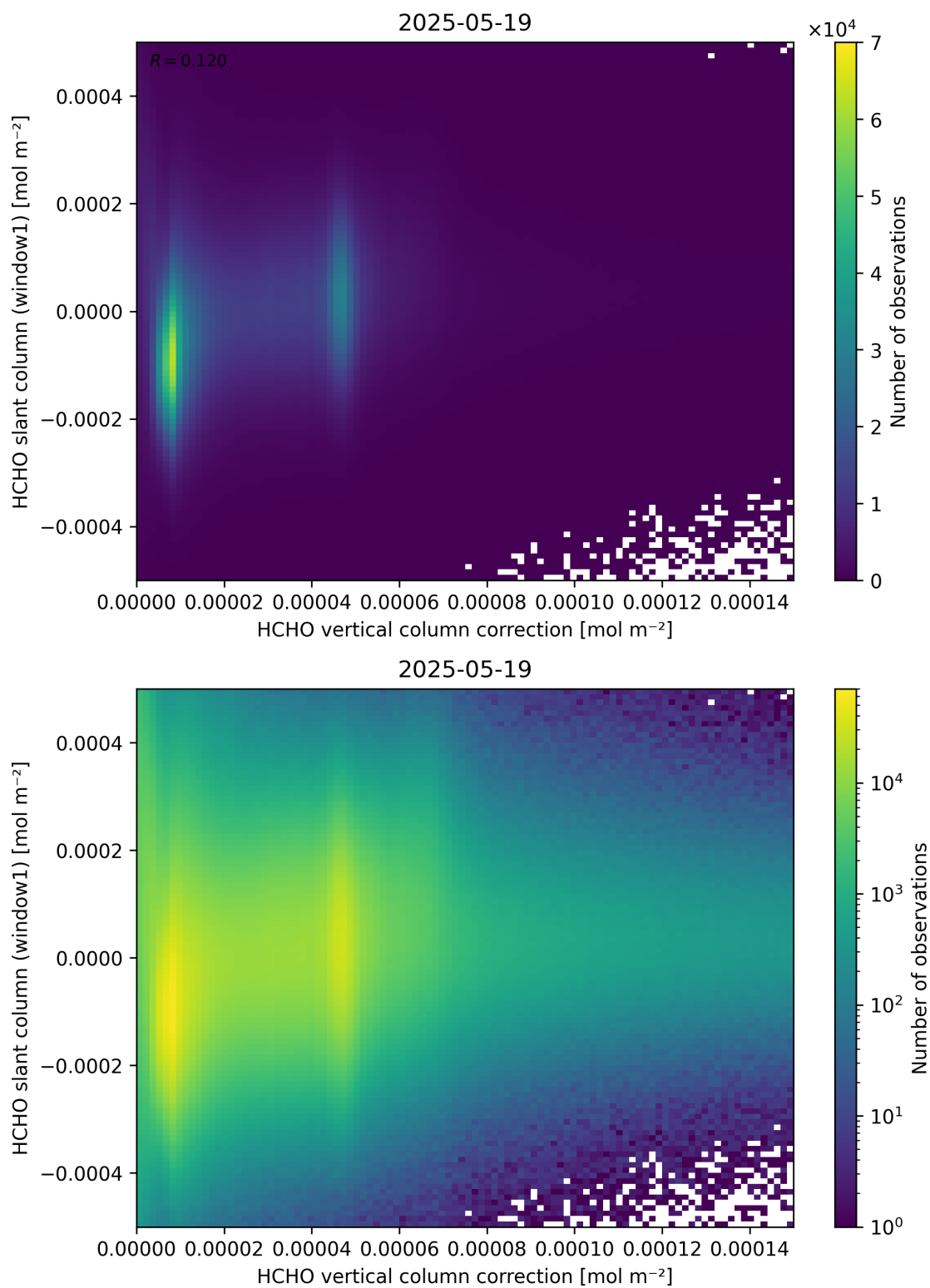
Figure 118: Scatter density plot of “HCHO vertical column correction” against “HCHO slant column (window1)” for 2025-05-18 to 2025-05-20.
