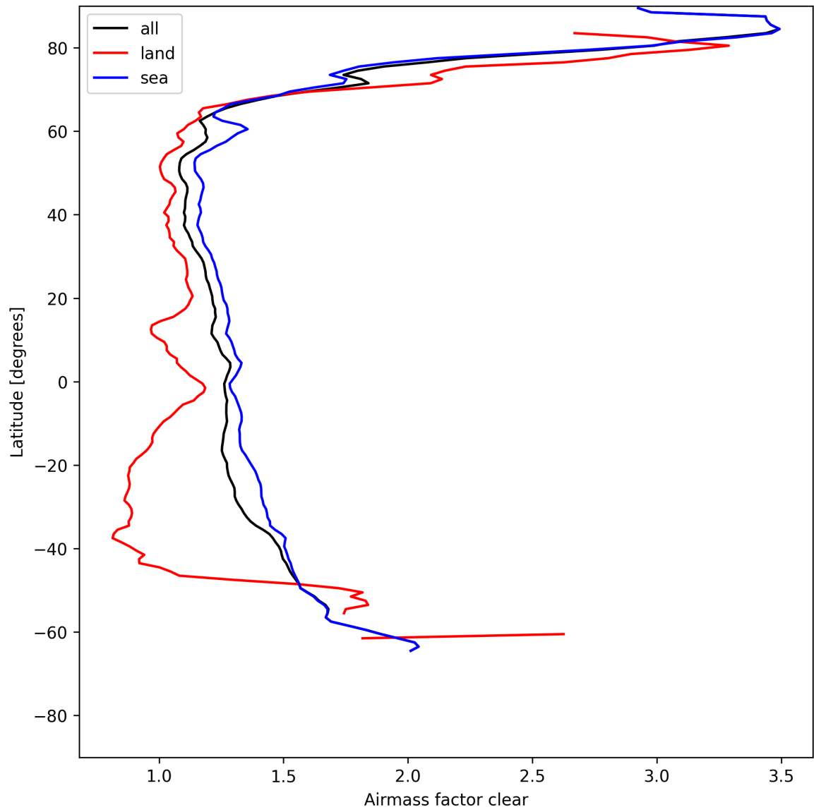
Figure 28: Zonal average of “Airmass factor clear” for 2025-05-18 to 2025-05-20.
