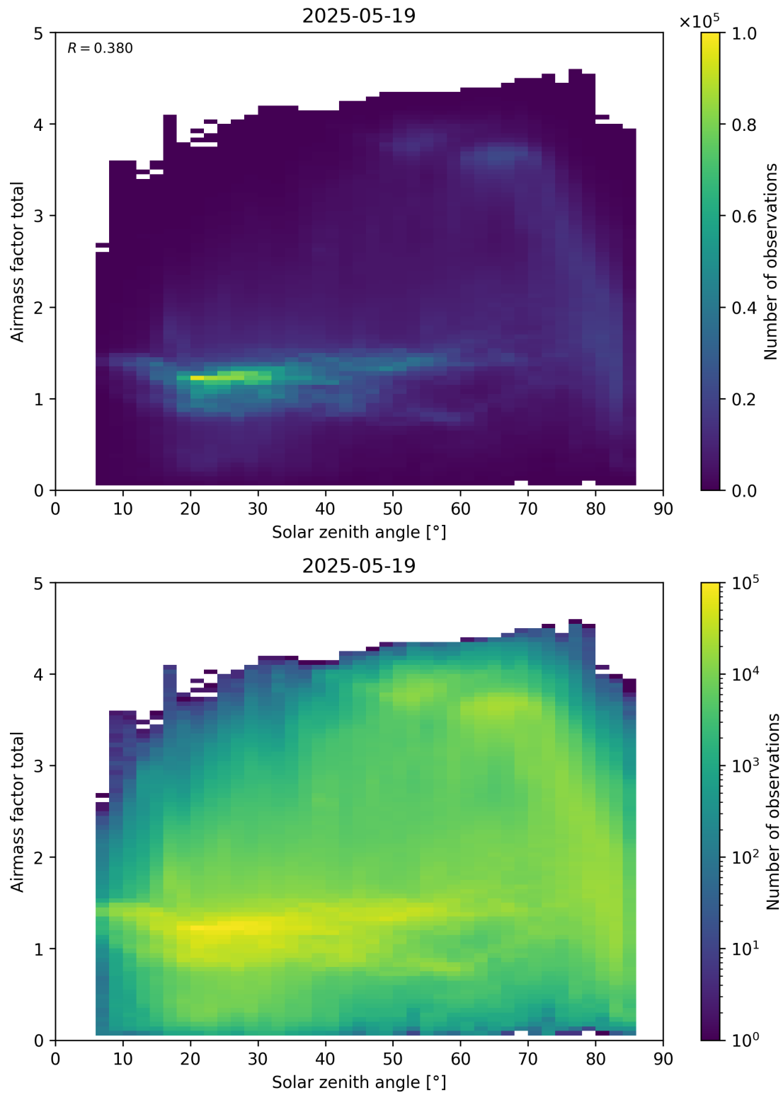
Figure 175: Scatter density plot of “Solar zenith angle” against “Airmass factor total” for 2025-05-18 to 2025-05-20.
