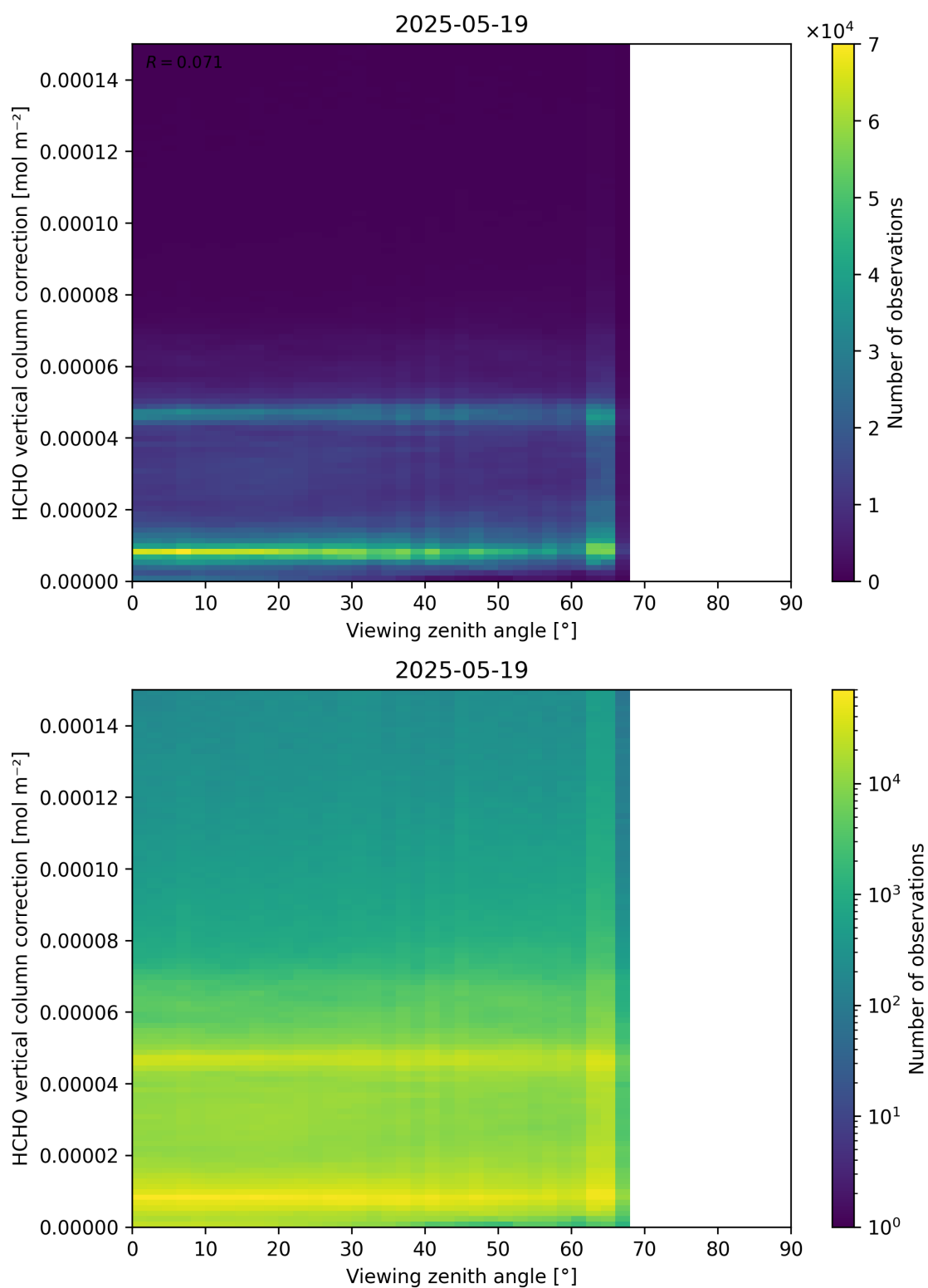
Figure 193: Scatter density plot of “Viewing zenith angle” against “HCHO vertical column correction” for 2025-05-18 to 2025-05-20.
