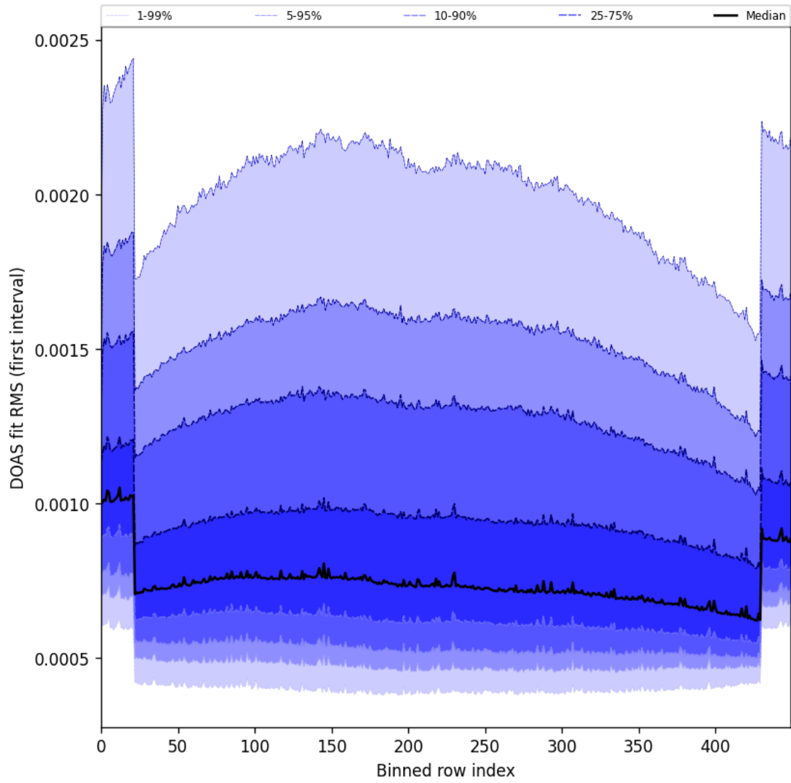
Figure 60: Along track statistics of “DOAS fit RMS (first interval)” for 2025-05-18 to 2025-05-20
