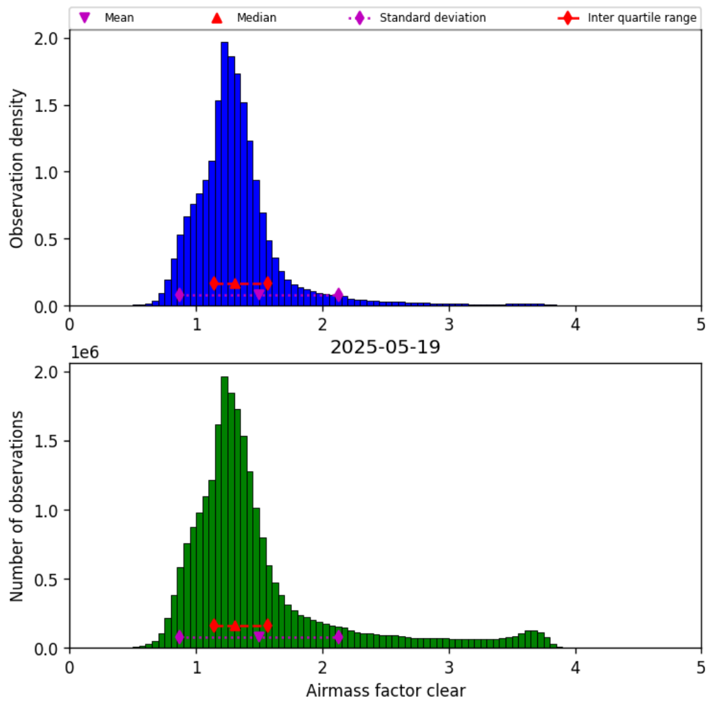
Figure 42: Histogram of “Airmass factor clear” for 2025-05-18 to 2025-05-20
