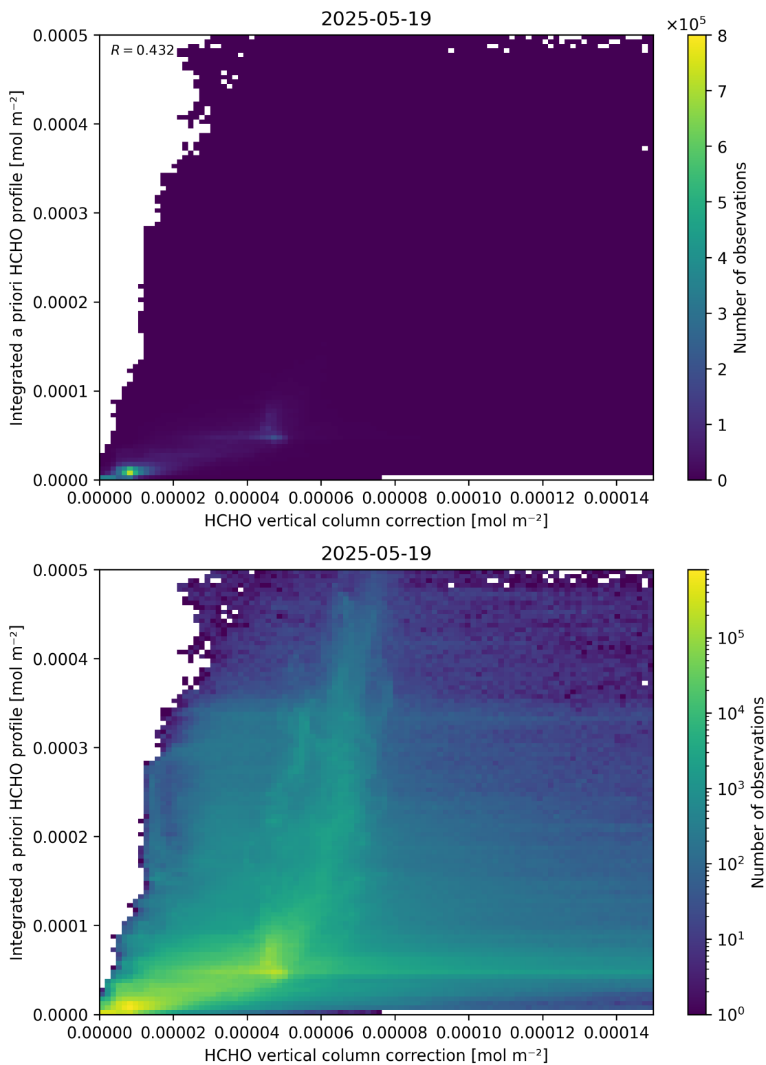
Figure 122: Scatter density plot of “HCHO vertical column correction” against “Integrated a priori HCHO profile” for 2025-05-18 to 2025-05-20.
