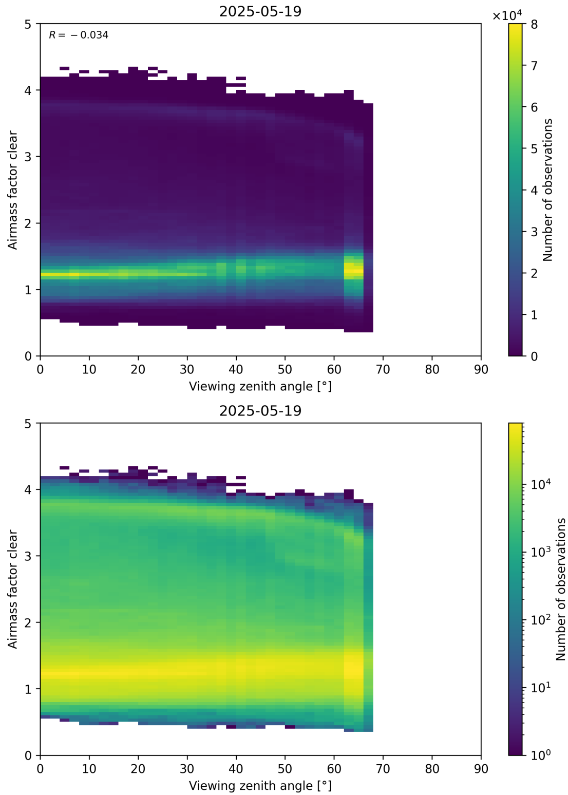
Figure 185: Scatter density plot of “Viewing zenith angle” against “Airmass factor clear” for 2025-05-18 to 2025-05-20.
