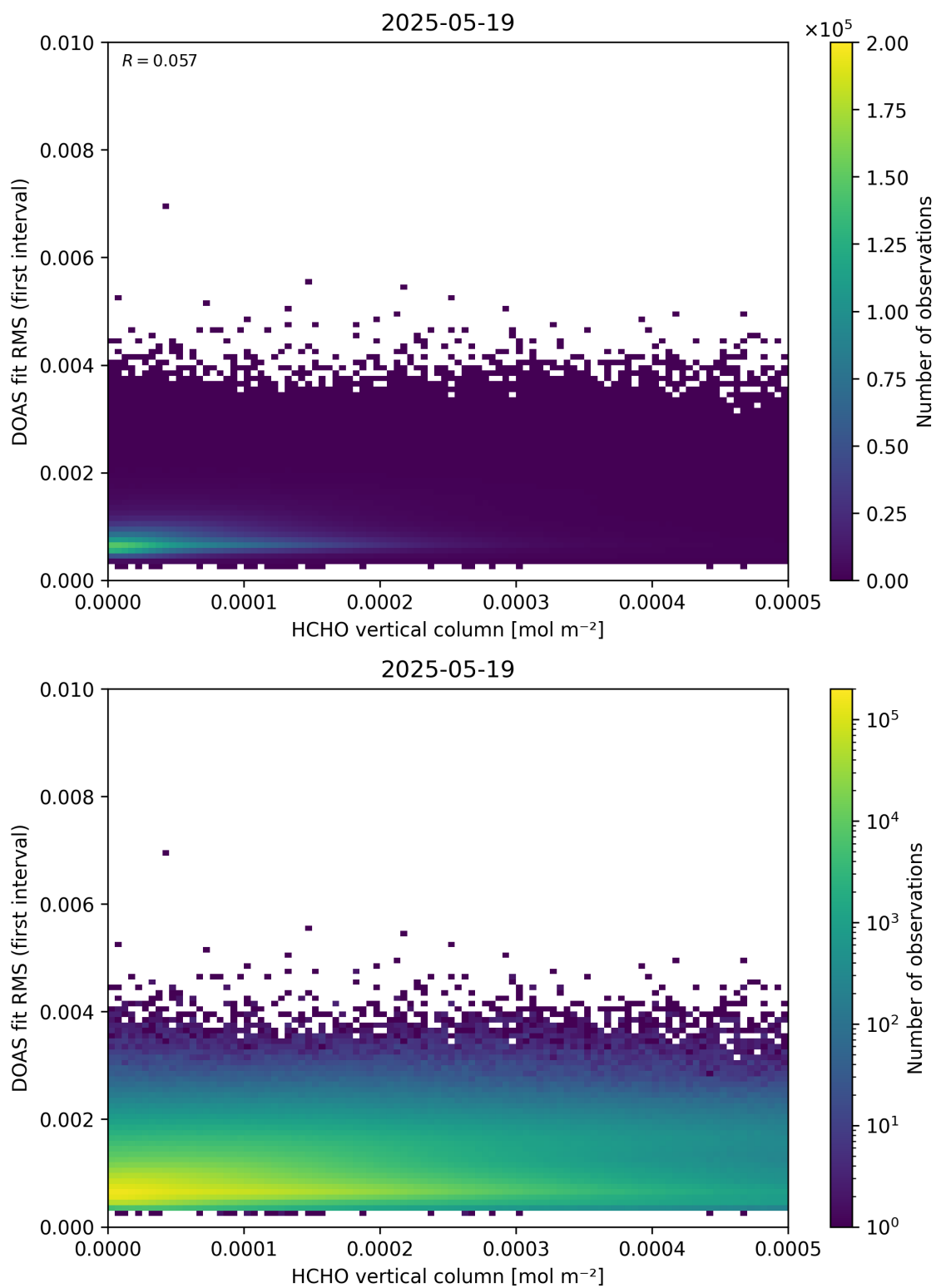
Figure 123: Scatter density plot of “HCHO vertical column” against “DOAS fit RMS (first interval)” for 2025-05-18 to 2025-05-20.
