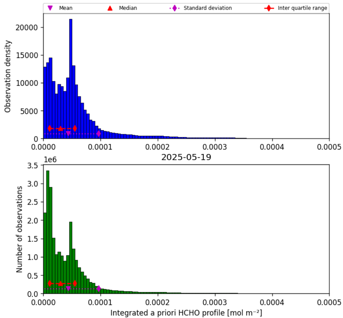
Figure 43: Histogram of “Integrated a priori HCHO profile” for 2025-05-18 to 2025-05-20
