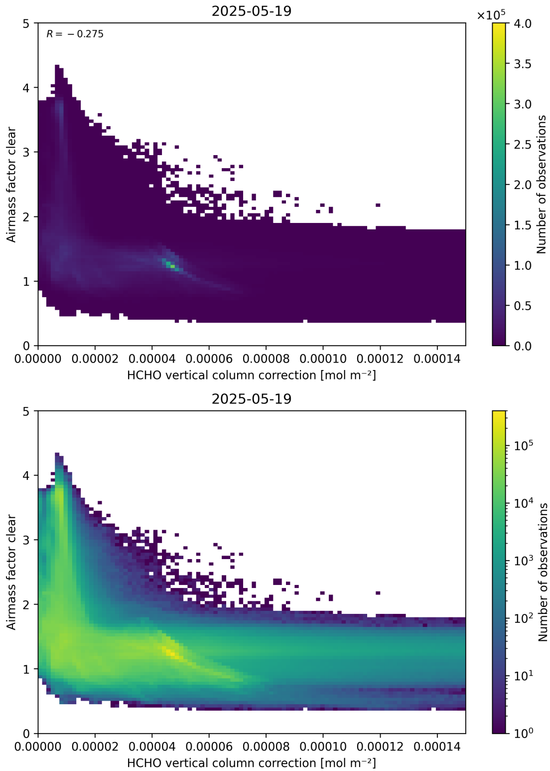
Figure 115: Scatter density plot of “HCHO vertical column correction” against “Airmass factor clear” for 2025-05-18 to 2025-05-20.
