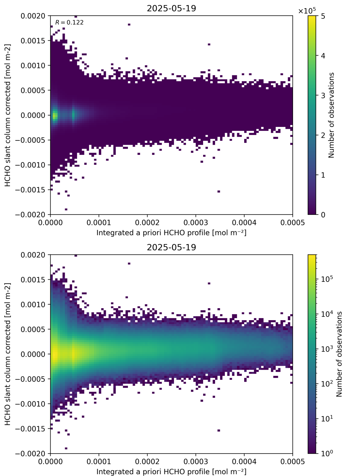
Figure 151: Scatter density plot of “Integrated a priori HCHO profile” against “HCHO slant column corrected” for 2025-05-18 to 2025-05-20.
