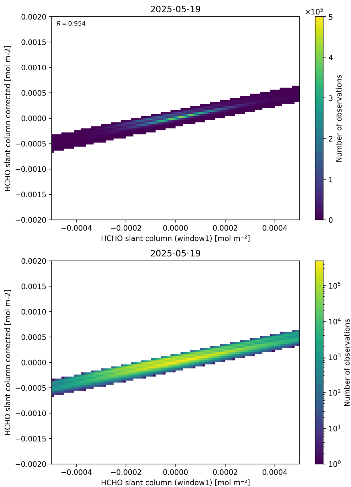
Figure 82: Scatter density plot of “HCHO slant column (window1)” against “HCHO slant column corrected” for 2025-05-18 to 2025-05-20.
