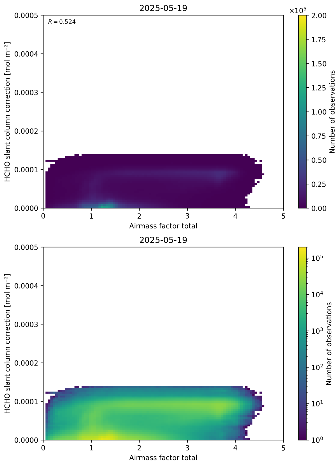
Figure 102: Scatter density plot of “Airmass factor total” against “HCHO slant column correction” for 2025-05-18 to 2025-05-20.
