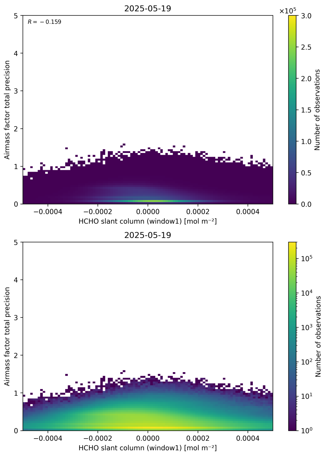
Figure 86: Scatter density plot of “HCHO slant column (window1)” against “Airmass factor total precision” for 2025-05-18 to 2025-05-20.
