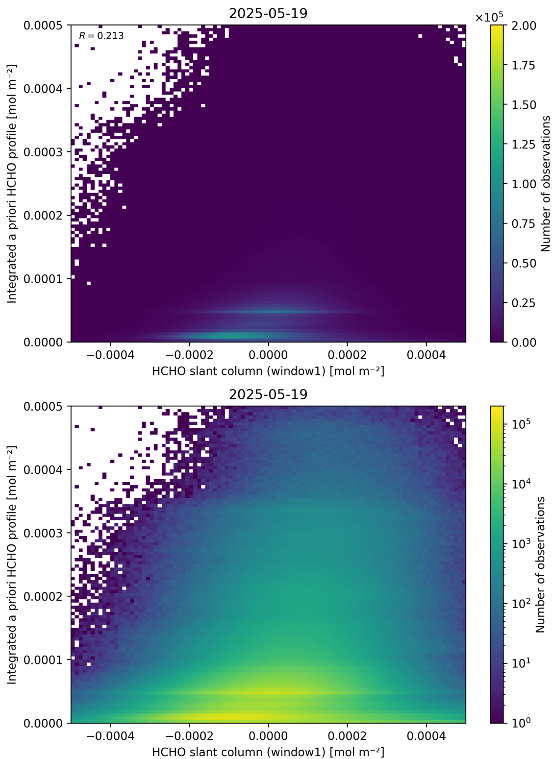
Figure 87: Scatter density plot of “HCHO slant column (window1)” against “Integrated a priori HCHO profile” for 2025-05-18 to 2025-05-20.
