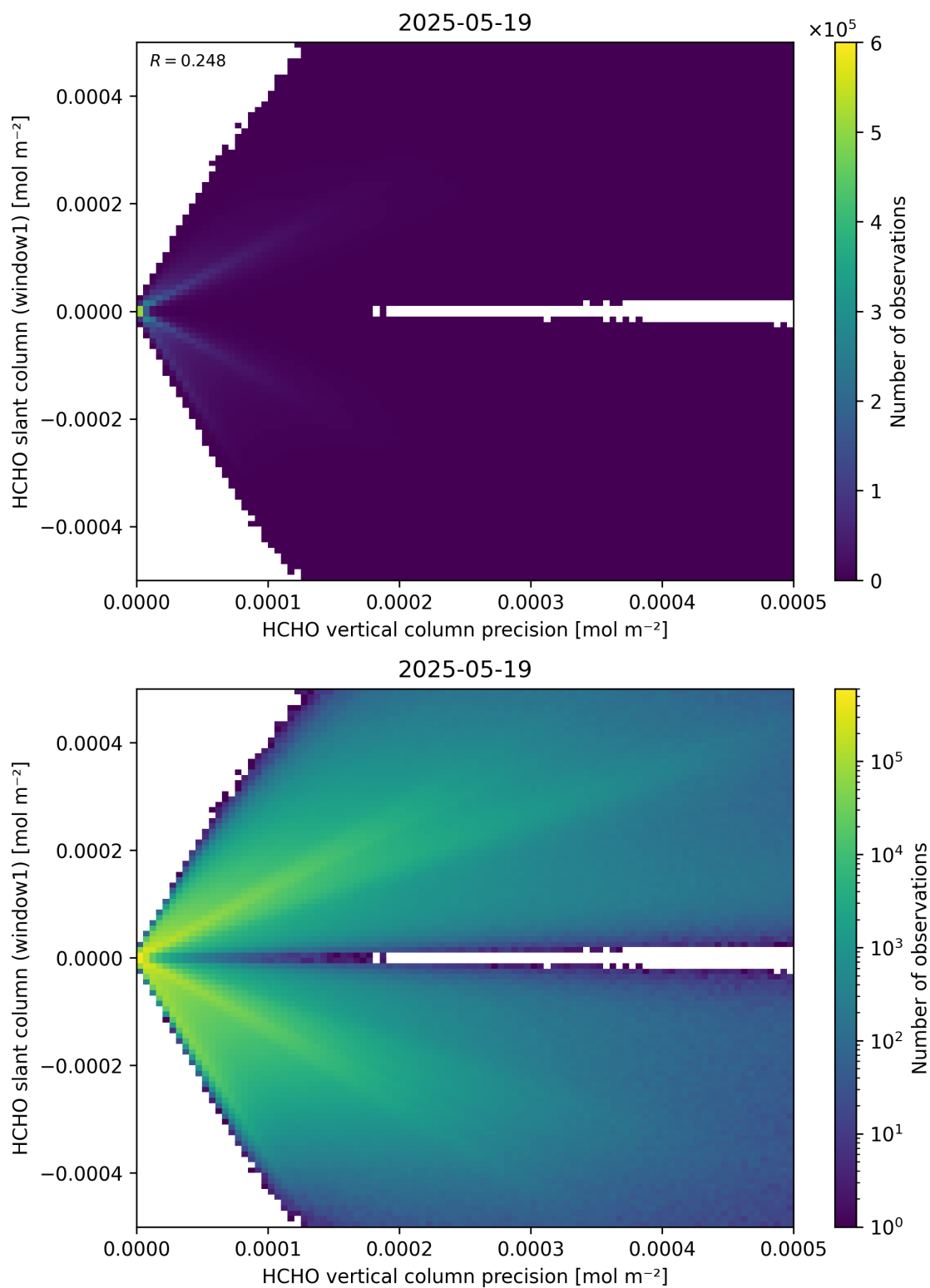
Figure 142: Scatter density plot of “HCHO vertical column precision” against “HCHO slant column (window1)” for 2025-05-18 to 2025-05-20.
