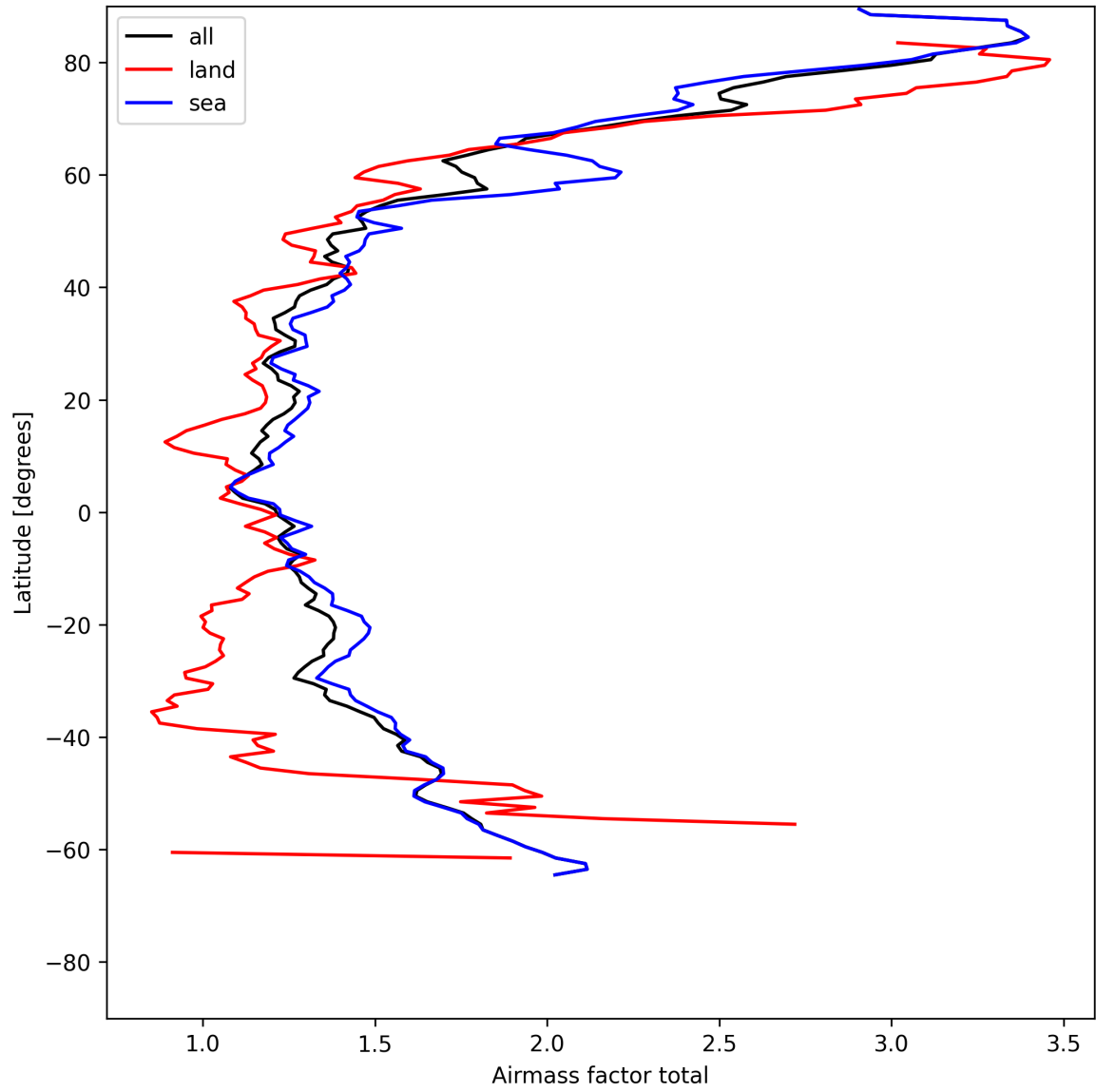
Figure 26: Zonal average of “Airmass factor total” for 2025-05-18 to 2025-05-20.
