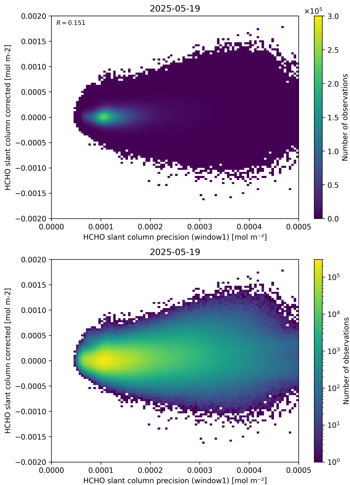
Figure 92: Scatter density plot of “HCHO slant column precision (window1)” against “HCHO slant column corrected” for 2025-05-18 to 2025-05-20.
