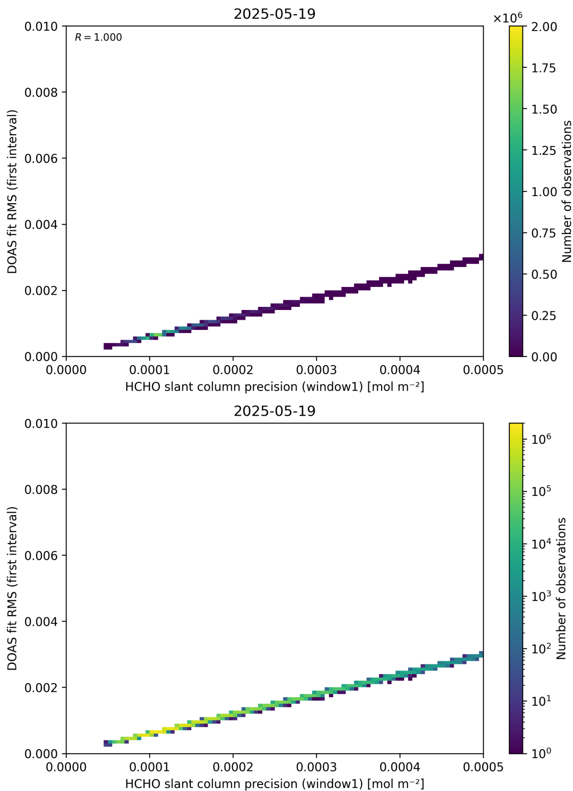
Figure 88: Scatter density plot of “HCHO slant column precision (window1)” against “DOAS fit RMS (first interval)” for 2025-05-18 to 2025-05-20.
