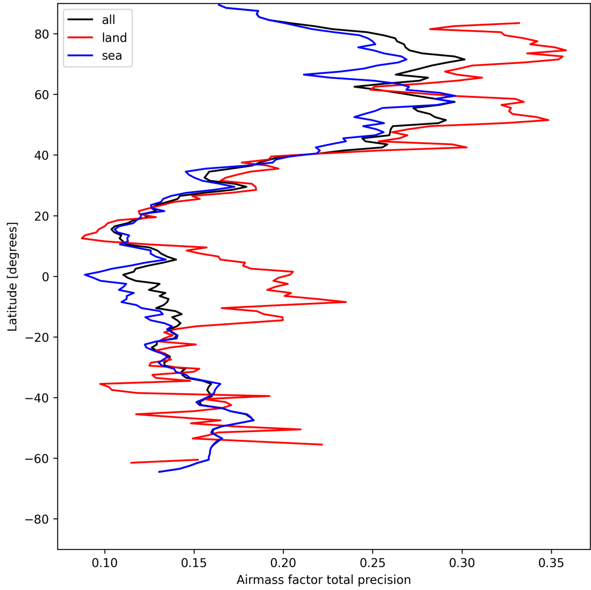
Figure 27: Zonal average of “Airmass factor total precision” for 2025-05-18 to 2025-05-20.
