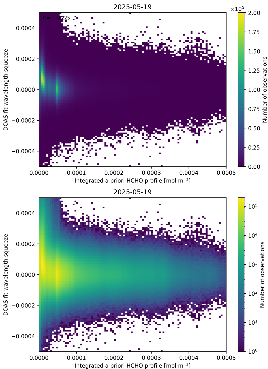
Figure 150: Scatter density plot of “Integrated a priori HCHO profile” against “DOAS fit wavelength squeeze” for 2025-05-18 to 2025-05-20.
