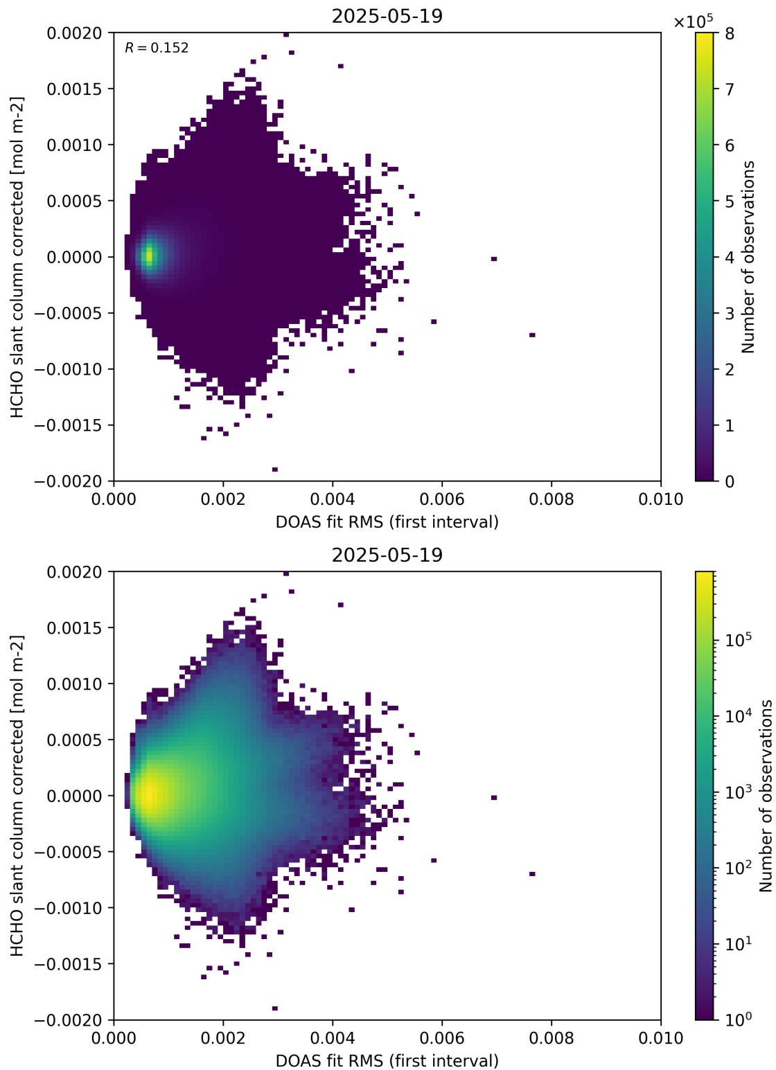
Figure 62: Scatter density plot of “DOAS fit RMS (first interval)” against “HCHO slant column corrected” for 2025-05-18 to 2025-05-20.
