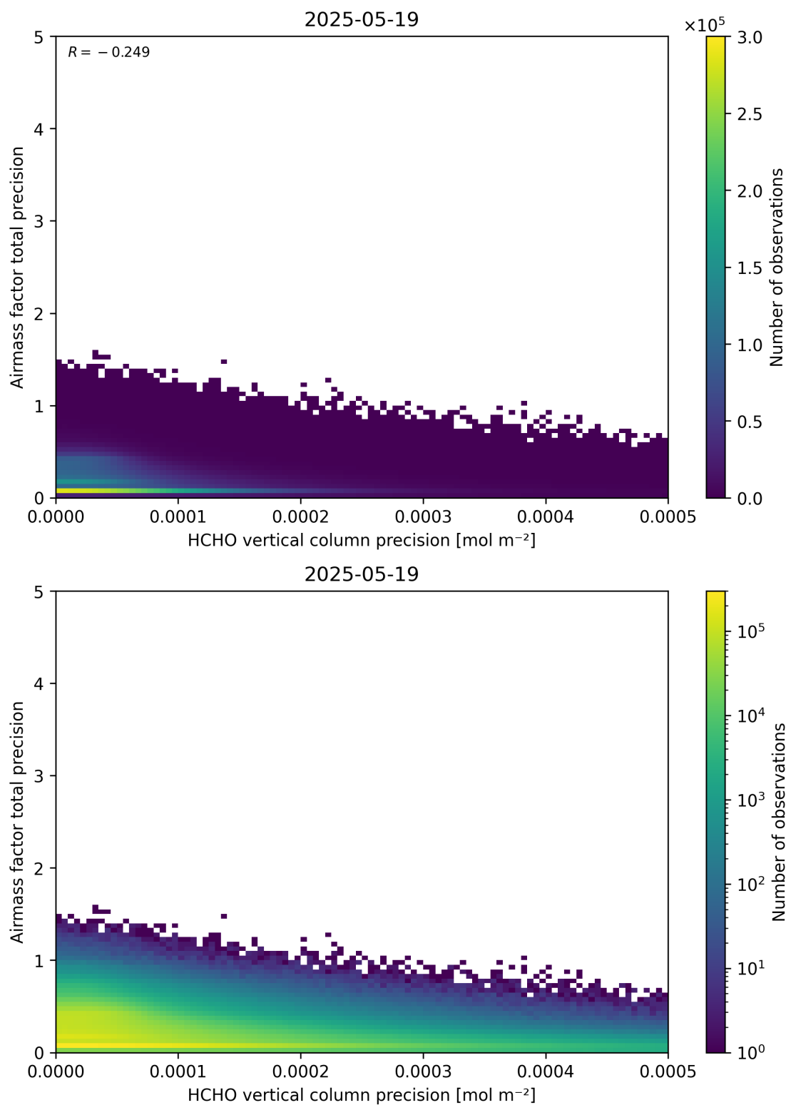
Figure 145: Scatter density plot of “HCHO vertical column precision” against “Airmass factor total precision” for 2025-05-18 to 2025-05-20.
