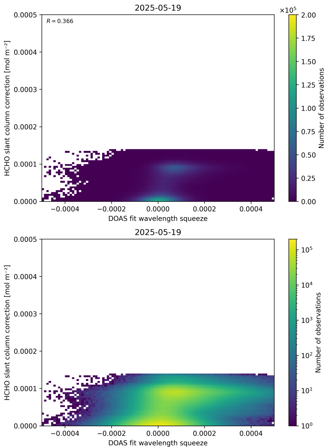
Figure 70: Scatter density plot of “DOAS fit wavelength squeeze” against “HCHO slant column correction” for 2025-05-18 to 2025-05-20.
