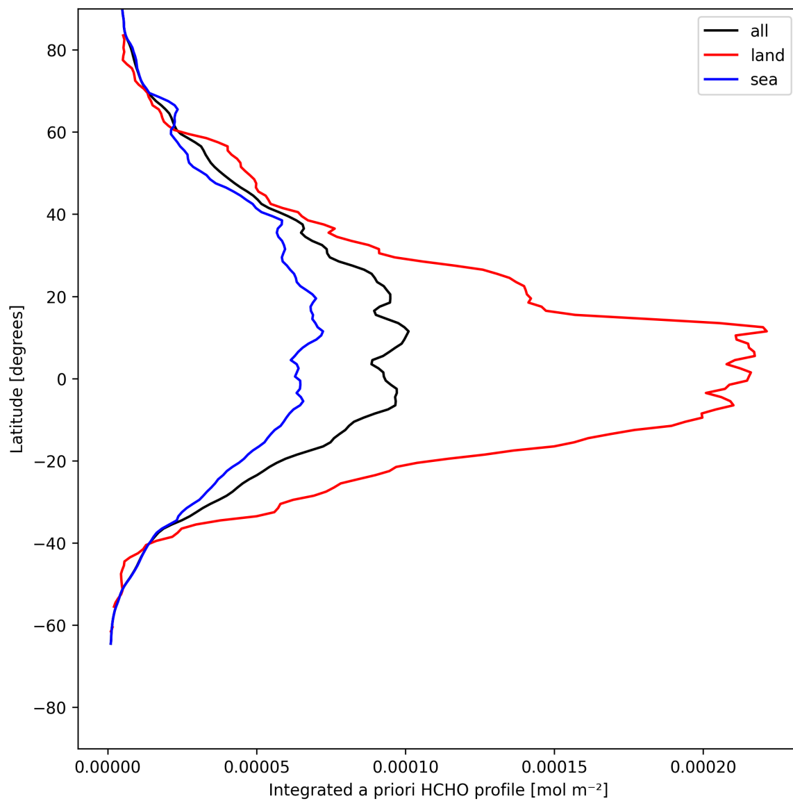
Figure 29: Zonal average of “Integrated a priori HCHO profile” for 2025-05-18 to 2025-05-20.
