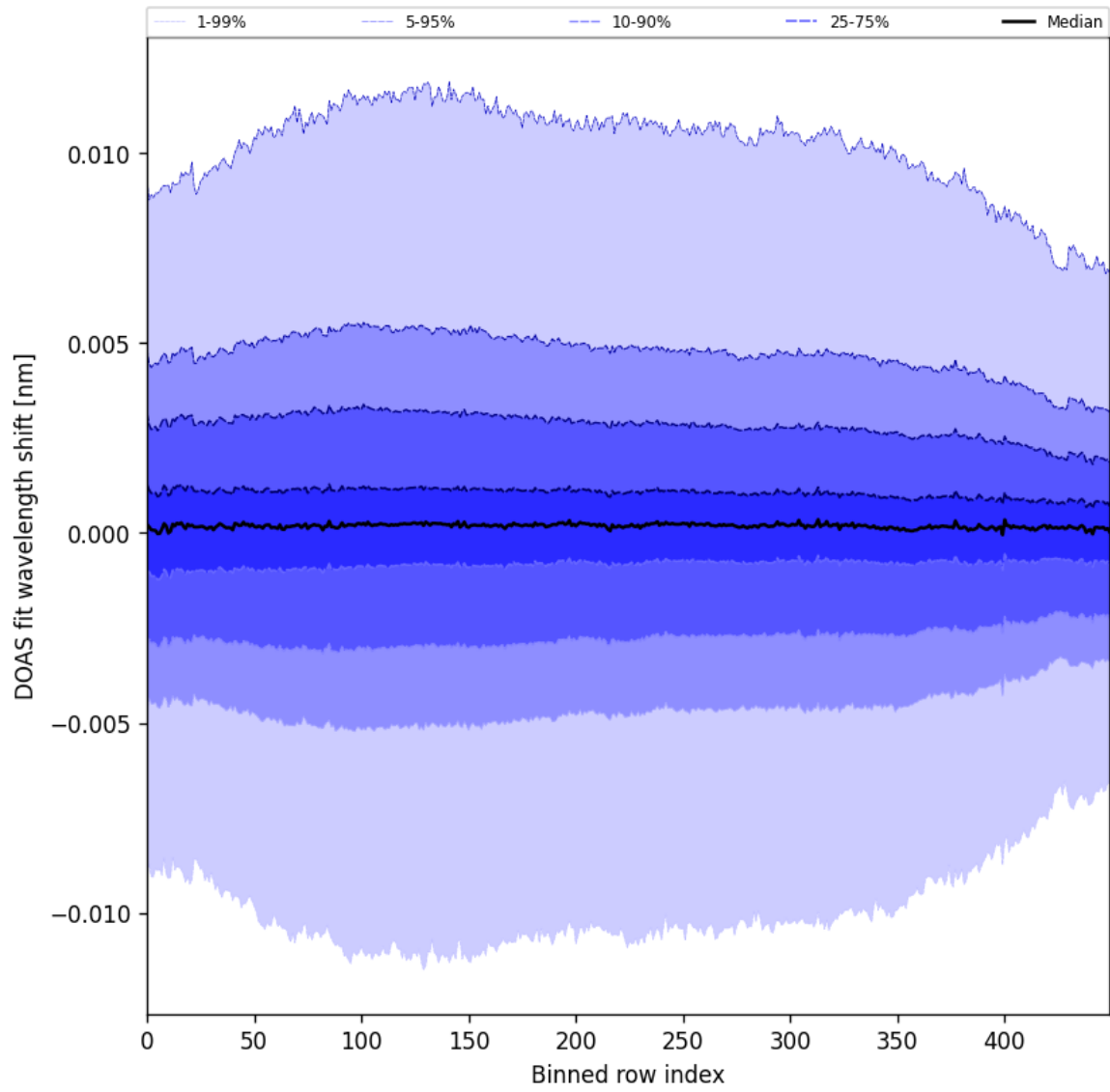
Figure 58: Along track statistics of “DOAS fit wavelength shift” for 2025-05-18 to 2025-05-20
