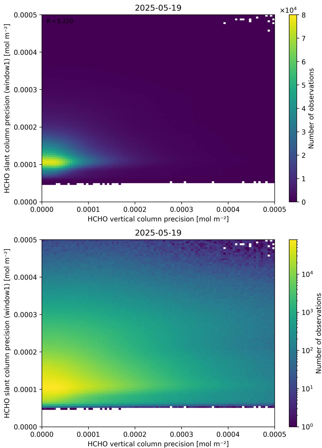
Figure 143: Scatter density plot of “HCHO vertical column precision” against “HCHO slant column precision (window1)” for 2025-05-18 to 2025-05-20.
