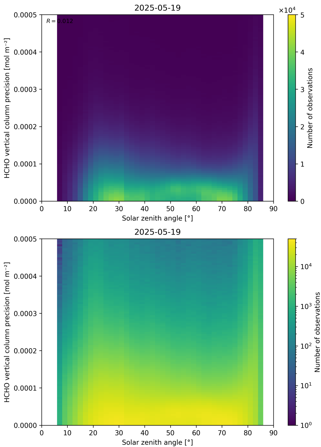
Figure 179: Scatter density plot of “Solar zenith angle” against “HCHO vertical column precision” for 2025-05-18 to 2025-05-20.
