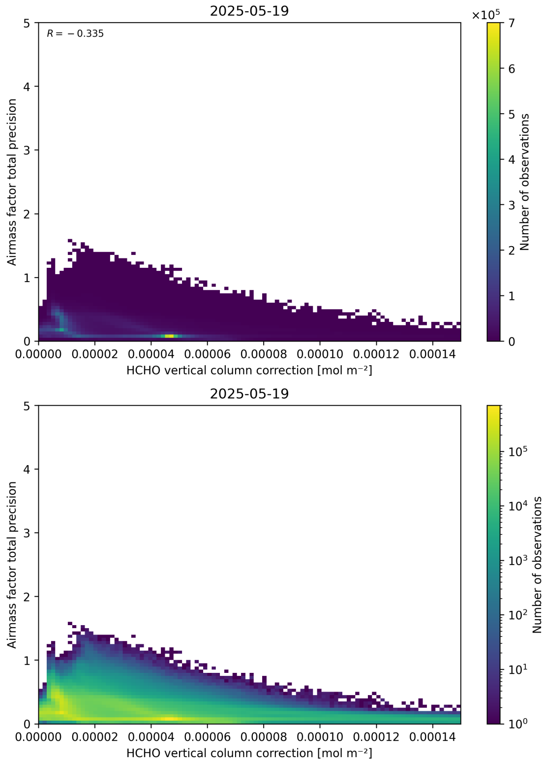
Figure 121: Scatter density plot of “HCHO vertical column correction” against “Airmass factor total precision” for 2025-05-18 to 2025-05-20.
