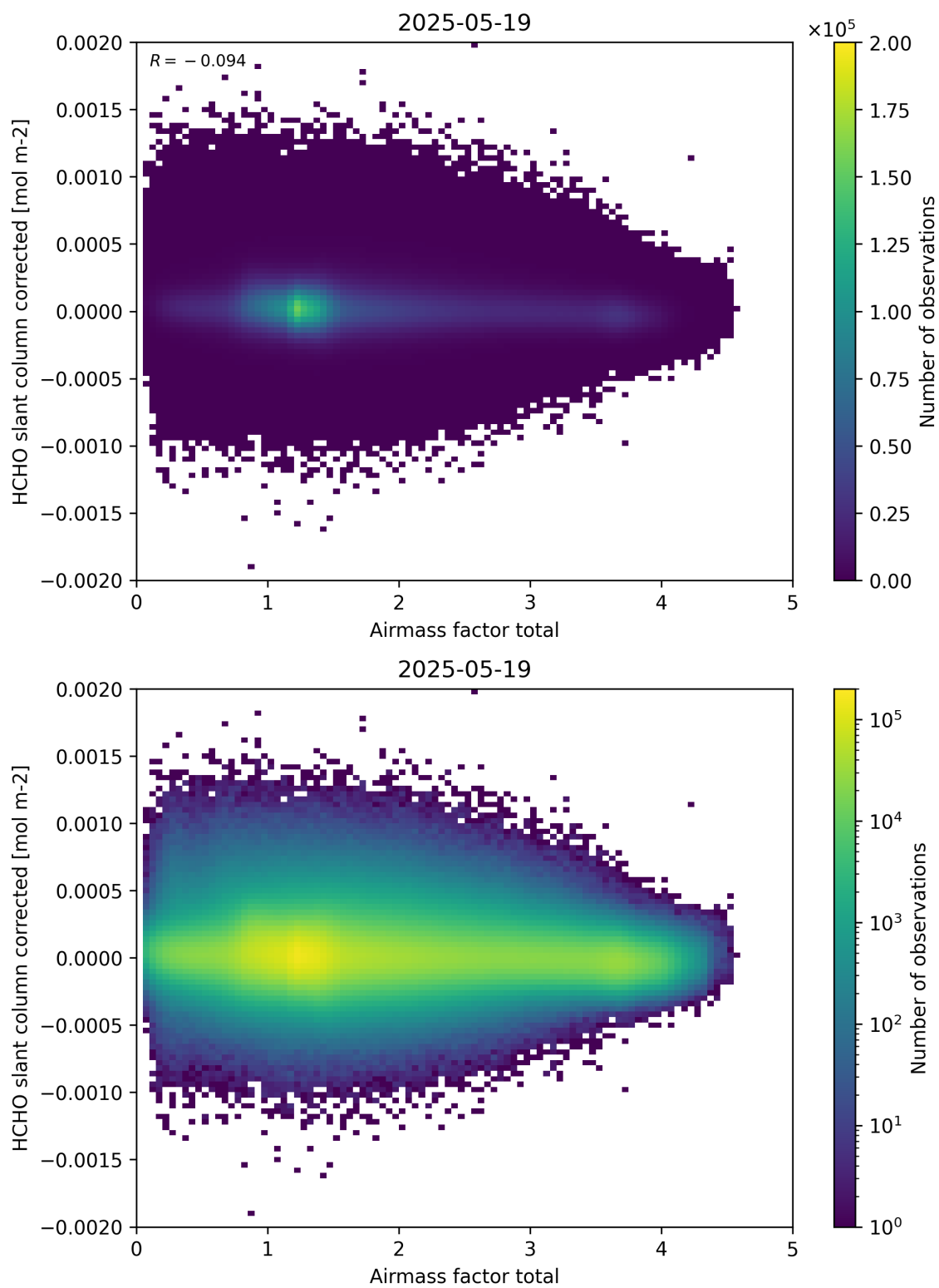
Figure 101: Scatter density plot of “Airmass factor total” against “HCHO slant column corrected” for 2025-05-18 to 2025-05-20.
