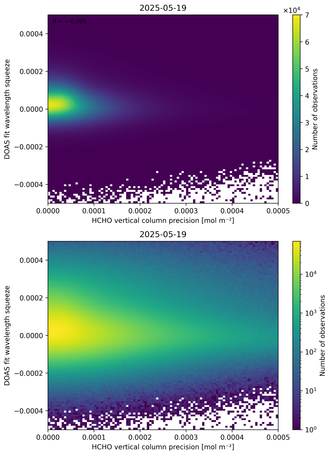
Figure 138: Scatter density plot of “HCHO vertical column precision” against “DOAS fit wavelength squeeze” for 2025-05-18 to 2025-05-20.
