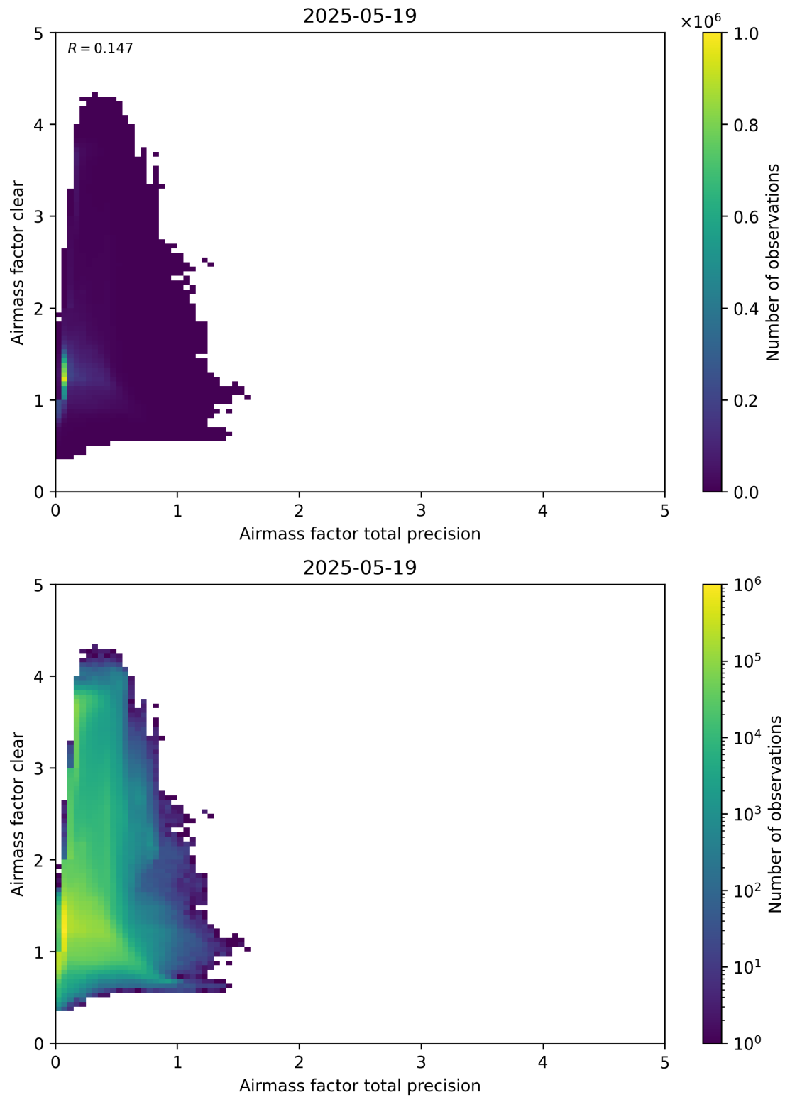
Figure 108: Scatter density plot of “Airmass factor total precision” against “Airmass factor clear” for 2025-05-18 to 2025-05-20.
