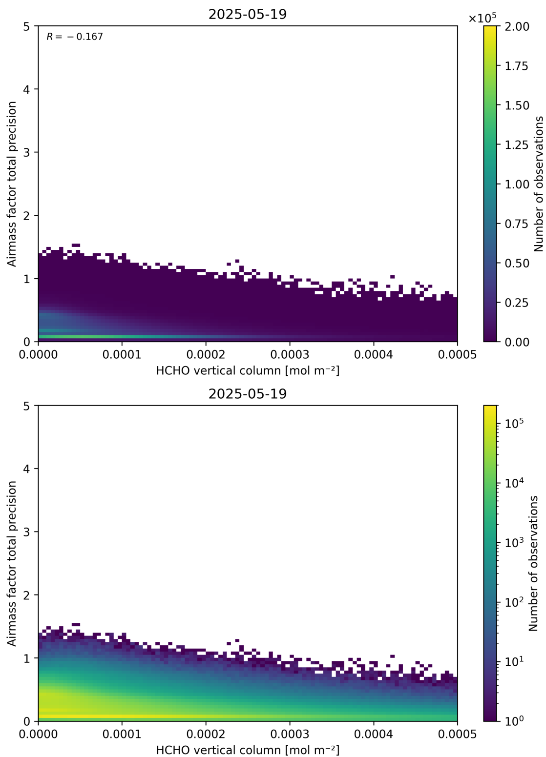
Figure 132: Scatter density plot of “HCHO vertical column” against “Airmass factor total precision” for 2025-05-18 to 2025-05-20.
