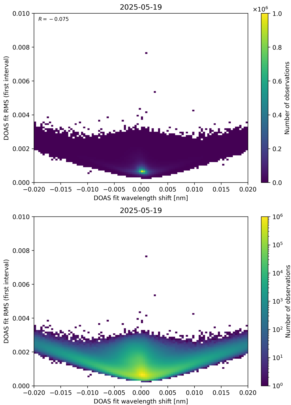
Figure 64: Scatter density plot of “DOAS fit wavelength shift” against “DOAS fit RMS (first interval)” for 2025-05-18 to 2025-05-20.
