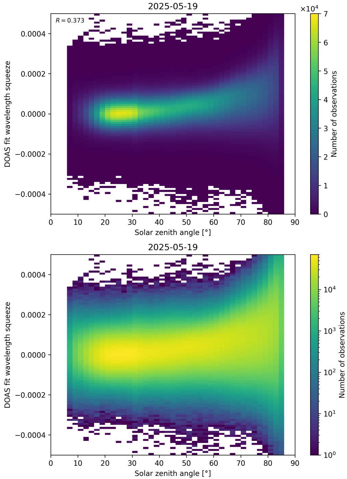
Figure 169: Scatter density plot of “Solar zenith angle” against “DOAS fit wavelength squeeze” for 2025-05-18 to 2025-05-20.
