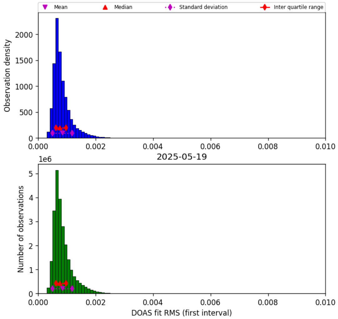
Figure 46: Histogram of “DOAS fit RMS (first interval)” for 2025-05-18 to 2025-05-20
