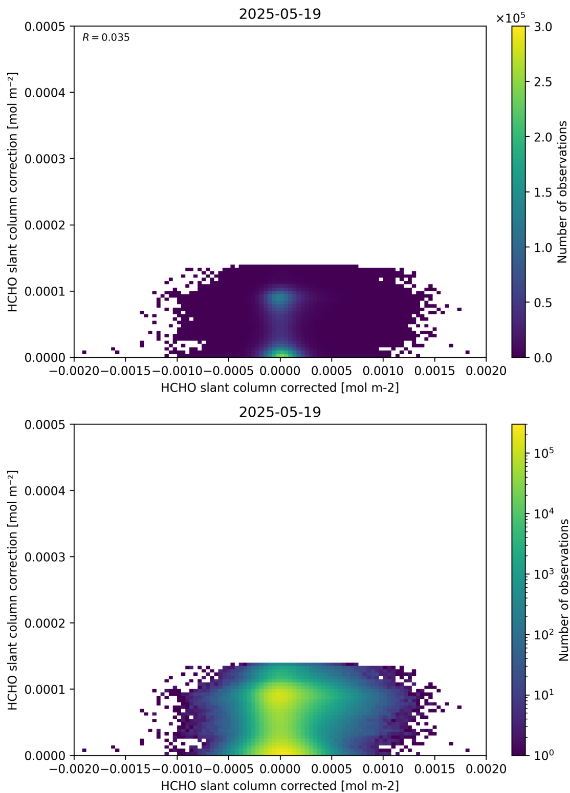
Figure 77: Scatter density plot of “HCHO slant column corrected” against “HCHO slant column correction” for 2025-05-18 to 2025-05-20.
