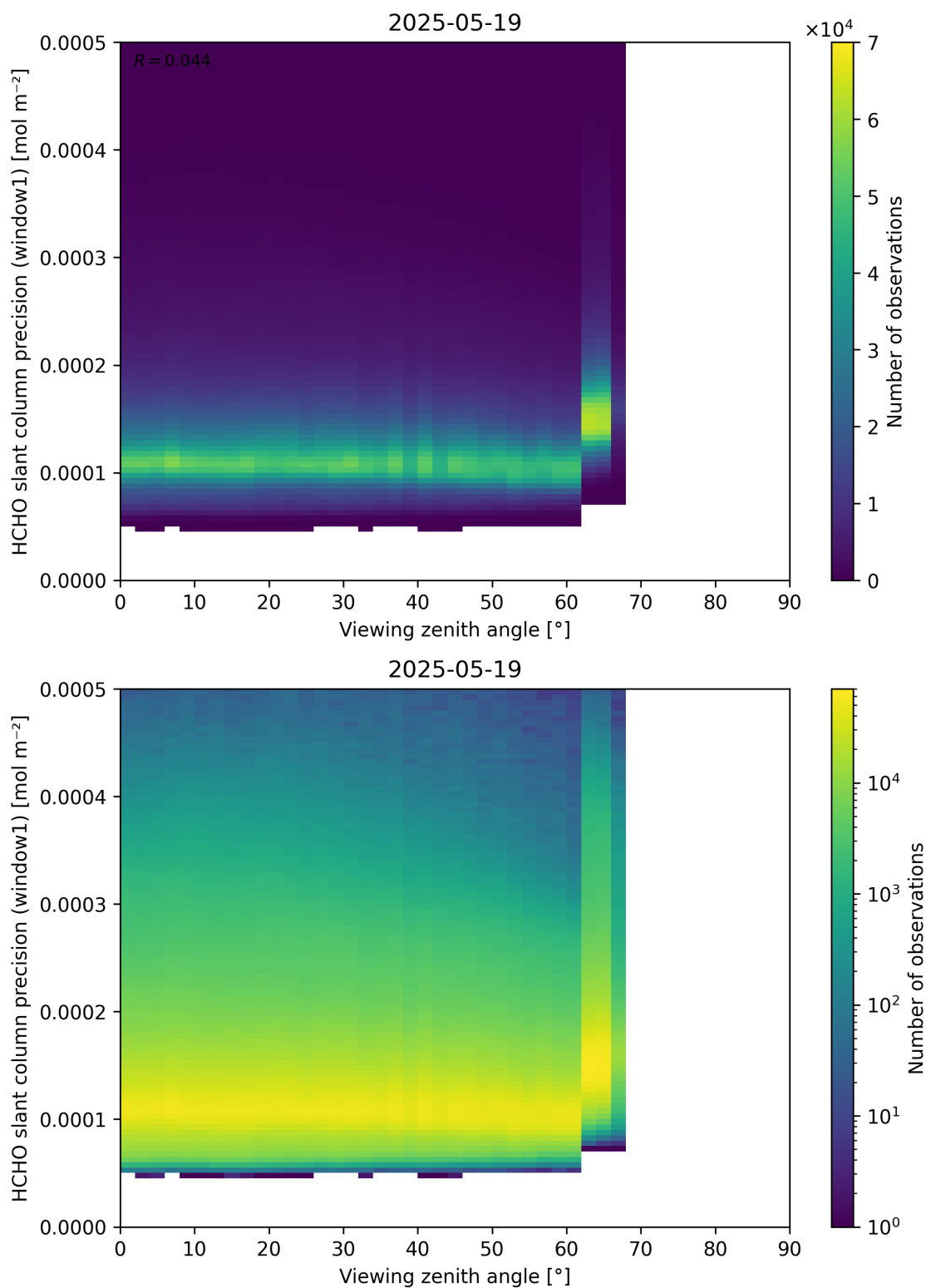
Figure 189: Scatter density plot of “Viewing zenith angle” against “HCHO slant column precision (window1)” for 2025-05-18 to 2025-05-20.
