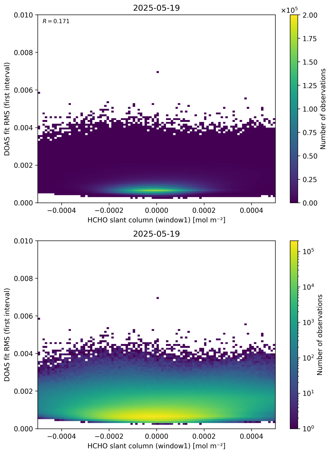
Figure 78: Scatter density plot of “HCHO slant column (window1)” against “DOAS fit RMS (first interval)” for 2025-05-18 to 2025-05-20.
