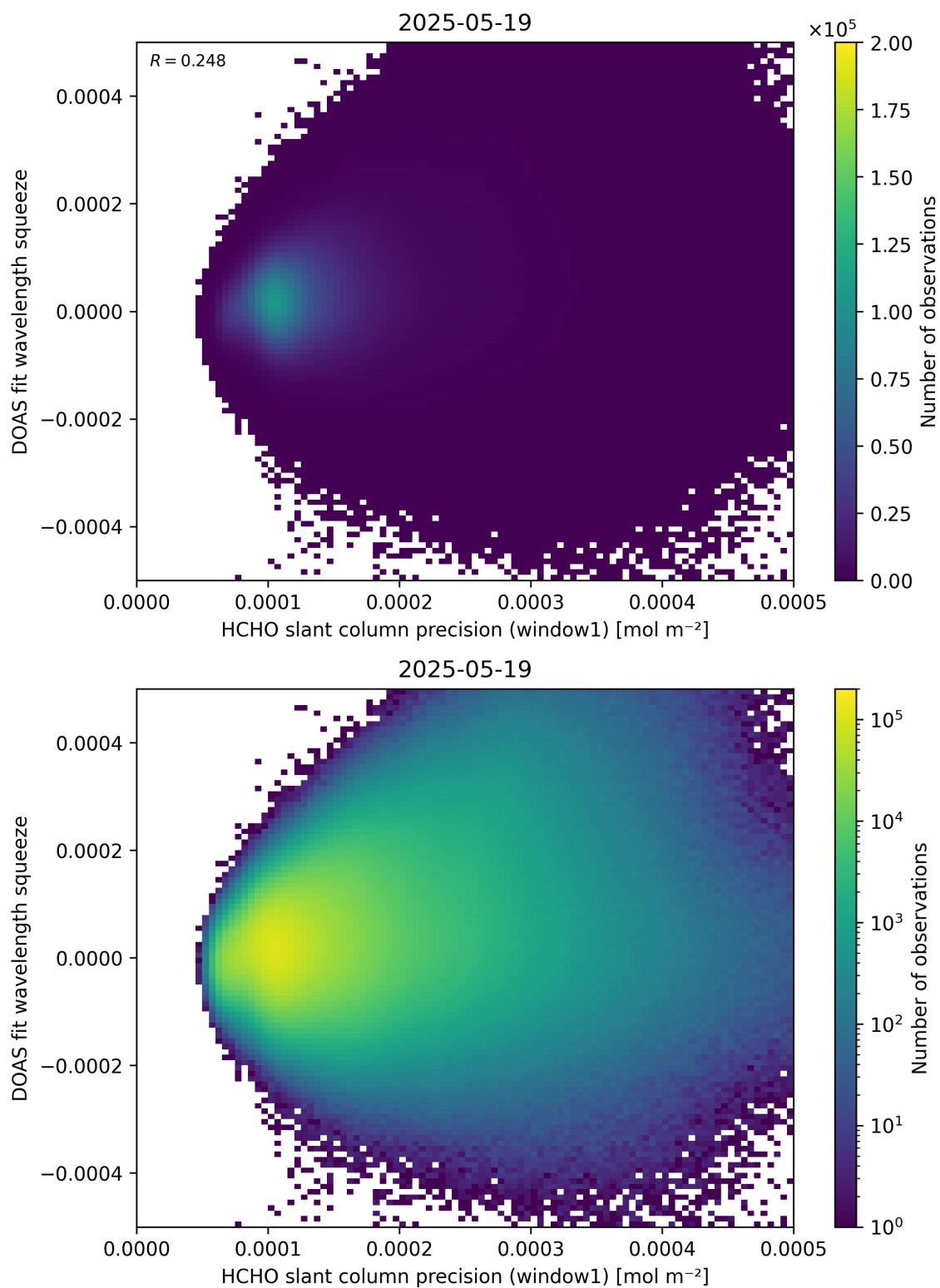
Figure 90: Scatter density plot of “HCHO slant column precision (window1)” against “DOAS fit wavelength squeeze” for 2025-05-18 to 2025-05-20.
