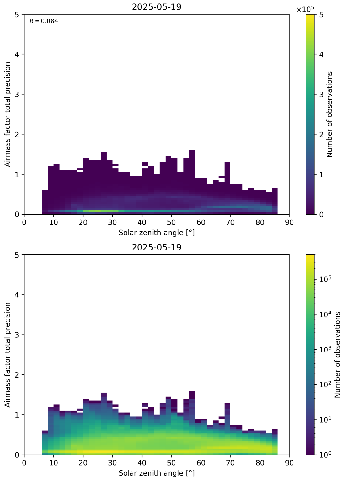
Figure 176: Scatter density plot of “Solar zenith angle” against “Airmass factor total precision” for 2025-05-18 to 2025-05-20.
