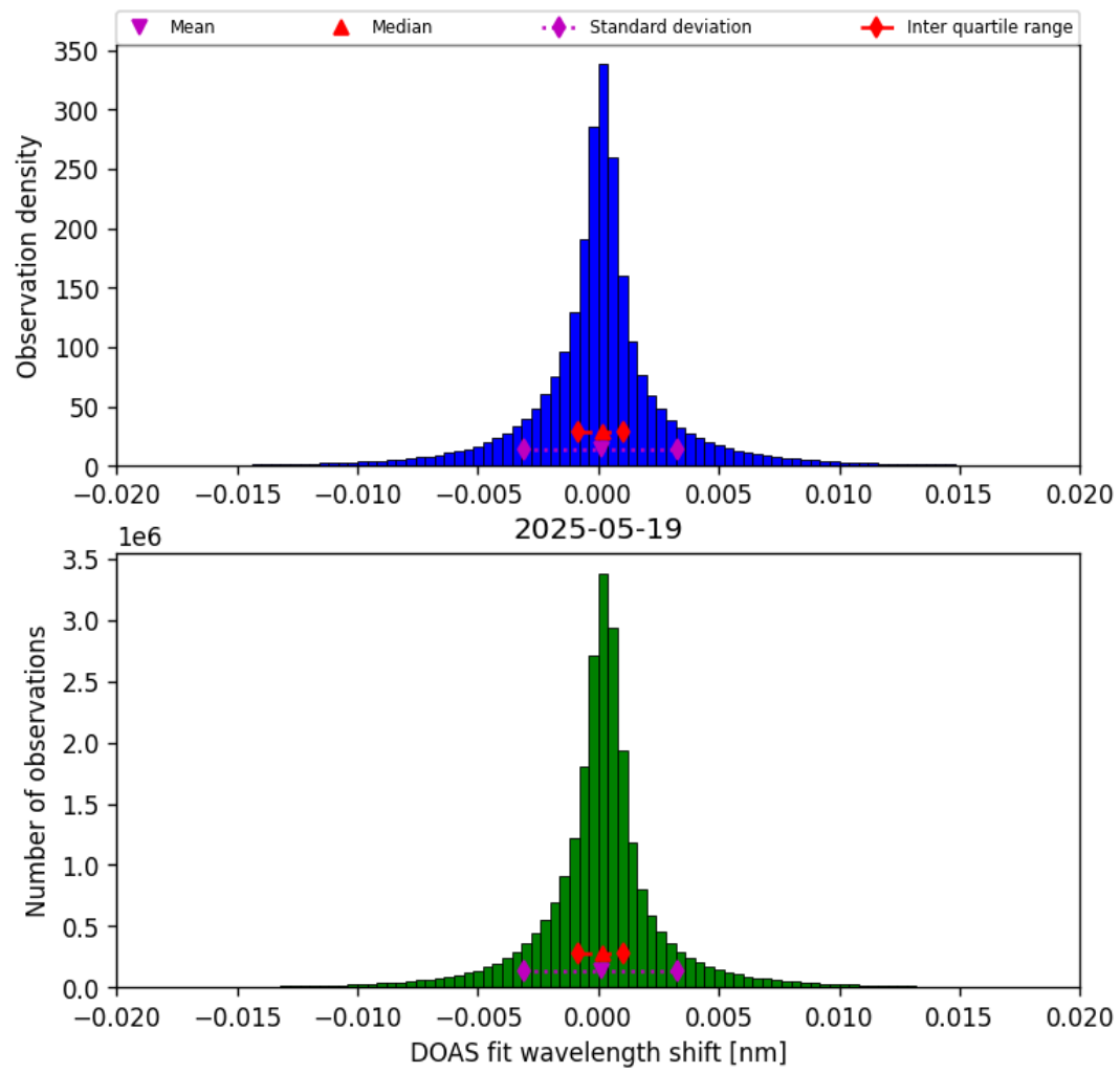
Figure 44: Histogram of “DOAS fit wavelength shift” for 2025-05-18 to 2025-05-20
