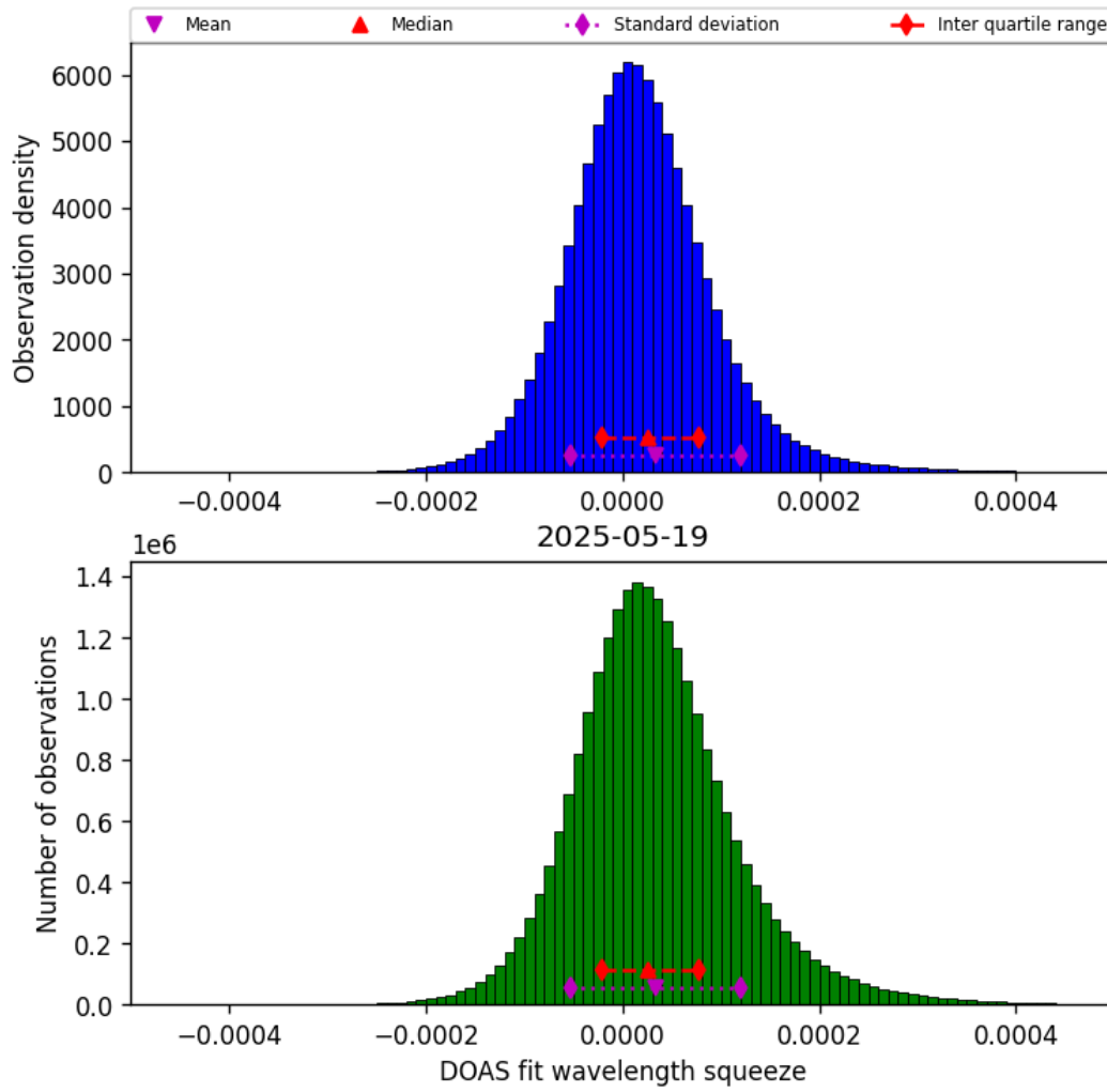
Figure 45: Histogram of “DOAS fit wavelength squeeze” for 2025-05-18 to 2025-05-20
