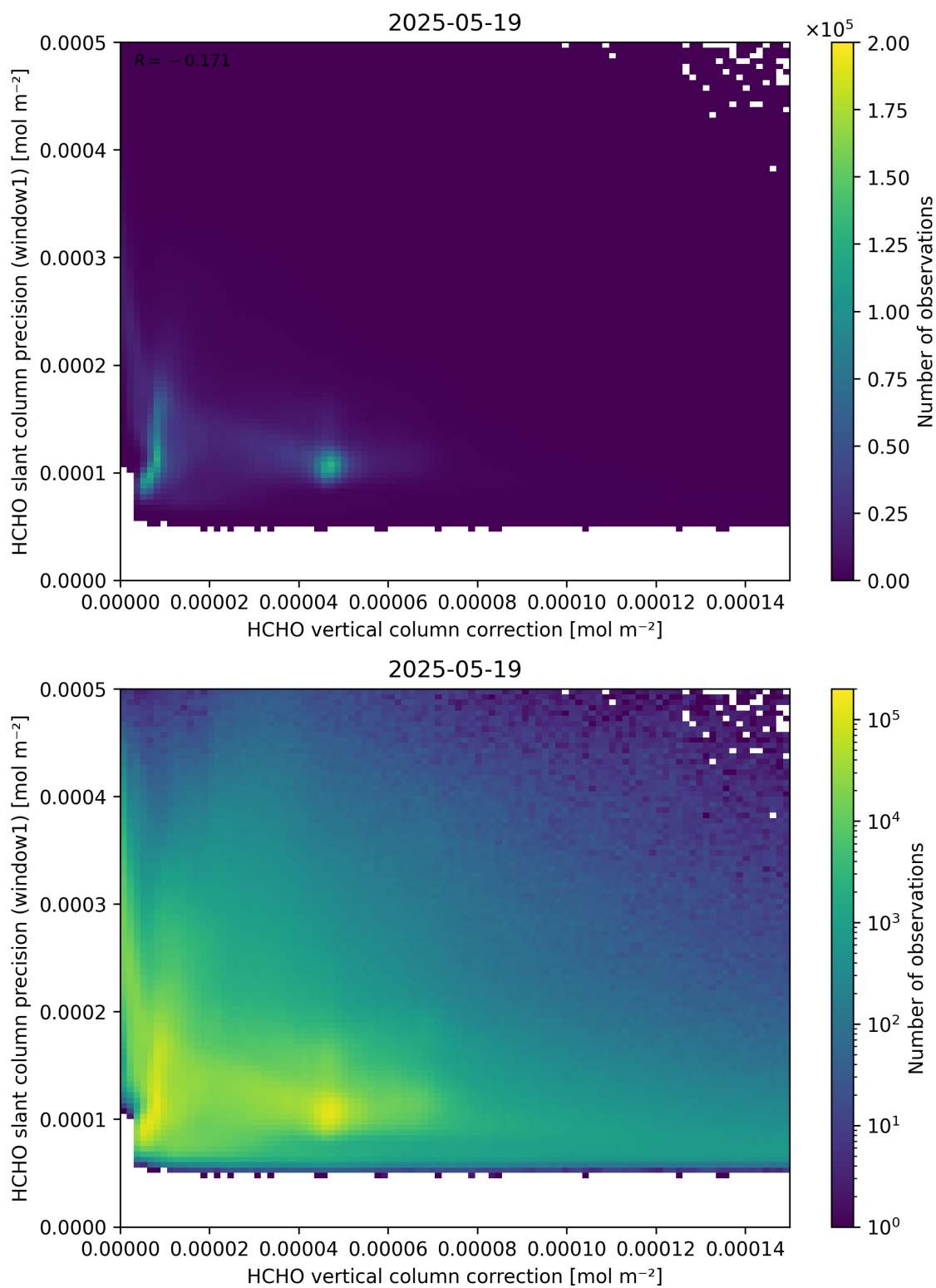
Figure 119: Scatter density plot of “HCHO vertical column correction” against “HCHO slant column precision (window1)” for 2025-05-18 to 2025-05-20.
