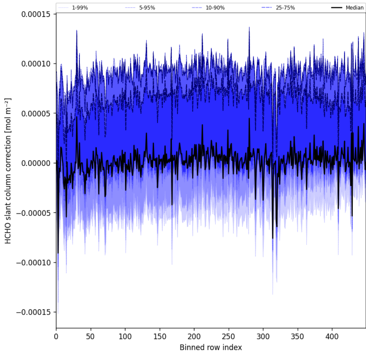
Figure 61: Along track statistics of "HCHO slant column correction" for 2025-05-18 to 2025-05-20
