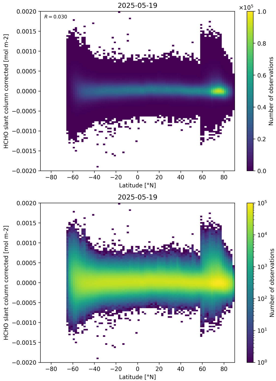
Figure 157: Scatter density plot of “Latitude” against “HCHO slant column corrected” for 2025-05-18 to 2025-05-20.
