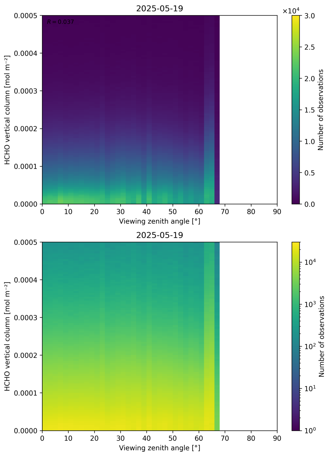
Figure 192: Scatter density plot of “Viewing zenith angle” against “HCHO vertical column” for 2025-05-18 to 2025-05-20.
