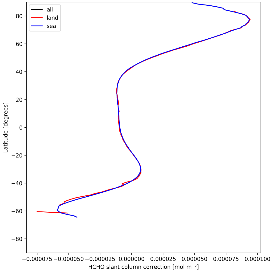
Figure 33: Zonal average of “HCHO slant column correction” for 2025-05-18 to 2025-05-20.
