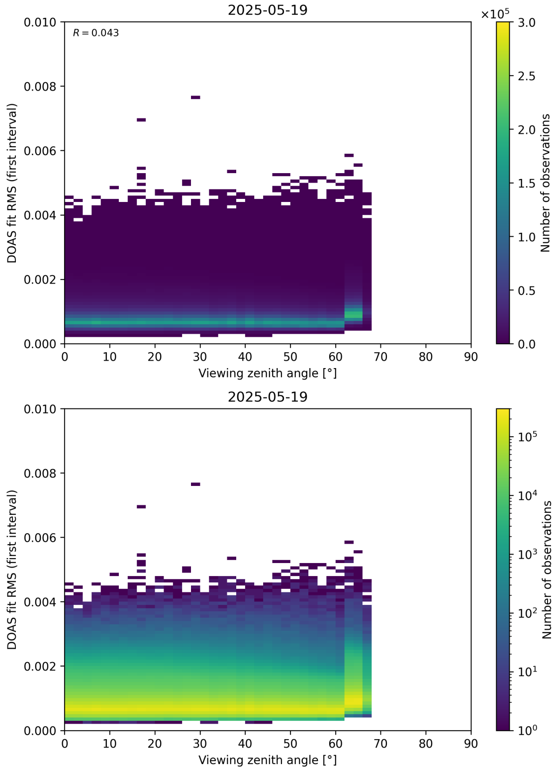
Figure 182: Scatter density plot of “Viewing zenith angle” against “DOAS fit RMS (first interval)” for 2025-05-18 to 2025-05-20.
