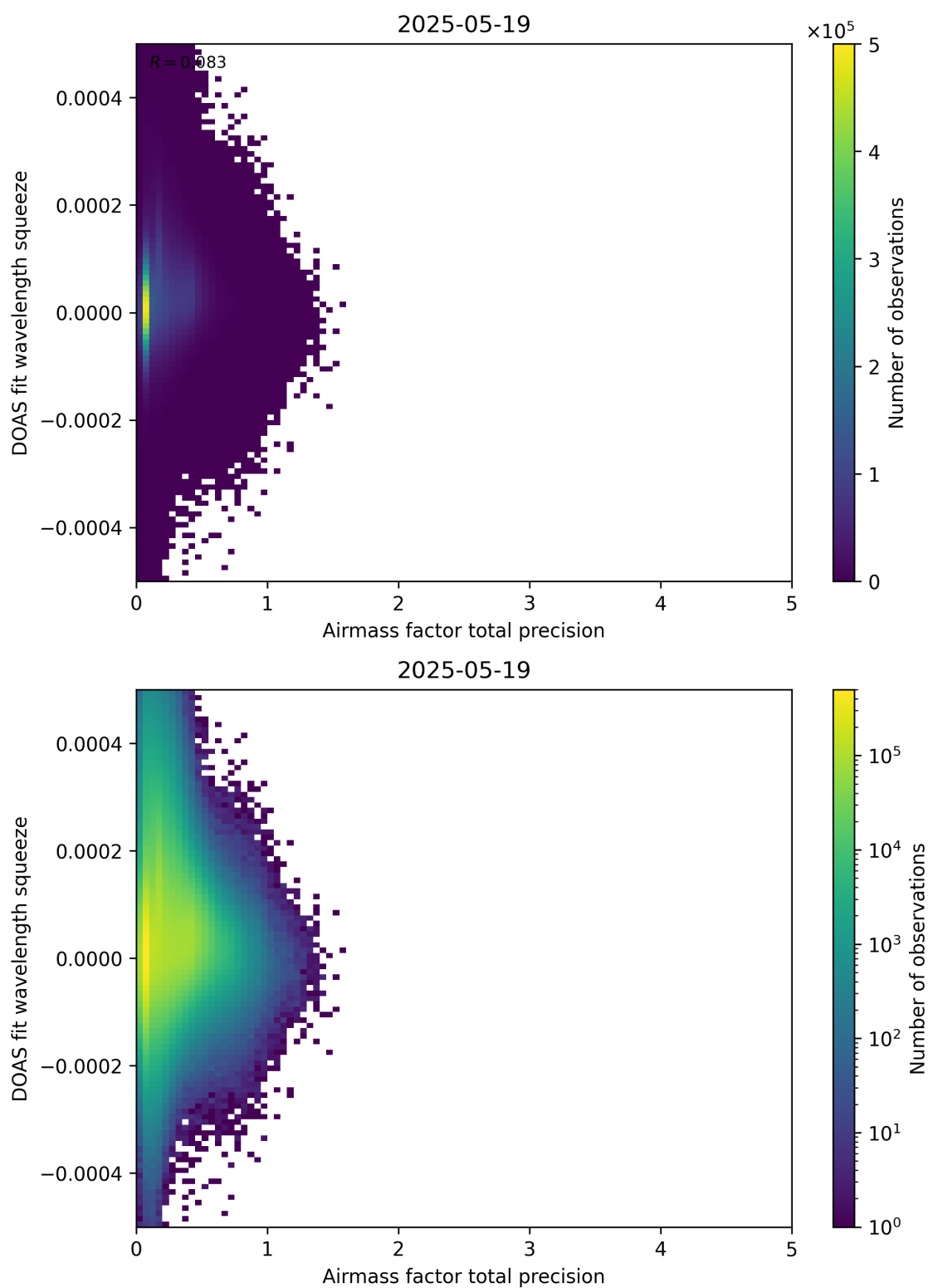
Figure 107: Scatter density plot of “Airmass factor total precision” against “DOAS fit wavelength squeeze” for 2025-05-18 to 2025-05-20.
