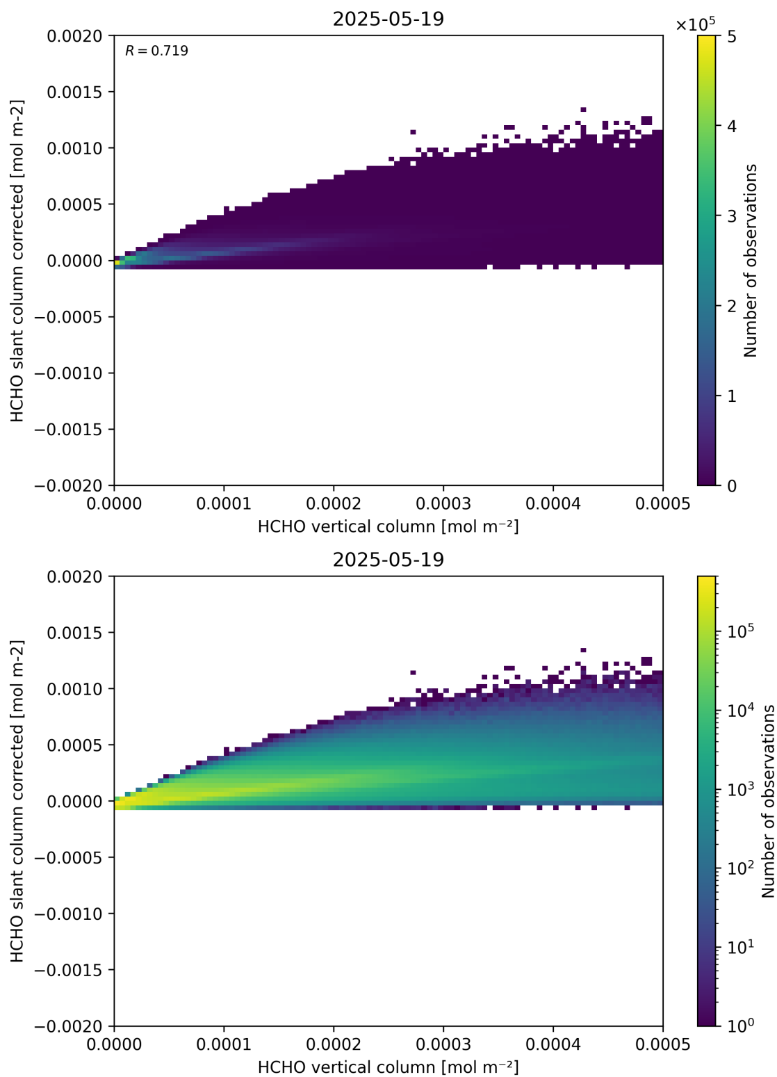
Figure 127: Scatter density plot of “HCHO vertical column” against “HCHO slant column corrected” for 2025-05-18 to 2025-05-20.
