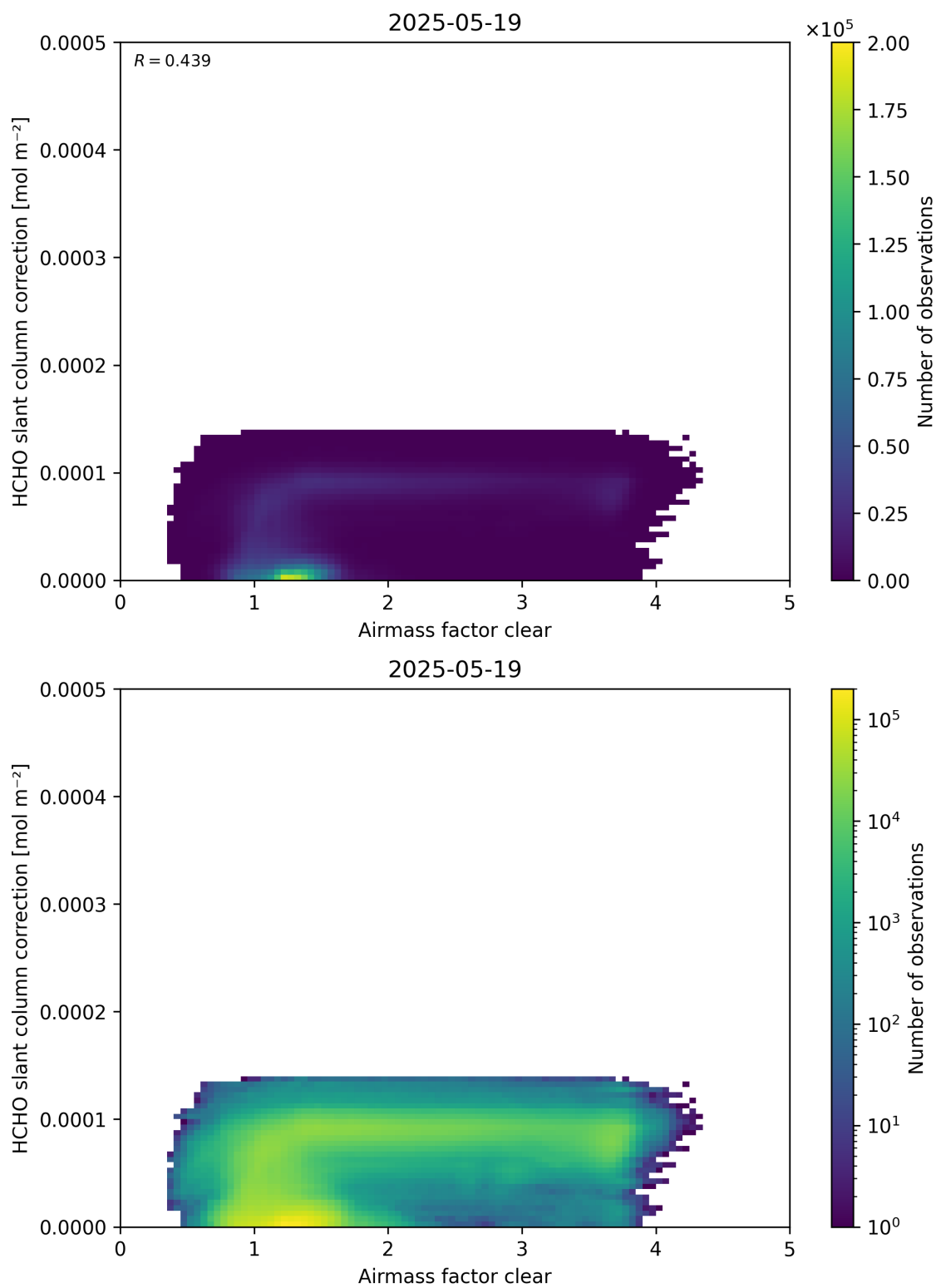
Figure 75: Scatter density plot of “Airmass factor clear” against “HCHO slant column correction” for 2025-05-18 to 2025-05-20.
