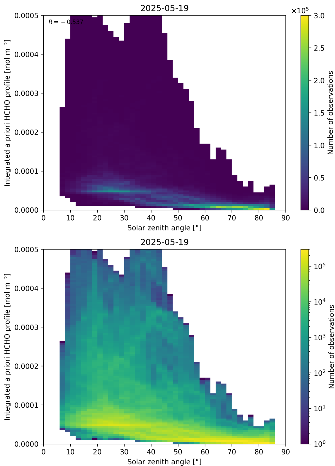
Figure 180: Scatter density plot of “Solar zenith angle” against “Integrated a priori HCHO profile” for 2025-05-18 to 2025-05-20.
