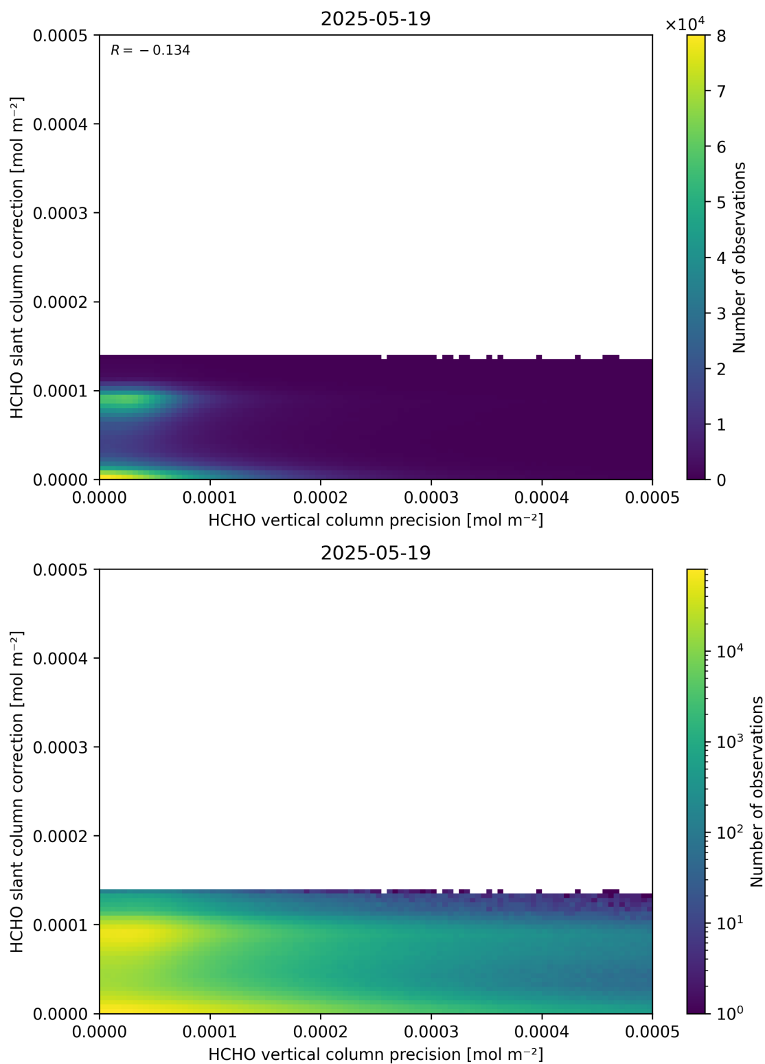
Figure 141: Scatter density plot of “HCHO vertical column precision” against “HCHO slant column correction” for 2025-05-18 to 2025-05-20.
