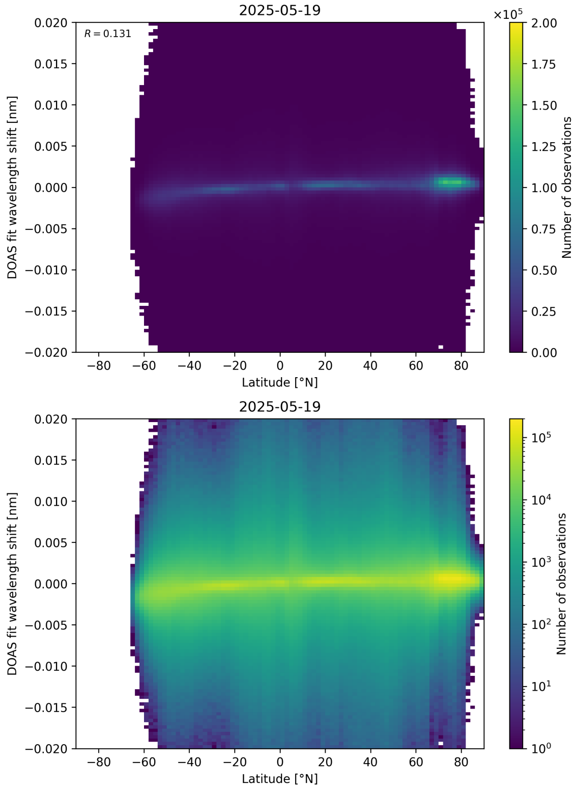
Figure 154: Scatter density plot of “Latitude” against “DOAS fit wavelength shift” for 2025-05-18 to 2025-05-20.
