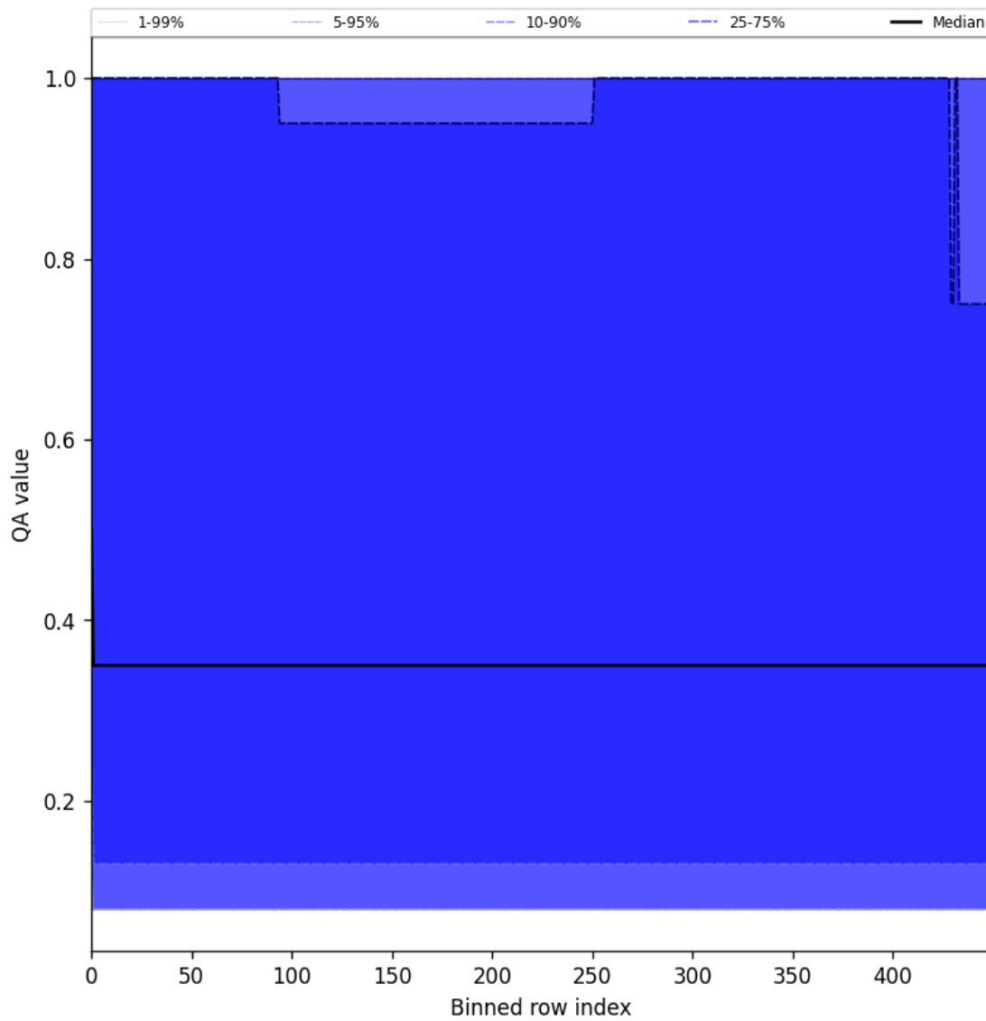
Figure 48: Along track statistics of “QA value” for 2025-05-18 to 2025-05-20
