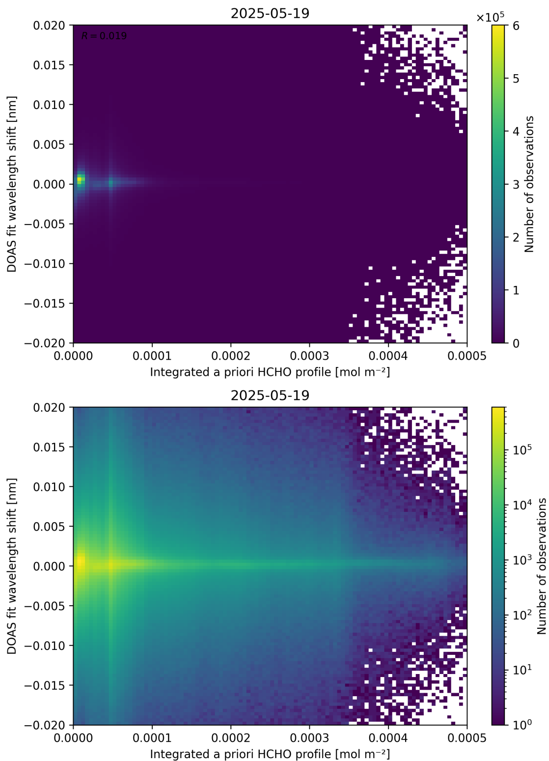
Figure 149: Scatter density plot of “Integrated a priori HCHO profile” against “DOAS fit wavelength shift” for 2025-05-18 to 2025-05-20.
