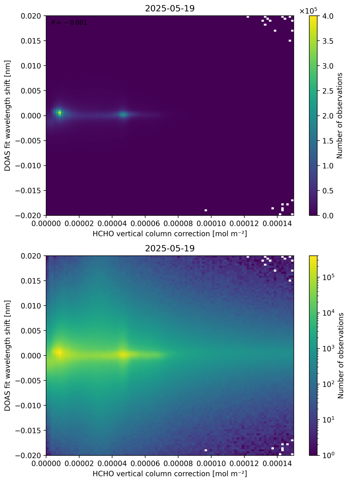
Figure 113: Scatter density plot of “HCHO vertical column correction” against “DOAS fit wavelength shift” for 2025-05-18 to 2025-05-20.
