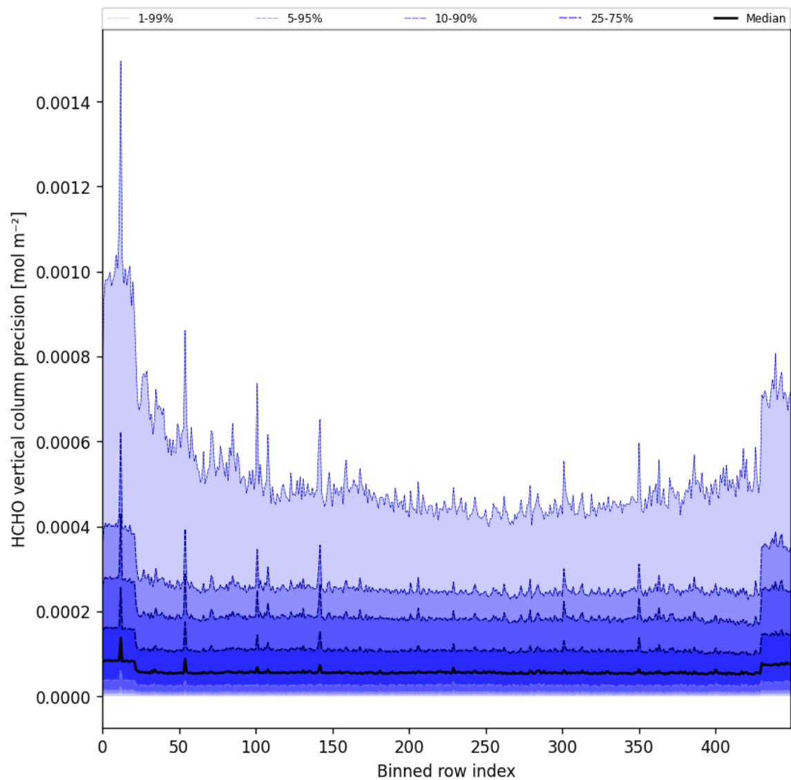
Figure 50: Along track statistics of “HCHO vertical column precision” for 2025-05-18 to 2025-05-20
