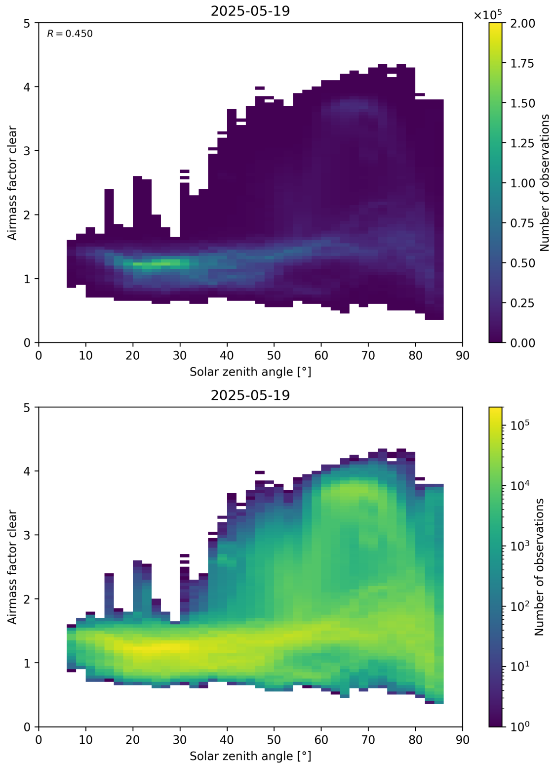
Figure 170: Scatter density plot of “Solar zenith angle” against “Airmass factor clear” for 2025-05-18 to 2025-05-20.
