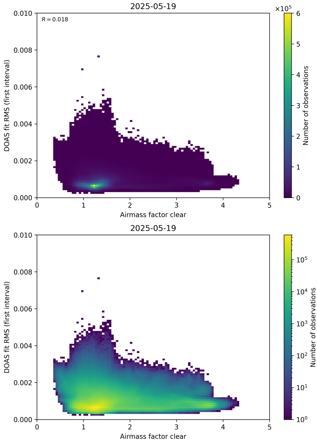
Figure 71: Scatter density plot of “Airmass factor clear” against “DOAS fit RMS (first interval)” for 2025-05-18 to 2025-05-20.
