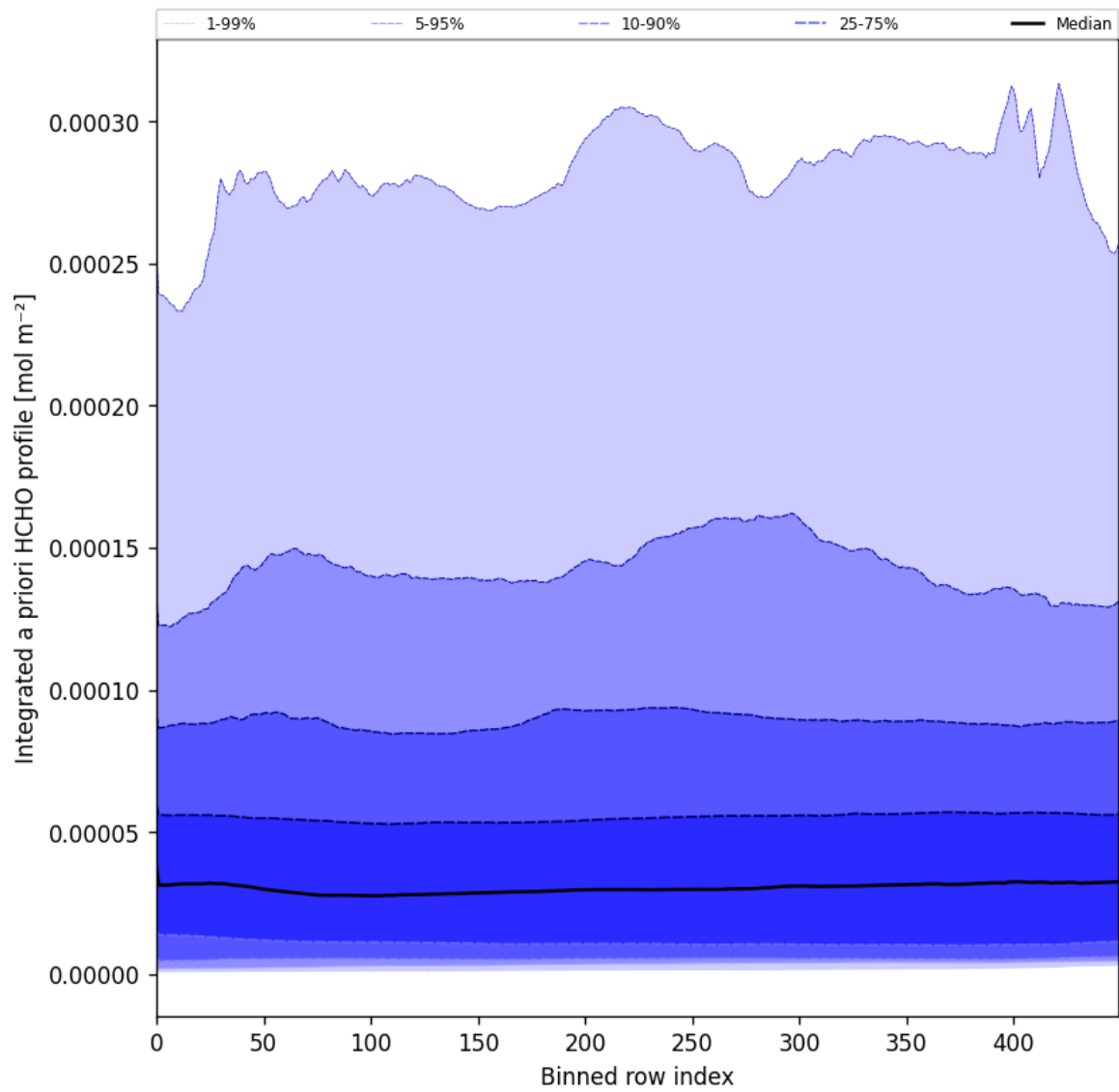
Figure 57: Along track statistics of "Integrated a priori HCHO profile" for 2025-05-18 to 2025-05-20
