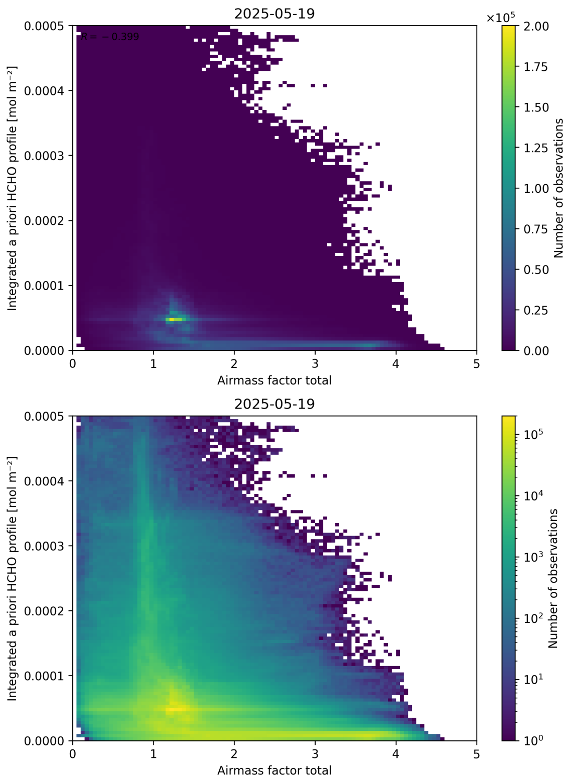
Figure 104: Scatter density plot of “Airmass factor total” against “Integrated a priori HCHO profile” for 2025-05-18 to 2025-05-20.
