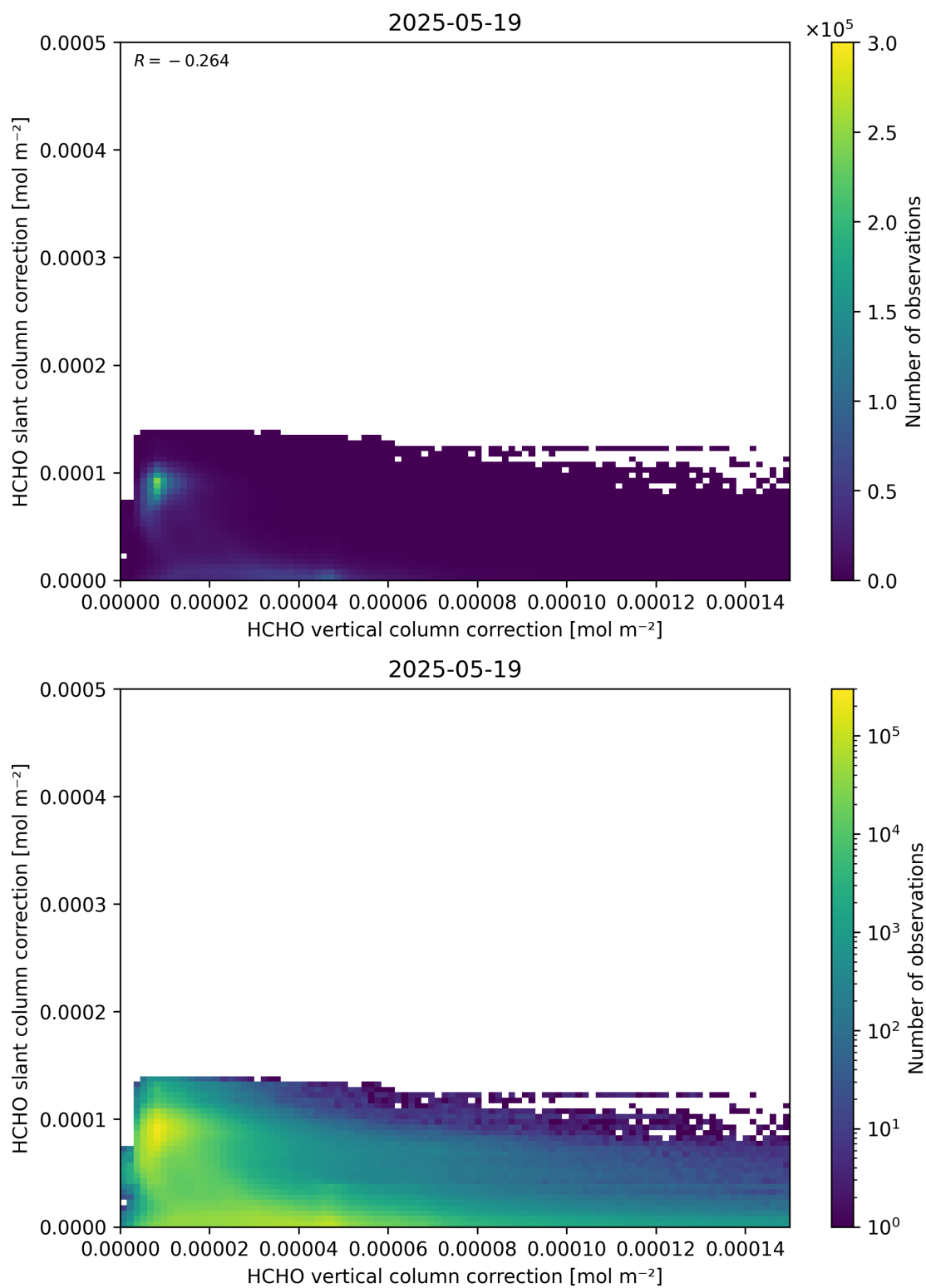
Figure 117: Scatter density plot of “HCHO vertical column correction” against “HCHO slant column correction” for 2025-05-18 to 2025-05-20.
