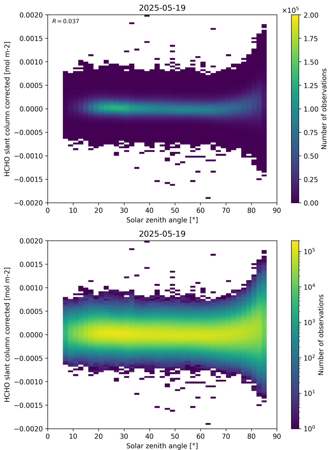
Figure 171: Scatter density plot of “Solar zenith angle” against “HCHO slant column corrected” for 2025-05-18 to 2025-05-20.
