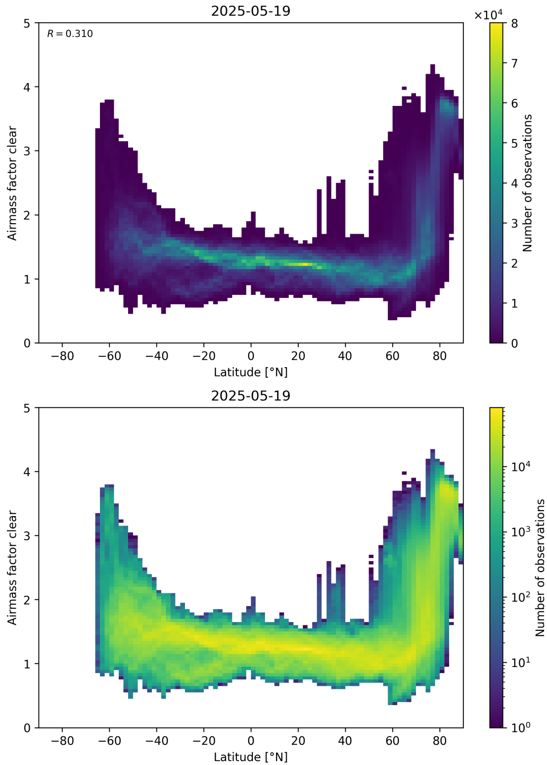
Figure 156: Scatter density plot of “Latitude” against “Airmass factor clear” for 2025-05-18 to 2025-05-20.
