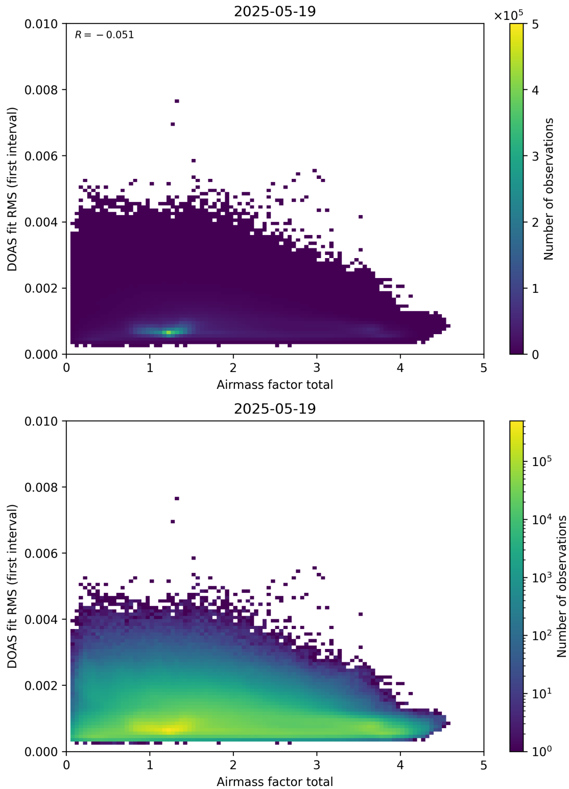
Figure 97: Scatter density plot of “Airmass factor total” against “DOAS fit RMS (first interval)” for 2025-05-18 to 2025-05-20.
