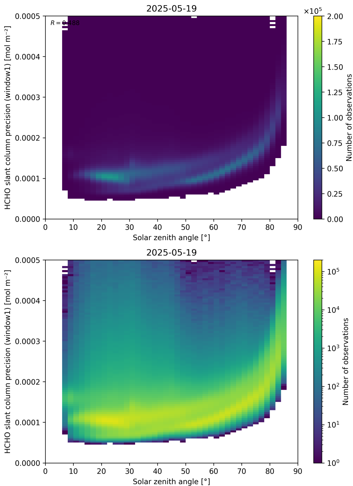
Figure 174: Scatter density plot of “Solar zenith angle” against “HCHO slant column precision (window1)” for 2025-05-18 to 2025-05-20.
