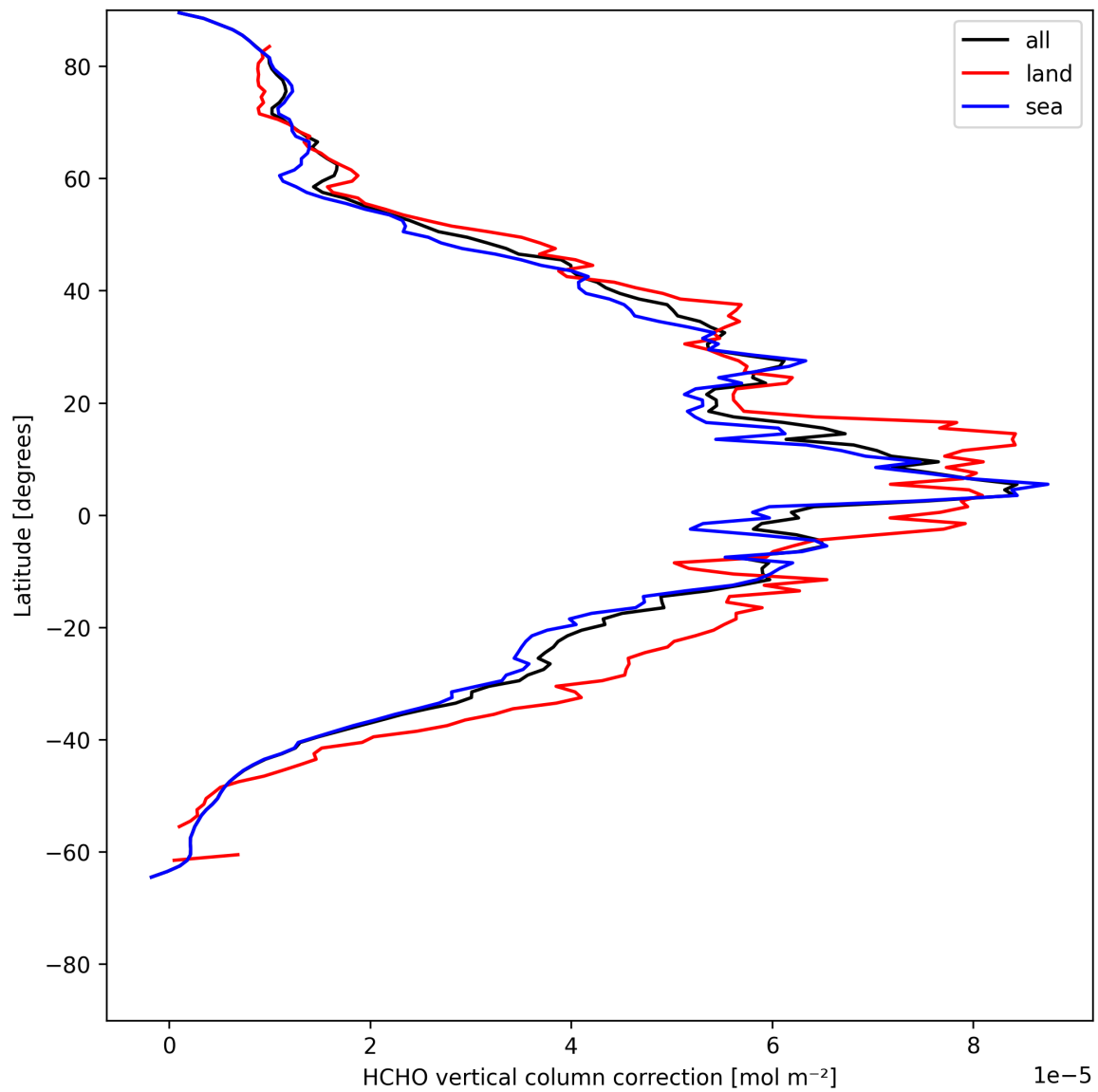
Figure 23: Zonal average of “HCHO vertical column correction” for 2025-05-18 to 2025-05-20.
