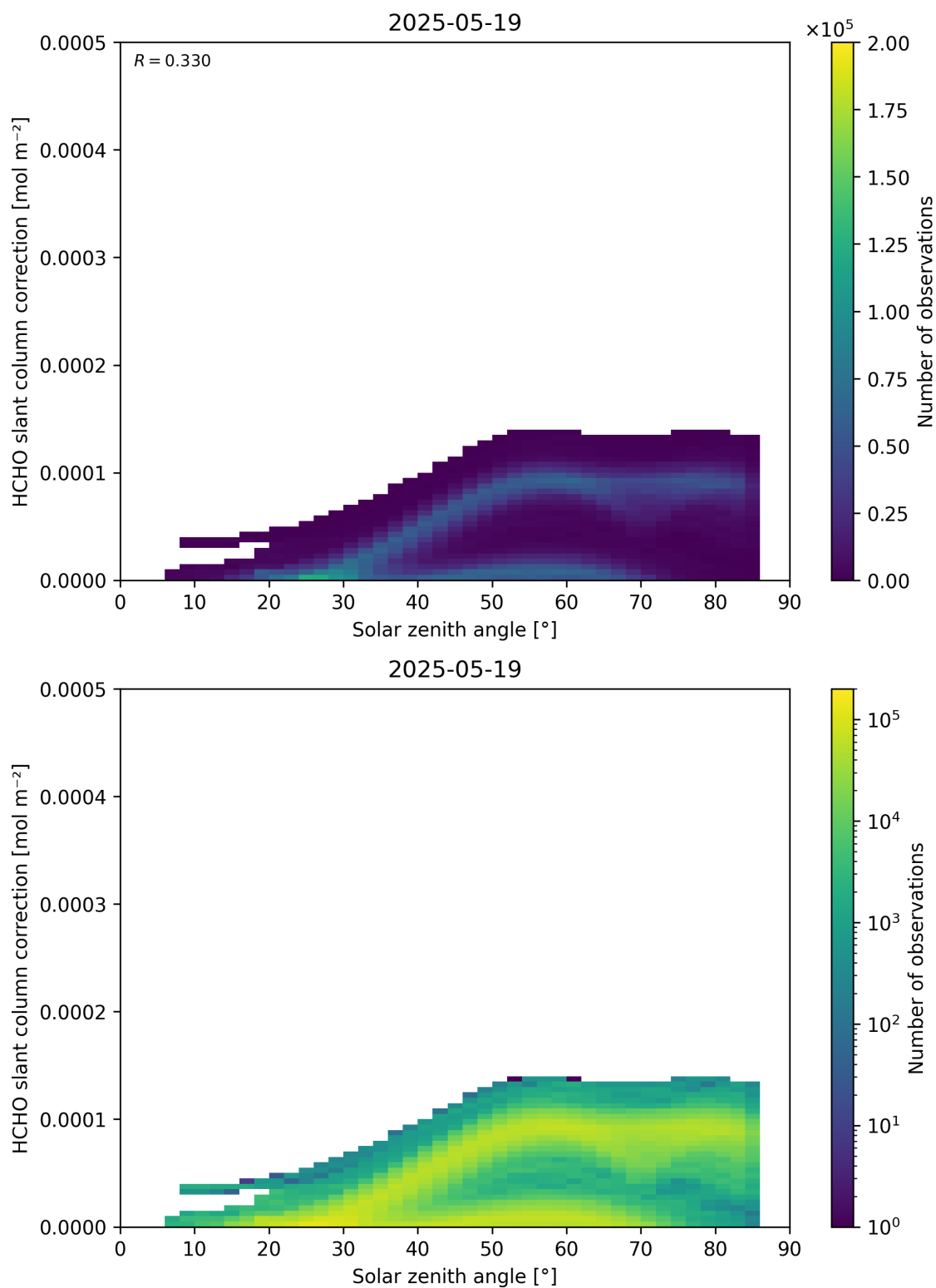
Figure 172: Scatter density plot of “Solar zenith angle” against “HCHO slant column correction” for 2025-05-18 to 2025-05-20.
