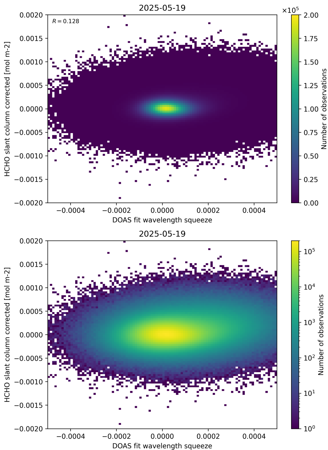
Figure 69: Scatter density plot of “DOAS fit wavelength squeeze” against “HCHO slant column corrected” for 2025-05-18 to 2025-05-20.
