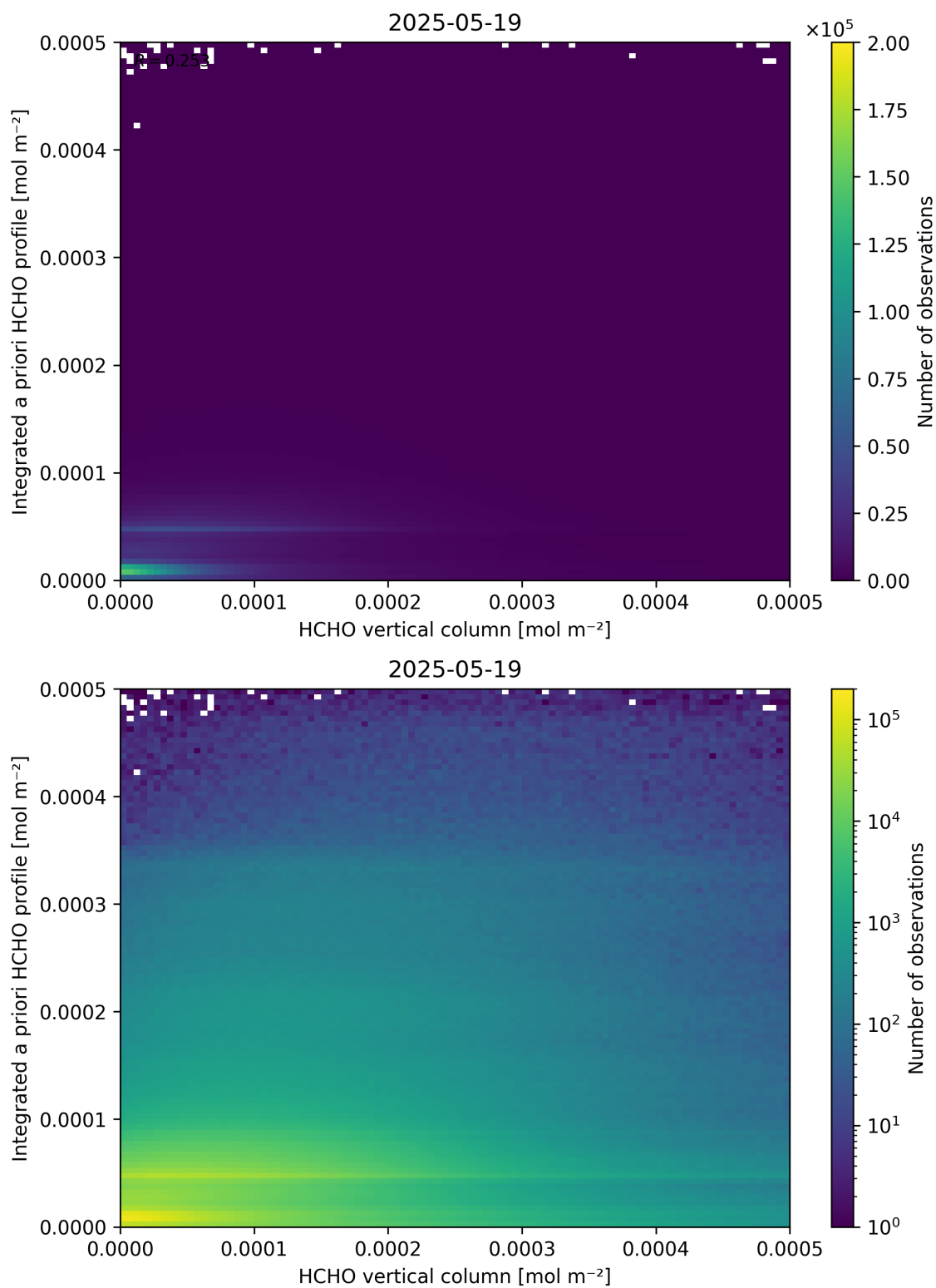
Figure 135: Scatter density plot of “HCHO vertical column” against “Integrated a priori HCHO profile” for 2025-05-18 to 2025-05-20.
