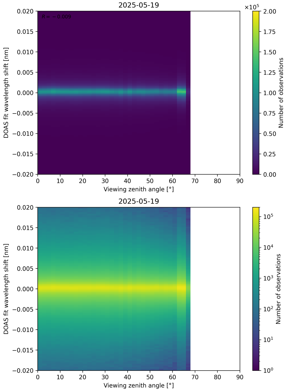
Figure 183: Scatter density plot of “Viewing zenith angle” against “DOAS fit wavelength shift” for 2025-05-18 to 2025-05-20.
