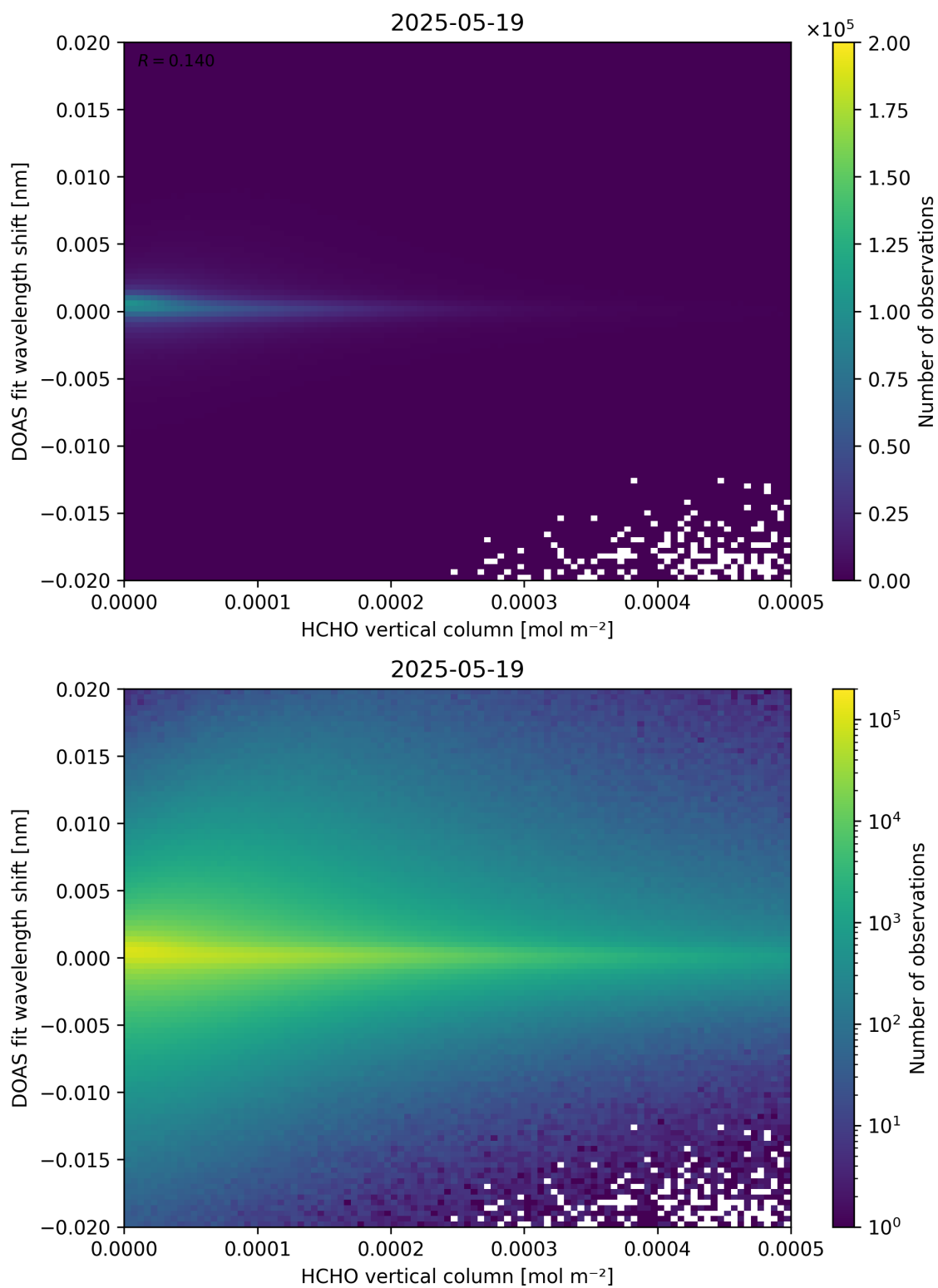
Figure 124: Scatter density plot of “HCHO vertical column” against “DOAS fit wavelength shift” for 2025-05-18 to 2025-05-20.
