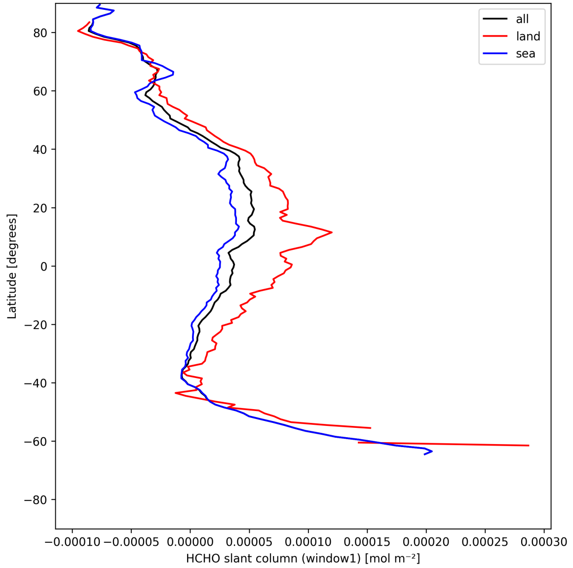
Figure 24: Zonal average of “HCHO slant column (window1)” for 2025-05-18 to 2025-05-20.
