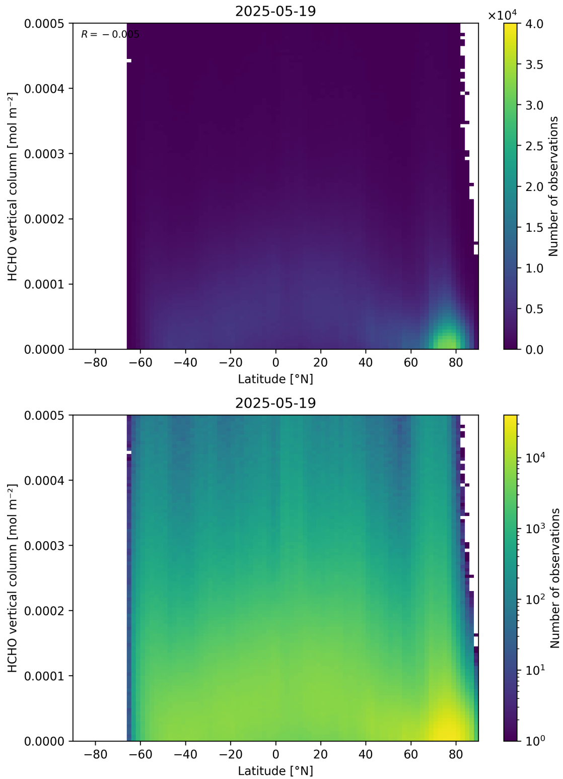
Figure 163: Scatter density plot of “Latitude” against “HCHO vertical column” for 2025-05-18 to 2025-05-20.
