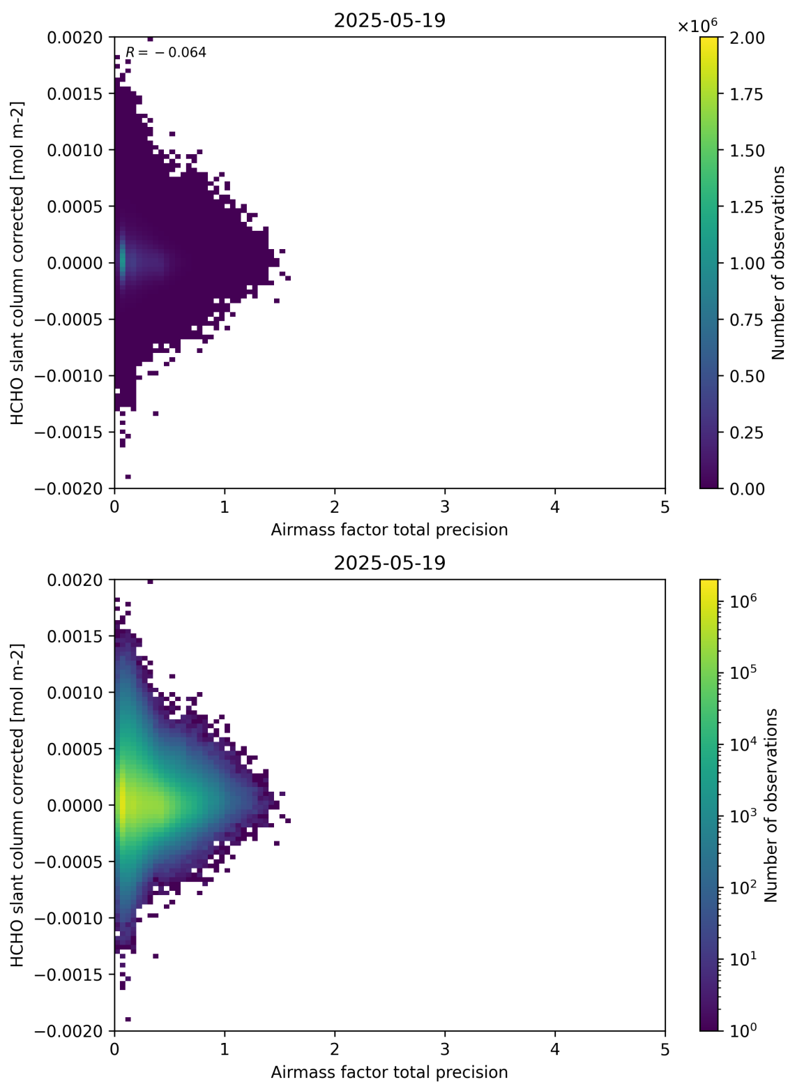
Figure 109: Scatter density plot of “Airmass factor total precision” against “HCHO slant column corrected” for 2025-05-18 to 2025-05-20.
