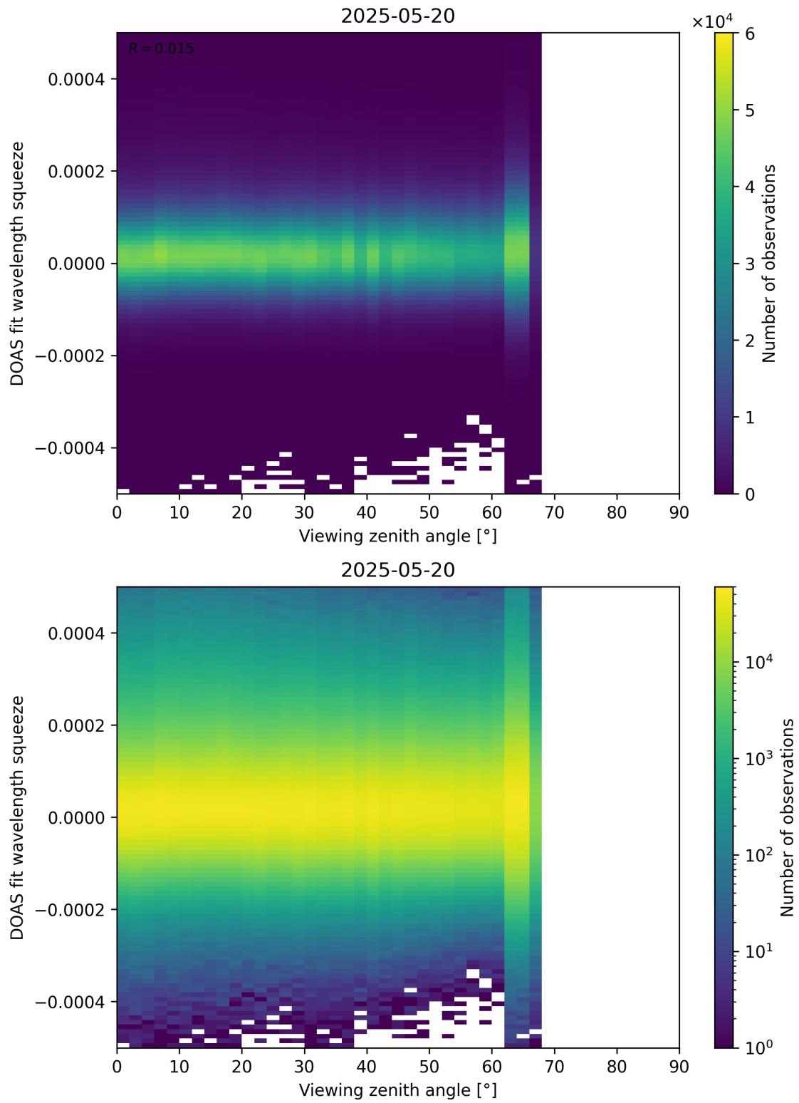
Figure 184: Scatter density plot of “Viewing zenith angle” against “DOAS fit wavelength squeeze” for 2025-05-19 to 2025-05-21.
