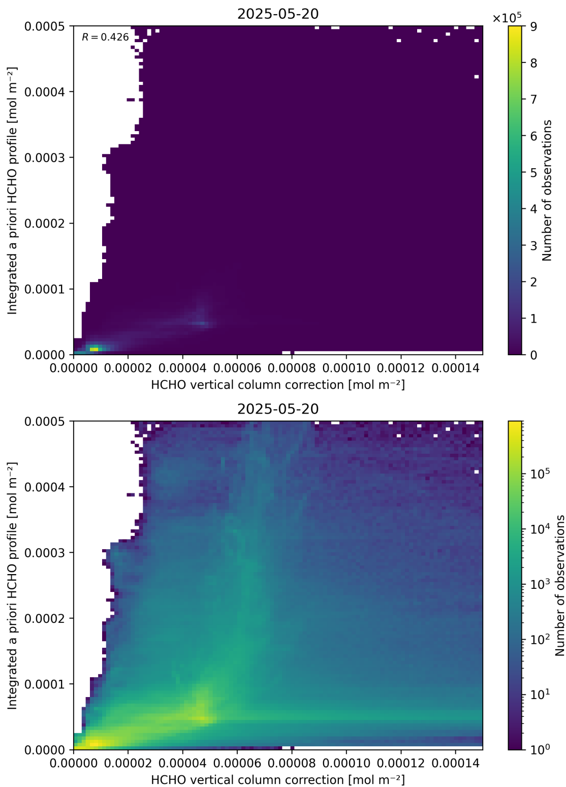
Figure 122: Scatter density plot of “HCHO vertical column correction” against “Integrated a priori HCHO profile” for 2025-05-19 to 2025-05-21.
