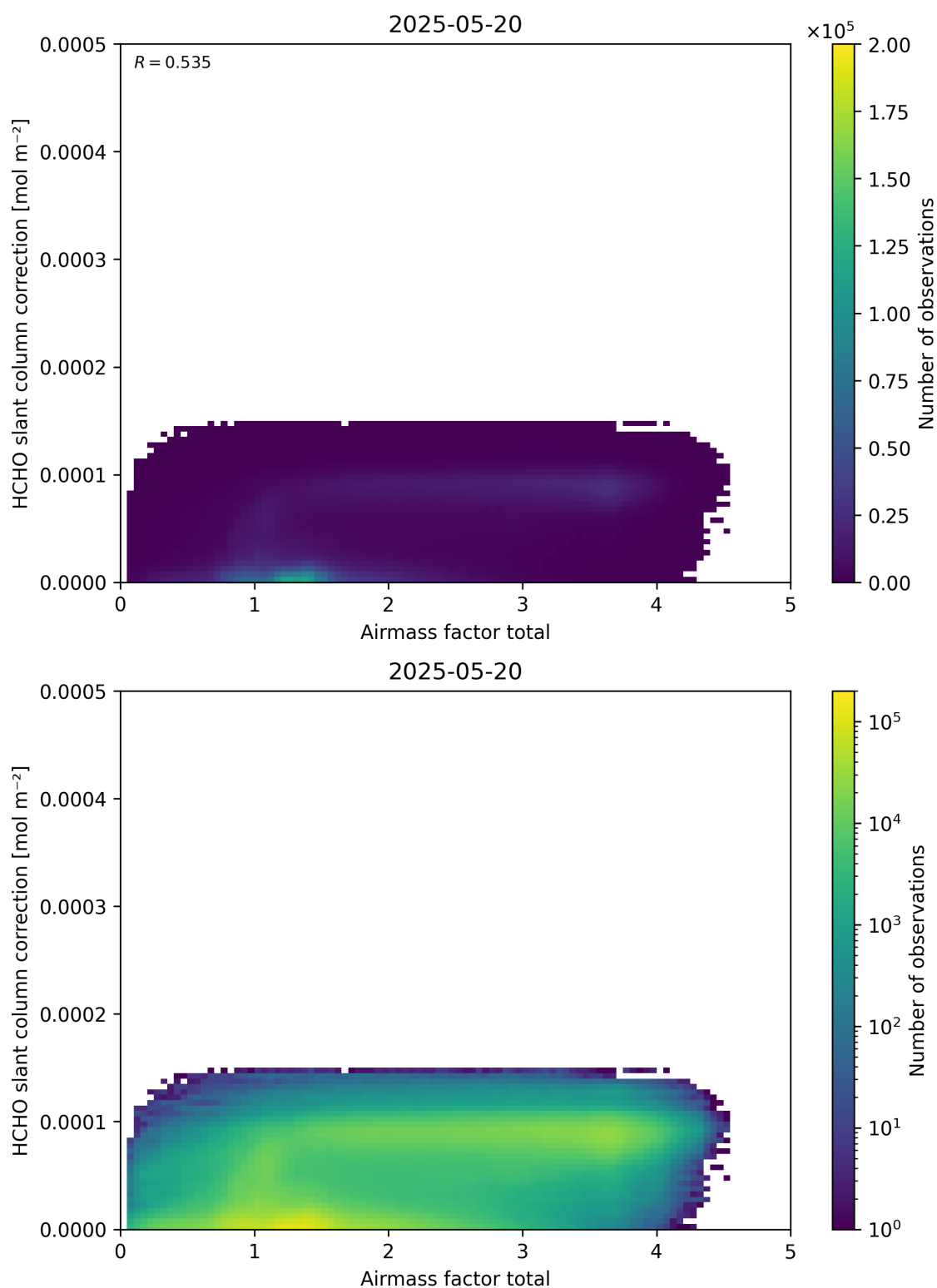
Figure 102: Scatter density plot of “Airmass factor total” against “HCHO slant column correction” for 2025-05-19 to 2025-05-21.
