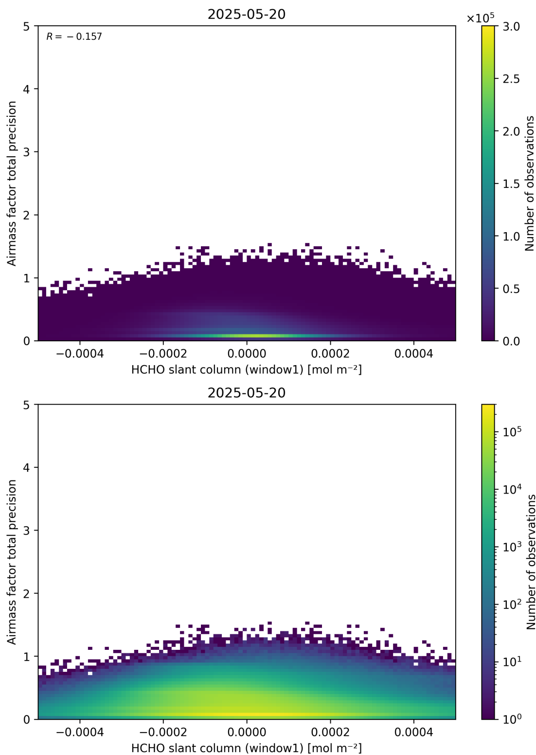
Figure 86: Scatter density plot of “HCHO slant column (window1)” against “Airmass factor total precision” for 2025-05-19 to 2025-05-21.
