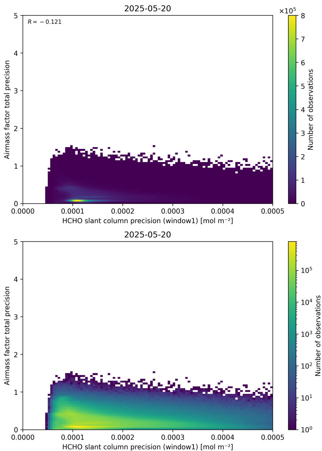
Figure 95: Scatter density plot of “HCHO slant column precision (window1)” against “Airmass factor total precision” for 2025-05-19 to 2025-05-21.
