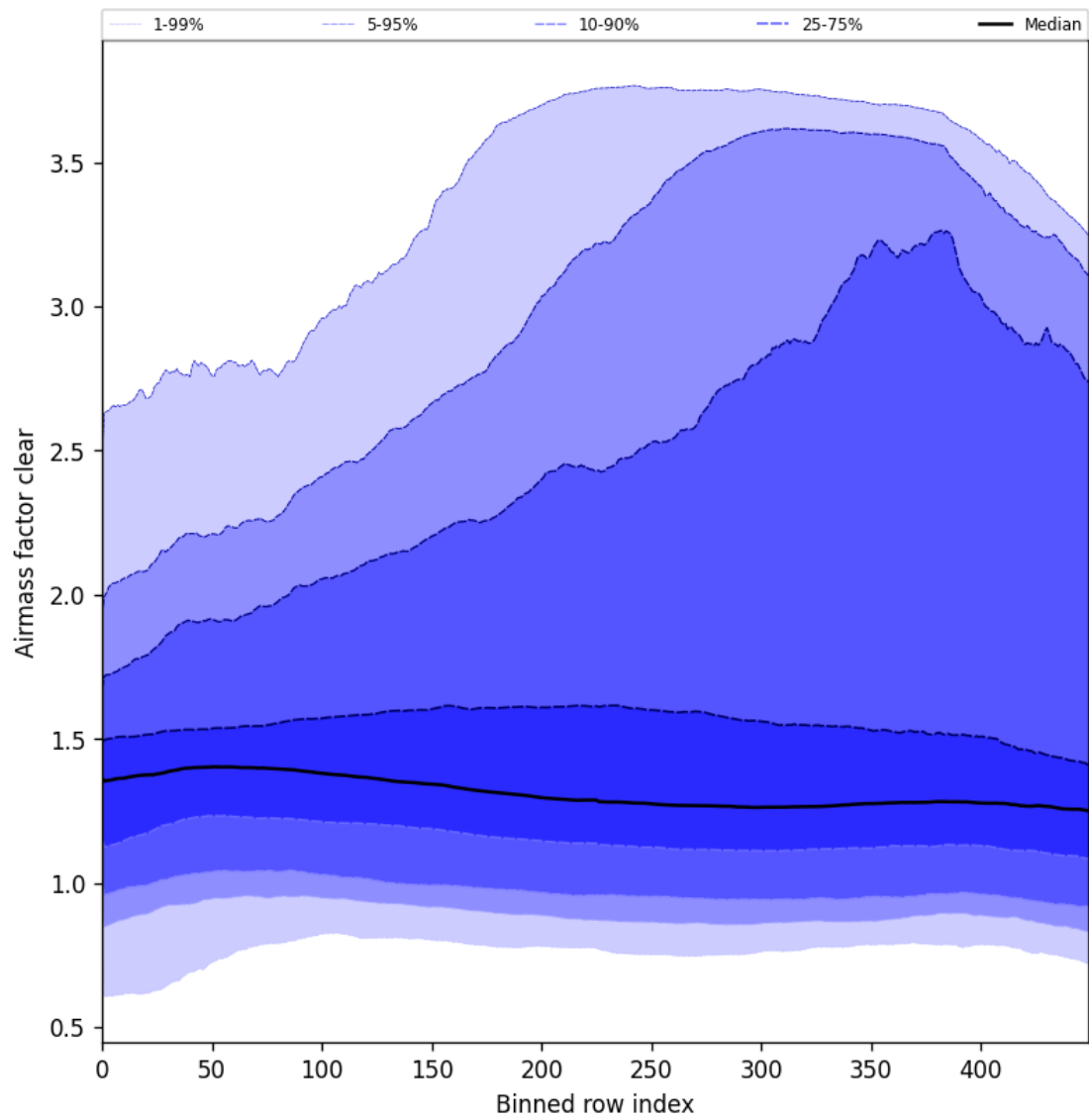
Figure 56: Along track statistics of “Airmass factor clear” for 2025-05-19 to 2025-05-21
