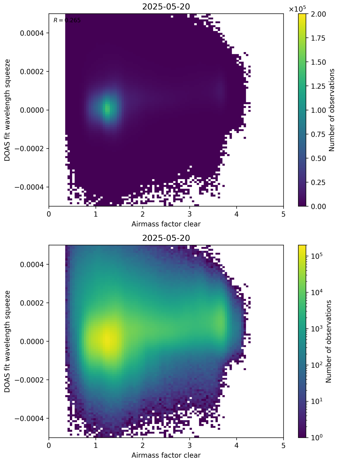
Figure 73: Scatter density plot of “Airmass factor clear” against “DOAS fit wavelength squeeze” for 2025-05-19 to 2025-05-21.
