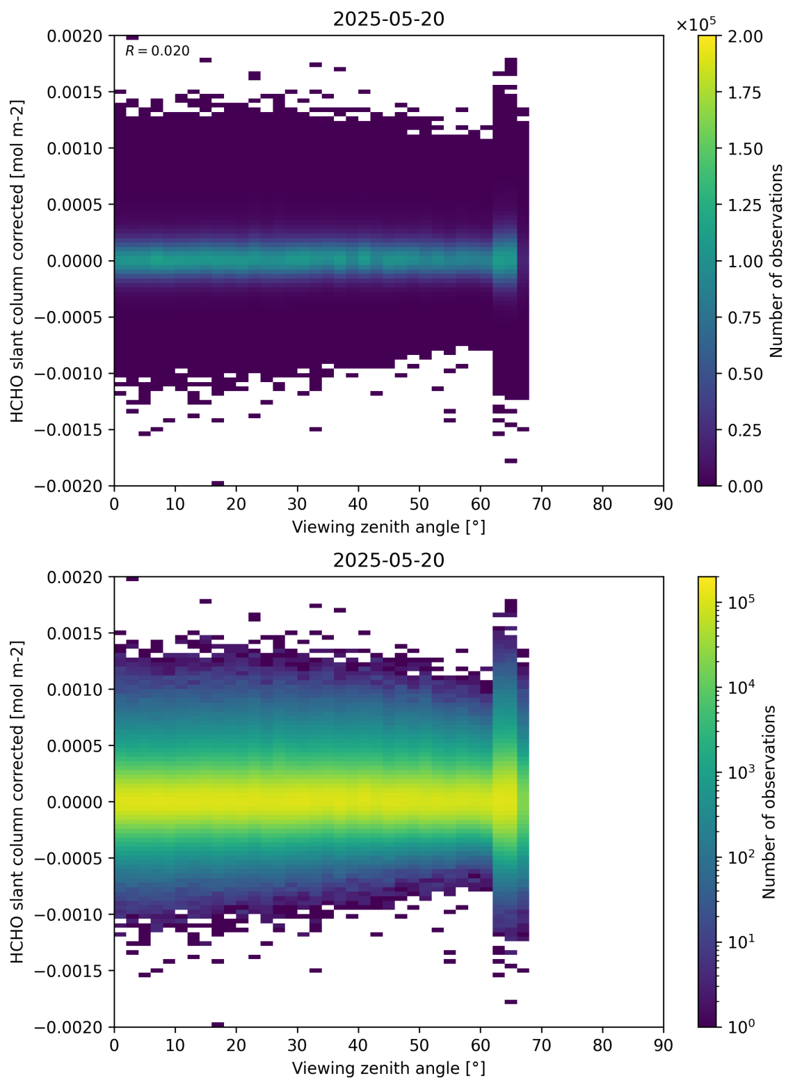
Figure 186: Scatter density plot of “Viewing zenith angle” against “HCHO slant column corrected” for 2025-05-19 to 2025-05-21.
