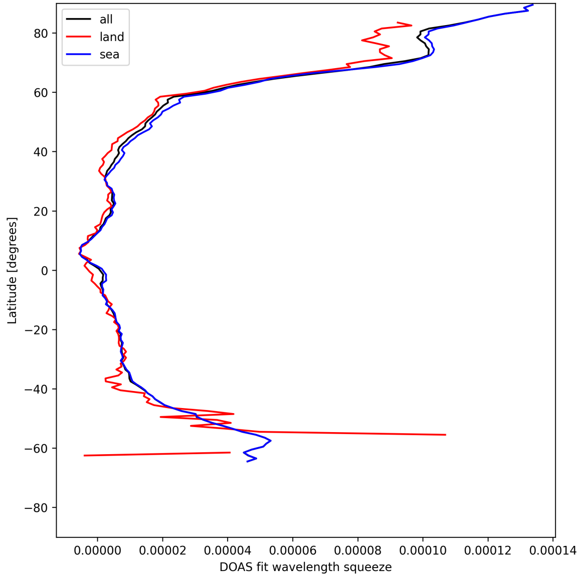
Figure 31: Zonal average of “DOAS fit wavelength squeeze” for 2025-05-19 to 2025-05-21.
