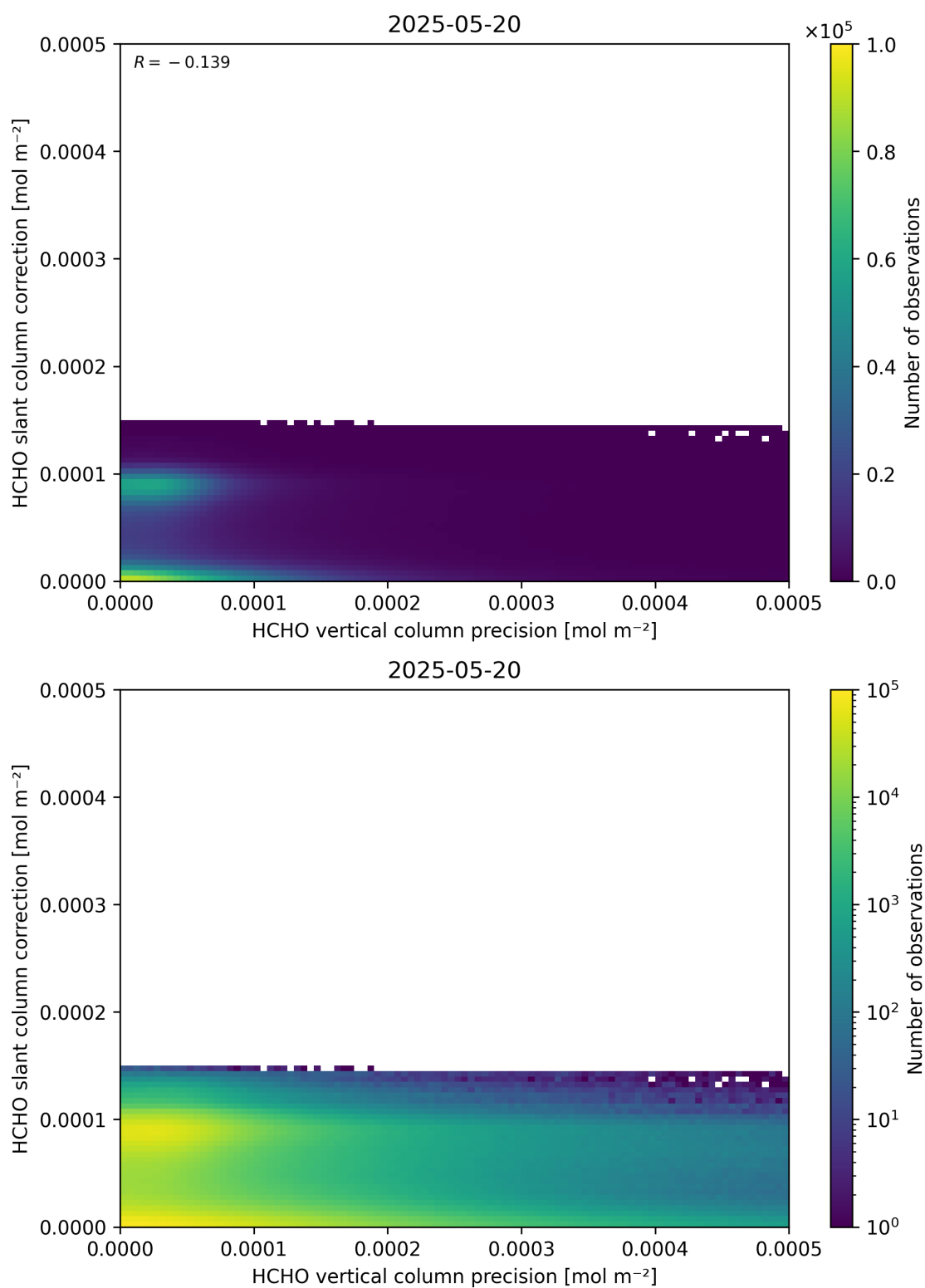
Figure 141: Scatter density plot of “HCHO vertical column precision” against “HCHO slant column correction” for 2025-05-19 to 2025-05-21.
