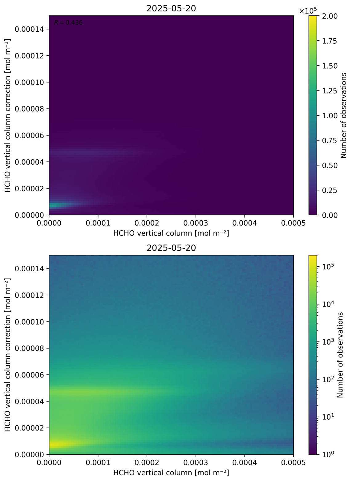
Figure 133: Scatter density plot of “HCHO vertical column” against “HCHO vertical column correction” for 2025-05-19 to 2025-05-21.
