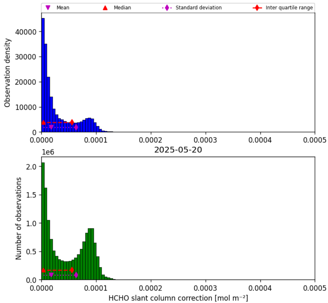
Figure 47: Histogram of “HCHO slant column correction” for 2025-05-19 to 2025-05-21
