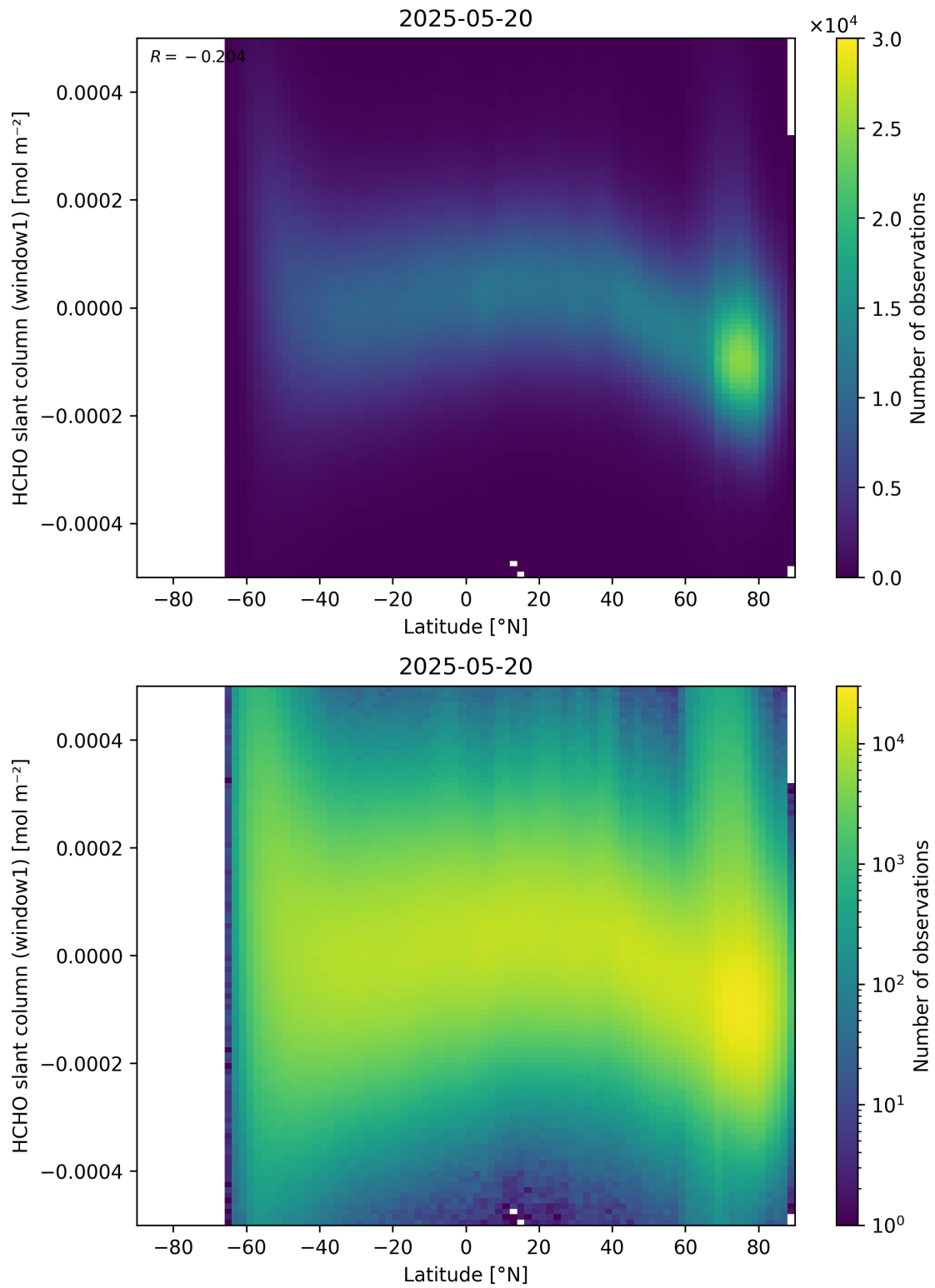
Figure 159: Scatter density plot of “Latitude” against “HCHO slant column (window1)” for 2025-05-19 to 2025-05-21.
