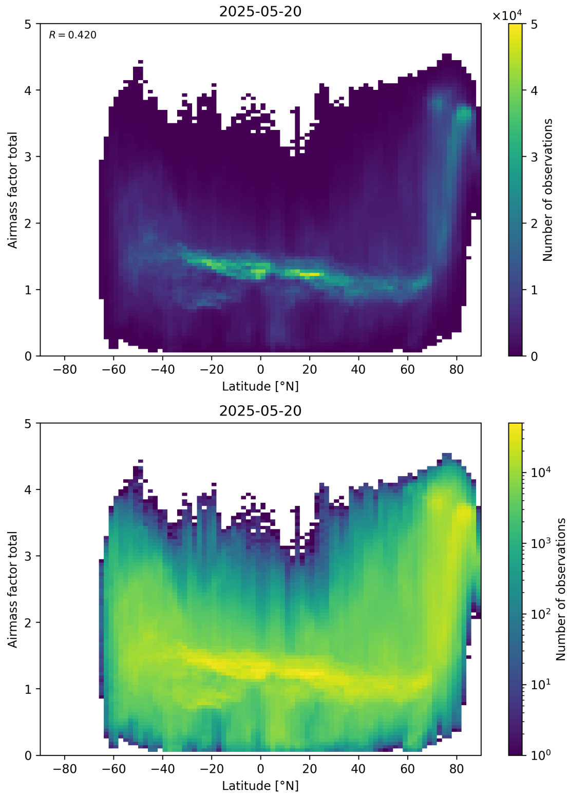
Figure 161: Scatter density plot of “Latitude” against “Airmass factor total” for 2025-05-19 to 2025-05-21.
