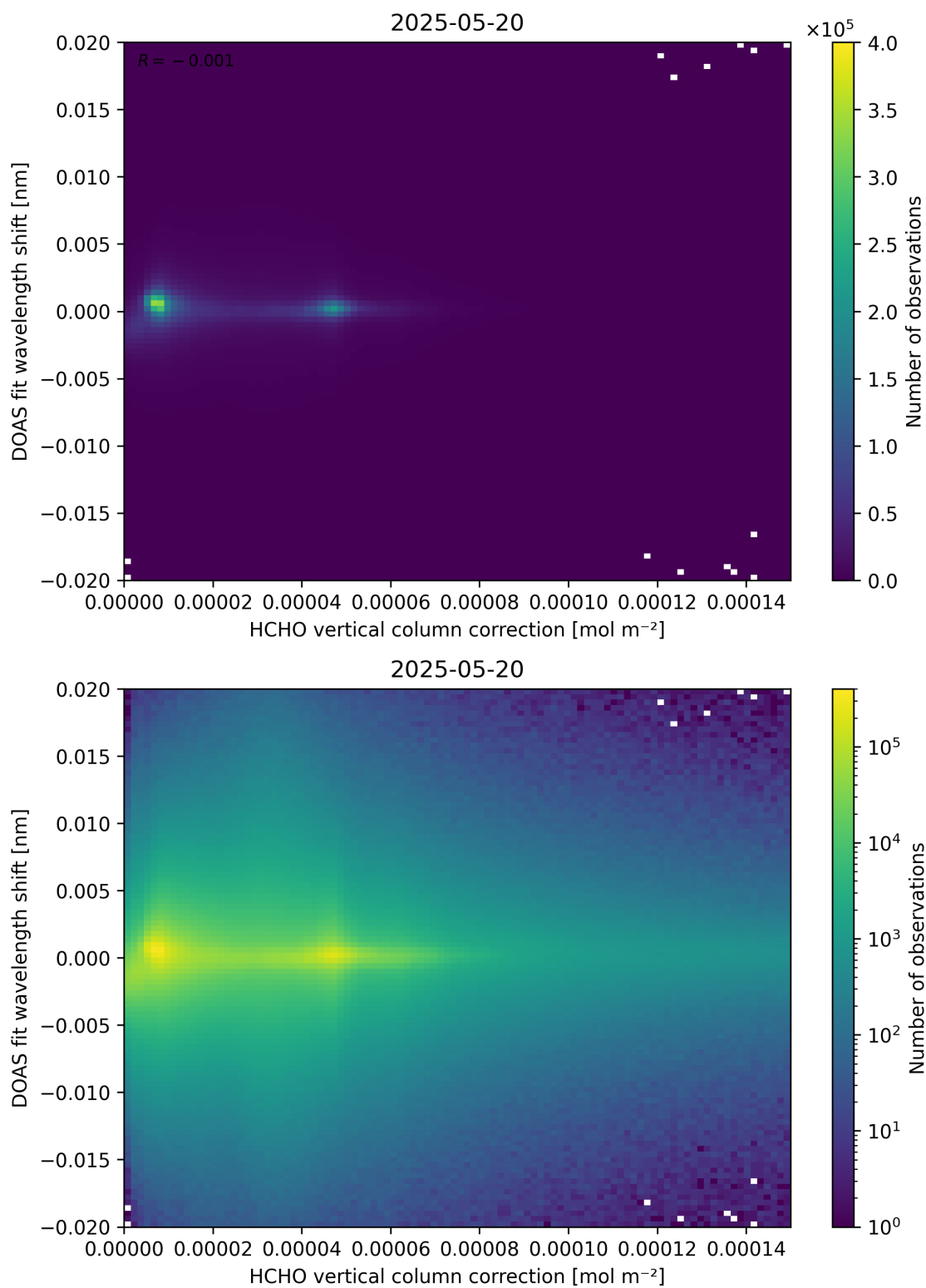
Figure 113: Scatter density plot of “HCHO vertical column correction” against “DOAS fit wavelength shift” for 2025-05-19 to 2025-05-21.
