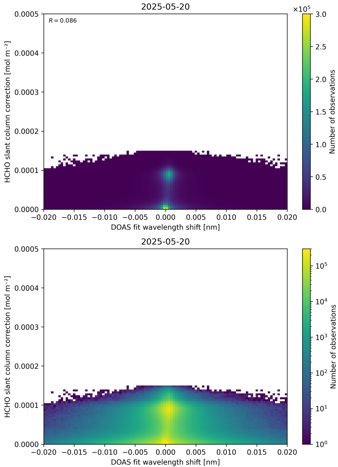
Figure 67: Scatter density plot of “DOAS fit wavelength shift” against “HCHO slant column correction” for 2025-05-19 to 2025-05-21.
