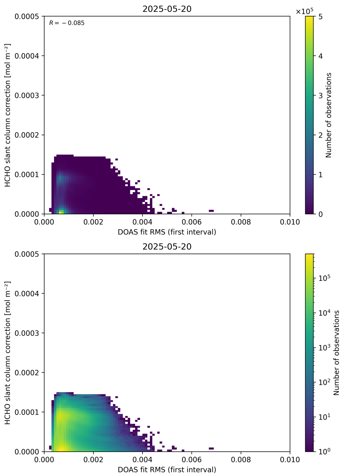
Figure 63: Scatter density plot of “DOAS fit RMS (first interval)” against “HCHO slant column correction” for 2025-05-19 to 2025-05-21.
