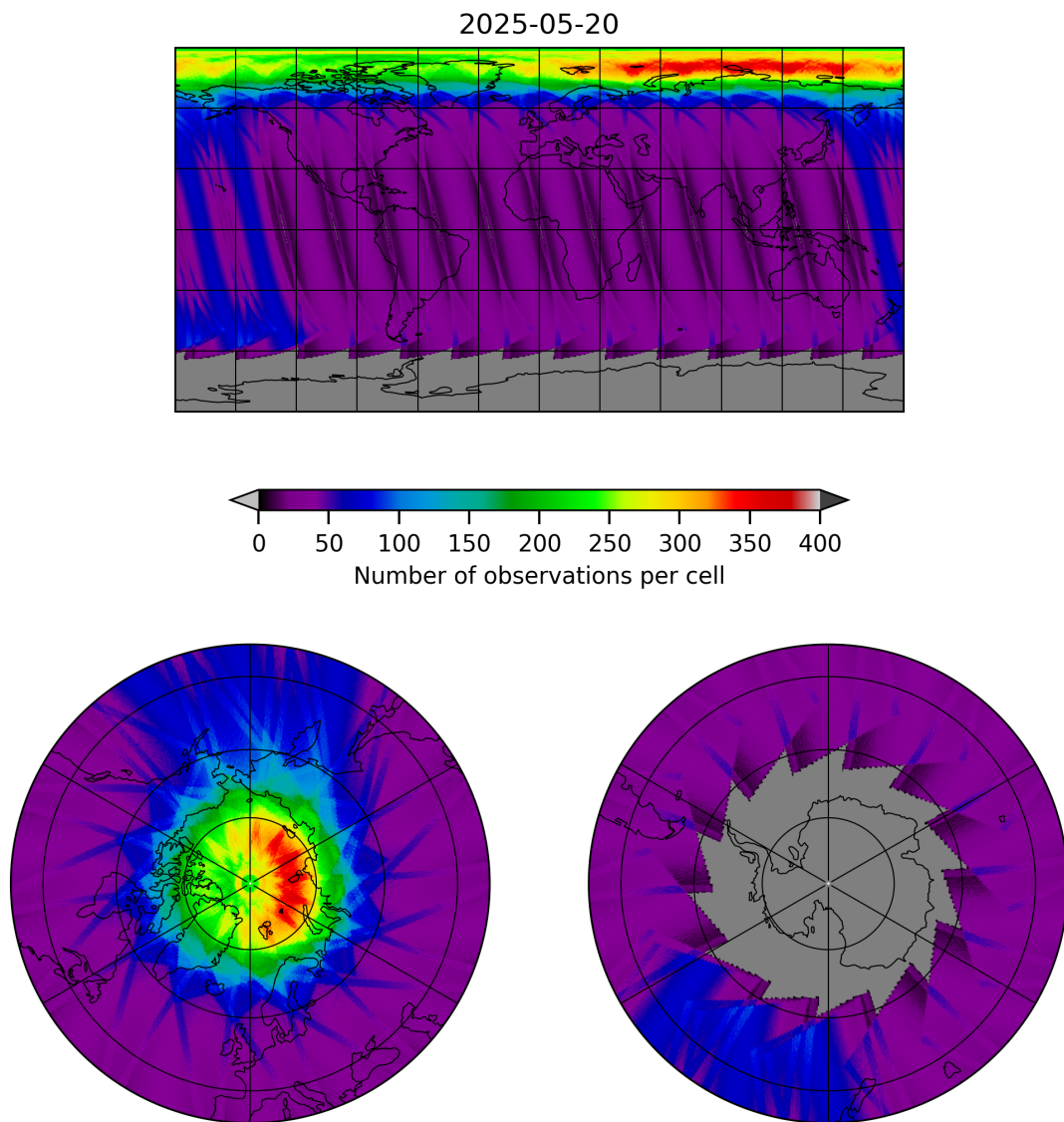
Figure 19: Map of the number of observations for 2025-05-19 to 2025-05-21
