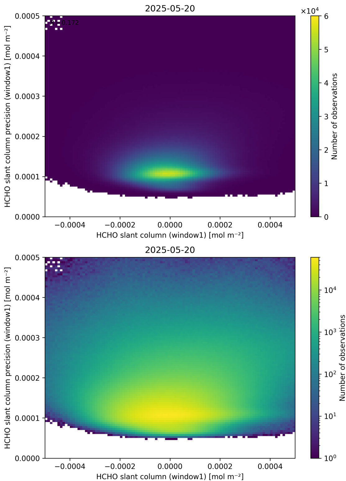
Figure 84: Scatter density plot of “HCHO slant column (window1)” against “HCHO slant column precision (window1)” for 2025-05-19 to 2025-05-21.
