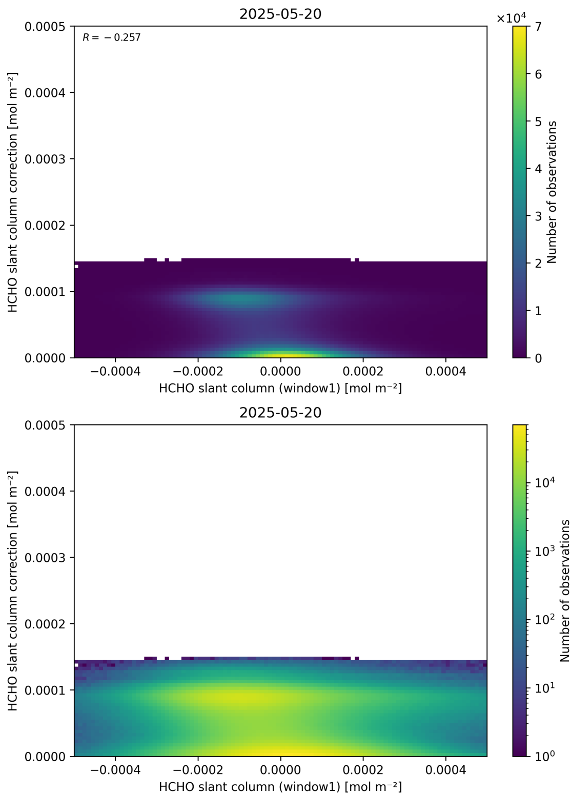
Figure 83: Scatter density plot of “HCHO slant column (window1)” against “HCHO slant column correction” for 2025-05-19 to 2025-05-21.
