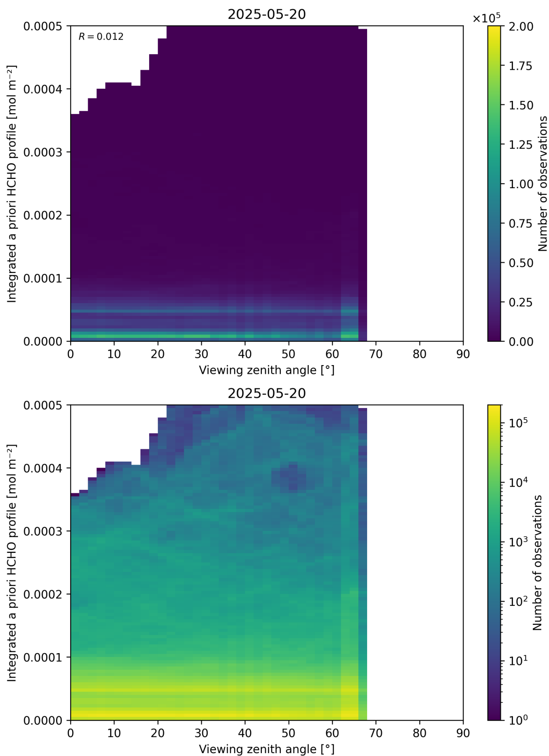
Figure 195: Scatter density plot of “Viewing zenith angle” against “Integrated a priori HCHO profile” for 2025-05-19 to 2025-05-21.
