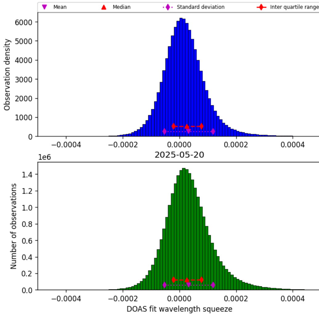
Figure 45: Histogram of “DOAS fit wavelength squeeze” for 2025-05-19 to 2025-05-21
