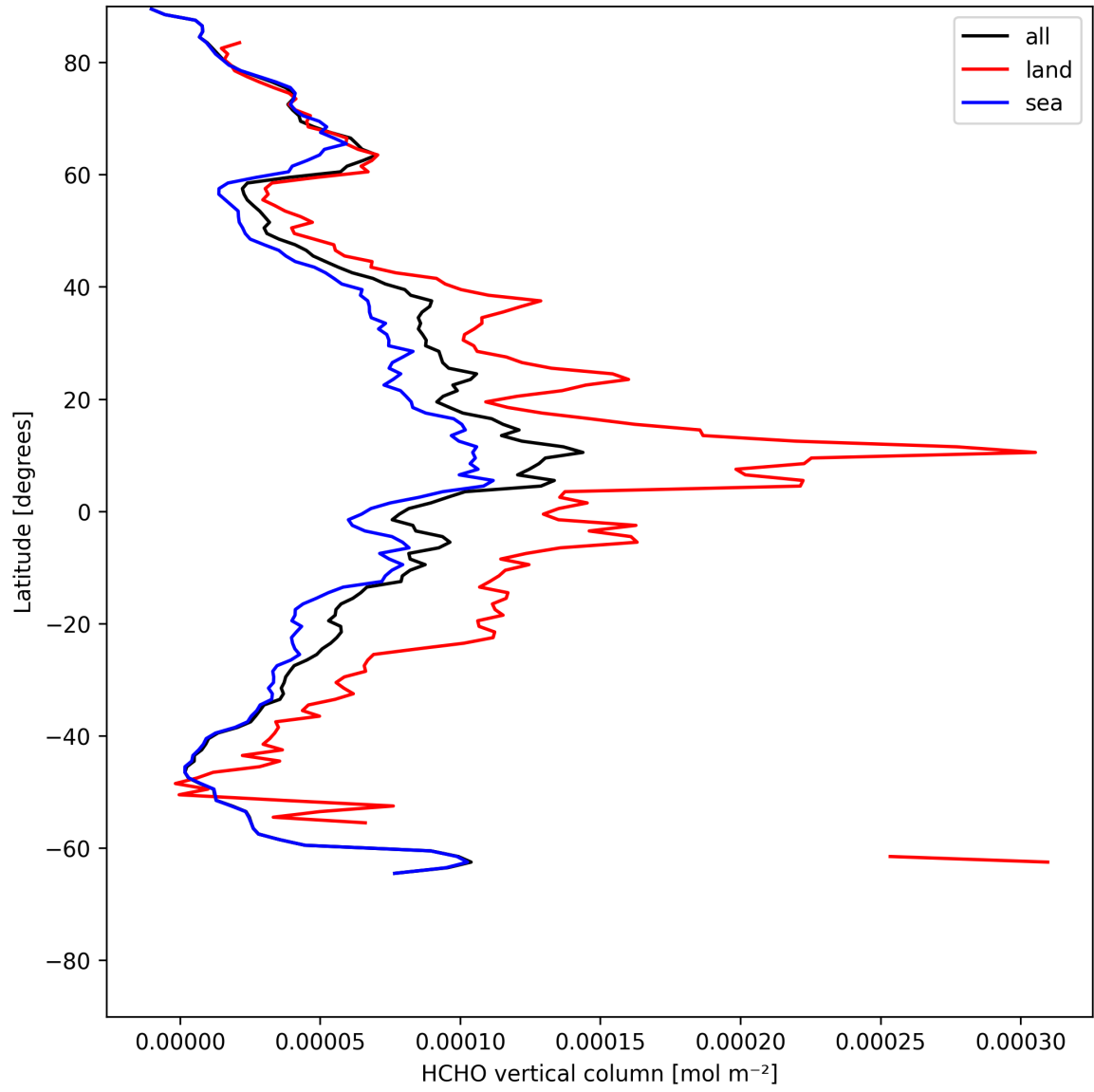
Figure 21: Zonal average of “HCHO vertical column” for 2025-05-19 to 2025-05-21.
