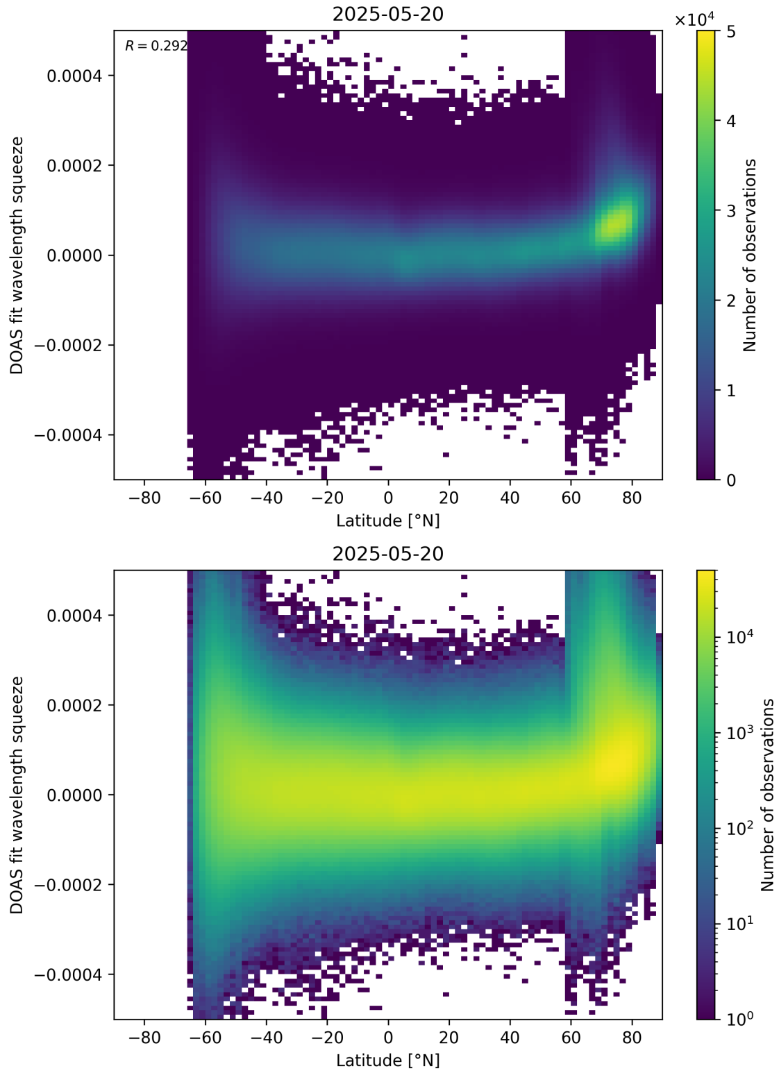
Figure 155: Scatter density plot of “Latitude” against “DOAS fit wavelength squeeze” for 2025-05-19 to 2025-05-21.
