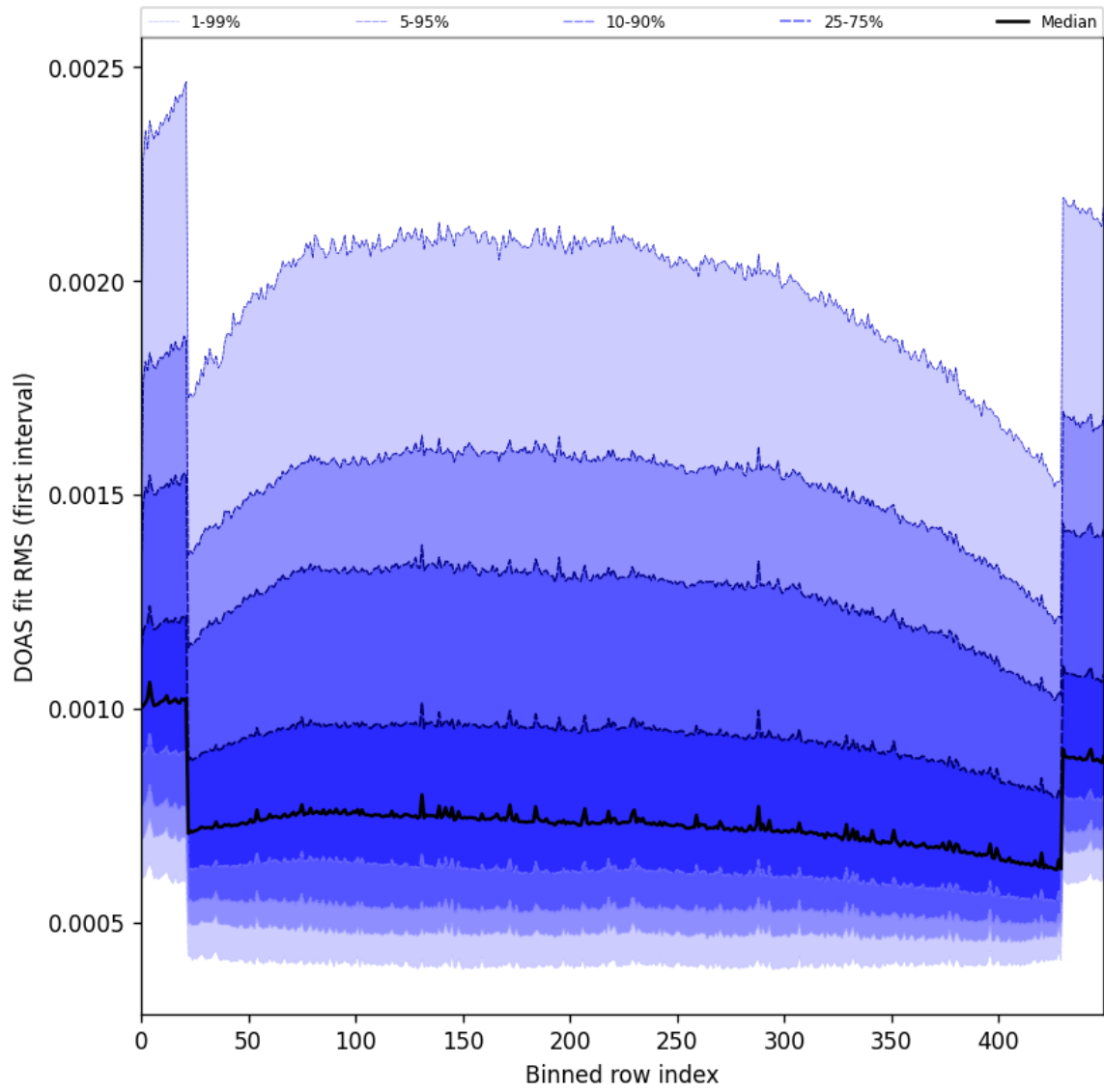
Figure 60: Along track statistics of “DOAS fit RMS (first interval)” for 2025-05-19 to 2025-05-21
