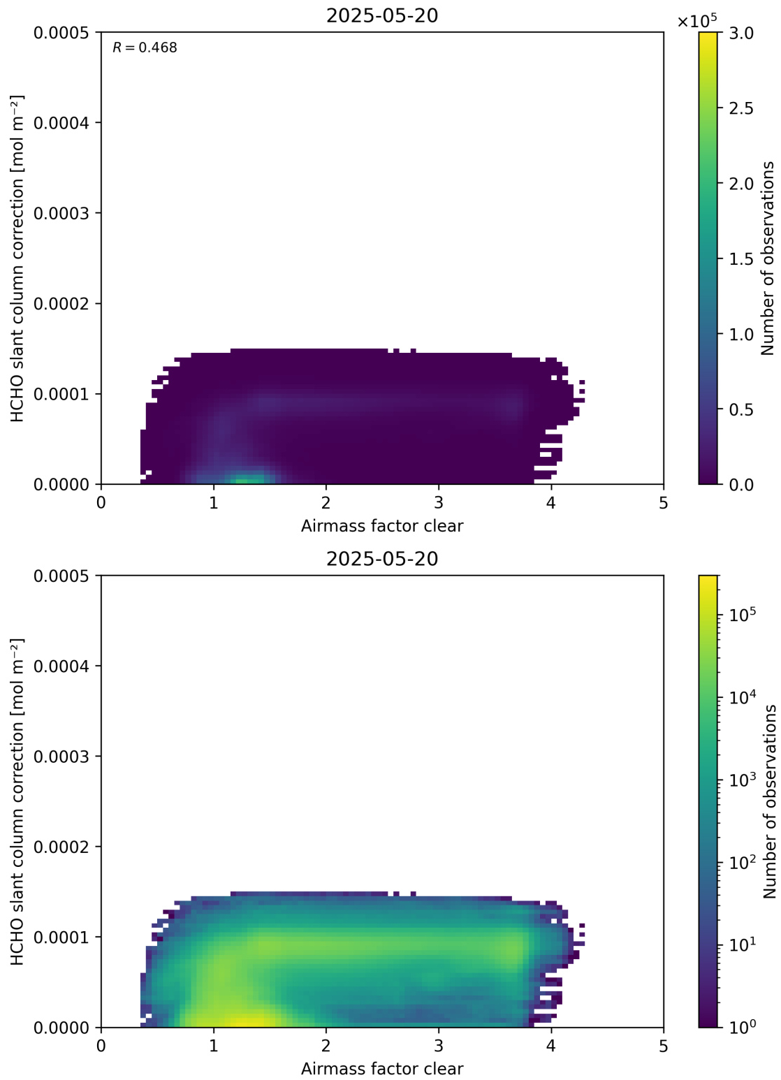
Figure 75: Scatter density plot of “Airmass factor clear” against “HCHO slant column correction” for 2025-05-19 to 2025-05-21.
