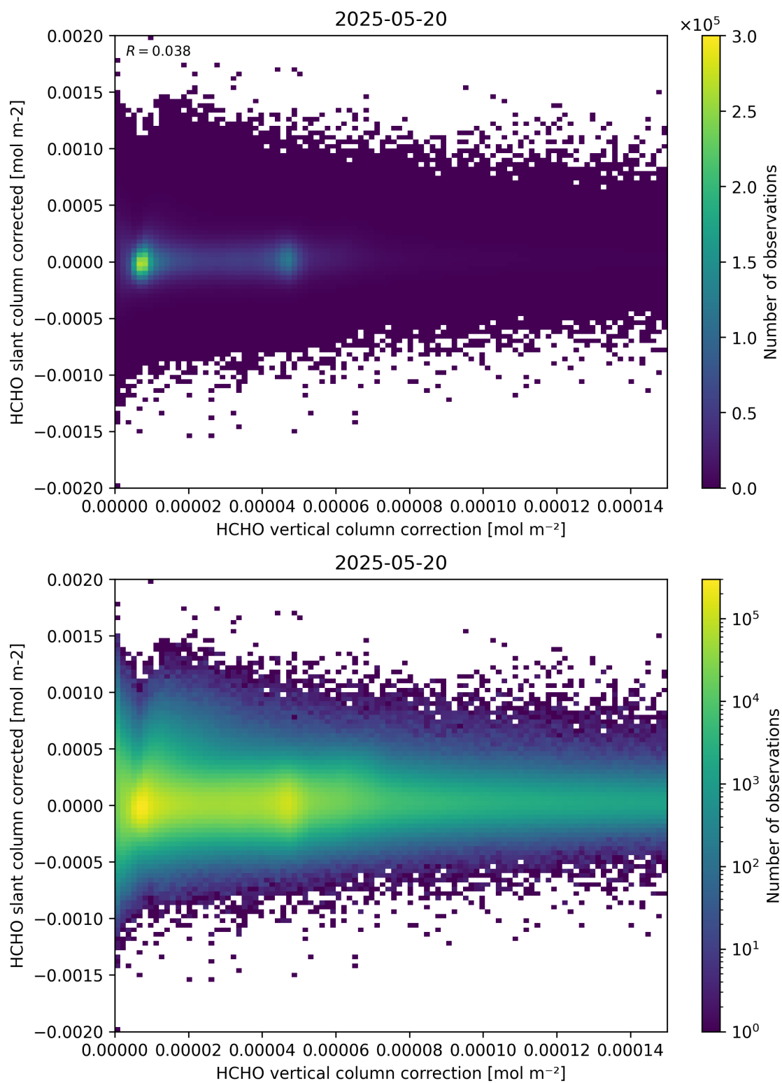
Figure 116: Scatter density plot of “HCHO vertical column correction” against “HCHO slant column corrected” for 2025-05-19 to 2025-05-21.
