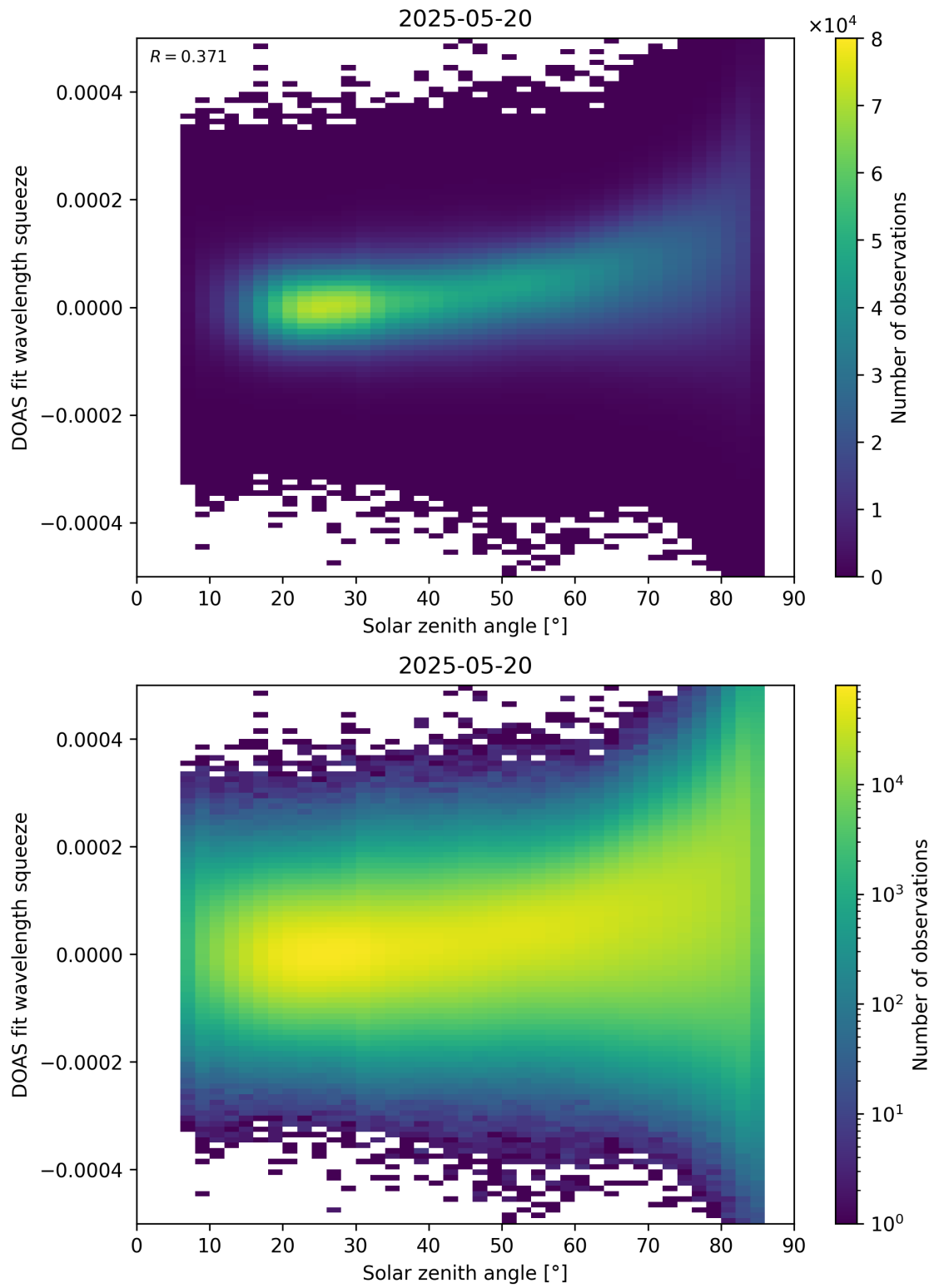
Figure 169: Scatter density plot of “Solar zenith angle” against “DOAS fit wavelength squeeze” for 2025-05-19 to 2025-05-21.
