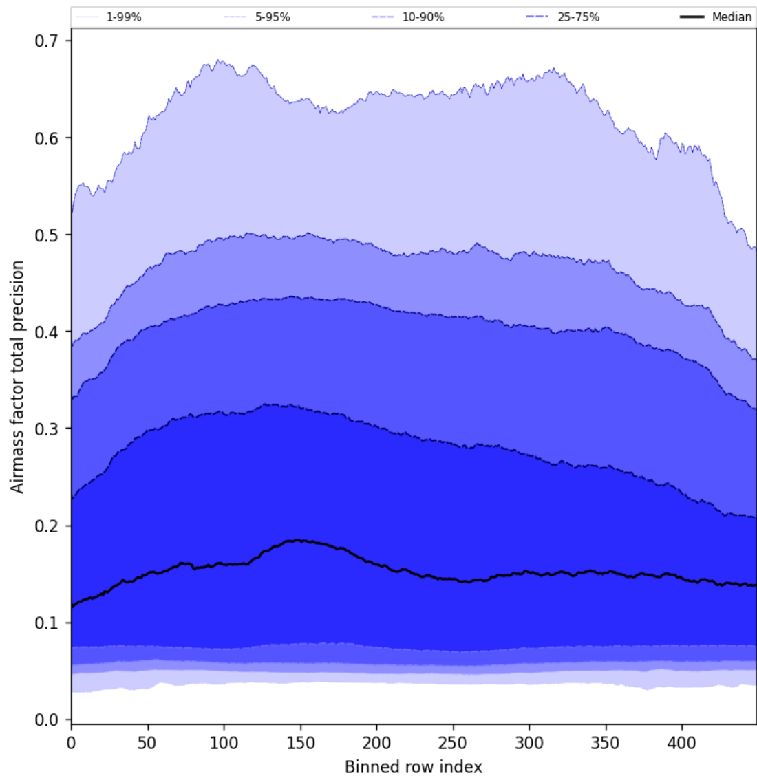
Figure 55: Along track statistics of “Airmass factor total precision” for 2025-05-19 to 2025-05-21
