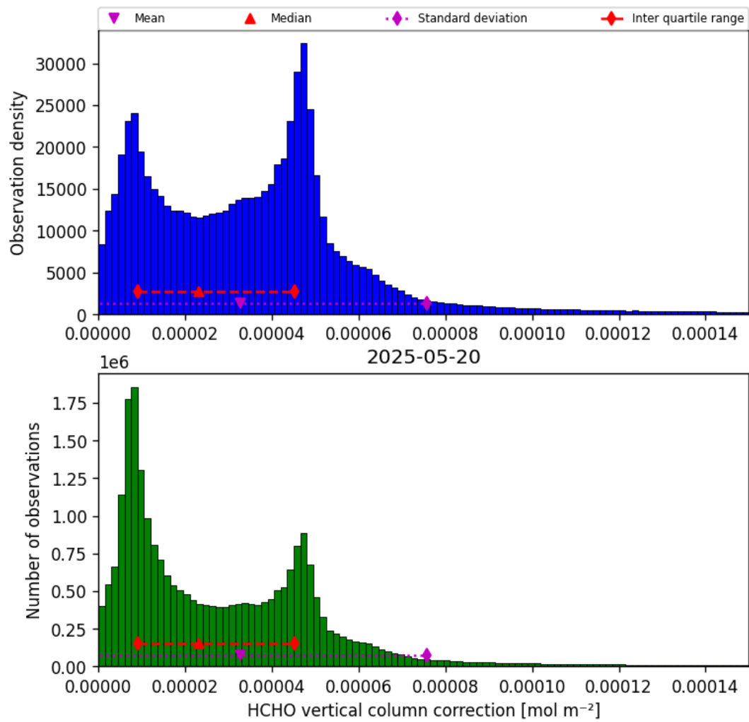
Figure 37: Histogram of “HCHO vertical column correction” for 2025-05-19 to 2025-05-21
