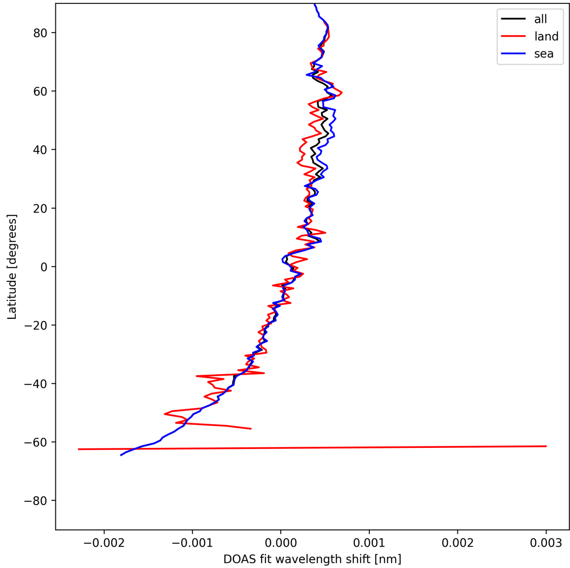
Figure 30: Zonal average of “DOAS fit wavelength shift” for 2025-05-19 to 2025-05-21.
