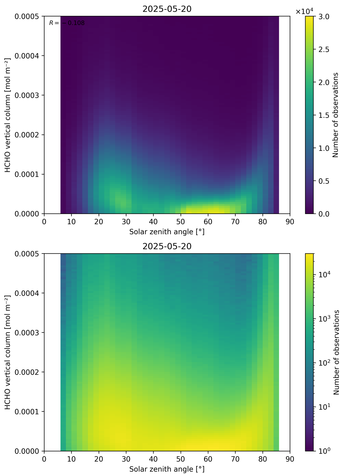
Figure 177: Scatter density plot of “Solar zenith angle” against “HCHO vertical column” for 2025-05-19 to 2025-05-21.
