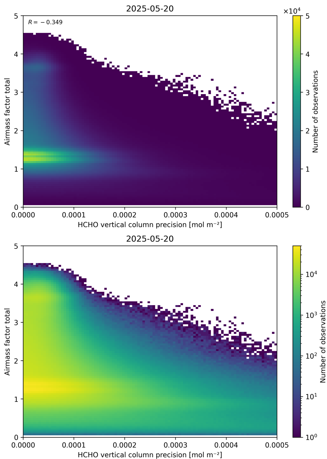
Figure 144: Scatter density plot of “HCHO vertical column precision” against “Airmass factor total” for 2025-05-19 to 2025-05-21.
