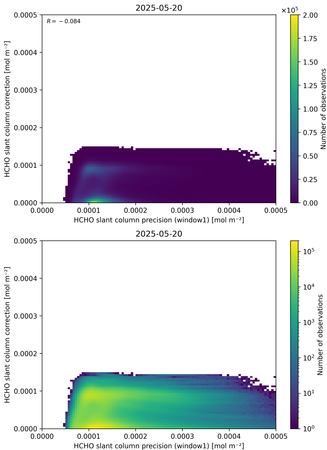
Figure 93: Scatter density plot of “HCHO slant column precision (window1)” against “HCHO slant column correction” for 2025-05-19 to 2025-05-21.
