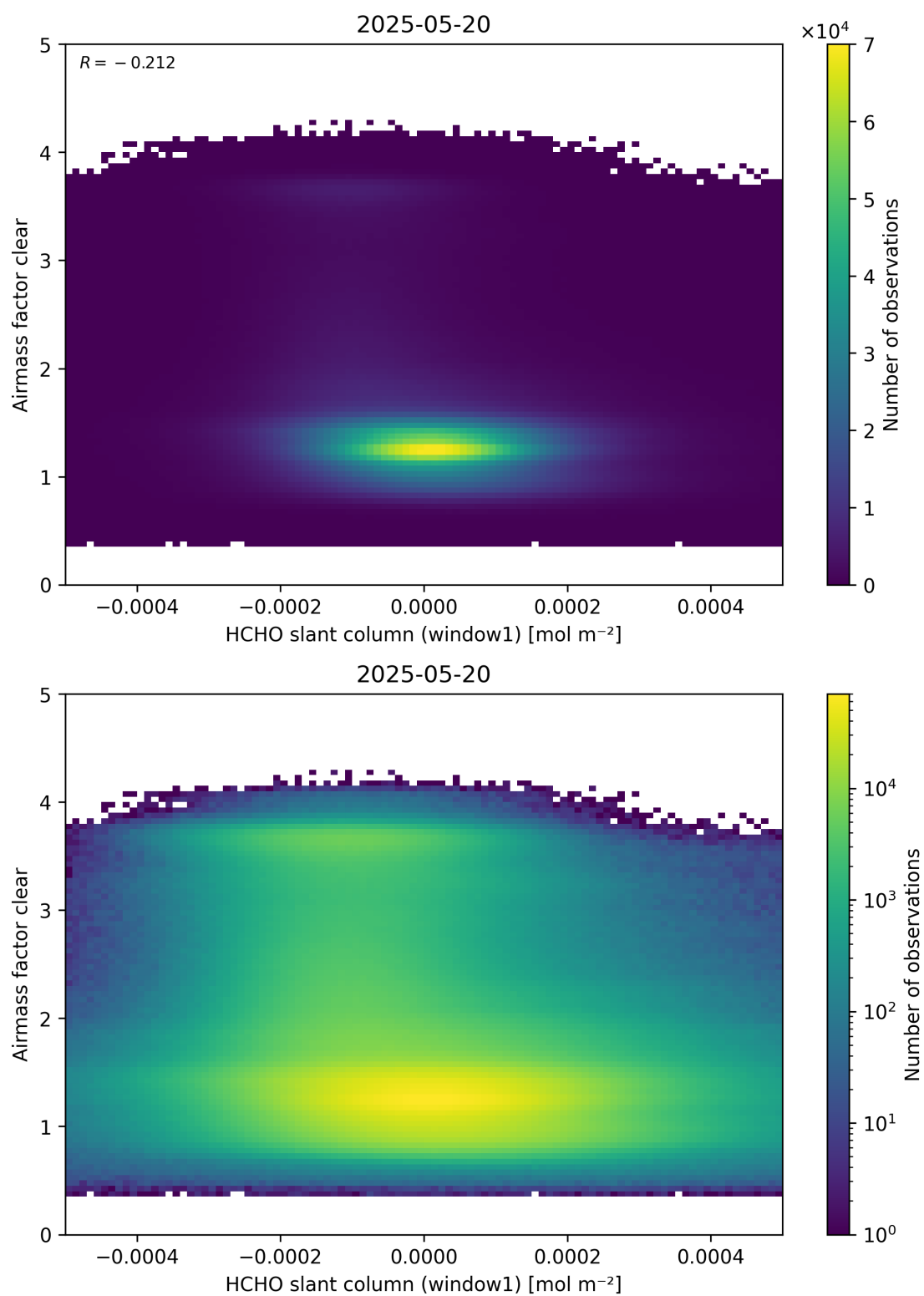
Figure 81: Scatter density plot of “HCHO slant column (window1)” against “Airmass factor clear” for 2025-05-19 to 2025-05-21.
