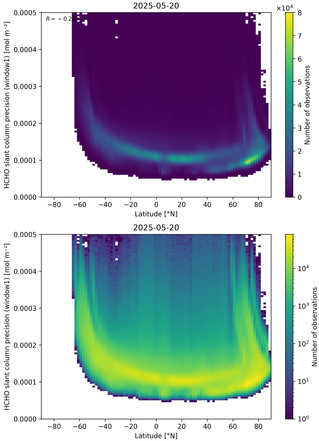
Figure 160: Scatter density plot of “Latitude” against “HCHO slant column precision (window1)” for 2025-05-19 to 2025-05-21.
