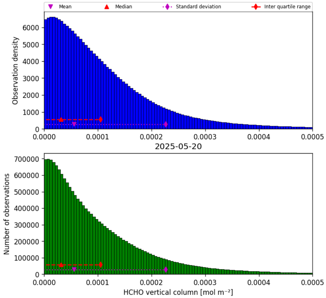
Figure 35: Histogram of “HCHO vertical column” for 2025-05-19 to 2025-05-21
