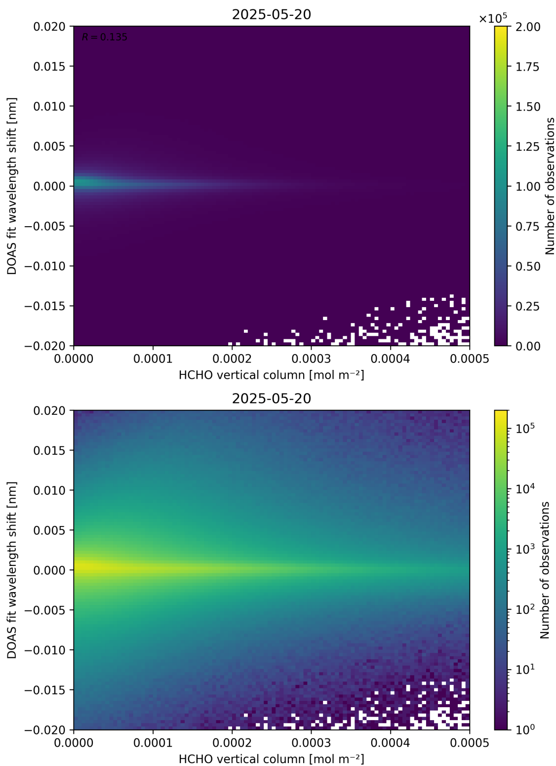
Figure 124: Scatter density plot of “HCHO vertical column” against “DOAS fit wavelength shift” for 2025-05-19 to 2025-05-21.
