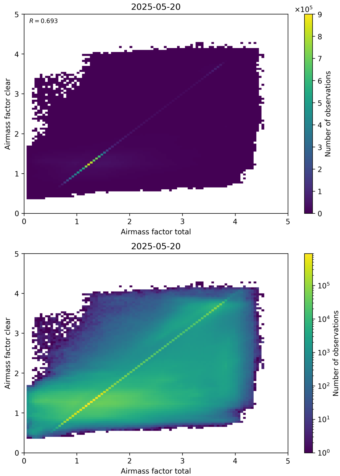
Figure 100: Scatter density plot of “Airmass factor total” against “Airmass factor clear” for 2025-05-19 to 2025-05-21.
