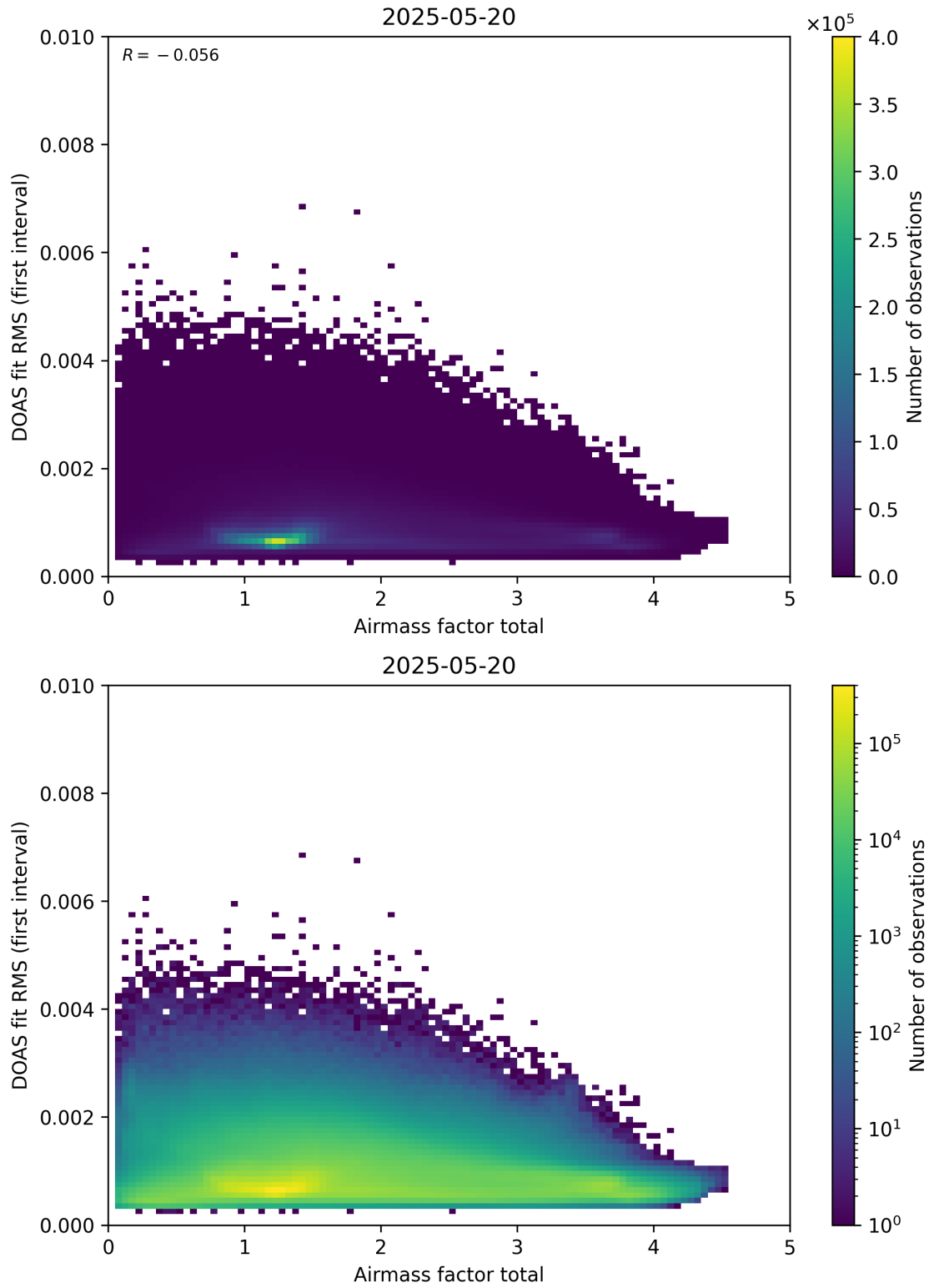
Figure 97: Scatter density plot of “Airmass factor total” against “DOAS fit RMS (first interval)” for 2025-05-19 to 2025-05-21.
