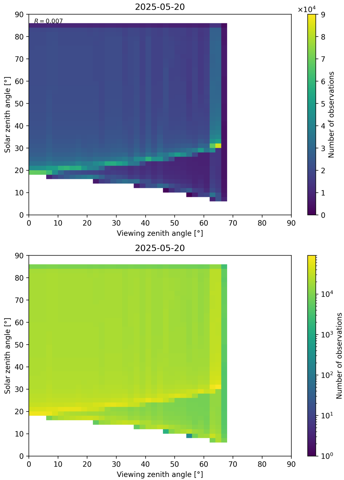
Figure 197: Scatter density plot of “Viewing zenith angle” against “Solar zenith angle” for 2025-05-19 to 2025-05-21.
