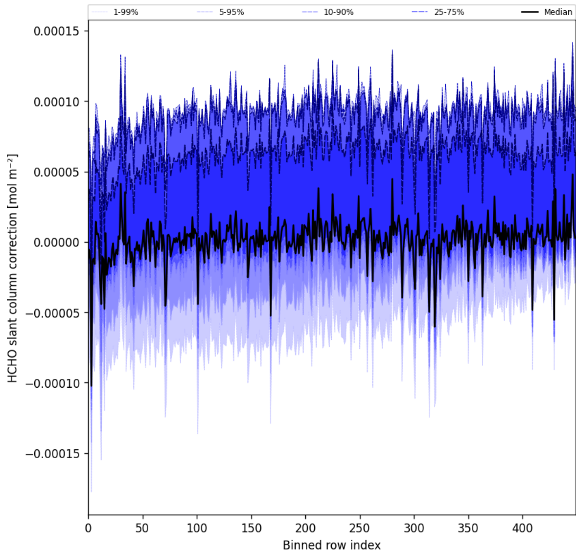
Figure 61: Along track statistics of "HCHO slant column correction" for 2025-05-19 to 2025-05-21
