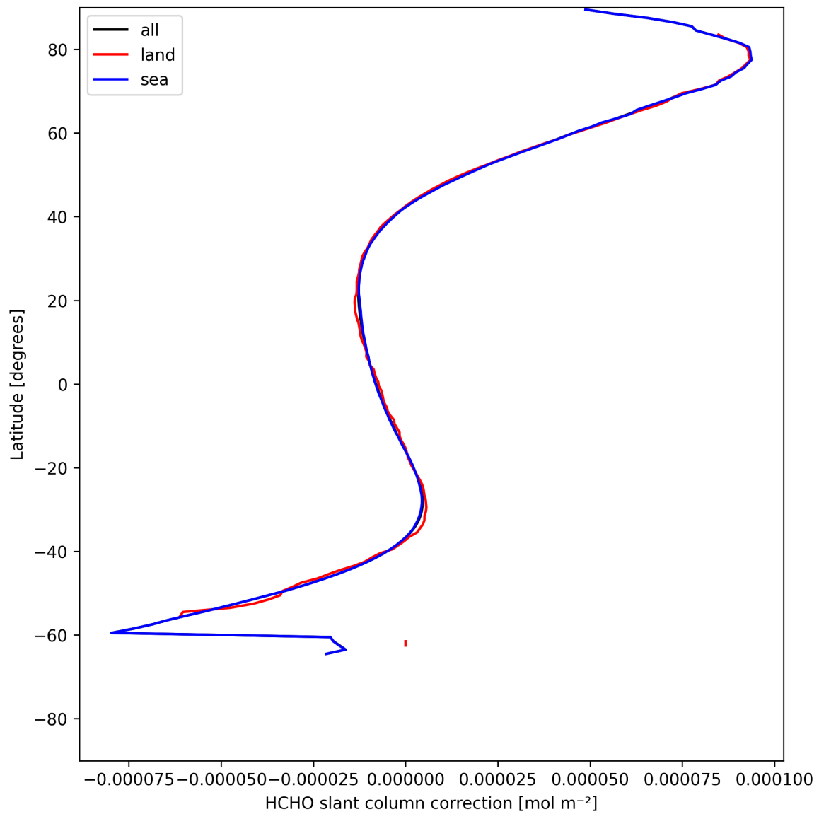
Figure 33: Zonal average of “HCHO slant column correction” for 2025-05-19 to 2025-05-21.
