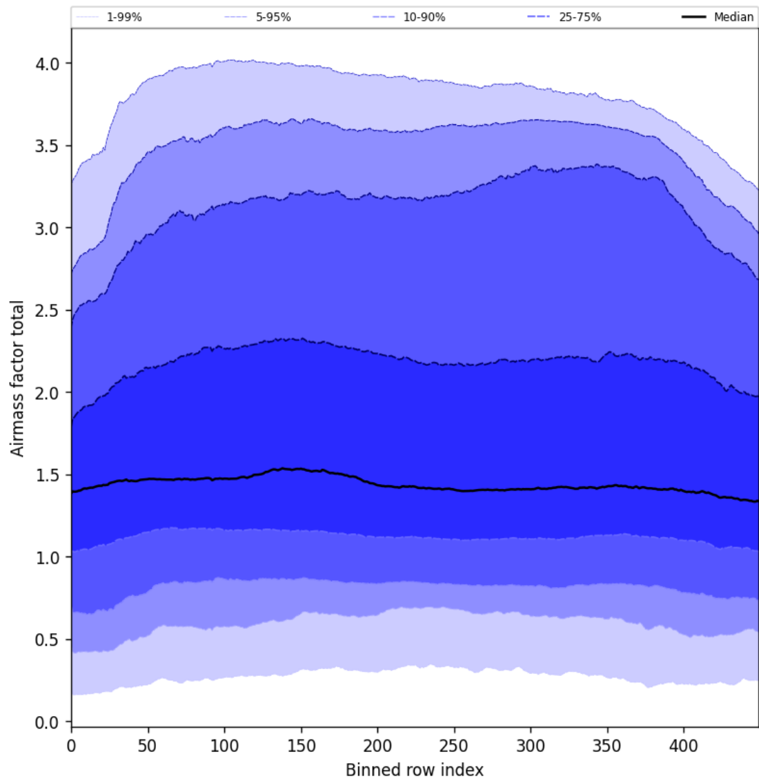
Figure 54: Along track statistics of “Airmass factor total” for 2025-05-19 to 2025-05-21
