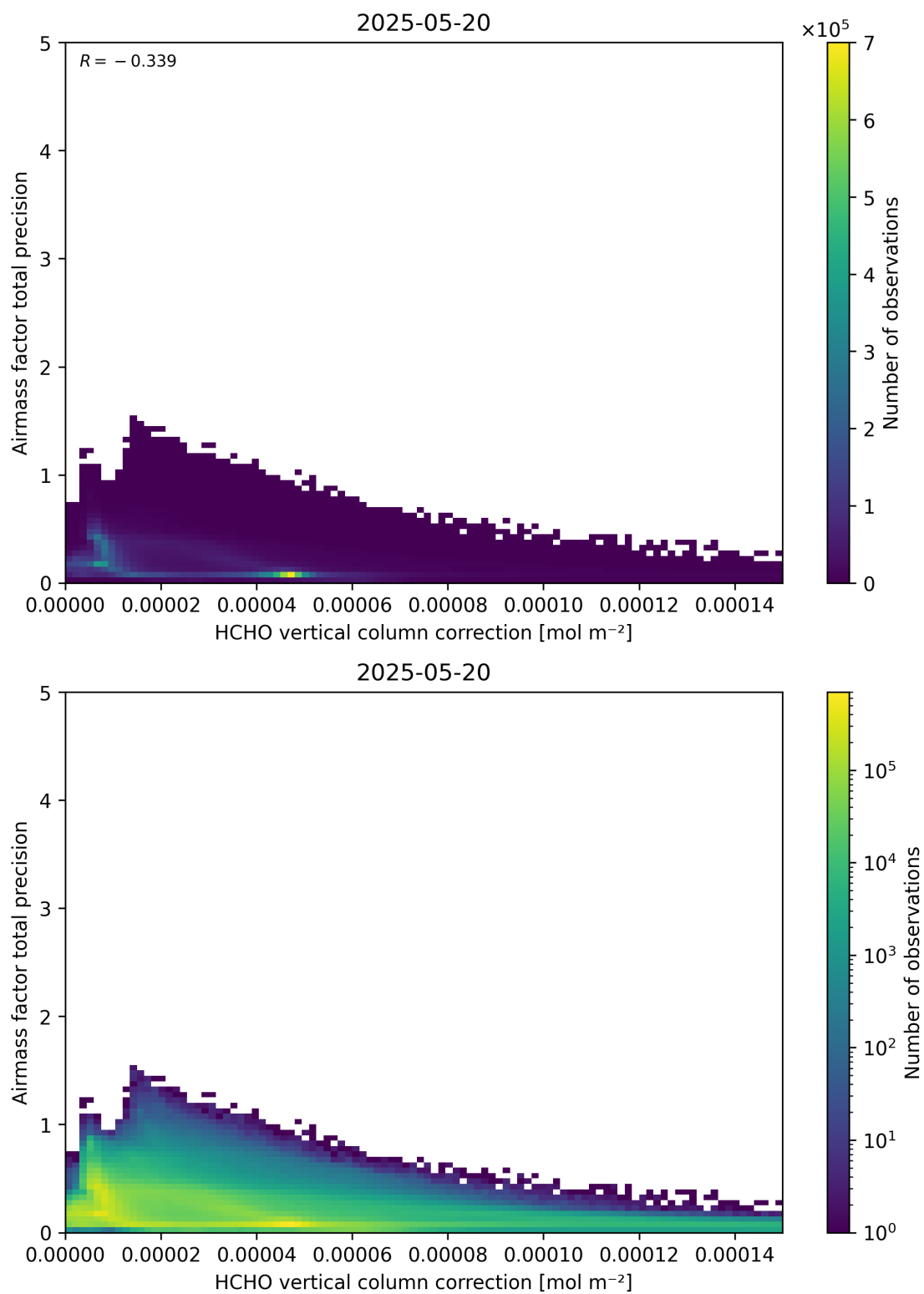
Figure 121: Scatter density plot of “HCHO vertical column correction” against “Airmass factor total precision” for 2025-05-19 to 2025-05-21.
