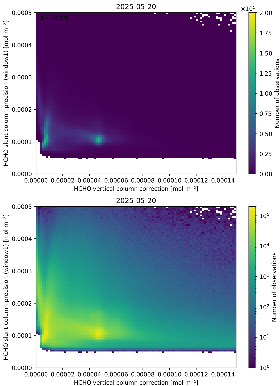
Figure 119: Scatter density plot of “HCHO vertical column correction” against “HCHO slant column precision (window1)” for 2025-05-19 to 2025-05-21.
