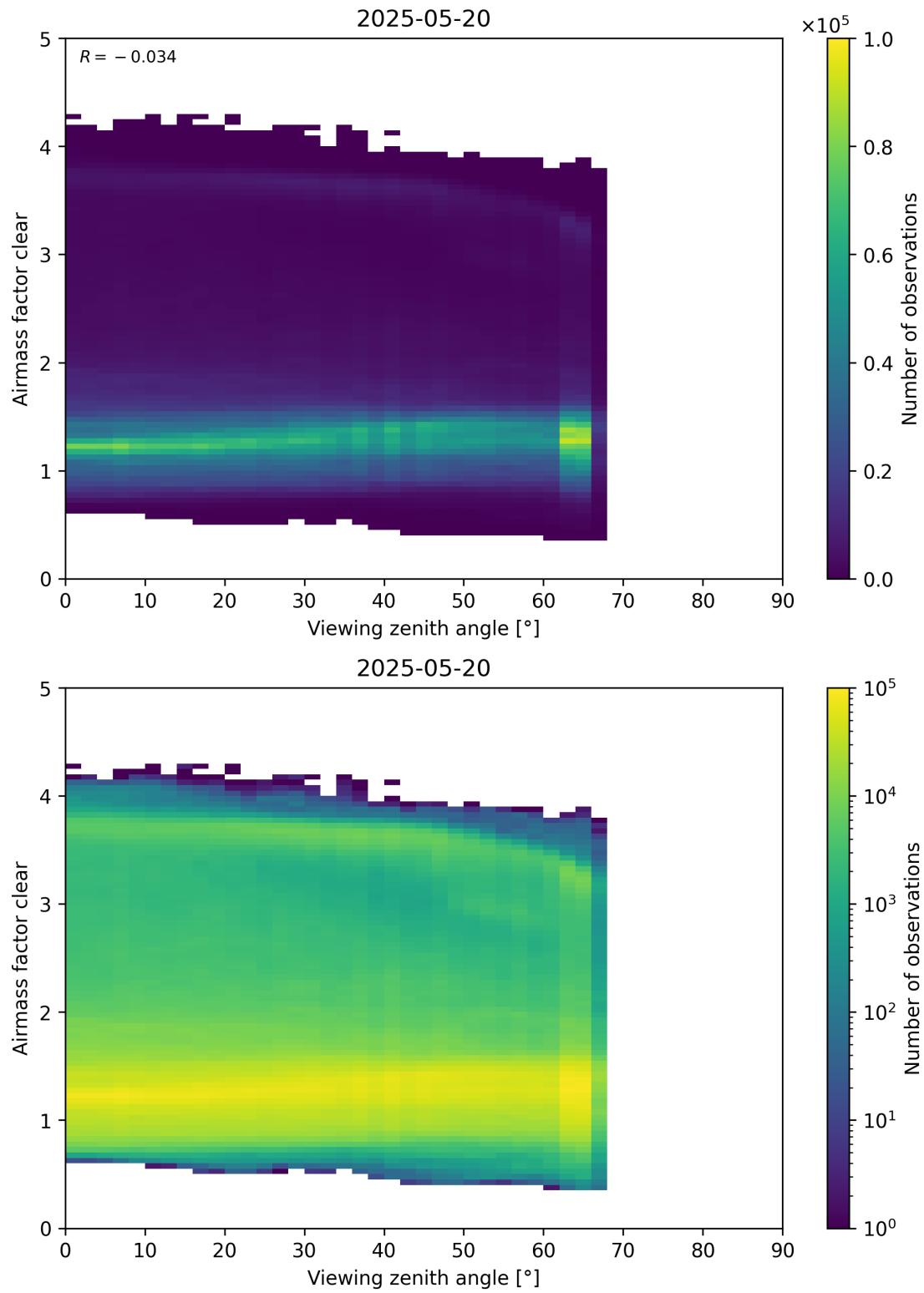
Figure 185: Scatter density plot of “Viewing zenith angle” against “Airmass factor clear” for 2025-05-19 to 2025-05-21.
