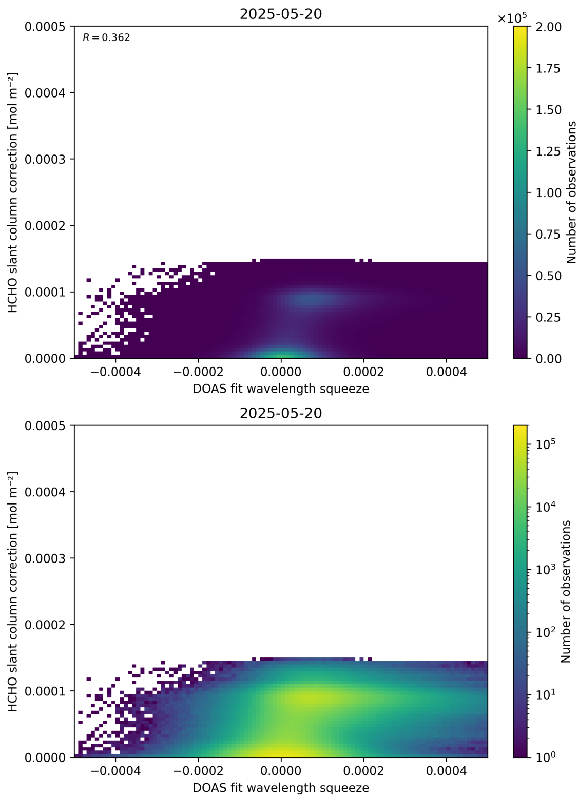
Figure 70: Scatter density plot of “DOAS fit wavelength squeeze” against “HCHO slant column correction” for 2025-05-19 to 2025-05-21.
