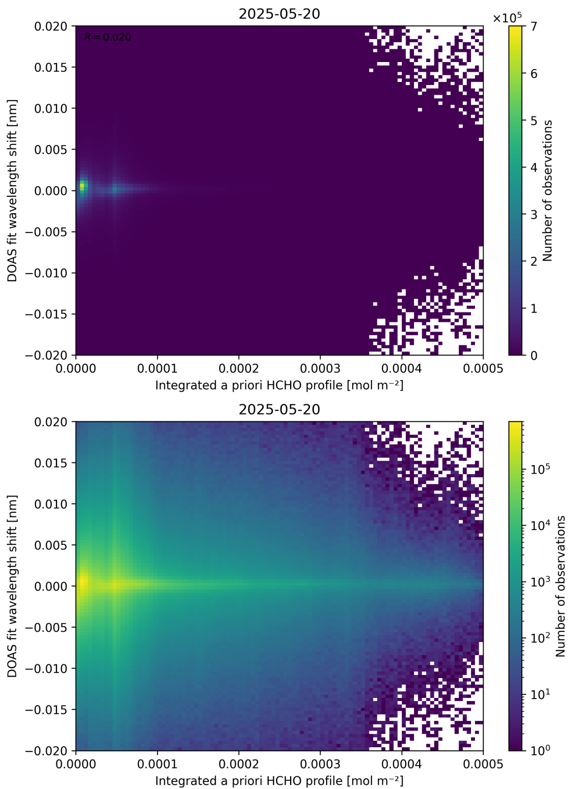
Figure 149: Scatter density plot of “Integrated a priori HCHO profile” against “DOAS fit wavelength shift” for 2025-05-19 to 2025-05-21.
