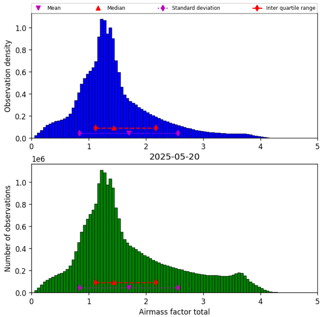
Figure 40: Histogram of “Airmass factor total” for 2025-05-19 to 2025-05-21
