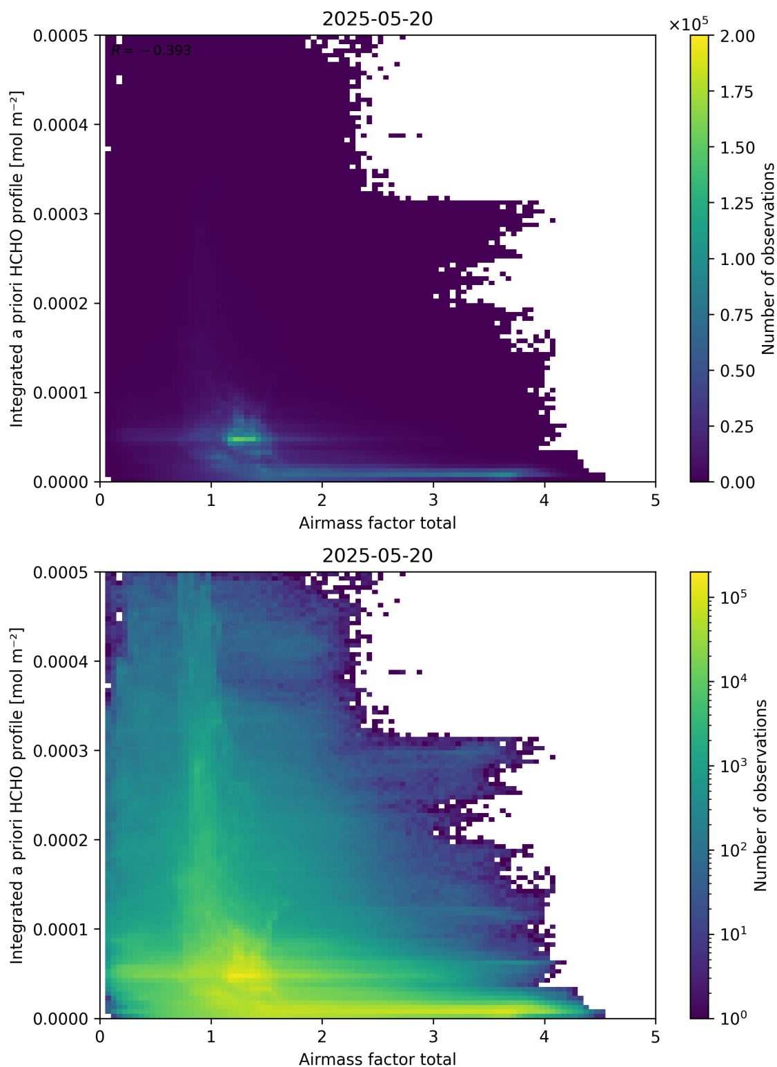
Figure 104: Scatter density plot of “Airmass factor total” against “Integrated a priori HCHO profile” for 2025-05-19 to 2025-05-21.
