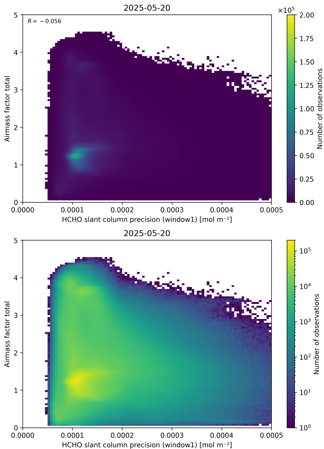
Figure 94: Scatter density plot of “HCHO slant column precision (window1)” against “Airmass factor total” for 2025-05-19 to 2025-05-21.
