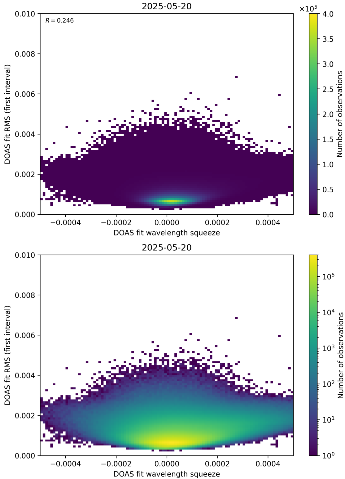
Figure 68: Scatter density plot of “DOAS fit wavelength squeeze” against “DOAS fit RMS (first interval)” for 2025-05-19 to 2025-05-21.
