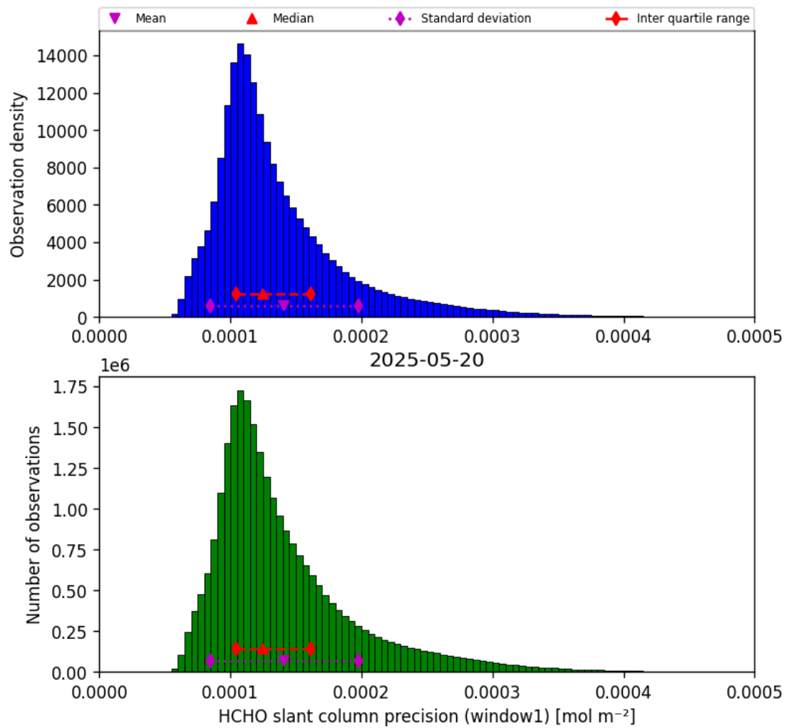
Figure 39: Histogram of “HCHO slant column precision (window1)” for 2025-05-19 to 2025-05-21
