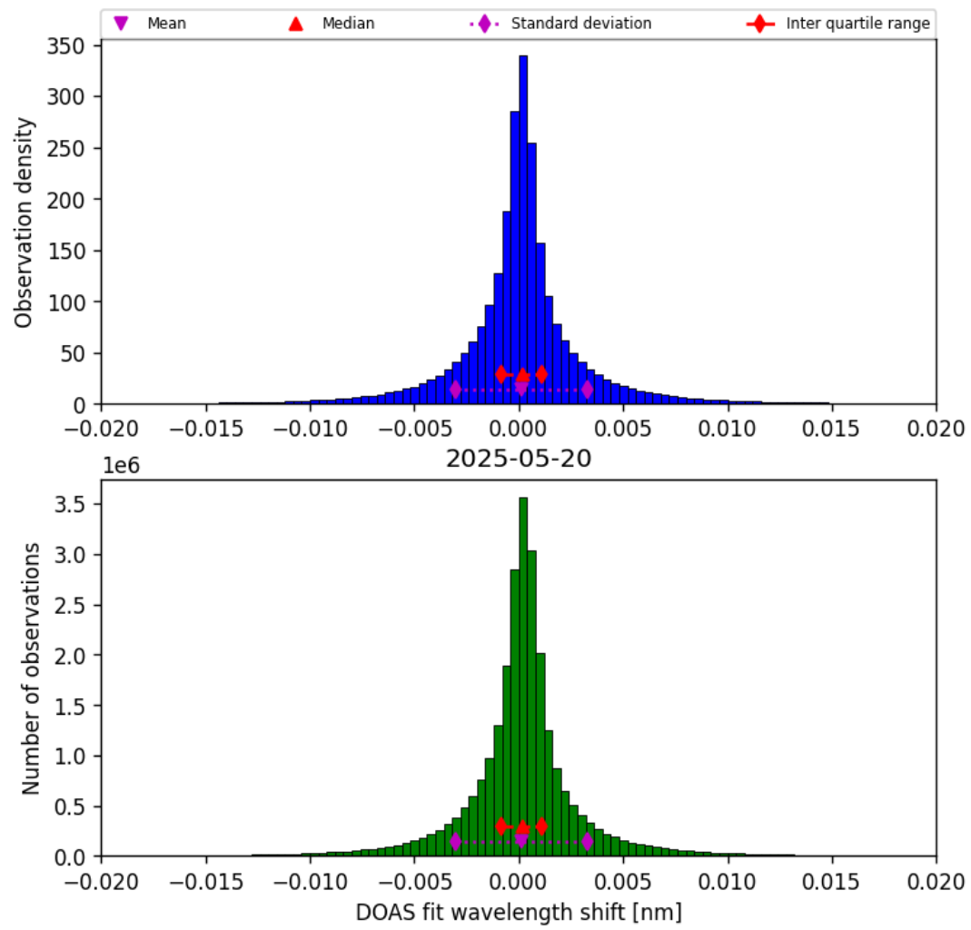
Figure 44: Histogram of “DOAS fit wavelength shift” for 2025-05-19 to 2025-05-21
