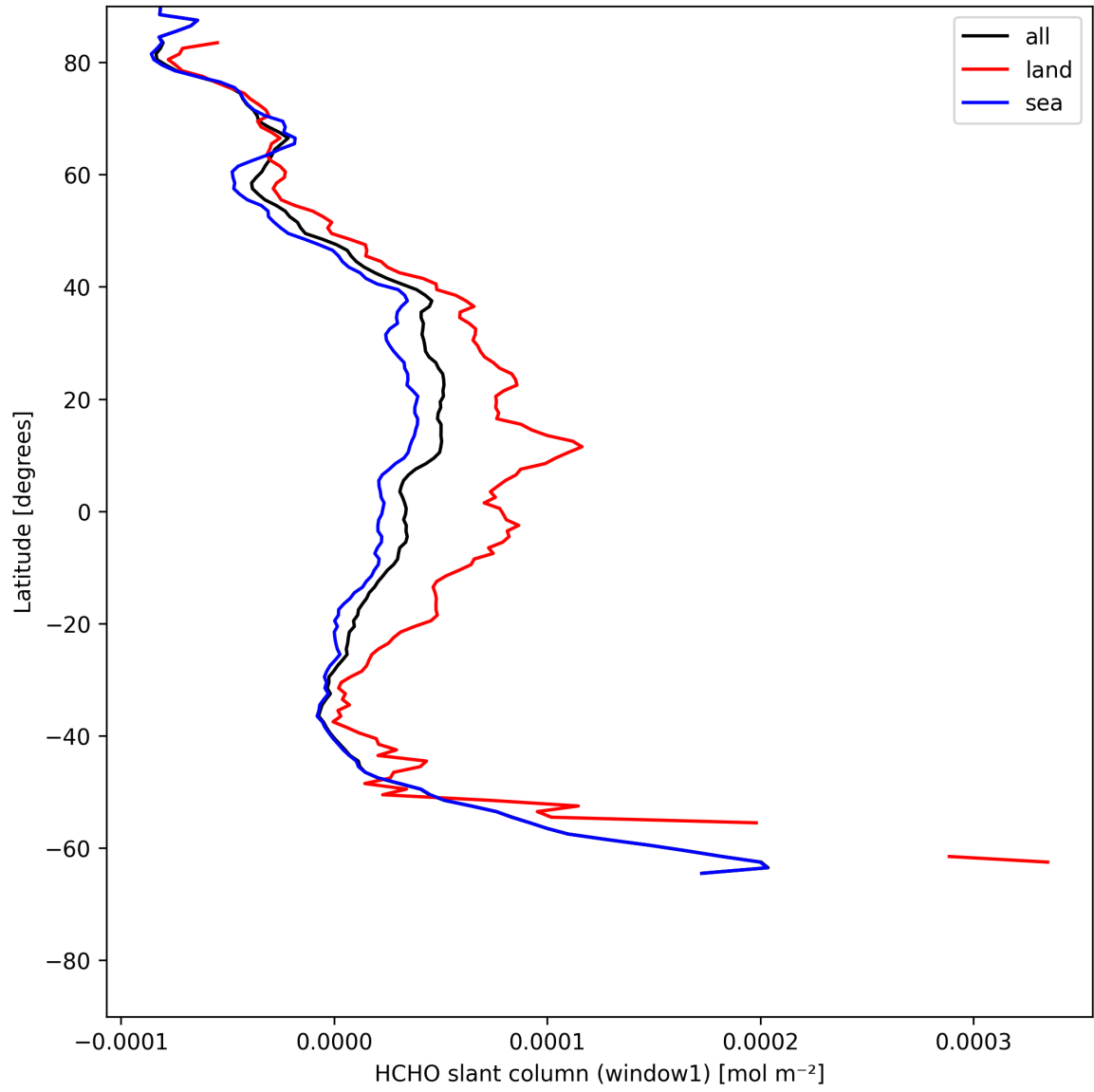
Figure 24: Zonal average of “HCHO slant column (window1)” for 2025-05-19 to 2025-05-21.
