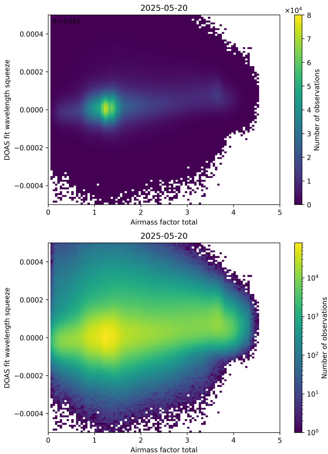
Figure 99: Scatter density plot of “Airmass factor total” against “DOAS fit wavelength squeeze” for 2025-05-19 to 2025-05-21.
