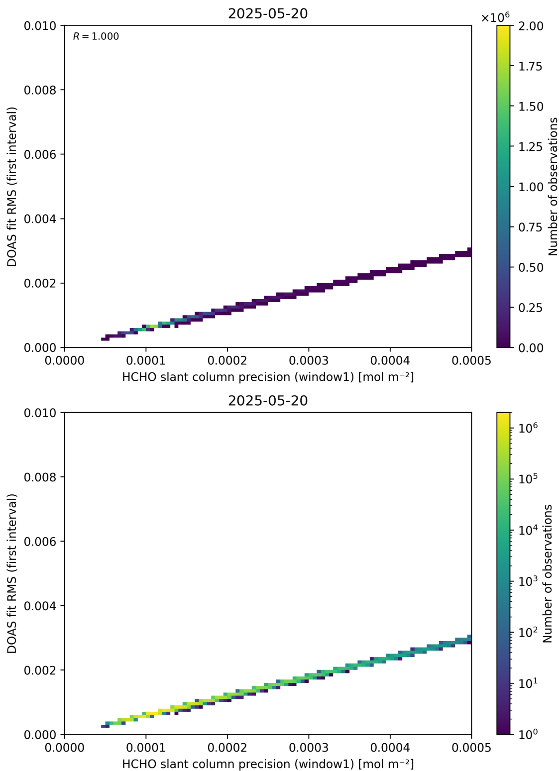
Figure 88: Scatter density plot of “HCHO slant column precision (window1)” against “DOAS fit RMS (first interval)” for 2025-05-19 to 2025-05-21.
