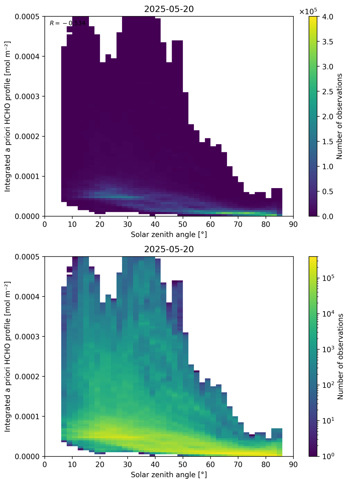
Figure 180: Scatter density plot of “Solar zenith angle” against “Integrated a priori HCHO profile” for 2025-05-19 to 2025-05-21.
