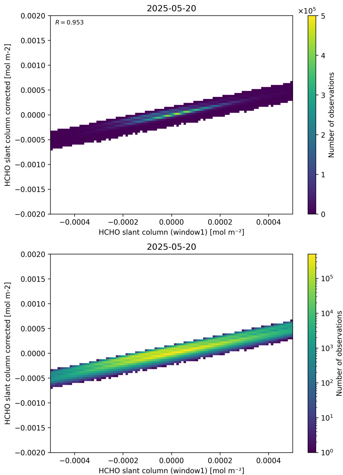
Figure 82: Scatter density plot of “HCHO slant column (window1)” against “HCHO slant column corrected” for 2025-05-19 to 2025-05-21.
