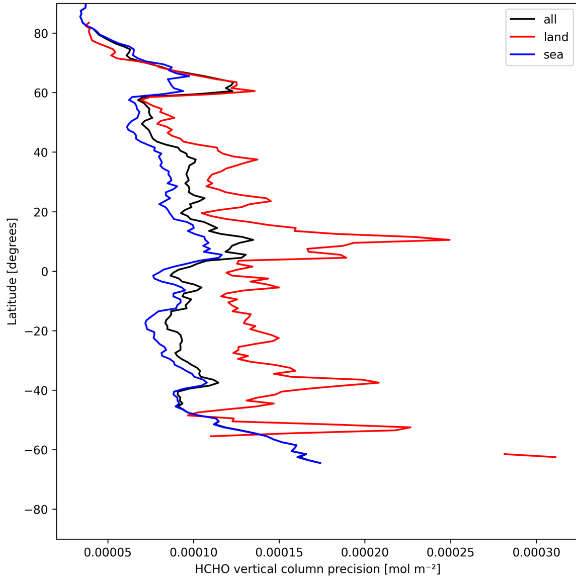
Figure 22: Zonal average of “HCHO vertical column precision” for 2025-05-19 to 2025-05-21.
