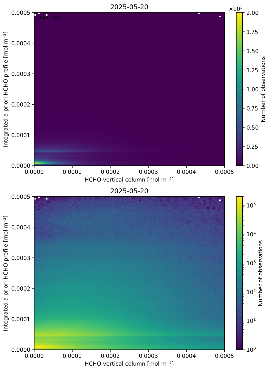
Figure 135: Scatter density plot of “HCHO vertical column” against “Integrated a priori HCHO profile” for 2025-05-19 to 2025-05-21.
