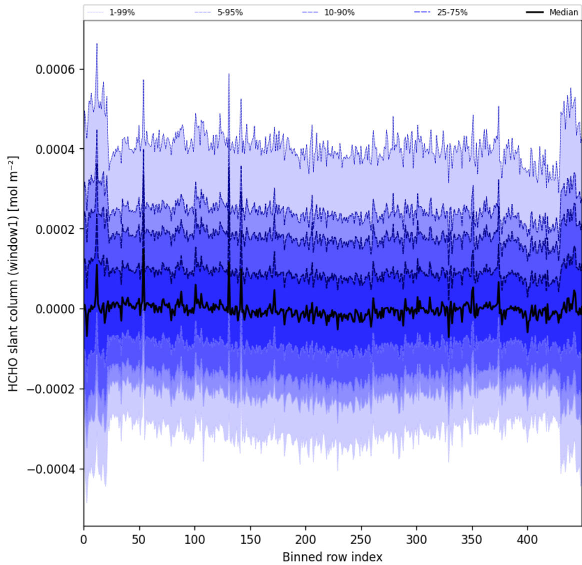
Figure 52: Along track statistics of “HCHO slant column (window1)” for 2025-05-19 to 2025-05-21
