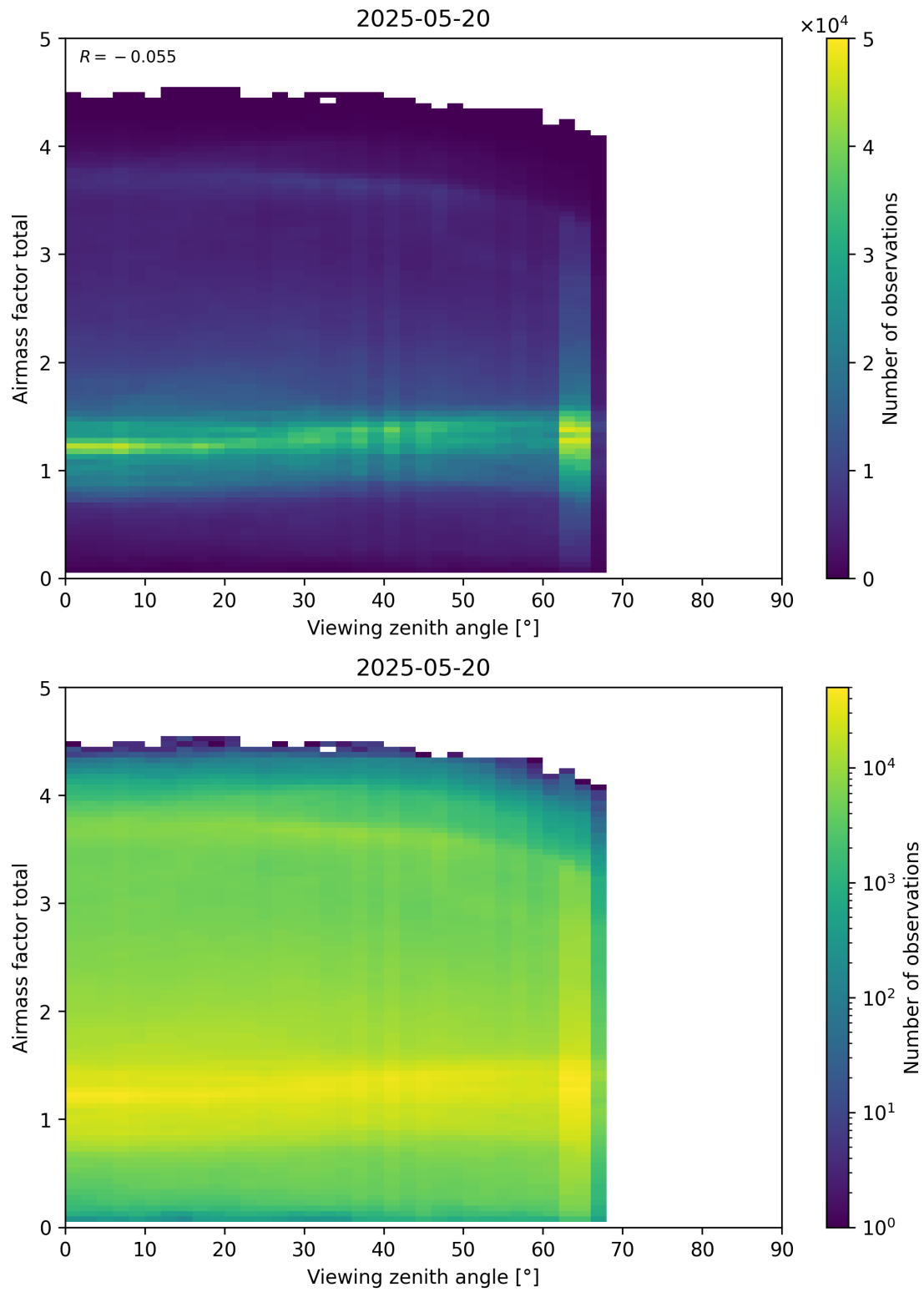
Figure 190: Scatter density plot of “Viewing zenith angle” against “Airmass factor total” for 2025-05-19 to 2025-05-21.
