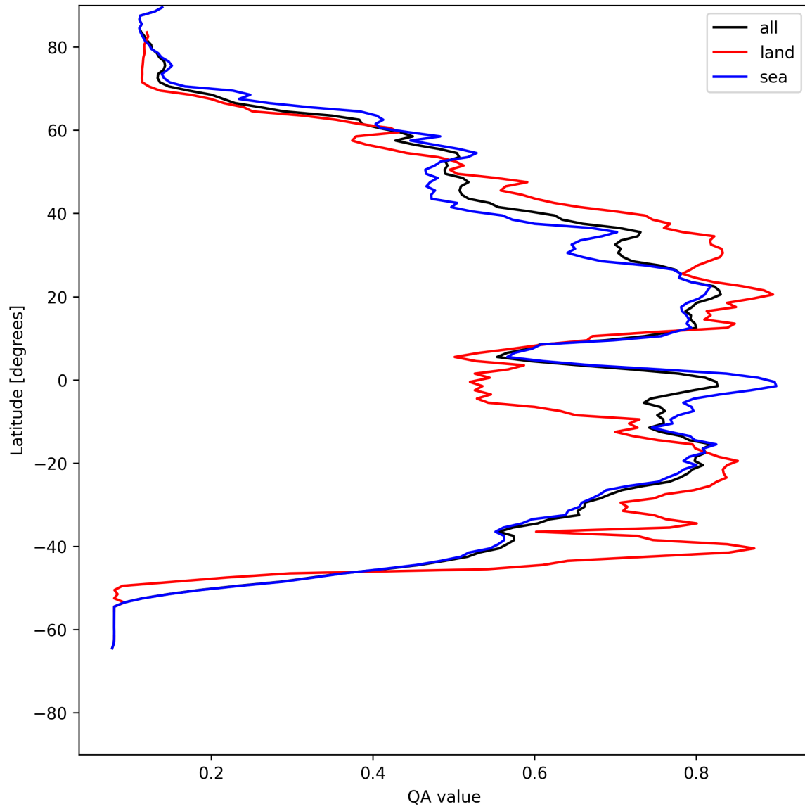
Figure 20: Zonal average of “QA value” for 2025-05-19 to 2025-05-21.
