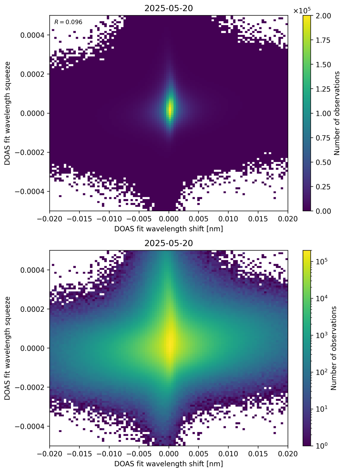
Figure 65: Scatter density plot of “DOAS fit wavelength shift” against “DOAS fit wavelength squeeze” for 2025-05-19 to 2025-05-21.
