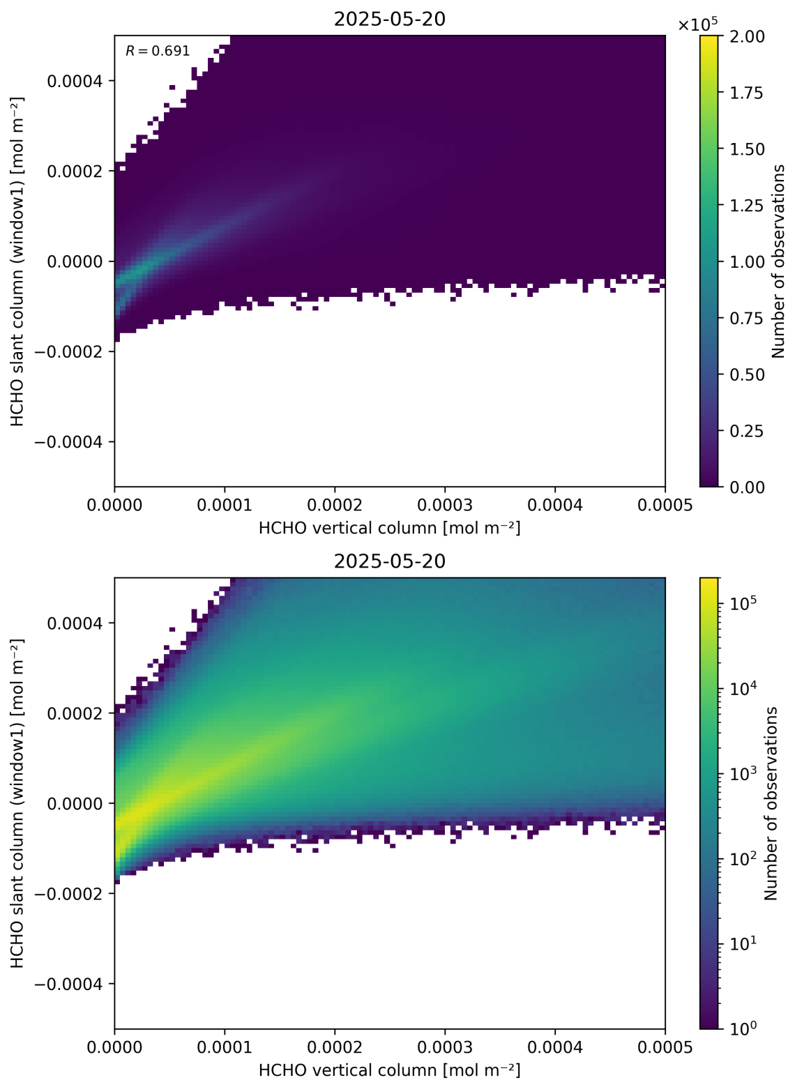
Figure 129: Scatter density plot of “HCHO vertical column” against “HCHO slant column (window1)” for 2025-05-19 to 2025-05-21.
