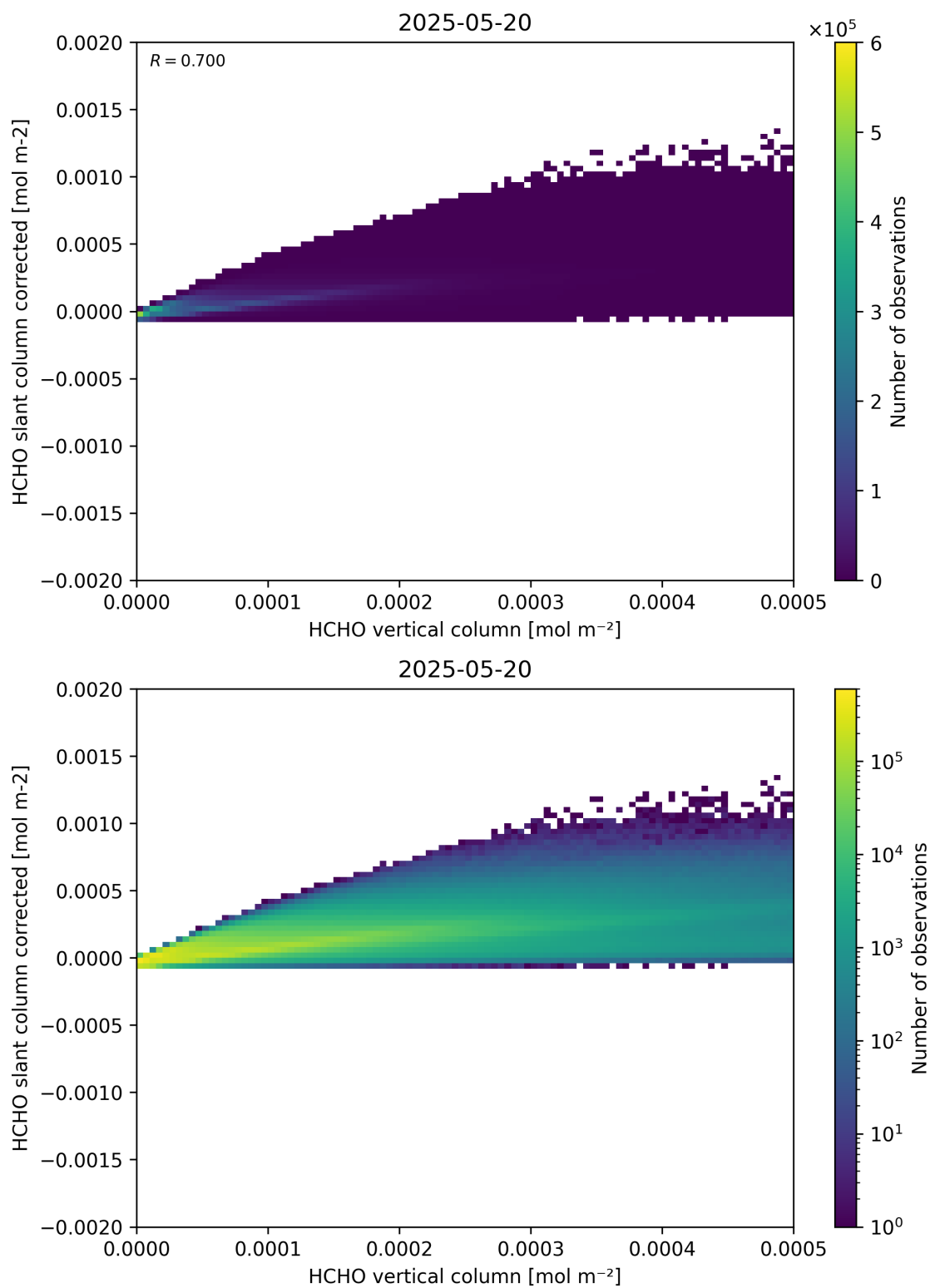
Figure 127: Scatter density plot of “HCHO vertical column” against “HCHO slant column corrected” for 2025-05-19 to 2025-05-21.
