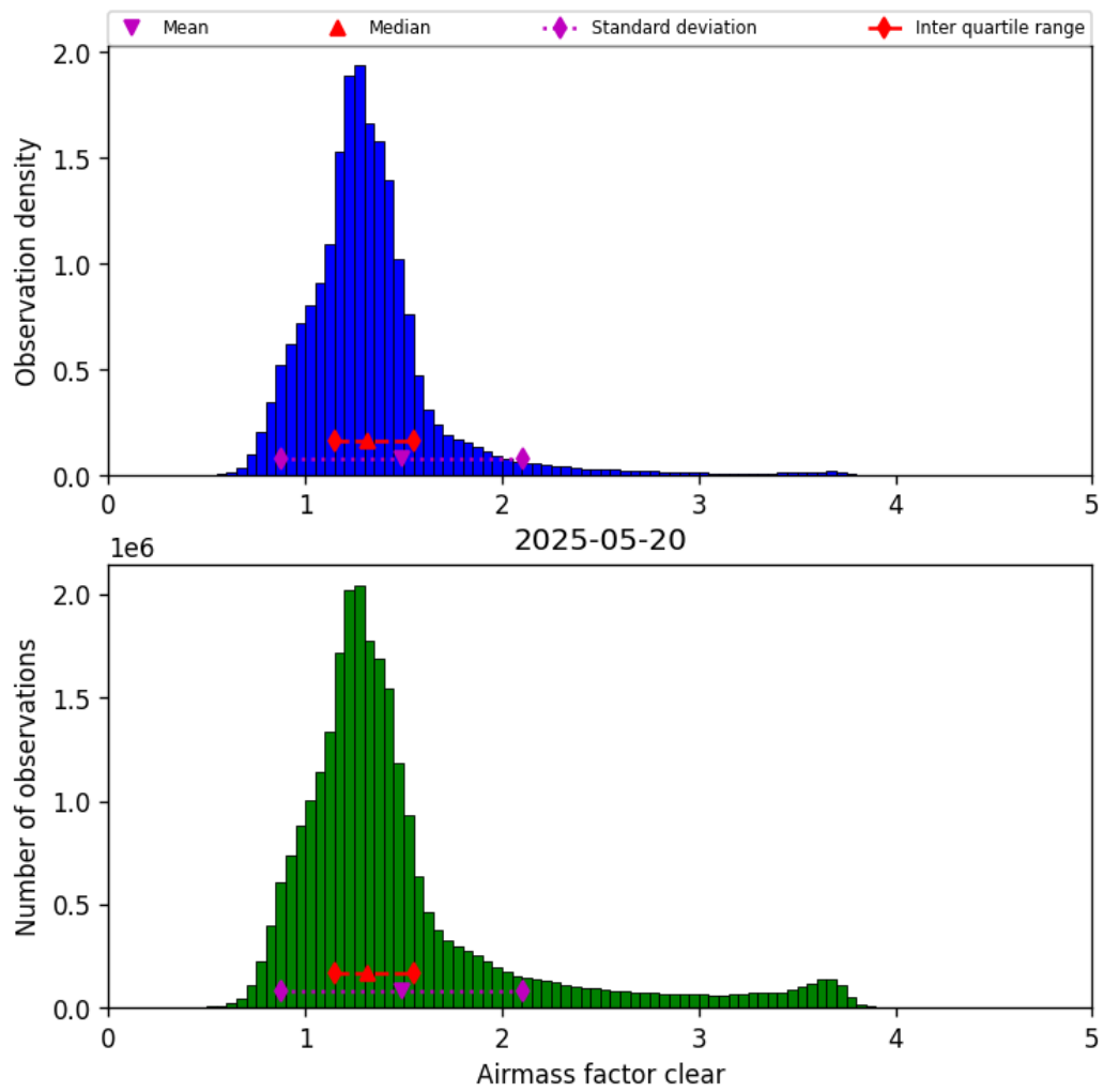
Figure 42: Histogram of “Airmass factor clear” for 2025-05-19 to 2025-05-21
