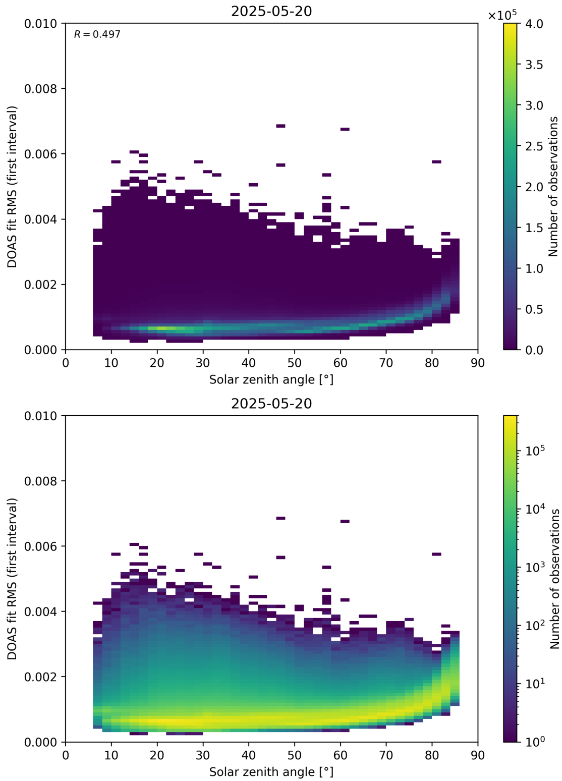
Figure 167: Scatter density plot of “Solar zenith angle” against “DOAS fit RMS (first interval)” for 2025-05-19 to 2025-05-21.
