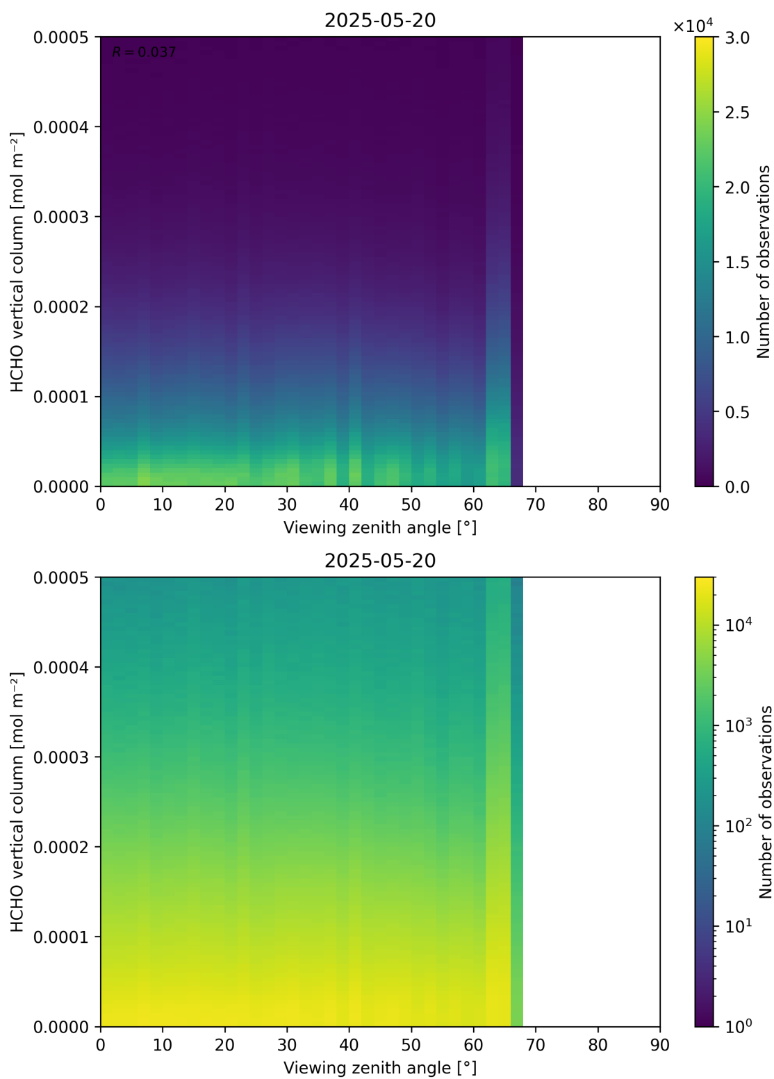
Figure 192: Scatter density plot of “Viewing zenith angle” against “HCHO vertical column” for 2025-05-19 to 2025-05-21.
