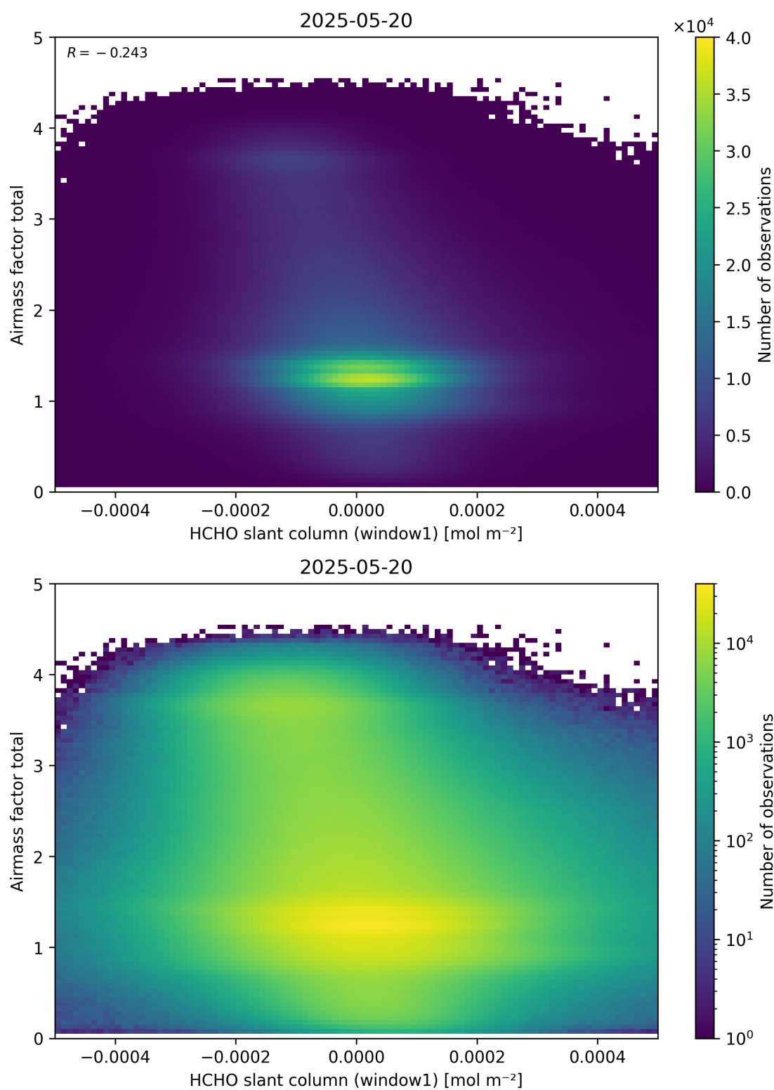
Figure 85: Scatter density plot of “HCHO slant column (window1)” against “Airmass factor total” for 2025-05-19 to 2025-05-21.
