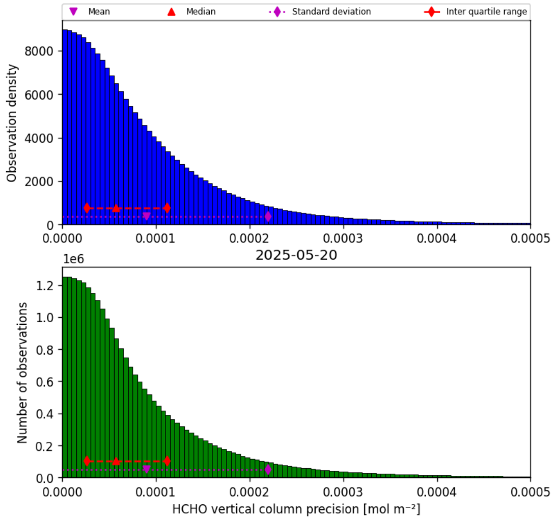
Figure 36: Histogram of “HCHO vertical column precision” for 2025-05-19 to 2025-05-21
