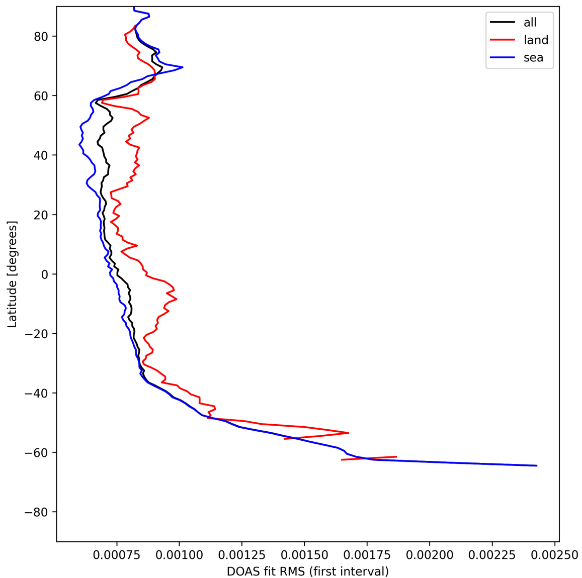
Figure 32: Zonal average of “DOAS fit RMS (first interval)” for 2025-05-19 to 2025-05-21.
