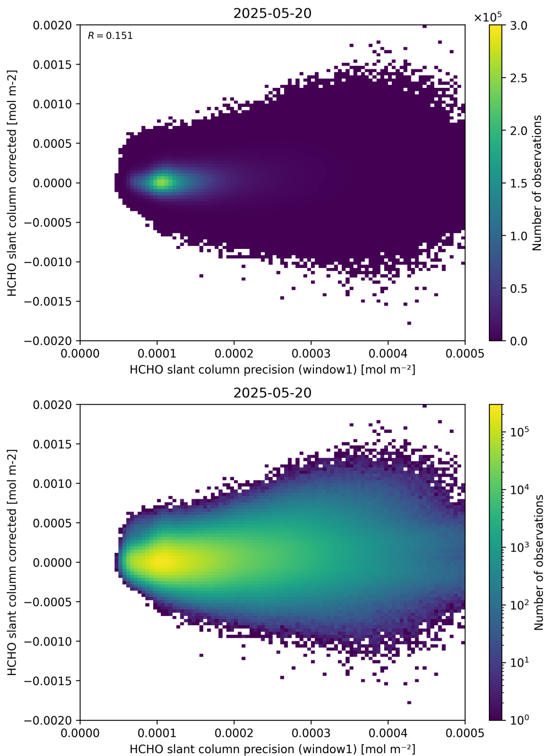
Figure 92: Scatter density plot of “HCHO slant column precision (window1)” against “HCHO slant column corrected” for 2025-05-19 to 2025-05-21.
