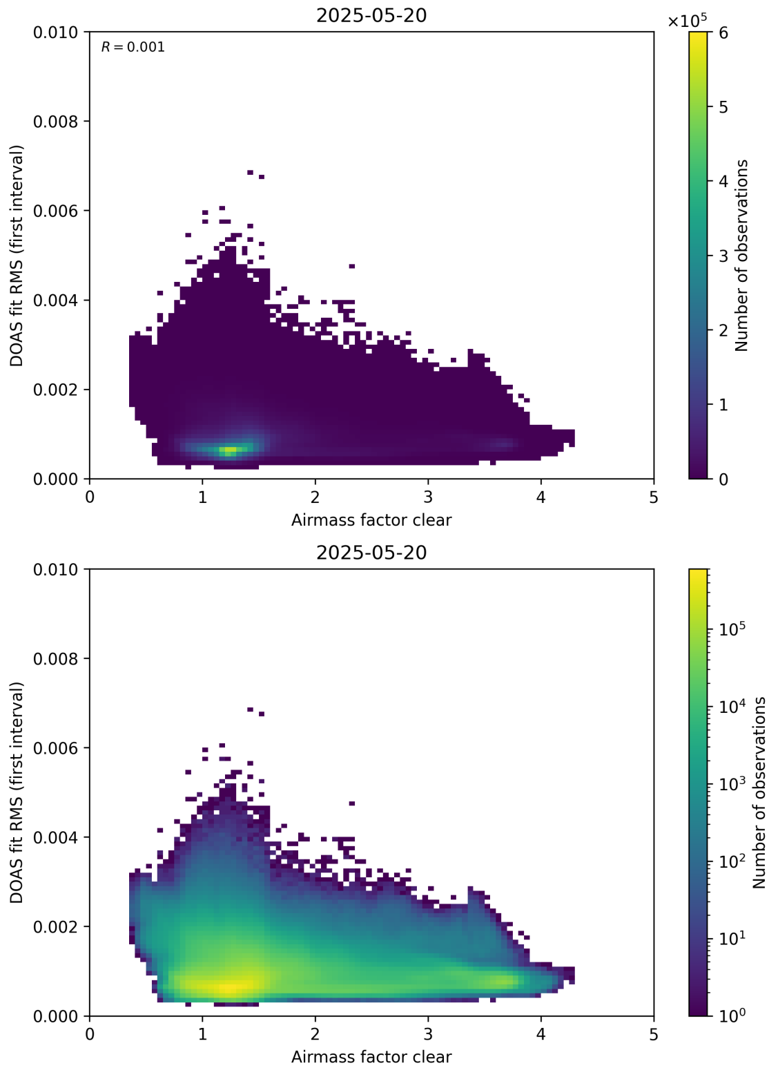
Figure 71: Scatter density plot of “Airmass factor clear” against “DOAS fit RMS (first interval)” for 2025-05-19 to 2025-05-21.
