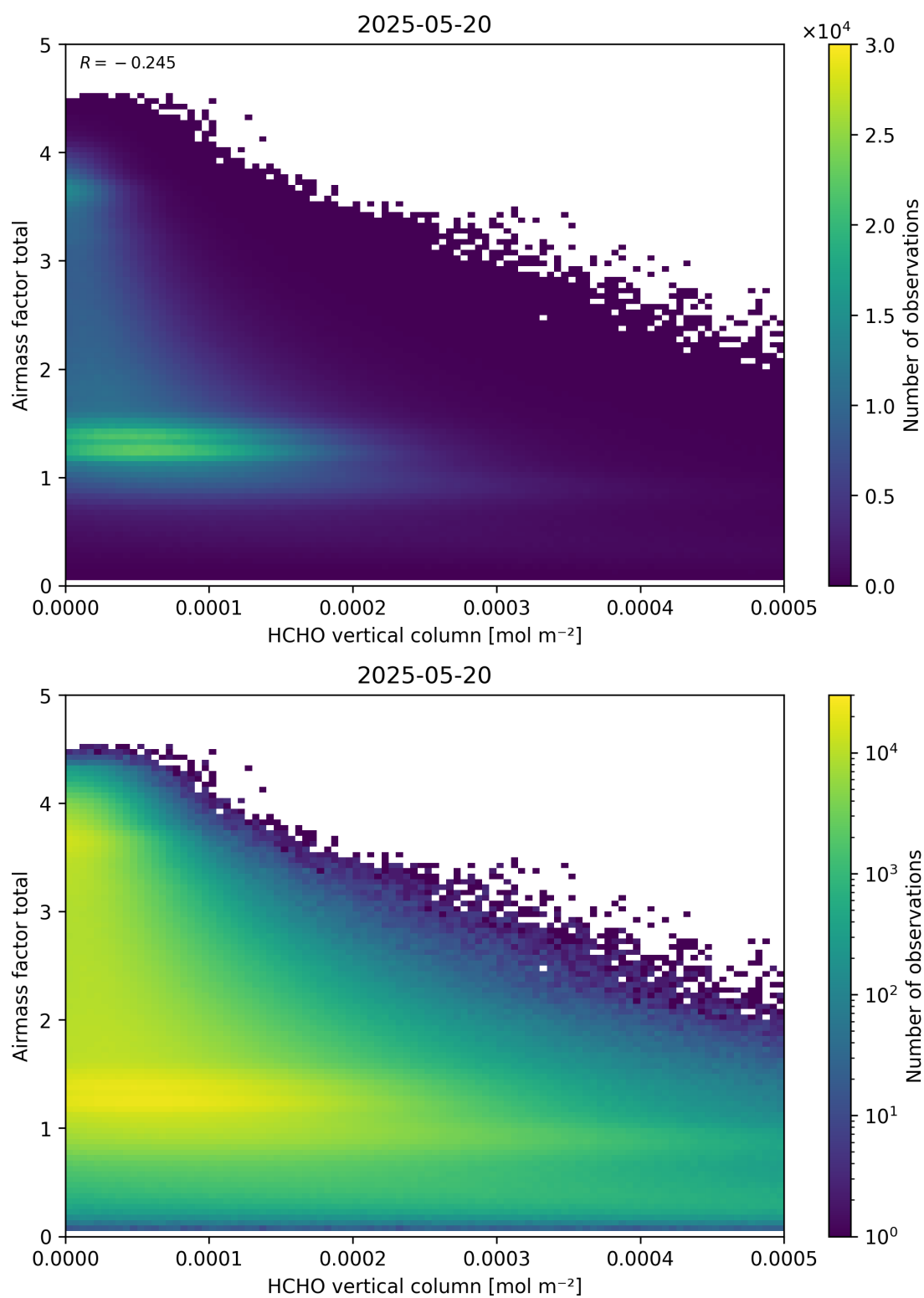
Figure 131: Scatter density plot of “HCHO vertical column” against “Airmass factor total” for 2025-05-19 to 2025-05-21.
