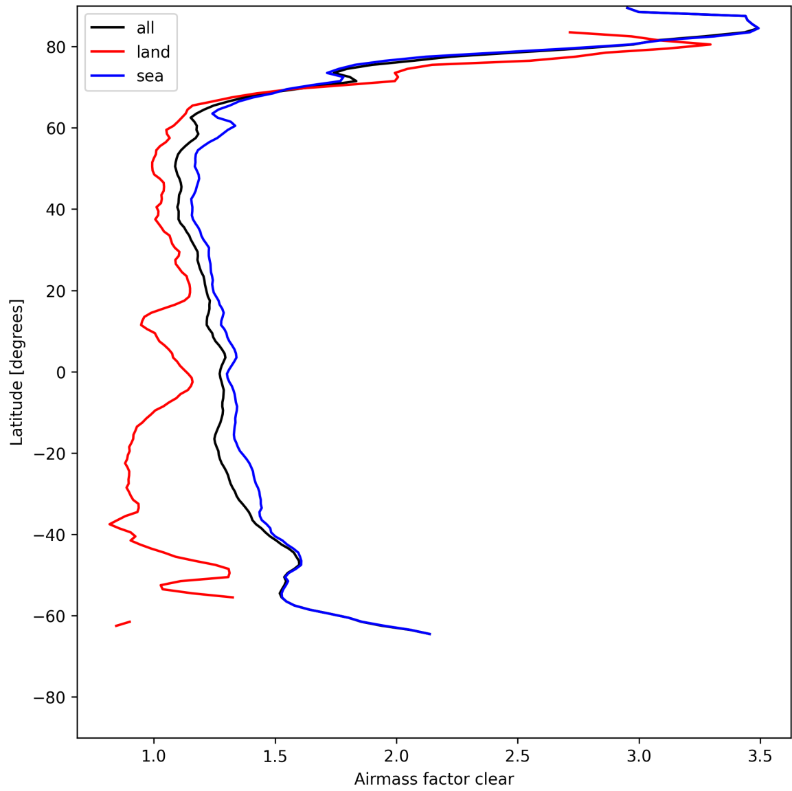
Figure 28: Zonal average of “Airmass factor clear” for 2025-05-19 to 2025-05-21.
