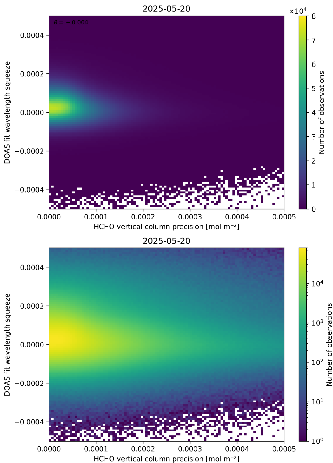
Figure 138: Scatter density plot of “HCHO vertical column precision” against “DOAS fit wavelength squeeze” for 2025-05-19 to 2025-05-21.
