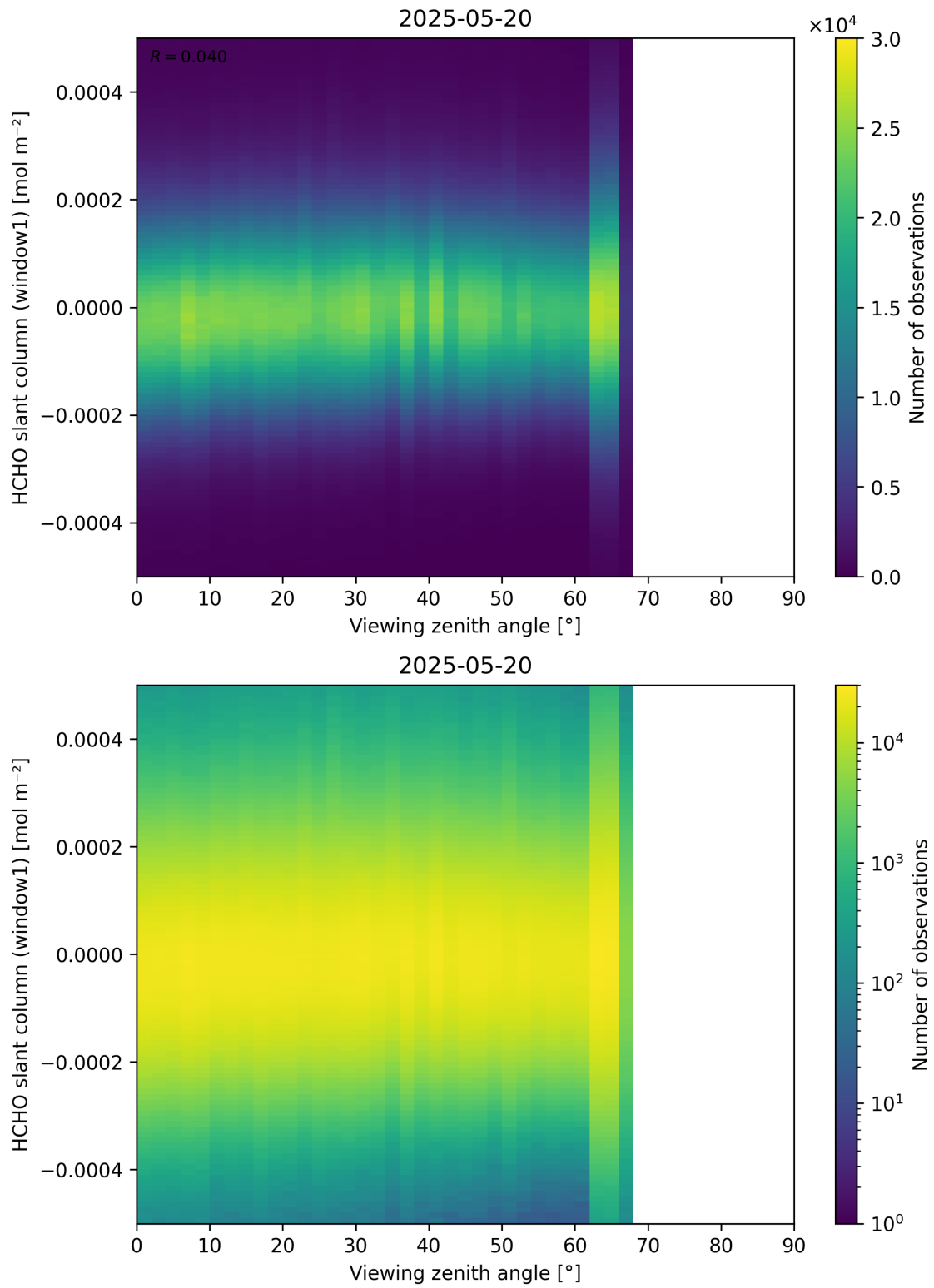
Figure 188: Scatter density plot of “Viewing zenith angle” against “HCHO slant column (window1)” for 2025-05-19 to 2025-05-21.
