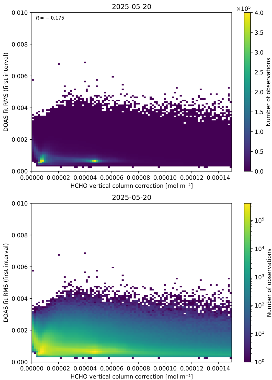
Figure 112: Scatter density plot of “HCHO vertical column correction” against “DOAS fit RMS (first interval)” for 2025-05-19 to 2025-05-21.
