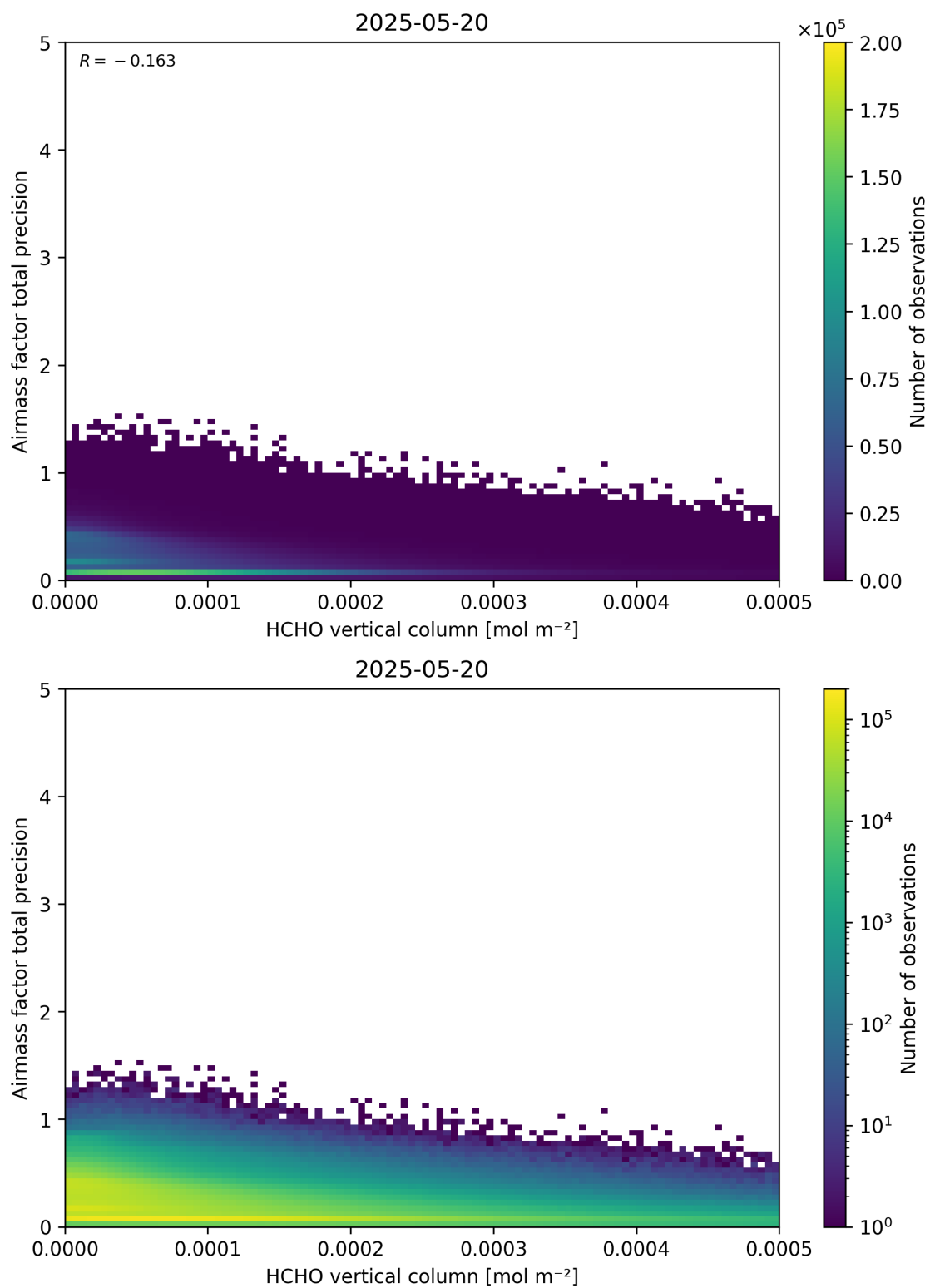
Figure 132: Scatter density plot of “HCHO vertical column” against “Airmass factor total precision” for 2025-05-19 to 2025-05-21.
