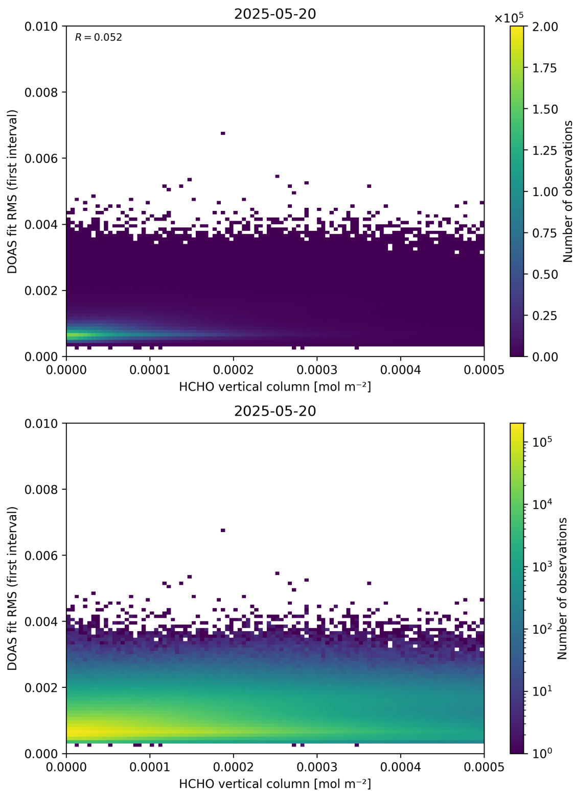
Figure 123: Scatter density plot of “HCHO vertical column” against “DOAS fit RMS (first interval)” for 2025-05-19 to 2025-05-21.
