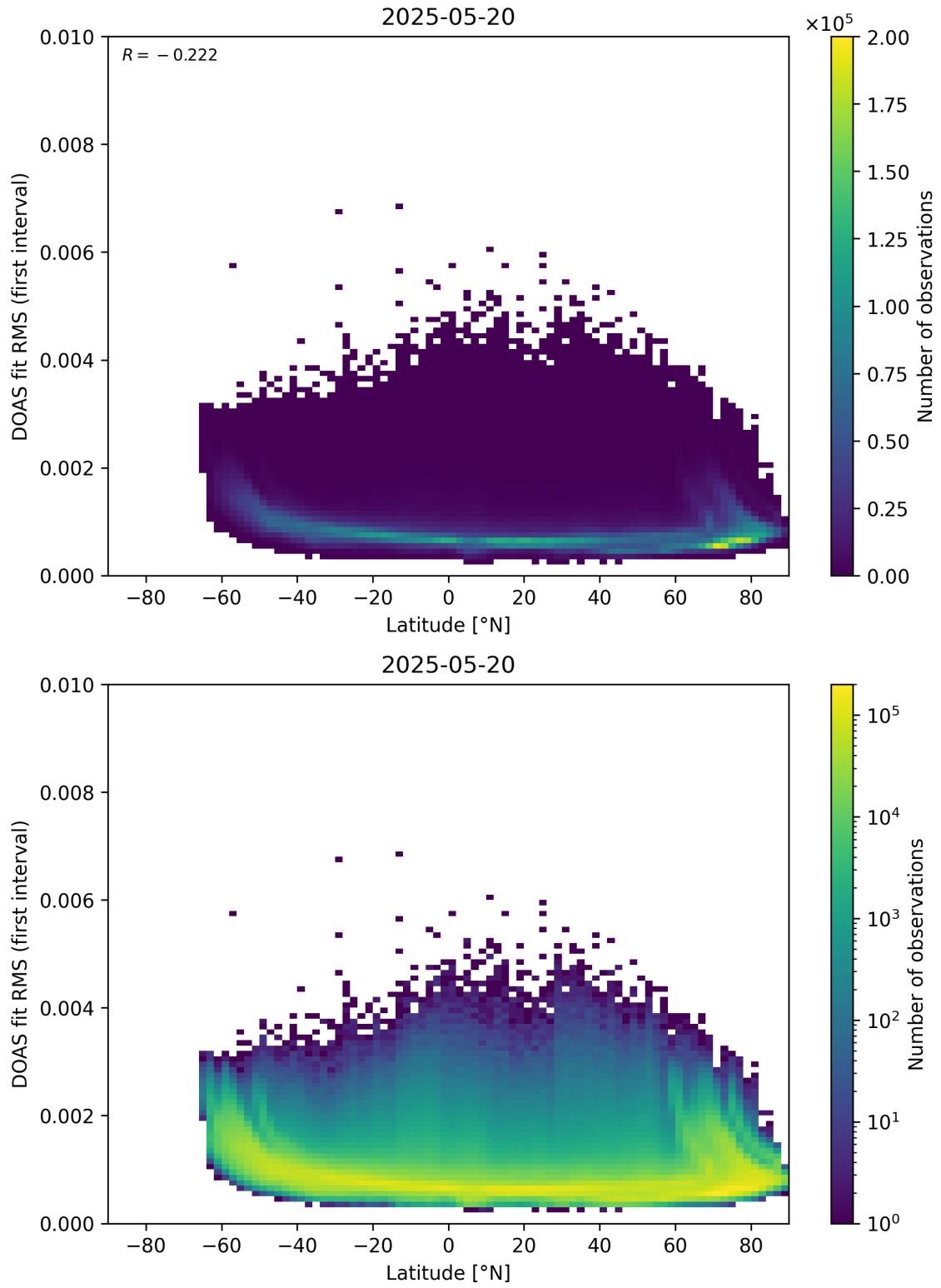
Figure 153: Scatter density plot of “Latitude” against “DOAS fit RMS (first interval)” for 2025-05-19 to 2025-05-21.
