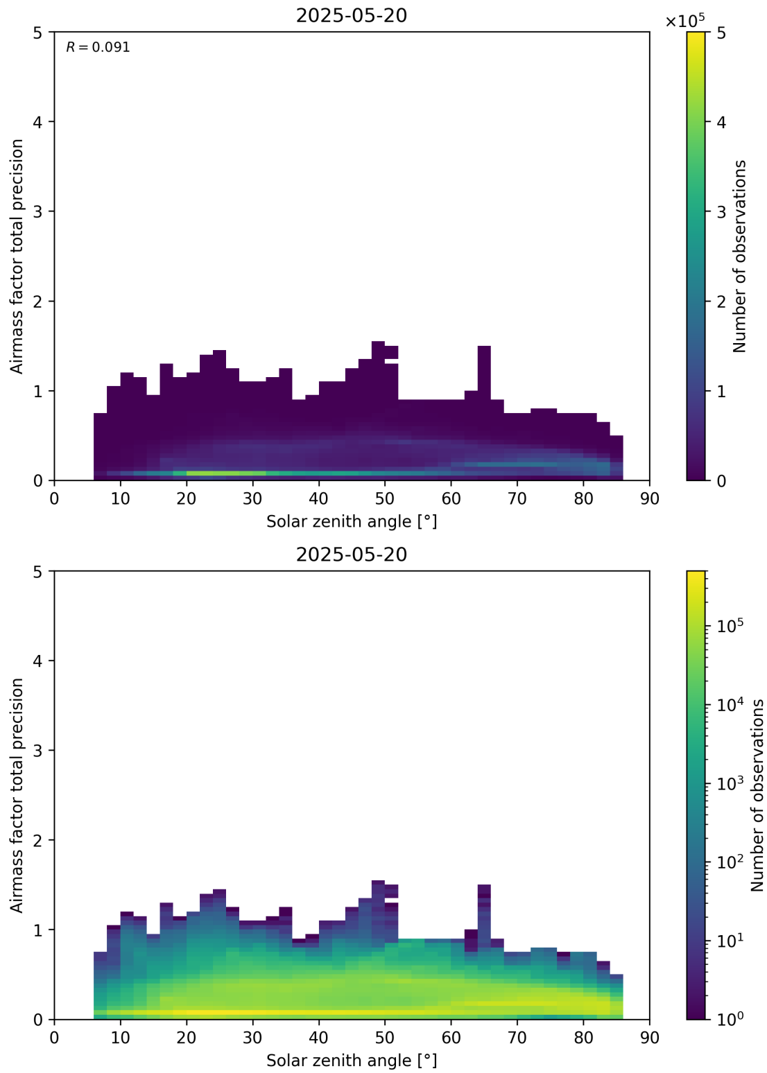
Figure 176: Scatter density plot of “Solar zenith angle” against “Airmass factor total precision” for 2025-05-19 to 2025-05-21.
