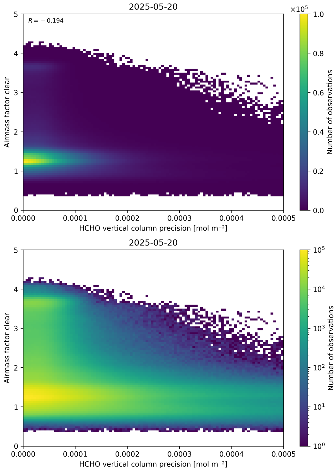
Figure 139: Scatter density plot of “HCHO vertical column precision” against “Airmass factor clear” for 2025-05-19 to 2025-05-21.
