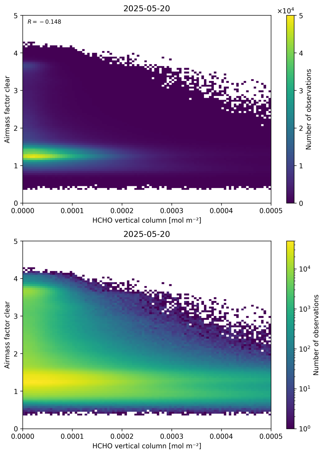
Figure 126: Scatter density plot of “HCHO vertical column” against “Airmass factor clear” for 2025-05-19 to 2025-05-21.
