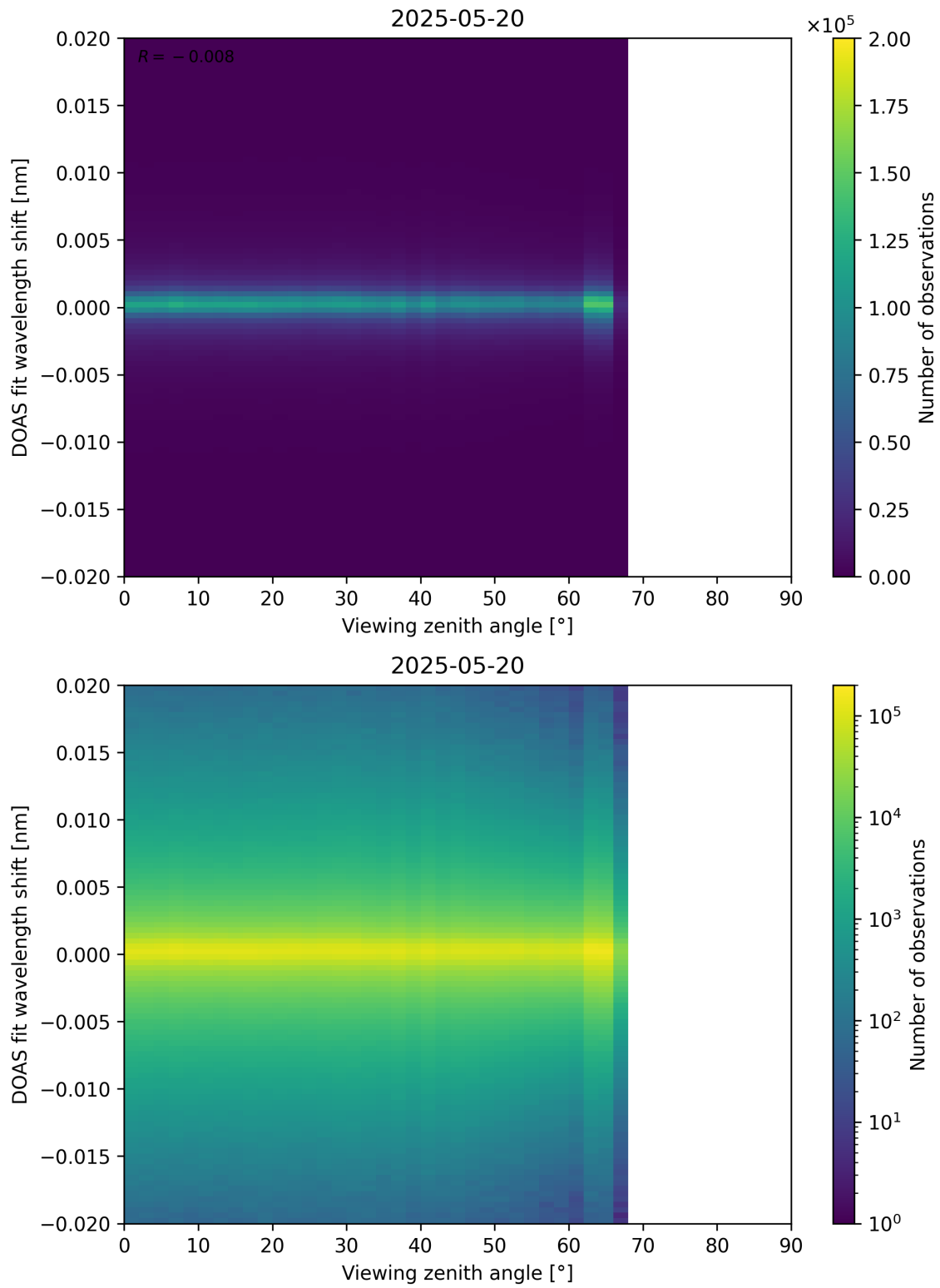
Figure 183: Scatter density plot of “Viewing zenith angle” against “DOAS fit wavelength shift” for 2025-05-19 to 2025-05-21.
