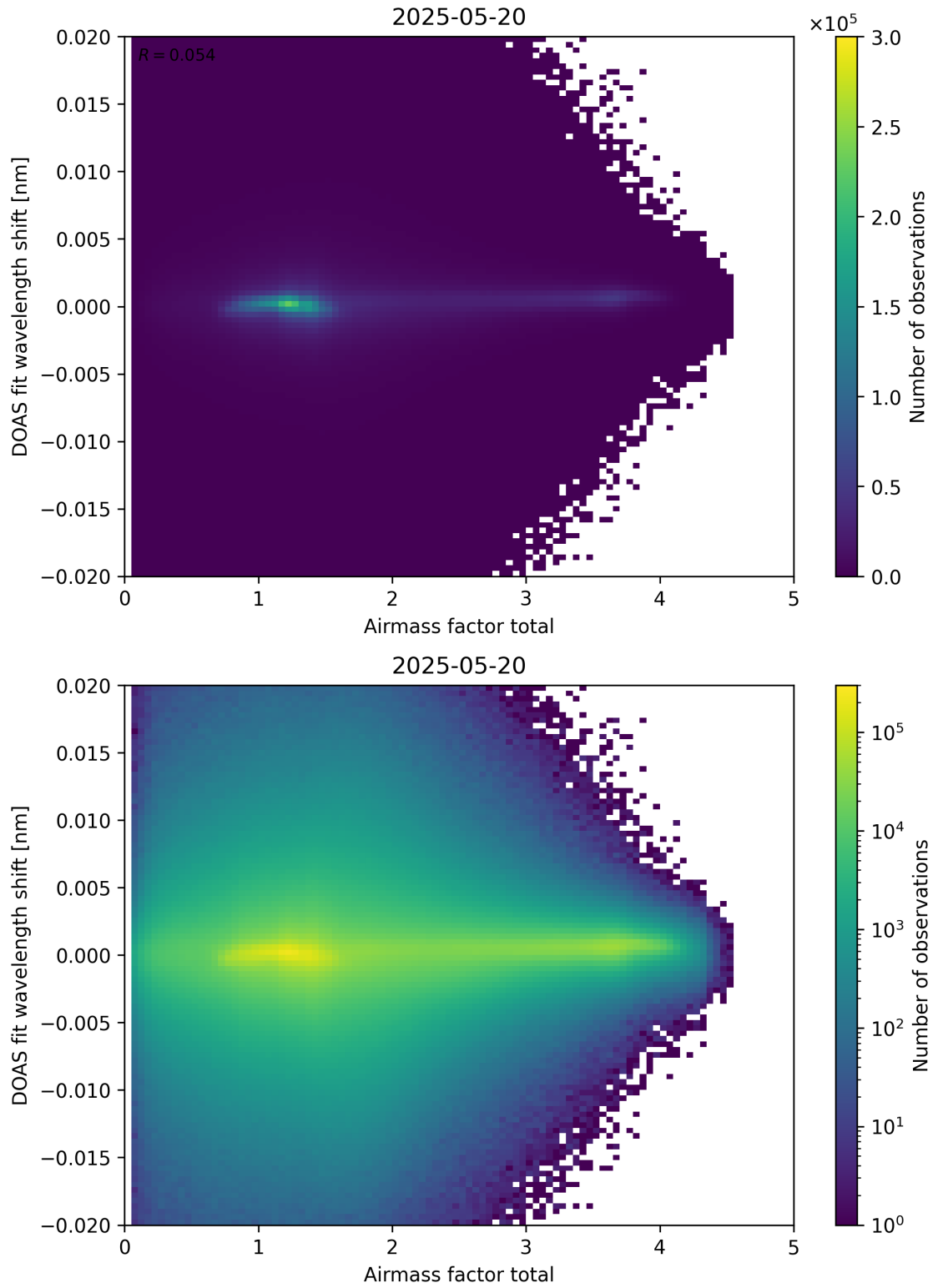
Figure 98: Scatter density plot of “Airmass factor total” against “DOAS fit wavelength shift” for 2025-05-19 to 2025-05-21.
