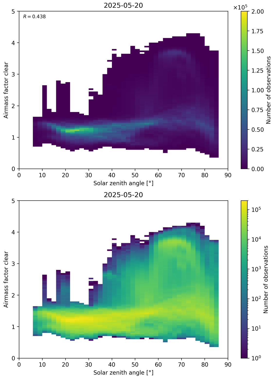
Figure 170: Scatter density plot of “Solar zenith angle” against “Airmass factor clear” for 2025-05-19 to 2025-05-21.
