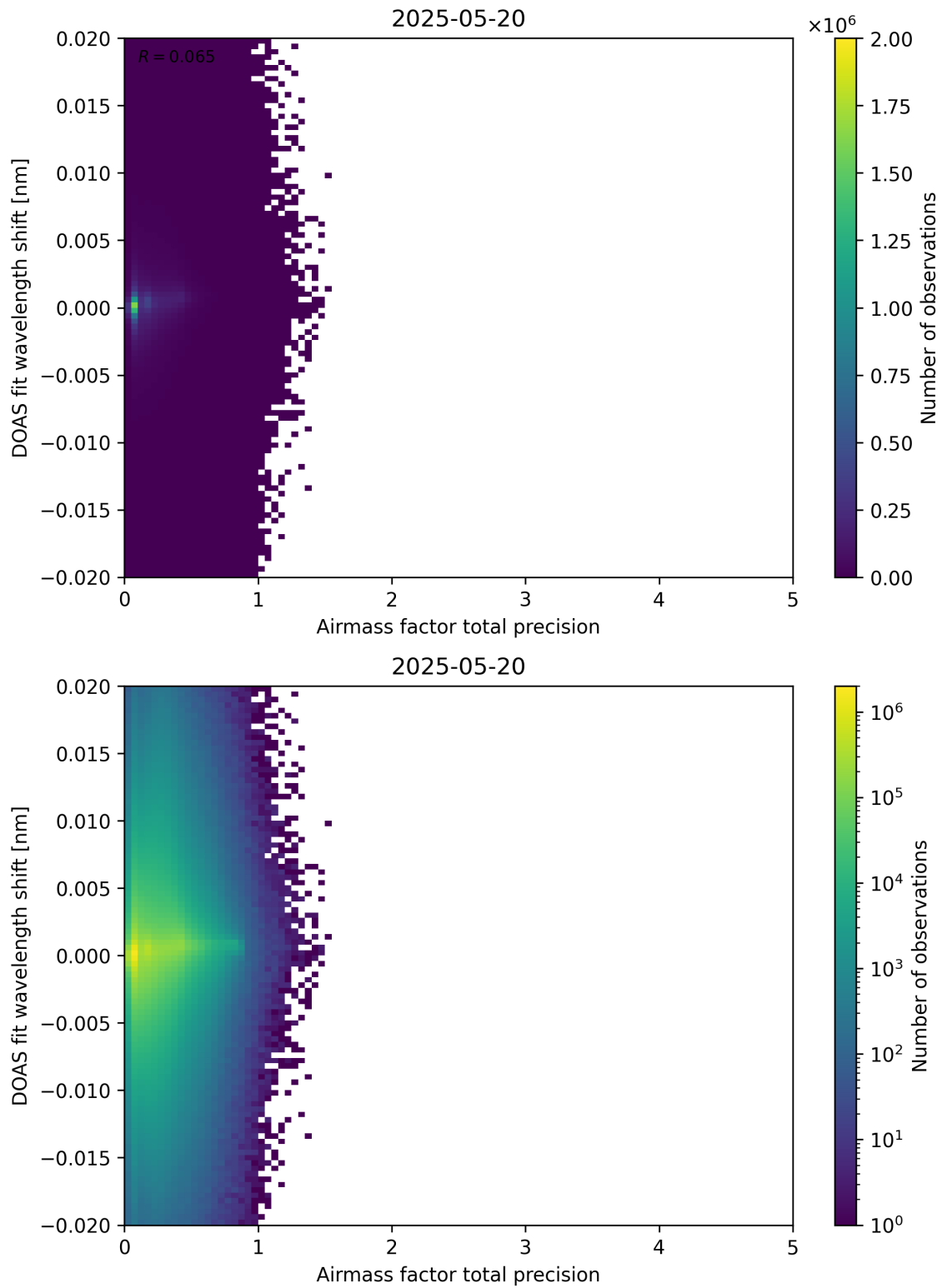
Figure 106: Scatter density plot of “Airmass factor total precision” against “DOAS fit wavelength shift” for 2025-05-19 to 2025-05-21.
