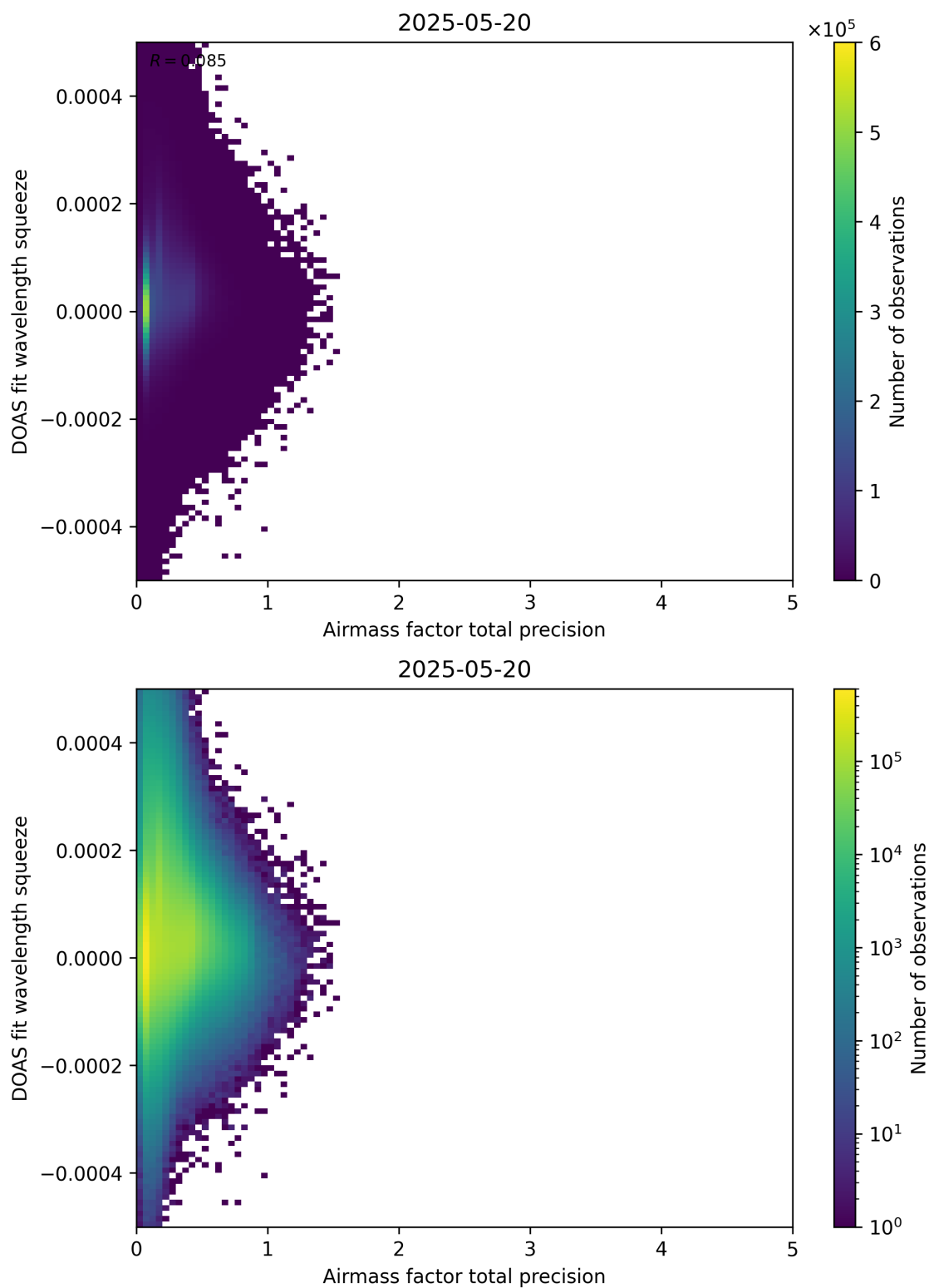
Figure 107: Scatter density plot of “Airmass factor total precision” against “DOAS fit wavelength squeeze” for 2025-05-19 to 2025-05-21.
