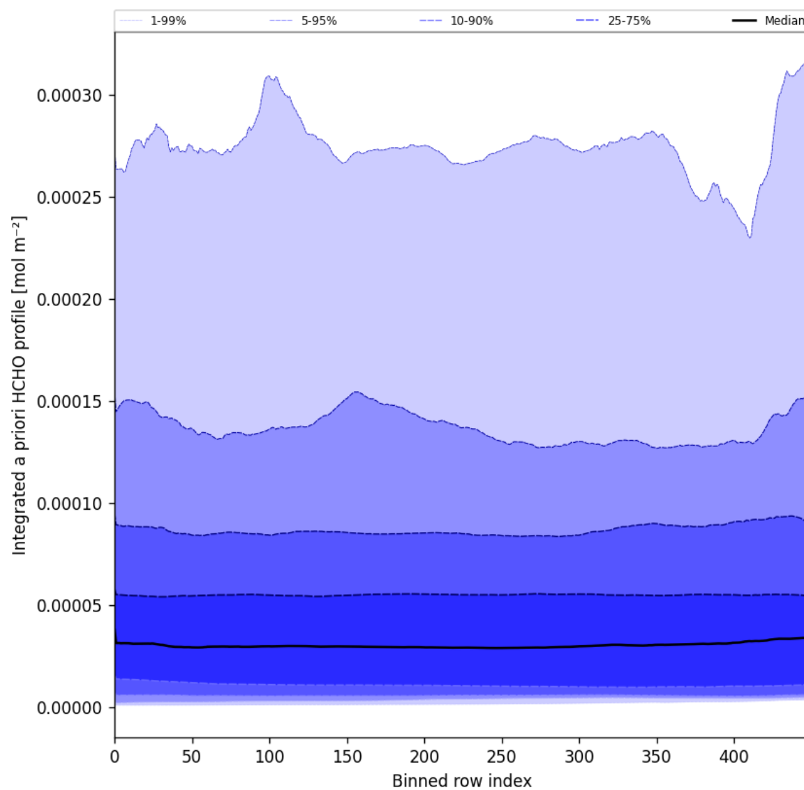
Figure 57: Along track statistics of “Integrated a priori HCHO profile” for 2025-05-19 to 2025-05-21
