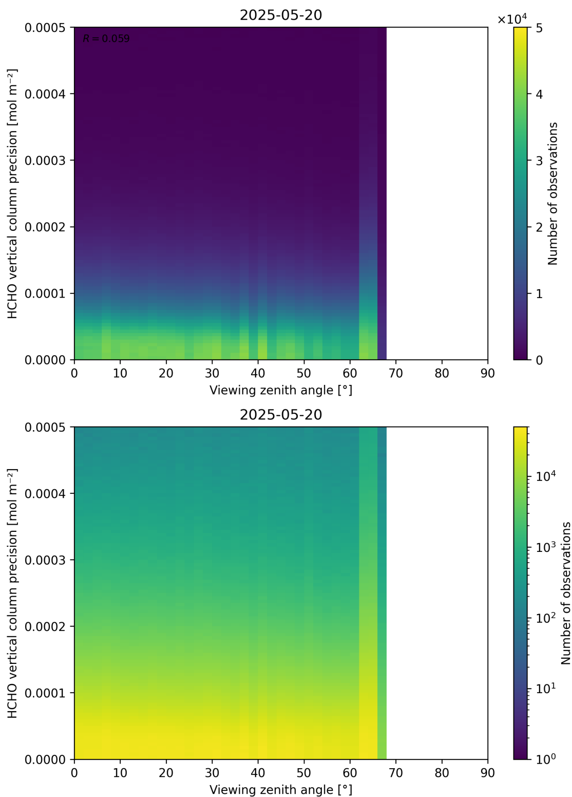
Figure 194: Scatter density plot of “Viewing zenith angle” against “HCHO vertical column precision” for 2025-05-19 to 2025-05-21.
