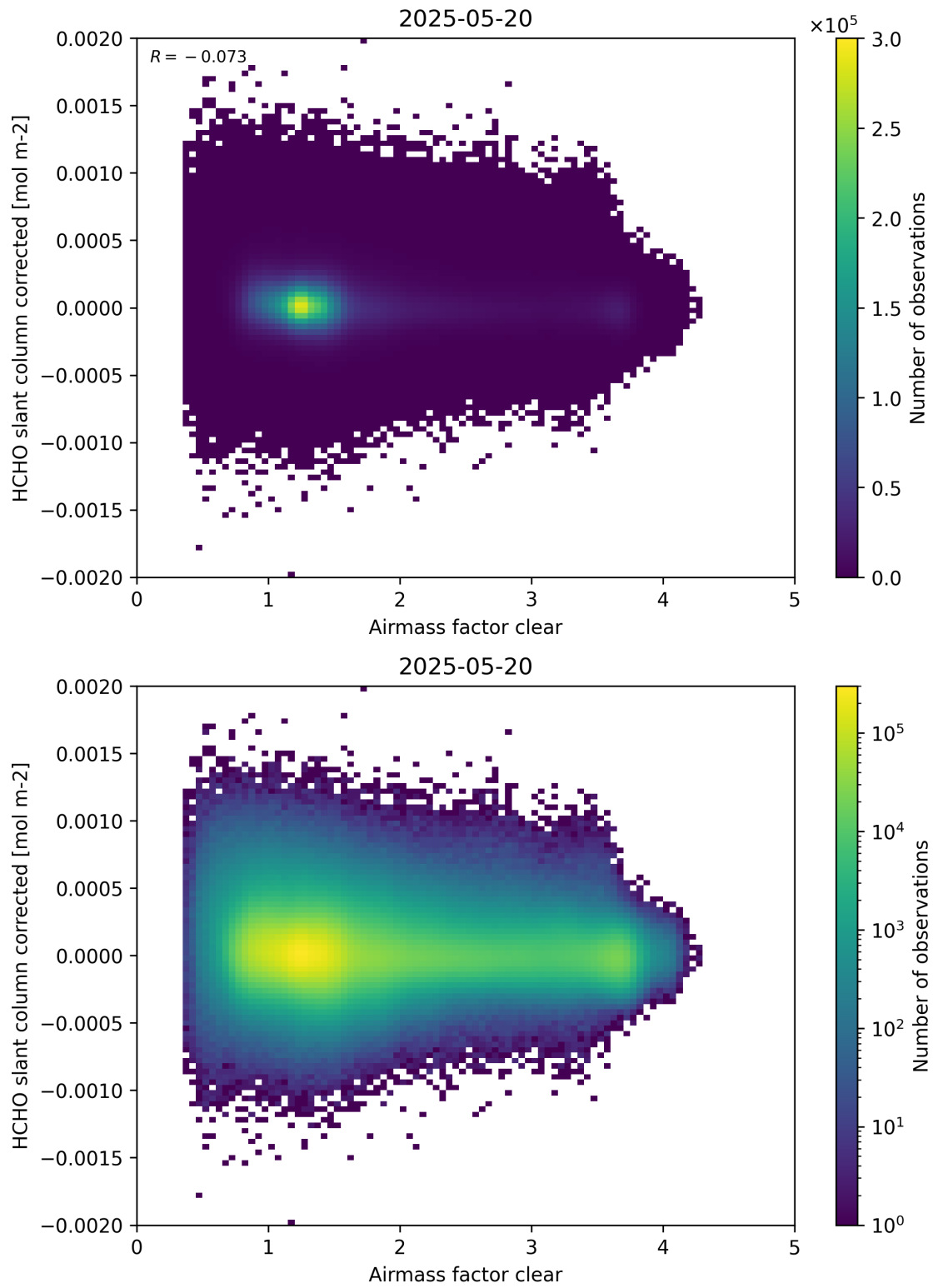
Figure 74: Scatter density plot of “Airmass factor clear” against “HCHO slant column corrected” for 2025-05-19 to 2025-05-21.
