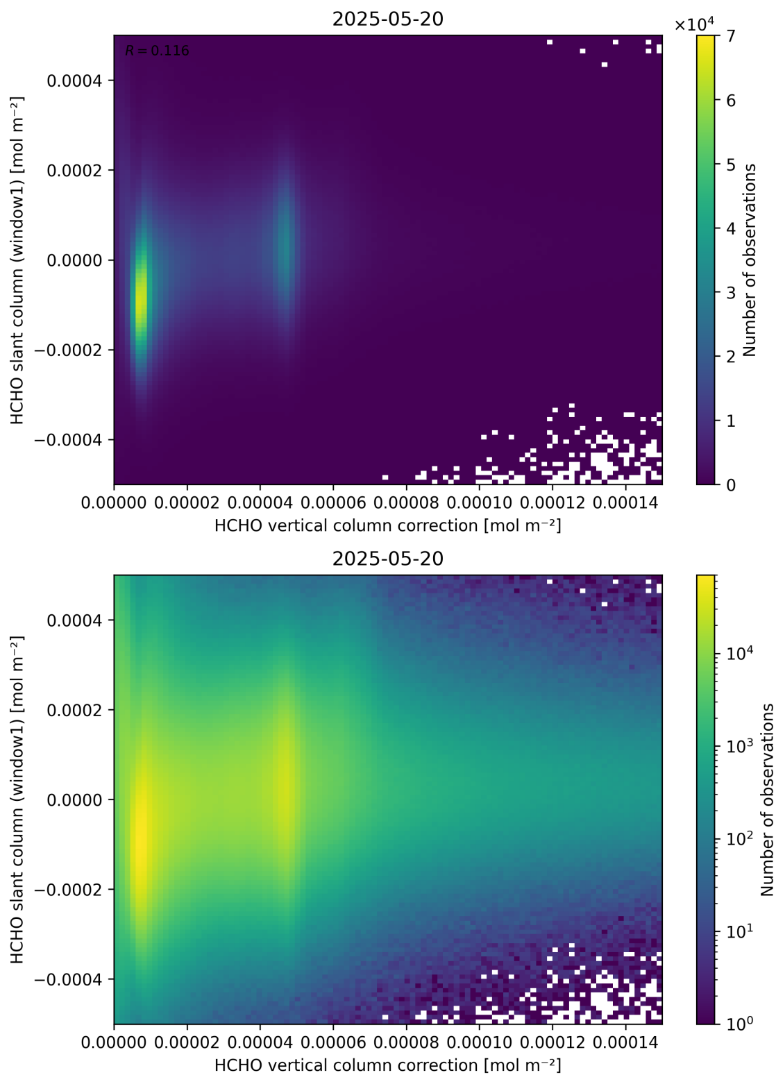
Figure 118: Scatter density plot of “HCHO vertical column correction” against “HCHO slant column (window1)” for 2025-05-19 to 2025-05-21.
