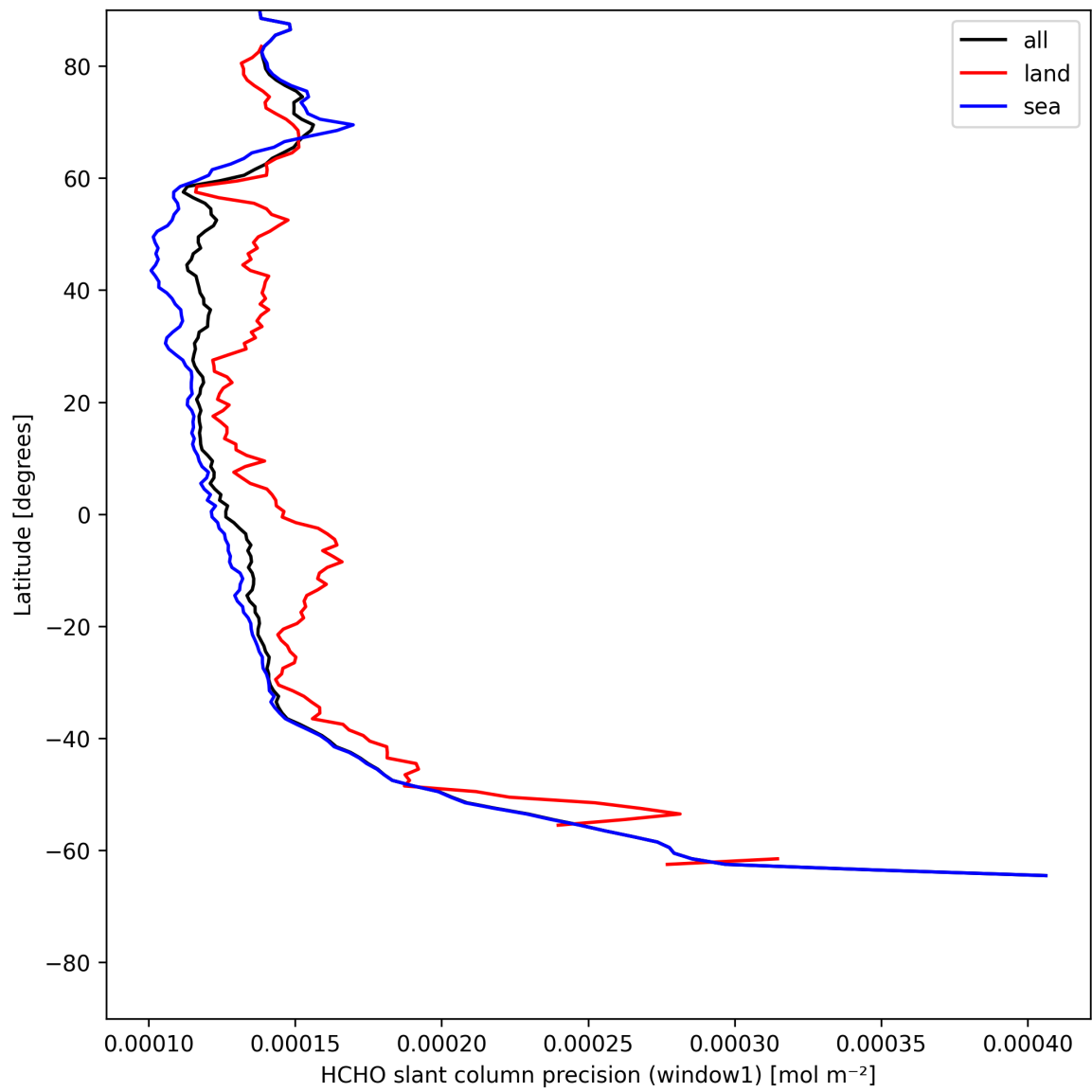
Figure 25: Zonal average of “HCHO slant column precision (window1)” for 2025-05-19 to 2025-05-21.
