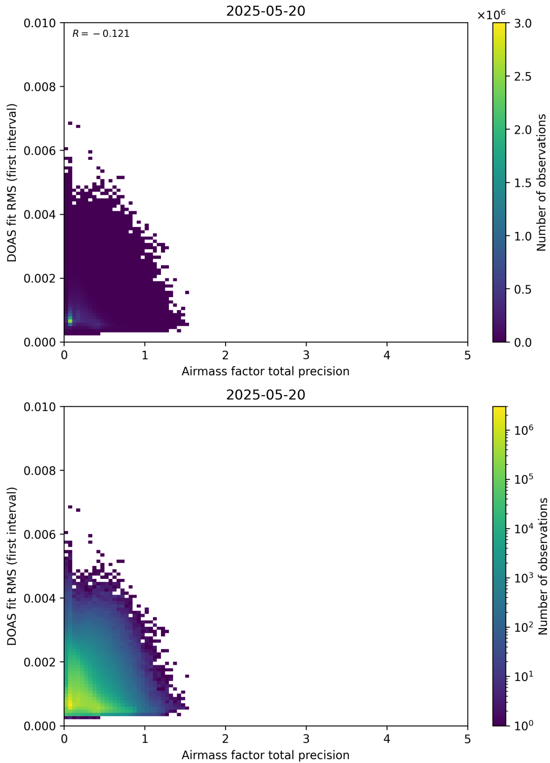
Figure 105: Scatter density plot of “Airmass factor total precision” against “DOAS fit RMS (first interval)” for 2025-05-19 to 2025-05-21.
