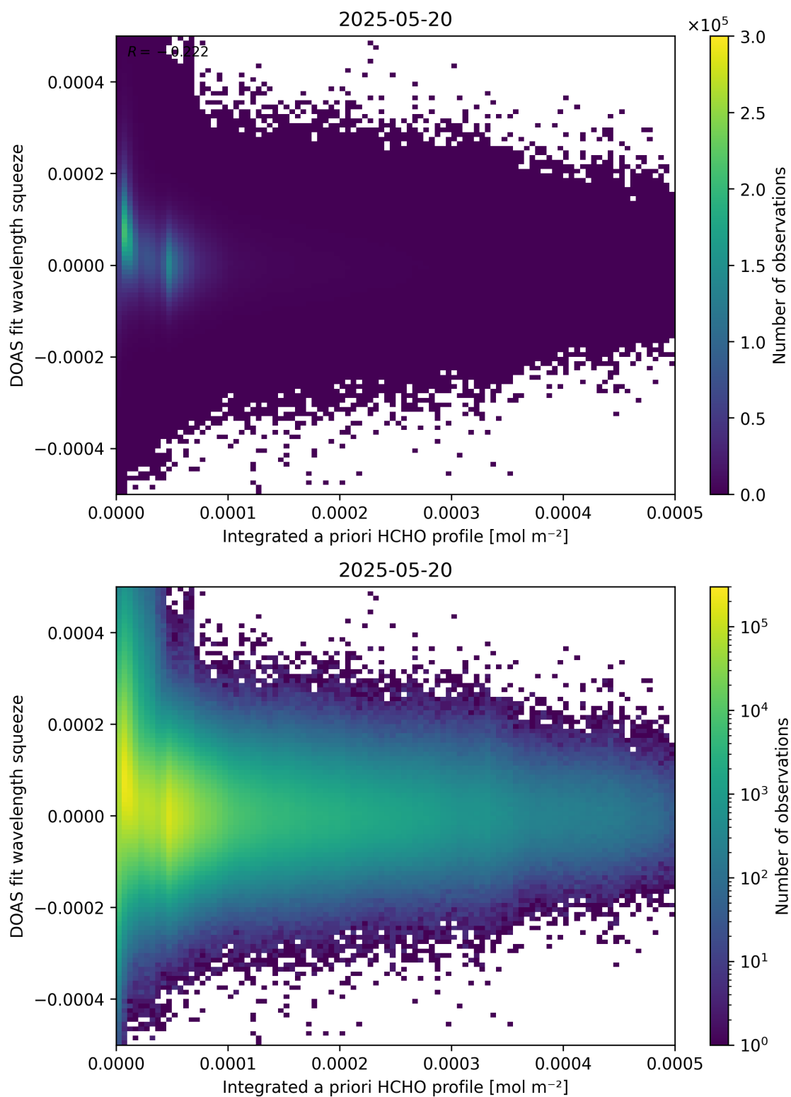
Figure 150: Scatter density plot of “Integrated a priori HCHO profile” against “DOAS fit wavelength squeeze” for 2025-05-19 to 2025-05-21.
