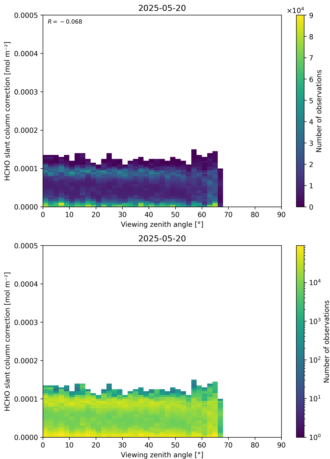
Figure 187: Scatter density plot of “Viewing zenith angle” against “HCHO slant column correction” for 2025-05-19 to 2025-05-21.
