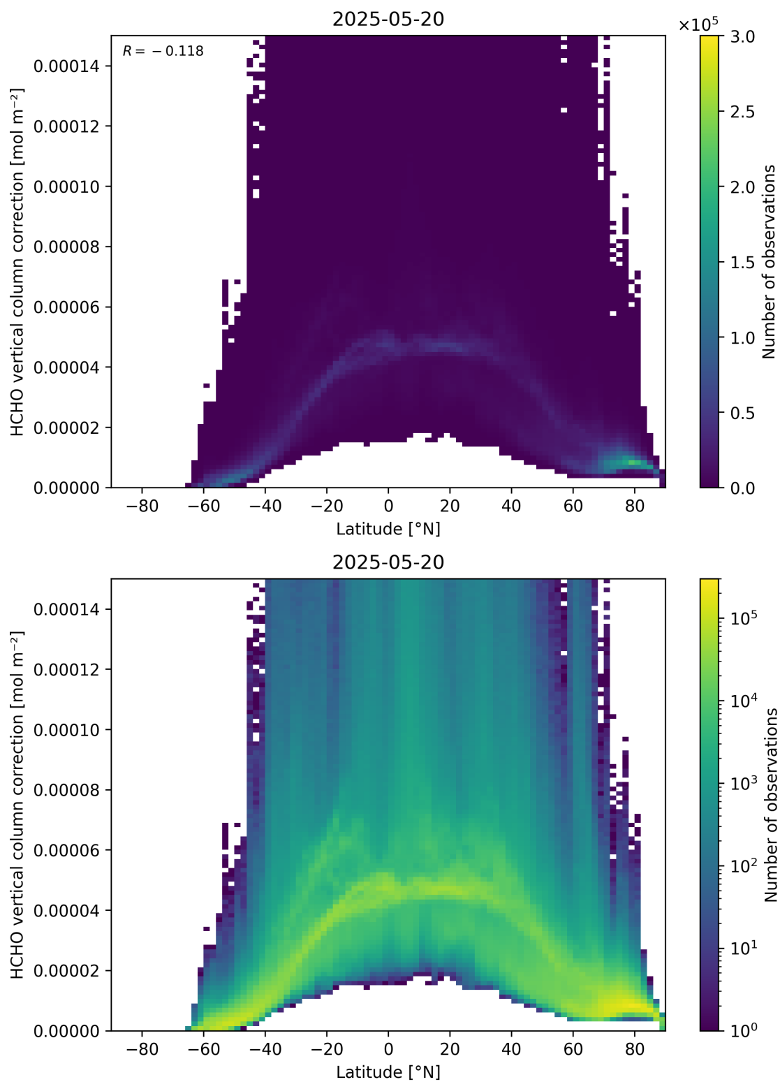
Figure 164: Scatter density plot of “Latitude” against “HCHO vertical column correction” for 2025-05-19 to 2025-05-21.
