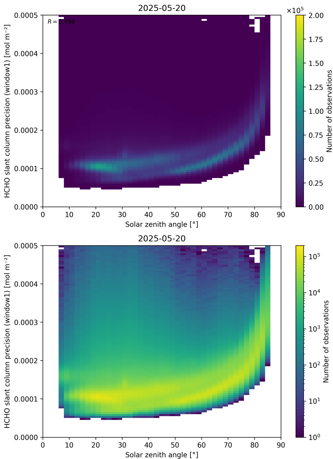
Figure 174: Scatter density plot of “Solar zenith angle” against “HCHO slant column precision (window1)” for 2025-05-19 to 2025-05-21.
