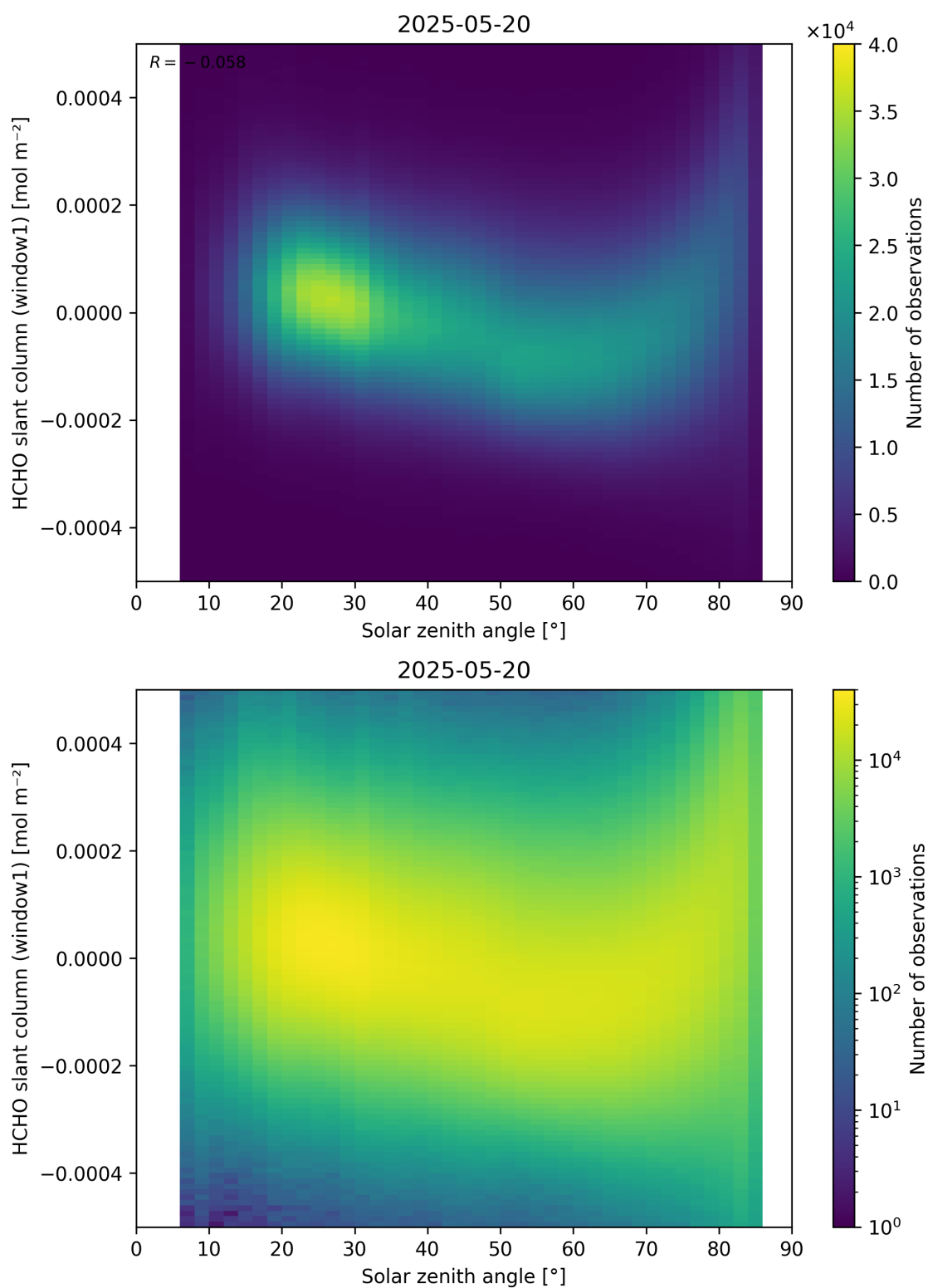
Figure 173: Scatter density plot of “Solar zenith angle” against “HCHO slant column (window1)” for 2025-05-19 to 2025-05-21.
