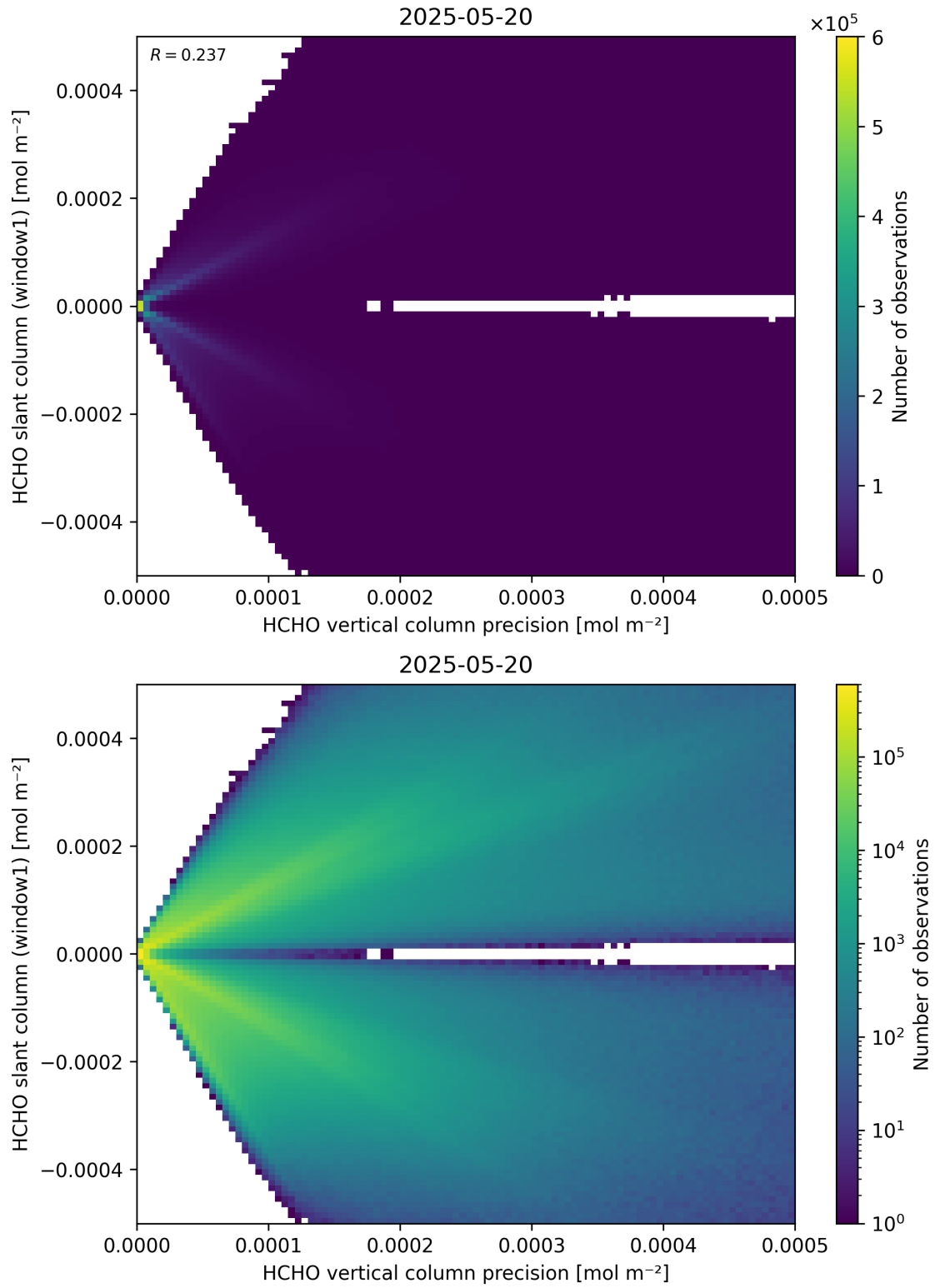
Figure 142: Scatter density plot of “HCHO vertical column precision” against “HCHO slant column (window1)” for 2025-05-19 to 2025-05-21.
