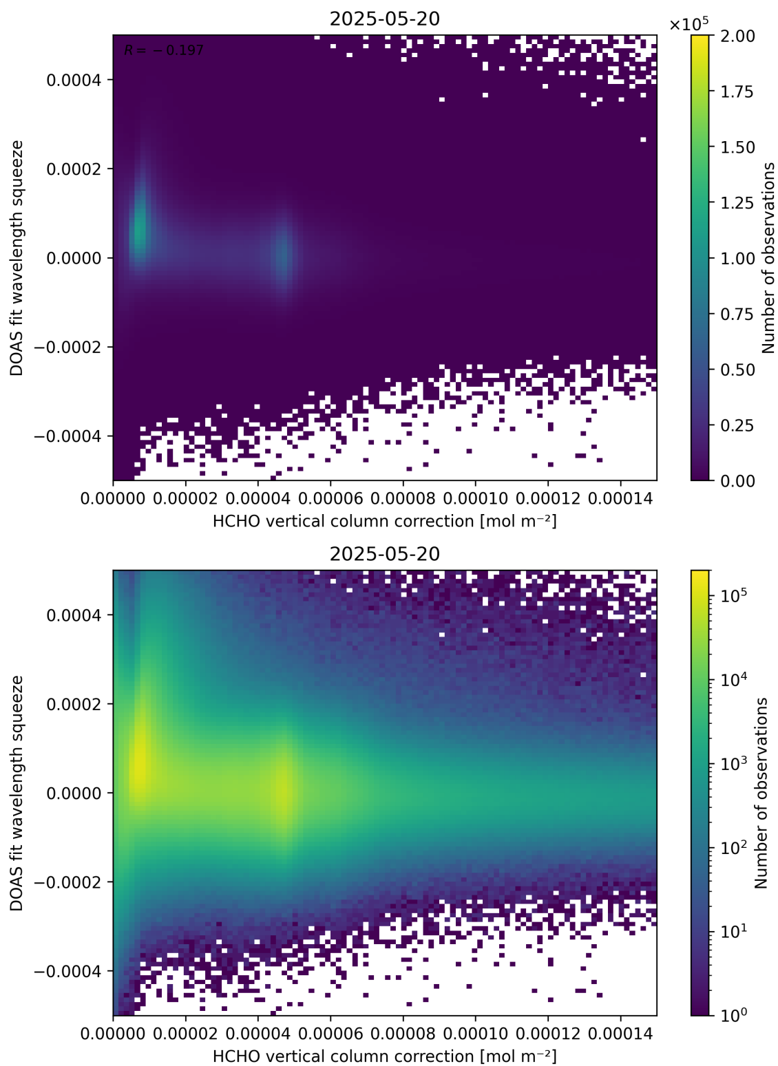
Figure 114: Scatter density plot of “HCHO vertical column correction” against “DOAS fit wavelength squeeze” for 2025-05-19 to 2025-05-21.
