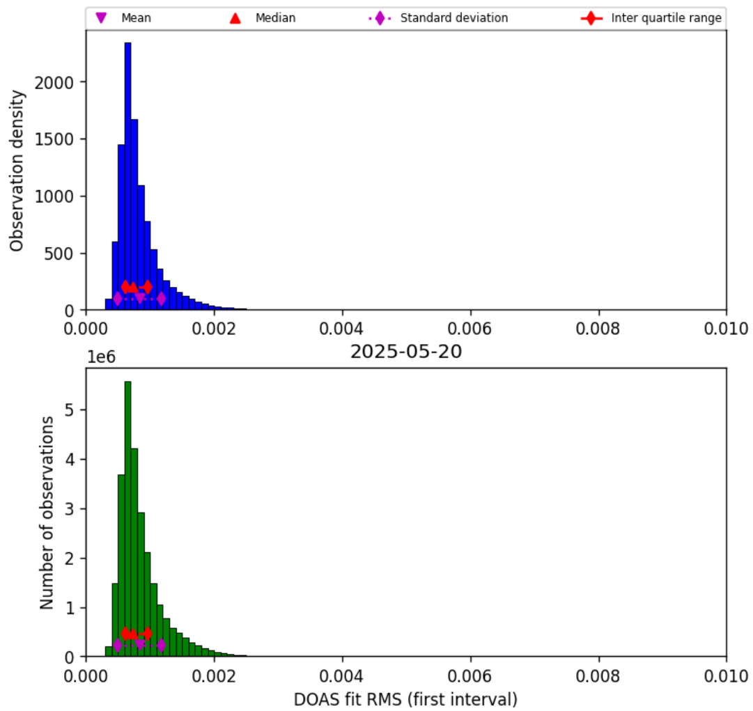
Figure 46: Histogram of “DOAS fit RMS (first interval)” for 2025-05-19 to 2025-05-21
