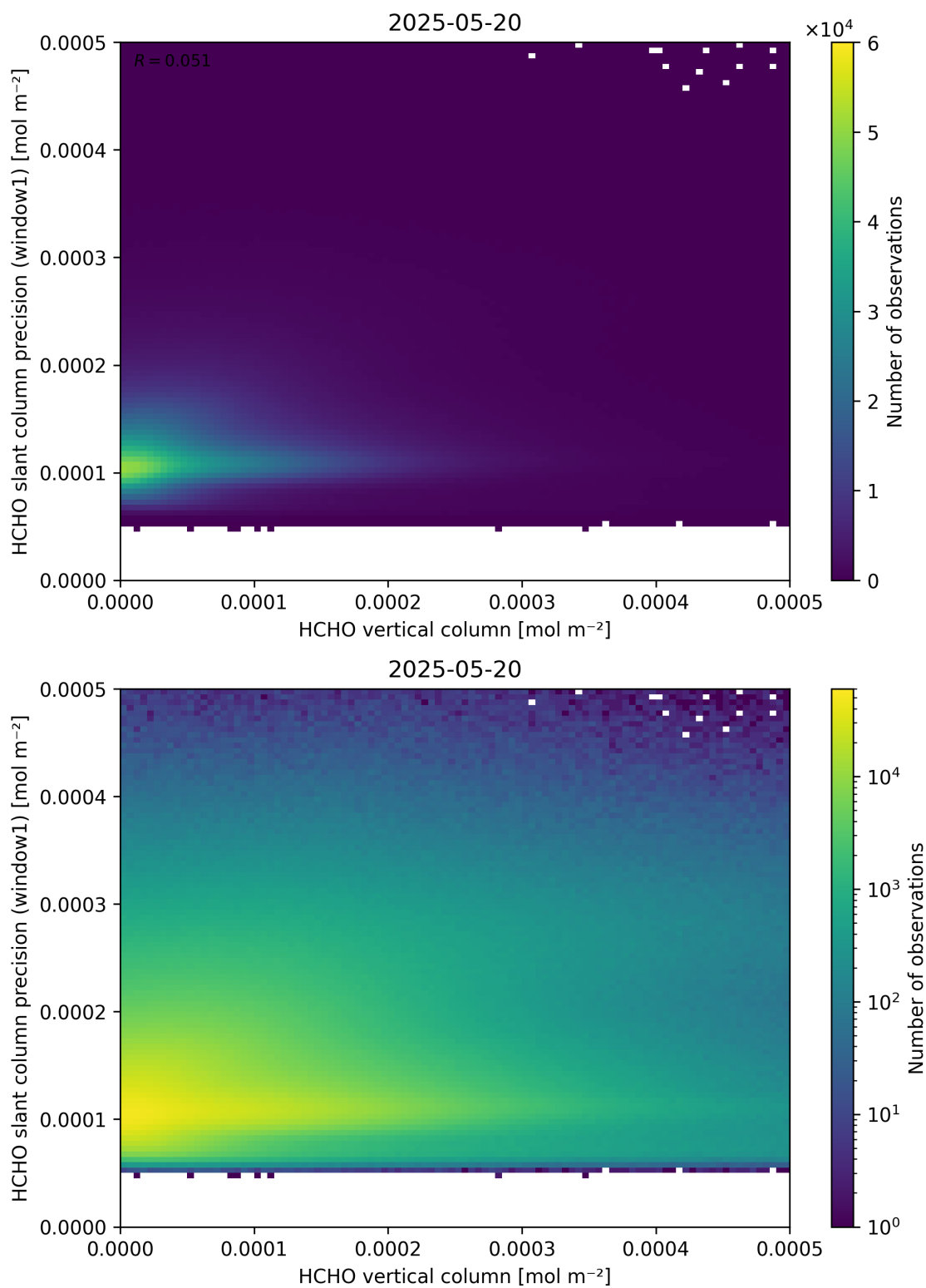
Figure 130: Scatter density plot of “HCHO vertical column” against “HCHO slant column precision (window1)” for 2025-05-19 to 2025-05-21.
