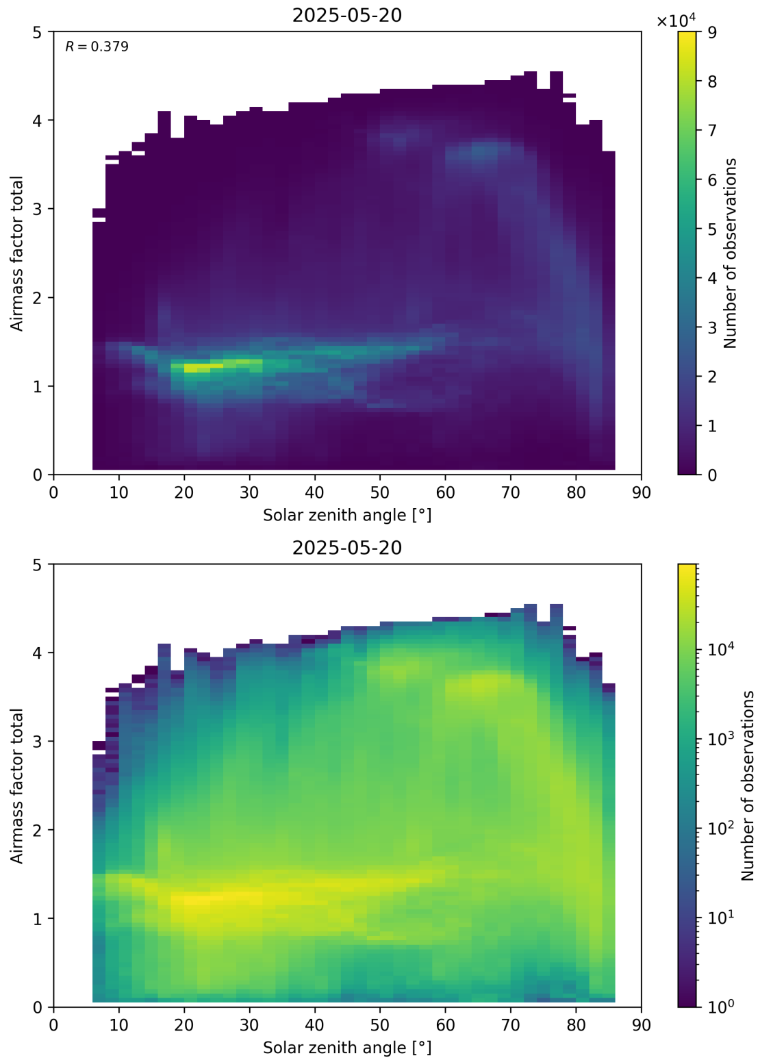
Figure 175: Scatter density plot of “Solar zenith angle” against “Airmass factor total” for 2025-05-19 to 2025-05-21.
