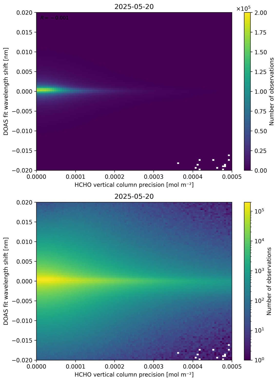
Figure 137: Scatter density plot of “HCHO vertical column precision” against “DOAS fit wavelength shift” for 2025-05-19 to 2025-05-21.
