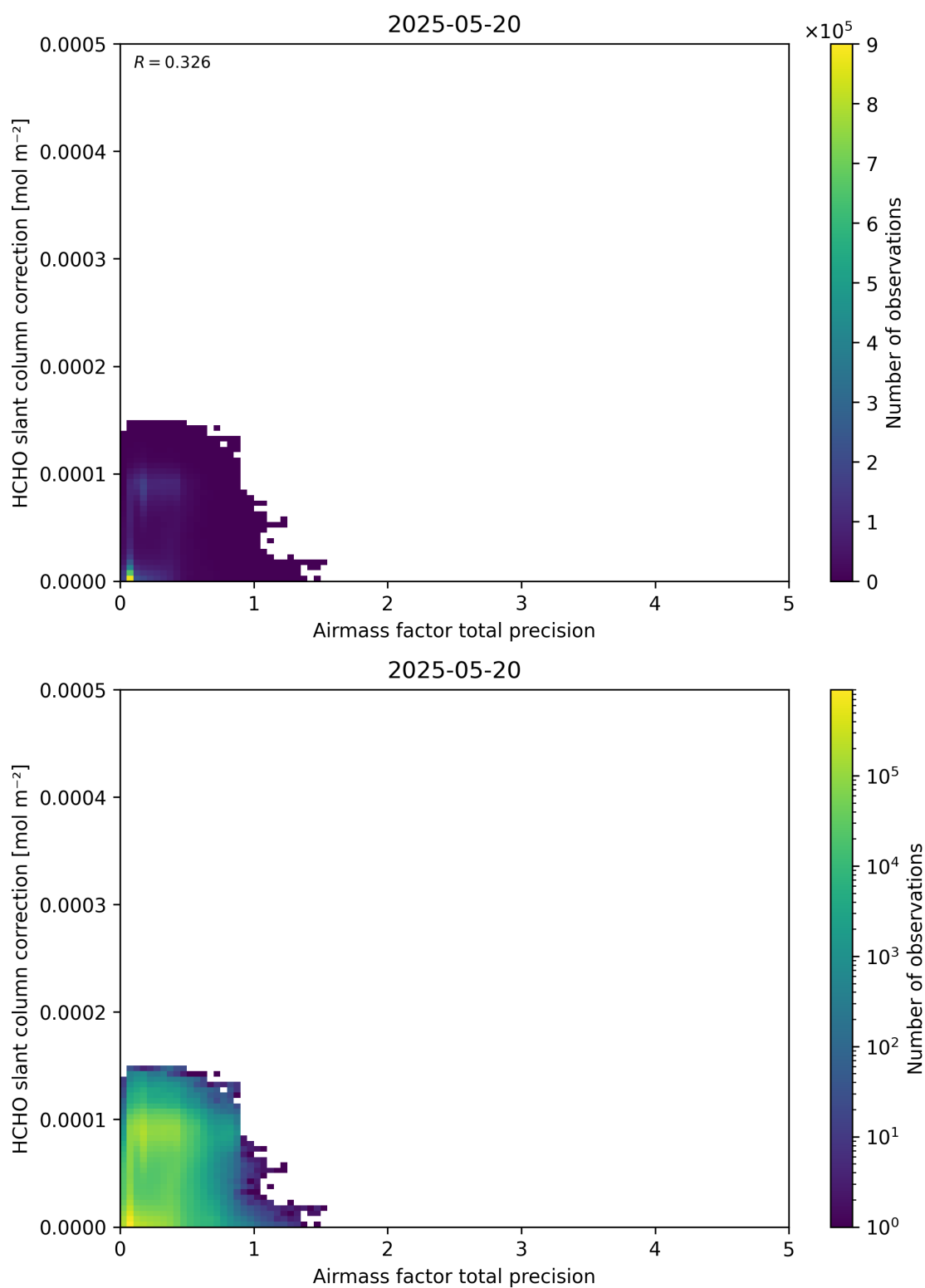
Figure 110: Scatter density plot of “Airmass factor total precision” against “HCHO slant column correction” for 2025-05-19 to 2025-05-21.
