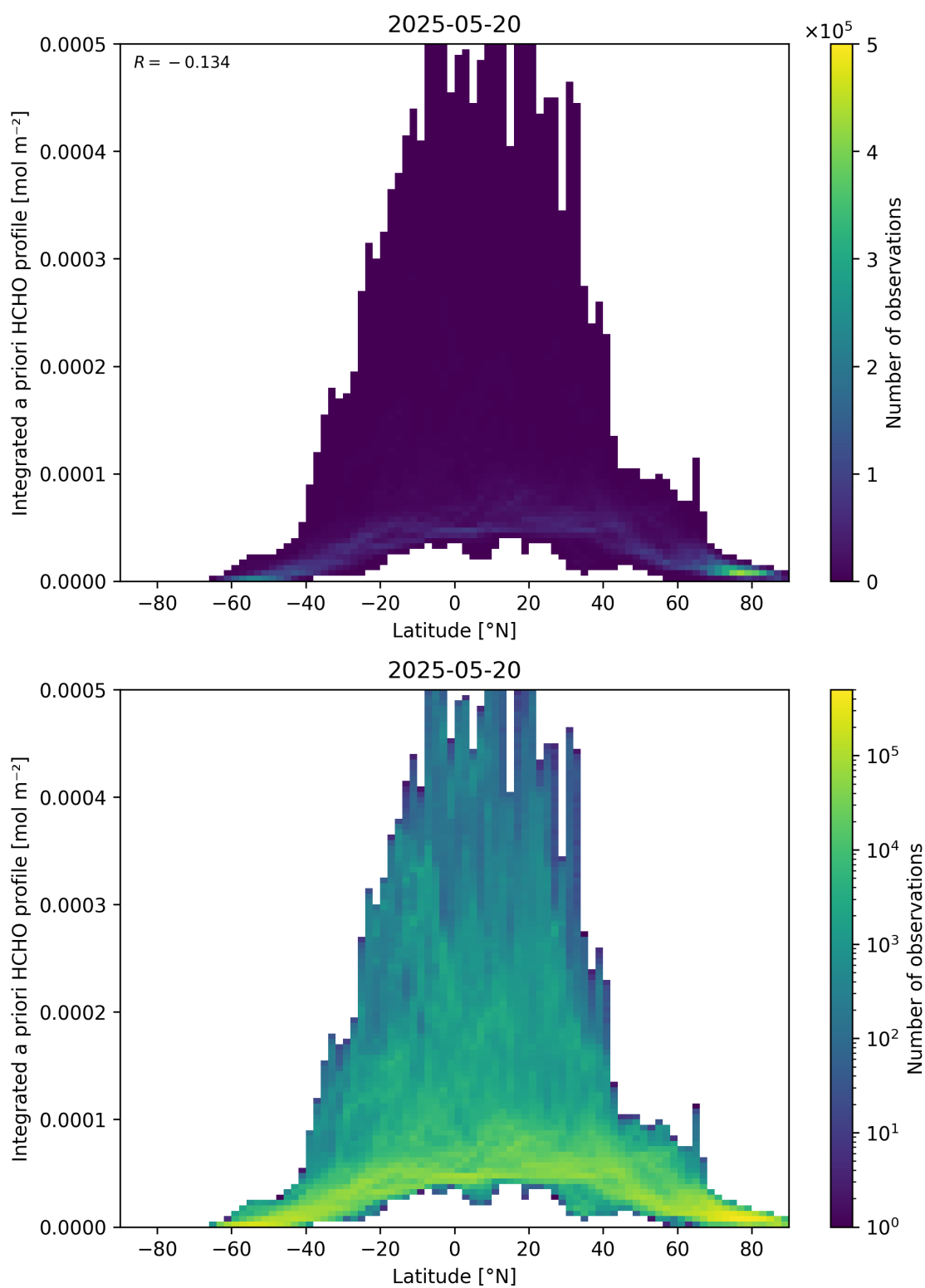
Figure 166: Scatter density plot of “Latitude” against “Integrated a priori HCHO profile” for 2025-05-19 to 2025-05-21.
