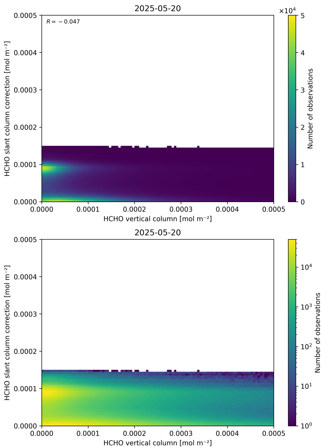
Figure 128: Scatter density plot of “HCHO vertical column” against “HCHO slant column correction” for 2025-05-19 to 2025-05-21.
