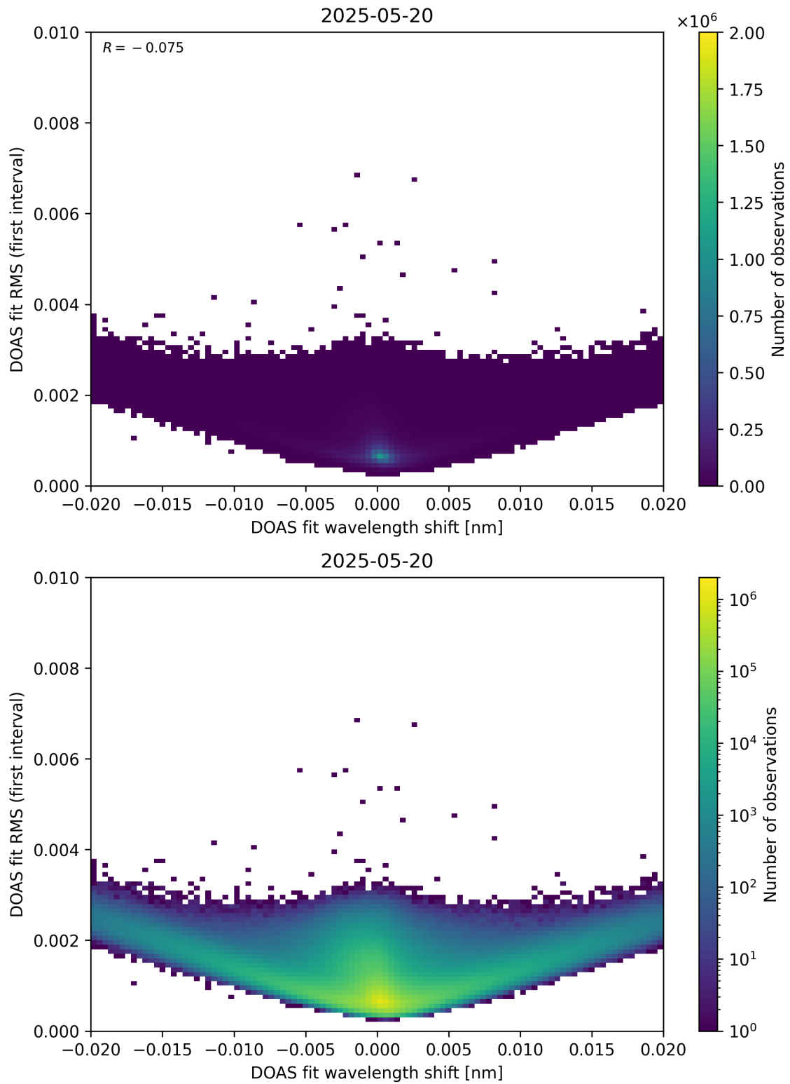
Figure 64: Scatter density plot of “DOAS fit wavelength shift” against “DOAS fit RMS (first interval)” for 2025-05-19 to 2025-05-21.
