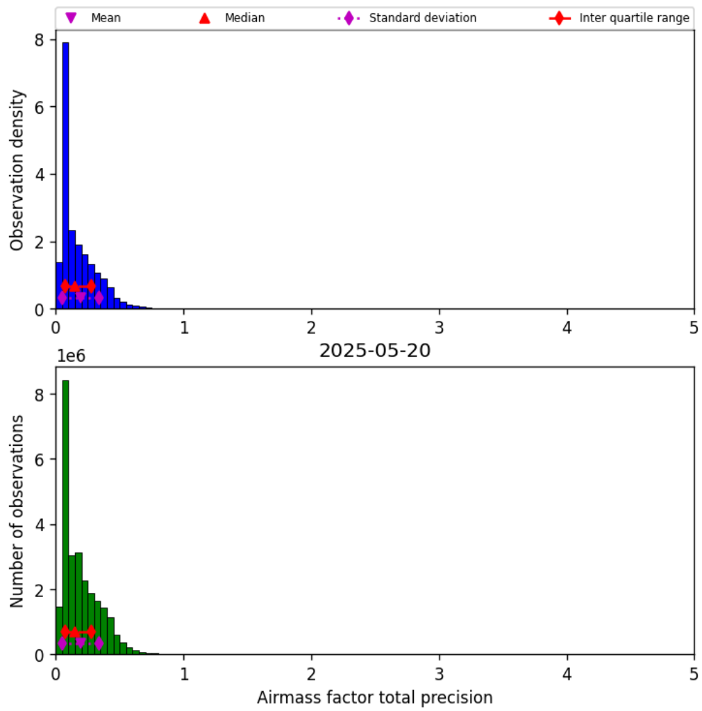
Figure 41: Histogram of “Airmass factor total precision” for 2025-05-19 to 2025-05-21
