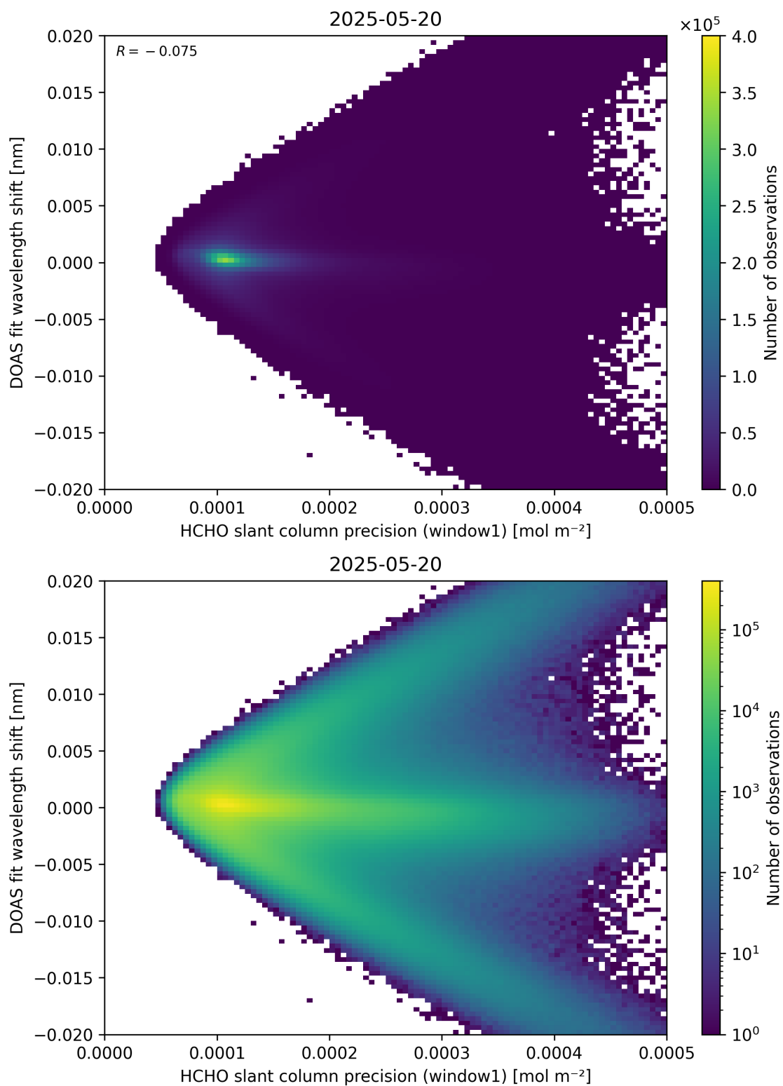
Figure 89: Scatter density plot of “HCHO slant column precision (window1)” against “DOAS fit wavelength shift” for 2025-05-19 to 2025-05-21.
