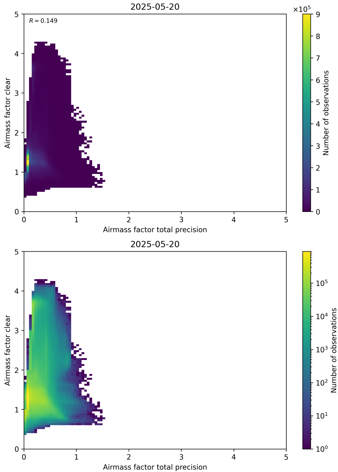
Figure 108: Scatter density plot of “Airmass factor total precision” against “Airmass factor clear” for 2025-05-19 to 2025-05-21.
