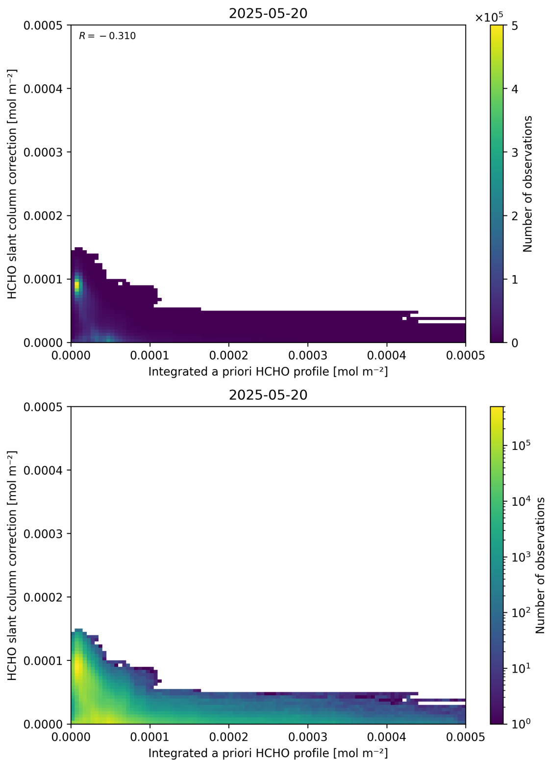
Figure 152: Scatter density plot of “Integrated a priori HCHO profile” against “HCHO slant column correction” for 2025-05-19 to 2025-05-21.
