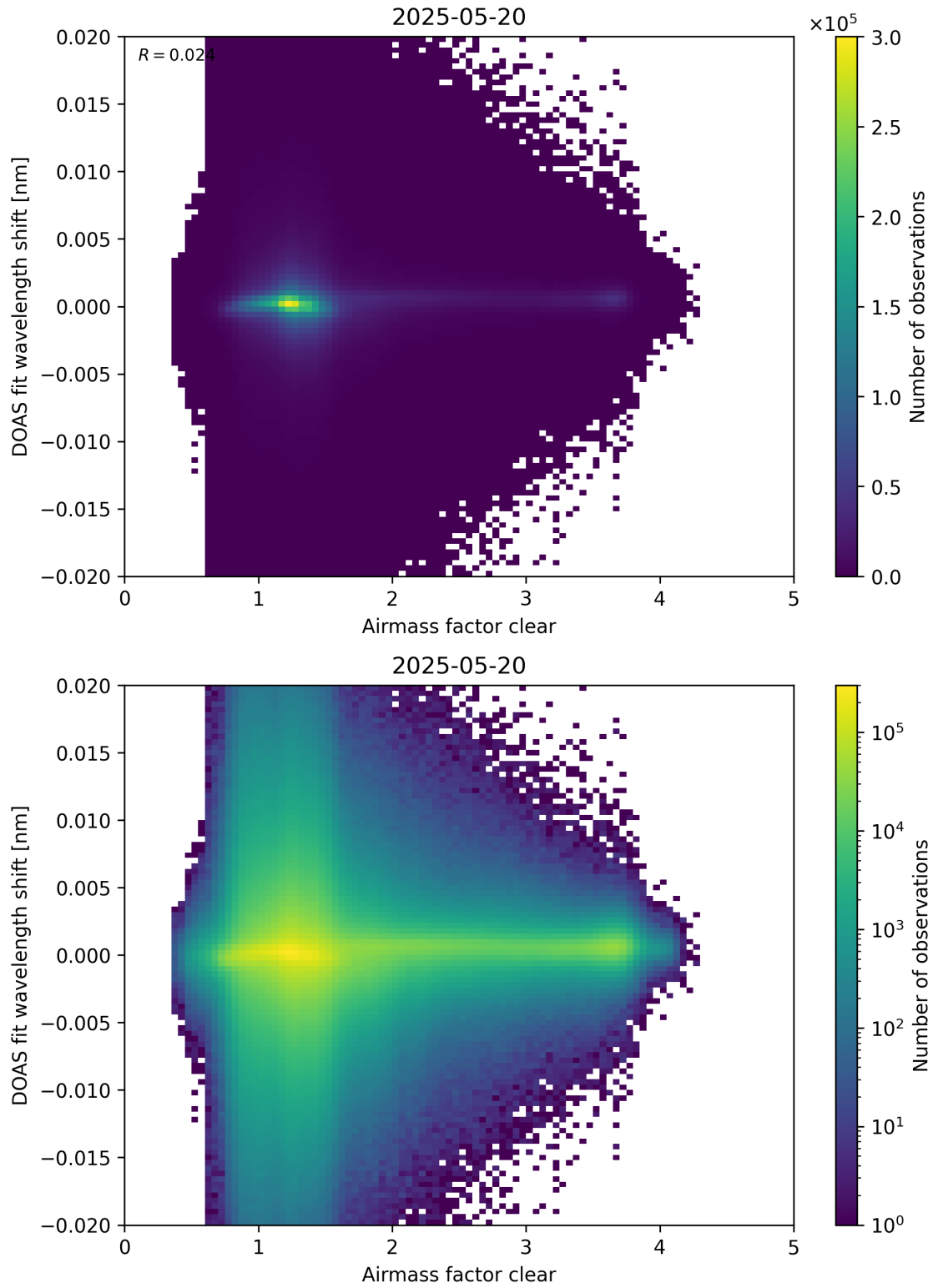
Figure 72: Scatter density plot of “Airmass factor clear” against “DOAS fit wavelength shift” for 2025-05-19 to 2025-05-21.
