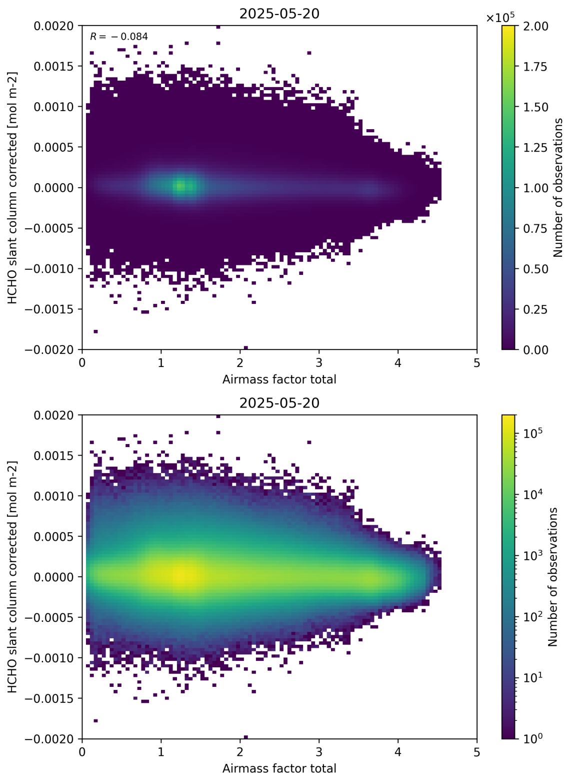
Figure 101: Scatter density plot of “Airmass factor total” against “HCHO slant column corrected” for 2025-05-19 to 2025-05-21.
