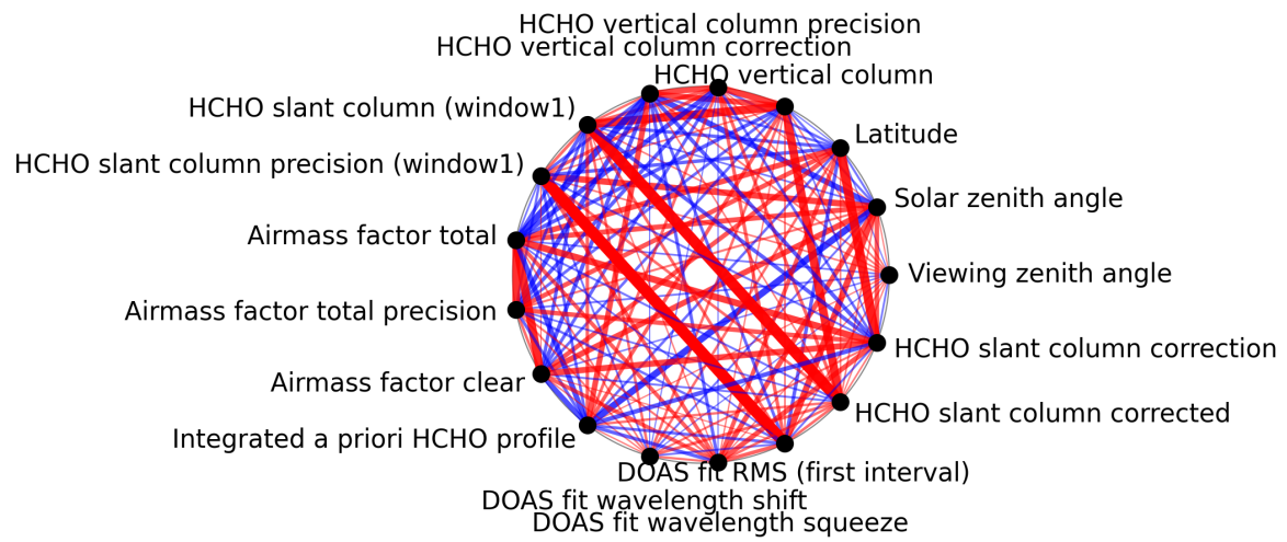
Figure 1: Map of correlation graph for 2025-05-19 to 2025-05-21.
