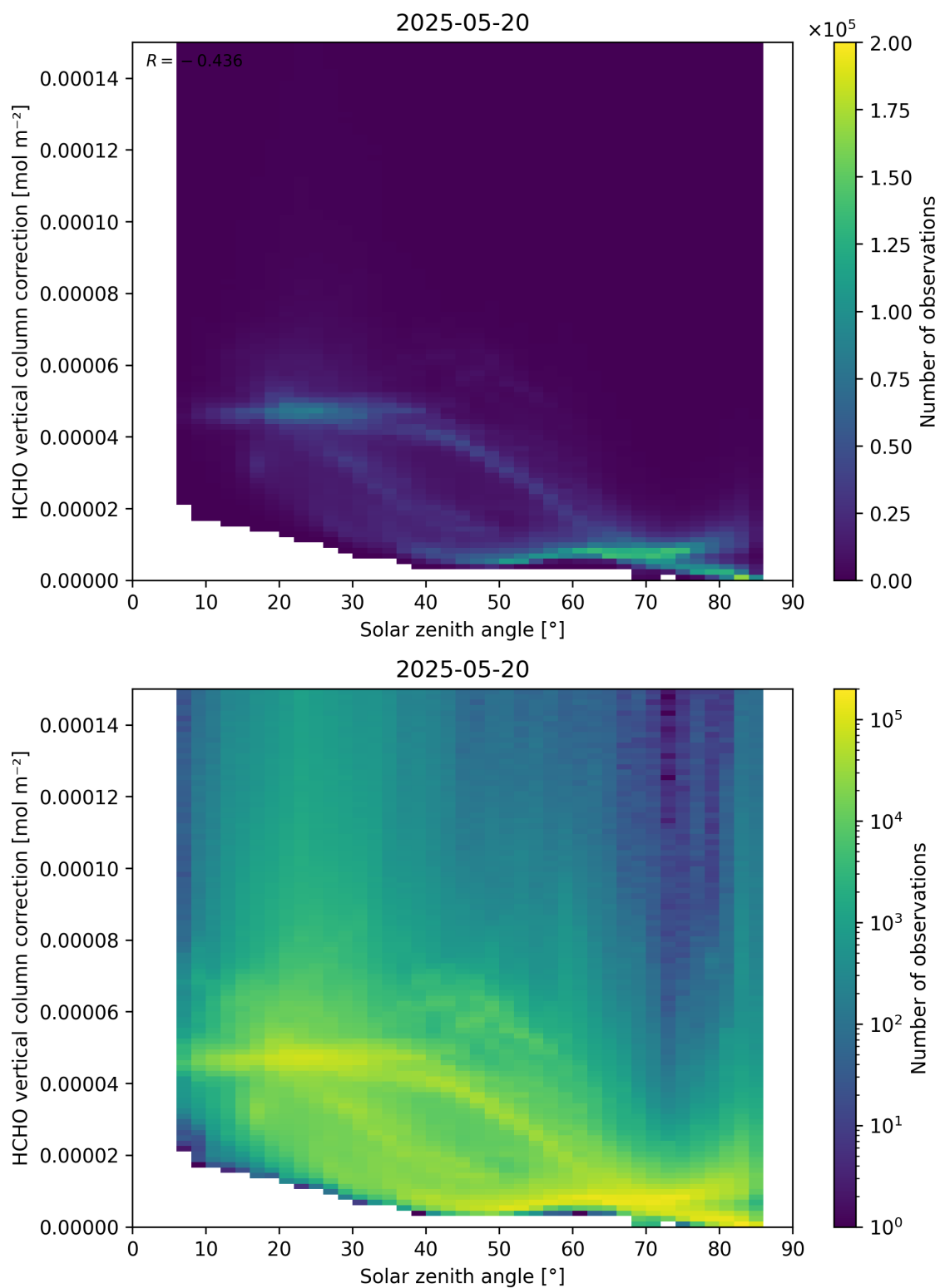
Figure 178: Scatter density plot of “Solar zenith angle” against “HCHO vertical column correction” for 2025-05-19 to 2025-05-21.
