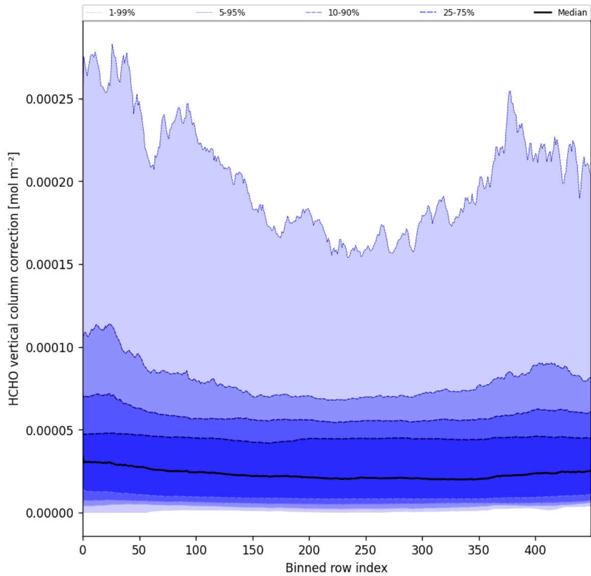
Figure 51: Along track statistics of “HCHO vertical column correction” for 2025-05-19 to 2025-05-21
