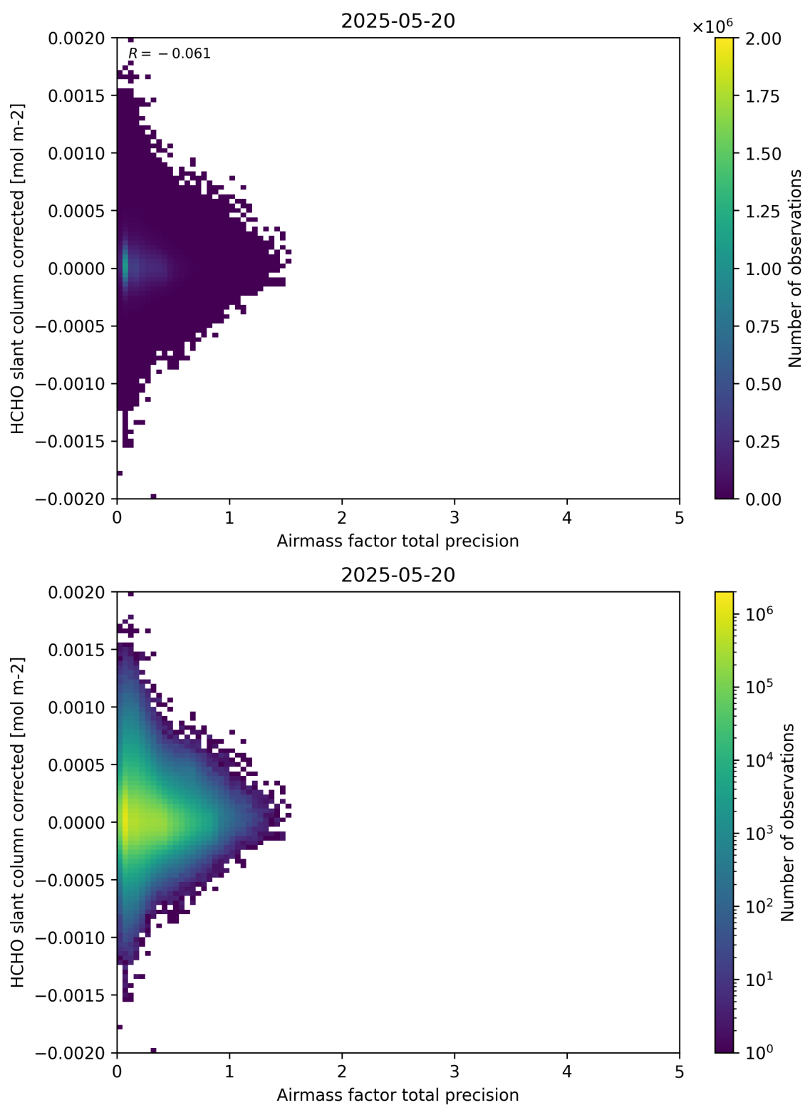
Figure 109: Scatter density plot of “Airmass factor total precision” against “HCHO slant column corrected” for 2025-05-19 to 2025-05-21.
