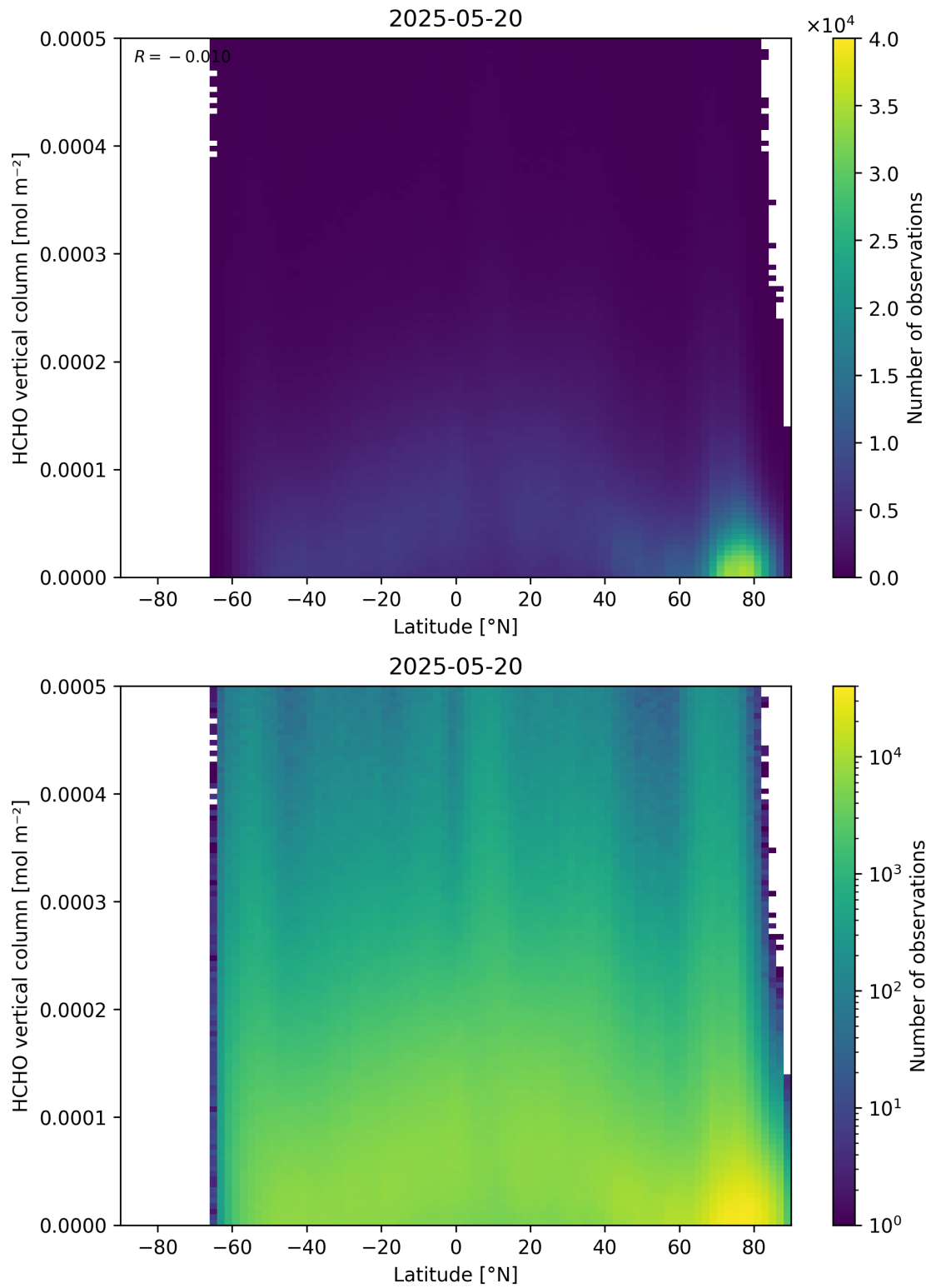
Figure 163: Scatter density plot of “Latitude” against “HCHO vertical column” for 2025-05-19 to 2025-05-21.
