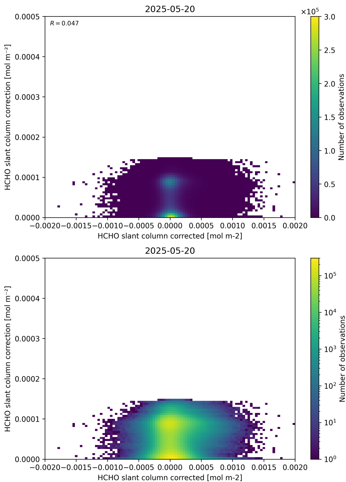
Figure 77: Scatter density plot of “HCHO slant column corrected” against “HCHO slant column correction” for 2025-05-19 to 2025-05-21.
