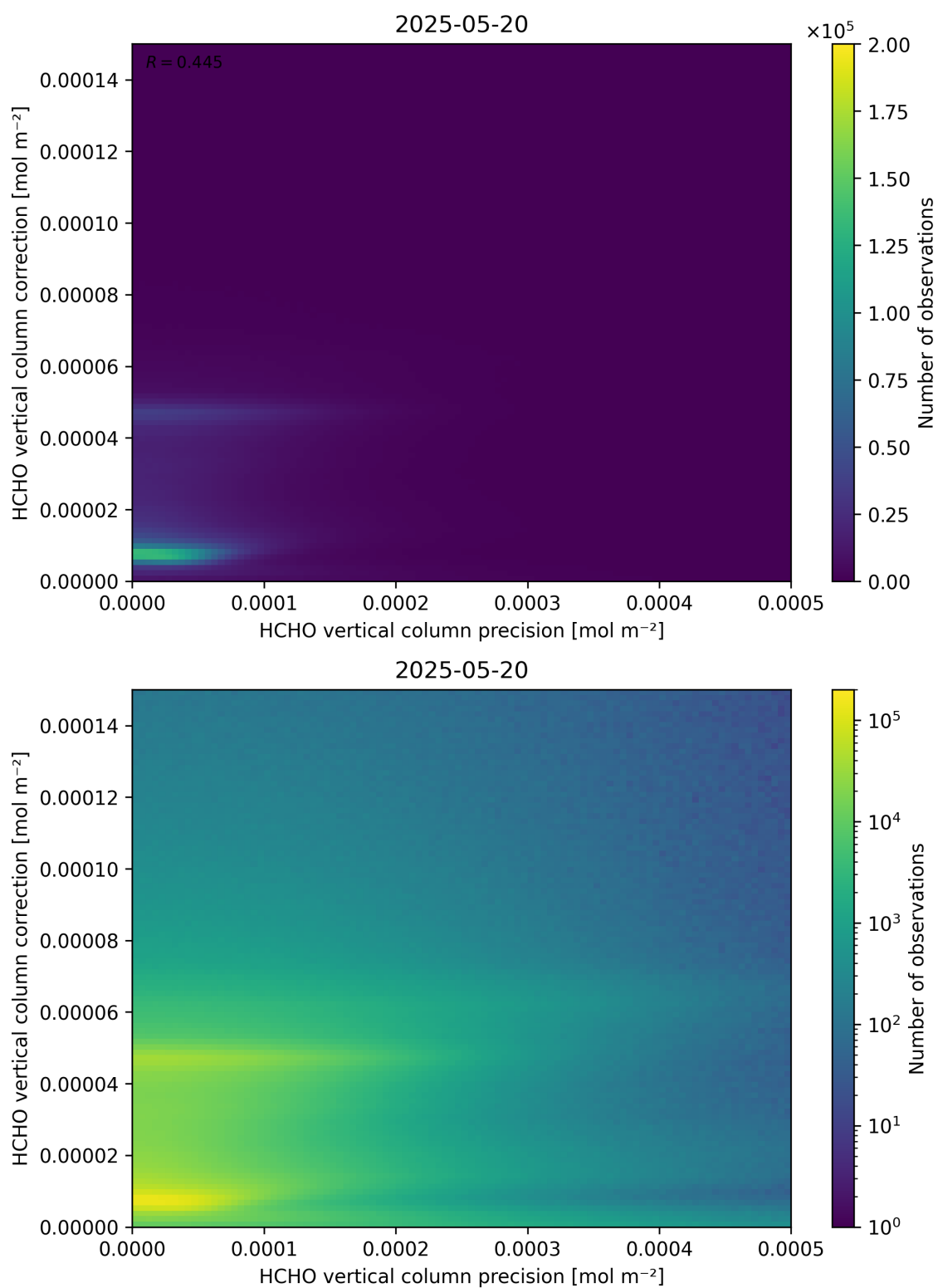
Figure 146: Scatter density plot of “HCHO vertical column precision” against “HCHO vertical column correction” for 2025-05-19 to 2025-05-21.
