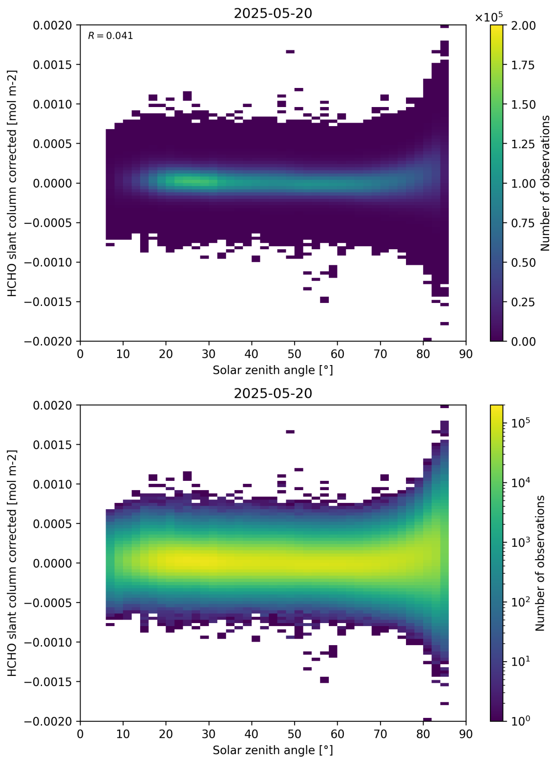
Figure 171: Scatter density plot of “Solar zenith angle” against “HCHO slant column corrected” for 2025-05-19 to 2025-05-21.
