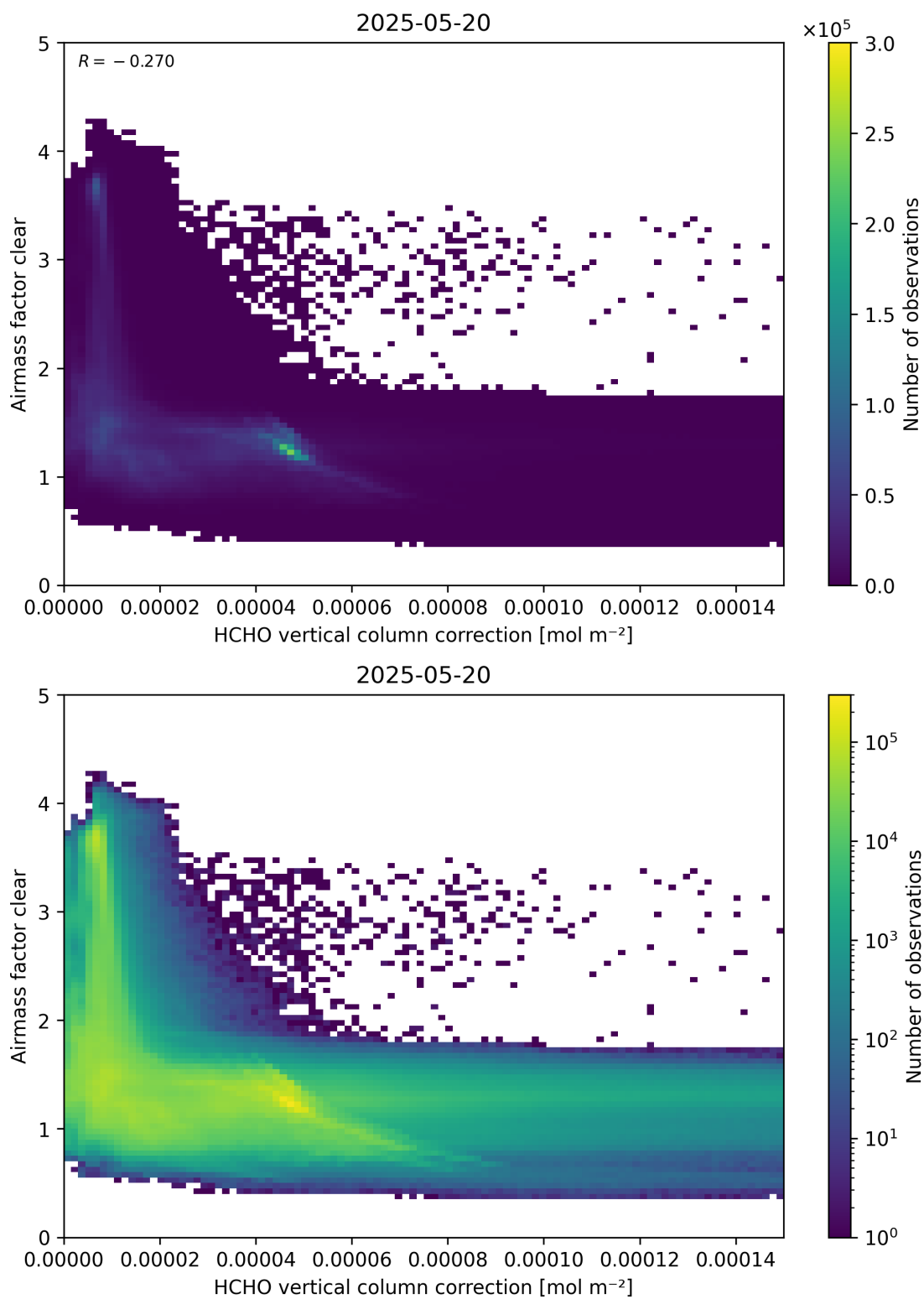
Figure 115: Scatter density plot of “HCHO vertical column correction” against “Airmass factor clear” for 2025-05-19 to 2025-05-21.
