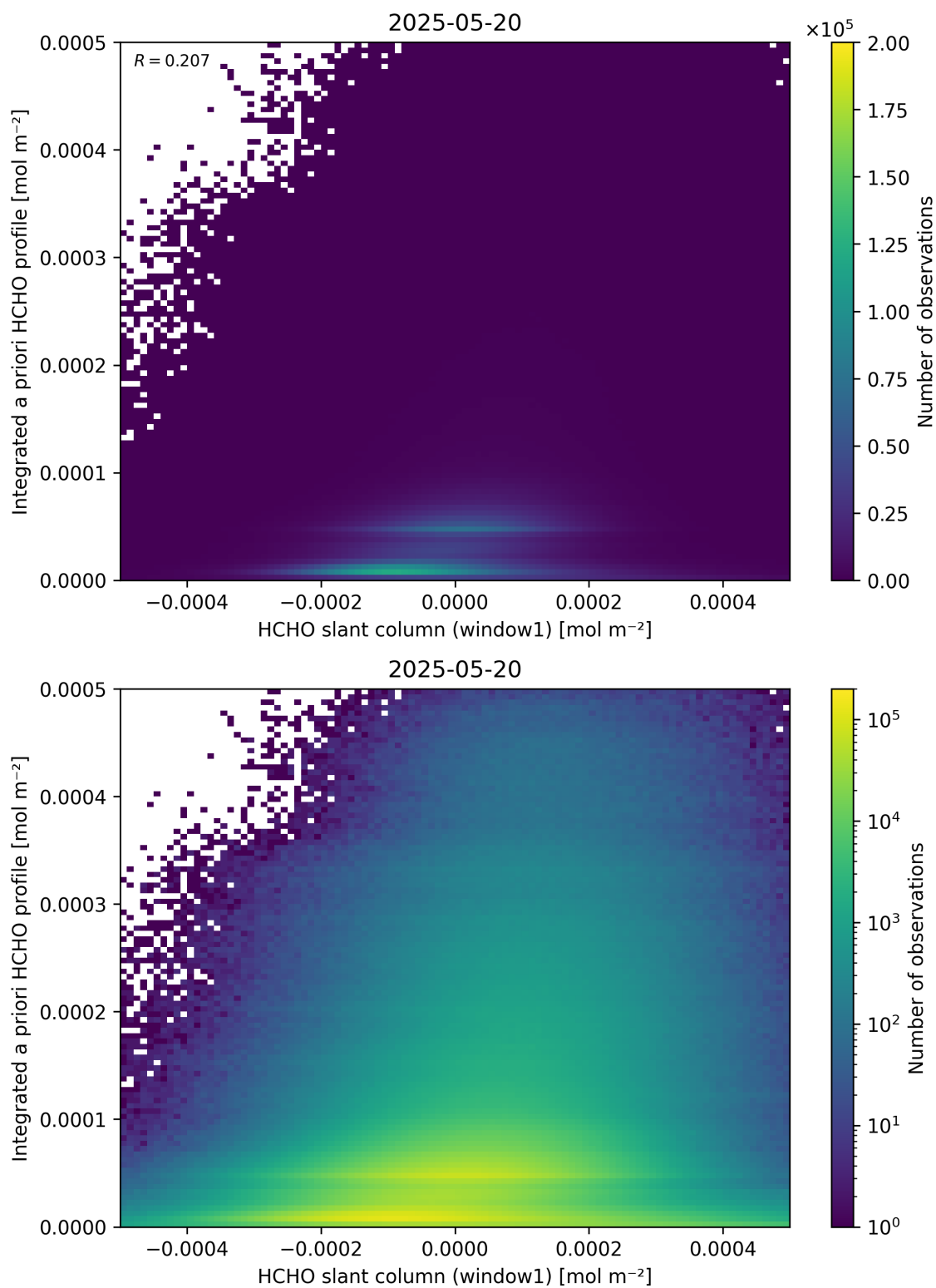
Figure 87: Scatter density plot of “HCHO slant column (window1)” against “Integrated a priori HCHO profile” for 2025-05-19 to 2025-05-21.
