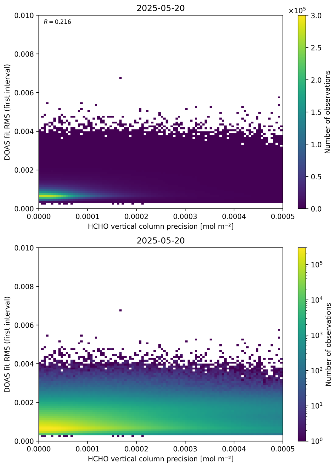
Figure 136: Scatter density plot of “HCHO vertical column precision” against “DOAS fit RMS (first interval)” for 2025-05-19 to 2025-05-21.
