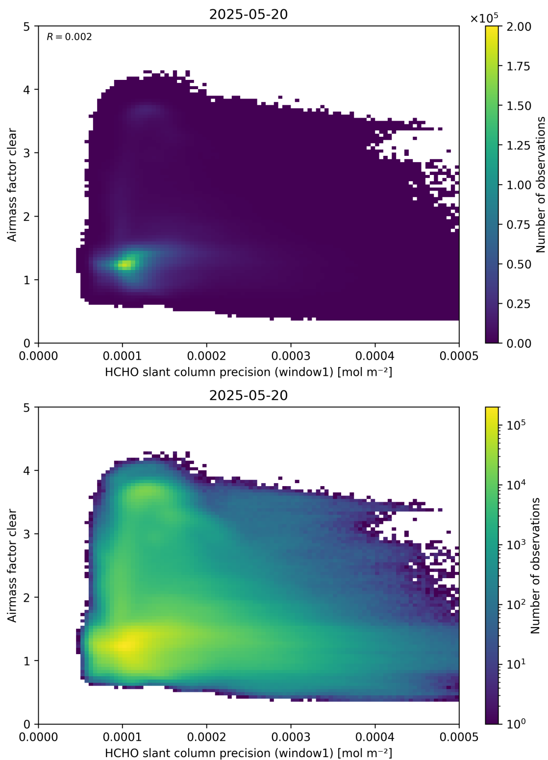
Figure 91: Scatter density plot of “HCHO slant column precision (window1)” against “Airmass factor clear” for 2025-05-19 to 2025-05-21.
