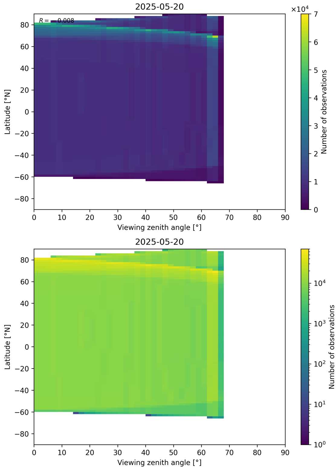
Figure 196: Scatter density plot of “Viewing zenith angle” against “Latitude” for 2025-05-19 to 2025-05-21.
