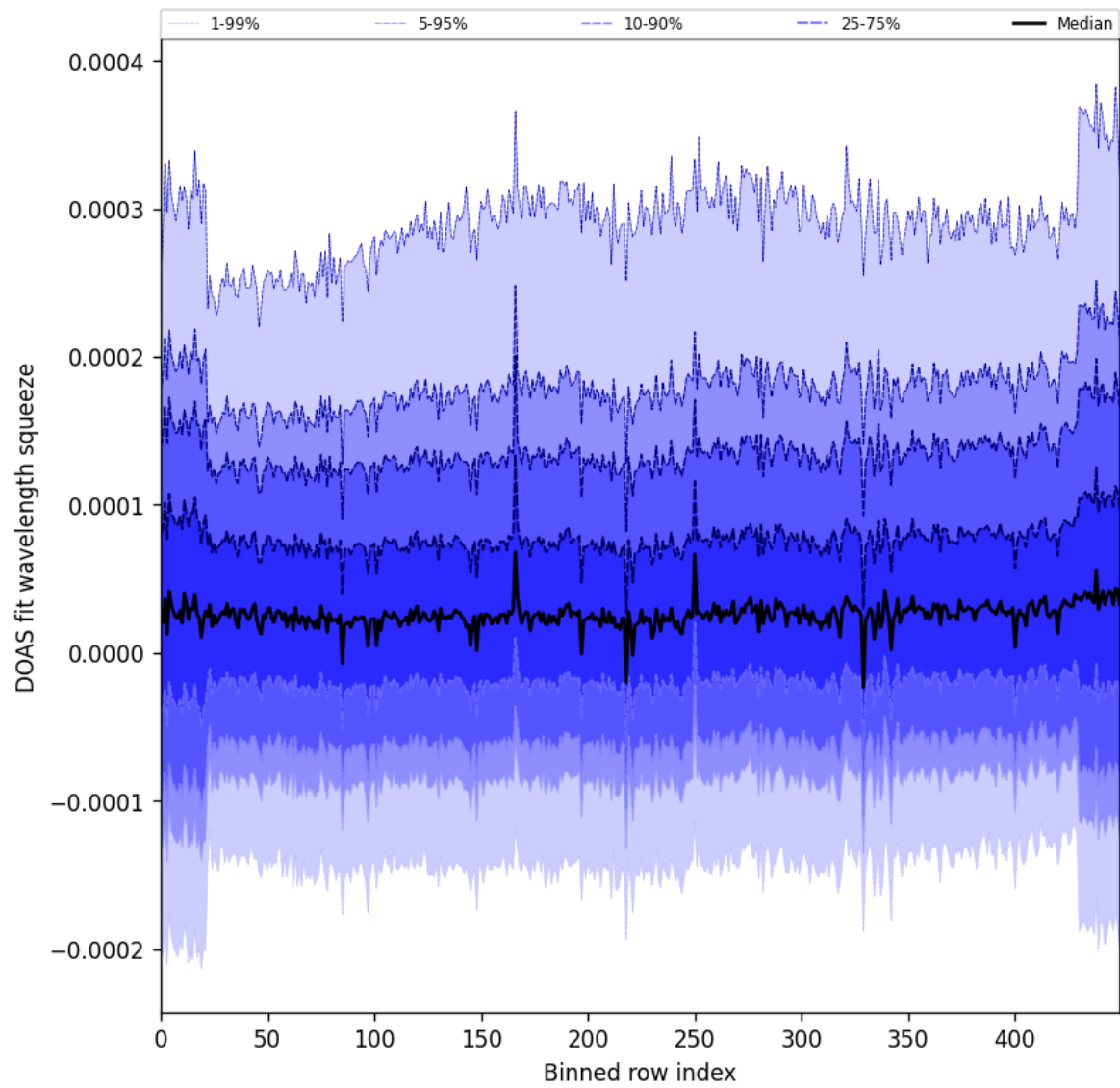
Figure 59: Along track statistics of “DOAS fit wavelength squeeze” for 2025-05-19 to 2025-05-21
