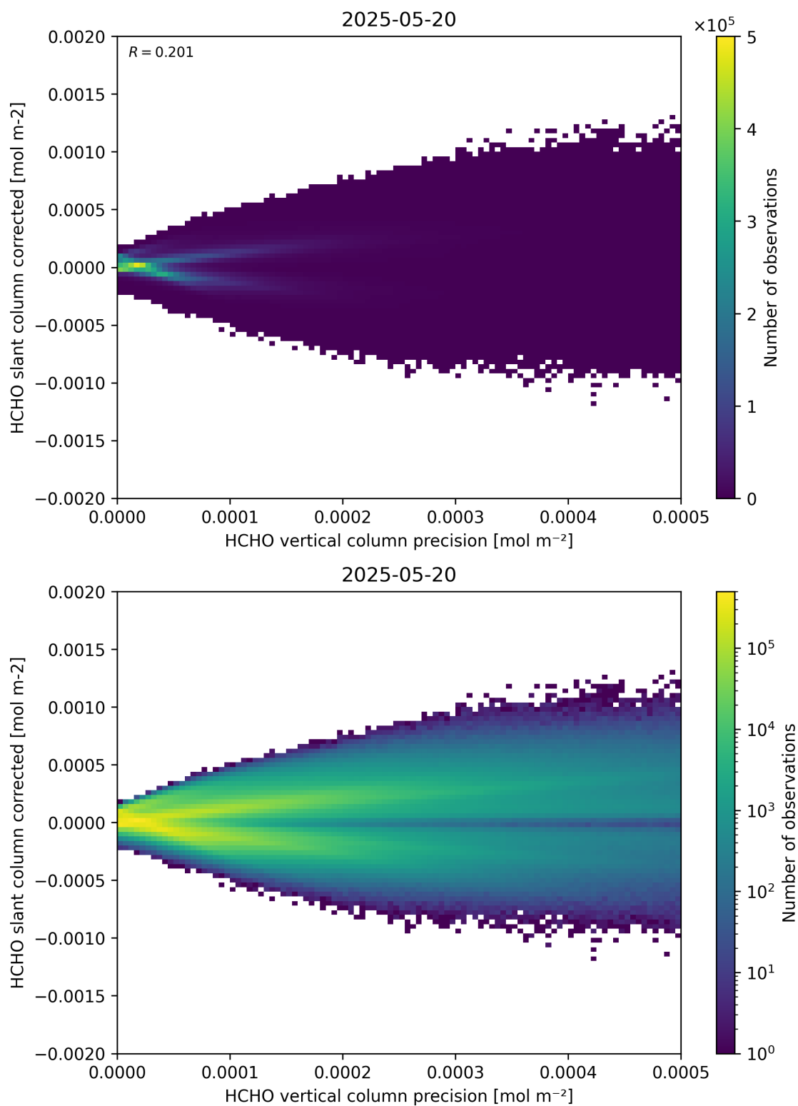
Figure 140: Scatter density plot of “HCHO vertical column precision” against “HCHO slant column corrected” for 2025-05-19 to 2025-05-21.
