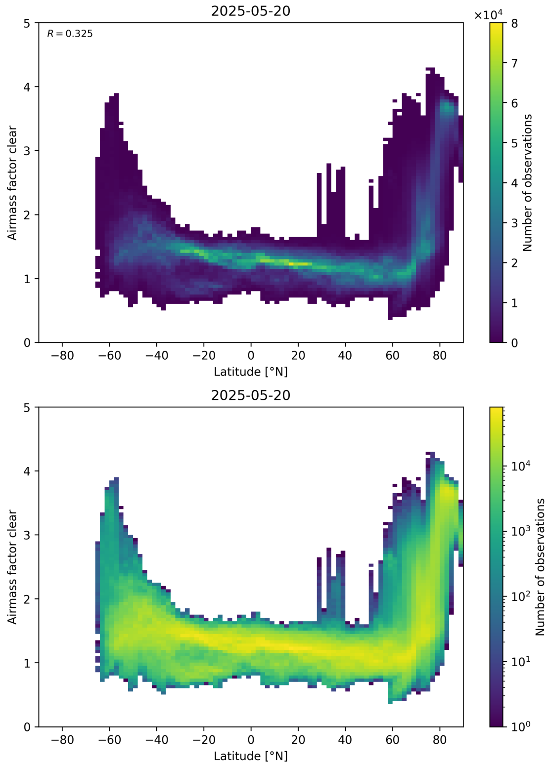
Figure 156: Scatter density plot of “Latitude” against “Airmass factor clear” for 2025-05-19 to 2025-05-21.
