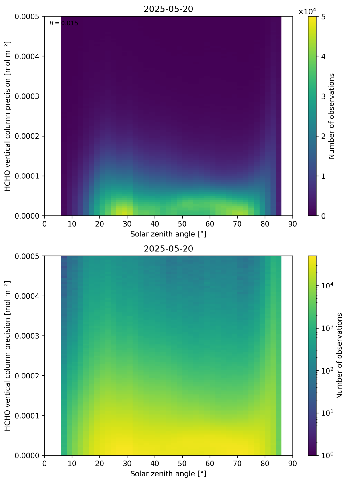
Figure 179: Scatter density plot of “Solar zenith angle” against “HCHO vertical column precision” for 2025-05-19 to 2025-05-21.
