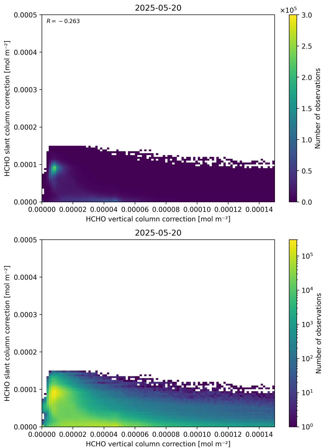
Figure 117: Scatter density plot of “HCHO vertical column correction” against “HCHO slant column correction” for 2025-05-19 to 2025-05-21.
