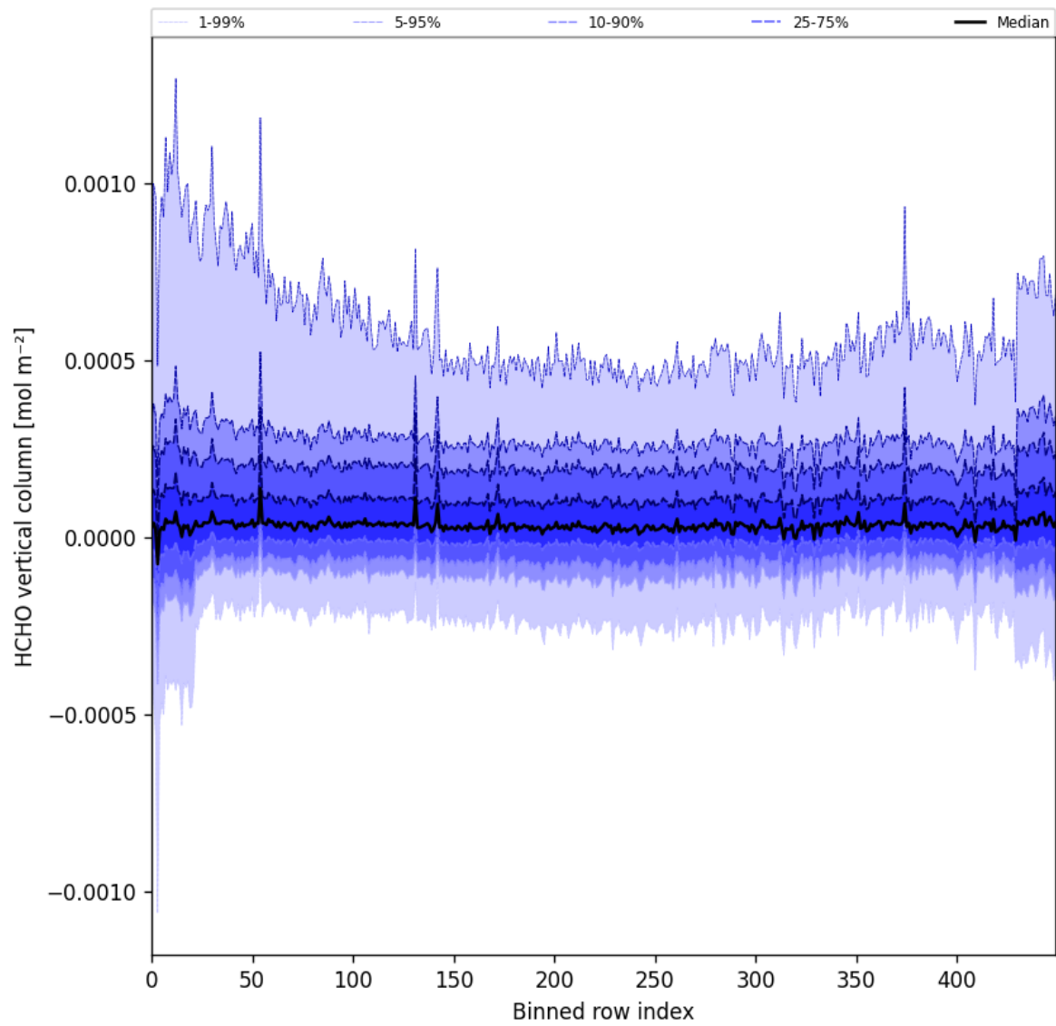
Figure 49: Along track statistics of “HCHO vertical column” for 2025-05-19 to 2025-05-21
