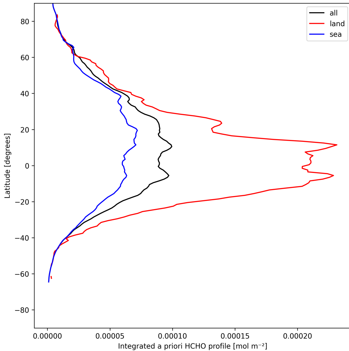
Figure 29: Zonal average of “Integrated a priori HCHO profile” for 2025-05-19 to 2025-05-21.
