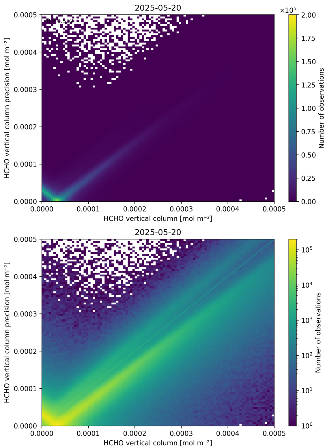
Figure 134: Scatter density plot of “HCHO vertical column” against “HCHO vertical column precision” for 2025-05-19 to 2025-05-21.
