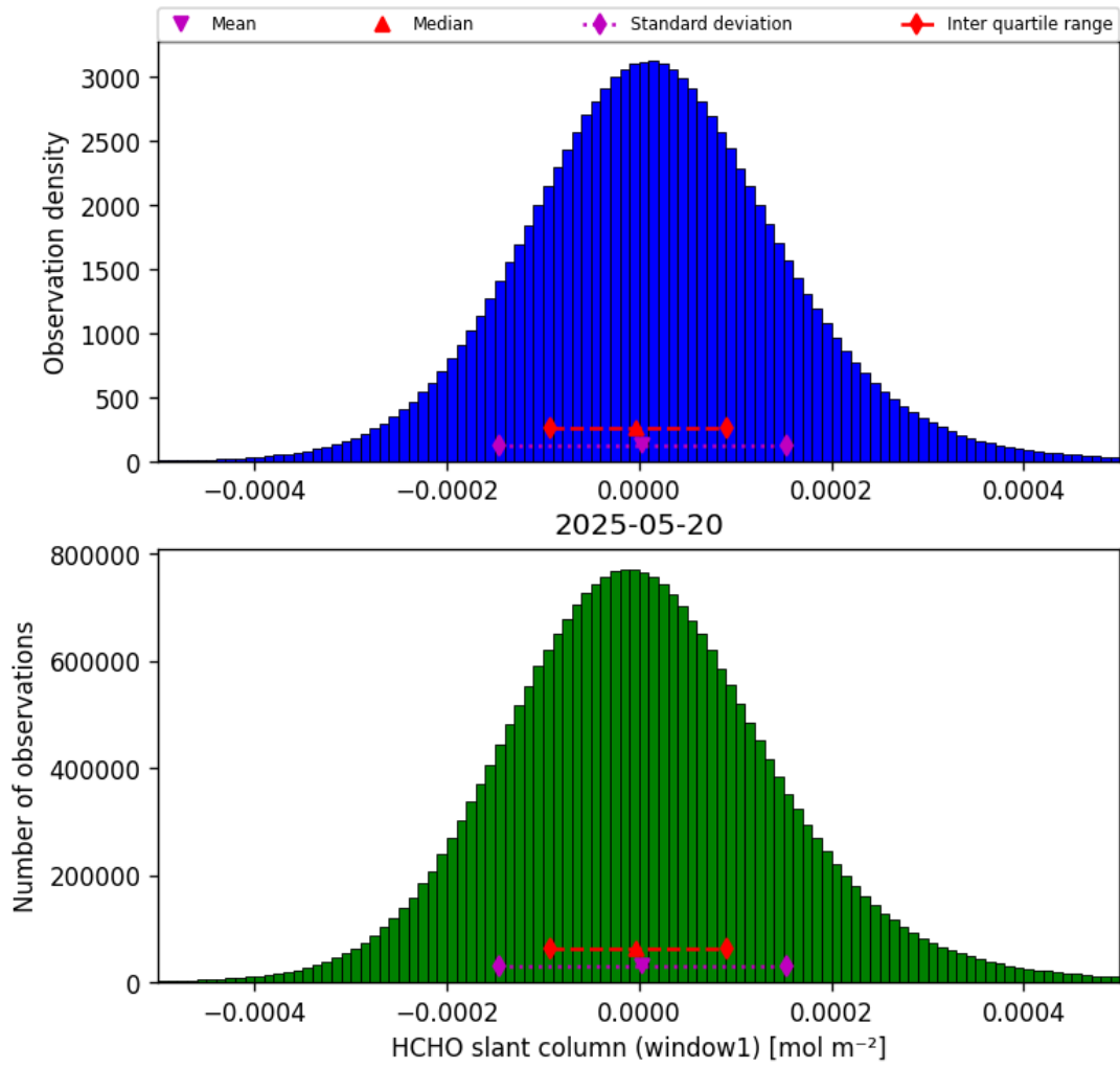
Figure 38: Histogram of “HCHO slant column (window1)” for 2025-05-19 to 2025-05-21
