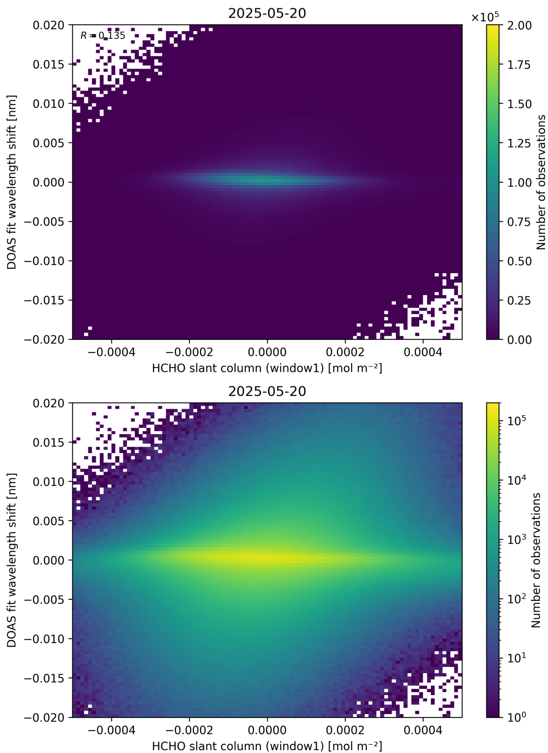
Figure 79: Scatter density plot of “HCHO slant column (window1)” against “DOAS fit wavelength shift” for 2025-05-19 to 2025-05-21.
