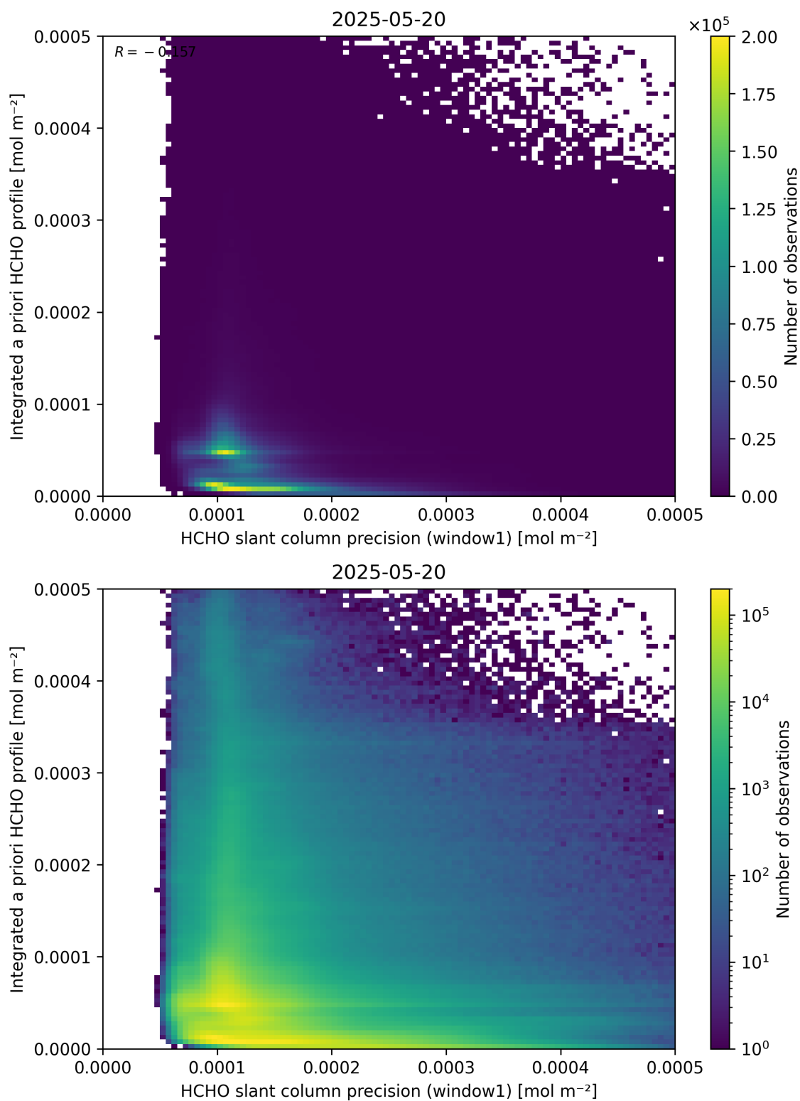
Figure 96: Scatter density plot of “HCHO slant column precision (window1)” against “Integrated a priori HCHO profile” for 2025-05-19 to 2025-05-21.
