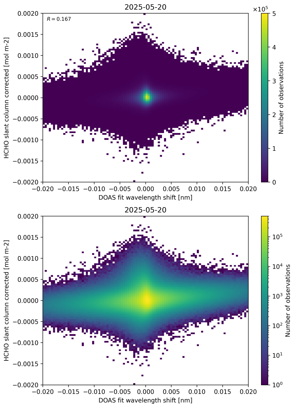
Figure 66: Scatter density plot of “DOAS fit wavelength shift” against “HCHO slant column corrected” for 2025-05-19 to 2025-05-21.
