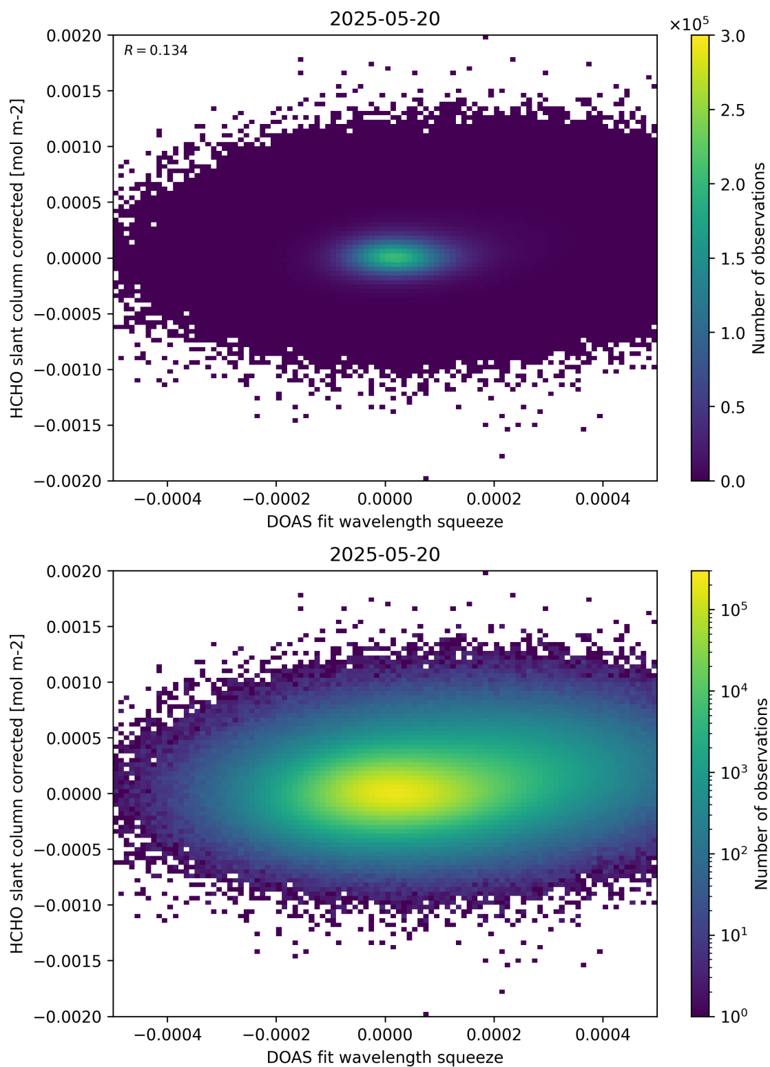
Figure 69: Scatter density plot of “DOAS fit wavelength squeeze” against “HCHO slant column corrected” for 2025-05-19 to 2025-05-21.
