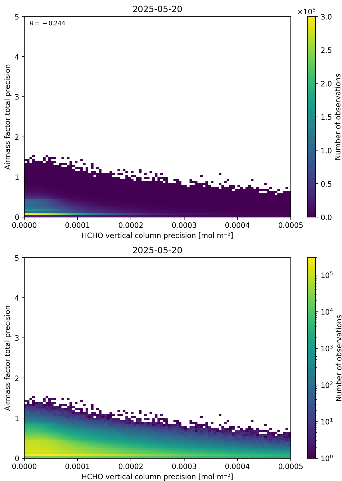
Figure 145: Scatter density plot of “HCHO vertical column precision” against “Airmass factor total precision” for 2025-05-19 to 2025-05-21.
