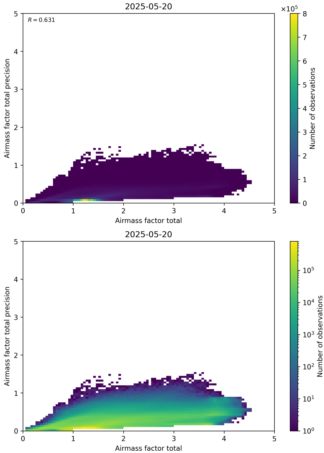
Figure 103: Scatter density plot of “Airmass factor total” against “Airmass factor total precision” for 2025-05-19 to 2025-05-21.
