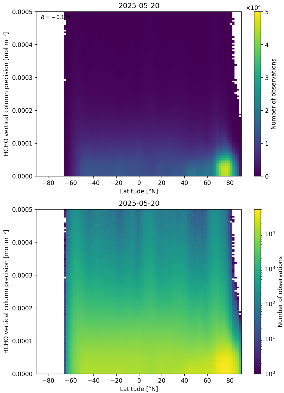
Figure 165: Scatter density plot of “Latitude” against “HCHO vertical column precision” for 2025-05-19 to 2025-05-21.
