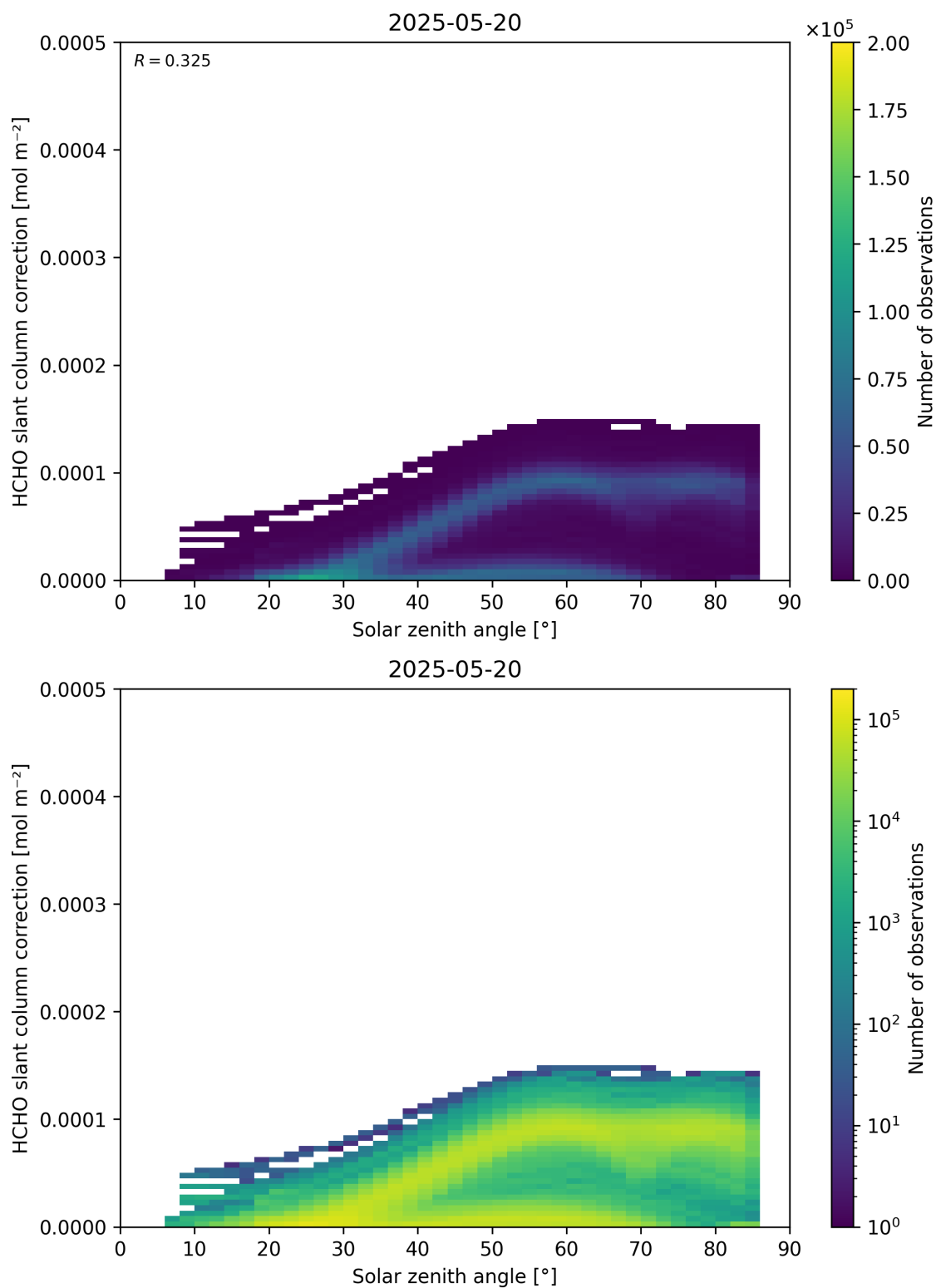
Figure 172: Scatter density plot of “Solar zenith angle” against “HCHO slant column correction” for 2025-05-19 to 2025-05-21.
