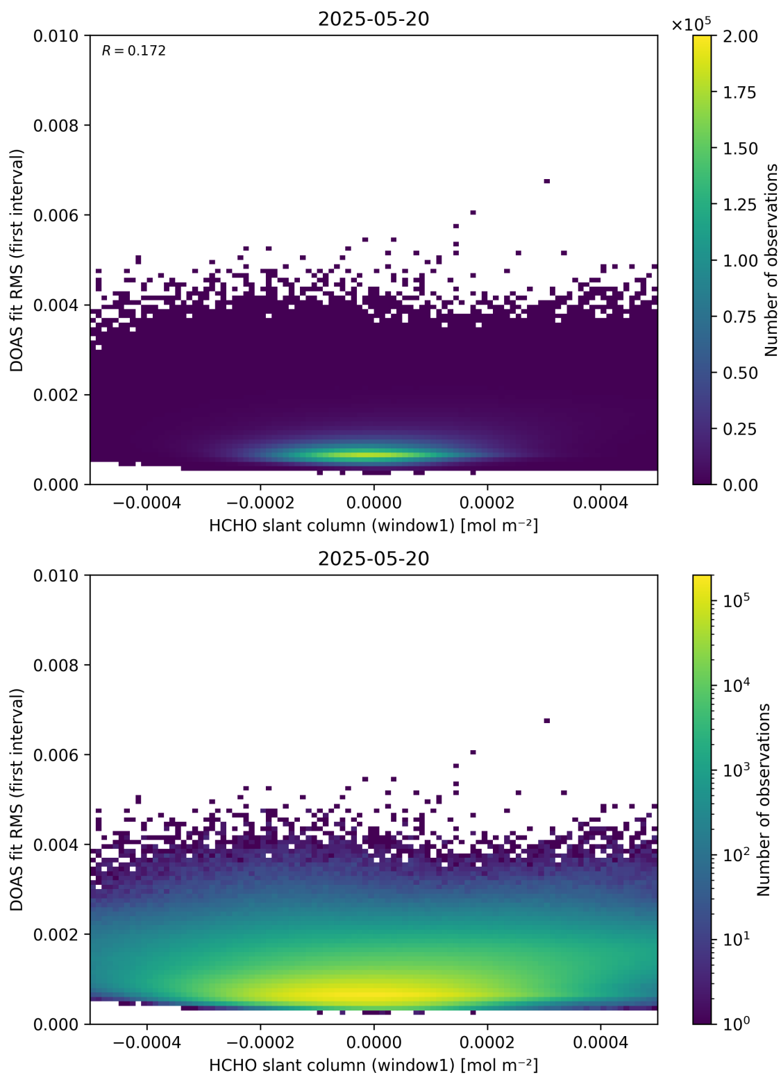
Figure 78: Scatter density plot of “HCHO slant column (window1)” against “DOAS fit RMS (first interval)” for 2025-05-19 to 2025-05-21.
