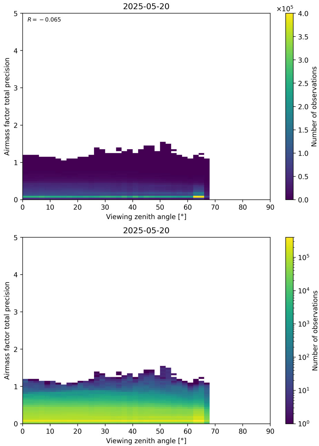
Figure 191: Scatter density plot of “Viewing zenith angle” against “Airmass factor total precision” for 2025-05-19 to 2025-05-21.
