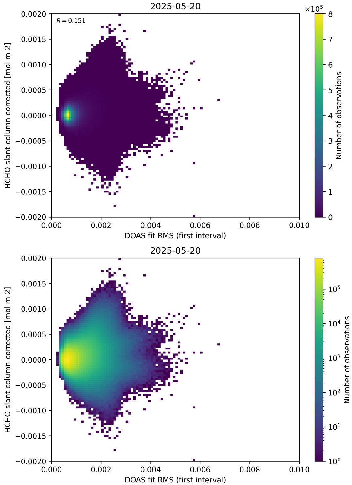
Figure 62: Scatter density plot of “DOAS fit RMS (first interval)” against “HCHO slant column corrected” for 2025-05-19 to 2025-05-21.
