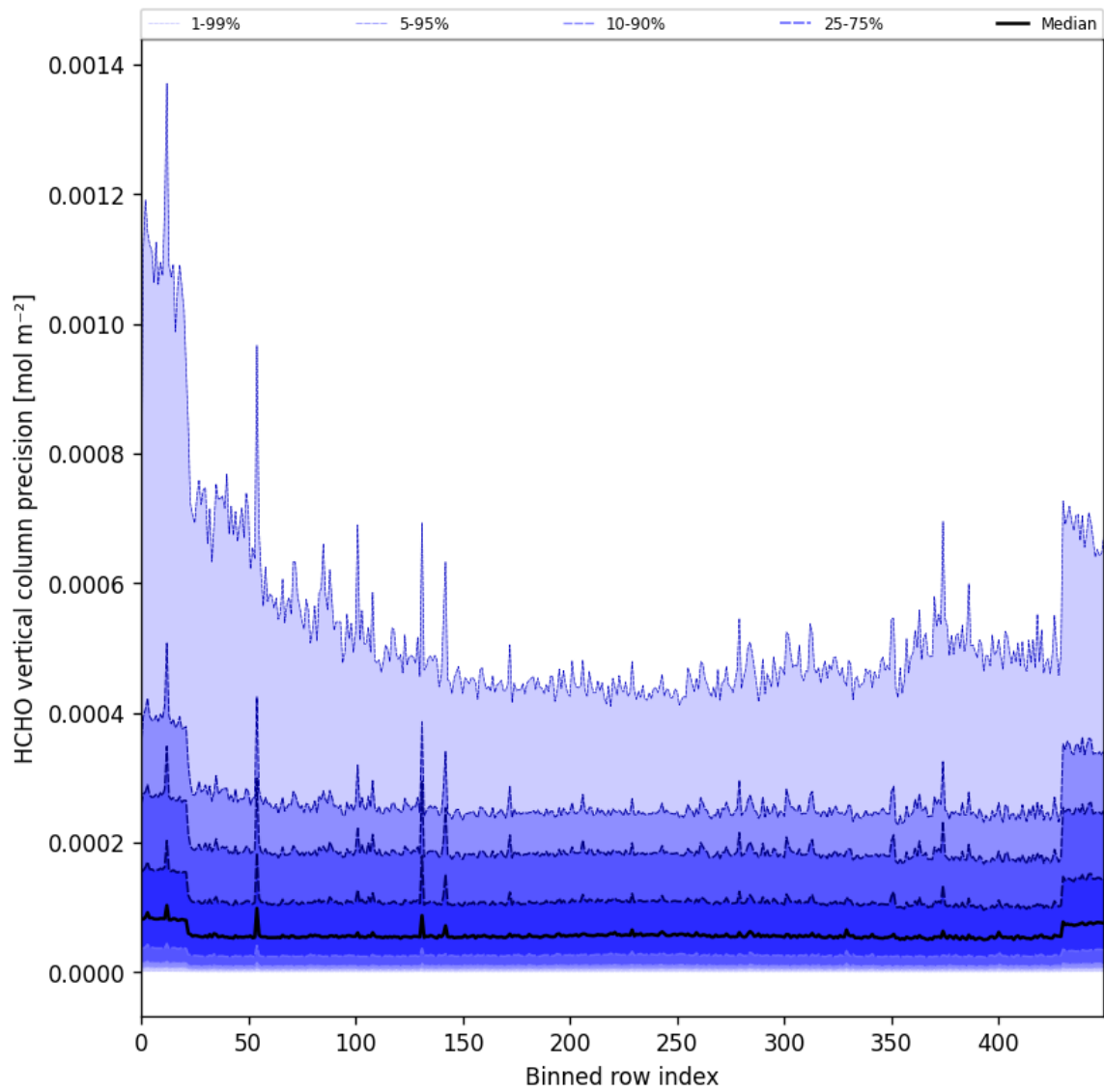
Figure 50: Along track statistics of “HCHO vertical column precision” for 2025-05-19 to 2025-05-21
