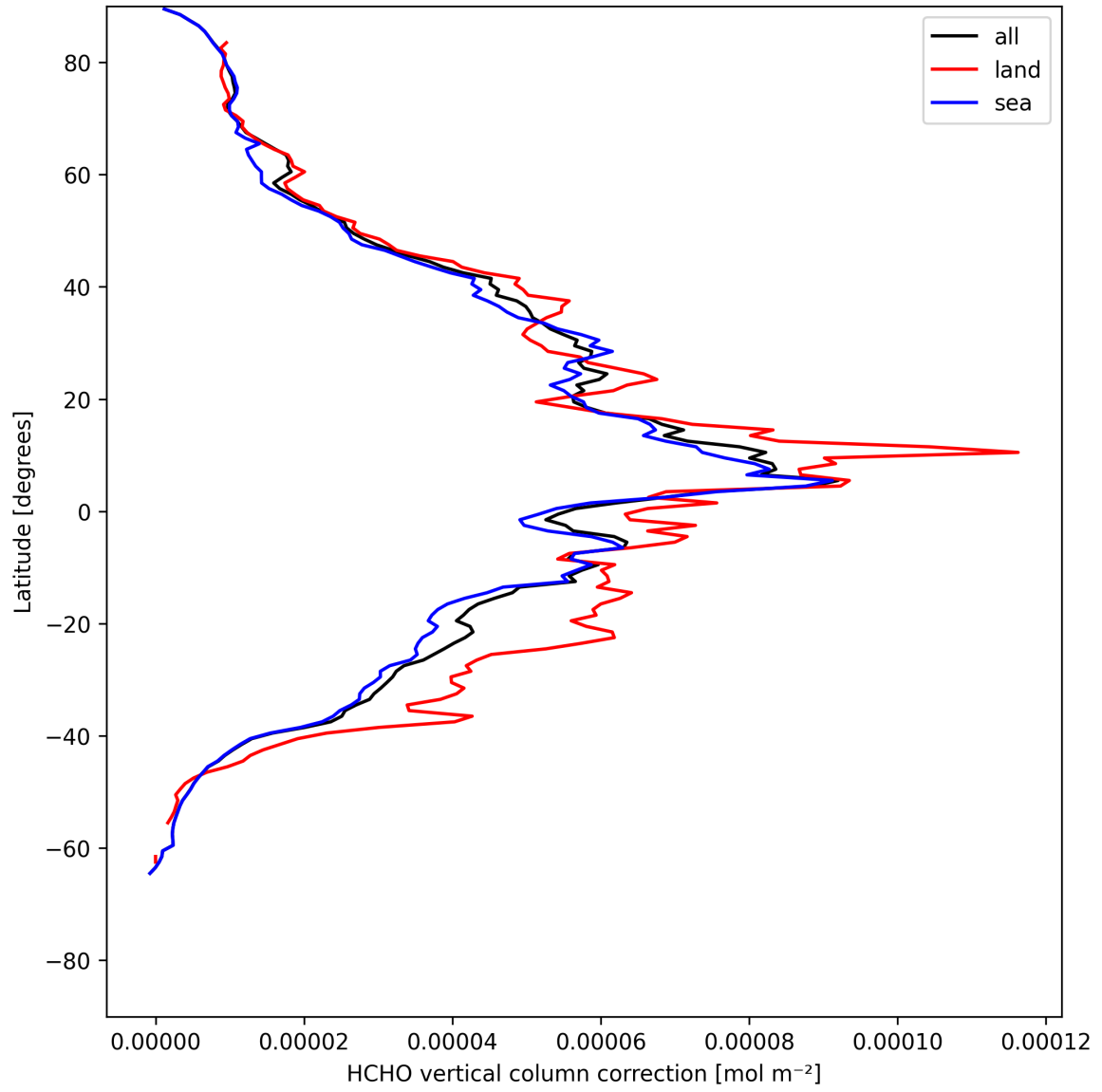
Figure 23: Zonal average of “HCHO vertical column correction” for 2025-05-19 to 2025-05-21.
