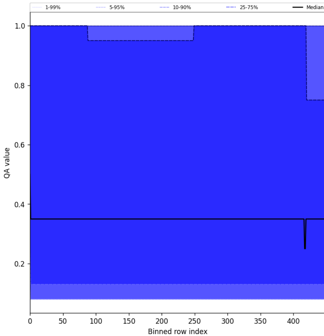
Figure 48: Along track statistics of “QA value” for 2025-05-19 to 2025-05-21
