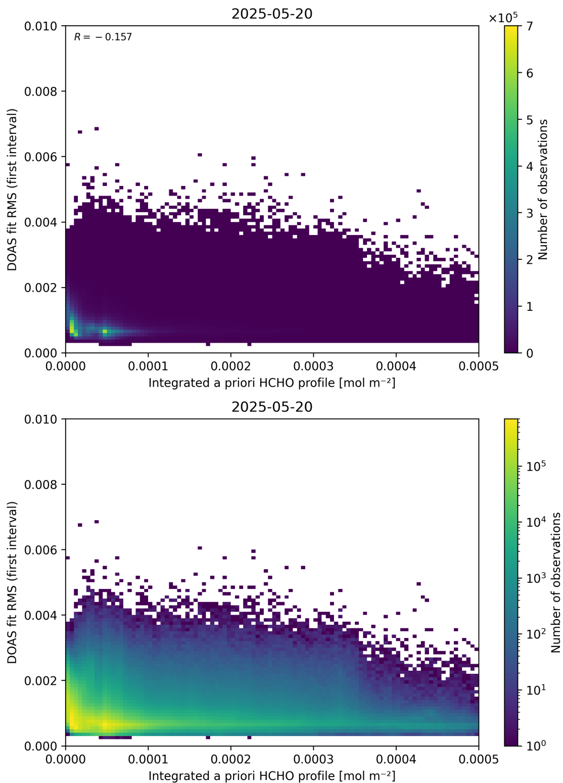
Figure 148: Scatter density plot of “Integrated a priori HCHO profile” against “DOAS fit RMS (first interval)” for 2025-05-19 to 2025-05-21.
