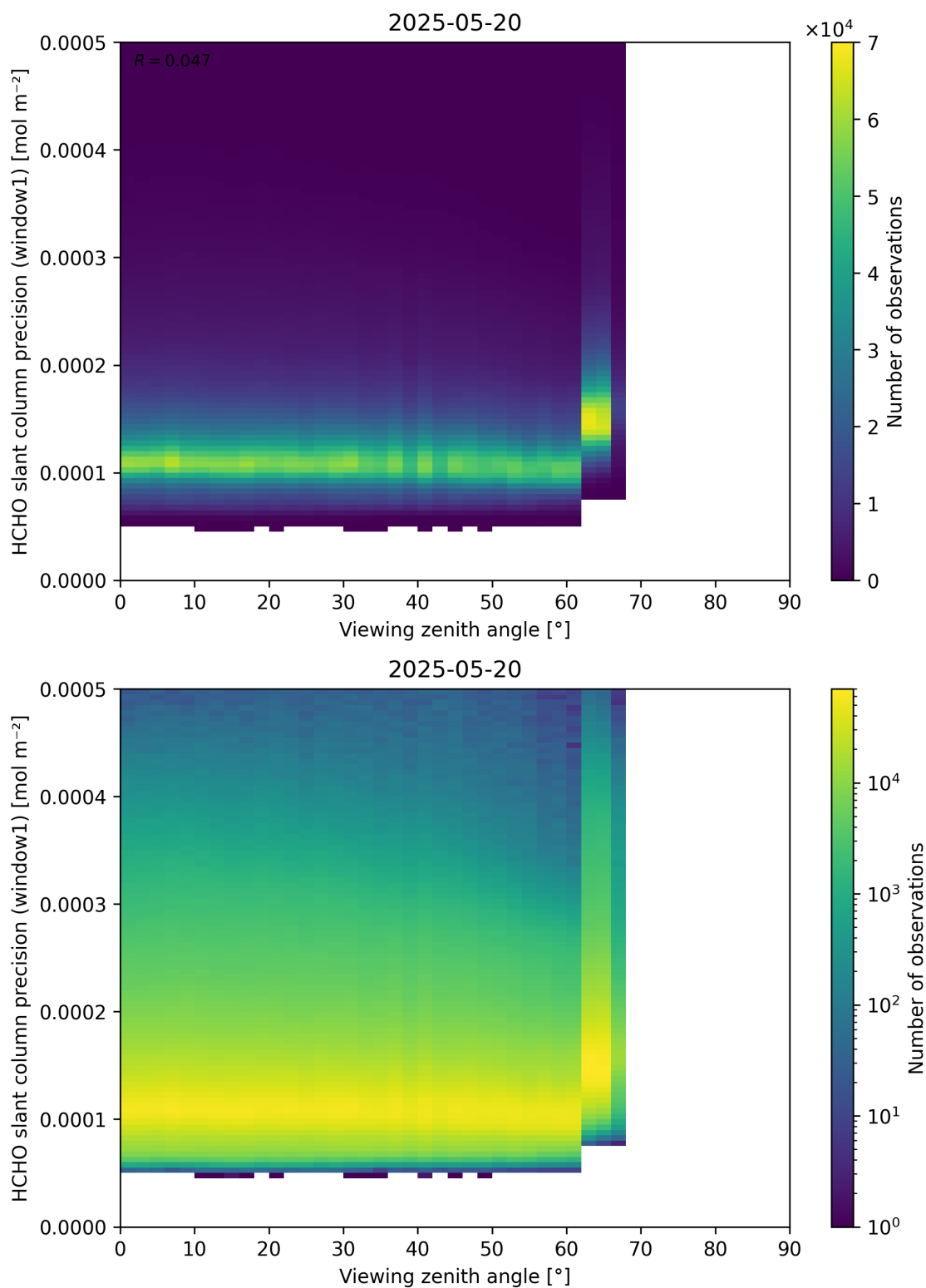
Figure 189: Scatter density plot of “Viewing zenith angle” against “HCHO slant column precision (window1)” for 2025-05-19 to 2025-05-21.
