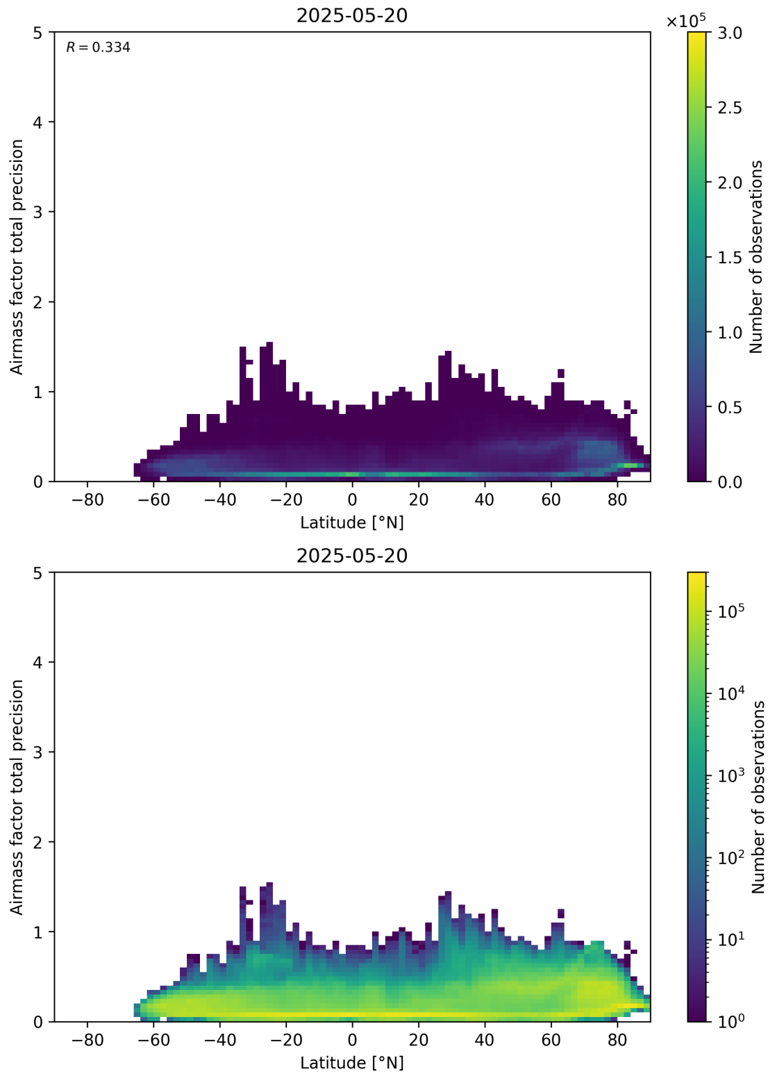
Figure 162: Scatter density plot of “Latitude” against “Airmass factor total precision” for 2025-05-19 to 2025-05-21.
