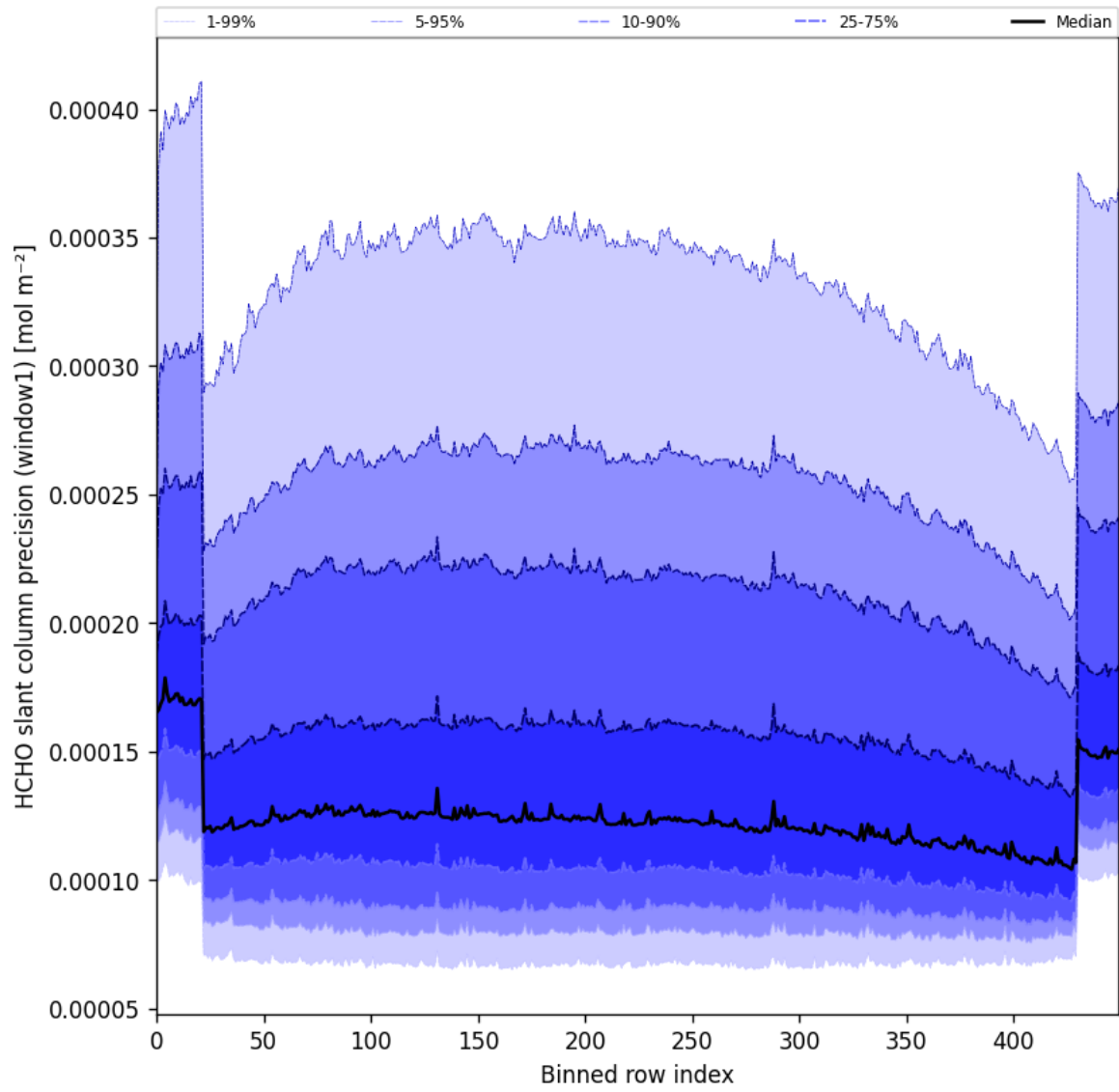
Figure 53: Along track statistics of “HCHO slant column precision (window1)” for 2025-05-19 to 2025-05-21
