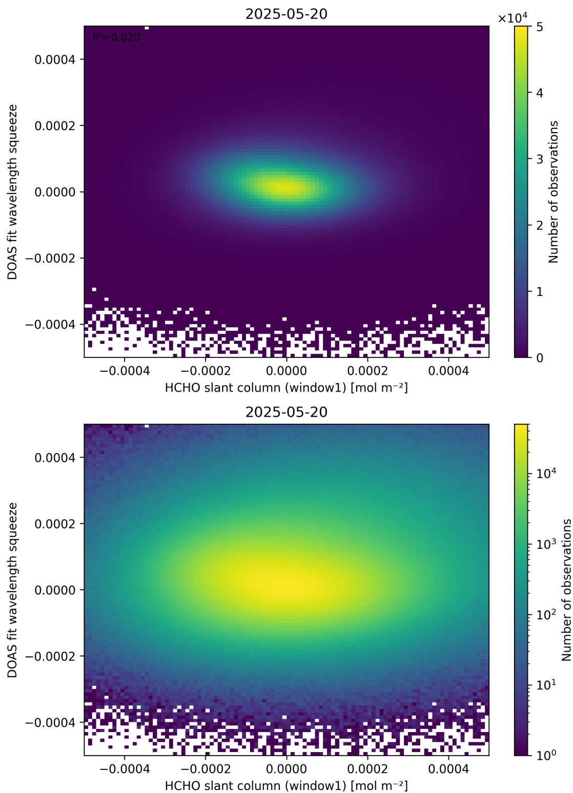
Figure 80: Scatter density plot of “HCHO slant column (window1)” against “DOAS fit wavelength squeeze” for 2025-05-19 to 2025-05-21.
