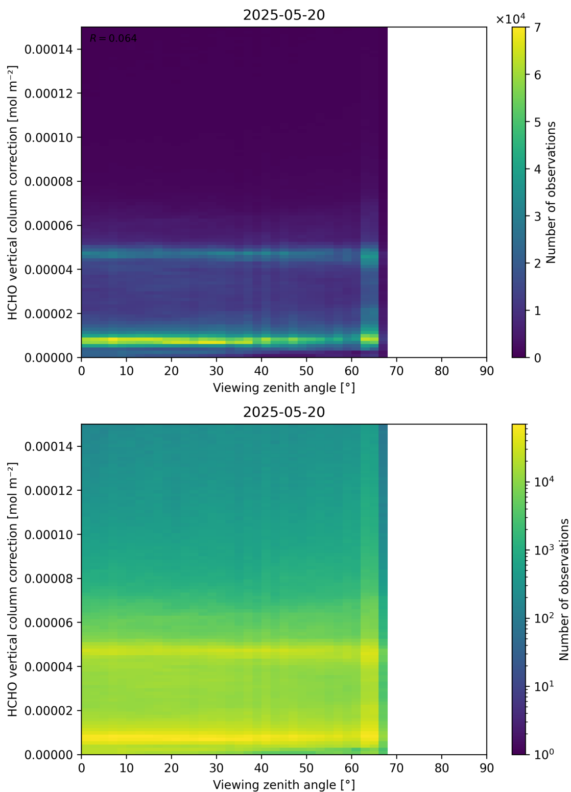
Figure 193: Scatter density plot of “Viewing zenith angle” against “HCHO vertical column correction” for 2025-05-19 to 2025-05-21.
