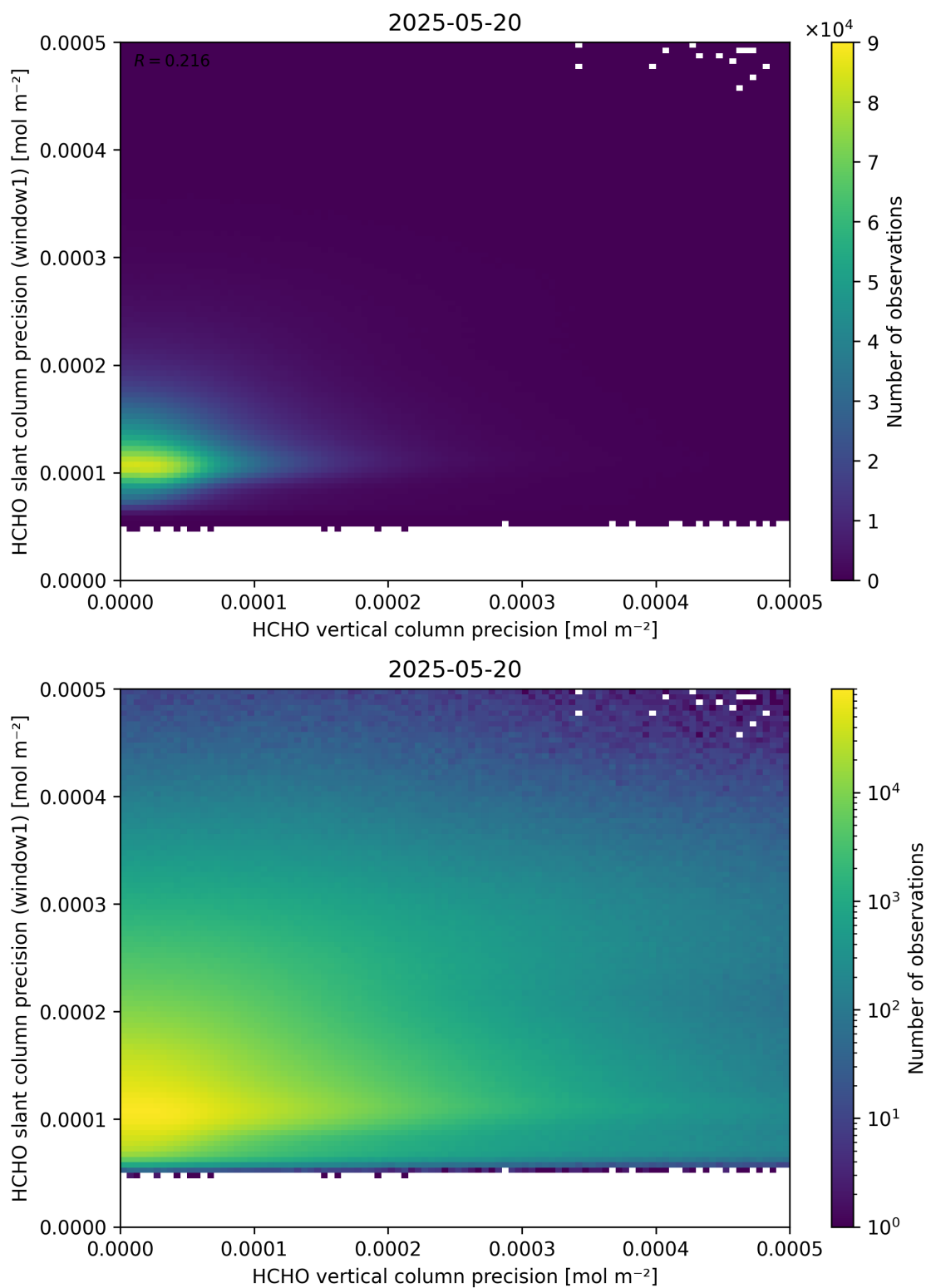
Figure 143: Scatter density plot of “HCHO vertical column precision” against “HCHO slant column precision (window1)” for 2025-05-19 to 2025-05-21.
