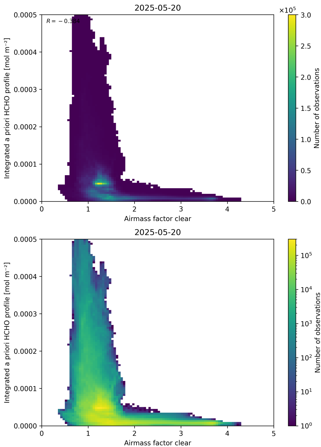
Figure 76: Scatter density plot of “Airmass factor clear” against “Integrated a priori HCHO profile” for 2025-05-19 to 2025-05-21.
