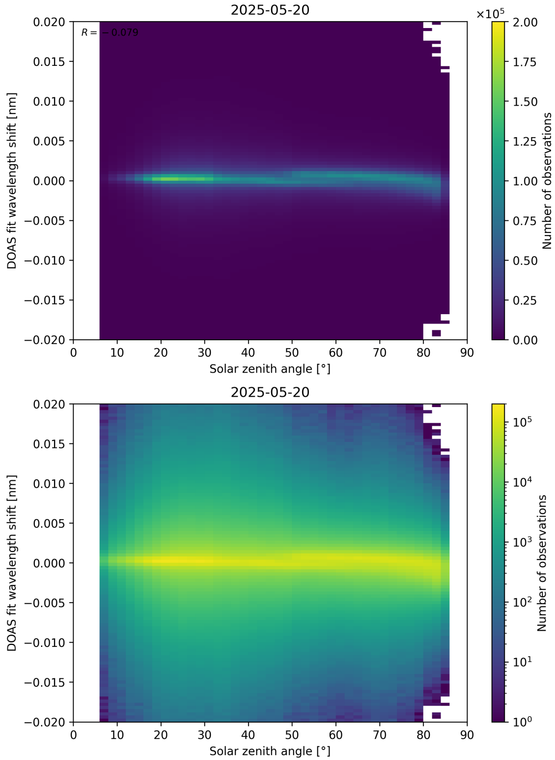
Figure 168: Scatter density plot of “Solar zenith angle” against “DOAS fit wavelength shift” for 2025-05-19 to 2025-05-21.
