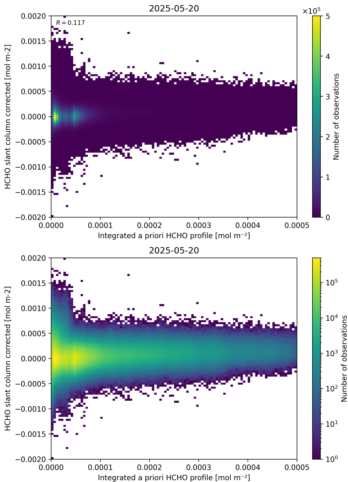
Figure 151: Scatter density plot of “Integrated a priori HCHO profile” against “HCHO slant column corrected” for 2025-05-19 to 2025-05-21.
