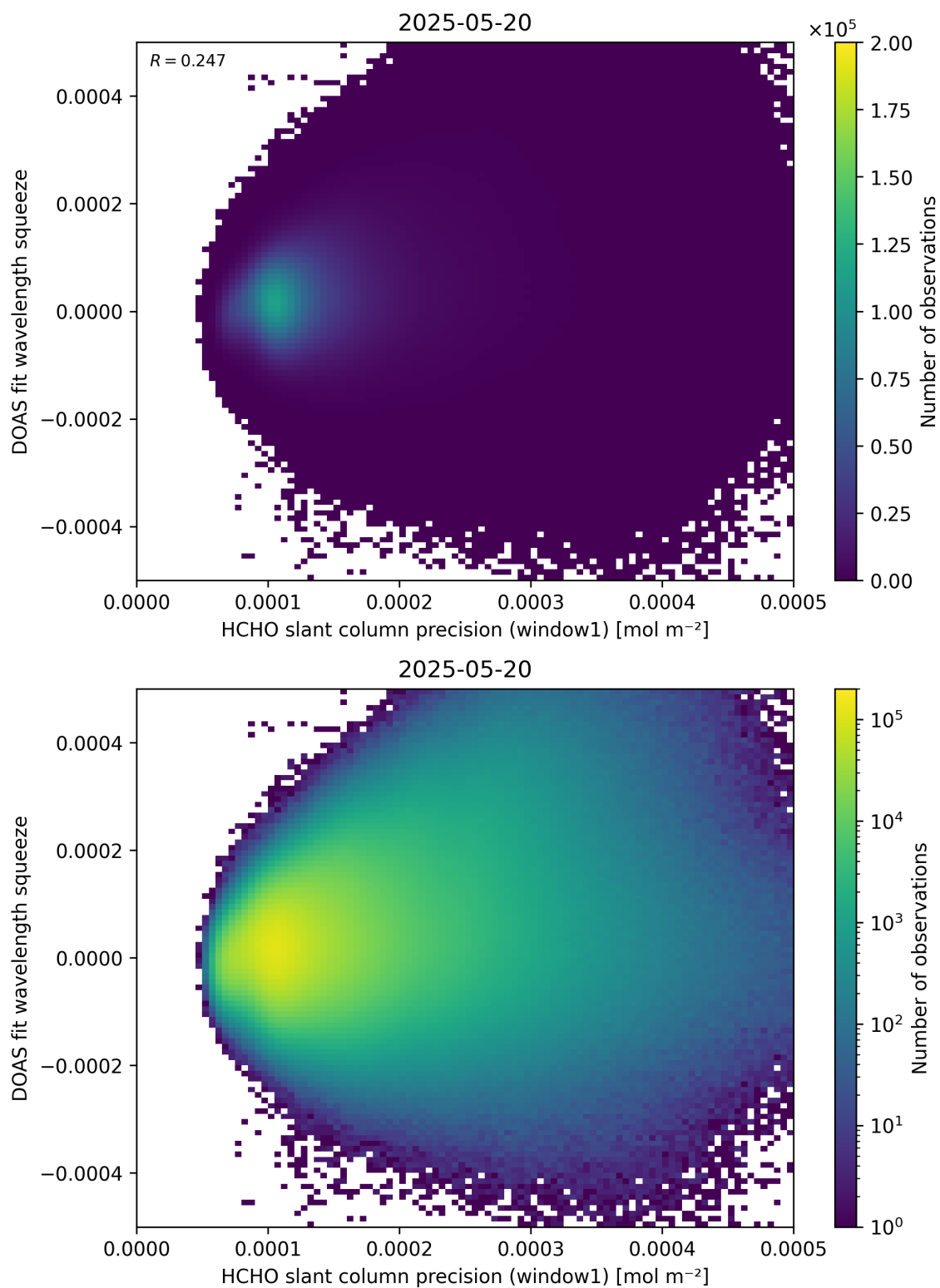
Figure 90: Scatter density plot of “HCHO slant column precision (window1)” against “DOAS fit wavelength squeeze” for 2025-05-19 to 2025-05-21.
