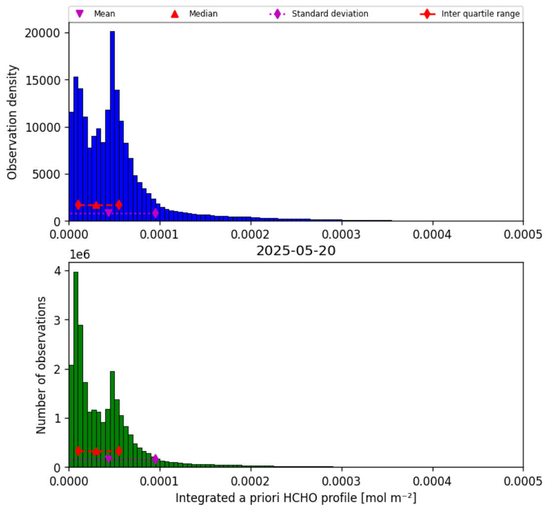
Figure 43: Histogram of “Integrated a priori HCHO profile” for 2025-05-19 to 2025-05-21
