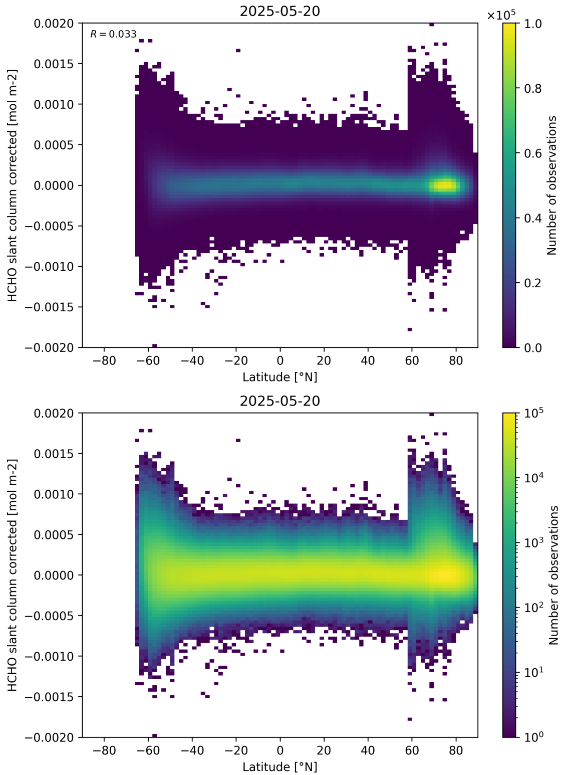
Figure 157: Scatter density plot of “Latitude” against “HCHO slant column corrected” for 2025-05-19 to 2025-05-21.
