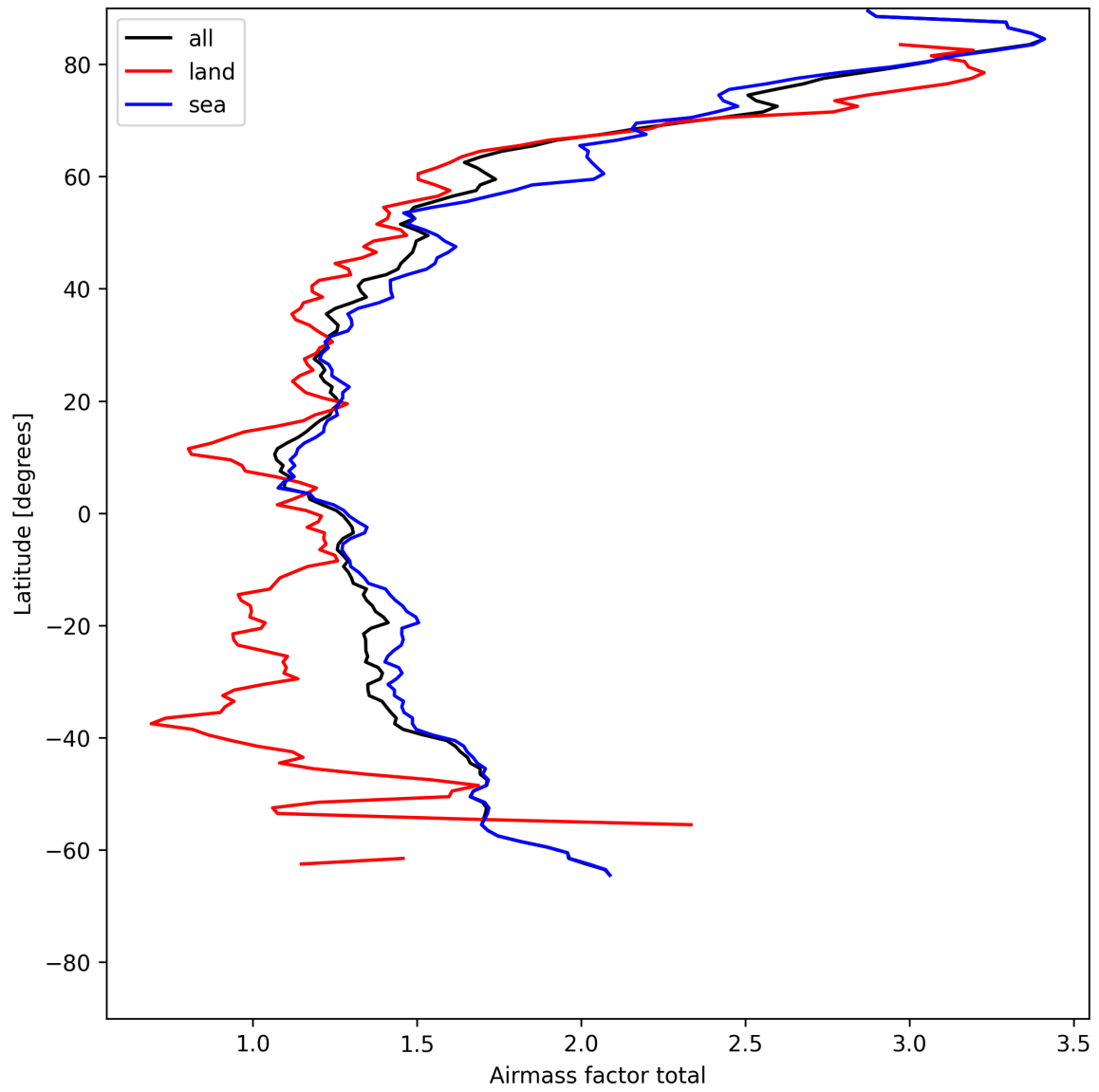
Figure 26: Zonal average of “Airmass factor total” for 2025-05-19 to 2025-05-21.
