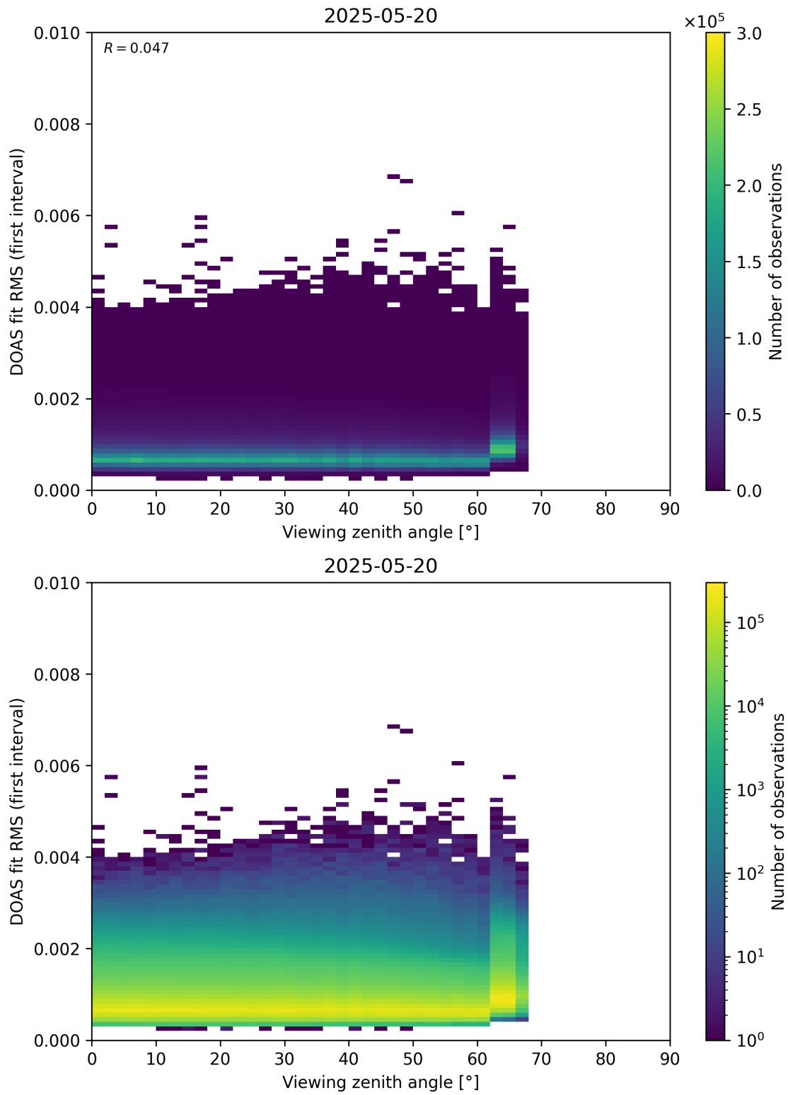
Figure 182: Scatter density plot of “Viewing zenith angle” against “DOAS fit RMS (first interval)” for 2025-05-19 to 2025-05-21.
