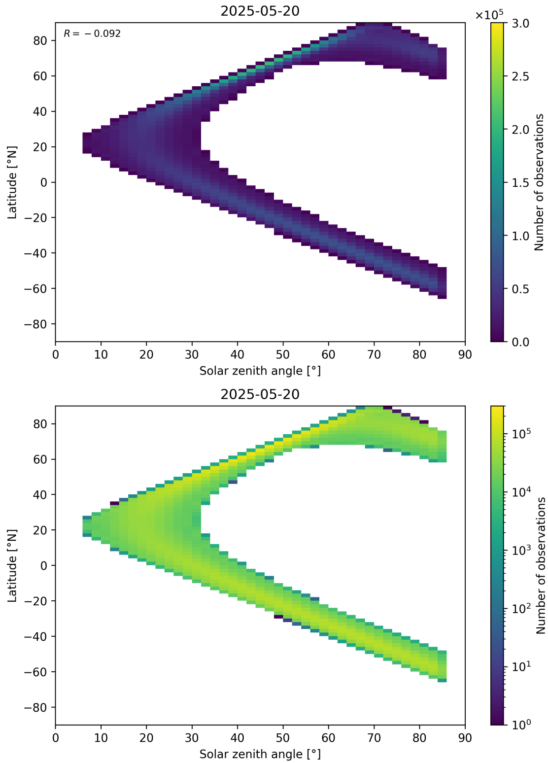
Figure 181: Scatter density plot of “Solar zenith angle” against “Latitude” for 2025-05-19 to 2025-05-21.
