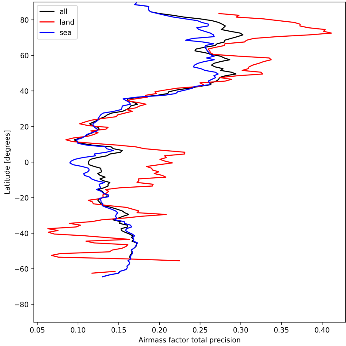
Figure 27: Zonal average of “Airmass factor total precision” for 2025-05-19 to 2025-05-21.
