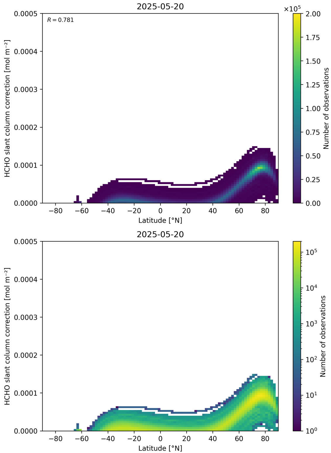
Figure 158: Scatter density plot of “Latitude” against “HCHO slant column correction” for 2025-05-19 to 2025-05-21.
