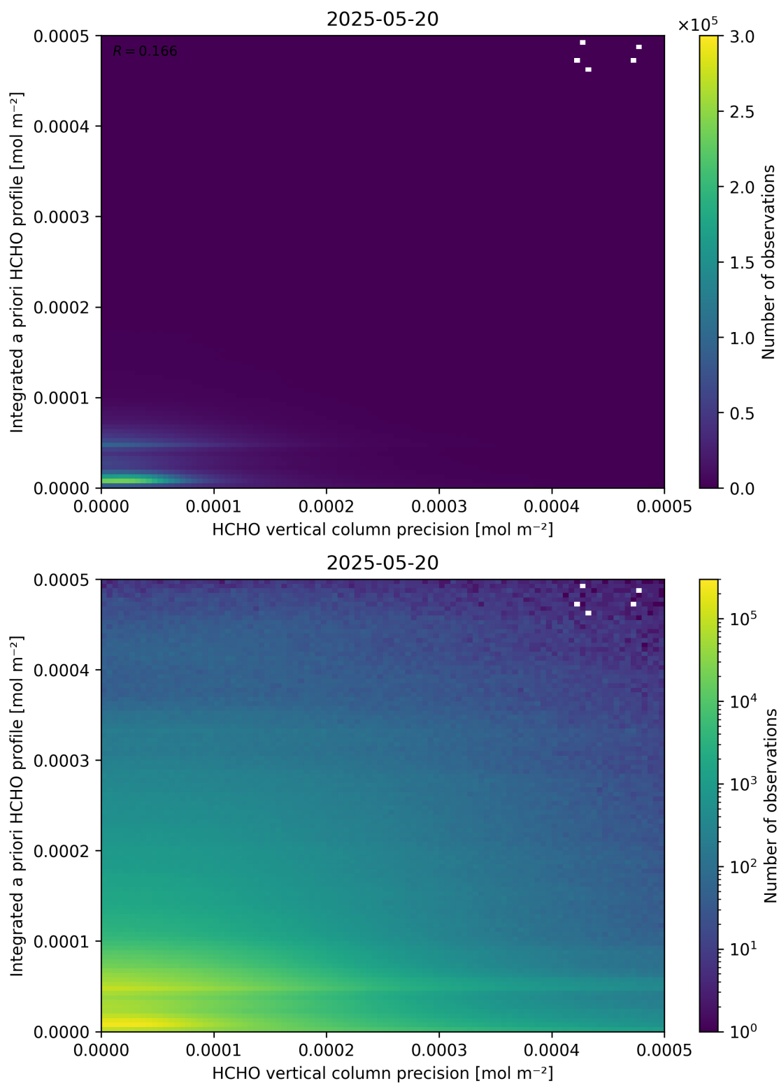
Figure 147: Scatter density plot of “HCHO vertical column precision” against “Integrated a priori HCHO profile” for 2025-05-19 to 2025-05-21.
