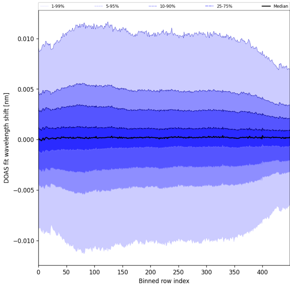
Figure 58: Along track statistics of “DOAS fit wavelength shift” for 2025-05-19 to 2025-05-21
