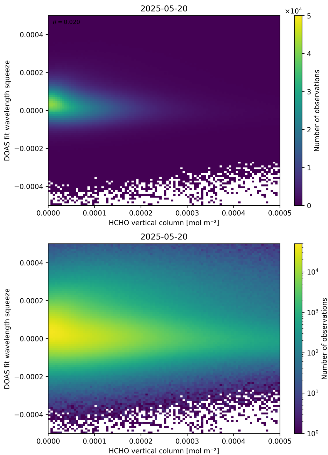
Figure 125: Scatter density plot of “HCHO vertical column” against “DOAS fit wavelength squeeze” for 2025-05-19 to 2025-05-21.
