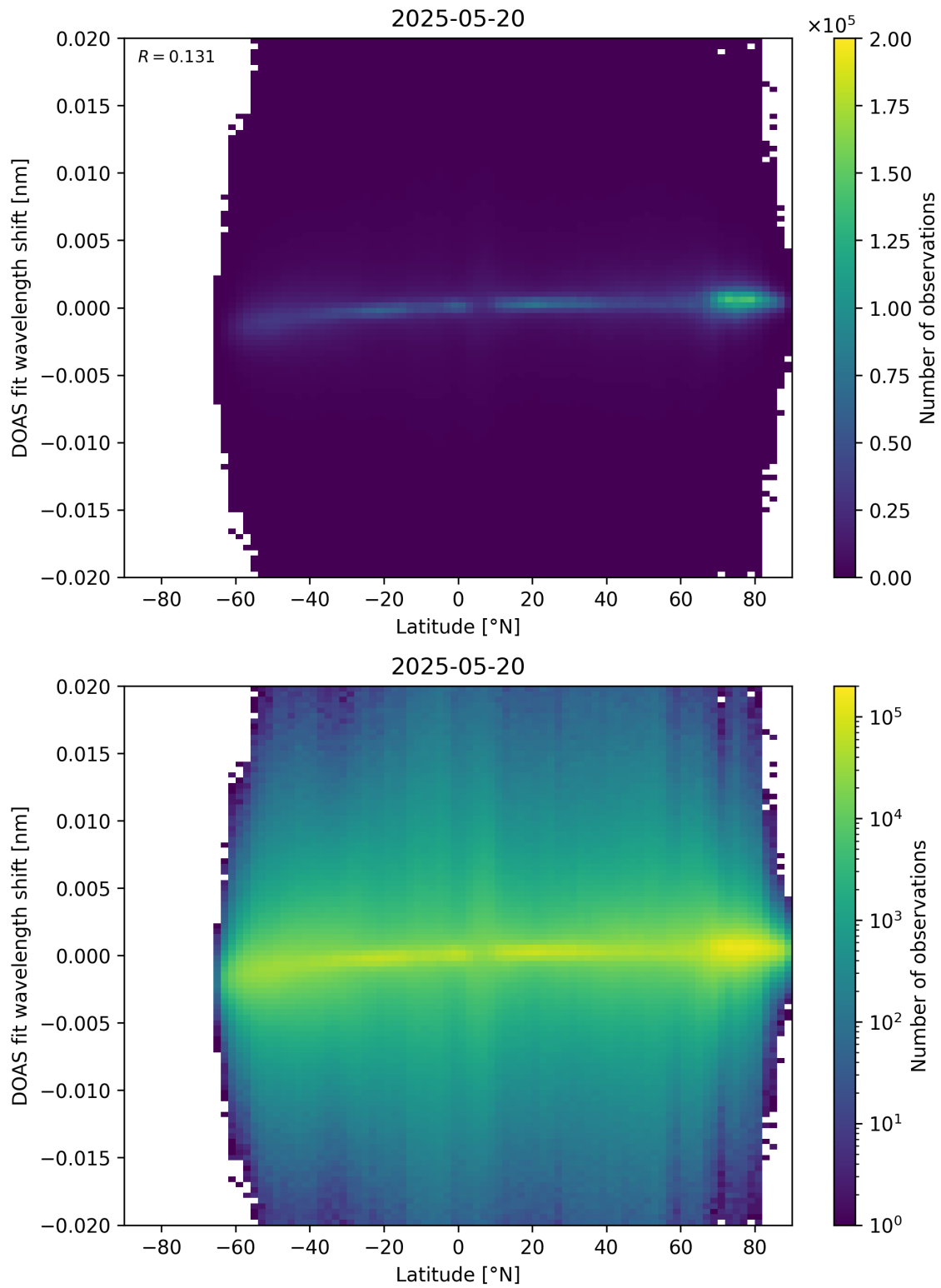
Figure 154: Scatter density plot of “Latitude” against “DOAS fit wavelength shift” for 2025-05-19 to 2025-05-21.
