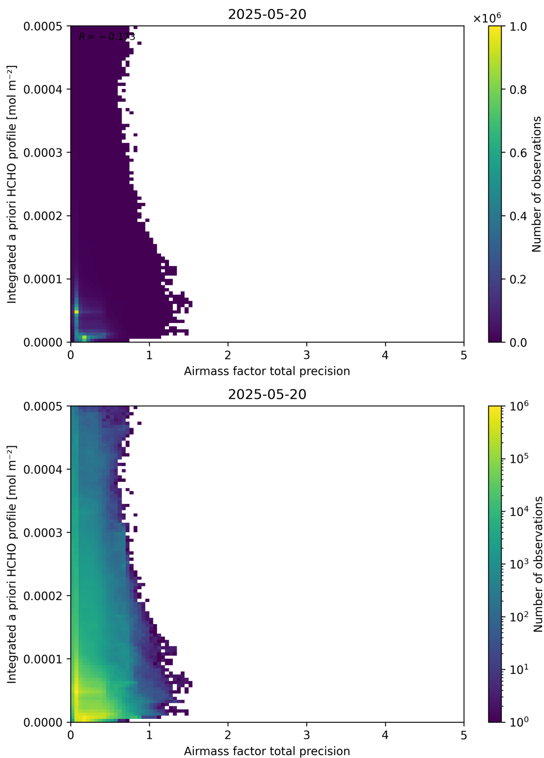
Figure 111: Scatter density plot of “Airmass factor total precision” against “Integrated a priori HCHO profile” for 2025-05-19 to 2025-05-21.
