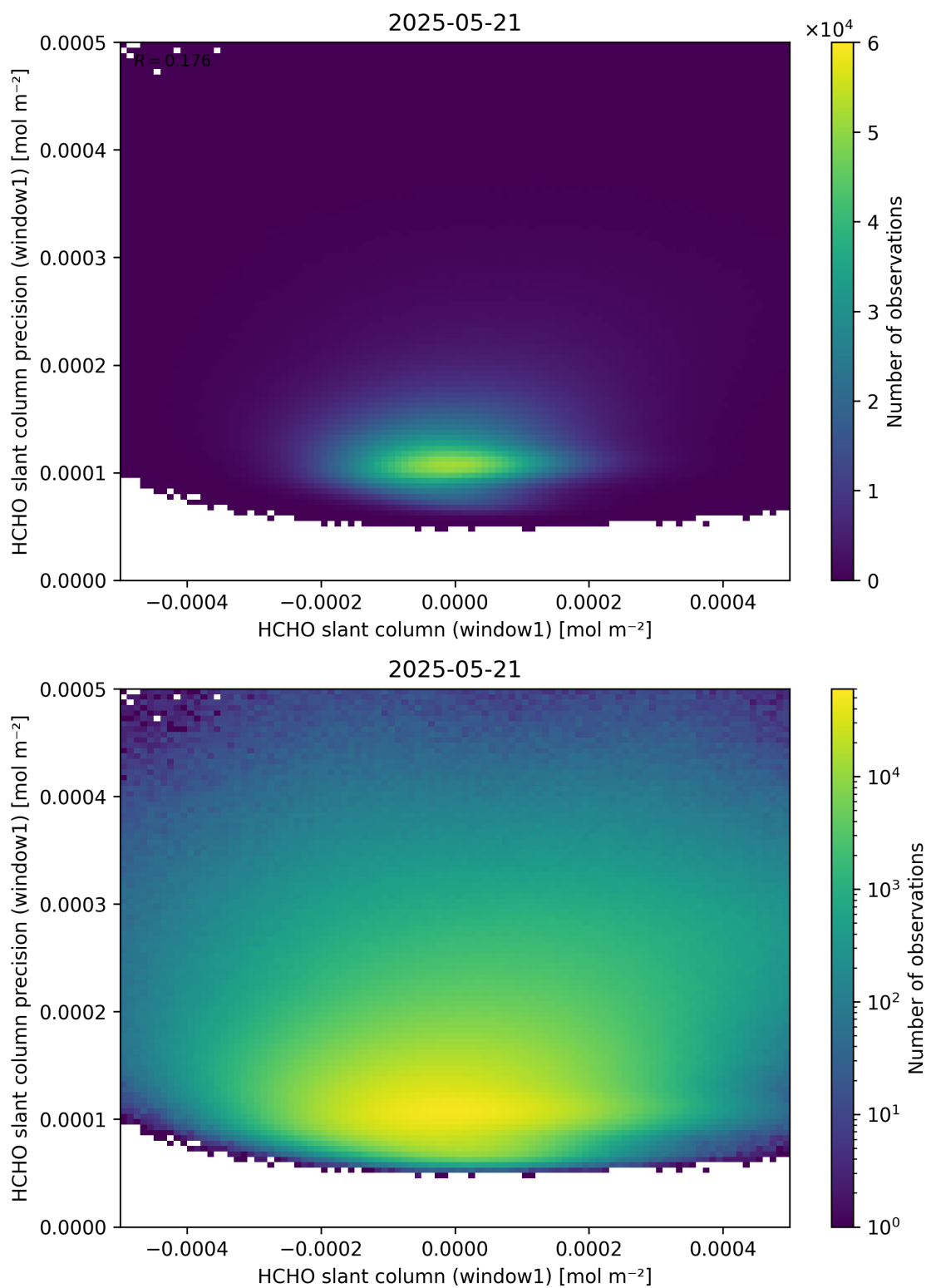
Figure 84: Scatter density plot of “HCHO slant column (window1)” against “HCHO slant column precision (window1)” for 2025-05-21 to 2025-05-22.
