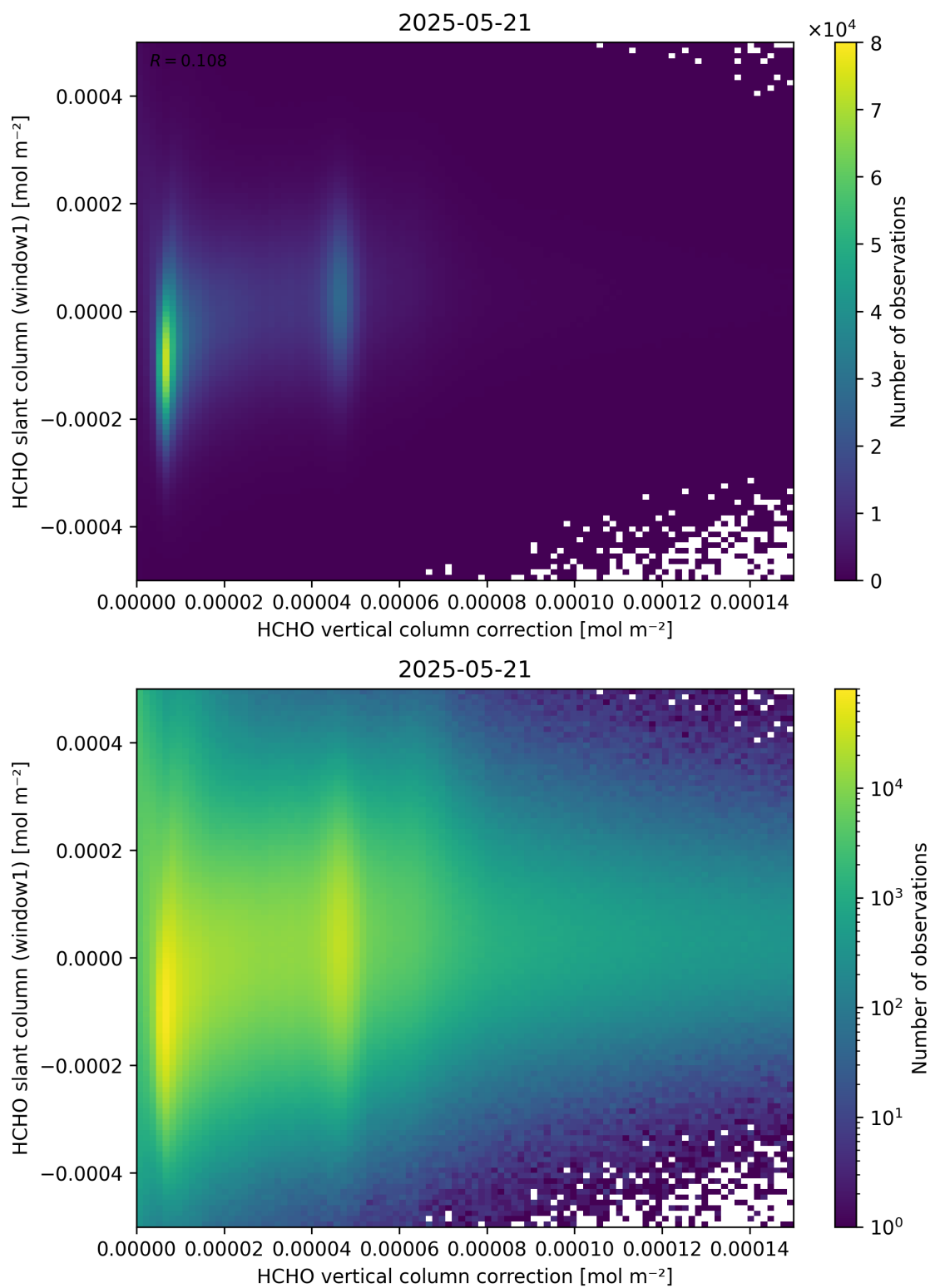
Figure 118: Scatter density plot of “HCHO vertical column correction” against “HCHO slant column (window1)” for 2025-05-21 to 2025-05-22.
