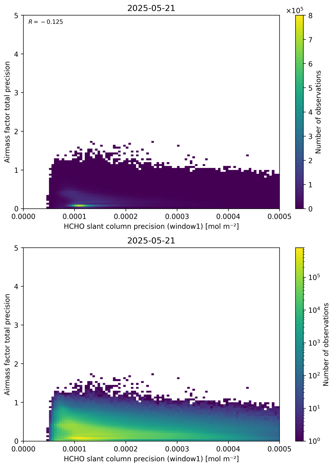
Figure 95: Scatter density plot of “HCHO slant column precision (window1)” against “Airmass factor total precision” for 2025-05-21 to 2025-05-22.
