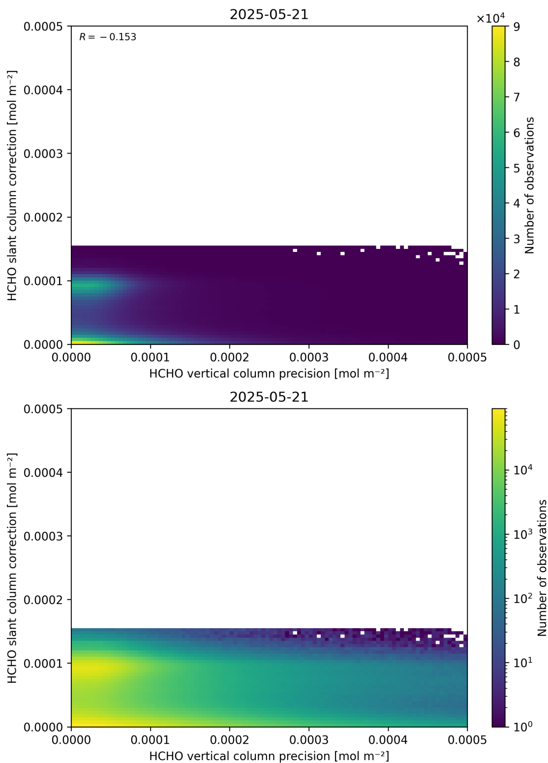
Figure 141: Scatter density plot of “HCHO vertical column precision” against “HCHO slant column correction” for 2025-05-21 to 2025-05-22.
