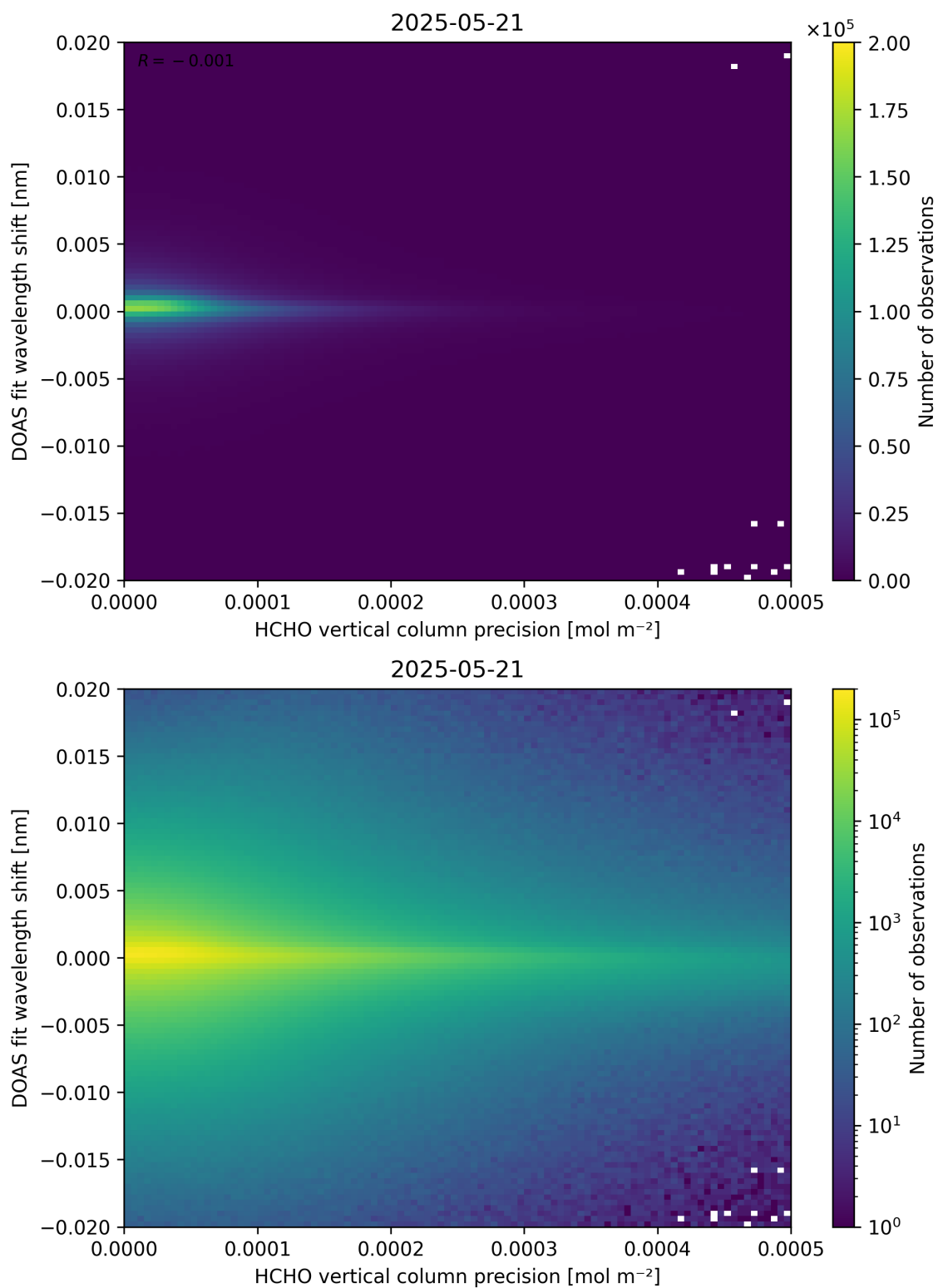
Figure 137: Scatter density plot of “HCHO vertical column precision” against “DOAS fit wavelength shift” for 2025-05-21 to 2025-05-22.
