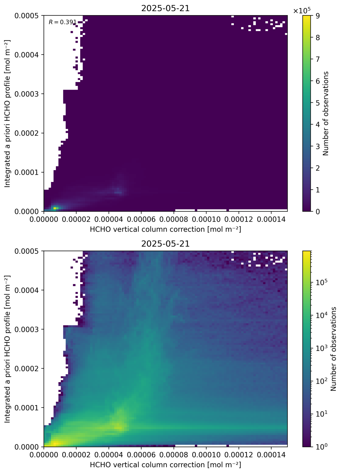
Figure 122: Scatter density plot of “HCHO vertical column correction” against “Integrated a priori HCHO profile” for 2025-05-21 to 2025-05-22.
