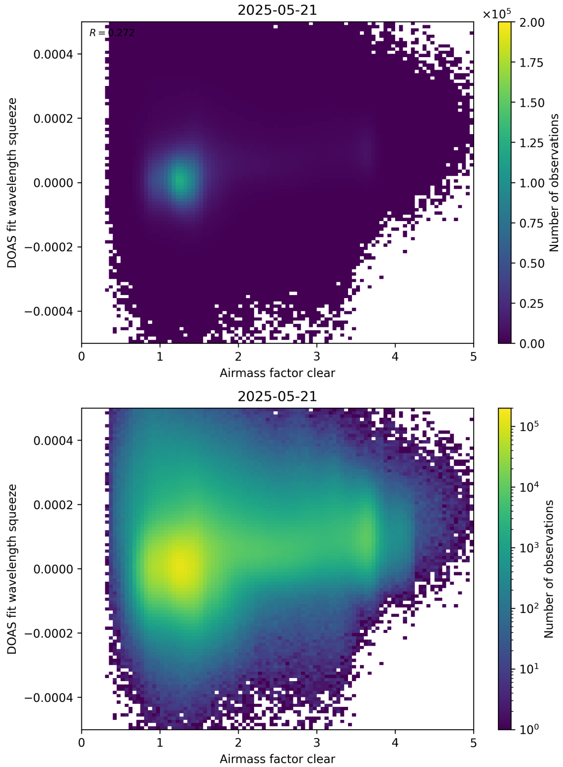
Figure 73: Scatter density plot of “Airmass factor clear” against “DOAS fit wavelength squeeze” for 2025-05-21 to 2025-05-22.
