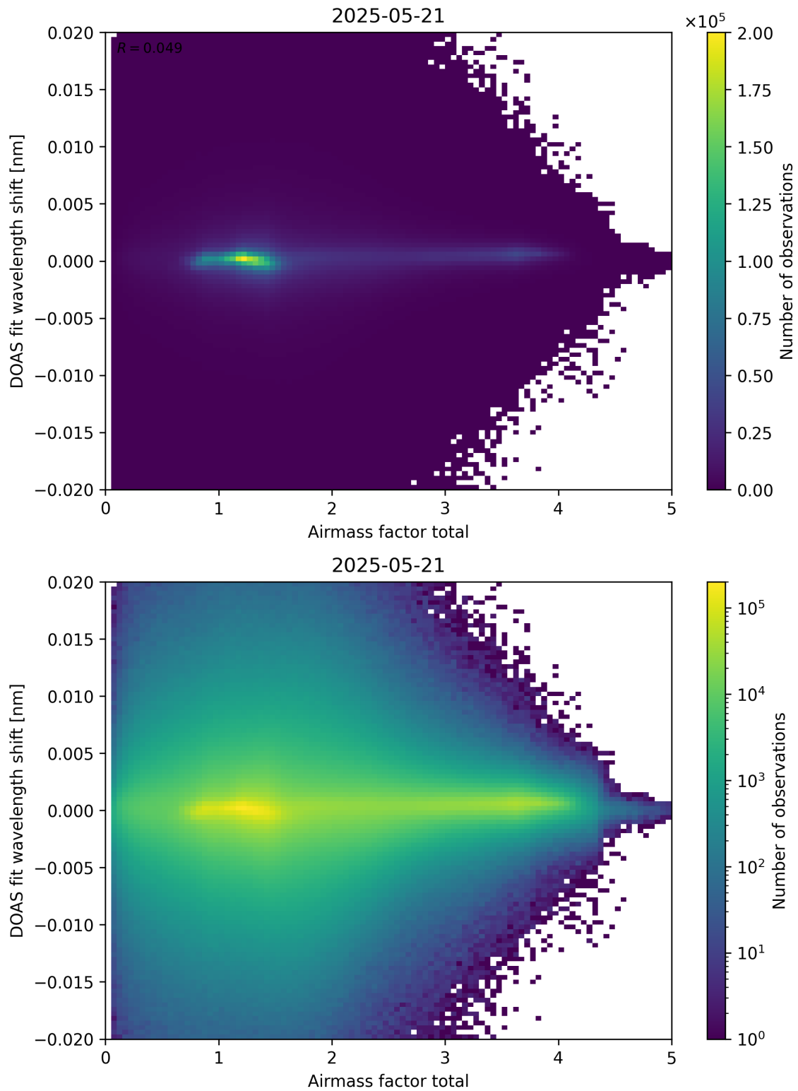
Figure 98: Scatter density plot of “Airmass factor total” against “DOAS fit wavelength shift” for 2025-05-21 to 2025-05-22.
