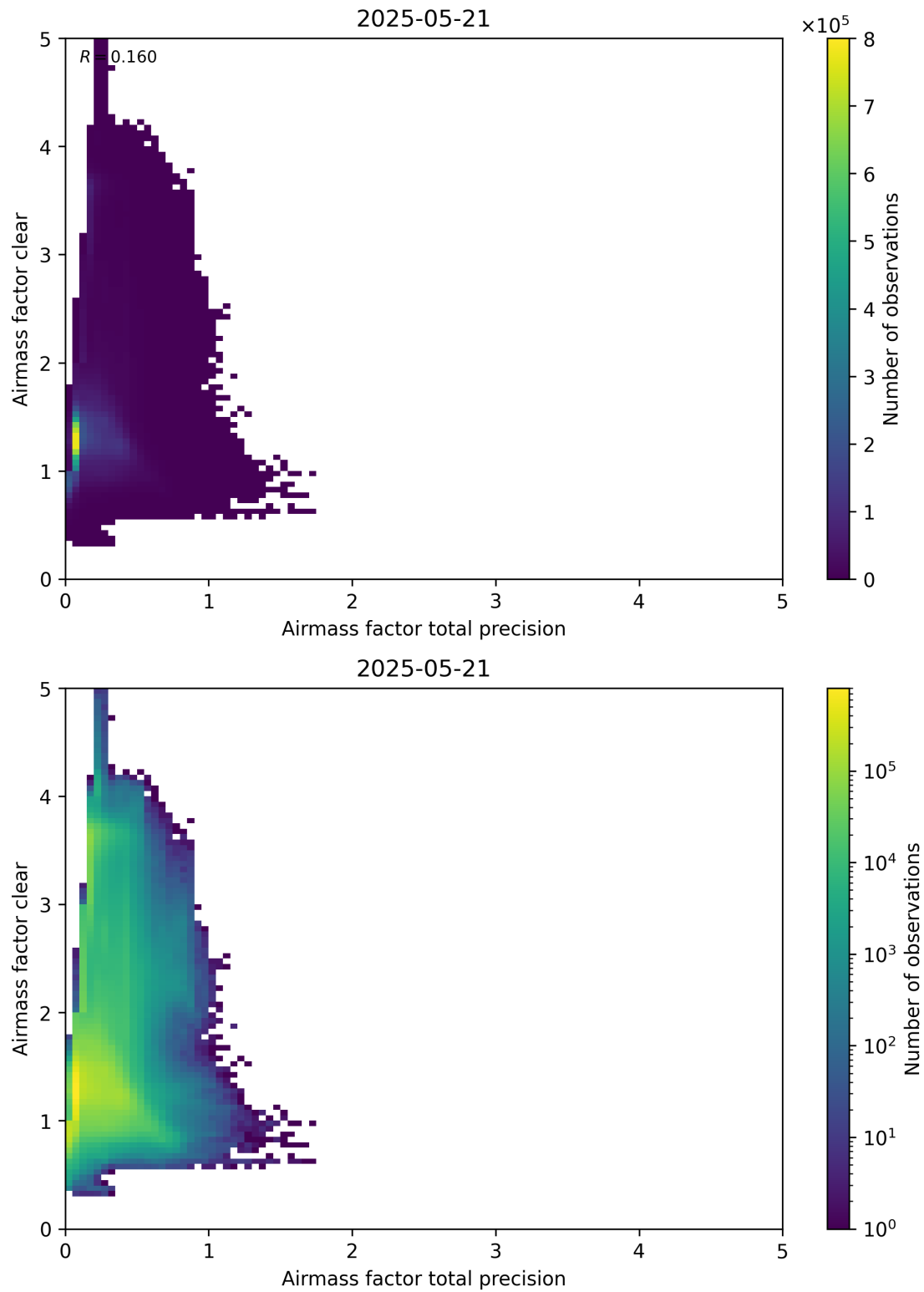
Figure 108: Scatter density plot of “Airmass factor total precision” against “Airmass factor clear” for 2025-05-21 to 2025-05-22.
