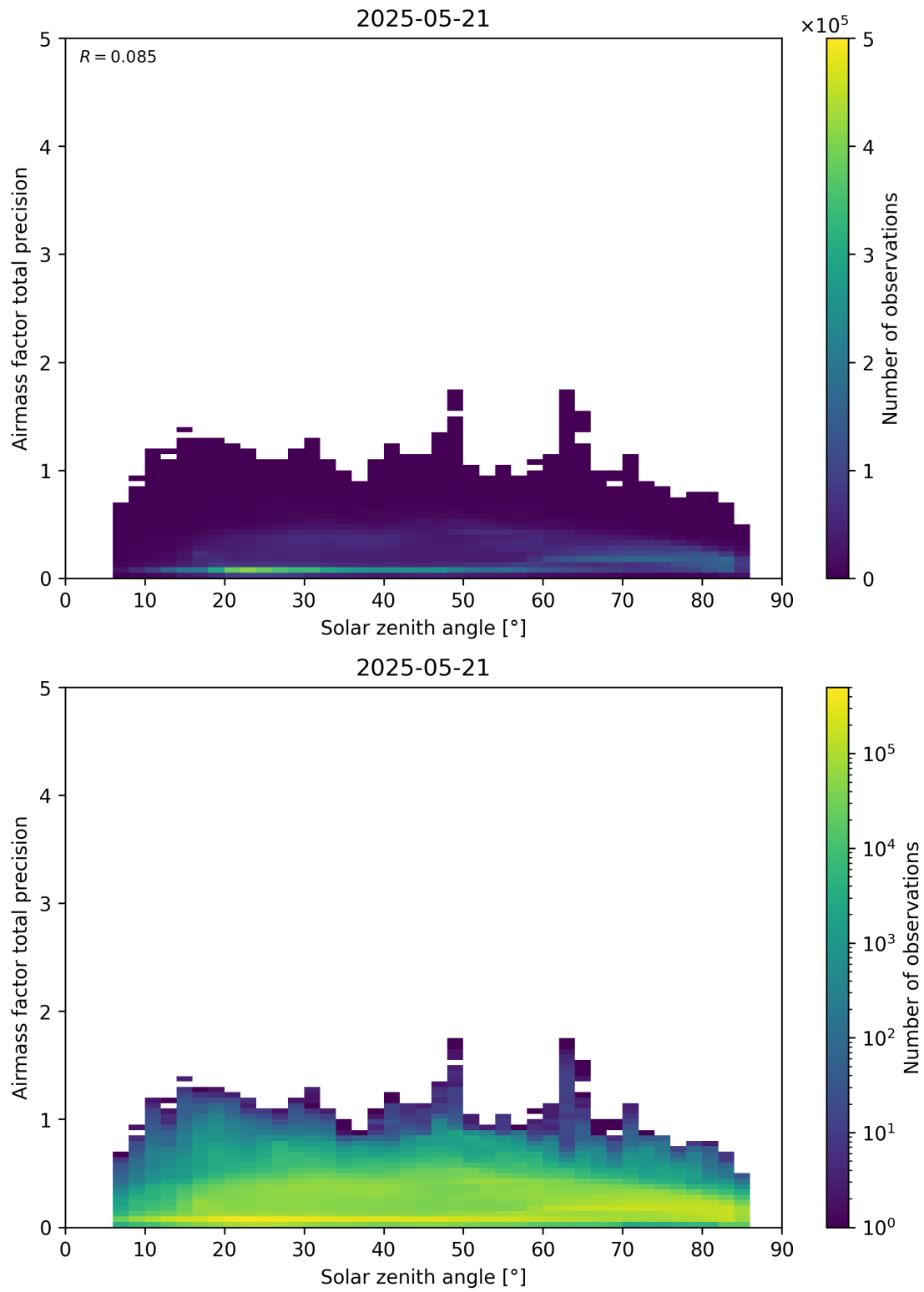
Figure 176: Scatter density plot of “Solar zenith angle” against “Airmass factor total precision” for 2025-05-21 to 2025-05-22.
