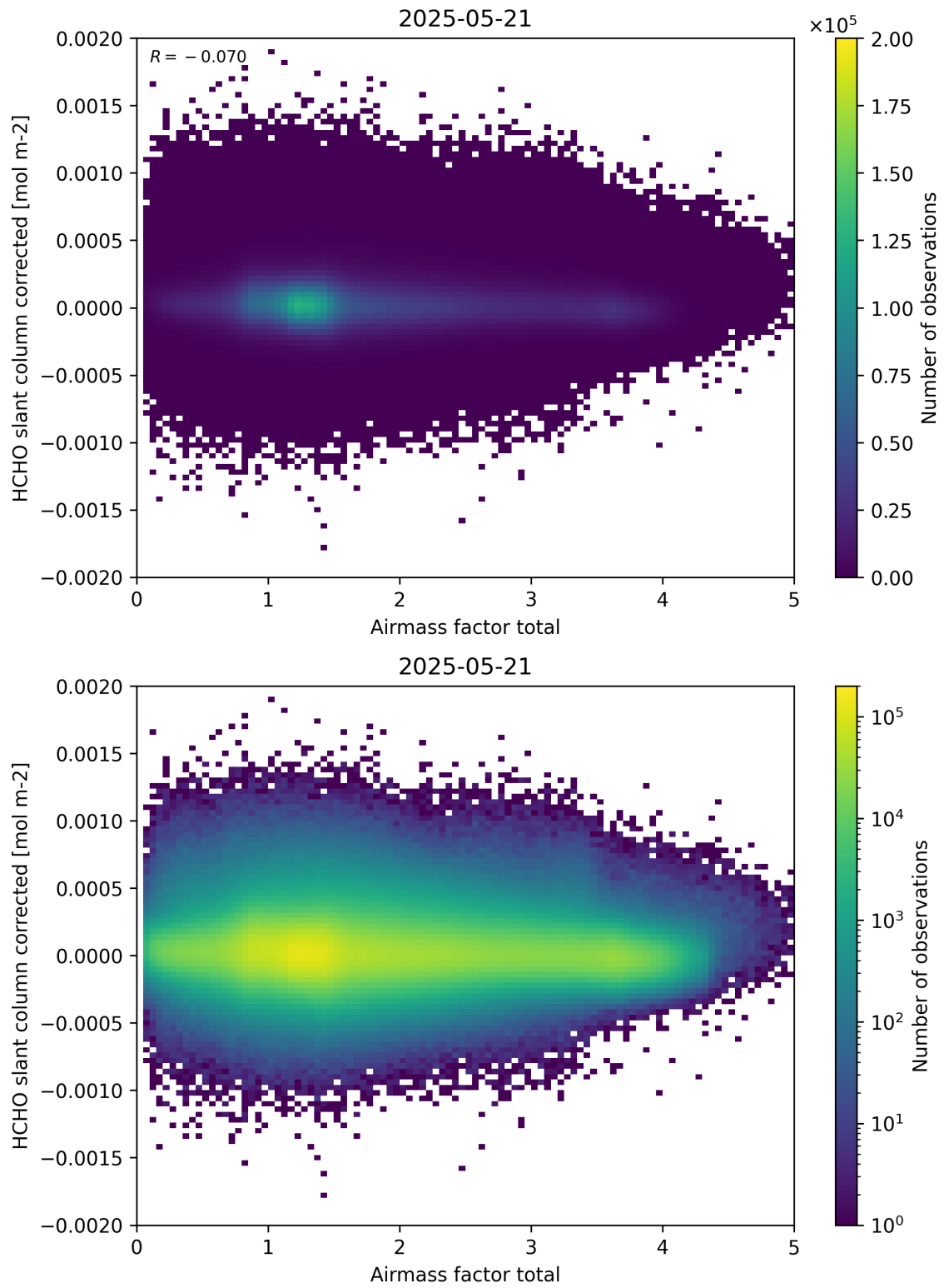
Figure 101: Scatter density plot of “Airmass factor total” against “HCHO slant column corrected” for 2025-05-21 to 2025-05-22.
