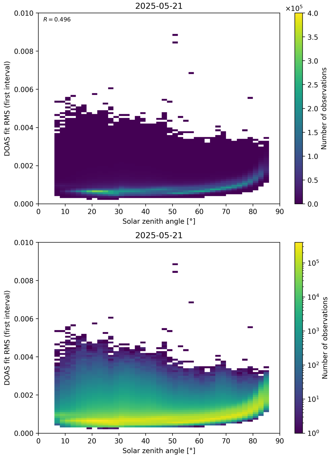
Figure 167: Scatter density plot of “Solar zenith angle” against “DOAS fit RMS (first interval)” for 2025-05-21 to 2025-05-22.
