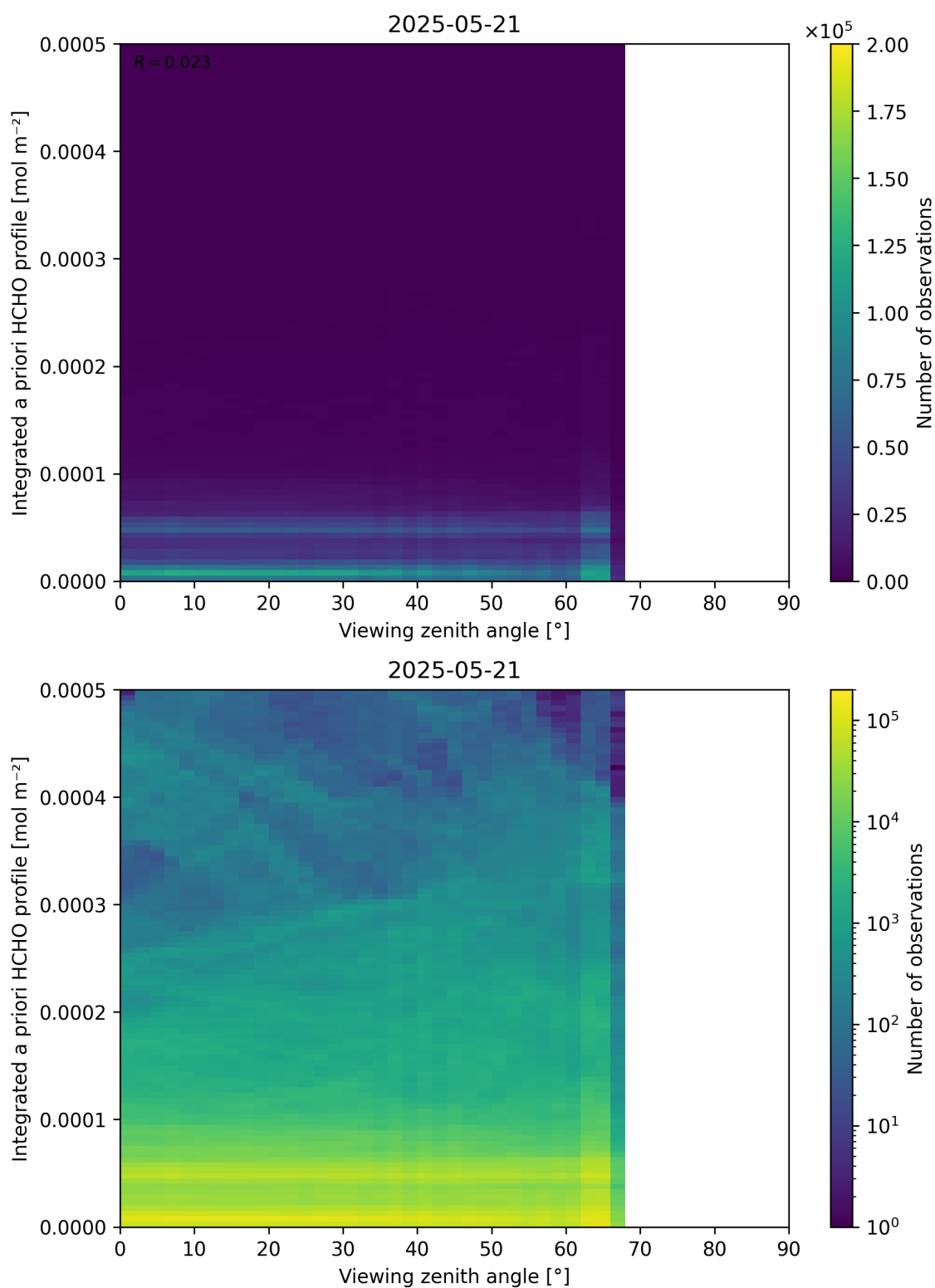
Figure 195: Scatter density plot of “Viewing zenith angle” against “Integrated a priori HCHO profile” for 2025-05-21 to 2025-05-22.
