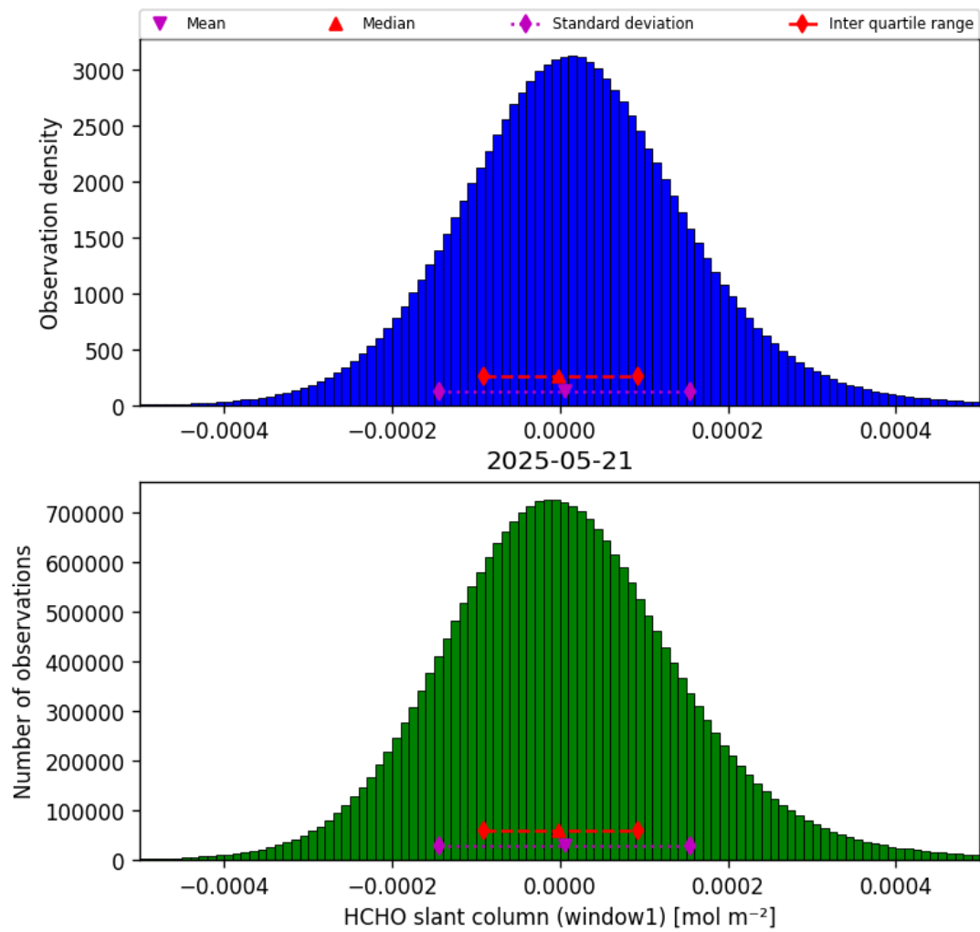
Figure 38: Histogram of “HCHO slant column (window1)” for 2025-05-21 to 2025-05-22
