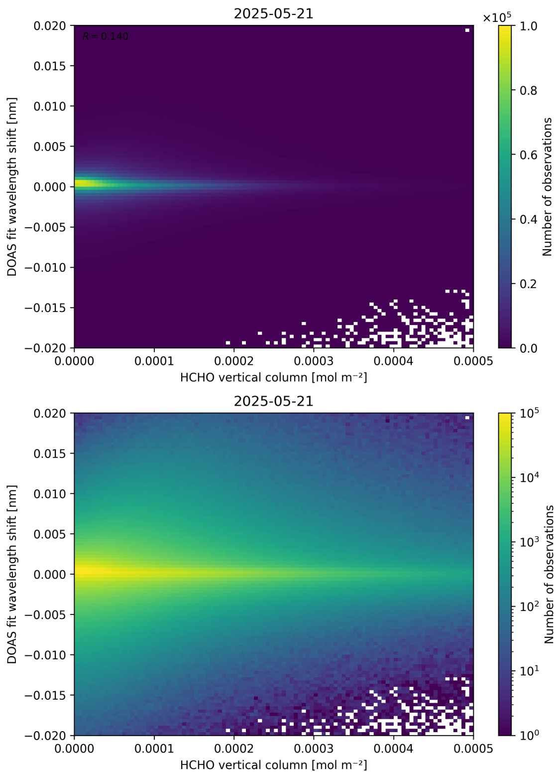
Figure 124: Scatter density plot of “HCHO vertical column” against “DOAS fit wavelength shift” for 2025-05-21 to 2025-05-22.
