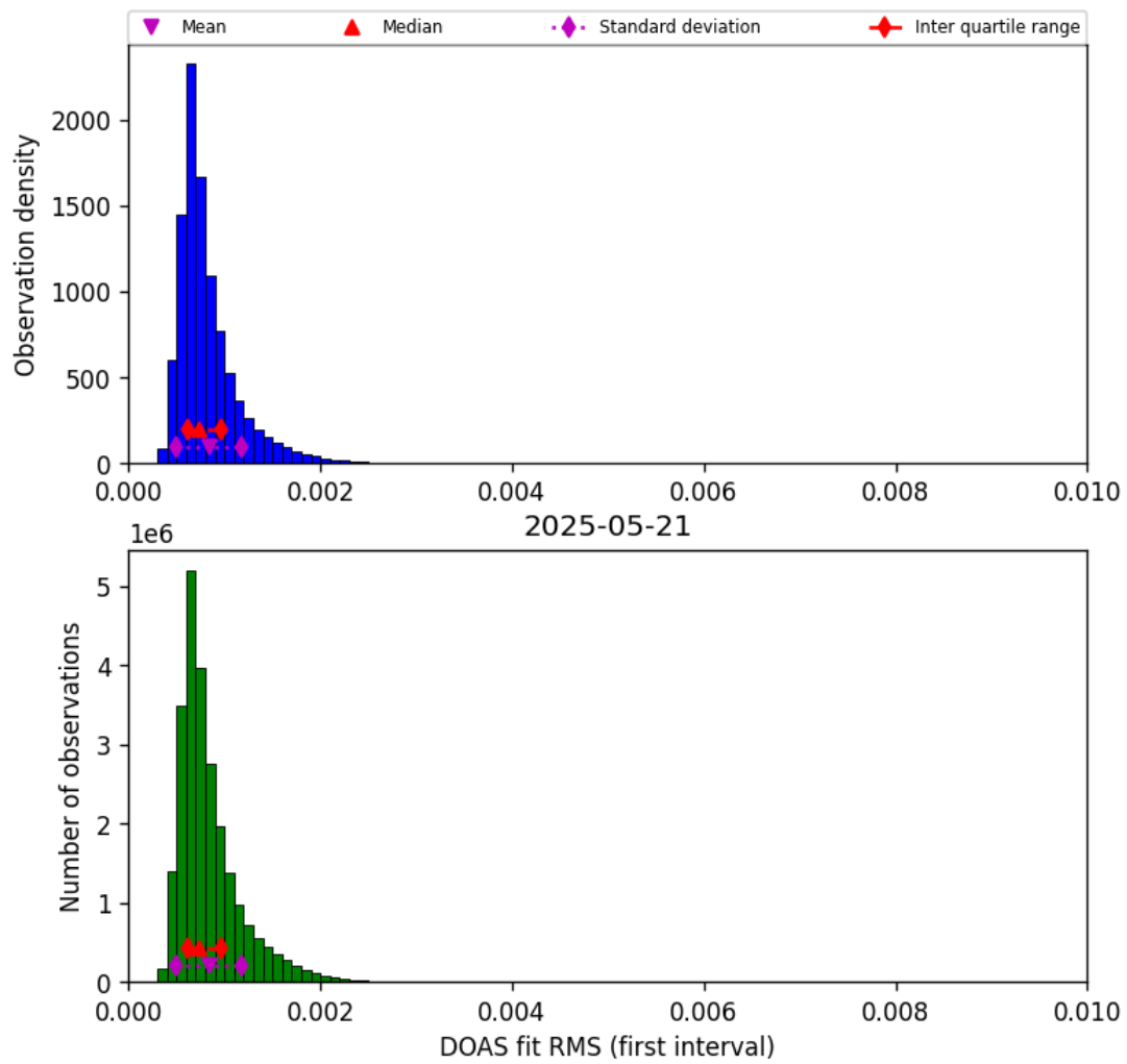
Figure 46: Histogram of “DOAS fit RMS (first interval)” for 2025-05-21 to 2025-05-22
