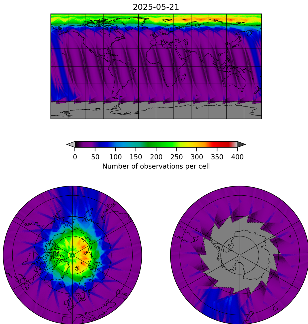
Figure 19: Map of the number of observations for 2025-05-21 to 2025-05-22
