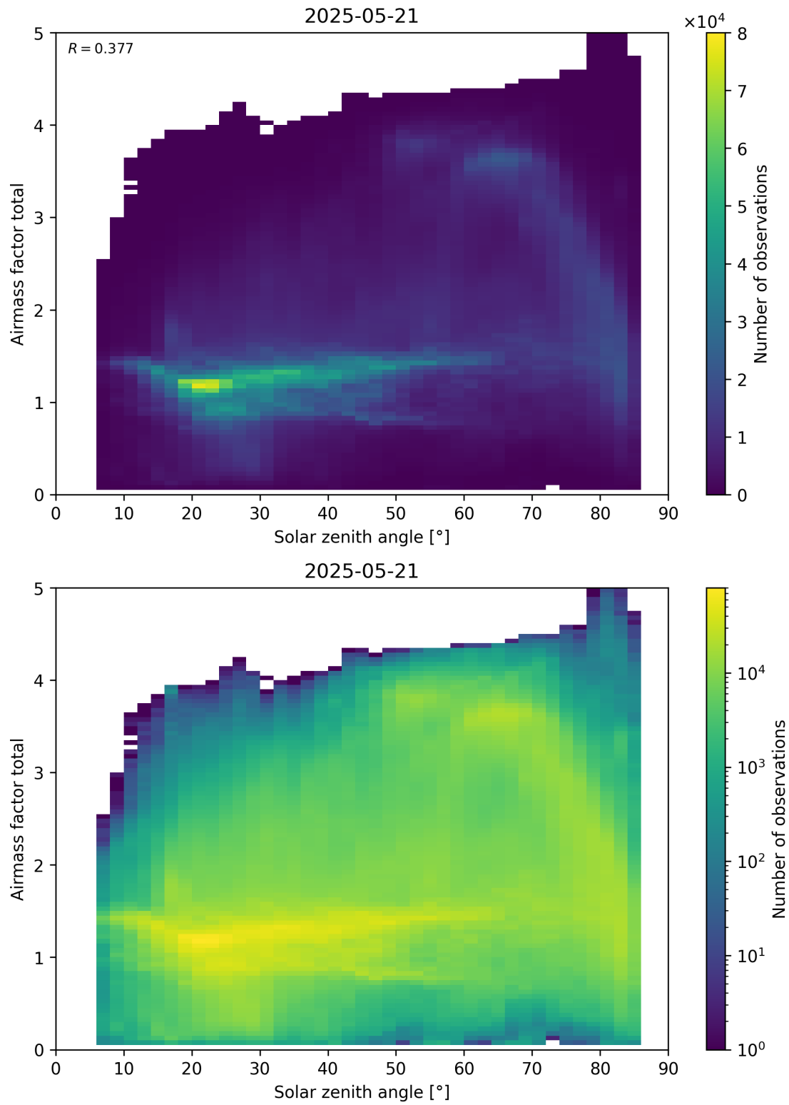
Figure 175: Scatter density plot of “Solar zenith angle” against “Airmass factor total” for 2025-05-21 to 2025-05-22.
