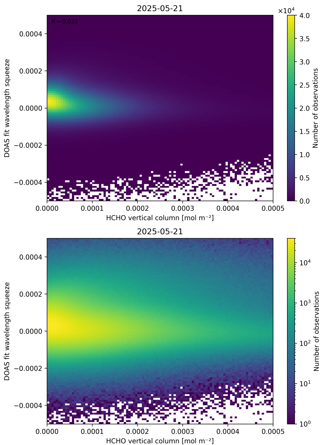
Figure 125: Scatter density plot of “HCHO vertical column” against “DOAS fit wavelength squeeze” for 2025-05-21 to 2025-05-22.
