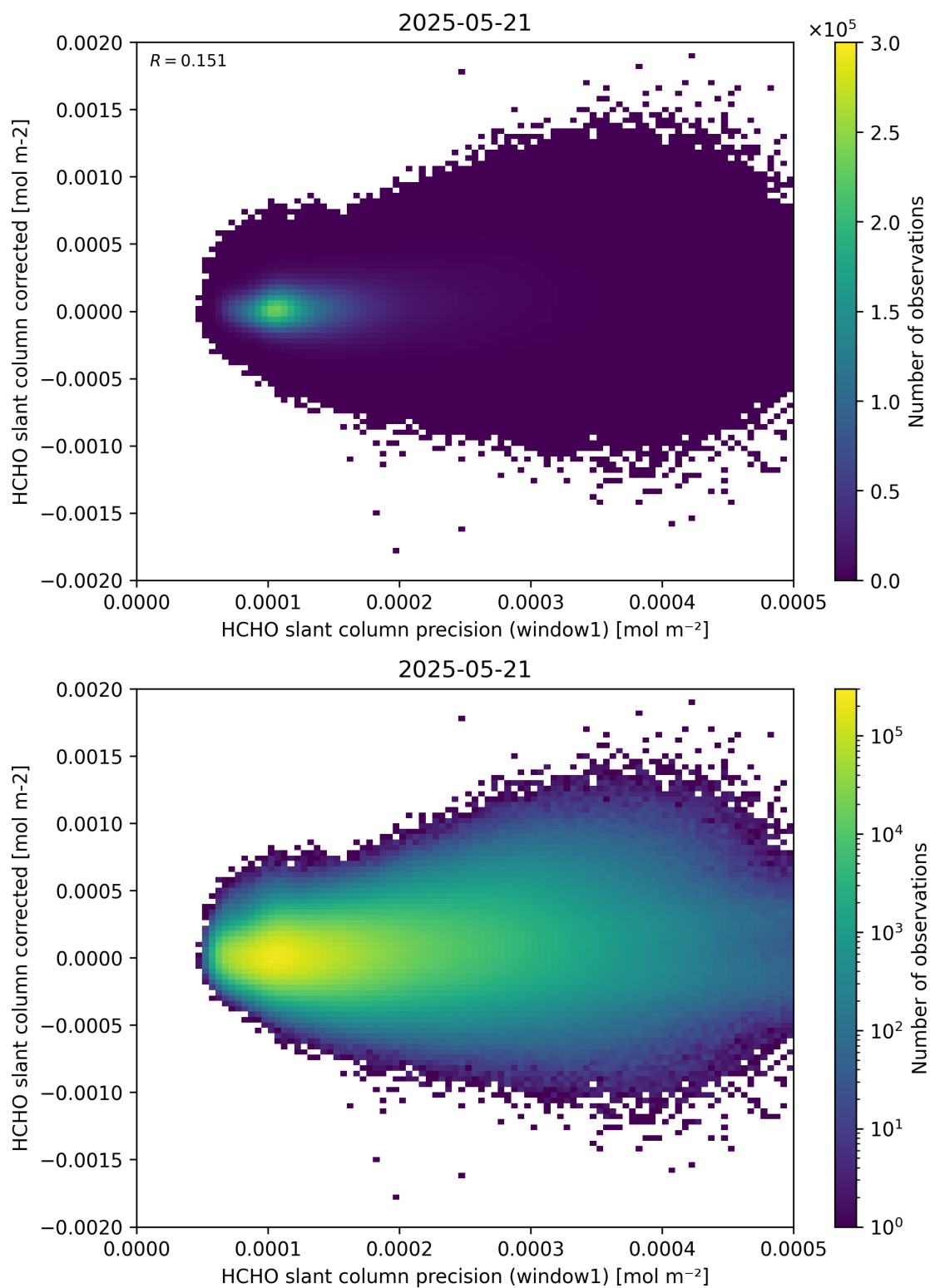
Figure 92: Scatter density plot of “HCHO slant column precision (window1)” against “HCHO slant column corrected” for 2025-05-21 to 2025-05-22.
