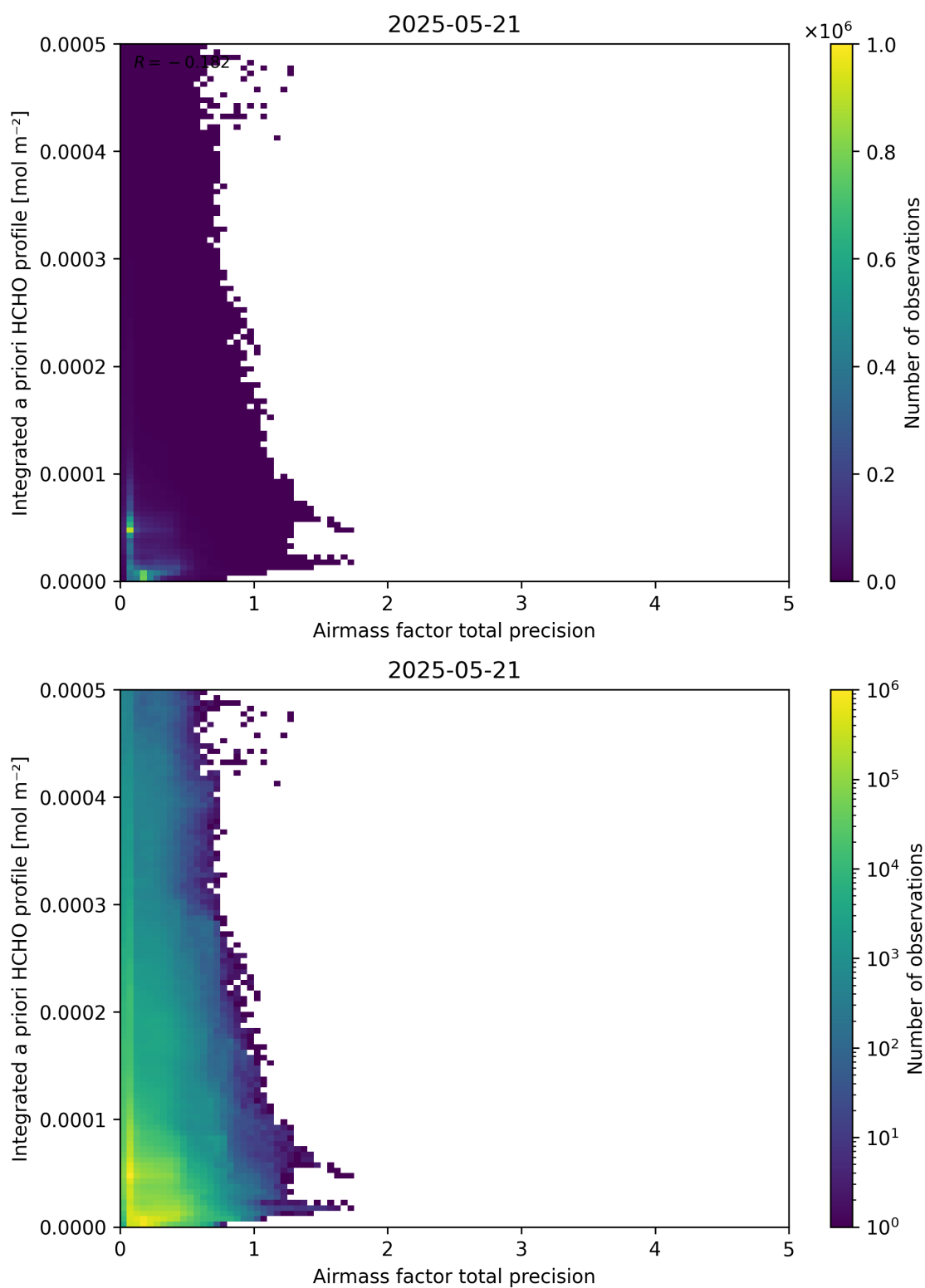
Figure 111: Scatter density plot of “Airmass factor total precision” against “Integrated a priori HCHO profile” for 2025-05-21 to 2025-05-22.
