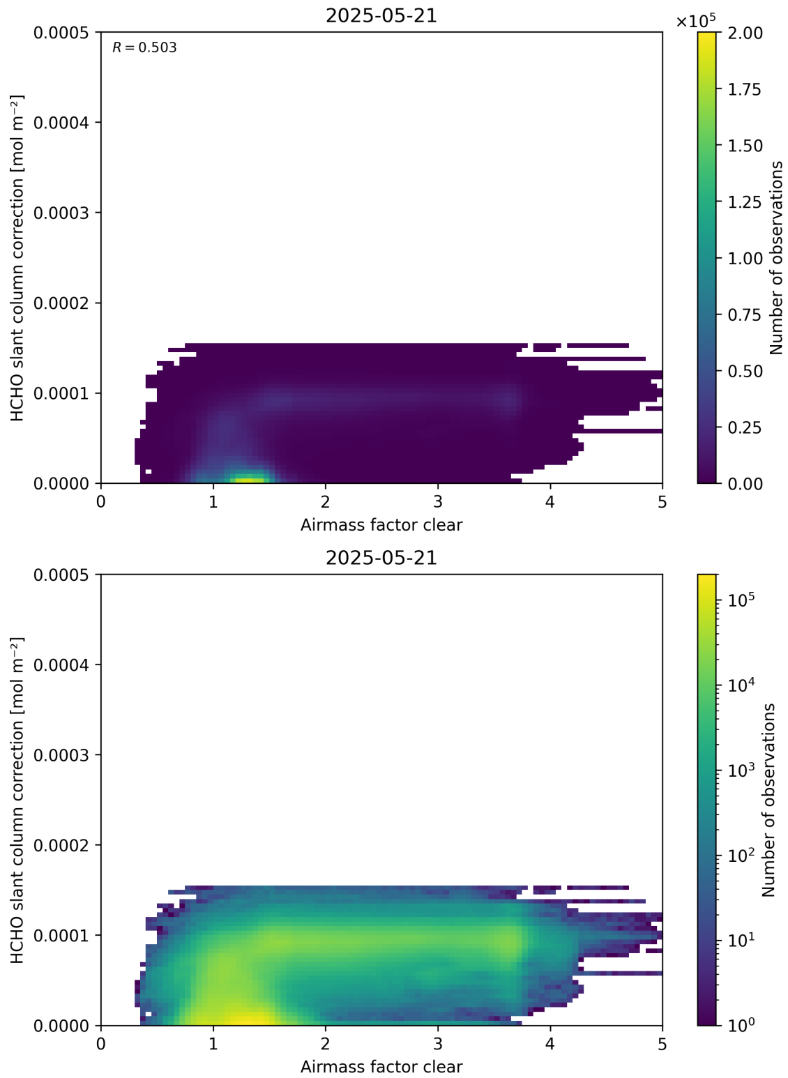
Figure 75: Scatter density plot of “Airmass factor clear” against “HCHO slant column correction” for 2025-05-21 to 2025-05-22.
