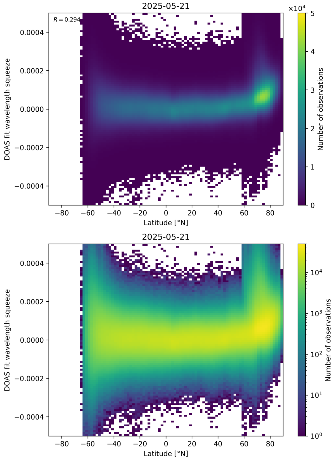
Figure 155: Scatter density plot of “Latitude” against “DOAS fit wavelength squeeze” for 2025-05-21 to 2025-05-22.
