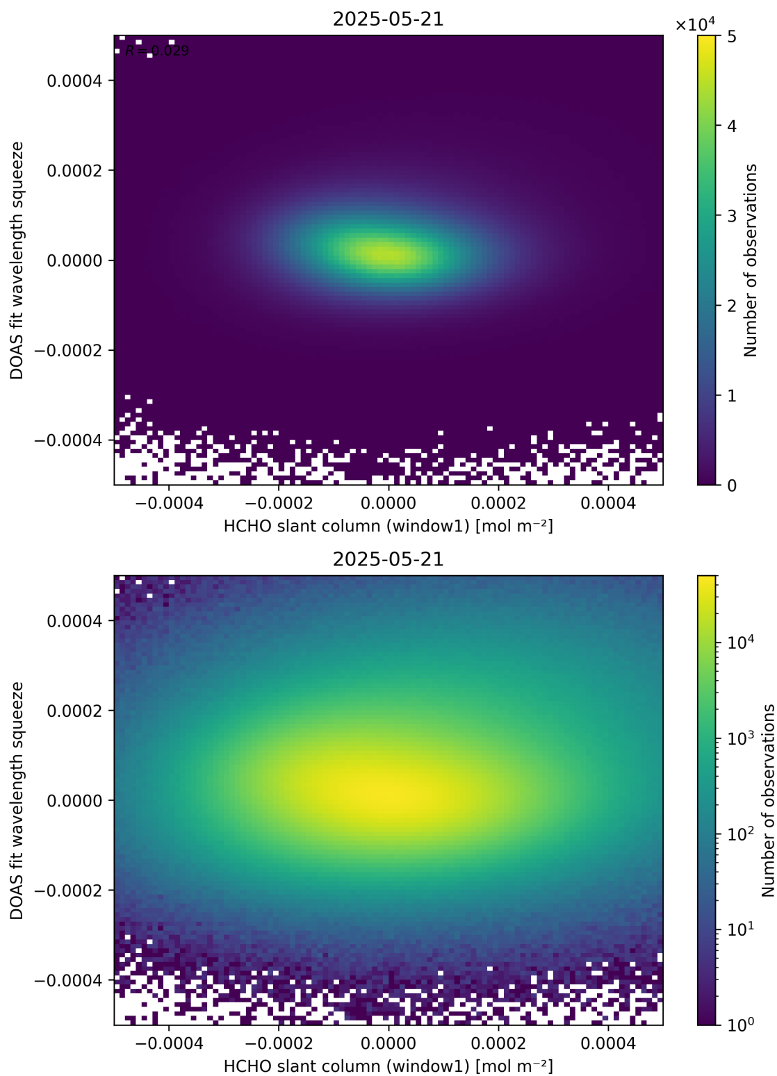
Figure 80: Scatter density plot of “HCHO slant column (window1)” against “DOAS fit wavelength squeeze” for 2025-05-21 to 2025-05-22.
