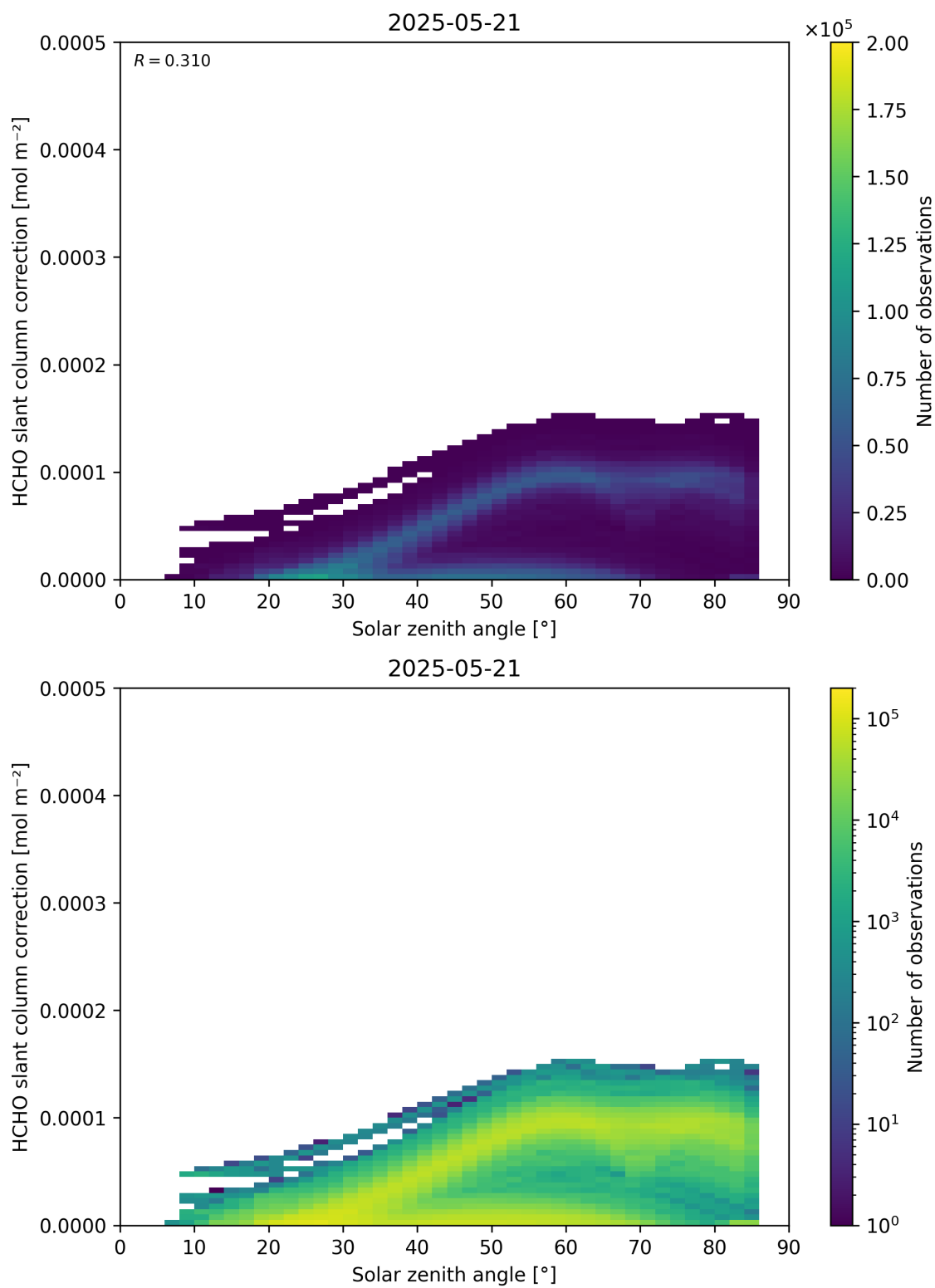
Figure 172: Scatter density plot of “Solar zenith angle” against “HCHO slant column correction” for 2025-05-21 to 2025-05-22.
