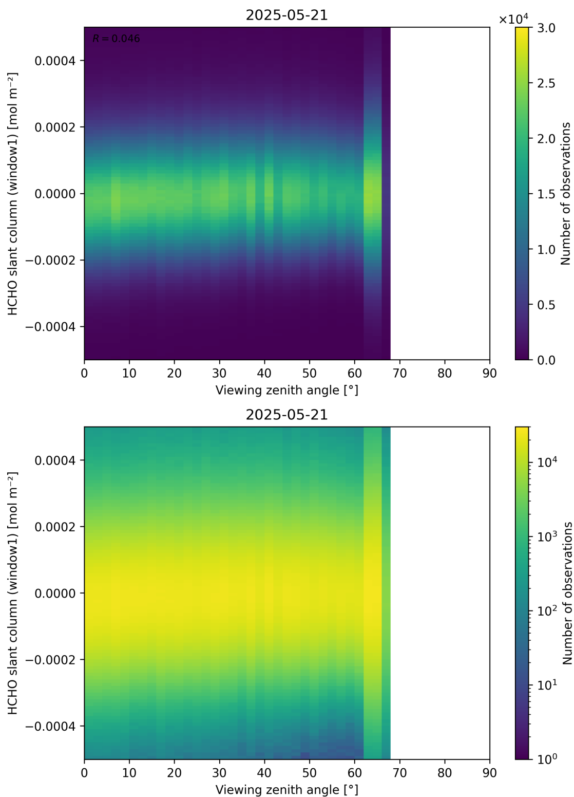
Figure 188: Scatter density plot of “Viewing zenith angle” against “HCHO slant column (window1)” for 2025-05-21 to 2025-05-22.
