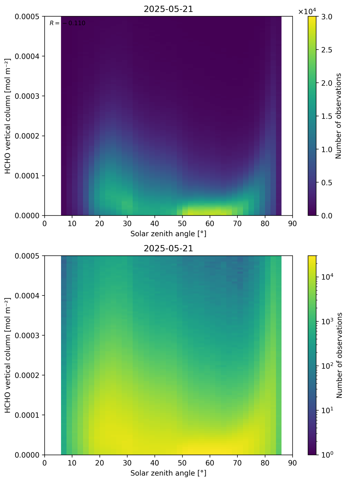
Figure 177: Scatter density plot of “Solar zenith angle” against “HCHO vertical column” for 2025-05-21 to 2025-05-22.
