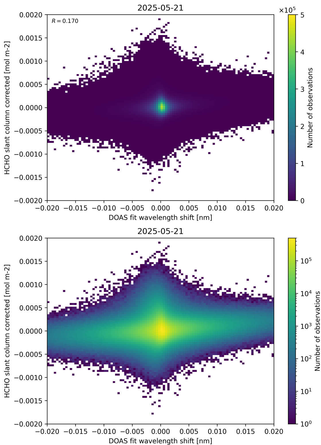
Figure 66: Scatter density plot of “DOAS fit wavelength shift” against “HCHO slant column corrected” for 2025-05-21 to 2025-05-22.
