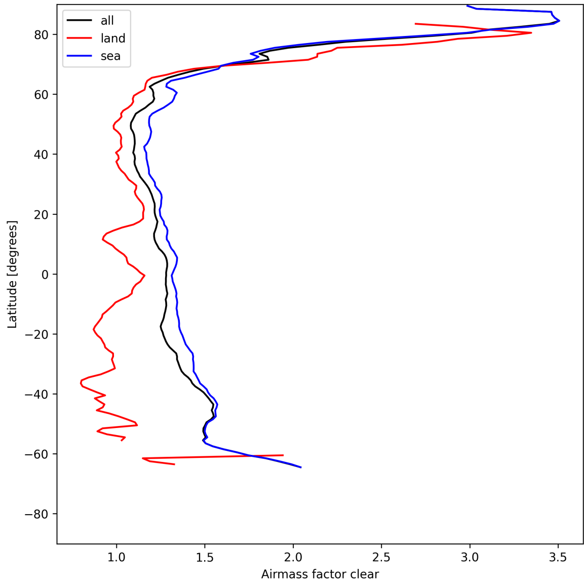
Figure 28: Zonal average of “Airmass factor clear” for 2025-05-21 to 2025-05-22.
