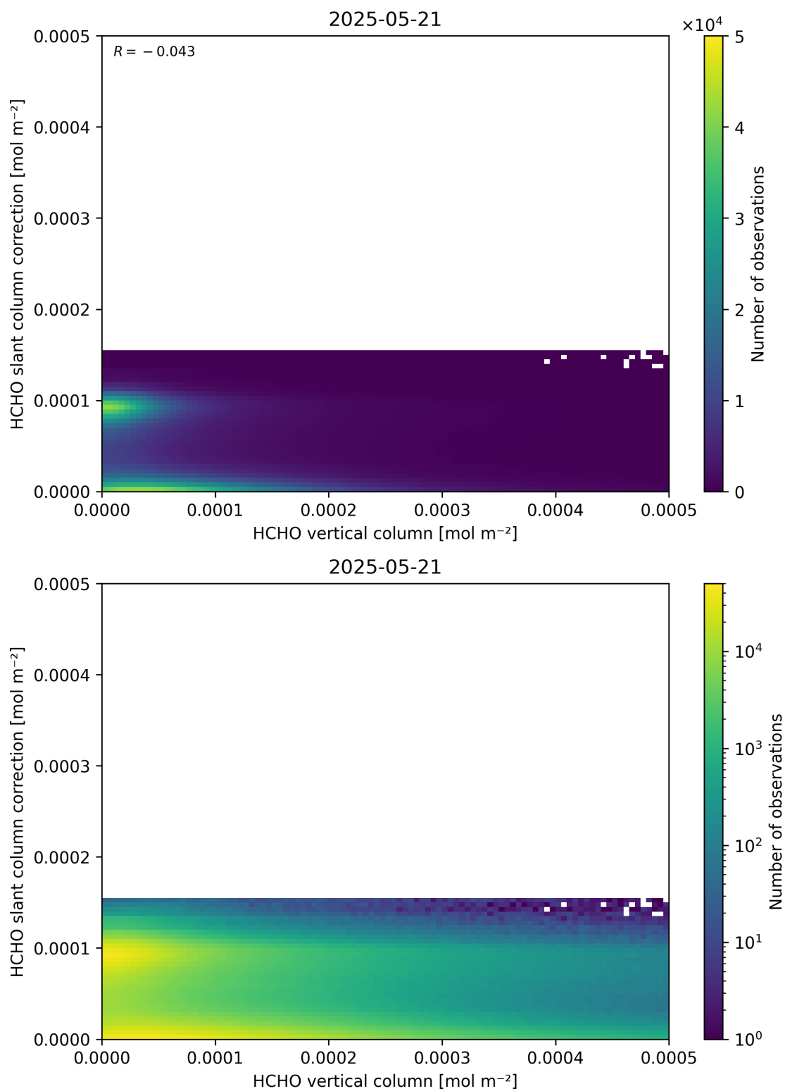
Figure 128: Scatter density plot of “HCHO vertical column” against “HCHO slant column correction” for 2025-05-21 to 2025-05-22.
