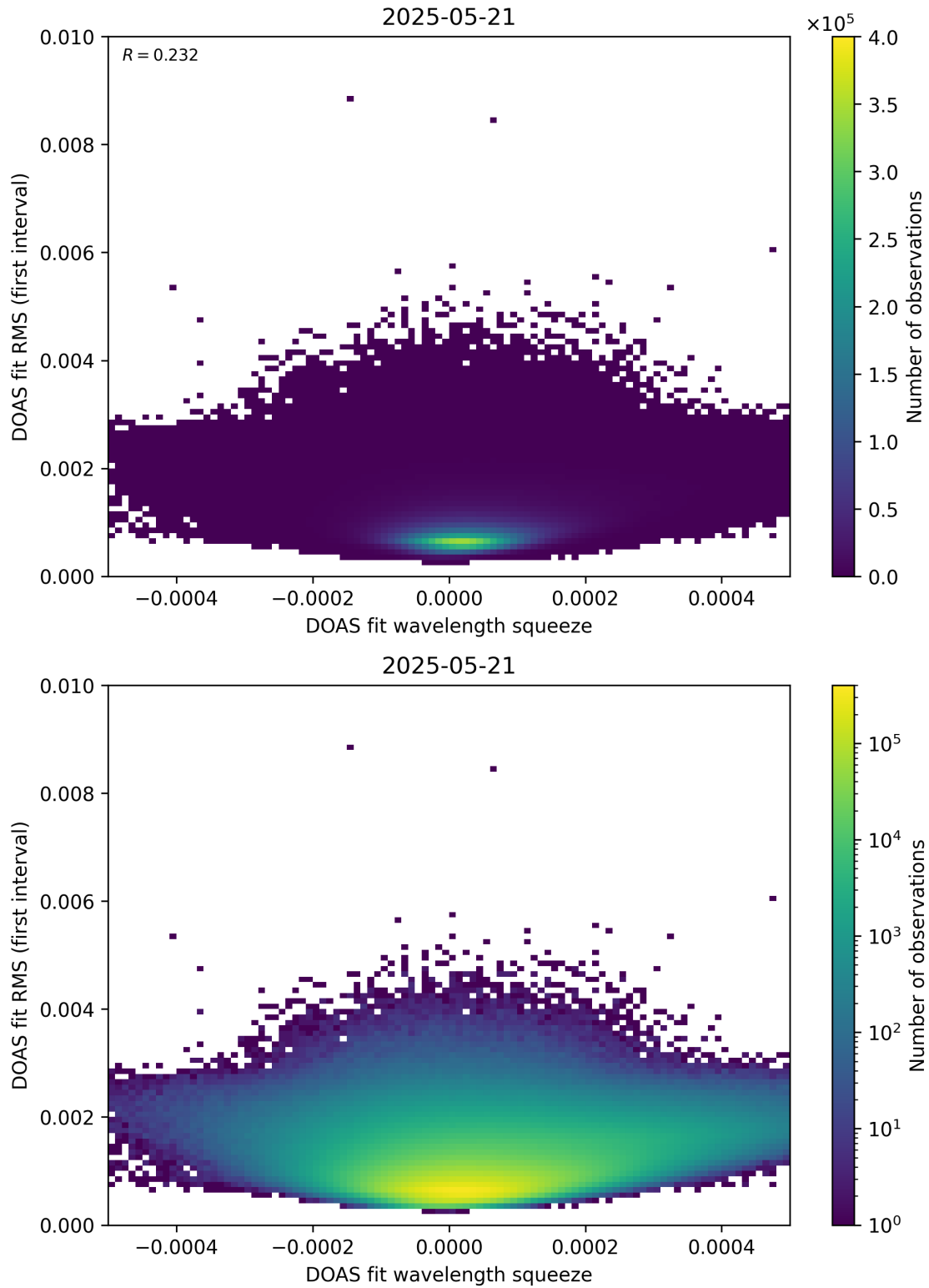
Figure 68: Scatter density plot of “DOAS fit wavelength squeeze” against “DOAS fit RMS (first interval)” for 2025-05-21 to 2025-05-22.
