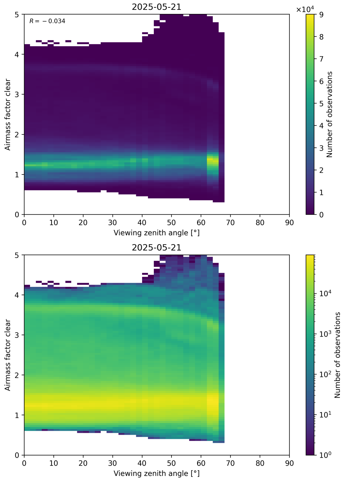
Figure 185: Scatter density plot of “Viewing zenith angle” against “Airmass factor clear” for 2025-05-21 to 2025-05-22.
