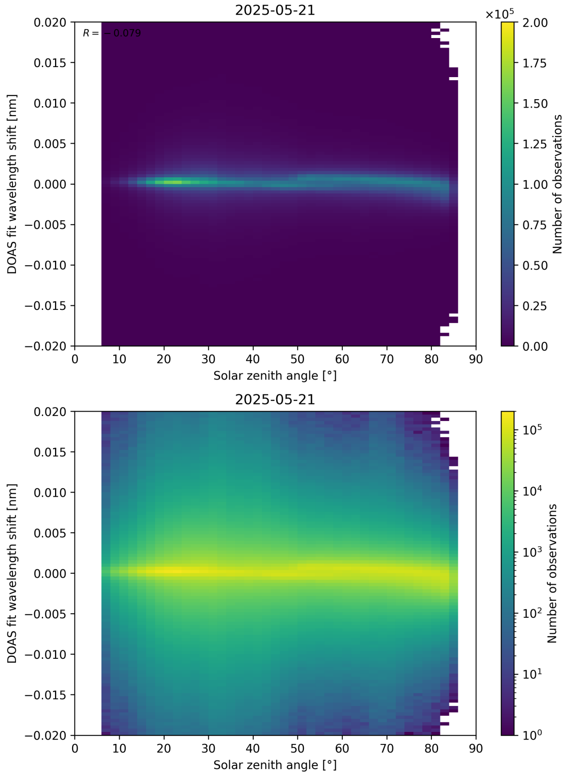
Figure 168: Scatter density plot of “Solar zenith angle” against “DOAS fit wavelength shift” for 2025-05-21 to 2025-05-22.
