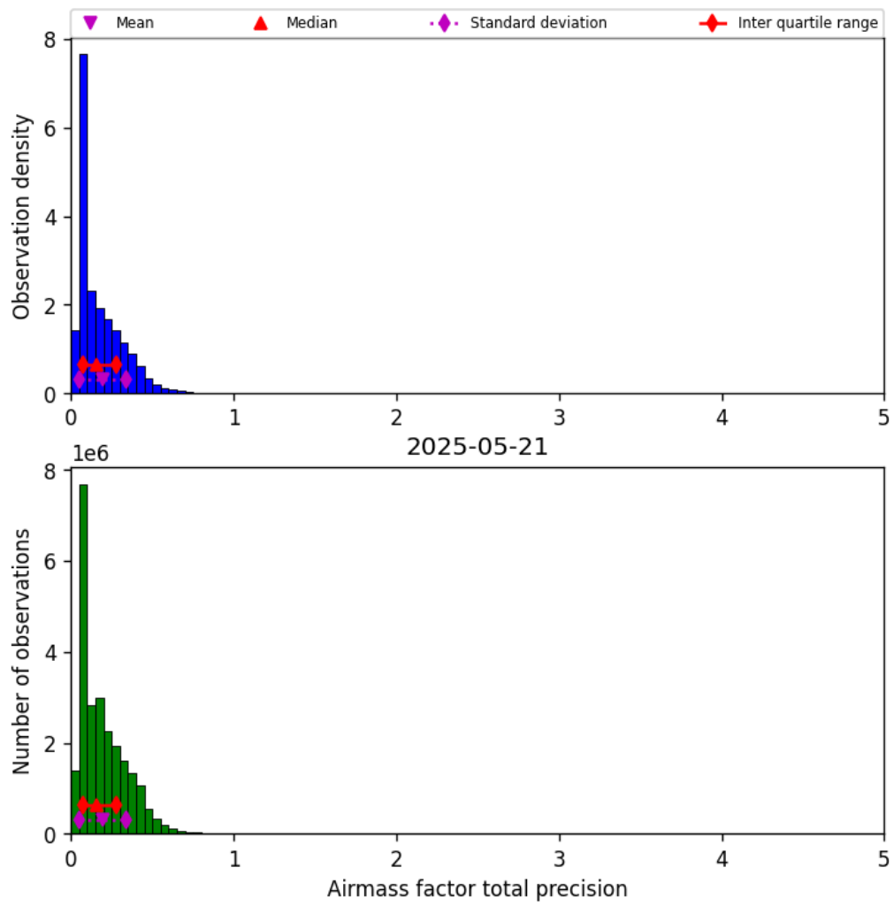
Figure 41: Histogram of “Airmass factor total precision” for 2025-05-21 to 2025-05-22
