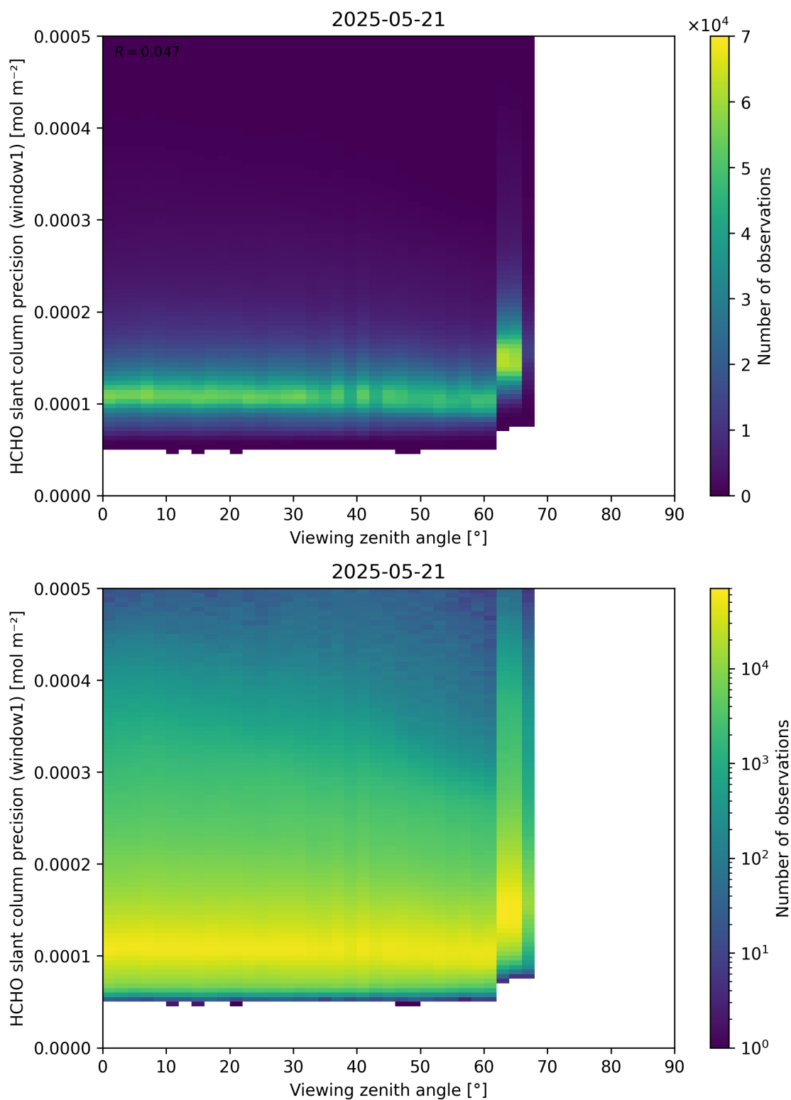
Figure 189: Scatter density plot of “Viewing zenith angle” against “HCHO slant column precision (window1)” for 2025-05-21 to 2025-05-22.
