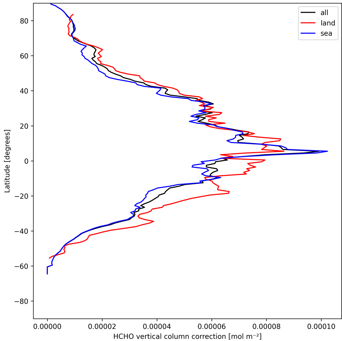
Figure 23: Zonal average of “HCHO vertical column correction” for 2025-05-21 to 2025-05-22.
