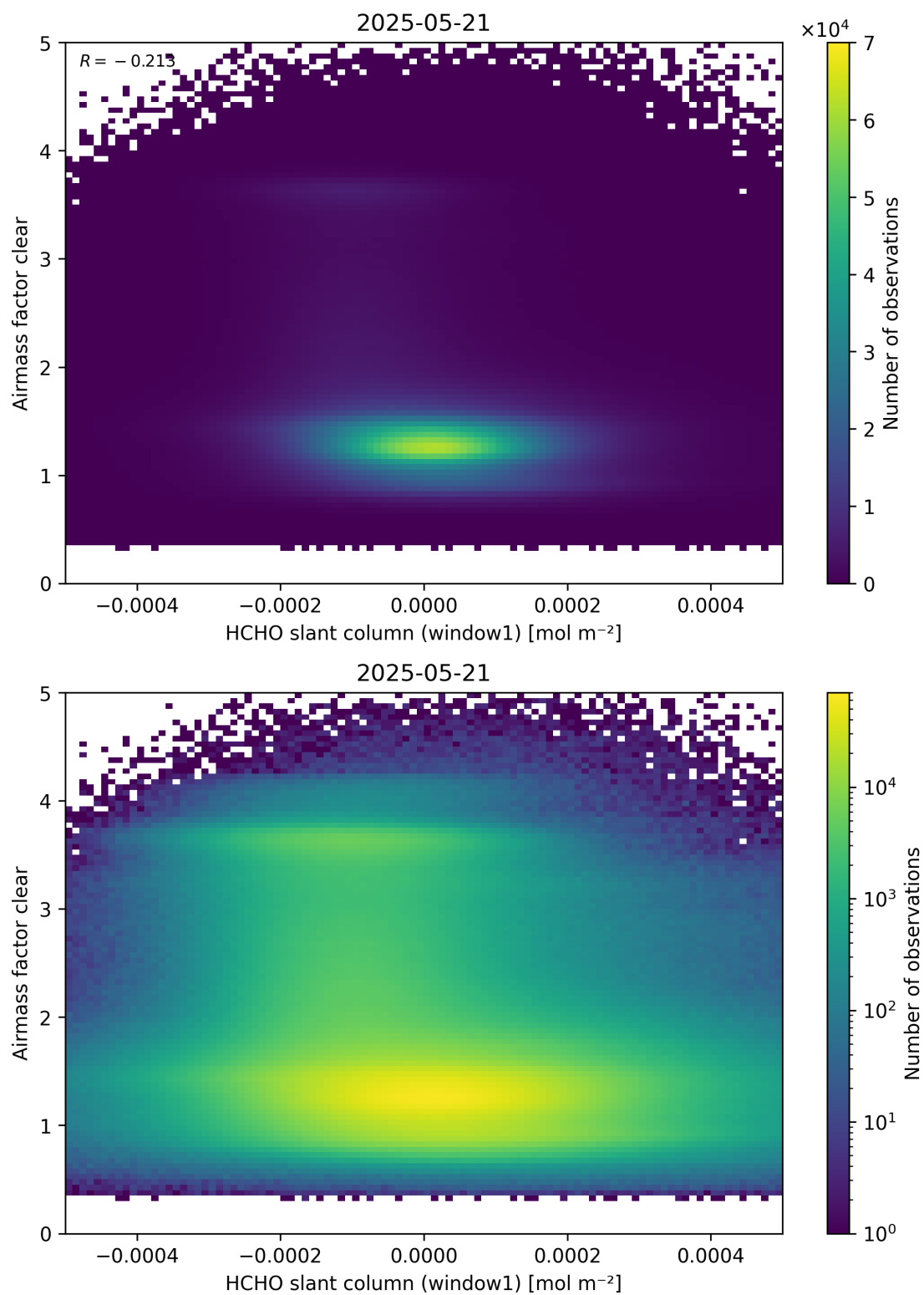
Figure 81: Scatter density plot of “HCHO slant column (window1)” against “Airmass factor clear” for 2025-05-21 to 2025-05-22.
