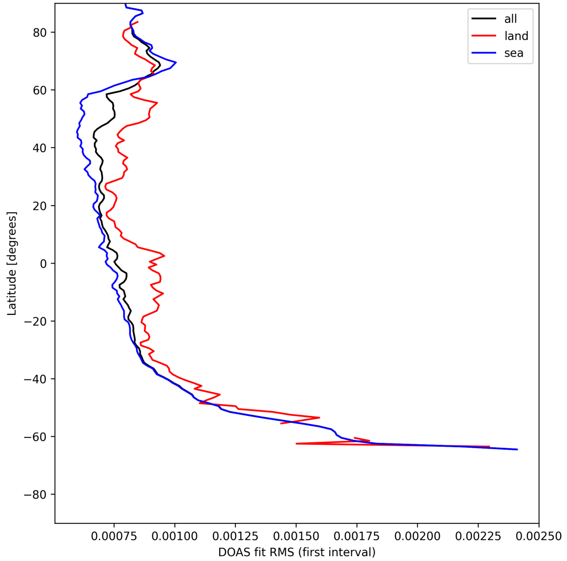
Figure 32: Zonal average of "DOAS fit RMS (first interval)" for 2025-05-21 to 2025-05-22.
