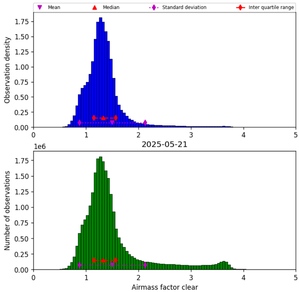
Figure 42: Histogram of “Airmass factor clear” for 2025-05-21 to 2025-05-22
