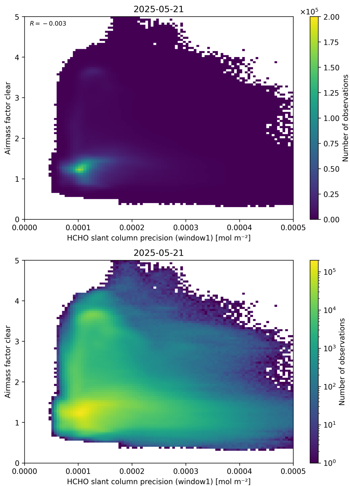
Figure 91: Scatter density plot of “HCHO slant column precision (window1)” against “Airmass factor clear” for 2025-05-21 to 2025-05-22.
