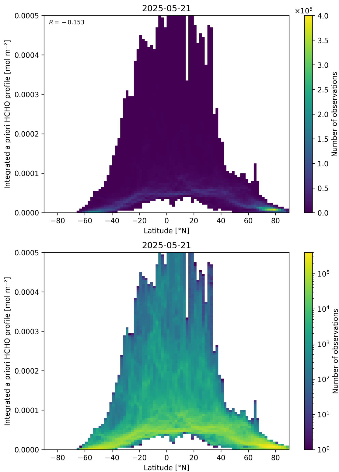
Figure 166: Scatter density plot of “Latitude” against “Integrated a priori HCHO profile” for 2025-05-21 to 2025-05-22.
