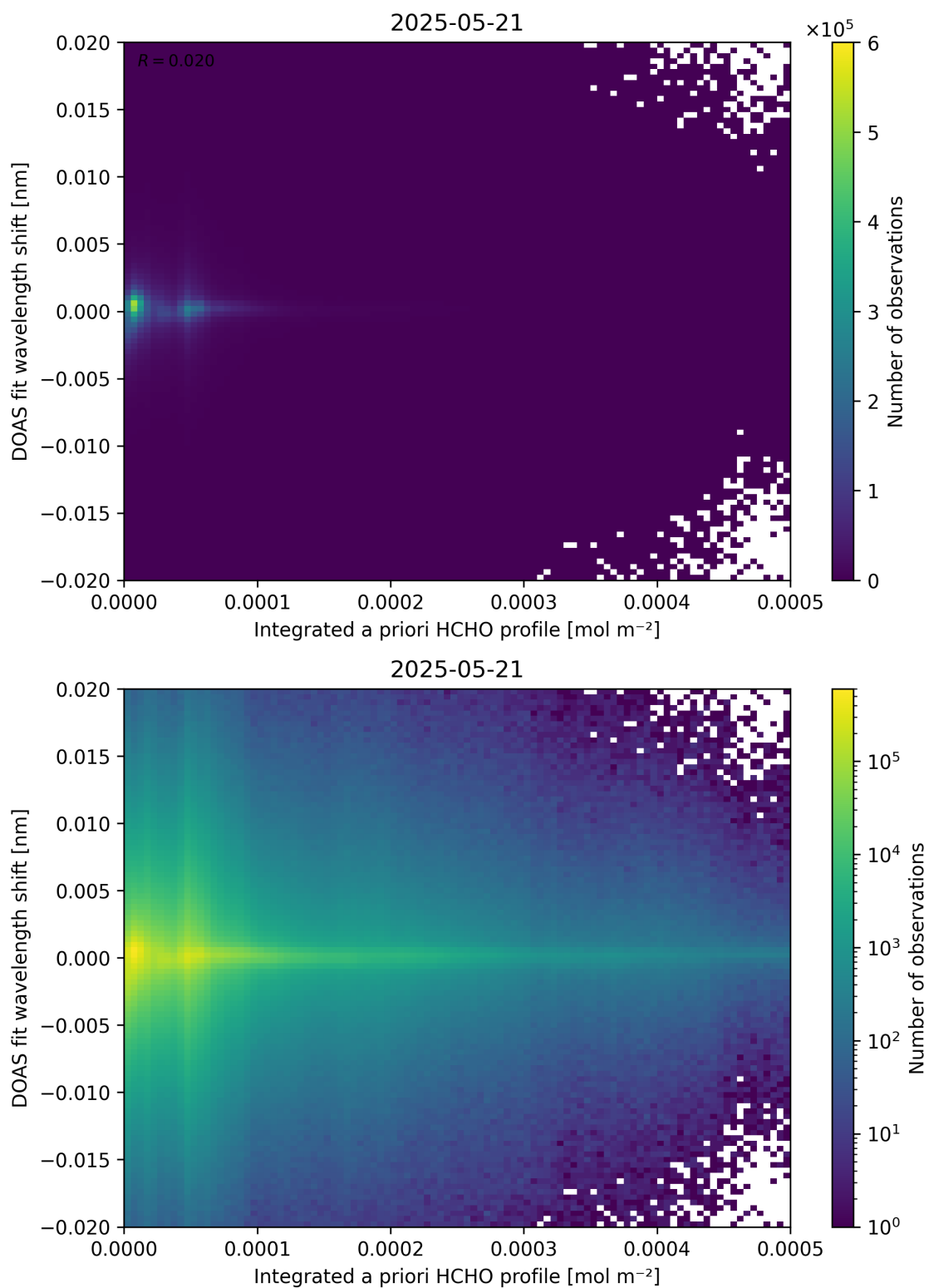
Figure 149: Scatter density plot of “Integrated a priori HCHO profile” against “DOAS fit wavelength shift” for 2025-05-21 to 2025-05-22.
