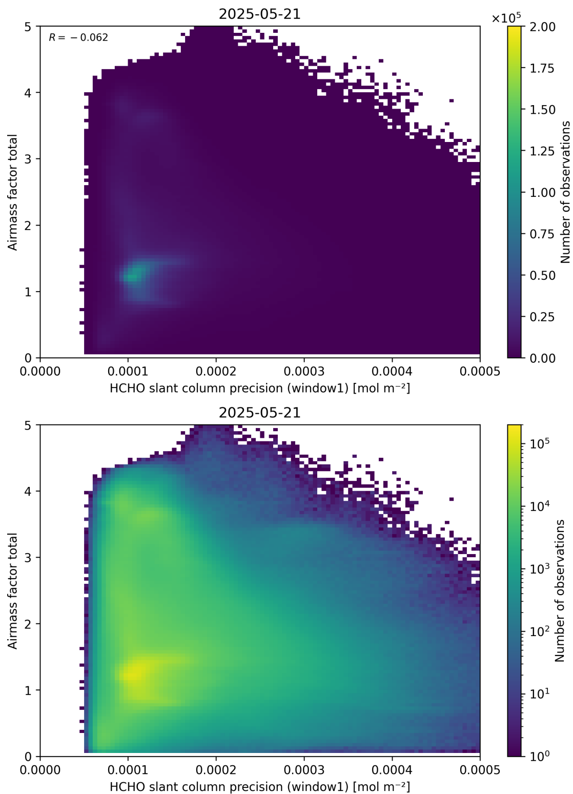
Figure 94: Scatter density plot of “HCHO slant column precision (window1)” against “Airmass factor total” for 2025-05-21 to 2025-05-22.
