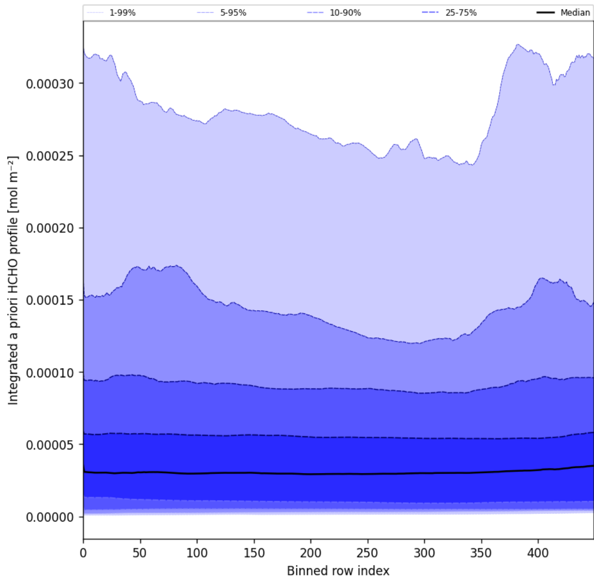
Figure 57: Along track statistics of “Integrated a priori HCHO profile” for 2025-05-21 to 2025-05-22
