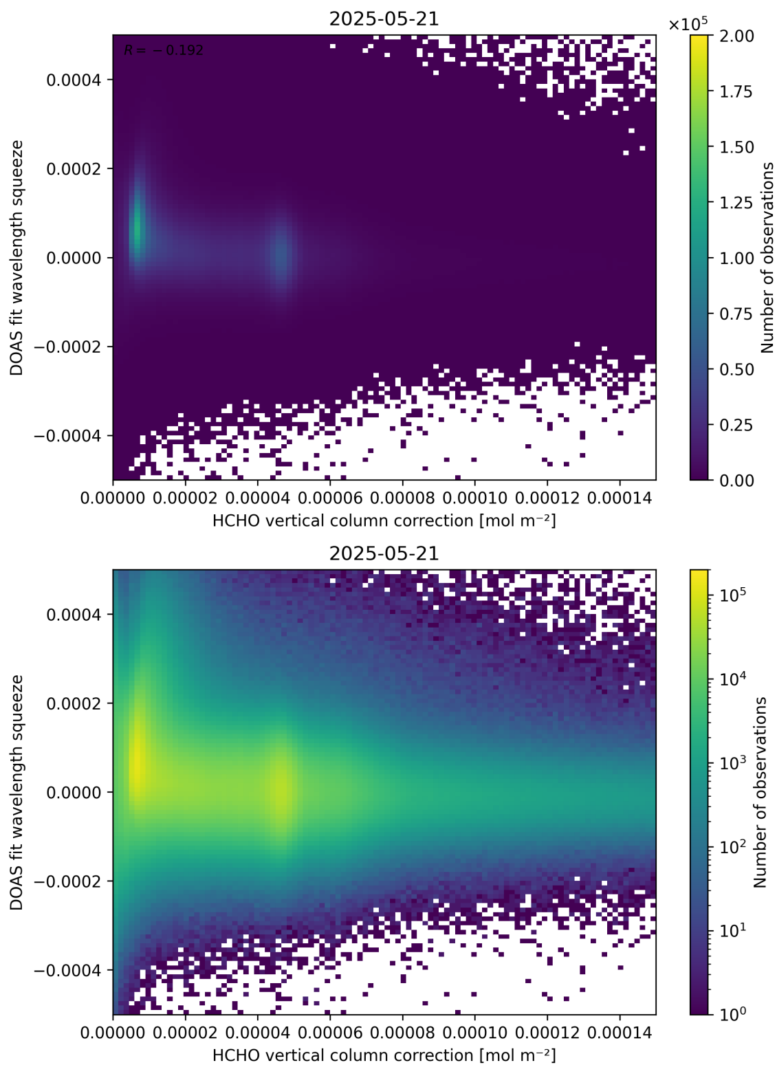
Figure 114: Scatter density plot of “HCHO vertical column correction” against “DOAS fit wavelength squeeze” for 2025-05-21 to 2025-05-22.
