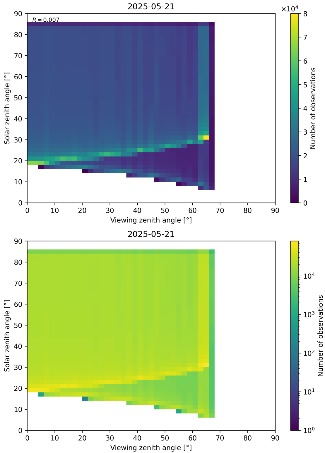
Figure 197: Scatter density plot of “Viewing zenith angle” against “Solar zenith angle” for 2025-05-21 to 2025-05-22.
