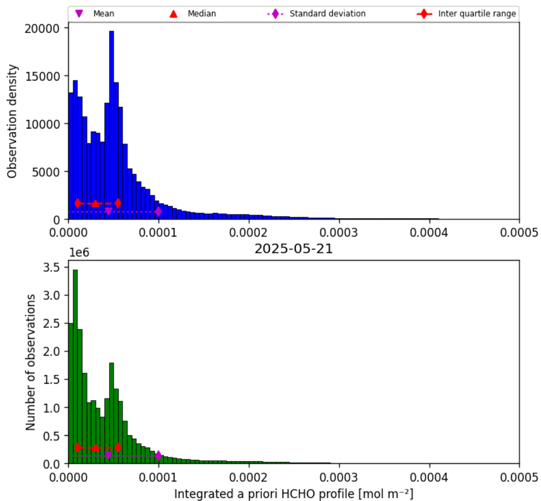
Figure 43: Histogram of “Integrated a priori HCHO profile” for 2025-05-21 to 2025-05-22
