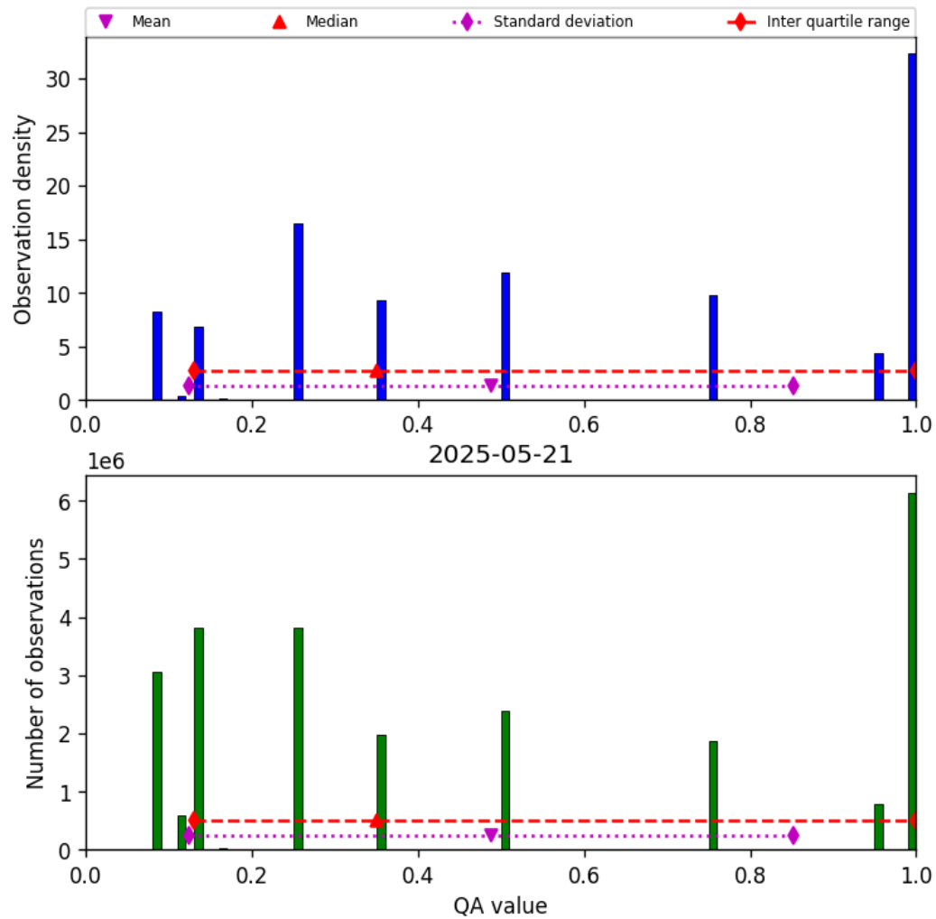
Figure 34: Histogram of “QA value” for 2025-05-21 to 2025-05-22
