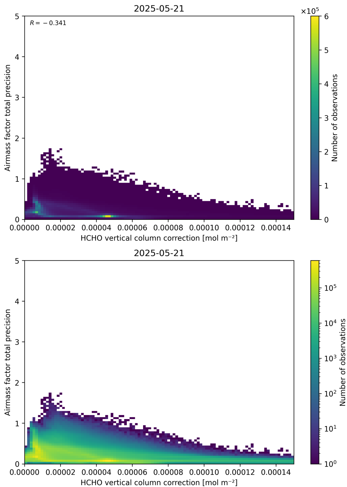
Figure 121: Scatter density plot of “HCHO vertical column correction” against “Airmass factor total precision” for 2025-05-21 to 2025-05-22.
