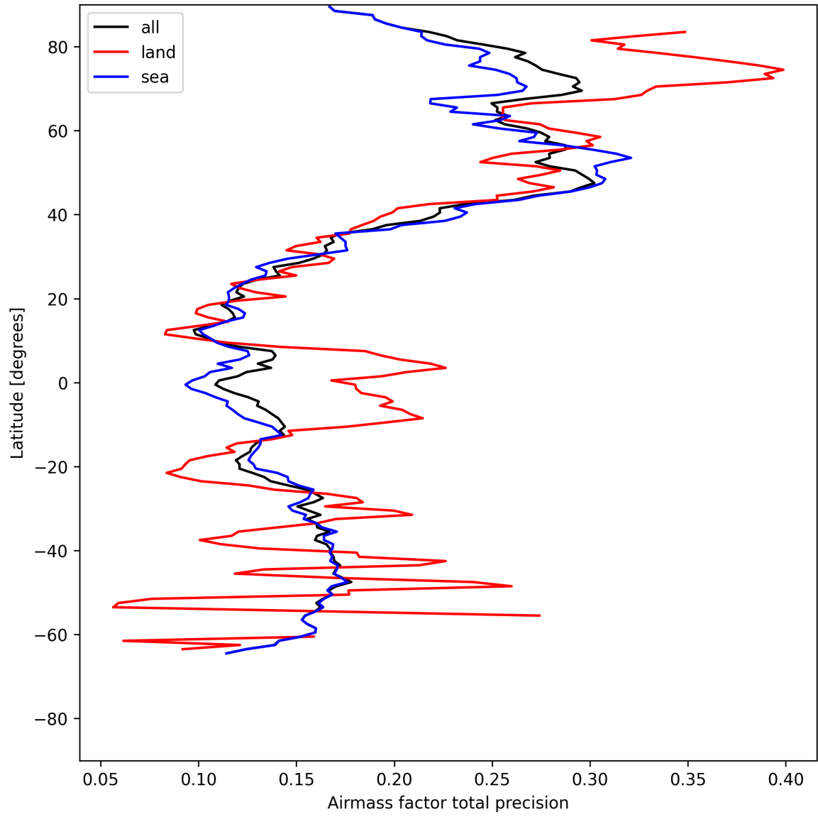
Figure 27: Zonal average of “Airmass factor total precision” for 2025-05-21 to 2025-05-22.
