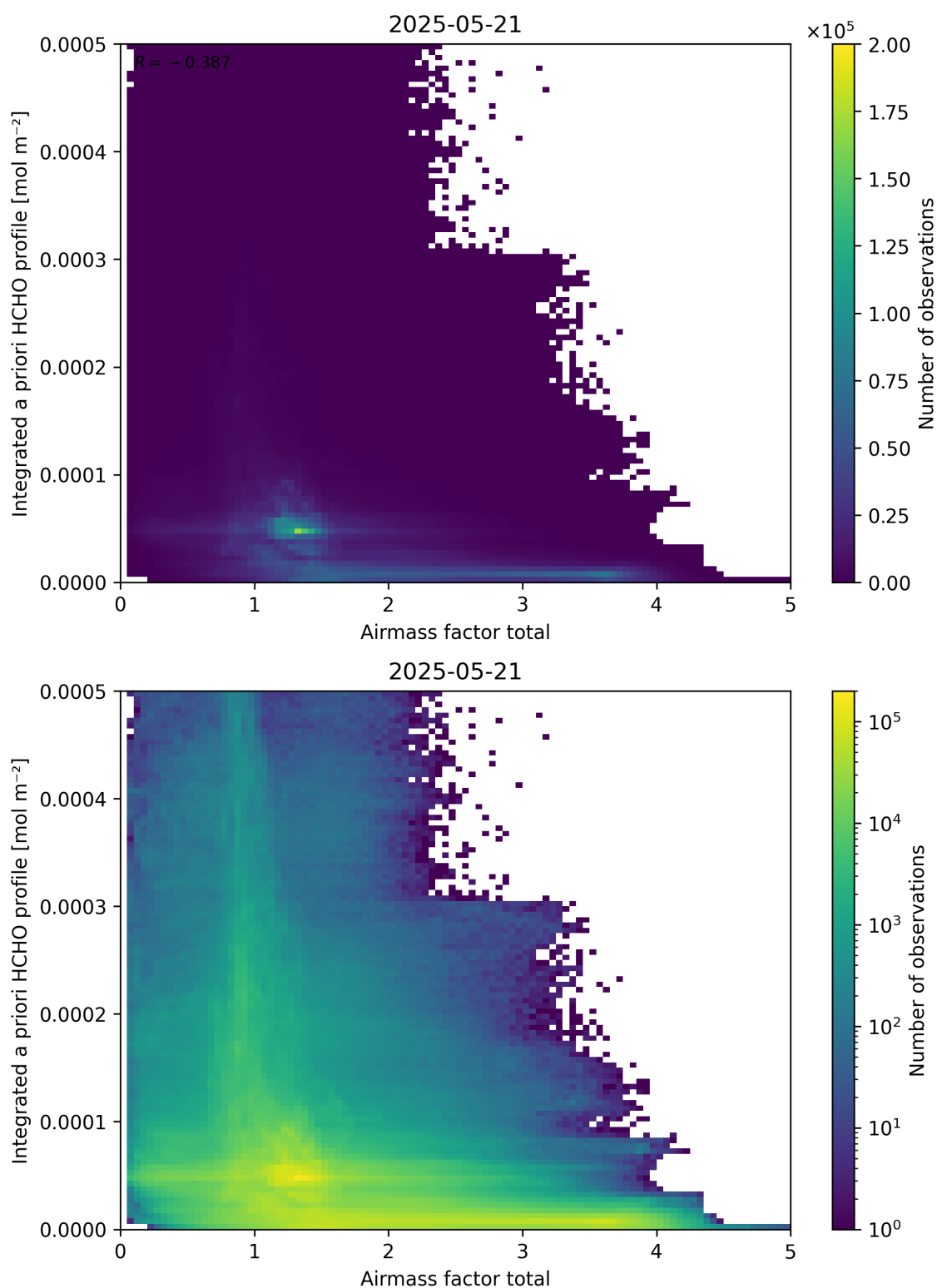
Figure 104: Scatter density plot of “Airmass factor total” against “Integrated a priori HCHO profile” for 2025-05-21 to 2025-05-22.
