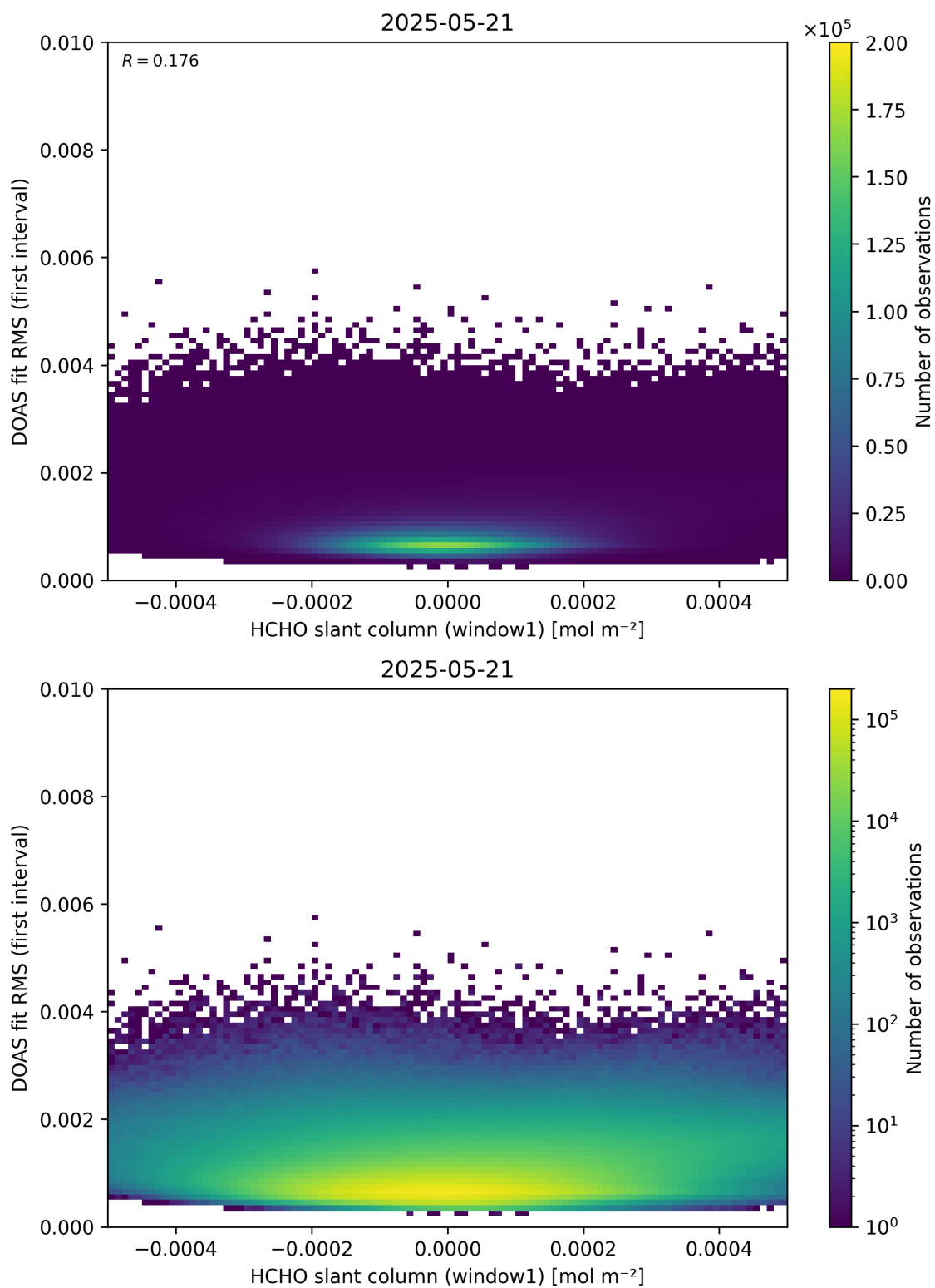
Figure 78: Scatter density plot of “HCHO slant column (window1)” against “DOAS fit RMS (first interval)” for 2025-05-21 to 2025-05-22.
