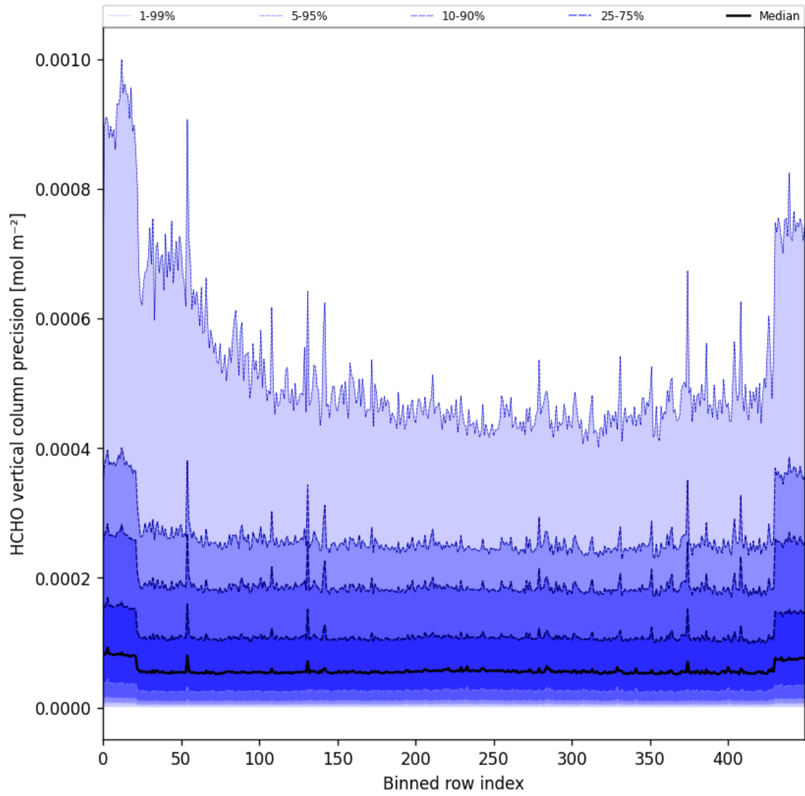
Figure 50: Along track statistics of “HCHO vertical column precision” for 2025-05-21 to 2025-05-22
