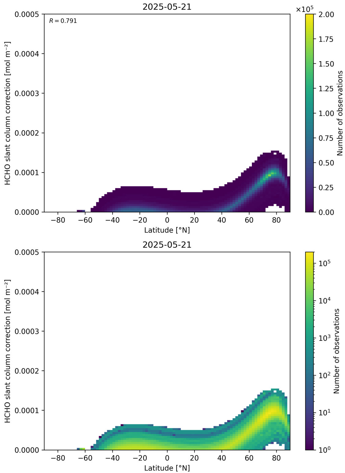
Figure 158: Scatter density plot of “Latitude” against “HCHO slant column correction” for 2025-05-21 to 2025-05-22.
