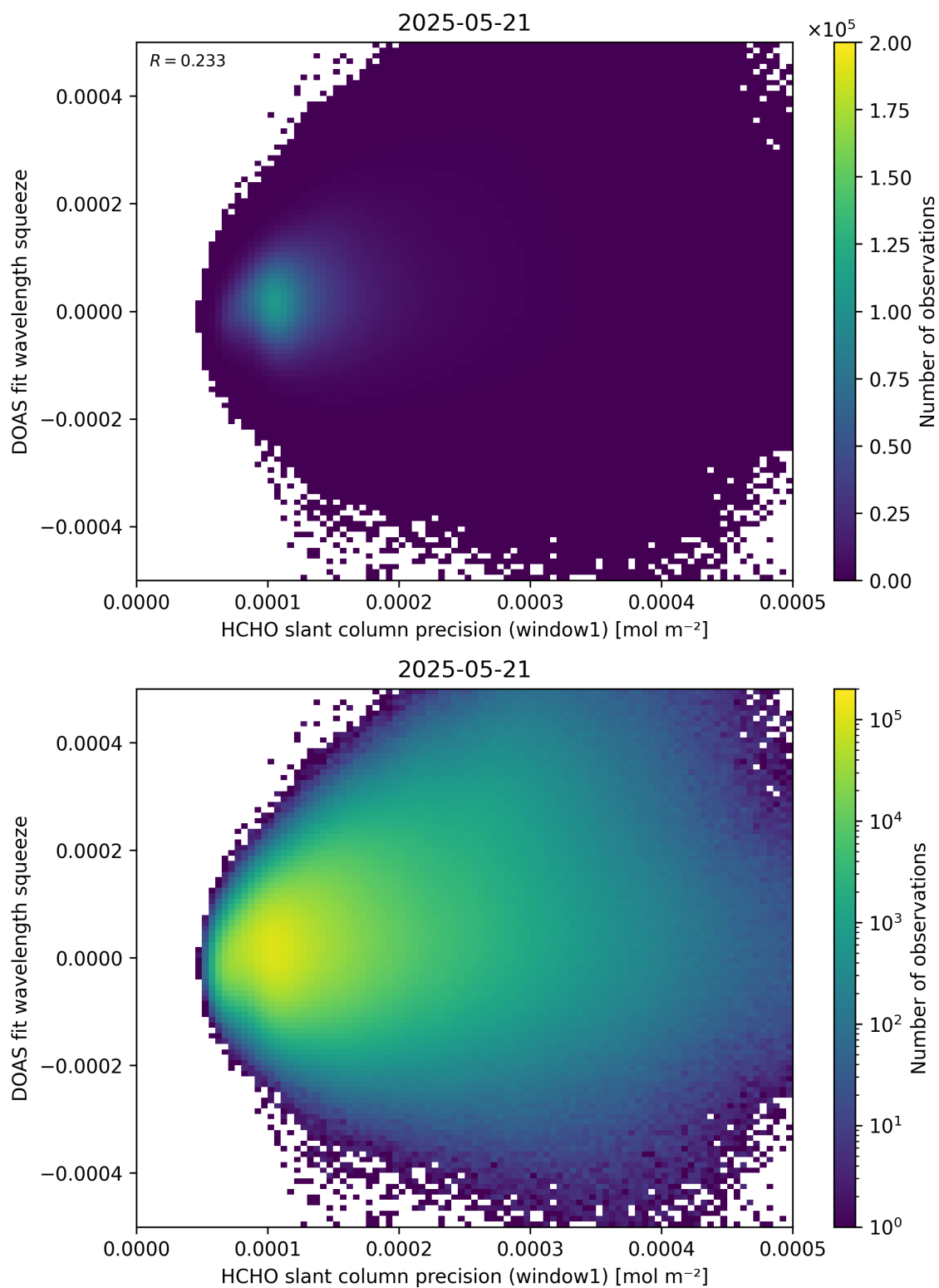
Figure 90: Scatter density plot of “HCHO slant column precision (window1)” against “DOAS fit wavelength squeeze” for 2025-05-21 to 2025-05-22.
