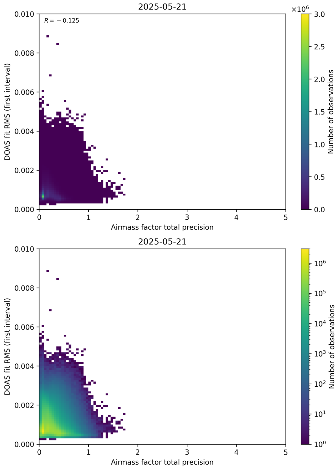
Figure 105: Scatter density plot of “Airmass factor total precision” against “DOAS fit RMS (first interval)” for 2025-05-21 to 2025-05-22.
