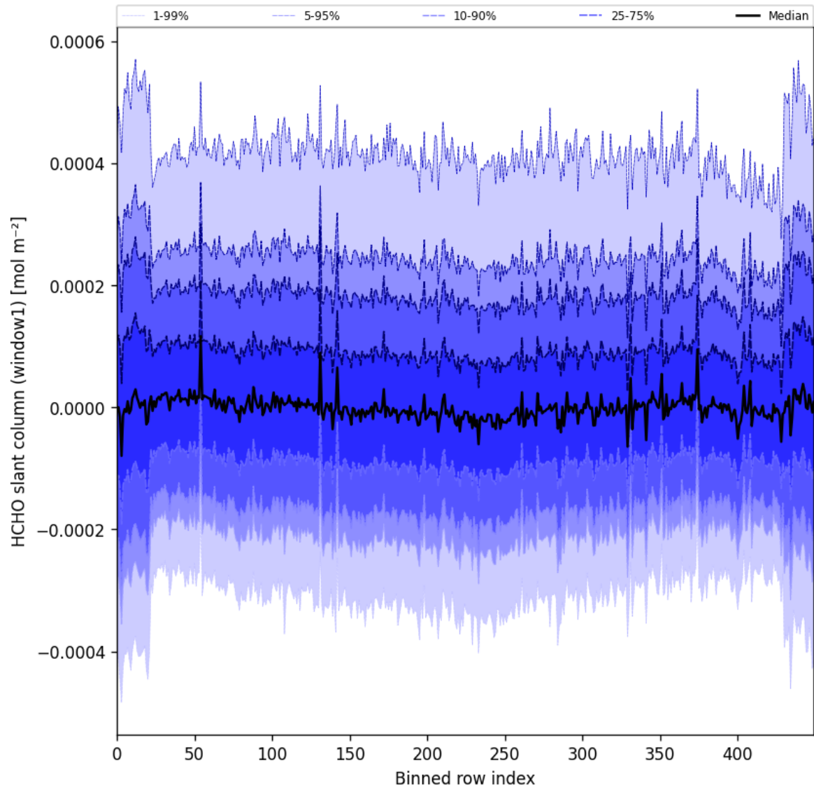
Figure 52: Along track statistics of “HCHO slant column (window1)” for 2025-05-21 to 2025-05-22
