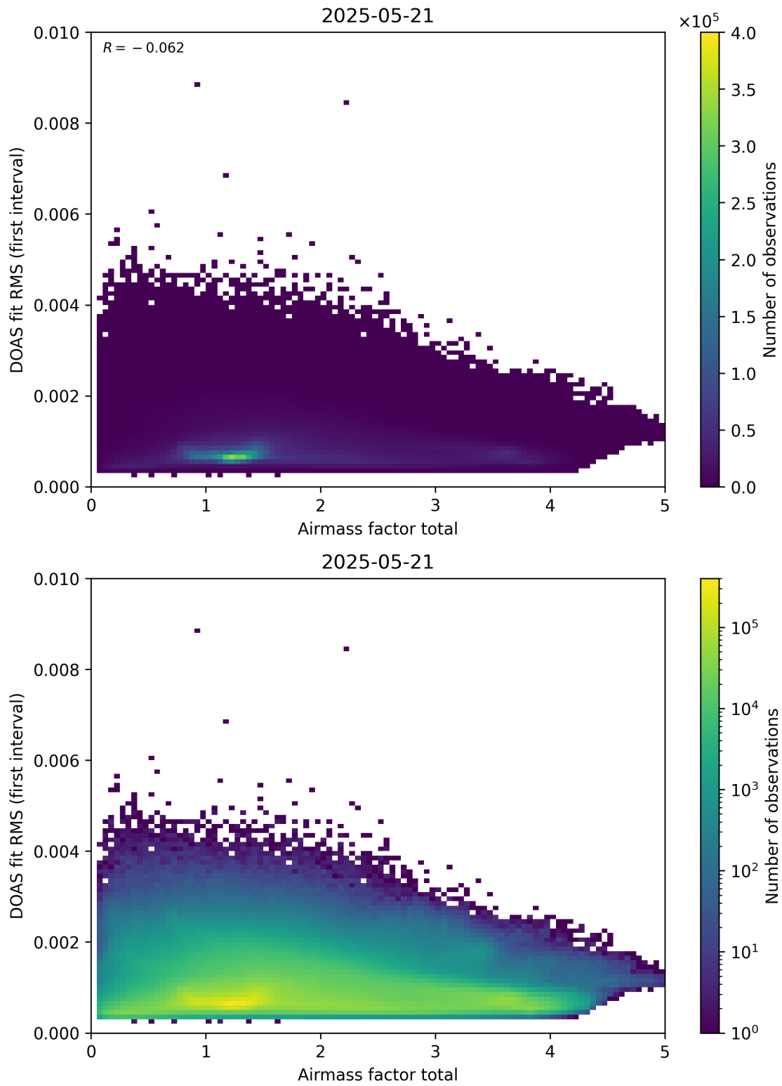
Figure 97: Scatter density plot of “Airmass factor total” against “DOAS fit RMS (first interval)” for 2025-05-21 to 2025-05-22.
