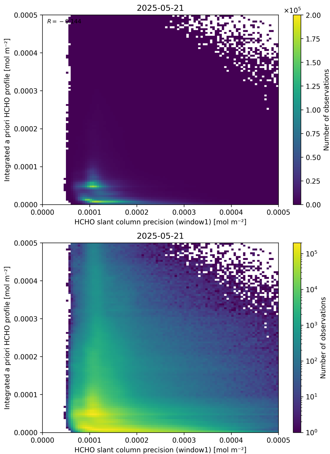
Figure 96: Scatter density plot of “HCHO slant column precision (window1)” against “Integrated a priori HCHO profile” for 2025-05-21 to 2025-05-22.
