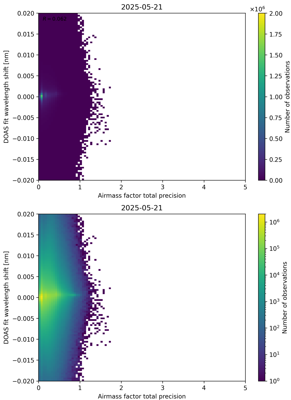
Figure 106: Scatter density plot of “Airmass factor total precision” against “DOAS fit wavelength shift” for 2025-05-21 to 2025-05-22.
