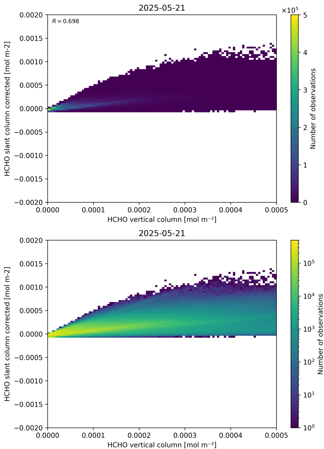
Figure 127: Scatter density plot of “HCHO vertical column” against “HCHO slant column corrected” for 2025-05-21 to 2025-05-22.
