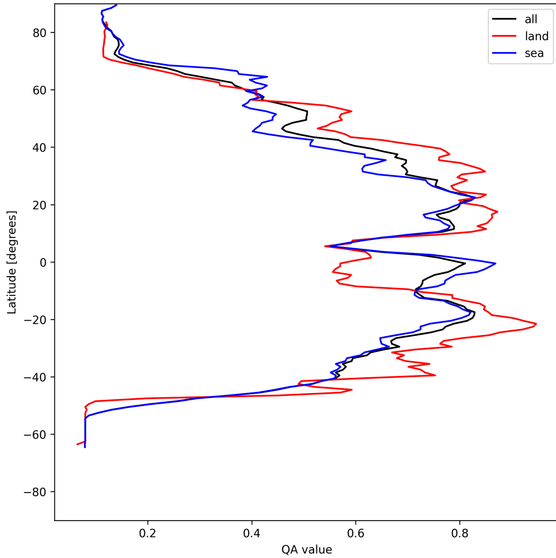
Figure 20: Zonal average of “QA value” for 2025-05-21 to 2025-05-22.
