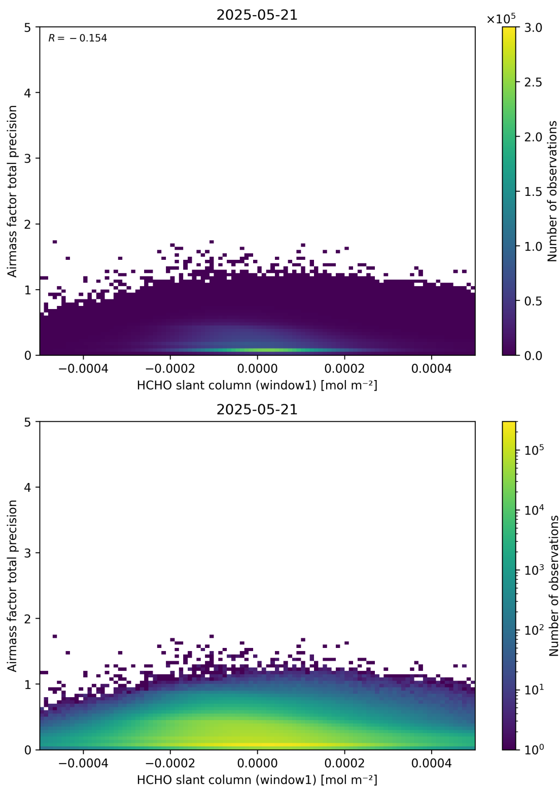
Figure 86: Scatter density plot of “HCHO slant column (window1)” against “Airmass factor total precision” for 2025-05-21 to 2025-05-22.
