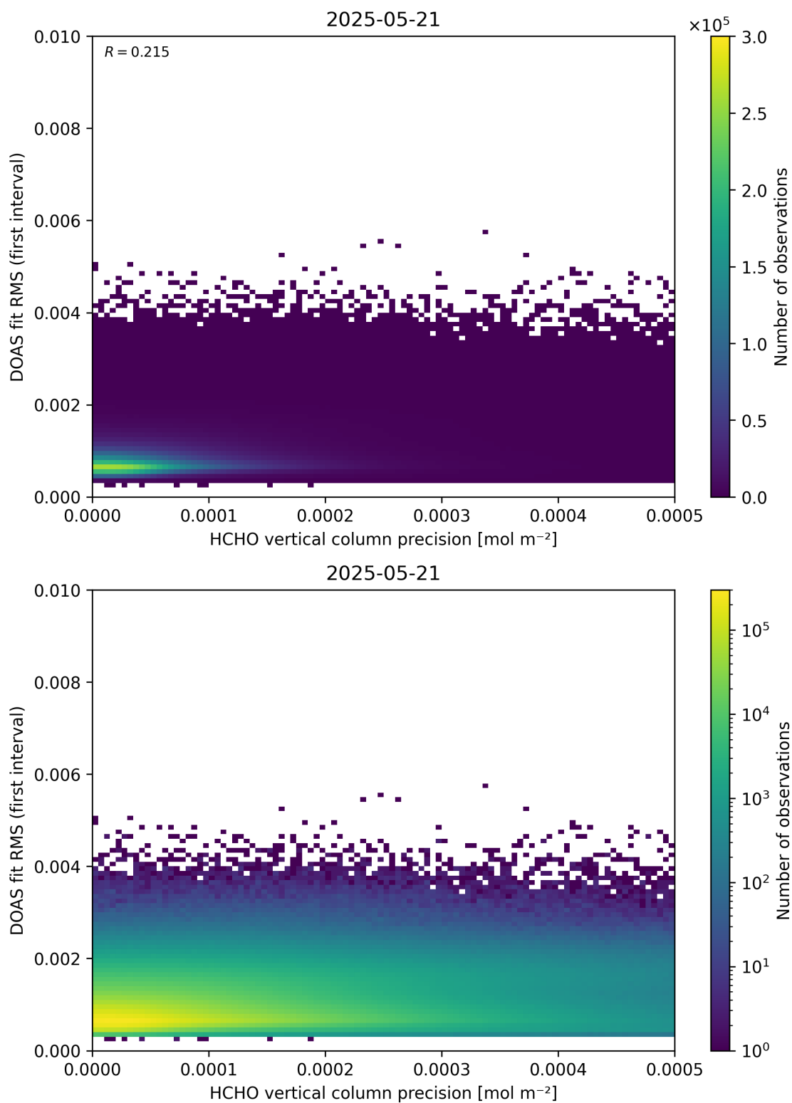
Figure 136: Scatter density plot of “HCHO vertical column precision” against “DOAS fit RMS (first interval)” for 2025-05-21 to 2025-05-22.
