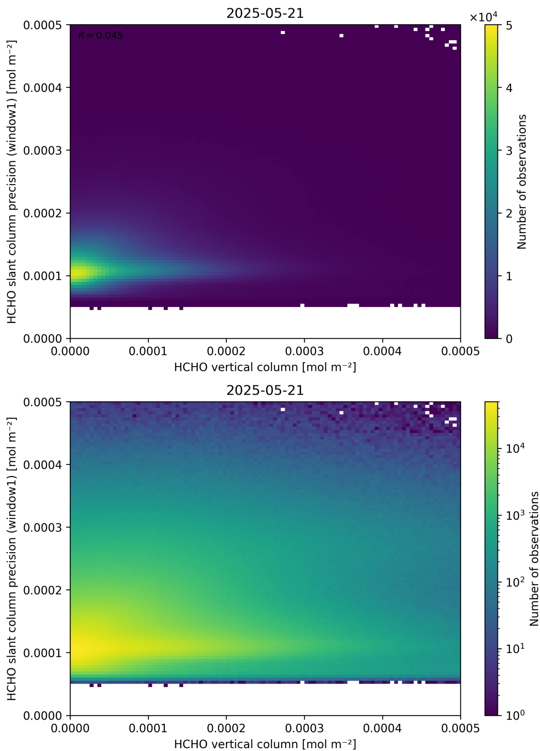
Figure 130: Scatter density plot of “HCHO vertical column” against “HCHO slant column precision (window1)” for 2025-05-21 to 2025-05-22.
