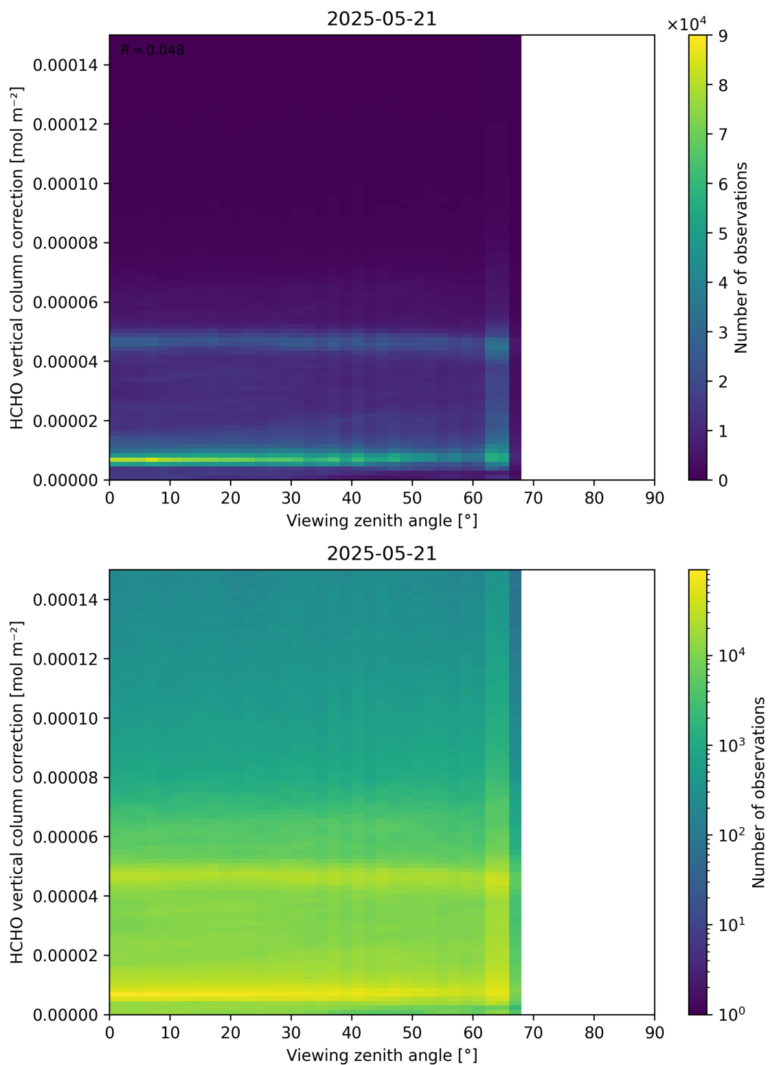
Figure 193: Scatter density plot of “Viewing zenith angle” against “HCHO vertical column correction” for 2025-05-21 to 2025-05-22.
