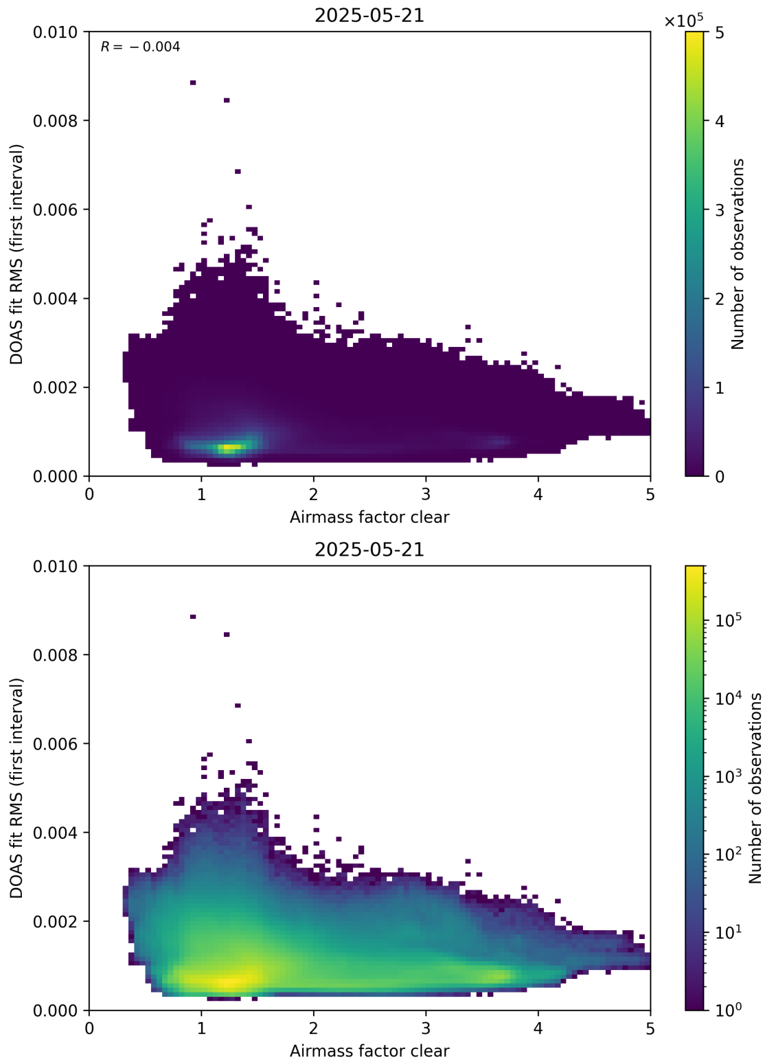
Figure 71: Scatter density plot of “Airmass factor clear” against “DOAS fit RMS (first interval)” for 2025-05-21 to 2025-05-22.
