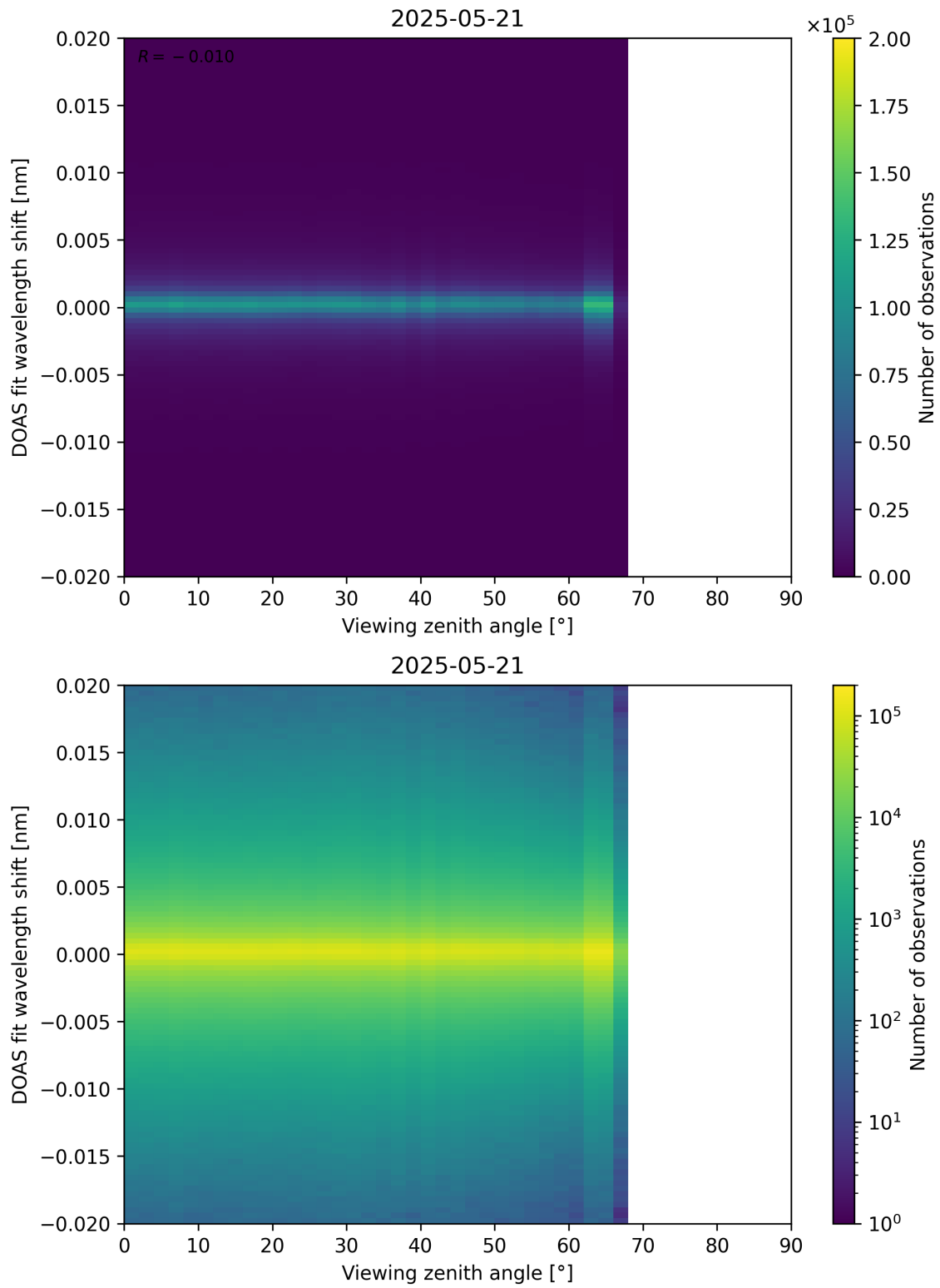
Figure 183: Scatter density plot of “Viewing zenith angle” against “DOAS fit wavelength shift” for 2025-05-21 to 2025-05-22.
