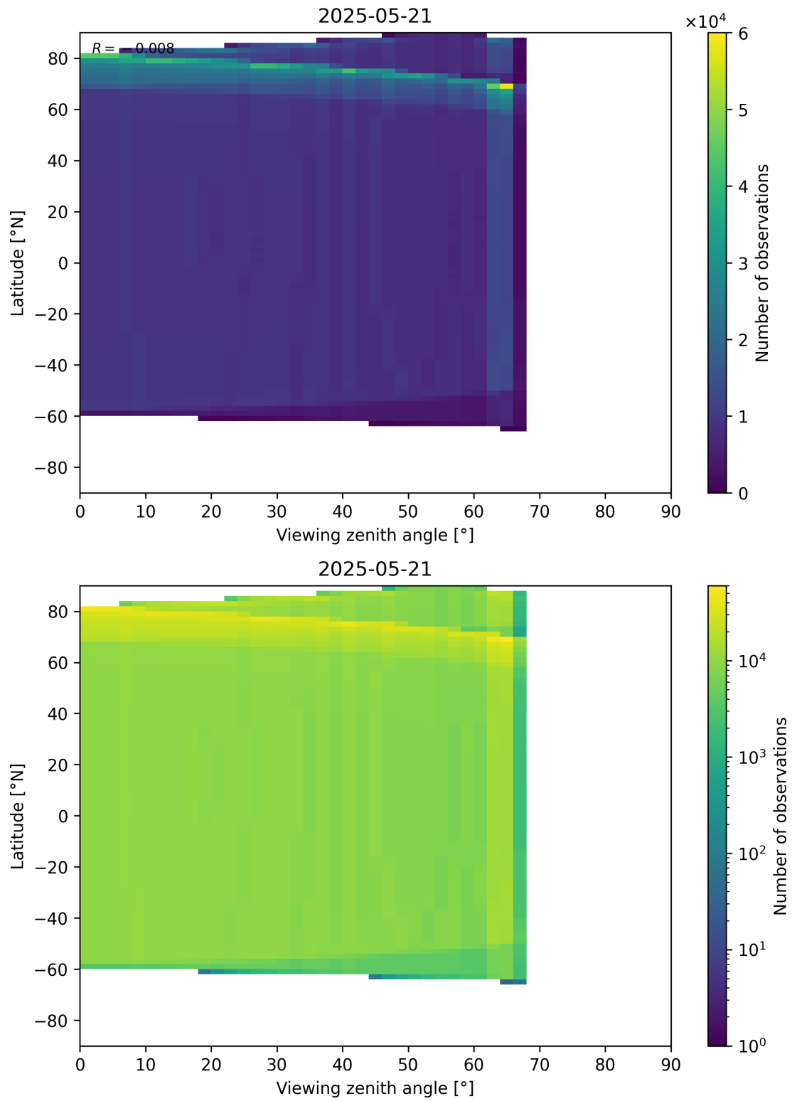
Figure 196: Scatter density plot of “Viewing zenith angle” against “Latitude” for 2025-05-21 to 2025-05-22.
