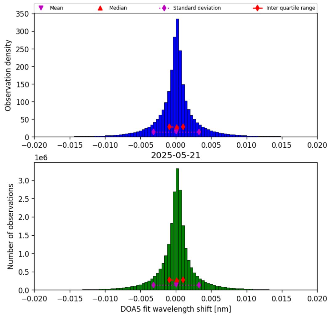
Figure 44: Histogram of “DOAS fit wavelength shift” for 2025-05-21 to 2025-05-22
