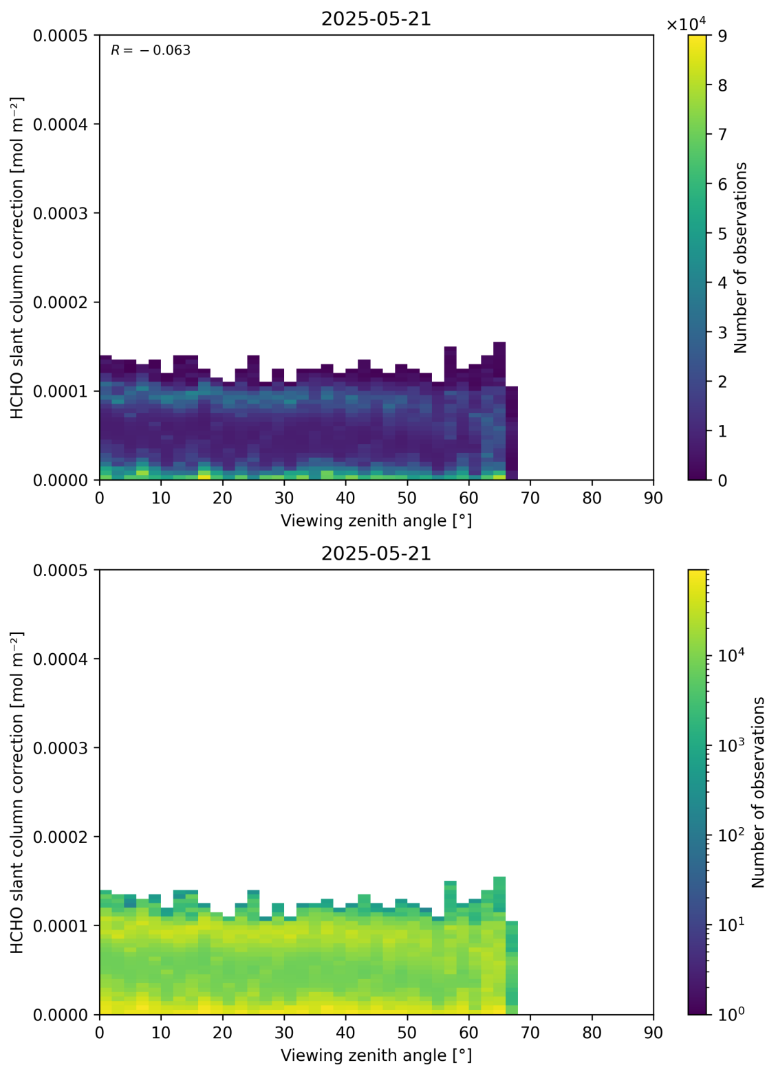
Figure 187: Scatter density plot of “Viewing zenith angle” against “HCHO slant column correction” for 2025-05-21 to 2025-05-22.
