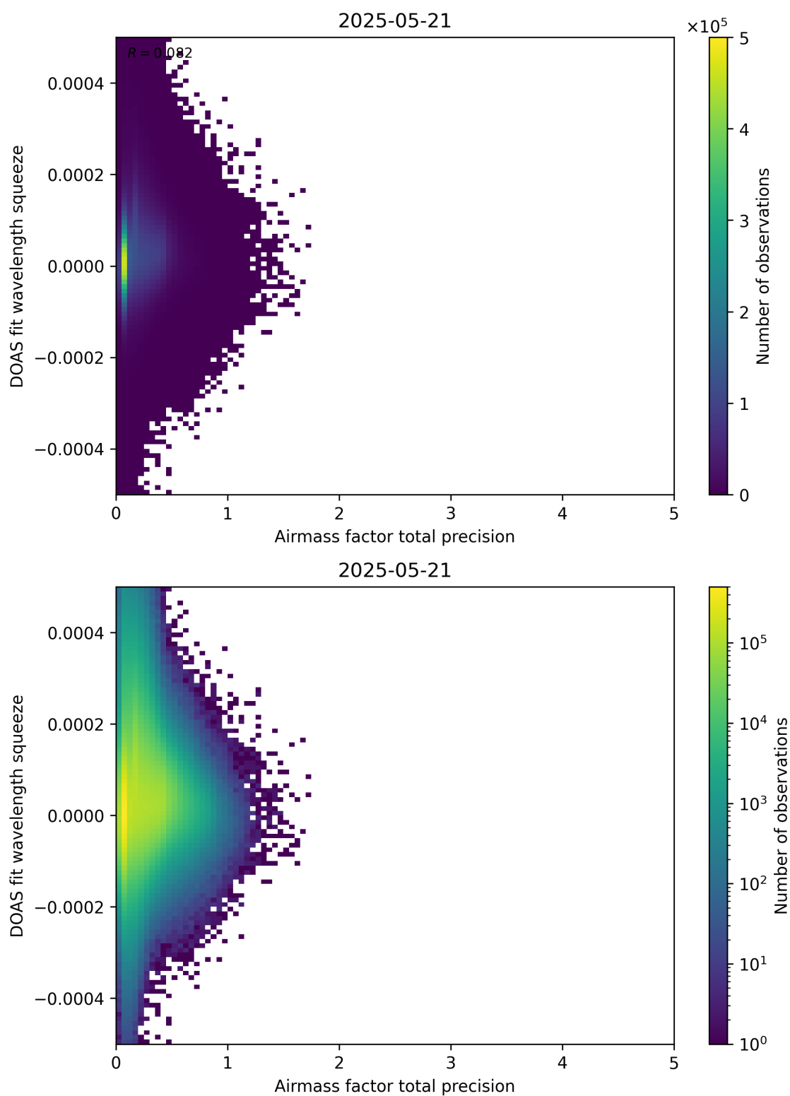
Figure 107: Scatter density plot of “Airmass factor total precision” against “DOAS fit wavelength squeeze” for 2025-05-21 to 2025-05-22.
