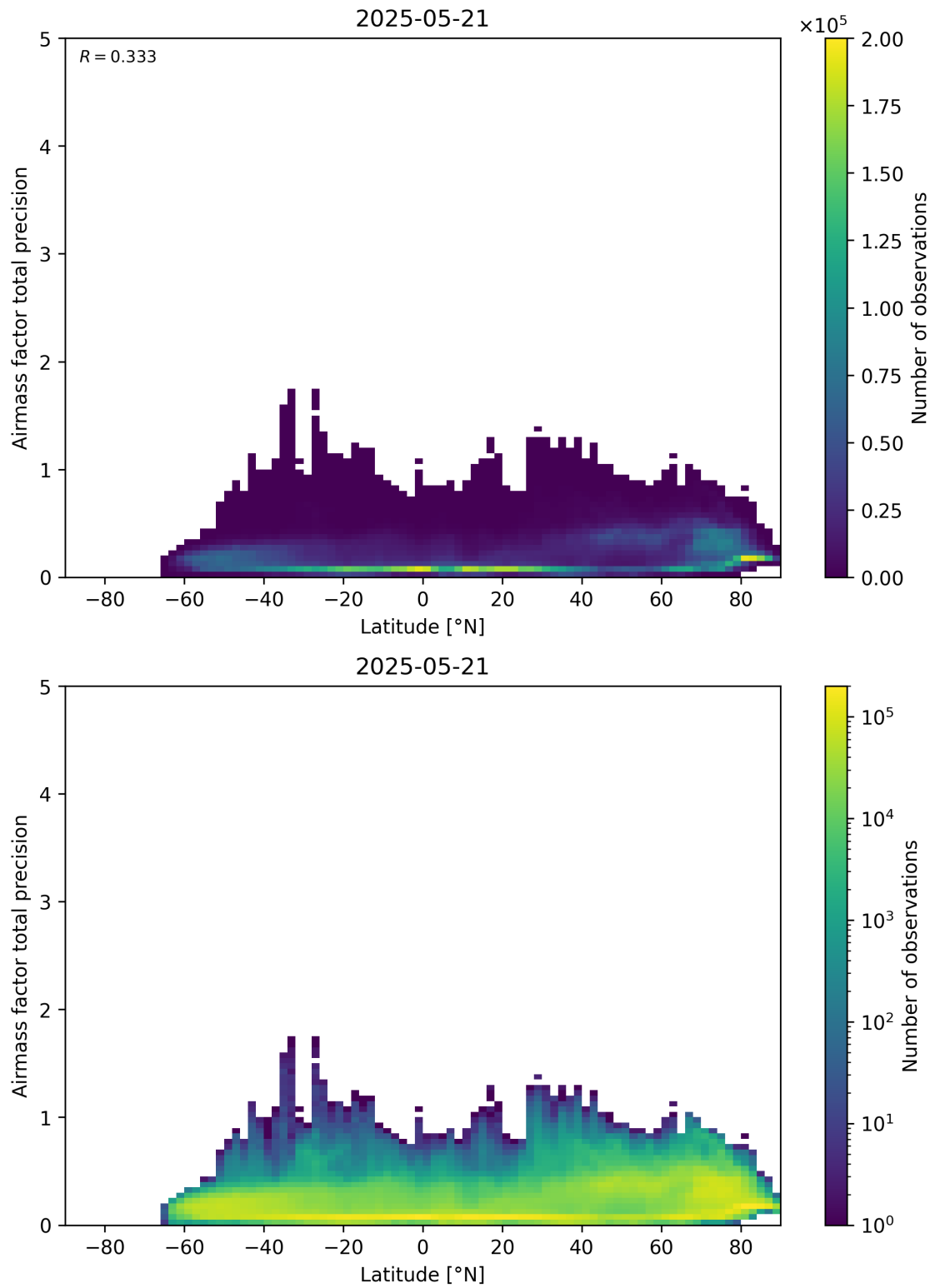
Figure 162: Scatter density plot of “Latitude” against “Airmass factor total precision” for 2025-05-21 to 2025-05-22.
