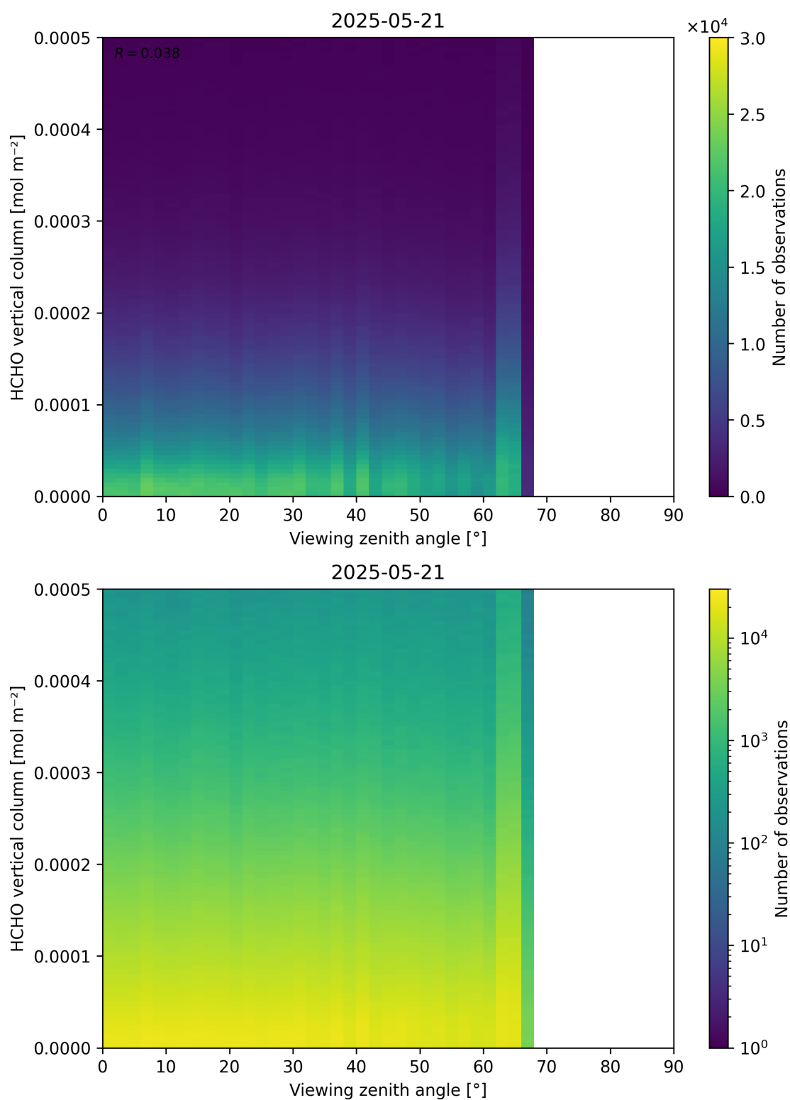
Figure 192: Scatter density plot of “Viewing zenith angle” against “HCHO vertical column” for 2025-05-21 to 2025-05-22.
