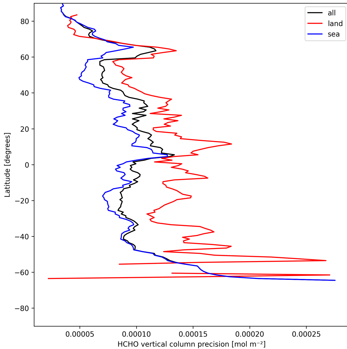
Figure 22: Zonal average of “HCHO vertical column precision” for 2025-05-21 to 2025-05-22.
