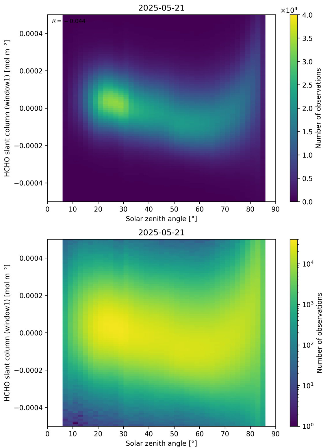
Figure 173: Scatter density plot of “Solar zenith angle” against “HCHO slant column (window1)” for 2025-05-21 to 2025-05-22.
