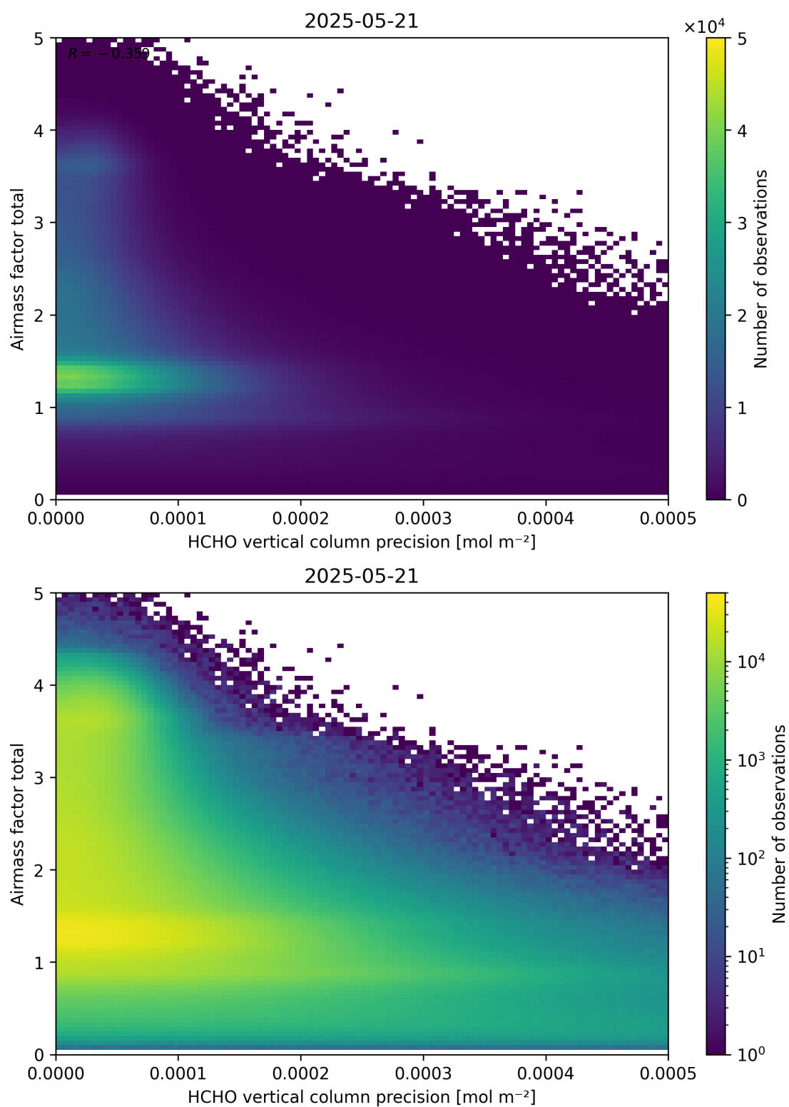
Figure 144: Scatter density plot of “HCHO vertical column precision” against “Airmass factor total” for 2025-05-21 to 2025-05-22.
