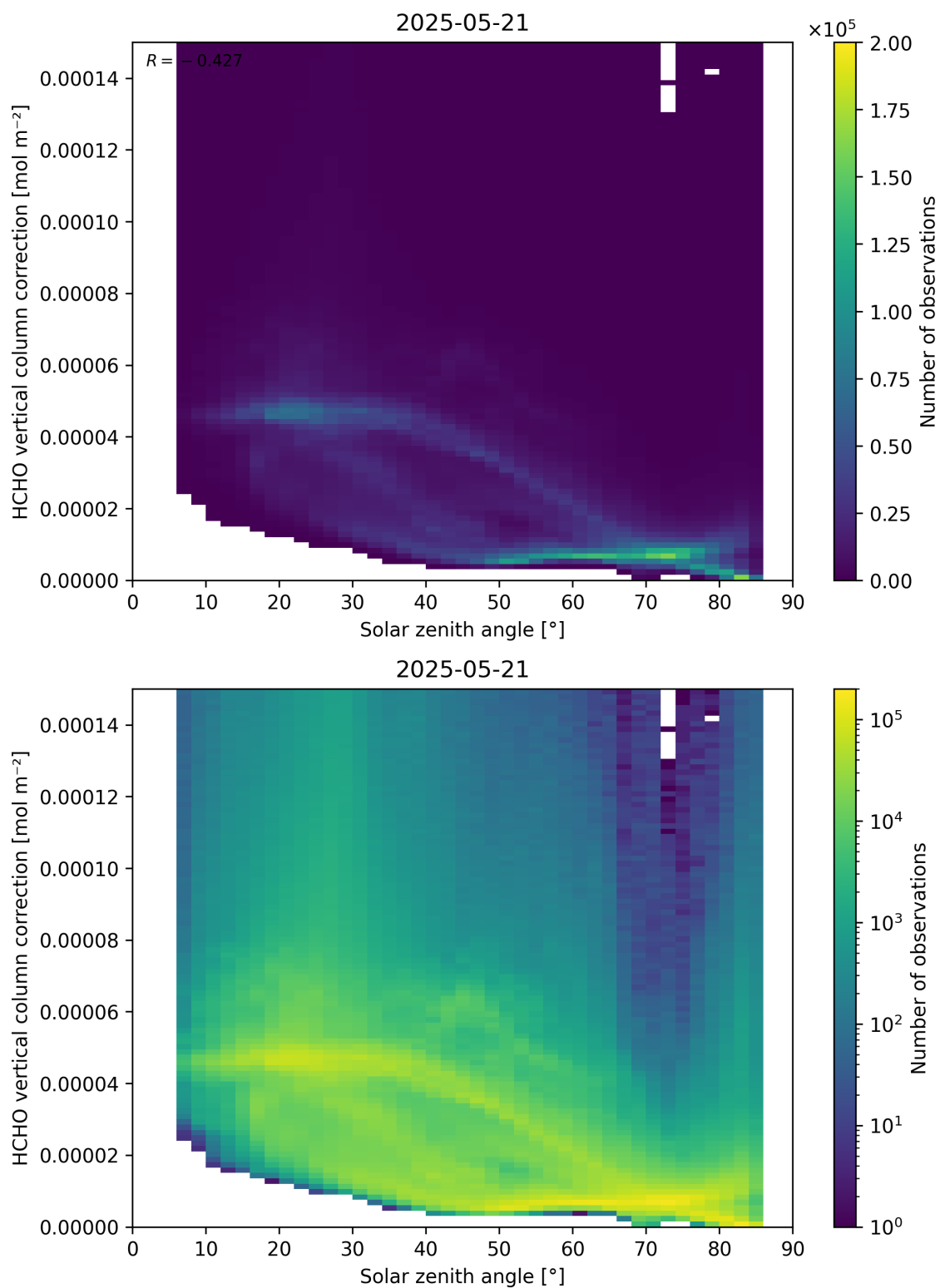
Figure 178: Scatter density plot of “Solar zenith angle” against “HCHO vertical column correction” for 2025-05-21 to 2025-05-22.
