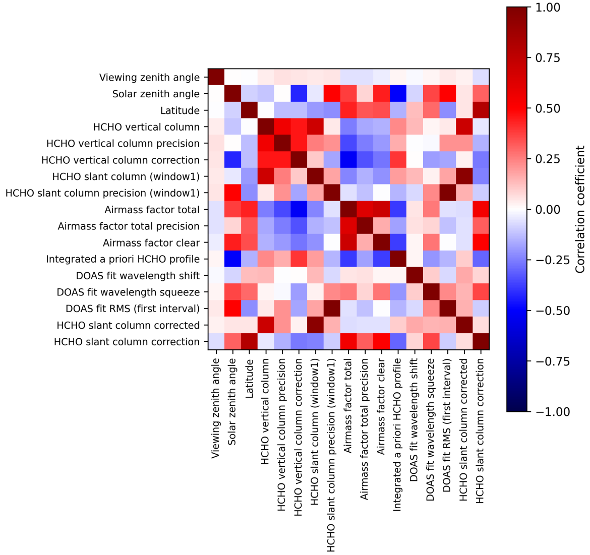
Figure 2: Map of correlation matrix for 2025-05-21 to 2025-05-22.
