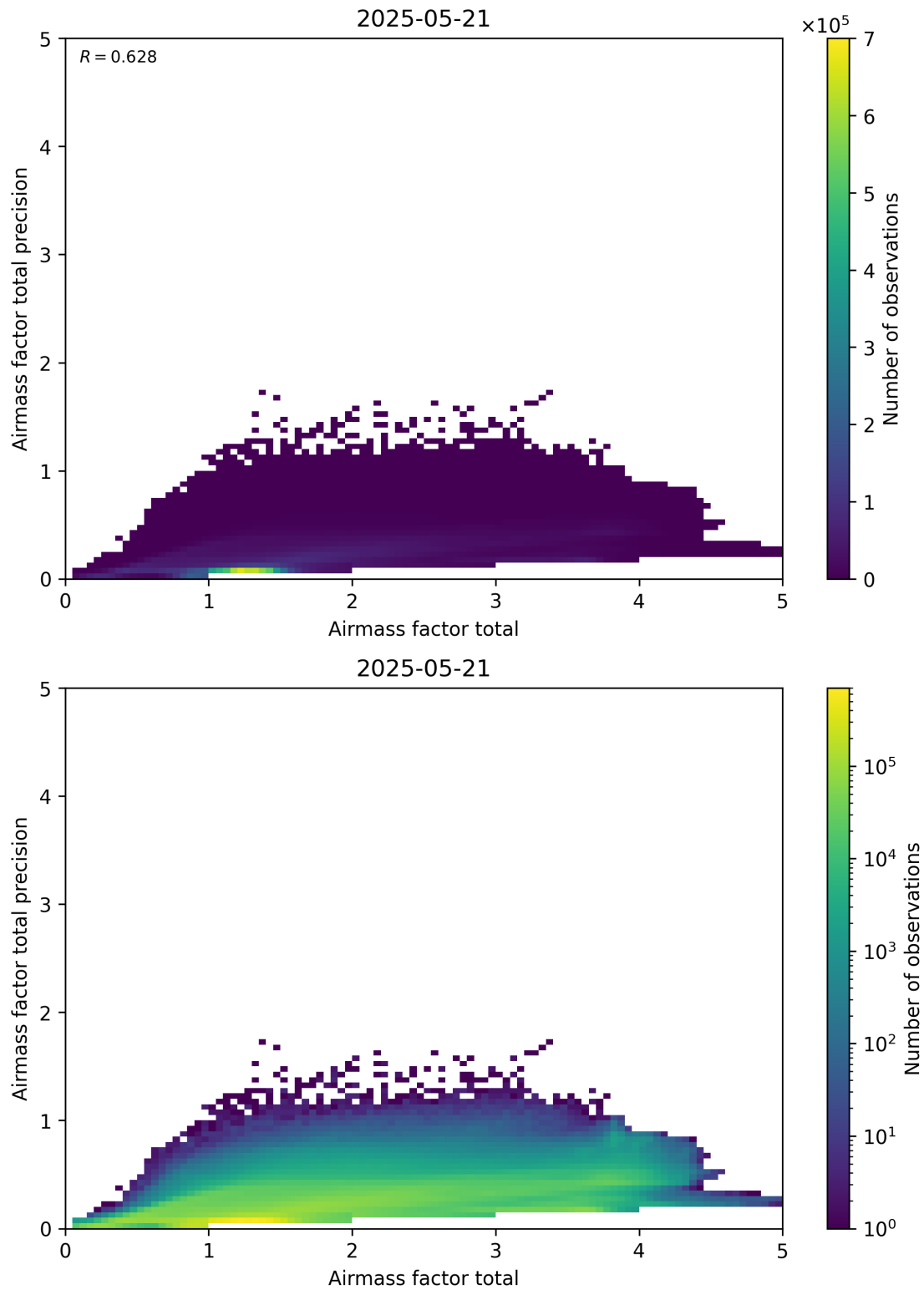
Figure 103: Scatter density plot of “Airmass factor total” against “Airmass factor total precision” for 2025-05-21 to 2025-05-22.
