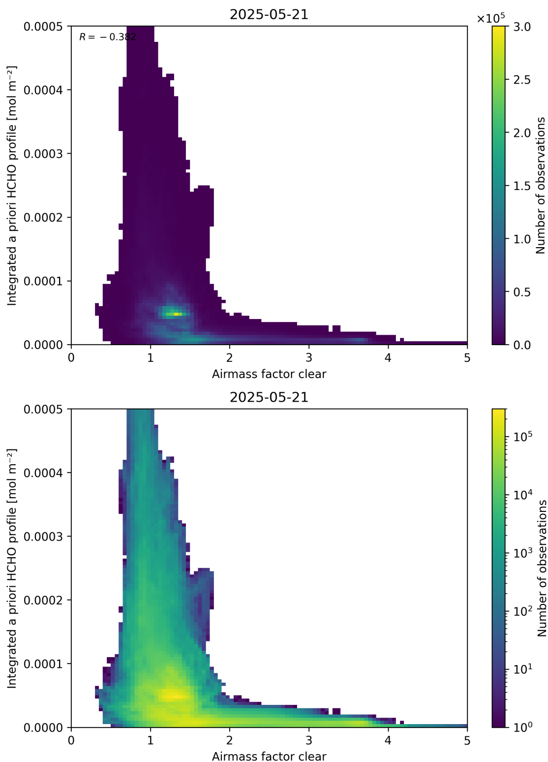
Figure 76: Scatter density plot of “Airmass factor clear” against “Integrated a priori HCHO profile” for 2025-05-21 to 2025-05-22.
