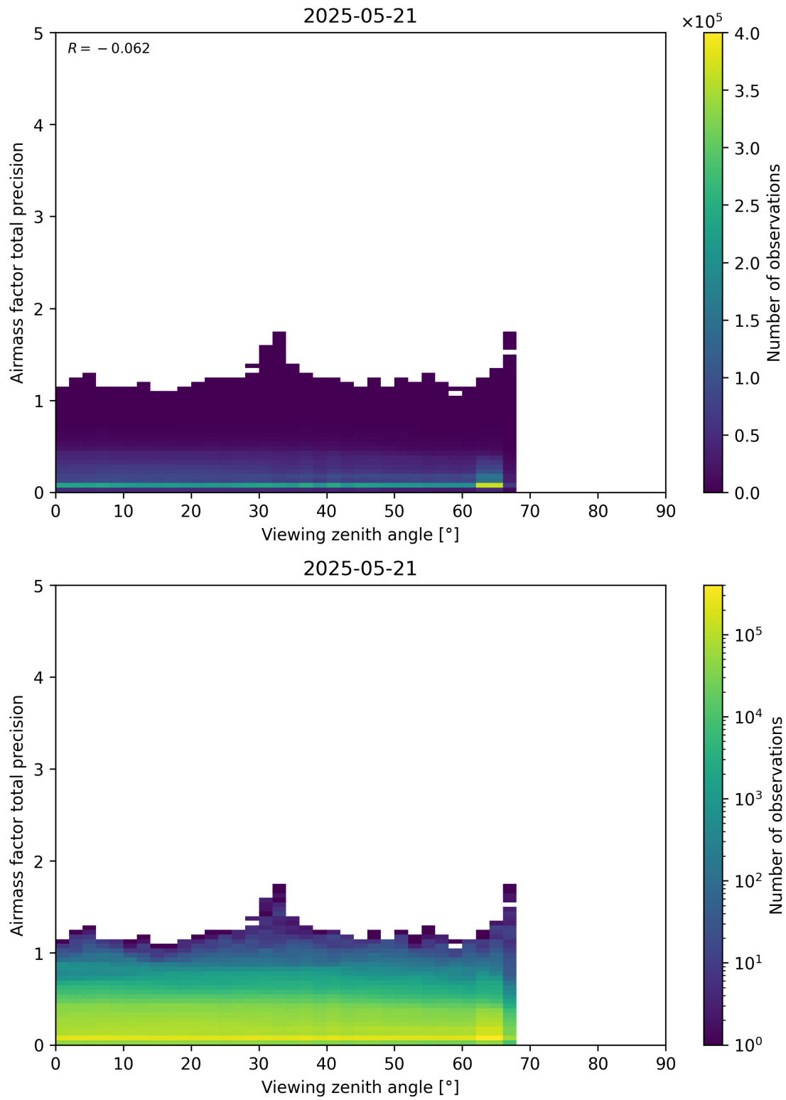
Figure 191: Scatter density plot of “Viewing zenith angle” against “Airmass factor total precision” for 2025-05-21 to 2025-05-22.
