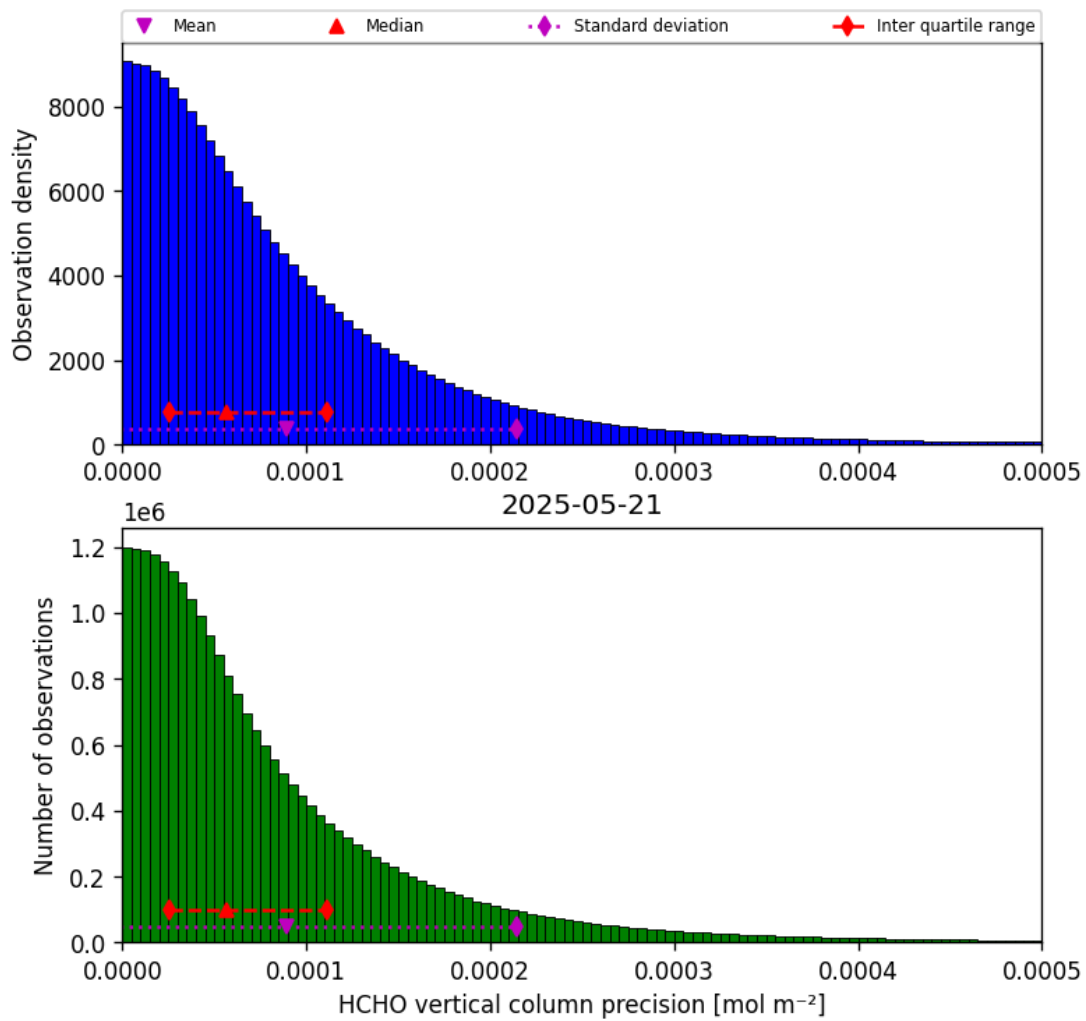
Figure 36: Histogram of “HCHO vertical column precision” for 2025-05-21 to 2025-05-22
