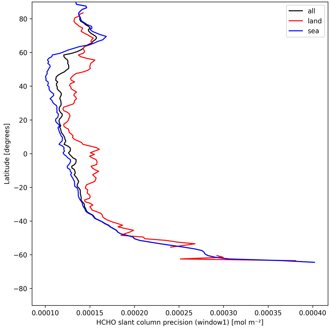
Figure 25: Zonal average of “HCHO slant column precision (window1)” for 2025-05-21 to 2025-05-22.
