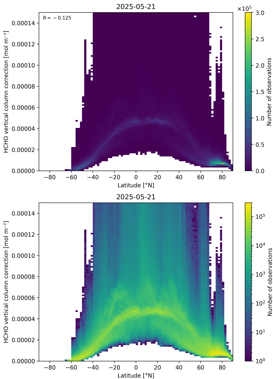
Figure 164: Scatter density plot of “Latitude” against “HCHO vertical column correction” for 2025-05-21 to 2025-05-22.
