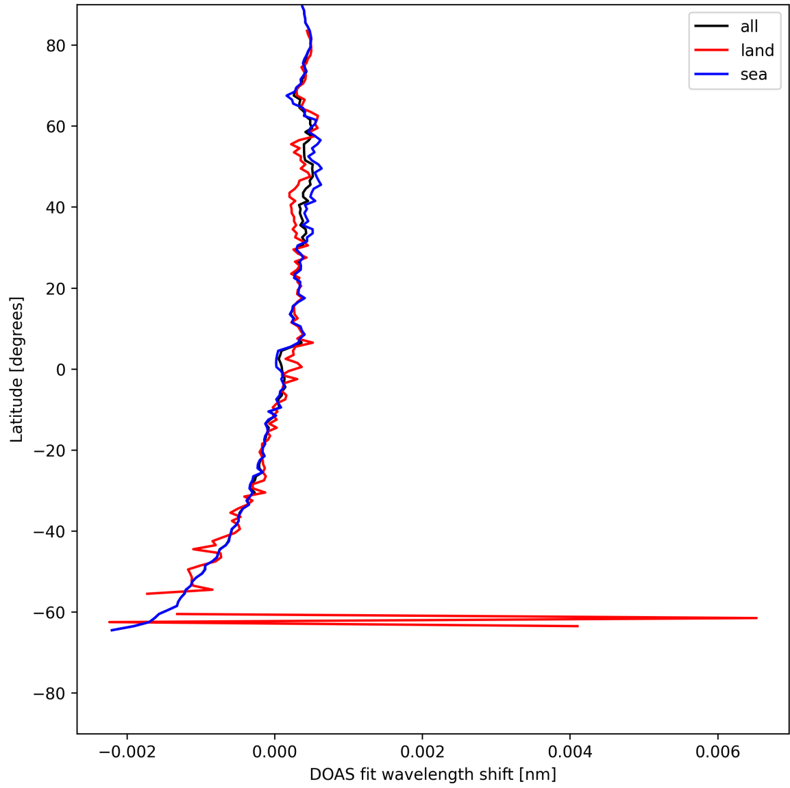
Figure 30: Zonal average of "DOAS fit wavelength shift" for 2025-05-21 to 2025-05-22.
