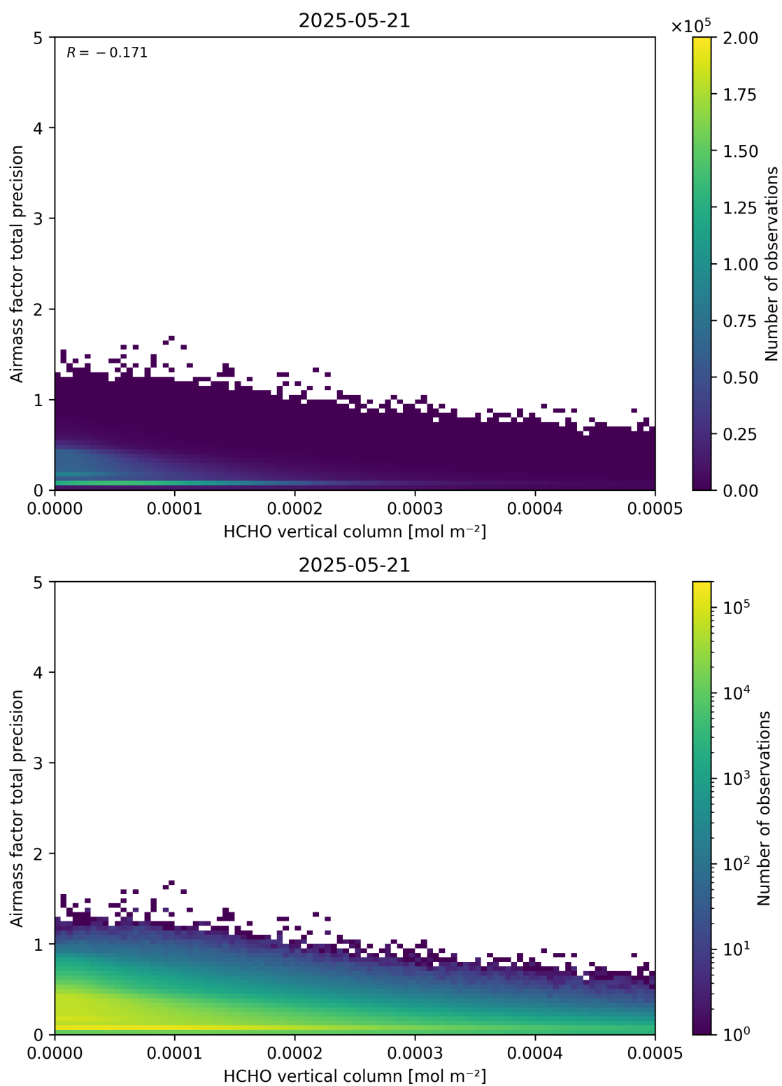
Figure 132: Scatter density plot of “HCHO vertical column” against “Airmass factor total precision” for 2025-05-21 to 2025-05-22.
