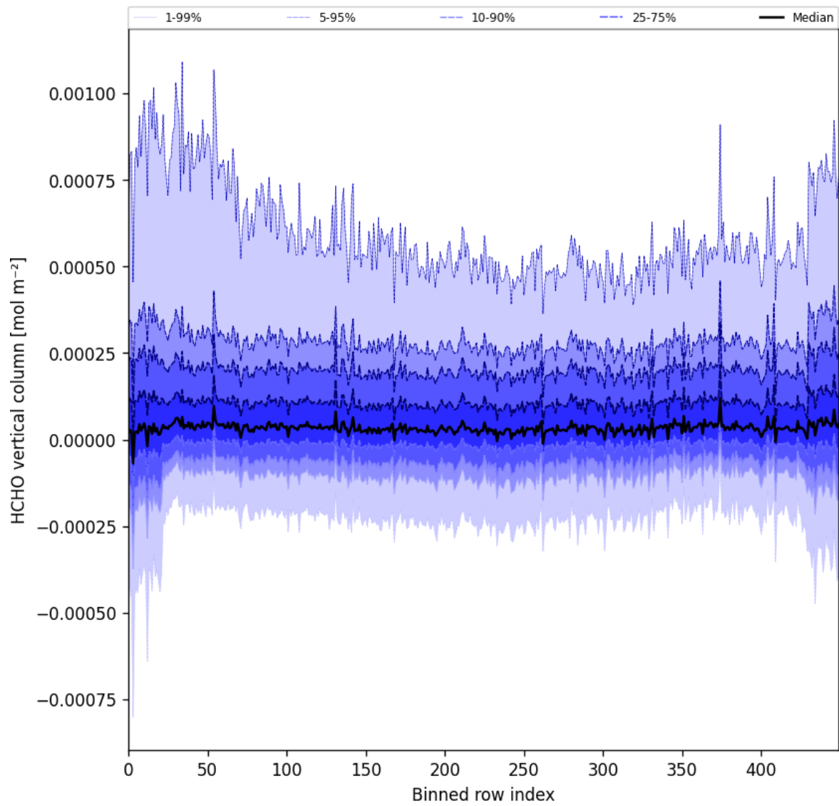
Figure 49: Along track statistics of “HCHO vertical column” for 2025-05-21 to 2025-05-22
