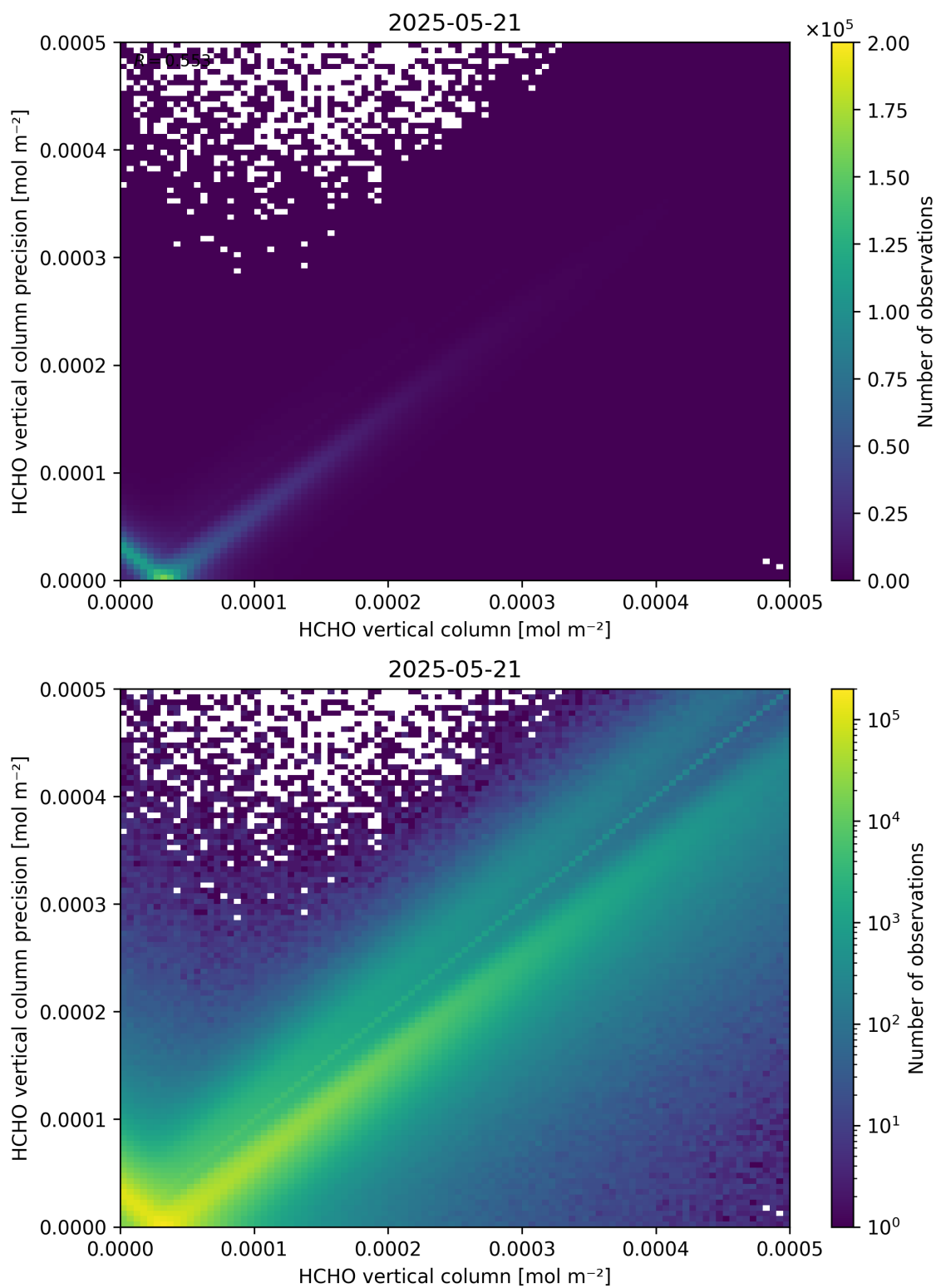
Figure 134: Scatter density plot of “HCHO vertical column” against “HCHO vertical column precision” for 2025-05-21 to 2025-05-22.
