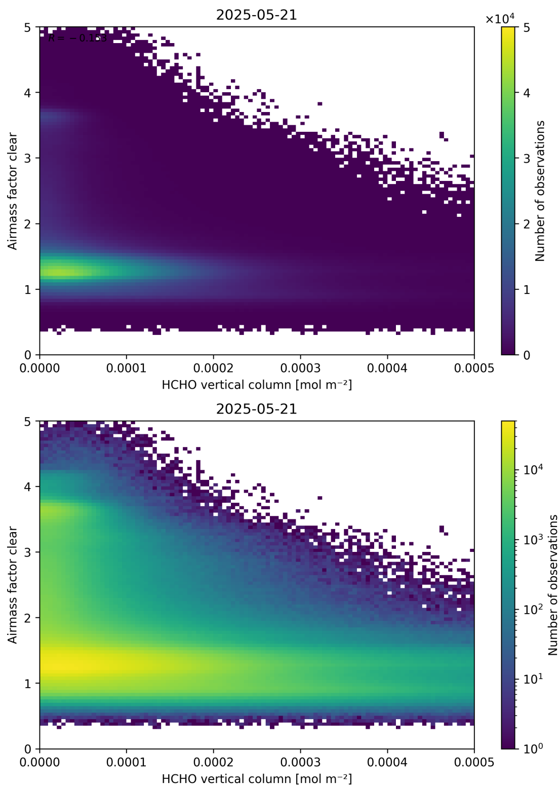
Figure 126: Scatter density plot of “HCHO vertical column” against “Airmass factor clear” for 2025-05-21 to 2025-05-22.
