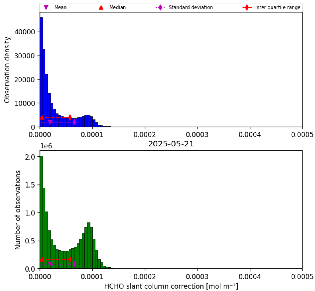
Figure 47: Histogram of “HCHO slant column correction” for 2025-05-21 to 2025-05-22
