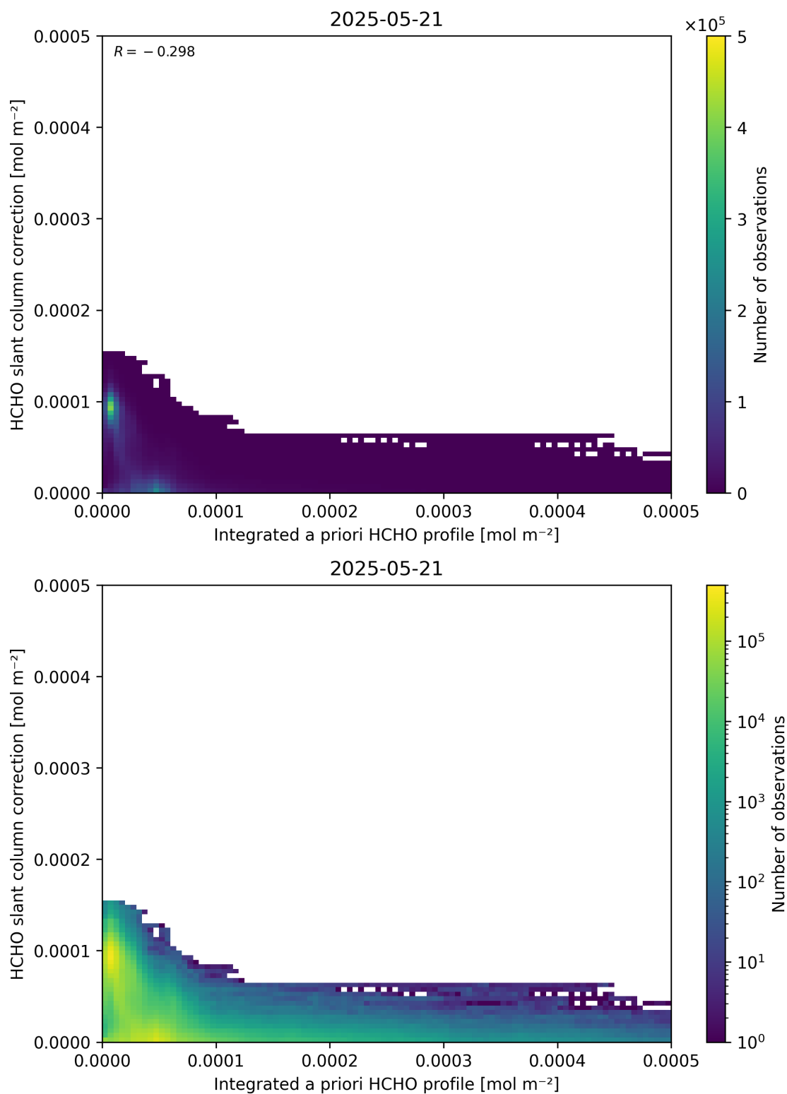
Figure 152: Scatter density plot of “Integrated a priori HCHO profile” against “HCHO slant column correction” for 2025-05-21 to 2025-05-22.
