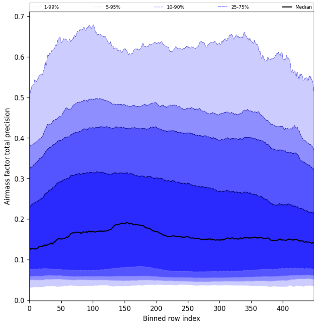
Figure 55: Along track statistics of “Airmass factor total precision” for 2025-05-21 to 2025-05-22
