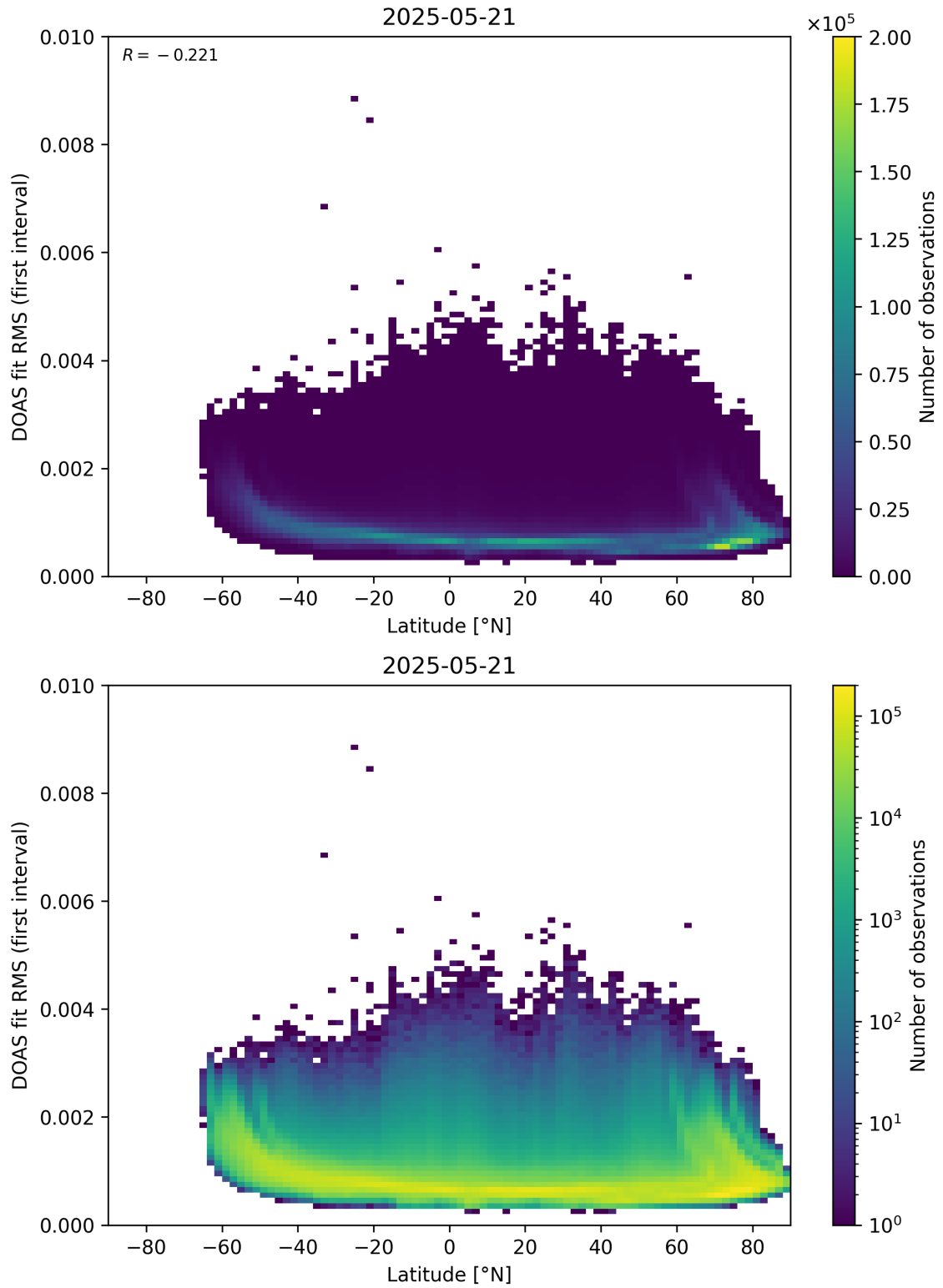
Figure 153: Scatter density plot of “Latitude” against “DOAS fit RMS (first interval)” for 2025-05-21 to 2025-05-22.
