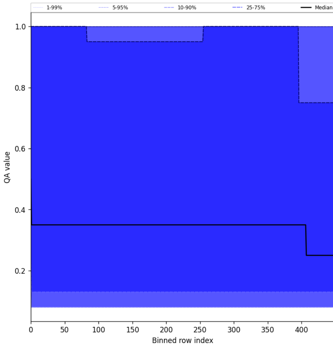
Figure 48: Along track statistics of “QA value” for 2025-05-21 to 2025-05-22
