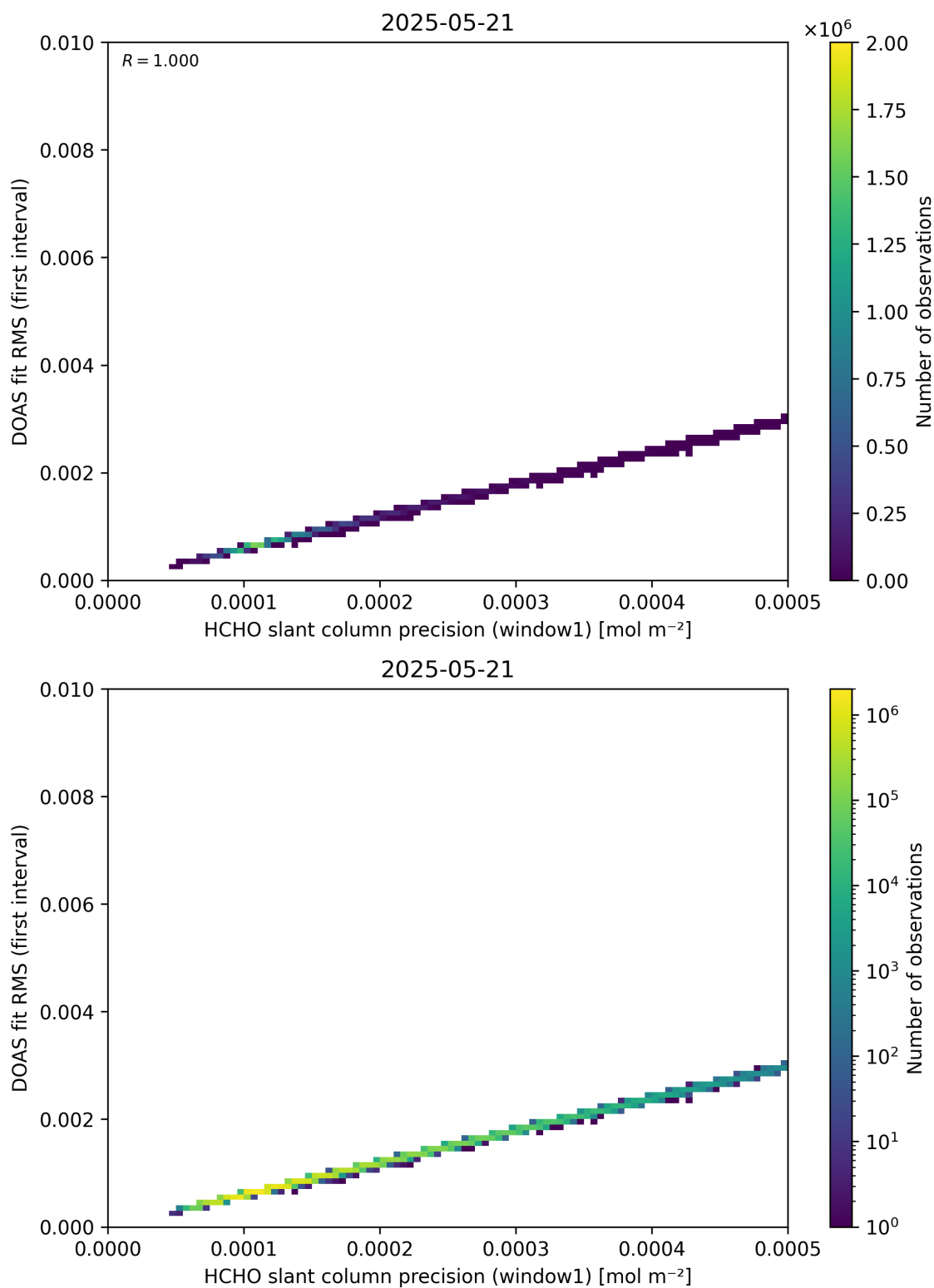
Figure 88: Scatter density plot of “HCHO slant column precision (window1)” against “DOAS fit RMS (first interval)” for 2025-05-21 to 2025-05-22.
