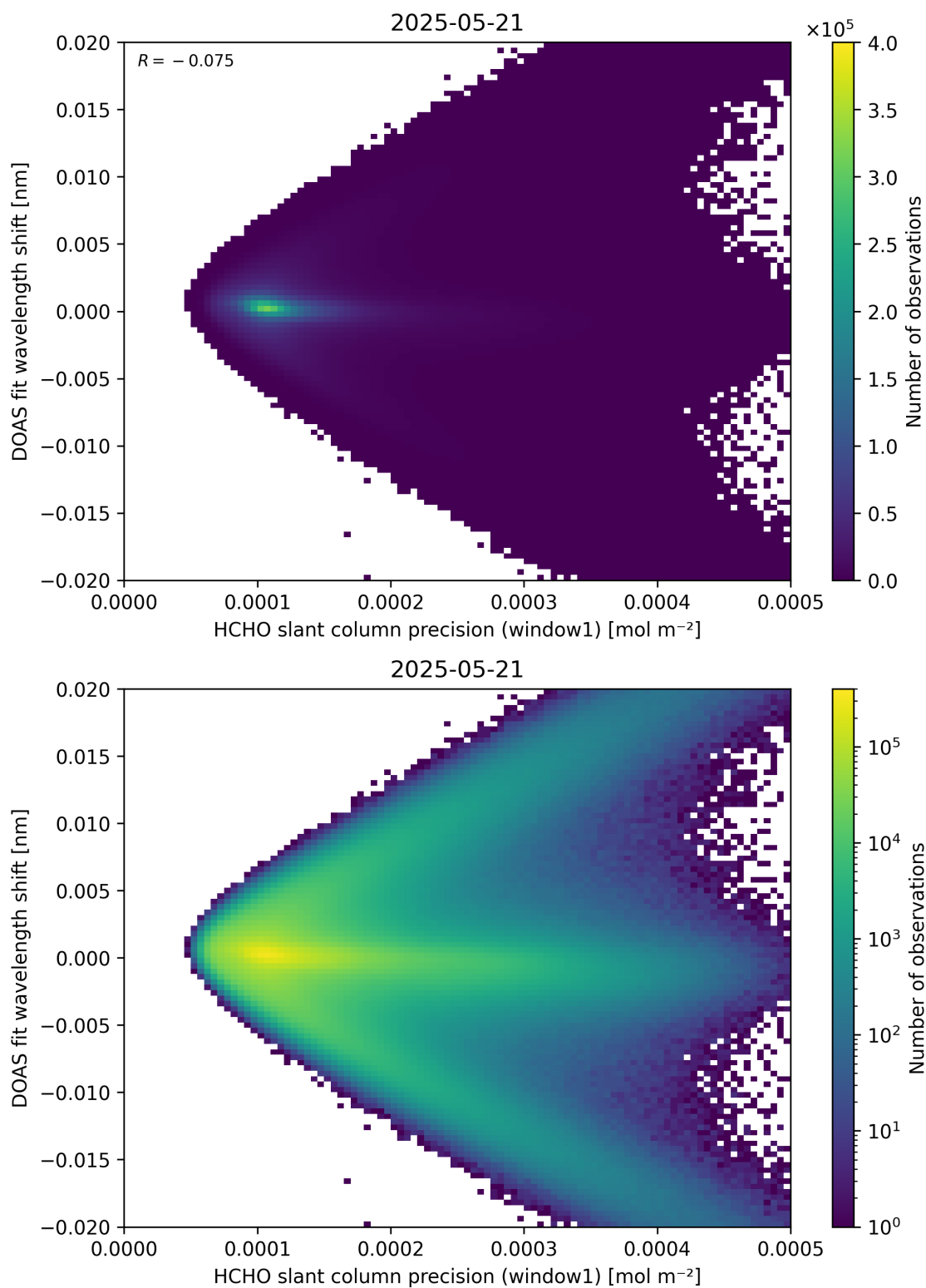
Figure 89: Scatter density plot of “HCHO slant column precision (window1)” against “DOAS fit wavelength shift” for 2025-05-21 to 2025-05-22.
