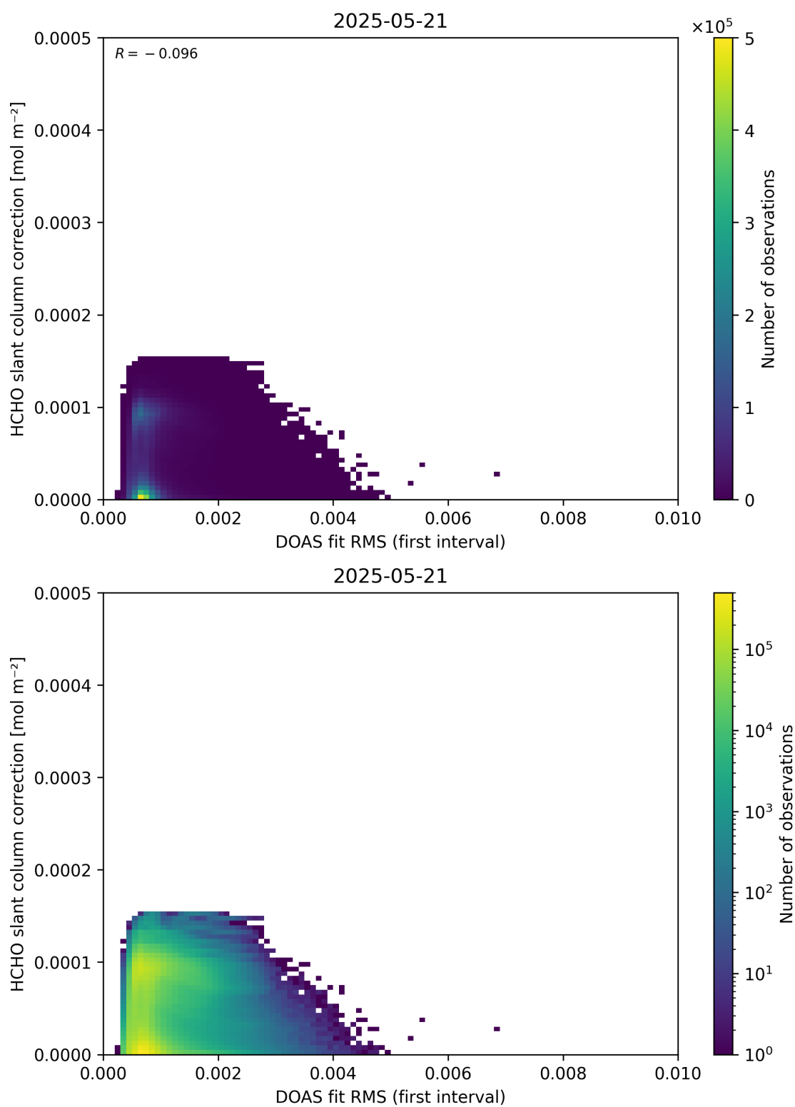
Figure 63: Scatter density plot of “DOAS fit RMS (first interval)” against “HCHO slant column correction” for 2025-05-21 to 2025-05-22.
