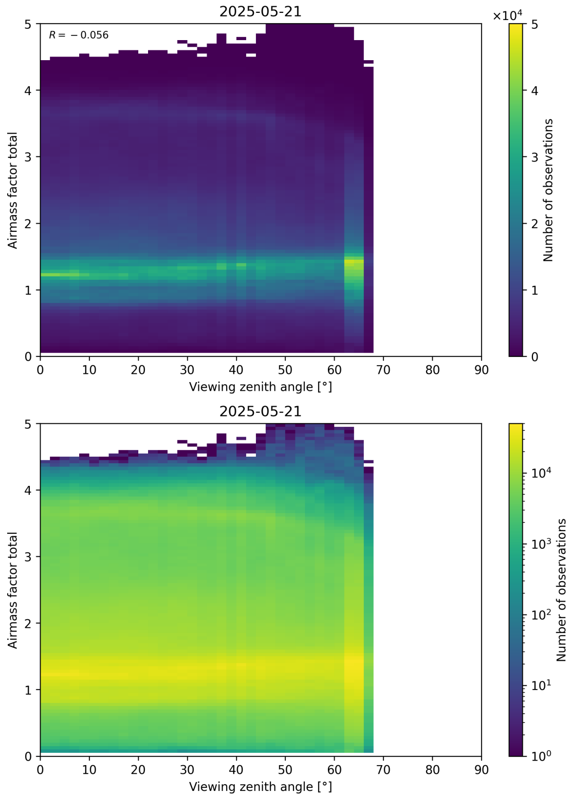
Figure 190: Scatter density plot of “Viewing zenith angle” against “Airmass factor total” for 2025-05-21 to 2025-05-22.
