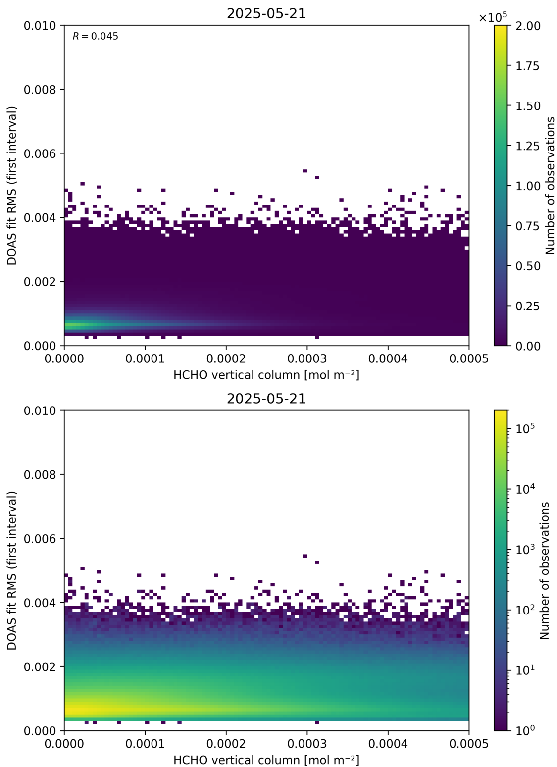
Figure 123: Scatter density plot of “HCHO vertical column” against “DOAS fit RMS (first interval)” for 2025-05-21 to 2025-05-22.
