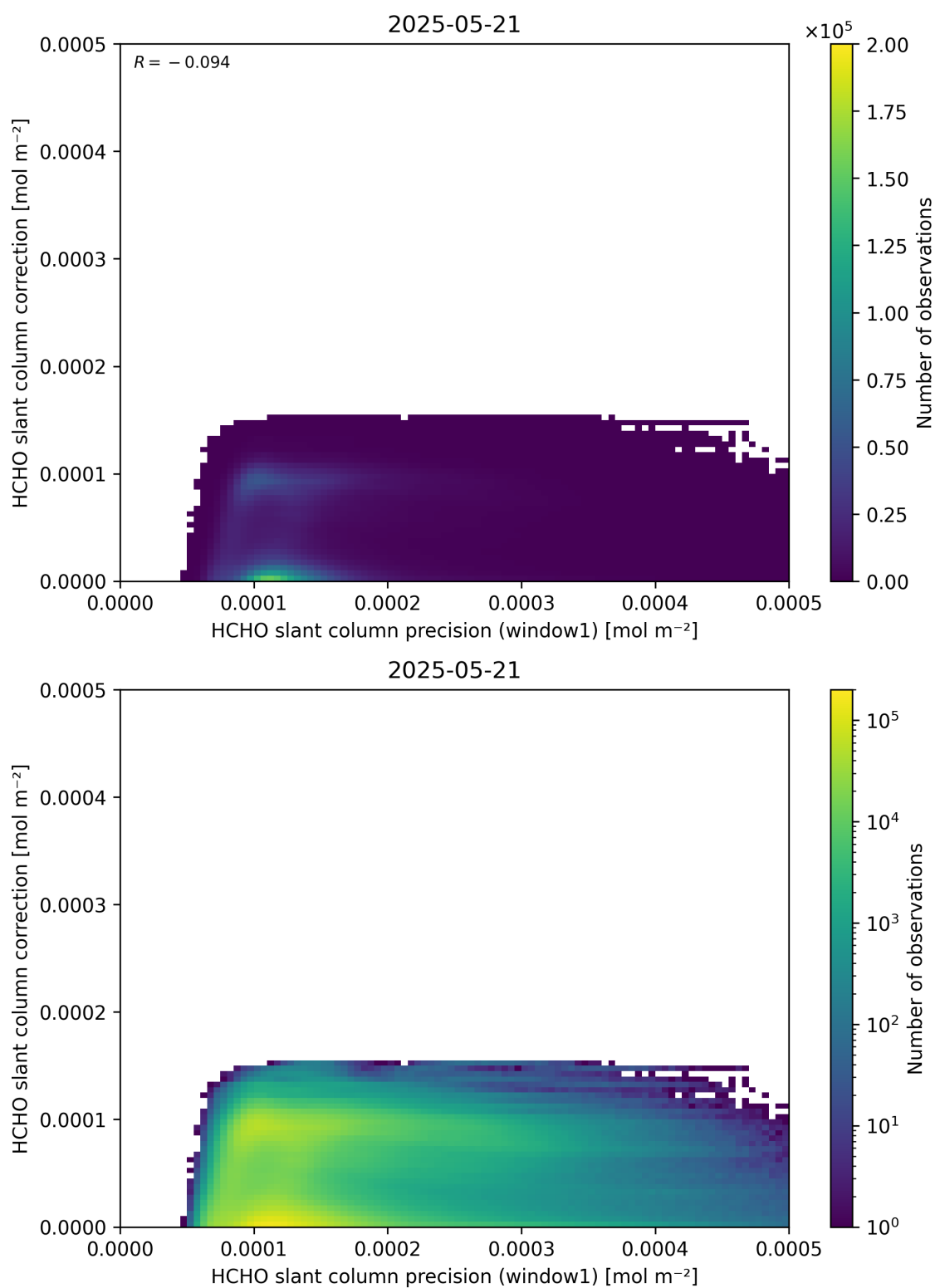
Figure 93: Scatter density plot of “HCHO slant column precision (window1)” against “HCHO slant column correction” for 2025-05-21 to 2025-05-22.
