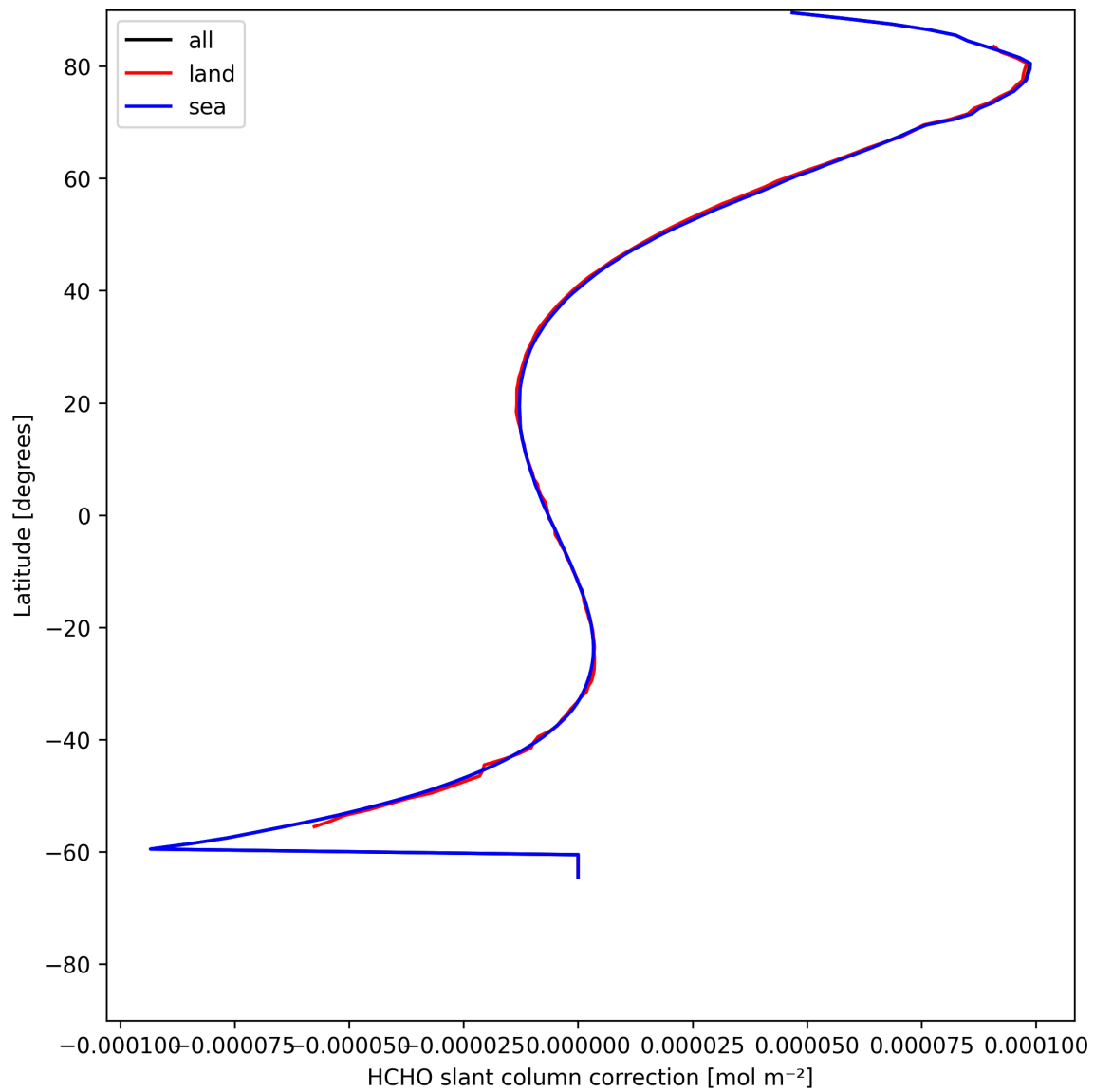
Figure 33: Zonal average of “HCHO slant column correction” for 2025-05-21 to 2025-05-22.
