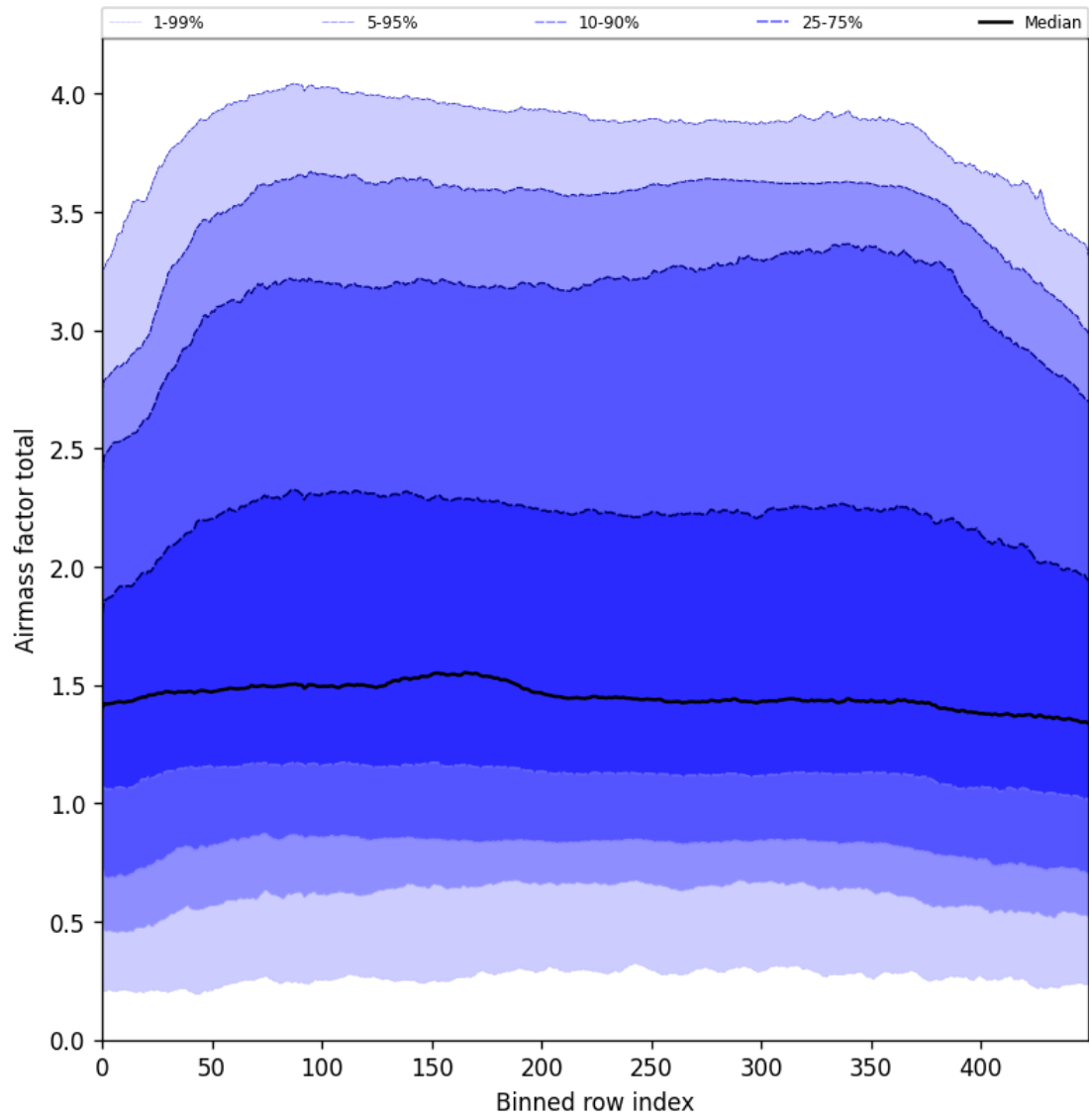
Figure 54: Along track statistics of “Airmass factor total” for 2025-05-21 to 2025-05-22
