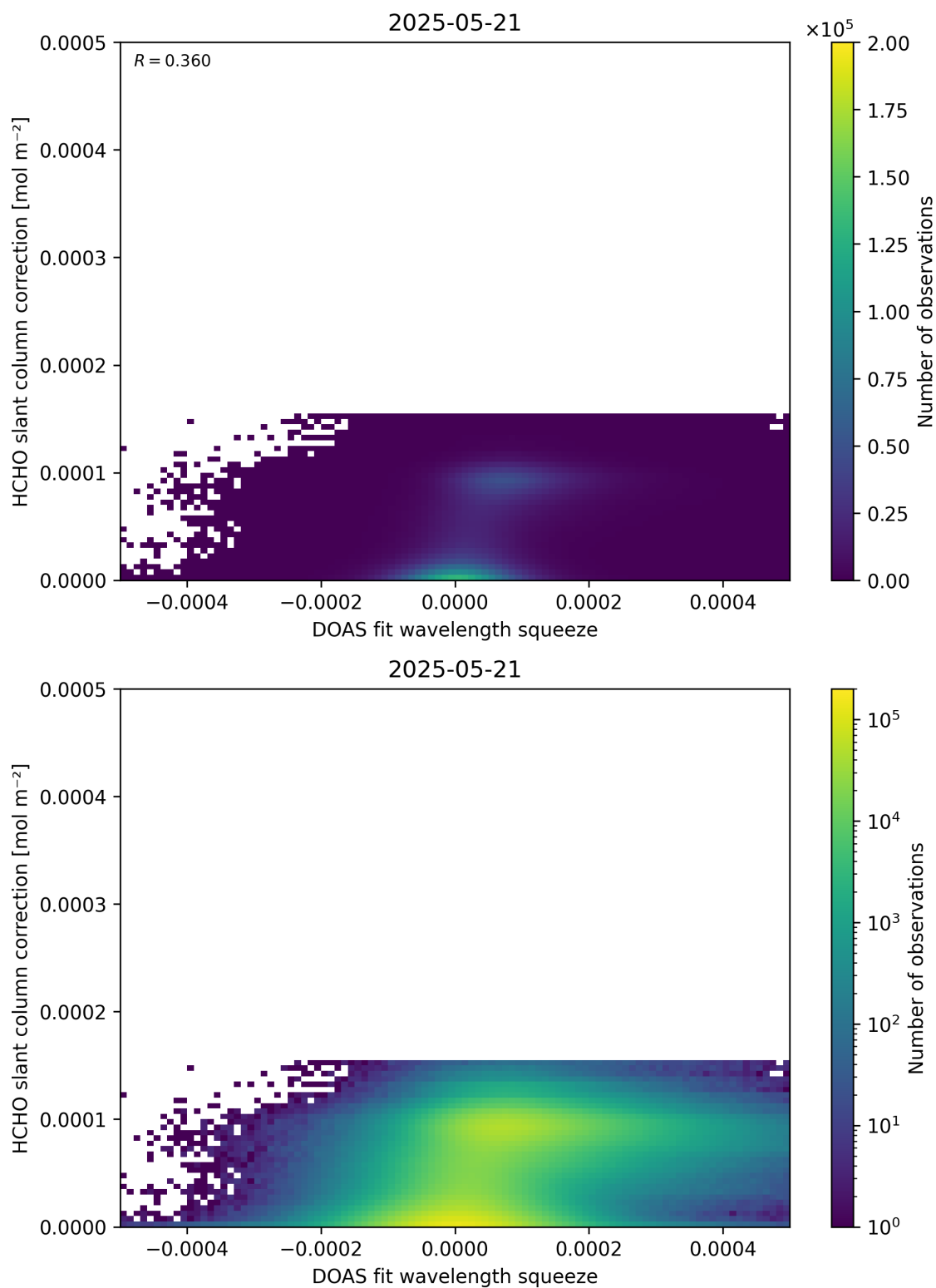
Figure 70: Scatter density plot of “DOAS fit wavelength squeeze” against “HCHO slant column correction” for 2025-05-21 to 2025-05-22.
