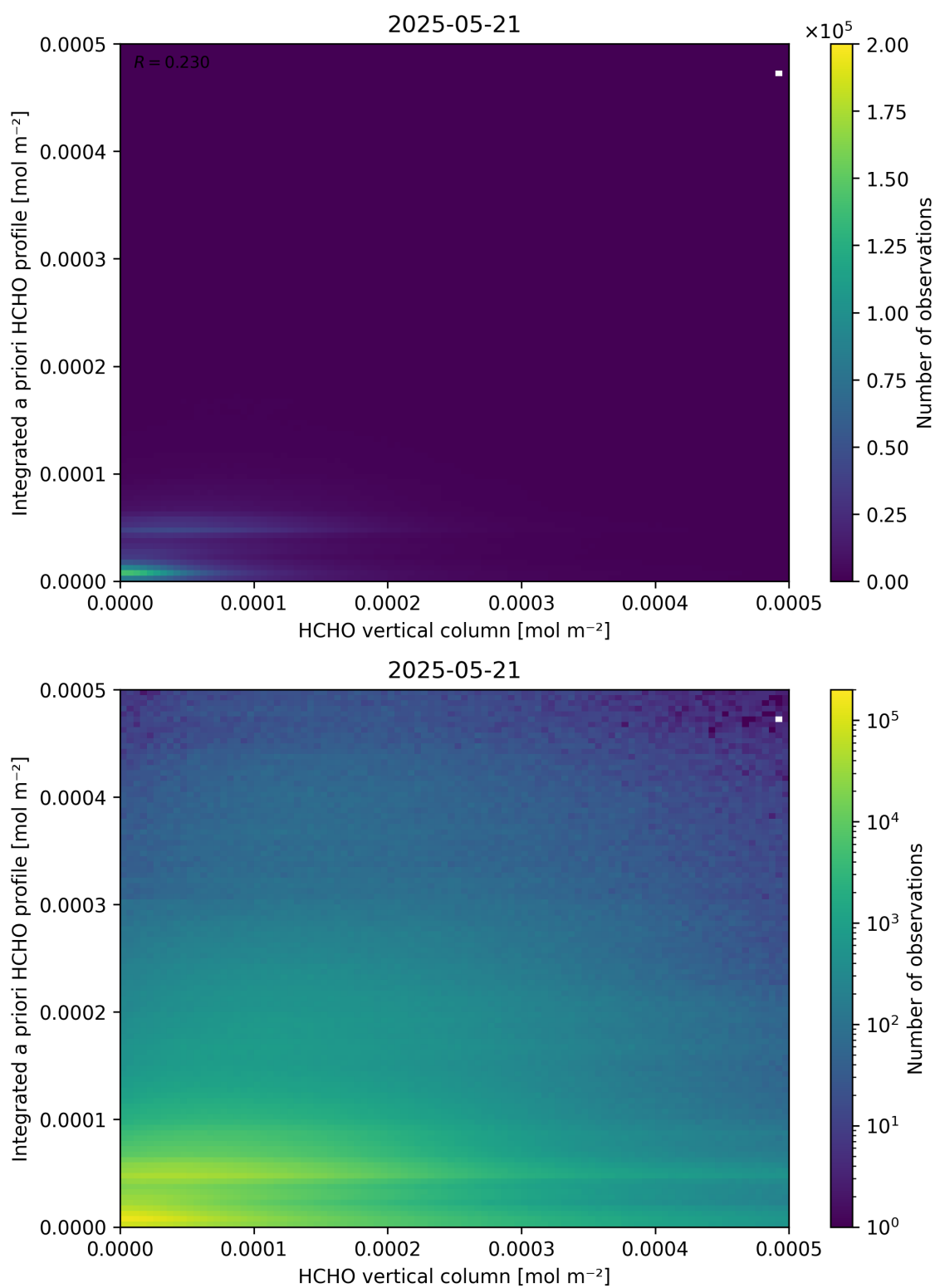
Figure 135: Scatter density plot of “HCHO vertical column” against “Integrated a priori HCHO profile” for 2025-05-21 to 2025-05-22.
