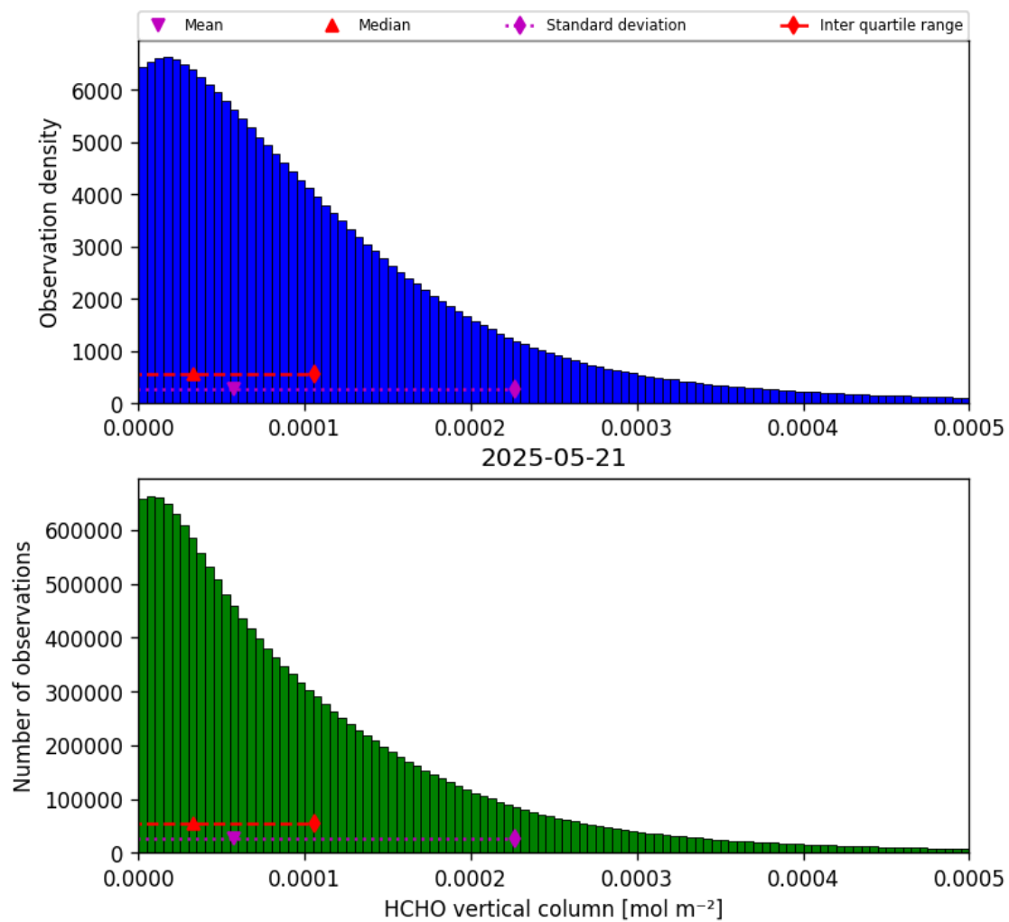
Figure 35: Histogram of “HCHO vertical column” for 2025-05-21 to 2025-05-22
