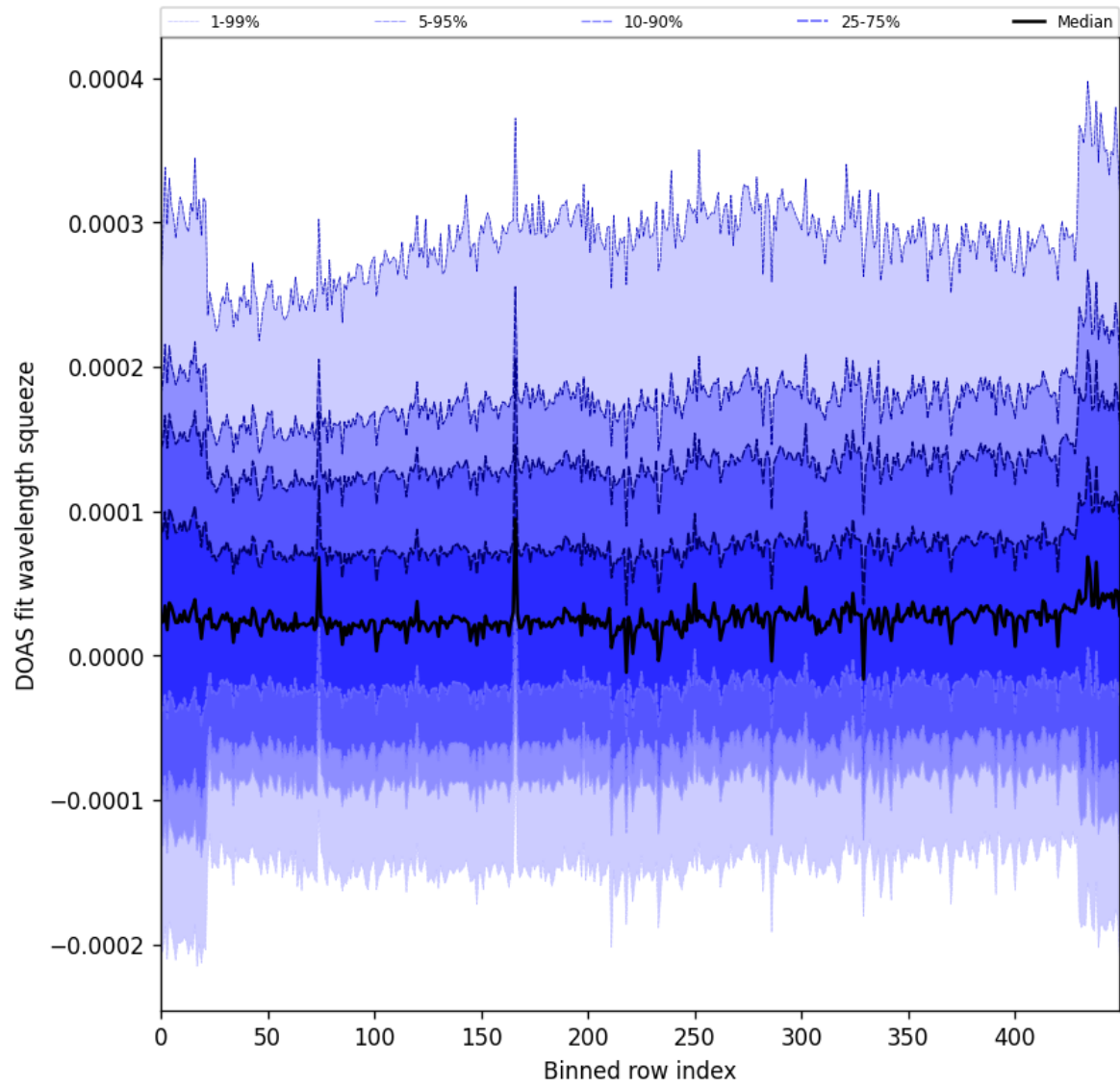
Figure 59: Along track statistics of “DOAS fit wavelength squeeze” for 2025-05-21 to 2025-05-22
