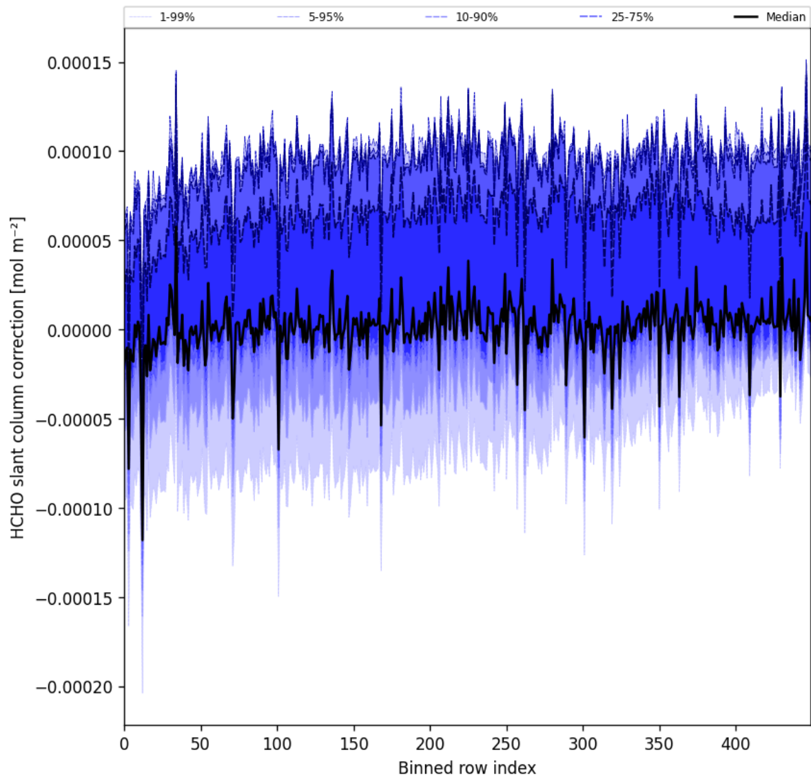
Figure 61: Along track statistics of "HCHO slant column correction" for 2025-05-21 to 2025-05-22
