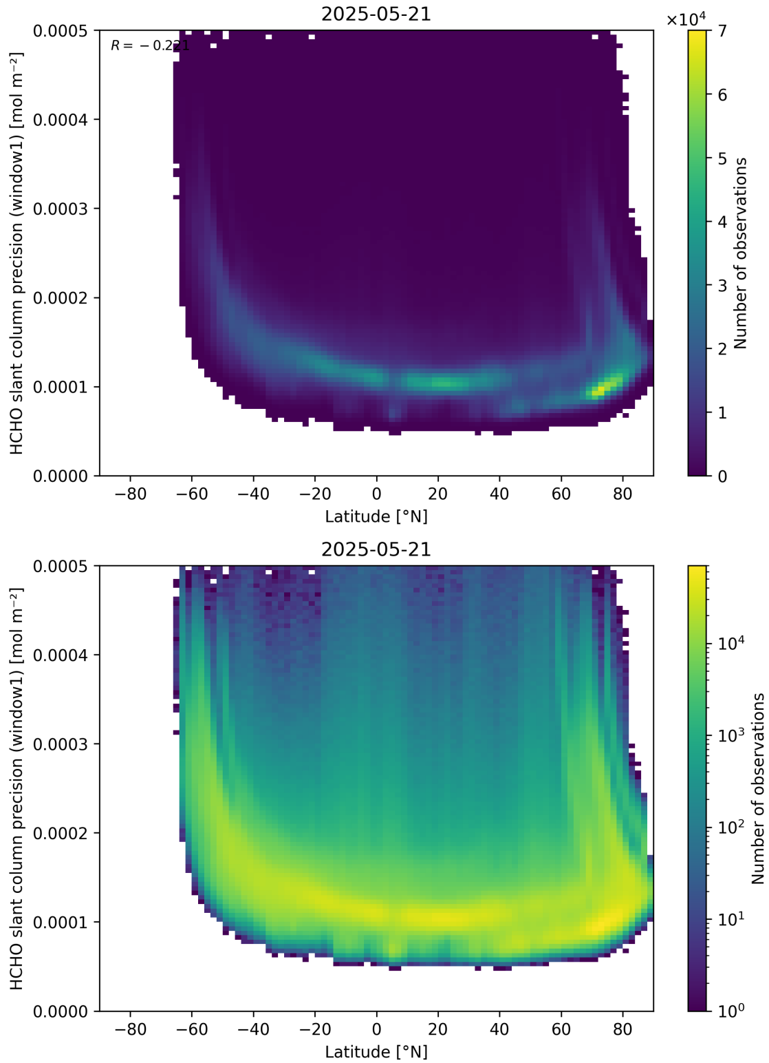
Figure 160: Scatter density plot of “Latitude” against “HCHO slant column precision (window1)” for 2025-05-21 to 2025-05-22.
