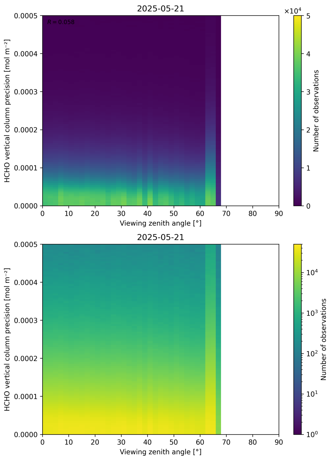
Figure 194: Scatter density plot of “Viewing zenith angle” against “HCHO vertical column precision” for 2025-05-21 to 2025-05-22.
