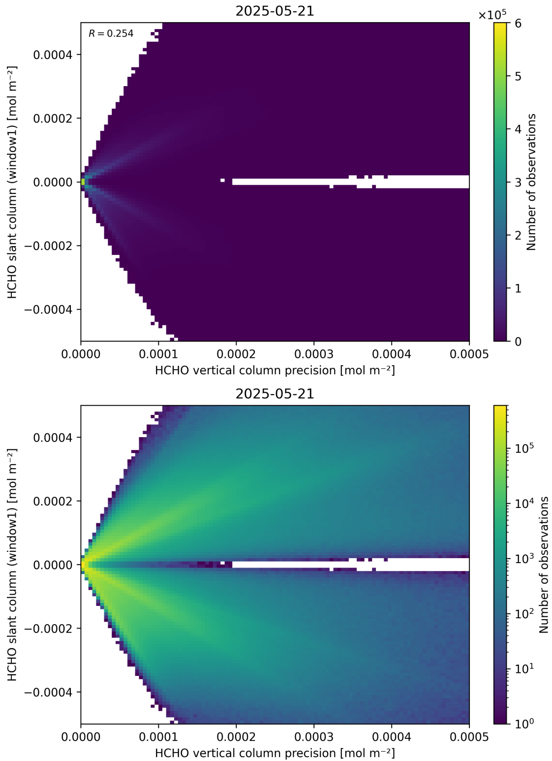
Figure 142: Scatter density plot of “HCHO vertical column precision” against “HCHO slant column (window1)” for 2025-05-21 to 2025-05-22.
