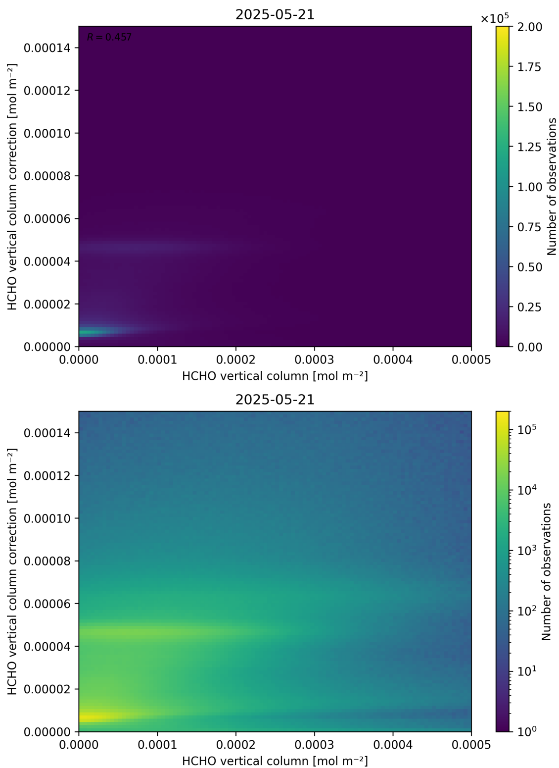
Figure 133: Scatter density plot of “HCHO vertical column” against “HCHO vertical column correction” for 2025-05-21 to 2025-05-22.
