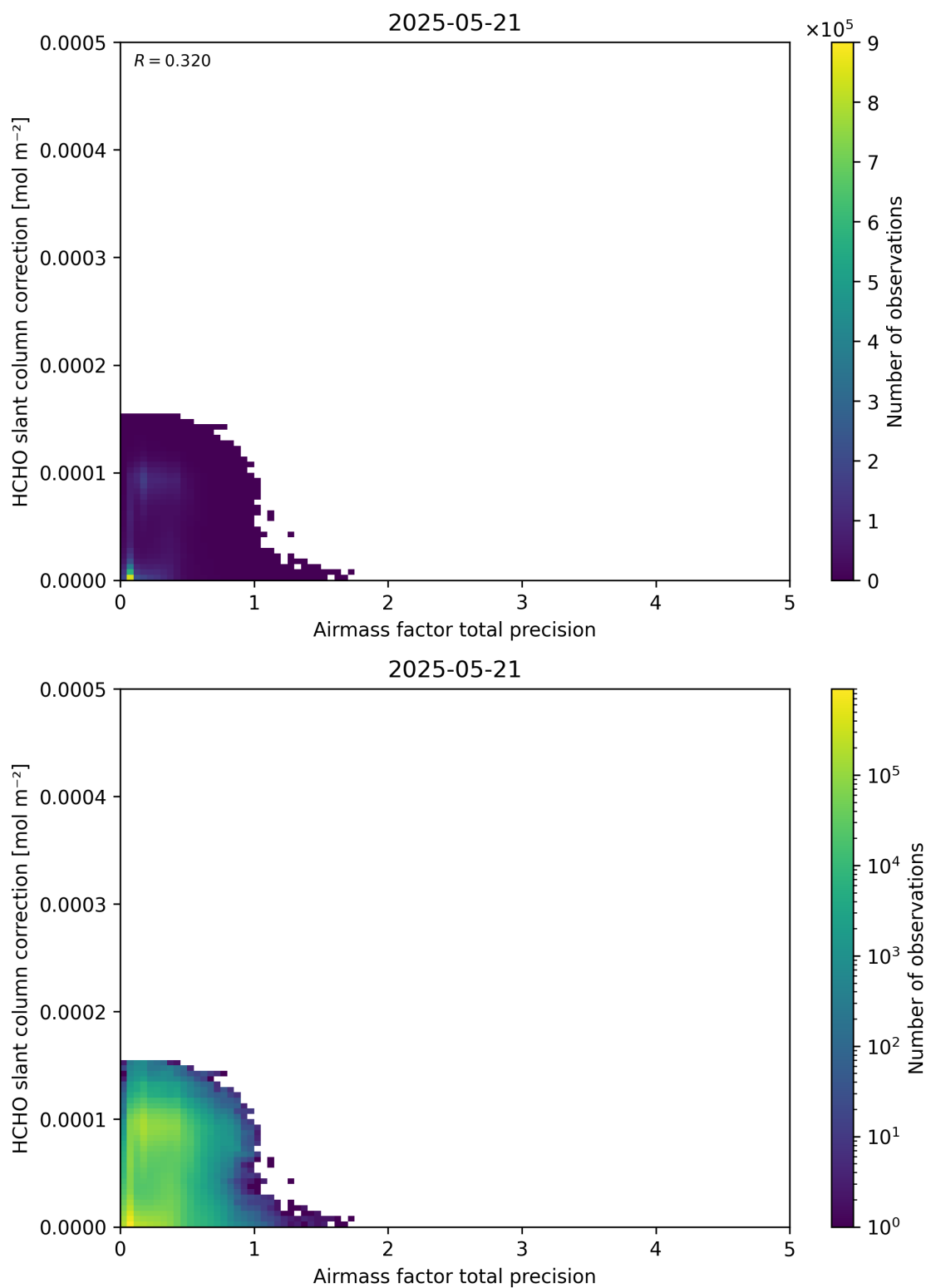
Figure 110: Scatter density plot of “Airmass factor total precision” against “HCHO slant column correction” for 2025-05-21 to 2025-05-22.
