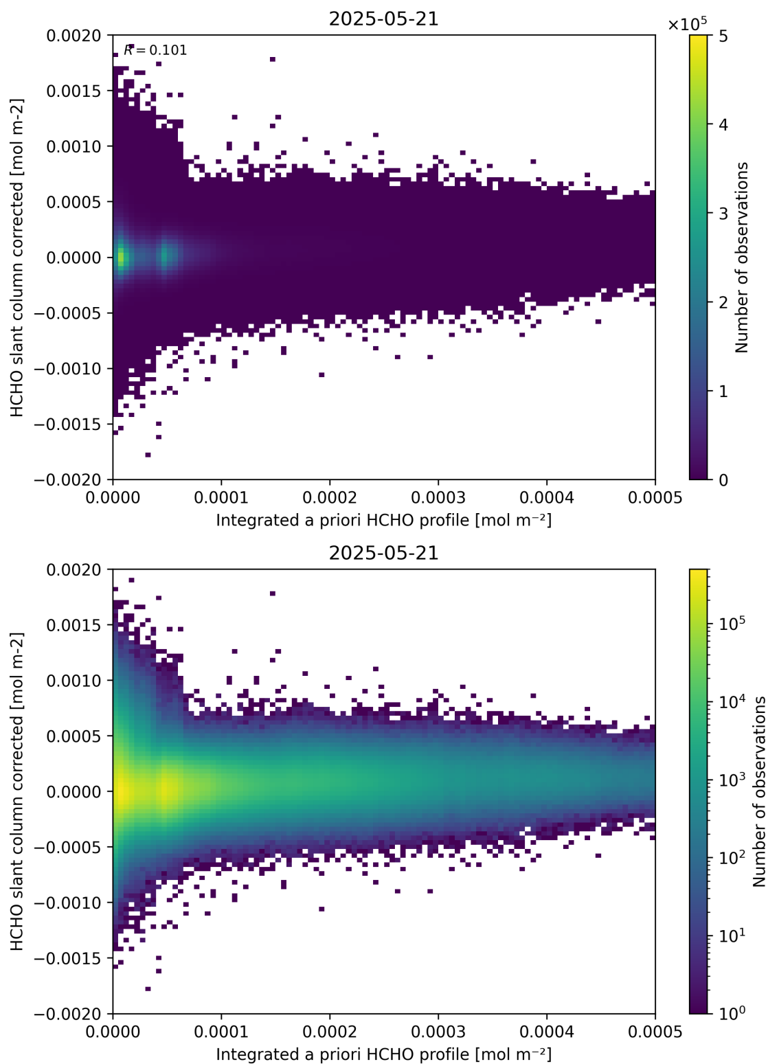
Figure 151: Scatter density plot of “Integrated a priori HCHO profile” against “HCHO slant column corrected” for 2025-05-21 to 2025-05-22.
