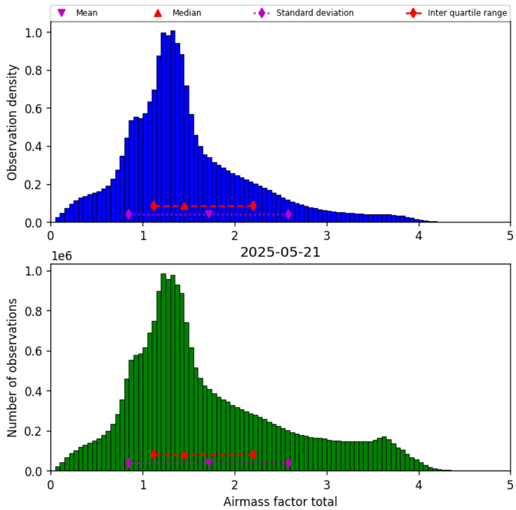
Figure 40: Histogram of “Airmass factor total” for 2025-05-21 to 2025-05-22
