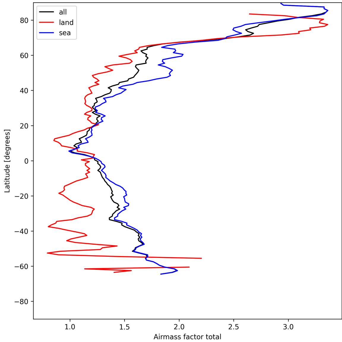
Figure 26: Zonal average of “Airmass factor total” for 2025-05-21 to 2025-05-22.
