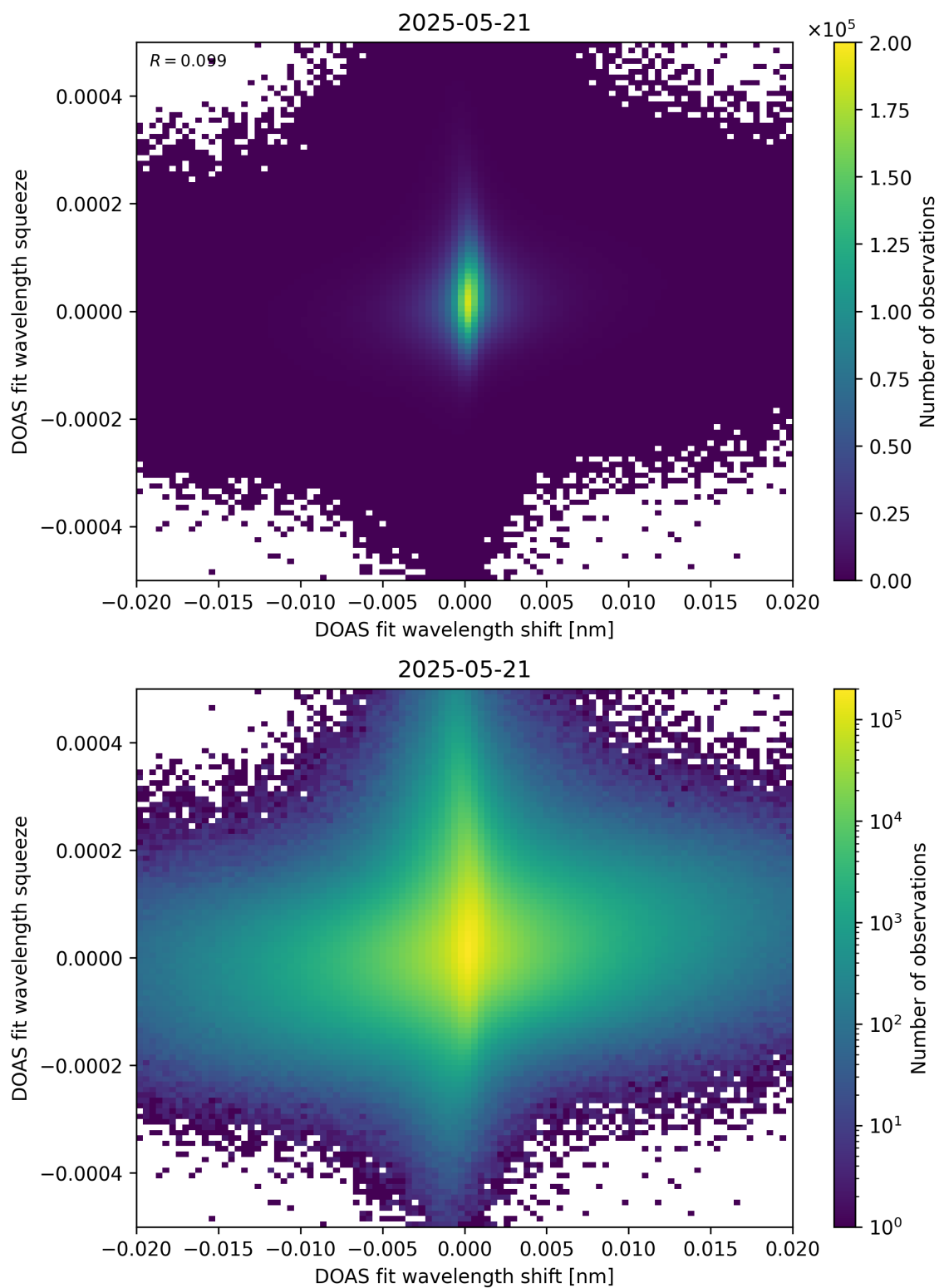
Figure 65: Scatter density plot of “DOAS fit wavelength shift” against “DOAS fit wavelength squeeze” for 2025-05-21 to 2025-05-22.
