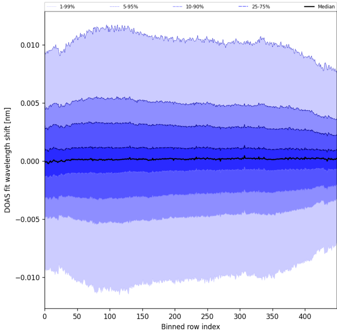
Figure 58: Along track statistics of “DOAS fit wavelength shift” for 2025-05-21 to 2025-05-22
