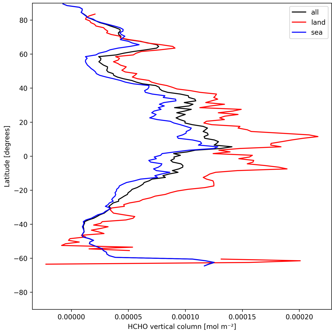
Figure 21: Zonal average of “HCHO vertical column” for 2025-05-21 to 2025-05-22.
