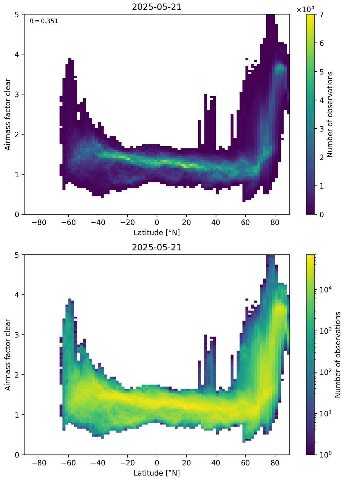
Figure 156: Scatter density plot of “Latitude” against “Airmass factor clear” for 2025-05-21 to 2025-05-22.
