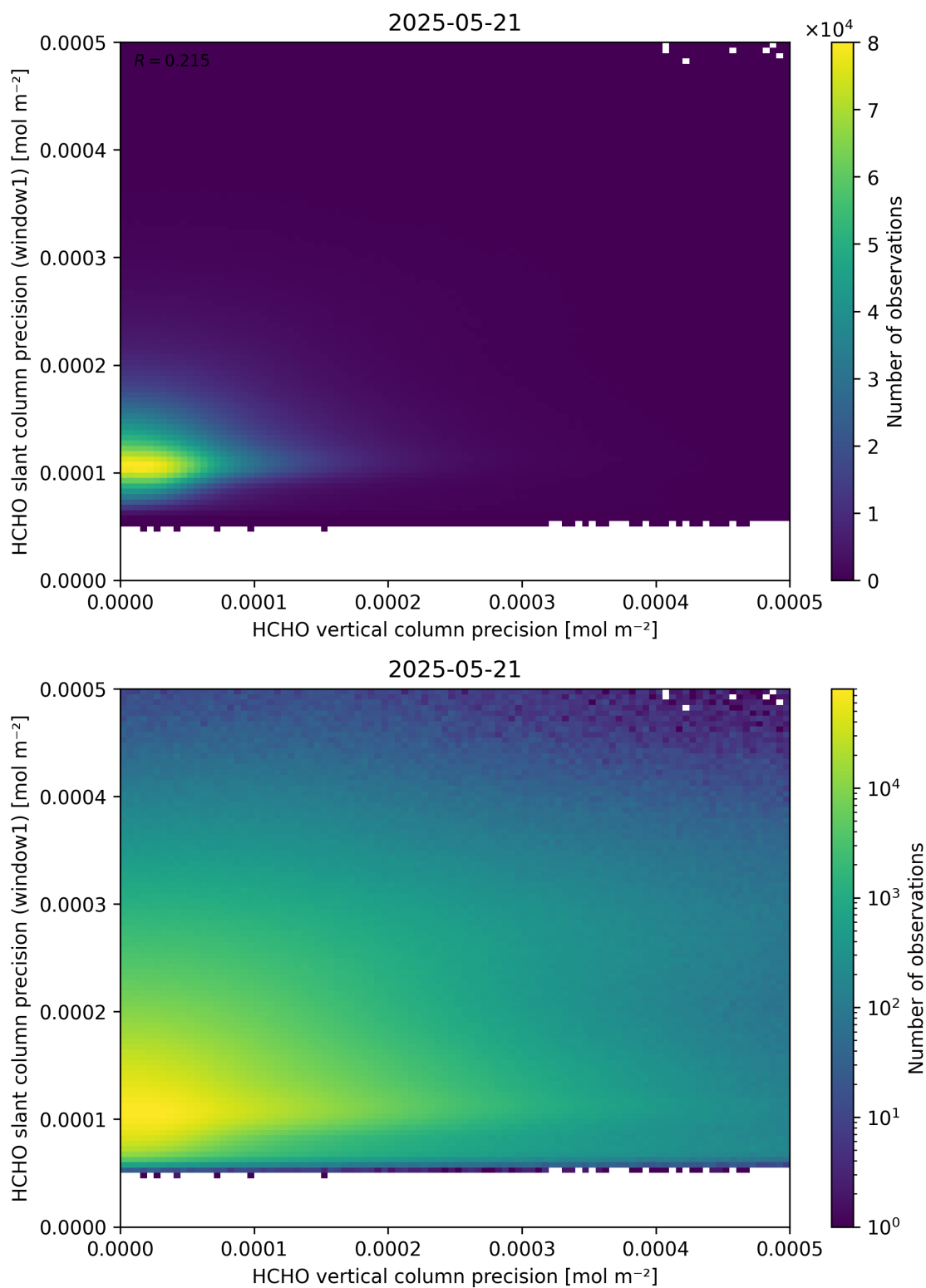
Figure 143: Scatter density plot of “HCHO vertical column precision” against “HCHO slant column precision (window1)” for 2025-05-21 to 2025-05-22.
