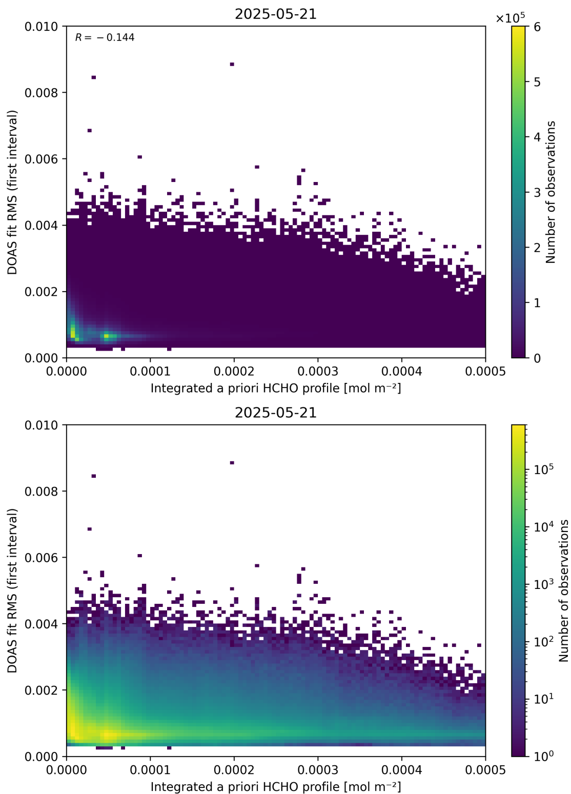
Figure 148: Scatter density plot of “Integrated a priori HCHO profile” against “DOAS fit RMS (first interval)” for 2025-05-21 to 2025-05-22.
