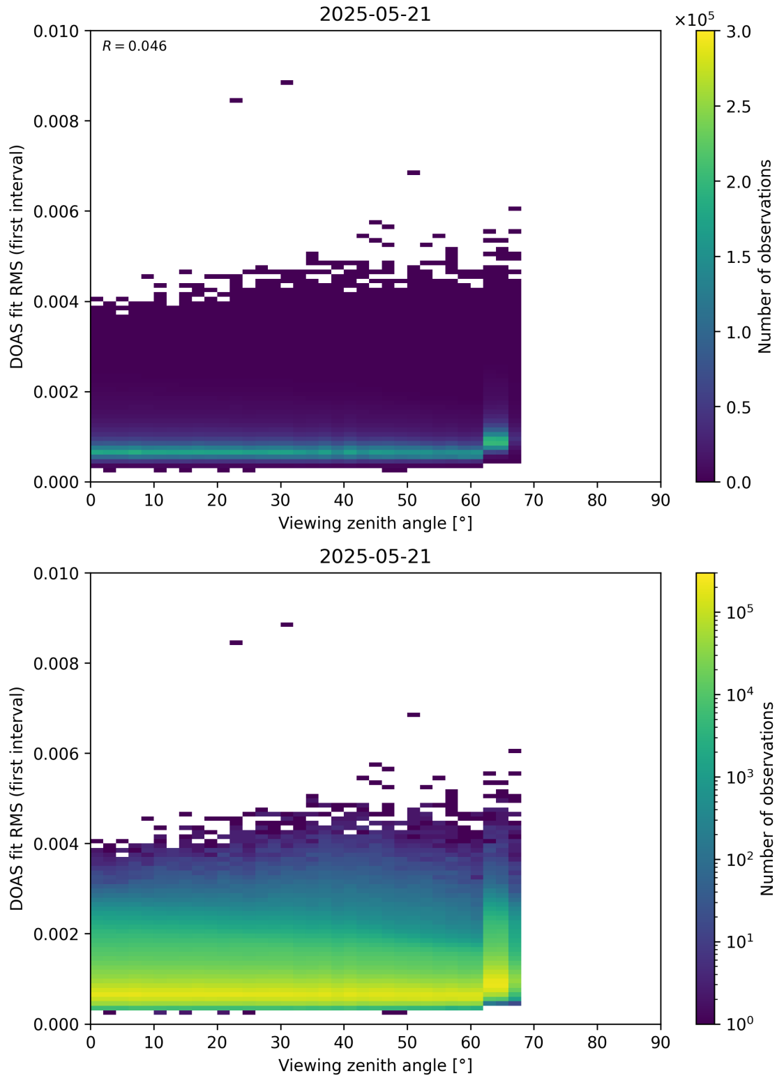
Figure 182: Scatter density plot of “Viewing zenith angle” against “DOAS fit RMS (first interval)” for 2025-05-21 to 2025-05-22.
