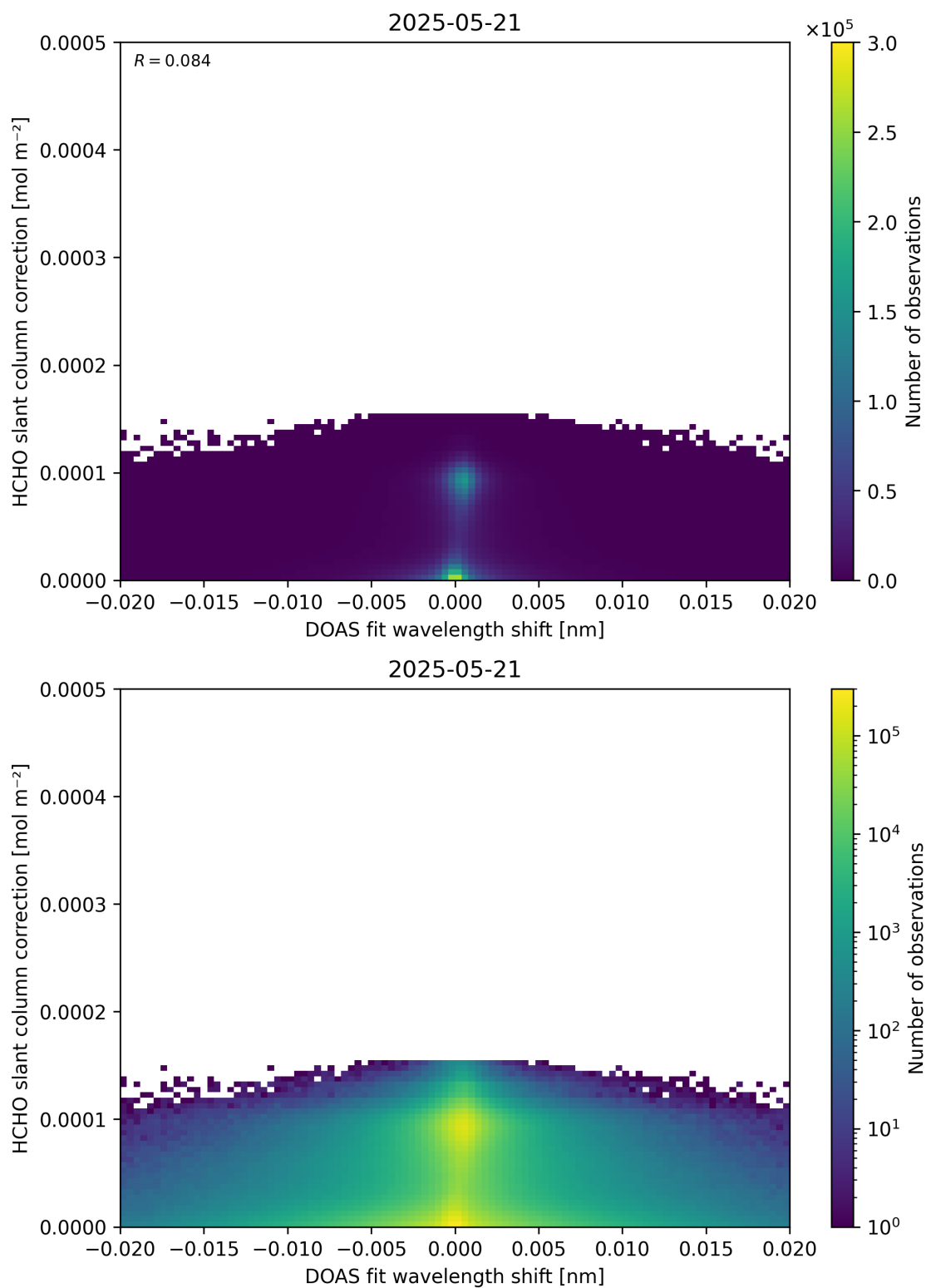
Figure 67: Scatter density plot of “DOAS fit wavelength shift” against “HCHO slant column correction” for 2025-05-21 to 2025-05-22.
