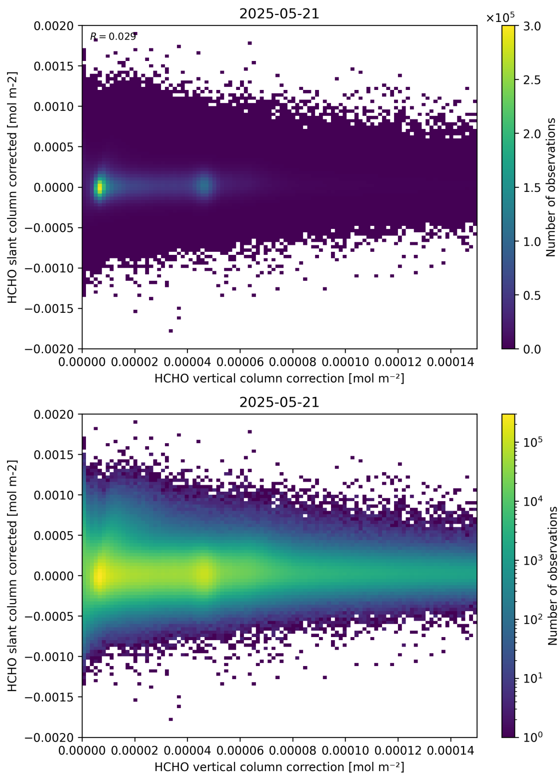
Figure 116: Scatter density plot of “HCHO vertical column correction” against “HCHO slant column corrected” for 2025-05-21 to 2025-05-22.
