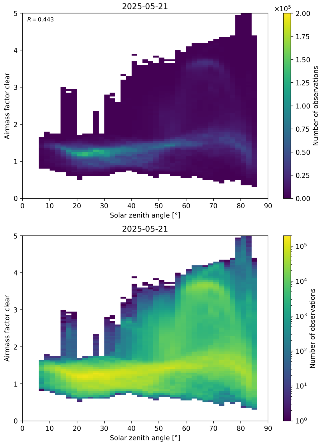
Figure 170: Scatter density plot of “Solar zenith angle” against “Airmass factor clear” for 2025-05-21 to 2025-05-22.
