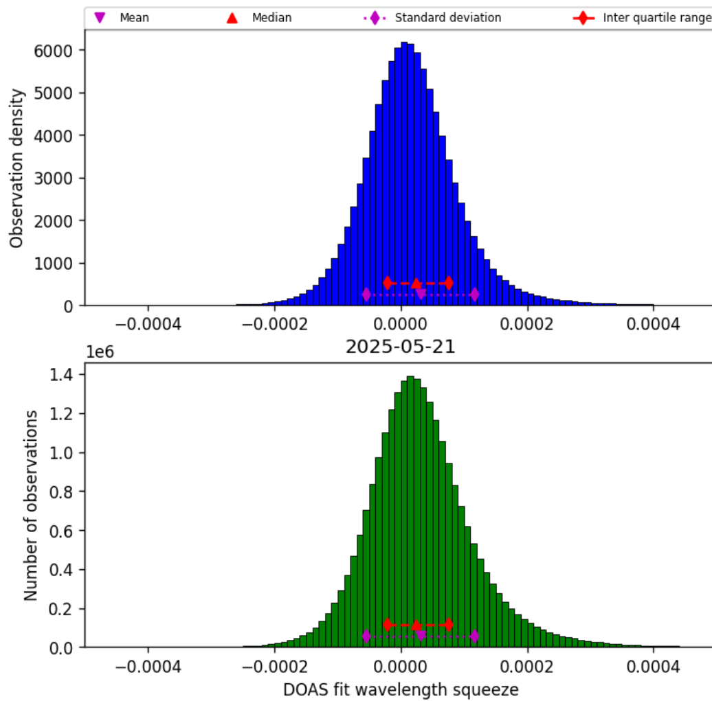
Figure 45: Histogram of “DOAS fit wavelength squeeze” for 2025-05-21 to 2025-05-22
