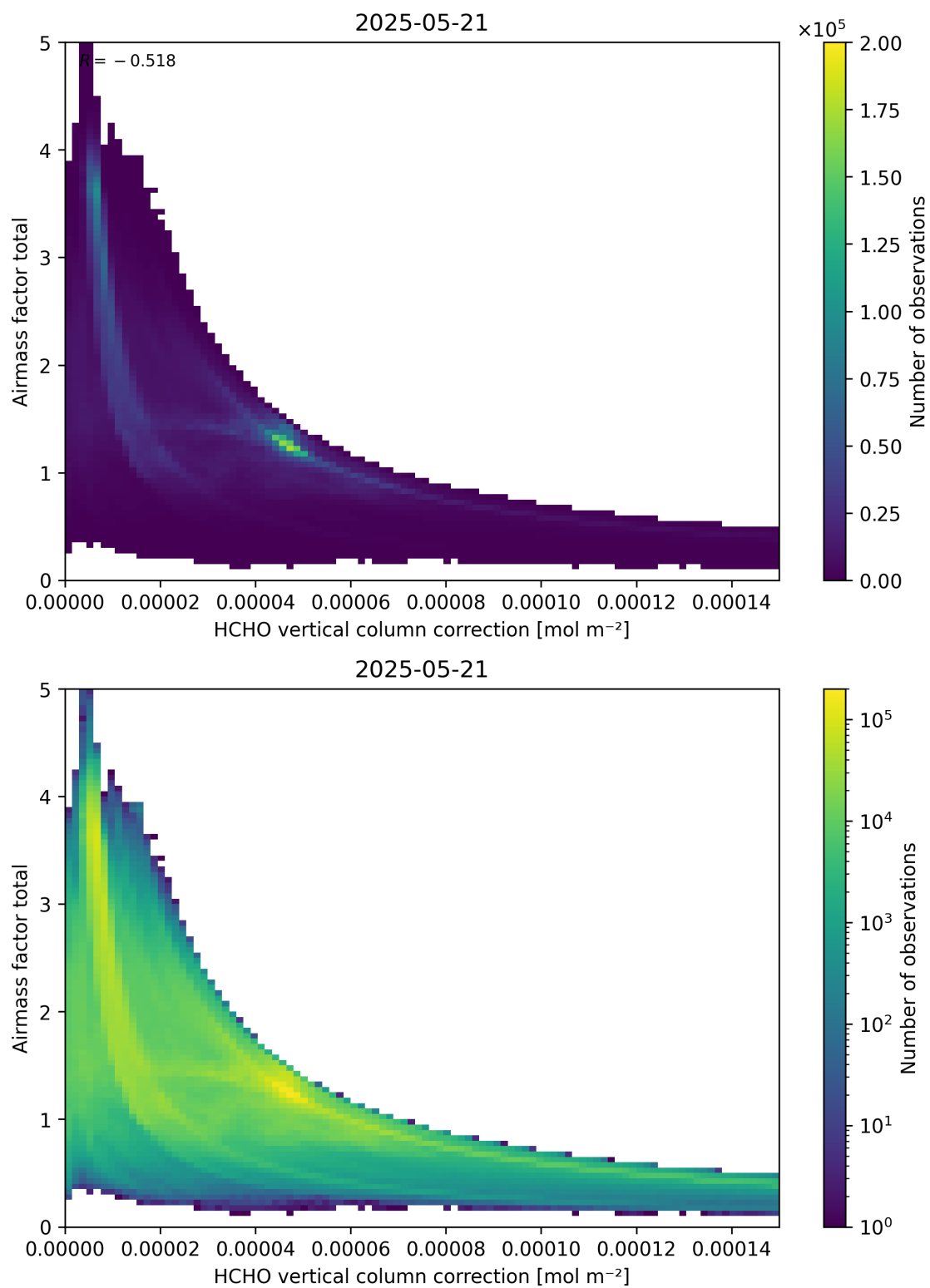
Figure 120: Scatter density plot of “HCHO vertical column correction” against “Airmass factor total” for 2025-05-21 to 2025-05-22.
