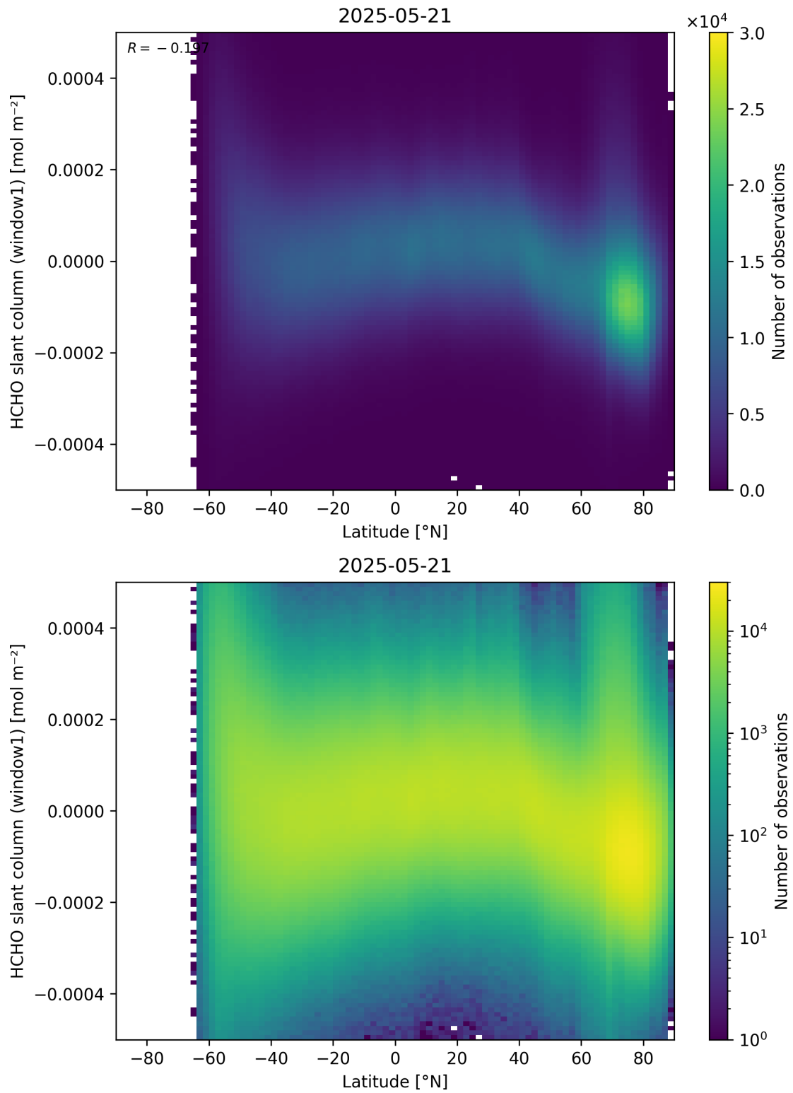
Figure 159: Scatter density plot of “Latitude” against “HCHO slant column (window1)” for 2025-05-21 to 2025-05-22.
