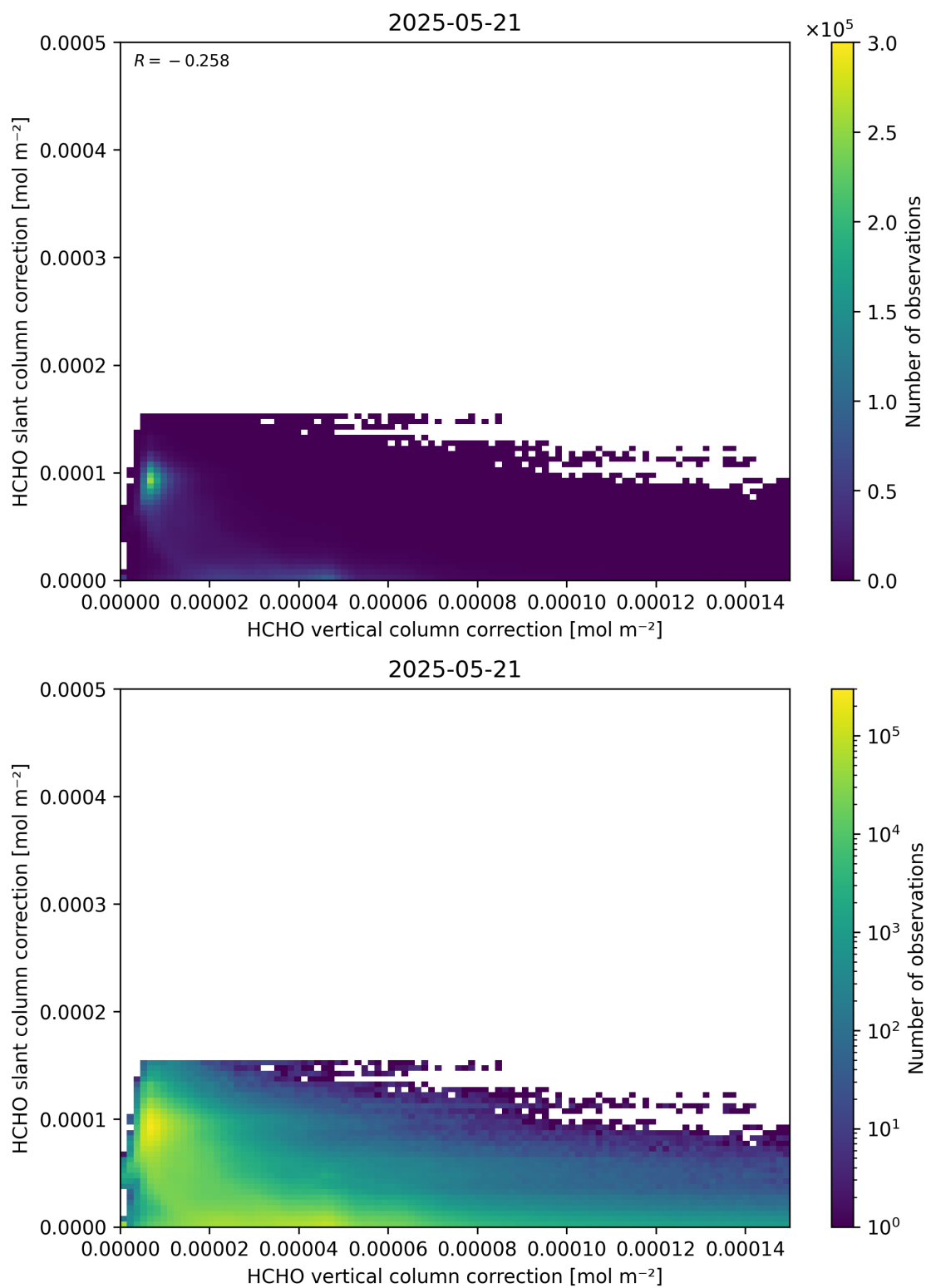
Figure 117: Scatter density plot of “HCHO vertical column correction” against “HCHO slant column correction” for 2025-05-21 to 2025-05-22.
