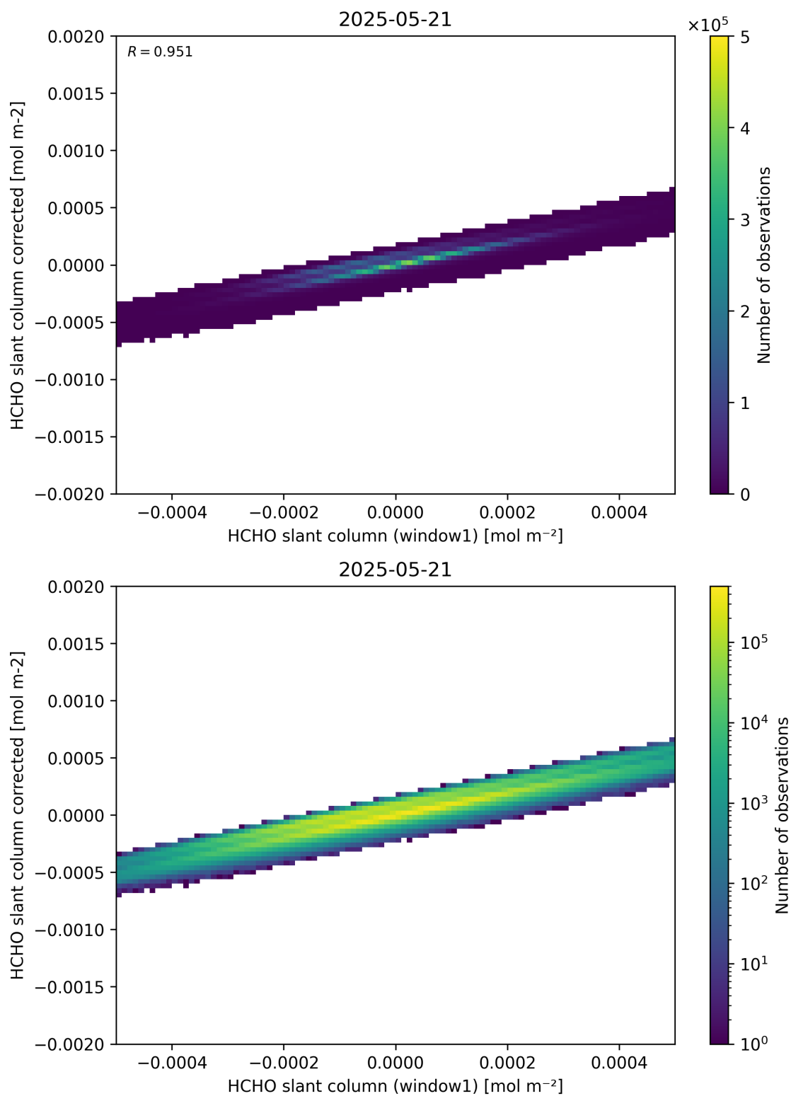
Figure 82: Scatter density plot of “HCHO slant column (window1)” against “HCHO slant column corrected” for 2025-05-21 to 2025-05-22.
