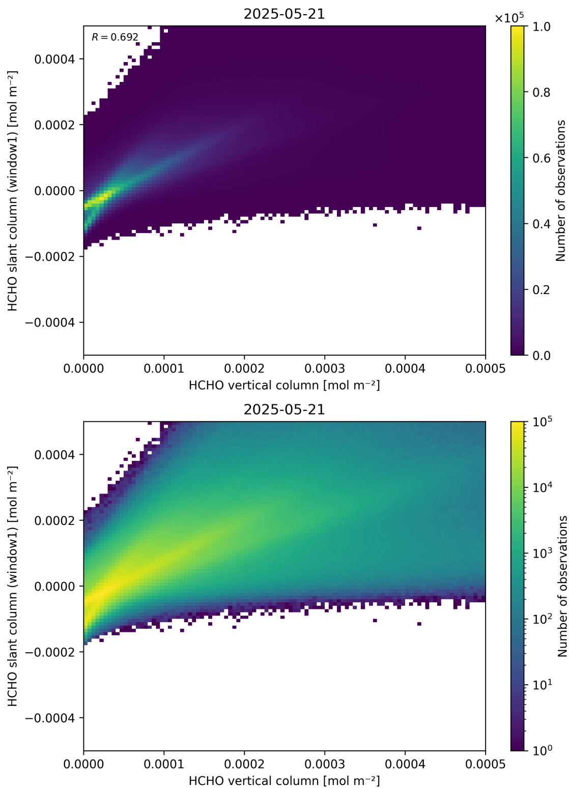
Figure 129: Scatter density plot of “HCHO vertical column” against “HCHO slant column (window1)” for 2025-05-21 to 2025-05-22.
