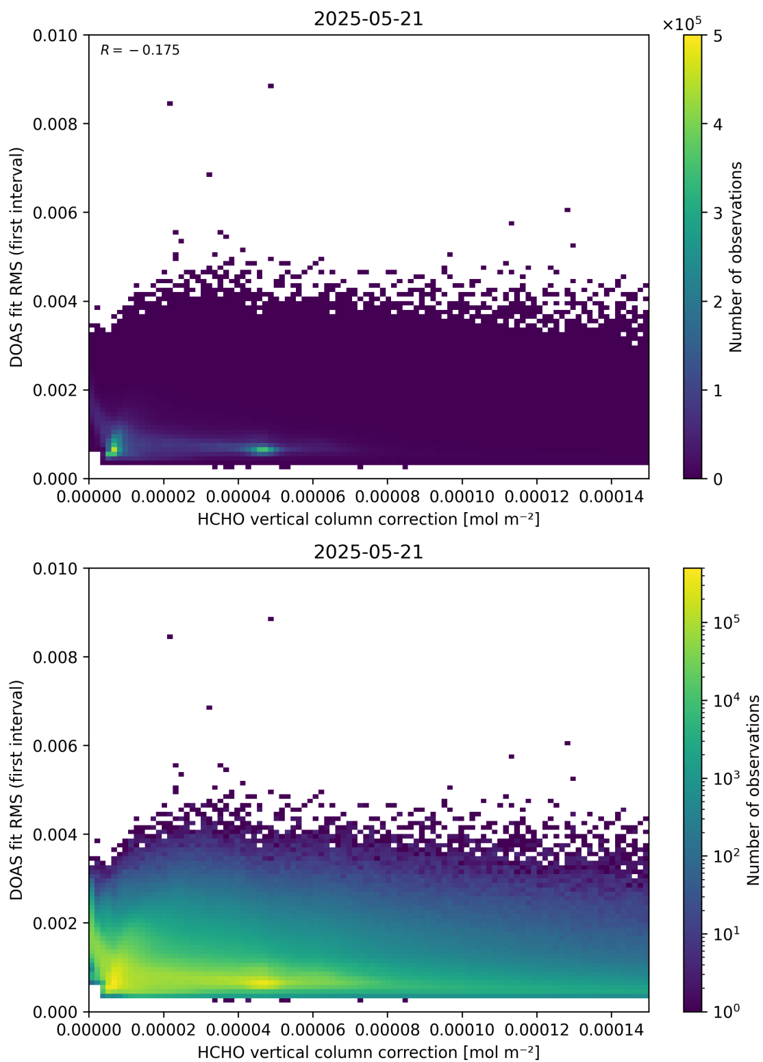
Figure 112: Scatter density plot of “HCHO vertical column correction” against “DOAS fit RMS (first interval)” for 2025-05-21 to 2025-05-22.
