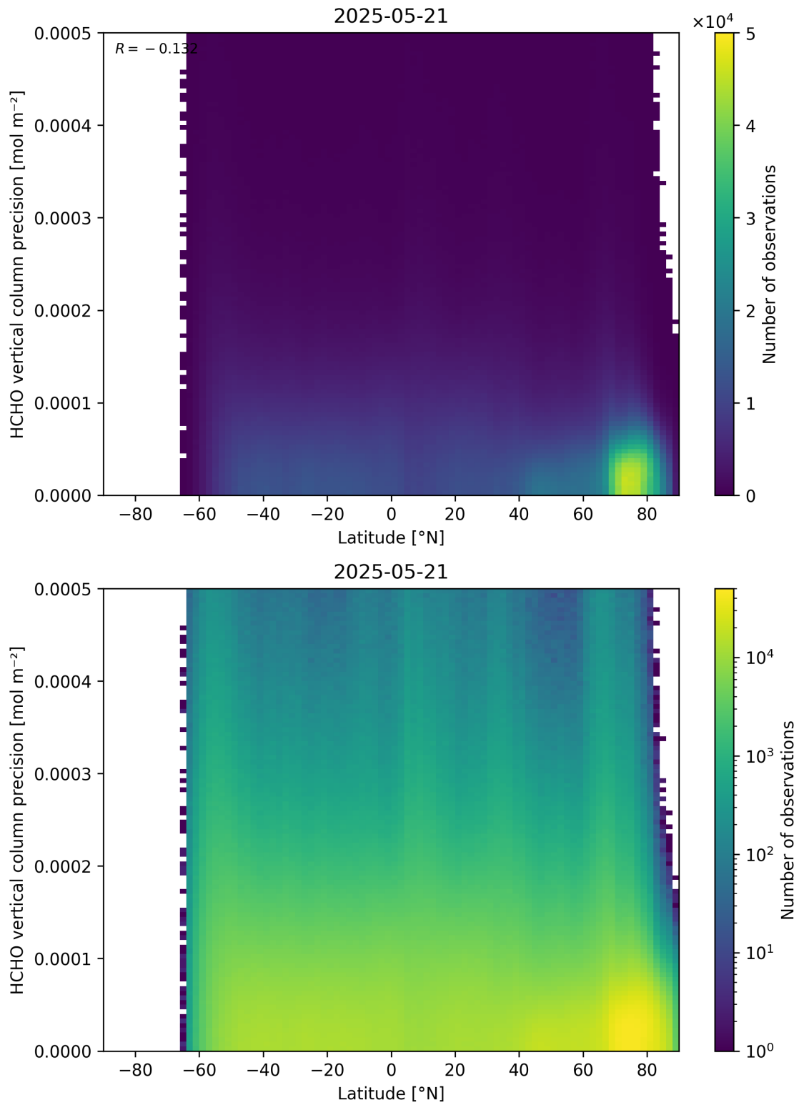
Figure 165: Scatter density plot of “Latitude” against “HCHO vertical column precision” for 2025-05-21 to 2025-05-22.
