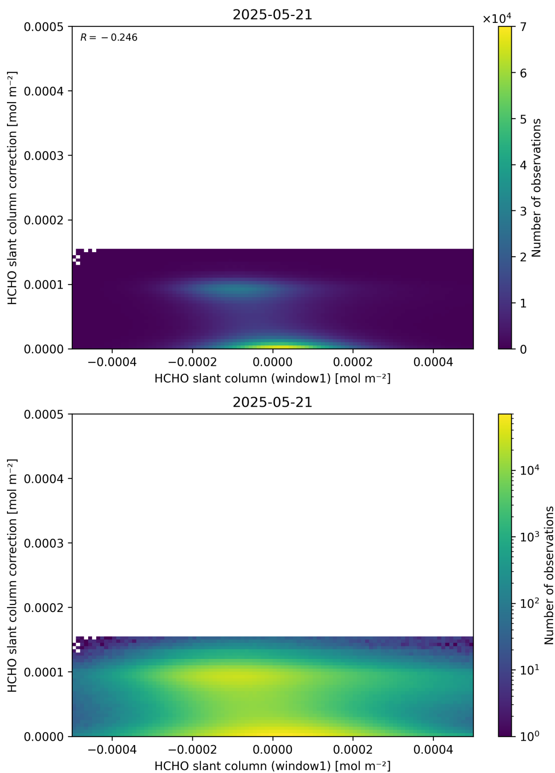
Figure 83: Scatter density plot of “HCHO slant column (window1)” against “HCHO slant column correction” for 2025-05-21 to 2025-05-22.
