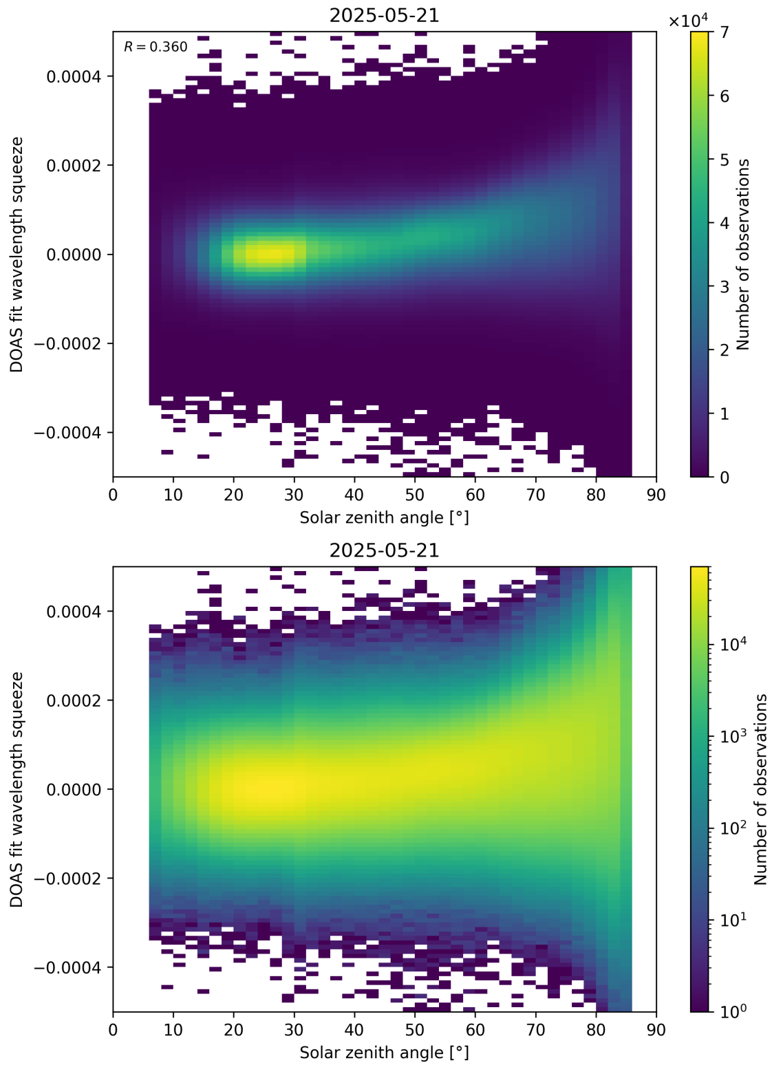
Figure 169: Scatter density plot of “Solar zenith angle” against “DOAS fit wavelength squeeze” for 2025-05-21 to 2025-05-22.
