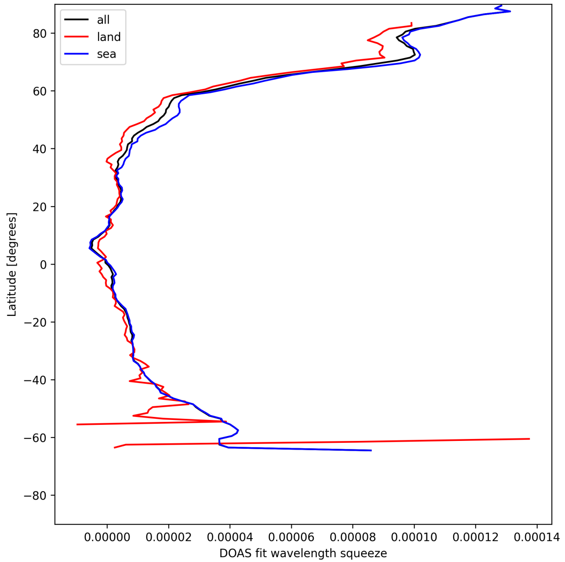
Figure 31: Zonal average of “DOAS fit wavelength squeeze” for 2025-05-21 to 2025-05-22.
