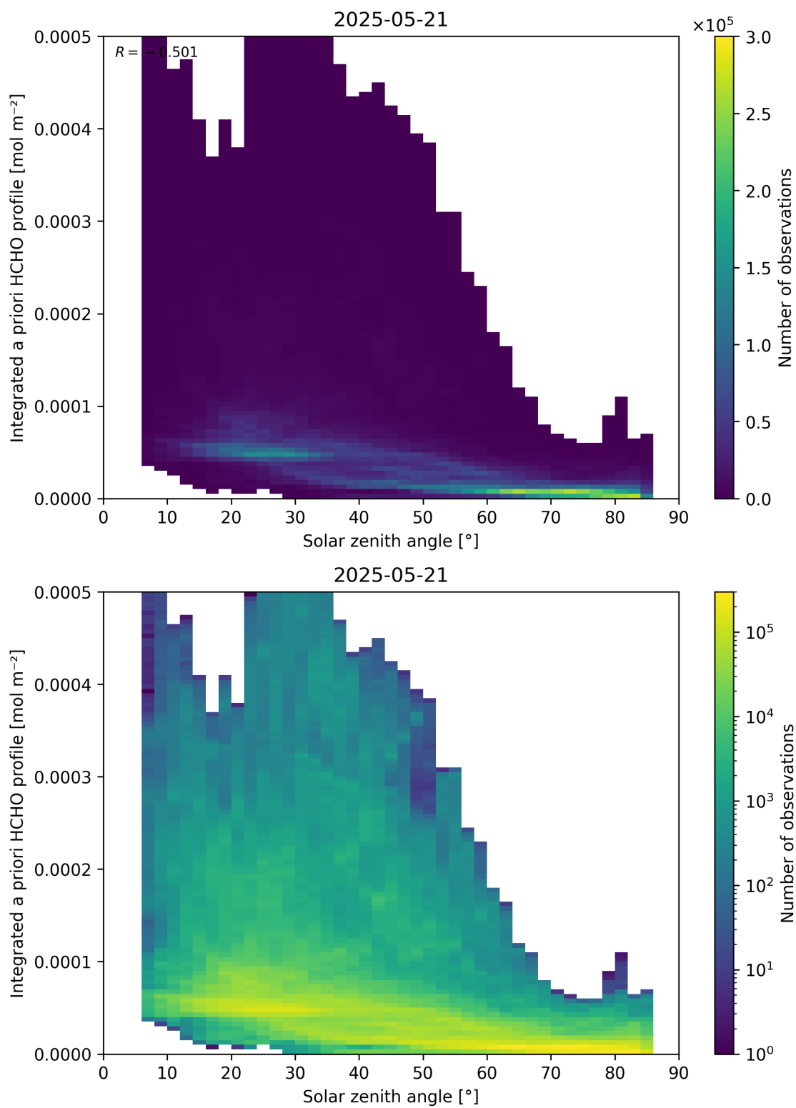
Figure 180: Scatter density plot of “Solar zenith angle” against “Integrated a priori HCHO profile” for 2025-05-21 to 2025-05-22.
