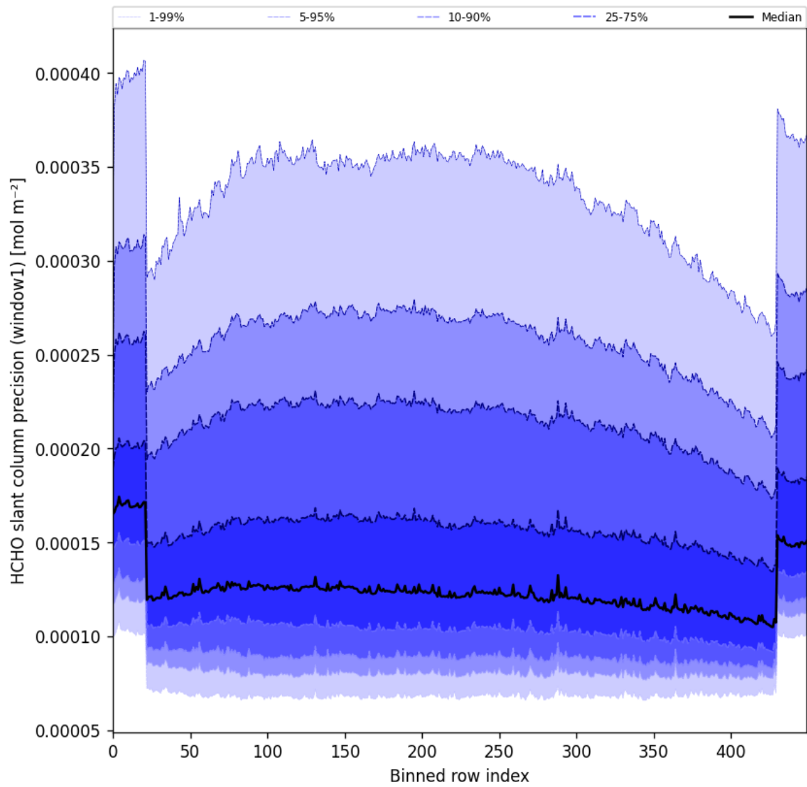
Figure 53: Along track statistics of “HCHO slant column precision (window1)” for 2025-05-21 to 2025-05-22
