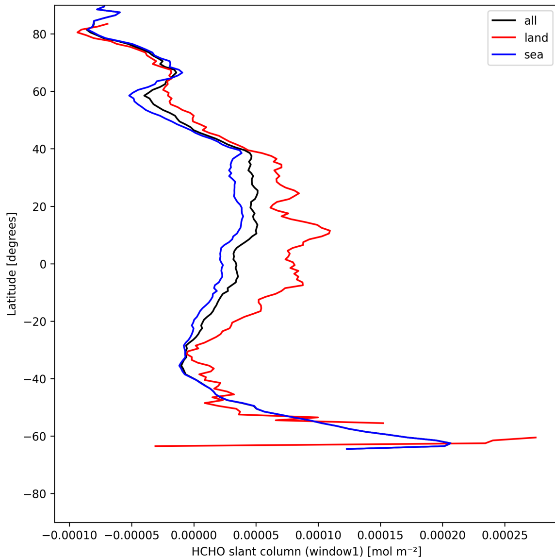
Figure 24: Zonal average of “HCHO slant column (window1)” for 2025-05-21 to 2025-05-22.
