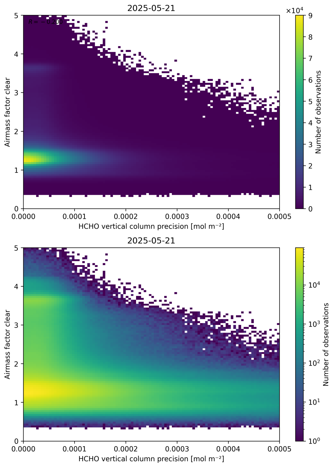
Figure 139: Scatter density plot of “HCHO vertical column precision” against “Airmass factor clear” for 2025-05-21 to 2025-05-22.
