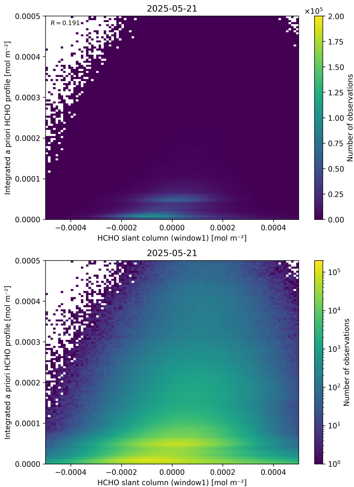
Figure 87: Scatter density plot of “HCHO slant column (window1)” against “Integrated a priori HCHO profile” for 2025-05-21 to 2025-05-22.
