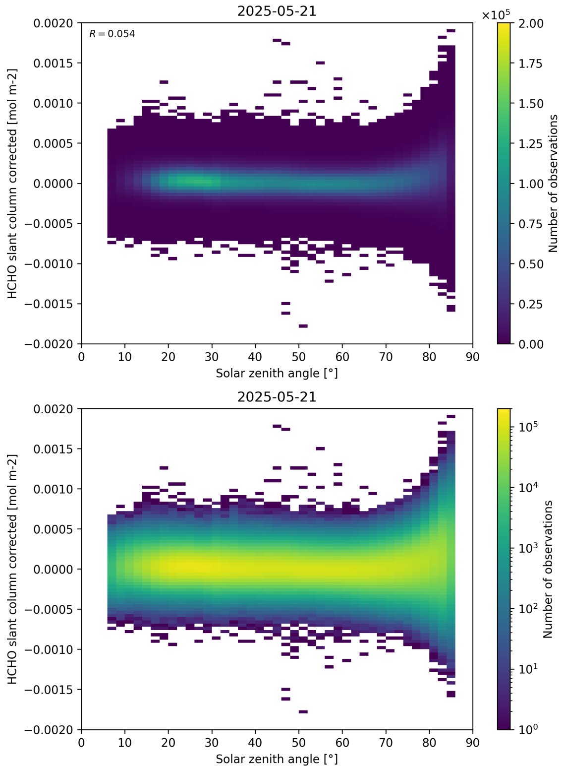
Figure 171: Scatter density plot of “Solar zenith angle” against “HCHO slant column corrected” for 2025-05-21 to 2025-05-22.
