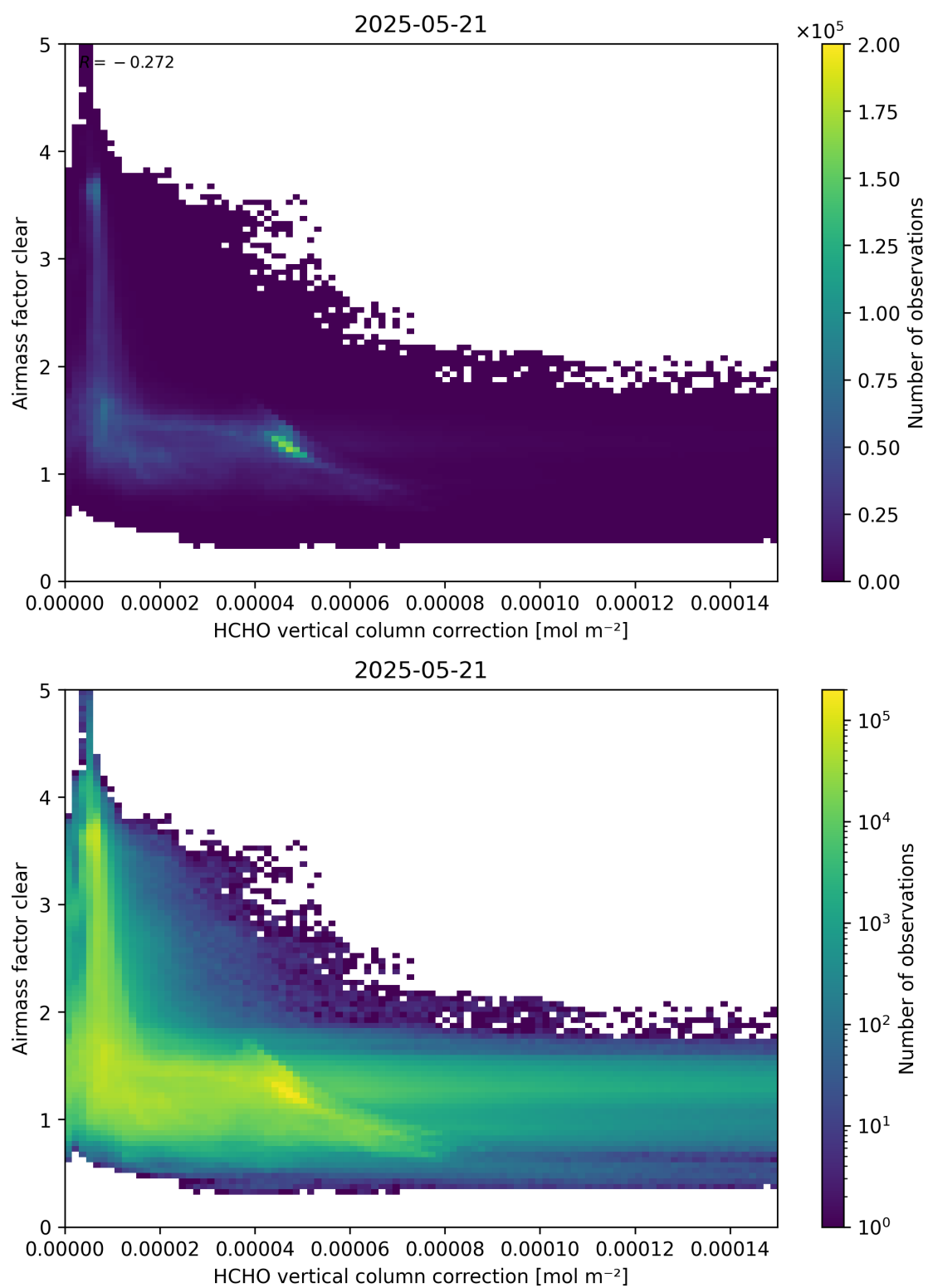
Figure 115: Scatter density plot of “HCHO vertical column correction” against “Airmass factor clear” for 2025-05-21 to 2025-05-22.
