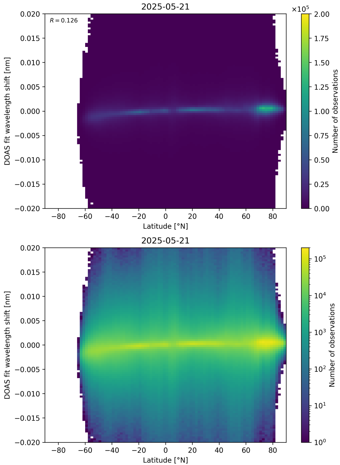
Figure 154: Scatter density plot of “Latitude” against “DOAS fit wavelength shift” for 2025-05-21 to 2025-05-22.
