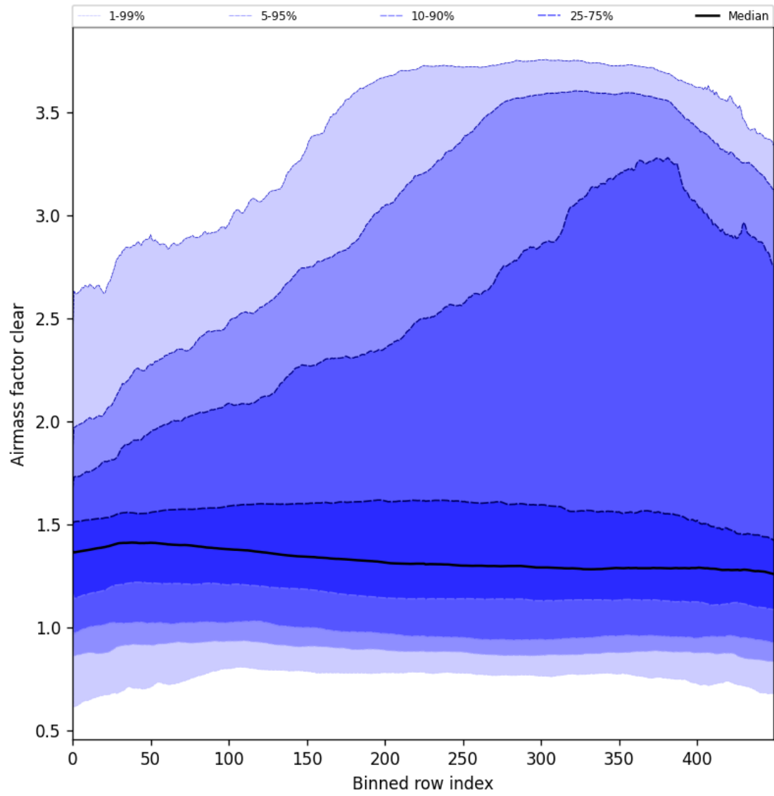
Figure 56: Along track statistics of “Airmass factor clear” for 2025-05-21 to 2025-05-22
