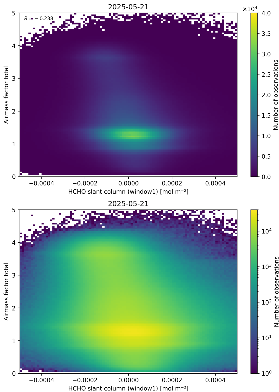
Figure 85: Scatter density plot of “HCHO slant column (window1)” against “Airmass factor total” for 2025-05-21 to 2025-05-22.
