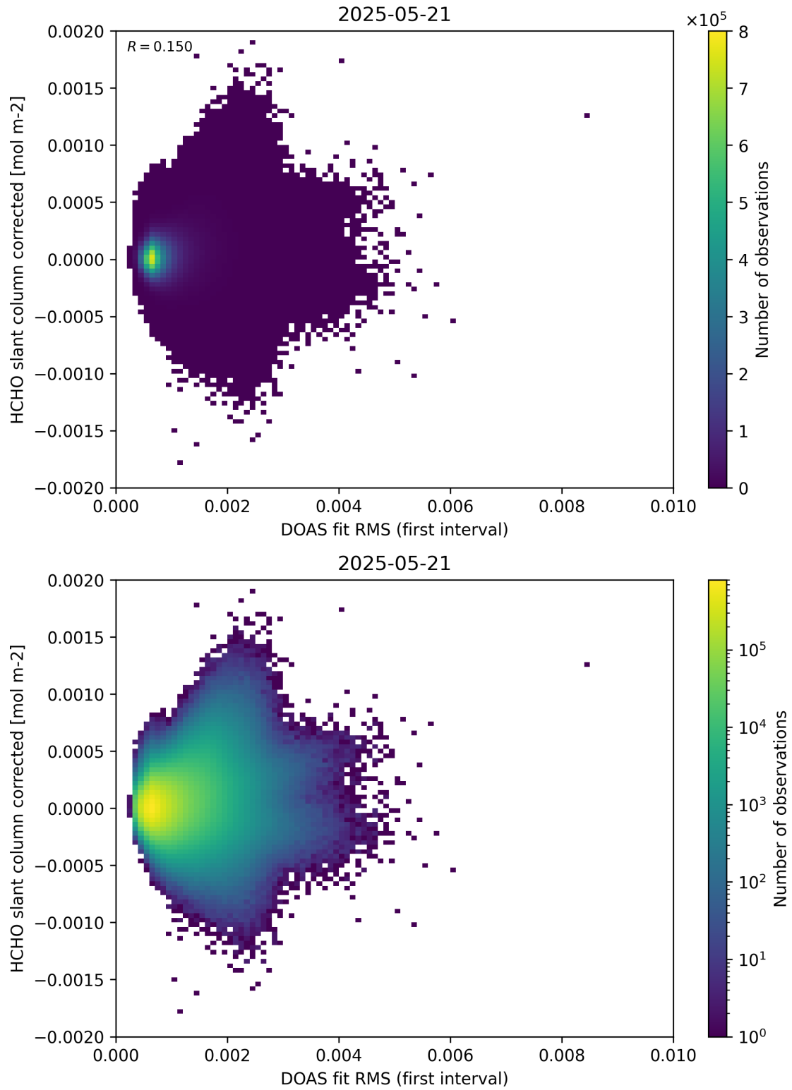
Figure 62: Scatter density plot of “DOAS fit RMS (first interval)” against “HCHO slant column corrected” for 2025-05-21 to 2025-05-22.
