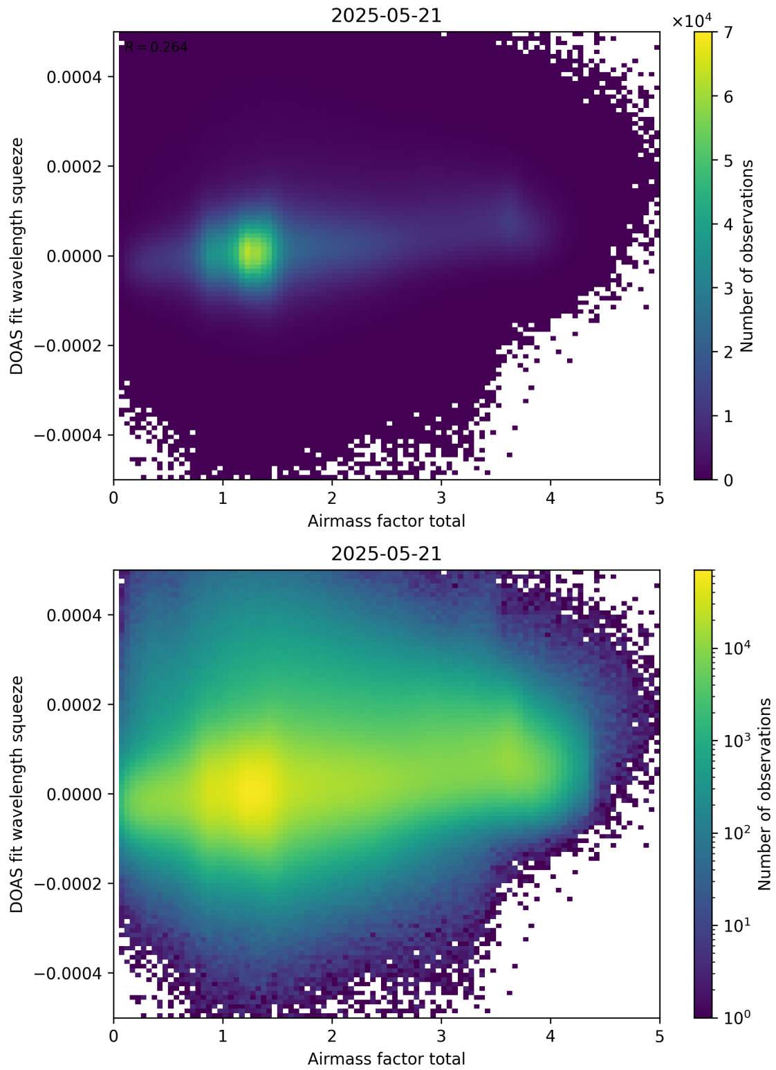
Figure 99: Scatter density plot of “Airmass factor total” against “DOAS fit wavelength squeeze” for 2025-05-21 to 2025-05-22.
