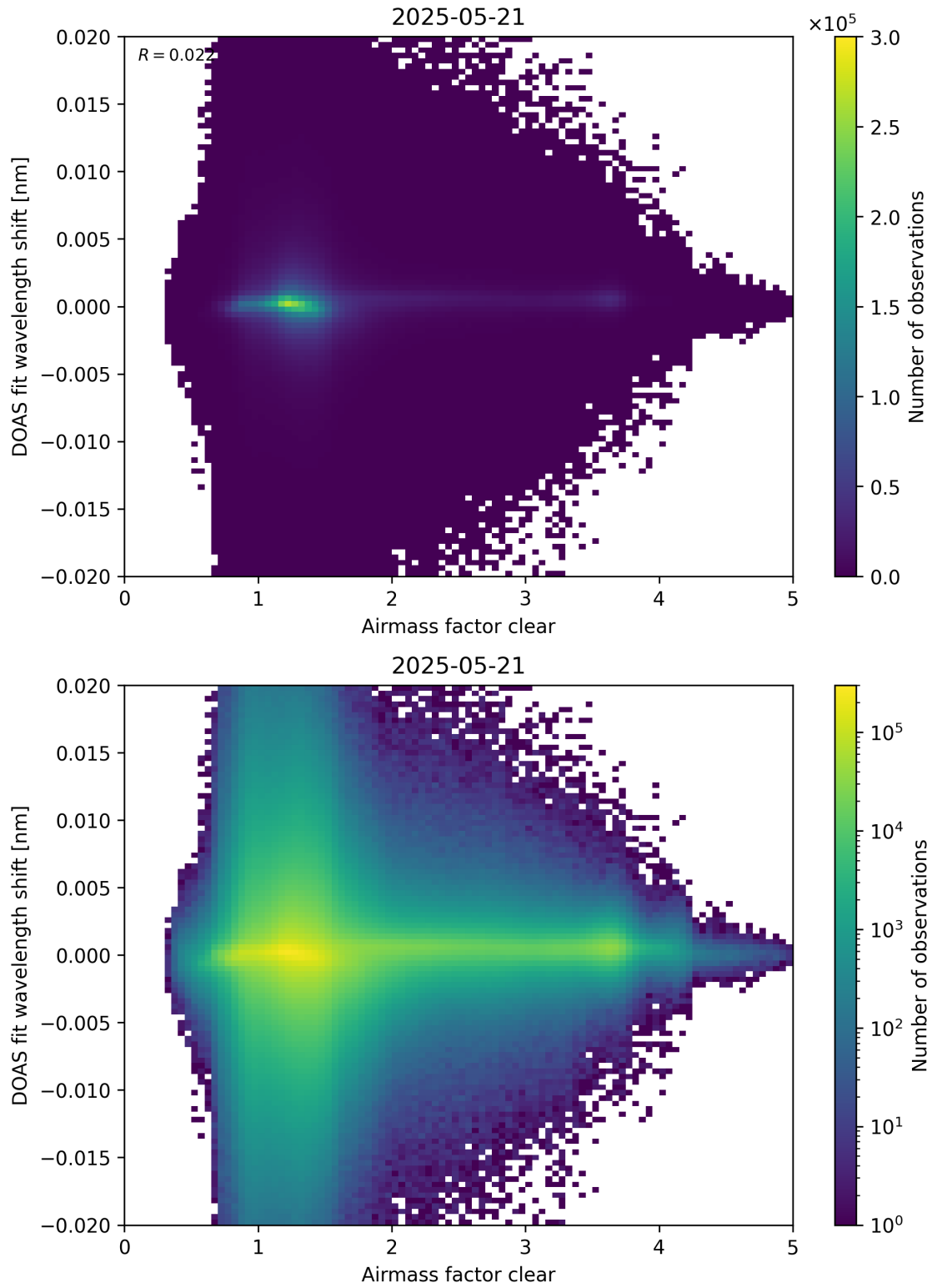
Figure 72: Scatter density plot of “Airmass factor clear” against “DOAS fit wavelength shift” for 2025-05-21 to 2025-05-22.
