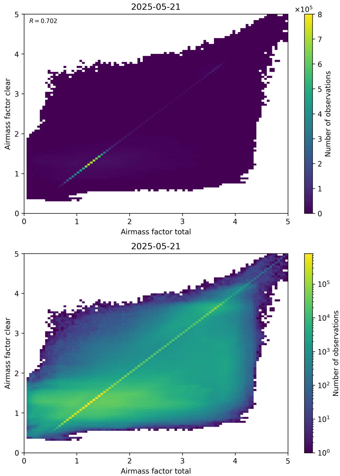
Figure 100: Scatter density plot of “Airmass factor total” against “Airmass factor clear” for 2025-05-21 to 2025-05-22.
