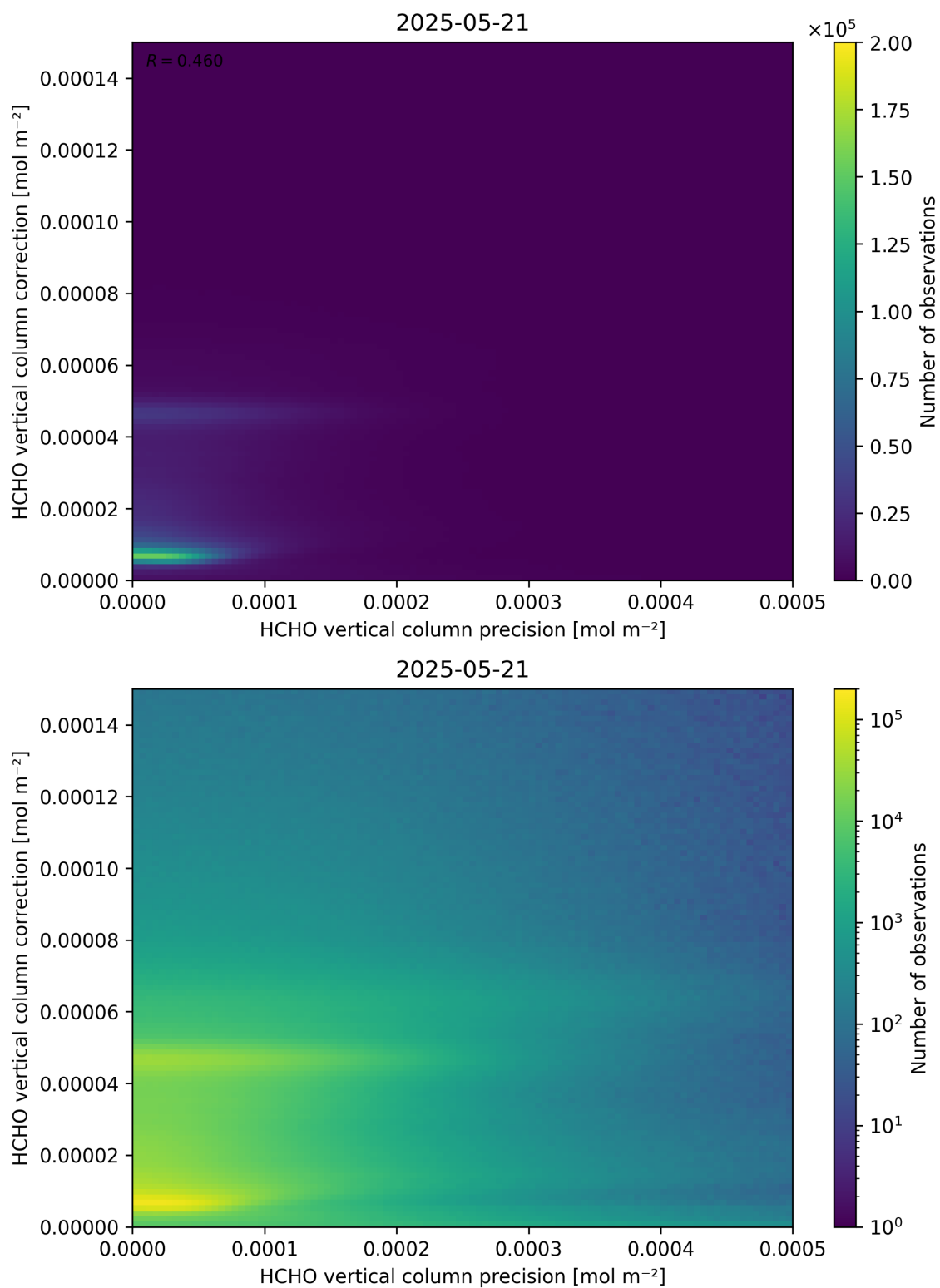
Figure 146: Scatter density plot of “HCHO vertical column precision” against “HCHO vertical column correction” for 2025-05-21 to 2025-05-22.
