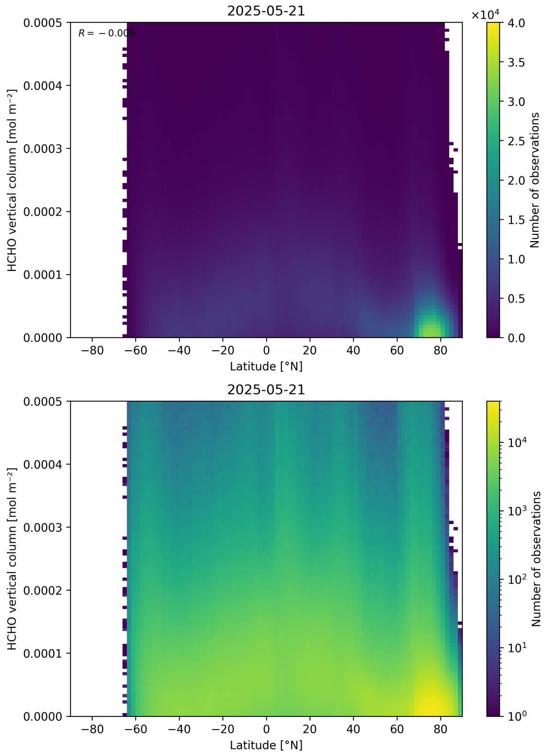
Figure 163: Scatter density plot of “Latitude” against “HCHO vertical column” for 2025-05-21 to 2025-05-22.
