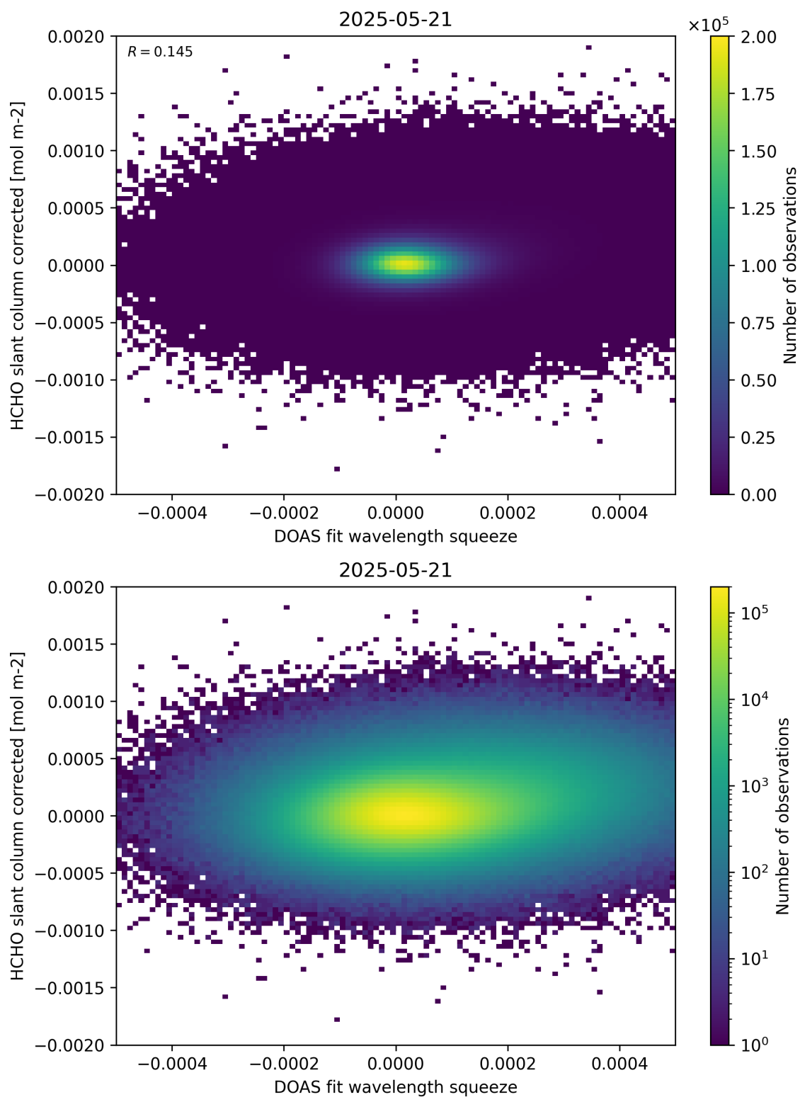
Figure 69: Scatter density plot of “DOAS fit wavelength squeeze” against “HCHO slant column corrected” for 2025-05-21 to 2025-05-22.
