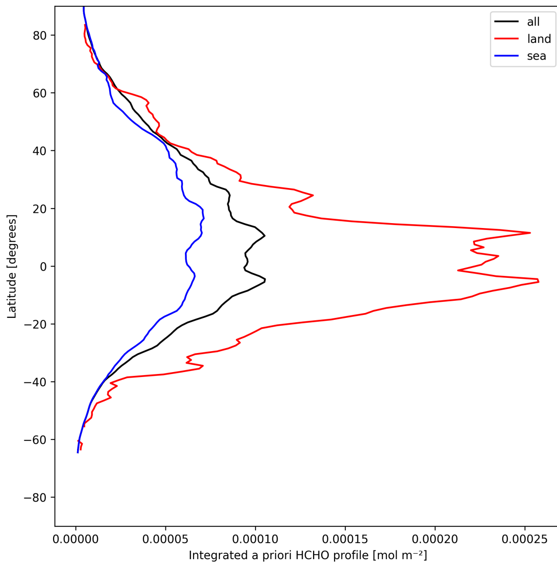
Figure 29: Zonal average of “Integrated a priori HCHO profile” for 2025-05-21 to 2025-05-22.
