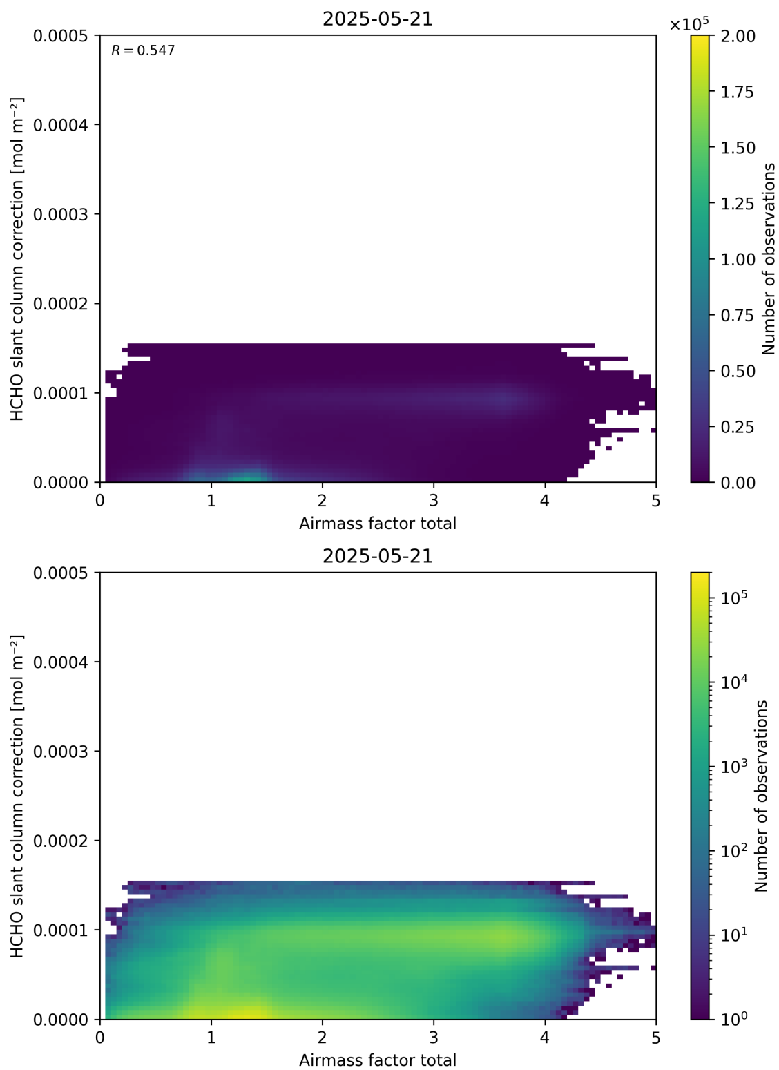
Figure 102: Scatter density plot of “Airmass factor total” against “HCHO slant column correction” for 2025-05-21 to 2025-05-22.
