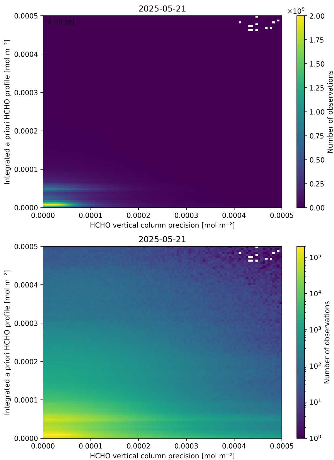
Figure 147: Scatter density plot of “HCHO vertical column precision” against “Integrated a priori HCHO profile” for 2025-05-21 to 2025-05-22.
