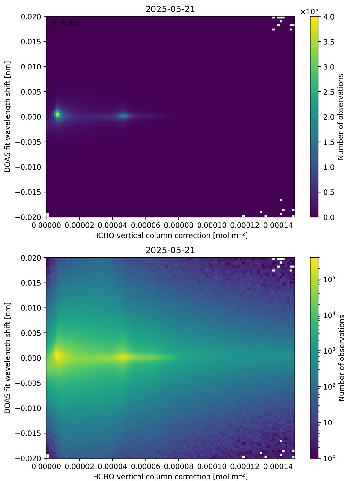
Figure 113: Scatter density plot of “HCHO vertical column correction” against “DOAS fit wavelength shift” for 2025-05-21 to 2025-05-22.
