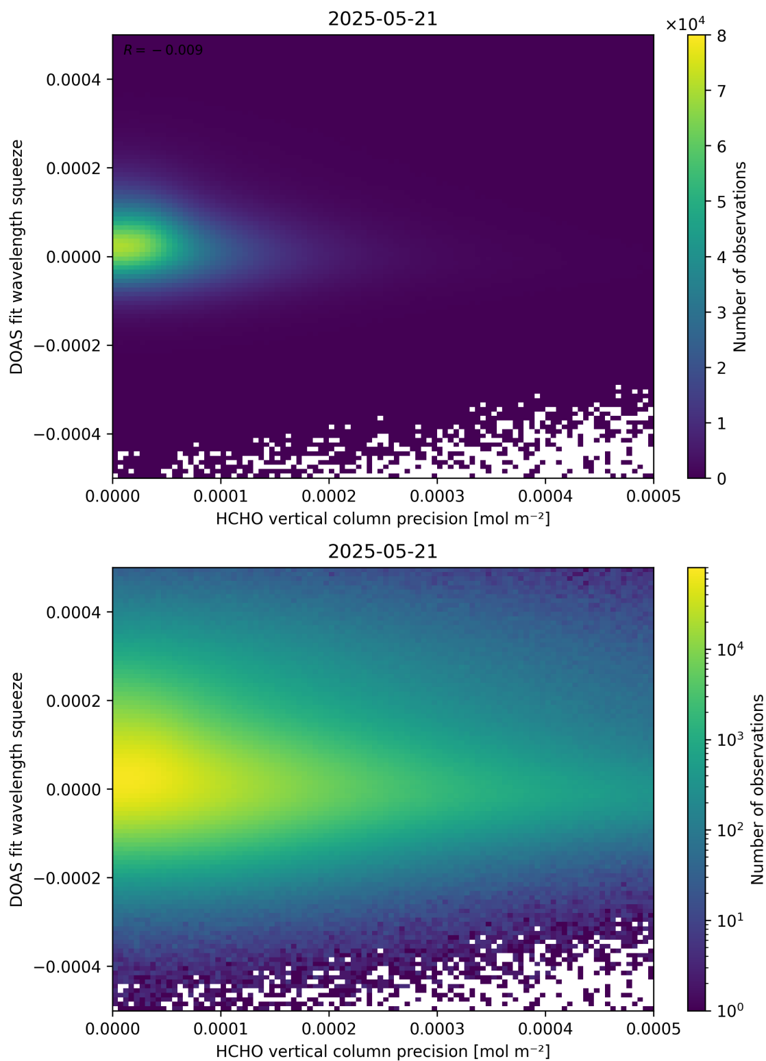
Figure 138: Scatter density plot of “HCHO vertical column precision” against “DOAS fit wavelength squeeze” for 2025-05-21 to 2025-05-22.
