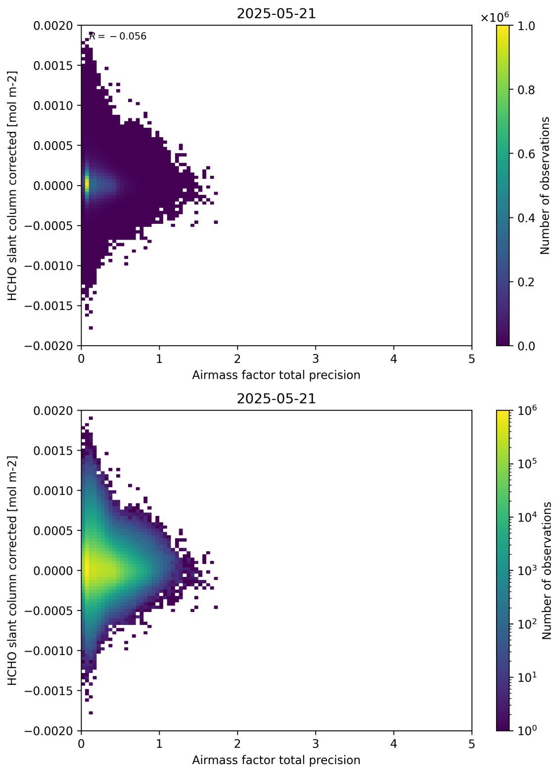
Figure 109: Scatter density plot of “Airmass factor total precision” against “HCHO slant column corrected” for 2025-05-21 to 2025-05-22.
