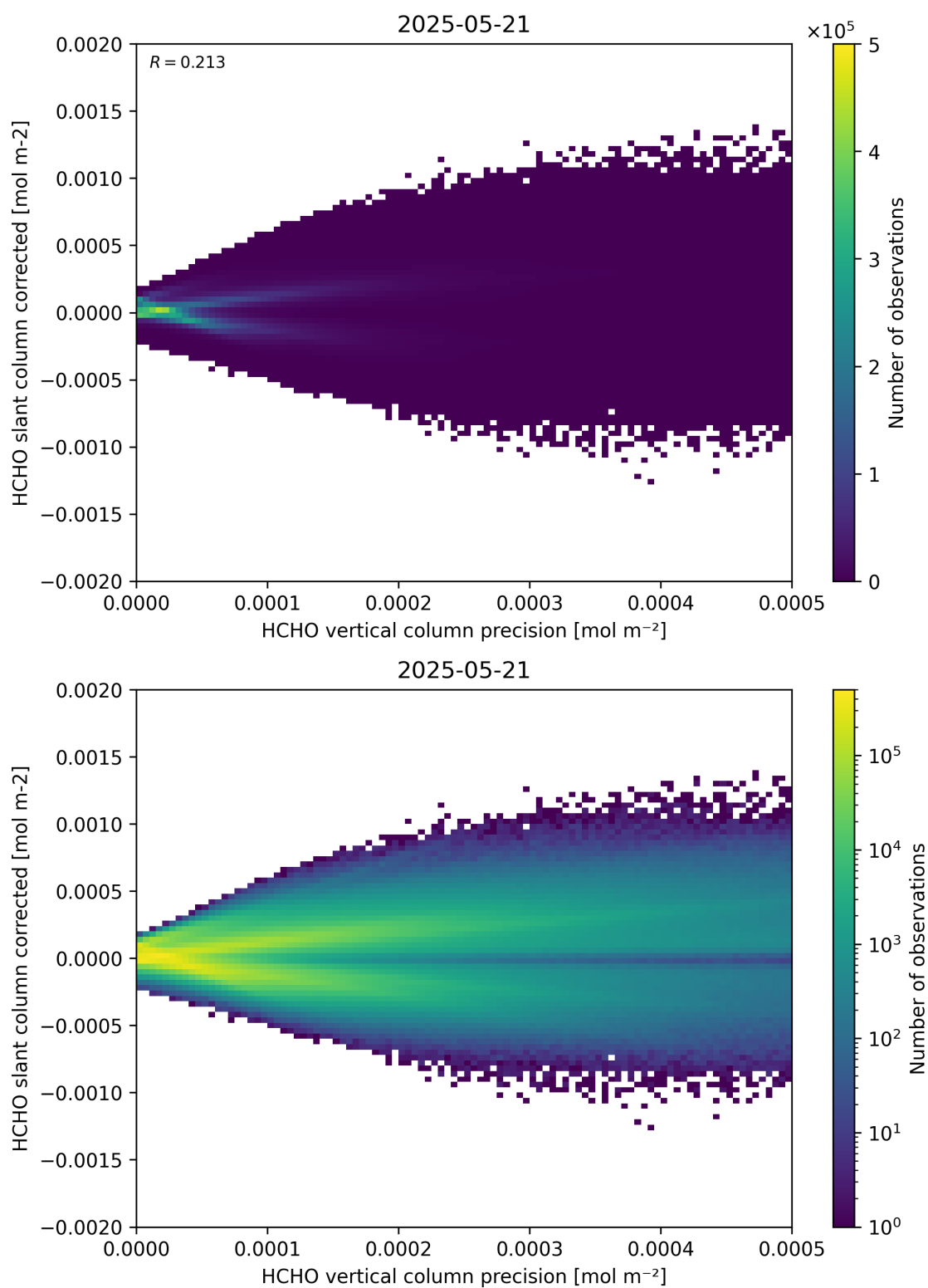
Figure 140: Scatter density plot of “HCHO vertical column precision” against “HCHO slant column corrected” for 2025-05-21 to 2025-05-22.
