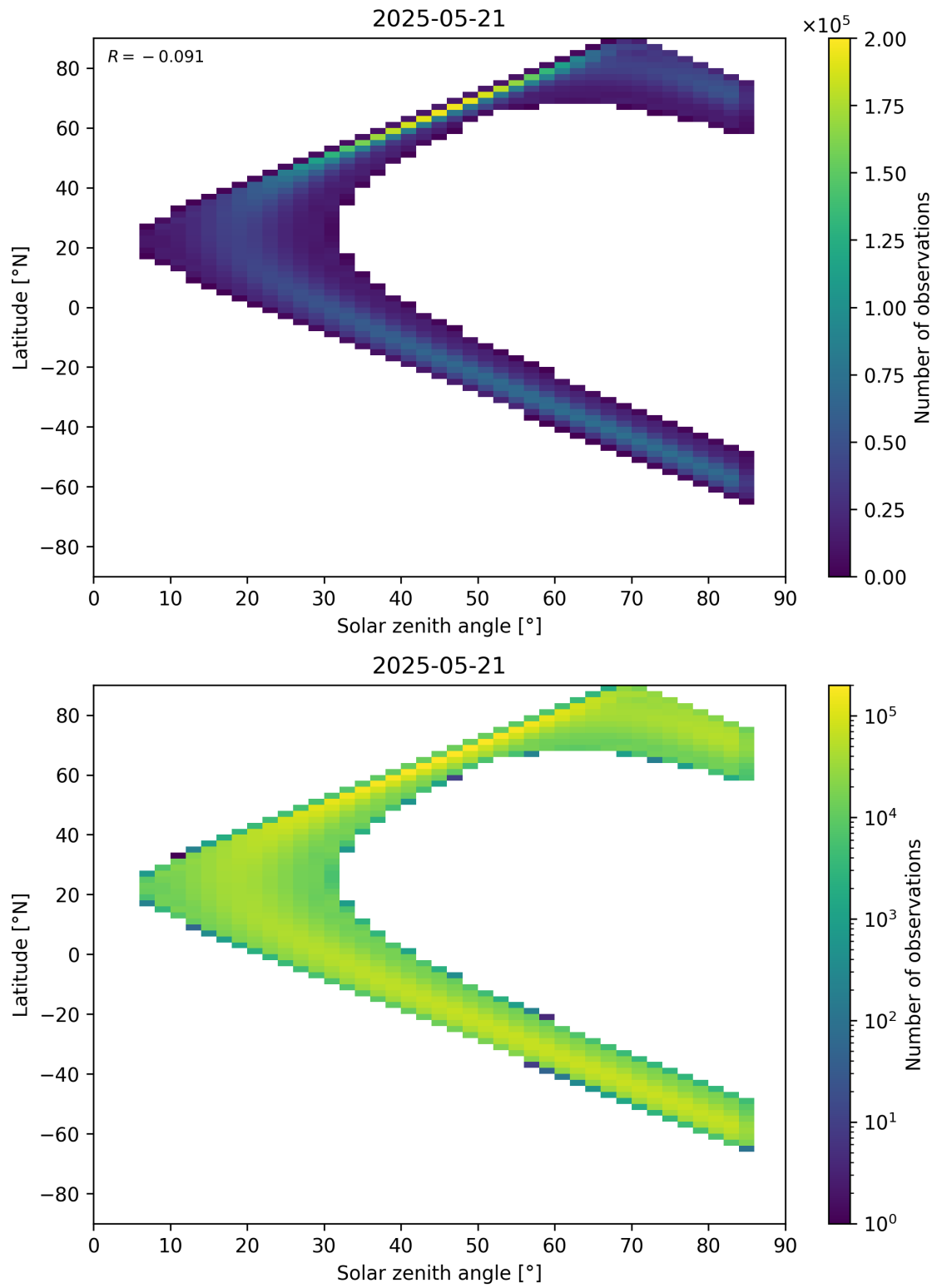
Figure 181: Scatter density plot of “Solar zenith angle” against “Latitude” for 2025-05-21 to 2025-05-22.
