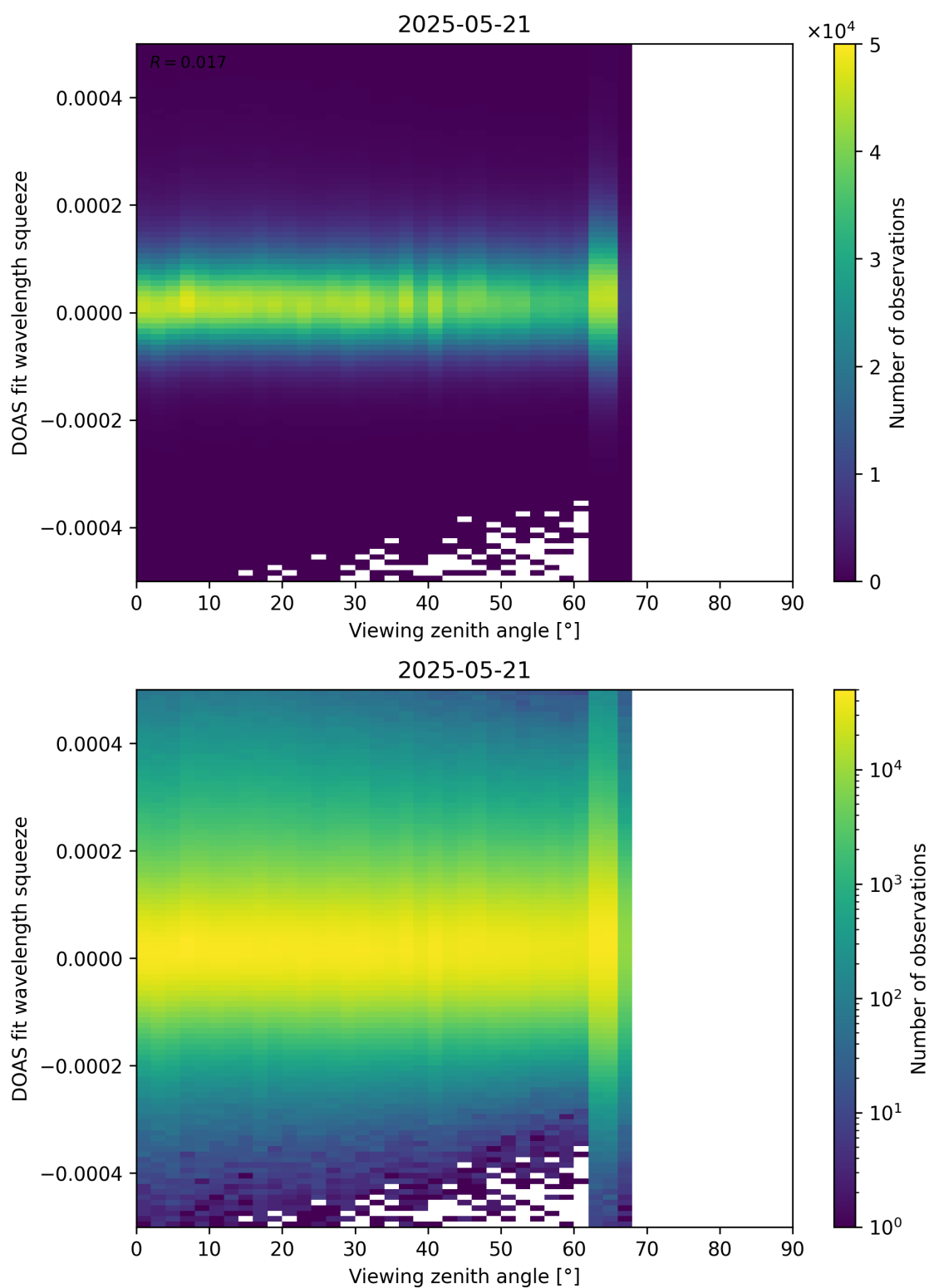
Figure 184: Scatter density plot of “Viewing zenith angle” against “DOAS fit wavelength squeeze” for 2025-05-21 to 2025-05-22.
