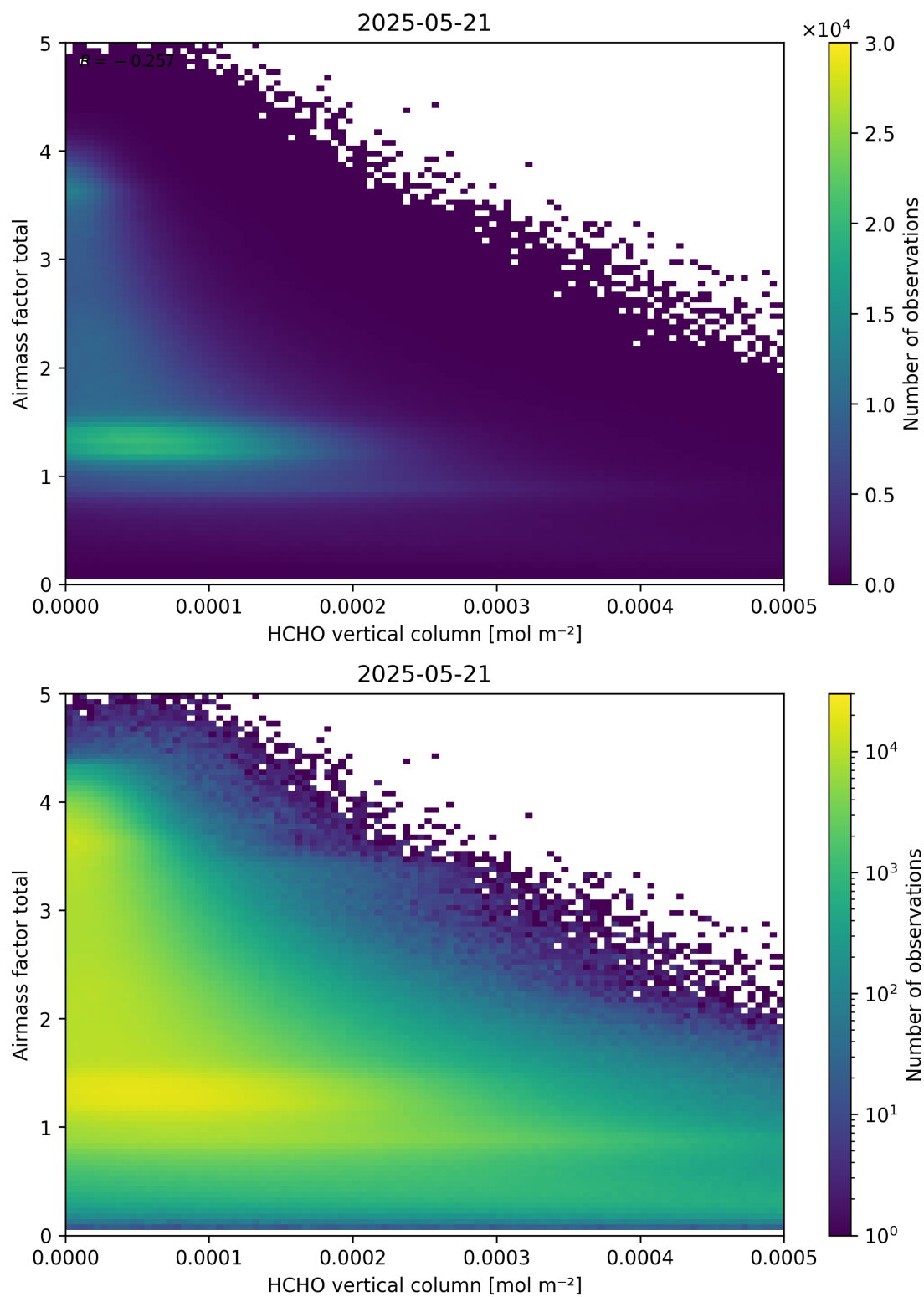
Figure 131: Scatter density plot of “HCHO vertical column” against “Airmass factor total” for 2025-05-21 to 2025-05-22.
