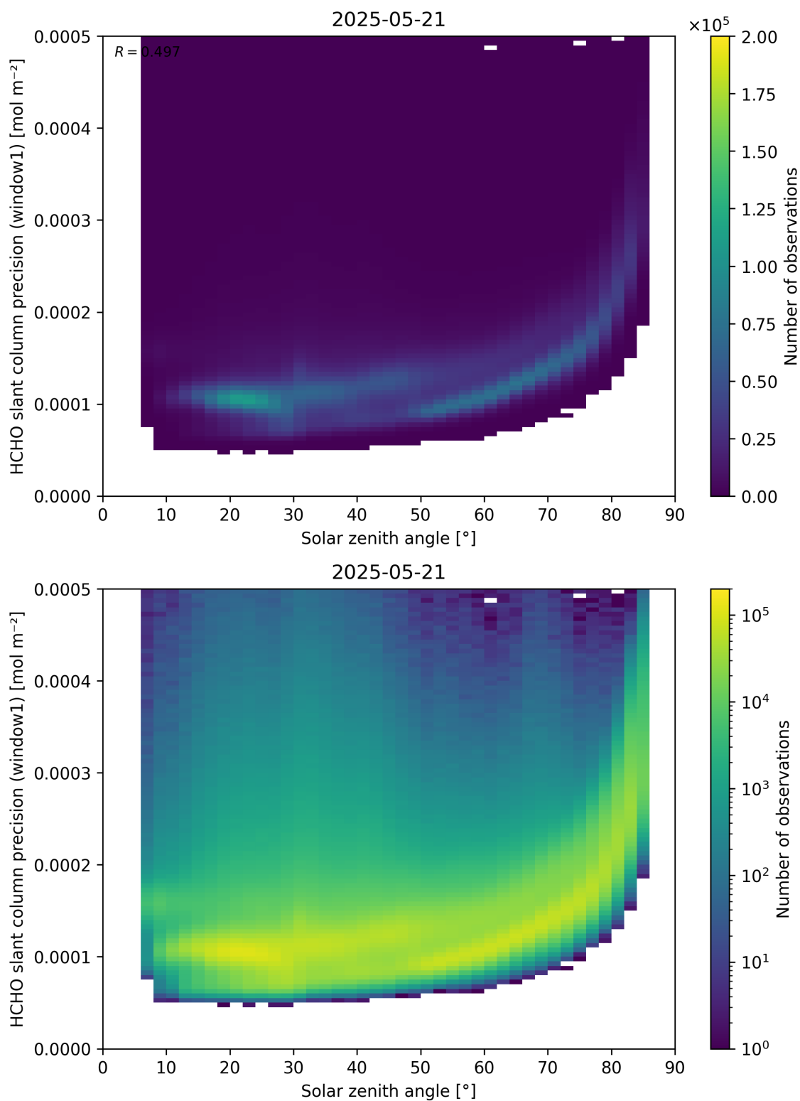
Figure 174: Scatter density plot of “Solar zenith angle” against “HCHO slant column precision (window1)” for 2025-05-21 to 2025-05-22.
