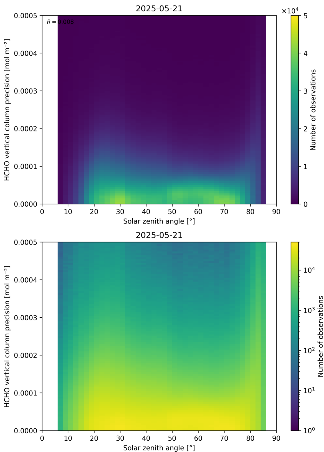
Figure 179: Scatter density plot of “Solar zenith angle” against “HCHO vertical column precision” for 2025-05-21 to 2025-05-22.
