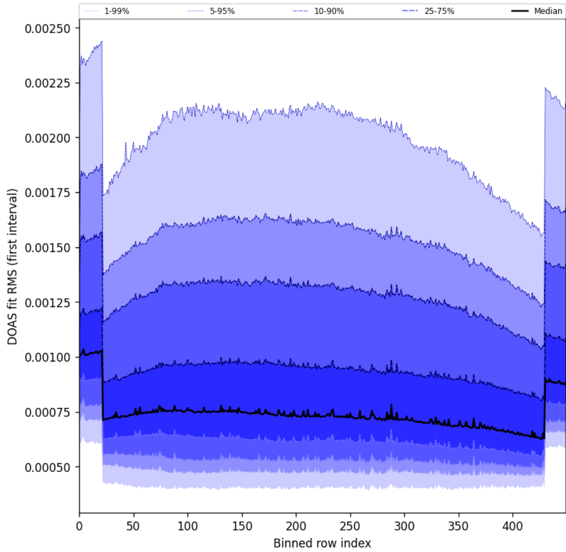
Figure 60: Along track statistics of “DOAS fit RMS (first interval)” for 2025-05-21 to 2025-05-22
