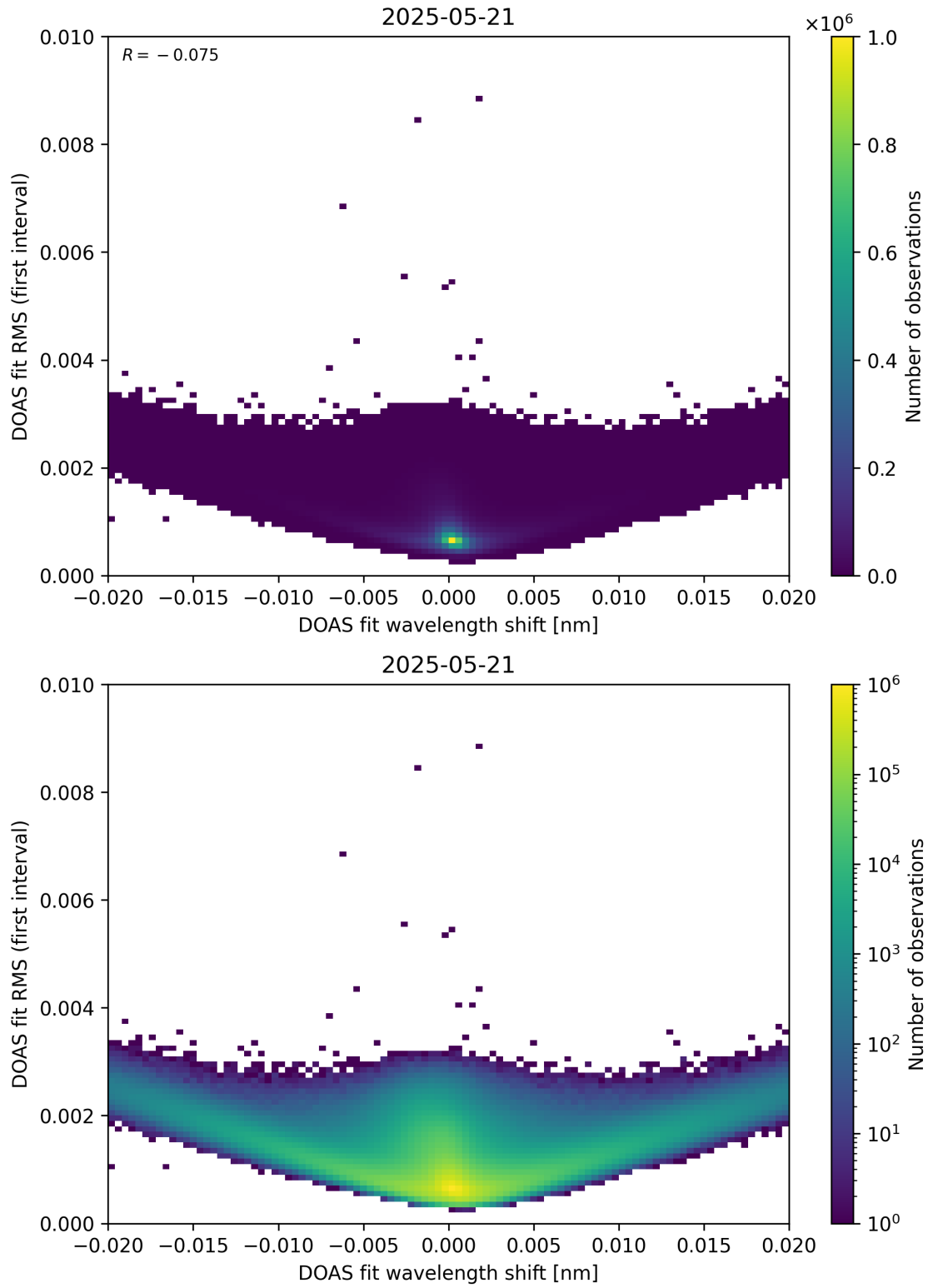
Figure 64: Scatter density plot of “DOAS fit wavelength shift” against “DOAS fit RMS (first interval)” for 2025-05-21 to 2025-05-22.
