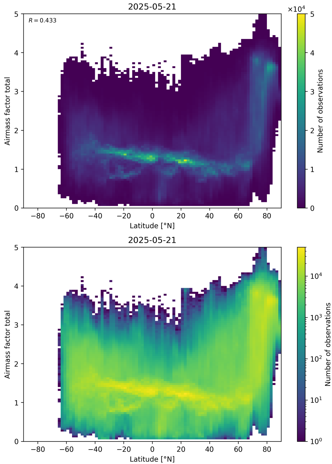
Figure 161: Scatter density plot of “Latitude” against “Airmass factor total” for 2025-05-21 to 2025-05-22.
