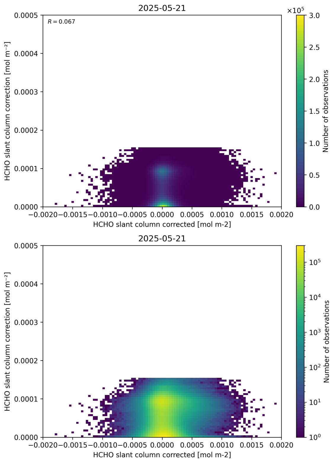
Figure 77: Scatter density plot of “HCHO slant column corrected” against “HCHO slant column correction” for 2025-05-21 to 2025-05-22.
