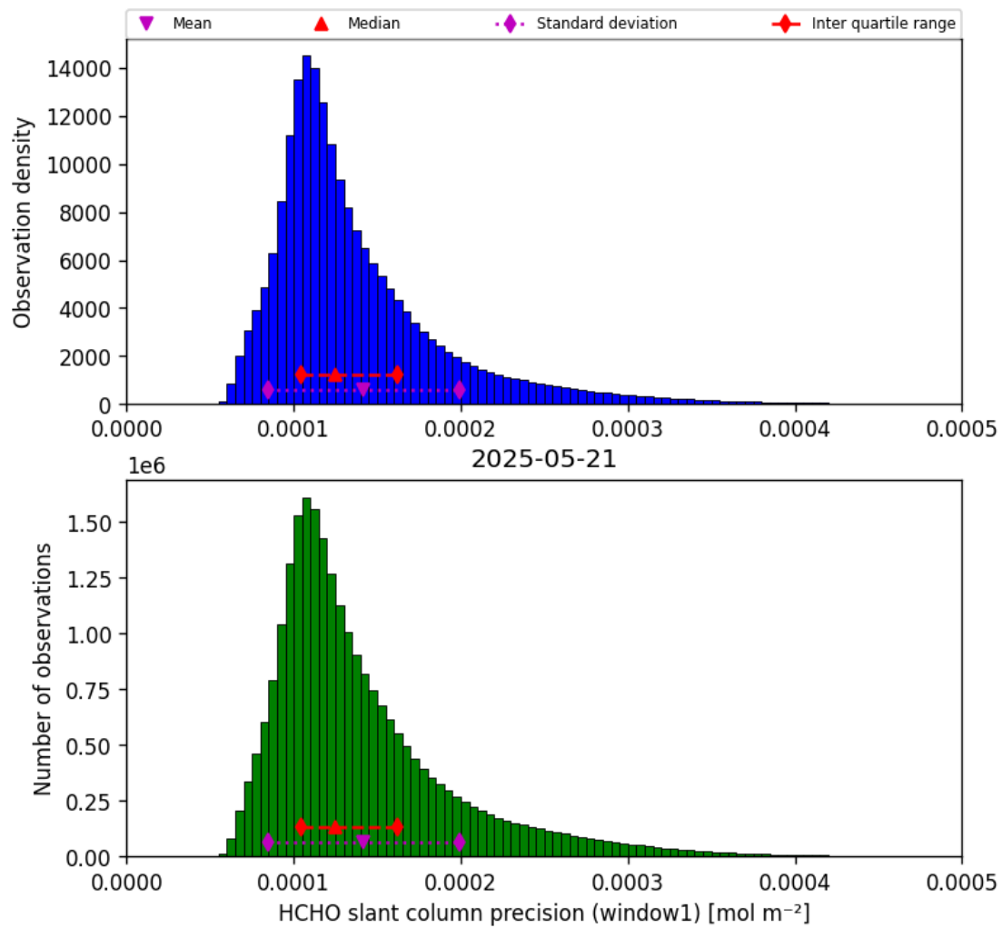
Figure 39: Histogram of “HCHO slant column precision (window1)” for 2025-05-21 to 2025-05-22
