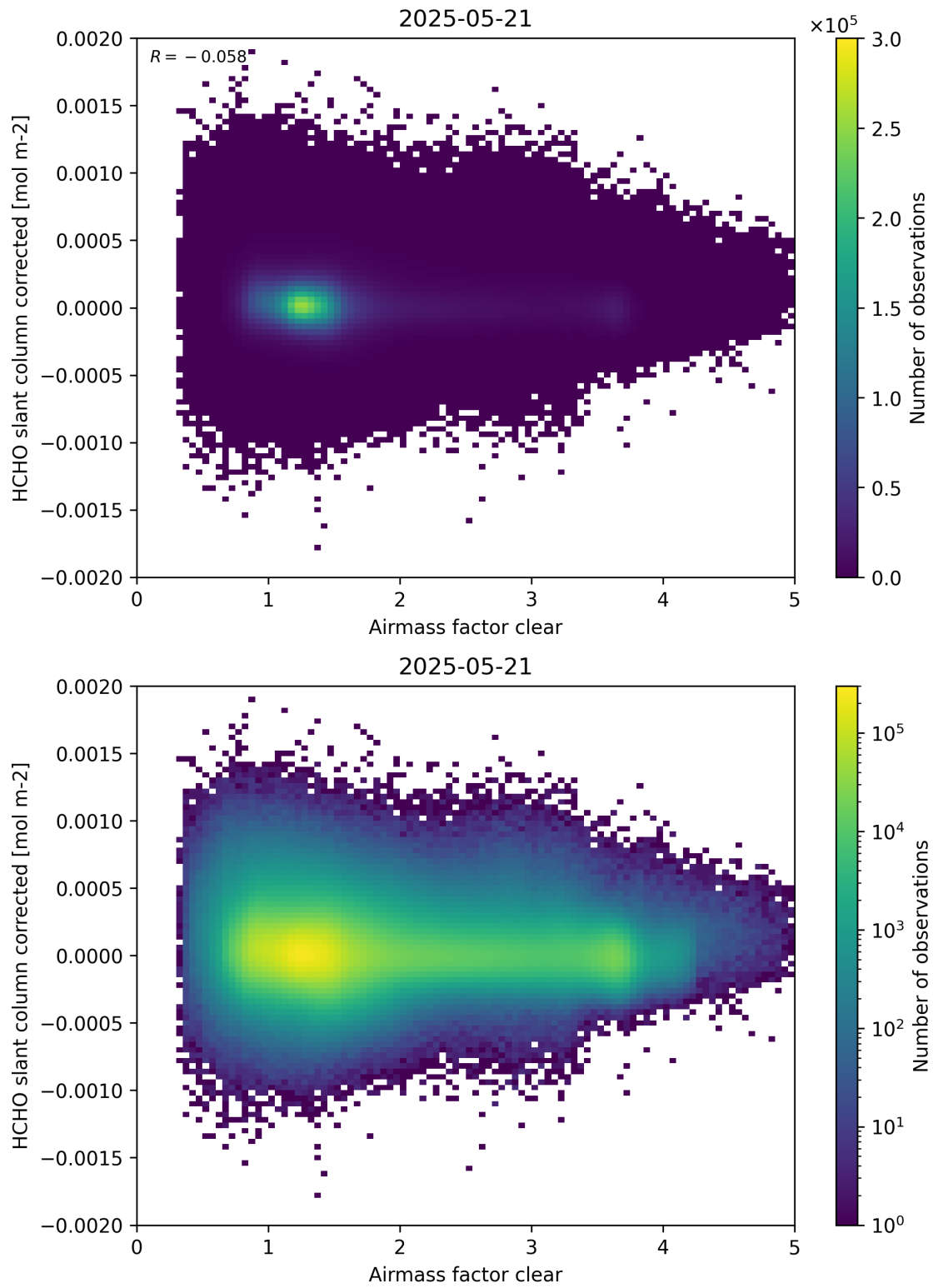
Figure 74: Scatter density plot of “Airmass factor clear” against “HCHO slant column corrected” for 2025-05-21 to 2025-05-22.
