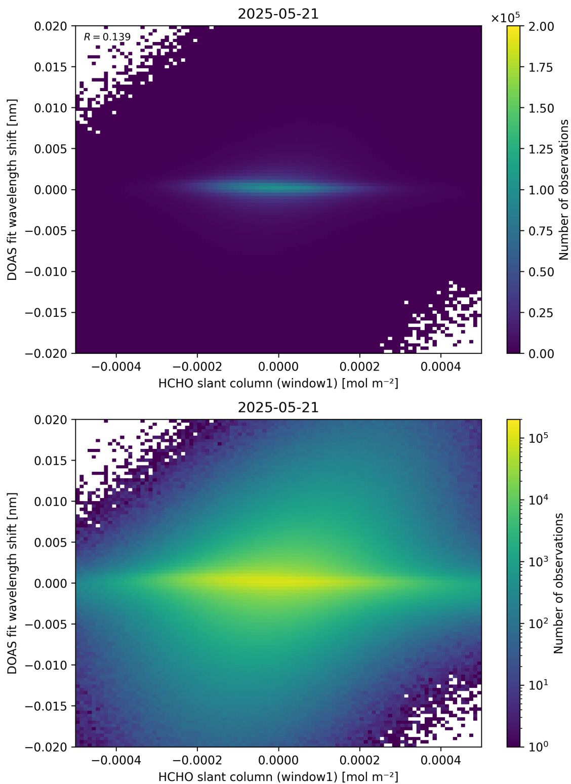
Figure 79: Scatter density plot of “HCHO slant column (window1)” against “DOAS fit wavelength shift” for 2025-05-21 to 2025-05-22.
