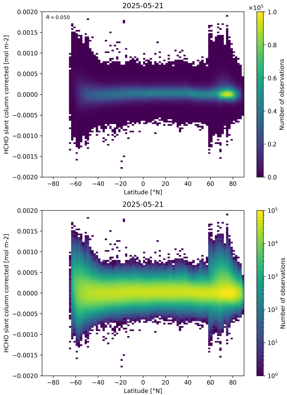
Figure 157: Scatter density plot of “Latitude” against “HCHO slant column corrected” for 2025-05-21 to 2025-05-22.
