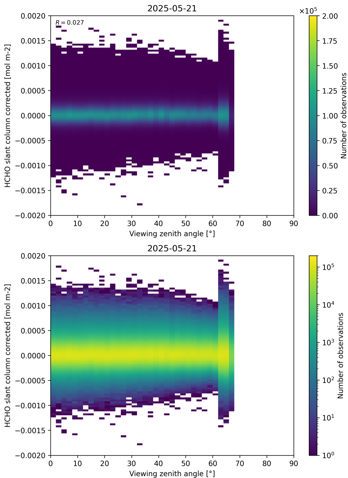
Figure 186: Scatter density plot of “Viewing zenith angle” against “HCHO slant column corrected” for 2025-05-21 to 2025-05-22.
