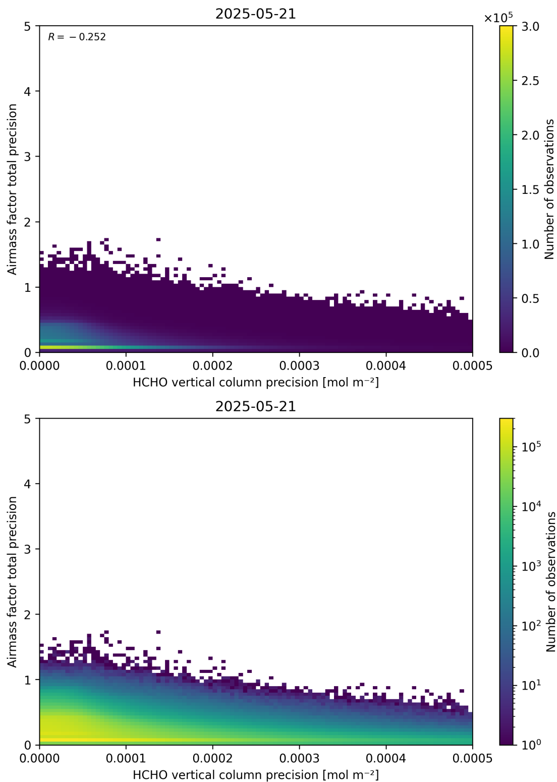
Figure 145: Scatter density plot of “HCHO vertical column precision” against “Airmass factor total precision” for 2025-05-21 to 2025-05-22.
