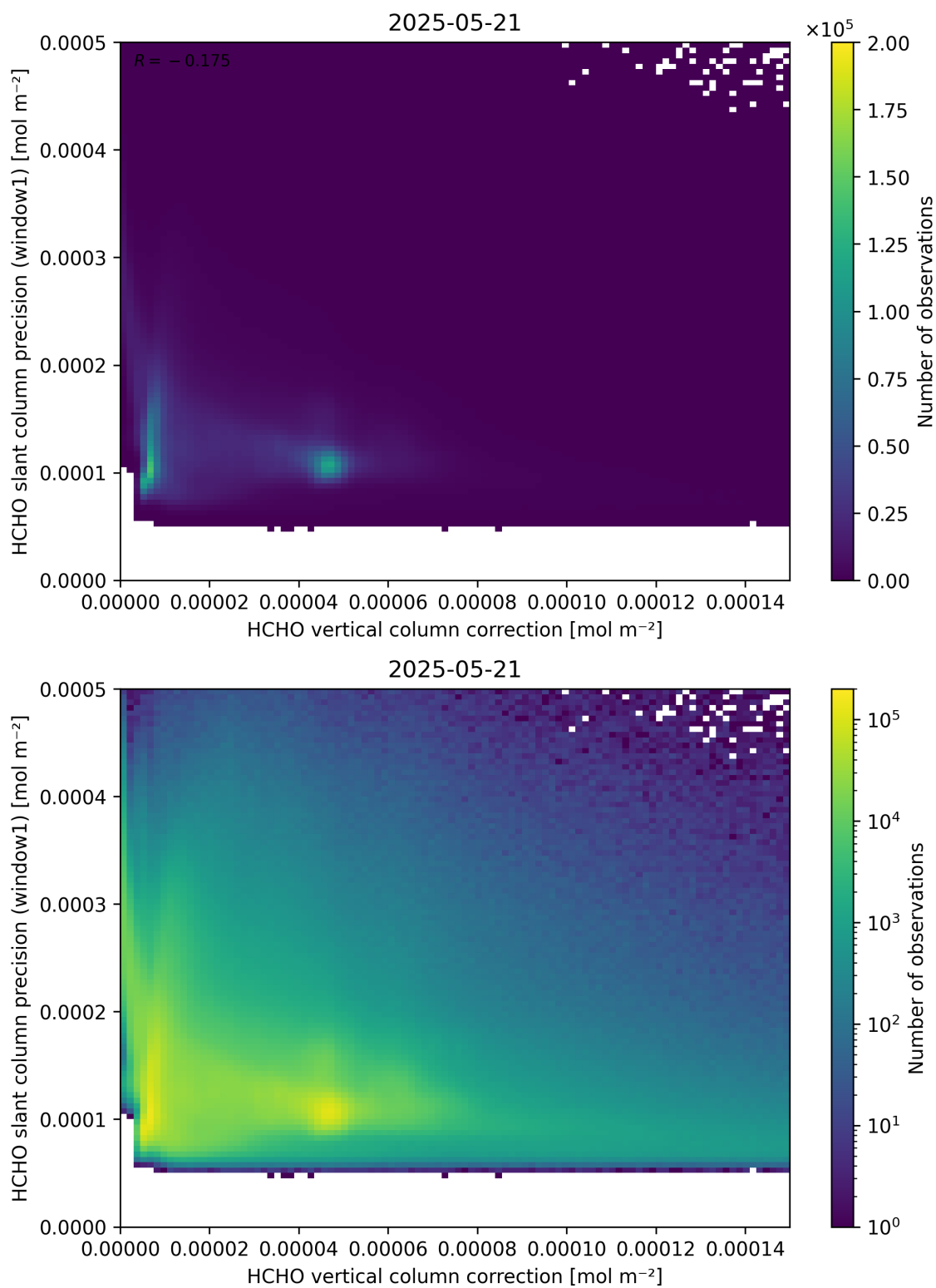
Figure 119: Scatter density plot of “HCHO vertical column correction” against “HCHO slant column precision (window1)” for 2025-05-21 to 2025-05-22.
