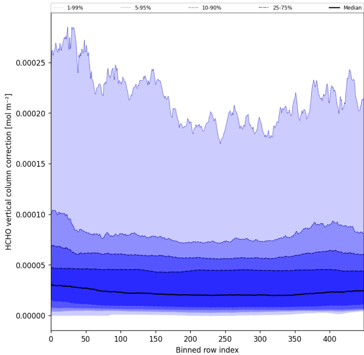
Figure 51: Along track statistics of “HCHO vertical column correction” for 2025-05-21 to 2025-05-22
