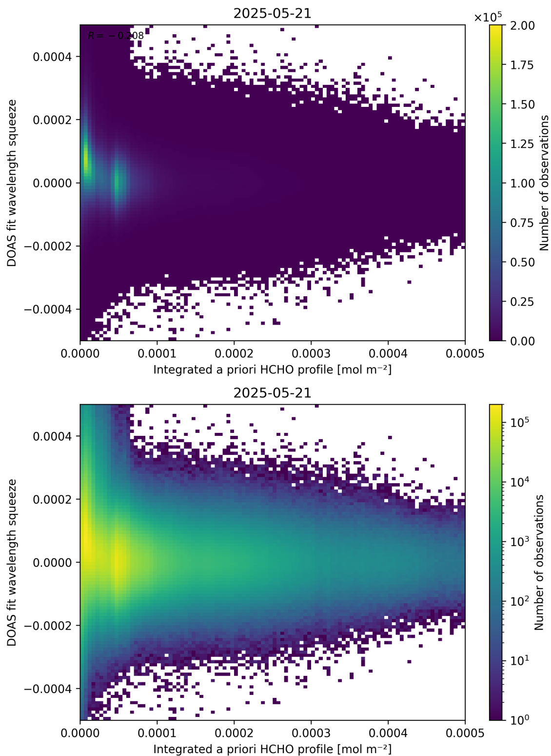
Figure 150: Scatter density plot of “Integrated a priori HCHO profile” against “DOAS fit wavelength squeeze” for 2025-05-21 to 2025-05-22.
