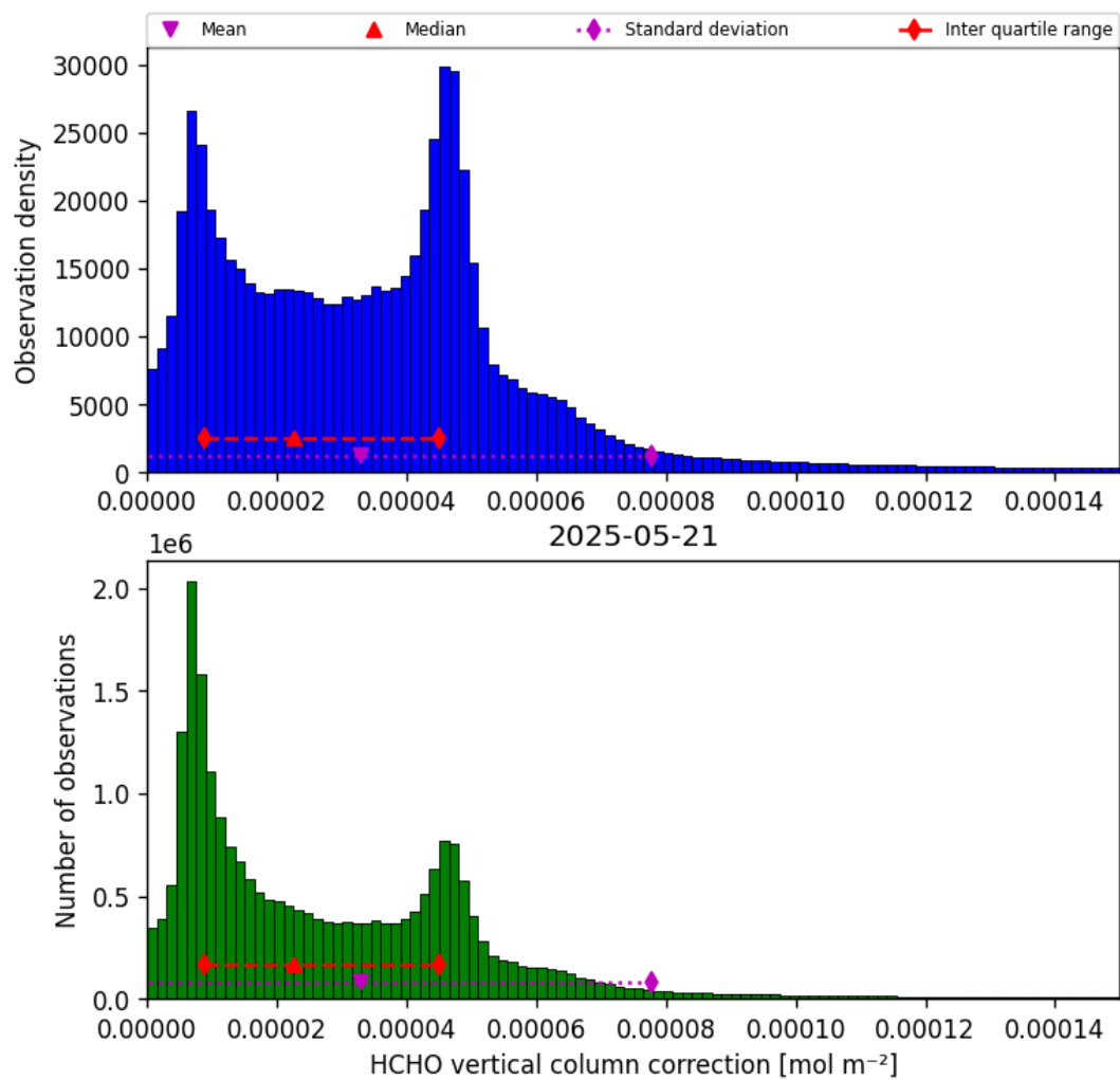
Figure 37: Histogram of “HCHO vertical column correction” for 2025-05-21 to 2025-05-22
