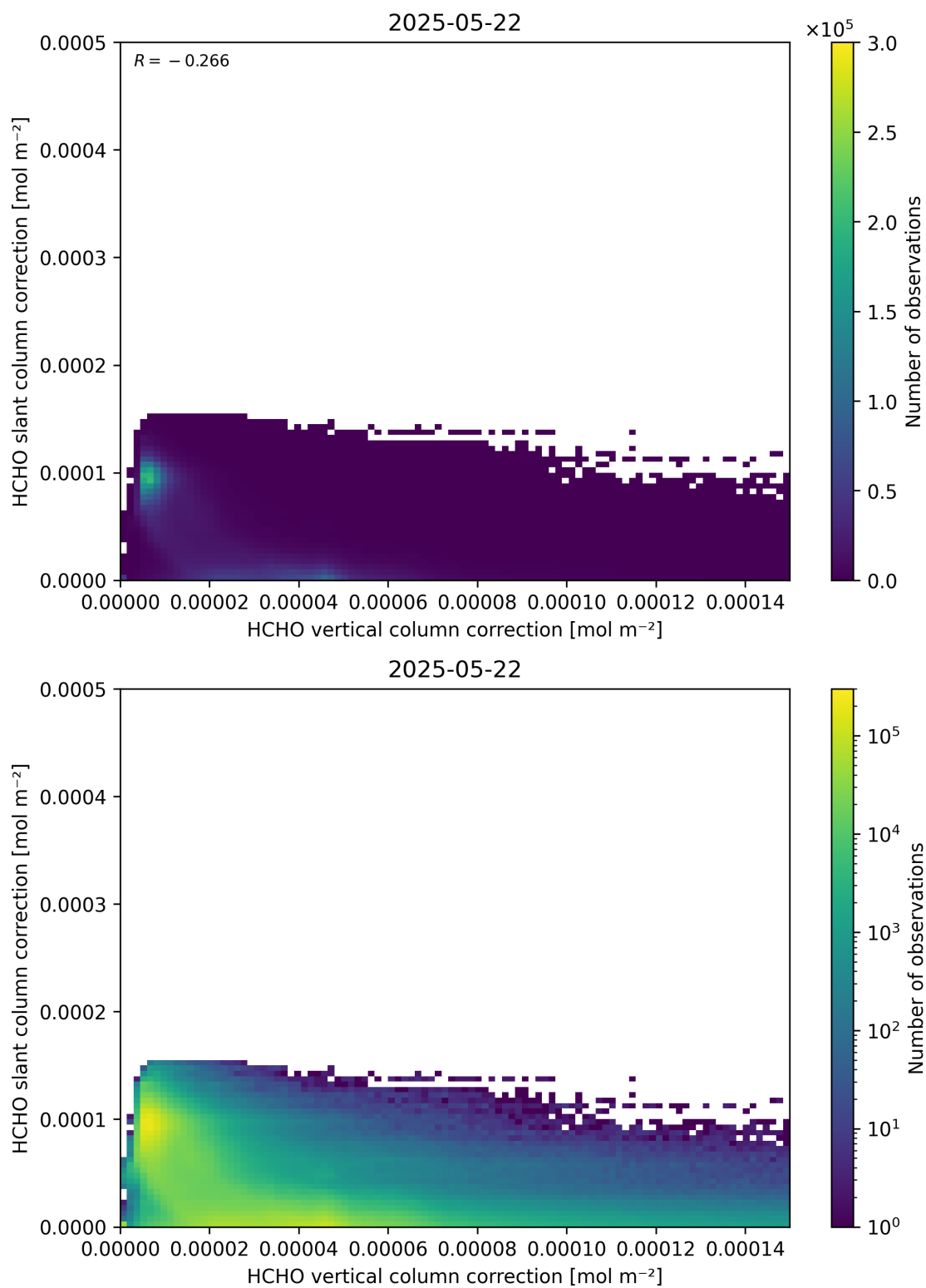
Figure 117: Scatter density plot of “HCHO vertical column correction” against “HCHO slant column correction” for 2025-05-21 to 2025-05-23.
