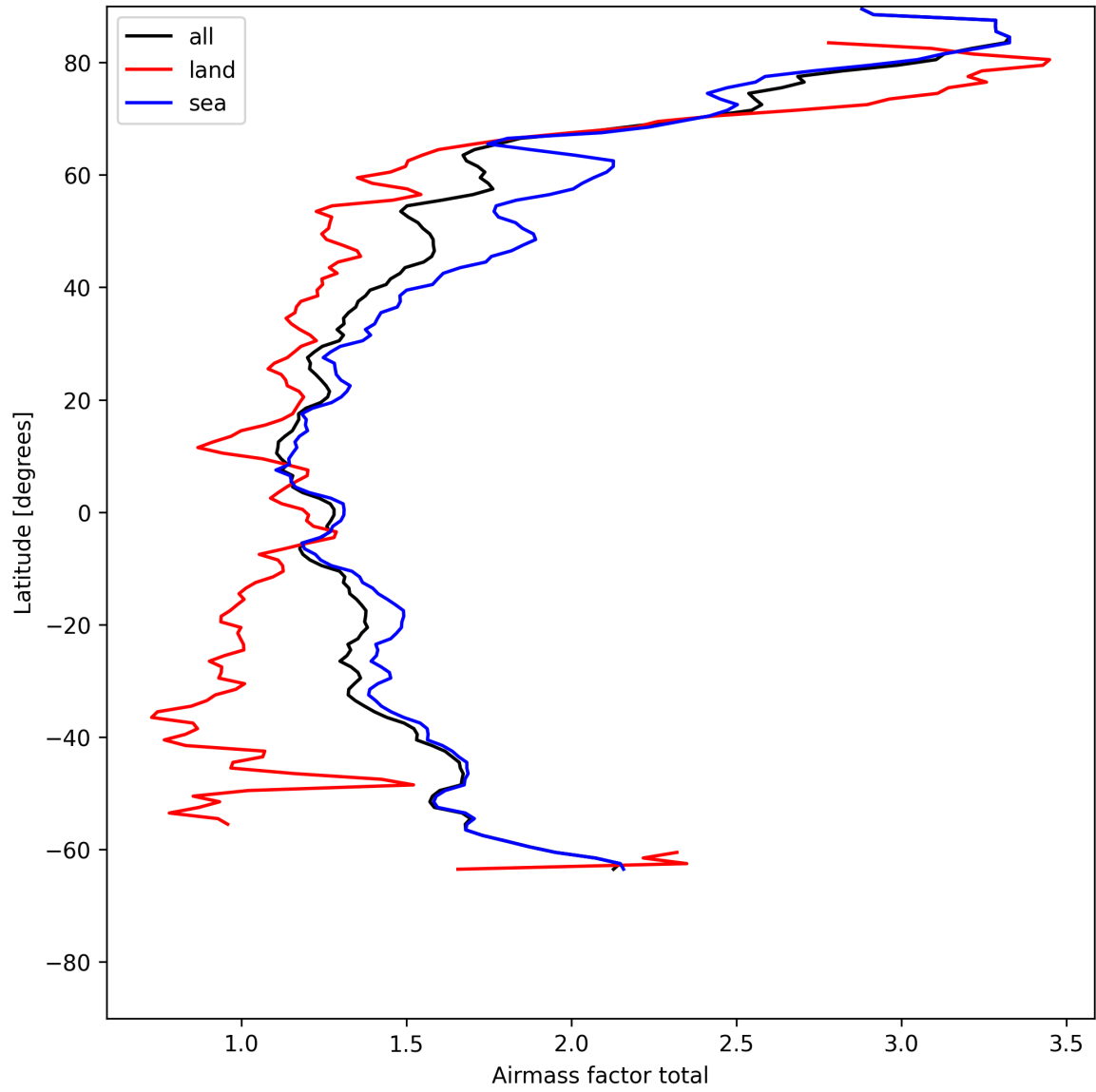
Figure 26: Zonal average of “Airmass factor total” for 2025-05-21 to 2025-05-23.
