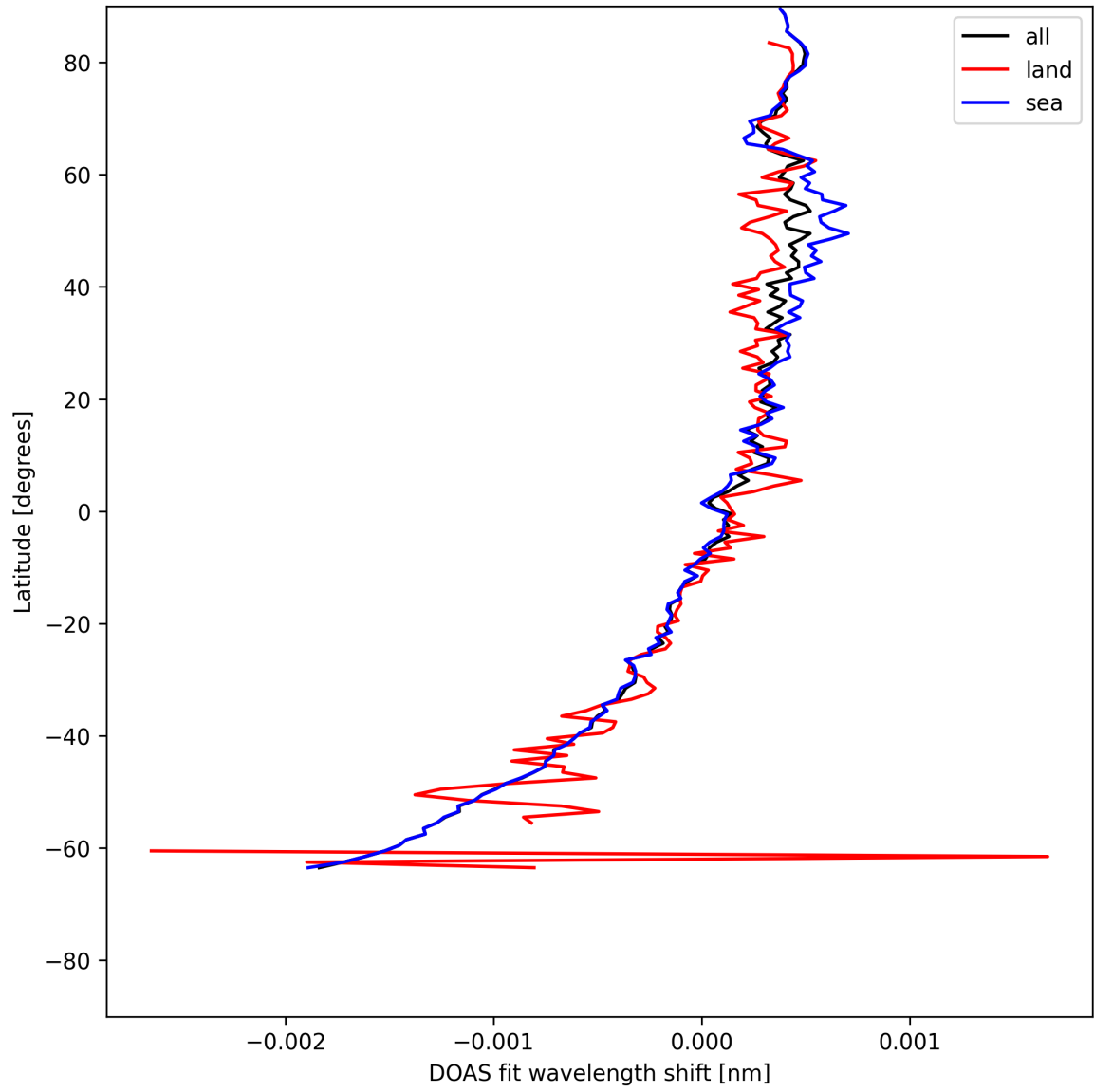
Figure 30: Zonal average of “DOAS fit wavelength shift” for 2025-05-21 to 2025-05-23.
