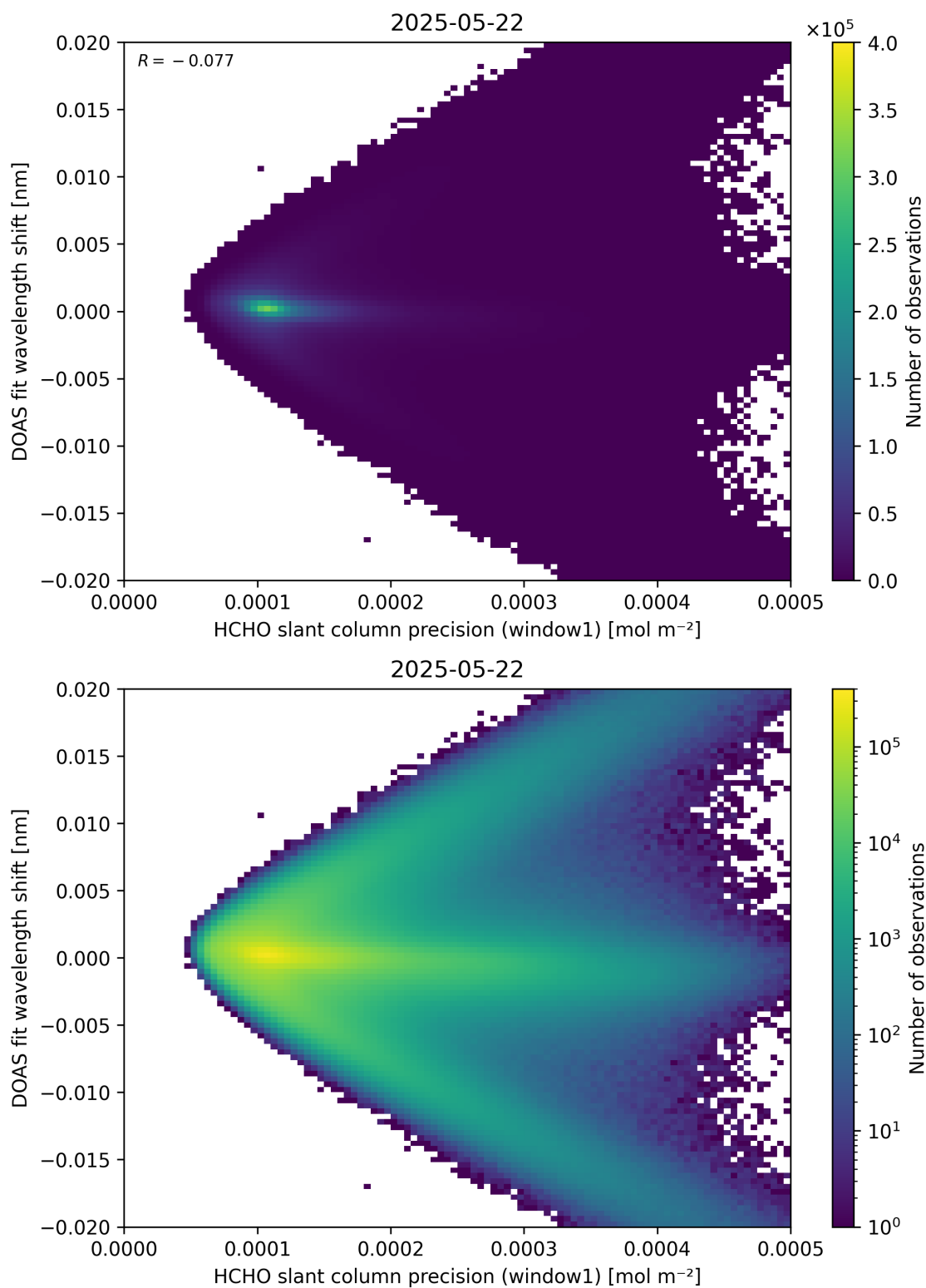
Figure 89: Scatter density plot of “HCHO slant column precision (window1)” against “DOAS fit wavelength shift” for 2025-05-21 to 2025-05-23.
