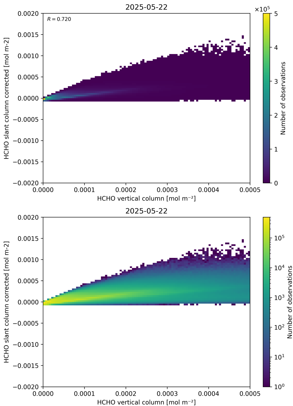
Figure 127: Scatter density plot of “HCHO vertical column” against “HCHO slant column corrected” for 2025-05-21 to 2025-05-23.
