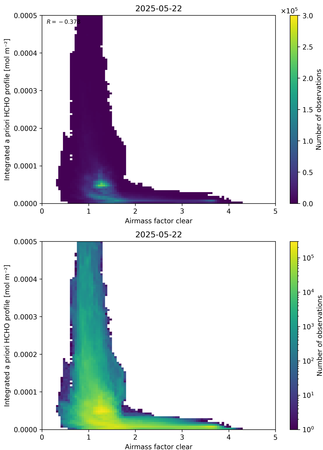
Figure 76: Scatter density plot of “Airmass factor clear” against “Integrated a priori HCHO profile” for 2025-05-21 to 2025-05-23.
