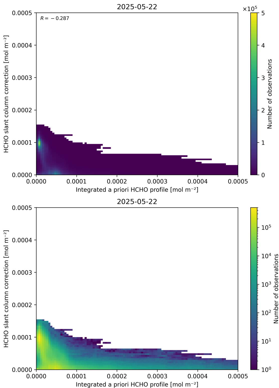
Figure 152: Scatter density plot of “Integrated a priori HCHO profile” against “HCHO slant column correction” for 2025-05-21 to 2025-05-23.
