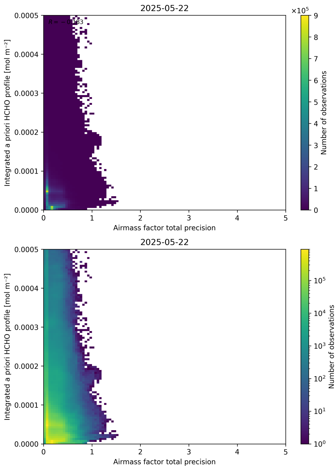
Figure 111: Scatter density plot of “Airmass factor total precision” against “Integrated a priori HCHO profile” for 2025-05-21 to 2025-05-23.
