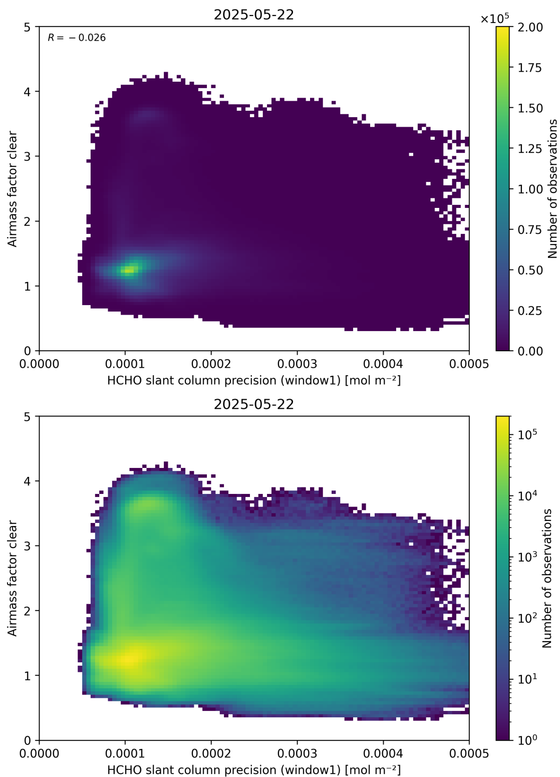
Figure 91: Scatter density plot of “HCHO slant column precision (window1)” against “Airmass factor clear” for 2025-05-21 to 2025-05-23.
