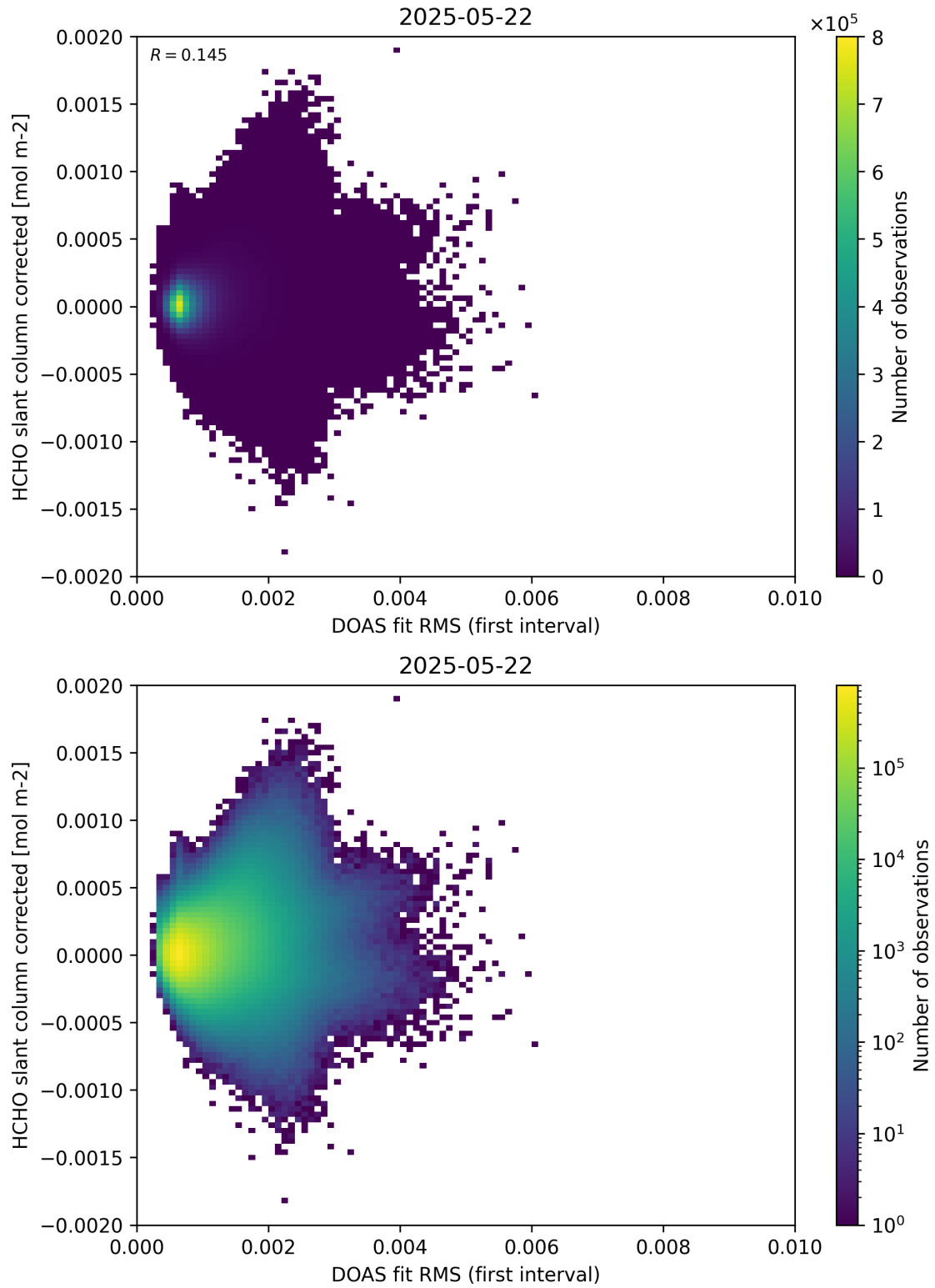
Figure 62: Scatter density plot of “DOAS fit RMS (first interval)” against “HCHO slant column corrected” for 2025-05-21 to 2025-05-23.
