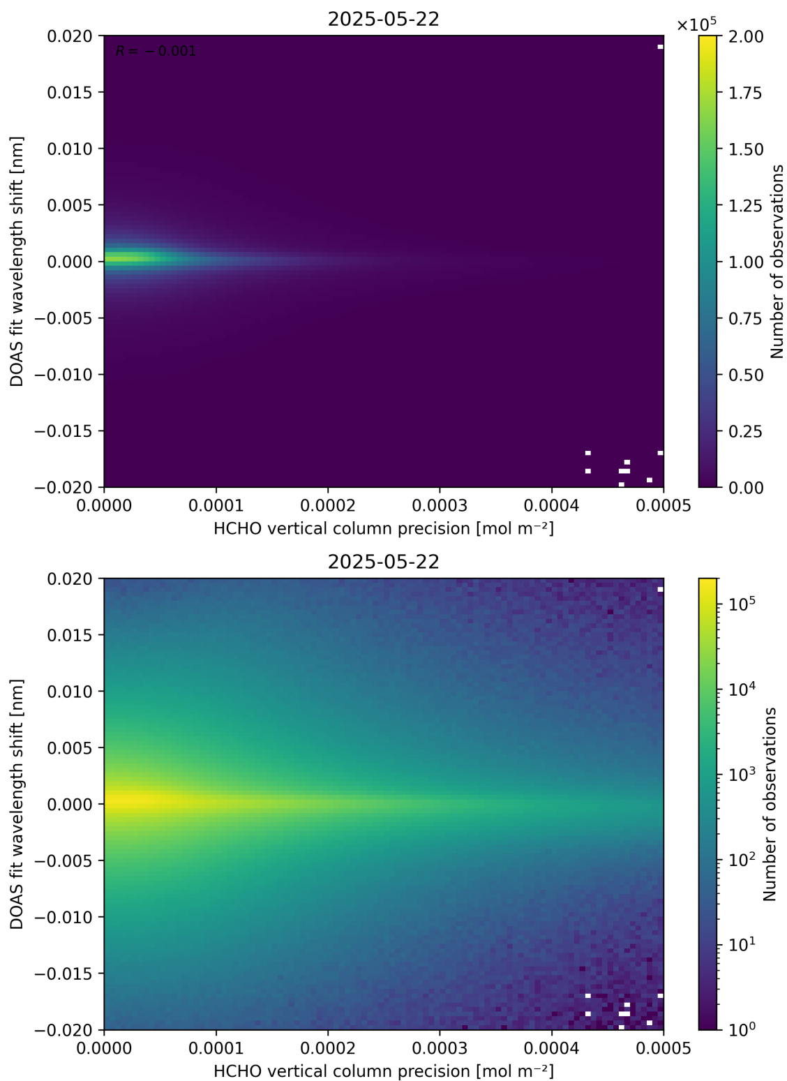
Figure 137: Scatter density plot of “HCHO vertical column precision” against “DOAS fit wavelength shift” for 2025-05-21 to 2025-05-23.
