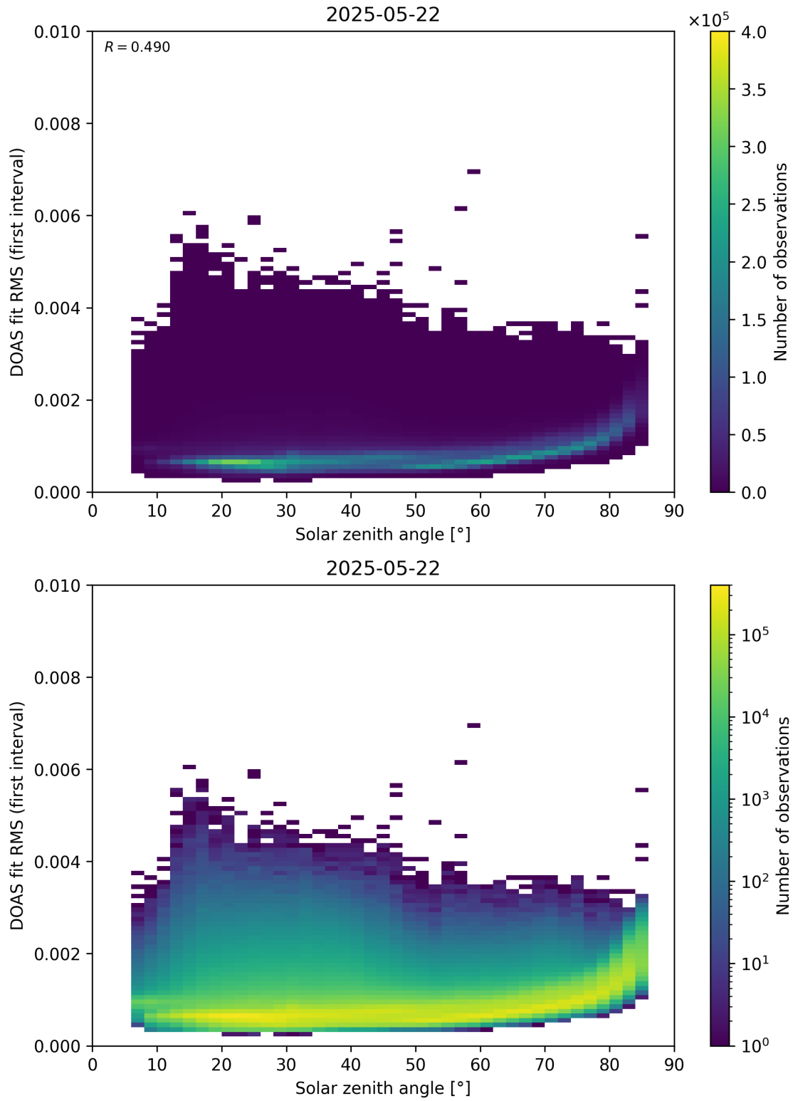
Figure 167: Scatter density plot of “Solar zenith angle” against “DOAS fit RMS (first interval)” for 2025-05-21 to 2025-05-23.
