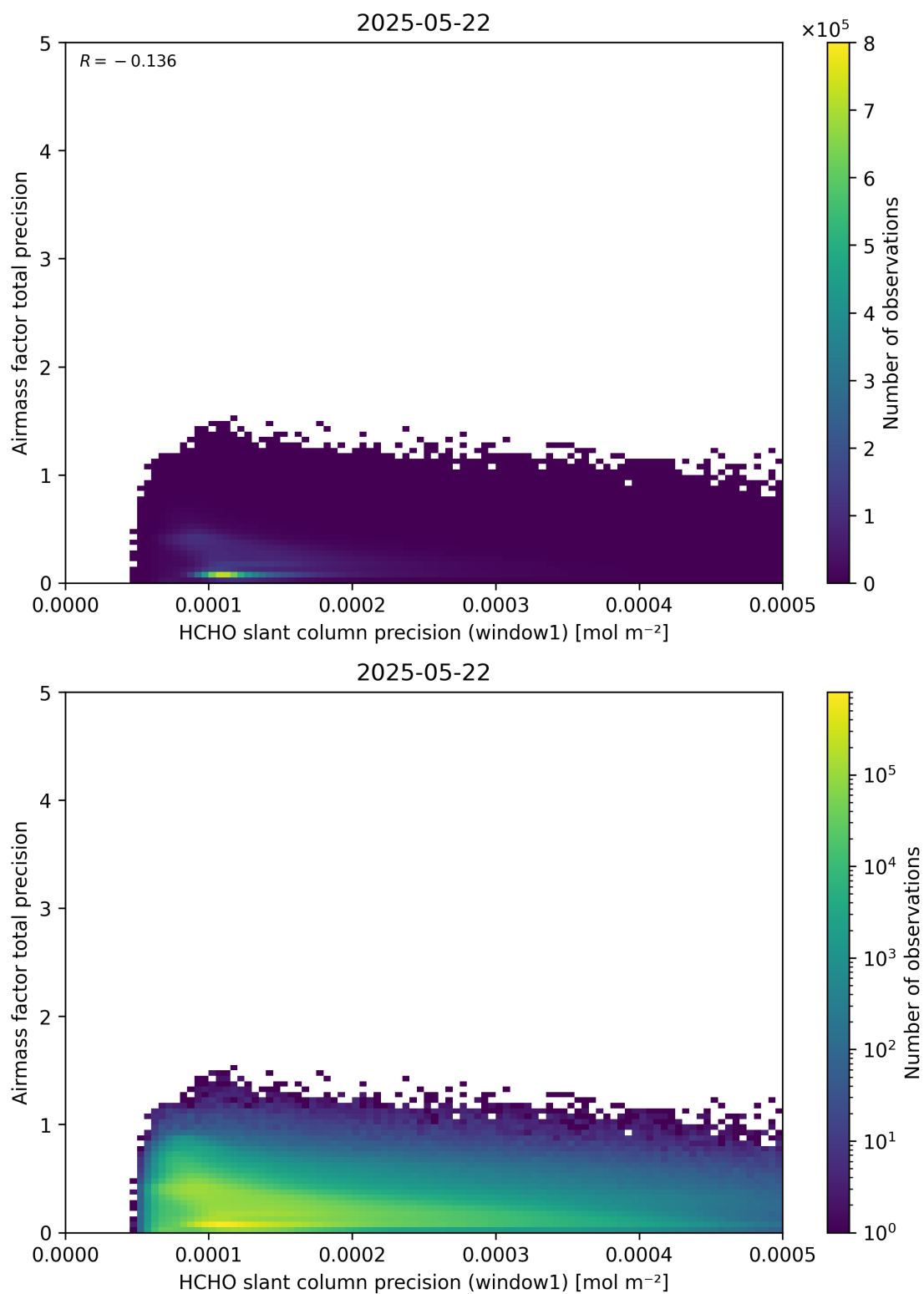
Figure 95: Scatter density plot of “HCHO slant column precision (window1)” against “Airmass factor total precision” for 2025-05-21 to 2025-05-23.
