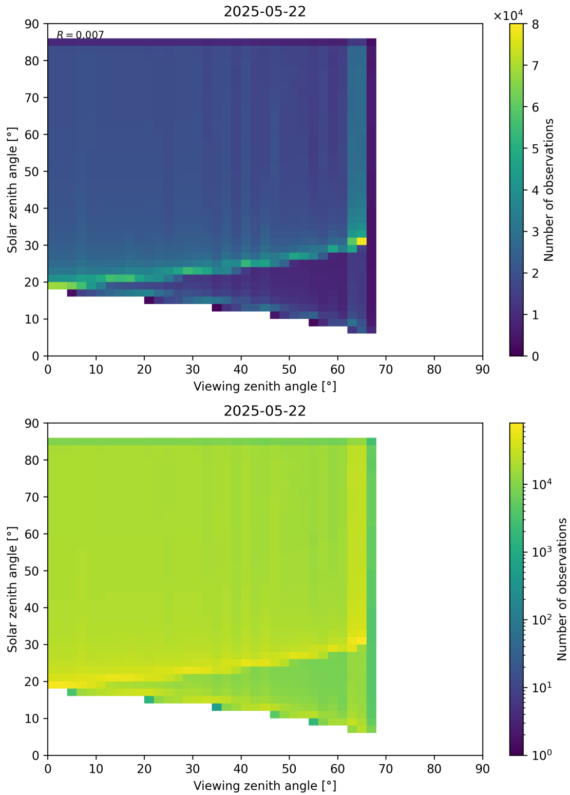
Figure 197: Scatter density plot of “Viewing zenith angle” against “Solar zenith angle” for 2025-05-21 to 2025-05-23.
