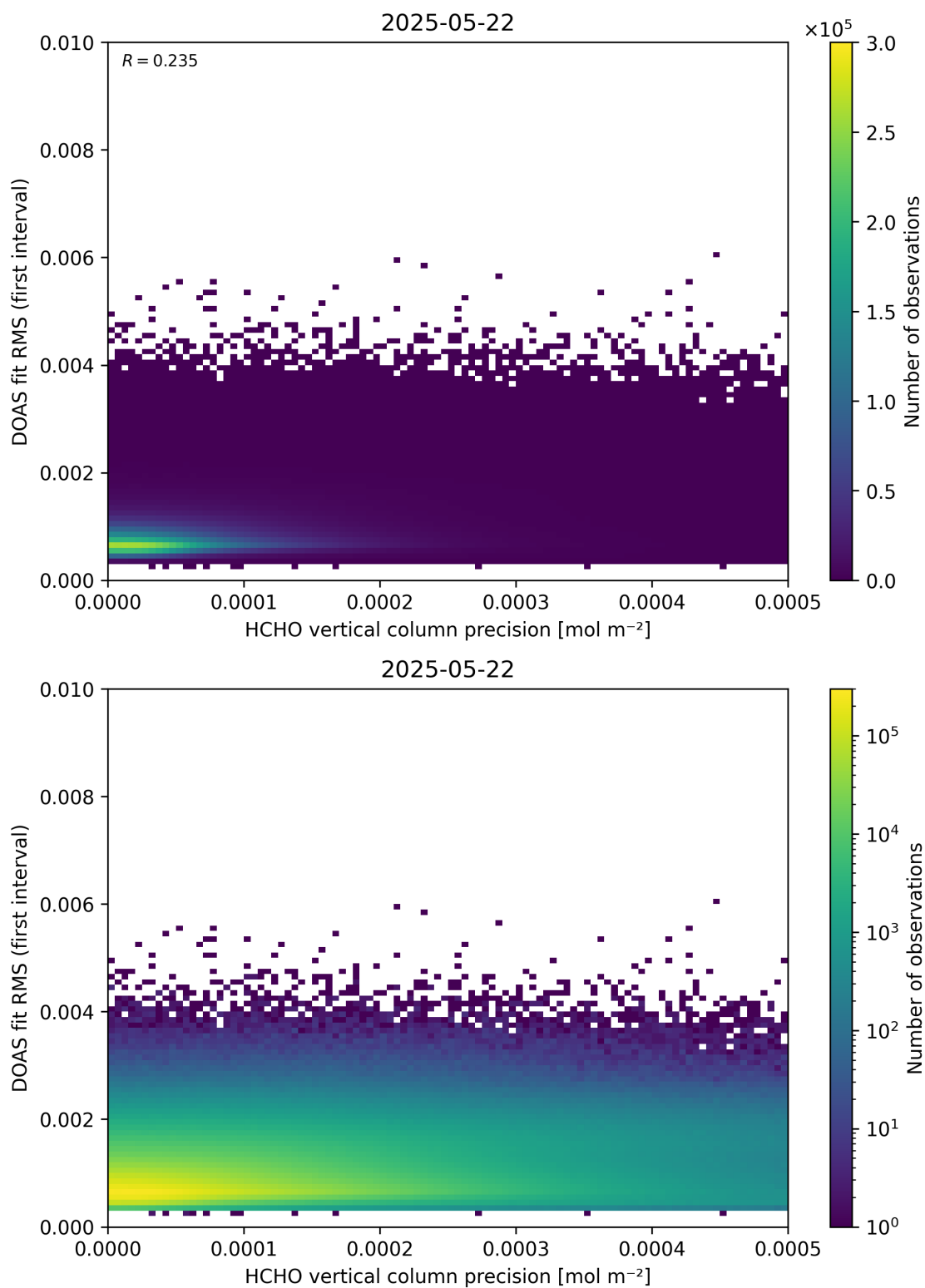
Figure 136: Scatter density plot of “HCHO vertical column precision” against “DOAS fit RMS (first interval)” for 2025-05-21 to 2025-05-23.
