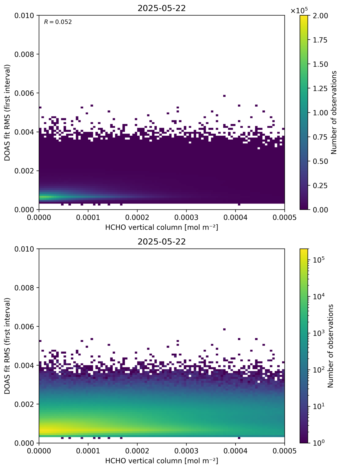
Figure 123: Scatter density plot of “HCHO vertical column” against “DOAS fit RMS (first interval)” for 2025-05-21 to 2025-05-23.
