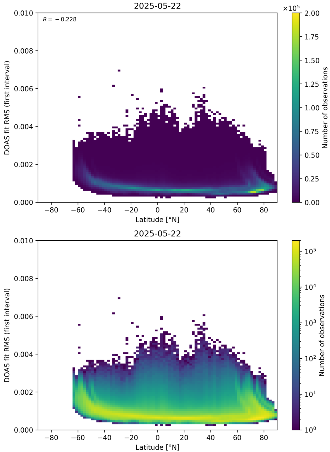
Figure 153: Scatter density plot of “Latitude” against “DOAS fit RMS (first interval)” for 2025-05-21 to 2025-05-23.
