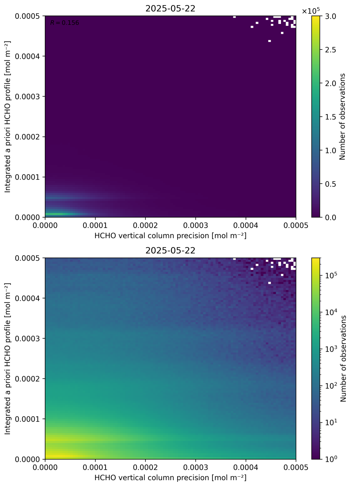
Figure 147: Scatter density plot of “HCHO vertical column precision” against “Integrated a priori HCHO profile” for 2025-05-21 to 2025-05-23.
