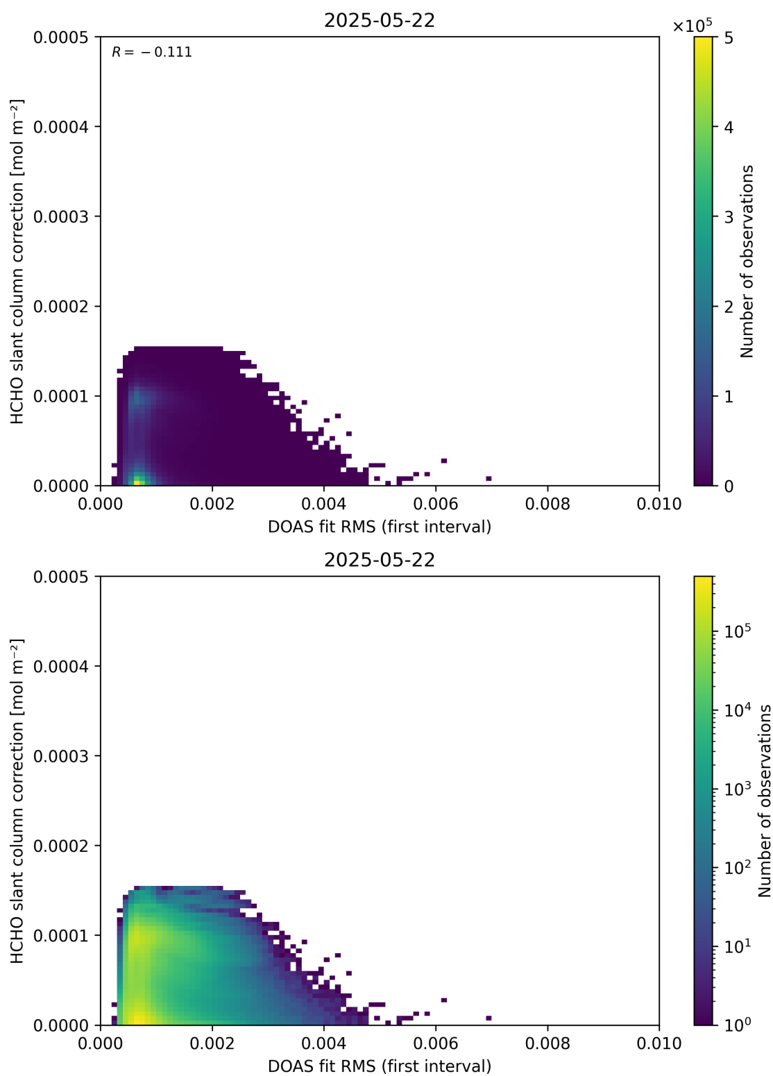
Figure 63: Scatter density plot of “DOAS fit RMS (first interval)” against “HCHO slant column correction” for 2025-05-21 to 2025-05-23.
