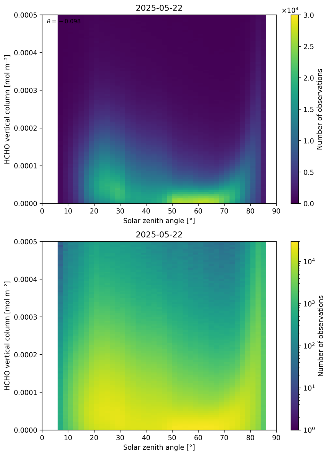
Figure 177: Scatter density plot of “Solar zenith angle” against “HCHO vertical column” for 2025-05-21 to 2025-05-23.
