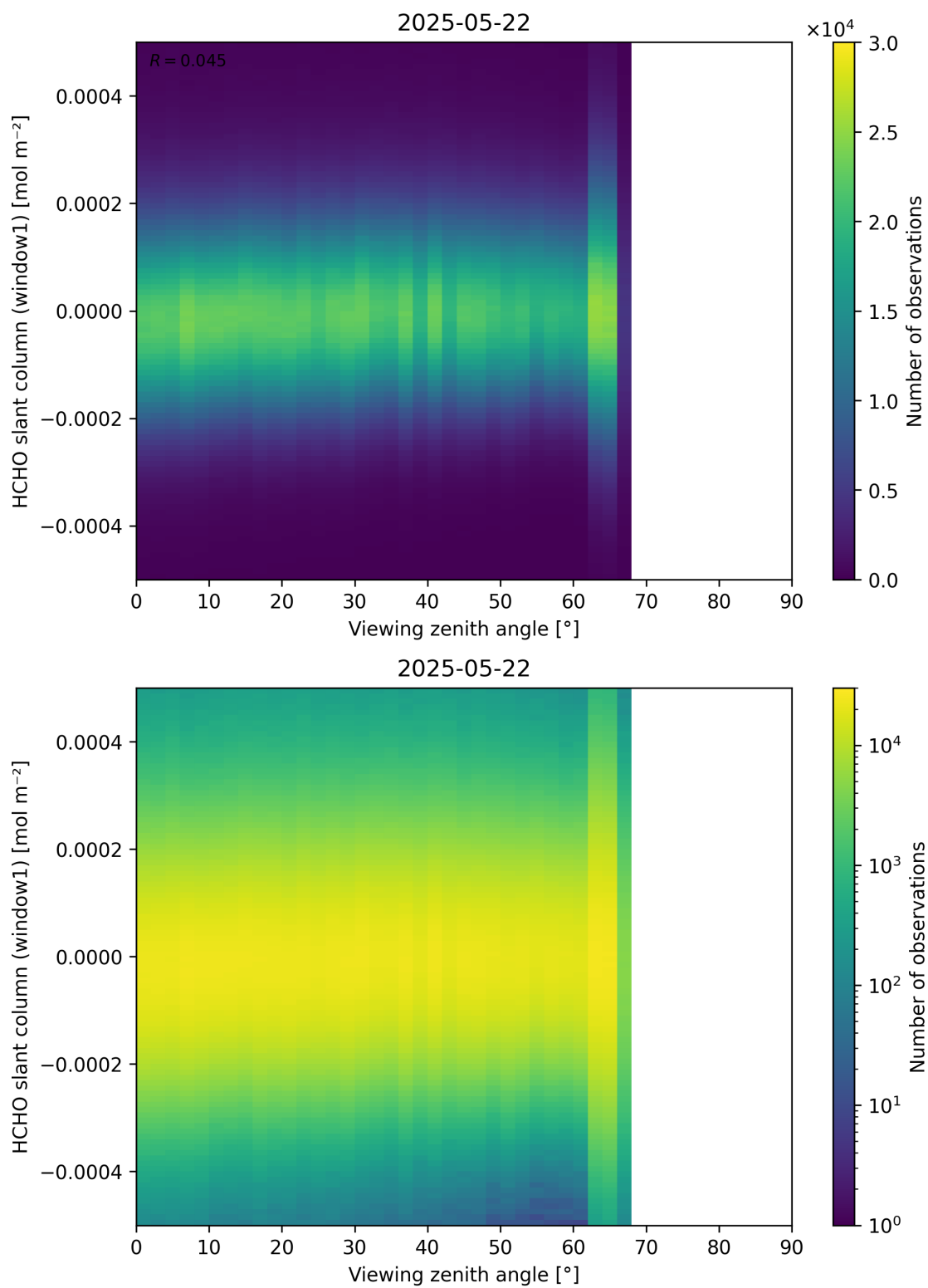
Figure 188: Scatter density plot of “Viewing zenith angle” against “HCHO slant column (window1)” for 2025-05-21 to 2025-05-23.
