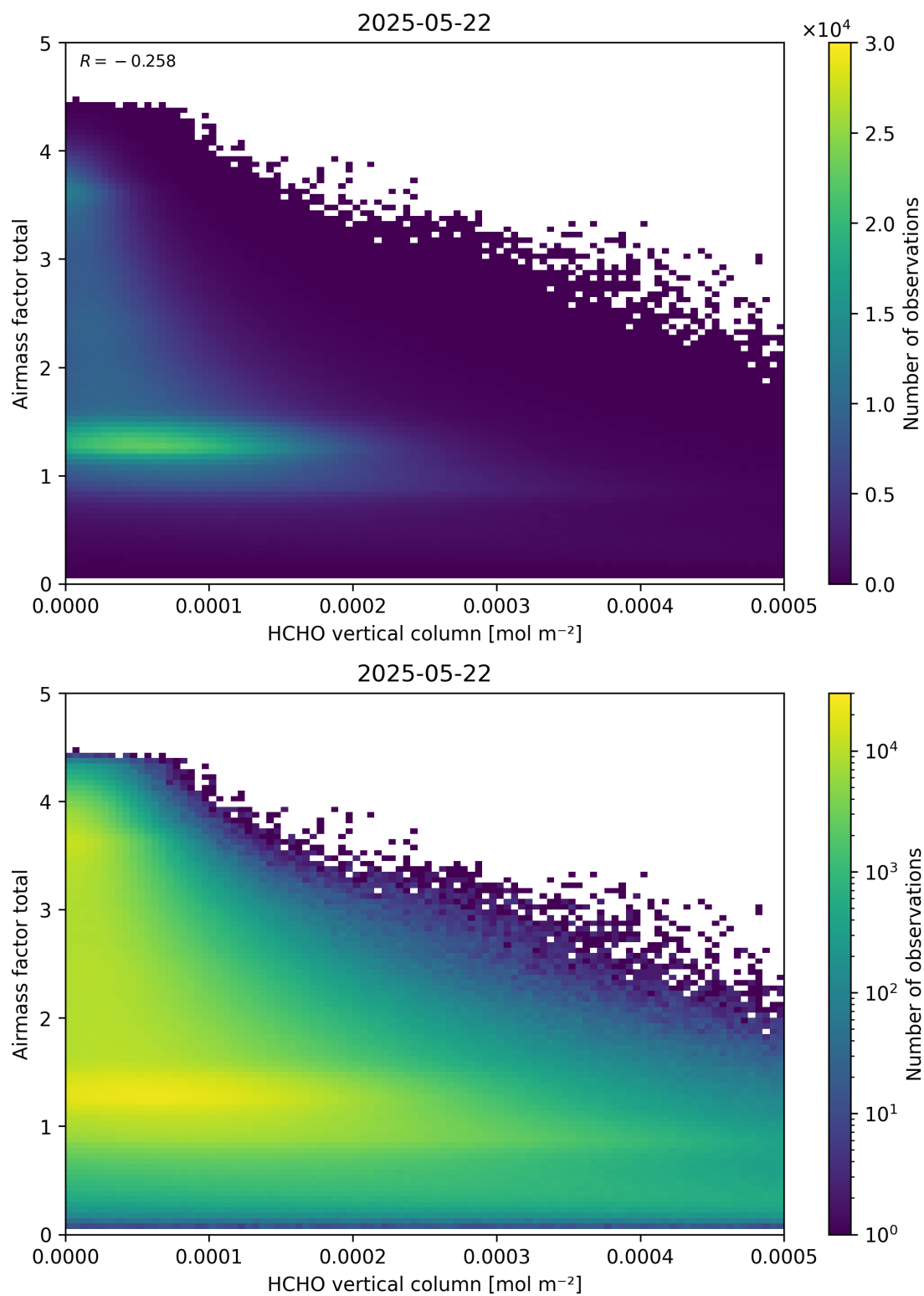
Figure 131: Scatter density plot of “HCHO vertical column” against “Airmass factor total” for 2025-05-21 to 2025-05-23.
