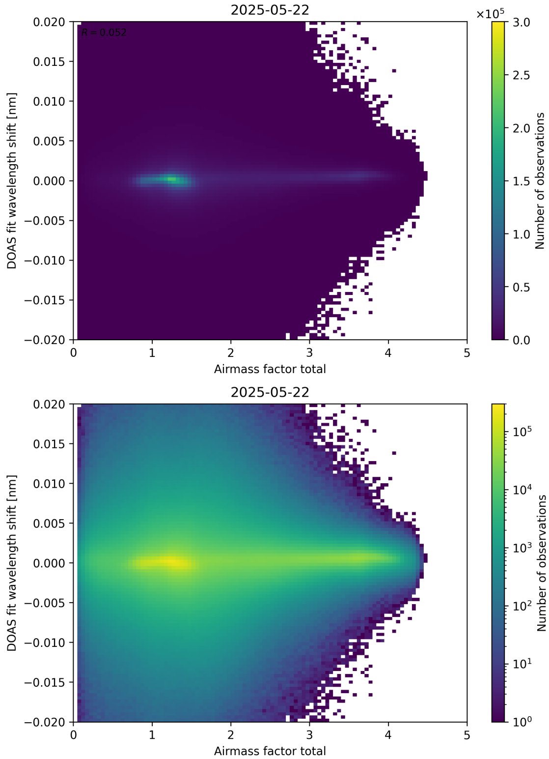
Figure 98: Scatter density plot of “Airmass factor total” against “DOAS fit wavelength shift” for 2025-05-21 to 2025-05-23.
