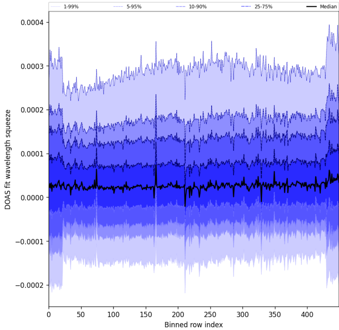
Figure 59: Along track statistics of “DOAS fit wavelength squeeze” for 2025-05-21 to 2025-05-23
