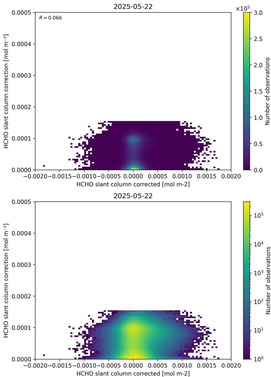
Figure 77: Scatter density plot of “HCHO slant column corrected” against “HCHO slant column correction” for 2025-05-21 to 2025-05-23.
