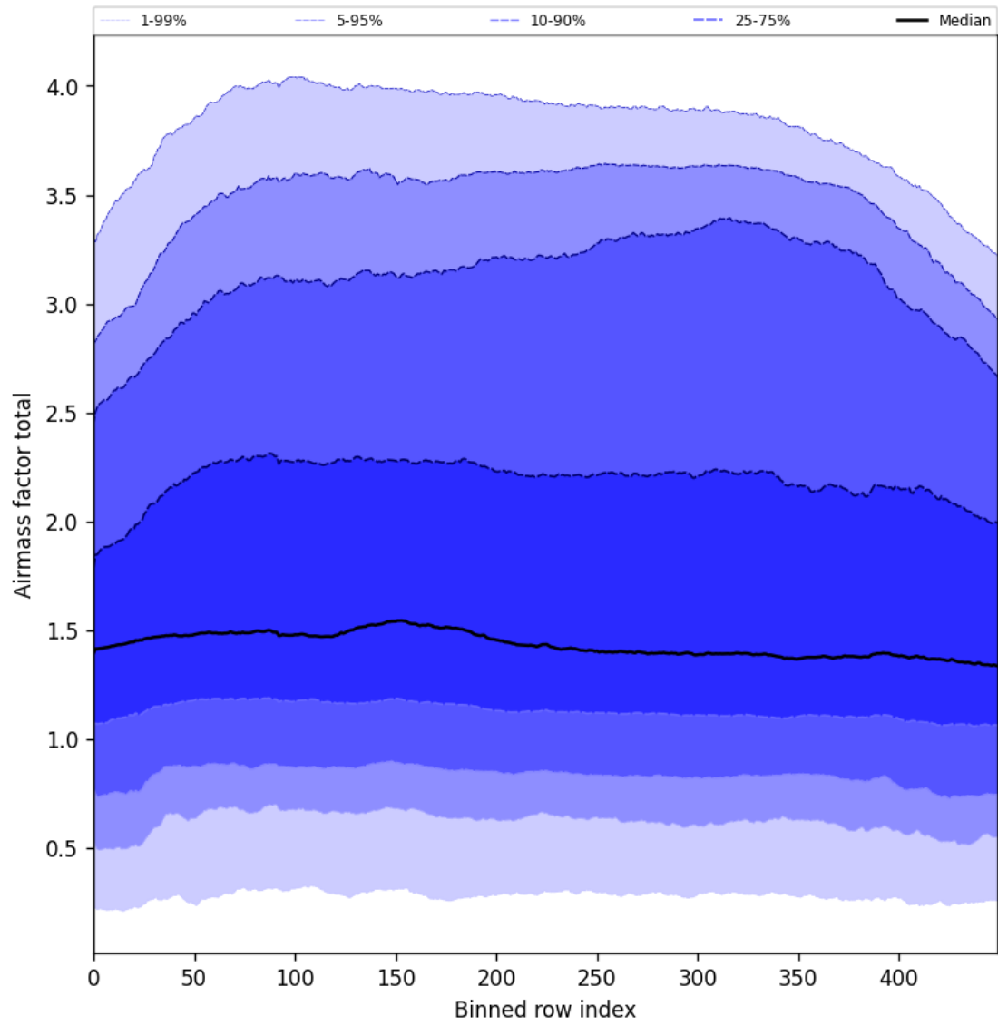
Figure 54: Along track statistics of “Airmass factor total” for 2025-05-21 to 2025-05-23
