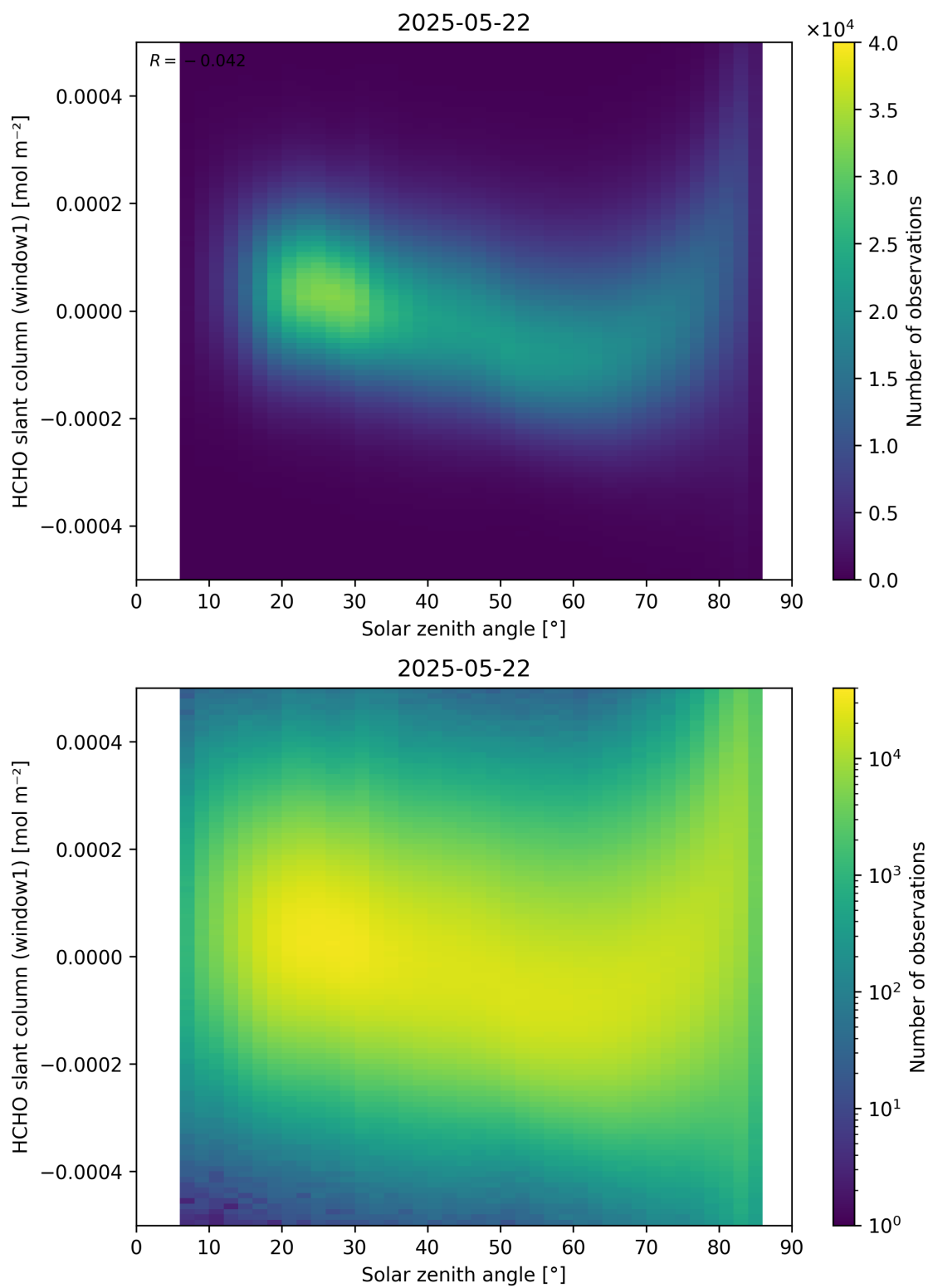
Figure 173: Scatter density plot of “Solar zenith angle” against “HCHO slant column (window1)” for 2025-05-21 to 2025-05-23.
