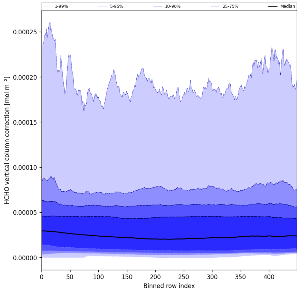
Figure 51: Along track statistics of “HCHO vertical column correction” for 2025-05-21 to 2025-05-23
