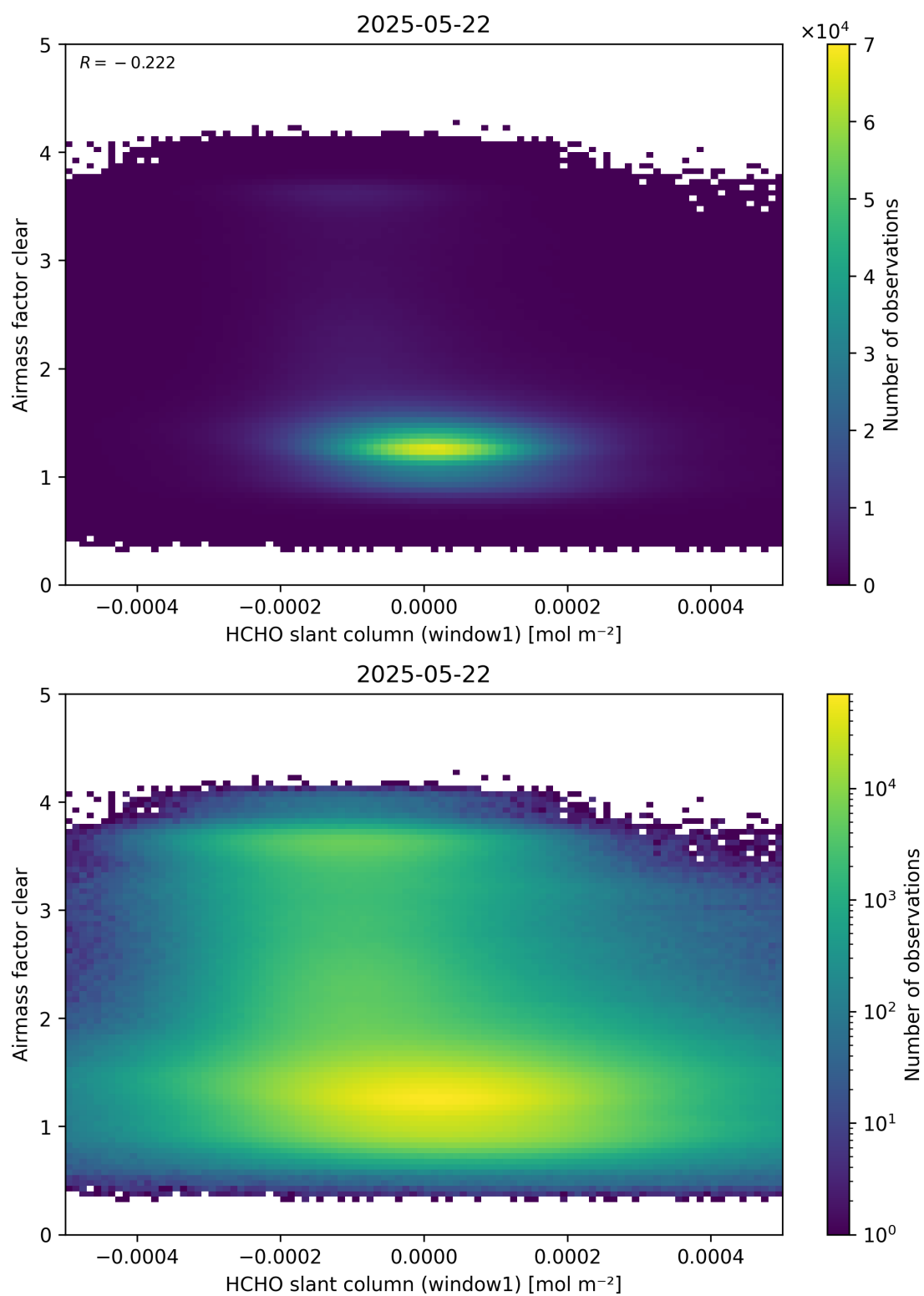
Figure 81: Scatter density plot of “HCHO slant column (window1)” against “Airmass factor clear” for 2025-05-21 to 2025-05-23.
