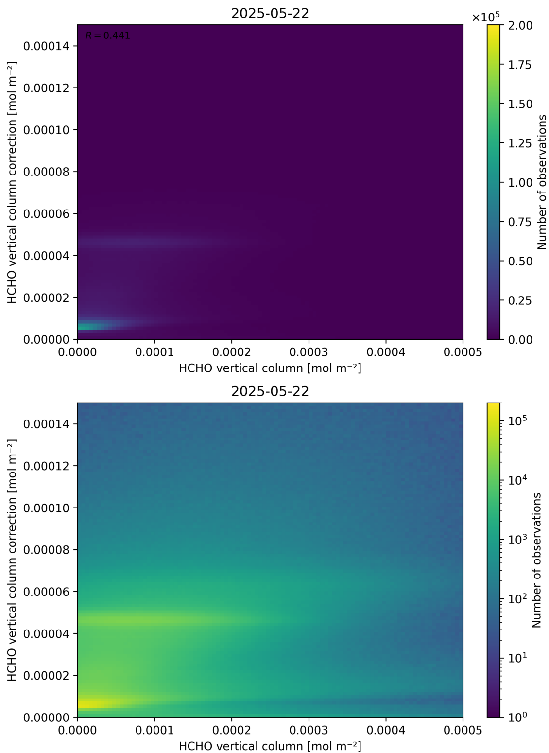
Figure 133: Scatter density plot of “HCHO vertical column” against “HCHO vertical column correction” for 2025-05-21 to 2025-05-23.
