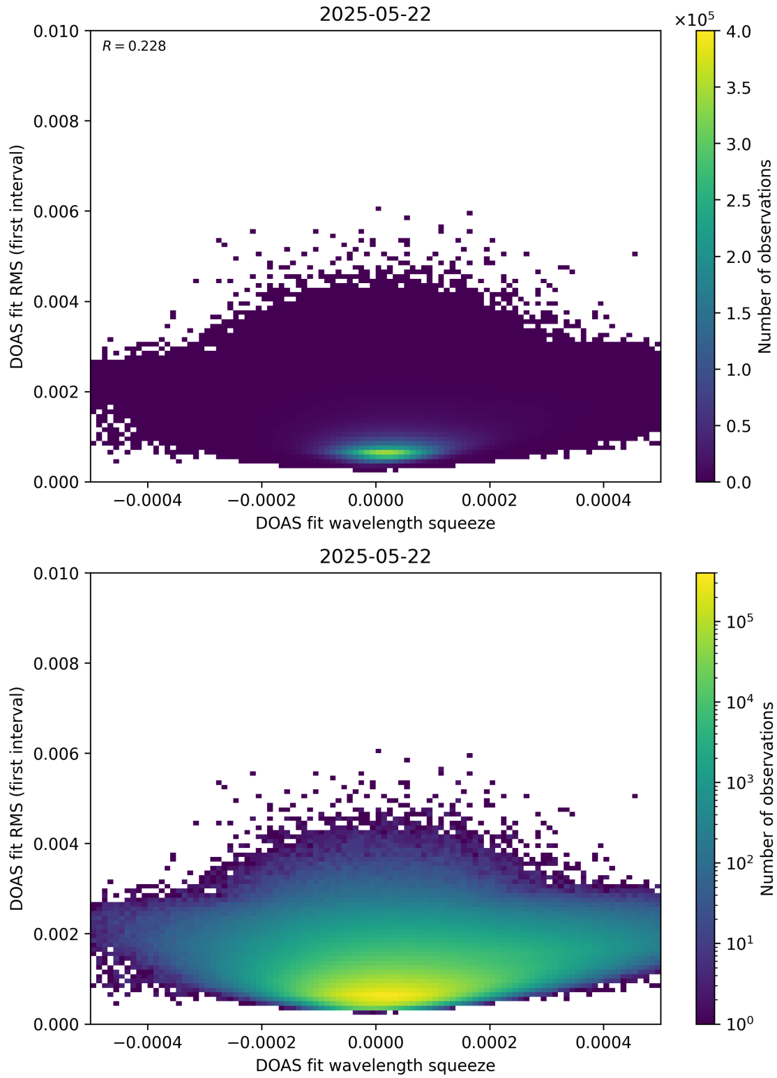
Figure 68: Scatter density plot of “DOAS fit wavelength squeeze” against “DOAS fit RMS (first interval)” for 2025-05-21 to 2025-05-23.
