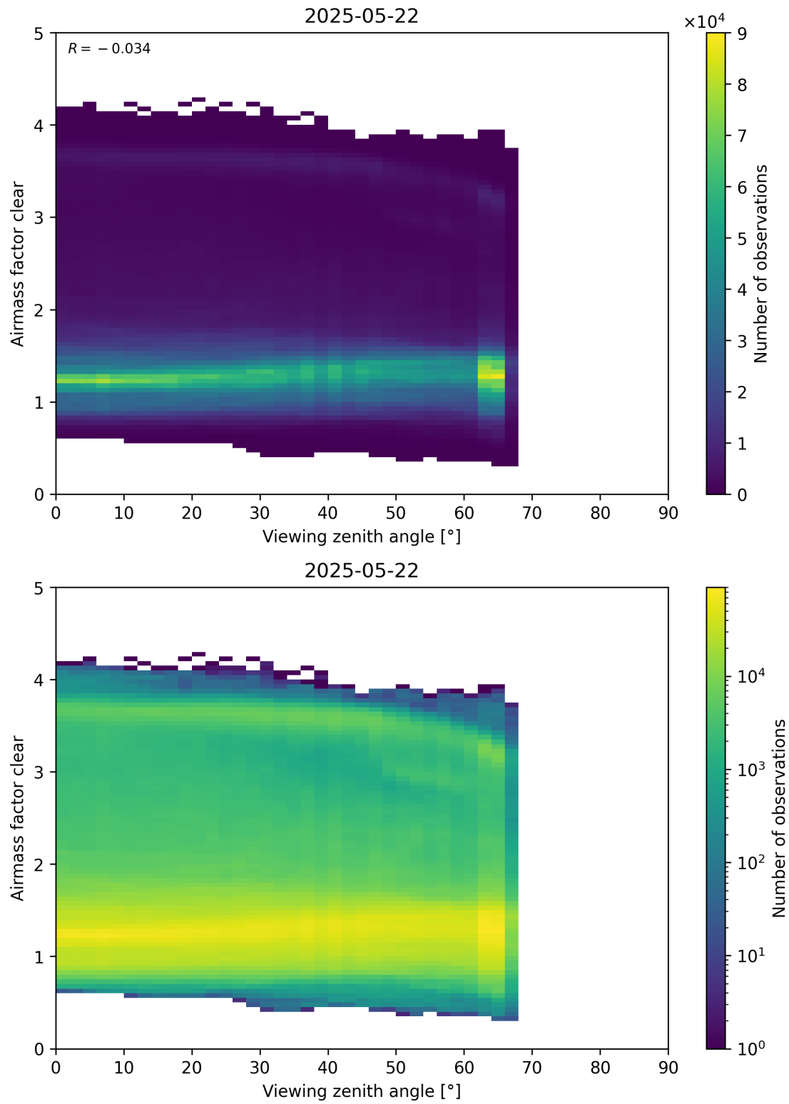
Figure 185: Scatter density plot of “Viewing zenith angle” against “Airmass factor clear” for 2025-05-21 to 2025-05-23.
