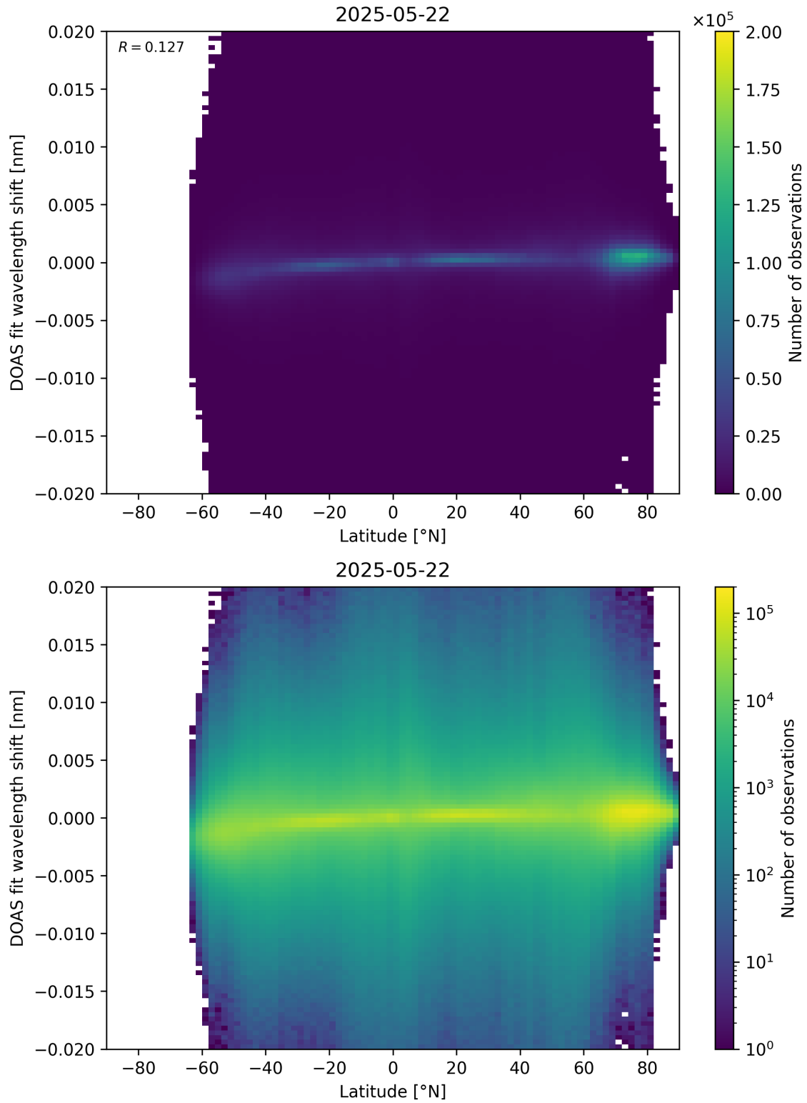
Figure 154: Scatter density plot of “Latitude” against “DOAS fit wavelength shift” for 2025-05-21 to 2025-05-23.
