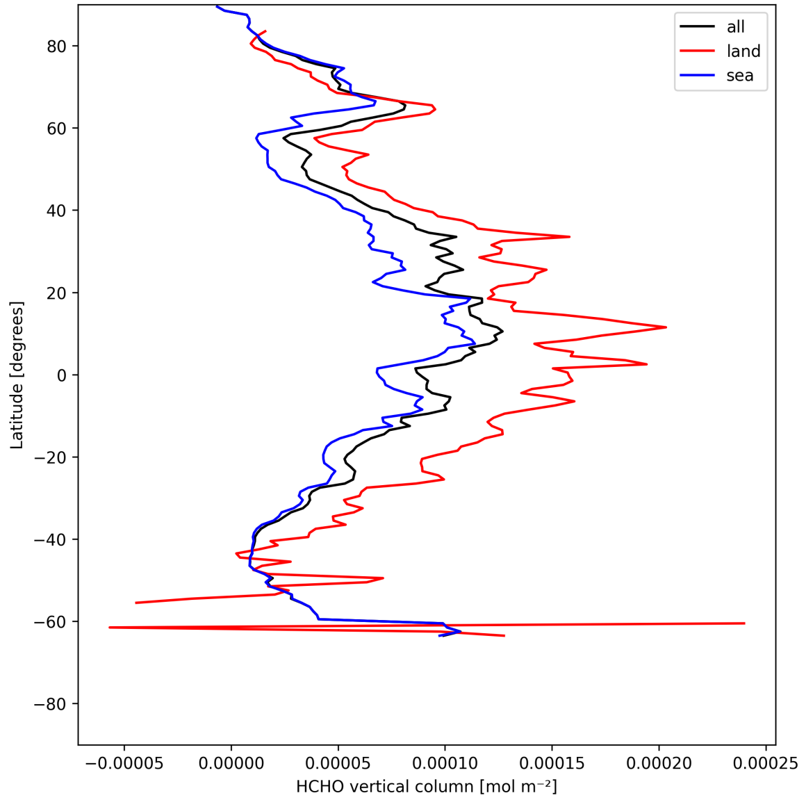
Figure 21: Zonal average of “HCHO vertical column” for 2025-05-21 to 2025-05-23.
