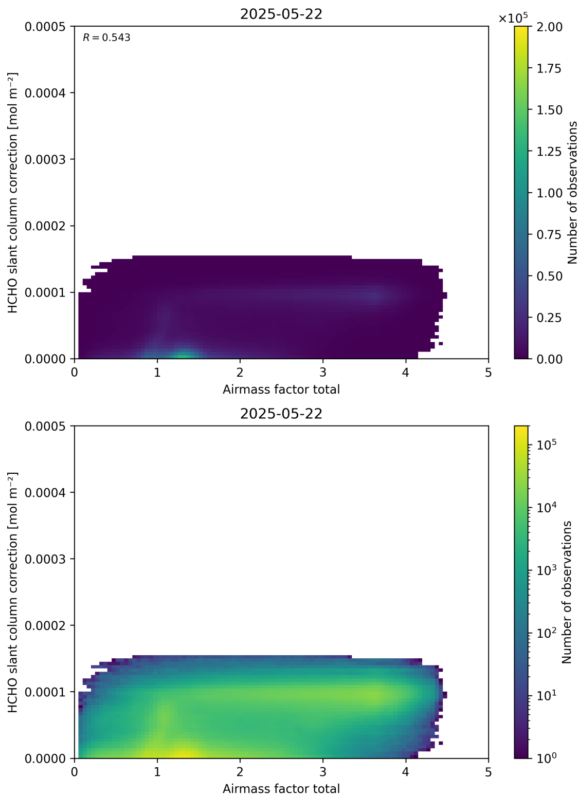
Figure 102: Scatter density plot of “Airmass factor total” against “HCHO slant column correction” for 2025-05-21 to 2025-05-23.
