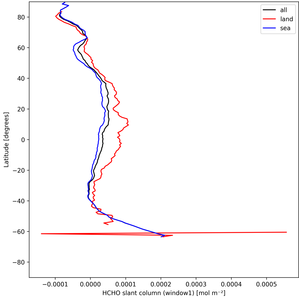
Figure 24: Zonal average of “HCHO slant column (window1)” for 2025-05-21 to 2025-05-23.
