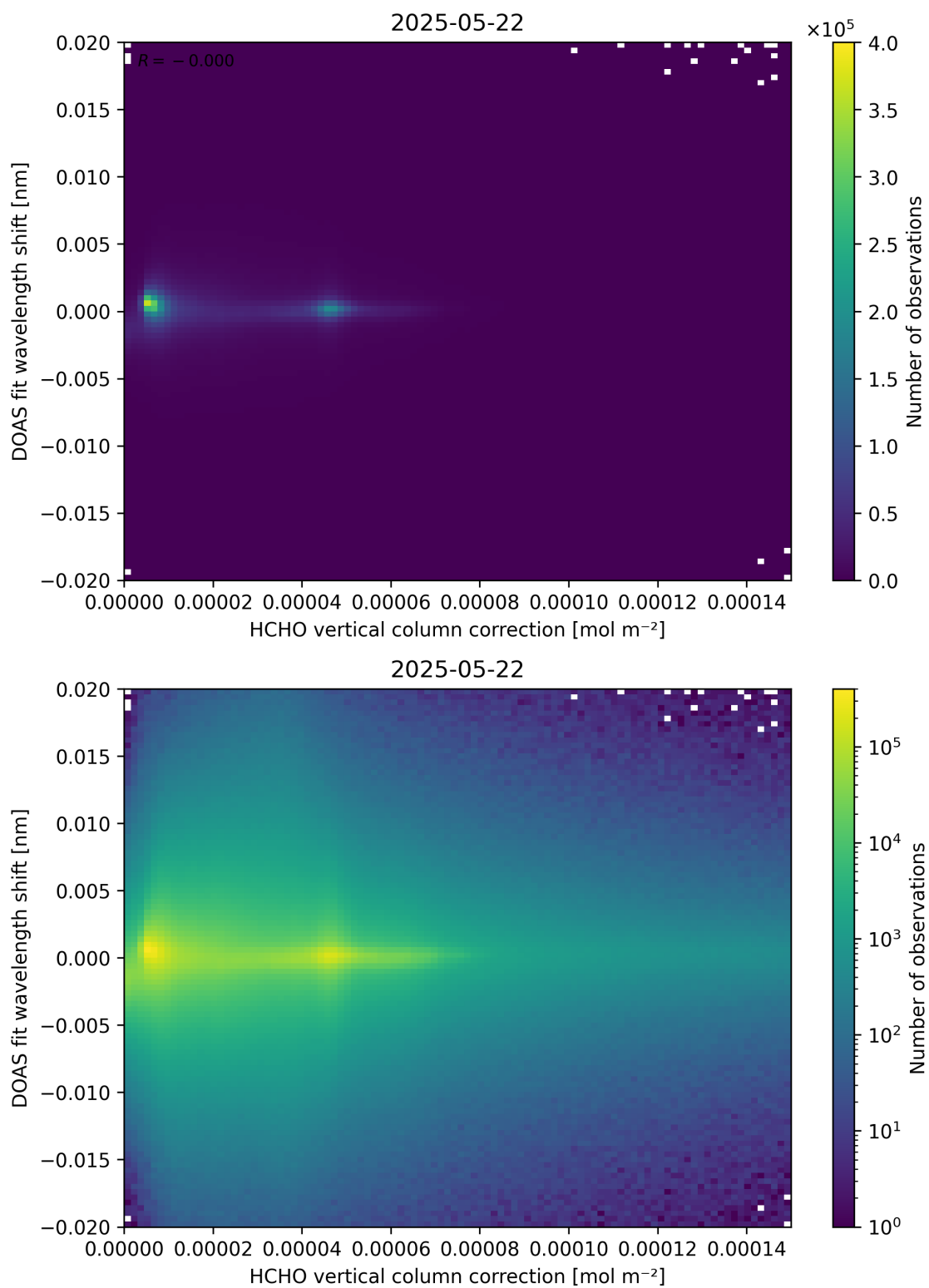
Figure 113: Scatter density plot of “HCHO vertical column correction” against “DOAS fit wavelength shift” for 2025-05-21 to 2025-05-23.
