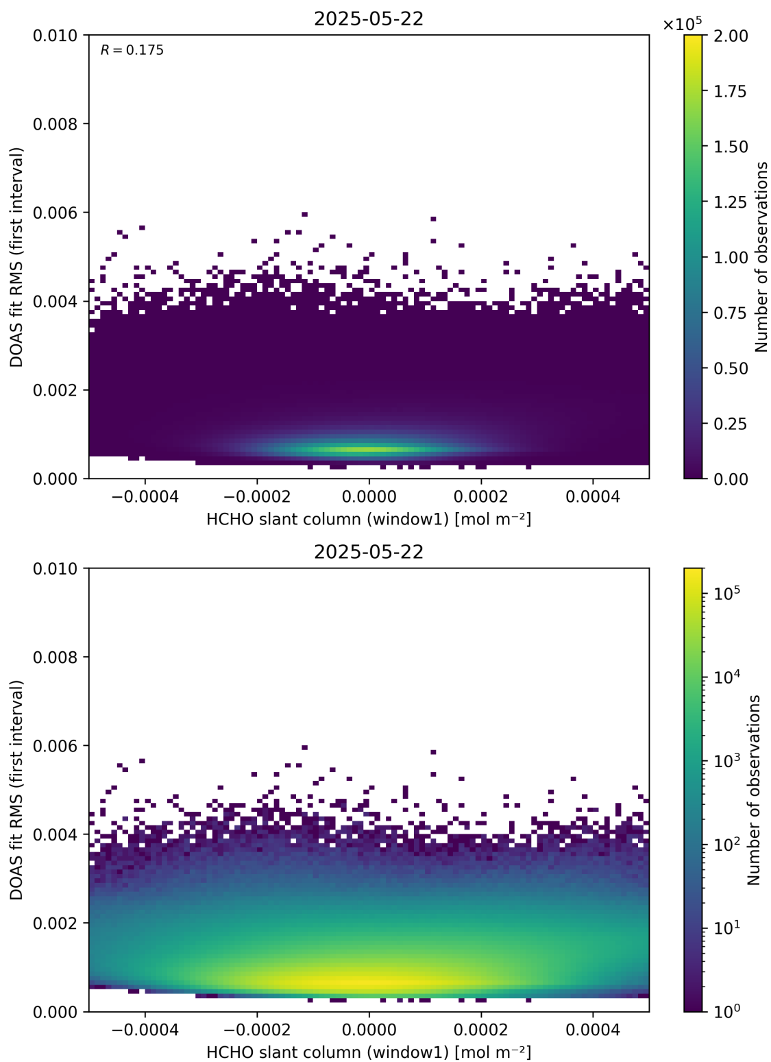
Figure 78: Scatter density plot of “HCHO slant column (window1)” against “DOAS fit RMS (first interval)” for 2025-05-21 to 2025-05-23.
