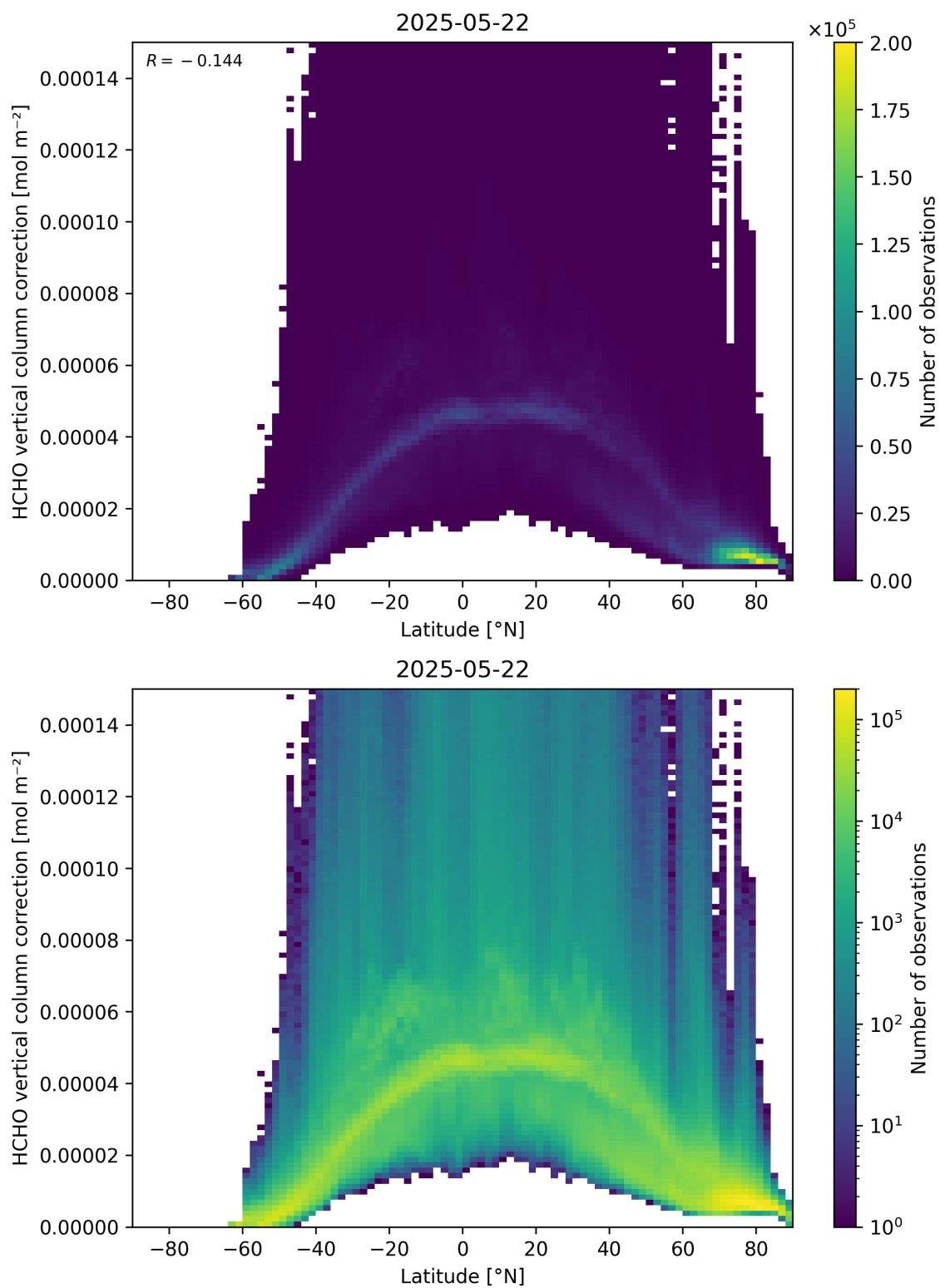
Figure 164: Scatter density plot of “Latitude” against “HCHO vertical column correction” for 2025-05-21 to 2025-05-23.
