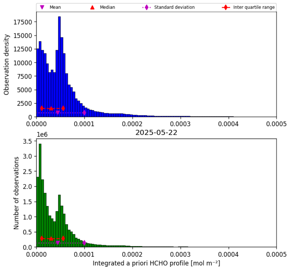
Figure 43: Histogram of “Integrated a priori HCHO profile” for 2025-05-21 to 2025-05-23
