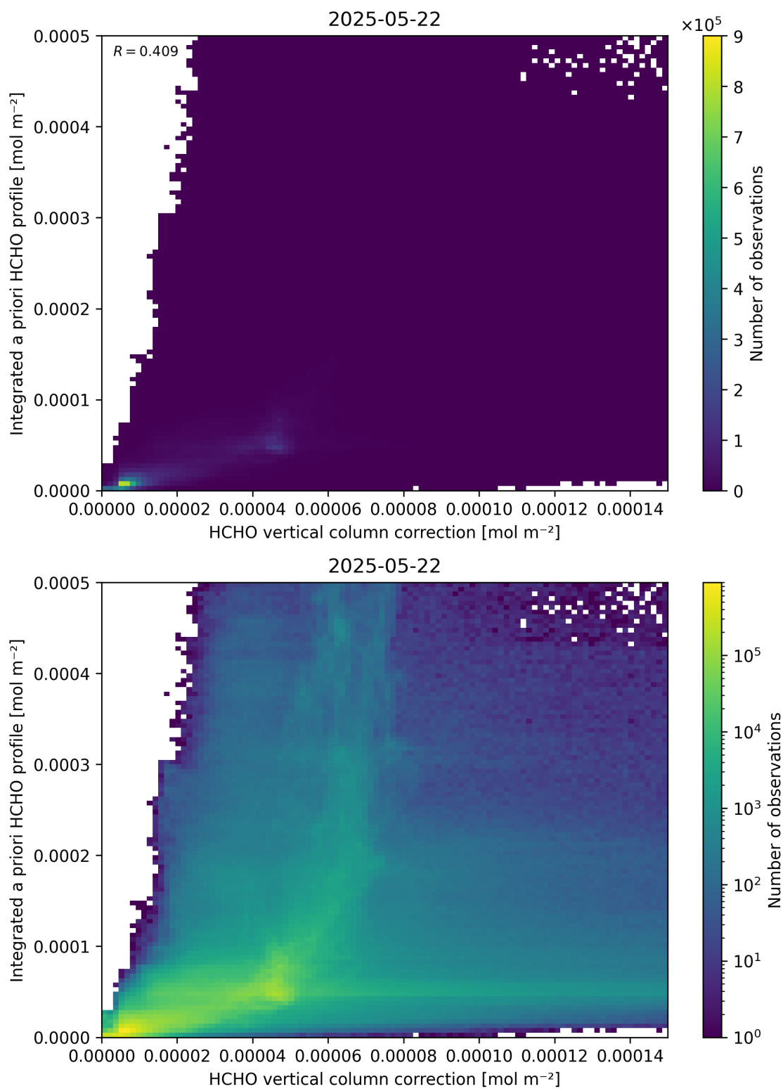
Figure 122: Scatter density plot of “HCHO vertical column correction” against “Integrated a priori HCHO profile” for 2025-05-21 to 2025-05-23.
