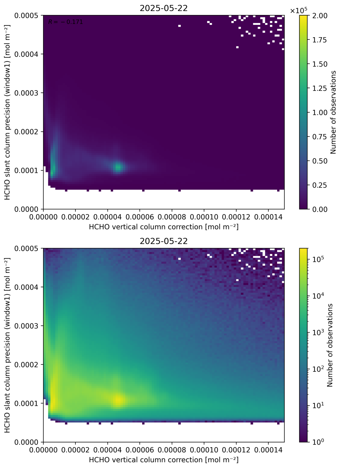
Figure 119: Scatter density plot of “HCHO vertical column correction” against “HCHO slant column precision (window1)” for 2025-05-21 to 2025-05-23.
