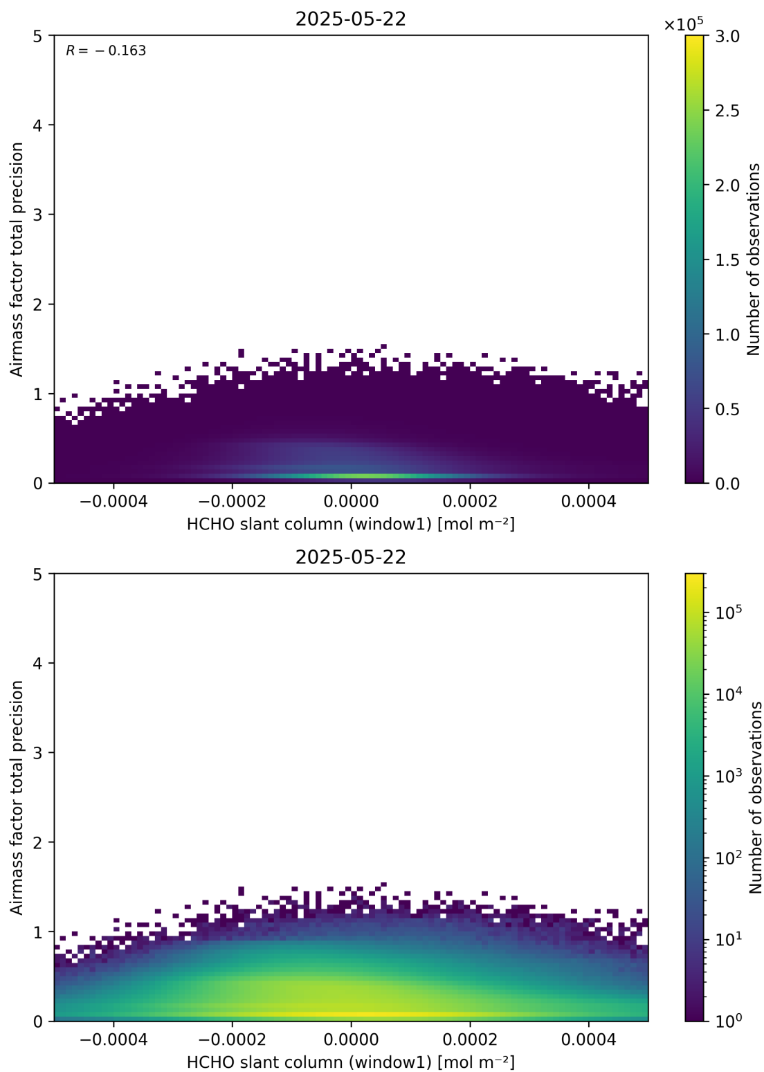
Figure 86: Scatter density plot of “HCHO slant column (window1)” against “Airmass factor total precision” for 2025-05-21 to 2025-05-23.
