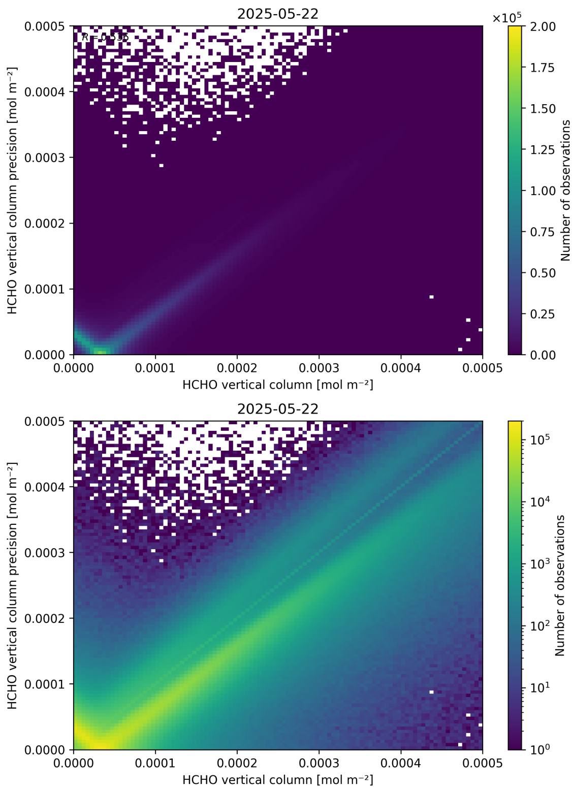
Figure 134: Scatter density plot of “HCHO vertical column” against “HCHO vertical column precision” for 2025-05-21 to 2025-05-23.
