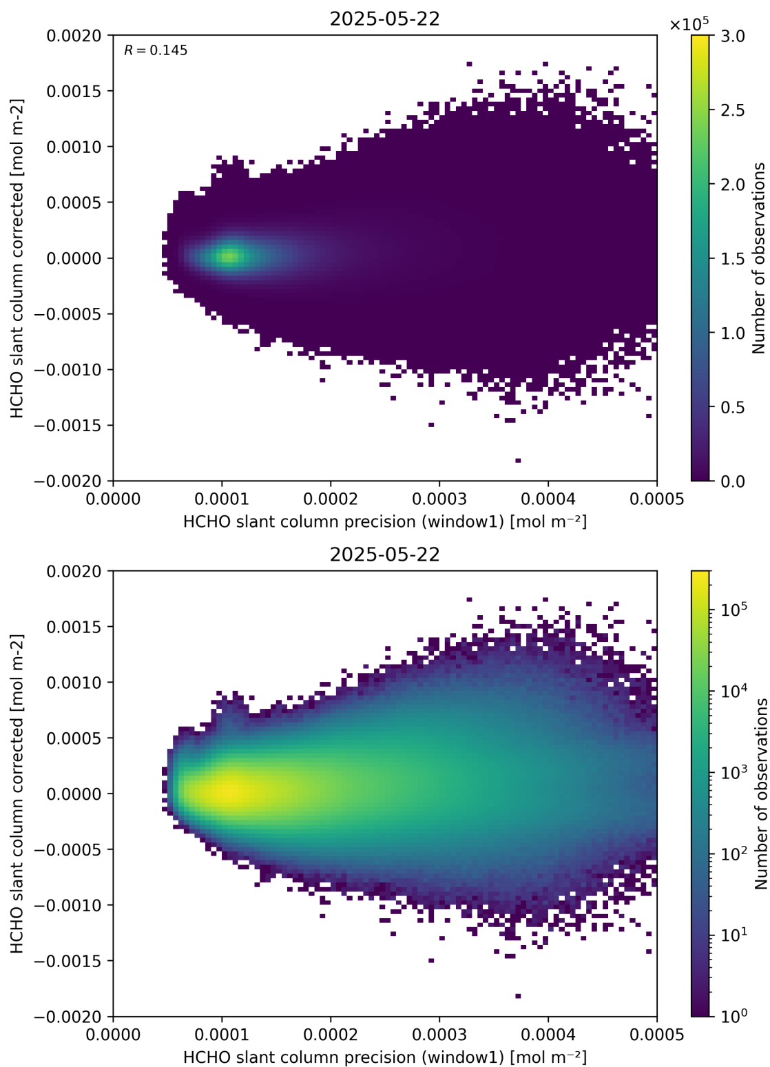
Figure 92: Scatter density plot of “HCHO slant column precision (window1)” against “HCHO slant column corrected” for 2025-05-21 to 2025-05-23.
