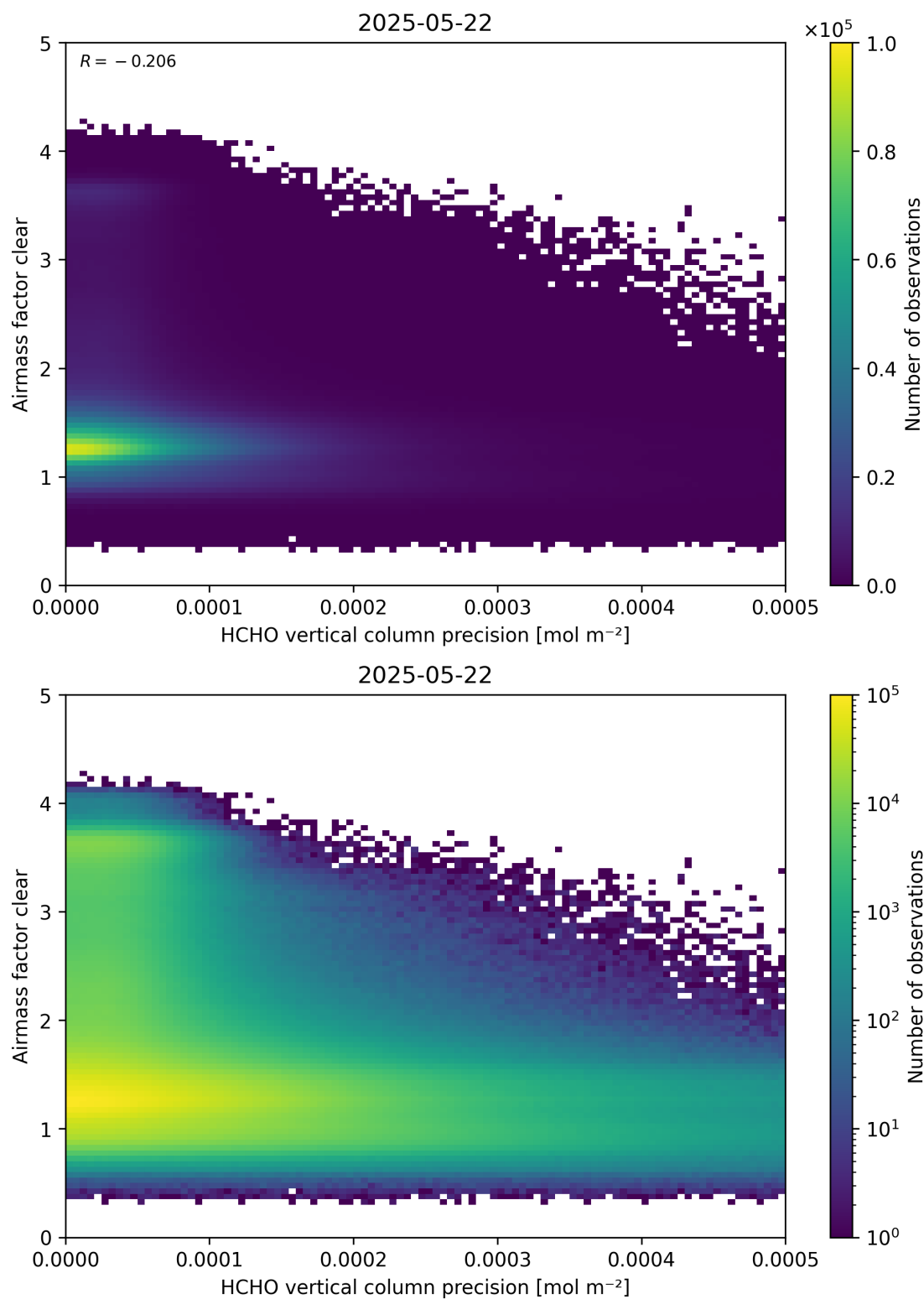
Figure 139: Scatter density plot of “HCHO vertical column precision” against “Airmass factor clear” for 2025-05-21 to 2025-05-23.
