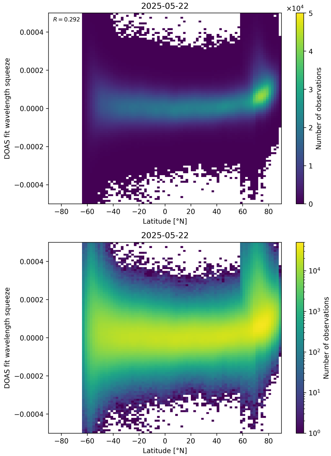
Figure 155: Scatter density plot of “Latitude” against “DOAS fit wavelength squeeze” for 2025-05-21 to 2025-05-23.
