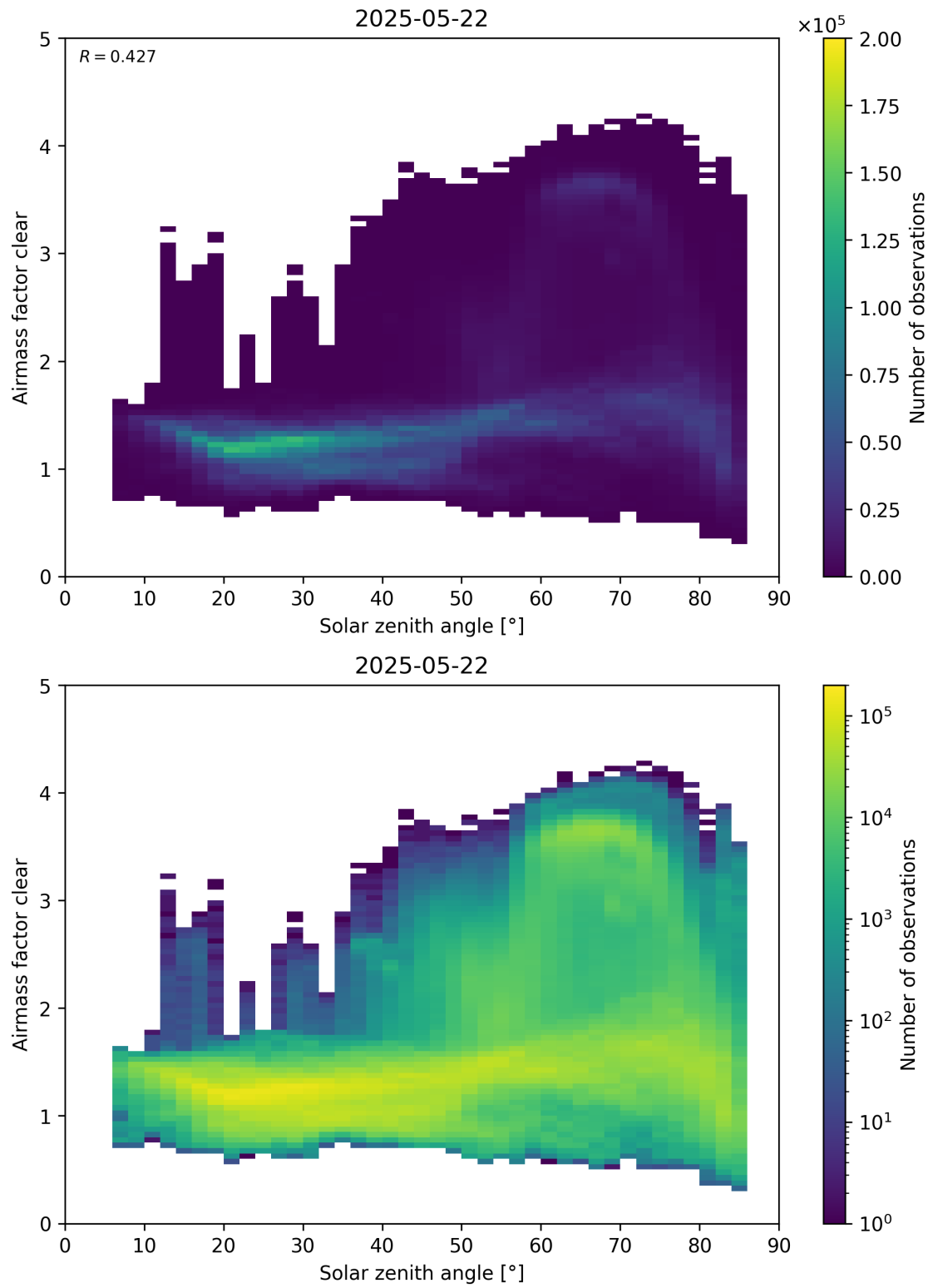
Figure 170: Scatter density plot of “Solar zenith angle” against “Airmass factor clear” for 2025-05-21 to 2025-05-23.
