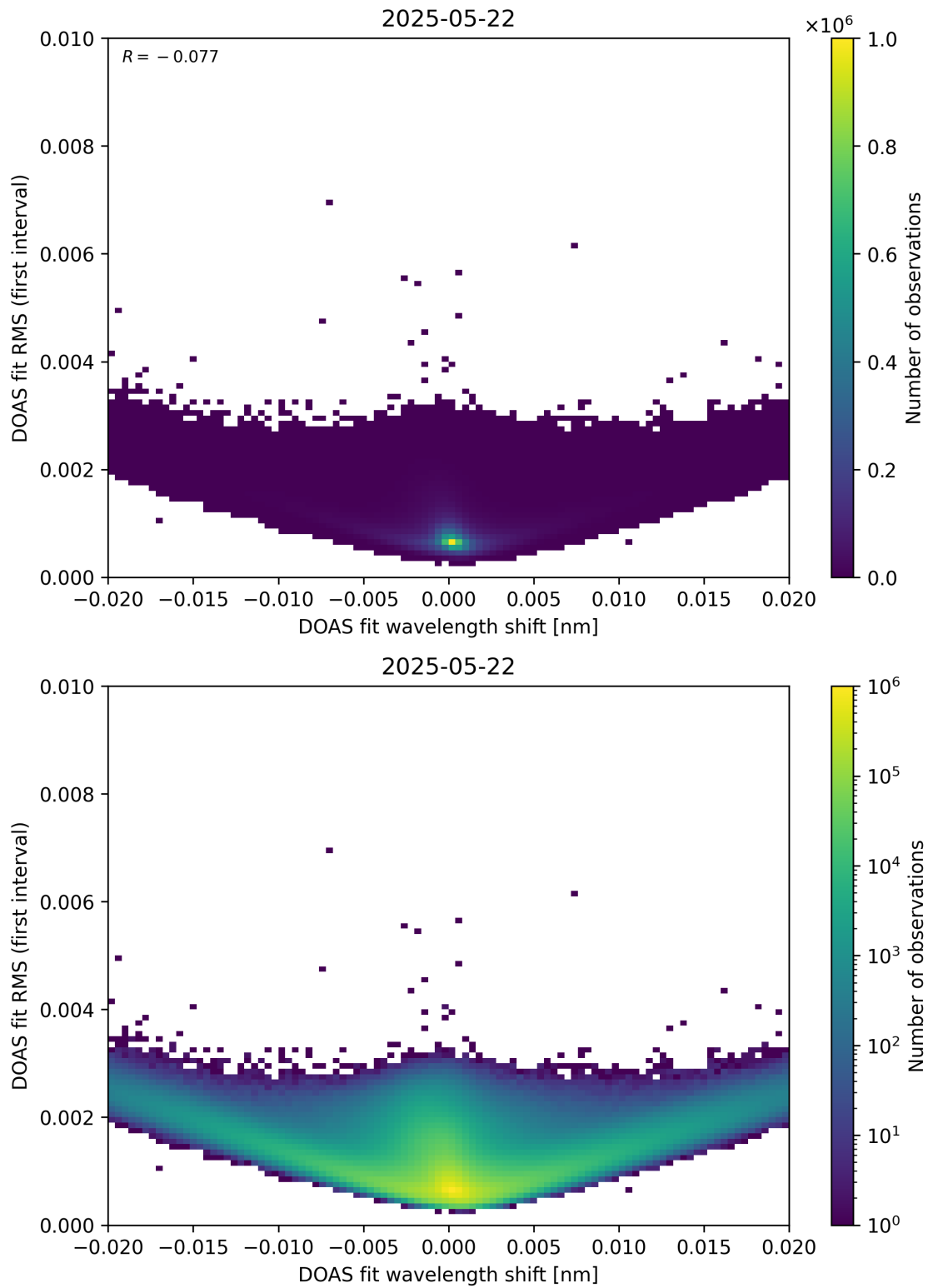
Figure 64: Scatter density plot of “DOAS fit wavelength shift” against “DOAS fit RMS (first interval)” for 2025-05-21 to 2025-05-23.
