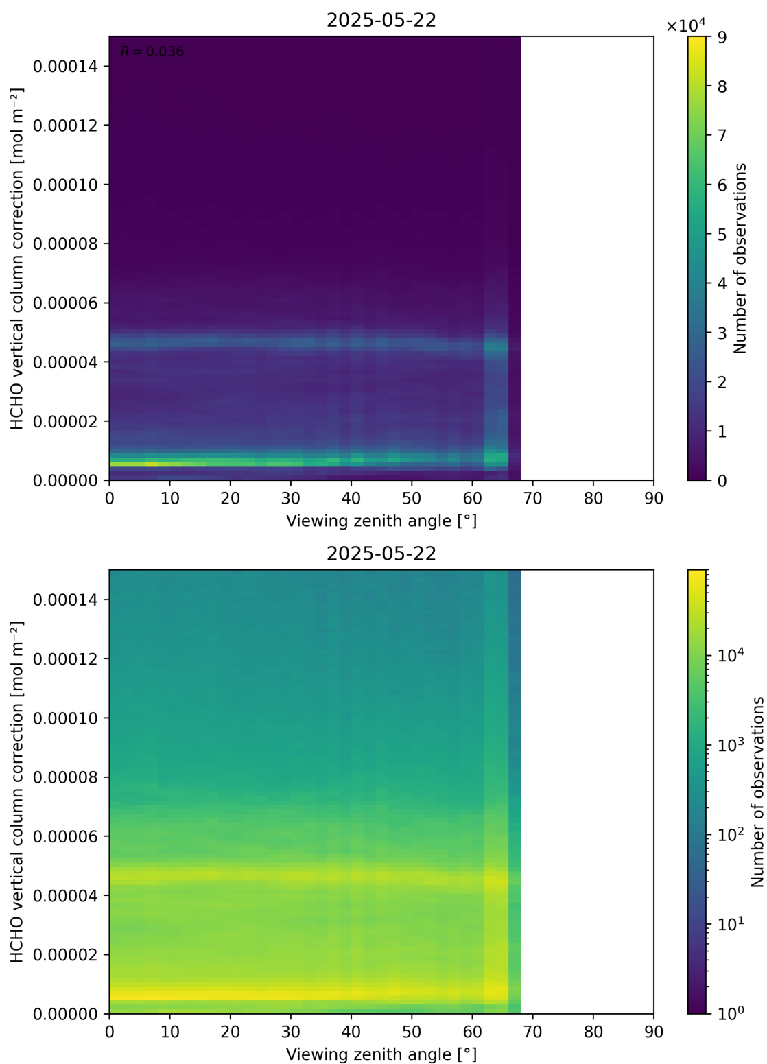
Figure 193: Scatter density plot of “Viewing zenith angle” against “HCHO vertical column correction” for 2025-05-21 to 2025-05-23.
