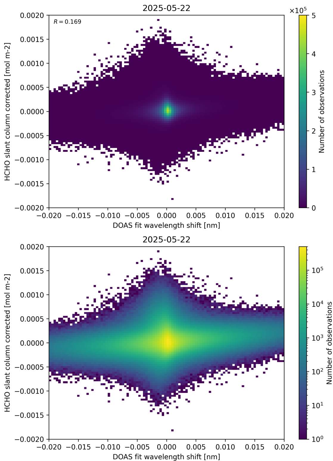
Figure 66: Scatter density plot of “DOAS fit wavelength shift” against “HCHO slant column corrected” for 2025-05-21 to 2025-05-23.
