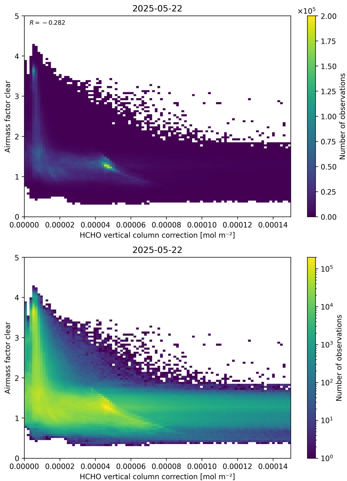
Figure 115: Scatter density plot of “HCHO vertical column correction” against “Airmass factor clear” for 2025-05-21 to 2025-05-23.
