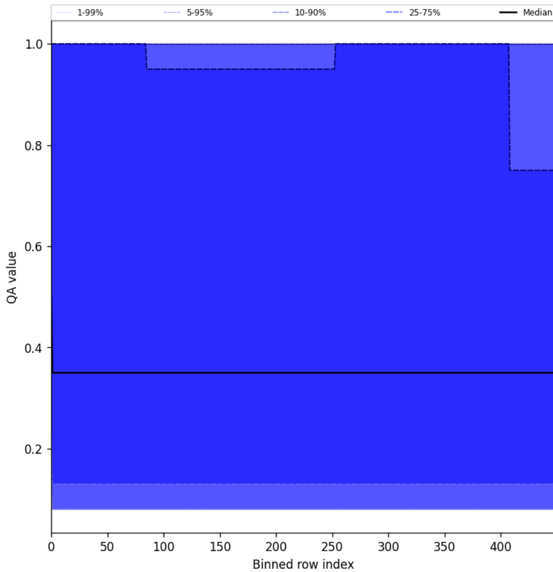
Figure 48: Along track statistics of “QA value” for 2025-05-21 to 2025-05-23
