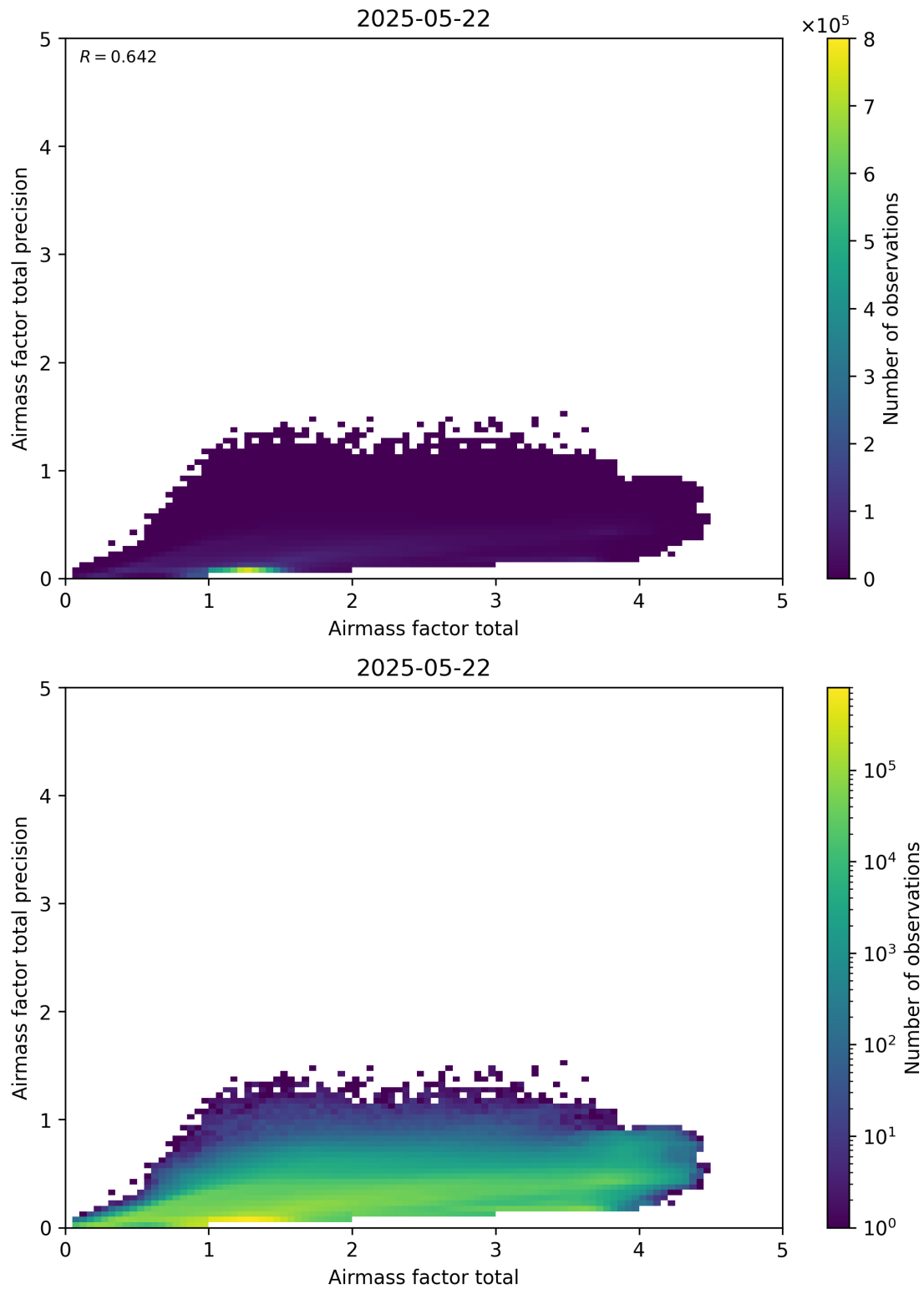
Figure 103: Scatter density plot of “Airmass factor total” against “Airmass factor total precision” for 2025-05-21 to 2025-05-23.
