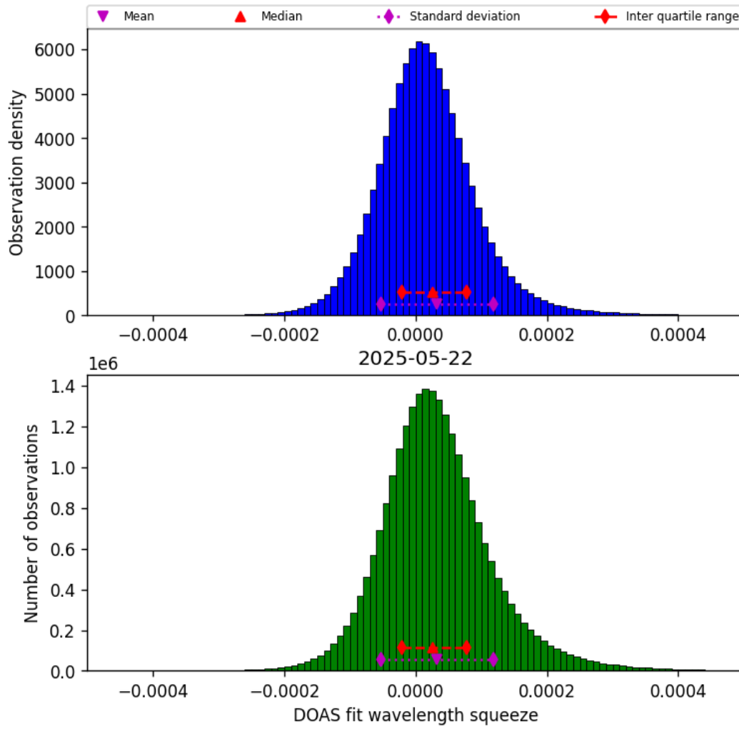
Figure 45: Histogram of “DOAS fit wavelength squeeze” for 2025-05-21 to 2025-05-23
