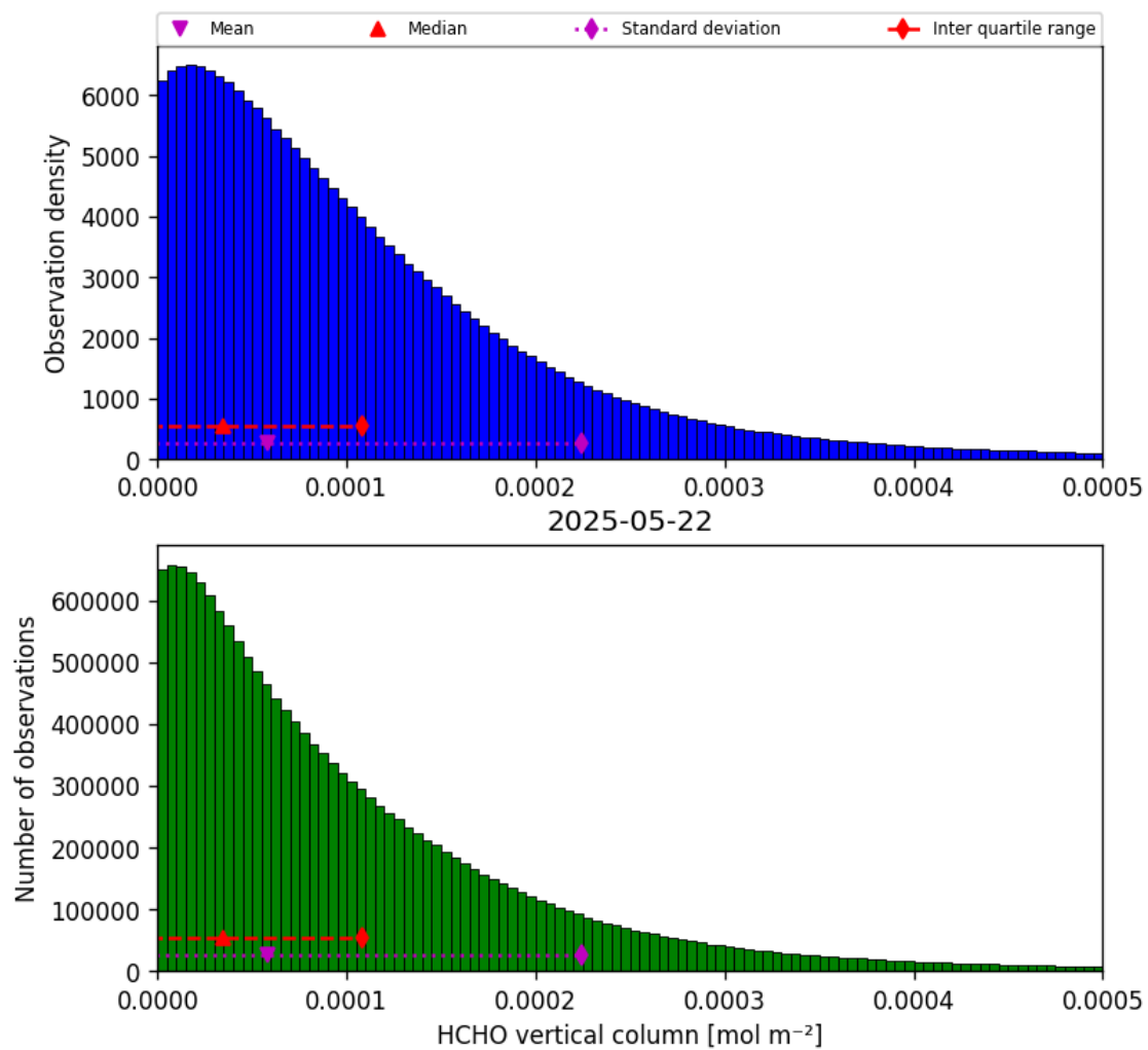
Figure 35: Histogram of “HCHO vertical column” for 2025-05-21 to 2025-05-23
