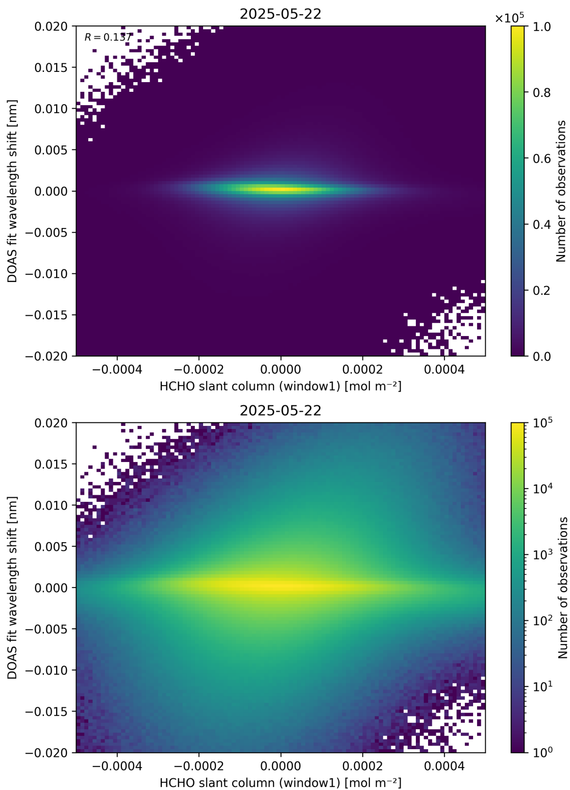
Figure 79: Scatter density plot of “HCHO slant column (window1)” against “DOAS fit wavelength shift” for 2025-05-21 to 2025-05-23.
