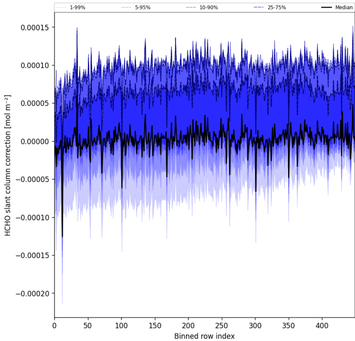
Figure 61: Along track statistics of “HCHO slant column correction” for 2025-05-21 to 2025-05-23
