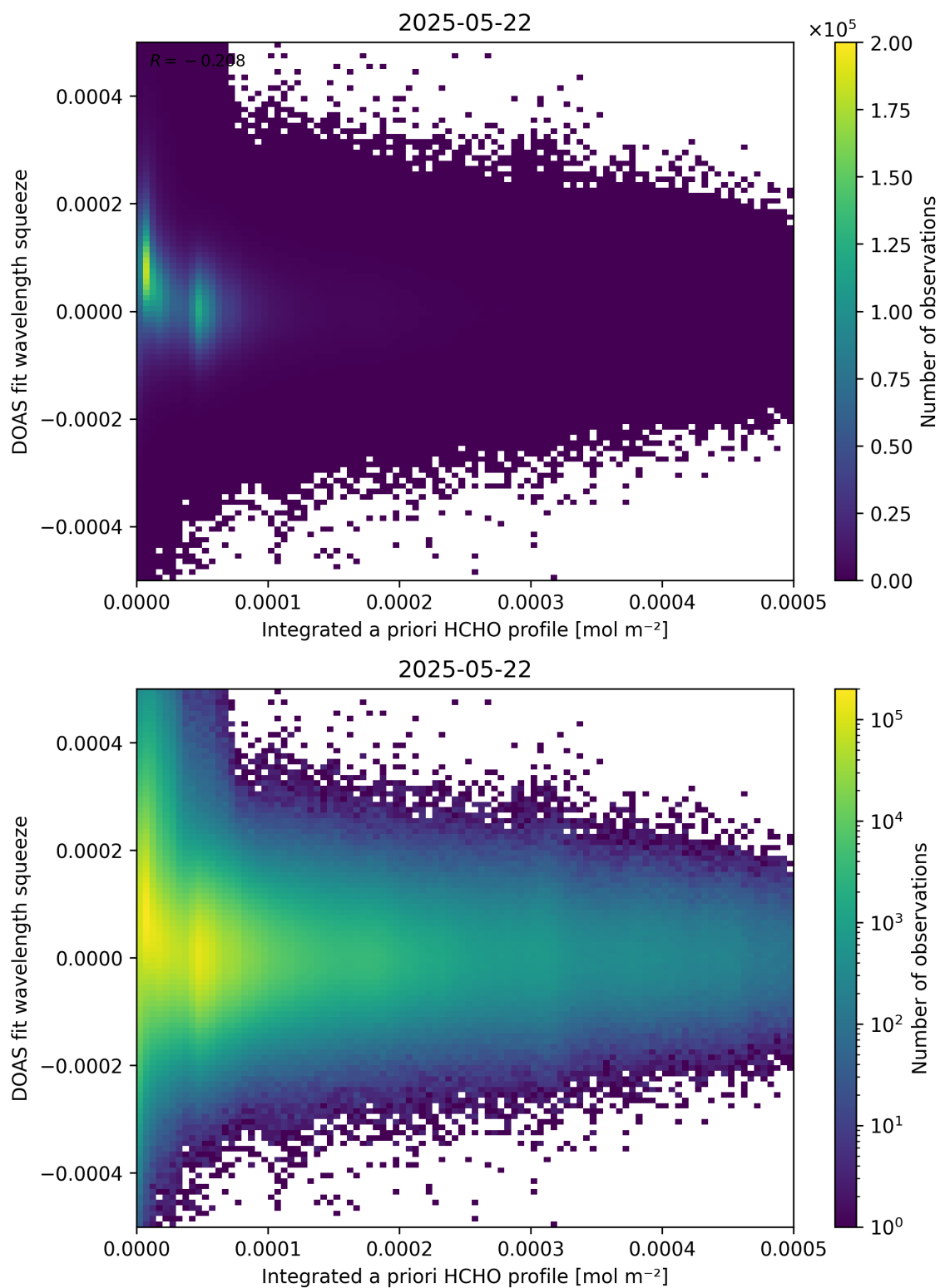
Figure 150: Scatter density plot of “Integrated a priori HCHO profile” against “DOAS fit wavelength squeeze” for 2025-05-21 to 2025-05-23.
