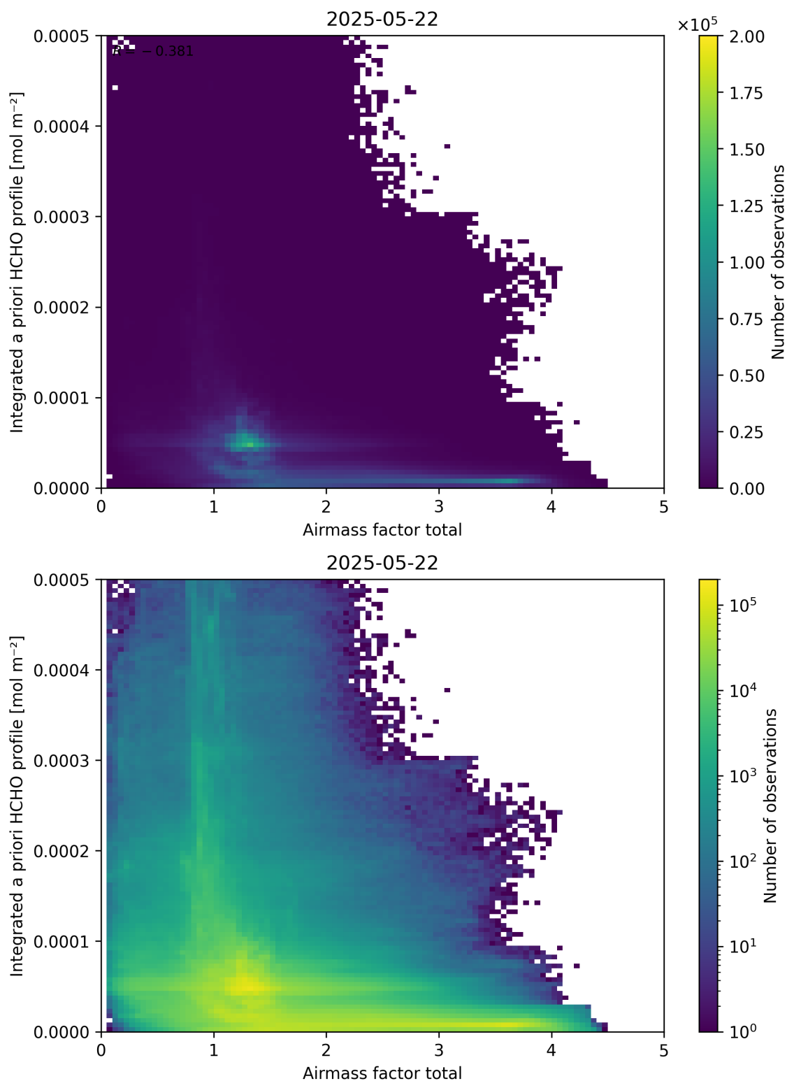
Figure 104: Scatter density plot of “Airmass factor total” against “Integrated a priori HCHO profile” for 2025-05-21 to 2025-05-23.
