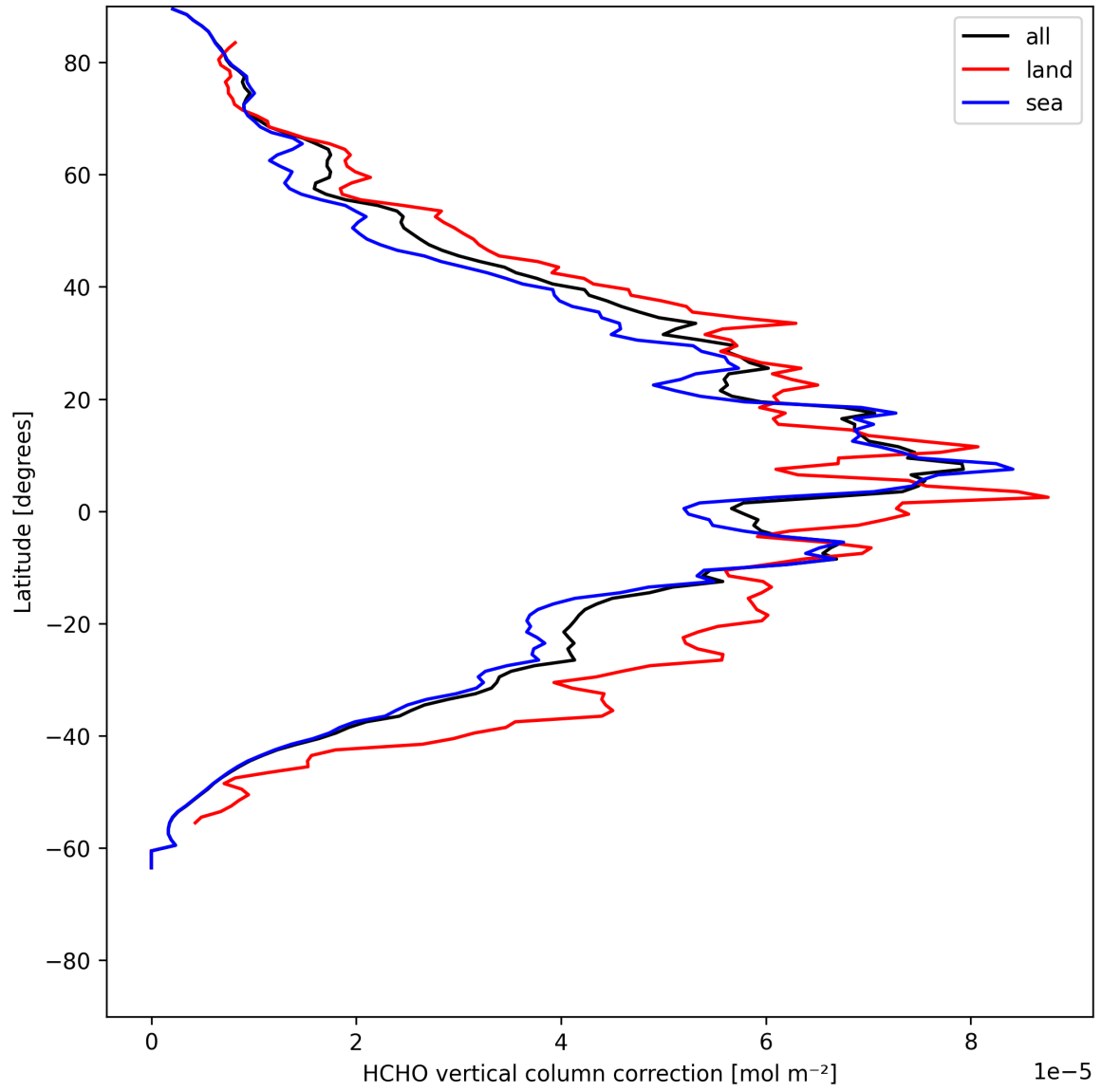
Figure 23: Zonal average of “HCHO vertical column correction” for 2025-05-21 to 2025-05-23.
