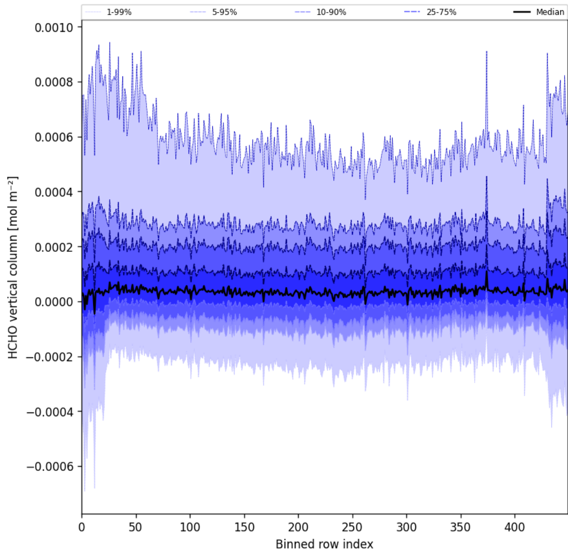
Figure 49: Along track statistics of “HCHO vertical column” for 2025-05-21 to 2025-05-23
