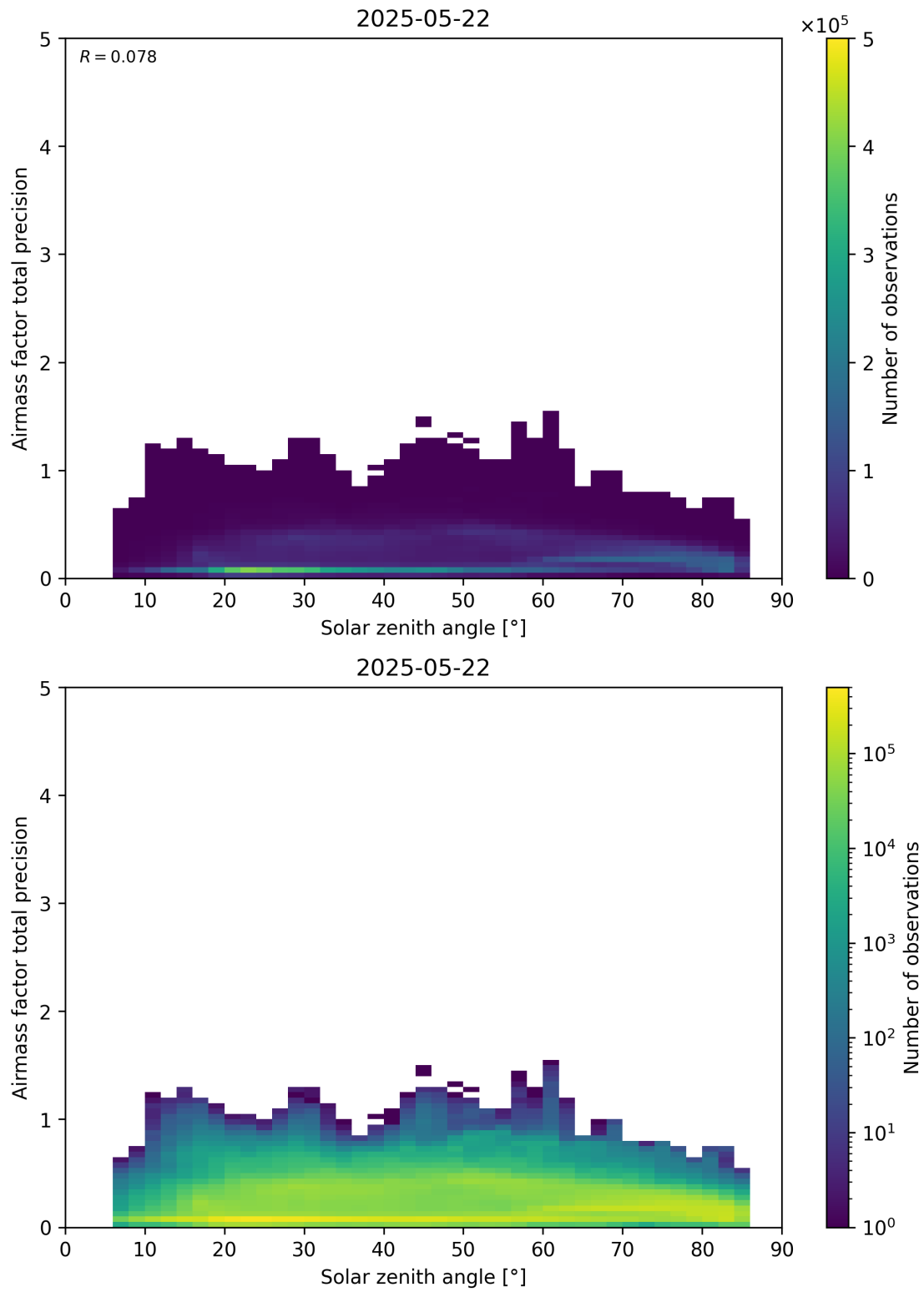
Figure 176: Scatter density plot of “Solar zenith angle” against “Airmass factor total precision” for 2025-05-21 to 2025-05-23.
