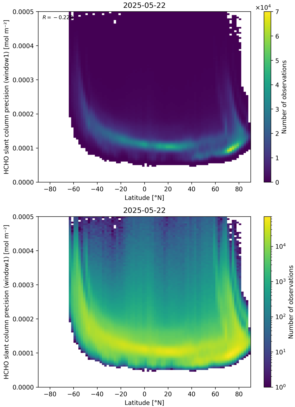
Figure 160: Scatter density plot of “Latitude” against “HCHO slant column precision (window1)” for 2025-05-21 to 2025-05-23.
