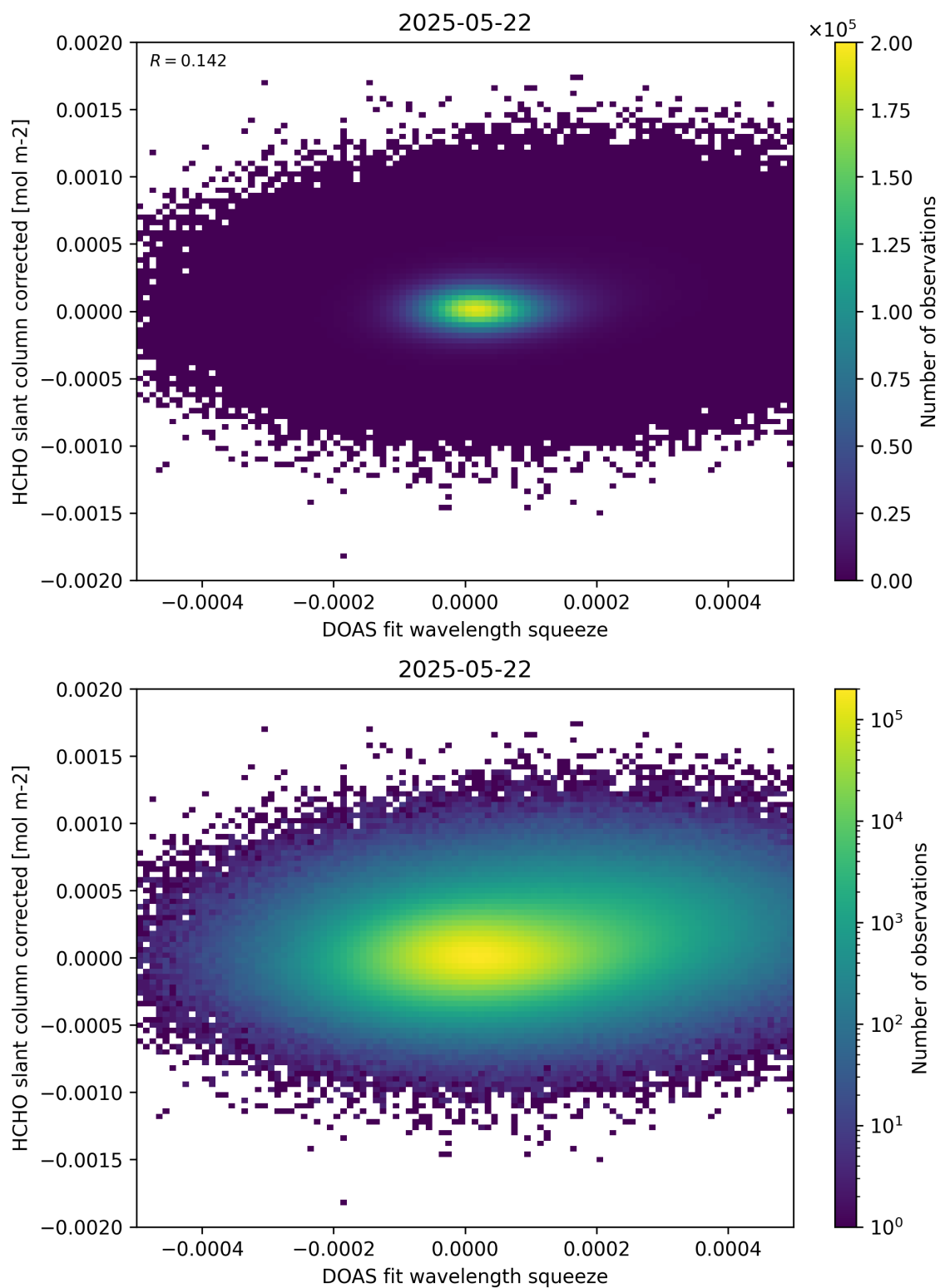
Figure 69: Scatter density plot of “DOAS fit wavelength squeeze” against “HCHO slant column corrected” for 2025-05-21 to 2025-05-23.
