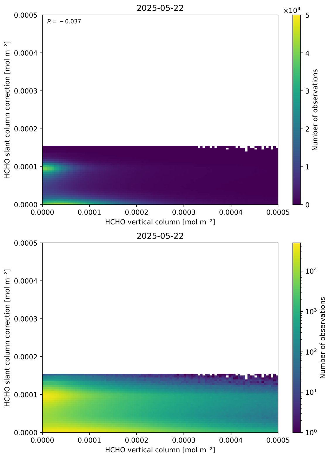
Figure 128: Scatter density plot of “HCHO vertical column” against “HCHO slant column correction” for 2025-05-21 to 2025-05-23.
