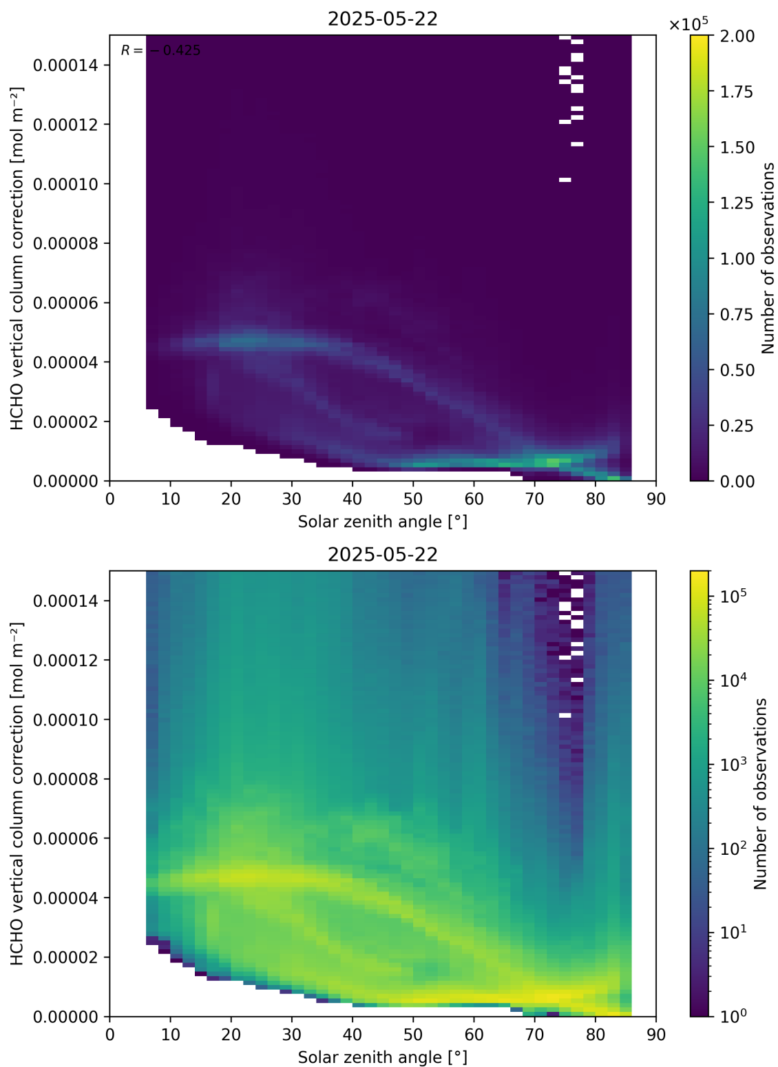
Figure 178: Scatter density plot of “Solar zenith angle” against “HCHO vertical column correction” for 2025-05-21 to 2025-05-23.
