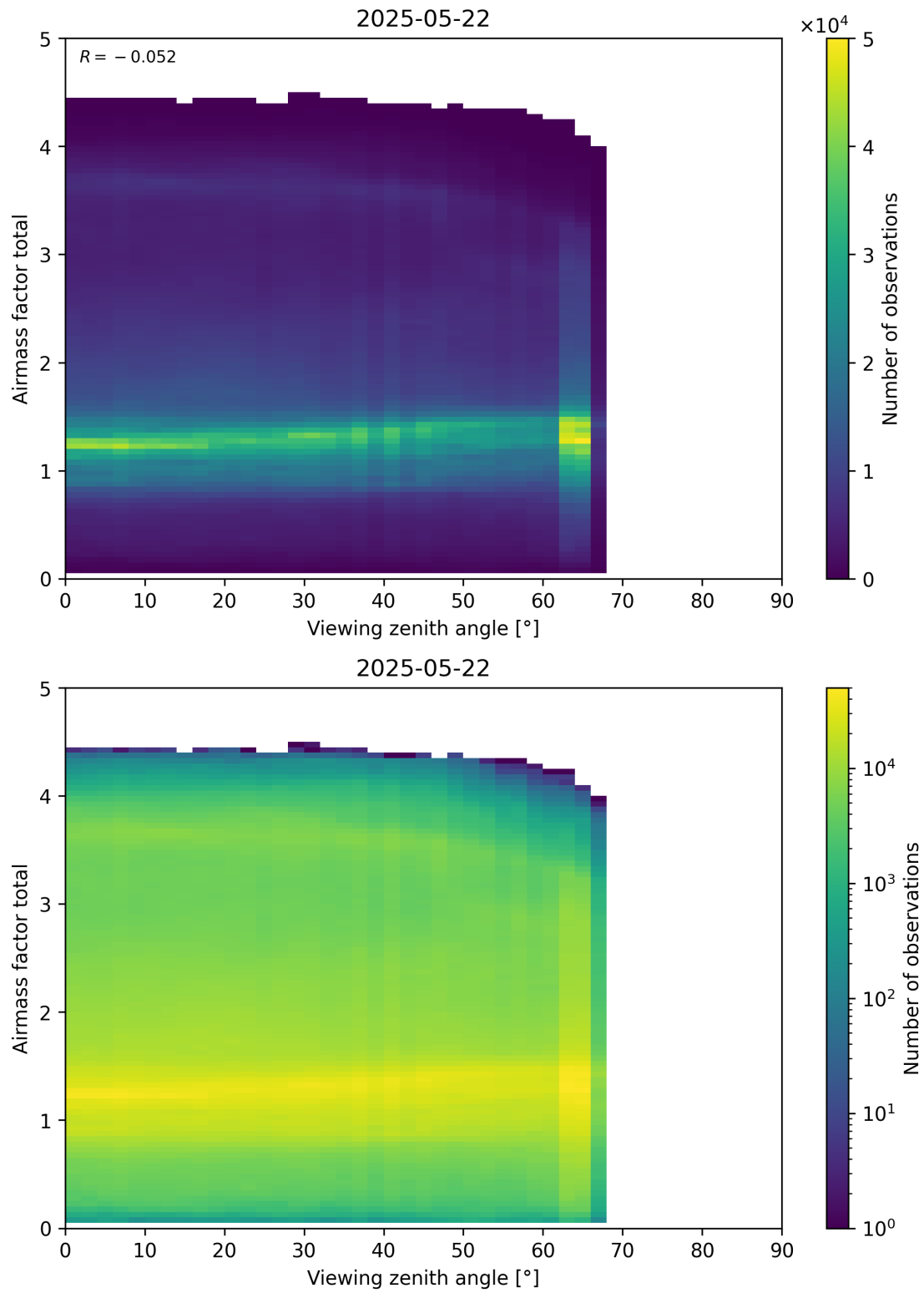
Figure 190: Scatter density plot of “Viewing zenith angle” against “Airmass factor total” for 2025-05-21 to 2025-05-23.
