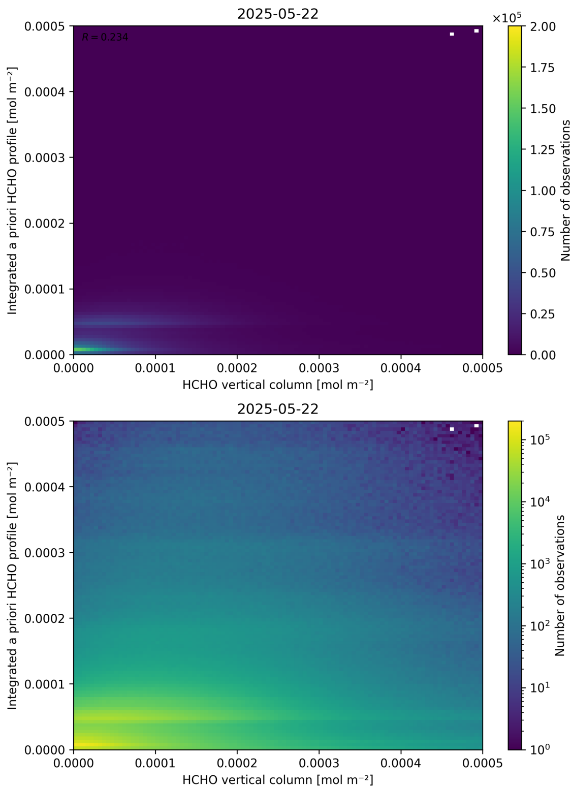
Figure 135: Scatter density plot of “HCHO vertical column” against “Integrated a priori HCHO profile” for 2025-05-21 to 2025-05-23.
