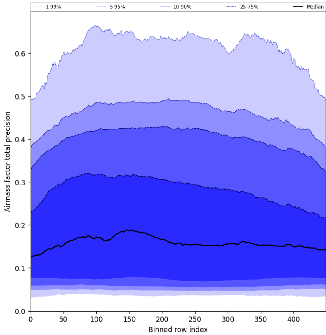
Figure 55: Along track statistics of “Airmass factor total precision” for 2025-05-21 to 2025-05-23
