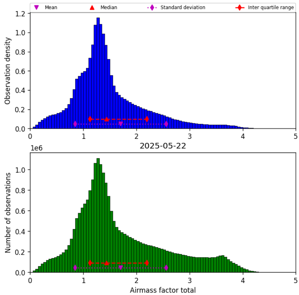
Figure 40: Histogram of “Airmass factor total” for 2025-05-21 to 2025-05-23
