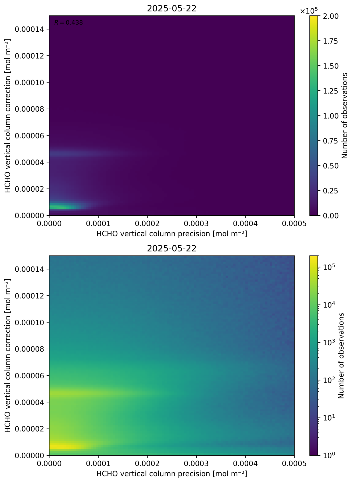
Figure 146: Scatter density plot of “HCHO vertical column precision” against “HCHO vertical column correction” for 2025-05-21 to 2025-05-23.
