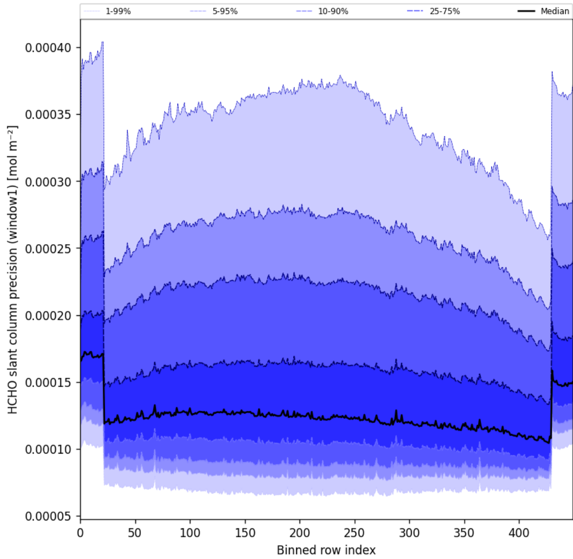
Figure 53: Along track statistics of “HCHO slant column precision (window1)” for 2025-05-21 to 2025-05-23
