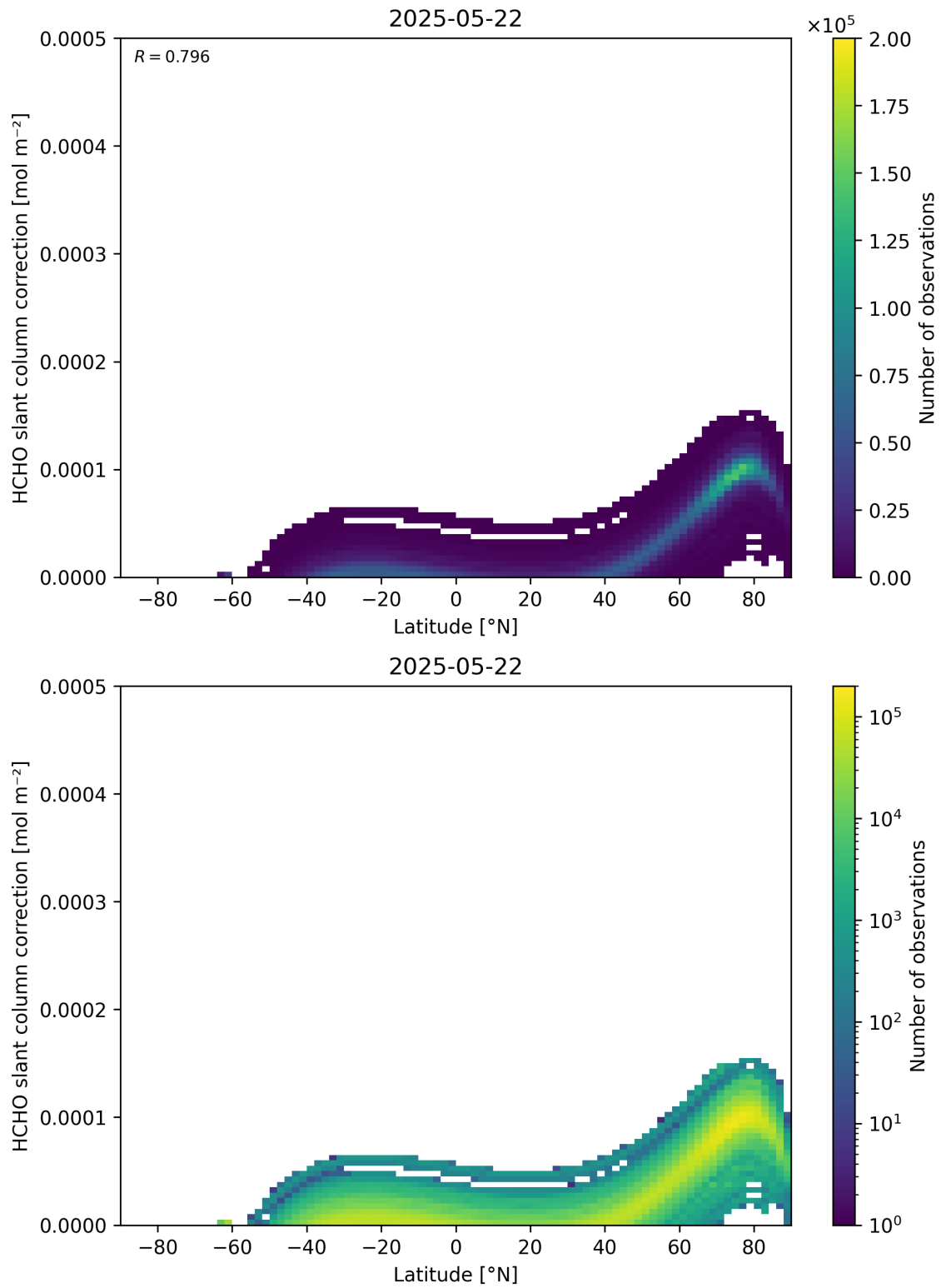
Figure 158: Scatter density plot of “Latitude” against “HCHO slant column correction” for 2025-05-21 to 2025-05-23.
