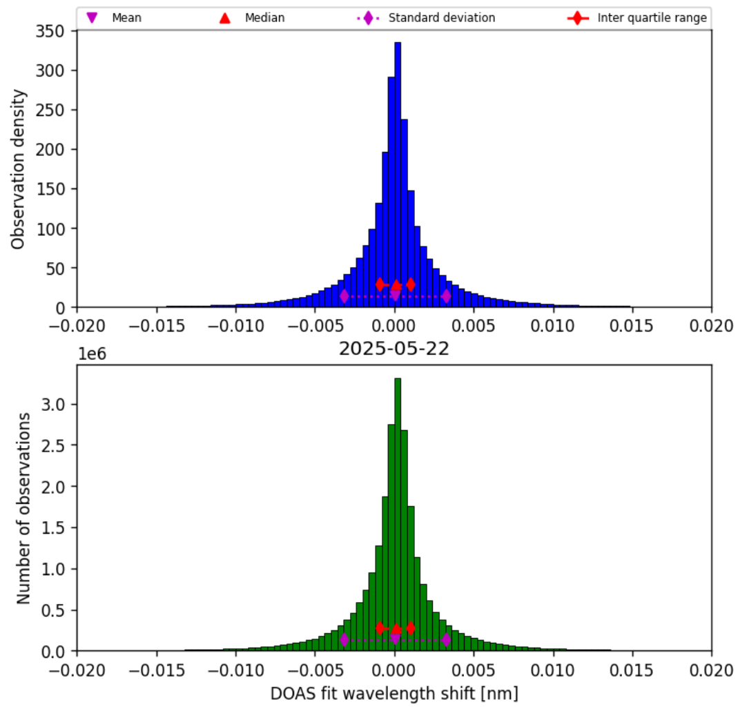
Figure 44: Histogram of “DOAS fit wavelength shift” for 2025-05-21 to 2025-05-23
