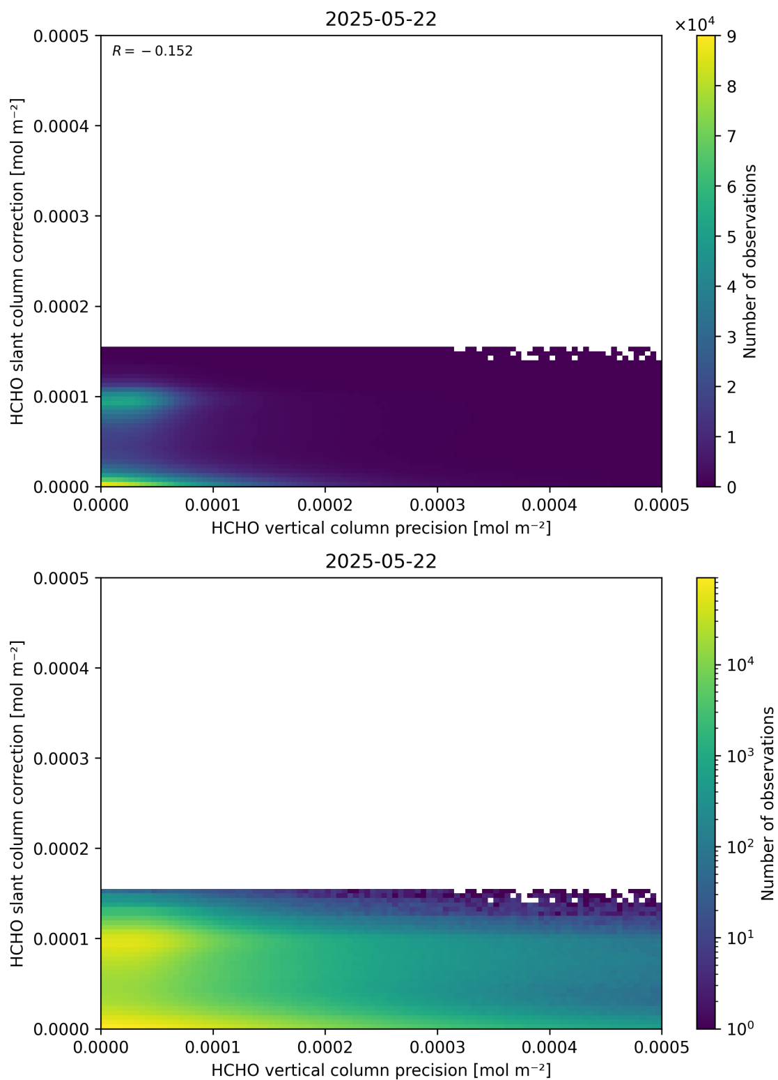
Figure 141: Scatter density plot of “HCHO vertical column precision” against “HCHO slant column correction” for 2025-05-21 to 2025-05-23.
