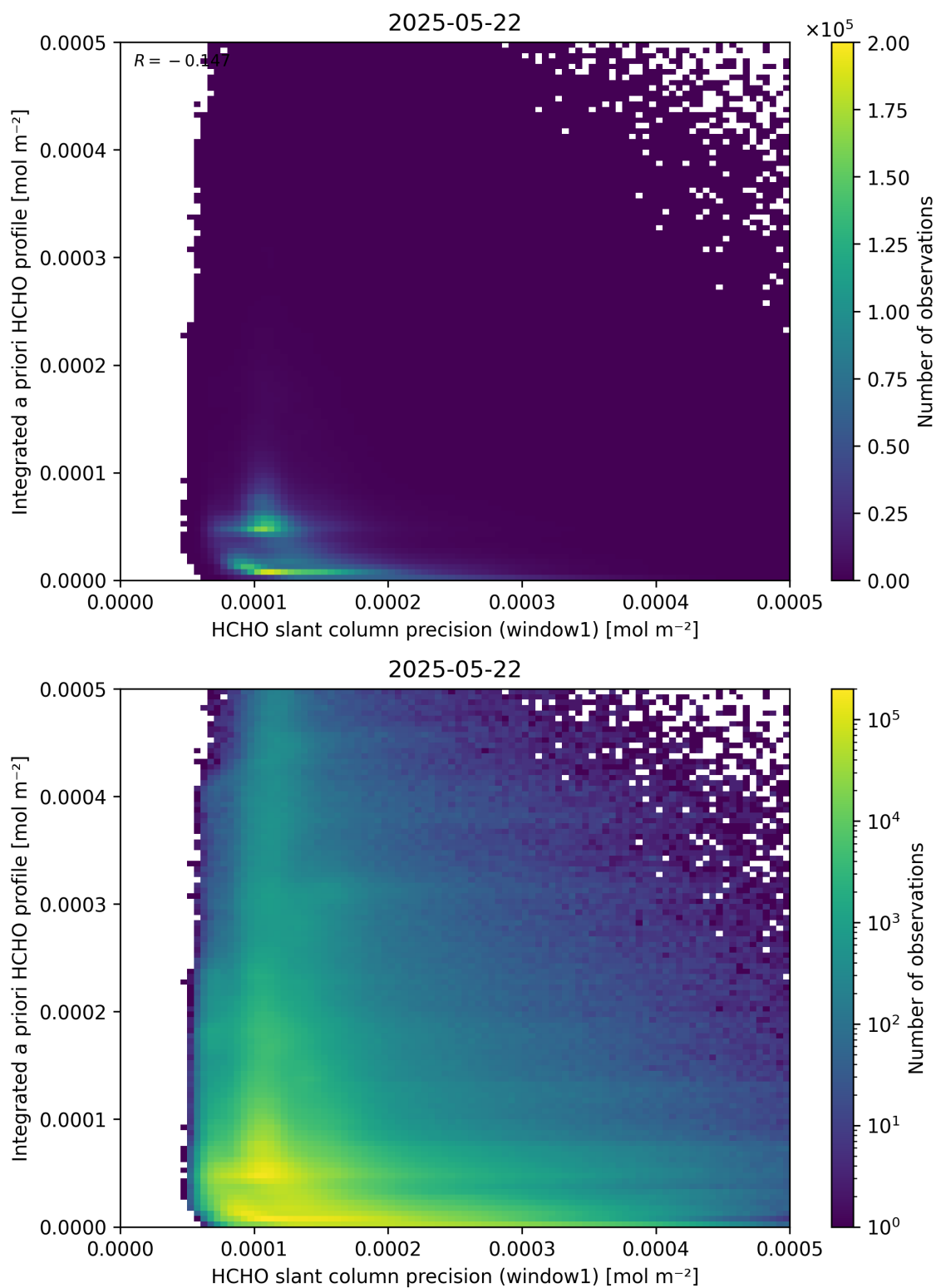
Figure 96: Scatter density plot of “HCHO slant column precision (window1)” against “Integrated a priori HCHO profile” for 2025-05-21 to 2025-05-23.
