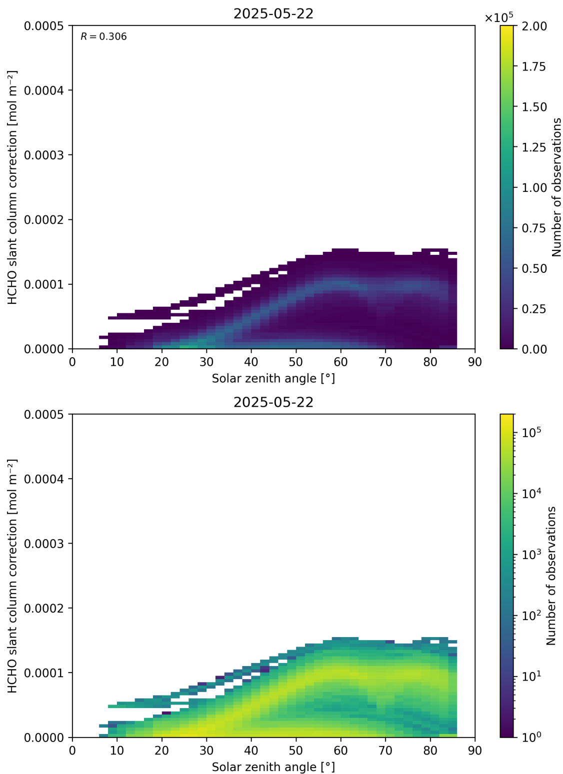
Figure 172: Scatter density plot of “Solar zenith angle” against “HCHO slant column correction” for 2025-05-21 to 2025-05-23.
