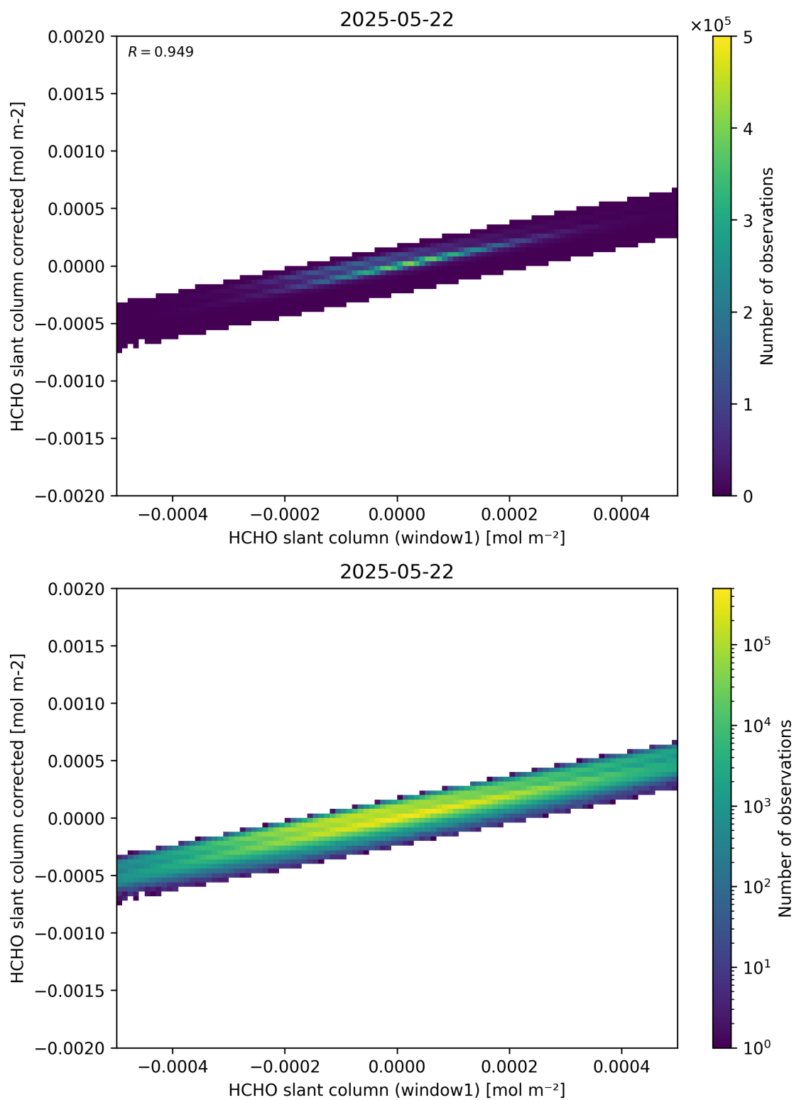
Figure 82: Scatter density plot of “HCHO slant column (window1)” against “HCHO slant column corrected” for 2025-05-21 to 2025-05-23.
