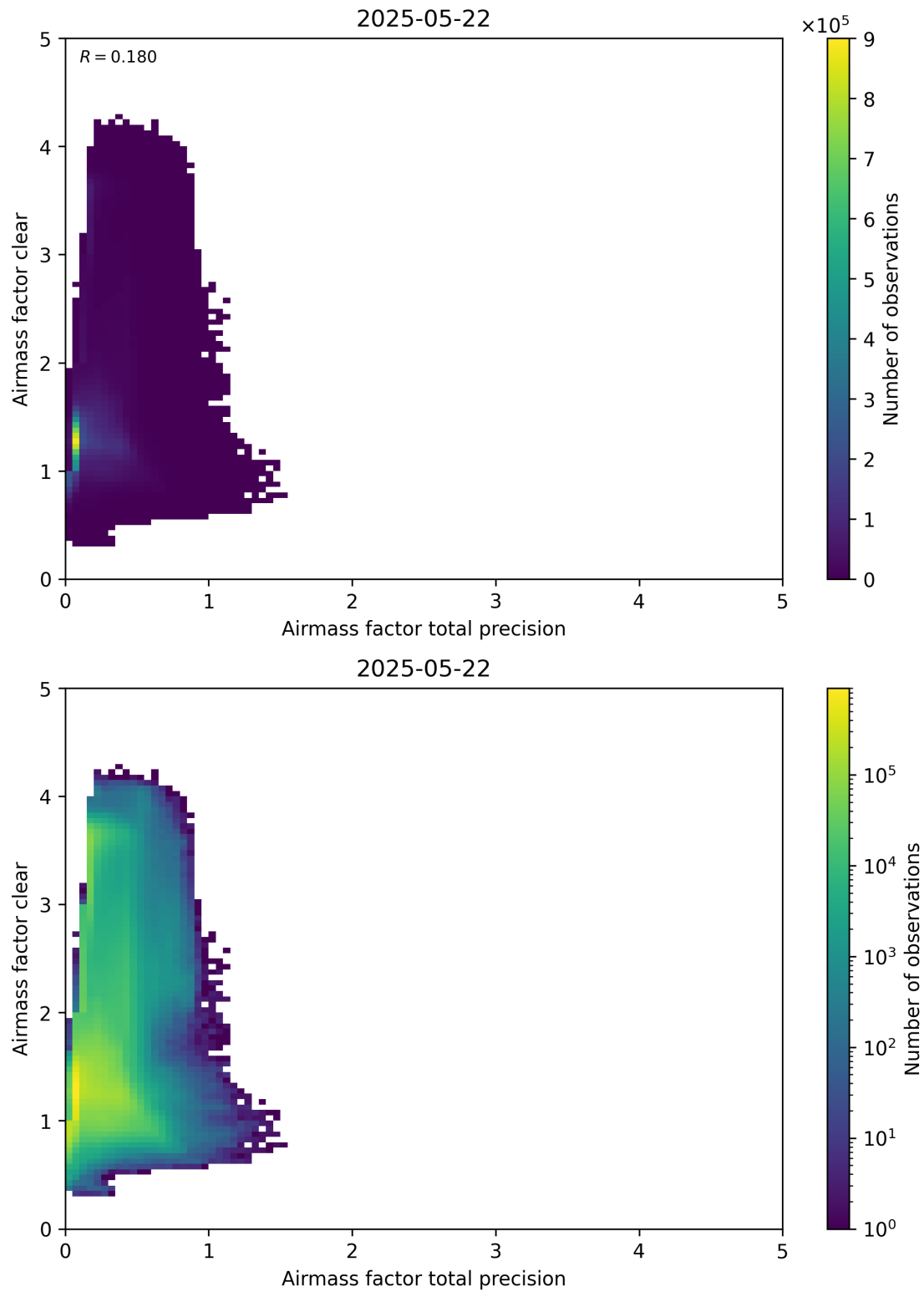
Figure 108: Scatter density plot of “Airmass factor total precision” against “Airmass factor clear” for 2025-05-21 to 2025-05-23.
