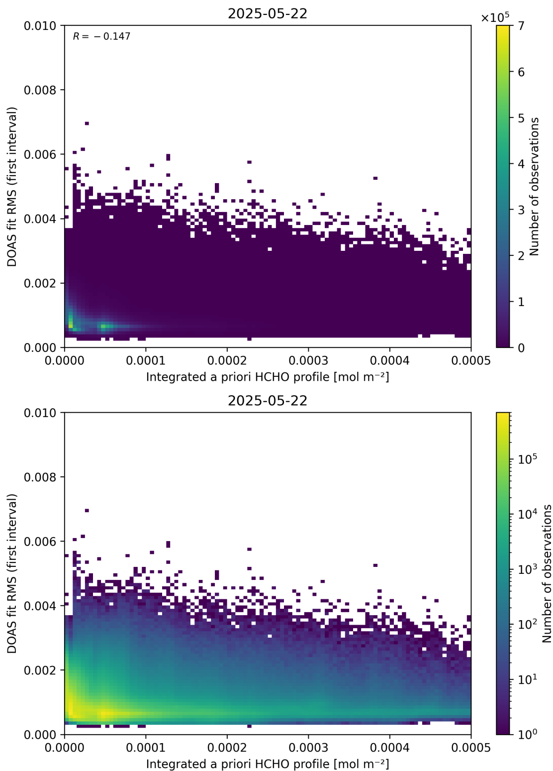
Figure 148: Scatter density plot of “Integrated a priori HCHO profile” against “DOAS fit RMS (first interval)” for 2025-05-21 to 2025-05-23.
