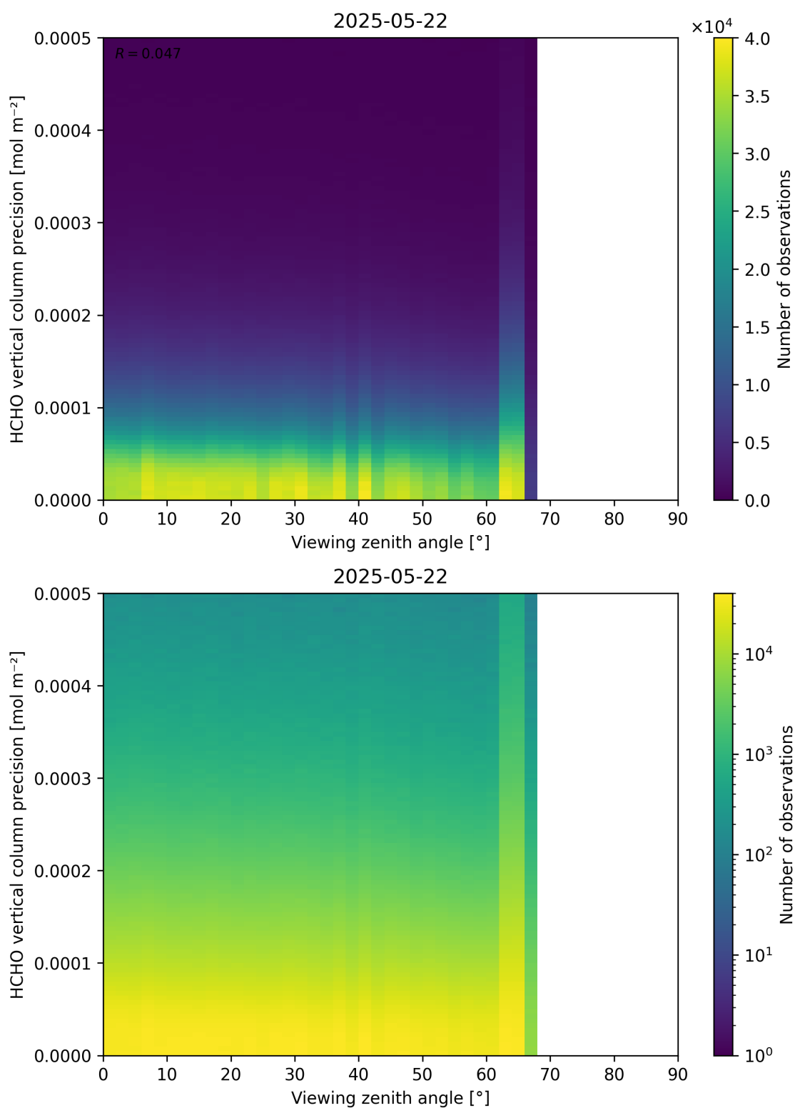
Figure 194: Scatter density plot of “Viewing zenith angle” against “HCHO vertical column precision” for 2025-05-21 to 2025-05-23.
