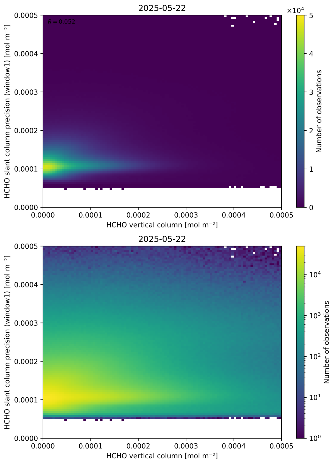
Figure 130: Scatter density plot of “HCHO vertical column” against “HCHO slant column precision (window1)” for 2025-05-21 to 2025-05-23.
