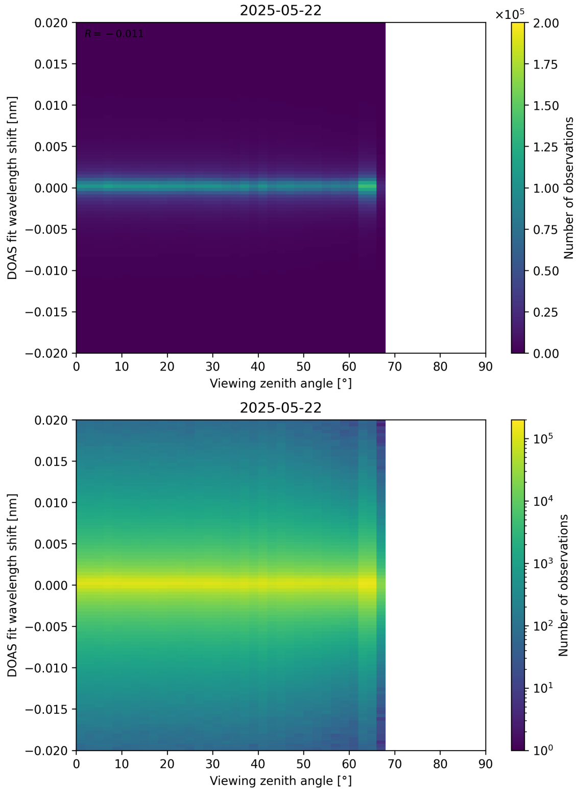
Figure 183: Scatter density plot of “Viewing zenith angle” against “DOAS fit wavelength shift” for 2025-05-21 to 2025-05-23.
