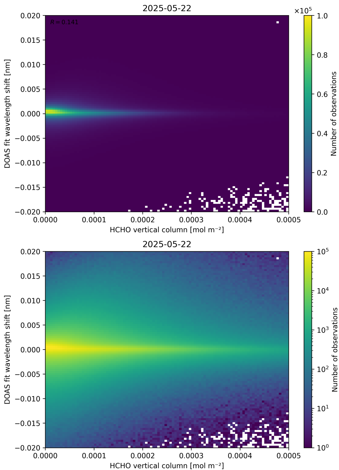
Figure 124: Scatter density plot of “HCHO vertical column” against “DOAS fit wavelength shift” for 2025-05-21 to 2025-05-23.
