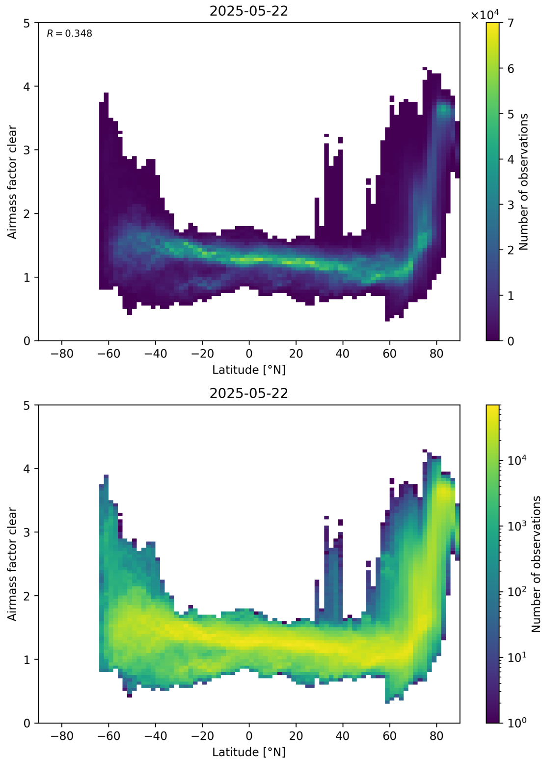
Figure 156: Scatter density plot of “Latitude” against “Airmass factor clear” for 2025-05-21 to 2025-05-23.
