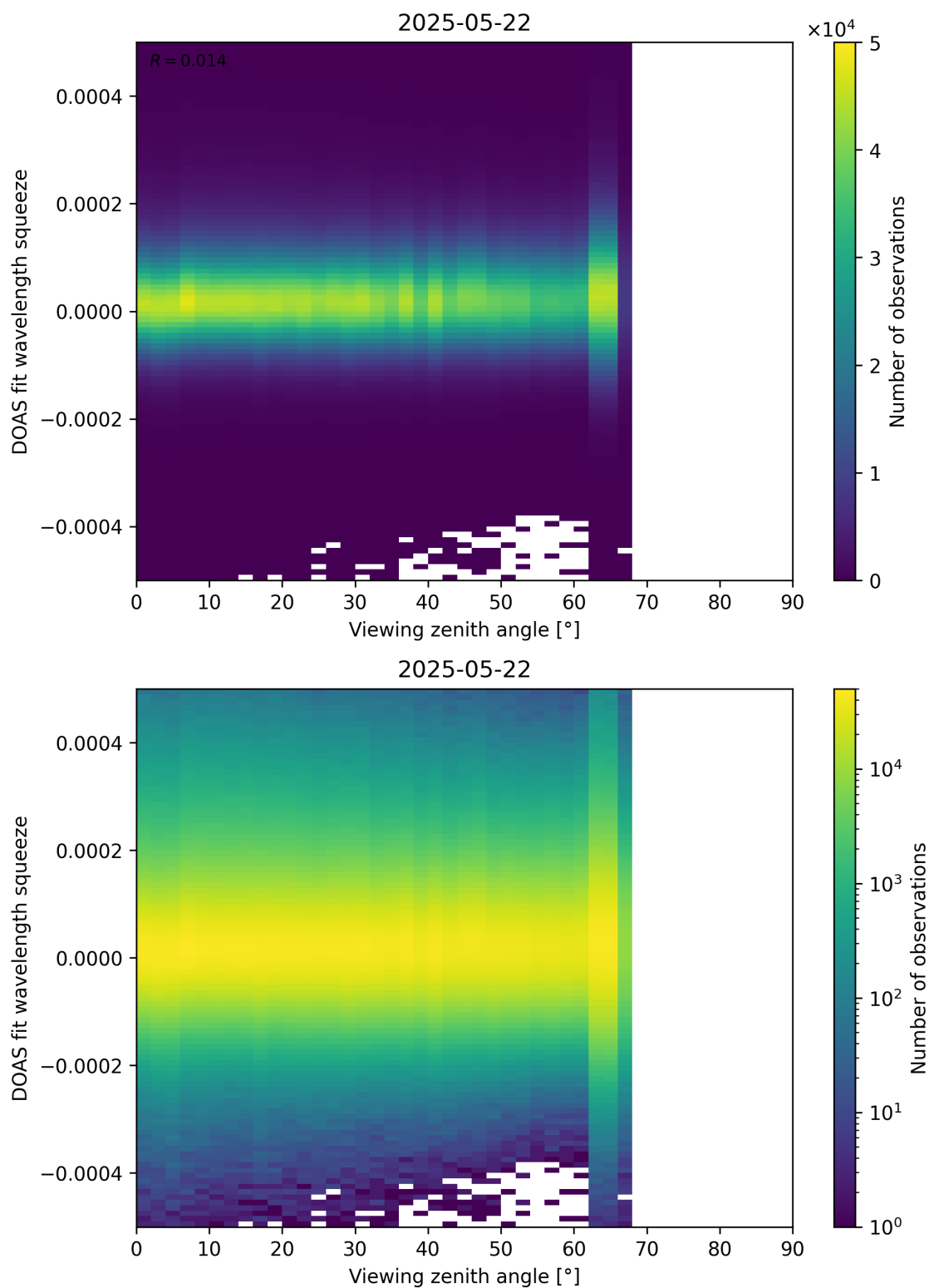
Figure 184: Scatter density plot of “Viewing zenith angle” against “DOAS fit wavelength squeeze” for 2025-05-21 to 2025-05-23.
