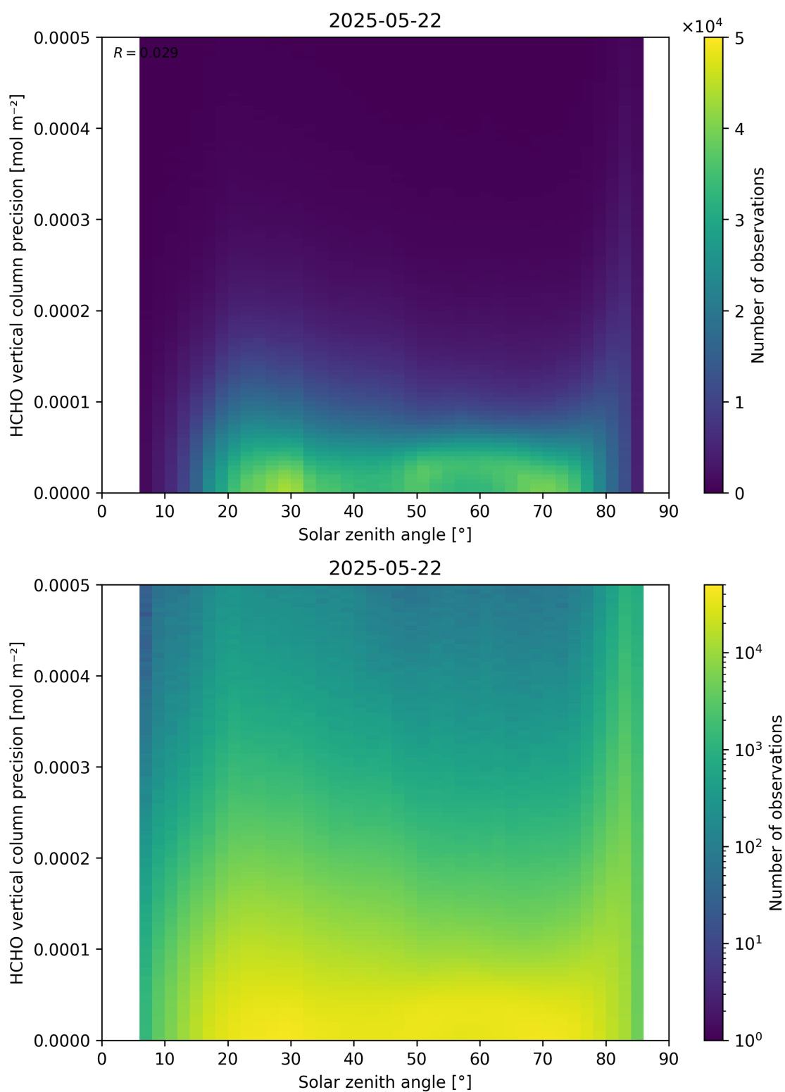
Figure 179: Scatter density plot of “Solar zenith angle” against “HCHO vertical column precision” for 2025-05-21 to 2025-05-23.
