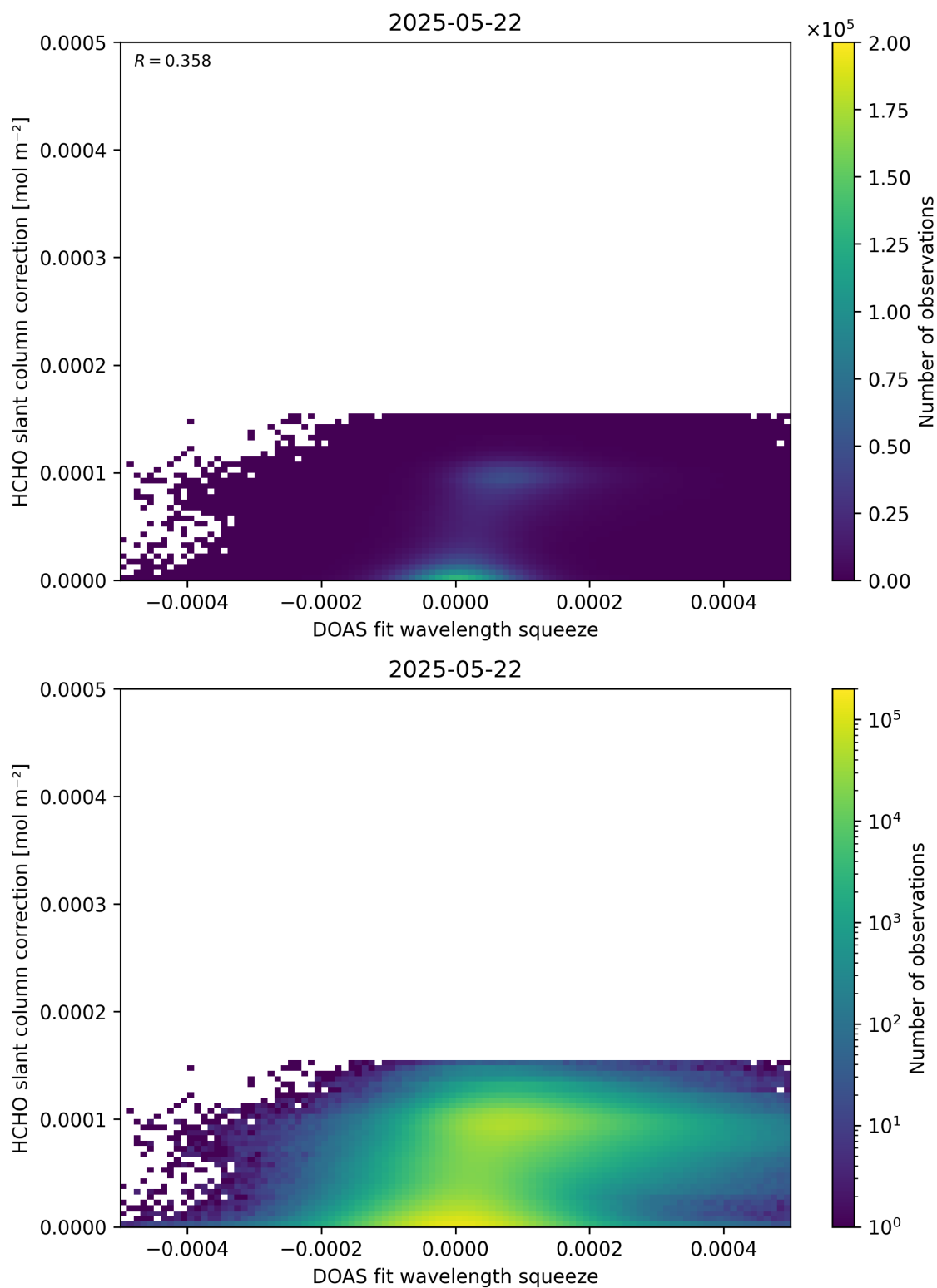
Figure 70: Scatter density plot of “DOAS fit wavelength squeeze” against “HCHO slant column correction” for 2025-05-21 to 2025-05-23.
