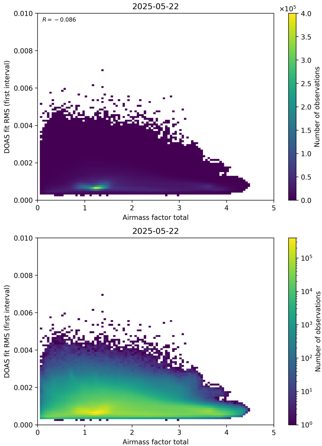
Figure 97: Scatter density plot of “Airmass factor total” against “DOAS fit RMS (first interval)” for 2025-05-21 to 2025-05-23.
