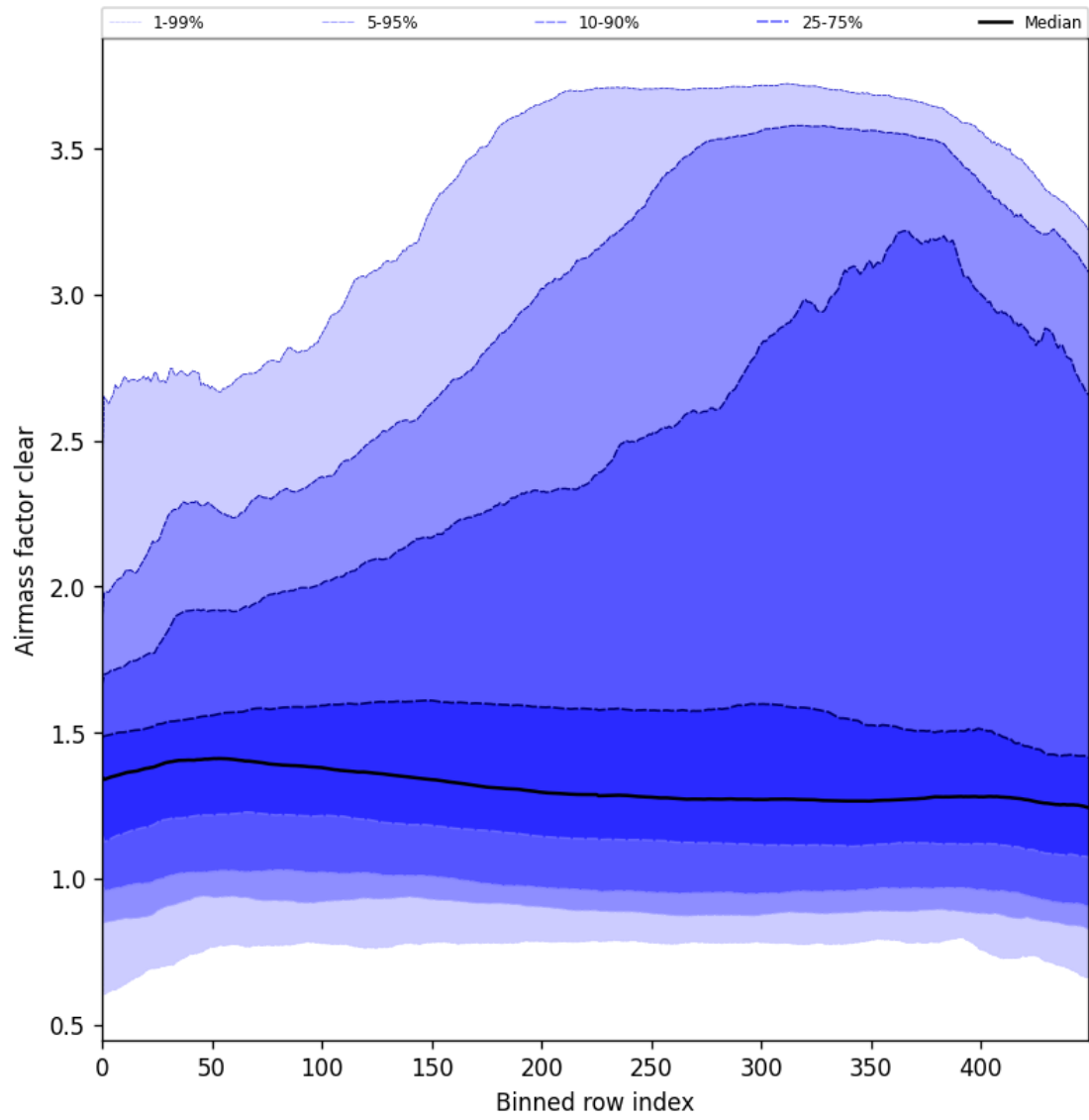
Figure 56: Along track statistics of “Airmass factor clear” for 2025-05-21 to 2025-05-23
