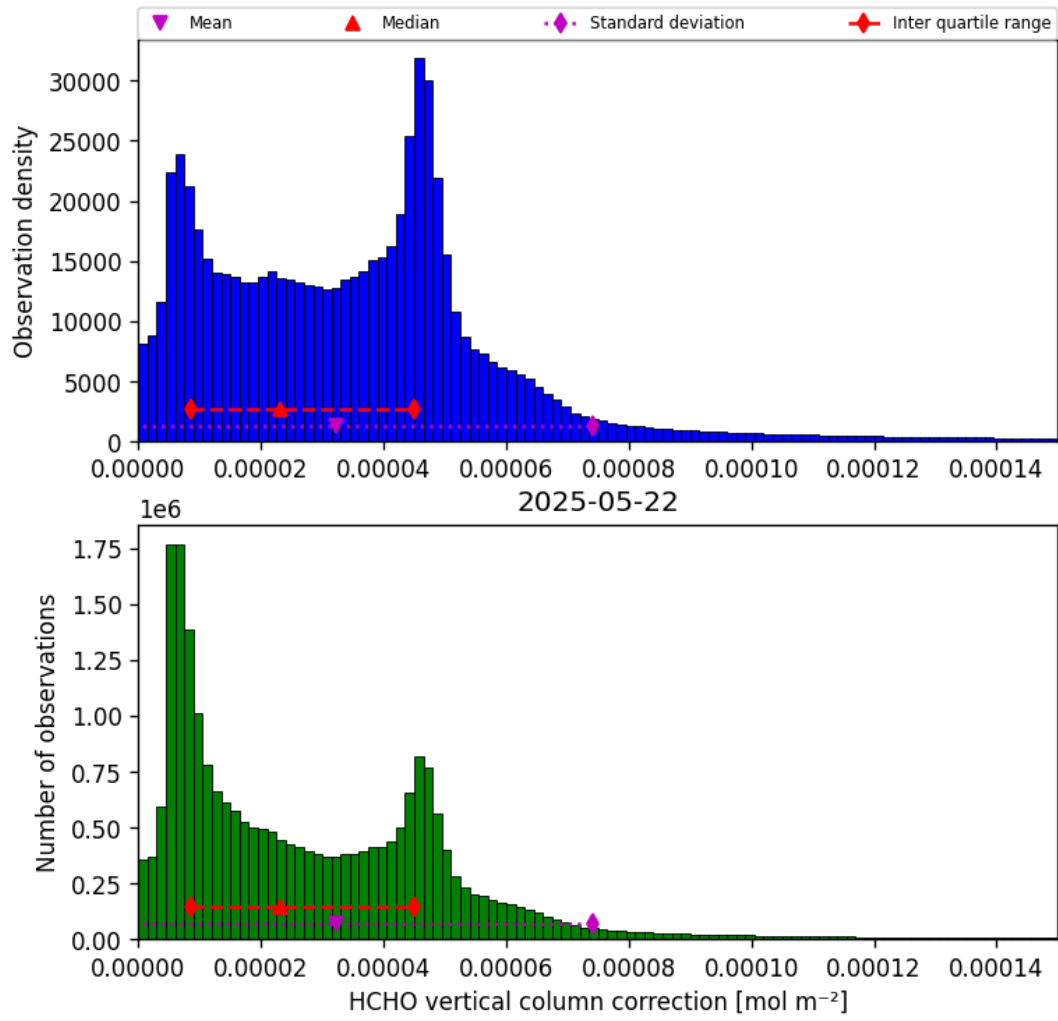
Figure 37: Histogram of “HCHO vertical column correction” for 2025-05-21 to 2025-05-23
