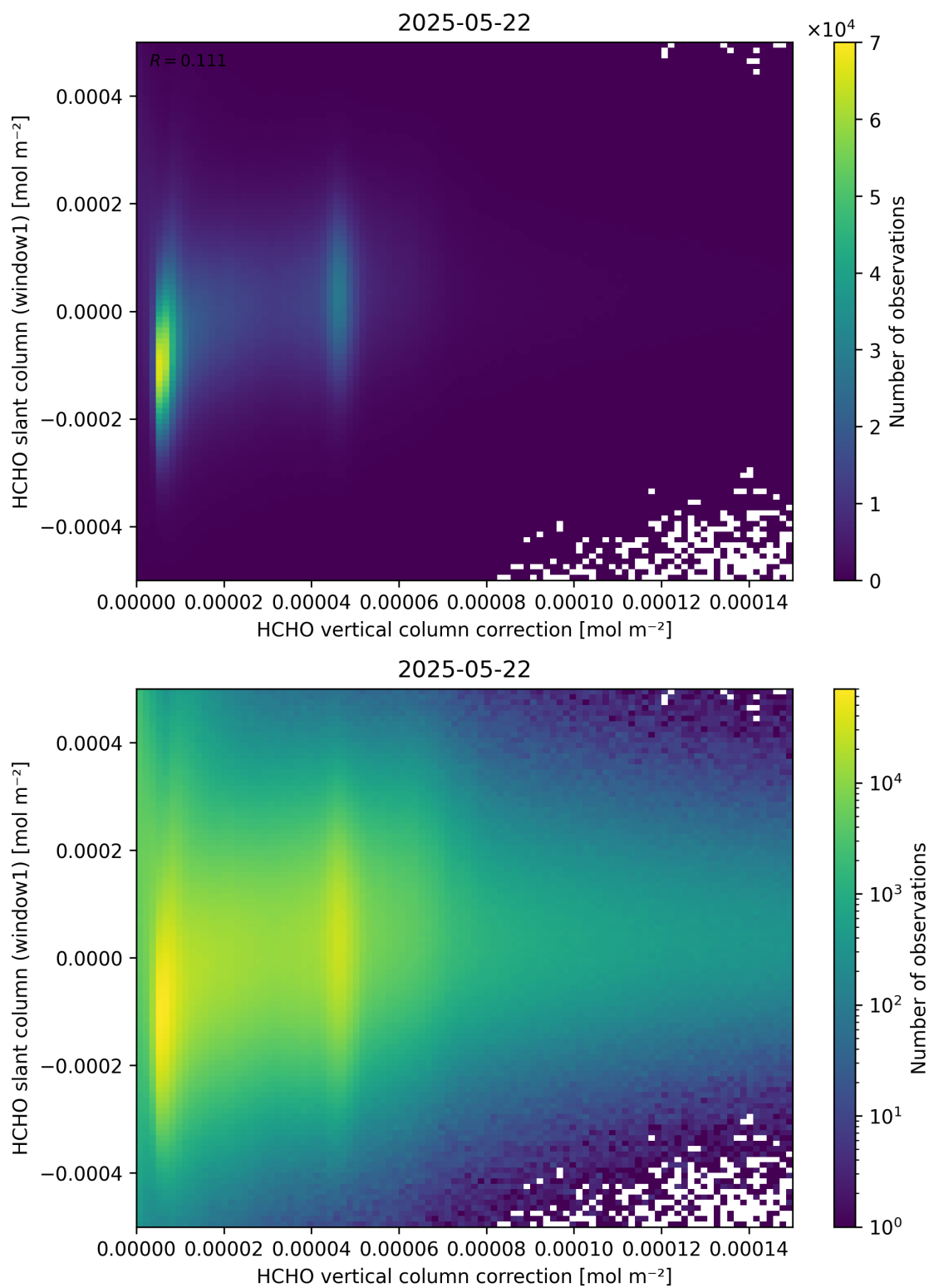
Figure 118: Scatter density plot of “HCHO vertical column correction” against “HCHO slant column (window1)” for 2025-05-21 to 2025-05-23.
