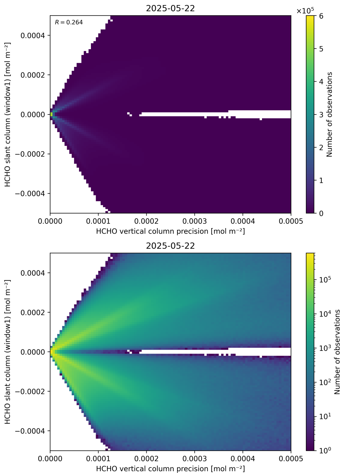
Figure 142: Scatter density plot of “HCHO vertical column precision” against “HCHO slant column (window1)” for 2025-05-21 to 2025-05-23.
