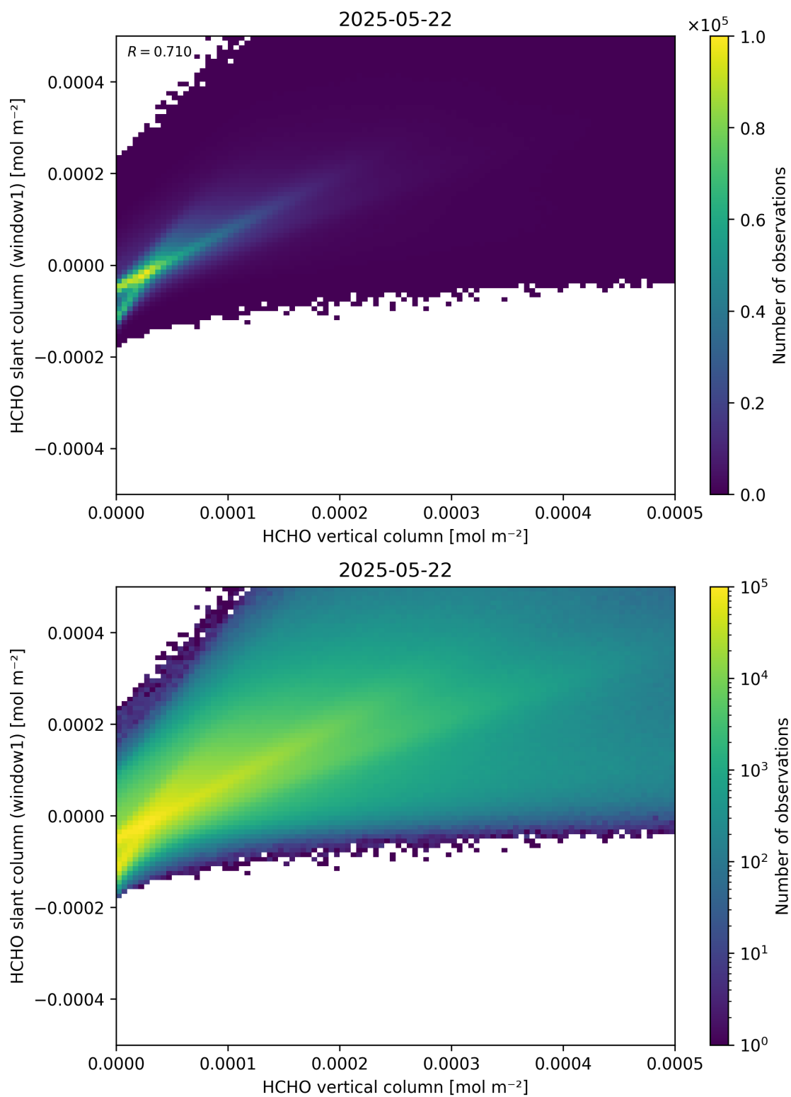
Figure 129: Scatter density plot of “HCHO vertical column” against “HCHO slant column (window1)” for 2025-05-21 to 2025-05-23.
