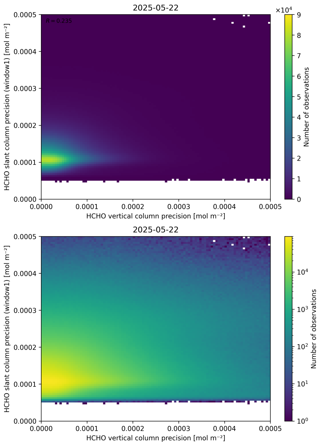
Figure 143: Scatter density plot of “HCHO vertical column precision” against “HCHO slant column precision (window1)” for 2025-05-21 to 2025-05-23.
