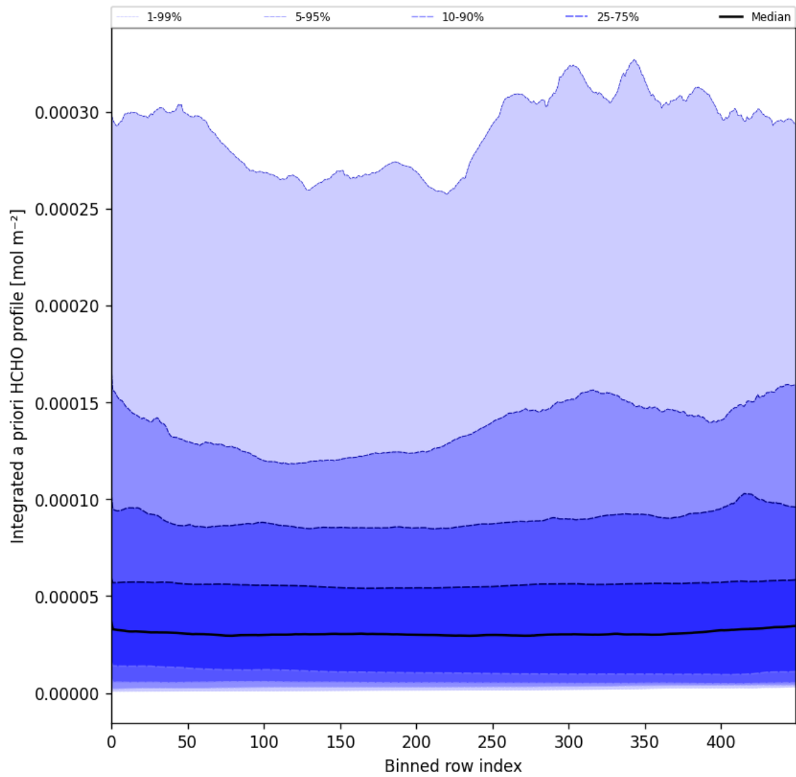
Figure 57: Along track statistics of “Integrated a priori HCHO profile” for 2025-05-21 to 2025-05-23
