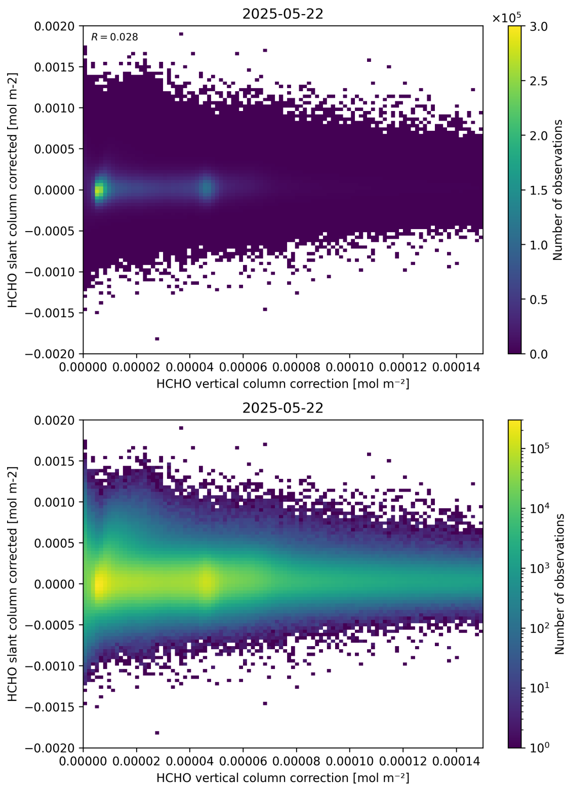
Figure 116: Scatter density plot of “HCHO vertical column correction” against “HCHO slant column corrected” for 2025-05-21 to 2025-05-23.
