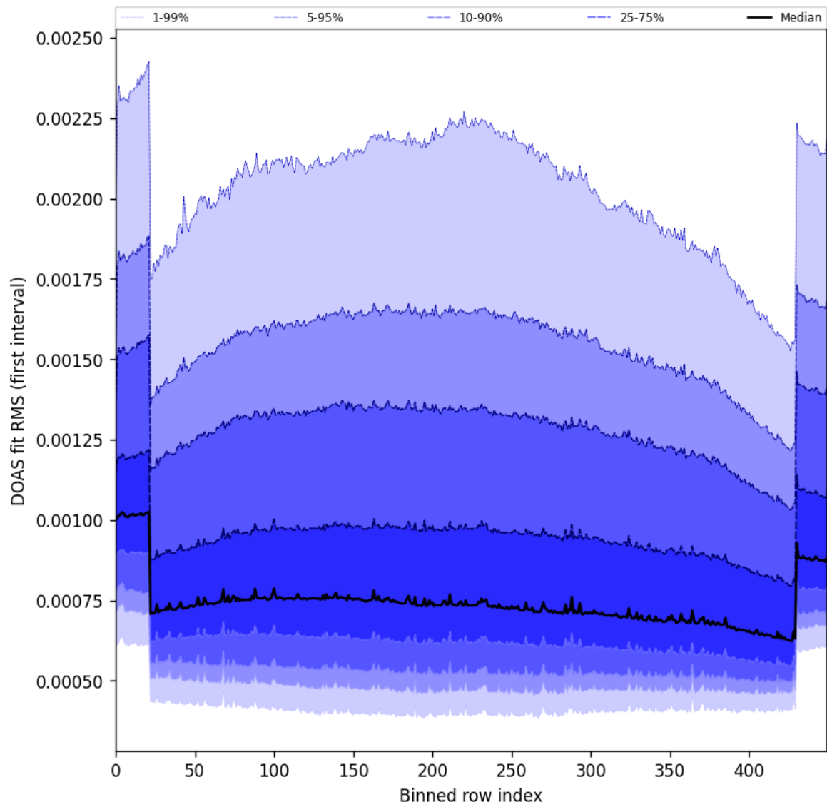
Figure 60: Along track statistics of “DOAS fit RMS (first interval)” for 2025-05-21 to 2025-05-23
