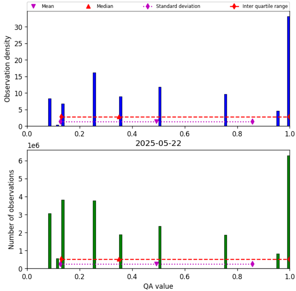
Figure 34: Histogram of “QA value” for 2025-05-21 to 2025-05-23
