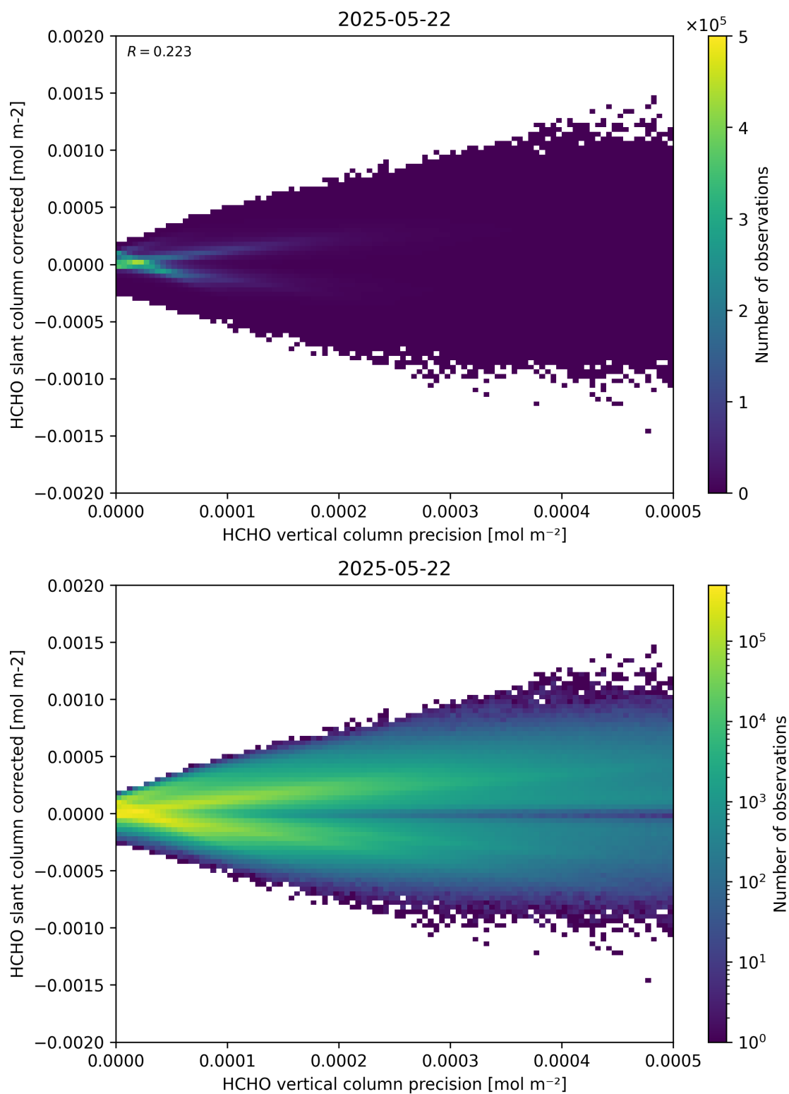
Figure 140: Scatter density plot of “HCHO vertical column precision” against “HCHO slant column corrected” for 2025-05-21 to 2025-05-23.
