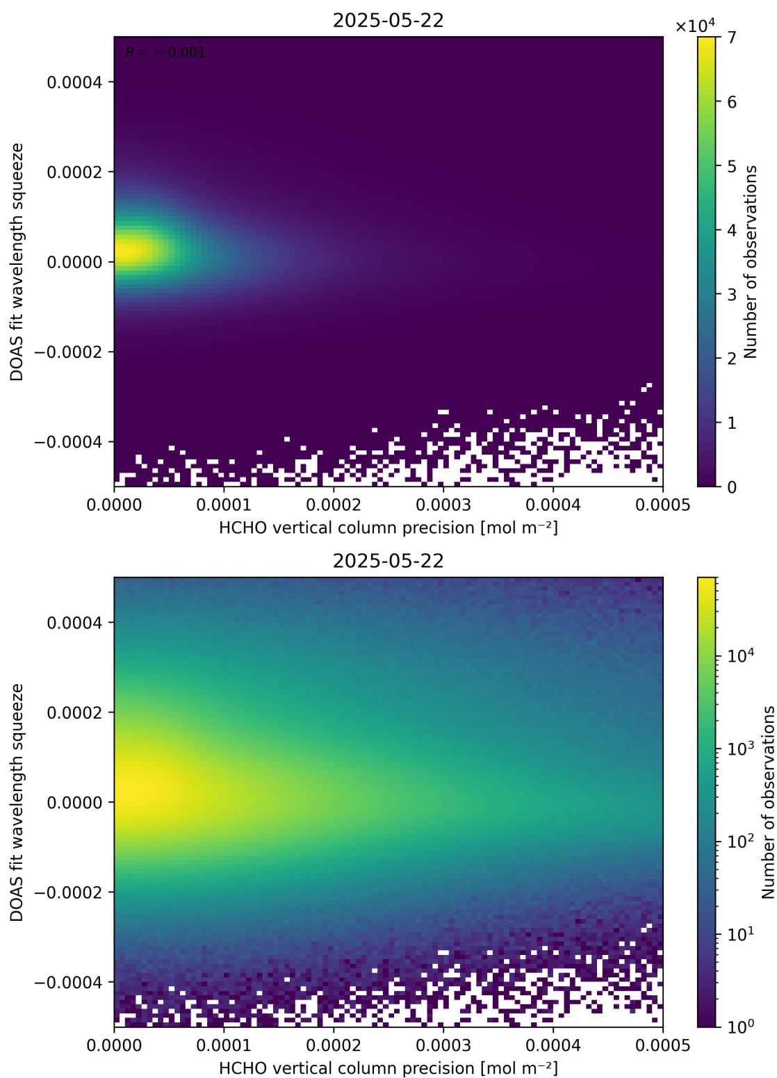
Figure 138: Scatter density plot of “HCHO vertical column precision” against “DOAS fit wavelength squeeze” for 2025-05-21 to 2025-05-23.
