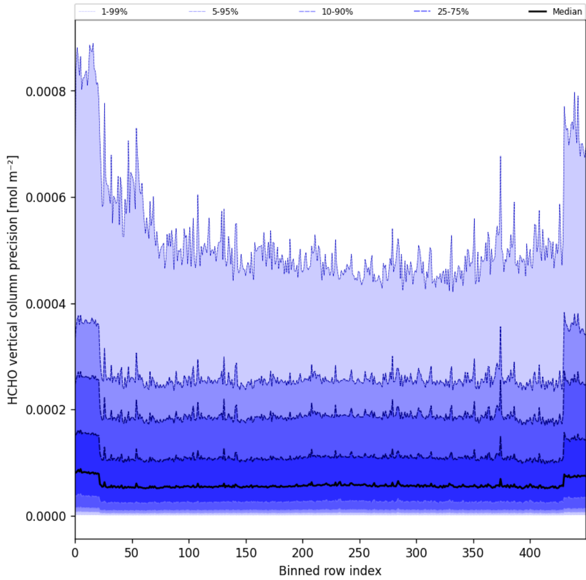
Figure 50: Along track statistics of “HCHO vertical column precision” for 2025-05-21 to 2025-05-23
