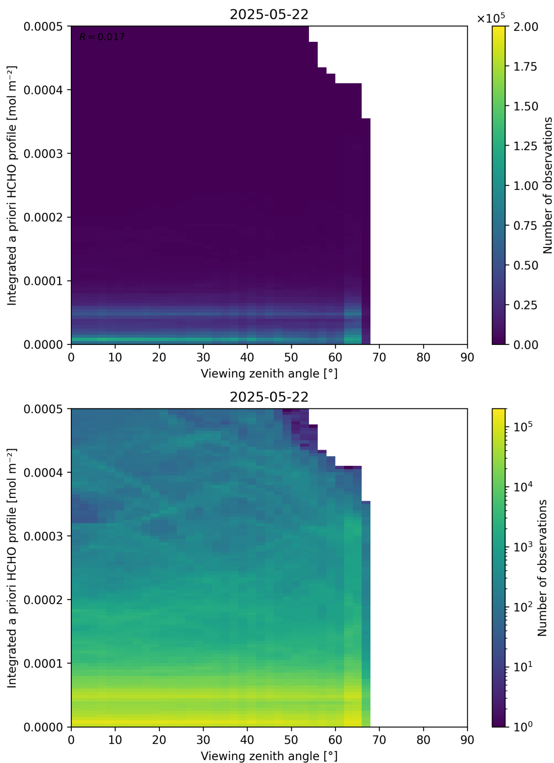
Figure 195: Scatter density plot of “Viewing zenith angle” against “Integrated a priori HCHO profile” for 2025-05-21 to 2025-05-23.
