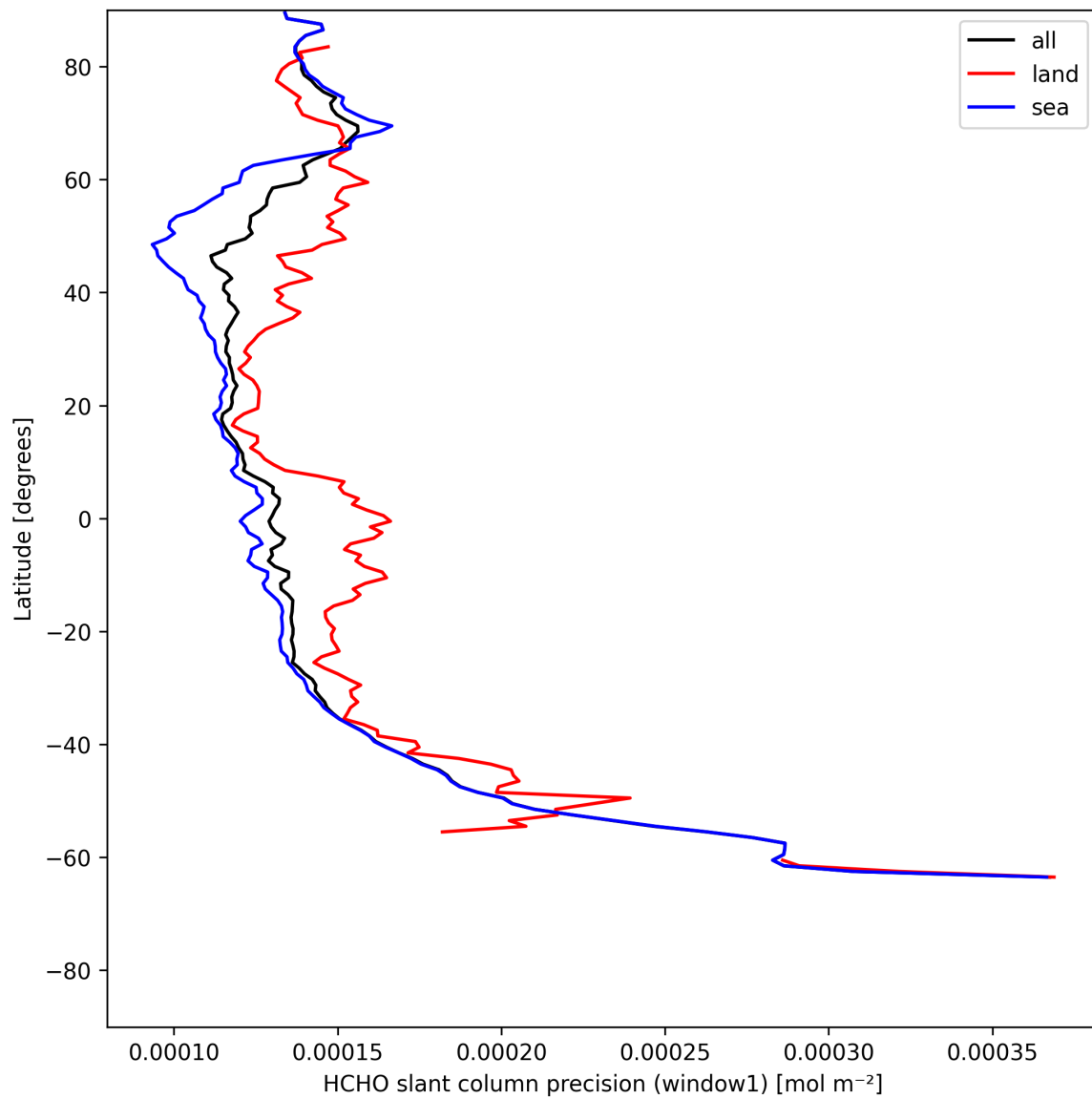
Figure 25: Zonal average of “HCHO slant column precision (window1)” for 2025-05-21 to 2025-05-23.
