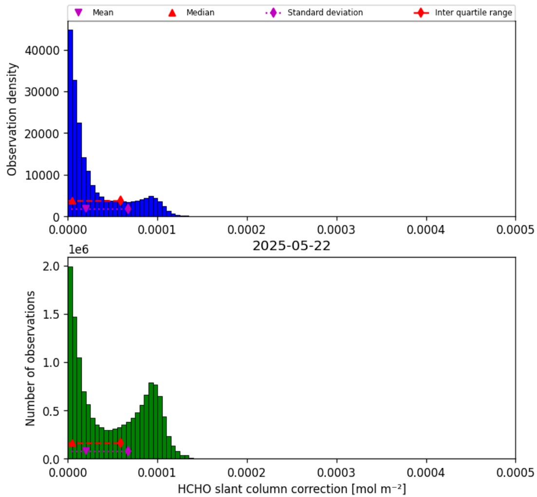
Figure 47: Histogram of “HCHO slant column correction” for 2025-05-21 to 2025-05-23
