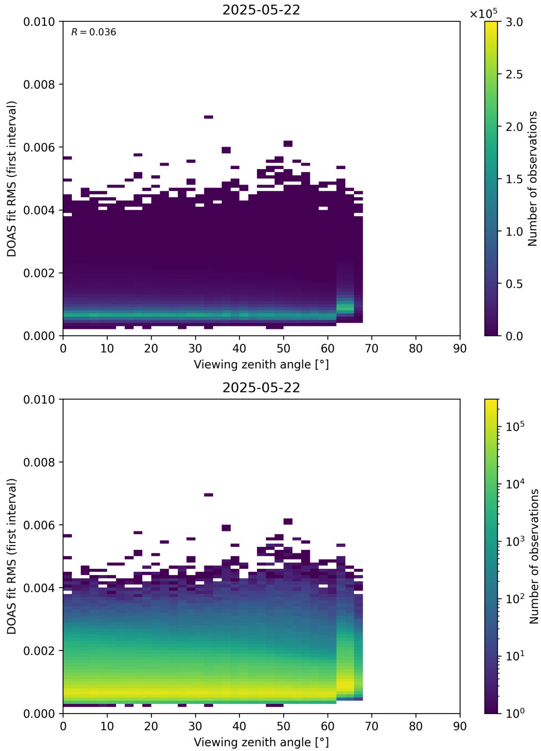
Figure 182: Scatter density plot of “Viewing zenith angle” against “DOAS fit RMS (first interval)” for 2025-05-21 to 2025-05-23.
