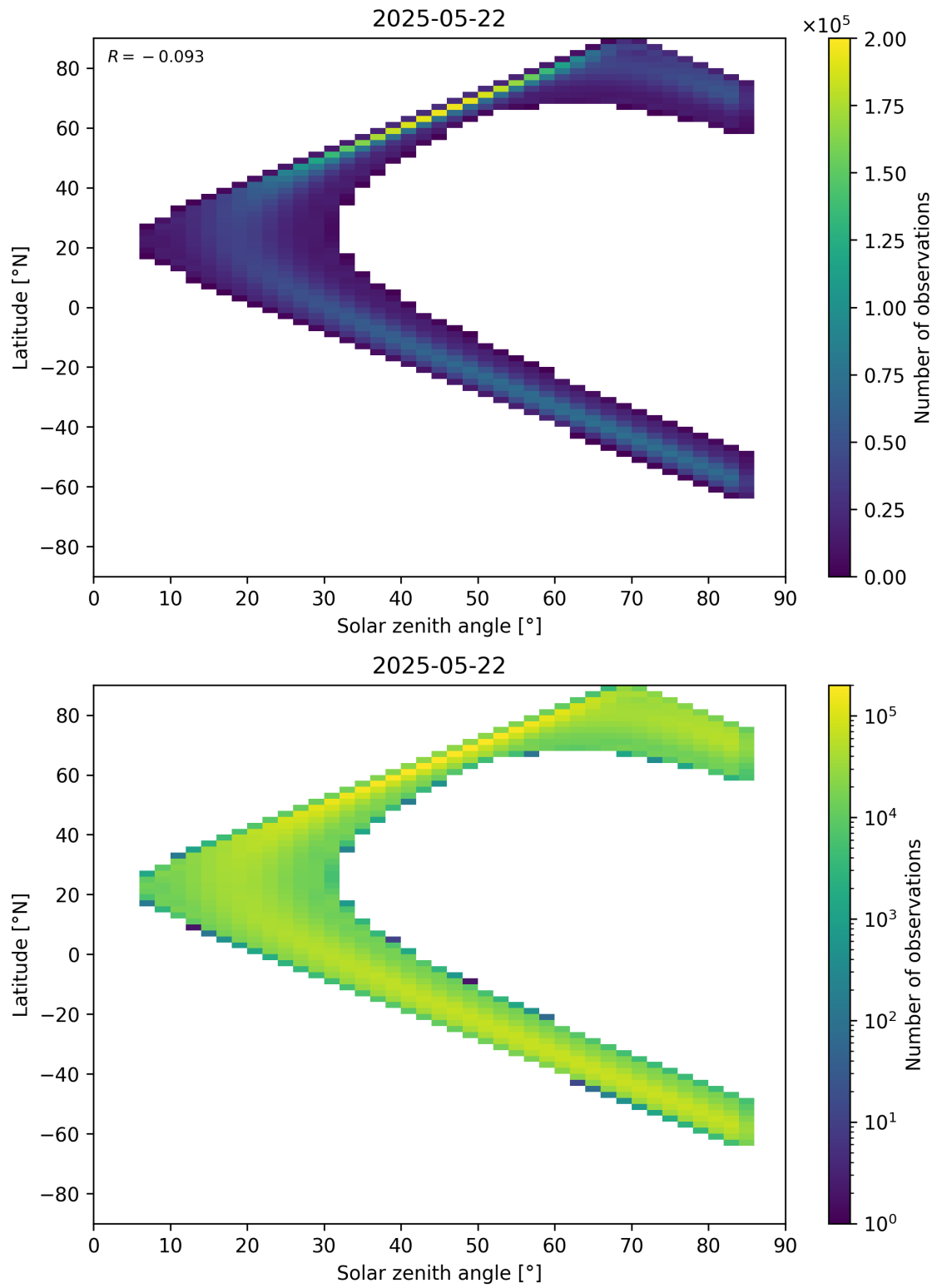
Figure 181: Scatter density plot of “Solar zenith angle” against “Latitude” for 2025-05-21 to 2025-05-23.
