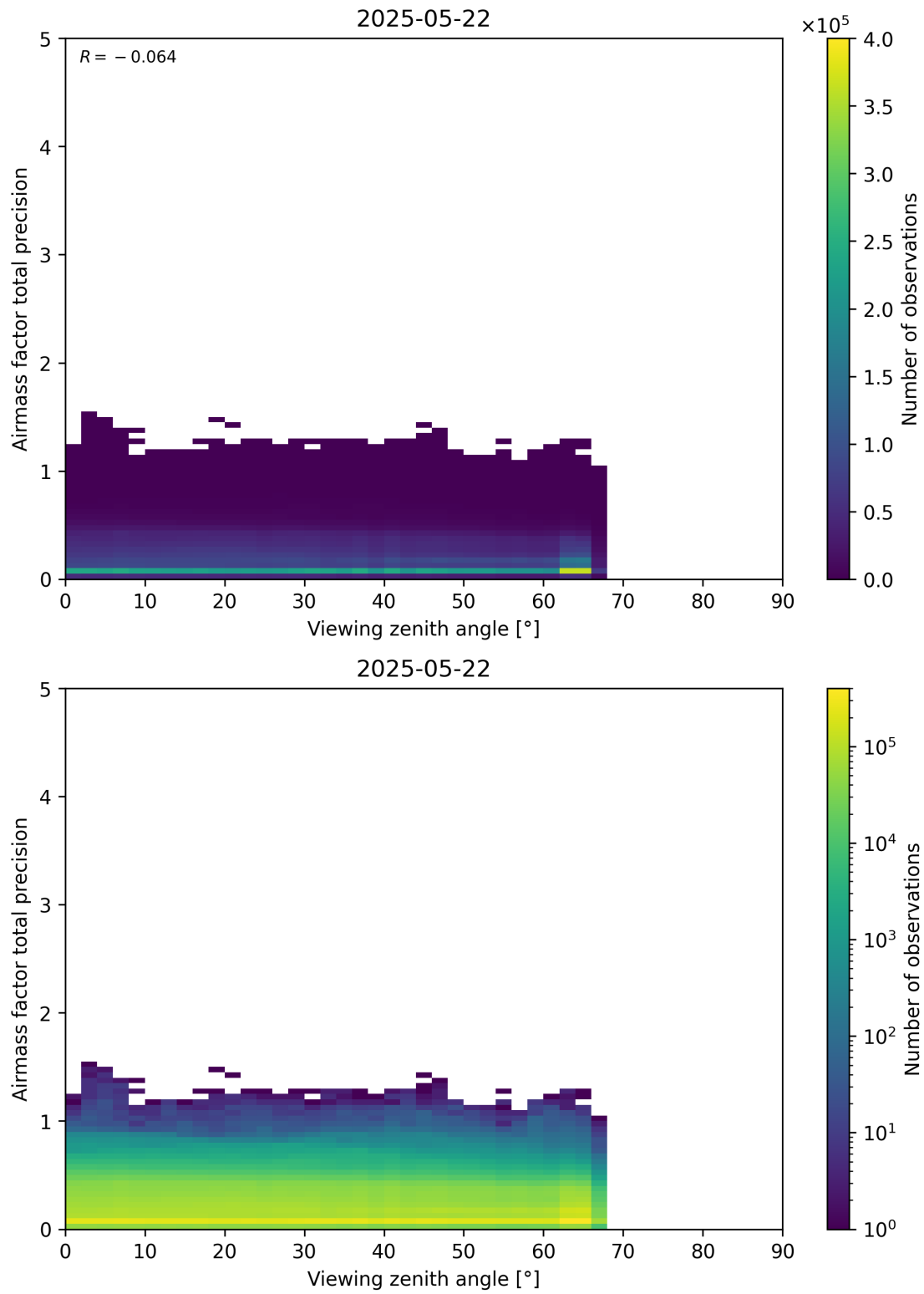
Figure 191: Scatter density plot of “Viewing zenith angle” against “Airmass factor total precision” for 2025-05-21 to 2025-05-23.
