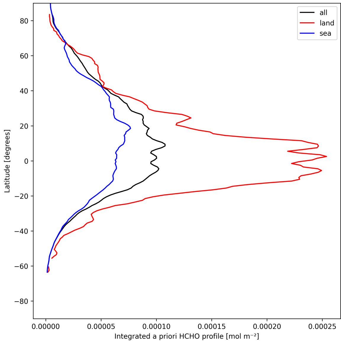
Figure 29: Zonal average of “Integrated a priori HCHO profile” for 2025-05-21 to 2025-05-23.
