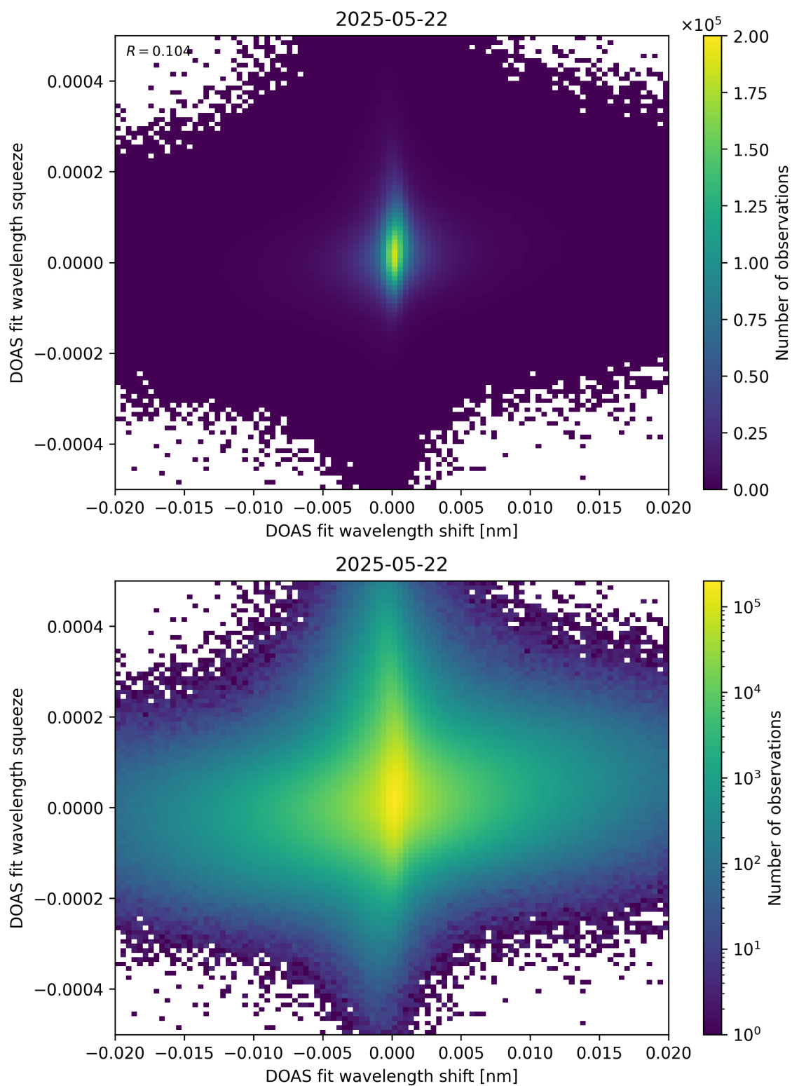
Figure 65: Scatter density plot of “DOAS fit wavelength shift” against “DOAS fit wavelength squeeze” for 2025-05-21 to 2025-05-23.
