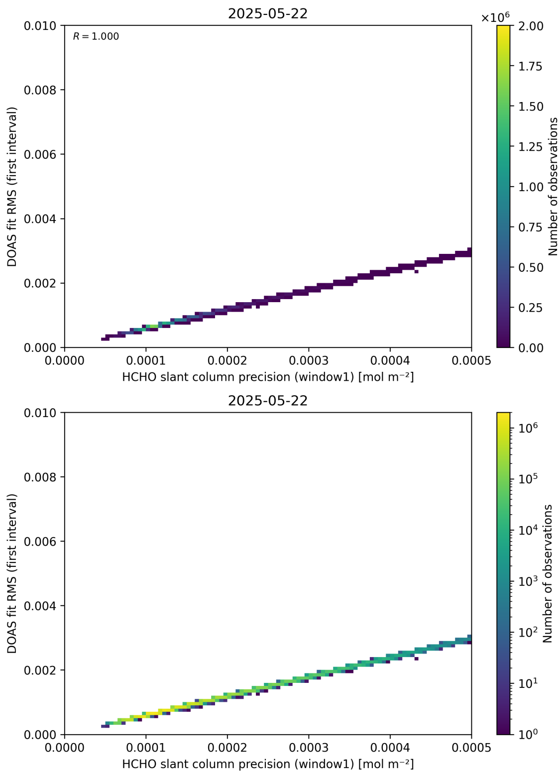
Figure 88: Scatter density plot of “HCHO slant column precision (window1)” against “DOAS fit RMS (first interval)” for 2025-05-21 to 2025-05-23.
