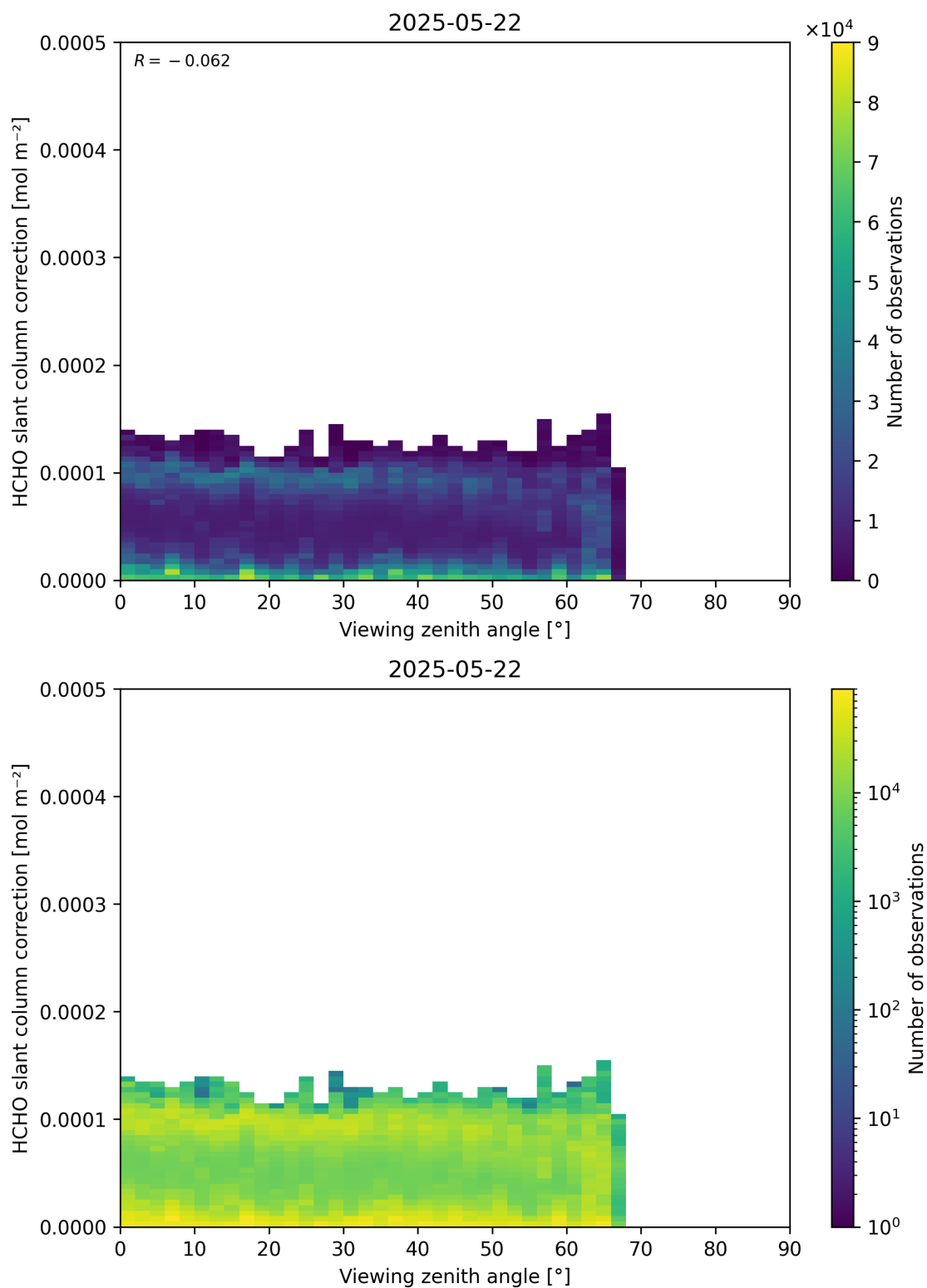
Figure 187: Scatter density plot of “Viewing zenith angle” against “HCHO slant column correction” for 2025-05-21 to 2025-05-23.
