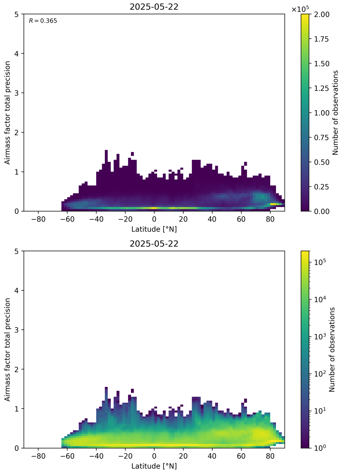
Figure 162: Scatter density plot of “Latitude” against “Airmass factor total precision” for 2025-05-21 to 2025-05-23.
