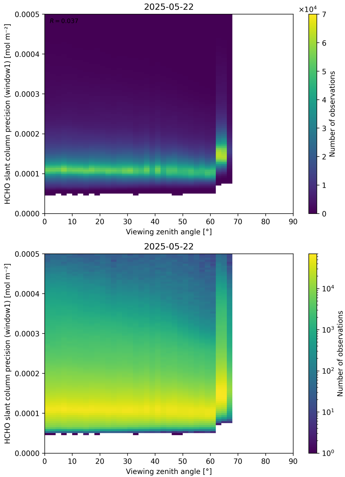
Figure 189: Scatter density plot of “Viewing zenith angle” against “HCHO slant column precision (window1)” for 2025-05-21 to 2025-05-23.
