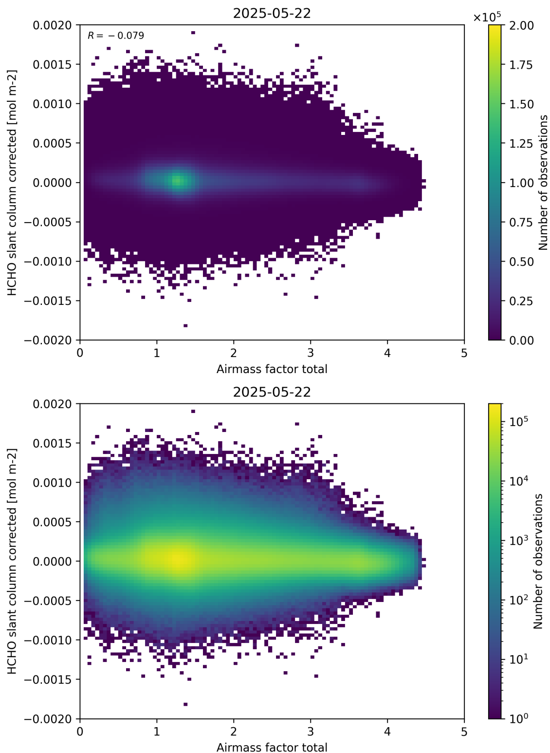
Figure 101: Scatter density plot of “Airmass factor total” against “HCHO slant column corrected” for 2025-05-21 to 2025-05-23.
