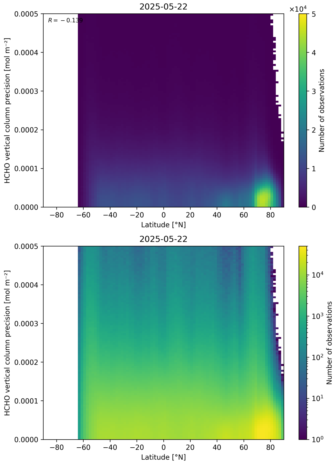
Figure 165: Scatter density plot of “Latitude” against “HCHO vertical column precision” for 2025-05-21 to 2025-05-23.
