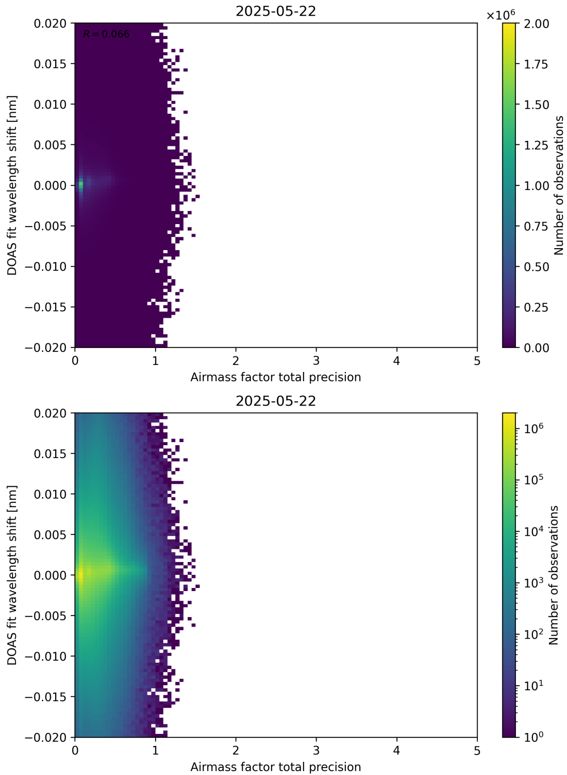
Figure 106: Scatter density plot of “Airmass factor total precision” against “DOAS fit wavelength shift” for 2025-05-21 to 2025-05-23.
