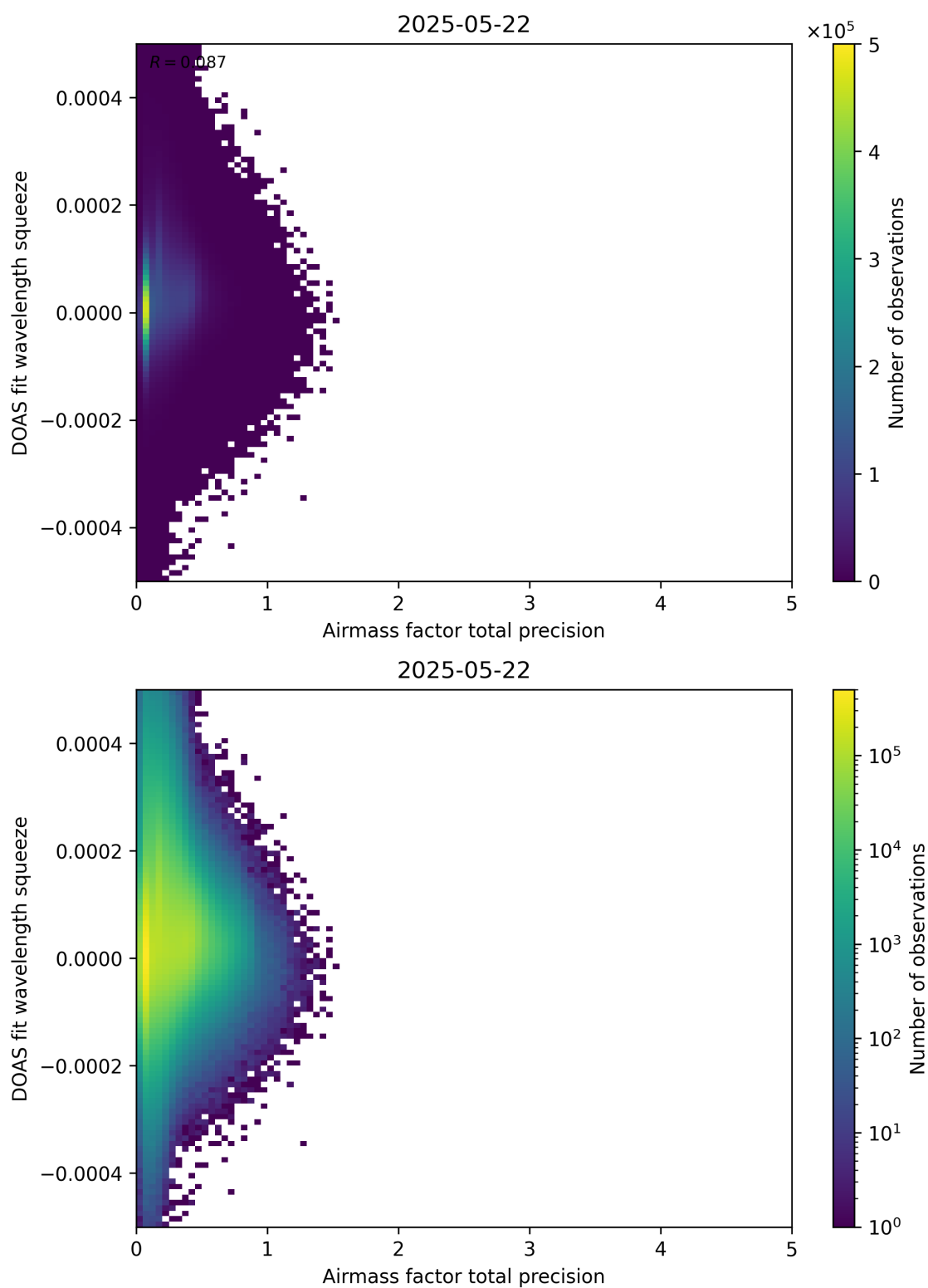
Figure 107: Scatter density plot of “Airmass factor total precision” against “DOAS fit wavelength squeeze” for 2025-05-21 to 2025-05-23.
