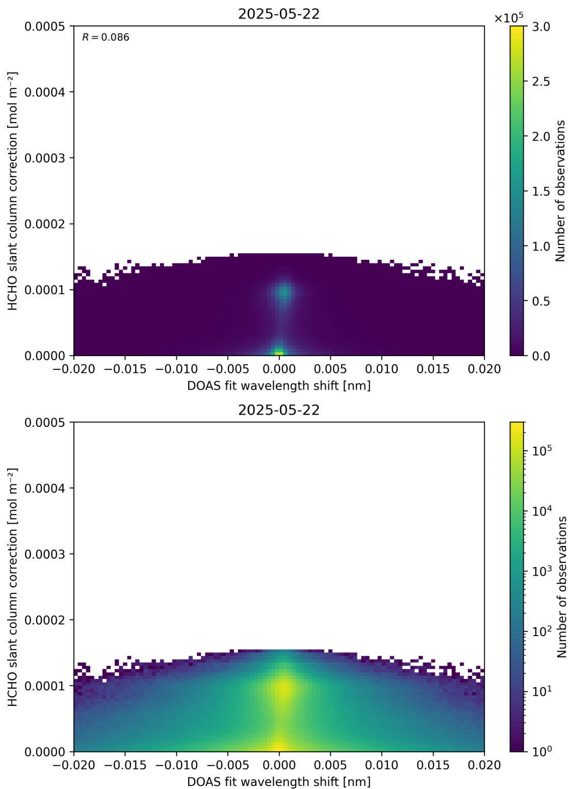
Figure 67: Scatter density plot of “DOAS fit wavelength shift” against “HCHO slant column correction” for 2025-05-21 to 2025-05-23.
