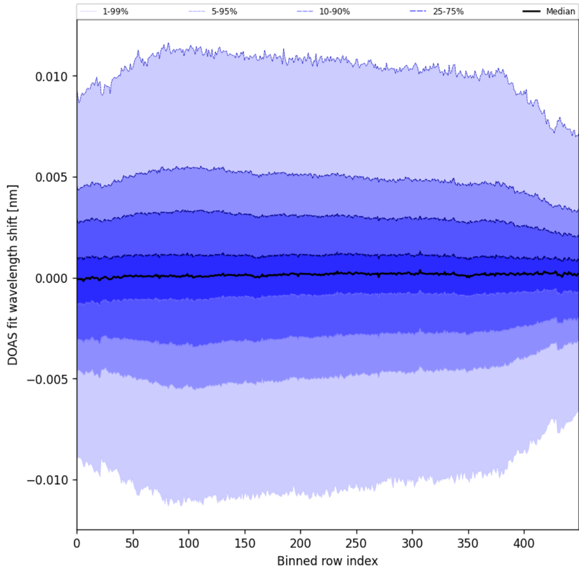
Figure 58: Along track statistics of “DOAS fit wavelength shift” for 2025-05-21 to 2025-05-23
