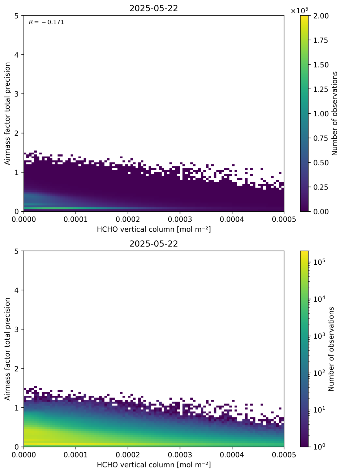
Figure 132: Scatter density plot of “HCHO vertical column” against “Airmass factor total precision” for 2025-05-21 to 2025-05-23.
