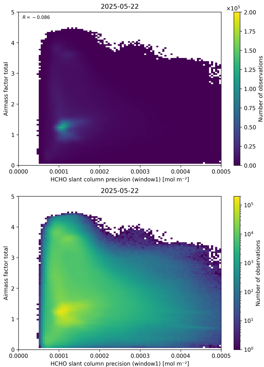
Figure 94: Scatter density plot of “HCHO slant column precision (window1)” against “Airmass factor total” for 2025-05-21 to 2025-05-23.
