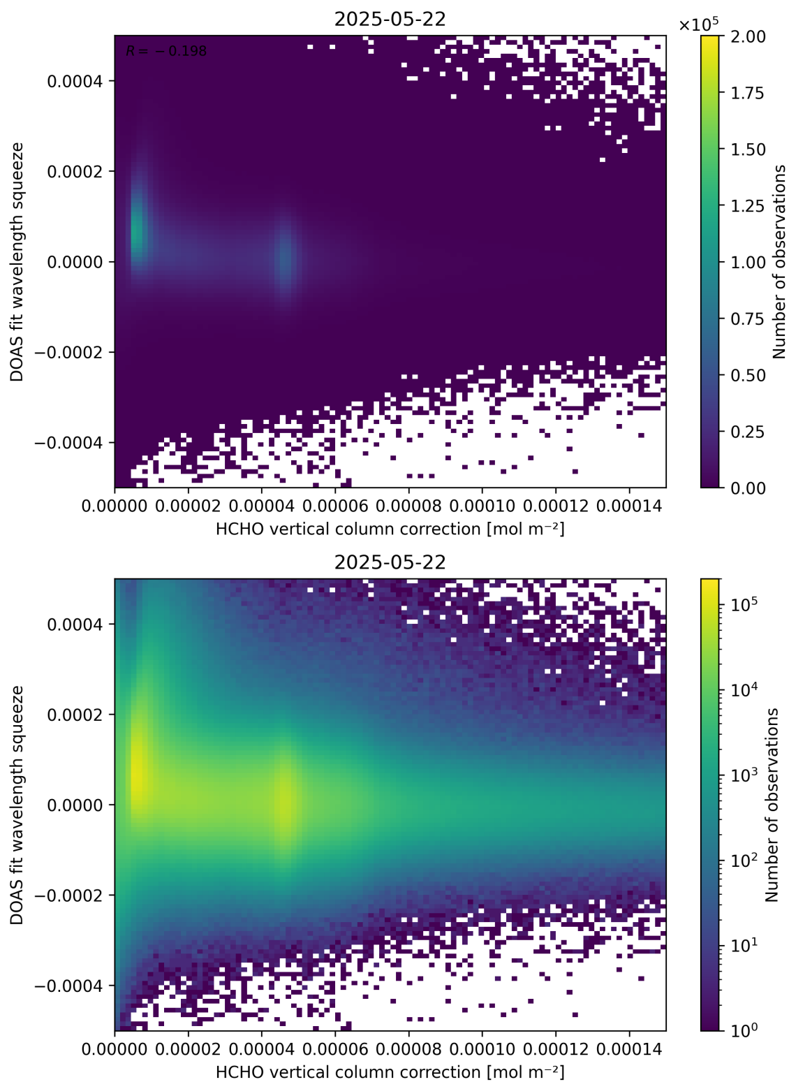
Figure 114: Scatter density plot of “HCHO vertical column correction” against “DOAS fit wavelength squeeze” for 2025-05-21 to 2025-05-23.
