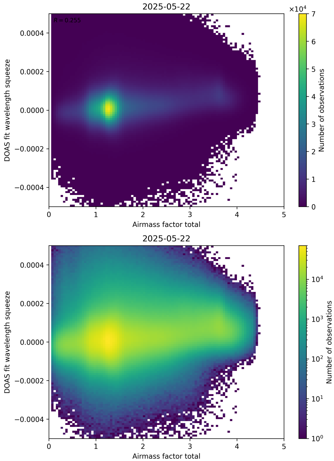
Figure 99: Scatter density plot of “Airmass factor total” against “DOAS fit wavelength squeeze” for 2025-05-21 to 2025-05-23.
