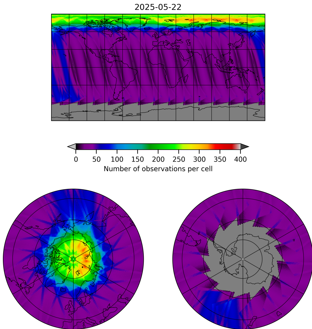
Figure 19: Map of the number of observations for 2025-05-21 to 2025-05-23
