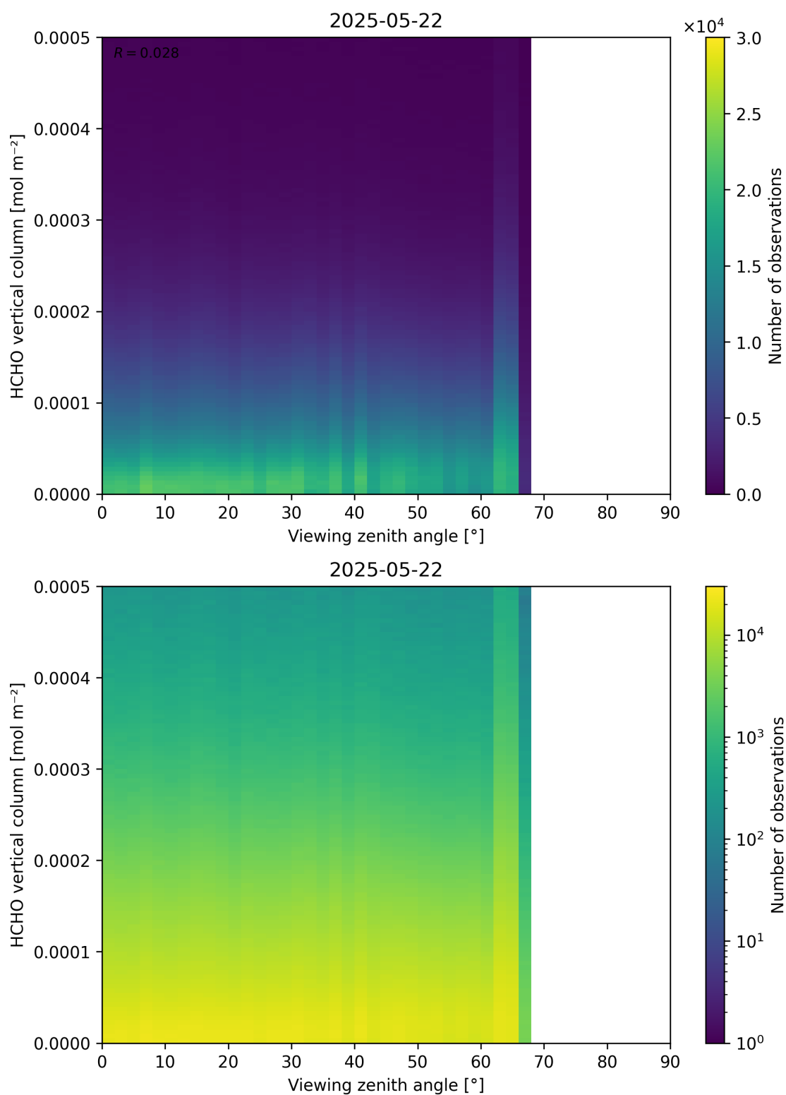
Figure 192: Scatter density plot of “Viewing zenith angle” against “HCHO vertical column” for 2025-05-21 to 2025-05-23.
