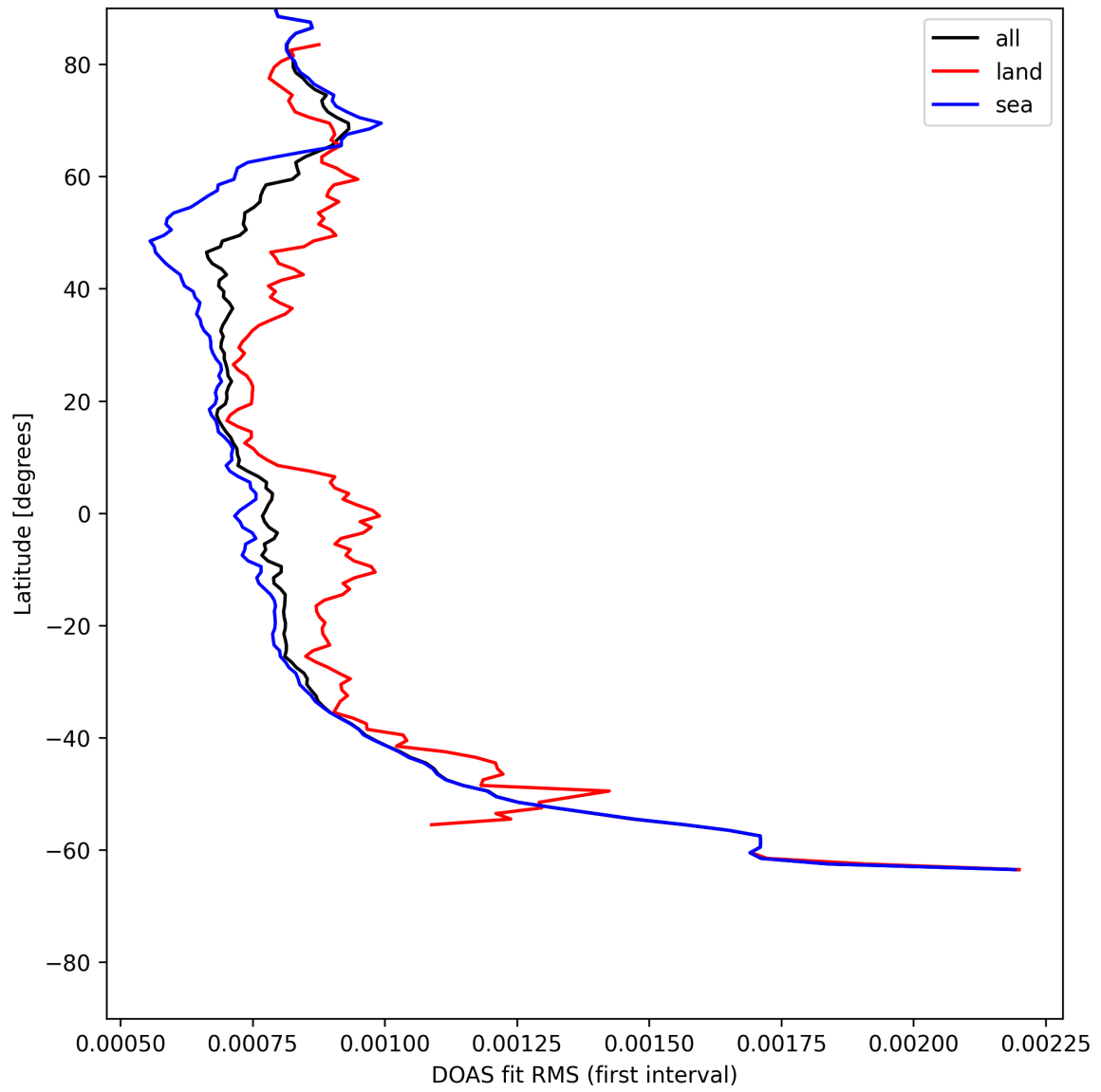
Figure 32: Zonal average of “DOAS fit RMS (first interval)” for 2025-05-21 to 2025-05-23.
