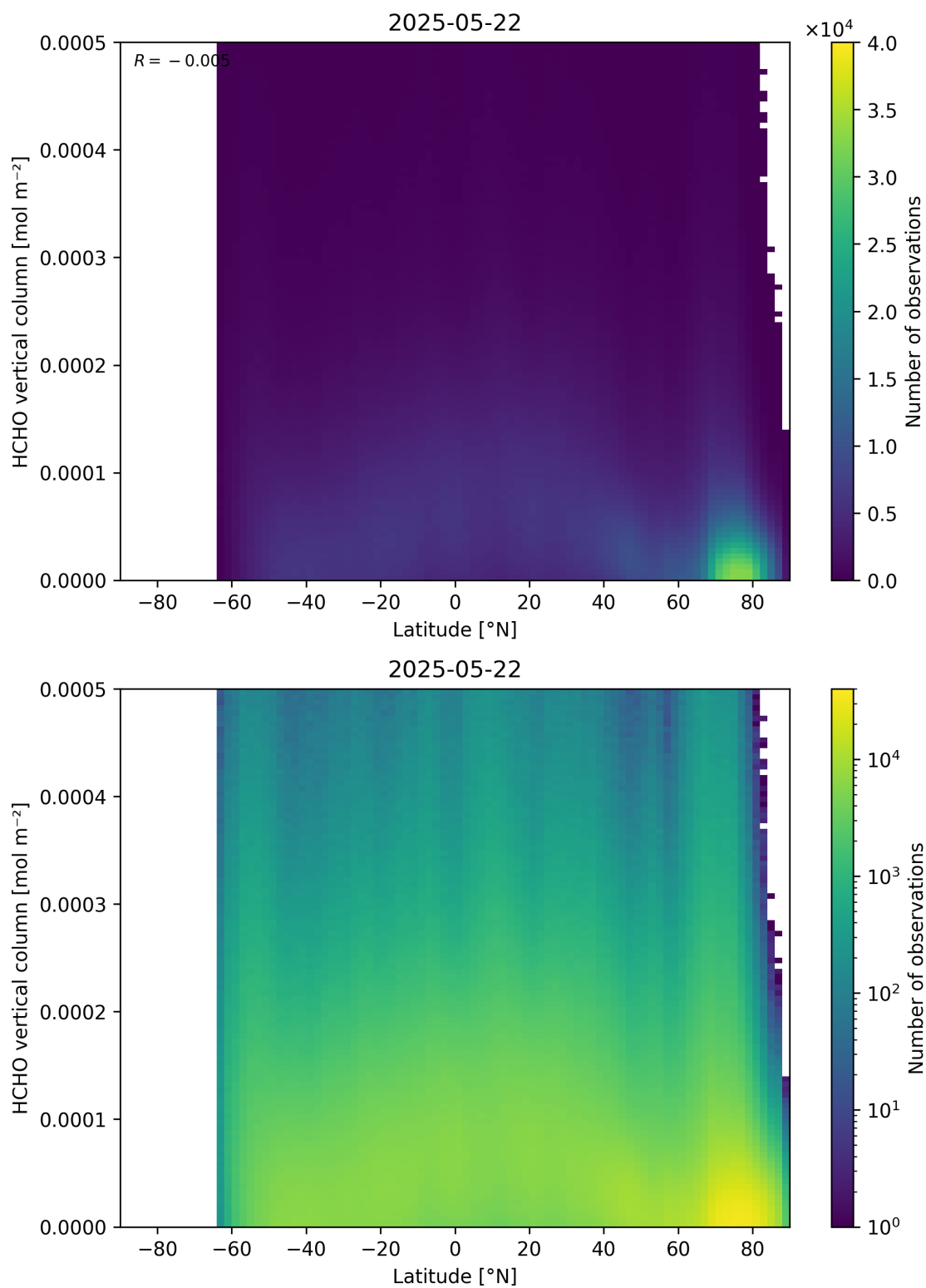
Figure 163: Scatter density plot of “Latitude” against “HCHO vertical column” for 2025-05-21 to 2025-05-23.
