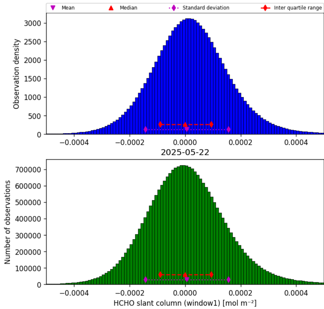
Figure 38: Histogram of “HCHO slant column (window1)” for 2025-05-21 to 2025-05-23
