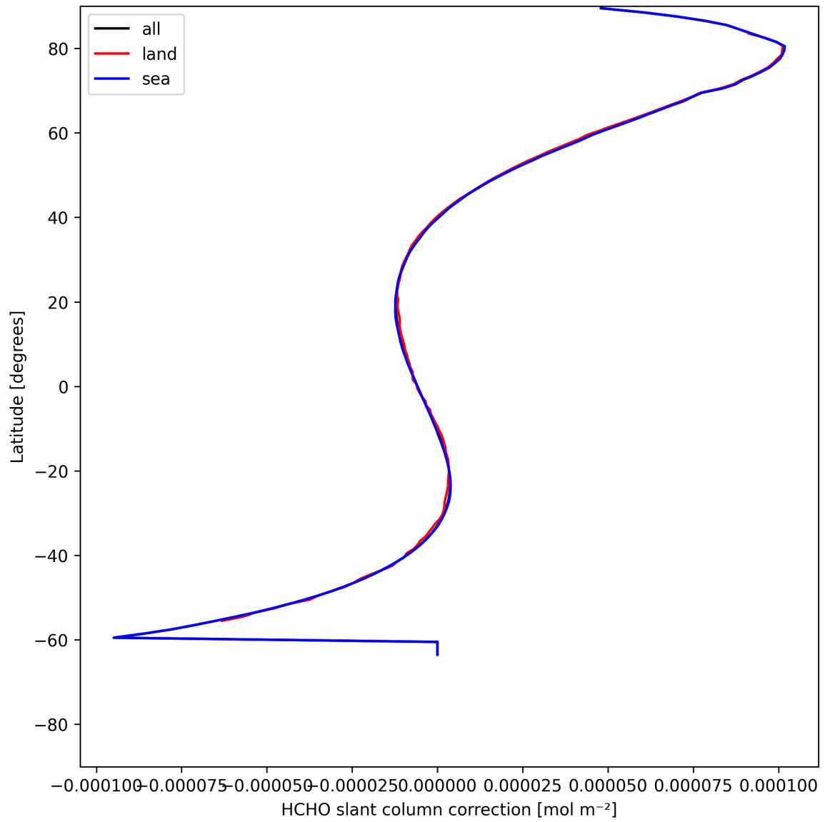
Figure 33: Zonal average of “HCHO slant column correction” for 2025-05-21 to 2025-05-23.
