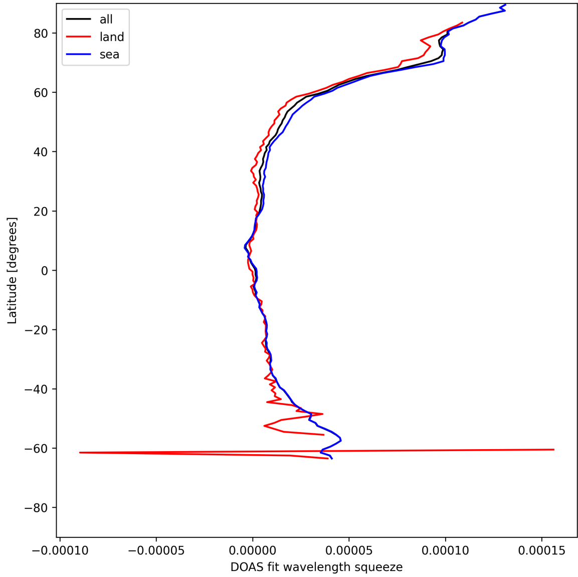
Figure 31: Zonal average of “DOAS fit wavelength squeeze” for 2025-05-21 to 2025-05-23.
