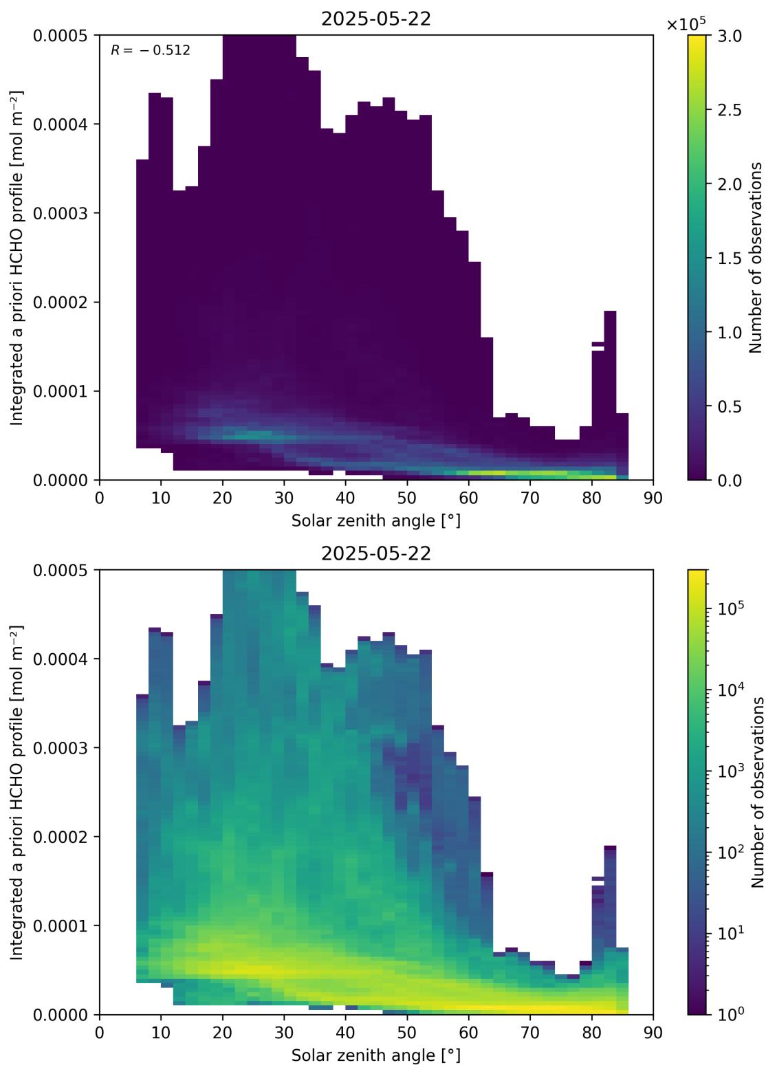
Figure 180: Scatter density plot of “Solar zenith angle” against “Integrated a priori HCHO profile” for 2025-05-21 to 2025-05-23.
