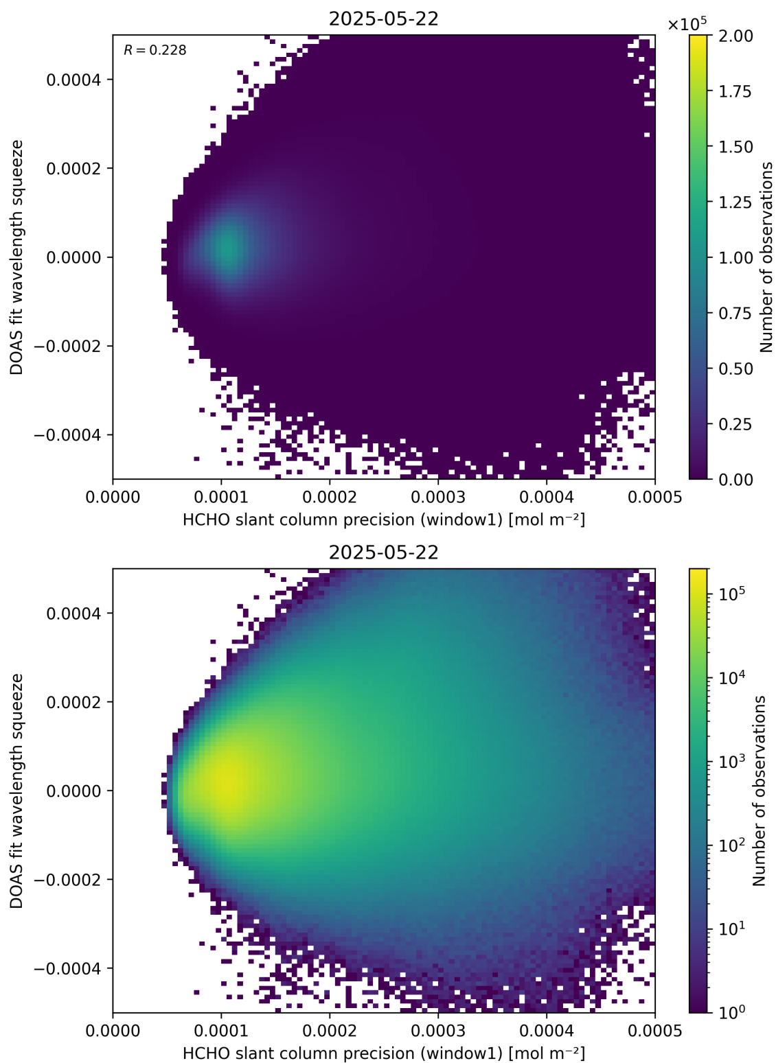
Figure 90: Scatter density plot of “HCHO slant column precision (window1)” against “DOAS fit wavelength squeeze” for 2025-05-21 to 2025-05-23.
