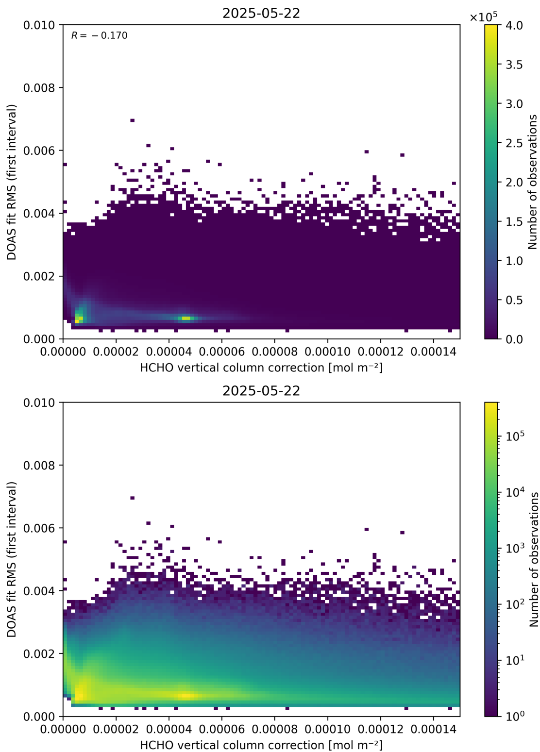
Figure 112: Scatter density plot of “HCHO vertical column correction” against “DOAS fit RMS (first interval)” for 2025-05-21 to 2025-05-23.
