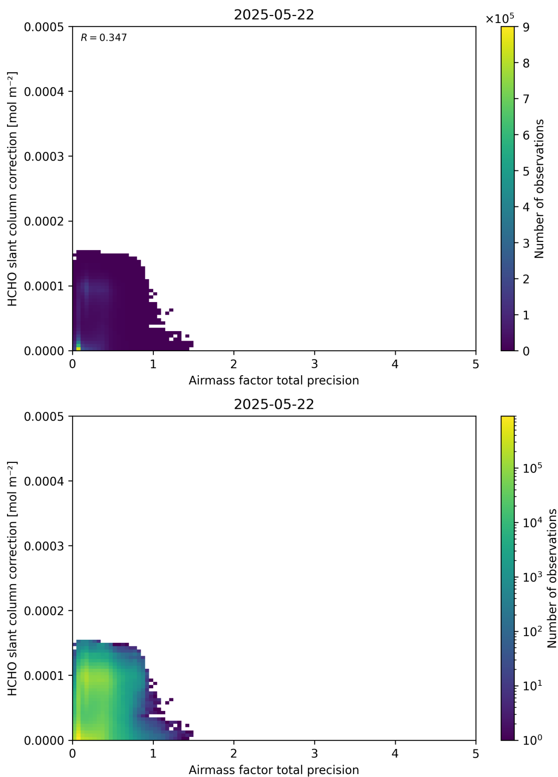
Figure 110: Scatter density plot of “Airmass factor total precision” against “HCHO slant column correction” for 2025-05-21 to 2025-05-23.
