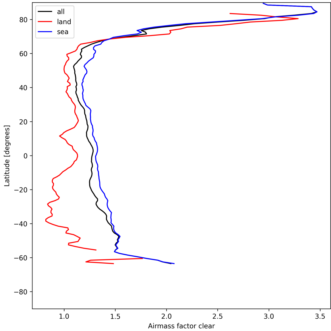
Figure 28: Zonal average of “Airmass factor clear” for 2025-05-21 to 2025-05-23.
