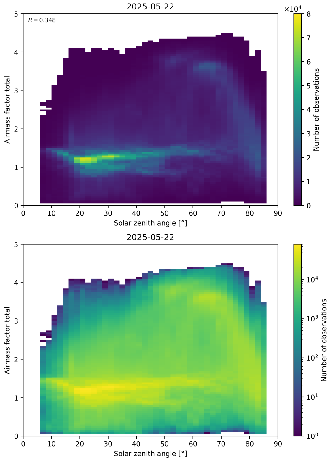
Figure 175: Scatter density plot of “Solar zenith angle” against “Airmass factor total” for 2025-05-21 to 2025-05-23.
