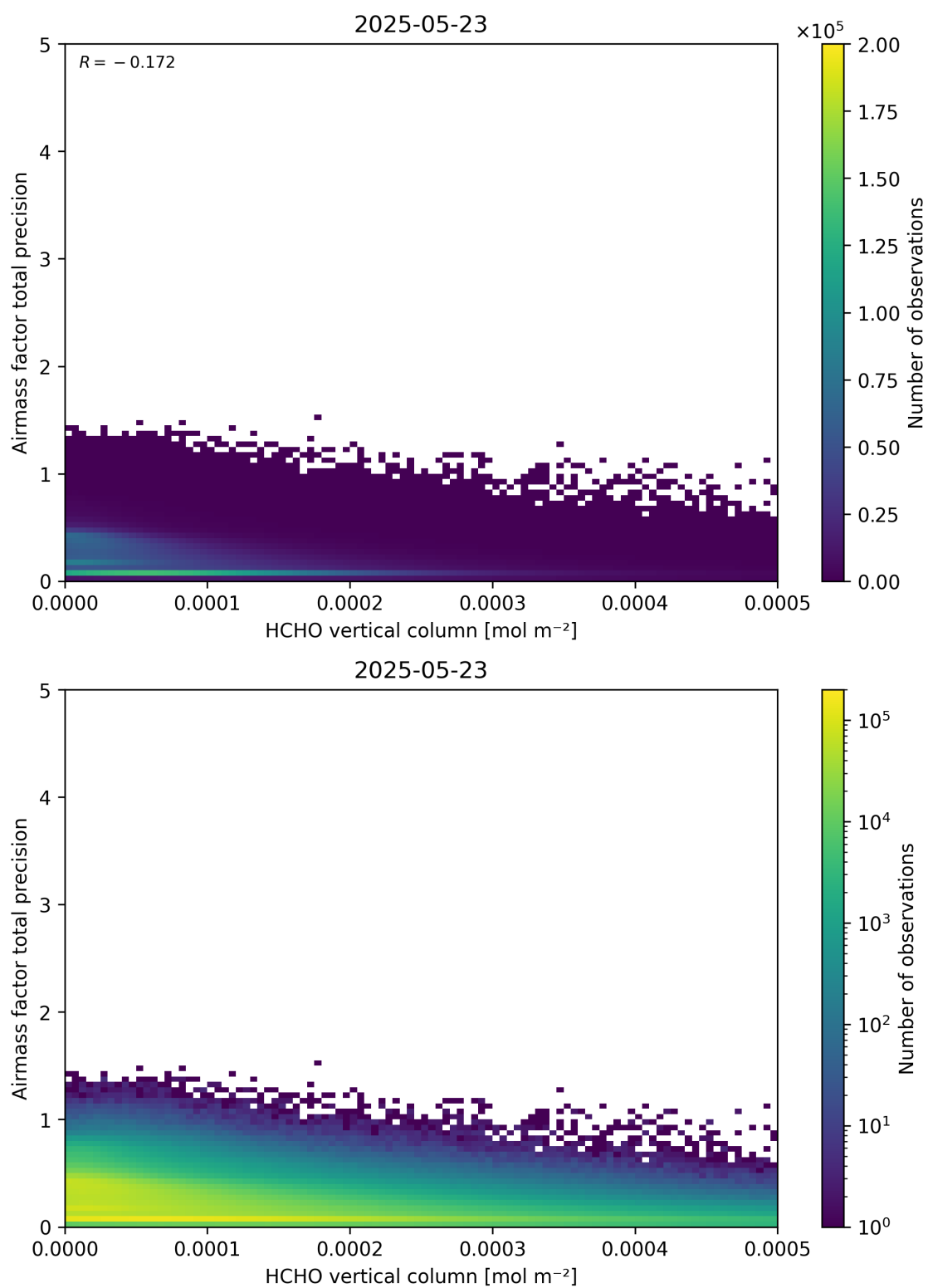
Figure 132: Scatter density plot of “HCHO vertical column” against “Airmass factor total precision” for 2025-05-22 to 2025-05-24.
