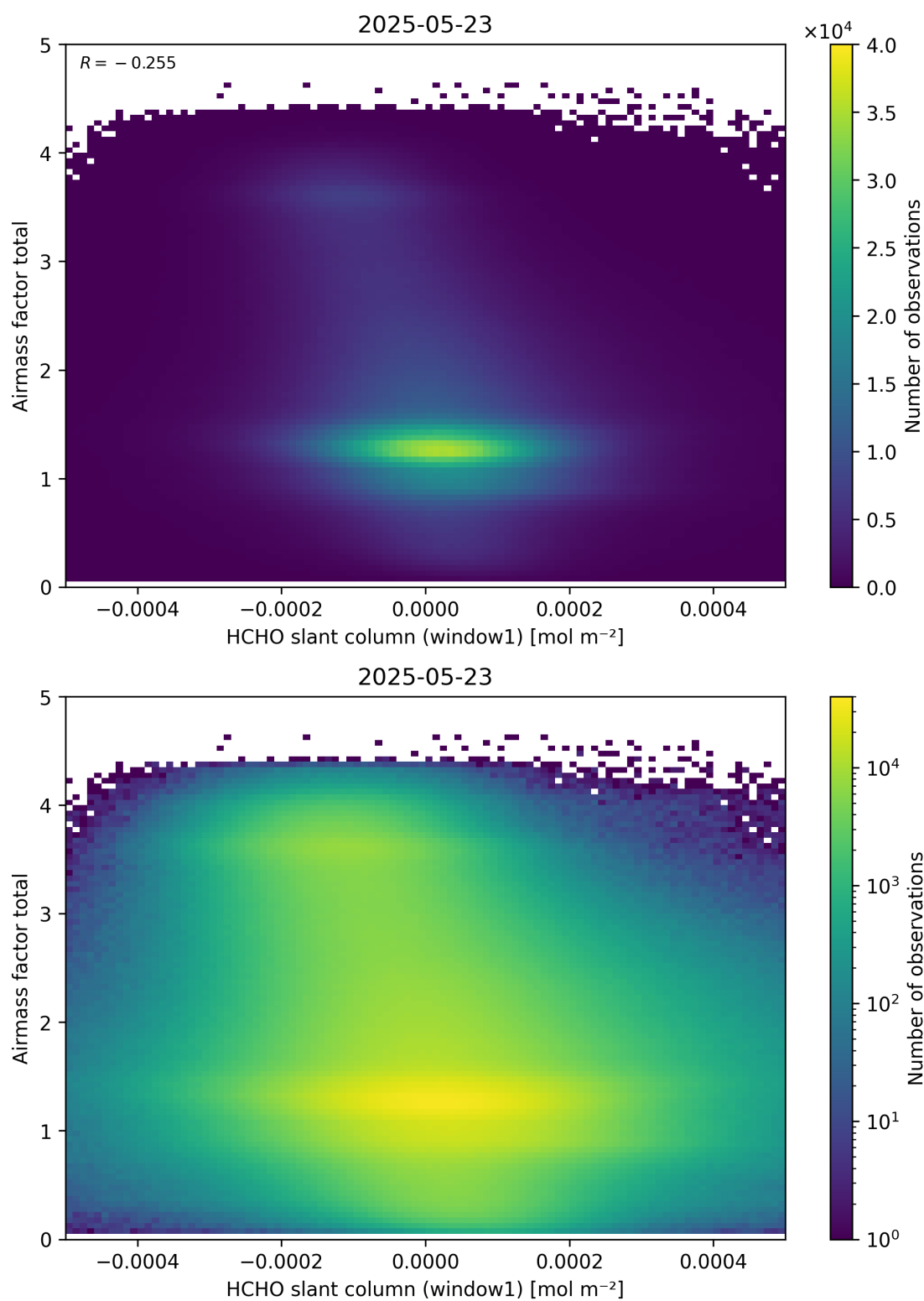
Figure 85: Scatter density plot of “HCHO slant column (window1)” against “Airmass factor total” for 2025-05-22 to 2025-05-24.
