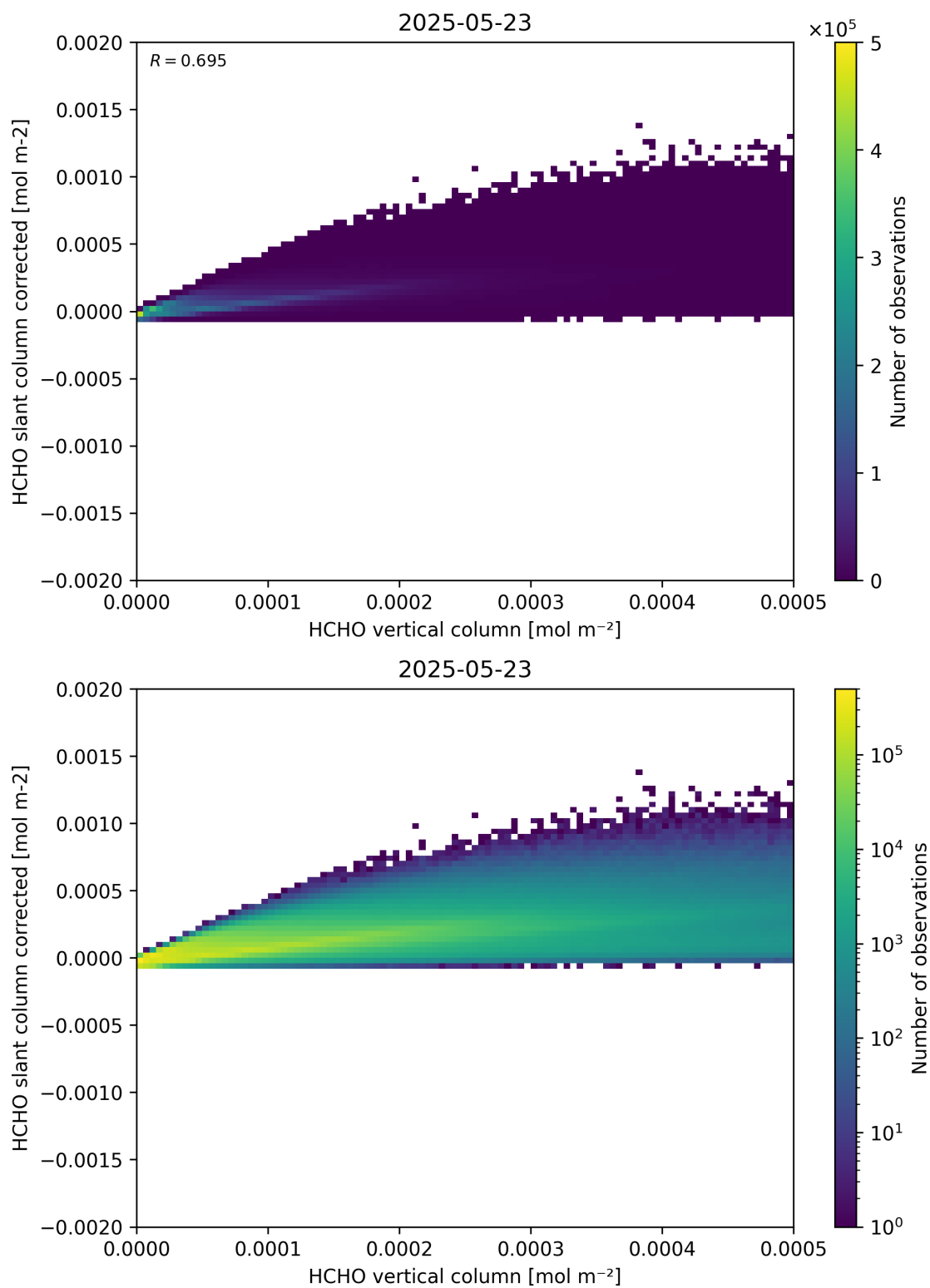
Figure 127: Scatter density plot of “HCHO vertical column” against “HCHO slant column corrected” for 2025-05-22 to 2025-05-24.
