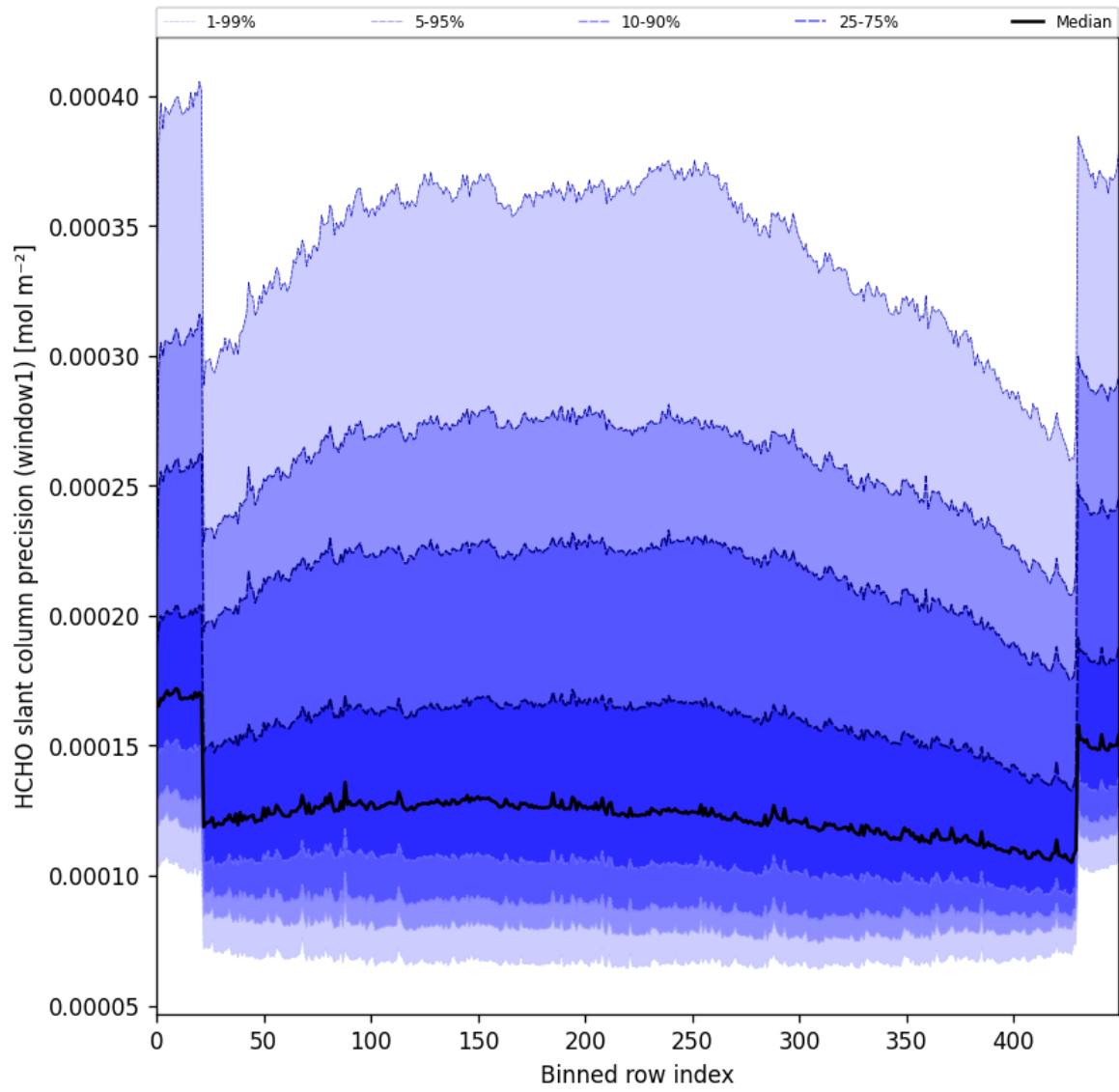
Figure 53: Along track statistics of “HCHO slant column precision (window1)” for 2025-05-22 to 2025-05-24
