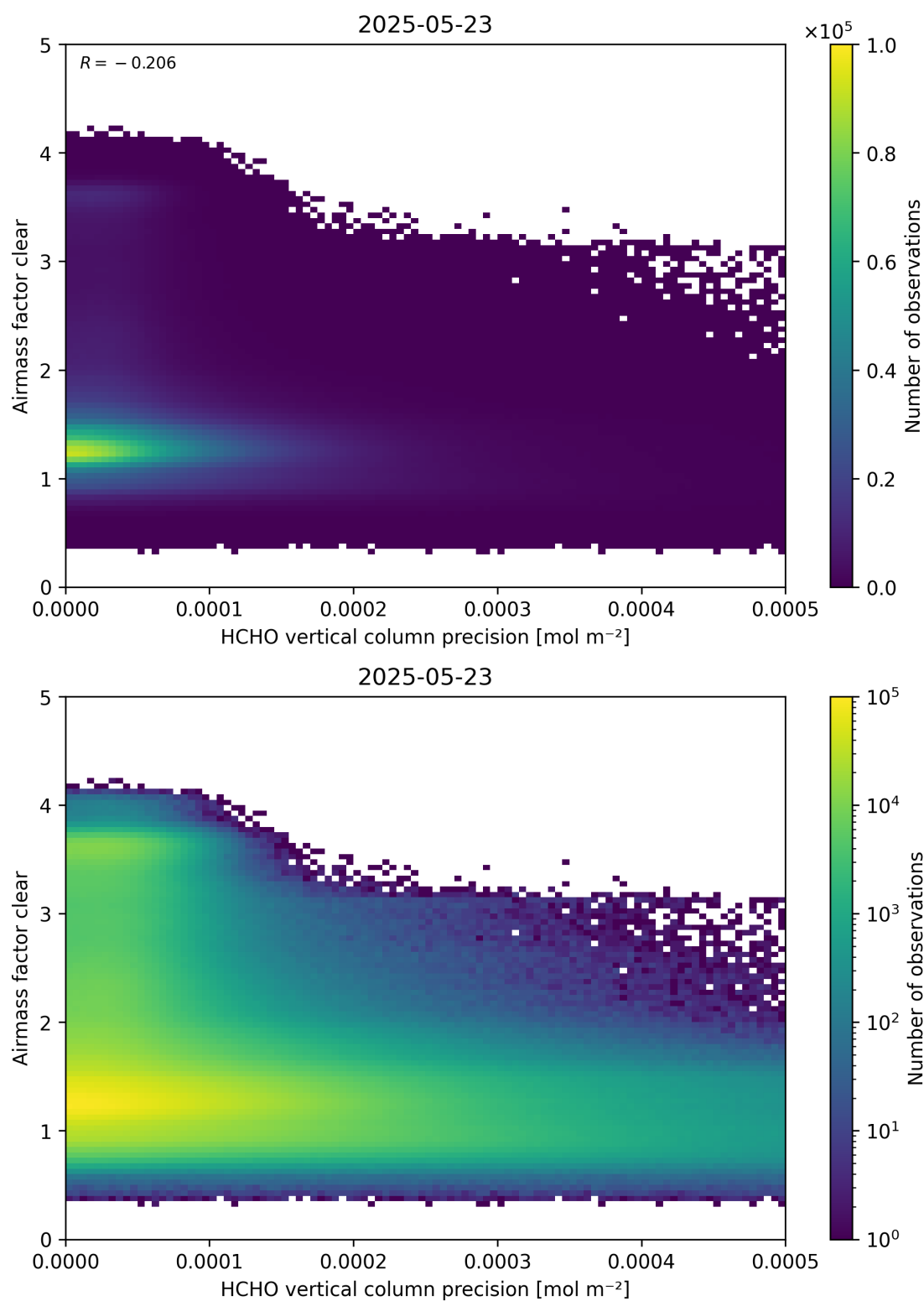
Figure 139: Scatter density plot of “HCHO vertical column precision” against “Airmass factor clear” for 2025-05-22 to 2025-05-24.
