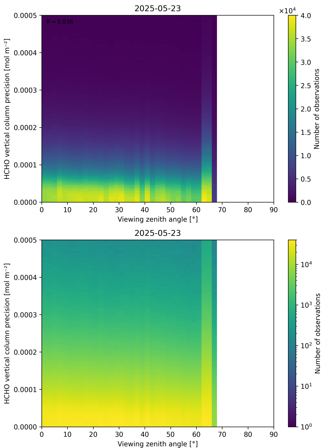
Figure 194: Scatter density plot of “Viewing zenith angle” against “HCHO vertical column precision” for 2025-05-22 to 2025-05-24.
