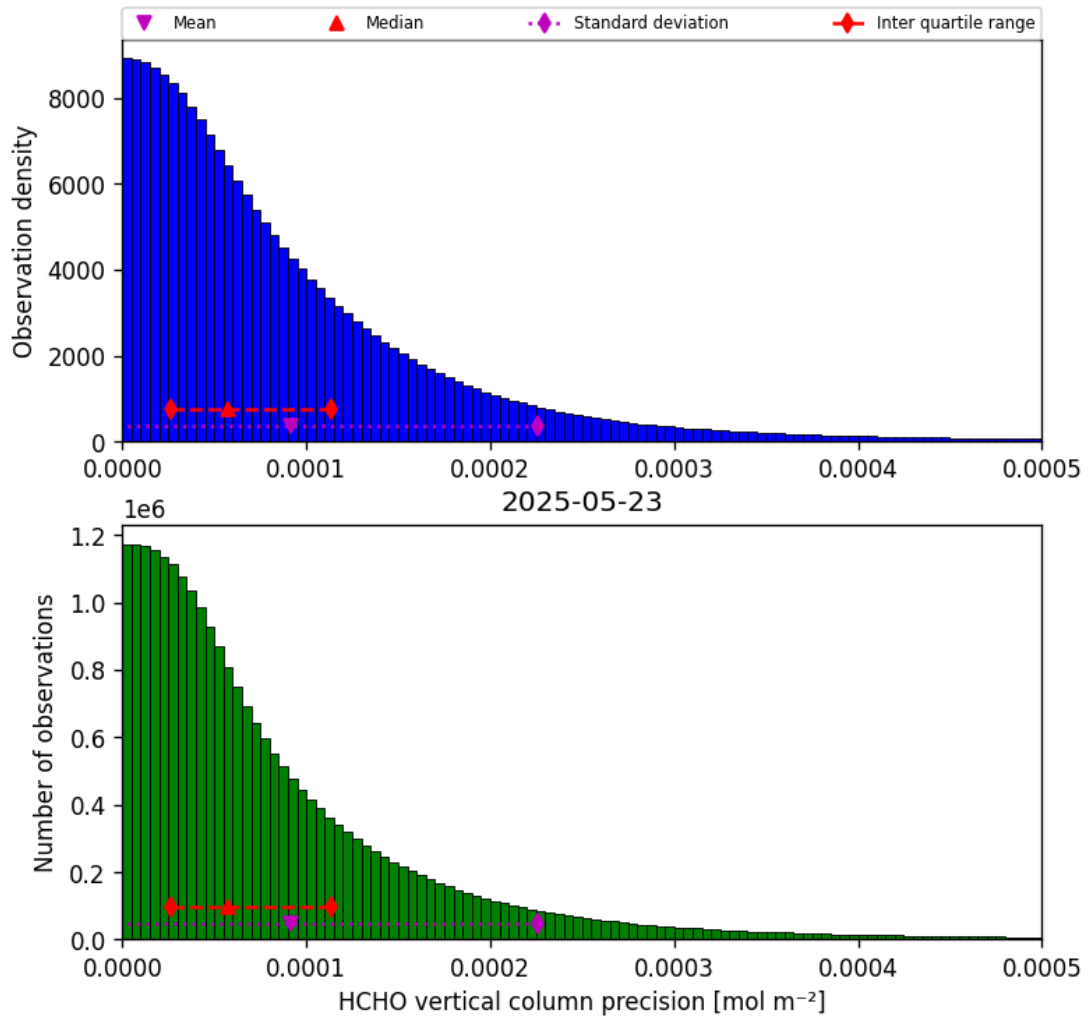
Figure 36: Histogram of “HCHO vertical column precision” for 2025-05-22 to 2025-05-24
