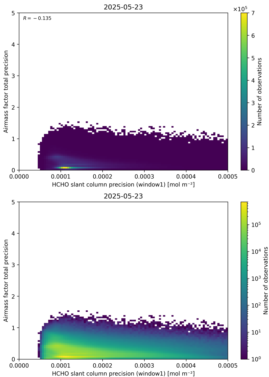
Figure 95: Scatter density plot of “HCHO slant column precision (window1)” against “Airmass factor total precision” for 2025-05-22 to 2025-05-24.
