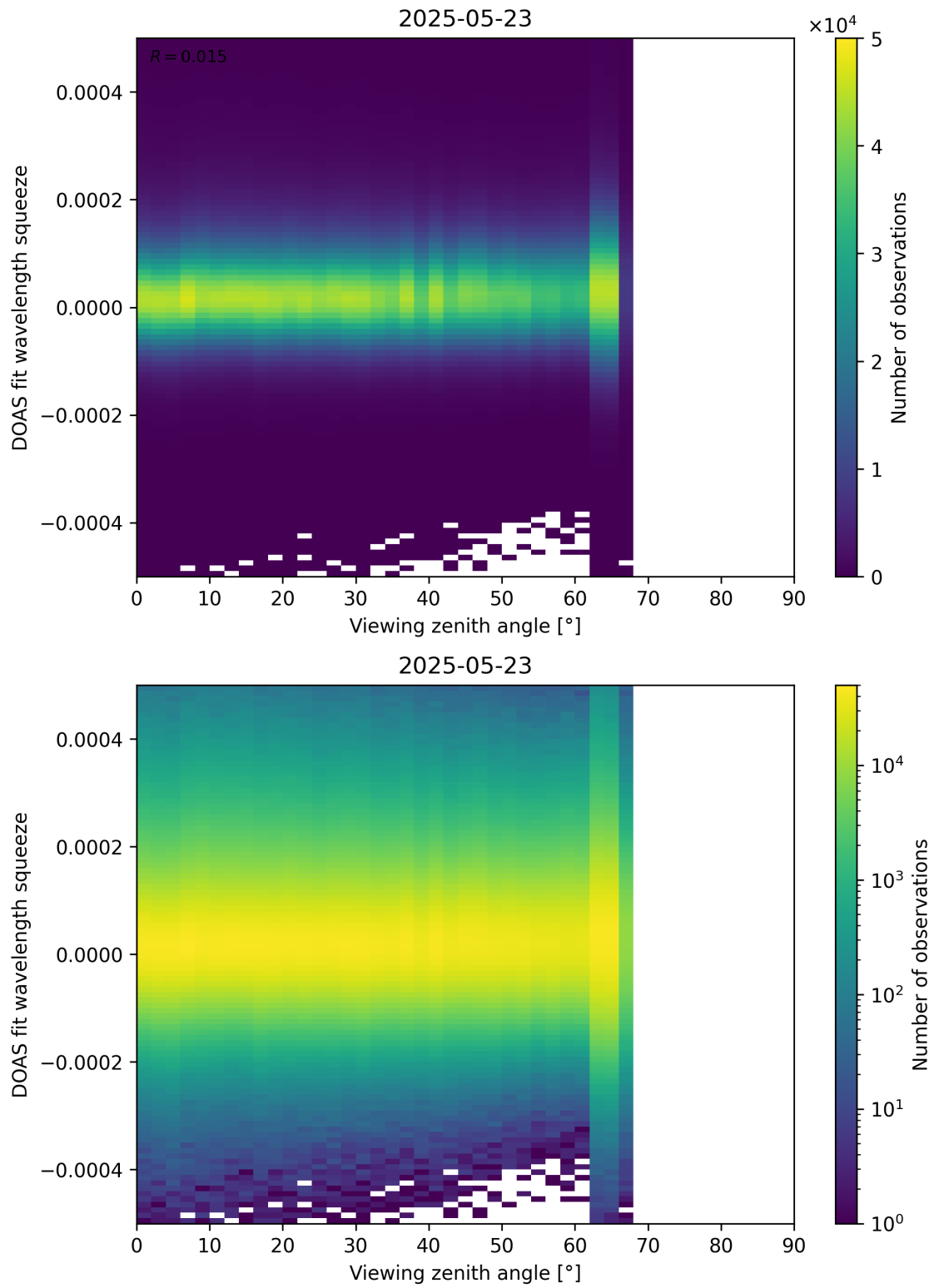
Figure 184: Scatter density plot of “Viewing zenith angle” against “DOAS fit wavelength squeeze” for 2025-05-22 to 2025-05-24.
