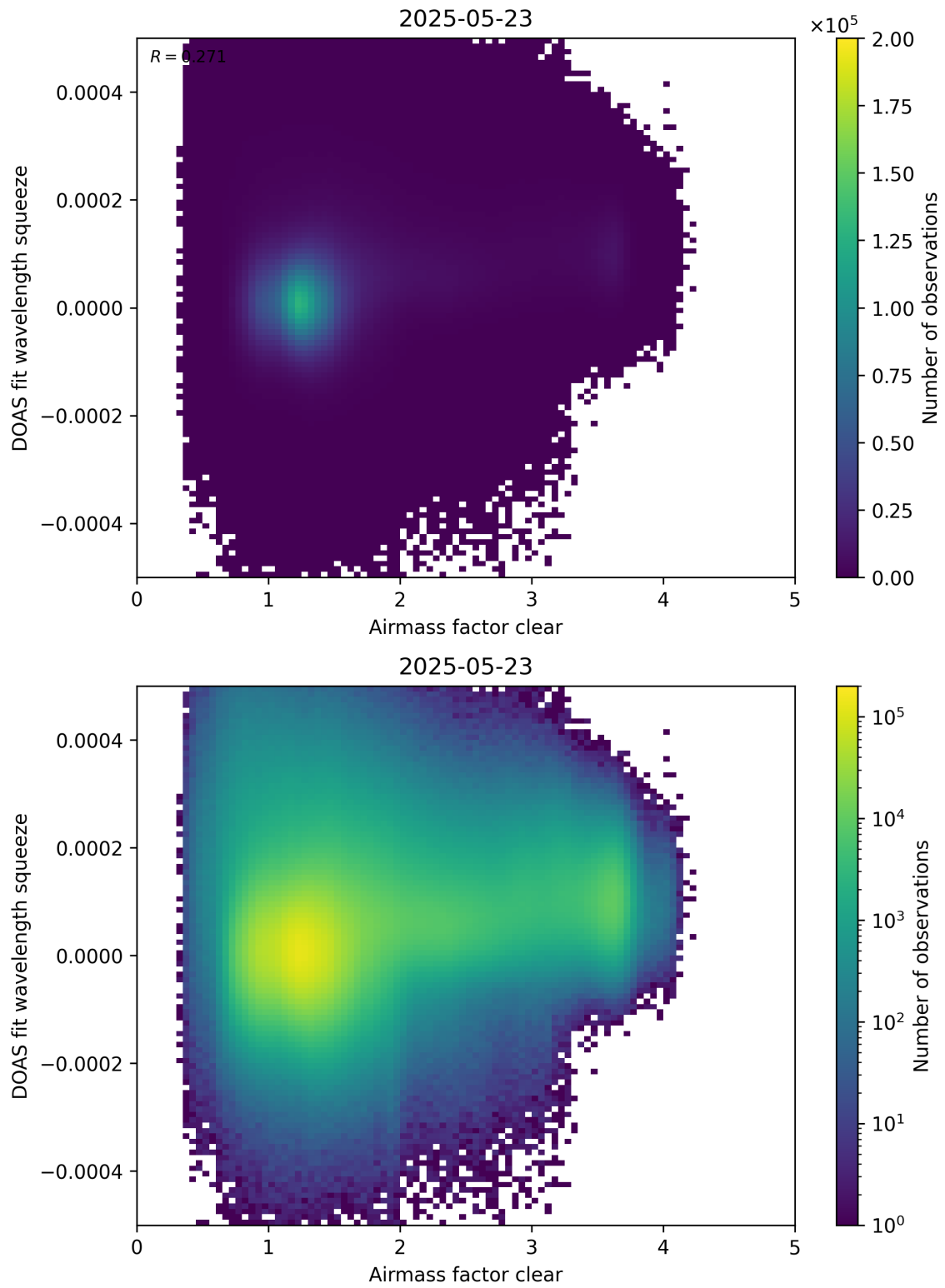
Figure 73: Scatter density plot of “Airmass factor clear” against “DOAS fit wavelength squeeze” for 2025-05-22 to 2025-05-24.
