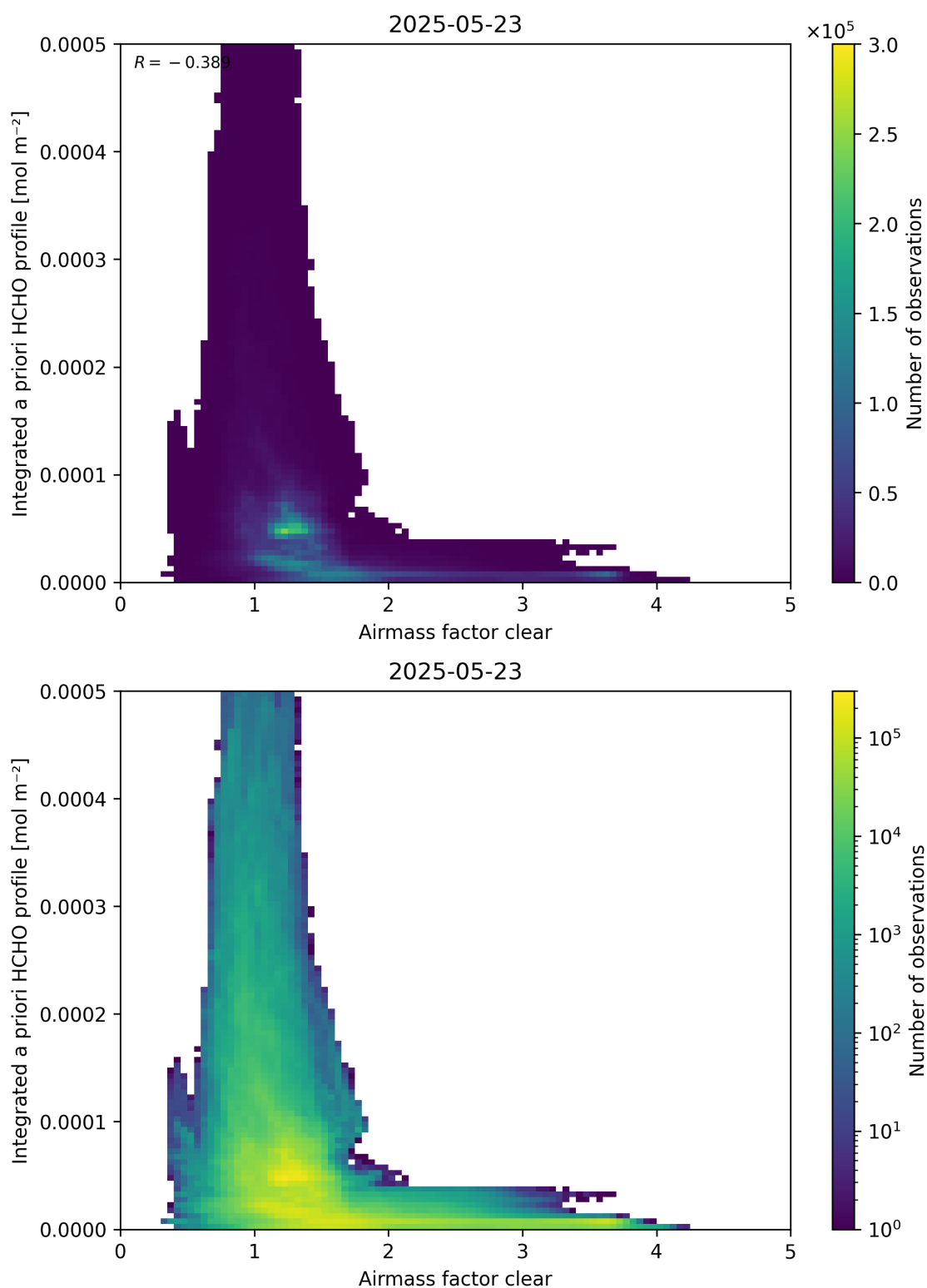
Figure 76: Scatter density plot of “Airmass factor clear” against “Integrated a priori HCHO profile” for 2025-05-22 to 2025-05-24.
