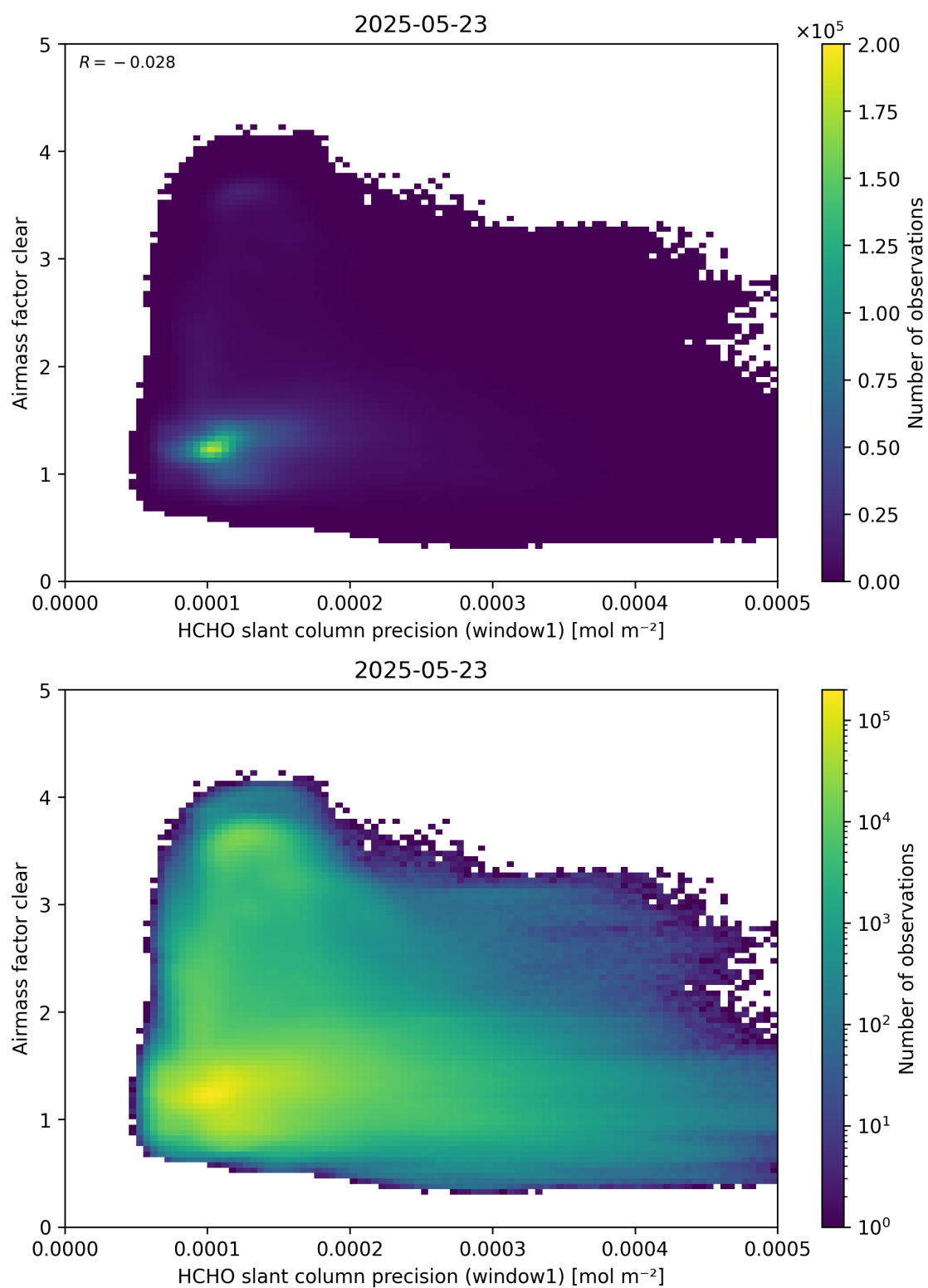
Figure 91: Scatter density plot of “HCHO slant column precision (window1)” against “Airmass factor clear” for 2025-05-22 to 2025-05-24.
