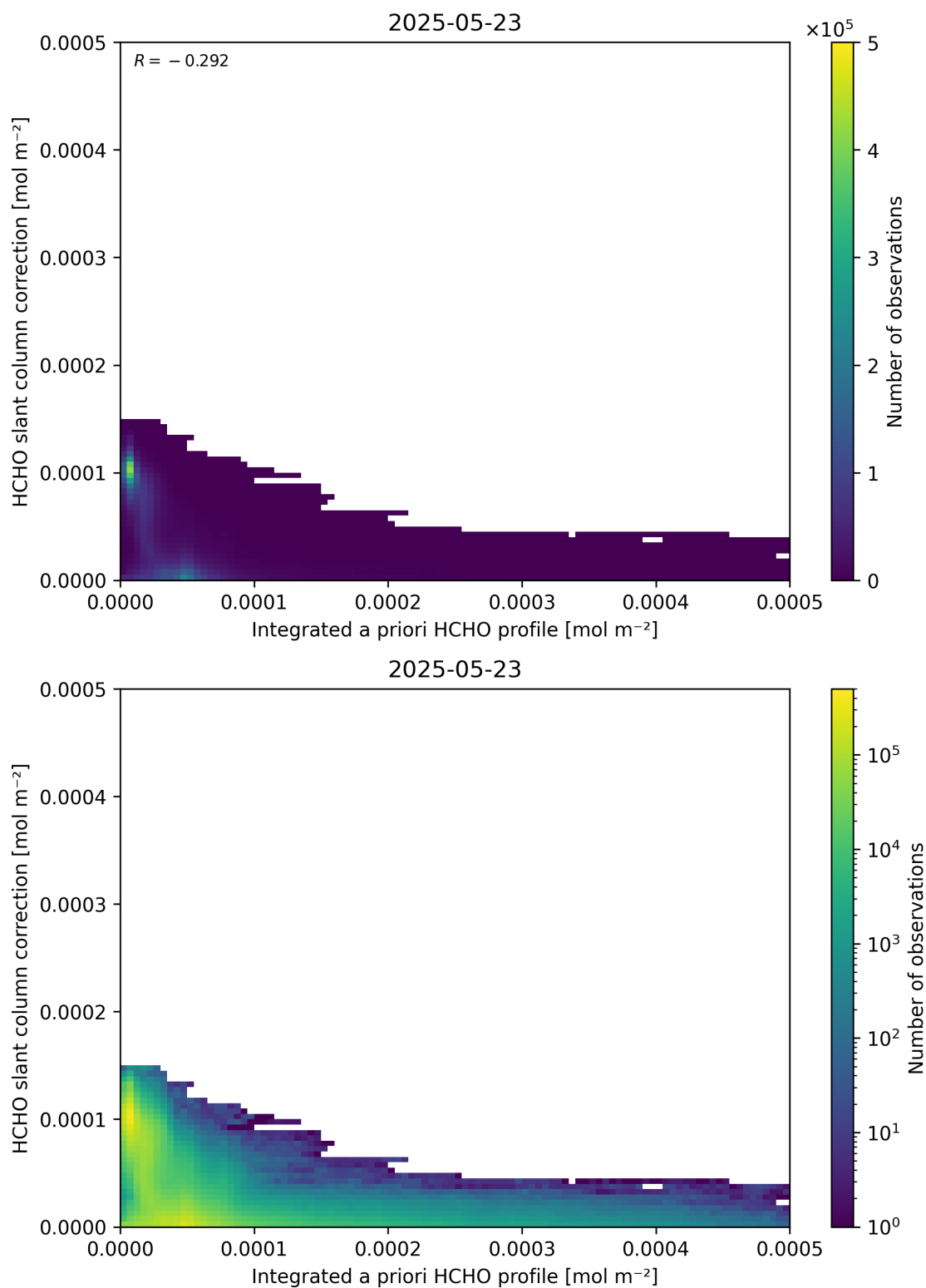
Figure 152: Scatter density plot of “Integrated a priori HCHO profile” against “HCHO slant column correction” for 2025-05-22 to 2025-05-24.
