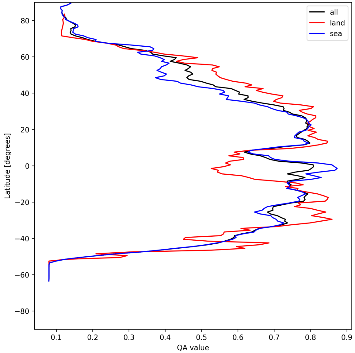
Figure 20: Zonal average of “QA value” for 2025-05-22 to 2025-05-24.
