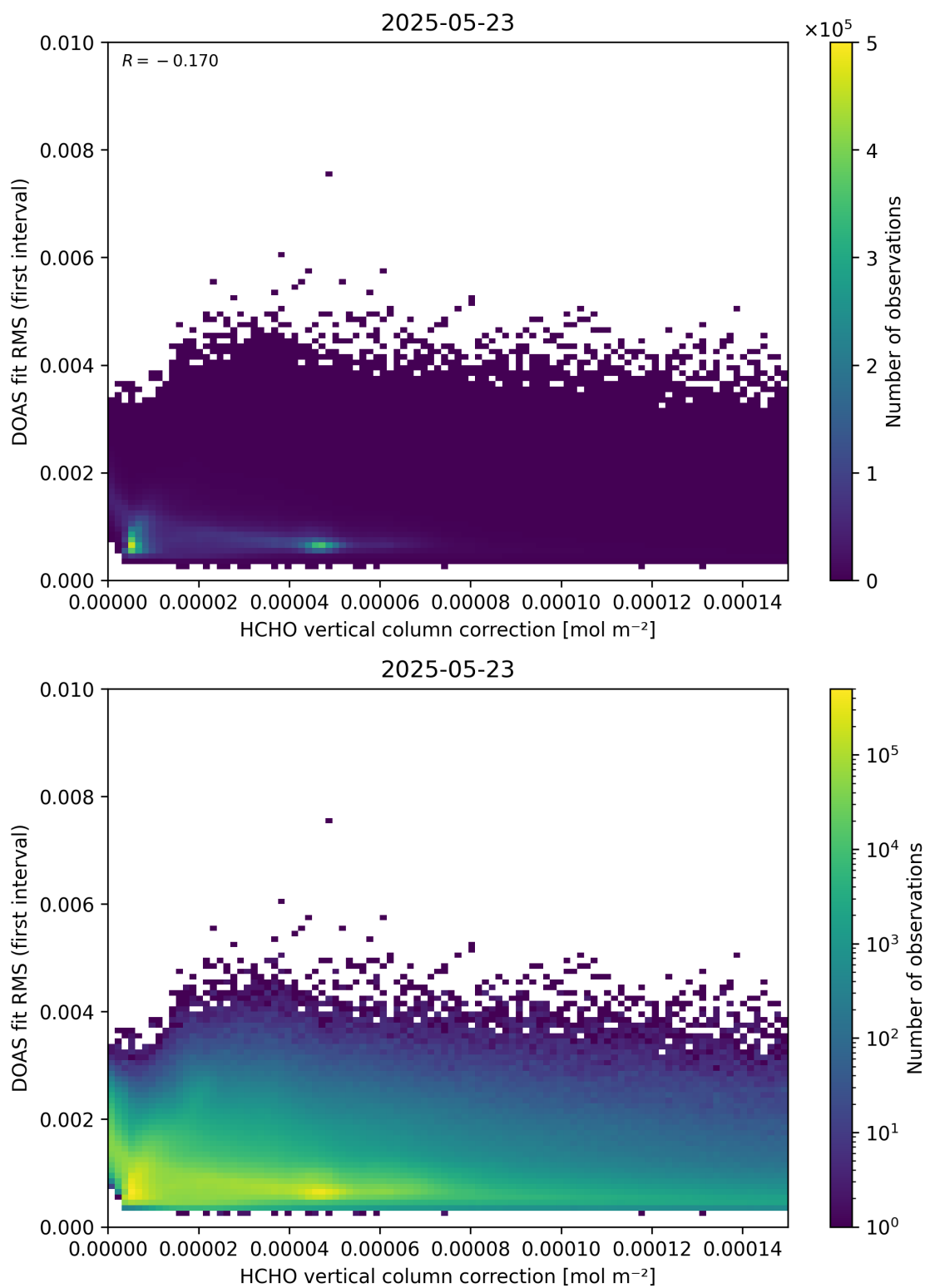
Figure 112: Scatter density plot of “HCHO vertical column correction” against “DOAS fit RMS (first interval)” for 2025-05-22 to 2025-05-24.
