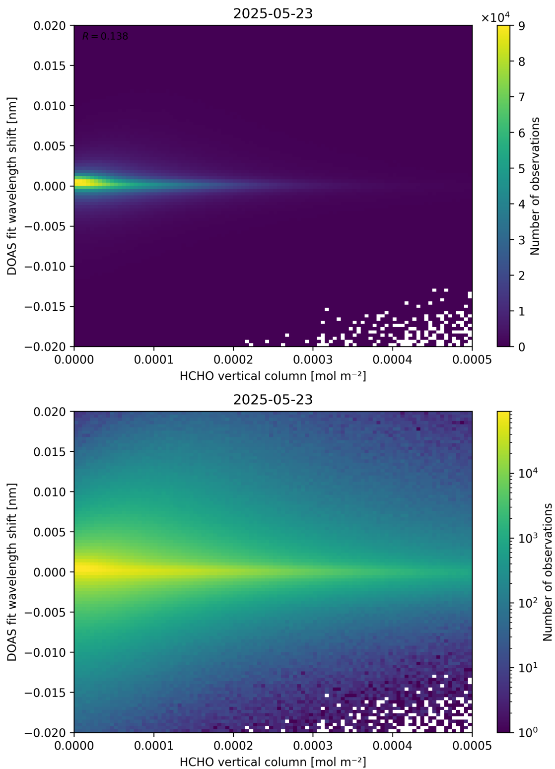
Figure 124: Scatter density plot of “HCHO vertical column” against “DOAS fit wavelength shift” for 2025-05-22 to 2025-05-24.
