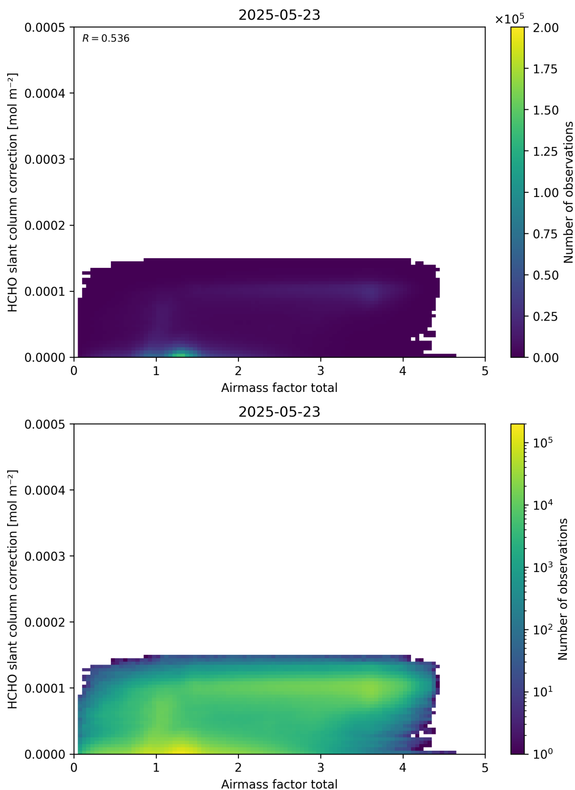
Figure 102: Scatter density plot of “Airmass factor total” against “HCHO slant column correction” for 2025-05-22 to 2025-05-24.
