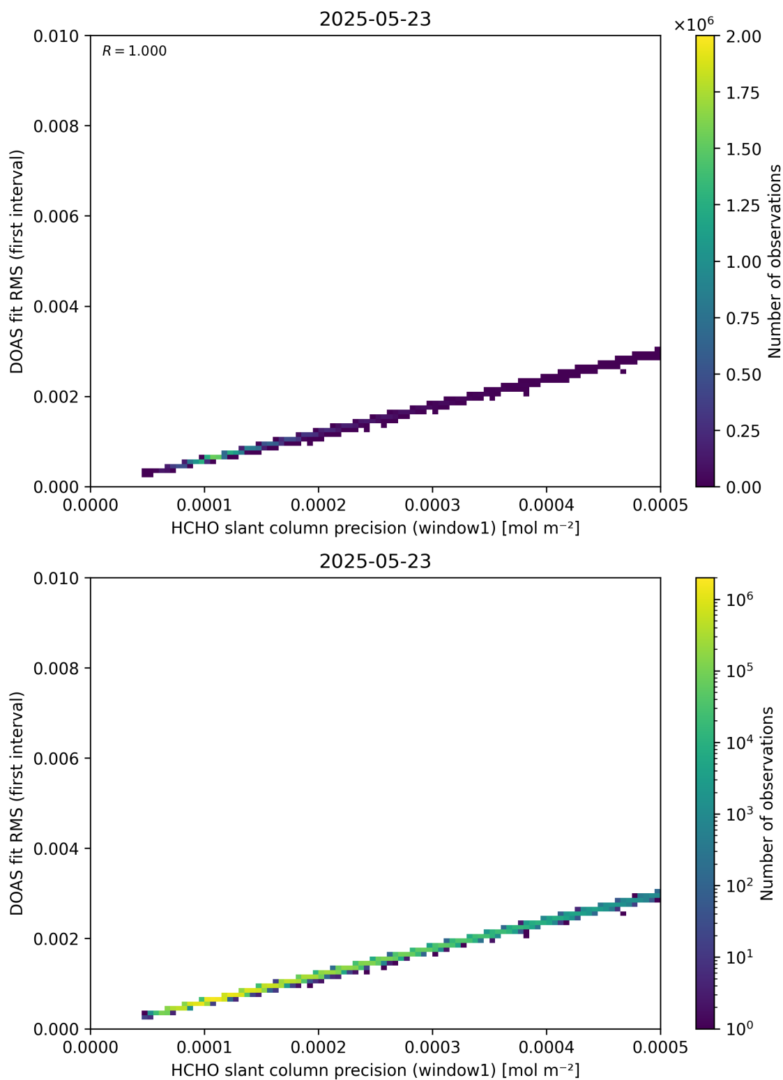
Figure 88: Scatter density plot of “HCHO slant column precision (window1)” against “DOAS fit RMS (first interval)” for 2025-05-22 to 2025-05-24.
