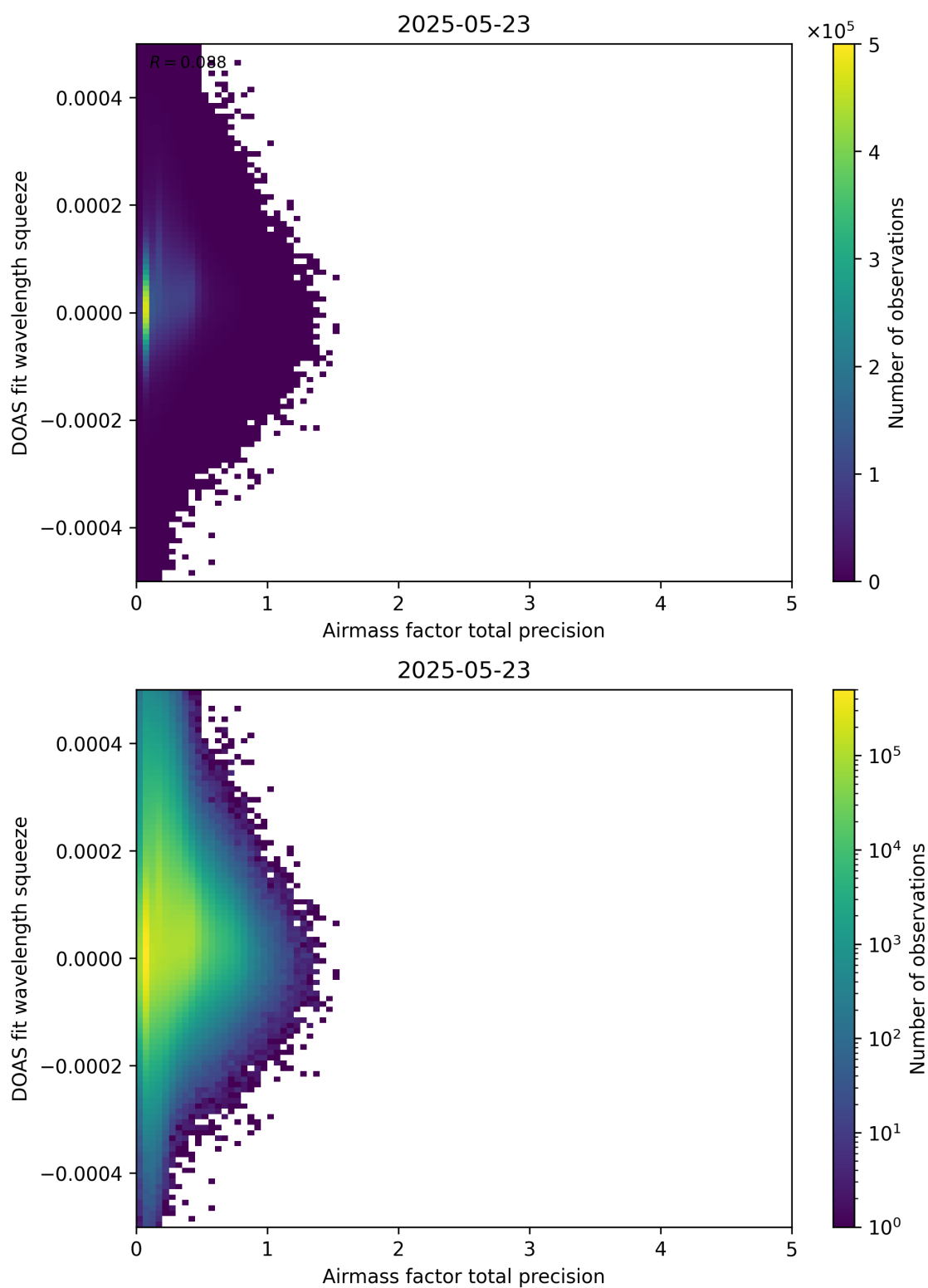
Figure 107: Scatter density plot of “Airmass factor total precision” against “DOAS fit wavelength squeeze” for 2025-05-22 to 2025-05-24.
