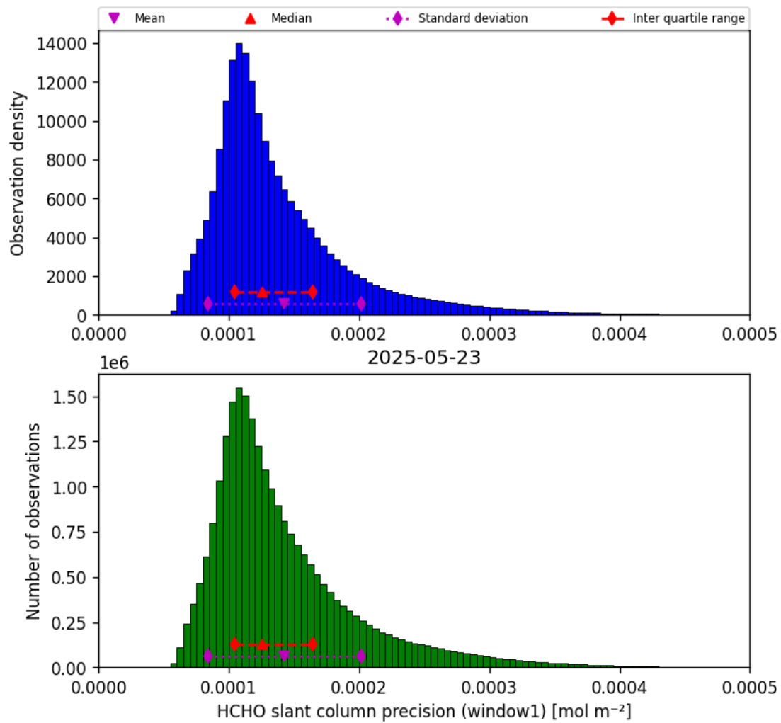
Figure 39: Histogram of “HCHO slant column precision (window1)” for 2025-05-22 to 2025-05-24
