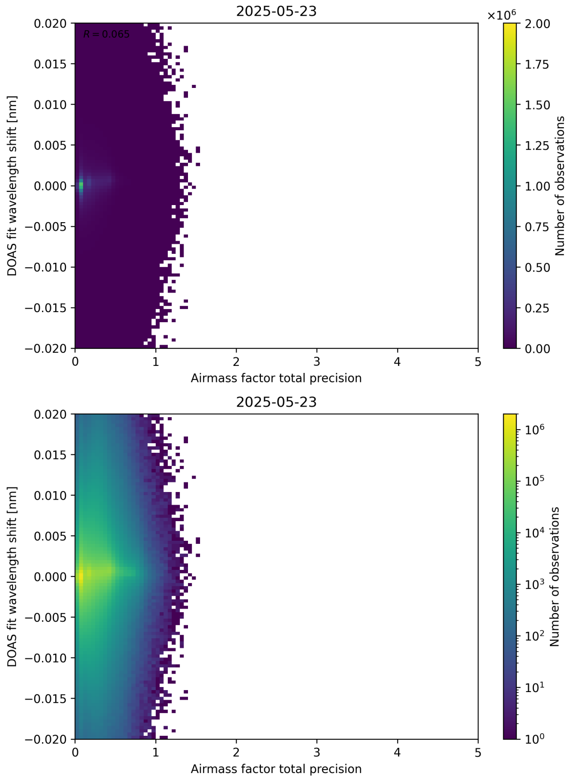
Figure 106: Scatter density plot of “Airmass factor total precision” against “DOAS fit wavelength shift” for 2025-05-22 to 2025-05-24.
