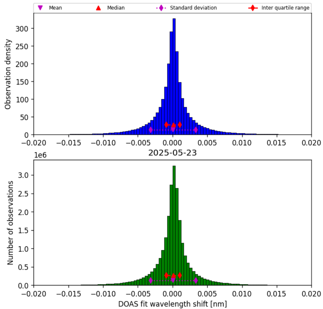
Figure 44: Histogram of “DOAS fit wavelength shift” for 2025-05-22 to 2025-05-24
