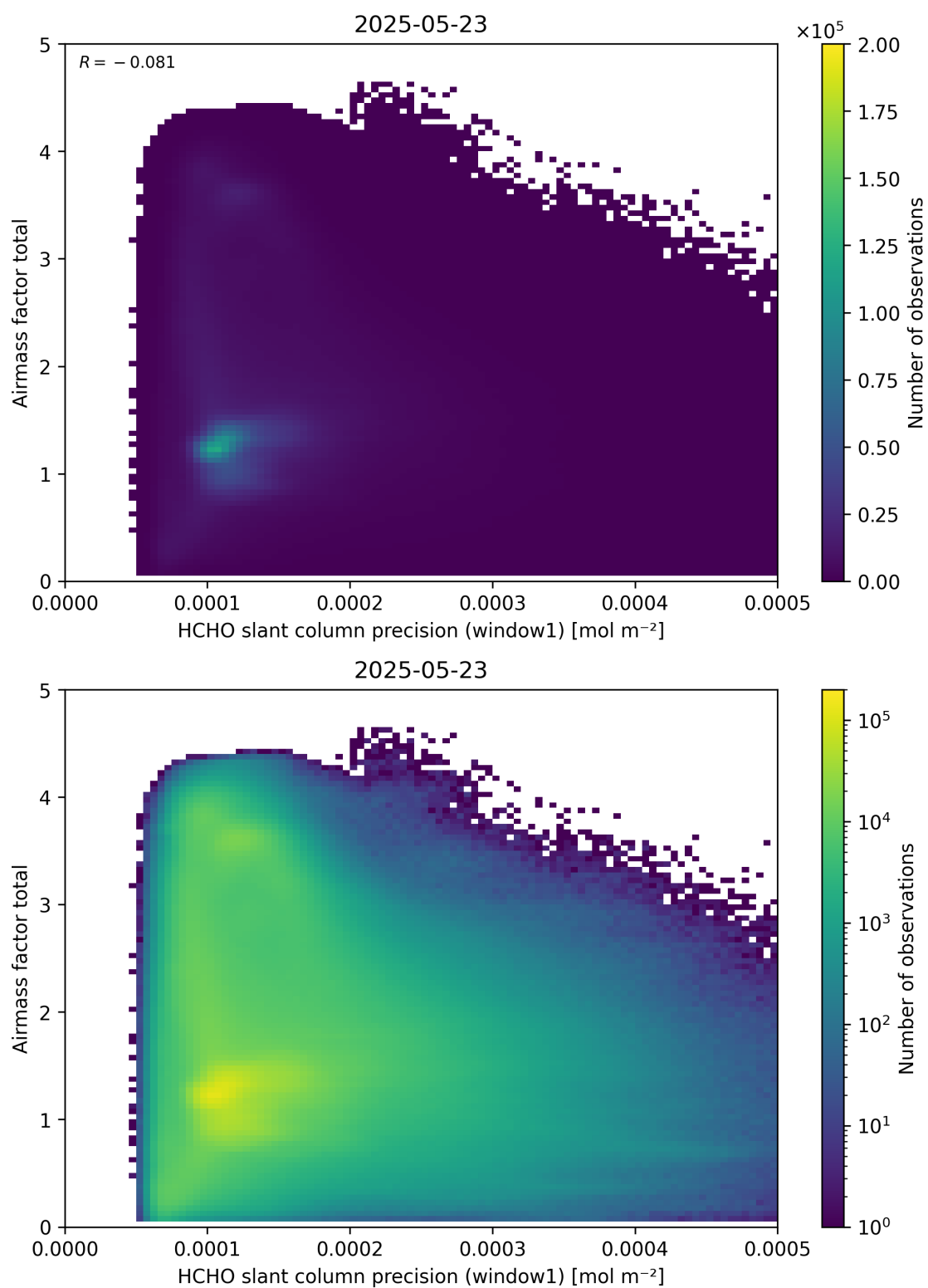
Figure 94: Scatter density plot of “HCHO slant column precision (window1)” against “Airmass factor total” for 2025-05-22 to 2025-05-24.
