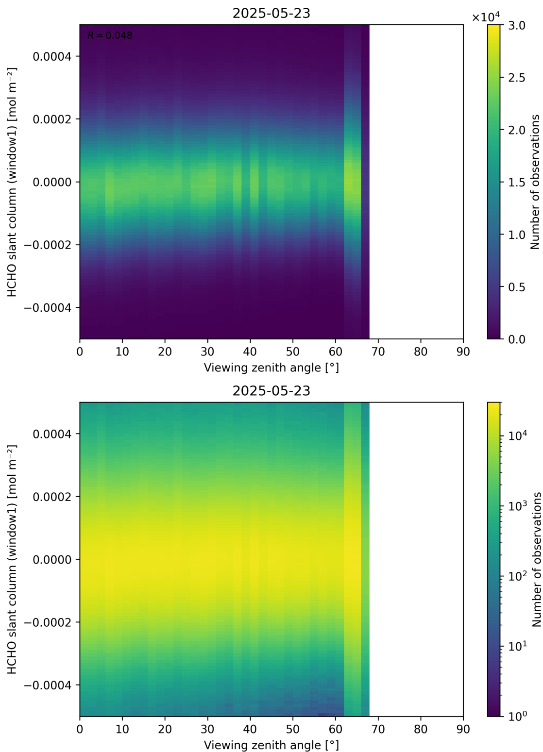
Figure 188: Scatter density plot of “Viewing zenith angle” against “HCHO slant column (window1)” for 2025-05-22 to 2025-05-24.
