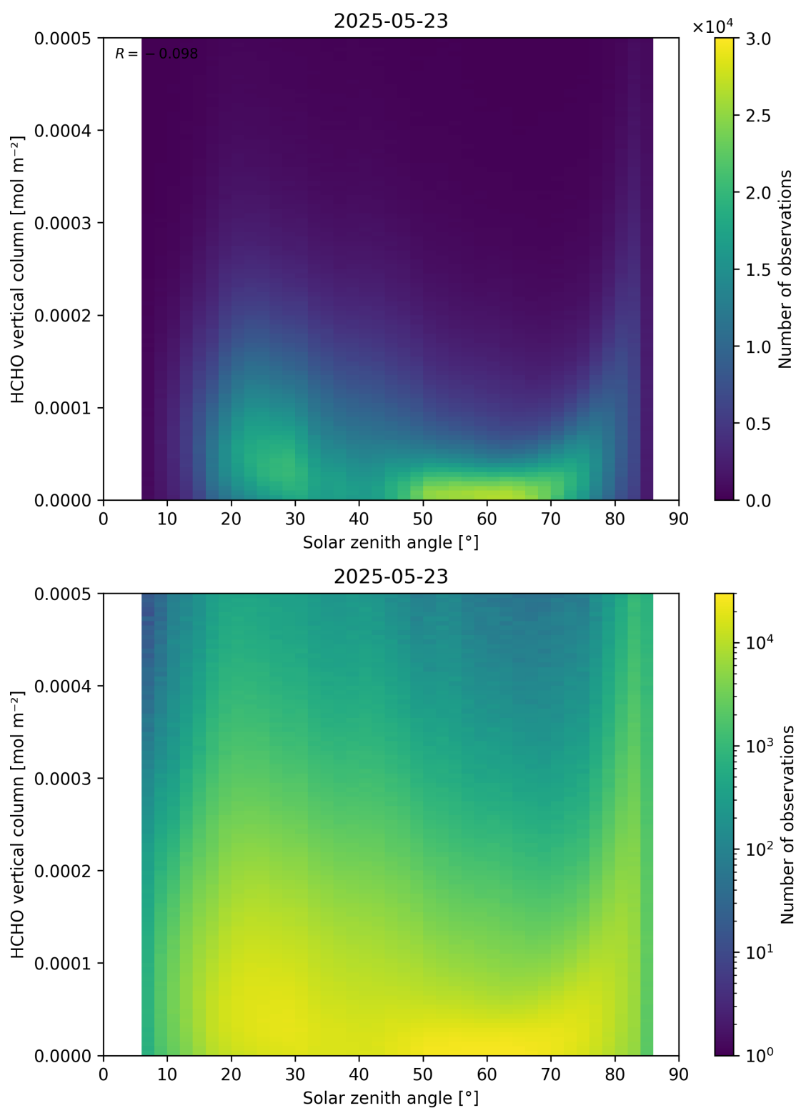
Figure 177: Scatter density plot of “Solar zenith angle” against “HCHO vertical column” for 2025-05-22 to 2025-05-24.
