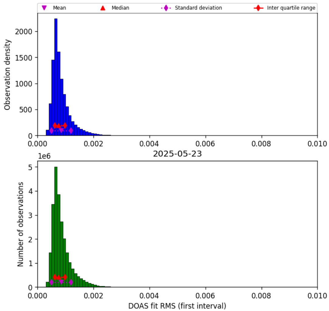
Figure 46: Histogram of “DOAS fit RMS (first interval)” for 2025-05-22 to 2025-05-24
