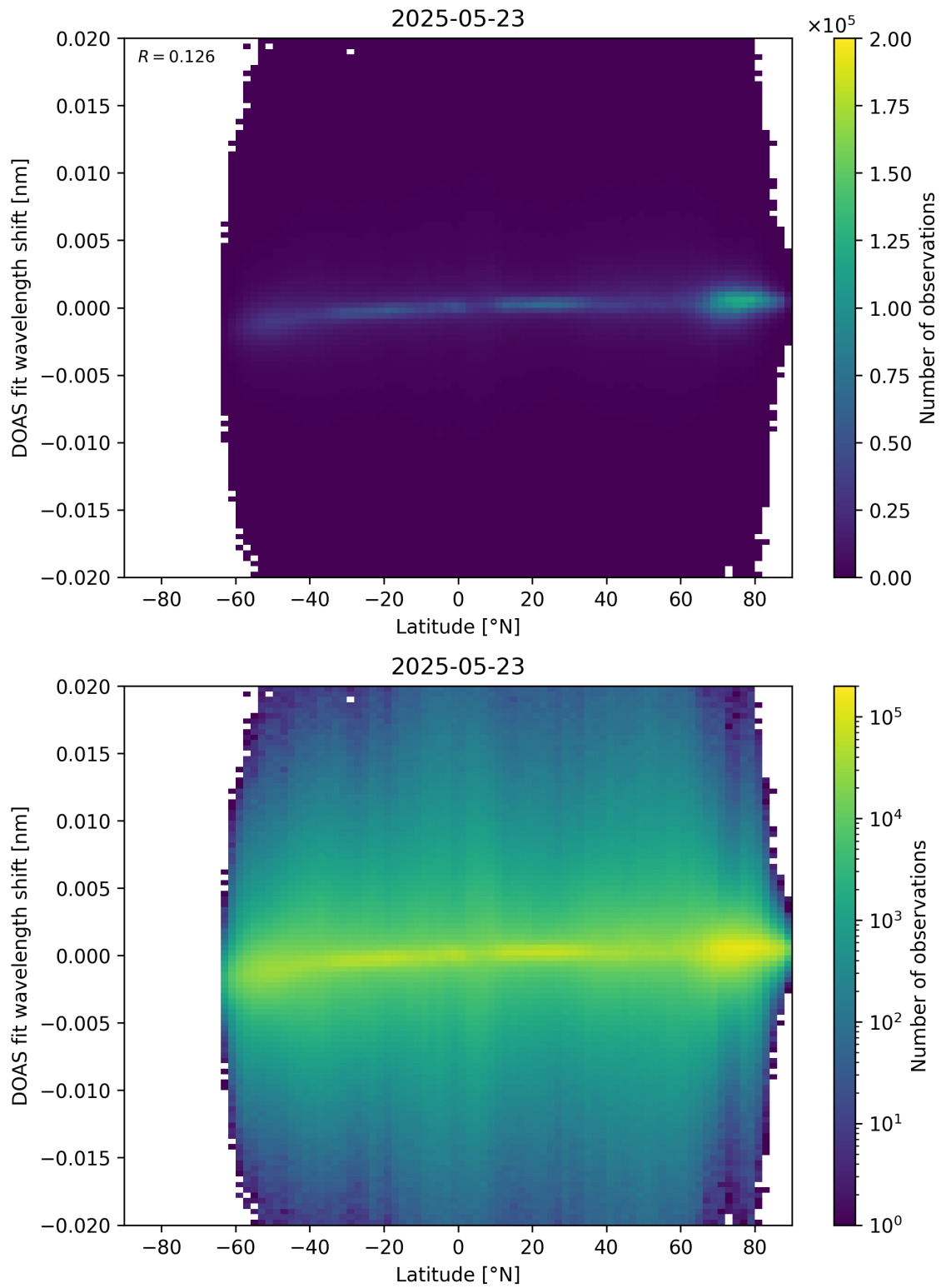
Figure 154: Scatter density plot of “Latitude” against “DOAS fit wavelength shift” for 2025-05-22 to 2025-05-24.
