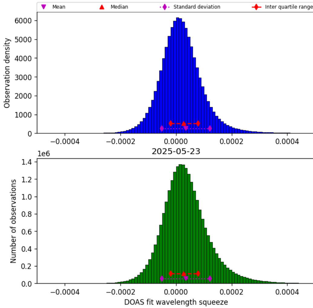
Figure 45: Histogram of “DOAS fit wavelength squeeze” for 2025-05-22 to 2025-05-24
