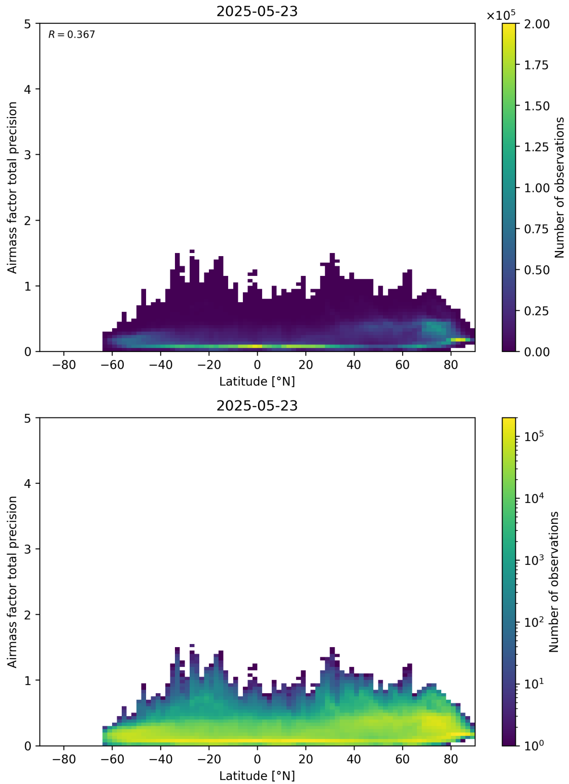
Figure 162: Scatter density plot of “Latitude” against “Airmass factor total precision” for 2025-05-22 to 2025-05-24.
