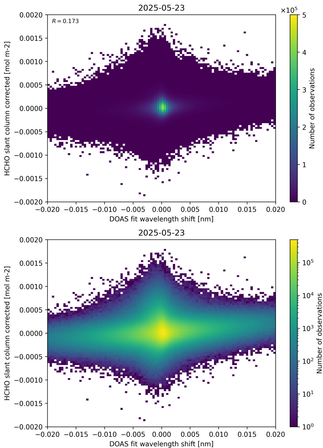
Figure 66: Scatter density plot of “DOAS fit wavelength shift” against “HCHO slant column corrected” for 2025-05-22 to 2025-05-24.
