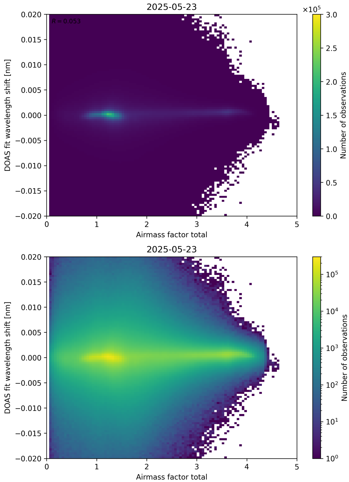
Figure 98: Scatter density plot of “Airmass factor total” against “DOAS fit wavelength shift” for 2025-05-22 to 2025-05-24.
