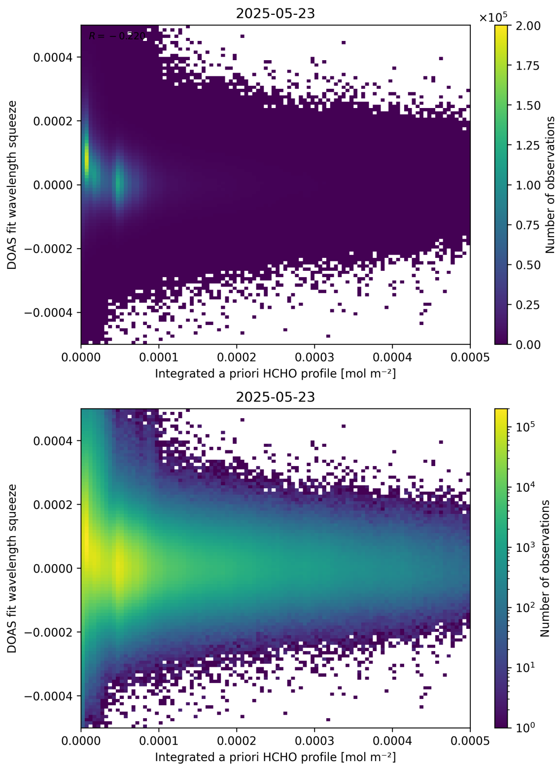
Figure 150: Scatter density plot of “Integrated a priori HCHO profile” against “DOAS fit wavelength squeeze” for 2025-05-22 to 2025-05-24.
