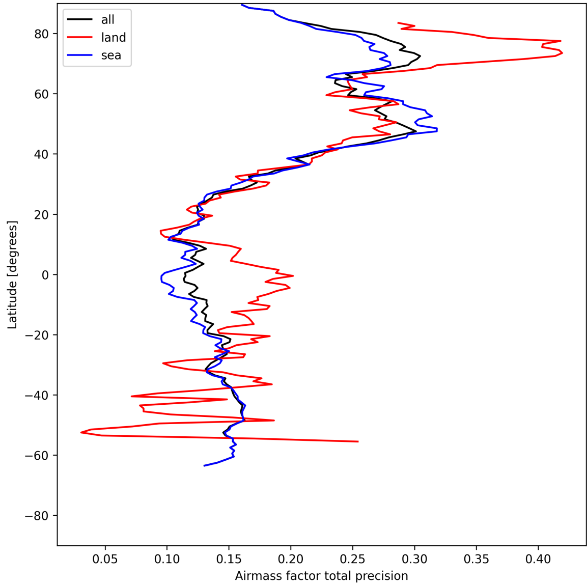
Figure 27: Zonal average of “Airmass factor total precision” for 2025-05-22 to 2025-05-24.
