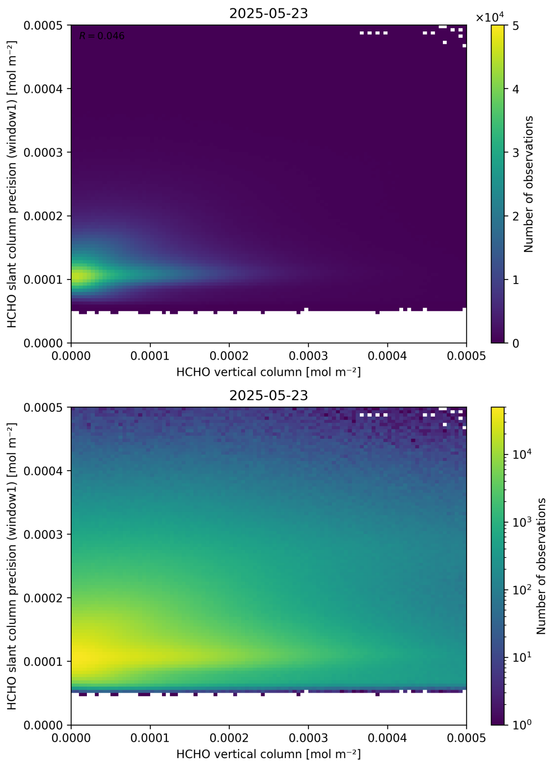
Figure 130: Scatter density plot of “HCHO vertical column” against “HCHO slant column precision (window1)” for 2025-05-22 to 2025-05-24.
