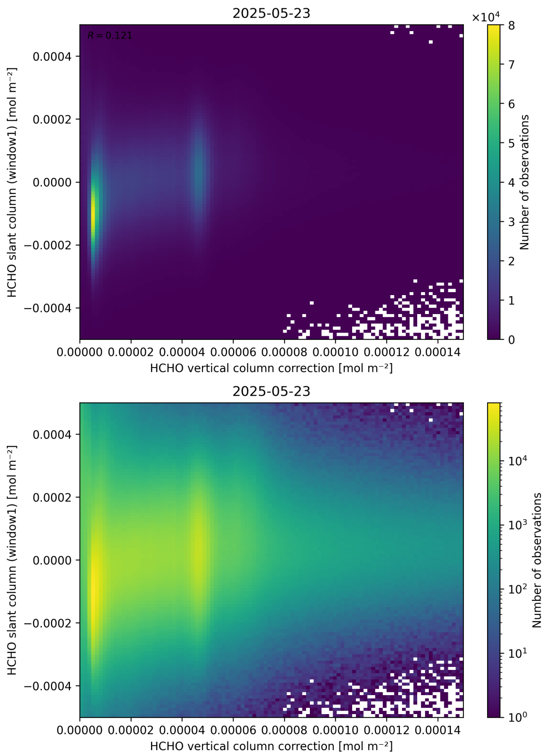
Figure 118: Scatter density plot of “HCHO vertical column correction” against “HCHO slant column (window1)” for 2025-05-22 to 2025-05-24.
