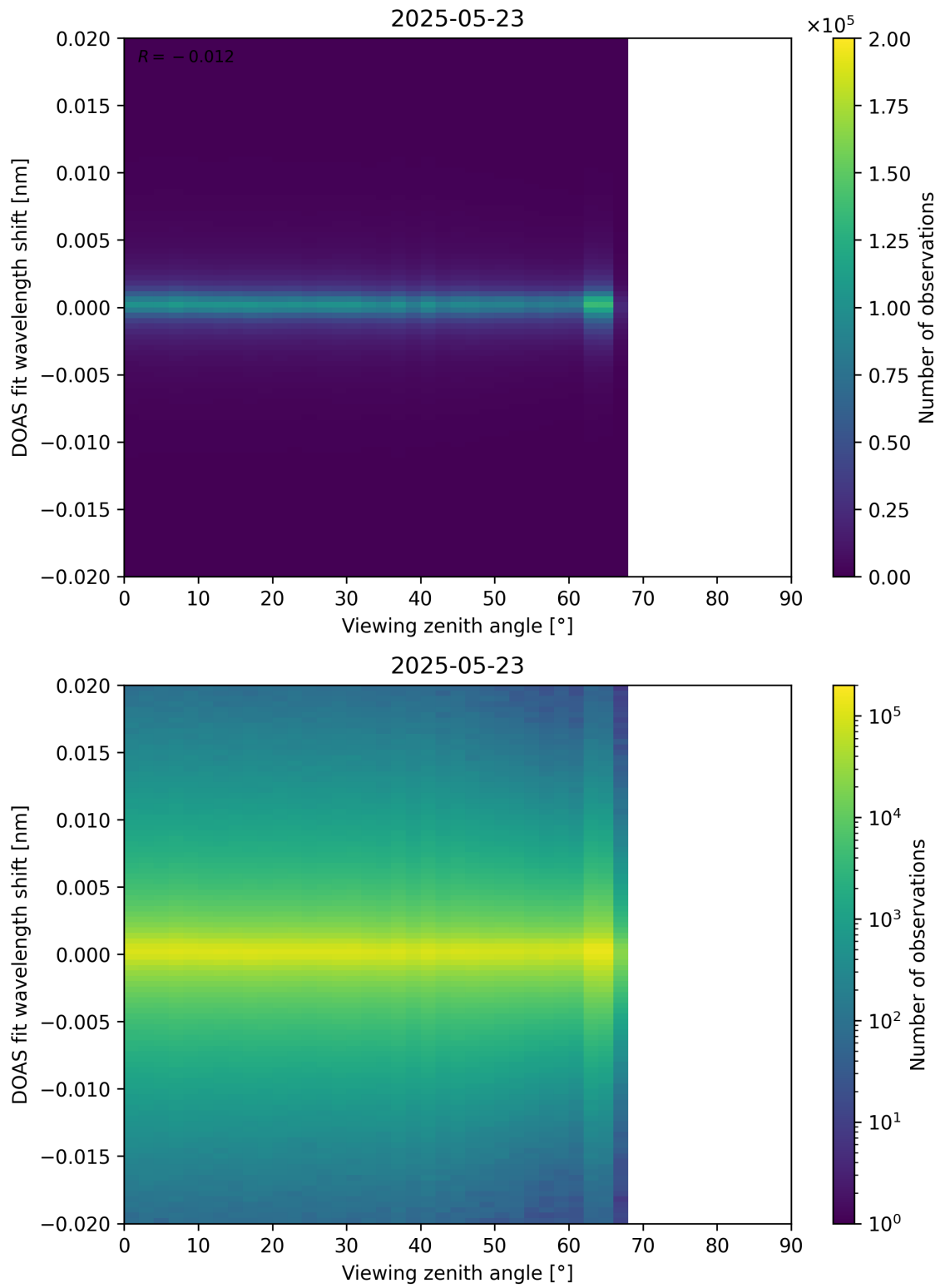
Figure 183: Scatter density plot of “Viewing zenith angle” against “DOAS fit wavelength shift” for 2025-05-22 to 2025-05-24.
