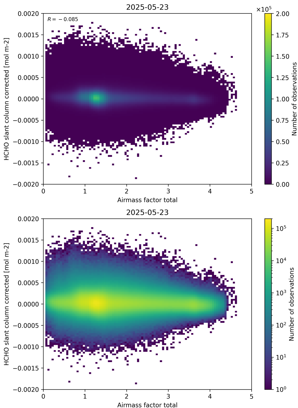
Figure 101: Scatter density plot of “Airmass factor total” against “HCHO slant column corrected” for 2025-05-22 to 2025-05-24.
