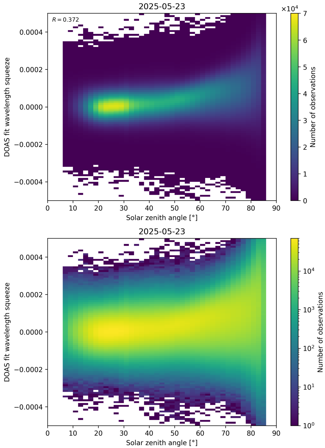
Figure 169: Scatter density plot of “Solar zenith angle” against “DOAS fit wavelength squeeze” for 2025-05-22 to 2025-05-24.
