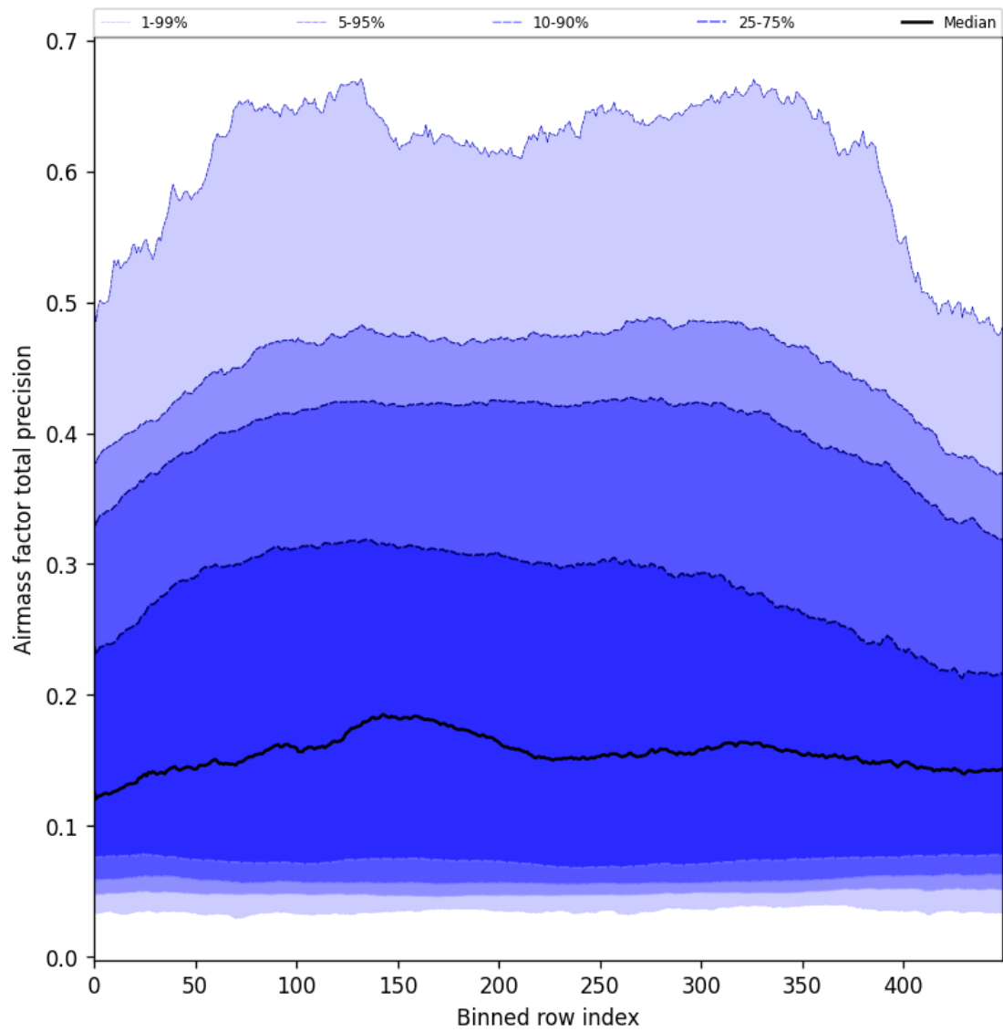
Figure 55: Along track statistics of “Airmass factor total precision” for 2025-05-22 to 2025-05-24
