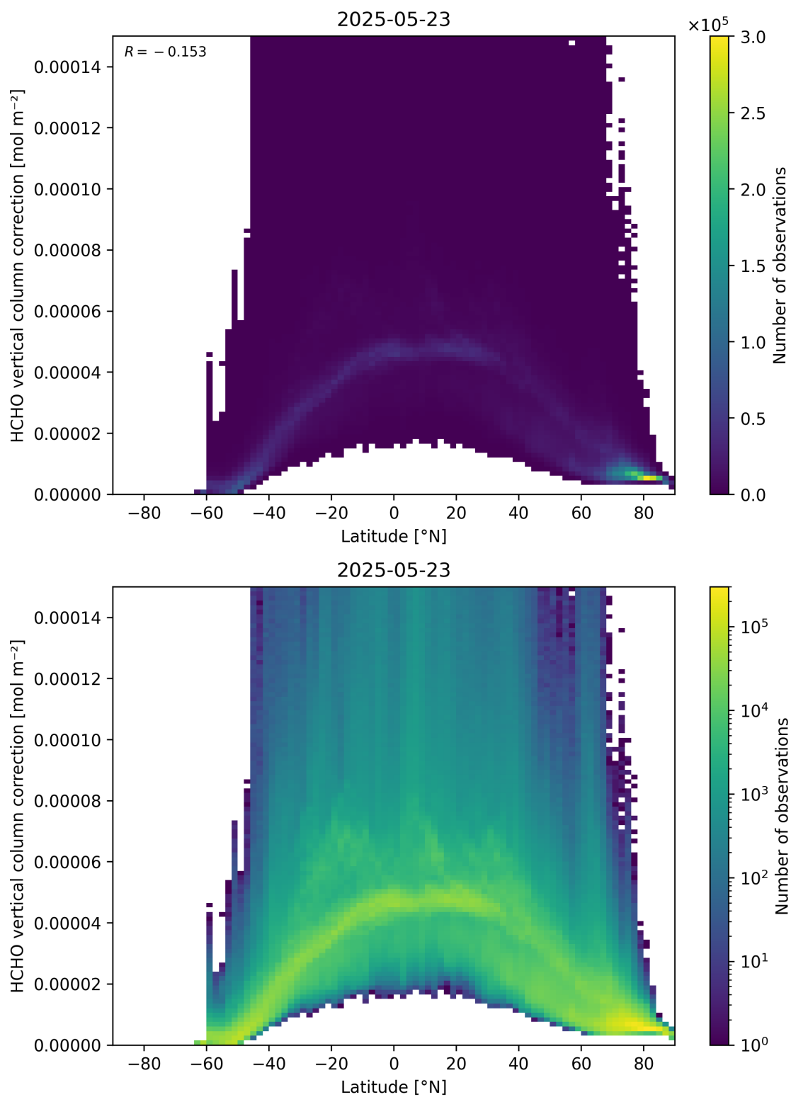
Figure 164: Scatter density plot of “Latitude” against “HCHO vertical column correction” for 2025-05-22 to 2025-05-24.
