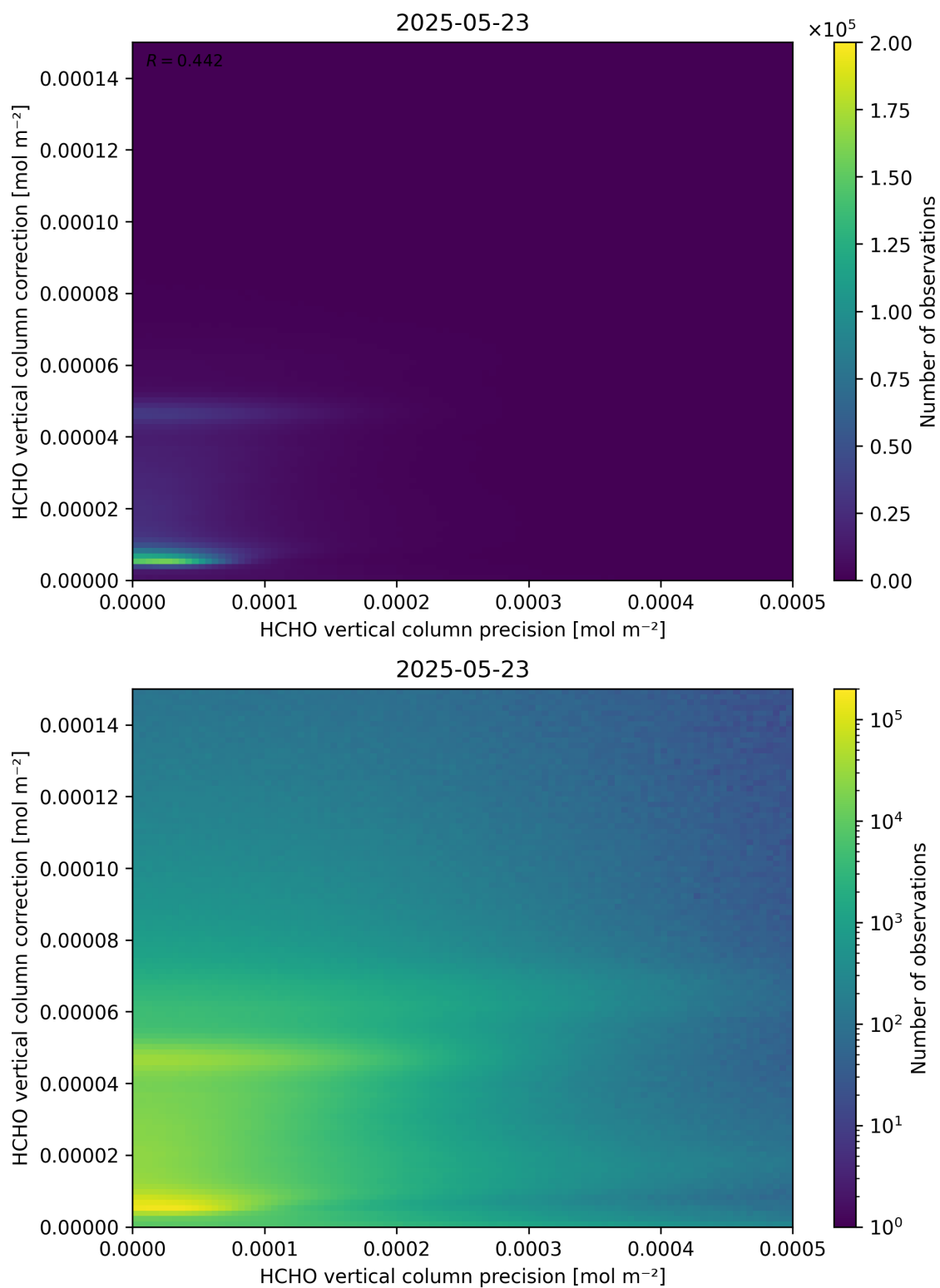
Figure 146: Scatter density plot of “HCHO vertical column precision” against “HCHO vertical column correction” for 2025-05-22 to 2025-05-24.
