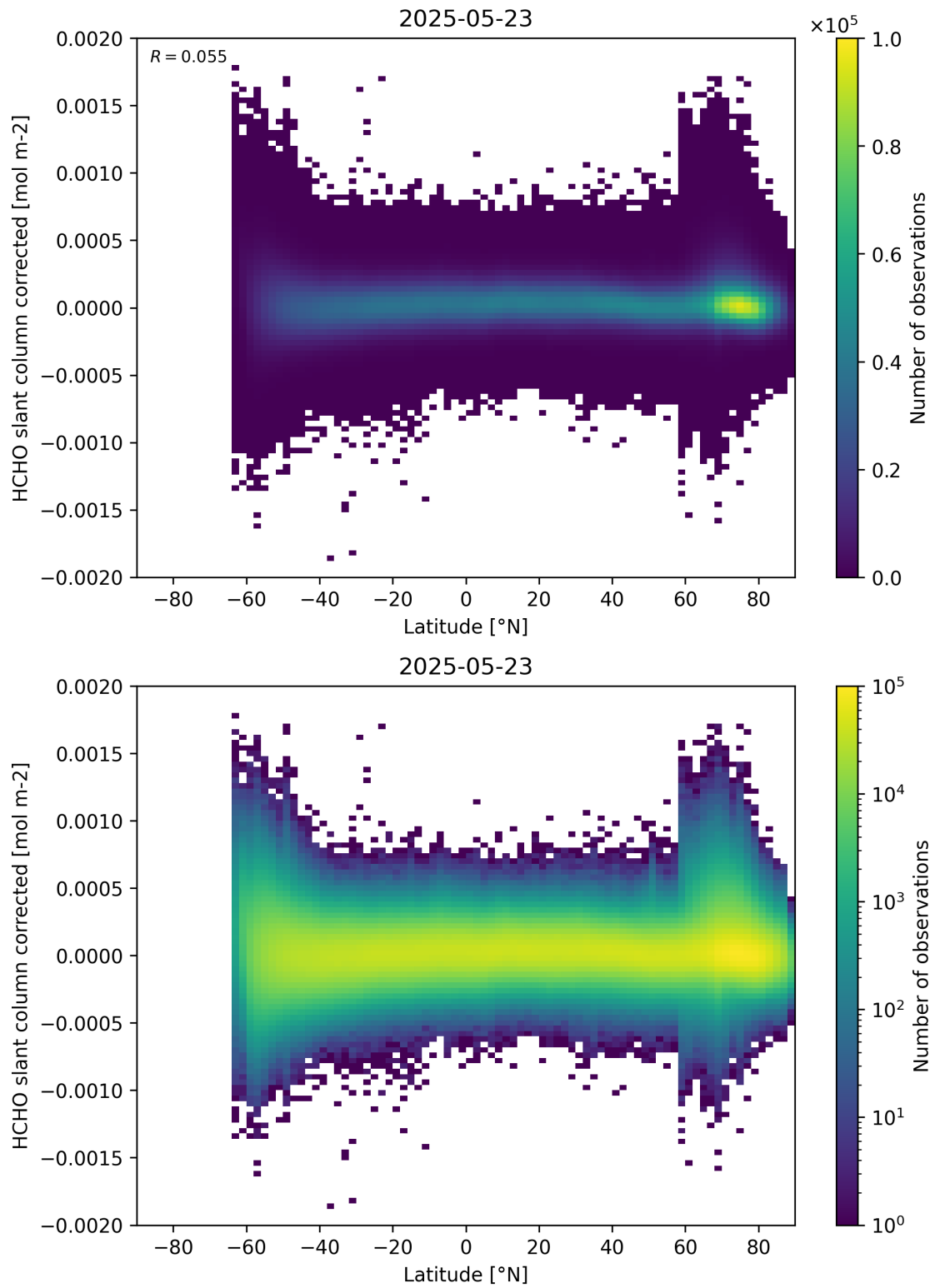
Figure 157: Scatter density plot of “Latitude” against “HCHO slant column corrected” for 2025-05-22 to 2025-05-24.
