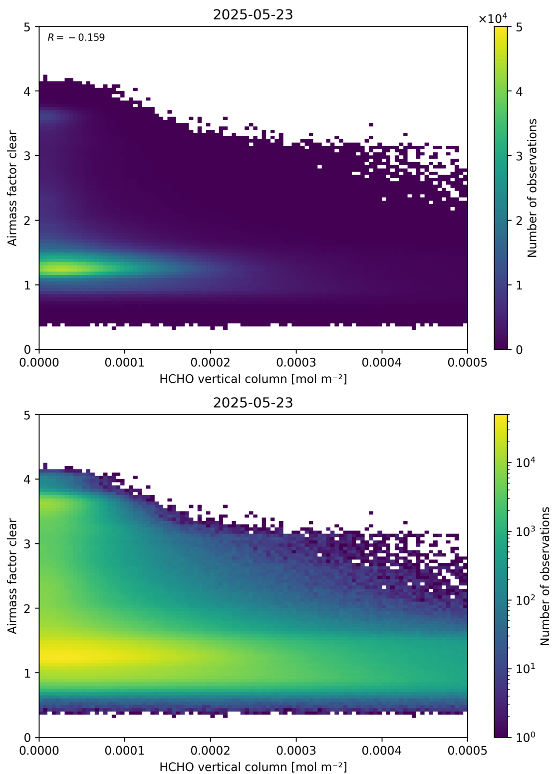
Figure 126: Scatter density plot of “HCHO vertical column” against “Airmass factor clear” for 2025-05-22 to 2025-05-24.
