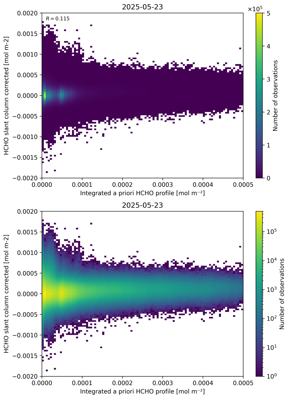
Figure 151: Scatter density plot of “Integrated a priori HCHO profile” against “HCHO slant column corrected” for 2025-05-22 to 2025-05-24.
