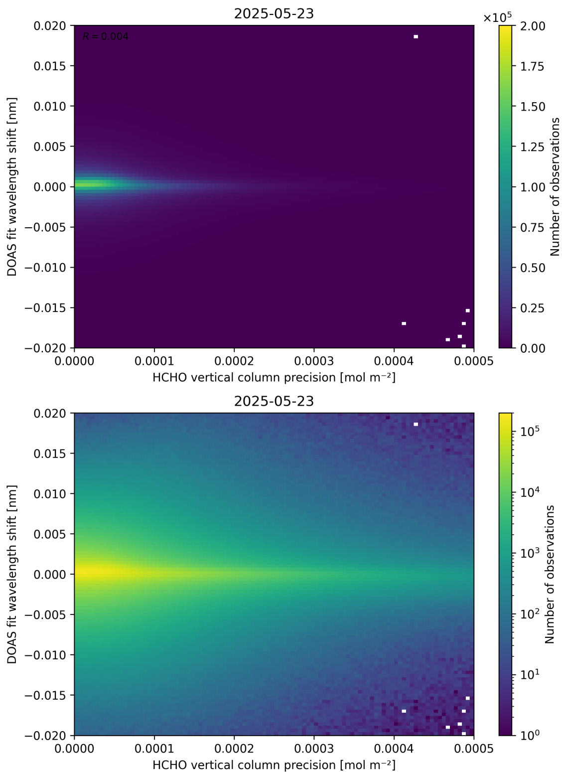
Figure 137: Scatter density plot of “HCHO vertical column precision” against “DOAS fit wavelength shift” for 2025-05-22 to 2025-05-24.
