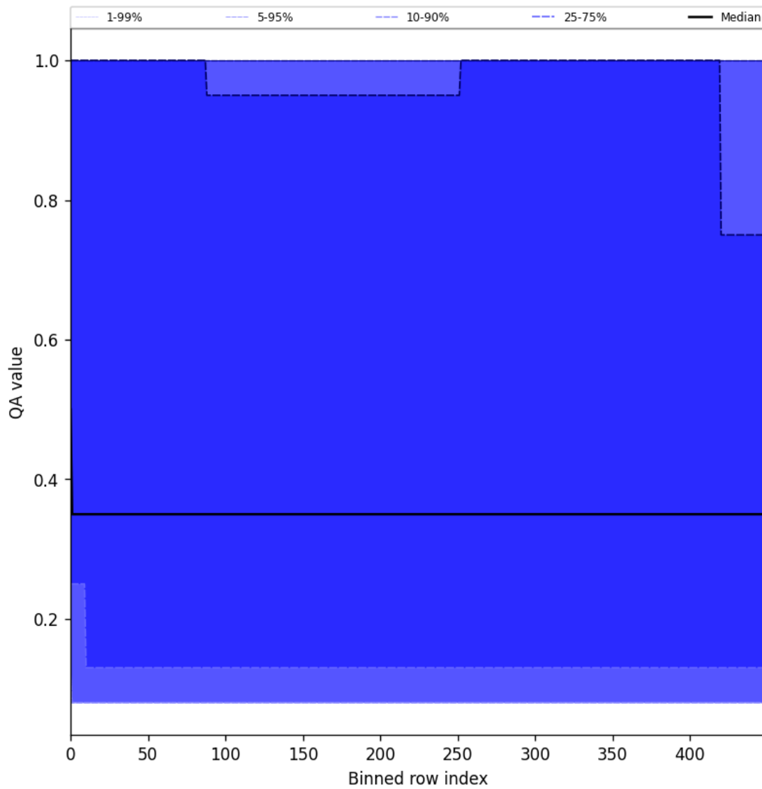
Figure 48: Along track statistics of “QA value” for 2025-05-22 to 2025-05-24
