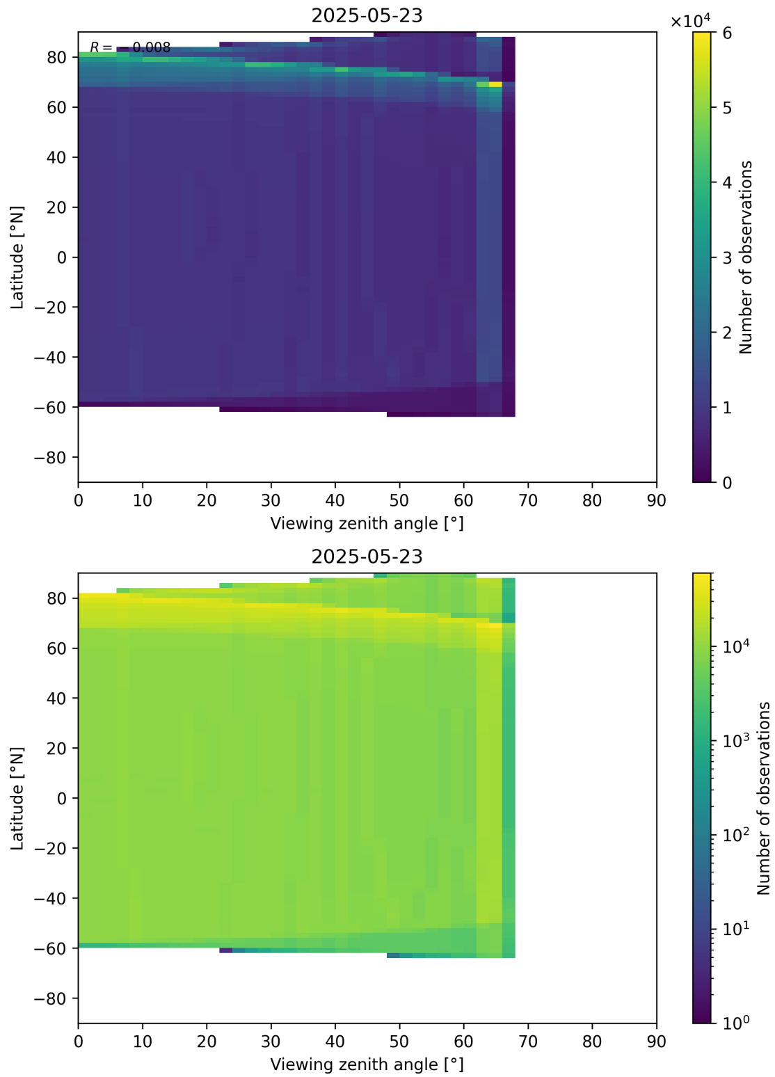
Figure 196: Scatter density plot of “Viewing zenith angle” against “Latitude” for 2025-05-22 to 2025-05-24.
