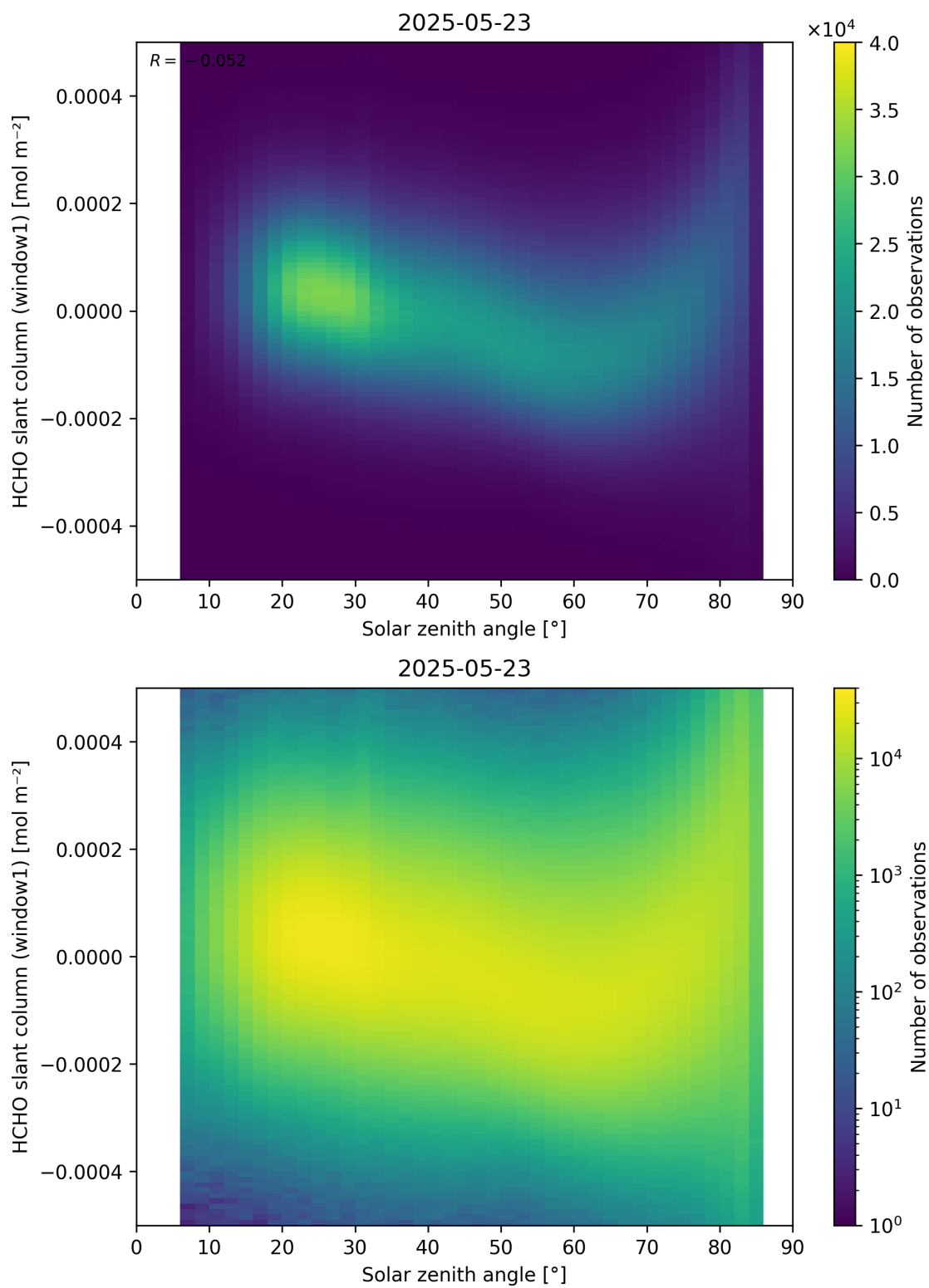
Figure 173: Scatter density plot of “Solar zenith angle” against “HCHO slant column (window1)” for 2025-05-22 to 2025-05-24.
