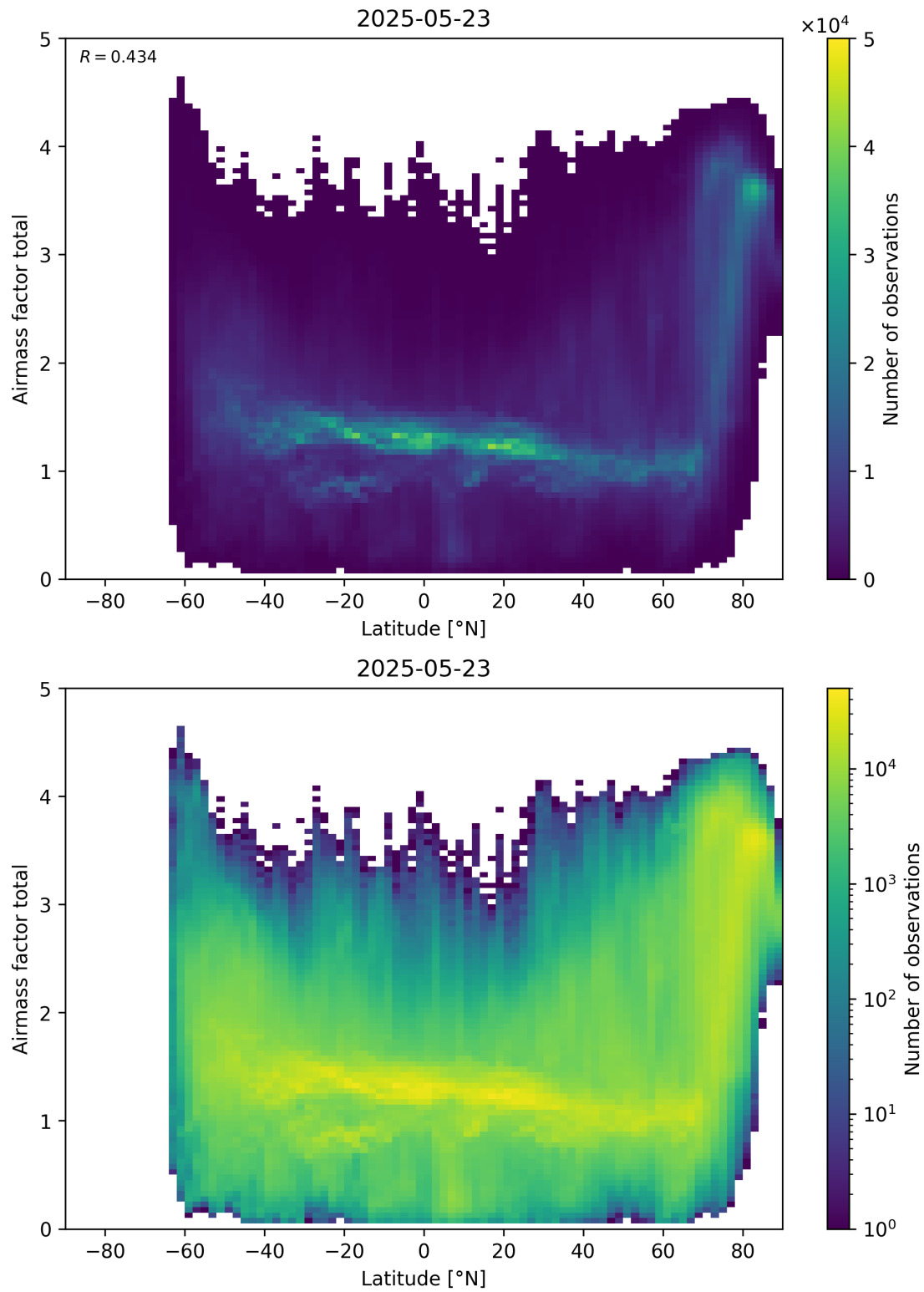
Figure 161: Scatter density plot of “Latitude” against “Airmass factor total” for 2025-05-22 to 2025-05-24.
