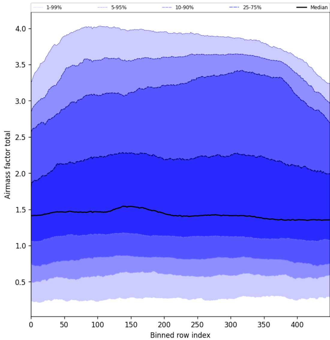
Figure 54: Along track statistics of “Airmass factor total” for 2025-05-22 to 2025-05-24
