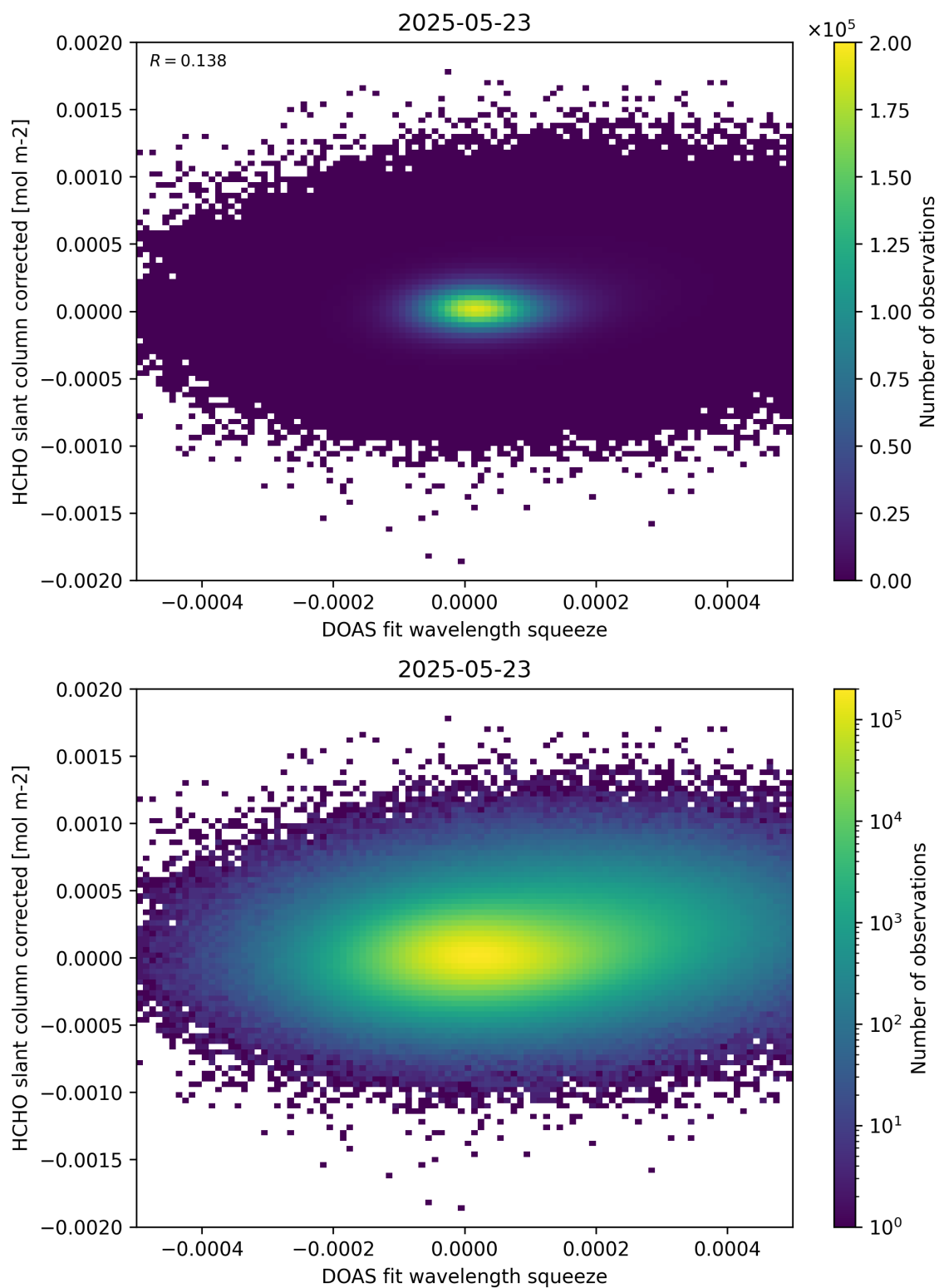
Figure 69: Scatter density plot of “DOAS fit wavelength squeeze” against “HCHO slant column corrected” for 2025-05-22 to 2025-05-24.
