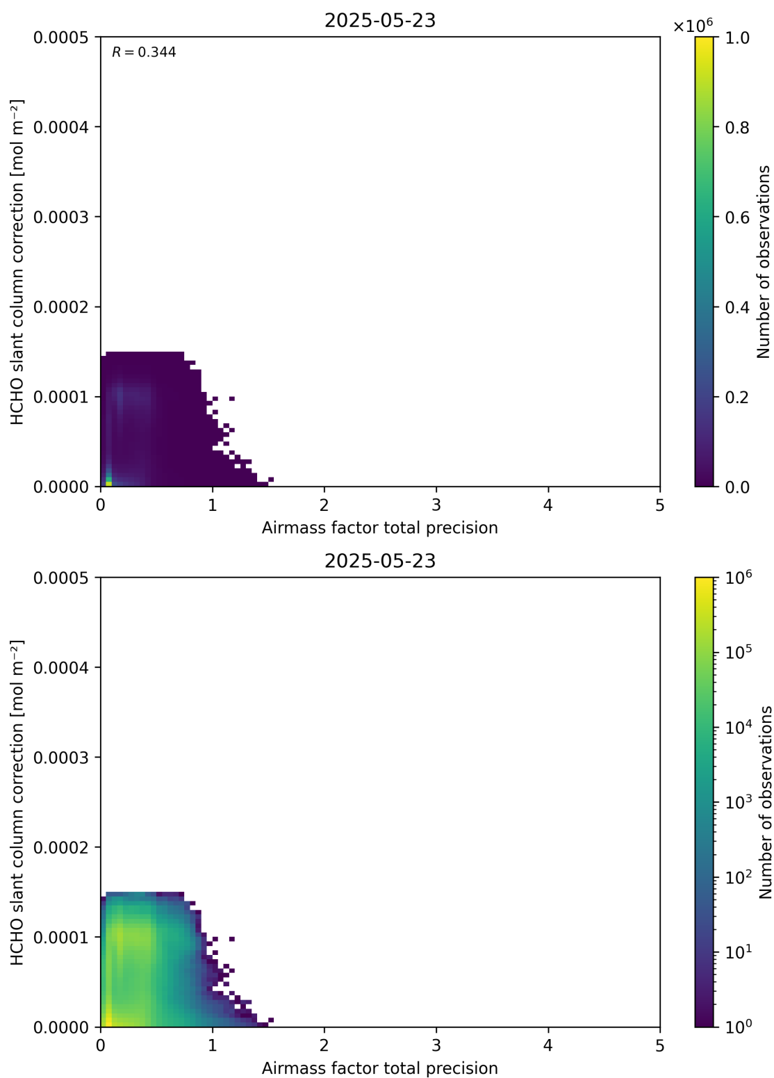
Figure 110: Scatter density plot of “Airmass factor total precision” against “HCHO slant column correction” for 2025-05-22 to 2025-05-24.
