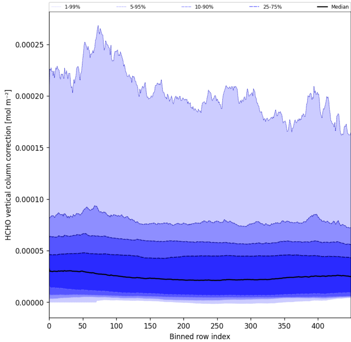
Figure 51: Along track statistics of “HCHO vertical column correction” for 2025-05-22 to 2025-05-24
