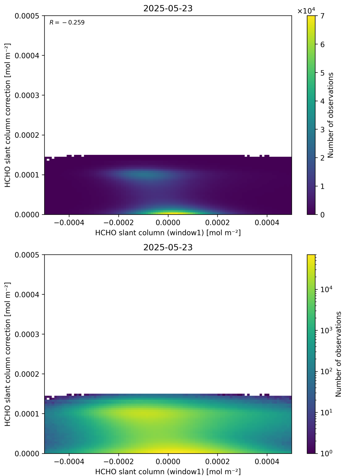
Figure 83: Scatter density plot of “HCHO slant column (window1)” against “HCHO slant column correction” for 2025-05-22 to 2025-05-24.
