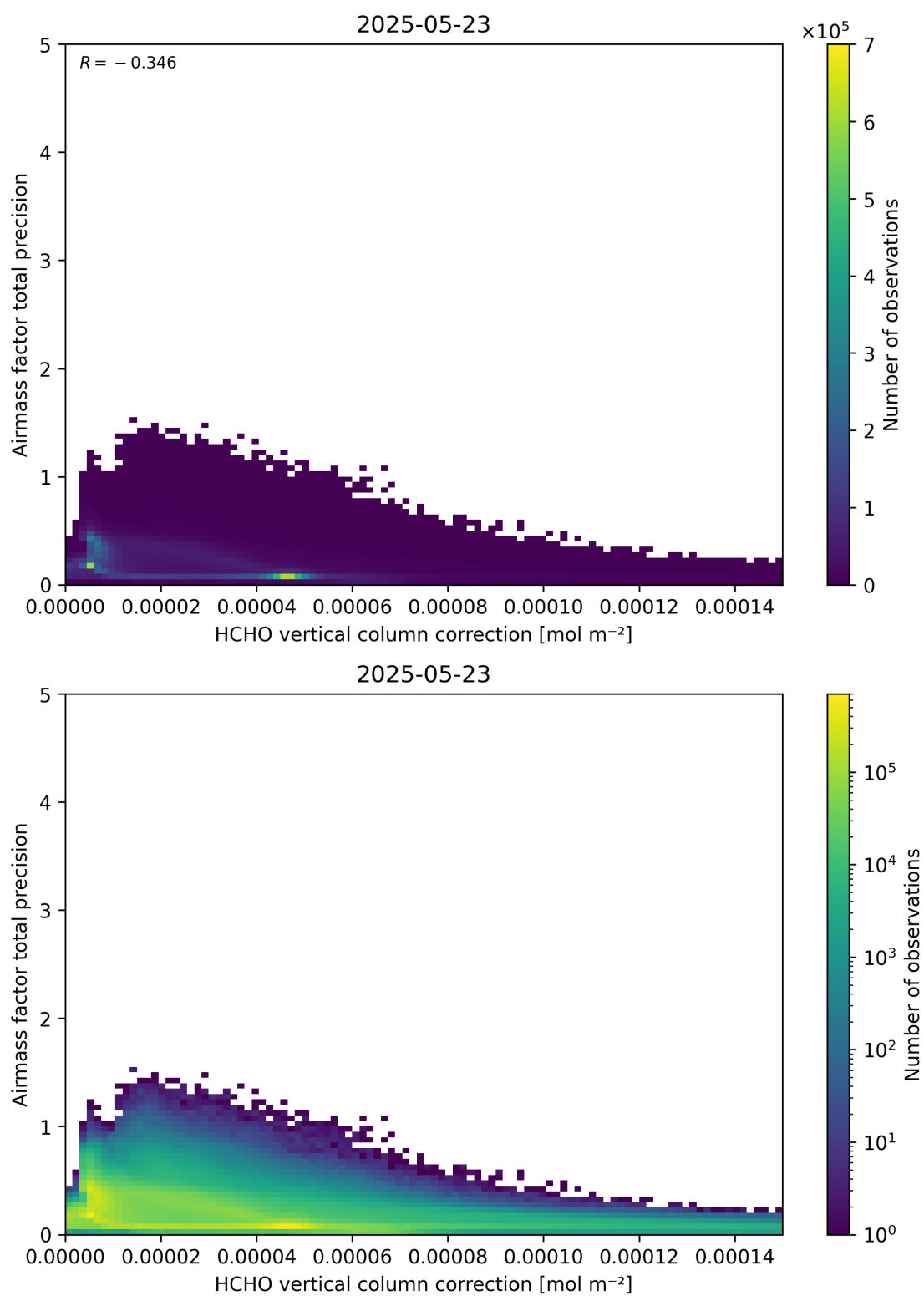
Figure 121: Scatter density plot of “HCHO vertical column correction” against “Airmass factor total precision” for 2025-05-22 to 2025-05-24.
