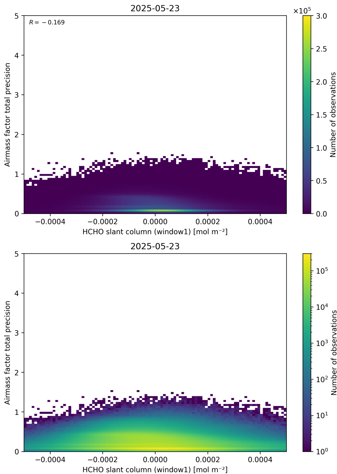
Figure 86: Scatter density plot of “HCHO slant column (window1)” against “Airmass factor total precision” for 2025-05-22 to 2025-05-24.
