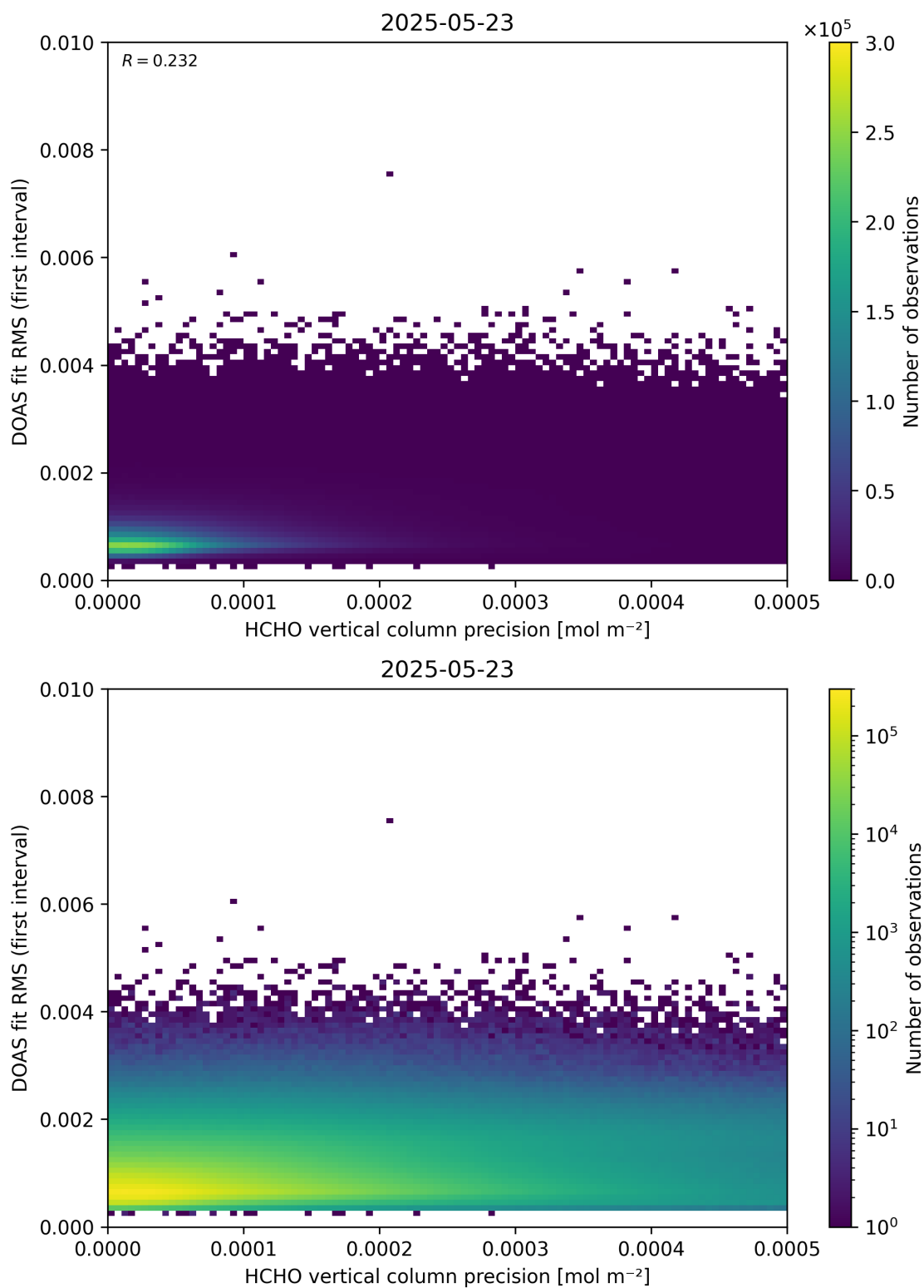
Figure 136: Scatter density plot of “HCHO vertical column precision” against “DOAS fit RMS (first interval)” for 2025-05-22 to 2025-05-24.
