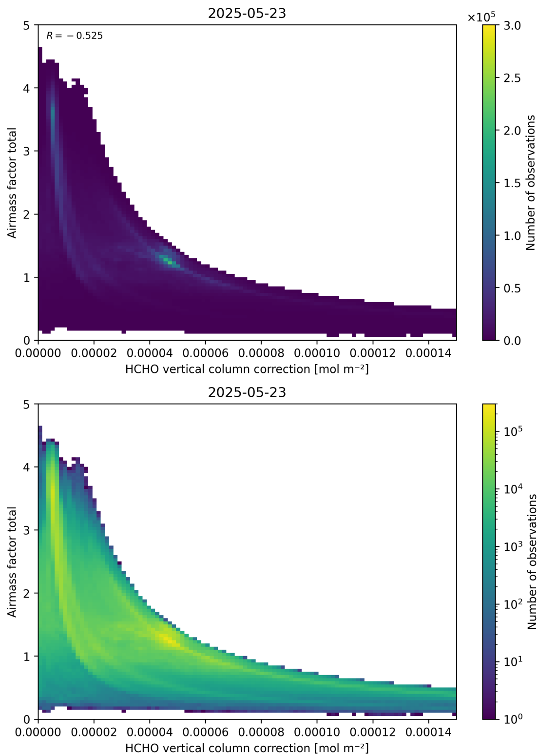
Figure 120: Scatter density plot of “HCHO vertical column correction” against “Airmass factor total” for 2025-05-22 to 2025-05-24.
