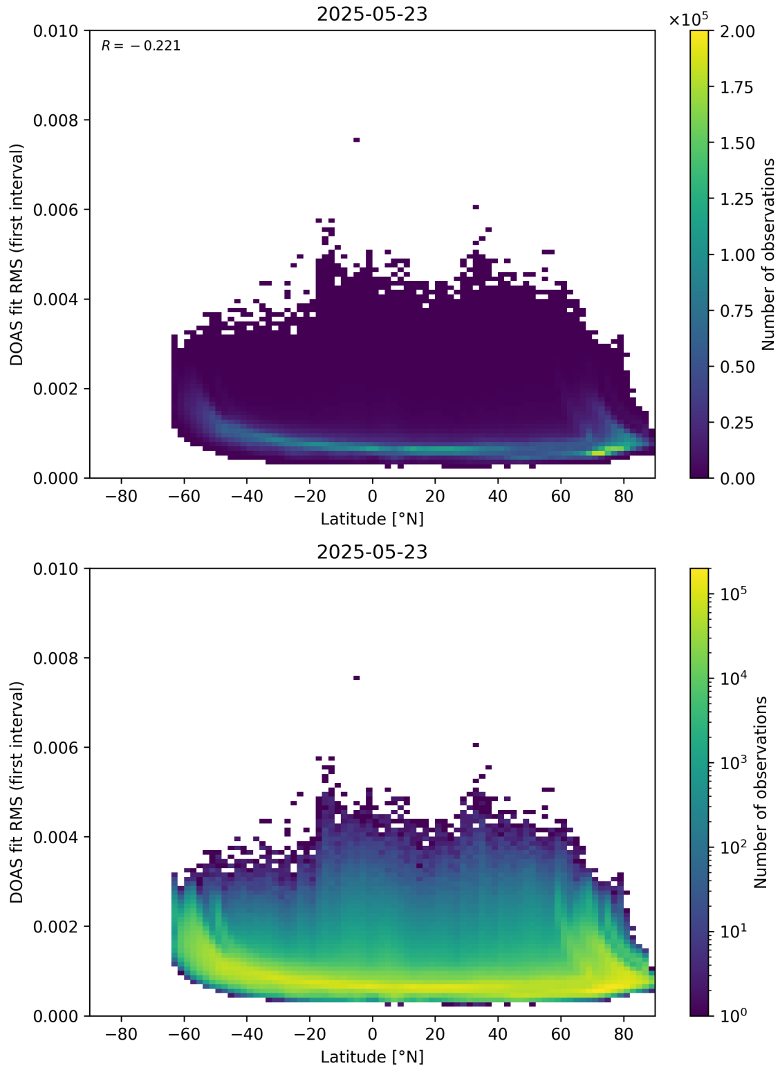
Figure 153: Scatter density plot of “Latitude” against “DOAS fit RMS (first interval)” for 2025-05-22 to 2025-05-24.
