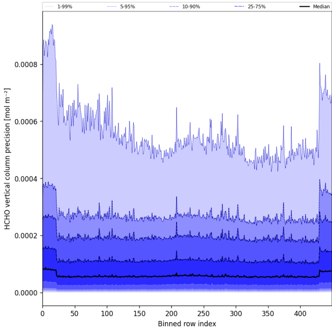
Figure 50: Along track statistics of "HCHO vertical column precision" for 2025-05-22 to 2025-05-24
