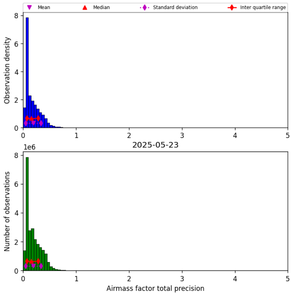
Figure 41: Histogram of “Airmass factor total precision” for 2025-05-22 to 2025-05-24
