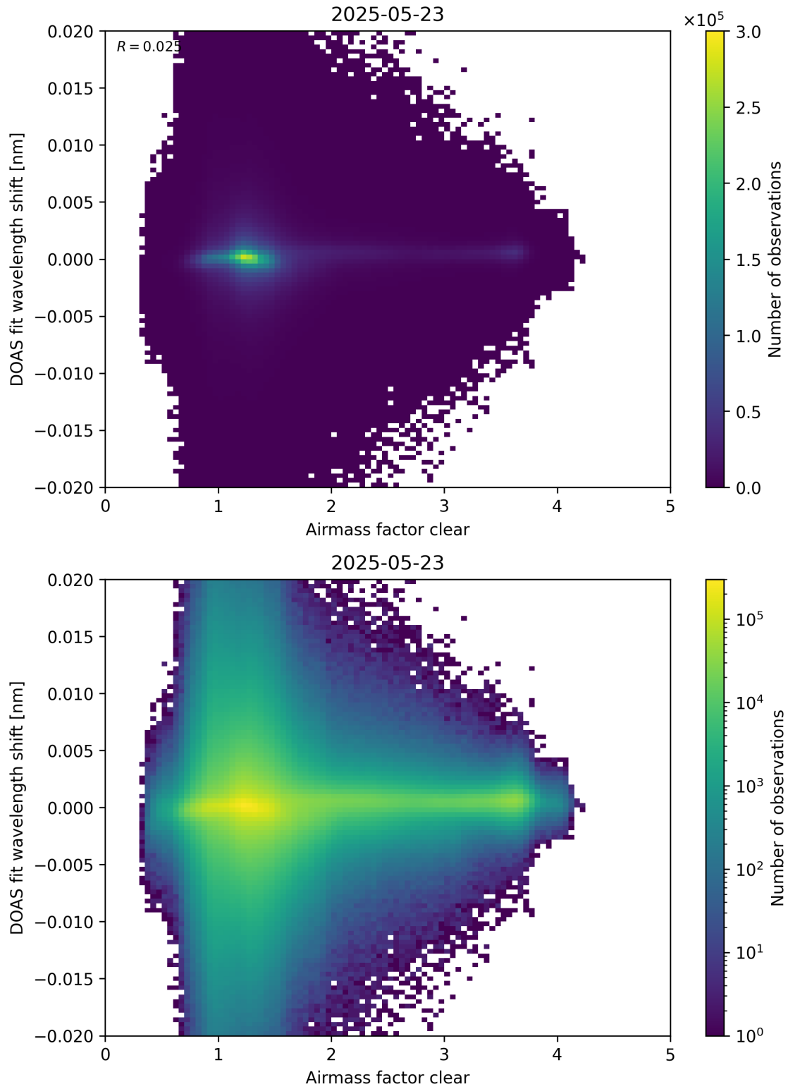
Figure 72: Scatter density plot of “Airmass factor clear” against “DOAS fit wavelength shift” for 2025-05-22 to 2025-05-24.
