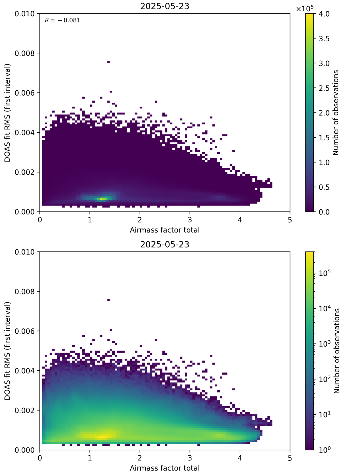
Figure 97: Scatter density plot of “Airmass factor total” against “DOAS fit RMS (first interval)” for 2025-05-22 to 2025-05-24.
