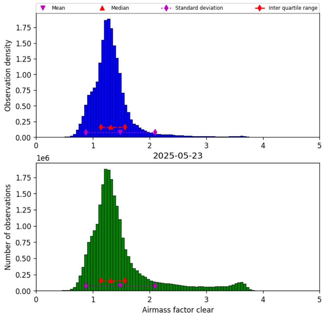
Figure 42: Histogram of “Airmass factor clear” for 2025-05-22 to 2025-05-24
