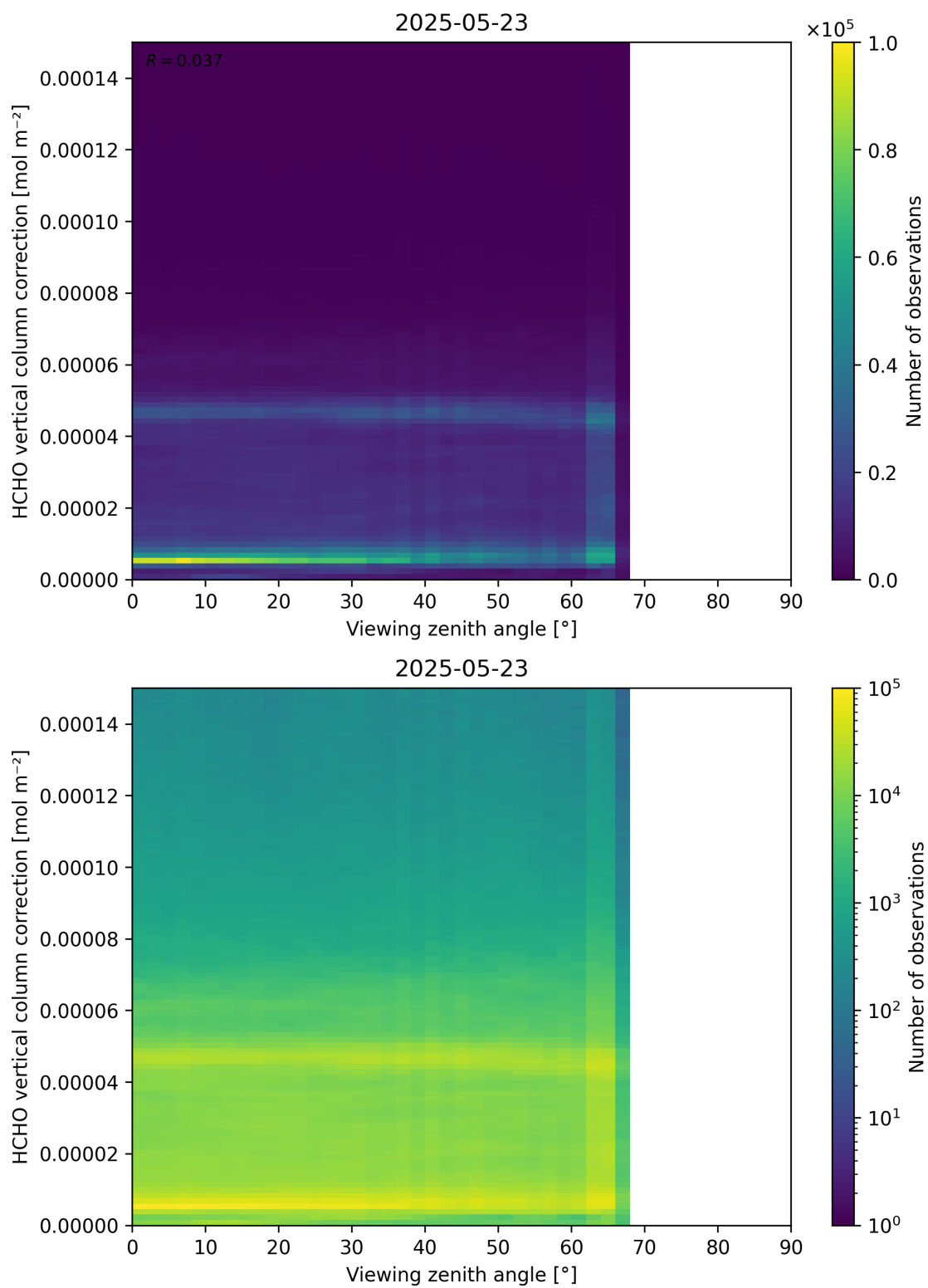
Figure 193: Scatter density plot of “Viewing zenith angle” against “HCHO vertical column correction” for 2025-05-22 to 2025-05-24.
