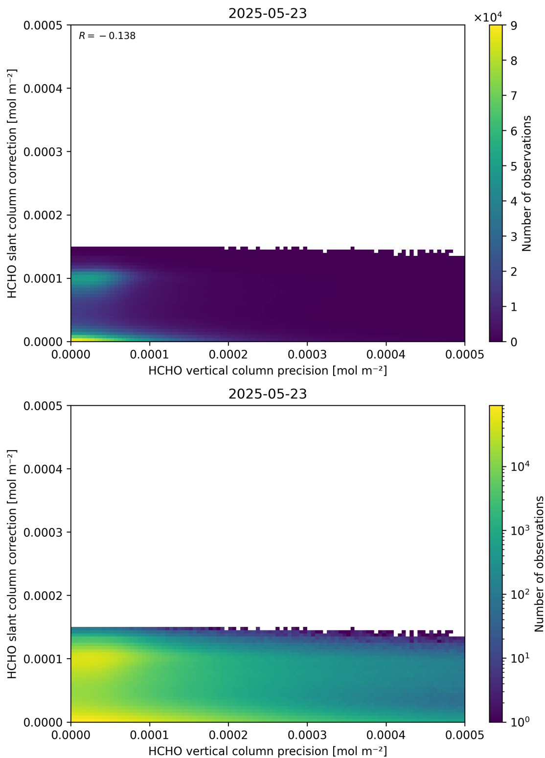
Figure 141: Scatter density plot of “HCHO vertical column precision” against “HCHO slant column correction” for 2025-05-22 to 2025-05-24.
