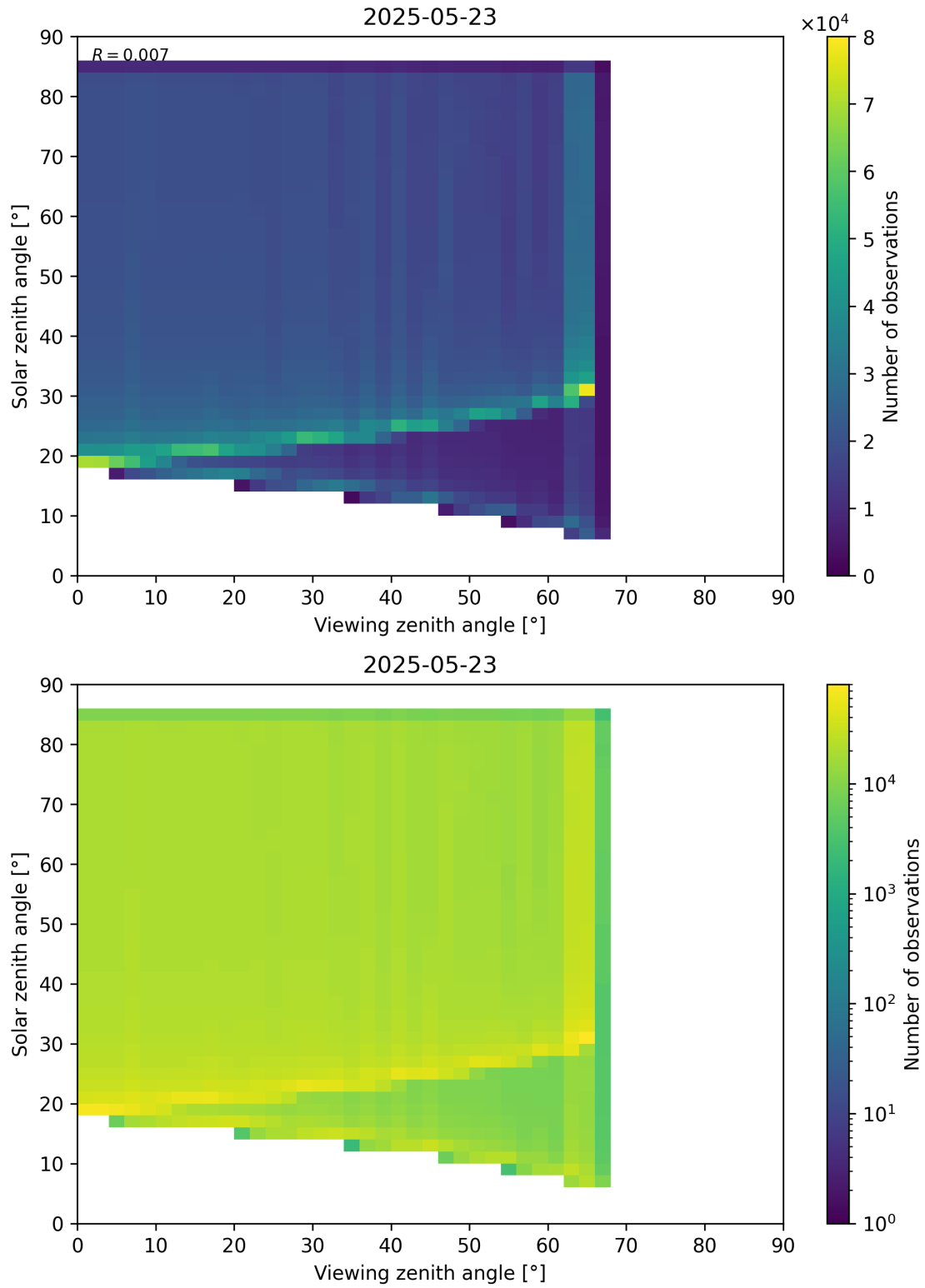
Figure 197: Scatter density plot of “Viewing zenith angle” against “Solar zenith angle” for 2025-05-22 to 2025-05-24.
