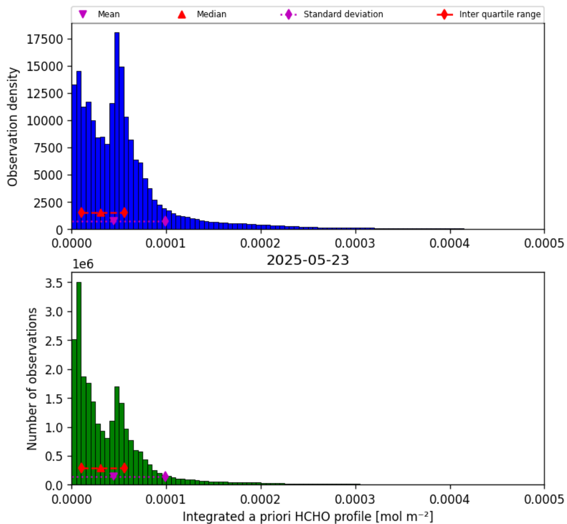
Figure 43: Histogram of “Integrated a priori HCHO profile” for 2025-05-22 to 2025-05-24
