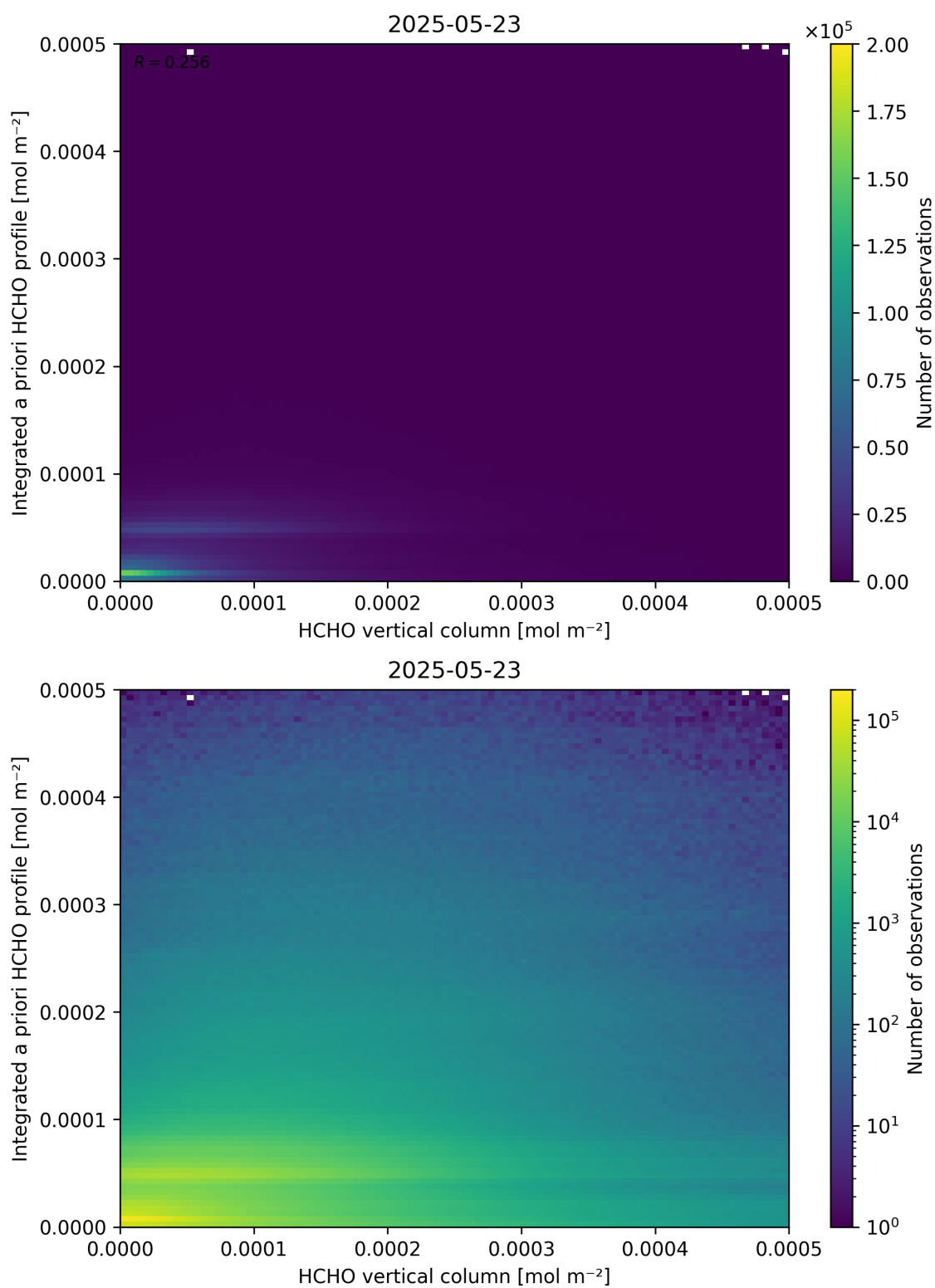
Figure 135: Scatter density plot of “HCHO vertical column” against “Integrated a priori HCHO profile” for 2025-05-22 to 2025-05-24.
