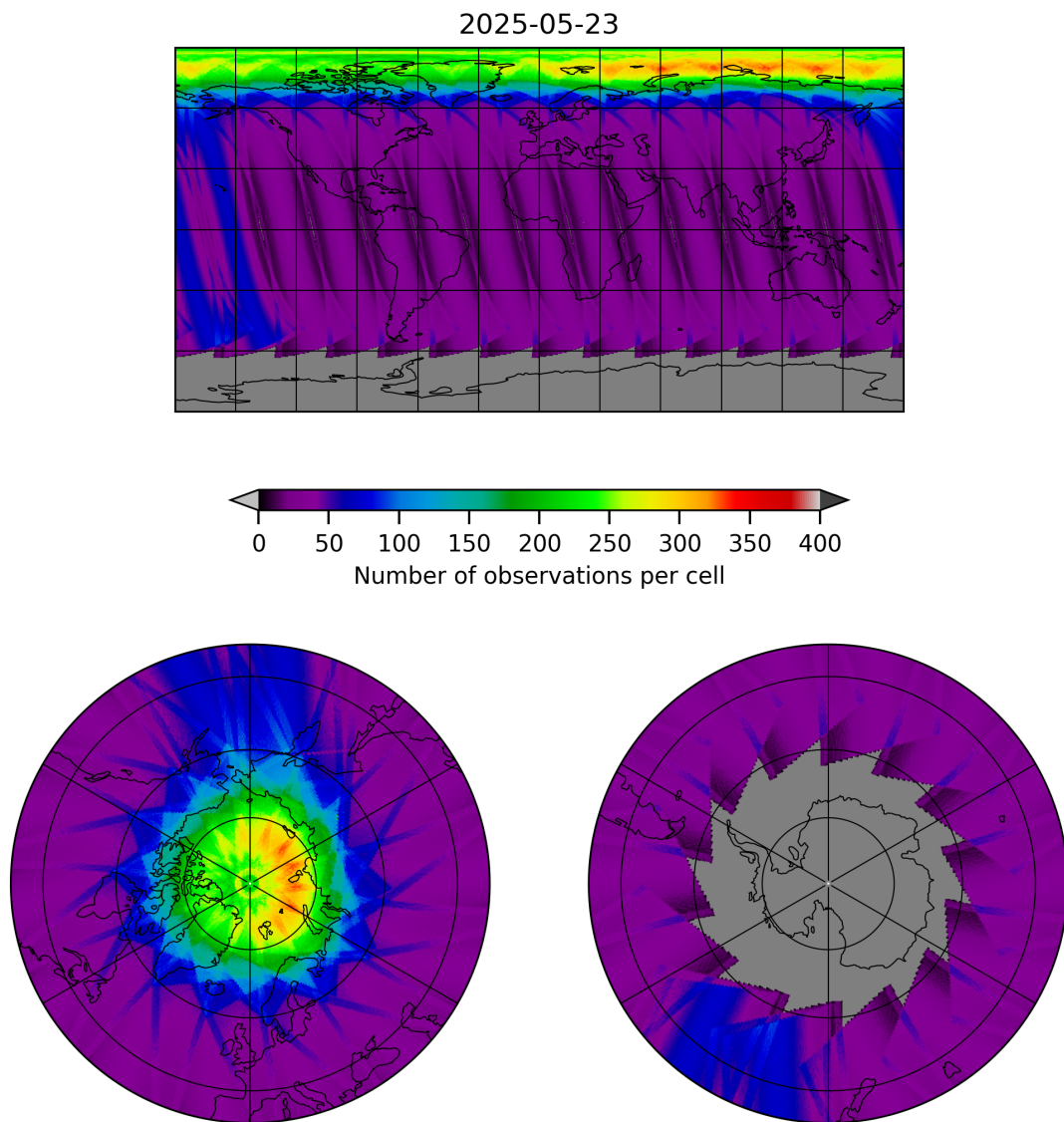
Figure 19: Map of the number of observations for 2025-05-22 to 2025-05-24
