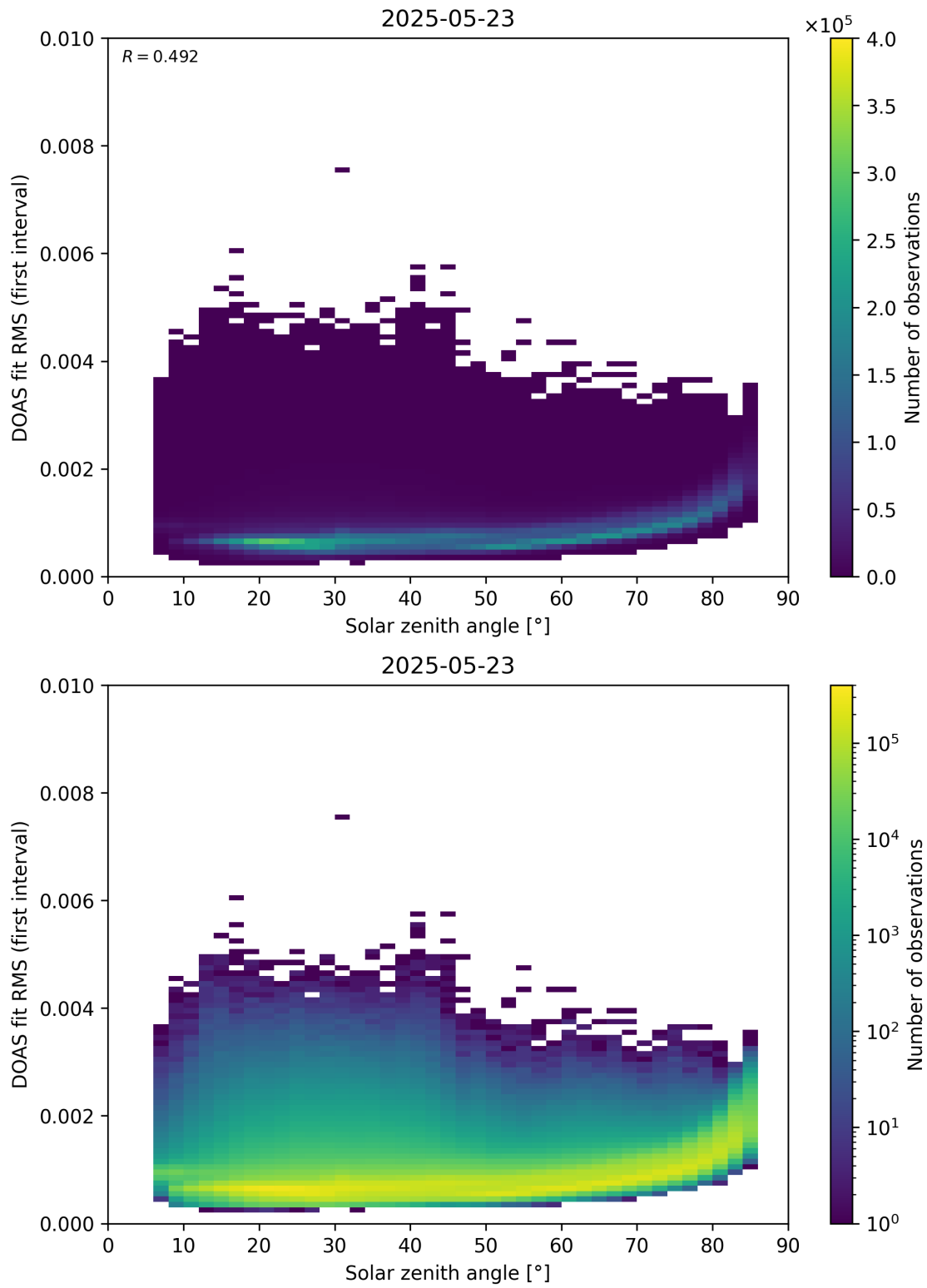
Figure 167: Scatter density plot of “Solar zenith angle” against “DOAS fit RMS (first interval)” for 2025-05-22 to 2025-05-24.
