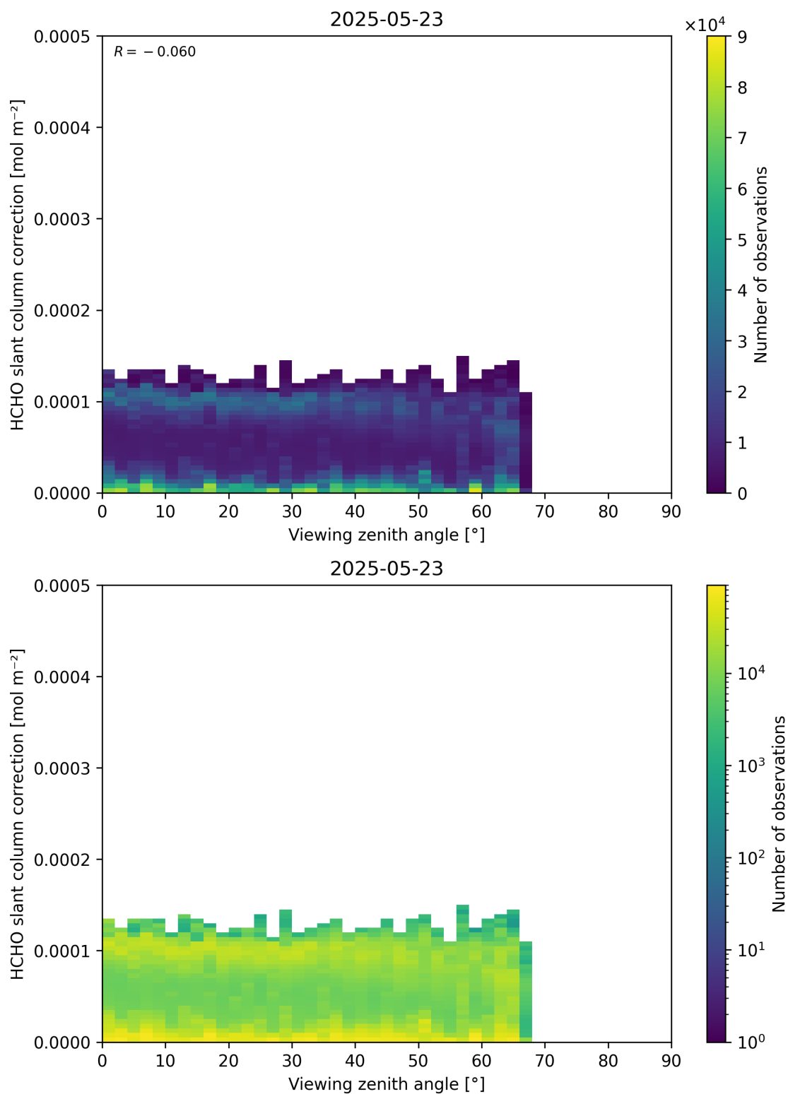
Figure 187: Scatter density plot of “Viewing zenith angle” against “HCHO slant column correction” for 2025-05-22 to 2025-05-24.
