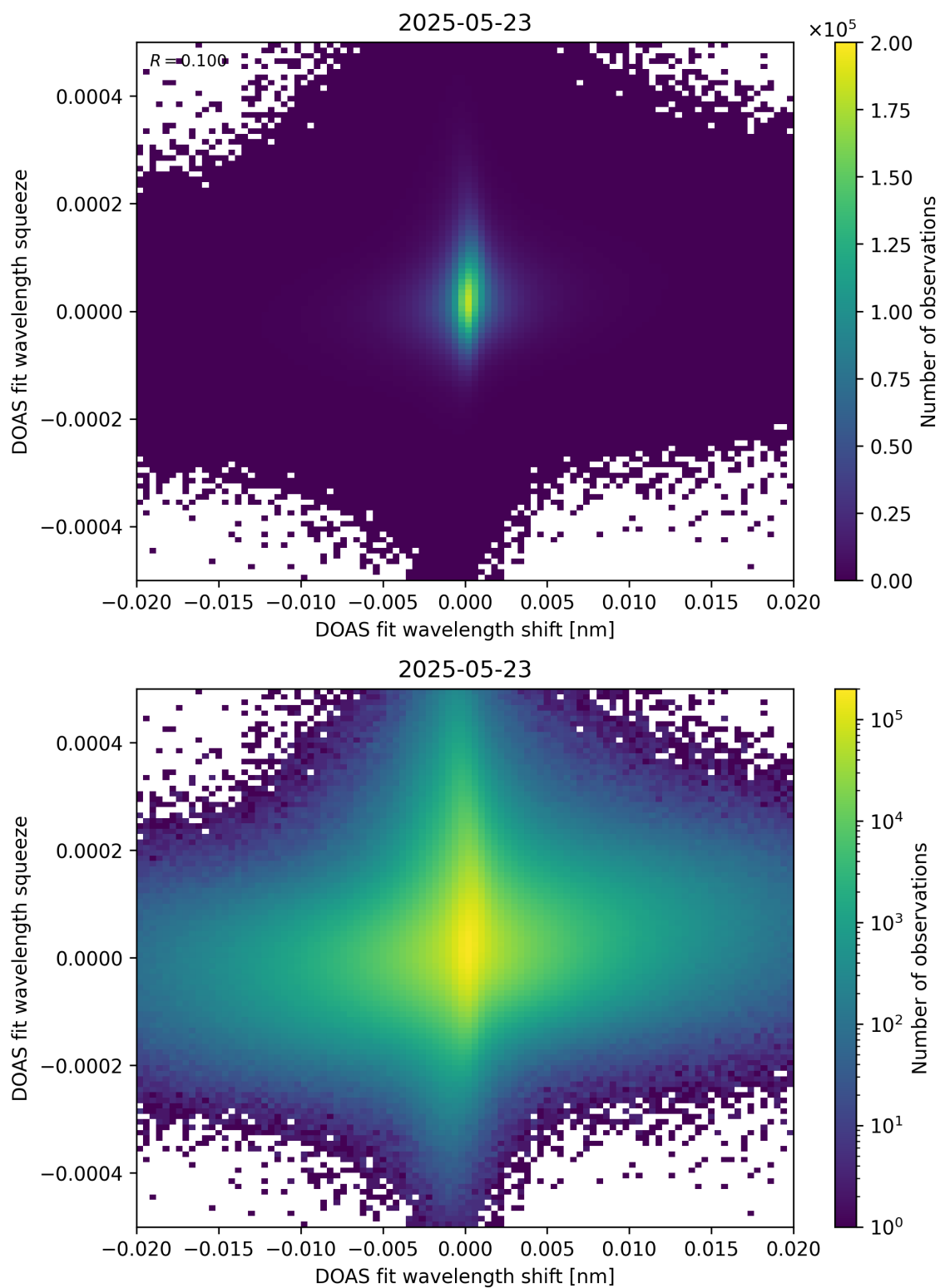
Figure 65: Scatter density plot of “DOAS fit wavelength shift” against “DOAS fit wavelength squeeze” for 2025-05-22 to 2025-05-24.
