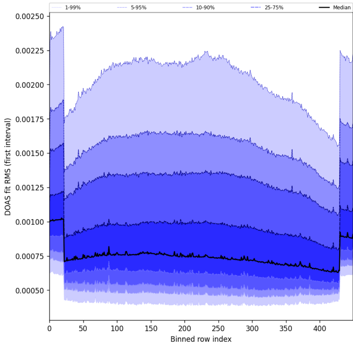
Figure 60: Along track statistics of “DOAS fit RMS (first interval)” for 2025-05-22 to 2025-05-24
