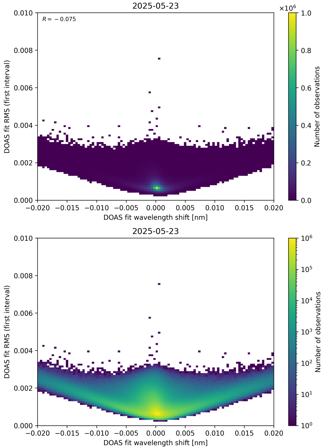
Figure 64: Scatter density plot of “DOAS fit wavelength shift” against “DOAS fit RMS (first interval)” for 2025-05-22 to 2025-05-24.
