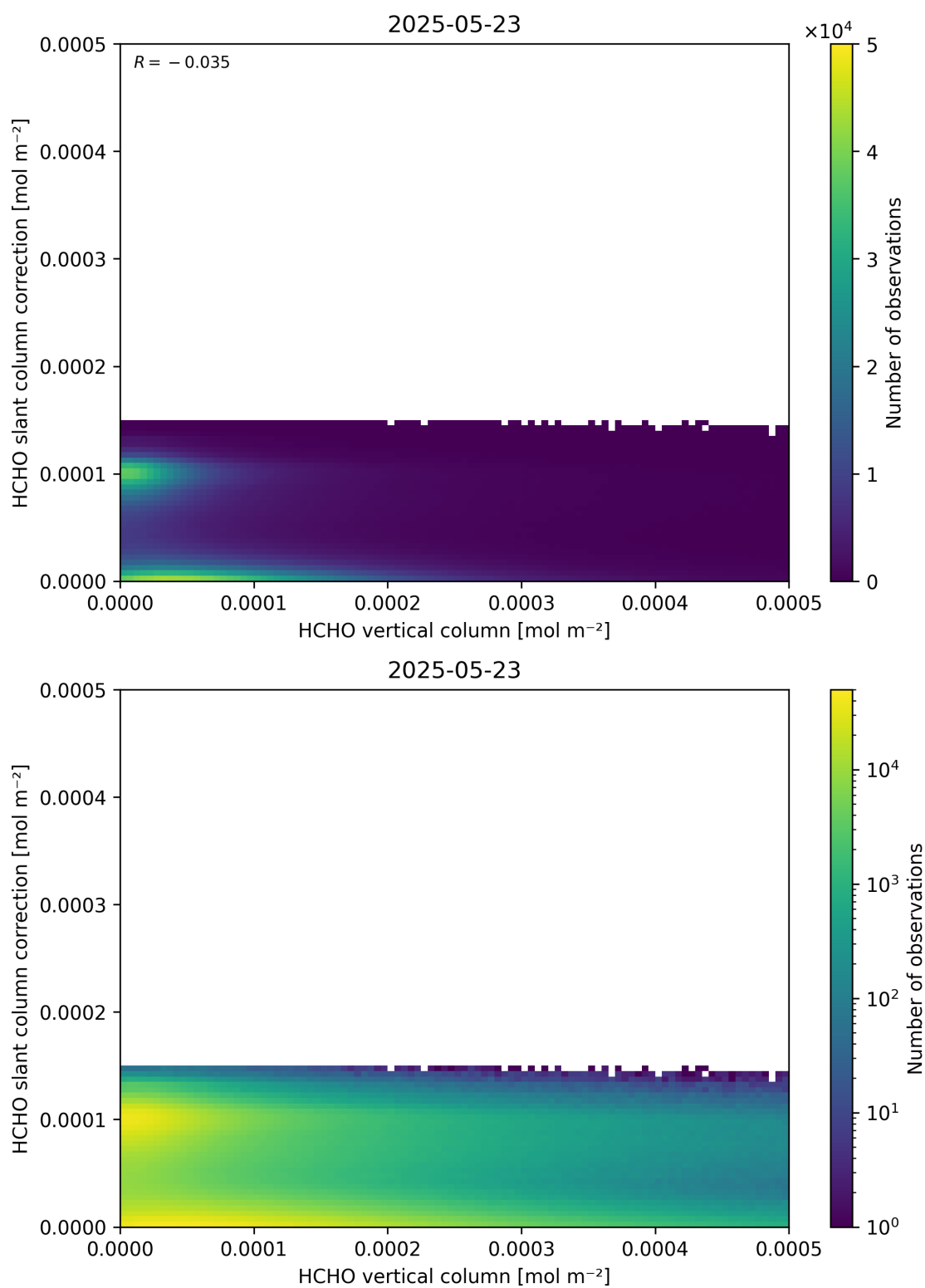
Figure 128: Scatter density plot of “HCHO vertical column” against “HCHO slant column correction” for 2025-05-22 to 2025-05-24.
