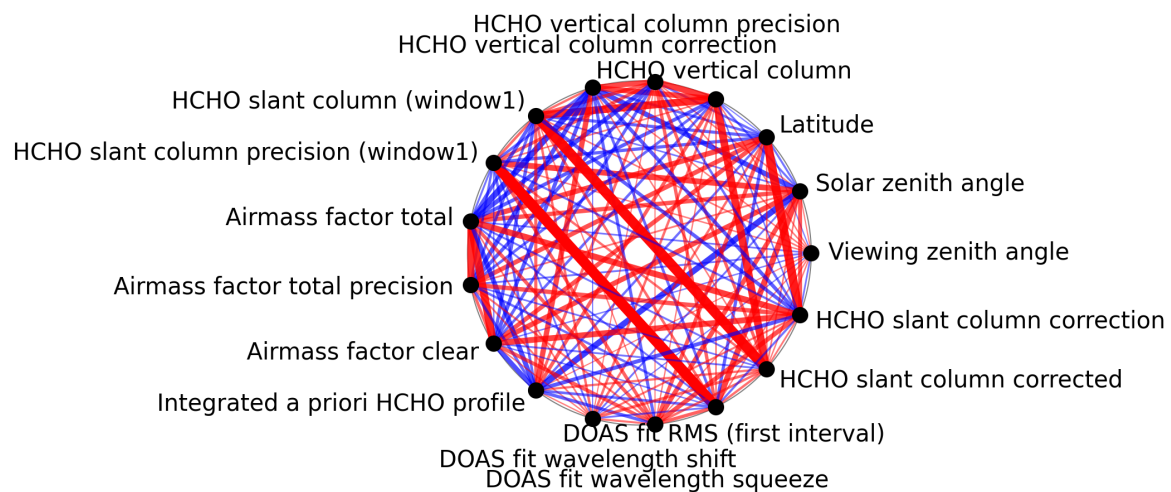
Figure 1: Map of correlation graph for 2025-05-22 to 2025-05-24.
