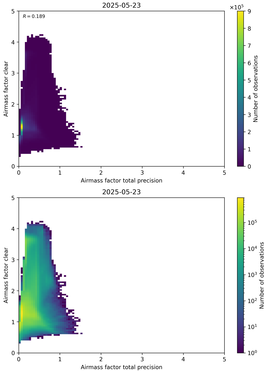
Figure 108: Scatter density plot of “Airmass factor total precision” against “Airmass factor clear” for 2025-05-22 to 2025-05-24.
