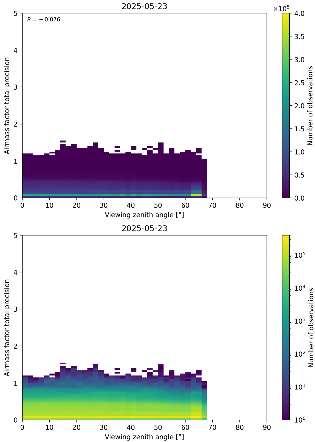
Figure 191: Scatter density plot of “Viewing zenith angle” against “Airmass factor total precision” for 2025-05-22 to 2025-05-24.
