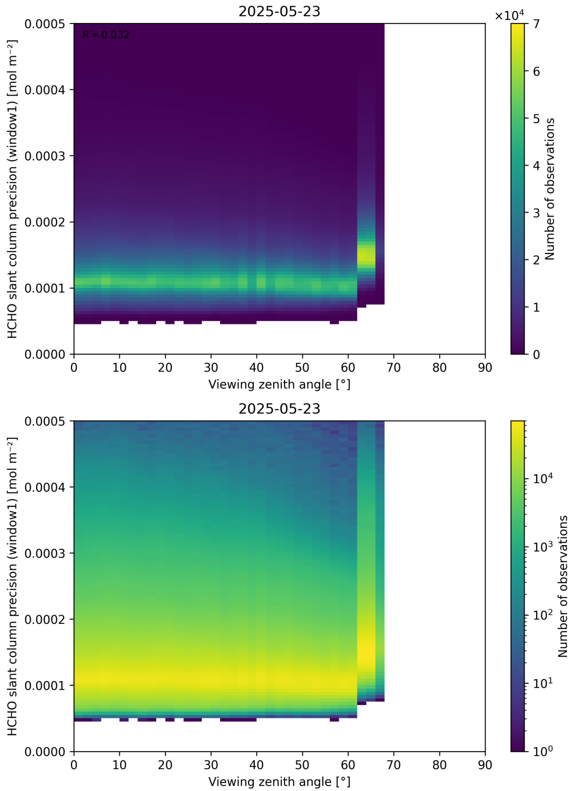
Figure 189: Scatter density plot of “Viewing zenith angle” against “HCHO slant column precision (window1)” for 2025-05-22 to 2025-05-24.
