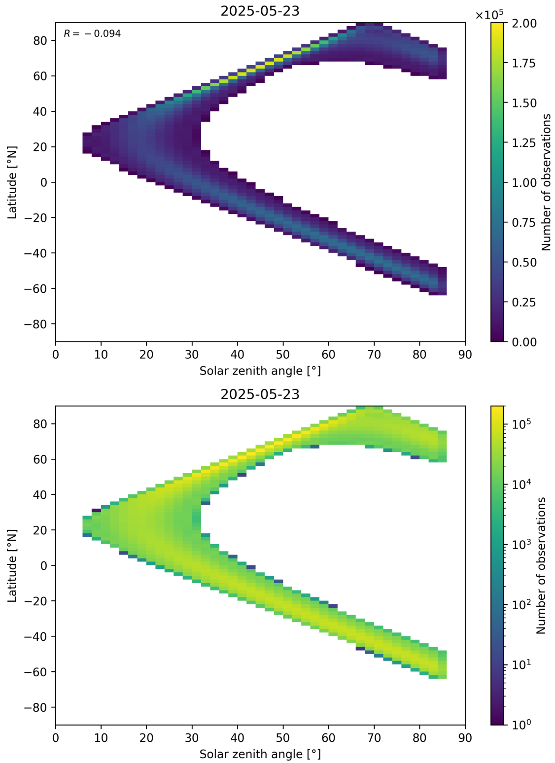
Figure 181: Scatter density plot of “Solar zenith angle” against “Latitude” for 2025-05-22 to 2025-05-24.
