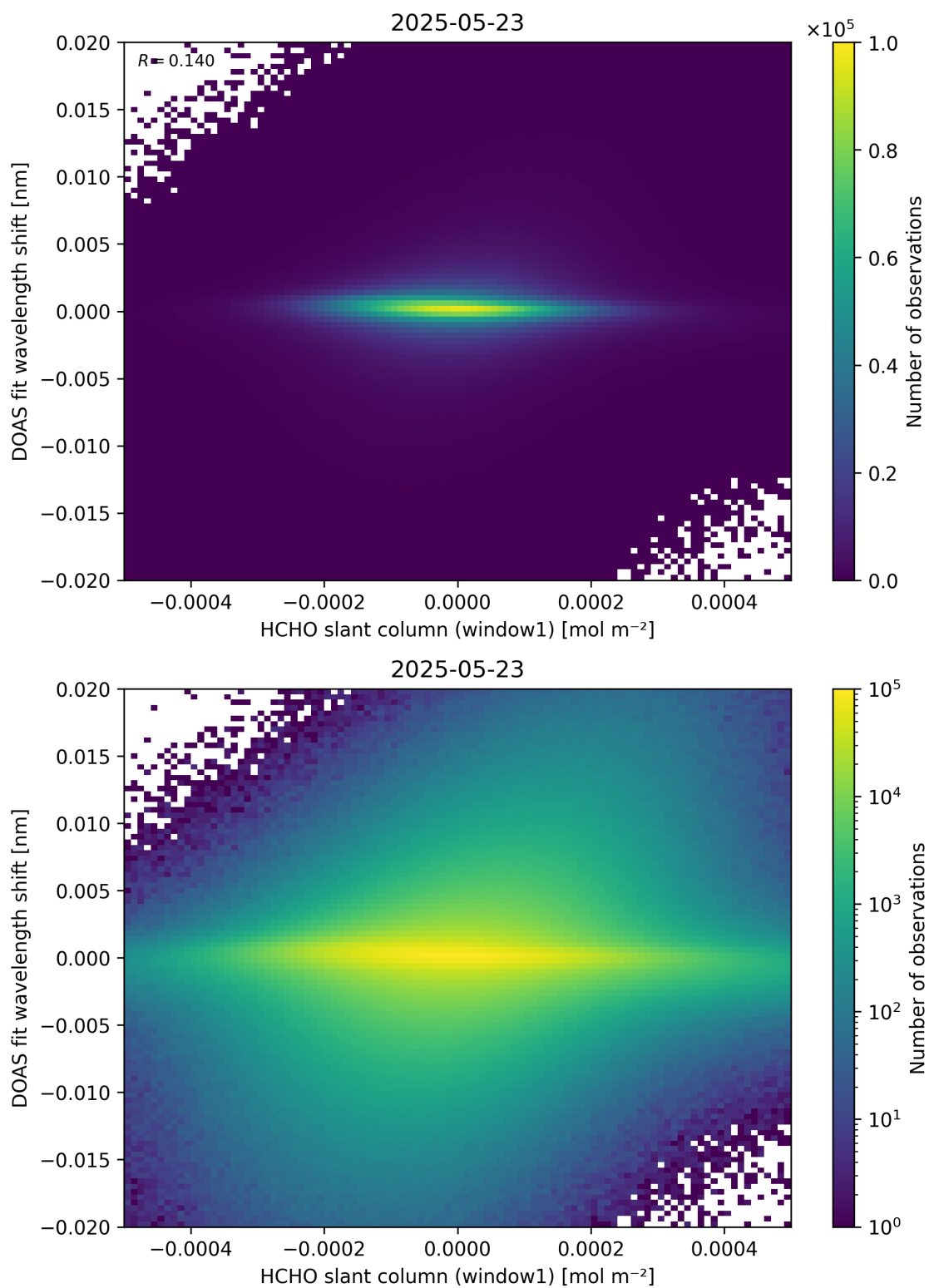
Figure 79: Scatter density plot of “HCHO slant column (window1)” against “DOAS fit wavelength shift” for 2025-05-22 to 2025-05-24.
