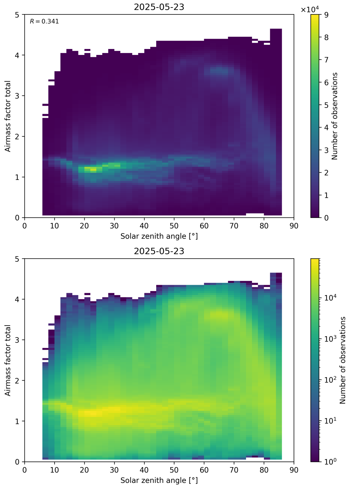
Figure 175: Scatter density plot of “Solar zenith angle” against “Airmass factor total” for 2025-05-22 to 2025-05-24.
