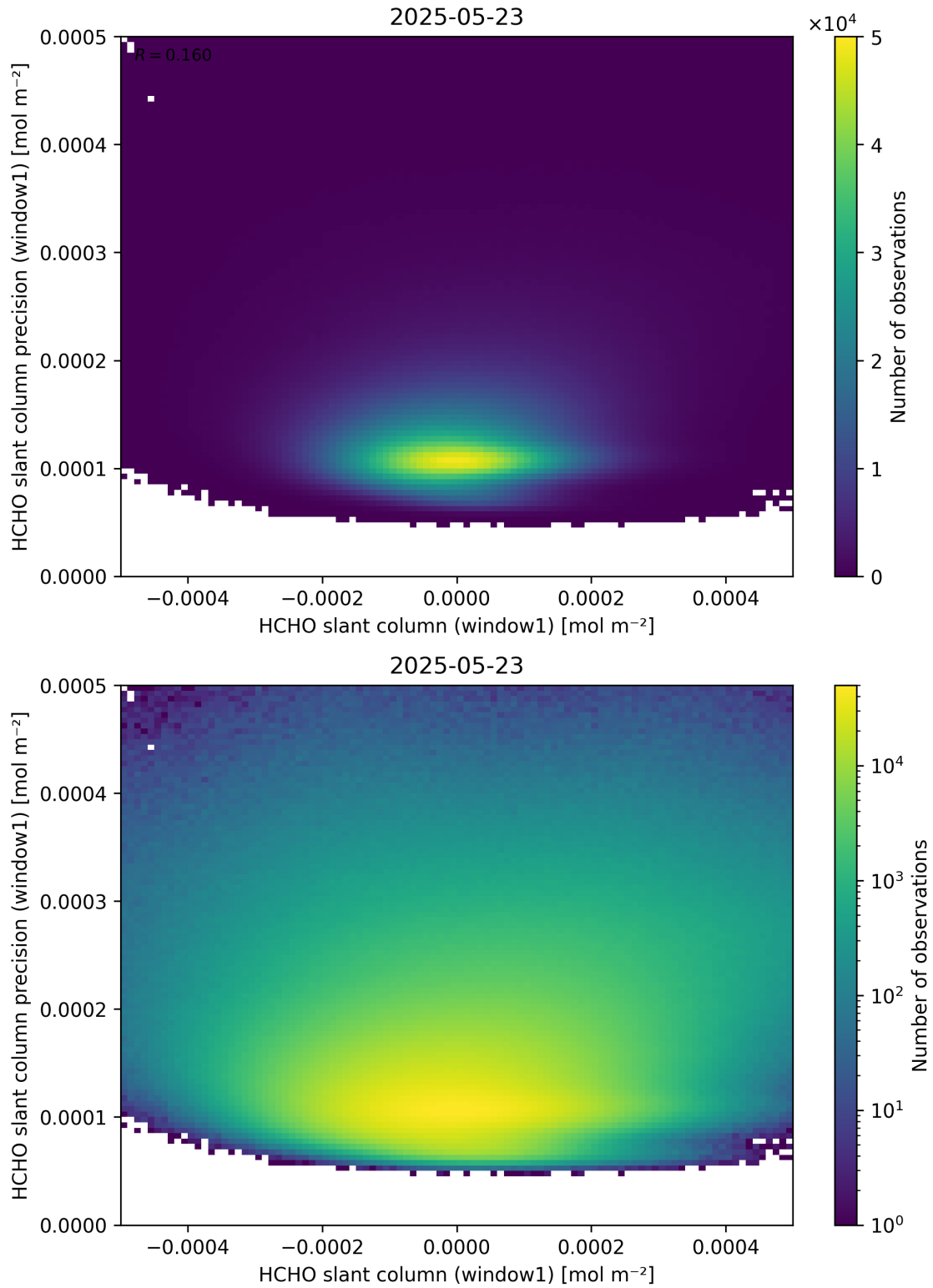
Figure 84: Scatter density plot of “HCHO slant column (window1)” against “HCHO slant column precision (window1)” for 2025-05-22 to 2025-05-24.
