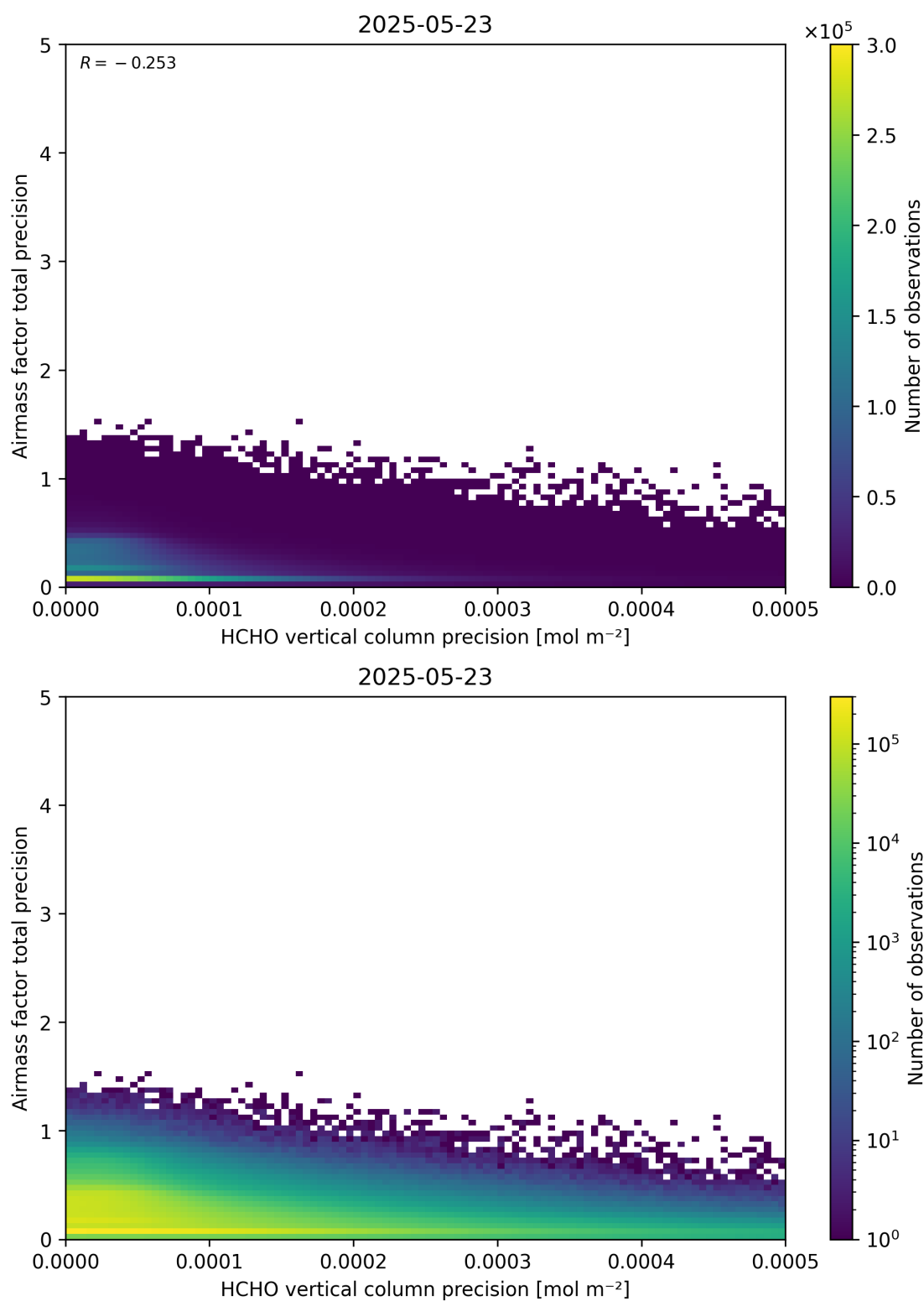
Figure 145: Scatter density plot of “HCHO vertical column precision” against “Airmass factor total precision” for 2025-05-22 to 2025-05-24.
