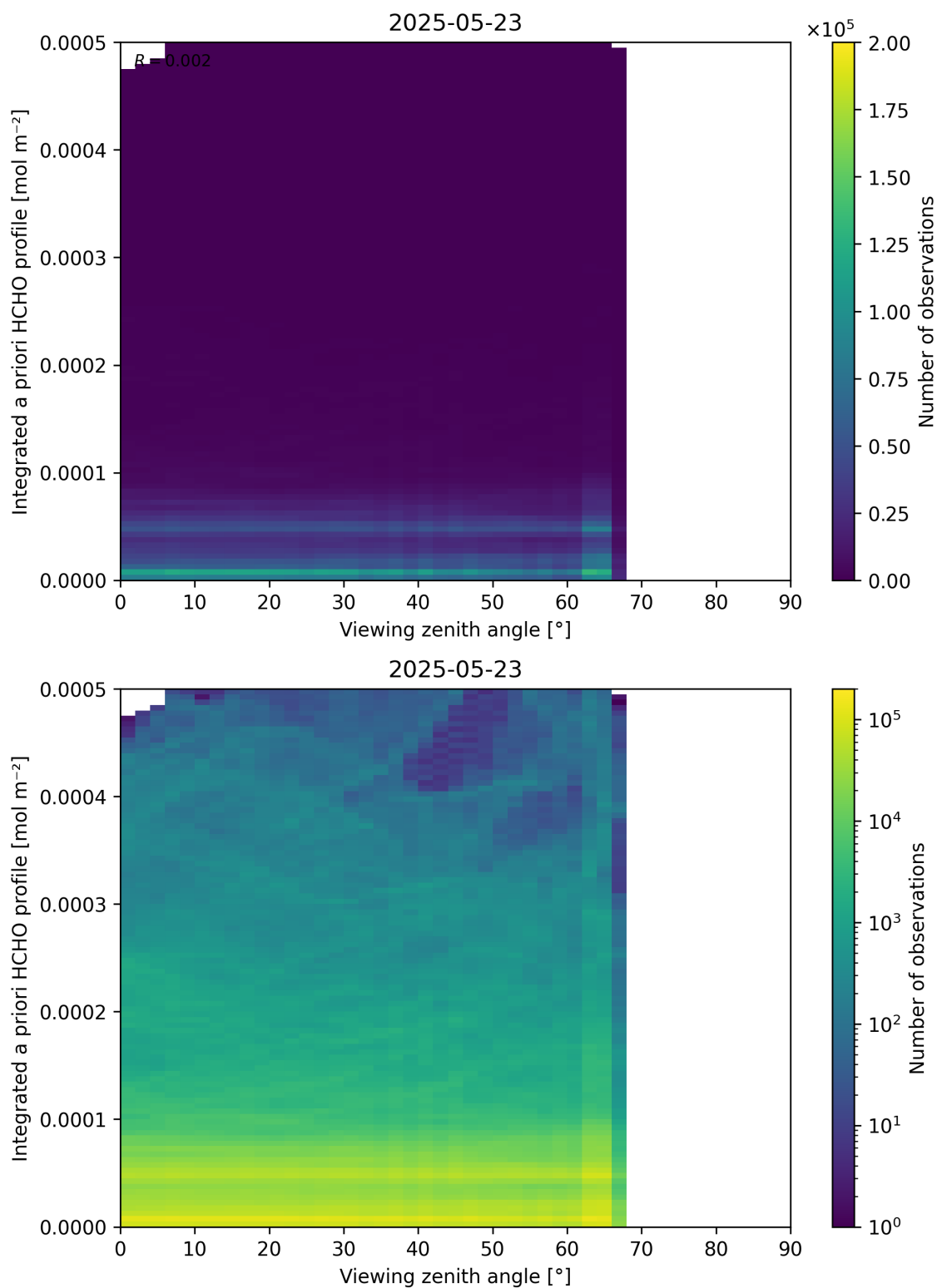
Figure 195: Scatter density plot of “Viewing zenith angle” against “Integrated a priori HCHO profile” for 2025-05-22 to 2025-05-24.
