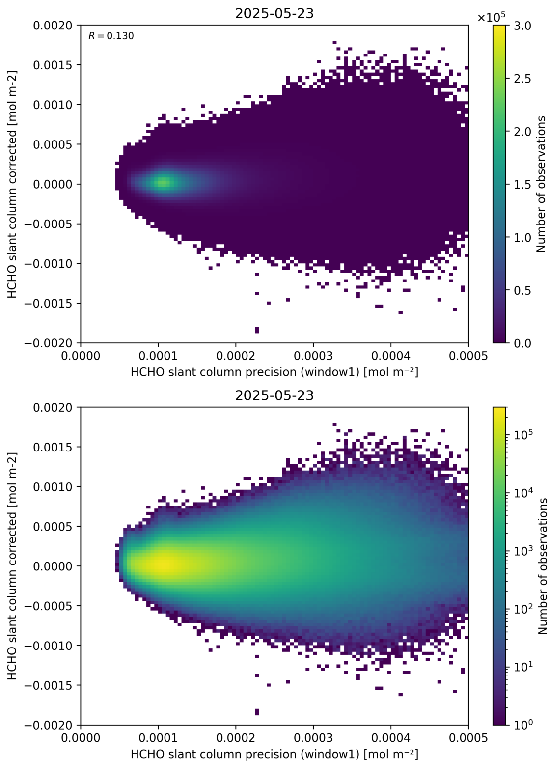
Figure 92: Scatter density plot of “HCHO slant column precision (window1)” against “HCHO slant column corrected” for 2025-05-22 to 2025-05-24.
