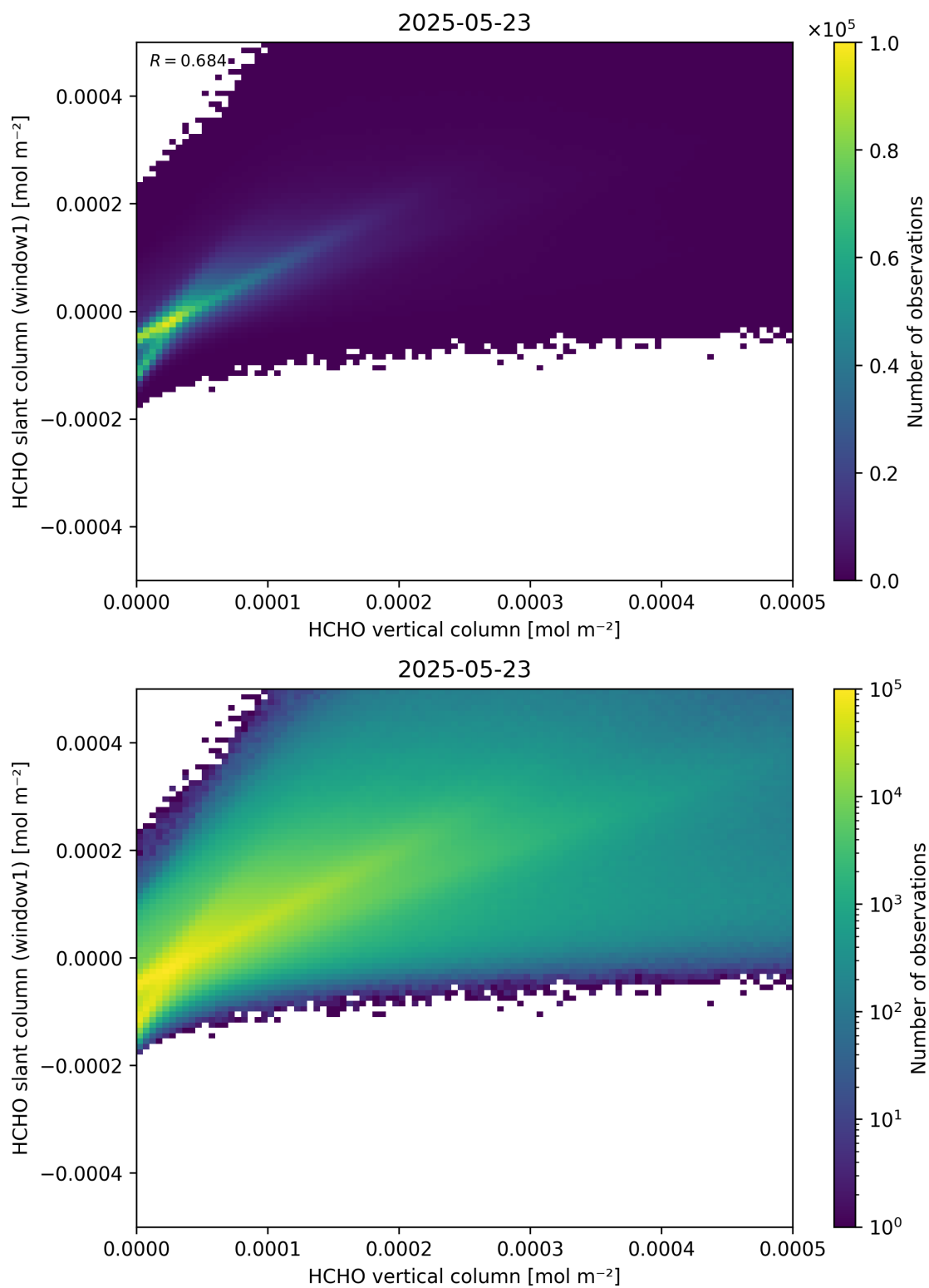
Figure 129: Scatter density plot of “HCHO vertical column” against “HCHO slant column (window1)” for 2025-05-22 to 2025-05-24.
