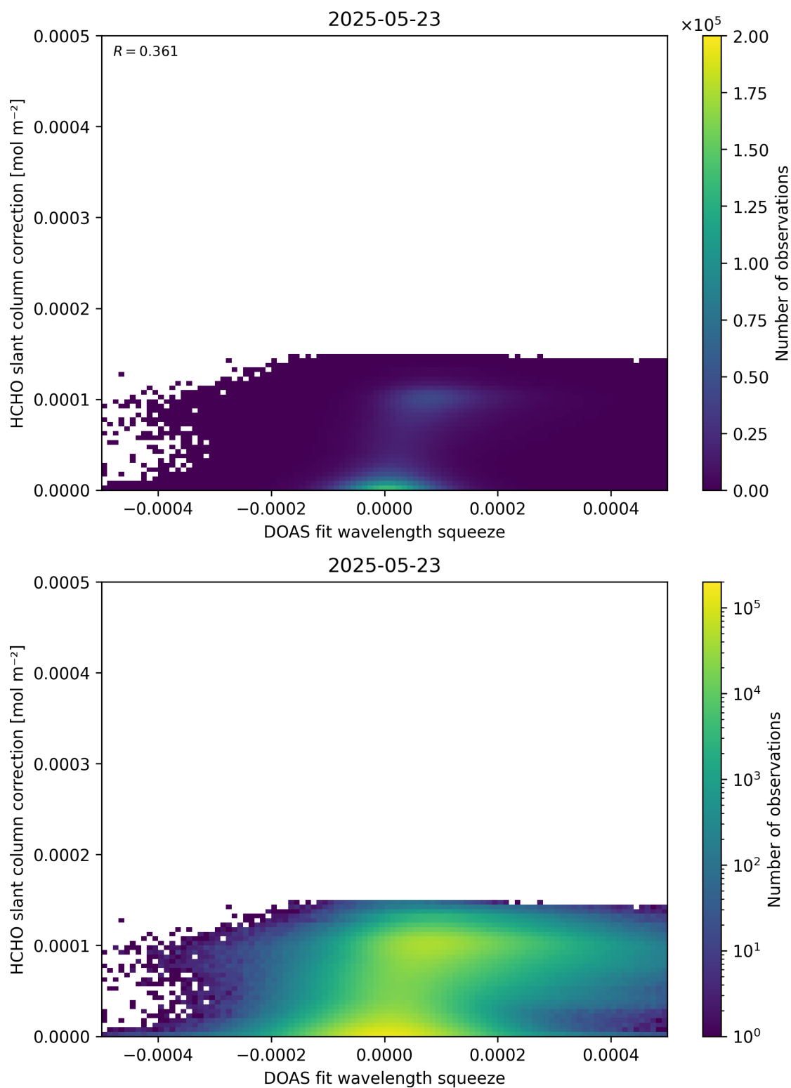
Figure 70: Scatter density plot of “DOAS fit wavelength squeeze” against “HCHO slant column correction” for 2025-05-22 to 2025-05-24.
