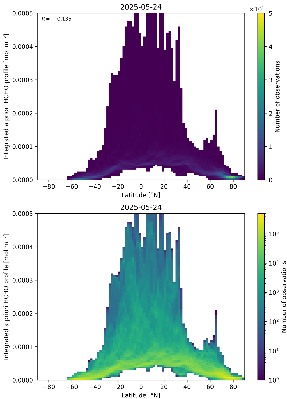
Figure 166: Scatter density plot of “Latitude” against “Integrated a priori HCHO profile” for 2025-05-23 to 2025-05-25.
