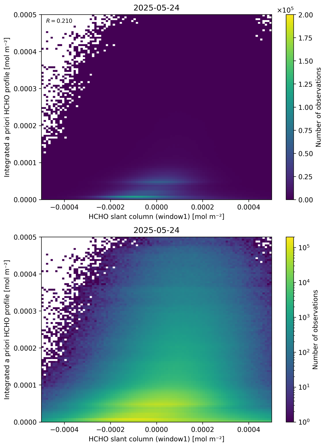
Figure 87: Scatter density plot of “HCHO slant column (window1)” against “Integrated a priori HCHO profile” for 2025-05-23 to 2025-05-25.
