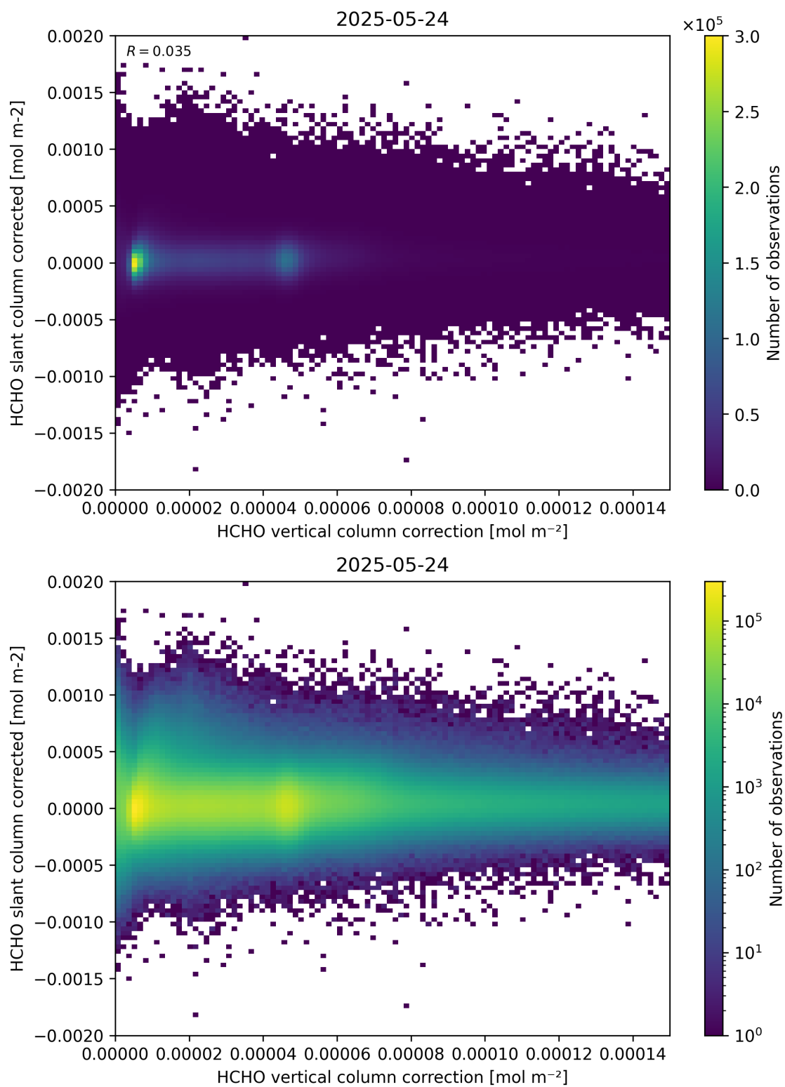
Figure 116: Scatter density plot of “HCHO vertical column correction” against “HCHO slant column corrected” for 2025-05-23 to 2025-05-25.
