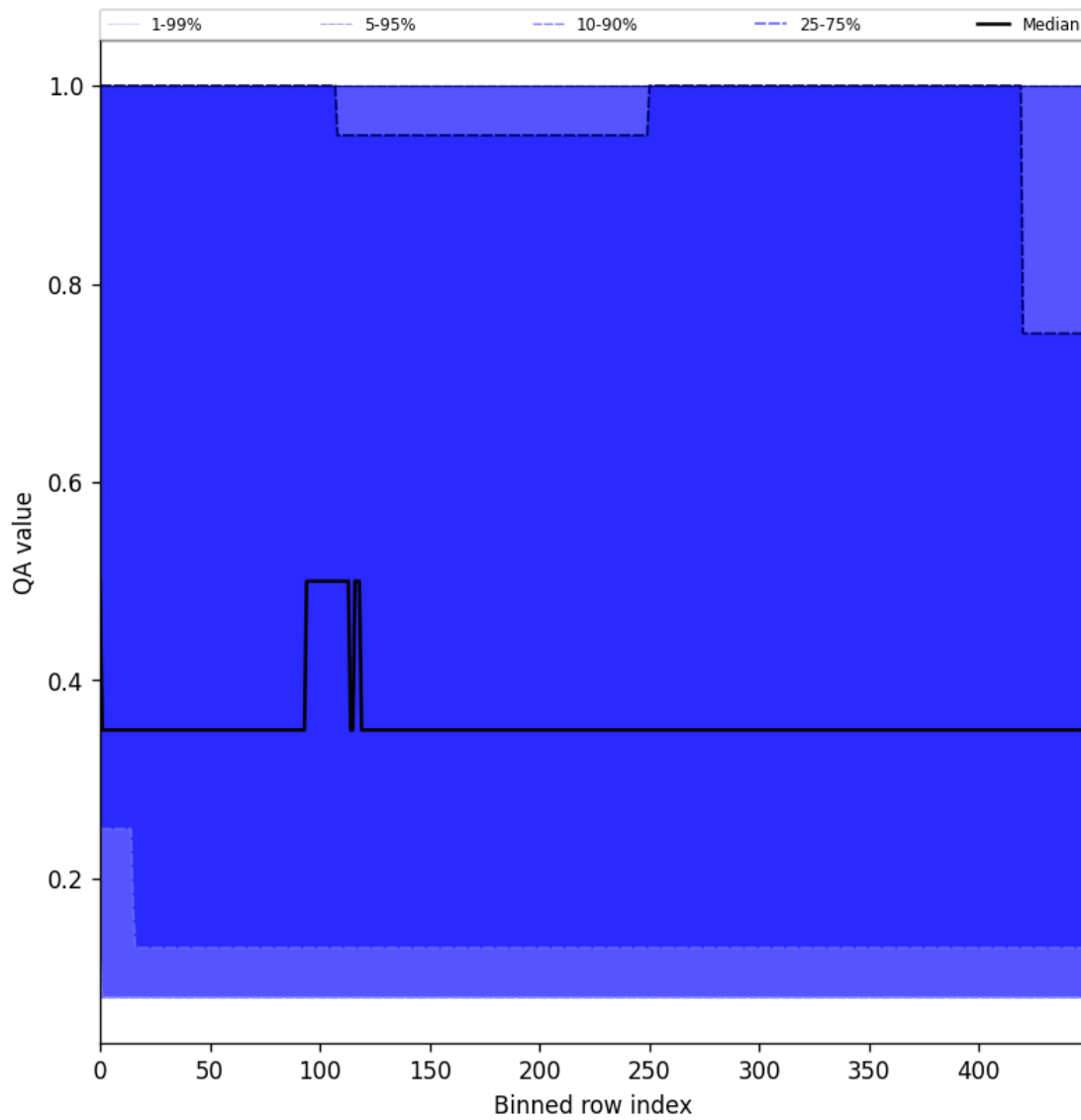
Figure 48: Along track statistics of “QA value” for 2025-05-23 to 2025-05-25
