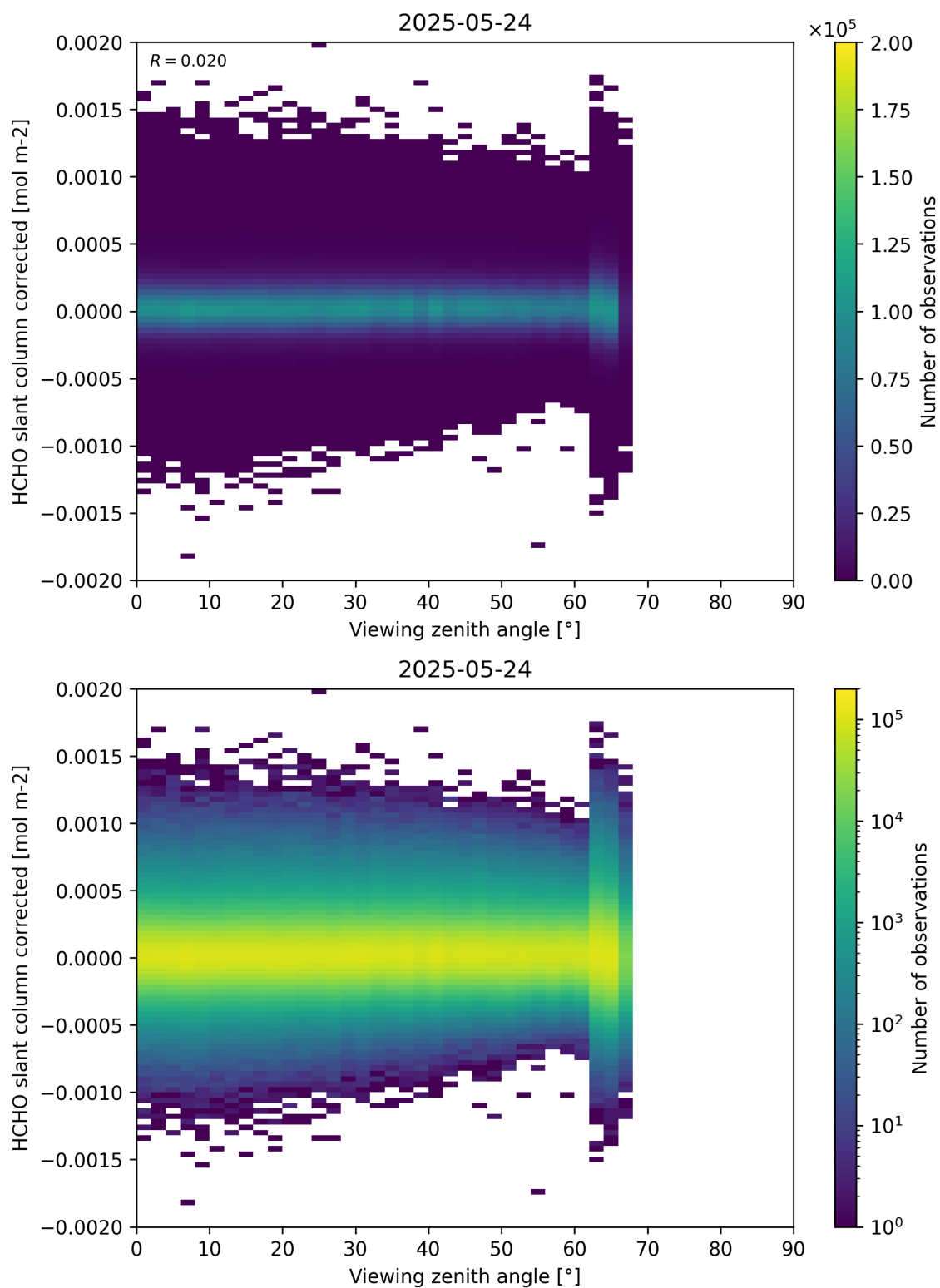
Figure 186: Scatter density plot of “Viewing zenith angle” against “HCHO slant column corrected” for 2025-05-23 to 2025-05-25.
