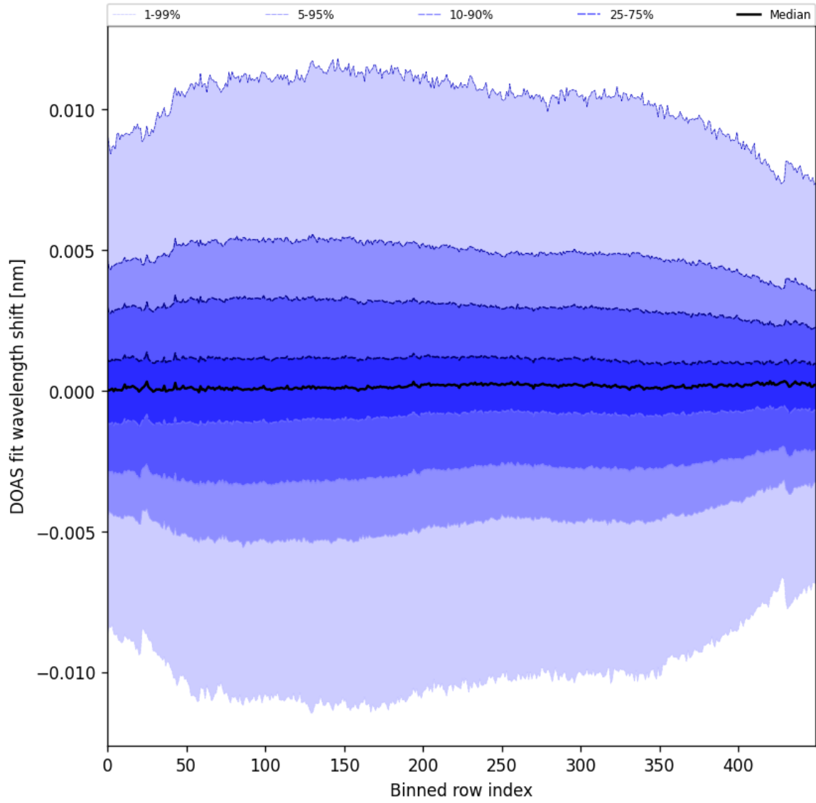
Figure 58: Along track statistics of “DOAS fit wavelength shift” for 2025-05-23 to 2025-05-25
