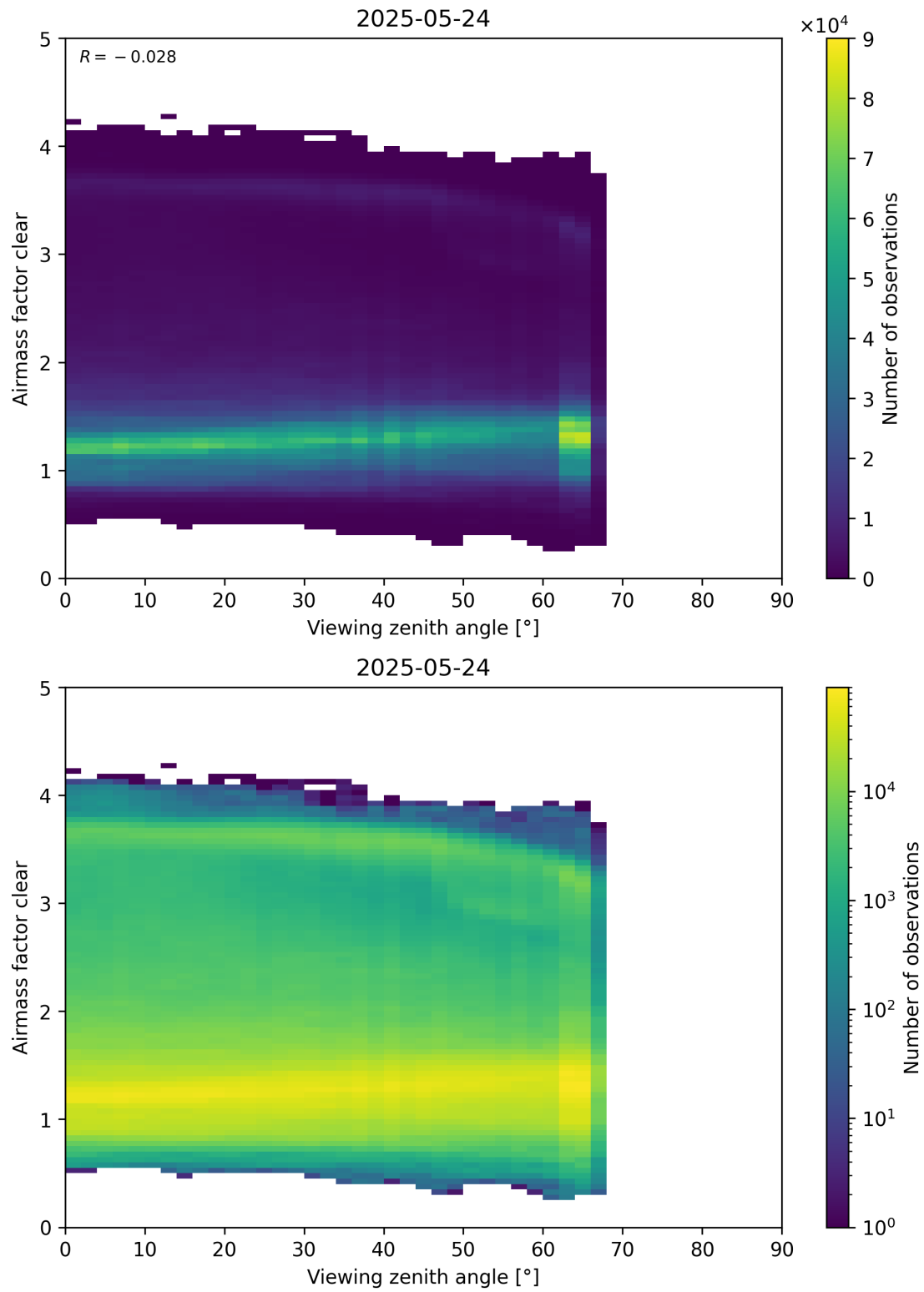
Figure 185: Scatter density plot of “Viewing zenith angle” against “Airmass factor clear” for 2025-05-23 to 2025-05-25.
