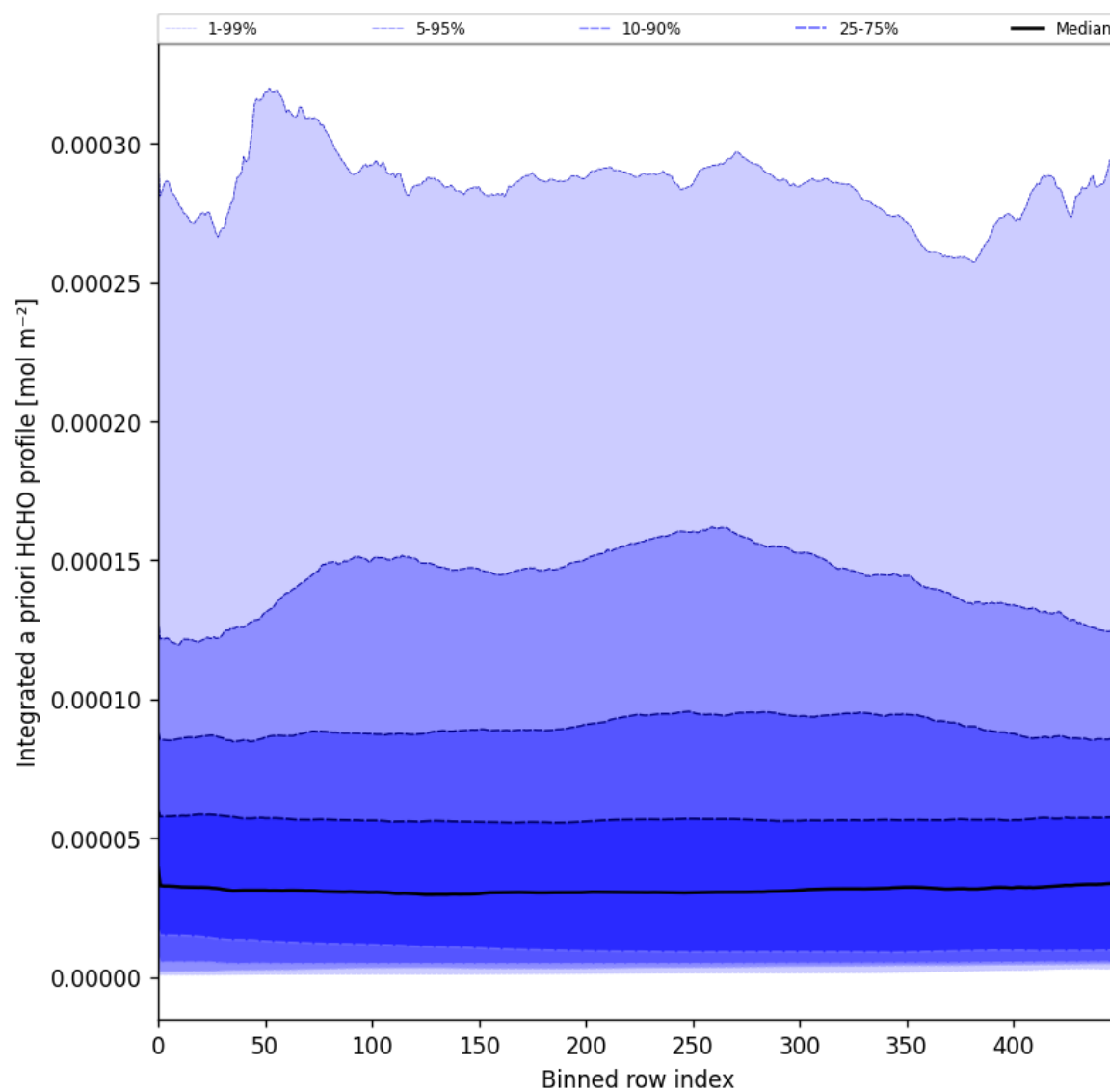
Figure 57: Along track statistics of "Integrated a priori HCHO profile" for 2025-05-23 to 2025-05-25
