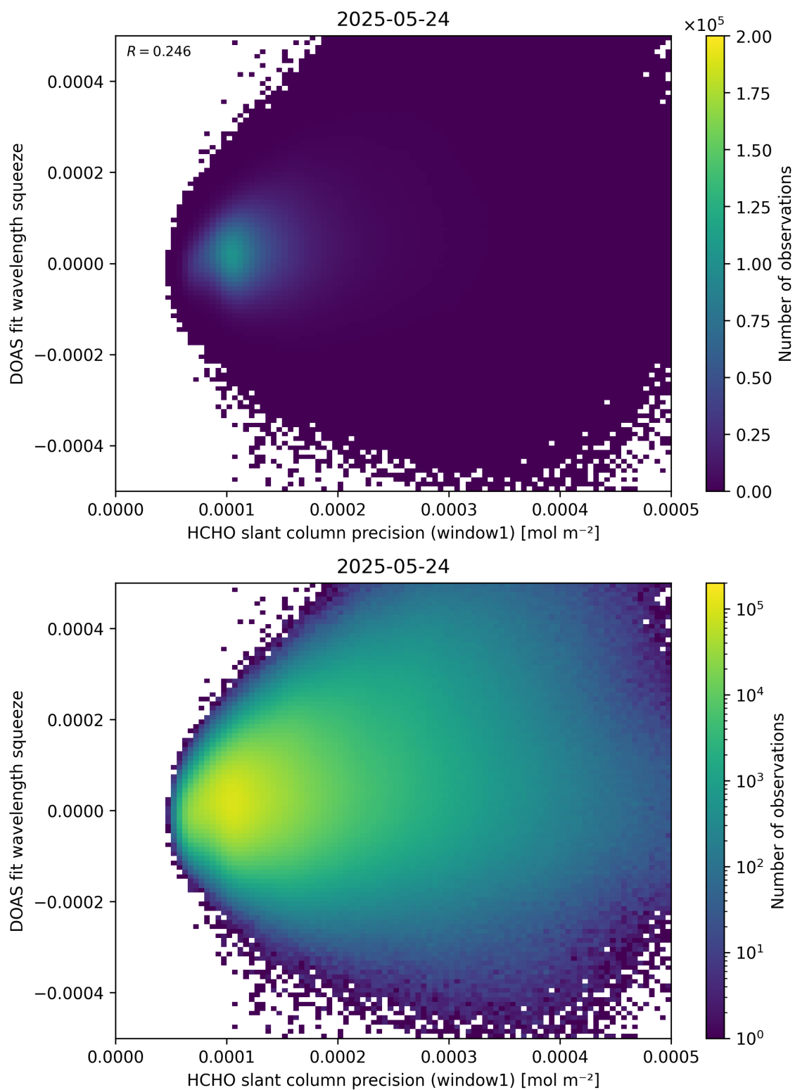
Figure 90: Scatter density plot of “HCHO slant column precision (window1)” against “DOAS fit wavelength squeeze” for 2025-05-23 to 2025-05-25.
