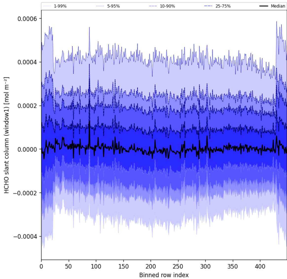
Figure 52: Along track statistics of “HCHO slant column (window1)” for 2025-05-23 to 2025-05-25
