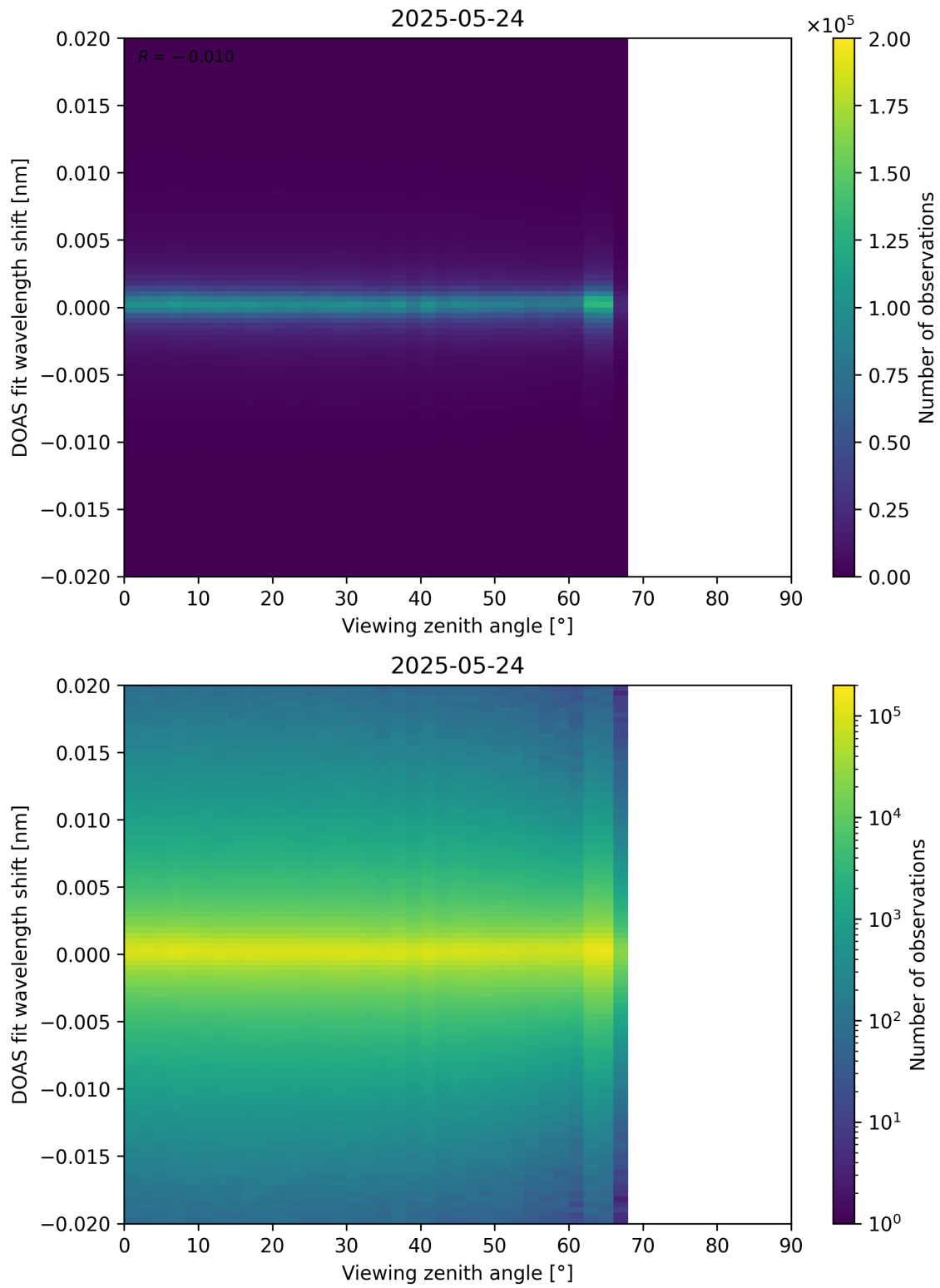
Figure 183: Scatter density plot of “Viewing zenith angle” against “DOAS fit wavelength shift” for 2025-05-23 to 2025-05-25.
