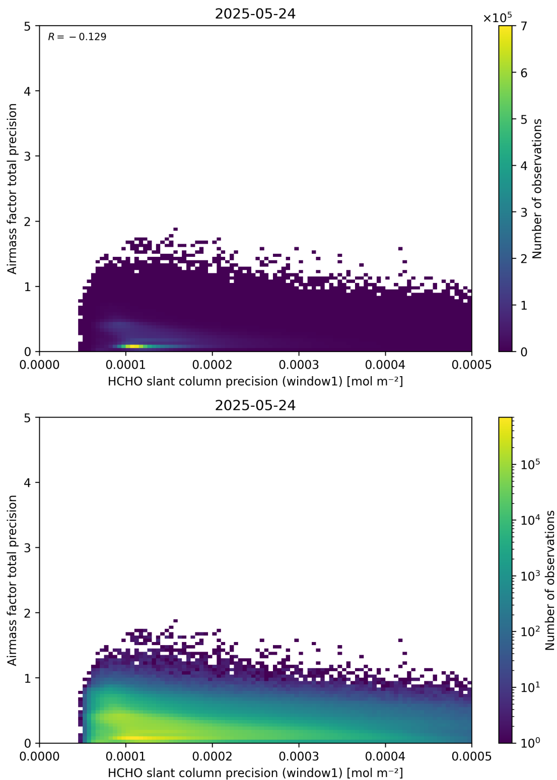
Figure 95: Scatter density plot of “HCHO slant column precision (window1)” against “Airmass factor total precision” for 2025-05-23 to 2025-05-25.
