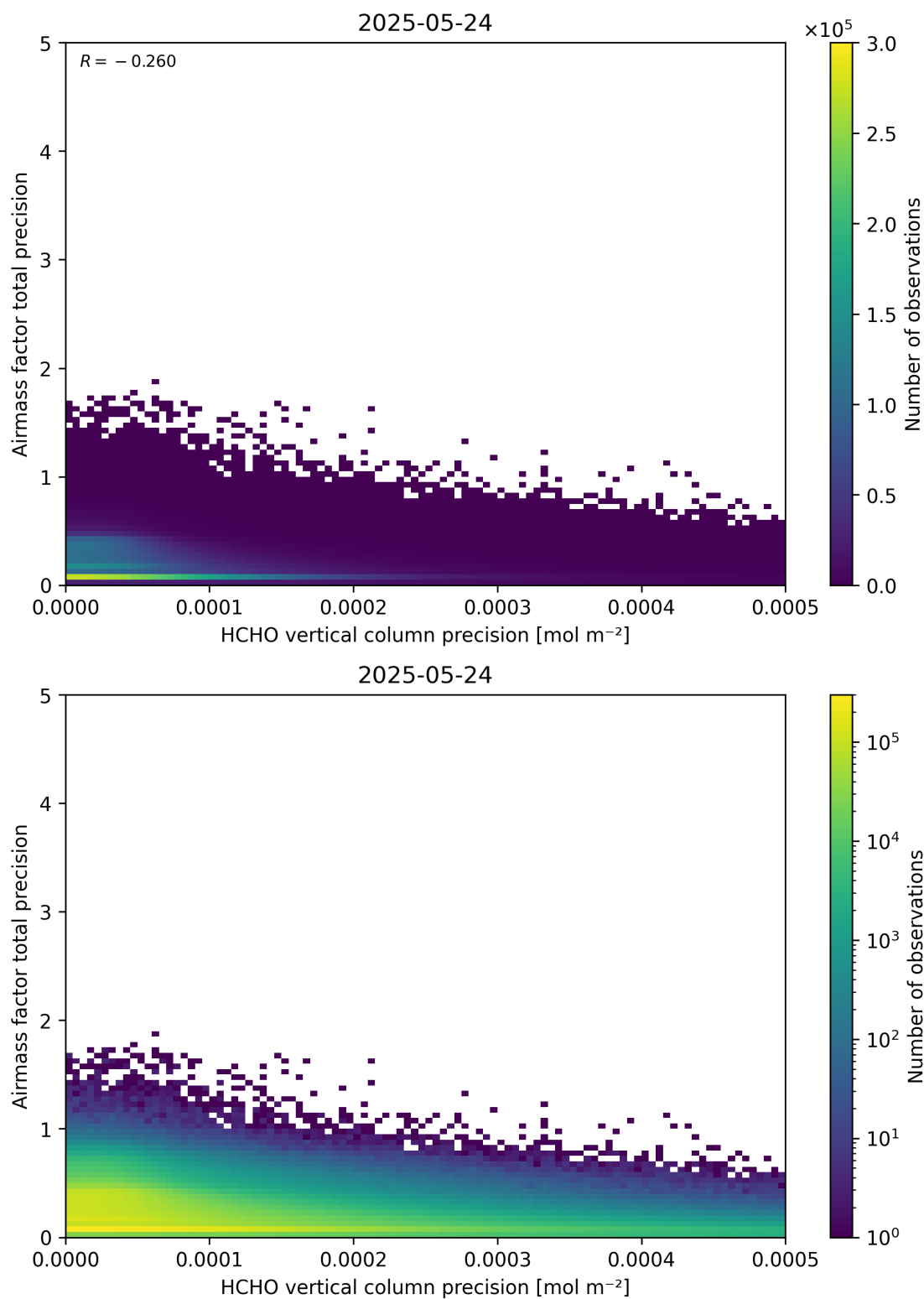
Figure 145: Scatter density plot of “HCHO vertical column precision” against “Airmass factor total precision” for 2025-05-23 to 2025-05-25.
