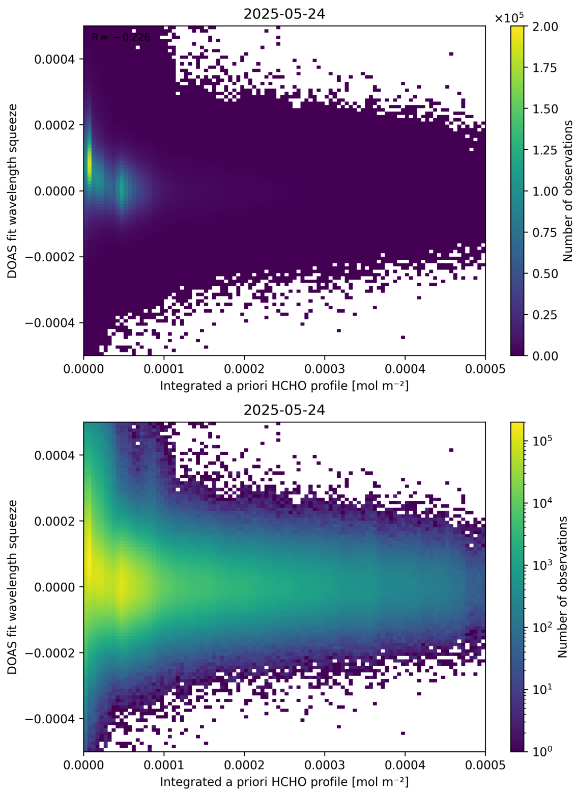
Figure 150: Scatter density plot of “Integrated a priori HCHO profile” against “DOAS fit wavelength squeeze” for 2025-05-23 to 2025-05-25.
