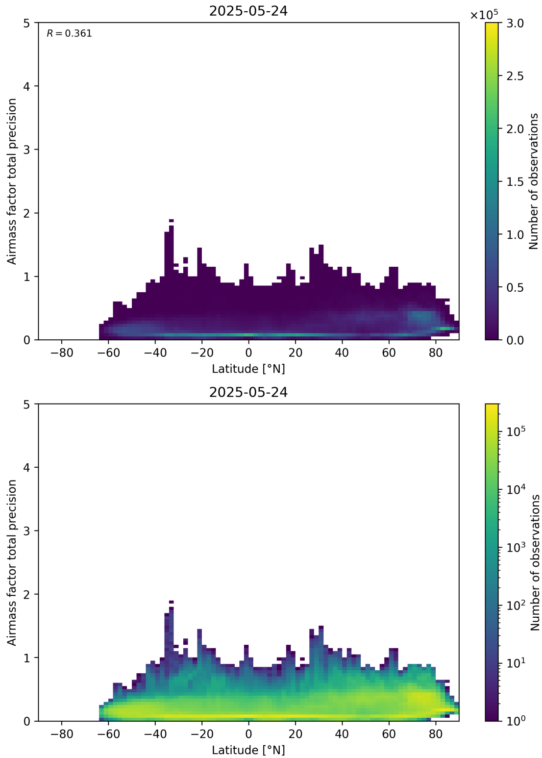
Figure 162: Scatter density plot of “Latitude” against “Airmass factor total precision” for 2025-05-23 to 2025-05-25.
