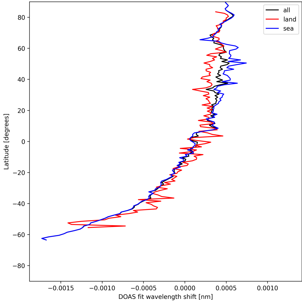
Figure 30: Zonal average of “DOAS fit wavelength shift” for 2025-05-23 to 2025-05-25.
