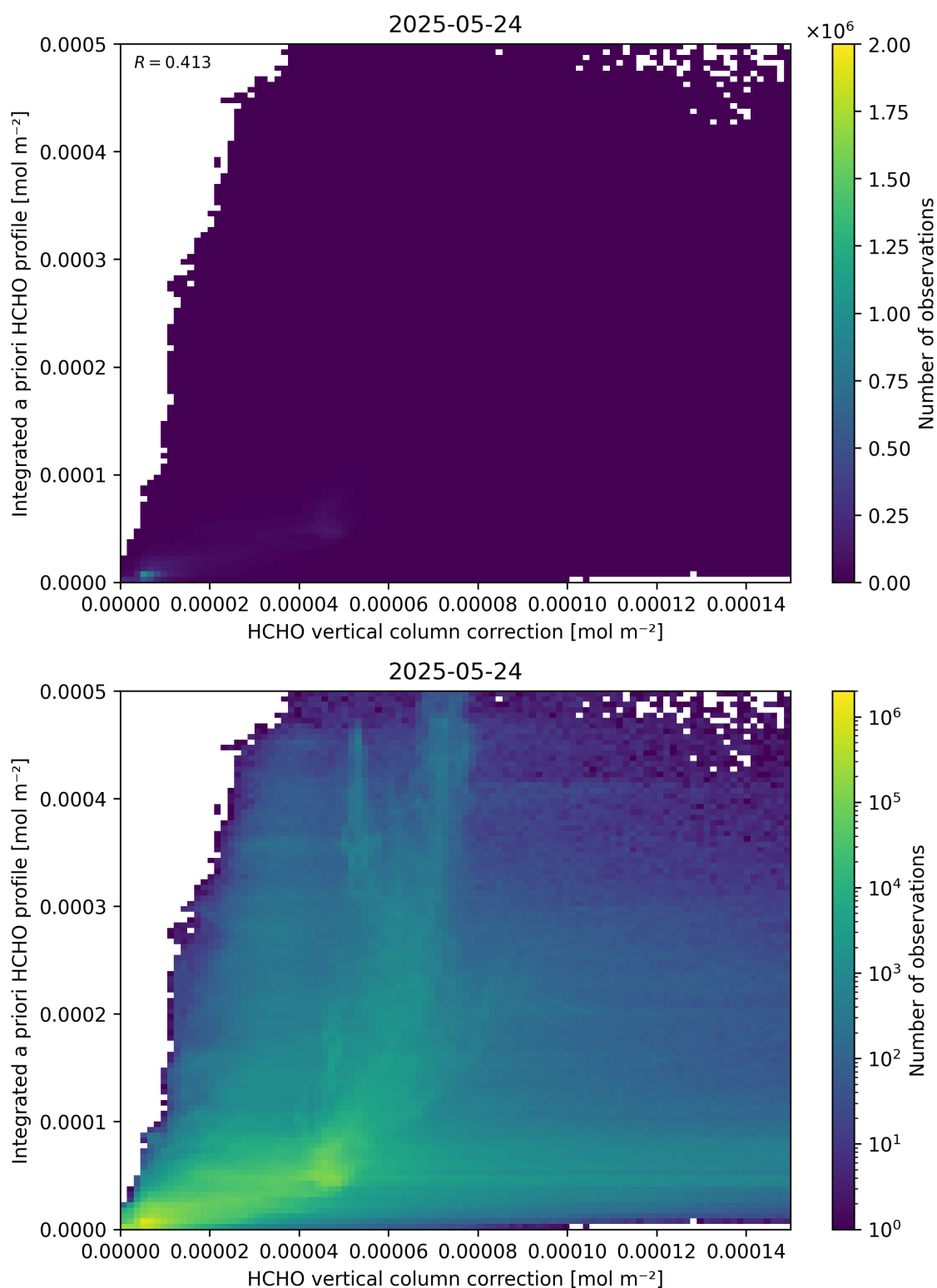
Figure 122: Scatter density plot of “HCHO vertical column correction” against “Integrated a priori HCHO profile” for 2025-05-23 to 2025-05-25.
