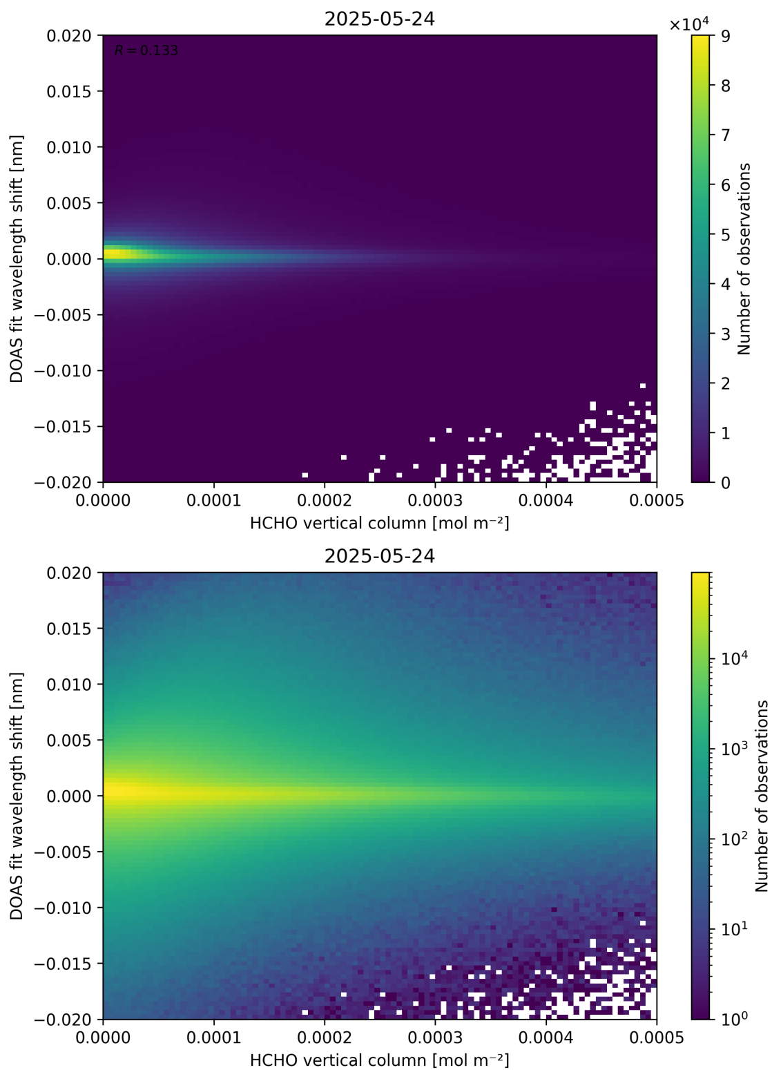
Figure 124: Scatter density plot of “HCHO vertical column” against “DOAS fit wavelength shift” for 2025-05-23 to 2025-05-25.
