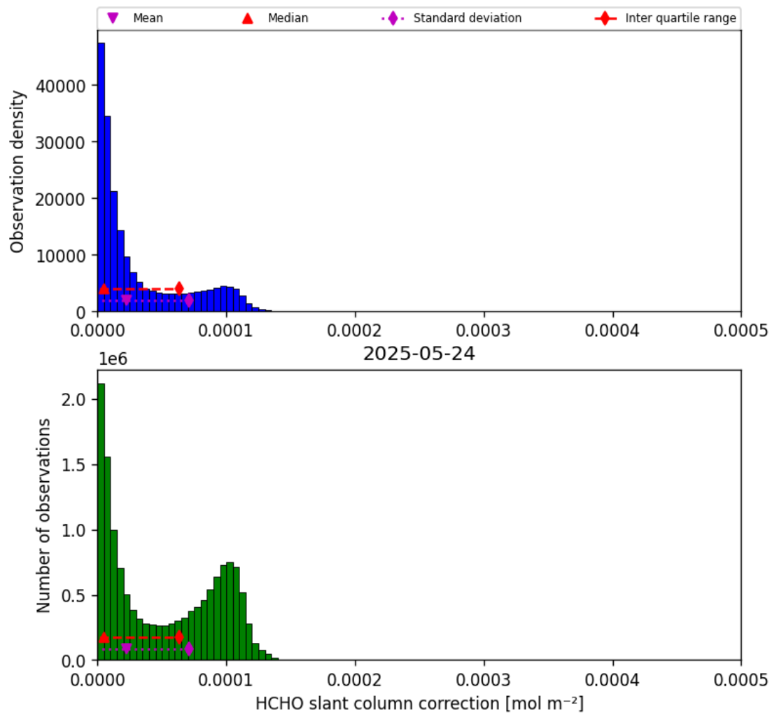
Figure 47: Histogram of “HCHO slant column correction” for 2025-05-23 to 2025-05-25
