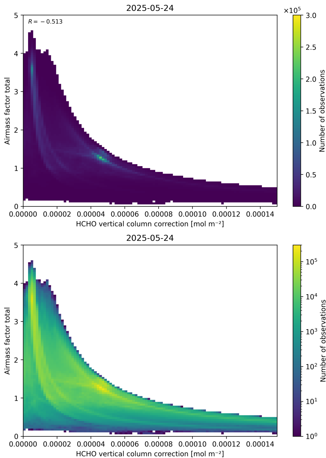
Figure 120: Scatter density plot of “HCHO vertical column correction” against “Airmass factor total” for 2025-05-23 to 2025-05-25.
