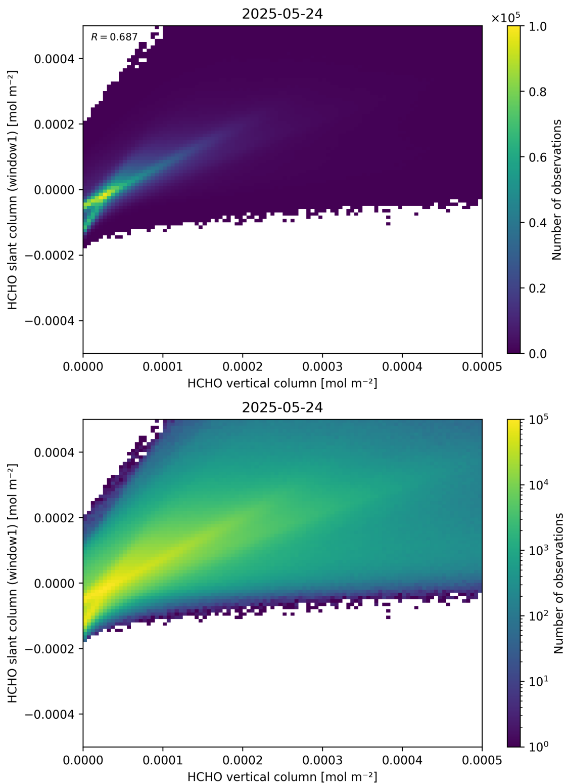
Figure 129: Scatter density plot of “HCHO vertical column” against “HCHO slant column (window1)” for 2025-05-23 to 2025-05-25.
