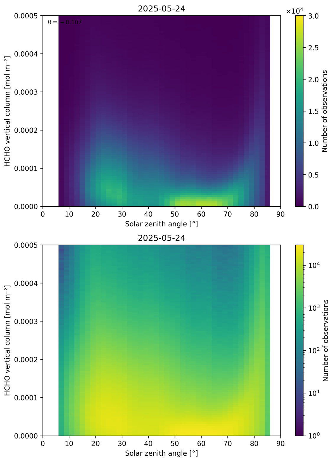
Figure 177: Scatter density plot of “Solar zenith angle” against “HCHO vertical column” for 2025-05-23 to 2025-05-25.
