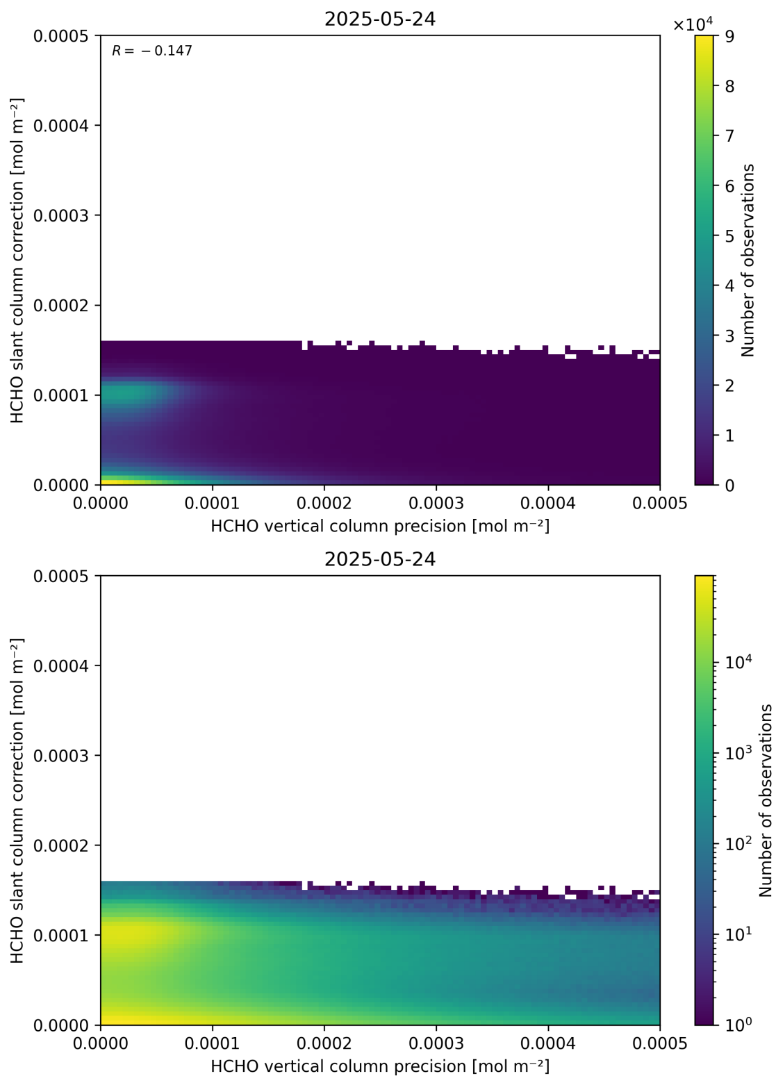
Figure 141: Scatter density plot of “HCHO vertical column precision” against “HCHO slant column correction” for 2025-05-23 to 2025-05-25.
