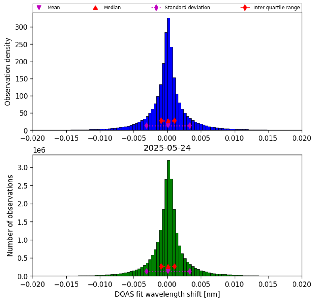
Figure 44: Histogram of “DOAS fit wavelength shift” for 2025-05-23 to 2025-05-25
