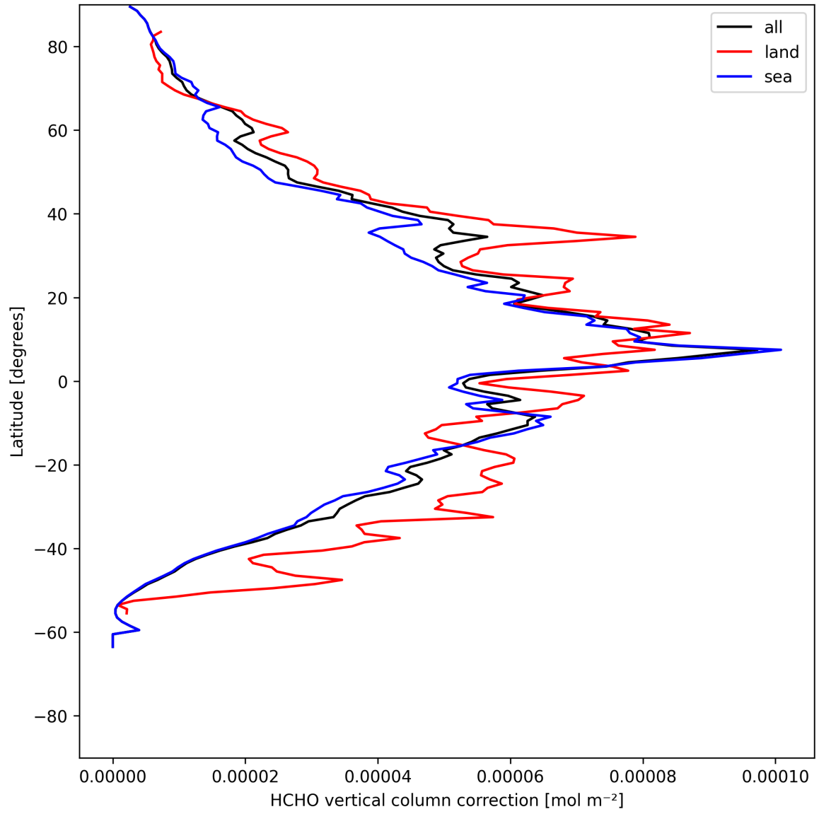
Figure 23: Zonal average of “HCHO vertical column correction” for 2025-05-23 to 2025-05-25.
