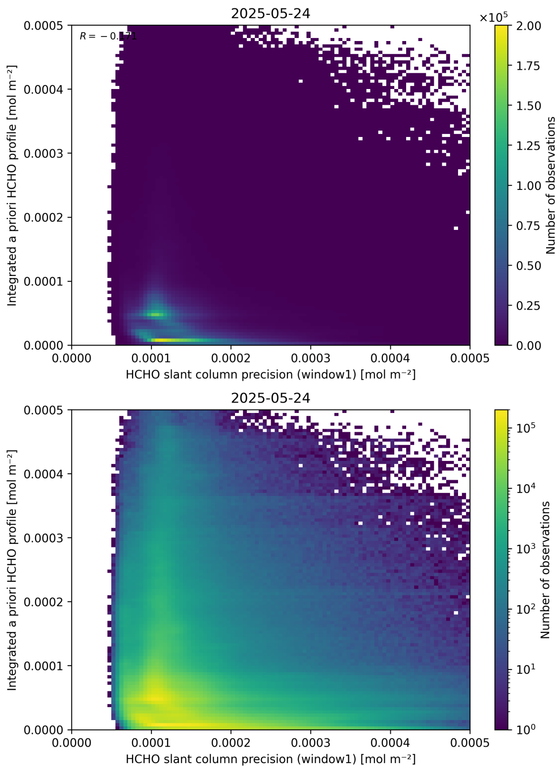
Figure 96: Scatter density plot of “HCHO slant column precision (window1)” against “Integrated a priori HCHO profile” for 2025-05-23 to 2025-05-25.
