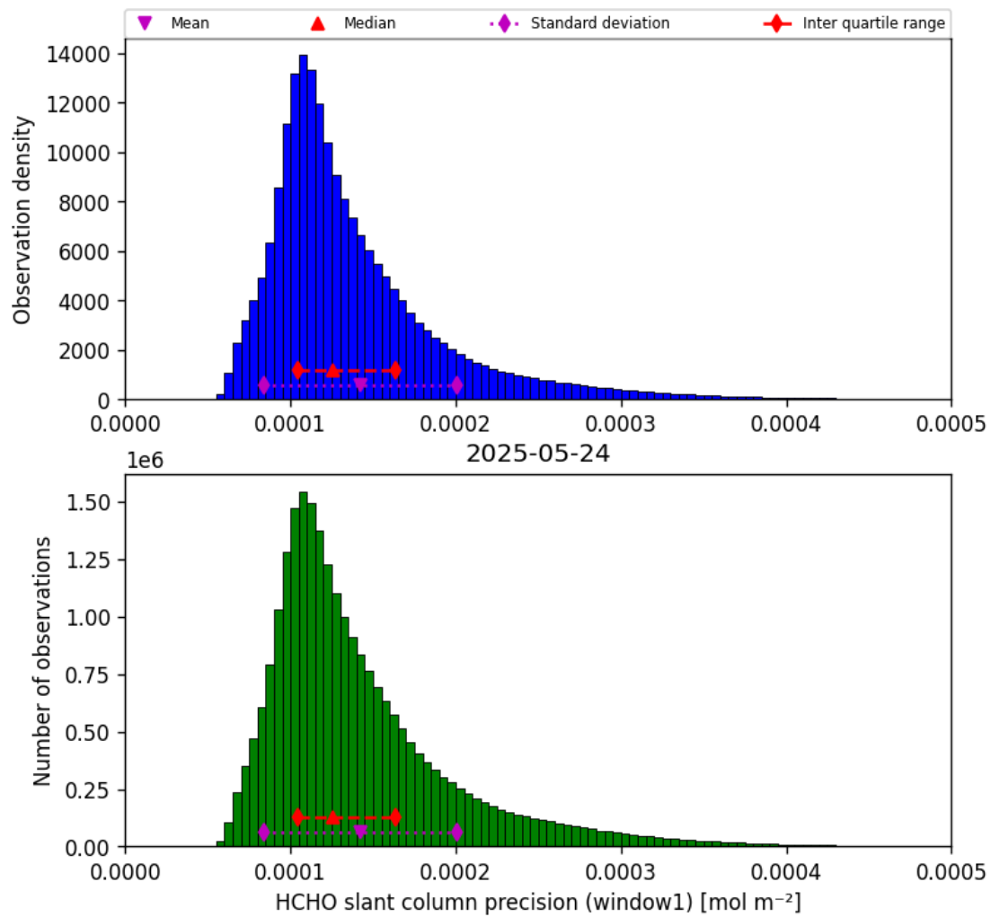
Figure 39: Histogram of “HCHO slant column precision (window1)” for 2025-05-23 to 2025-05-25
