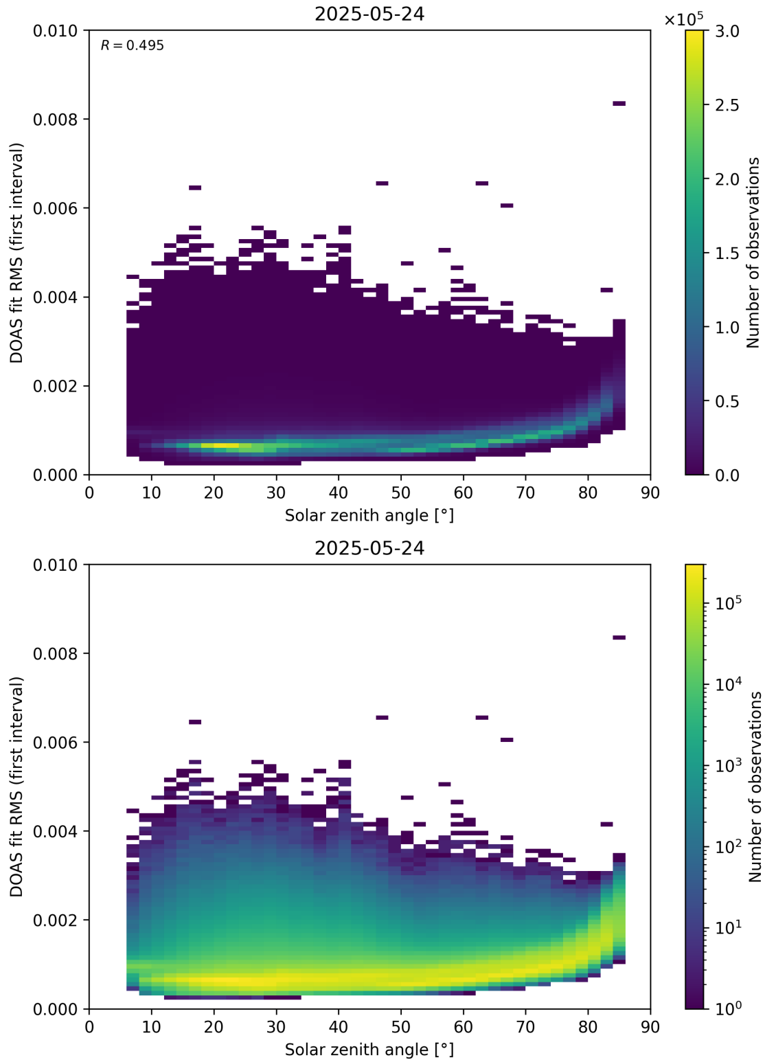
Figure 167: Scatter density plot of “Solar zenith angle” against “DOAS fit RMS (first interval)” for 2025-05-23 to 2025-05-25.
