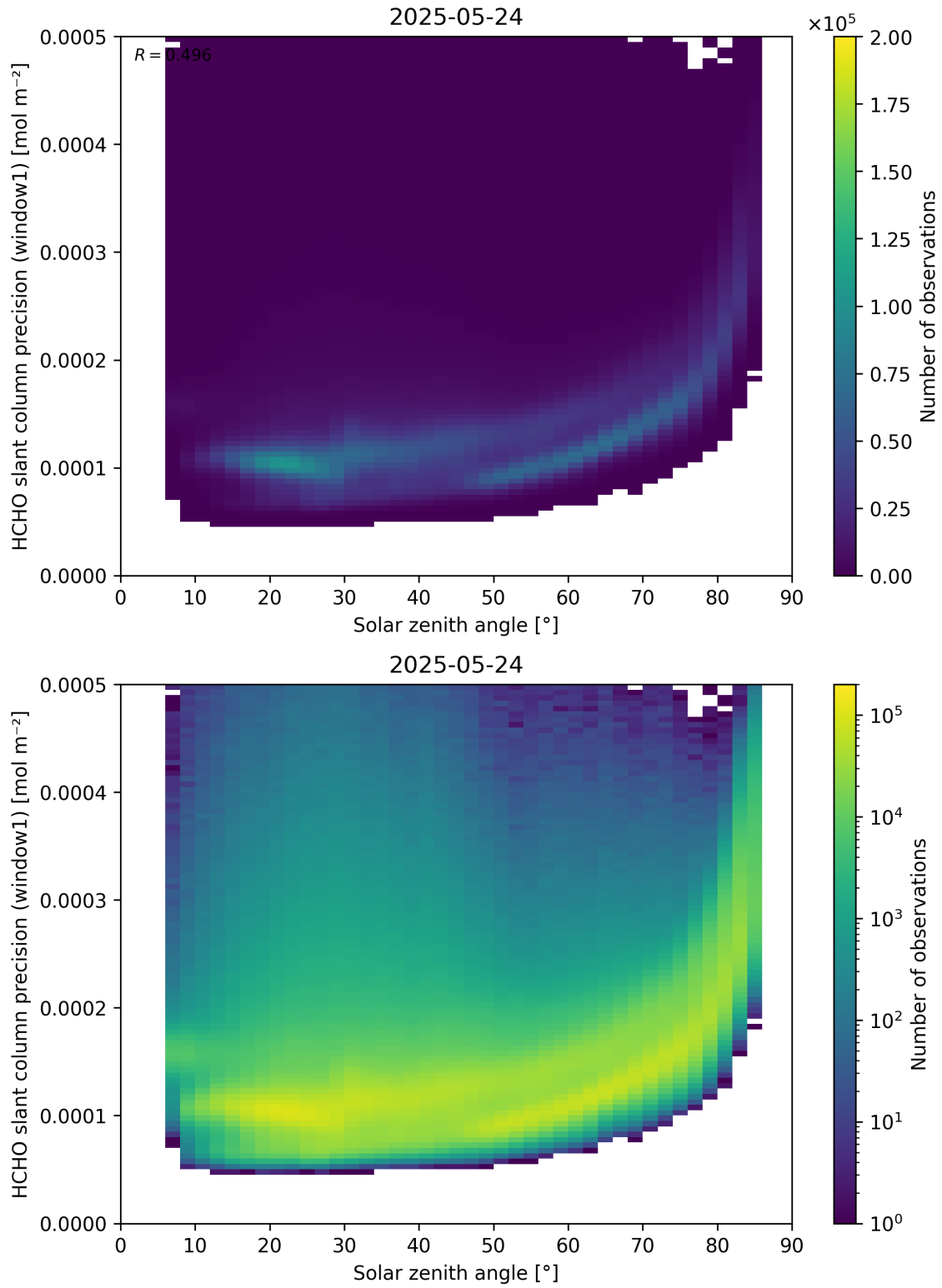
Figure 174: Scatter density plot of “Solar zenith angle” against “HCHO slant column precision (window1)” for 2025-05-23 to 2025-05-25.
