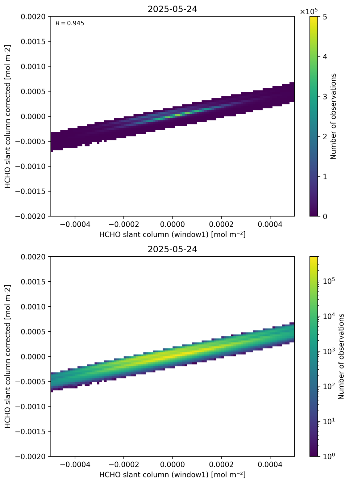
Figure 82: Scatter density plot of “HCHO slant column (window1)” against “HCHO slant column corrected” for 2025-05-23 to 2025-05-25.
