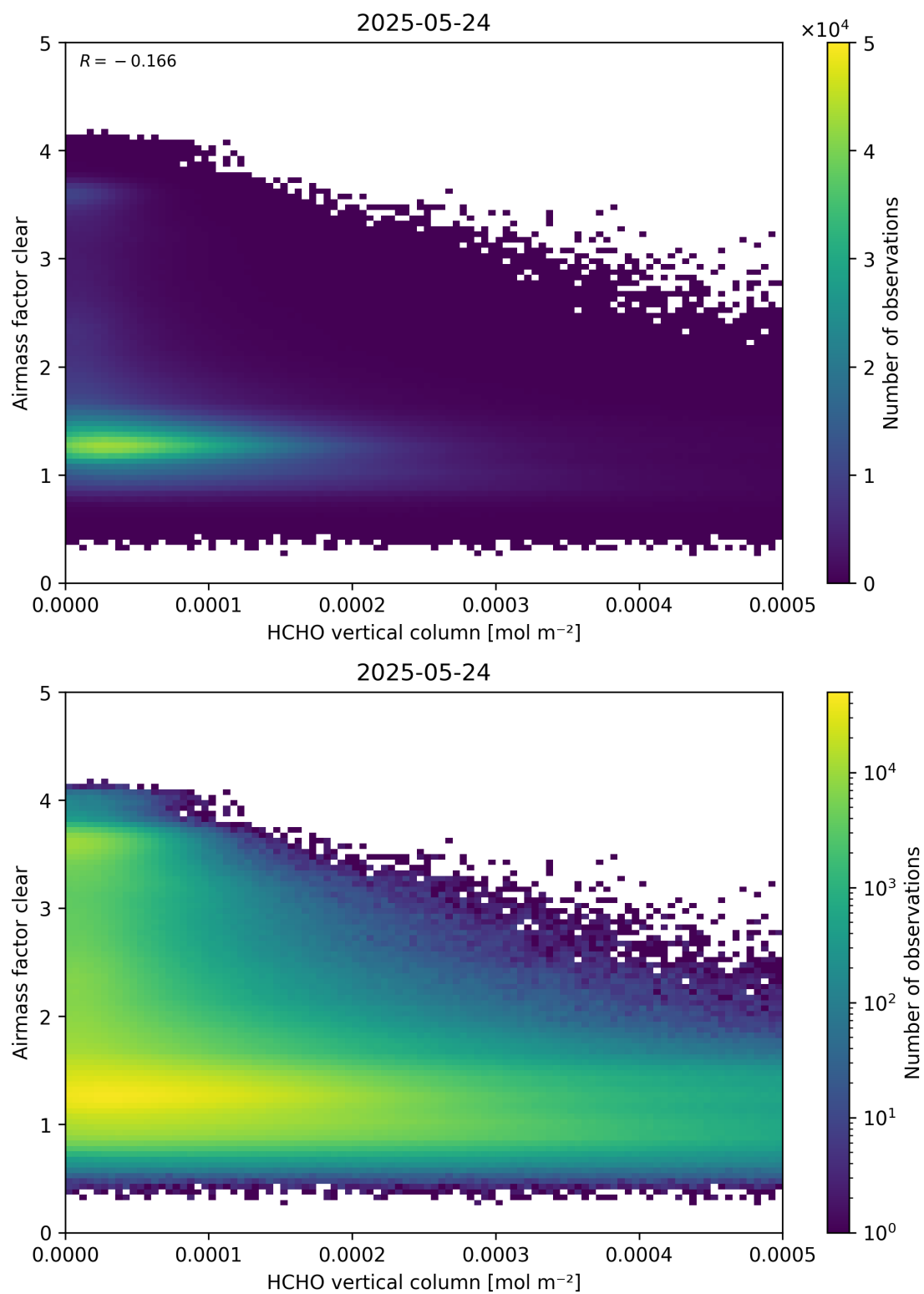
Figure 126: Scatter density plot of “HCHO vertical column” against “Airmass factor clear” for 2025-05-23 to 2025-05-25.
