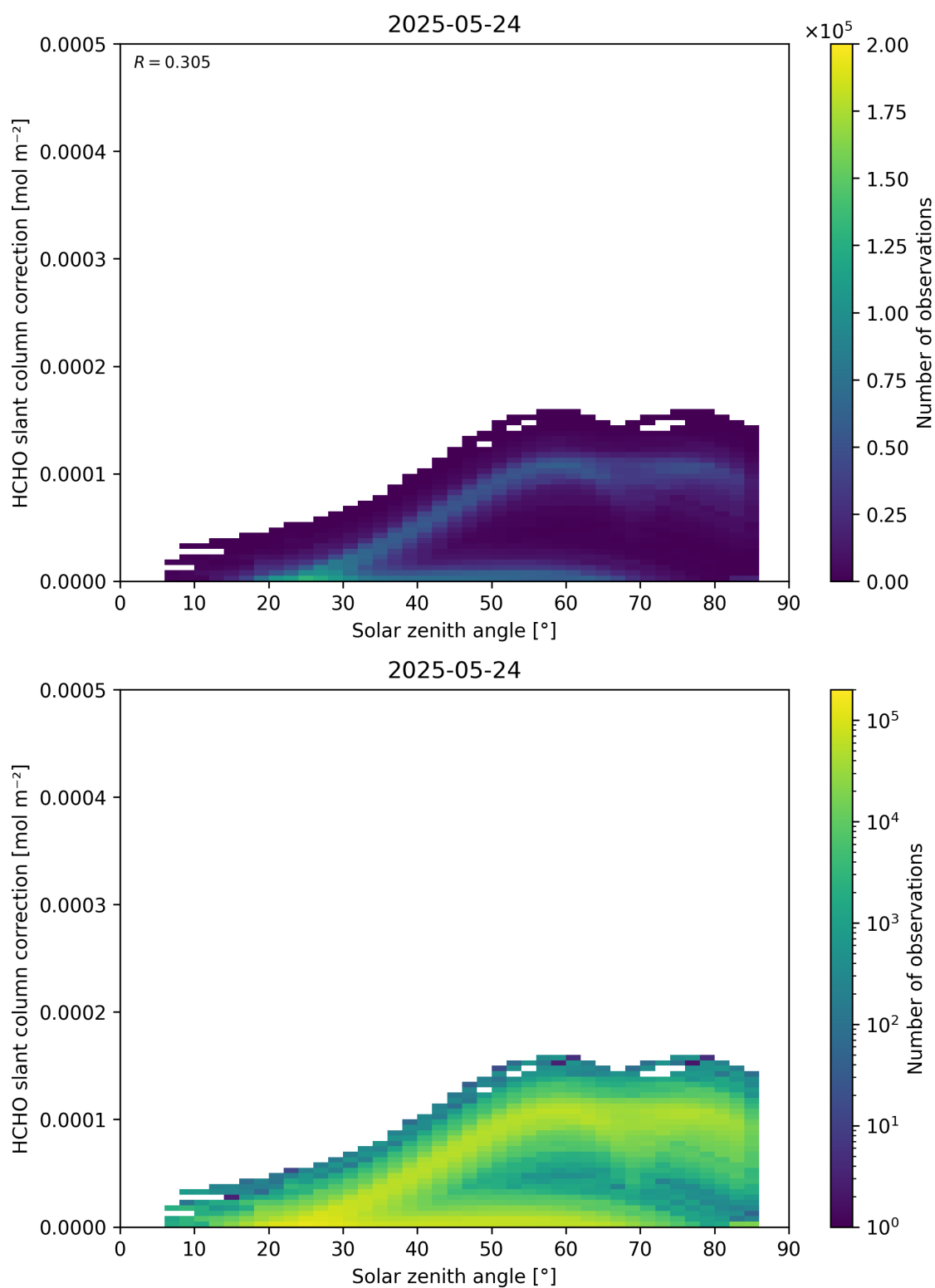
Figure 172: Scatter density plot of “Solar zenith angle” against “HCHO slant column correction” for 2025-05-23 to 2025-05-25.
