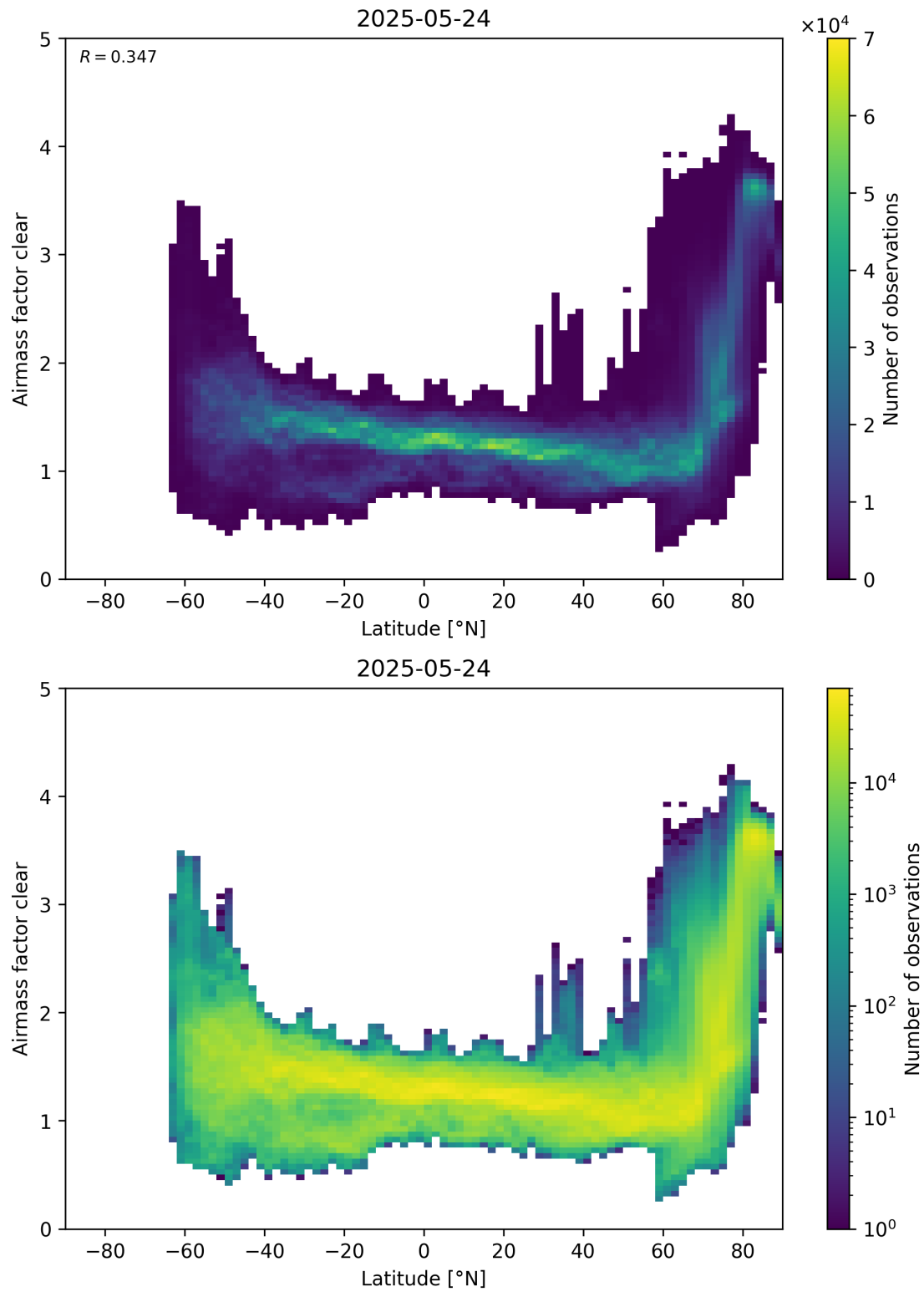
Figure 156: Scatter density plot of “Latitude” against “Airmass factor clear” for 2025-05-23 to 2025-05-25.
