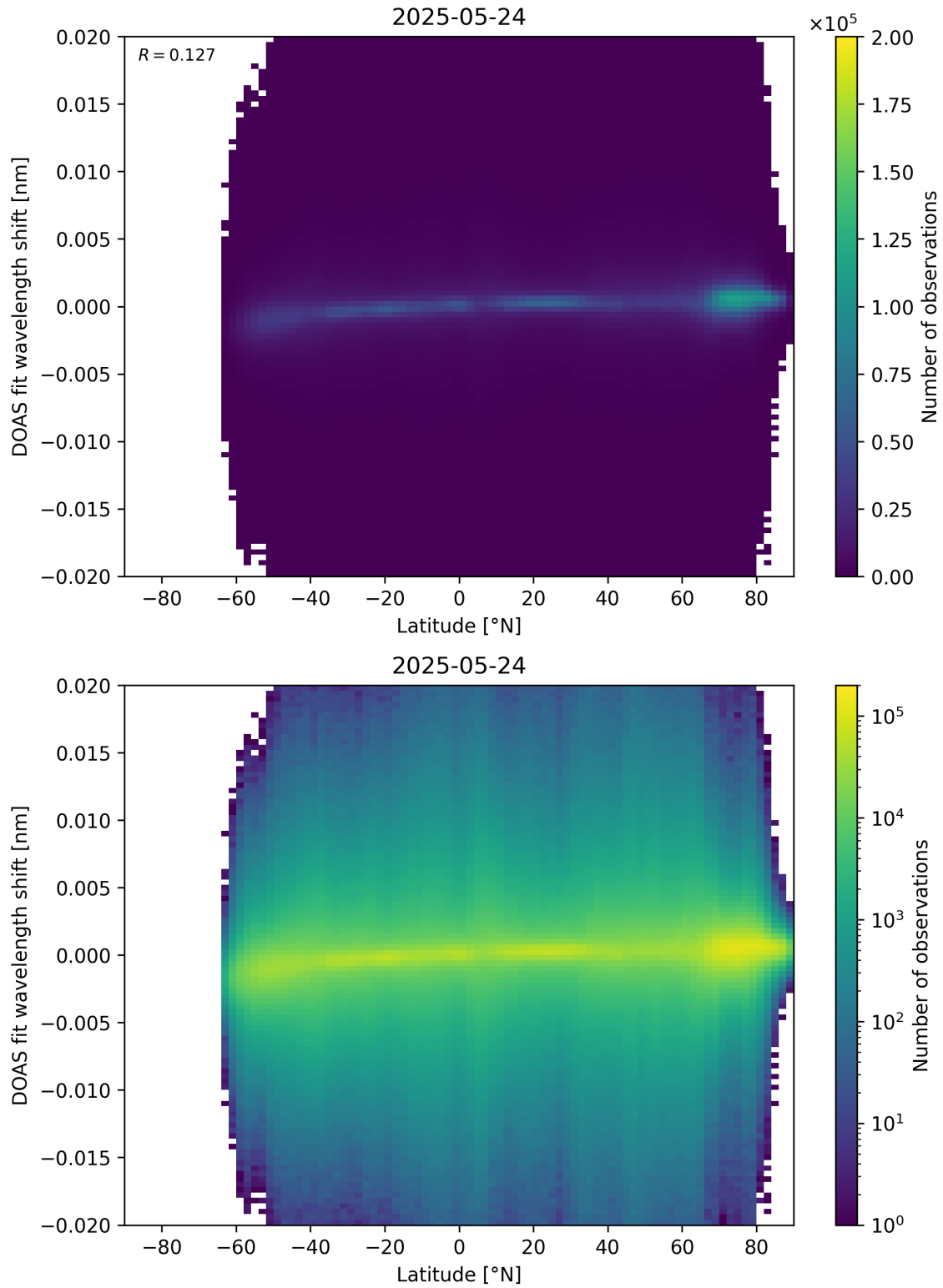
Figure 154: Scatter density plot of “Latitude” against “DOAS fit wavelength shift” for 2025-05-23 to 2025-05-25.
