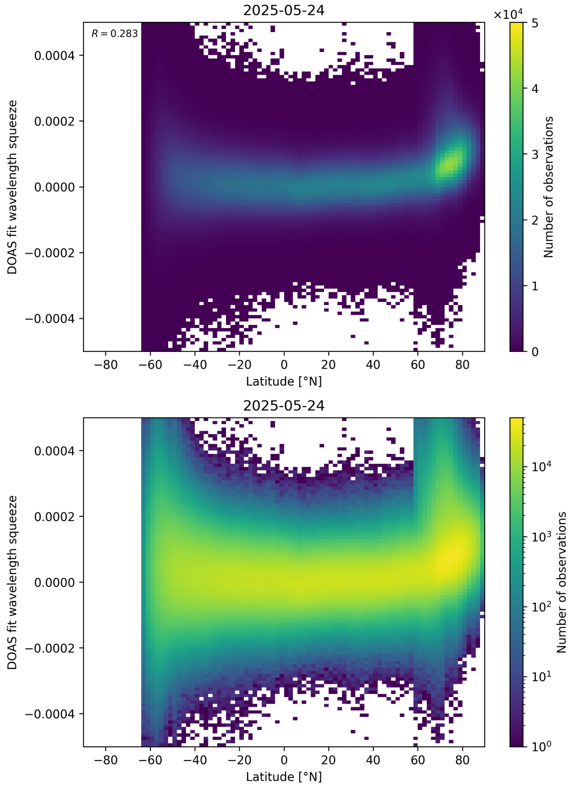
Figure 155: Scatter density plot of “Latitude” against “DOAS fit wavelength squeeze” for 2025-05-23 to 2025-05-25.
