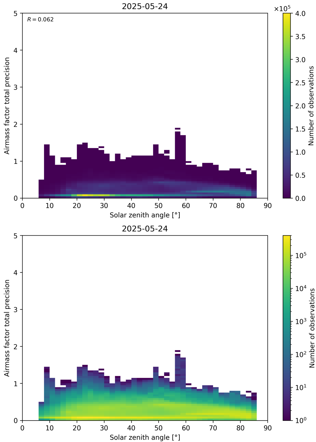
Figure 176: Scatter density plot of “Solar zenith angle” against “Airmass factor total precision” for 2025-05-23 to 2025-05-25.
