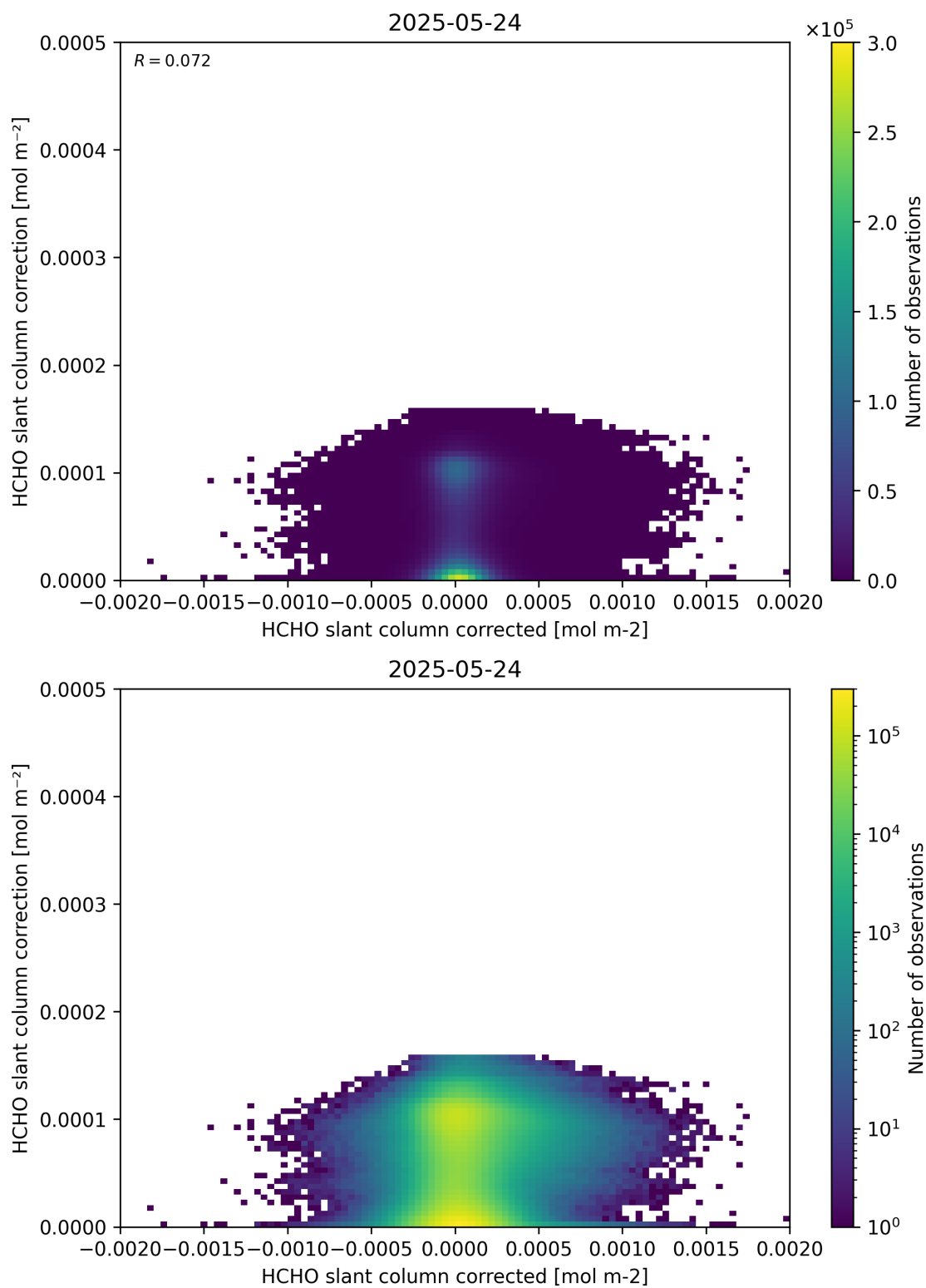
Figure 77: Scatter density plot of “HCHO slant column corrected” against “HCHO slant column correction” for 2025-05-23 to 2025-05-25.
