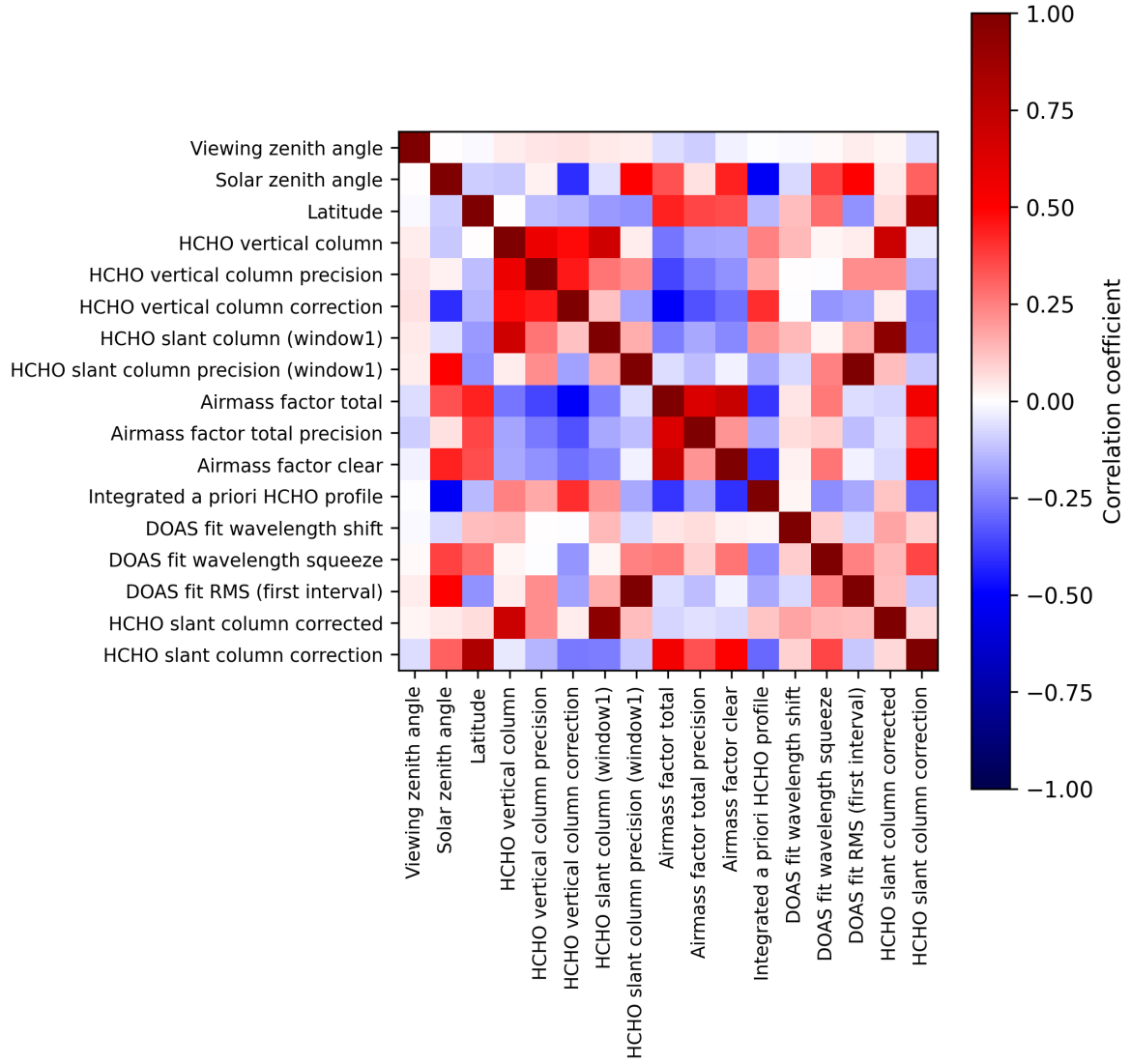
Figure 2: Map of correlation matrix for 2025-05-23 to 2025-05-25.
