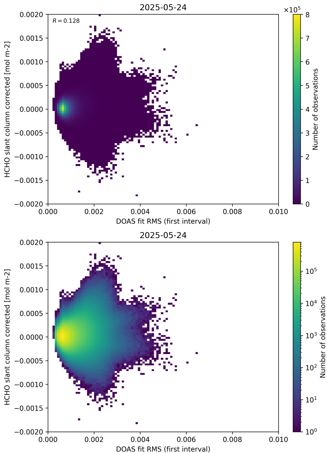
Figure 62: Scatter density plot of “DOAS fit RMS (first interval)” against “HCHO slant column corrected” for 2025-05-23 to 2025-05-25.
