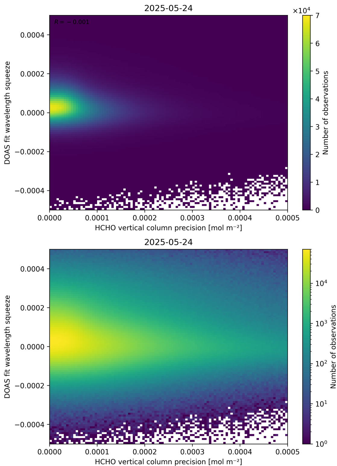
Figure 138: Scatter density plot of “HCHO vertical column precision” against “DOAS fit wavelength squeeze” for 2025-05-23 to 2025-05-25.
