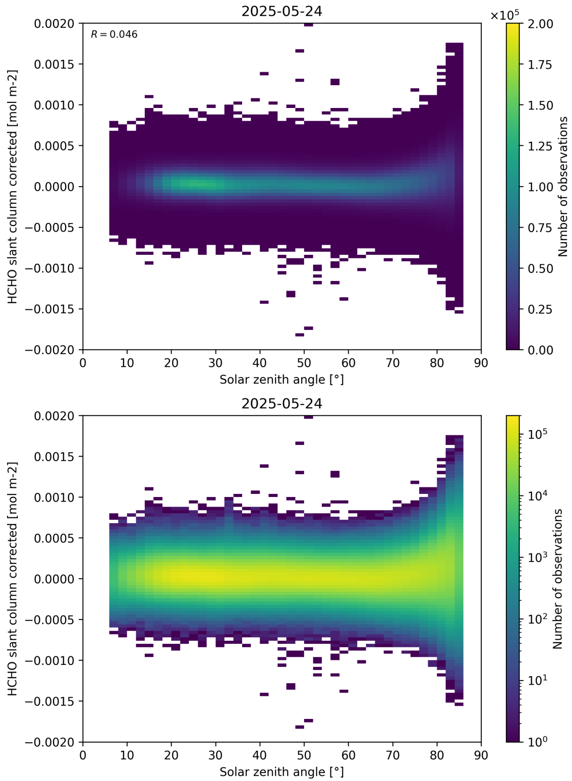
Figure 171: Scatter density plot of “Solar zenith angle” against “HCHO slant column corrected” for 2025-05-23 to 2025-05-25.
