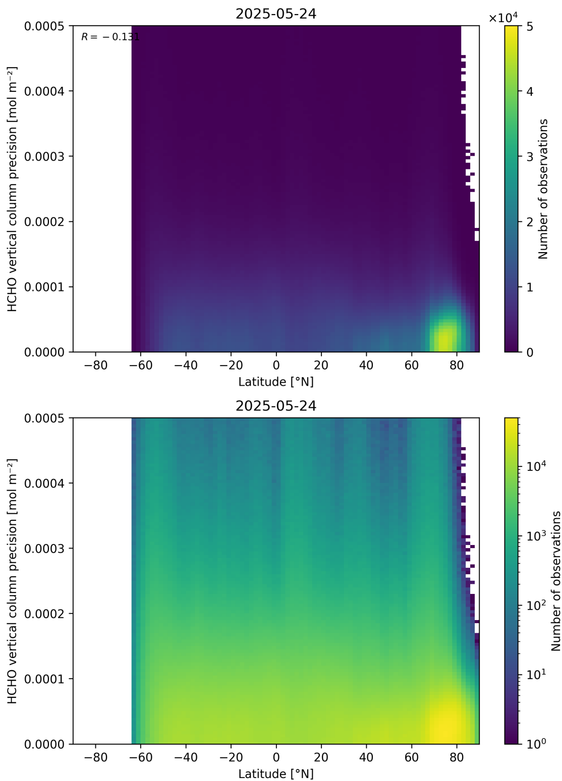
Figure 165: Scatter density plot of “Latitude” against “HCHO vertical column precision” for 2025-05-23 to 2025-05-25.
