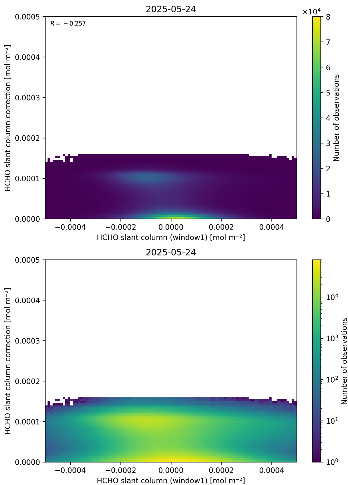
Figure 83: Scatter density plot of “HCHO slant column (window1)” against “HCHO slant column correction” for 2025-05-23 to 2025-05-25.
