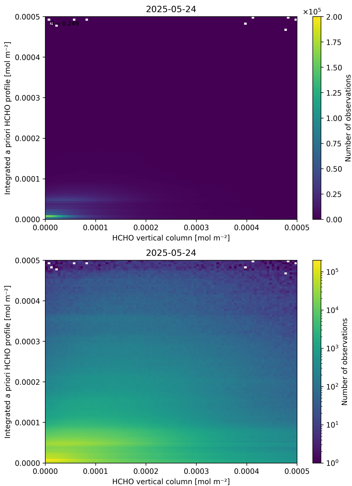
Figure 135: Scatter density plot of “HCHO vertical column” against “Integrated a priori HCHO profile” for 2025-05-23 to 2025-05-25.
