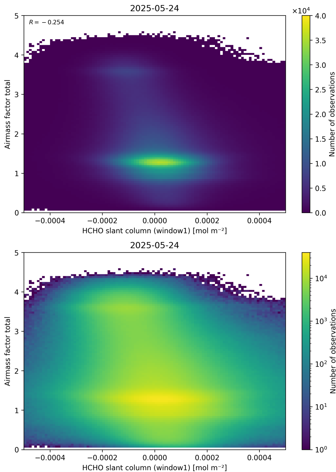
Figure 85: Scatter density plot of “HCHO slant column (window1)” against “Airmass factor total” for 2025-05-23 to 2025-05-25.
