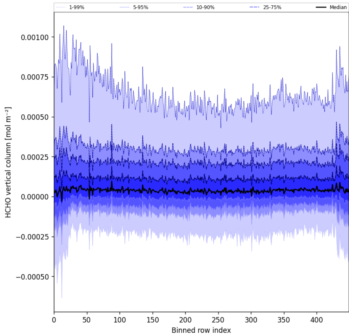
Figure 49: Along track statistics of “HCHO vertical column” for 2025-05-23 to 2025-05-25
