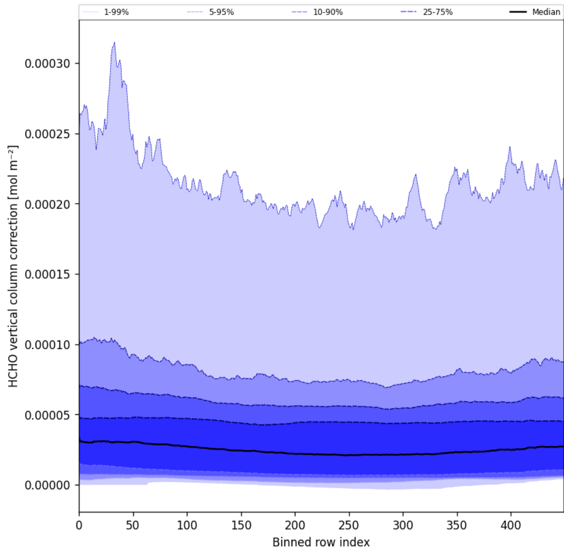
Figure 51: Along track statistics of "HCHO vertical column correction" for 2025-05-23 to 2025-05-25
