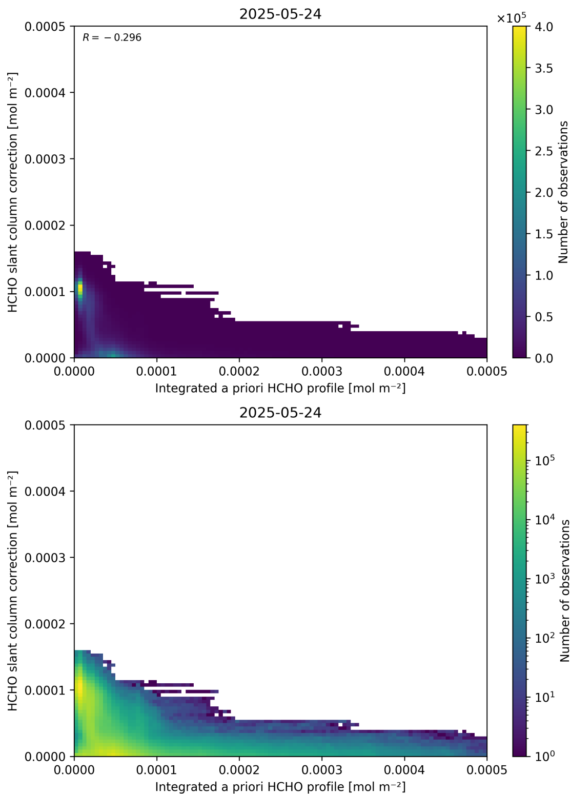
Figure 152: Scatter density plot of “Integrated a priori HCHO profile” against “HCHO slant column correction” for 2025-05-23 to 2025-05-25.
