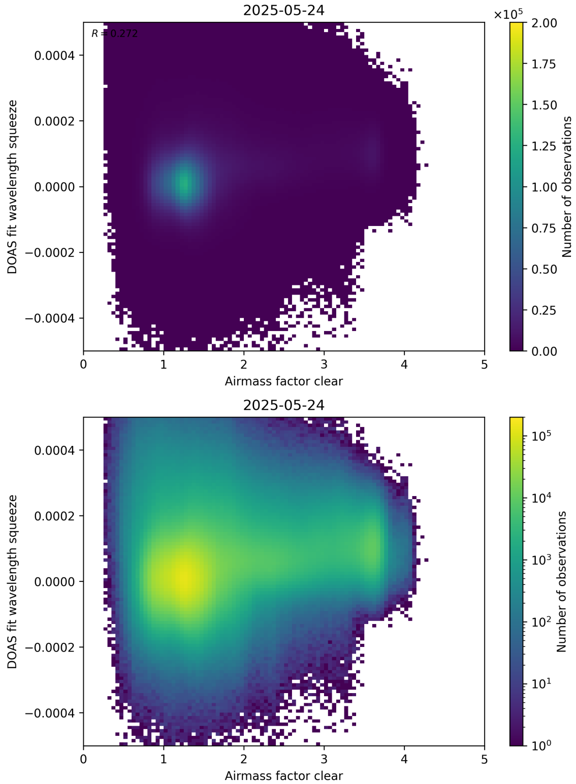
Figure 73: Scatter density plot of “Airmass factor clear” against “DOAS fit wavelength squeeze” for 2025-05-23 to 2025-05-25.
