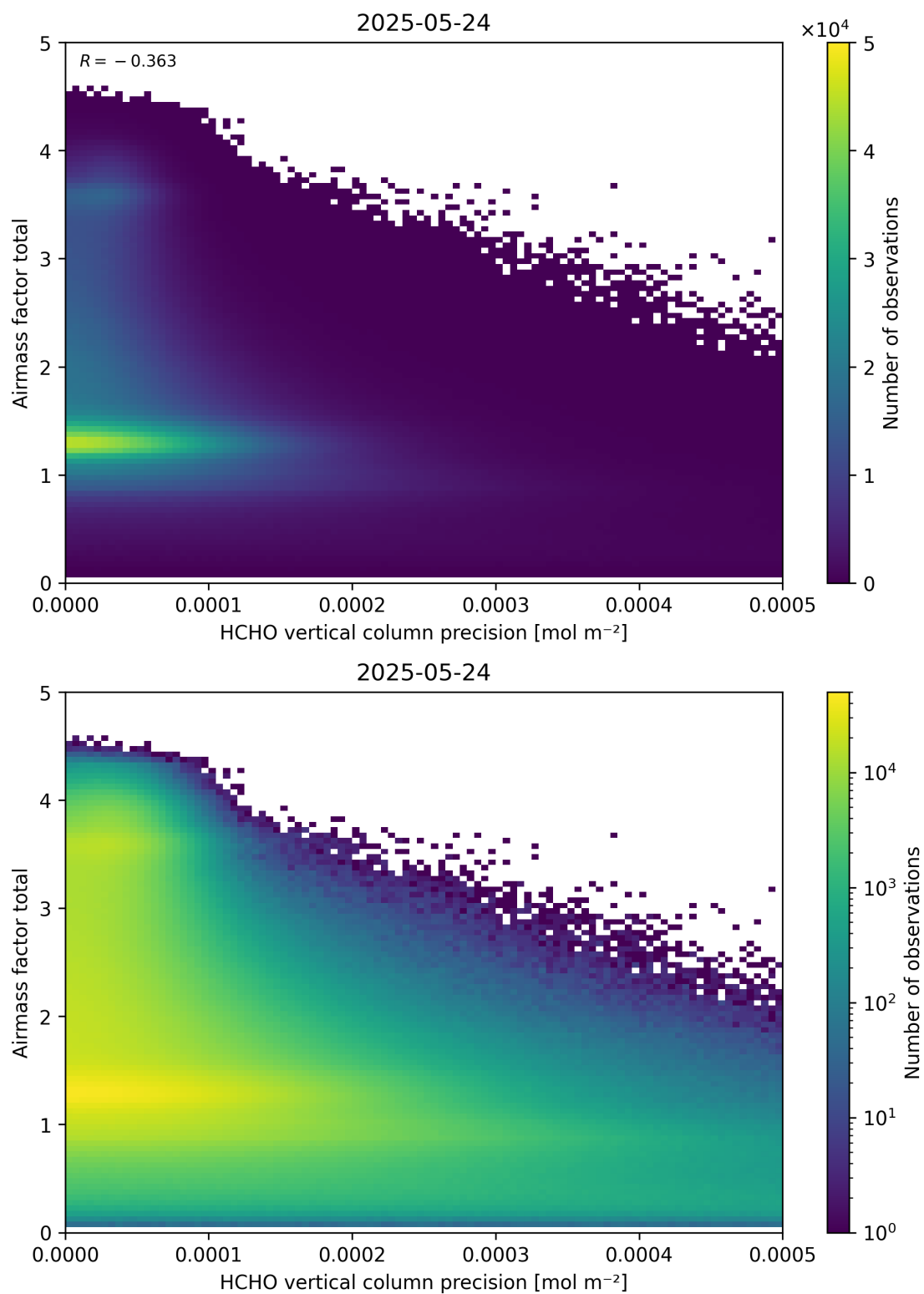
Figure 144: Scatter density plot of “HCHO vertical column precision” against “Airmass factor total” for 2025-05-23 to 2025-05-25.
