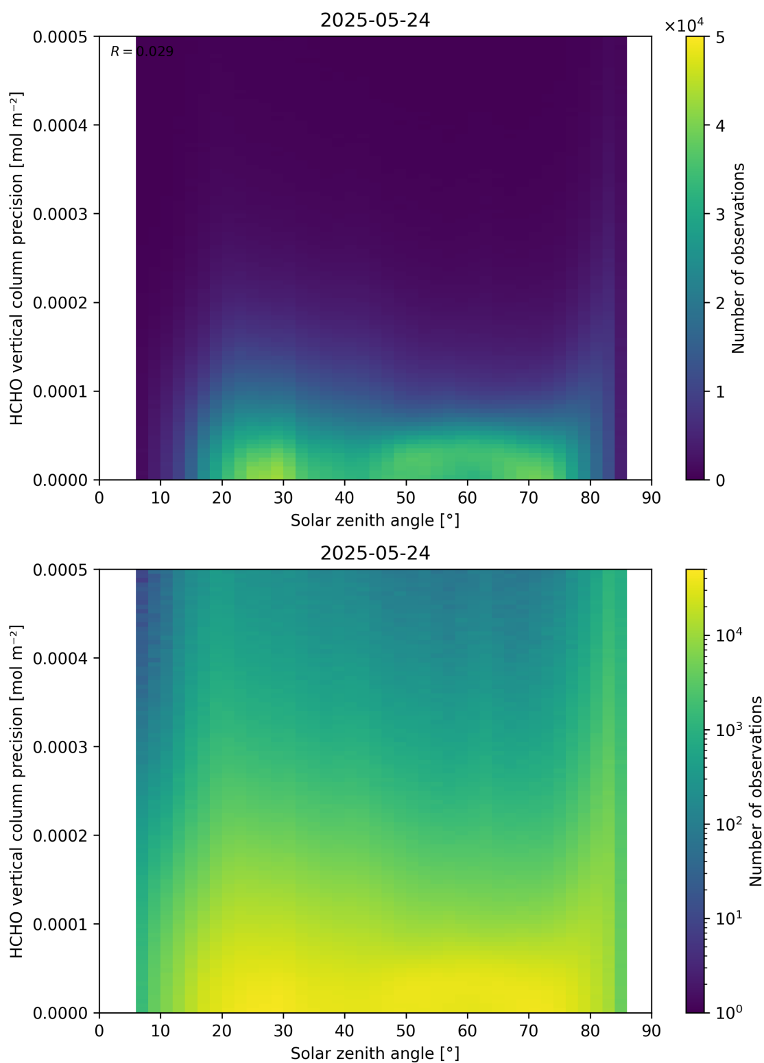
Figure 179: Scatter density plot of “Solar zenith angle” against “HCHO vertical column precision” for 2025-05-23 to 2025-05-25.
