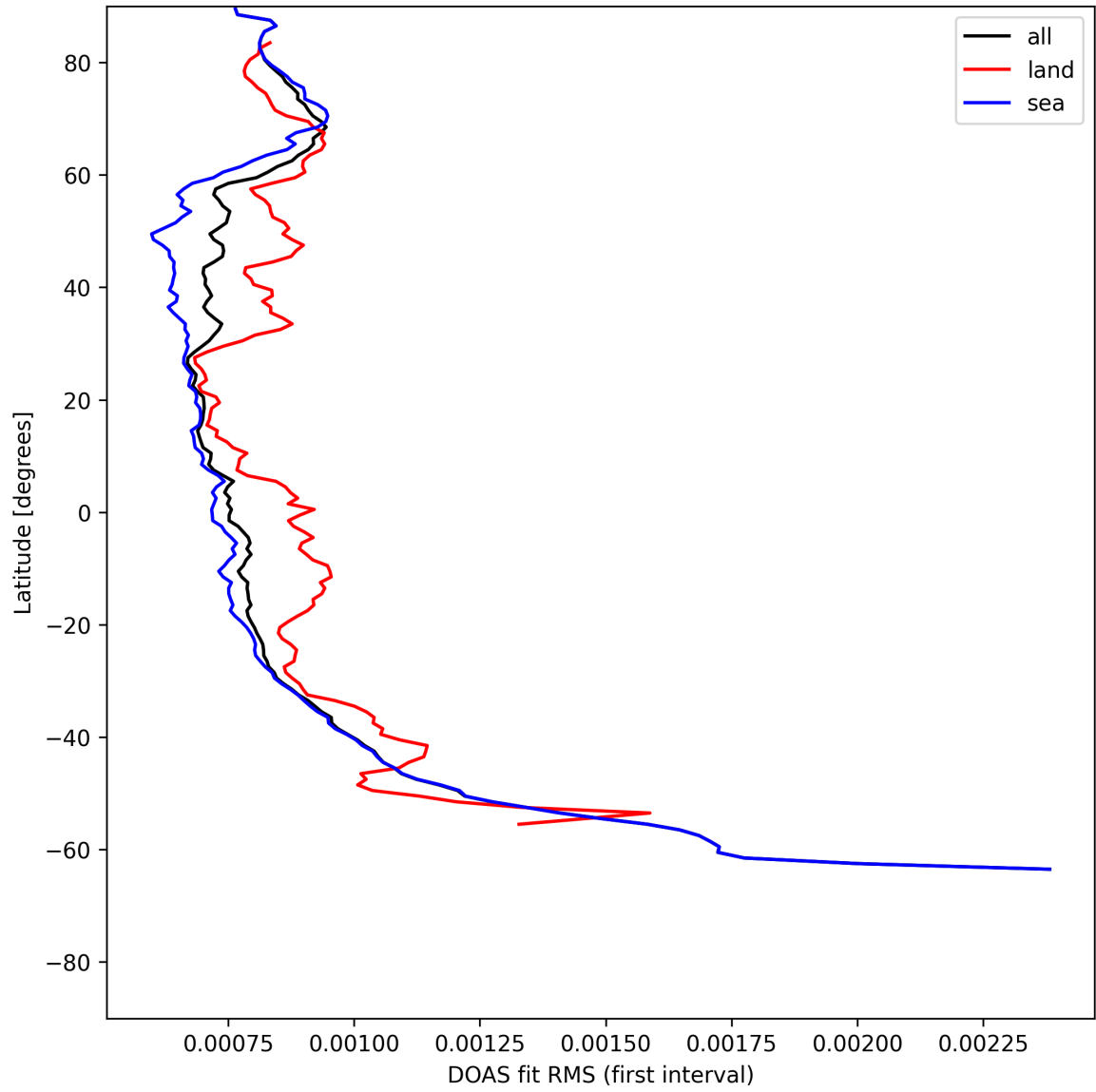
Figure 32: Zonal average of “DOAS fit RMS (first interval)” for 2025-05-23 to 2025-05-25.
