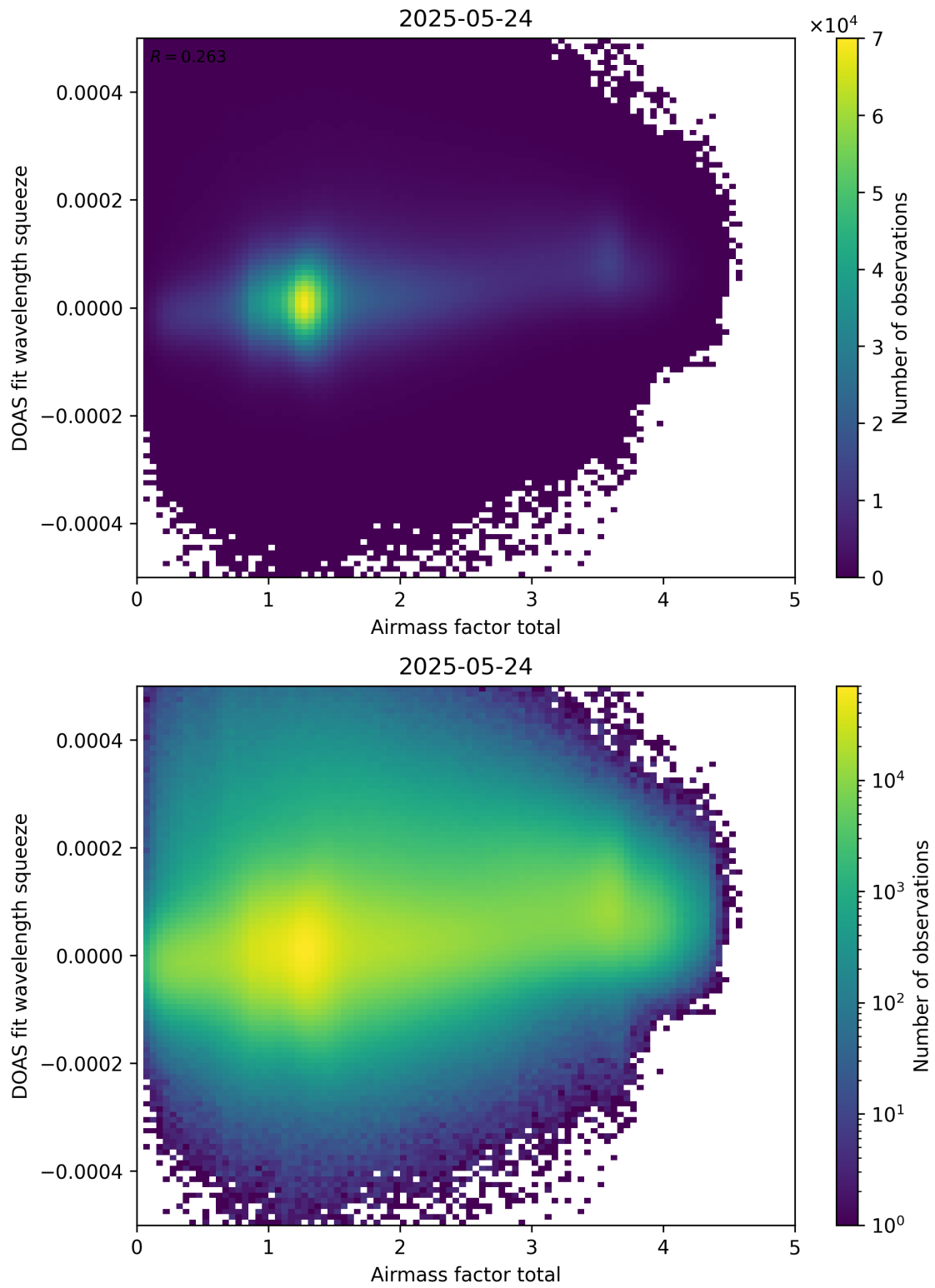
Figure 99: Scatter density plot of “Airmass factor total” against “DOAS fit wavelength squeeze” for 2025-05-23 to 2025-05-25.
