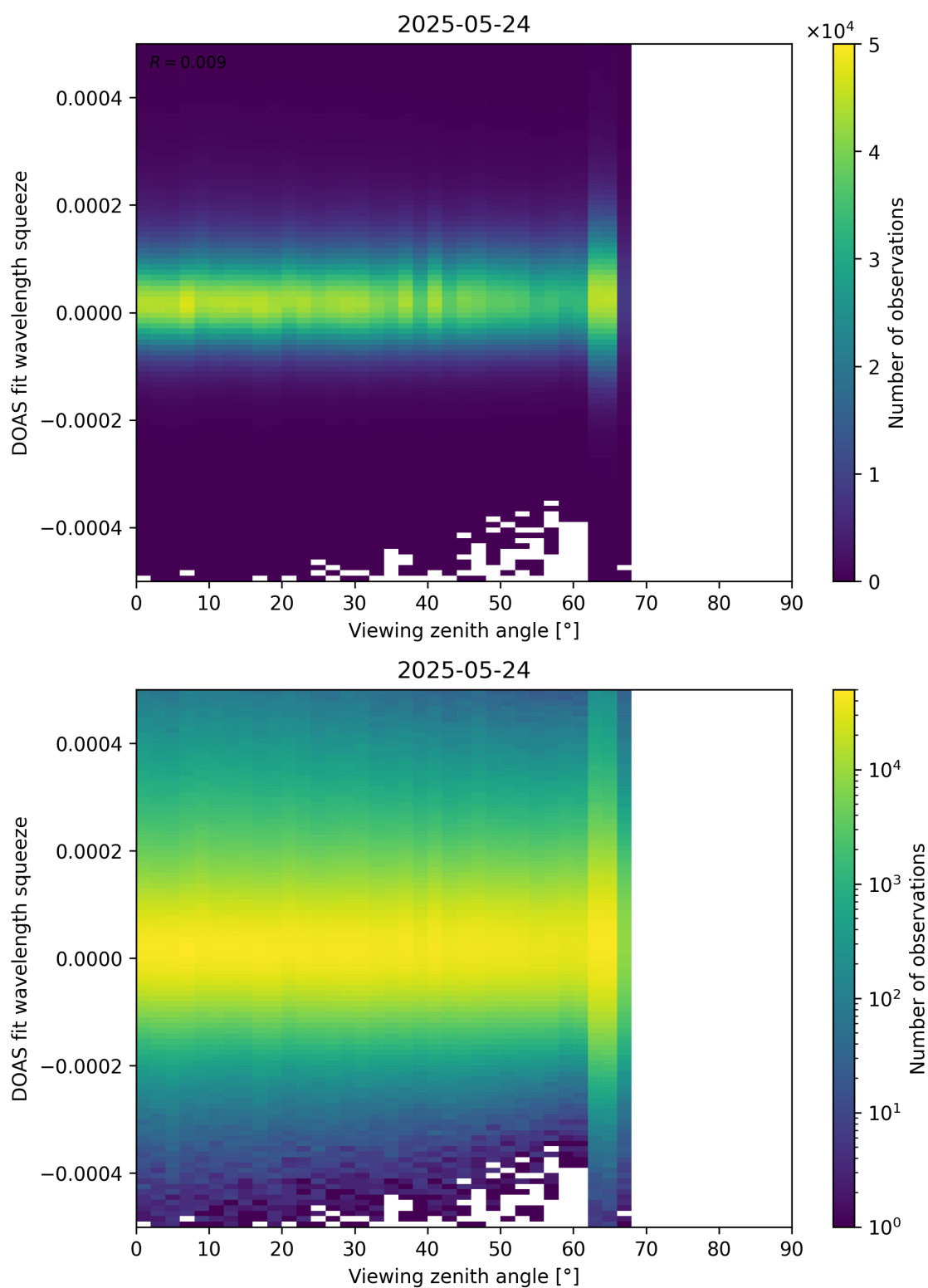
Figure 184: Scatter density plot of “Viewing zenith angle” against “DOAS fit wavelength squeeze” for 2025-05-23 to 2025-05-25.
