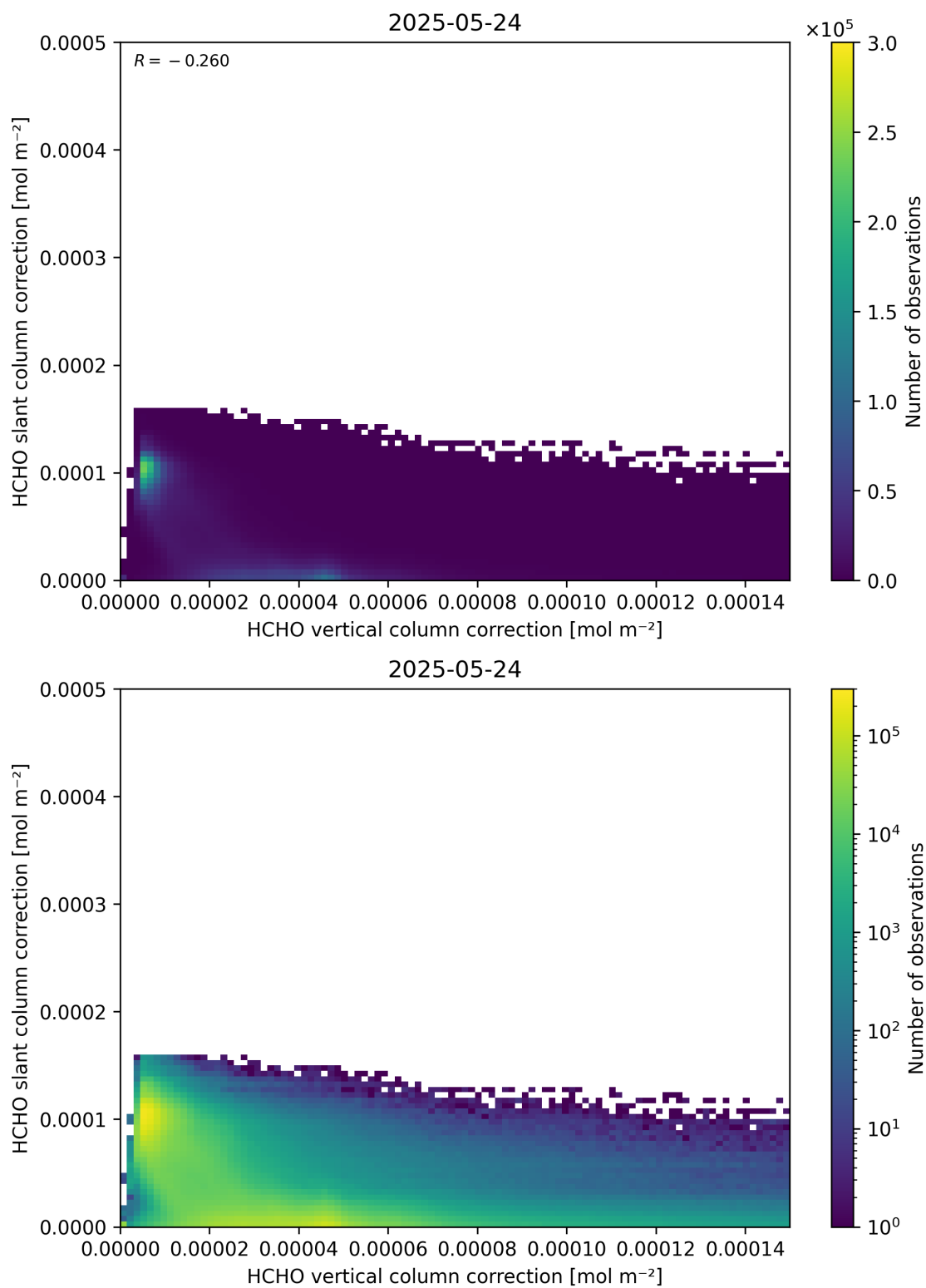
Figure 117: Scatter density plot of “HCHO vertical column correction” against “HCHO slant column correction” for 2025-05-23 to 2025-05-25.
