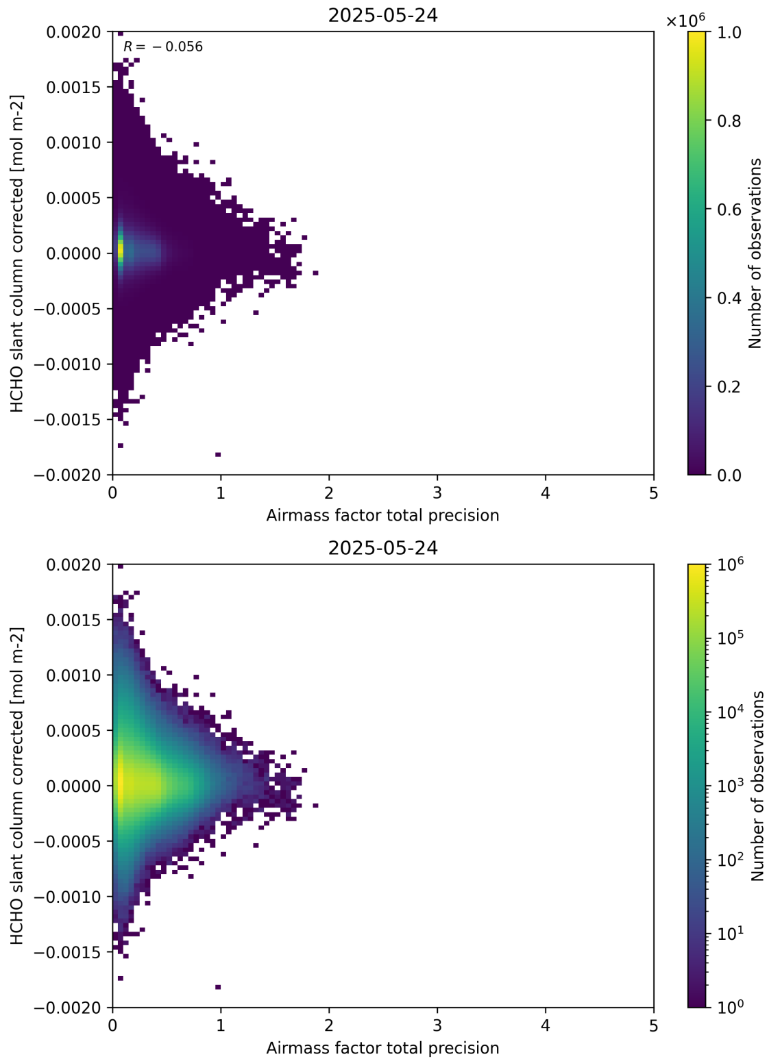
Figure 109: Scatter density plot of “Airmass factor total precision” against “HCHO slant column corrected” for 2025-05-23 to 2025-05-25.
