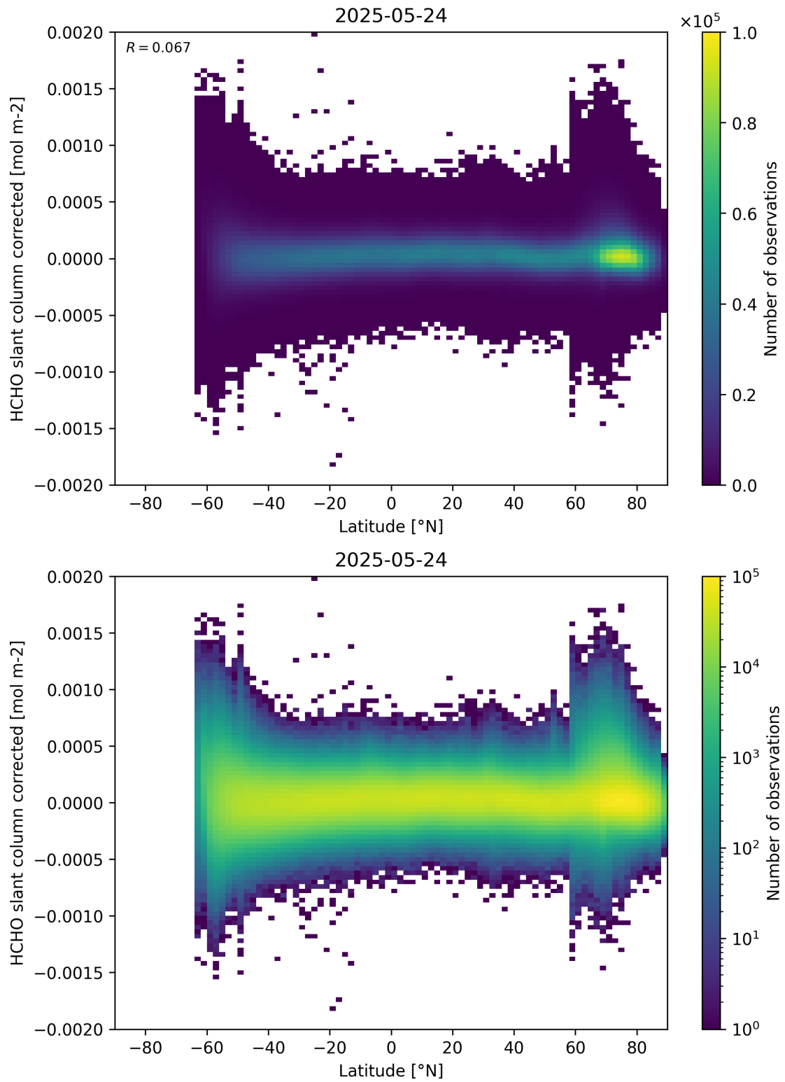
Figure 157: Scatter density plot of “Latitude” against “HCHO slant column corrected” for 2025-05-23 to 2025-05-25.
