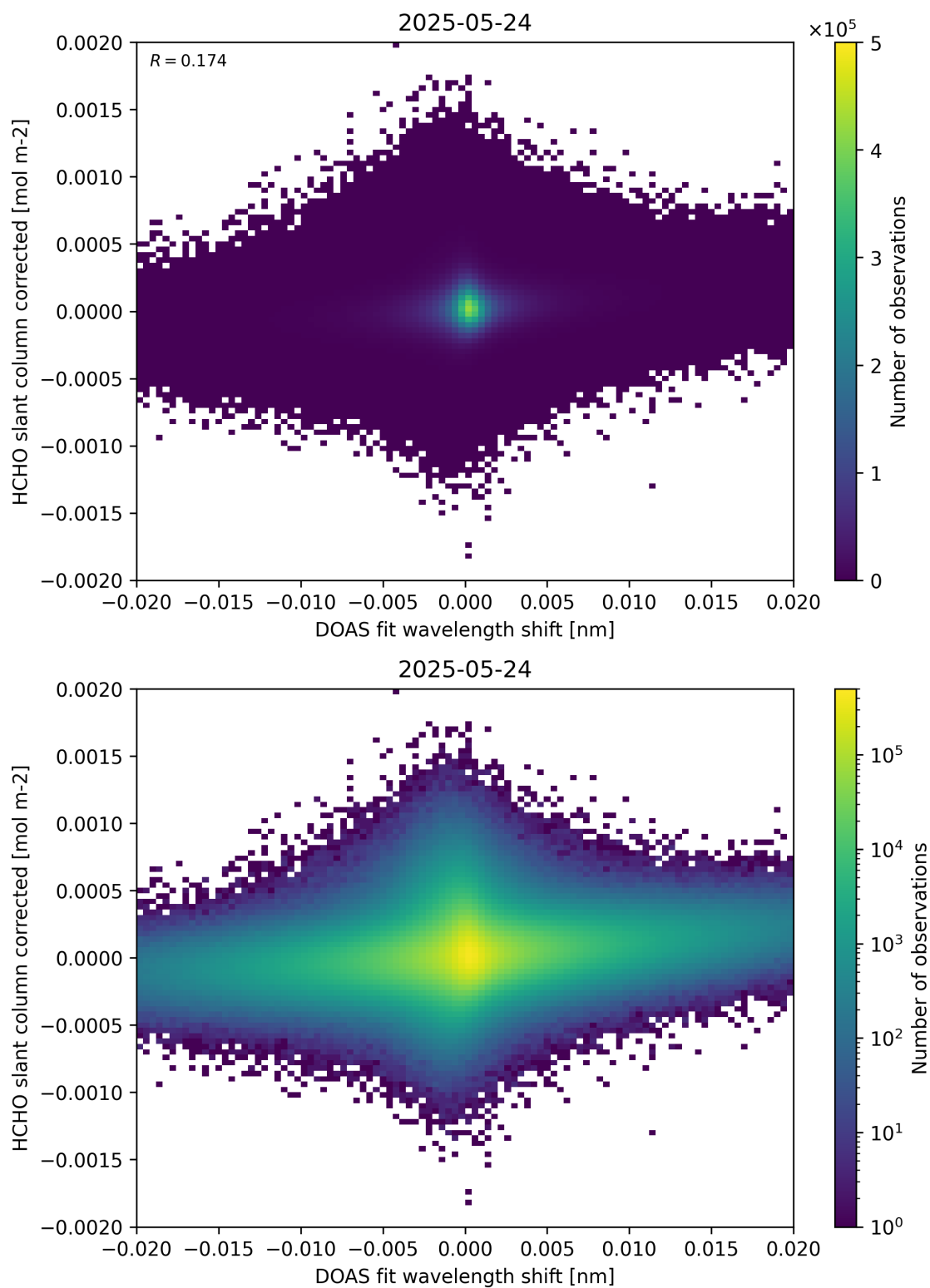
Figure 66: Scatter density plot of “DOAS fit wavelength shift” against “HCHO slant column corrected” for 2025-05-23 to 2025-05-25.
