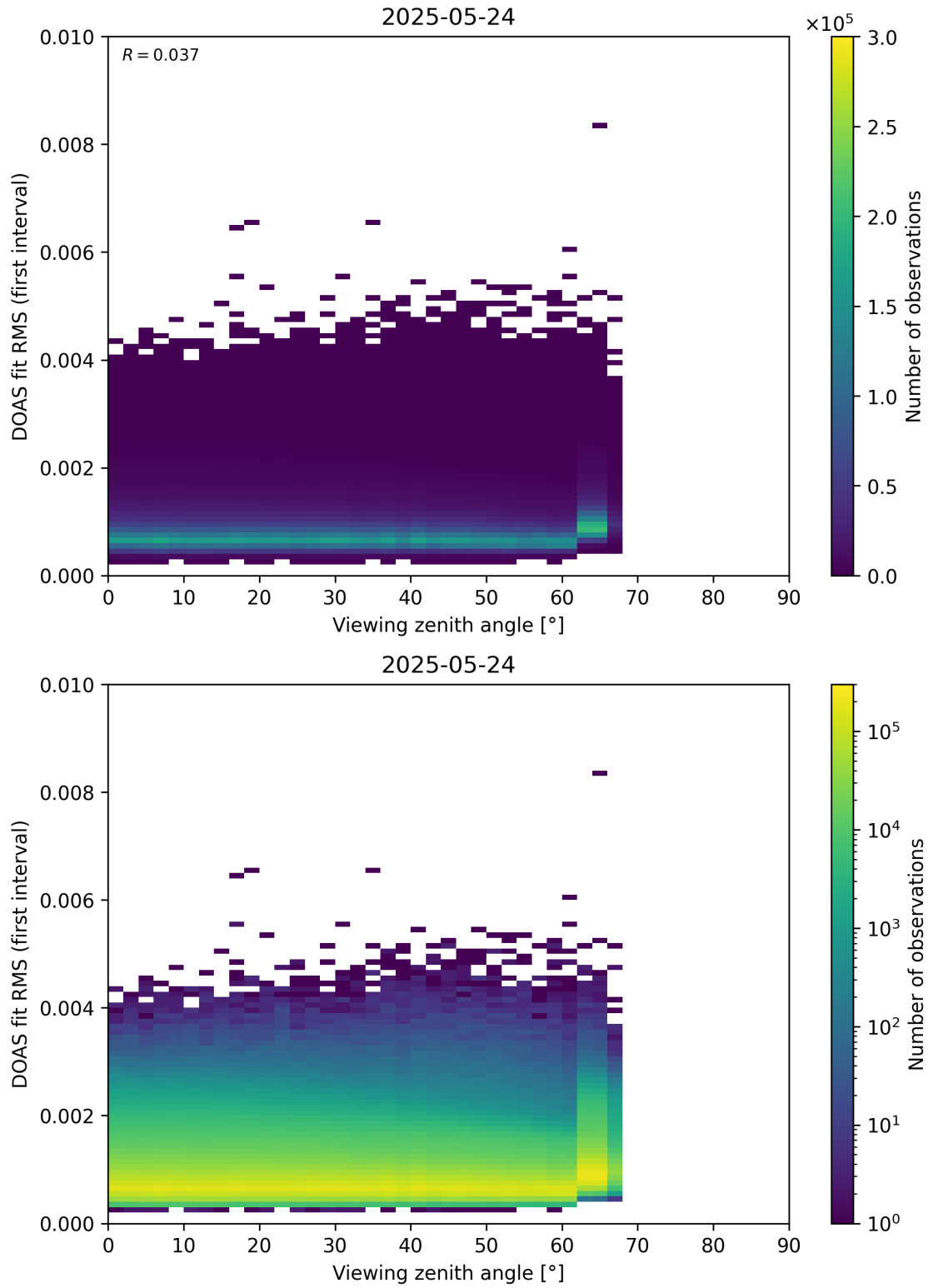
Figure 182: Scatter density plot of “Viewing zenith angle” against “DOAS fit RMS (first interval)” for 2025-05-23 to 2025-05-25.
