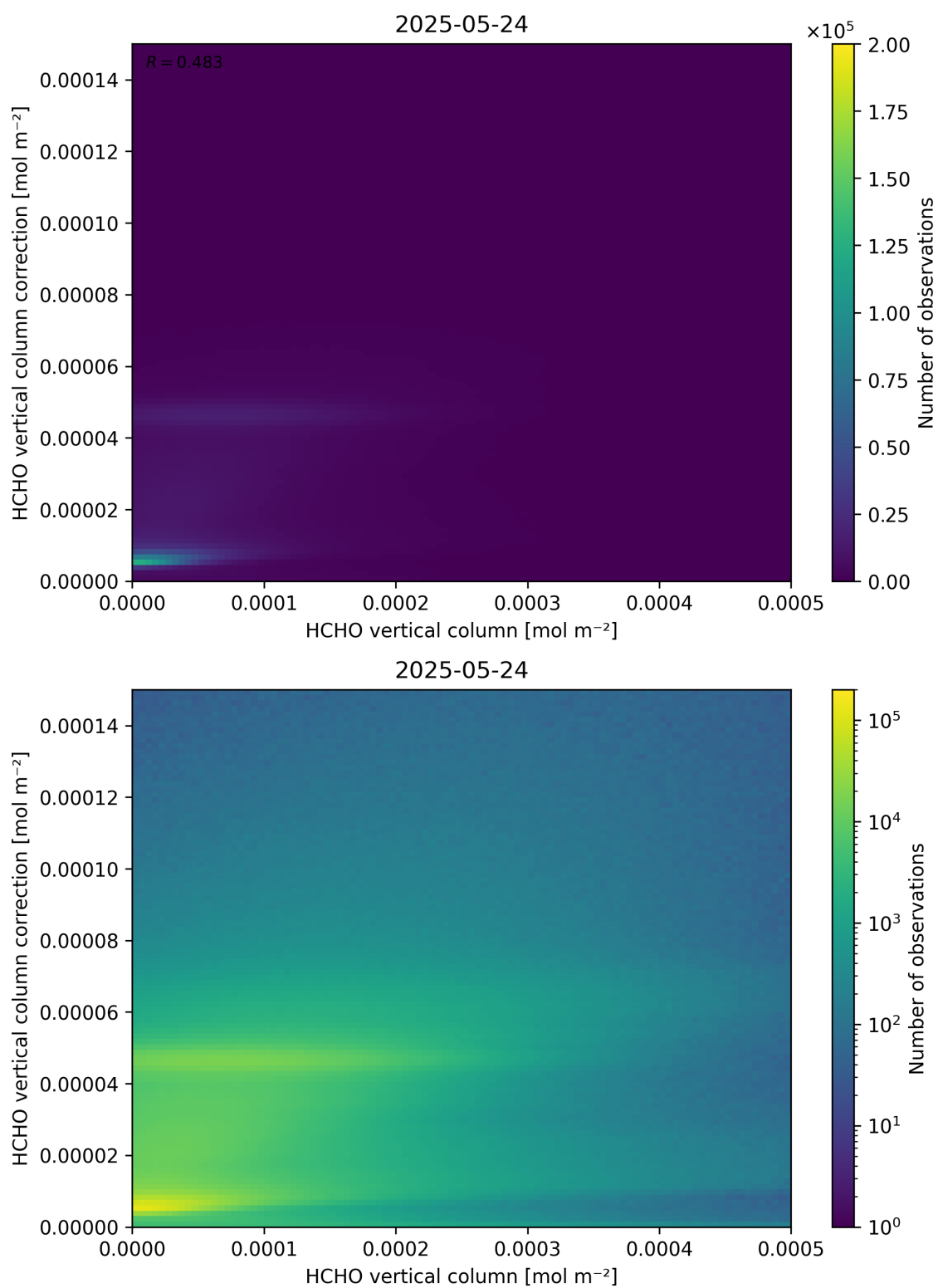
Figure 133: Scatter density plot of “HCHO vertical column” against “HCHO vertical column correction” for 2025-05-23 to 2025-05-25.
