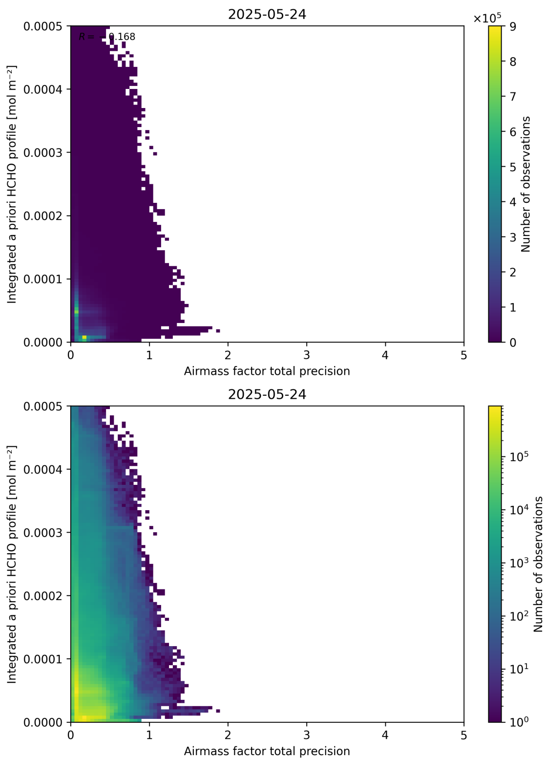
Figure 111: Scatter density plot of “Airmass factor total precision” against “Integrated a priori HCHO profile” for 2025-05-23 to 2025-05-25.
