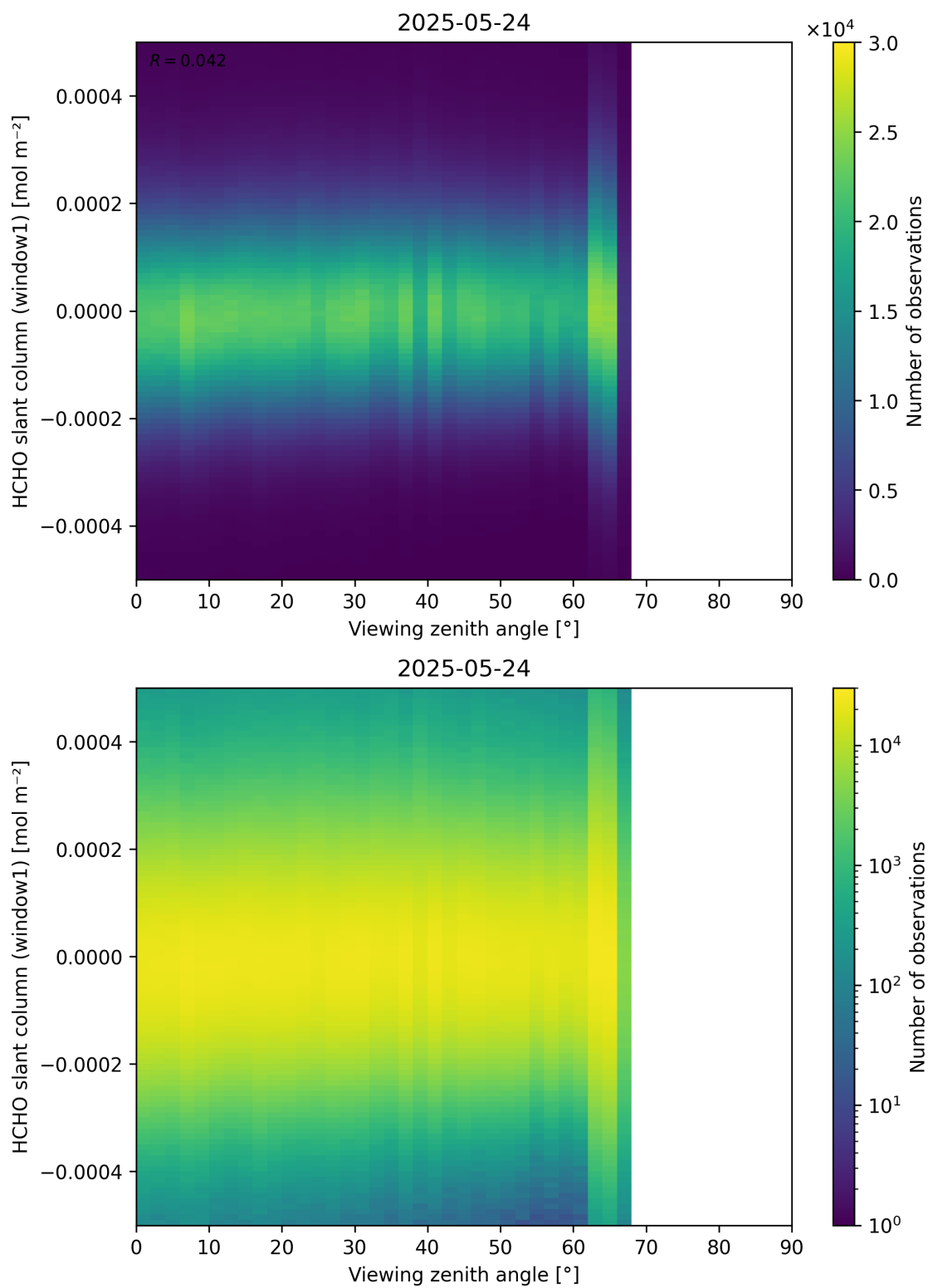
Figure 188: Scatter density plot of “Viewing zenith angle” against “HCHO slant column (window1)” for 2025-05-23 to 2025-05-25.
