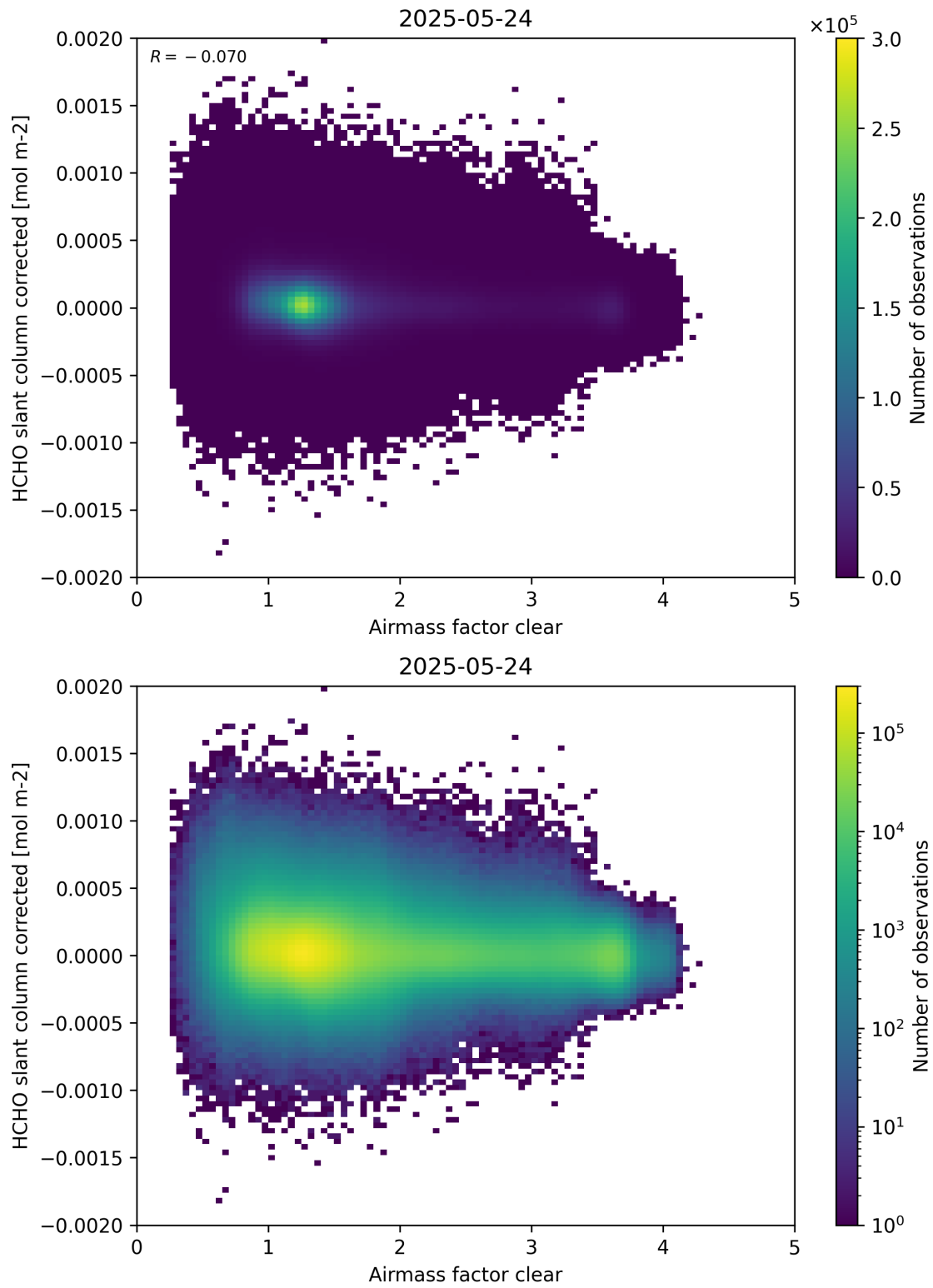
Figure 74: Scatter density plot of “Airmass factor clear” against “HCHO slant column corrected” for 2025-05-23 to 2025-05-25.
