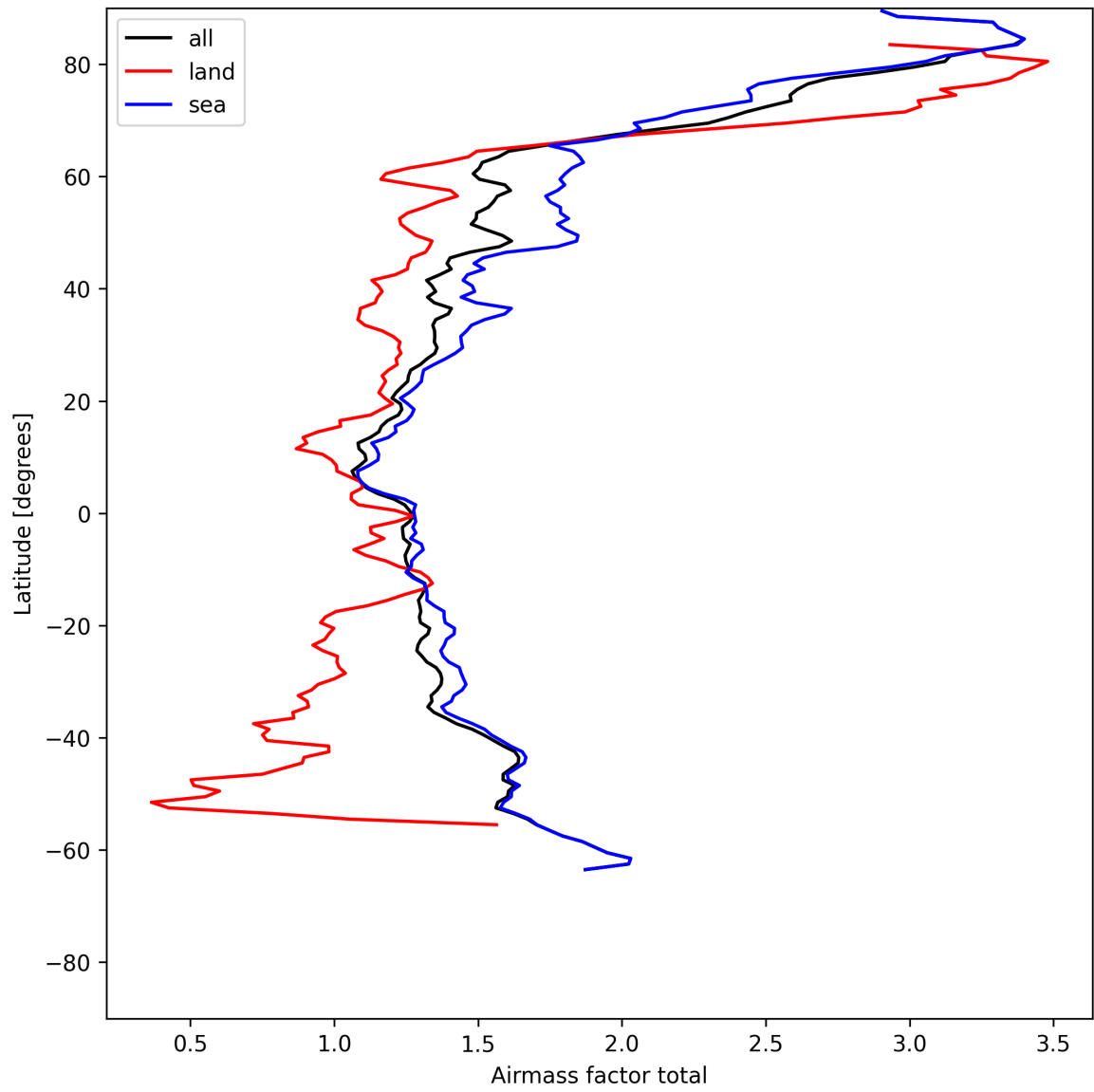
Figure 26: Zonal average of “Airmass factor total” for 2025-05-23 to 2025-05-25.
