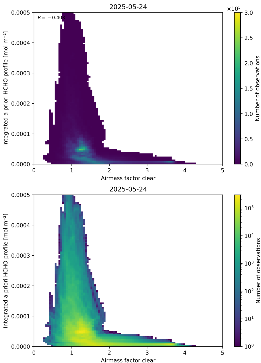
Figure 76: Scatter density plot of “Airmass factor clear” against “Integrated a priori HCHO profile” for 2025-05-23 to 2025-05-25.
