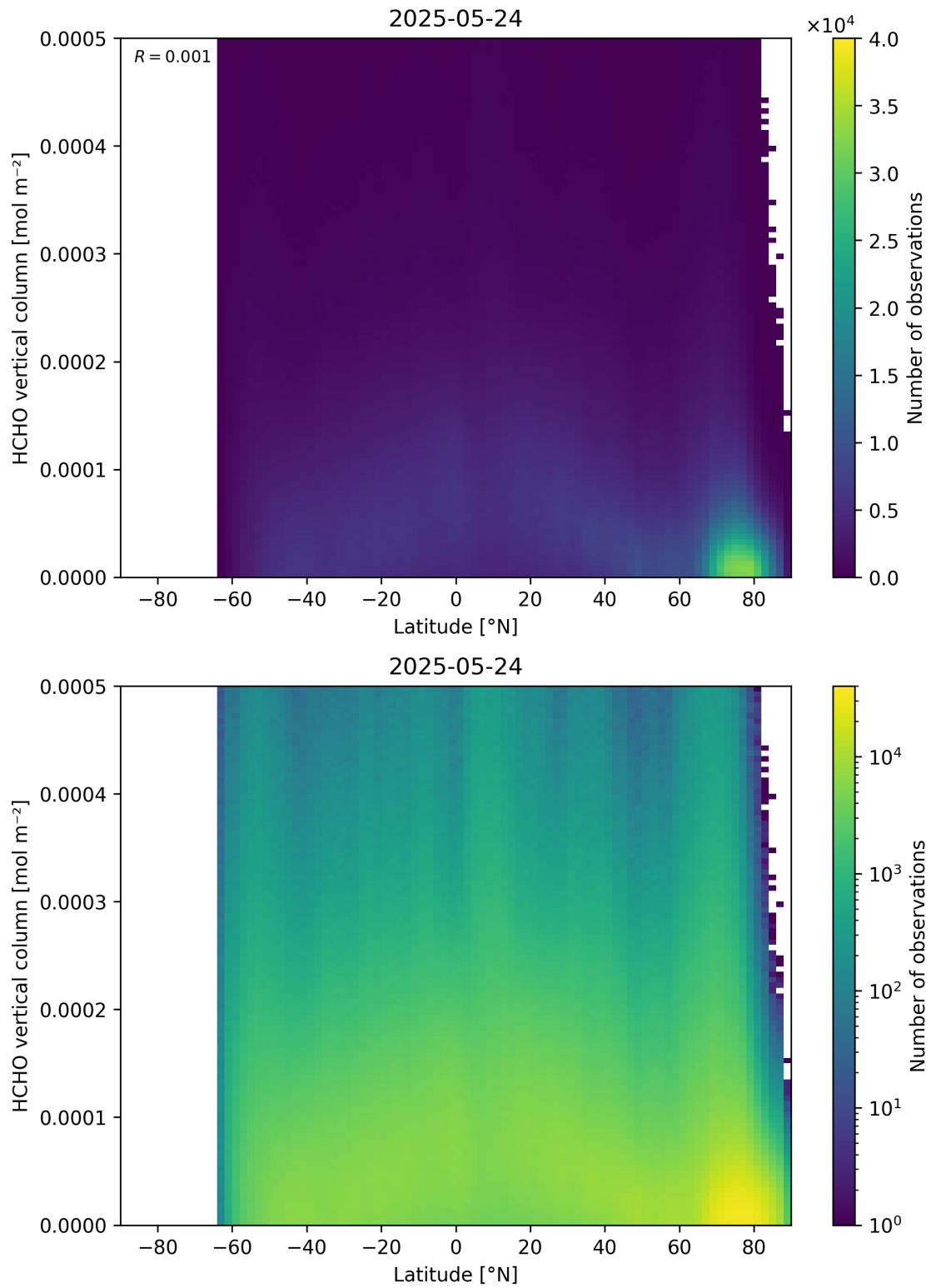
Figure 163: Scatter density plot of “Latitude” against “HCHO vertical column” for 2025-05-23 to 2025-05-25.
