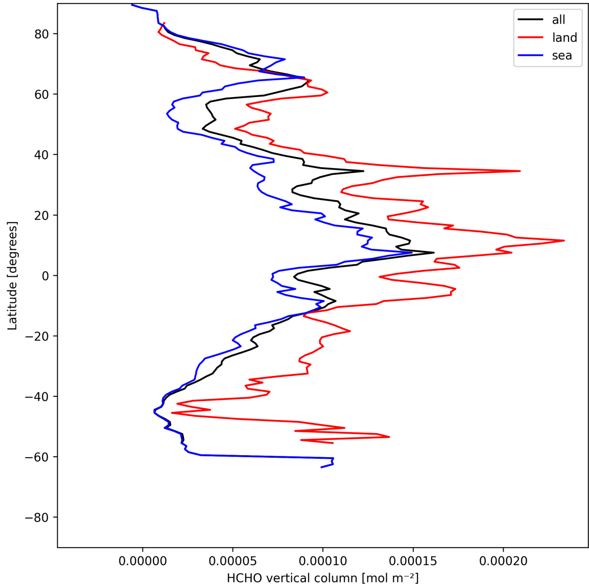
Figure 21: Zonal average of “HCHO vertical column” for 2025-05-23 to 2025-05-25.
