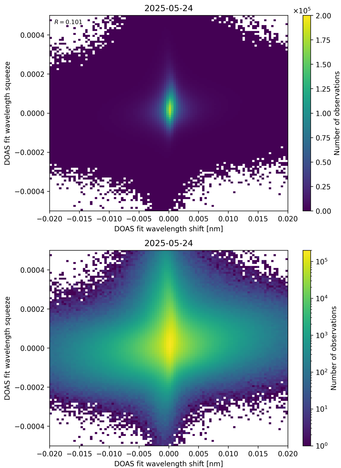
Figure 65: Scatter density plot of “DOAS fit wavelength shift” against “DOAS fit wavelength squeeze” for 2025-05-23 to 2025-05-25.
