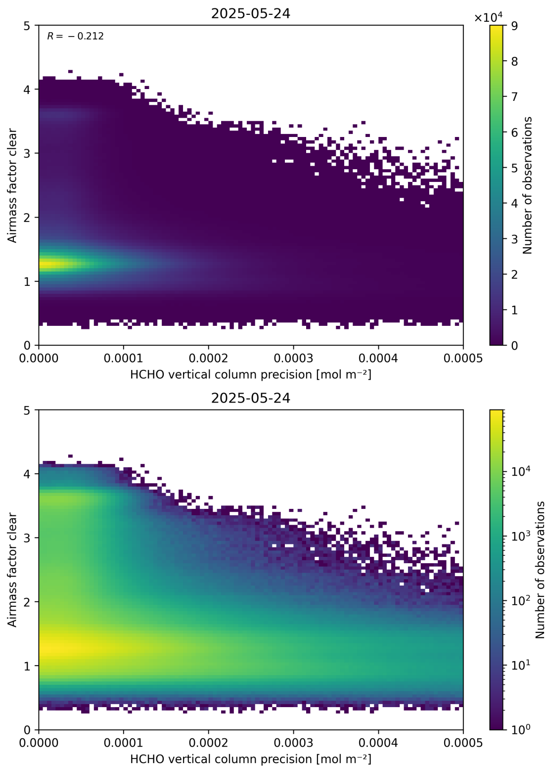
Figure 139: Scatter density plot of “HCHO vertical column precision” against “Airmass factor clear” for 2025-05-23 to 2025-05-25.
