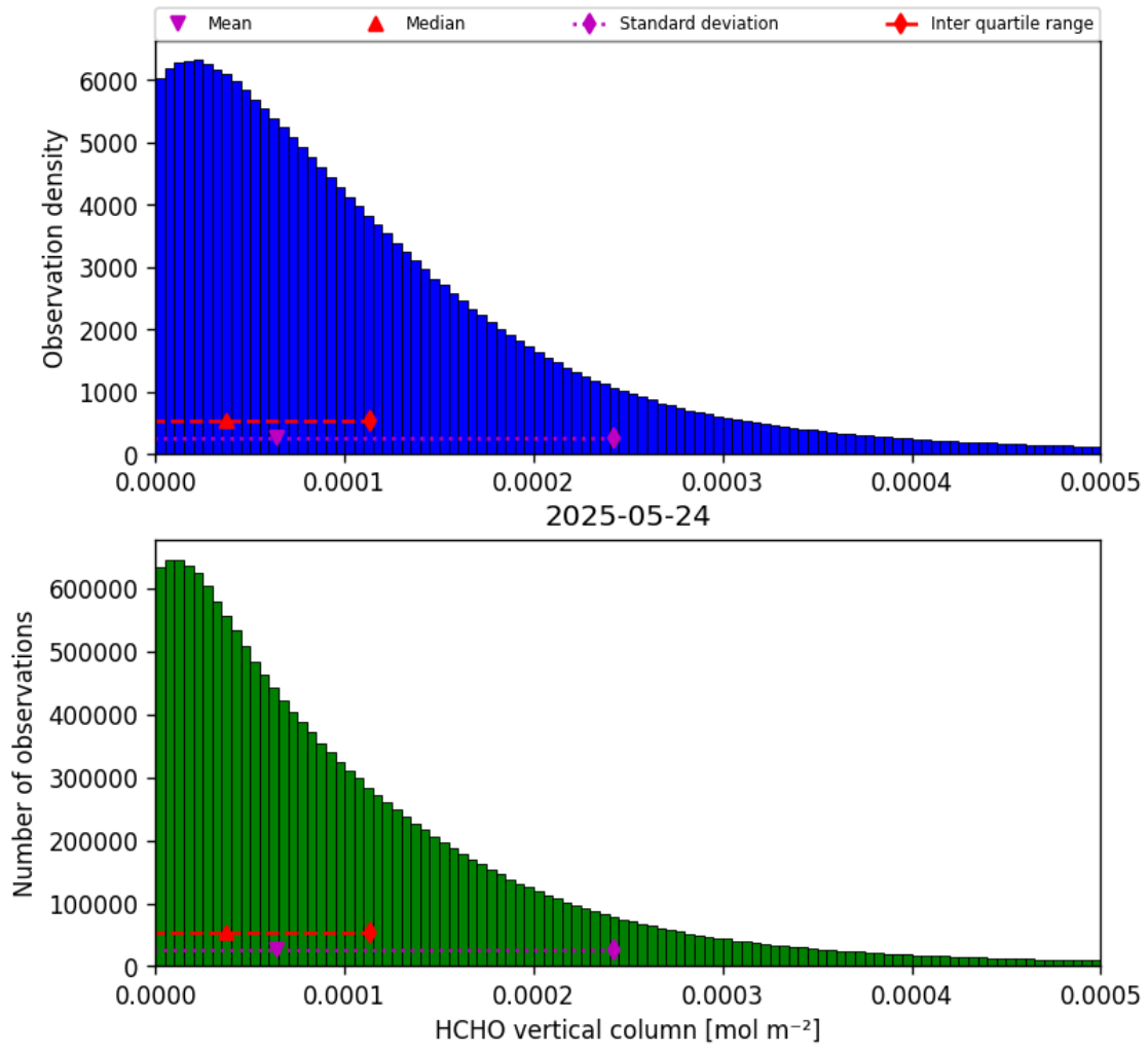
Figure 35: Histogram of “HCHO vertical column” for 2025-05-23 to 2025-05-25
