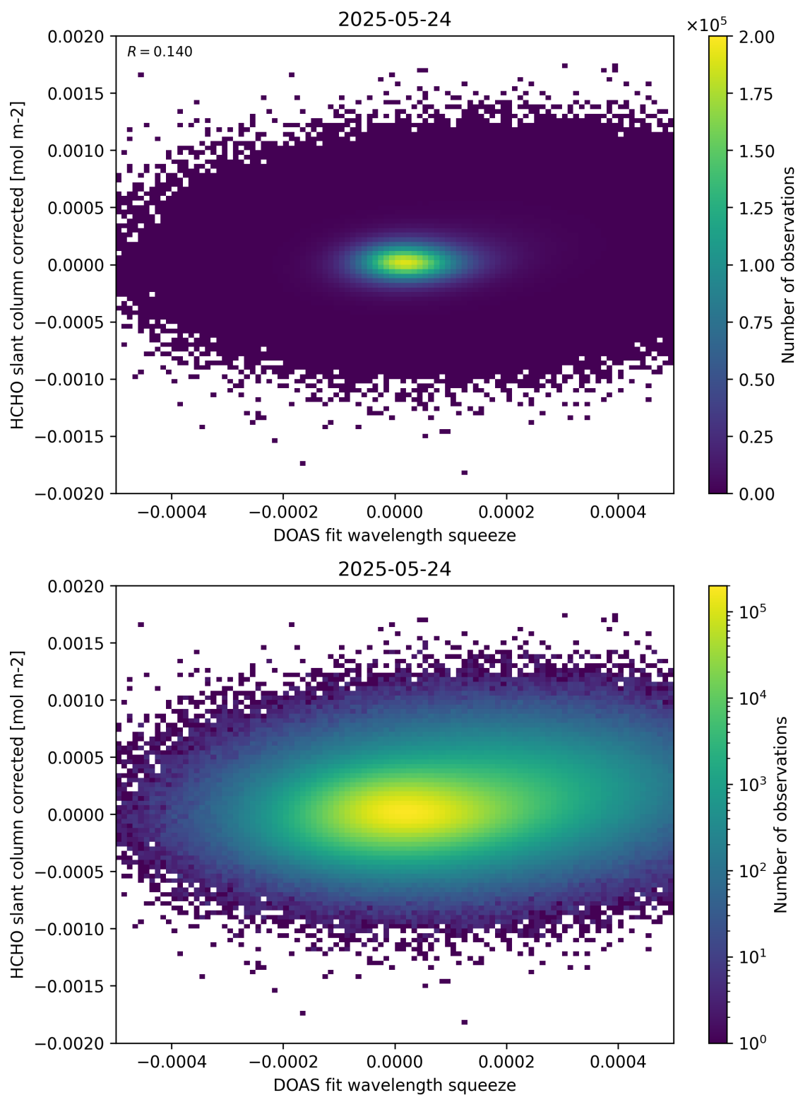
Figure 69: Scatter density plot of “DOAS fit wavelength squeeze” against “HCHO slant column corrected” for 2025-05-23 to 2025-05-25.
