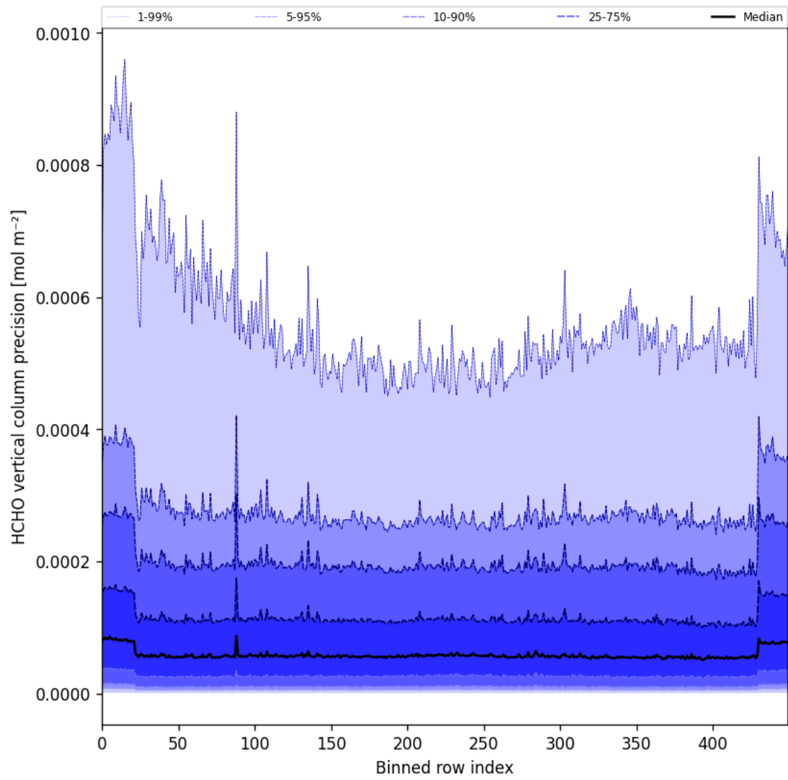
Figure 50: Along track statistics of “HCHO vertical column precision” for 2025-05-23 to 2025-05-25
