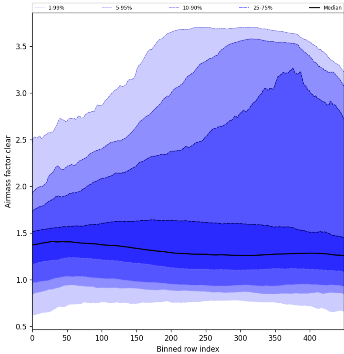
Figure 56: Along track statistics of “Airmass factor clear” for 2025-05-23 to 2025-05-25
