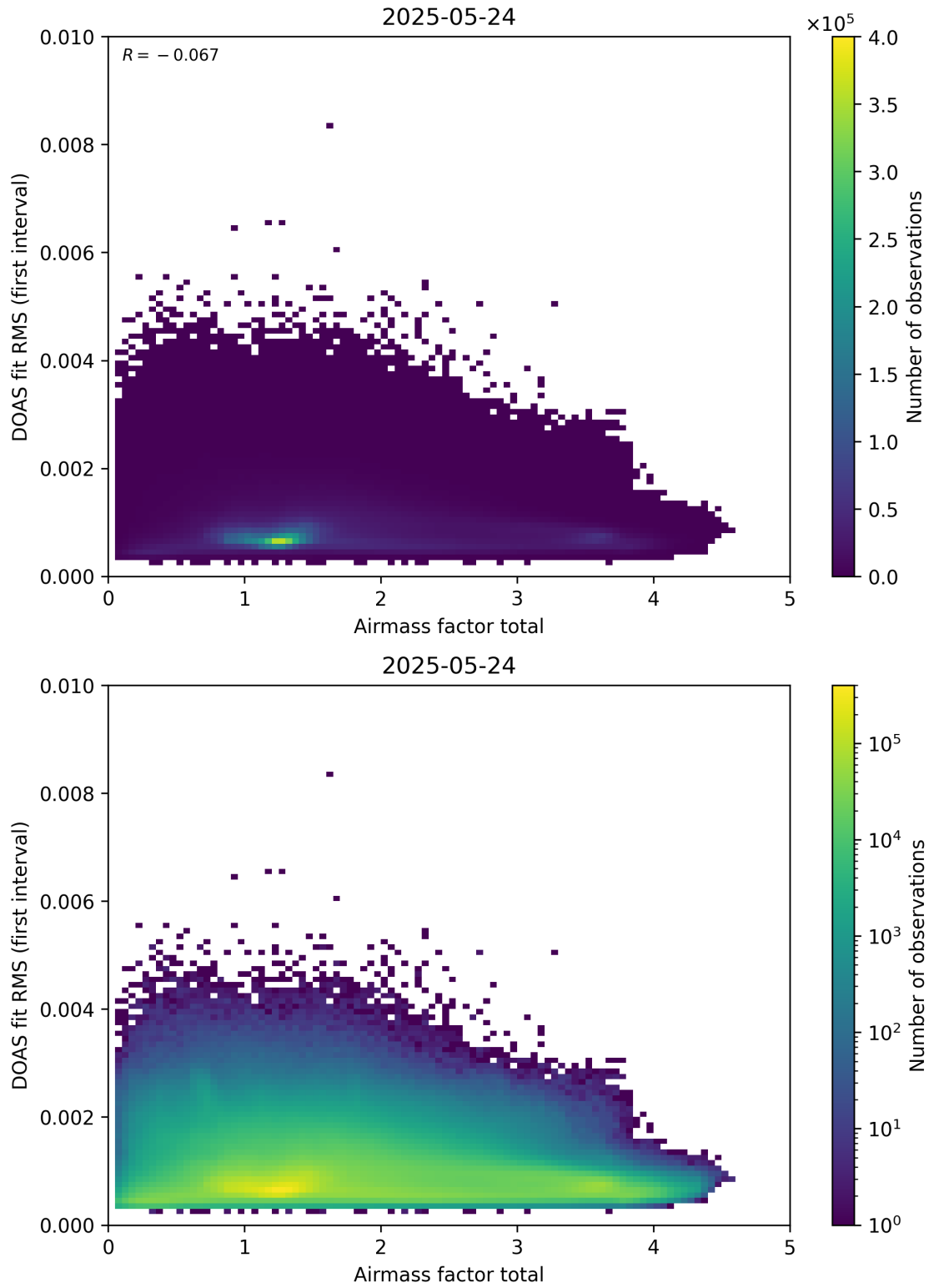
Figure 97: Scatter density plot of “Airmass factor total” against “DOAS fit RMS (first interval)” for 2025-05-23 to 2025-05-25.
