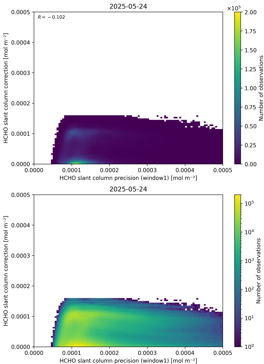
Figure 93: Scatter density plot of “HCHO slant column precision (window1)” against “HCHO slant column correction” for 2025-05-23 to 2025-05-25.
