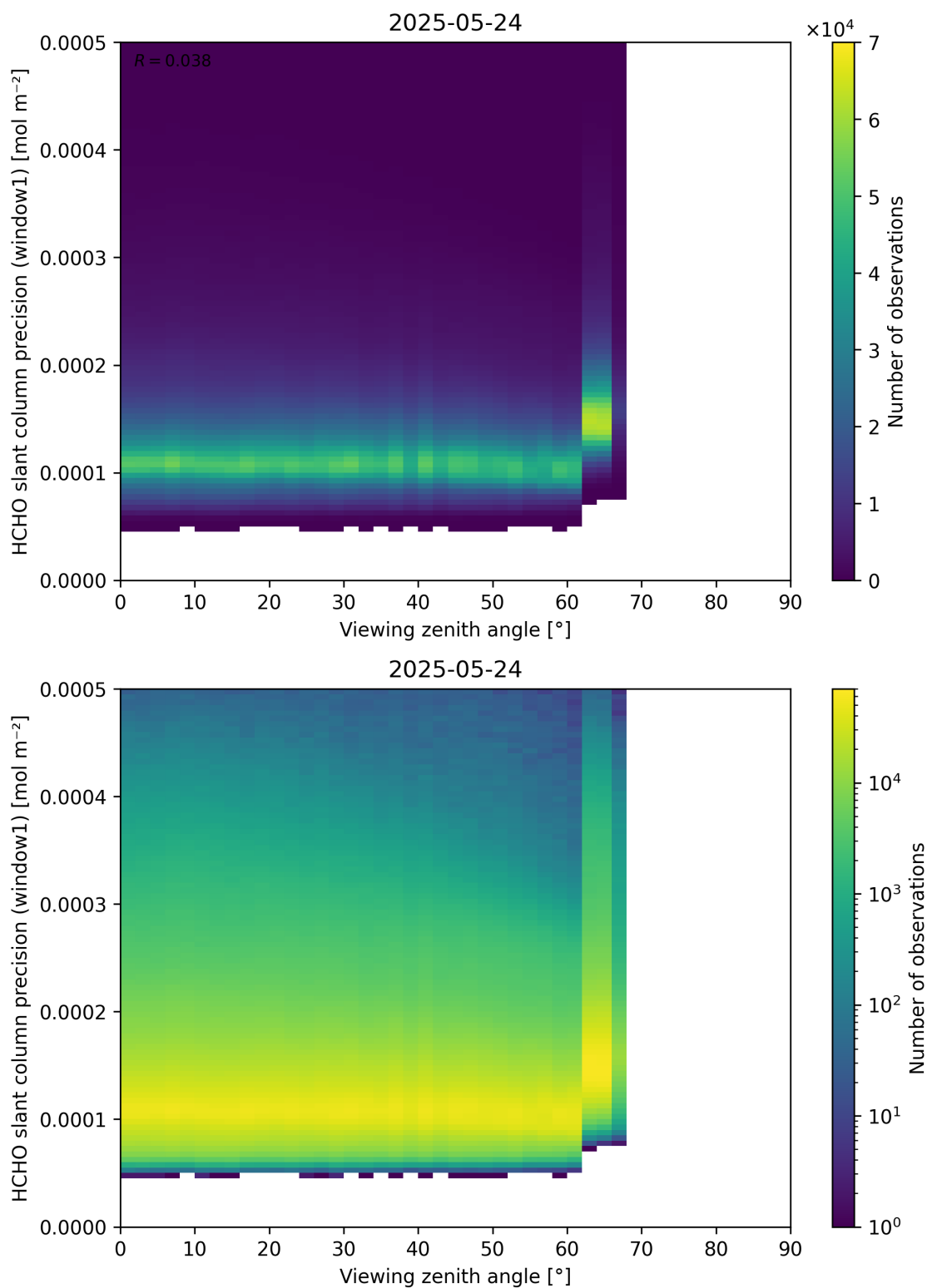
Figure 189: Scatter density plot of “Viewing zenith angle” against “HCHO slant column precision (window1)” for 2025-05-23 to 2025-05-25.
