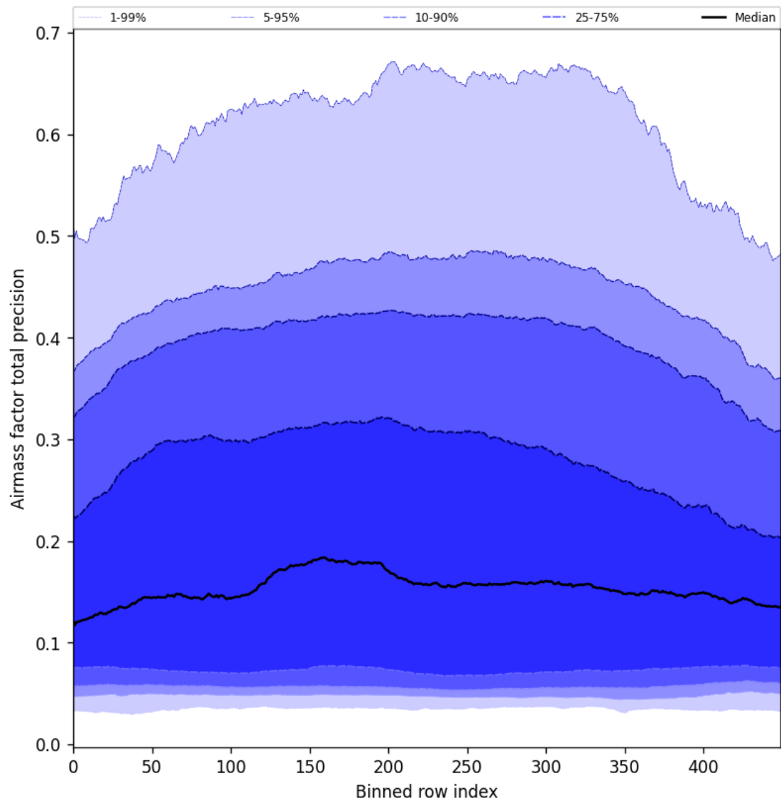
Figure 55: Along track statistics of “Airmass factor total precision” for 2025-05-23 to 2025-05-25
