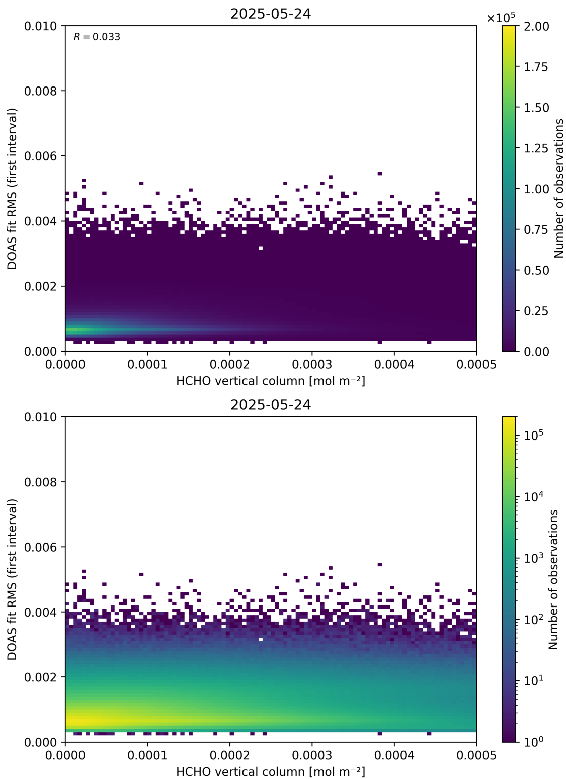
Figure 123: Scatter density plot of “HCHO vertical column” against “DOAS fit RMS (first interval)” for 2025-05-23 to 2025-05-25.
