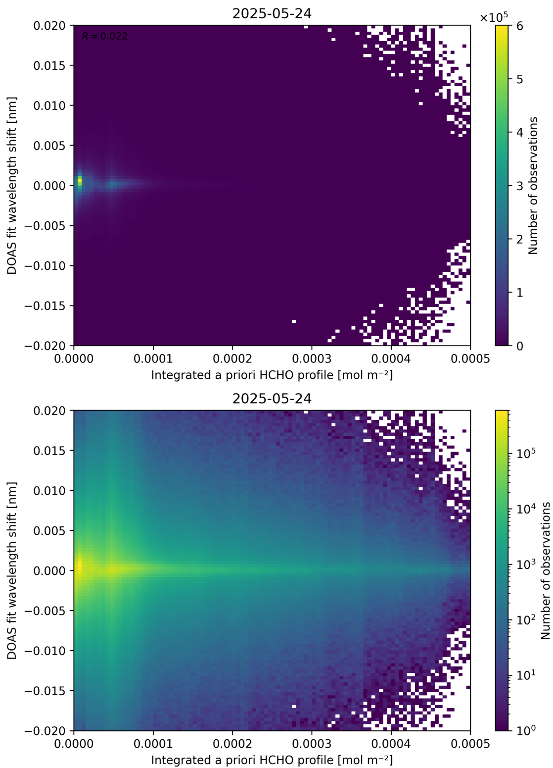
Figure 149: Scatter density plot of “Integrated a priori HCHO profile” against “DOAS fit wavelength shift” for 2025-05-23 to 2025-05-25.
