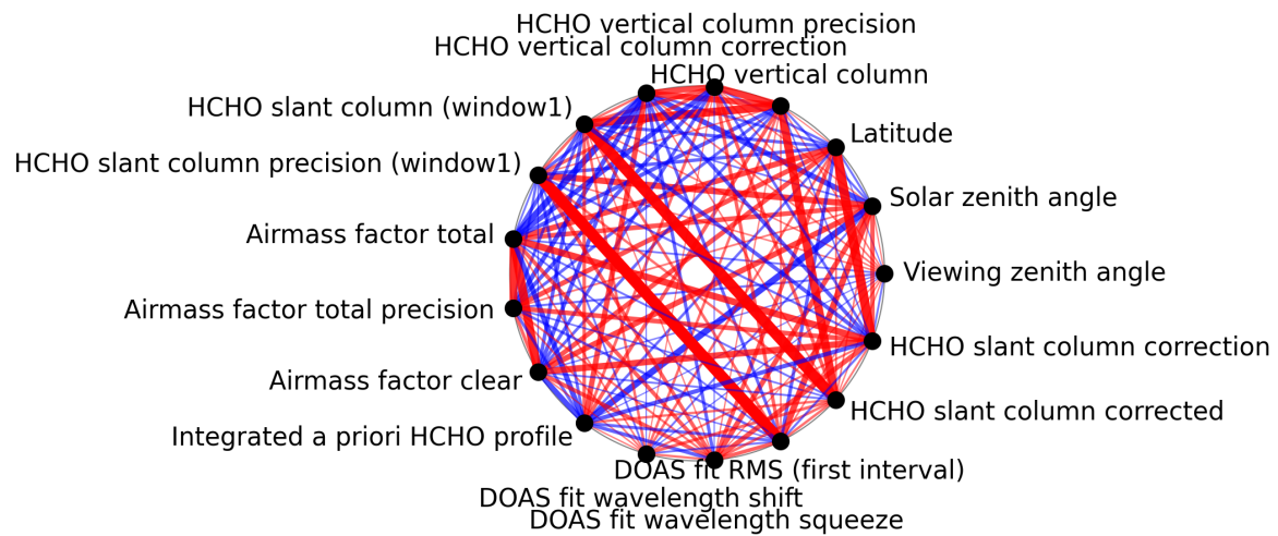
Figure 1: Map of correlation graph for 2025-05-23 to 2025-05-25.
