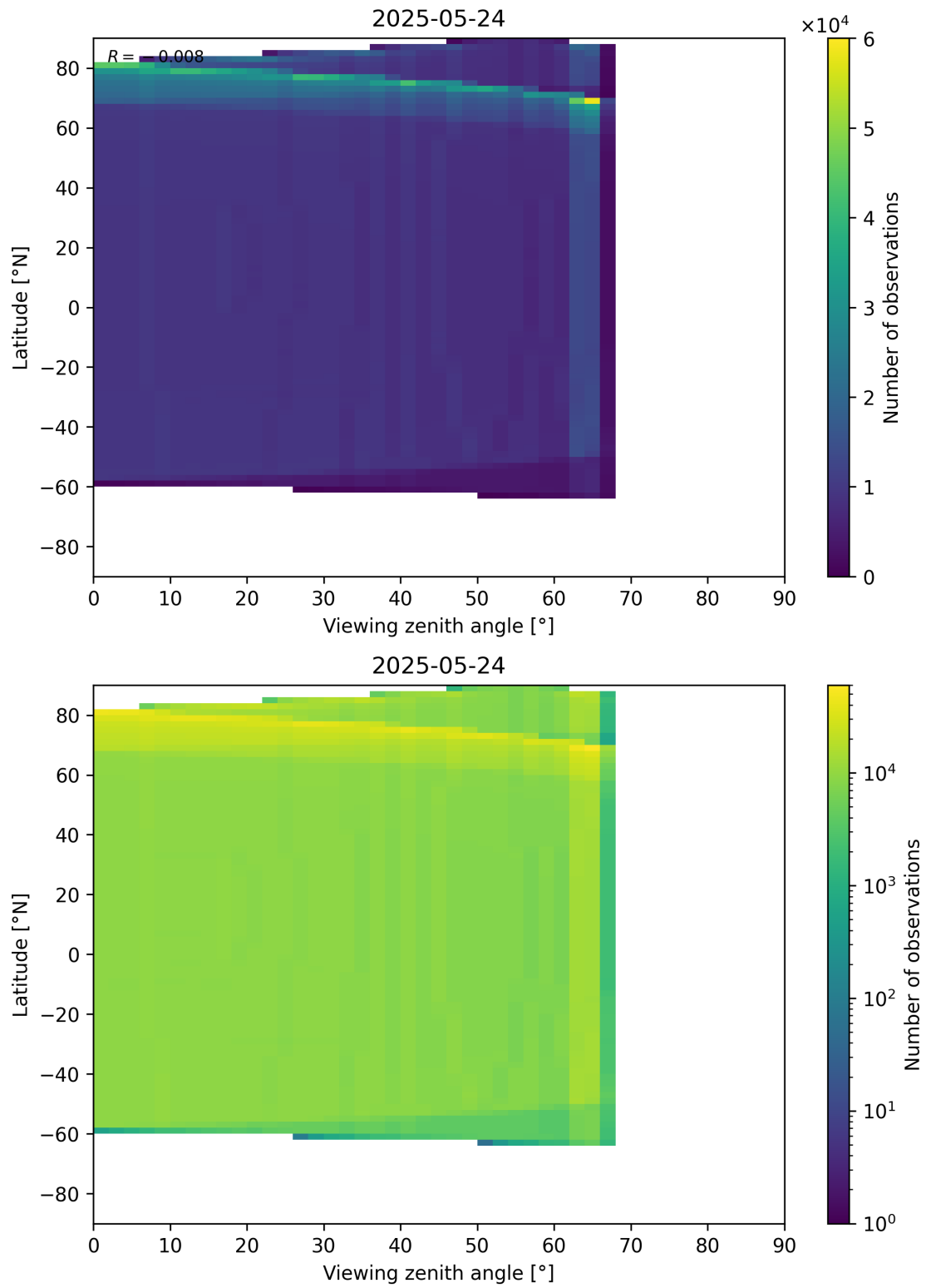
Figure 196: Scatter density plot of “Viewing zenith angle” against “Latitude” for 2025-05-23 to 2025-05-25.
