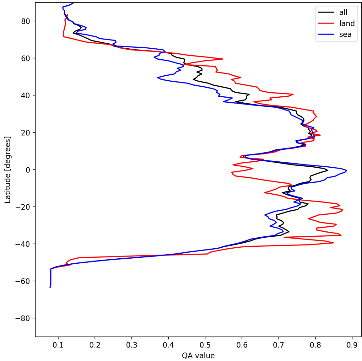
Figure 20: Zonal average of “QA value” for 2025-05-23 to 2025-05-25.
