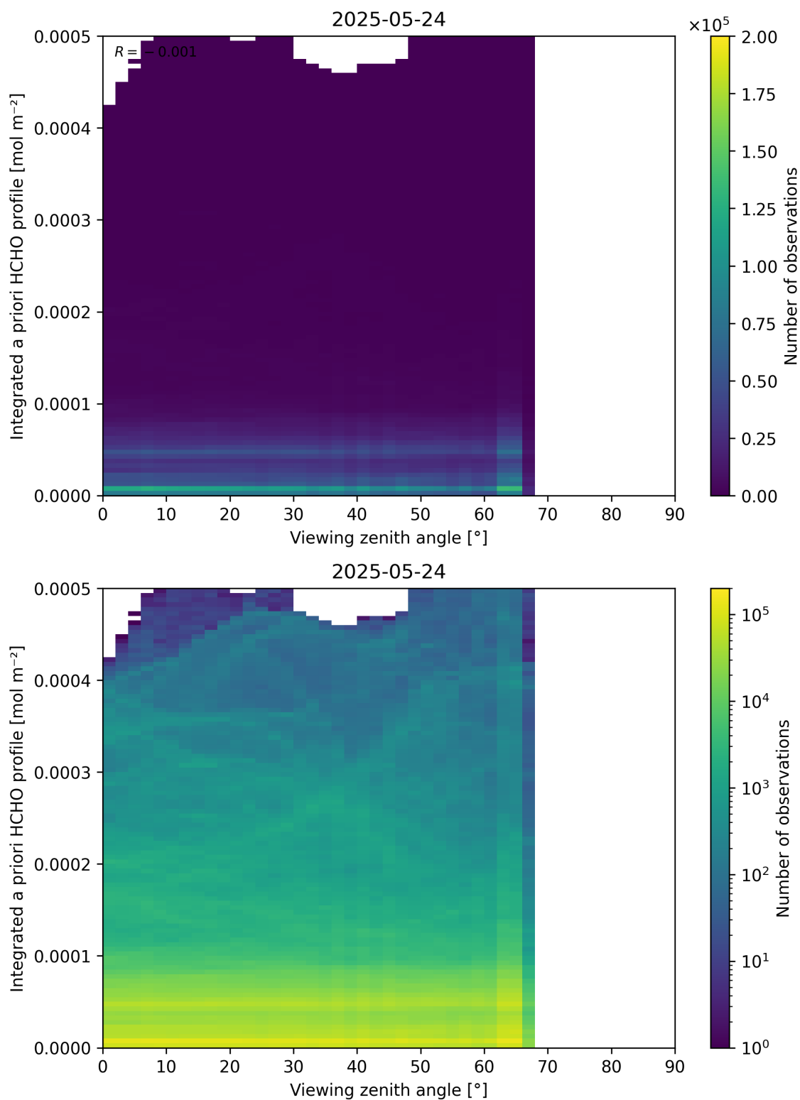
Figure 195: Scatter density plot of “Viewing zenith angle” against “Integrated a priori HCHO profile” for 2025-05-23 to 2025-05-25.
