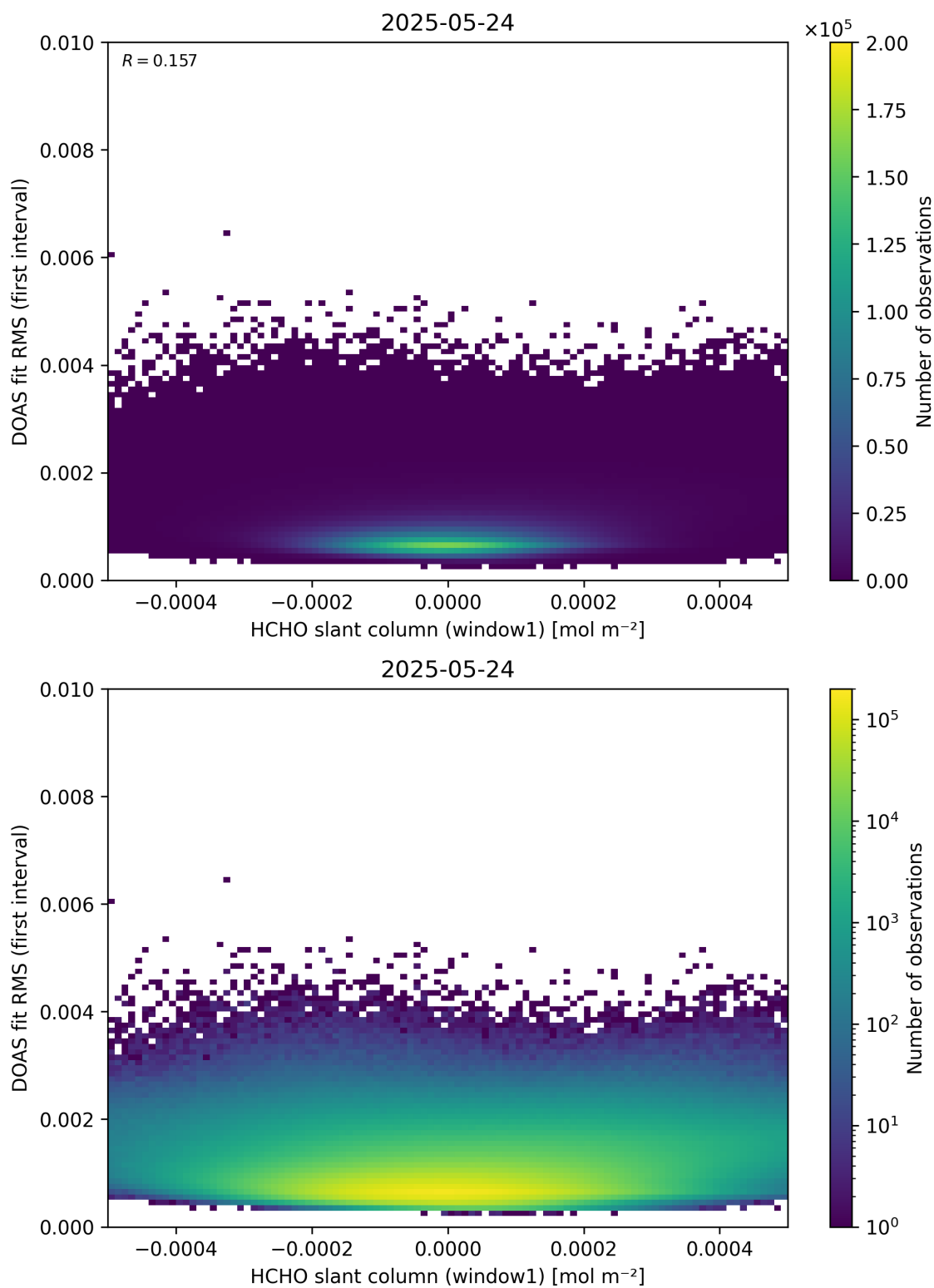
Figure 78: Scatter density plot of “HCHO slant column (window1)” against “DOAS fit RMS (first interval)” for 2025-05-23 to 2025-05-25.
