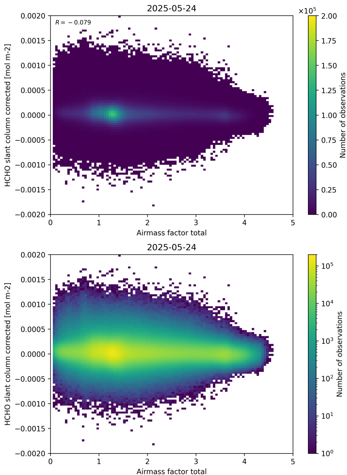
Figure 101: Scatter density plot of “Airmass factor total” against “HCHO slant column corrected” for 2025-05-23 to 2025-05-25.
