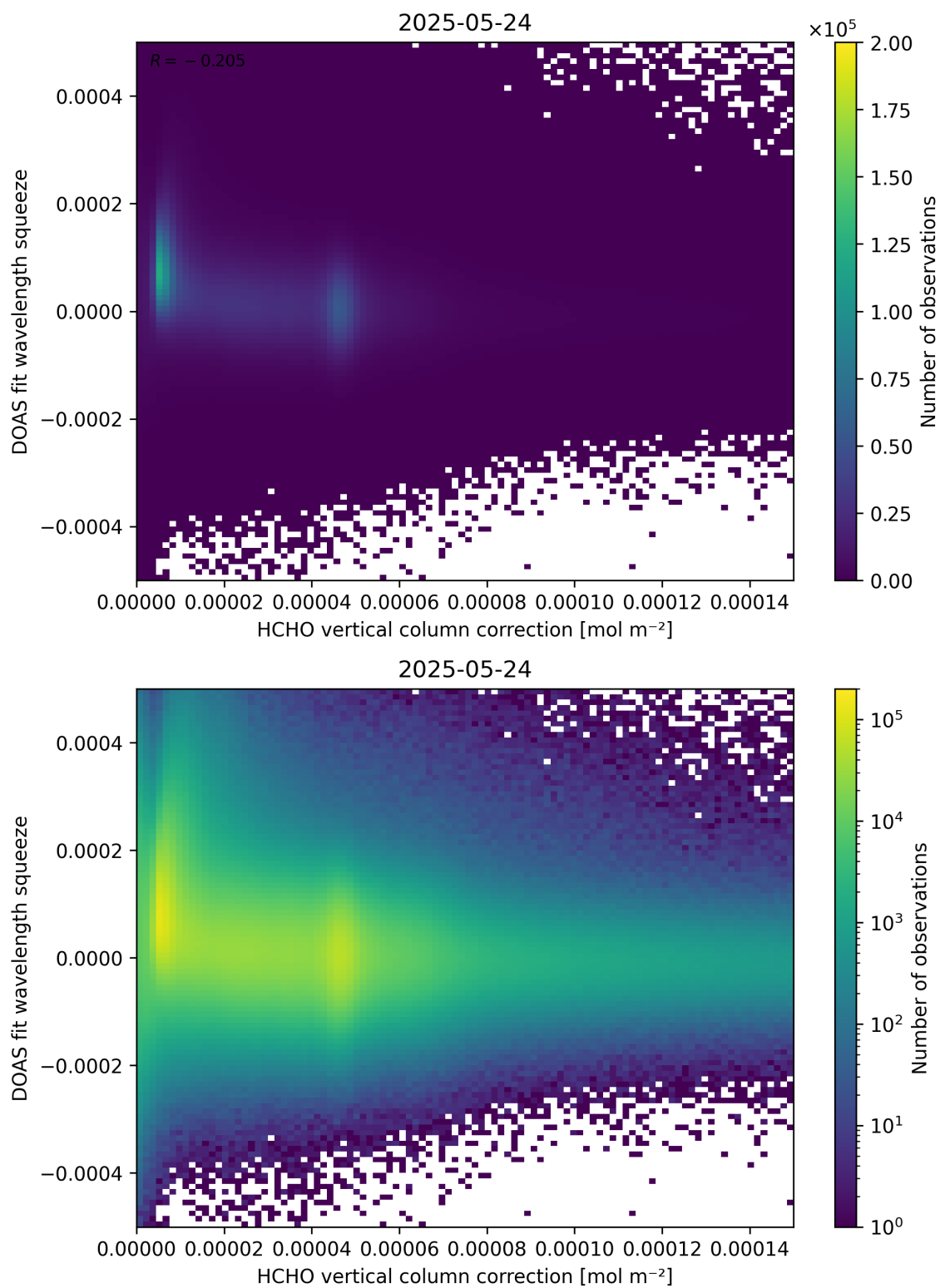
Figure 114: Scatter density plot of “HCHO vertical column correction” against “DOAS fit wavelength squeeze” for 2025-05-23 to 2025-05-25.
