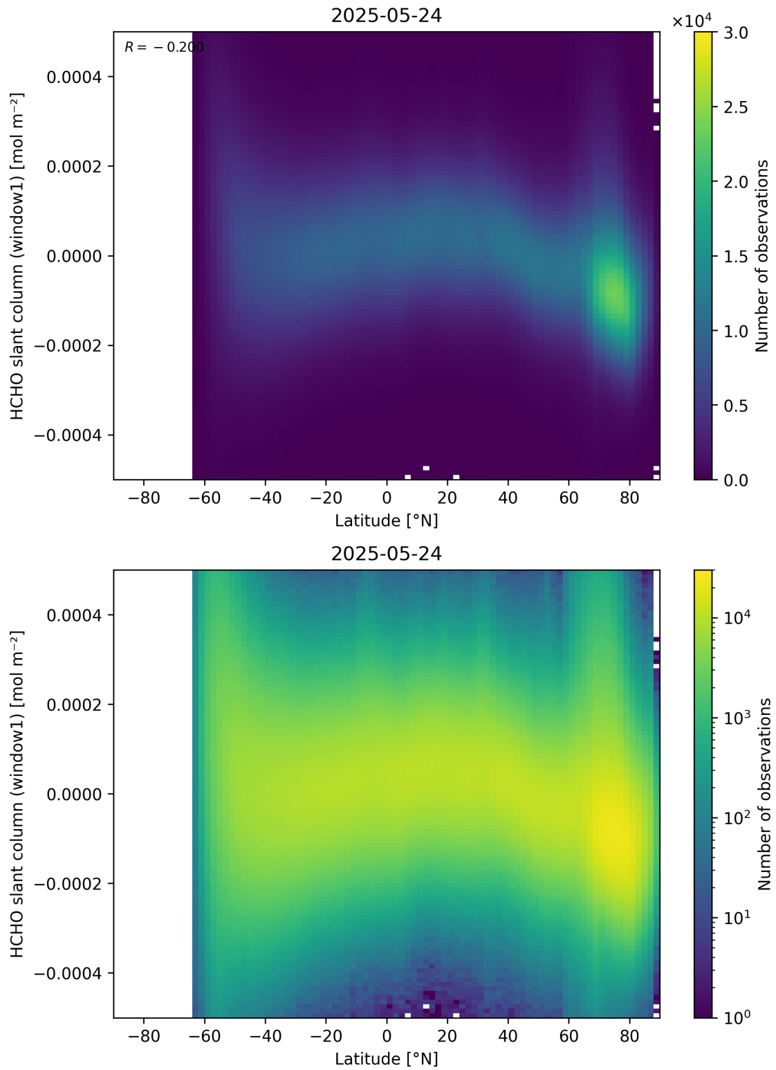
Figure 159: Scatter density plot of “Latitude” against “HCHO slant column (window1)” for 2025-05-23 to 2025-05-25.
