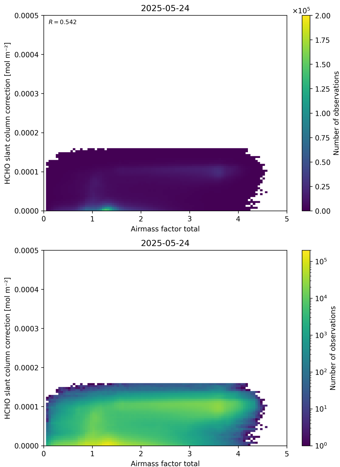
Figure 102: Scatter density plot of “Airmass factor total” against “HCHO slant column correction” for 2025-05-23 to 2025-05-25.
