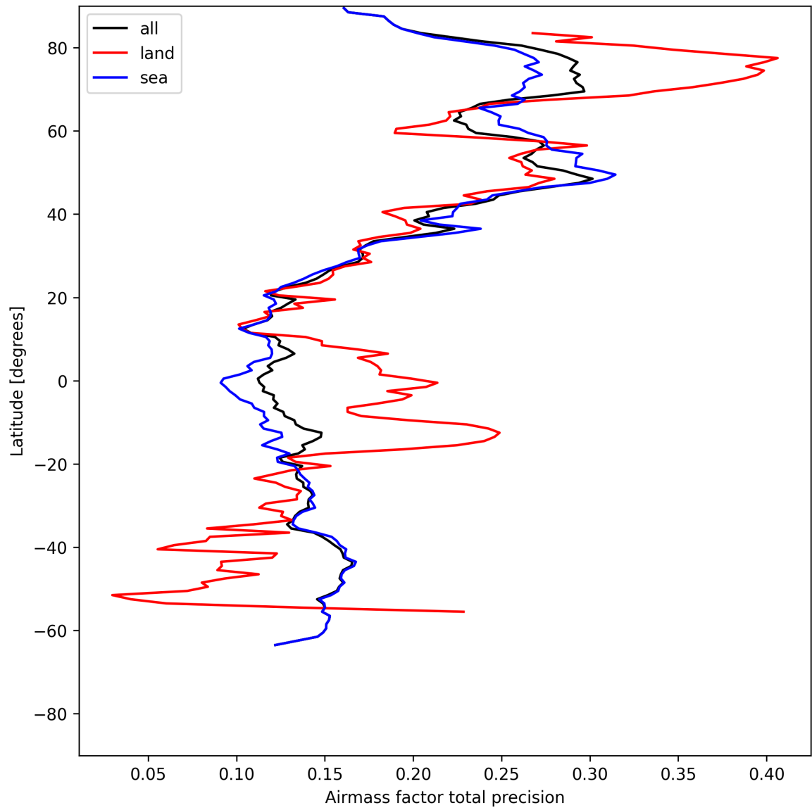
Figure 27: Zonal average of “Airmass factor total precision” for 2025-05-23 to 2025-05-25.
