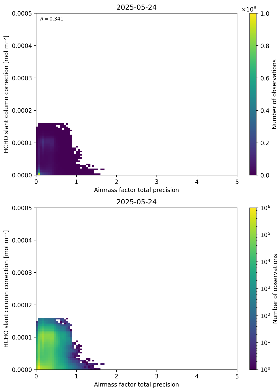
Figure 110: Scatter density plot of “Airmass factor total precision” against “HCHO slant column correction” for 2025-05-23 to 2025-05-25.
