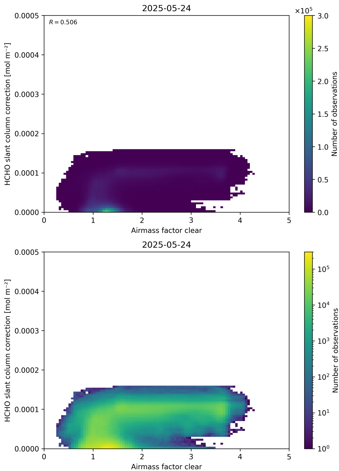
Figure 75: Scatter density plot of “Airmass factor clear” against “HCHO slant column correction” for 2025-05-23 to 2025-05-25.
