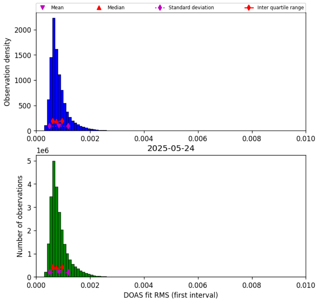
Figure 46: Histogram of “DOAS fit RMS (first interval)” for 2025-05-23 to 2025-05-25
