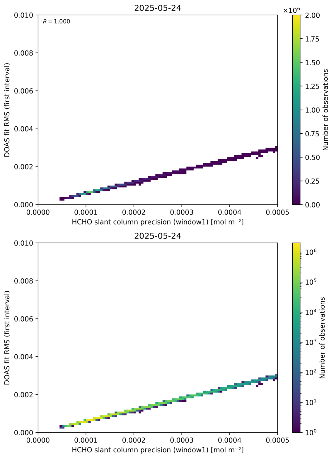
Figure 88: Scatter density plot of “HCHO slant column precision (window1)” against “DOAS fit RMS (first interval)” for 2025-05-23 to 2025-05-25.
