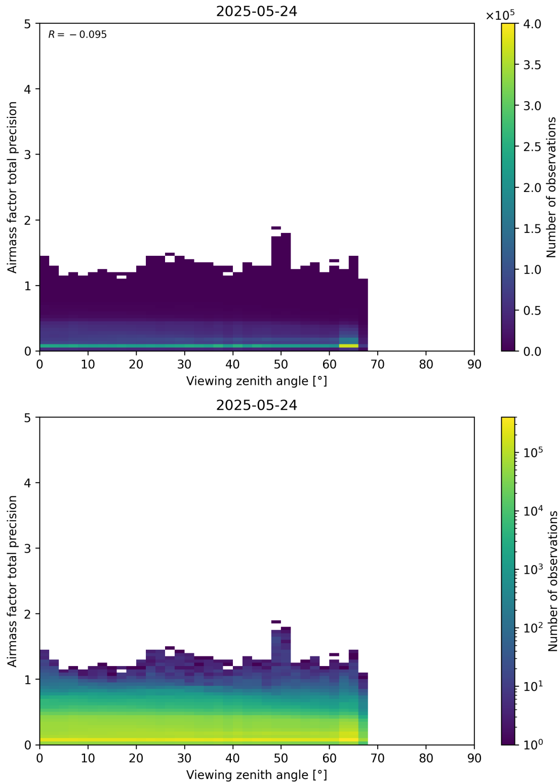
Figure 191: Scatter density plot of “Viewing zenith angle” against “Airmass factor total precision” for 2025-05-23 to 2025-05-25.
