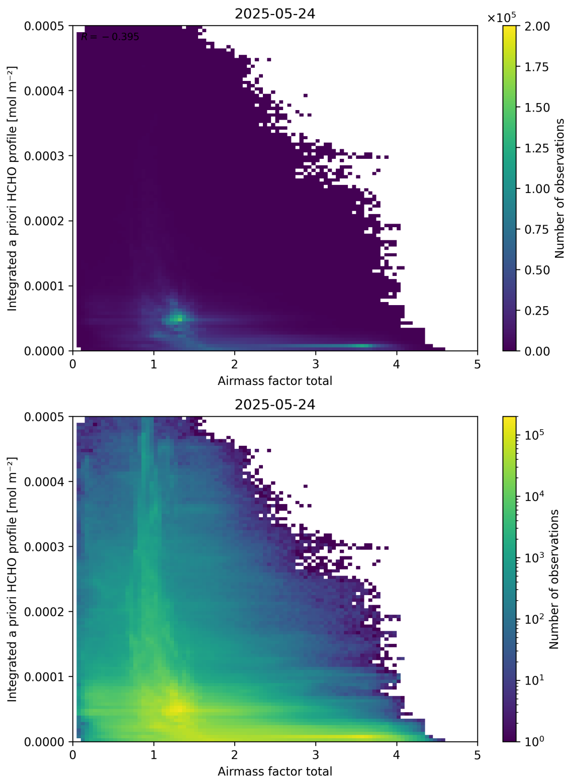
Figure 104: Scatter density plot of “Airmass factor total” against “Integrated a priori HCHO profile” for 2025-05-23 to 2025-05-25.
