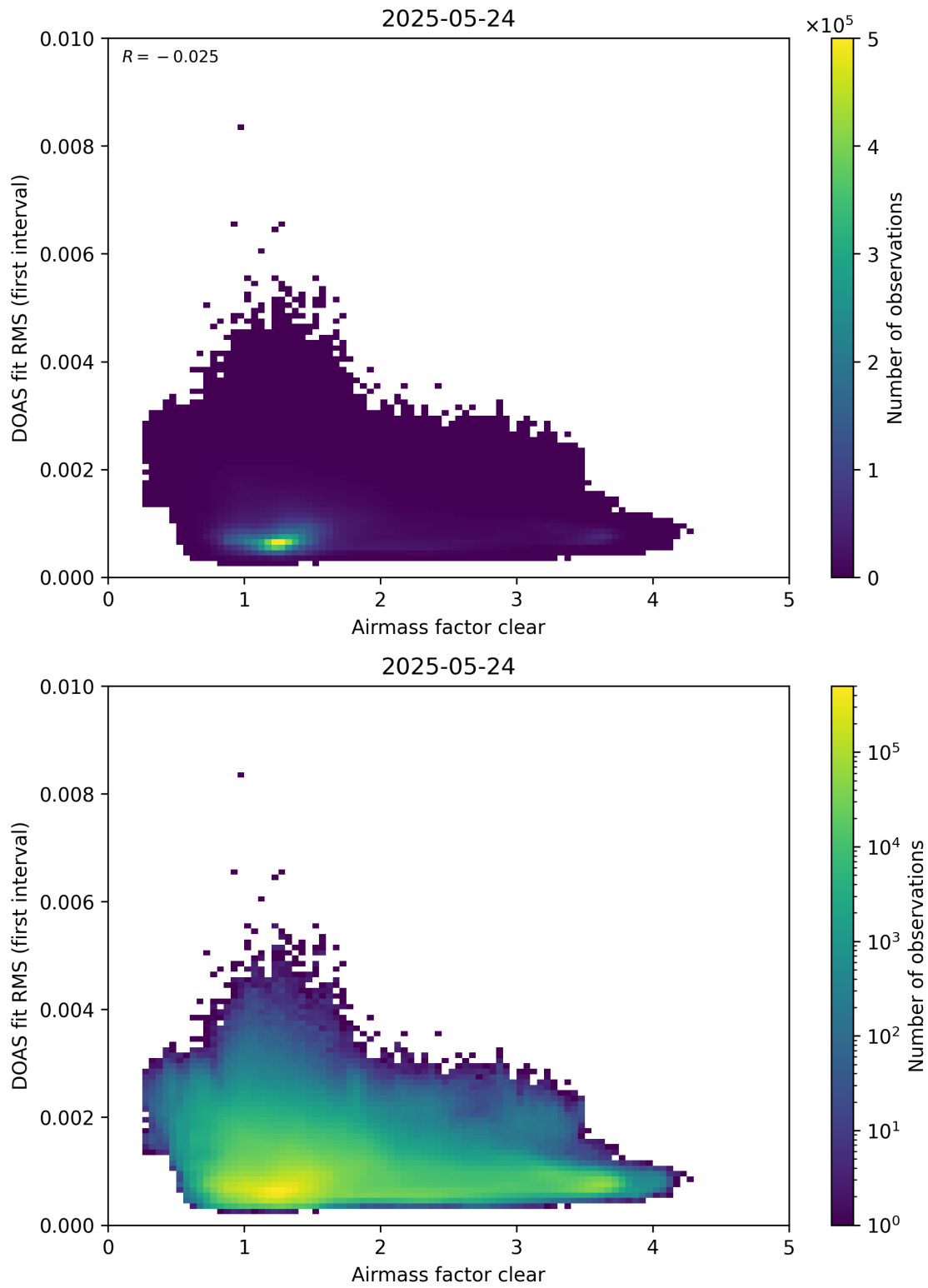
Figure 71: Scatter density plot of “Airmass factor clear” against “DOAS fit RMS (first interval)” for 2025-05-23 to 2025-05-25.
