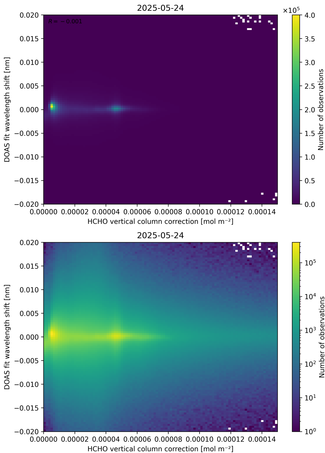
Figure 113: Scatter density plot of “HCHO vertical column correction” against “DOAS fit wavelength shift” for 2025-05-23 to 2025-05-25.
