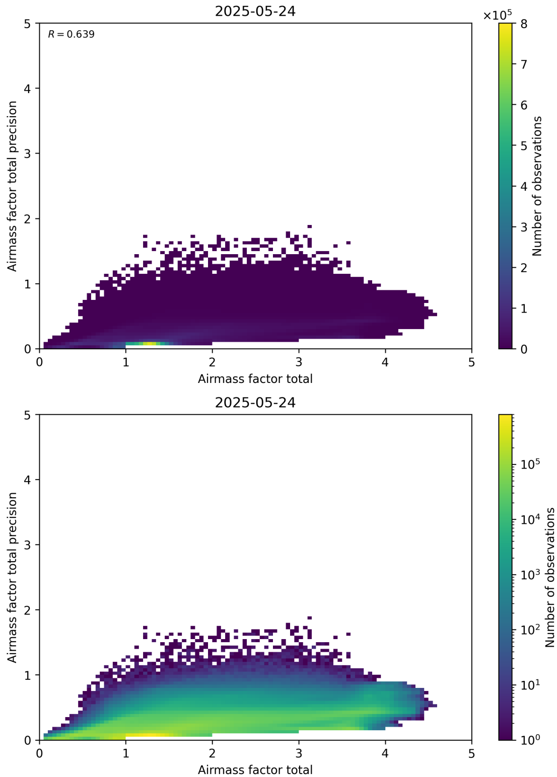
Figure 103: Scatter density plot of “Airmass factor total” against “Airmass factor total precision” for 2025-05-23 to 2025-05-25.
