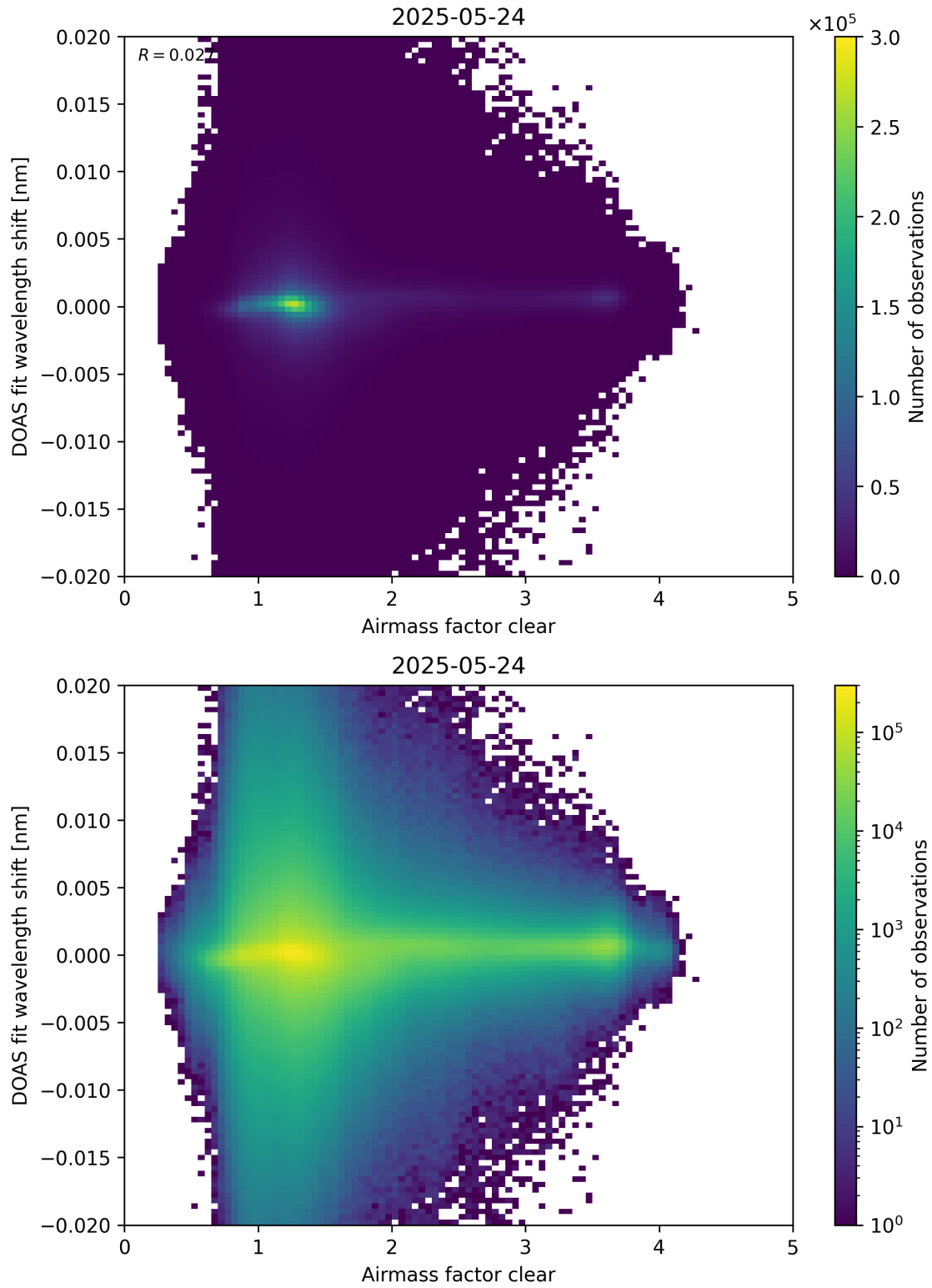
Figure 72: Scatter density plot of “Airmass factor clear” against “DOAS fit wavelength shift” for 2025-05-23 to 2025-05-25.
