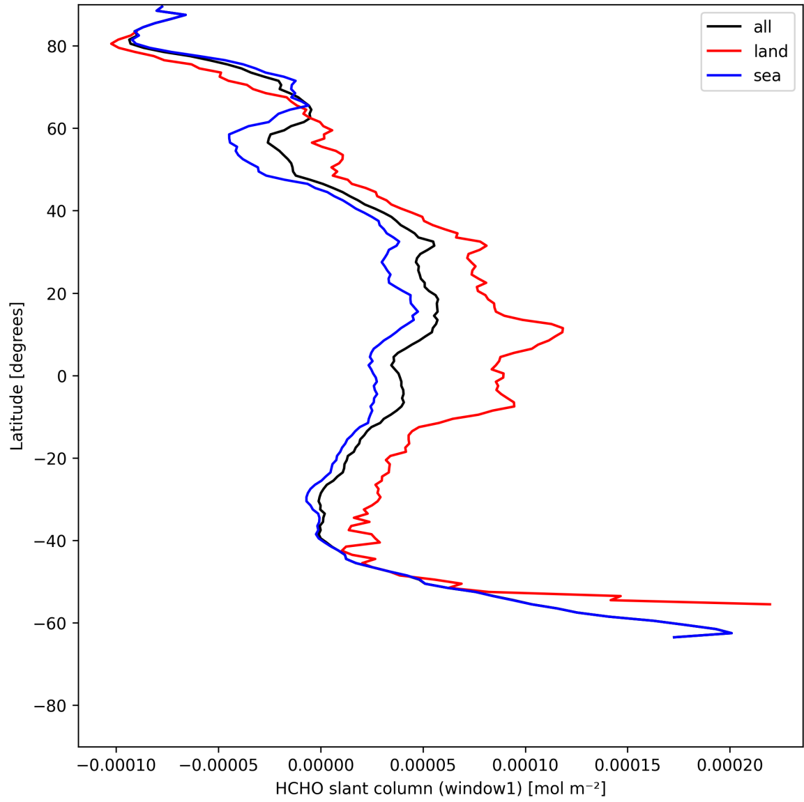
Figure 24: Zonal average of “HCHO slant column (window1)” for 2025-05-23 to 2025-05-25.
