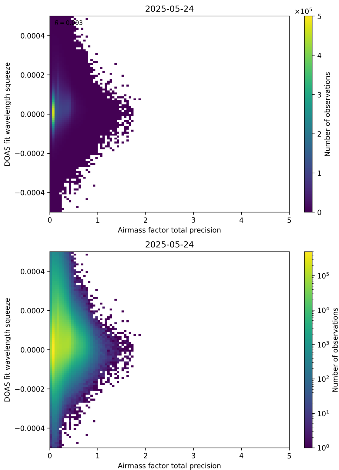
Figure 107: Scatter density plot of “Airmass factor total precision” against “DOAS fit wavelength squeeze” for 2025-05-23 to 2025-05-25.
