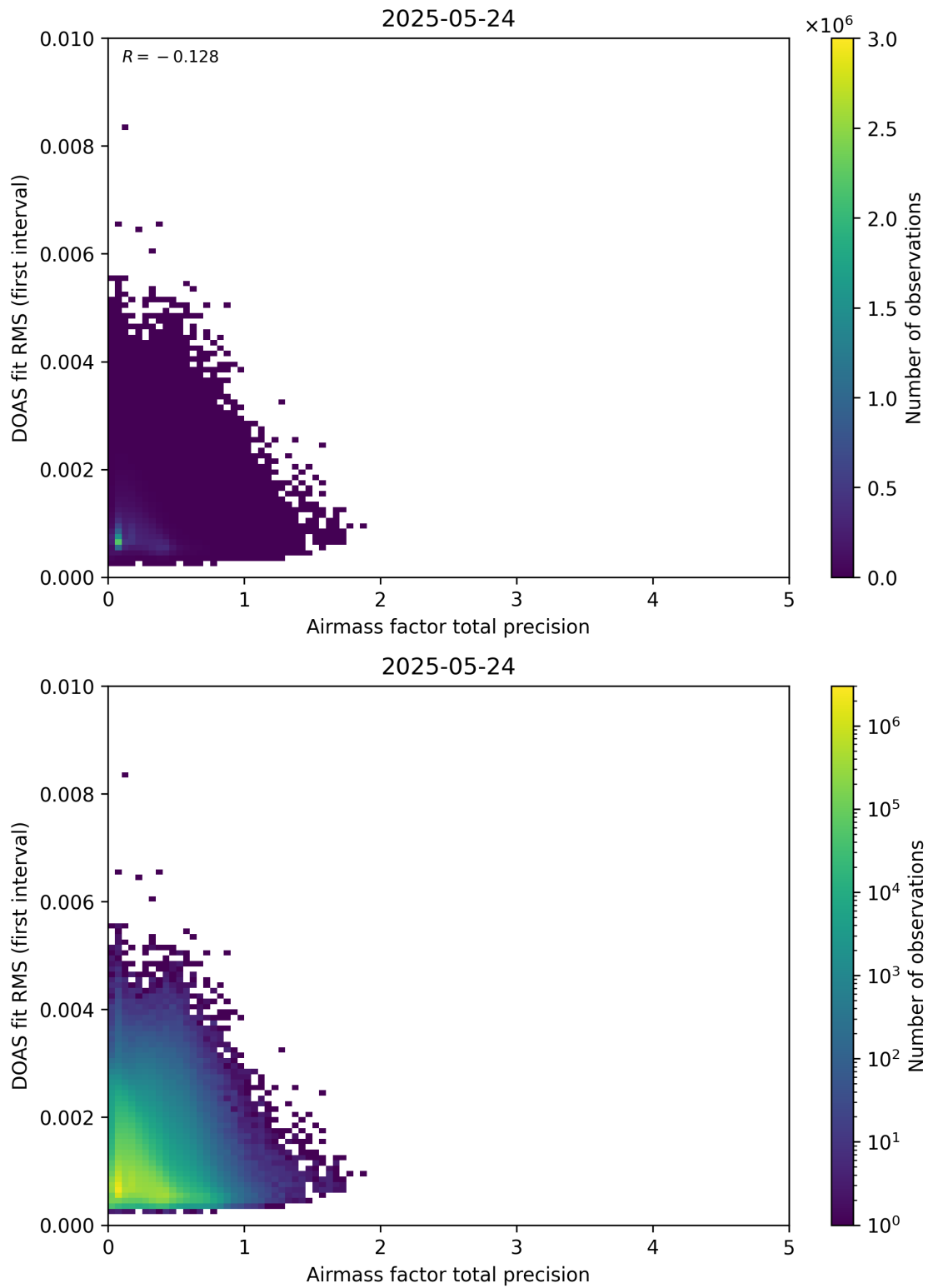
Figure 105: Scatter density plot of “Airmass factor total precision” against “DOAS fit RMS (first interval)” for 2025-05-23 to 2025-05-25.
