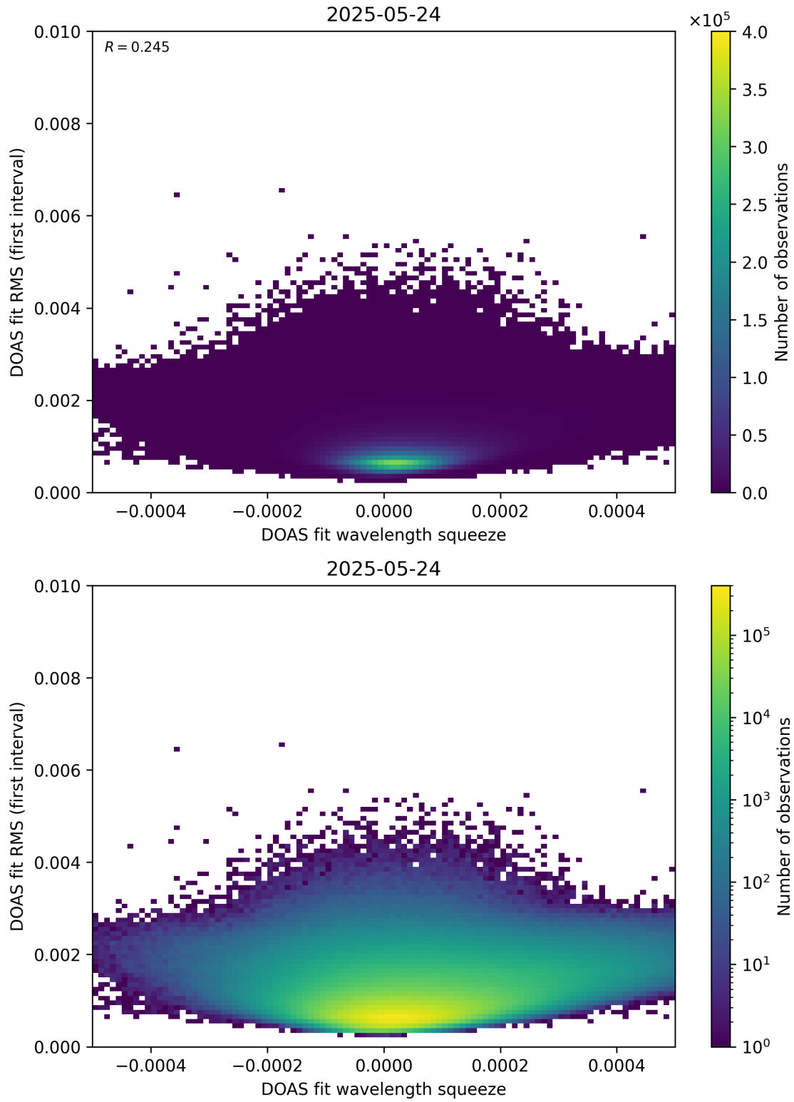
Figure 68: Scatter density plot of “DOAS fit wavelength squeeze” against “DOAS fit RMS (first interval)” for 2025-05-23 to 2025-05-25.
