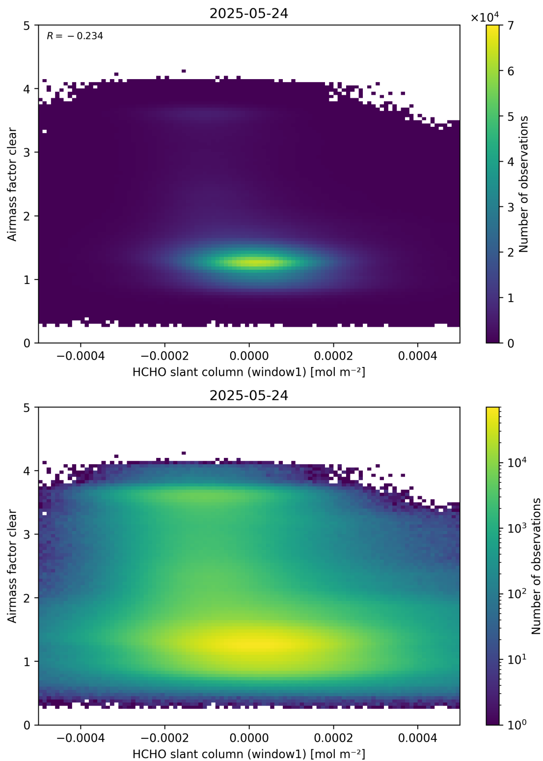
Figure 81: Scatter density plot of “HCHO slant column (window1)” against “Airmass factor clear” for 2025-05-23 to 2025-05-25.
