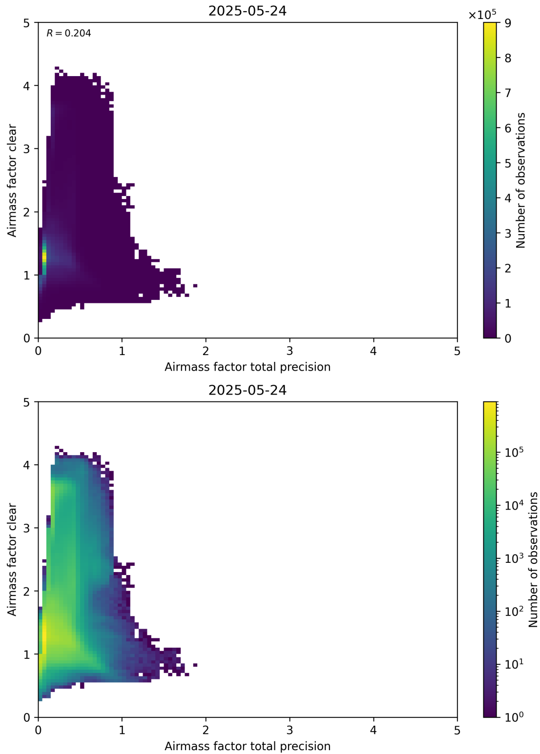
Figure 108: Scatter density plot of “Airmass factor total precision” against “Airmass factor clear” for 2025-05-23 to 2025-05-25.
