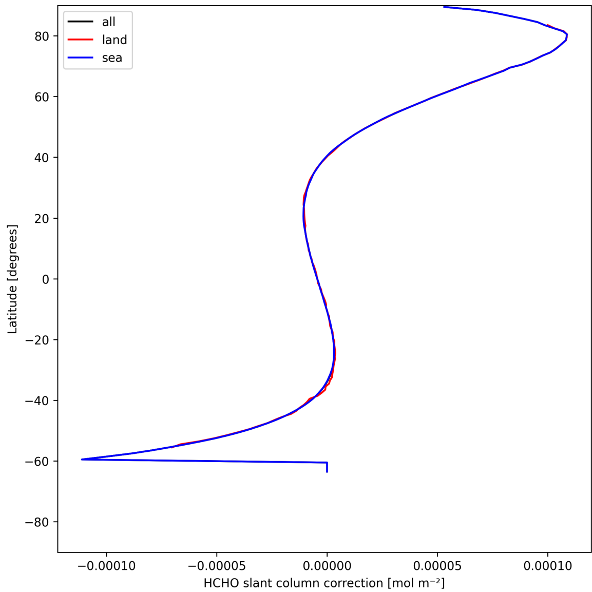
Figure 33: Zonal average of “HCHO slant column correction” for 2025-05-23 to 2025-05-25.
