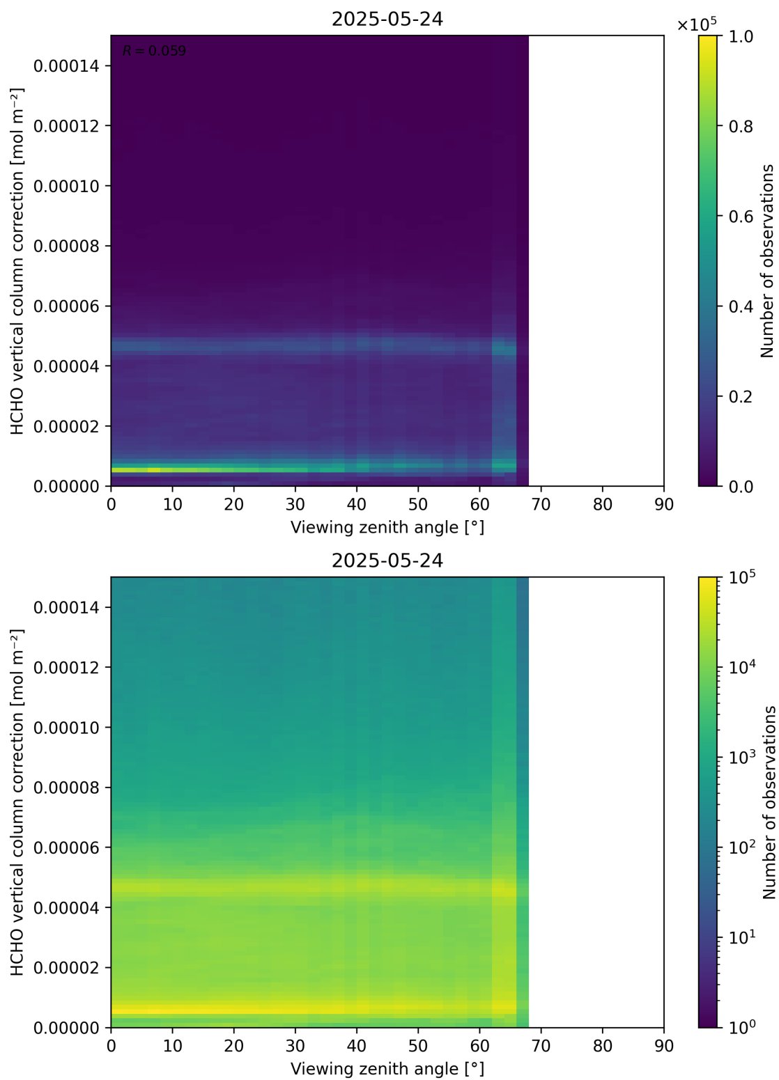
Figure 193: Scatter density plot of “Viewing zenith angle” against “HCHO vertical column correction” for 2025-05-23 to 2025-05-25.
