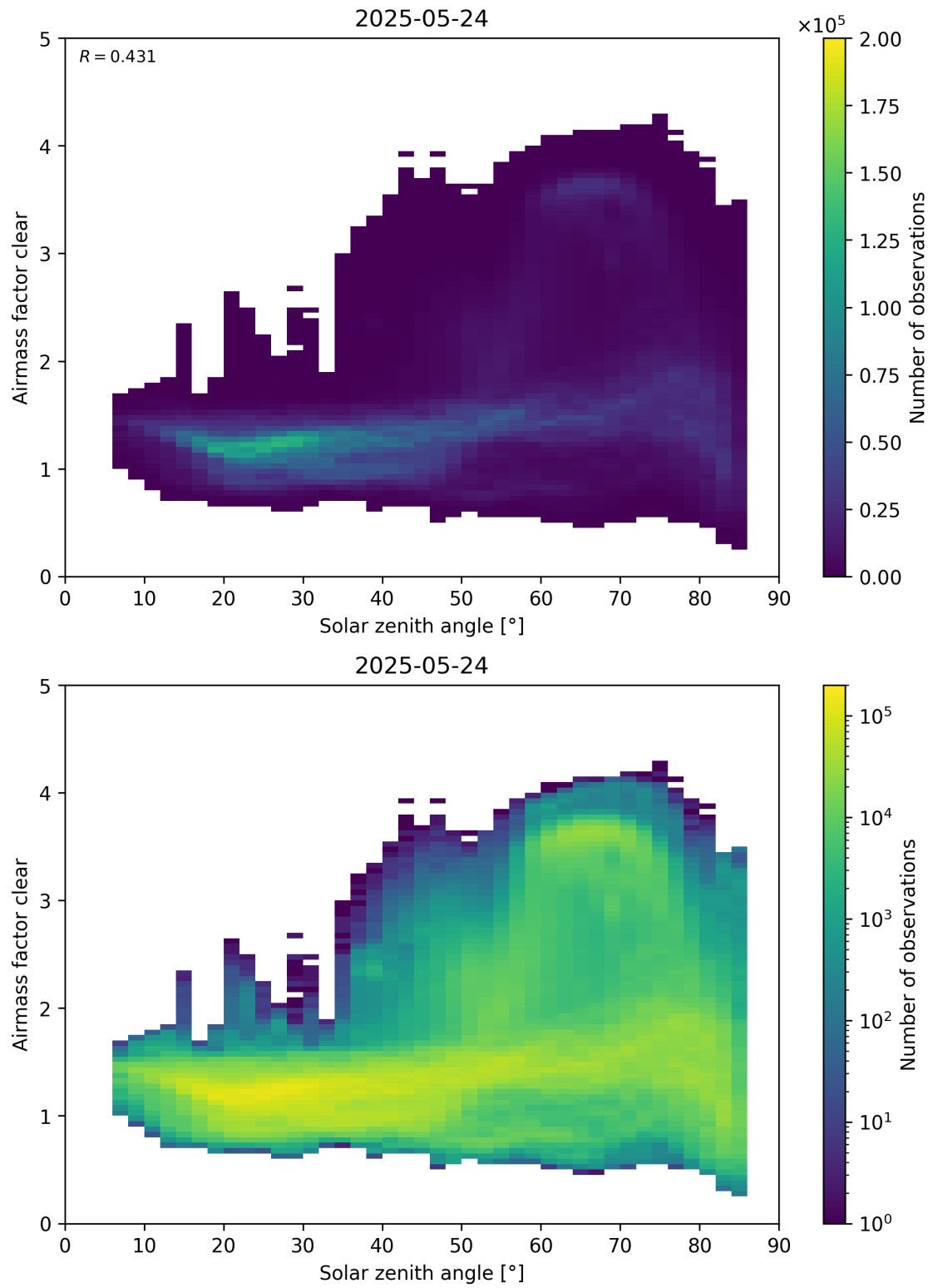
Figure 170: Scatter density plot of “Solar zenith angle” against “Airmass factor clear” for 2025-05-23 to 2025-05-25.
