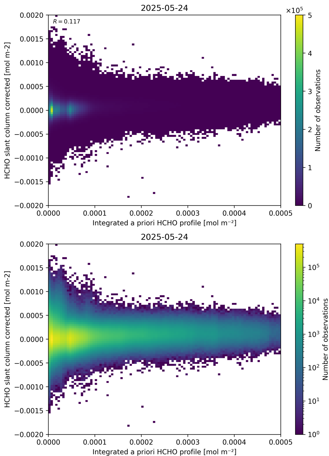
Figure 151: Scatter density plot of “Integrated a priori HCHO profile” against “HCHO slant column corrected” for 2025-05-23 to 2025-05-25.
