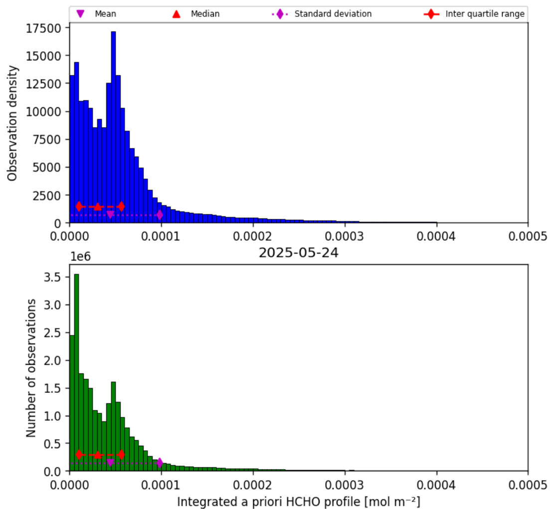
Figure 43: Histogram of “Integrated a priori HCHO profile” for 2025-05-23 to 2025-05-25
