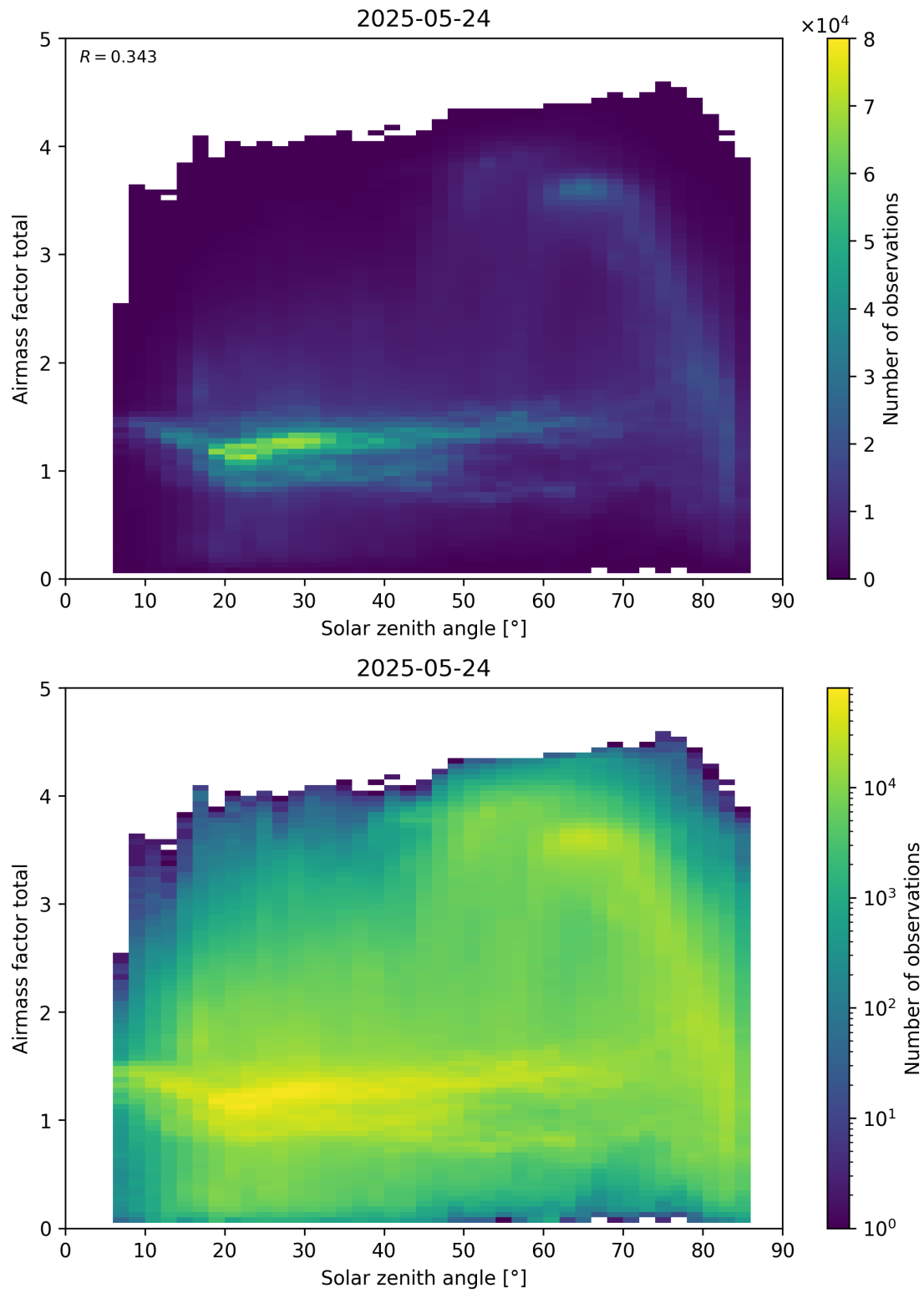
Figure 175: Scatter density plot of “Solar zenith angle” against “Airmass factor total” for 2025-05-23 to 2025-05-25.
