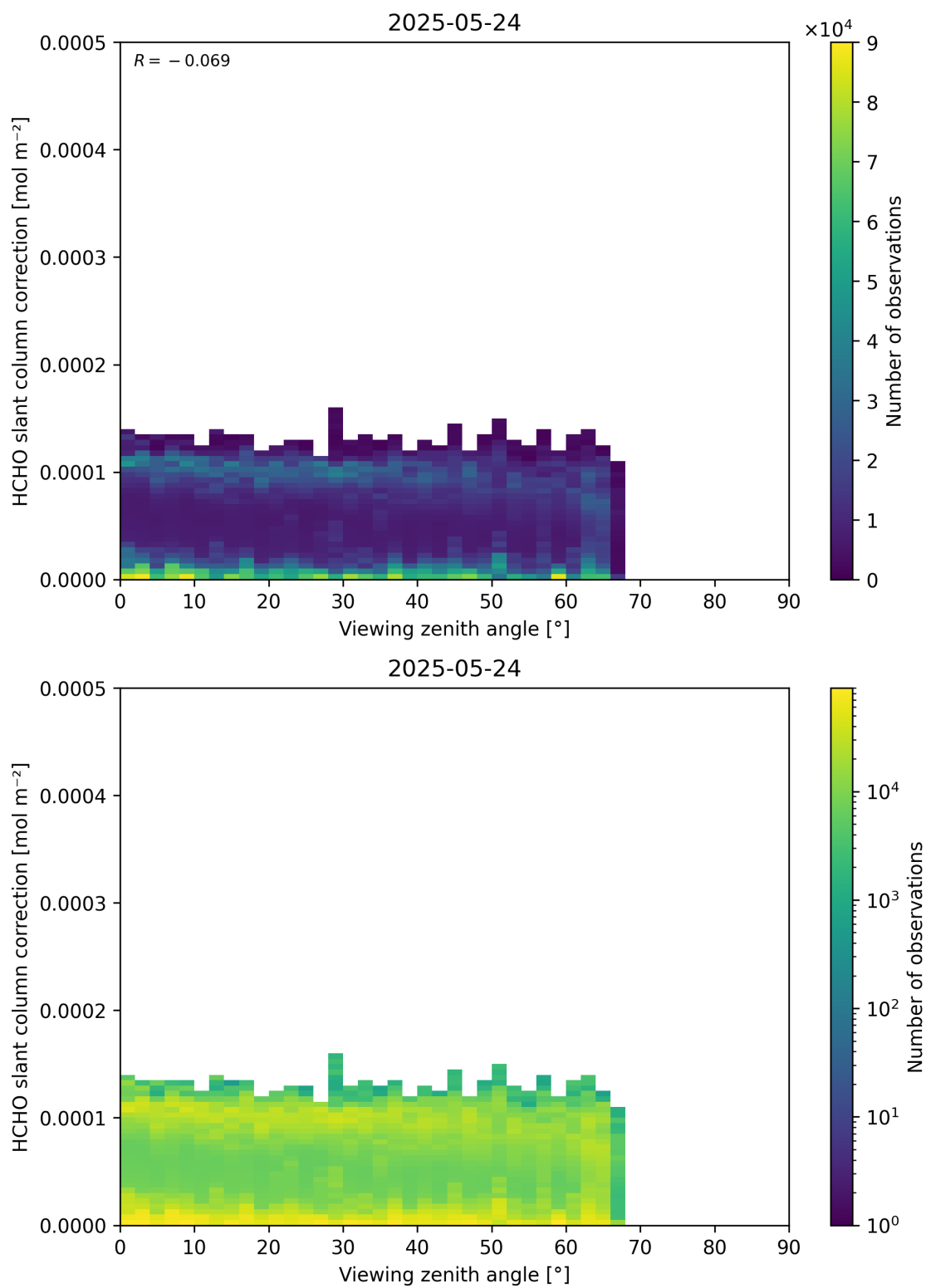
Figure 187: Scatter density plot of “Viewing zenith angle” against “HCHO slant column correction” for 2025-05-23 to 2025-05-25.
