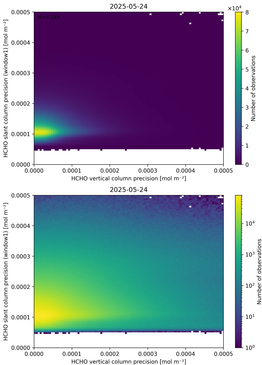
Figure 143: Scatter density plot of “HCHO vertical column precision” against “HCHO slant column precision (window1)” for 2025-05-23 to 2025-05-25.
