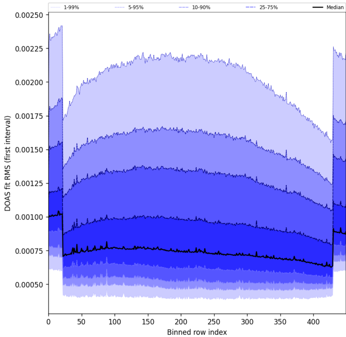
Figure 60: Along track statistics of “DOAS fit RMS (first interval)” for 2025-05-23 to 2025-05-25
