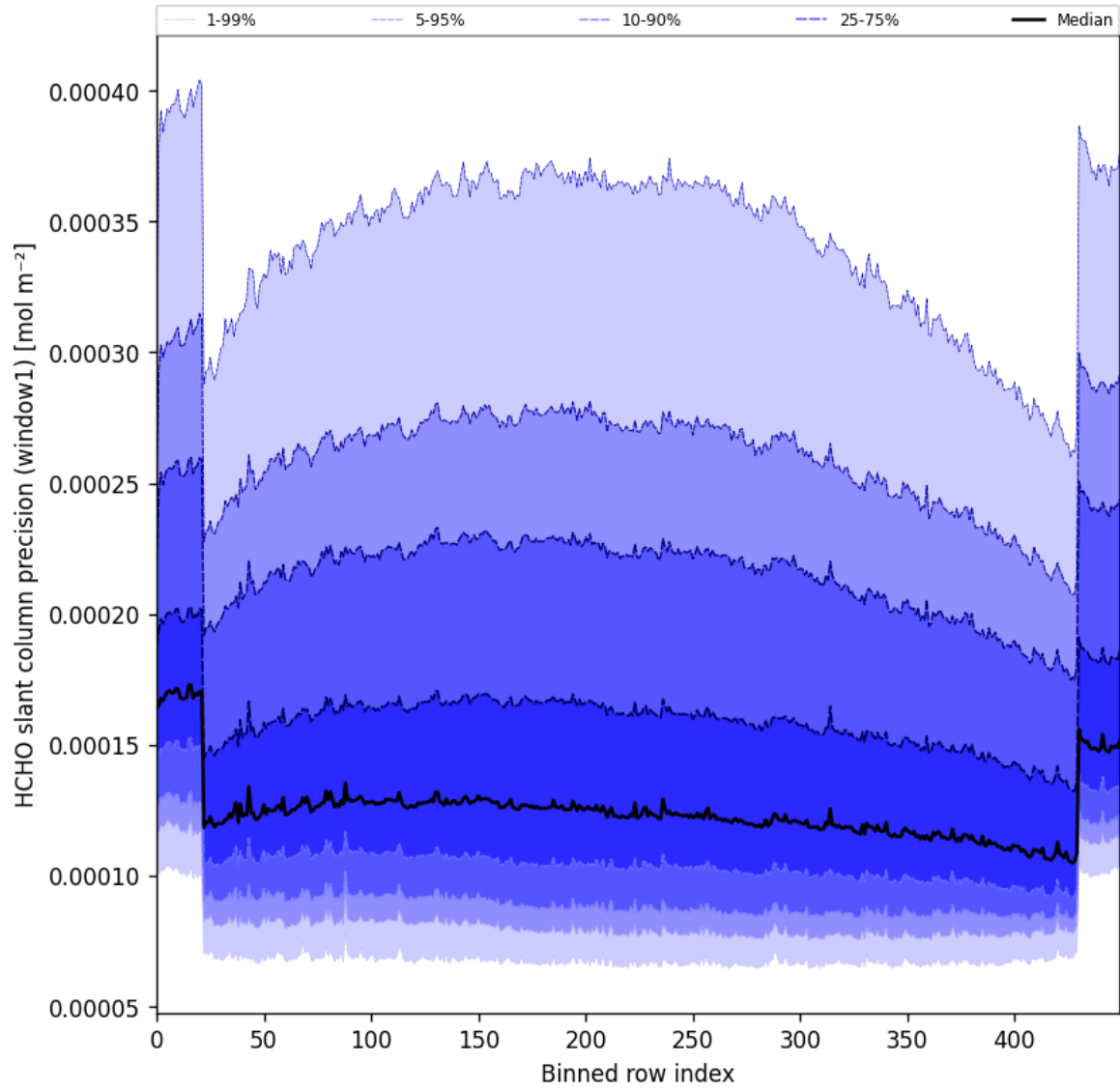
Figure 53: Along track statistics of “HCHO slant column precision (window1)” for 2025-05-23 to 2025-05-25
