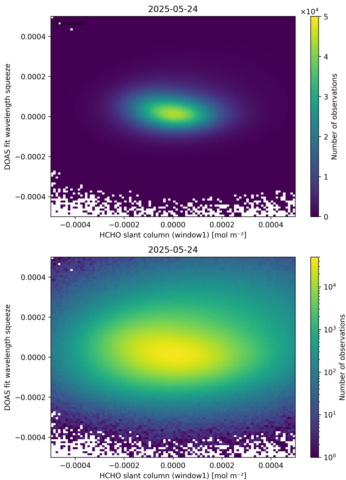
Figure 80: Scatter density plot of “HCHO slant column (window1)” against “DOAS fit wavelength squeeze” for 2025-05-23 to 2025-05-25.
