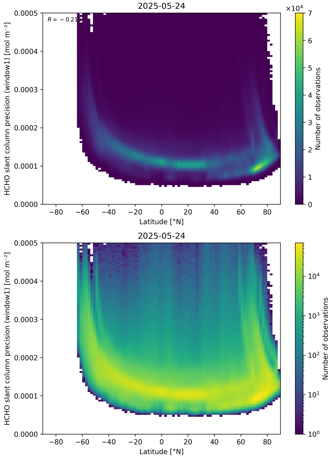
Figure 160: Scatter density plot of “Latitude” against “HCHO slant column precision (window1)” for 2025-05-23 to 2025-05-25.
