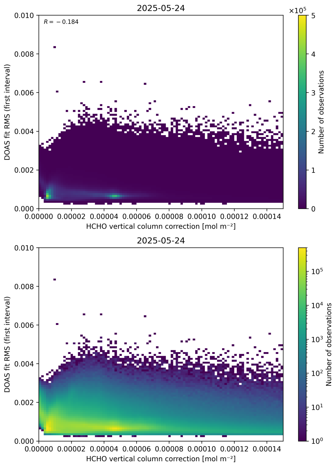
Figure 112: Scatter density plot of “HCHO vertical column correction” against “DOAS fit RMS (first interval)” for 2025-05-23 to 2025-05-25.
