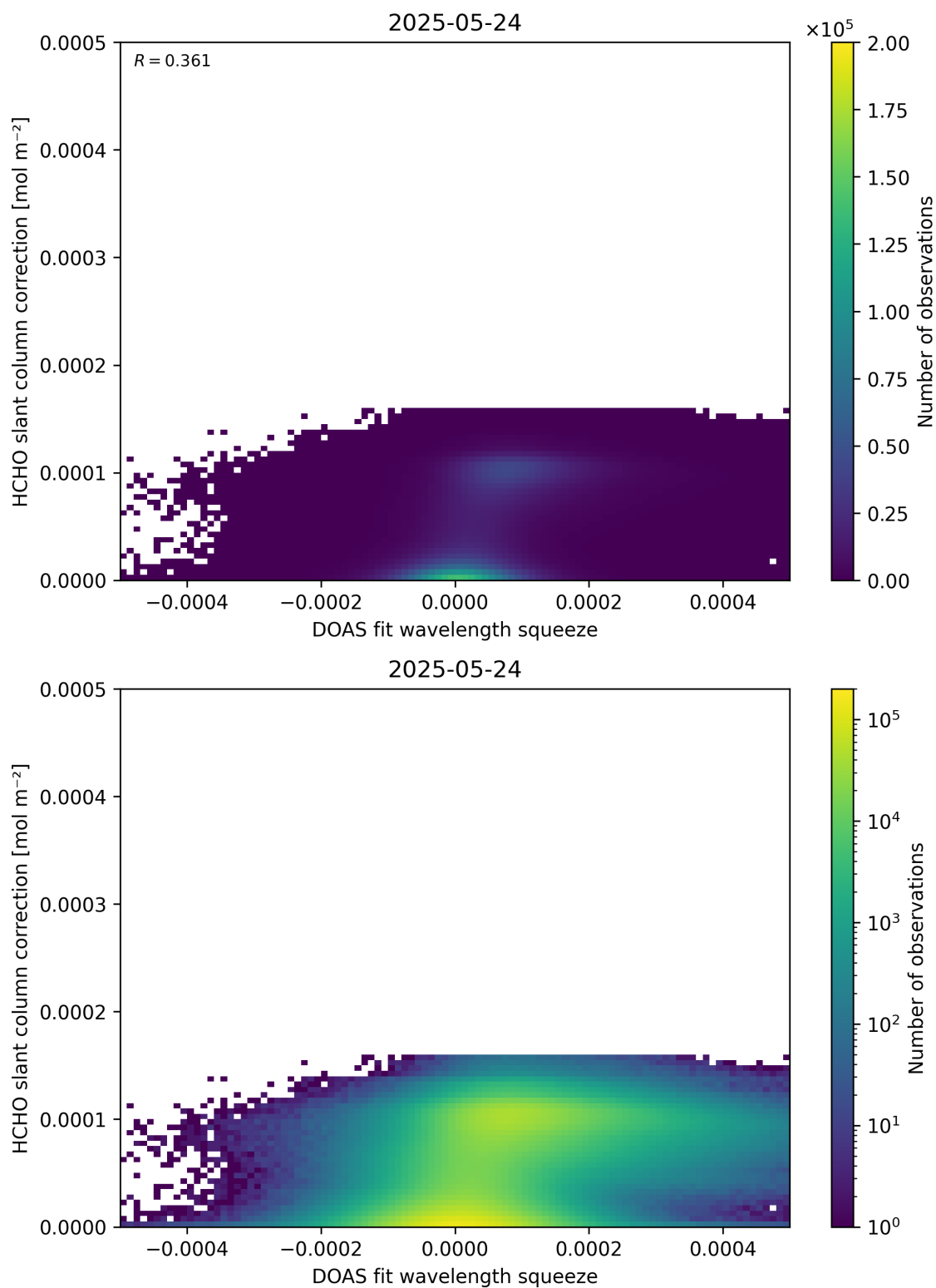
Figure 70: Scatter density plot of “DOAS fit wavelength squeeze” against “HCHO slant column correction” for 2025-05-23 to 2025-05-25.
