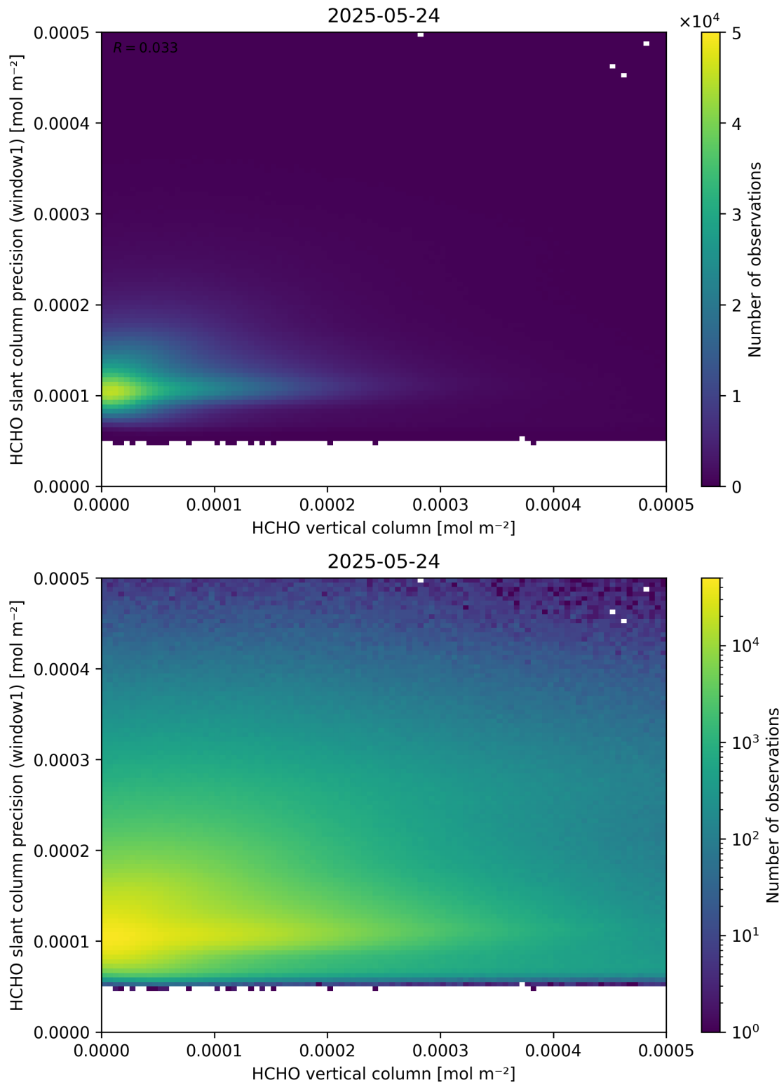
Figure 130: Scatter density plot of “HCHO vertical column” against “HCHO slant column precision (window1)” for 2025-05-23 to 2025-05-25.
