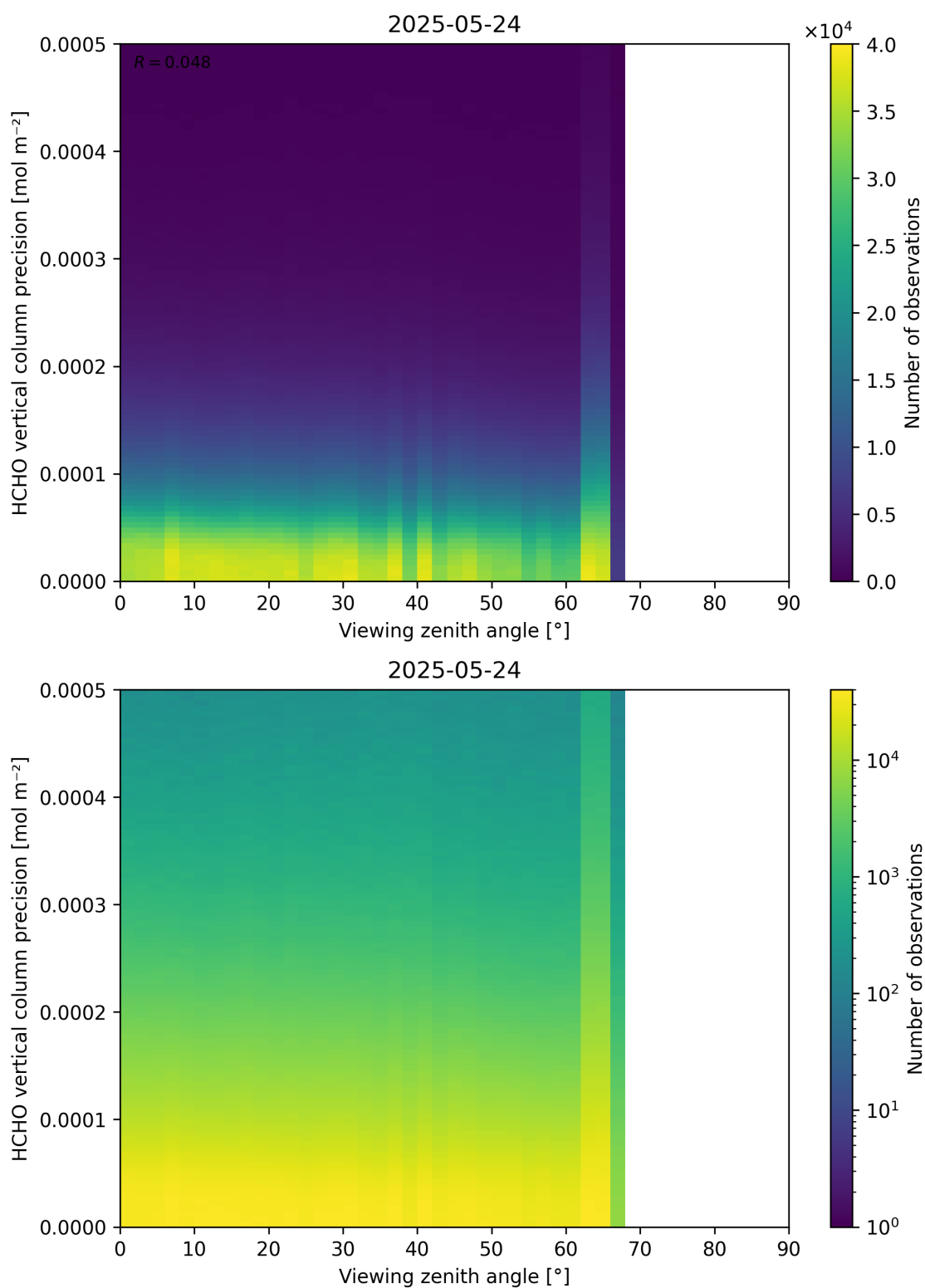
Figure 194: Scatter density plot of “Viewing zenith angle” against “HCHO vertical column precision” for 2025-05-23 to 2025-05-25.
