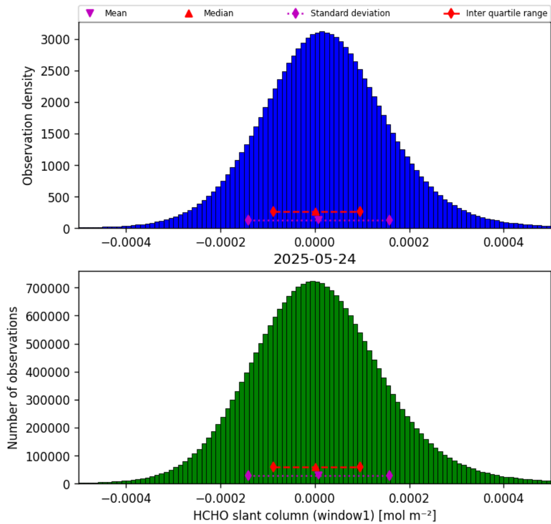
Figure 38: Histogram of “HCHO slant column (window1)” for 2025-05-23 to 2025-05-25
