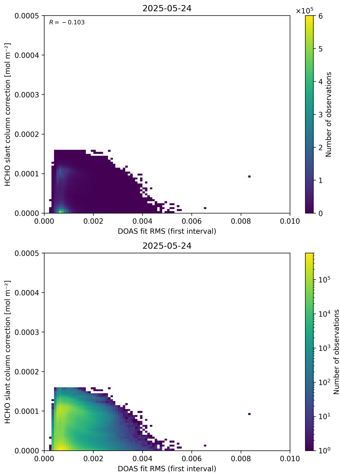
Figure 63: Scatter density plot of “DOAS fit RMS (first interval)” against “HCHO slant column correction” for 2025-05-23 to 2025-05-25.
