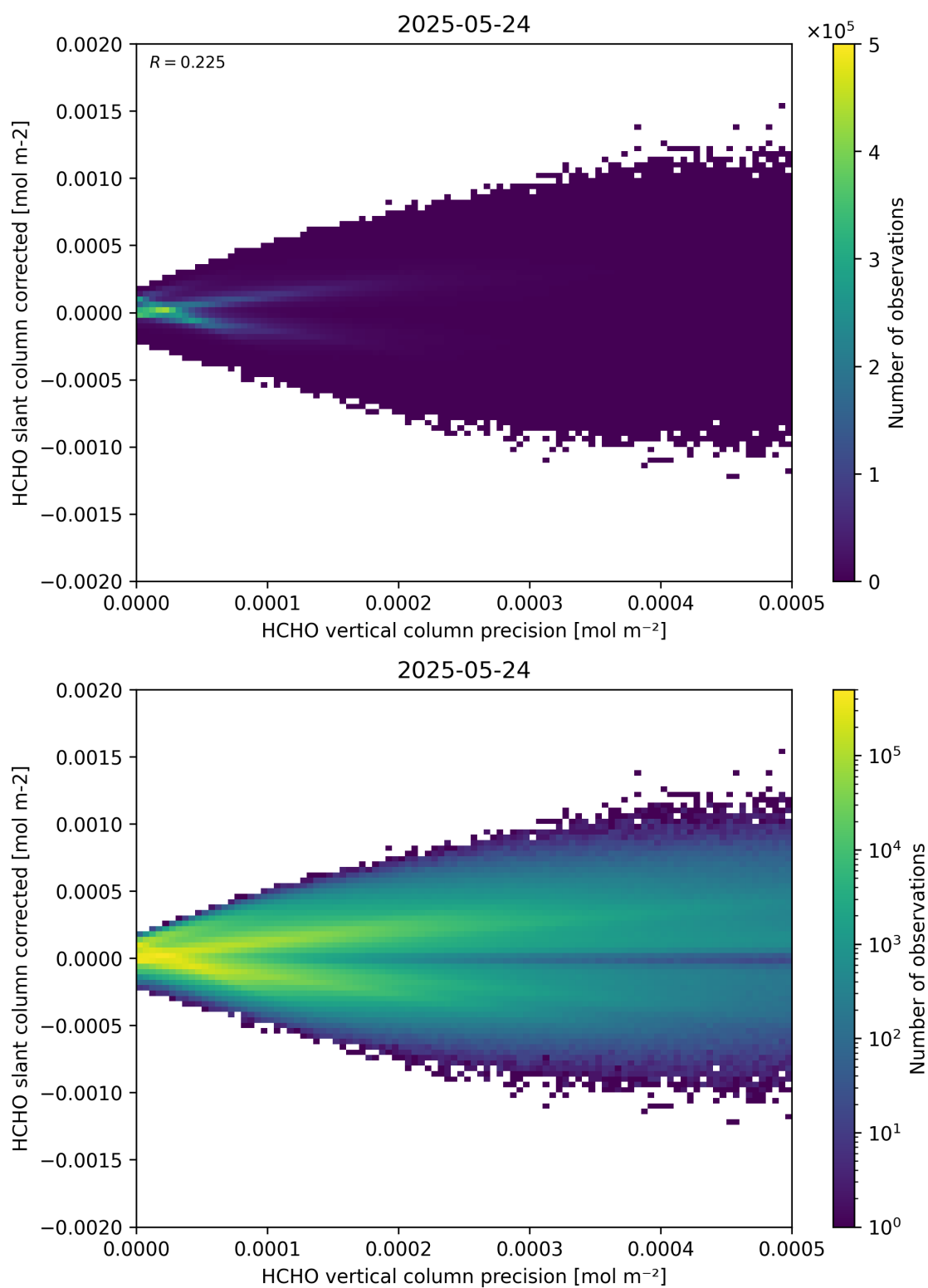
Figure 140: Scatter density plot of “HCHO vertical column precision” against “HCHO slant column corrected” for 2025-05-23 to 2025-05-25.
