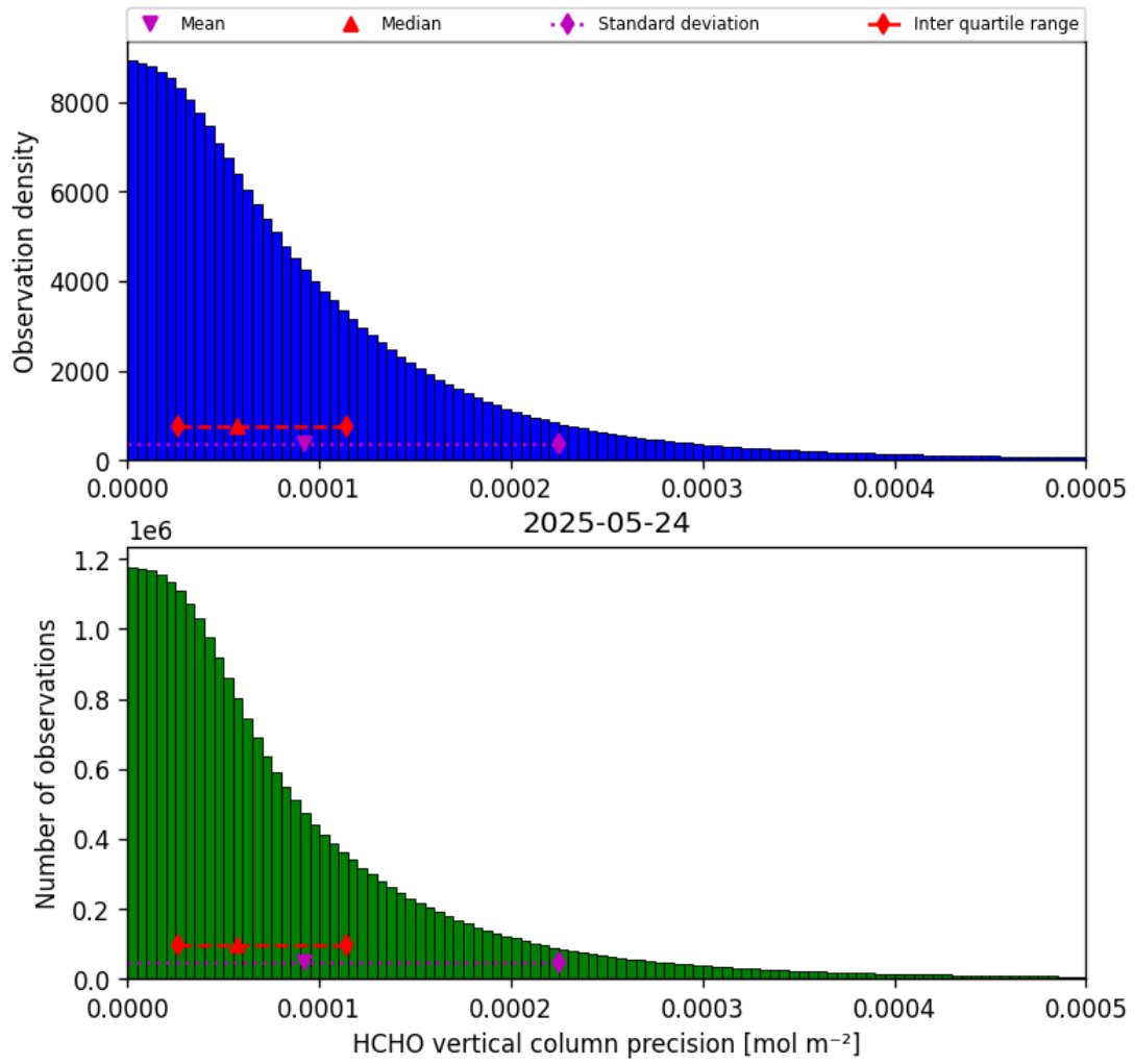
Figure 36: Histogram of “HCHO vertical column precision” for 2025-05-23 to 2025-05-25
