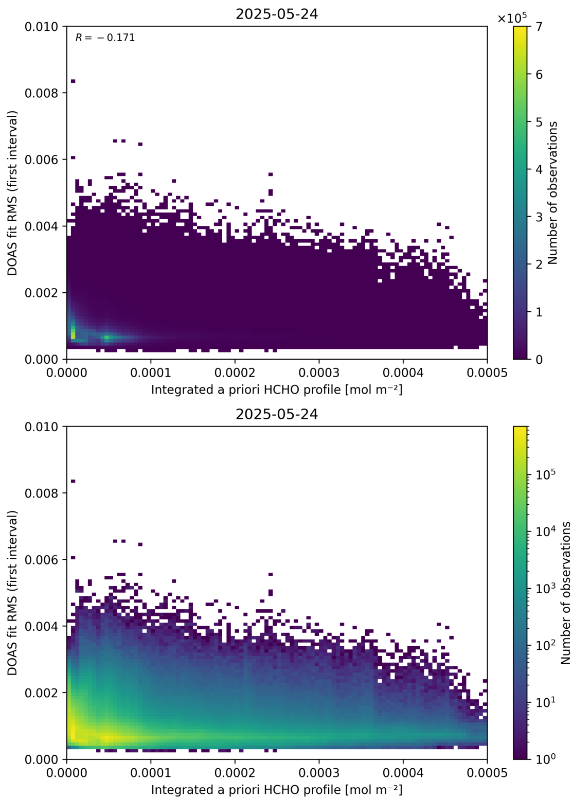
Figure 148: Scatter density plot of “Integrated a priori HCHO profile” against “DOAS fit RMS (first interval)” for 2025-05-23 to 2025-05-25.
