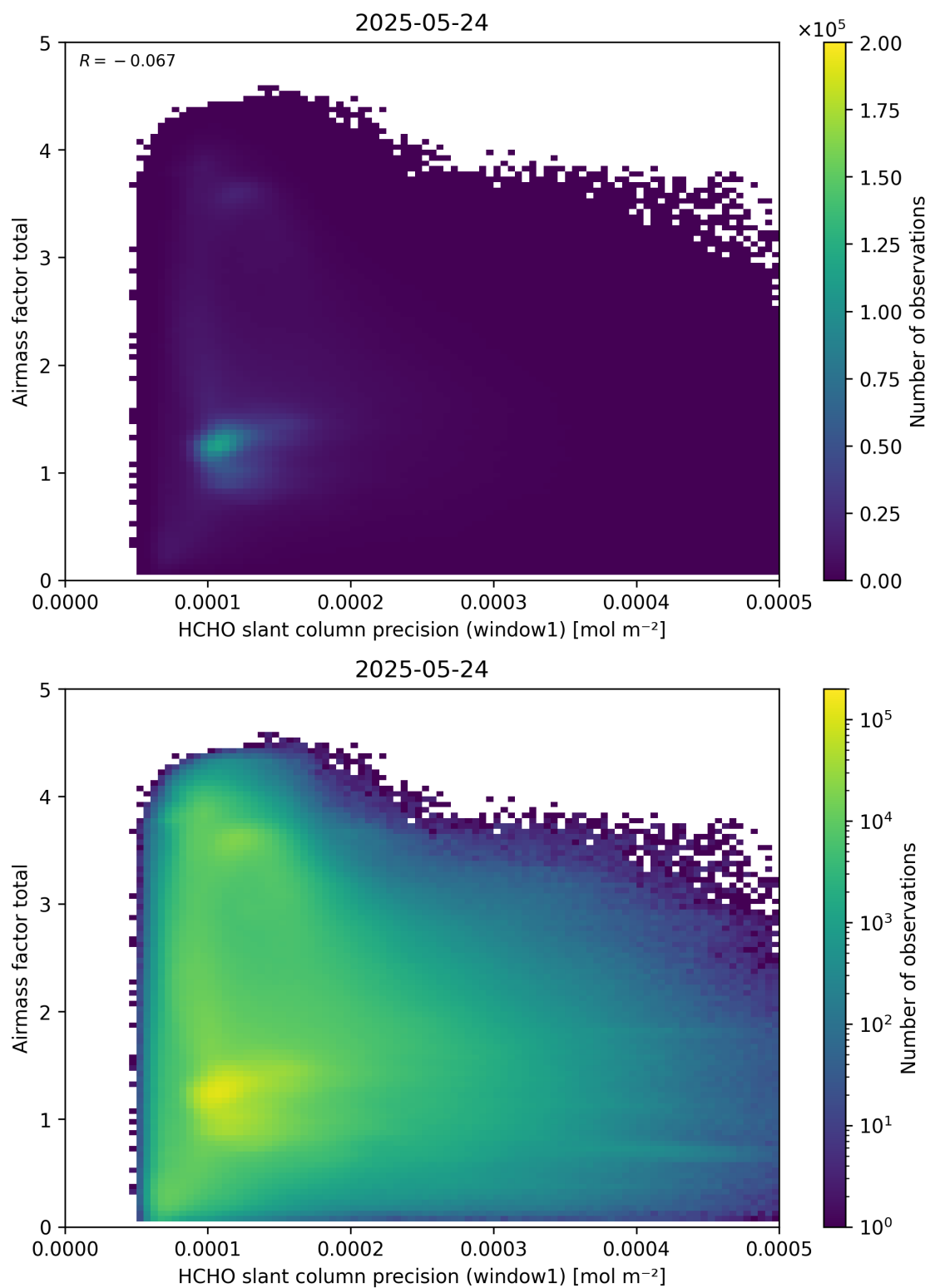
Figure 94: Scatter density plot of “HCHO slant column precision (window1)” against “Airmass factor total” for 2025-05-23 to 2025-05-25.
