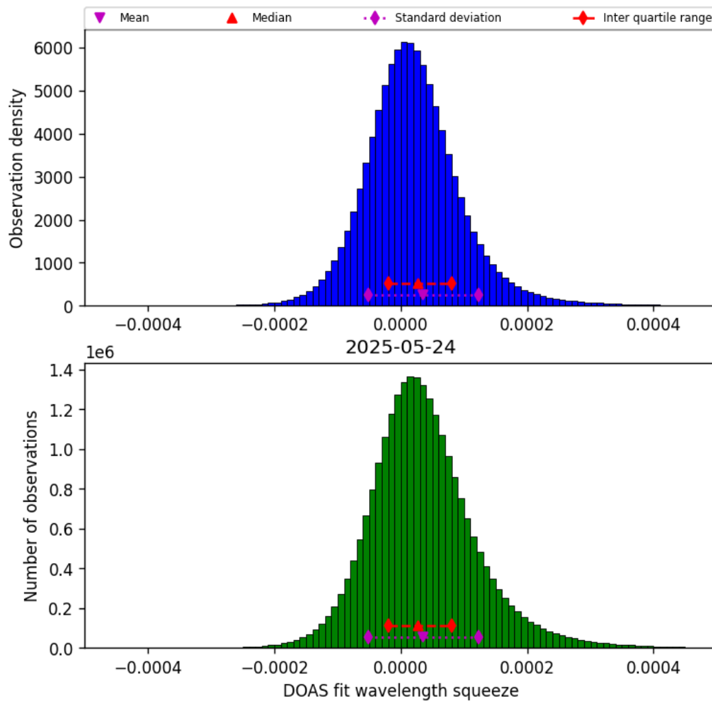
Figure 45: Histogram of “DOAS fit wavelength squeeze” for 2025-05-23 to 2025-05-25
