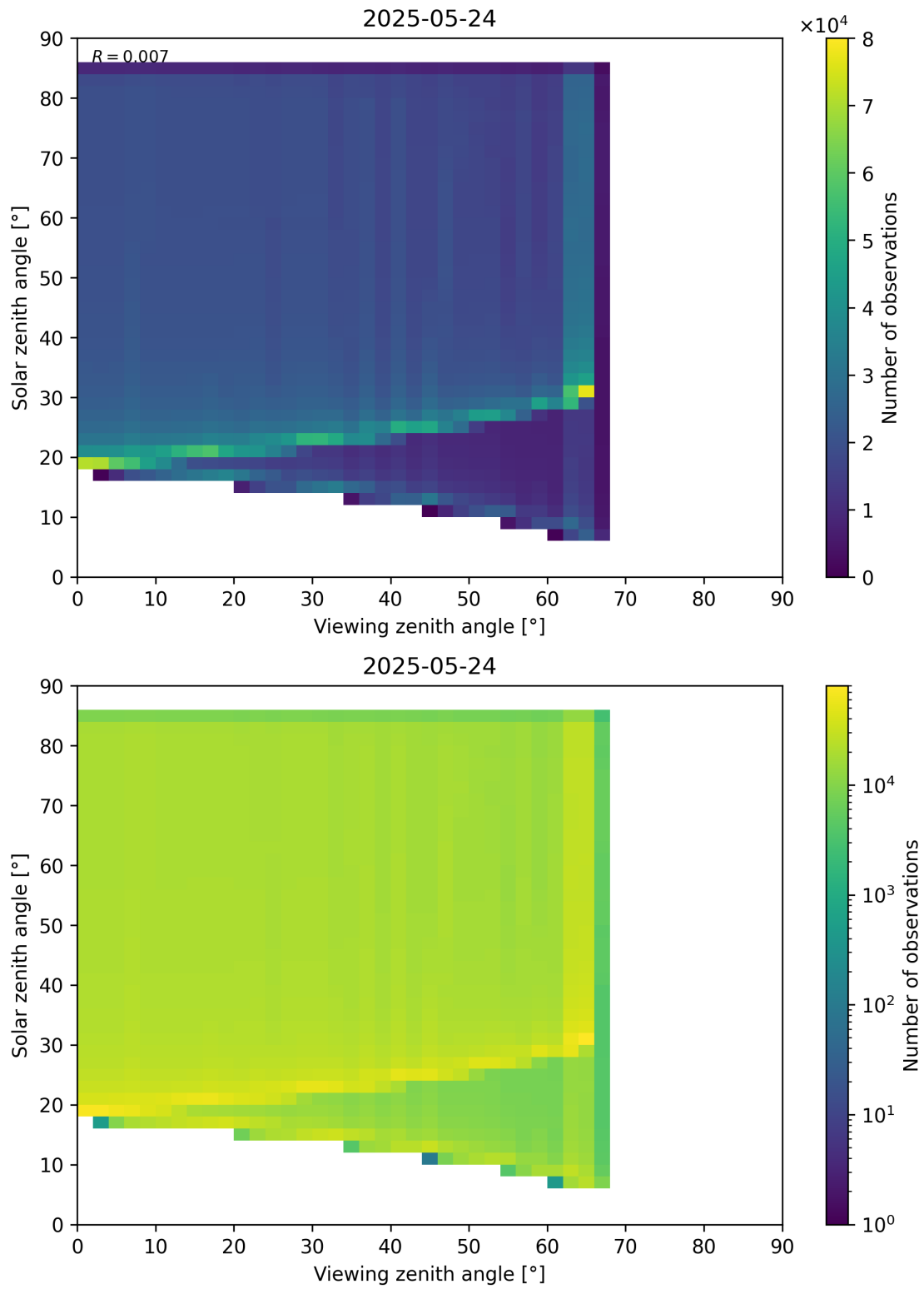
Figure 197: Scatter density plot of “Viewing zenith angle” against “Solar zenith angle” for 2025-05-23 to 2025-05-25.
