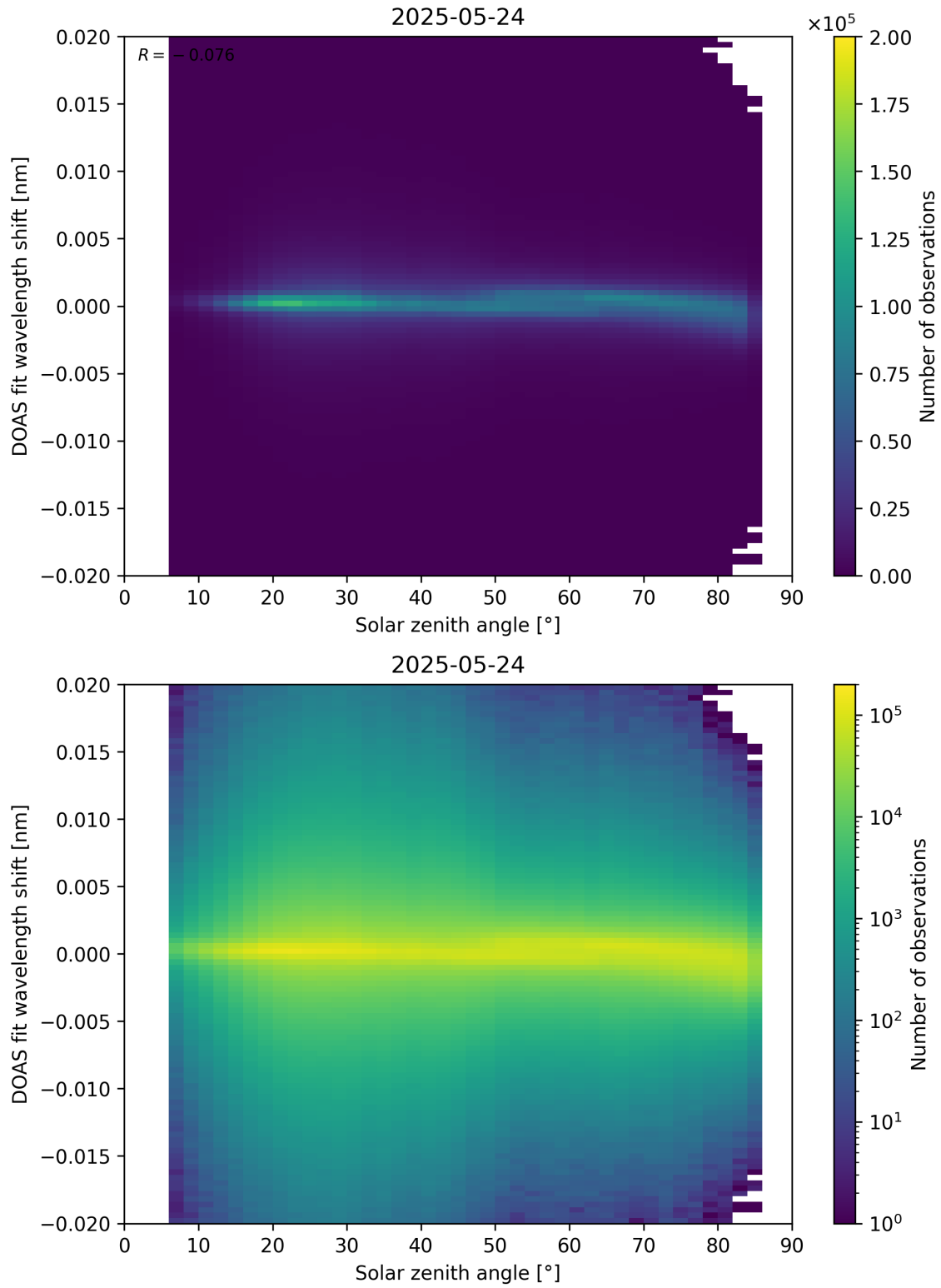
Figure 168: Scatter density plot of “Solar zenith angle” against “DOAS fit wavelength shift” for 2025-05-23 to 2025-05-25.
