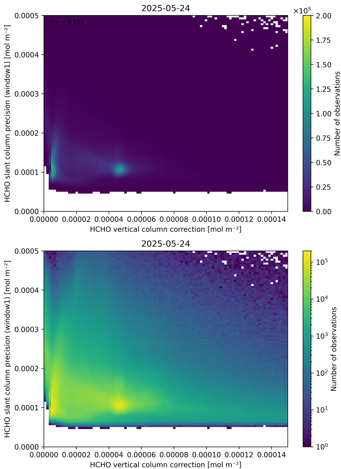
Figure 119: Scatter density plot of “HCHO vertical column correction” against “HCHO slant column precision (window1)” for 2025-05-23 to 2025-05-25.
