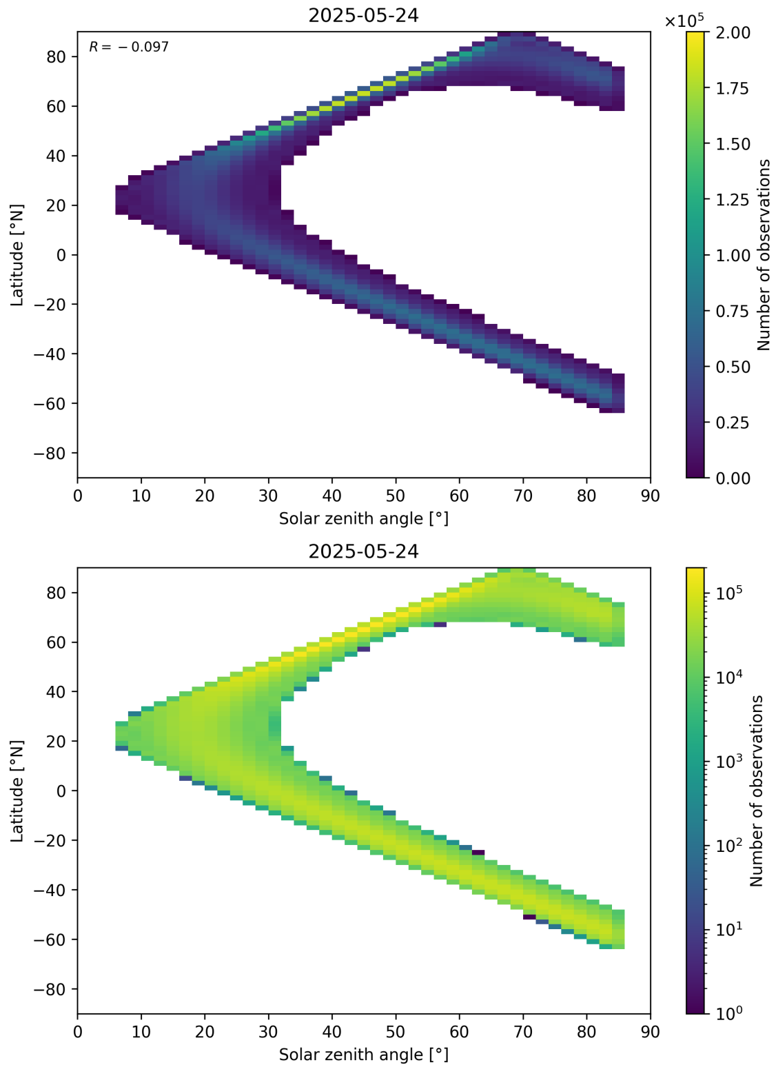
Figure 181: Scatter density plot of “Solar zenith angle” against “Latitude” for 2025-05-23 to 2025-05-25.
