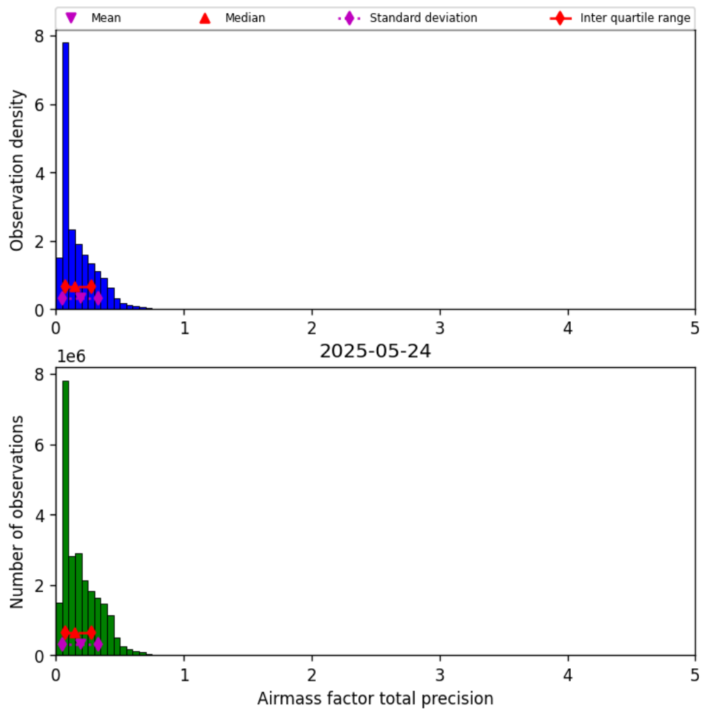
Figure 41: Histogram of “Airmass factor total precision” for 2025-05-23 to 2025-05-25
