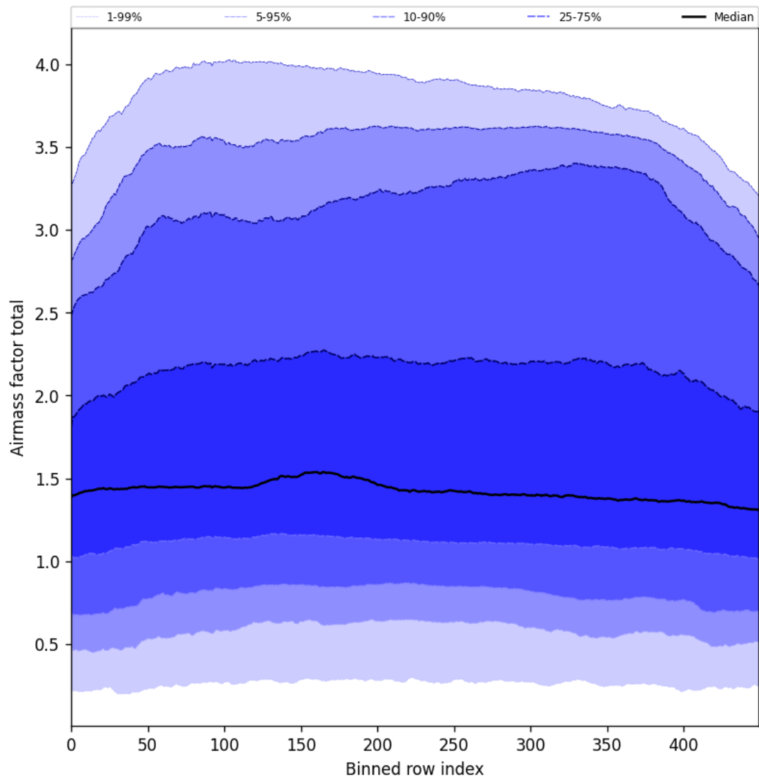
Figure 54: Along track statistics of “Airmass factor total” for 2025-05-23 to 2025-05-25
