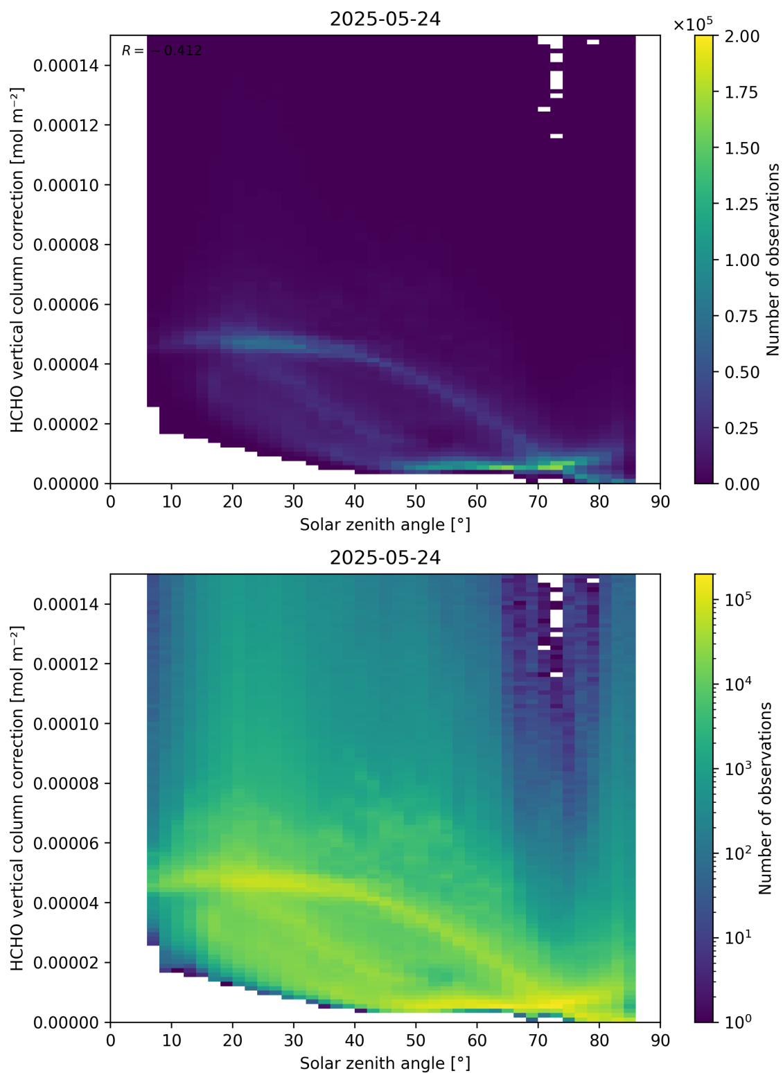
Figure 178: Scatter density plot of “Solar zenith angle” against “HCHO vertical column correction” for 2025-05-23 to 2025-05-25.
