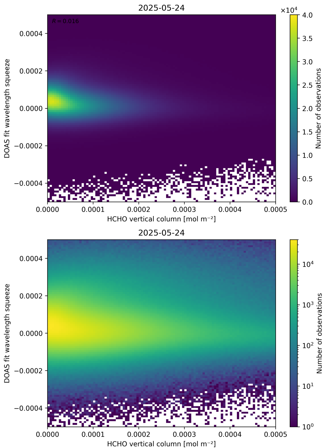
Figure 125: Scatter density plot of “HCHO vertical column” against “DOAS fit wavelength squeeze” for 2025-05-23 to 2025-05-25.
