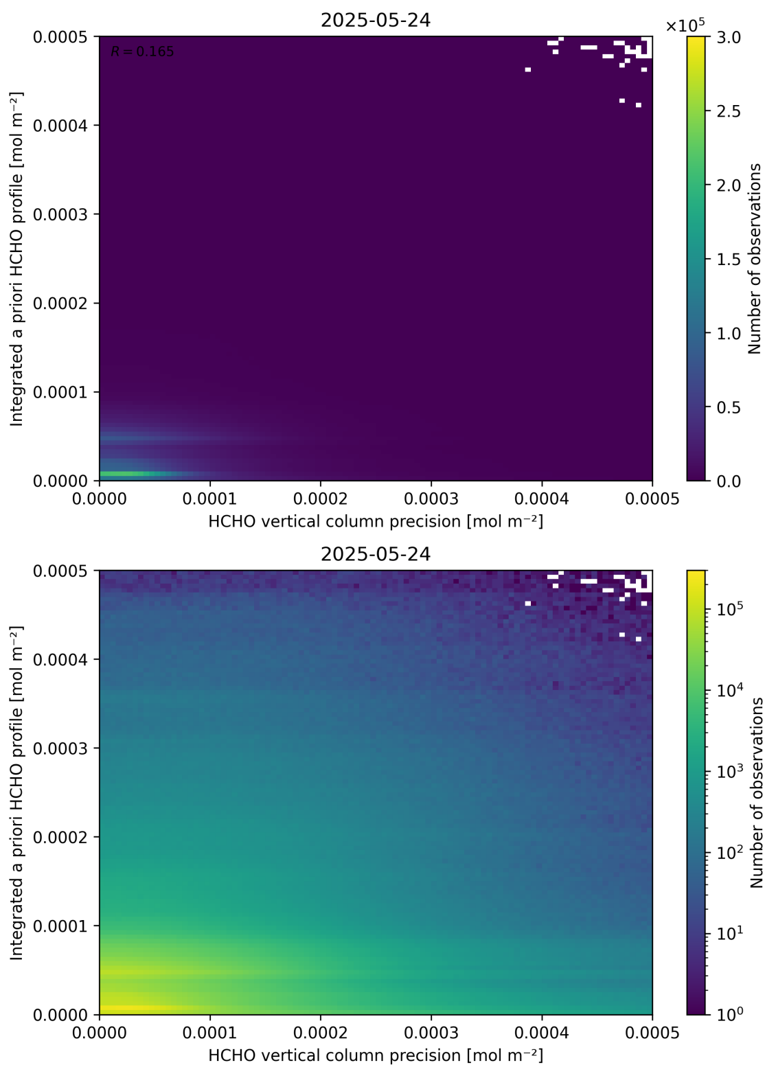
Figure 147: Scatter density plot of “HCHO vertical column precision” against “Integrated a priori HCHO profile” for 2025-05-23 to 2025-05-25.
