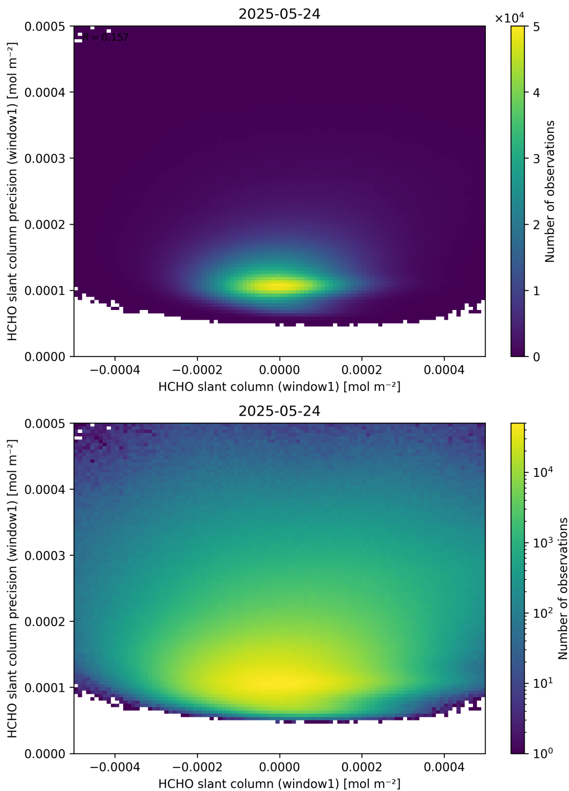
Figure 84: Scatter density plot of “HCHO slant column (window1)” against “HCHO slant column precision (window1)” for 2025-05-23 to 2025-05-25.
