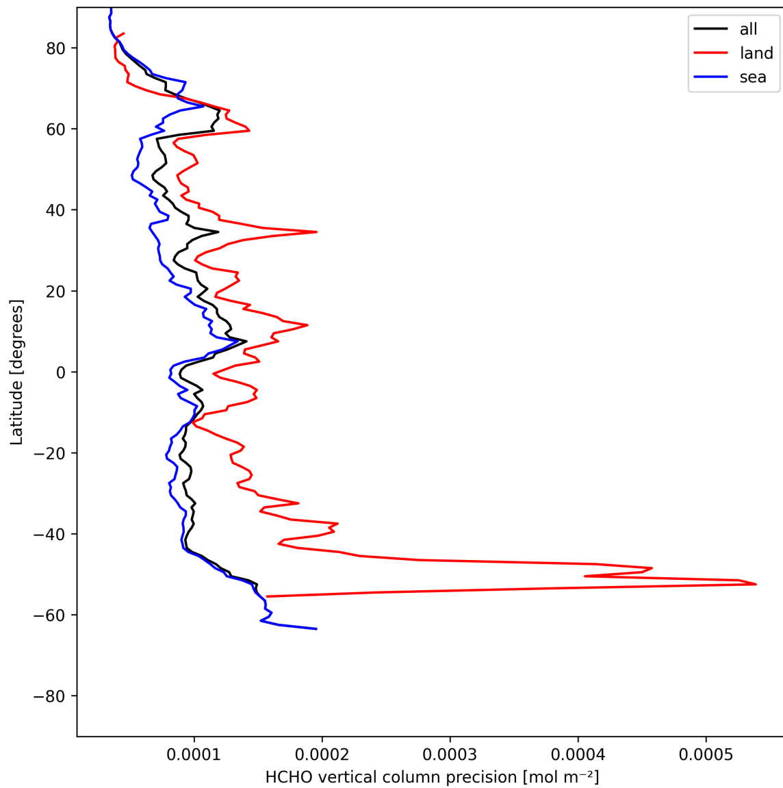
Figure 22: Zonal average of “HCHO vertical column precision” for 2025-05-23 to 2025-05-25.
