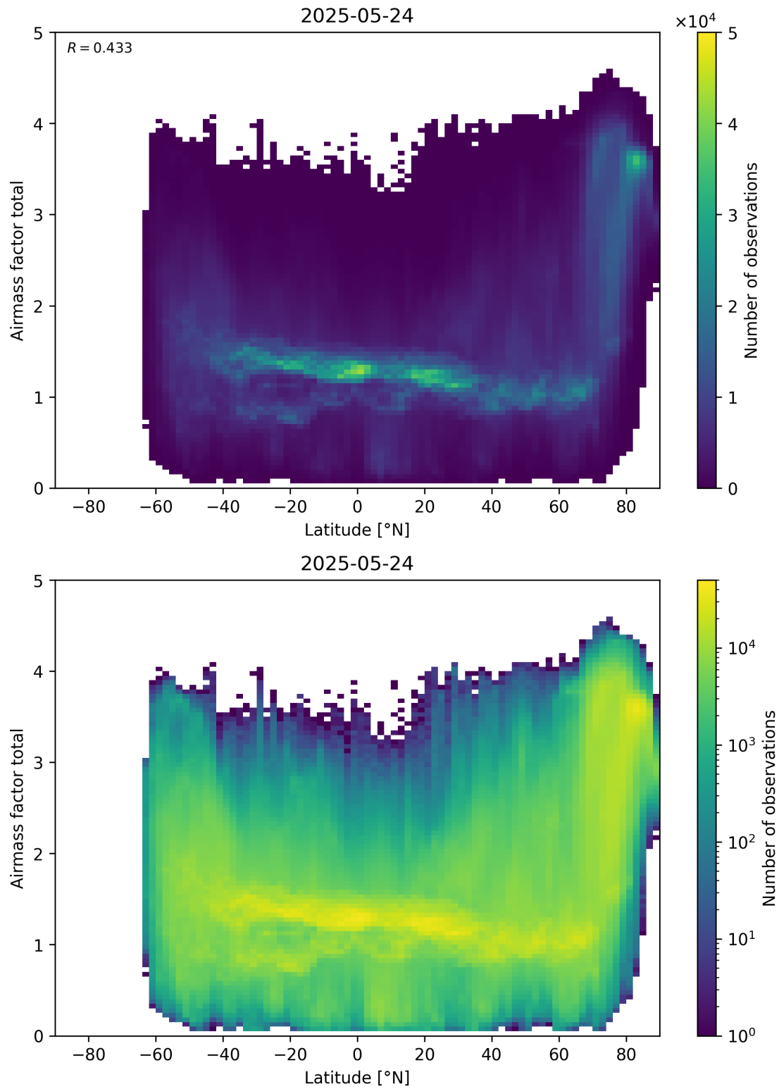
Figure 161: Scatter density plot of “Latitude” against “Airmass factor total” for 2025-05-23 to 2025-05-25.
