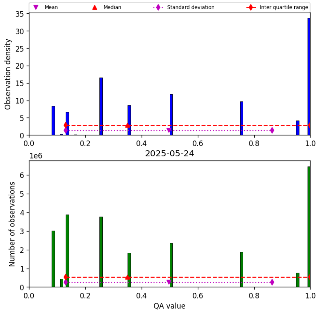
Figure 34: Histogram of “QA value” for 2025-05-23 to 2025-05-25
