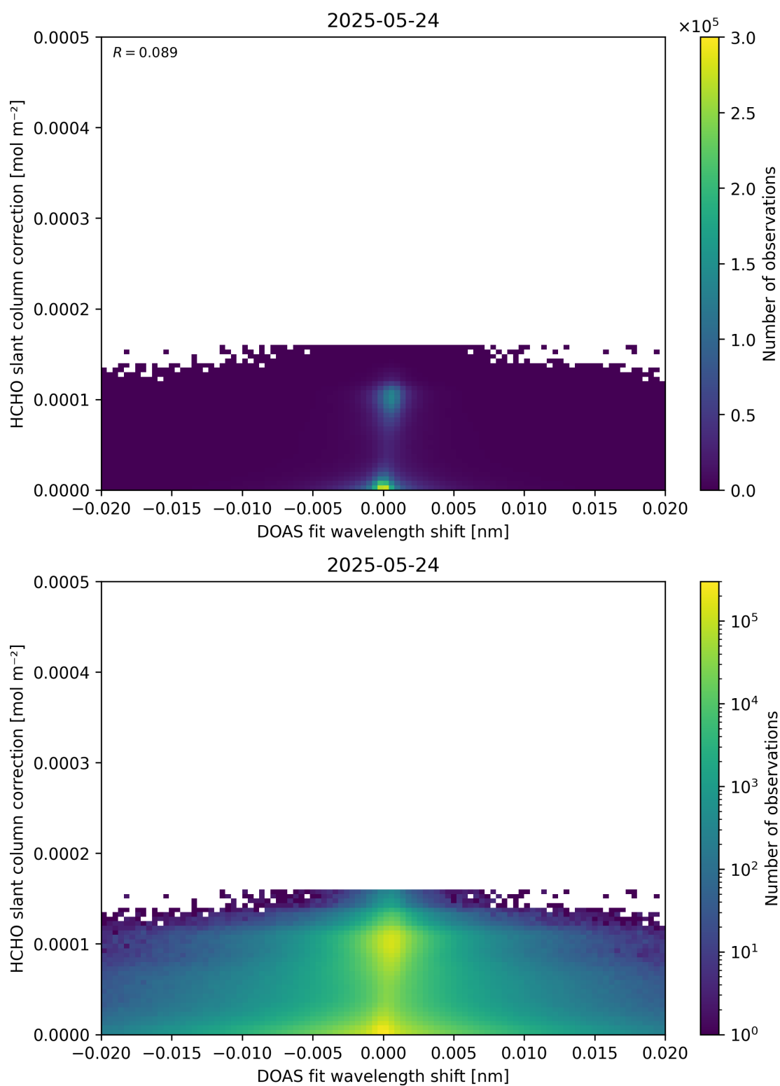
Figure 67: Scatter density plot of “DOAS fit wavelength shift” against “HCHO slant column correction” for 2025-05-23 to 2025-05-25.
