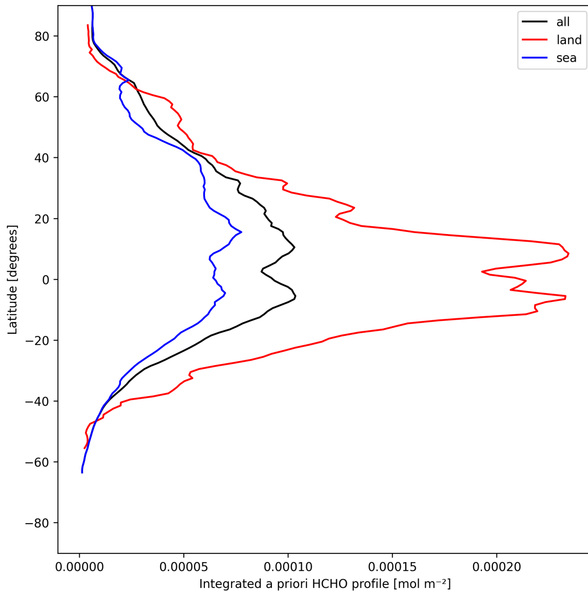
Figure 29: Zonal average of “Integrated a priori HCHO profile” for 2025-05-23 to 2025-05-25.
