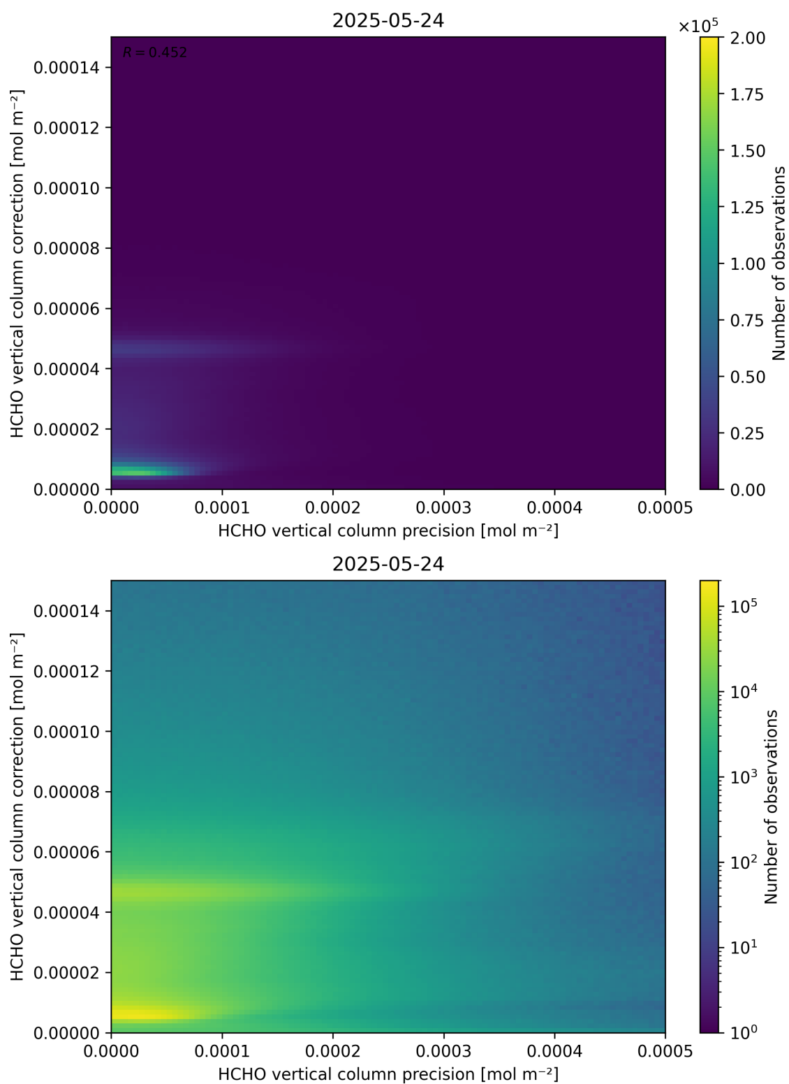
Figure 146: Scatter density plot of “HCHO vertical column precision” against “HCHO vertical column correction” for 2025-05-23 to 2025-05-25.
