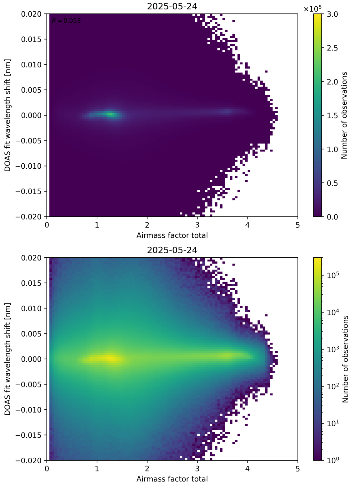
Figure 98: Scatter density plot of “Airmass factor total” against “DOAS fit wavelength shift” for 2025-05-23 to 2025-05-25.
