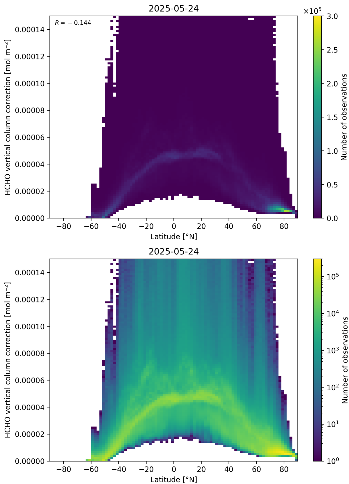
Figure 164: Scatter density plot of “Latitude” against “HCHO vertical column correction” for 2025-05-23 to 2025-05-25.
