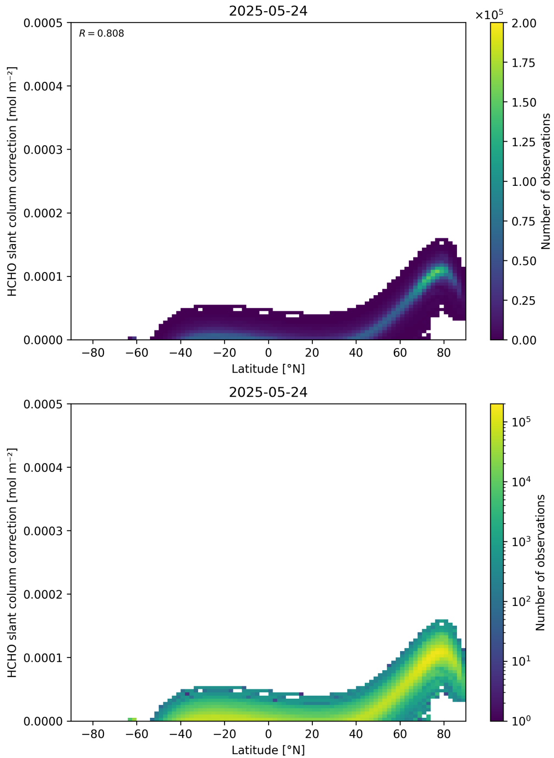
Figure 158: Scatter density plot of “Latitude” against “HCHO slant column correction” for 2025-05-23 to 2025-05-25.
