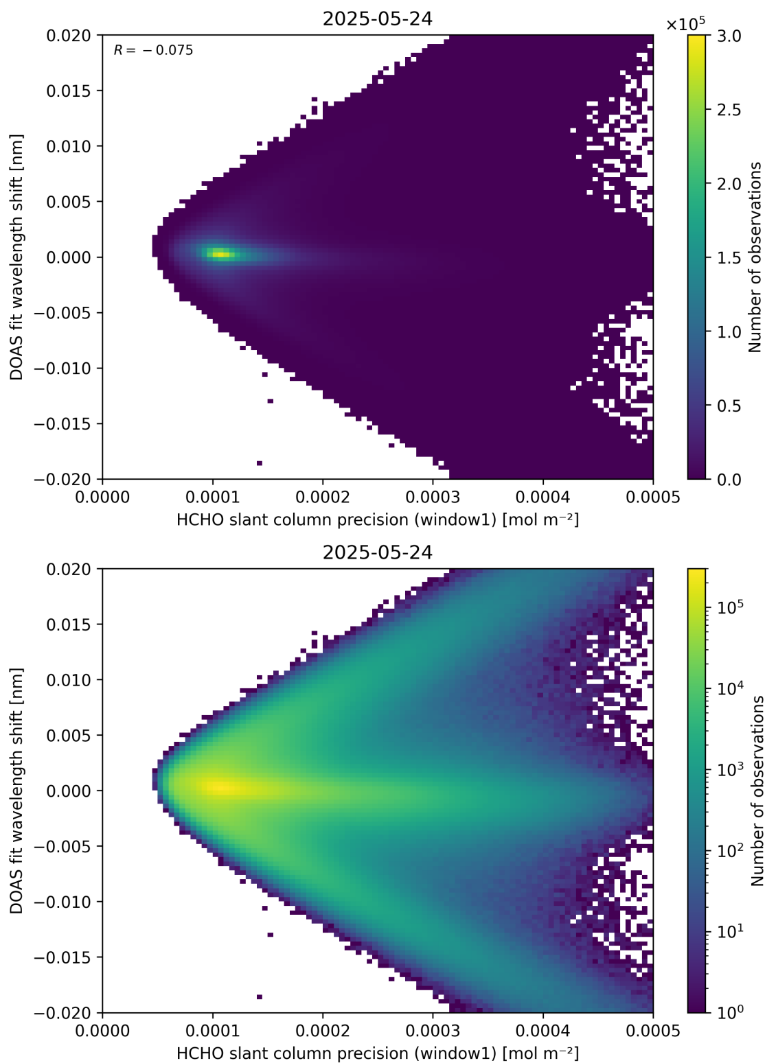
Figure 89: Scatter density plot of “HCHO slant column precision (window1)” against “DOAS fit wavelength shift” for 2025-05-23 to 2025-05-25.
