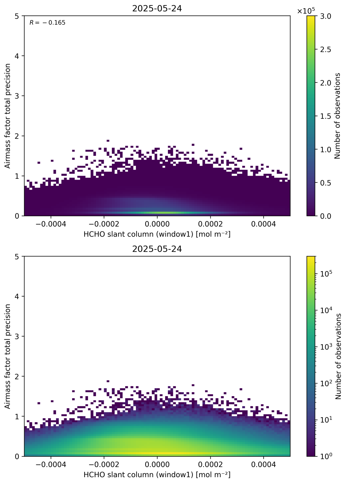
Figure 86: Scatter density plot of “HCHO slant column (window1)” against “Airmass factor total precision” for 2025-05-23 to 2025-05-25.
