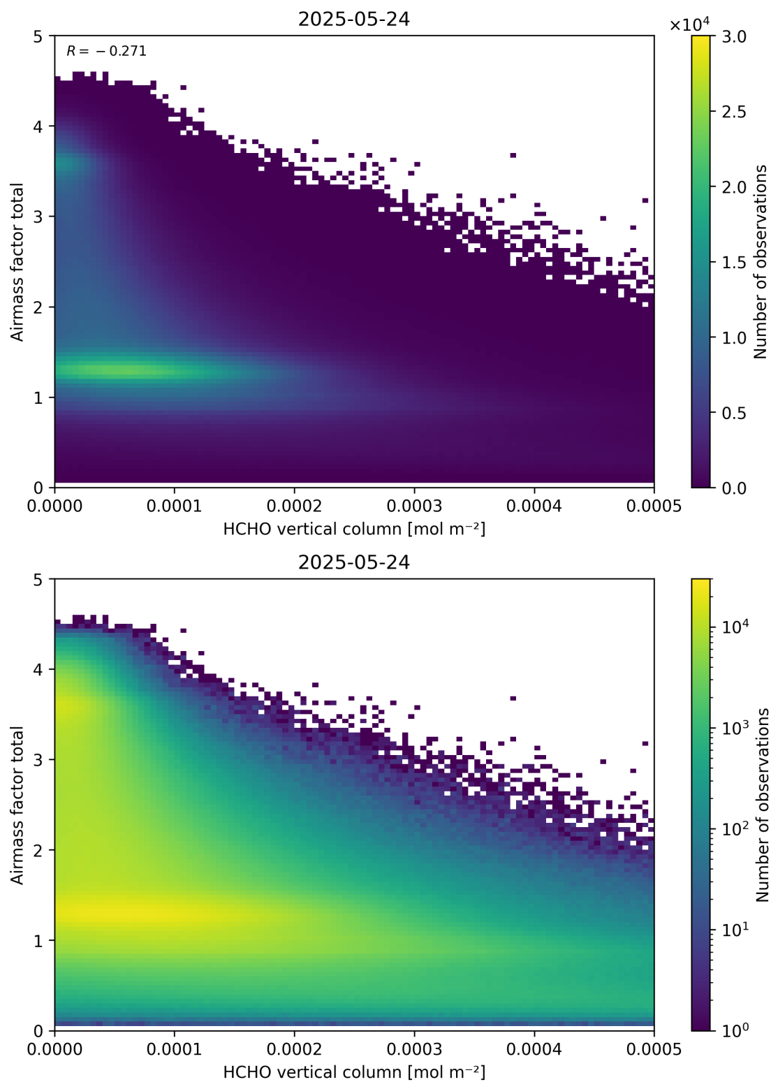
Figure 131: Scatter density plot of “HCHO vertical column” against “Airmass factor total” for 2025-05-23 to 2025-05-25.
