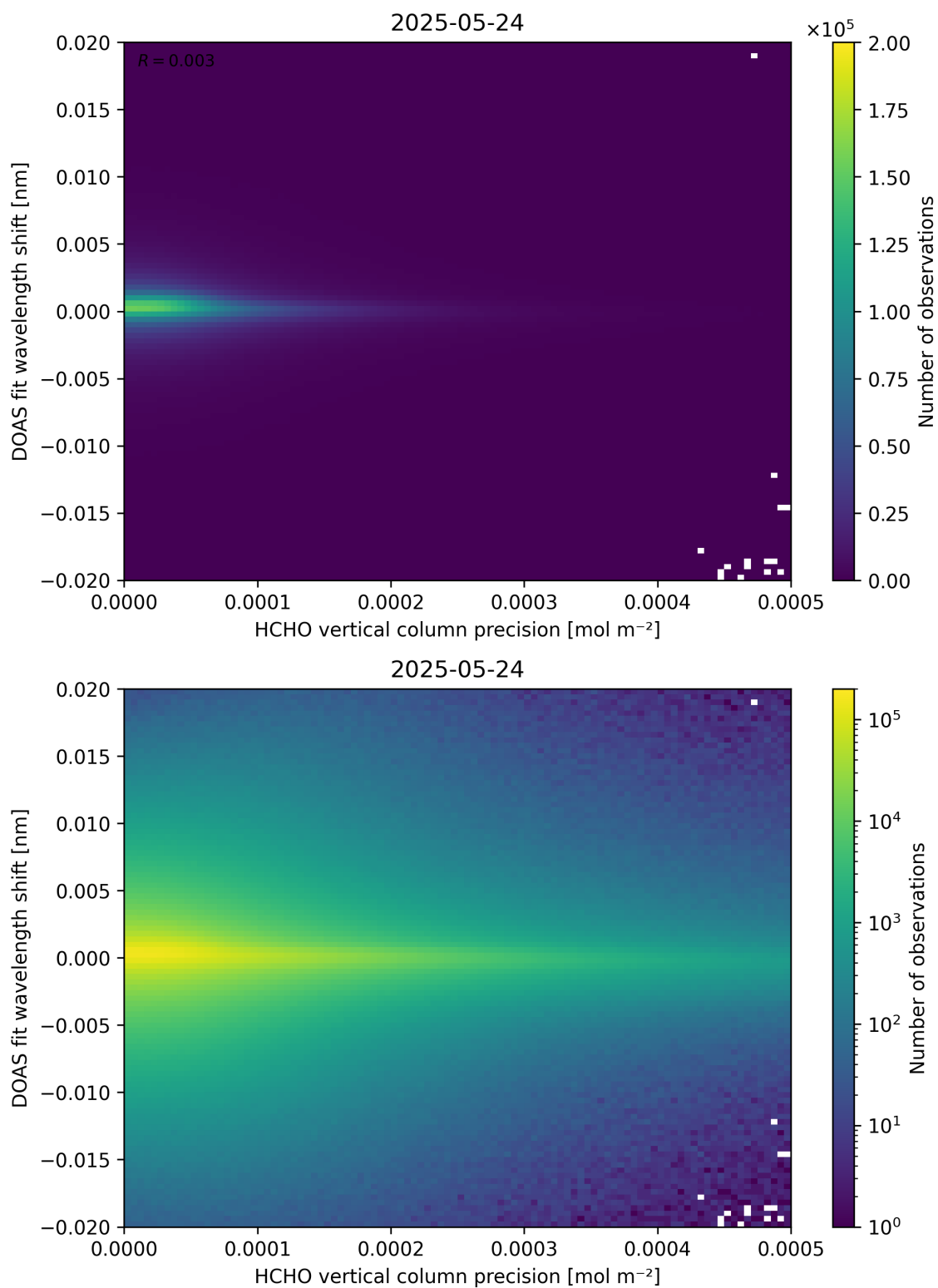
Figure 137: Scatter density plot of “HCHO vertical column precision” against “DOAS fit wavelength shift” for 2025-05-23 to 2025-05-25.
