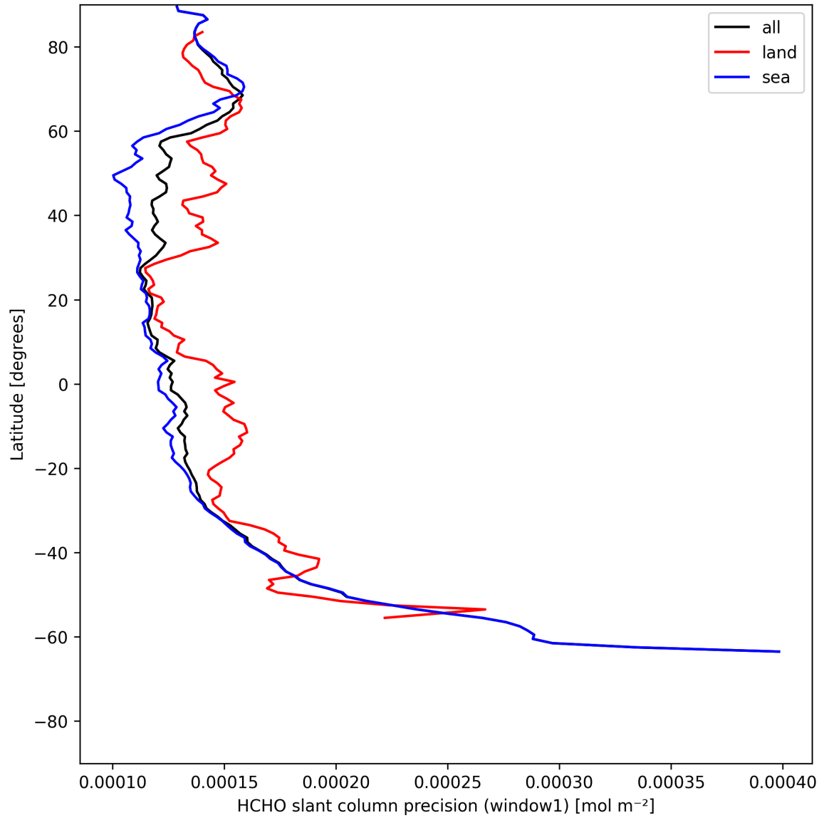
Figure 25: Zonal average of “HCHO slant column precision (window1)” for 2025-05-23 to 2025-05-25.
