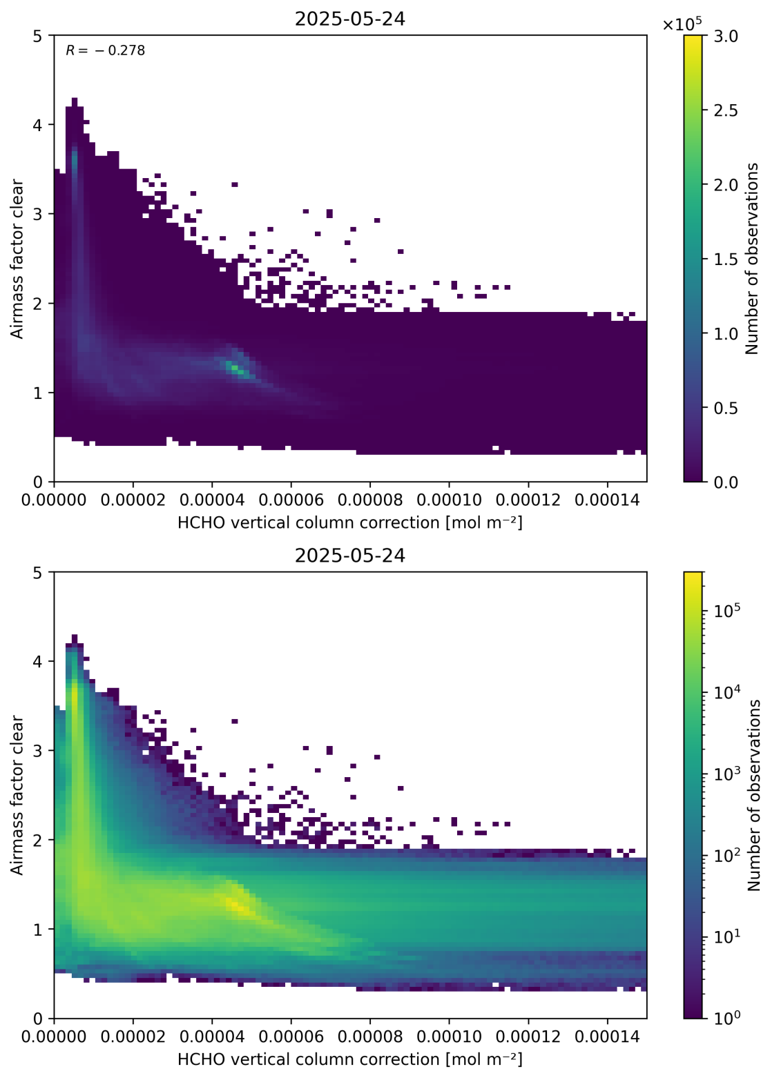
Figure 115: Scatter density plot of “HCHO vertical column correction” against “Airmass factor clear” for 2025-05-23 to 2025-05-25.
