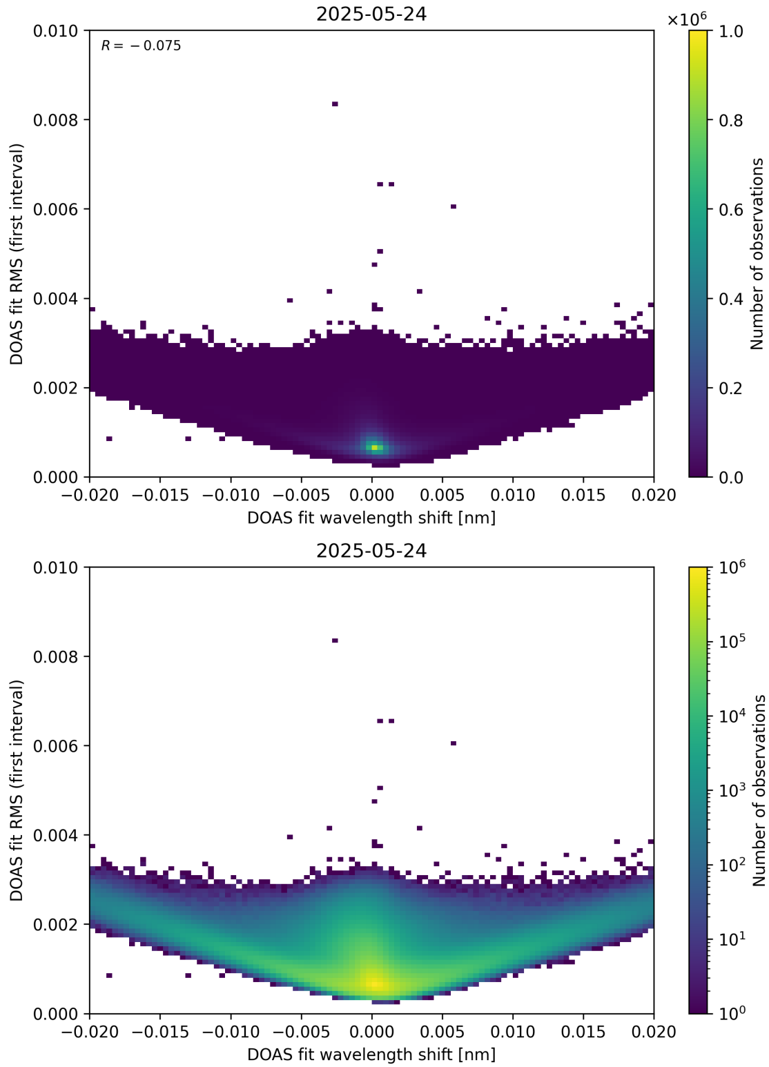
Figure 64: Scatter density plot of “DOAS fit wavelength shift” against “DOAS fit RMS (first interval)” for 2025-05-23 to 2025-05-25.
