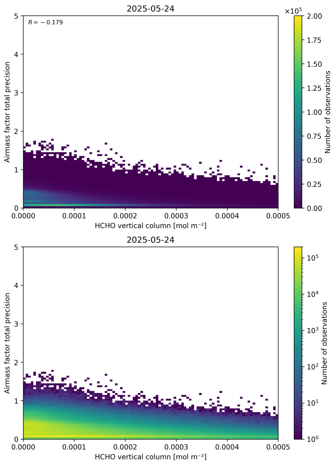
Figure 132: Scatter density plot of “HCHO vertical column” against “Airmass factor total precision” for 2025-05-23 to 2025-05-25.
