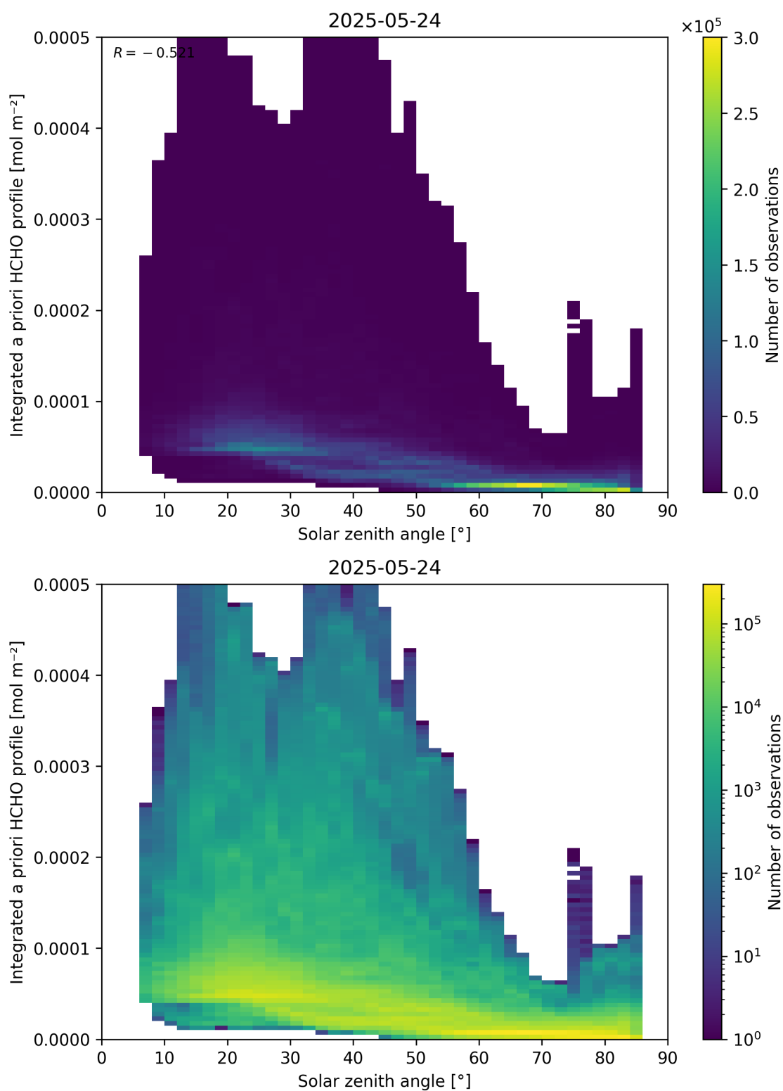
Figure 180: Scatter density plot of “Solar zenith angle” against “Integrated a priori HCHO profile” for 2025-05-23 to 2025-05-25.
