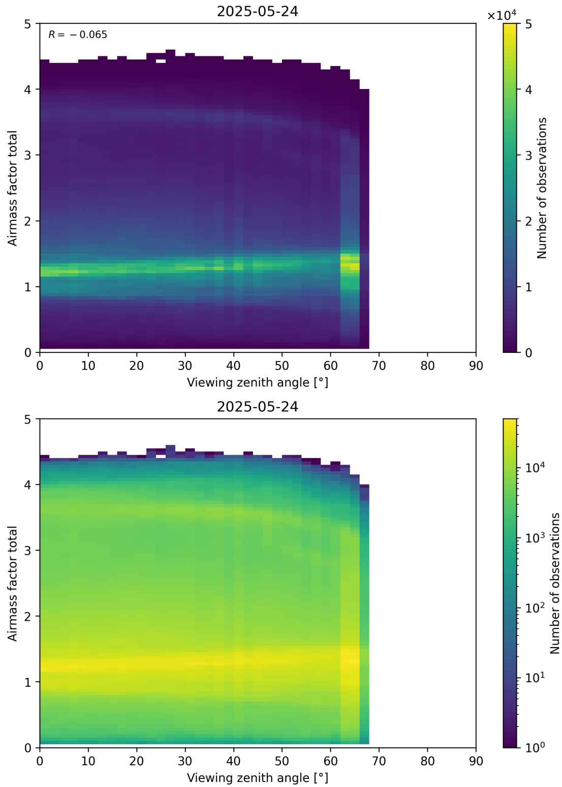
Figure 190: Scatter density plot of “Viewing zenith angle” against “Airmass factor total” for 2025-05-23 to 2025-05-25.
