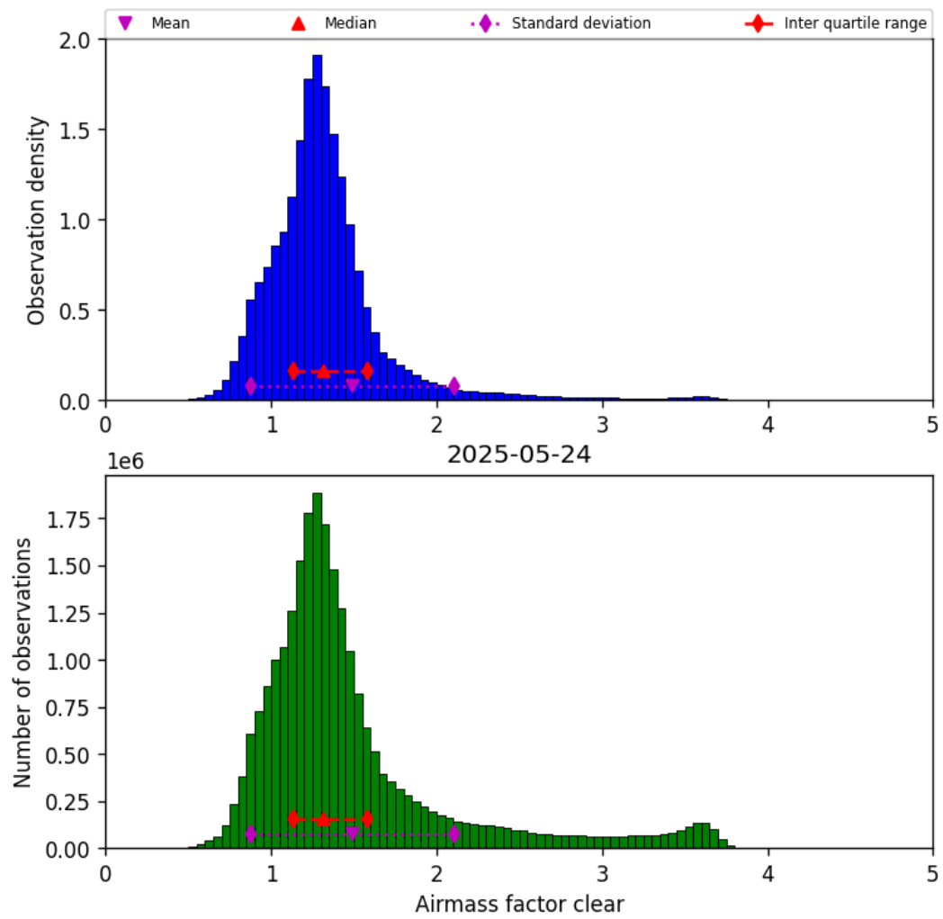
Figure 42: Histogram of “Airmass factor clear” for 2025-05-23 to 2025-05-25
