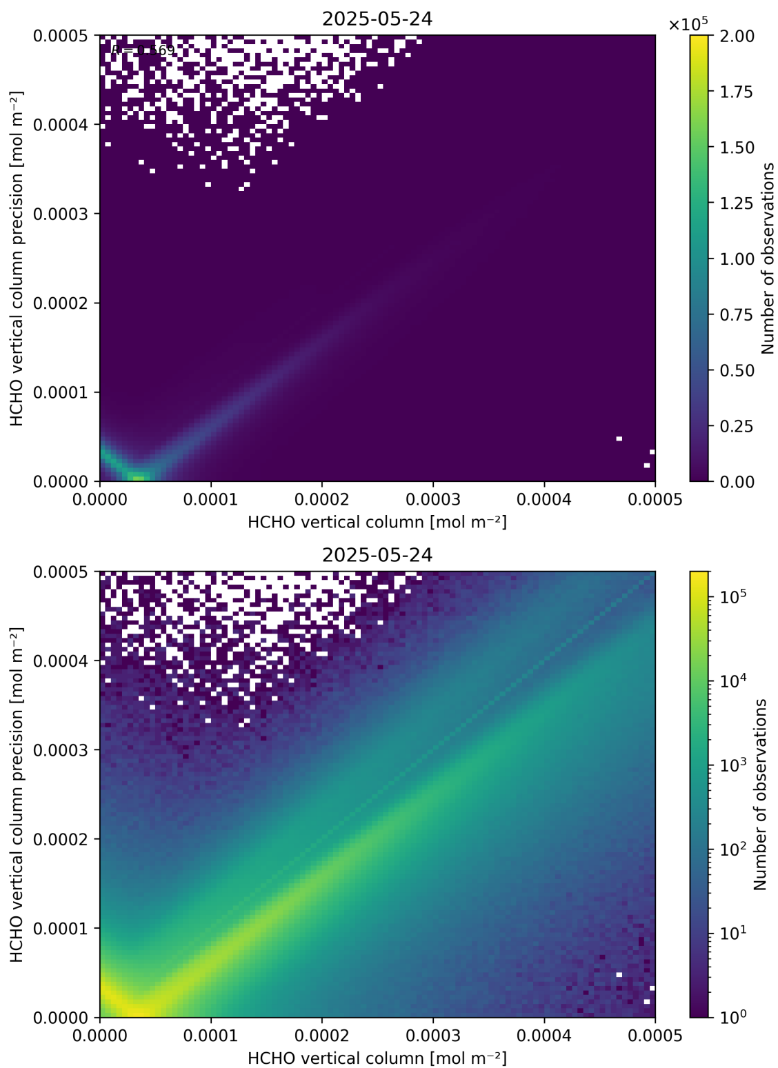
Figure 134: Scatter density plot of “HCHO vertical column” against “HCHO vertical column precision” for 2025-05-23 to 2025-05-25.
