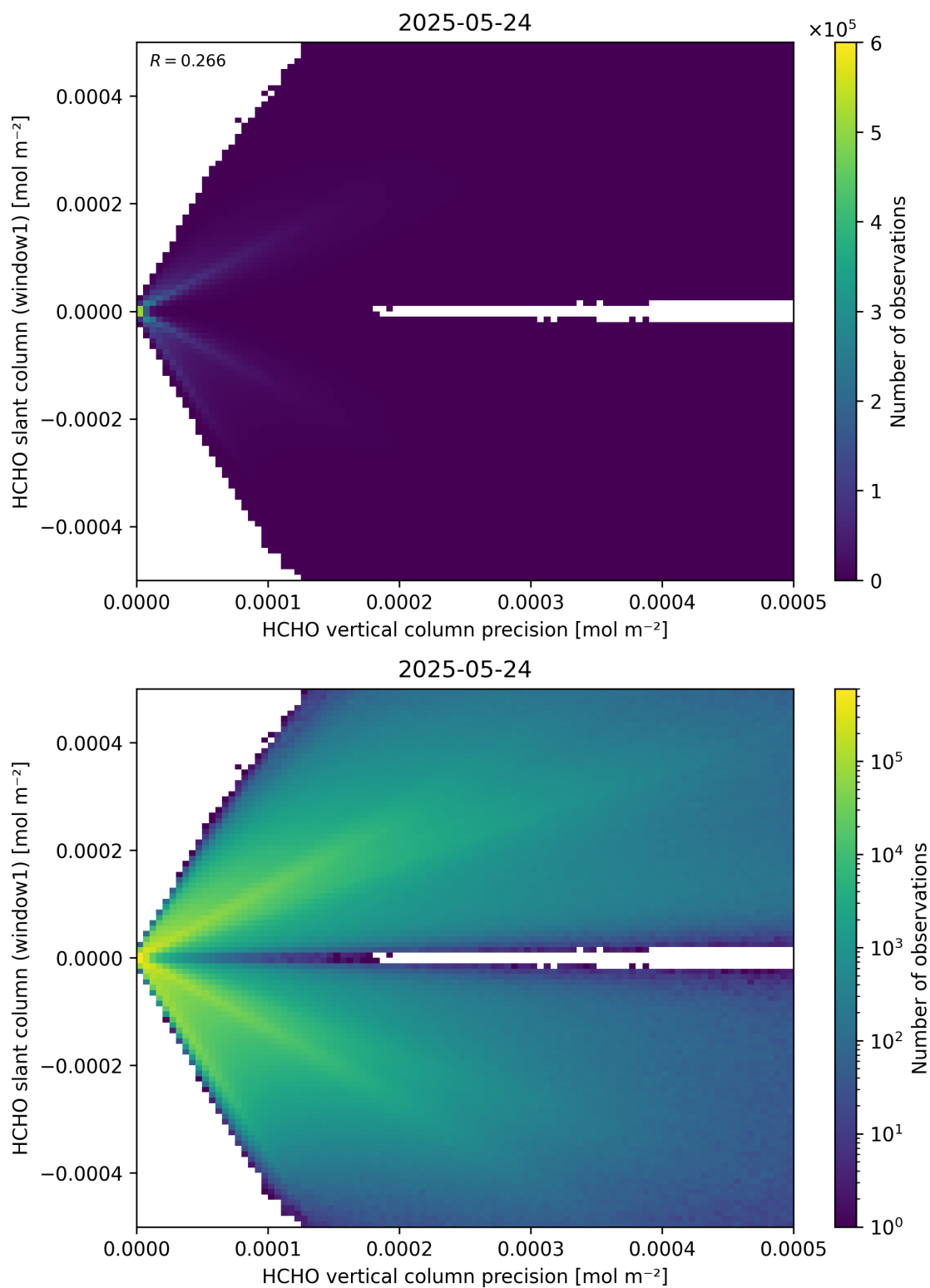
Figure 142: Scatter density plot of “HCHO vertical column precision” against “HCHO slant column (window1)” for 2025-05-23 to 2025-05-25.
