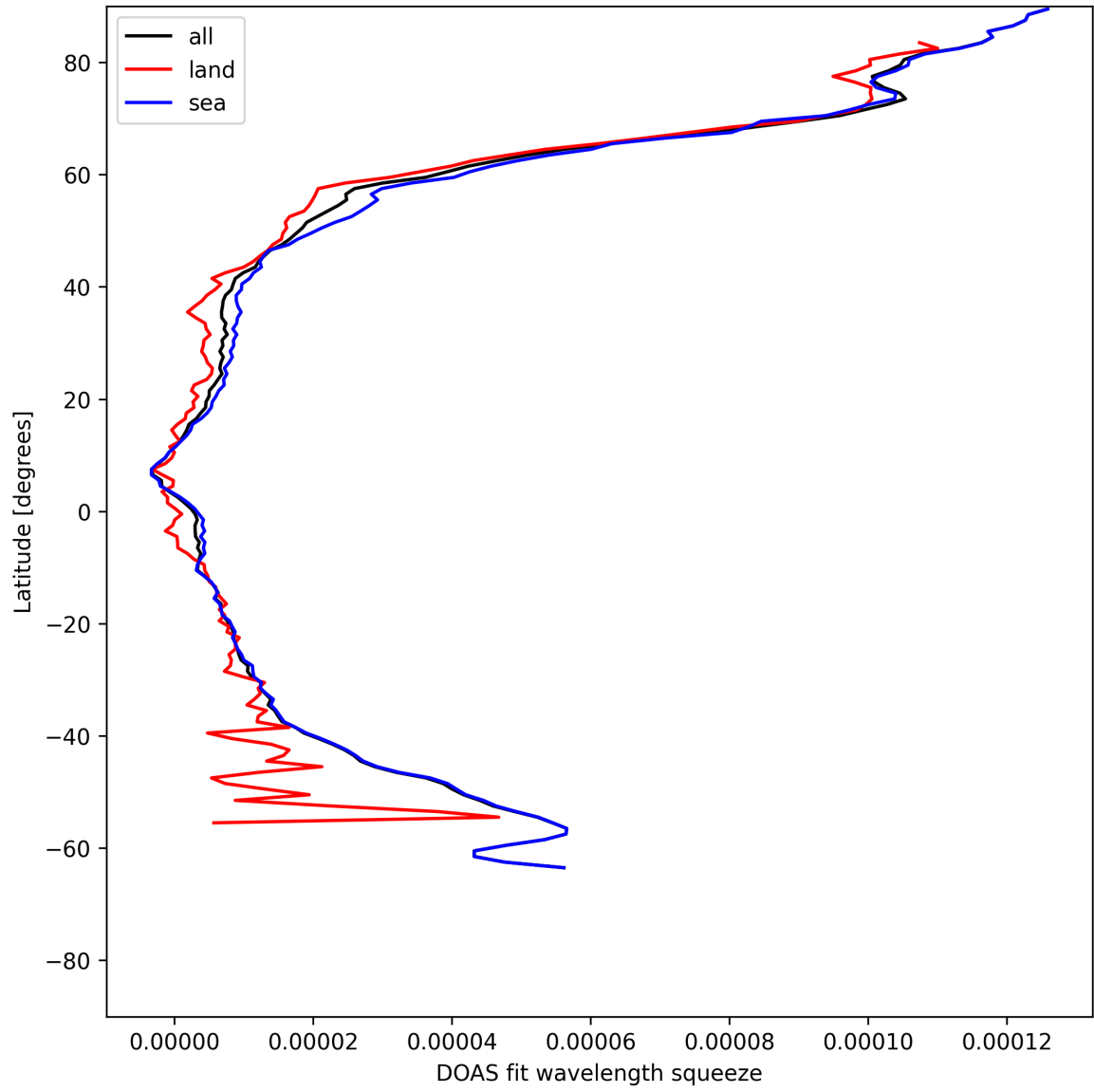
Figure 31: Zonal average of “DOAS fit wavelength squeeze” for 2025-05-23 to 2025-05-25.
