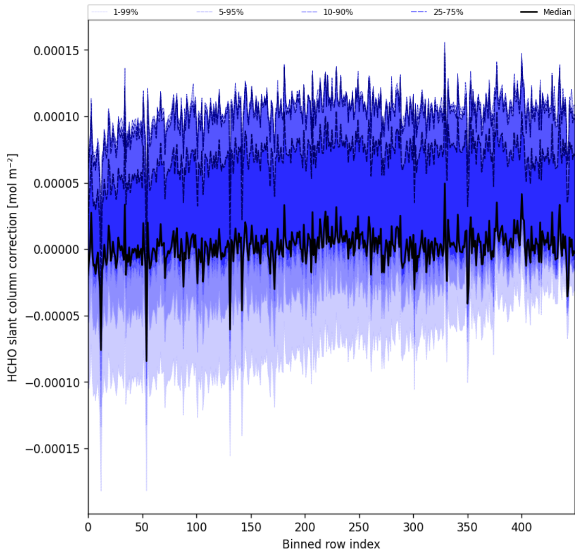
Figure 61: Along track statistics of "HCHO slant column correction" for 2025-05-23 to 2025-05-25
