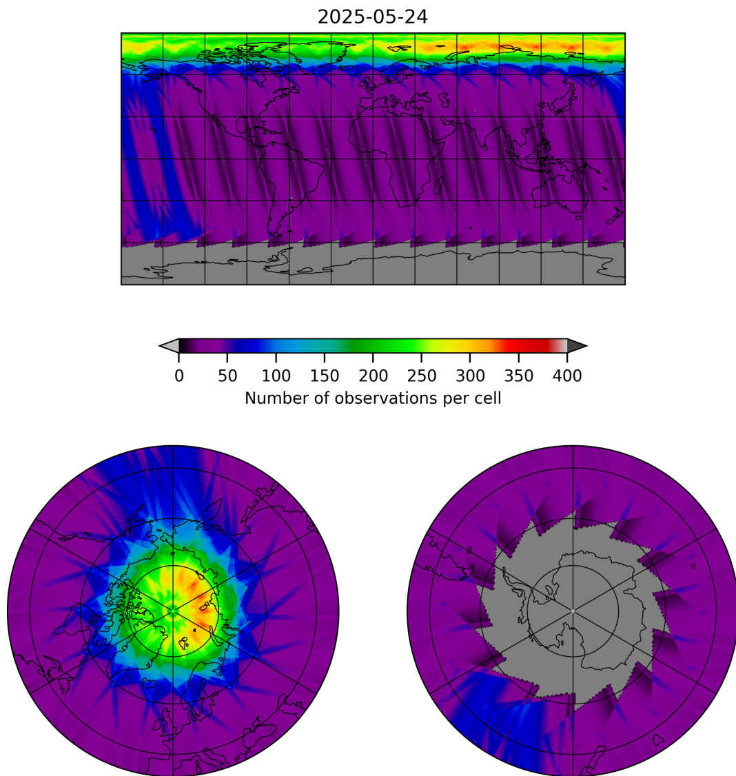
Figure 19: Map of the number of observations for 2025-05-23 to 2025-05-25
