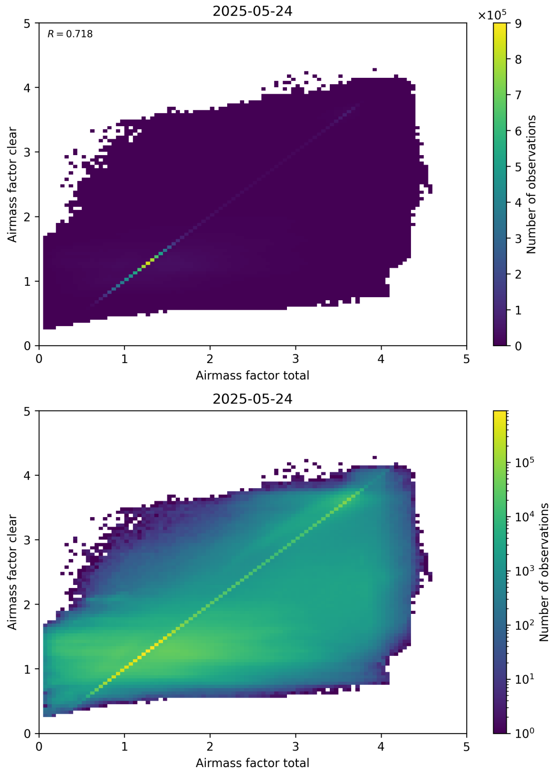
Figure 100: Scatter density plot of “Airmass factor total” against “Airmass factor clear” for 2025-05-23 to 2025-05-25.
