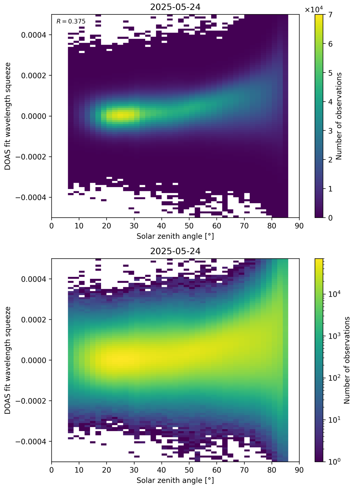
Figure 169: Scatter density plot of “Solar zenith angle” against “DOAS fit wavelength squeeze” for 2025-05-23 to 2025-05-25.
