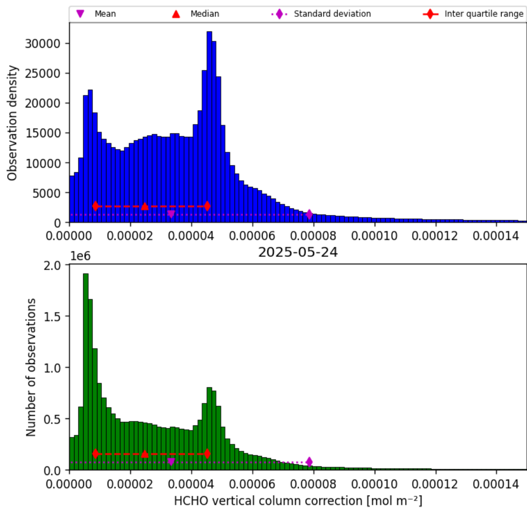
Figure 37: Histogram of “HCHO vertical column correction” for 2025-05-23 to 2025-05-25
