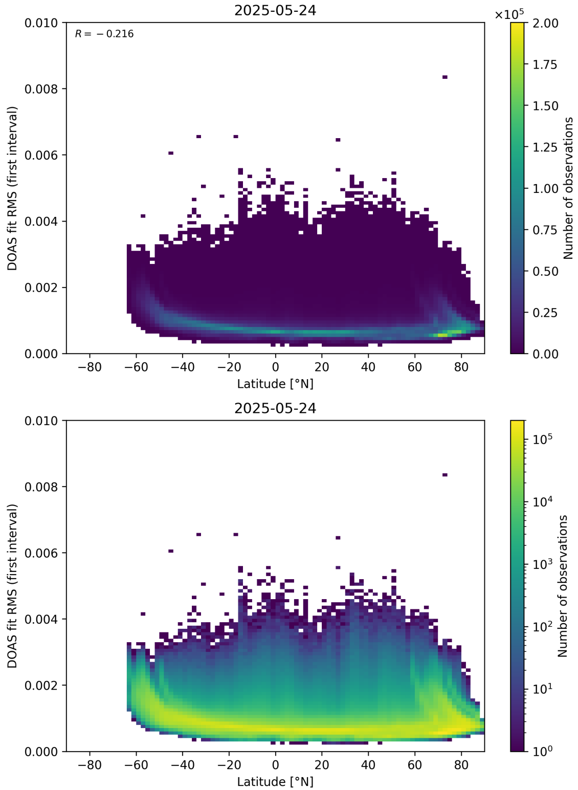
Figure 153: Scatter density plot of “Latitude” against “DOAS fit RMS (first interval)” for 2025-05-23 to 2025-05-25.
