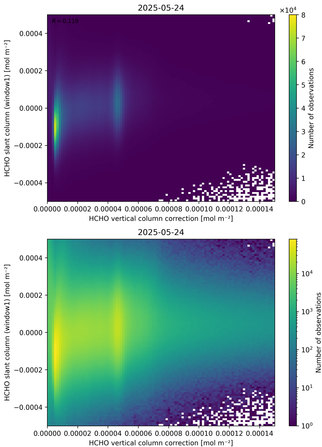
Figure 118: Scatter density plot of “HCHO vertical column correction” against “HCHO slant column (window1)” for 2025-05-23 to 2025-05-25.
