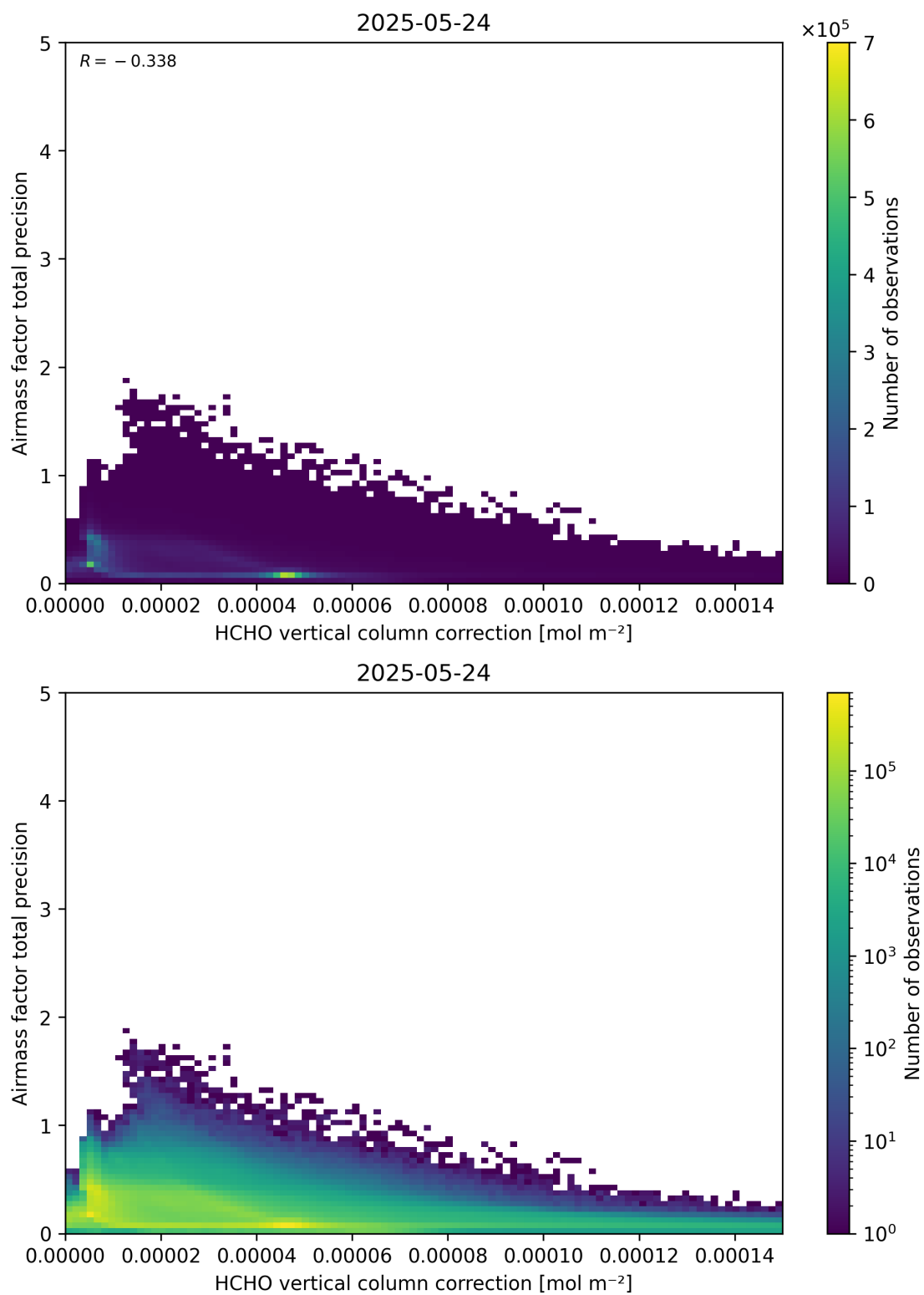
Figure 121: Scatter density plot of “HCHO vertical column correction” against “Airmass factor total precision” for 2025-05-23 to 2025-05-25.
