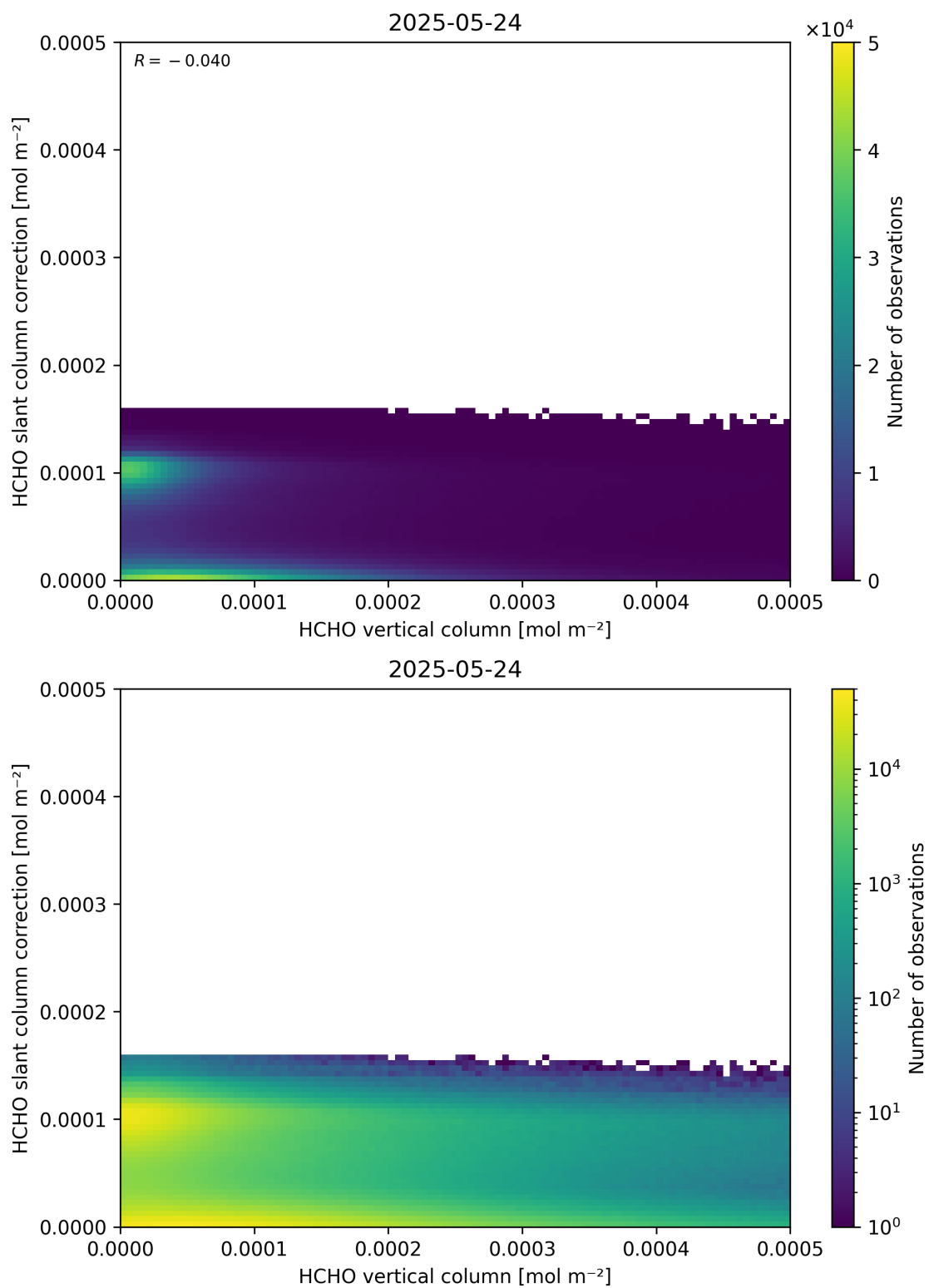
Figure 128: Scatter density plot of “HCHO vertical column” against “HCHO slant column correction” for 2025-05-23 to 2025-05-25.
