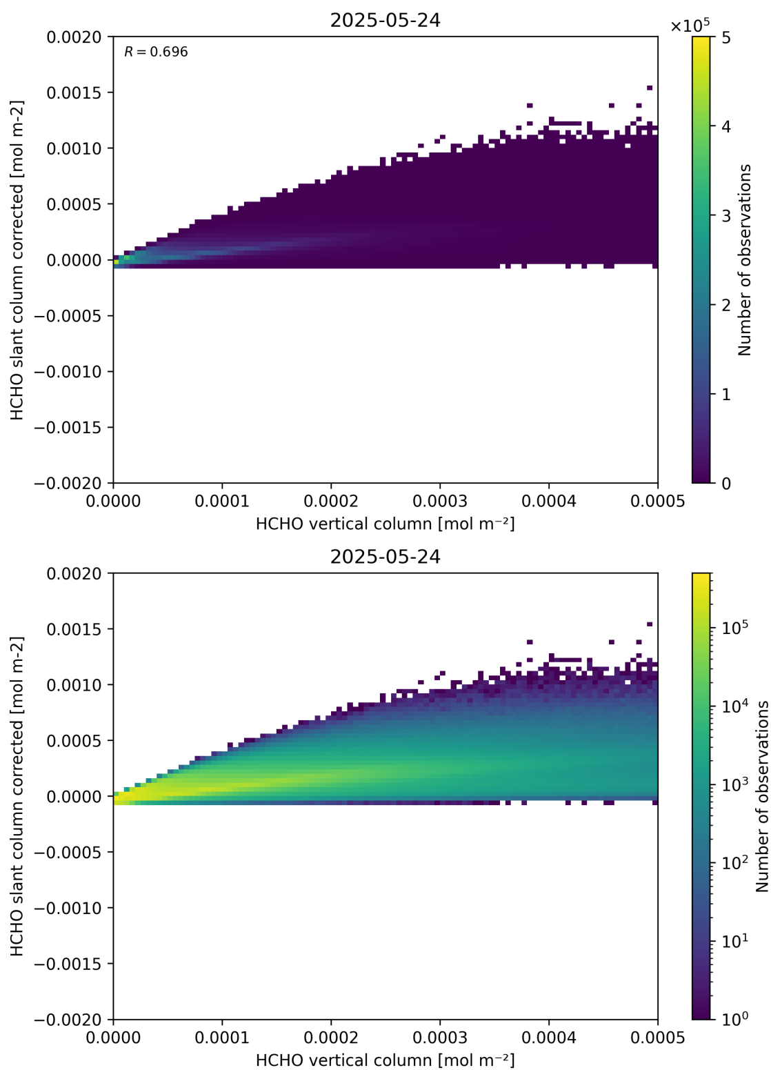
Figure 127: Scatter density plot of “HCHO vertical column” against “HCHO slant column corrected” for 2025-05-23 to 2025-05-25.
