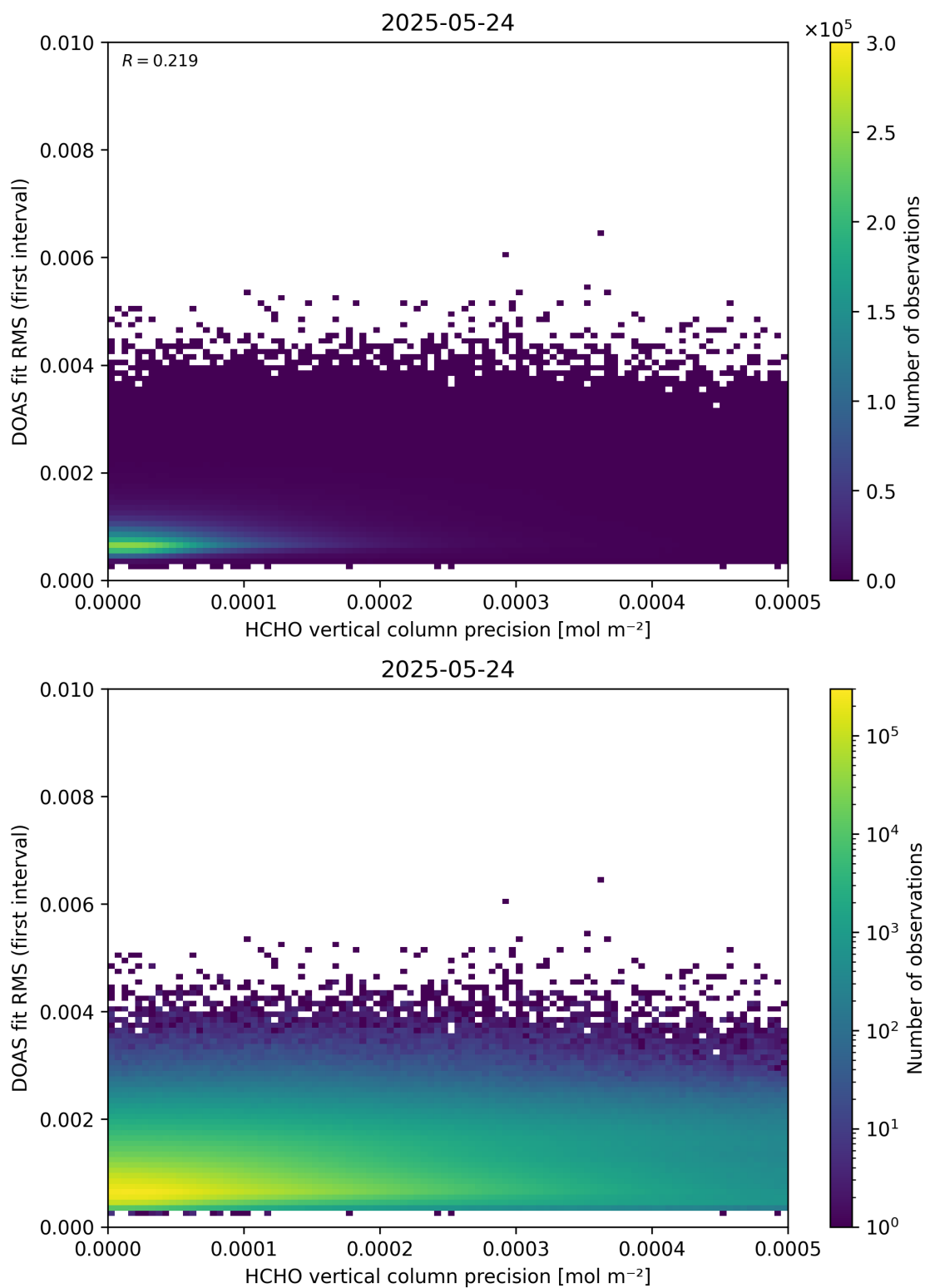
Figure 136: Scatter density plot of “HCHO vertical column precision” against “DOAS fit RMS (first interval)” for 2025-05-23 to 2025-05-25.
