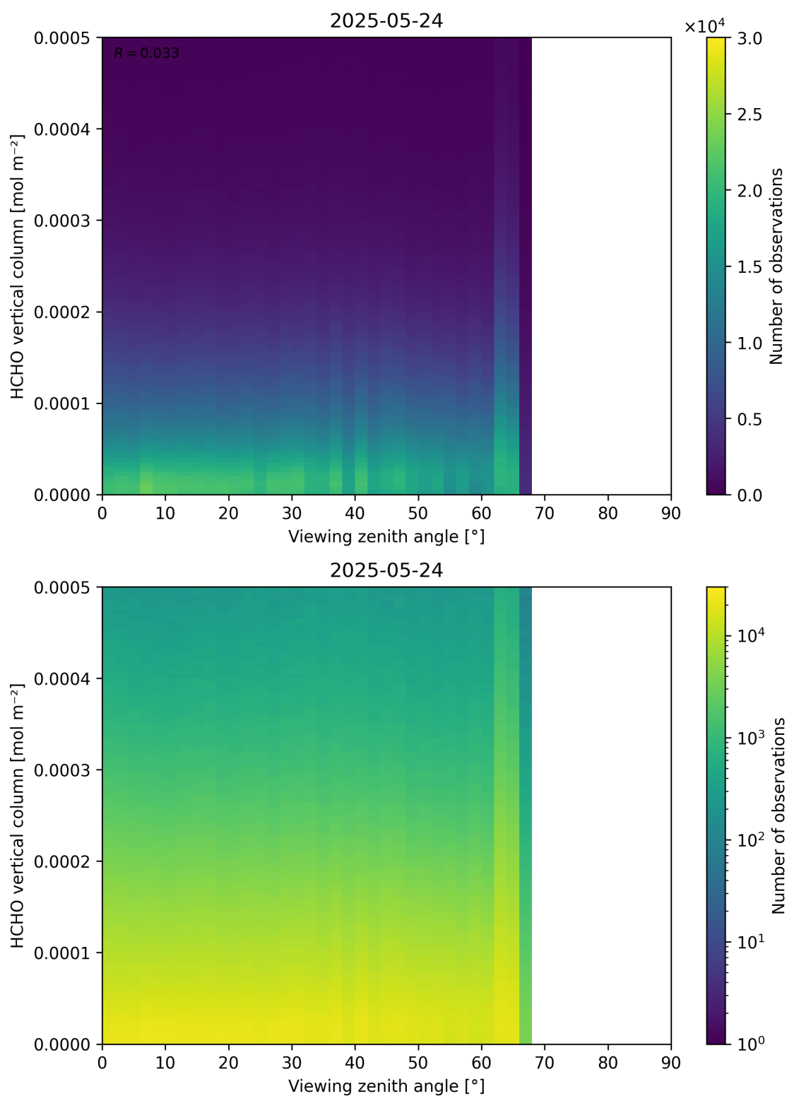
Figure 192: Scatter density plot of “Viewing zenith angle” against “HCHO vertical column” for 2025-05-23 to 2025-05-25.
