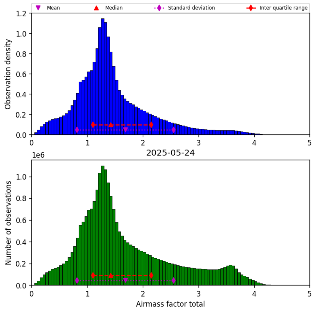
Figure 40: Histogram of “Airmass factor total” for 2025-05-23 to 2025-05-25
