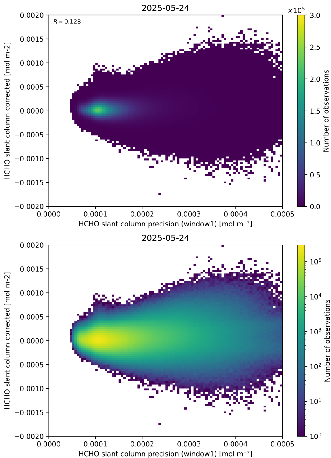
Figure 92: Scatter density plot of “HCHO slant column precision (window1)” against “HCHO slant column corrected” for 2025-05-23 to 2025-05-25.
