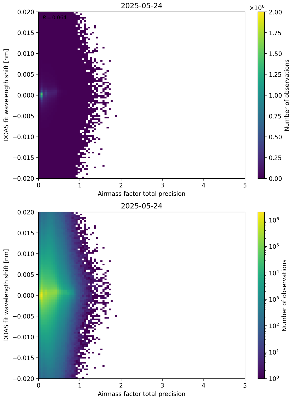
Figure 106: Scatter density plot of “Airmass factor total precision” against “DOAS fit wavelength shift” for 2025-05-23 to 2025-05-25.
