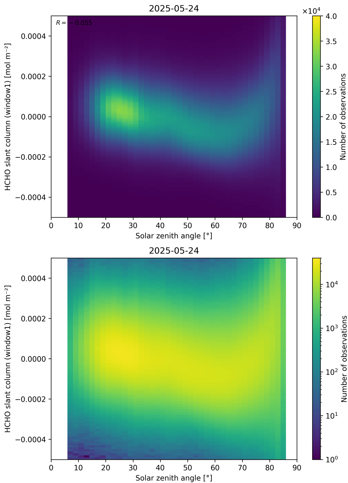
Figure 173: Scatter density plot of “Solar zenith angle” against “HCHO slant column (window1)” for 2025-05-23 to 2025-05-25.
