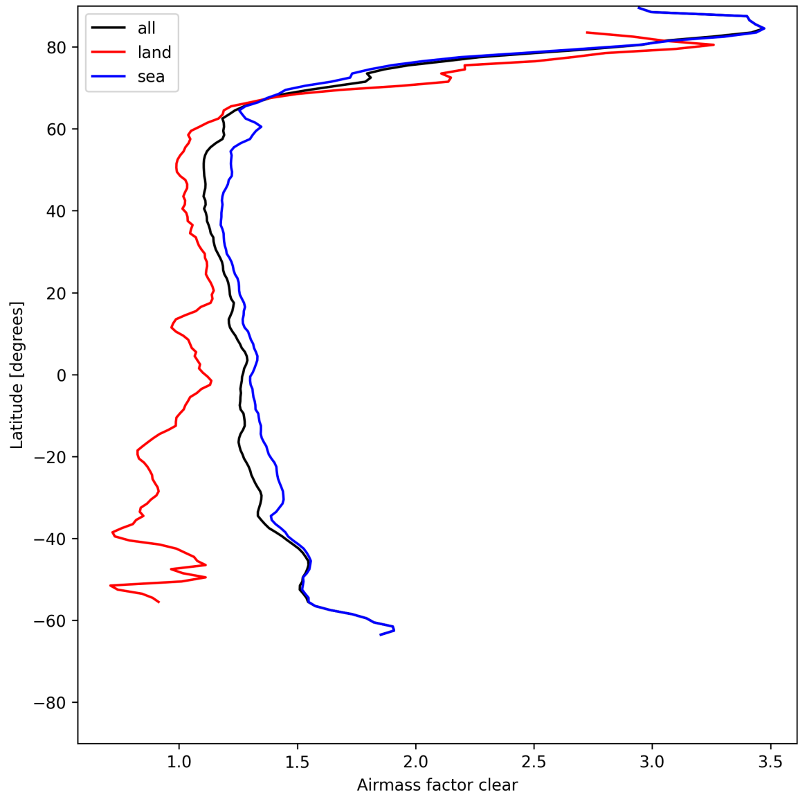
Figure 28: Zonal average of “Airmass factor clear” for 2025-05-23 to 2025-05-25.
