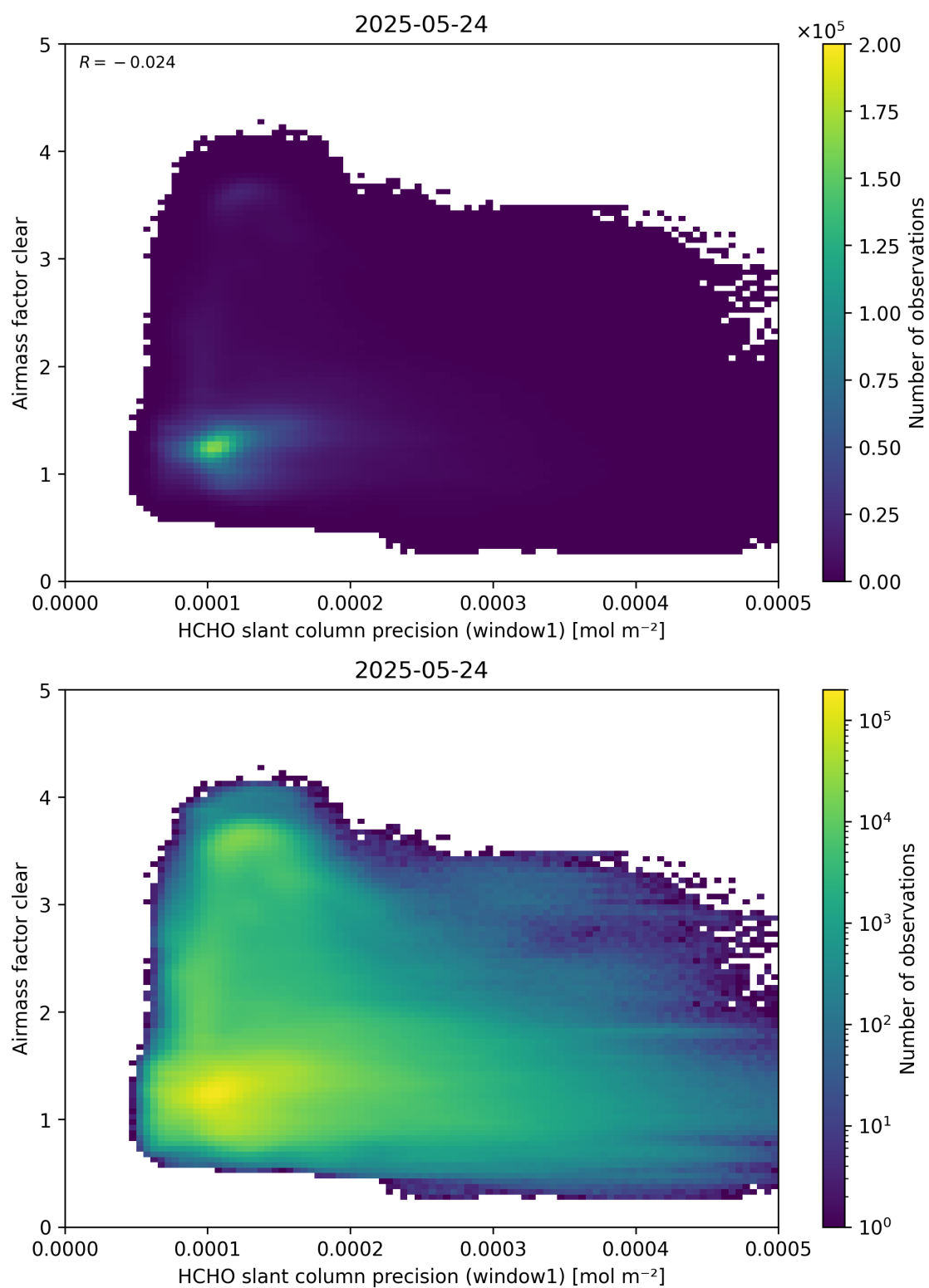
Figure 91: Scatter density plot of “HCHO slant column precision (window1)” against “Airmass factor clear” for 2025-05-23 to 2025-05-25.
