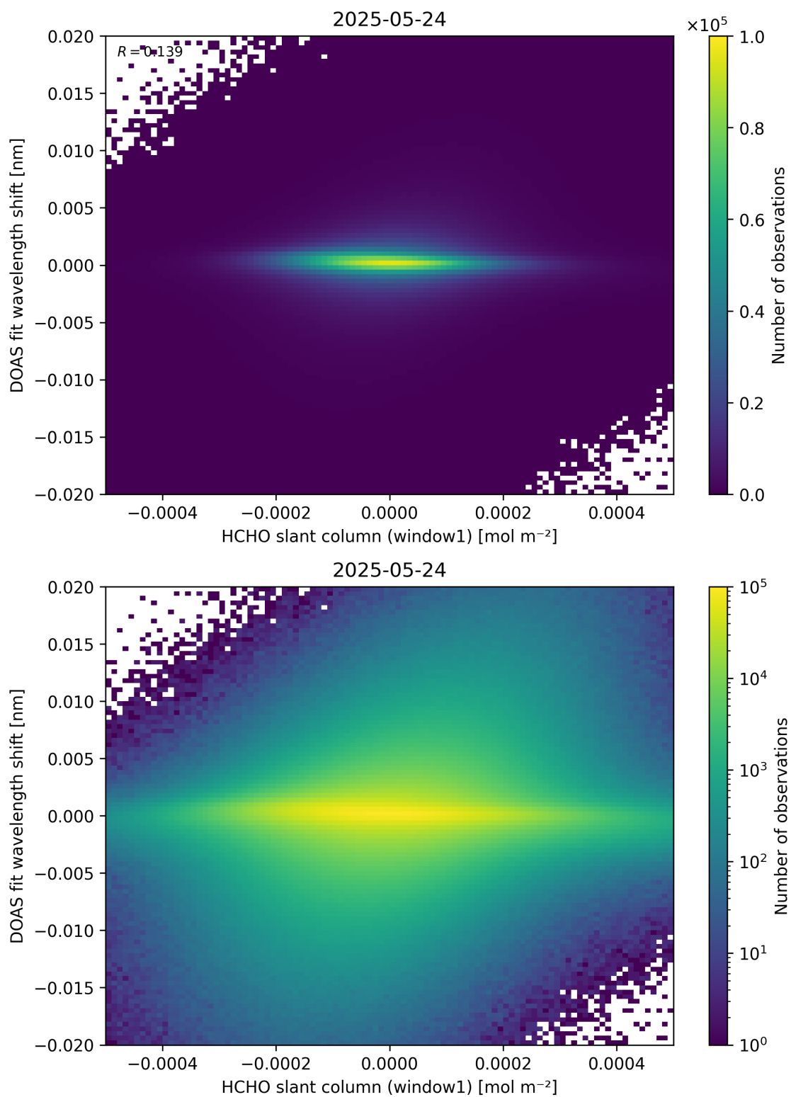
Figure 79: Scatter density plot of “HCHO slant column (window1)” against “DOAS fit wavelength shift” for 2025-05-23 to 2025-05-25.
