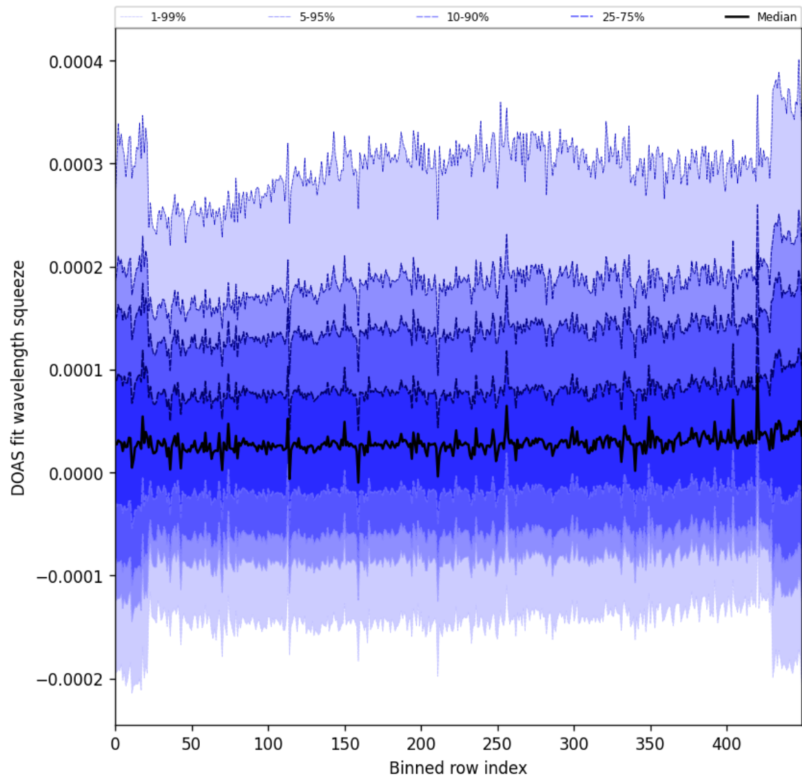
Figure 59: Along track statistics of “DOAS fit wavelength squeeze” for 2025-05-23 to 2025-05-25
