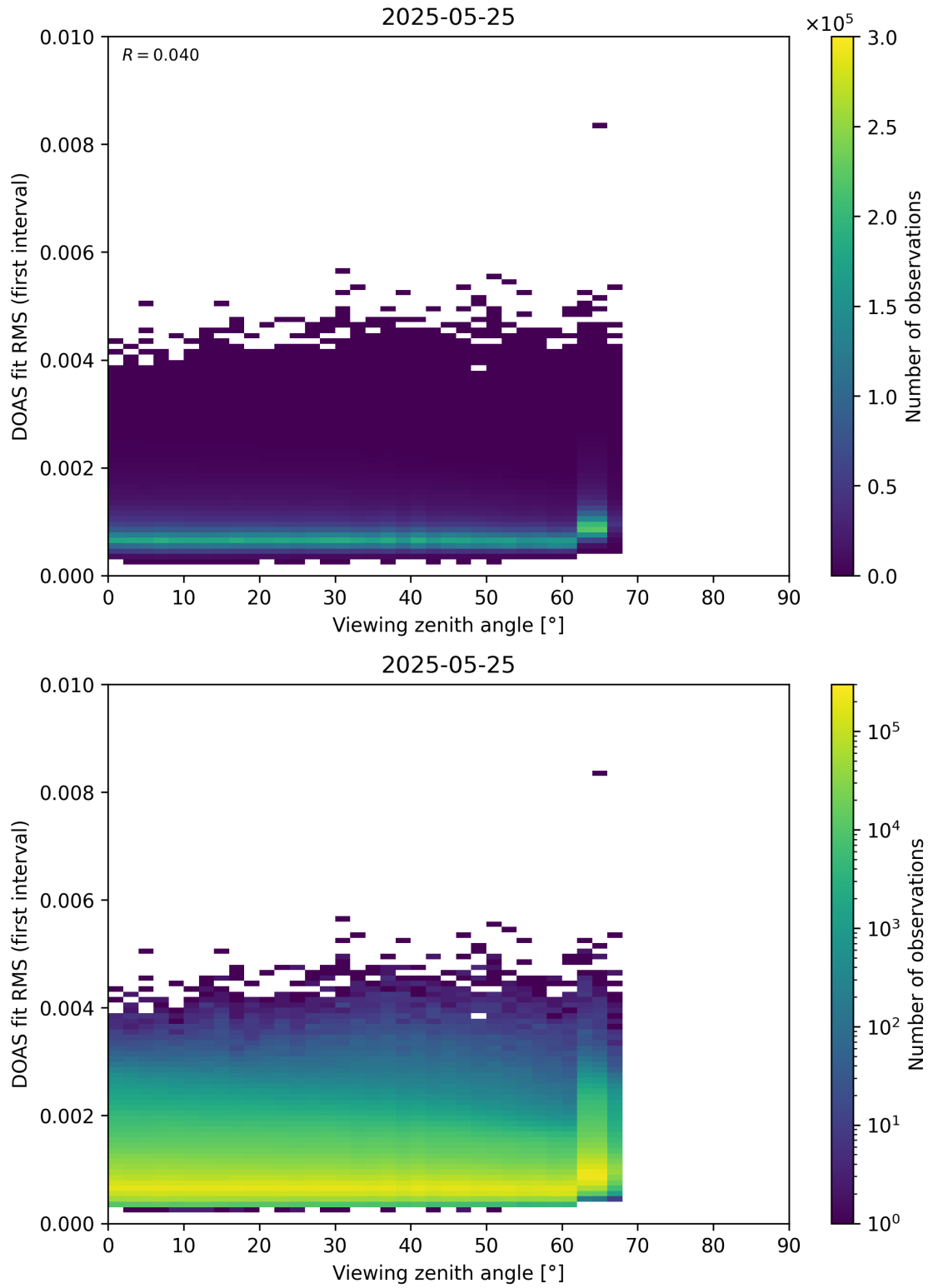
Figure 182: Scatter density plot of “Viewing zenith angle” against “DOAS fit RMS (first interval)” for 2025-05-24 to 2025-05-26.
