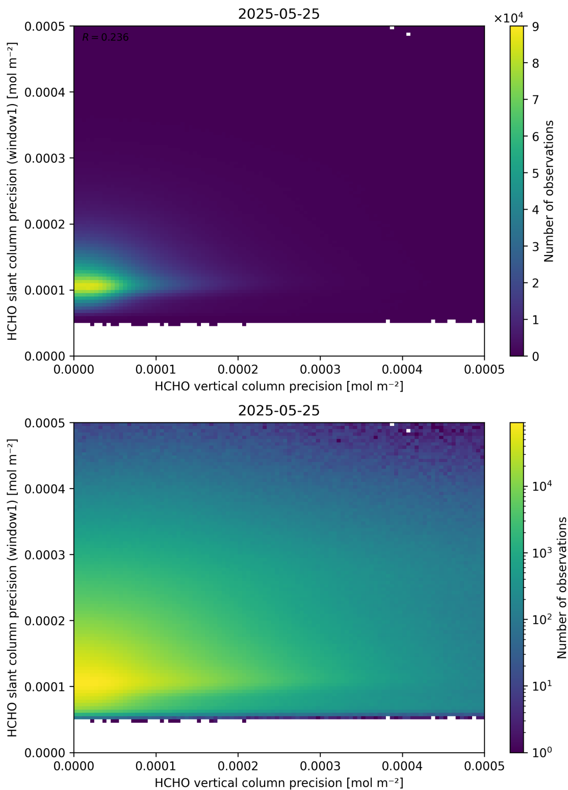
Figure 143: Scatter density plot of “HCHO vertical column precision” against “HCHO slant column precision (window1)” for 2025-05-24 to 2025-05-26.
