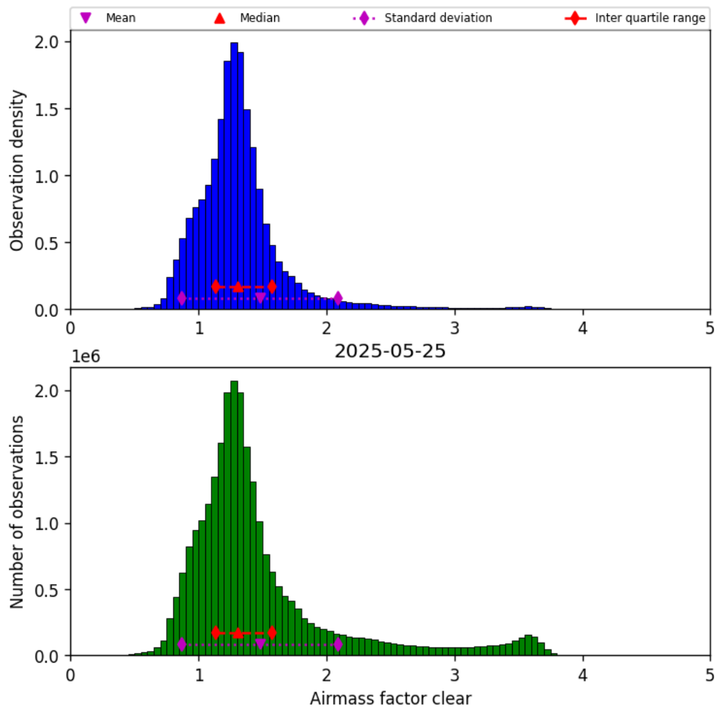
Figure 42: Histogram of “Airmass factor clear” for 2025-05-24 to 2025-05-26
