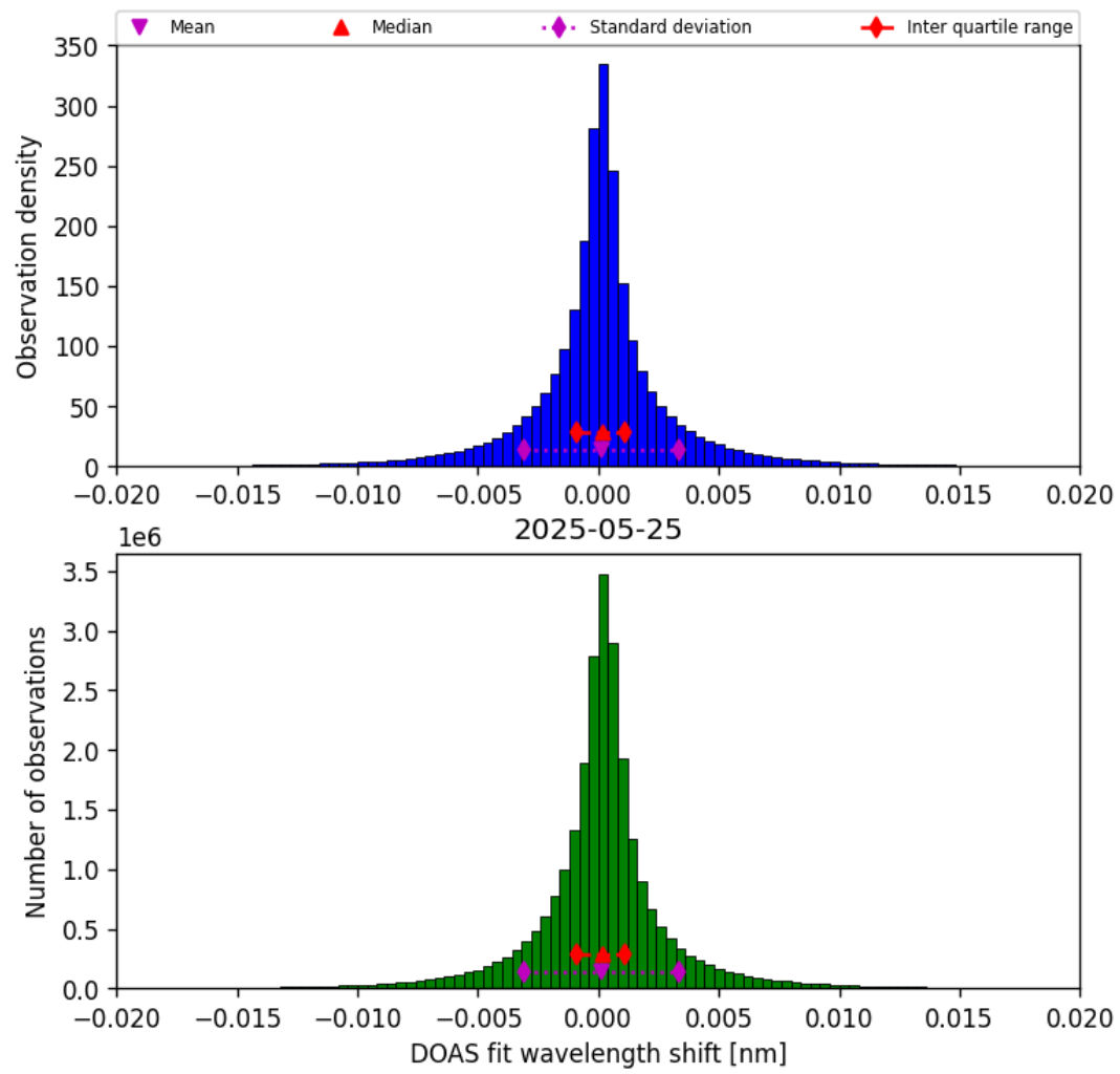
Figure 44: Histogram of “DOAS fit wavelength shift” for 2025-05-24 to 2025-05-26
