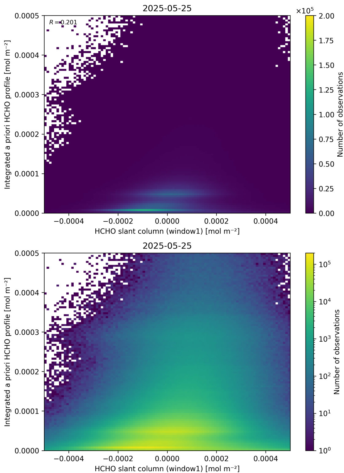
Figure 87: Scatter density plot of “HCHO slant column (window1)” against “Integrated a priori HCHO profile” for 2025-05-24 to 2025-05-26.
