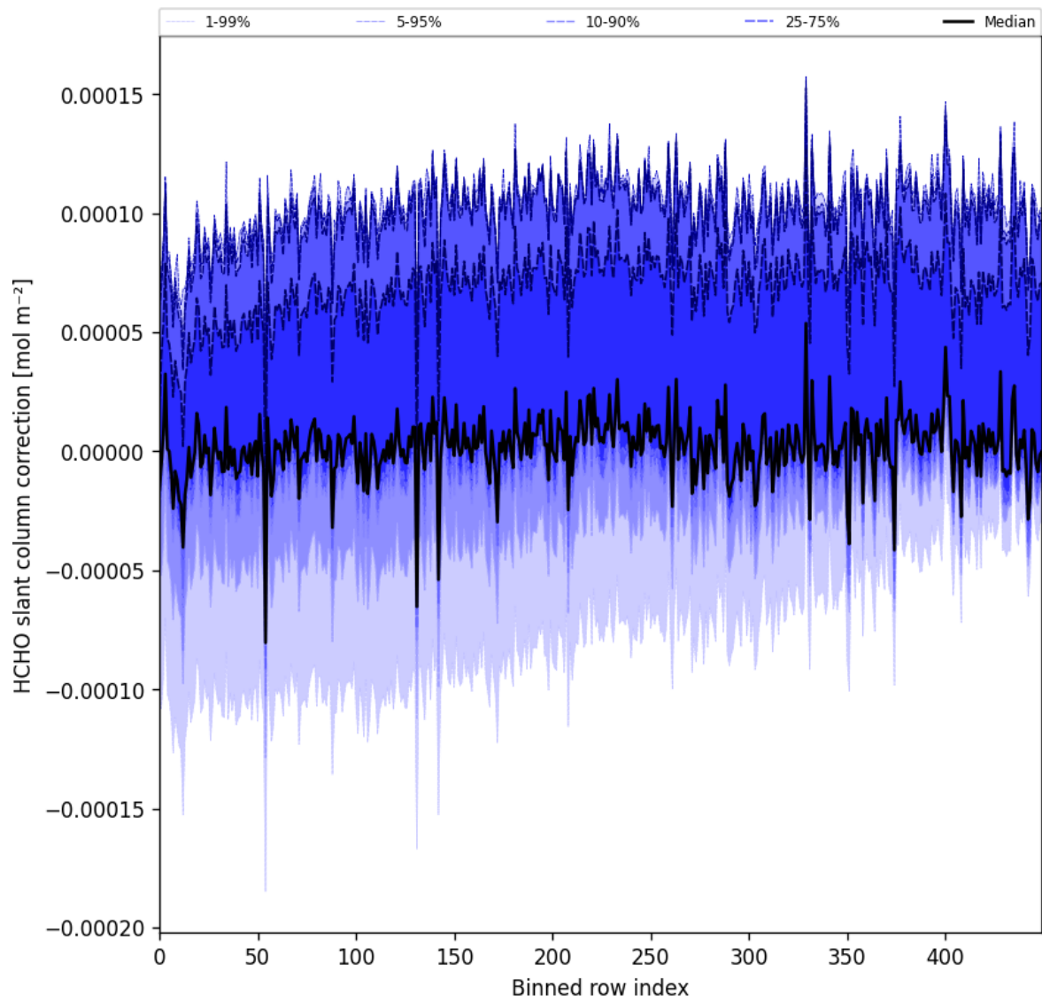
Figure 61: Along track statistics of “HCHO slant column correction” for 2025-05-24 to 2025-05-26
