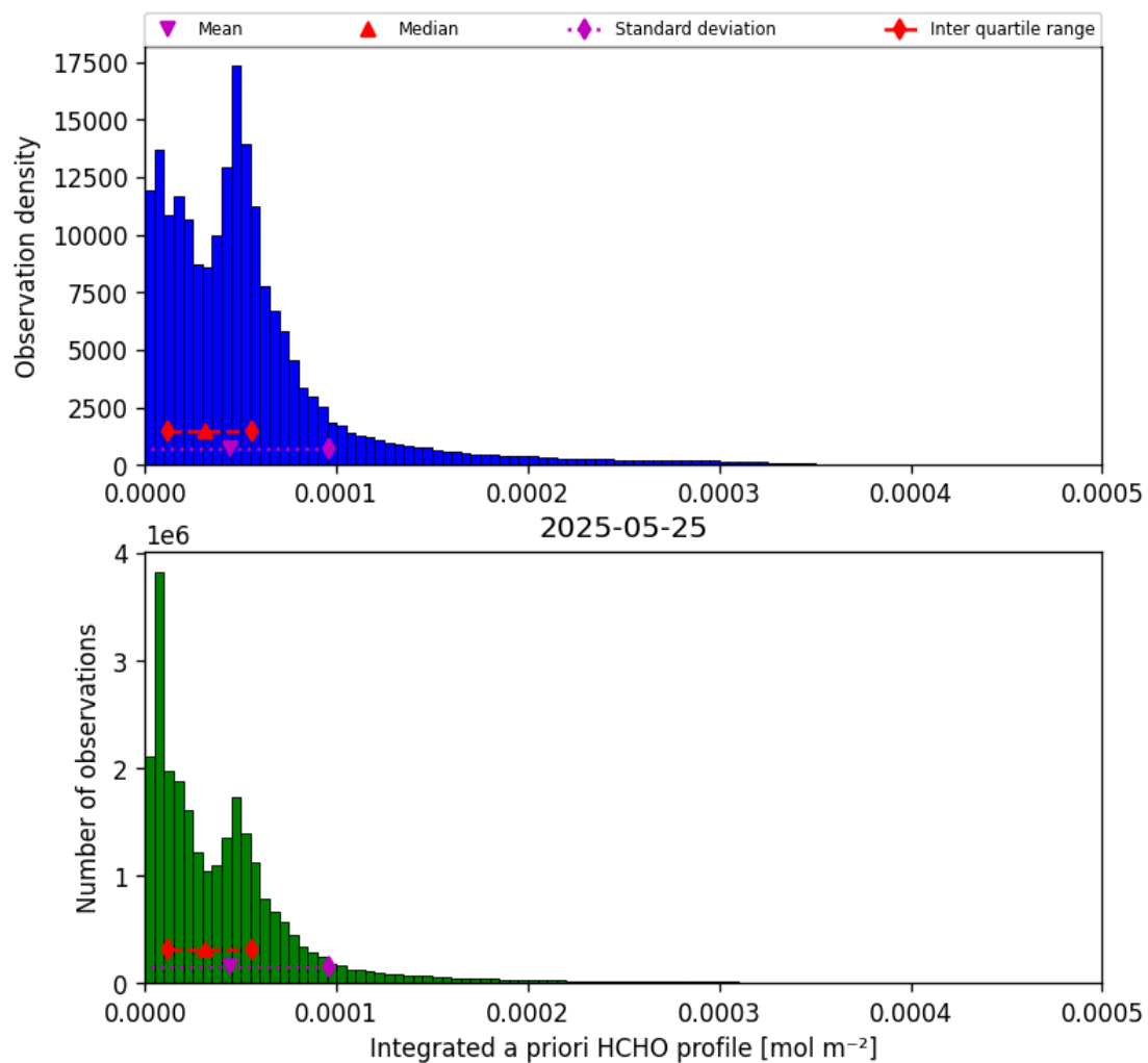
Figure 43: Histogram of “Integrated a priori HCHO profile” for 2025-05-24 to 2025-05-26
