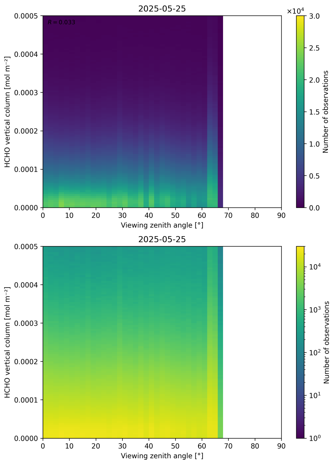
Figure 192: Scatter density plot of “Viewing zenith angle” against “HCHO vertical column” for 2025-05-24 to 2025-05-26.
