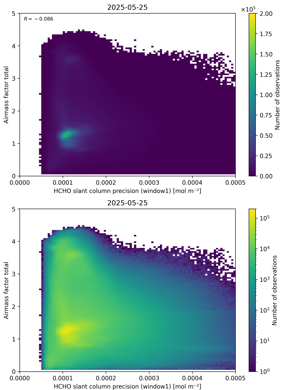
Figure 94: Scatter density plot of “HCHO slant column precision (window1)” against “Airmass factor total” for 2025-05-24 to 2025-05-26.
