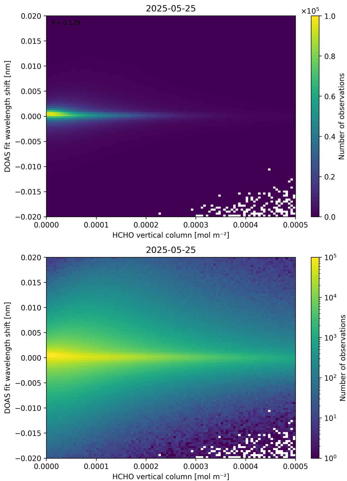
Figure 124: Scatter density plot of “HCHO vertical column” against “DOAS fit wavelength shift” for 2025-05-24 to 2025-05-26.
