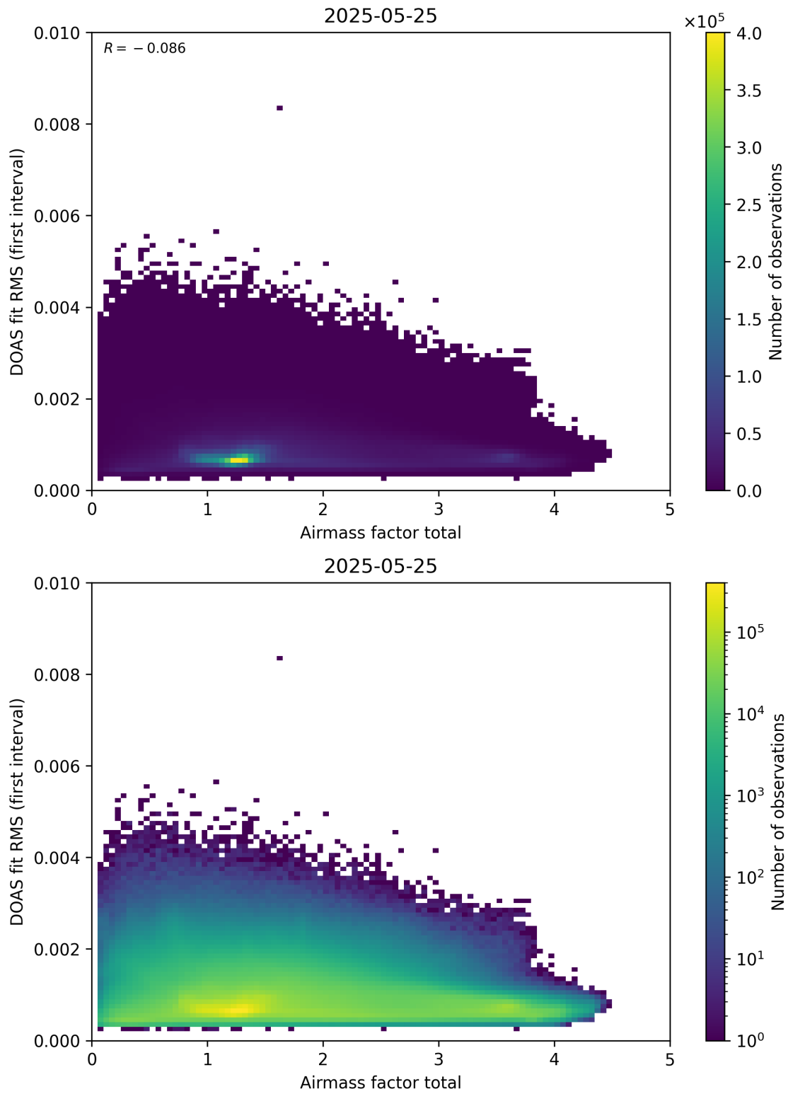
Figure 97: Scatter density plot of “Airmass factor total” against “DOAS fit RMS (first interval)” for 2025-05-24 to 2025-05-26.
