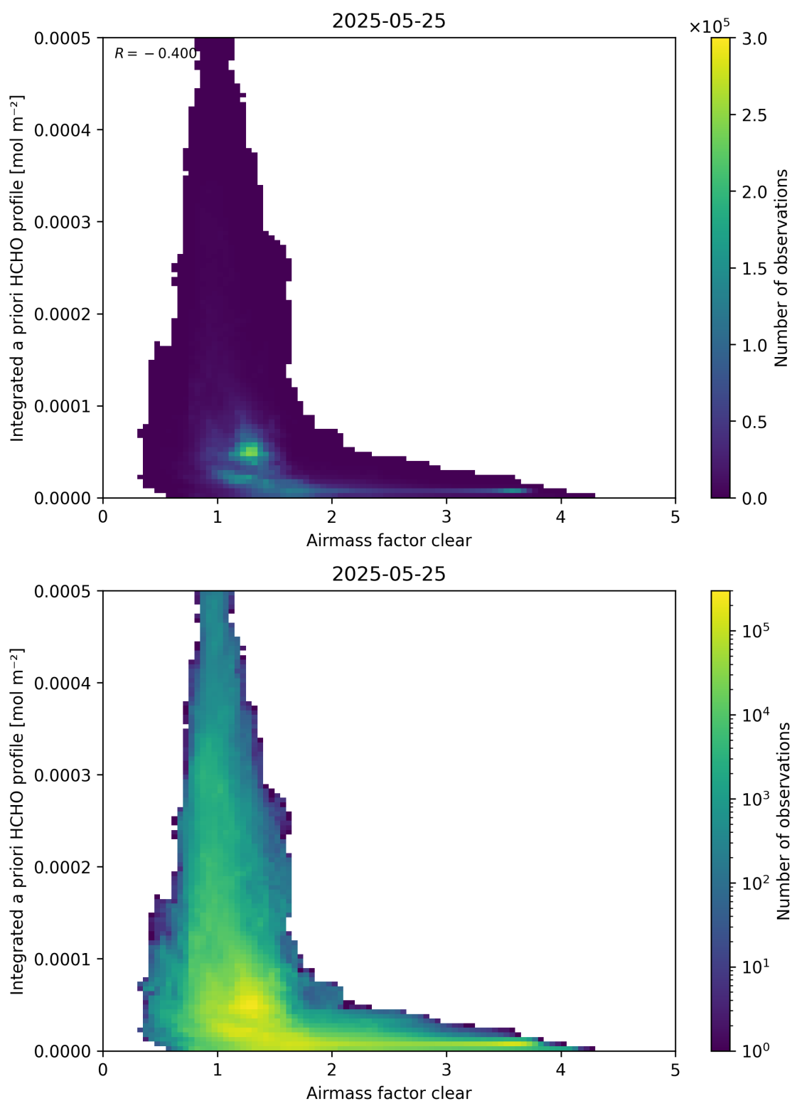
Figure 76: Scatter density plot of “Airmass factor clear” against “Integrated a priori HCHO profile” for 2025-05-24 to 2025-05-26.
