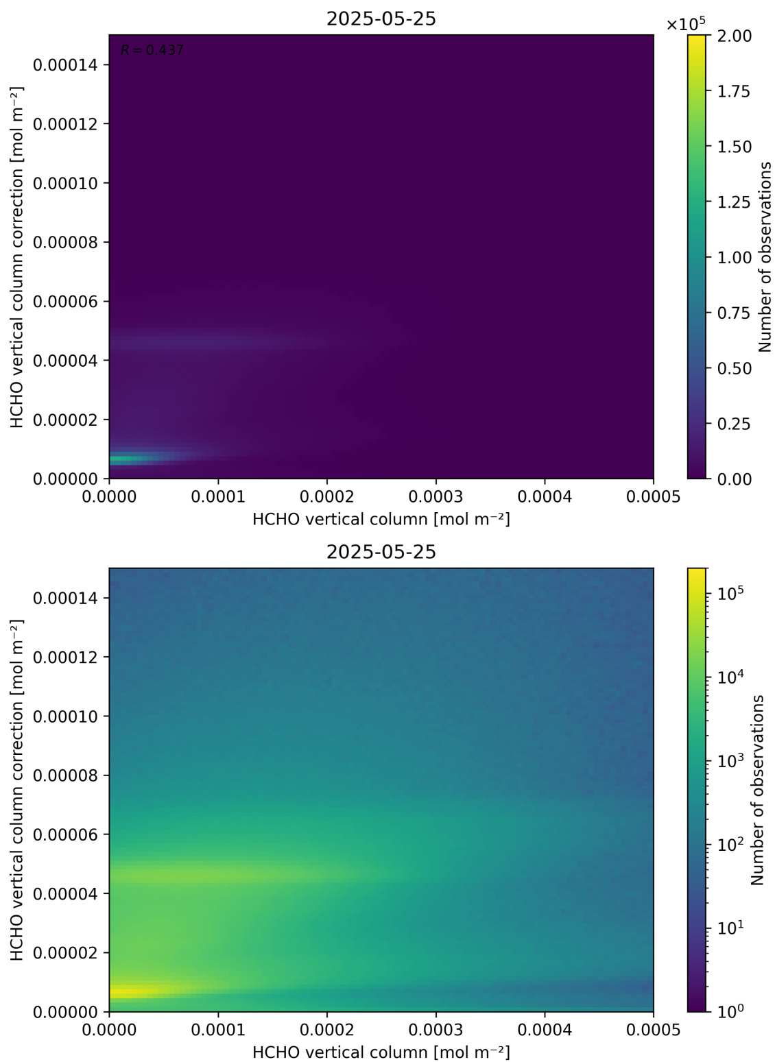
Figure 133: Scatter density plot of “HCHO vertical column” against “HCHO vertical column correction” for 2025-05-24 to 2025-05-26.
