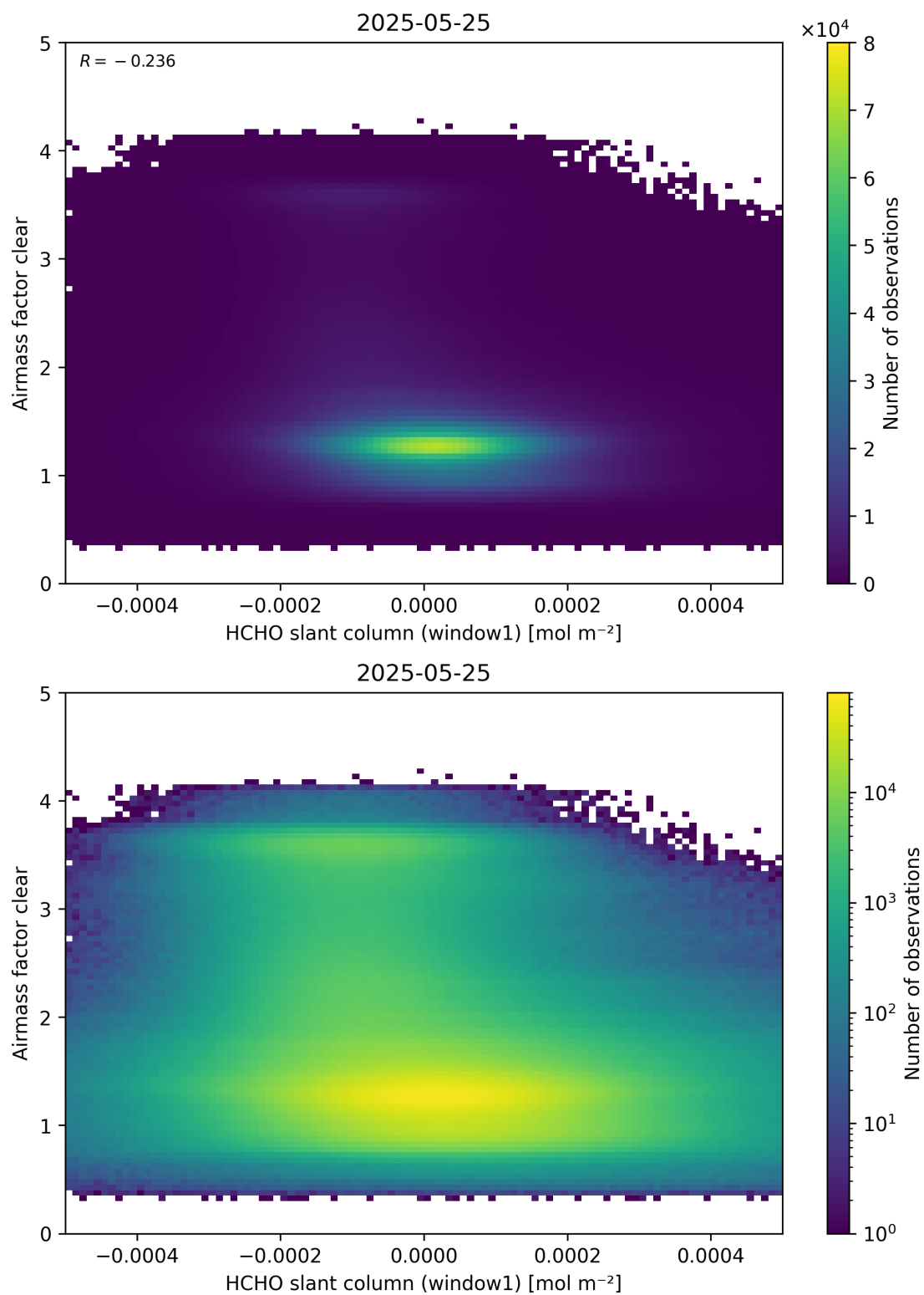
Figure 81: Scatter density plot of “HCHO slant column (window1)” against “Airmass factor clear” for 2025-05-24 to 2025-05-26.
