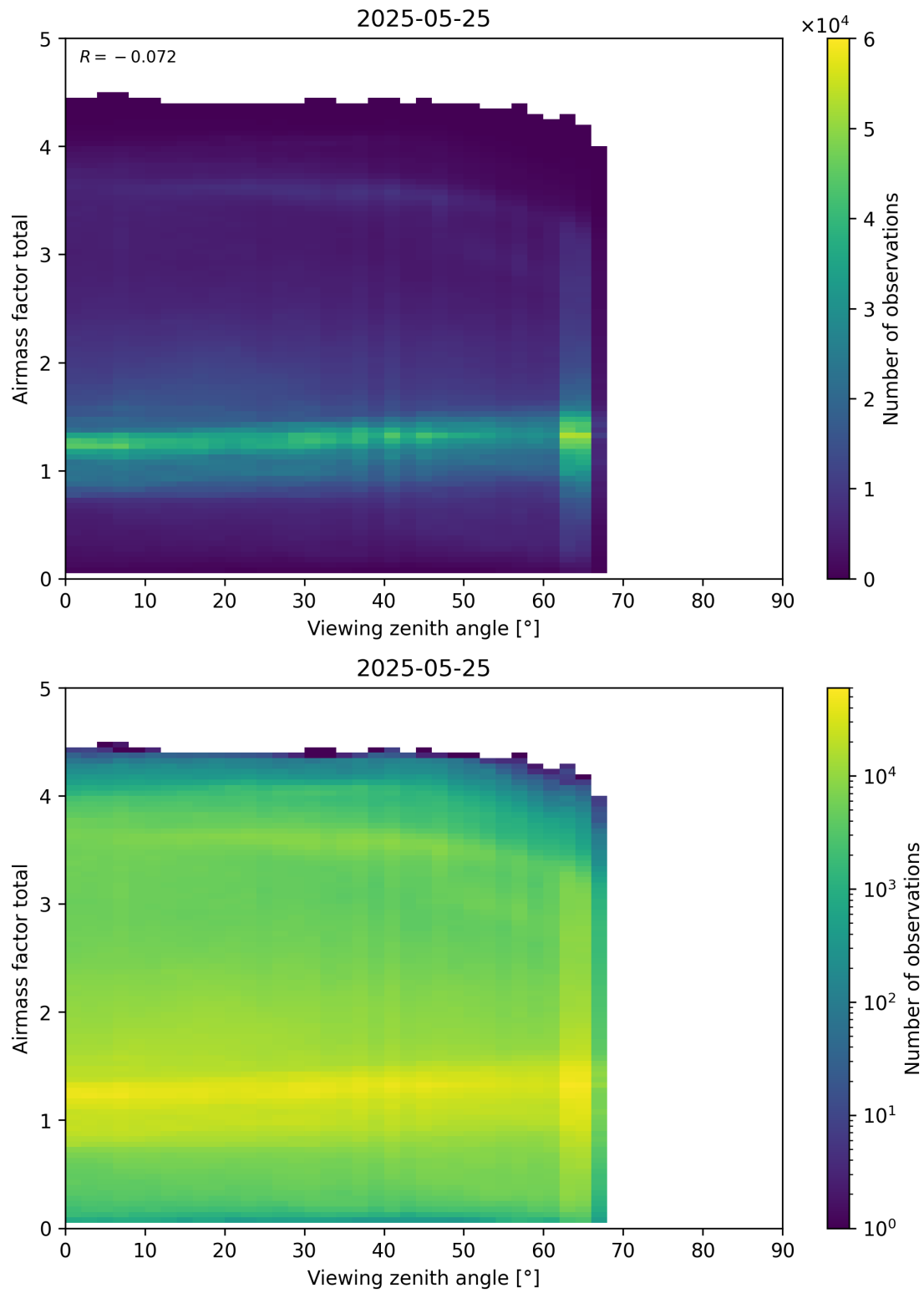
Figure 190: Scatter density plot of “Viewing zenith angle” against “Airmass factor total” for 2025-05-24 to 2025-05-26.
