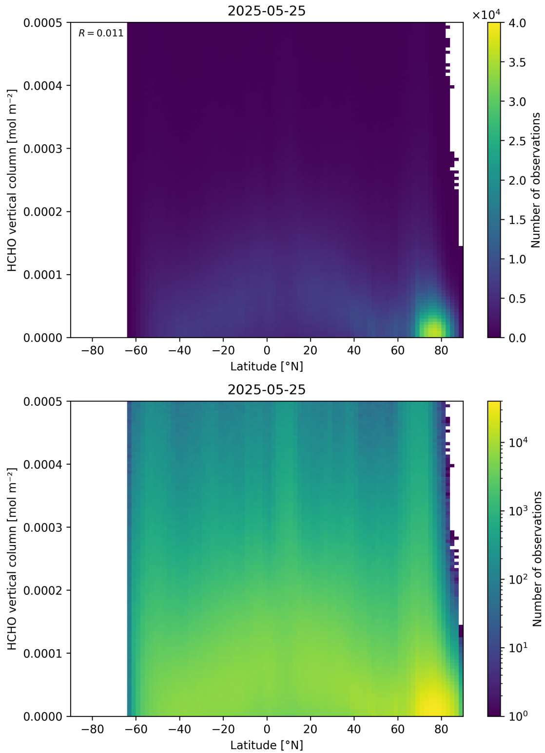
Figure 163: Scatter density plot of “Latitude” against “HCHO vertical column” for 2025-05-24 to 2025-05-26.
