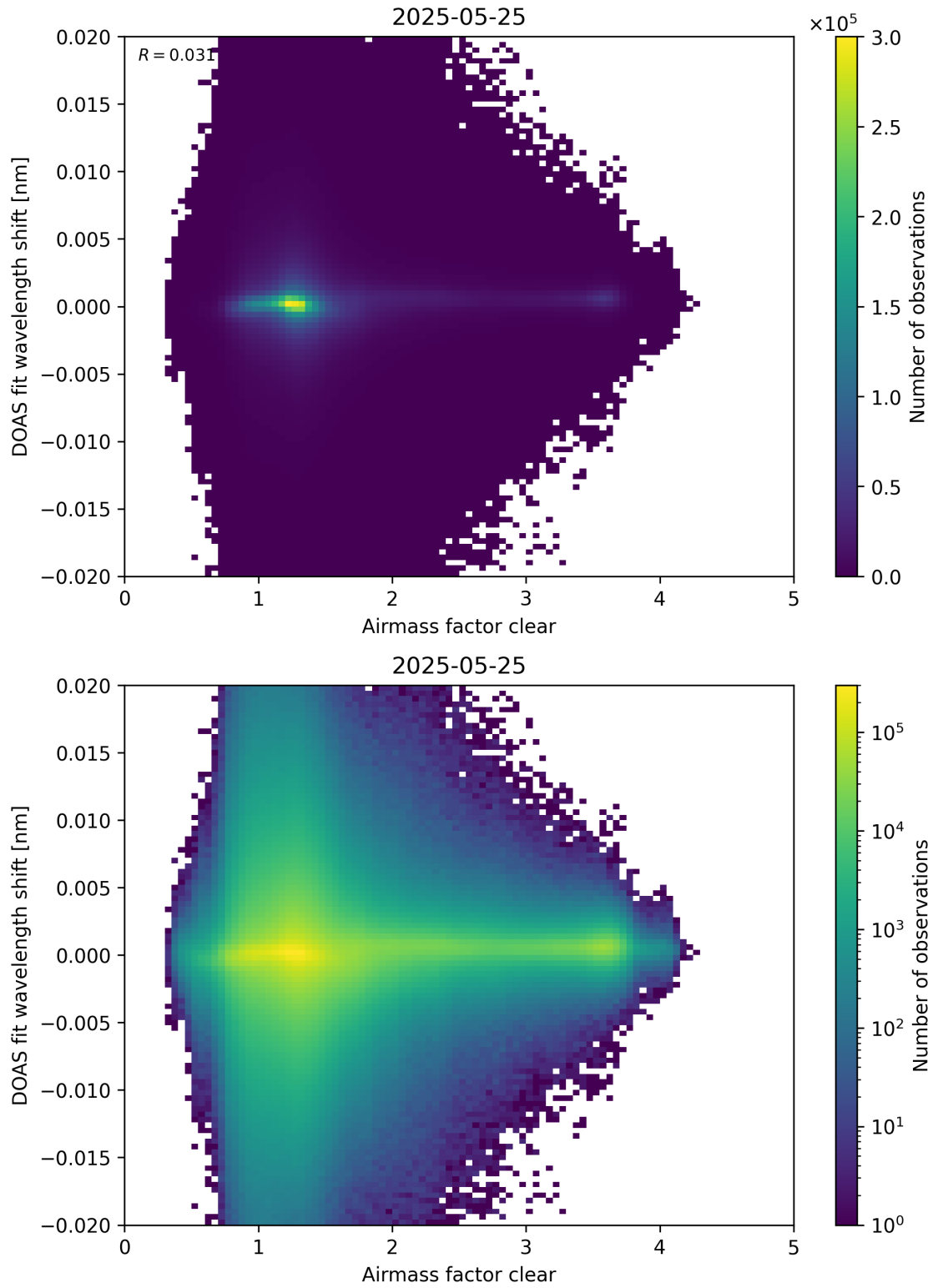
Figure 72: Scatter density plot of “Airmass factor clear” against “DOAS fit wavelength shift” for 2025-05-24 to 2025-05-26.
