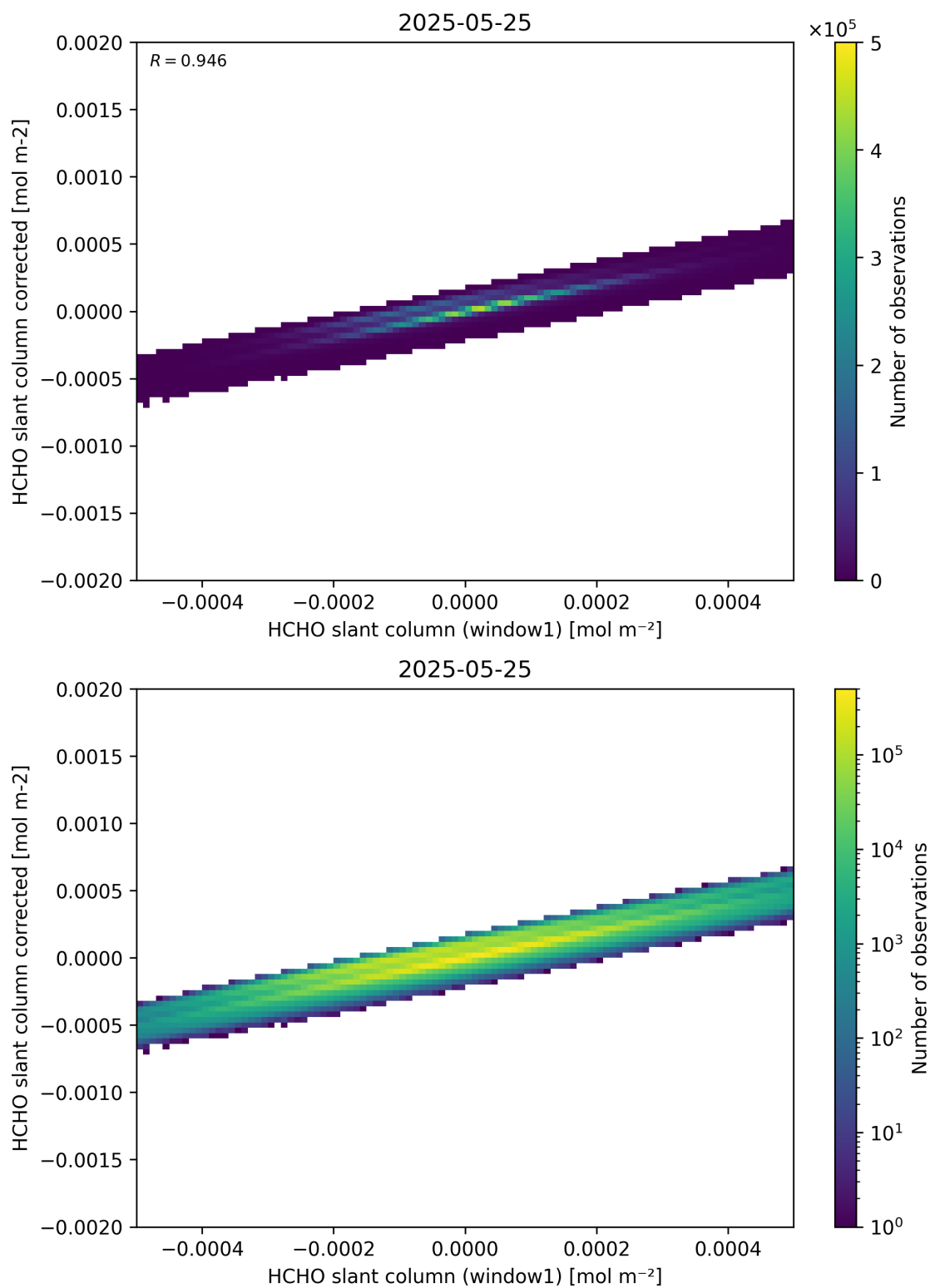
Figure 82: Scatter density plot of “HCHO slant column (window1)” against “HCHO slant column corrected” for 2025-05-24 to 2025-05-26.
