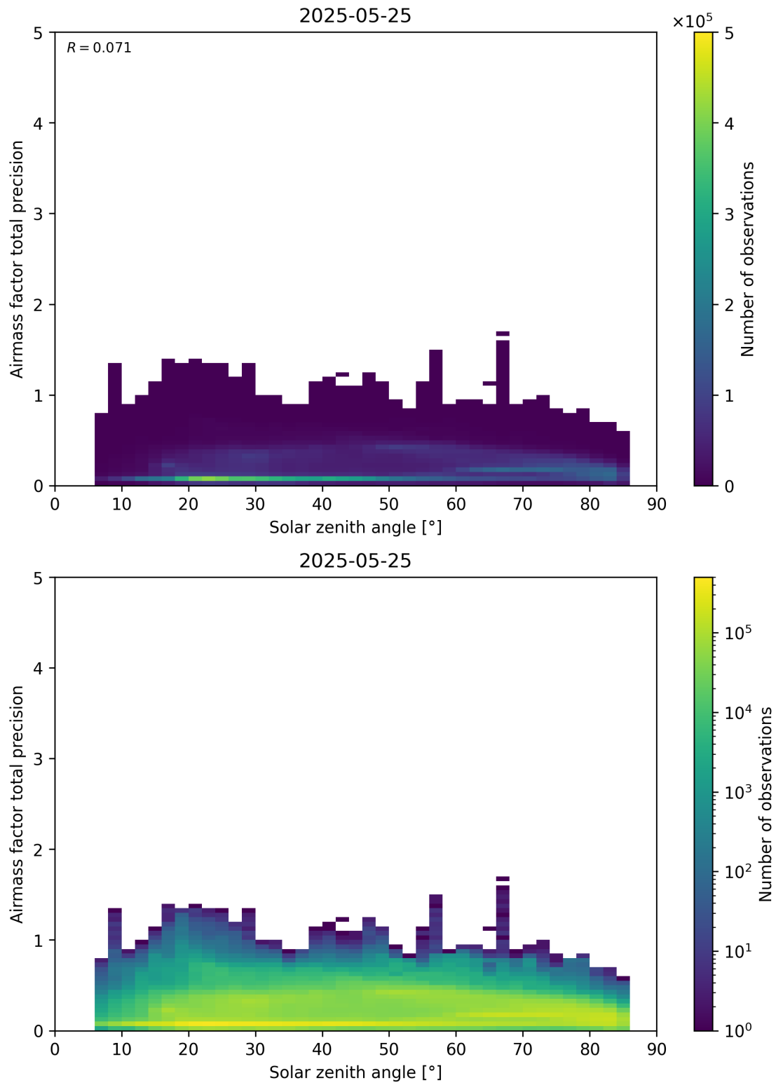
Figure 176: Scatter density plot of “Solar zenith angle” against “Airmass factor total precision” for 2025-05-24 to 2025-05-26.
