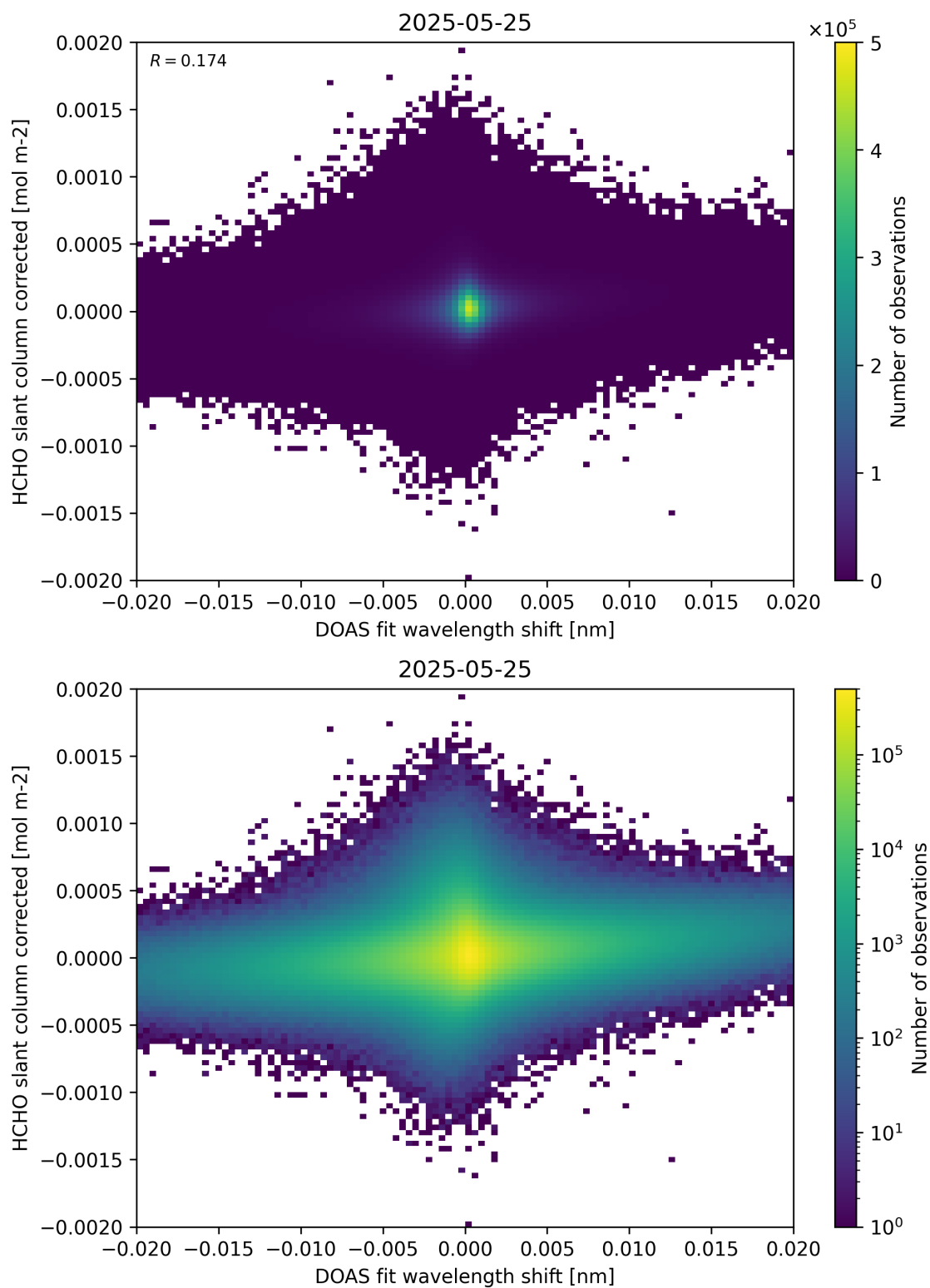
Figure 66: Scatter density plot of “DOAS fit wavelength shift” against “HCHO slant column corrected” for 2025-05-24 to 2025-05-26.
