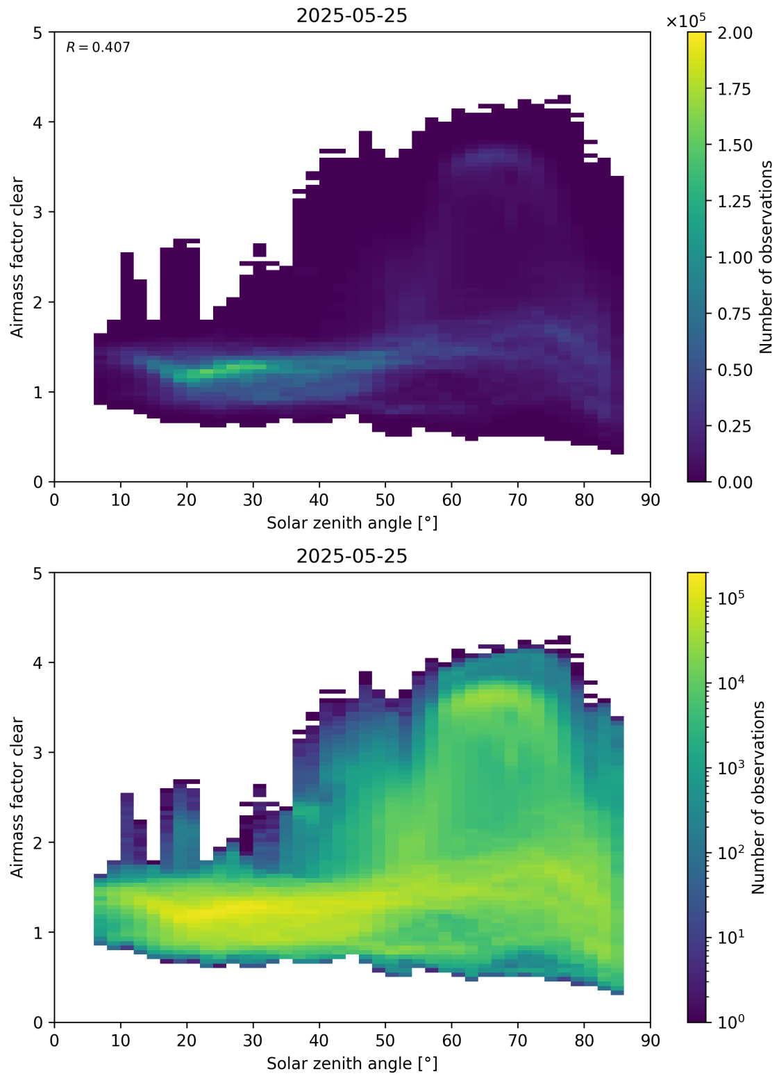
Figure 170: Scatter density plot of “Solar zenith angle” against “Airmass factor clear” for 2025-05-24 to 2025-05-26.
