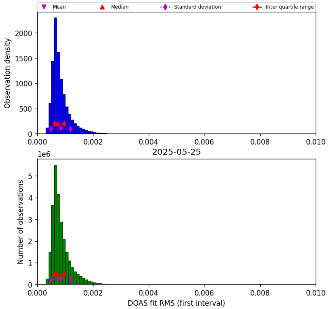
Figure 46: Histogram of “DOAS fit RMS (first interval)” for 2025-05-24 to 2025-05-26
