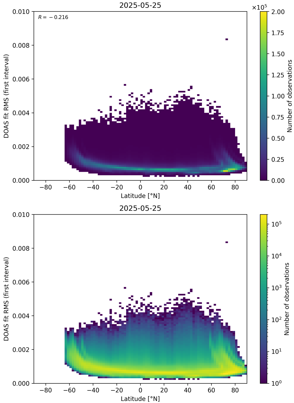
Figure 153: Scatter density plot of “Latitude” against “DOAS fit RMS (first interval)” for 2025-05-24 to 2025-05-26.
