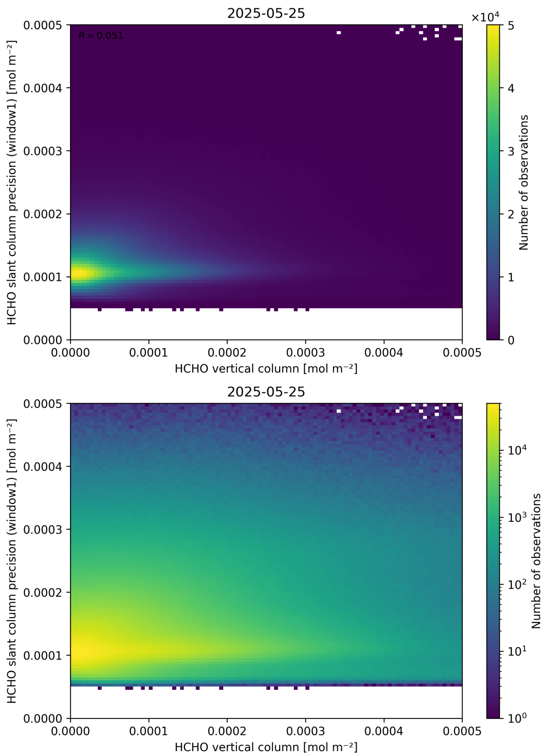
Figure 130: Scatter density plot of “HCHO vertical column” against “HCHO slant column precision (window1)” for 2025-05-24 to 2025-05-26.
