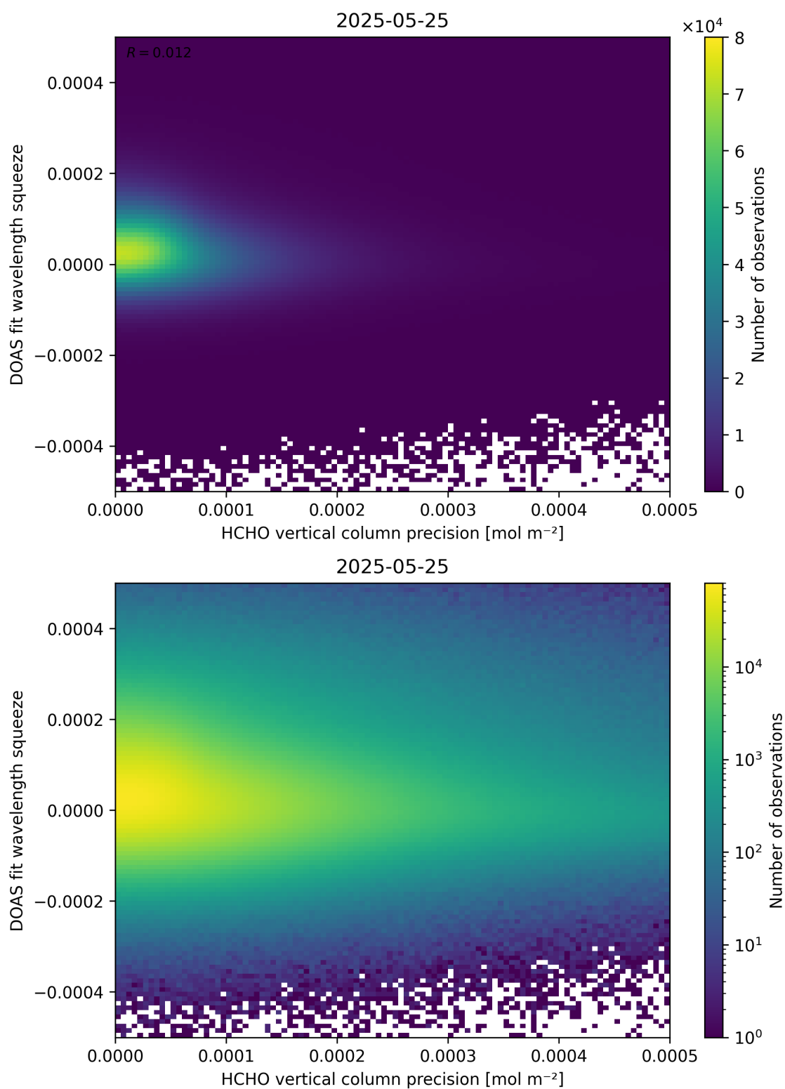
Figure 138: Scatter density plot of “HCHO vertical column precision” against “DOAS fit wavelength squeeze” for 2025-05-24 to 2025-05-26.
