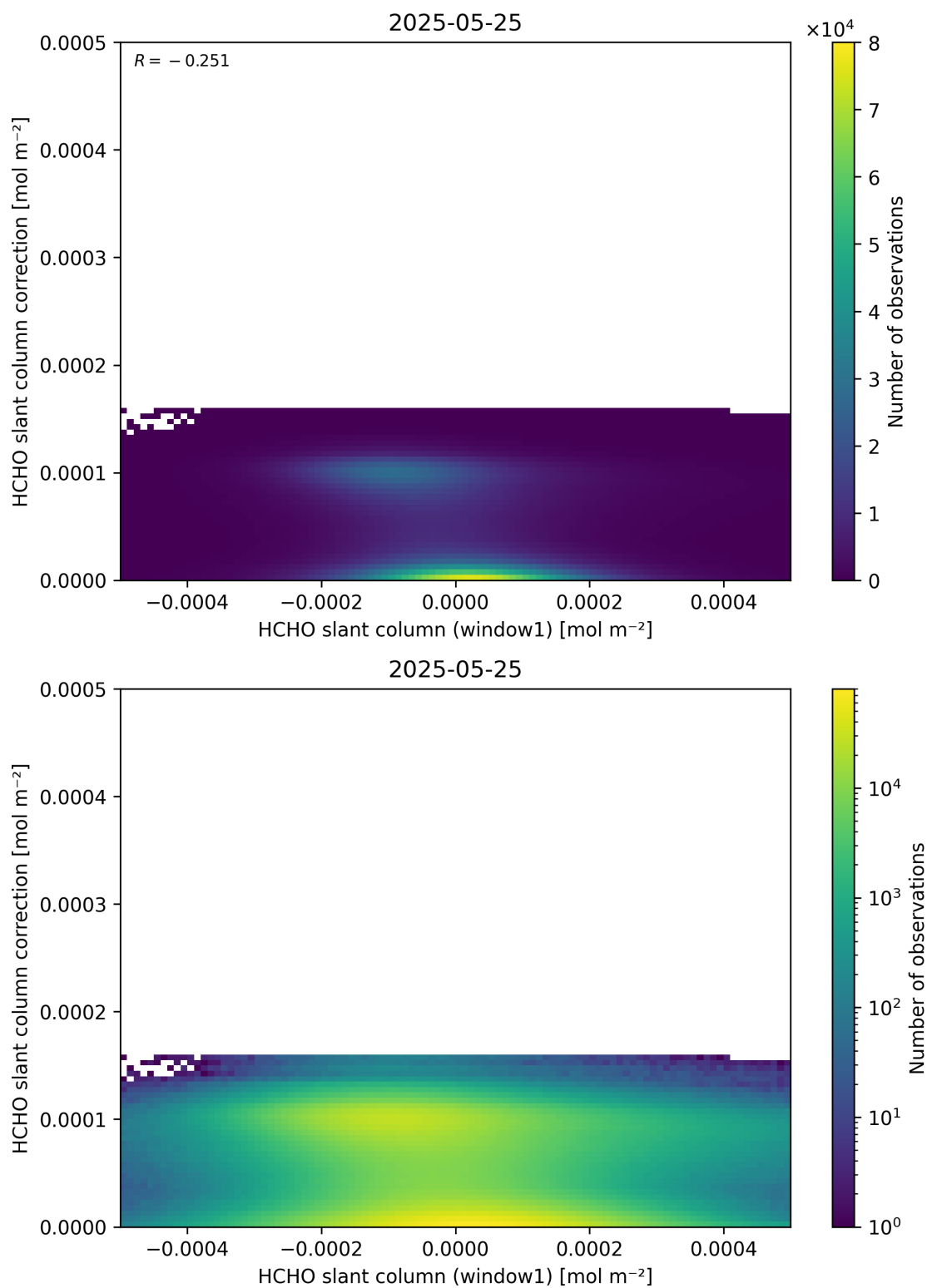
Figure 83: Scatter density plot of “HCHO slant column (window1)” against “HCHO slant column correction” for 2025-05-24 to 2025-05-26.
