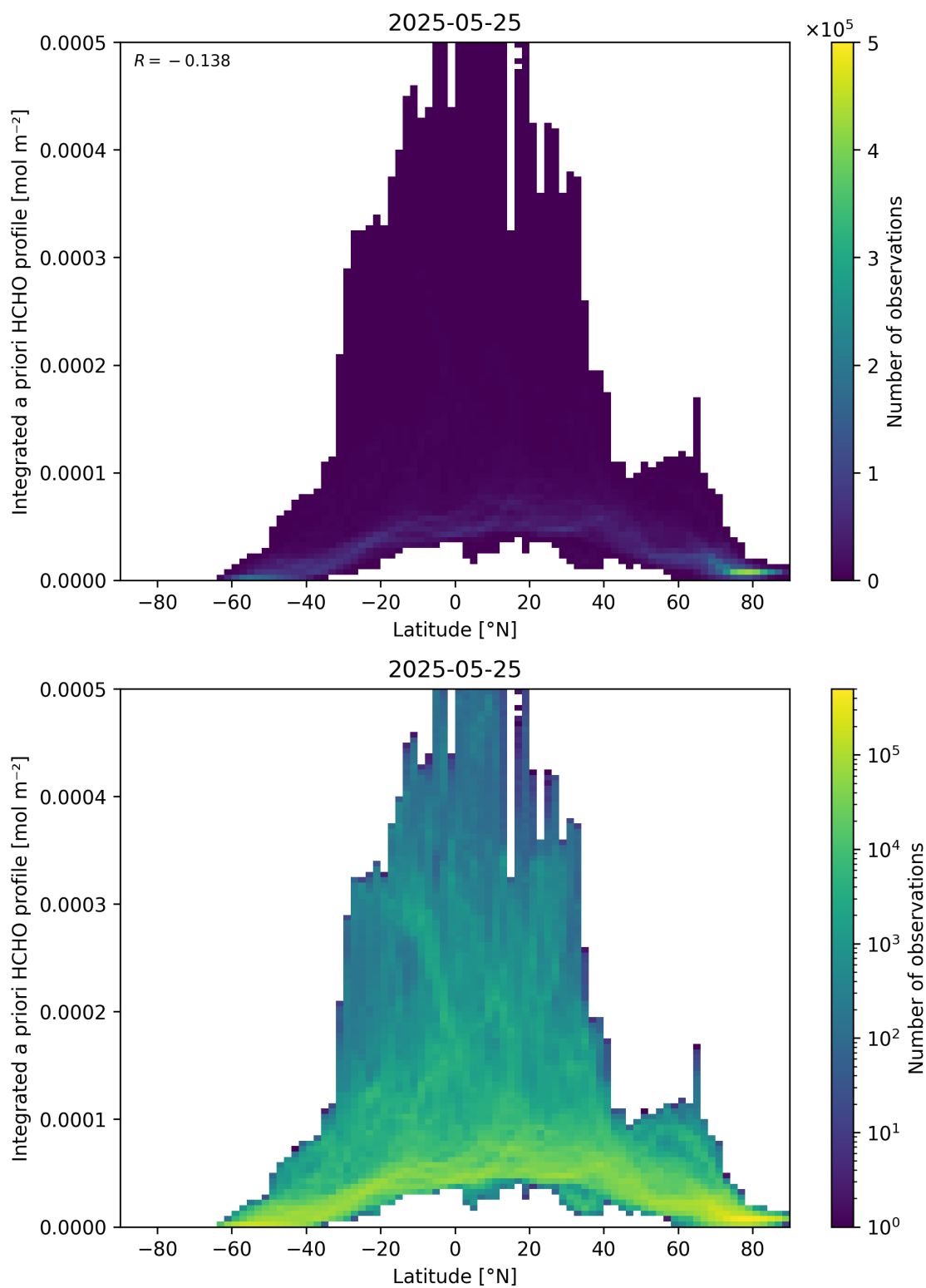
Figure 166: Scatter density plot of “Latitude” against “Integrated a priori HCHO profile” for 2025-05-24 to 2025-05-26.
