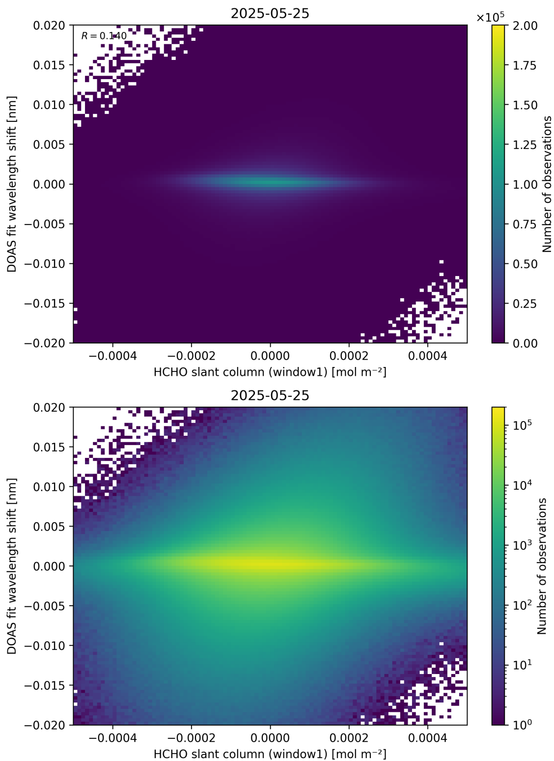
Figure 79: Scatter density plot of “HCHO slant column (window1)” against “DOAS fit wavelength shift” for 2025-05-24 to 2025-05-26.
