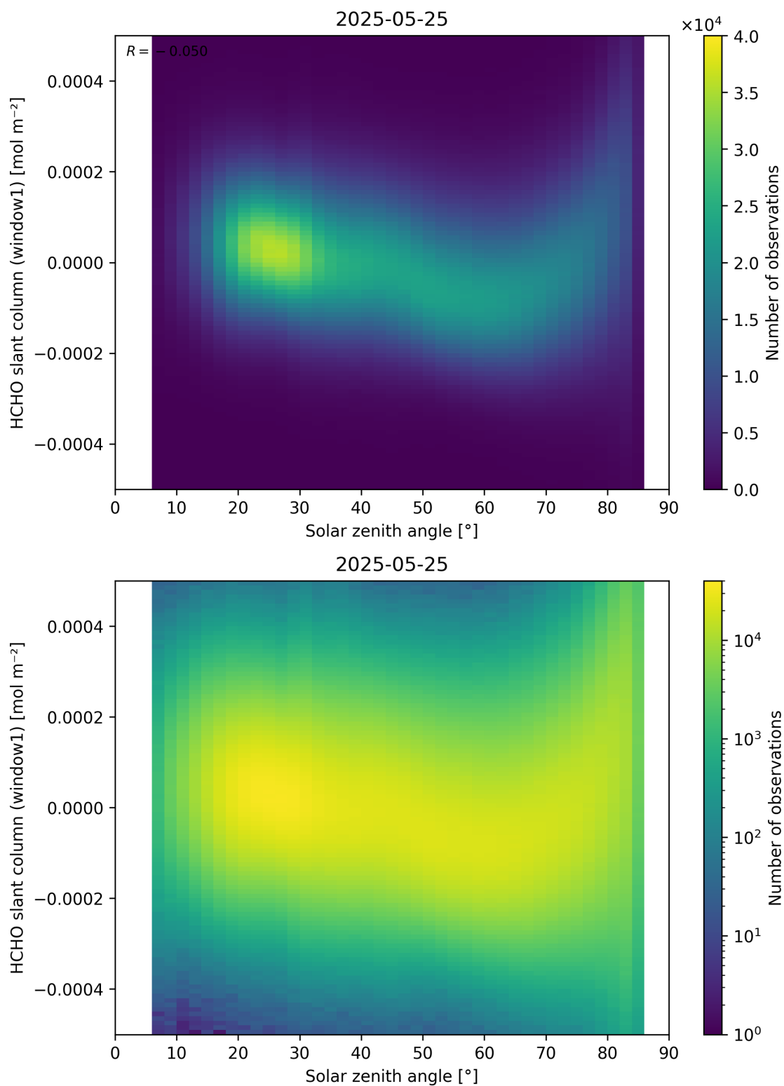
Figure 173: Scatter density plot of “Solar zenith angle” against “HCHO slant column (window1)” for 2025-05-24 to 2025-05-26.
