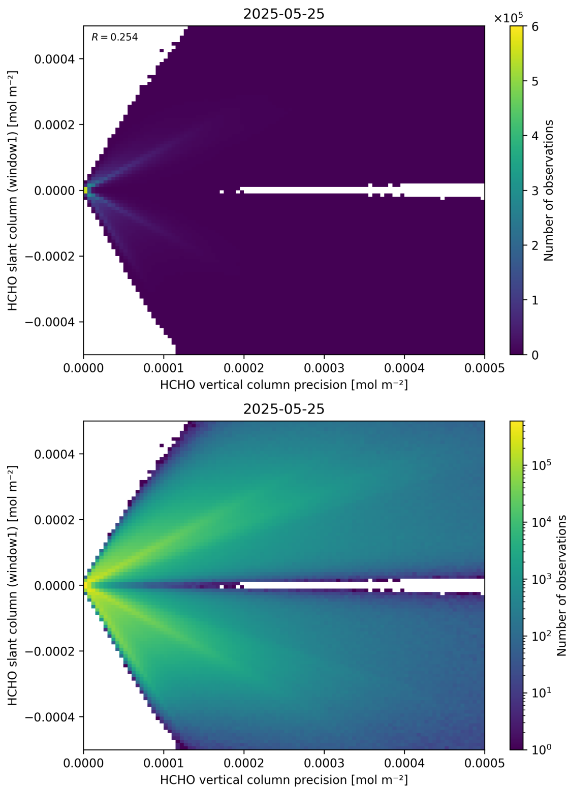
Figure 142: Scatter density plot of “HCHO vertical column precision” against “HCHO slant column (window1)” for 2025-05-24 to 2025-05-26.
