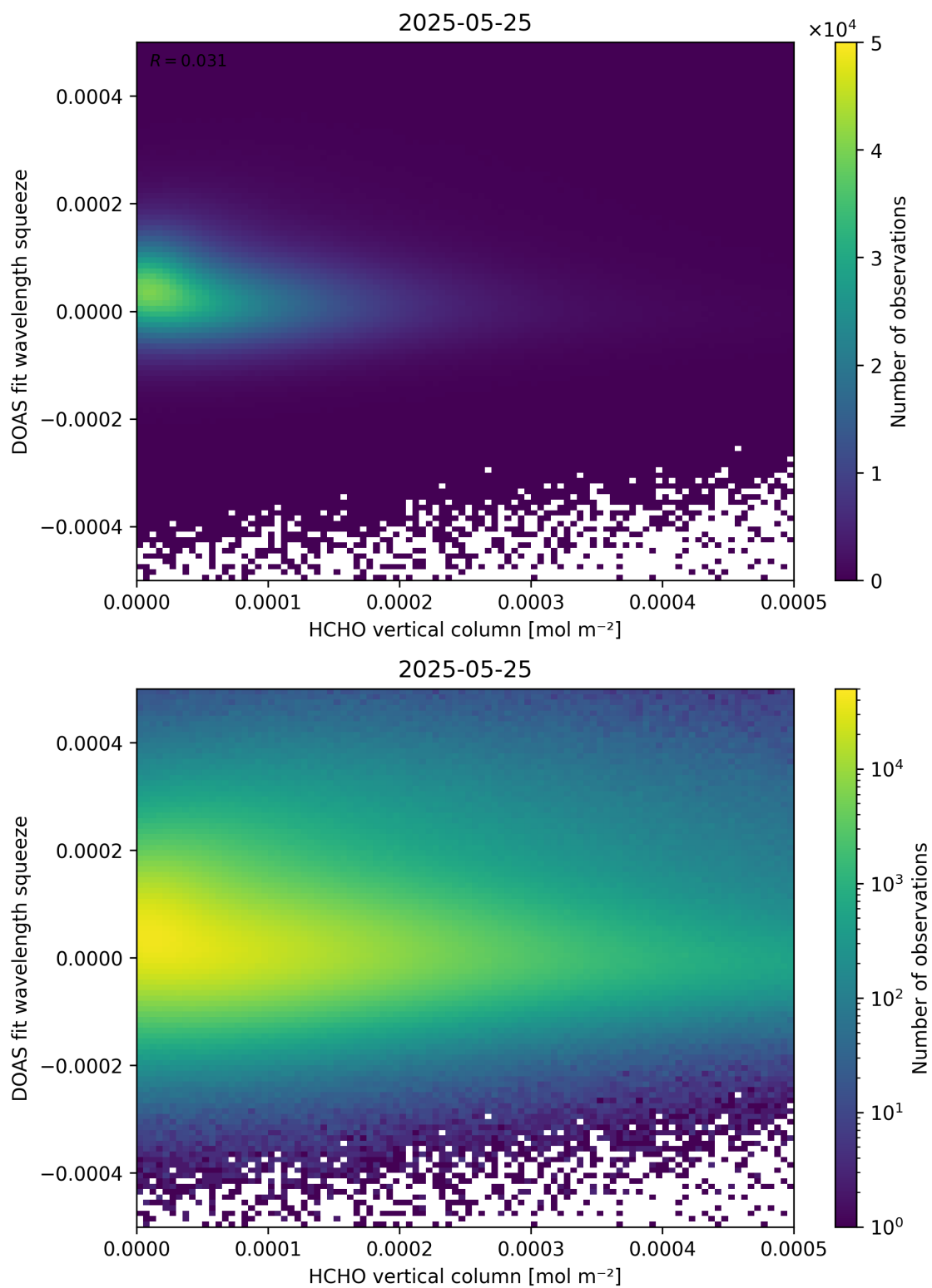
Figure 125: Scatter density plot of “HCHO vertical column” against “DOAS fit wavelength squeeze” for 2025-05-24 to 2025-05-26.
