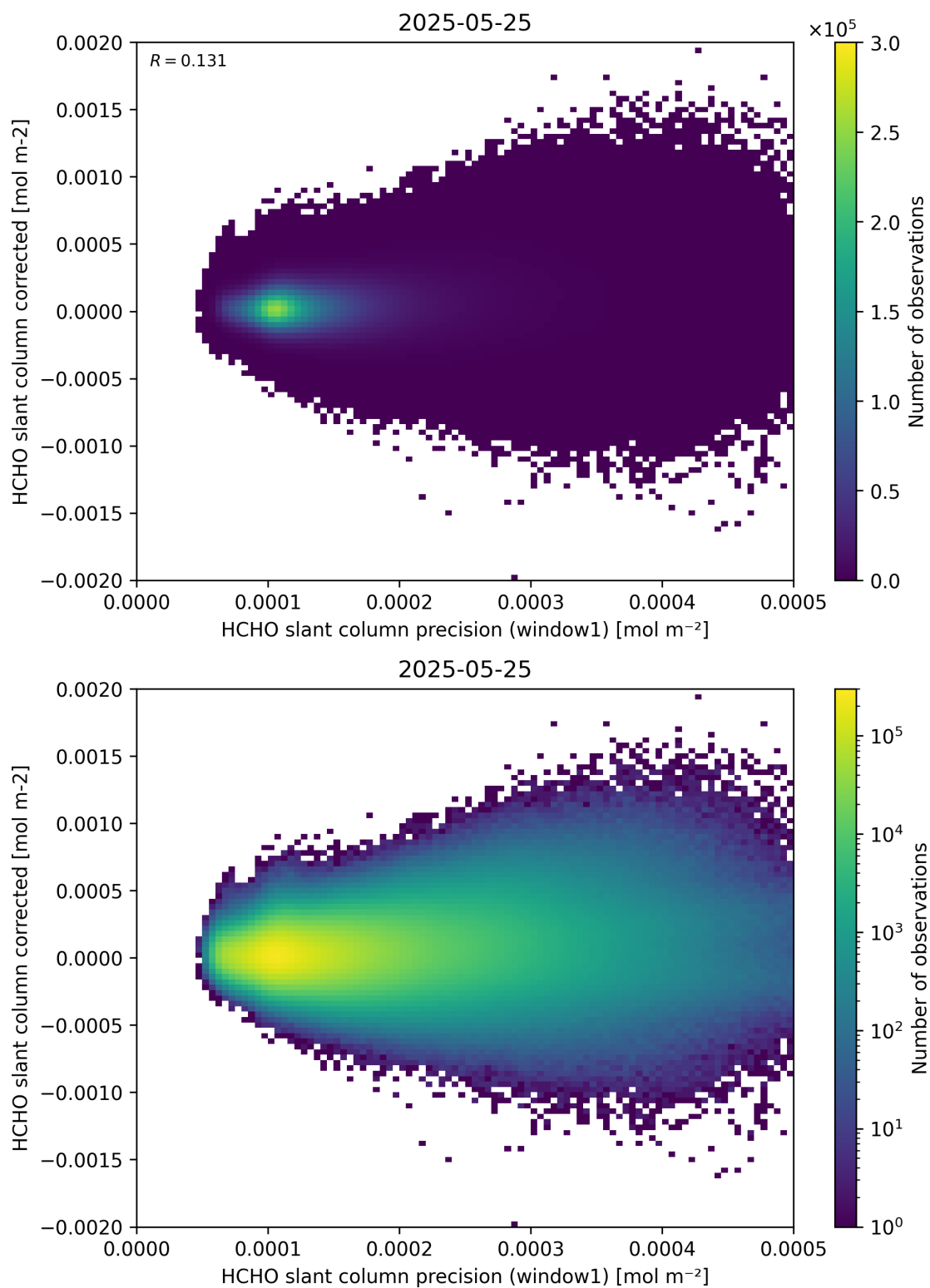
Figure 92: Scatter density plot of “HCHO slant column precision (window1)” against “HCHO slant column corrected” for 2025-05-24 to 2025-05-26.
