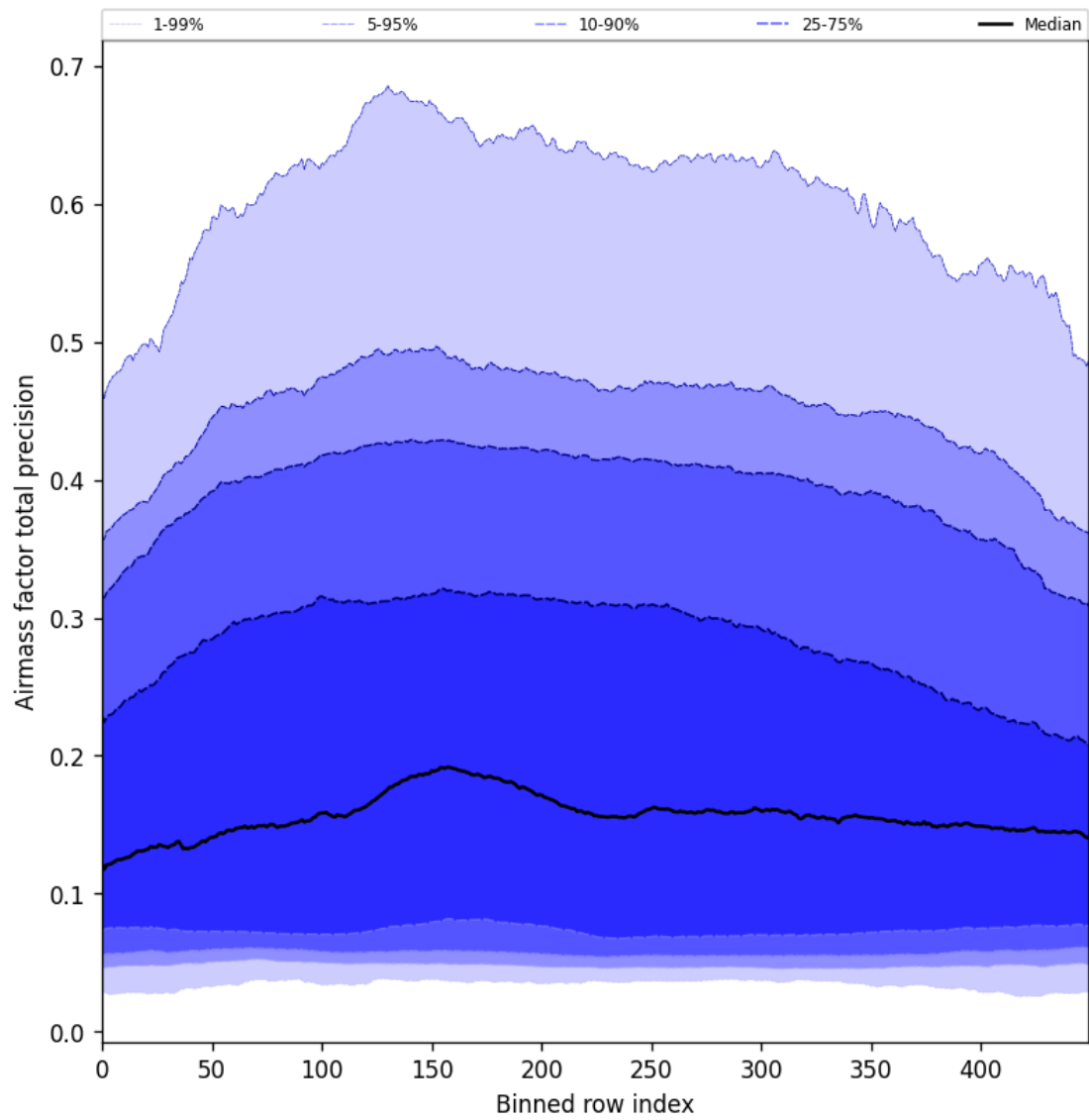
Figure 55: Along track statistics of “Airmass factor total precision” for 2025-05-24 to 2025-05-26
