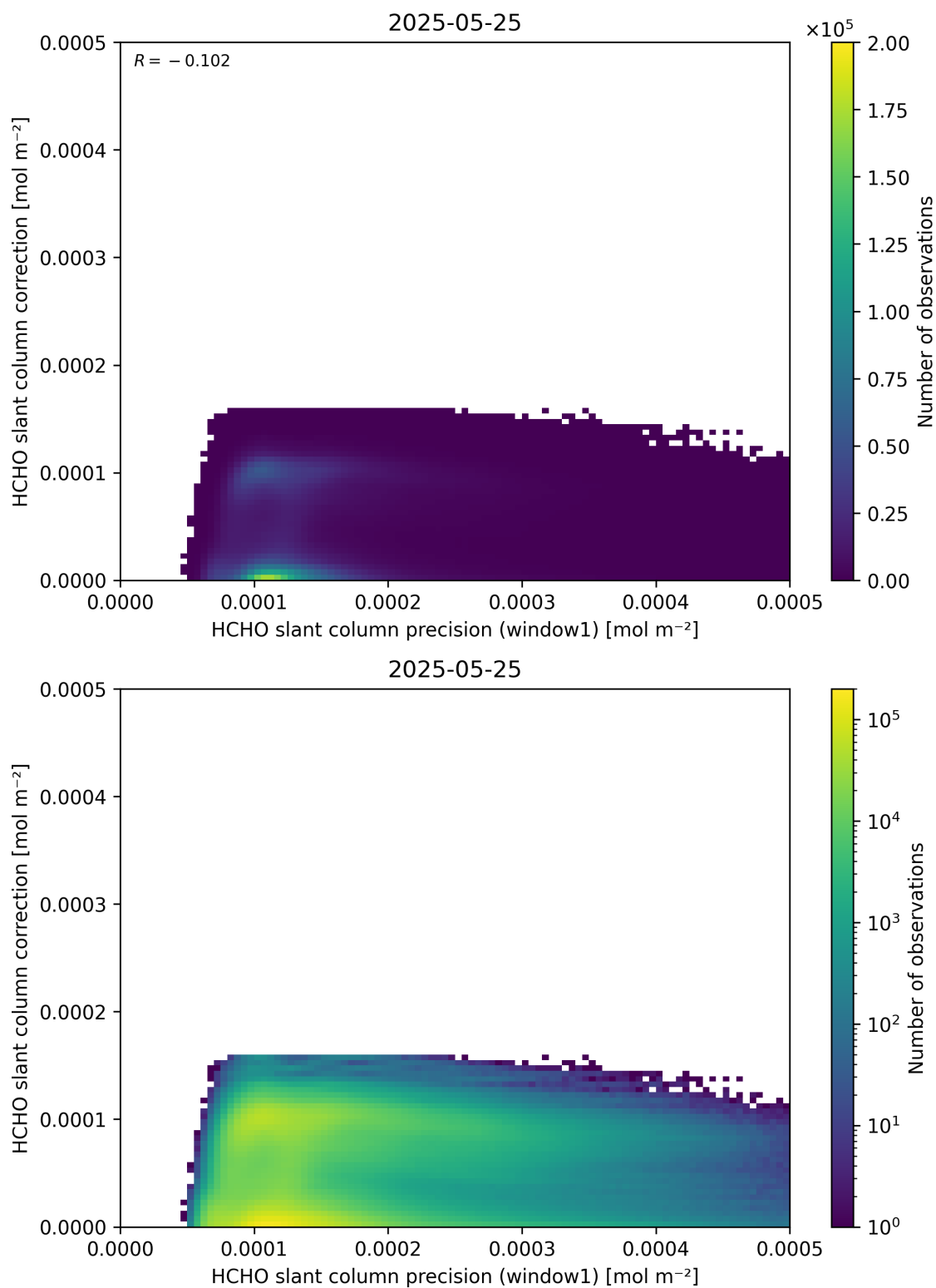
Figure 93: Scatter density plot of “HCHO slant column precision (window1)” against “HCHO slant column correction” for 2025-05-24 to 2025-05-26.
