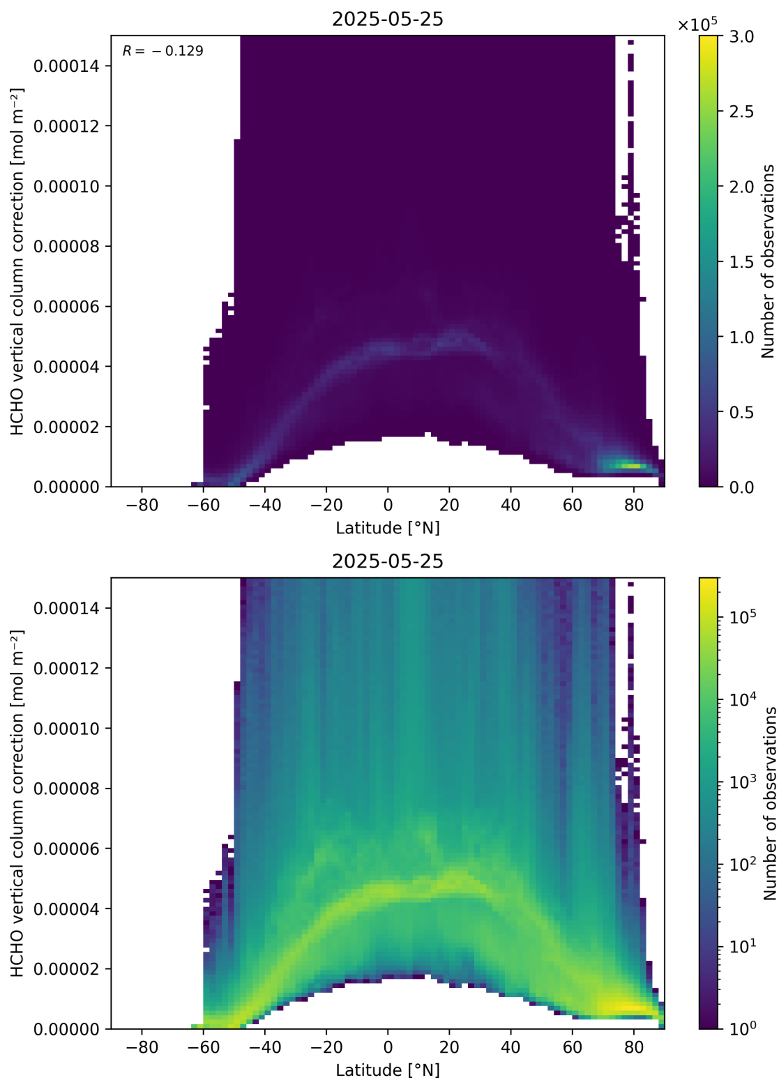
Figure 164: Scatter density plot of “Latitude” against “HCHO vertical column correction” for 2025-05-24 to 2025-05-26.
