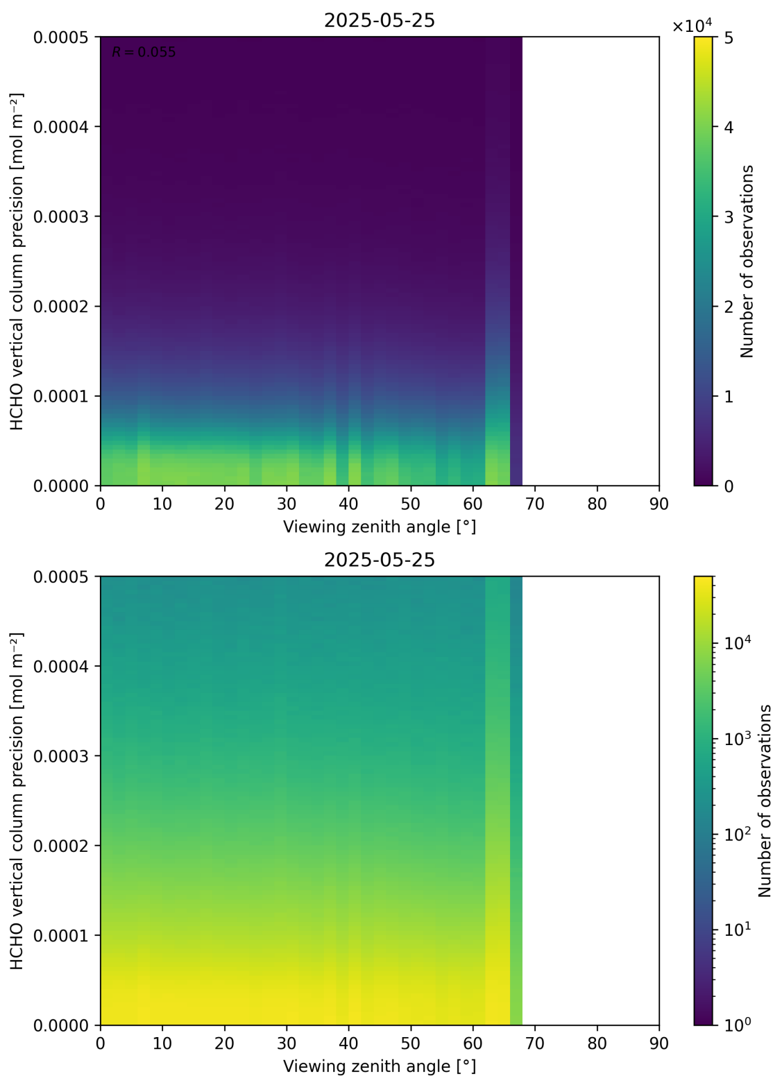
Figure 194: Scatter density plot of “Viewing zenith angle” against “HCHO vertical column precision” for 2025-05-24 to 2025-05-26.
