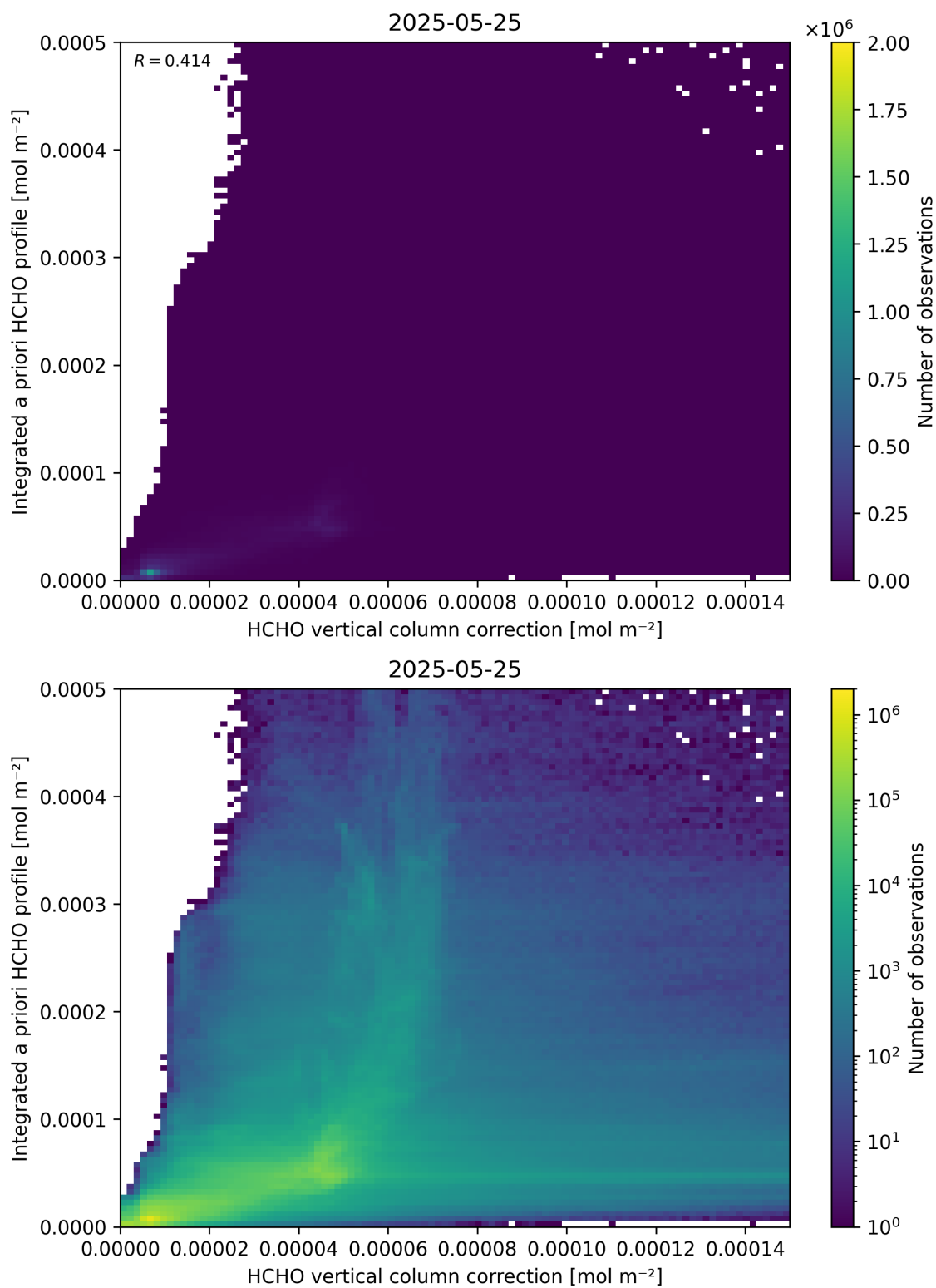
Figure 122: Scatter density plot of “HCHO vertical column correction” against “Integrated a priori HCHO profile” for 2025-05-24 to 2025-05-26.
