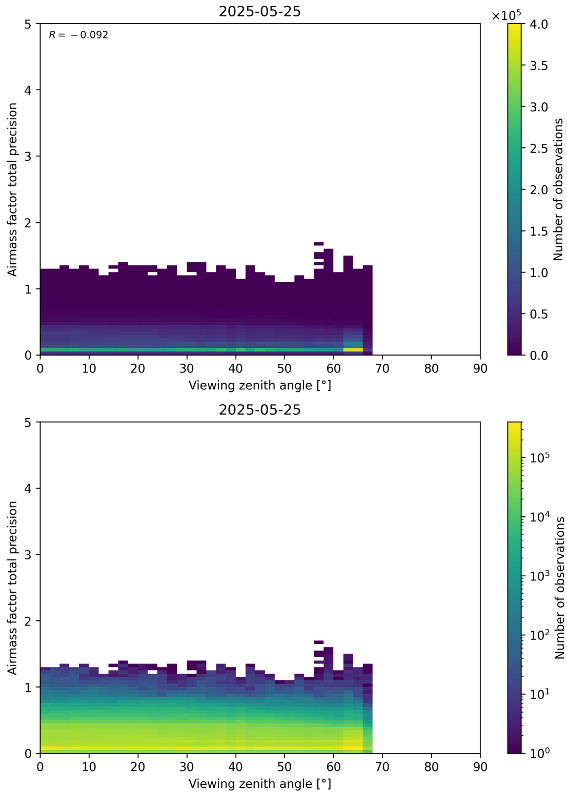
Figure 191: Scatter density plot of “Viewing zenith angle” against “Airmass factor total precision” for 2025-05-24 to 2025-05-26.
