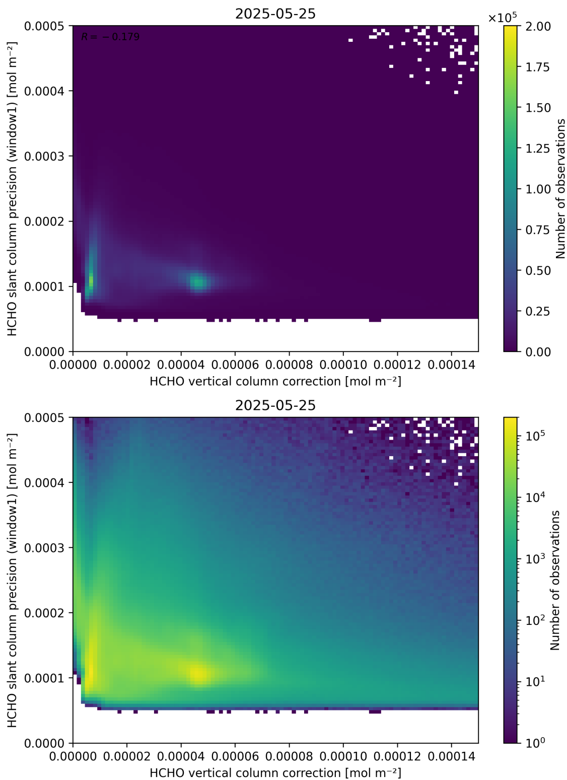
Figure 119: Scatter density plot of “HCHO vertical column correction” against “HCHO slant column precision (window1)” for 2025-05-24 to 2025-05-26.
