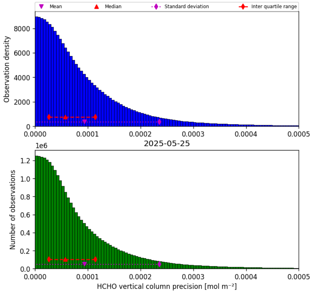
Figure 36: Histogram of “HCHO vertical column precision” for 2025-05-24 to 2025-05-26
