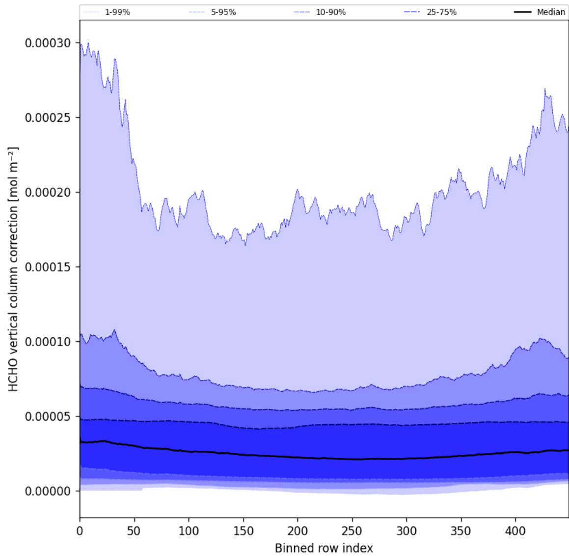
Figure 51: Along track statistics of “HCHO vertical column correction” for 2025-05-24 to 2025-05-26
