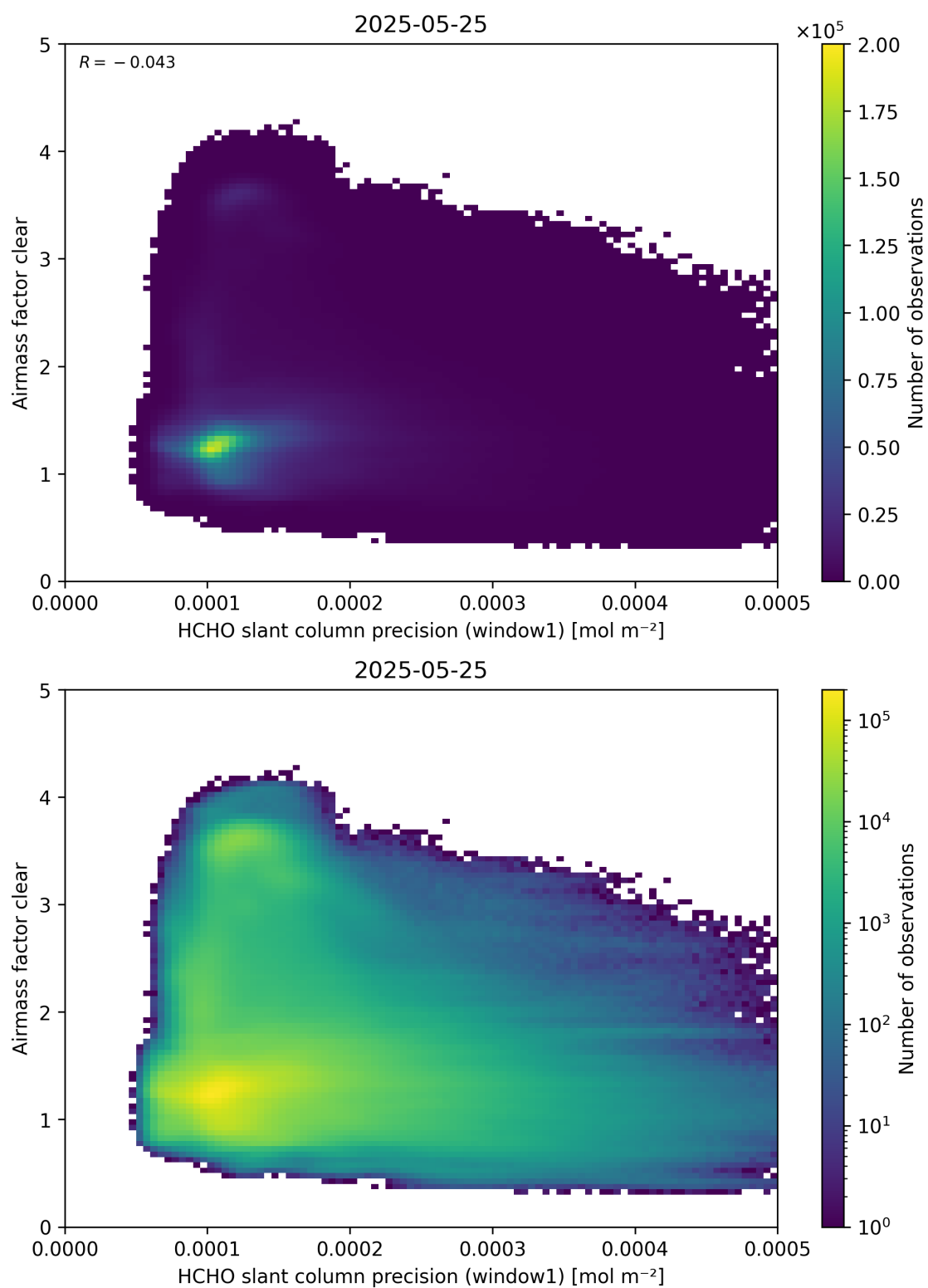
Figure 91: Scatter density plot of “HCHO slant column precision (window1)” against “Airmass factor clear” for 2025-05-24 to 2025-05-26.
