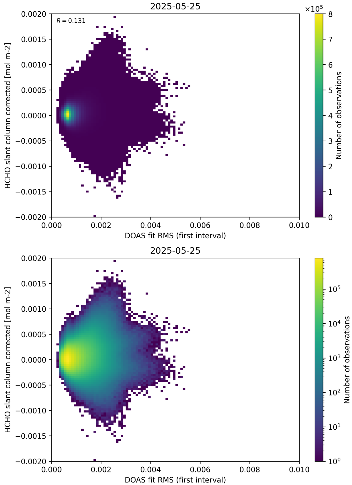
Figure 62: Scatter density plot of “DOAS fit RMS (first interval)” against “HCHO slant column corrected” for 2025-05-24 to 2025-05-26.
