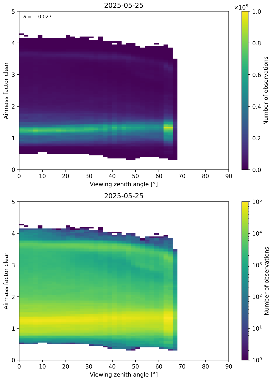
Figure 185: Scatter density plot of “Viewing zenith angle” against “Airmass factor clear” for 2025-05-24 to 2025-05-26.
