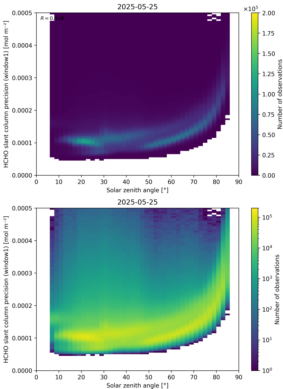
Figure 174: Scatter density plot of “Solar zenith angle” against “HCHO slant column precision (window1)” for 2025-05-24 to 2025-05-26.
