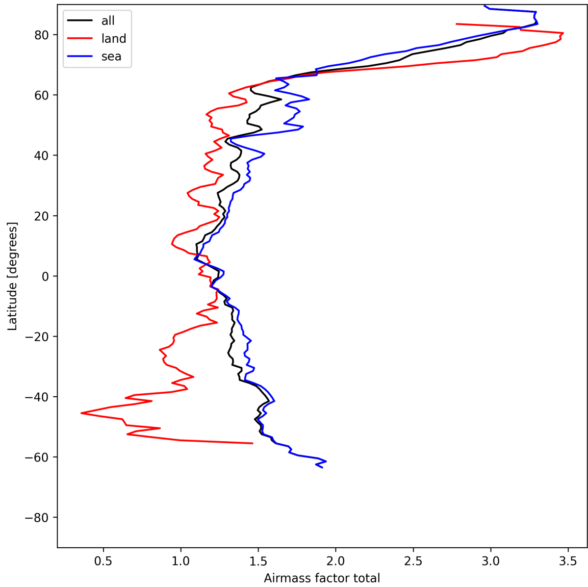
Figure 26: Zonal average of “Airmass factor total” for 2025-05-24 to 2025-05-26.
