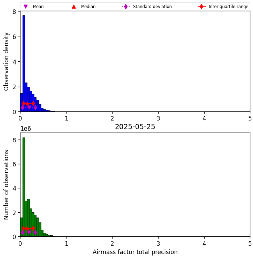
Figure 41: Histogram of “Airmass factor total precision” for 2025-05-24 to 2025-05-26
