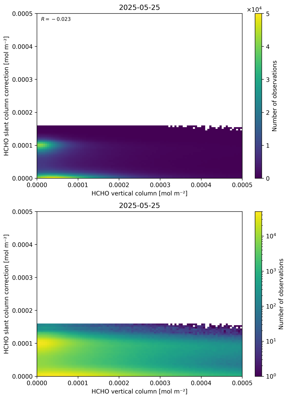
Figure 128: Scatter density plot of “HCHO vertical column” against “HCHO slant column correction” for 2025-05-24 to 2025-05-26.
