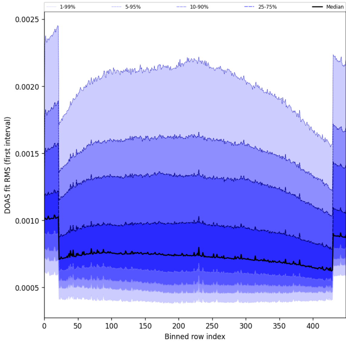
Figure 60: Along track statistics of “DOAS fit RMS (first interval)” for 2025-05-24 to 2025-05-26
