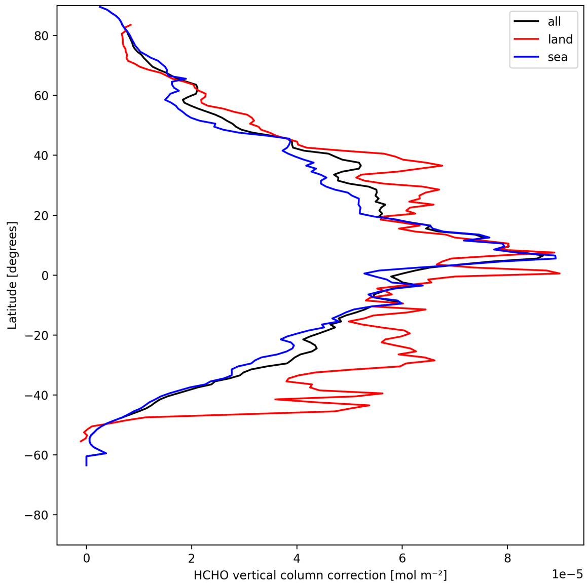
Figure 23: Zonal average of “HCHO vertical column correction” for 2025-05-24 to 2025-05-26.
