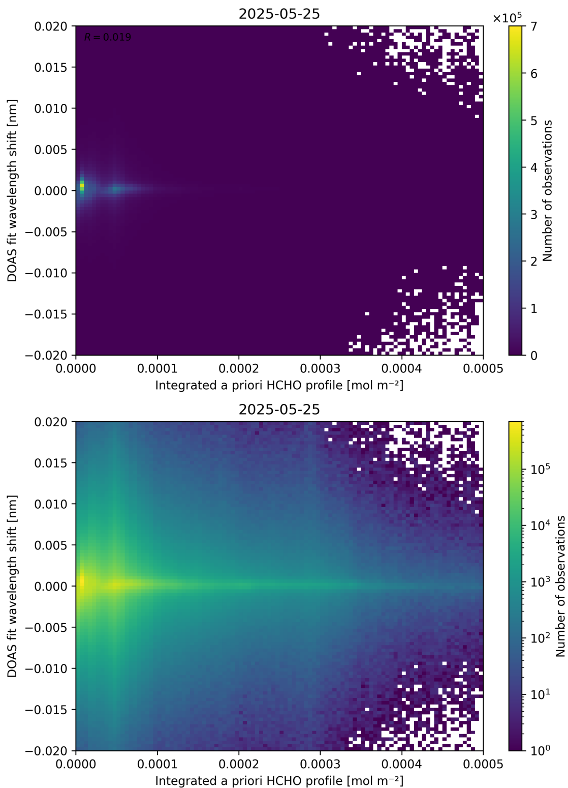
Figure 149: Scatter density plot of “Integrated a priori HCHO profile” against “DOAS fit wavelength shift” for 2025-05-24 to 2025-05-26.
