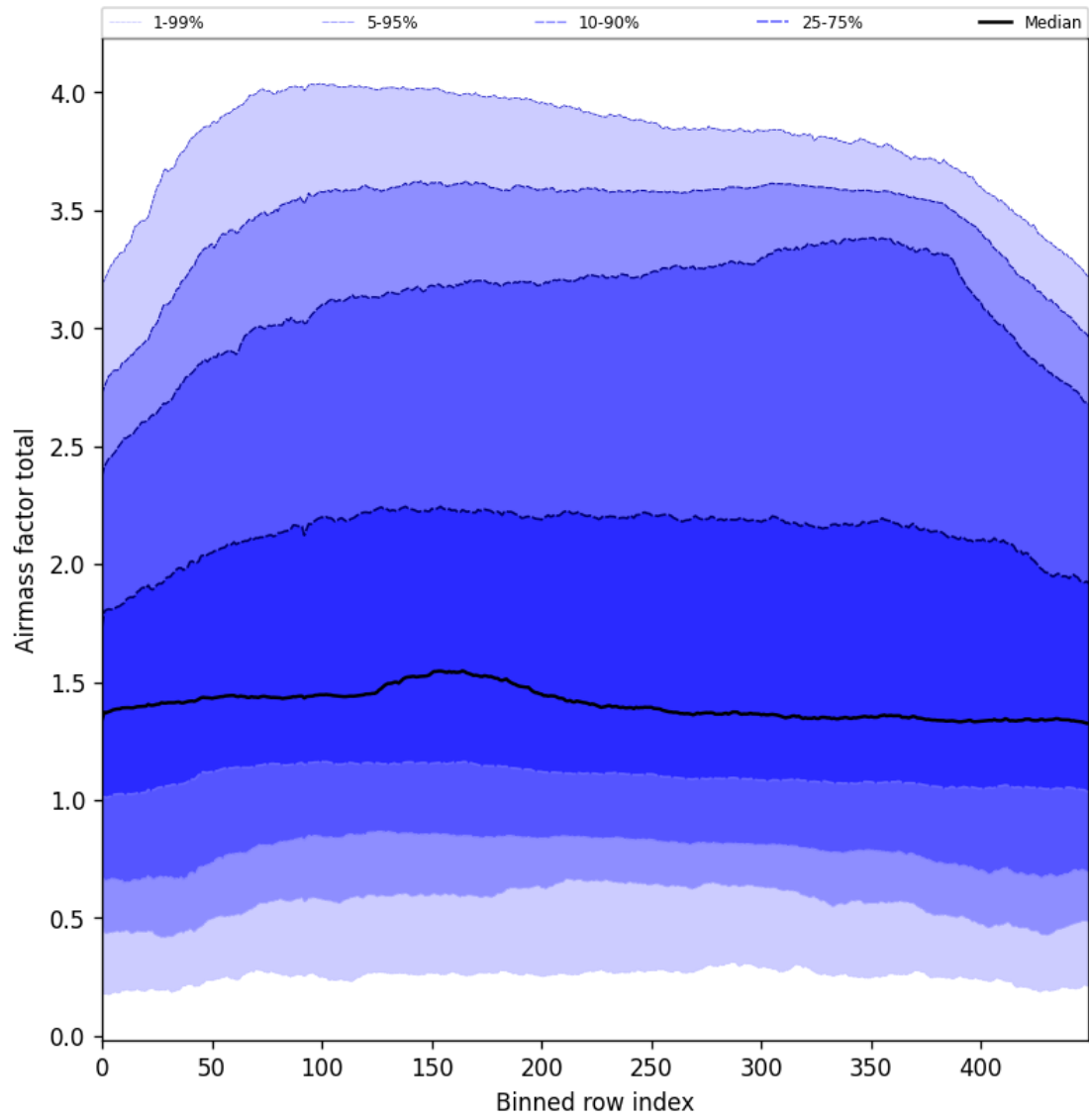
Figure 54: Along track statistics of “Airmass factor total” for 2025-05-24 to 2025-05-26
