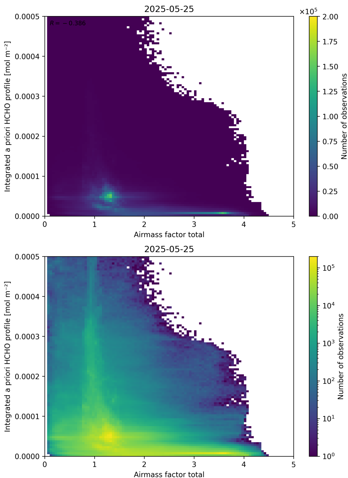
Figure 104: Scatter density plot of “Airmass factor total” against “Integrated a priori HCHO profile” for 2025-05-24 to 2025-05-26.
