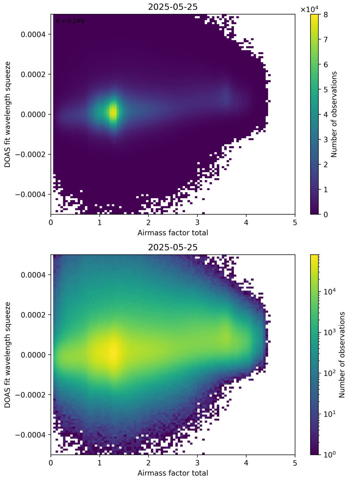
Figure 99: Scatter density plot of “Airmass factor total” against “DOAS fit wavelength squeeze” for 2025-05-24 to 2025-05-26.
