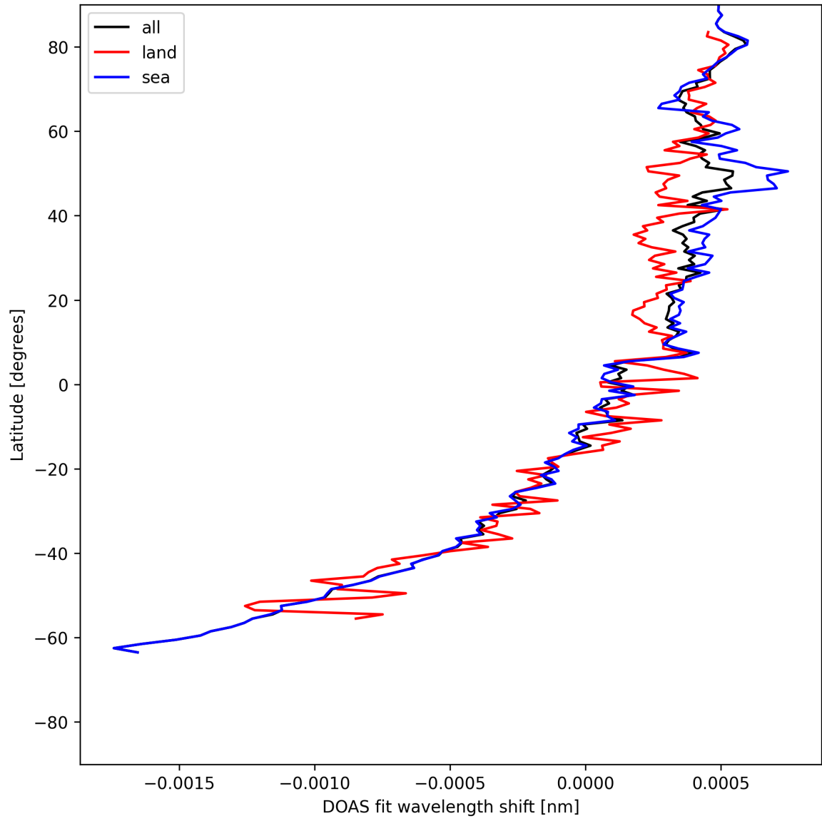
Figure 30: Zonal average of “DOAS fit wavelength shift” for 2025-05-24 to 2025-05-26.
