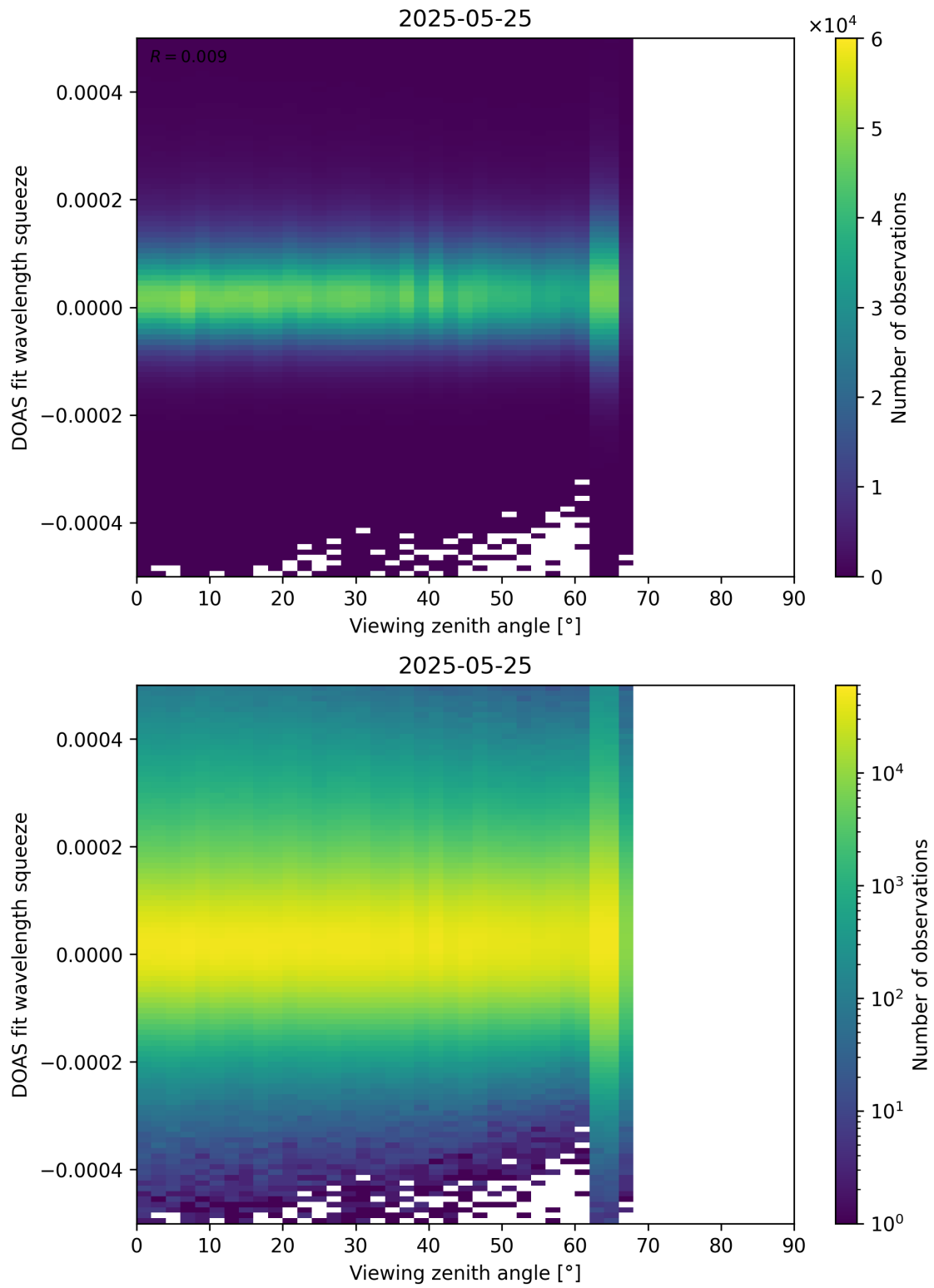
Figure 184: Scatter density plot of “Viewing zenith angle” against “DOAS fit wavelength squeeze” for 2025-05-24 to 2025-05-26.
