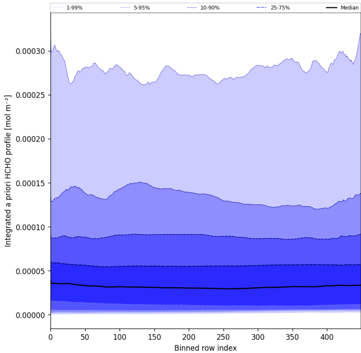
Figure 57: Along track statistics of "Integrated a priori HCHO profile" for 2025-05-24 to 2025-05-26
