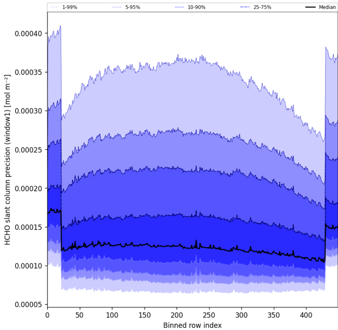
Figure 53: Along track statistics of “HCHO slant column precision (window1)” for 2025-05-24 to 2025-05-26
