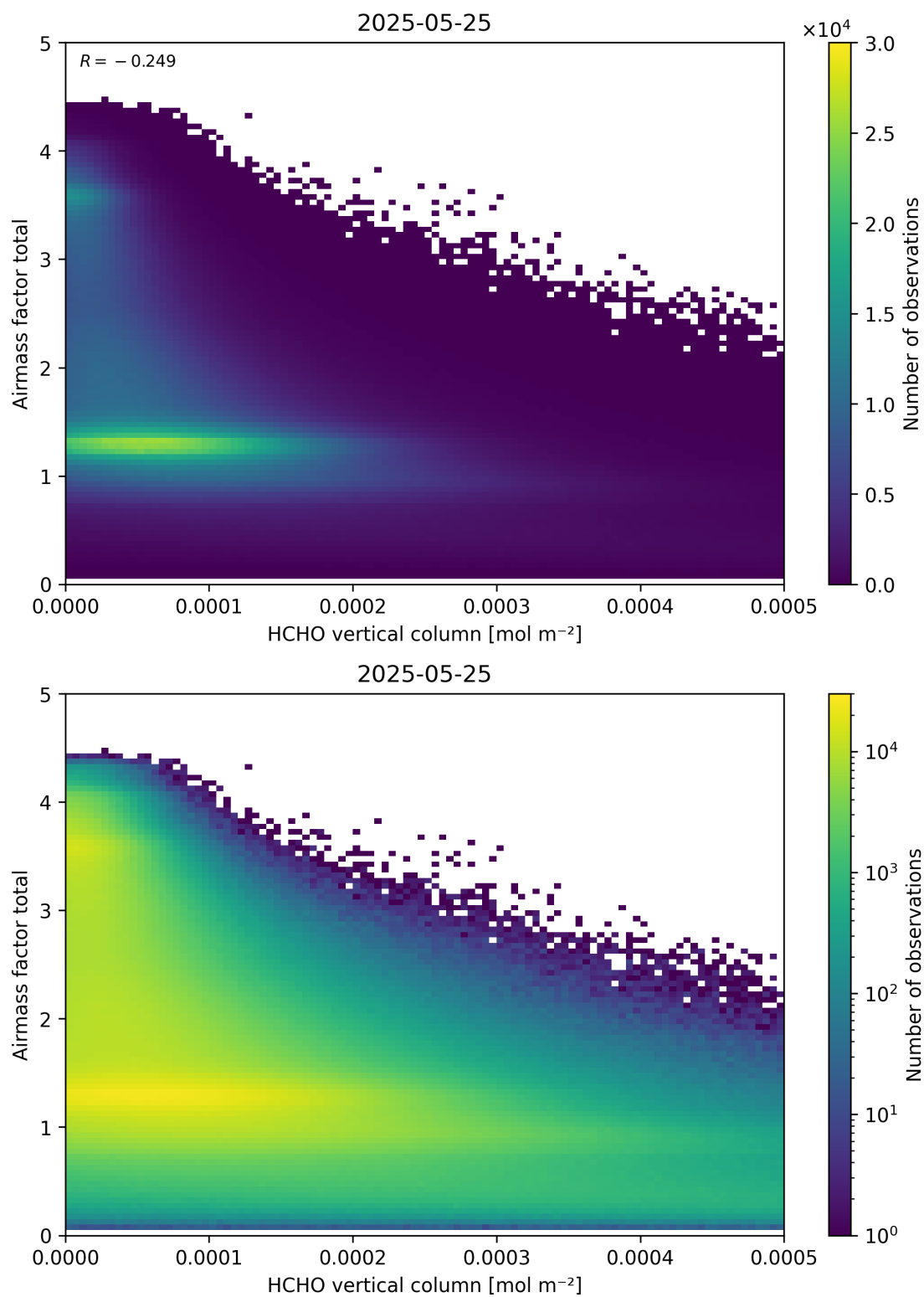
Figure 131: Scatter density plot of “HCHO vertical column” against “Airmass factor total” for 2025-05-24 to 2025-05-26.
