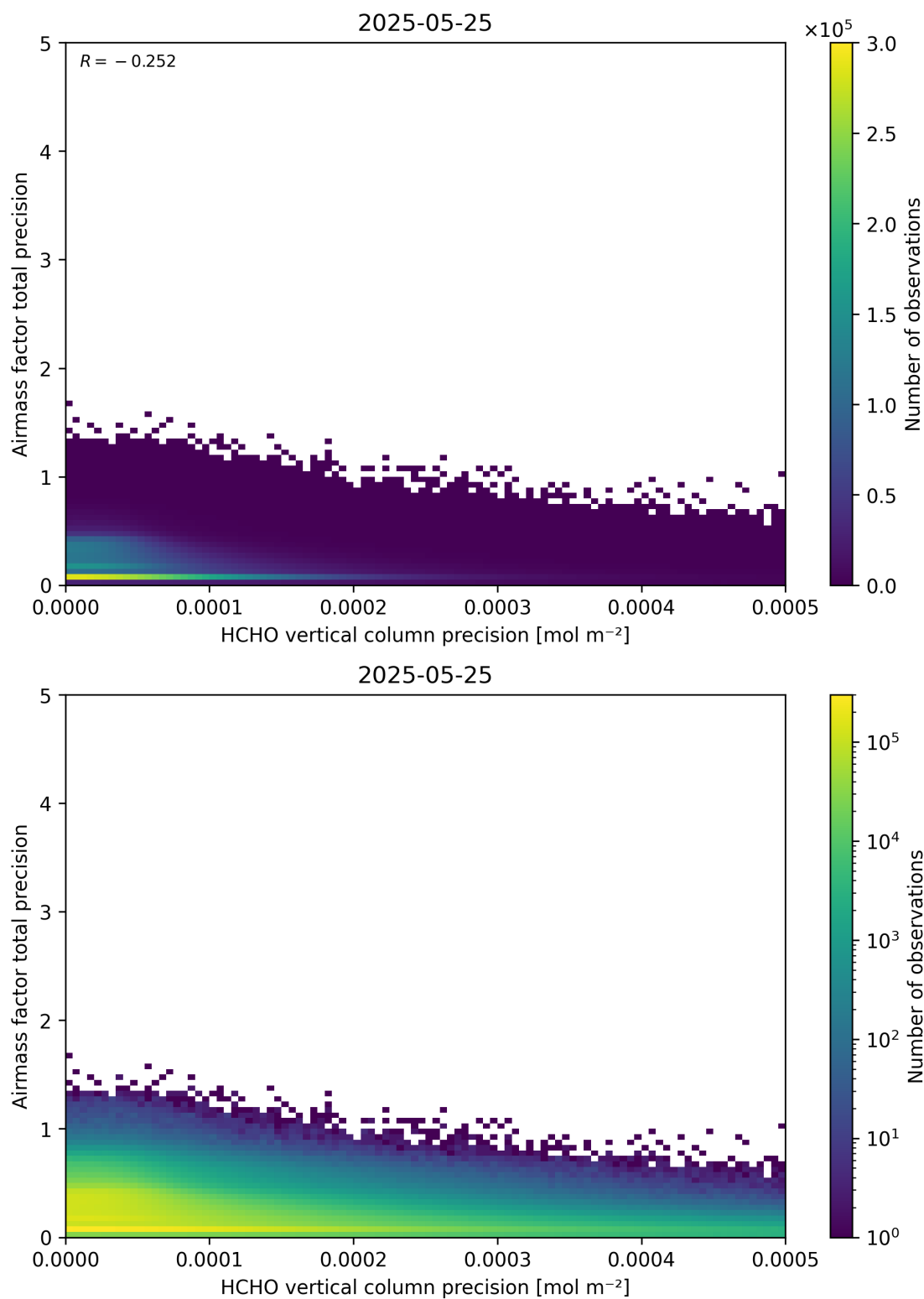
Figure 145: Scatter density plot of “HCHO vertical column precision” against “Airmass factor total precision” for 2025-05-24 to 2025-05-26.
