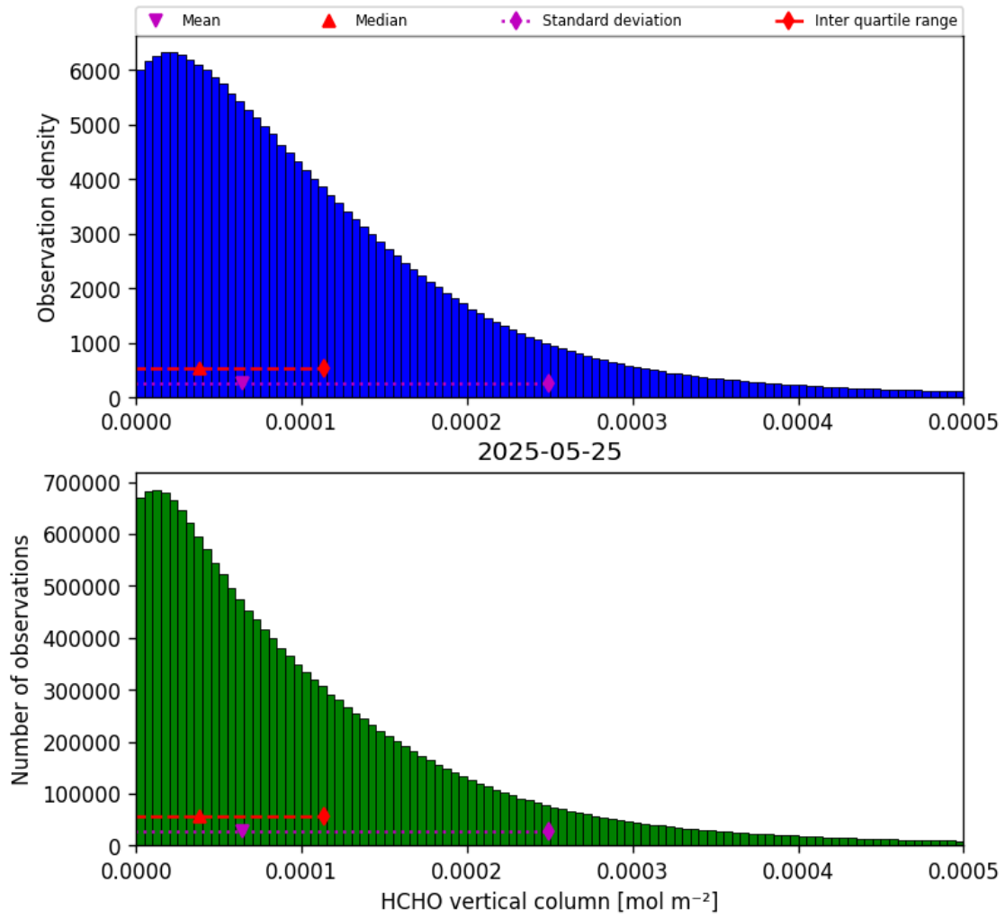
Figure 35: Histogram of “HCHO vertical column” for 2025-05-24 to 2025-05-26
