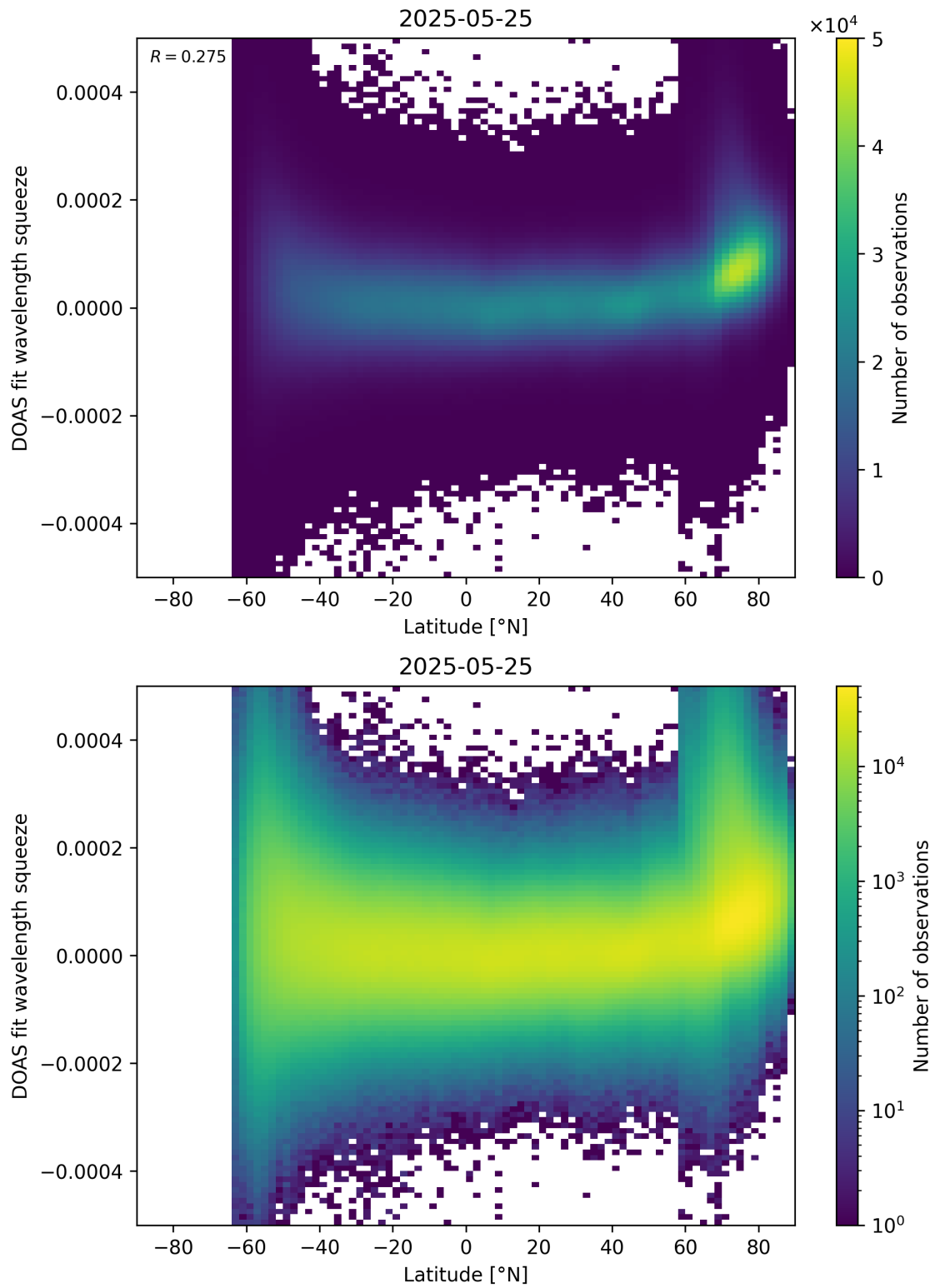
Figure 155: Scatter density plot of “Latitude” against “DOAS fit wavelength squeeze” for 2025-05-24 to 2025-05-26.
