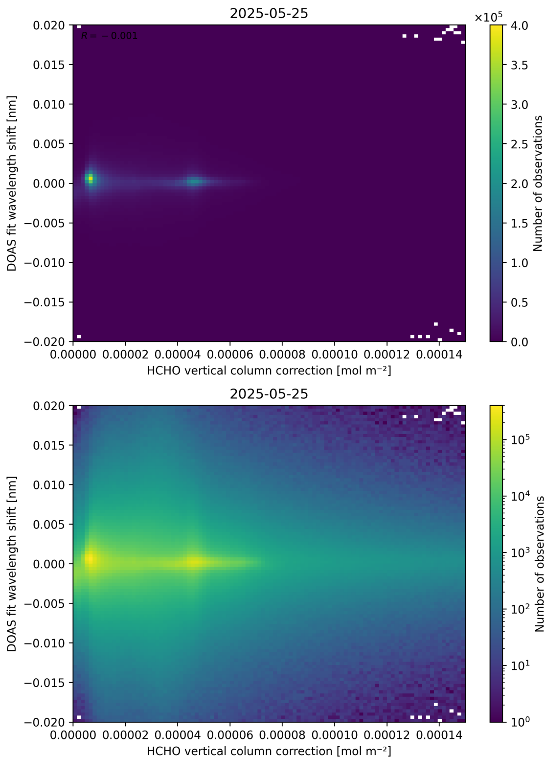
Figure 113: Scatter density plot of “HCHO vertical column correction” against “DOAS fit wavelength shift” for 2025-05-24 to 2025-05-26.
