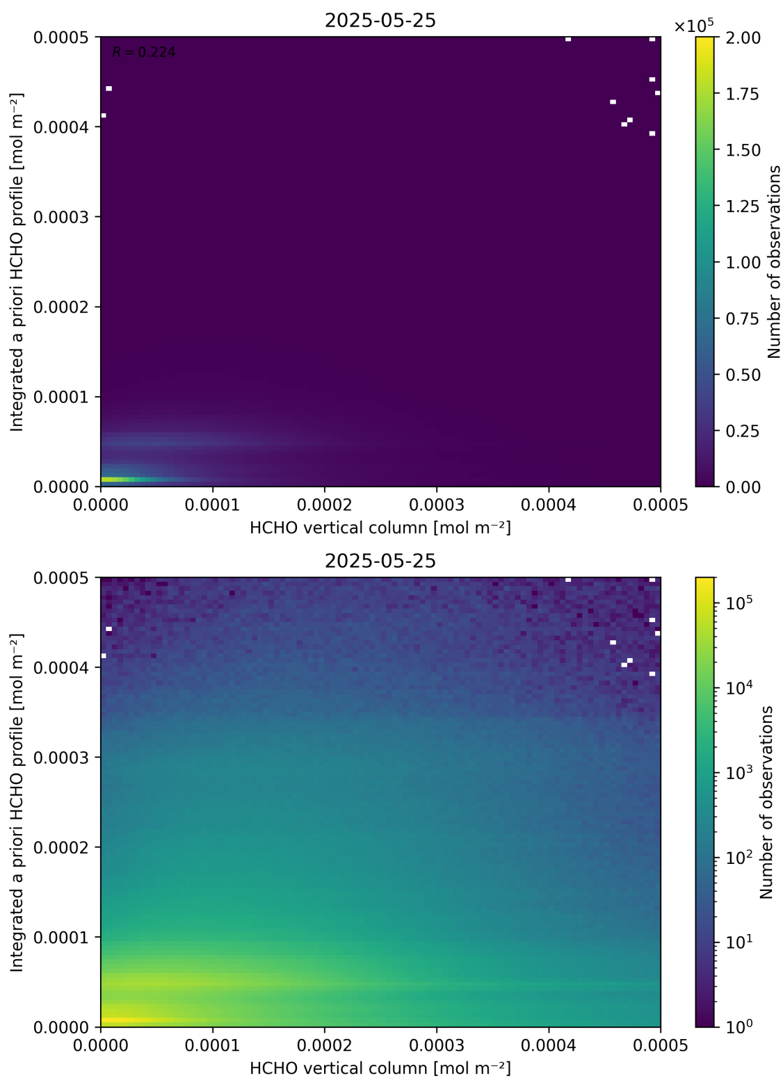
Figure 135: Scatter density plot of “HCHO vertical column” against “Integrated a priori HCHO profile” for 2025-05-24 to 2025-05-26.
