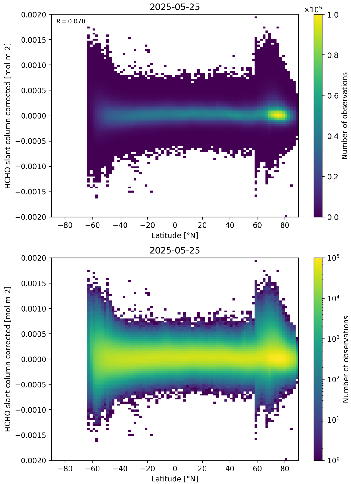
Figure 157: Scatter density plot of “Latitude” against “HCHO slant column corrected” for 2025-05-24 to 2025-05-26.
