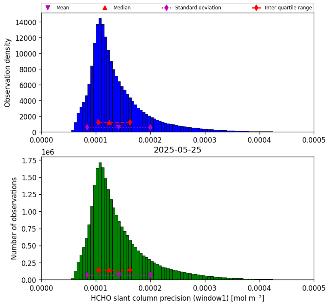
Figure 39: Histogram of “HCHO slant column precision (window1)” for 2025-05-24 to 2025-05-26
