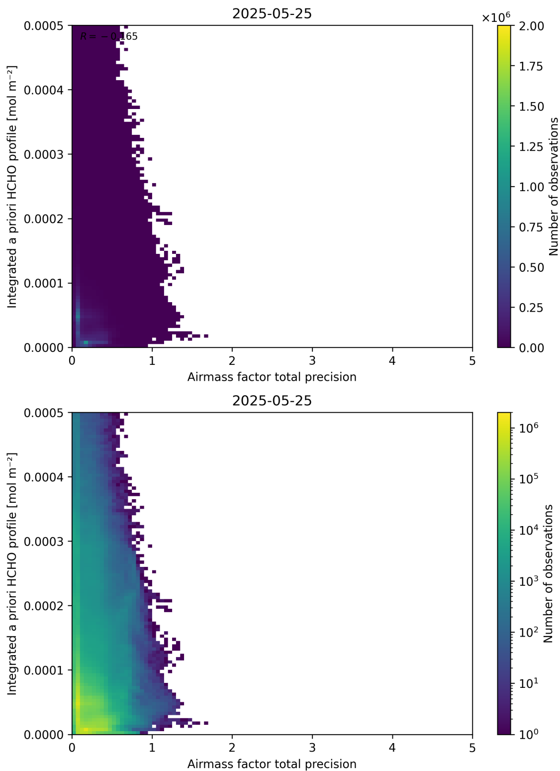
Figure 111: Scatter density plot of “Airmass factor total precision” against “Integrated a priori HCHO profile” for 2025-05-24 to 2025-05-26.
