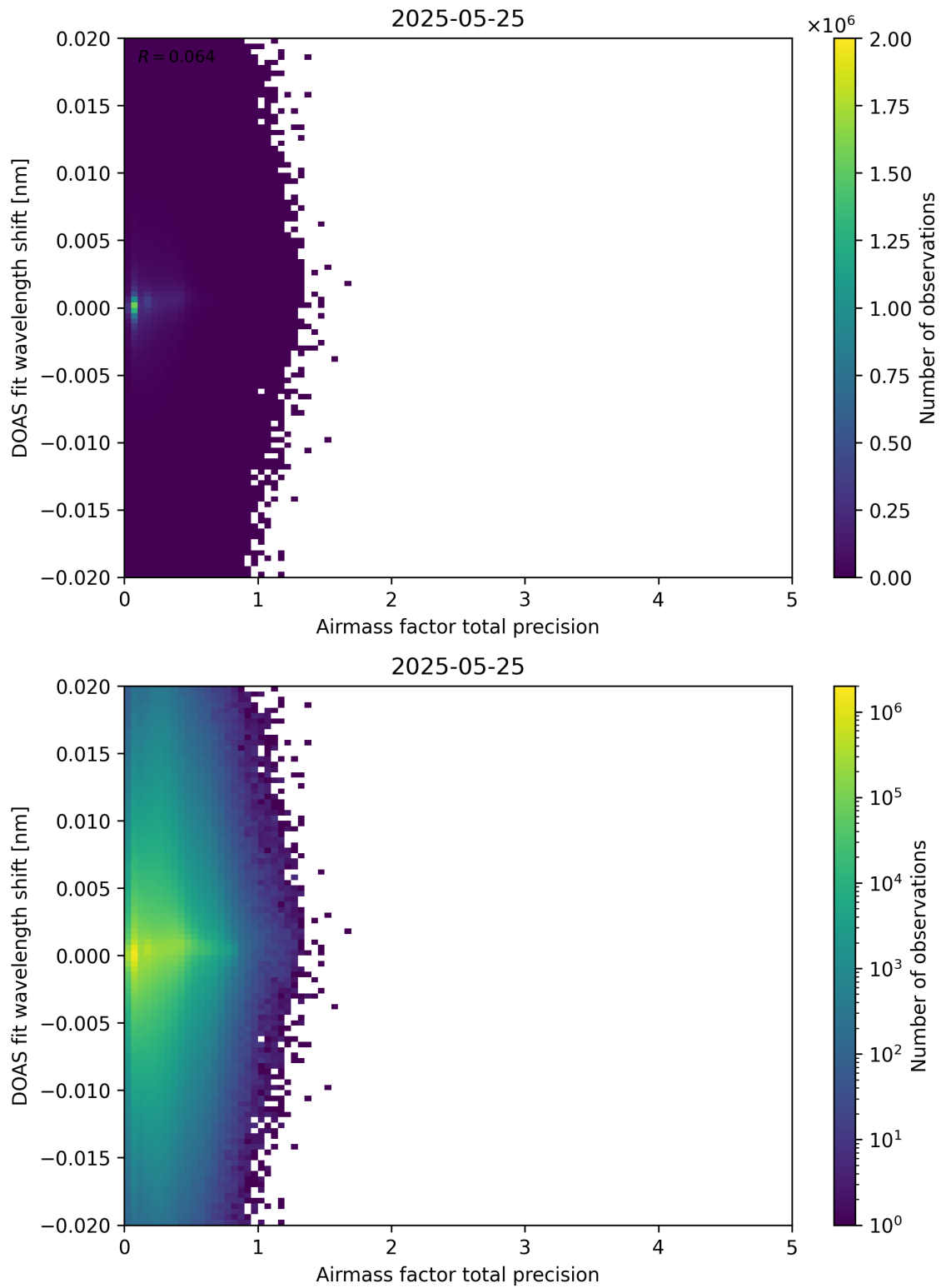
Figure 106: Scatter density plot of “Airmass factor total precision” against “DOAS fit wavelength shift” for 2025-05-24 to 2025-05-26.
