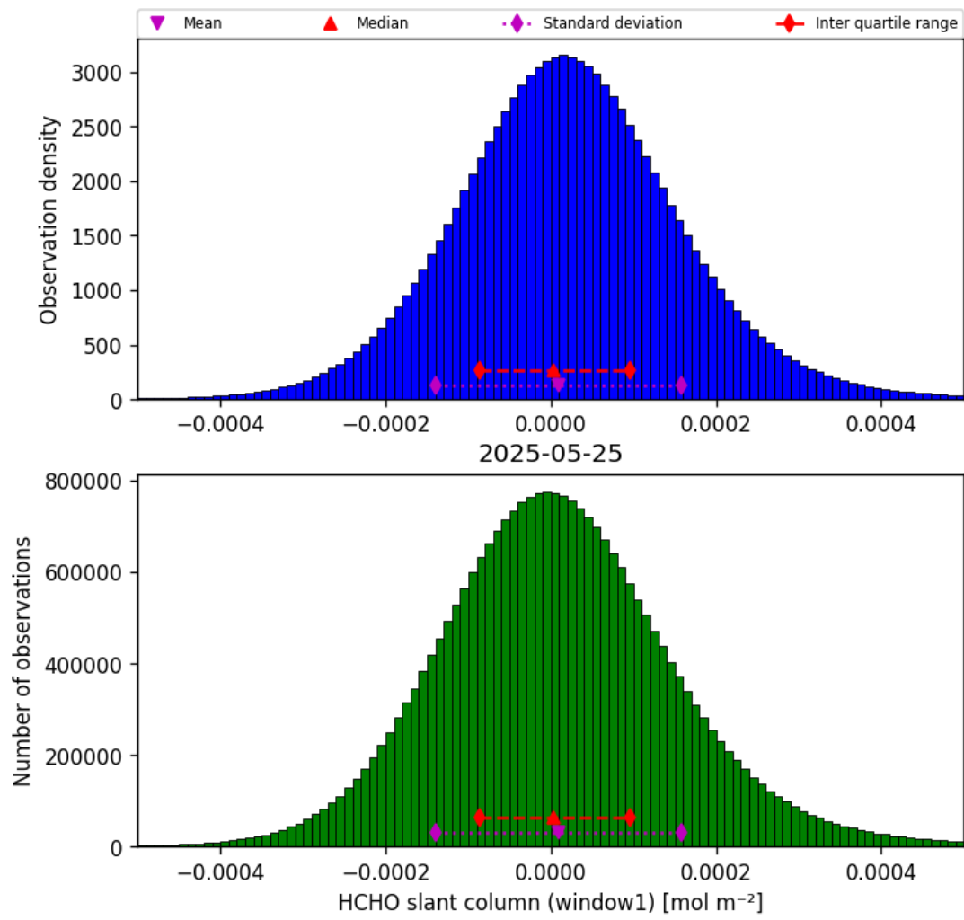
Figure 38: Histogram of “HCHO slant column (window1)” for 2025-05-24 to 2025-05-26
