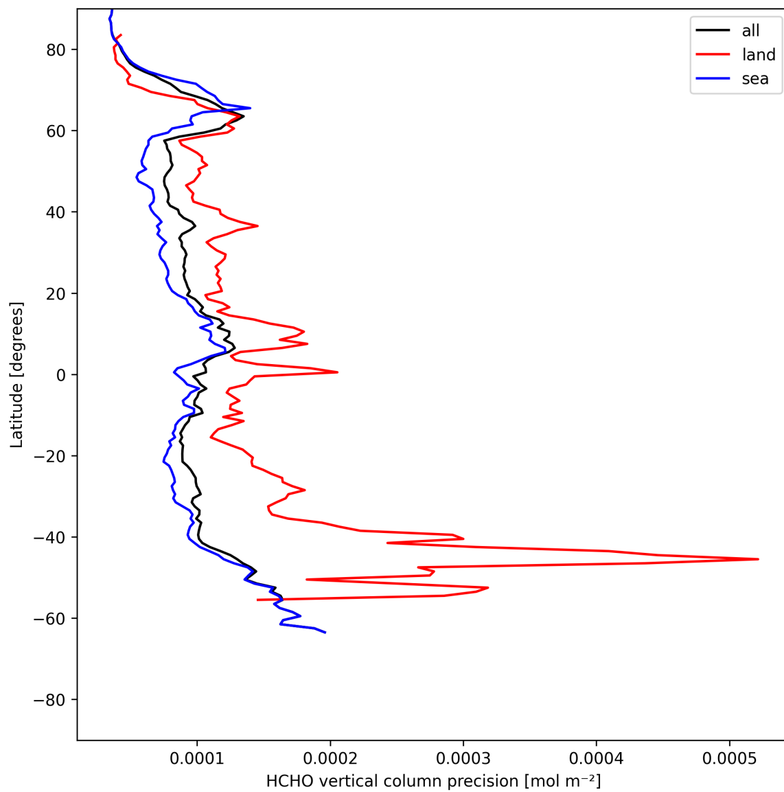
Figure 22: Zonal average of “HCHO vertical column precision” for 2025-05-24 to 2025-05-26.
