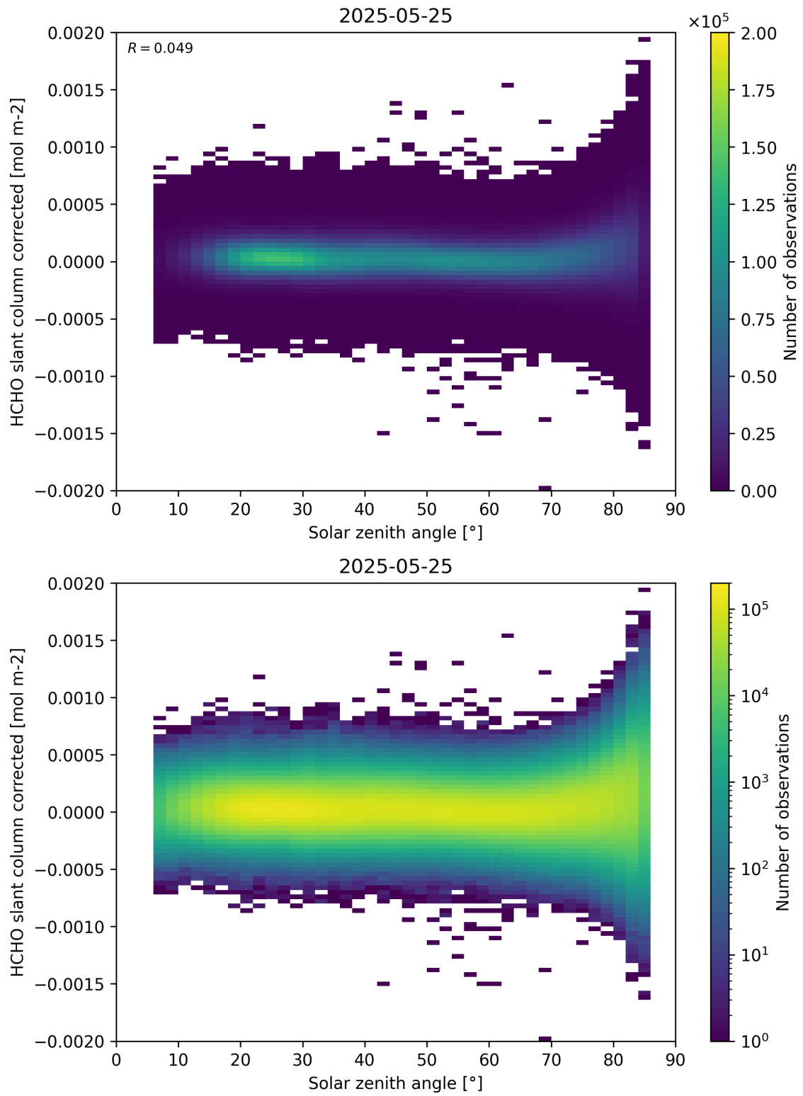
Figure 171: Scatter density plot of “Solar zenith angle” against “HCHO slant column corrected” for 2025-05-24 to 2025-05-26.
