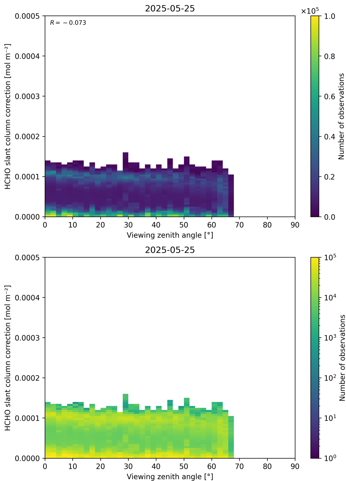
Figure 187: Scatter density plot of “Viewing zenith angle” against “HCHO slant column correction” for 2025-05-24 to 2025-05-26.
