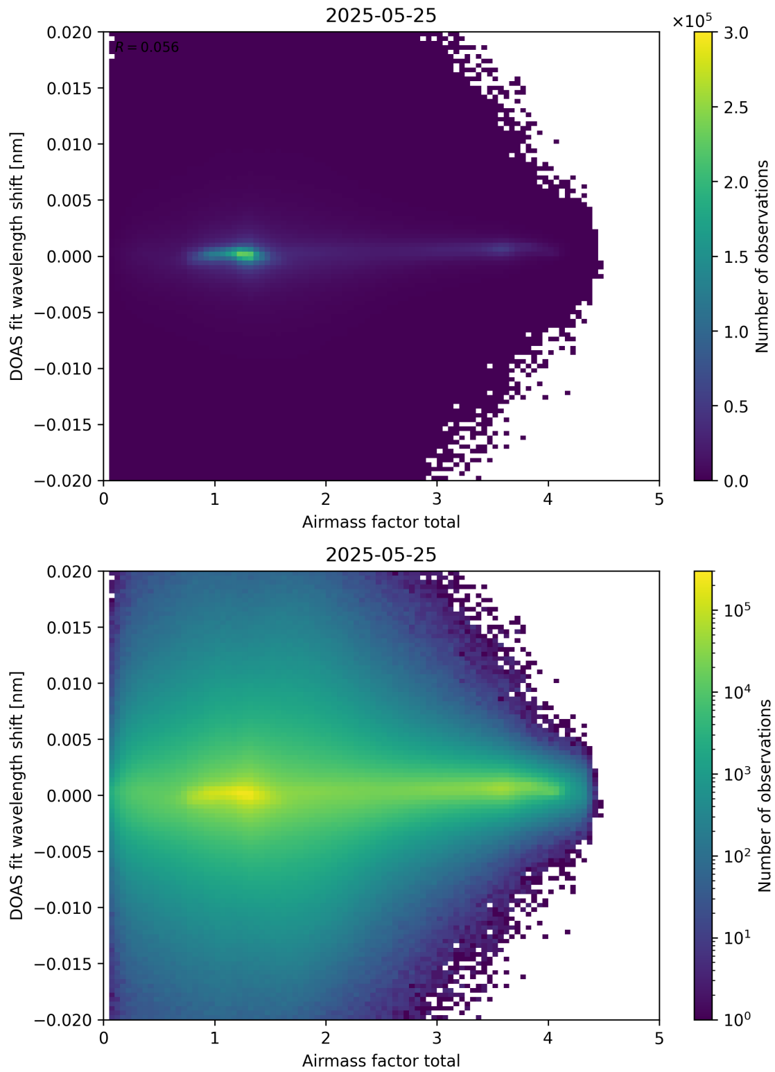
Figure 98: Scatter density plot of “Airmass factor total” against “DOAS fit wavelength shift” for 2025-05-24 to 2025-05-26.
