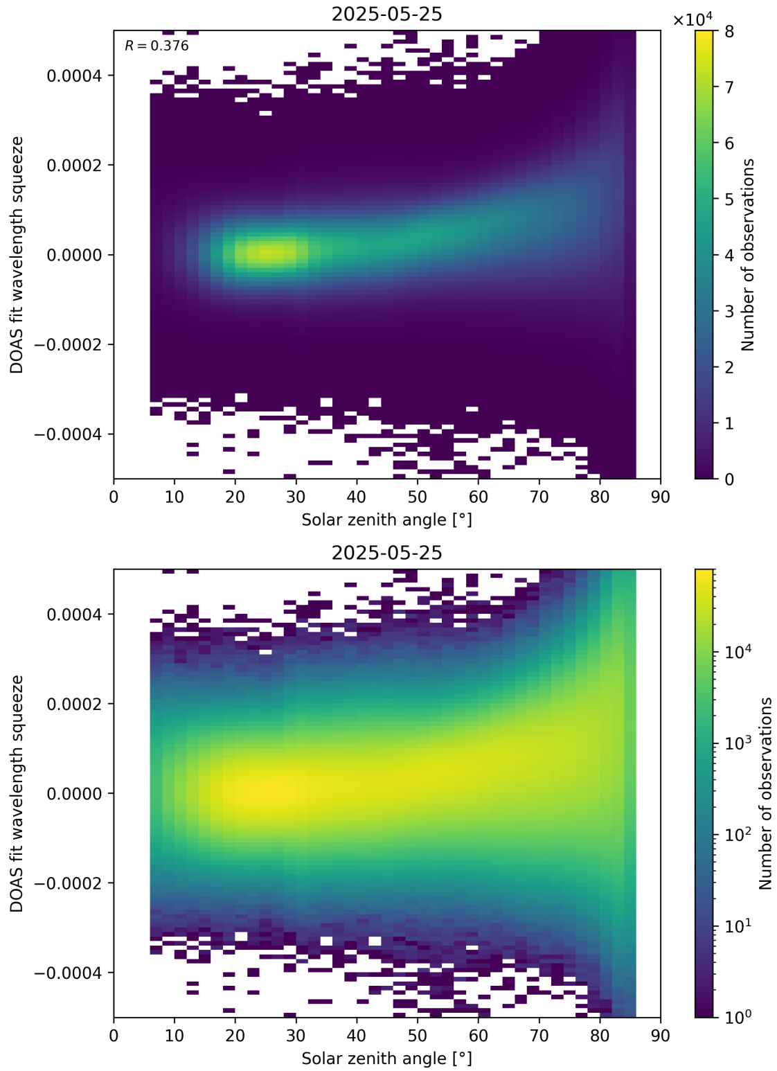
Figure 169: Scatter density plot of “Solar zenith angle” against “DOAS fit wavelength squeeze” for 2025-05-24 to 2025-05-26.
