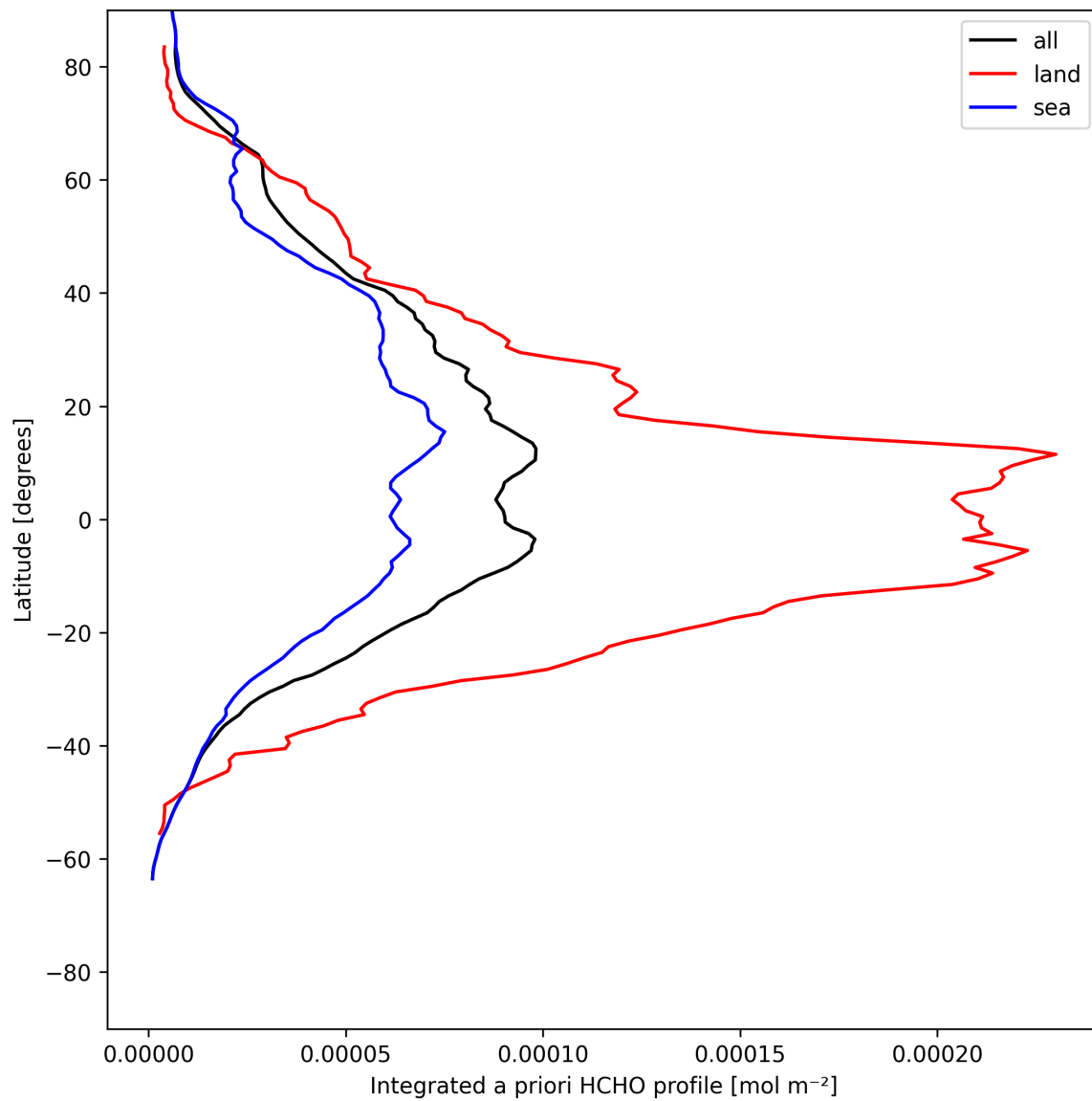
Figure 29: Zonal average of “Integrated a priori HCHO profile” for 2025-05-24 to 2025-05-26.
