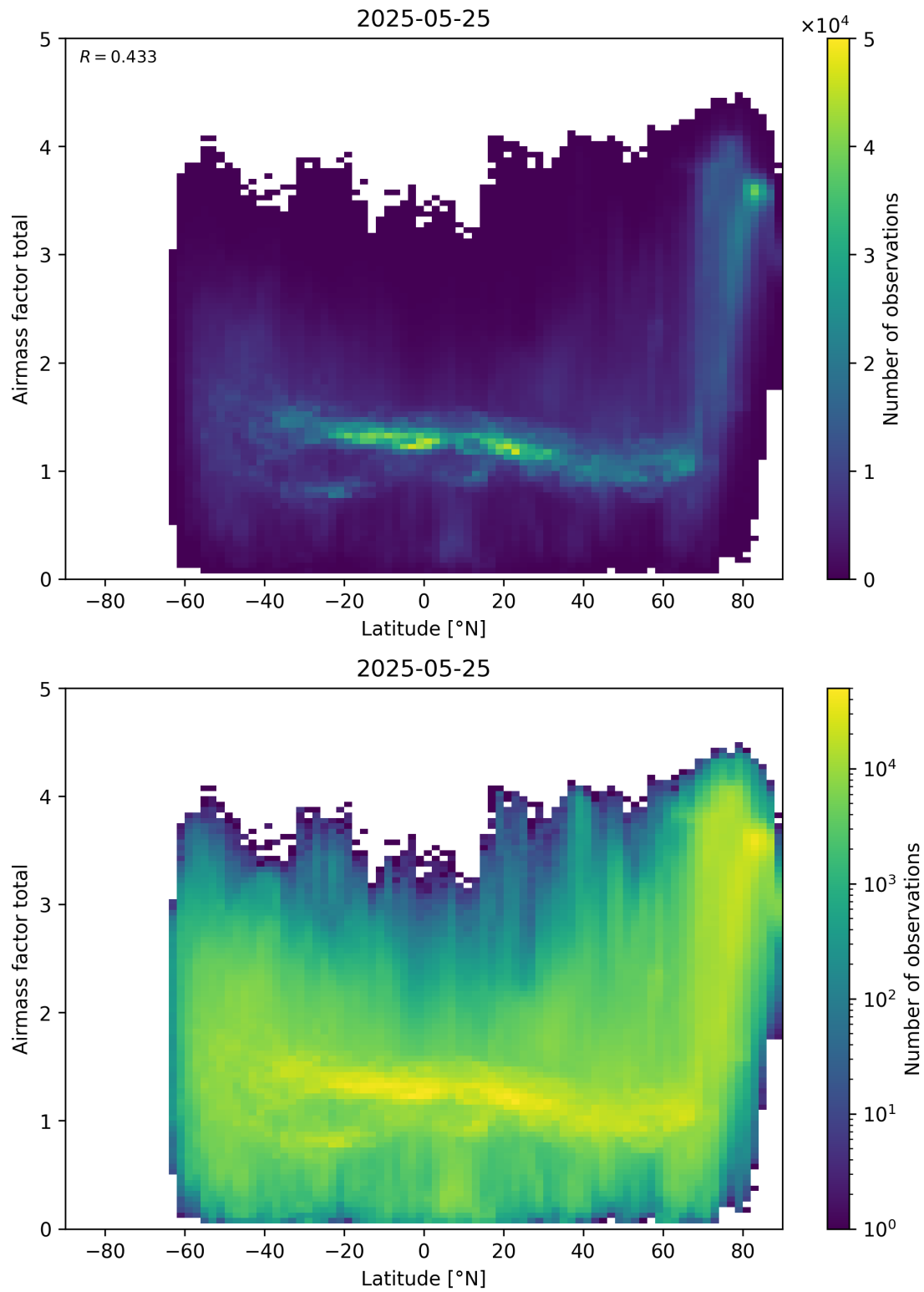
Figure 161: Scatter density plot of “Latitude” against “Airmass factor total” for 2025-05-24 to 2025-05-26.
