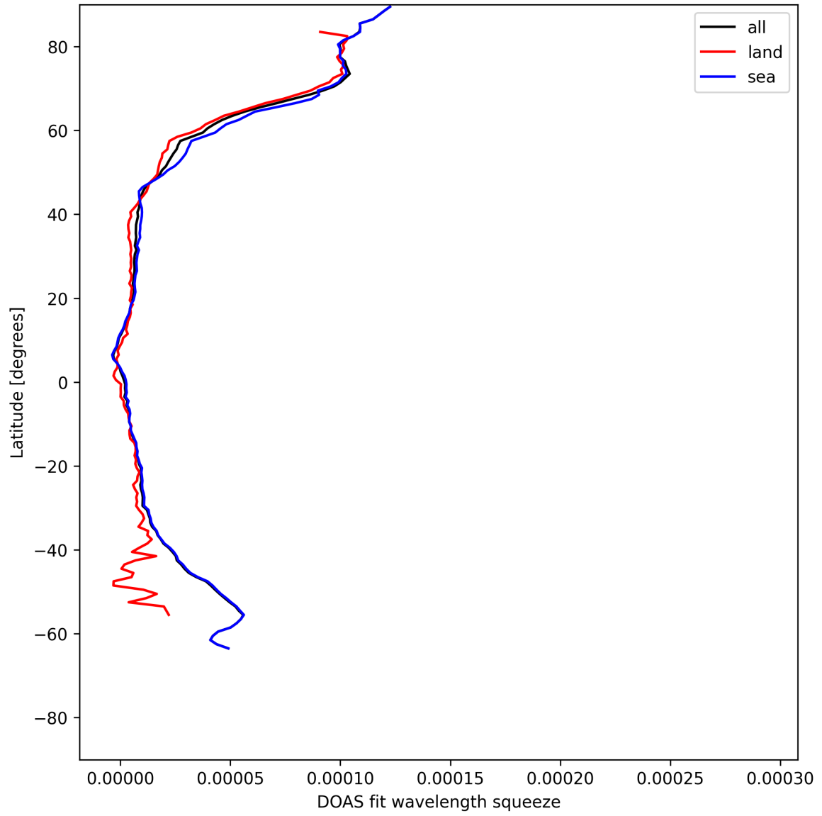
Figure 31: Zonal average of “DOAS fit wavelength squeeze” for 2025-05-24 to 2025-05-26.
