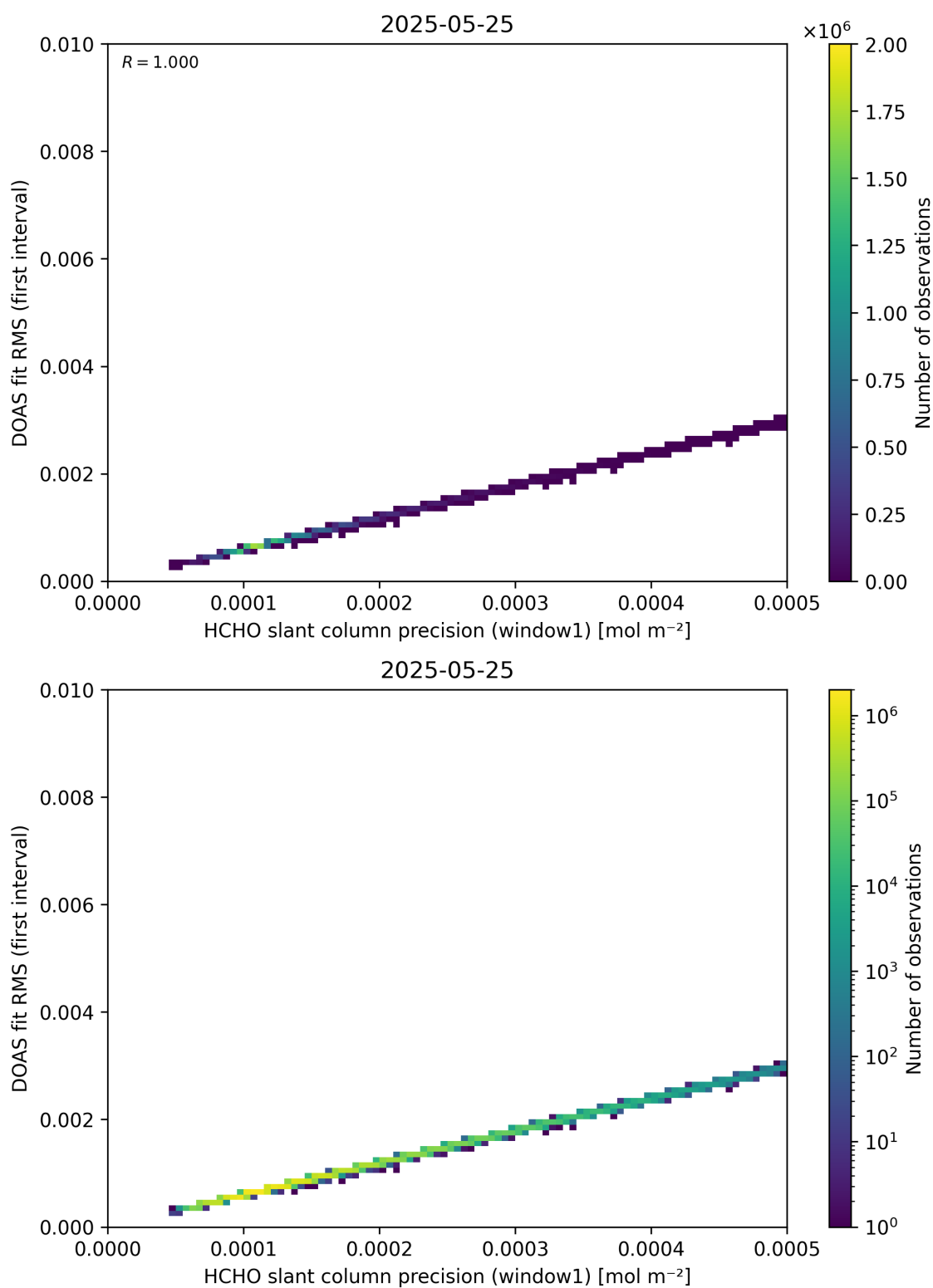
Figure 88: Scatter density plot of “HCHO slant column precision (window1)” against “DOAS fit RMS (first interval)” for 2025-05-24 to 2025-05-26.
