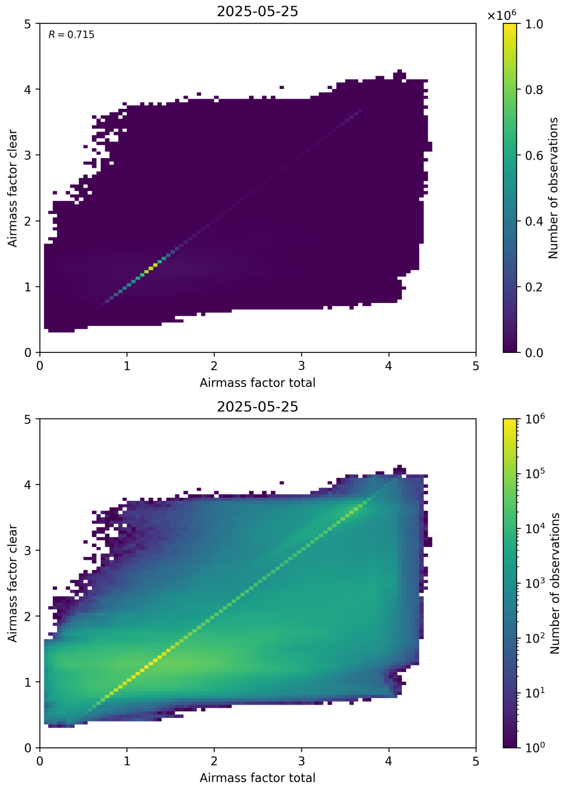
Figure 100: Scatter density plot of “Airmass factor total” against “Airmass factor clear” for 2025-05-24 to 2025-05-26.
