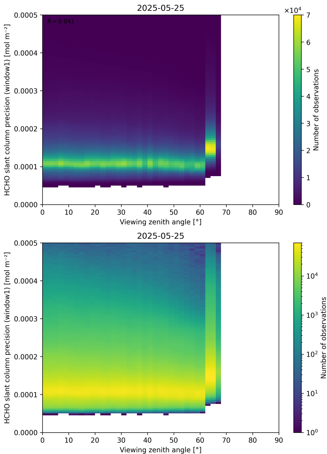
Figure 189: Scatter density plot of “Viewing zenith angle” against “HCHO slant column precision (window1)” for 2025-05-24 to 2025-05-26.
