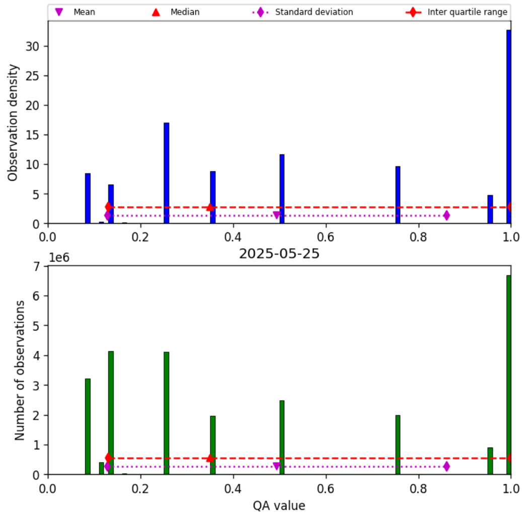
Figure 34: Histogram of “QA value” for 2025-05-24 to 2025-05-26
