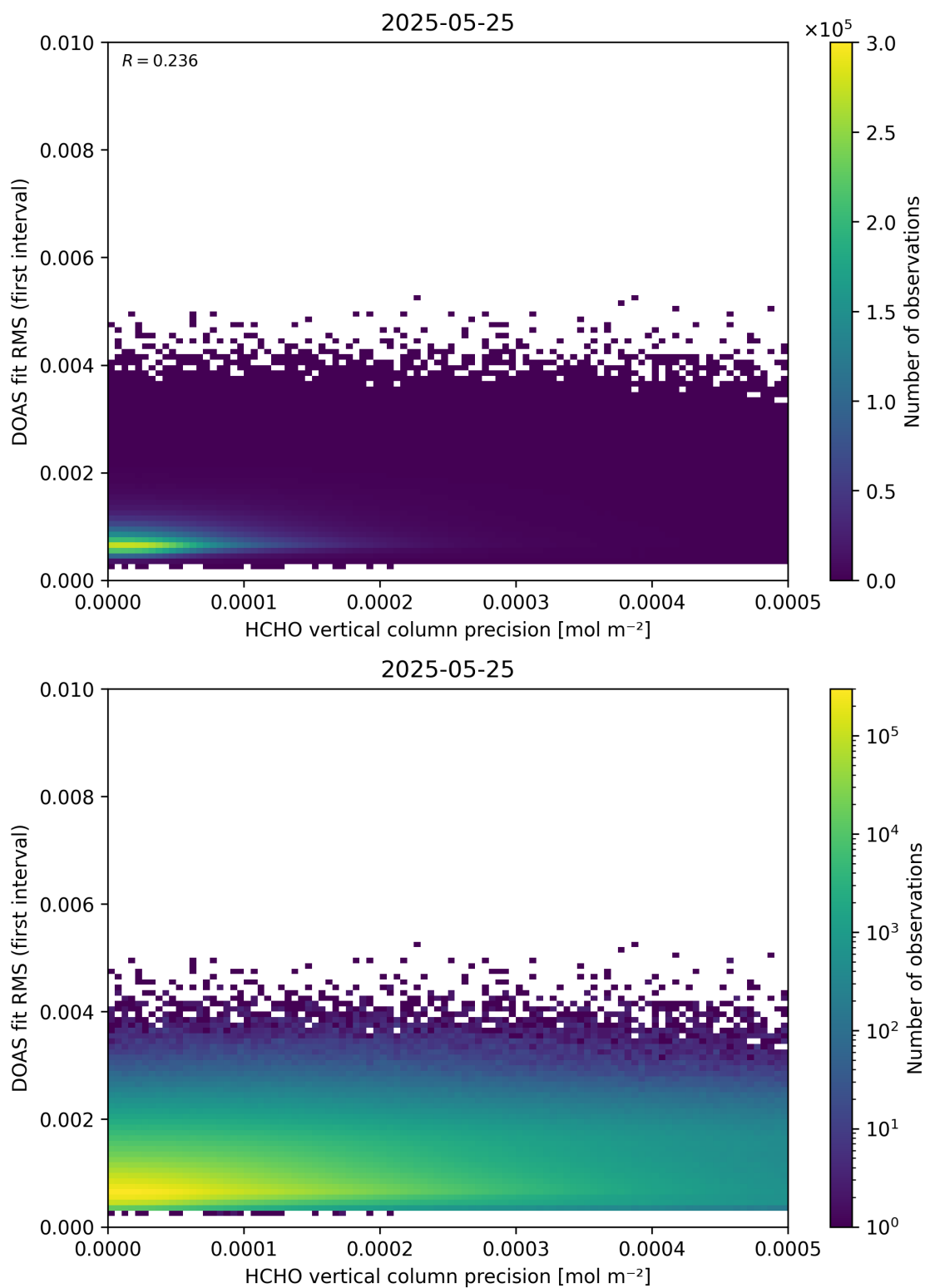
Figure 136: Scatter density plot of “HCHO vertical column precision” against “DOAS fit RMS (first interval)” for 2025-05-24 to 2025-05-26.
