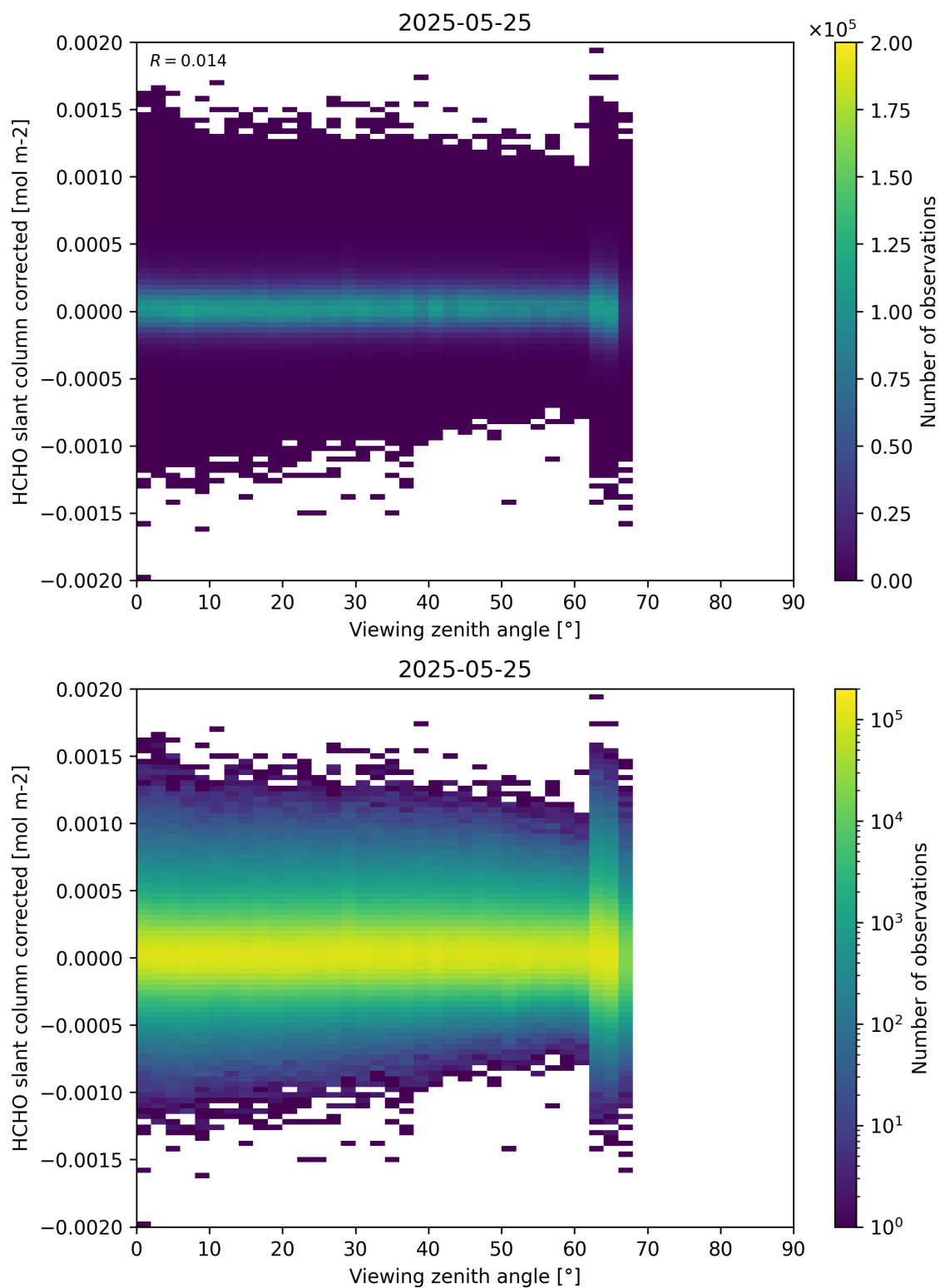
Figure 186: Scatter density plot of “Viewing zenith angle” against “HCHO slant column corrected” for 2025-05-24 to 2025-05-26.
