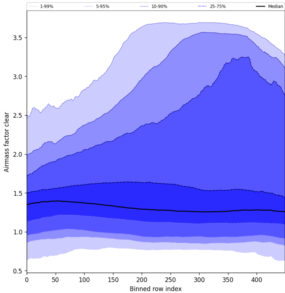
Figure 56: Along track statistics of “Airmass factor clear” for 2025-05-24 to 2025-05-26
