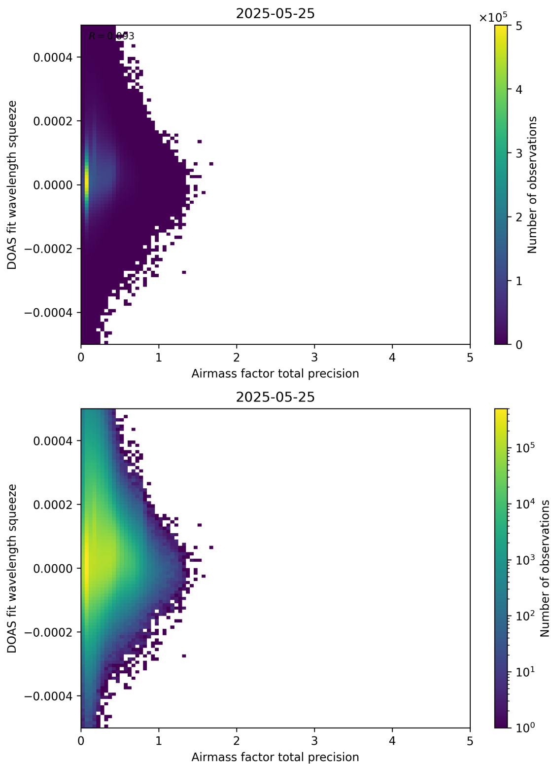
Figure 107: Scatter density plot of “Airmass factor total precision” against “DOAS fit wavelength squeeze” for 2025-05-24 to 2025-05-26.
