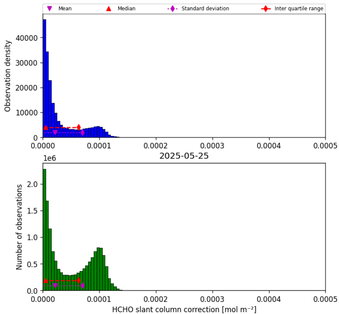
Figure 47: Histogram of “HCHO slant column correction” for 2025-05-24 to 2025-05-26
