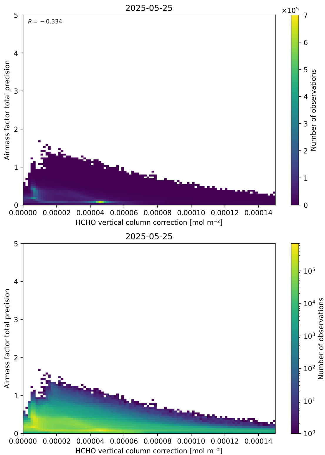
Figure 121: Scatter density plot of “HCHO vertical column correction” against “Airmass factor total precision” for 2025-05-24 to 2025-05-26.
