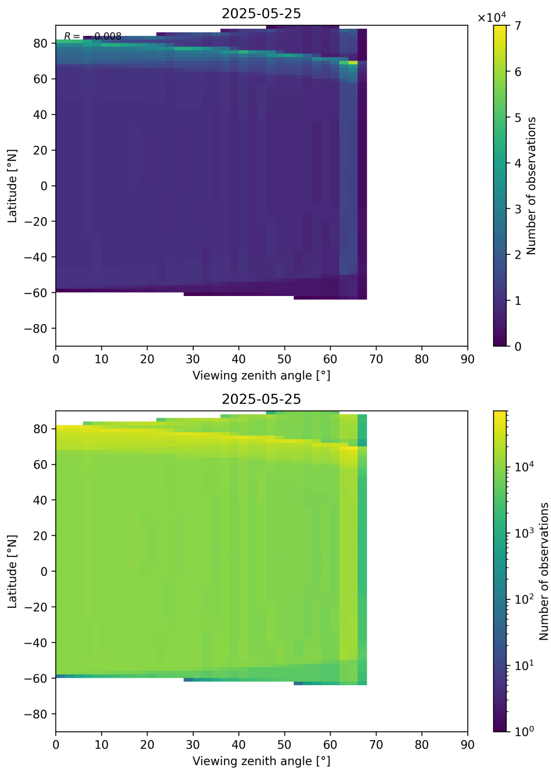
Figure 196: Scatter density plot of “Viewing zenith angle” against “Latitude” for 2025-05-24 to 2025-05-26.
