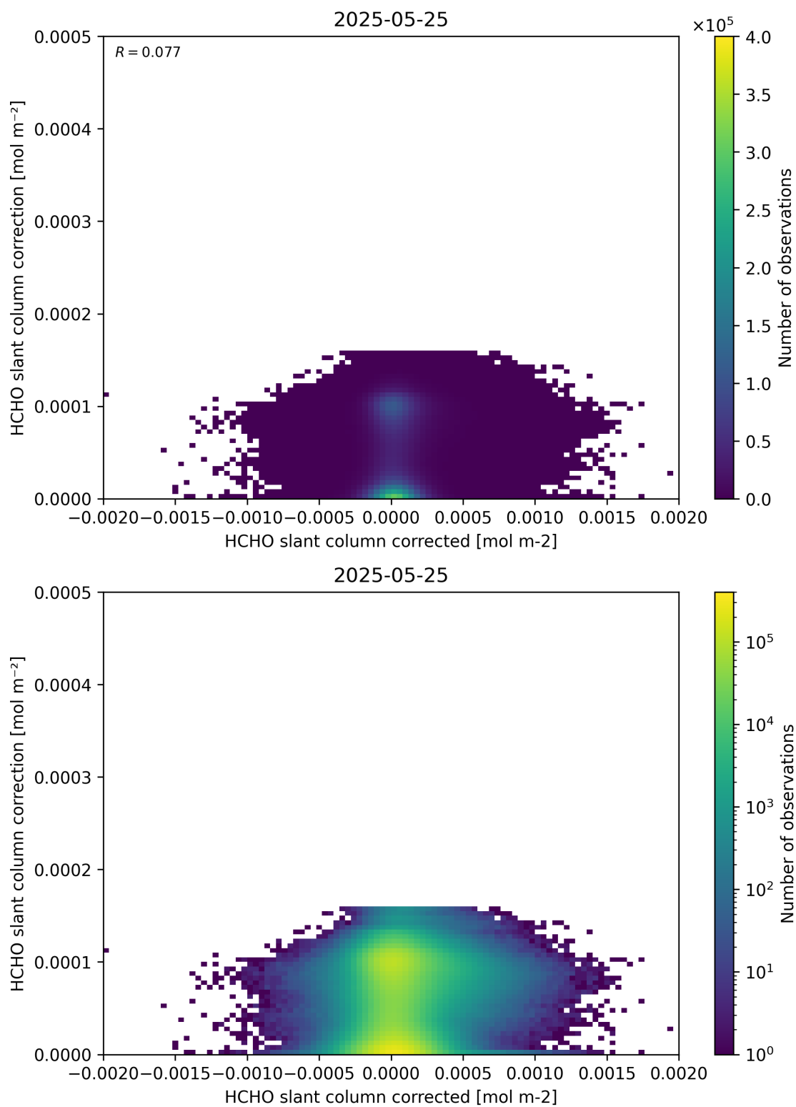
Figure 77: Scatter density plot of “HCHO slant column corrected” against “HCHO slant column correction” for 2025-05-24 to 2025-05-26.
