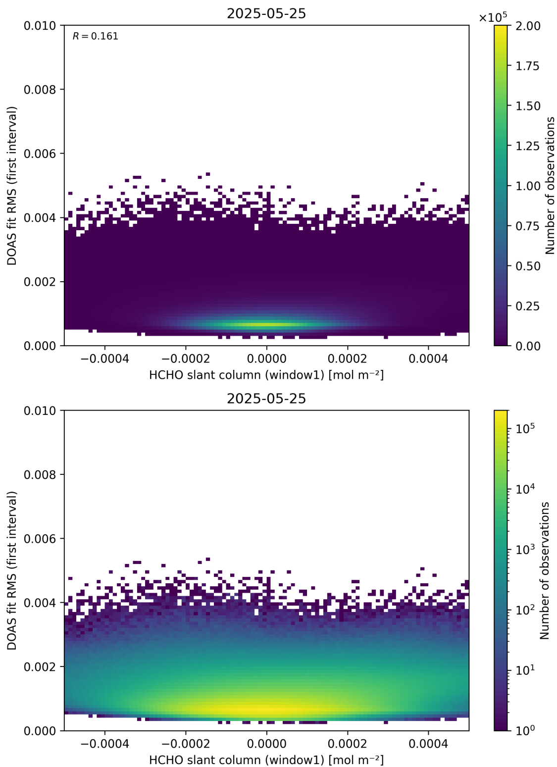
Figure 78: Scatter density plot of “HCHO slant column (window1)” against “DOAS fit RMS (first interval)” for 2025-05-24 to 2025-05-26.
