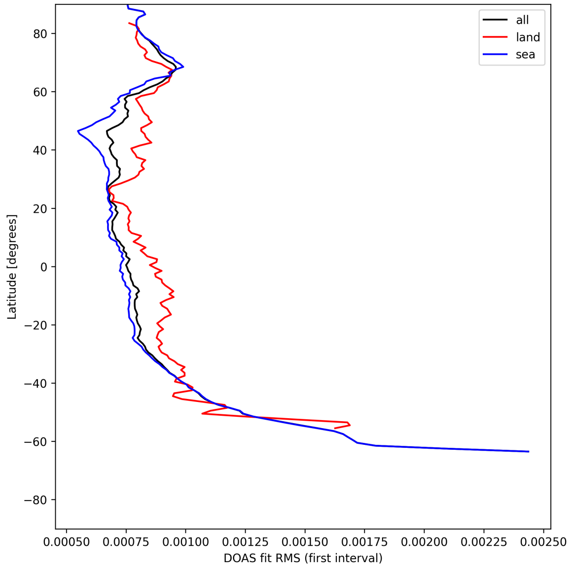
Figure 32: Zonal average of “DOAS fit RMS (first interval)” for 2025-05-24 to 2025-05-26.
