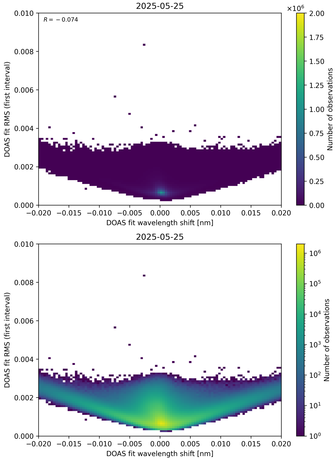
Figure 64: Scatter density plot of “DOAS fit wavelength shift” against “DOAS fit RMS (first interval)” for 2025-05-24 to 2025-05-26.
