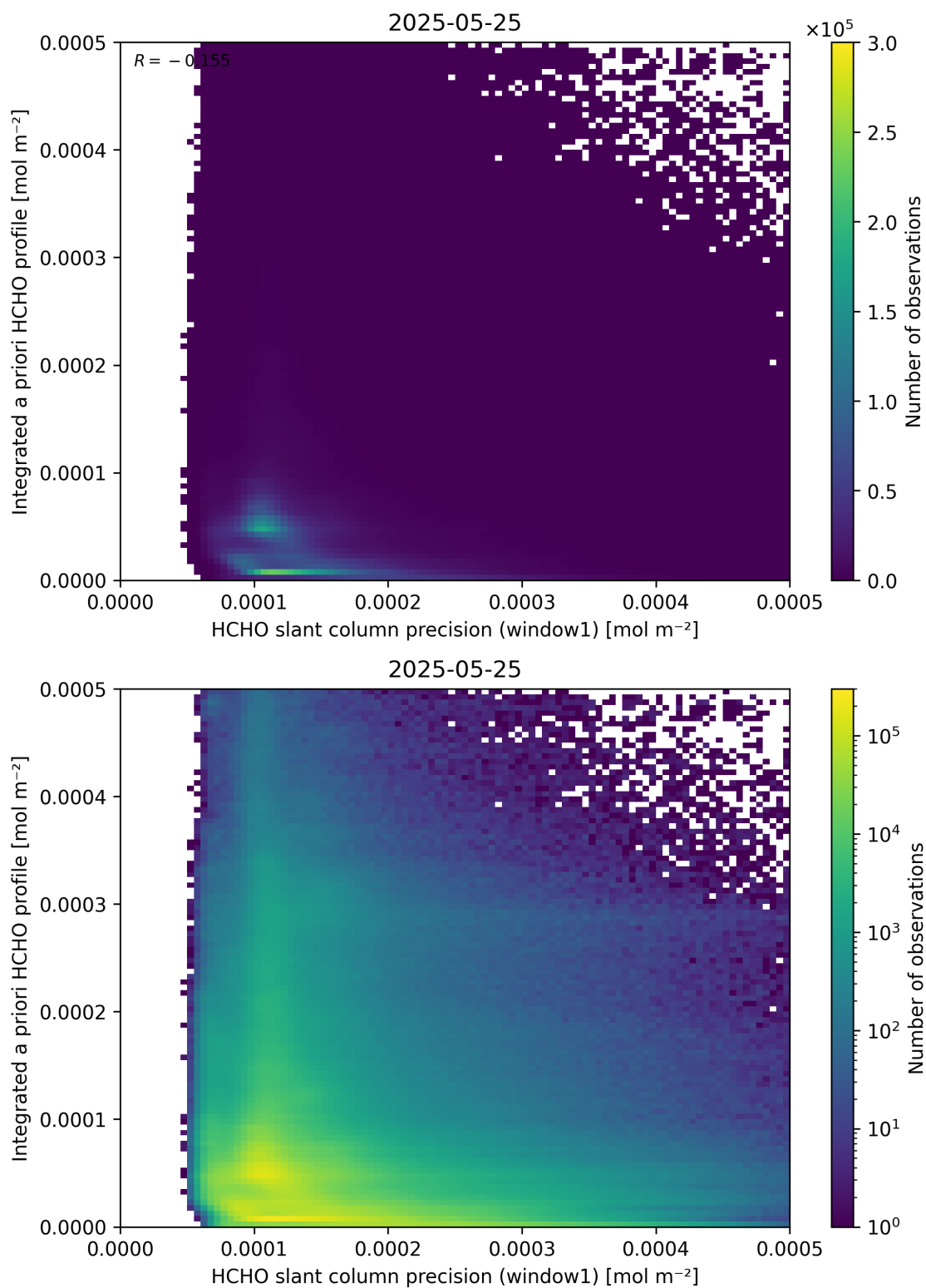
Figure 96: Scatter density plot of “HCHO slant column precision (window1)” against “Integrated a priori HCHO profile” for 2025-05-24 to 2025-05-26.
