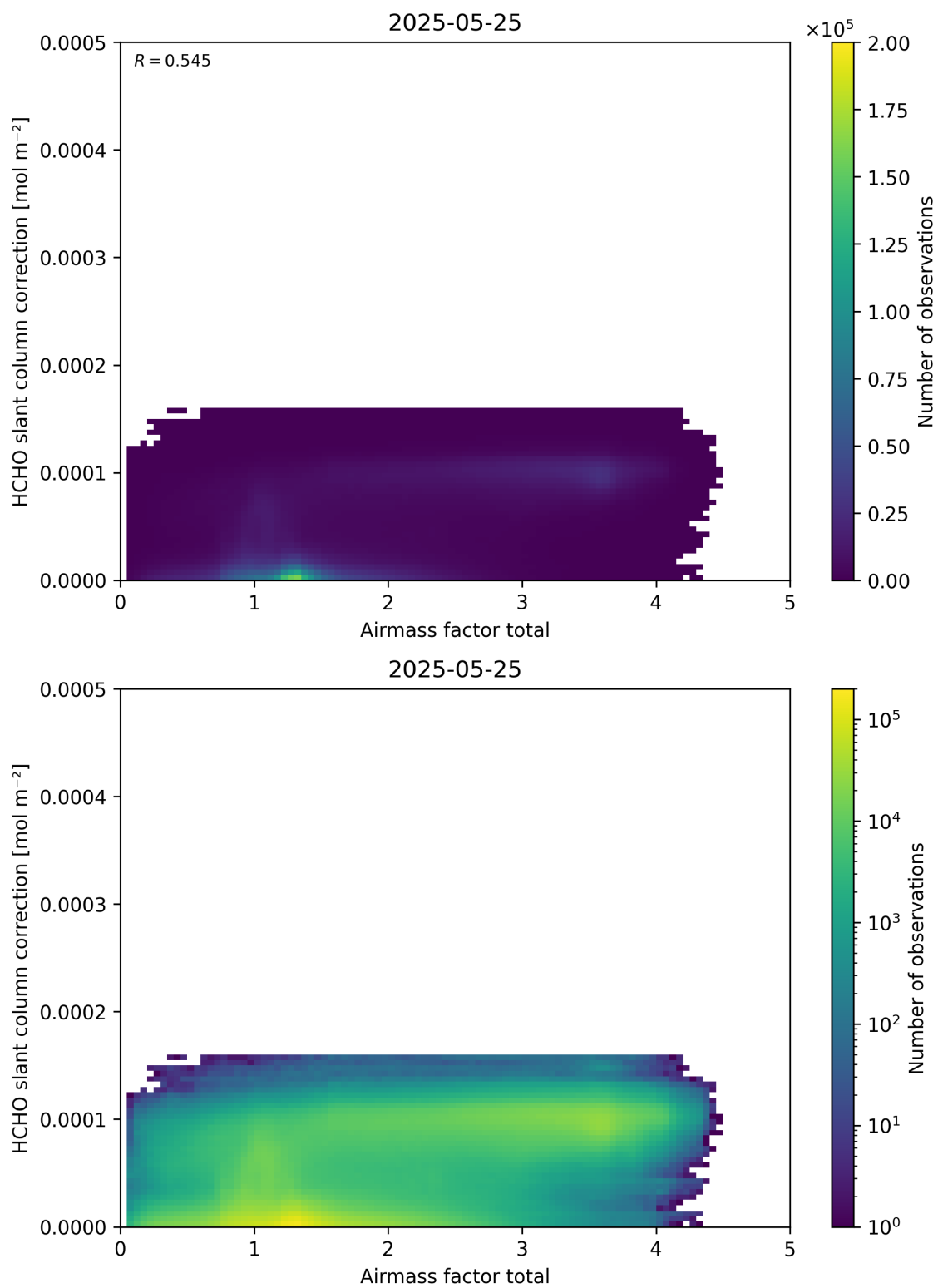
Figure 102: Scatter density plot of “Airmass factor total” against “HCHO slant column correction” for 2025-05-24 to 2025-05-26.
