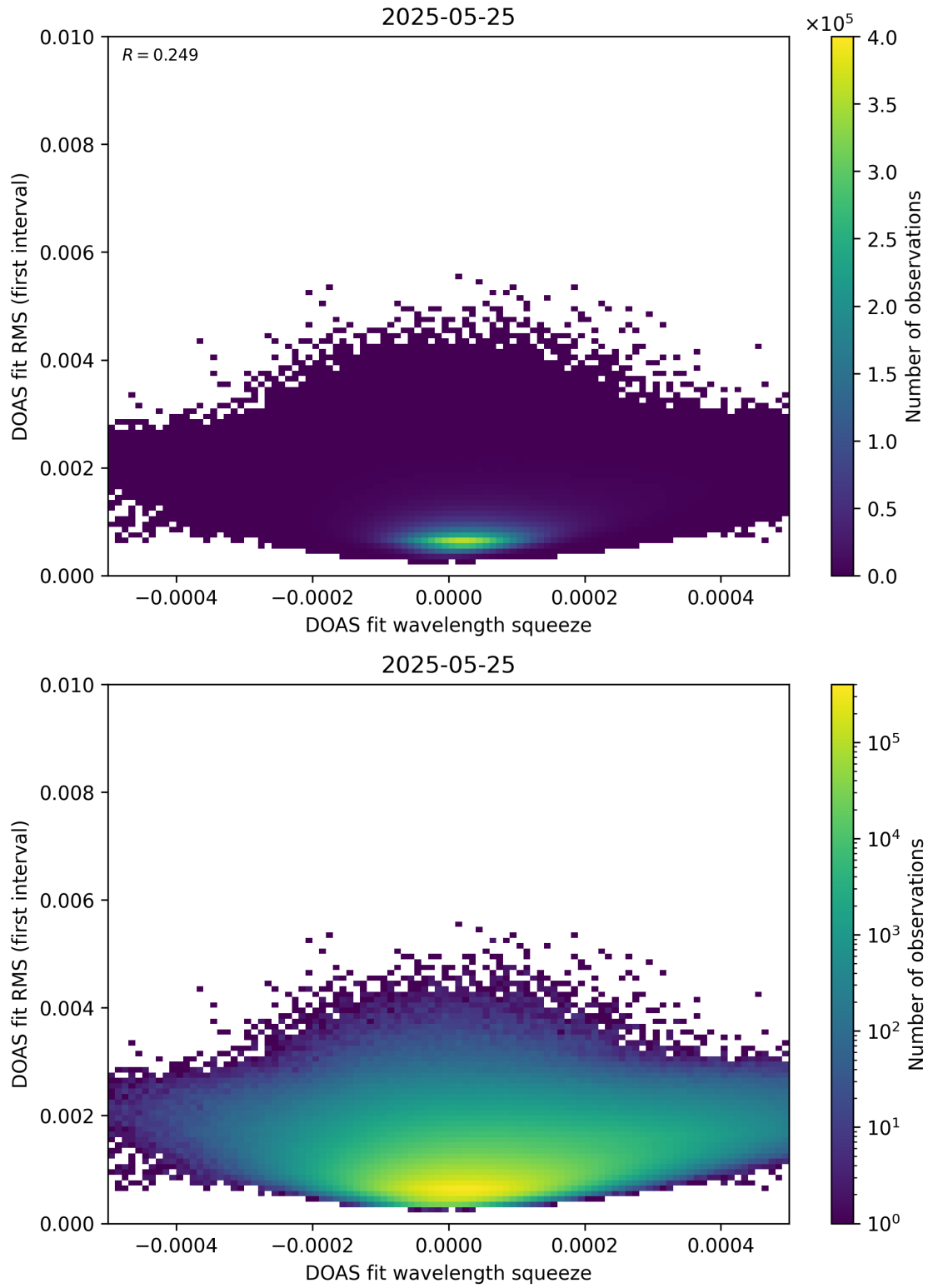
Figure 68: Scatter density plot of “DOAS fit wavelength squeeze” against “DOAS fit RMS (first interval)” for 2025-05-24 to 2025-05-26.
