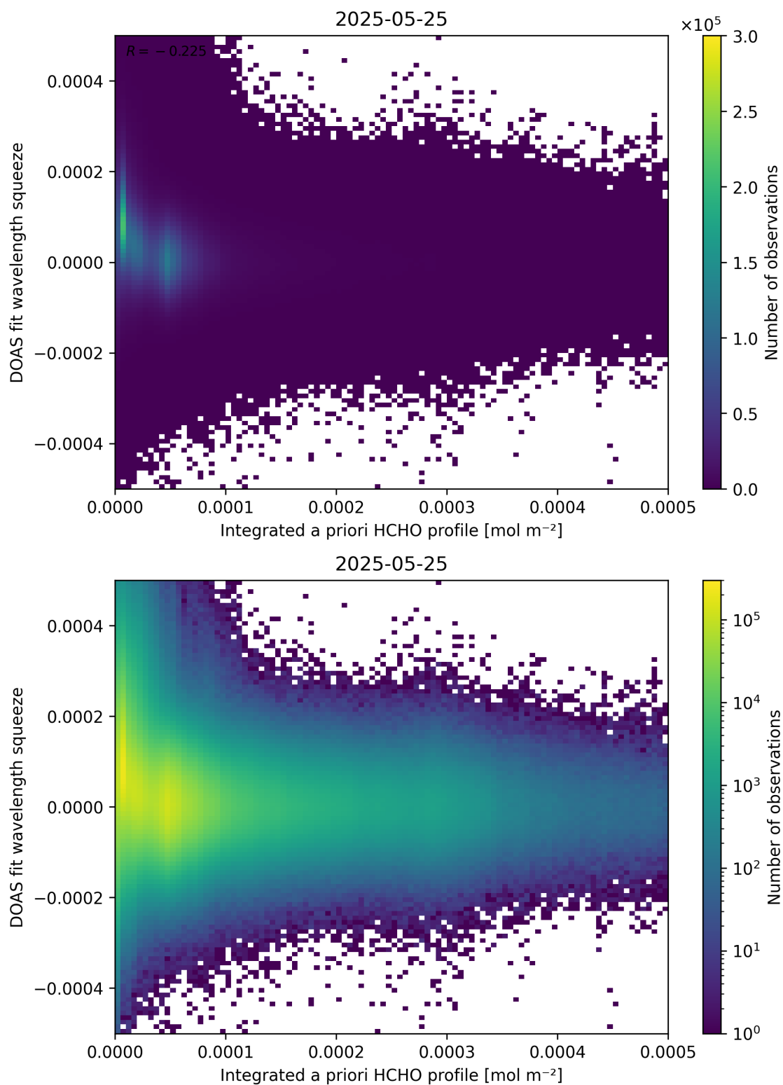
Figure 150: Scatter density plot of “Integrated a priori HCHO profile” against “DOAS fit wavelength squeeze” for 2025-05-24 to 2025-05-26.
