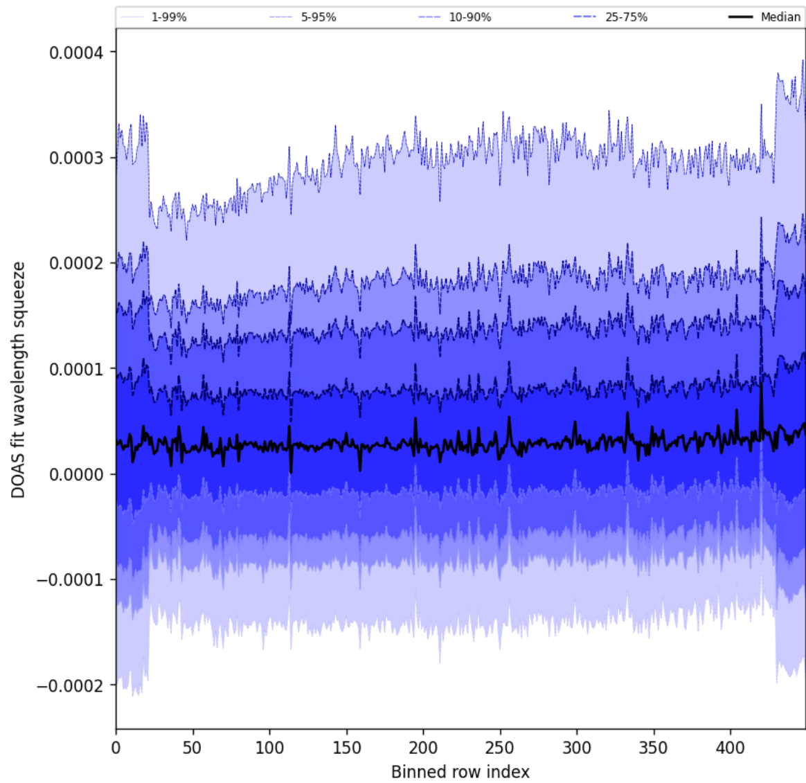
Figure 59: Along track statistics of “DOAS fit wavelength squeeze” for 2025-05-24 to 2025-05-26
