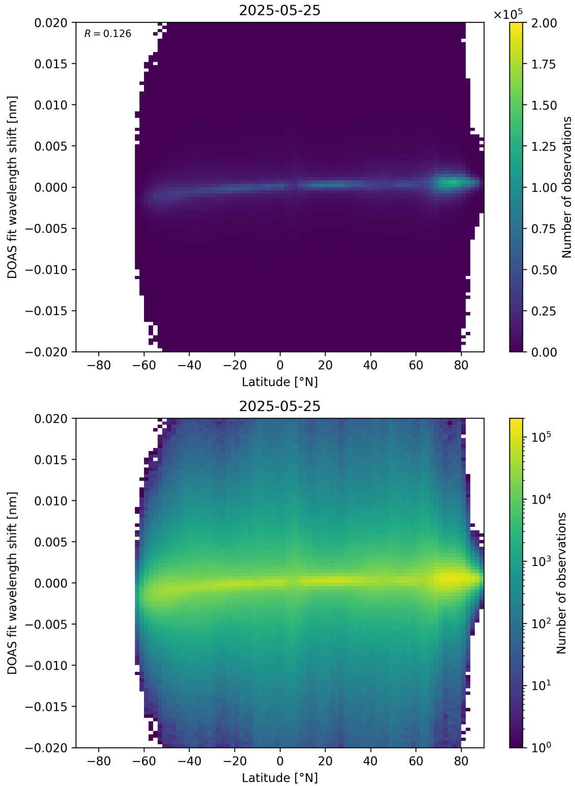
Figure 154: Scatter density plot of “Latitude” against “DOAS fit wavelength shift” for 2025-05-24 to 2025-05-26.
