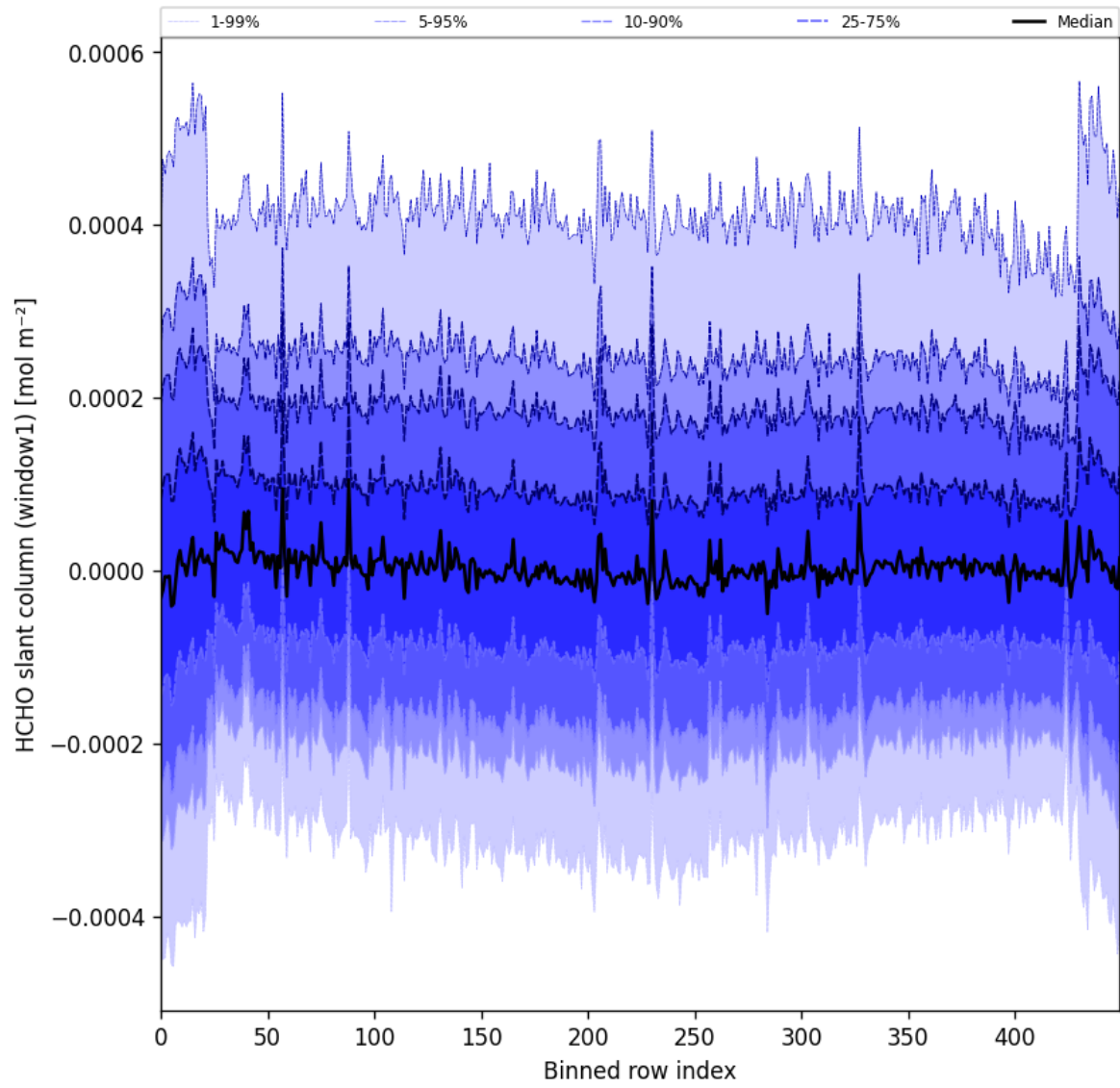
Figure 52: Along track statistics of “HCHO slant column (window1)” for 2025-05-24 to 2025-05-26
