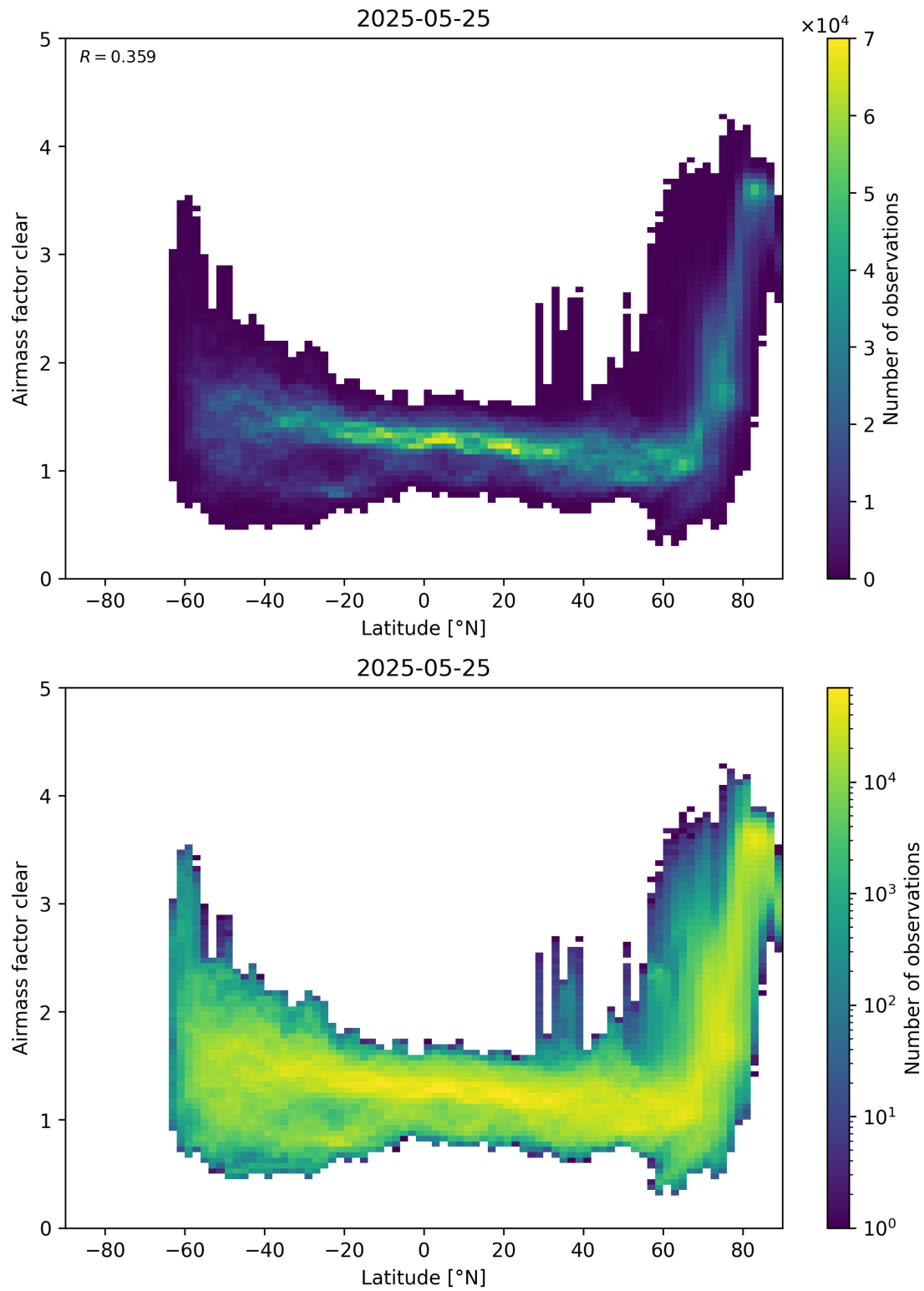
Figure 156: Scatter density plot of “Latitude” against “Airmass factor clear” for 2025-05-24 to 2025-05-26.
