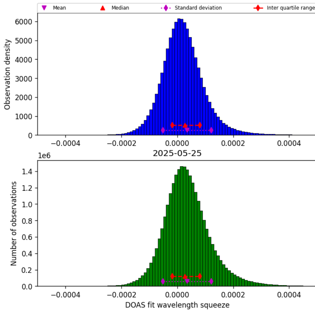
Figure 45: Histogram of “DOAS fit wavelength squeeze” for 2025-05-24 to 2025-05-26
