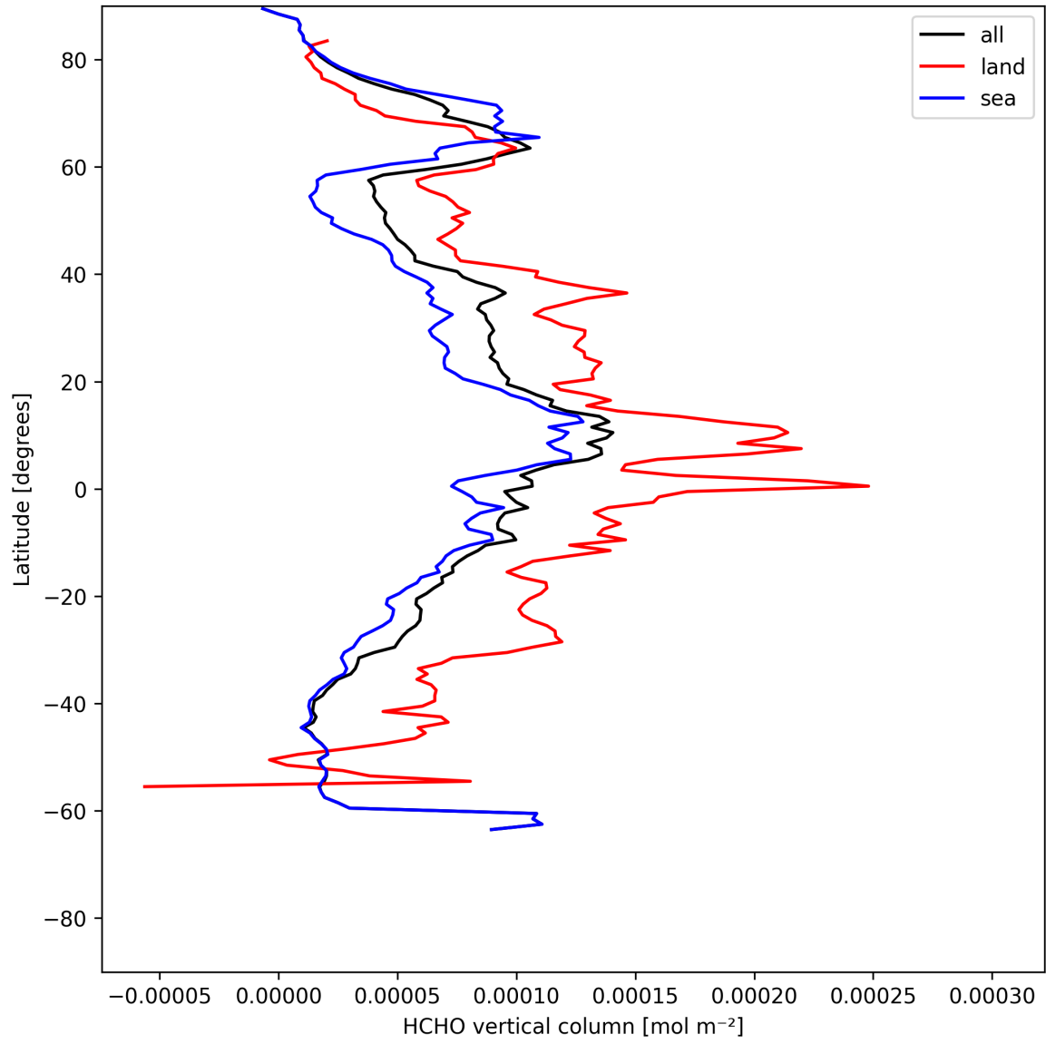
Figure 21: Zonal average of “HCHO vertical column” for 2025-05-24 to 2025-05-26.
