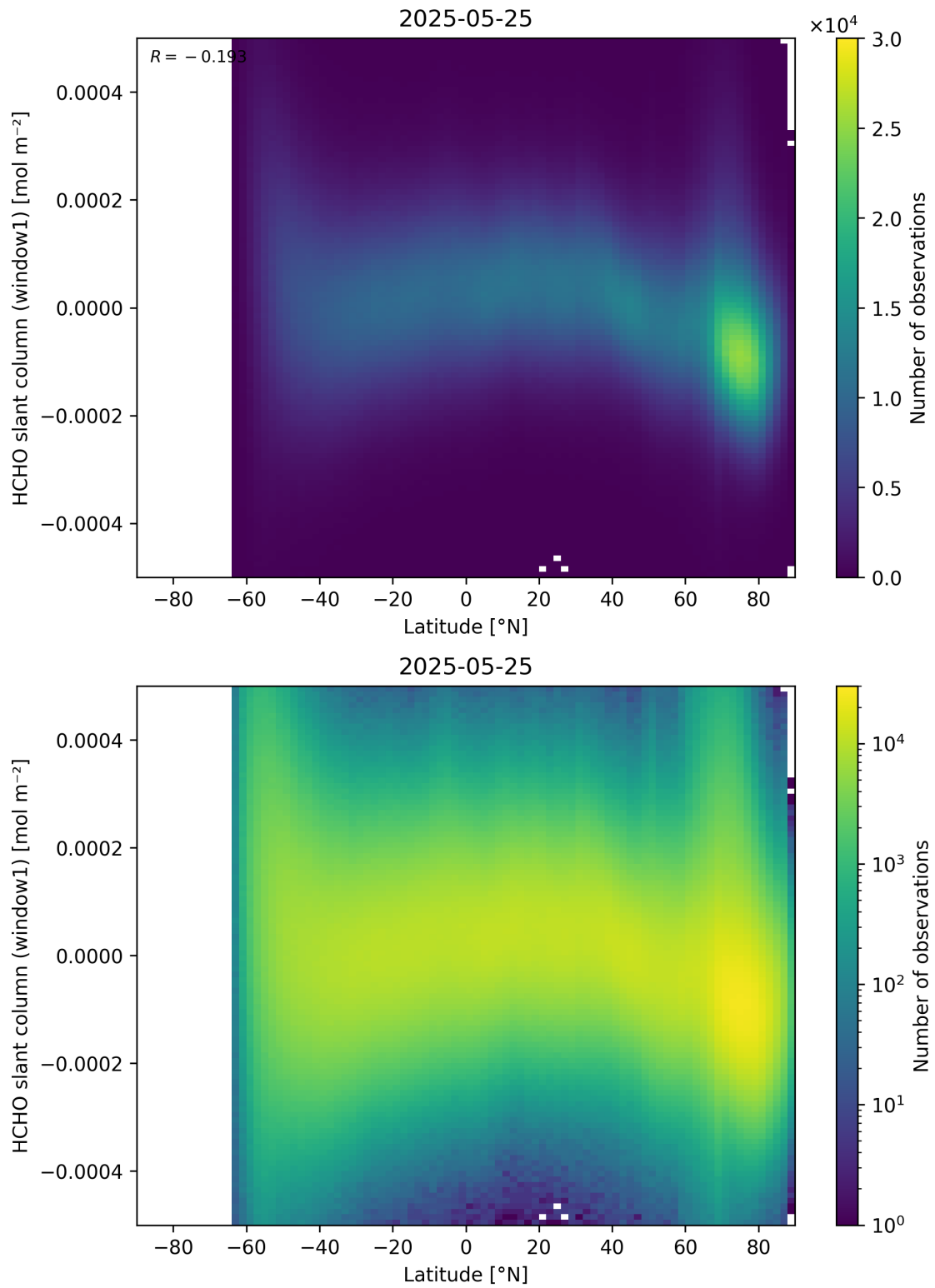
Figure 159: Scatter density plot of “Latitude” against “HCHO slant column (window1)” for 2025-05-24 to 2025-05-26.
