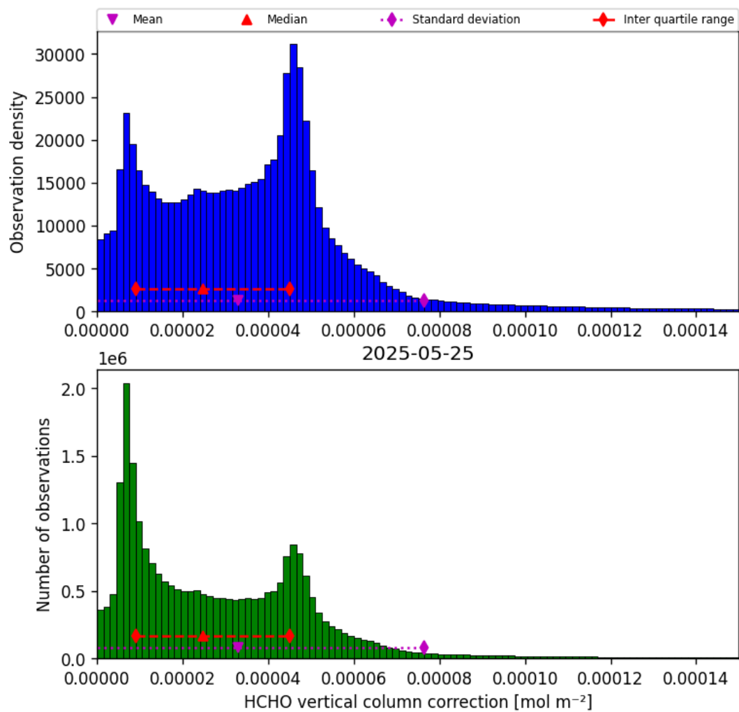
Figure 37: Histogram of “HCHO vertical column correction” for 2025-05-24 to 2025-05-26
