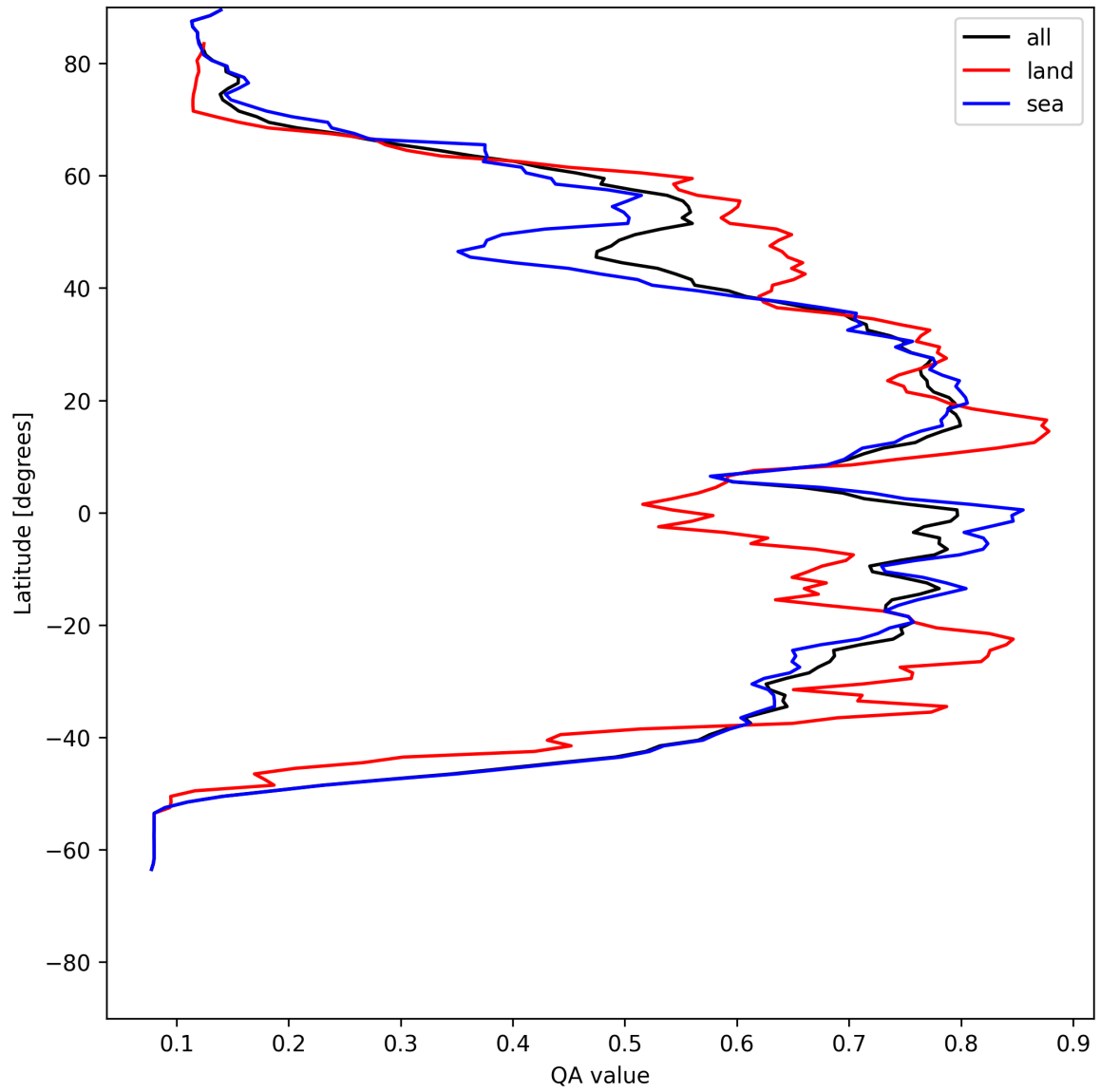
Figure 20: Zonal average of “QA value” for 2025-05-24 to 2025-05-26.
