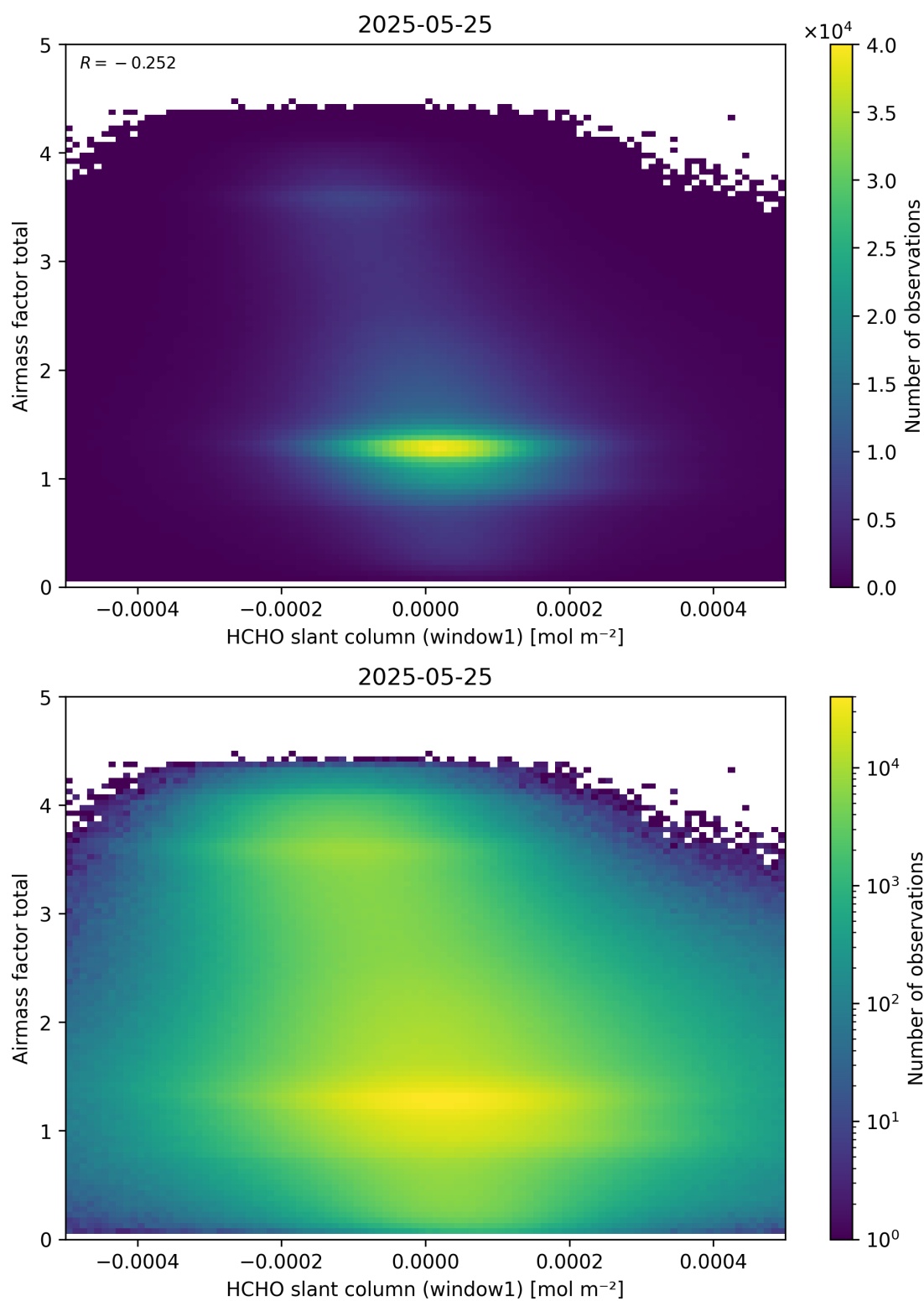
Figure 85: Scatter density plot of “HCHO slant column (window1)” against “Airmass factor total” for 2025-05-24 to 2025-05-26.
