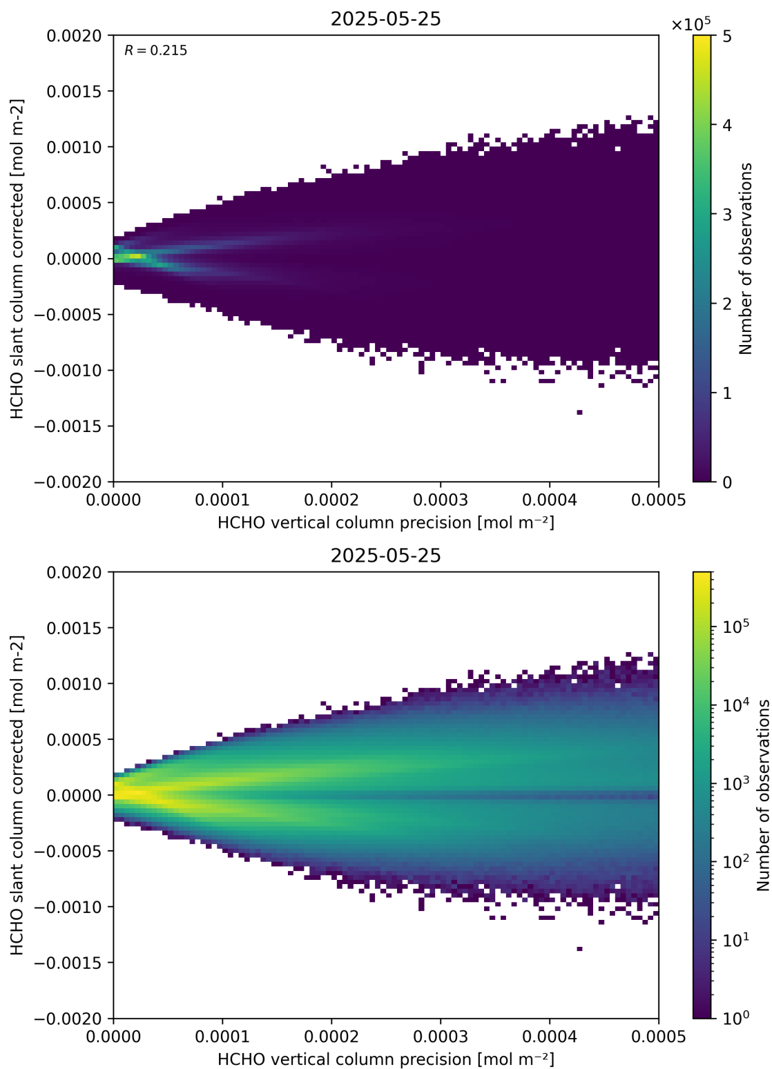
Figure 140: Scatter density plot of “HCHO vertical column precision” against “HCHO slant column corrected” for 2025-05-24 to 2025-05-26.
