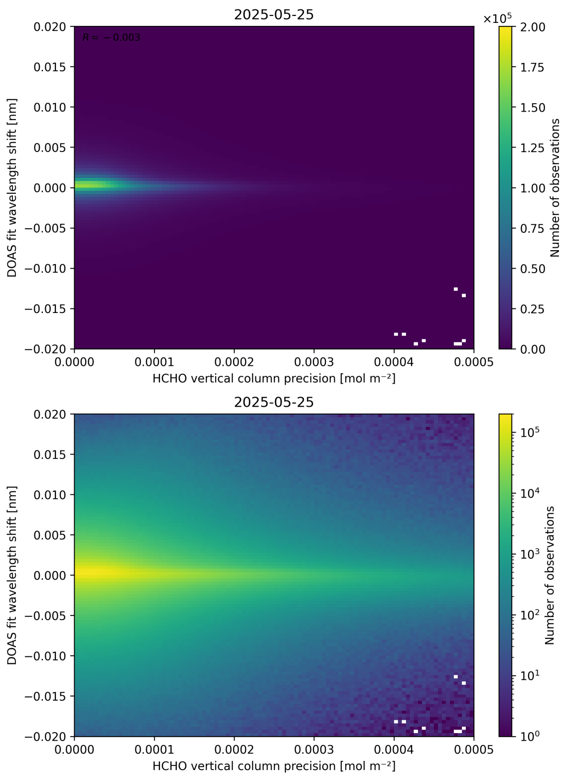
Figure 137: Scatter density plot of “HCHO vertical column precision” against “DOAS fit wavelength shift” for 2025-05-24 to 2025-05-26.
