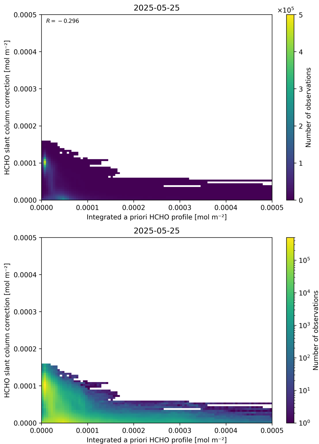
Figure 152: Scatter density plot of “Integrated a priori HCHO profile” against “HCHO slant column correction” for 2025-05-24 to 2025-05-26.
