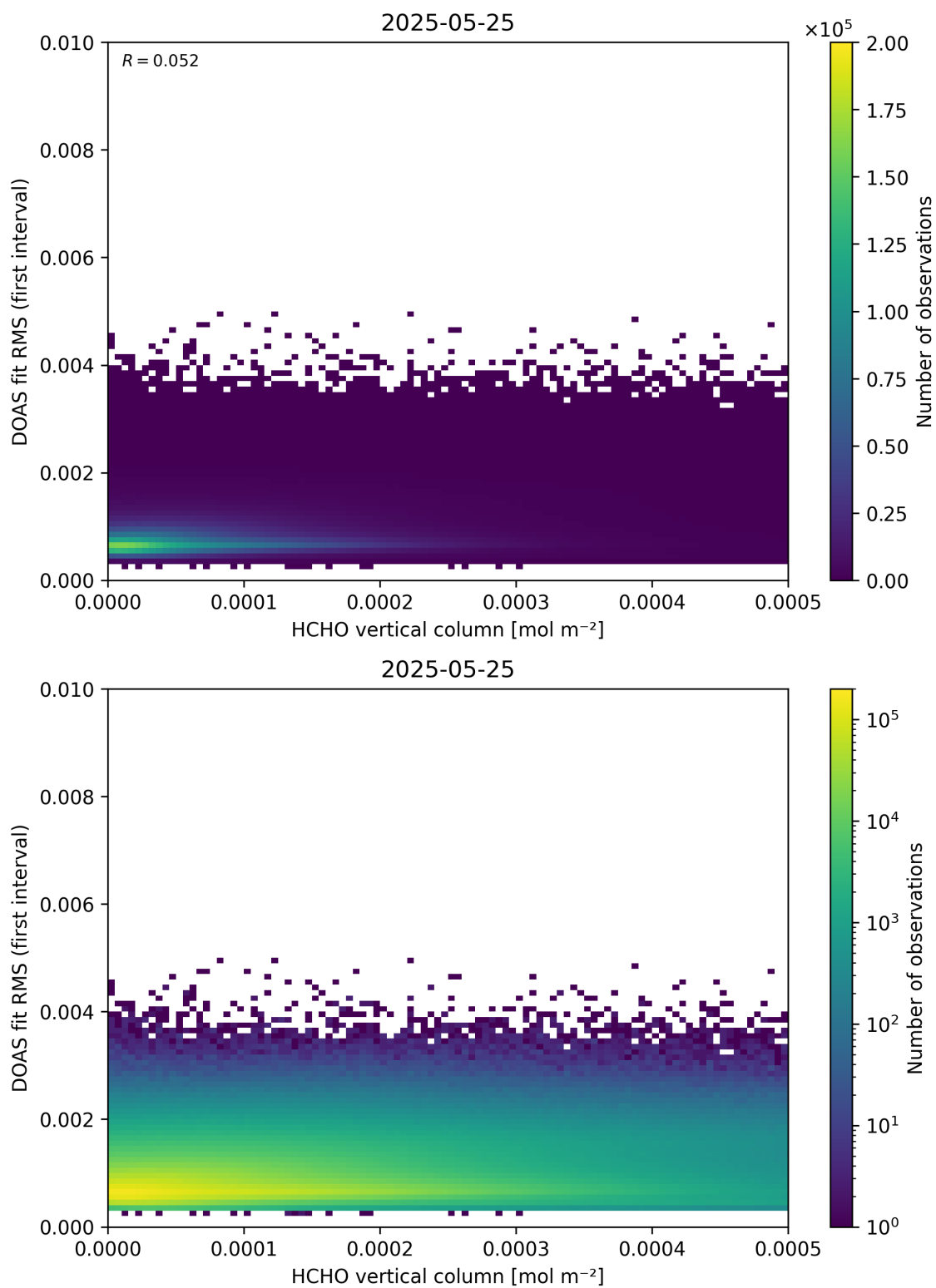
Figure 123: Scatter density plot of “HCHO vertical column” against “DOAS fit RMS (first interval)” for 2025-05-24 to 2025-05-26.
