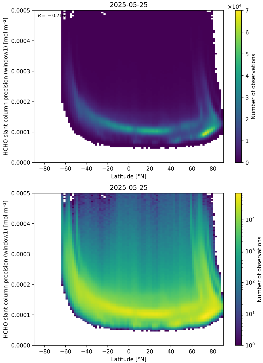
Figure 160: Scatter density plot of “Latitude” against “HCHO slant column precision (window1)” for 2025-05-24 to 2025-05-26.
