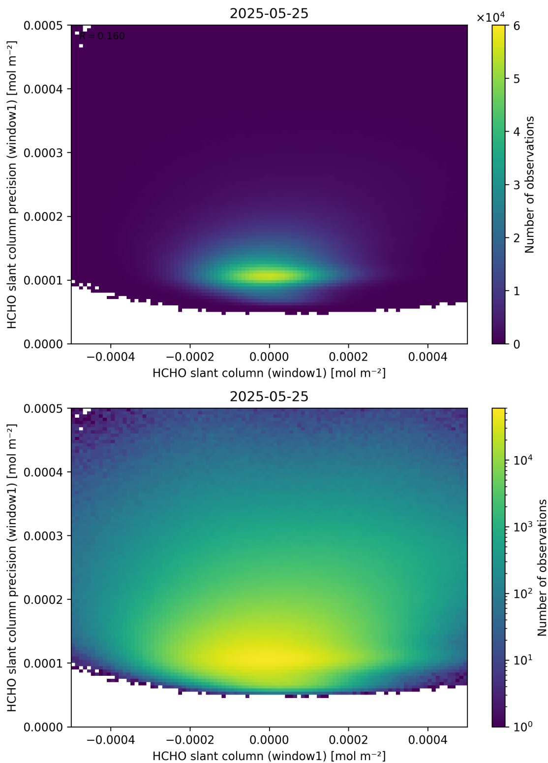
Figure 84: Scatter density plot of “HCHO slant column (window1)” against “HCHO slant column precision (window1)” for 2025-05-24 to 2025-05-26.
