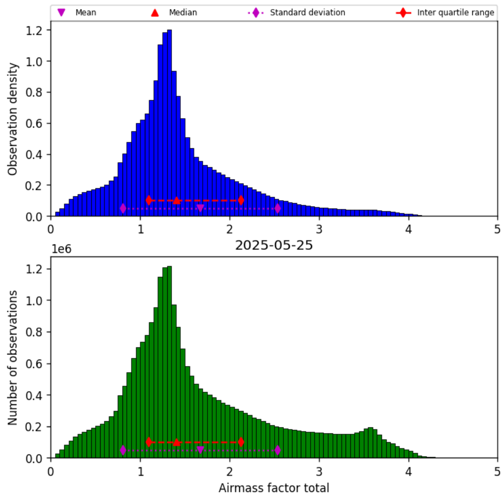
Figure 40: Histogram of “Airmass factor total” for 2025-05-24 to 2025-05-26
