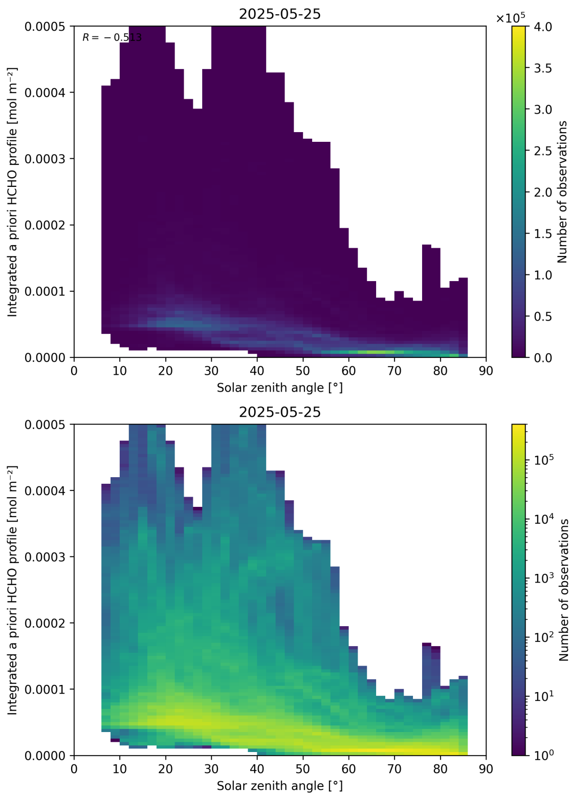
Figure 180: Scatter density plot of “Solar zenith angle” against “Integrated a priori HCHO profile” for 2025-05-24 to 2025-05-26.
