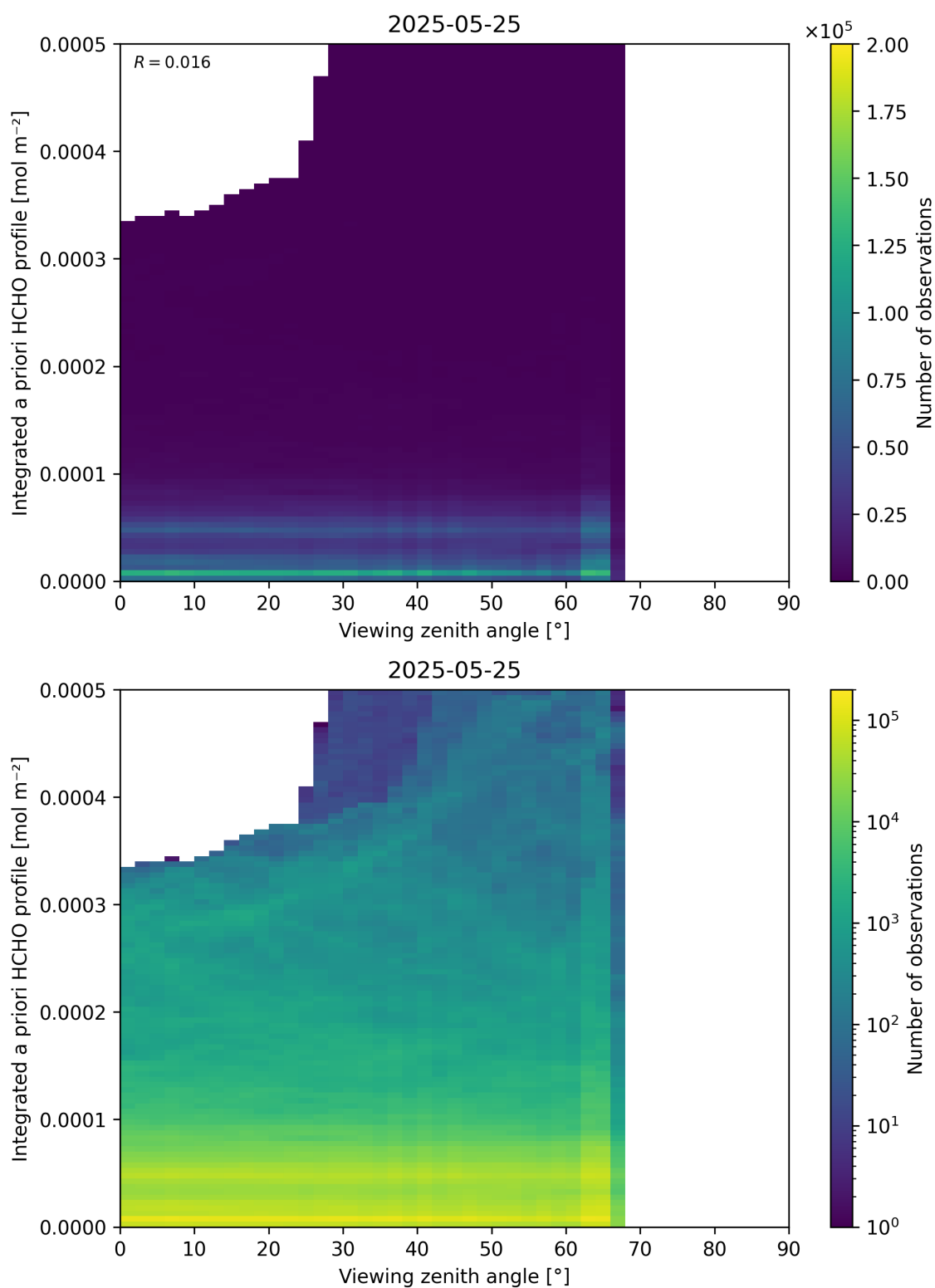
Figure 195: Scatter density plot of “Viewing zenith angle” against “Integrated a priori HCHO profile” for 2025-05-24 to 2025-05-26.
