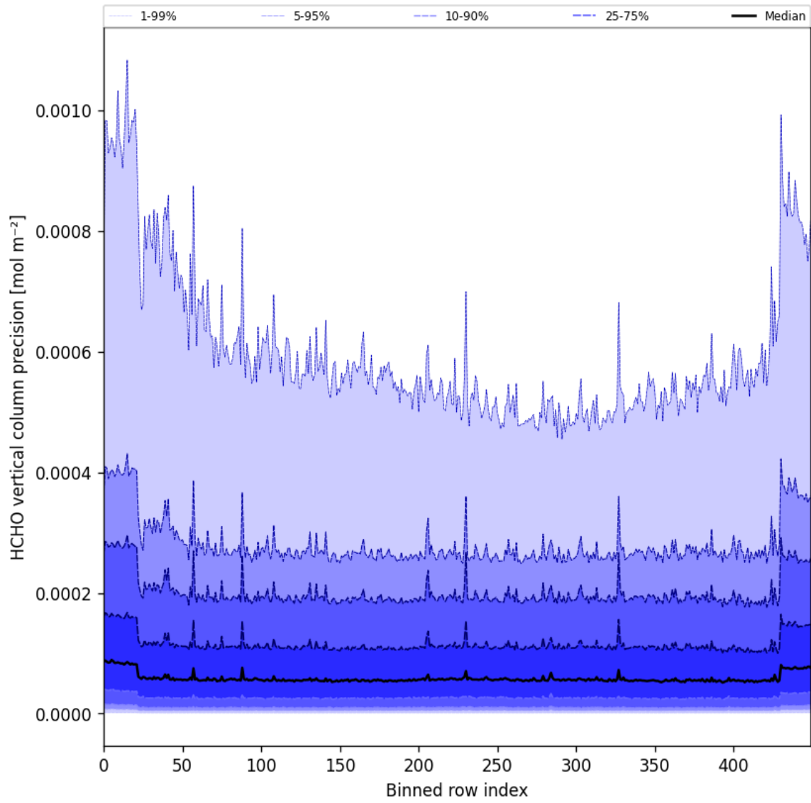
Figure 50: Along track statistics of “HCHO vertical column precision” for 2025-05-24 to 2025-05-26
