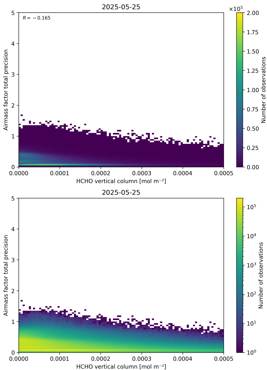
Figure 132: Scatter density plot of “HCHO vertical column” against “Airmass factor total precision” for 2025-05-24 to 2025-05-26.
