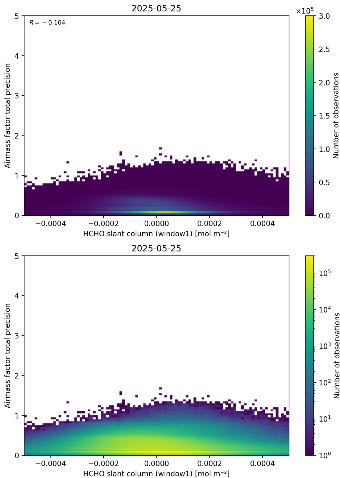
Figure 86: Scatter density plot of “HCHO slant column (window1)” against “Airmass factor total precision” for 2025-05-24 to 2025-05-26.
