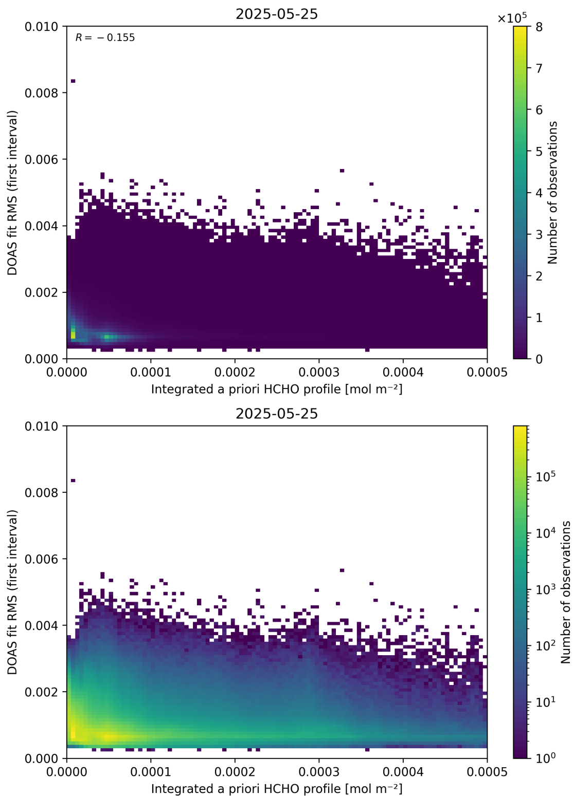
Figure 148: Scatter density plot of “Integrated a priori HCHO profile” against “DOAS fit RMS (first interval)” for 2025-05-24 to 2025-05-26.
