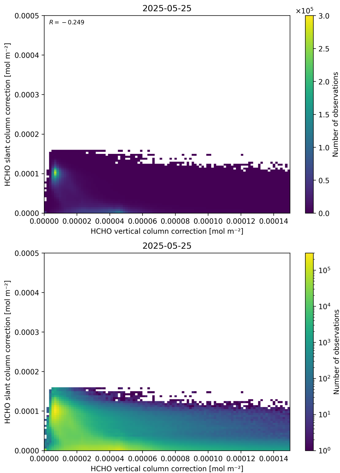
Figure 117: Scatter density plot of “HCHO vertical column correction” against “HCHO slant column correction” for 2025-05-24 to 2025-05-26.
