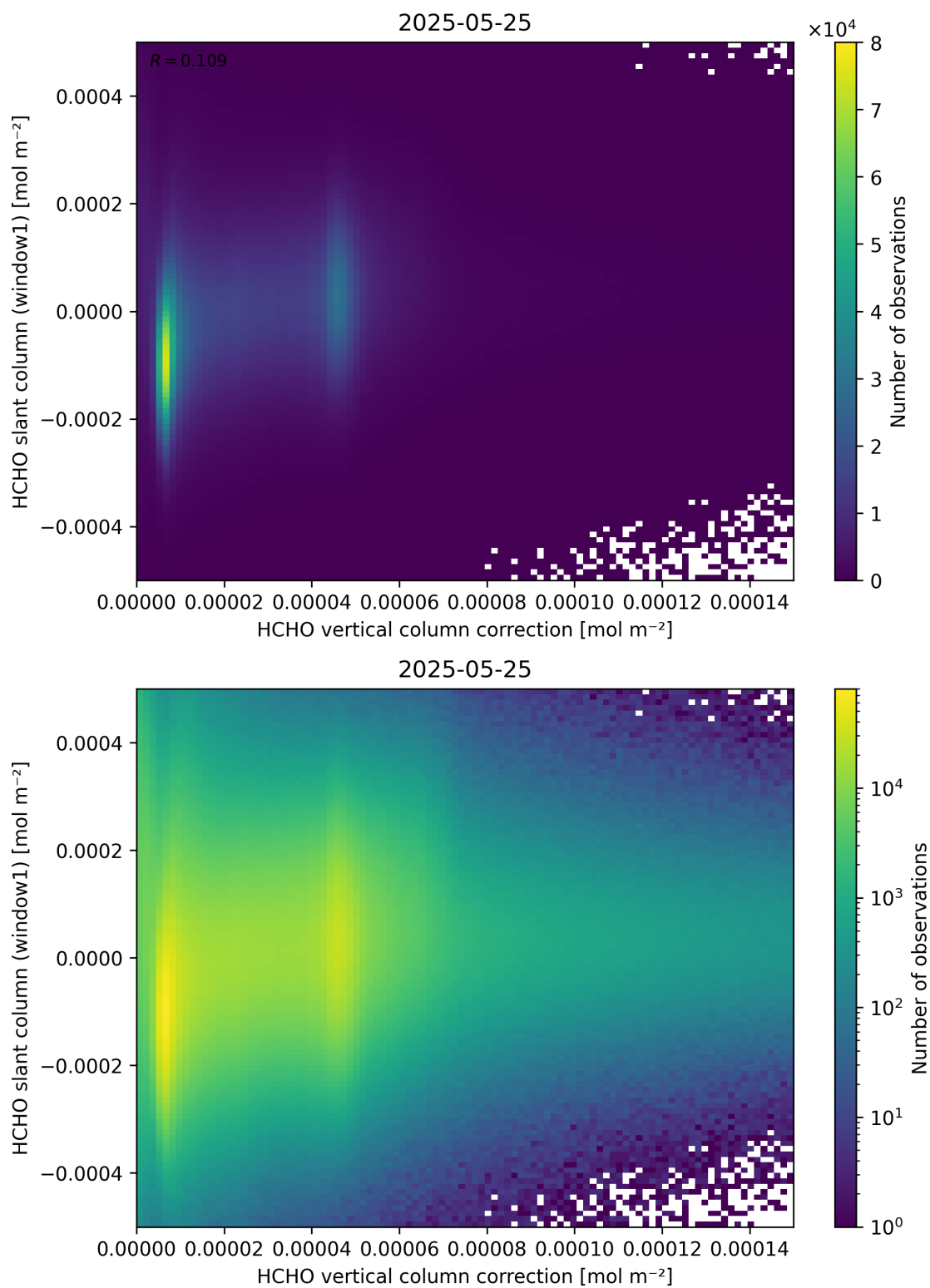
Figure 118: Scatter density plot of “HCHO vertical column correction” against “HCHO slant column (window1)” for 2025-05-24 to 2025-05-26.
