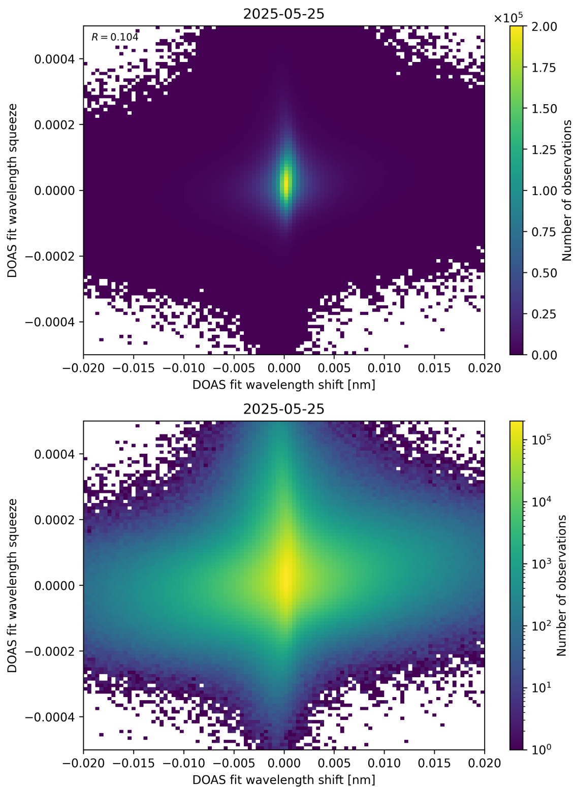
Figure 65: Scatter density plot of “DOAS fit wavelength shift” against “DOAS fit wavelength squeeze” for 2025-05-24 to 2025-05-26.
