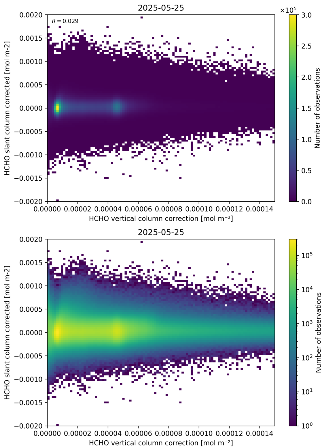
Figure 116: Scatter density plot of “HCHO vertical column correction” against “HCHO slant column corrected” for 2025-05-24 to 2025-05-26.
