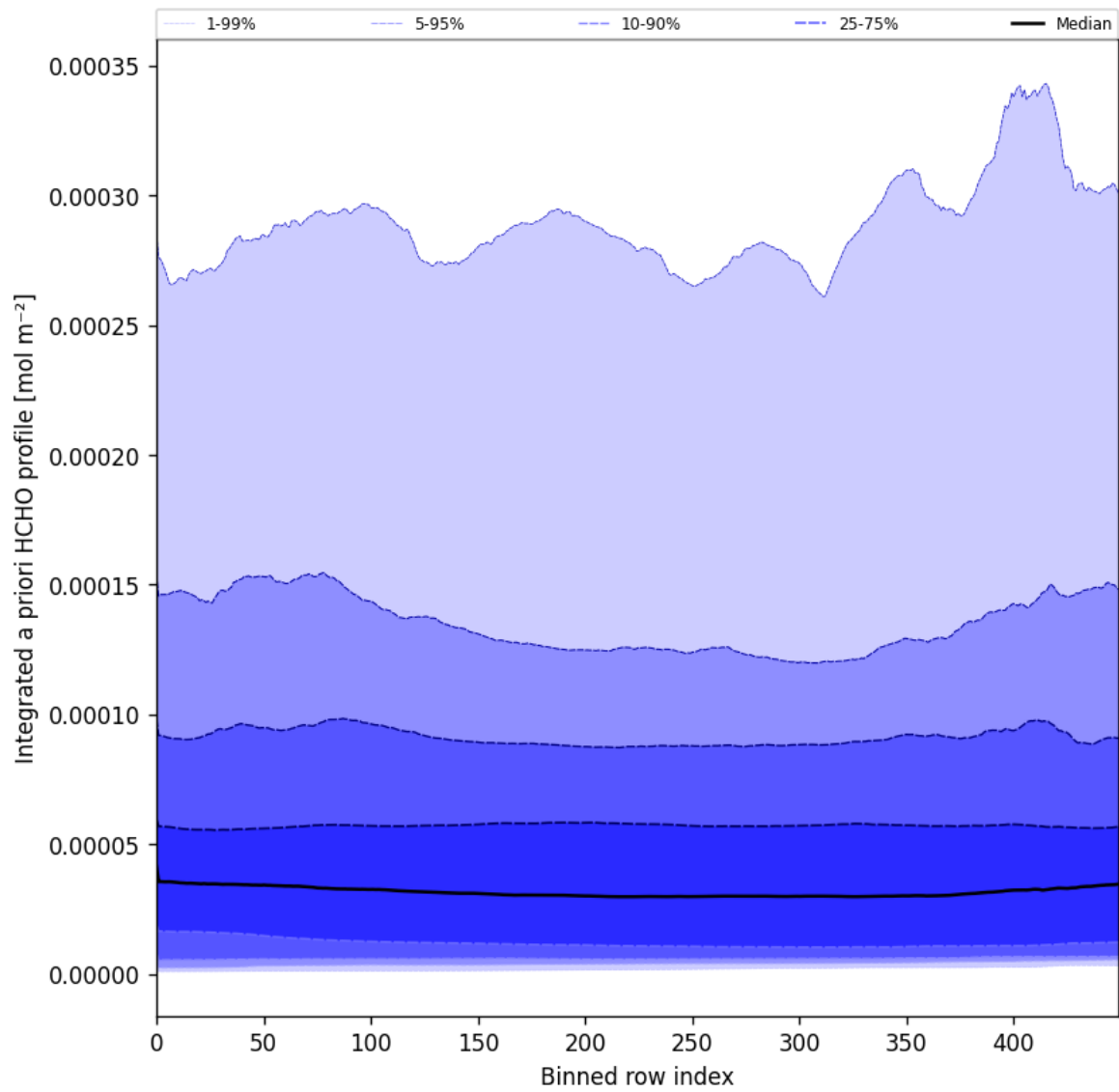
Figure 57: Along track statistics of “Integrated a priori HCHO profile” for 2025-05-26 to 2025-05-27
