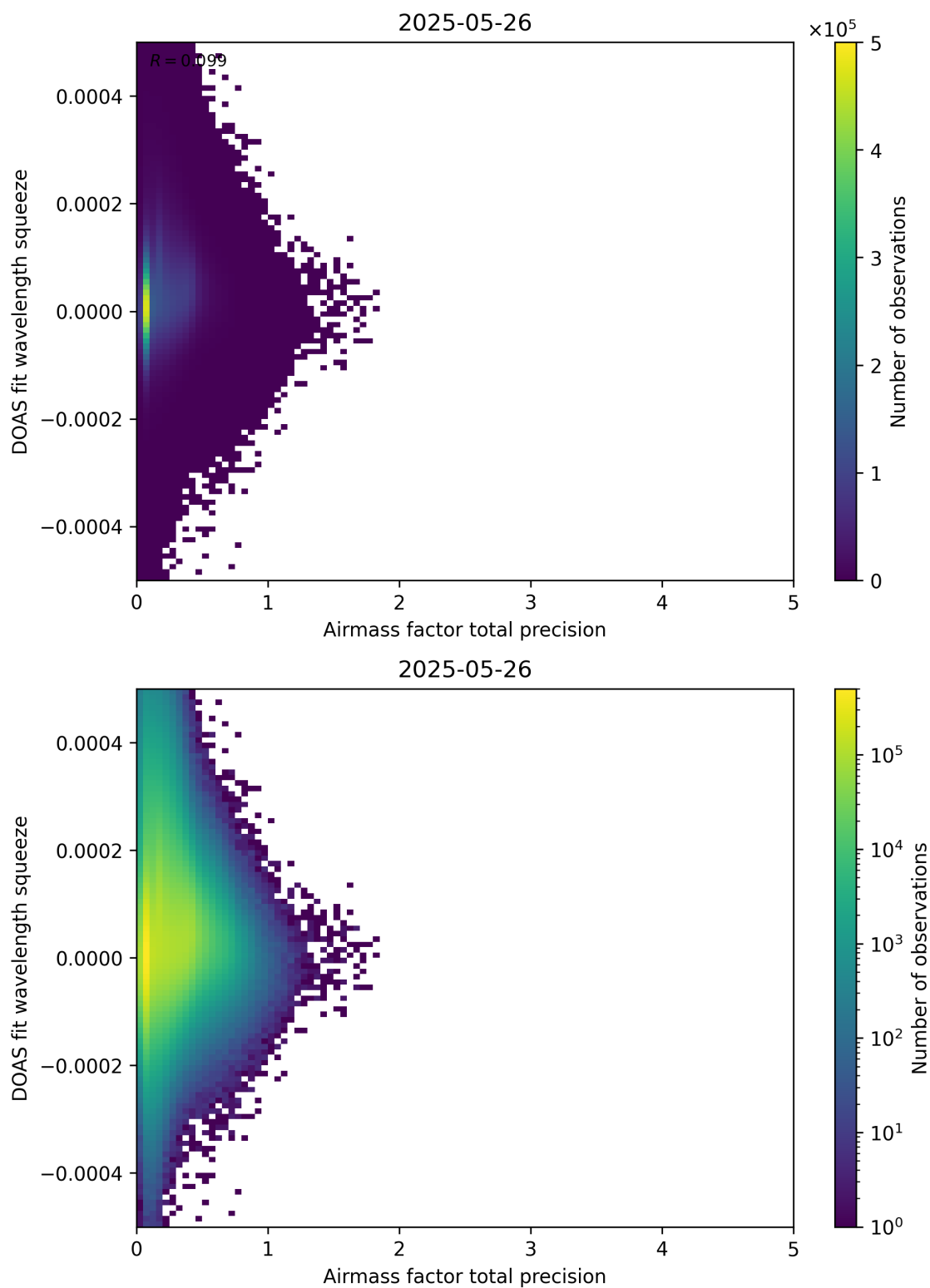
Figure 107: Scatter density plot of “Airmass factor total precision” against “DOAS fit wavelength squeeze” for 2025-05-26 to 2025-05-27.
