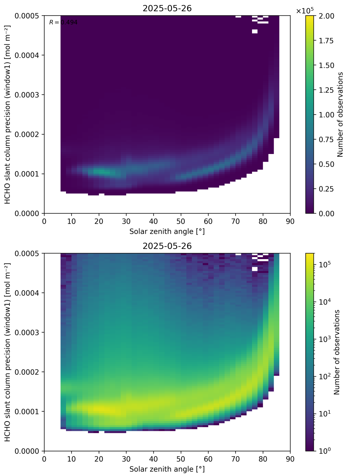
Figure 174: Scatter density plot of “Solar zenith angle” against “HCHO slant column precision (window1)” for 2025-05-26 to 2025-05-27.
