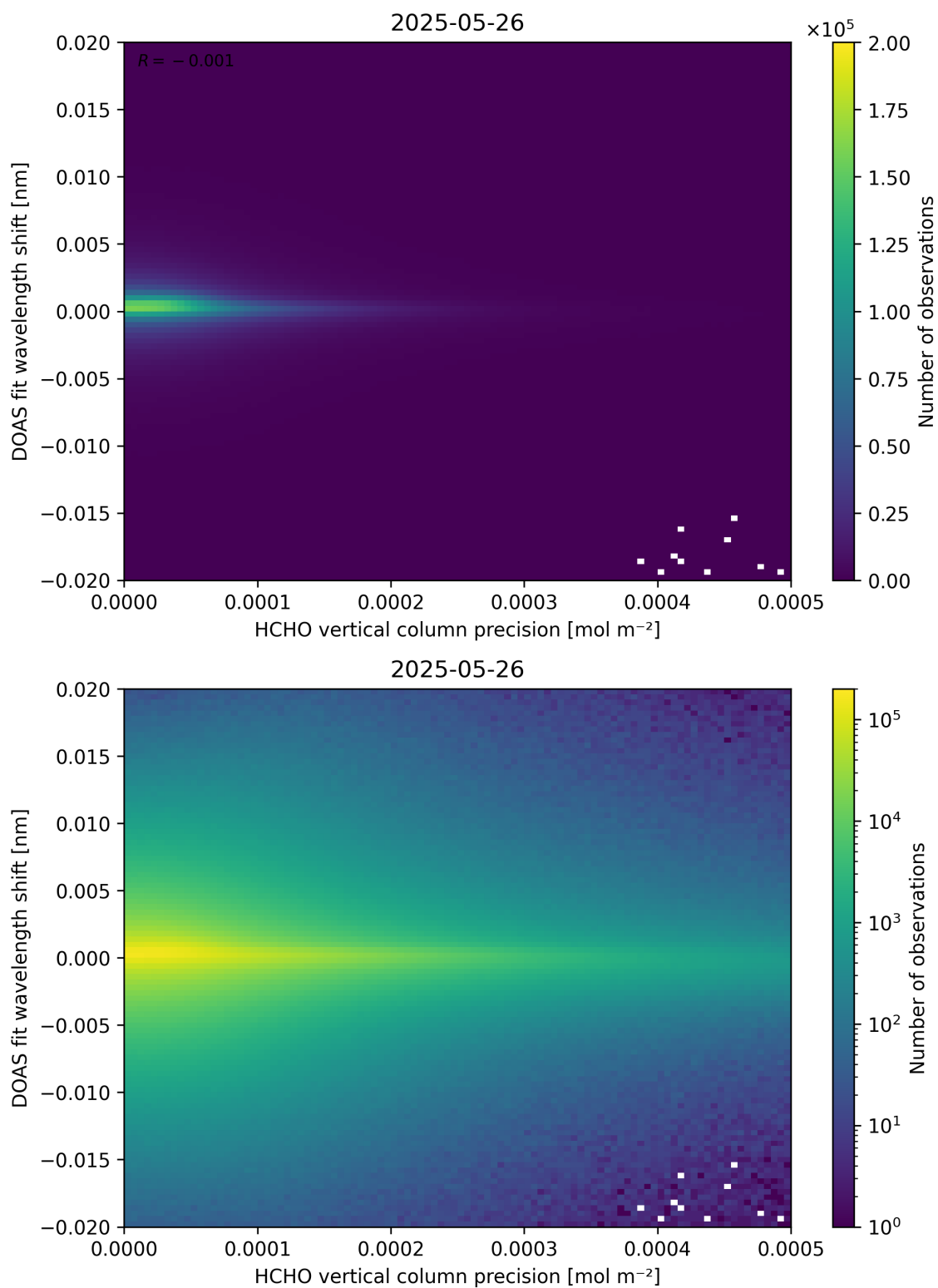
Figure 137: Scatter density plot of “HCHO vertical column precision” against “DOAS fit wavelength shift” for 2025-05-26 to 2025-05-27.
