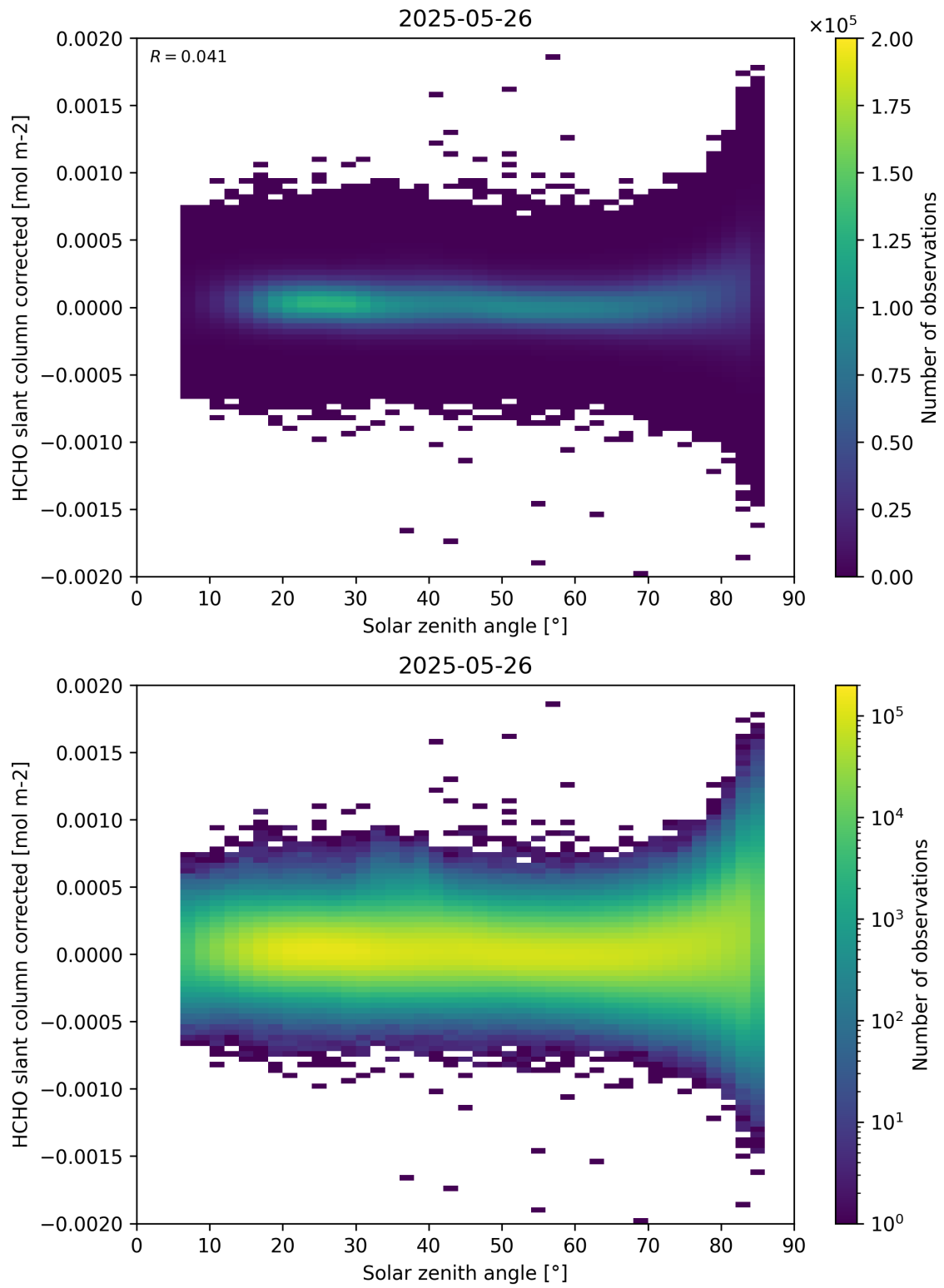
Figure 171: Scatter density plot of “Solar zenith angle” against “HCHO slant column corrected” for 2025-05-26 to 2025-05-27.
