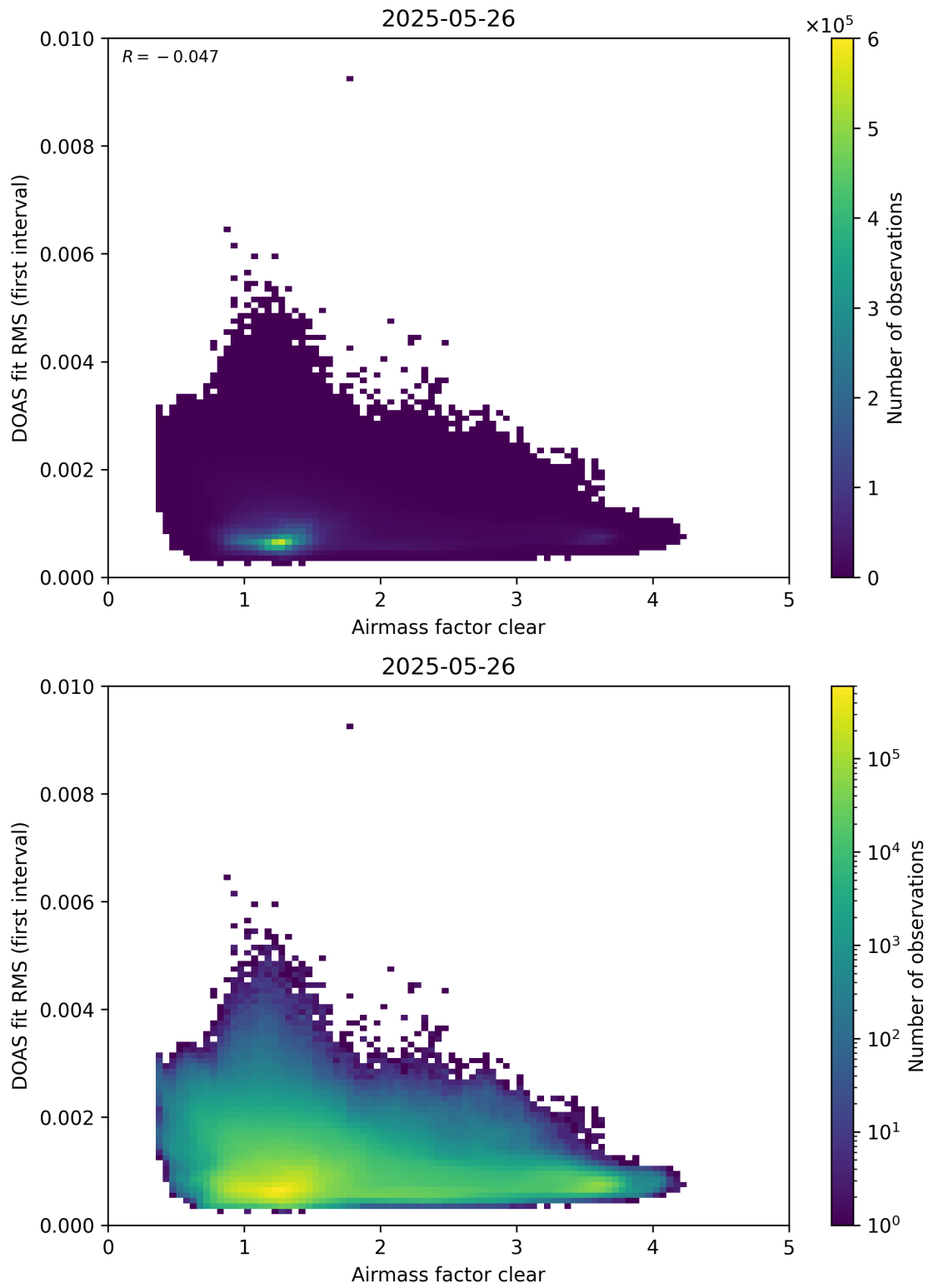
Figure 71: Scatter density plot of “Airmass factor clear” against “DOAS fit RMS (first interval)” for 2025-05-26 to 2025-05-27.
