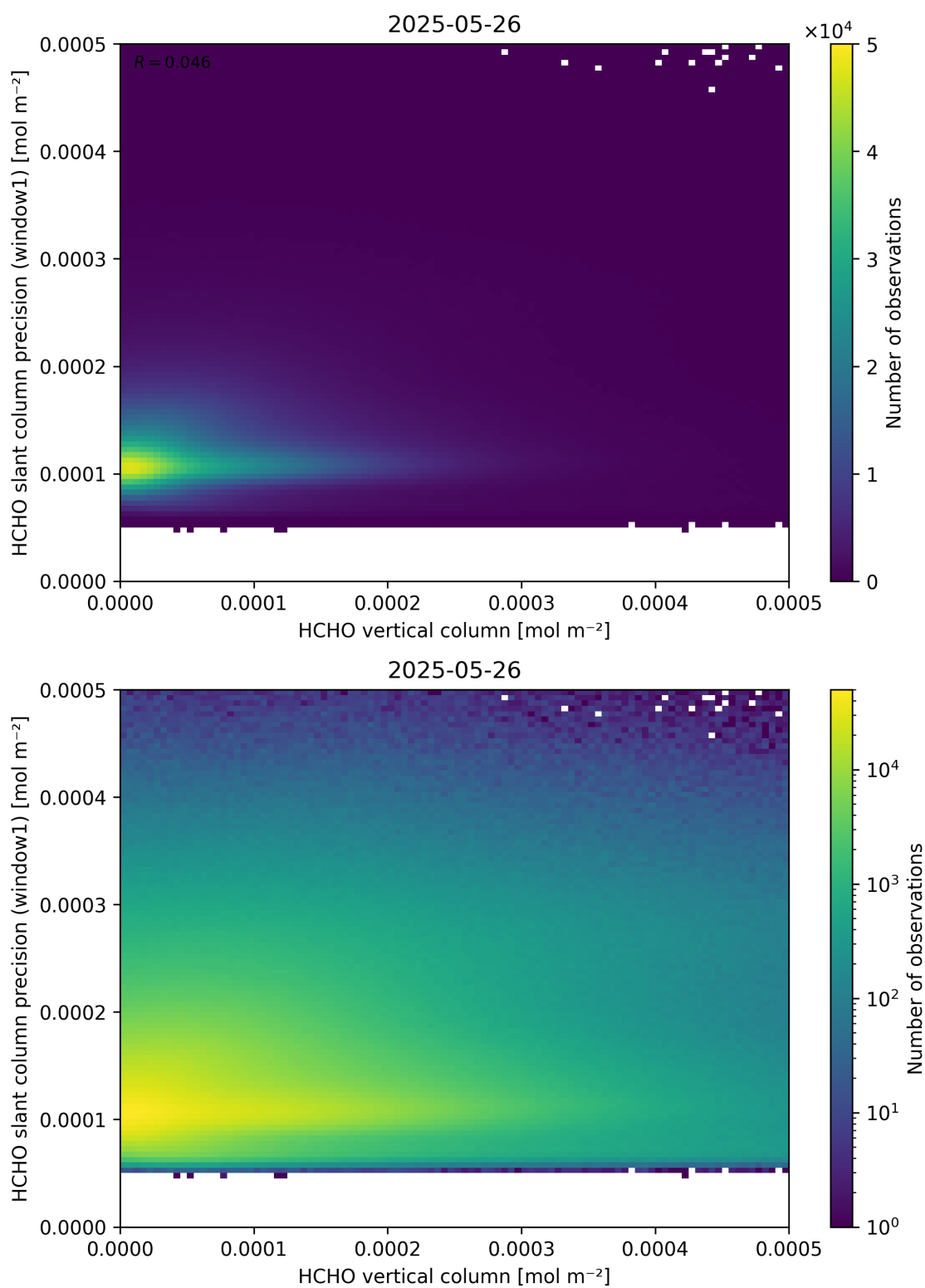
Figure 130: Scatter density plot of “HCHO vertical column” against “HCHO slant column precision (window1)” for 2025-05-26 to 2025-05-27.
