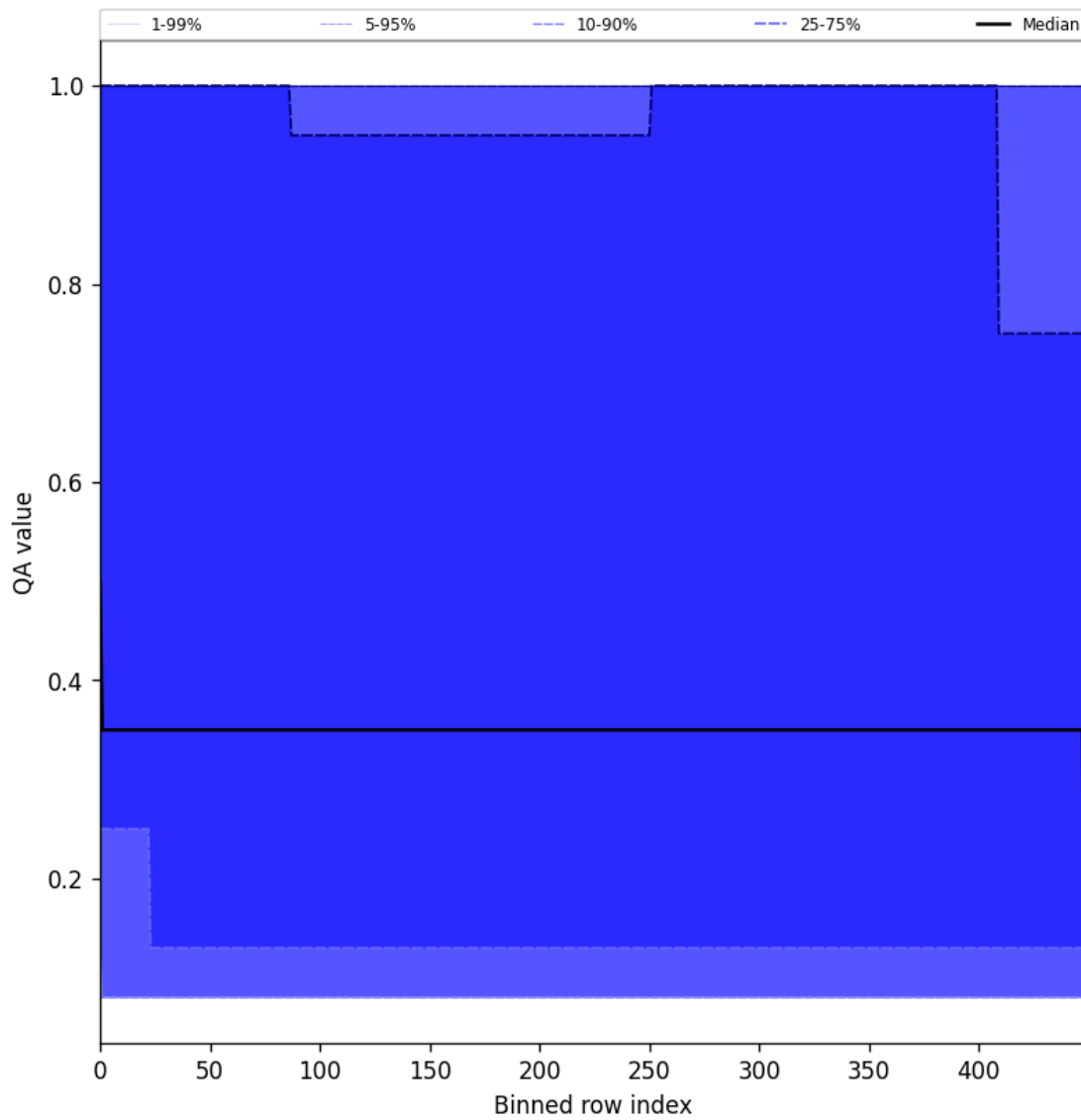
Figure 48: Along track statistics of “QA value” for 2025-05-26 to 2025-05-27
