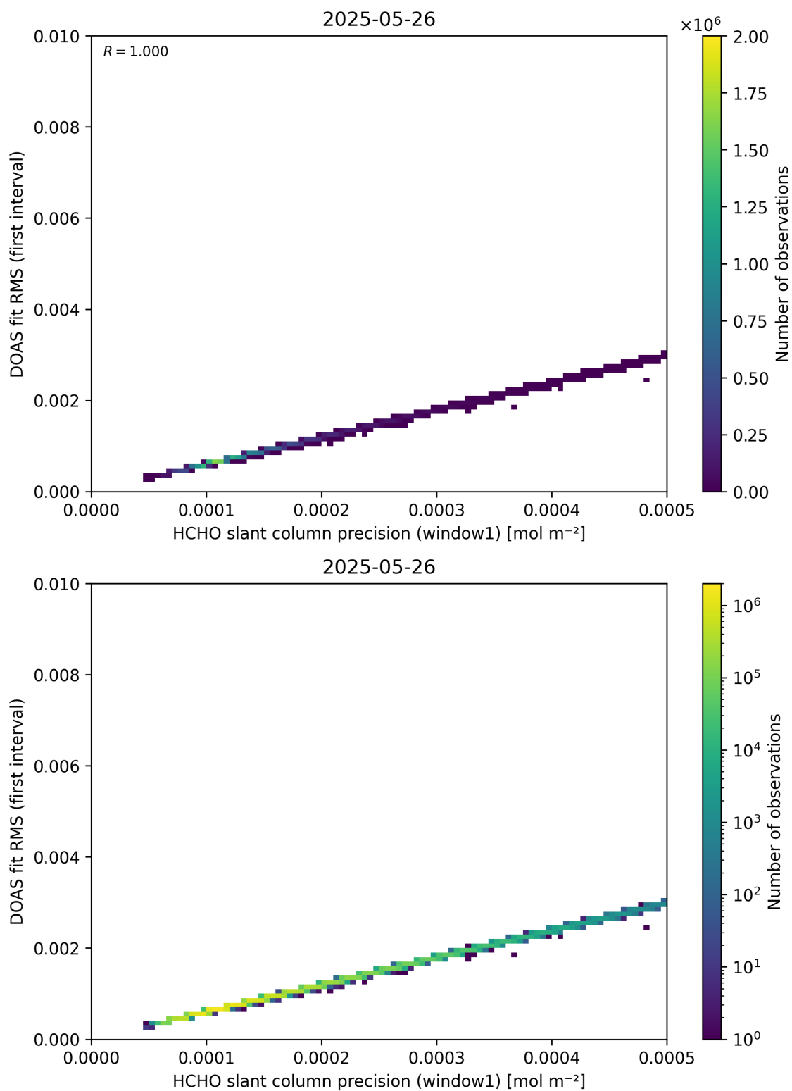
Figure 88: Scatter density plot of “HCHO slant column precision (window1)” against “DOAS fit RMS (first interval)” for 2025-05-26 to 2025-05-27.
