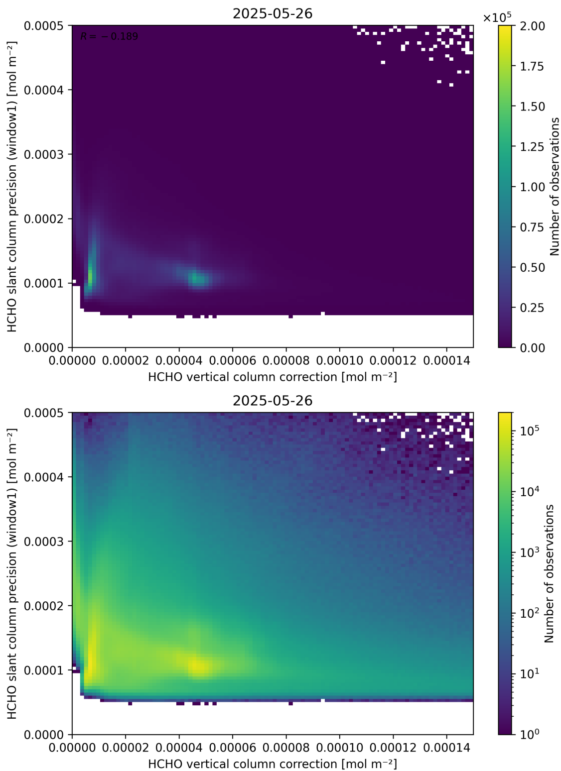
Figure 119: Scatter density plot of “HCHO vertical column correction” against “HCHO slant column precision (window1)” for 2025-05-26 to 2025-05-27.
