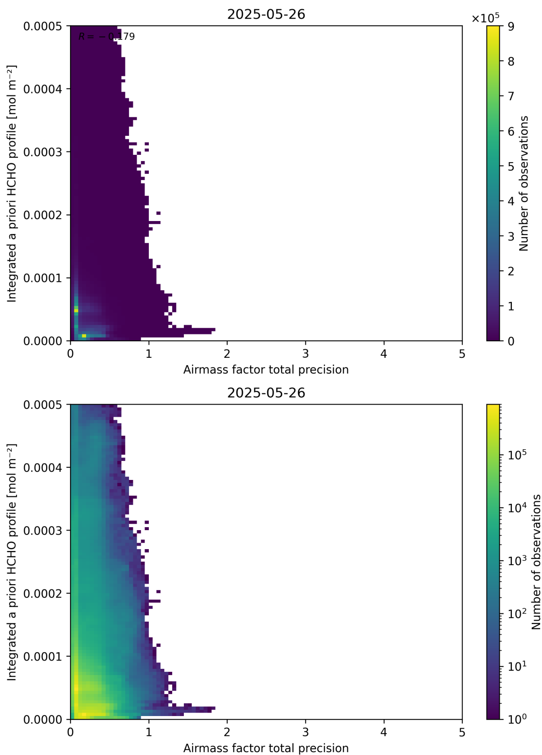
Figure 111: Scatter density plot of “Airmass factor total precision” against “Integrated a priori HCHO profile” for 2025-05-26 to 2025-05-27.
