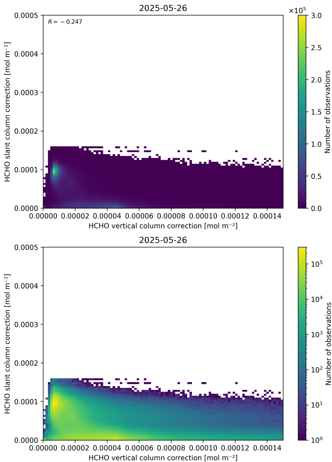
Figure 117: Scatter density plot of “HCHO vertical column correction” against “HCHO slant column correction” for 2025-05-26 to 2025-05-27.
