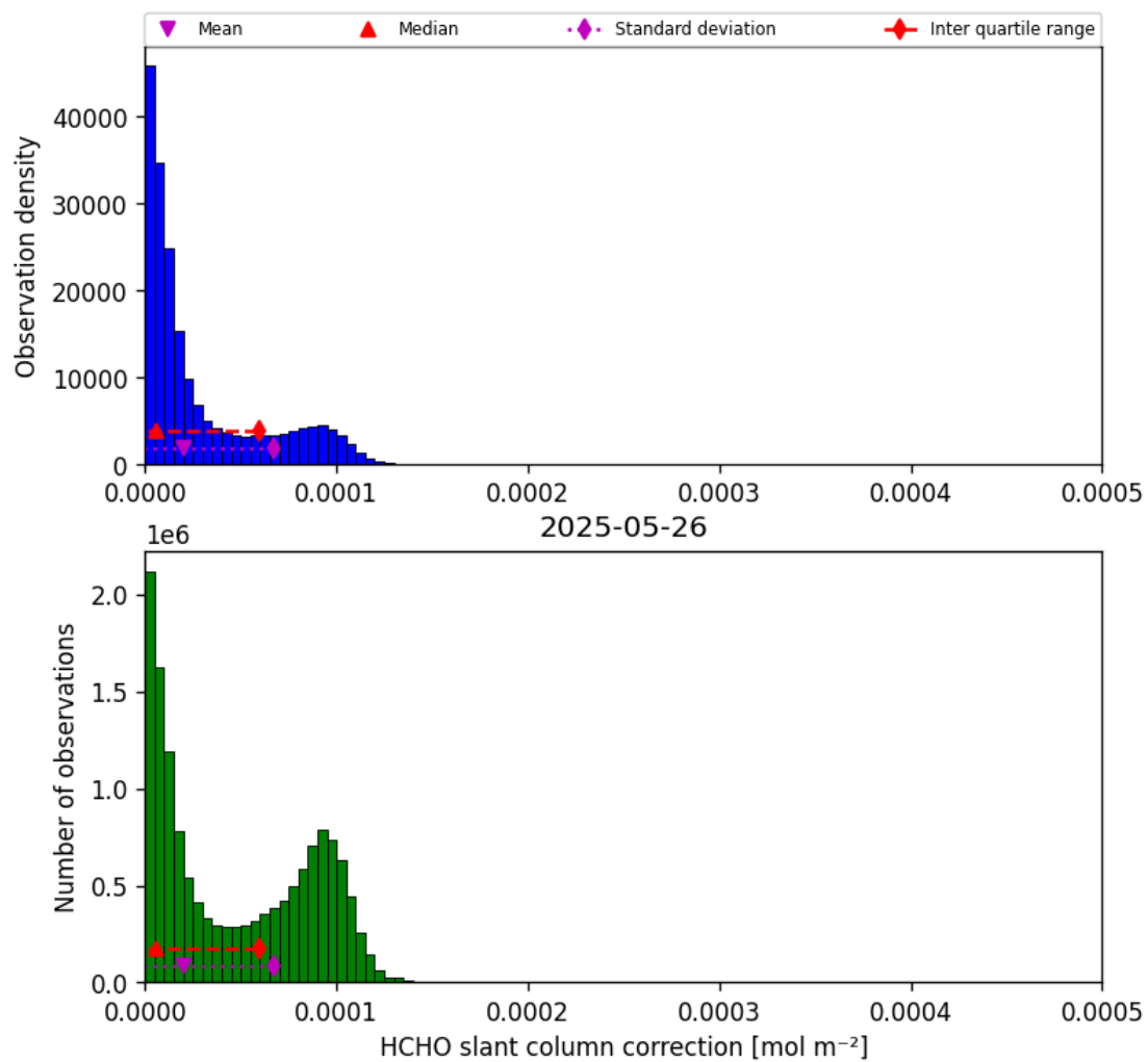
Figure 47: Histogram of “HCHO slant column correction” for 2025-05-26 to 2025-05-27
