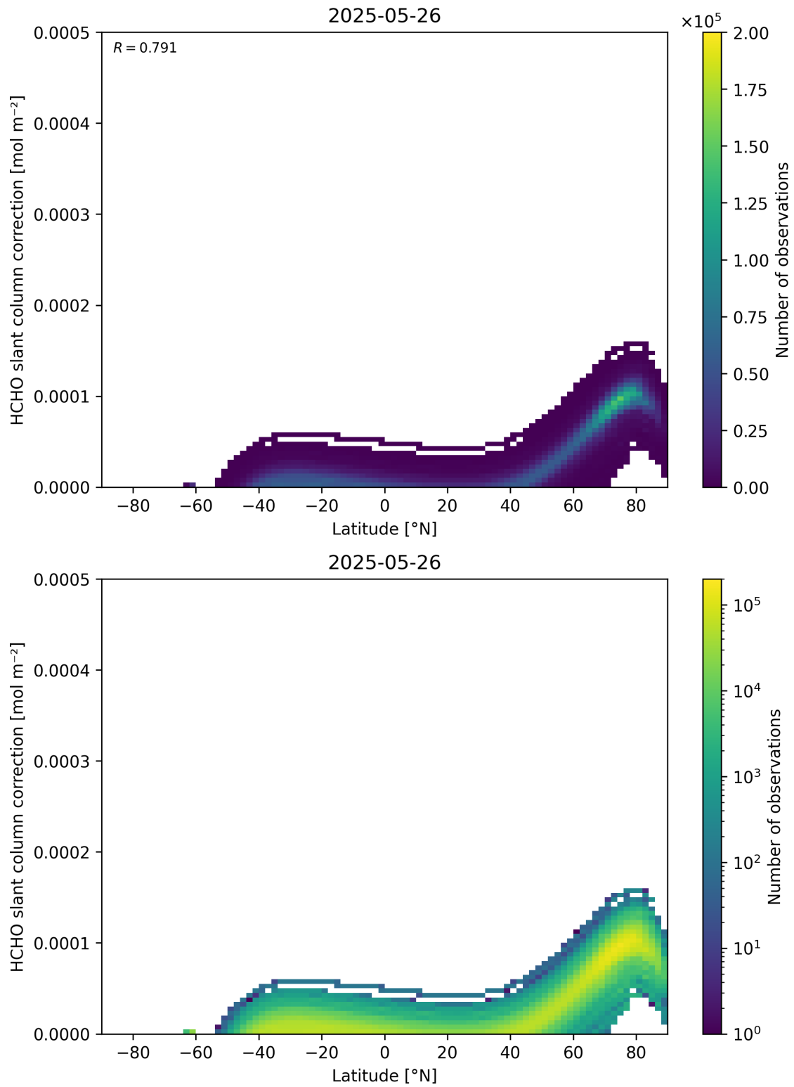
Figure 158: Scatter density plot of “Latitude” against “HCHO slant column correction” for 2025-05-26 to 2025-05-27.
