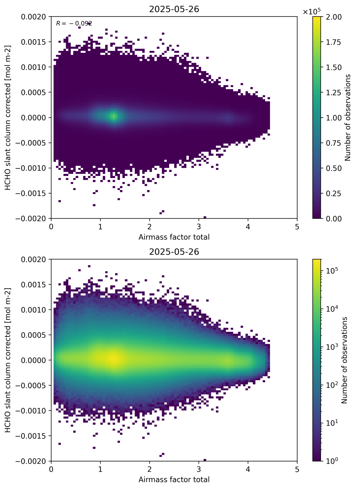
Figure 101: Scatter density plot of “Airmass factor total” against “HCHO slant column corrected” for 2025-05-26 to 2025-05-27.
