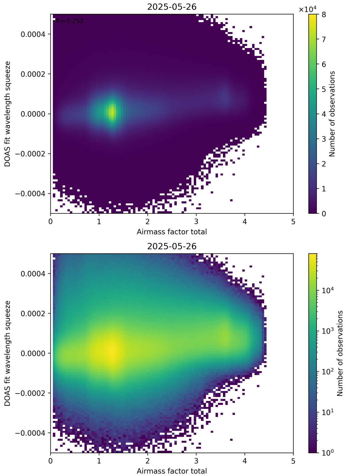
Figure 99: Scatter density plot of “Airmass factor total” against “DOAS fit wavelength squeeze” for 2025-05-26 to 2025-05-27.
