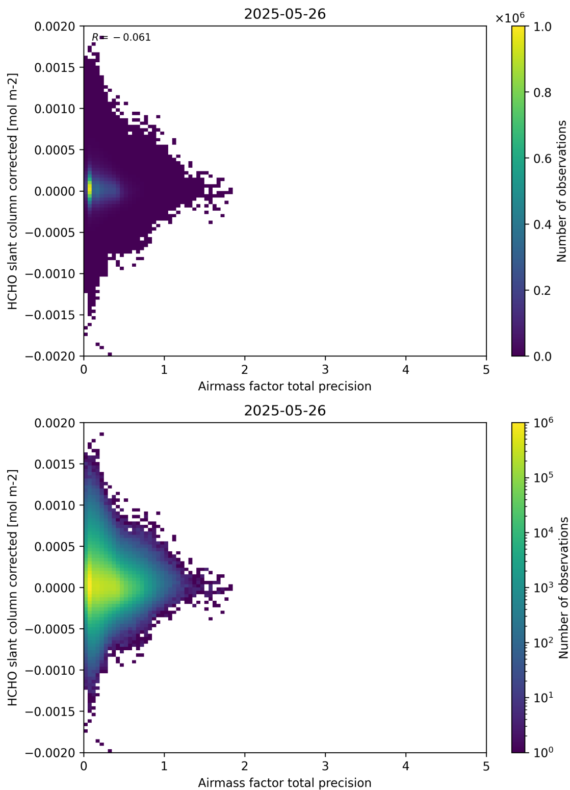
Figure 109: Scatter density plot of “Airmass factor total precision” against “HCHO slant column corrected” for 2025-05-26 to 2025-05-27.
