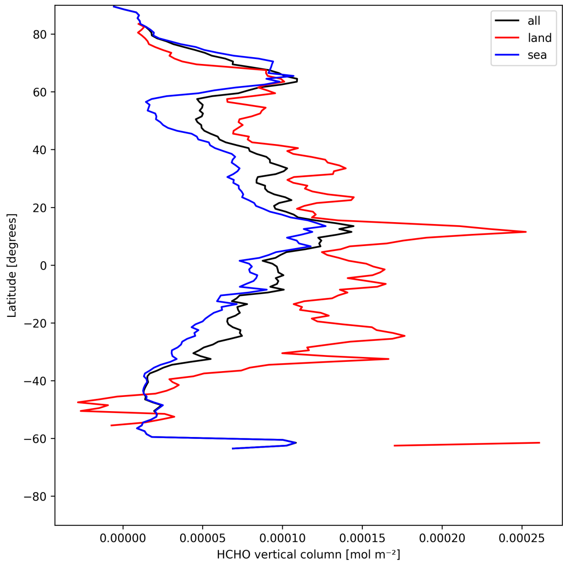
Figure 21: Zonal average of “HCHO vertical column” for 2025-05-26 to 2025-05-27.
