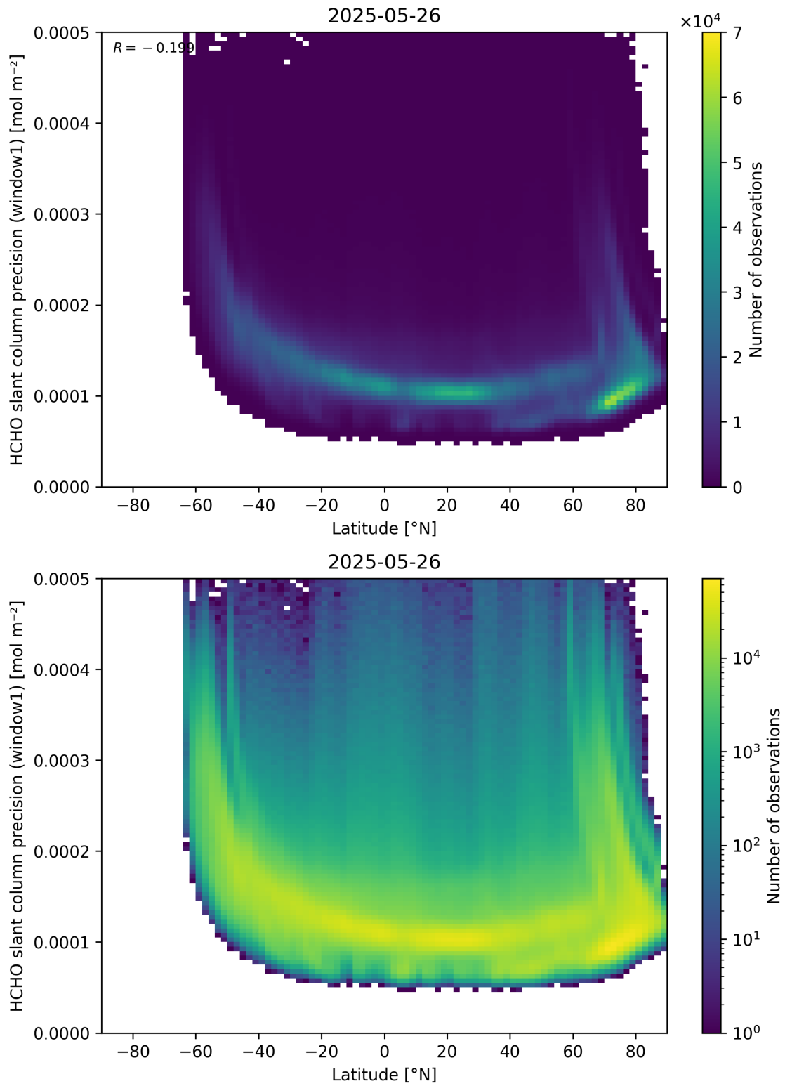
Figure 160: Scatter density plot of “Latitude” against “HCHO slant column precision (window1)” for 2025-05-26 to 2025-05-27.
