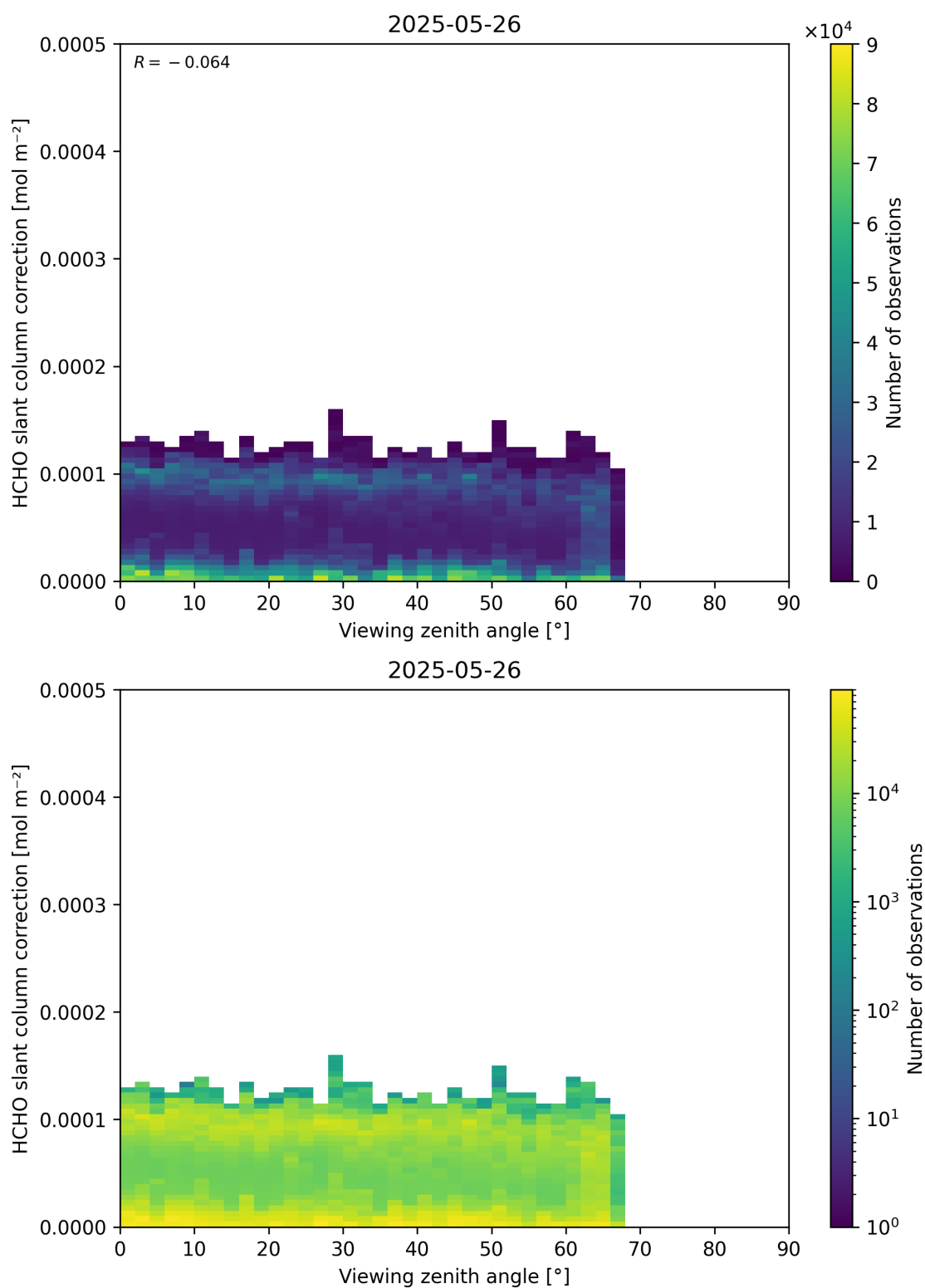
Figure 187: Scatter density plot of “Viewing zenith angle” against “HCHO slant column correction” for 2025-05-26 to 2025-05-27.
