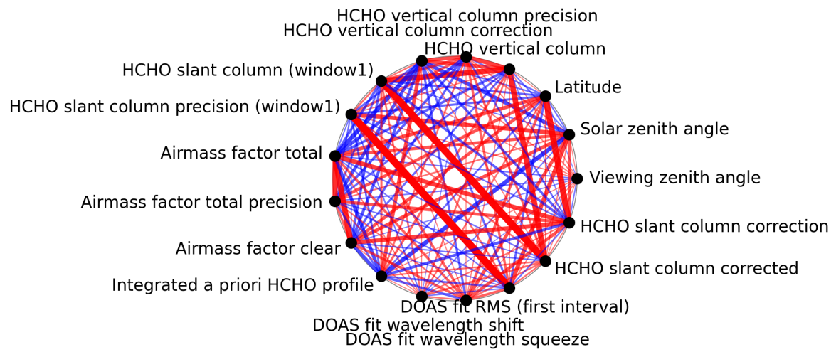
Figure 1: Map of correlation graph for 2025-05-26 to 2025-05-27.
