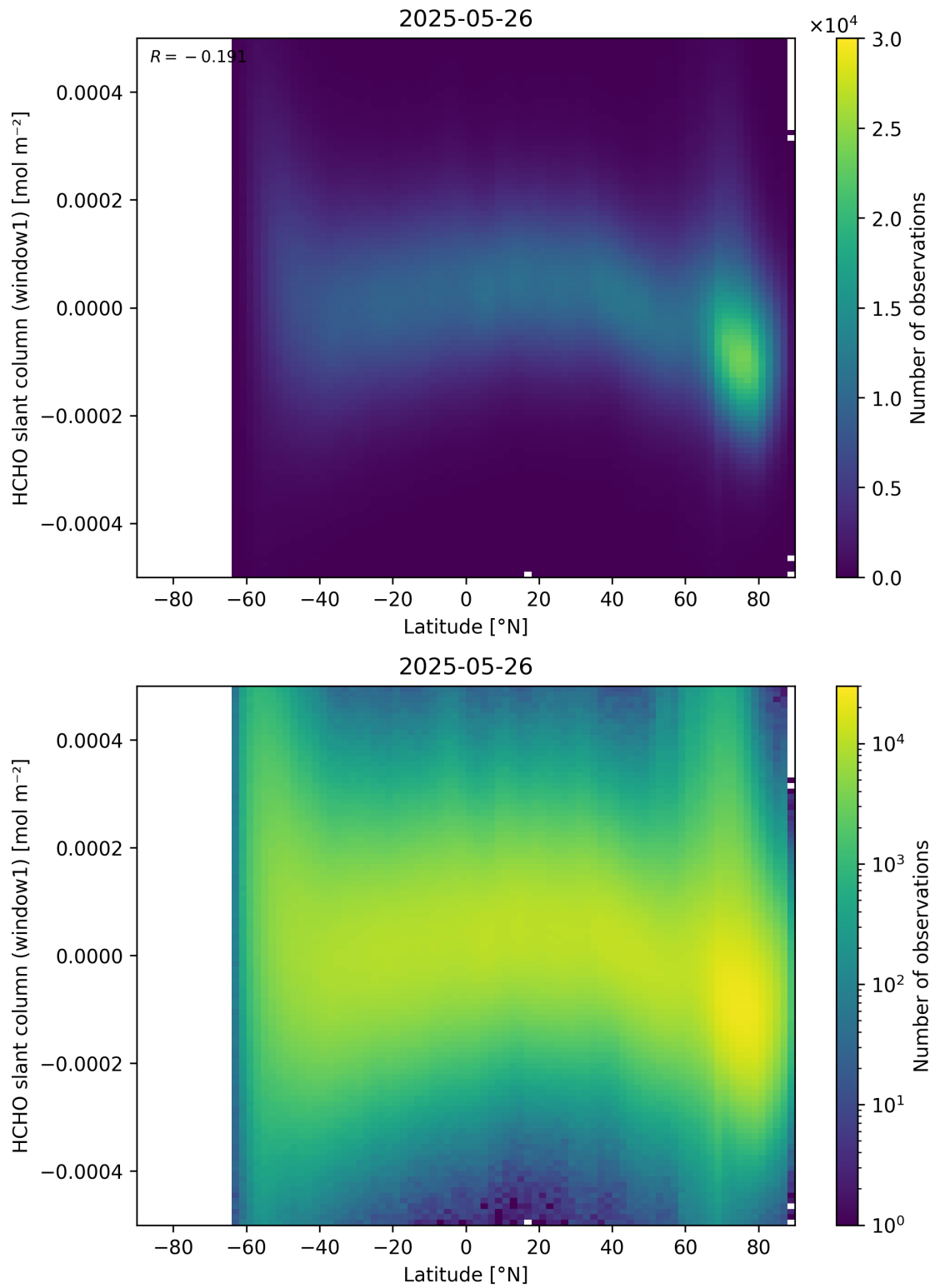
Figure 159: Scatter density plot of “Latitude” against “HCHO slant column (window1)” for 2025-05-26 to 2025-05-27.
