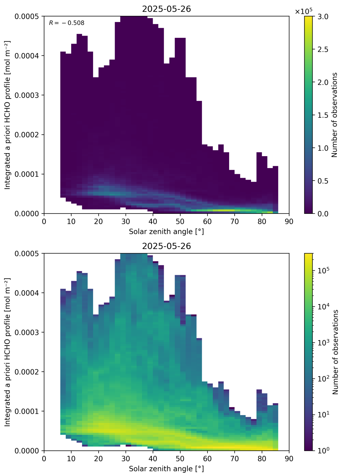
Figure 180: Scatter density plot of “Solar zenith angle” against “Integrated a priori HCHO profile” for 2025-05-26 to 2025-05-27.
