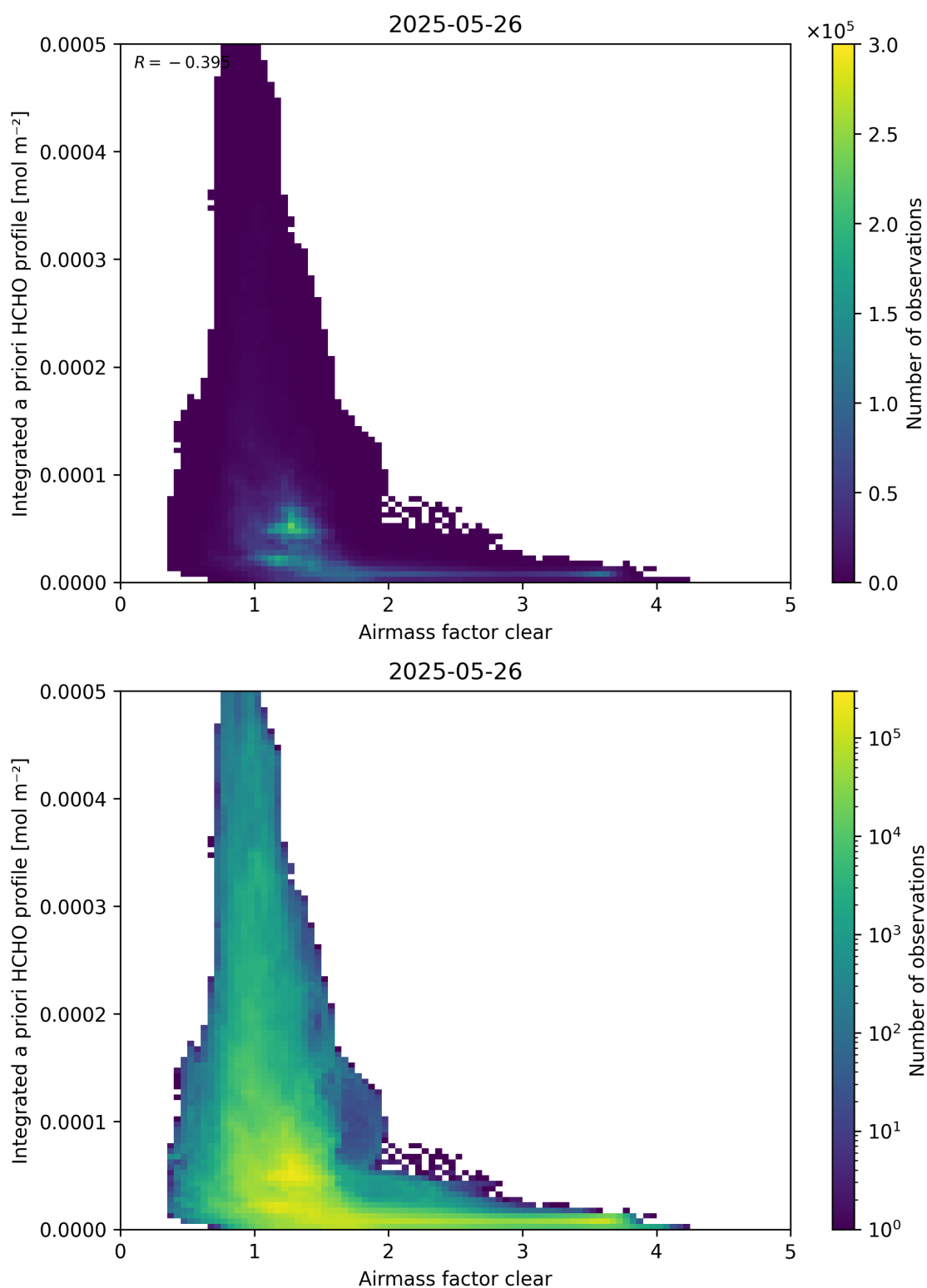
Figure 76: Scatter density plot of “Airmass factor clear” against “Integrated a priori HCHO profile” for 2025-05-26 to 2025-05-27.
