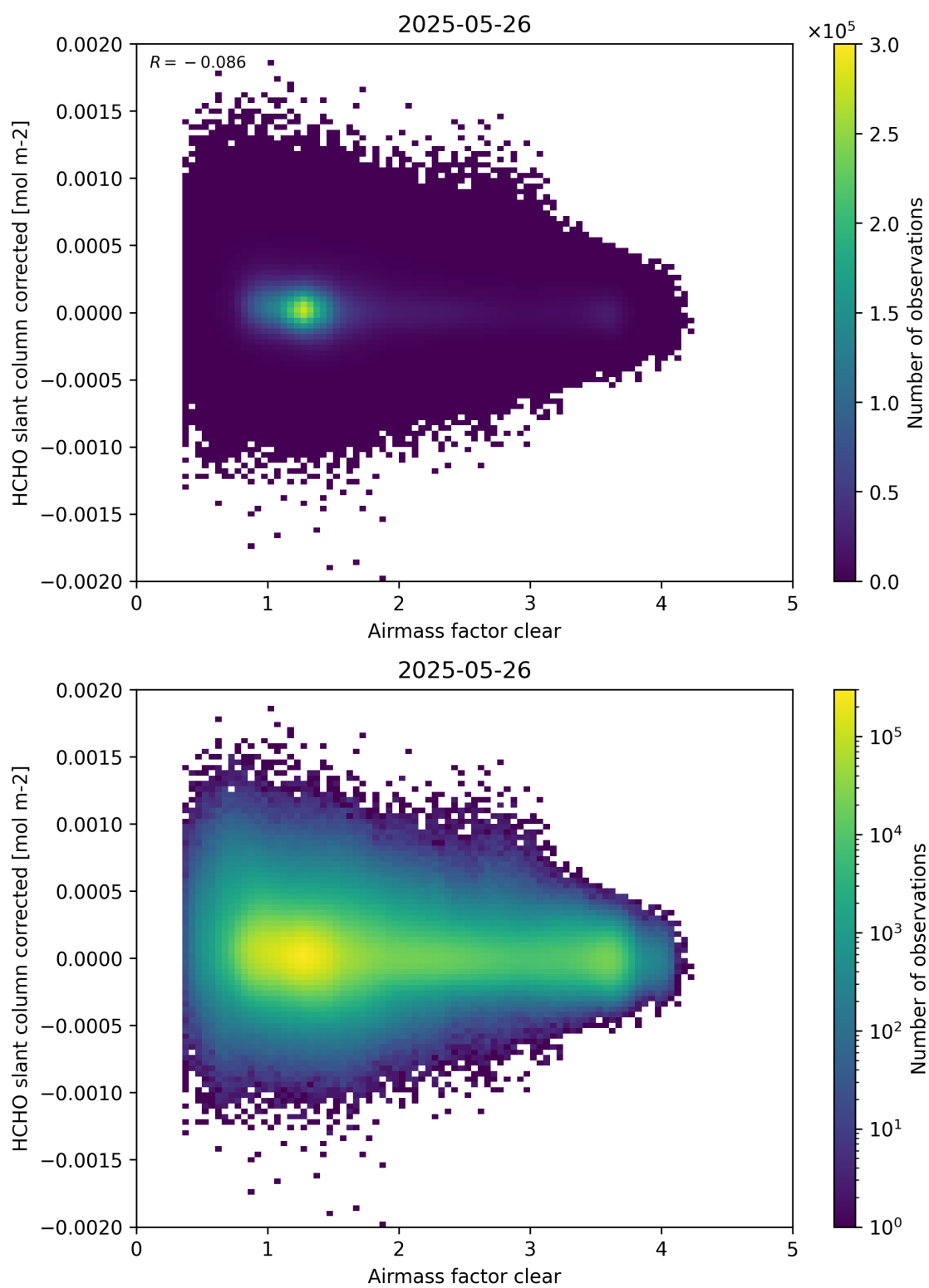
Figure 74: Scatter density plot of “Airmass factor clear” against “HCHO slant column corrected” for 2025-05-26 to 2025-05-27.
