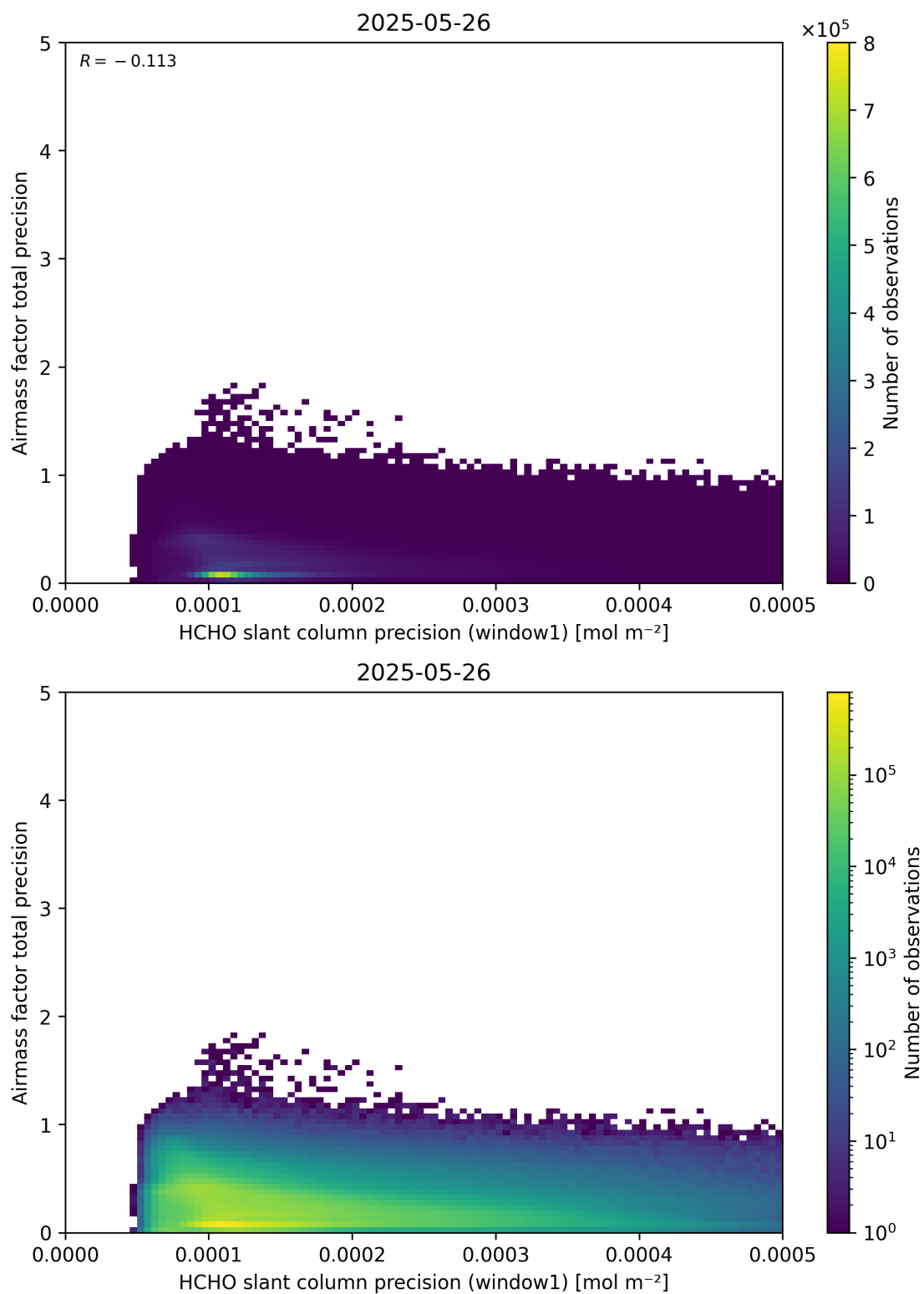
Figure 95: Scatter density plot of “HCHO slant column precision (window1)” against “Airmass factor total precision” for 2025-05-26 to 2025-05-27.
