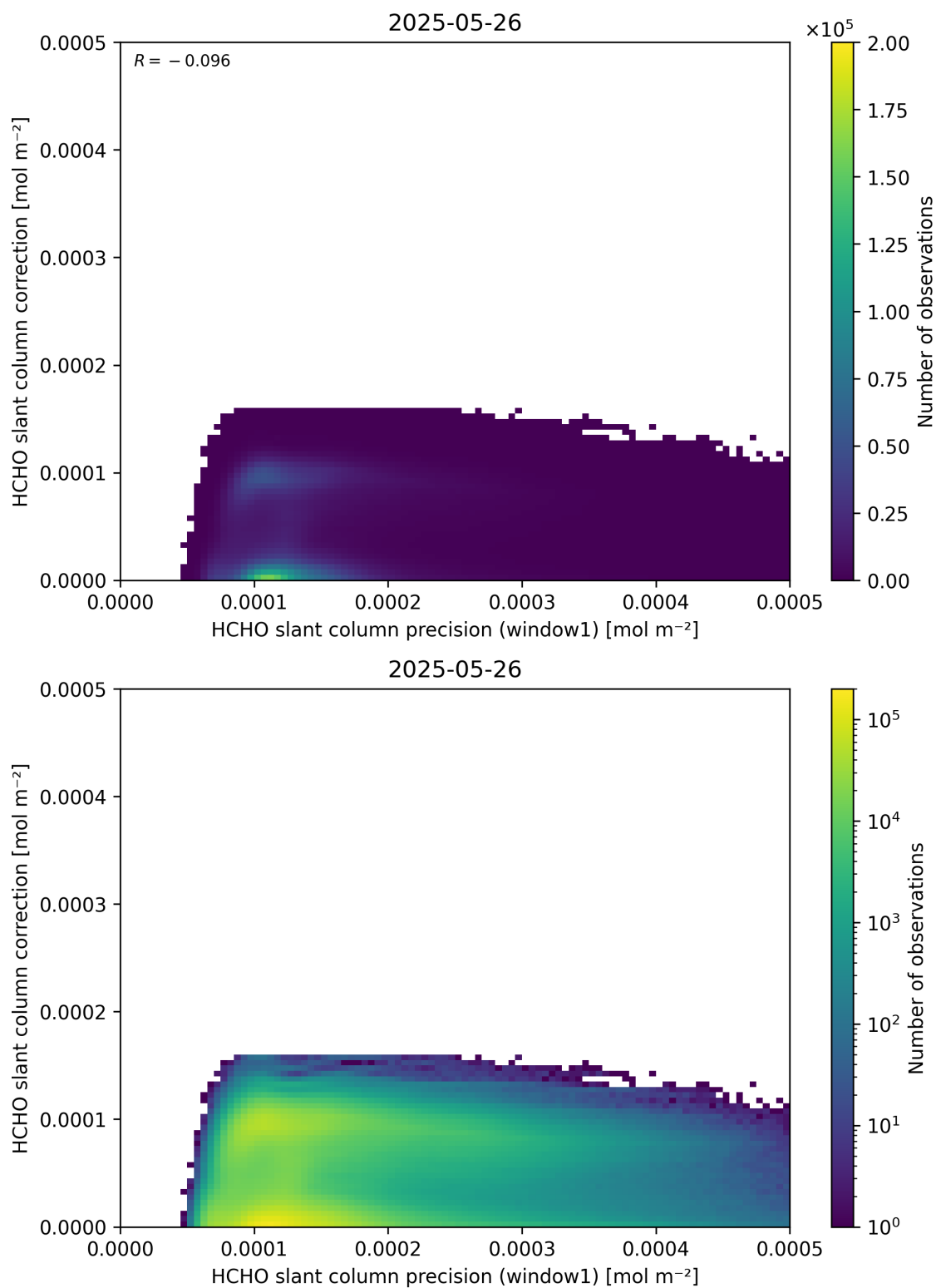
Figure 93: Scatter density plot of “HCHO slant column precision (window1)” against “HCHO slant column correction” for 2025-05-26 to 2025-05-27.
