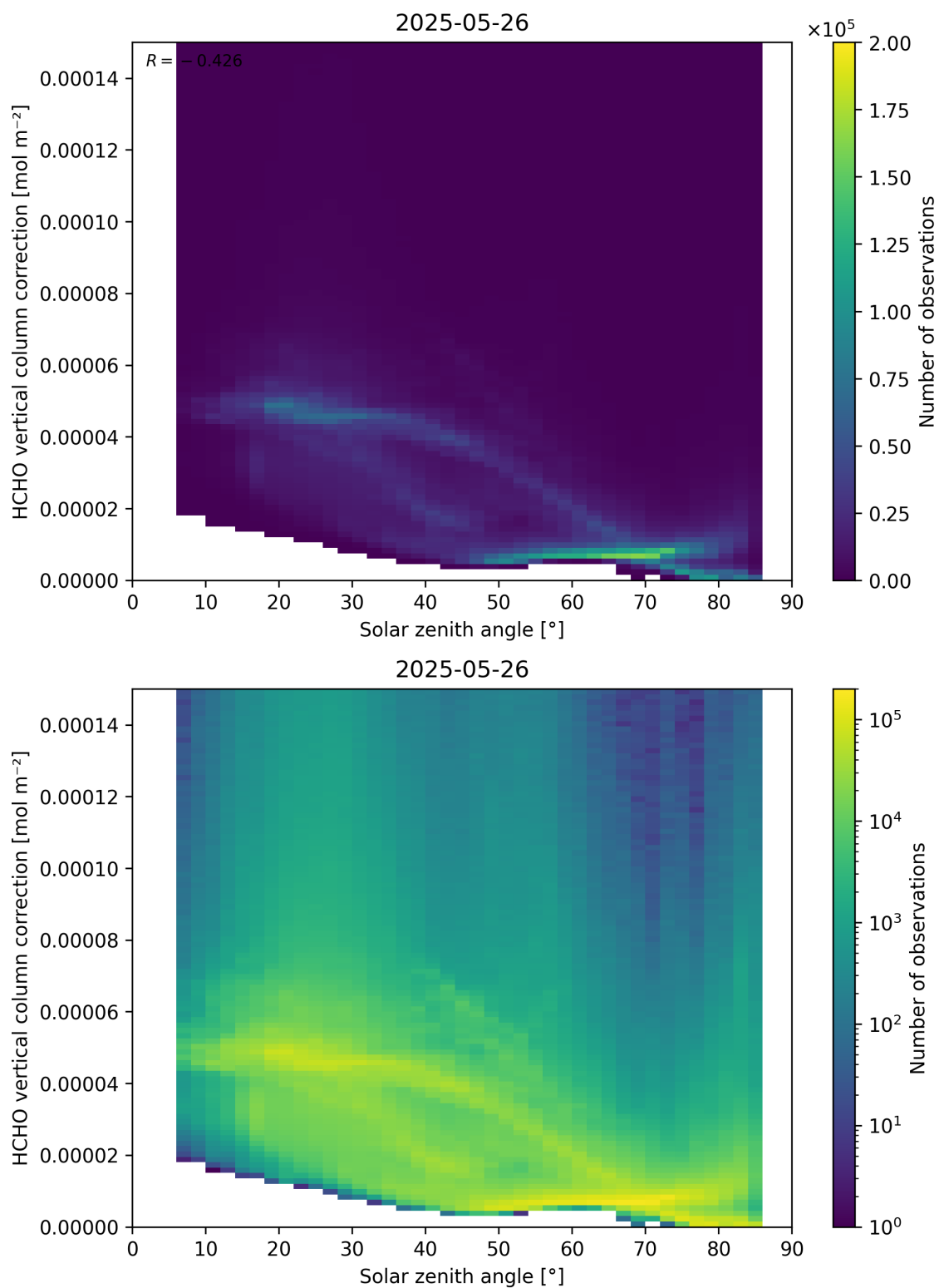
Figure 178: Scatter density plot of “Solar zenith angle” against “HCHO vertical column correction” for 2025-05-26 to 2025-05-27.
