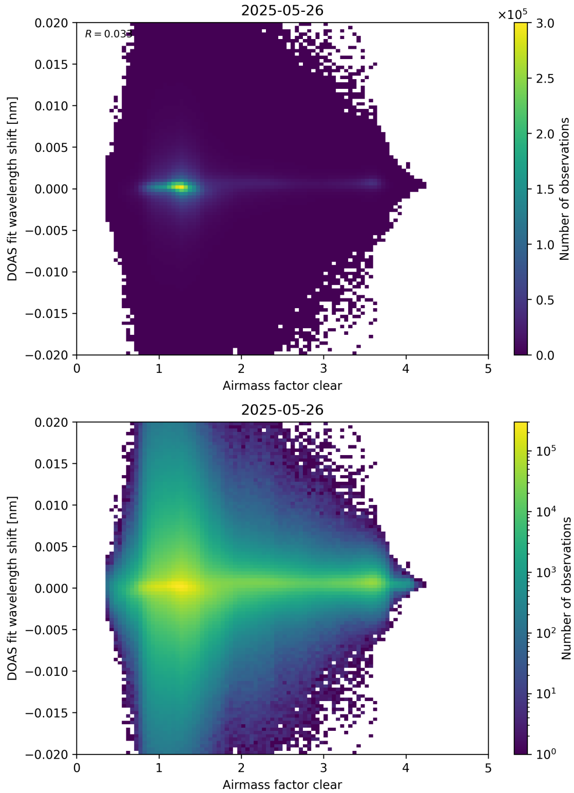
Figure 72: Scatter density plot of “Airmass factor clear” against “DOAS fit wavelength shift” for 2025-05-26 to 2025-05-27.
