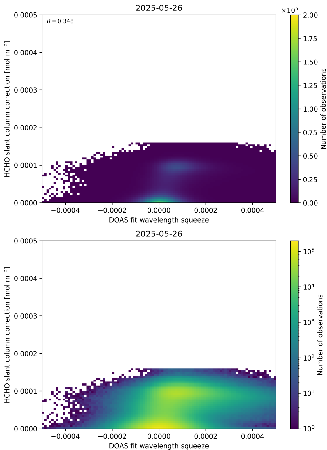
Figure 70: Scatter density plot of “DOAS fit wavelength squeeze” against “HCHO slant column correction” for 2025-05-26 to 2025-05-27.
