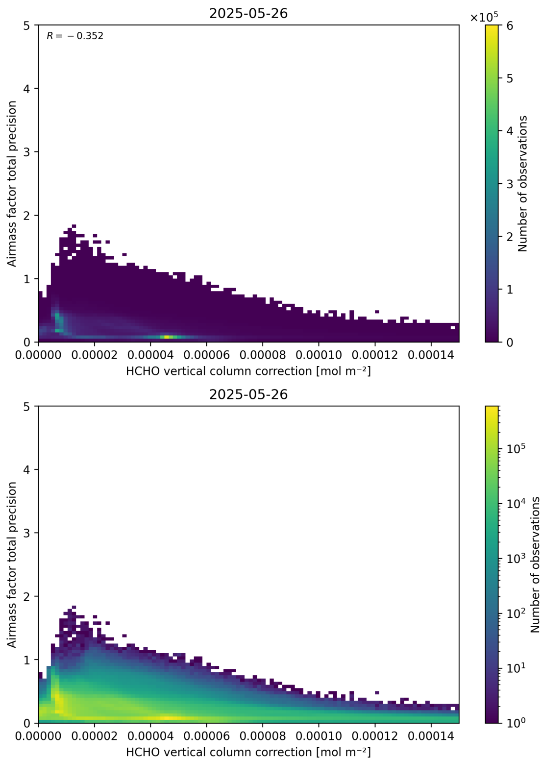
Figure 121: Scatter density plot of “HCHO vertical column correction” against “Airmass factor total precision” for 2025-05-26 to 2025-05-27.
