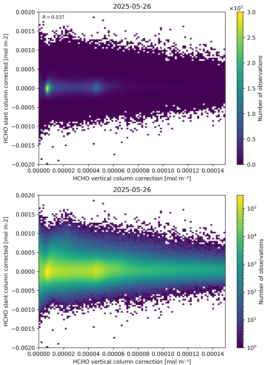
Figure 116: Scatter density plot of “HCHO vertical column correction” against “HCHO slant column corrected” for 2025-05-26 to 2025-05-27.
