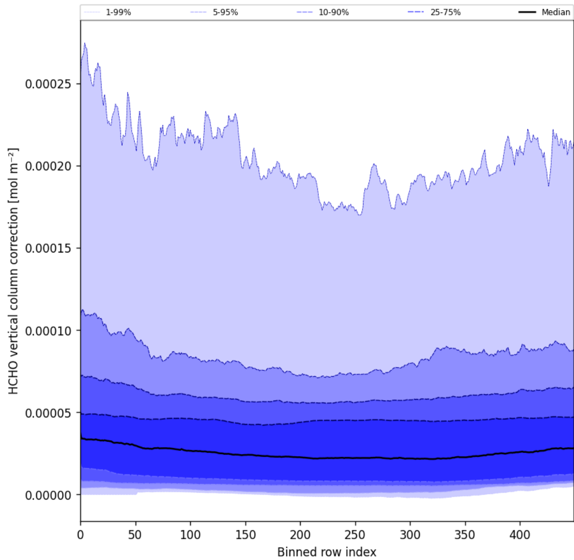
Figure 51: Along track statistics of “HCHO vertical column correction” for 2025-05-26 to 2025-05-27
