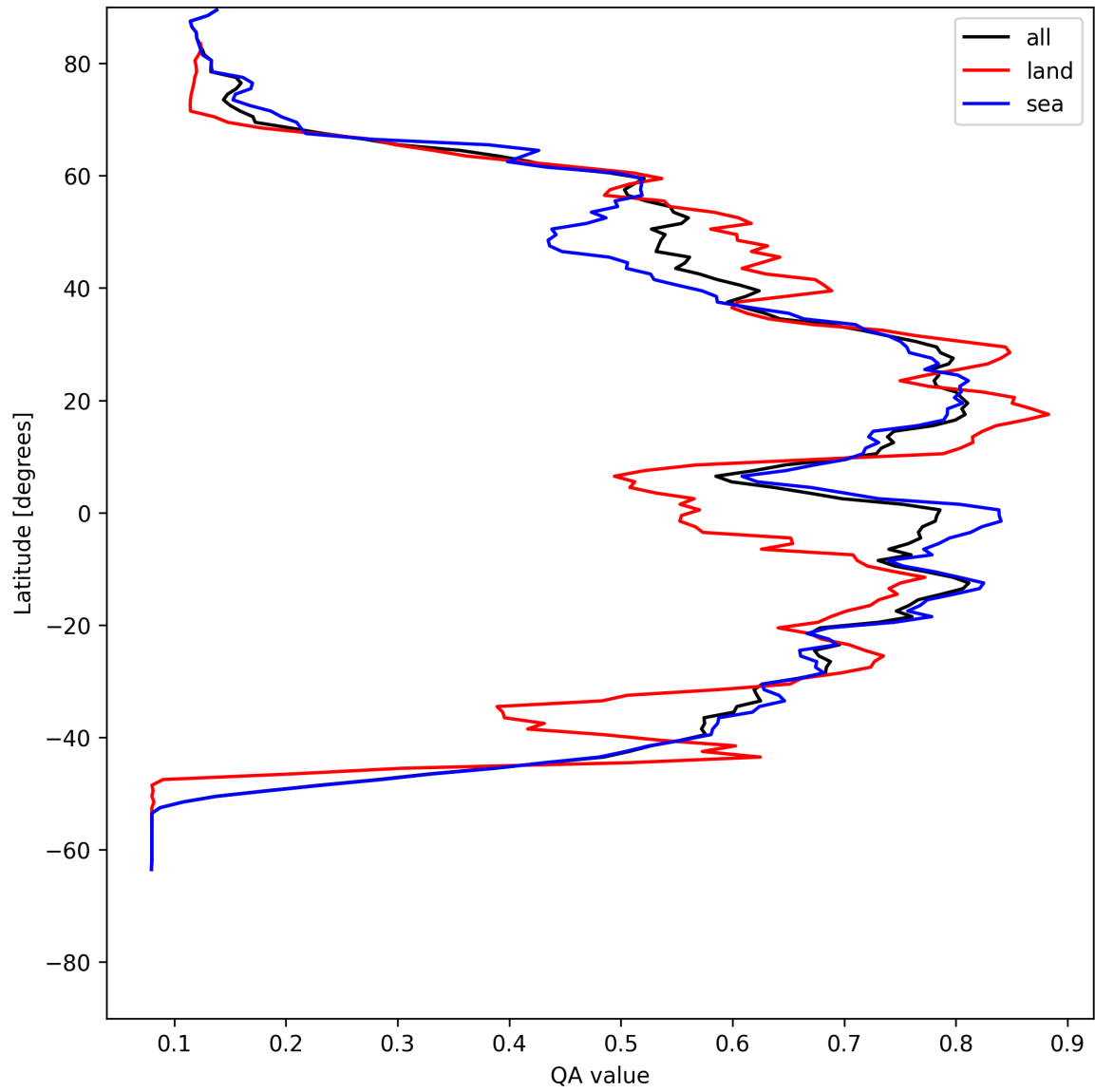
Figure 20: Zonal average of “QA value” for 2025-05-26 to 2025-05-27.
