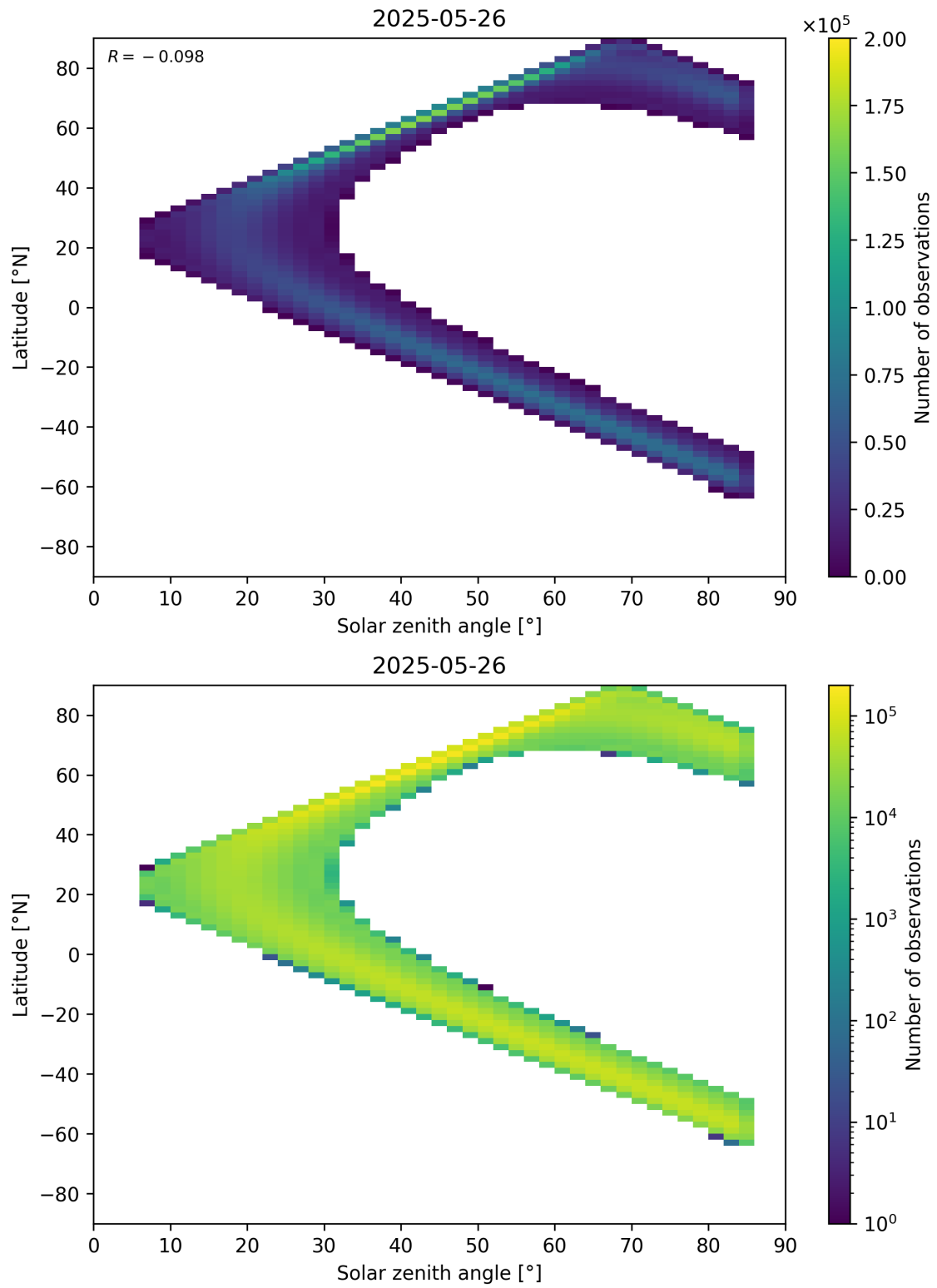
Figure 181: Scatter density plot of “Solar zenith angle” against “Latitude” for 2025-05-26 to 2025-05-27.
