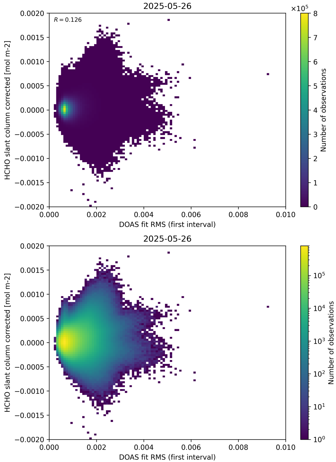
Figure 62: Scatter density plot of “DOAS fit RMS (first interval)” against “HCHO slant column corrected” for 2025-05-26 to 2025-05-27.
