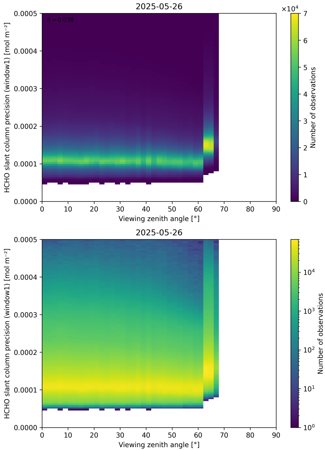
Figure 189: Scatter density plot of “Viewing zenith angle” against “HCHO slant column precision (window1)” for 2025-05-26 to 2025-05-27.
