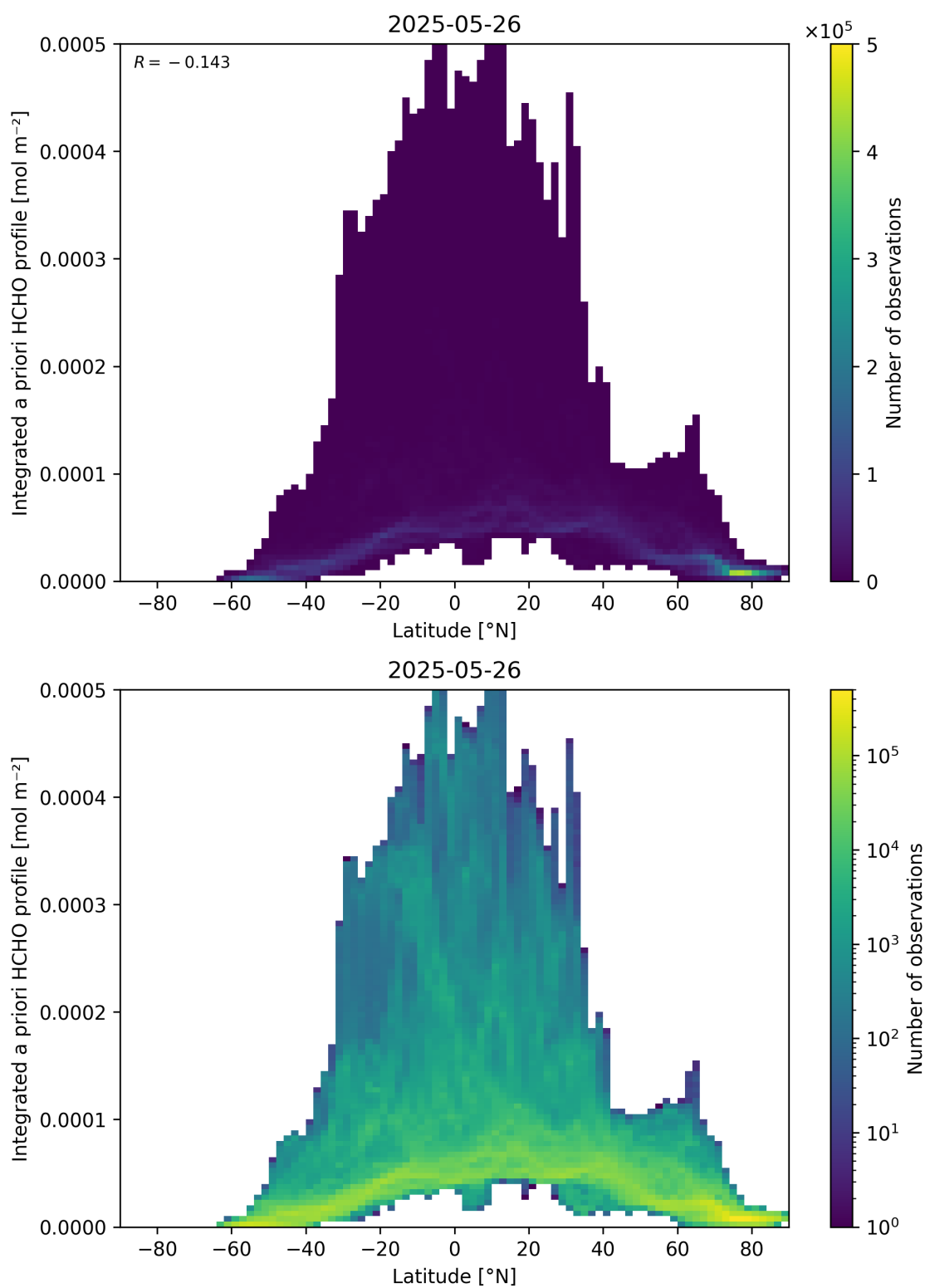
Figure 166: Scatter density plot of “Latitude” against “Integrated a priori HCHO profile” for 2025-05-26 to 2025-05-27.
