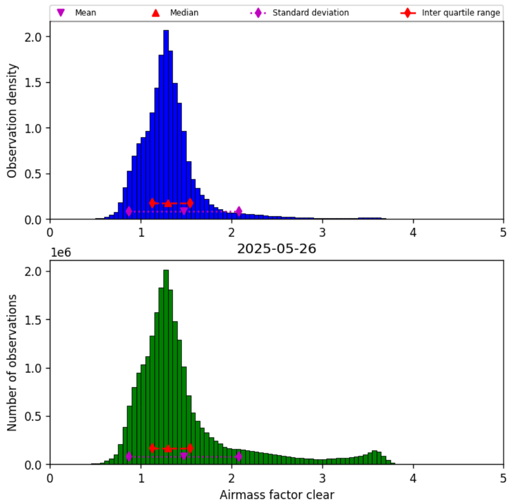
Figure 42: Histogram of “Airmass factor clear” for 2025-05-26 to 2025-05-27
