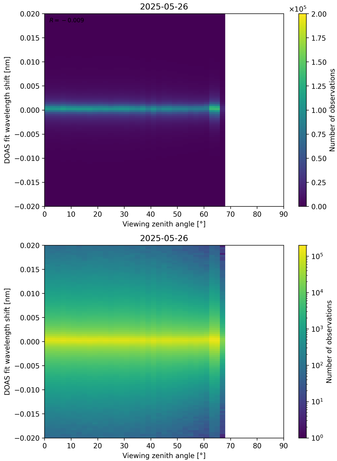
Figure 183: Scatter density plot of “Viewing zenith angle” against “DOAS fit wavelength shift” for 2025-05-26 to 2025-05-27.
