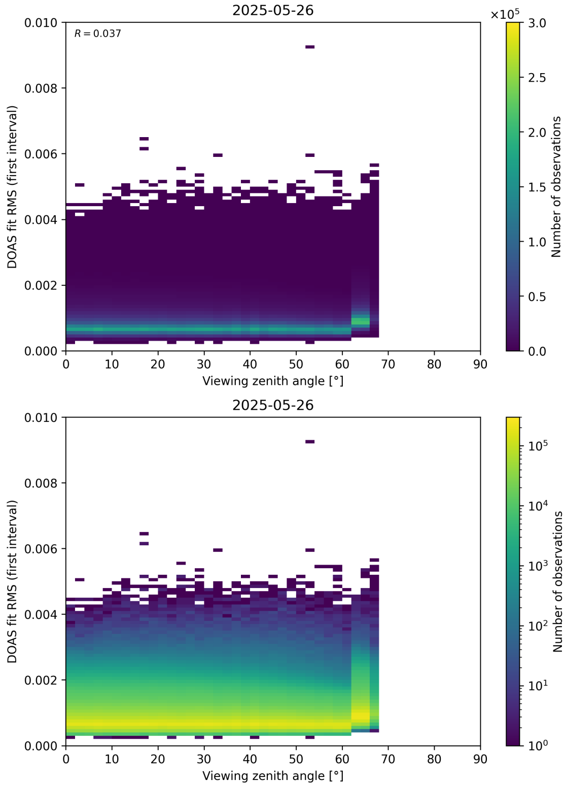
Figure 182: Scatter density plot of “Viewing zenith angle” against “DOAS fit RMS (first interval)” for 2025-05-26 to 2025-05-27.
