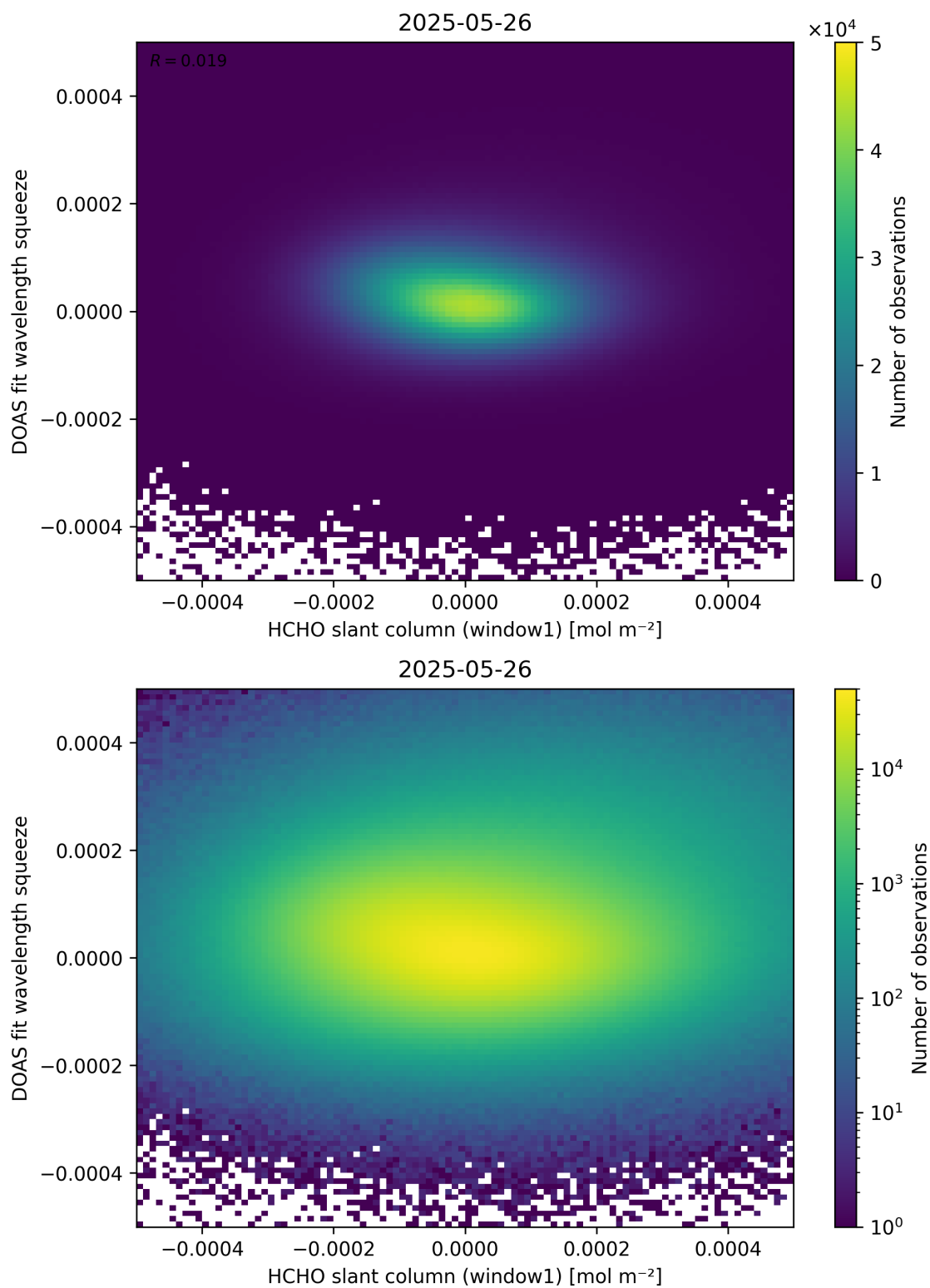
Figure 80: Scatter density plot of “HCHO slant column (window1)” against “DOAS fit wavelength squeeze” for 2025-05-26 to 2025-05-27.
