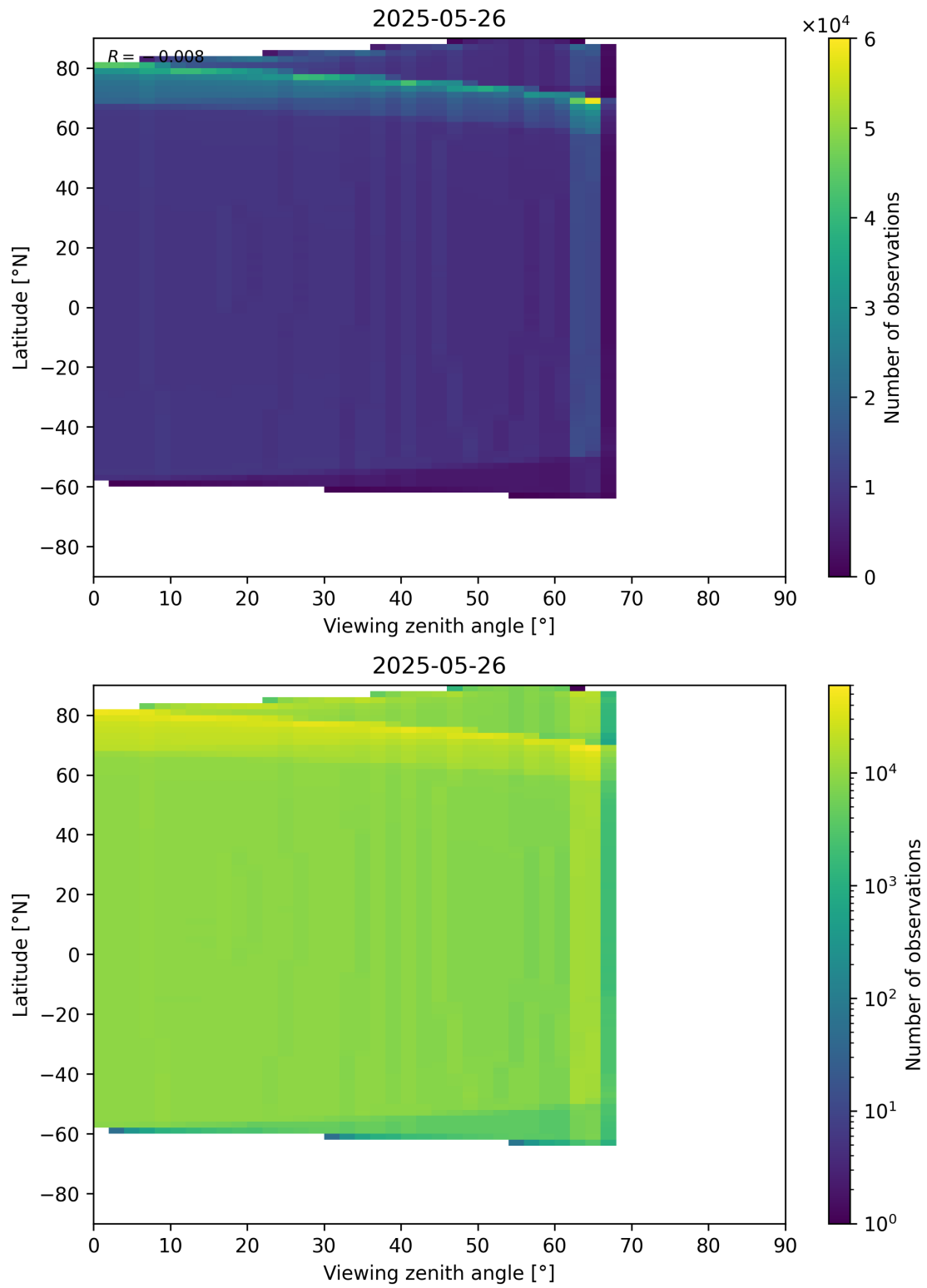
Figure 196: Scatter density plot of “Viewing zenith angle” against “Latitude” for 2025-05-26 to 2025-05-27.
