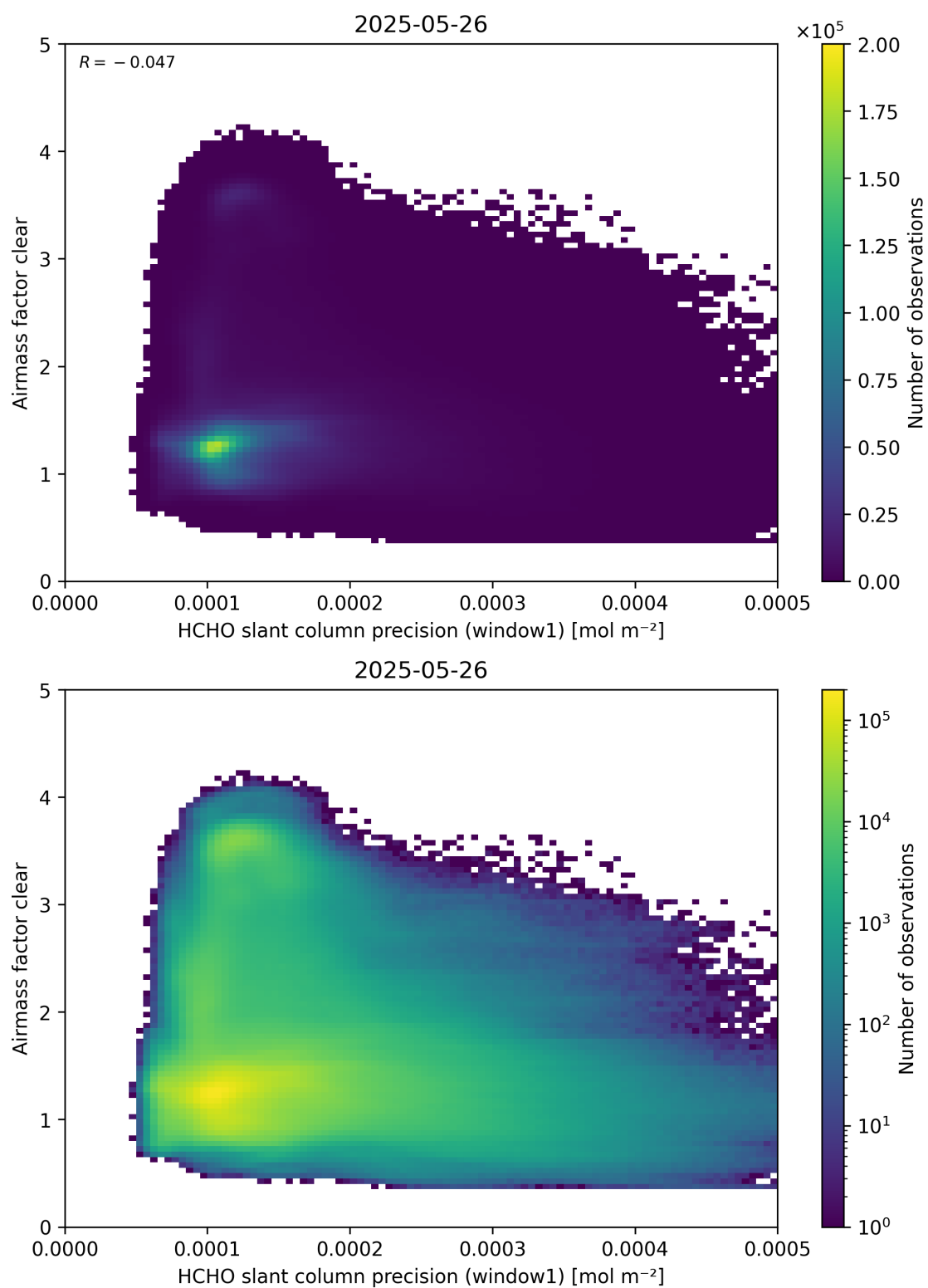
Figure 91: Scatter density plot of “HCHO slant column precision (window1)” against “Airmass factor clear” for 2025-05-26 to 2025-05-27.
