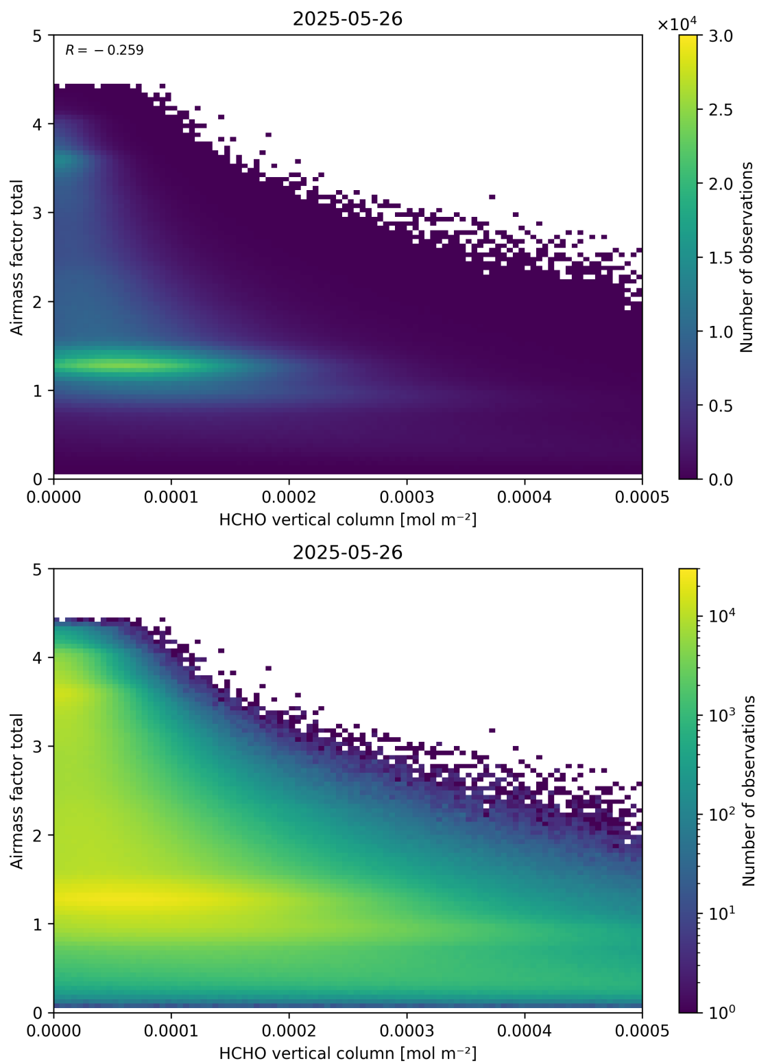
Figure 131: Scatter density plot of “HCHO vertical column” against “Airmass factor total” for 2025-05-26 to 2025-05-27.
