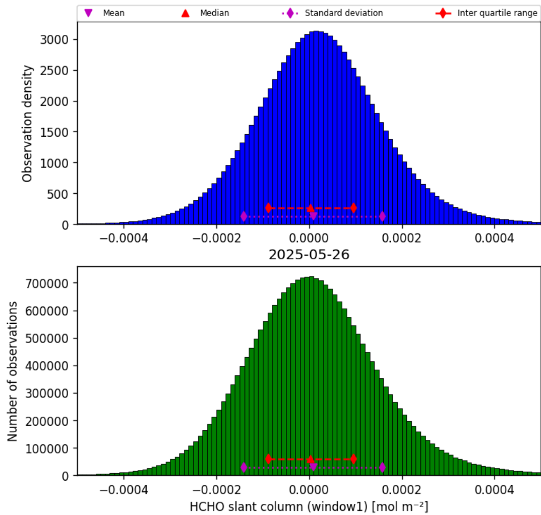
Figure 38: Histogram of “HCHO slant column (window1)” for 2025-05-26 to 2025-05-27
