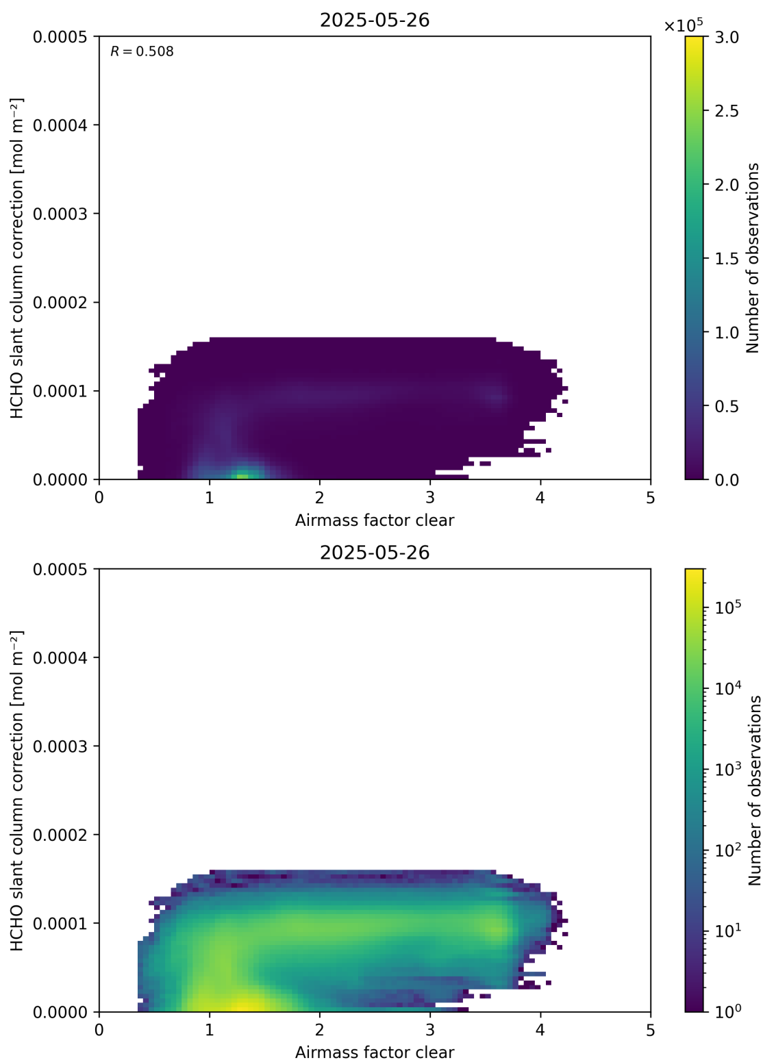
Figure 75: Scatter density plot of “Airmass factor clear” against “HCHO slant column correction” for 2025-05-26 to 2025-05-27.
