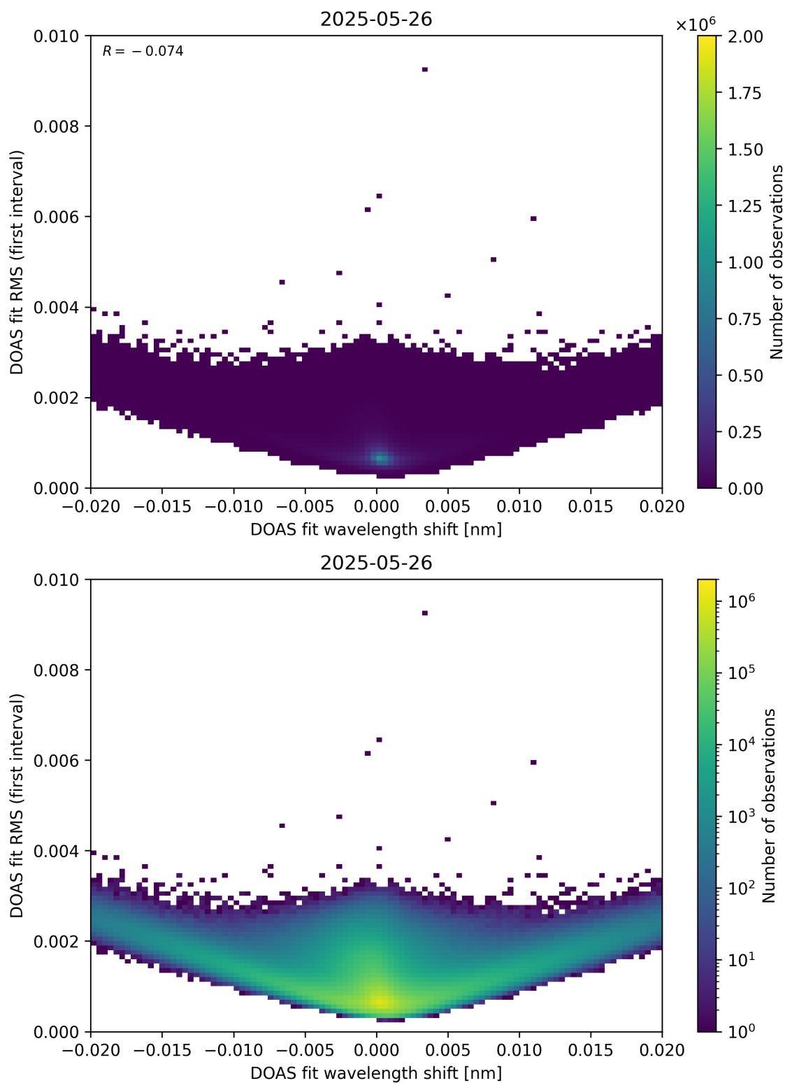
Figure 64: Scatter density plot of “DOAS fit wavelength shift” against “DOAS fit RMS (first interval)” for 2025-05-26 to 2025-05-27.
