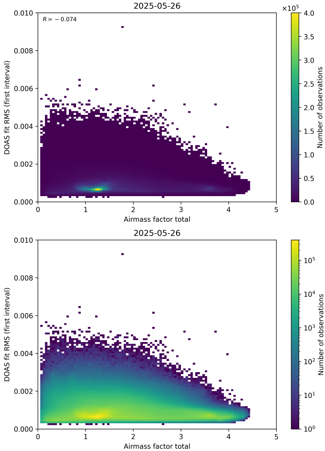
Figure 97: Scatter density plot of “Airmass factor total” against “DOAS fit RMS (first interval)” for 2025-05-26 to 2025-05-27.
