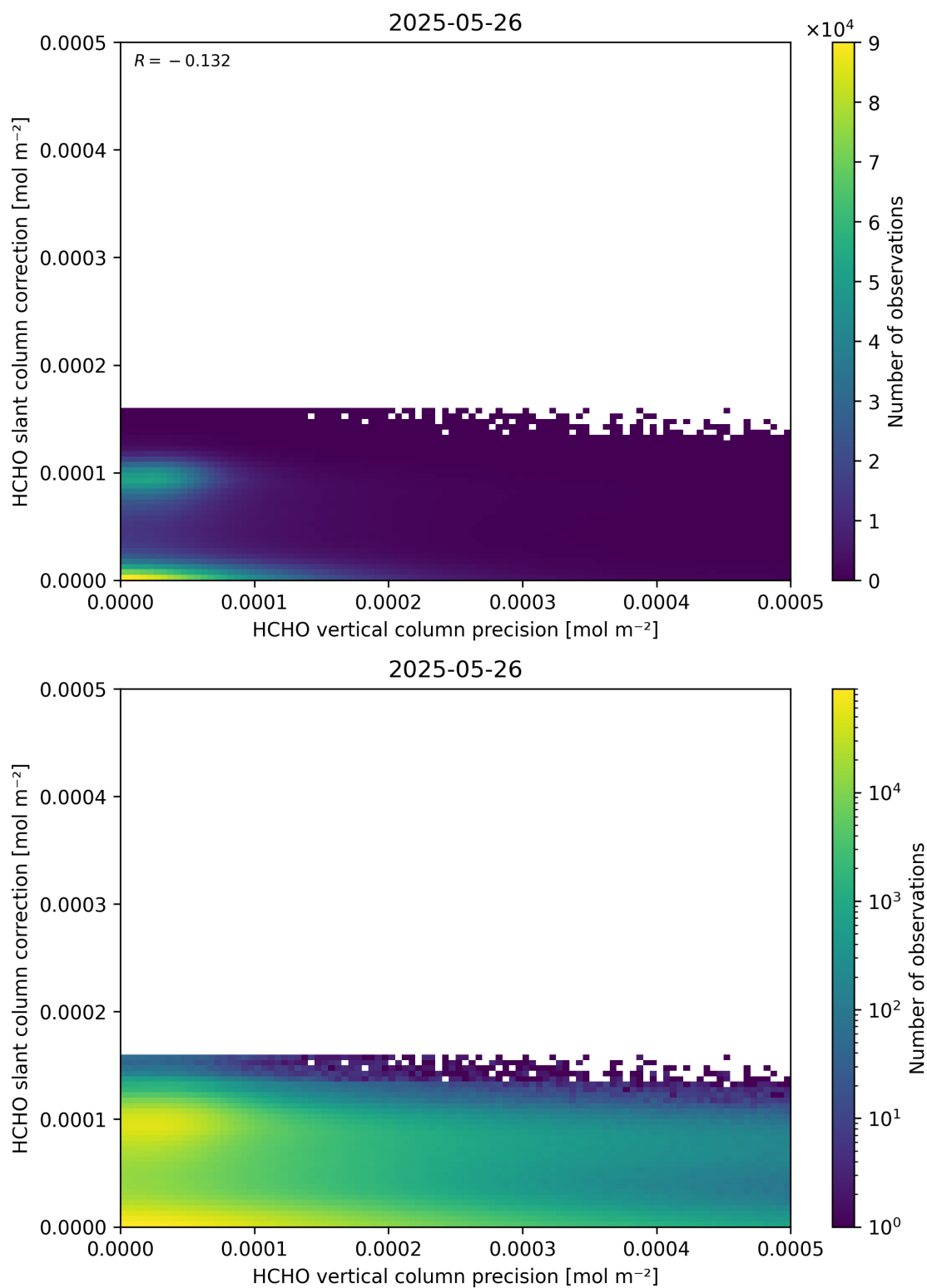
Figure 141: Scatter density plot of “HCHO vertical column precision” against “HCHO slant column correction” for 2025-05-26 to 2025-05-27.
