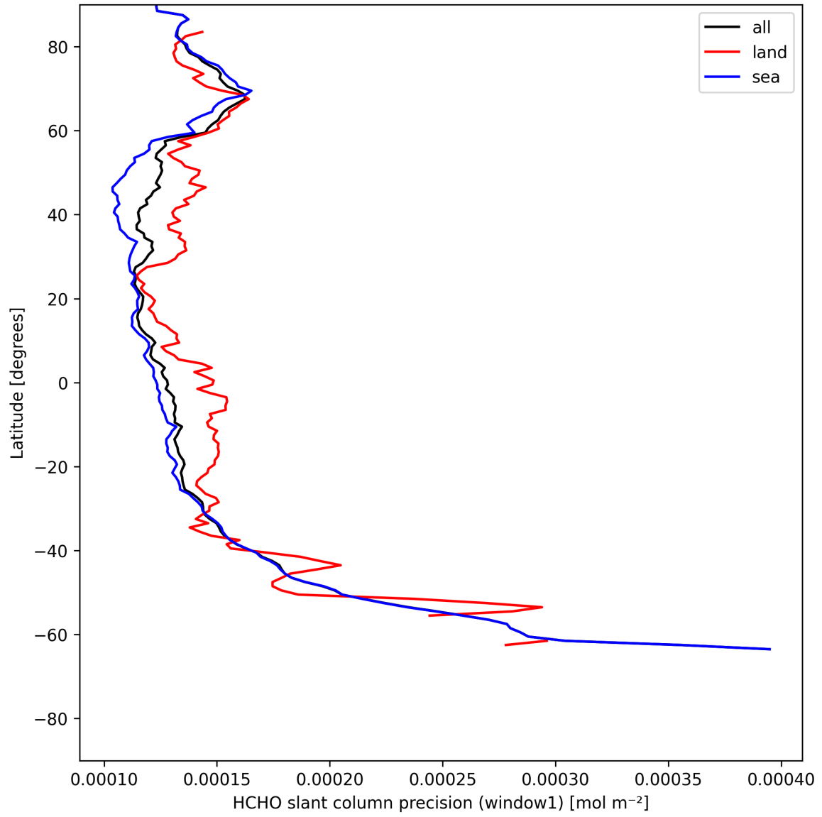
Figure 25: Zonal average of “HCHO slant column precision (window1)” for 2025-05-26 to 2025-05-27.
