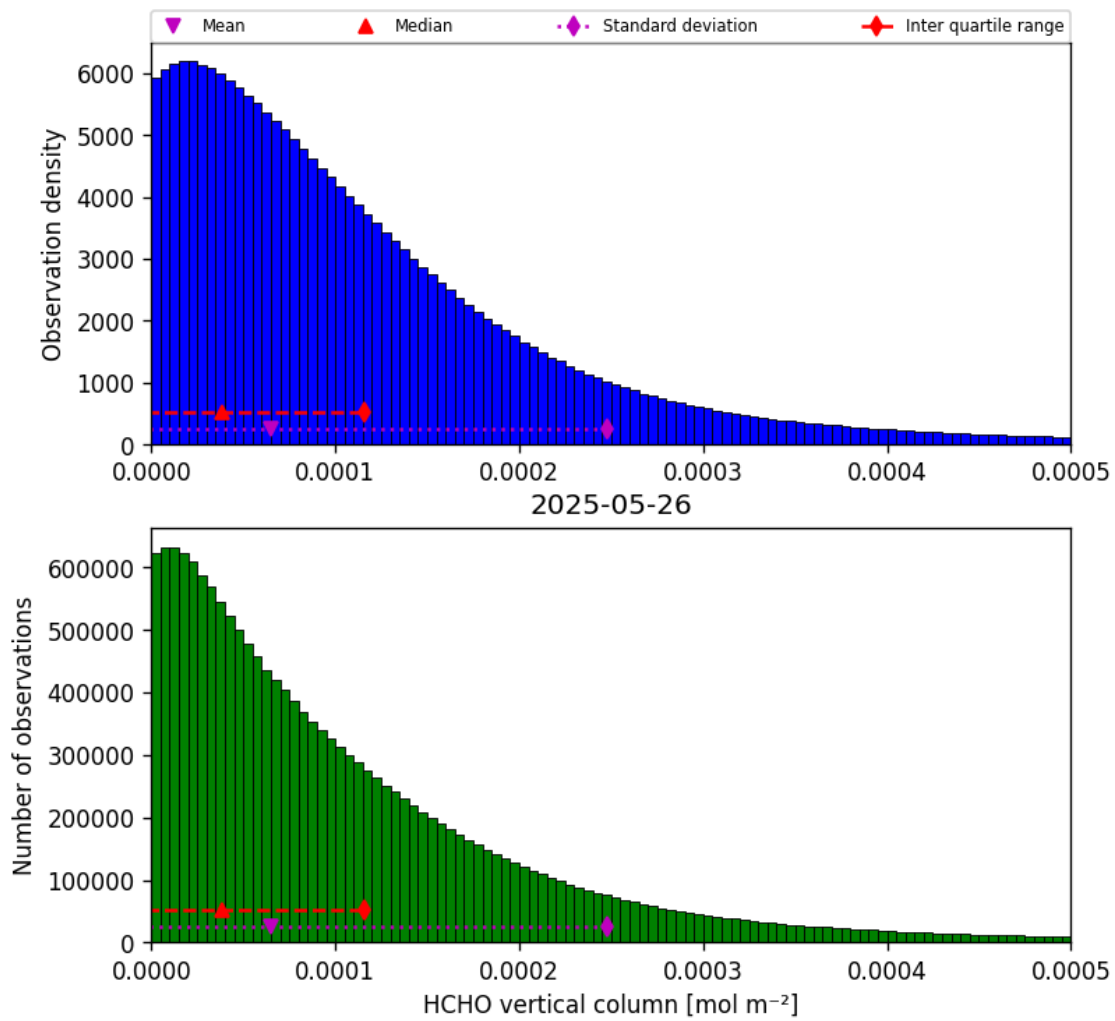
Figure 35: Histogram of “HCHO vertical column” for 2025-05-26 to 2025-05-27
