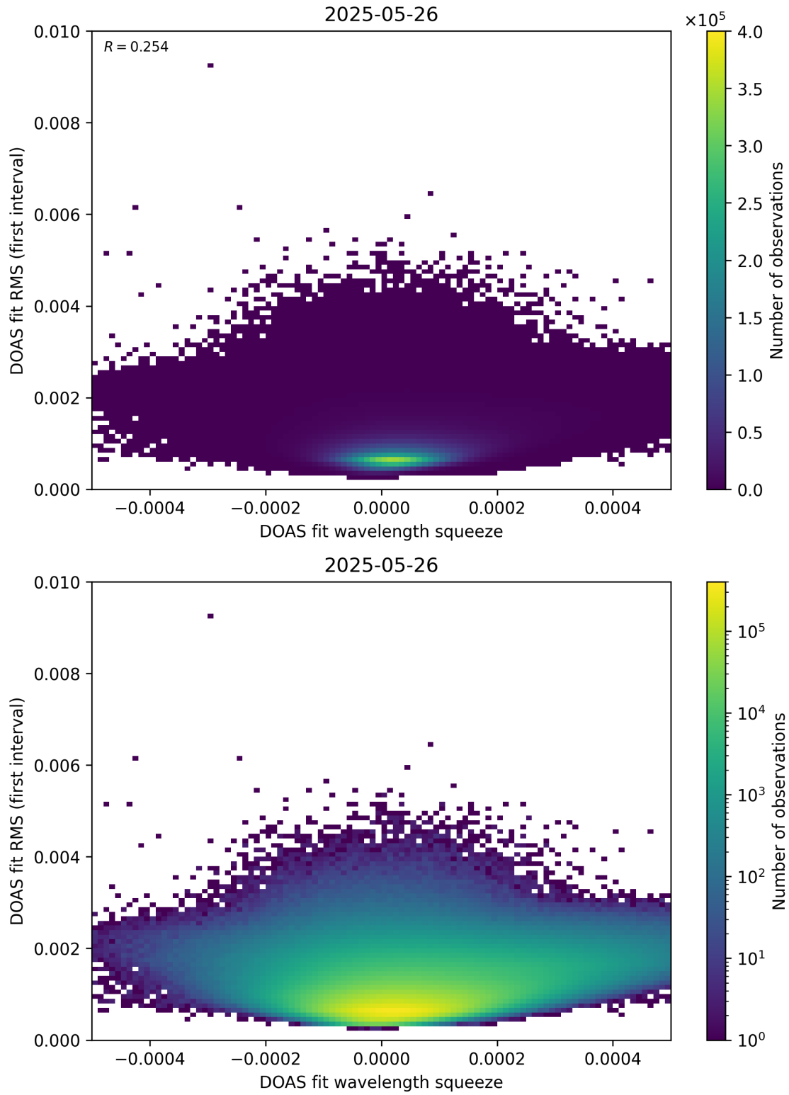
Figure 68: Scatter density plot of “DOAS fit wavelength squeeze” against “DOAS fit RMS (first interval)” for 2025-05-26 to 2025-05-27.
