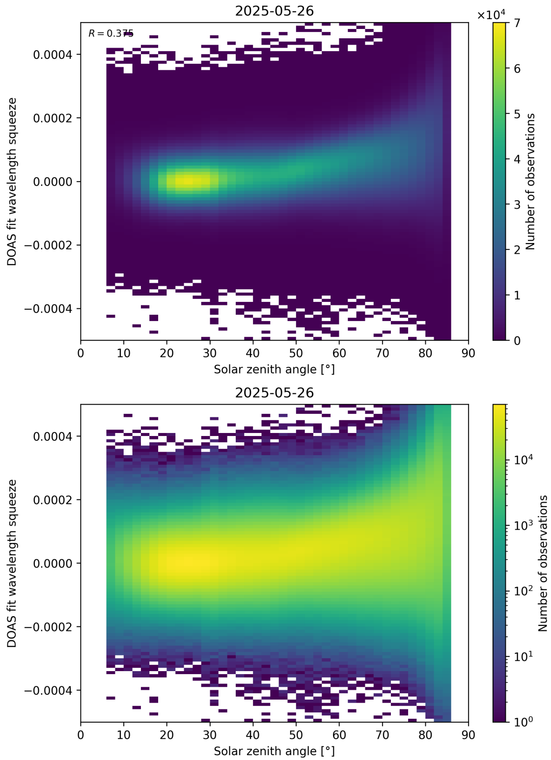
Figure 169: Scatter density plot of “Solar zenith angle” against “DOAS fit wavelength squeeze” for 2025-05-26 to 2025-05-27.
