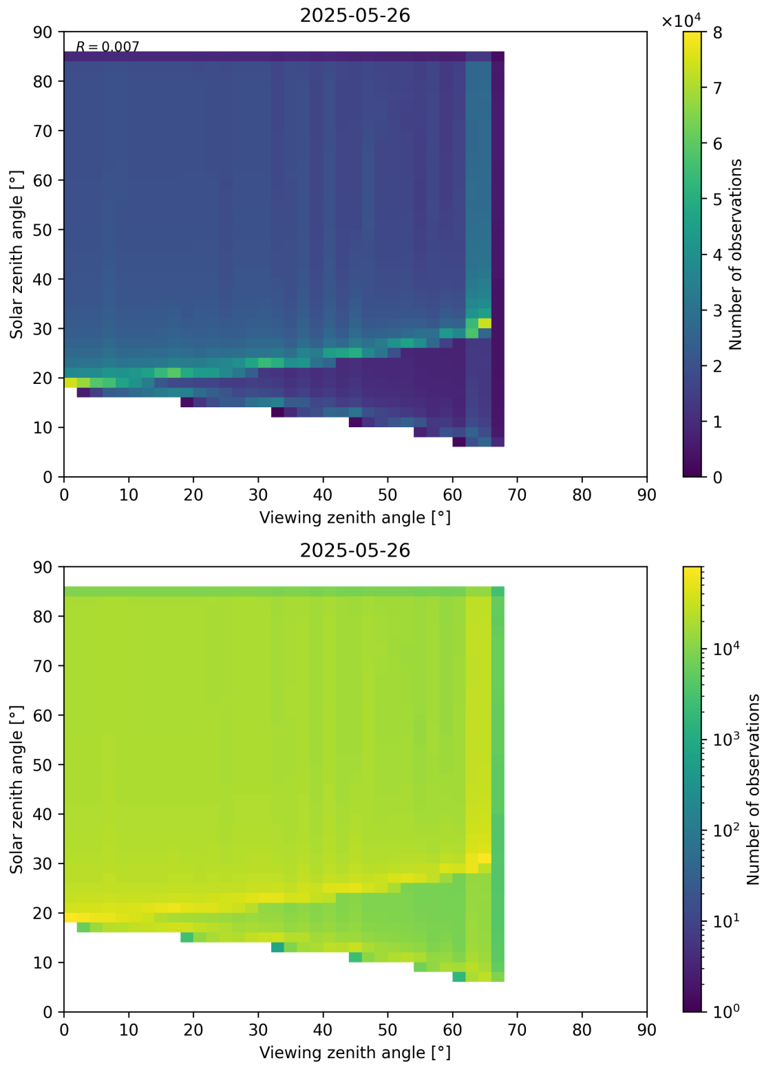
Figure 197: Scatter density plot of “Viewing zenith angle” against “Solar zenith angle” for 2025-05-26 to 2025-05-27.
