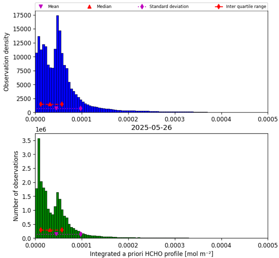
Figure 43: Histogram of “Integrated a priori HCHO profile” for 2025-05-26 to 2025-05-27
