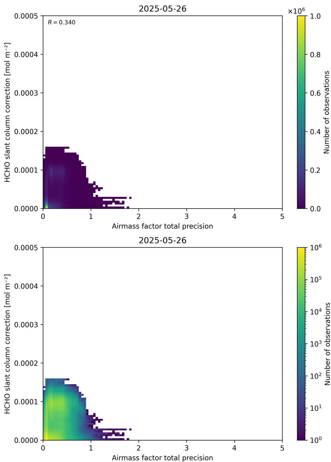
Figure 110: Scatter density plot of “Airmass factor total precision” against “HCHO slant column correction” for 2025-05-26 to 2025-05-27.
