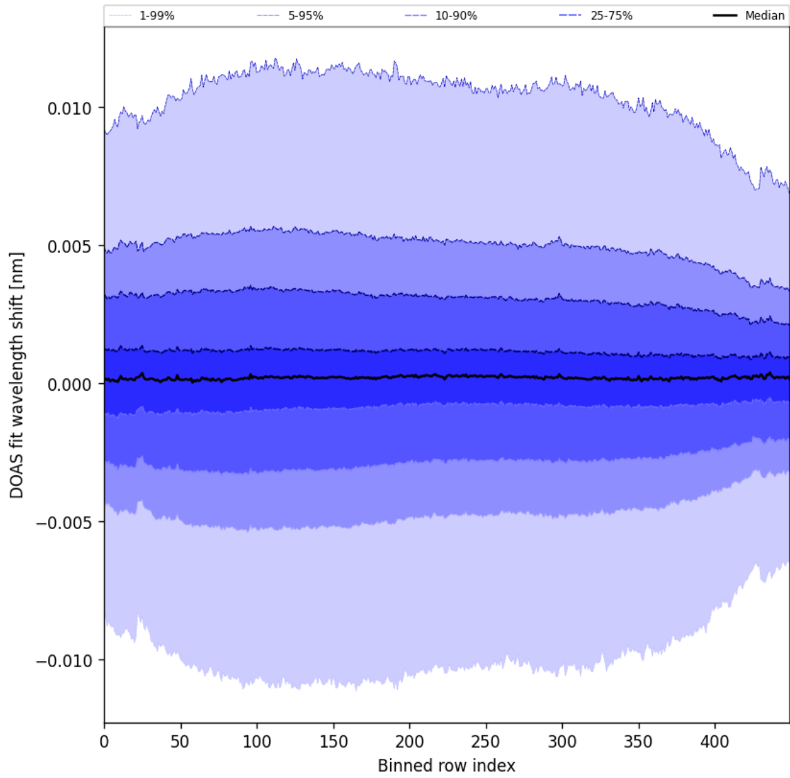
Figure 58: Along track statistics of “DOAS fit wavelength shift” for 2025-05-26 to 2025-05-27
