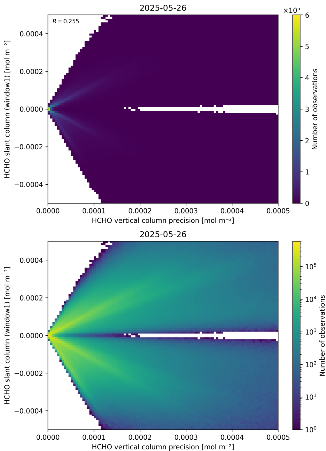
Figure 142: Scatter density plot of “HCHO vertical column precision” against “HCHO slant column (window1)” for 2025-05-26 to 2025-05-27.
