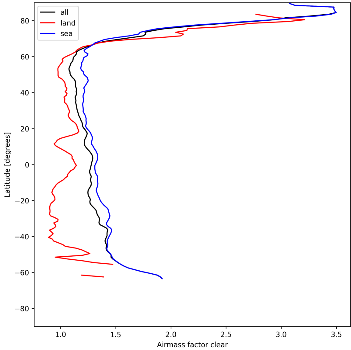
Figure 28: Zonal average of “Airmass factor clear” for 2025-05-26 to 2025-05-27.
