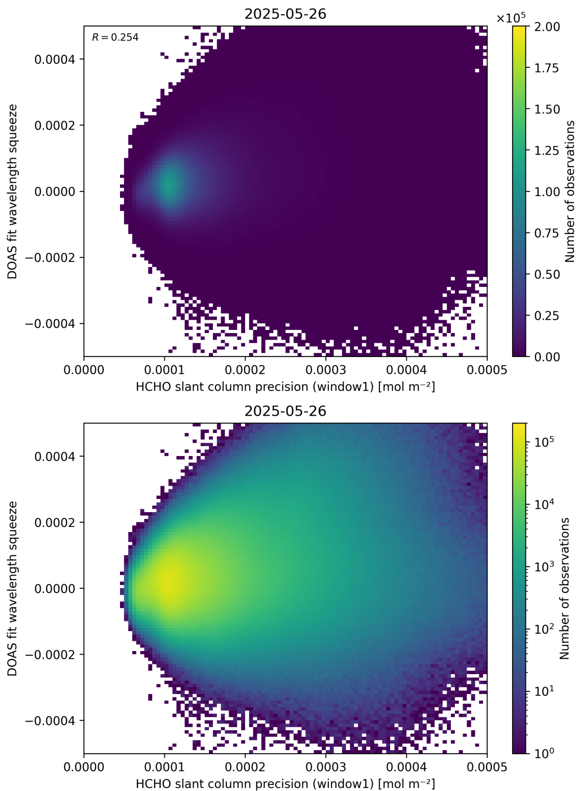
Figure 90: Scatter density plot of “HCHO slant column precision (window1)” against “DOAS fit wavelength squeeze” for 2025-05-26 to 2025-05-27.
