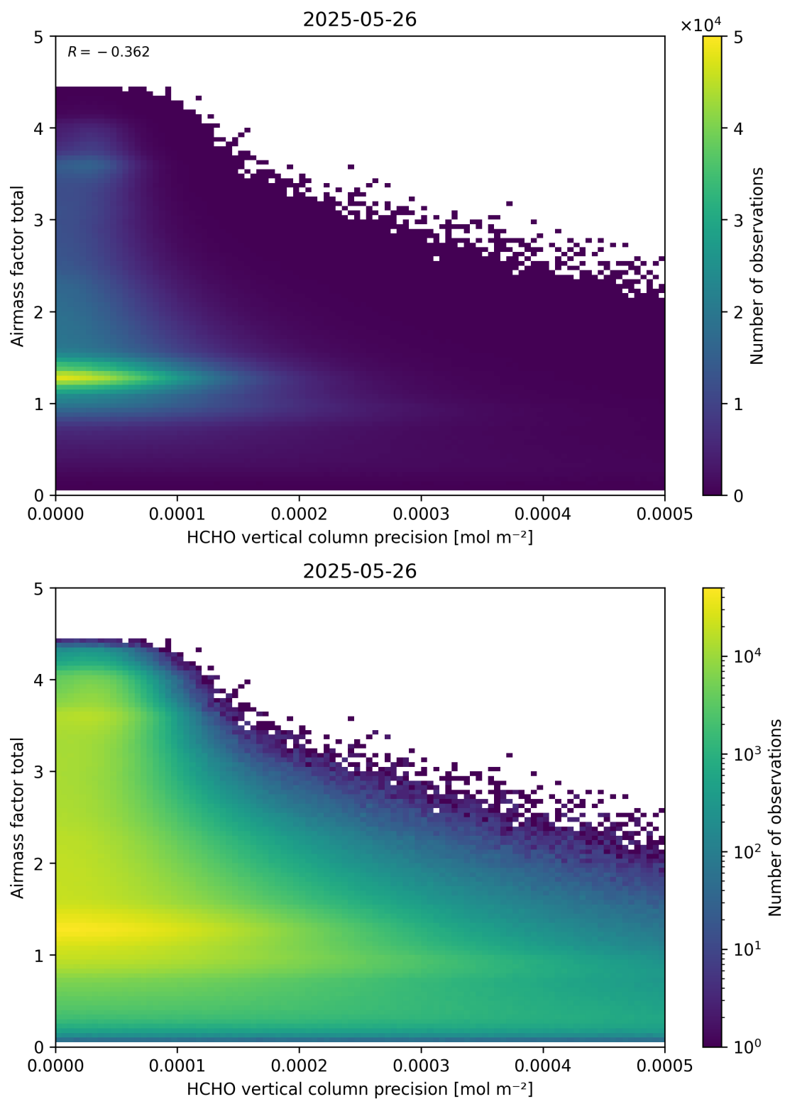
Figure 144: Scatter density plot of “HCHO vertical column precision” against “Airmass factor total” for 2025-05-26 to 2025-05-27.
