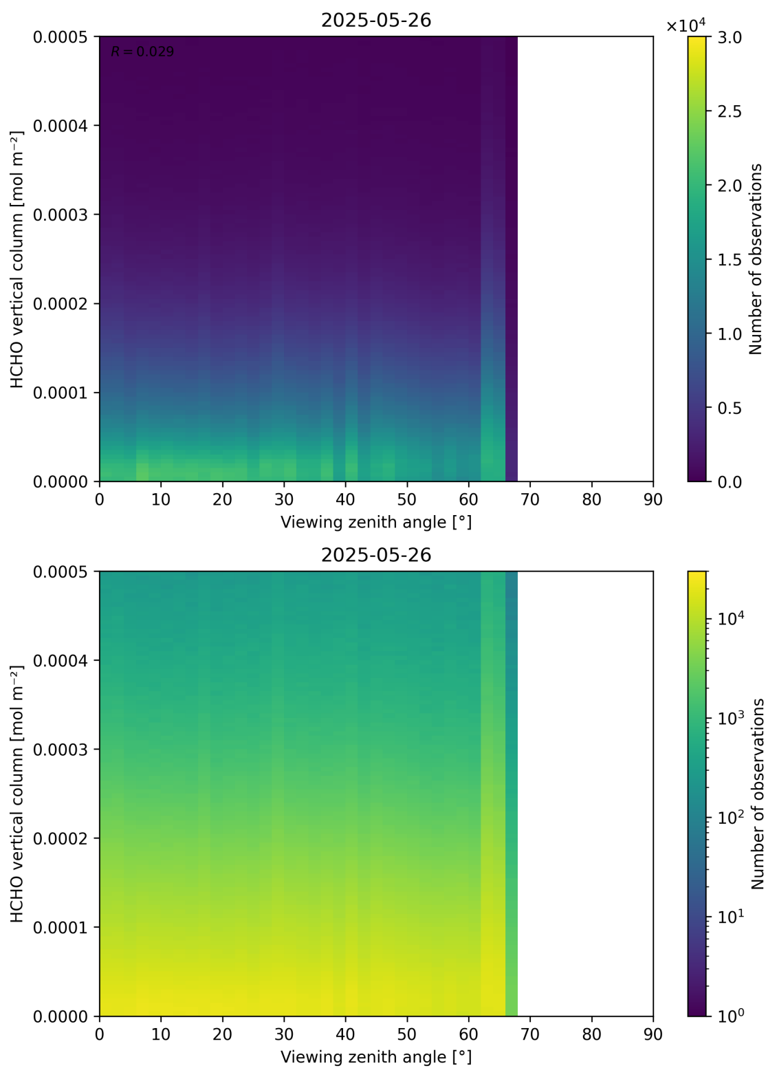
Figure 192: Scatter density plot of “Viewing zenith angle” against “HCHO vertical column” for 2025-05-26 to 2025-05-27.
