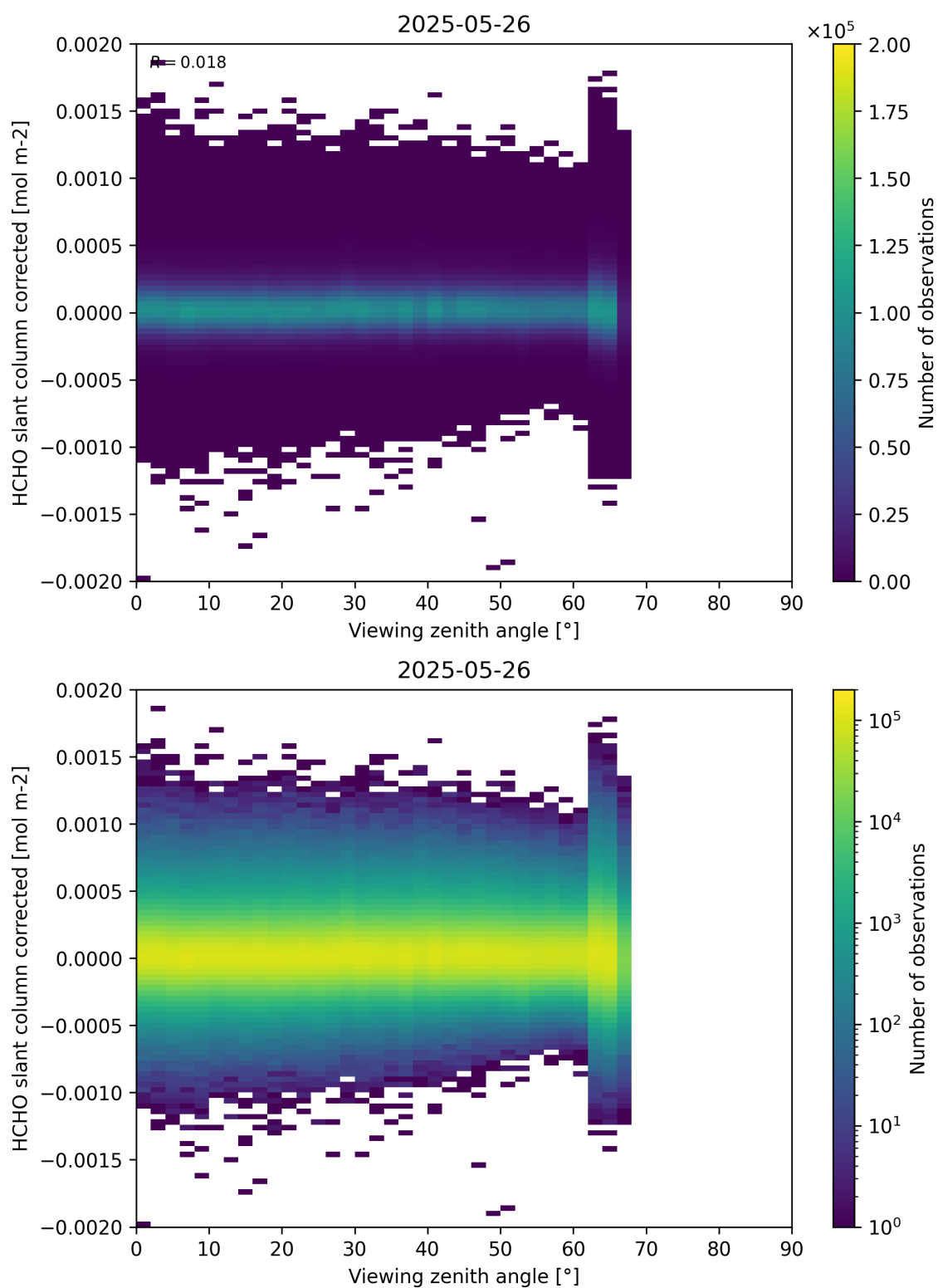
Figure 186: Scatter density plot of “Viewing zenith angle” against “HCHO slant column corrected” for 2025-05-26 to 2025-05-27.
