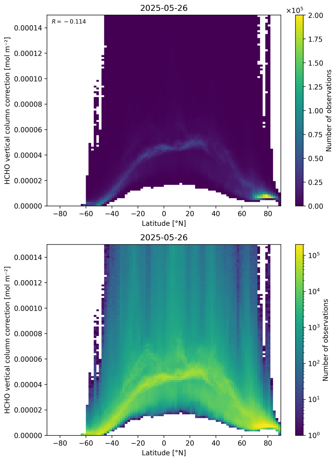
Figure 164: Scatter density plot of “Latitude” against “HCHO vertical column correction” for 2025-05-26 to 2025-05-27.
