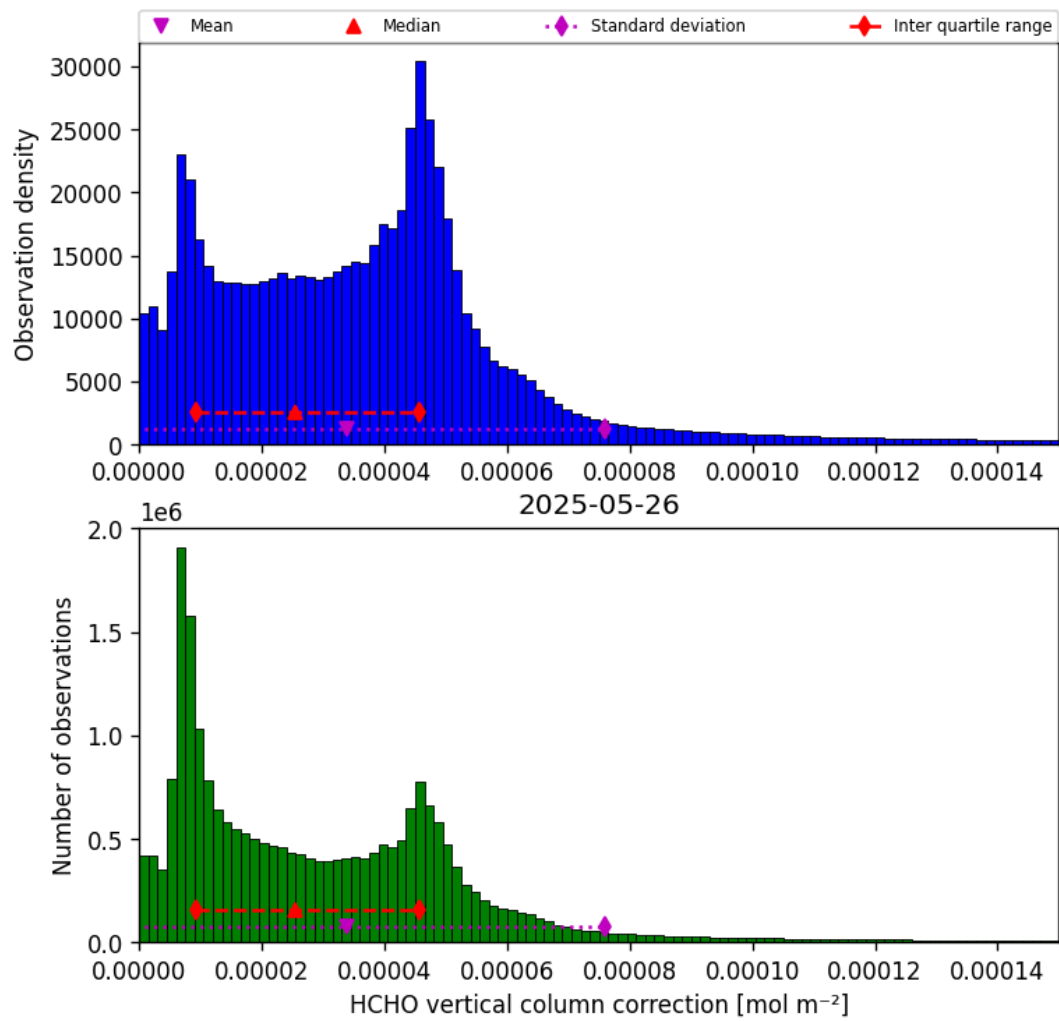
Figure 37: Histogram of “HCHO vertical column correction” for 2025-05-26 to 2025-05-27
