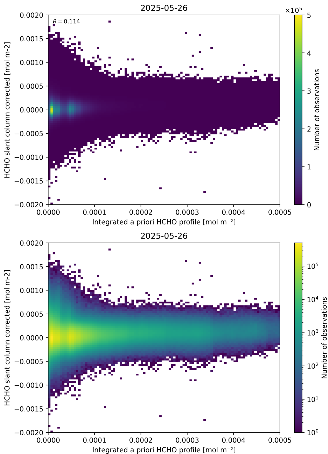
Figure 151: Scatter density plot of “Integrated a priori HCHO profile” against “HCHO slant column corrected” for 2025-05-26 to 2025-05-27.
