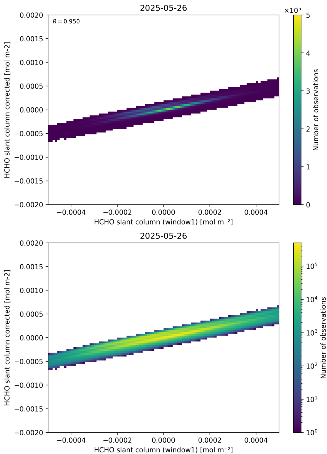
Figure 82: Scatter density plot of “HCHO slant column (window1)” against “HCHO slant column corrected” for 2025-05-26 to 2025-05-27.
