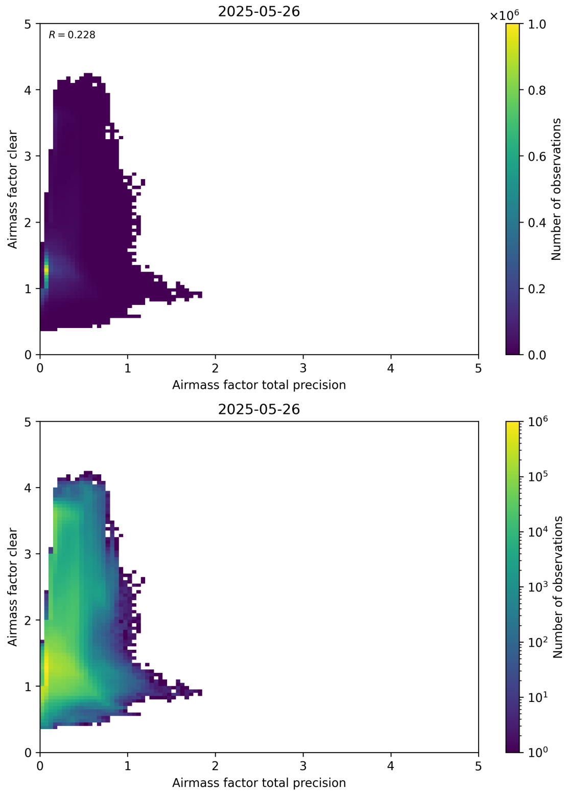
Figure 108: Scatter density plot of “Airmass factor total precision” against “Airmass factor clear” for 2025-05-26 to 2025-05-27.
