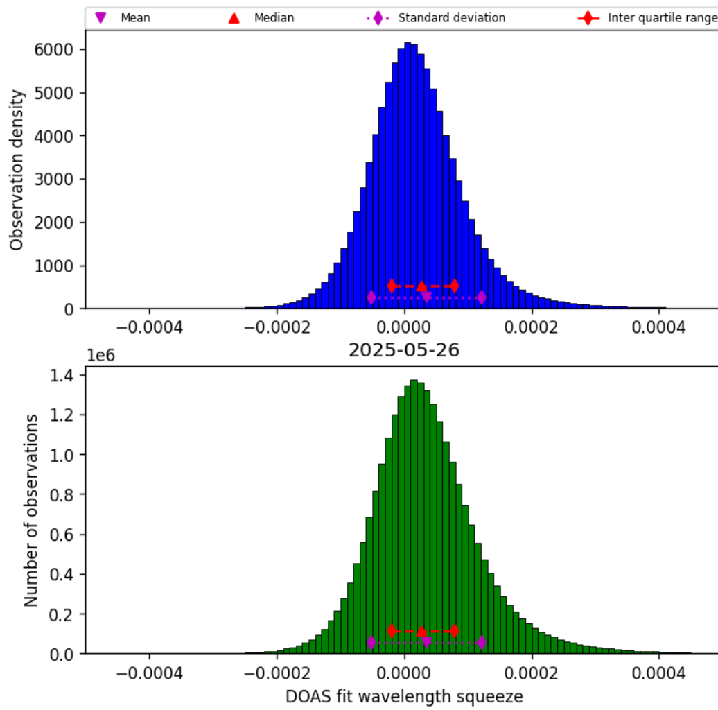
Figure 45: Histogram of “DOAS fit wavelength squeeze” for 2025-05-26 to 2025-05-27
