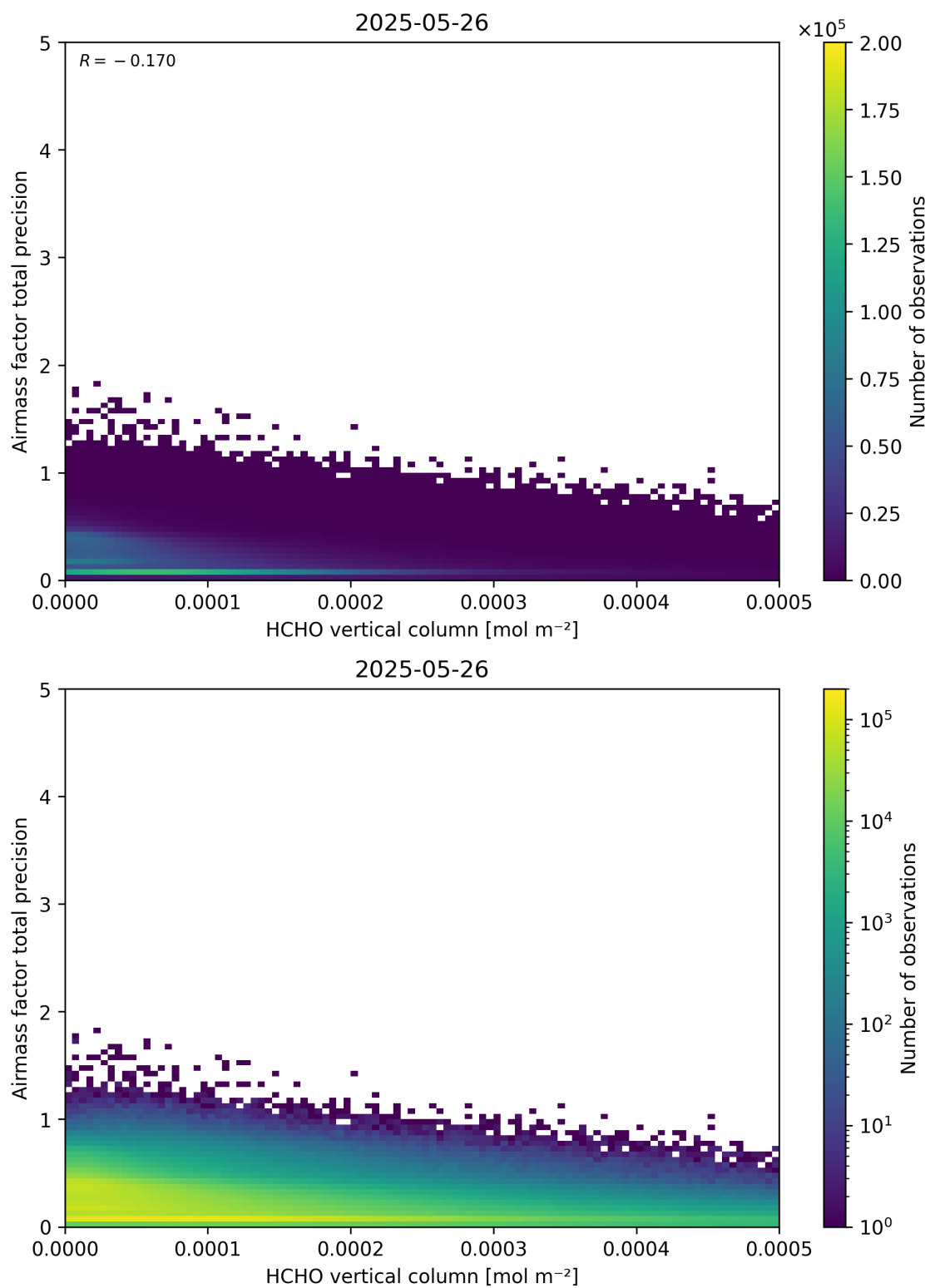
Figure 132: Scatter density plot of “HCHO vertical column” against “Airmass factor total precision” for 2025-05-26 to 2025-05-27.
