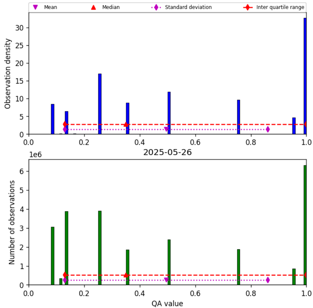
Figure 34: Histogram of “QA value” for 2025-05-26 to 2025-05-27
