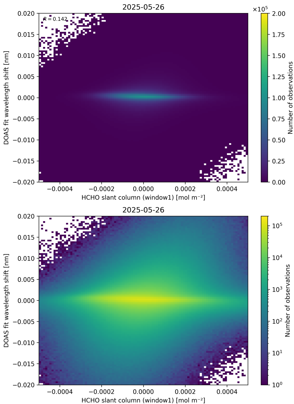
Figure 79: Scatter density plot of “HCHO slant column (window1)” against “DOAS fit wavelength shift” for 2025-05-26 to 2025-05-27.
