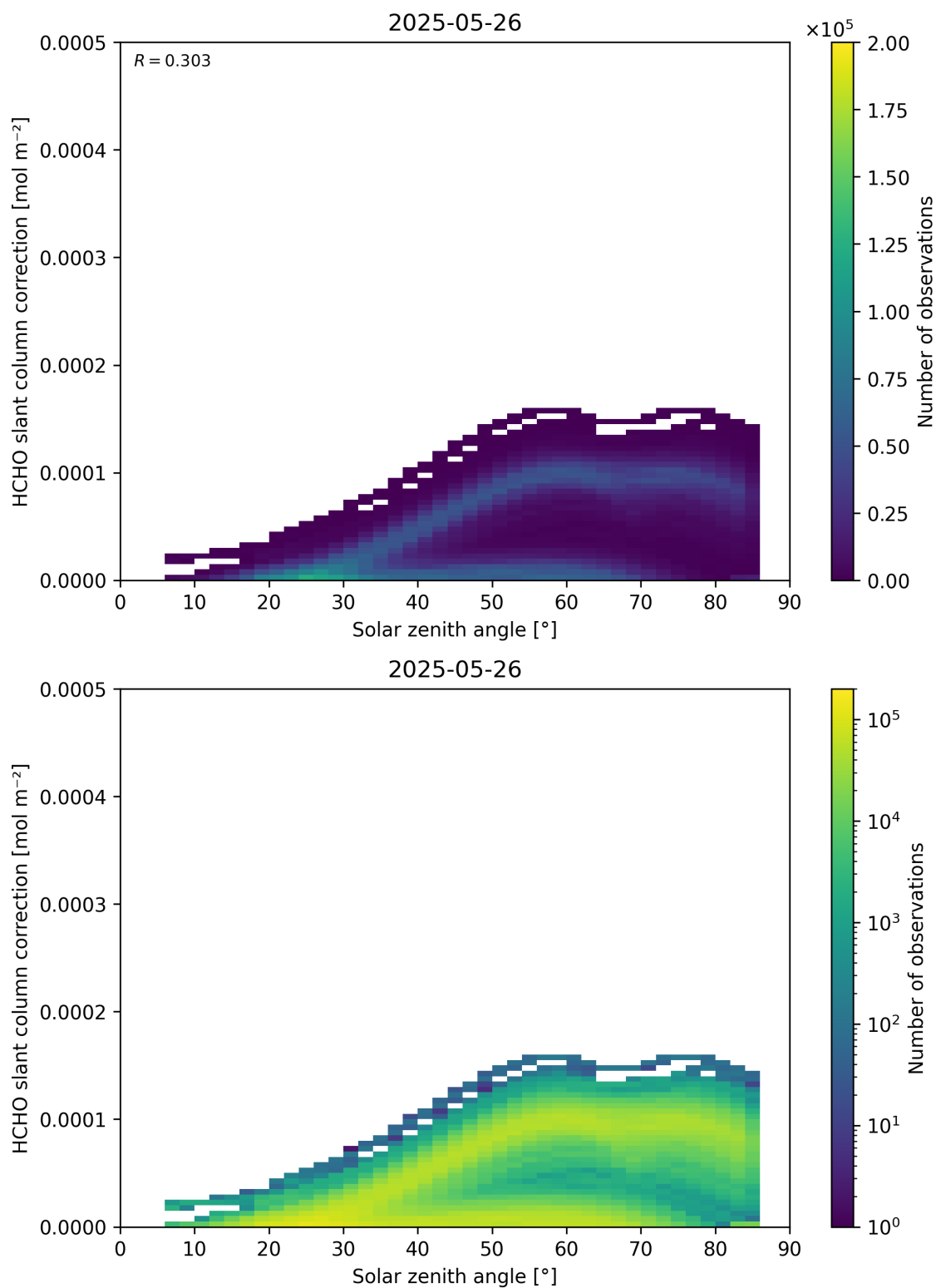
Figure 172: Scatter density plot of “Solar zenith angle” against “HCHO slant column correction” for 2025-05-26 to 2025-05-27.
