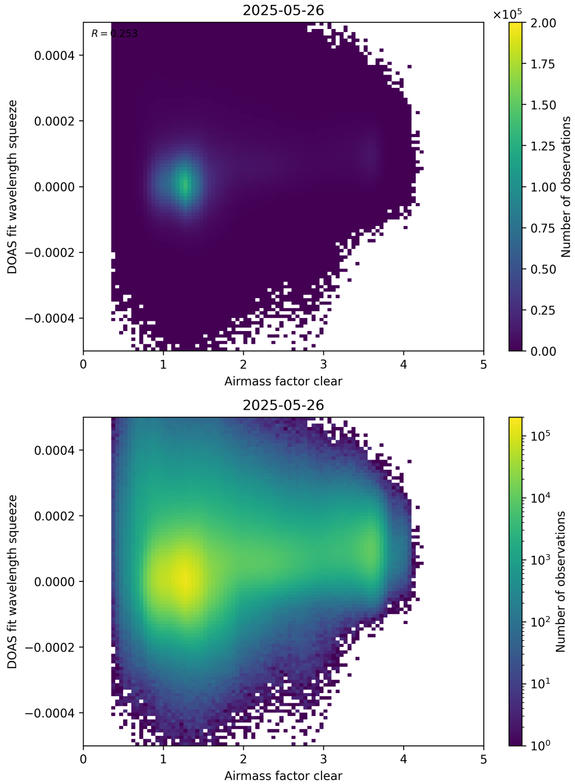
Figure 73: Scatter density plot of “Airmass factor clear” against “DOAS fit wavelength squeeze” for 2025-05-26 to 2025-05-27.
