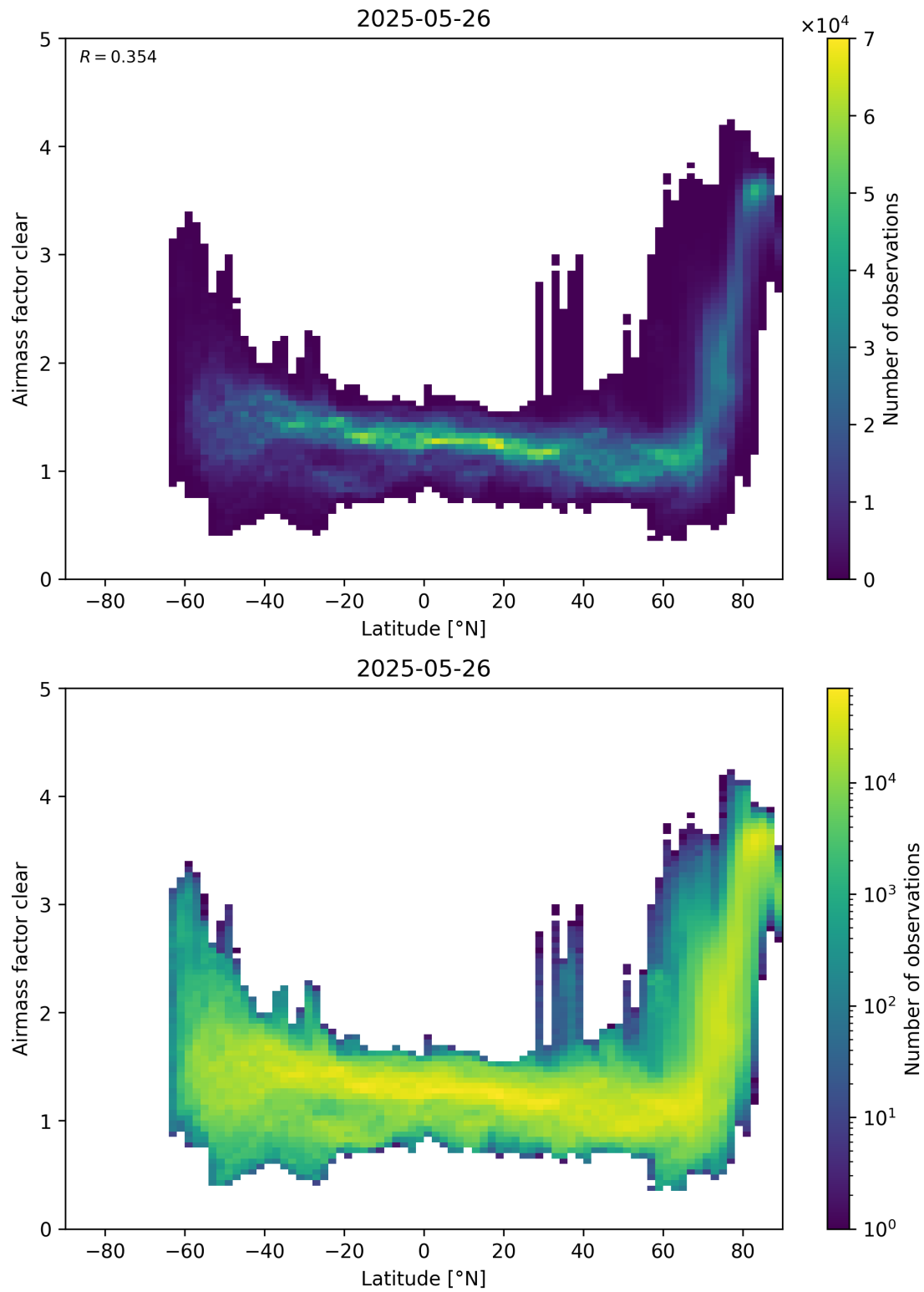
Figure 156: Scatter density plot of “Latitude” against “Airmass factor clear” for 2025-05-26 to 2025-05-27.
