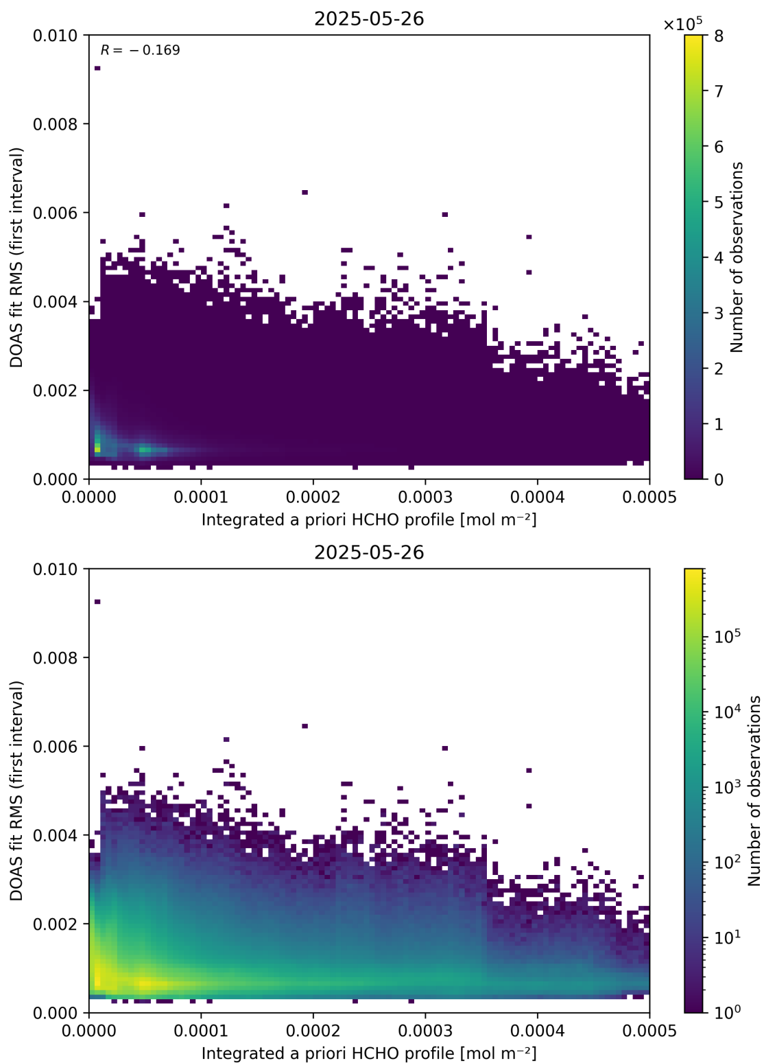
Figure 148: Scatter density plot of “Integrated a priori HCHO profile” against “DOAS fit RMS (first interval)” for 2025-05-26 to 2025-05-27.
