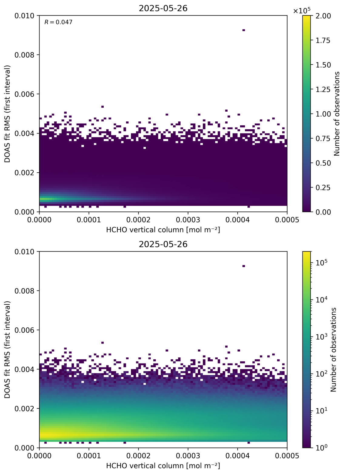
Figure 123: Scatter density plot of “HCHO vertical column” against “DOAS fit RMS (first interval)” for 2025-05-26 to 2025-05-27.
