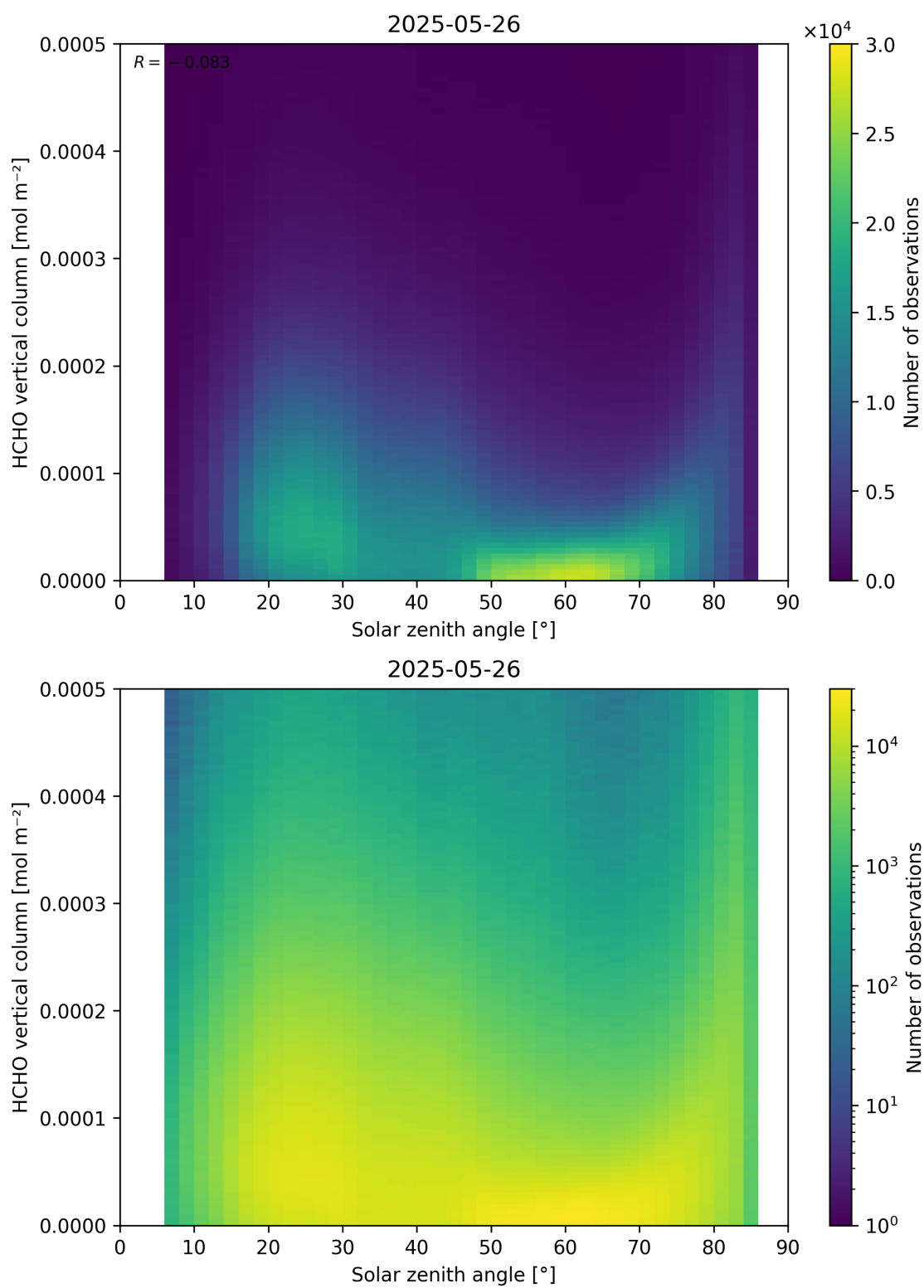
Figure 177: Scatter density plot of “Solar zenith angle” against “HCHO vertical column” for 2025-05-26 to 2025-05-27.
