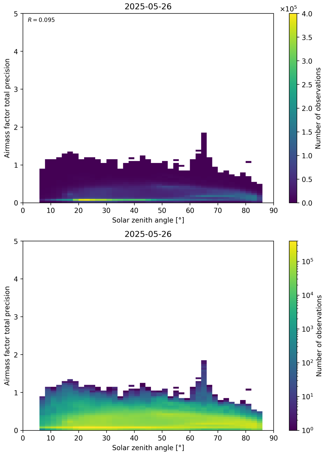
Figure 176: Scatter density plot of “Solar zenith angle” against “Airmass factor total precision” for 2025-05-26 to 2025-05-27.
