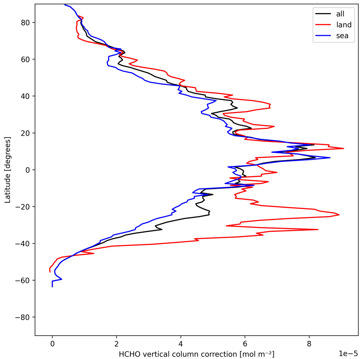
Figure 23: Zonal average of “HCHO vertical column correction” for 2025-05-26 to 2025-05-27.
