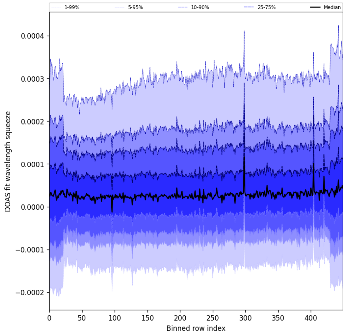
Figure 59: Along track statistics of “DOAS fit wavelength squeeze” for 2025-05-26 to 2025-05-27
