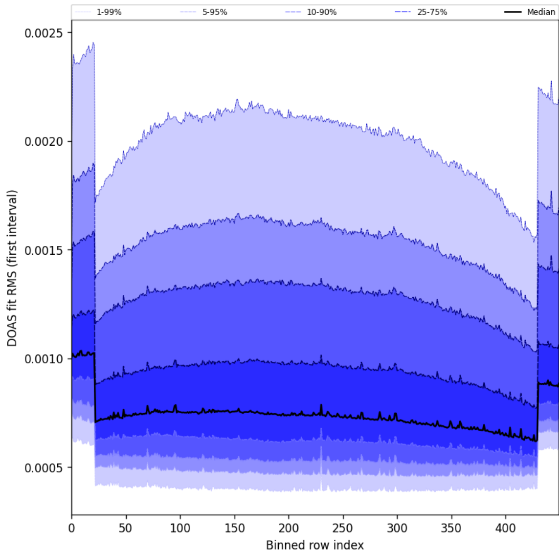
Figure 60: Along track statistics of “DOAS fit RMS (first interval)” for 2025-05-26 to 2025-05-27
