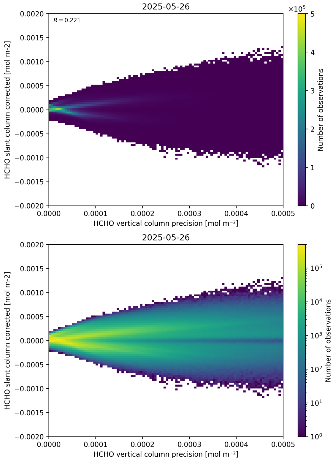
Figure 140: Scatter density plot of “HCHO vertical column precision” against “HCHO slant column corrected” for 2025-05-26 to 2025-05-27.
