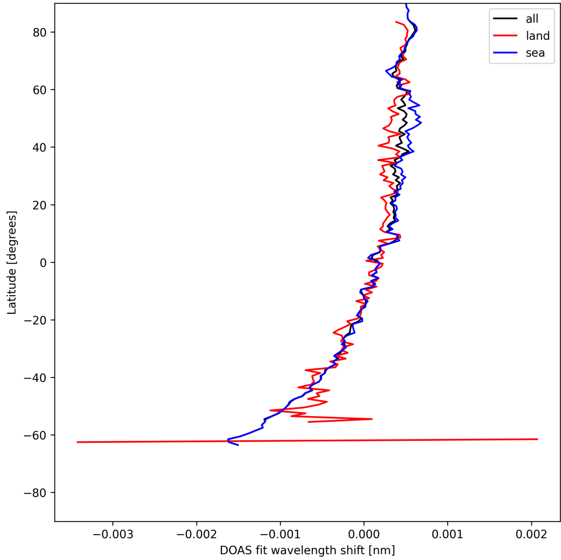
Figure 30: Zonal average of "DOAS fit wavelength shift" for 2025-05-26 to 2025-05-27.
