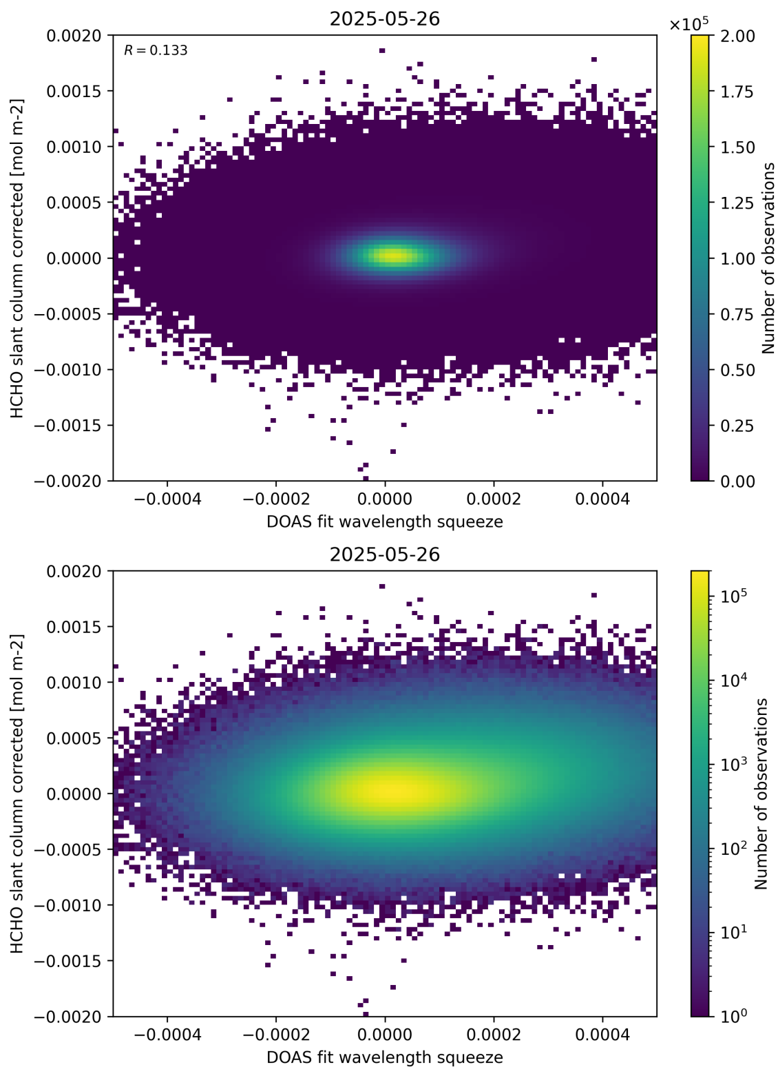
Figure 69: Scatter density plot of “DOAS fit wavelength squeeze” against “HCHO slant column corrected” for 2025-05-26 to 2025-05-27.
