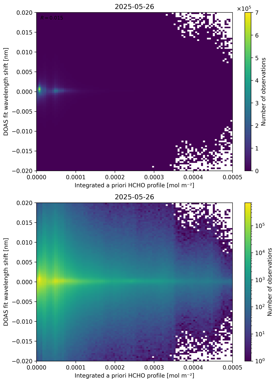
Figure 149: Scatter density plot of “Integrated a priori HCHO profile” against “DOAS fit wavelength shift” for 2025-05-26 to 2025-05-27.
