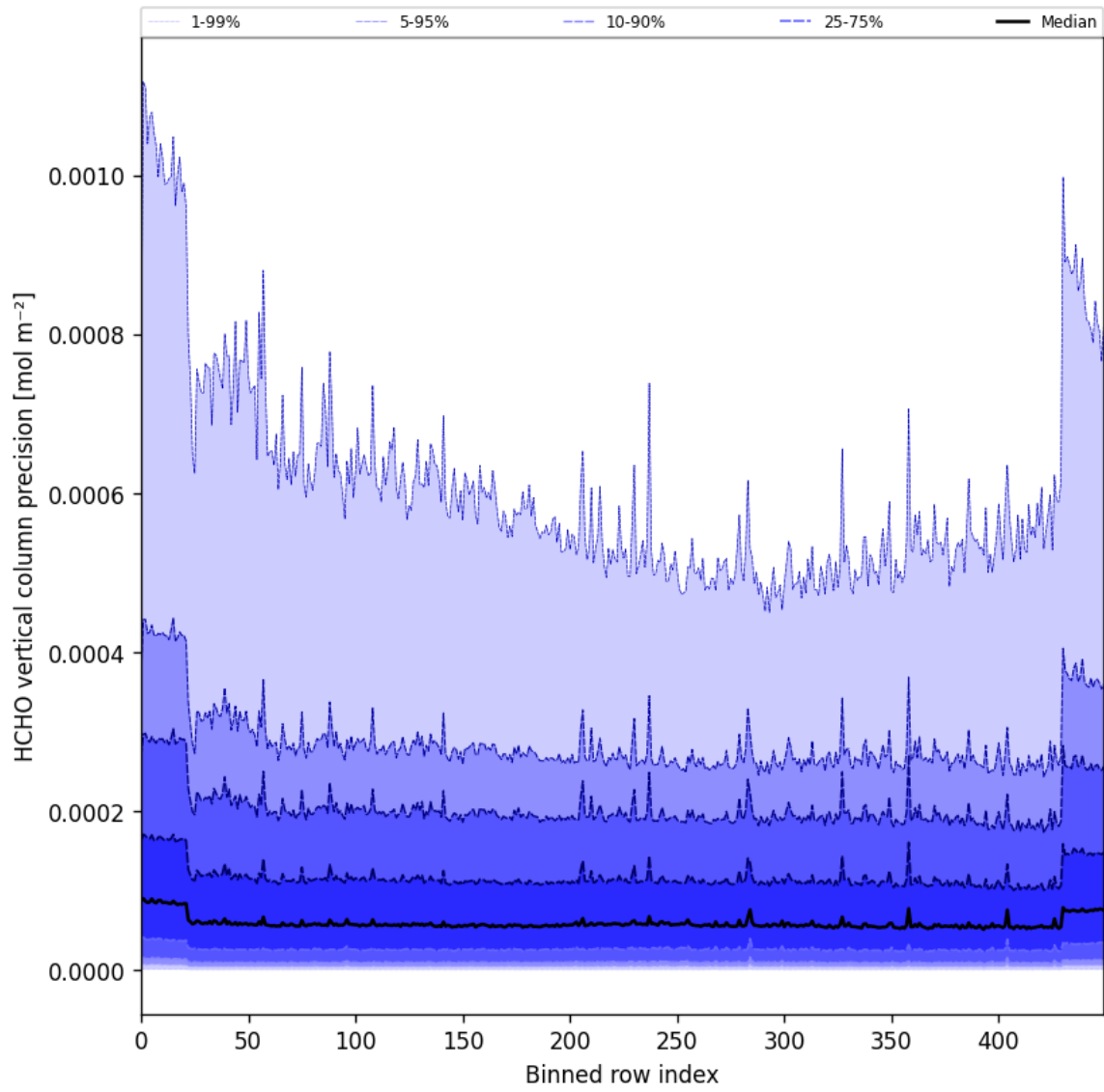
Figure 50: Along track statistics of “HCHO vertical column precision” for 2025-05-26 to 2025-05-27
