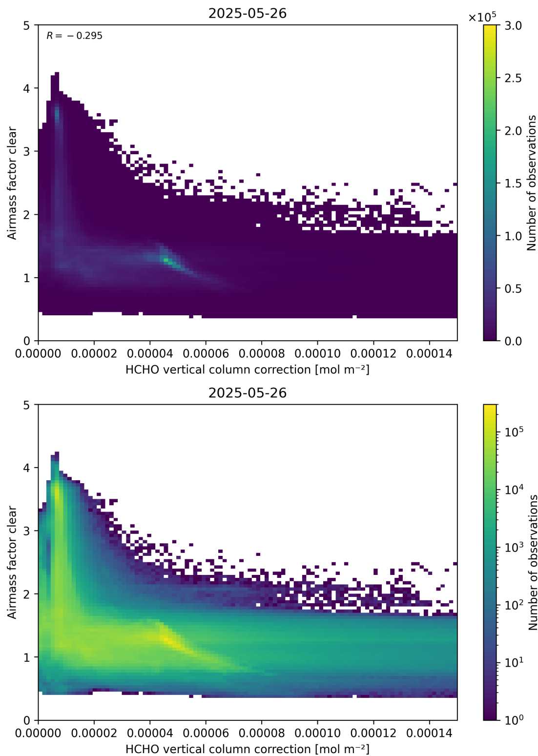
Figure 115: Scatter density plot of “HCHO vertical column correction” against “Airmass factor clear” for 2025-05-26 to 2025-05-27.
