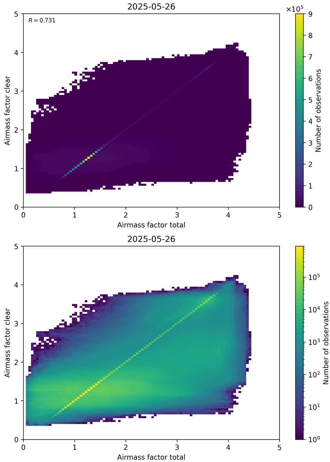
Figure 100: Scatter density plot of “Airmass factor total” against “Airmass factor clear” for 2025-05-26 to 2025-05-27.
