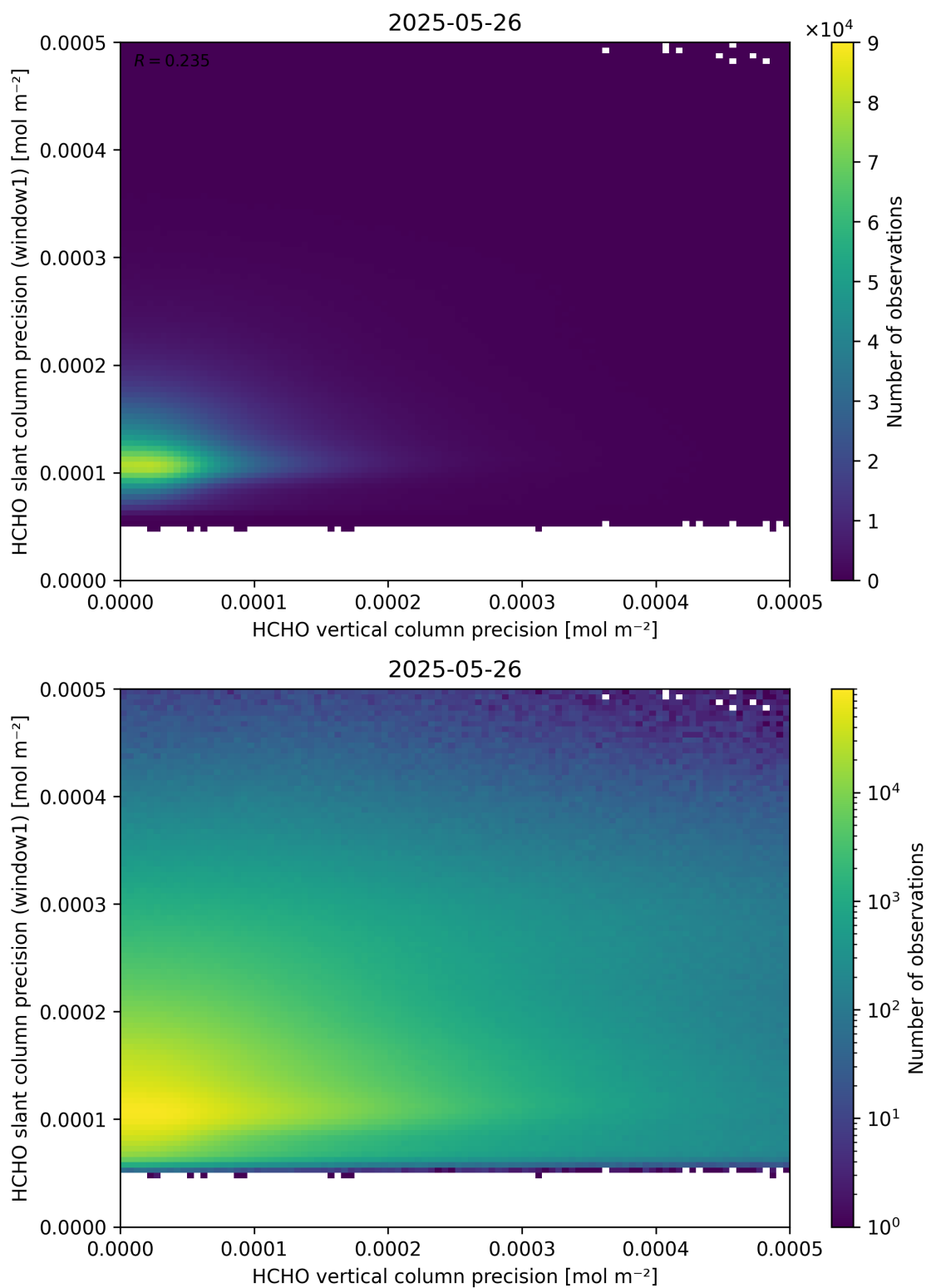
Figure 143: Scatter density plot of “HCHO vertical column precision” against “HCHO slant column precision (window1)” for 2025-05-26 to 2025-05-27.
