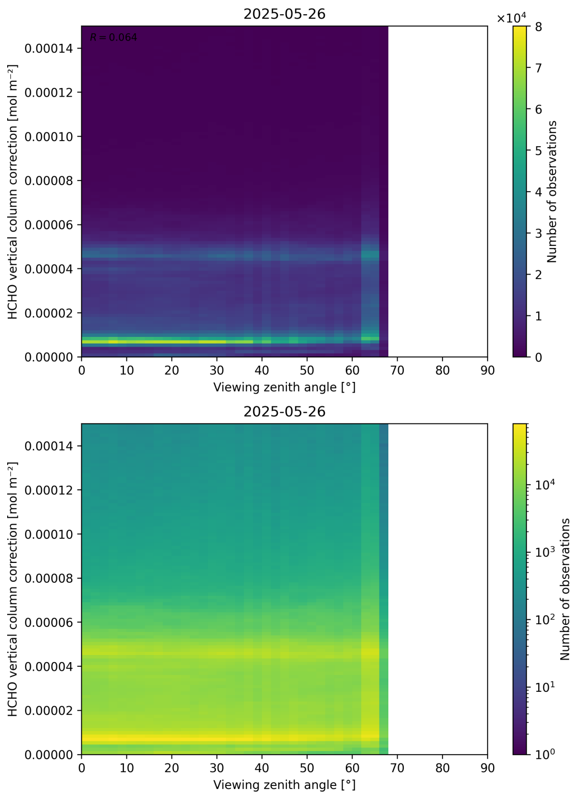
Figure 193: Scatter density plot of “Viewing zenith angle” against “HCHO vertical column correction” for 2025-05-26 to 2025-05-27.
