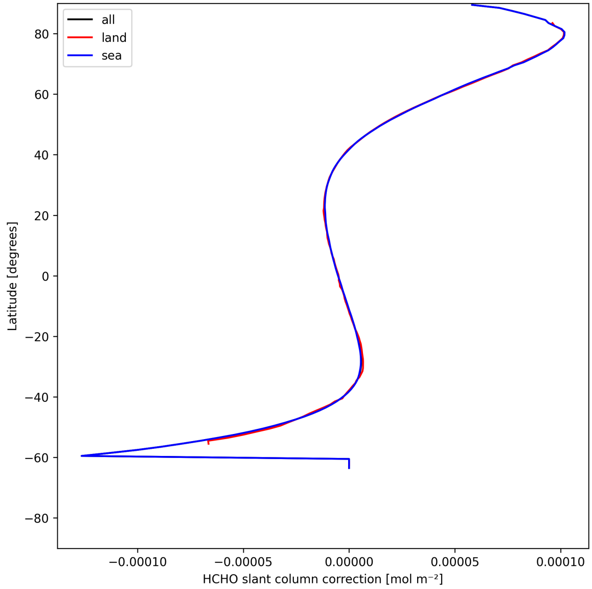
Figure 33: Zonal average of “HCHO slant column correction” for 2025-05-26 to 2025-05-27.
