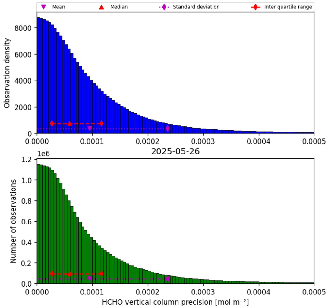
Figure 36: Histogram of “HCHO vertical column precision” for 2025-05-26 to 2025-05-27
