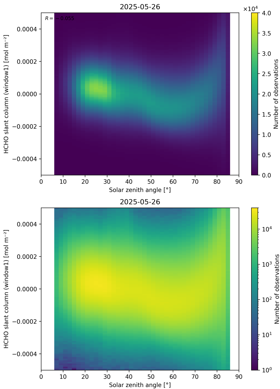
Figure 173: Scatter density plot of “Solar zenith angle” against “HCHO slant column (window1)” for 2025-05-26 to 2025-05-27.
