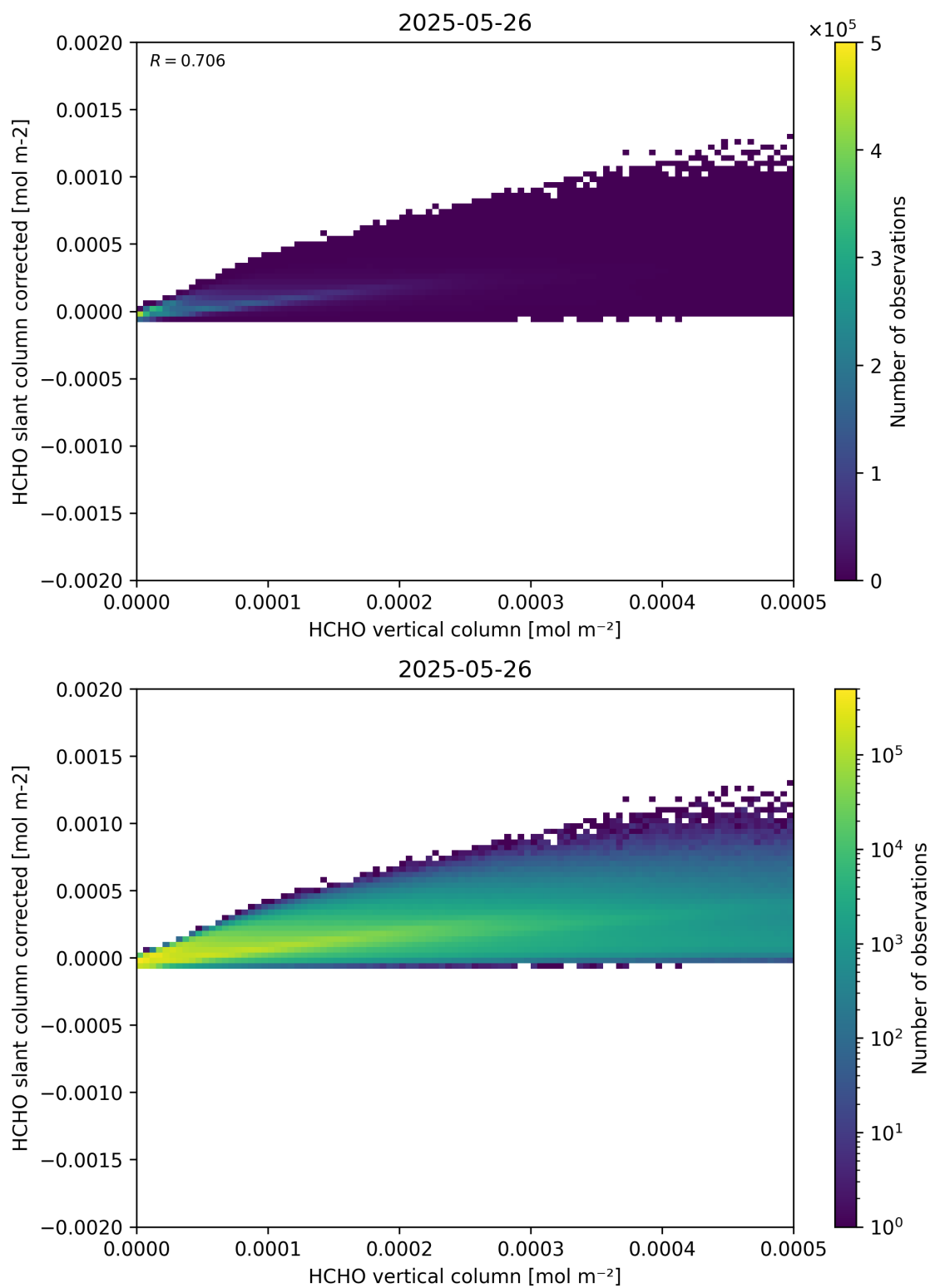
Figure 127: Scatter density plot of “HCHO vertical column” against “HCHO slant column corrected” for 2025-05-26 to 2025-05-27.
