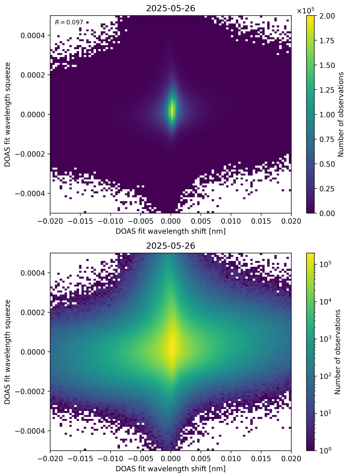
Figure 65: Scatter density plot of “DOAS fit wavelength shift” against “DOAS fit wavelength squeeze” for 2025-05-26 to 2025-05-27.
