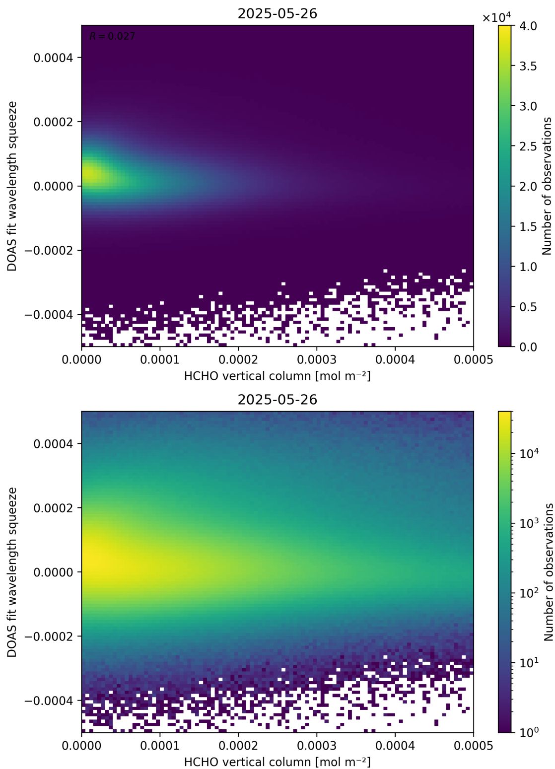
Figure 125: Scatter density plot of “HCHO vertical column” against “DOAS fit wavelength squeeze” for 2025-05-26 to 2025-05-27.
