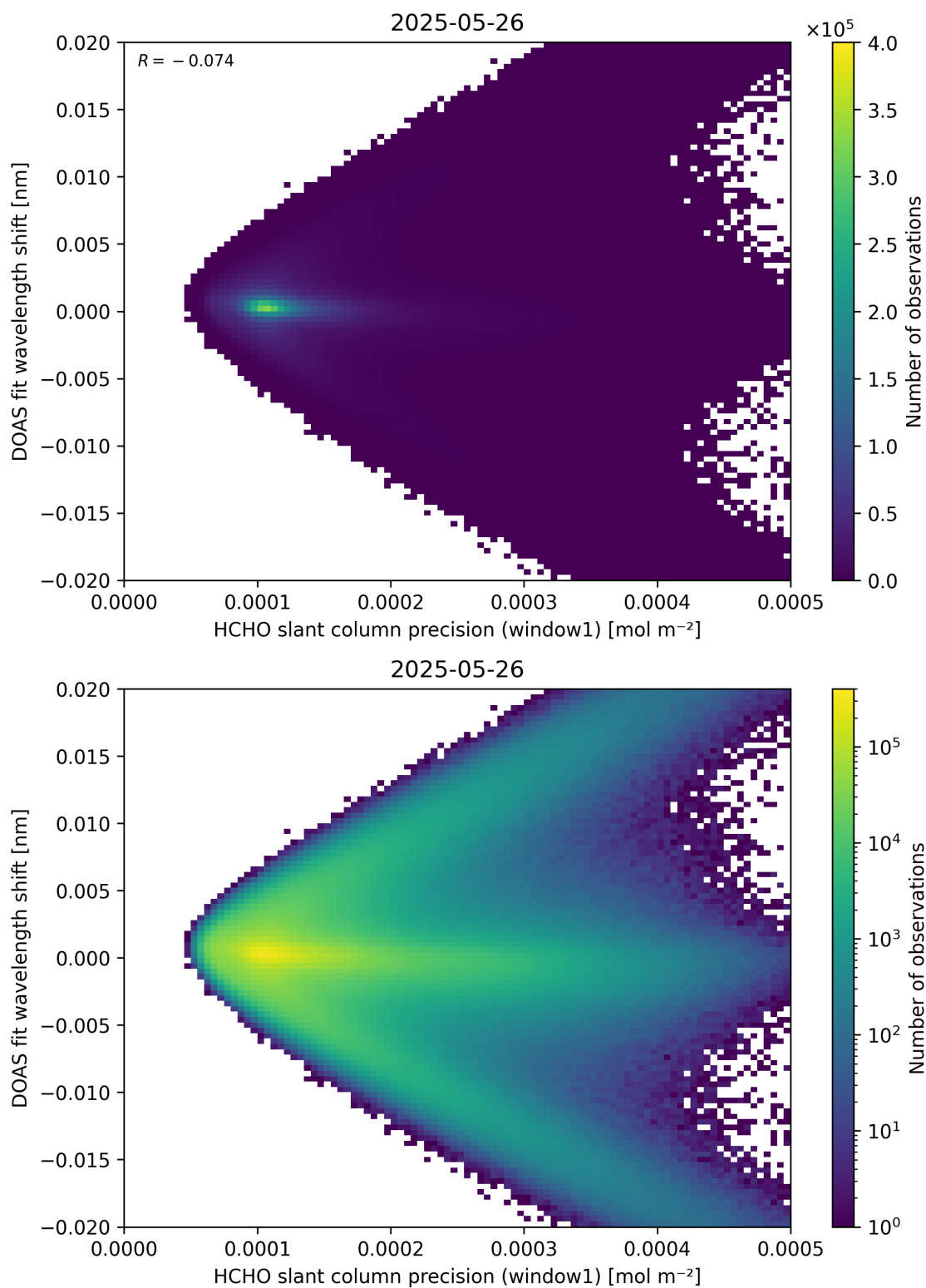
Figure 89: Scatter density plot of “HCHO slant column precision (window1)” against “DOAS fit wavelength shift” for 2025-05-26 to 2025-05-27.
