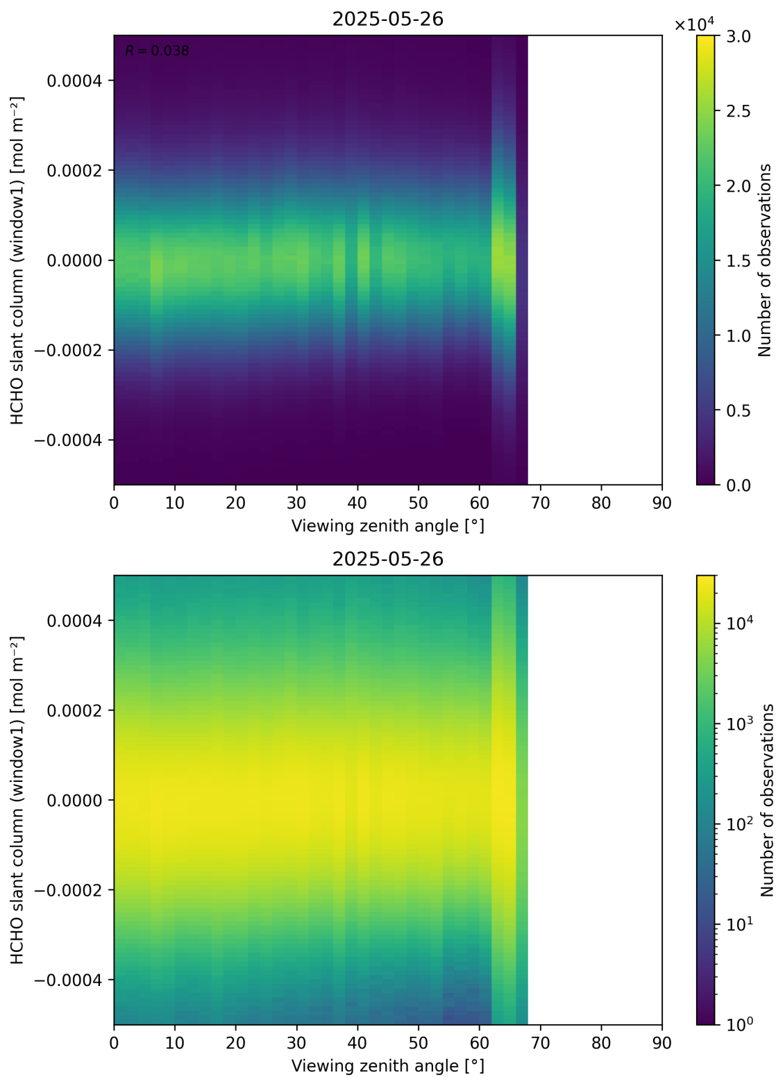
Figure 188: Scatter density plot of “Viewing zenith angle” against “HCHO slant column (window1)” for 2025-05-26 to 2025-05-27.
