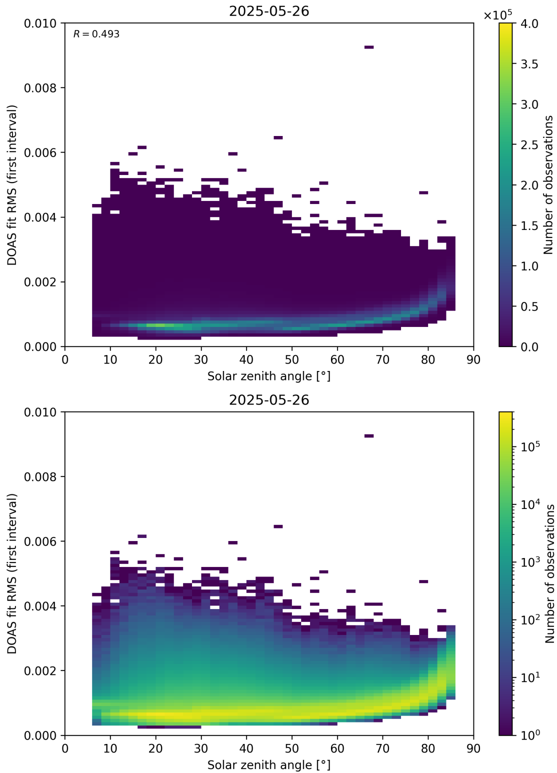
Figure 167: Scatter density plot of “Solar zenith angle” against “DOAS fit RMS (first interval)” for 2025-05-26 to 2025-05-27.
