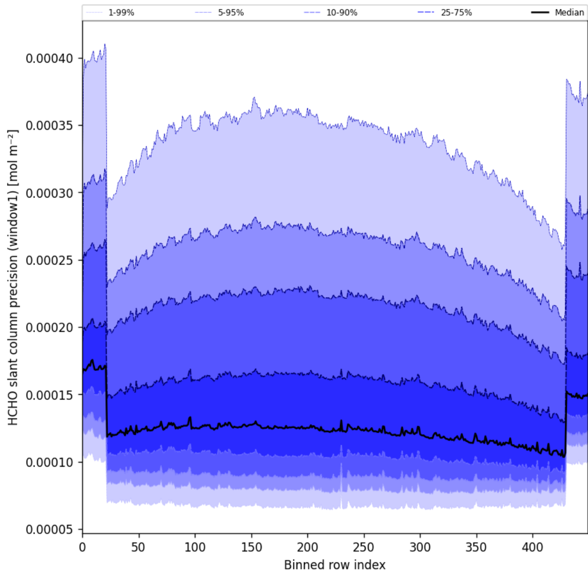
Figure 53: Along track statistics of “HCHO slant column precision (window1)” for 2025-05-26 to 2025-05-27
