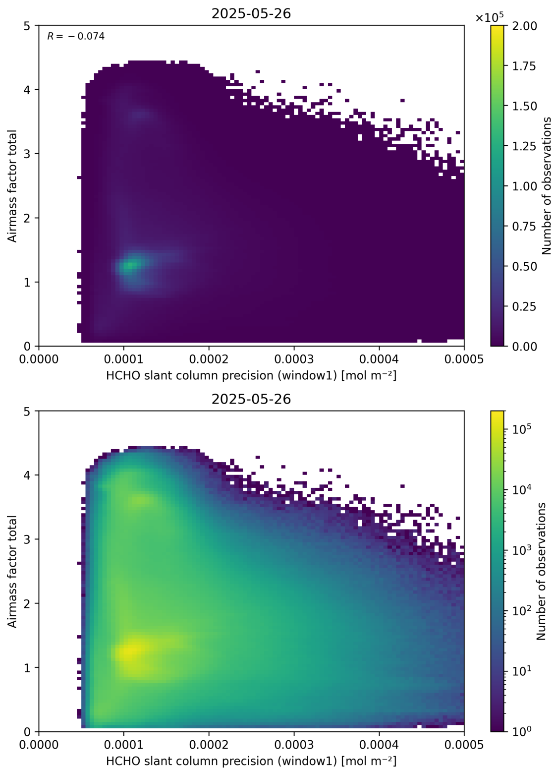
Figure 94: Scatter density plot of “HCHO slant column precision (window1)” against “Airmass factor total” for 2025-05-26 to 2025-05-27.
