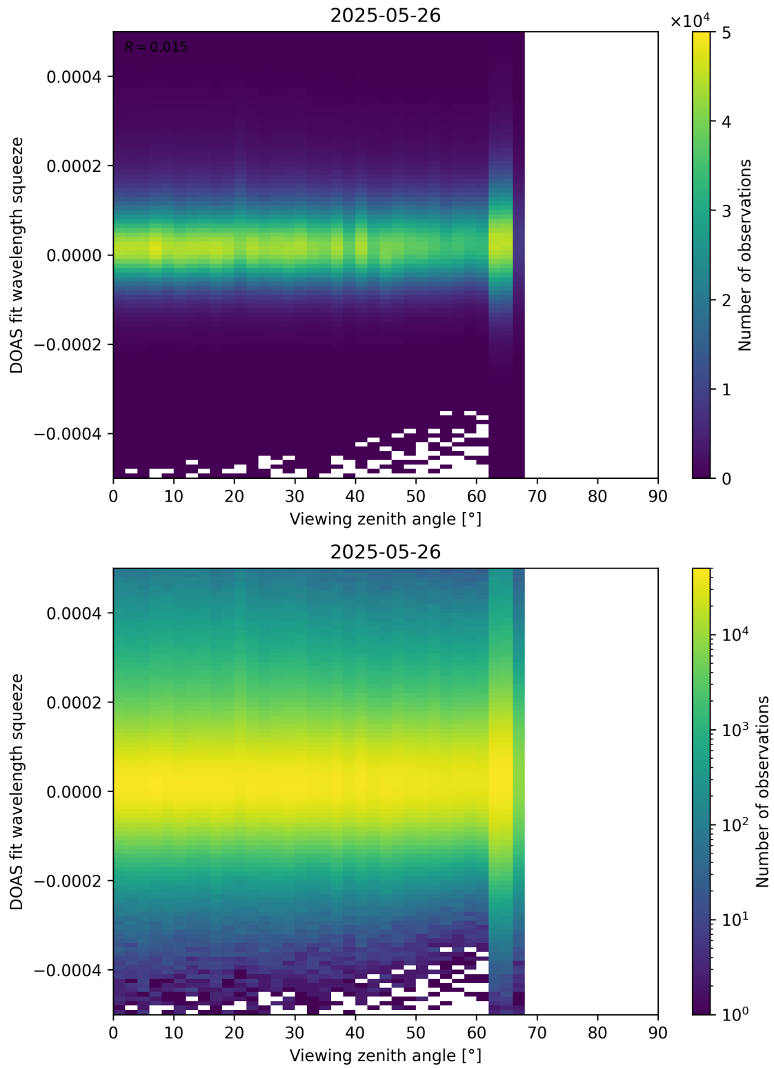
Figure 184: Scatter density plot of “Viewing zenith angle” against “DOAS fit wavelength squeeze” for 2025-05-26 to 2025-05-27.
