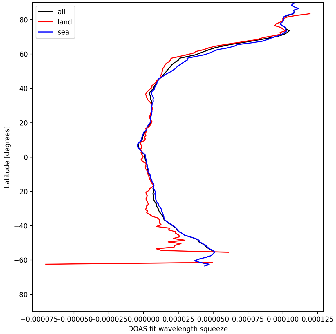
Figure 31: Zonal average of “DOAS fit wavelength squeeze” for 2025-05-26 to 2025-05-27.
