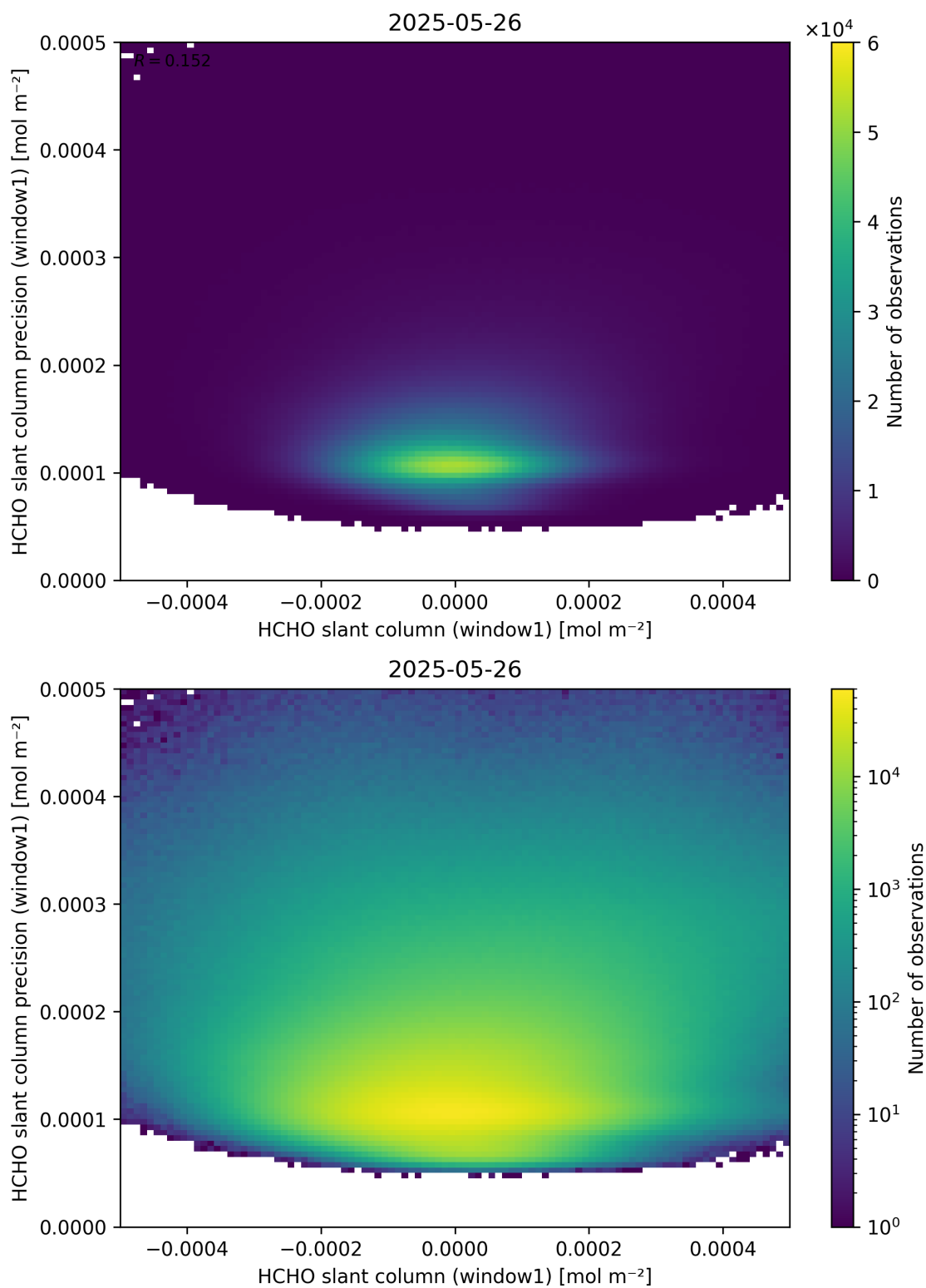
Figure 84: Scatter density plot of “HCHO slant column (window1)” against “HCHO slant column precision (window1)” for 2025-05-26 to 2025-05-27.
