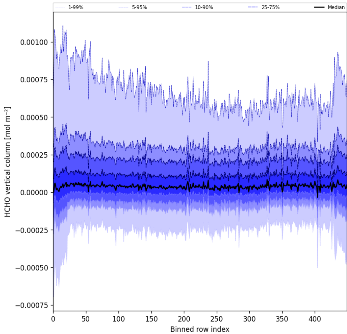
Figure 49: Along track statistics of “HCHO vertical column” for 2025-05-26 to 2025-05-27
