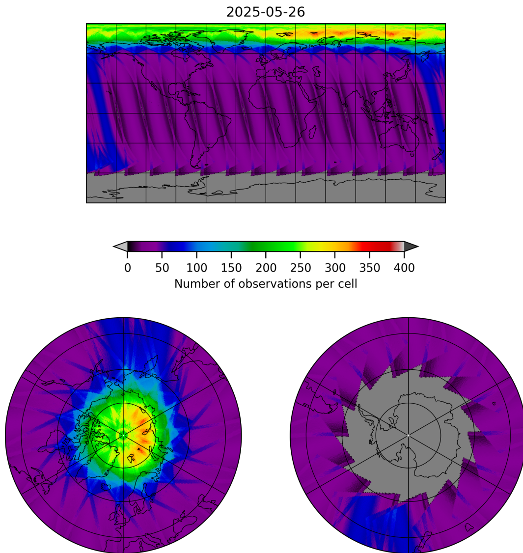
Figure 19: Map of the number of observations for 2025-05-26 to 2025-05-27
