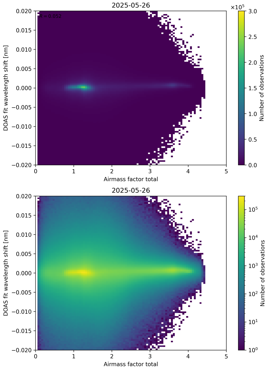
Figure 98: Scatter density plot of “Airmass factor total” against “DOAS fit wavelength shift” for 2025-05-26 to 2025-05-27.
