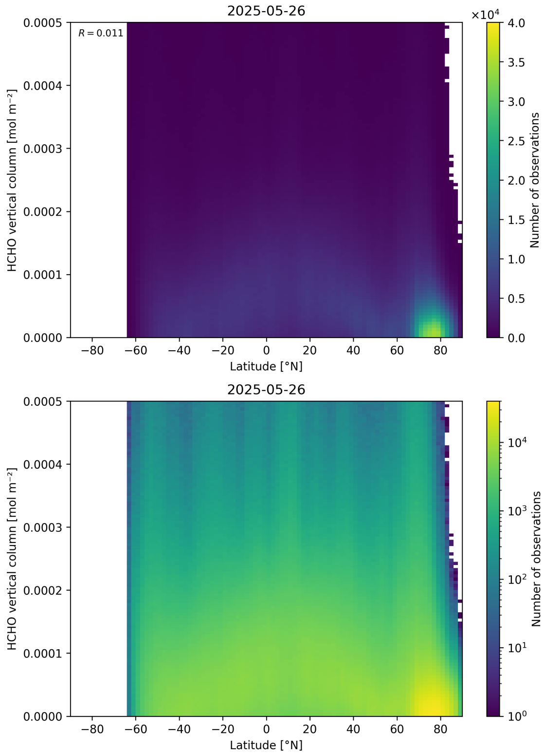
Figure 163: Scatter density plot of “Latitude” against “HCHO vertical column” for 2025-05-26 to 2025-05-27.
