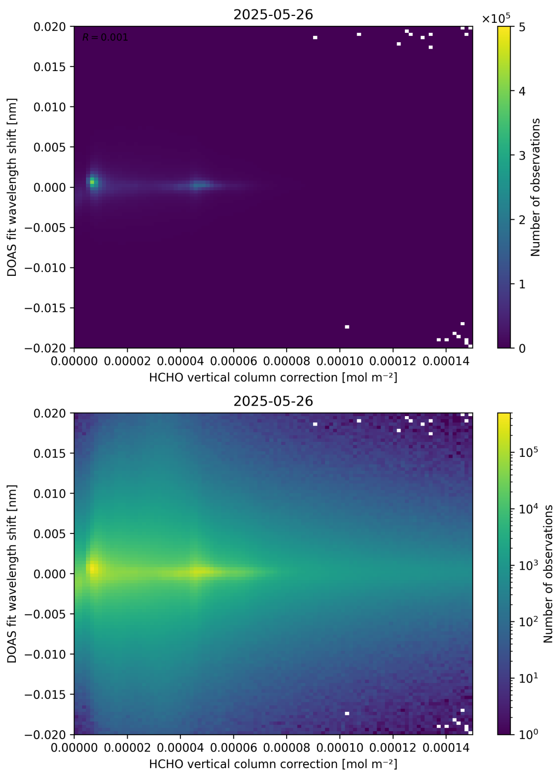
Figure 113: Scatter density plot of “HCHO vertical column correction” against “DOAS fit wavelength shift” for 2025-05-26 to 2025-05-27.
