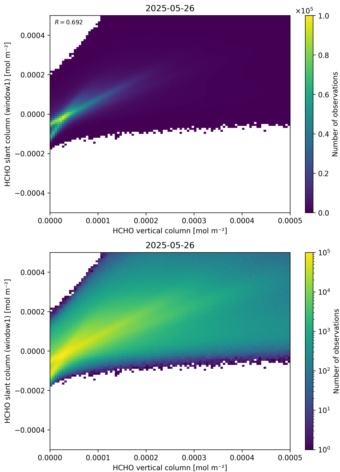
Figure 129: Scatter density plot of “HCHO vertical column” against “HCHO slant column (window1)” for 2025-05-26 to 2025-05-27.
