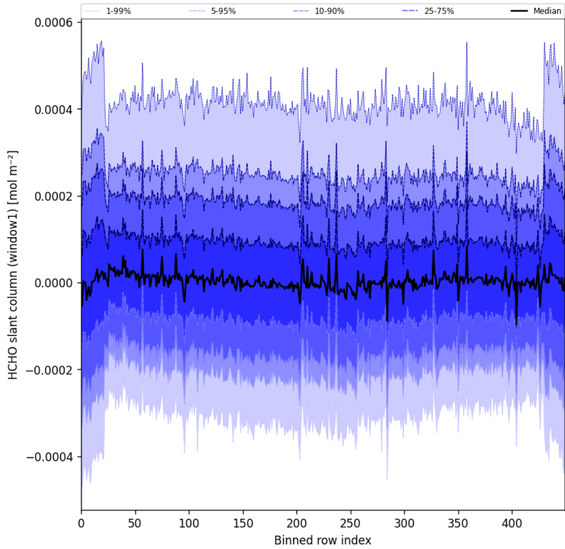
Figure 52: Along track statistics of “HCHO slant column (window1)” for 2025-05-26 to 2025-05-27
