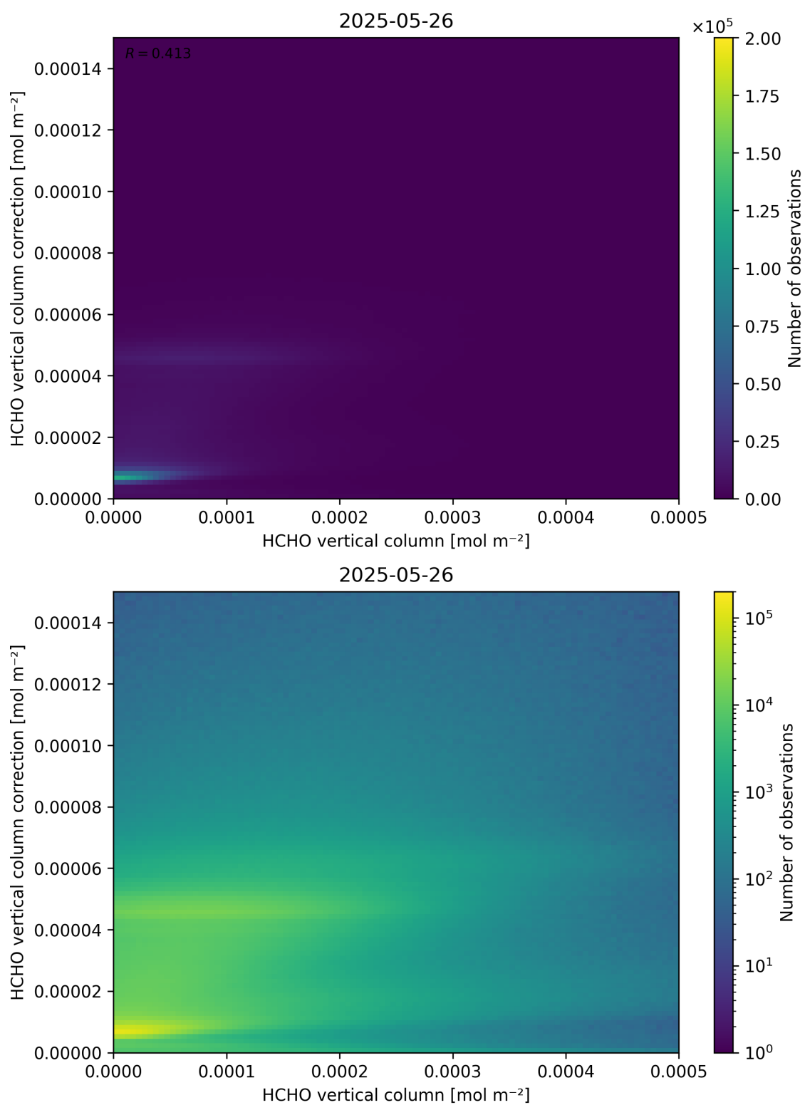
Figure 133: Scatter density plot of “HCHO vertical column” against “HCHO vertical column correction” for 2025-05-26 to 2025-05-27.
