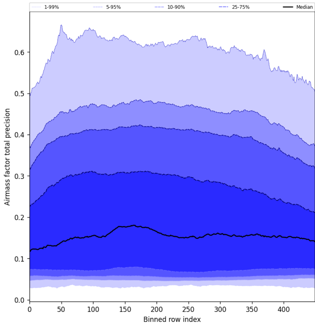
Figure 55: Along track statistics of “Airmass factor total precision” for 2025-05-26 to 2025-05-27
