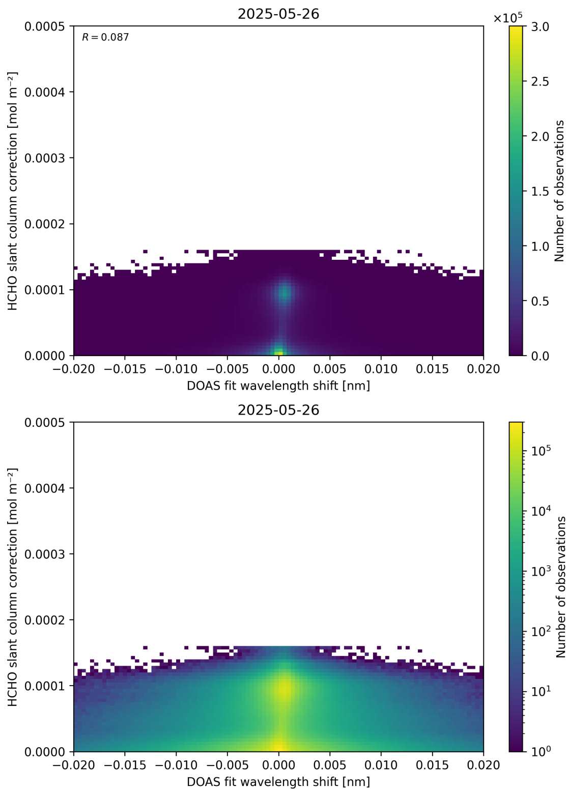
Figure 67: Scatter density plot of “DOAS fit wavelength shift” against “HCHO slant column correction” for 2025-05-26 to 2025-05-27.
