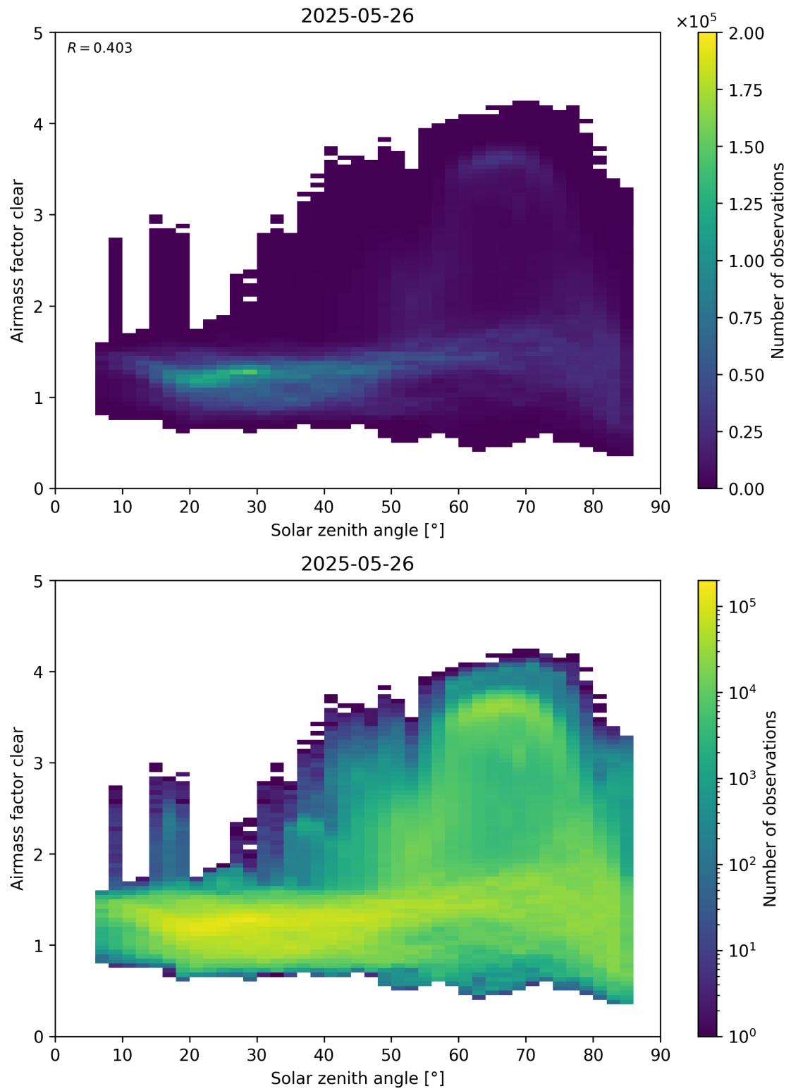
Figure 170: Scatter density plot of “Solar zenith angle” against “Airmass factor clear” for 2025-05-26 to 2025-05-27.
