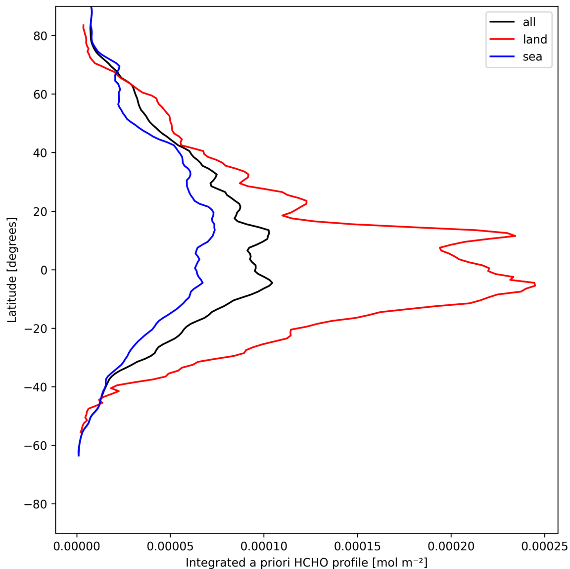
Figure 29: Zonal average of “Integrated a priori HCHO profile” for 2025-05-26 to 2025-05-27.
