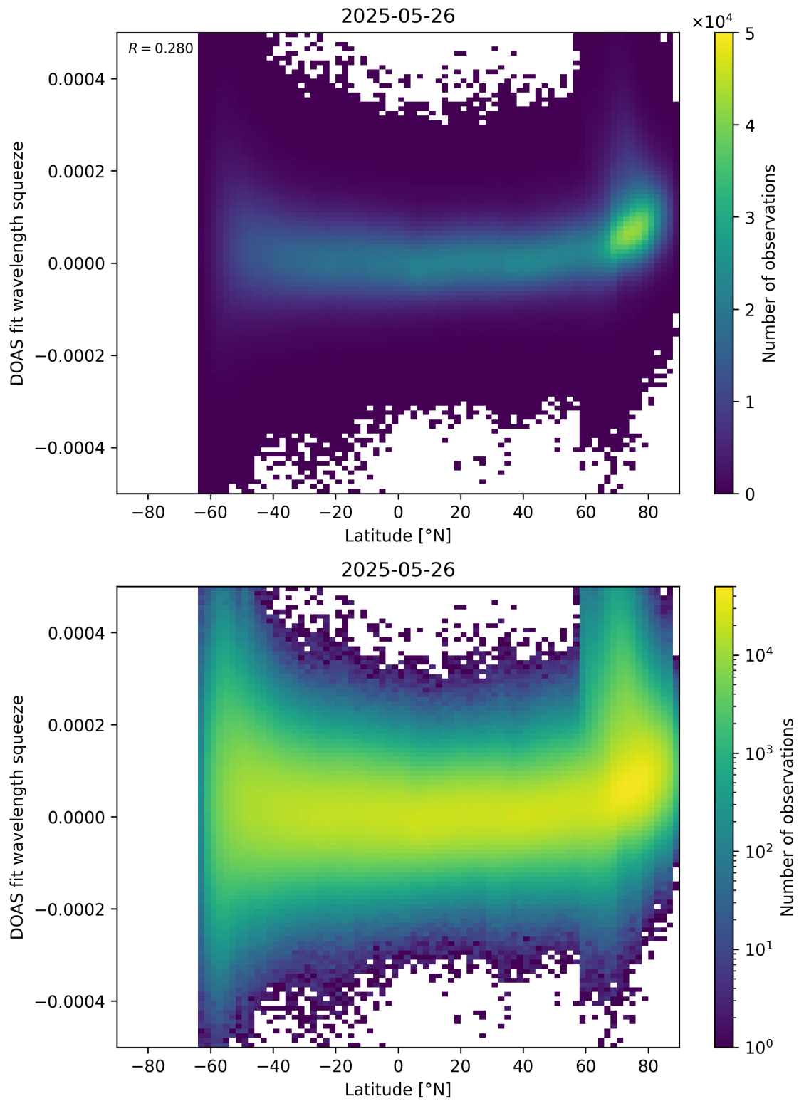
Figure 155: Scatter density plot of “Latitude” against “DOAS fit wavelength squeeze” for 2025-05-26 to 2025-05-27.
