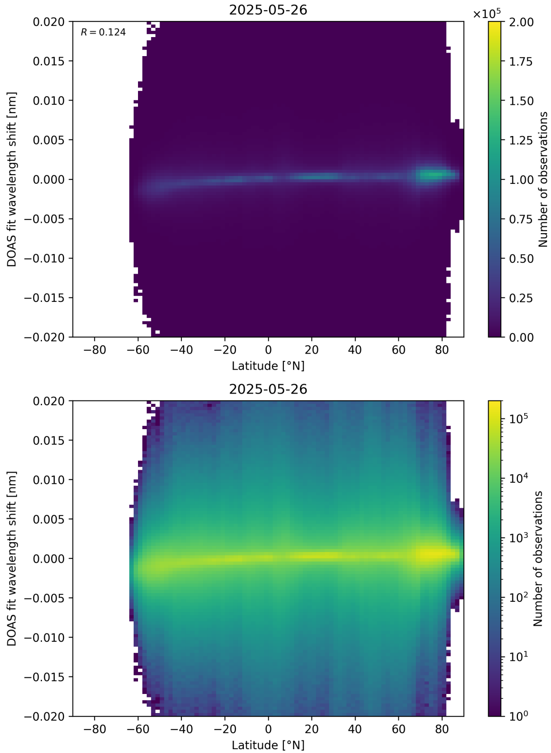
Figure 154: Scatter density plot of “Latitude” against “DOAS fit wavelength shift” for 2025-05-26 to 2025-05-27.
