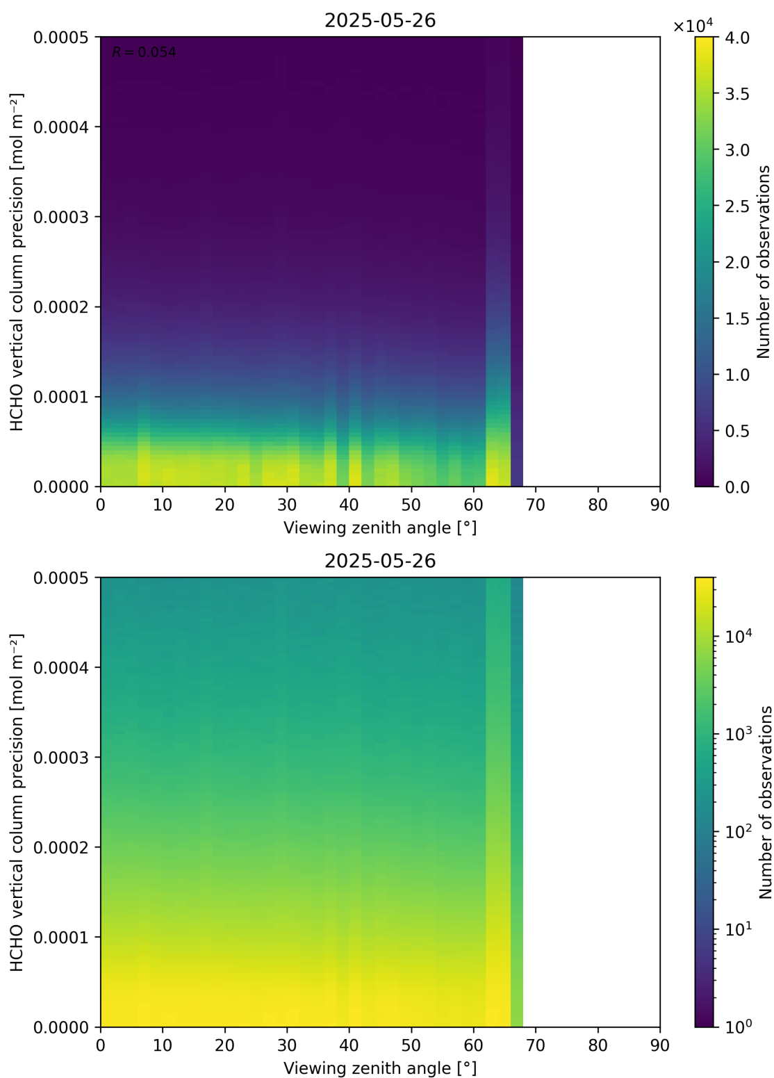
Figure 194: Scatter density plot of “Viewing zenith angle” against “HCHO vertical column precision” for 2025-05-26 to 2025-05-27.
