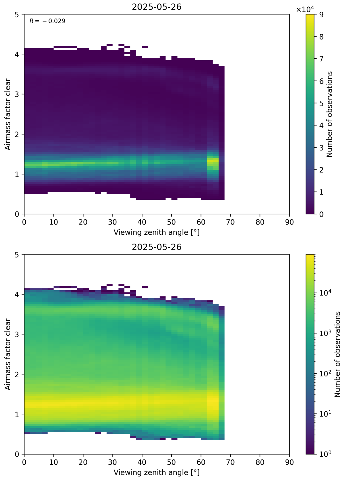
Figure 185: Scatter density plot of “Viewing zenith angle” against “Airmass factor clear” for 2025-05-26 to 2025-05-27.
