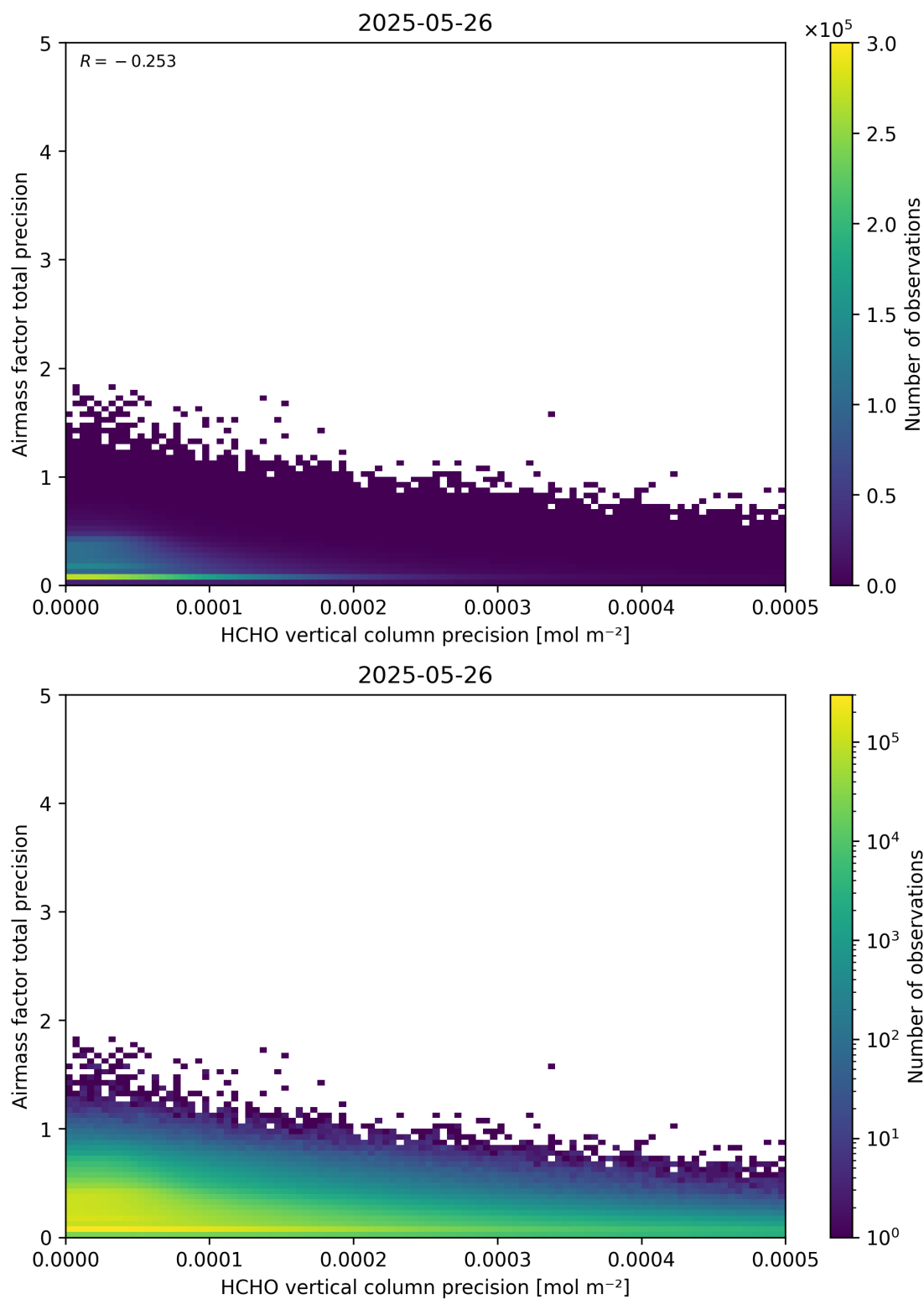
Figure 145: Scatter density plot of “HCHO vertical column precision” against “Airmass factor total precision” for 2025-05-26 to 2025-05-27.
