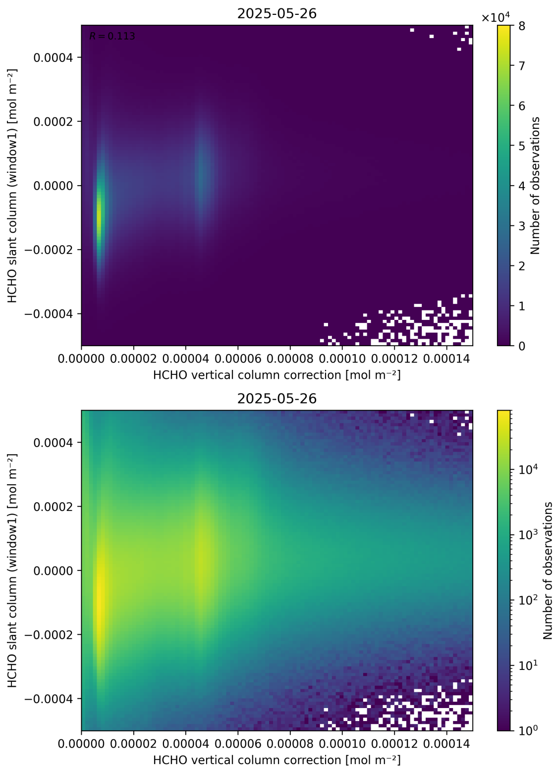
Figure 118: Scatter density plot of “HCHO vertical column correction” against “HCHO slant column (window1)” for 2025-05-26 to 2025-05-27.
