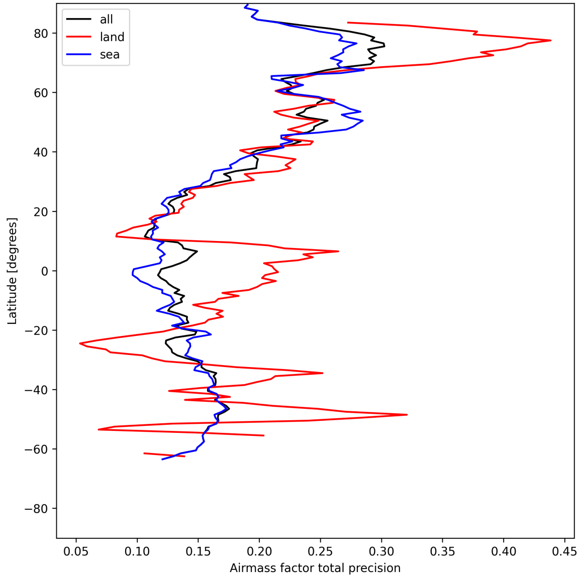
Figure 27: Zonal average of “Airmass factor total precision” for 2025-05-26 to 2025-05-27.
