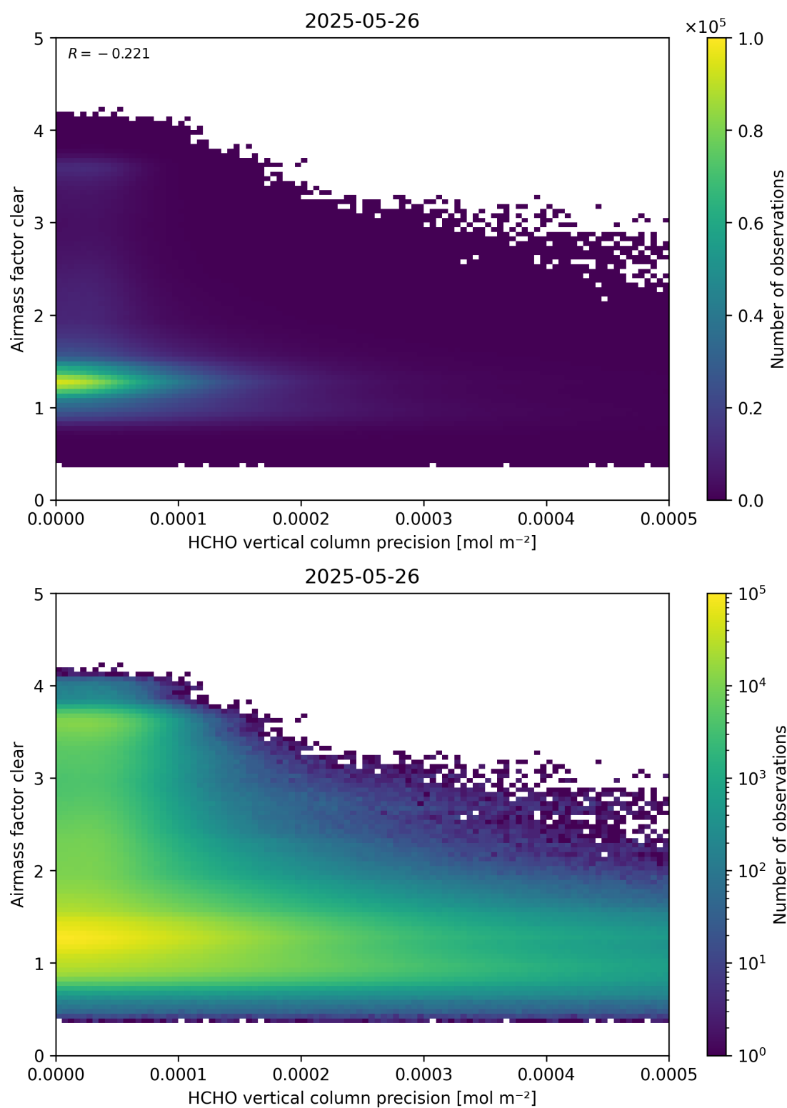
Figure 139: Scatter density plot of “HCHO vertical column precision” against “Airmass factor clear” for 2025-05-26 to 2025-05-27.
