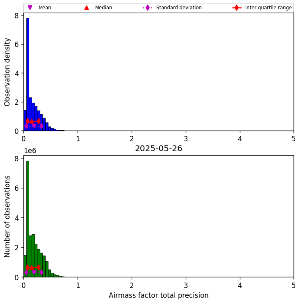
Figure 41: Histogram of “Airmass factor total precision” for 2025-05-26 to 2025-05-27
