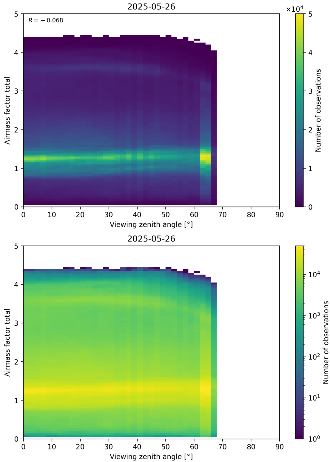
Figure 190: Scatter density plot of “Viewing zenith angle” against “Airmass factor total” for 2025-05-26 to 2025-05-27.
