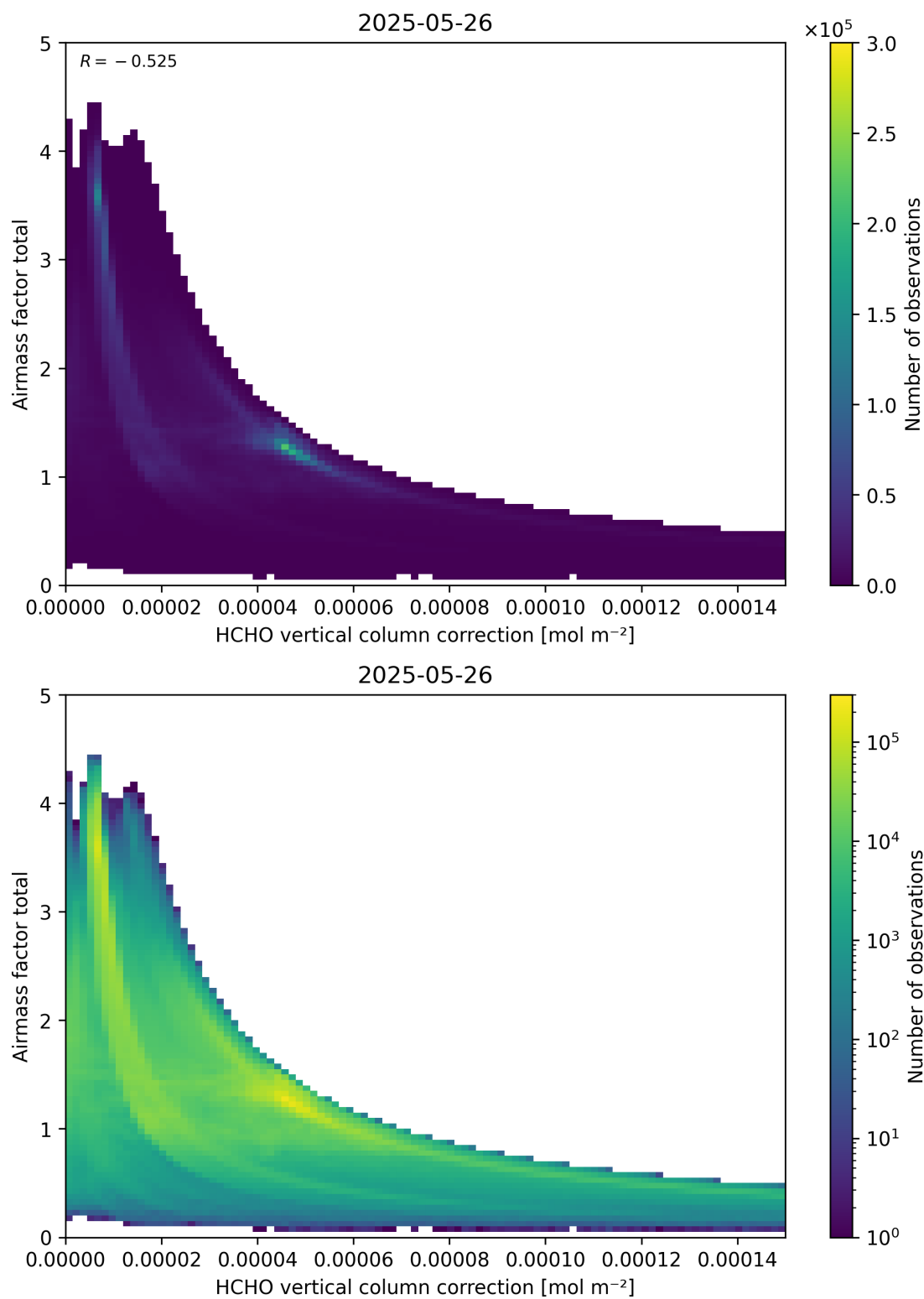
Figure 120: Scatter density plot of “HCHO vertical column correction” against “Airmass factor total” for 2025-05-26 to 2025-05-27.
