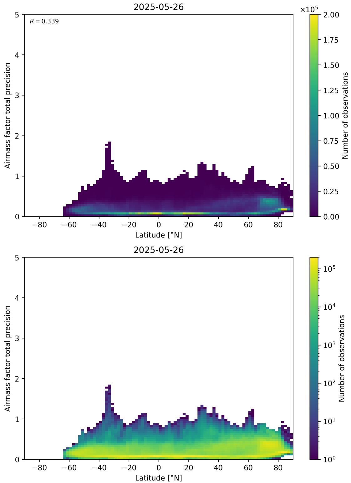
Figure 162: Scatter density plot of “Latitude” against “Airmass factor total precision” for 2025-05-26 to 2025-05-27.
