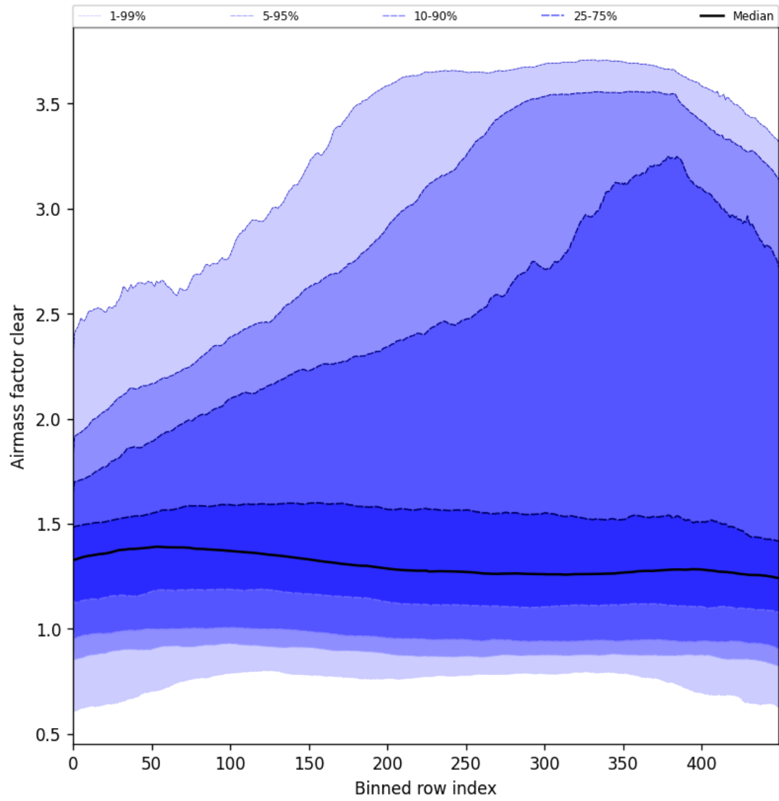
Figure 56: Along track statistics of “Airmass factor clear” for 2025-05-26 to 2025-05-27
