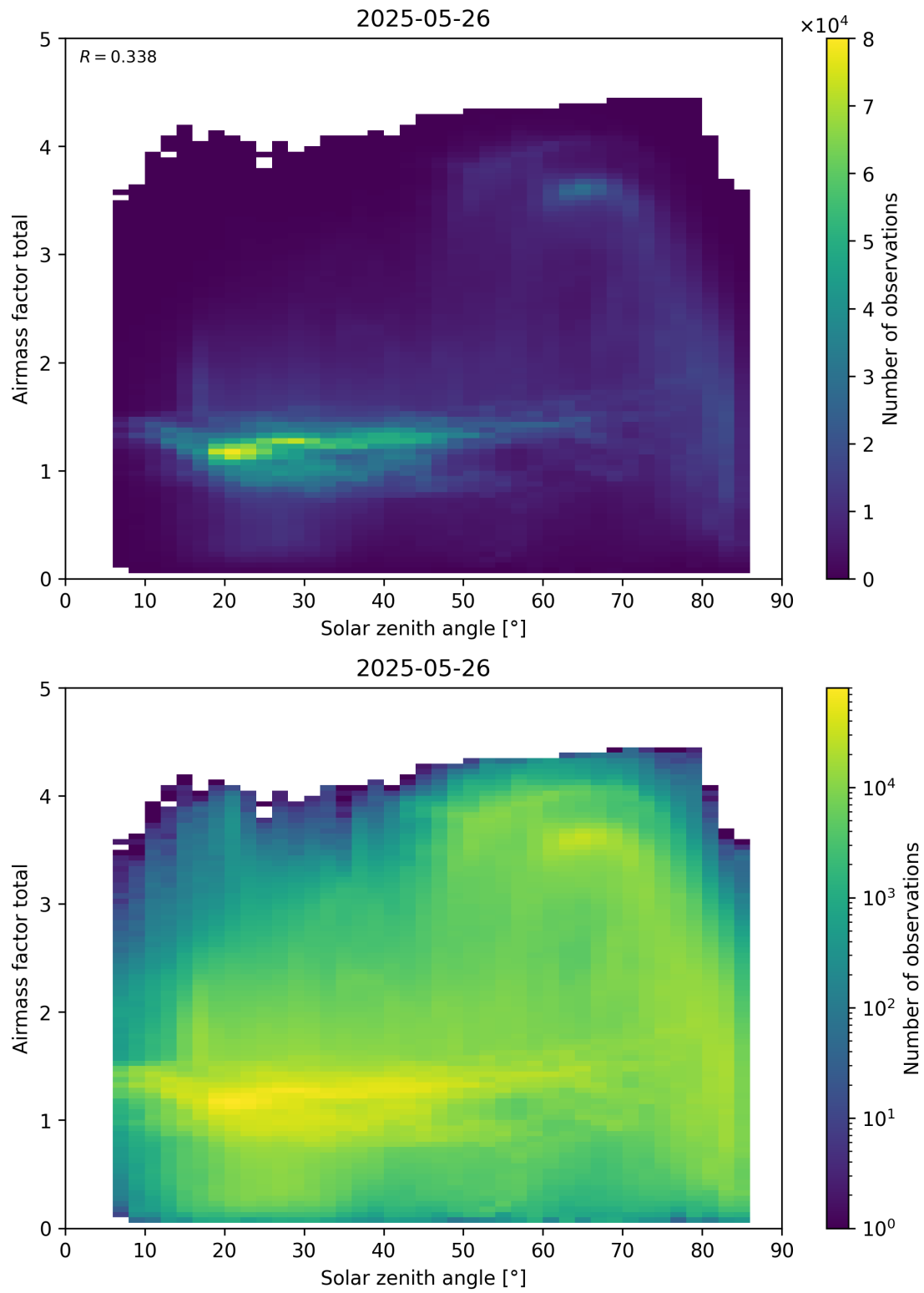
Figure 175: Scatter density plot of “Solar zenith angle” against “Airmass factor total” for 2025-05-26 to 2025-05-27.
