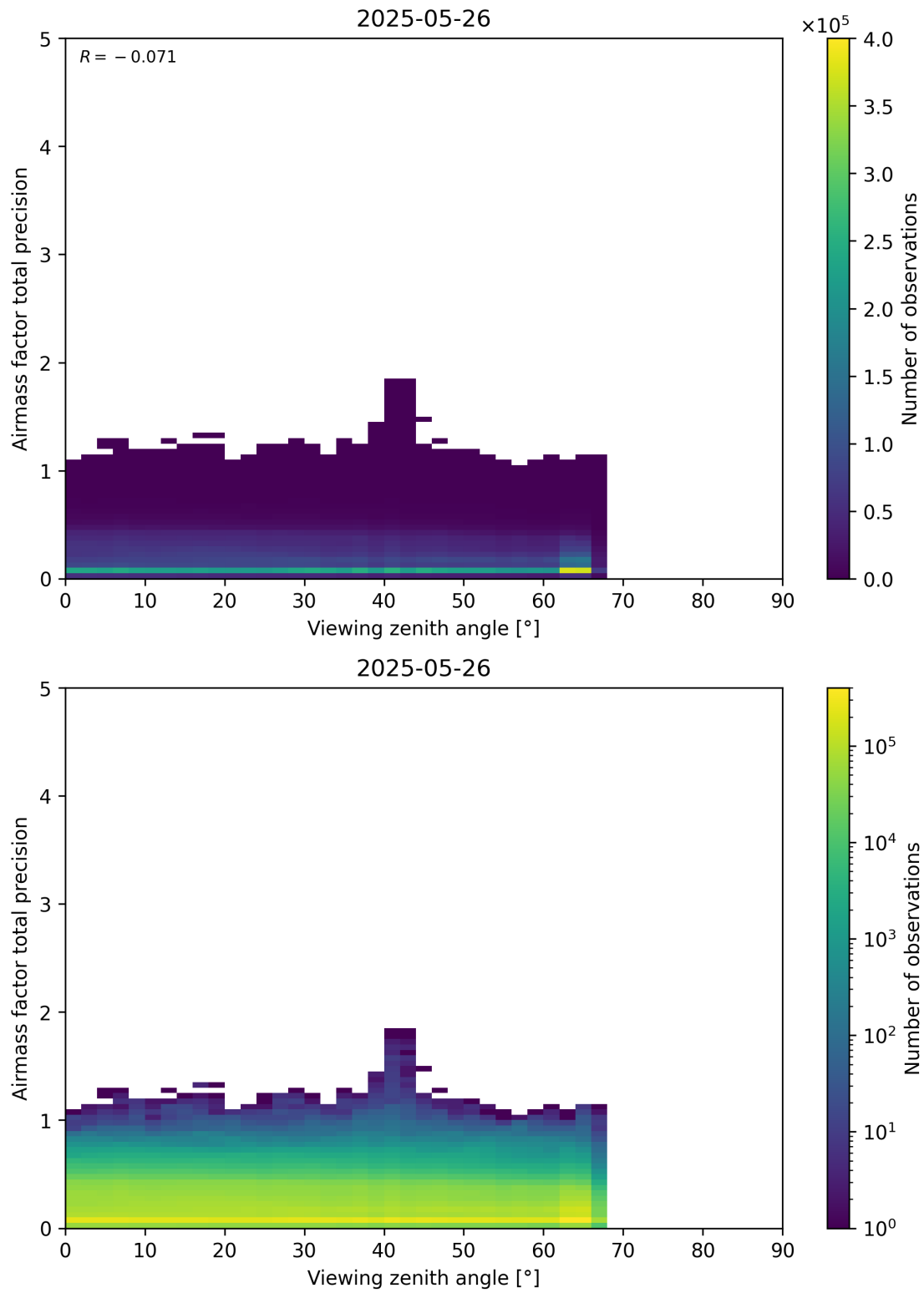
Figure 191: Scatter density plot of “Viewing zenith angle” against “Airmass factor total precision” for 2025-05-26 to 2025-05-27.
