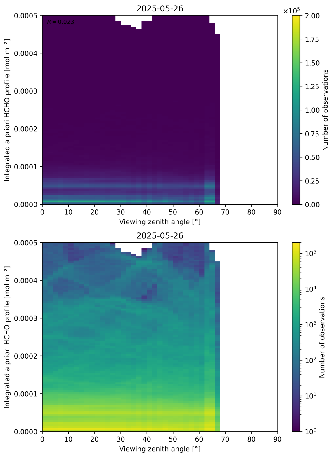
Figure 195: Scatter density plot of “Viewing zenith angle” against “Integrated a priori HCHO profile” for 2025-05-26 to 2025-05-27.
