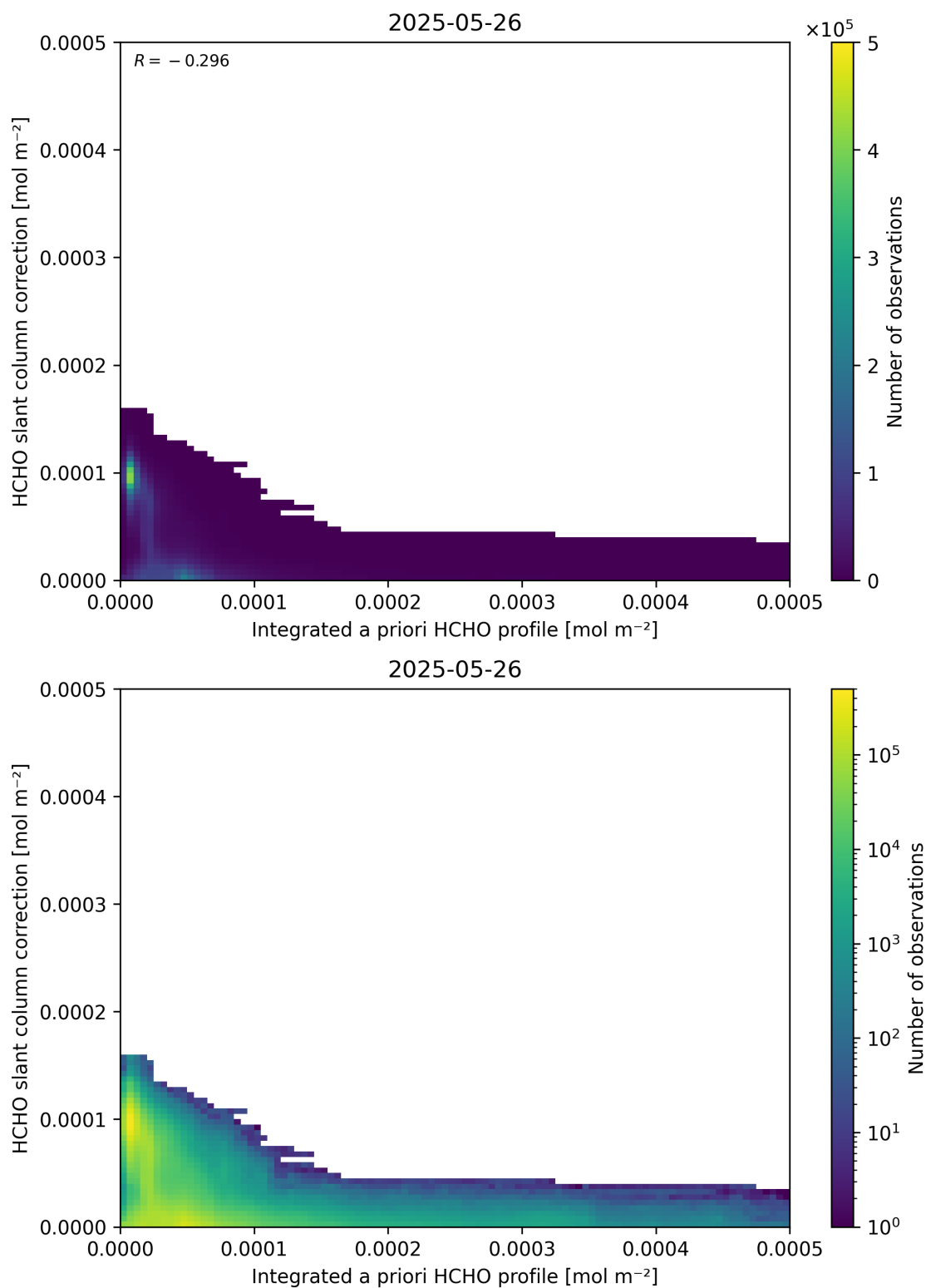
Figure 152: Scatter density plot of “Integrated a priori HCHO profile” against “HCHO slant column correction” for 2025-05-26 to 2025-05-27.
