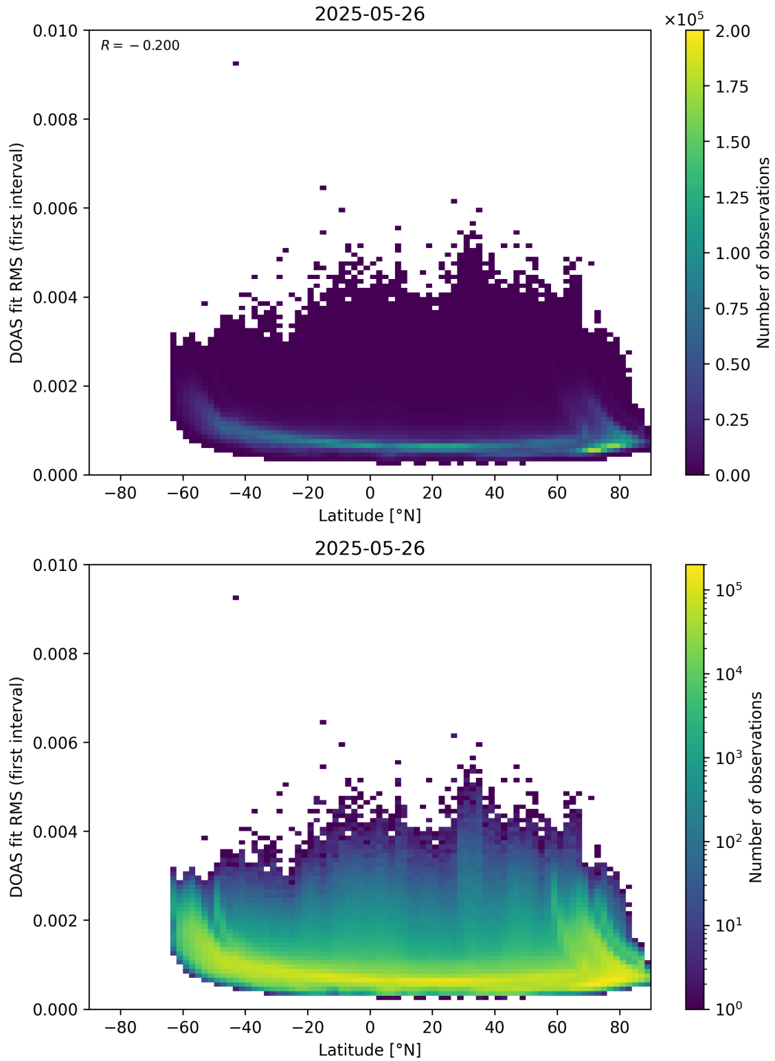
Figure 153: Scatter density plot of “Latitude” against “DOAS fit RMS (first interval)” for 2025-05-26 to 2025-05-27.
