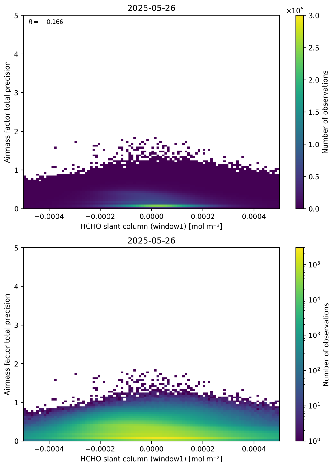
Figure 86: Scatter density plot of “HCHO slant column (window1)” against “Airmass factor total precision” for 2025-05-26 to 2025-05-27.
