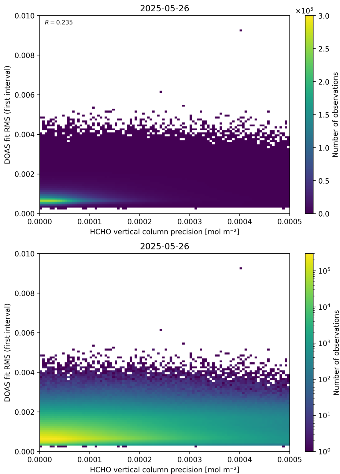
Figure 136: Scatter density plot of “HCHO vertical column precision” against “DOAS fit RMS (first interval)” for 2025-05-26 to 2025-05-27.
