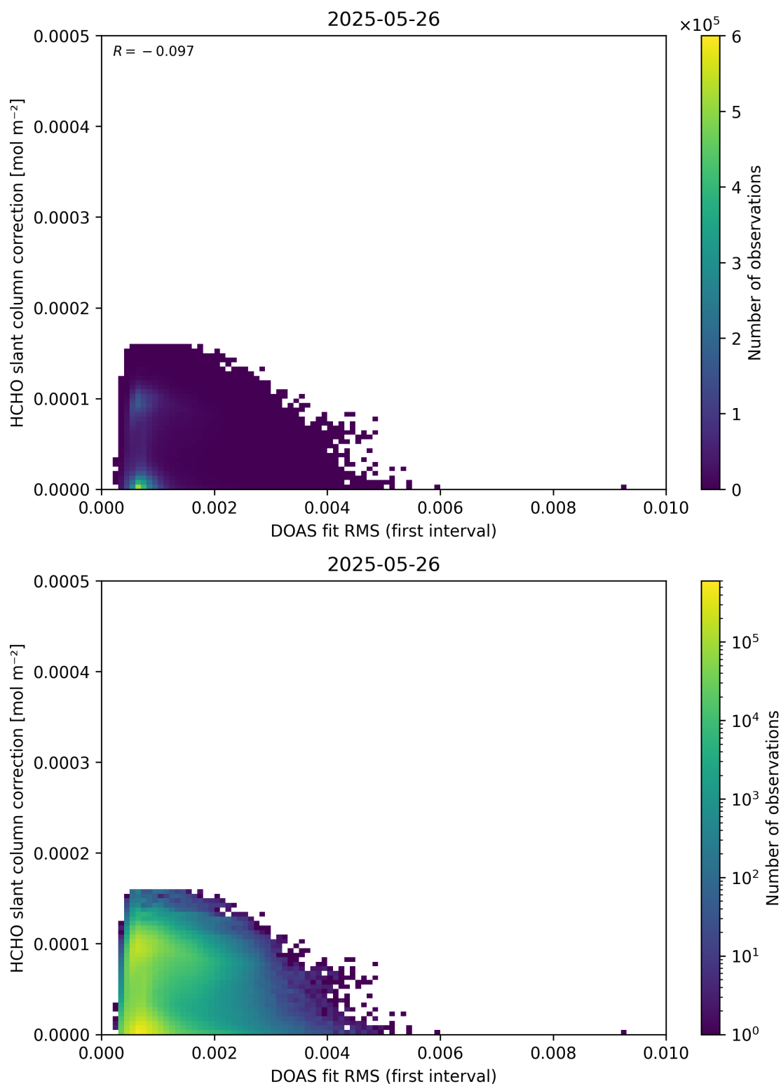
Figure 63: Scatter density plot of “DOAS fit RMS (first interval)” against “HCHO slant column correction” for 2025-05-26 to 2025-05-27.
