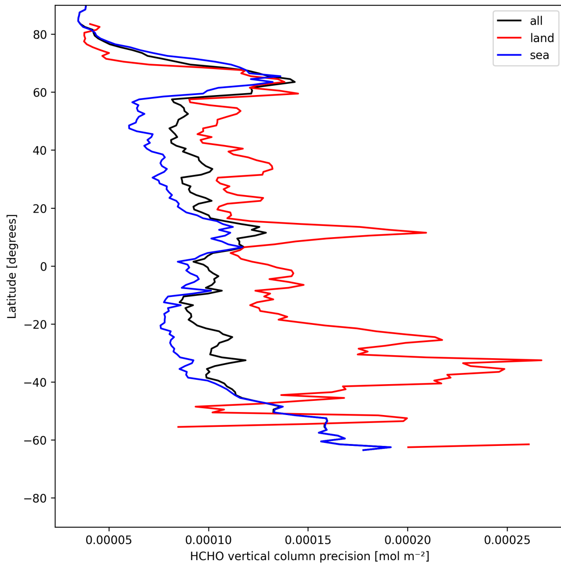
Figure 22: Zonal average of “HCHO vertical column precision” for 2025-05-26 to 2025-05-27.
