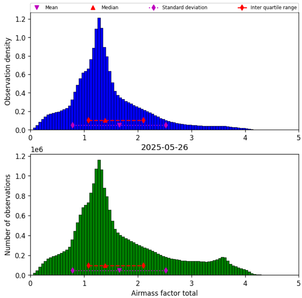
Figure 40: Histogram of “Airmass factor total” for 2025-05-26 to 2025-05-27
