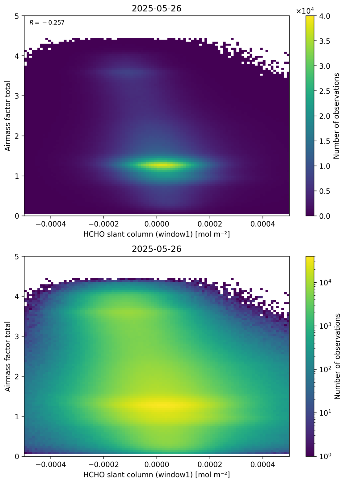
Figure 85: Scatter density plot of “HCHO slant column (window1)” against “Airmass factor total” for 2025-05-26 to 2025-05-27.
