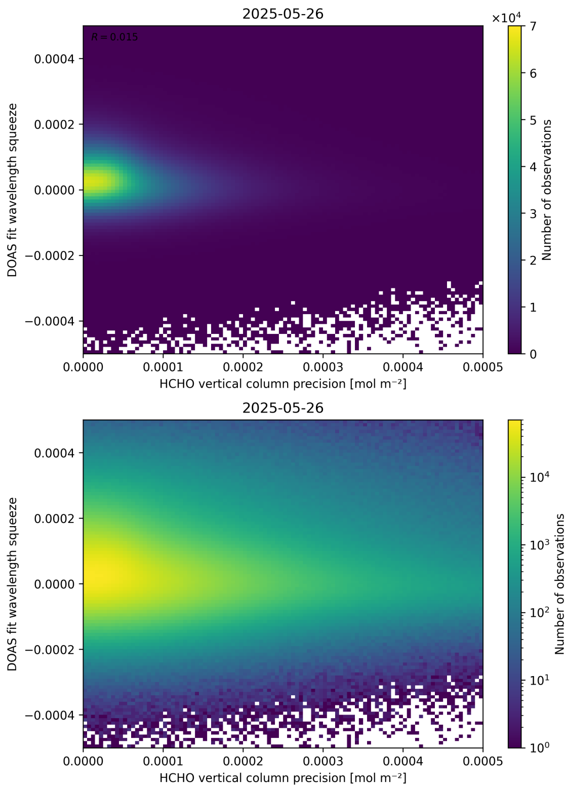
Figure 138: Scatter density plot of “HCHO vertical column precision” against “DOAS fit wavelength squeeze” for 2025-05-26 to 2025-05-27.
