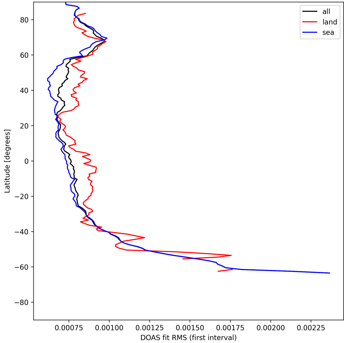
Figure 32: Zonal average of "DOAS fit RMS (first interval)" for 2025-05-26 to 2025-05-27.
