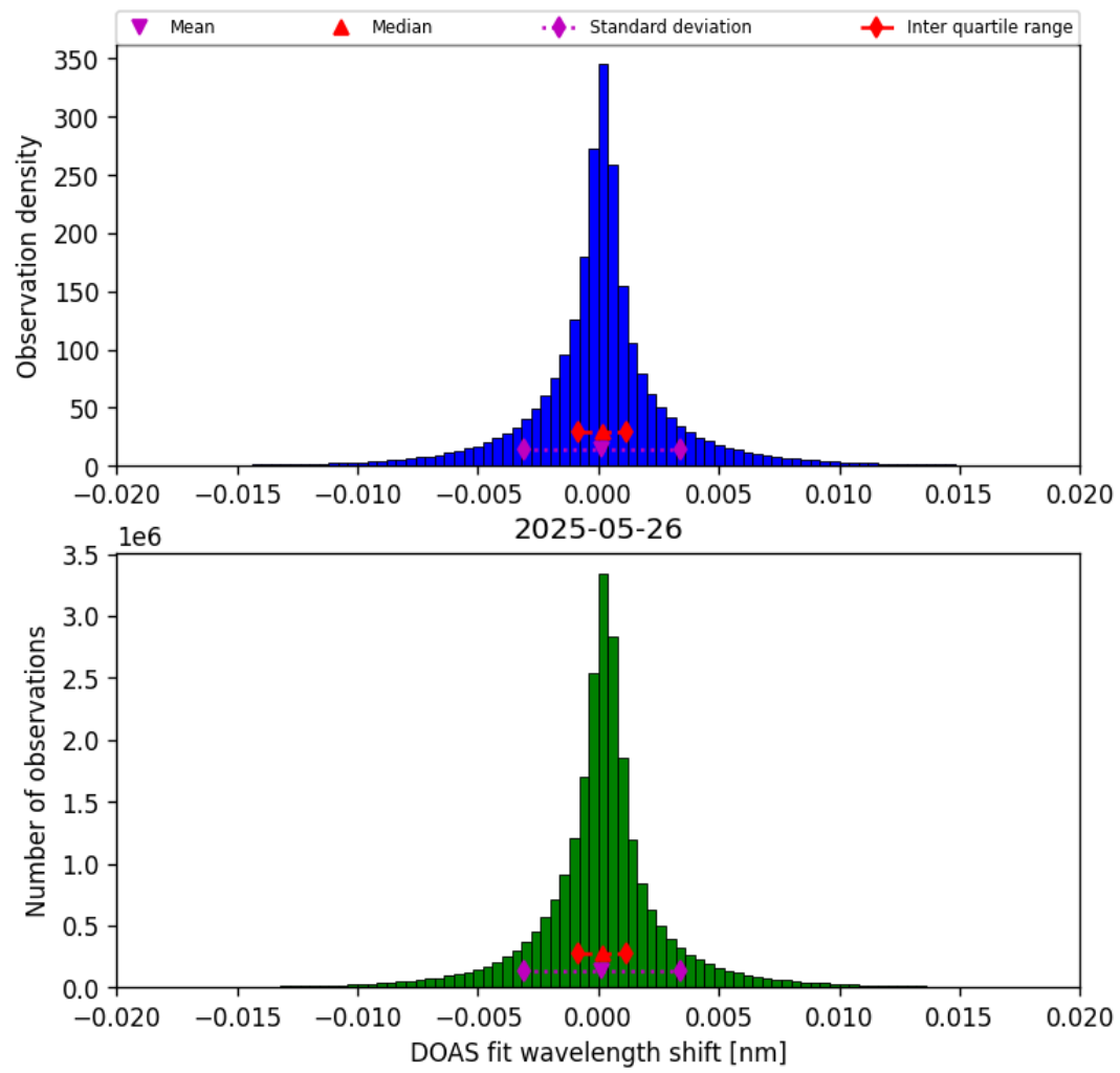
Figure 44: Histogram of “DOAS fit wavelength shift” for 2025-05-26 to 2025-05-27
