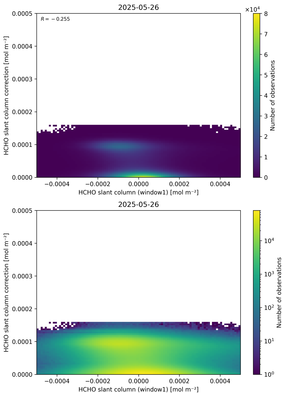
Figure 83: Scatter density plot of “HCHO slant column (window1)” against “HCHO slant column correction” for 2025-05-26 to 2025-05-27.
