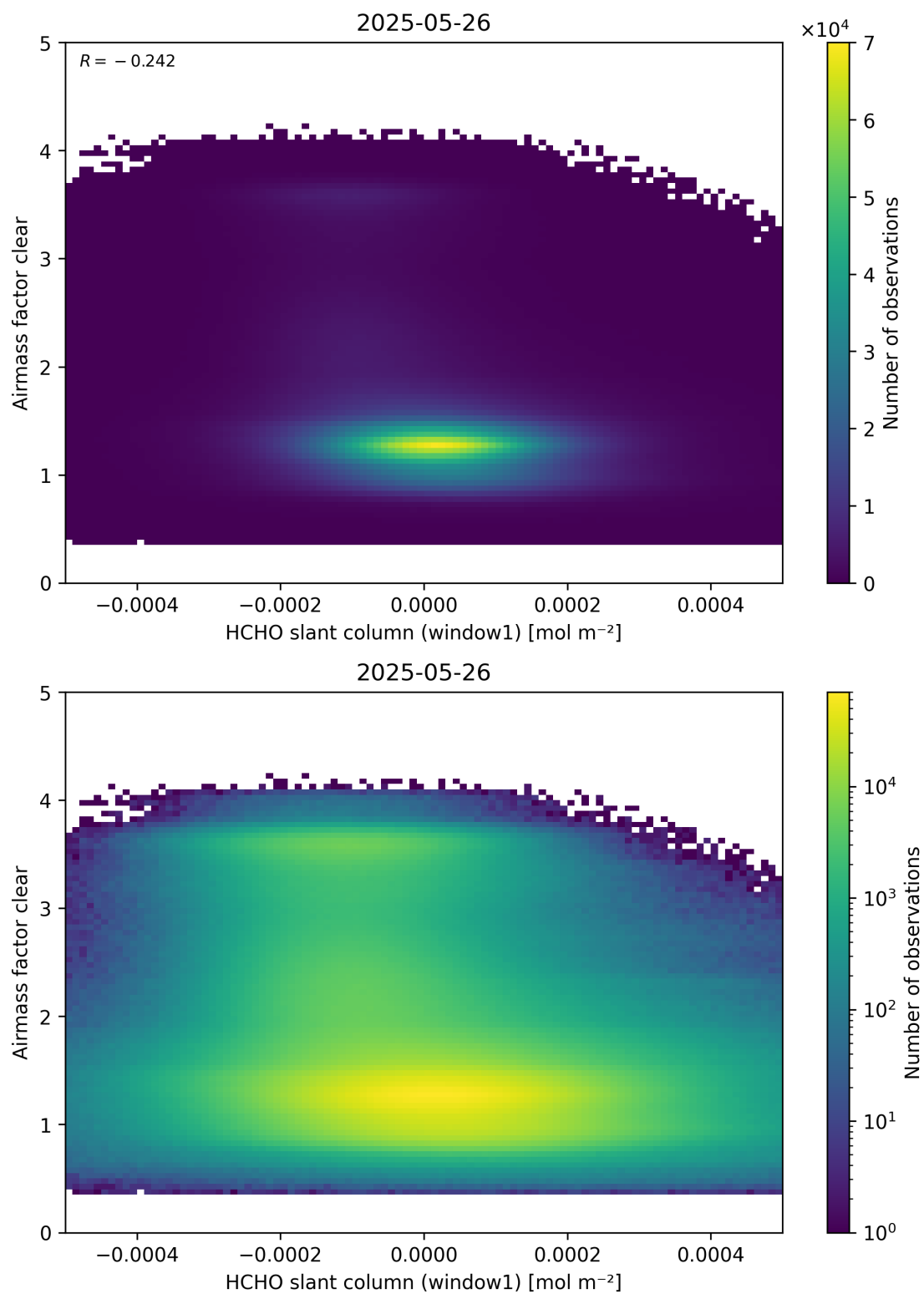
Figure 81: Scatter density plot of “HCHO slant column (window1)” against “Airmass factor clear” for 2025-05-26 to 2025-05-27.
