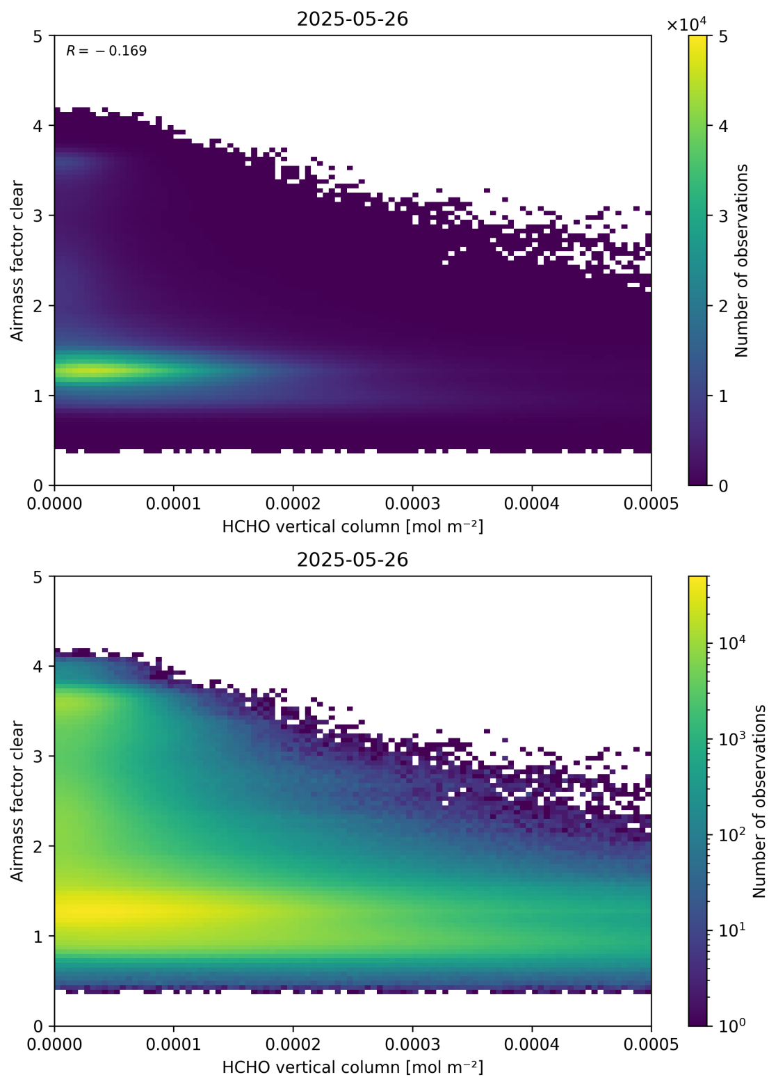
Figure 126: Scatter density plot of “HCHO vertical column” against “Airmass factor clear” for 2025-05-26 to 2025-05-27.
