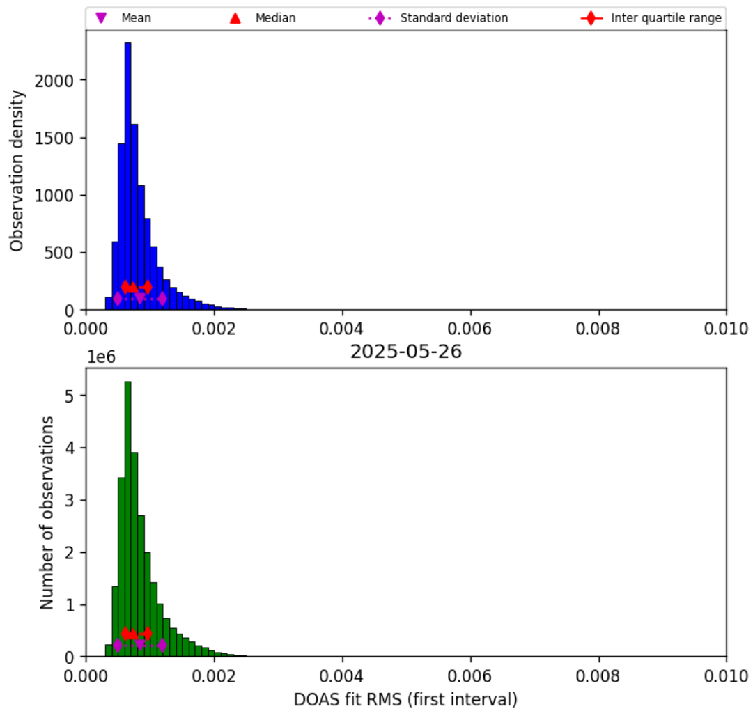
Figure 46: Histogram of “DOAS fit RMS (first interval)” for 2025-05-26 to 2025-05-27
