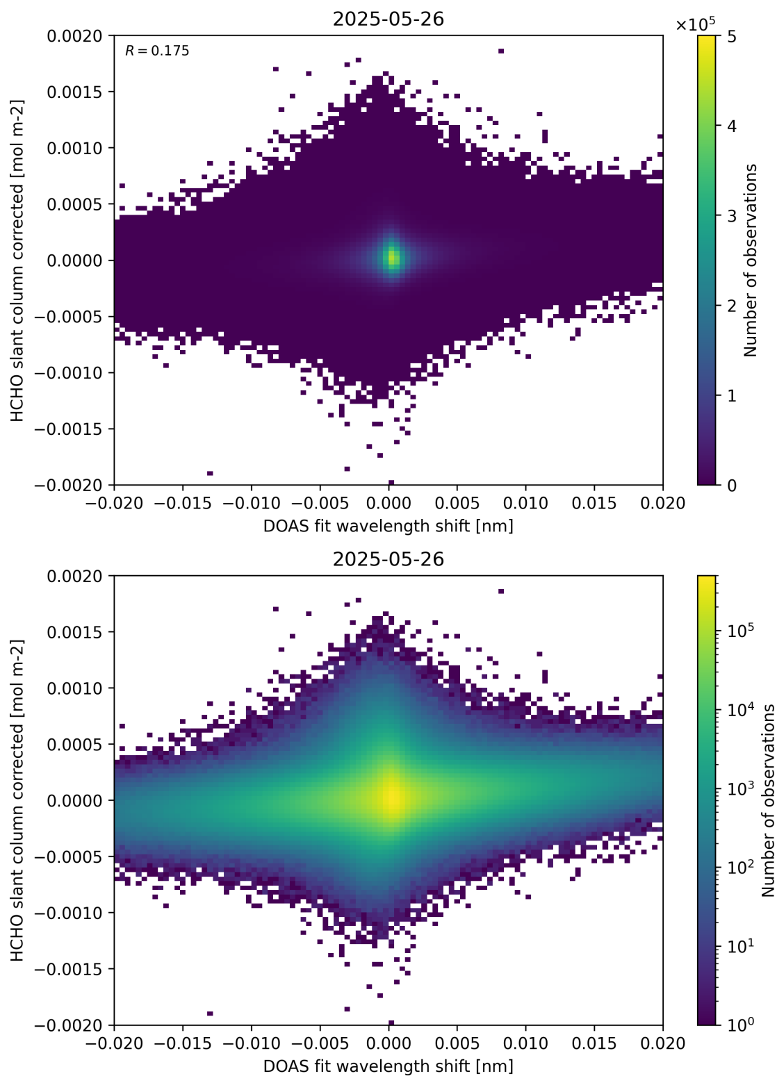
Figure 66: Scatter density plot of “DOAS fit wavelength shift” against “HCHO slant column corrected” for 2025-05-26 to 2025-05-27.
