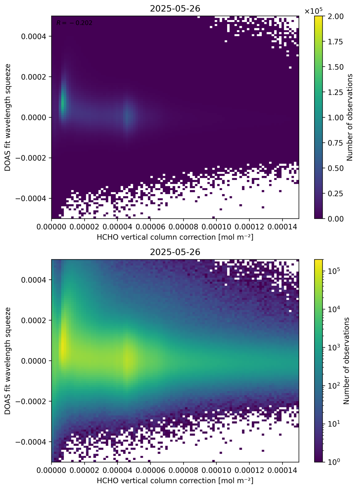
Figure 114: Scatter density plot of “HCHO vertical column correction” against “DOAS fit wavelength squeeze” for 2025-05-26 to 2025-05-27.
