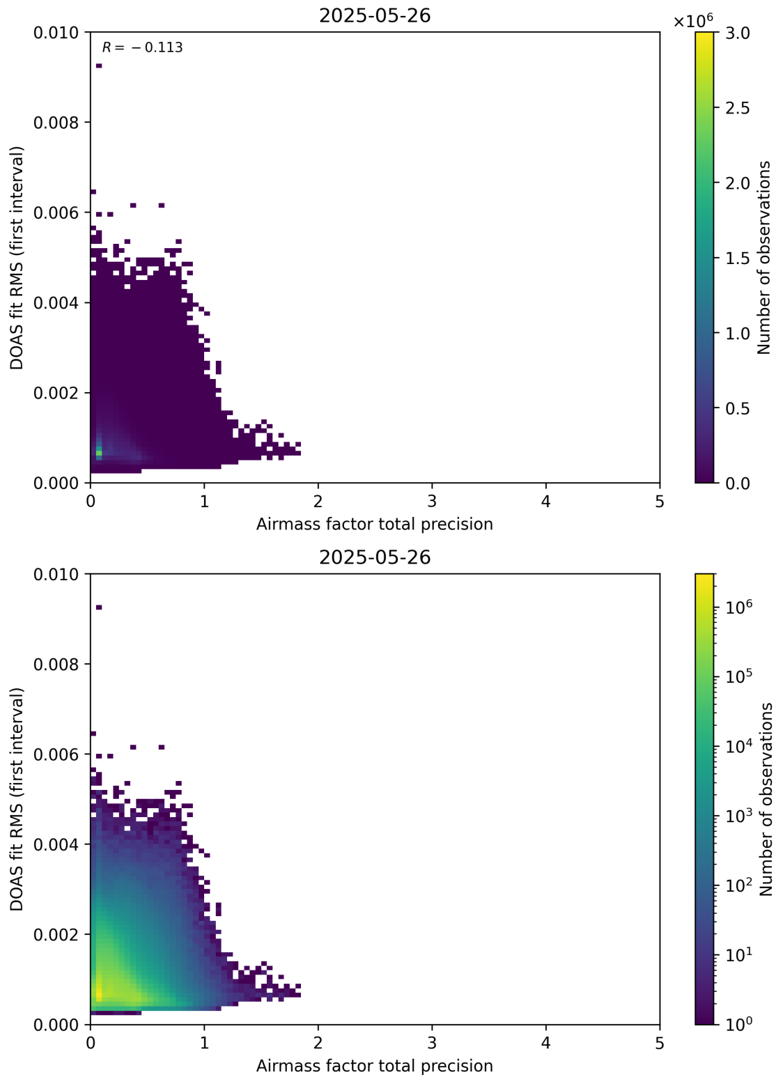
Figure 105: Scatter density plot of “Airmass factor total precision” against “DOAS fit RMS (first interval)” for 2025-05-26 to 2025-05-27.
