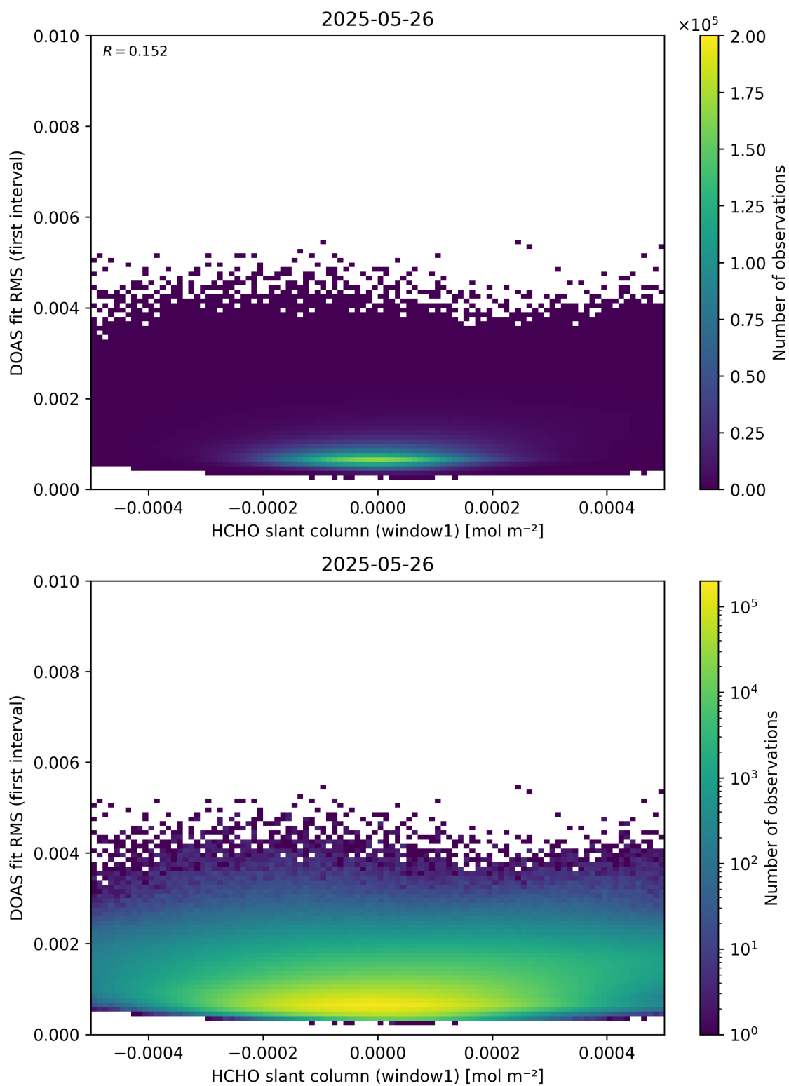
Figure 78: Scatter density plot of “HCHO slant column (window1)” against “DOAS fit RMS (first interval)” for 2025-05-26 to 2025-05-27.
