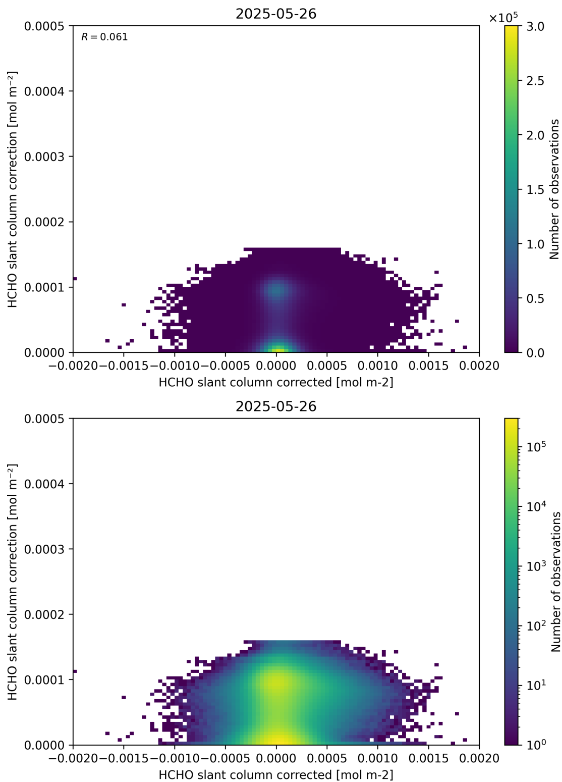
Figure 77: Scatter density plot of “HCHO slant column corrected” against “HCHO slant column correction” for 2025-05-26 to 2025-05-27.
