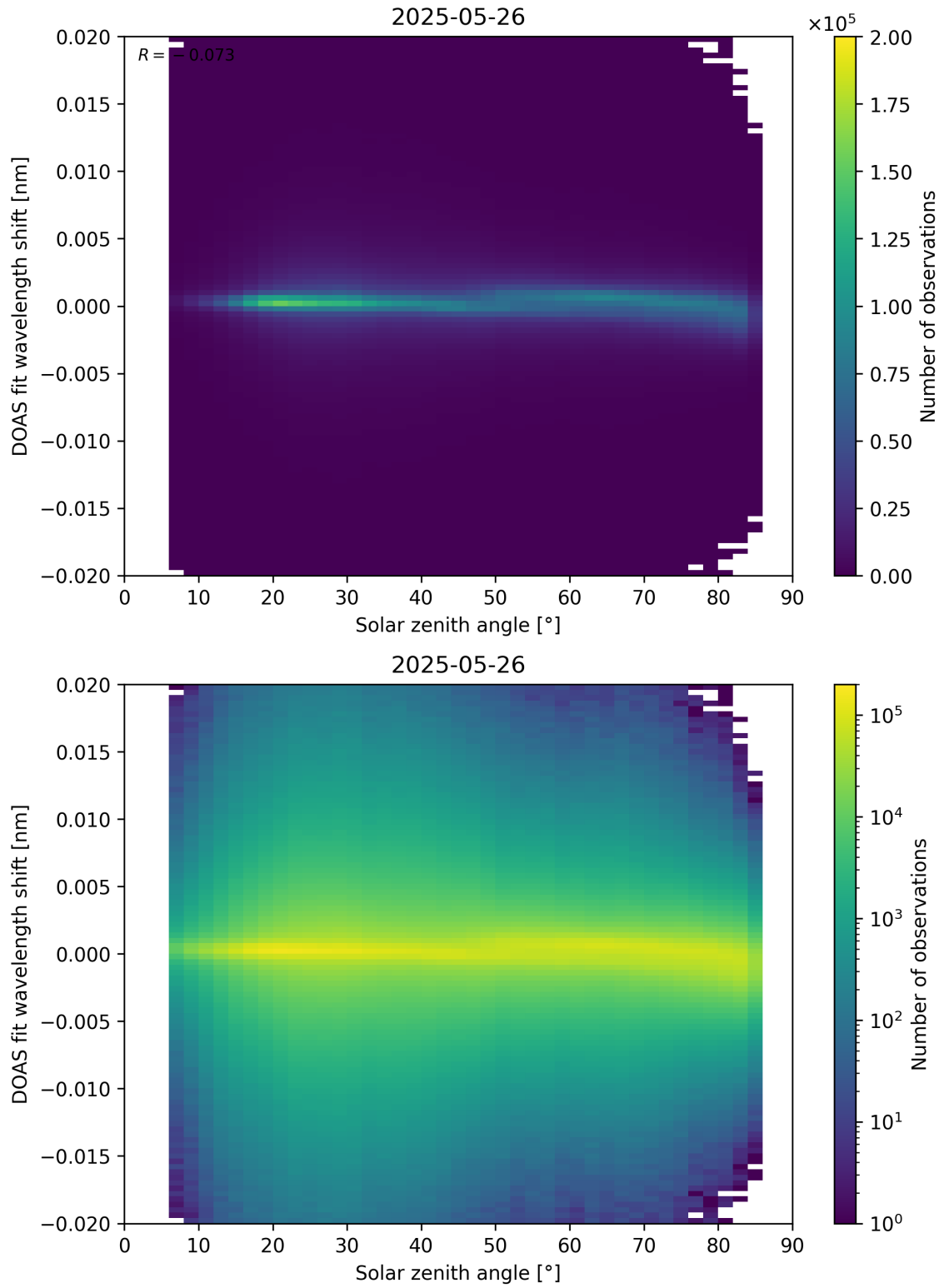
Figure 168: Scatter density plot of “Solar zenith angle” against “DOAS fit wavelength shift” for 2025-05-26 to 2025-05-27.
