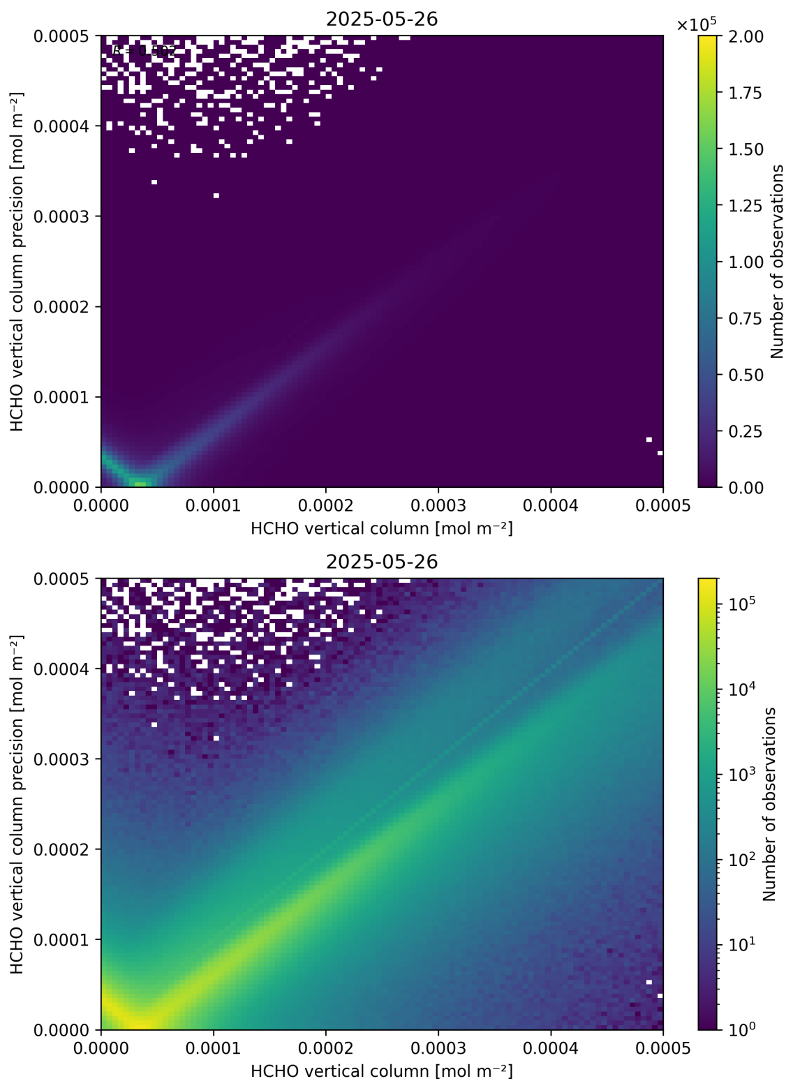
Figure 134: Scatter density plot of “HCHO vertical column” against “HCHO vertical column precision” for 2025-05-26 to 2025-05-27.
