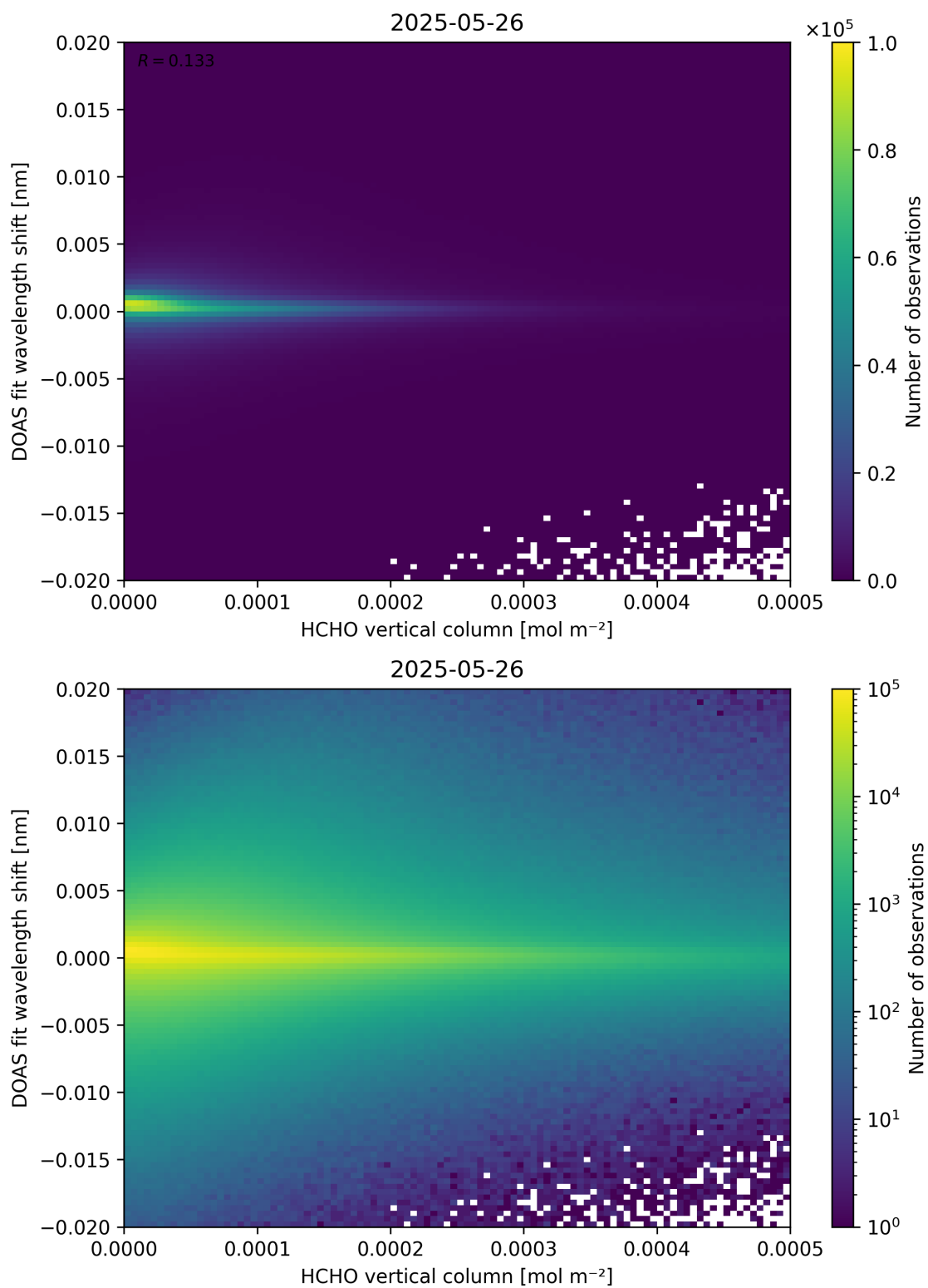
Figure 124: Scatter density plot of “HCHO vertical column” against “DOAS fit wavelength shift” for 2025-05-26 to 2025-05-27.
