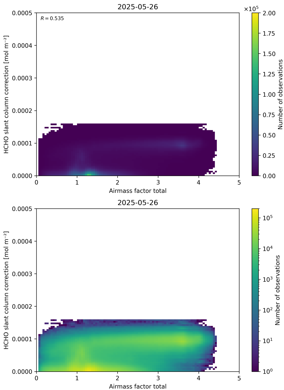
Figure 102: Scatter density plot of “Airmass factor total” against “HCHO slant column correction” for 2025-05-26 to 2025-05-27.
