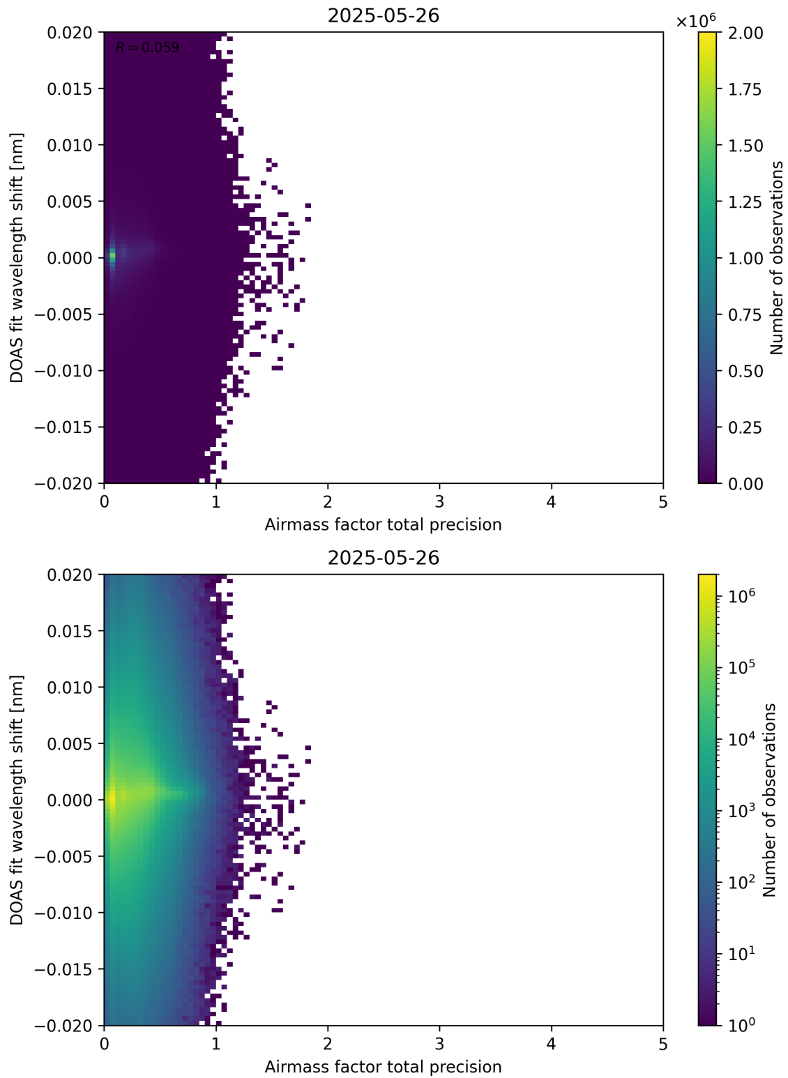
Figure 106: Scatter density plot of “Airmass factor total precision” against “DOAS fit wavelength shift” for 2025-05-26 to 2025-05-27.
