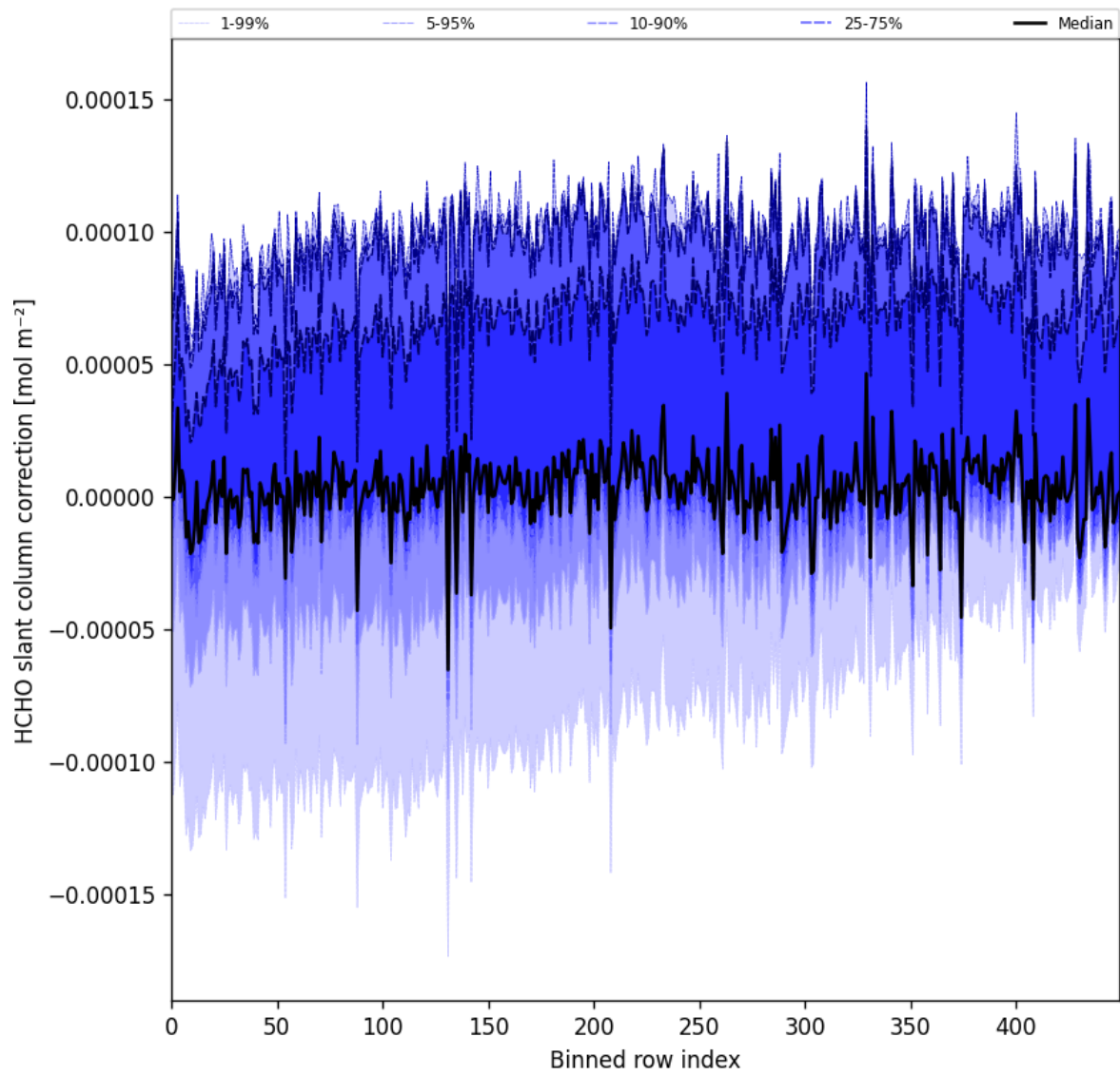
Figure 61: Along track statistics of “HCHO slant column correction” for 2025-05-26 to 2025-05-27
