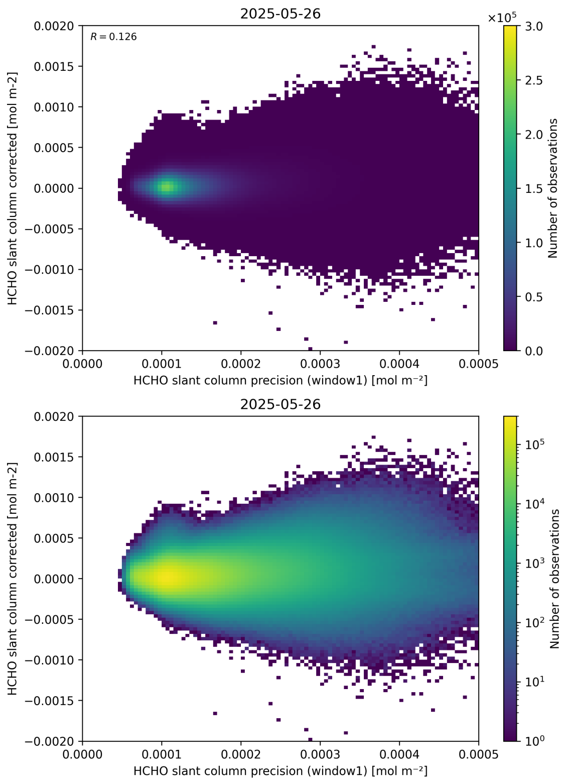
Figure 92: Scatter density plot of “HCHO slant column precision (window1)” against “HCHO slant column corrected” for 2025-05-26 to 2025-05-27.
