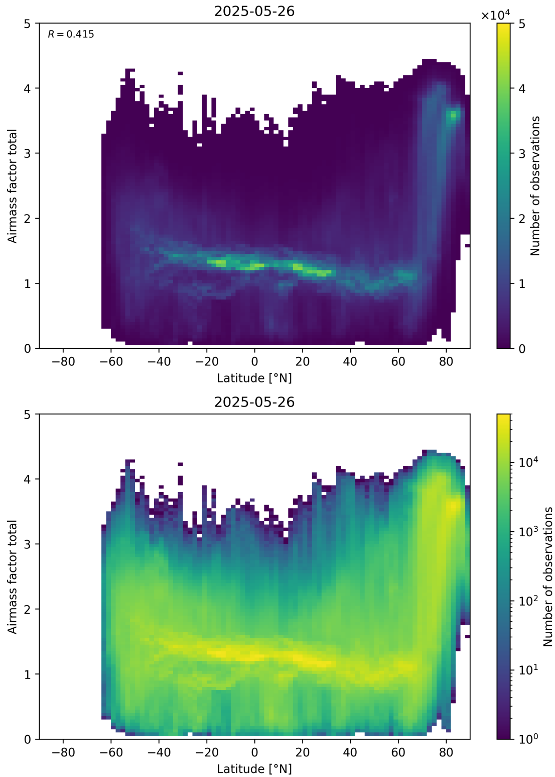
Figure 161: Scatter density plot of “Latitude” against “Airmass factor total” for 2025-05-26 to 2025-05-27.
