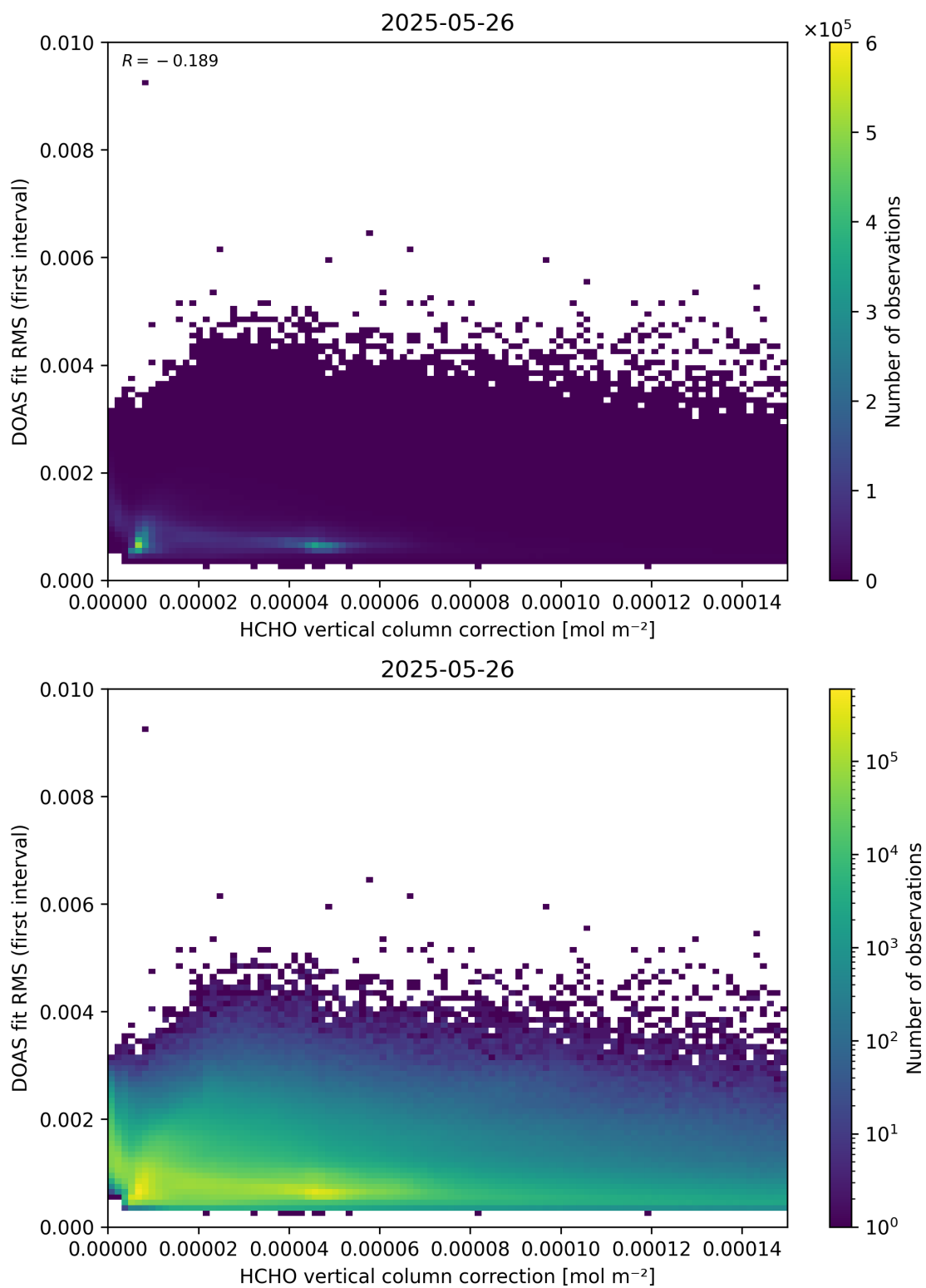
Figure 112: Scatter density plot of “HCHO vertical column correction” against “DOAS fit RMS (first interval)” for 2025-05-26 to 2025-05-27.
