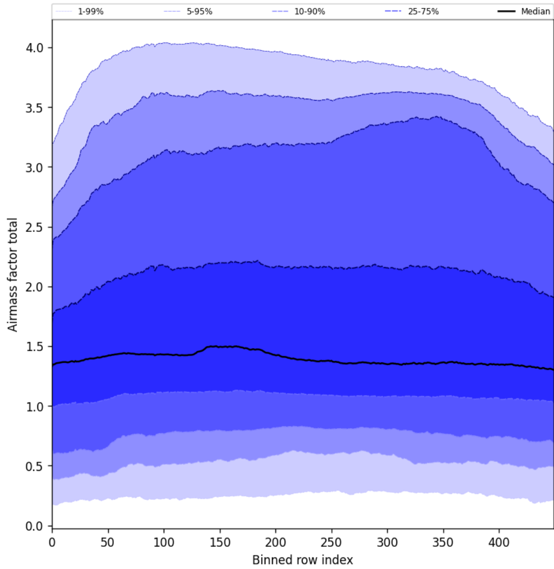
Figure 54: Along track statistics of “Airmass factor total” for 2025-05-26 to 2025-05-27
