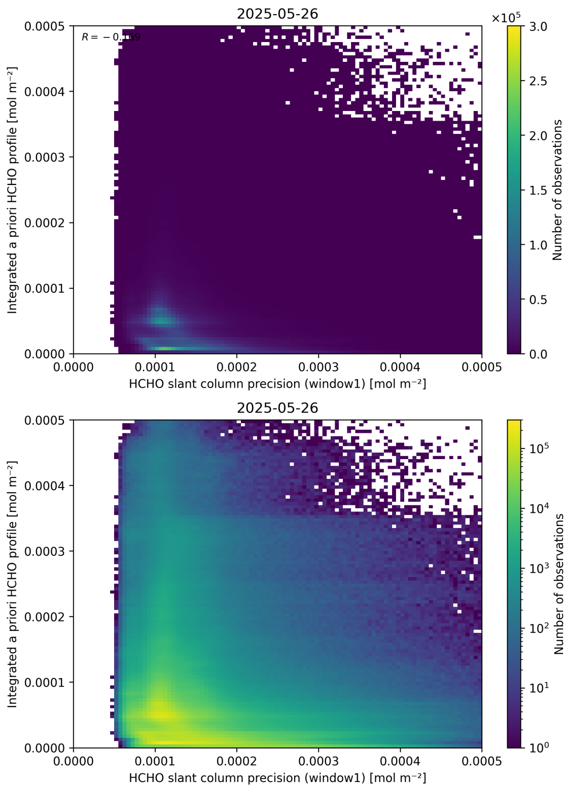
Figure 96: Scatter density plot of “HCHO slant column precision (window1)” against “Integrated a priori HCHO profile” for 2025-05-26 to 2025-05-27.
