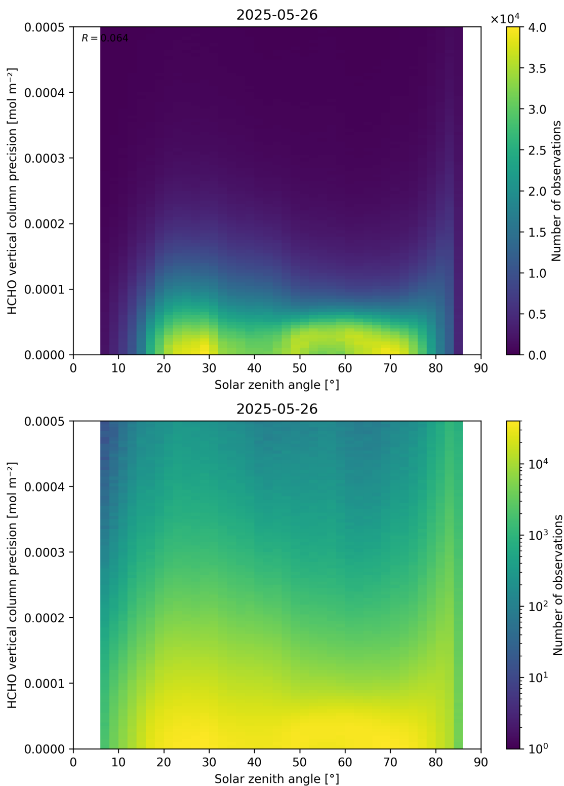
Figure 179: Scatter density plot of “Solar zenith angle” against “HCHO vertical column precision” for 2025-05-26 to 2025-05-27.
