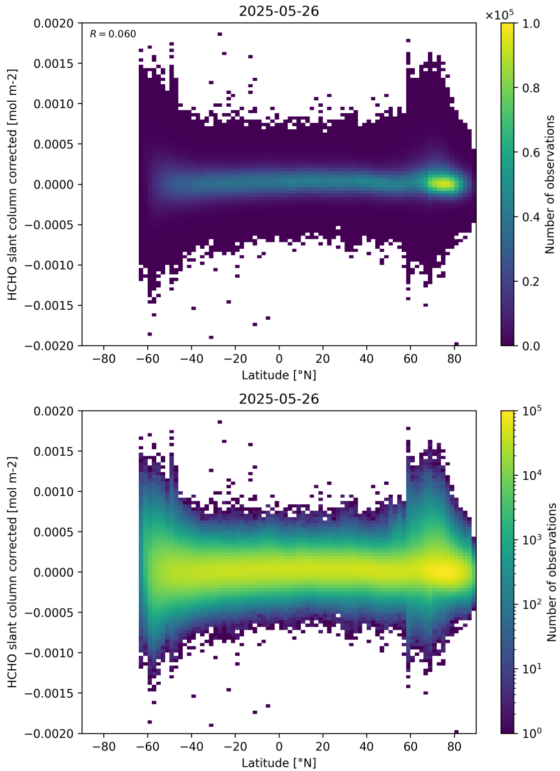
Figure 157: Scatter density plot of “Latitude” against “HCHO slant column corrected” for 2025-05-26 to 2025-05-27.
