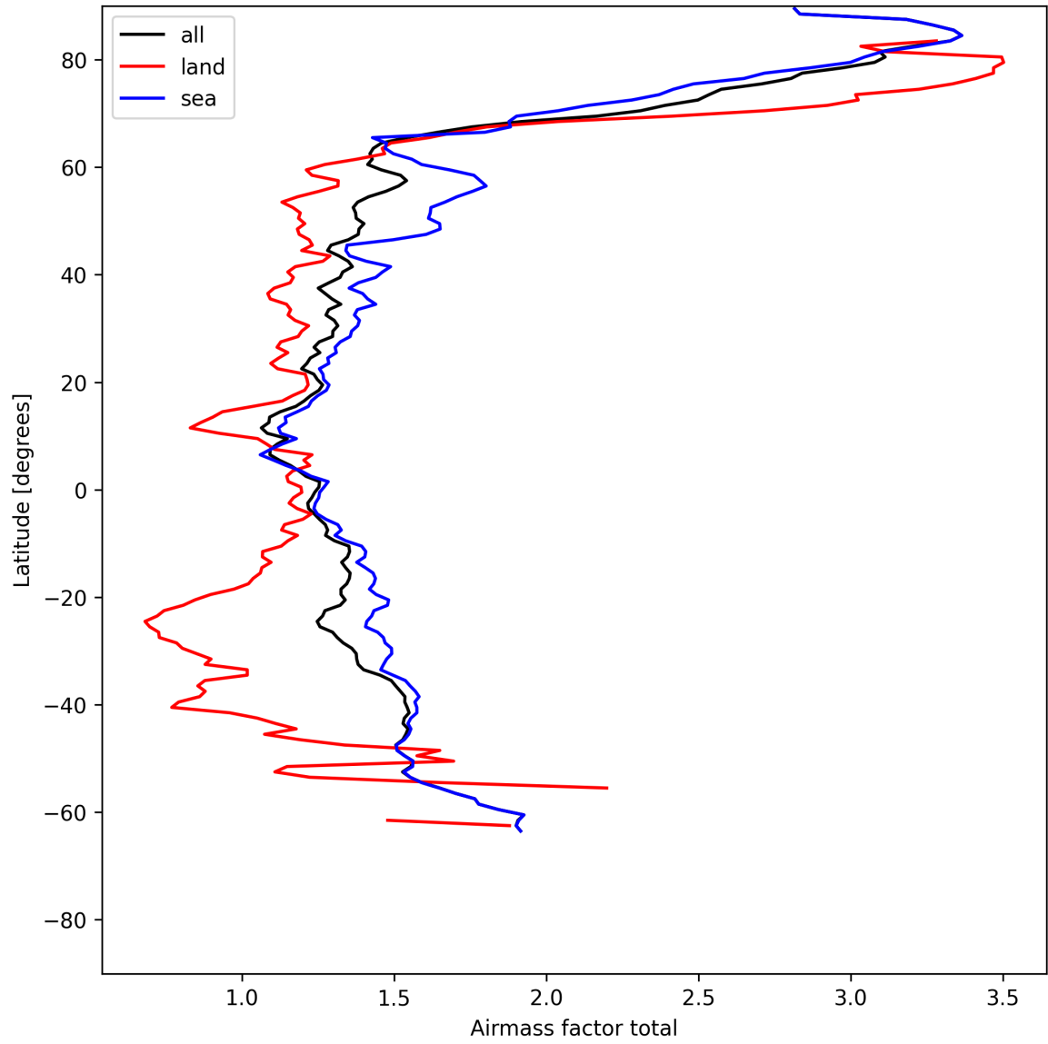
Figure 26: Zonal average of “Airmass factor total” for 2025-05-26 to 2025-05-27.
