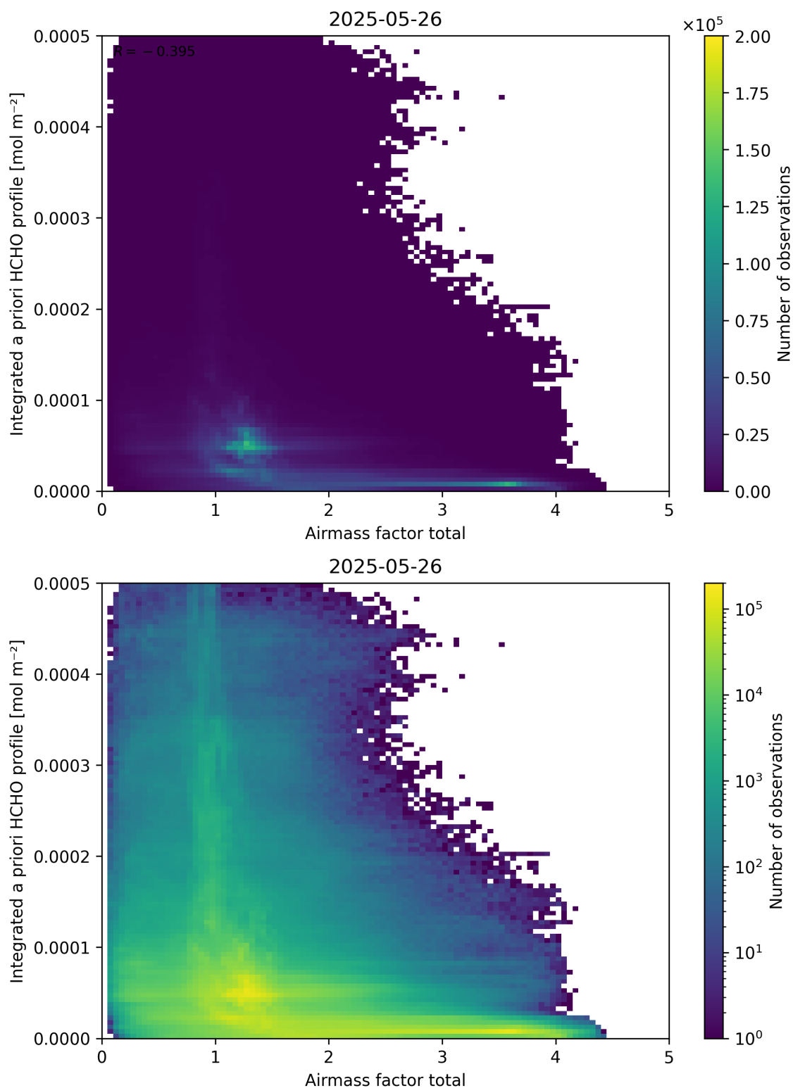
Figure 104: Scatter density plot of “Airmass factor total” against “Integrated a priori HCHO profile” for 2025-05-26 to 2025-05-27.
