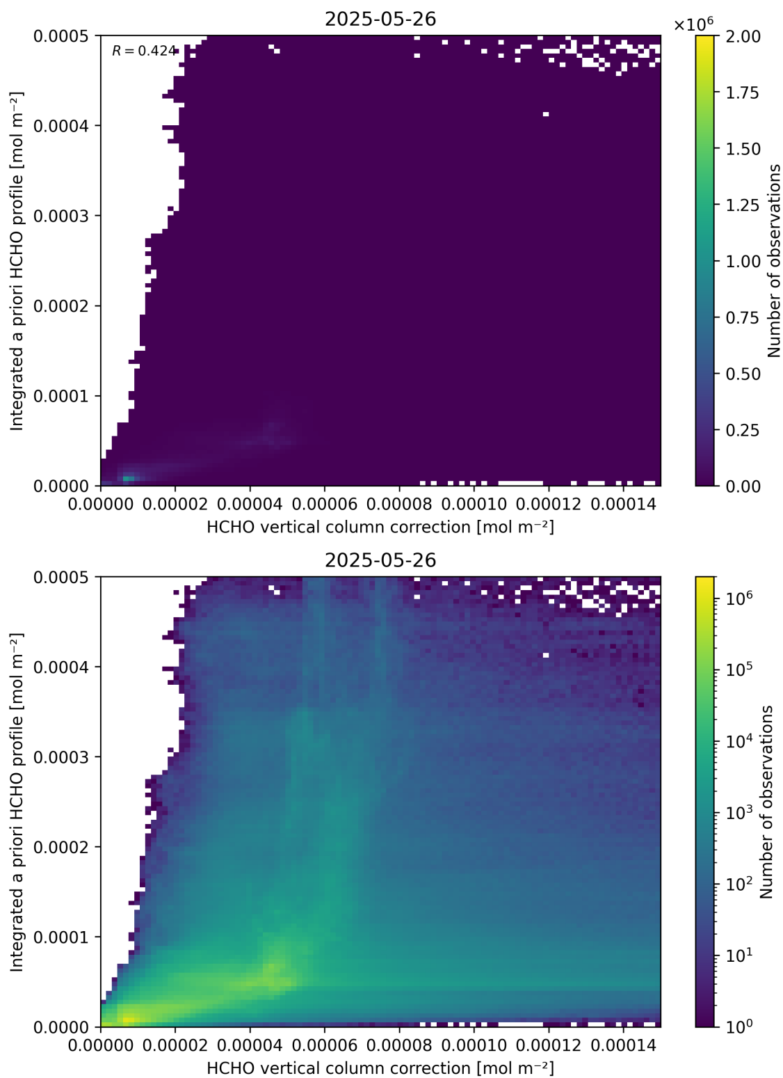
Figure 122: Scatter density plot of “HCHO vertical column correction” against “Integrated a priori HCHO profile” for 2025-05-26 to 2025-05-27.
