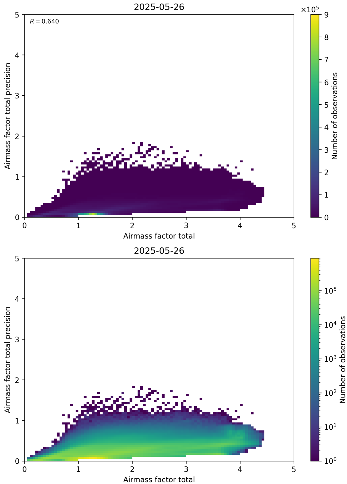
Figure 103: Scatter density plot of “Airmass factor total” against “Airmass factor total precision” for 2025-05-26 to 2025-05-27.
