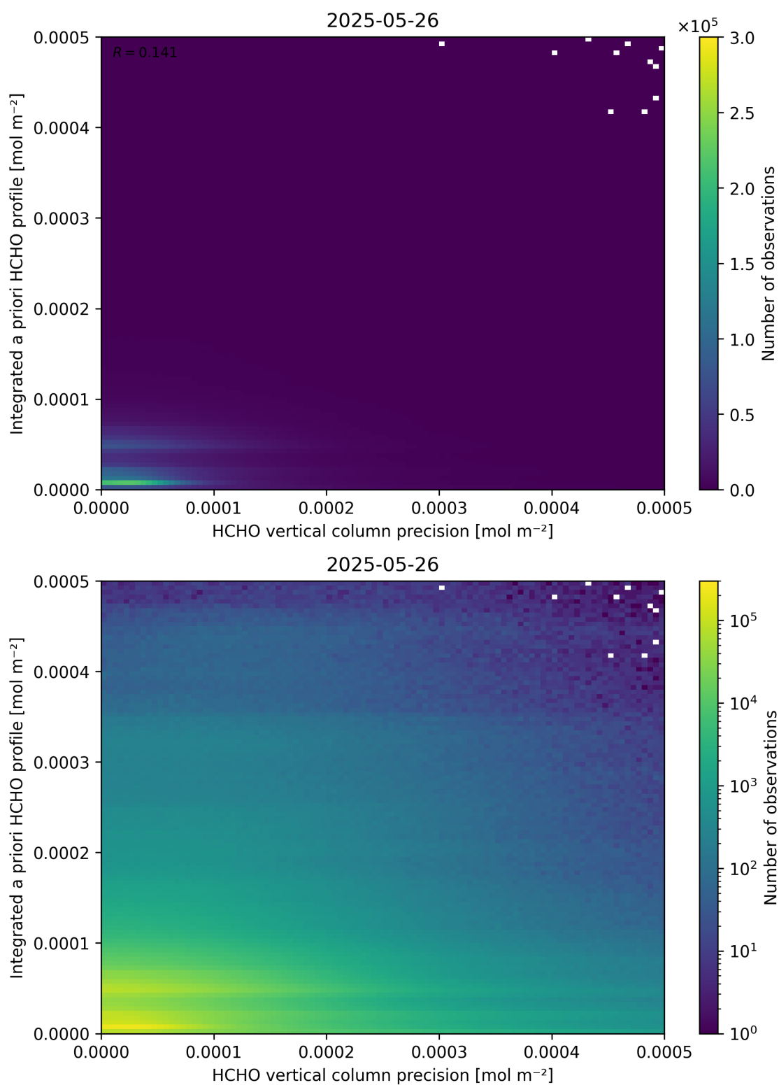
Figure 147: Scatter density plot of “HCHO vertical column precision” against “Integrated a priori HCHO profile” for 2025-05-26 to 2025-05-27.
