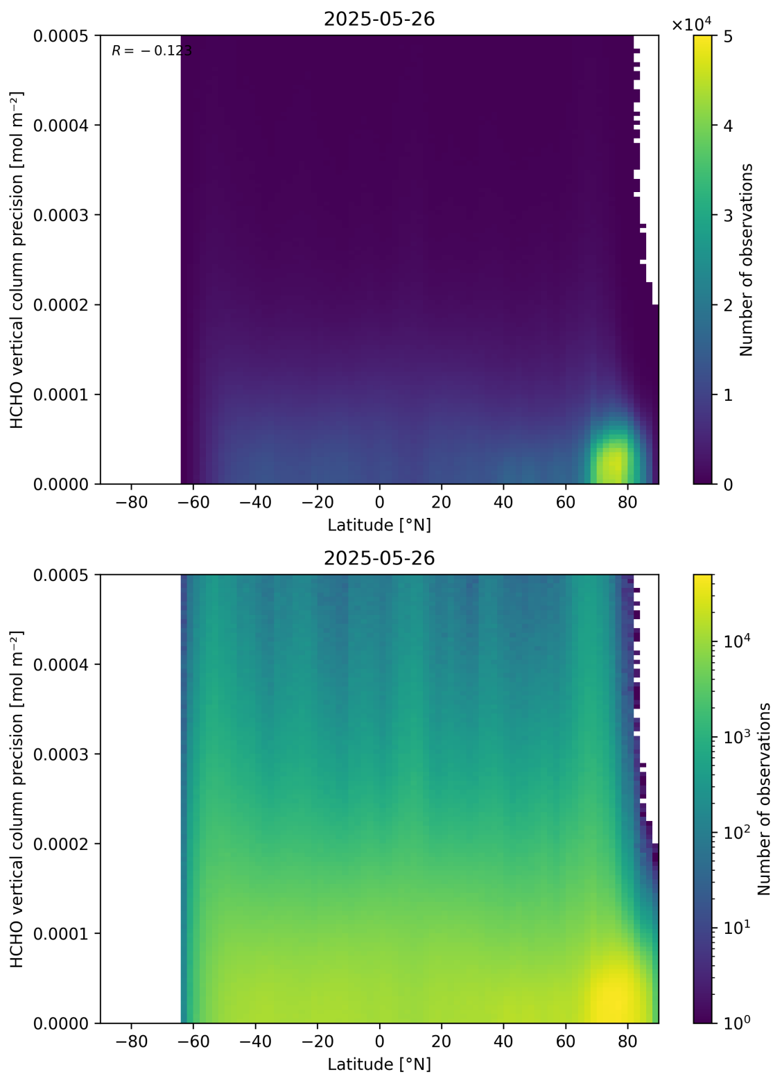
Figure 165: Scatter density plot of “Latitude” against “HCHO vertical column precision” for 2025-05-26 to 2025-05-27.
