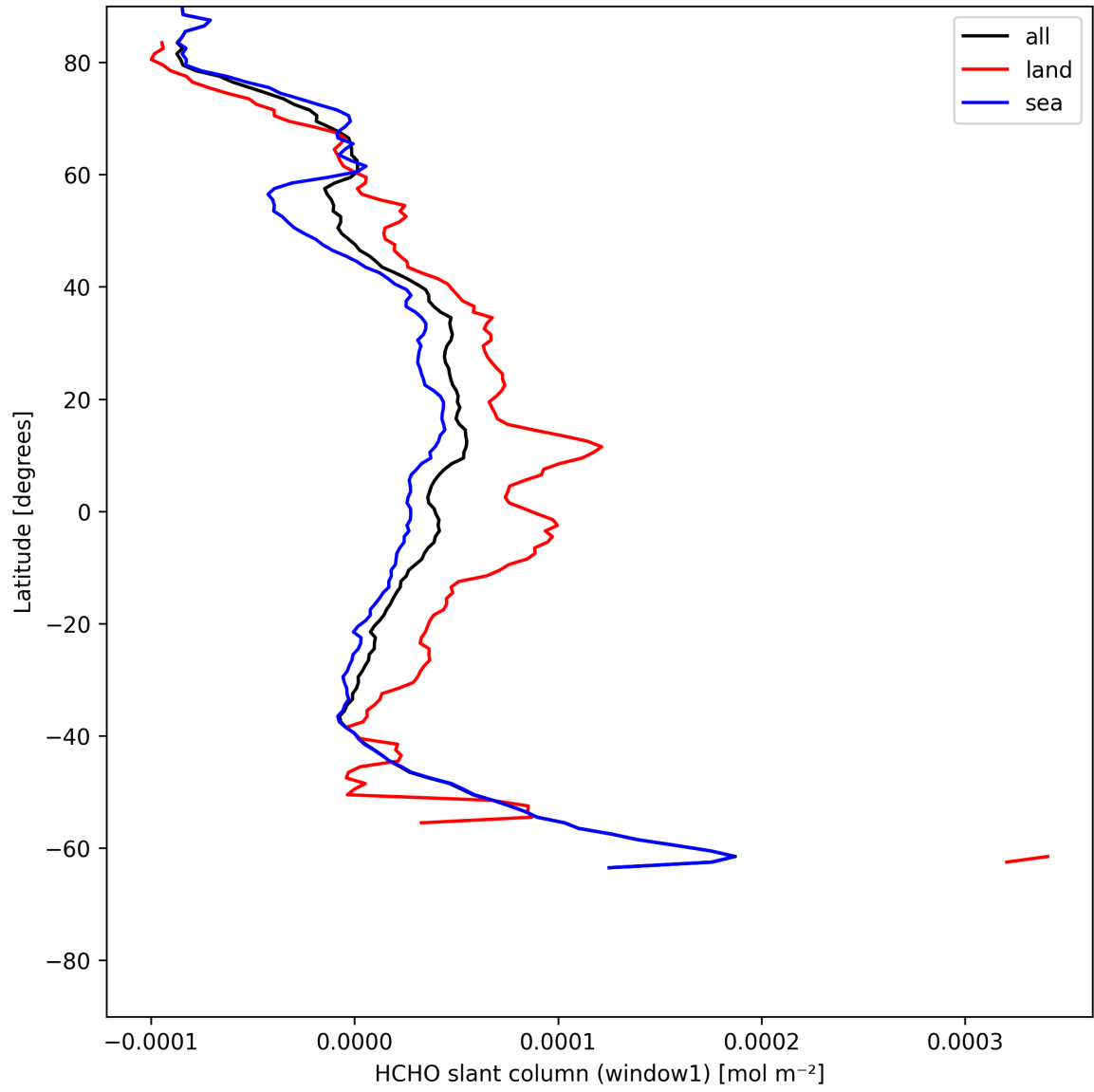
Figure 24: Zonal average of “HCHO slant column (window1)” for 2025-05-26 to 2025-05-27.
