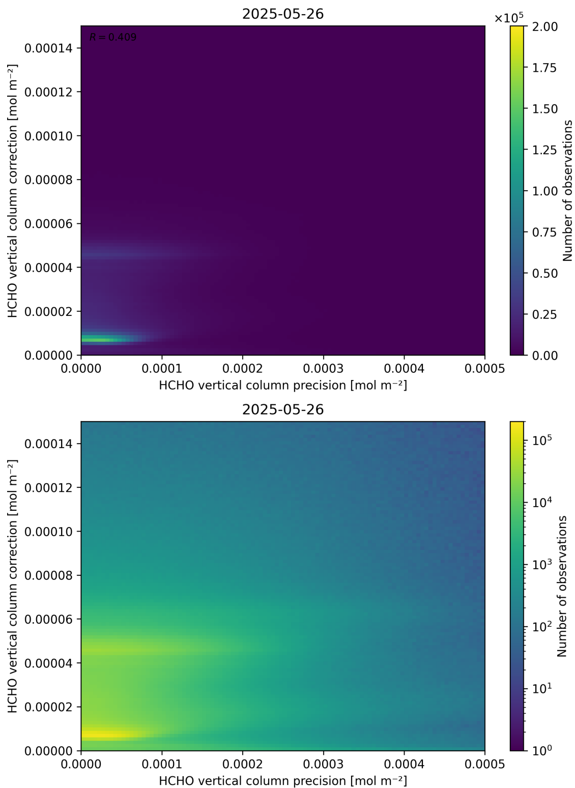
Figure 146: Scatter density plot of “HCHO vertical column precision” against “HCHO vertical column correction” for 2025-05-26 to 2025-05-27.
