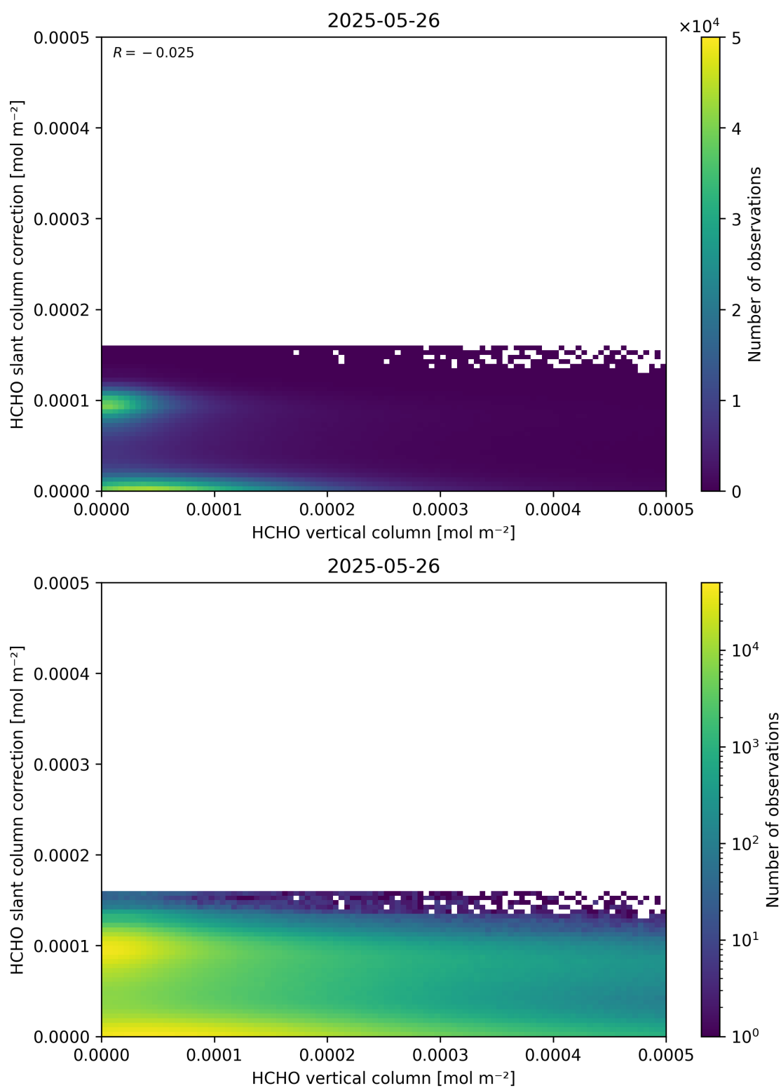
Figure 128: Scatter density plot of “HCHO vertical column” against “HCHO slant column correction” for 2025-05-26 to 2025-05-27.
