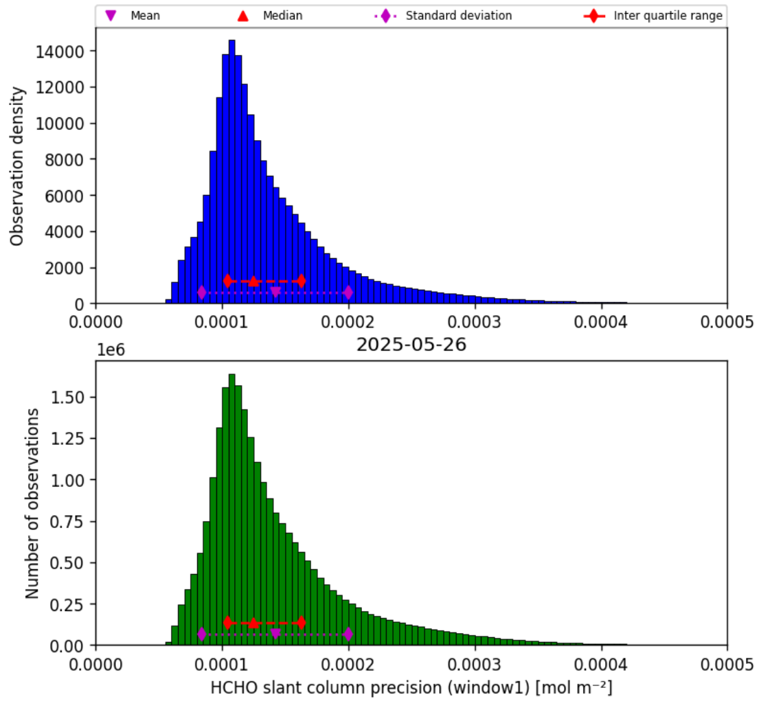
Figure 39: Histogram of “HCHO slant column precision (window1)” for 2025-05-26 to 2025-05-27
