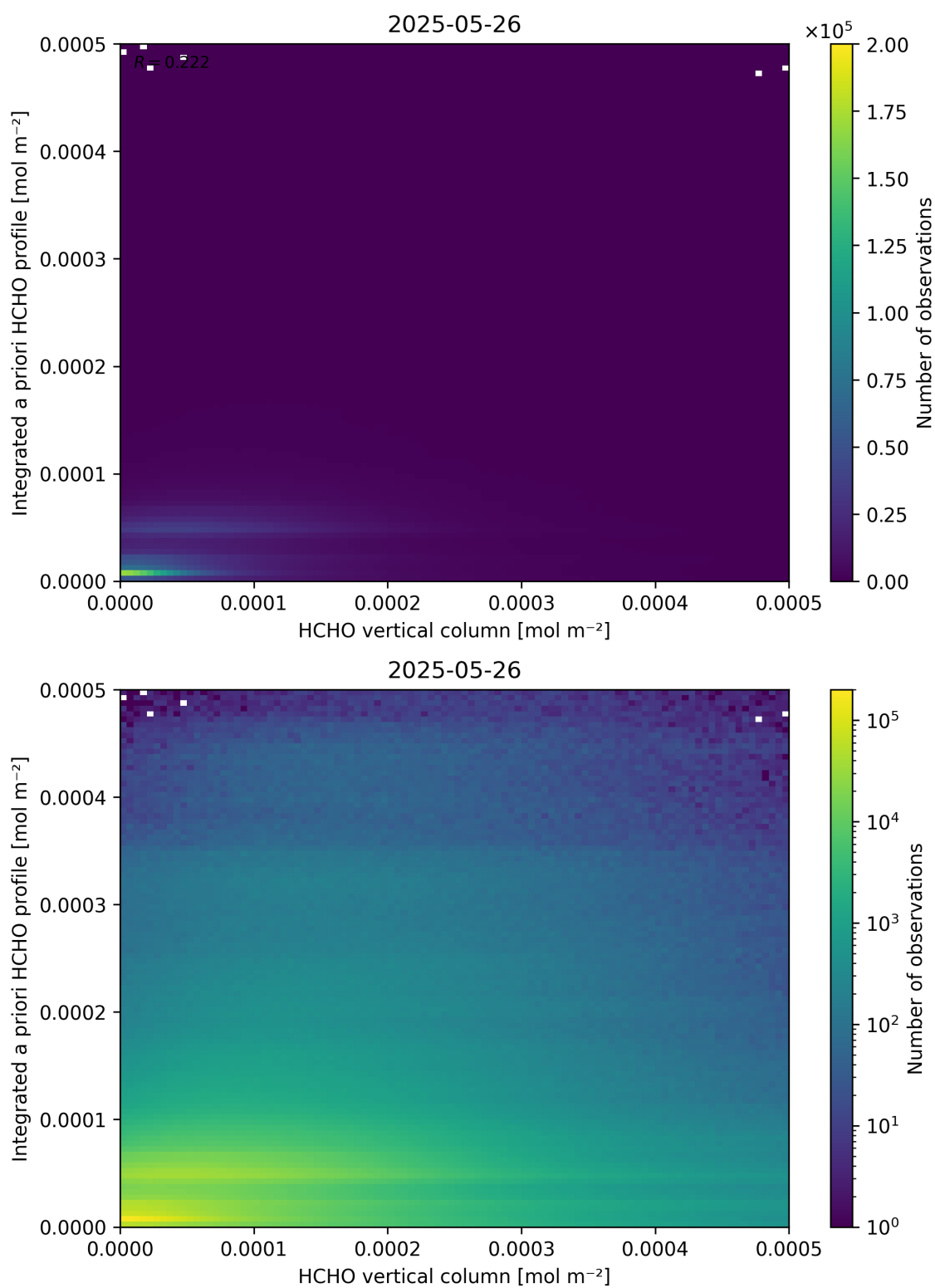
Figure 135: Scatter density plot of “HCHO vertical column” against “Integrated a priori HCHO profile” for 2025-05-26 to 2025-05-27.
