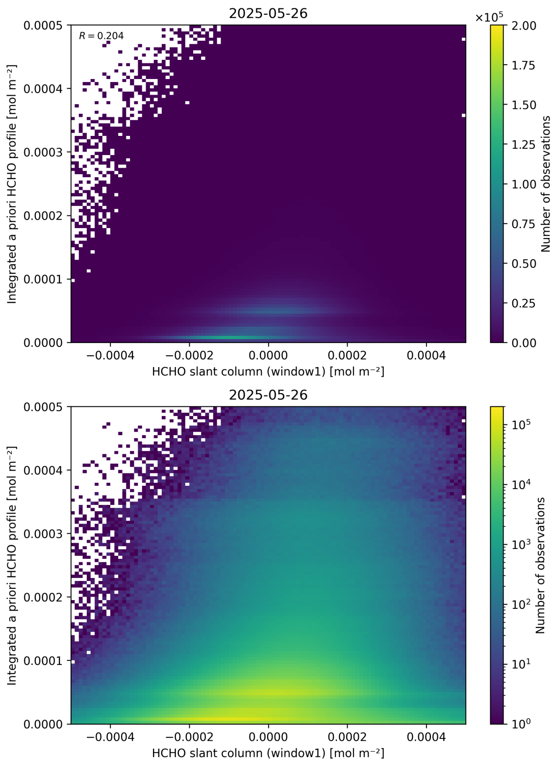
Figure 87: Scatter density plot of “HCHO slant column (window1)” against “Integrated a priori HCHO profile” for 2025-05-26 to 2025-05-27.
