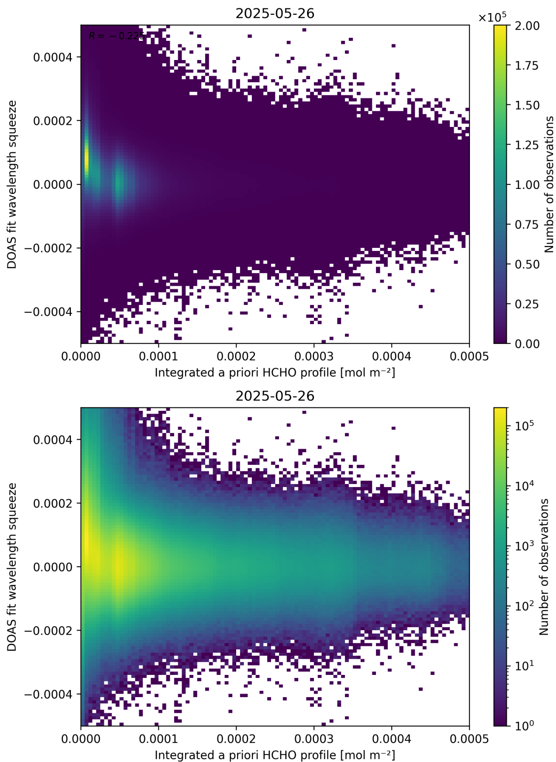
Figure 150: Scatter density plot of “Integrated a priori HCHO profile” against “DOAS fit wavelength squeeze” for 2025-05-26 to 2025-05-27.
