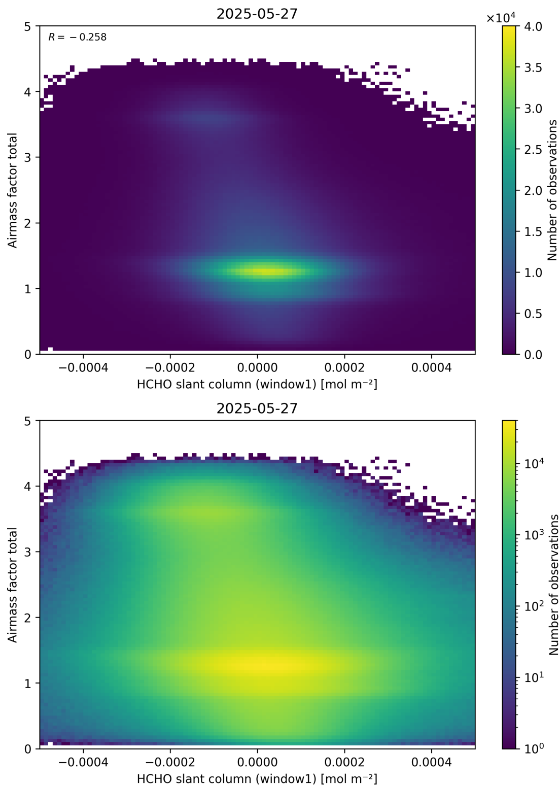
Figure 85: Scatter density plot of “HCHO slant column (window1)” against “Airmass factor total” for 2025-05-26 to 2025-05-28.
