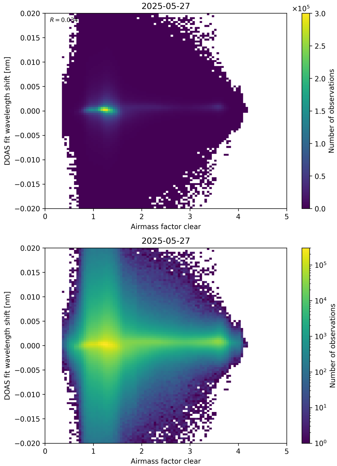
Figure 72: Scatter density plot of “Airmass factor clear” against “DOAS fit wavelength shift” for 2025-05-26 to 2025-05-28.
