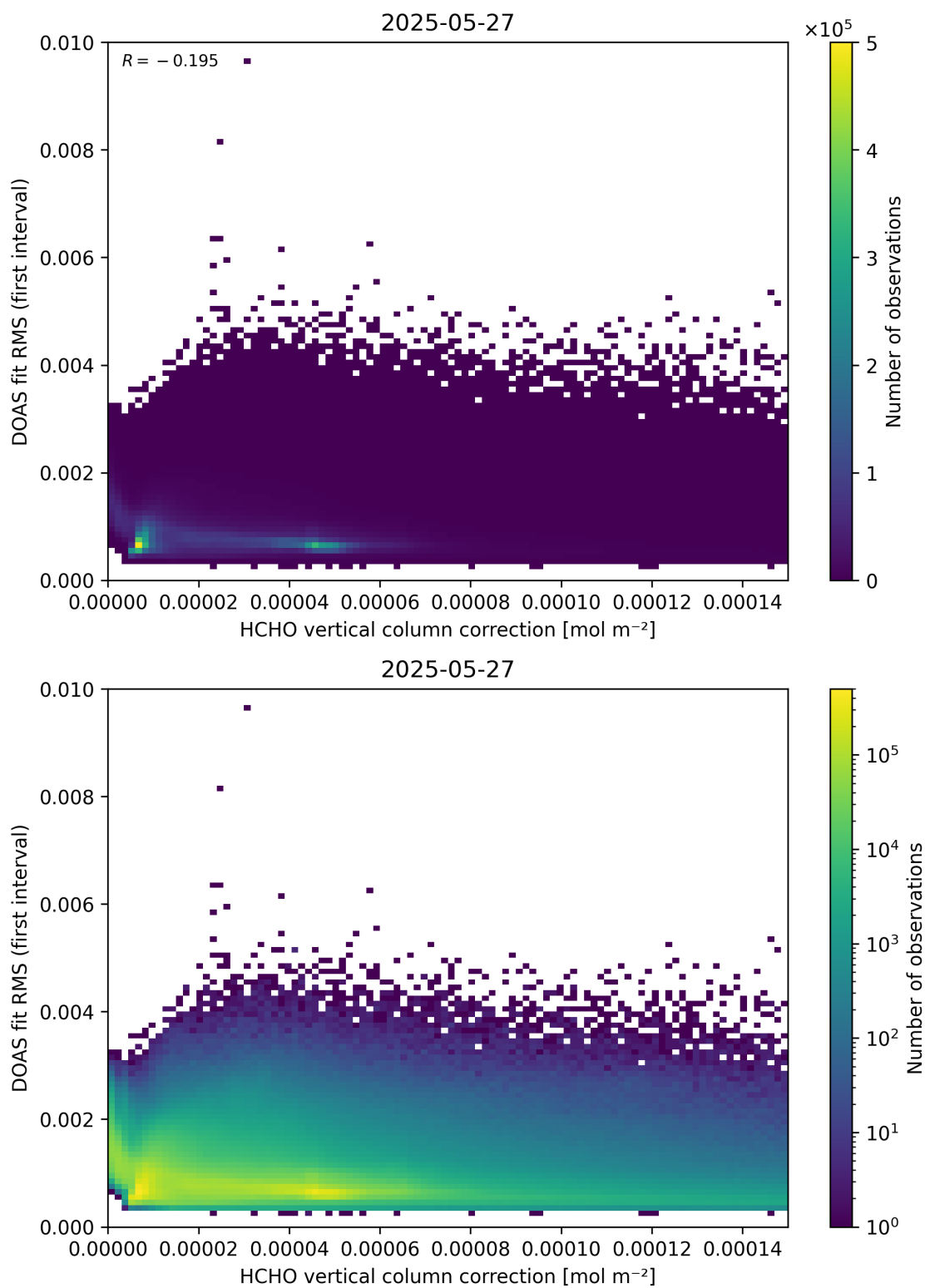
Figure 112: Scatter density plot of “HCHO vertical column correction” against “DOAS fit RMS (first interval)” for 2025-05-26 to 2025-05-28.
