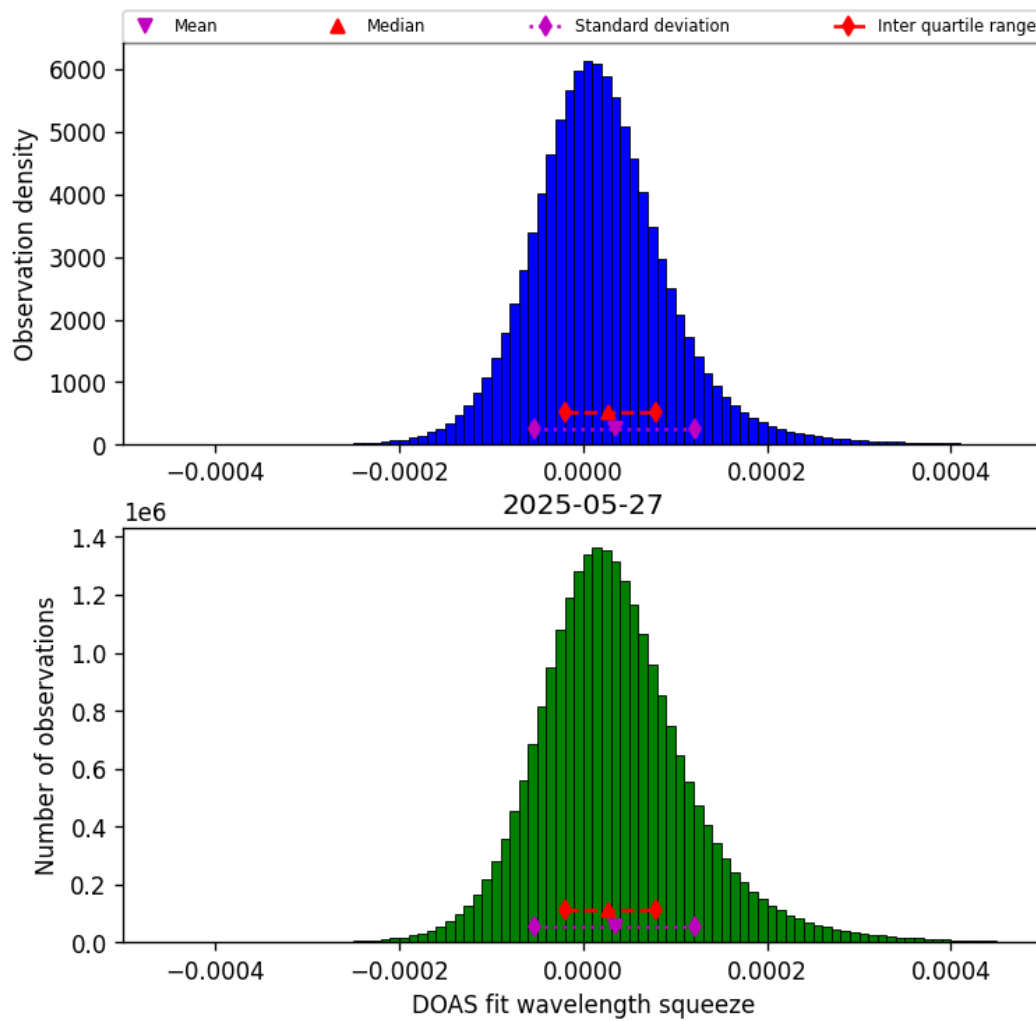
Figure 45: Histogram of “DOAS fit wavelength squeeze” for 2025-05-26 to 2025-05-28
