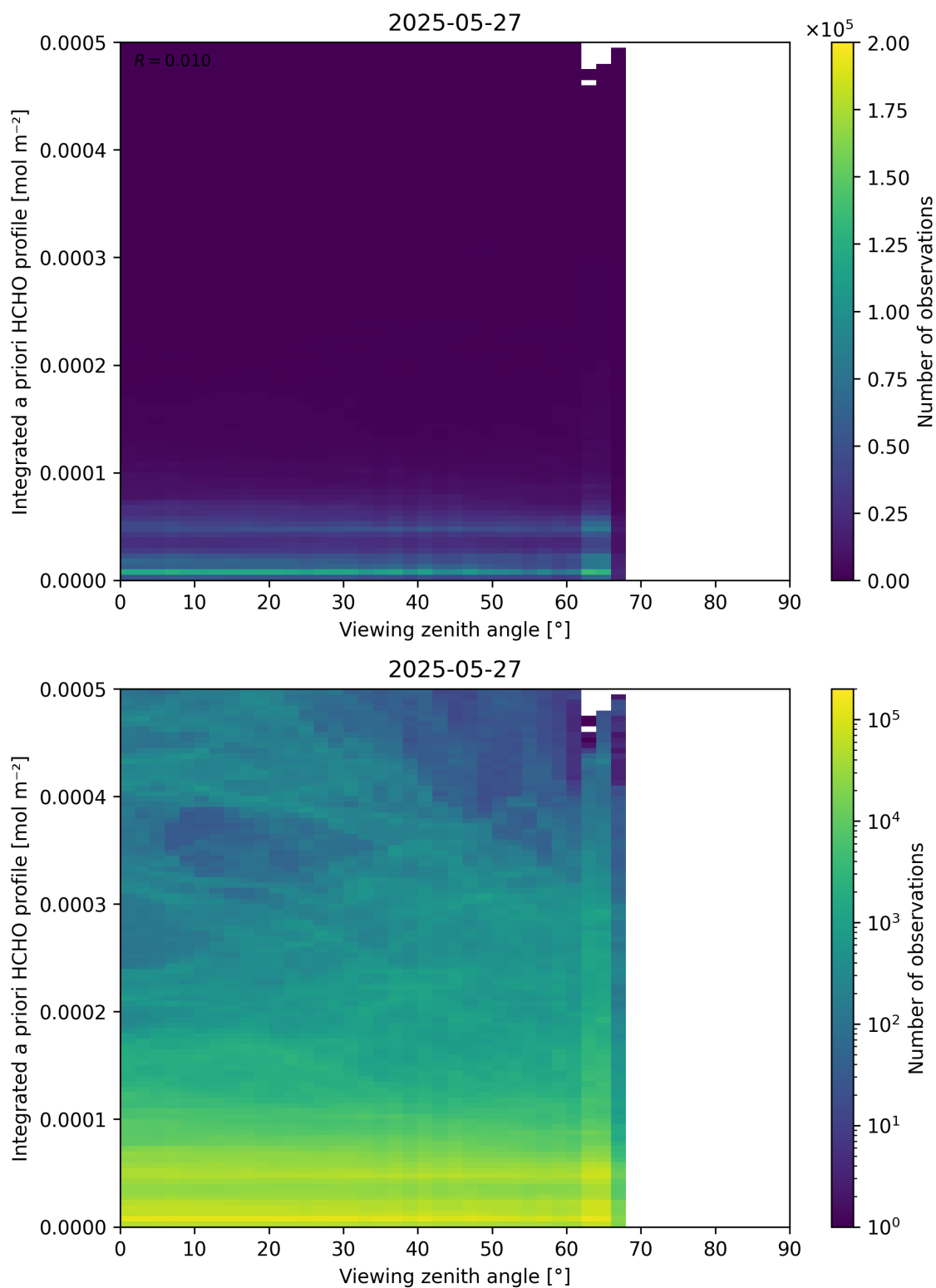
Figure 195: Scatter density plot of “Viewing zenith angle” against “Integrated a priori HCHO profile” for 2025-05-26 to 2025-05-28.
