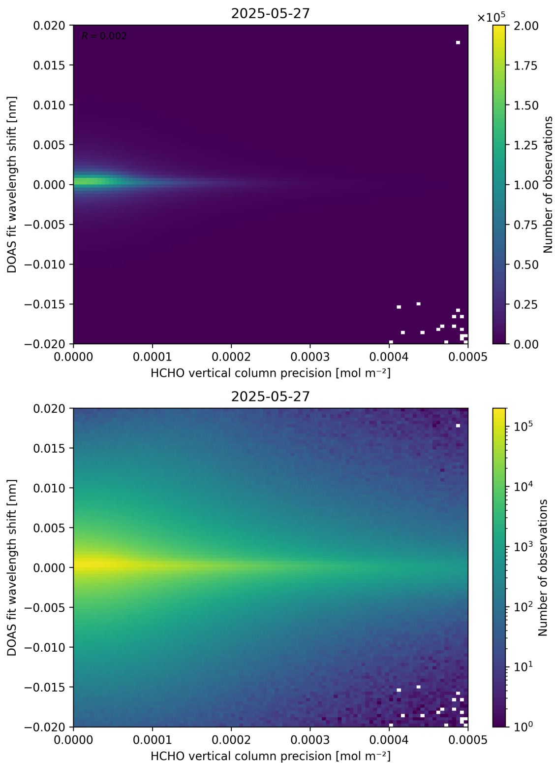
Figure 137: Scatter density plot of “HCHO vertical column precision” against “DOAS fit wavelength shift” for 2025-05-26 to 2025-05-28.
