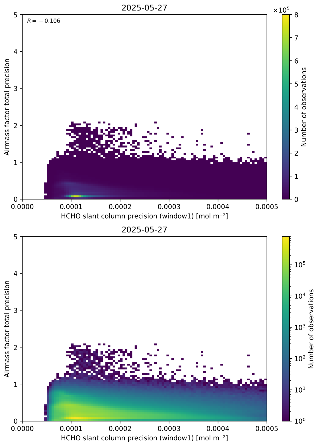
Figure 95: Scatter density plot of “HCHO slant column precision (window1)” against “Airmass factor total precision” for 2025-05-26 to 2025-05-28.
