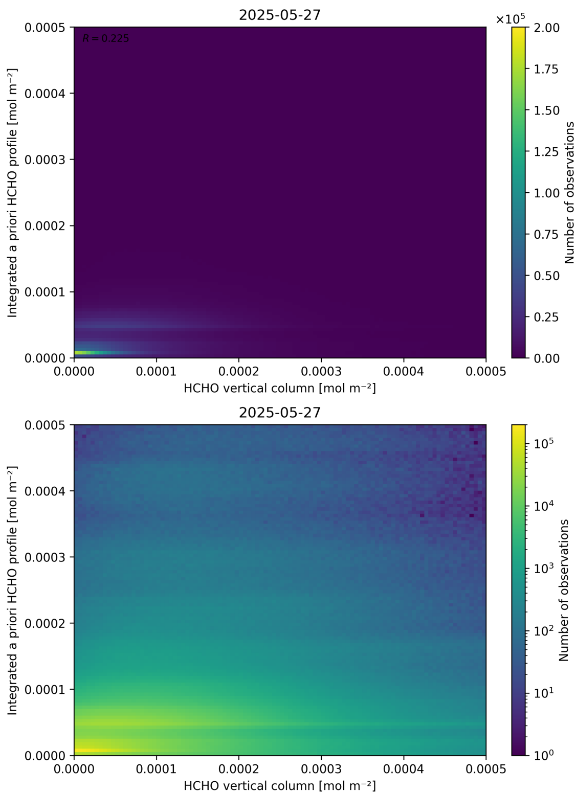
Figure 135: Scatter density plot of “HCHO vertical column” against “Integrated a priori HCHO profile” for 2025-05-26 to 2025-05-28.
