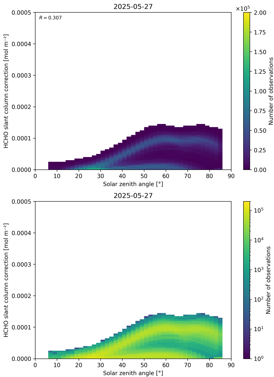
Figure 172: Scatter density plot of “Solar zenith angle” against “HCHO slant column correction” for 2025-05-26 to 2025-05-28.
