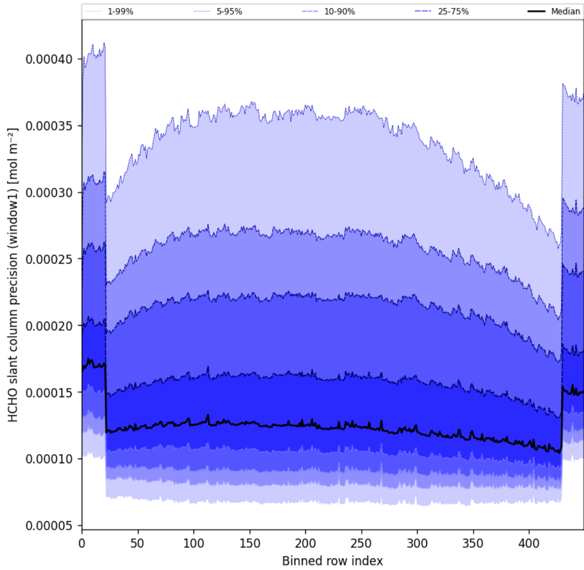
Figure 53: Along track statistics of “HCHO slant column precision (window1)” for 2025-05-26 to 2025-05-28
