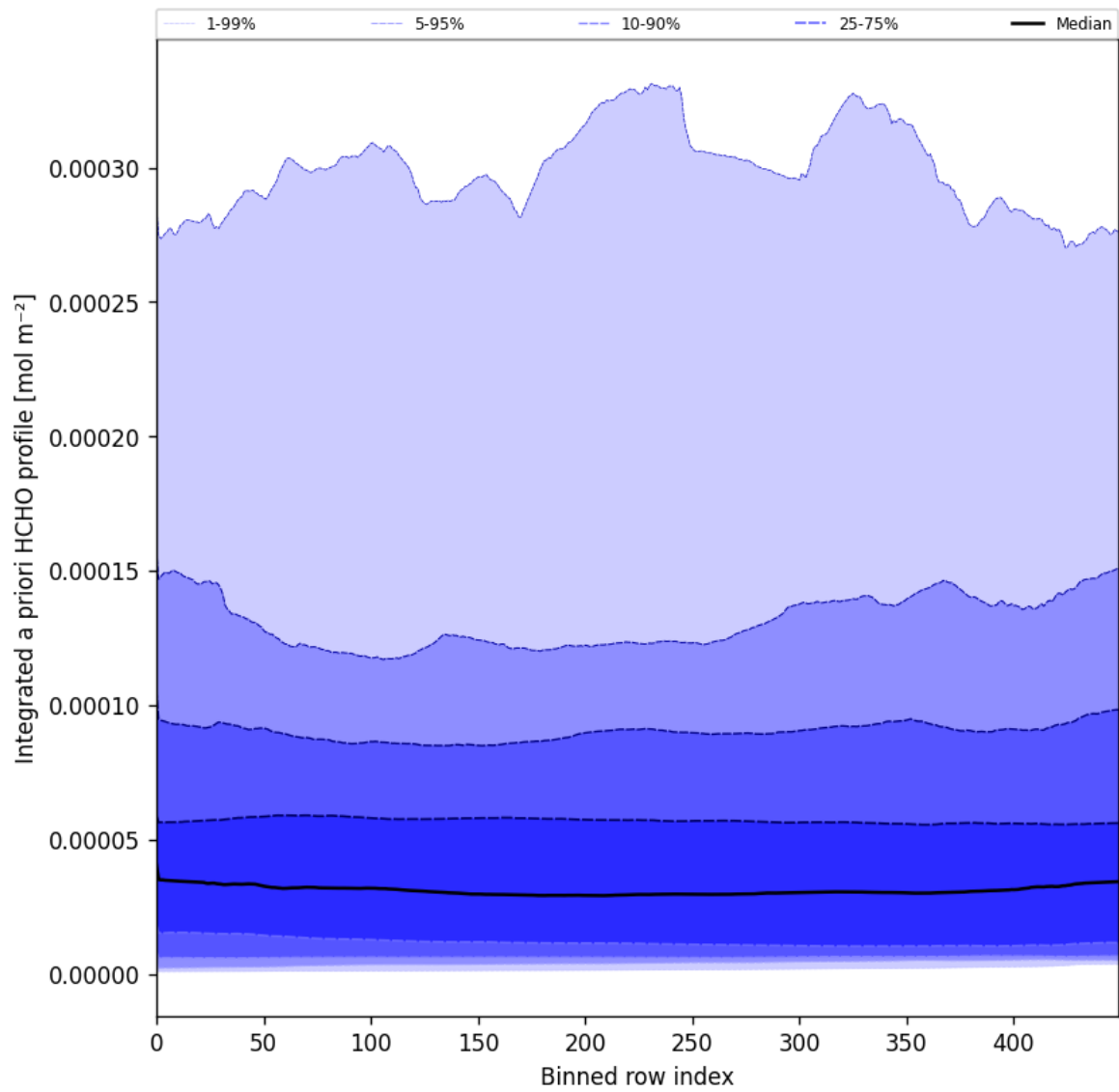
Figure 57: Along track statistics of “Integrated a priori HCHO profile” for 2025-05-26 to 2025-05-28
