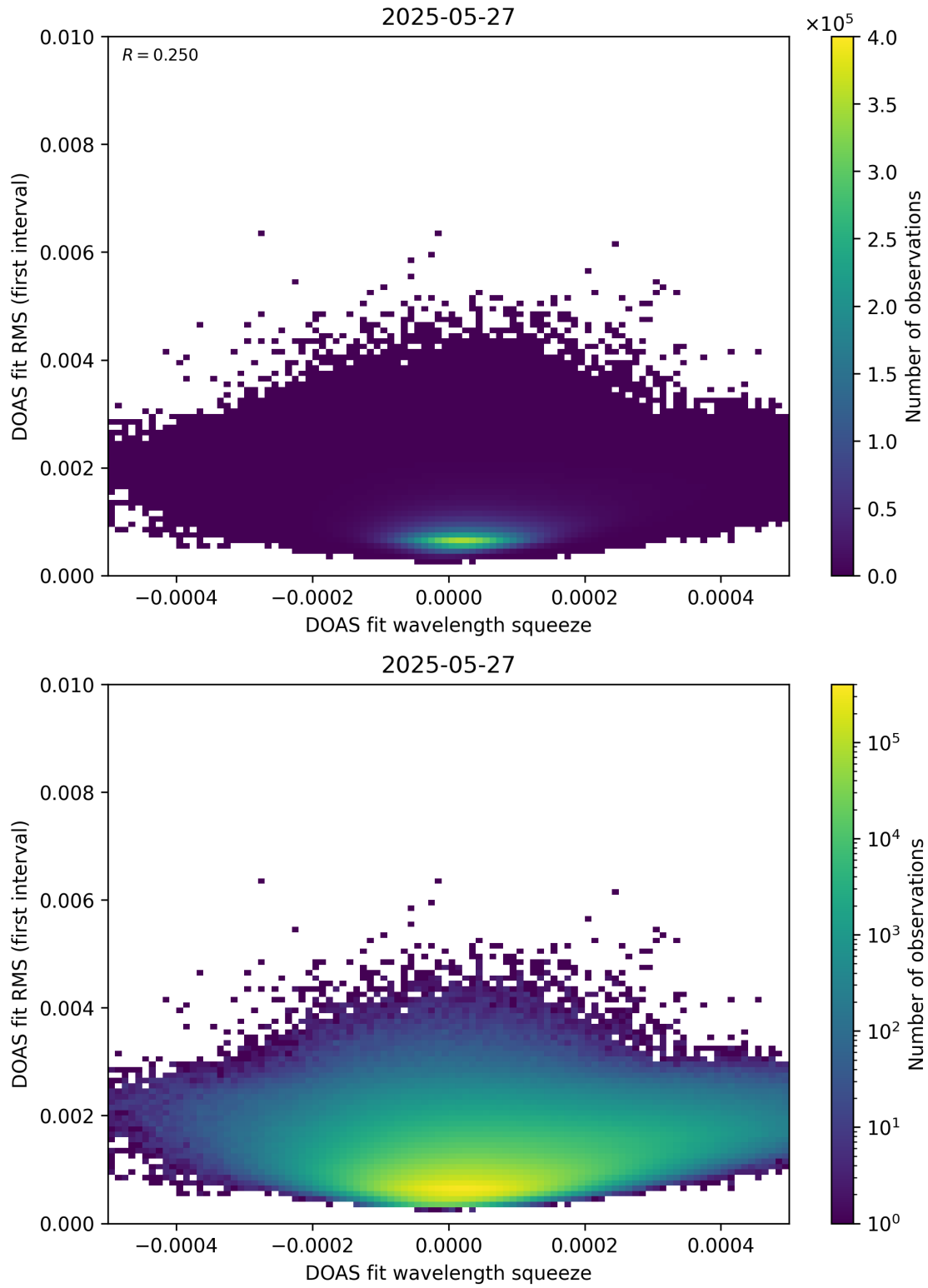
Figure 68: Scatter density plot of “DOAS fit wavelength squeeze” against “DOAS fit RMS (first interval)” for 2025-05-26 to 2025-05-28.
