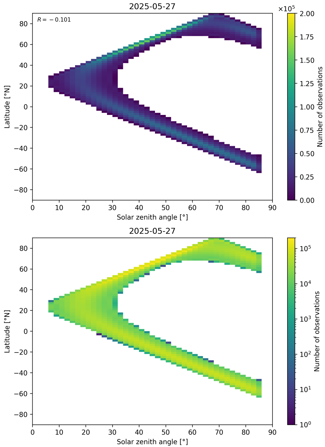
Figure 181: Scatter density plot of “Solar zenith angle” against “Latitude” for 2025-05-26 to 2025-05-28.
