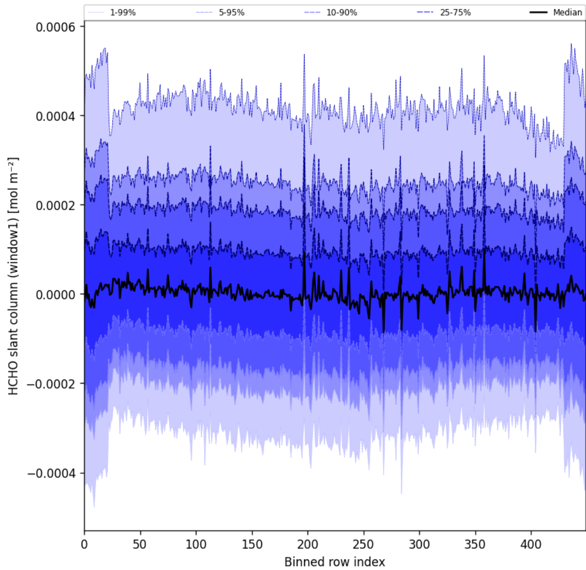
Figure 52: Along track statistics of “HCHO slant column (window1)” for 2025-05-26 to 2025-05-28
