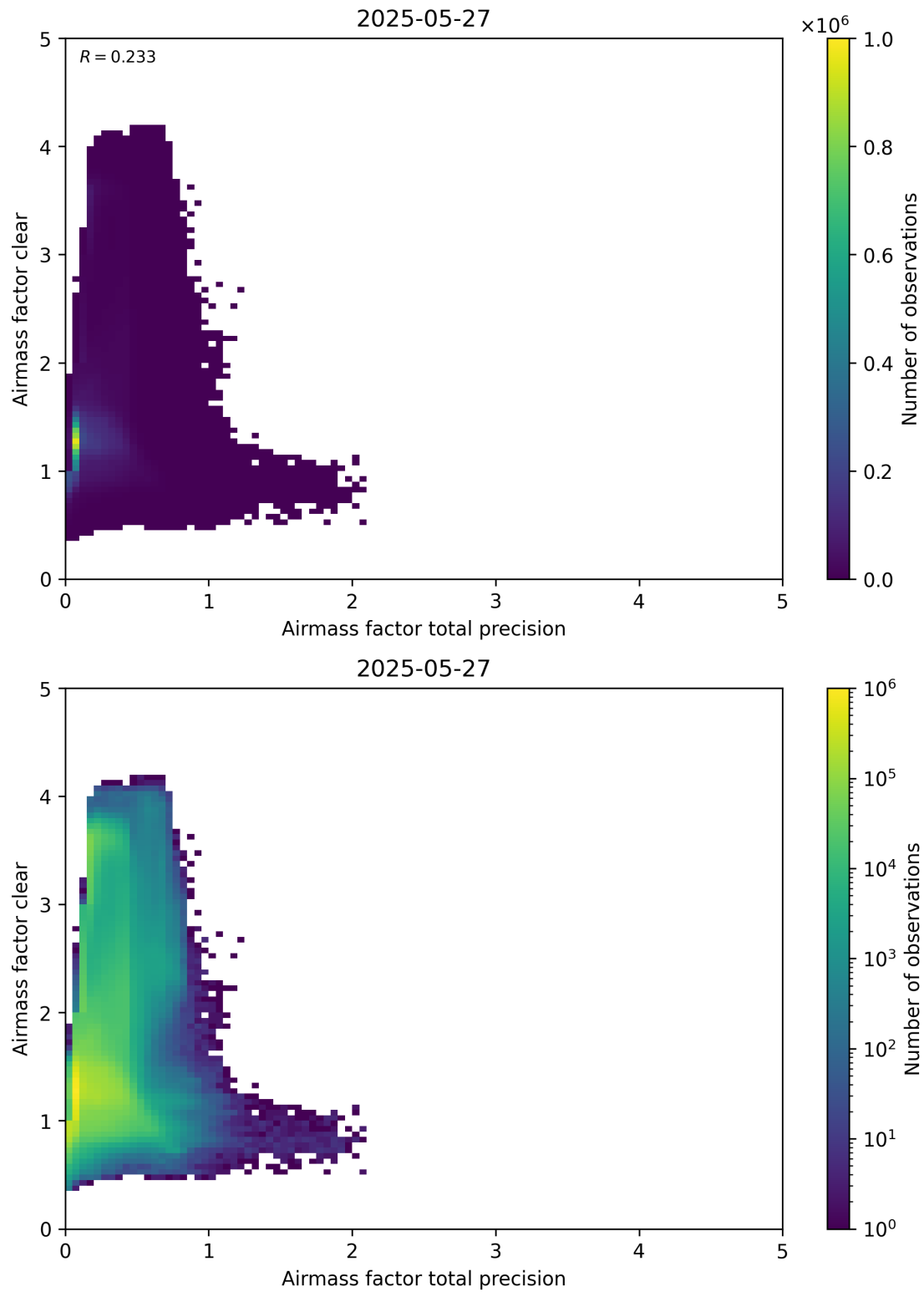
Figure 108: Scatter density plot of “Airmass factor total precision” against “Airmass factor clear” for 2025-05-26 to 2025-05-28.
