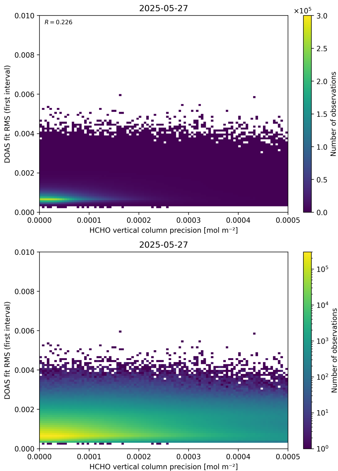
Figure 136: Scatter density plot of “HCHO vertical column precision” against “DOAS fit RMS (first interval)” for 2025-05-26 to 2025-05-28.
