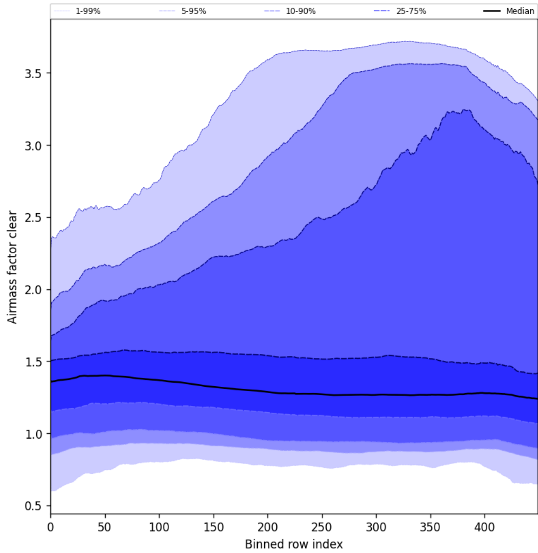
Figure 56: Along track statistics of “Airmass factor clear” for 2025-05-26 to 2025-05-28
