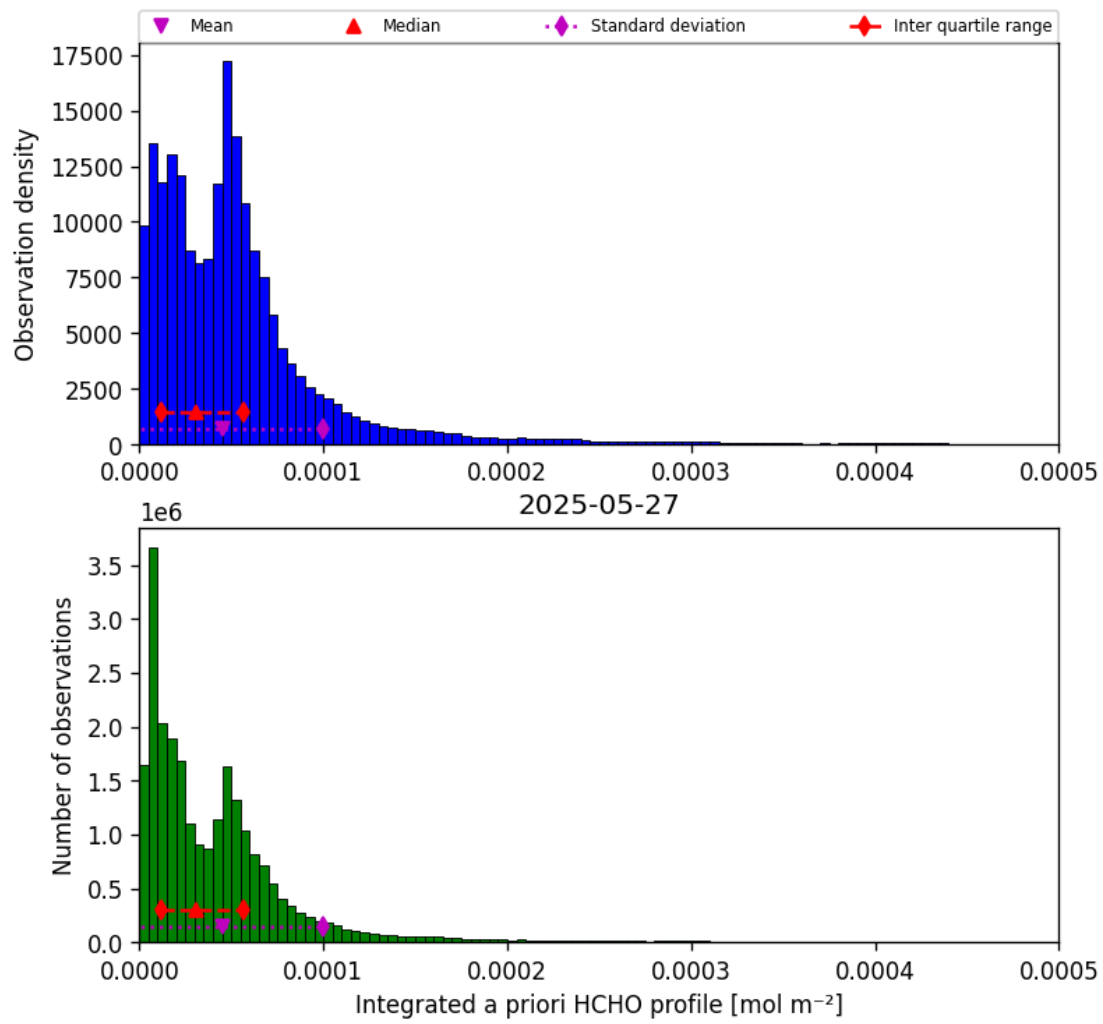
Figure 43: Histogram of “Integrated a priori HCHO profile” for 2025-05-26 to 2025-05-28
