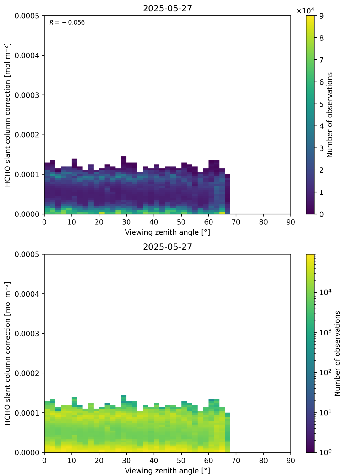
Figure 187: Scatter density plot of “Viewing zenith angle” against “HCHO slant column correction” for 2025-05-26 to 2025-05-28.
