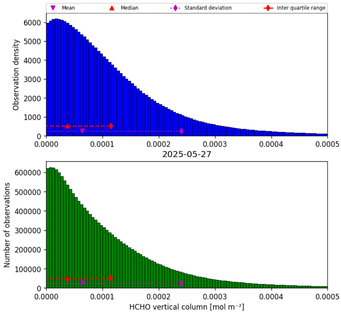
Figure 35: Histogram of “HCHO vertical column” for 2025-05-26 to 2025-05-28
