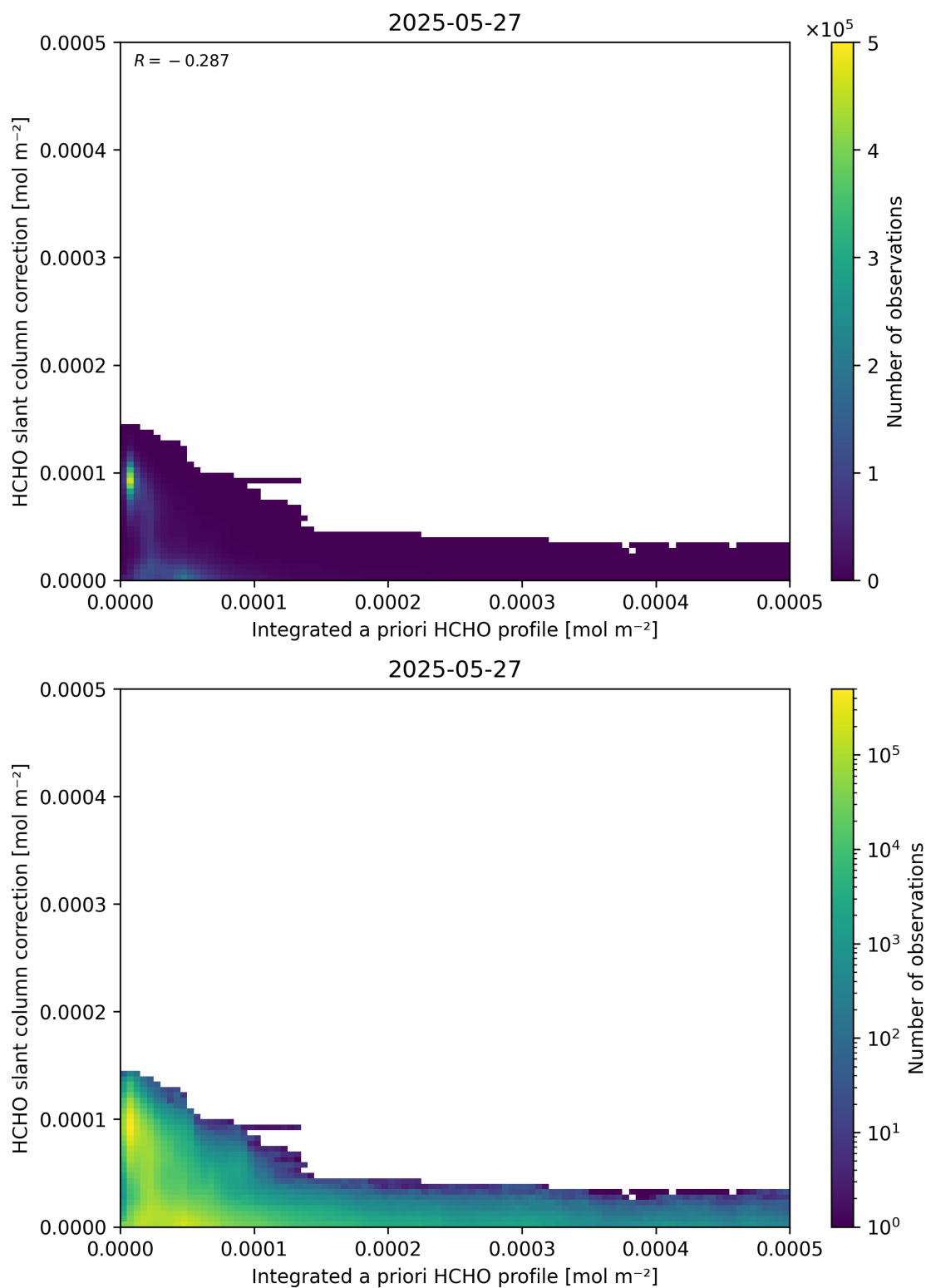
Figure 152: Scatter density plot of “Integrated a priori HCHO profile” against “HCHO slant column correction” for 2025-05-26 to 2025-05-28.
