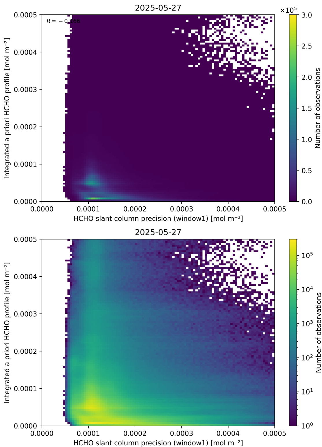
Figure 96: Scatter density plot of “HCHO slant column precision (window1)” against “Integrated a priori HCHO profile” for 2025-05-26 to 2025-05-28.
