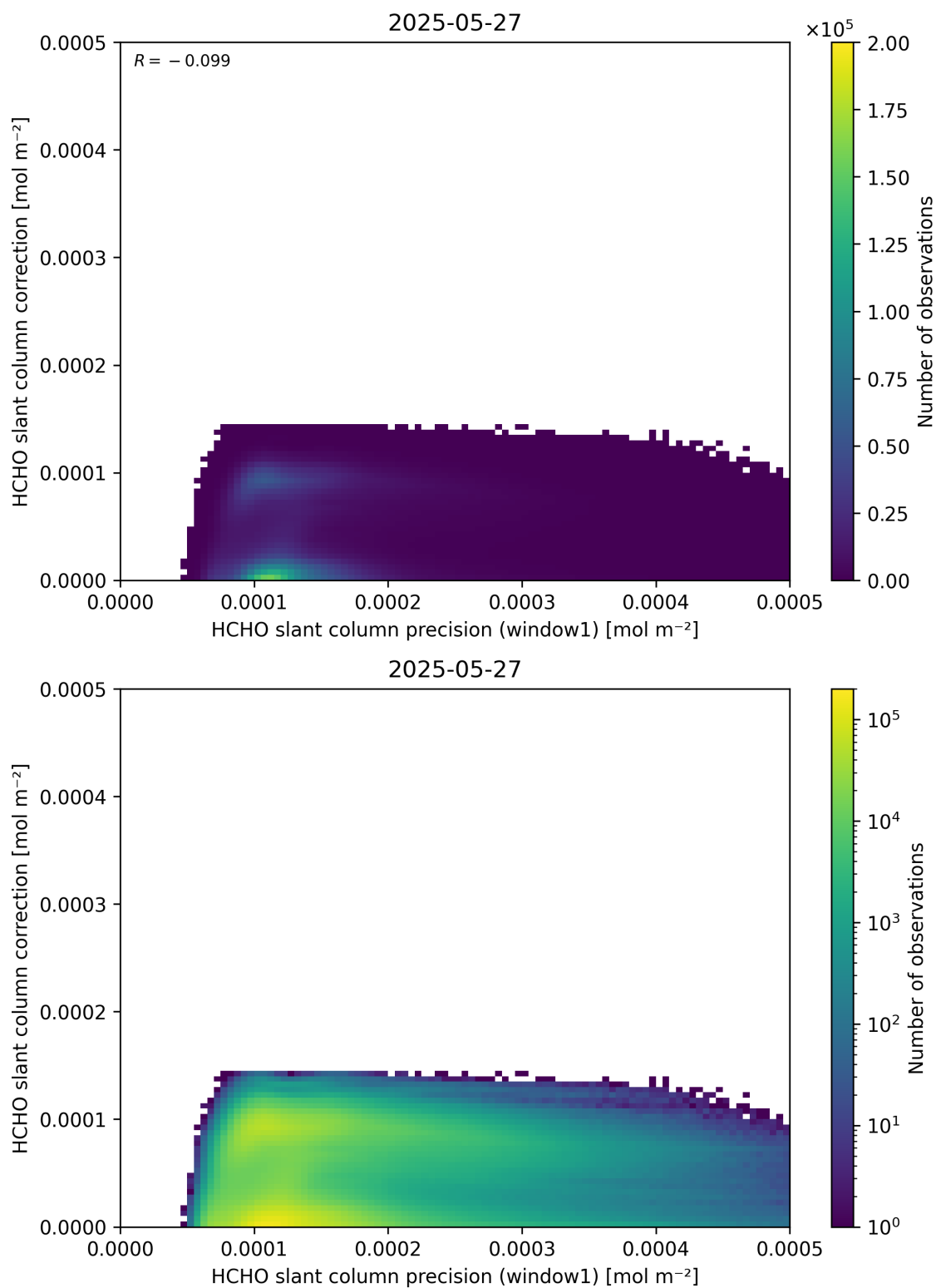
Figure 93: Scatter density plot of “HCHO slant column precision (window1)” against “HCHO slant column correction” for 2025-05-26 to 2025-05-28.
