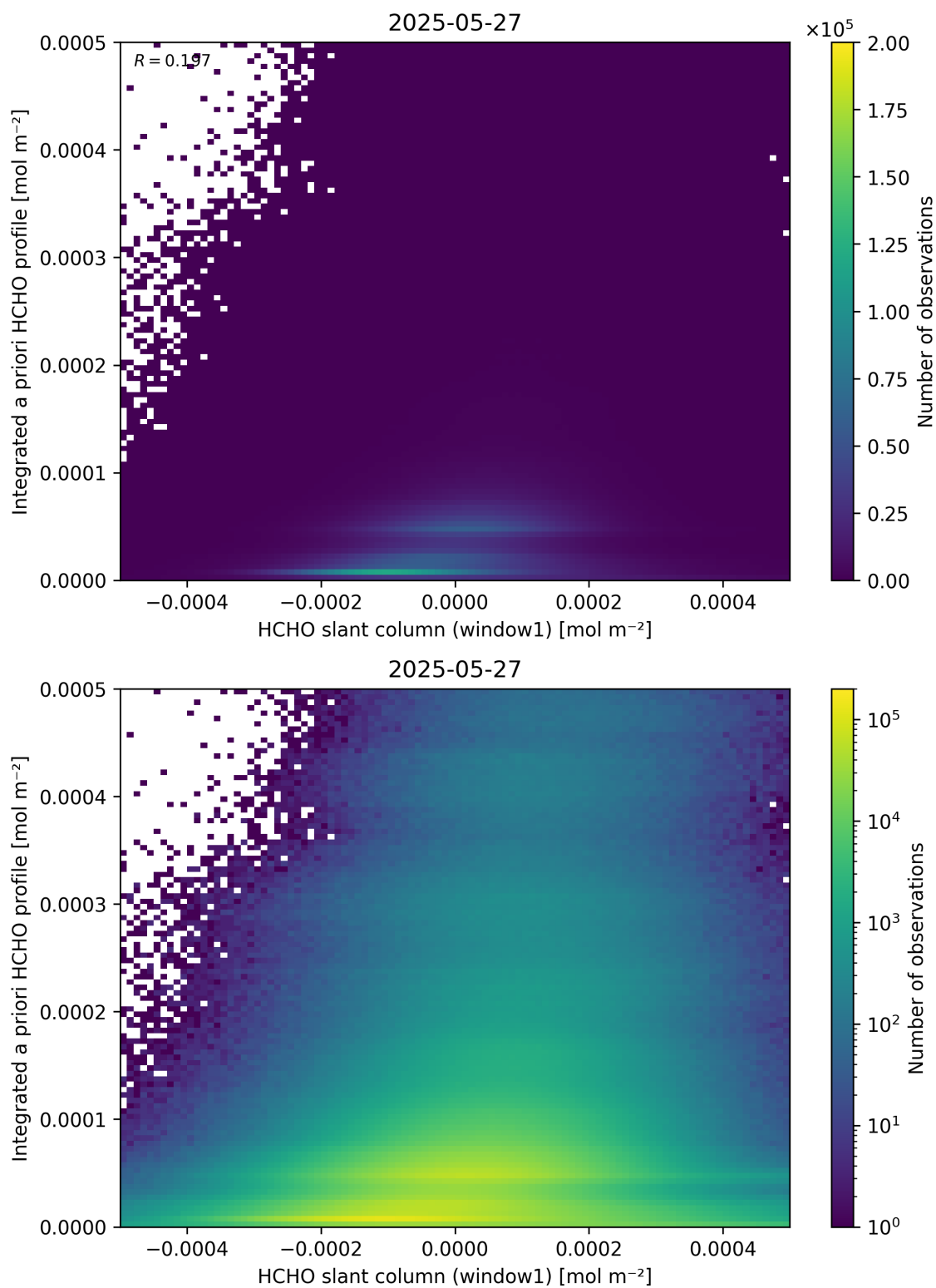
Figure 87: Scatter density plot of “HCHO slant column (window1)” against “Integrated a priori HCHO profile” for 2025-05-26 to 2025-05-28.
