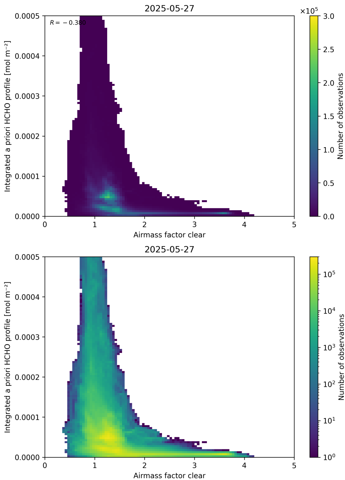
Figure 76: Scatter density plot of “Airmass factor clear” against “Integrated a priori HCHO profile” for 2025-05-26 to 2025-05-28.
