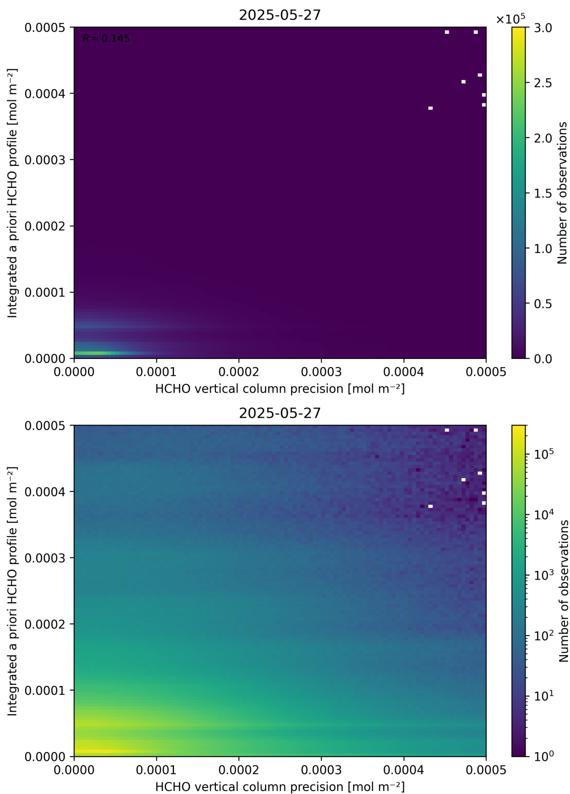
Figure 147: Scatter density plot of “HCHO vertical column precision” against “Integrated a priori HCHO profile” for 2025-05-26 to 2025-05-28.
