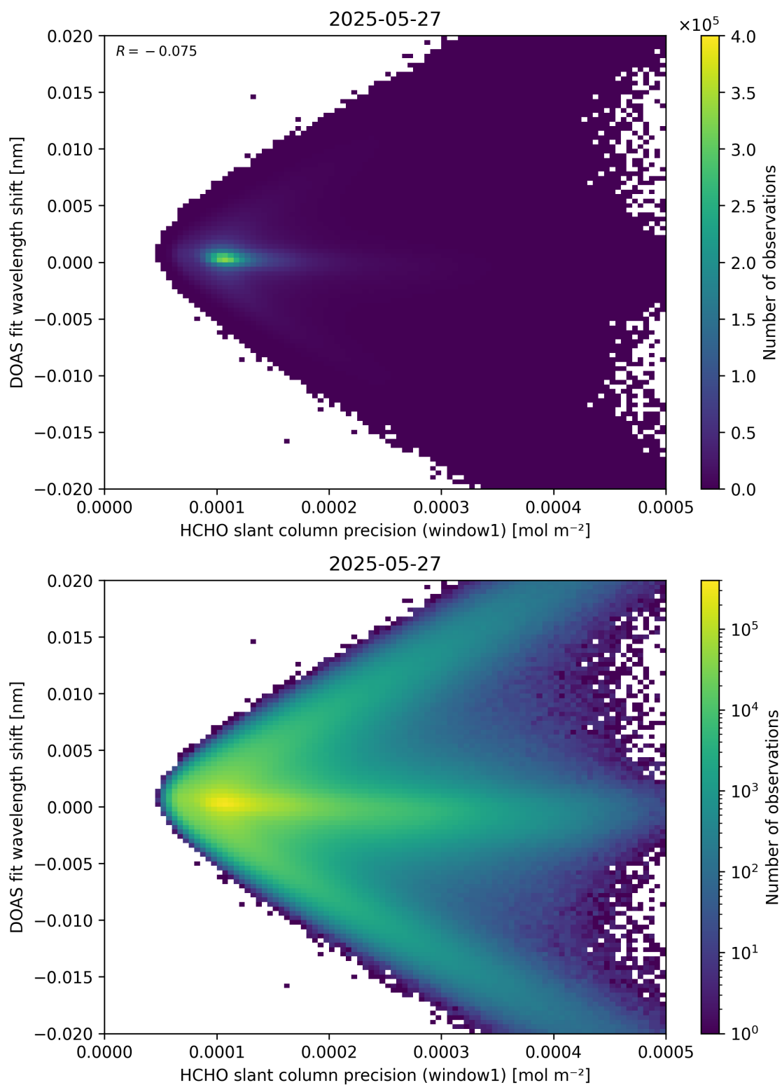
Figure 89: Scatter density plot of “HCHO slant column precision (window1)” against “DOAS fit wavelength shift” for 2025-05-26 to 2025-05-28.
