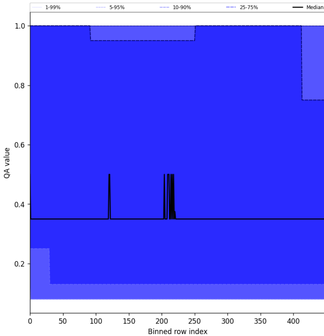
Figure 48: Along track statistics of “QA value” for 2025-05-26 to 2025-05-28
