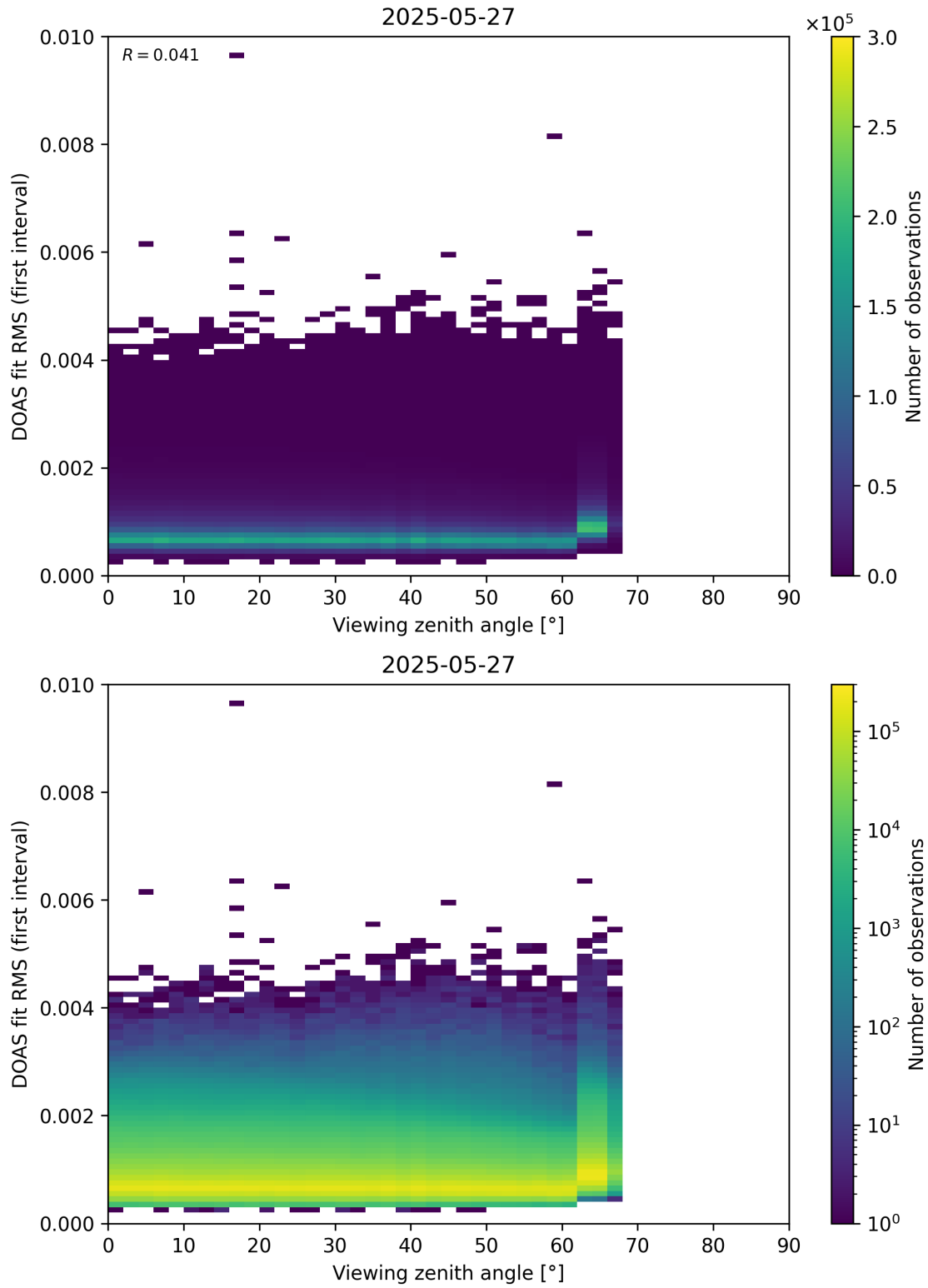
Figure 182: Scatter density plot of “Viewing zenith angle” against “DOAS fit RMS (first interval)” for 2025-05-26 to 2025-05-28.
