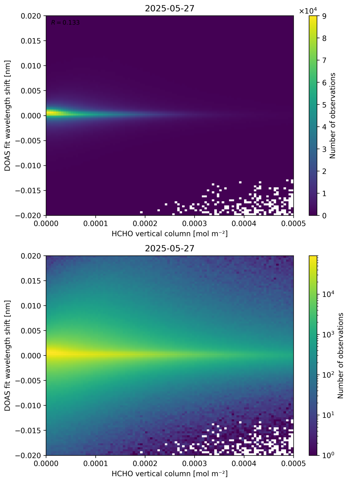
Figure 124: Scatter density plot of “HCHO vertical column” against “DOAS fit wavelength shift” for 2025-05-26 to 2025-05-28.
