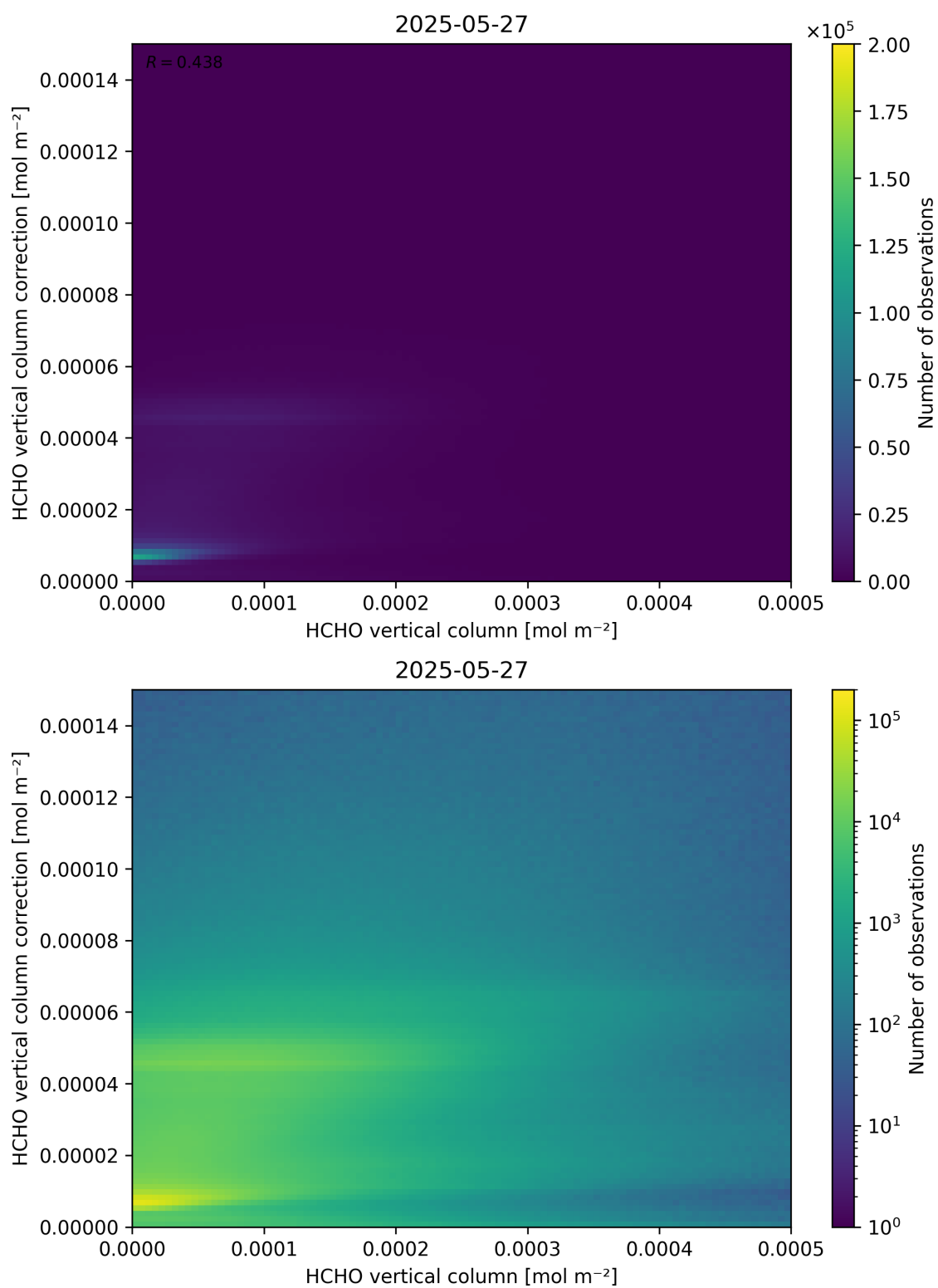
Figure 133: Scatter density plot of “HCHO vertical column” against “HCHO vertical column correction” for 2025-05-26 to 2025-05-28.
