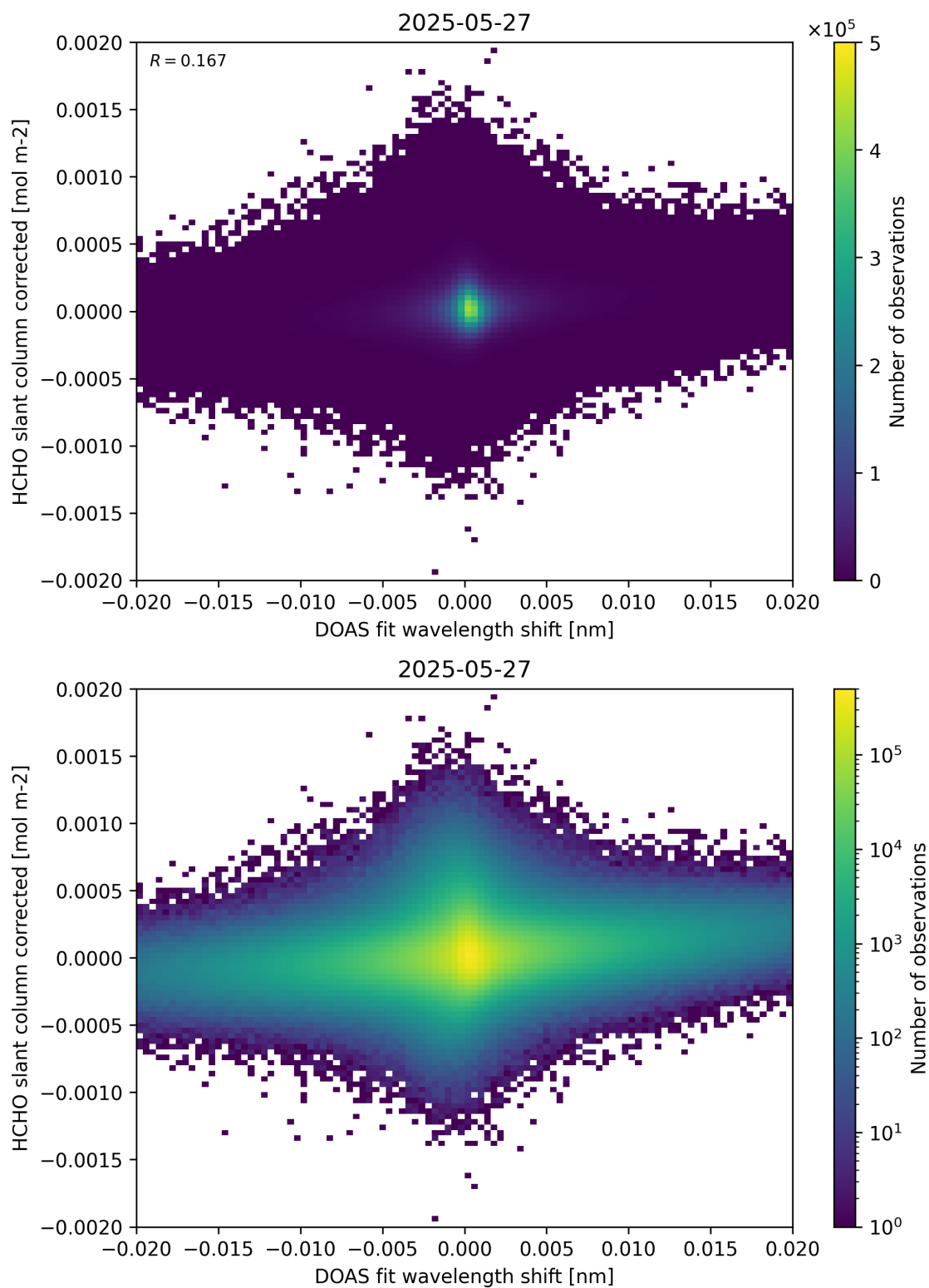
Figure 66: Scatter density plot of “DOAS fit wavelength shift” against “HCHO slant column corrected” for 2025-05-26 to 2025-05-28.
