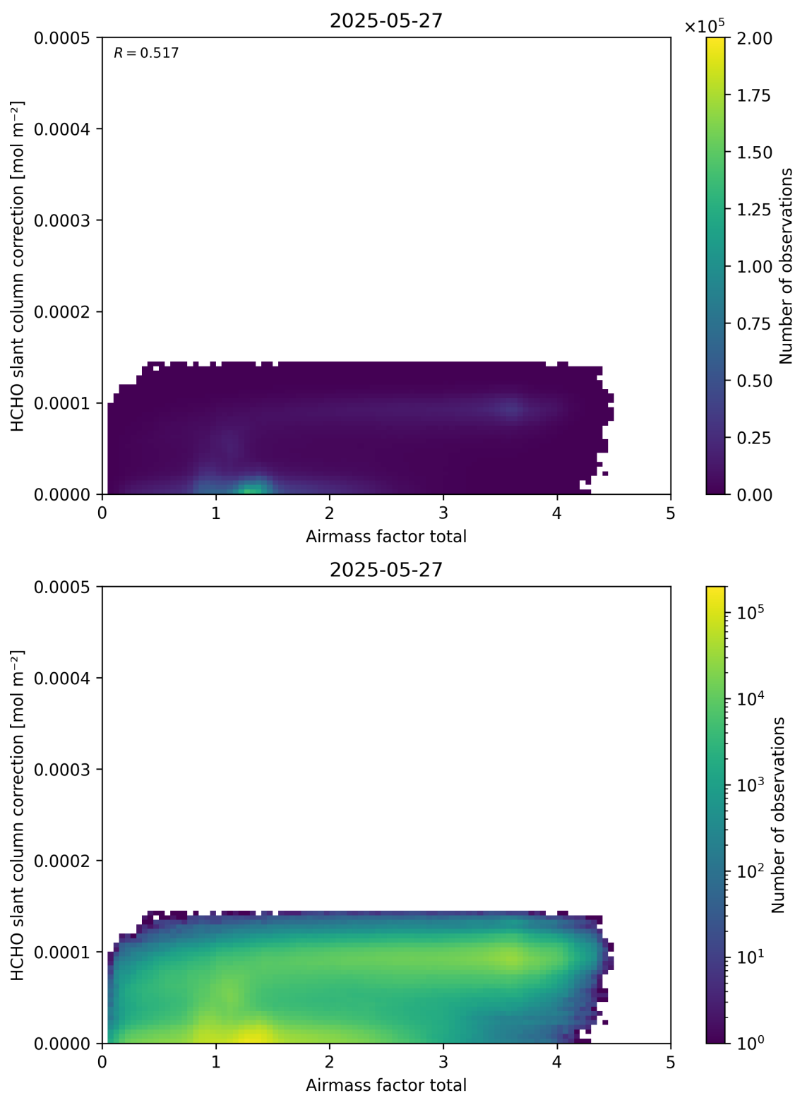
Figure 102: Scatter density plot of “Airmass factor total” against “HCHO slant column correction” for 2025-05-26 to 2025-05-28.
