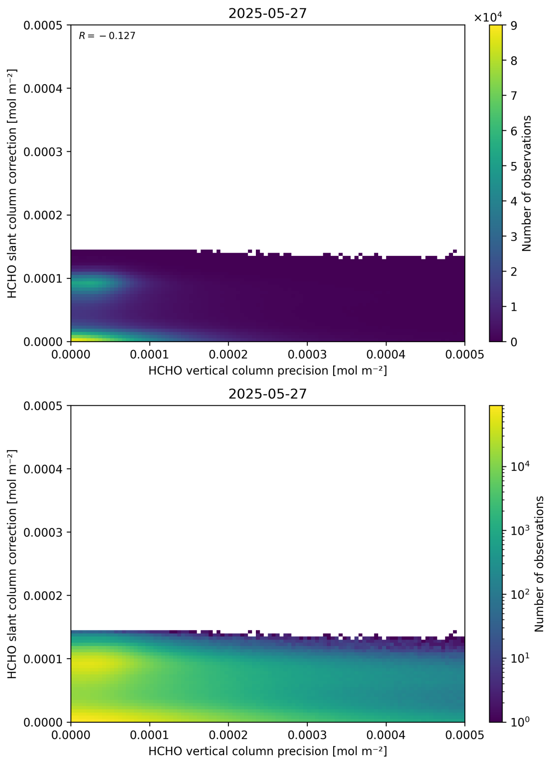
Figure 141: Scatter density plot of “HCHO vertical column precision” against “HCHO slant column correction” for 2025-05-26 to 2025-05-28.
