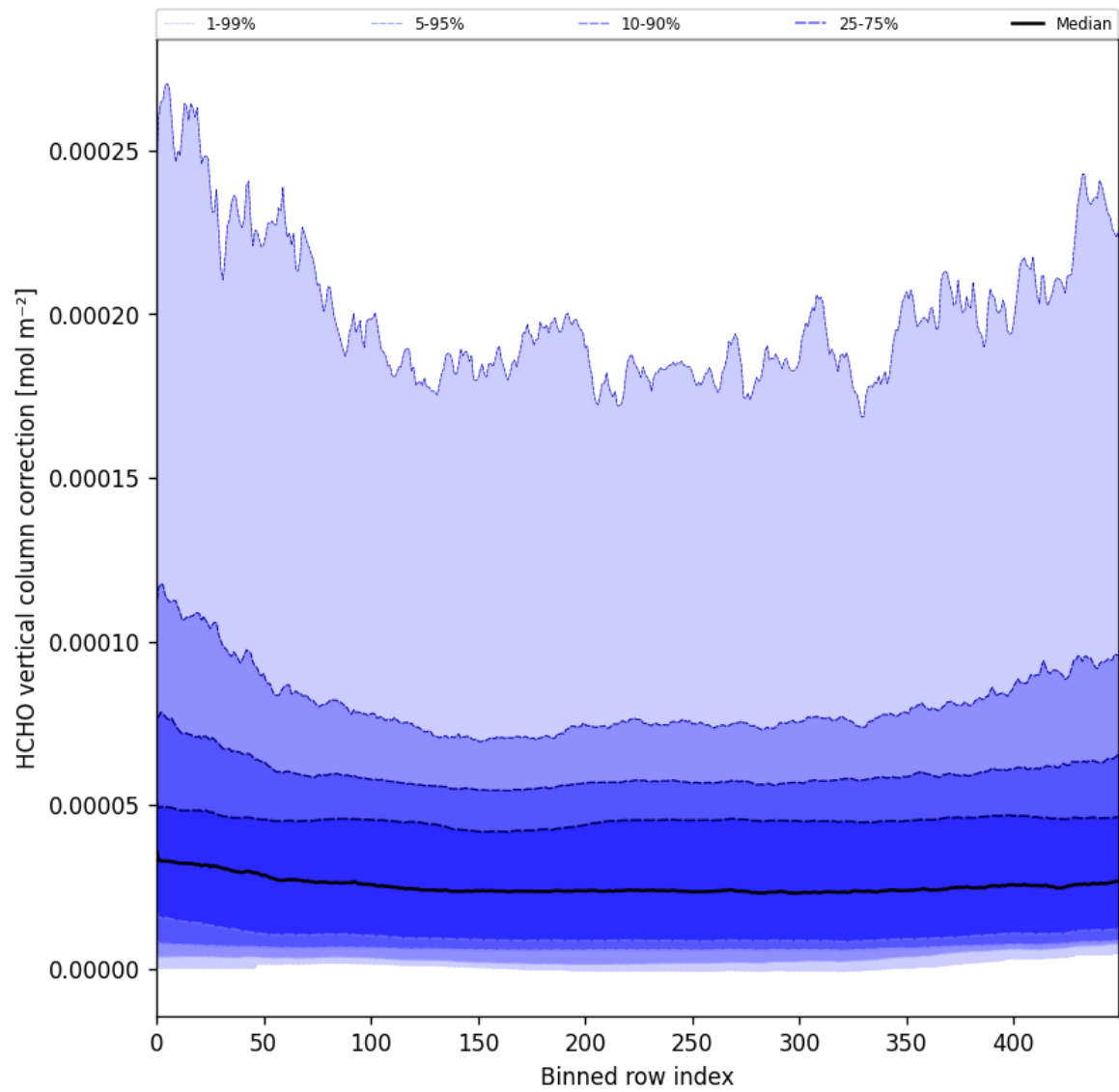
Figure 51: Along track statistics of “HCHO vertical column correction” for 2025-05-26 to 2025-05-28
