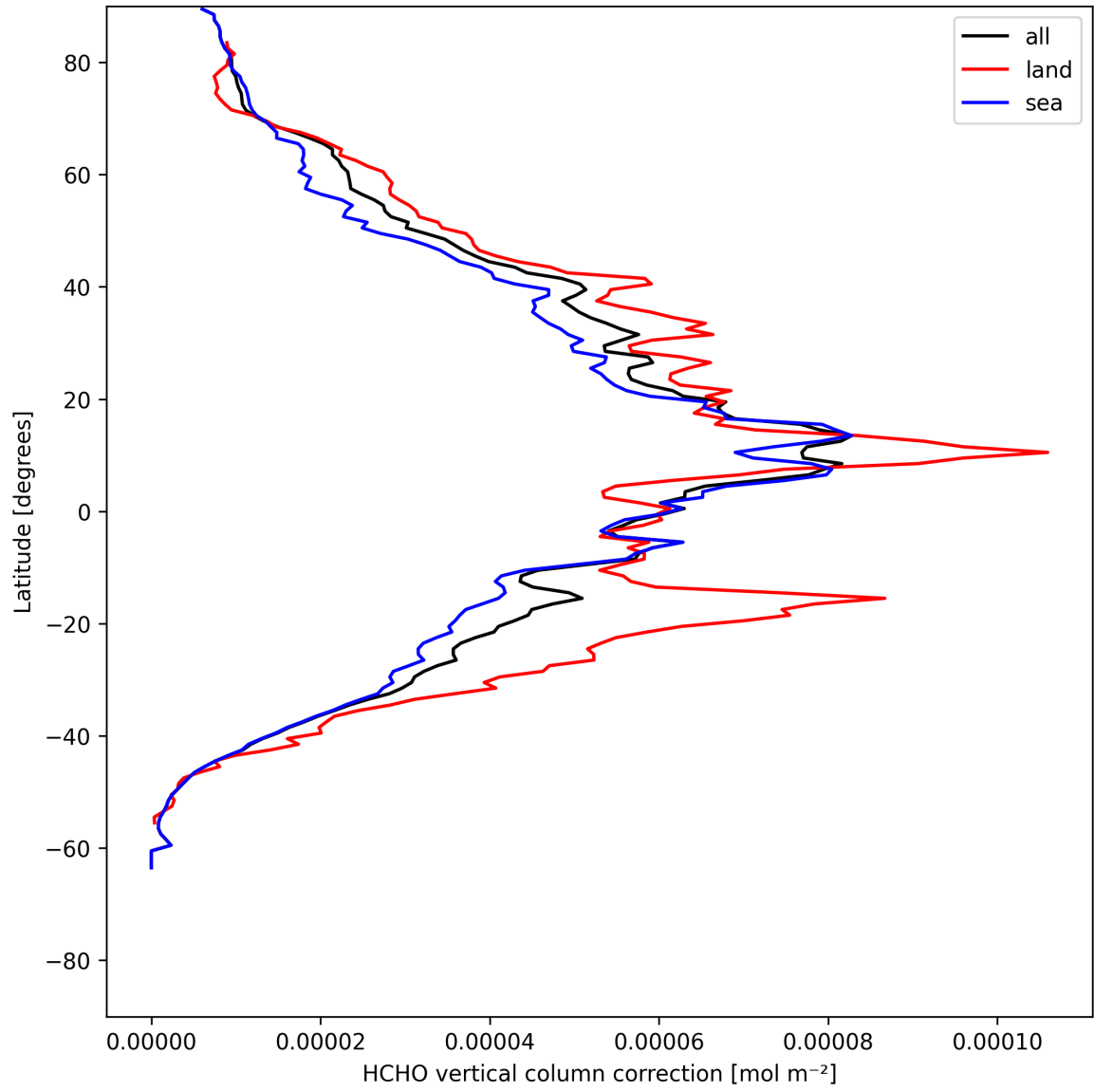
Figure 23: Zonal average of “HCHO vertical column correction” for 2025-05-26 to 2025-05-28.
