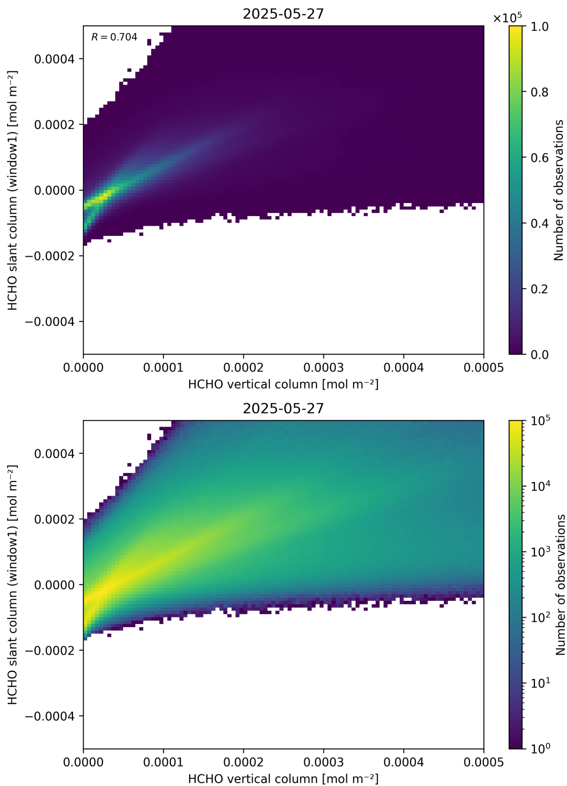
Figure 129: Scatter density plot of “HCHO vertical column” against “HCHO slant column (window1)” for 2025-05-26 to 2025-05-28.
