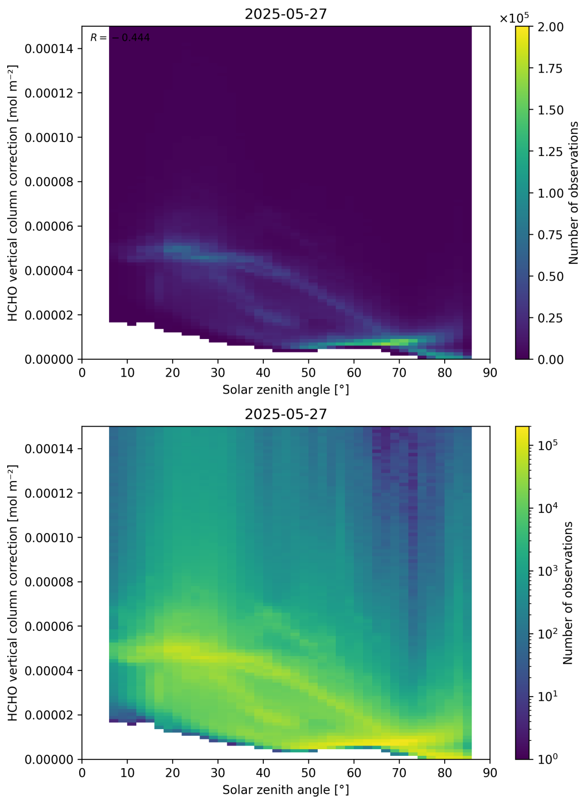
Figure 178: Scatter density plot of “Solar zenith angle” against “HCHO vertical column correction” for 2025-05-26 to 2025-05-28.
