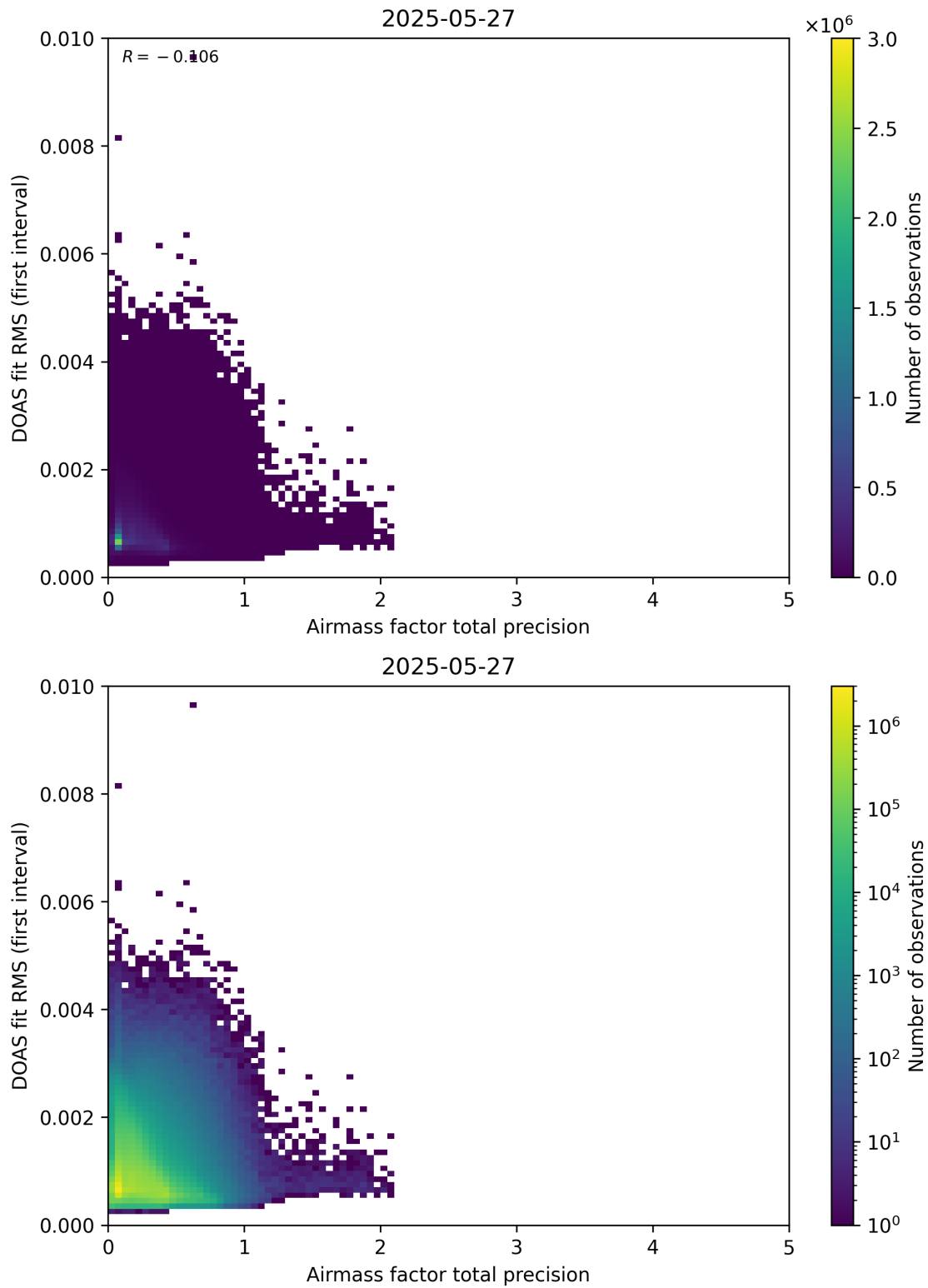
Figure 105: Scatter density plot of “Airmass factor total precision” against “DOAS fit RMS (first interval)” for 2025-05-26 to 2025-05-28.
