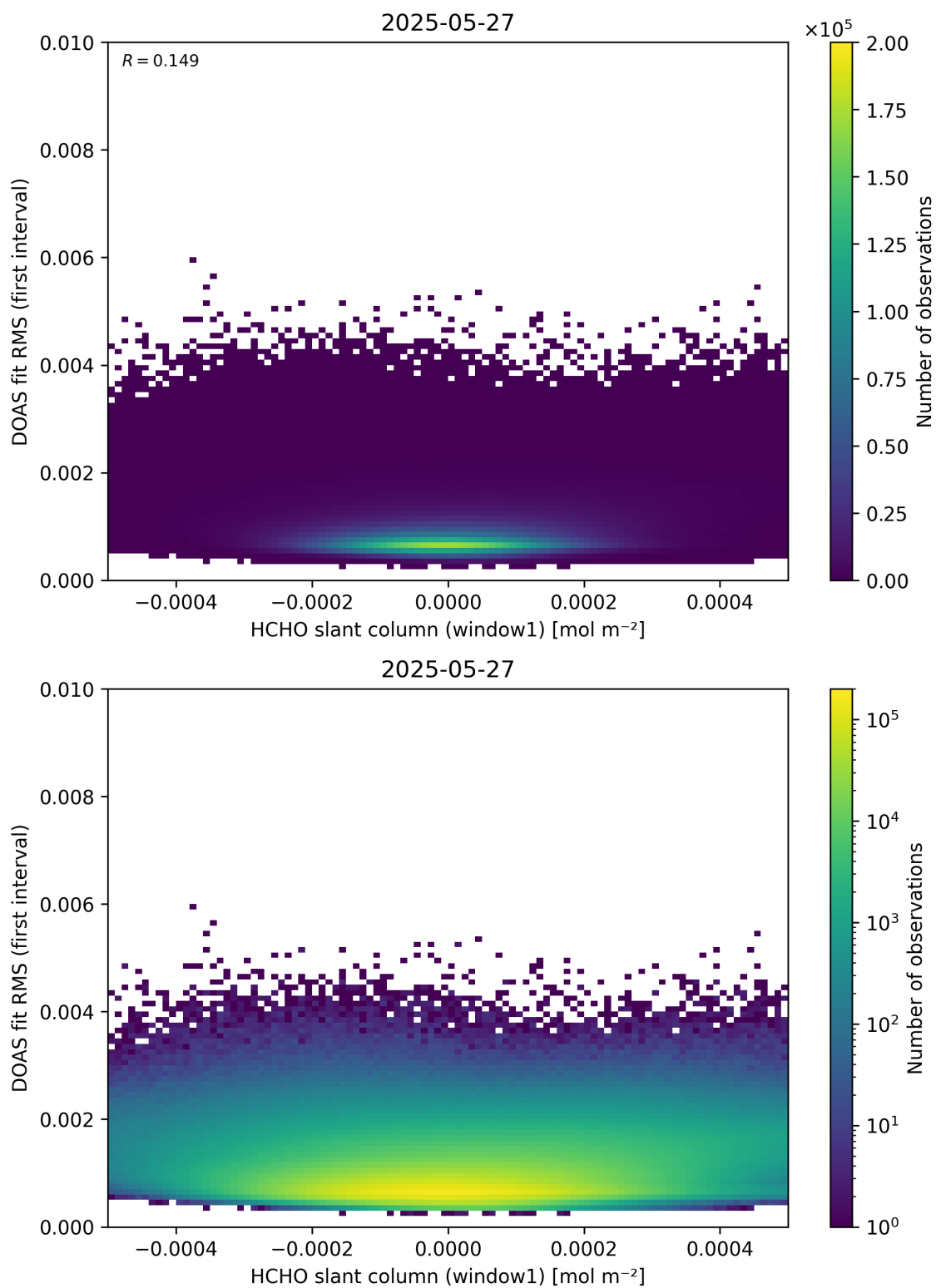
Figure 78: Scatter density plot of “HCHO slant column (window1)” against “DOAS fit RMS (first interval)” for 2025-05-26 to 2025-05-28.
