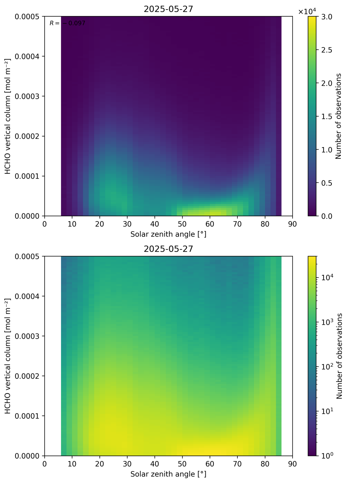
Figure 177: Scatter density plot of “Solar zenith angle” against “HCHO vertical column” for 2025-05-26 to 2025-05-28.
