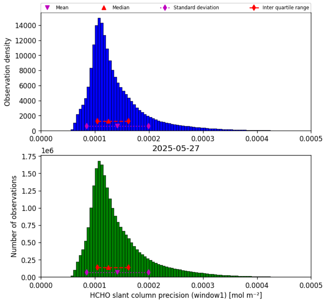
Figure 39: Histogram of “HCHO slant column precision (window1)” for 2025-05-26 to 2025-05-28
