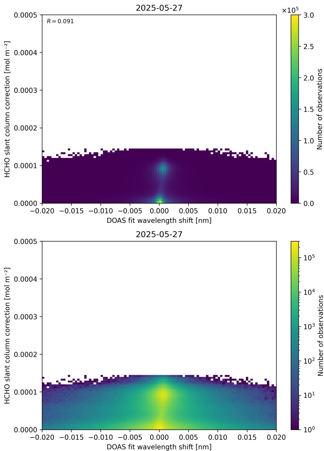
Figure 67: Scatter density plot of “DOAS fit wavelength shift” against “HCHO slant column correction” for 2025-05-26 to 2025-05-28.
