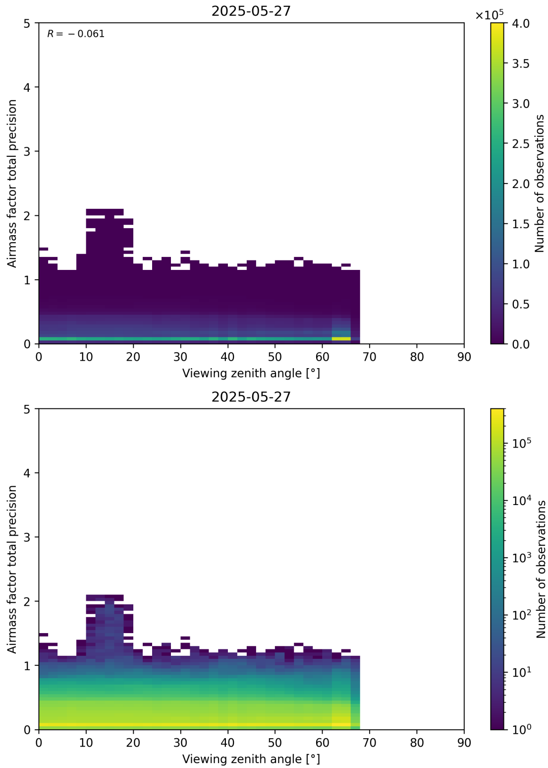
Figure 191: Scatter density plot of “Viewing zenith angle” against “Airmass factor total precision” for 2025-05-26 to 2025-05-28.
