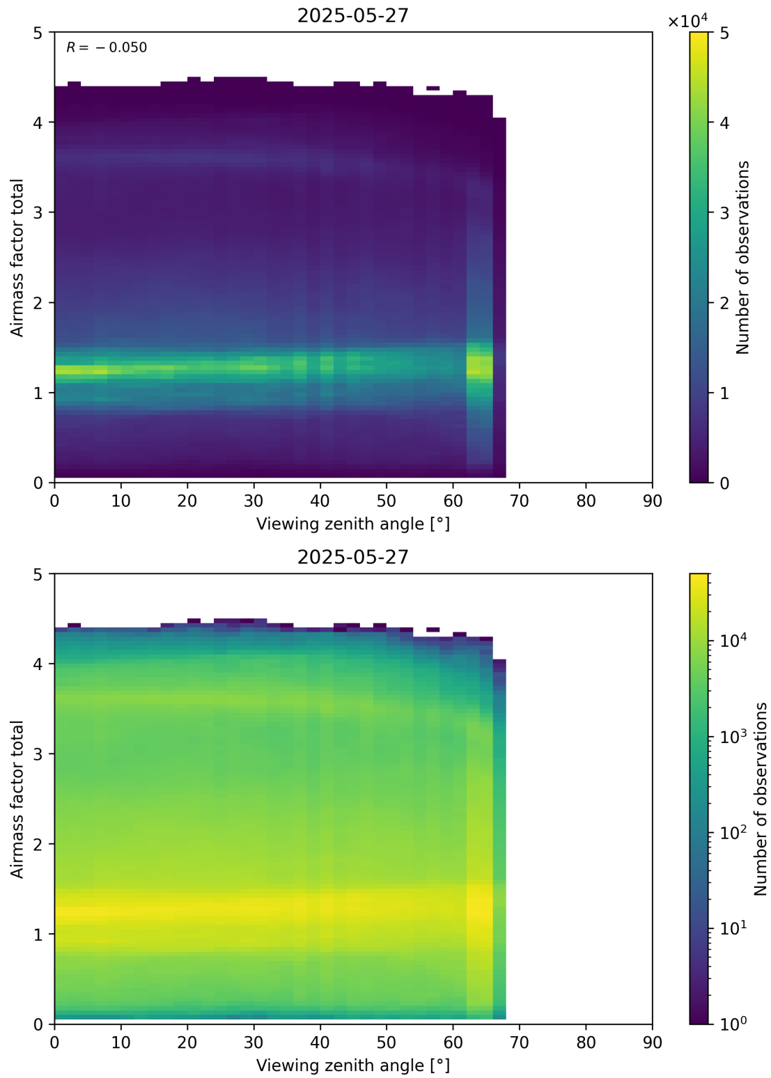
Figure 190: Scatter density plot of “Viewing zenith angle” against “Airmass factor total” for 2025-05-26 to 2025-05-28.
