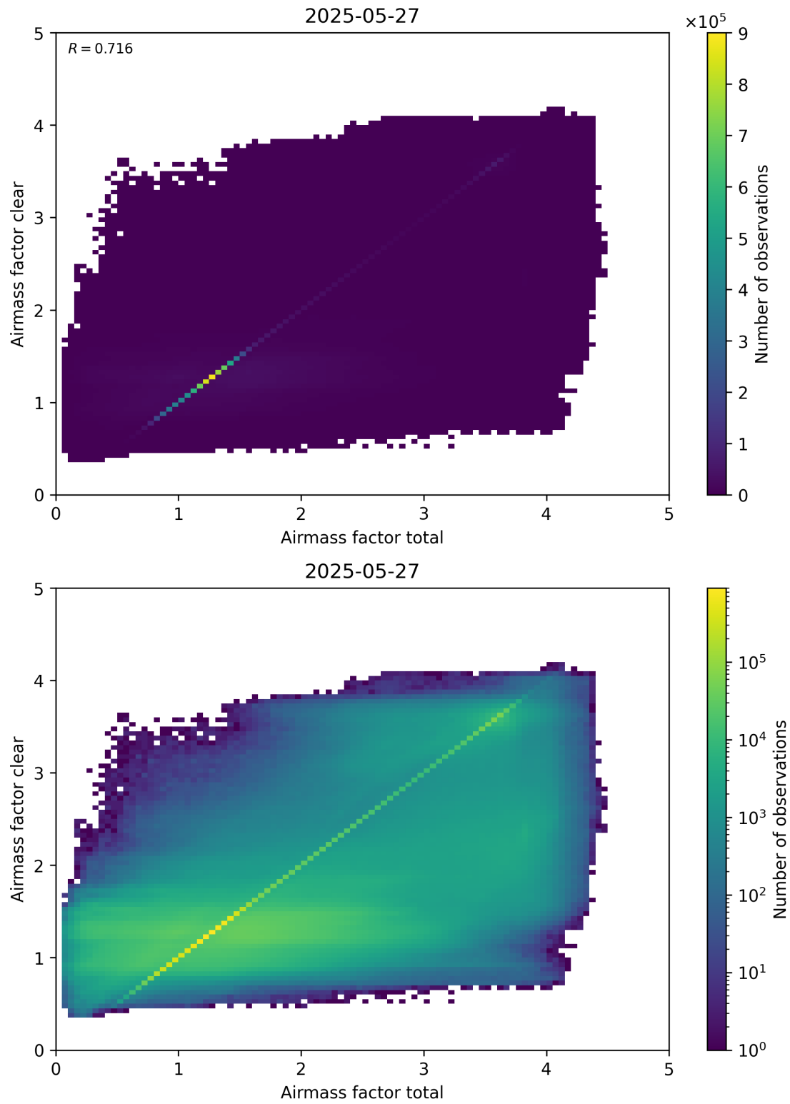
Figure 100: Scatter density plot of “Airmass factor total” against “Airmass factor clear” for 2025-05-26 to 2025-05-28.
