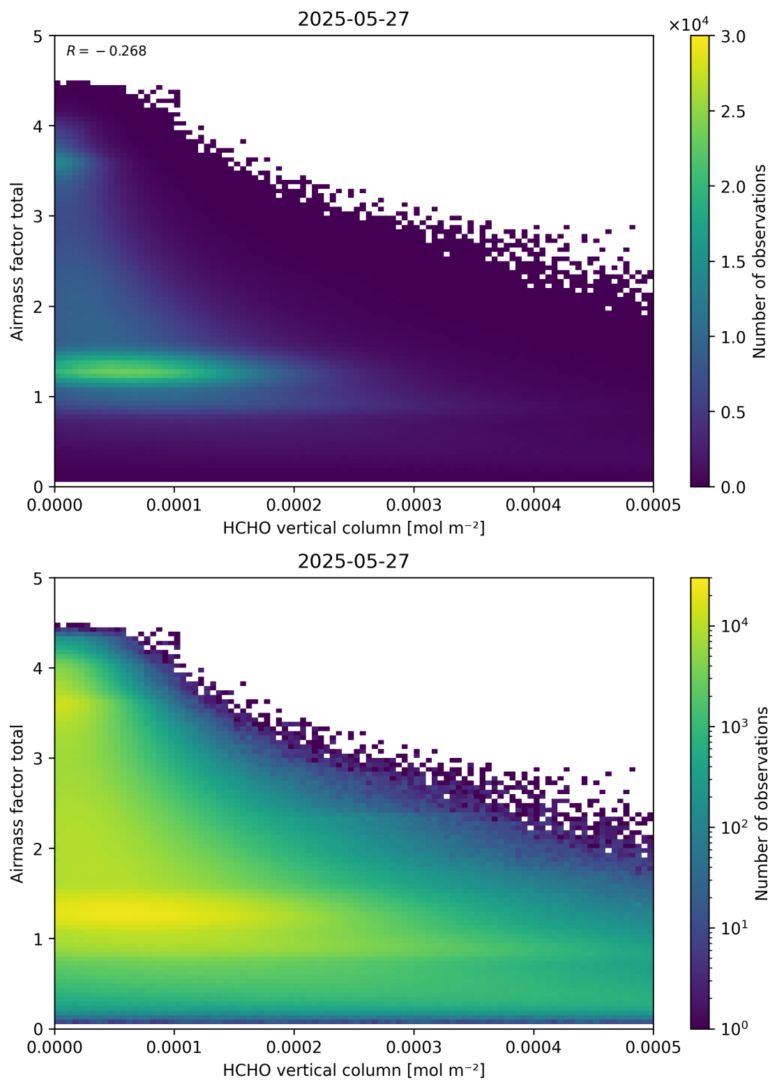
Figure 131: Scatter density plot of “HCHO vertical column” against “Airmass factor total” for 2025-05-26 to 2025-05-28.
