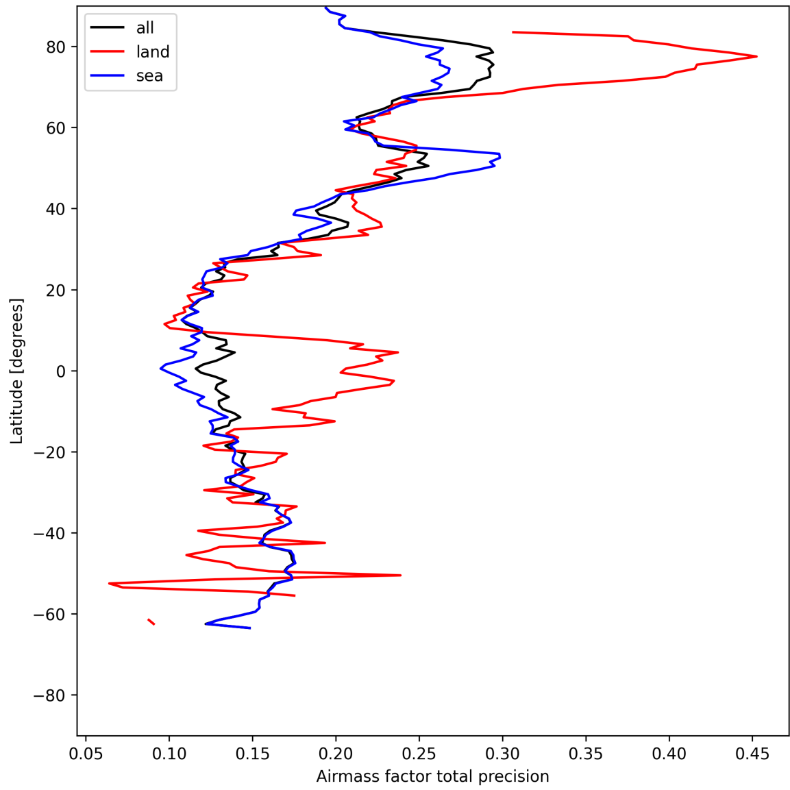
Figure 27: Zonal average of “Airmass factor total precision” for 2025-05-26 to 2025-05-28.
