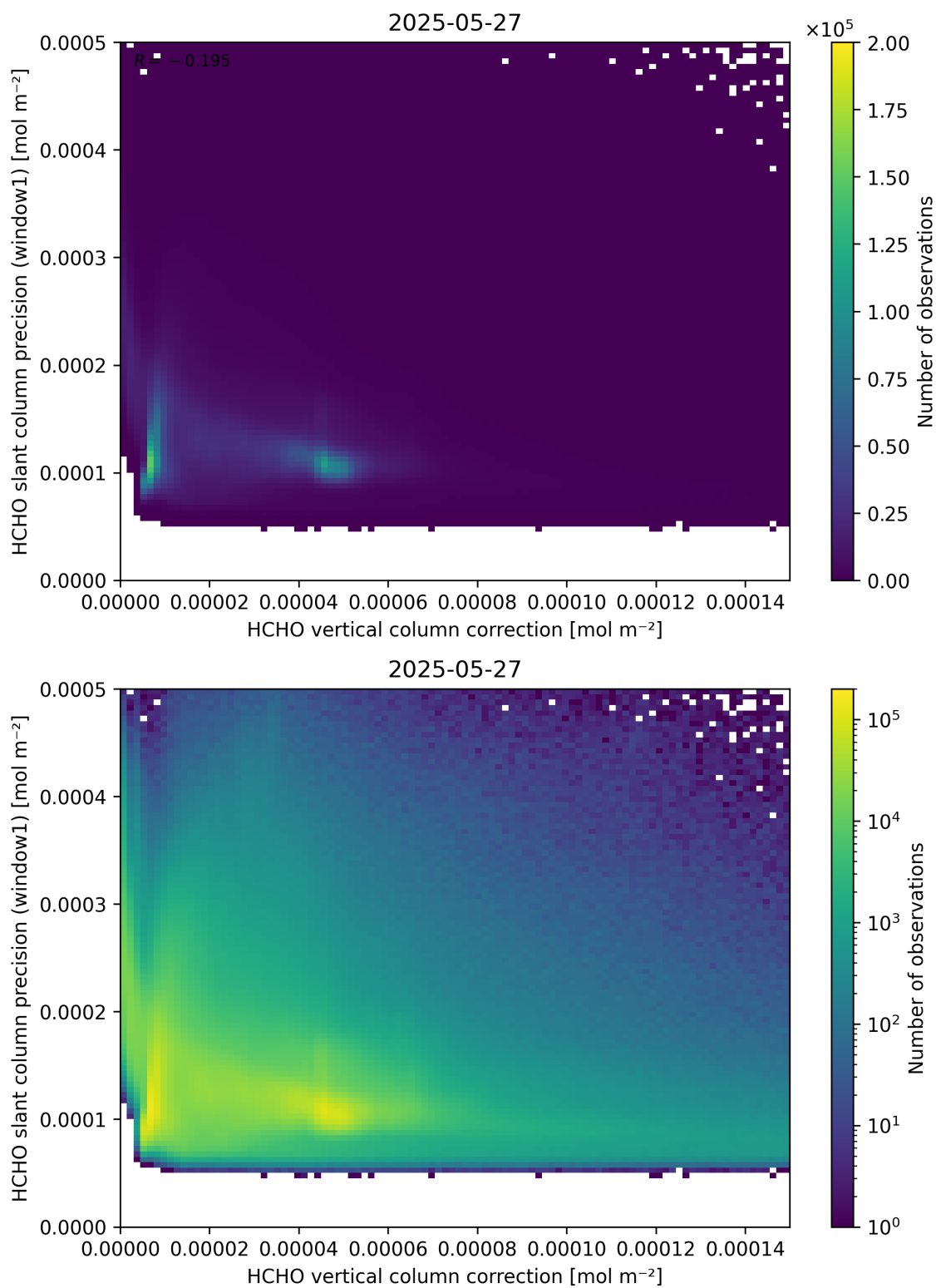
Figure 119: Scatter density plot of “HCHO vertical column correction” against “HCHO slant column precision (window1)” for 2025-05-26 to 2025-05-28.
