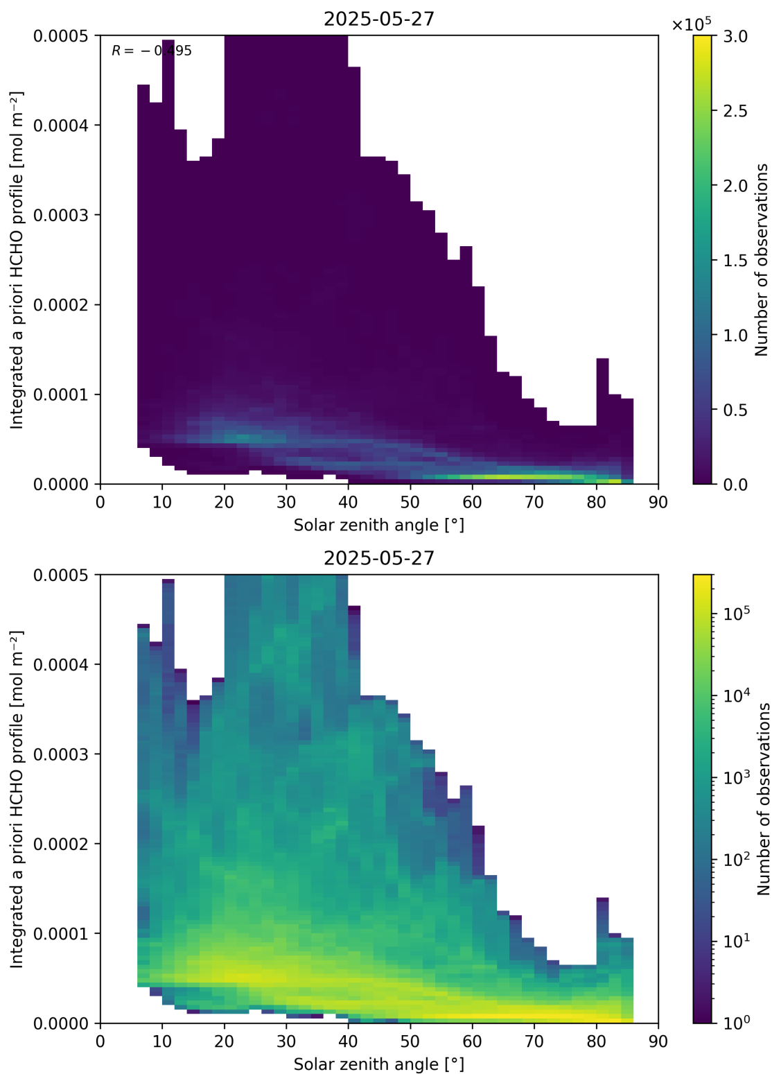
Figure 180: Scatter density plot of “Solar zenith angle” against “Integrated a priori HCHO profile” for 2025-05-26 to 2025-05-28.
