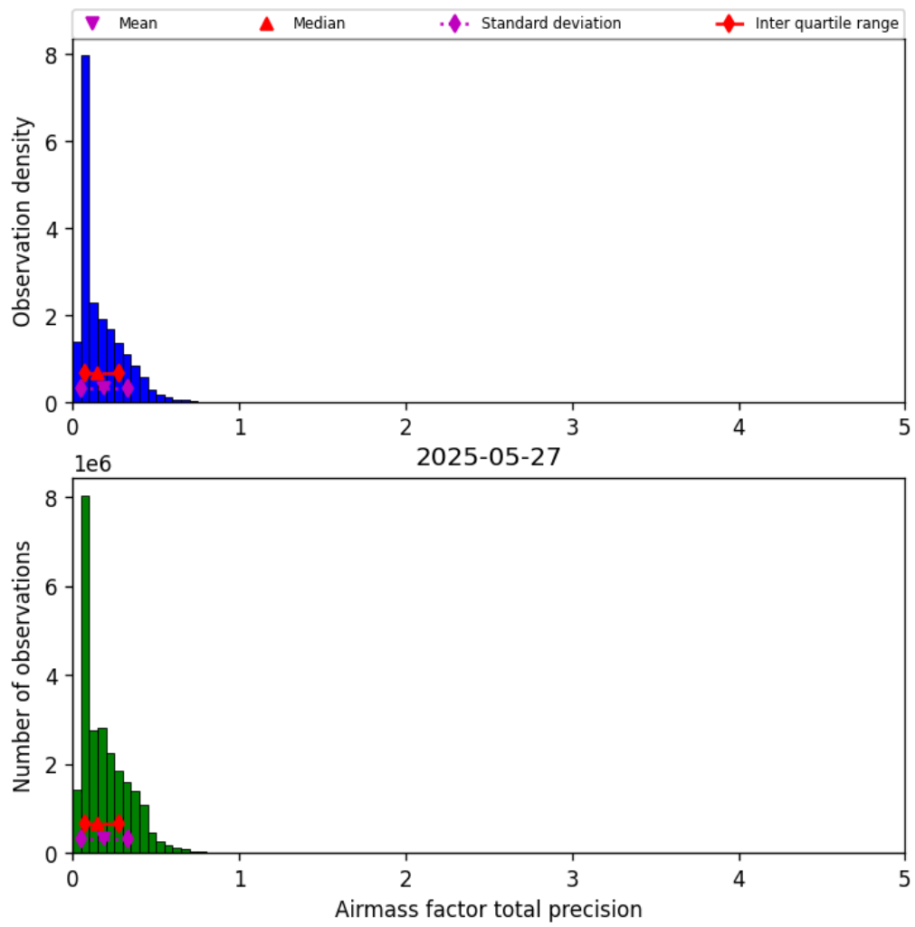
Figure 41: Histogram of “Airmass factor total precision” for 2025-05-26 to 2025-05-28
