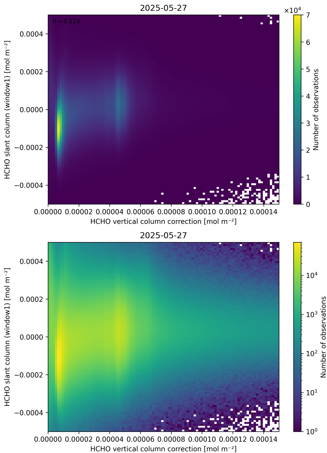
Figure 118: Scatter density plot of “HCHO vertical column correction” against “HCHO slant column (window1)” for 2025-05-26 to 2025-05-28.
