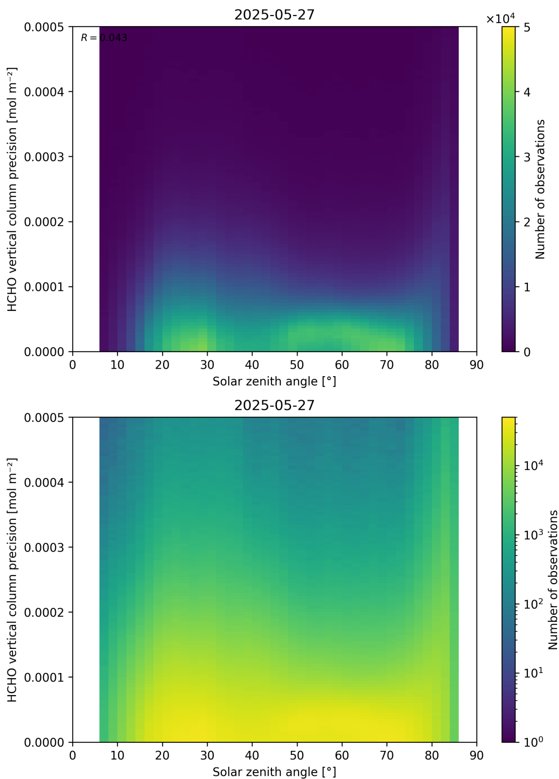
Figure 179: Scatter density plot of “Solar zenith angle” against “HCHO vertical column precision” for 2025-05-26 to 2025-05-28.
