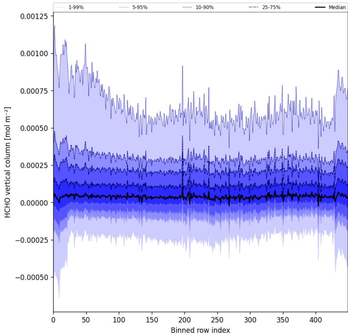
Figure 49: Along track statistics of “HCHO vertical column” for 2025-05-26 to 2025-05-28
