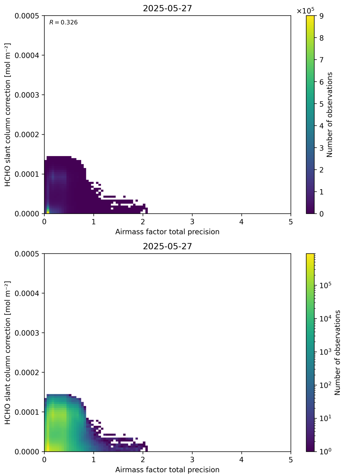
Figure 110: Scatter density plot of “Airmass factor total precision” against “HCHO slant column correction” for 2025-05-26 to 2025-05-28.
