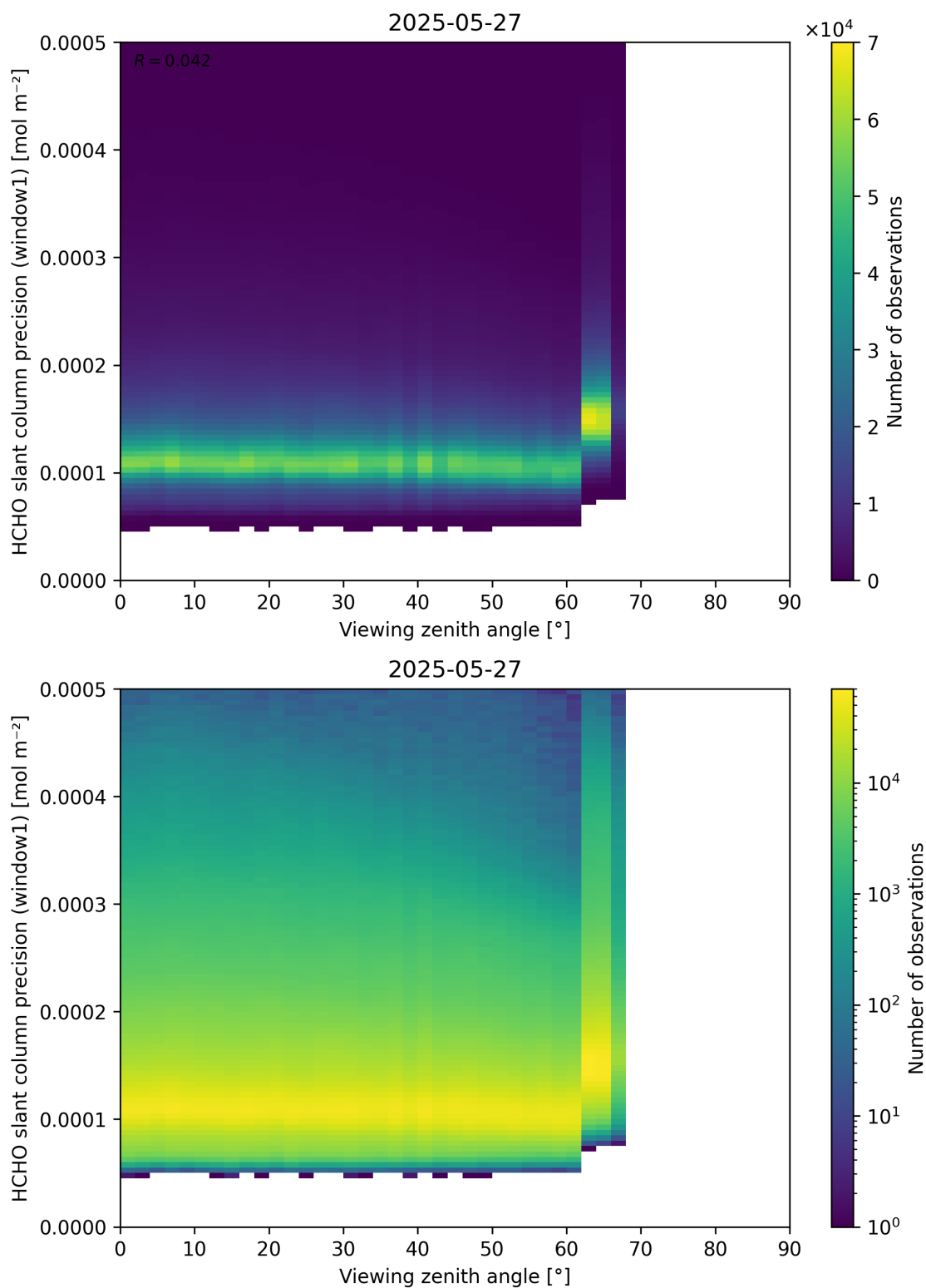
Figure 189: Scatter density plot of “Viewing zenith angle” against “HCHO slant column precision (window1)” for 2025-05-26 to 2025-05-28.
