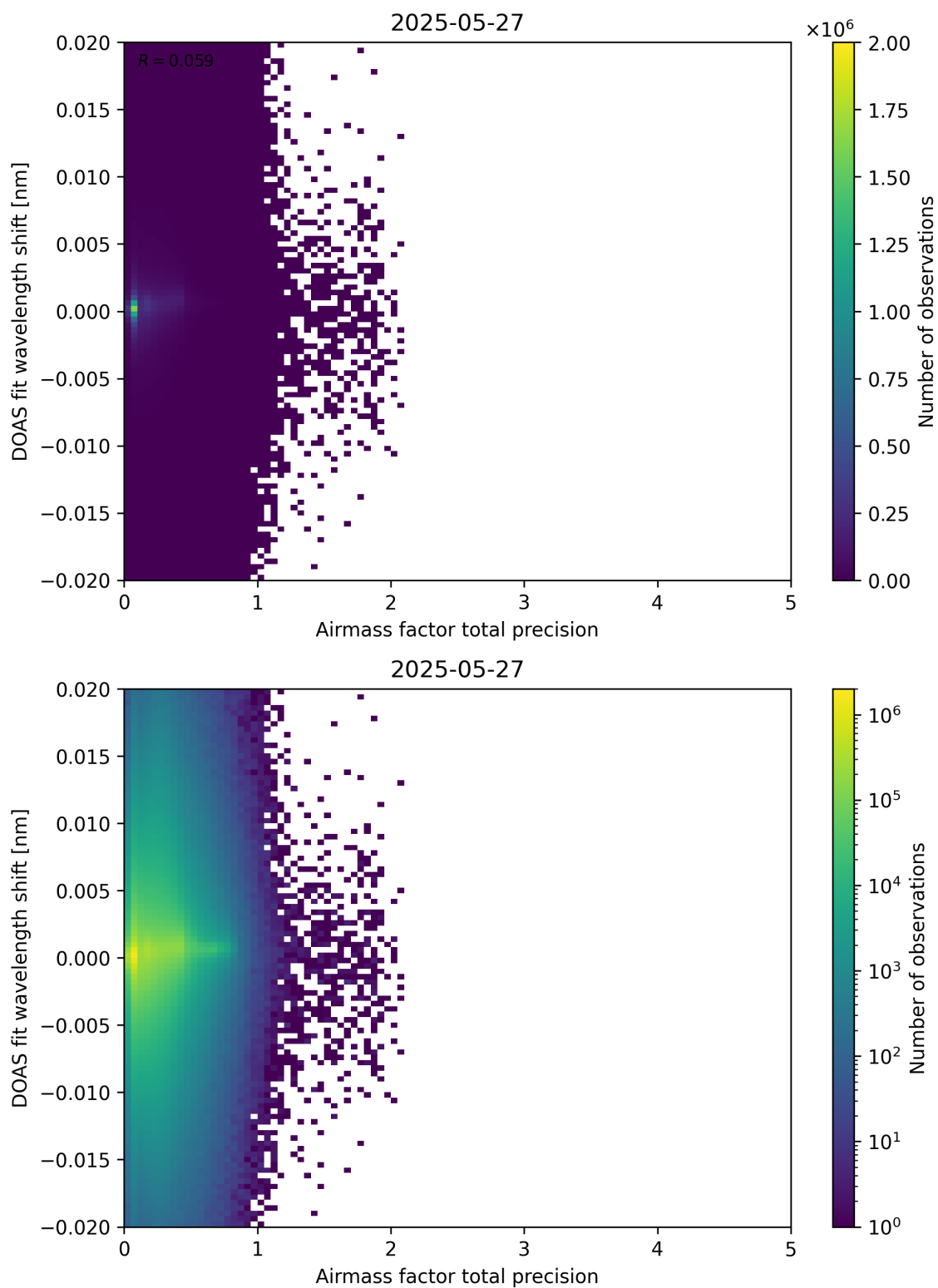
Figure 106: Scatter density plot of “Airmass factor total precision” against “DOAS fit wavelength shift” for 2025-05-26 to 2025-05-28.
