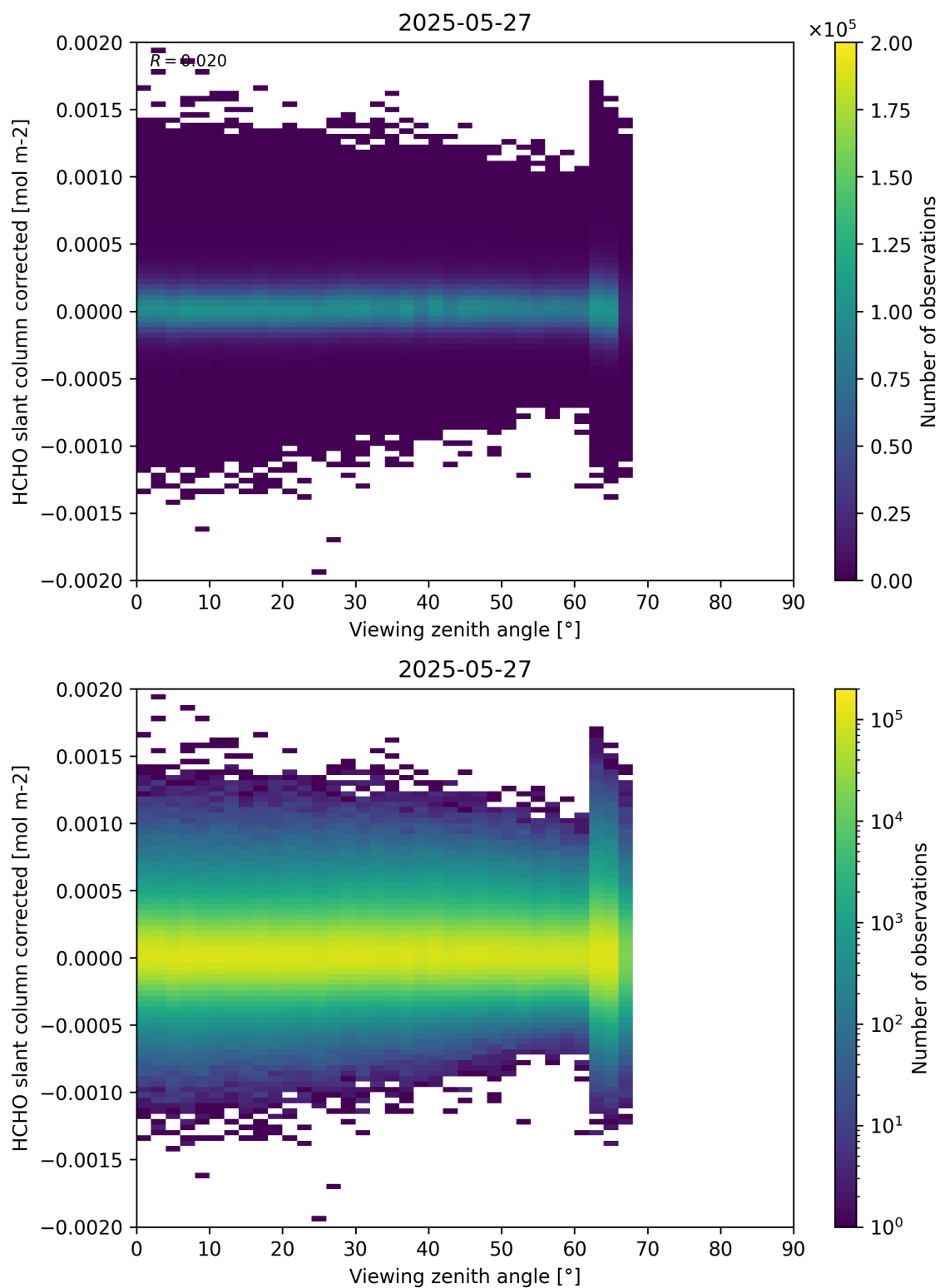
Figure 186: Scatter density plot of “Viewing zenith angle” against “HCHO slant column corrected” for 2025-05-26 to 2025-05-28.
