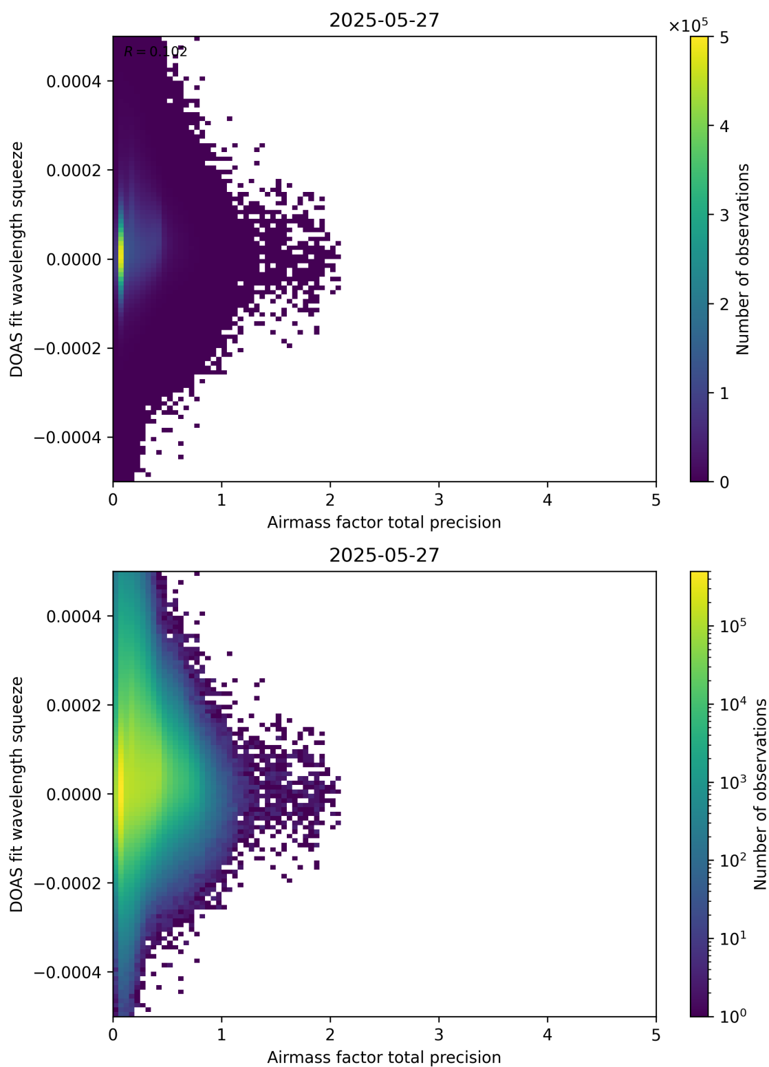
Figure 107: Scatter density plot of “Airmass factor total precision” against “DOAS fit wavelength squeeze” for 2025-05-26 to 2025-05-28.
