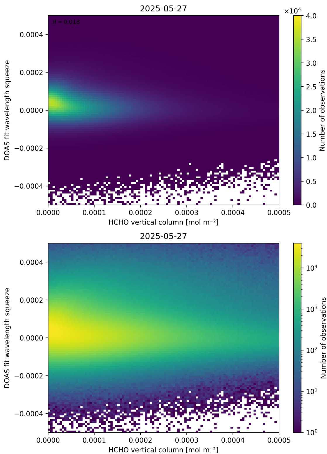
Figure 125: Scatter density plot of “HCHO vertical column” against “DOAS fit wavelength squeeze” for 2025-05-26 to 2025-05-28.
