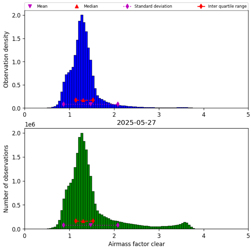
Figure 42: Histogram of “Airmass factor clear” for 2025-05-26 to 2025-05-28
