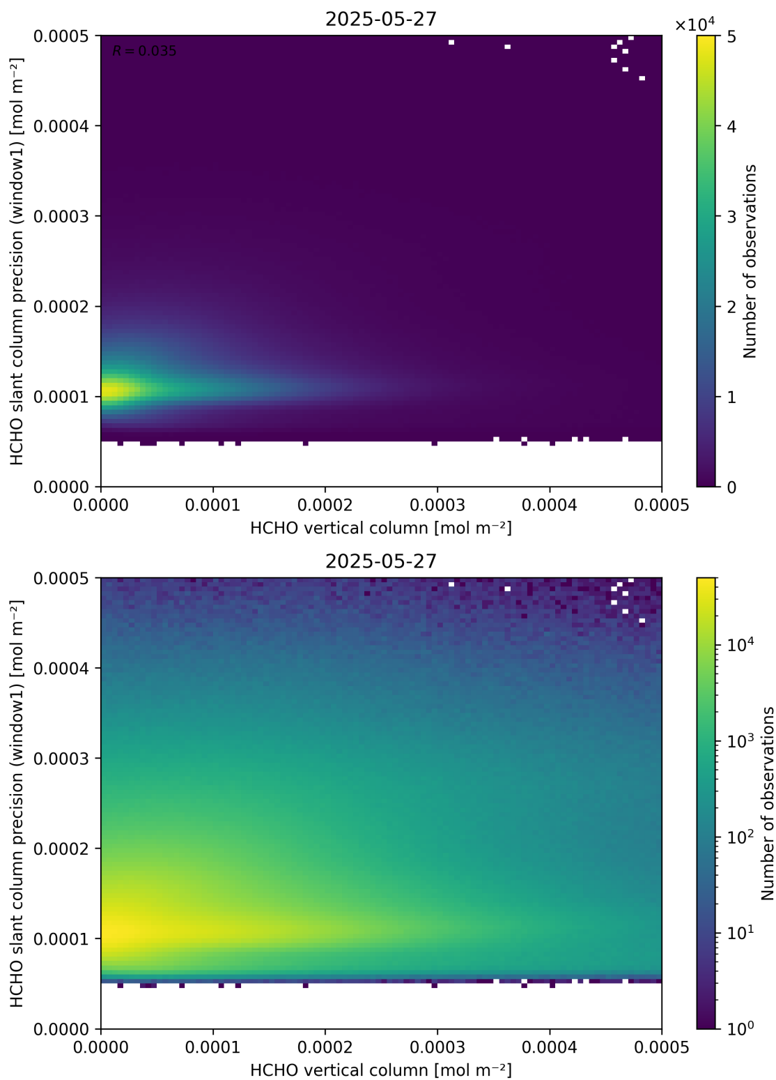
Figure 130: Scatter density plot of “HCHO vertical column” against “HCHO slant column precision (window1)” for 2025-05-26 to 2025-05-28.
