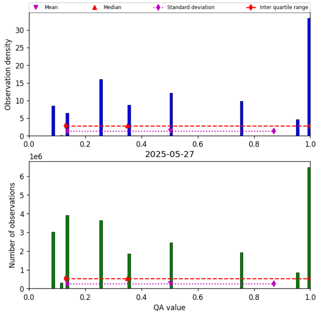
Figure 34: Histogram of “QA value” for 2025-05-26 to 2025-05-28
