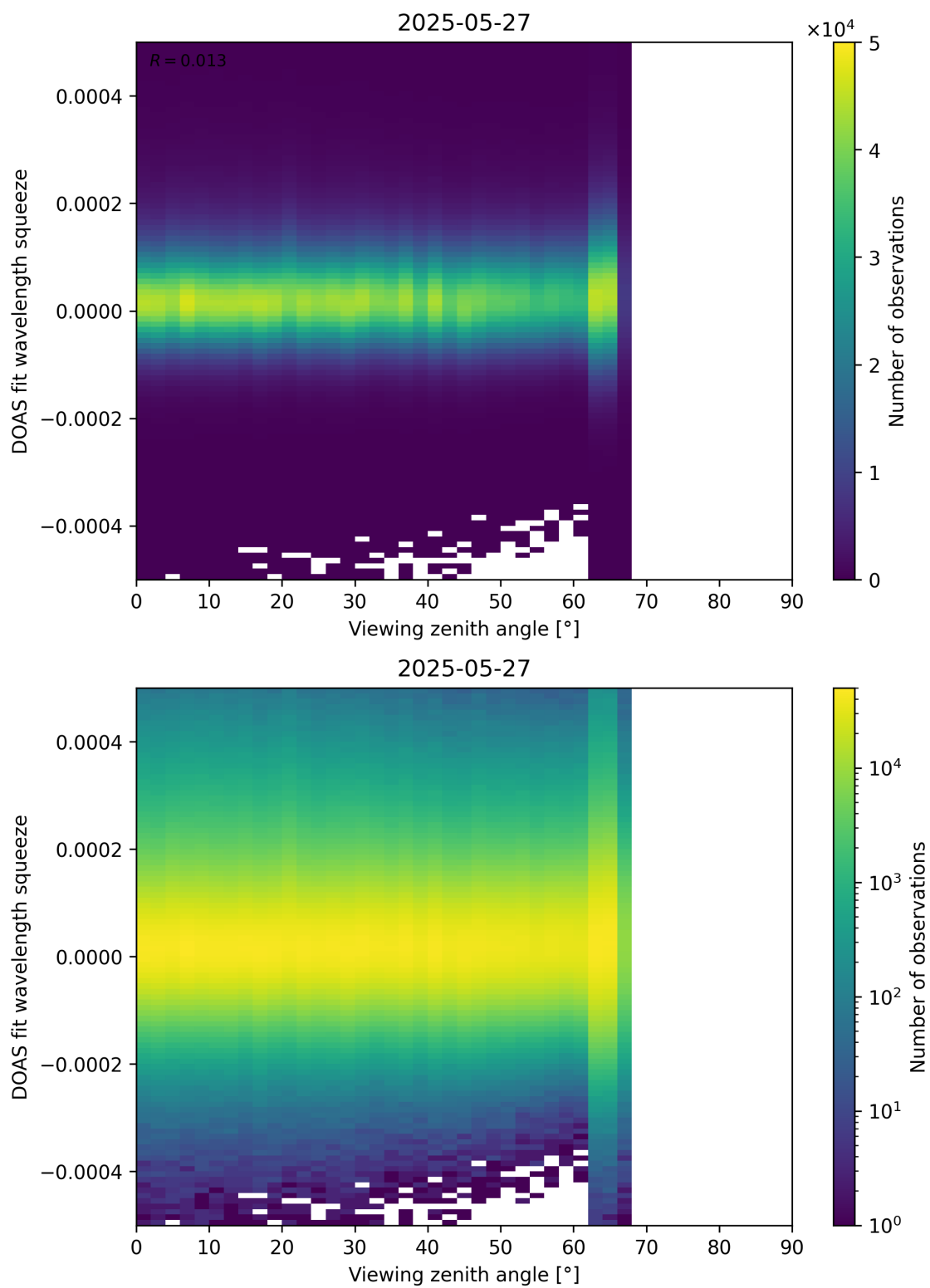
Figure 184: Scatter density plot of “Viewing zenith angle” against “DOAS fit wavelength squeeze” for 2025-05-26 to 2025-05-28.
