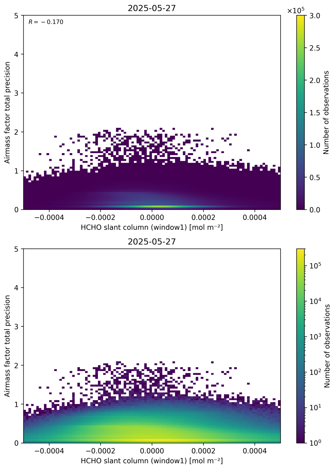
Figure 86: Scatter density plot of “HCHO slant column (window1)” against “Airmass factor total precision” for 2025-05-26 to 2025-05-28.
