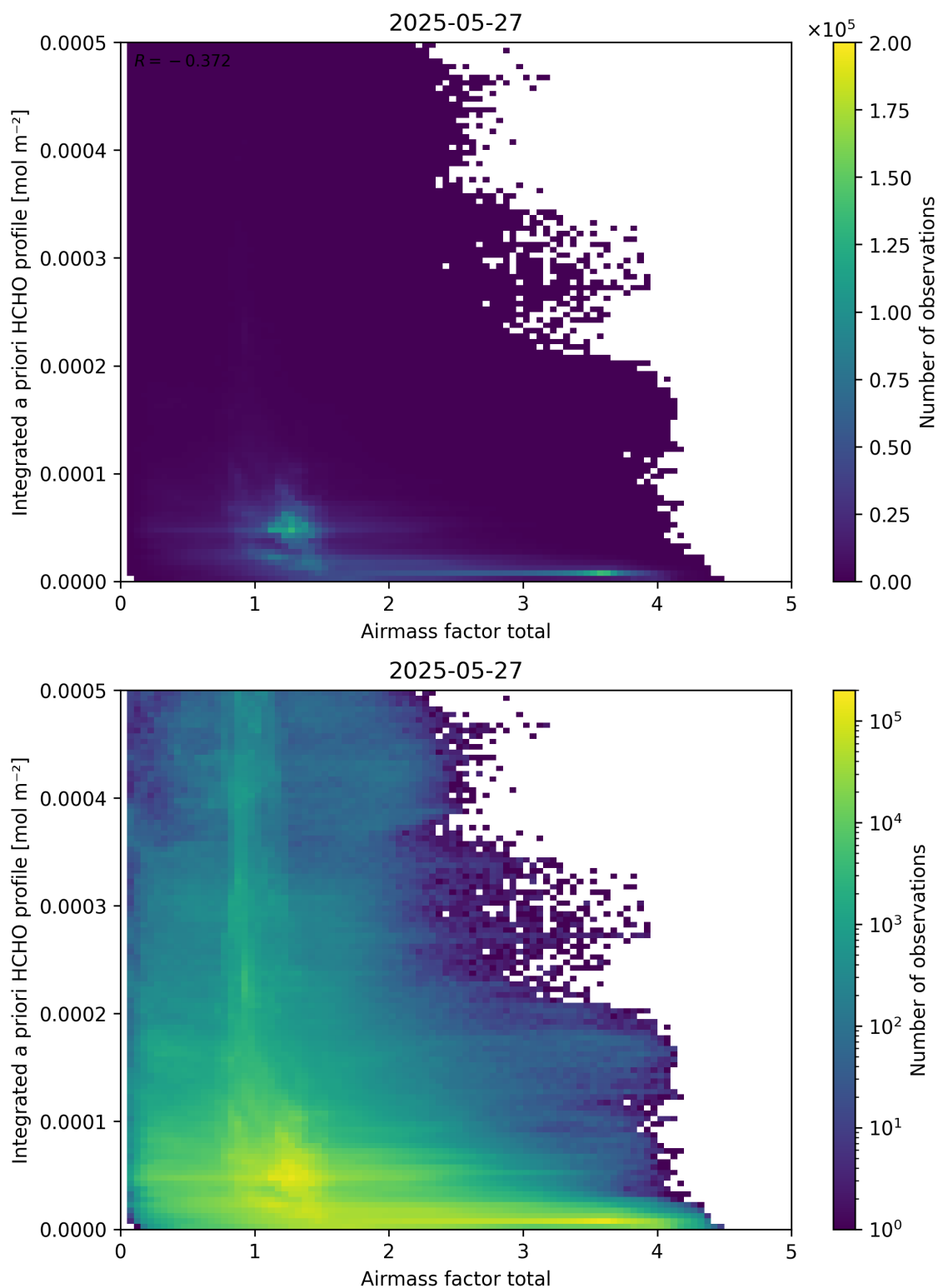
Figure 104: Scatter density plot of “Airmass factor total” against “Integrated a priori HCHO profile” for 2025-05-26 to 2025-05-28.
