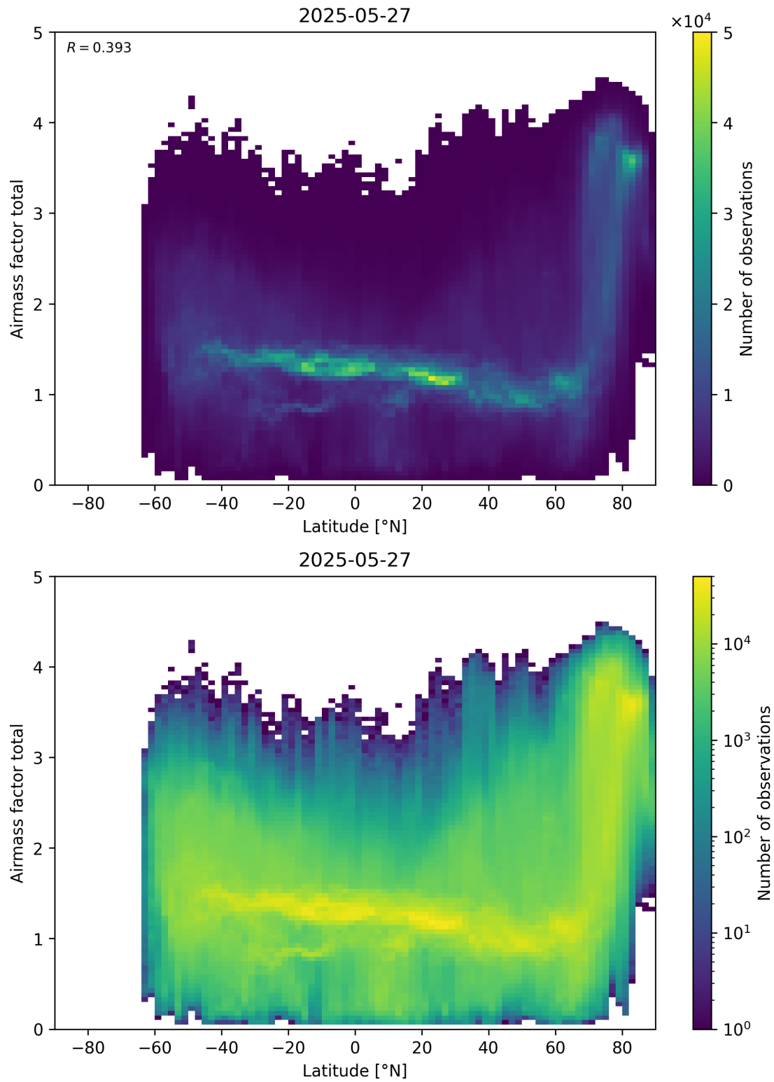
Figure 161: Scatter density plot of “Latitude” against “Airmass factor total” for 2025-05-26 to 2025-05-28.
