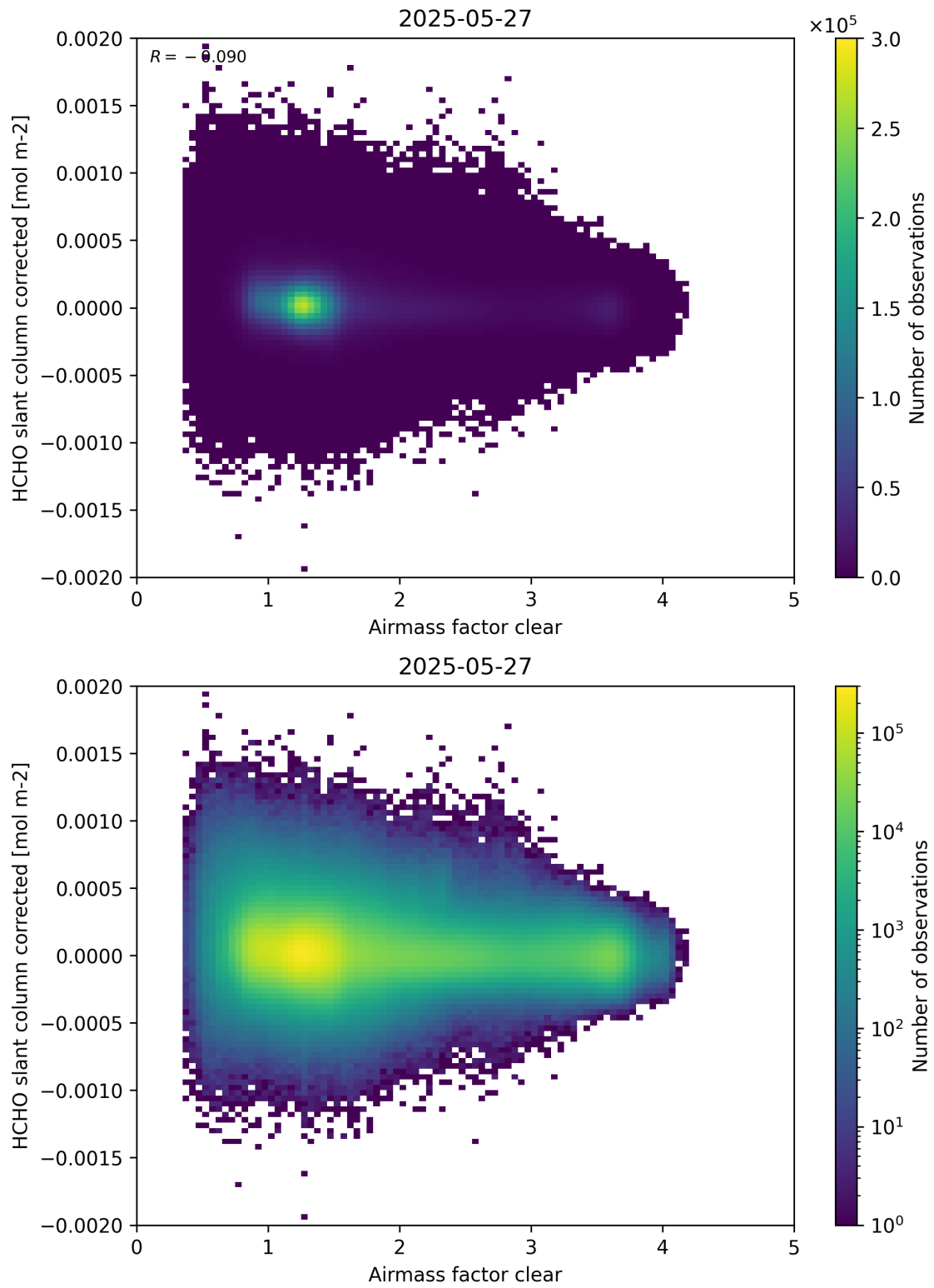
Figure 74: Scatter density plot of “Airmass factor clear” against “HCHO slant column corrected” for 2025-05-26 to 2025-05-28.
