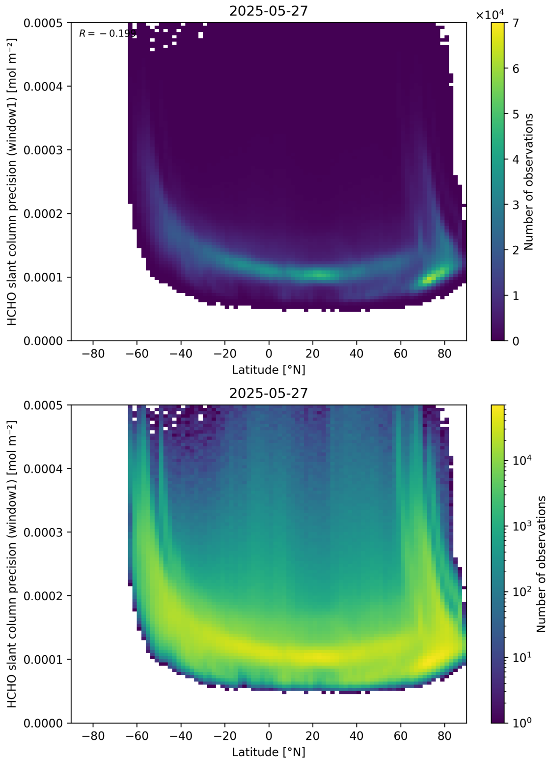
Figure 160: Scatter density plot of “Latitude” against “HCHO slant column precision (window1)” for 2025-05-26 to 2025-05-28.
