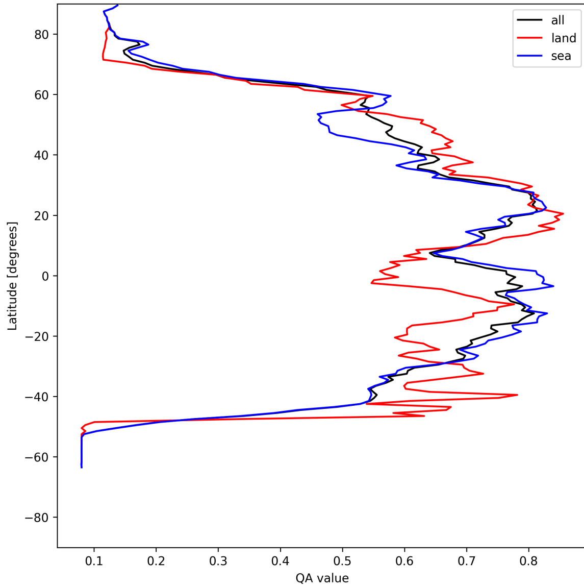
Figure 20: Zonal average of “QA value” for 2025-05-26 to 2025-05-28.
