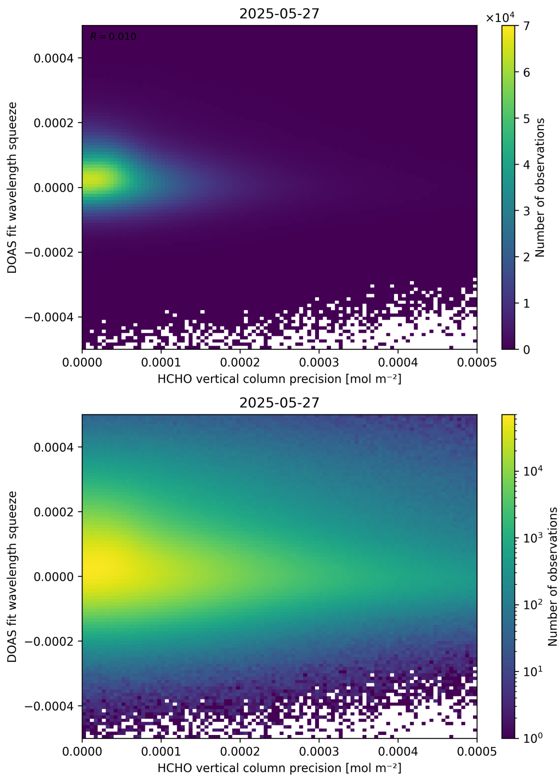
Figure 138: Scatter density plot of “HCHO vertical column precision” against “DOAS fit wavelength squeeze” for 2025-05-26 to 2025-05-28.
