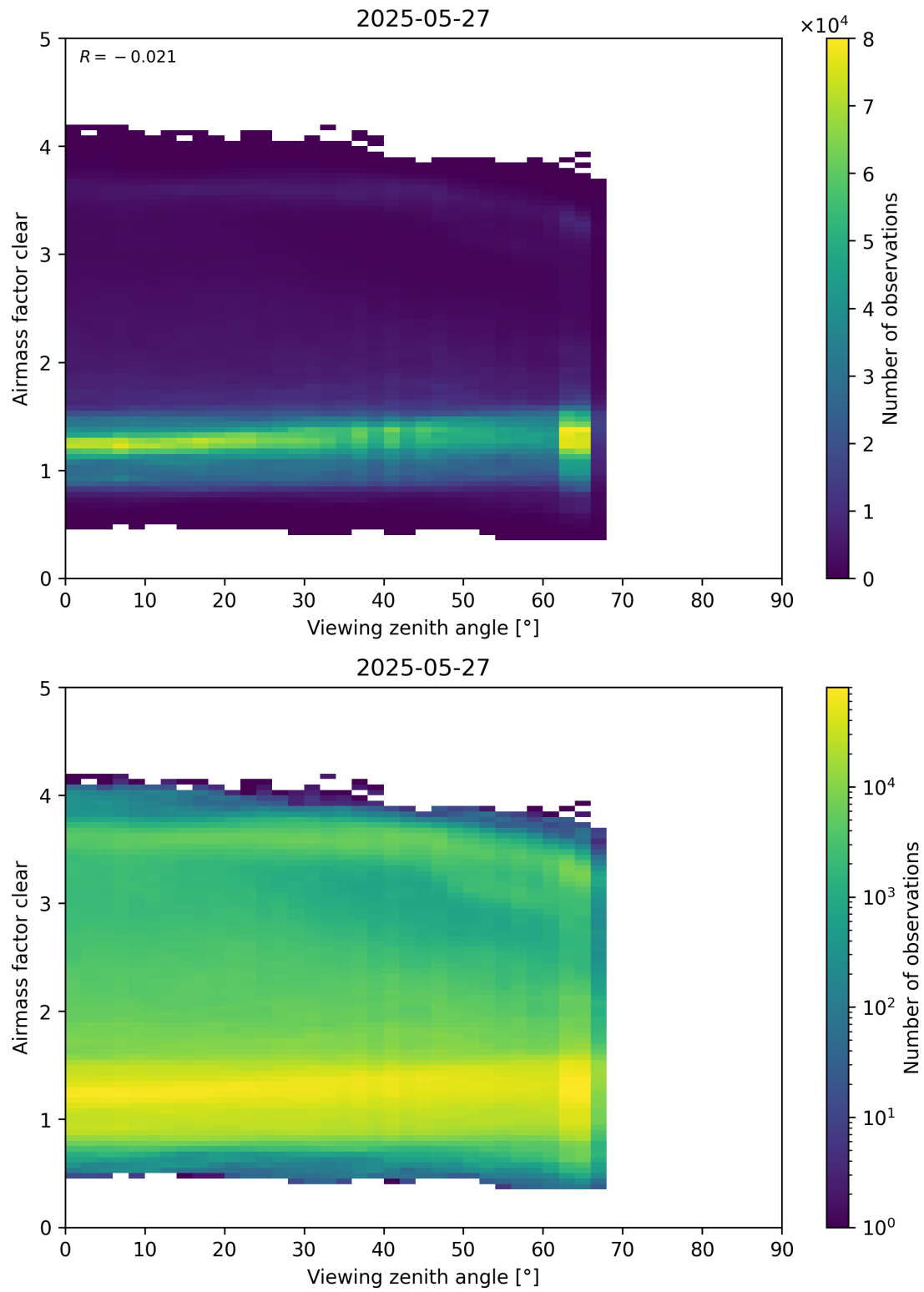
Figure 185: Scatter density plot of “Viewing zenith angle” against “Airmass factor clear” for 2025-05-26 to 2025-05-28.
