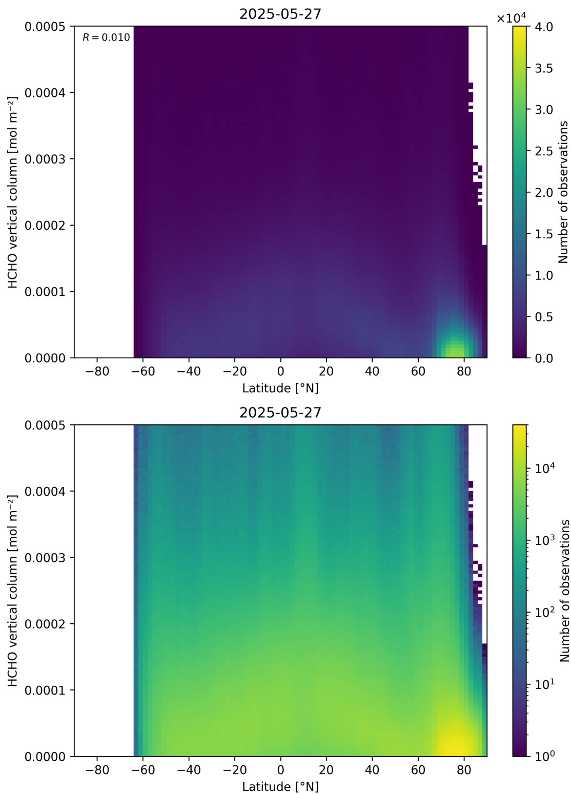
Figure 163: Scatter density plot of “Latitude” against “HCHO vertical column” for 2025-05-26 to 2025-05-28.
