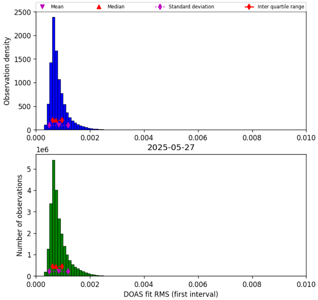
Figure 46: Histogram of “DOAS fit RMS (first interval)” for 2025-05-26 to 2025-05-28
