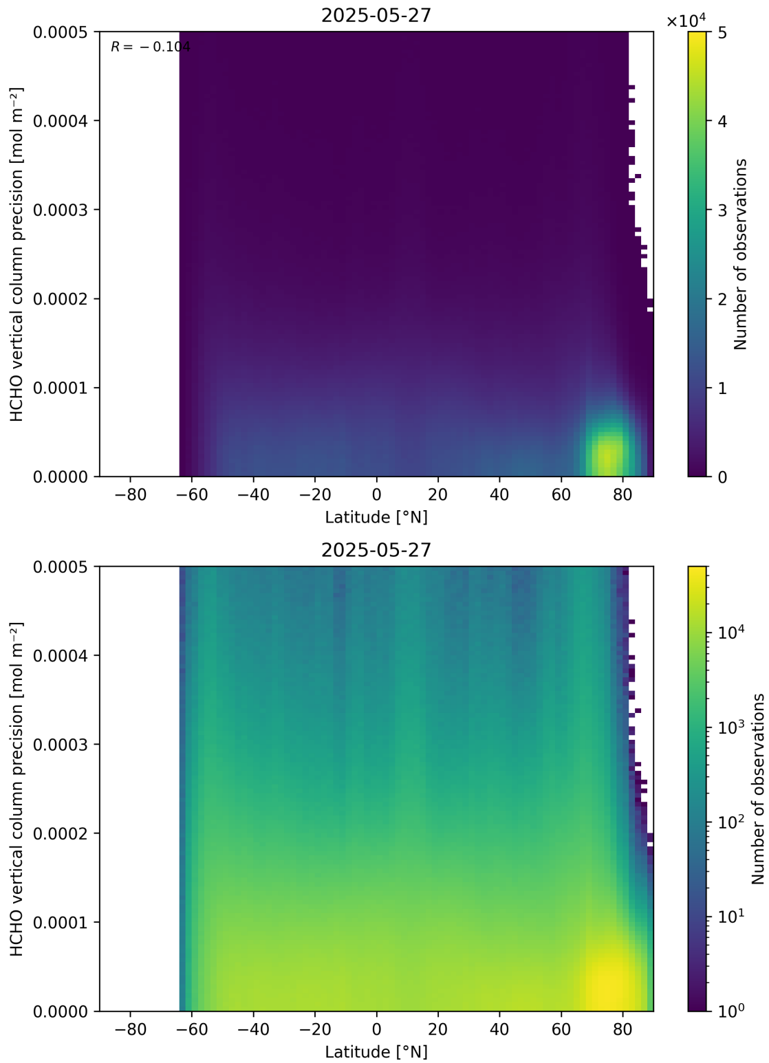
Figure 165: Scatter density plot of “Latitude” against “HCHO vertical column precision” for 2025-05-26 to 2025-05-28.
