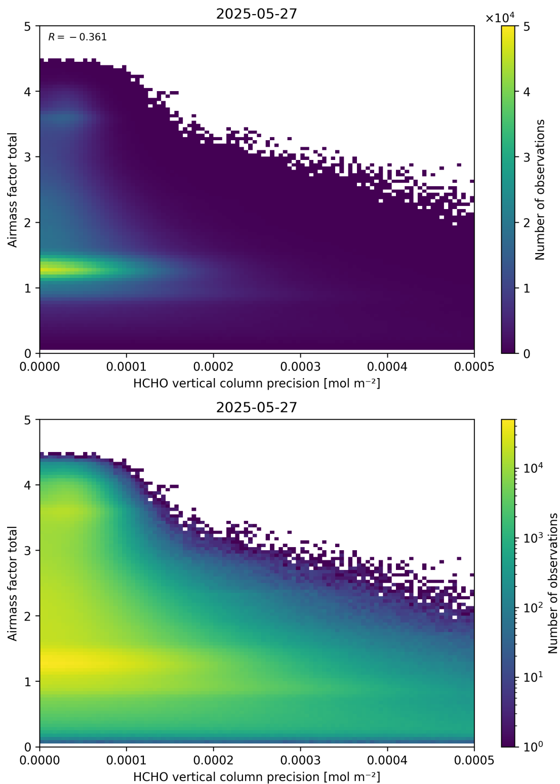
Figure 144: Scatter density plot of “HCHO vertical column precision” against “Airmass factor total” for 2025-05-26 to 2025-05-28.
