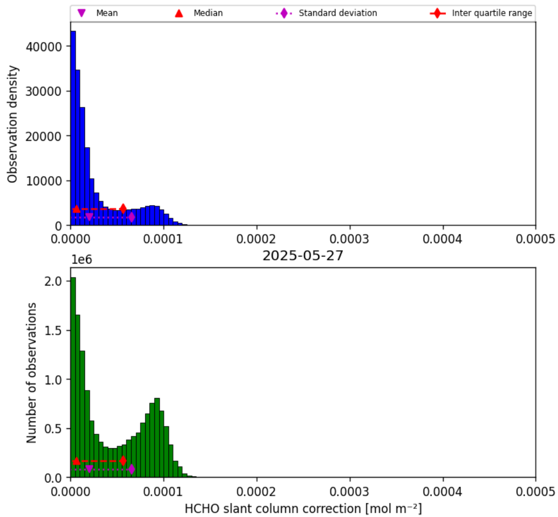
Figure 47: Histogram of “HCHO slant column correction” for 2025-05-26 to 2025-05-28
