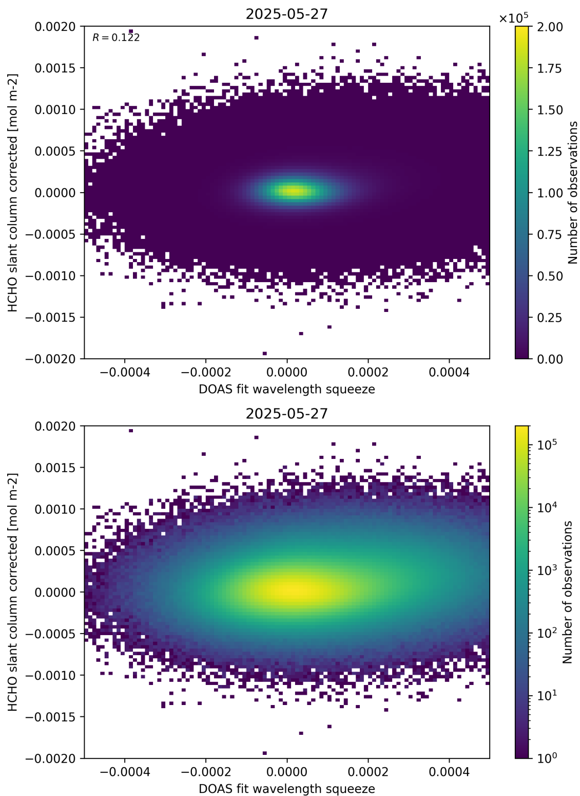
Figure 69: Scatter density plot of “DOAS fit wavelength squeeze” against “HCHO slant column corrected” for 2025-05-26 to 2025-05-28.
