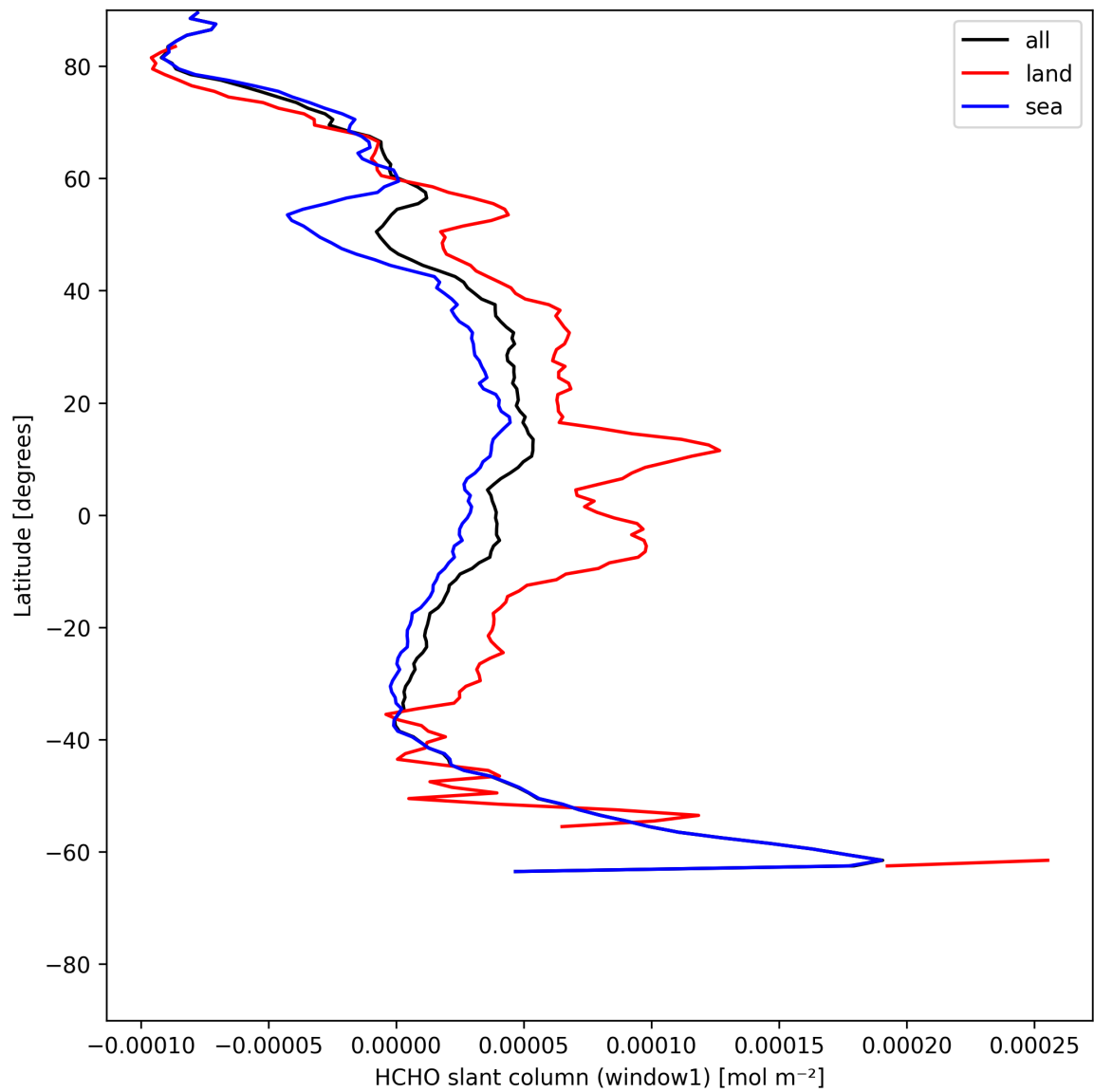
Figure 24: Zonal average of “HCHO slant column (window1)” for 2025-05-26 to 2025-05-28.
