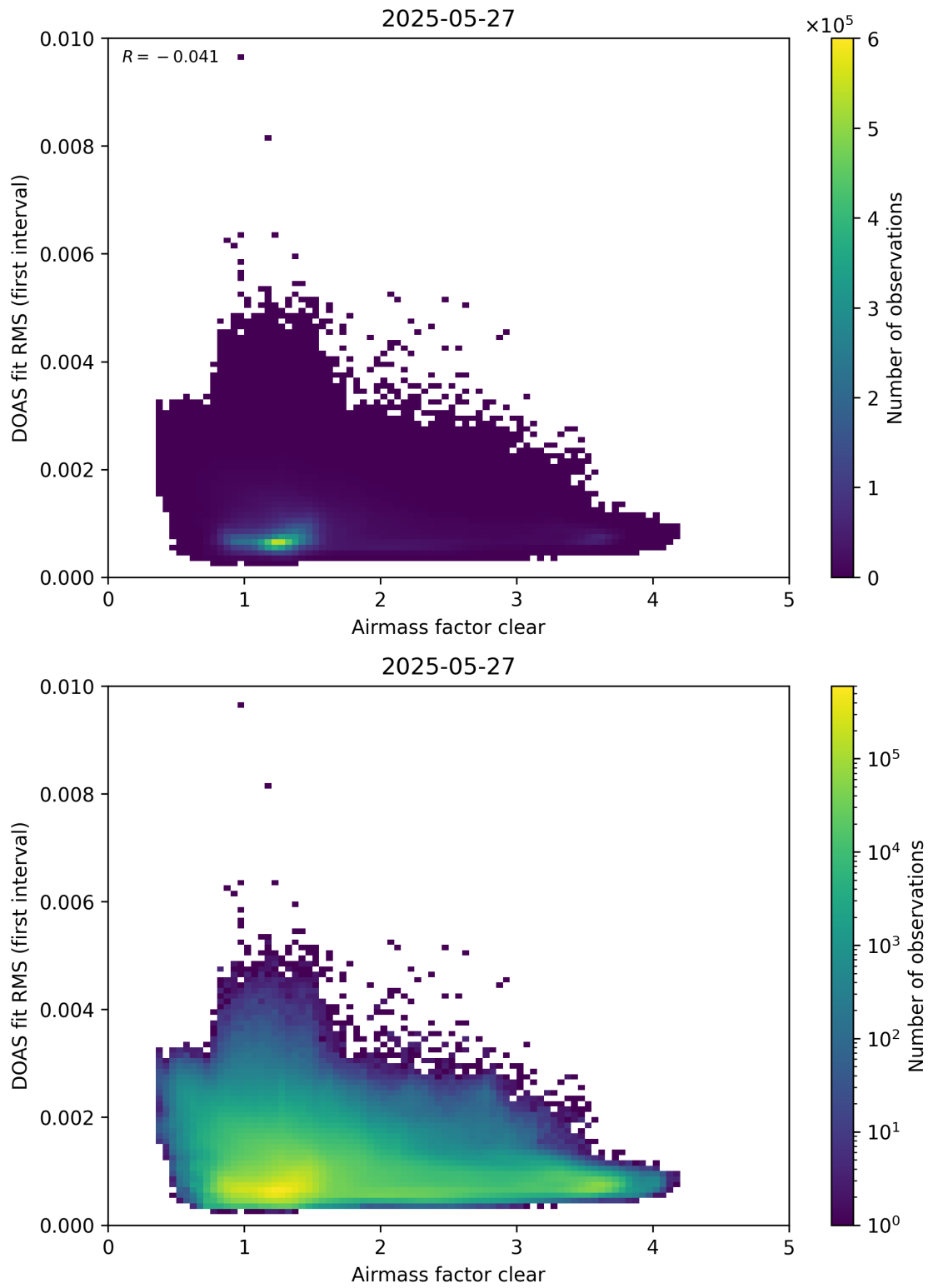
Figure 71: Scatter density plot of “Airmass factor clear” against “DOAS fit RMS (first interval)” for 2025-05-26 to 2025-05-28.
