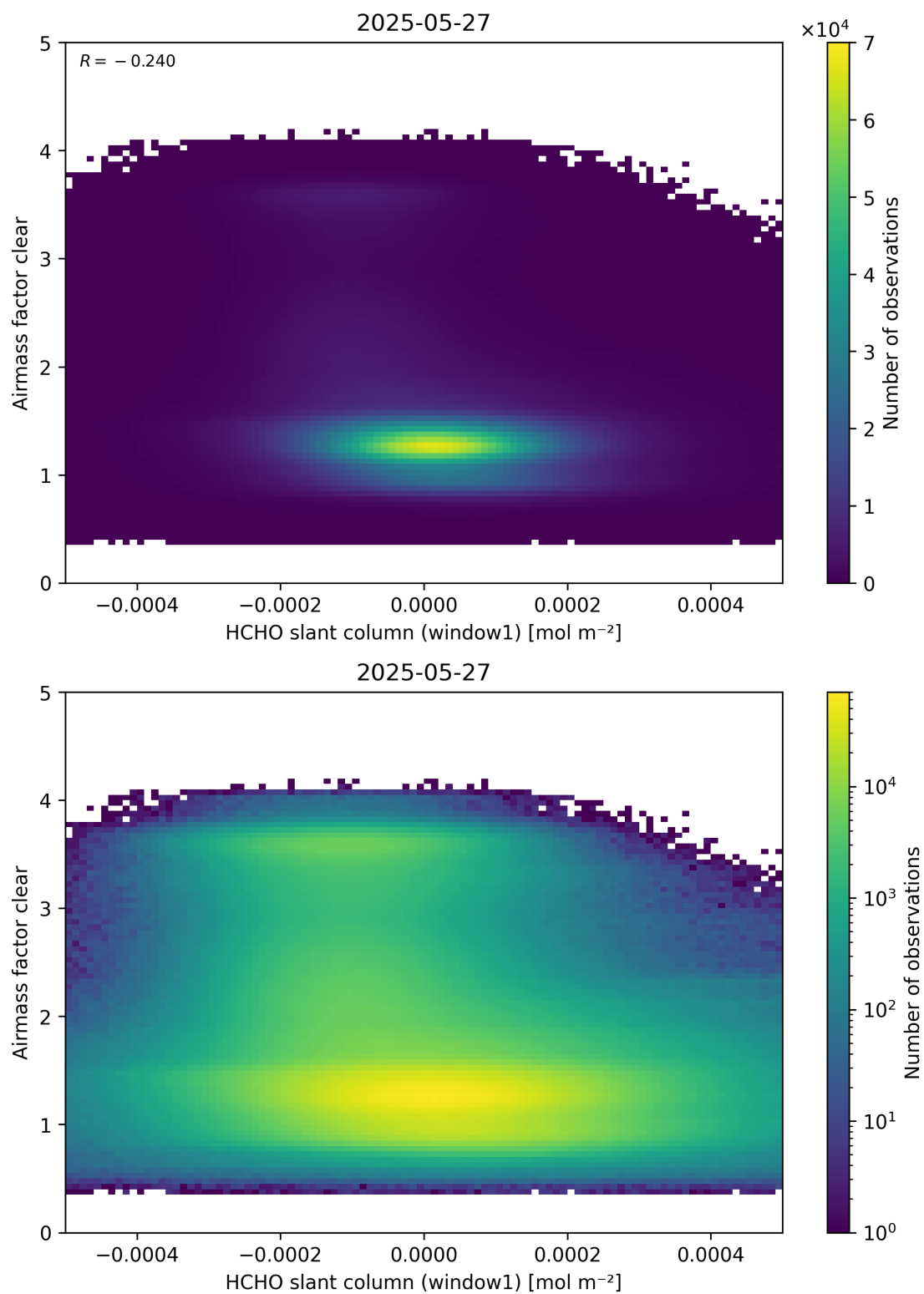
Figure 81: Scatter density plot of “HCHO slant column (window1)” against “Airmass factor clear” for 2025-05-26 to 2025-05-28.
