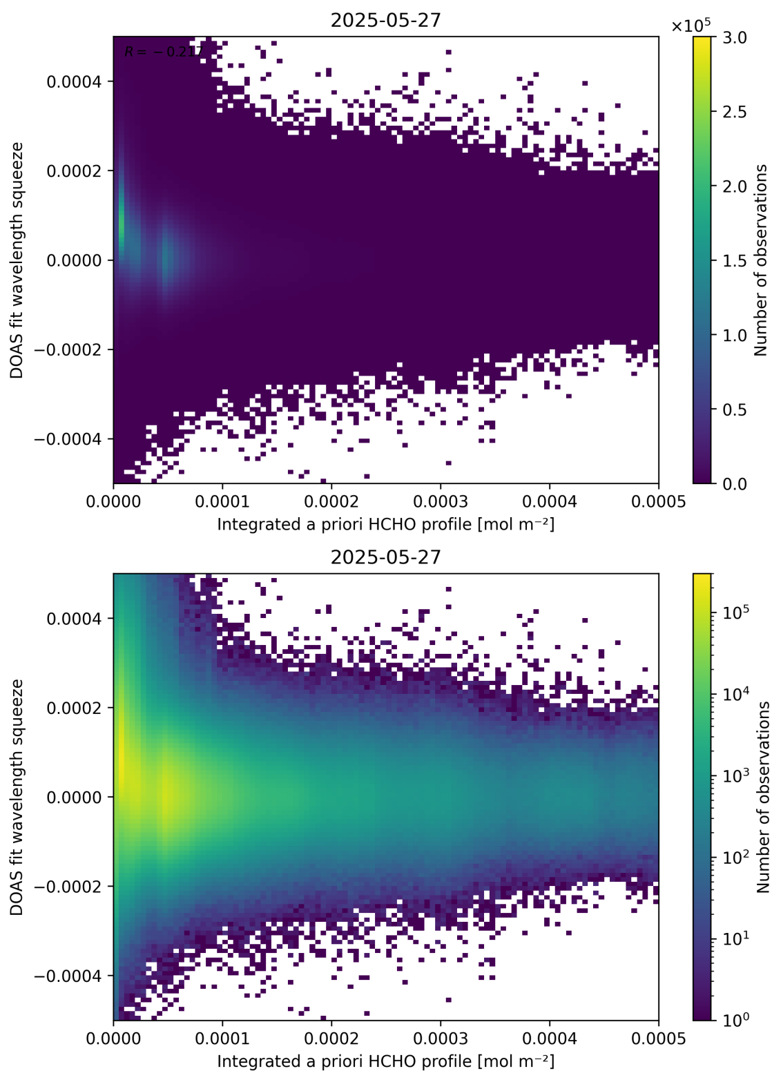
Figure 150: Scatter density plot of “Integrated a priori HCHO profile” against “DOAS fit wavelength squeeze” for 2025-05-26 to 2025-05-28.
