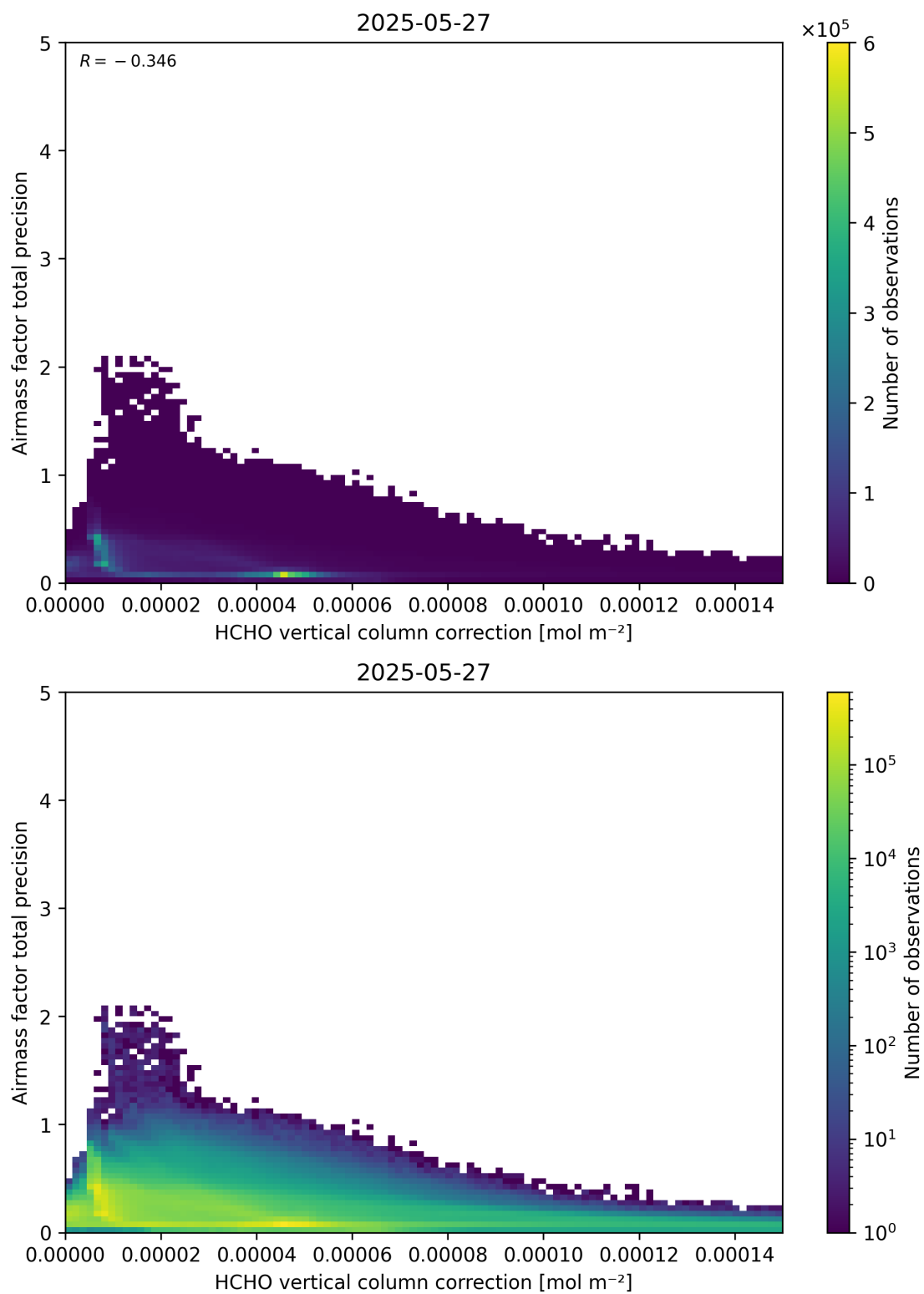
Figure 121: Scatter density plot of “HCHO vertical column correction” against “Airmass factor total precision” for 2025-05-26 to 2025-05-28.
