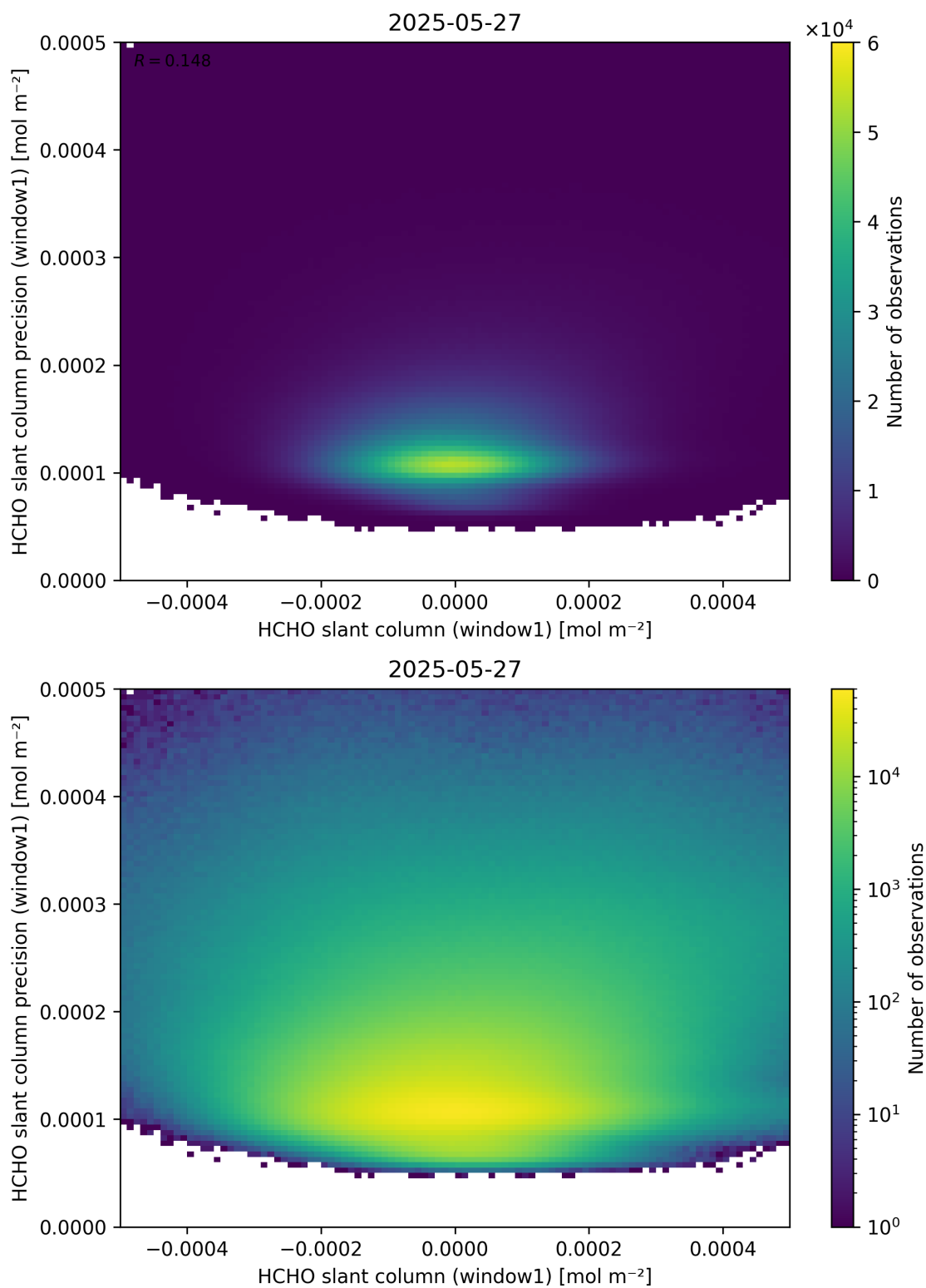
Figure 84: Scatter density plot of “HCHO slant column (window1)” against “HCHO slant column precision (window1)” for 2025-05-26 to 2025-05-28.
