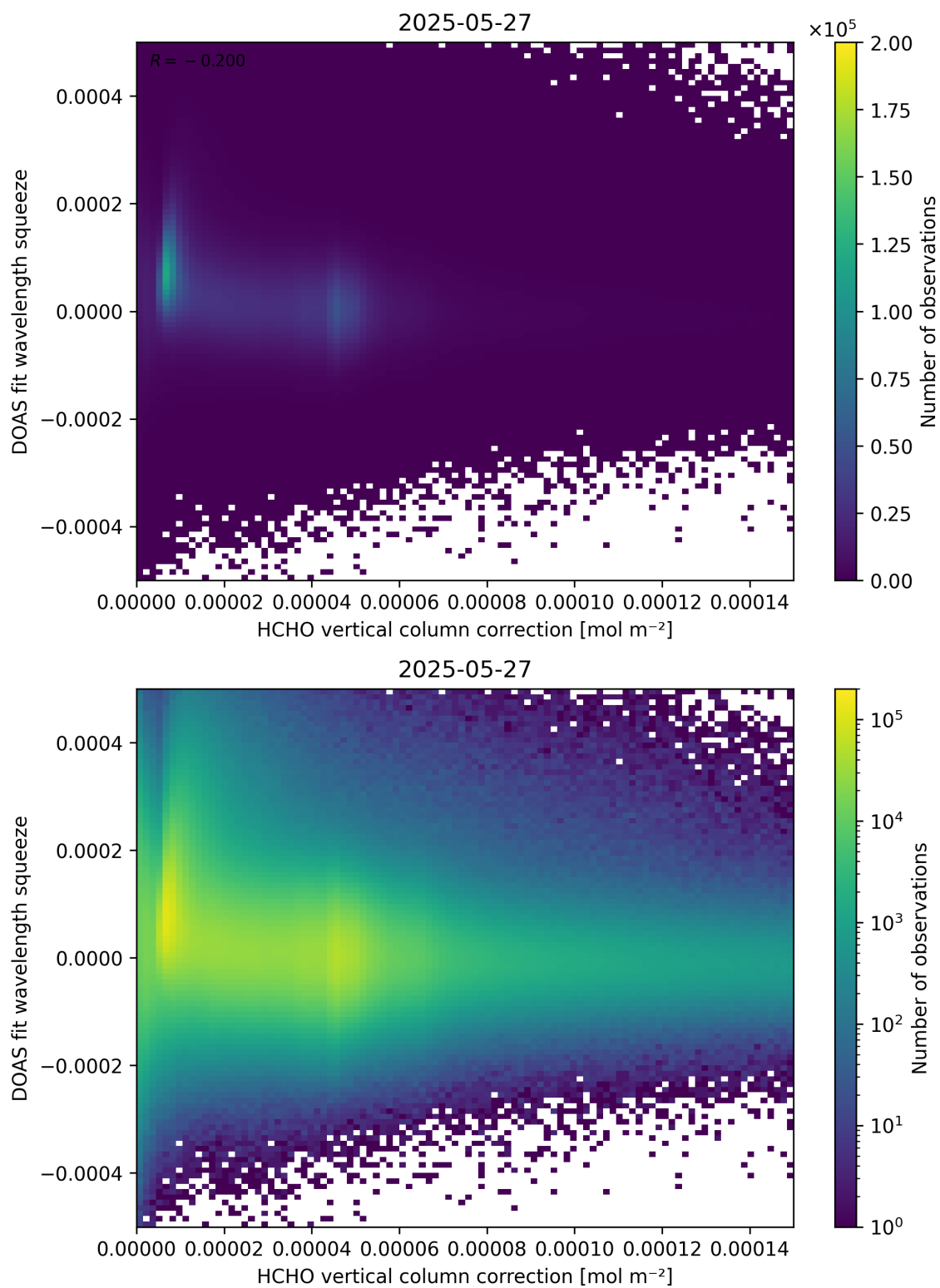
Figure 114: Scatter density plot of “HCHO vertical column correction” against “DOAS fit wavelength squeeze” for 2025-05-26 to 2025-05-28.
