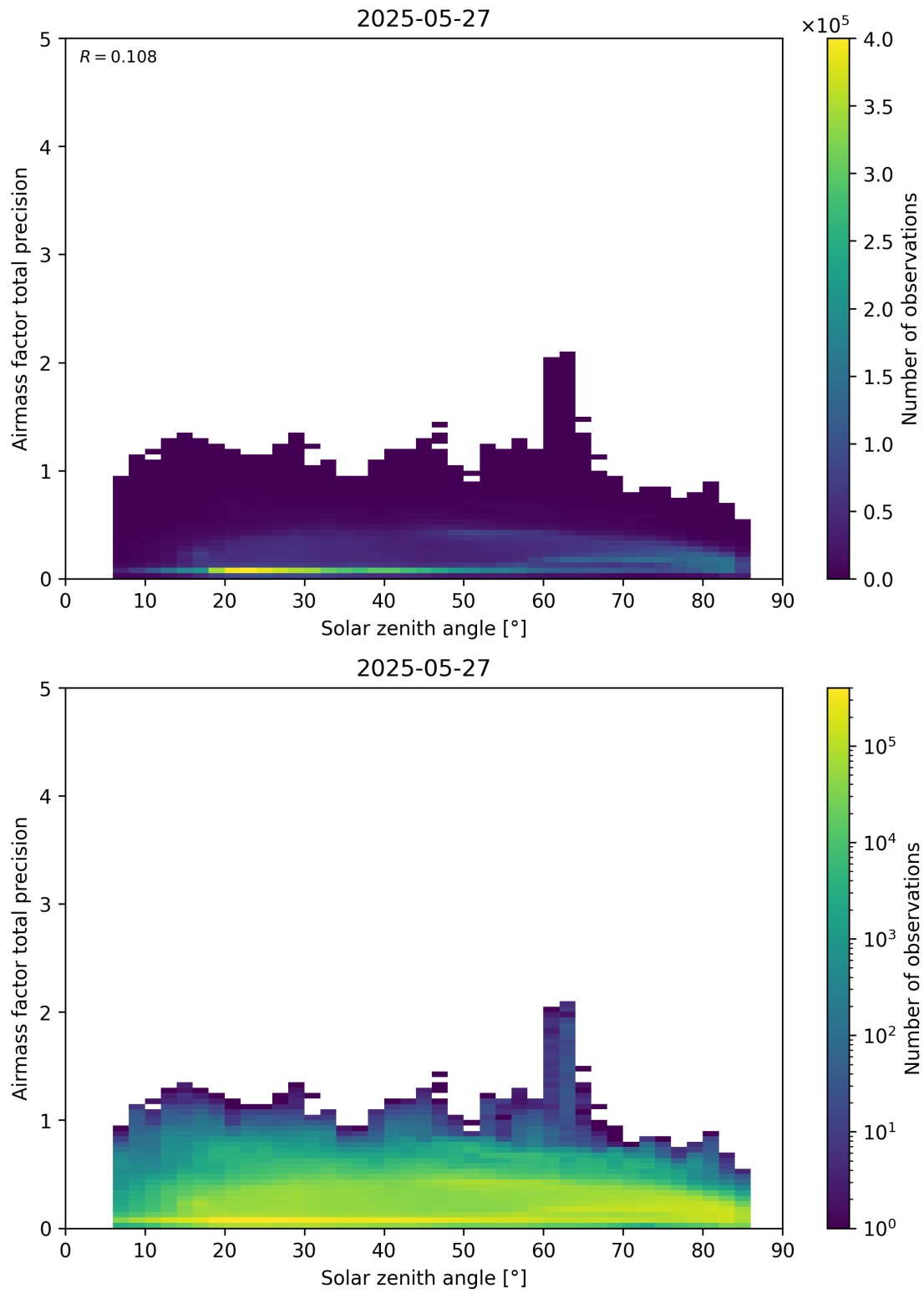
Figure 176: Scatter density plot of “Solar zenith angle” against “Airmass factor total precision” for 2025-05-26 to 2025-05-28.
