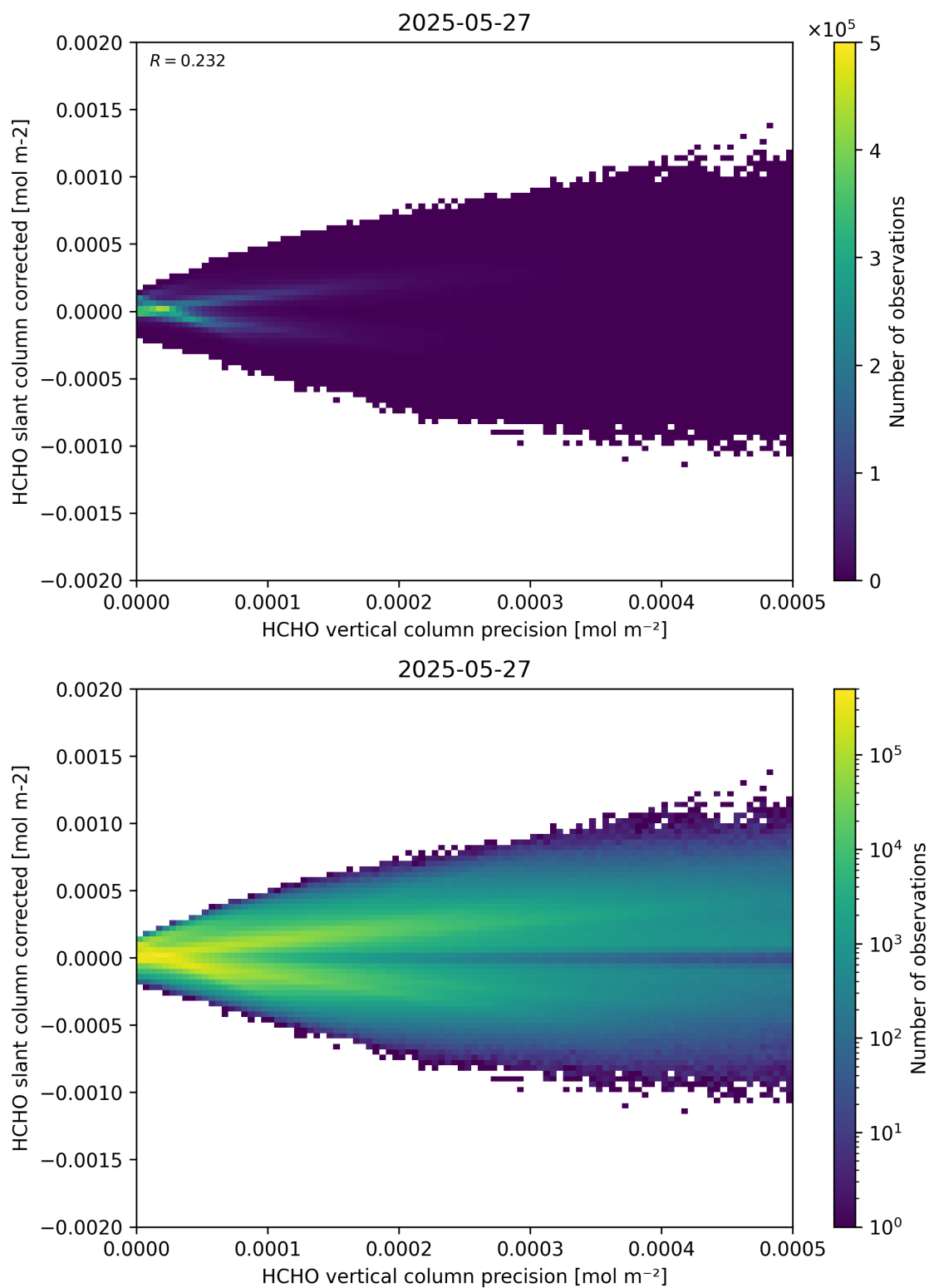
Figure 140: Scatter density plot of “HCHO vertical column precision” against “HCHO slant column corrected” for 2025-05-26 to 2025-05-28.
