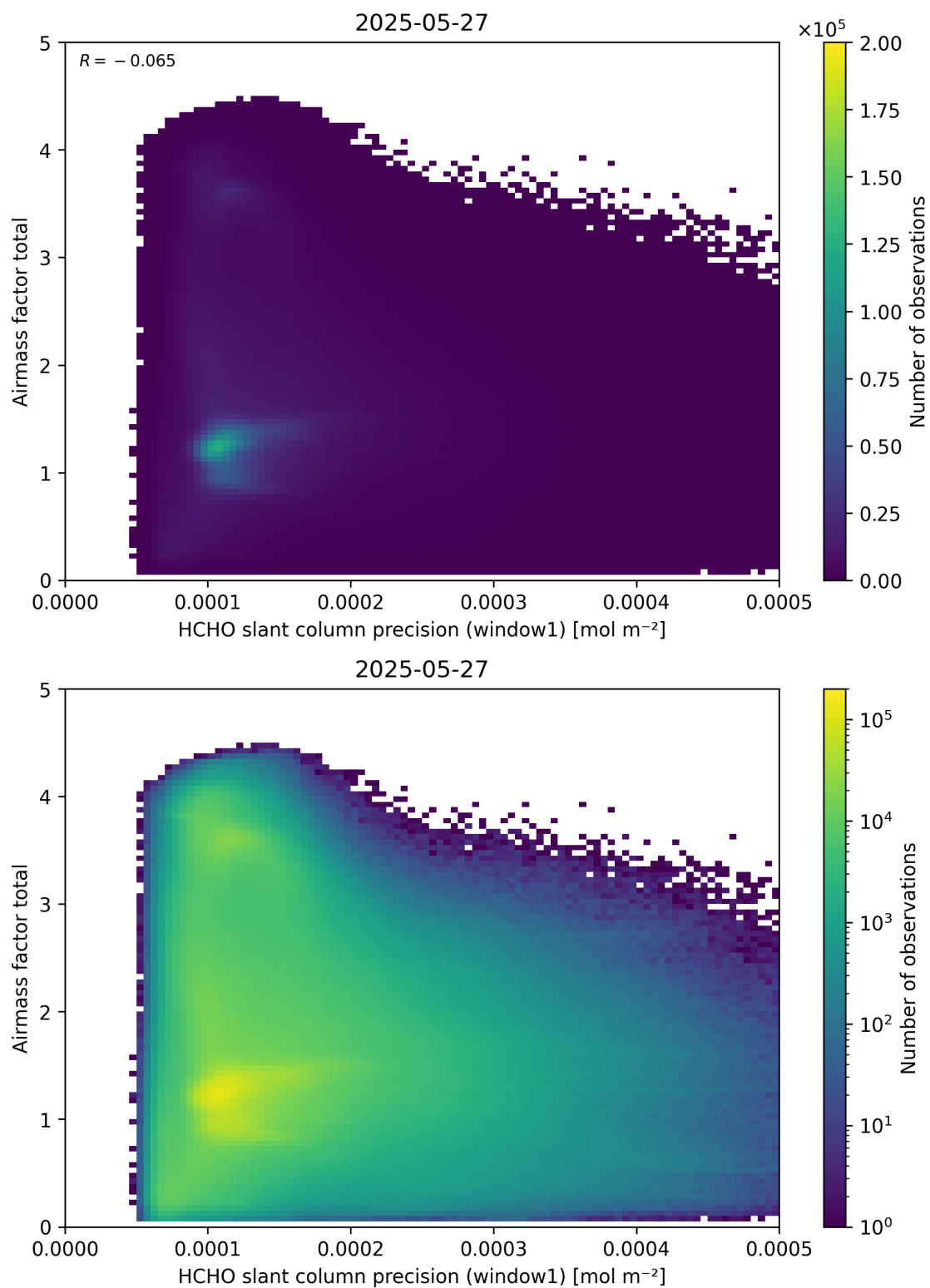
Figure 94: Scatter density plot of “HCHO slant column precision (window1)” against “Airmass factor total” for 2025-05-26 to 2025-05-28.
