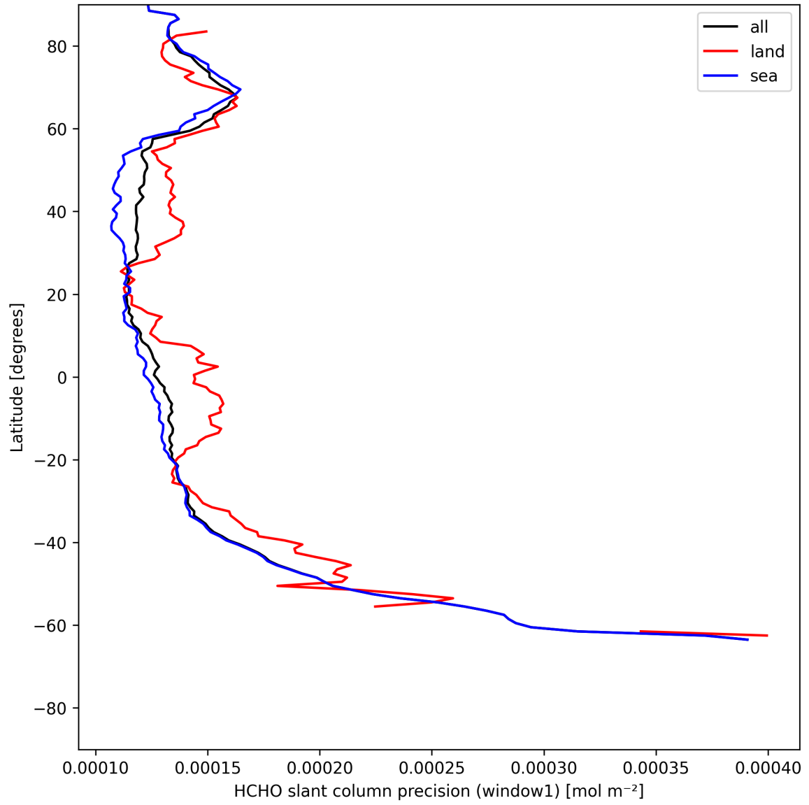
Figure 25: Zonal average of “HCHO slant column precision (window1)” for 2025-05-26 to 2025-05-28.
