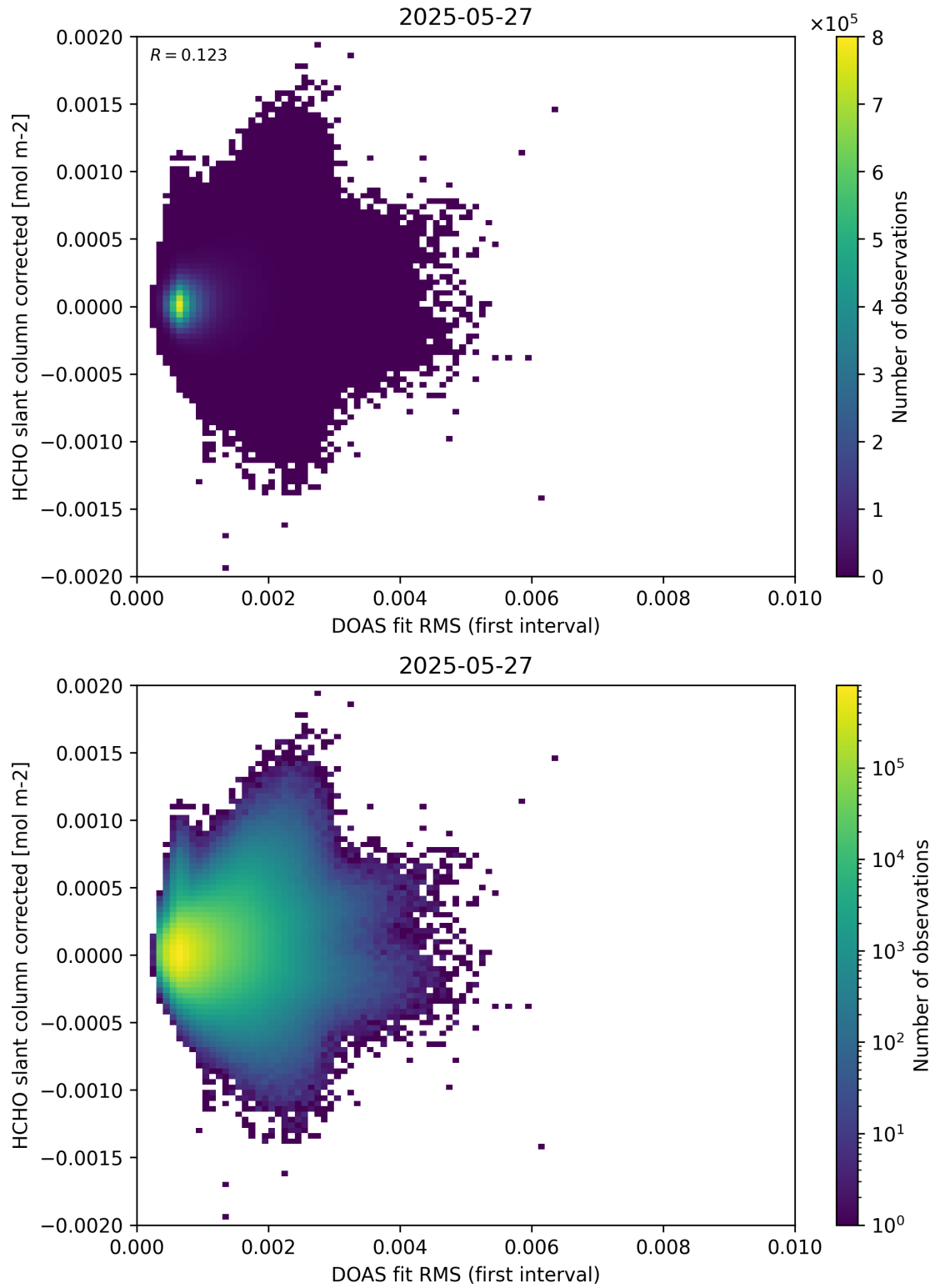
Figure 62: Scatter density plot of “DOAS fit RMS (first interval)” against “HCHO slant column corrected” for 2025-05-26 to 2025-05-28.
