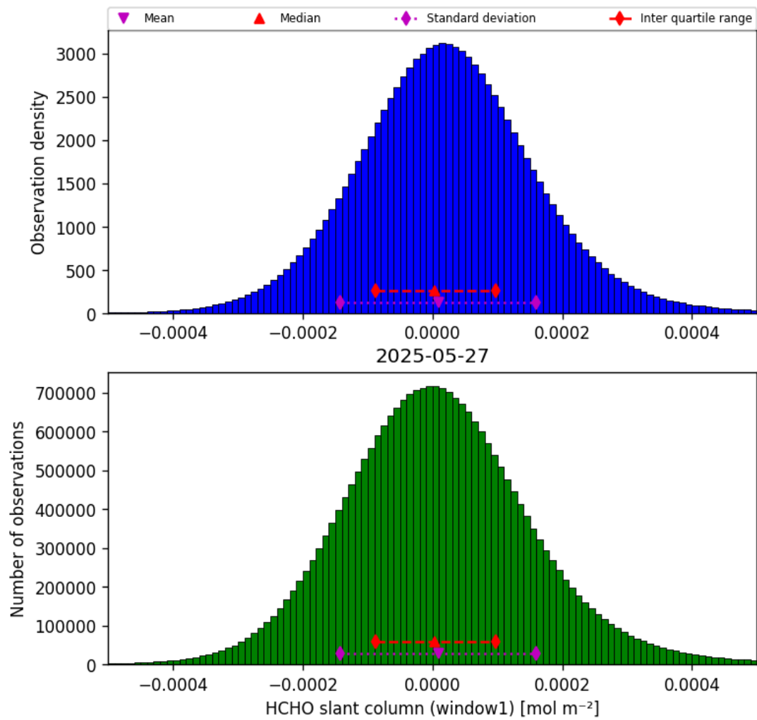
Figure 38: Histogram of “HCHO slant column (window1)” for 2025-05-26 to 2025-05-28
