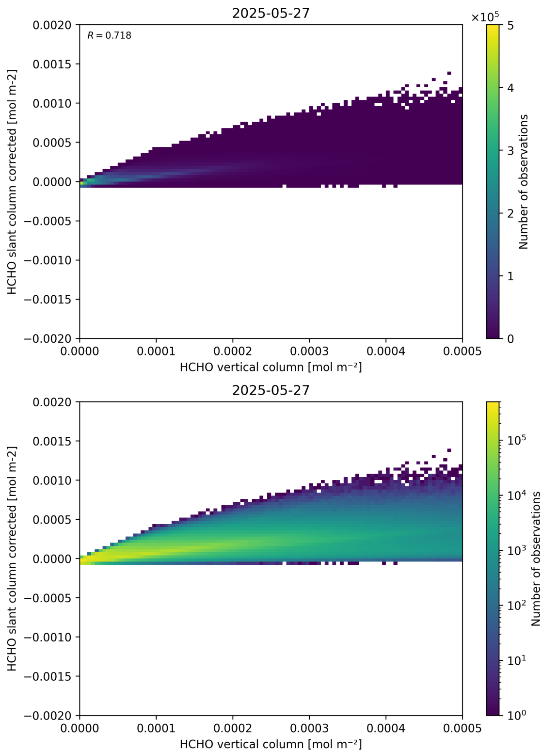
Figure 127: Scatter density plot of “HCHO vertical column” against “HCHO slant column corrected” for 2025-05-26 to 2025-05-28.
