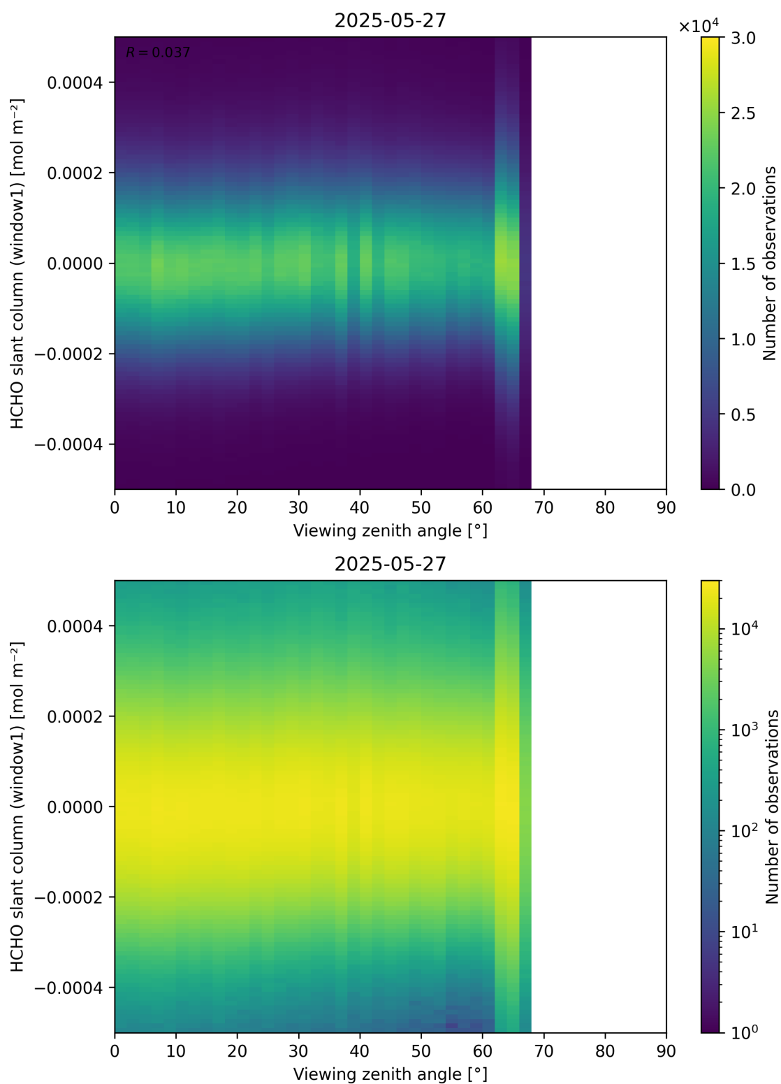
Figure 188: Scatter density plot of “Viewing zenith angle” against “HCHO slant column (window1)” for 2025-05-26 to 2025-05-28.
