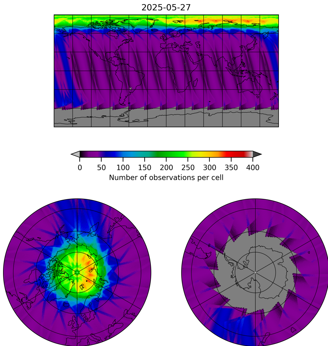
Figure 19: Map of the number of observations for 2025-05-26 to 2025-05-28
