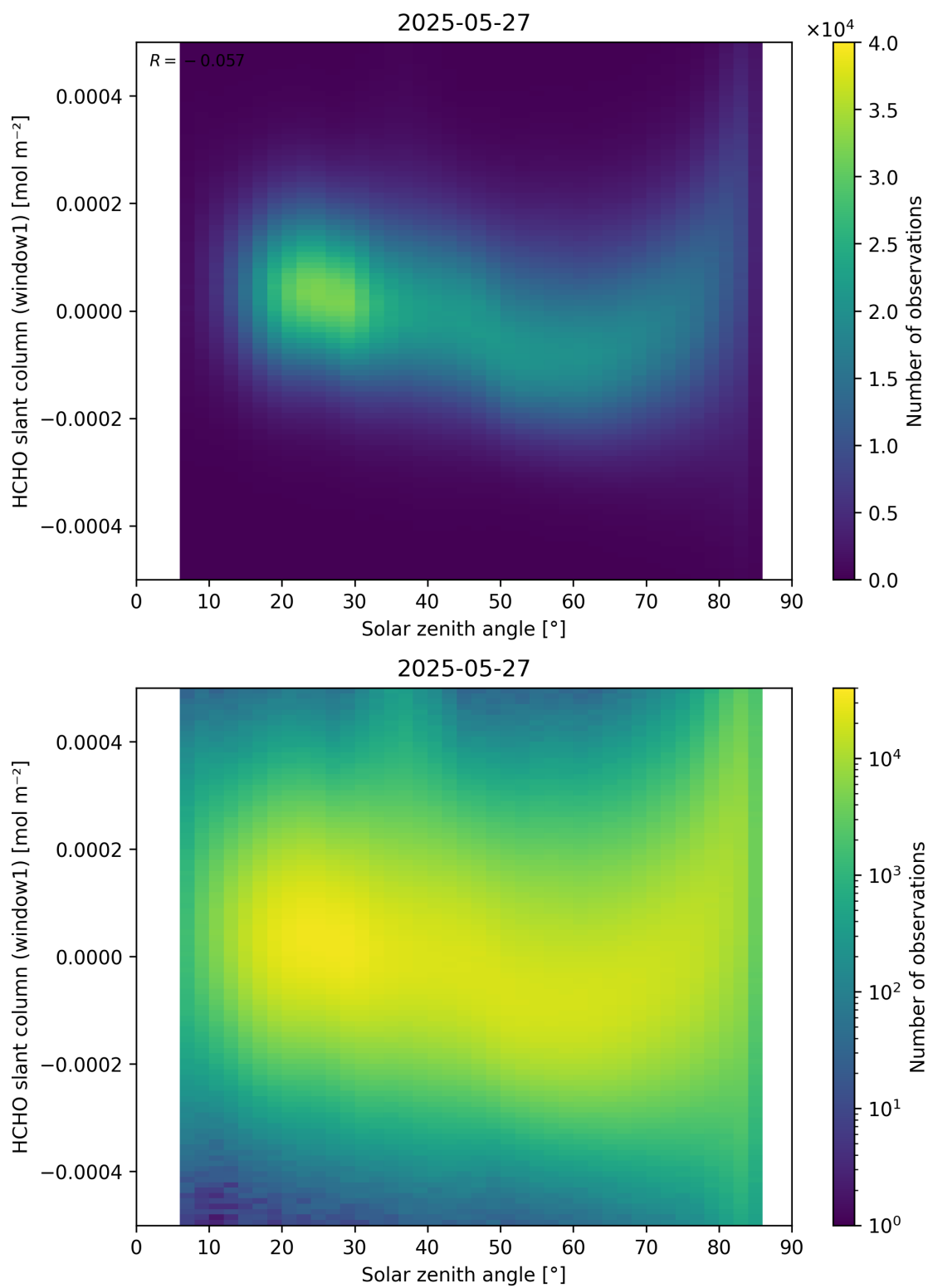
Figure 173: Scatter density plot of “Solar zenith angle” against “HCHO slant column (window1)” for 2025-05-26 to 2025-05-28.
