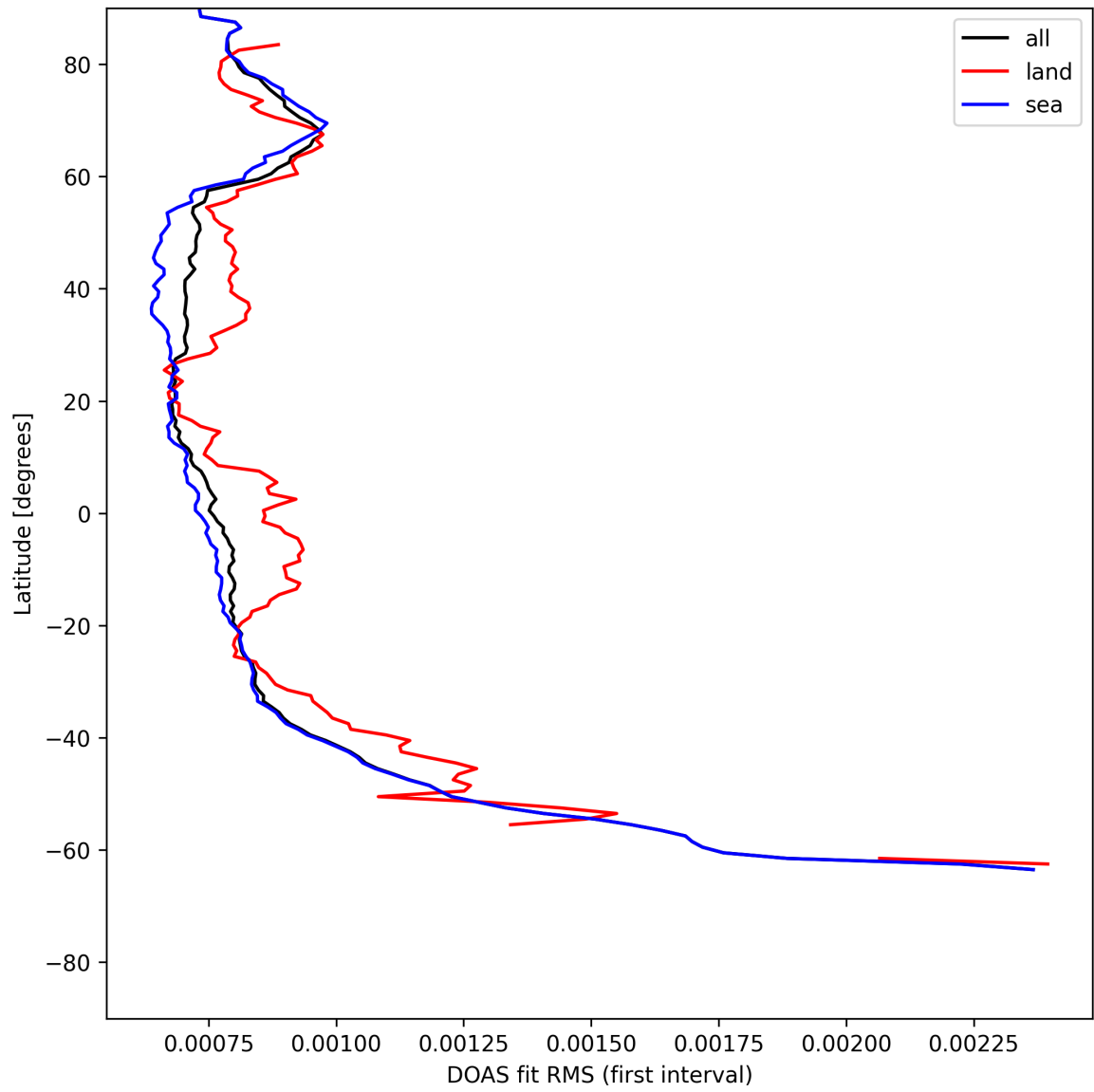
Figure 32: Zonal average of "DOAS fit RMS (first interval)" for 2025-05-26 to 2025-05-28.
