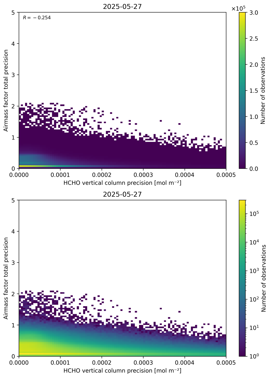
Figure 145: Scatter density plot of “HCHO vertical column precision” against “Airmass factor total precision” for 2025-05-26 to 2025-05-28.
