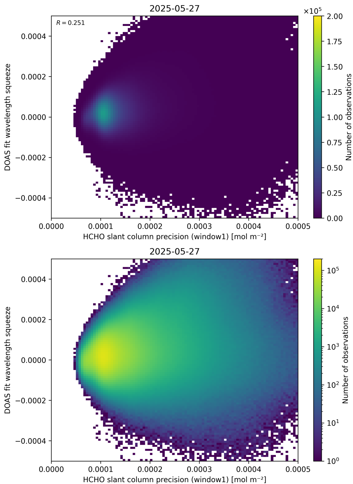
Figure 90: Scatter density plot of “HCHO slant column precision (window1)” against “DOAS fit wavelength squeeze” for 2025-05-26 to 2025-05-28.
