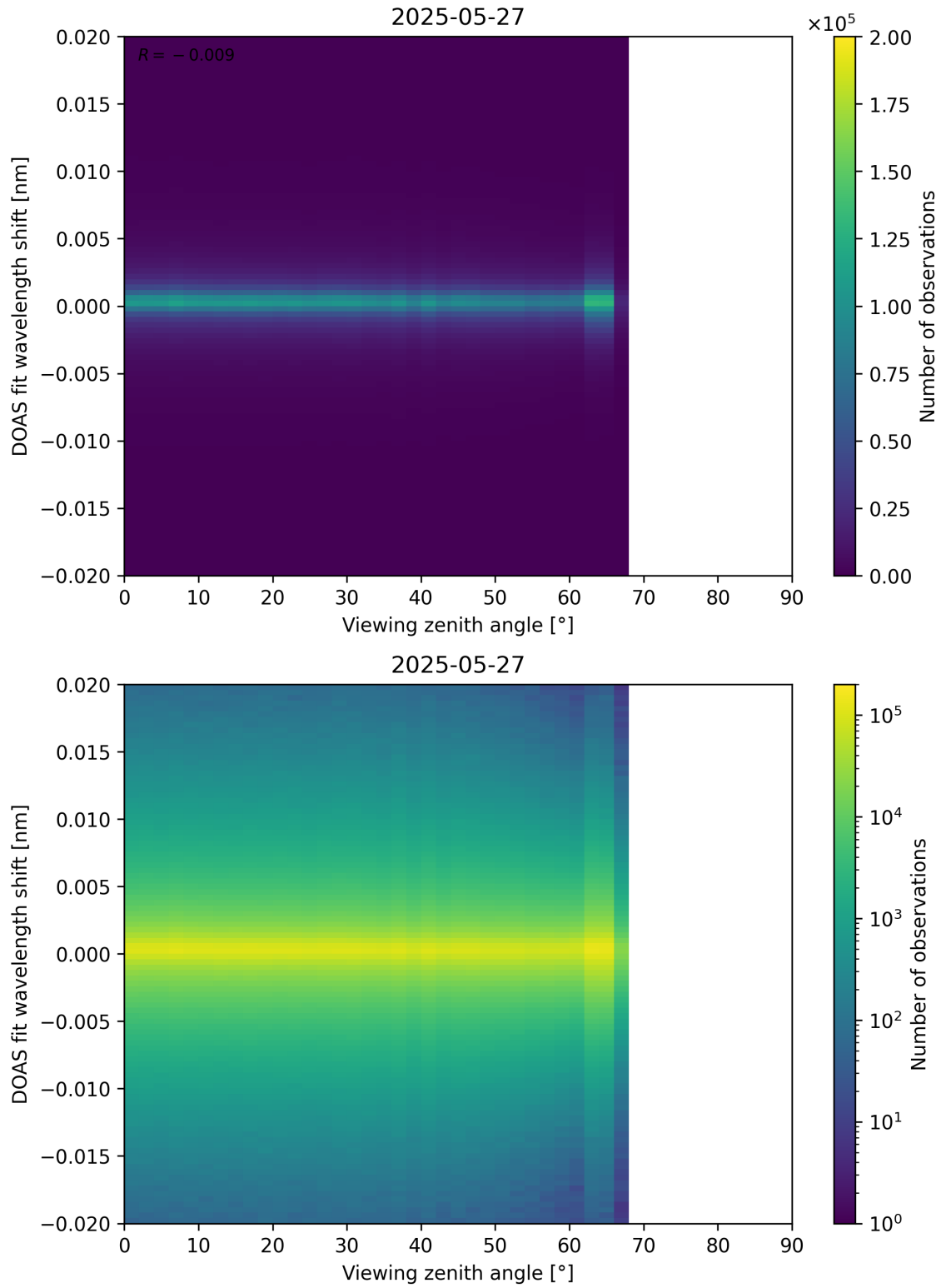
Figure 183: Scatter density plot of “Viewing zenith angle” against “DOAS fit wavelength shift” for 2025-05-26 to 2025-05-28.
