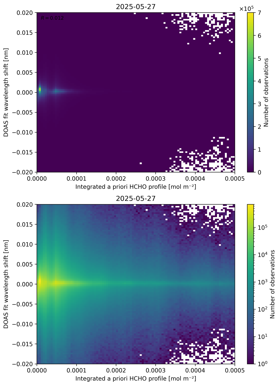
Figure 149: Scatter density plot of “Integrated a priori HCHO profile” against “DOAS fit wavelength shift” for 2025-05-26 to 2025-05-28.
