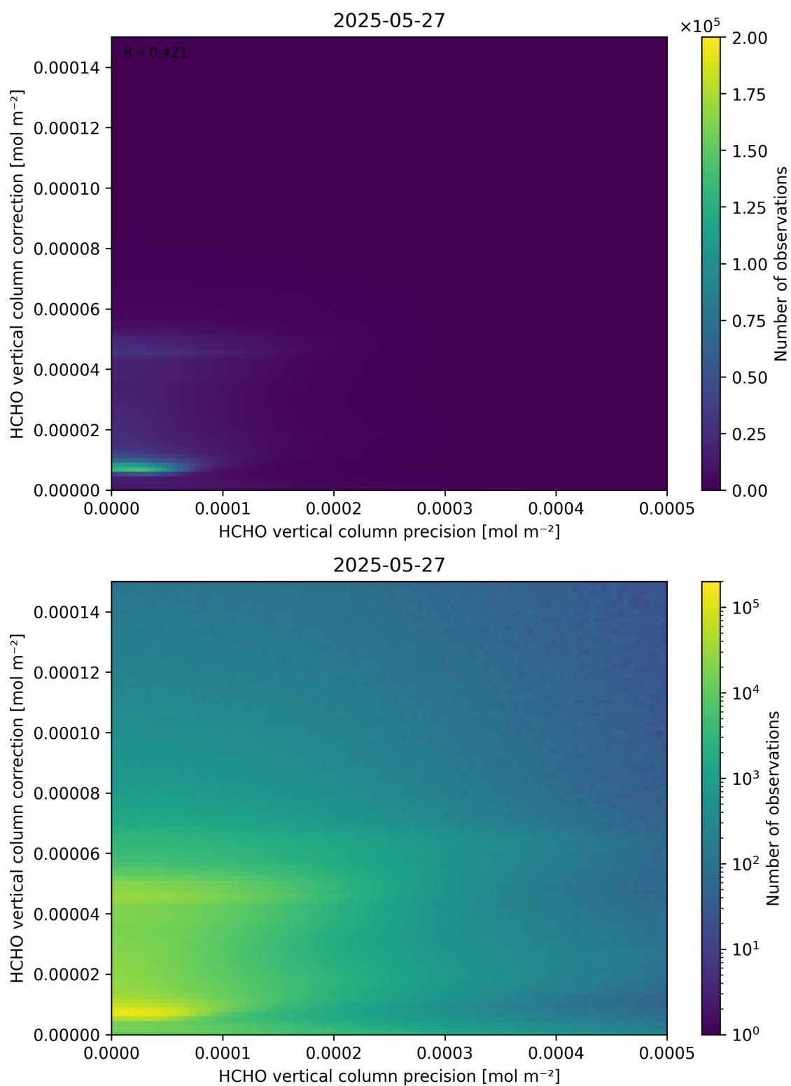
Figure 146: Scatter density plot of “HCHO vertical column precision” against “HCHO vertical column correction” for 2025-05-26 to 2025-05-28.
