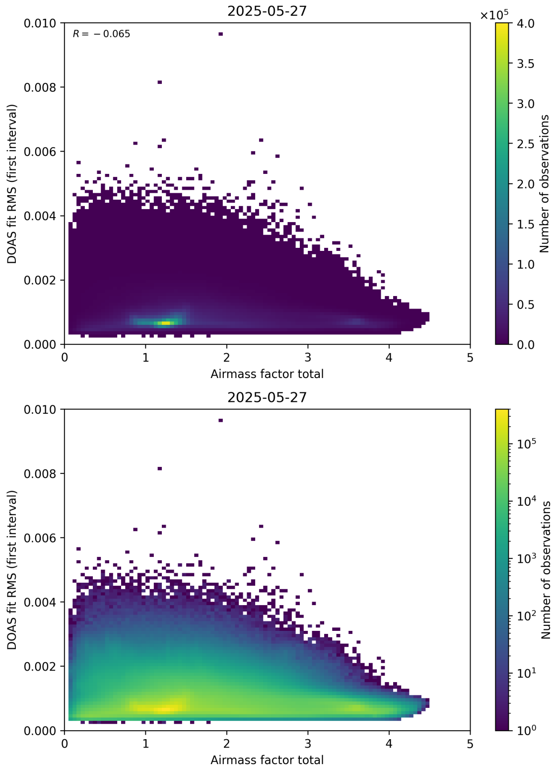
Figure 97: Scatter density plot of “Airmass factor total” against “DOAS fit RMS (first interval)” for 2025-05-26 to 2025-05-28.
