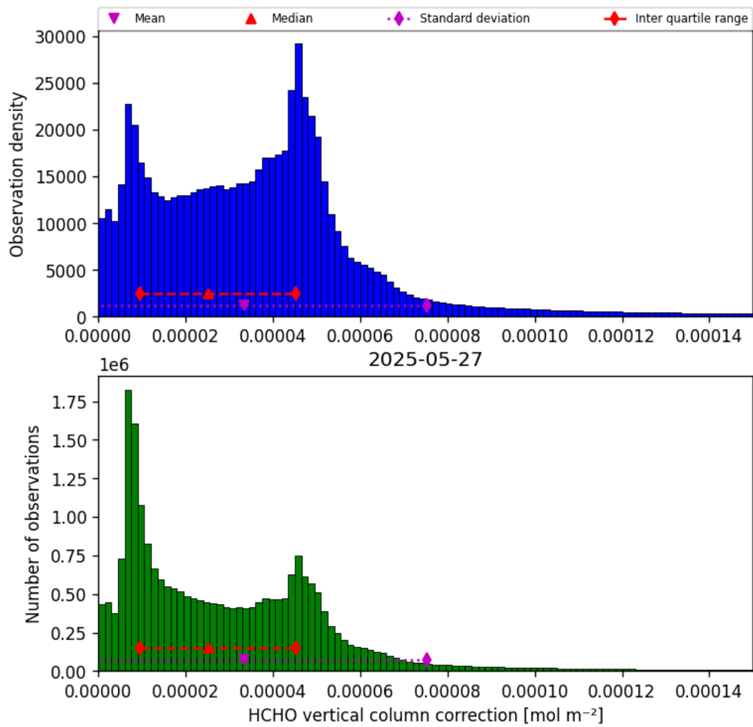
Figure 37: Histogram of “HCHO vertical column correction” for 2025-05-26 to 2025-05-28
