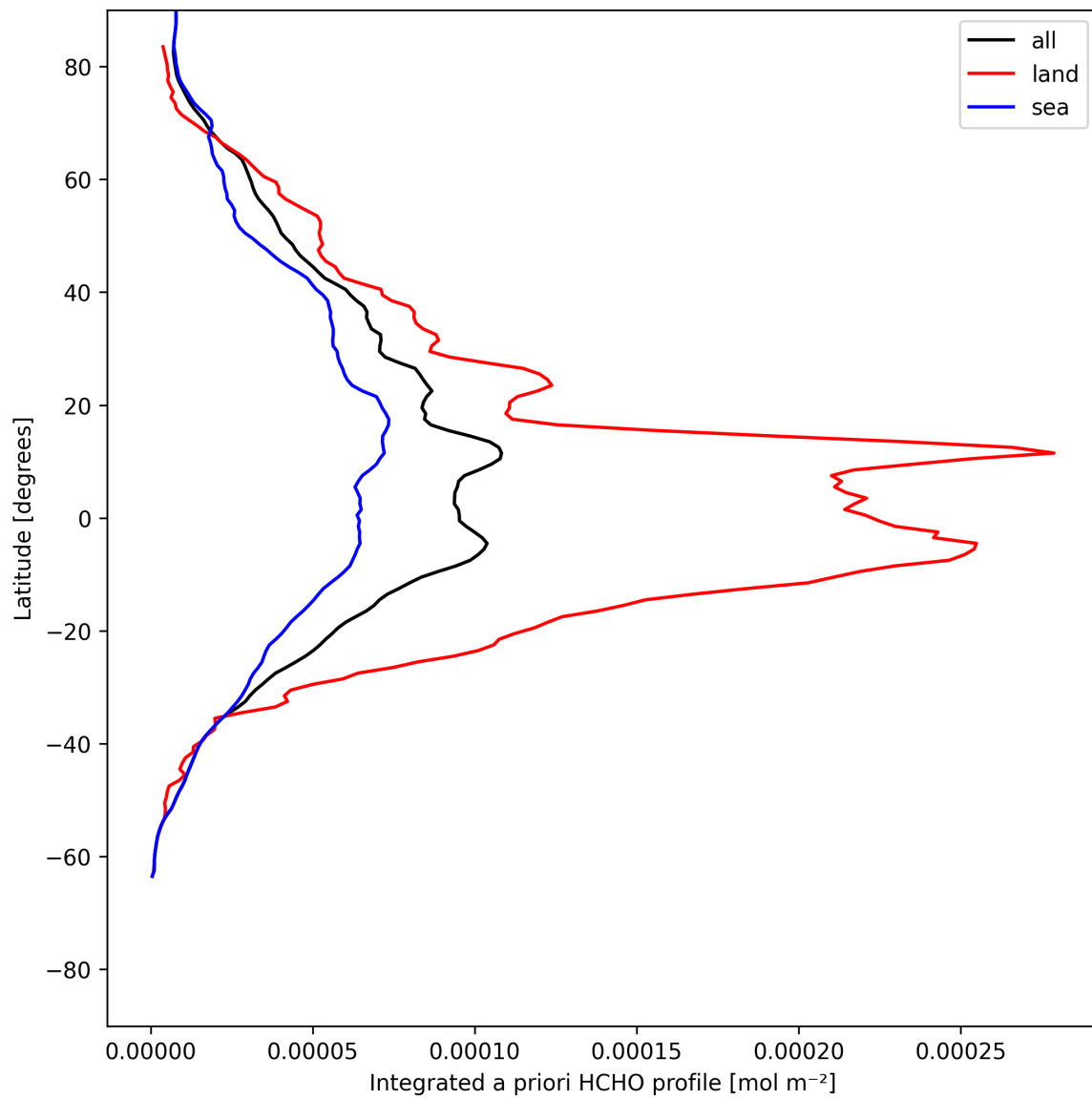
Figure 29: Zonal average of “Integrated a priori HCHO profile” for 2025-05-26 to 2025-05-28.
