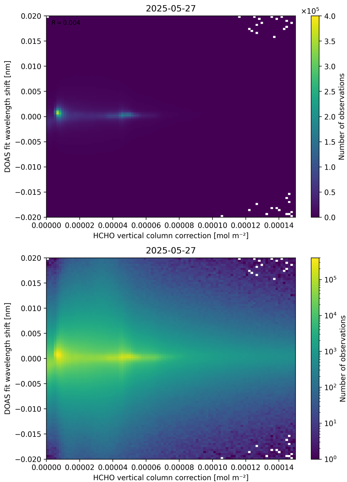
Figure 113: Scatter density plot of “HCHO vertical column correction” against “DOAS fit wavelength shift” for 2025-05-26 to 2025-05-28.
