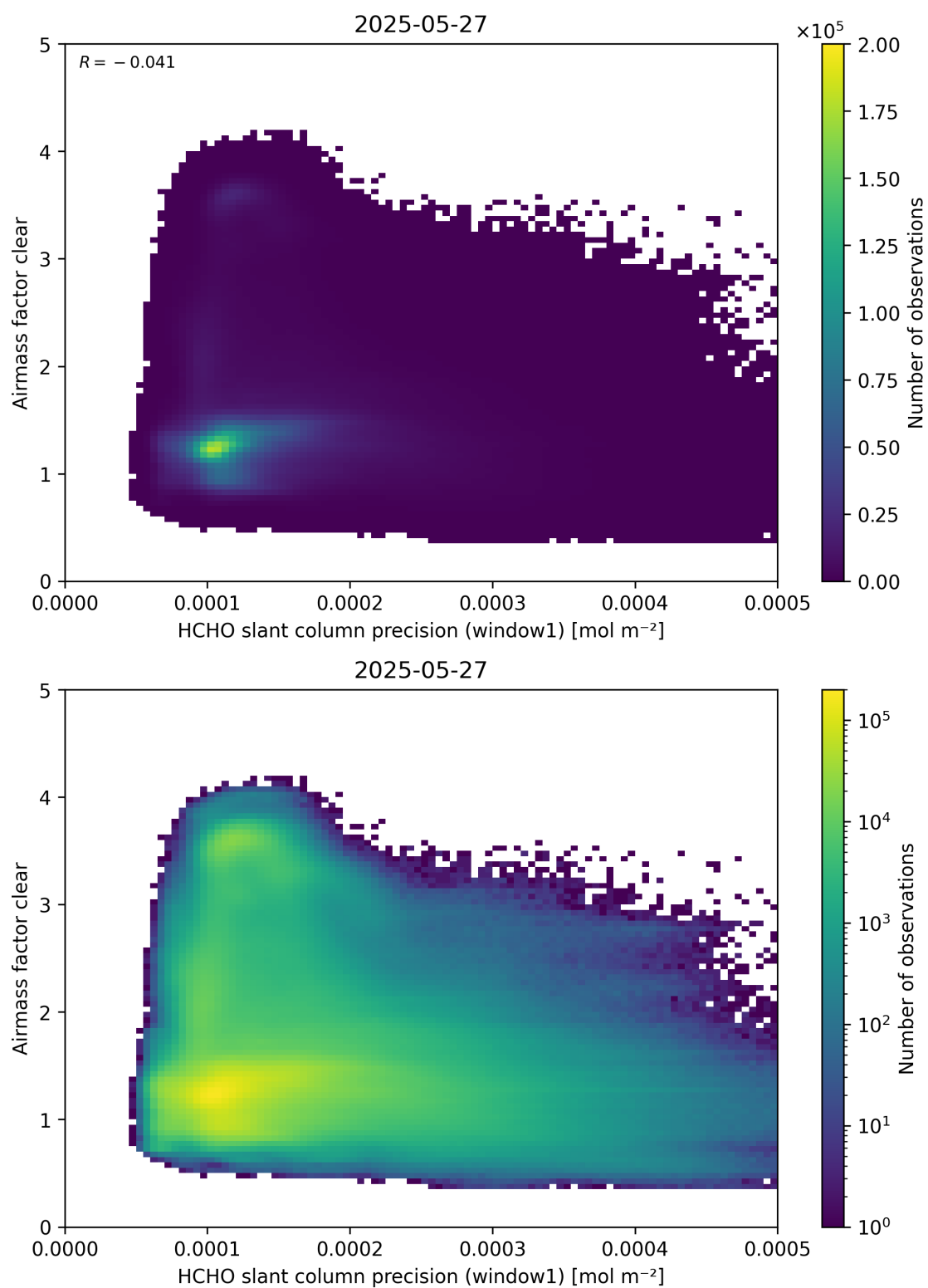
Figure 91: Scatter density plot of “HCHO slant column precision (window1)” against “Airmass factor clear” for 2025-05-26 to 2025-05-28.
