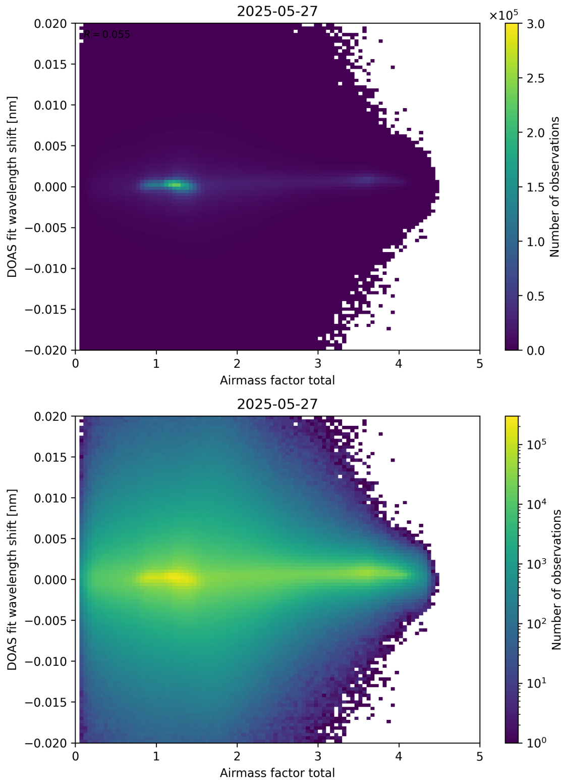
Figure 98: Scatter density plot of “Airmass factor total” against “DOAS fit wavelength shift” for 2025-05-26 to 2025-05-28.
