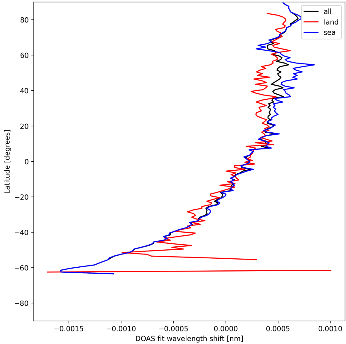
Figure 30: Zonal average of “DOAS fit wavelength shift” for 2025-05-26 to 2025-05-28.
