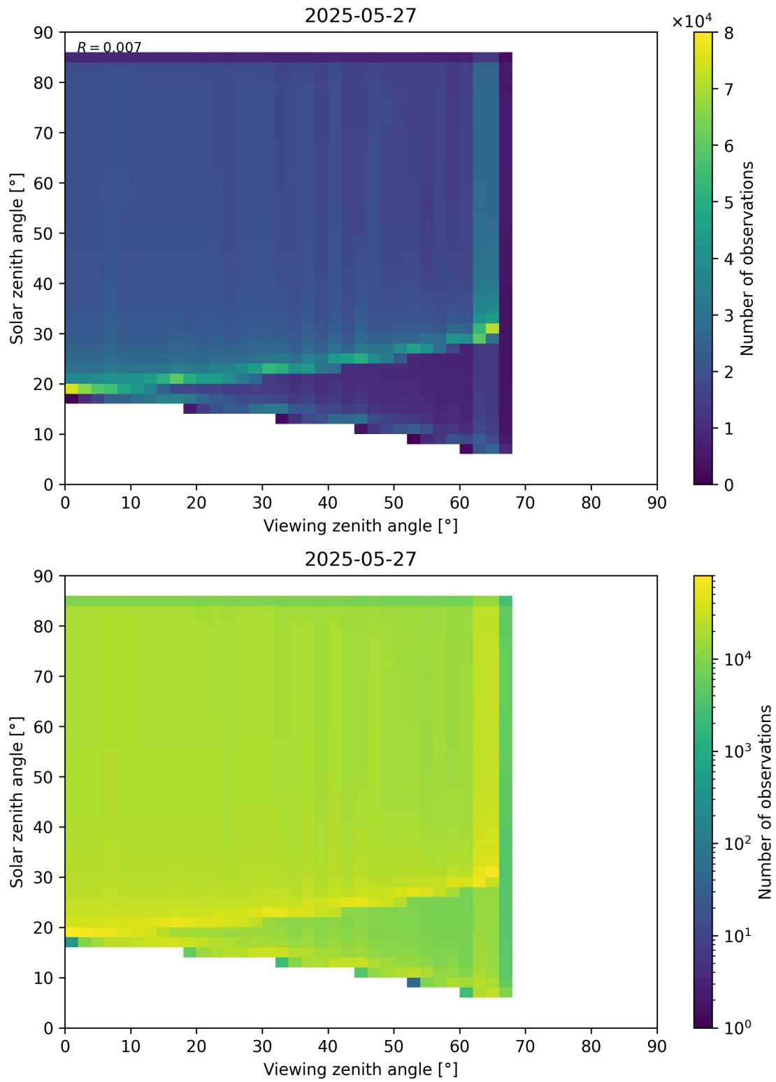
Figure 197: Scatter density plot of “Viewing zenith angle” against “Solar zenith angle” for 2025-05-26 to 2025-05-28.
