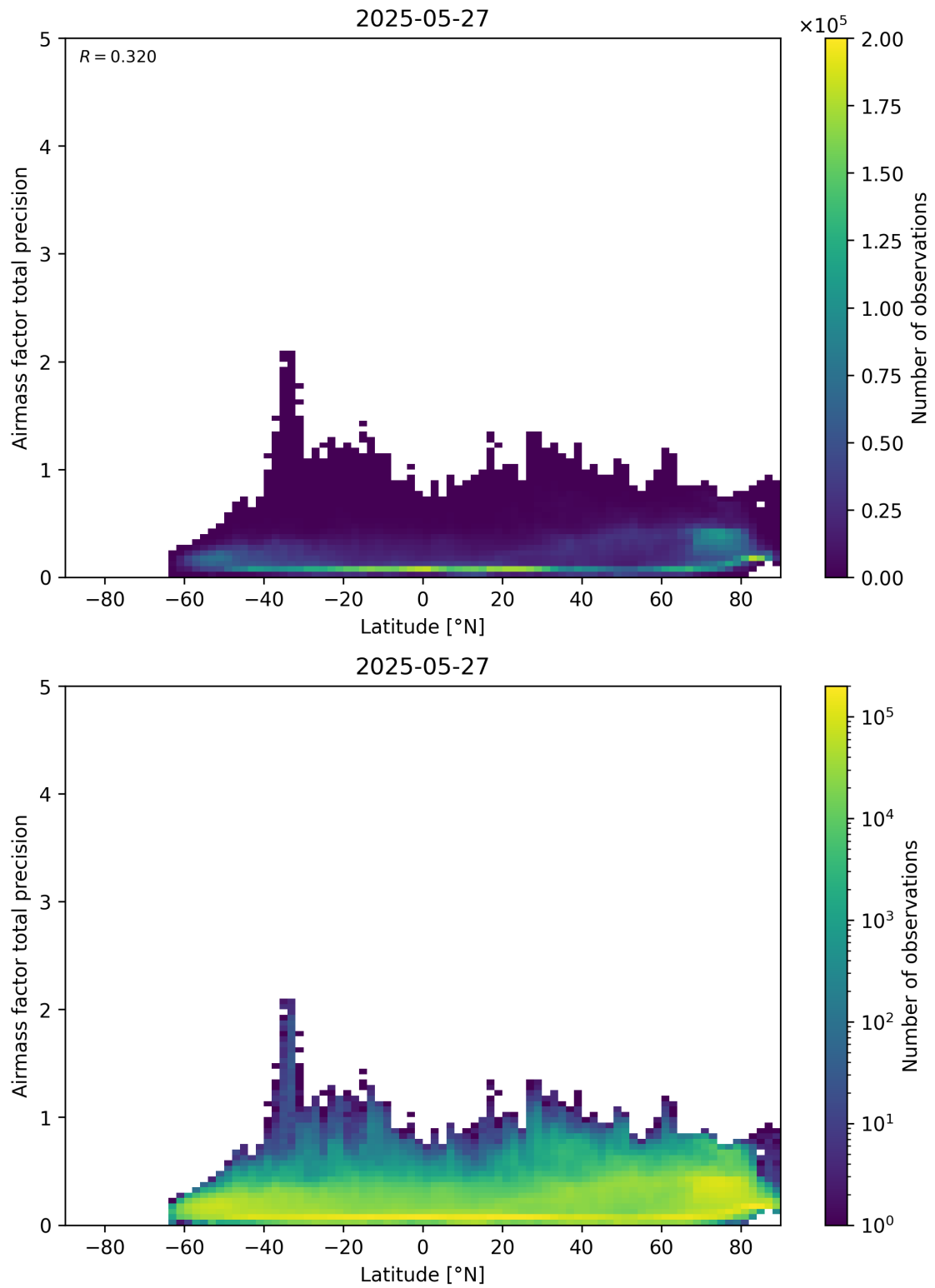
Figure 162: Scatter density plot of “Latitude” against “Airmass factor total precision” for 2025-05-26 to 2025-05-28.
