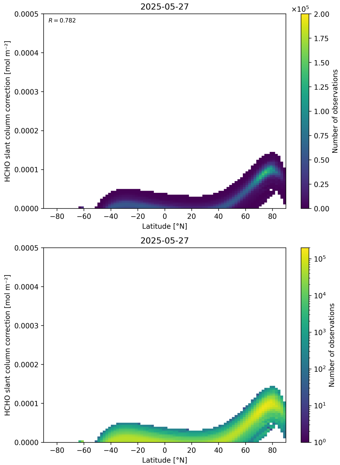
Figure 158: Scatter density plot of “Latitude” against “HCHO slant column correction” for 2025-05-26 to 2025-05-28.
