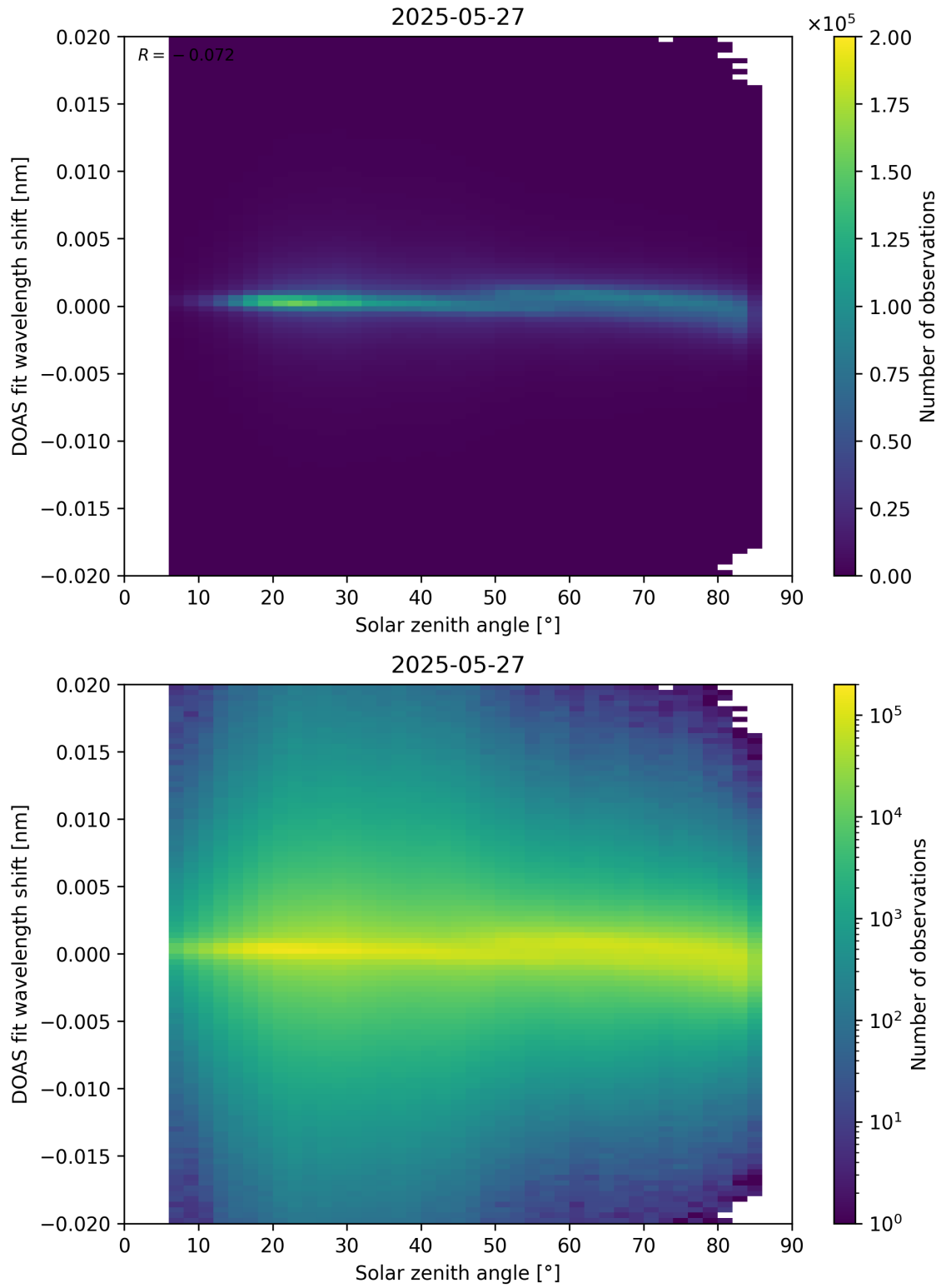
Figure 168: Scatter density plot of “Solar zenith angle” against “DOAS fit wavelength shift” for 2025-05-26 to 2025-05-28.
