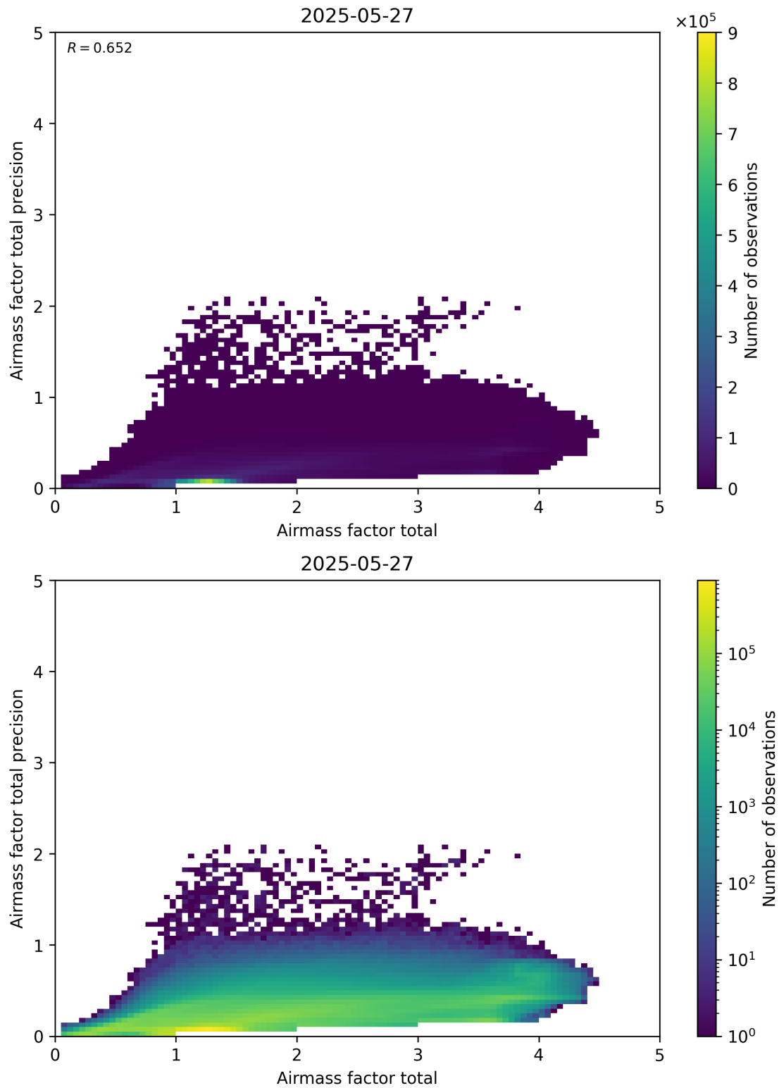
Figure 103: Scatter density plot of “Airmass factor total” against “Airmass factor total precision” for 2025-05-26 to 2025-05-28.
