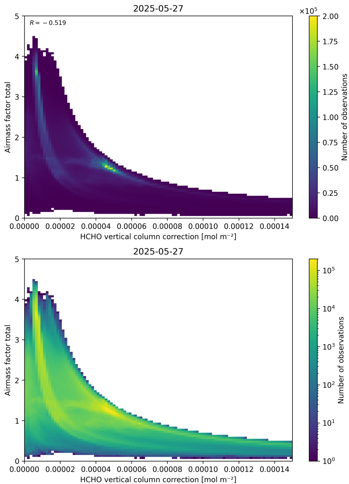
Figure 120: Scatter density plot of “HCHO vertical column correction” against “Airmass factor total” for 2025-05-26 to 2025-05-28.
