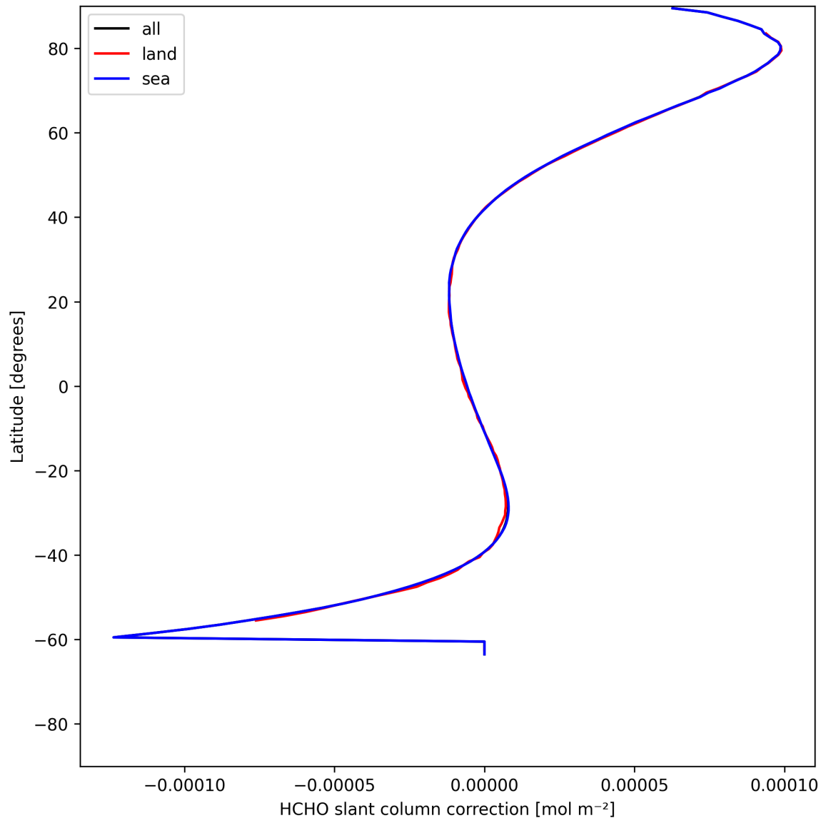
Figure 33: Zonal average of “HCHO slant column correction” for 2025-05-26 to 2025-05-28.
