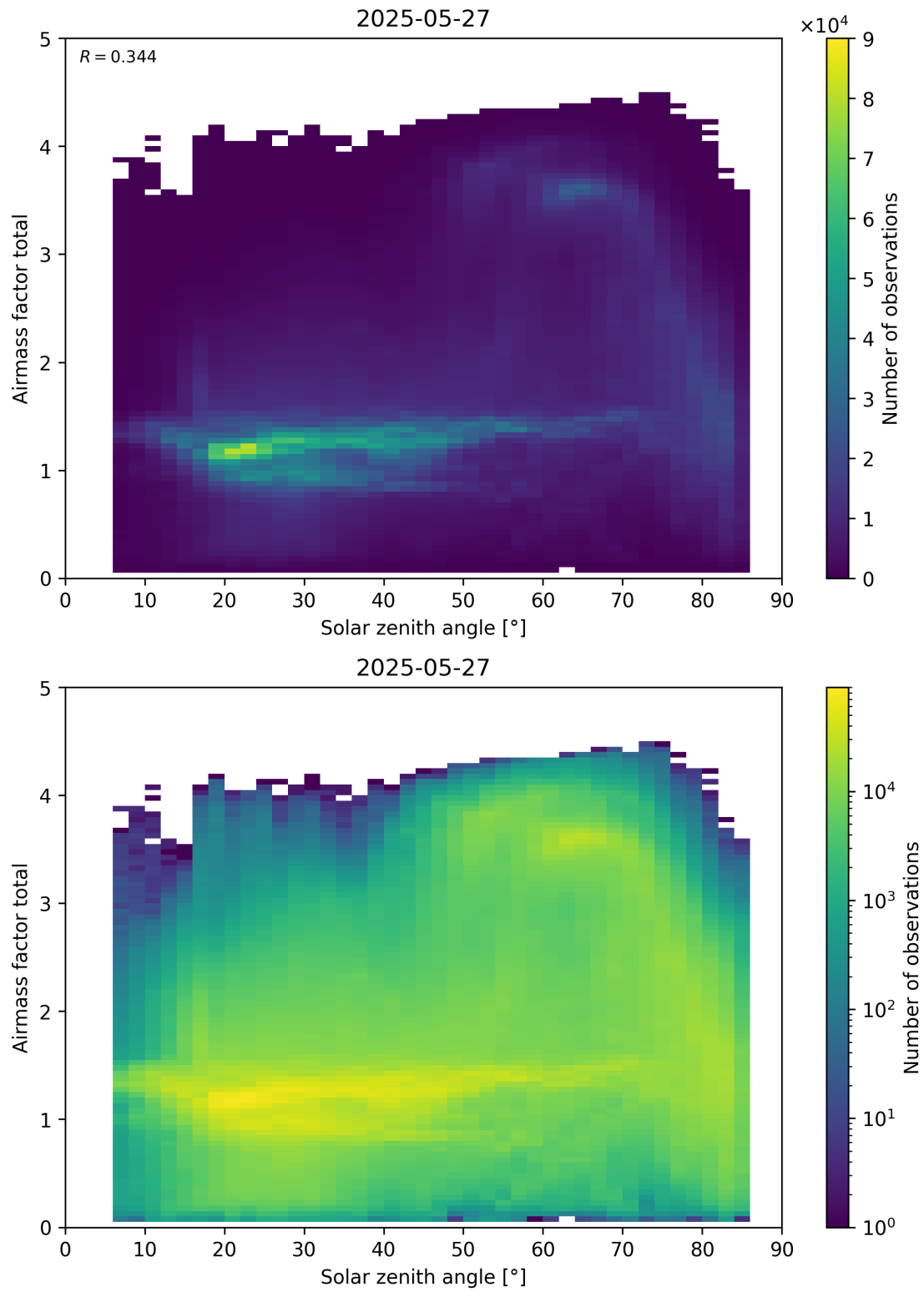
Figure 175: Scatter density plot of “Solar zenith angle” against “Airmass factor total” for 2025-05-26 to 2025-05-28.
