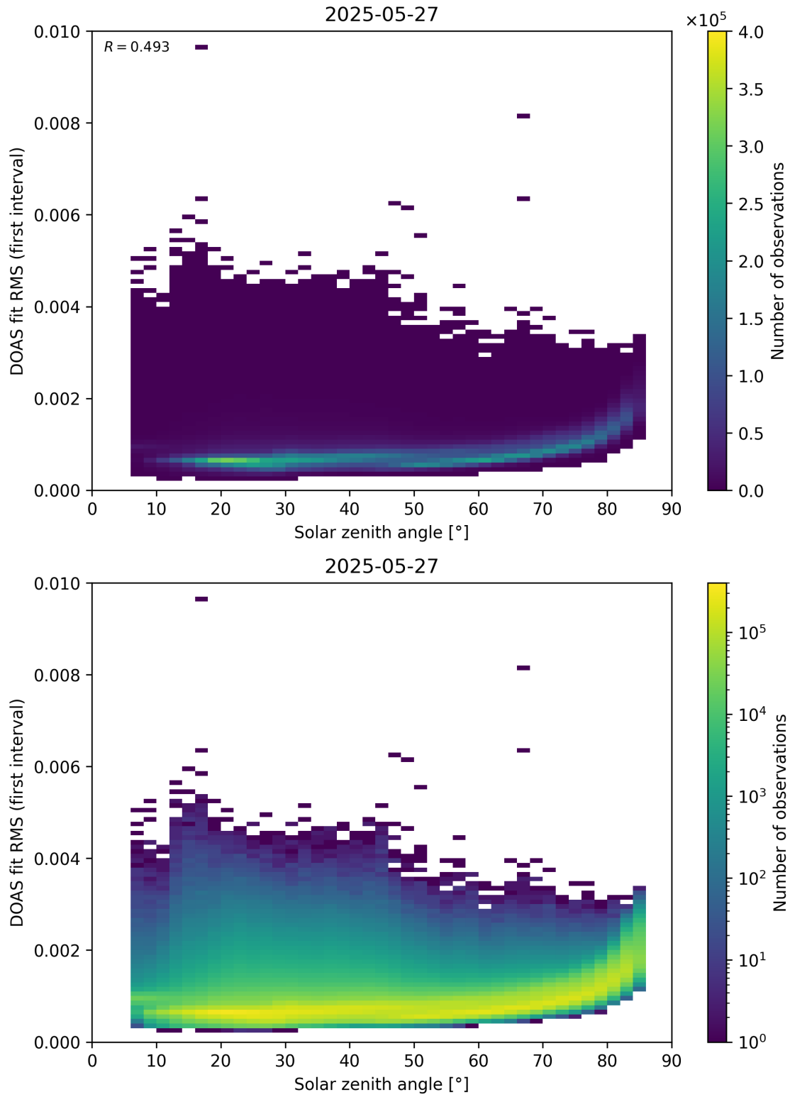
Figure 167: Scatter density plot of “Solar zenith angle” against “DOAS fit RMS (first interval)” for 2025-05-26 to 2025-05-28.
