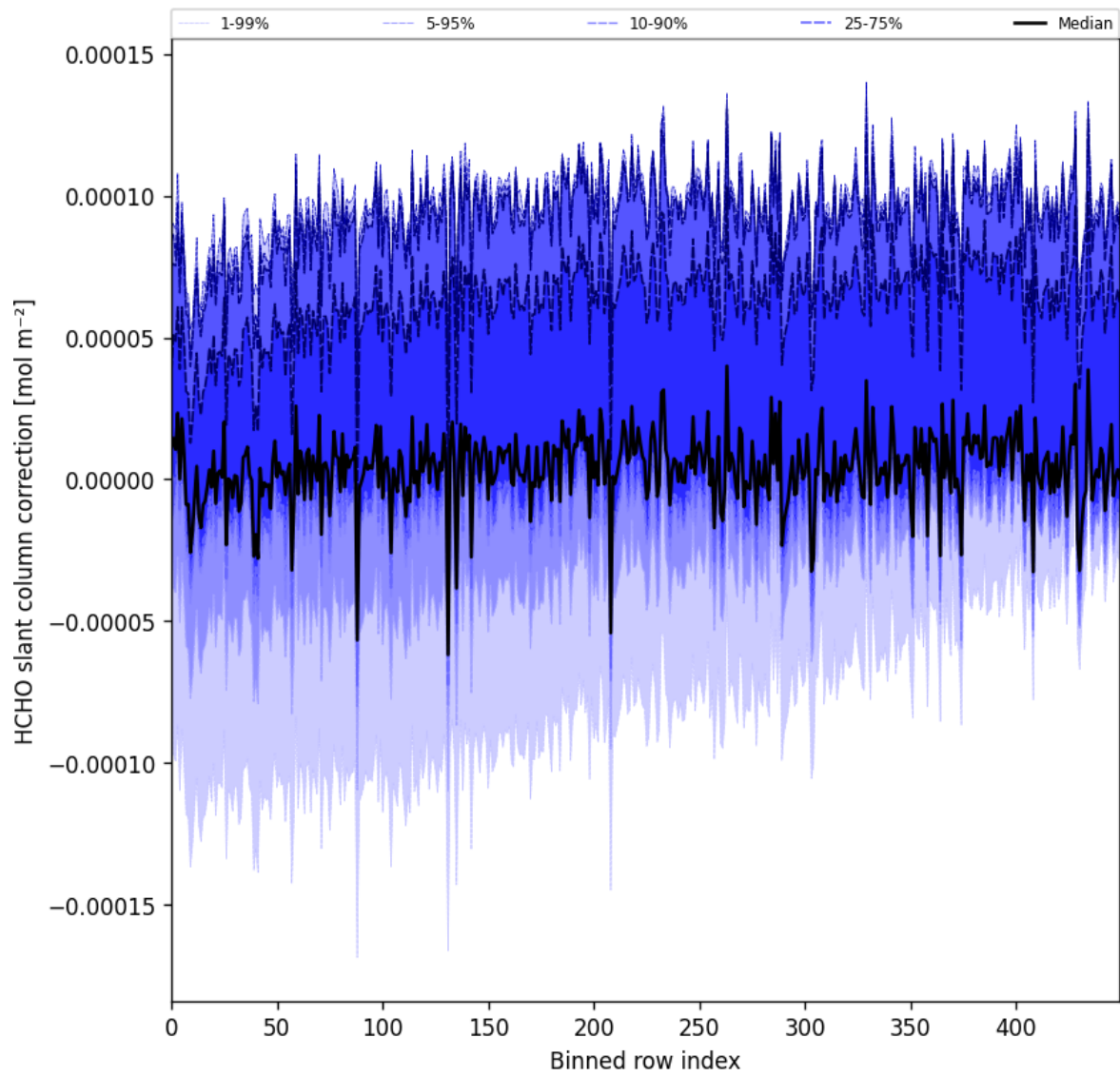
Figure 61: Along track statistics of "HCHO slant column correction" for 2025-05-26 to 2025-05-28
