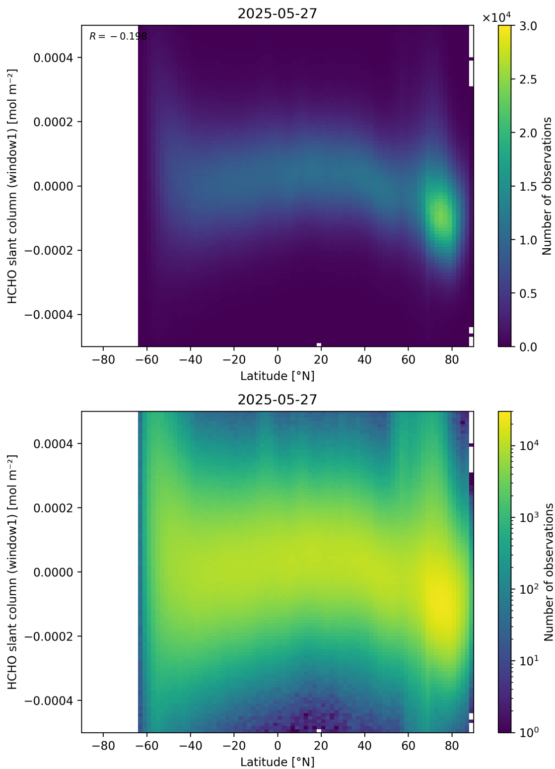
Figure 159: Scatter density plot of “Latitude” against “HCHO slant column (window1)” for 2025-05-26 to 2025-05-28.
