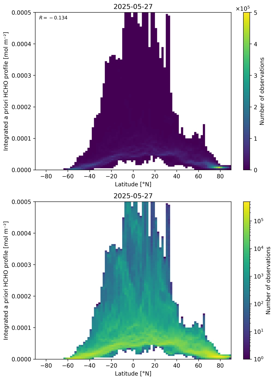
Figure 166: Scatter density plot of “Latitude” against “Integrated a priori HCHO profile” for 2025-05-26 to 2025-05-28.
