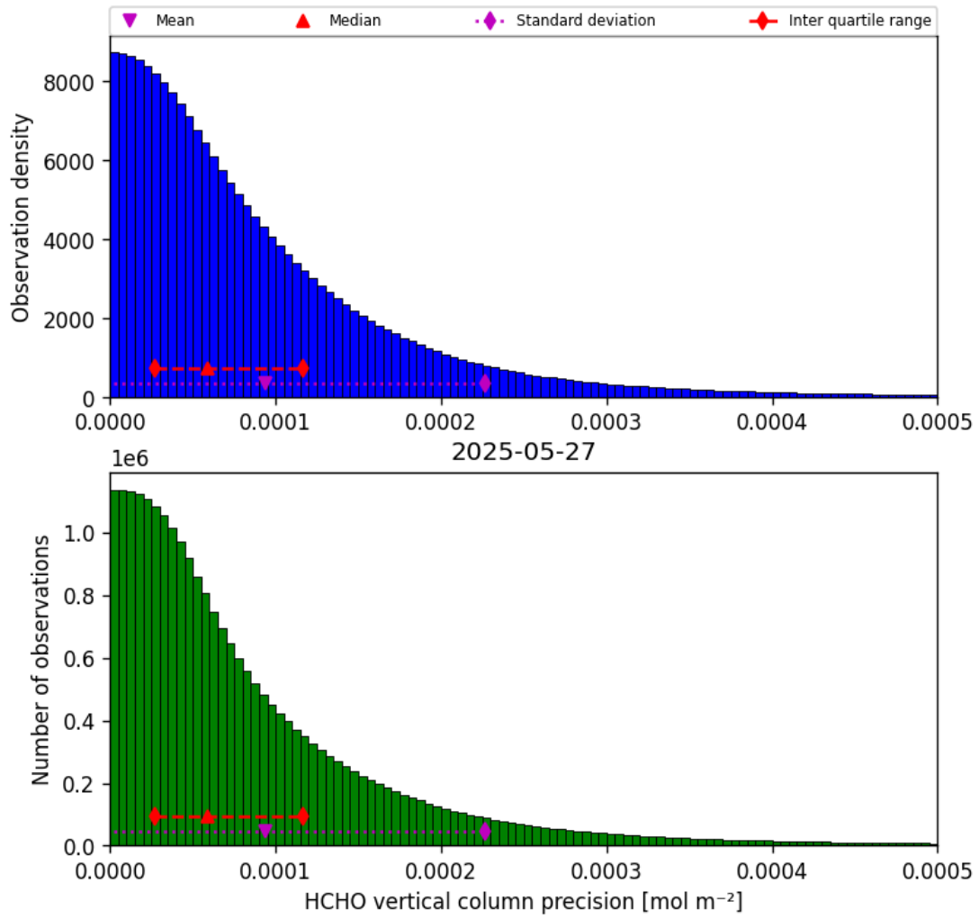
Figure 36: Histogram of “HCHO vertical column precision” for 2025-05-26 to 2025-05-28
