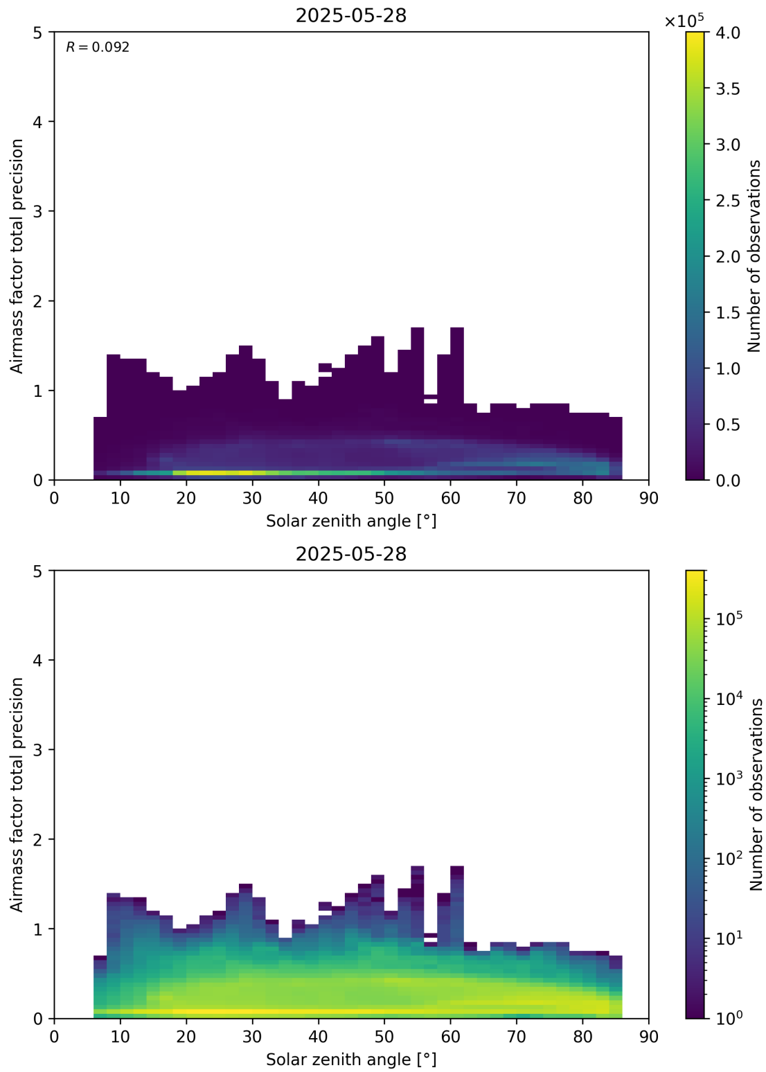
Figure 176: Scatter density plot of “Solar zenith angle” against “Airmass factor total precision” for 2025-05-27 to 2025-05-29.
