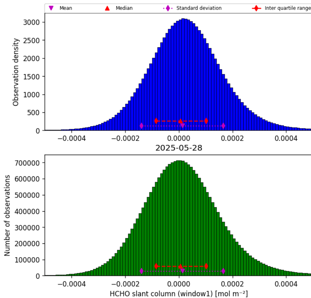
Figure 38: Histogram of “HCHO slant column (window1)” for 2025-05-27 to 2025-05-29
