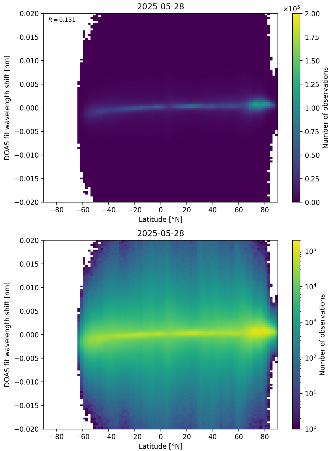
Figure 154: Scatter density plot of “Latitude” against “DOAS fit wavelength shift” for 2025-05-27 to 2025-05-29.
