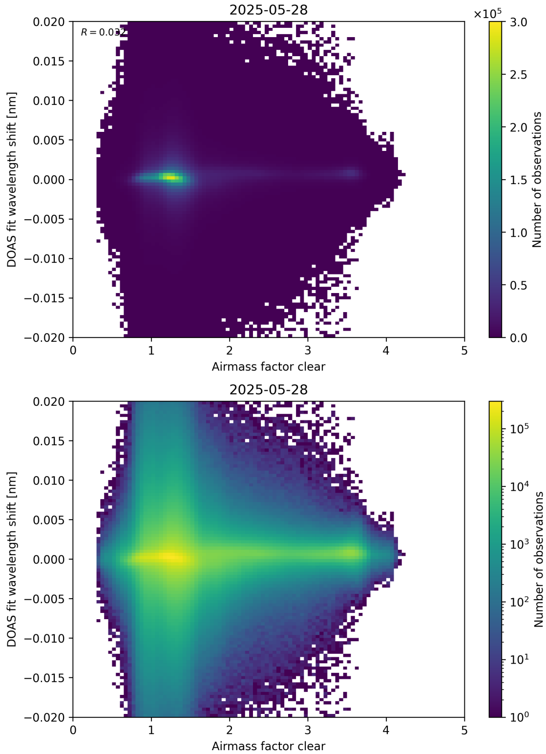
Figure 72: Scatter density plot of “Airmass factor clear” against “DOAS fit wavelength shift” for 2025-05-27 to 2025-05-29.
