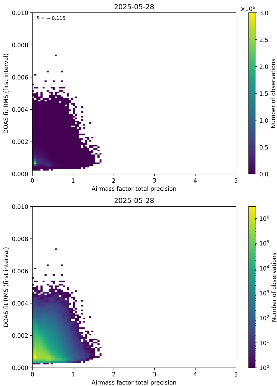
Figure 105: Scatter density plot of “Airmass factor total precision” against “DOAS fit RMS (first interval)” for 2025-05-27 to 2025-05-29.
