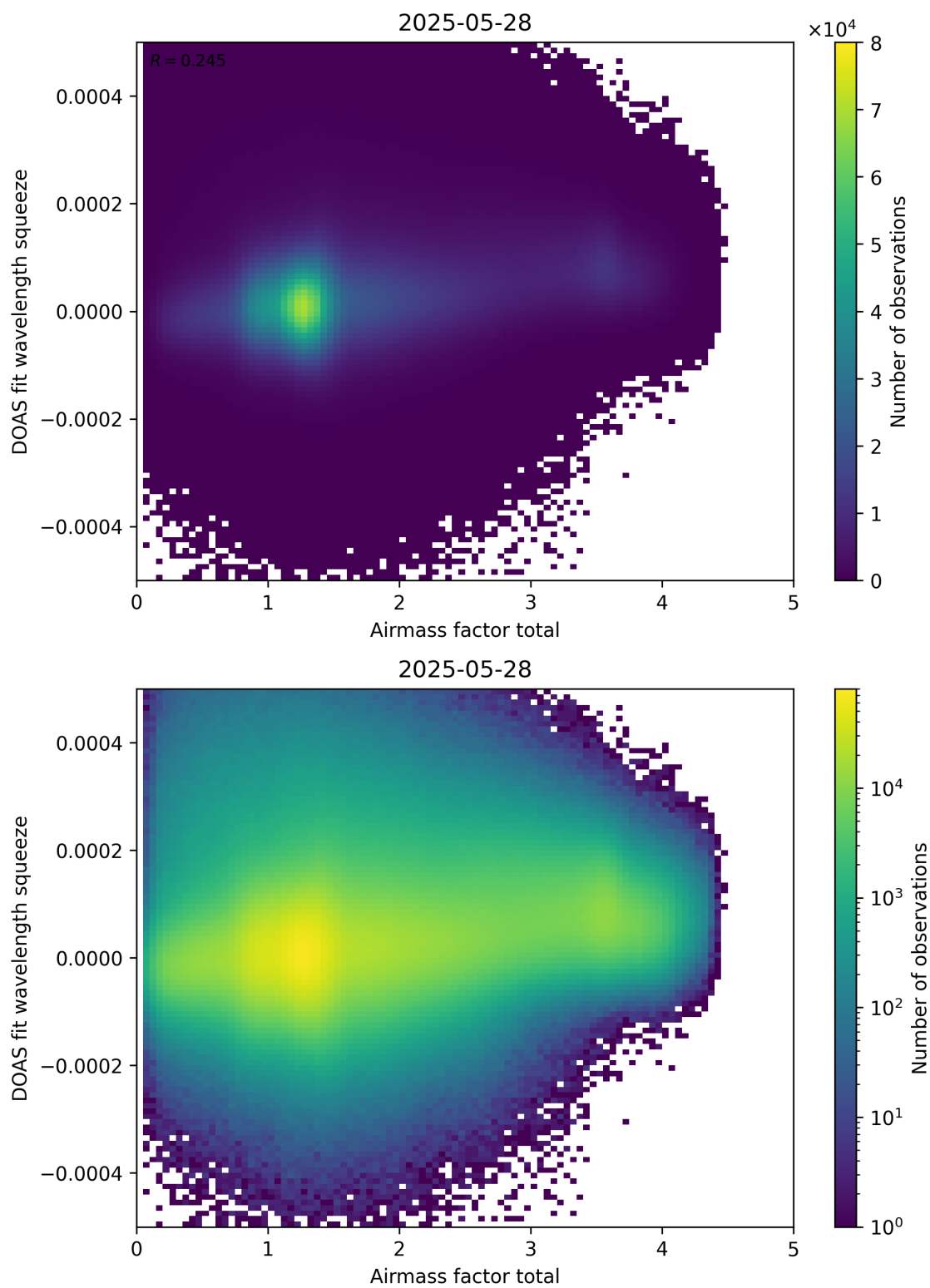
Figure 99: Scatter density plot of “Airmass factor total” against “DOAS fit wavelength squeeze” for 2025-05-27 to 2025-05-29.
