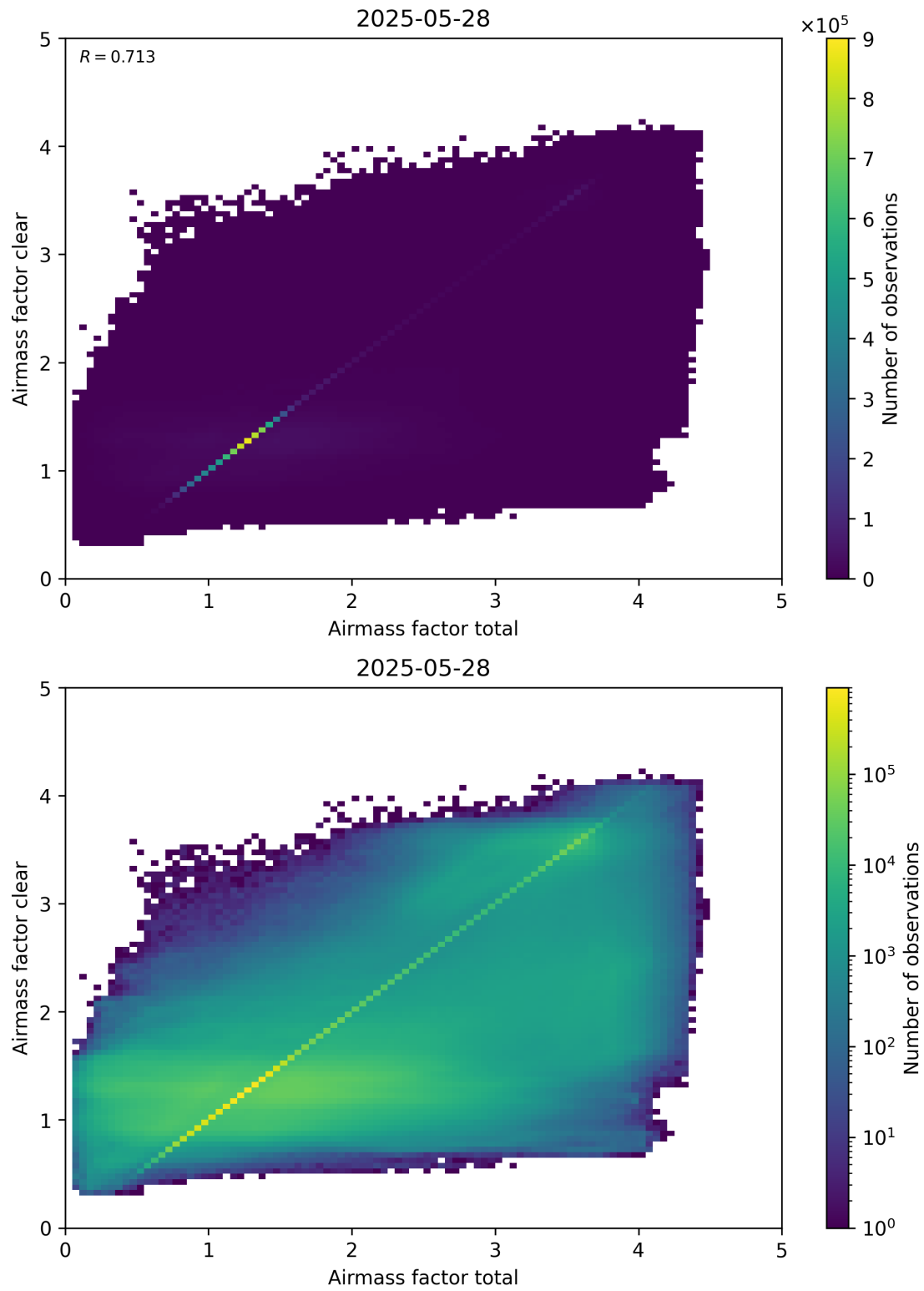
Figure 100: Scatter density plot of “Airmass factor total” against “Airmass factor clear” for 2025-05-27 to 2025-05-29.
