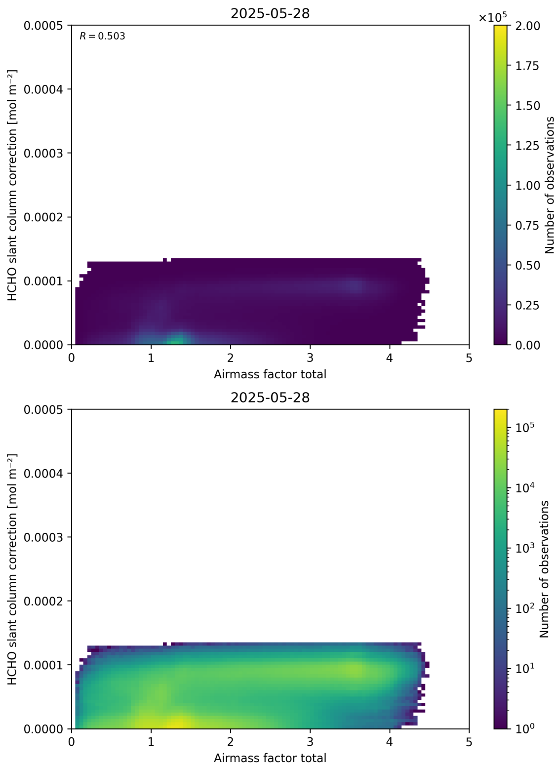
Figure 102: Scatter density plot of “Airmass factor total” against “HCHO slant column correction” for 2025-05-27 to 2025-05-29.
