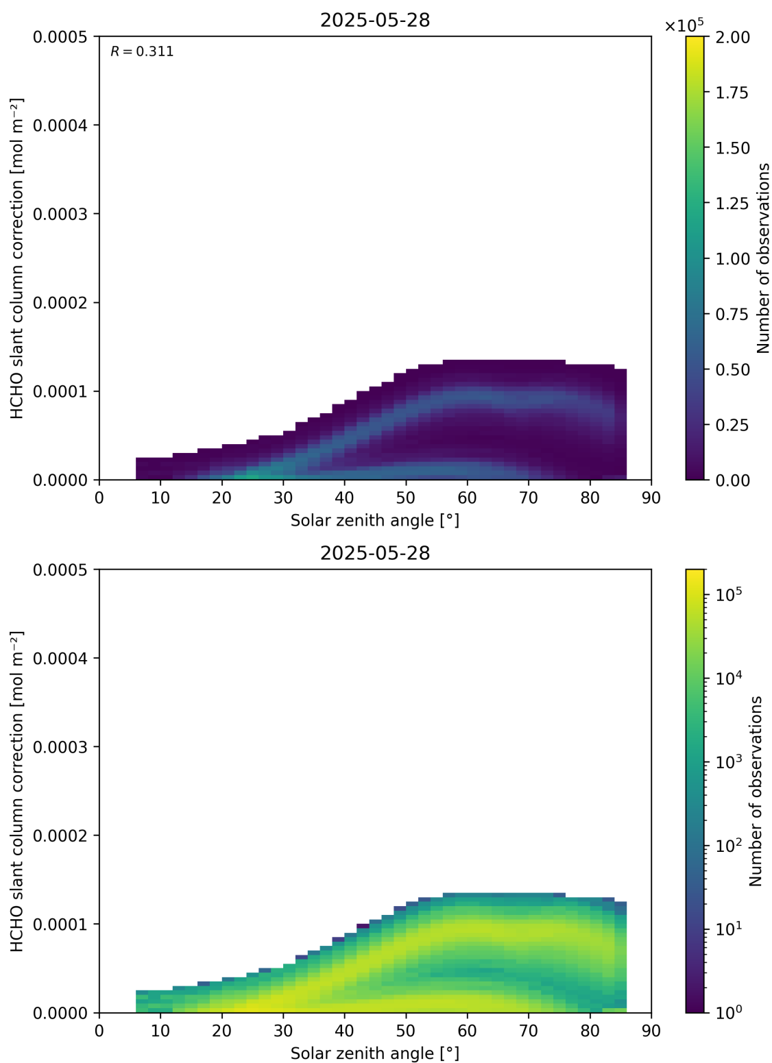
Figure 172: Scatter density plot of “Solar zenith angle” against “HCHO slant column correction” for 2025-05-27 to 2025-05-29.
