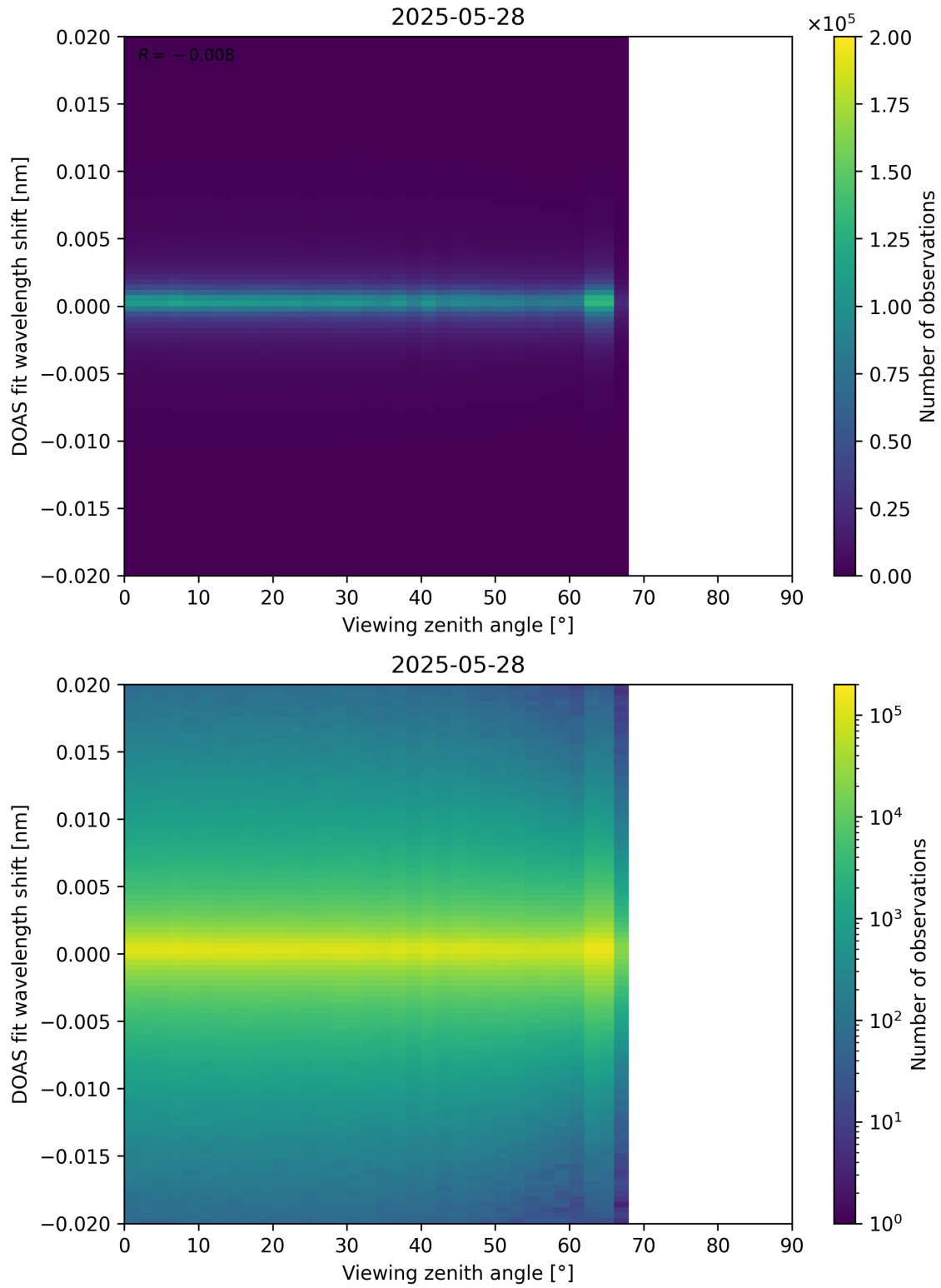
Figure 183: Scatter density plot of “Viewing zenith angle” against “DOAS fit wavelength shift” for 2025-05-27 to 2025-05-29.
