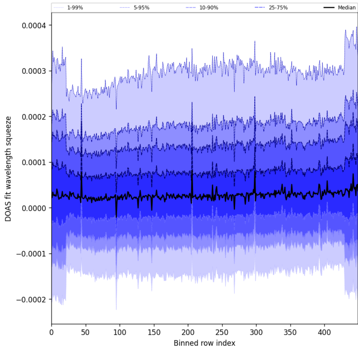
Figure 59: Along track statistics of “DOAS fit wavelength squeeze” for 2025-05-27 to 2025-05-29
