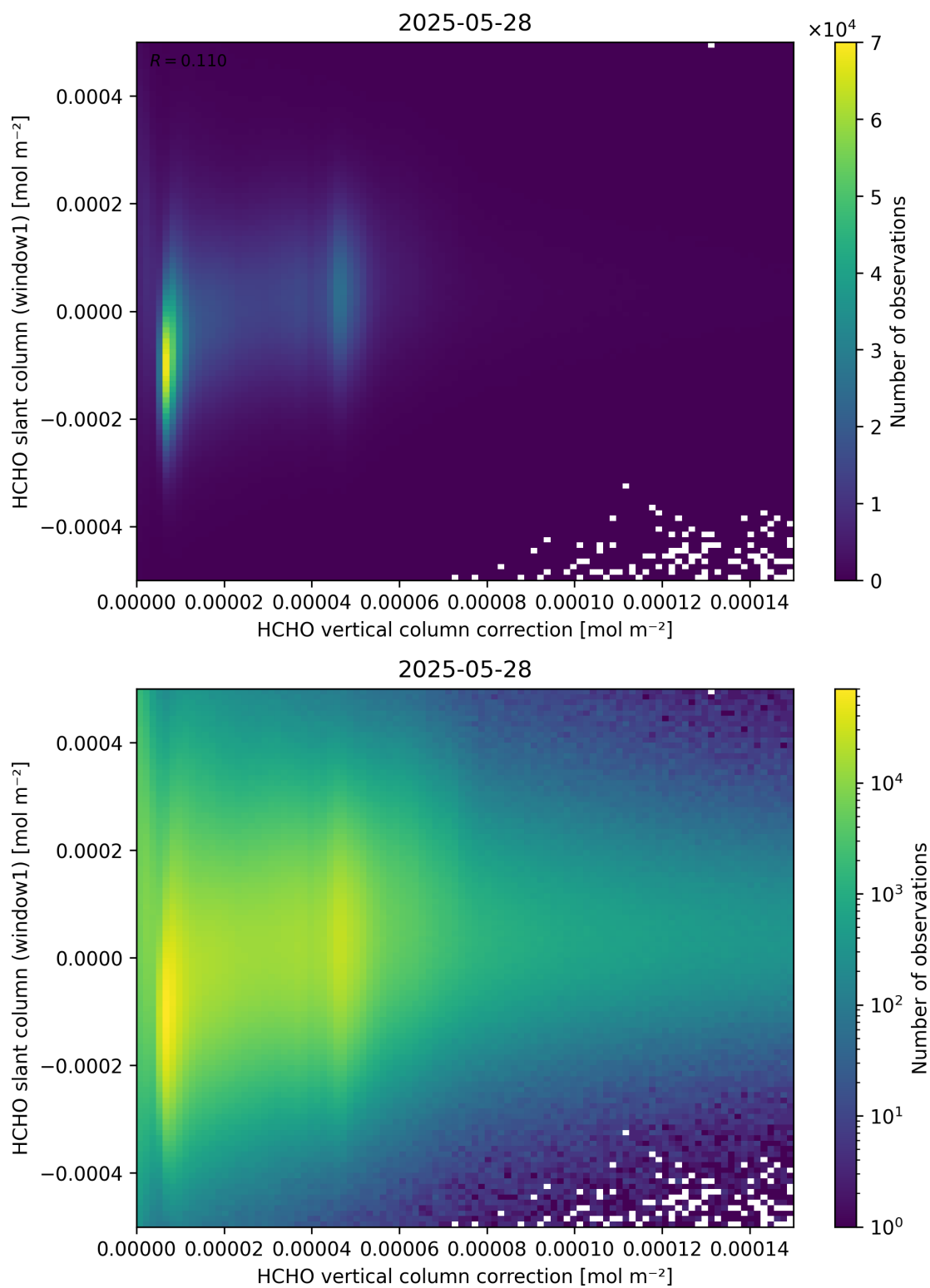
Figure 118: Scatter density plot of “HCHO vertical column correction” against “HCHO slant column (window1)” for 2025-05-27 to 2025-05-29.
