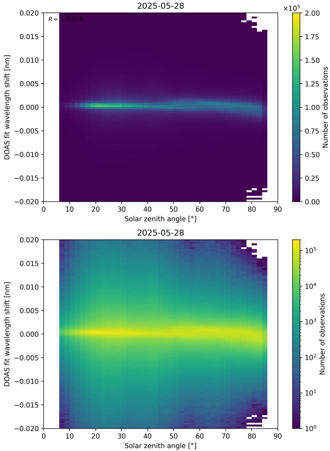
Figure 168: Scatter density plot of “Solar zenith angle” against “DOAS fit wavelength shift” for 2025-05-27 to 2025-05-29.
