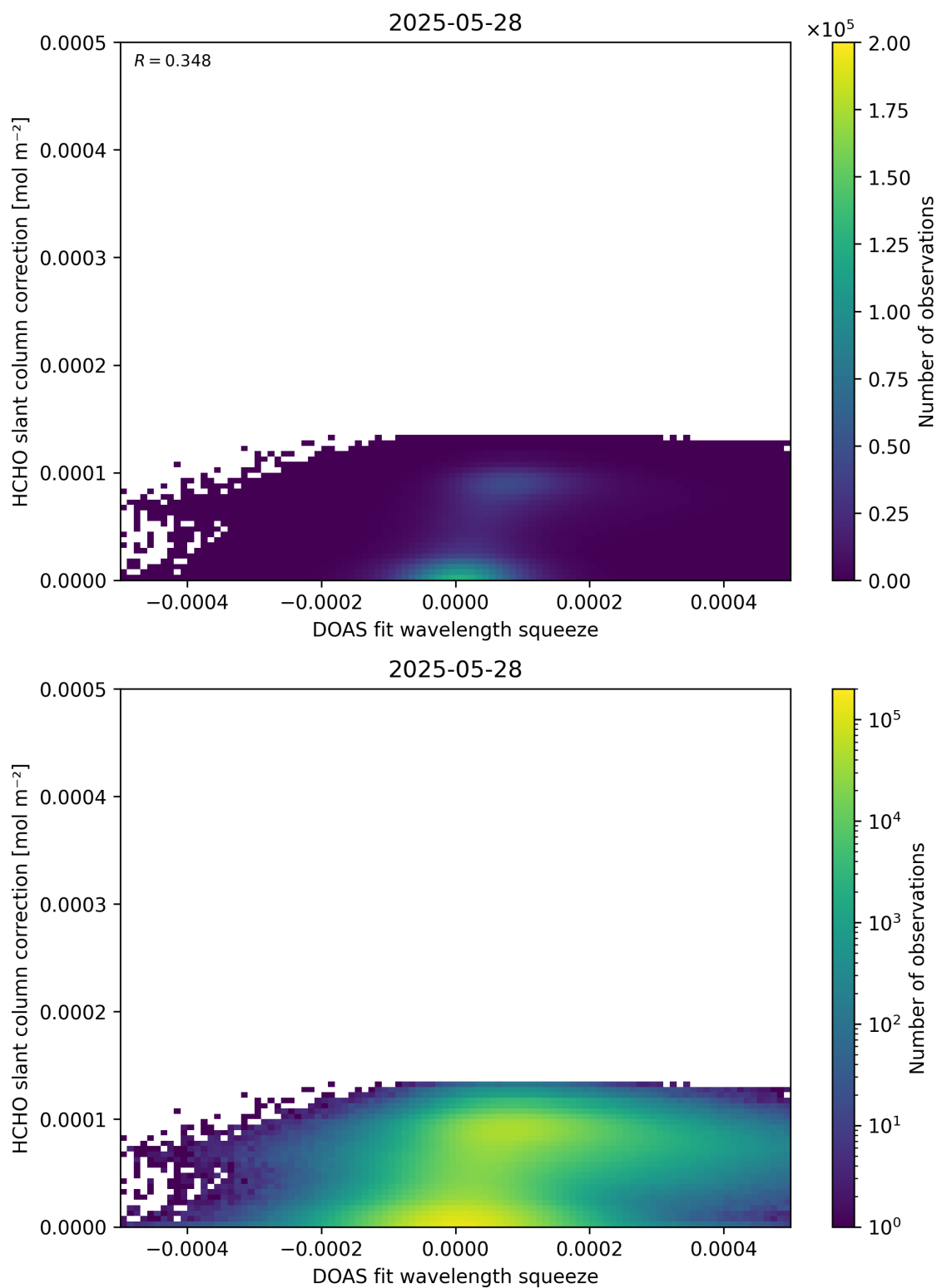
Figure 70: Scatter density plot of “DOAS fit wavelength squeeze” against “HCHO slant column correction” for 2025-05-27 to 2025-05-29.
