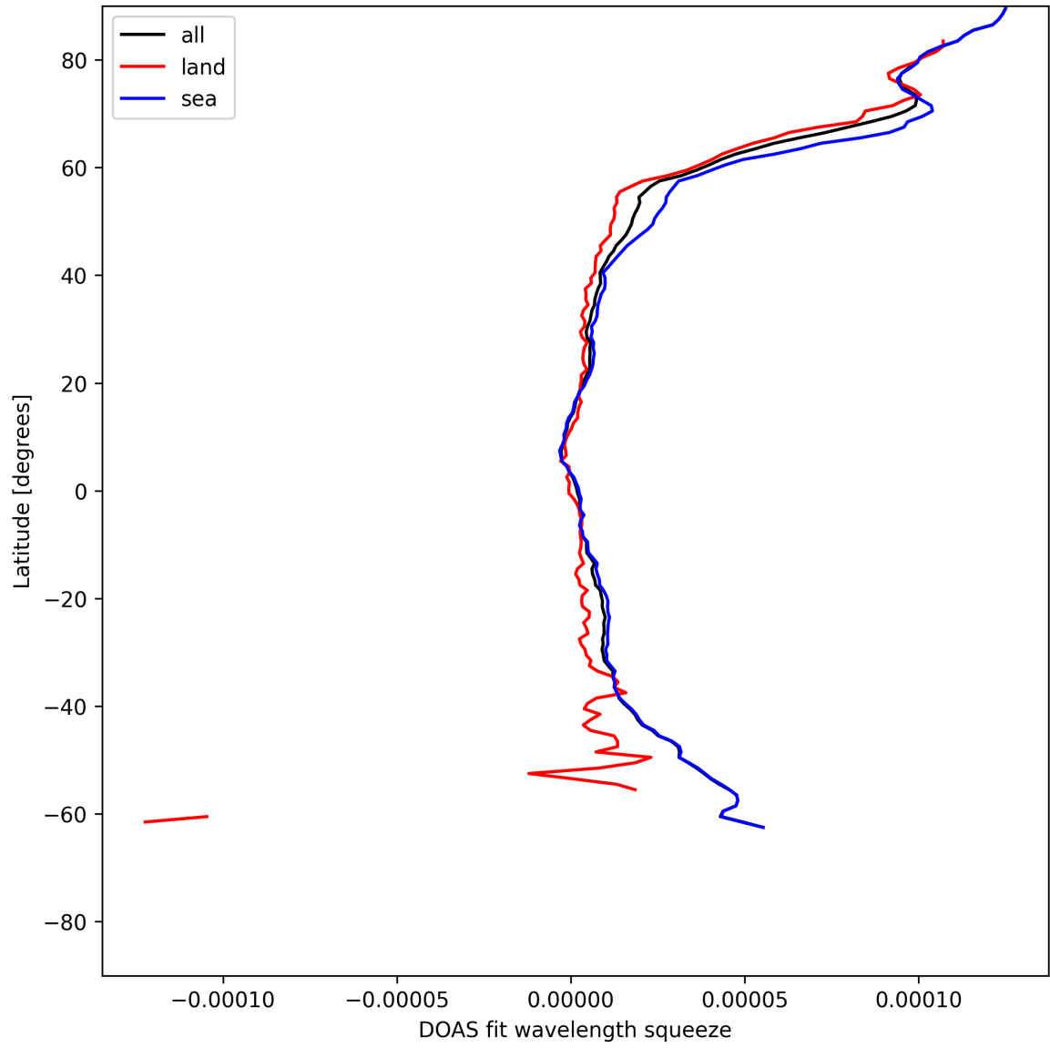
Figure 31: Zonal average of “DOAS fit wavelength squeeze” for 2025-05-27 to 2025-05-29.
