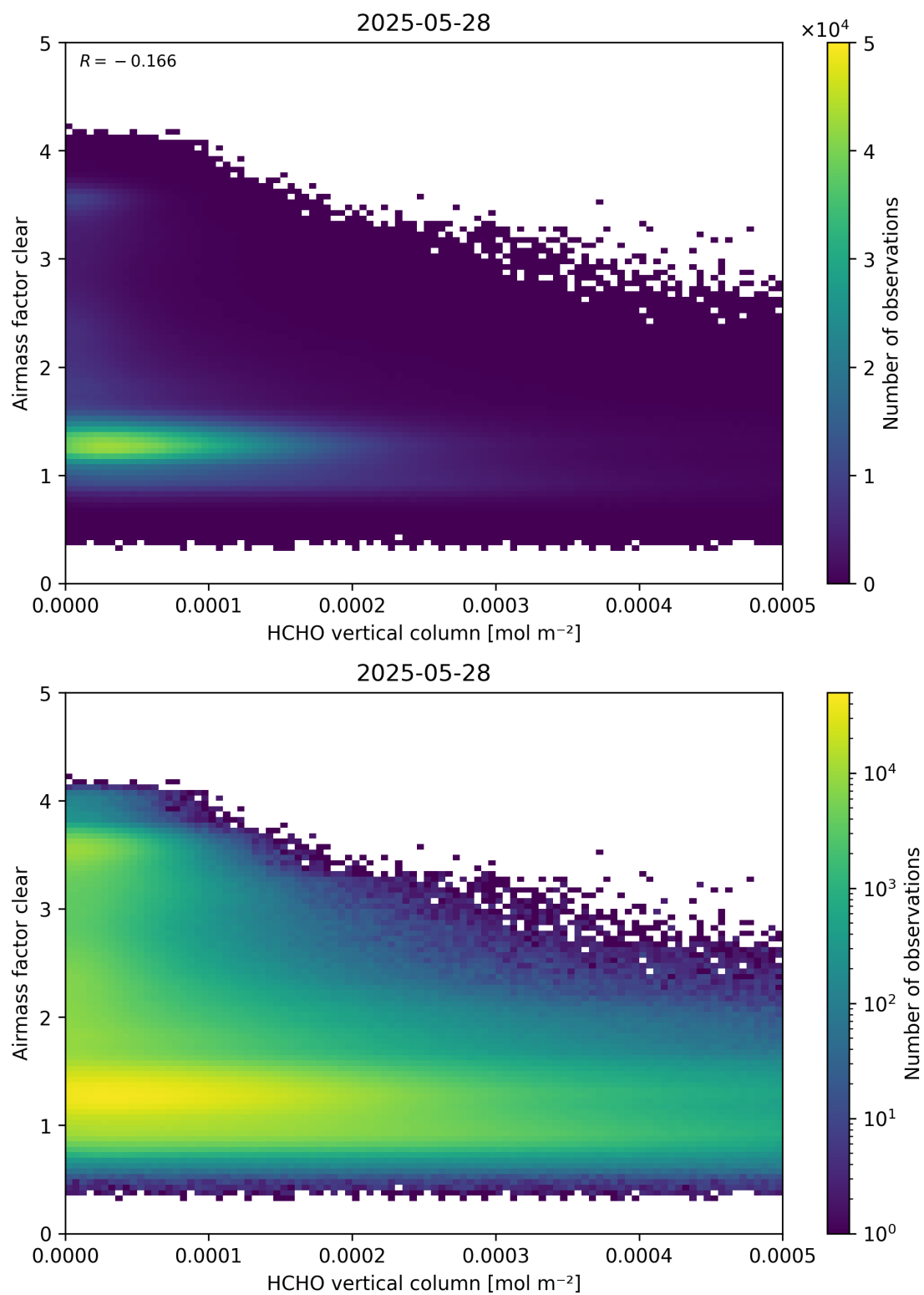
Figure 126: Scatter density plot of “HCHO vertical column” against “Airmass factor clear” for 2025-05-27 to 2025-05-29.
