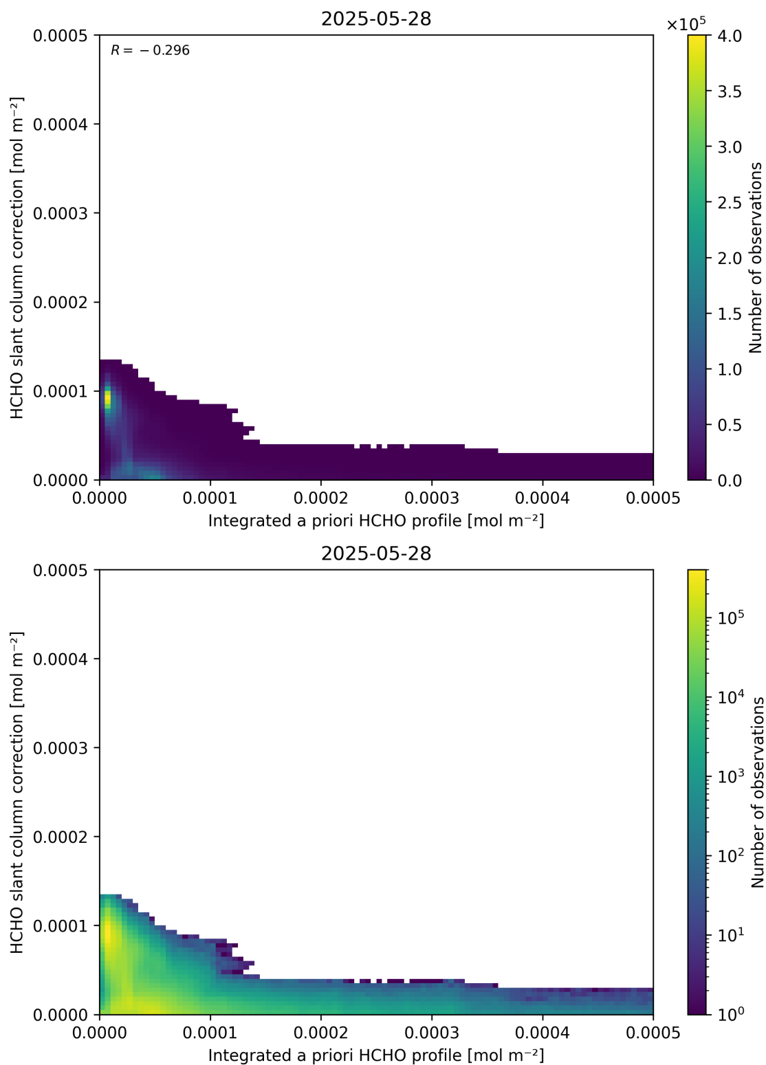
Figure 152: Scatter density plot of “Integrated a priori HCHO profile” against “HCHO slant column correction” for 2025-05-27 to 2025-05-29.
