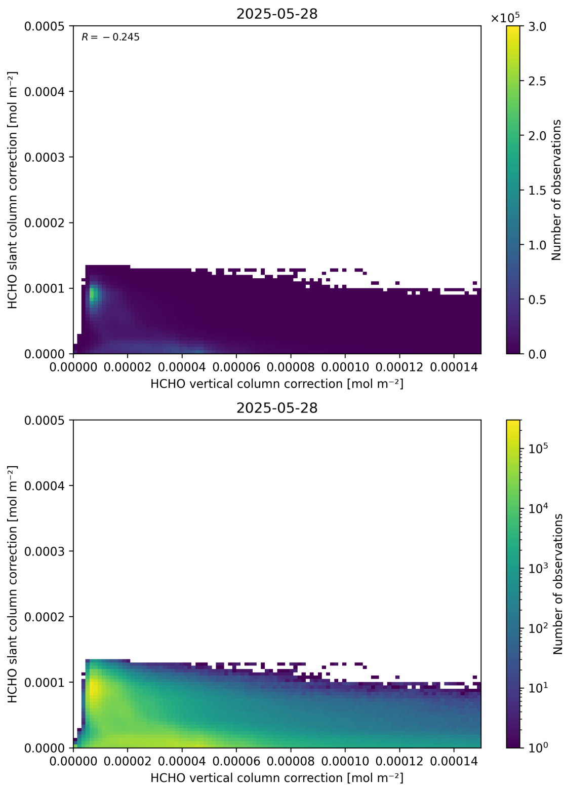
Figure 117: Scatter density plot of “HCHO vertical column correction” against “HCHO slant column correction” for 2025-05-27 to 2025-05-29.
