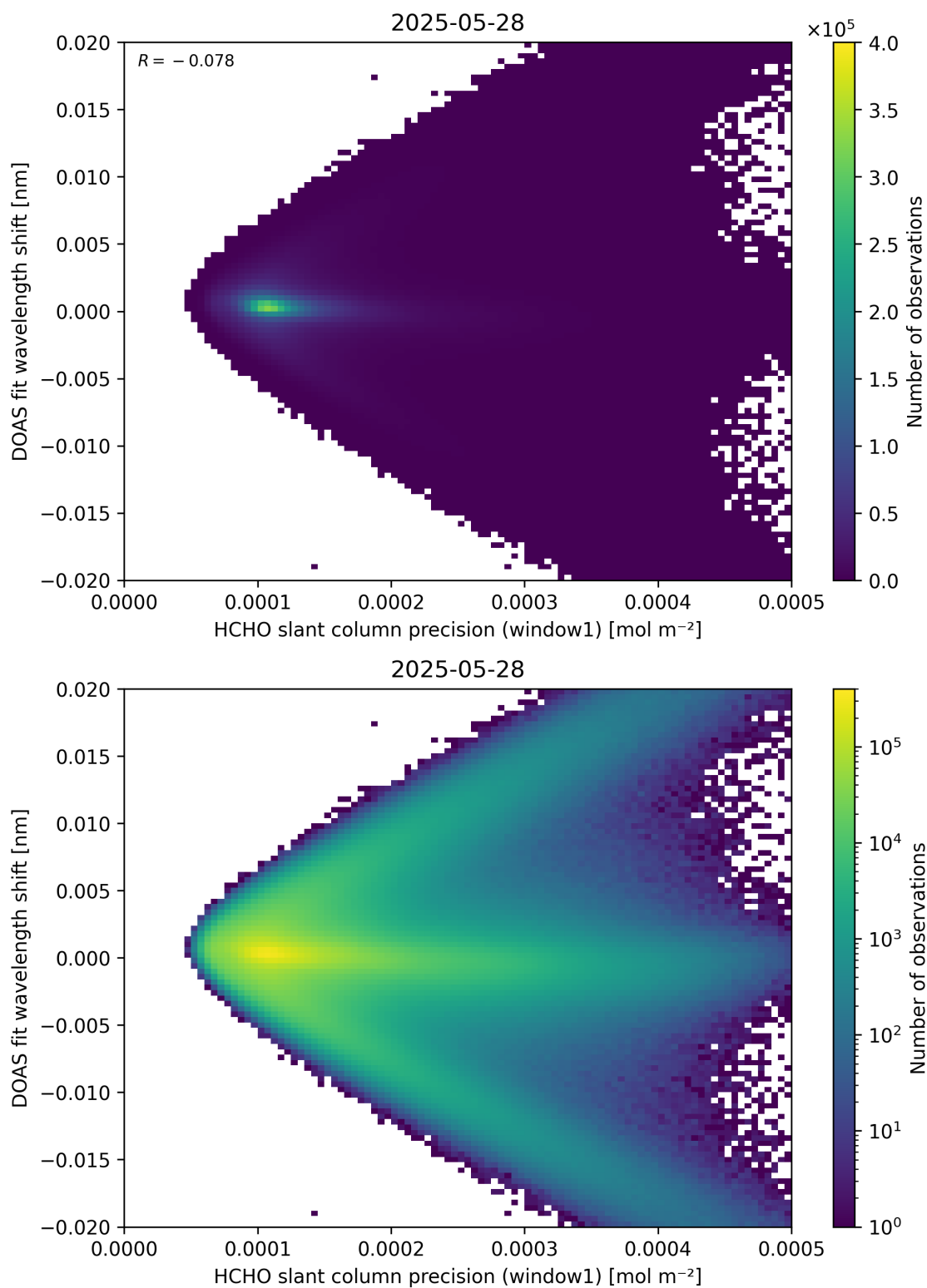
Figure 89: Scatter density plot of “HCHO slant column precision (window1)” against “DOAS fit wavelength shift” for 2025-05-27 to 2025-05-29.
