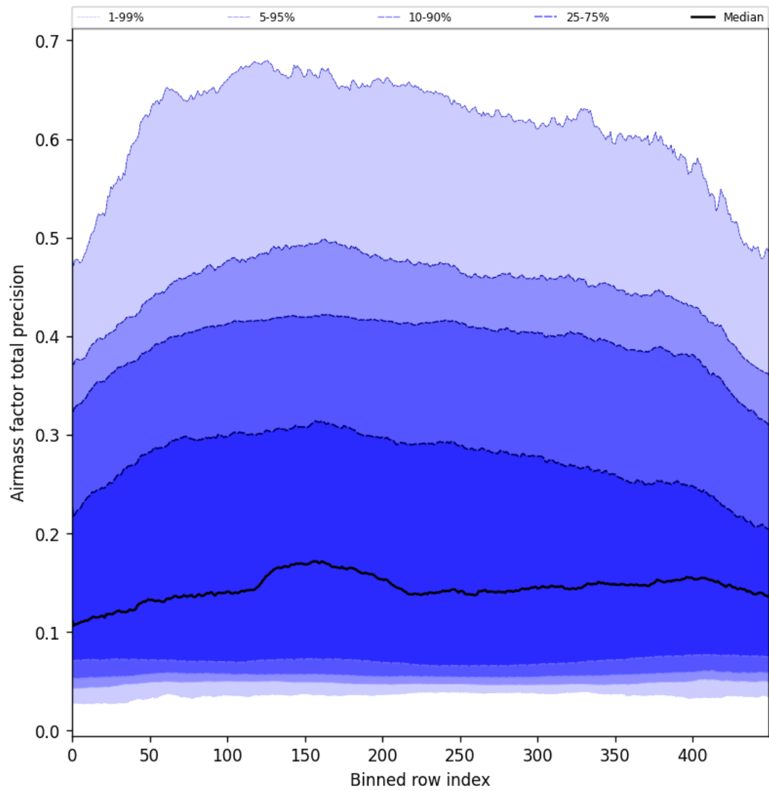
Figure 55: Along track statistics of “Airmass factor total precision” for 2025-05-27 to 2025-05-29
