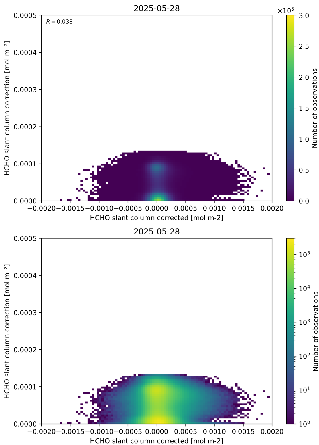
Figure 77: Scatter density plot of “HCHO slant column corrected” against “HCHO slant column correction” for 2025-05-27 to 2025-05-29.
