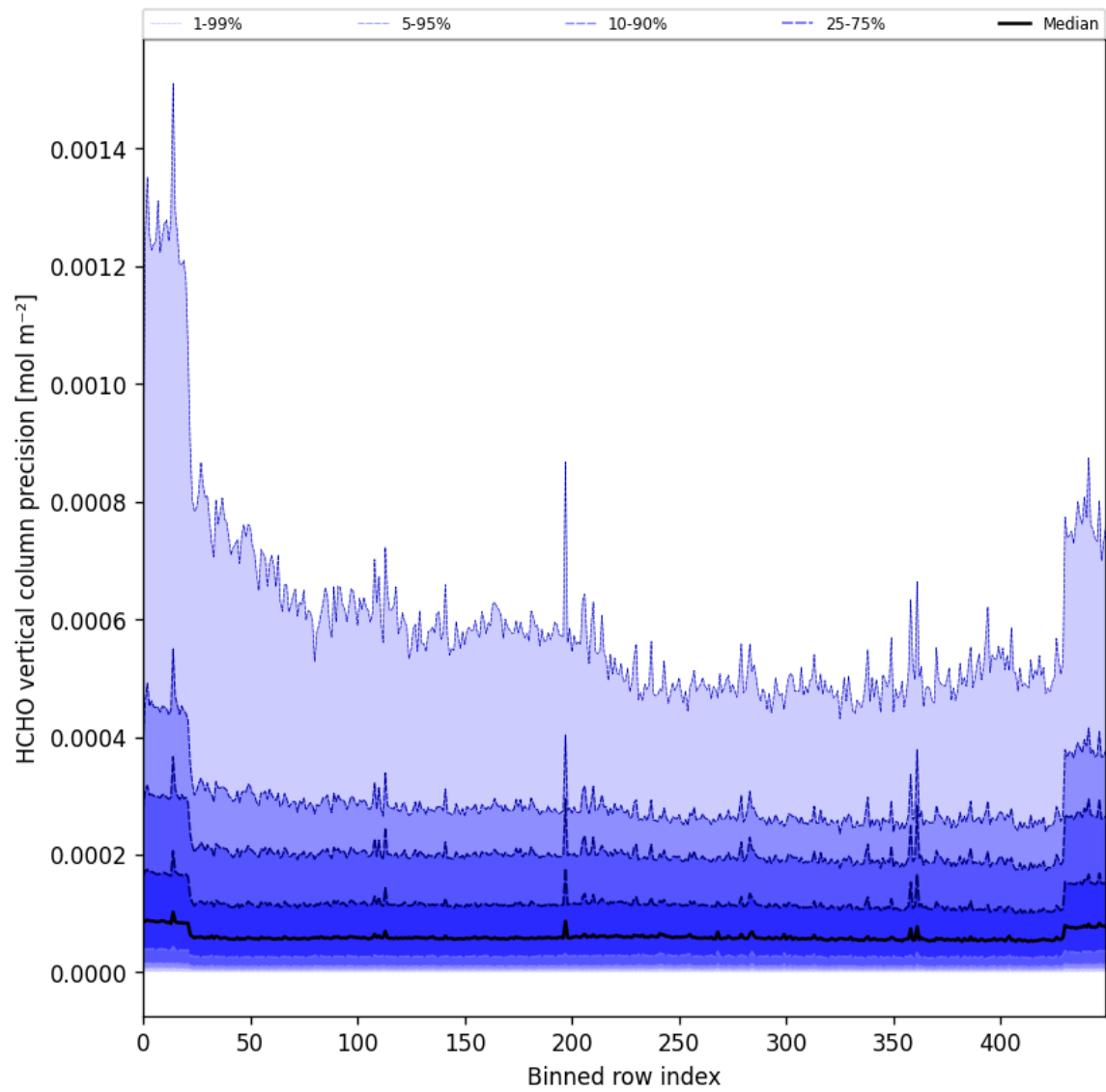
Figure 50: Along track statistics of “HCHO vertical column precision” for 2025-05-27 to 2025-05-29
