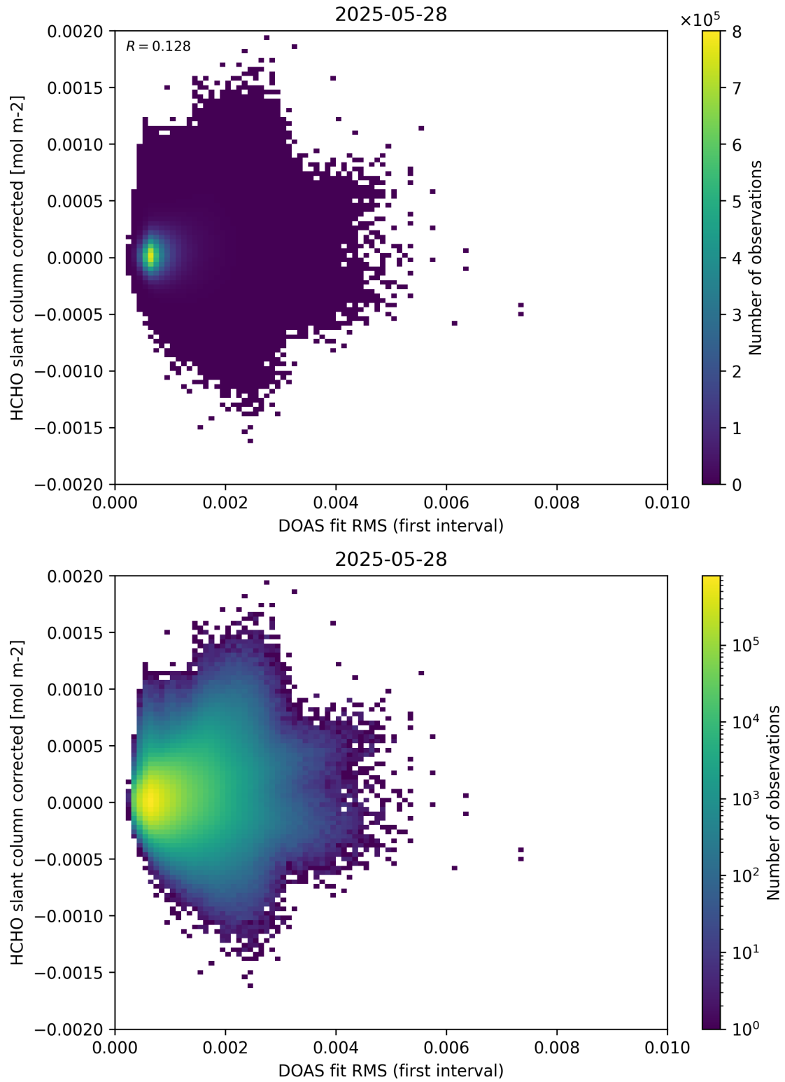
Figure 62: Scatter density plot of “DOAS fit RMS (first interval)” against “HCHO slant column corrected” for 2025-05-27 to 2025-05-29.
