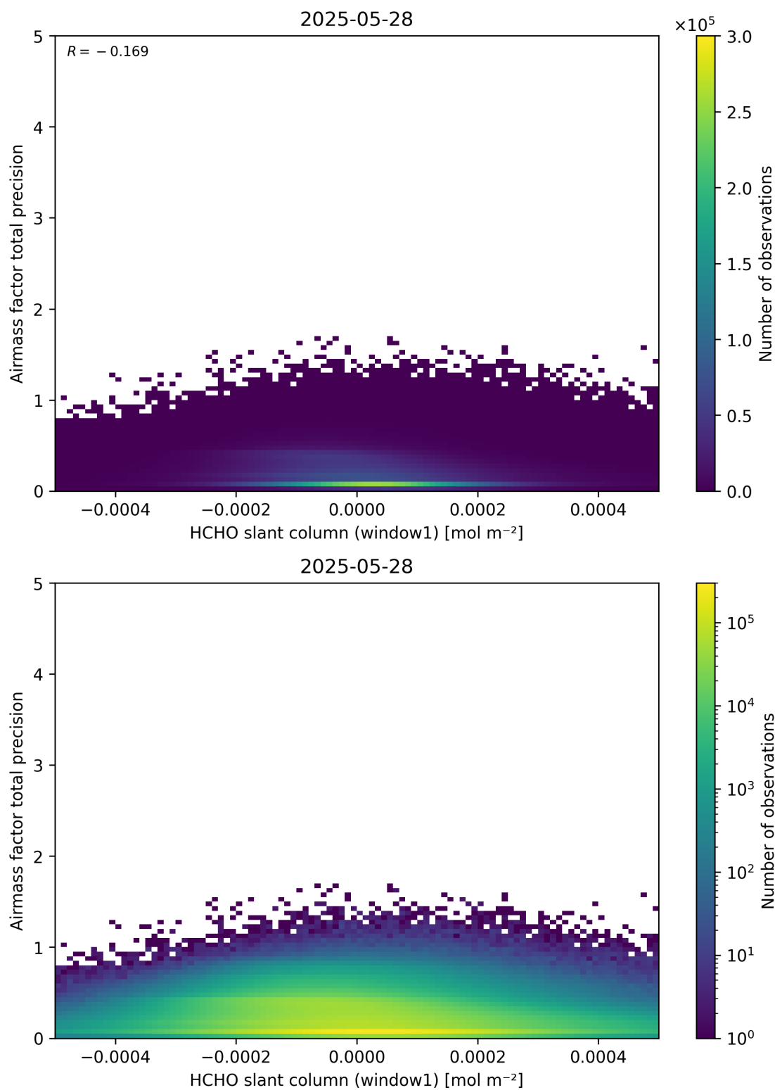
Figure 86: Scatter density plot of “HCHO slant column (window1)” against “Airmass factor total precision” for 2025-05-27 to 2025-05-29.
