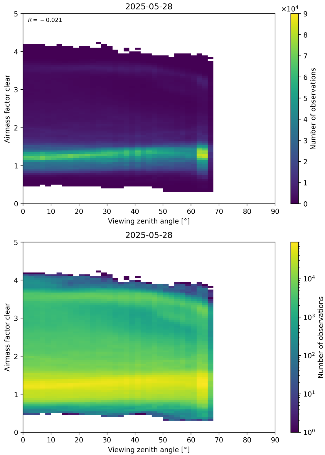
Figure 185: Scatter density plot of “Viewing zenith angle” against “Airmass factor clear” for 2025-05-27 to 2025-05-29.
