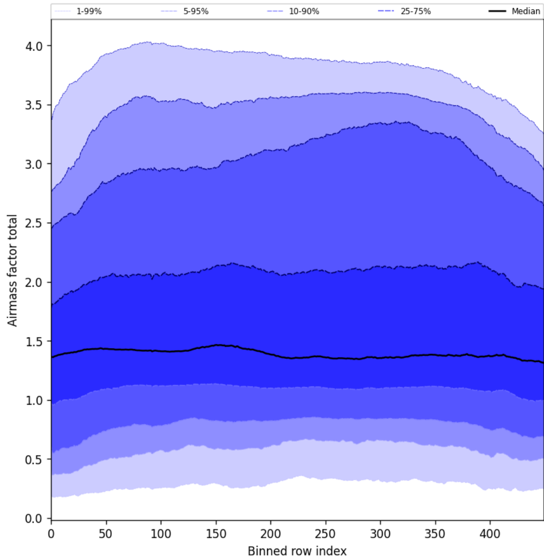
Figure 54: Along track statistics of “Airmass factor total” for 2025-05-27 to 2025-05-29
