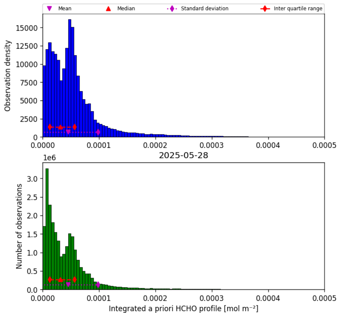
Figure 43: Histogram of “Integrated a priori HCHO profile” for 2025-05-27 to 2025-05-29
