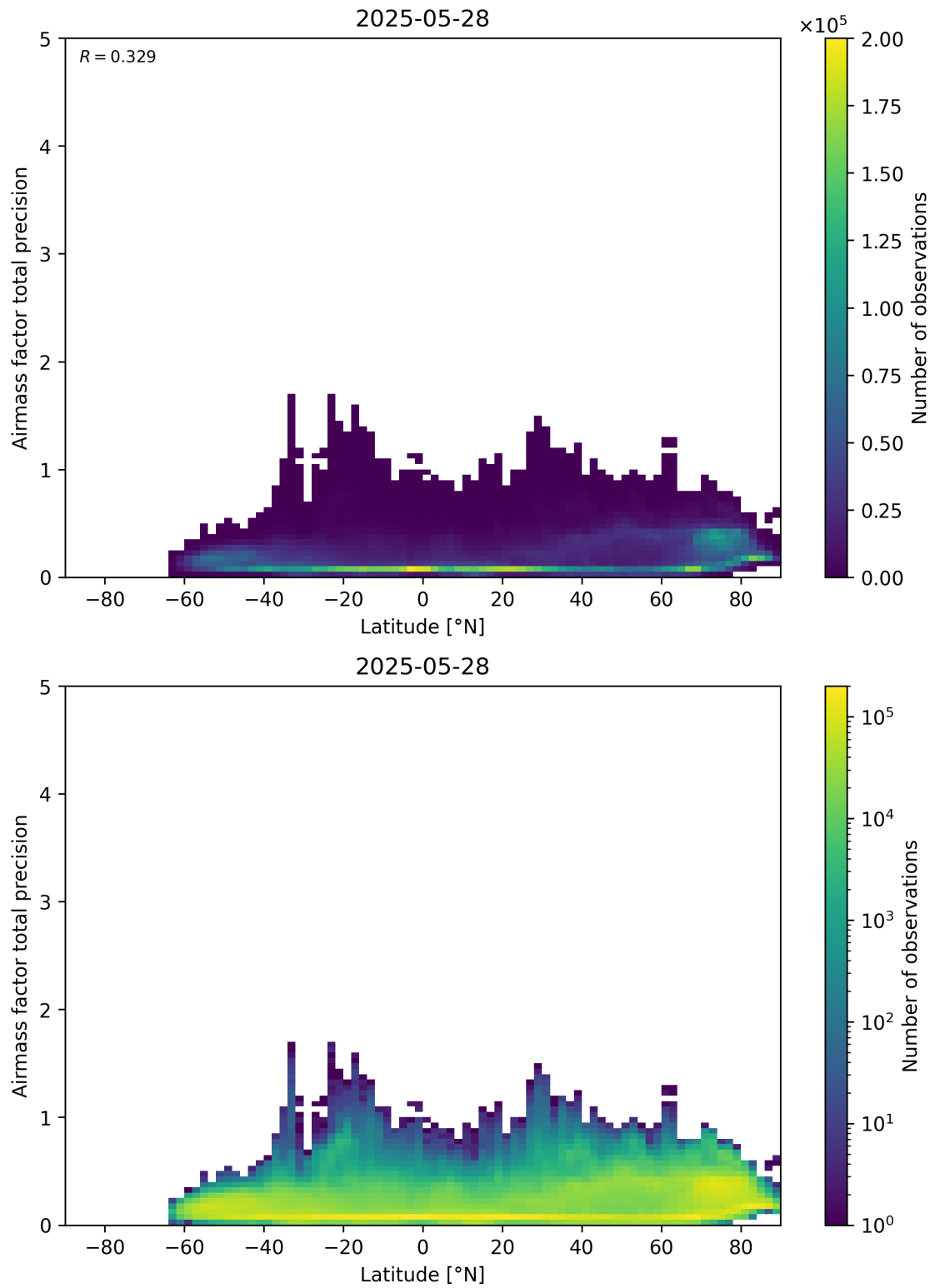
Figure 162: Scatter density plot of “Latitude” against “Airmass factor total precision” for 2025-05-27 to 2025-05-29.
