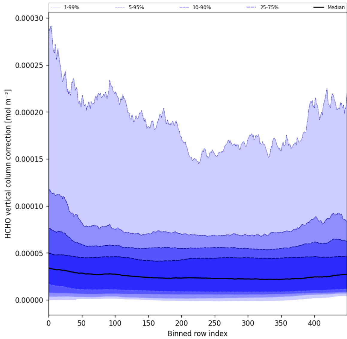
Figure 51: Along track statistics of “HCHO vertical column correction” for 2025-05-27 to 2025-05-29
