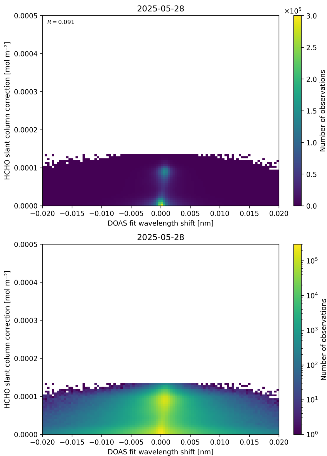
Figure 67: Scatter density plot of “DOAS fit wavelength shift” against “HCHO slant column correction” for 2025-05-27 to 2025-05-29.
