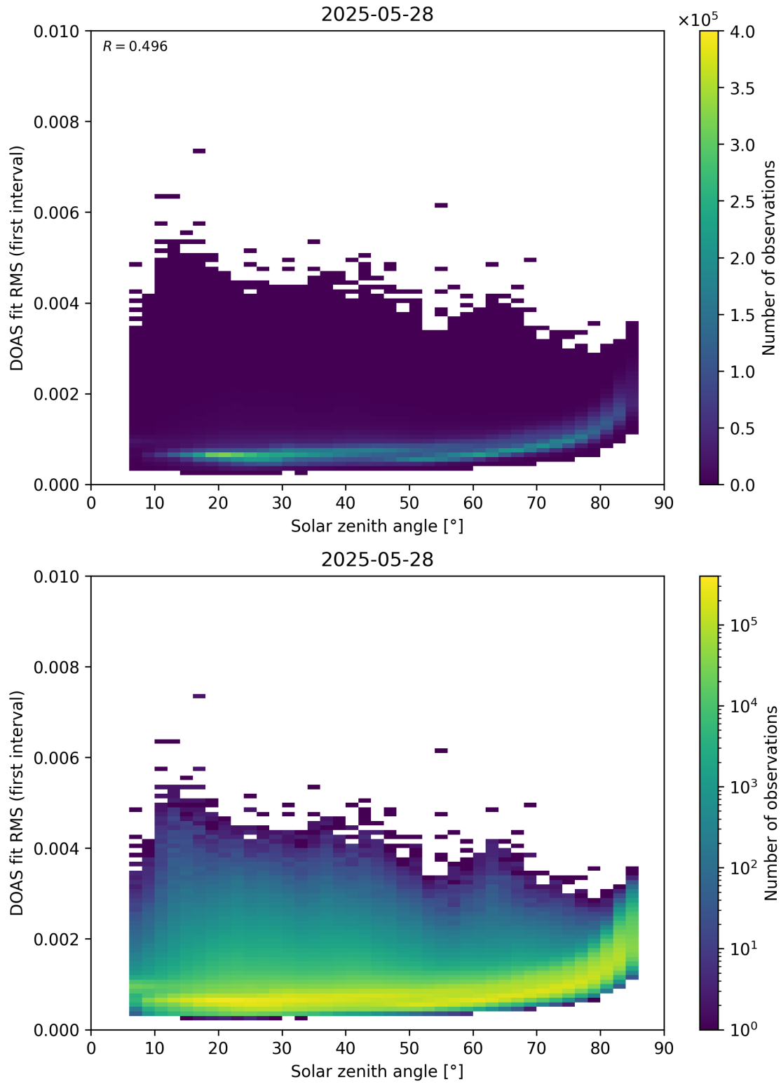
Figure 167: Scatter density plot of “Solar zenith angle” against “DOAS fit RMS (first interval)” for 2025-05-27 to 2025-05-29.
