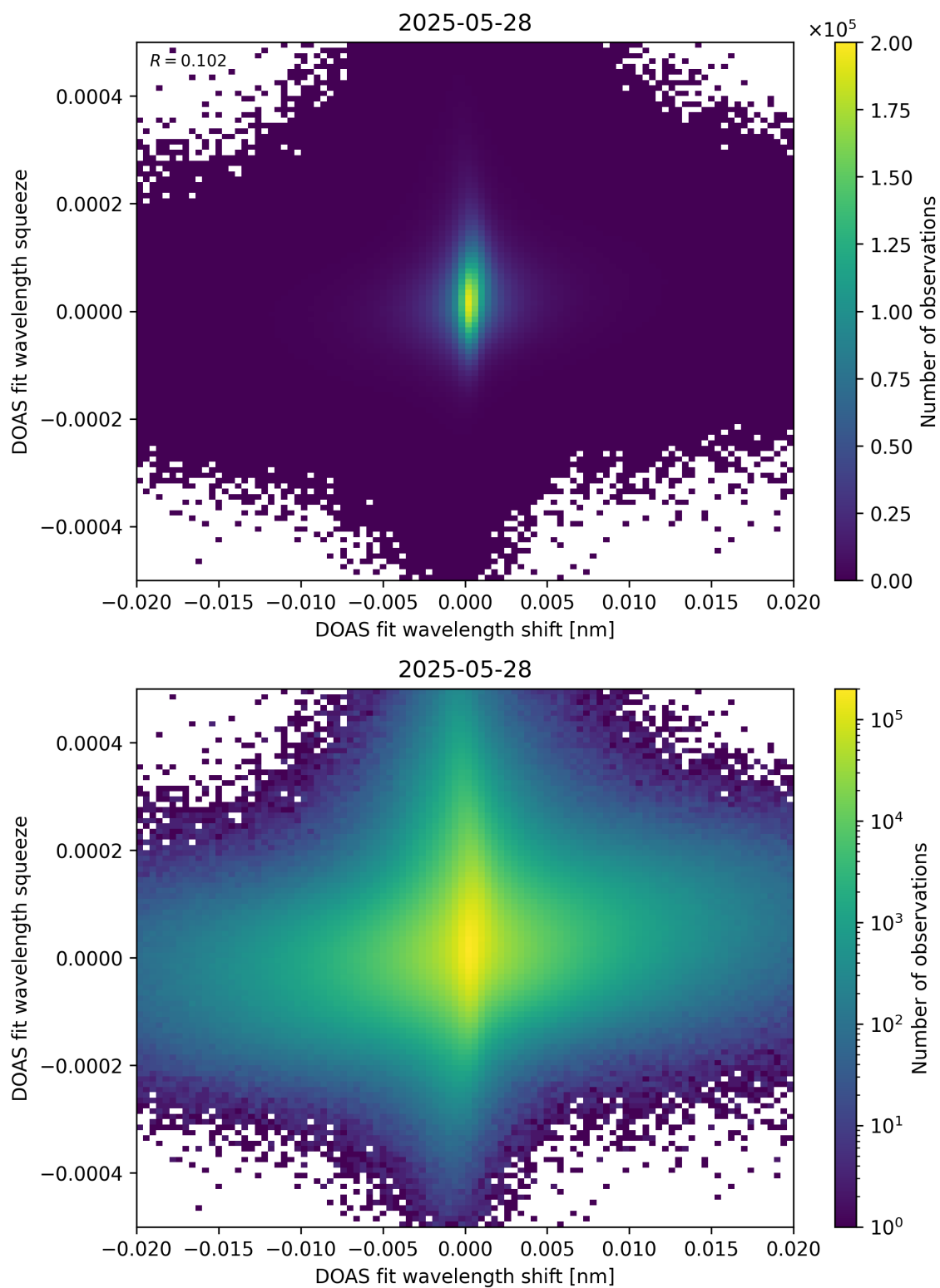
Figure 65: Scatter density plot of “DOAS fit wavelength shift” against “DOAS fit wavelength squeeze” for 2025-05-27 to 2025-05-29.
