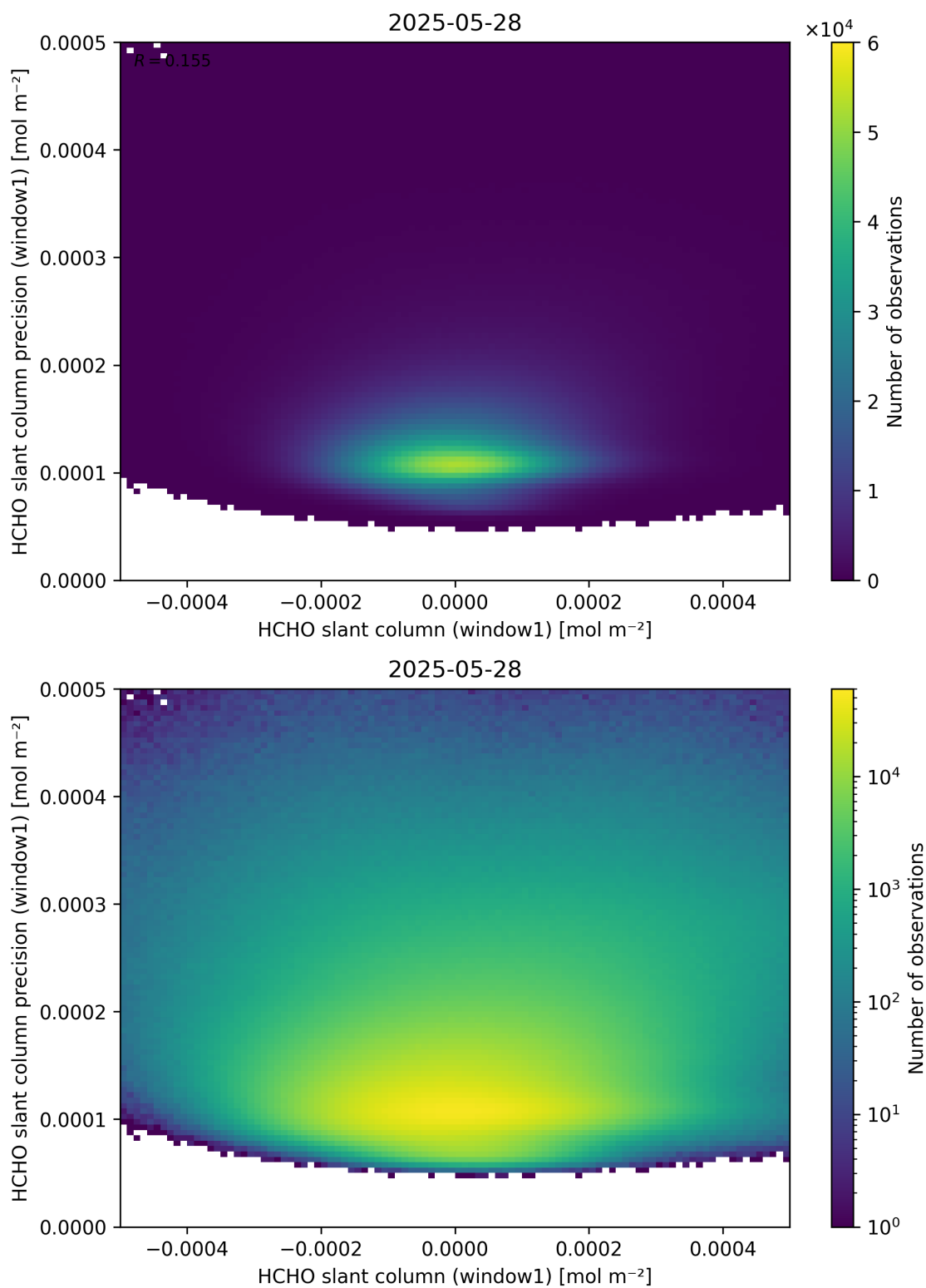
Figure 84: Scatter density plot of “HCHO slant column (window1)” against “HCHO slant column precision (window1)” for 2025-05-27 to 2025-05-29.
