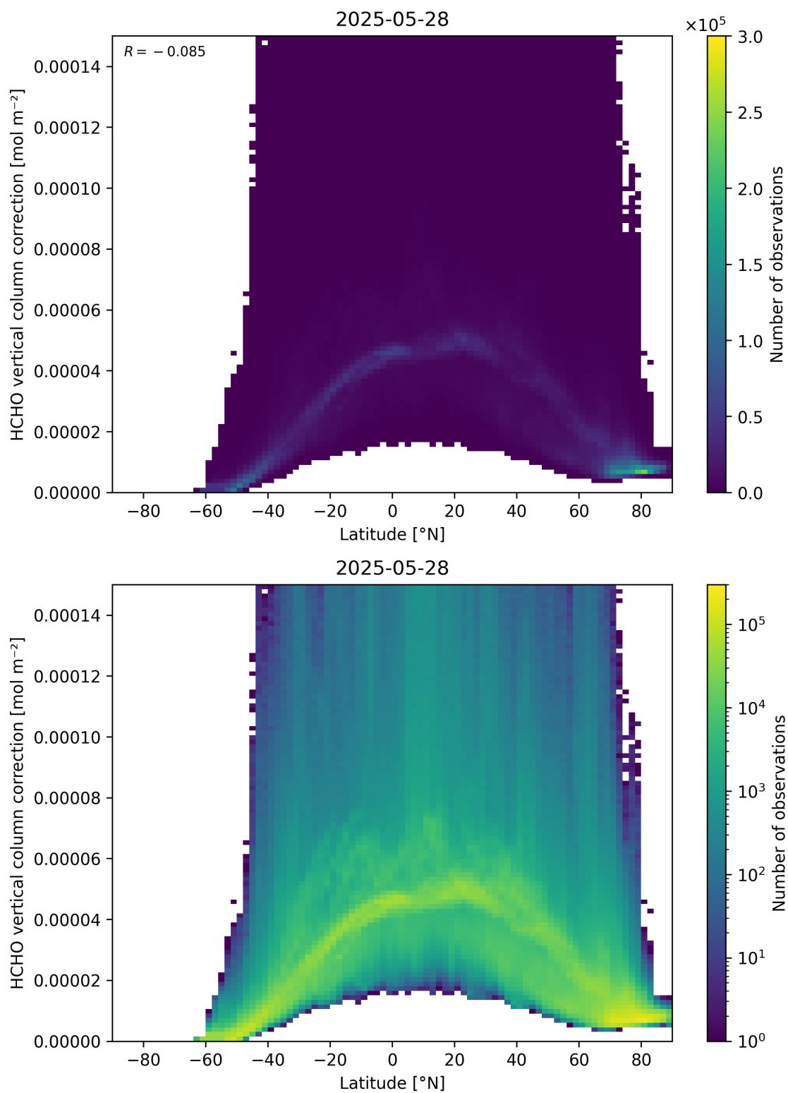
Figure 164: Scatter density plot of “Latitude” against “HCHO vertical column correction” for 2025-05-27 to 2025-05-29.
