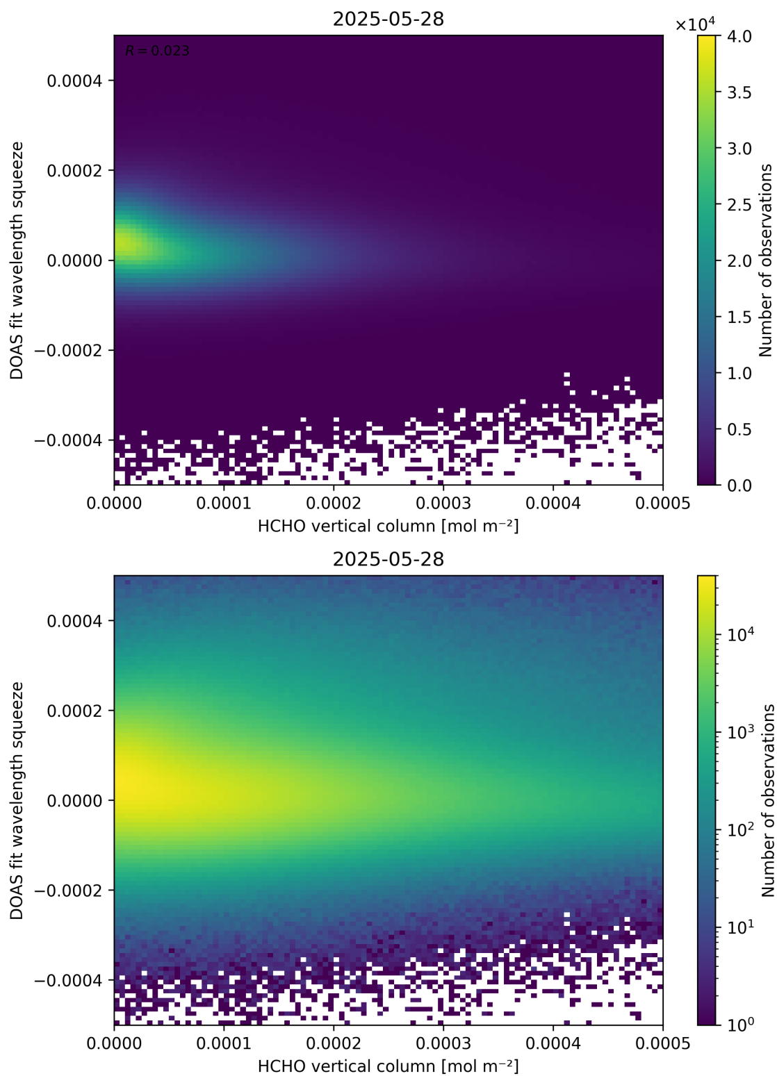
Figure 125: Scatter density plot of “HCHO vertical column” against “DOAS fit wavelength squeeze” for 2025-05-27 to 2025-05-29.
