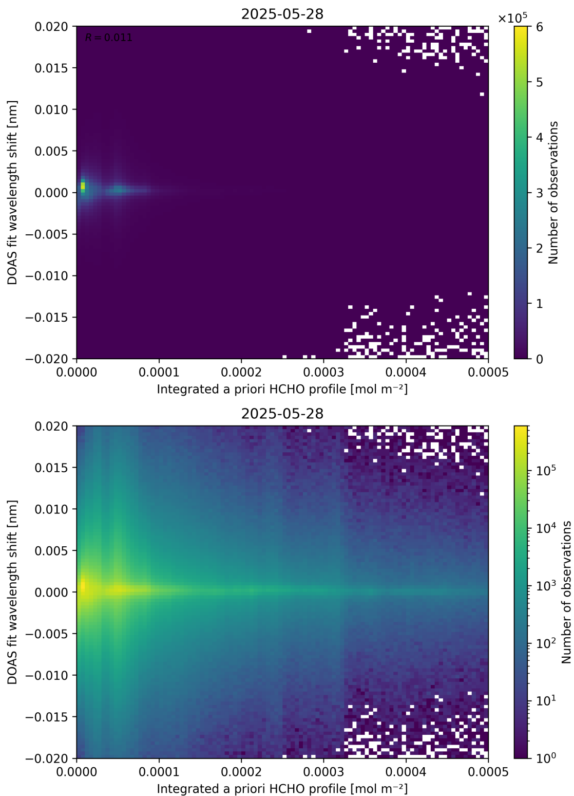
Figure 149: Scatter density plot of “Integrated a priori HCHO profile” against “DOAS fit wavelength shift” for 2025-05-27 to 2025-05-29.
