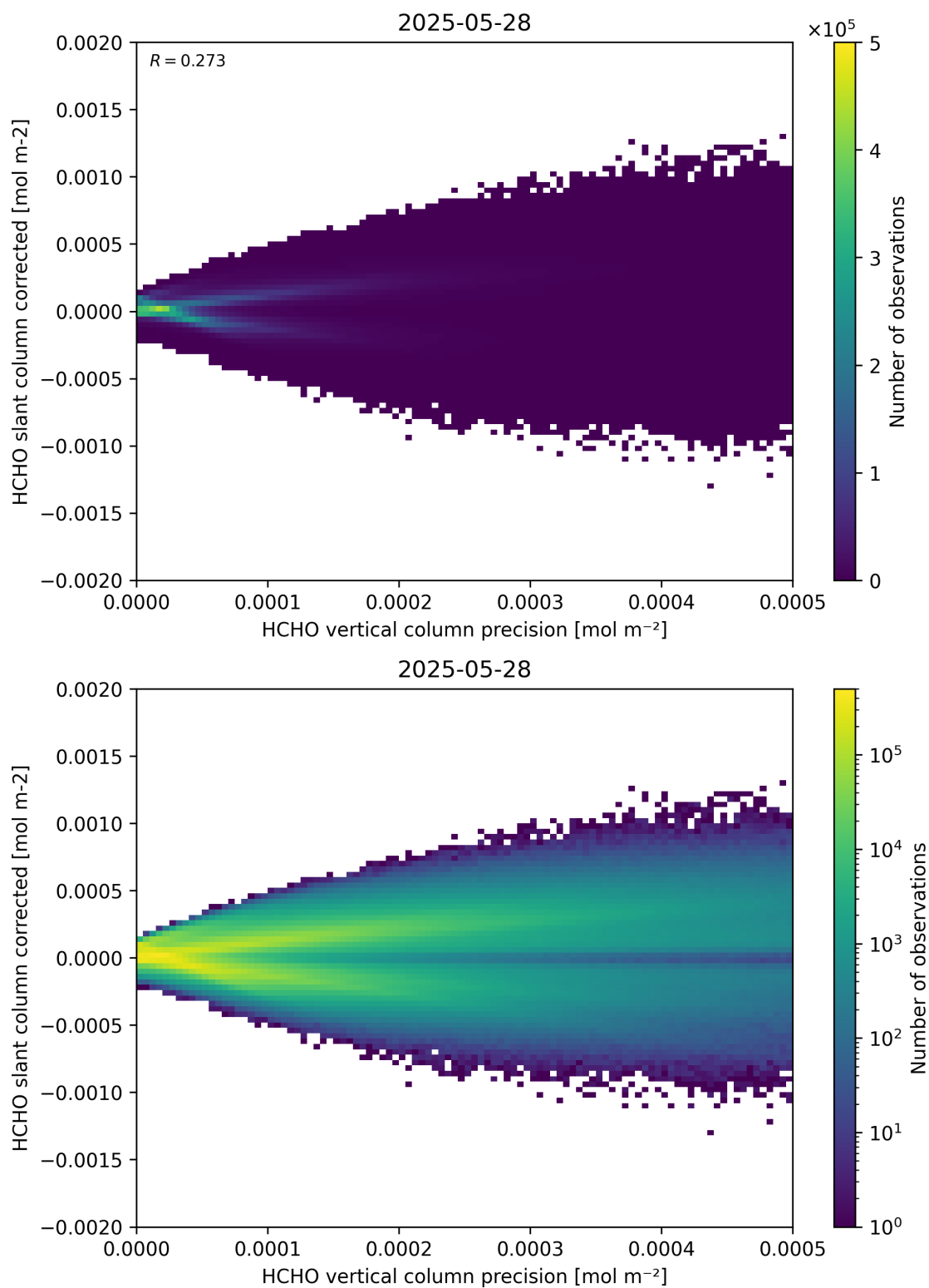
Figure 140: Scatter density plot of “HCHO vertical column precision” against “HCHO slant column corrected” for 2025-05-27 to 2025-05-29.
