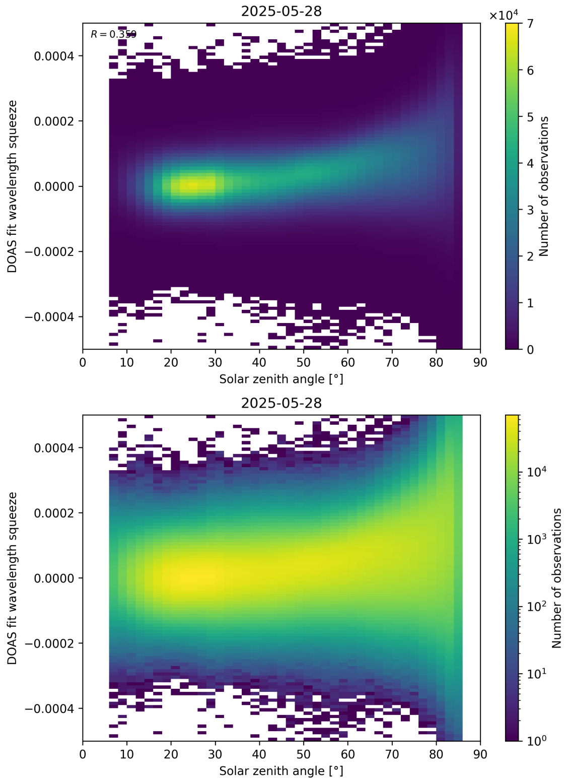
Figure 169: Scatter density plot of “Solar zenith angle” against “DOAS fit wavelength squeeze” for 2025-05-27 to 2025-05-29.
