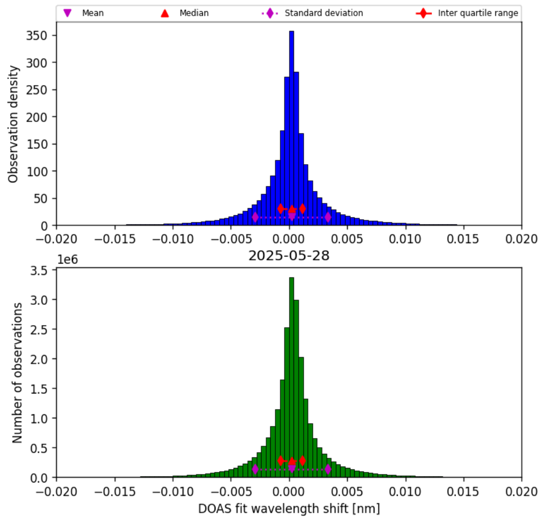
Figure 44: Histogram of “DOAS fit wavelength shift” for 2025-05-27 to 2025-05-29
