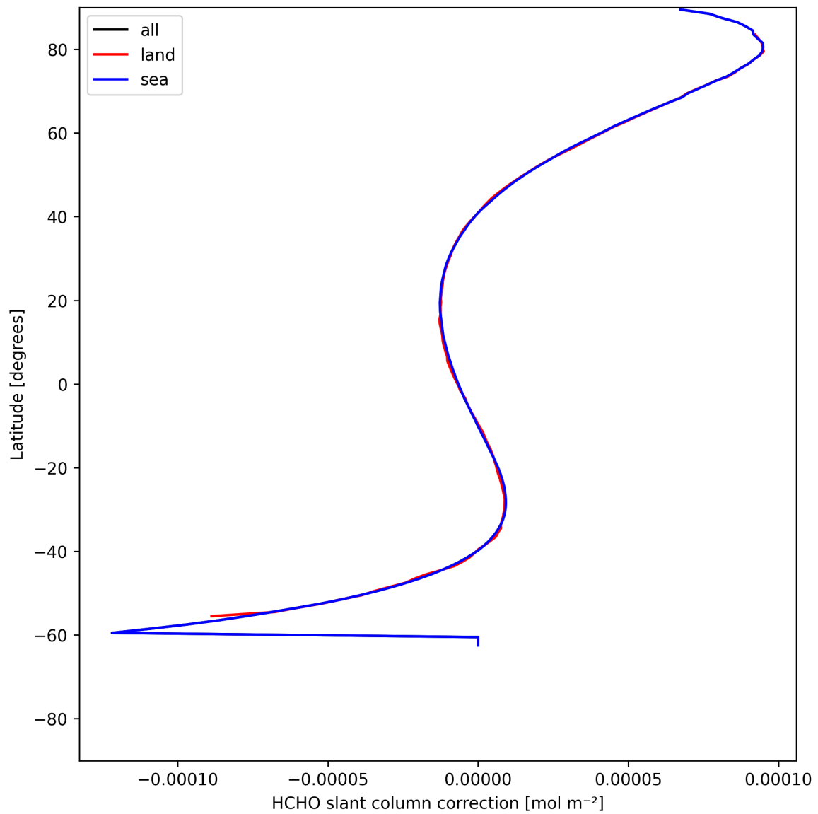
Figure 33: Zonal average of “HCHO slant column correction” for 2025-05-27 to 2025-05-29.
