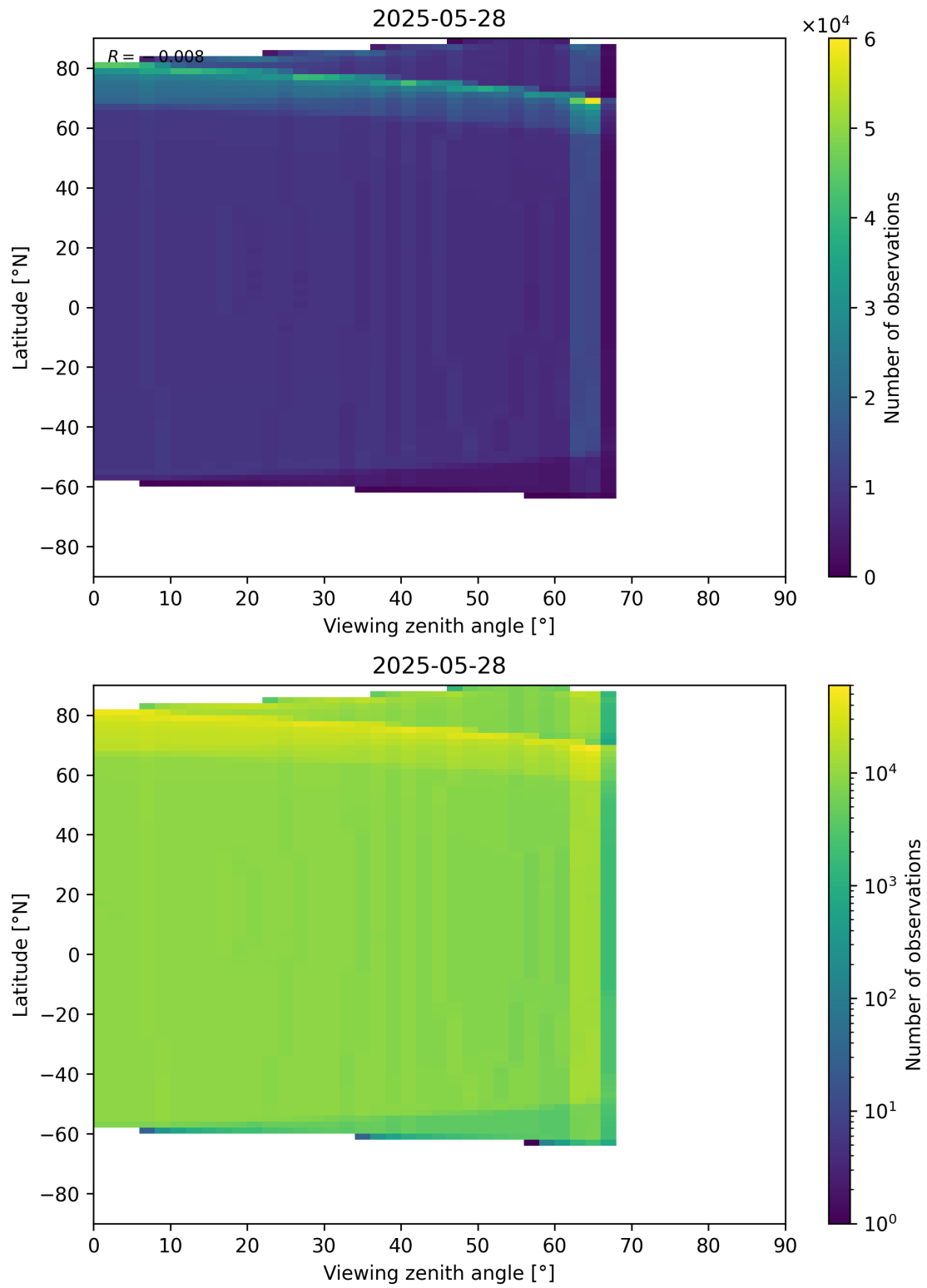
Figure 196: Scatter density plot of “Viewing zenith angle” against “Latitude” for 2025-05-27 to 2025-05-29.
