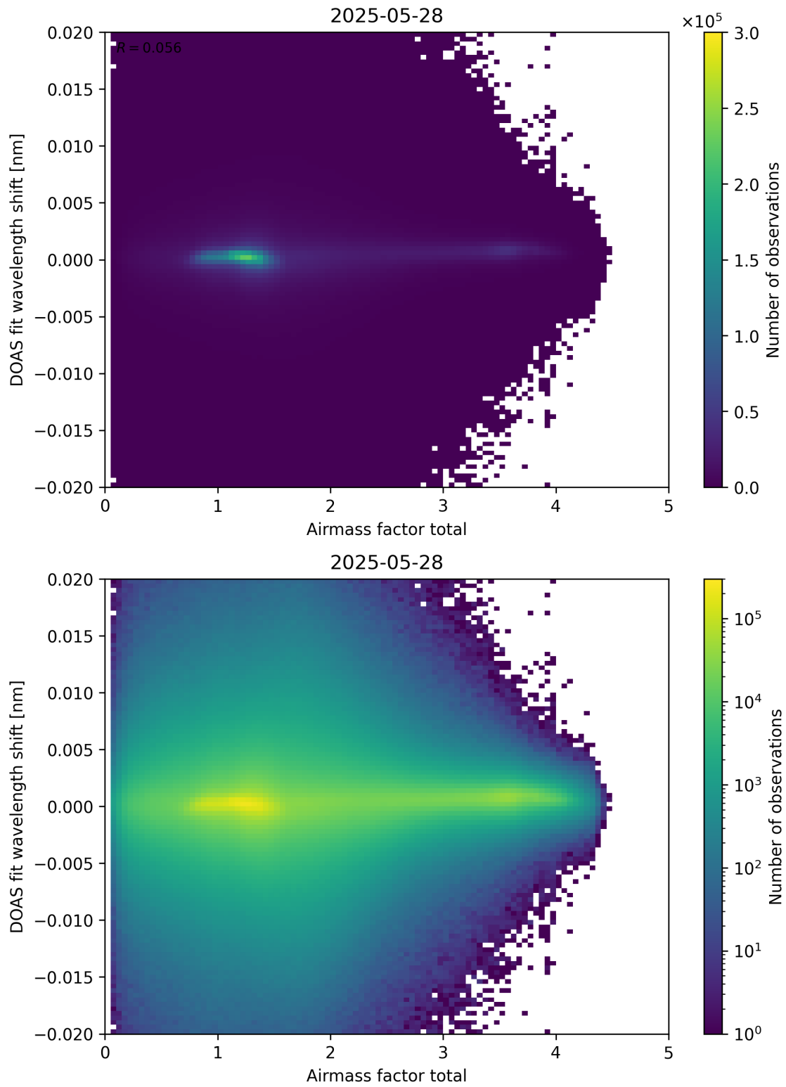
Figure 98: Scatter density plot of “Airmass factor total” against “DOAS fit wavelength shift” for 2025-05-27 to 2025-05-29.
