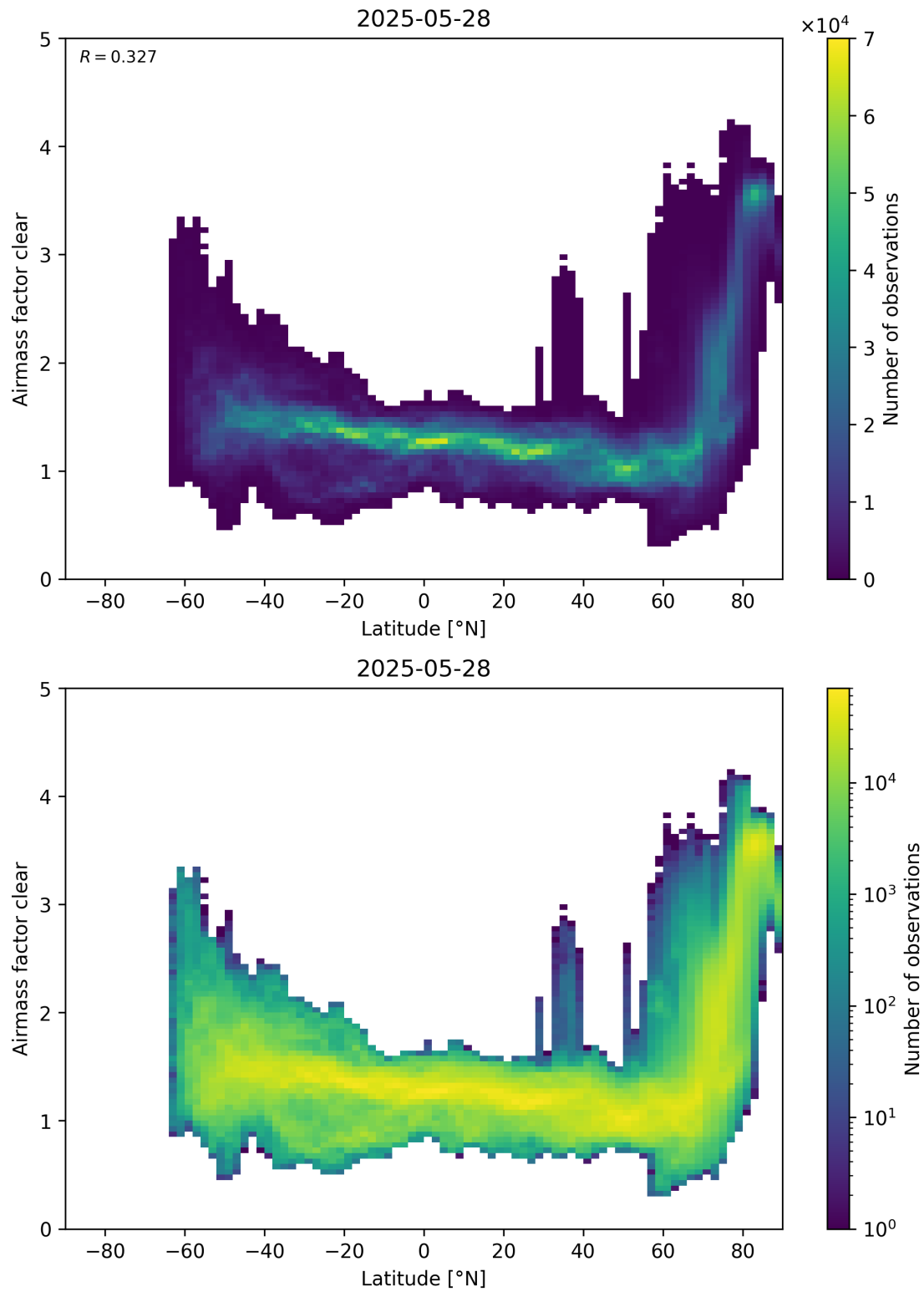
Figure 156: Scatter density plot of “Latitude” against “Airmass factor clear” for 2025-05-27 to 2025-05-29.
