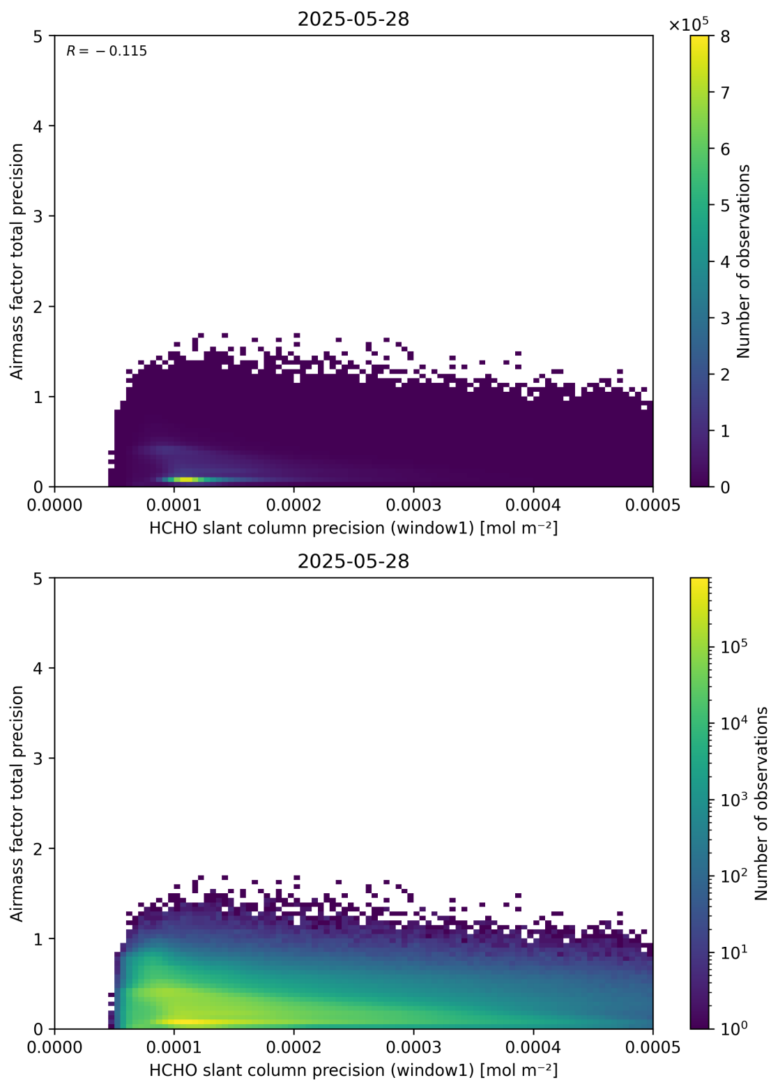
Figure 95: Scatter density plot of “HCHO slant column precision (window1)” against “Airmass factor total precision” for 2025-05-27 to 2025-05-29.
