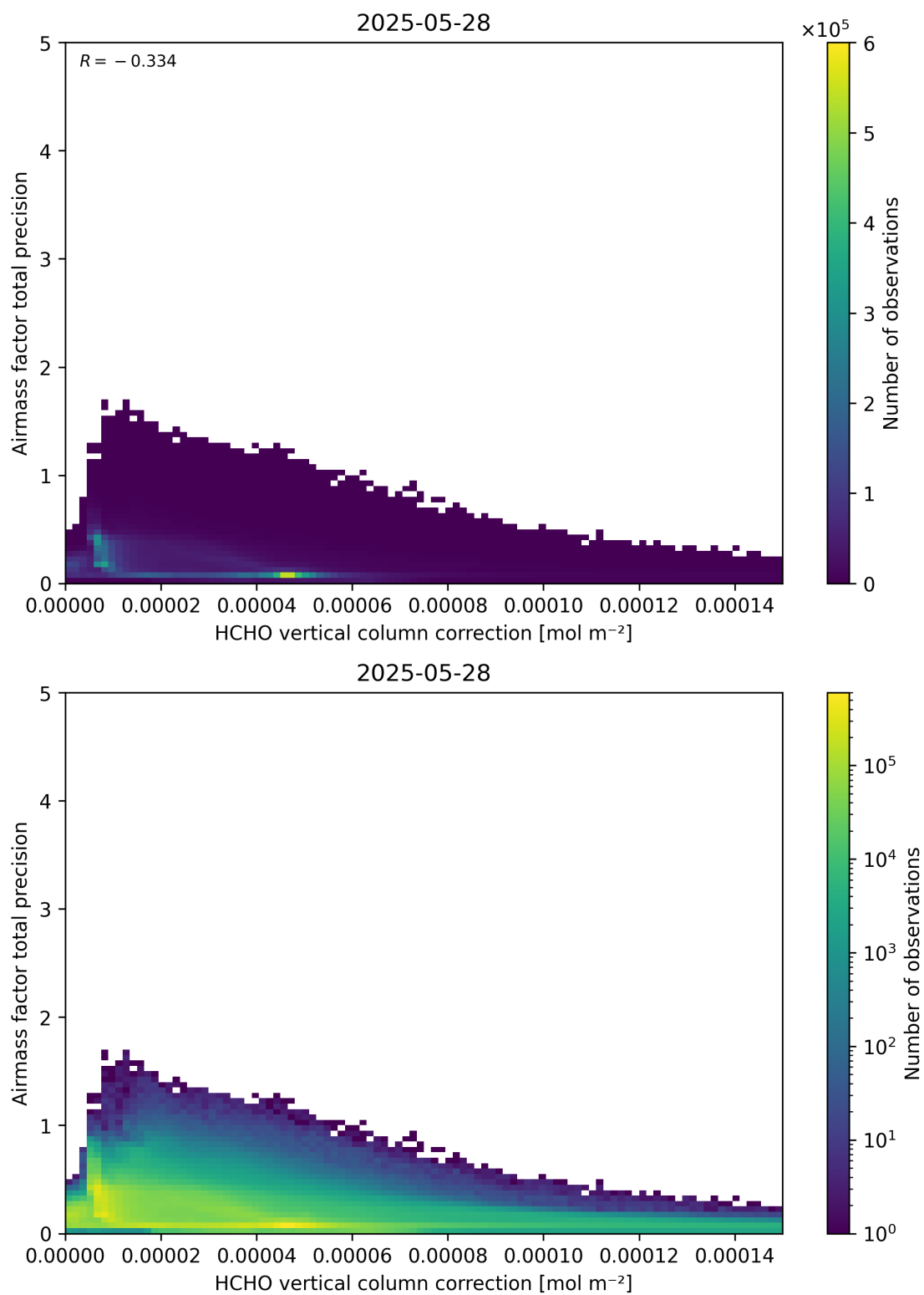
Figure 121: Scatter density plot of “HCHO vertical column correction” against “Airmass factor total precision” for 2025-05-27 to 2025-05-29.
