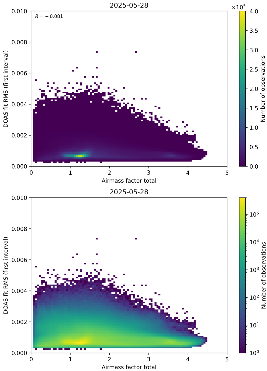
Figure 97: Scatter density plot of “Airmass factor total” against “DOAS fit RMS (first interval)” for 2025-05-27 to 2025-05-29.
