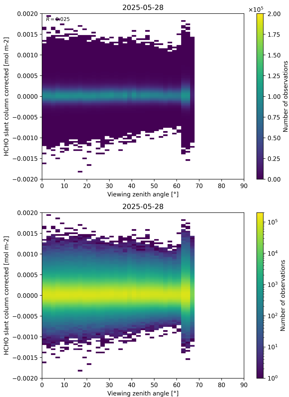
Figure 186: Scatter density plot of “Viewing zenith angle” against “HCHO slant column corrected” for 2025-05-27 to 2025-05-29.
