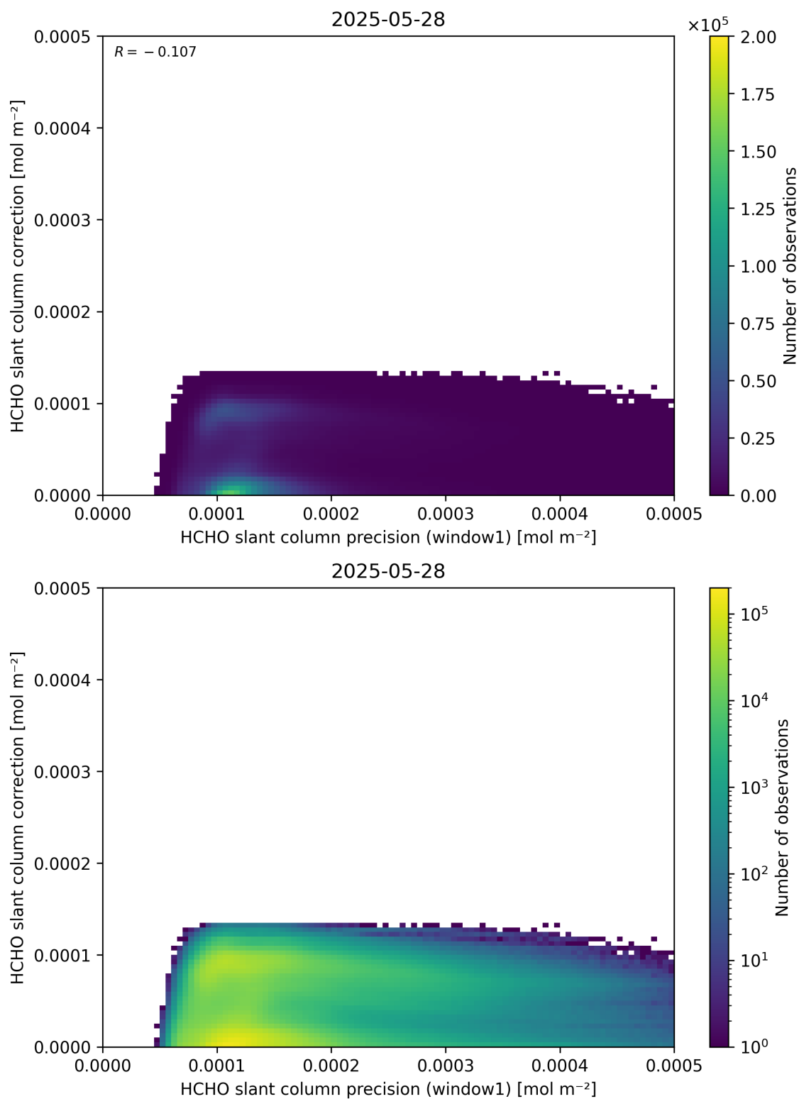
Figure 93: Scatter density plot of “HCHO slant column precision (window1)” against “HCHO slant column correction” for 2025-05-27 to 2025-05-29.
