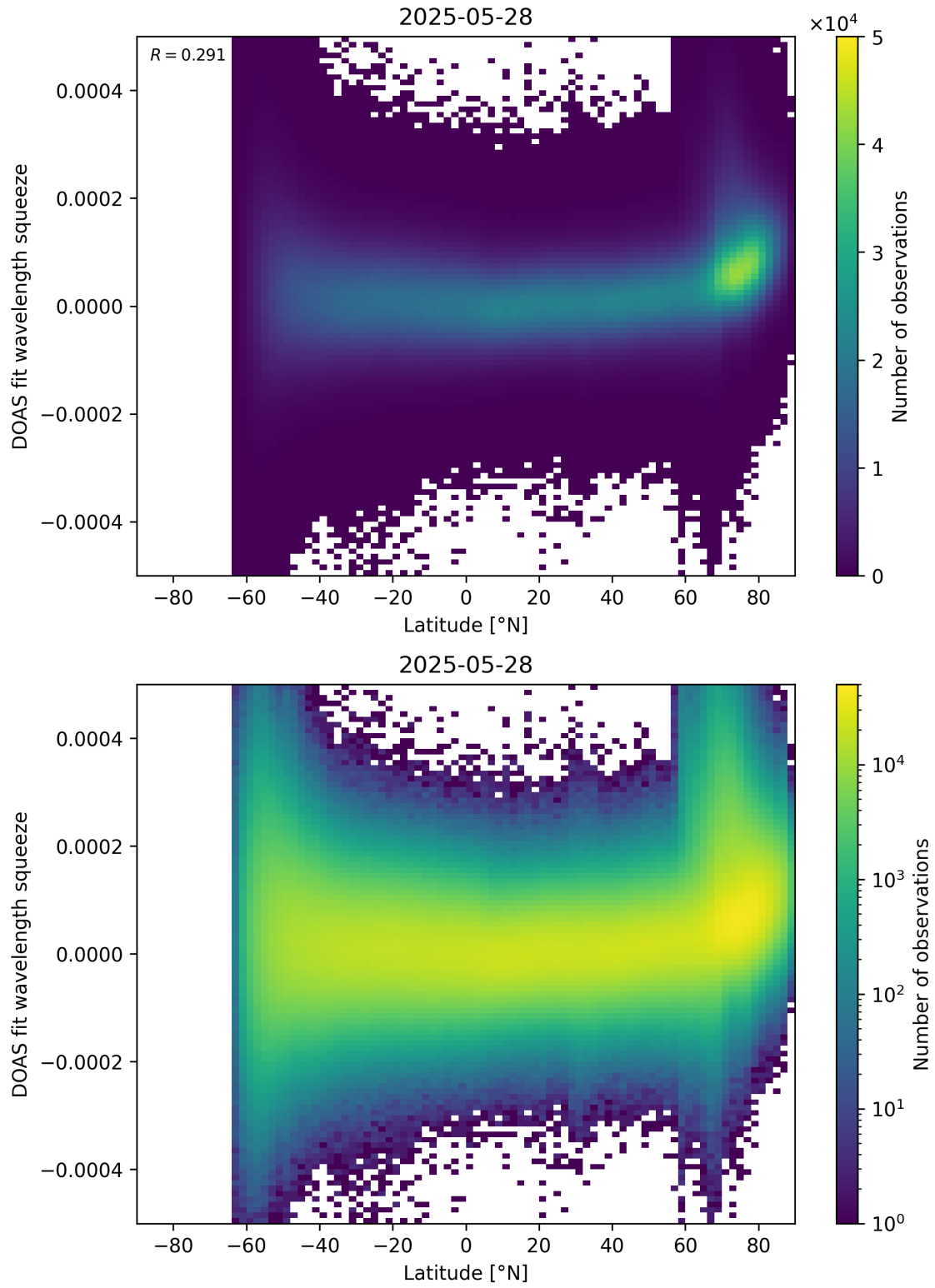
Figure 155: Scatter density plot of “Latitude” against “DOAS fit wavelength squeeze” for 2025-05-27 to 2025-05-29.
