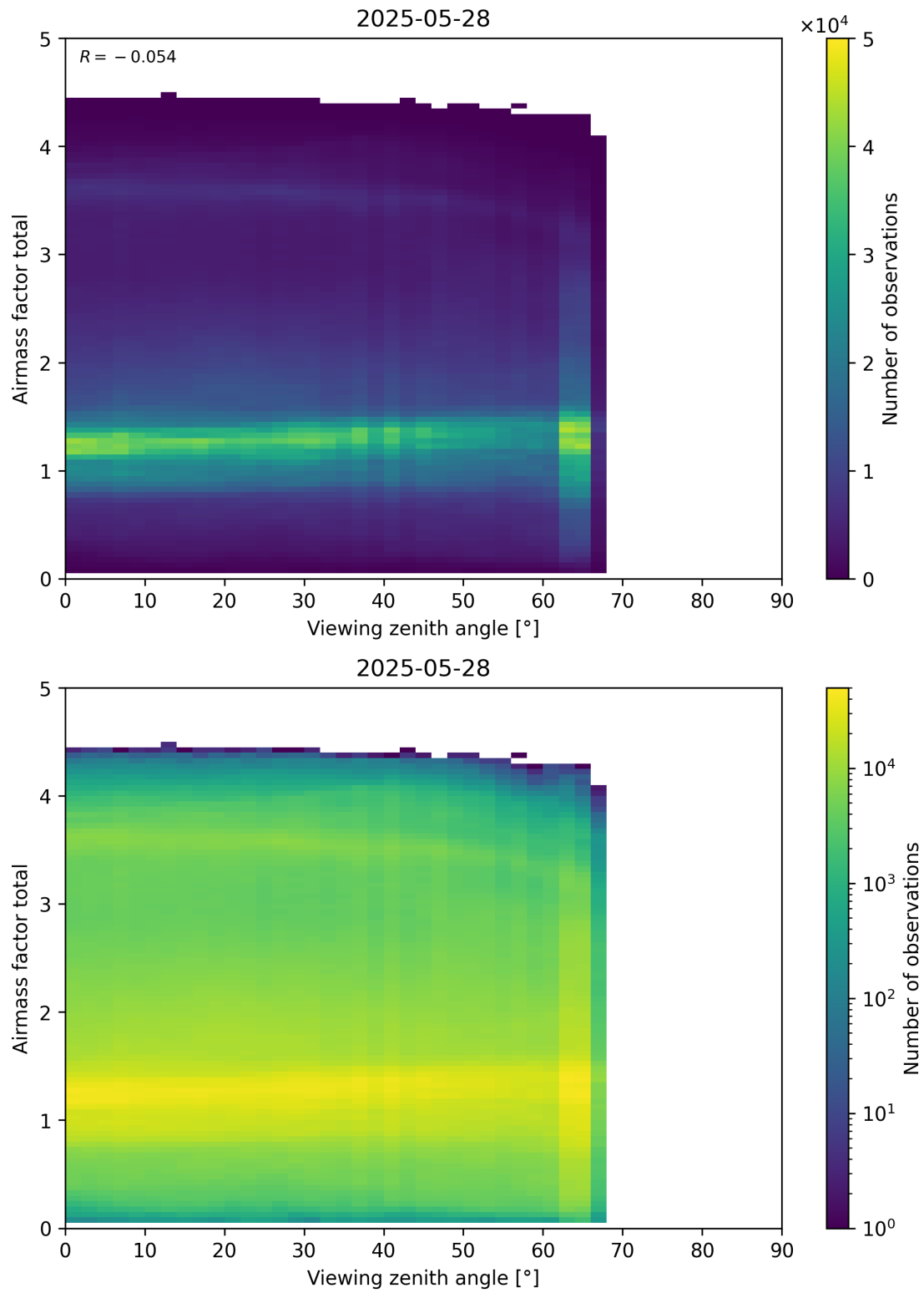
Figure 190: Scatter density plot of “Viewing zenith angle” against “Airmass factor total” for 2025-05-27 to 2025-05-29.
