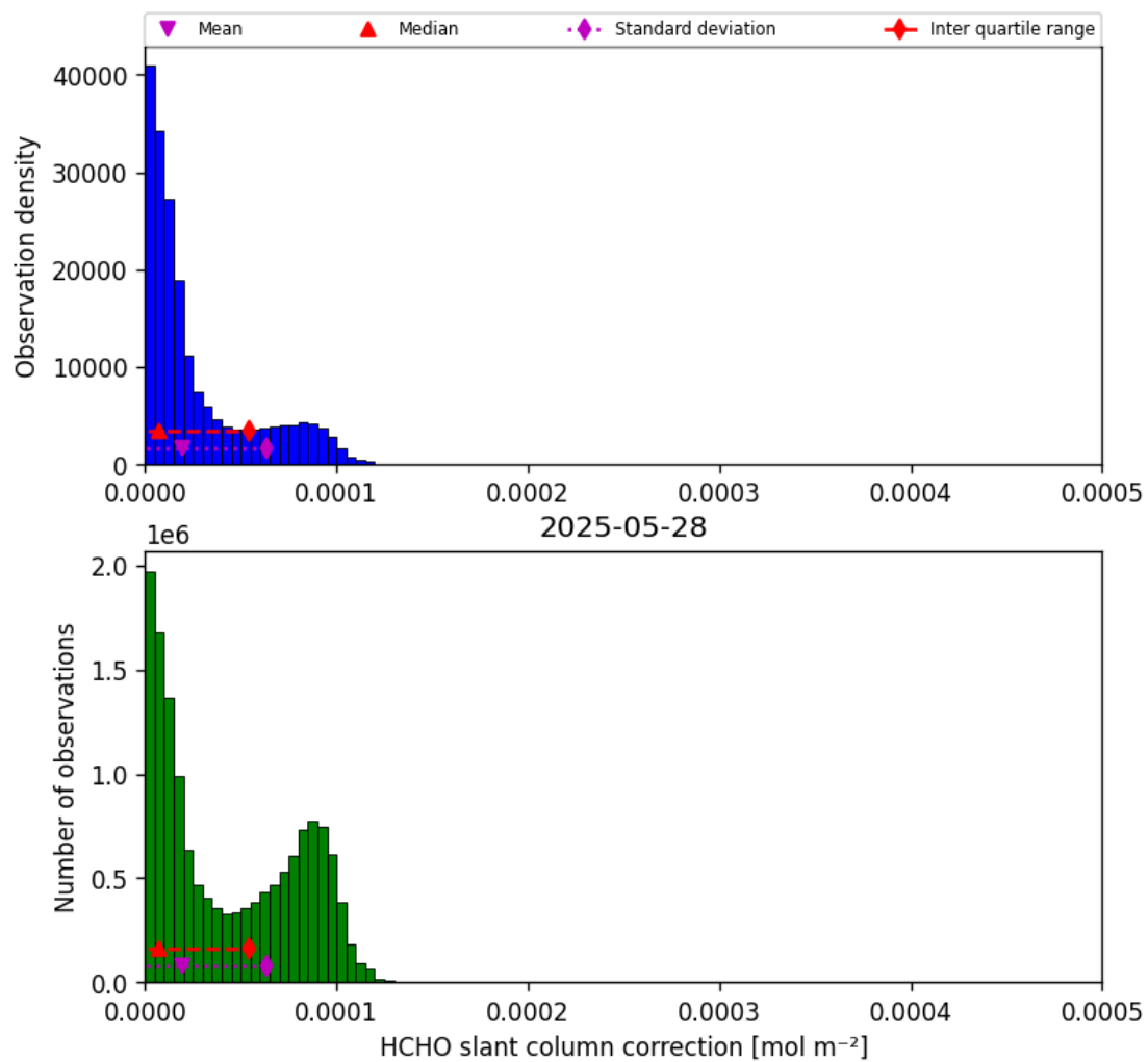
Figure 47: Histogram of “HCHO slant column correction” for 2025-05-27 to 2025-05-29
