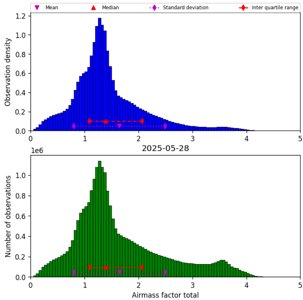
Figure 40: Histogram of “Airmass factor total” for 2025-05-27 to 2025-05-29
