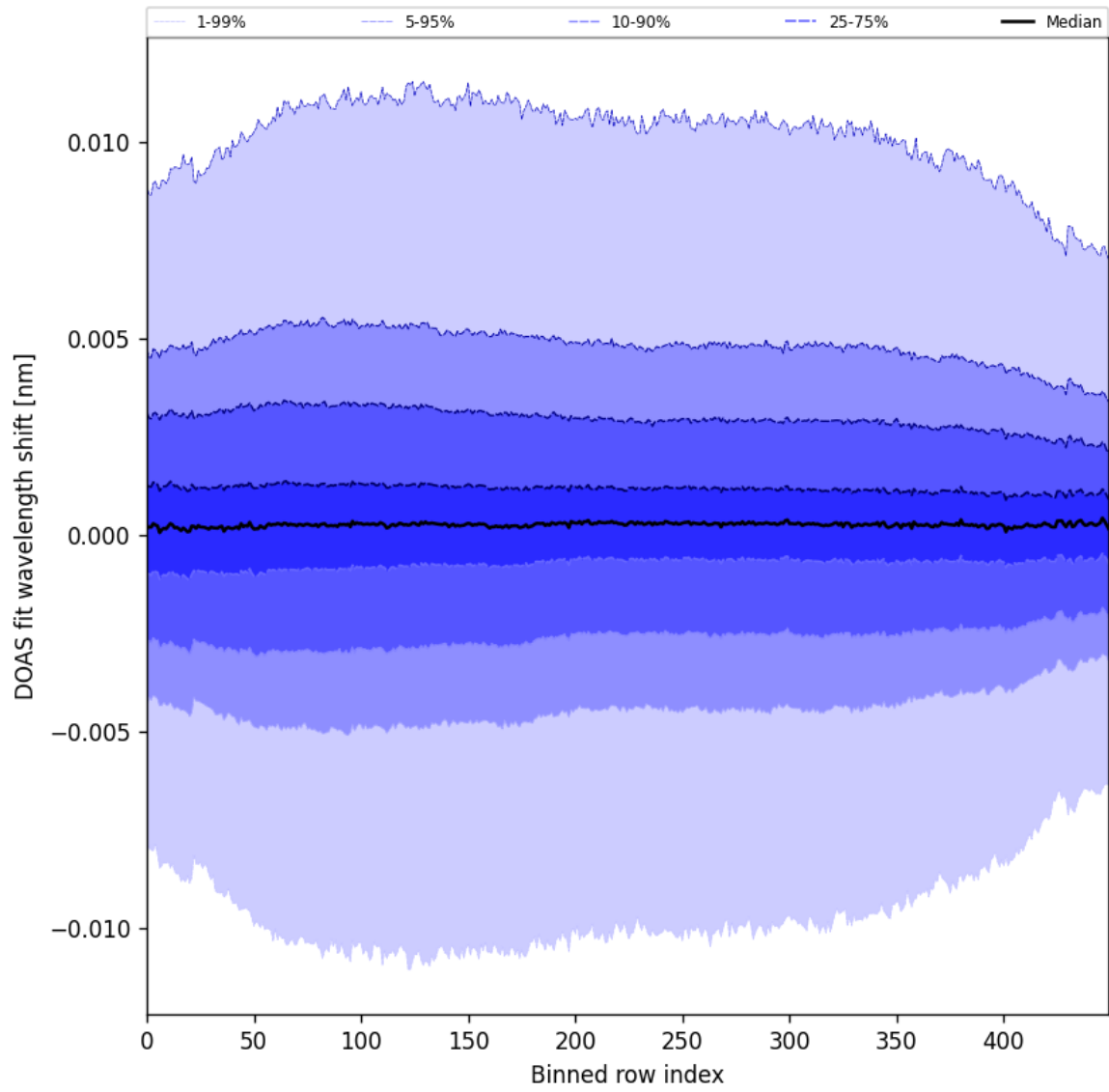
Figure 58: Along track statistics of “DOAS fit wavelength shift” for 2025-05-27 to 2025-05-29
