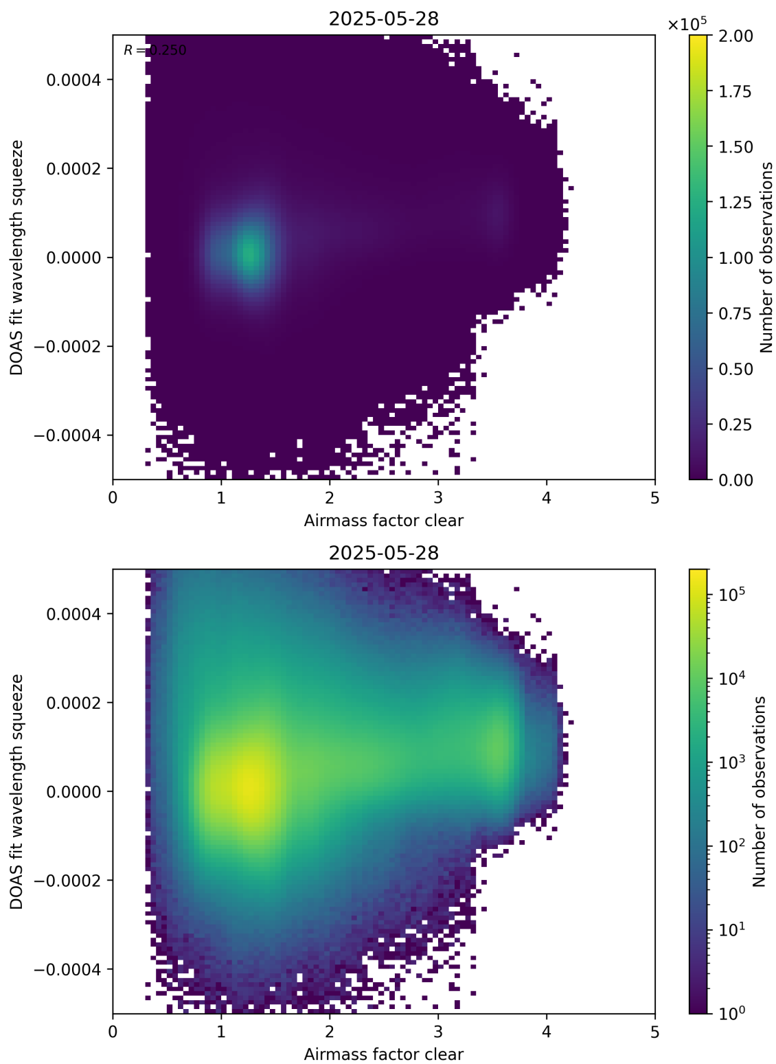
Figure 73: Scatter density plot of “Airmass factor clear” against “DOAS fit wavelength squeeze” for 2025-05-27 to 2025-05-29.
