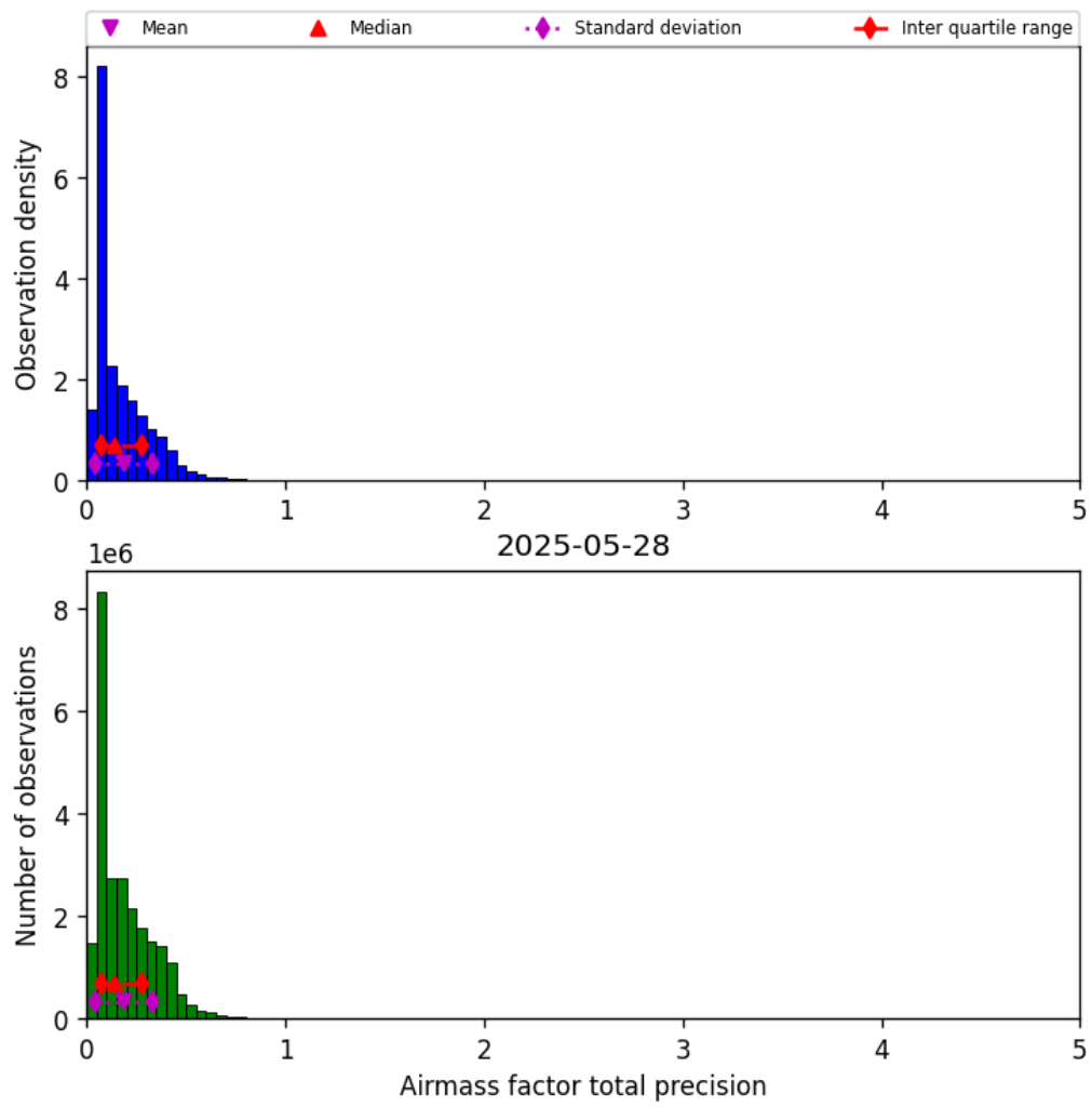
Figure 41: Histogram of “Airmass factor total precision” for 2025-05-27 to 2025-05-29
