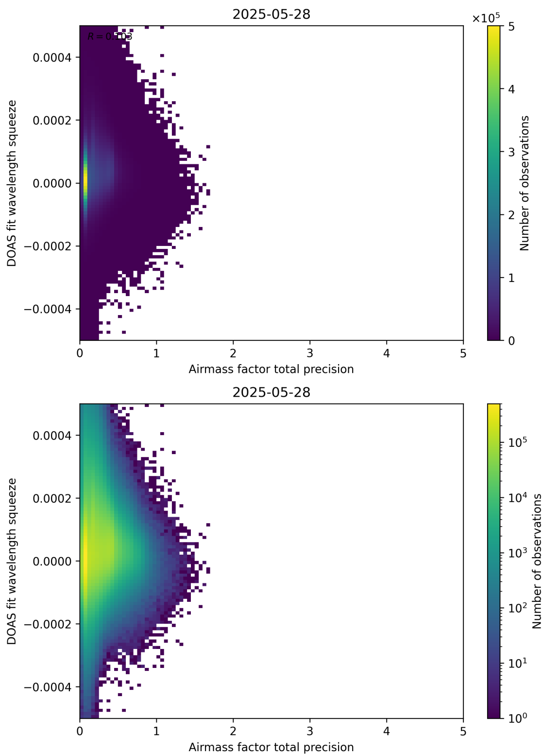
Figure 107: Scatter density plot of “Airmass factor total precision” against “DOAS fit wavelength squeeze” for 2025-05-27 to 2025-05-29.
