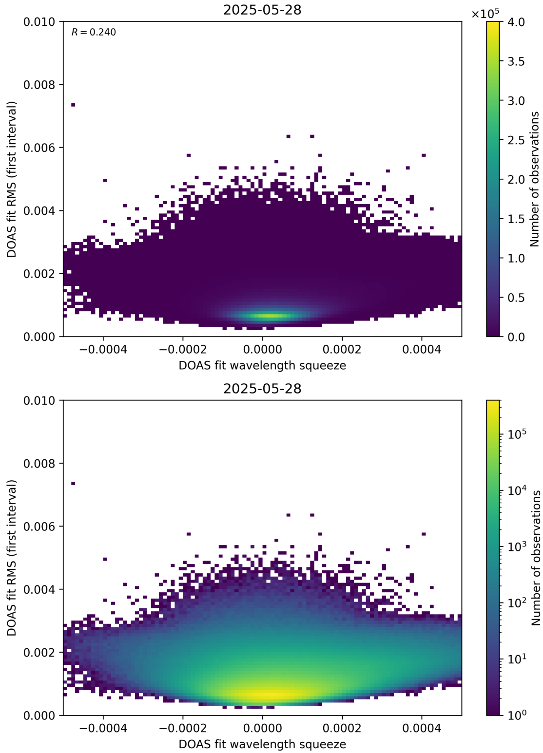
Figure 68: Scatter density plot of “DOAS fit wavelength squeeze” against “DOAS fit RMS (first interval)” for 2025-05-27 to 2025-05-29.
