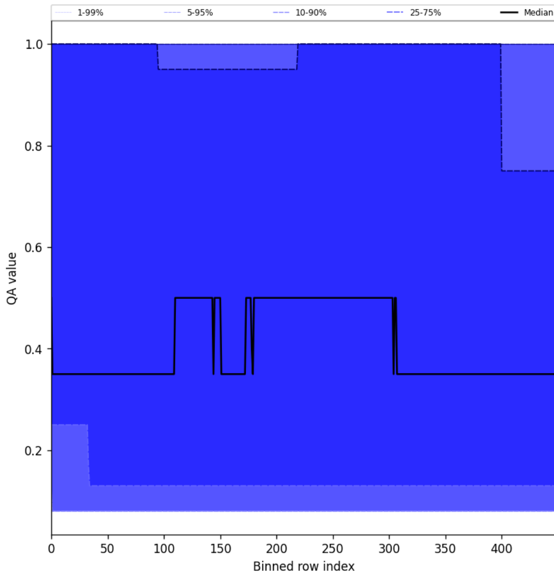
Figure 48: Along track statistics of “QA value” for 2025-05-27 to 2025-05-29
