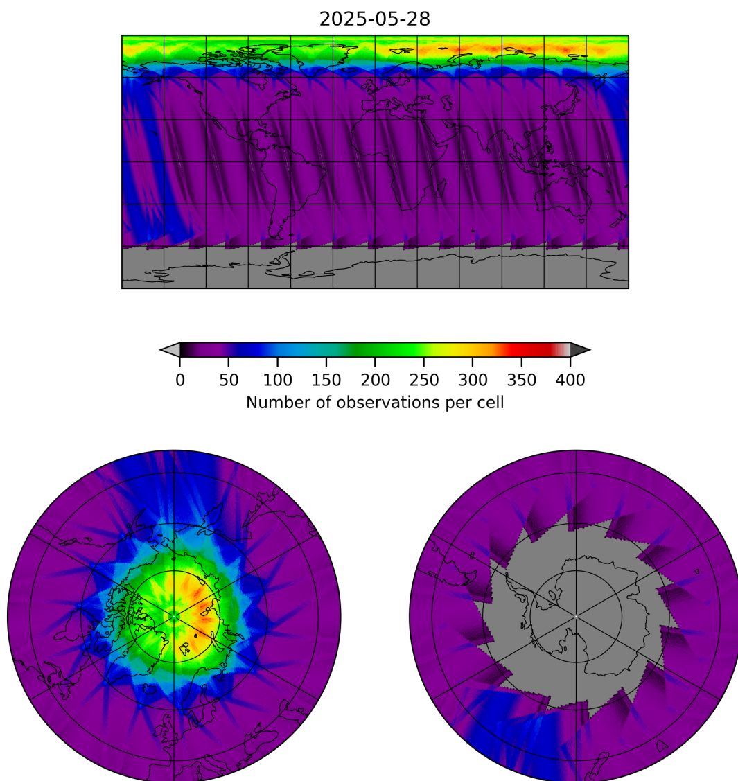
Figure 19: Map of the number of observations for 2025-05-27 to 2025-05-29
