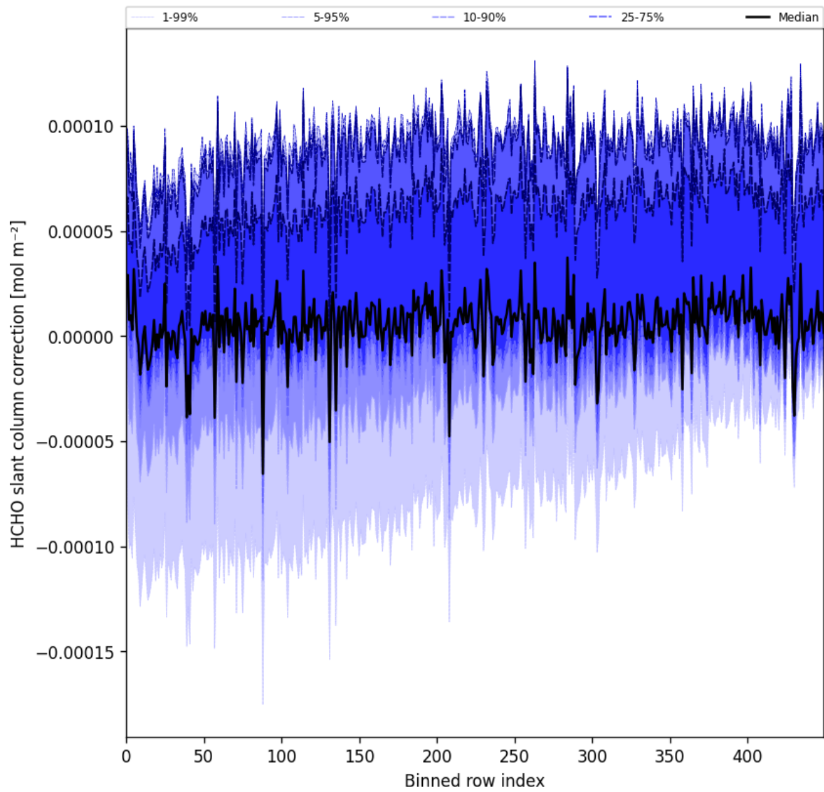
Figure 61: Along track statistics of “HCHO slant column correction” for 2025-05-27 to 2025-05-29
