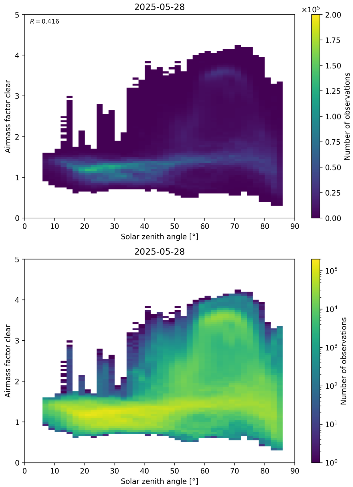
Figure 170: Scatter density plot of “Solar zenith angle” against “Airmass factor clear” for 2025-05-27 to 2025-05-29.
