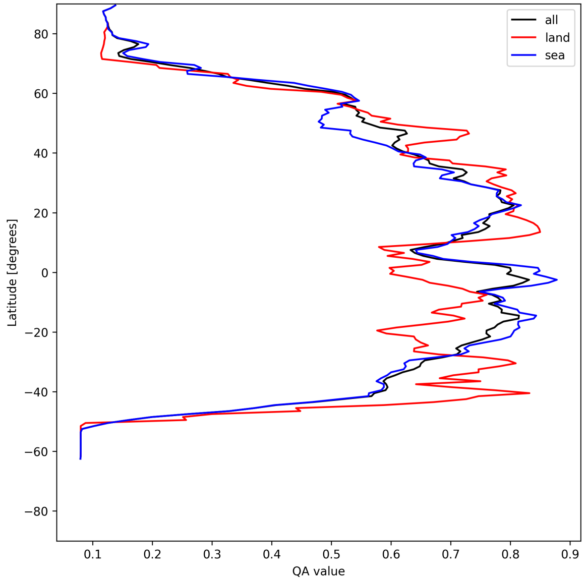
Figure 20: Zonal average of “QA value” for 2025-05-27 to 2025-05-29.
