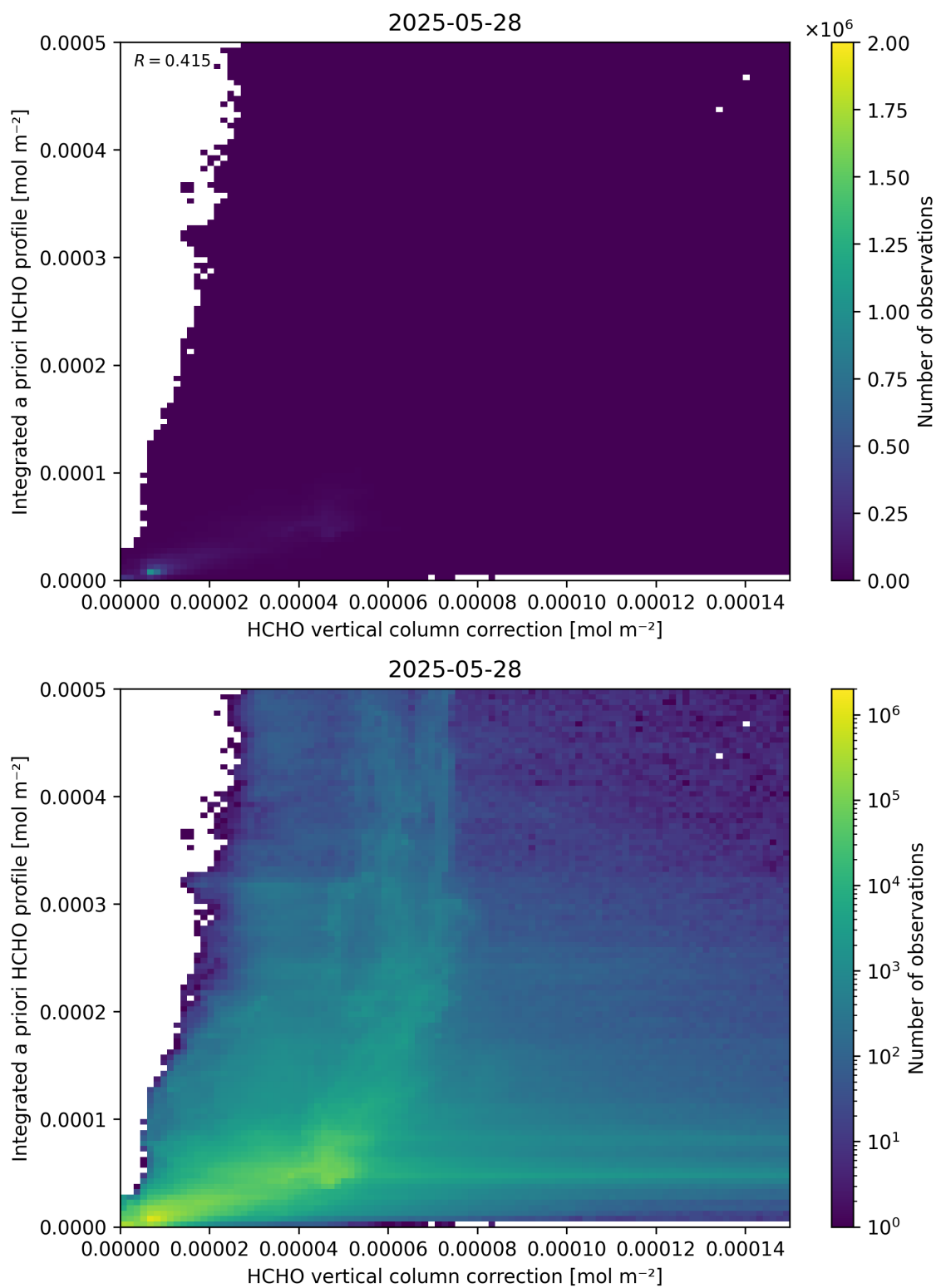
Figure 122: Scatter density plot of “HCHO vertical column correction” against “Integrated a priori HCHO profile” for 2025-05-27 to 2025-05-29.
