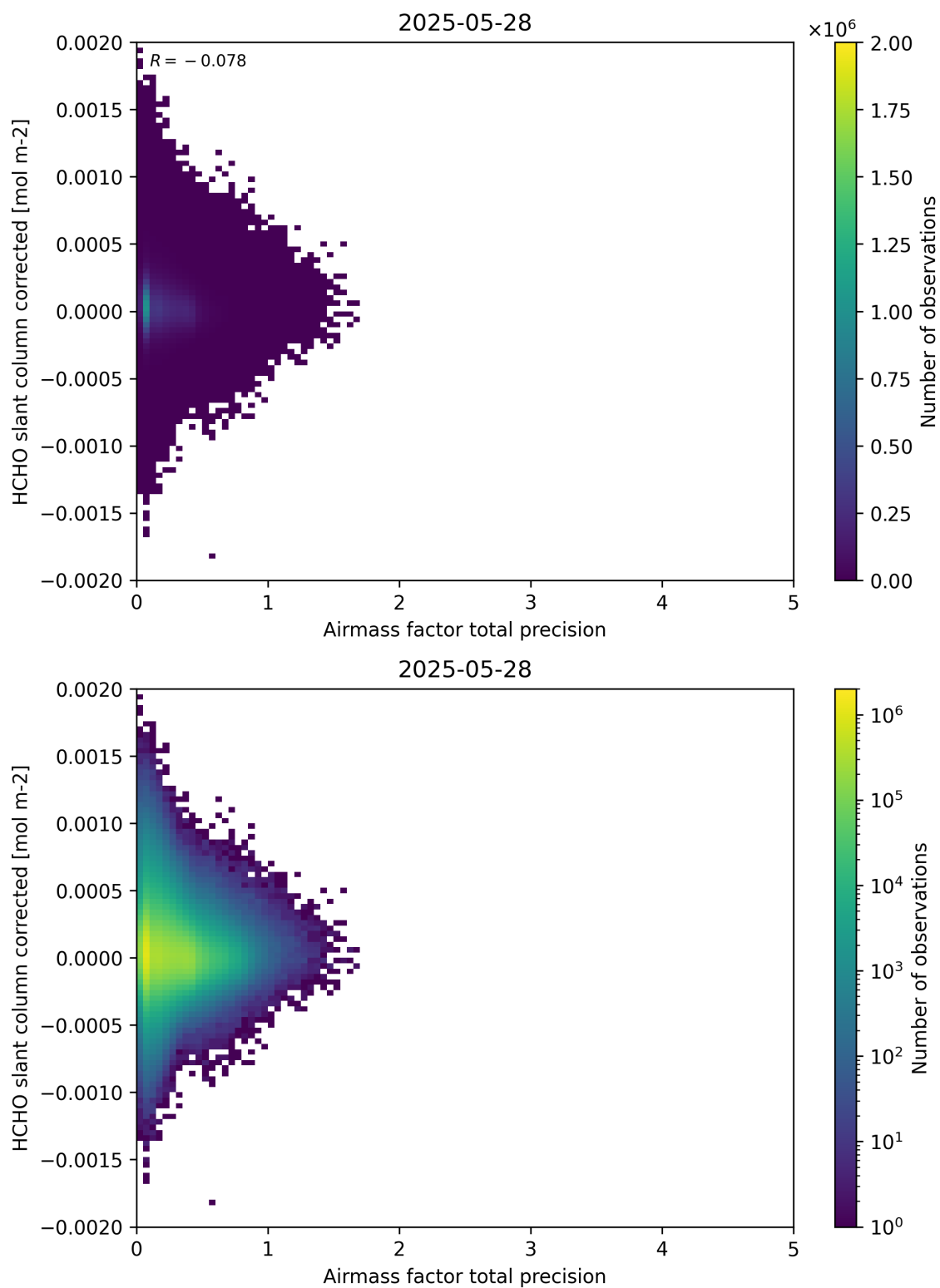
Figure 109: Scatter density plot of “Airmass factor total precision” against “HCHO slant column corrected” for 2025-05-27 to 2025-05-29.
