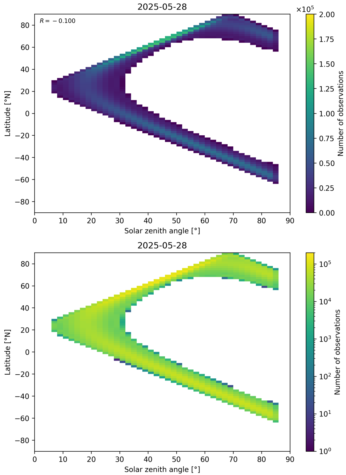
Figure 181: Scatter density plot of “Solar zenith angle” against “Latitude” for 2025-05-27 to 2025-05-29.
