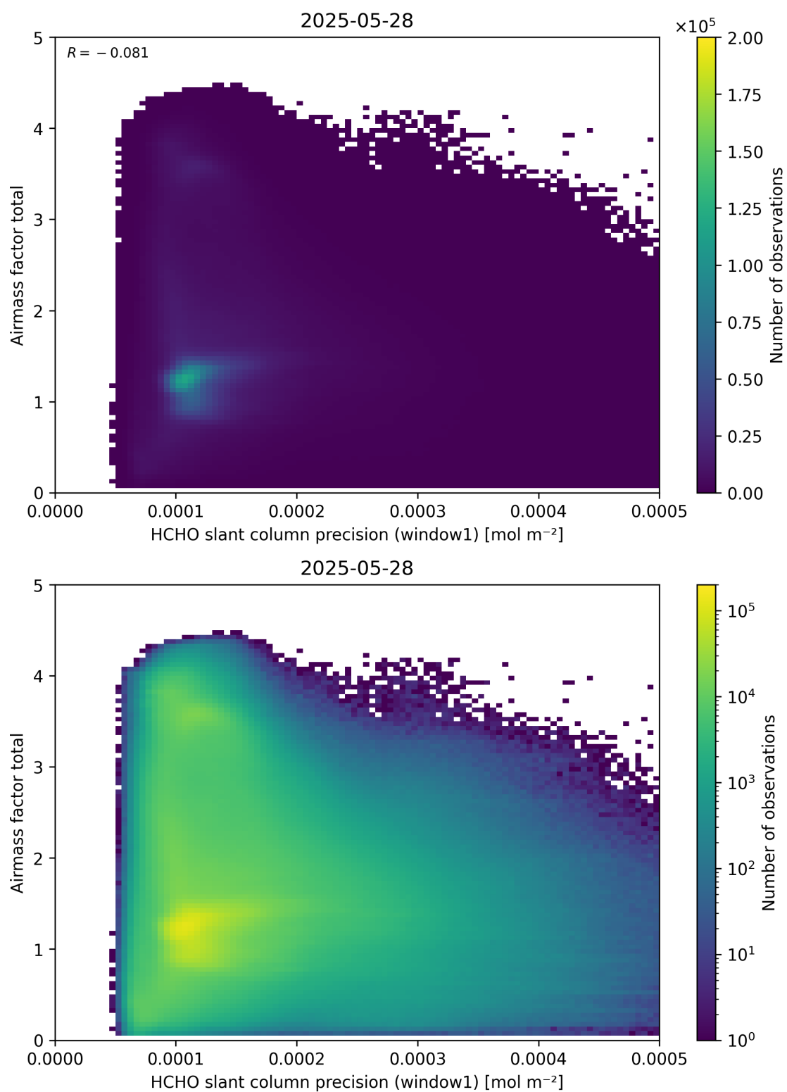
Figure 94: Scatter density plot of “HCHO slant column precision (window1)” against “Airmass factor total” for 2025-05-27 to 2025-05-29.
