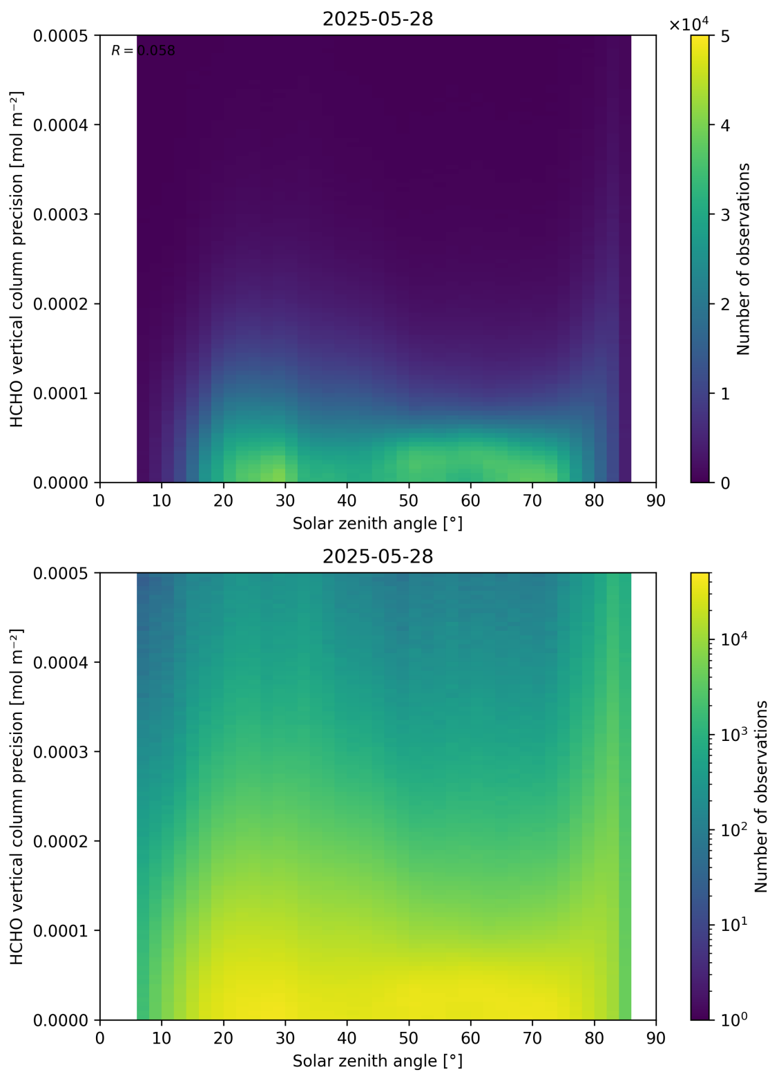
Figure 179: Scatter density plot of “Solar zenith angle” against “HCHO vertical column precision” for 2025-05-27 to 2025-05-29.
