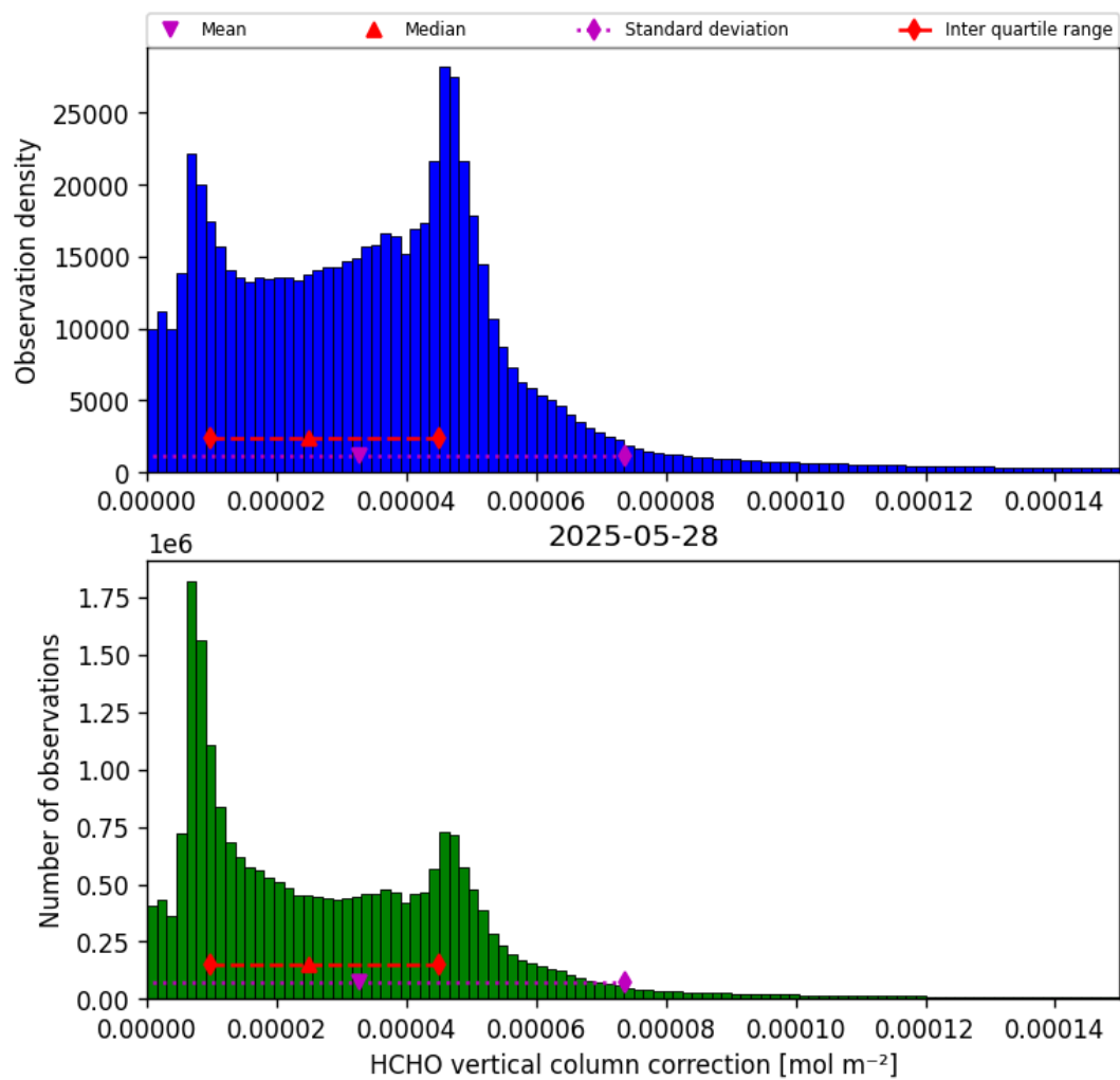
Figure 37: Histogram of “HCHO vertical column correction” for 2025-05-27 to 2025-05-29
