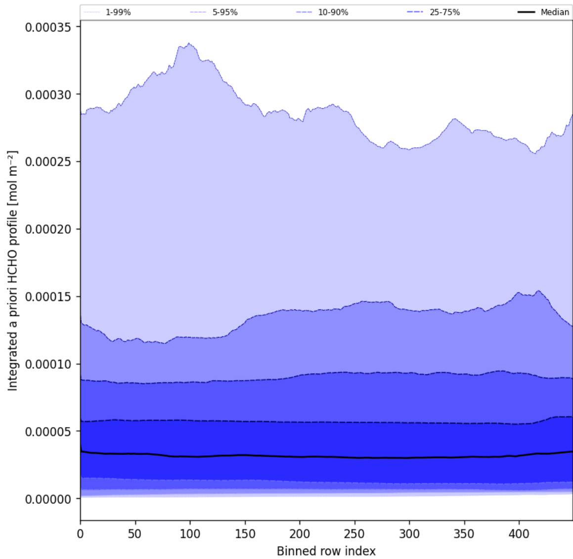
Figure 57: Along track statistics of "Integrated a priori HCHO profile" for 2025-05-27 to 2025-05-29
