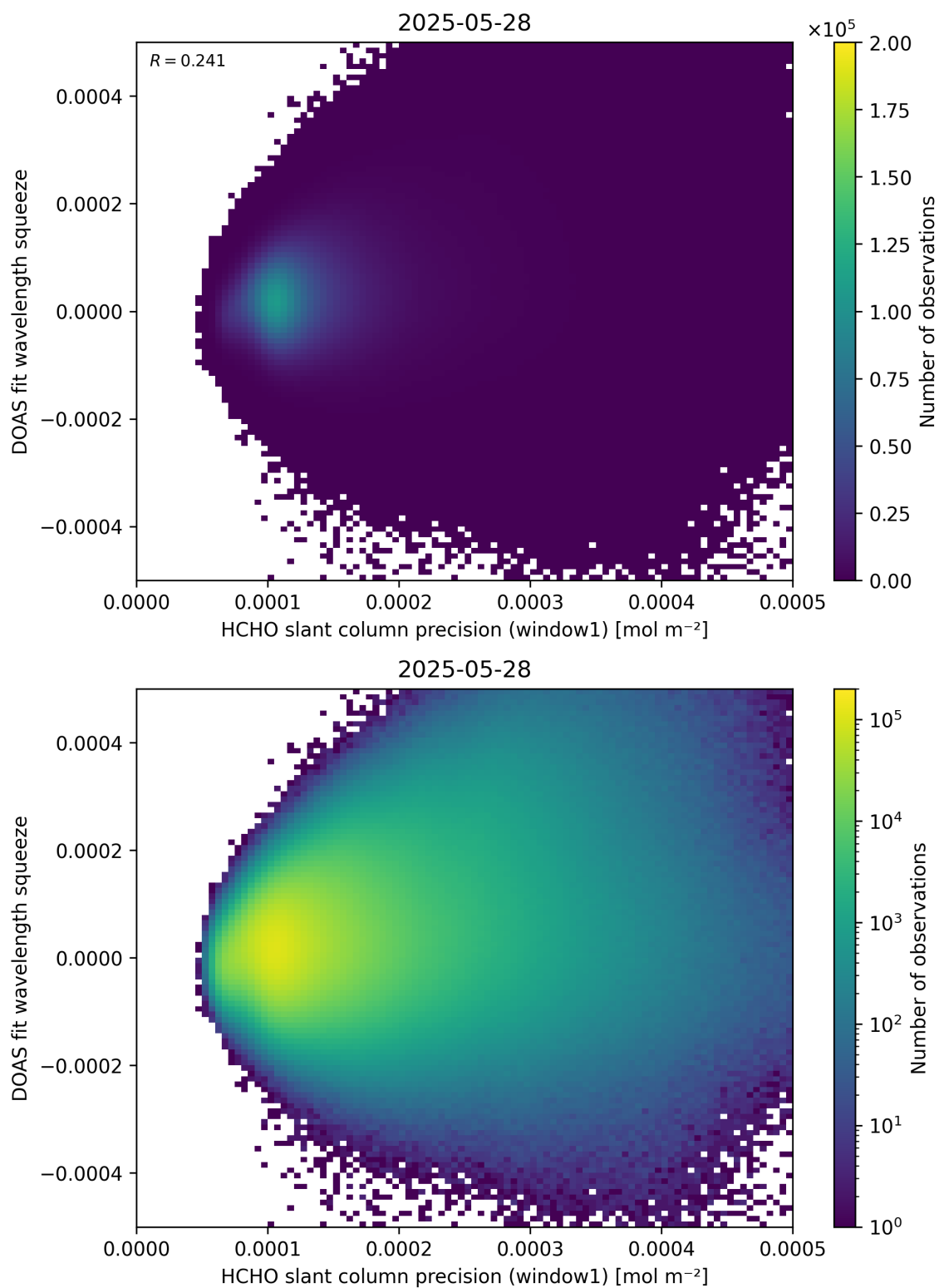
Figure 90: Scatter density plot of “HCHO slant column precision (window1)” against “DOAS fit wavelength squeeze” for 2025-05-27 to 2025-05-29.
