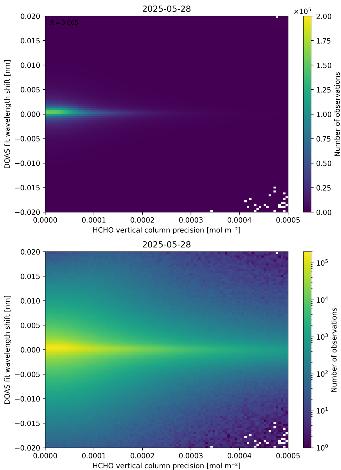
Figure 137: Scatter density plot of “HCHO vertical column precision” against “DOAS fit wavelength shift” for 2025-05-27 to 2025-05-29.
