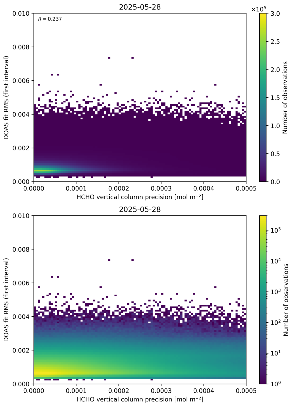
Figure 136: Scatter density plot of “HCHO vertical column precision” against “DOAS fit RMS (first interval)” for 2025-05-27 to 2025-05-29.
