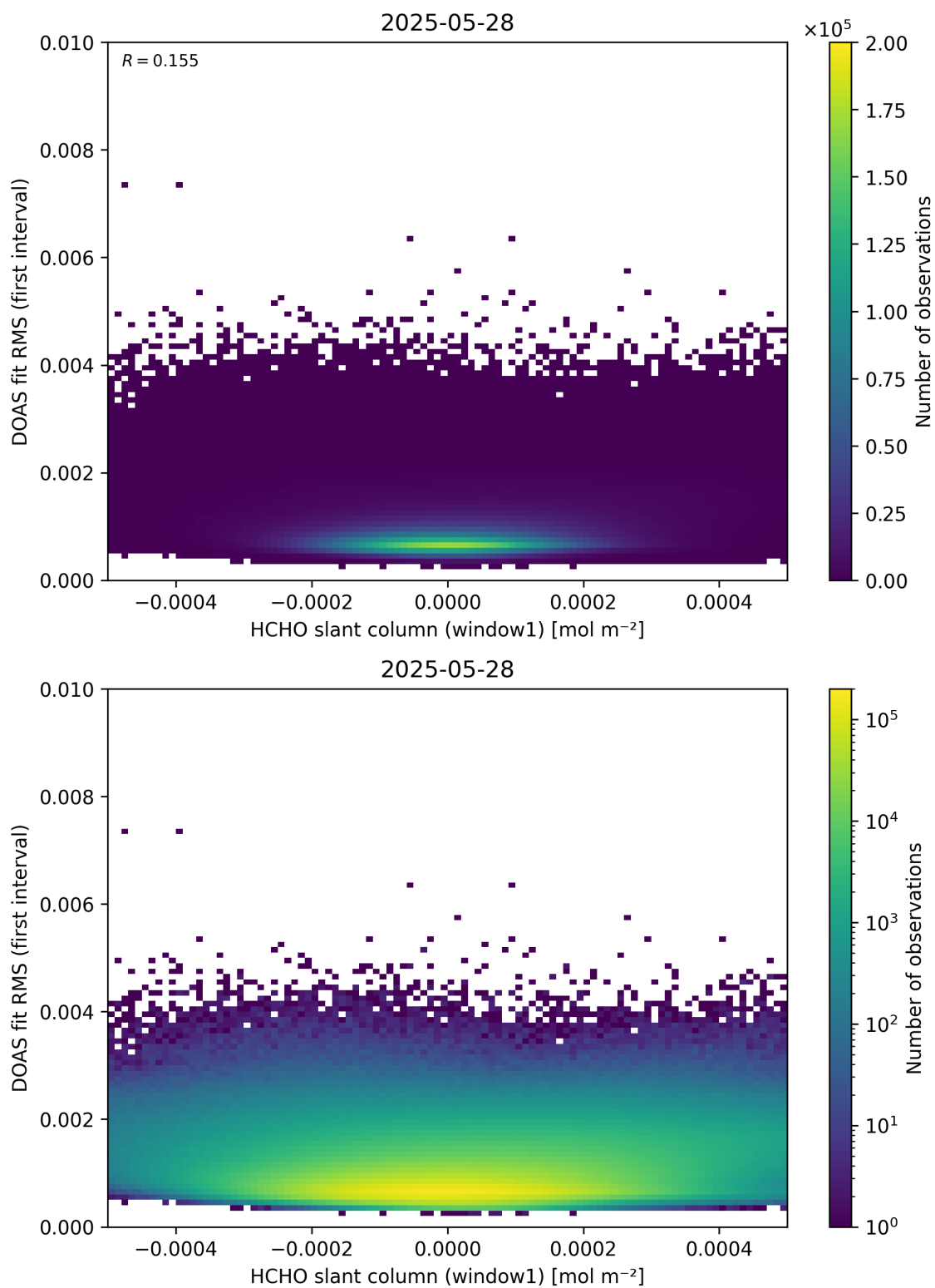
Figure 78: Scatter density plot of “HCHO slant column (window1)” against “DOAS fit RMS (first interval)” for 2025-05-27 to 2025-05-29.
