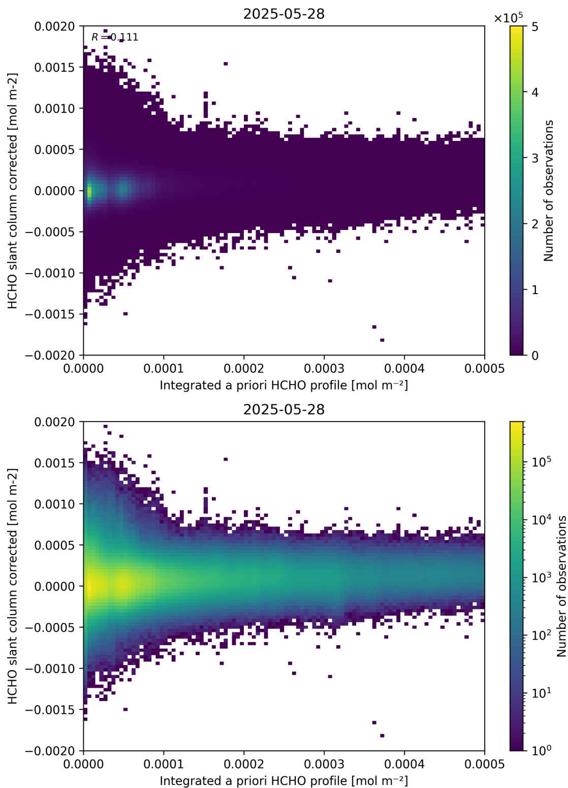
Figure 151: Scatter density plot of “Integrated a priori HCHO profile” against “HCHO slant column corrected” for 2025-05-27 to 2025-05-29.
