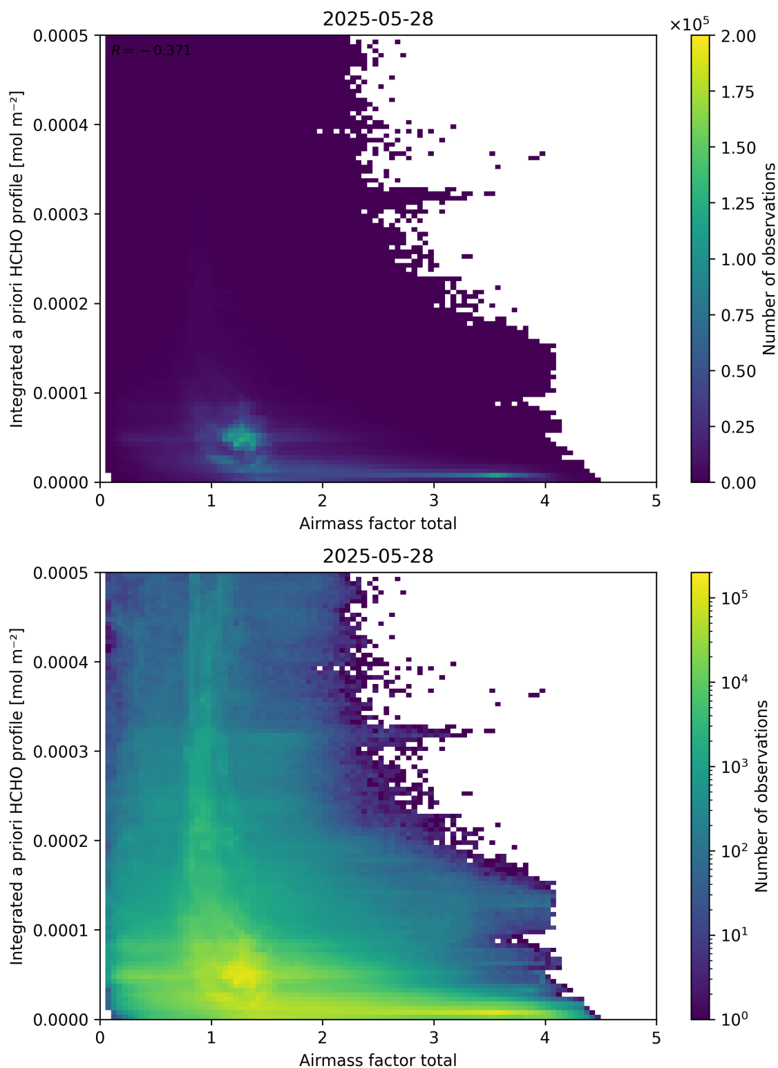
Figure 104: Scatter density plot of “Airmass factor total” against “Integrated a priori HCHO profile” for 2025-05-27 to 2025-05-29.
