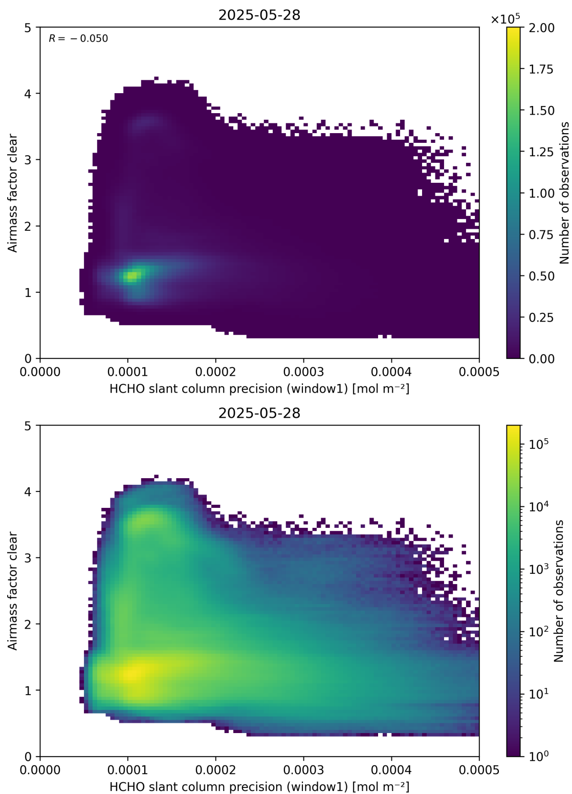
Figure 91: Scatter density plot of “HCHO slant column precision (window1)” against “Airmass factor clear” for 2025-05-27 to 2025-05-29.
