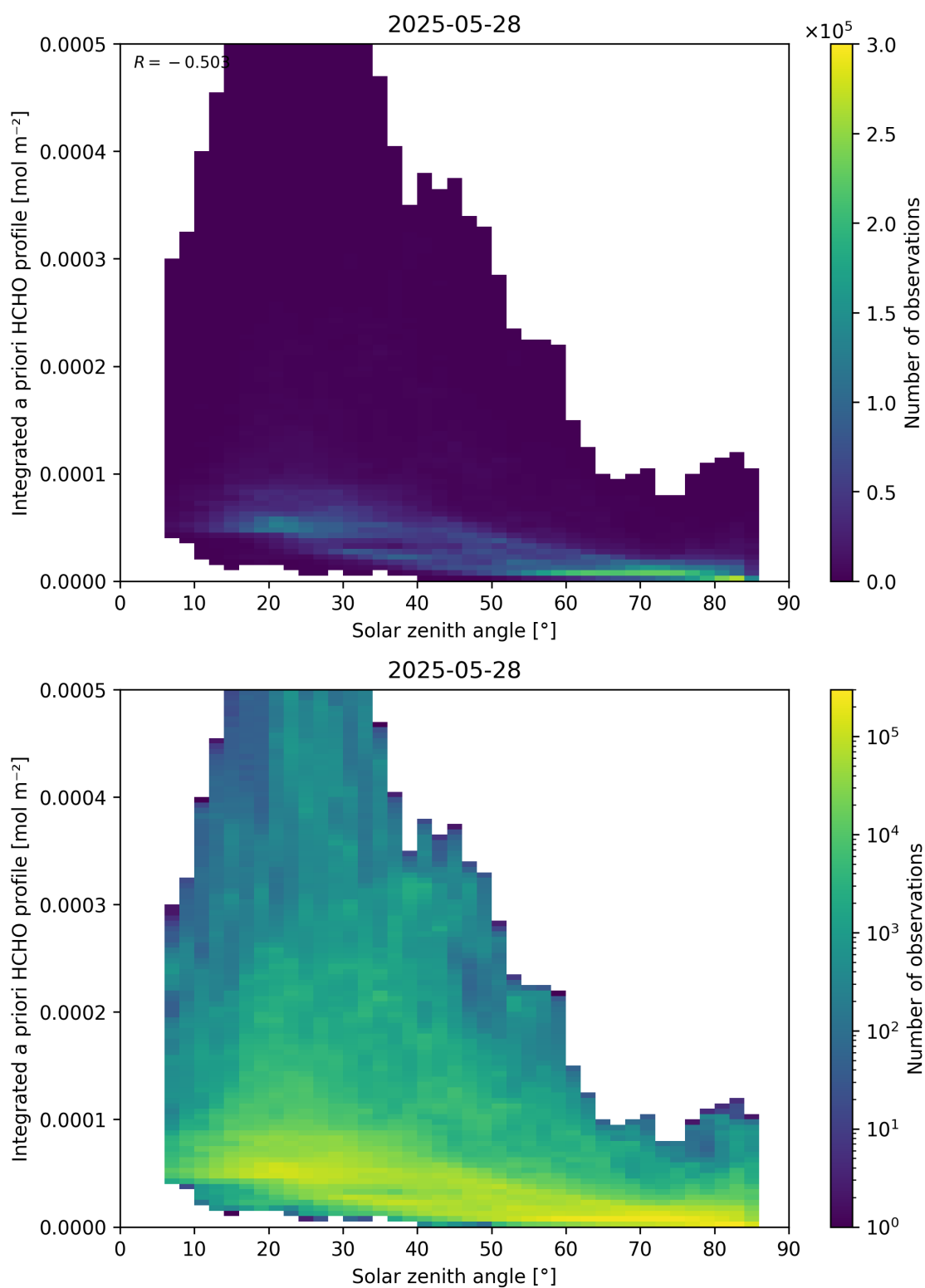
Figure 180: Scatter density plot of “Solar zenith angle” against “Integrated a priori HCHO profile” for 2025-05-27 to 2025-05-29.
