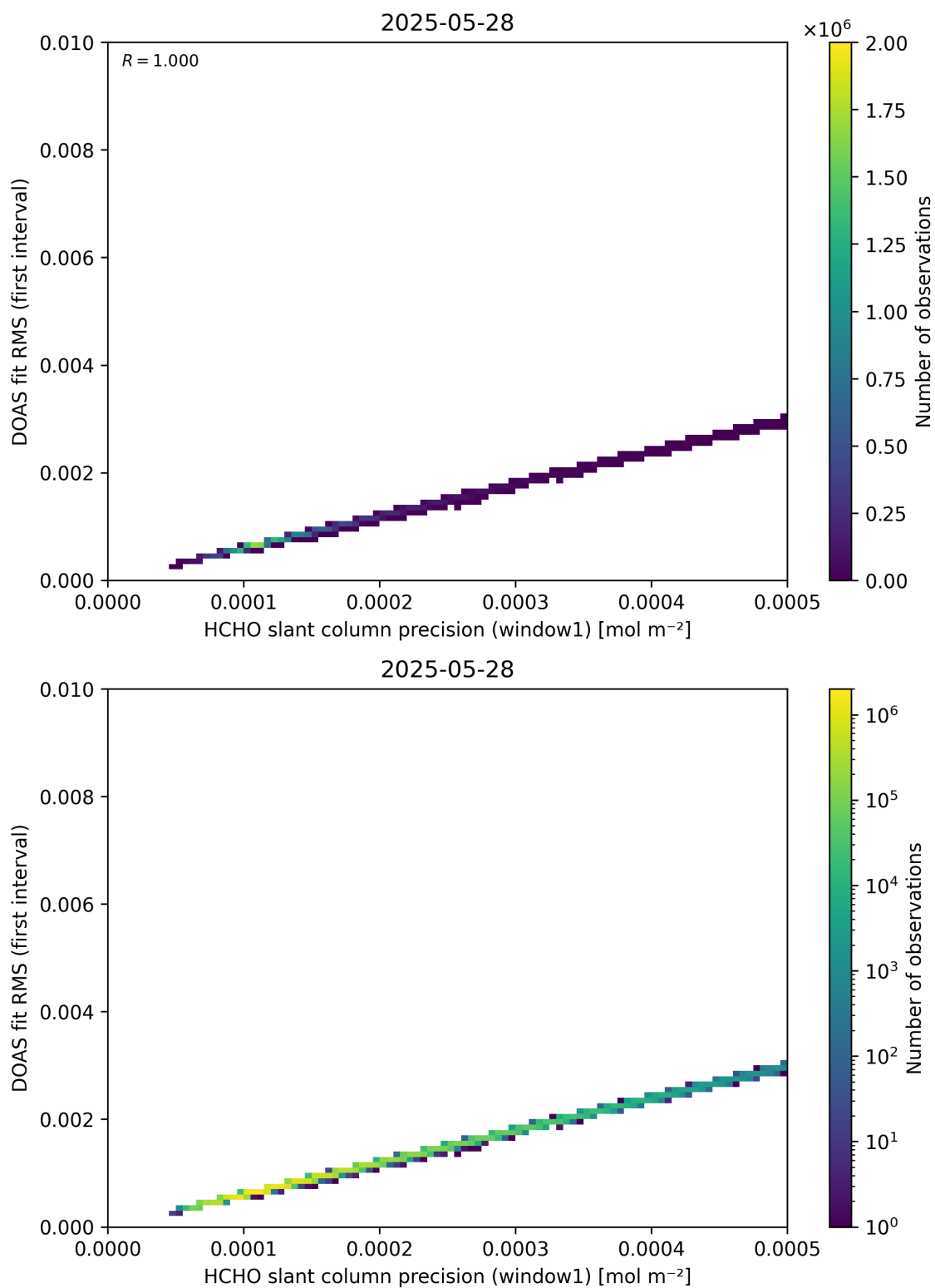
Figure 88: Scatter density plot of “HCHO slant column precision (window1)” against “DOAS fit RMS (first interval)” for 2025-05-27 to 2025-05-29.
