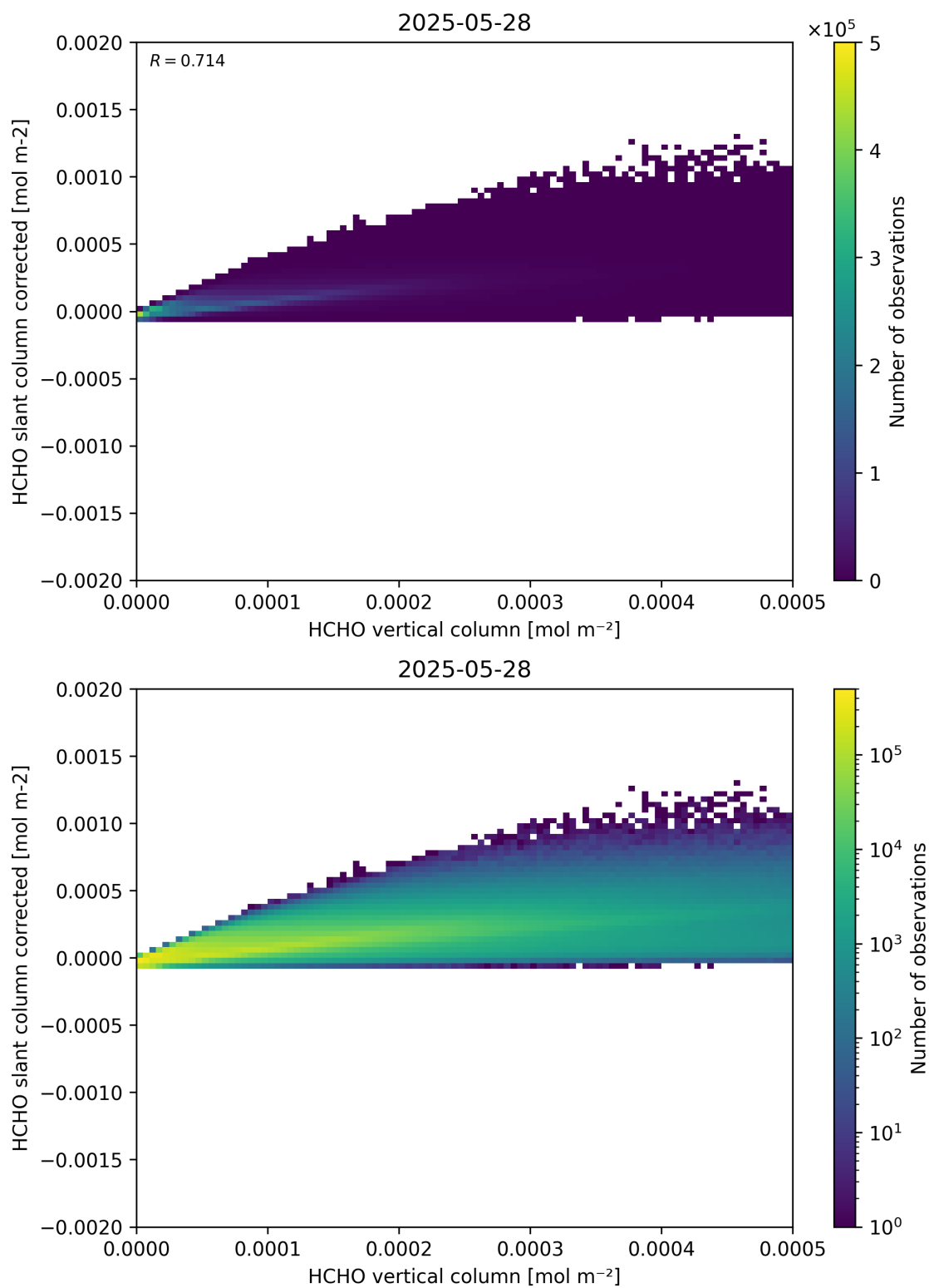
Figure 127: Scatter density plot of “HCHO vertical column” against “HCHO slant column corrected” for 2025-05-27 to 2025-05-29.
