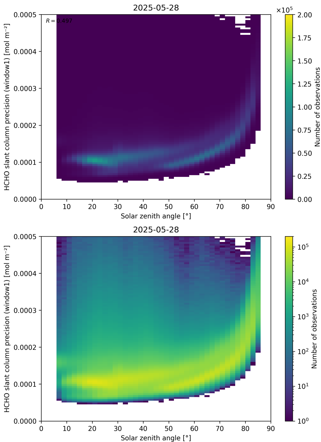
Figure 174: Scatter density plot of “Solar zenith angle” against “HCHO slant column precision (window1)” for 2025-05-27 to 2025-05-29.
