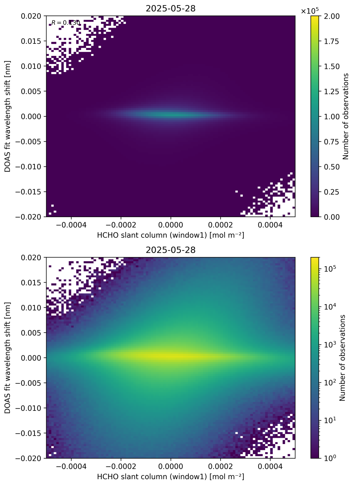
Figure 79: Scatter density plot of “HCHO slant column (window1)” against “DOAS fit wavelength shift” for 2025-05-27 to 2025-05-29.
