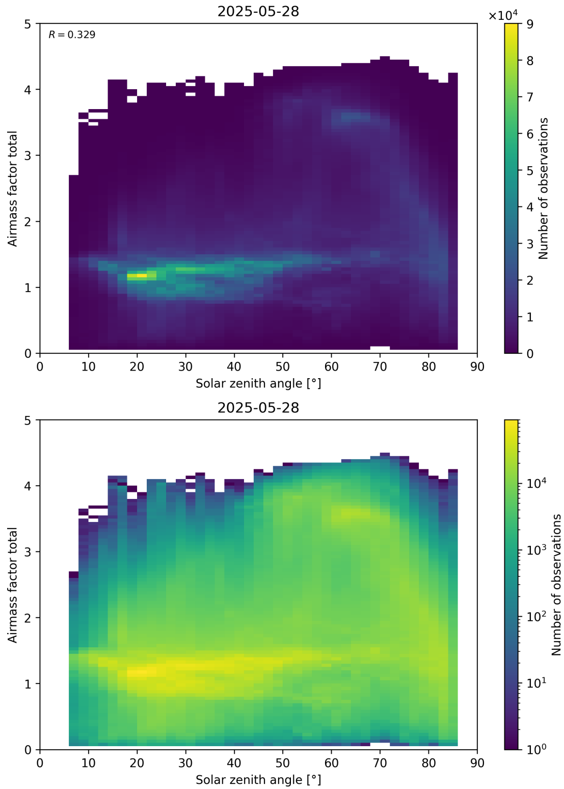
Figure 175: Scatter density plot of “Solar zenith angle” against “Airmass factor total” for 2025-05-27 to 2025-05-29.
