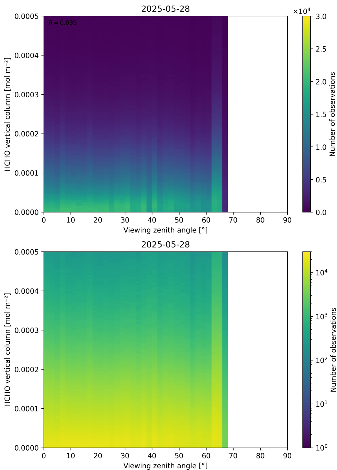
Figure 192: Scatter density plot of “Viewing zenith angle” against “HCHO vertical column” for 2025-05-27 to 2025-05-29.
