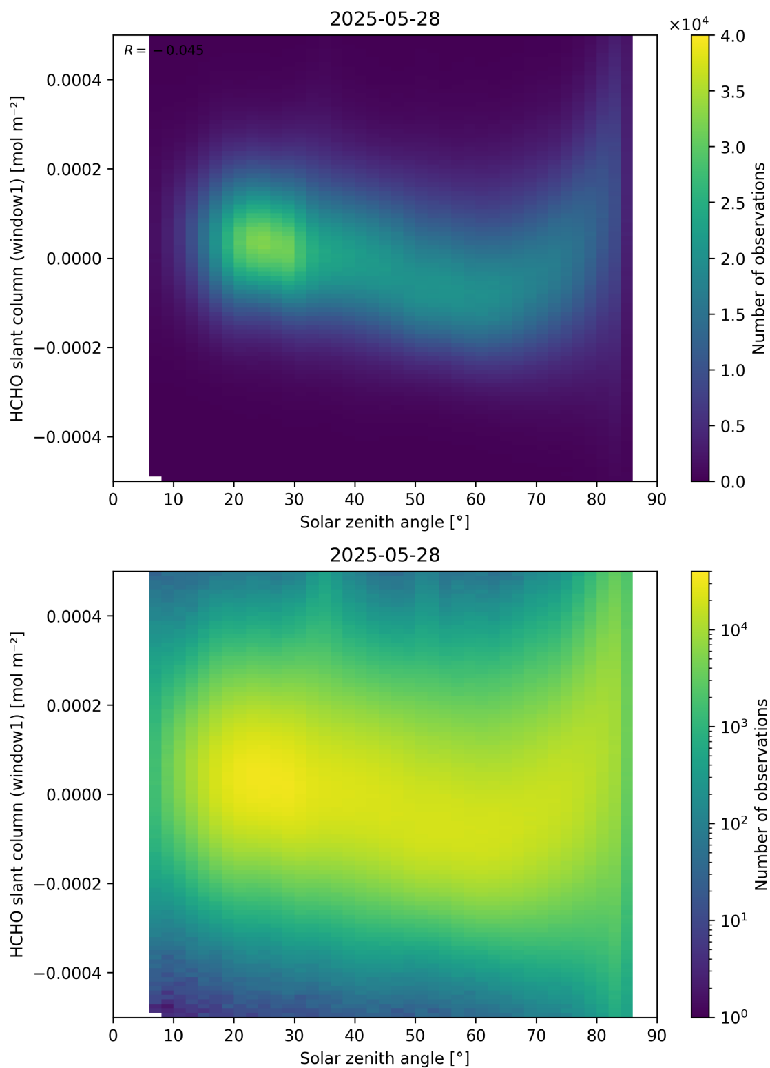
Figure 173: Scatter density plot of “Solar zenith angle” against “HCHO slant column (window1)” for 2025-05-27 to 2025-05-29.
