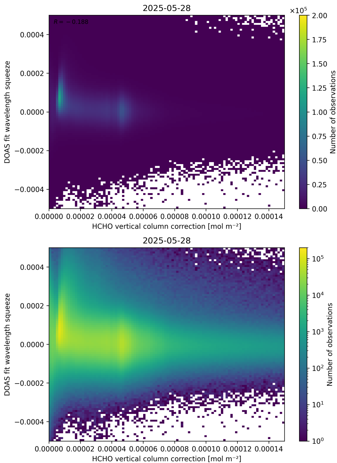
Figure 114: Scatter density plot of “HCHO vertical column correction” against “DOAS fit wavelength squeeze” for 2025-05-27 to 2025-05-29.
