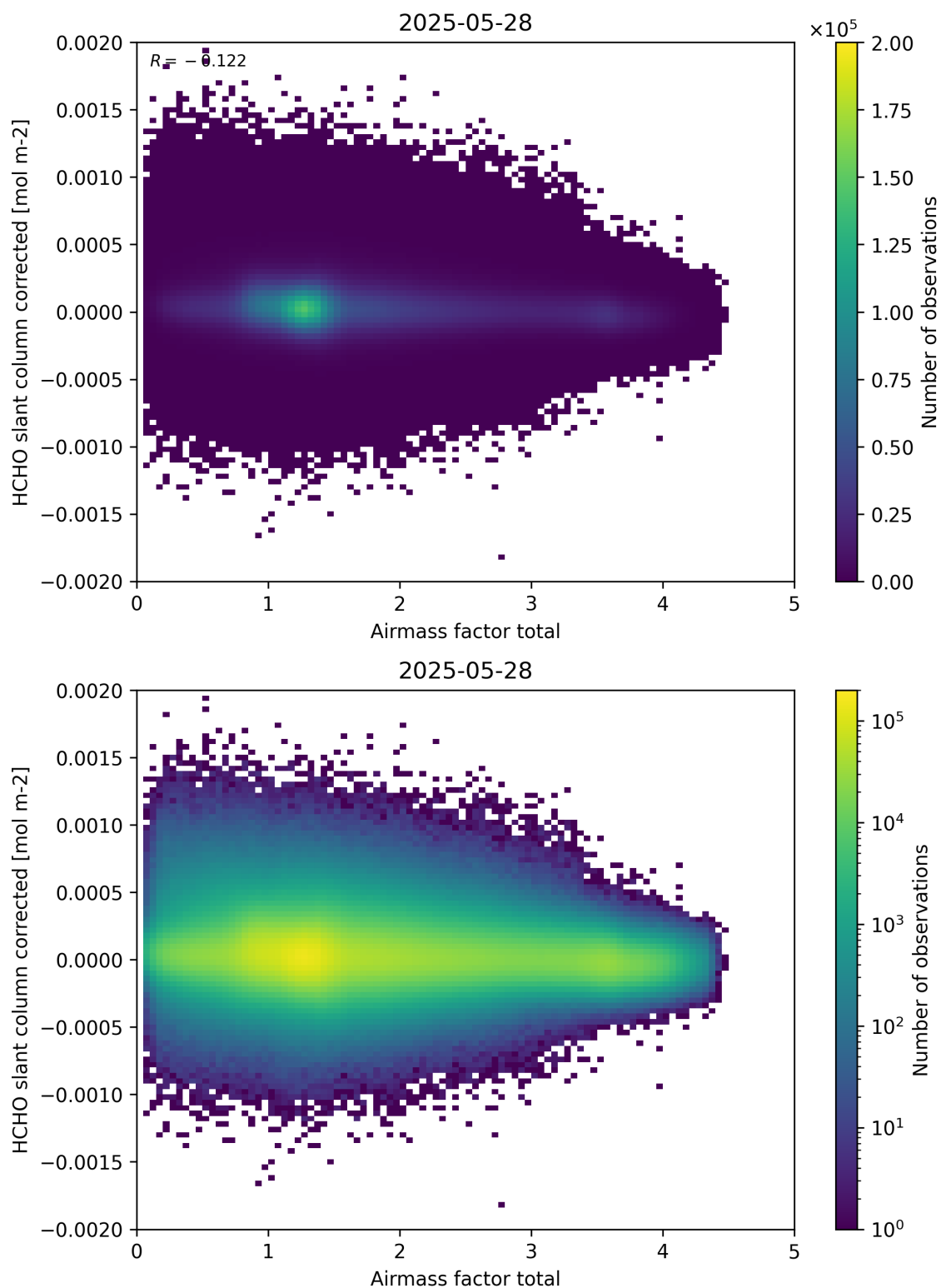
Figure 101: Scatter density plot of “Airmass factor total” against “HCHO slant column corrected” for 2025-05-27 to 2025-05-29.
