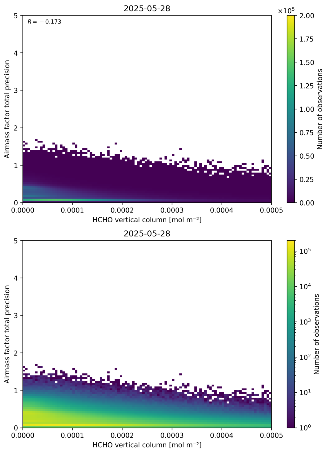
Figure 132: Scatter density plot of “HCHO vertical column” against “Airmass factor total precision” for 2025-05-27 to 2025-05-29.
