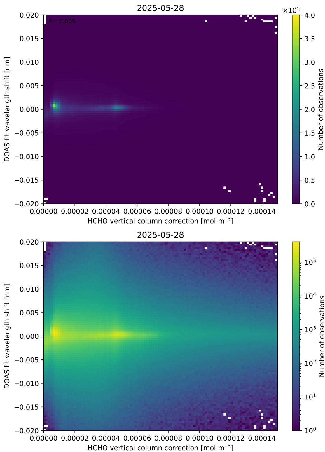
Figure 113: Scatter density plot of “HCHO vertical column correction” against “DOAS fit wavelength shift” for 2025-05-27 to 2025-05-29.
