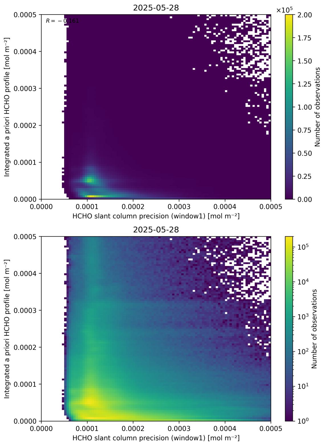
Figure 96: Scatter density plot of “HCHO slant column precision (window1)” against “Integrated a priori HCHO profile” for 2025-05-27 to 2025-05-29.
