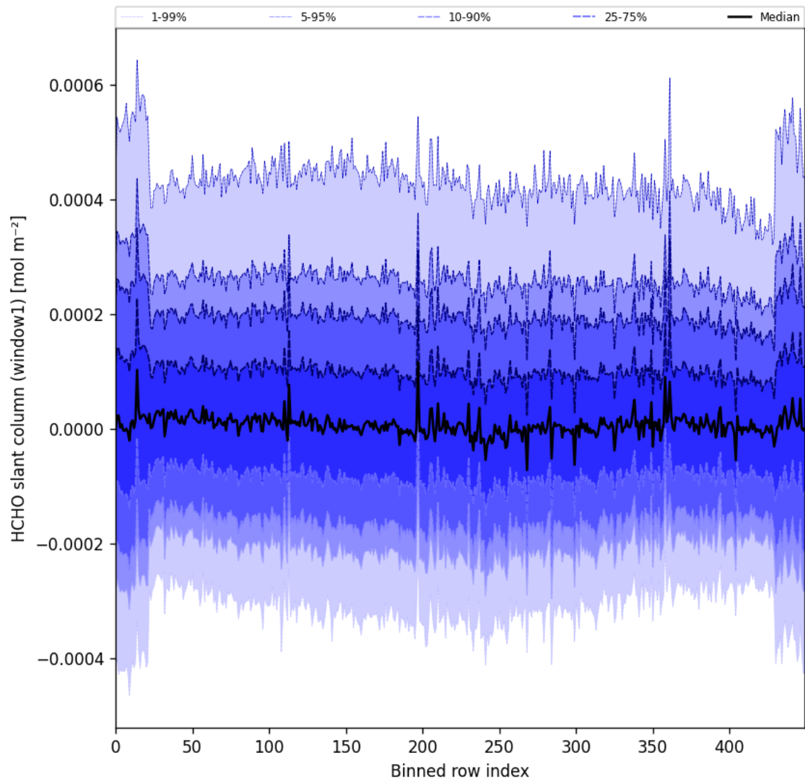
Figure 52: Along track statistics of “HCHO slant column (window1)” for 2025-05-27 to 2025-05-29
