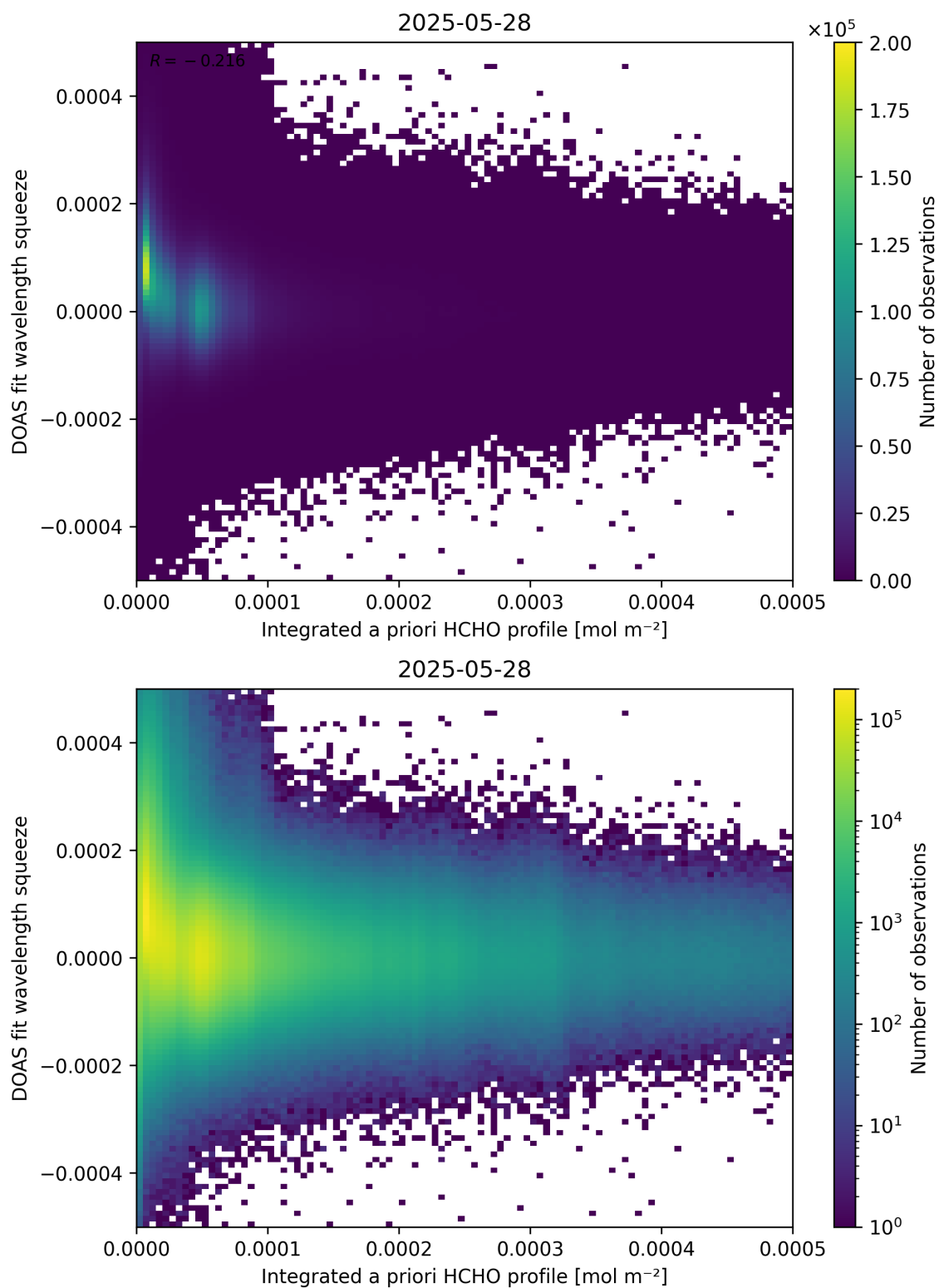
Figure 150: Scatter density plot of “Integrated a priori HCHO profile” against “DOAS fit wavelength squeeze” for 2025-05-27 to 2025-05-29.
