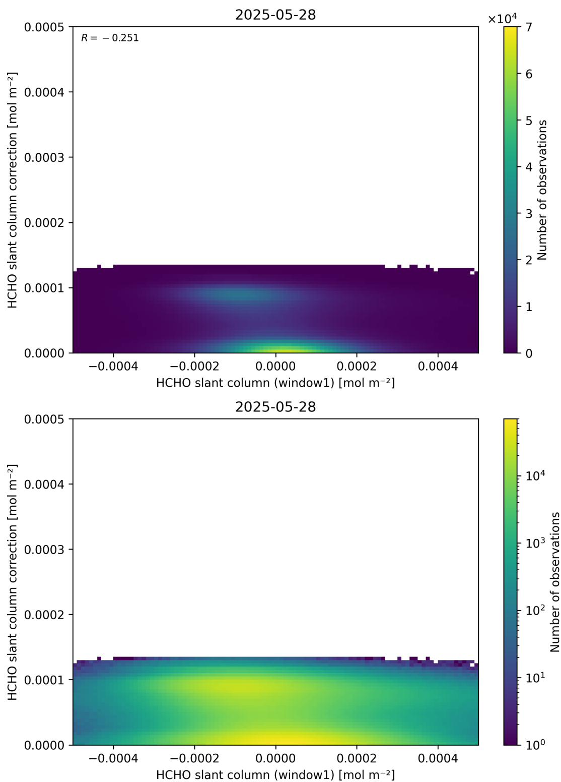
Figure 83: Scatter density plot of “HCHO slant column (window1)” against “HCHO slant column correction” for 2025-05-27 to 2025-05-29.
