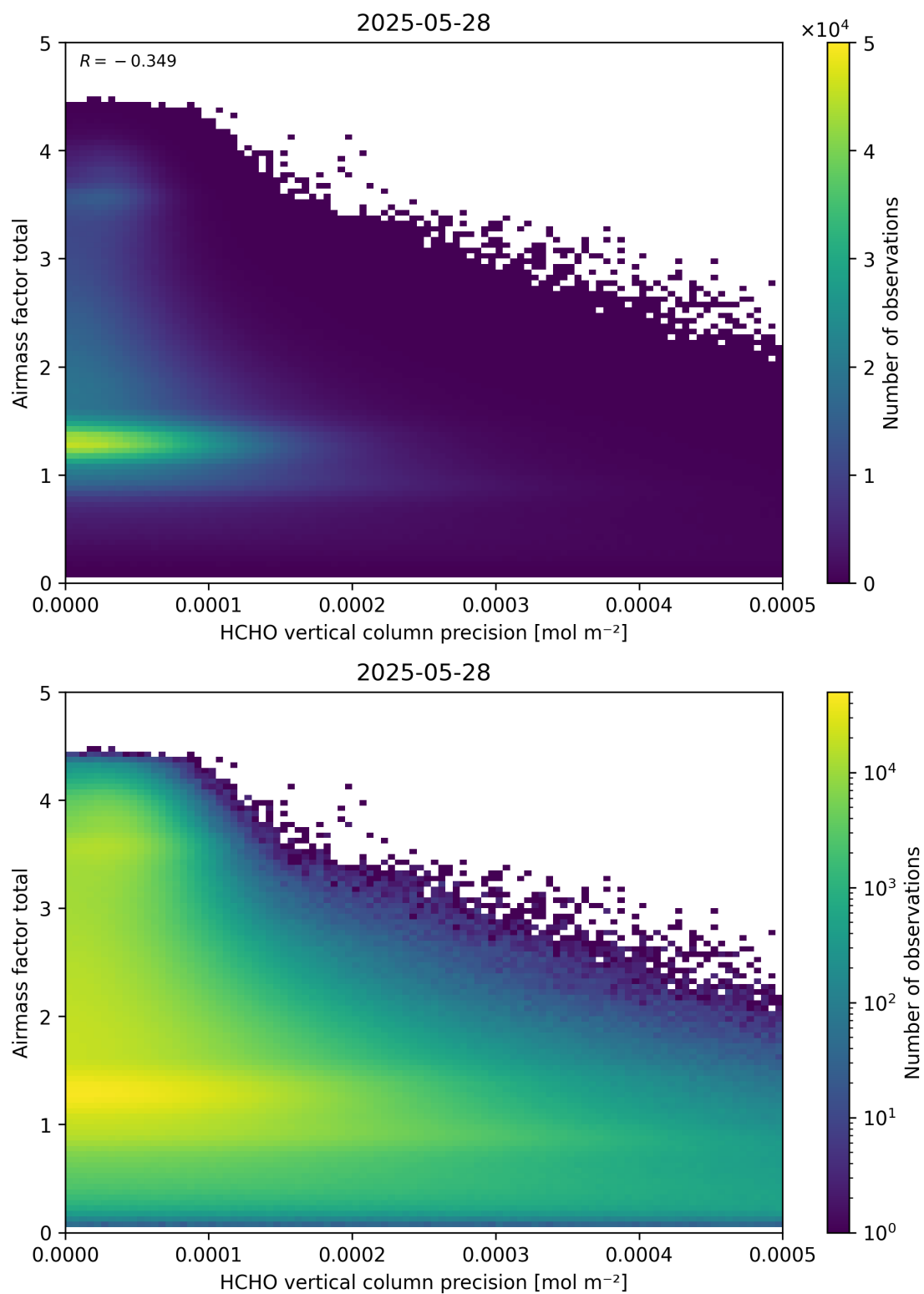
Figure 144: Scatter density plot of “HCHO vertical column precision” against “Airmass factor total” for 2025-05-27 to 2025-05-29.
