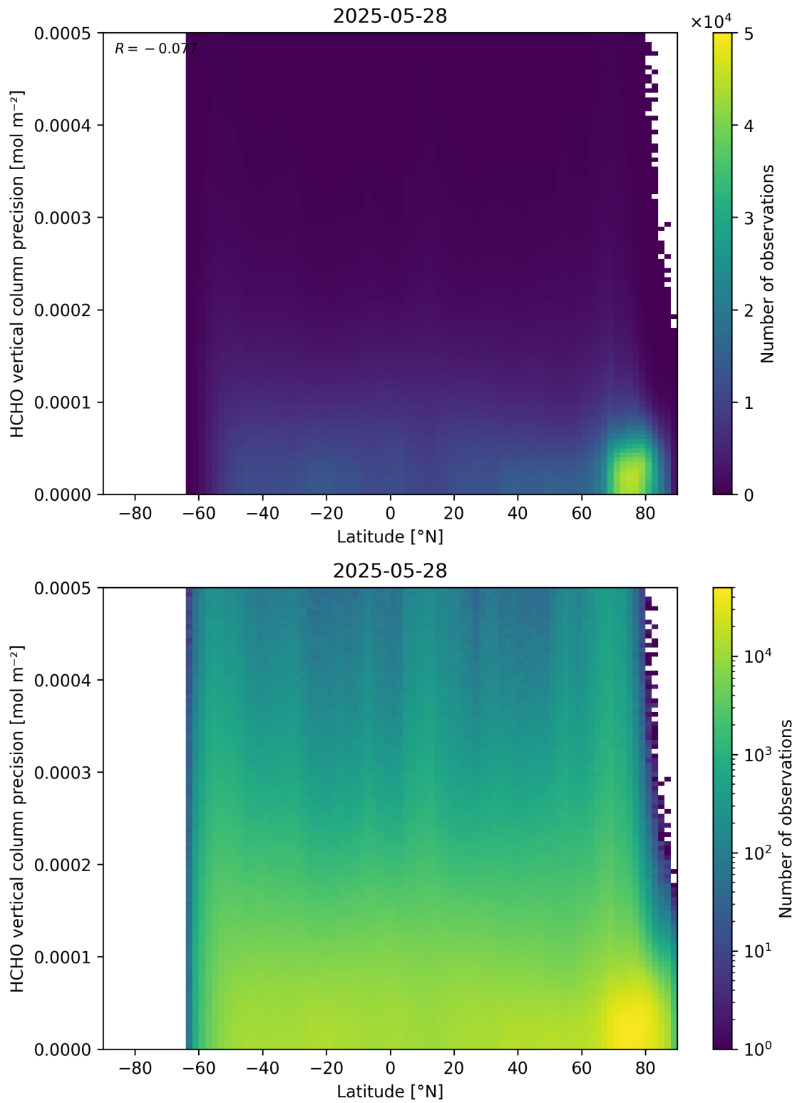
Figure 165: Scatter density plot of “Latitude” against “HCHO vertical column precision” for 2025-05-27 to 2025-05-29.
