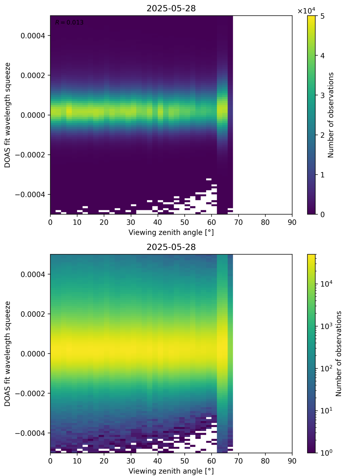
Figure 184: Scatter density plot of “Viewing zenith angle” against “DOAS fit wavelength squeeze” for 2025-05-27 to 2025-05-29.
