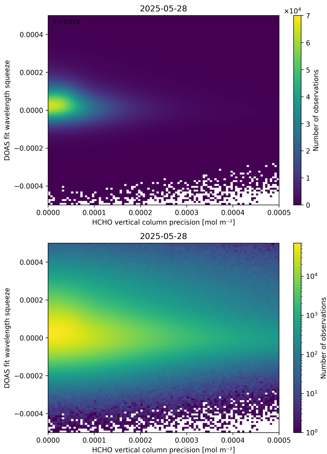
Figure 138: Scatter density plot of “HCHO vertical column precision” against “DOAS fit wavelength squeeze” for 2025-05-27 to 2025-05-29.
