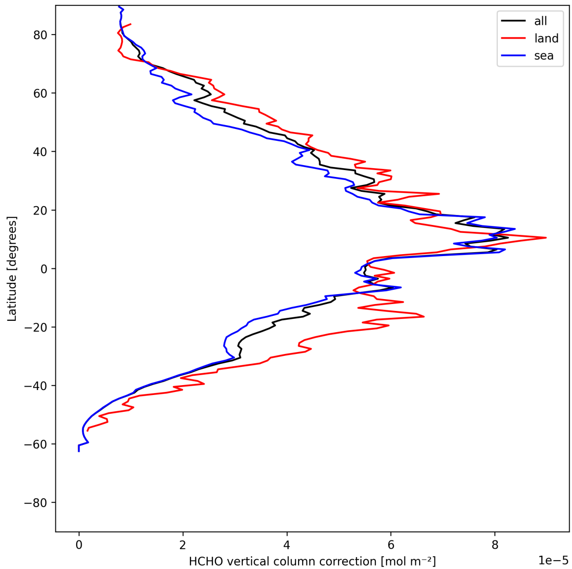
Figure 23: Zonal average of “HCHO vertical column correction” for 2025-05-27 to 2025-05-29.
