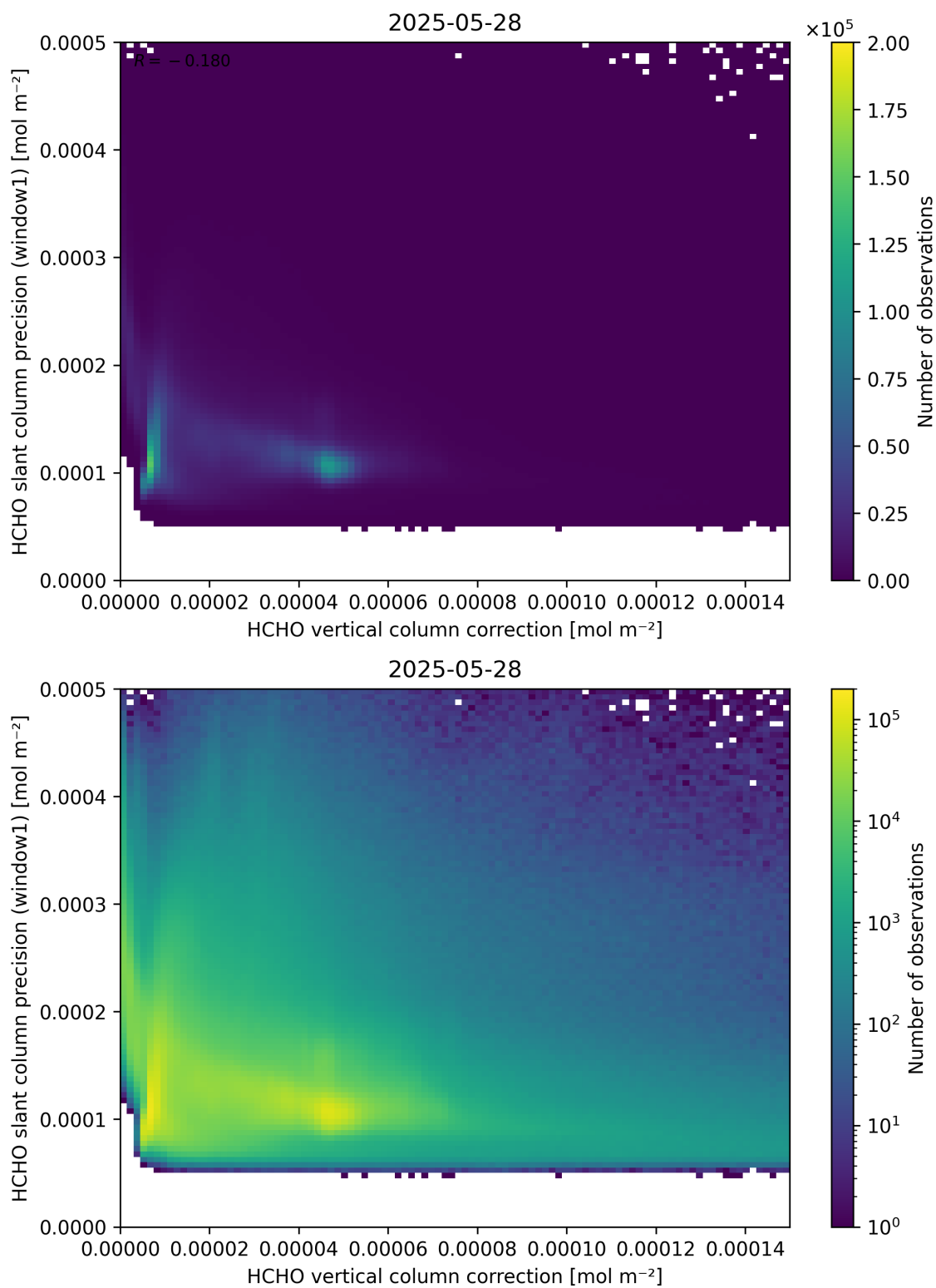
Figure 119: Scatter density plot of “HCHO vertical column correction” against “HCHO slant column precision (window1)” for 2025-05-27 to 2025-05-29.
