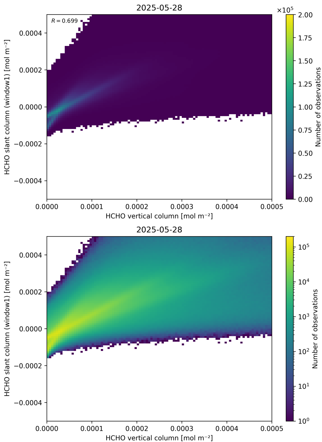
Figure 129: Scatter density plot of “HCHO vertical column” against “HCHO slant column (window1)” for 2025-05-27 to 2025-05-29.
