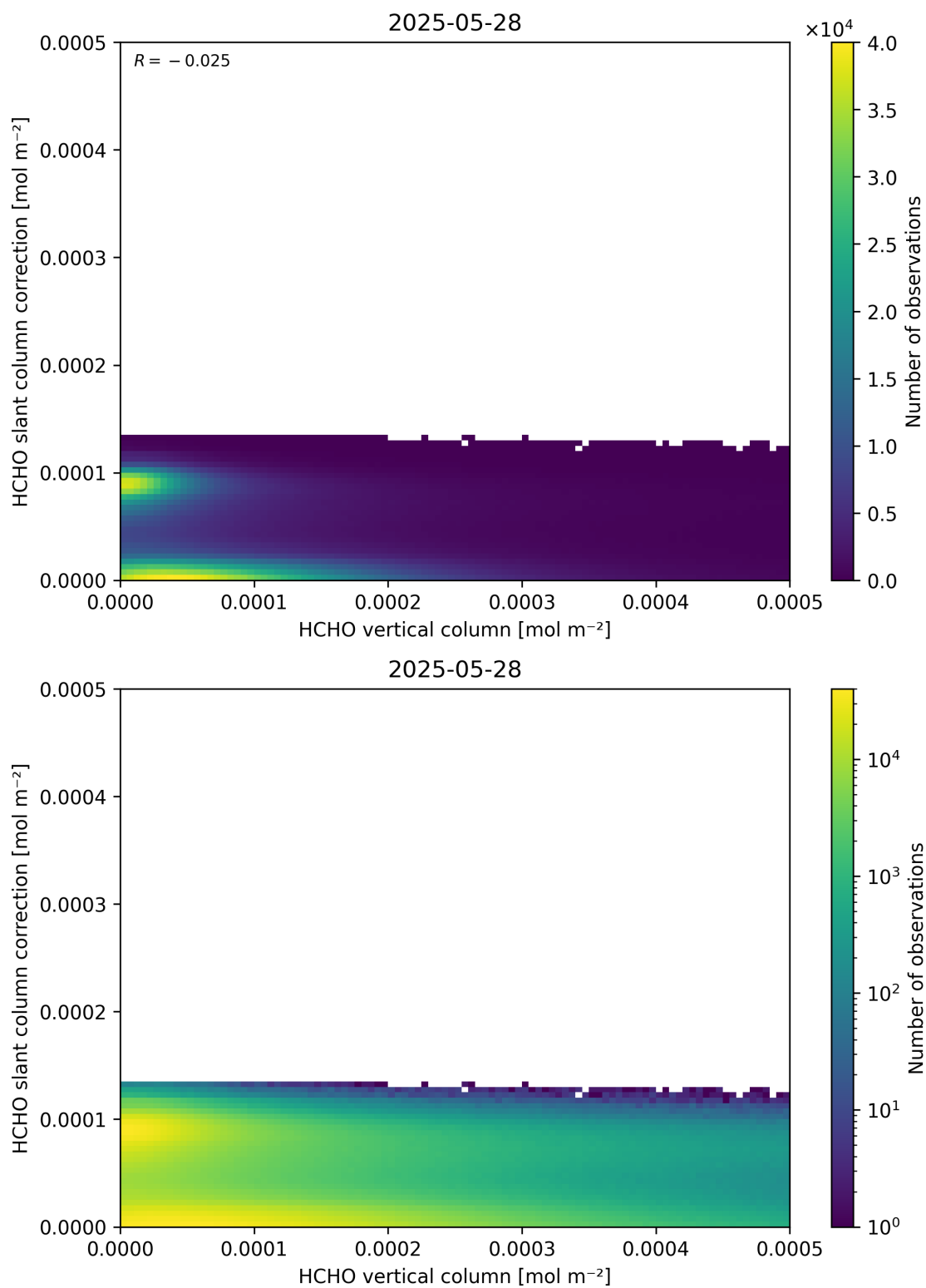
Figure 128: Scatter density plot of “HCHO vertical column” against “HCHO slant column correction” for 2025-05-27 to 2025-05-29.
