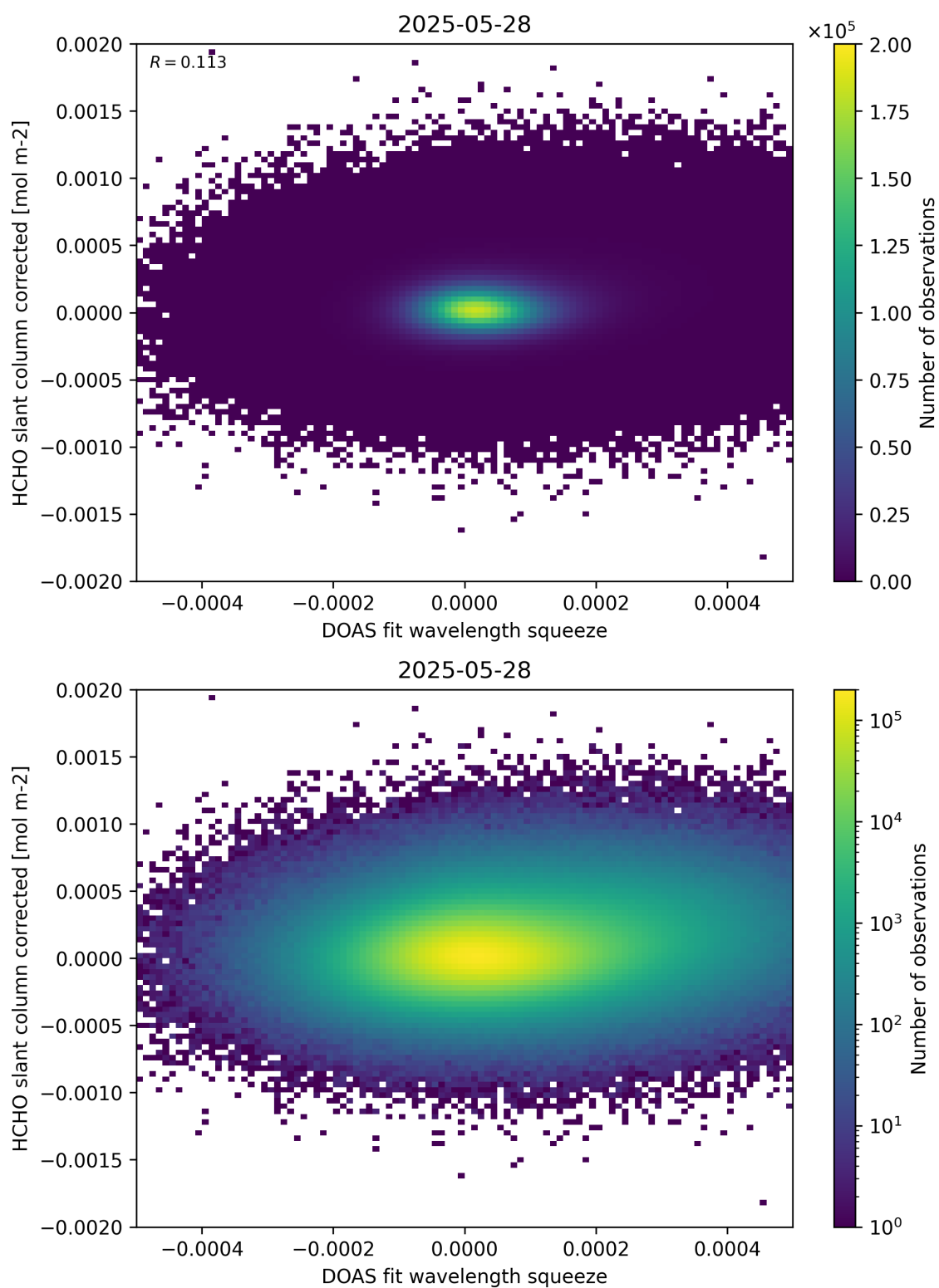
Figure 69: Scatter density plot of “DOAS fit wavelength squeeze” against “HCHO slant column corrected” for 2025-05-27 to 2025-05-29.
