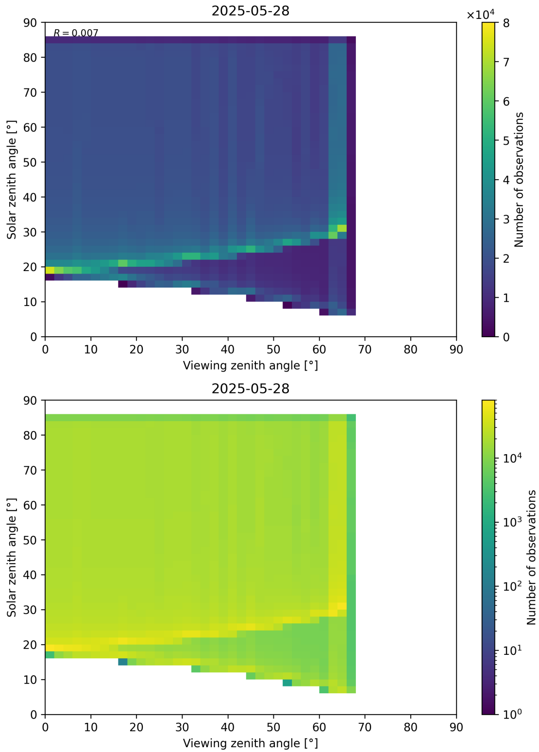
Figure 197: Scatter density plot of “Viewing zenith angle” against “Solar zenith angle” for 2025-05-27 to 2025-05-29.
