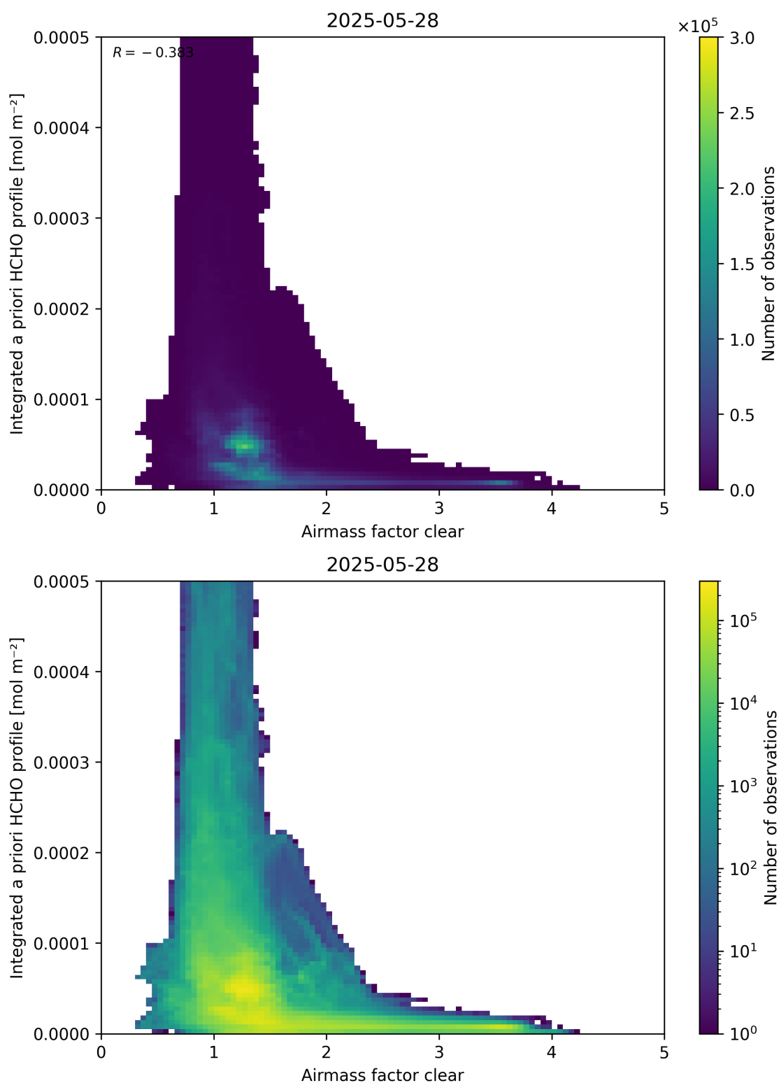
Figure 76: Scatter density plot of “Airmass factor clear” against “Integrated a priori HCHO profile” for 2025-05-27 to 2025-05-29.
