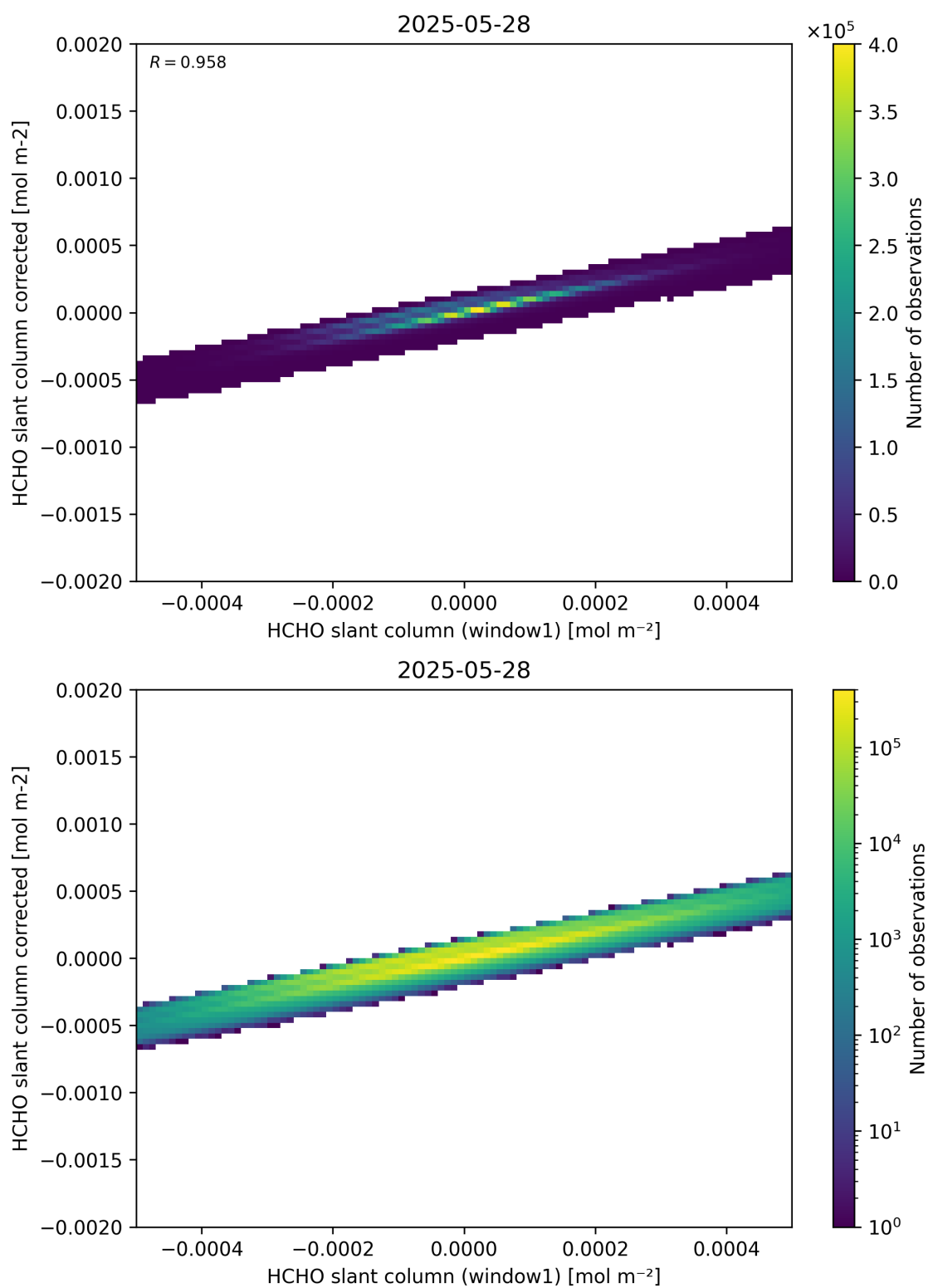
Figure 82: Scatter density plot of “HCHO slant column (window1)” against “HCHO slant column corrected” for 2025-05-27 to 2025-05-29.
