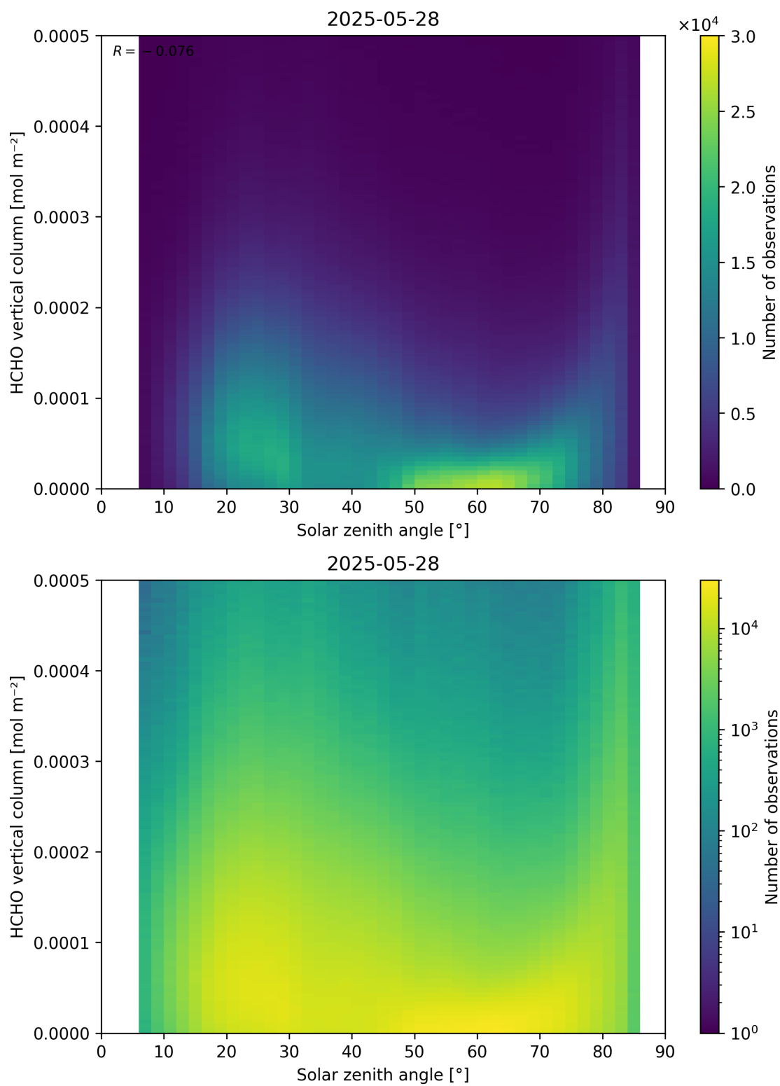
Figure 177: Scatter density plot of “Solar zenith angle” against “HCHO vertical column” for 2025-05-27 to 2025-05-29.
