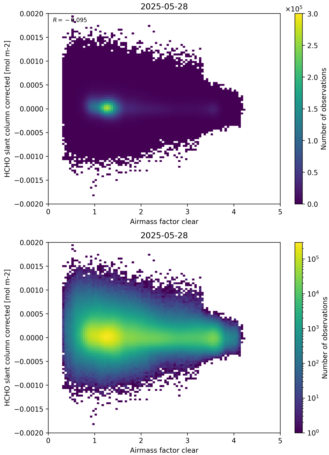
Figure 74: Scatter density plot of “Airmass factor clear” against “HCHO slant column corrected” for 2025-05-27 to 2025-05-29.
