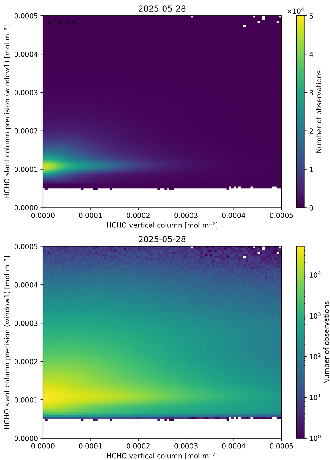
Figure 130: Scatter density plot of “HCHO vertical column” against “HCHO slant column precision (window1)” for 2025-05-27 to 2025-05-29.
