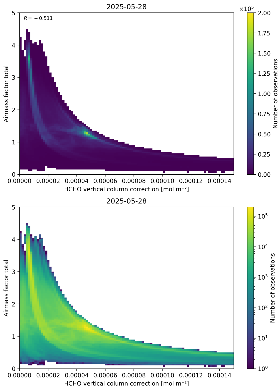
Figure 120: Scatter density plot of “HCHO vertical column correction” against “Airmass factor total” for 2025-05-27 to 2025-05-29.
