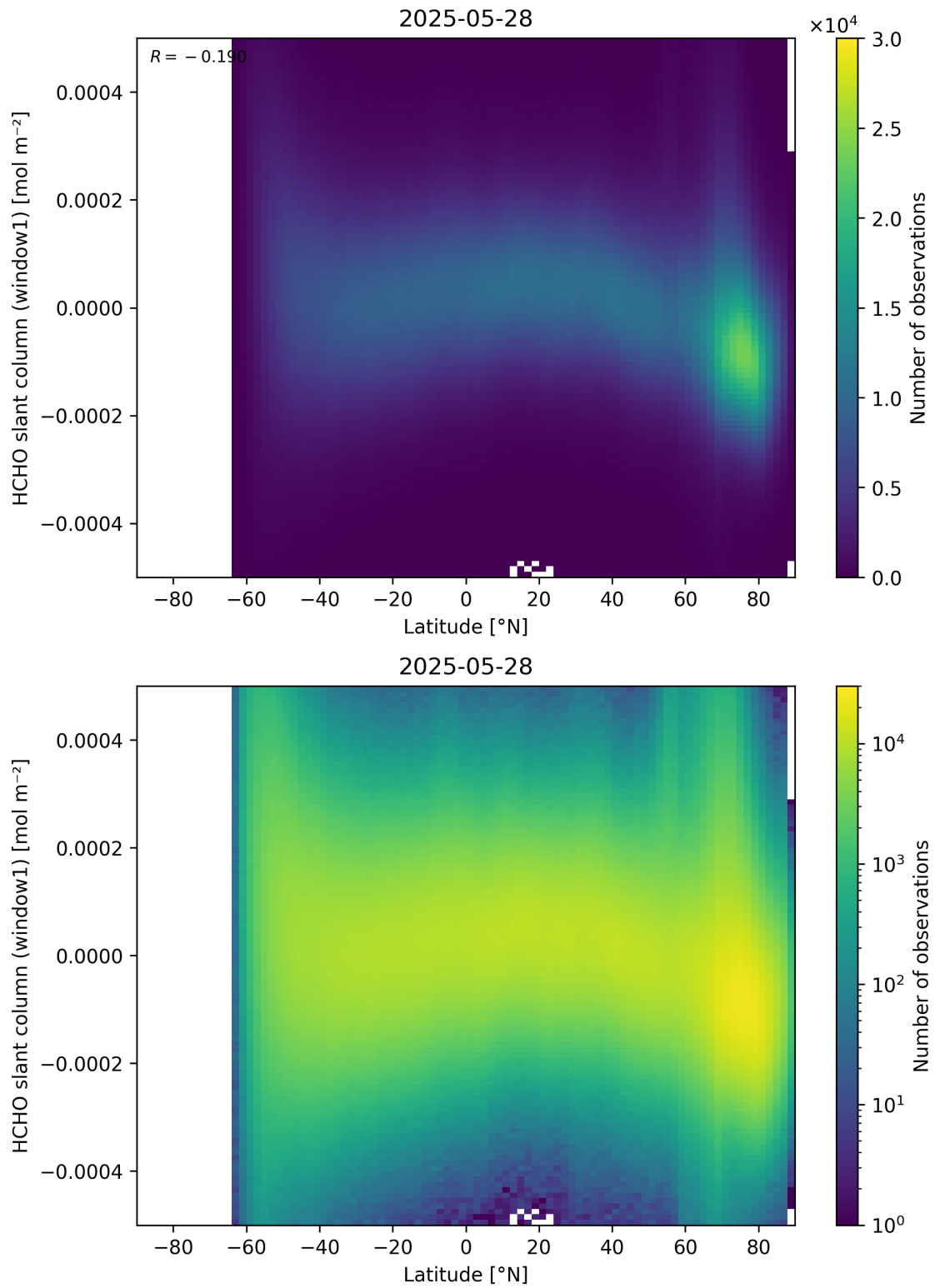
Figure 159: Scatter density plot of “Latitude” against “HCHO slant column (window1)” for 2025-05-27 to 2025-05-29.
