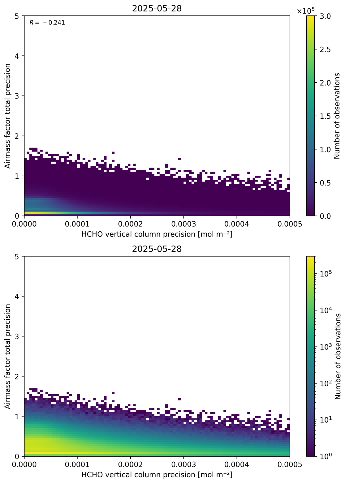
Figure 145: Scatter density plot of “HCHO vertical column precision” against “Airmass factor total precision” for 2025-05-27 to 2025-05-29.
