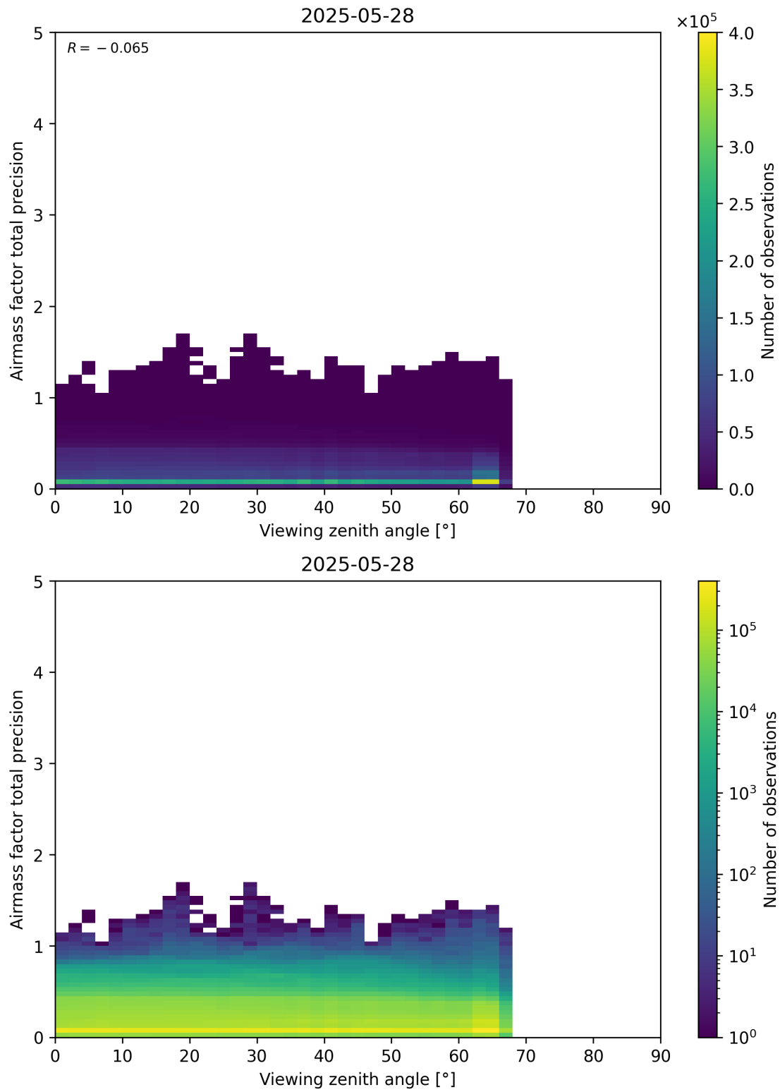
Figure 191: Scatter density plot of “Viewing zenith angle” against “Airmass factor total precision” for 2025-05-27 to 2025-05-29.
