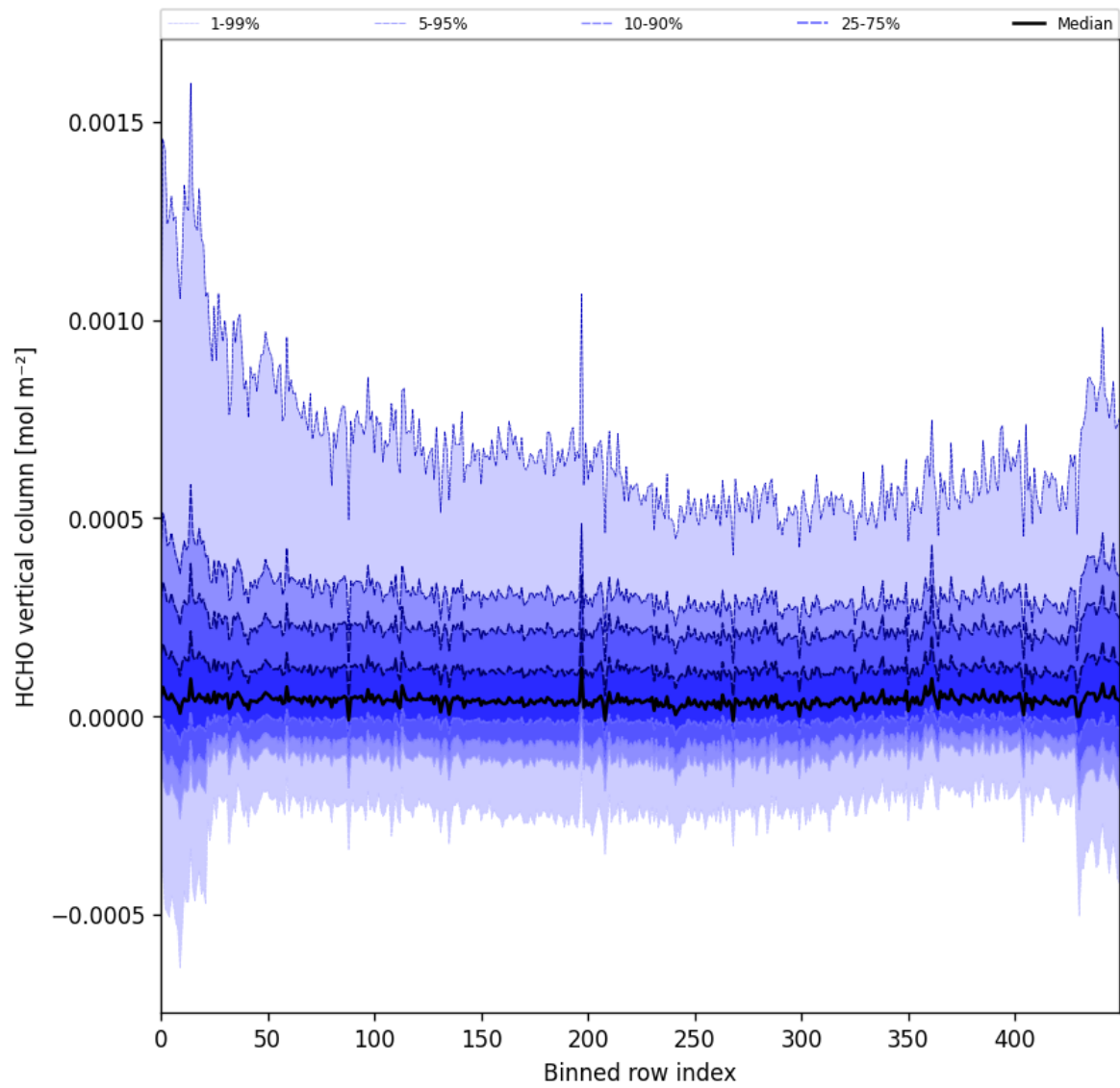
Figure 49: Along track statistics of “HCHO vertical column” for 2025-05-27 to 2025-05-29
