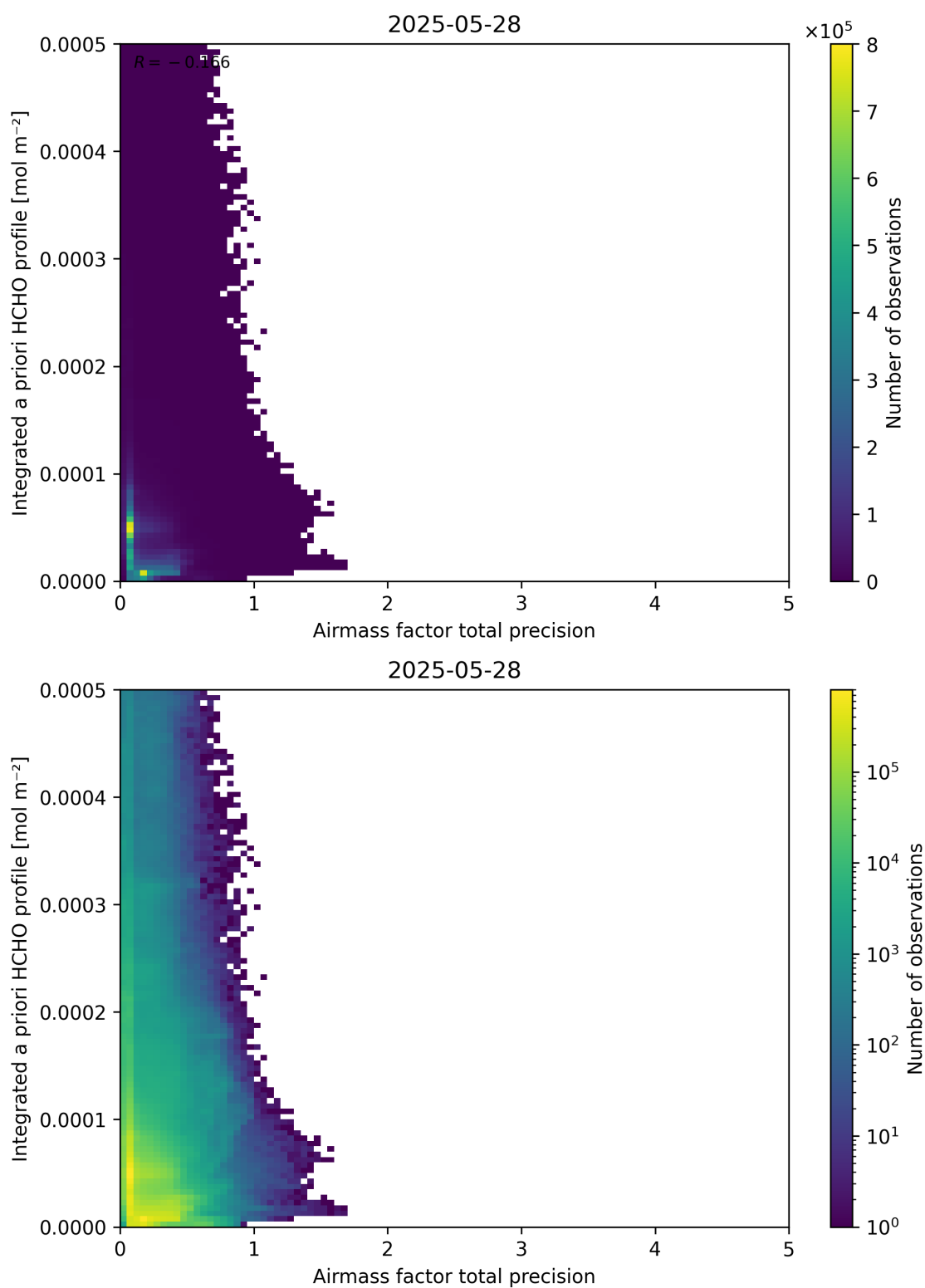
Figure 111: Scatter density plot of “Airmass factor total precision” against “Integrated a priori HCHO profile” for 2025-05-27 to 2025-05-29.
