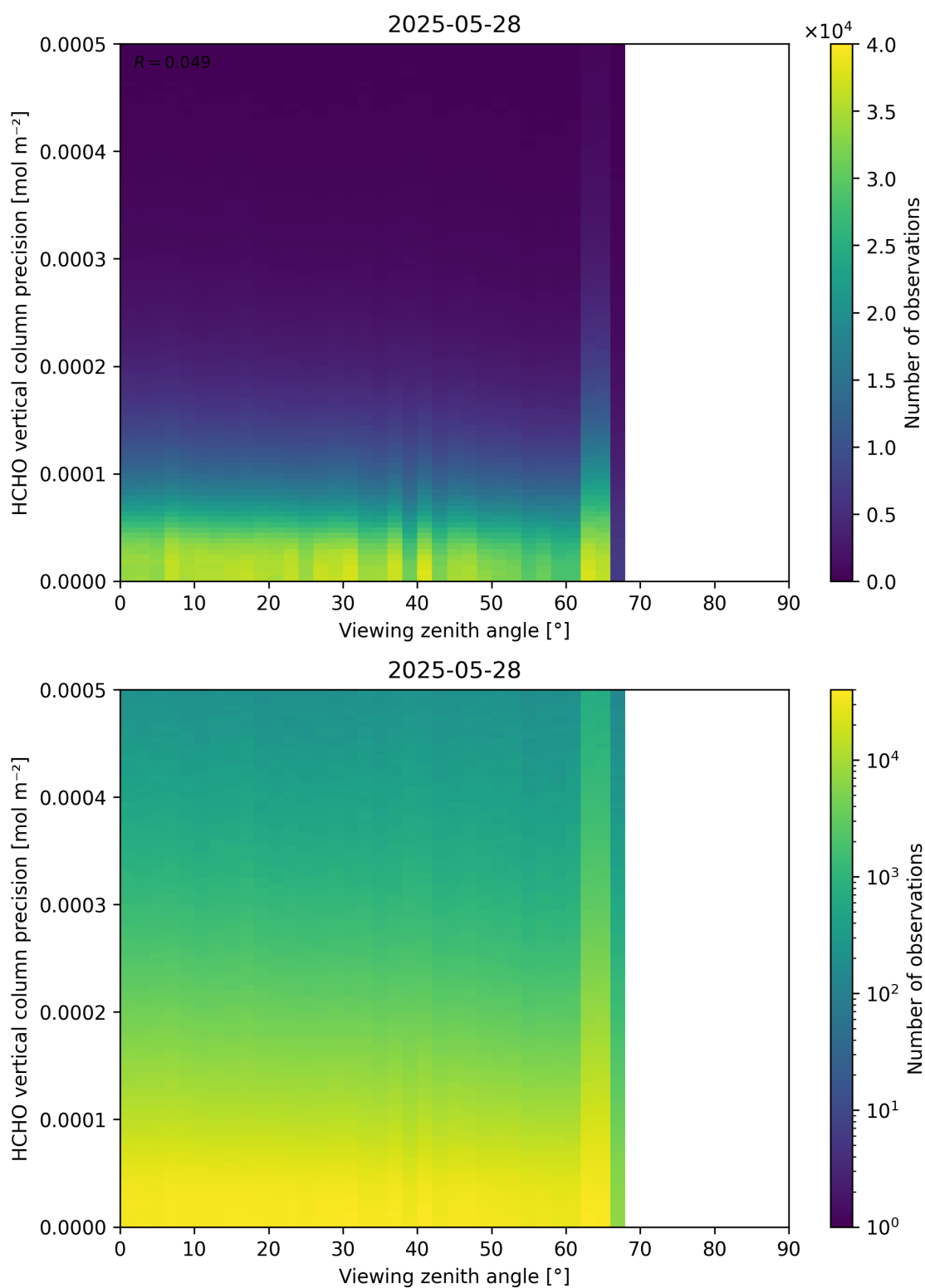
Figure 194: Scatter density plot of “Viewing zenith angle” against “HCHO vertical column precision” for 2025-05-27 to 2025-05-29.
