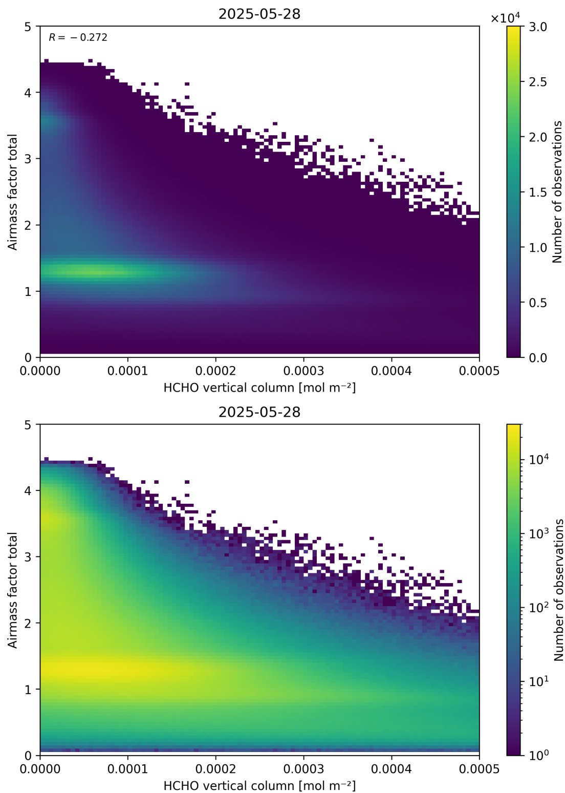
Figure 131: Scatter density plot of “HCHO vertical column” against “Airmass factor total” for 2025-05-27 to 2025-05-29.
