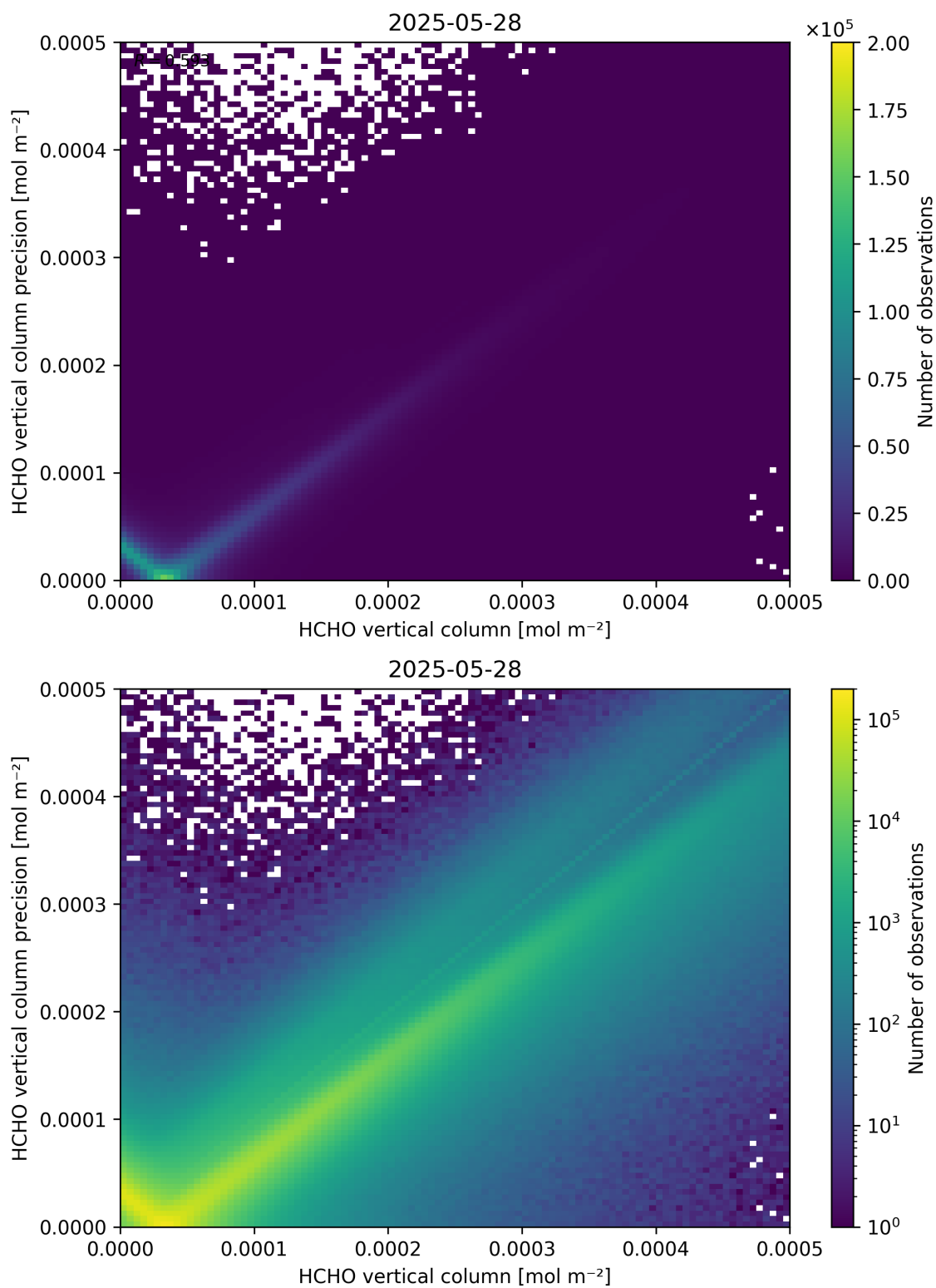
Figure 134: Scatter density plot of “HCHO vertical column” against “HCHO vertical column precision” for 2025-05-27 to 2025-05-29.
