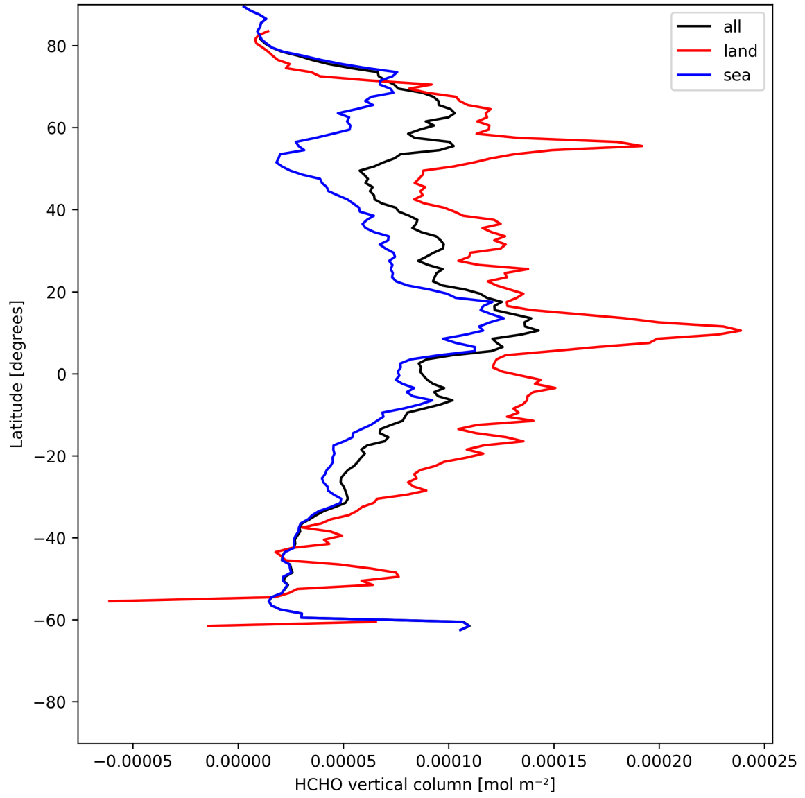
Figure 21: Zonal average of “HCHO vertical column” for 2025-05-27 to 2025-05-29.
