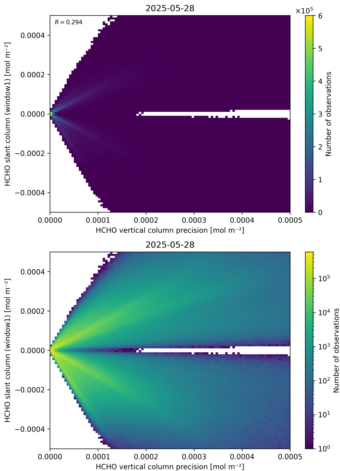
Figure 142: Scatter density plot of “HCHO vertical column precision” against “HCHO slant column (window1)” for 2025-05-27 to 2025-05-29.
