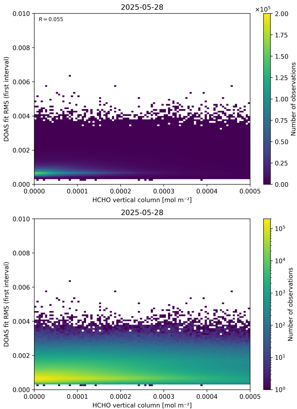
Figure 123: Scatter density plot of “HCHO vertical column” against “DOAS fit RMS (first interval)” for 2025-05-27 to 2025-05-29.
