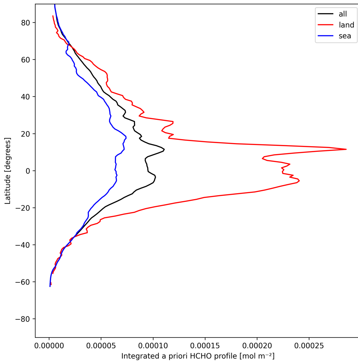
Figure 29: Zonal average of “Integrated a priori HCHO profile” for 2025-05-27 to 2025-05-29.
