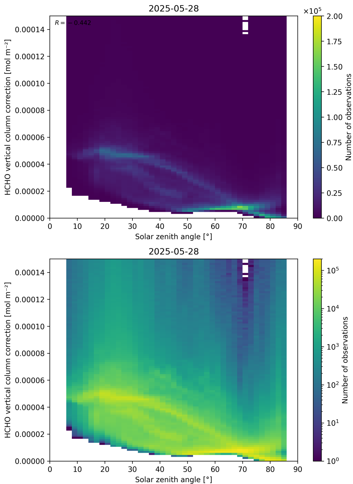
Figure 178: Scatter density plot of “Solar zenith angle” against “HCHO vertical column correction” for 2025-05-27 to 2025-05-29.
