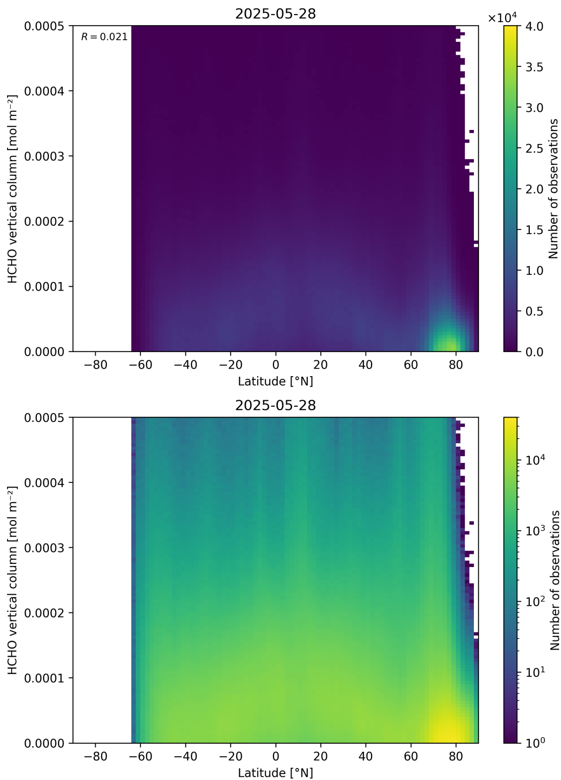
Figure 163: Scatter density plot of “Latitude” against “HCHO vertical column” for 2025-05-27 to 2025-05-29.
