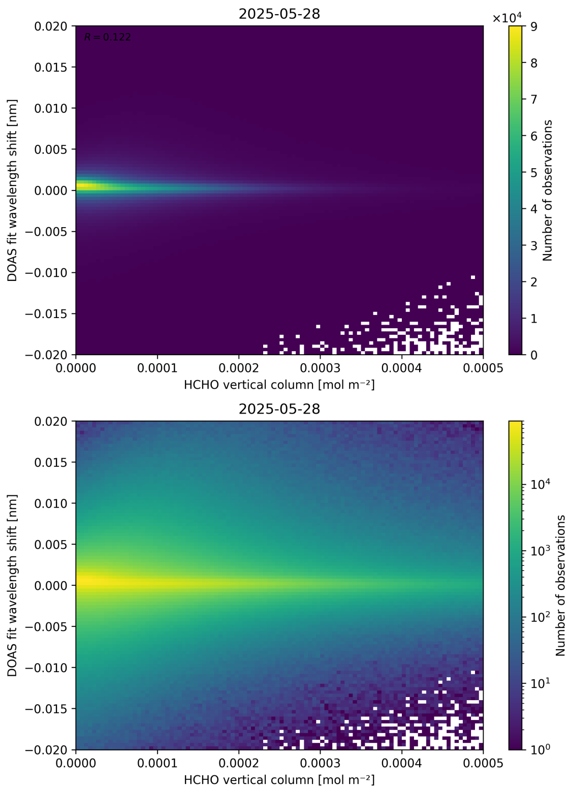
Figure 124: Scatter density plot of “HCHO vertical column” against “DOAS fit wavelength shift” for 2025-05-27 to 2025-05-29.
