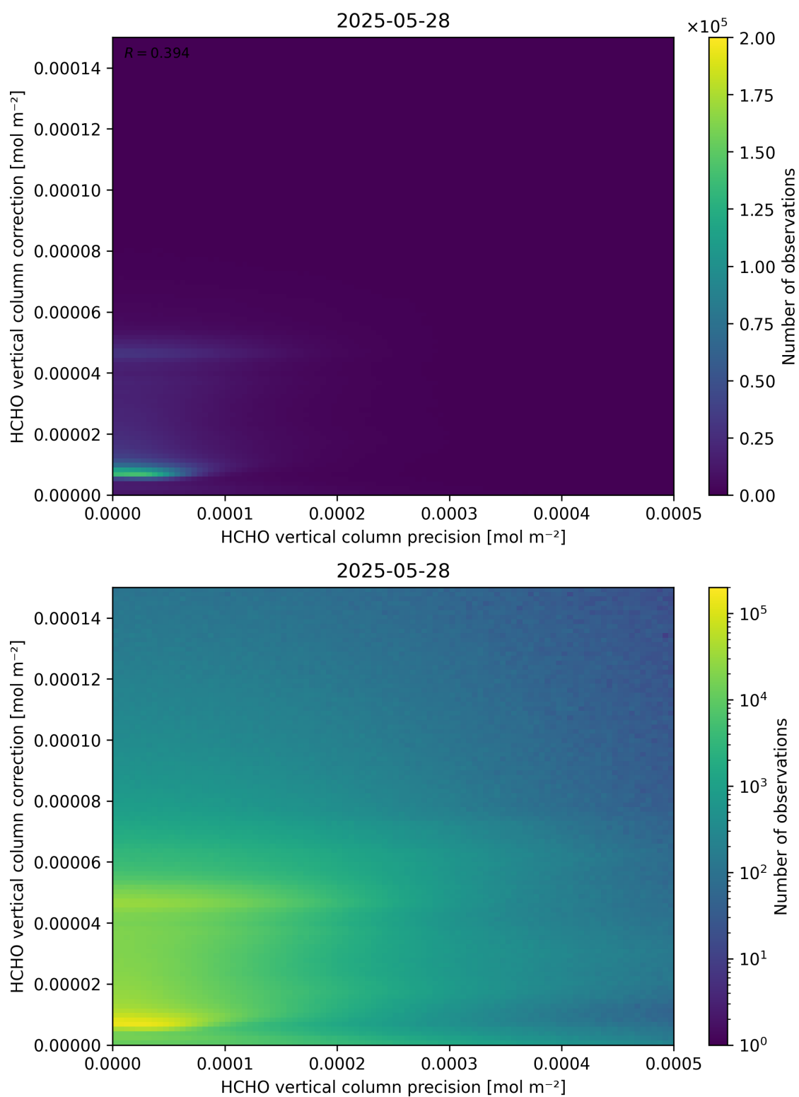
Figure 146: Scatter density plot of “HCHO vertical column precision” against “HCHO vertical column correction” for 2025-05-27 to 2025-05-29.
