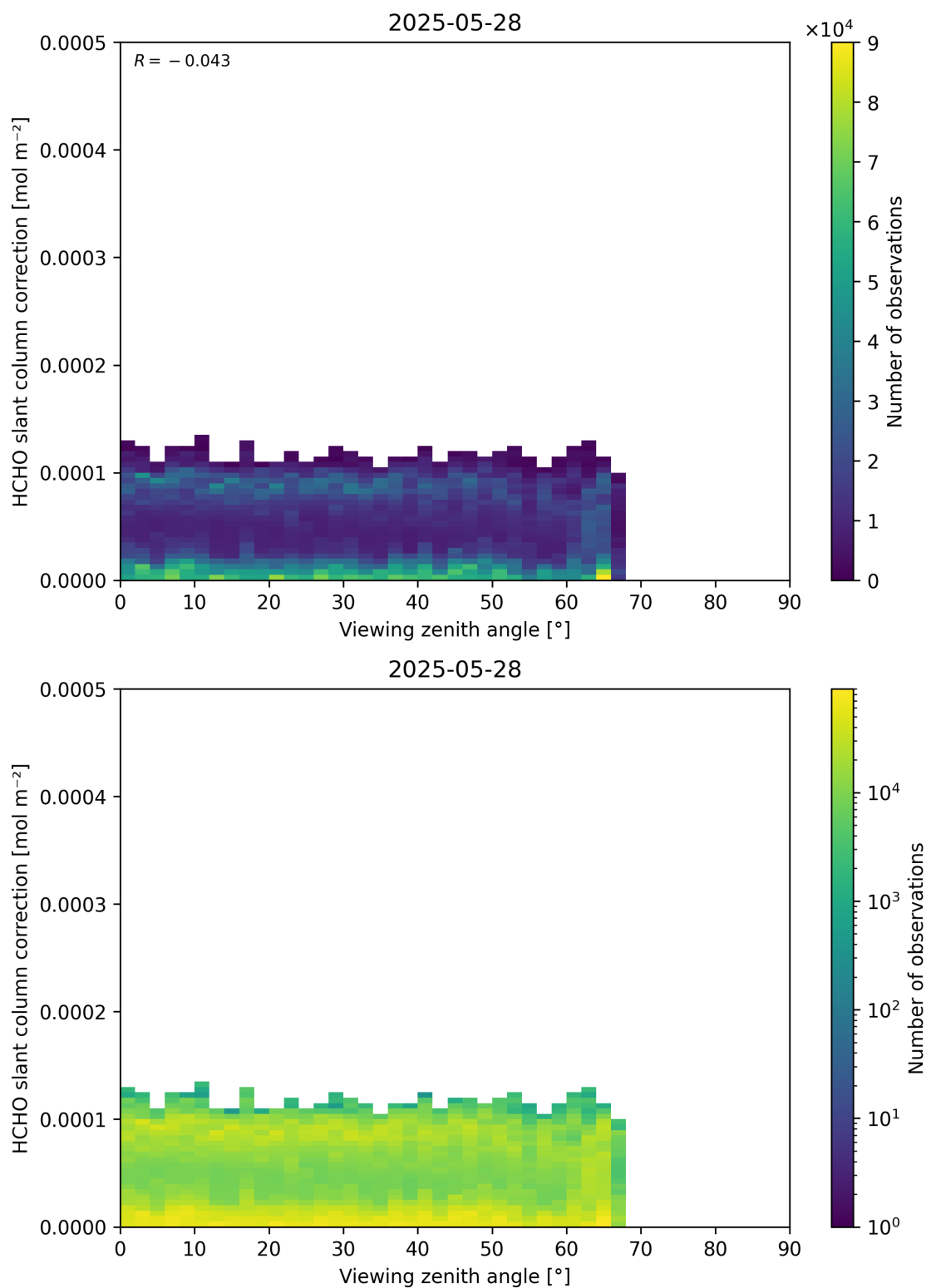
Figure 187: Scatter density plot of “Viewing zenith angle” against “HCHO slant column correction” for 2025-05-27 to 2025-05-29.
