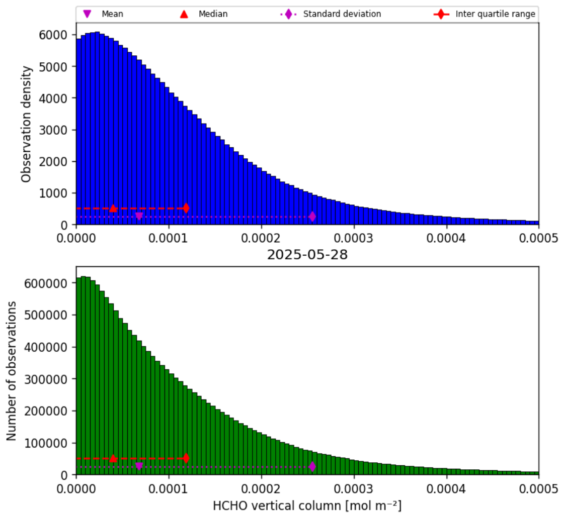
Figure 35: Histogram of “HCHO vertical column” for 2025-05-27 to 2025-05-29
