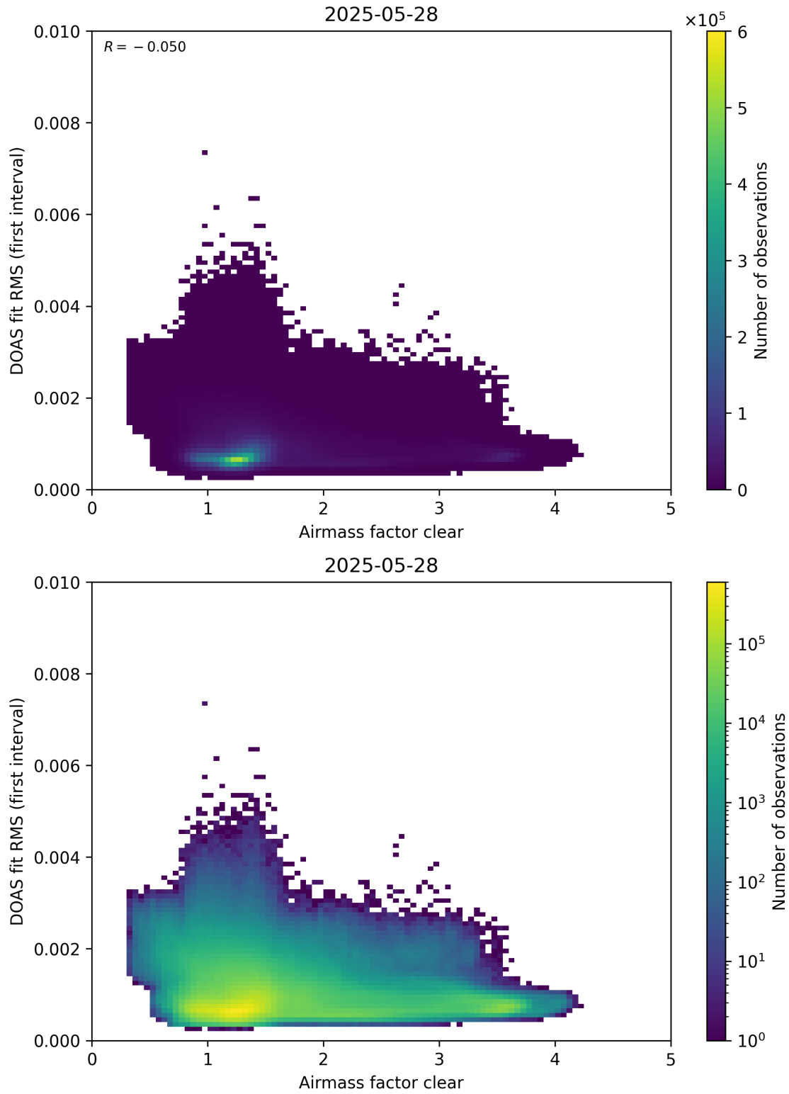
Figure 71: Scatter density plot of “Airmass factor clear” against “DOAS fit RMS (first interval)” for 2025-05-27 to 2025-05-29.
