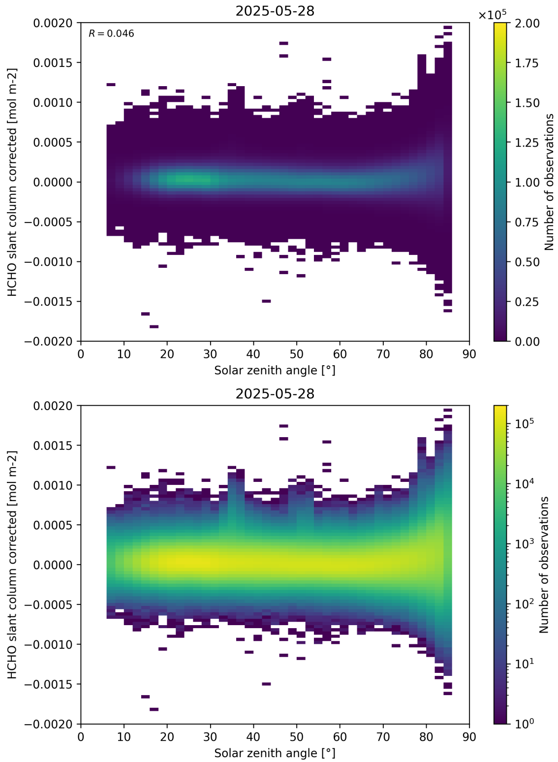
Figure 171: Scatter density plot of “Solar zenith angle” against “HCHO slant column corrected” for 2025-05-27 to 2025-05-29.
