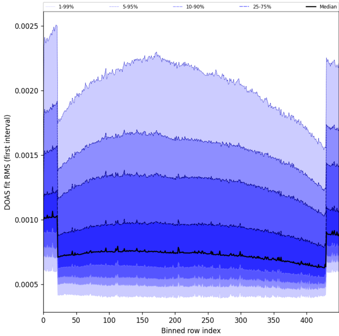
Figure 60: Along track statistics of “DOAS fit RMS (first interval)” for 2025-05-27 to 2025-05-29
