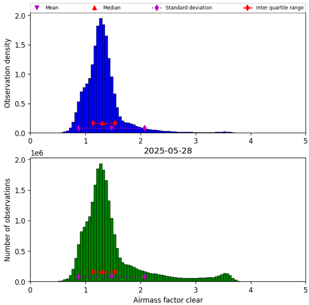
Figure 42: Histogram of “Airmass factor clear” for 2025-05-27 to 2025-05-29
