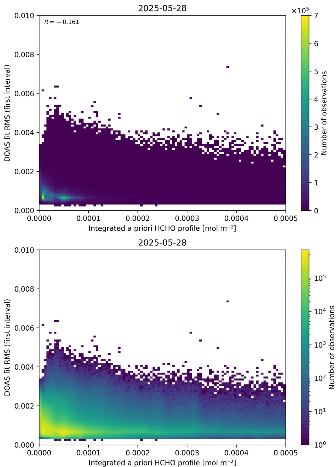
Figure 148: Scatter density plot of “Integrated a priori HCHO profile” against “DOAS fit RMS (first interval)” for 2025-05-27 to 2025-05-29.
