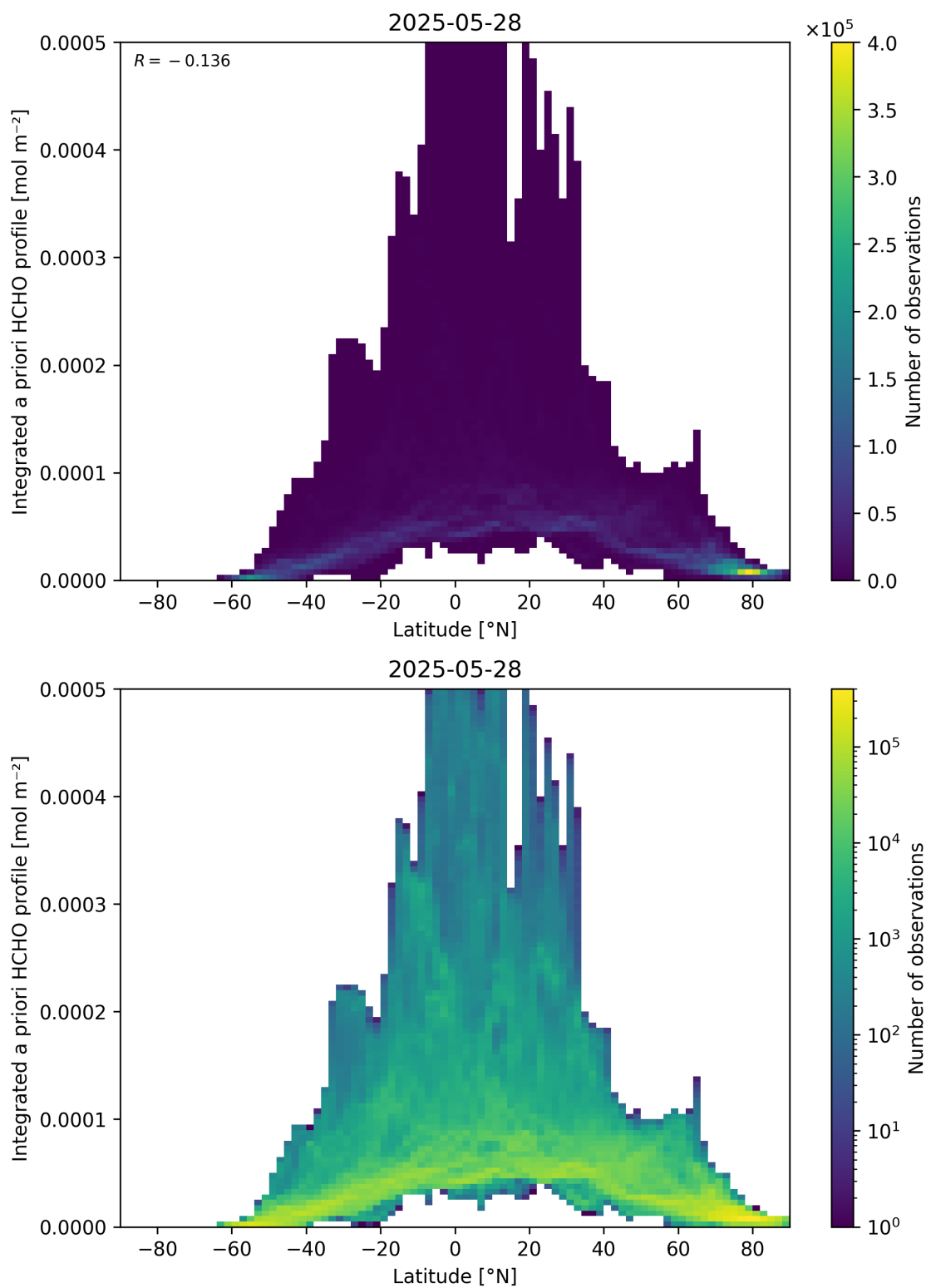
Figure 166: Scatter density plot of “Latitude” against “Integrated a priori HCHO profile” for 2025-05-27 to 2025-05-29.
