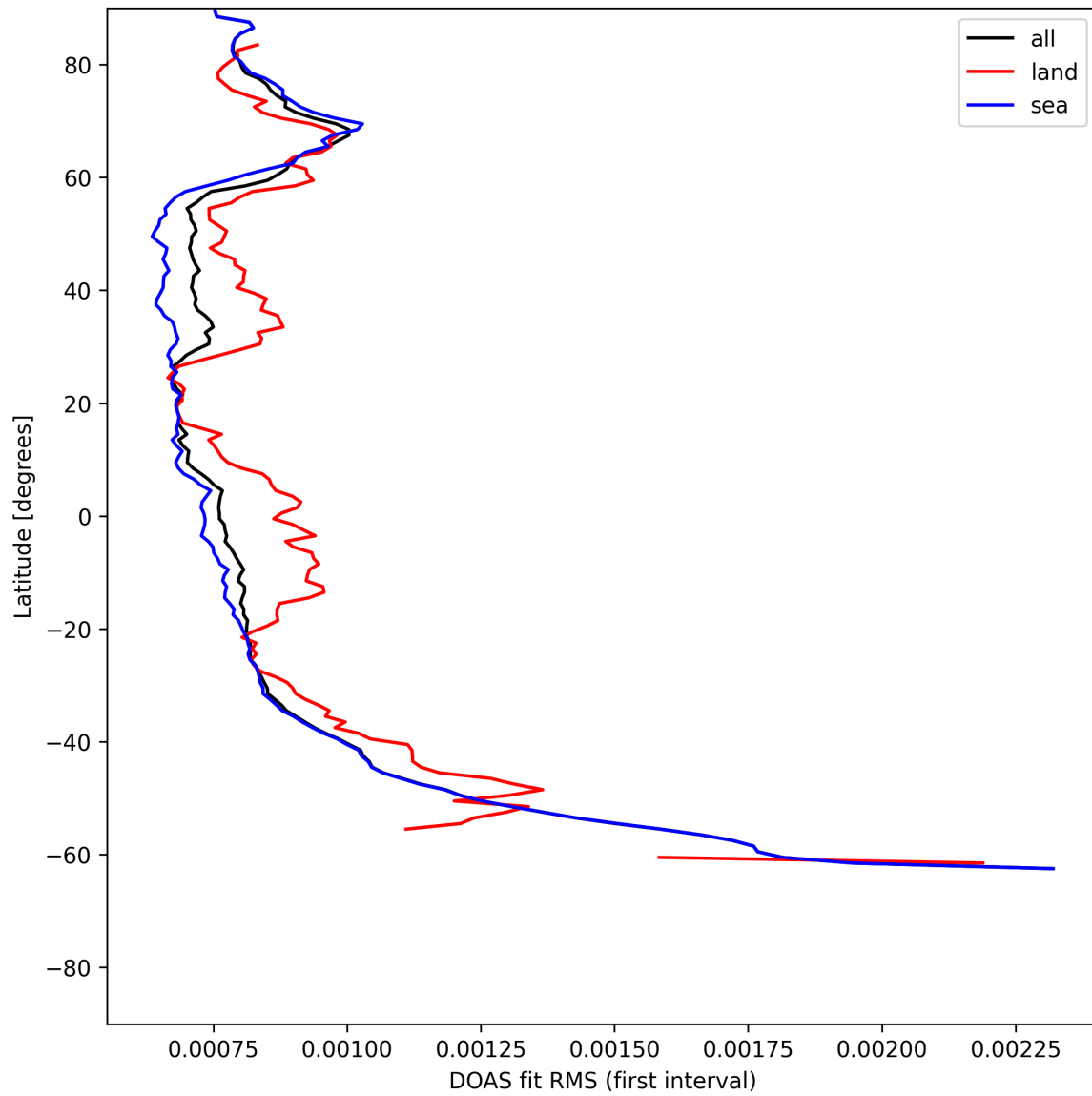
Figure 32: Zonal average of “DOAS fit RMS (first interval)” for 2025-05-27 to 2025-05-29.
