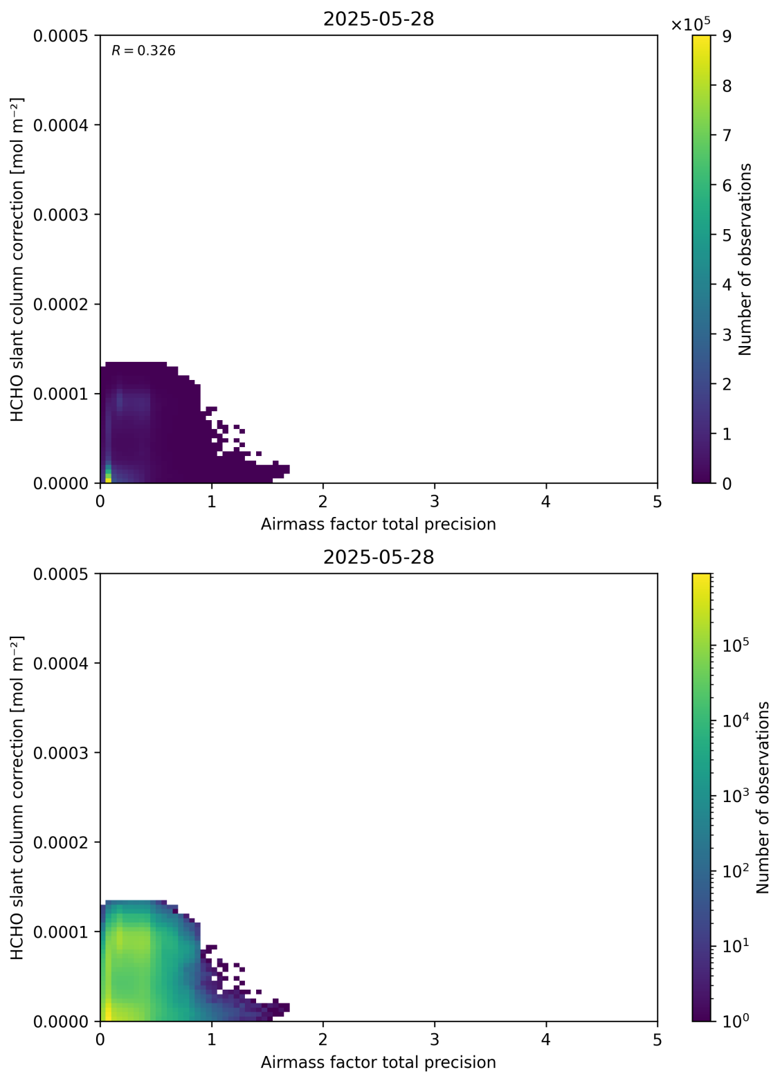
Figure 110: Scatter density plot of “Airmass factor total precision” against “HCHO slant column correction” for 2025-05-27 to 2025-05-29.
