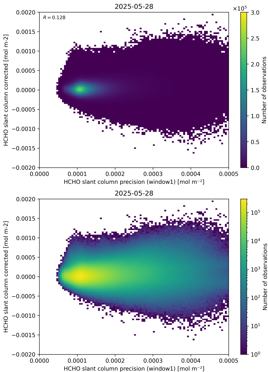
Figure 92: Scatter density plot of “HCHO slant column precision (window1)” against “HCHO slant column corrected” for 2025-05-27 to 2025-05-29.
