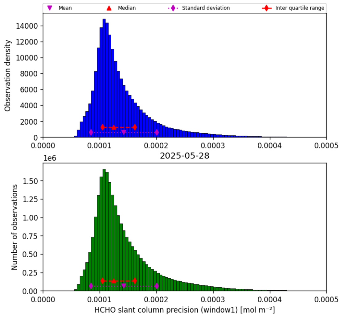
Figure 39: Histogram of “HCHO slant column precision (window1)” for 2025-05-27 to 2025-05-29
