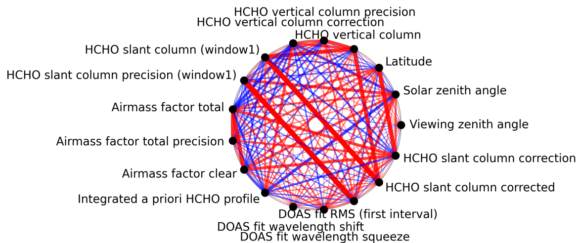
Figure 1: Map of correlation graph for 2025-05-27 to 2025-05-29.
