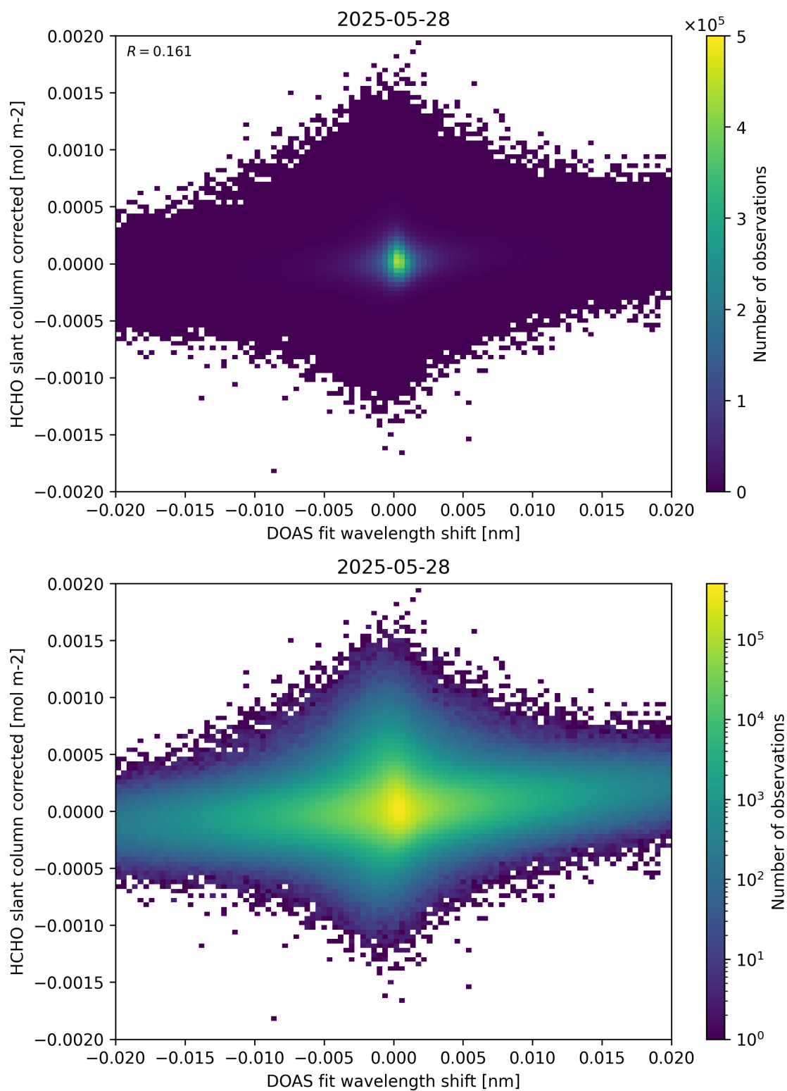
Figure 66: Scatter density plot of “DOAS fit wavelength shift” against “HCHO slant column corrected” for 2025-05-27 to 2025-05-29.
