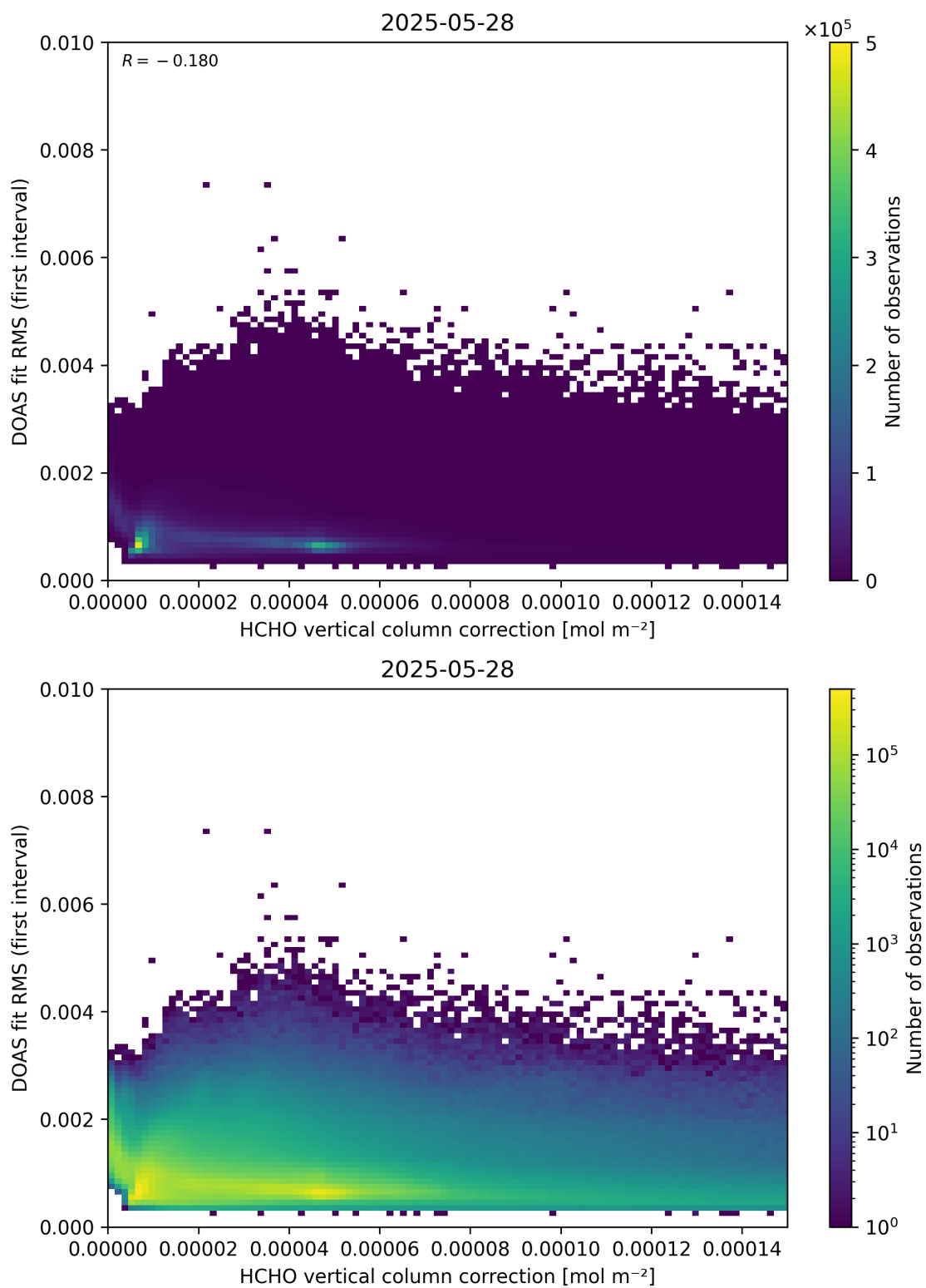
Figure 112: Scatter density plot of “HCHO vertical column correction” against “DOAS fit RMS (first interval)” for 2025-05-27 to 2025-05-29.
