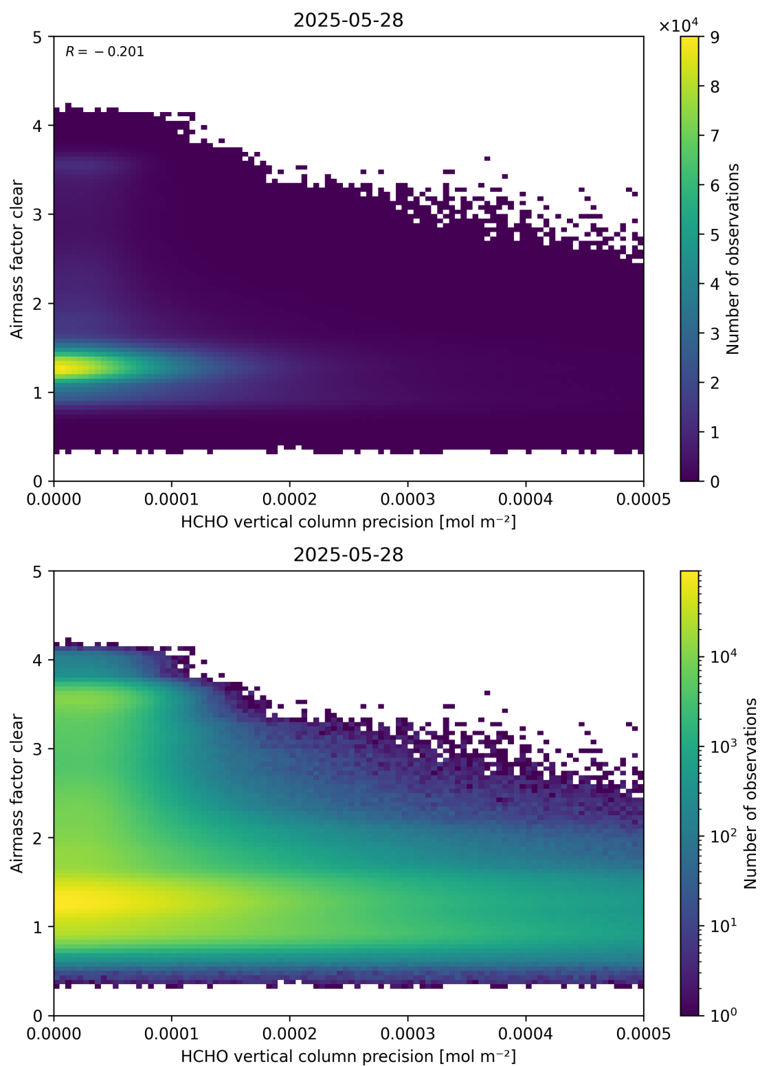
Figure 139: Scatter density plot of “HCHO vertical column precision” against “Airmass factor clear” for 2025-05-27 to 2025-05-29.
