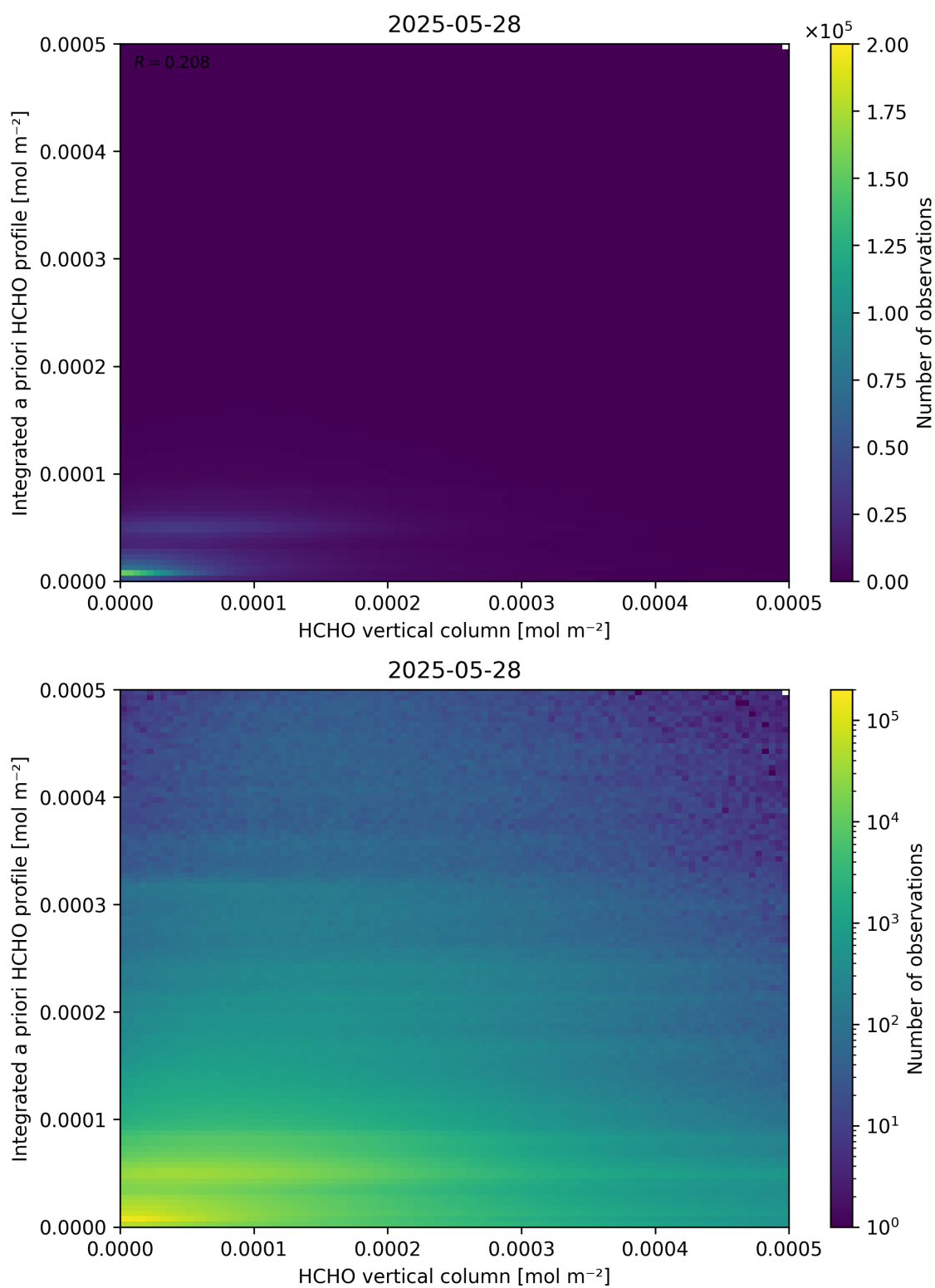
Figure 135: Scatter density plot of “HCHO vertical column” against “Integrated a priori HCHO profile” for 2025-05-27 to 2025-05-29.
