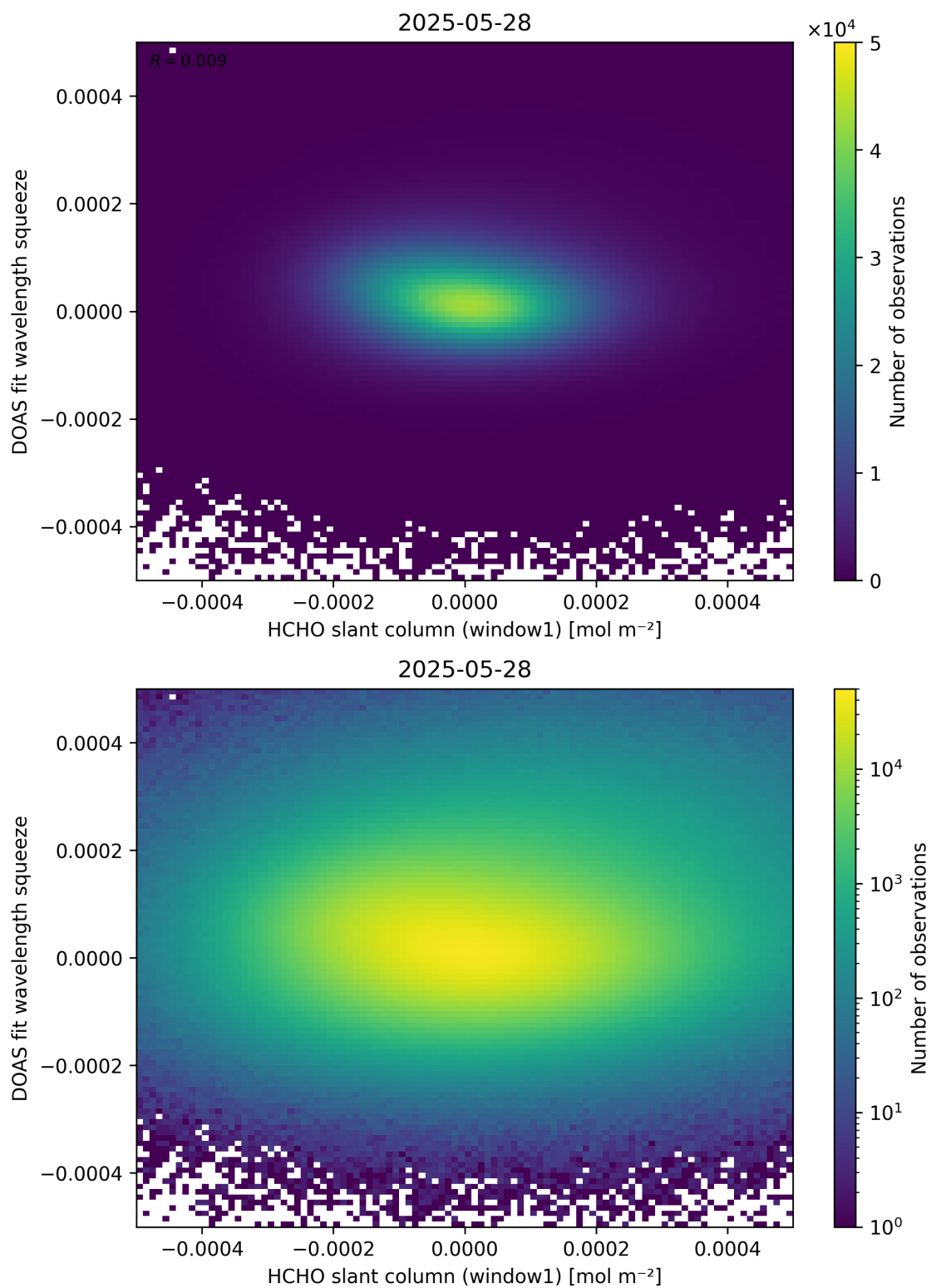
Figure 80: Scatter density plot of “HCHO slant column (window1)” against “DOAS fit wavelength squeeze” for 2025-05-27 to 2025-05-29.
