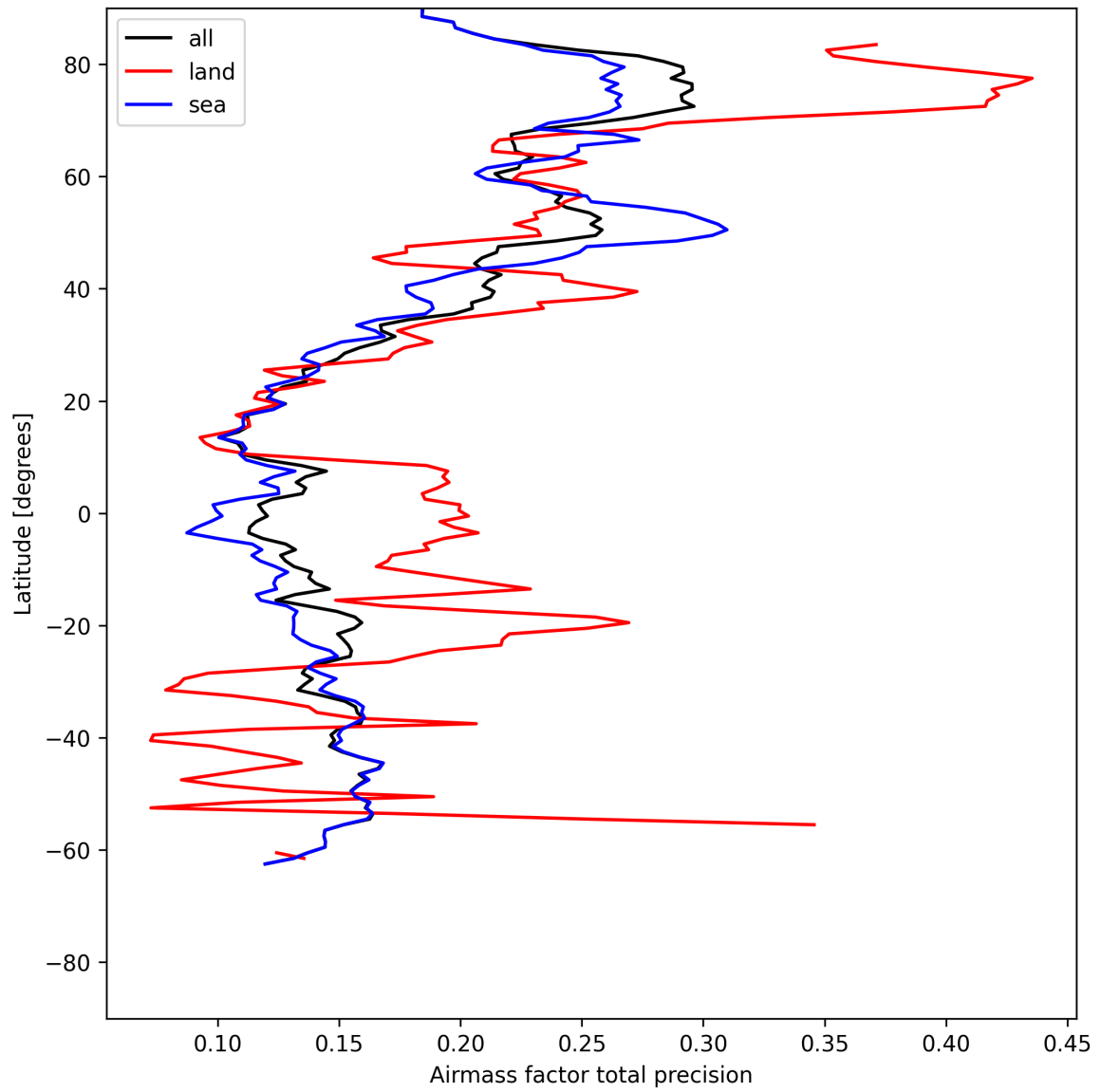
Figure 27: Zonal average of “Airmass factor total precision” for 2025-05-27 to 2025-05-29.
