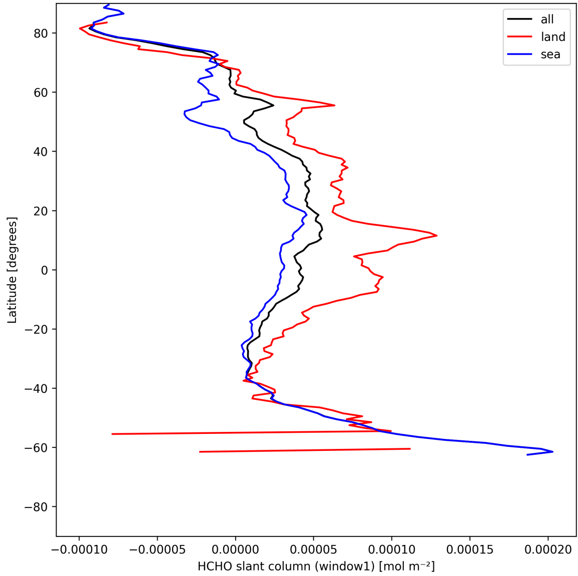
Figure 24: Zonal average of “HCHO slant column (window1)” for 2025-05-27 to 2025-05-29.
