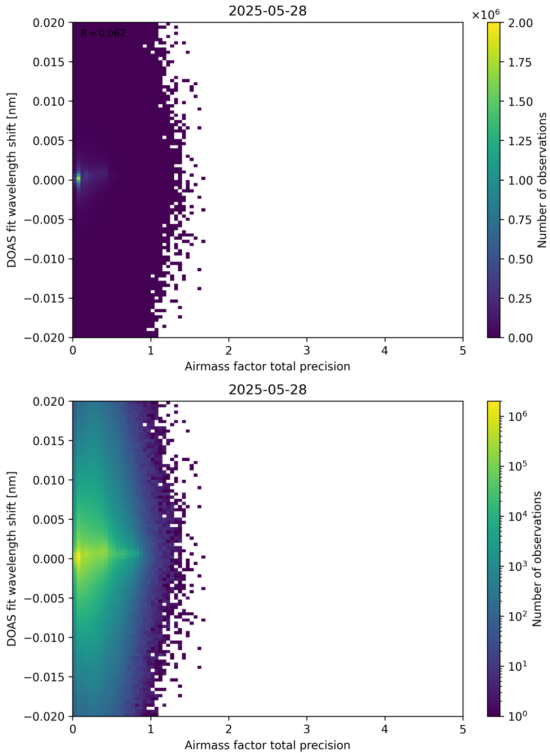
Figure 106: Scatter density plot of “Airmass factor total precision” against “DOAS fit wavelength shift” for 2025-05-27 to 2025-05-29.
