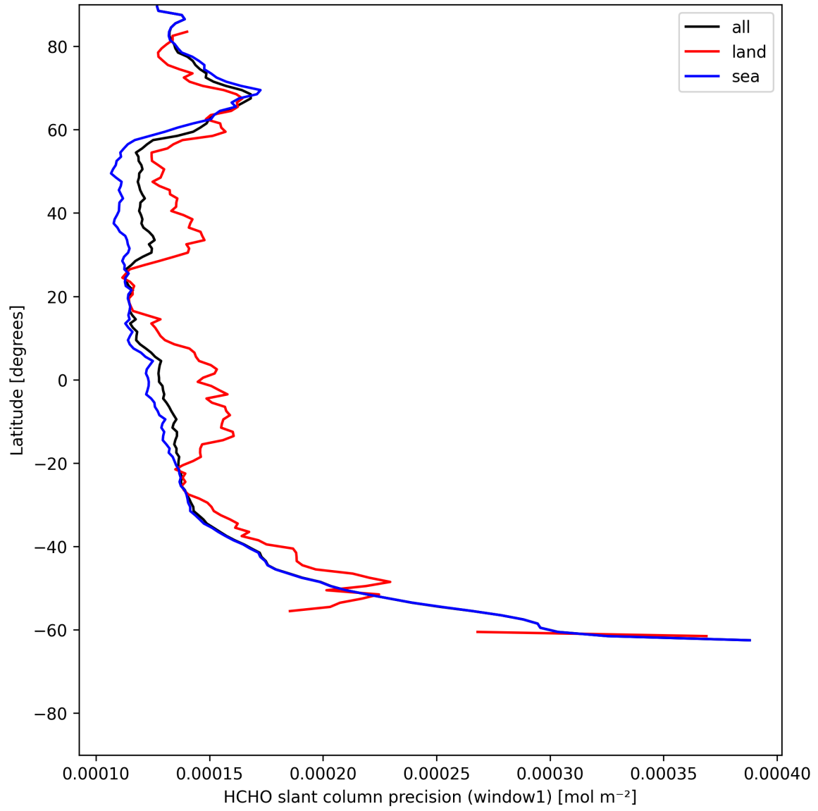
Figure 25: Zonal average of "HCHO slant column precision (window1)" for 2025-05-27 to 2025-05-29.
