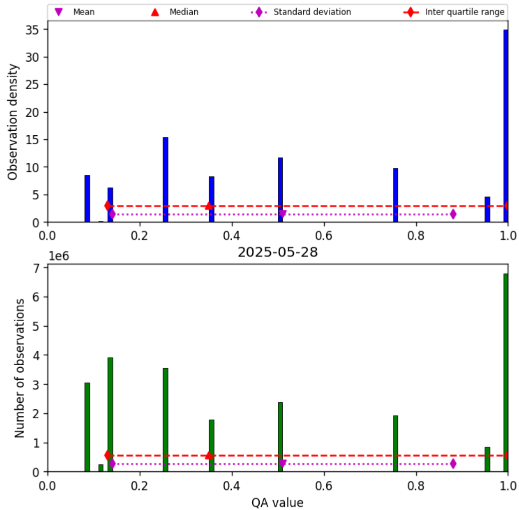
Figure 34: Histogram of “QA value” for 2025-05-27 to 2025-05-29
