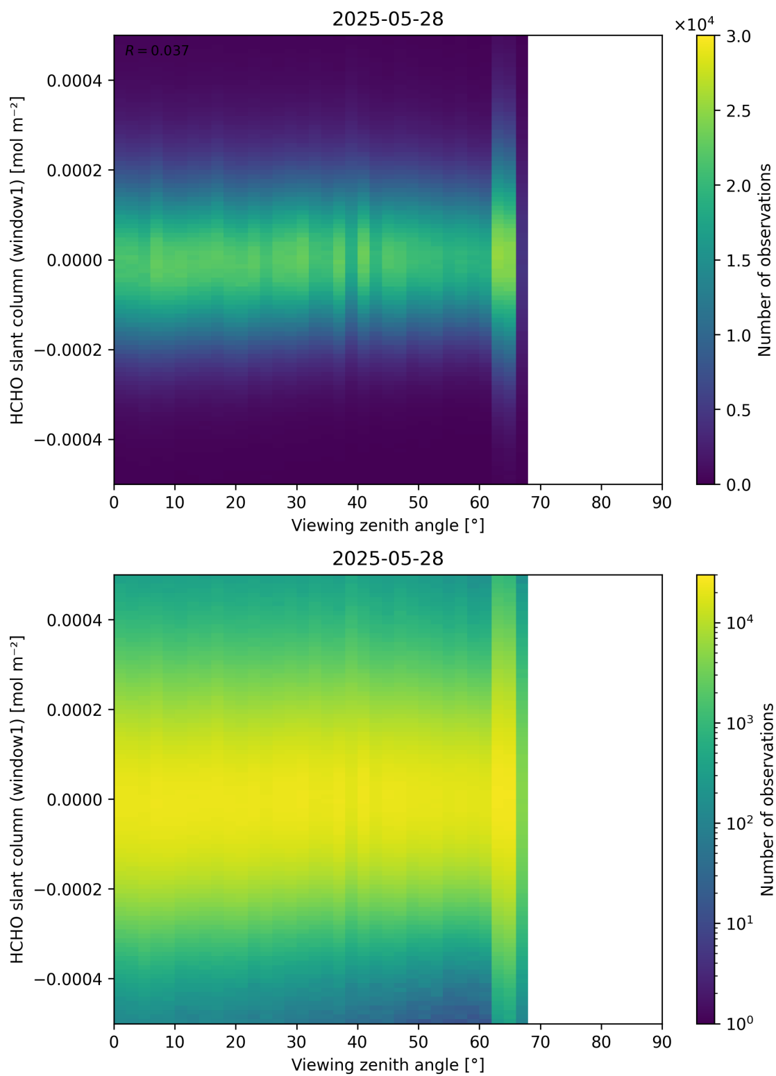
Figure 188: Scatter density plot of “Viewing zenith angle” against “HCHO slant column (window1)” for 2025-05-27 to 2025-05-29.
