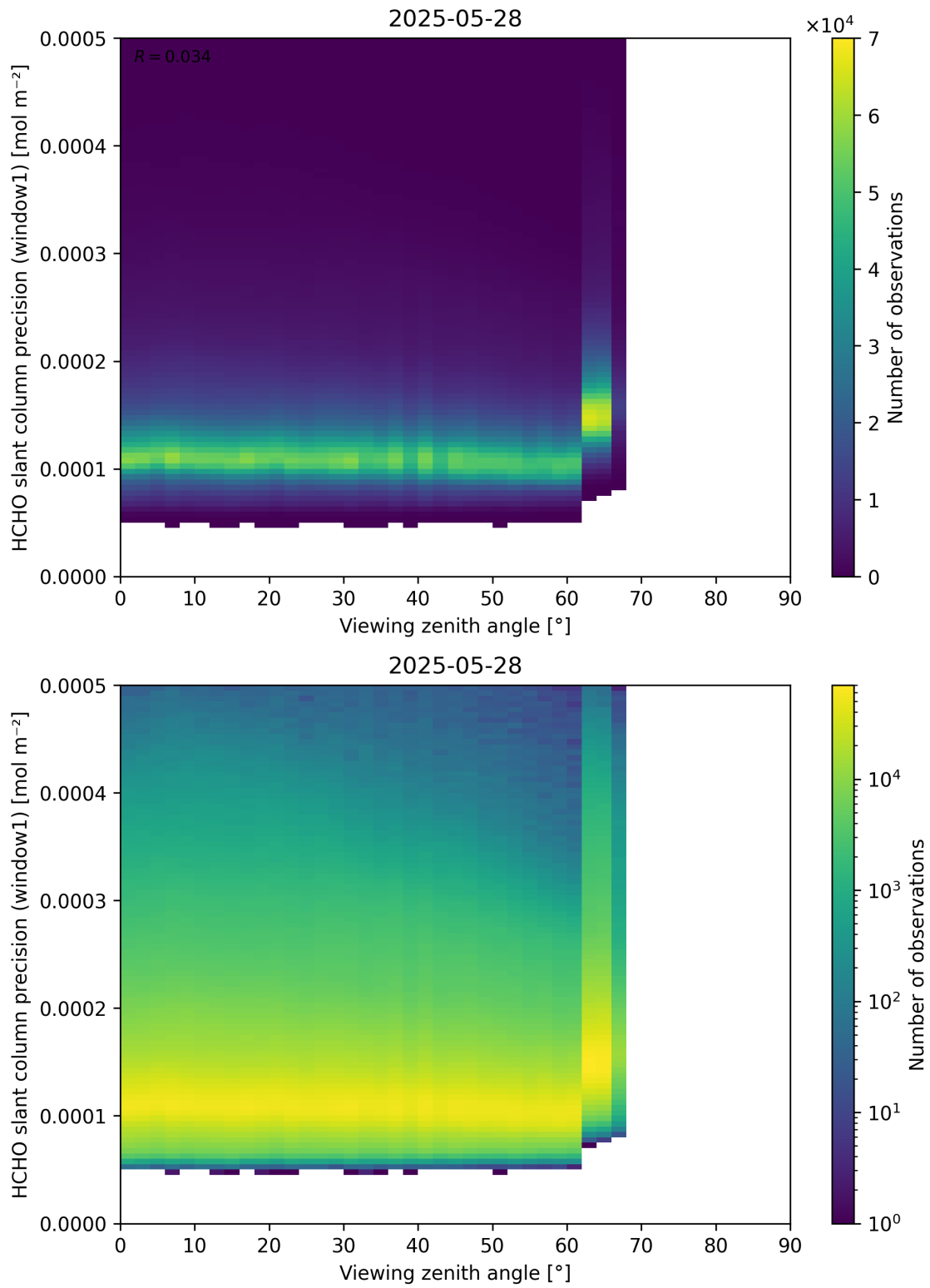
Figure 189: Scatter density plot of “Viewing zenith angle” against “HCHO slant column precision (window1)” for 2025-05-27 to 2025-05-29.
