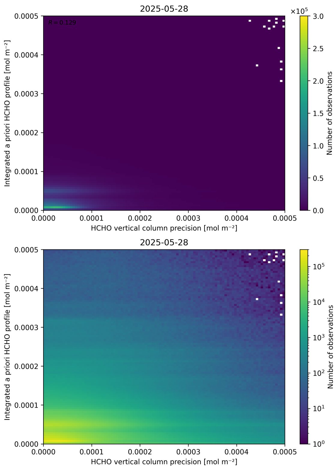
Figure 147: Scatter density plot of “HCHO vertical column precision” against “Integrated a priori HCHO profile” for 2025-05-27 to 2025-05-29.
