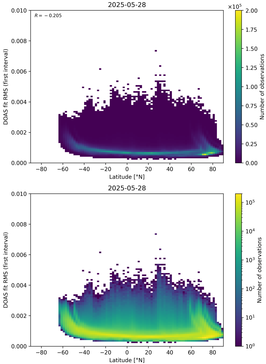
Figure 153: Scatter density plot of “Latitude” against “DOAS fit RMS (first interval)” for 2025-05-27 to 2025-05-29.
