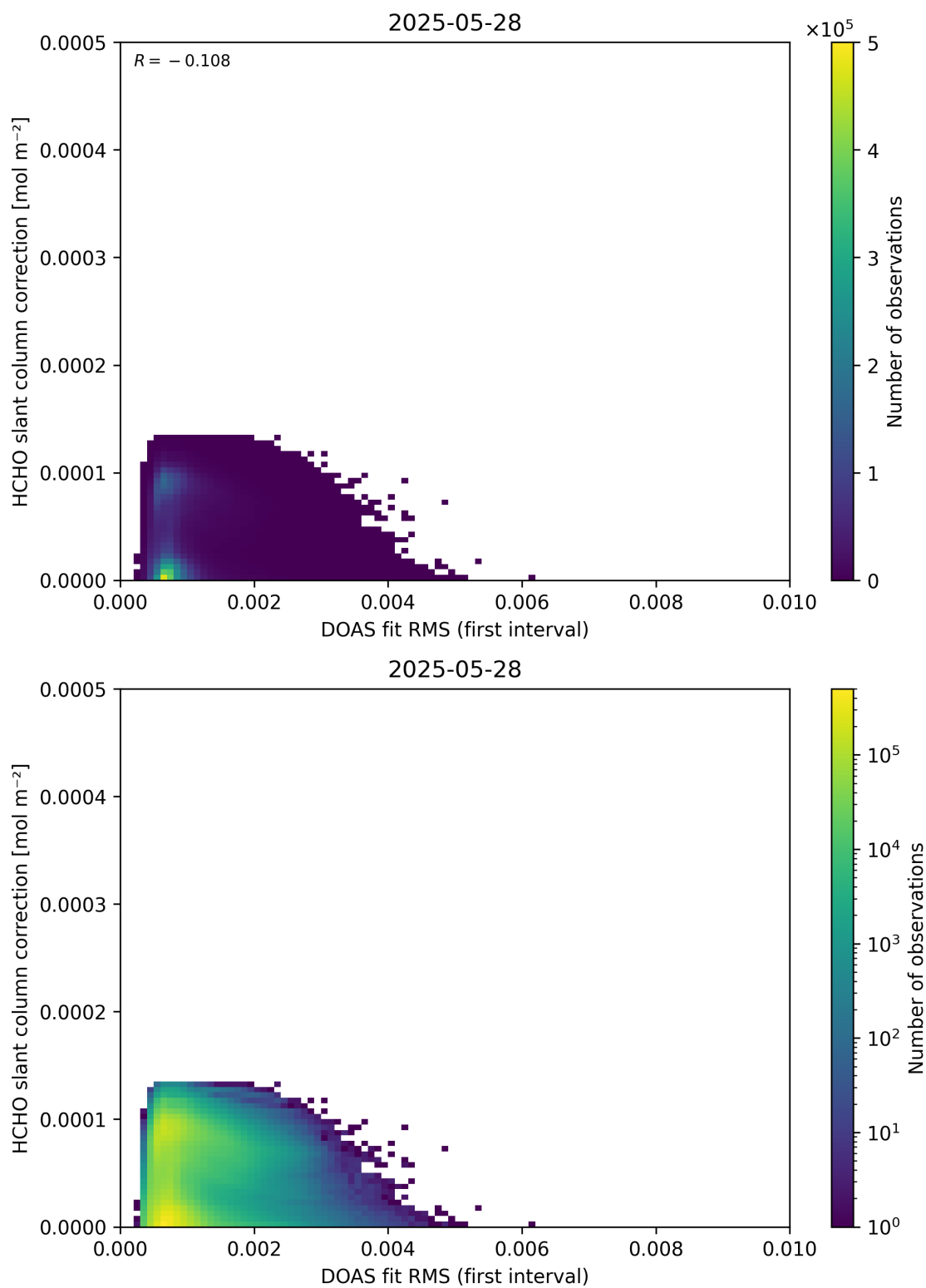
Figure 63: Scatter density plot of “DOAS fit RMS (first interval)” against “HCHO slant column correction” for 2025-05-27 to 2025-05-29.
