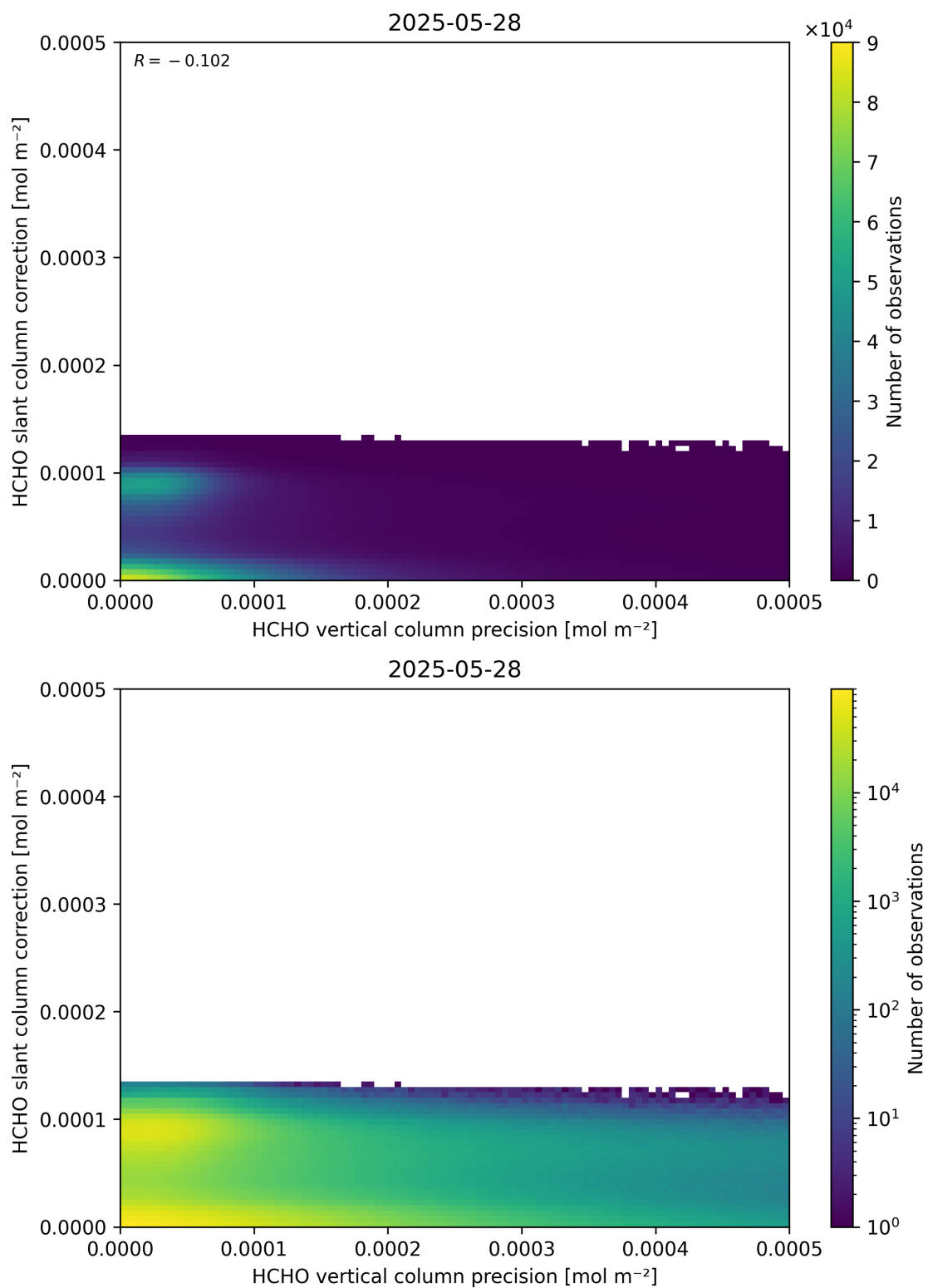
Figure 141: Scatter density plot of “HCHO vertical column precision” against “HCHO slant column correction” for 2025-05-27 to 2025-05-29.
