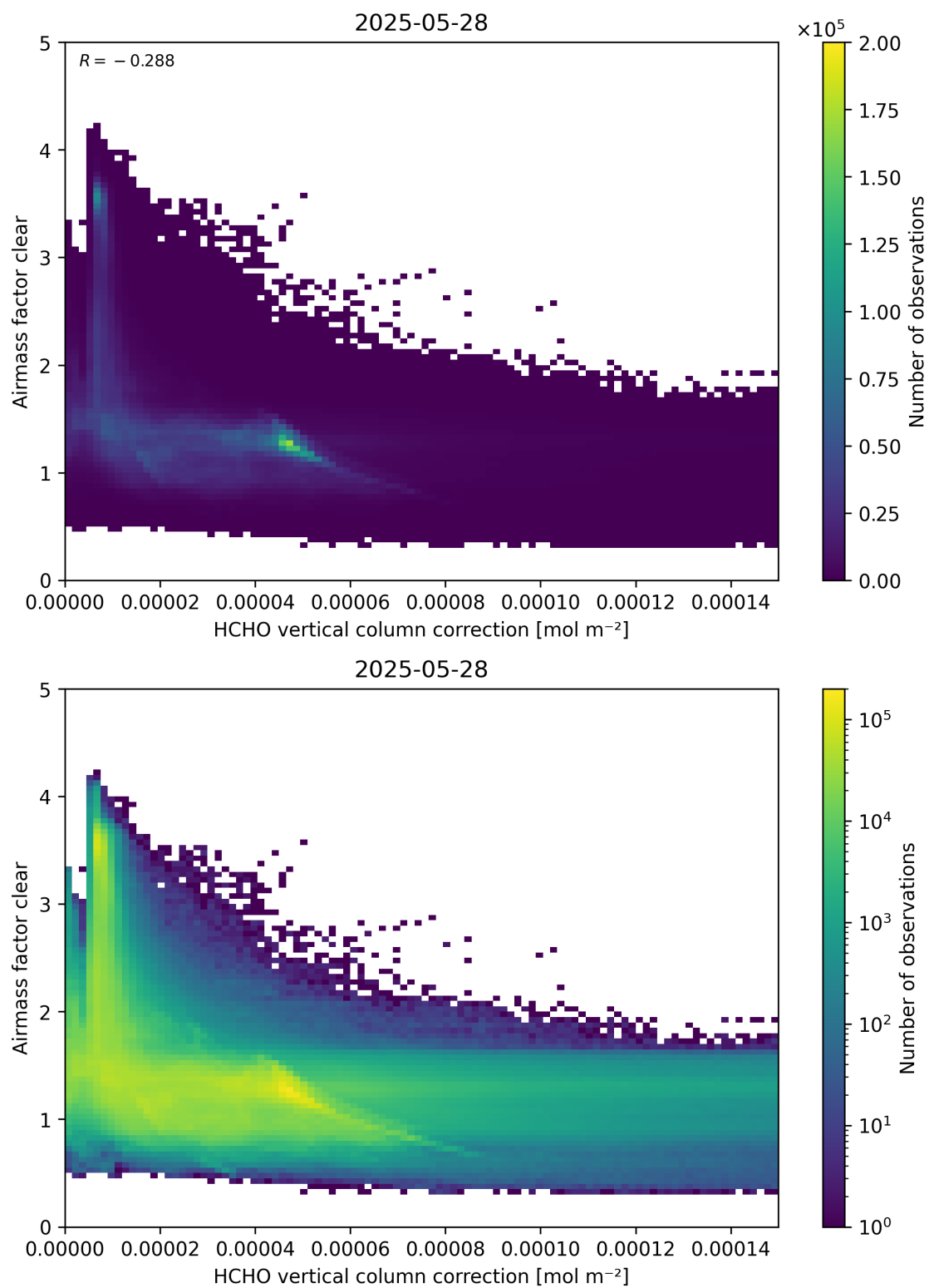
Figure 115: Scatter density plot of “HCHO vertical column correction” against “Airmass factor clear” for 2025-05-27 to 2025-05-29.
