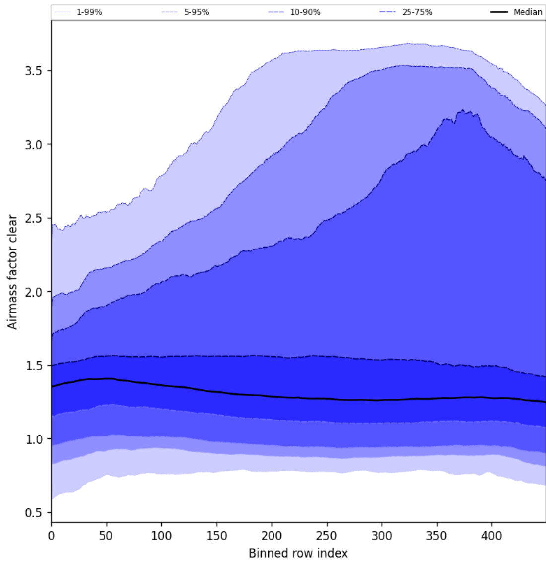
Figure 56: Along track statistics of “Airmass factor clear” for 2025-05-27 to 2025-05-29
