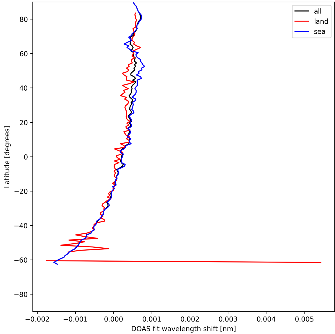
Figure 30: Zonal average of "DOAS fit wavelength shift" for 2025-05-27 to 2025-05-29.
