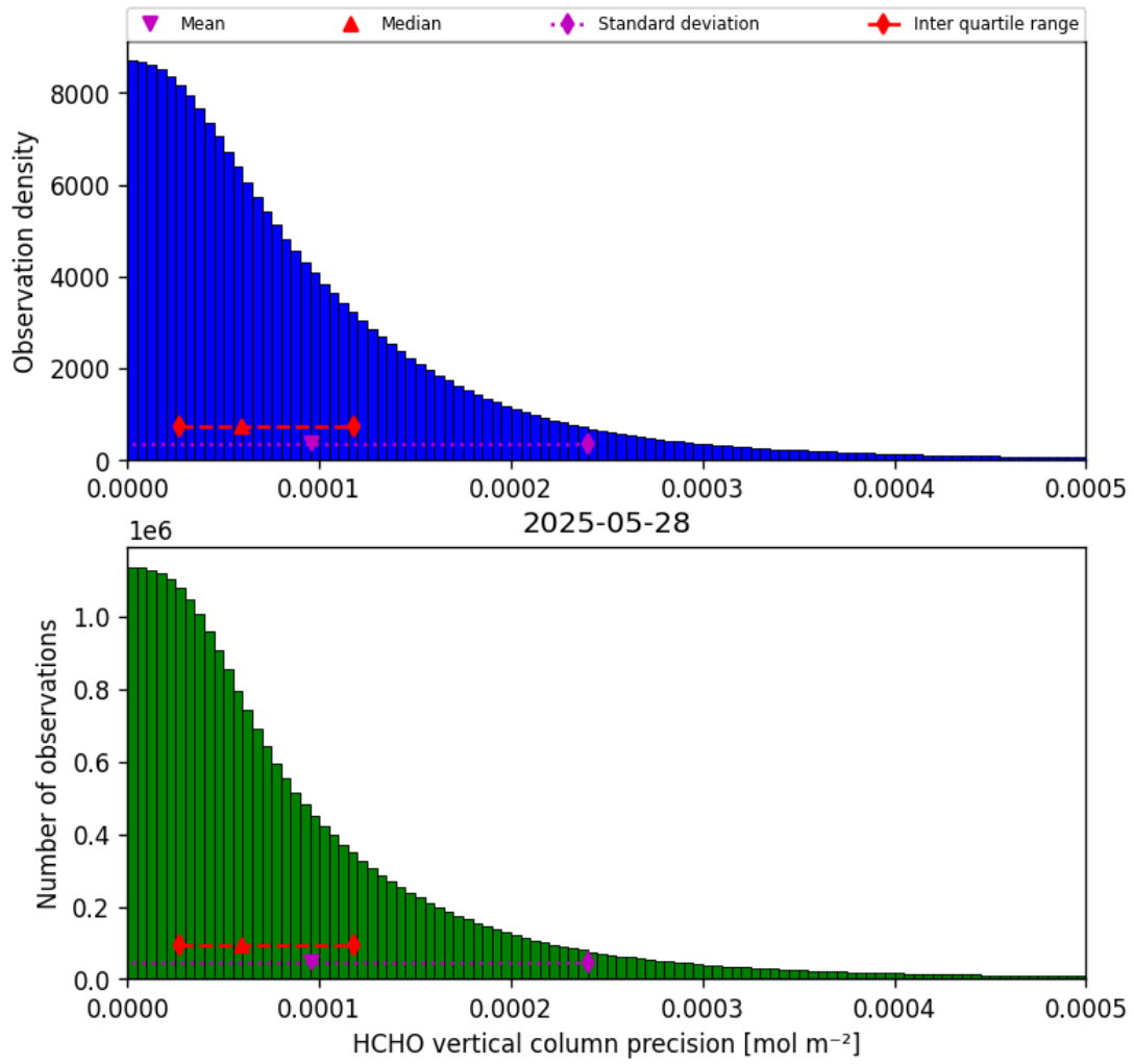
Figure 36: Histogram of “HCHO vertical column precision” for 2025-05-27 to 2025-05-29
