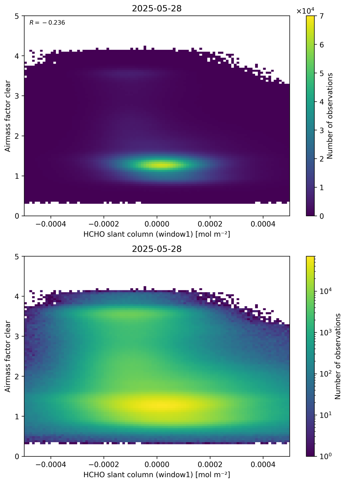
Figure 81: Scatter density plot of “HCHO slant column (window1)” against “Airmass factor clear” for 2025-05-27 to 2025-05-29.
