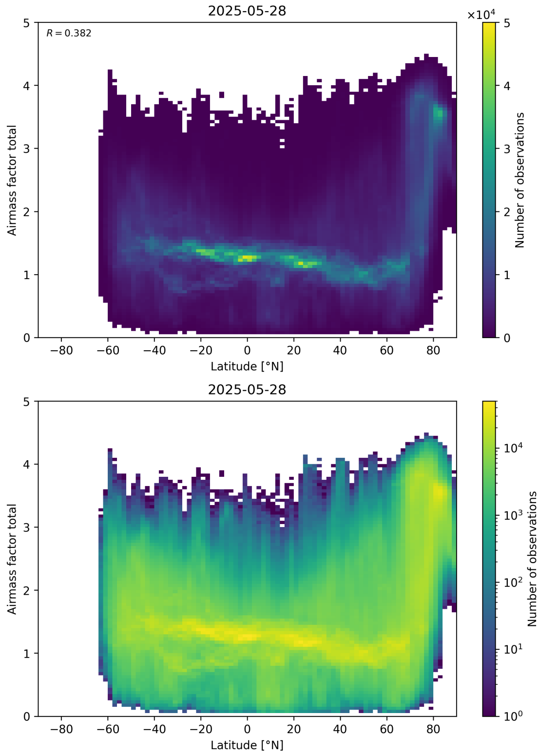
Figure 161: Scatter density plot of “Latitude” against “Airmass factor total” for 2025-05-27 to 2025-05-29.
