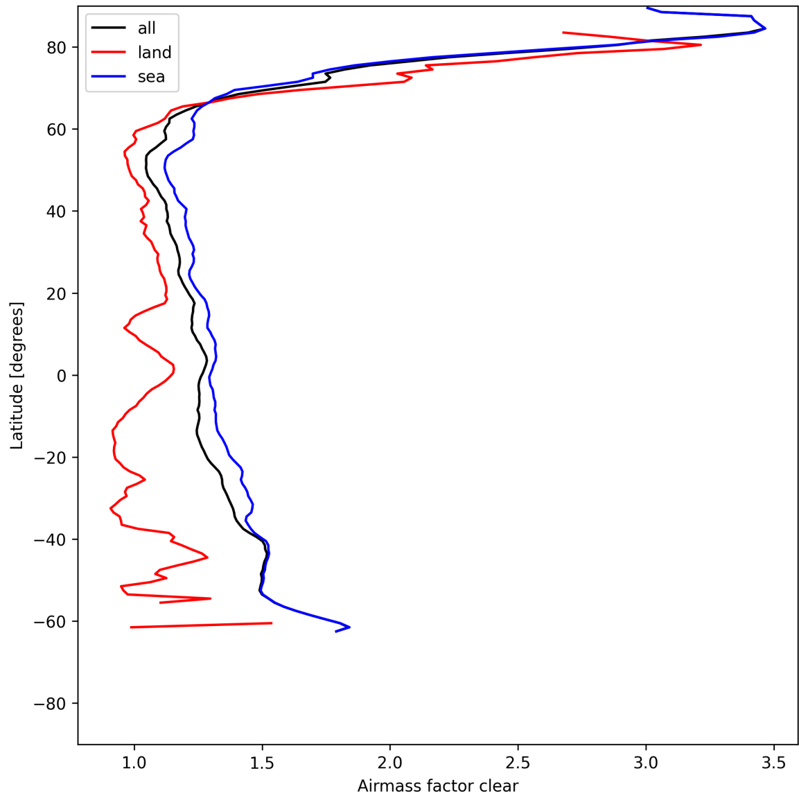
Figure 28: Zonal average of “Airmass factor clear” for 2025-05-27 to 2025-05-29.
