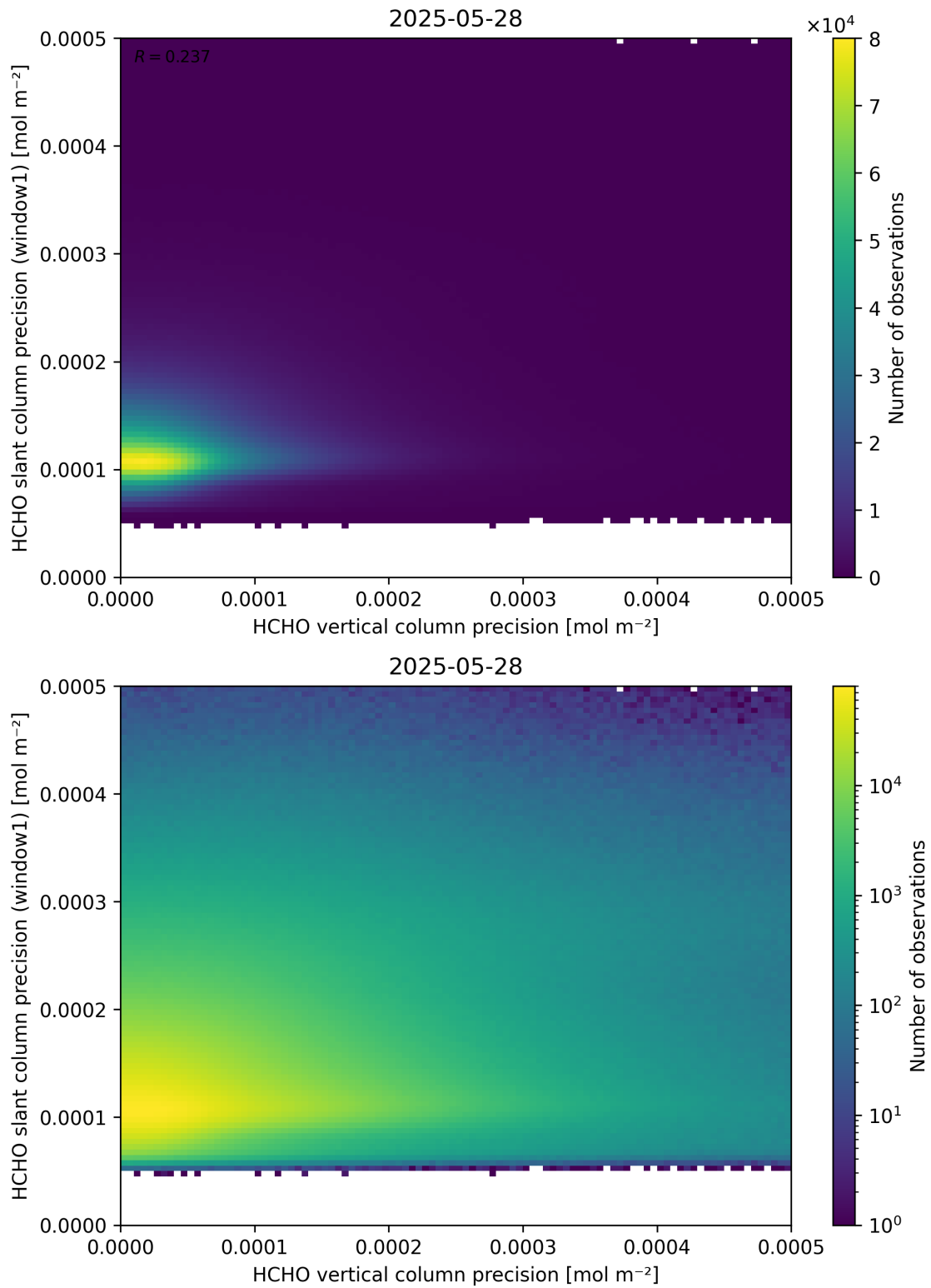
Figure 143: Scatter density plot of “HCHO vertical column precision” against “HCHO slant column precision (window1)” for 2025-05-27 to 2025-05-29.
