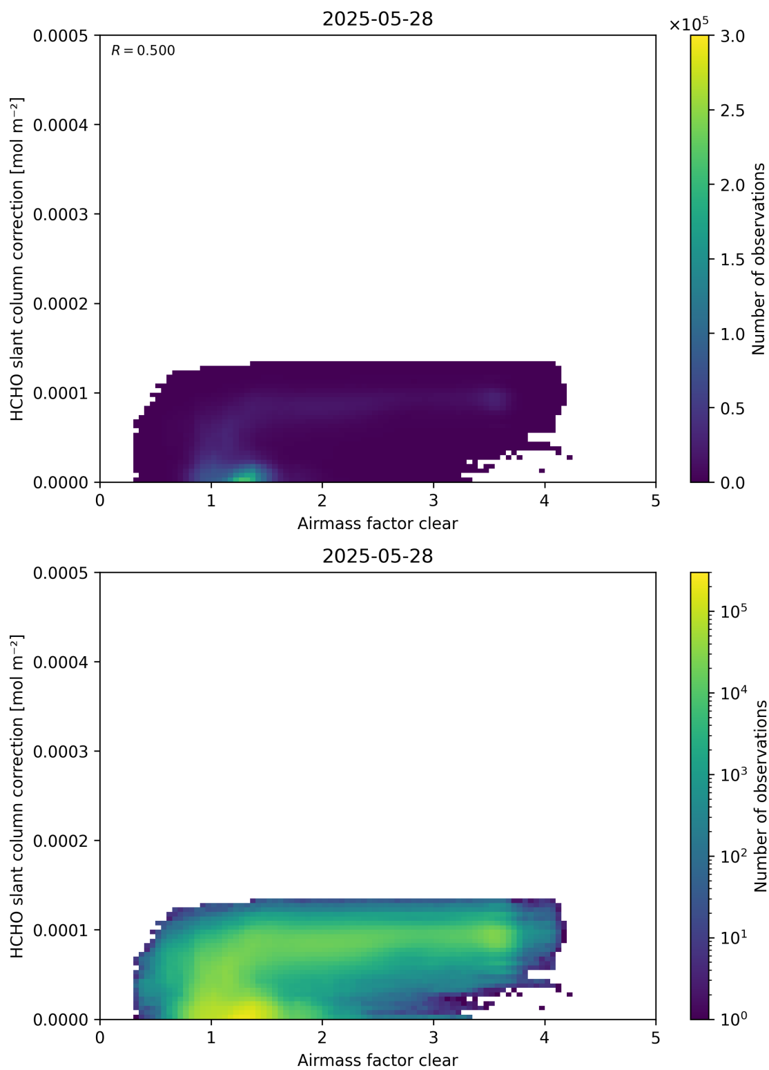
Figure 75: Scatter density plot of “Airmass factor clear” against “HCHO slant column correction” for 2025-05-27 to 2025-05-29.
