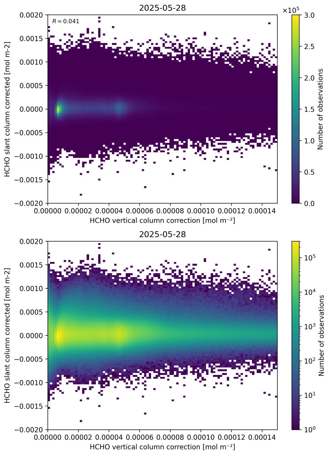
Figure 116: Scatter density plot of “HCHO vertical column correction” against “HCHO slant column corrected” for 2025-05-27 to 2025-05-29.
