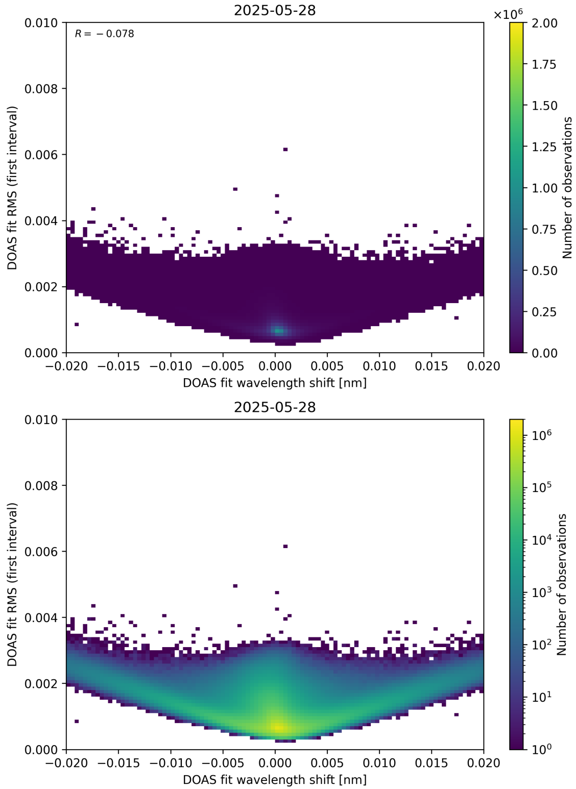
Figure 64: Scatter density plot of “DOAS fit wavelength shift” against “DOAS fit RMS (first interval)” for 2025-05-27 to 2025-05-29.
