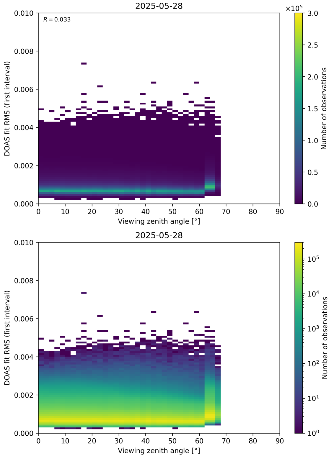
Figure 182: Scatter density plot of “Viewing zenith angle” against “DOAS fit RMS (first interval)” for 2025-05-27 to 2025-05-29.
