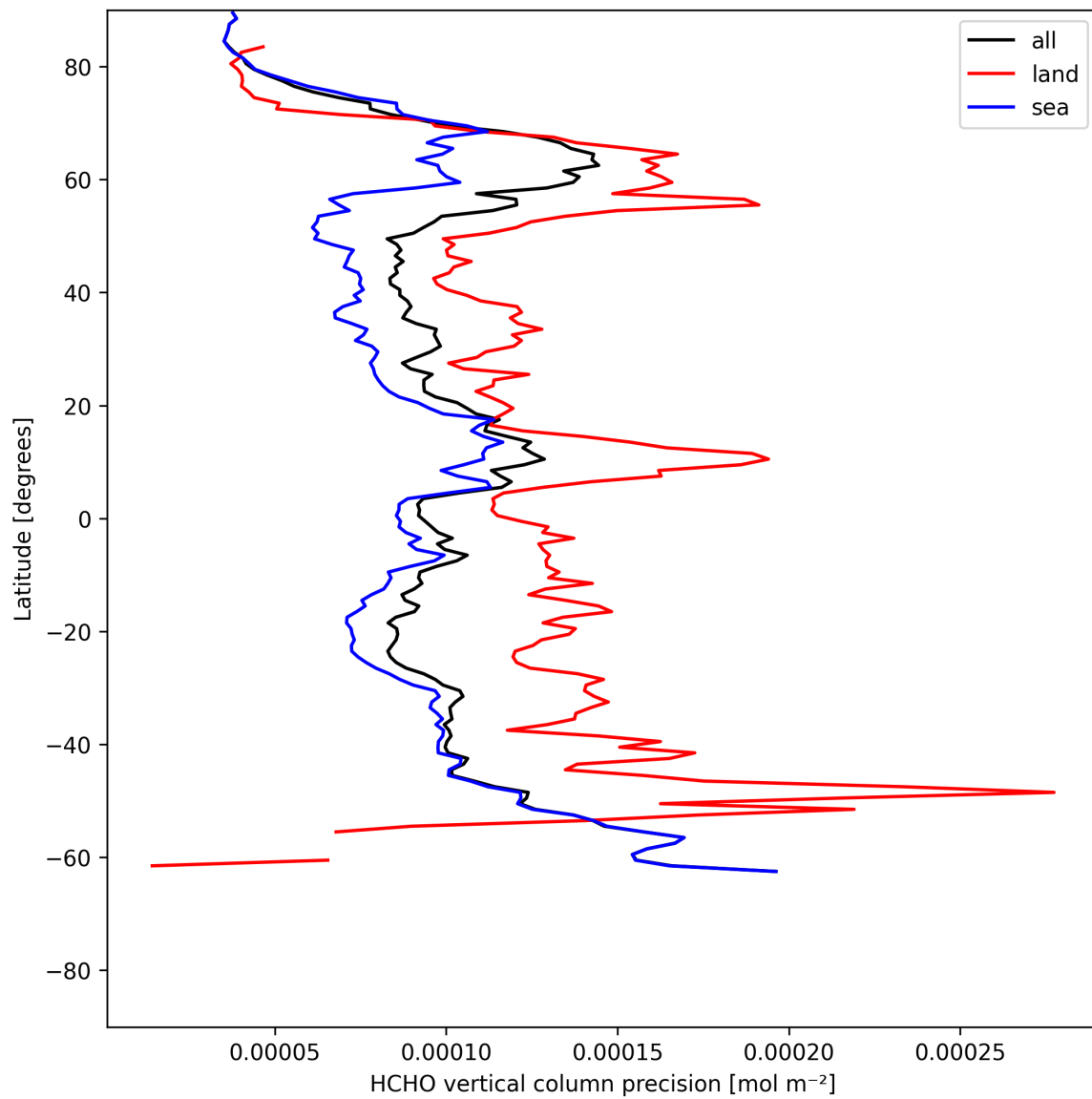
Figure 22: Zonal average of “HCHO vertical column precision” for 2025-05-27 to 2025-05-29.
