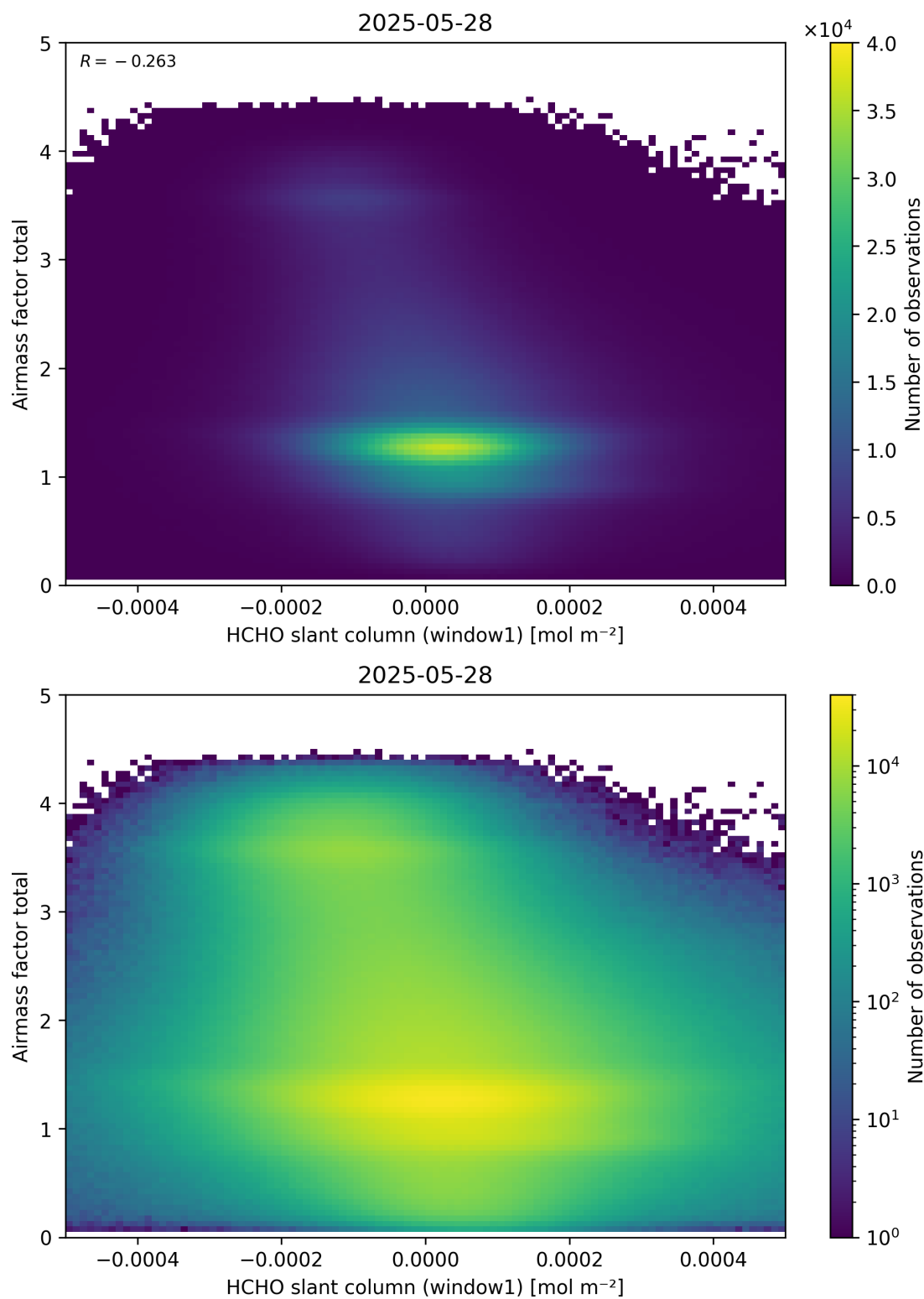
Figure 85: Scatter density plot of “HCHO slant column (window1)” against “Airmass factor total” for 2025-05-27 to 2025-05-29.
