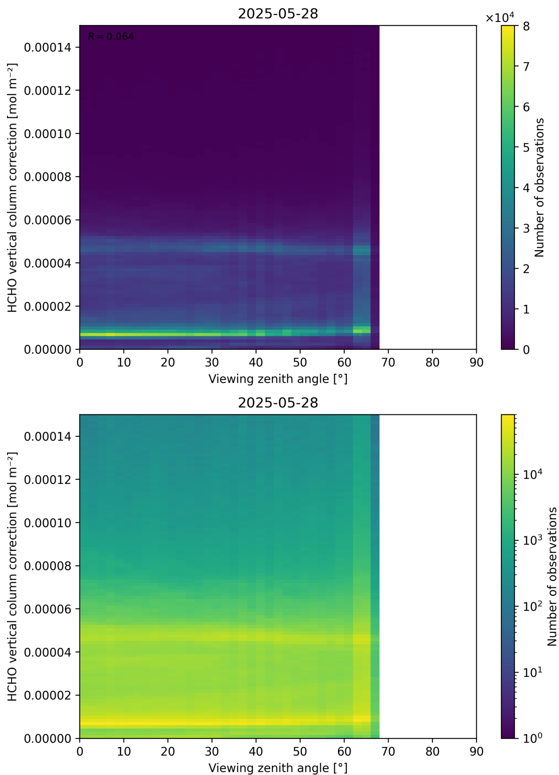
Figure 193: Scatter density plot of “Viewing zenith angle” against “HCHO vertical column correction” for 2025-05-27 to 2025-05-29.
