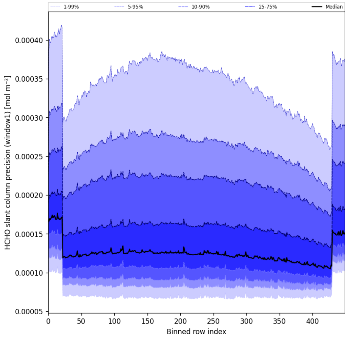
Figure 53: Along track statistics of “HCHO slant column precision (window1)” for 2025-05-27 to 2025-05-29
