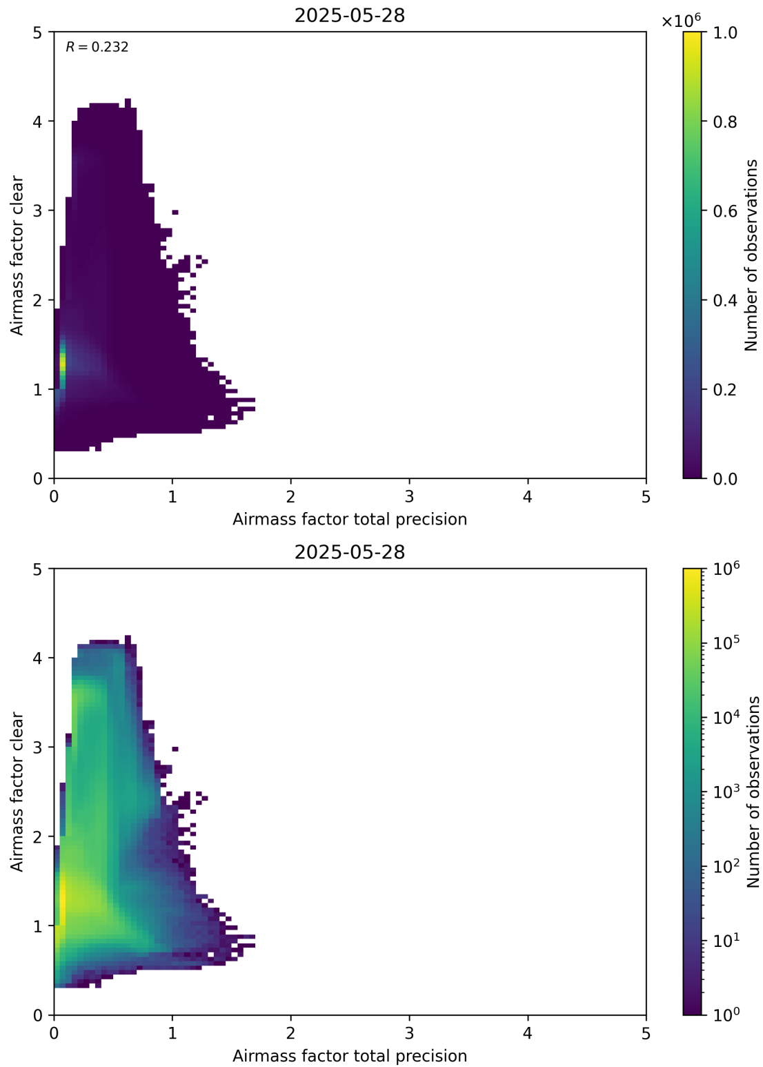
Figure 108: Scatter density plot of “Airmass factor total precision” against “Airmass factor clear” for 2025-05-27 to 2025-05-29.
