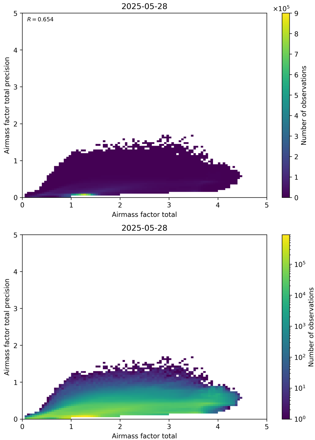
Figure 103: Scatter density plot of “Airmass factor total” against “Airmass factor total precision” for 2025-05-27 to 2025-05-29.
