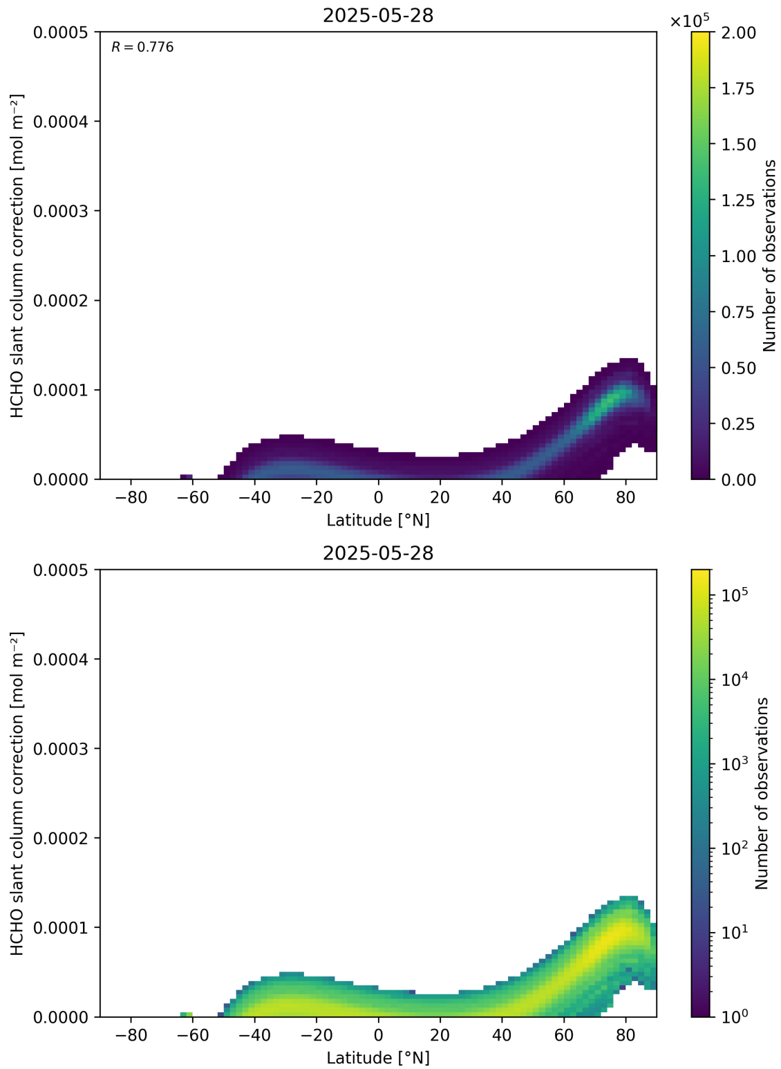
Figure 158: Scatter density plot of “Latitude” against “HCHO slant column correction” for 2025-05-27 to 2025-05-29.
