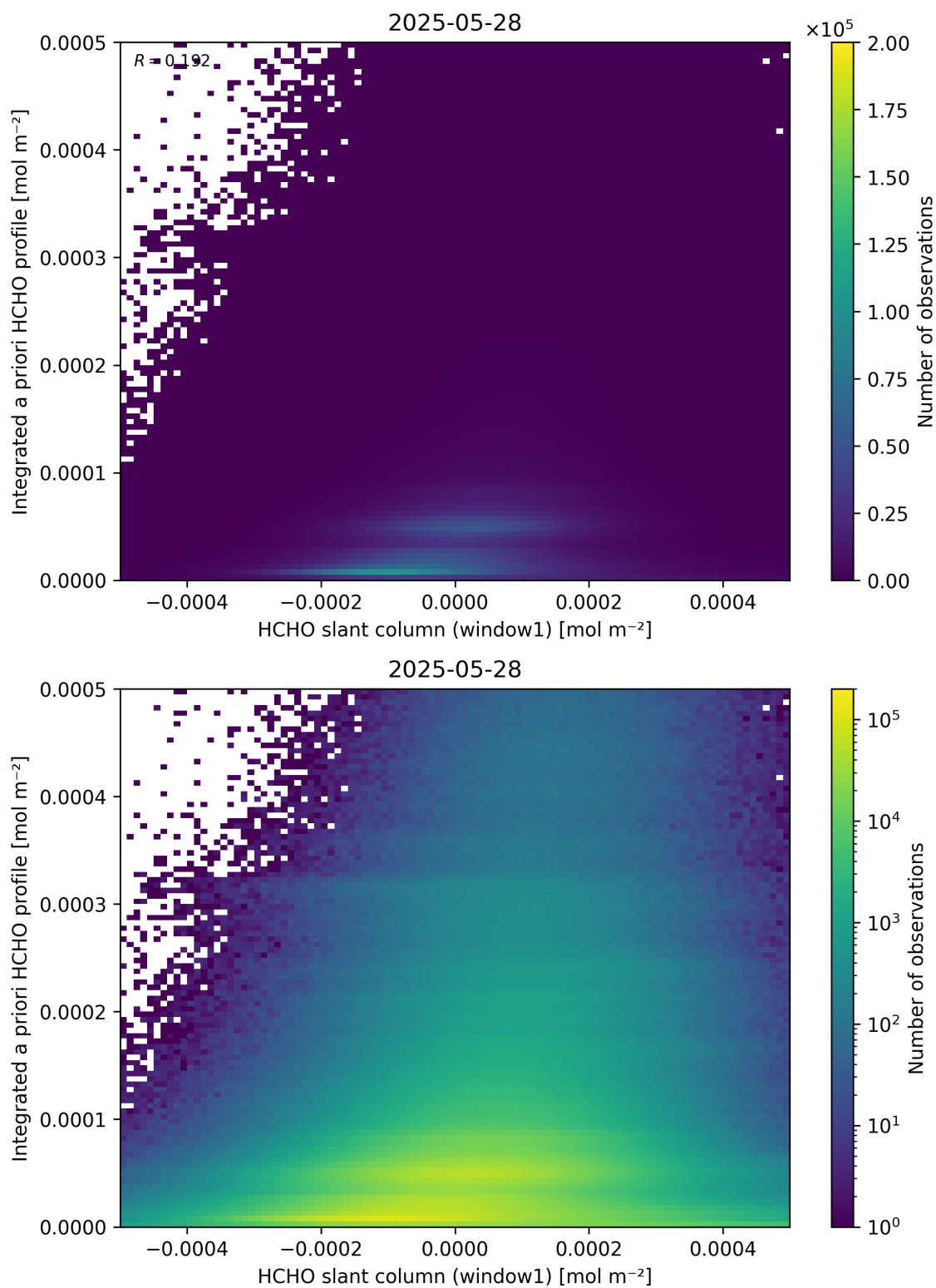
Figure 87: Scatter density plot of “HCHO slant column (window1)” against “Integrated a priori HCHO profile” for 2025-05-27 to 2025-05-29.
