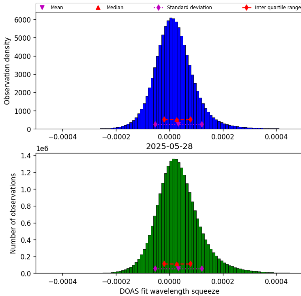
Figure 45: Histogram of “DOAS fit wavelength squeeze” for 2025-05-27 to 2025-05-29
