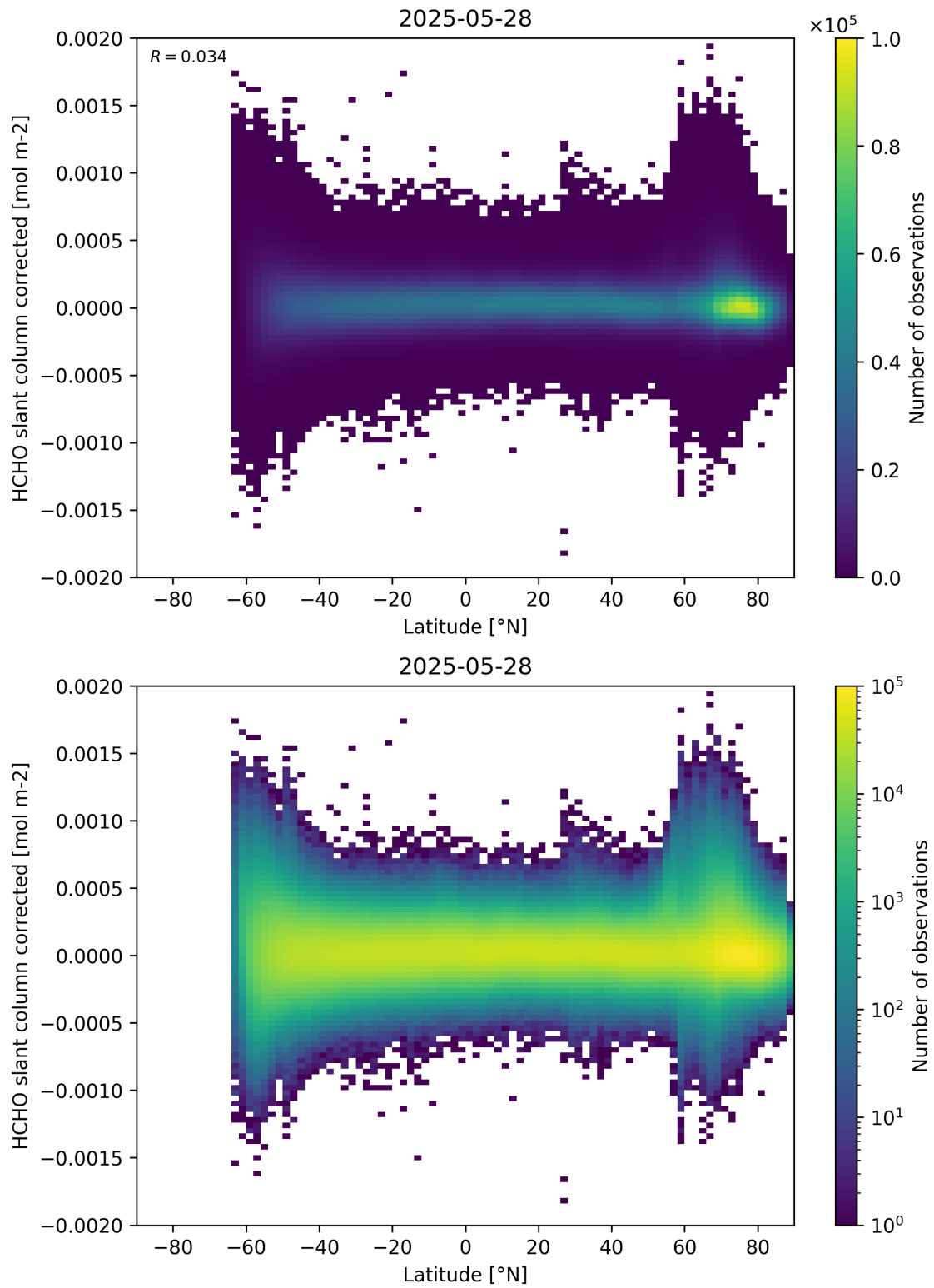
Figure 157: Scatter density plot of “Latitude” against “HCHO slant column corrected” for 2025-05-27 to 2025-05-29.
