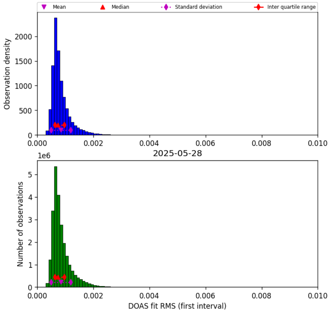
Figure 46: Histogram of “DOAS fit RMS (first interval)” for 2025-05-27 to 2025-05-29
