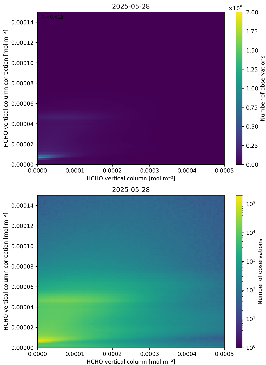
Figure 133: Scatter density plot of “HCHO vertical column” against “HCHO vertical column correction” for 2025-05-27 to 2025-05-29.
