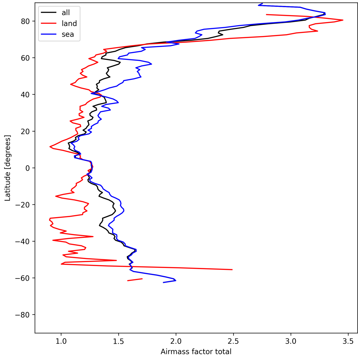
Figure 26: Zonal average of “Airmass factor total” for 2025-05-27 to 2025-05-29.
