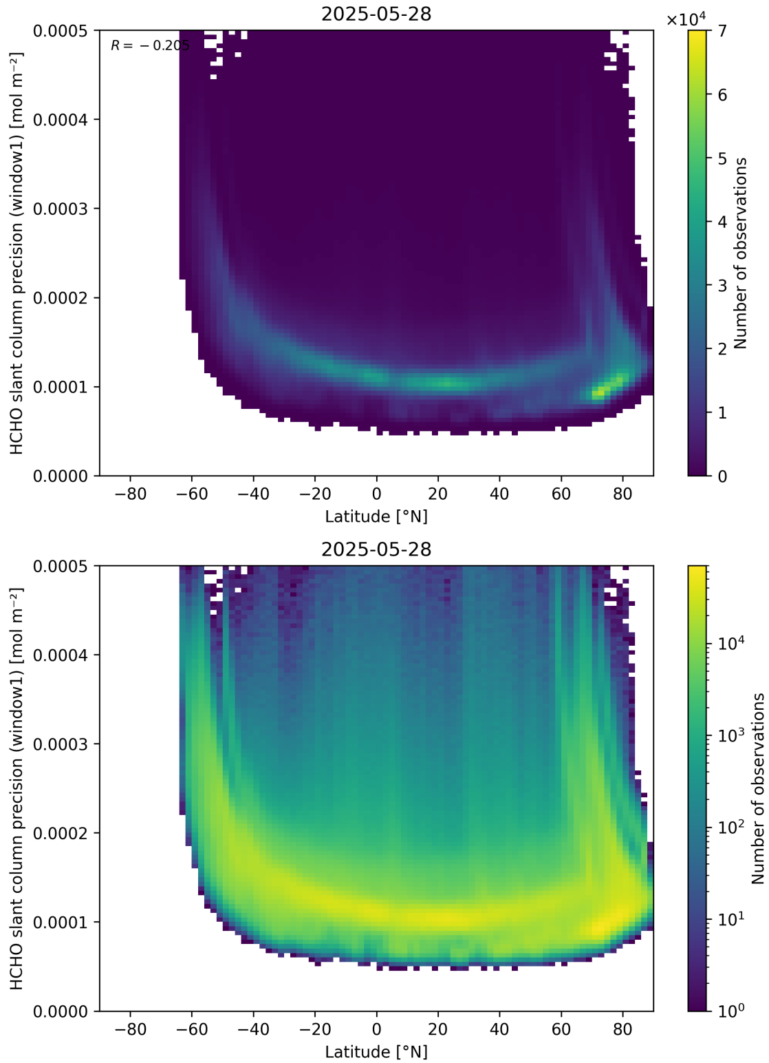
Figure 160: Scatter density plot of “Latitude” against “HCHO slant column precision (window1)” for 2025-05-27 to 2025-05-29.
