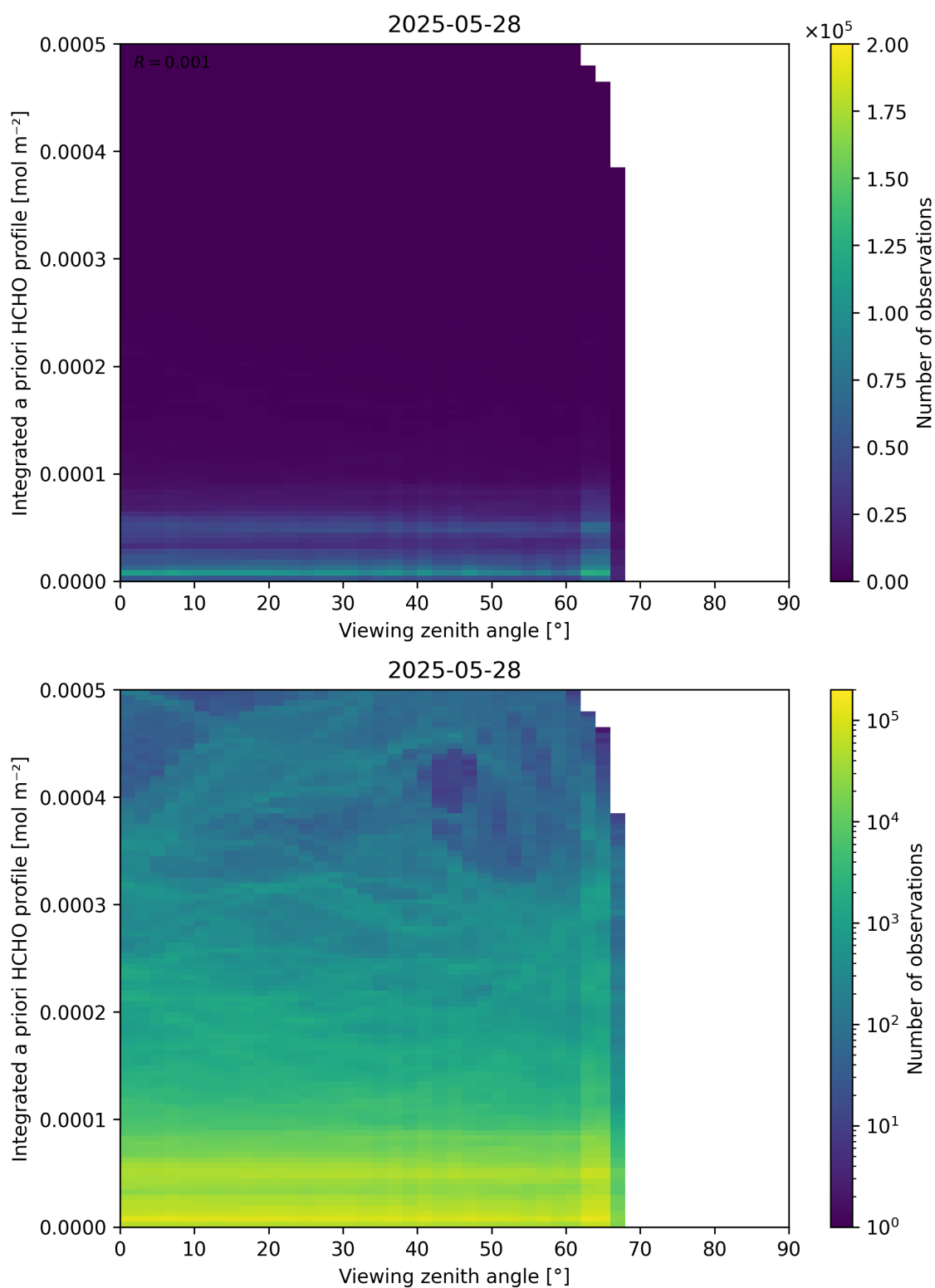
Figure 195: Scatter density plot of “Viewing zenith angle” against “Integrated a priori HCHO profile” for 2025-05-27 to 2025-05-29.
