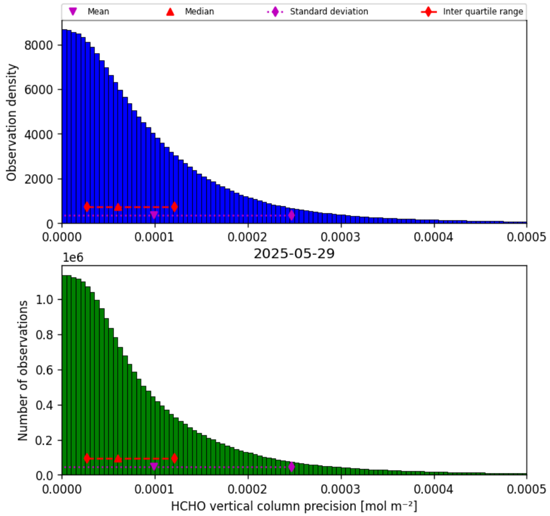
Figure 36: Histogram of “HCHO vertical column precision” for 2025-05-28 to 2025-05-30
