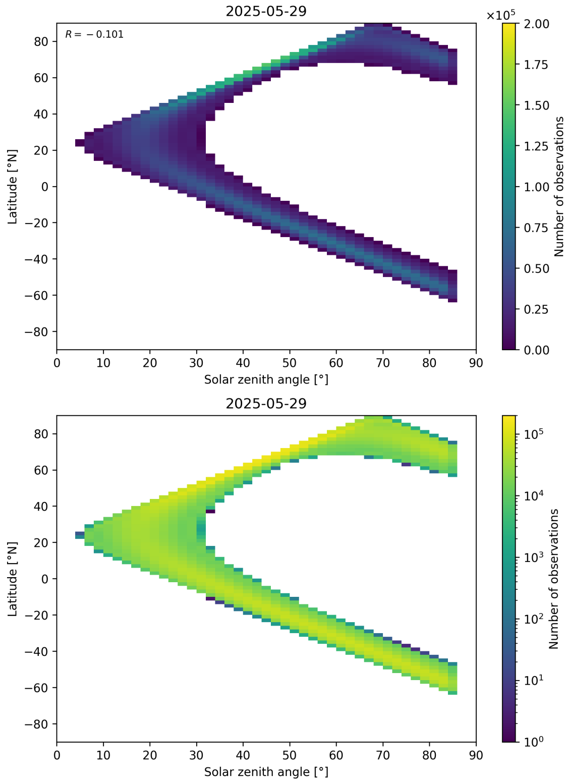
Figure 181: Scatter density plot of “Solar zenith angle” against “Latitude” for 2025-05-28 to 2025-05-30.
