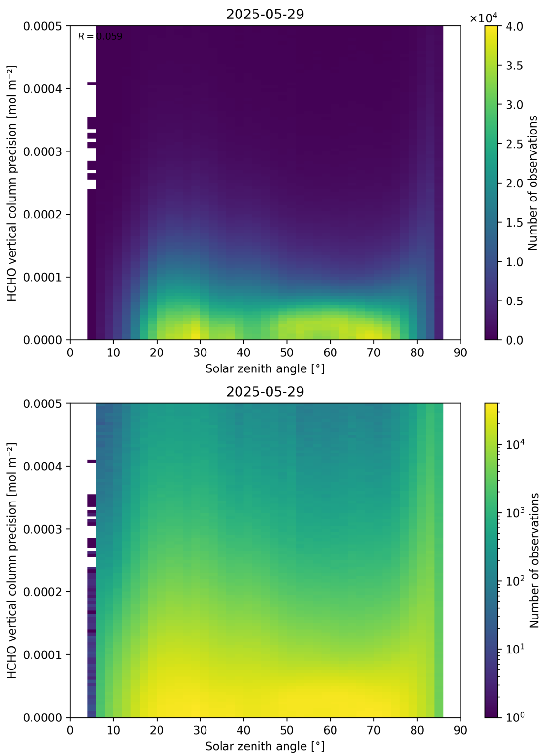
Figure 179: Scatter density plot of “Solar zenith angle” against “HCHO vertical column precision” for 2025-05-28 to 2025-05-30.
