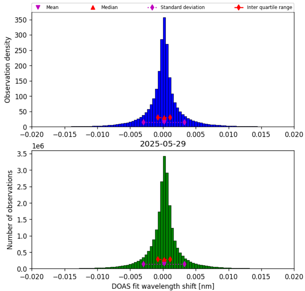
Figure 44: Histogram of “DOAS fit wavelength shift” for 2025-05-28 to 2025-05-30
