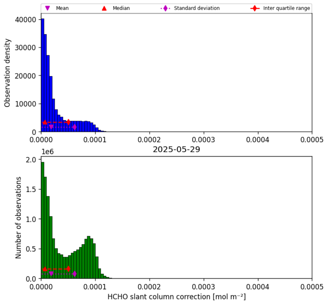
Figure 47: Histogram of “HCHO slant column correction” for 2025-05-28 to 2025-05-30
