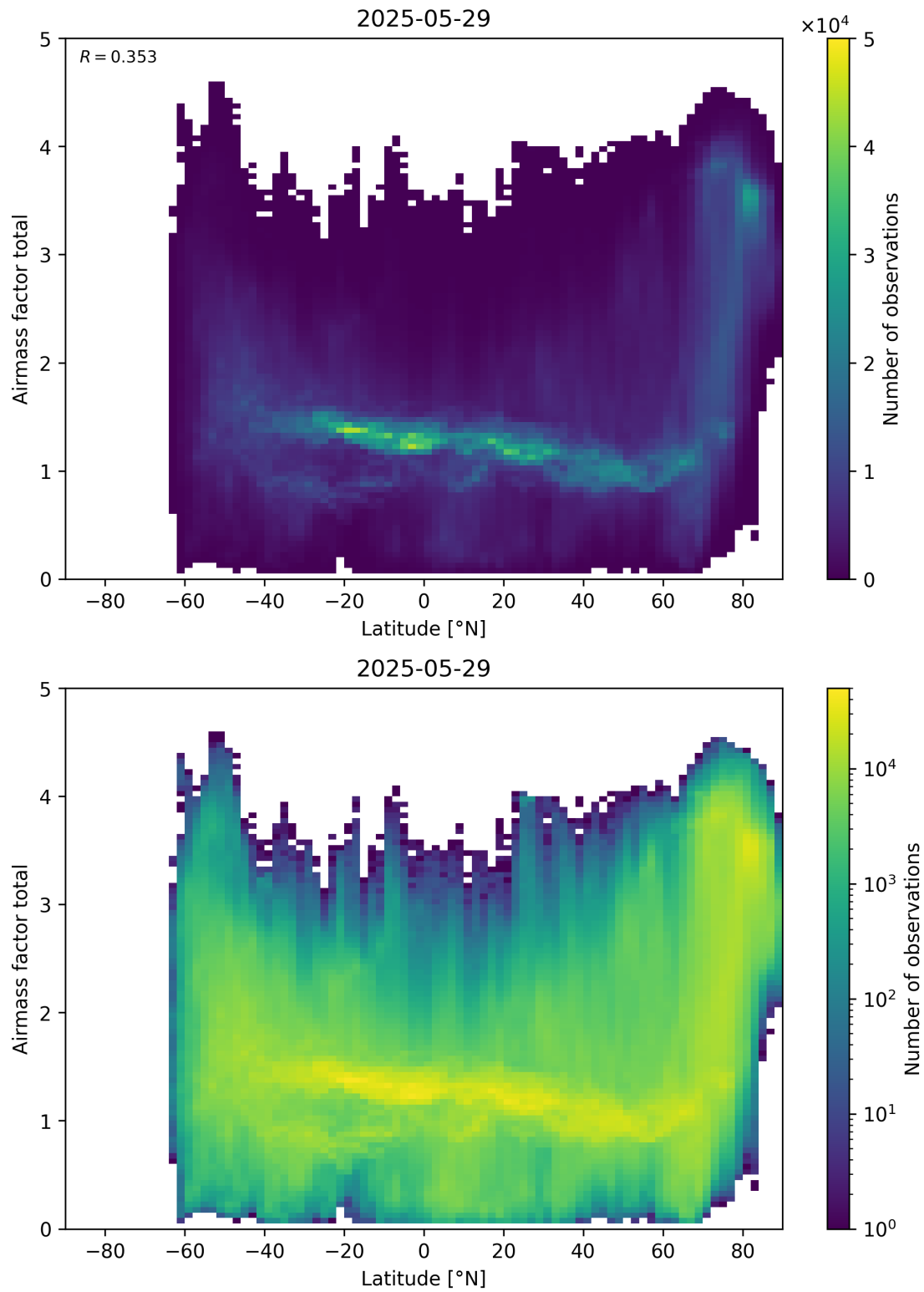
Figure 161: Scatter density plot of “Latitude” against “Airmass factor total” for 2025-05-28 to 2025-05-30.
