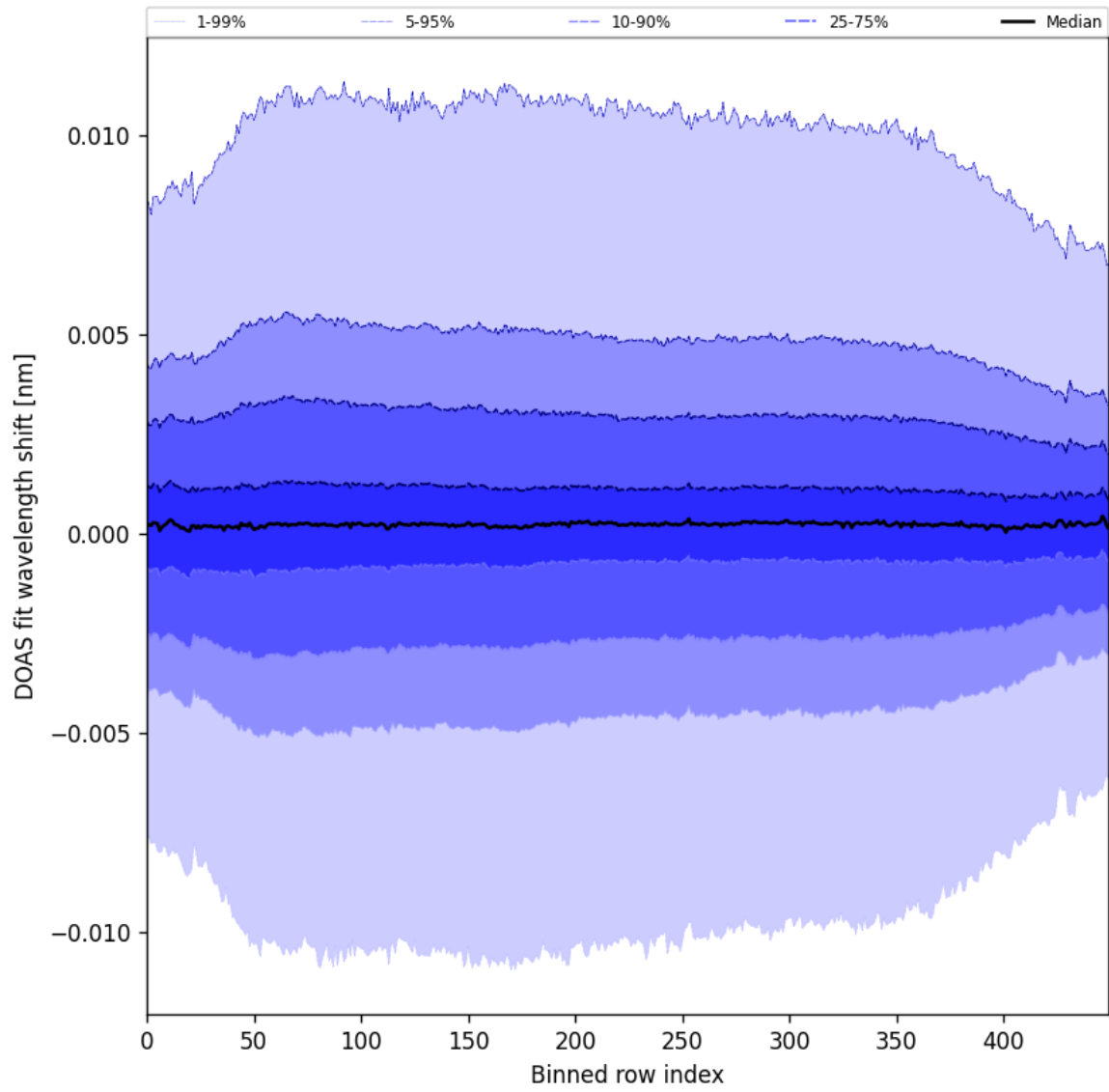
Figure 58: Along track statistics of “DOAS fit wavelength shift” for 2025-05-28 to 2025-05-30
