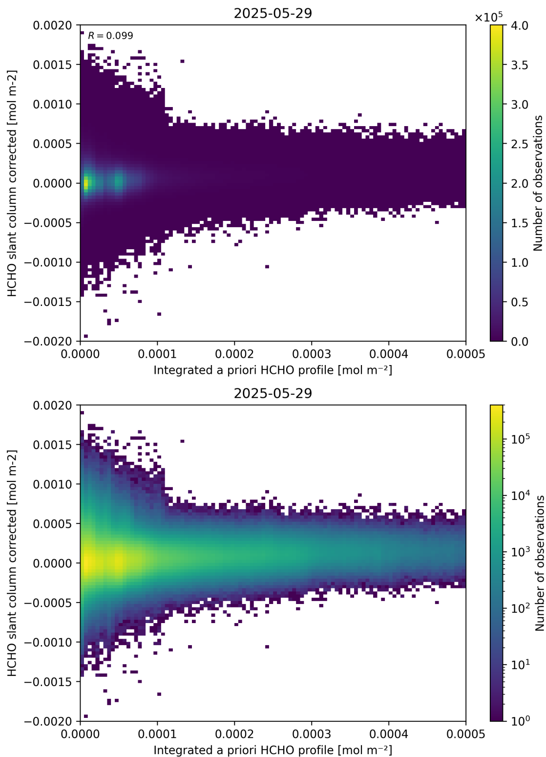
Figure 151: Scatter density plot of “Integrated a priori HCHO profile” against “HCHO slant column corrected” for 2025-05-28 to 2025-05-30.
