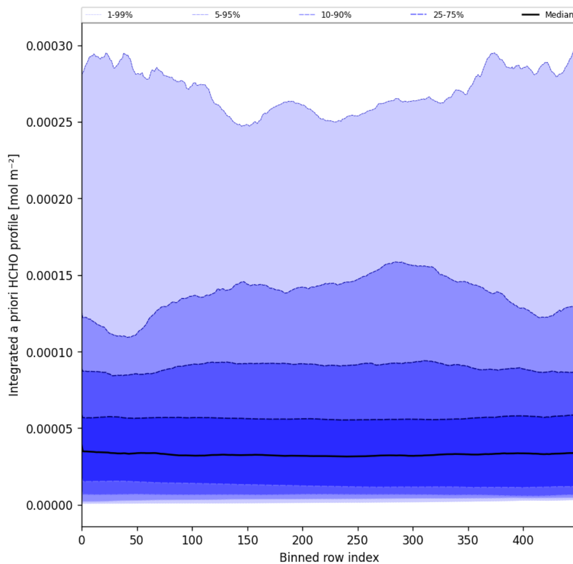
Figure 57: Along track statistics of “Integrated a priori HCHO profile” for 2025-05-28 to 2025-05-30
