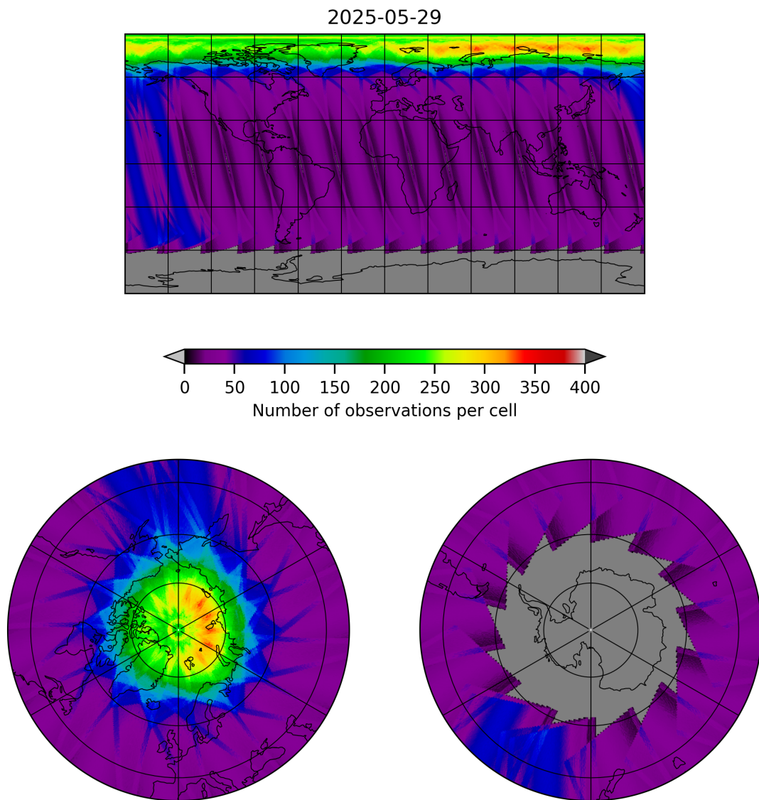
Figure 19: Map of the number of observations for 2025-05-28 to 2025-05-30
