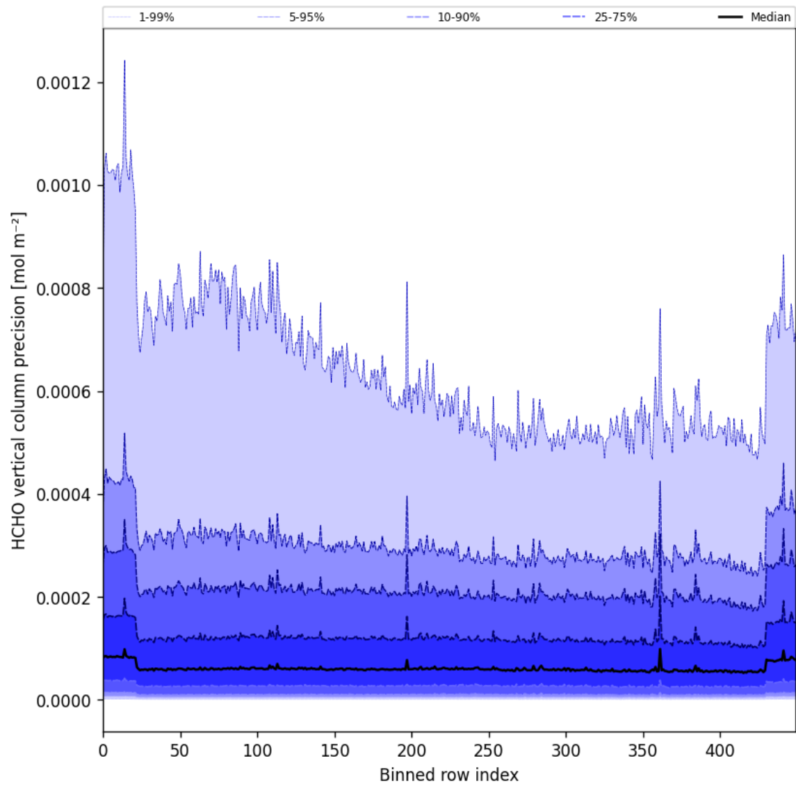
Figure 50: Along track statistics of “HCHO vertical column precision” for 2025-05-28 to 2025-05-30
