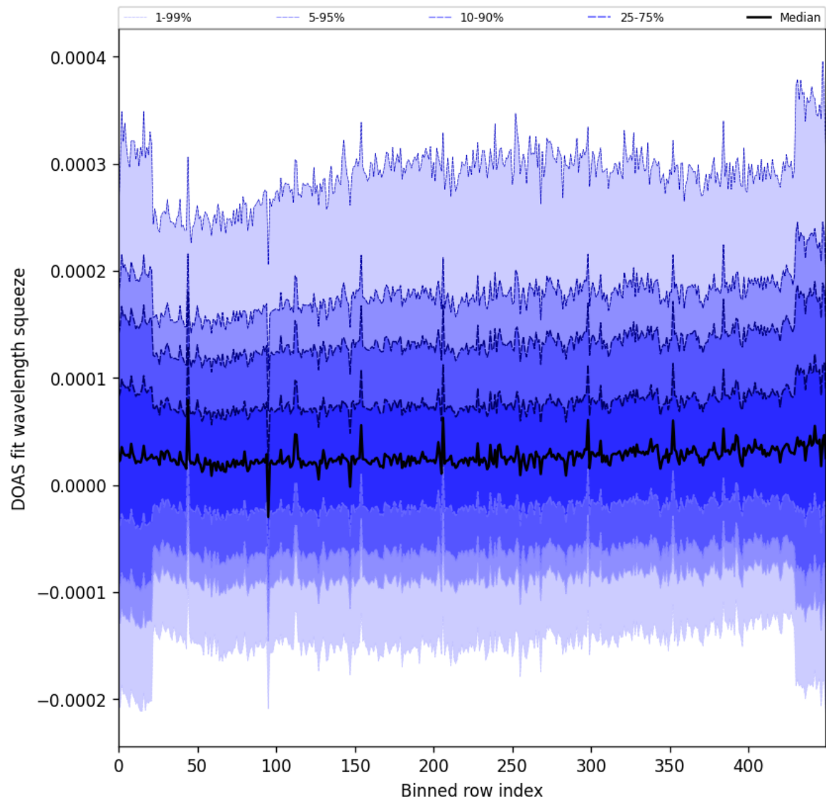
Figure 59: Along track statistics of “DOAS fit wavelength squeeze” for 2025-05-28 to 2025-05-30
