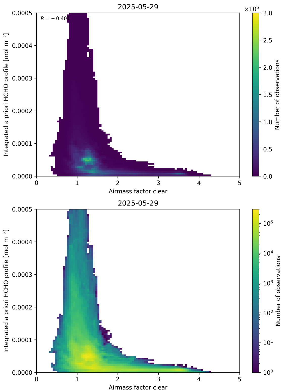
Figure 76: Scatter density plot of “Airmass factor clear” against “Integrated a priori HCHO profile” for 2025-05-28 to 2025-05-30.
