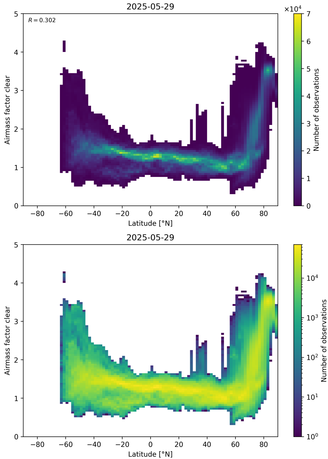
Figure 156: Scatter density plot of “Latitude” against “Airmass factor clear” for 2025-05-28 to 2025-05-30.
