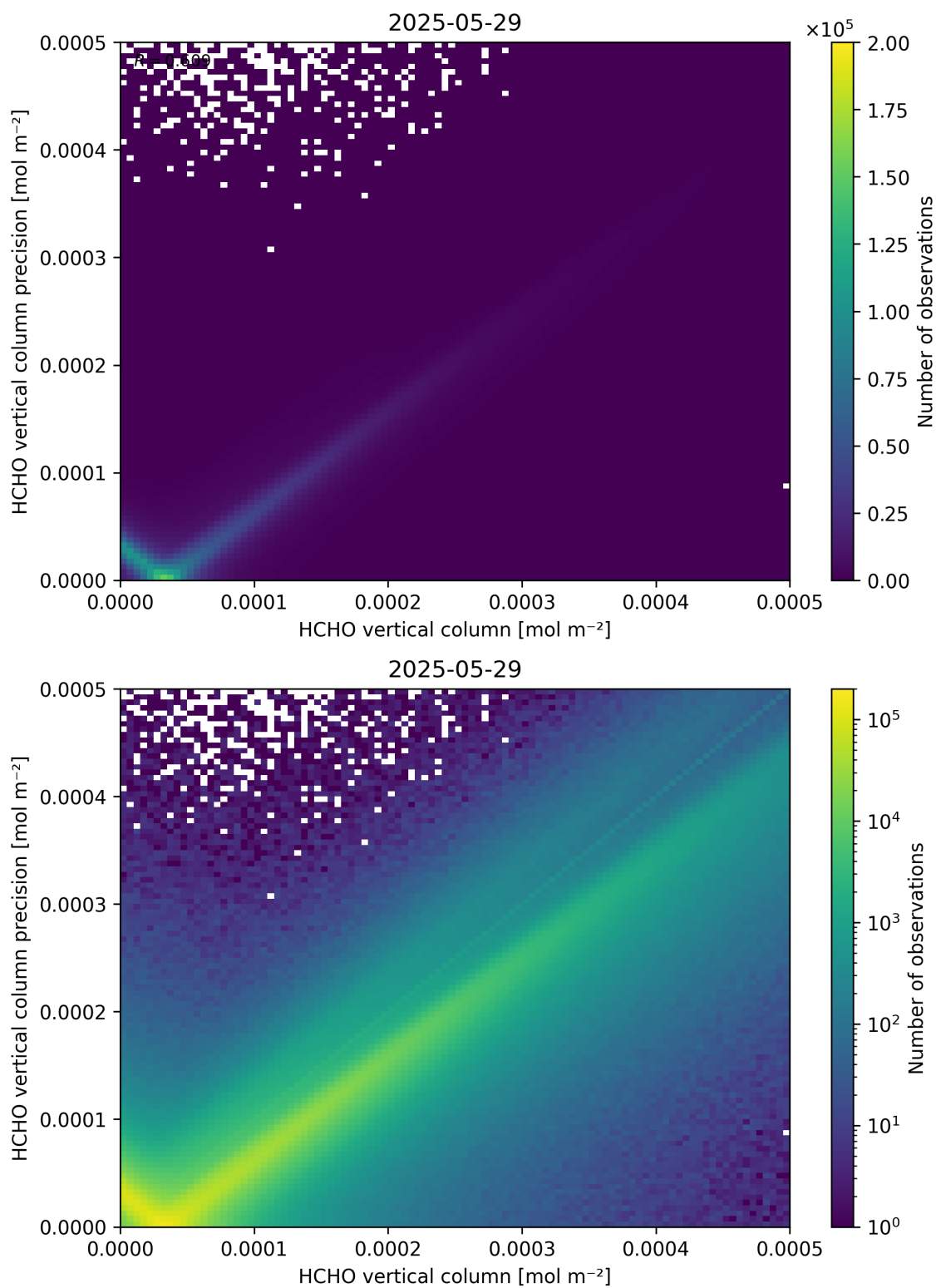
Figure 134: Scatter density plot of “HCHO vertical column” against “HCHO vertical column precision” for 2025-05-28 to 2025-05-30.
