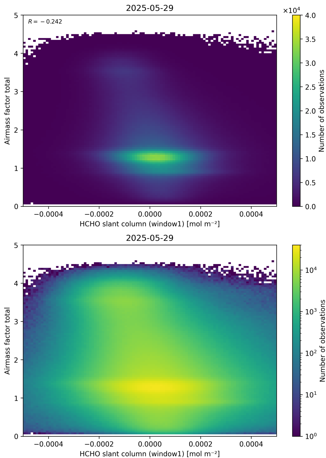
Figure 85: Scatter density plot of “HCHO slant column (window1)” against “Airmass factor total” for 2025-05-28 to 2025-05-30.
