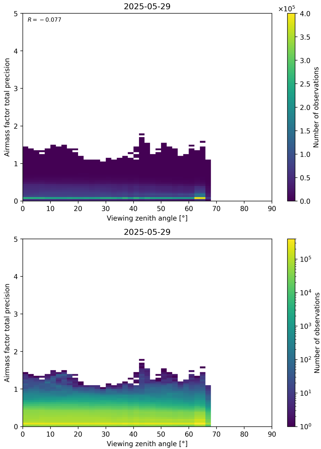
Figure 191: Scatter density plot of “Viewing zenith angle” against “Airmass factor total precision” for 2025-05-28 to 2025-05-30.
