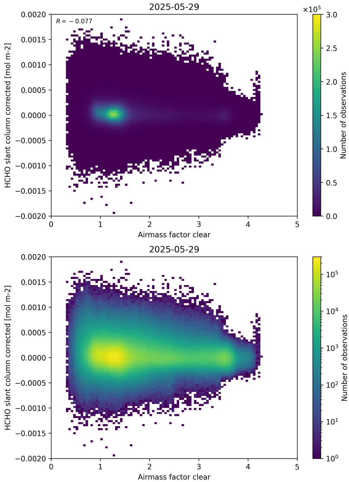
Figure 74: Scatter density plot of “Airmass factor clear” against “HCHO slant column corrected” for 2025-05-28 to 2025-05-30.
