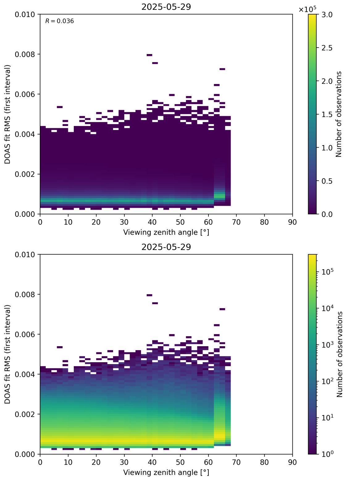
Figure 182: Scatter density plot of “Viewing zenith angle” against “DOAS fit RMS (first interval)” for 2025-05-28 to 2025-05-30.
