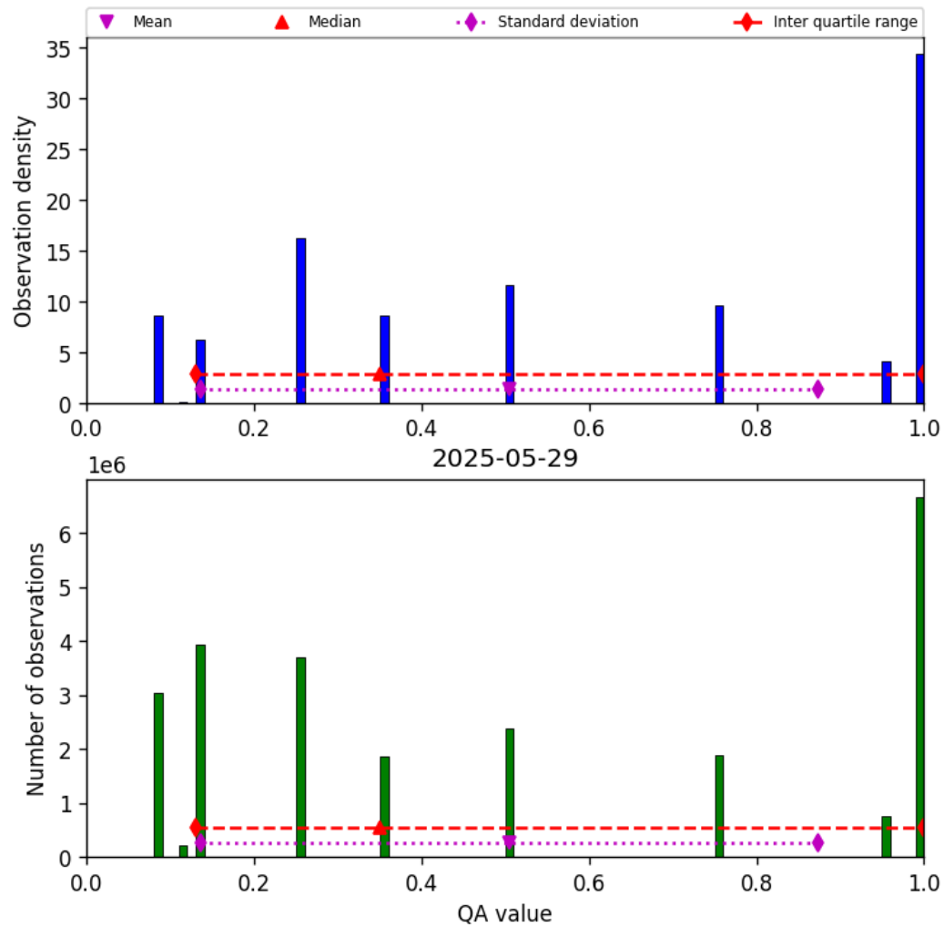
Figure 34: Histogram of “QA value” for 2025-05-28 to 2025-05-30
