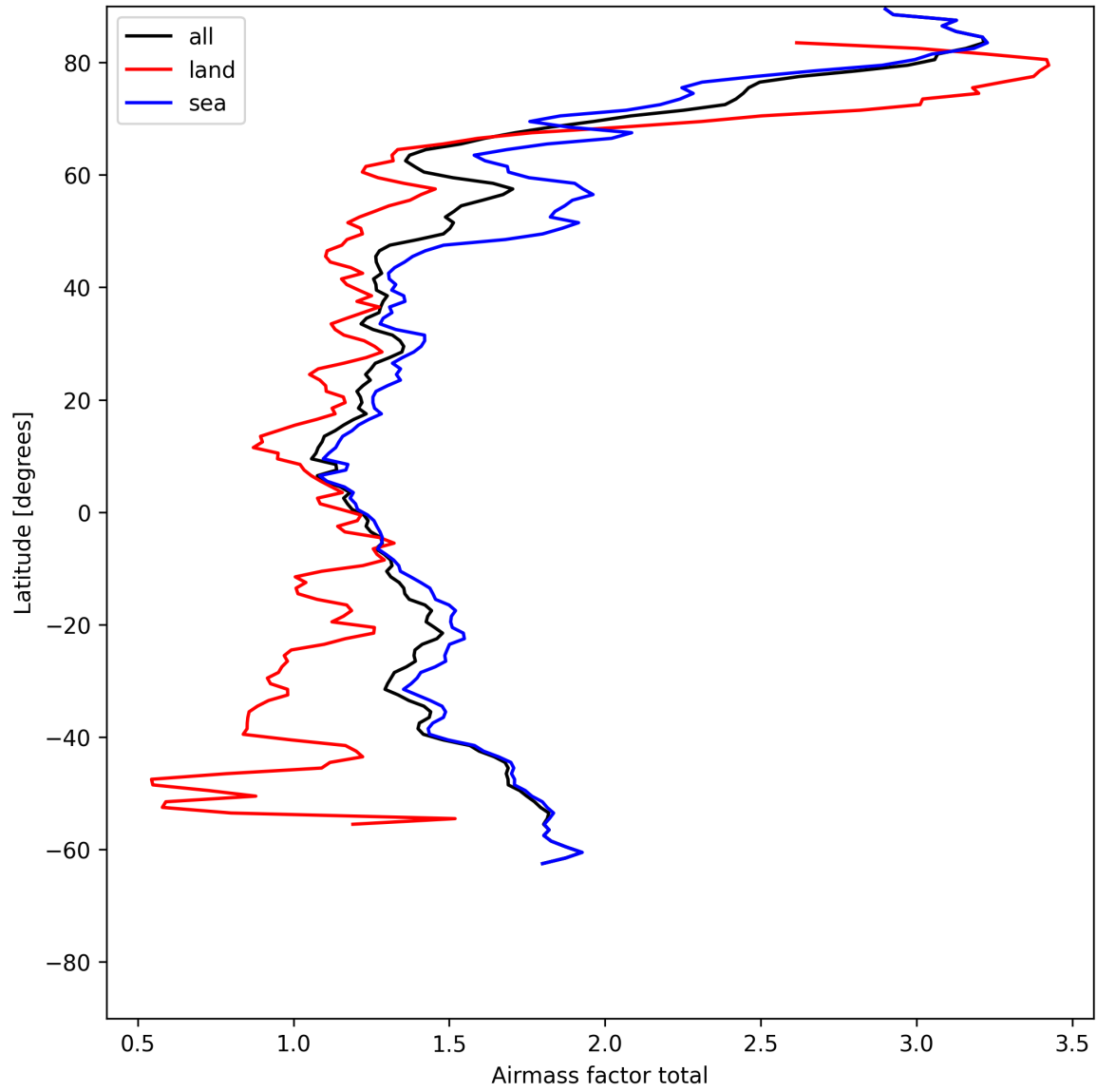
Figure 26: Zonal average of “Airmass factor total” for 2025-05-28 to 2025-05-30.
