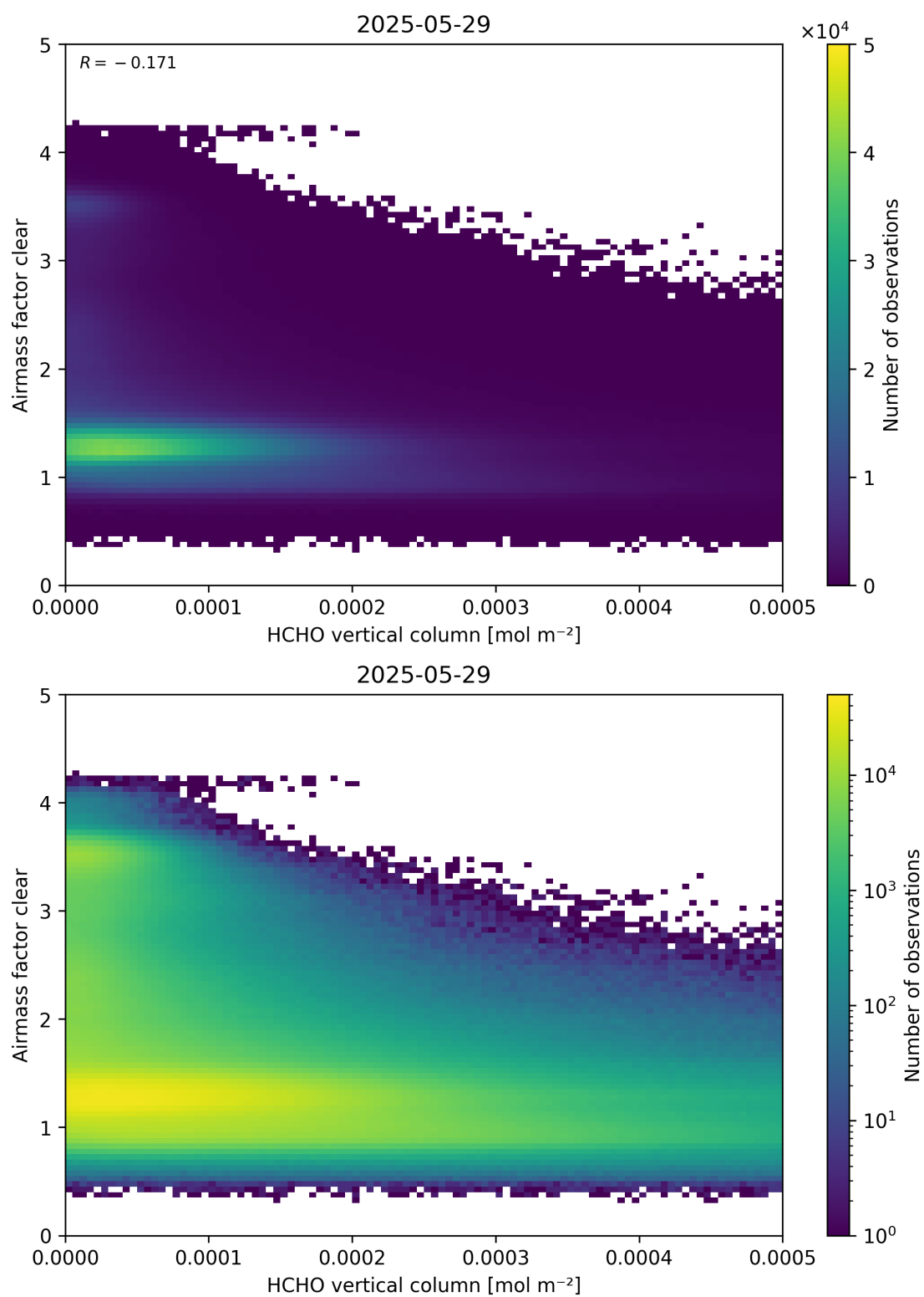
Figure 126: Scatter density plot of “HCHO vertical column” against “Airmass factor clear” for 2025-05-28 to 2025-05-30.
