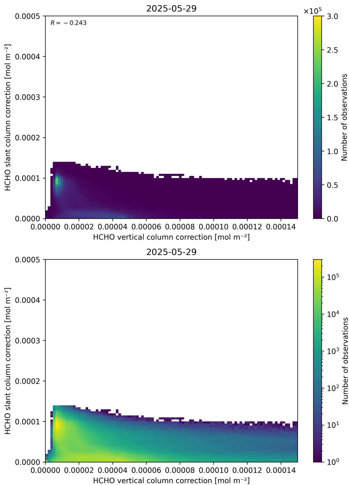
Figure 117: Scatter density plot of “HCHO vertical column correction” against “HCHO slant column correction” for 2025-05-28 to 2025-05-30.
