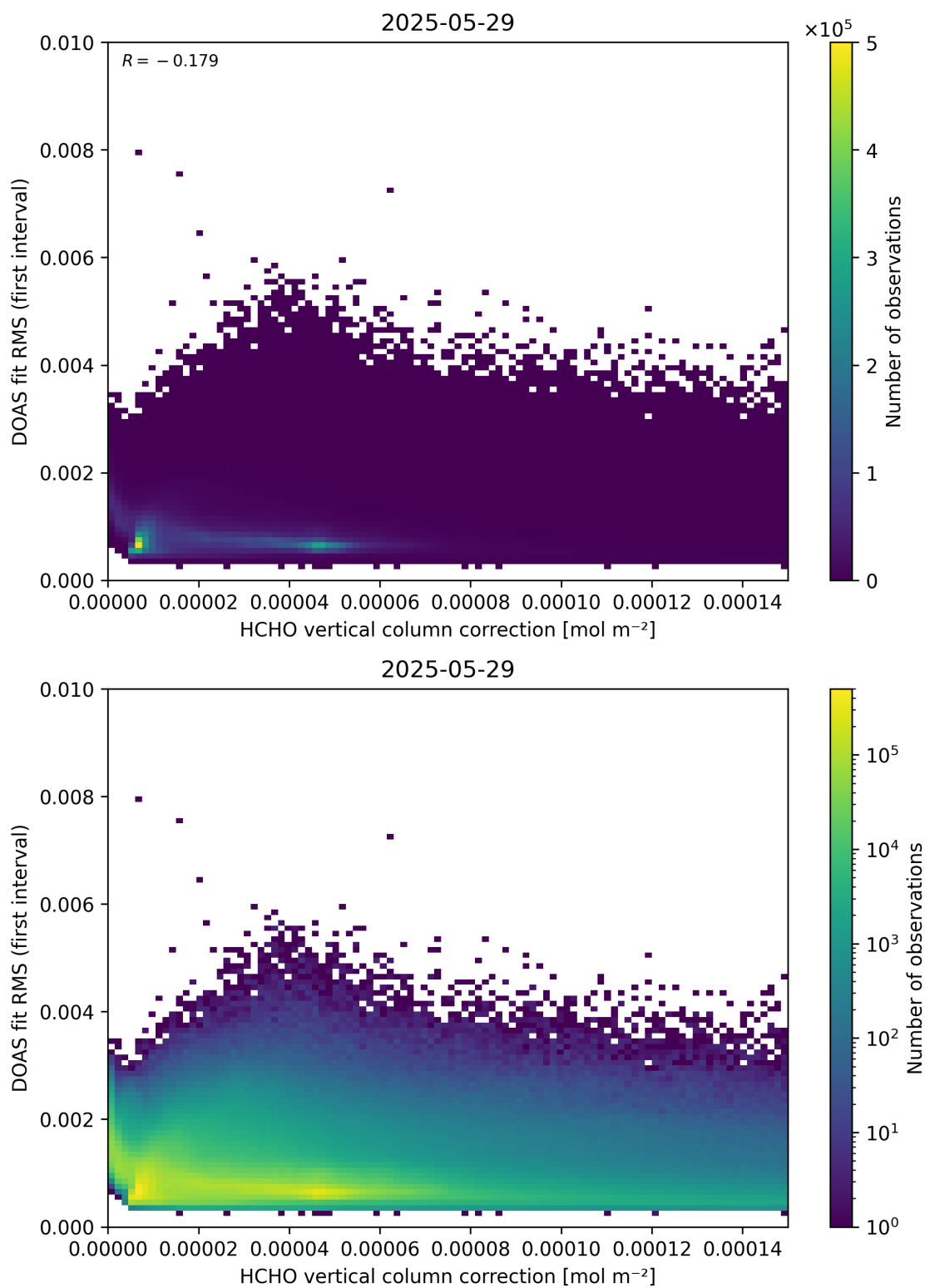
Figure 112: Scatter density plot of “HCHO vertical column correction” against “DOAS fit RMS (first interval)” for 2025-05-28 to 2025-05-30.
