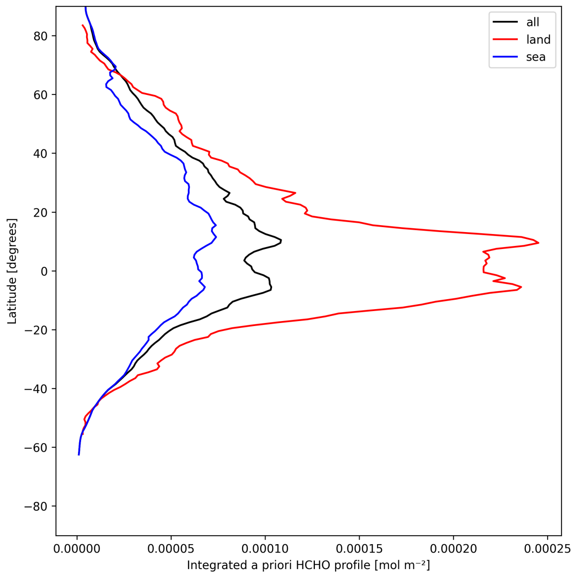
Figure 29: Zonal average of “Integrated a priori HCHO profile” for 2025-05-28 to 2025-05-30.
