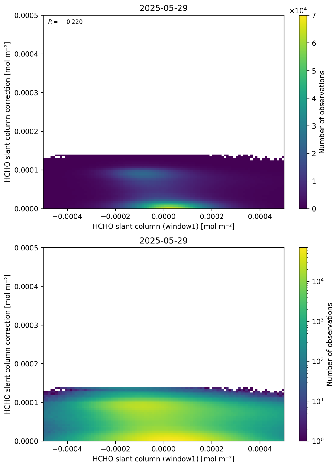
Figure 83: Scatter density plot of “HCHO slant column (window1)” against “HCHO slant column correction” for 2025-05-28 to 2025-05-30.
