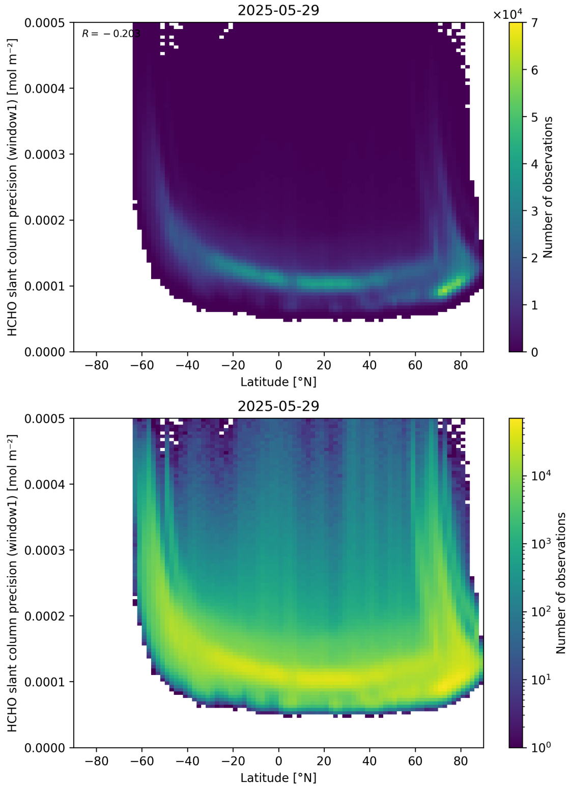
Figure 160: Scatter density plot of “Latitude” against “HCHO slant column precision (window1)” for 2025-05-28 to 2025-05-30.
