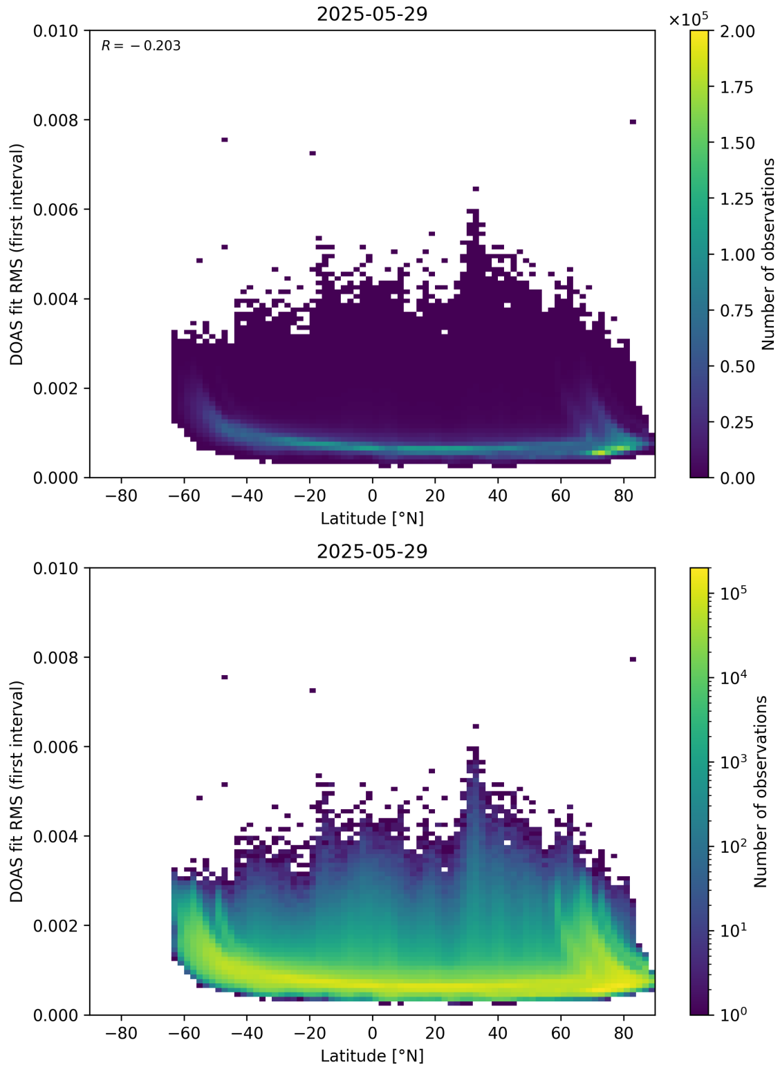
Figure 153: Scatter density plot of “Latitude” against “DOAS fit RMS (first interval)” for 2025-05-28 to 2025-05-30.
