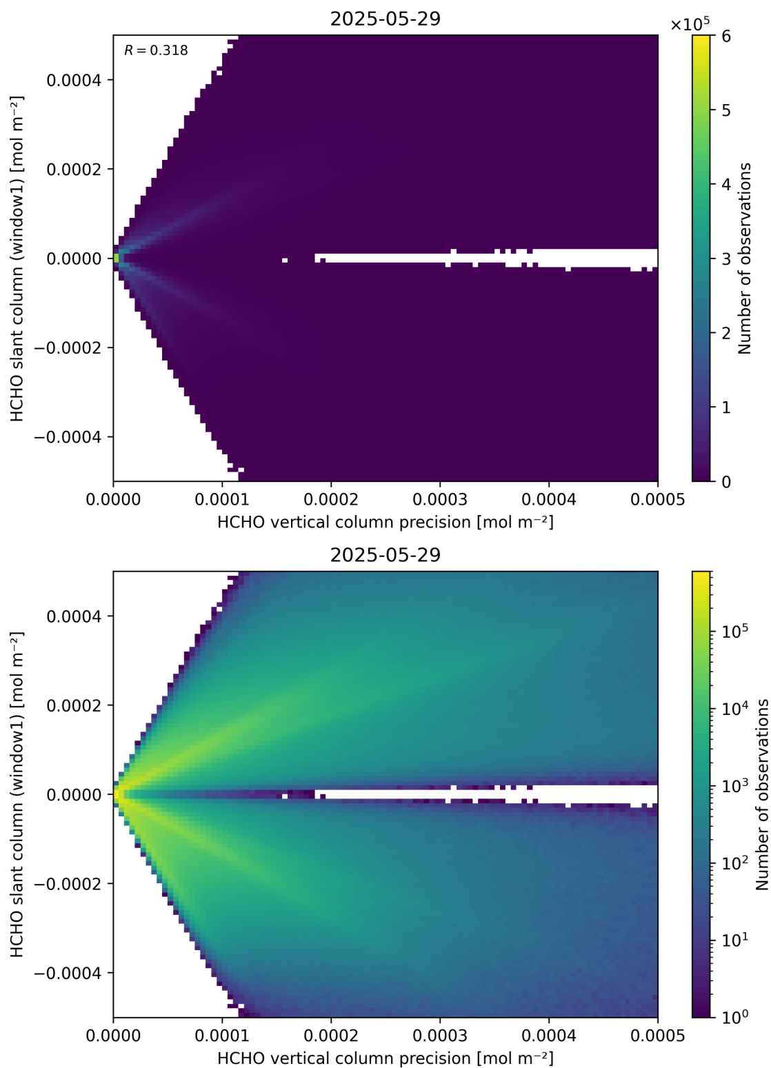
Figure 142: Scatter density plot of “HCHO vertical column precision” against “HCHO slant column (window1)” for 2025-05-28 to 2025-05-30.
