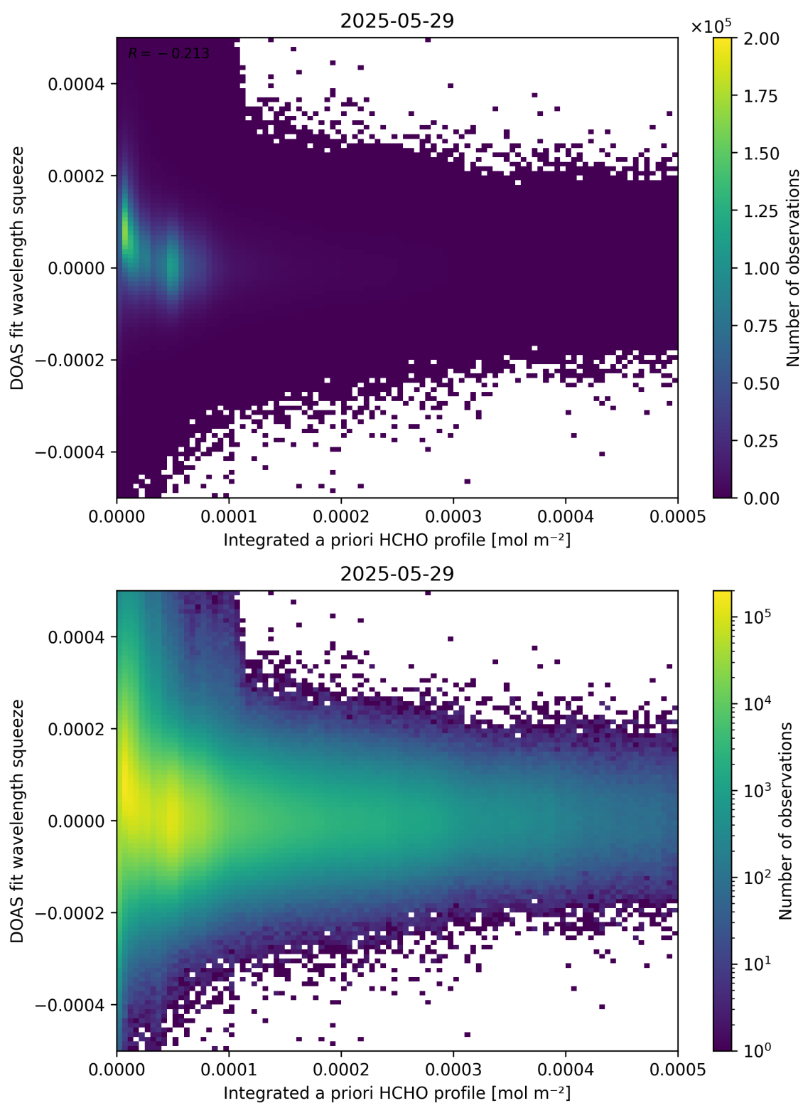
Figure 150: Scatter density plot of “Integrated a priori HCHO profile” against “DOAS fit wavelength squeeze” for 2025-05-28 to 2025-05-30.
