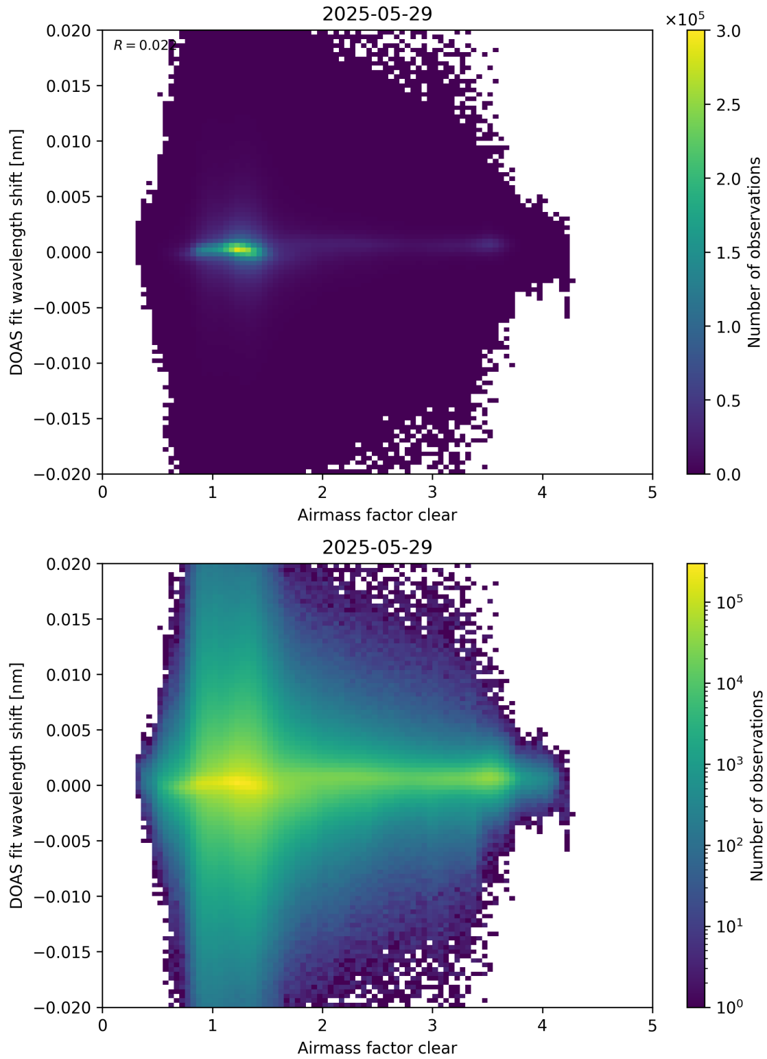
Figure 72: Scatter density plot of “Airmass factor clear” against “DOAS fit wavelength shift” for 2025-05-28 to 2025-05-30.
