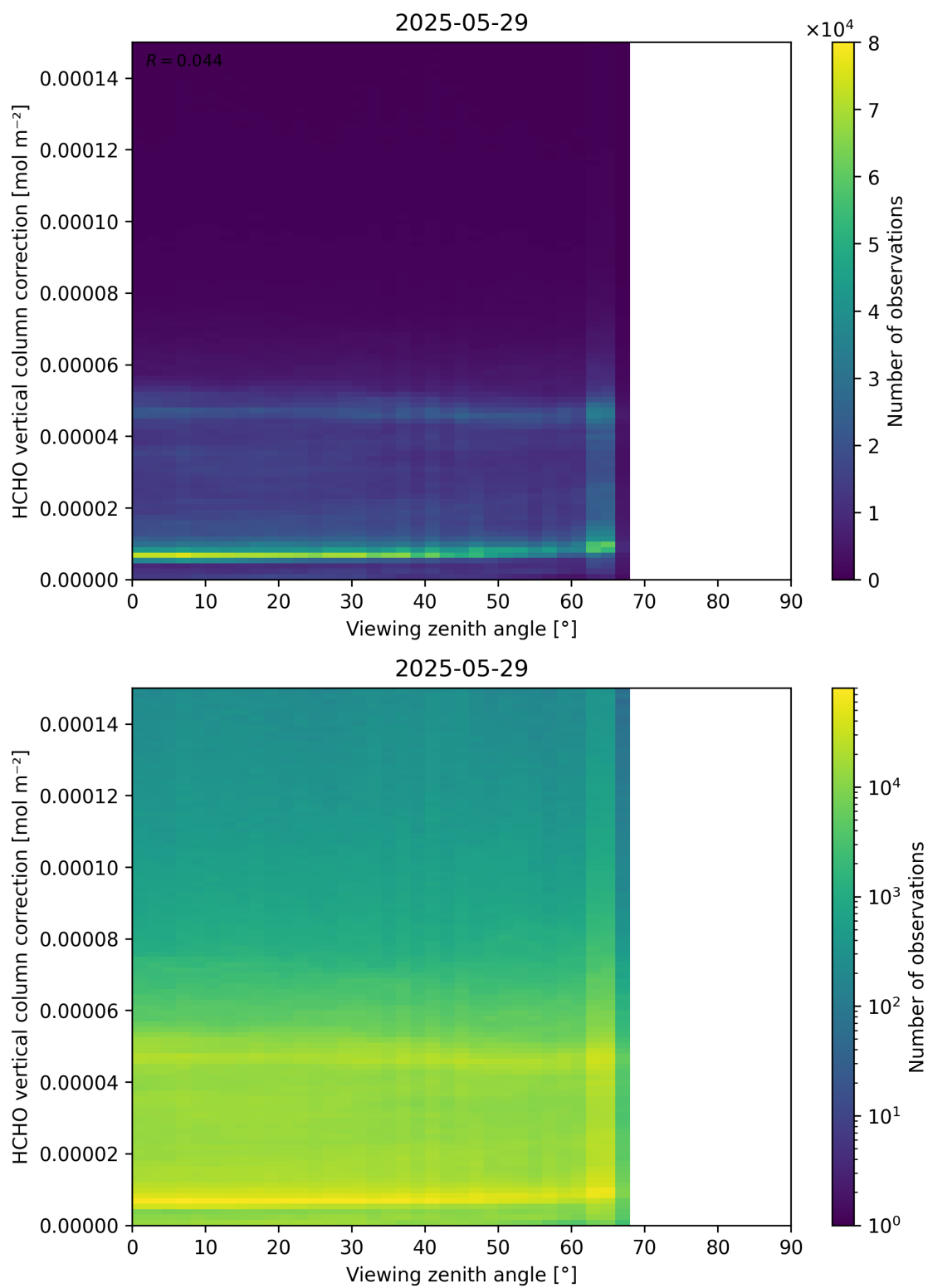
Figure 193: Scatter density plot of “Viewing zenith angle” against “HCHO vertical column correction” for 2025-05-28 to 2025-05-30.
