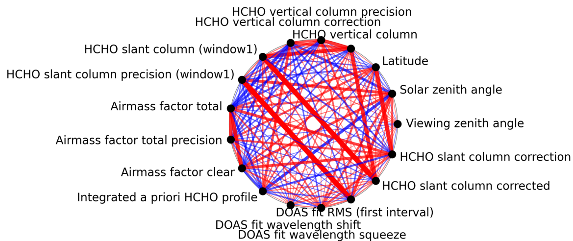
Figure 1: Map of correlation graph for 2025-05-28 to 2025-05-30.
