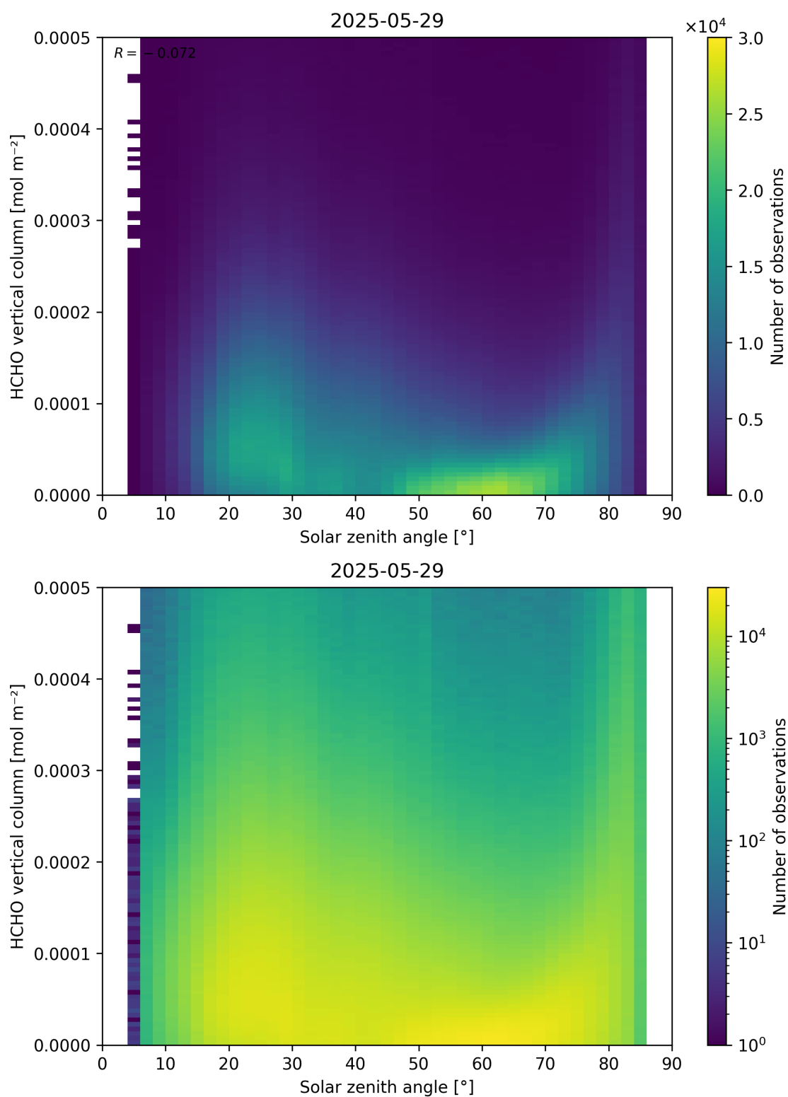
Figure 177: Scatter density plot of “Solar zenith angle” against “HCHO vertical column” for 2025-05-28 to 2025-05-30.
