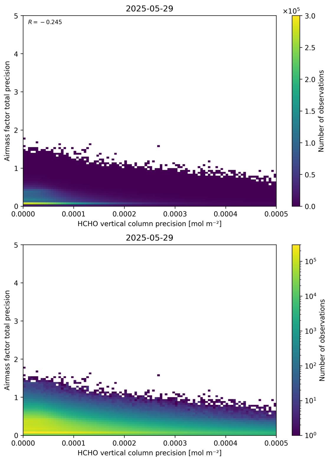
Figure 145: Scatter density plot of “HCHO vertical column precision” against “Airmass factor total precision” for 2025-05-28 to 2025-05-30.
