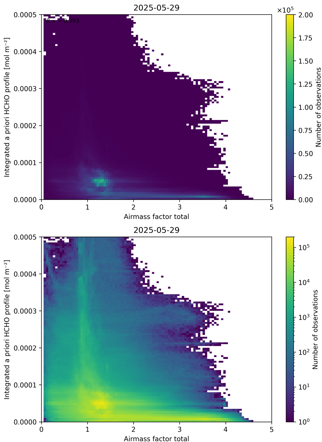
Figure 104: Scatter density plot of “Airmass factor total” against “Integrated a priori HCHO profile” for 2025-05-28 to 2025-05-30.
