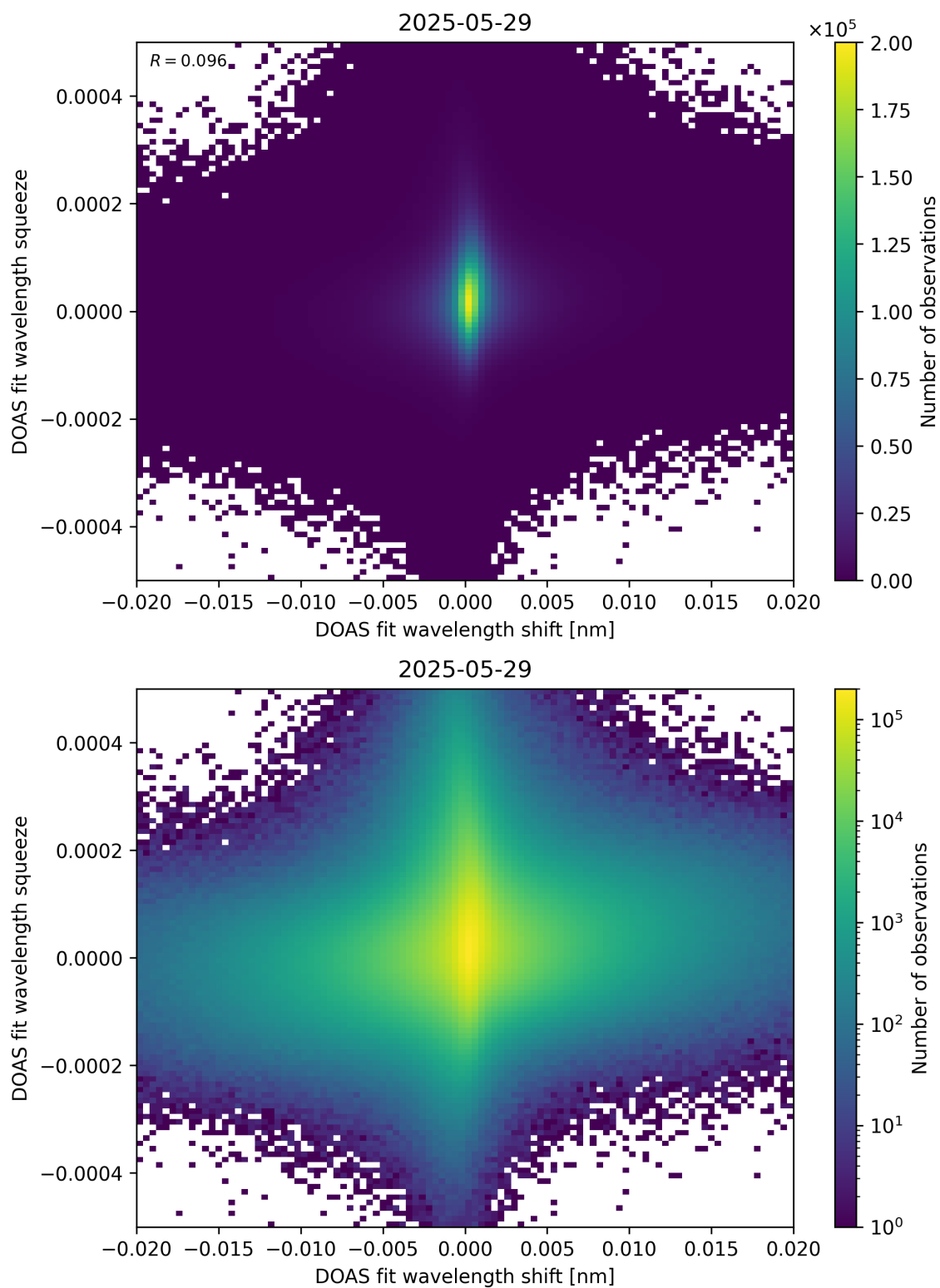
Figure 65: Scatter density plot of “DOAS fit wavelength shift” against “DOAS fit wavelength squeeze” for 2025-05-28 to 2025-05-30.
