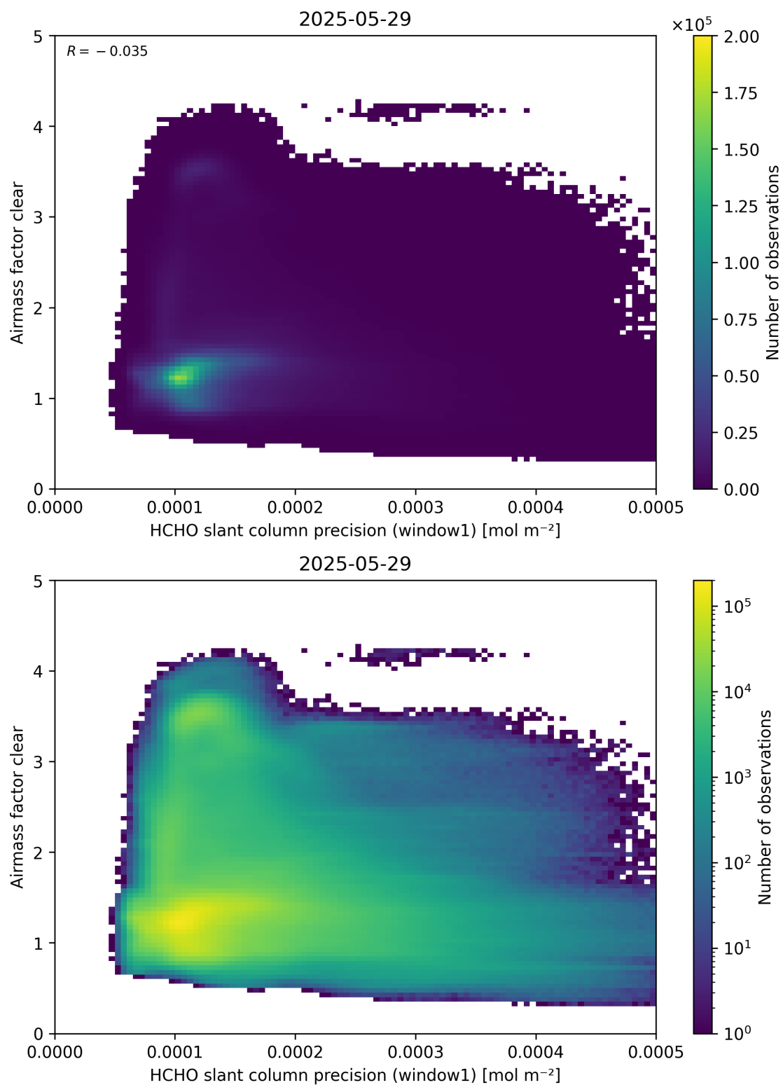
Figure 91: Scatter density plot of “HCHO slant column precision (window1)” against “Airmass factor clear” for 2025-05-28 to 2025-05-30.
