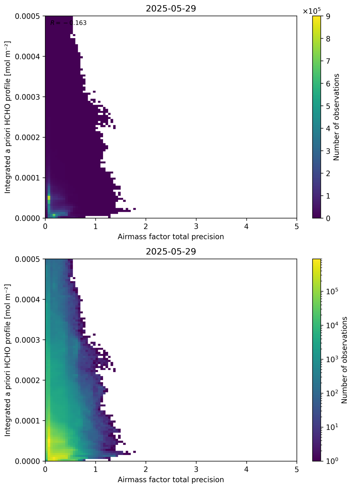
Figure 111: Scatter density plot of “Airmass factor total precision” against “Integrated a priori HCHO profile” for 2025-05-28 to 2025-05-30.
