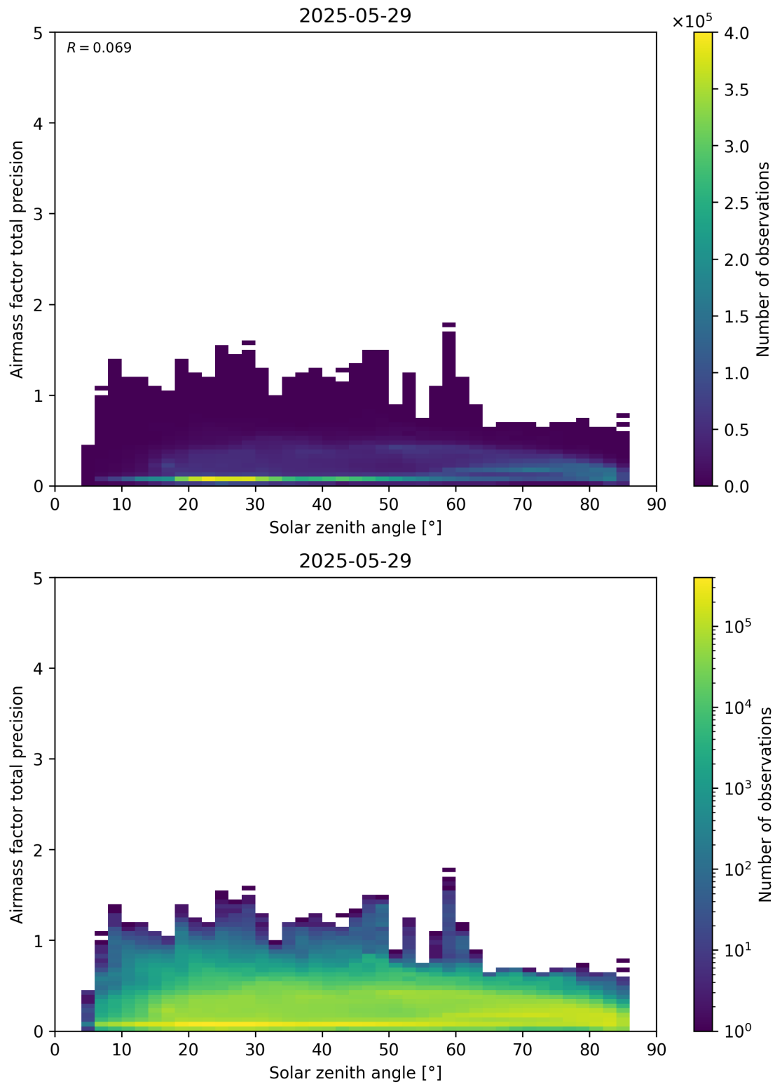
Figure 176: Scatter density plot of “Solar zenith angle” against “Airmass factor total precision” for 2025-05-28 to 2025-05-30.
