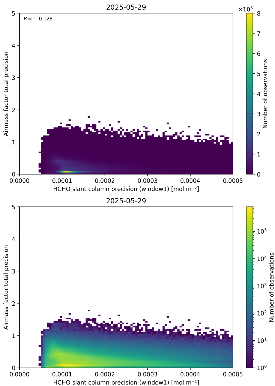
Figure 95: Scatter density plot of “HCHO slant column precision (window1)” against “Airmass factor total precision” for 2025-05-28 to 2025-05-30.
