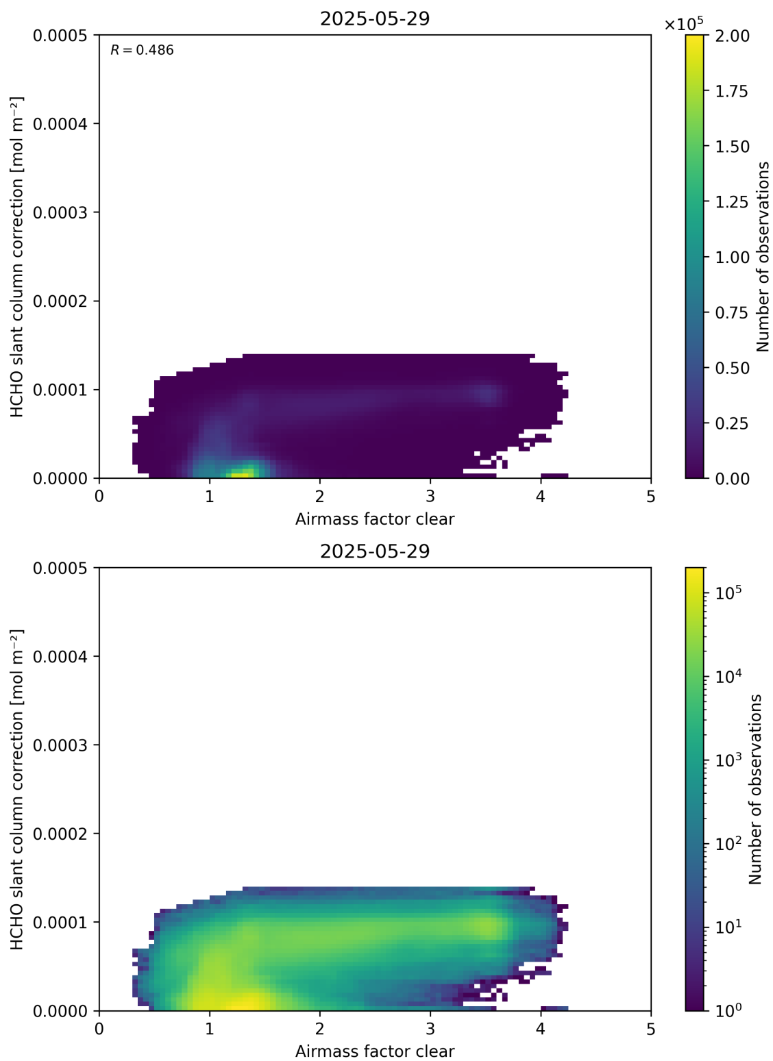
Figure 75: Scatter density plot of “Airmass factor clear” against “HCHO slant column correction” for 2025-05-28 to 2025-05-30.
