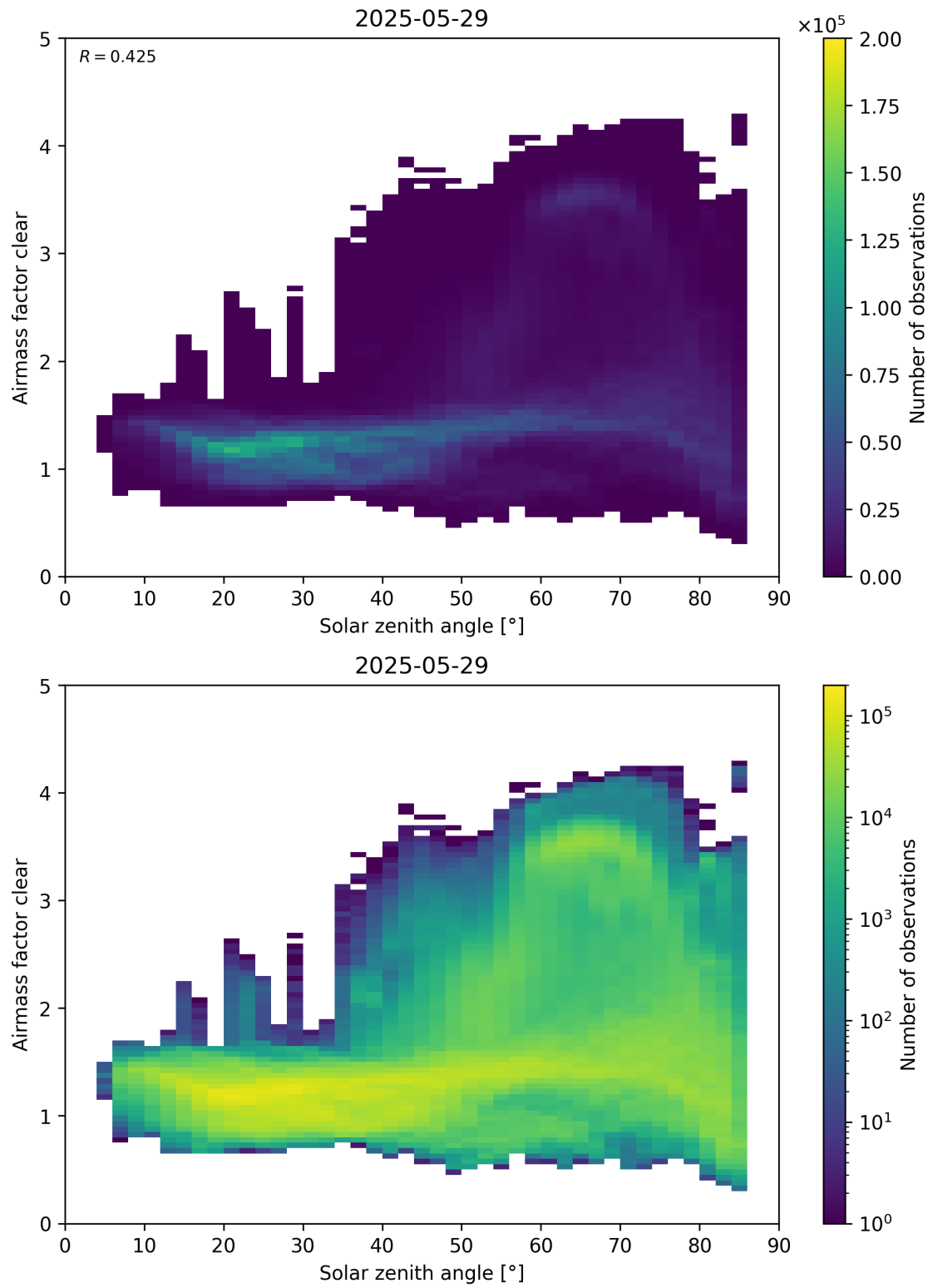
Figure 170: Scatter density plot of “Solar zenith angle” against “Airmass factor clear” for 2025-05-28 to 2025-05-30.
