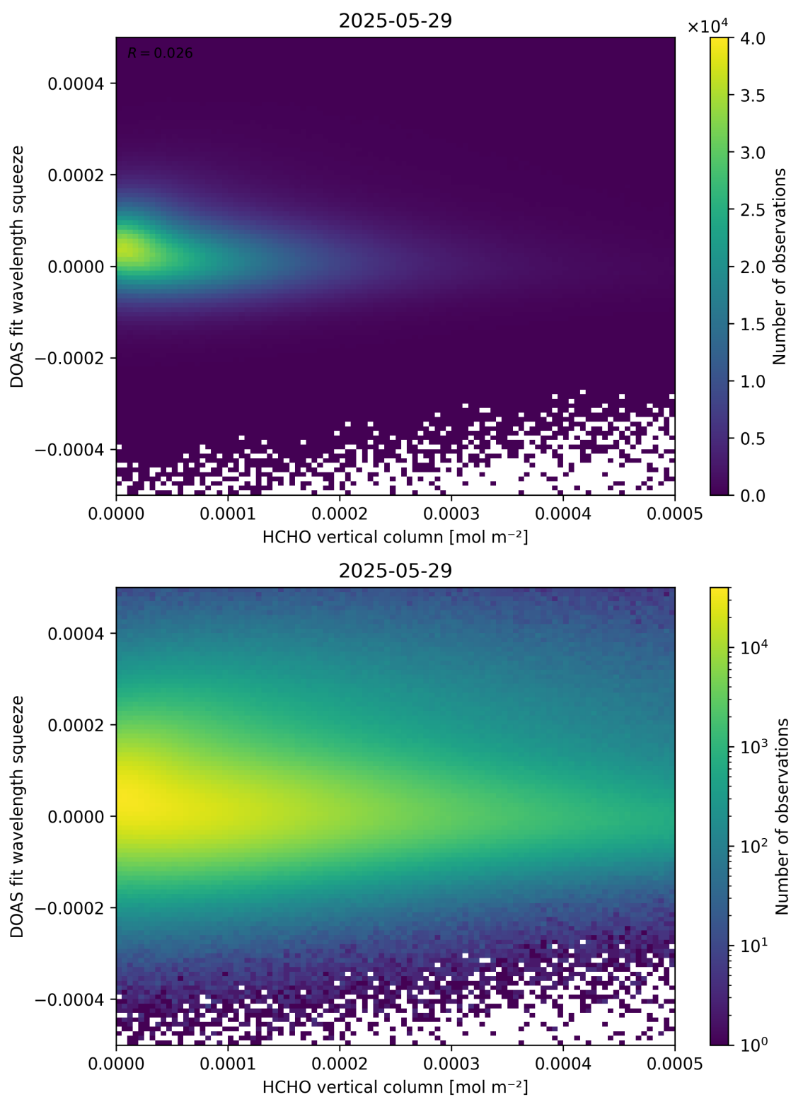
Figure 125: Scatter density plot of “HCHO vertical column” against “DOAS fit wavelength squeeze” for 2025-05-28 to 2025-05-30.
