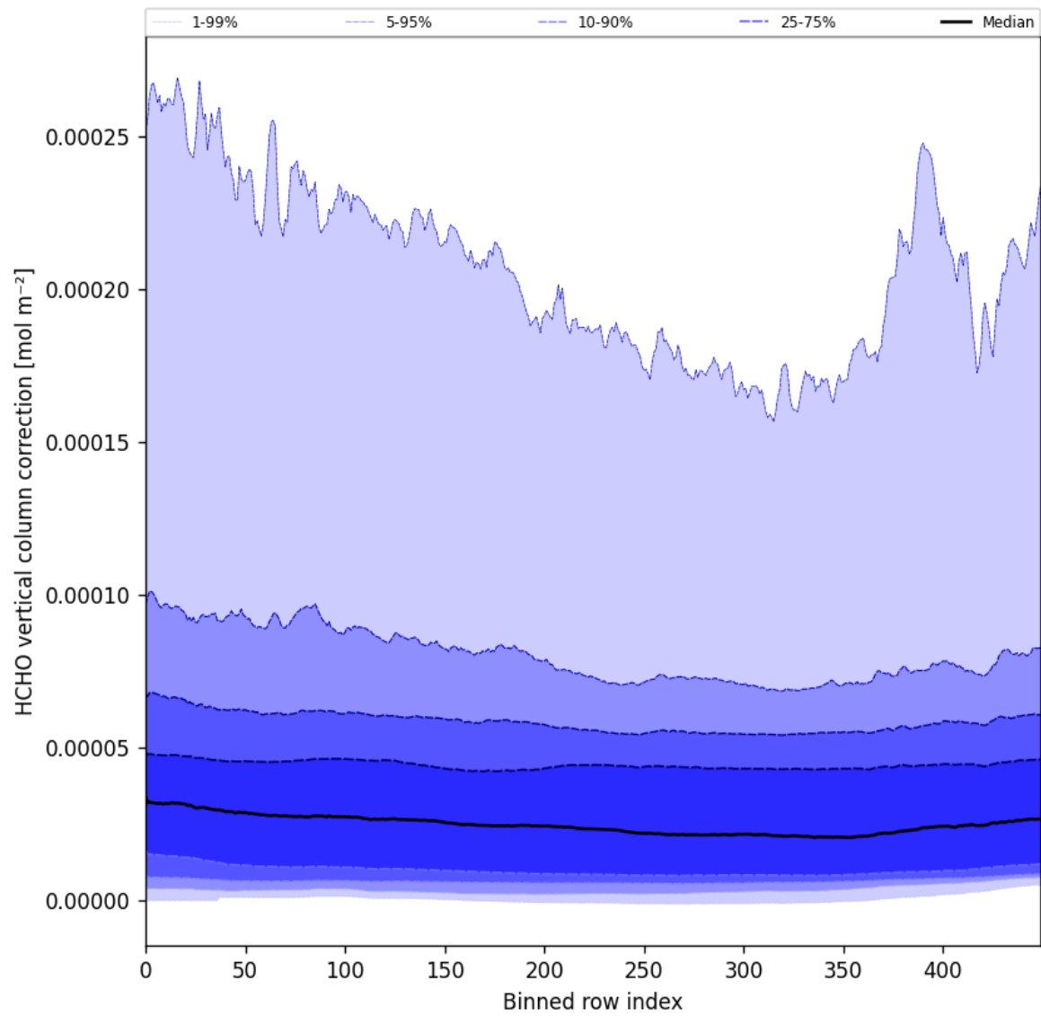
Figure 51: Along track statistics of “HCHO vertical column correction” for 2025-05-28 to 2025-05-30
