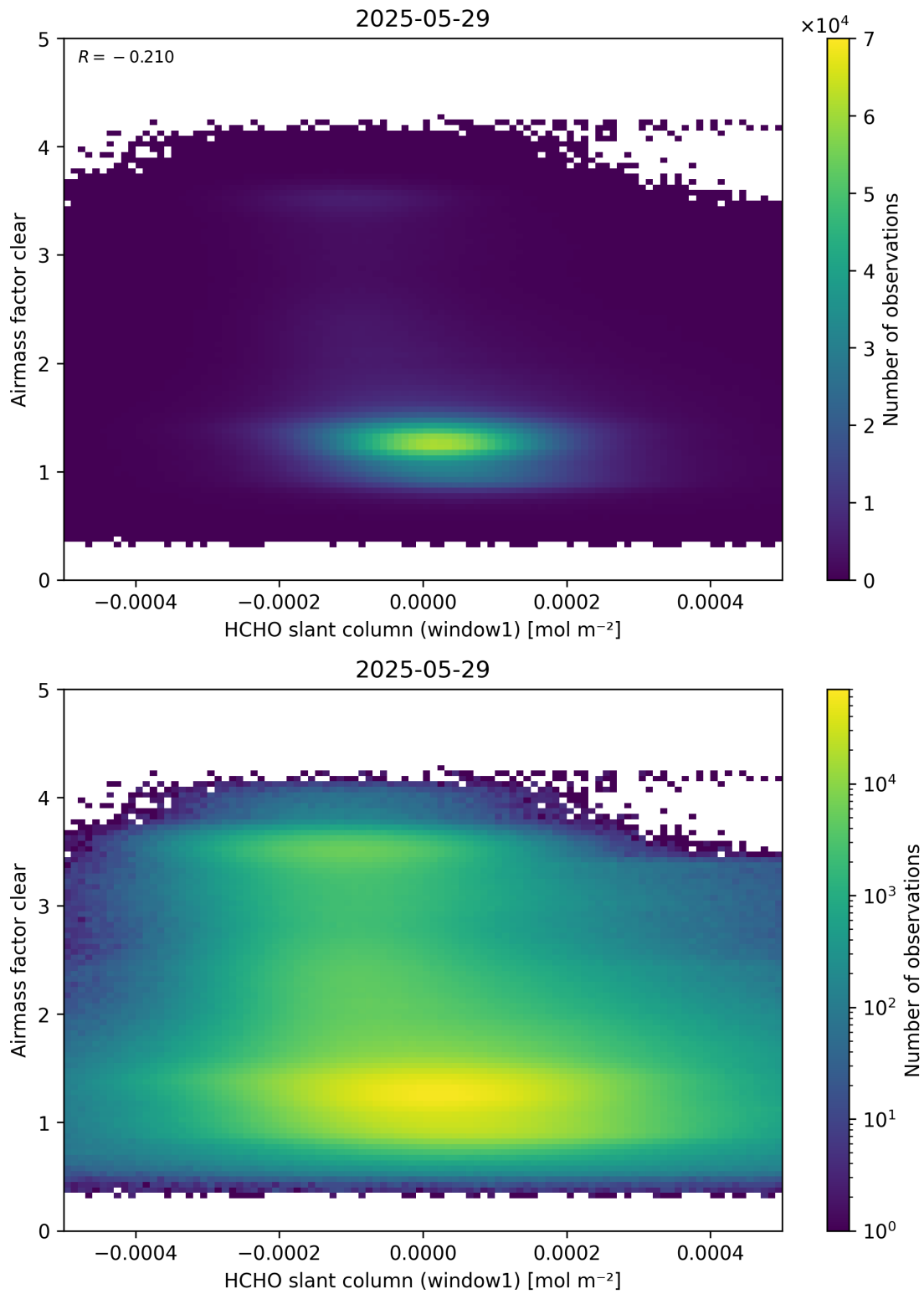
Figure 81: Scatter density plot of “HCHO slant column (window1)” against “Airmass factor clear” for 2025-05-28 to 2025-05-30.
