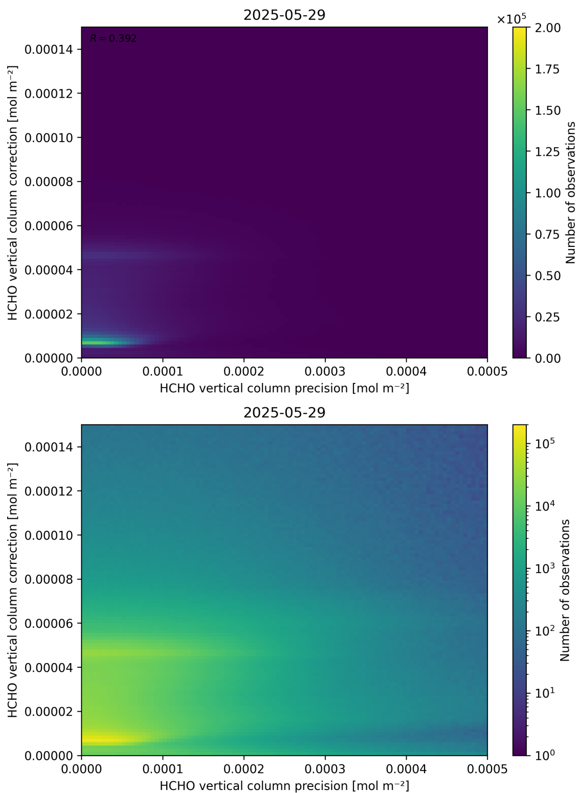
Figure 146: Scatter density plot of “HCHO vertical column precision” against “HCHO vertical column correction” for 2025-05-28 to 2025-05-30.
