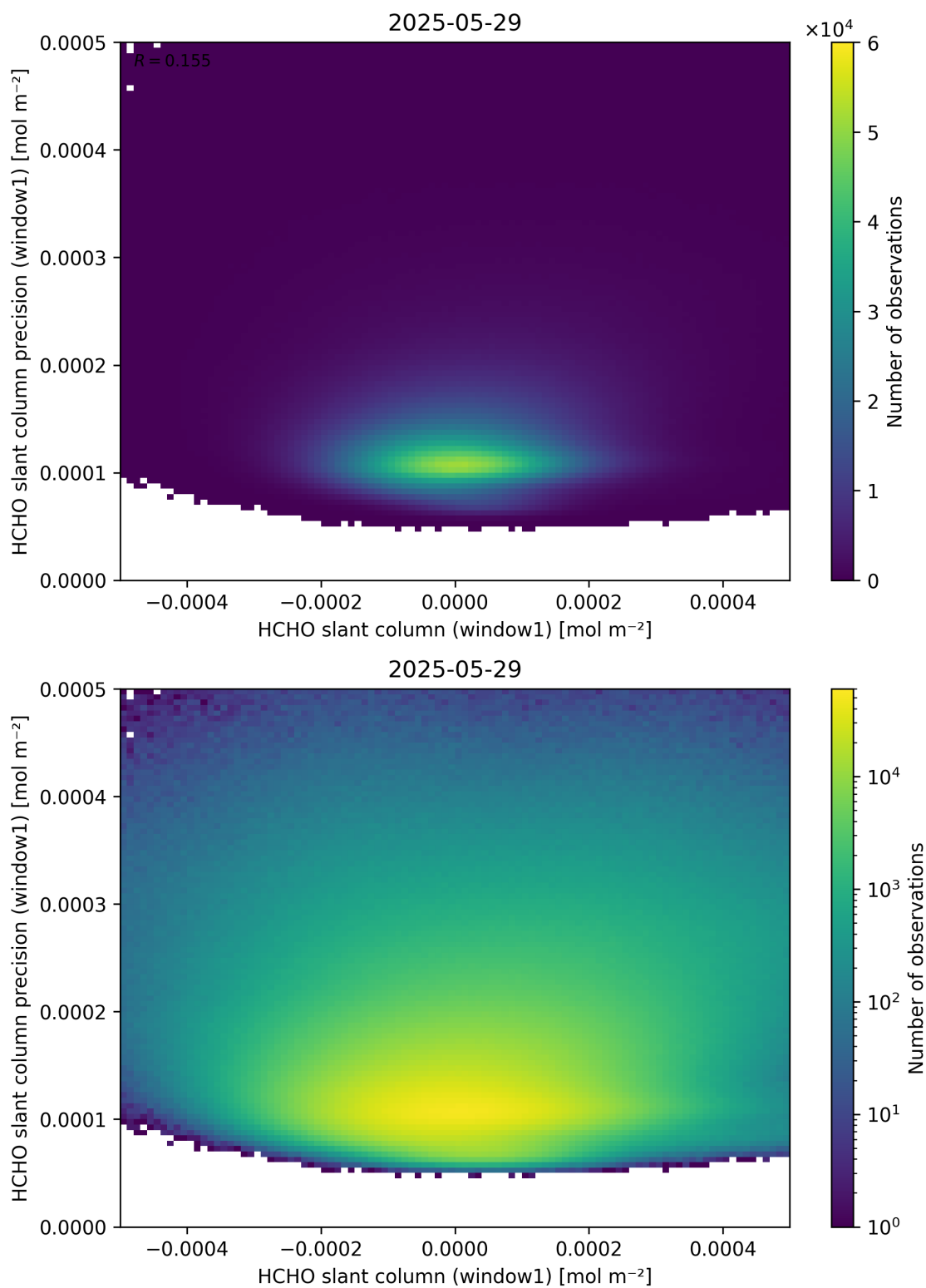
Figure 84: Scatter density plot of “HCHO slant column (window1)” against “HCHO slant column precision (window1)” for 2025-05-28 to 2025-05-30.
