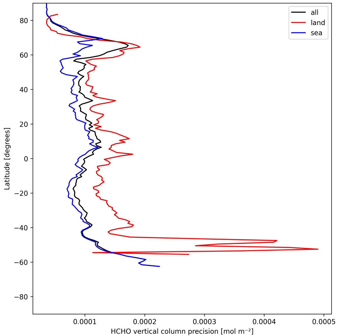
Figure 22: Zonal average of “HCHO vertical column precision” for 2025-05-28 to 2025-05-30.
