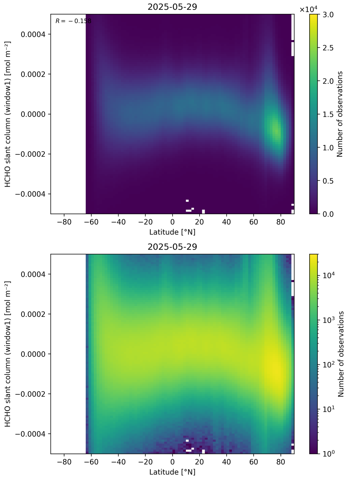
Figure 159: Scatter density plot of “Latitude” against “HCHO slant column (window1)” for 2025-05-28 to 2025-05-30.
