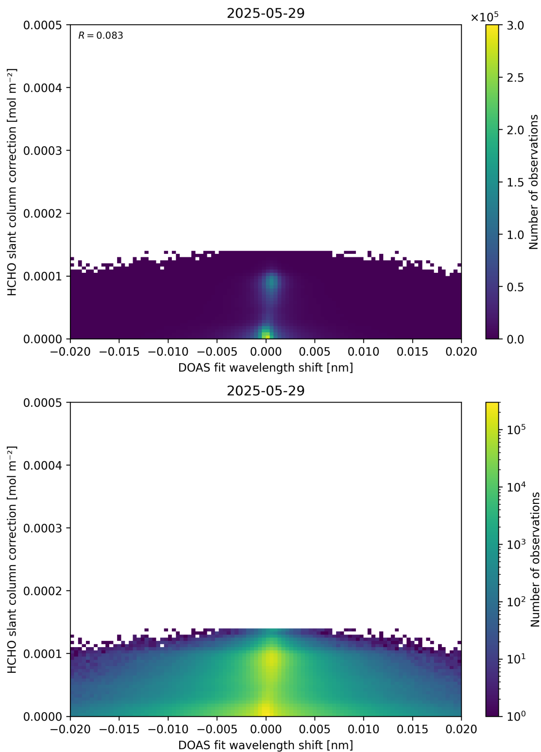
Figure 67: Scatter density plot of “DOAS fit wavelength shift” against “HCHO slant column correction” for 2025-05-28 to 2025-05-30.
