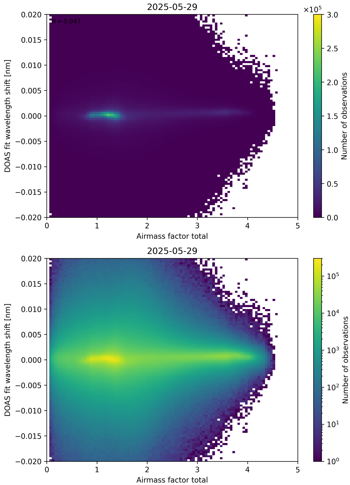
Figure 98: Scatter density plot of “Airmass factor total” against “DOAS fit wavelength shift” for 2025-05-28 to 2025-05-30.
