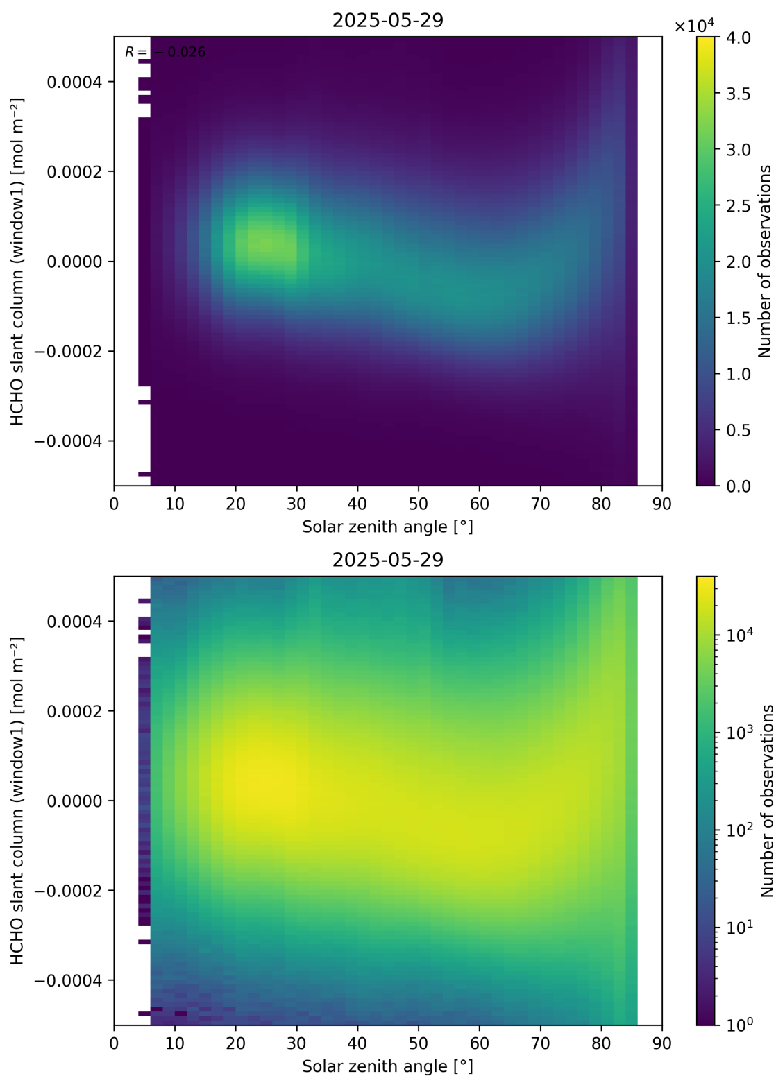
Figure 173: Scatter density plot of “Solar zenith angle” against “HCHO slant column (window1)” for 2025-05-28 to 2025-05-30.
