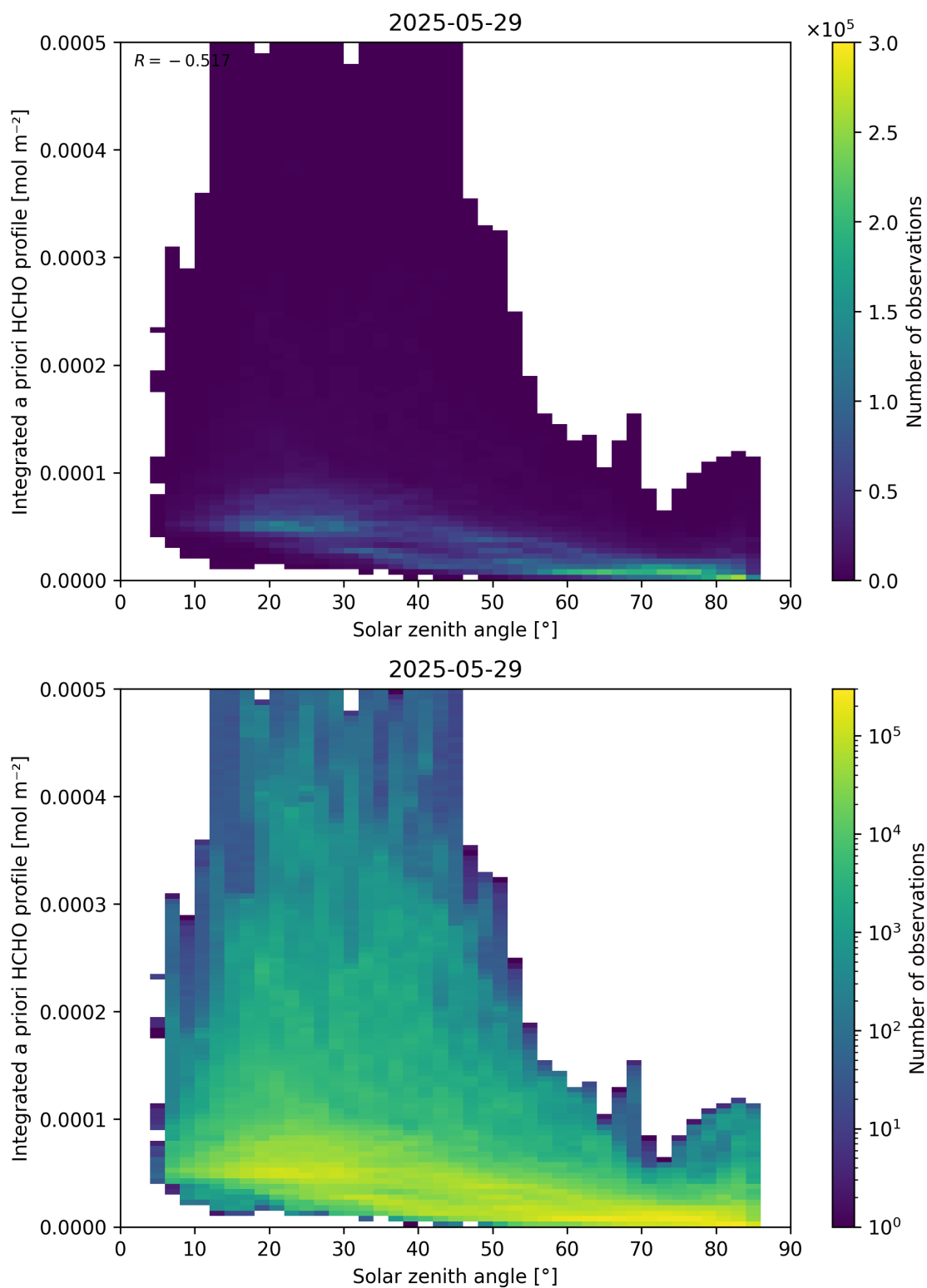
Figure 180: Scatter density plot of “Solar zenith angle” against “Integrated a priori HCHO profile” for 2025-05-28 to 2025-05-30.
