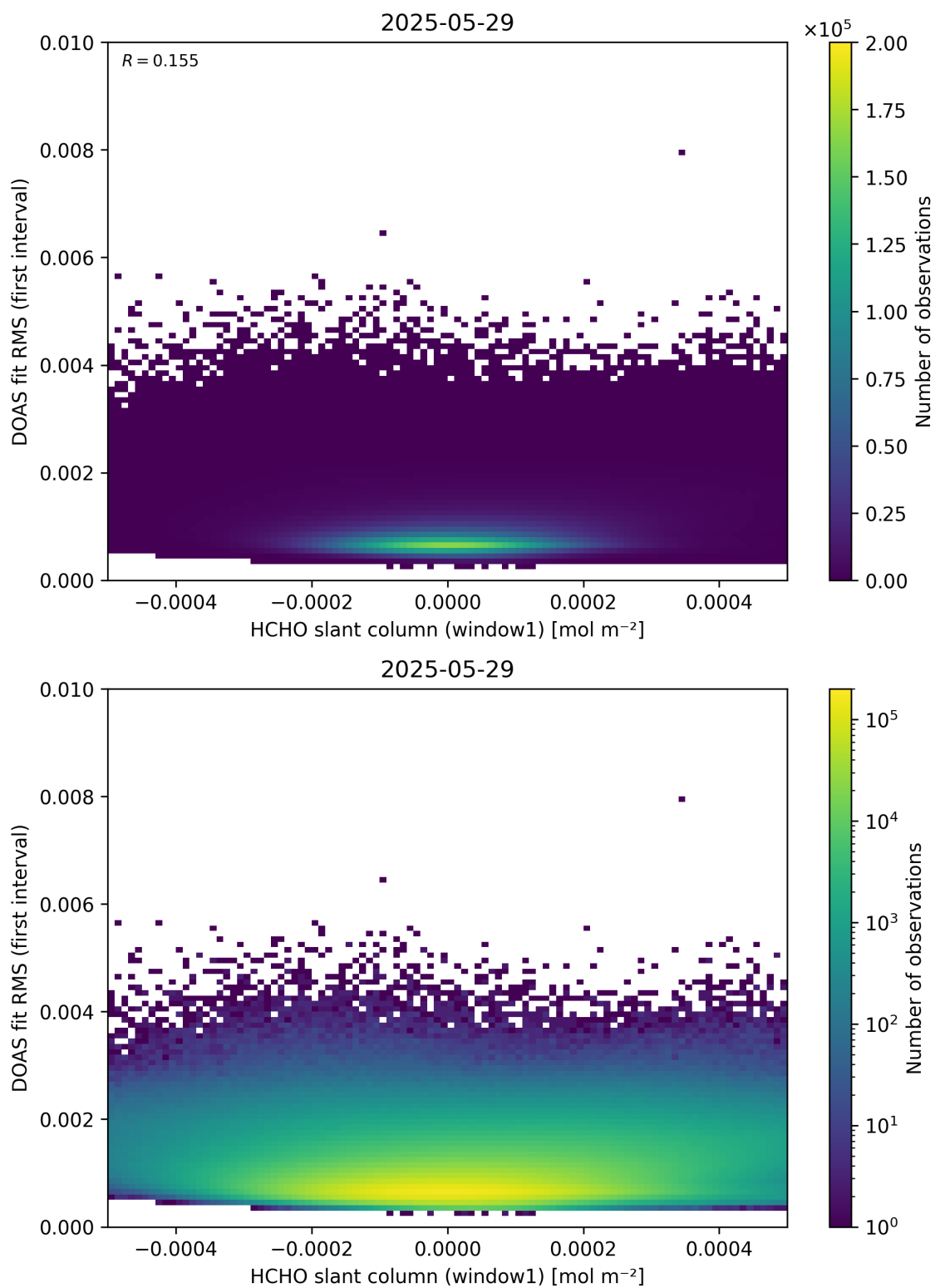
Figure 78: Scatter density plot of “HCHO slant column (window1)” against “DOAS fit RMS (first interval)” for 2025-05-28 to 2025-05-30.
