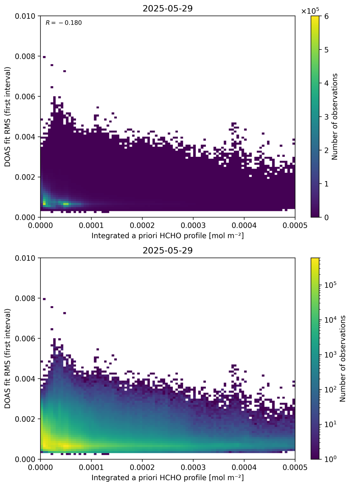
Figure 148: Scatter density plot of “Integrated a priori HCHO profile” against “DOAS fit RMS (first interval)” for 2025-05-28 to 2025-05-30.
