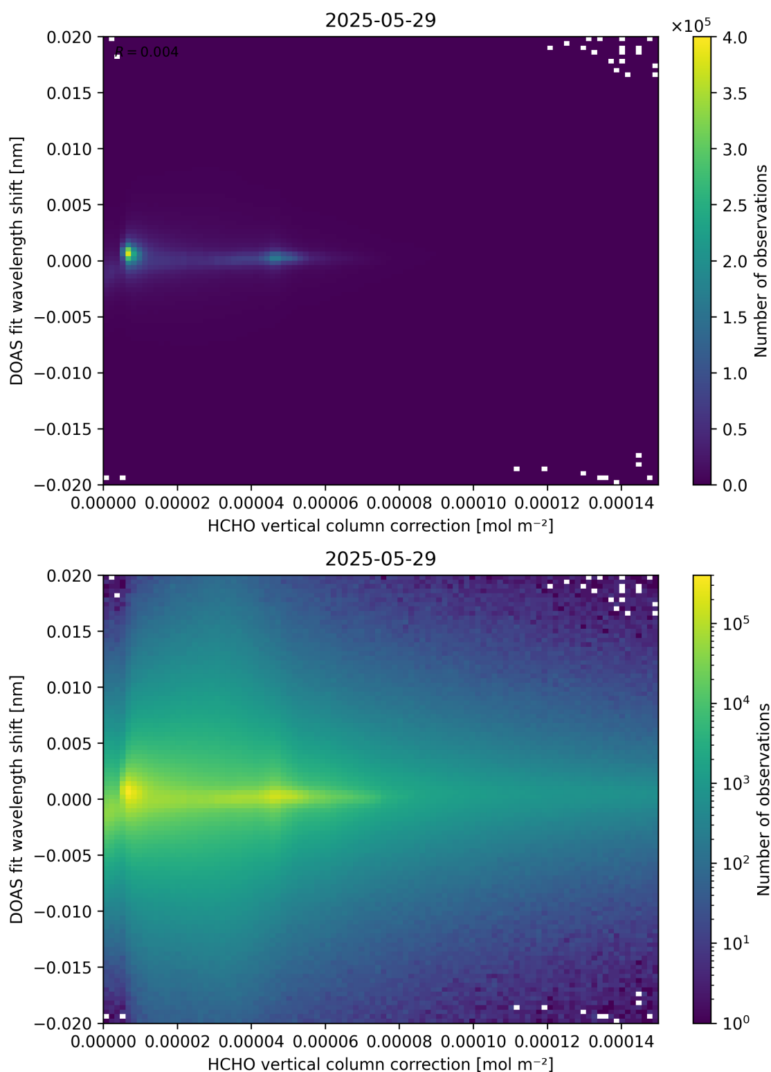
Figure 113: Scatter density plot of “HCHO vertical column correction” against “DOAS fit wavelength shift” for 2025-05-28 to 2025-05-30.
