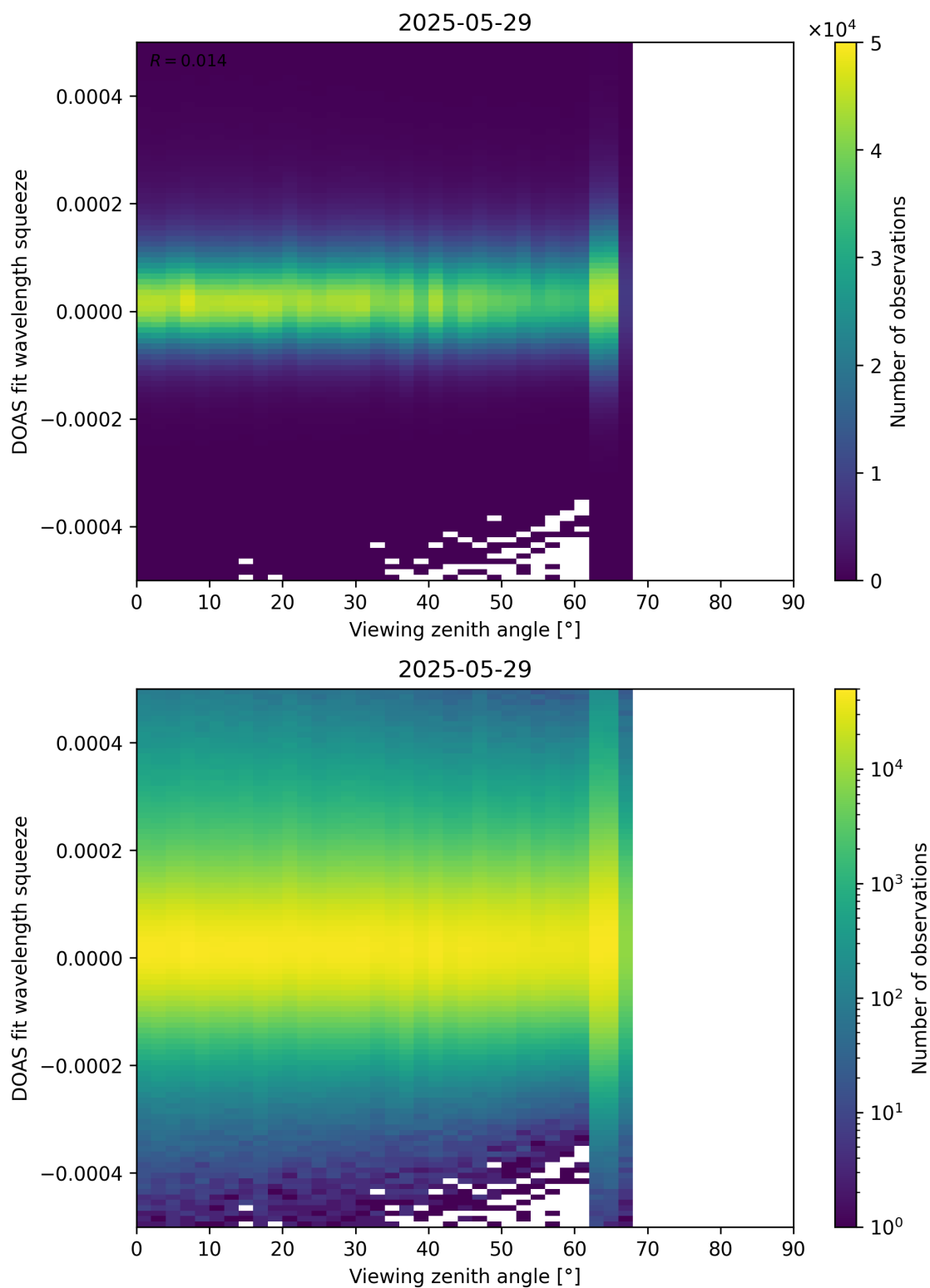
Figure 184: Scatter density plot of “Viewing zenith angle” against “DOAS fit wavelength squeeze” for 2025-05-28 to 2025-05-30.
