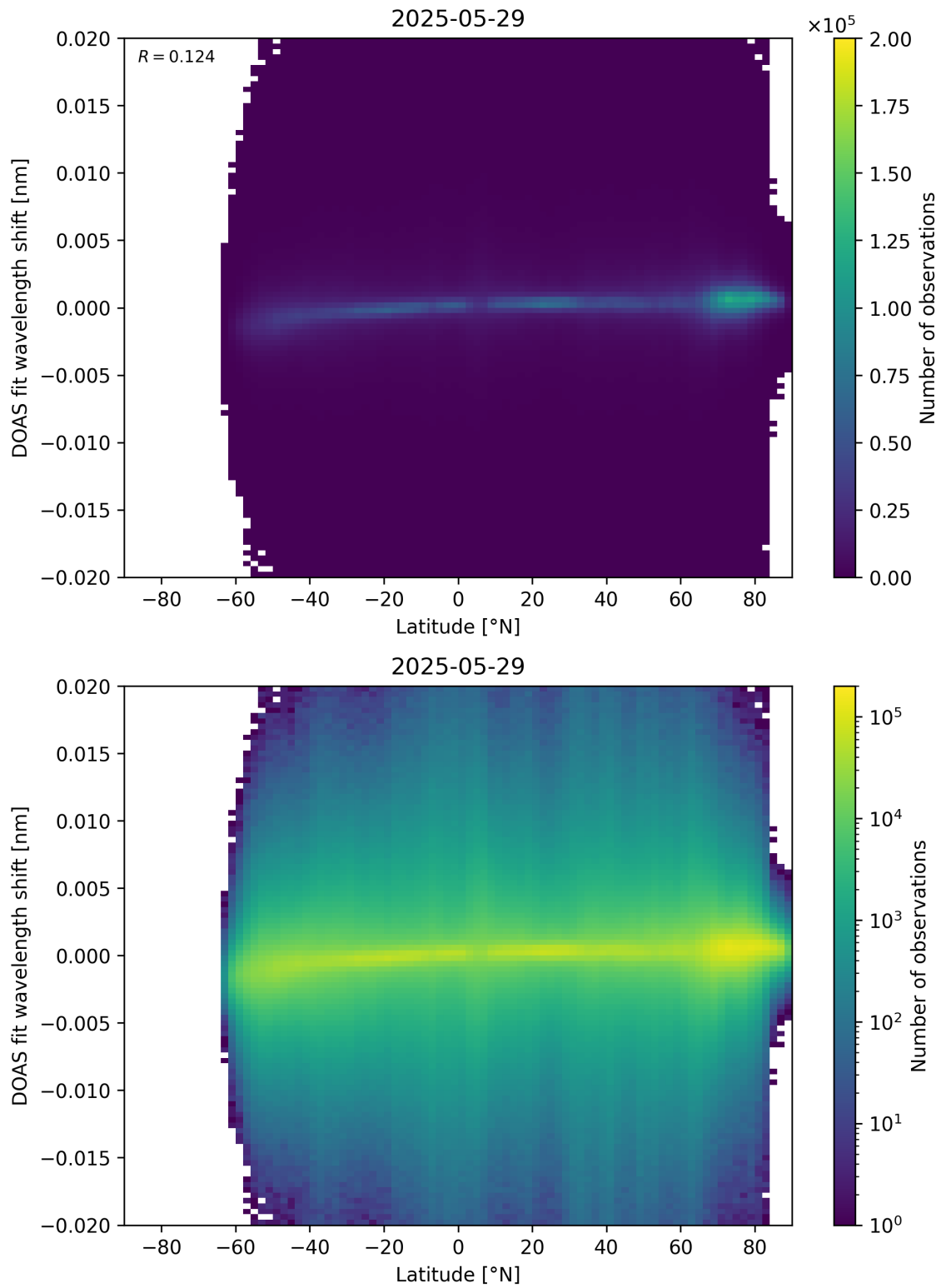
Figure 154: Scatter density plot of “Latitude” against “DOAS fit wavelength shift” for 2025-05-28 to 2025-05-30.
