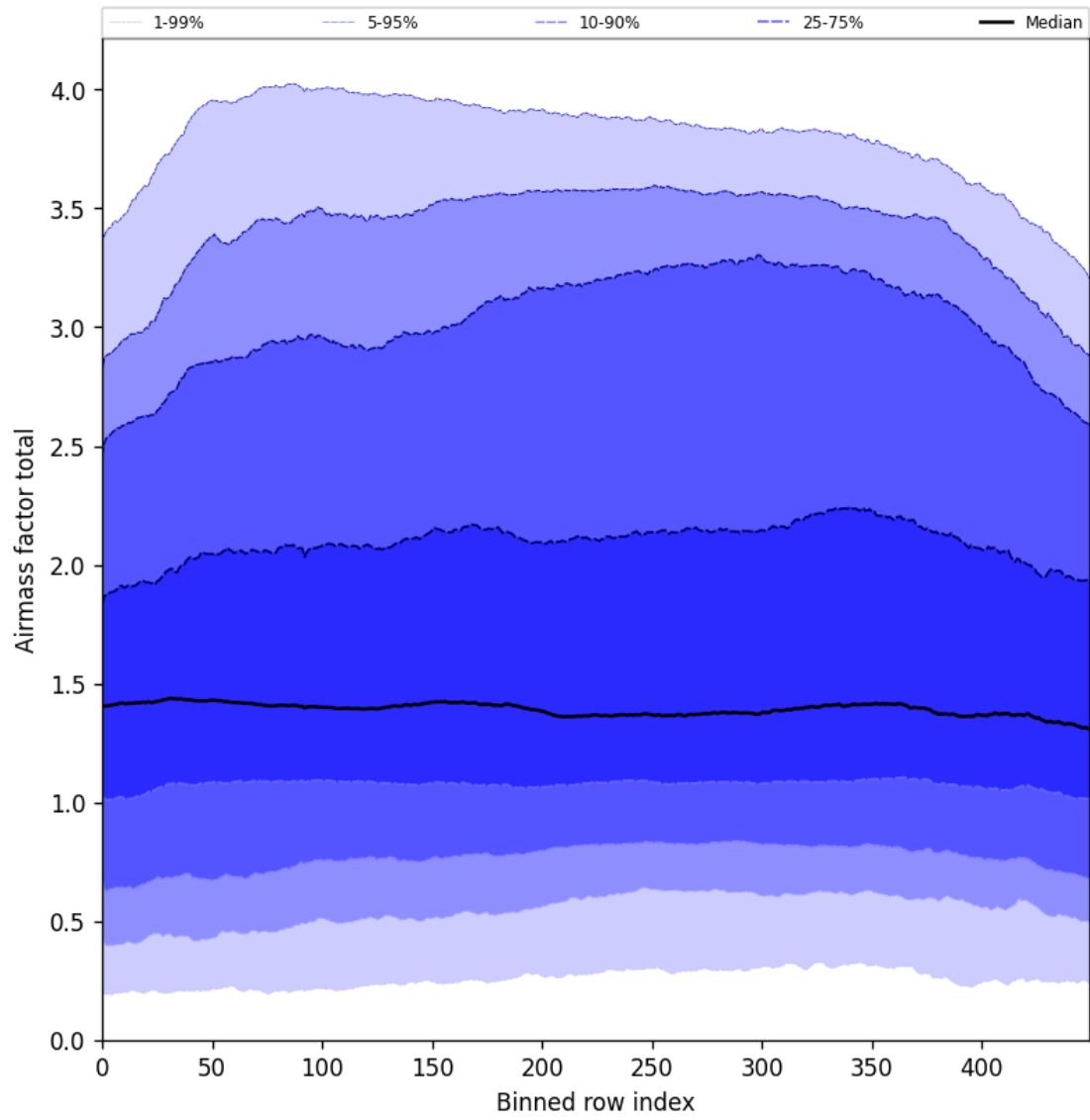
Figure 54: Along track statistics of “Airmass factor total” for 2025-05-28 to 2025-05-30
