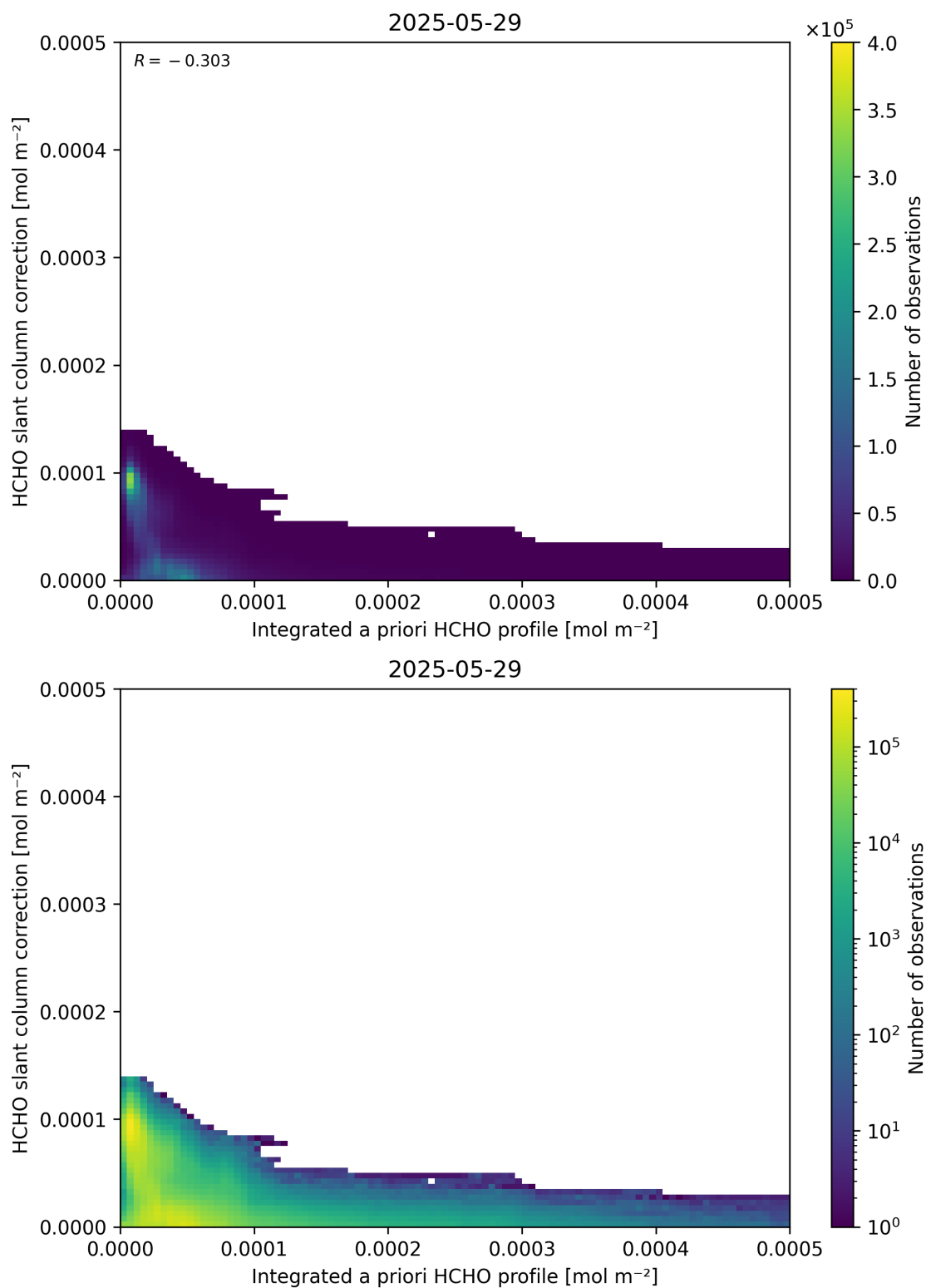
Figure 152: Scatter density plot of “Integrated a priori HCHO profile” against “HCHO slant column correction” for 2025-05-28 to 2025-05-30.
