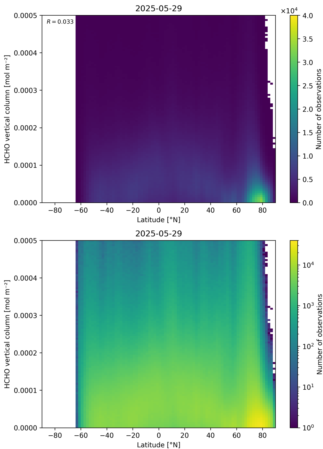
Figure 163: Scatter density plot of “Latitude” against “HCHO vertical column” for 2025-05-28 to 2025-05-30.
