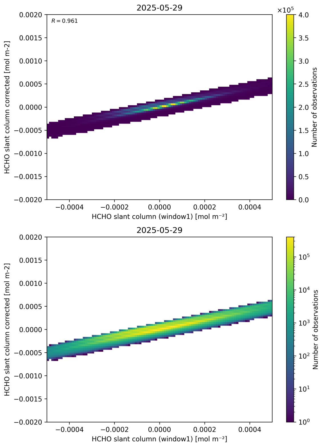
Figure 82: Scatter density plot of “HCHO slant column (window1)” against “HCHO slant column corrected” for 2025-05-28 to 2025-05-30.
