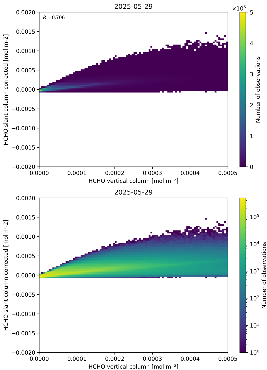
Figure 127: Scatter density plot of “HCHO vertical column” against “HCHO slant column corrected” for 2025-05-28 to 2025-05-30.
