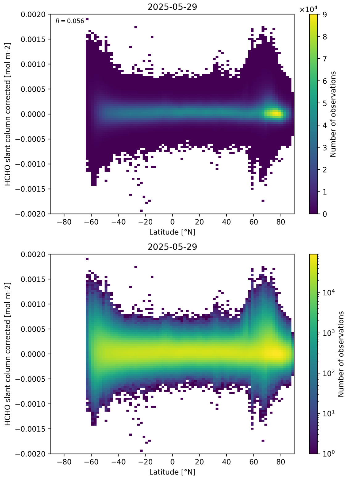
Figure 157: Scatter density plot of “Latitude” against “HCHO slant column corrected” for 2025-05-28 to 2025-05-30.
