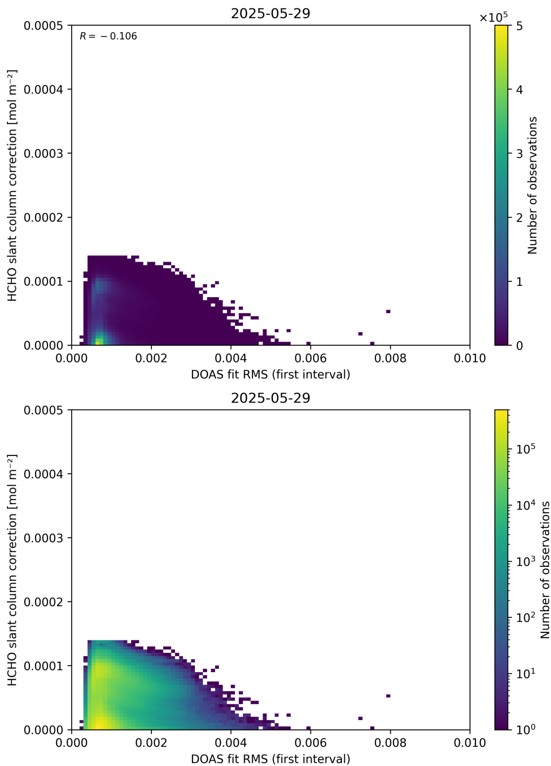
Figure 63: Scatter density plot of “DOAS fit RMS (first interval)” against “HCHO slant column correction” for 2025-05-28 to 2025-05-30.
