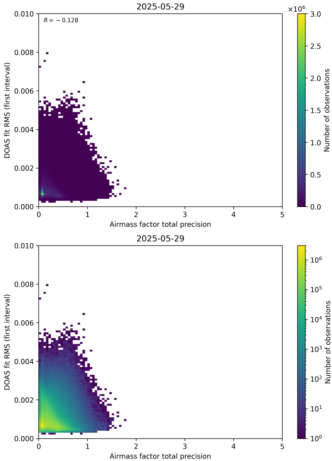
Figure 105: Scatter density plot of “Airmass factor total precision” against “DOAS fit RMS (first interval)” for 2025-05-28 to 2025-05-30.
