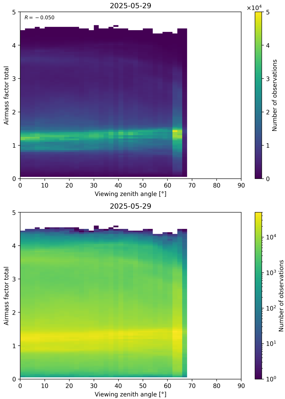
Figure 190: Scatter density plot of “Viewing zenith angle” against “Airmass factor total” for 2025-05-28 to 2025-05-30.
