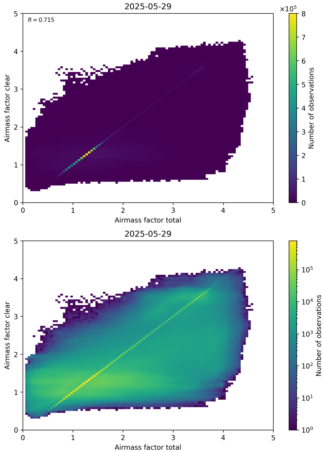
Figure 100: Scatter density plot of “Airmass factor total” against “Airmass factor clear” for 2025-05-28 to 2025-05-30.
