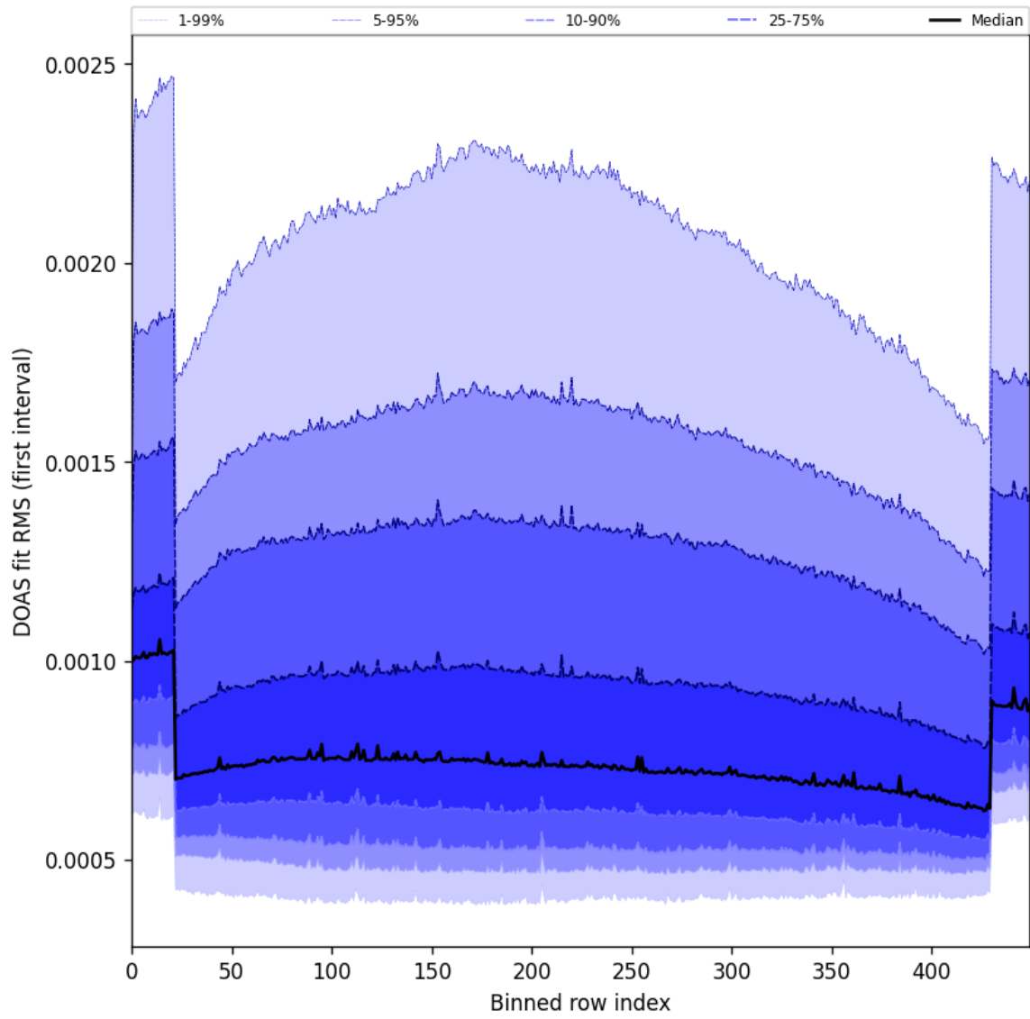
Figure 60: Along track statistics of “DOAS fit RMS (first interval)” for 2025-05-28 to 2025-05-30
