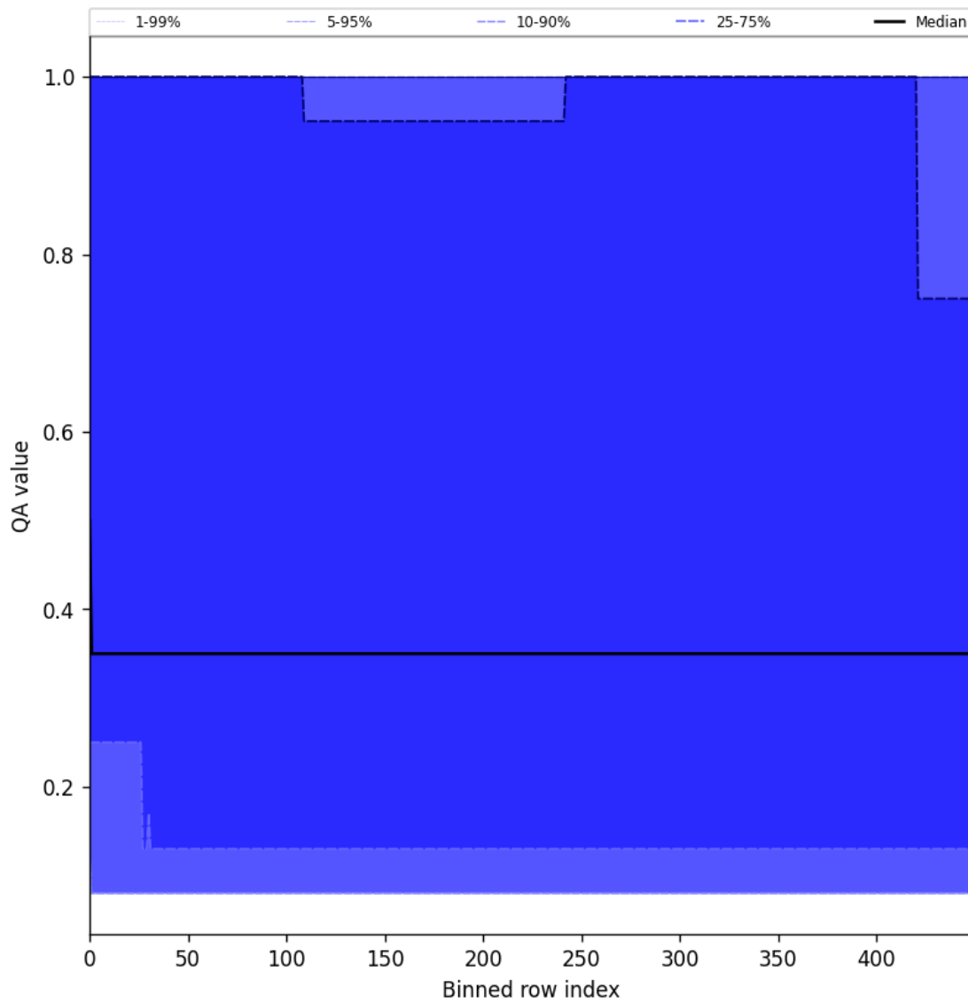
Figure 48: Along track statistics of “QA value” for 2025-05-28 to 2025-05-30
