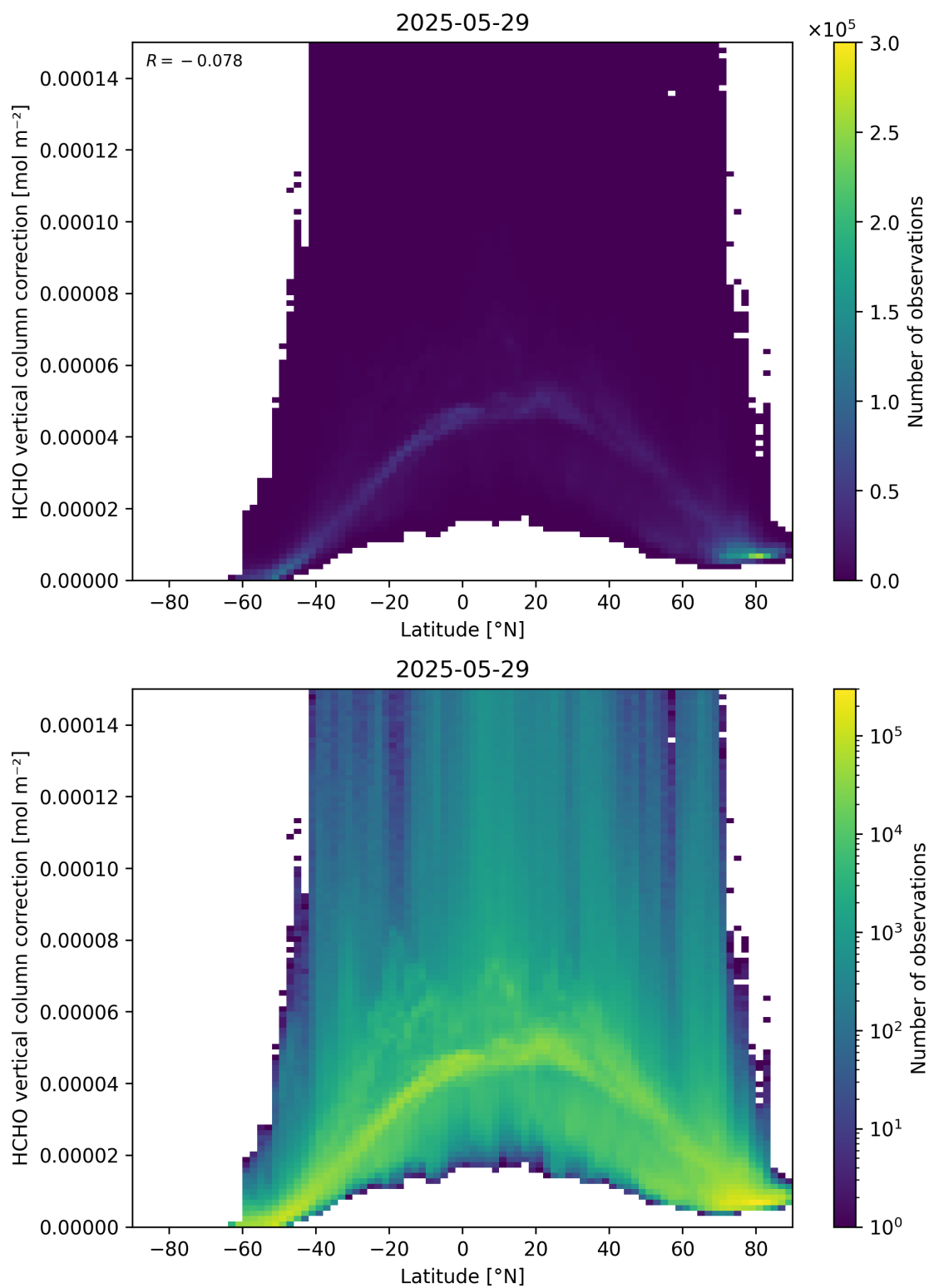
Figure 164: Scatter density plot of “Latitude” against “HCHO vertical column correction” for 2025-05-28 to 2025-05-30.
