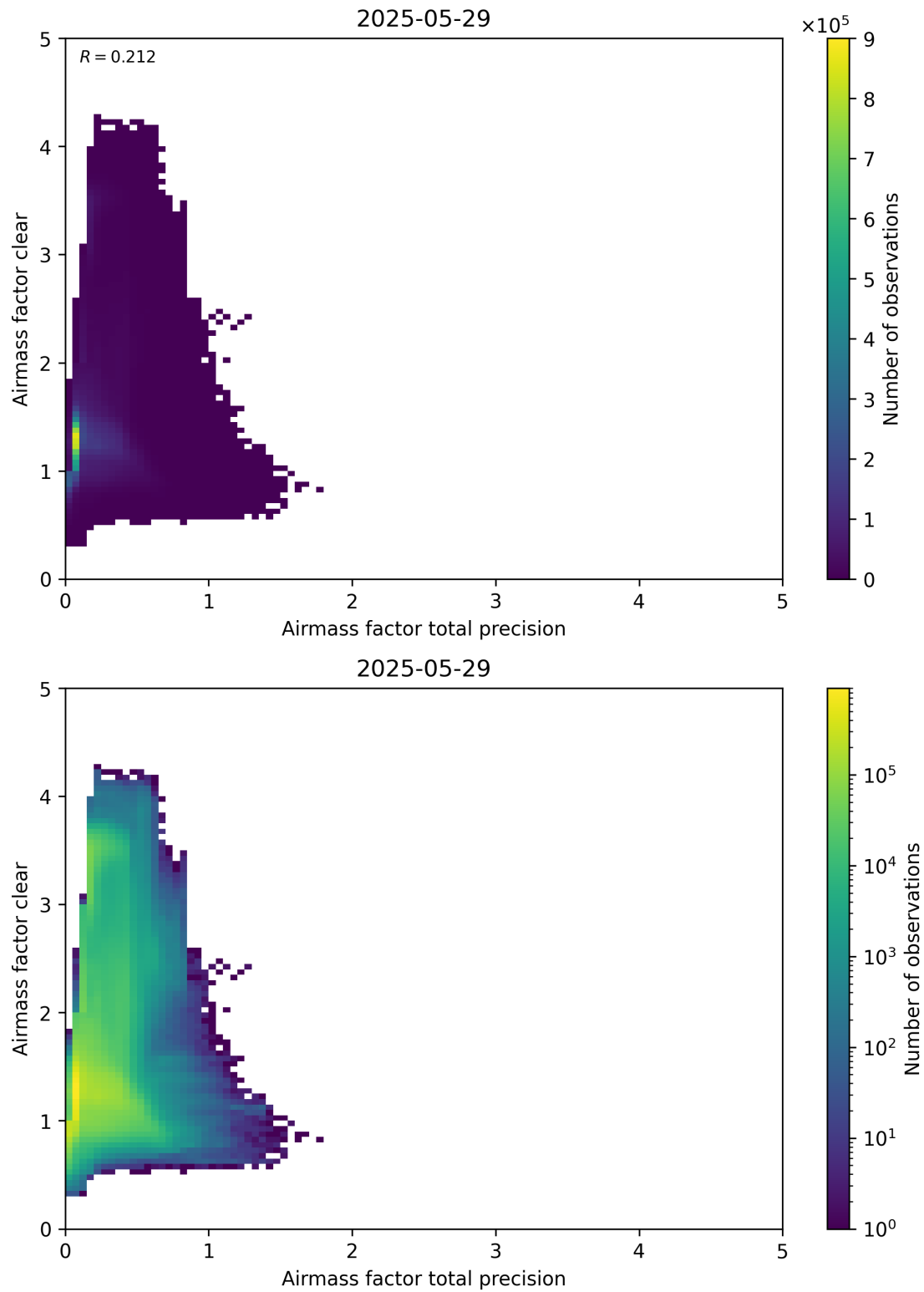
Figure 108: Scatter density plot of “Airmass factor total precision” against “Airmass factor clear” for 2025-05-28 to 2025-05-30.
