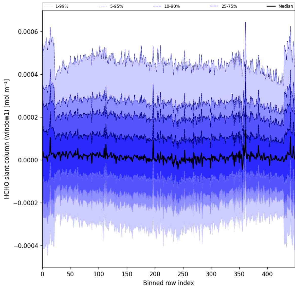
Figure 52: Along track statistics of “HCHO slant column (window1)” for 2025-05-28 to 2025-05-30
