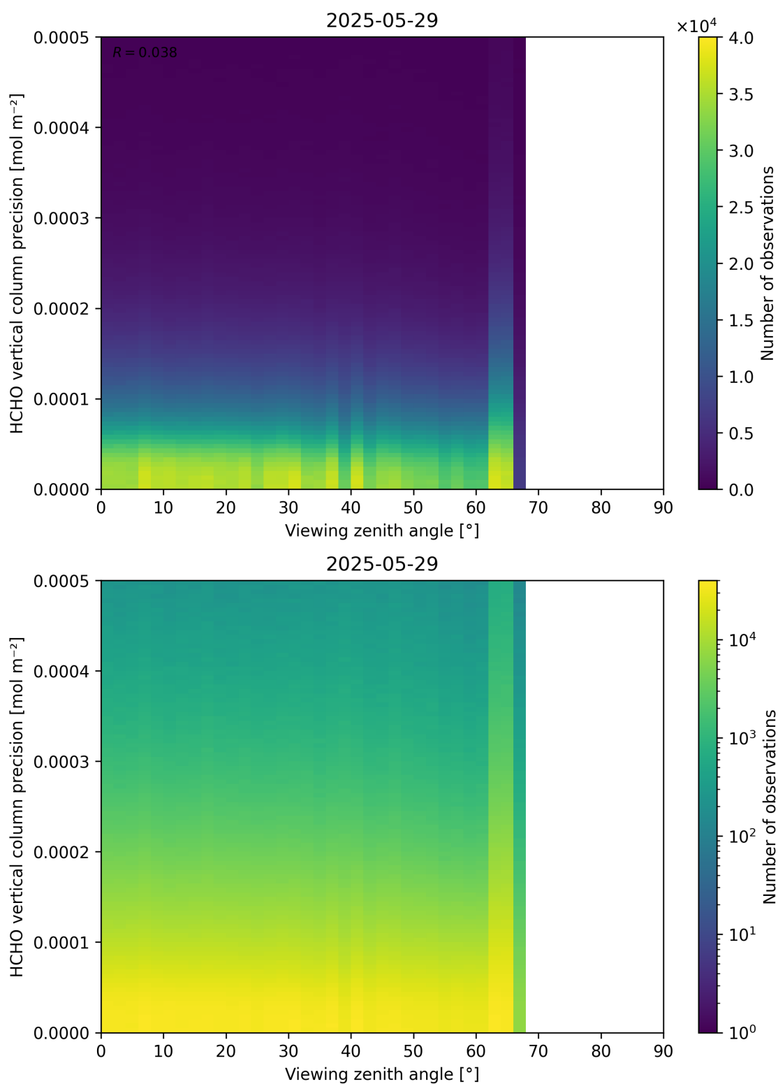
Figure 194: Scatter density plot of “Viewing zenith angle” against “HCHO vertical column precision” for 2025-05-28 to 2025-05-30.
