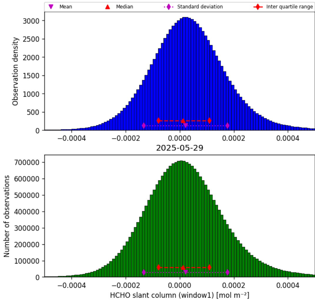
Figure 38: Histogram of “HCHO slant column (window1)” for 2025-05-28 to 2025-05-30
