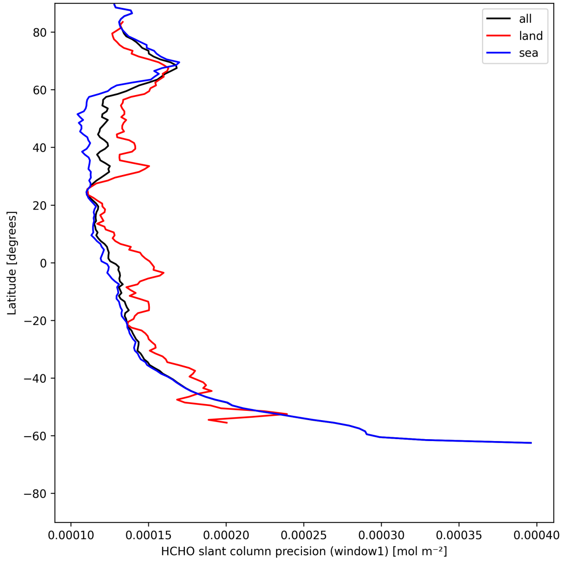
Figure 25: Zonal average of “HCHO slant column precision (window1)” for 2025-05-28 to 2025-05-30.
