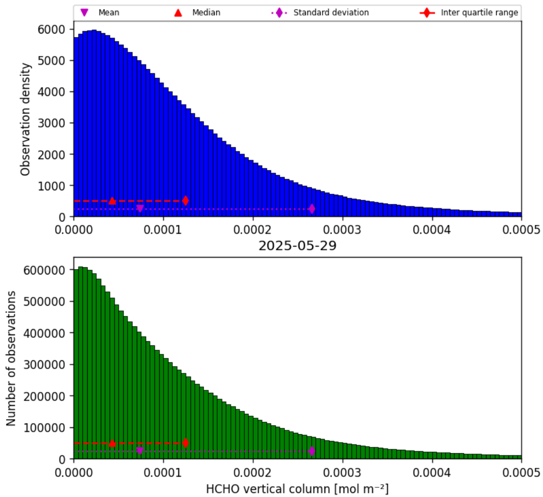
Figure 35: Histogram of “HCHO vertical column” for 2025-05-28 to 2025-05-30
