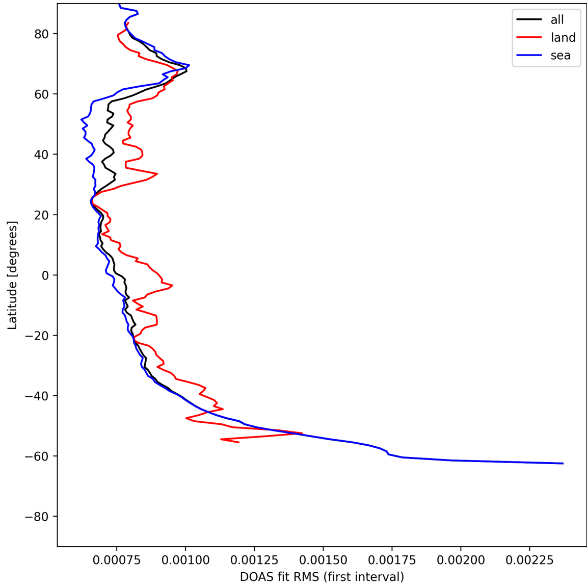
Figure 32: Zonal average of “DOAS fit RMS (first interval)” for 2025-05-28 to 2025-05-30.
