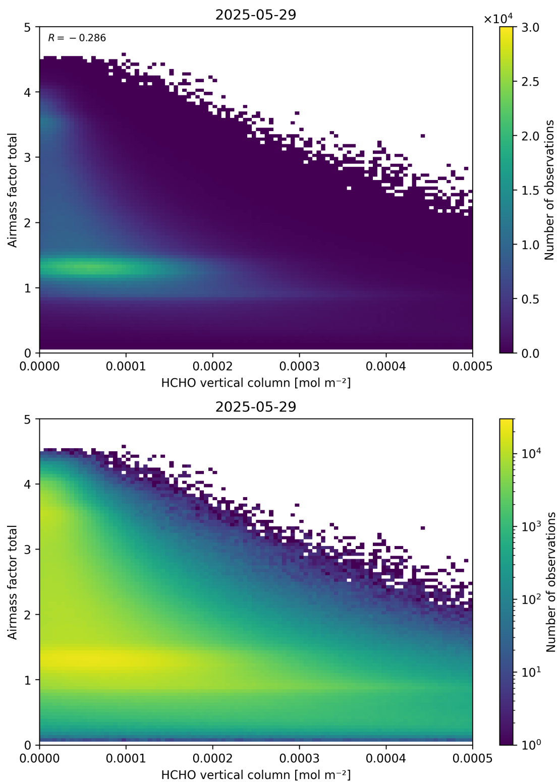
Figure 131: Scatter density plot of “HCHO vertical column” against “Airmass factor total” for 2025-05-28 to 2025-05-30.
