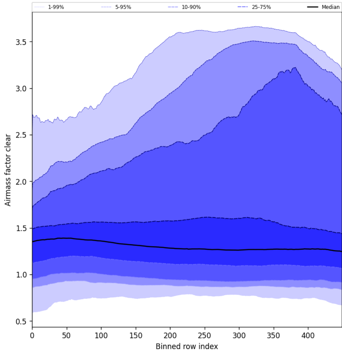
Figure 56: Along track statistics of “Airmass factor clear” for 2025-05-28 to 2025-05-30
