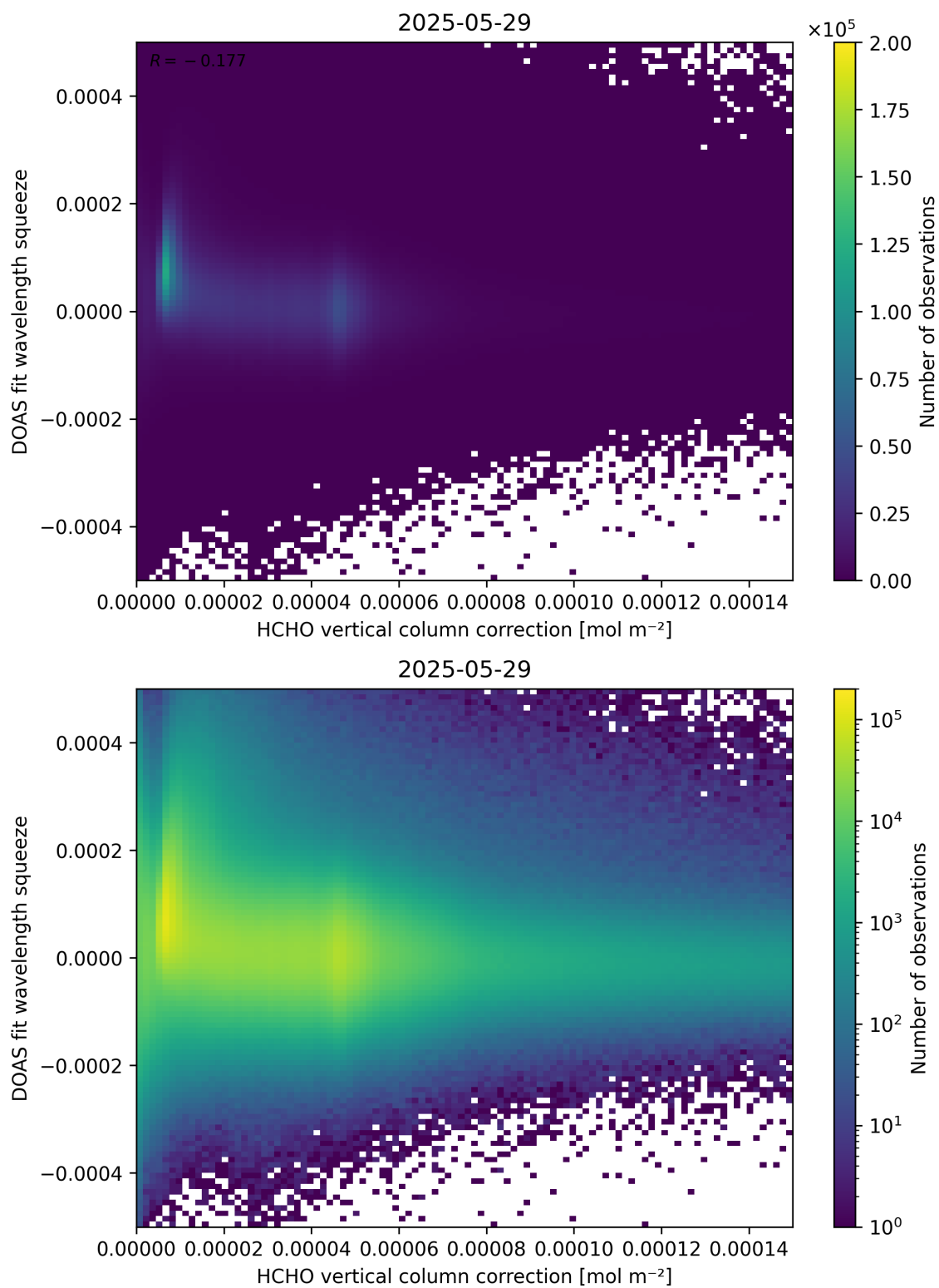
Figure 114: Scatter density plot of “HCHO vertical column correction” against “DOAS fit wavelength squeeze” for 2025-05-28 to 2025-05-30.
