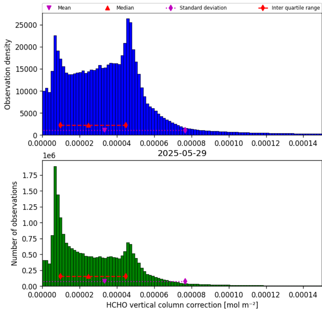
Figure 37: Histogram of “HCHO vertical column correction” for 2025-05-28 to 2025-05-30
