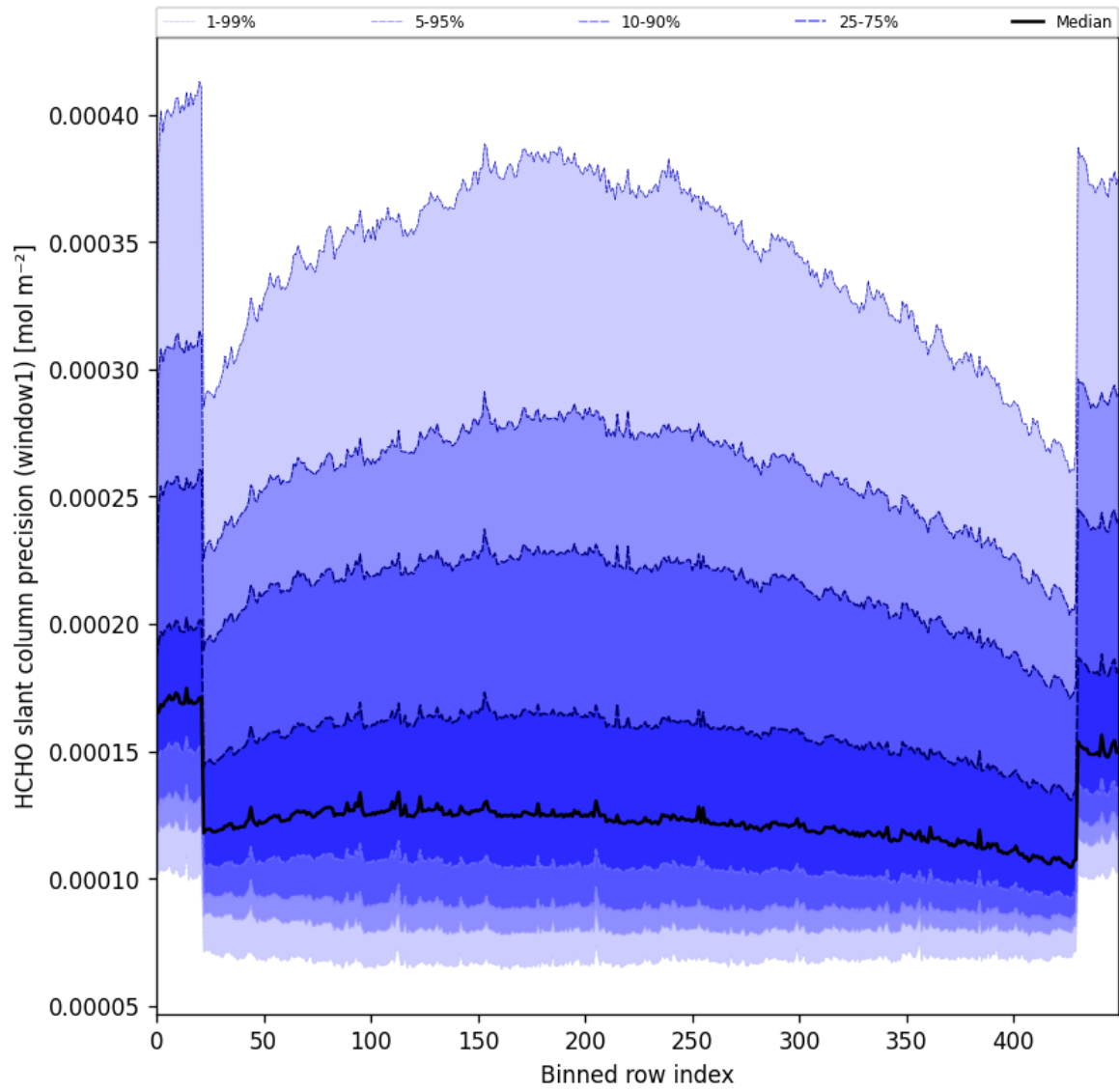
Figure 53: Along track statistics of “HCHO slant column precision (window1)” for 2025-05-28 to 2025-05-30
