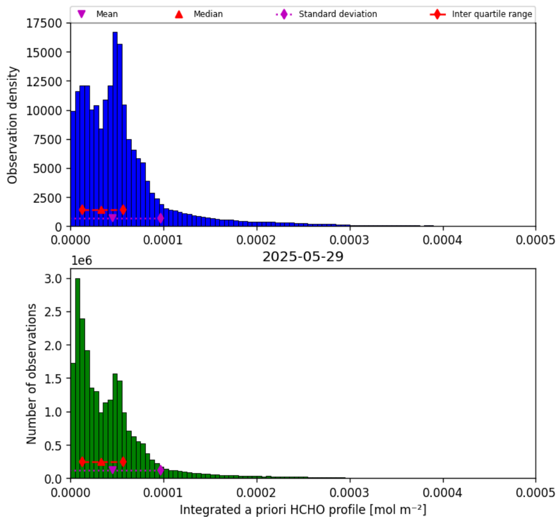
Figure 43: Histogram of “Integrated a priori HCHO profile” for 2025-05-28 to 2025-05-30
