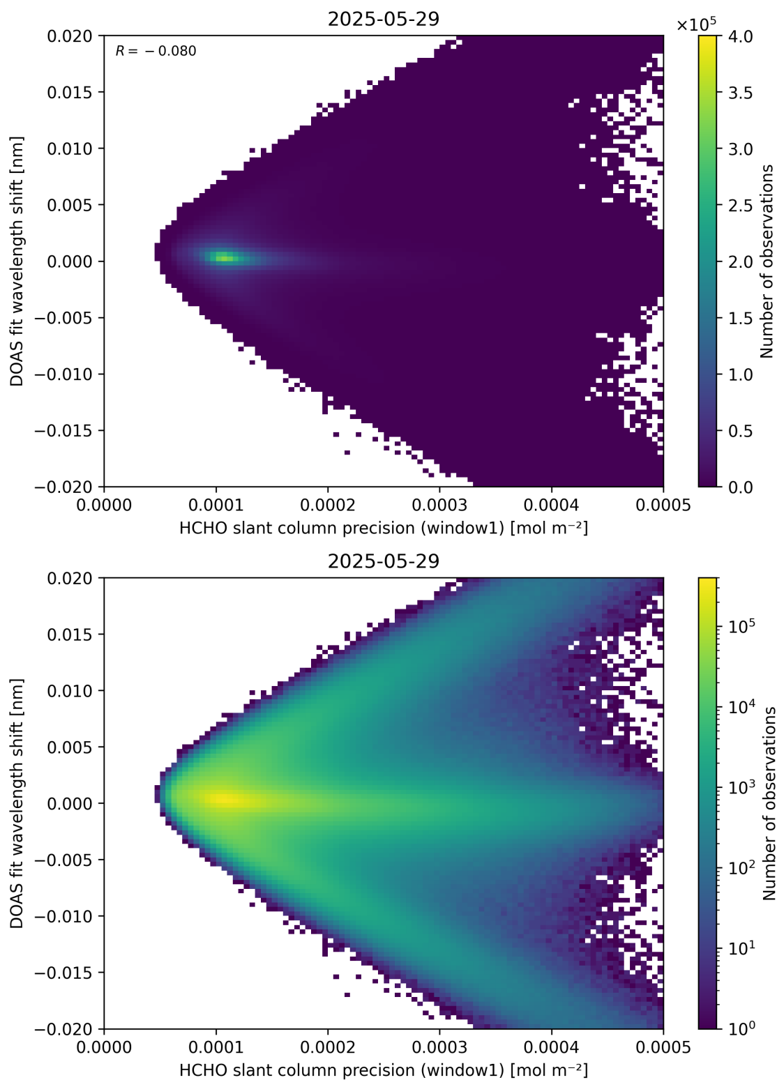
Figure 89: Scatter density plot of “HCHO slant column precision (window1)” against “DOAS fit wavelength shift” for 2025-05-28 to 2025-05-30.
