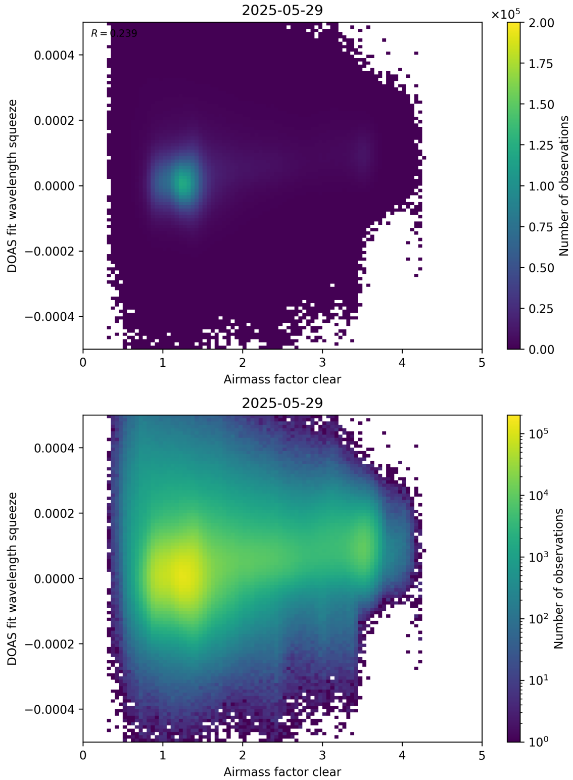
Figure 73: Scatter density plot of “Airmass factor clear” against “DOAS fit wavelength squeeze” for 2025-05-28 to 2025-05-30.
