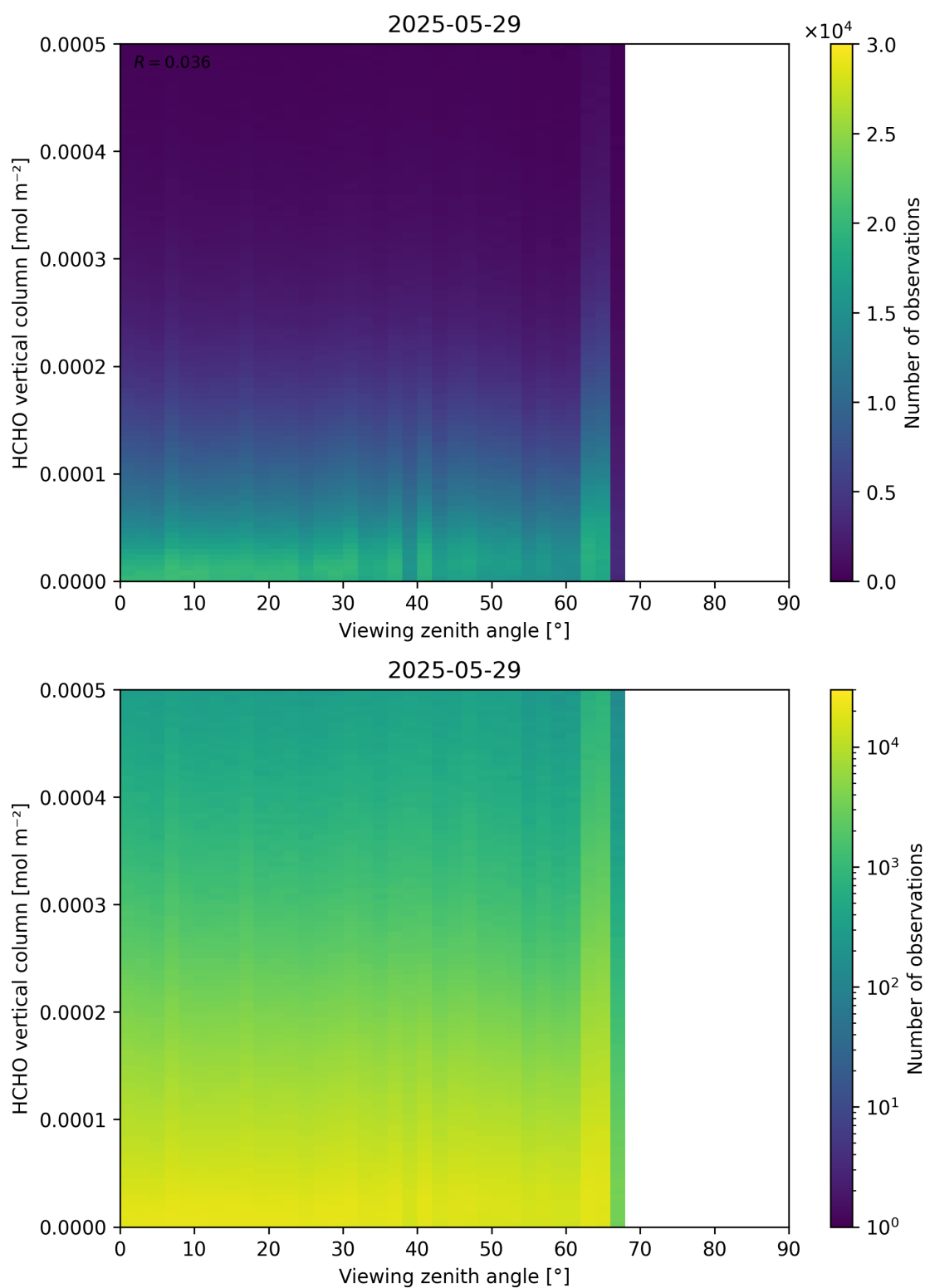
Figure 192: Scatter density plot of “Viewing zenith angle” against “HCHO vertical column” for 2025-05-28 to 2025-05-30.
