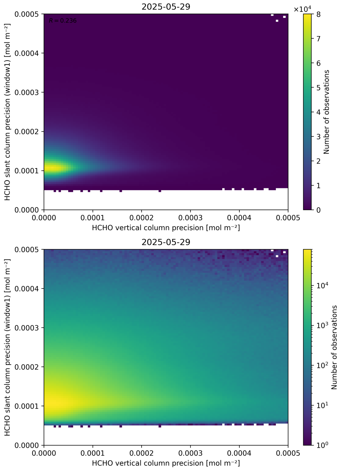
Figure 143: Scatter density plot of “HCHO vertical column precision” against “HCHO slant column precision (window1)” for 2025-05-28 to 2025-05-30.
