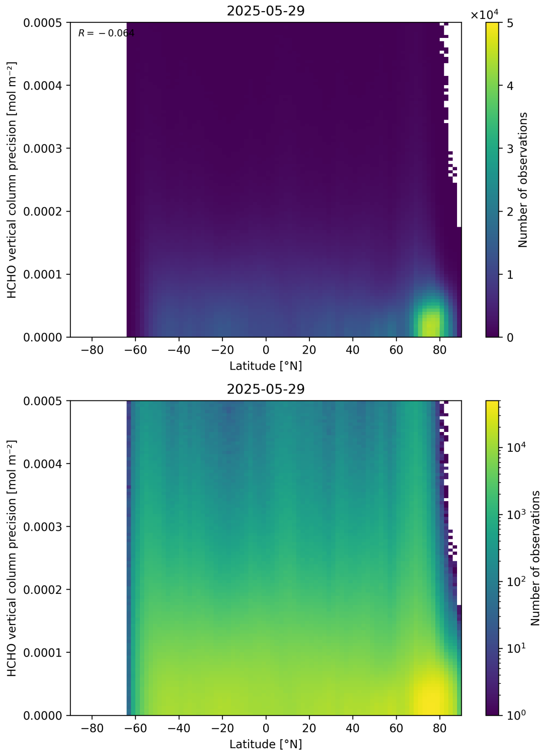
Figure 165: Scatter density plot of “Latitude” against “HCHO vertical column precision” for 2025-05-28 to 2025-05-30.
