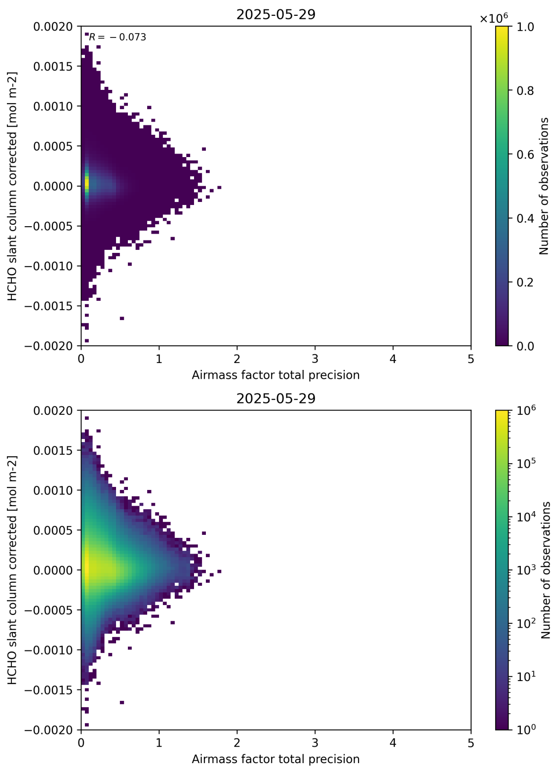
Figure 109: Scatter density plot of “Airmass factor total precision” against “HCHO slant column corrected” for 2025-05-28 to 2025-05-30.
