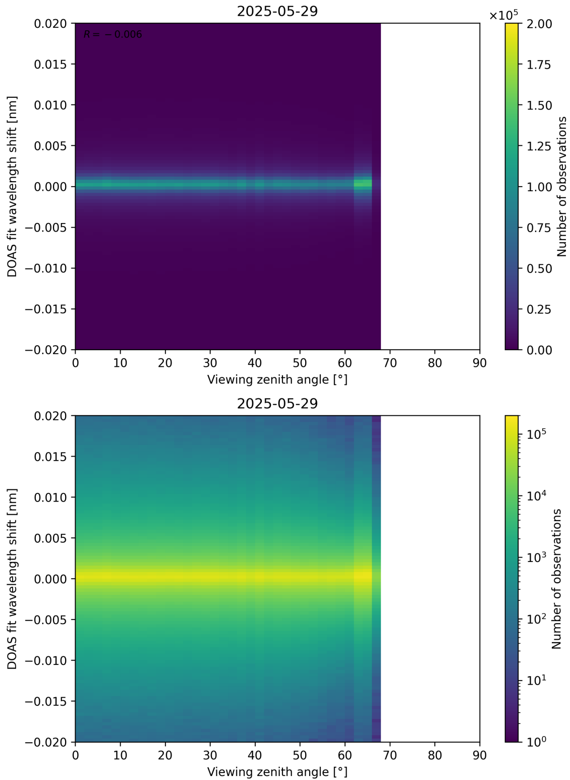
Figure 183: Scatter density plot of “Viewing zenith angle” against “DOAS fit wavelength shift” for 2025-05-28 to 2025-05-30.
