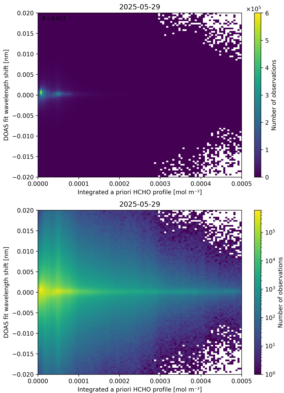
Figure 149: Scatter density plot of “Integrated a priori HCHO profile” against “DOAS fit wavelength shift” for 2025-05-28 to 2025-05-30.
