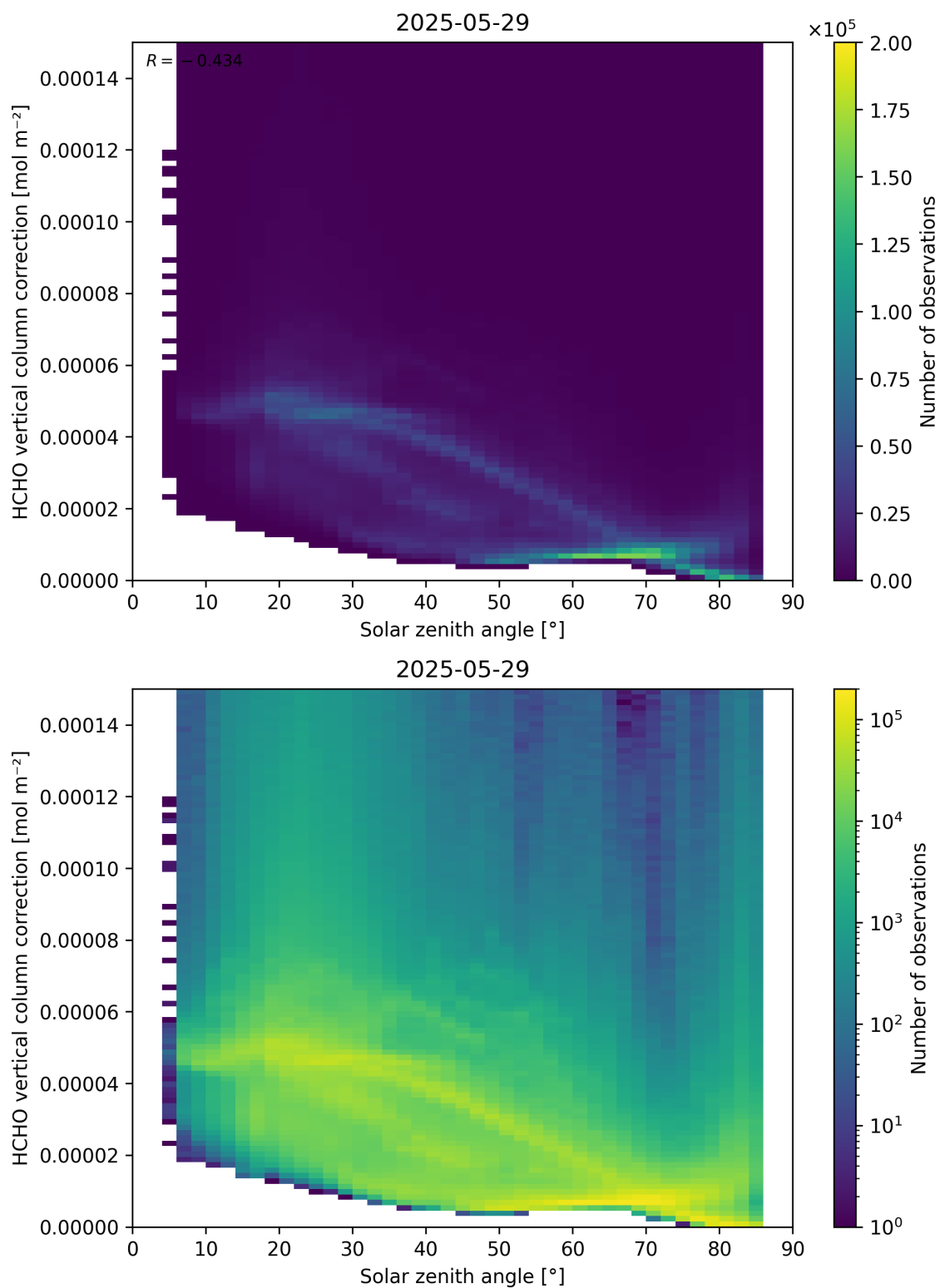
Figure 178: Scatter density plot of “Solar zenith angle” against “HCHO vertical column correction” for 2025-05-28 to 2025-05-30.
