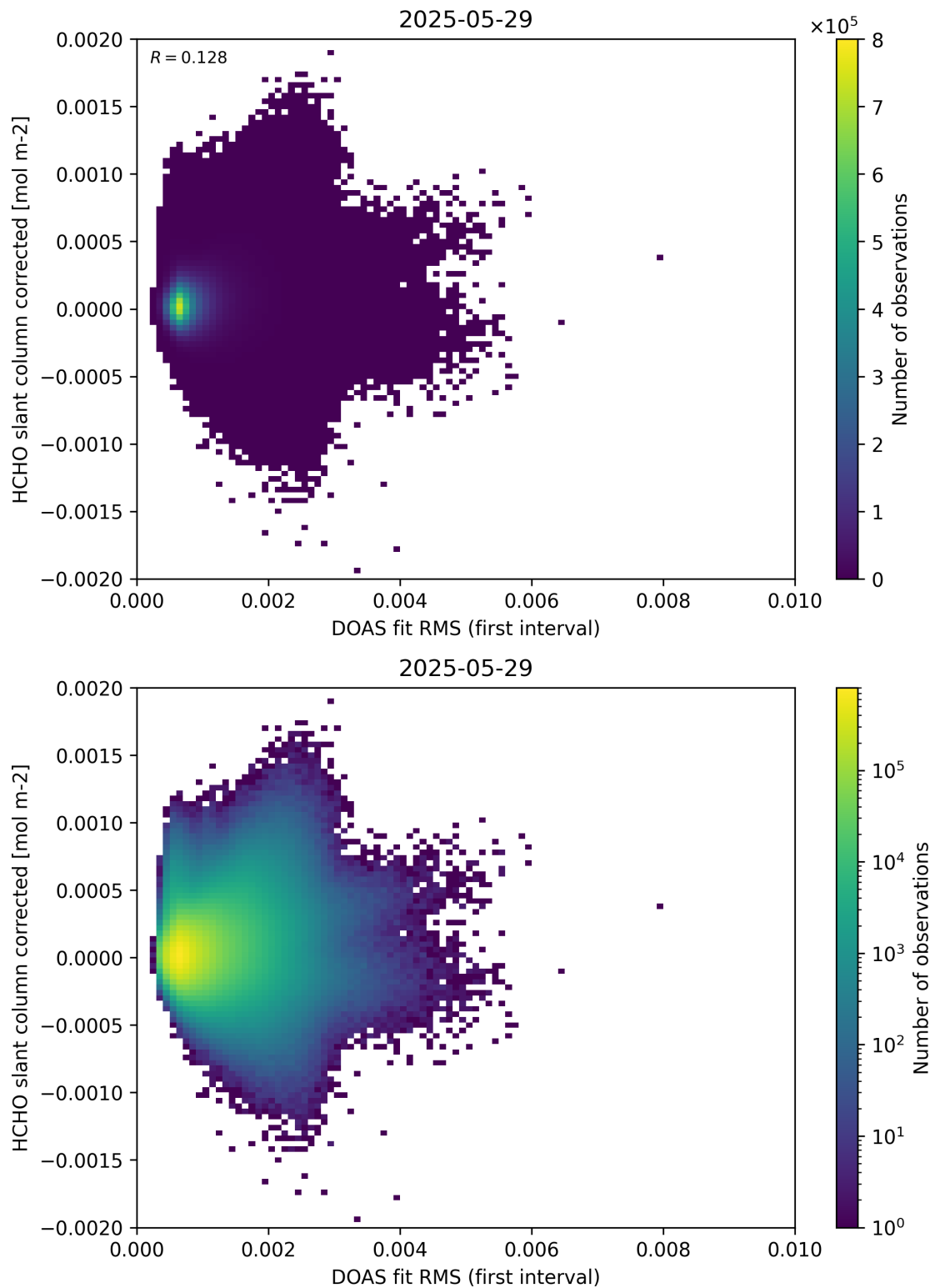
Figure 62: Scatter density plot of “DOAS fit RMS (first interval)” against “HCHO slant column corrected” for 2025-05-28 to 2025-05-30.
