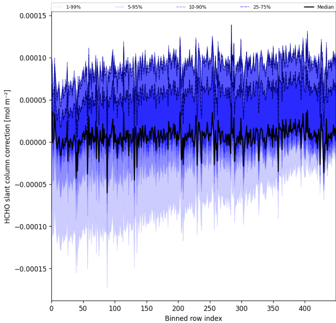
Figure 61: Along track statistics of “HCHO slant column correction” for 2025-05-28 to 2025-05-30
