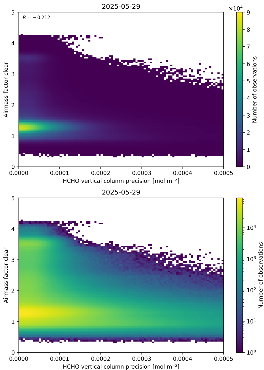
Figure 139: Scatter density plot of “HCHO vertical column precision” against “Airmass factor clear” for 2025-05-28 to 2025-05-30.
