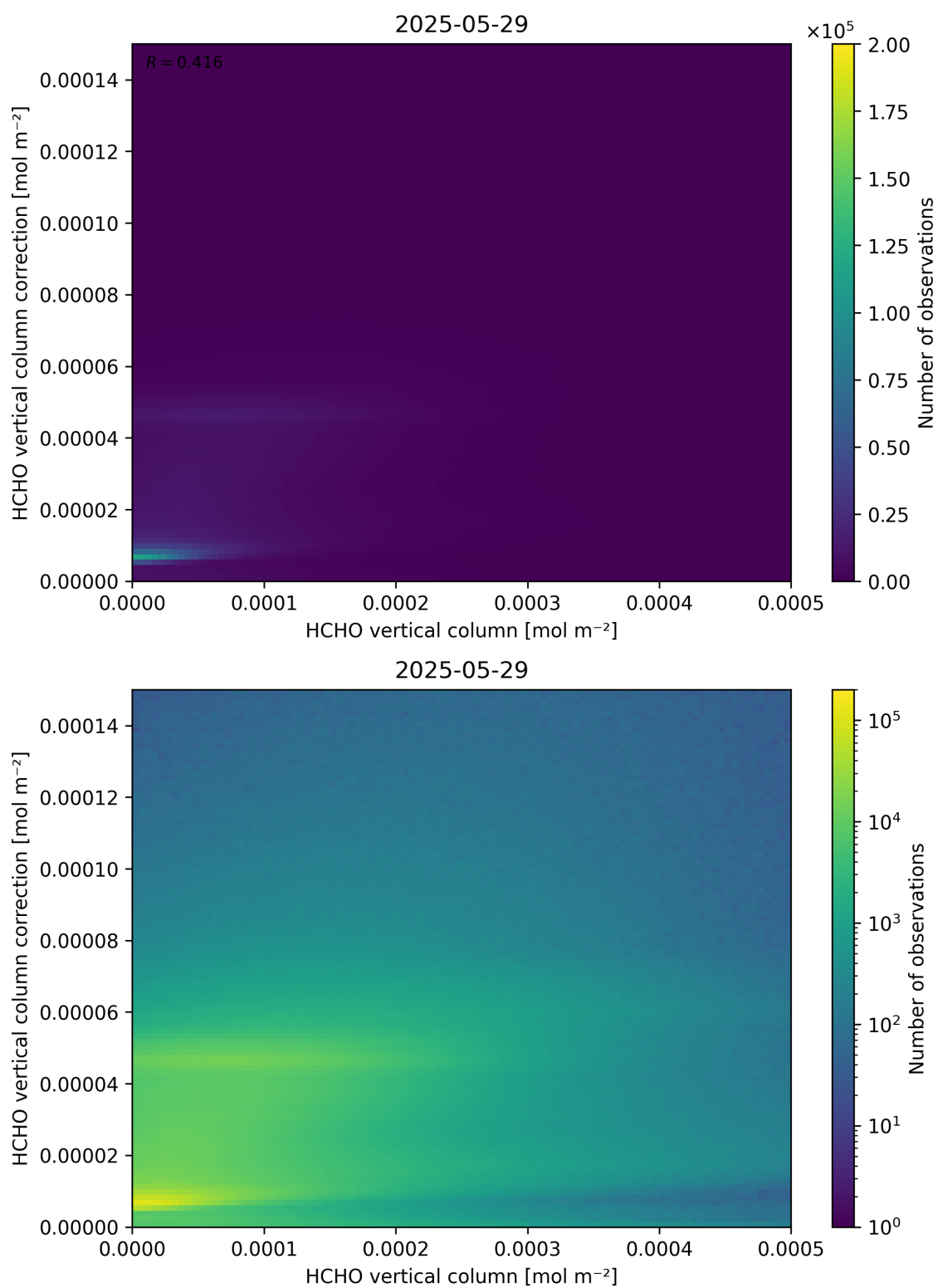
Figure 133: Scatter density plot of “HCHO vertical column” against “HCHO vertical column correction” for 2025-05-28 to 2025-05-30.
