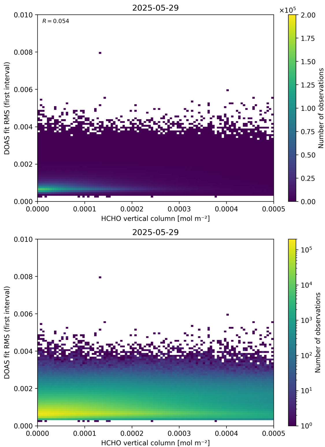
Figure 123: Scatter density plot of “HCHO vertical column” against “DOAS fit RMS (first interval)” for 2025-05-28 to 2025-05-30.
