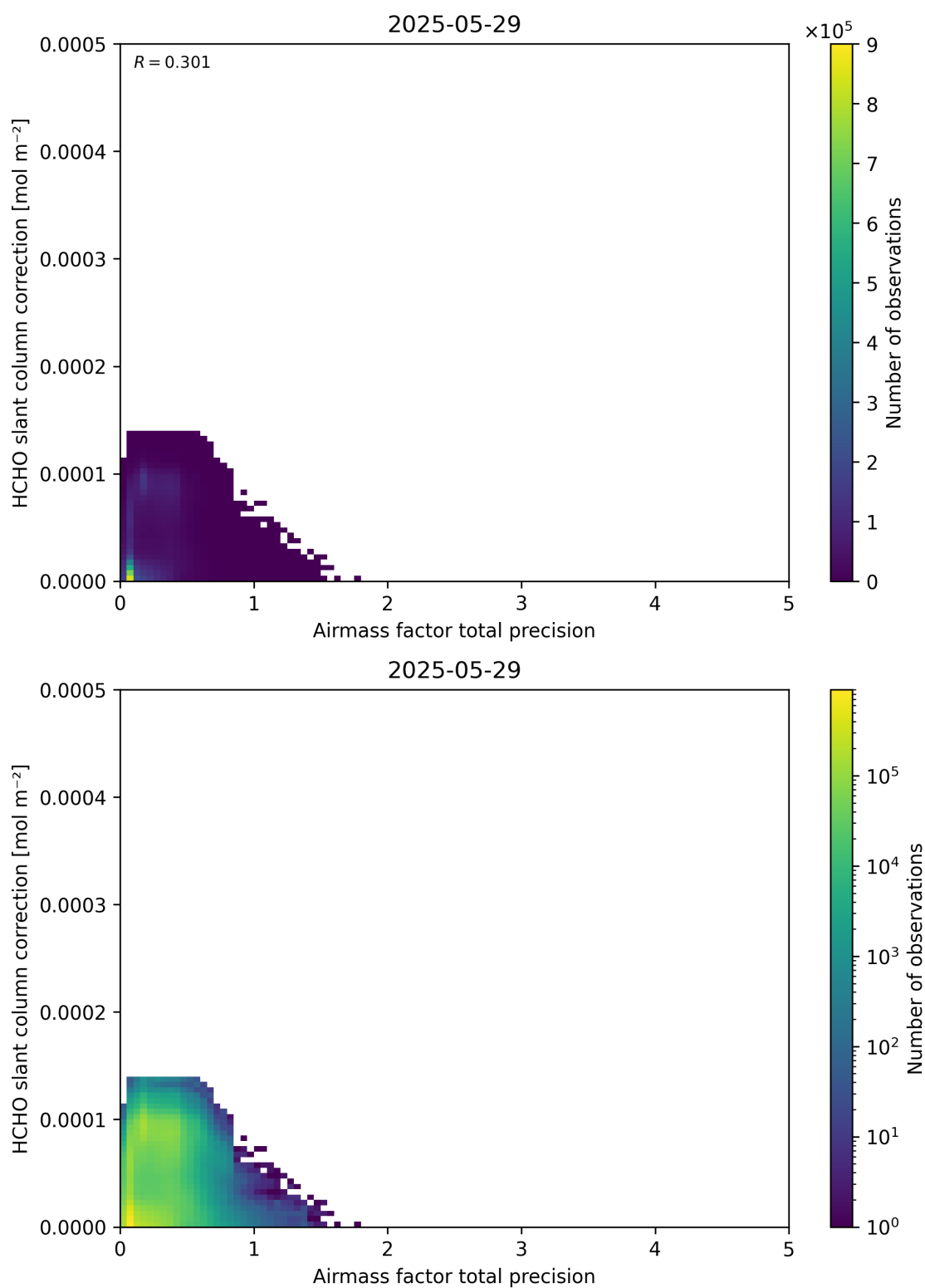
Figure 110: Scatter density plot of “Airmass factor total precision” against “HCHO slant column correction” for 2025-05-28 to 2025-05-30.
