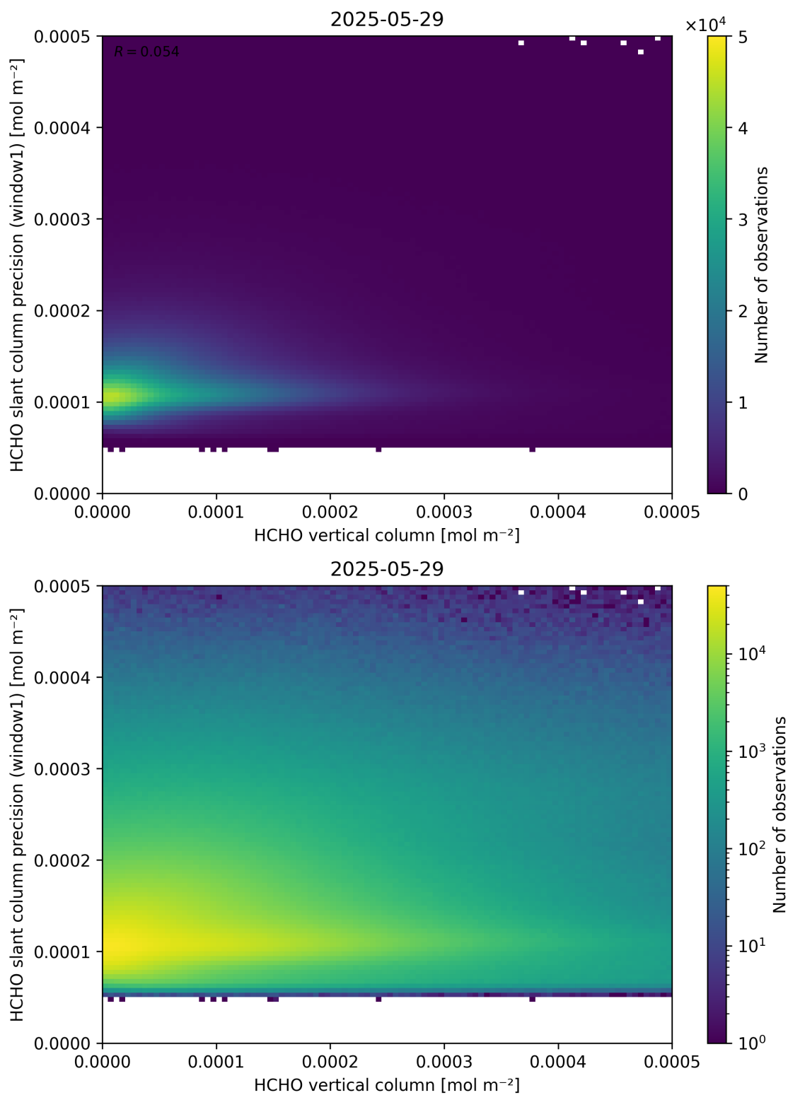
Figure 130: Scatter density plot of “HCHO vertical column” against “HCHO slant column precision (window1)” for 2025-05-28 to 2025-05-30.
