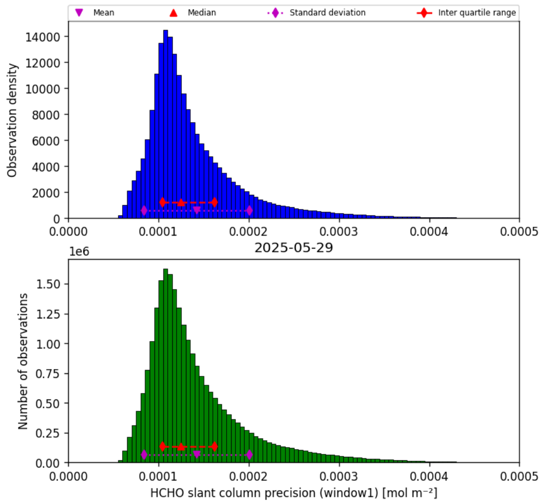
Figure 39: Histogram of “HCHO slant column precision (window1)” for 2025-05-28 to 2025-05-30
