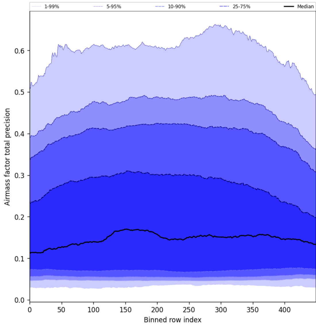
Figure 55: Along track statistics of “Airmass factor total precision” for 2025-05-28 to 2025-05-30
