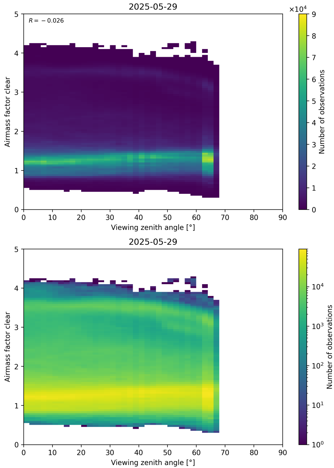
Figure 185: Scatter density plot of “Viewing zenith angle” against “Airmass factor clear” for 2025-05-28 to 2025-05-30.
