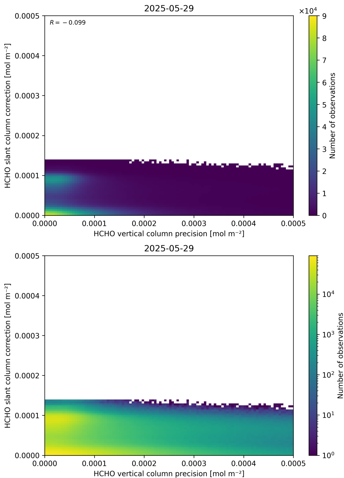
Figure 141: Scatter density plot of “HCHO vertical column precision” against “HCHO slant column correction” for 2025-05-28 to 2025-05-30.
