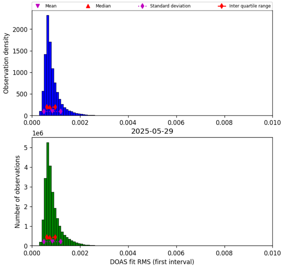
Figure 46: Histogram of “DOAS fit RMS (first interval)” for 2025-05-28 to 2025-05-30
