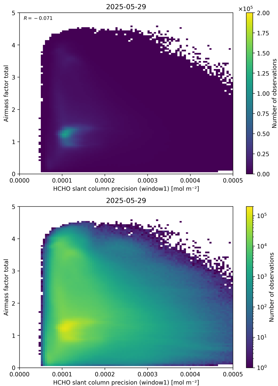
Figure 94: Scatter density plot of “HCHO slant column precision (window1)” against “Airmass factor total” for 2025-05-28 to 2025-05-30.
