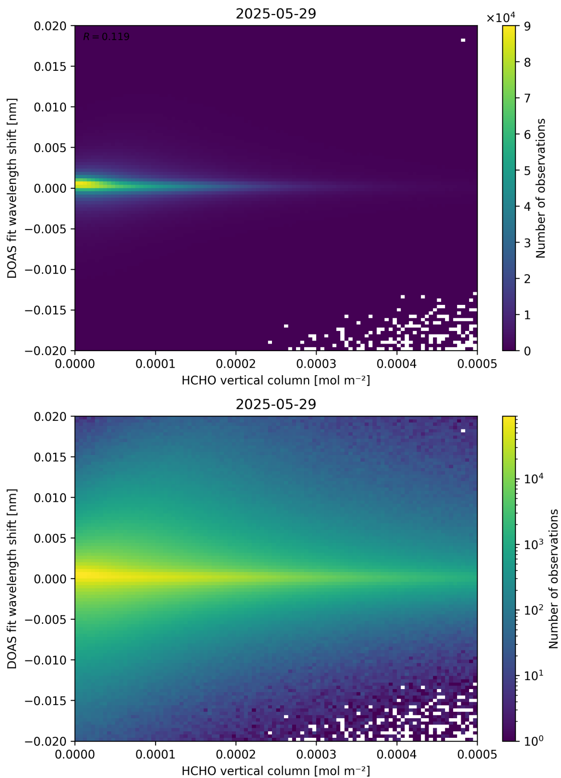
Figure 124: Scatter density plot of “HCHO vertical column” against “DOAS fit wavelength shift” for 2025-05-28 to 2025-05-30.
