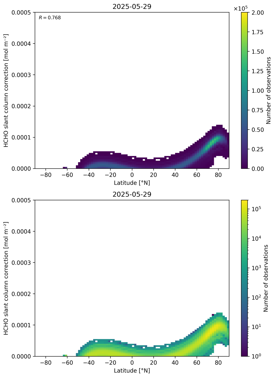
Figure 158: Scatter density plot of “Latitude” against “HCHO slant column correction” for 2025-05-28 to 2025-05-30.
