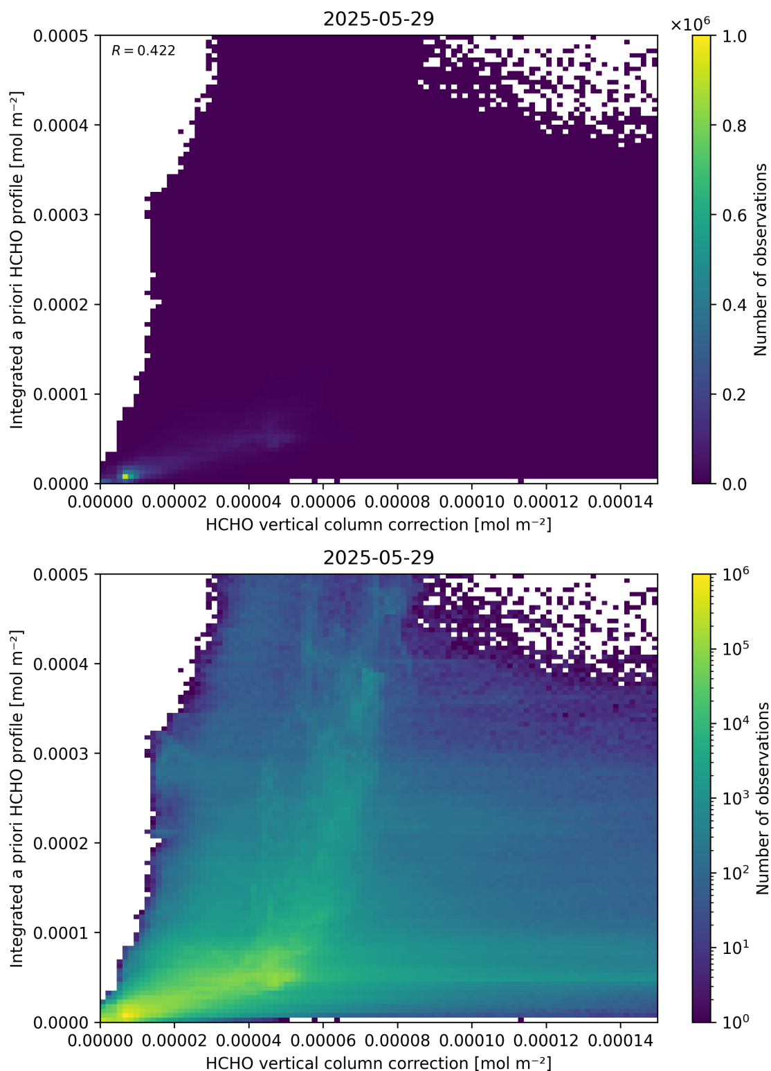
Figure 122: Scatter density plot of “HCHO vertical column correction” against “Integrated a priori HCHO profile” for 2025-05-28 to 2025-05-30.
