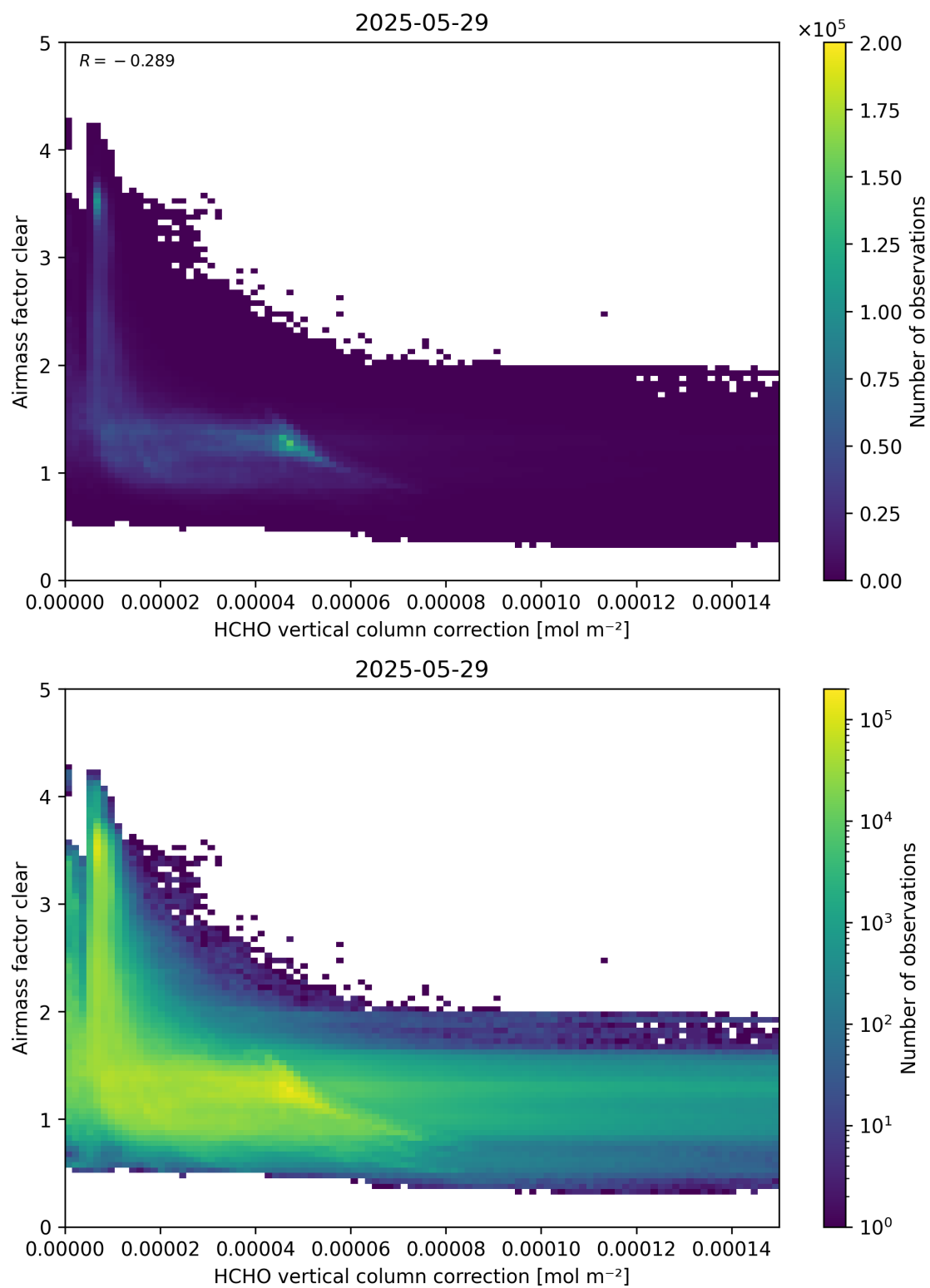
Figure 115: Scatter density plot of “HCHO vertical column correction” against “Airmass factor clear” for 2025-05-28 to 2025-05-30.
