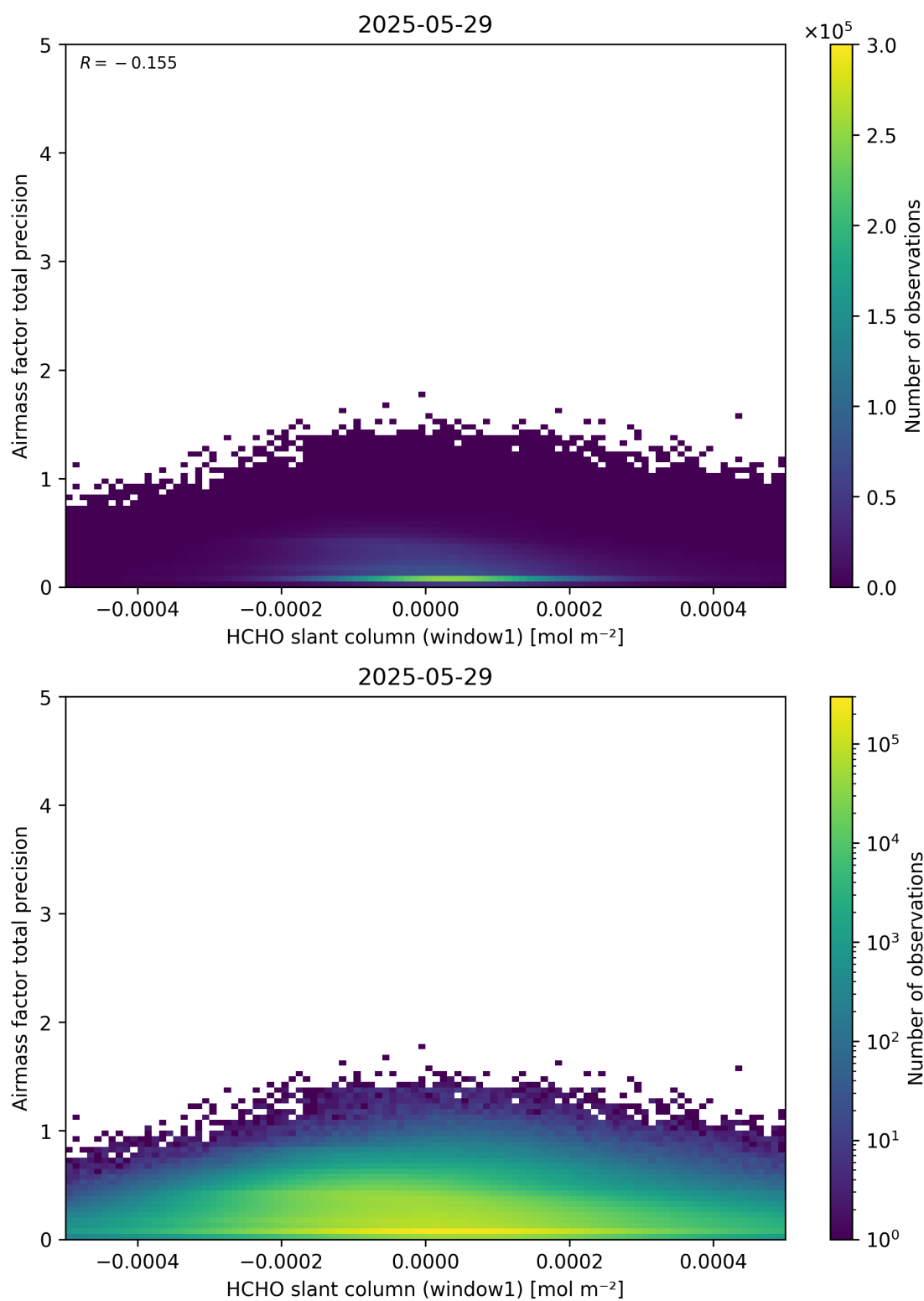
Figure 86: Scatter density plot of “HCHO slant column (window1)” against “Airmass factor total precision” for 2025-05-28 to 2025-05-30.
