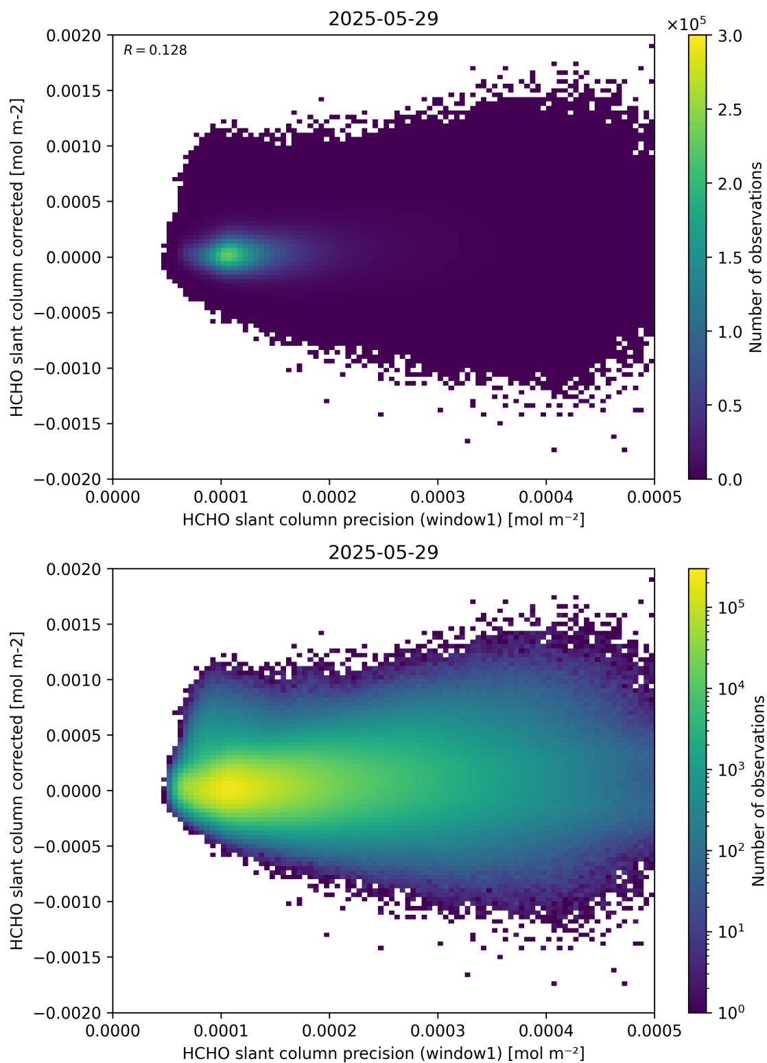
Figure 92: Scatter density plot of “HCHO slant column precision (window1)” against “HCHO slant column corrected” for 2025-05-28 to 2025-05-30.
