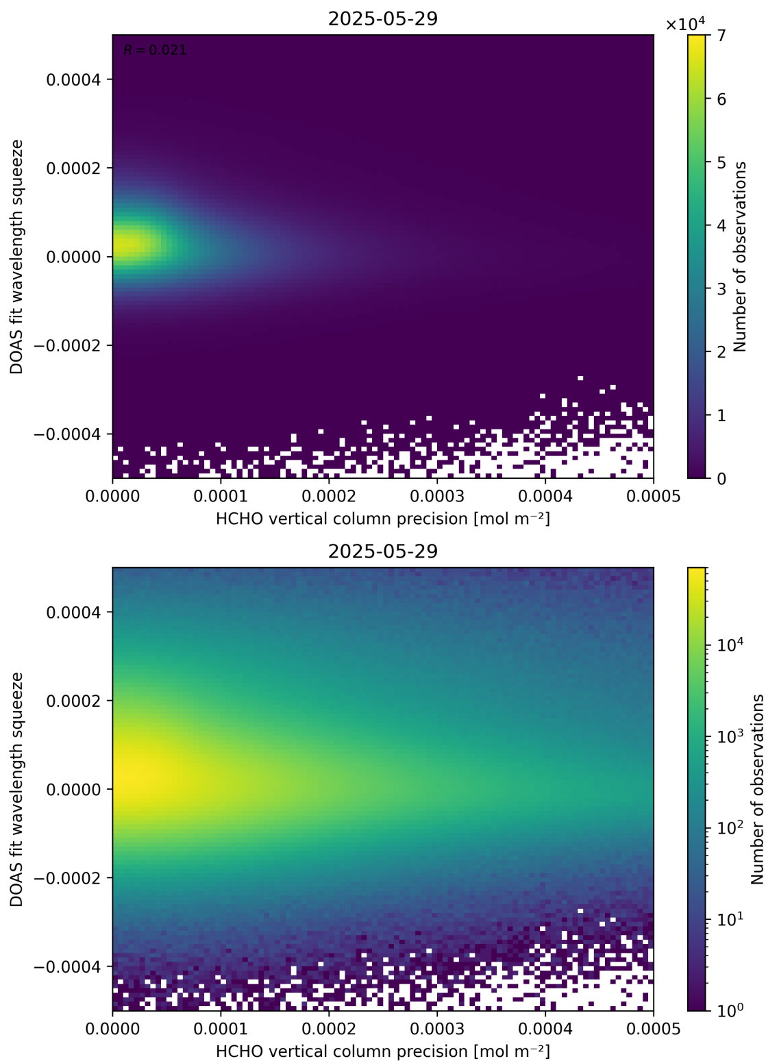
Figure 138: Scatter density plot of “HCHO vertical column precision” against “DOAS fit wavelength squeeze” for 2025-05-28 to 2025-05-30.
