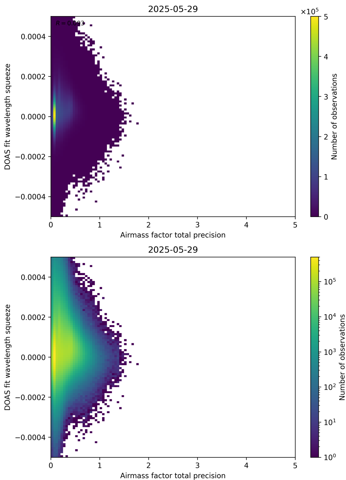
Figure 107: Scatter density plot of “Airmass factor total precision” against “DOAS fit wavelength squeeze” for 2025-05-28 to 2025-05-30.
