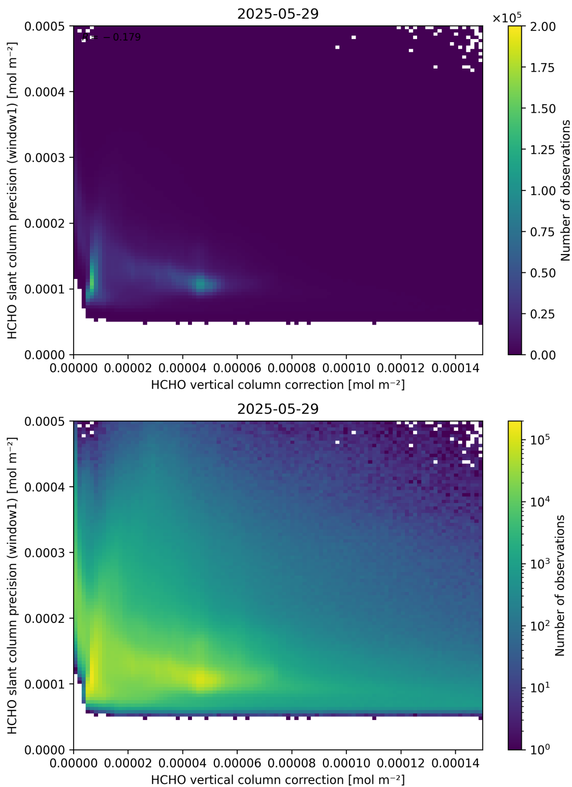
Figure 119: Scatter density plot of “HCHO vertical column correction” against “HCHO slant column precision (window1)” for 2025-05-28 to 2025-05-30.
