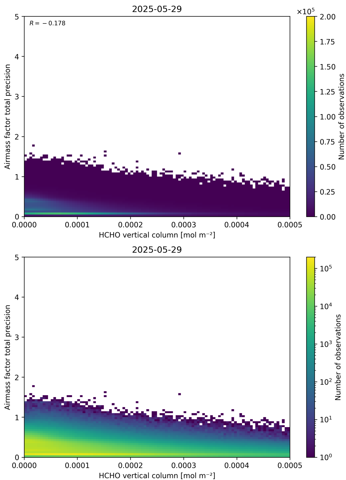
Figure 132: Scatter density plot of “HCHO vertical column” against “Airmass factor total precision” for 2025-05-28 to 2025-05-30.
