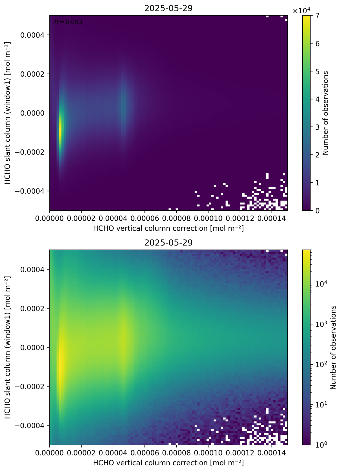
Figure 118: Scatter density plot of “HCHO vertical column correction” against “HCHO slant column (window1)” for 2025-05-28 to 2025-05-30.
