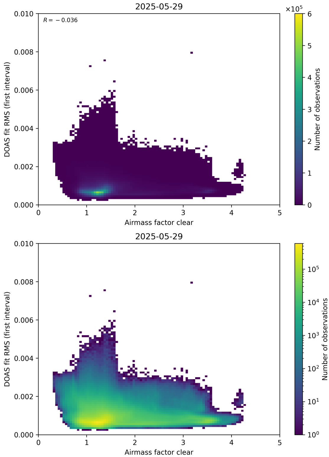
Figure 71: Scatter density plot of “Airmass factor clear” against “DOAS fit RMS (first interval)” for 2025-05-28 to 2025-05-30.
