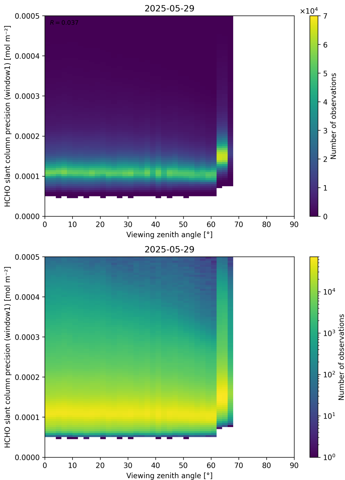
Figure 189: Scatter density plot of “Viewing zenith angle” against “HCHO slant column precision (window1)” for 2025-05-28 to 2025-05-30.
