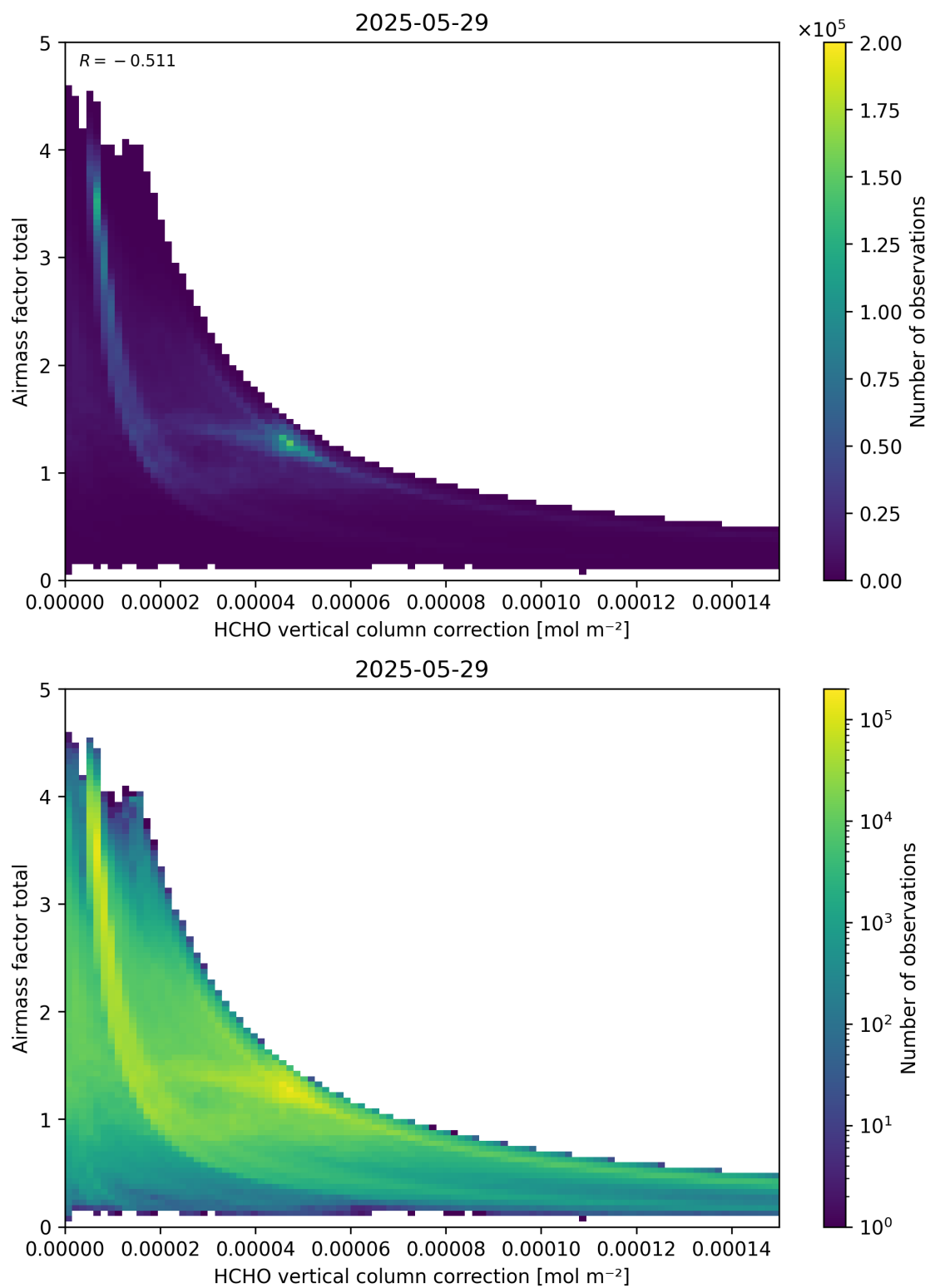
Figure 120: Scatter density plot of “HCHO vertical column correction” against “Airmass factor total” for 2025-05-28 to 2025-05-30.
