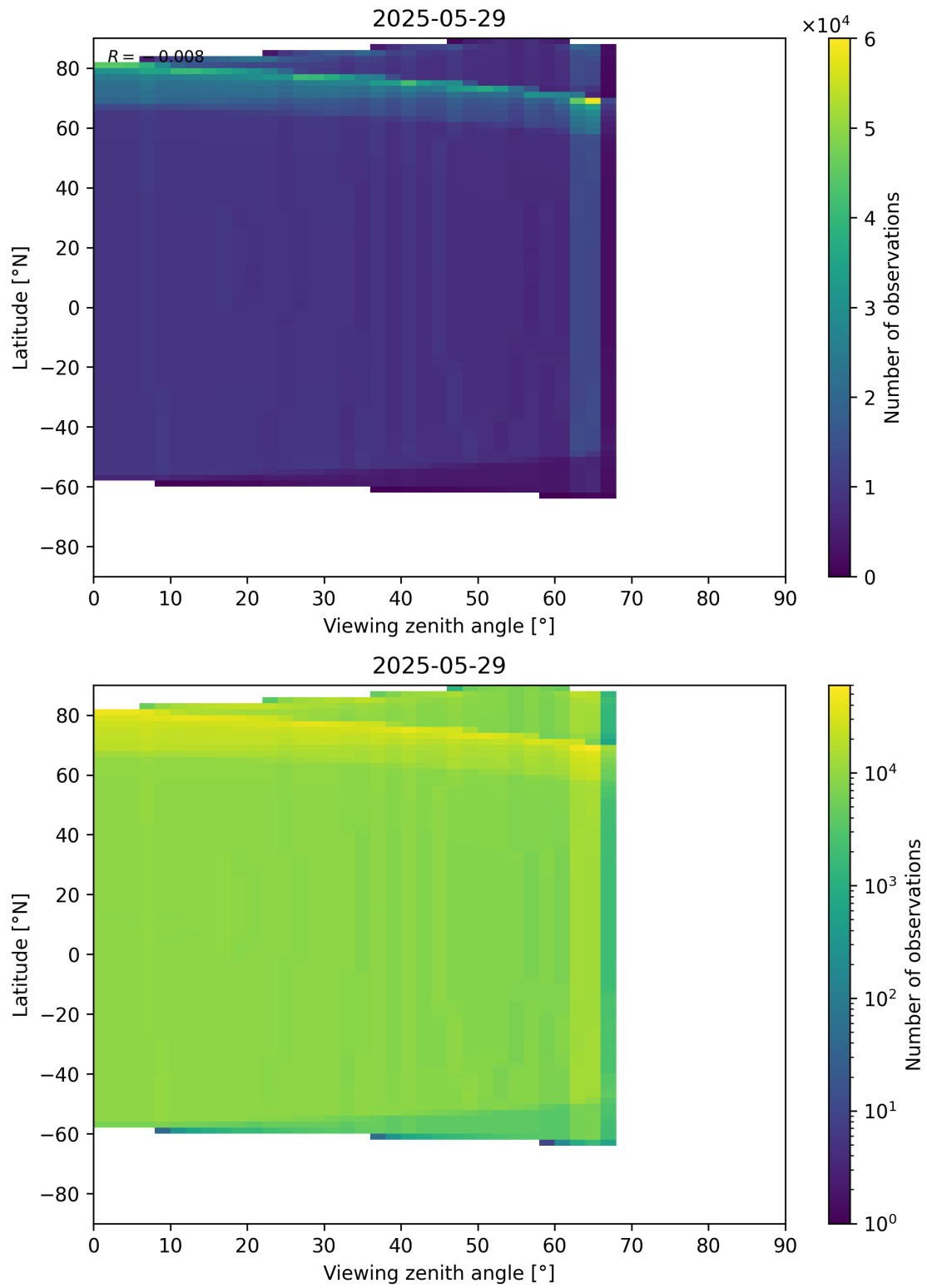
Figure 196: Scatter density plot of “Viewing zenith angle” against “Latitude” for 2025-05-28 to 2025-05-30.
