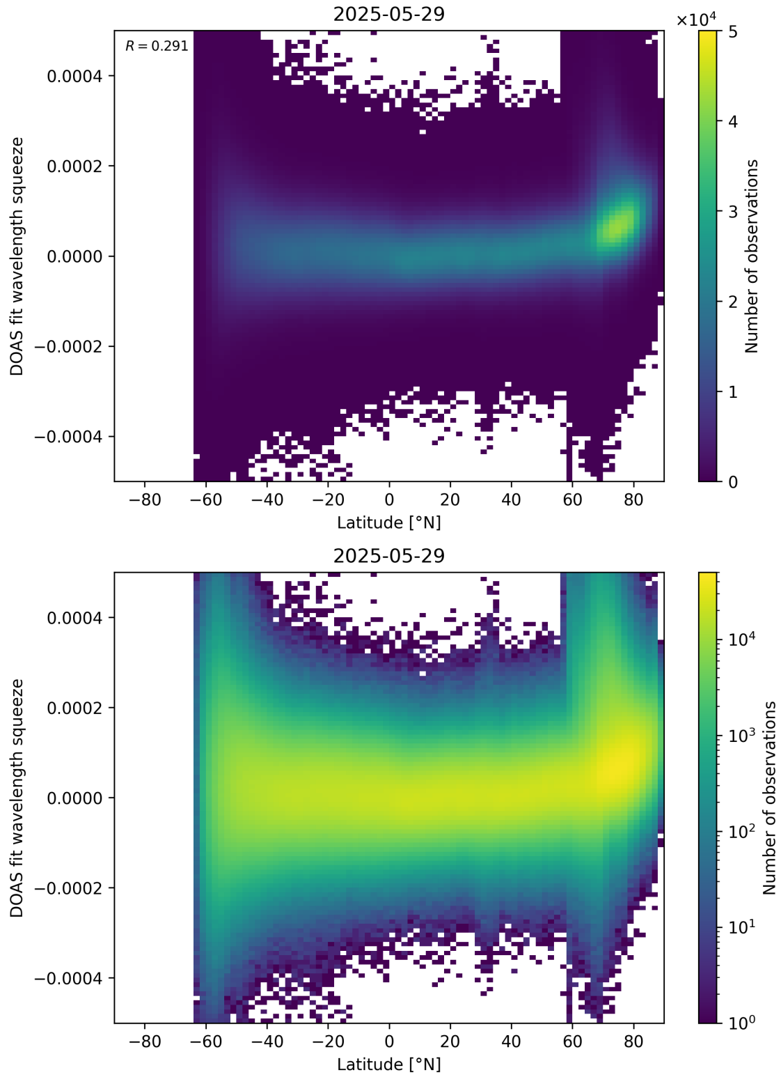
Figure 155: Scatter density plot of “Latitude” against “DOAS fit wavelength squeeze” for 2025-05-28 to 2025-05-30.
