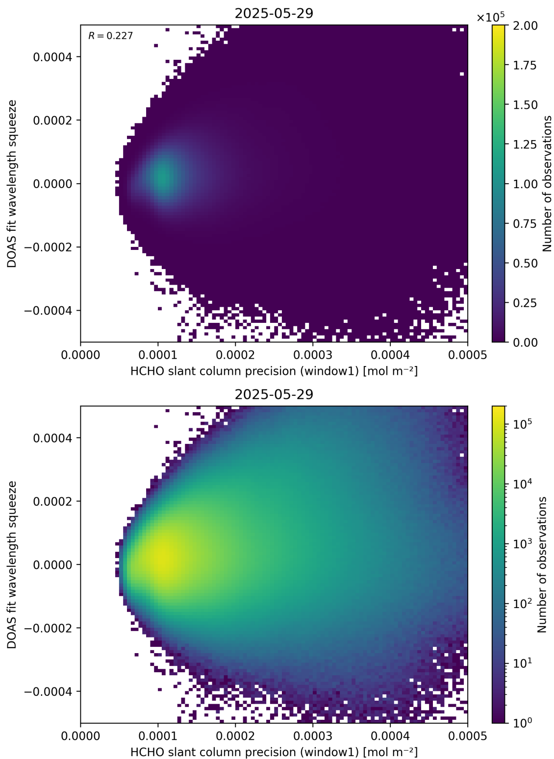
Figure 90: Scatter density plot of “HCHO slant column precision (window1)” against “DOAS fit wavelength squeeze” for 2025-05-28 to 2025-05-30.
