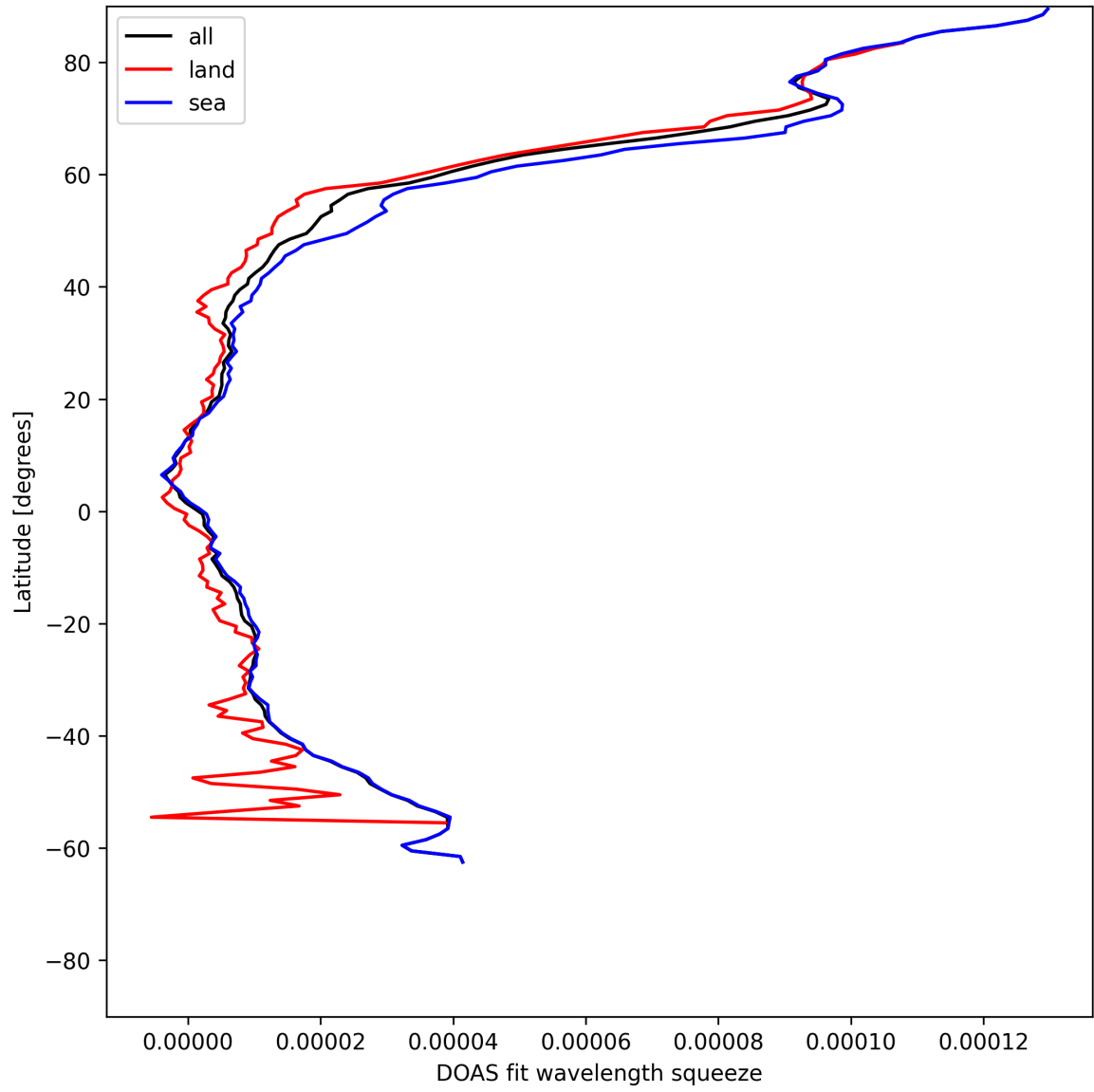
Figure 31: Zonal average of “DOAS fit wavelength squeeze” for 2025-05-28 to 2025-05-30.
