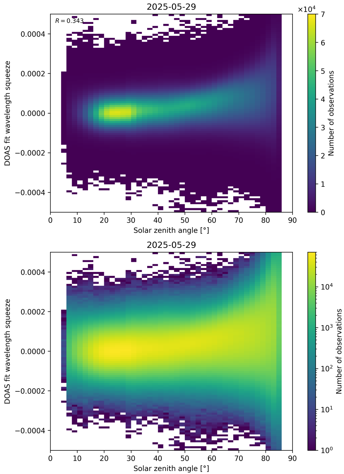
Figure 169: Scatter density plot of “Solar zenith angle” against “DOAS fit wavelength squeeze” for 2025-05-28 to 2025-05-30.
