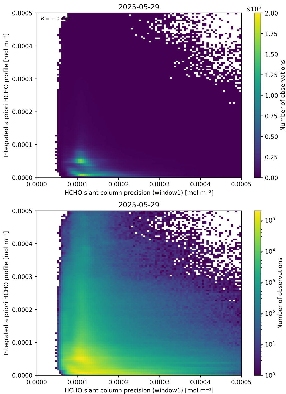
Figure 96: Scatter density plot of “HCHO slant column precision (window1)” against “Integrated a priori HCHO profile” for 2025-05-28 to 2025-05-30.
