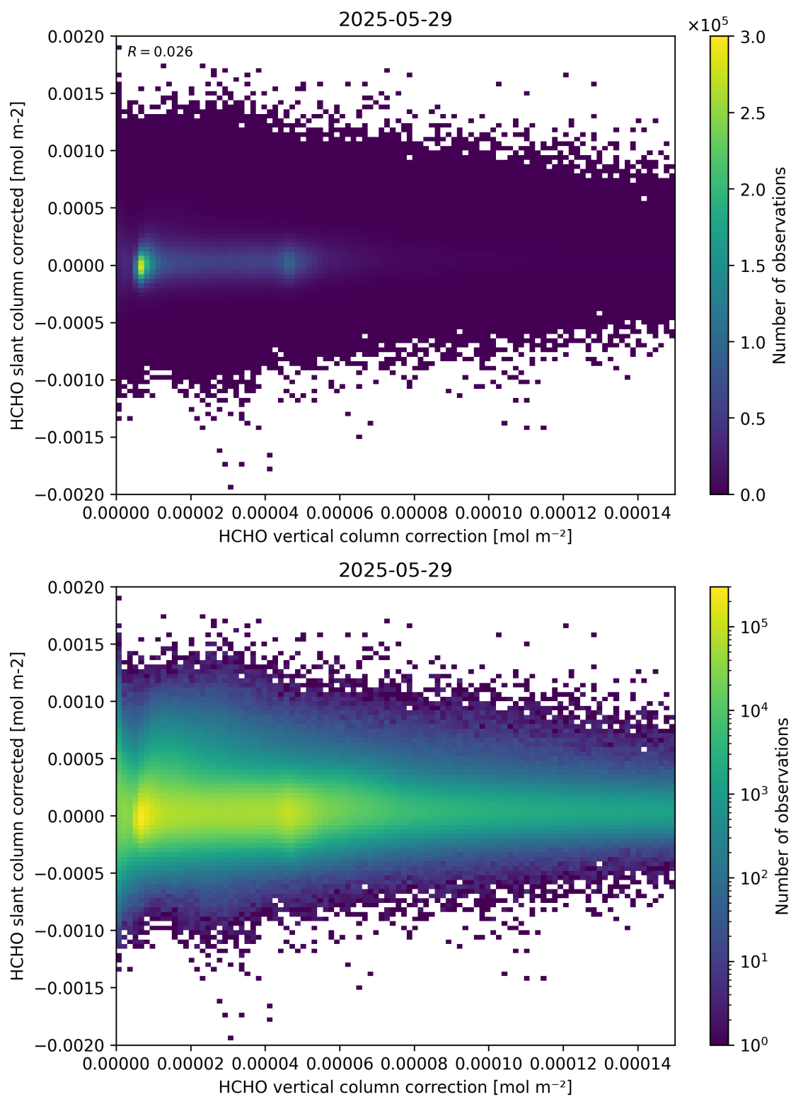
Figure 116: Scatter density plot of “HCHO vertical column correction” against “HCHO slant column corrected” for 2025-05-28 to 2025-05-30.
