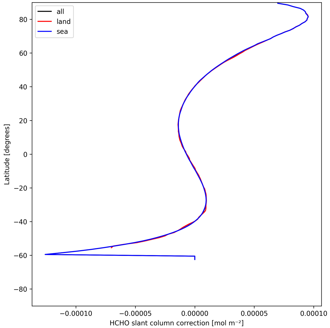
Figure 33: Zonal average of “HCHO slant column correction” for 2025-05-28 to 2025-05-30.
