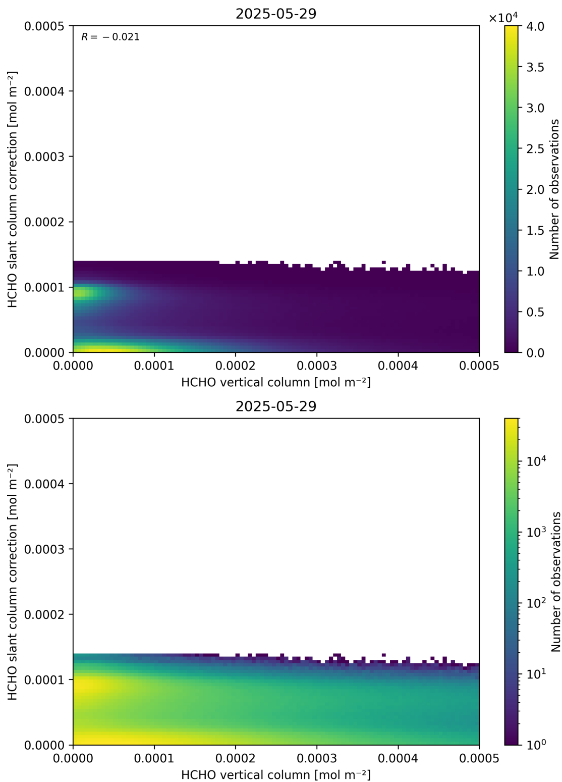
Figure 128: Scatter density plot of “HCHO vertical column” against “HCHO slant column correction” for 2025-05-28 to 2025-05-30.
