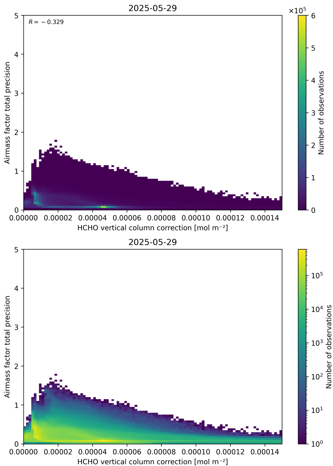
Figure 121: Scatter density plot of “HCHO vertical column correction” against “Airmass factor total precision” for 2025-05-28 to 2025-05-30.
