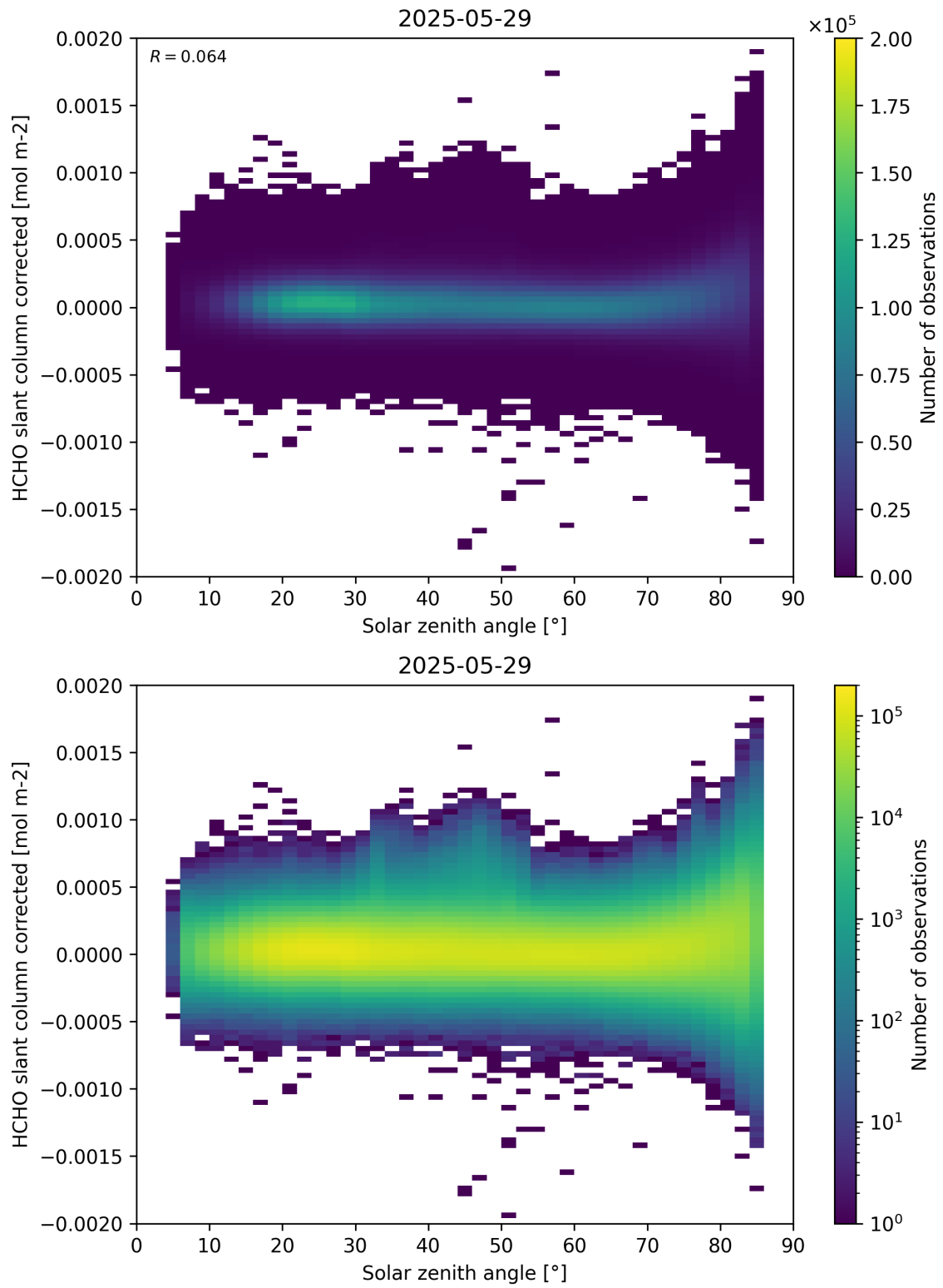
Figure 171: Scatter density plot of “Solar zenith angle” against “HCHO slant column corrected” for 2025-05-28 to 2025-05-30.
