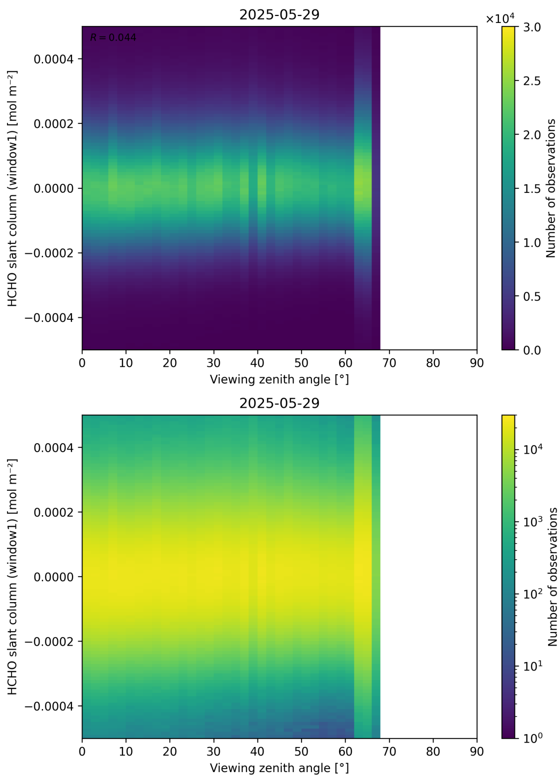
Figure 188: Scatter density plot of “Viewing zenith angle” against “HCHO slant column (window1)” for 2025-05-28 to 2025-05-30.
