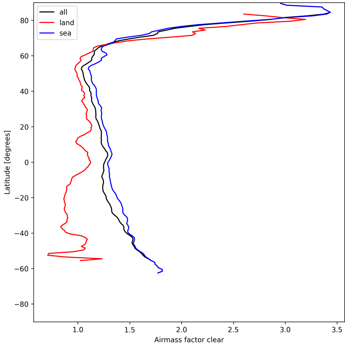
Figure 28: Zonal average of “Airmass factor clear” for 2025-05-28 to 2025-05-30.
