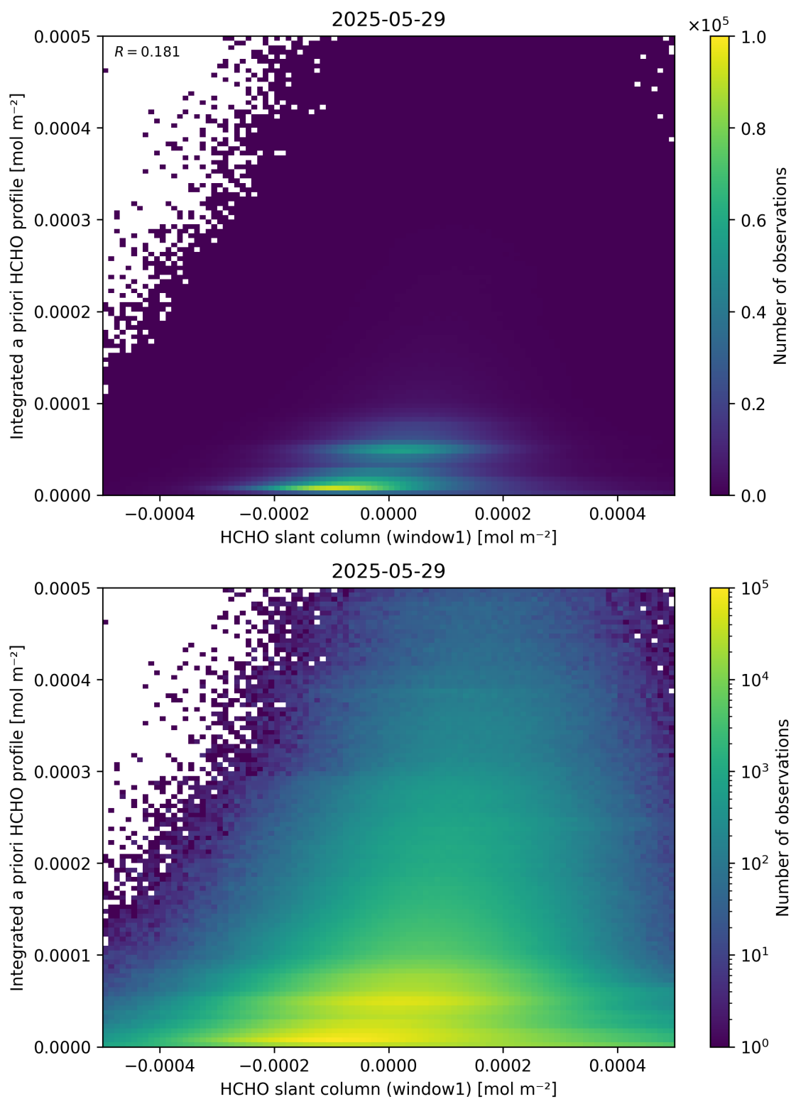
Figure 87: Scatter density plot of “HCHO slant column (window1)” against “Integrated a priori HCHO profile” for 2025-05-28 to 2025-05-30.
