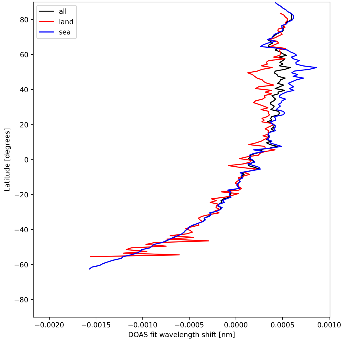
Figure 30: Zonal average of “DOAS fit wavelength shift” for 2025-05-28 to 2025-05-30.
