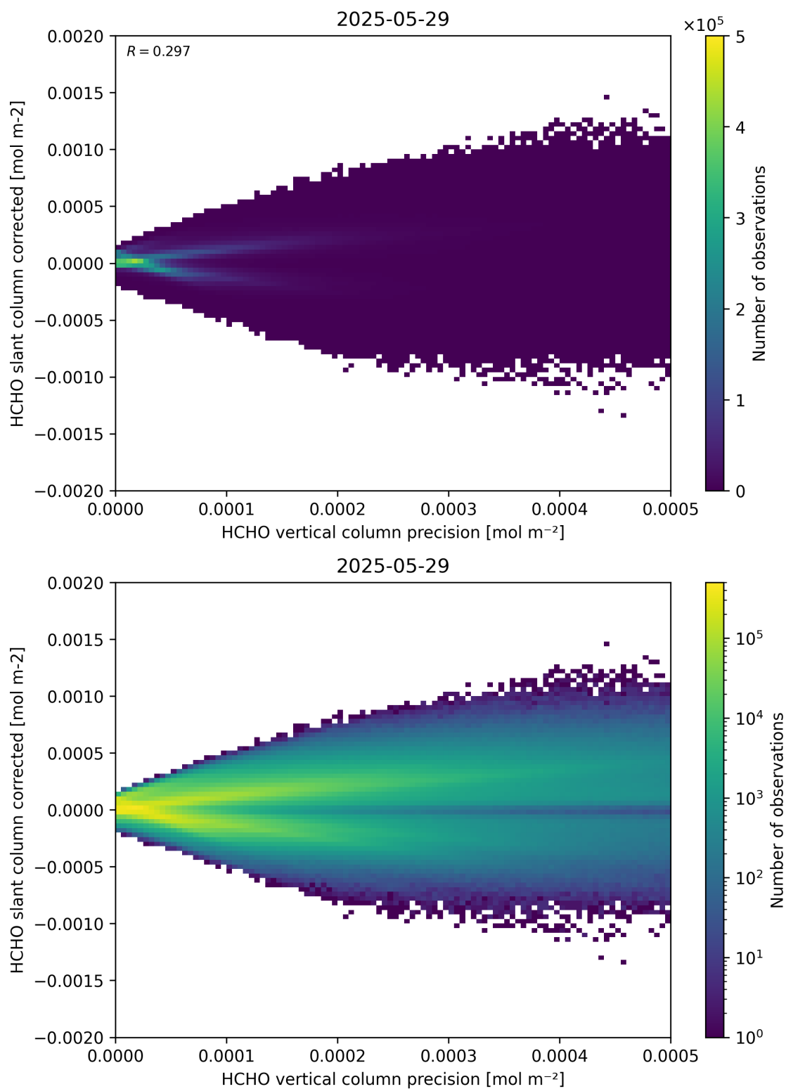
Figure 140: Scatter density plot of “HCHO vertical column precision” against “HCHO slant column corrected” for 2025-05-28 to 2025-05-30.
