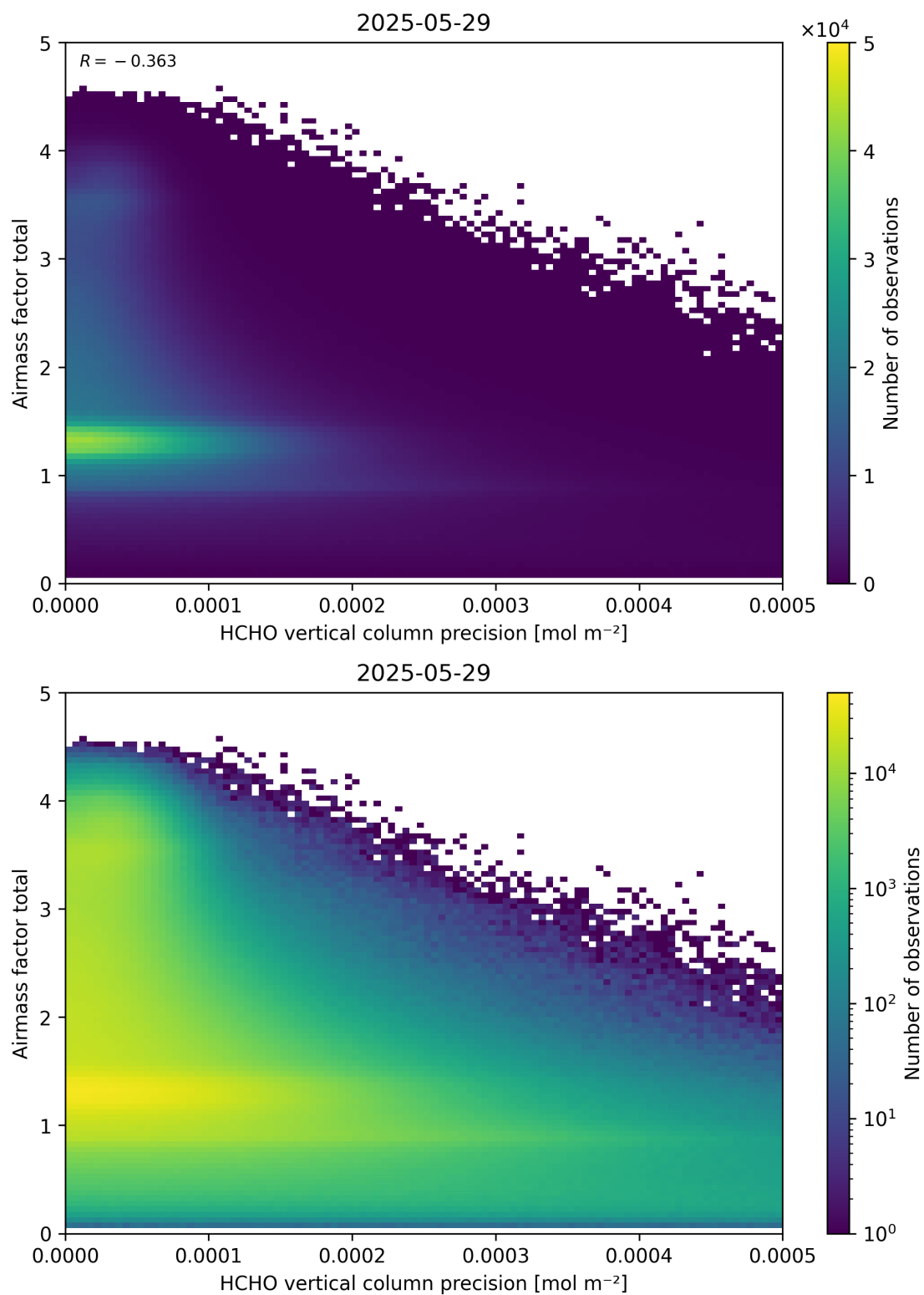
Figure 144: Scatter density plot of “HCHO vertical column precision” against “Airmass factor total” for 2025-05-28 to 2025-05-30.
