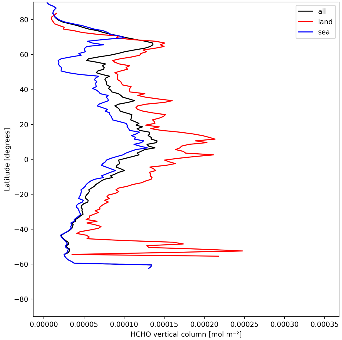
Figure 21: Zonal average of “HCHO vertical column” for 2025-05-28 to 2025-05-30.
