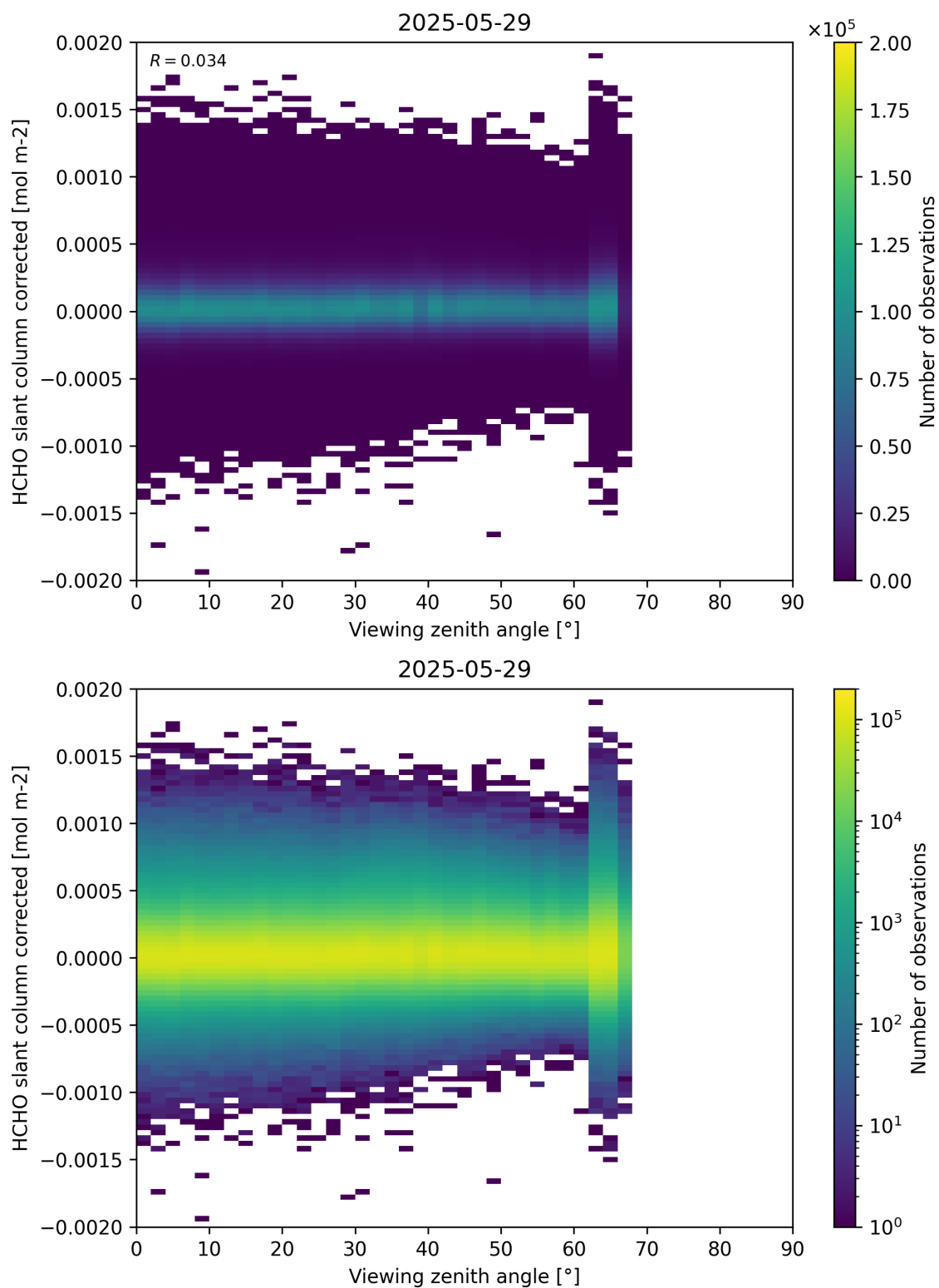
Figure 186: Scatter density plot of “Viewing zenith angle” against “HCHO slant column corrected” for 2025-05-28 to 2025-05-30.
