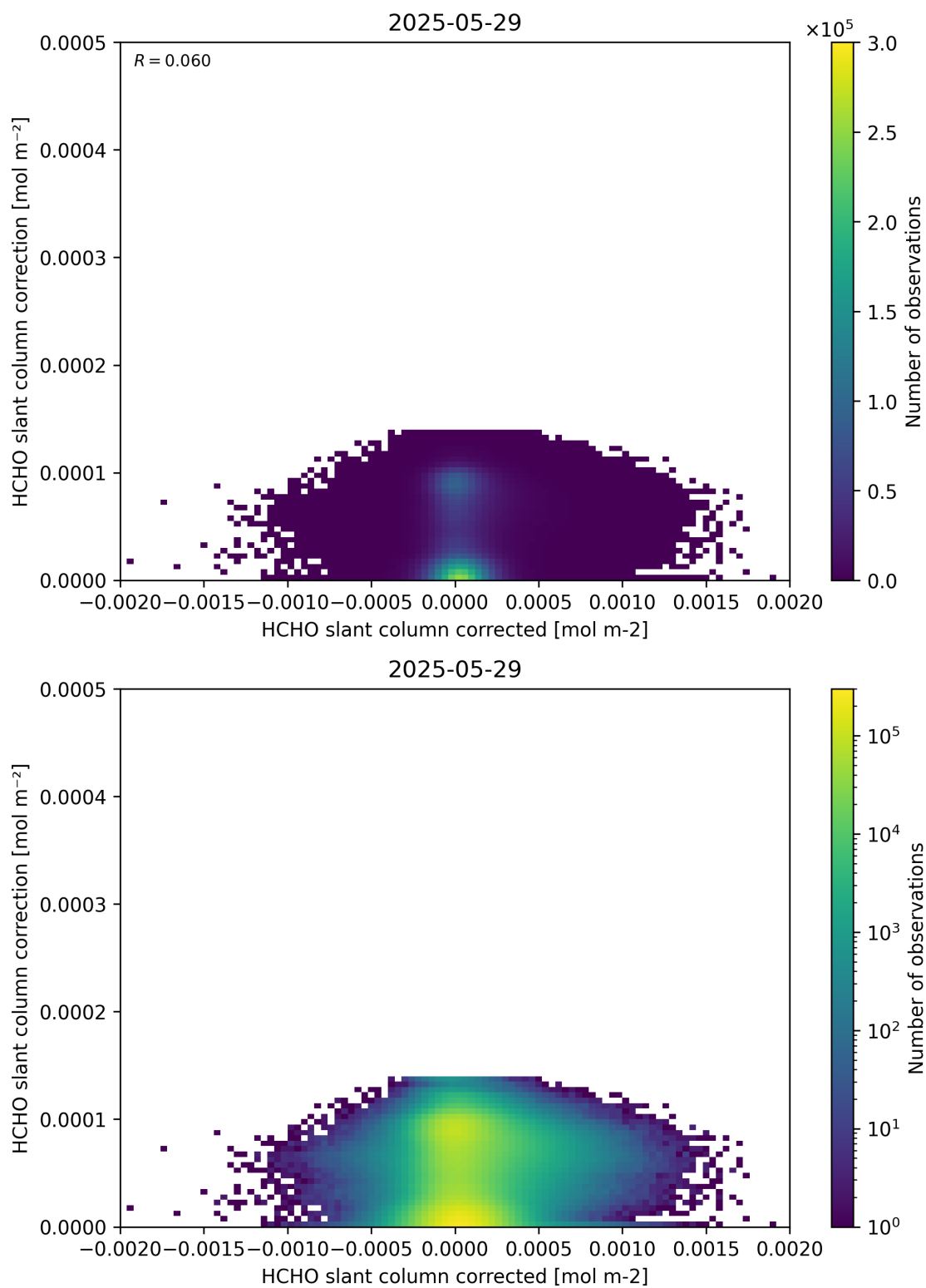
Figure 77: Scatter density plot of “HCHO slant column corrected” against “HCHO slant column correction” for 2025-05-28 to 2025-05-30.
