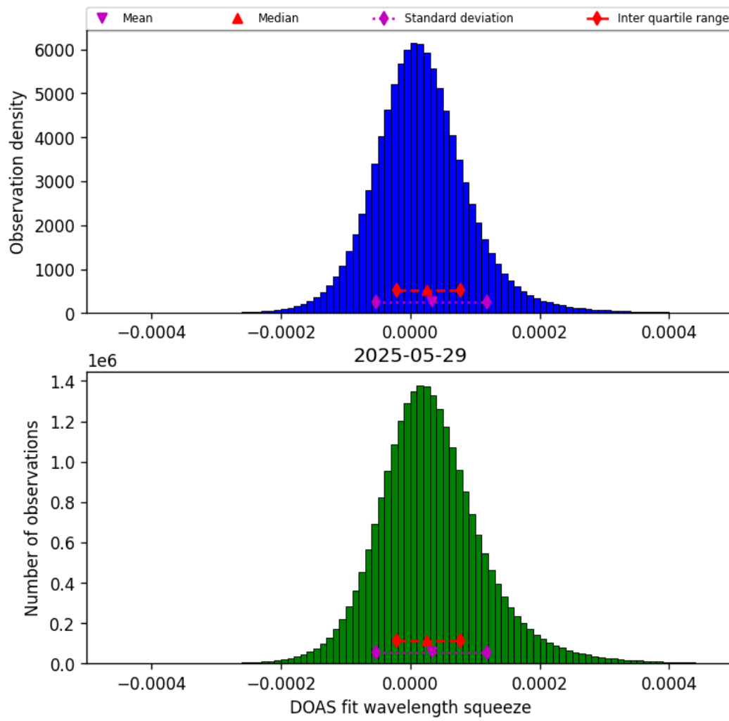
Figure 45: Histogram of “DOAS fit wavelength squeeze” for 2025-05-28 to 2025-05-30
