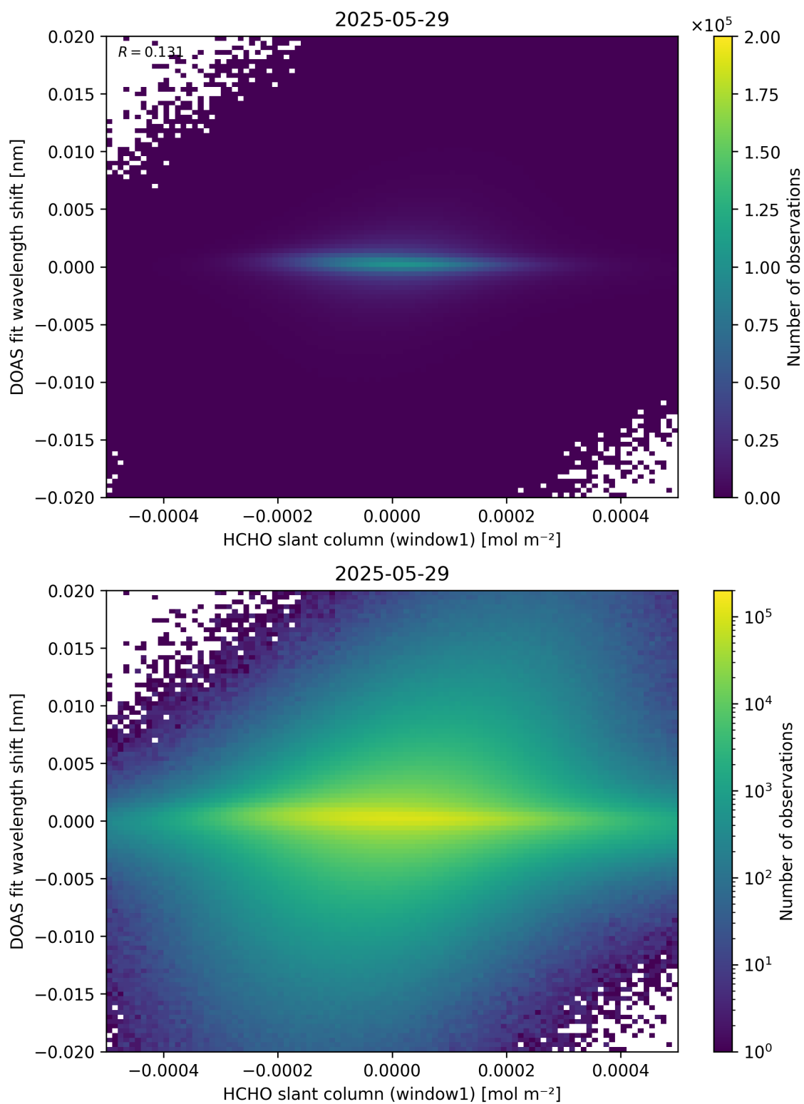
Figure 79: Scatter density plot of “HCHO slant column (window1)” against “DOAS fit wavelength shift” for 2025-05-28 to 2025-05-30.
