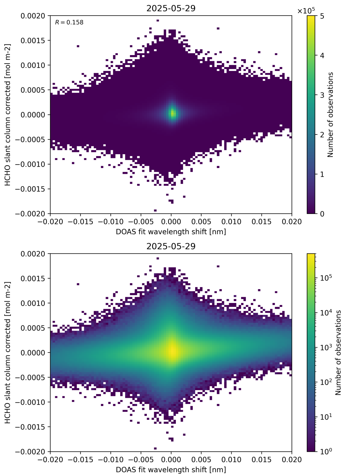
Figure 66: Scatter density plot of “DOAS fit wavelength shift” against “HCHO slant column corrected” for 2025-05-28 to 2025-05-30.
