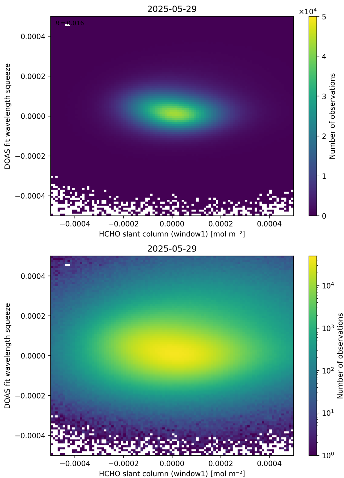
Figure 80: Scatter density plot of “HCHO slant column (window1)” against “DOAS fit wavelength squeeze” for 2025-05-28 to 2025-05-30.
