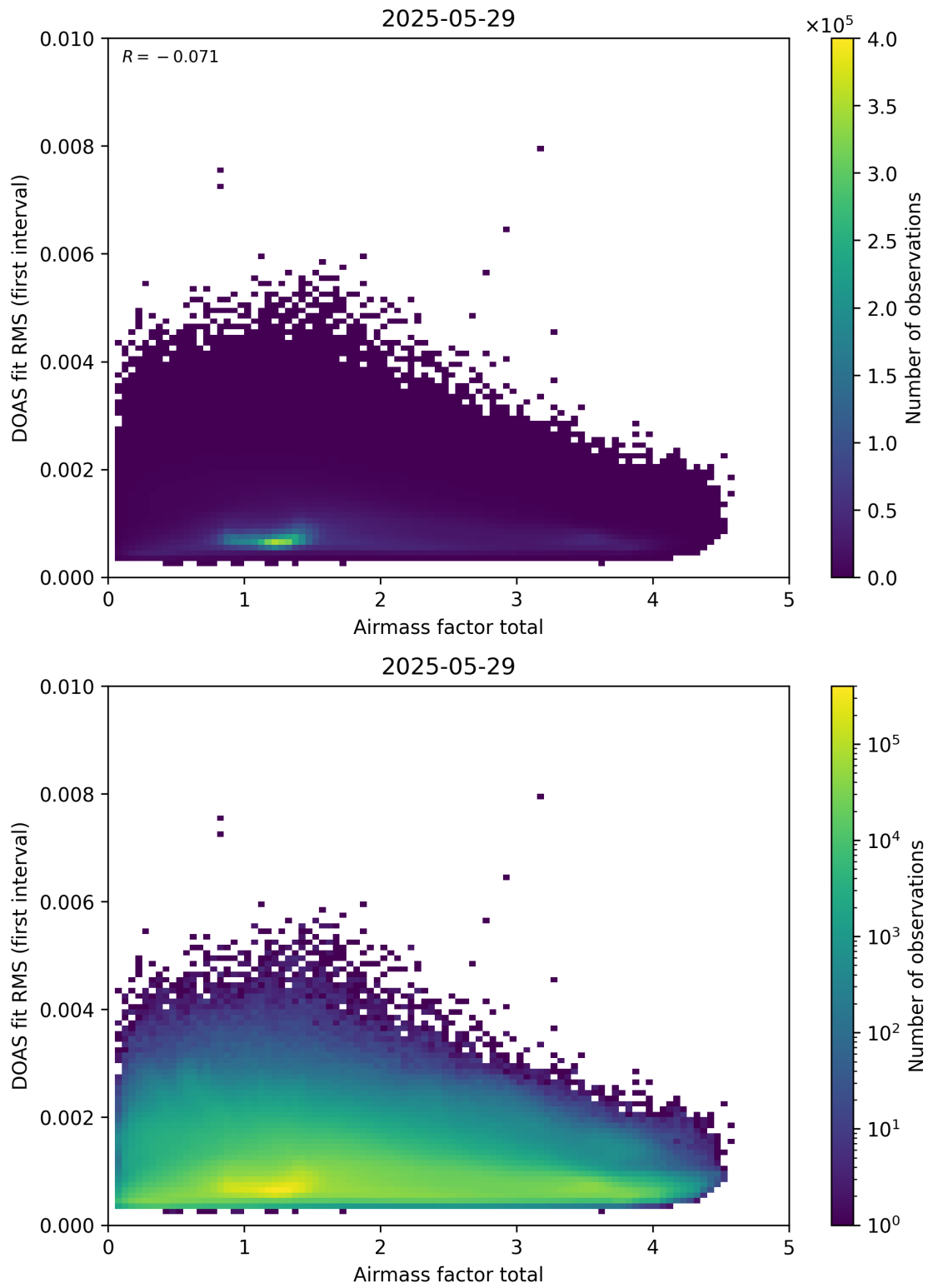
Figure 97: Scatter density plot of “Airmass factor total” against “DOAS fit RMS (first interval)” for 2025-05-28 to 2025-05-30.
