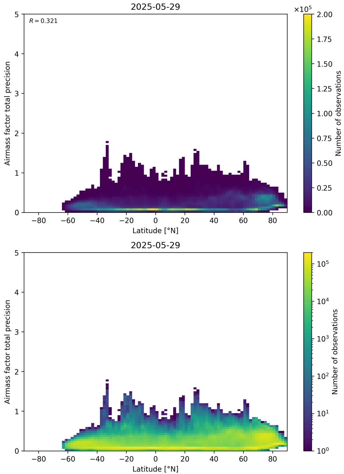
Figure 162: Scatter density plot of “Latitude” against “Airmass factor total precision” for 2025-05-28 to 2025-05-30.
