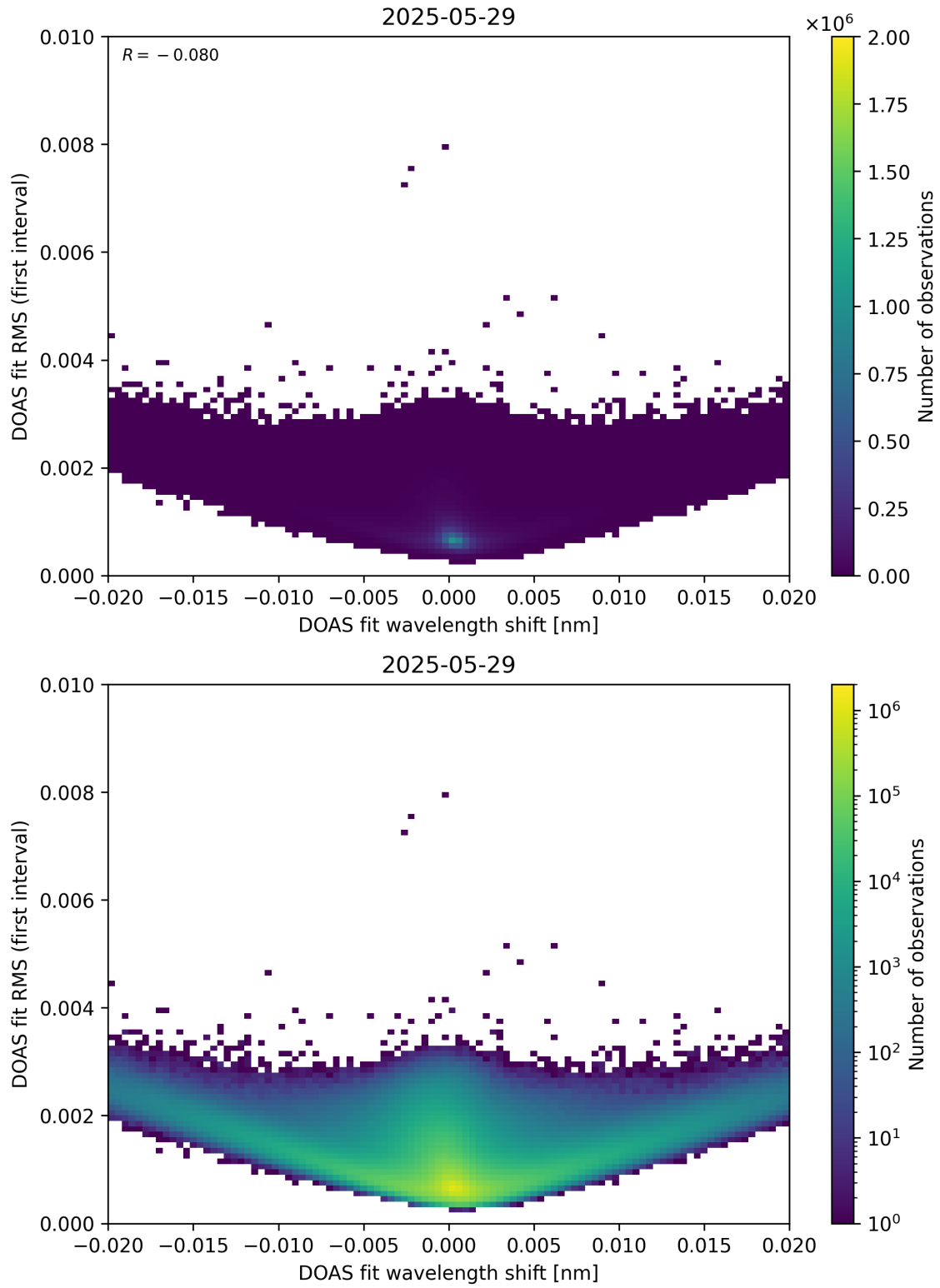
Figure 64: Scatter density plot of “DOAS fit wavelength shift” against “DOAS fit RMS (first interval)” for 2025-05-28 to 2025-05-30.
