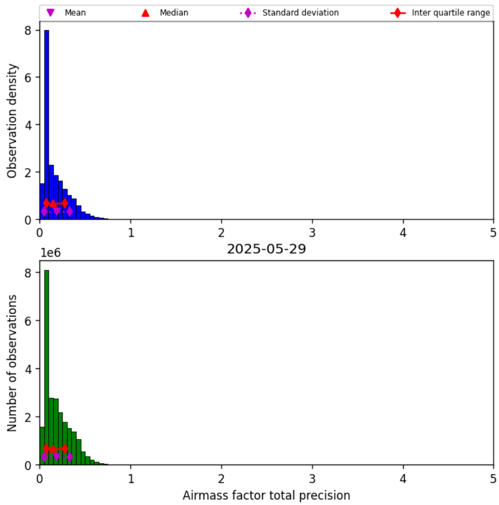
Figure 41: Histogram of “Airmass factor total precision” for 2025-05-28 to 2025-05-30
