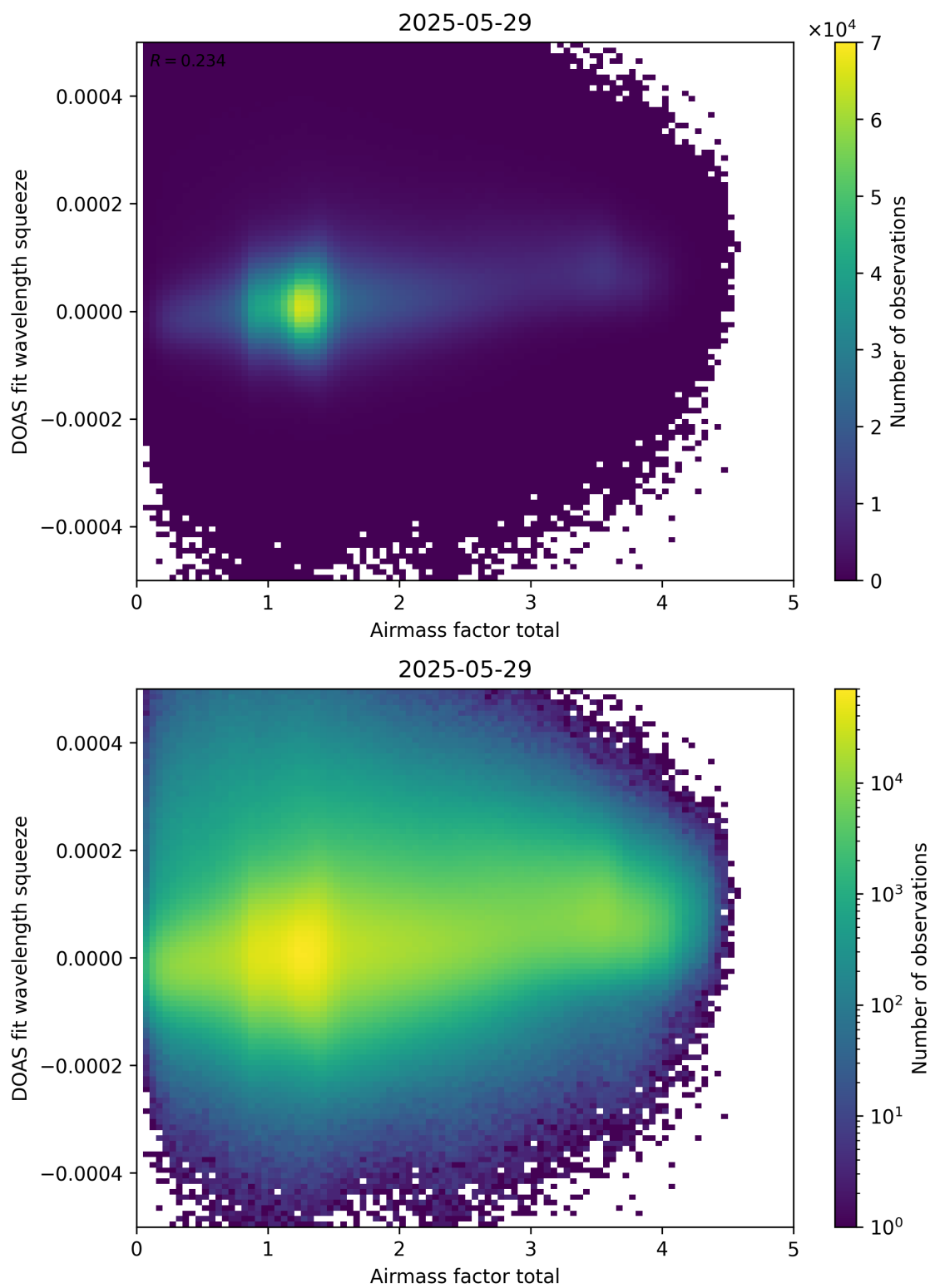
Figure 99: Scatter density plot of “Airmass factor total” against “DOAS fit wavelength squeeze” for 2025-05-28 to 2025-05-30.
