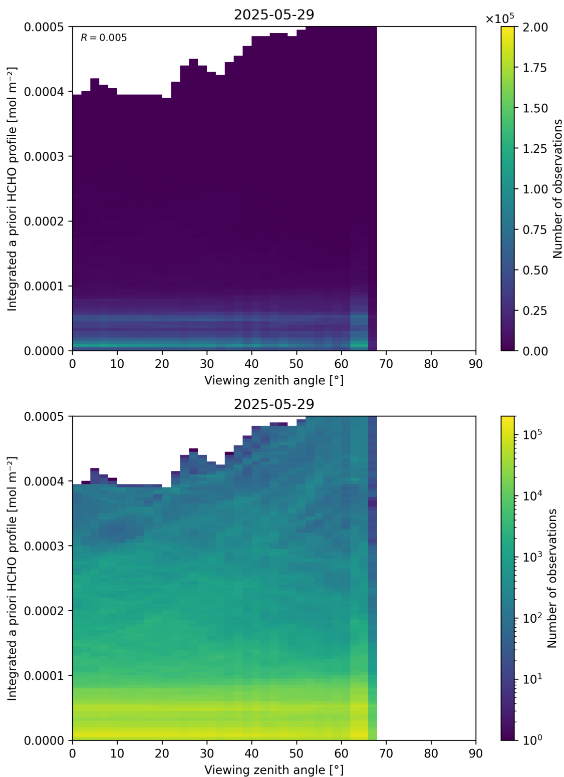
Figure 195: Scatter density plot of “Viewing zenith angle” against “Integrated a priori HCHO profile” for 2025-05-28 to 2025-05-30.
