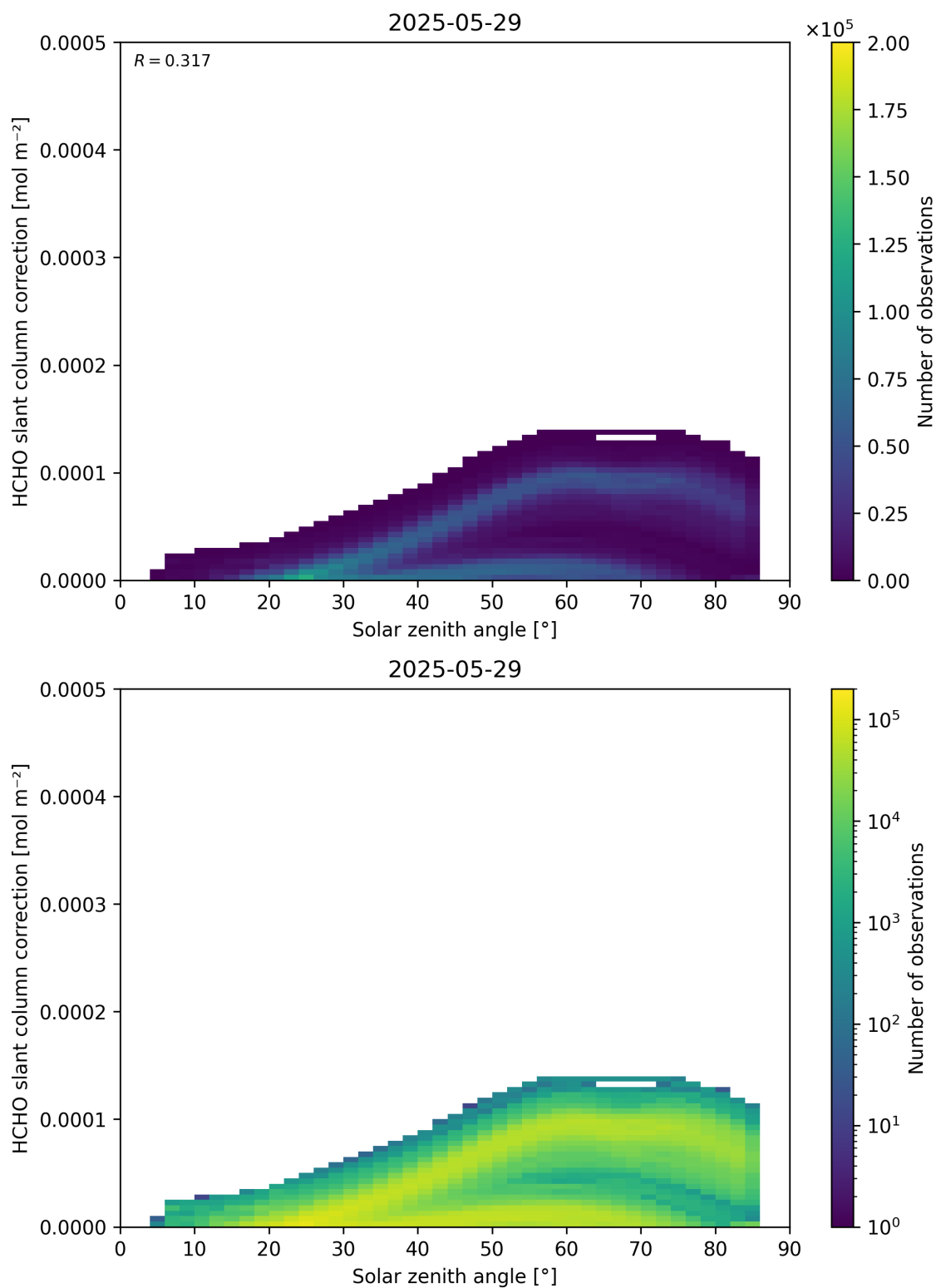
Figure 172: Scatter density plot of “Solar zenith angle” against “HCHO slant column correction” for 2025-05-28 to 2025-05-30.
