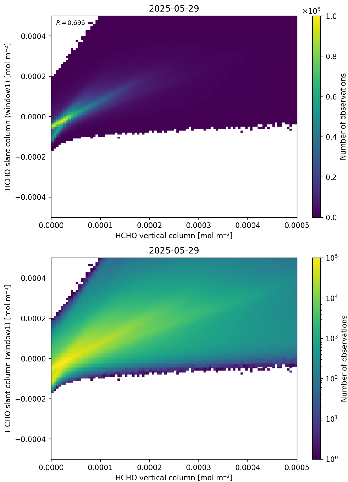
Figure 129: Scatter density plot of “HCHO vertical column” against “HCHO slant column (window1)” for 2025-05-28 to 2025-05-30.
