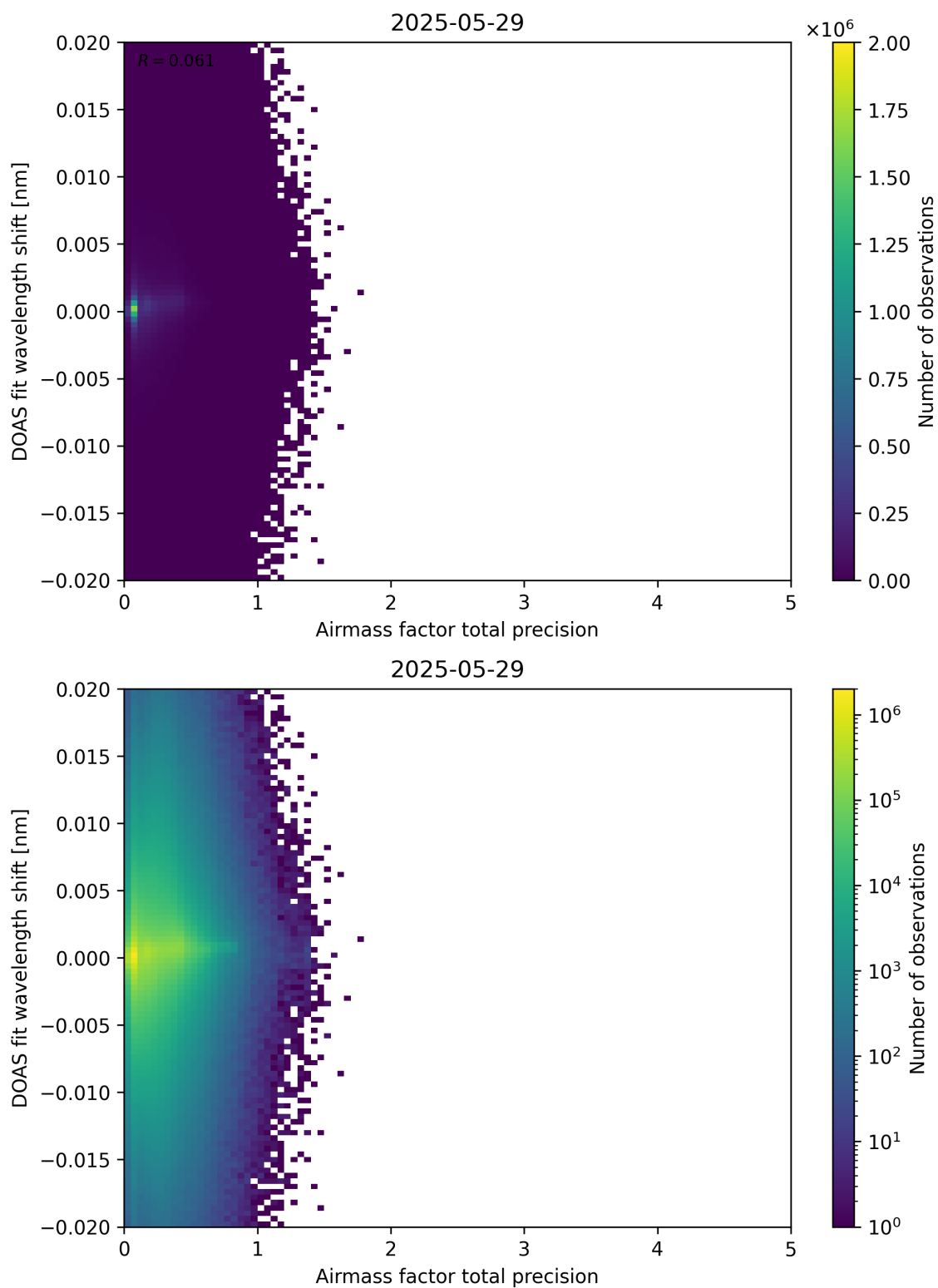
Figure 106: Scatter density plot of “Airmass factor total precision” against “DOAS fit wavelength shift” for 2025-05-28 to 2025-05-30.
