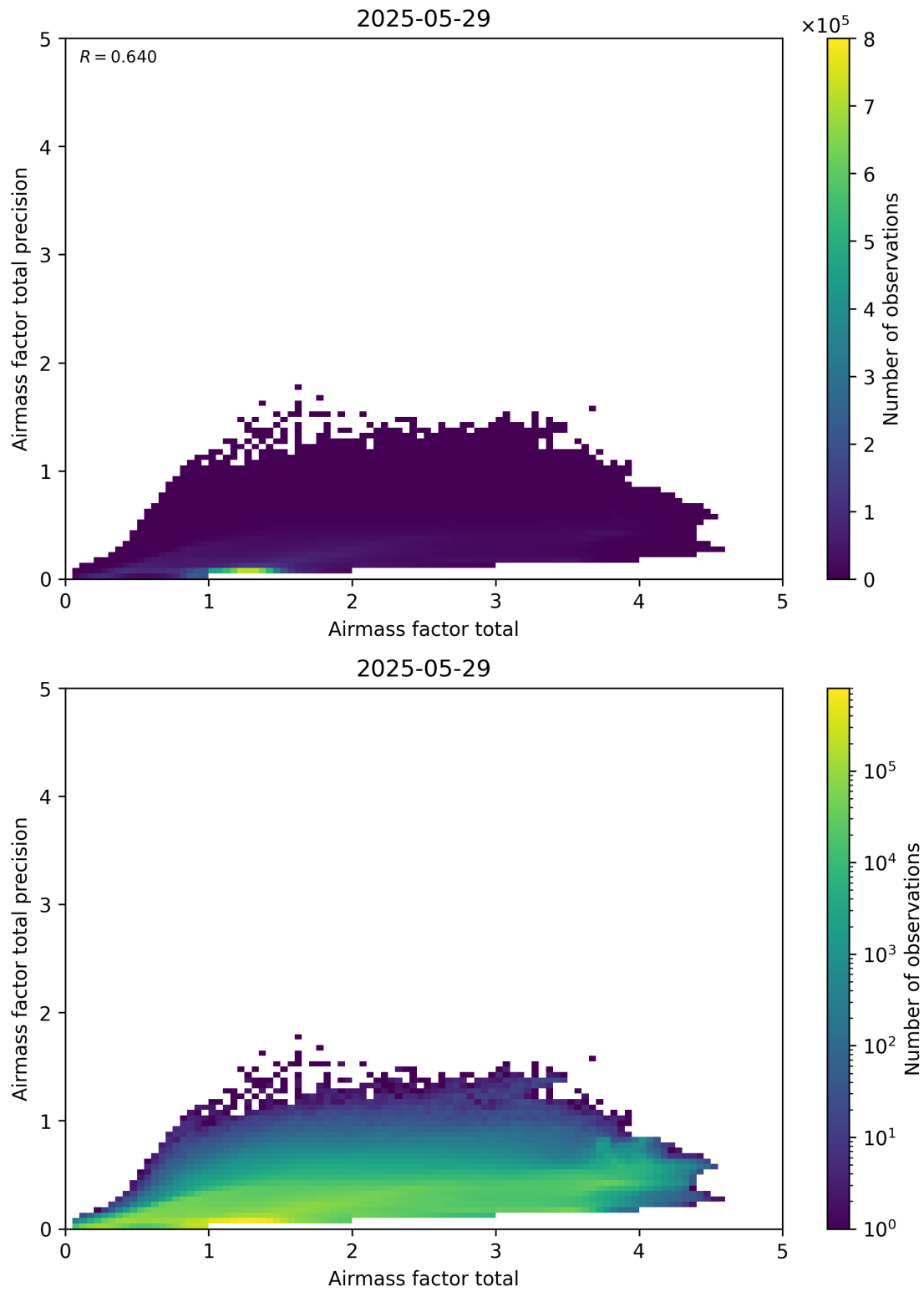
Figure 103: Scatter density plot of “Airmass factor total” against “Airmass factor total precision” for 2025-05-28 to 2025-05-30.
