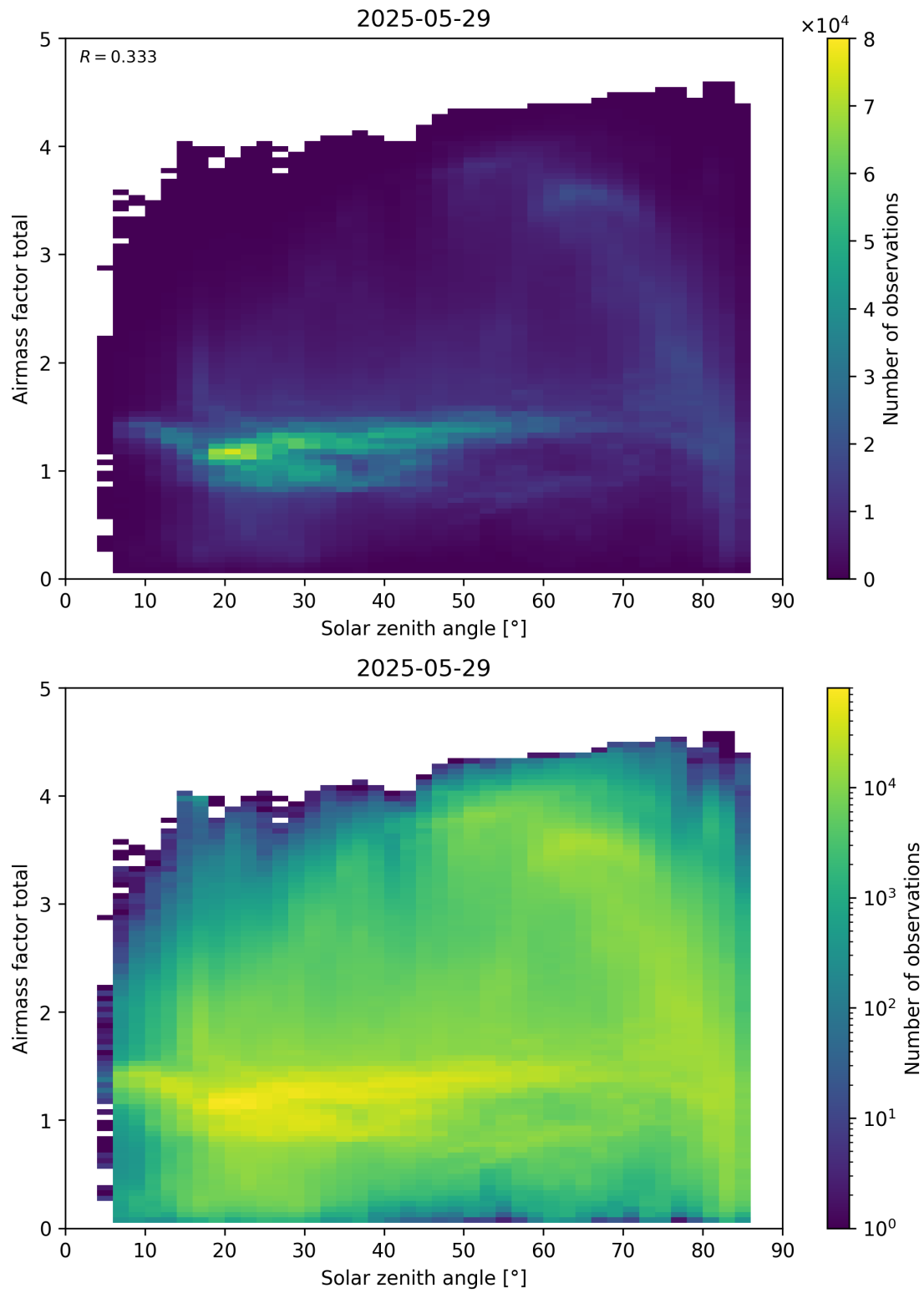
Figure 175: Scatter density plot of “Solar zenith angle” against “Airmass factor total” for 2025-05-28 to 2025-05-30.
