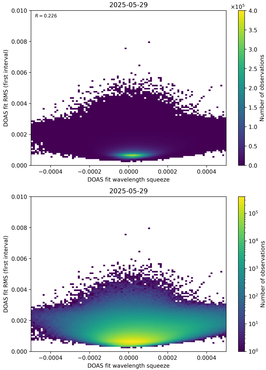
Figure 68: Scatter density plot of “DOAS fit wavelength squeeze” against “DOAS fit RMS (first interval)” for 2025-05-28 to 2025-05-30.
