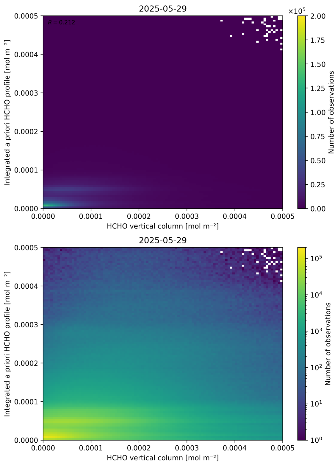
Figure 135: Scatter density plot of “HCHO vertical column” against “Integrated a priori HCHO profile” for 2025-05-28 to 2025-05-30.
