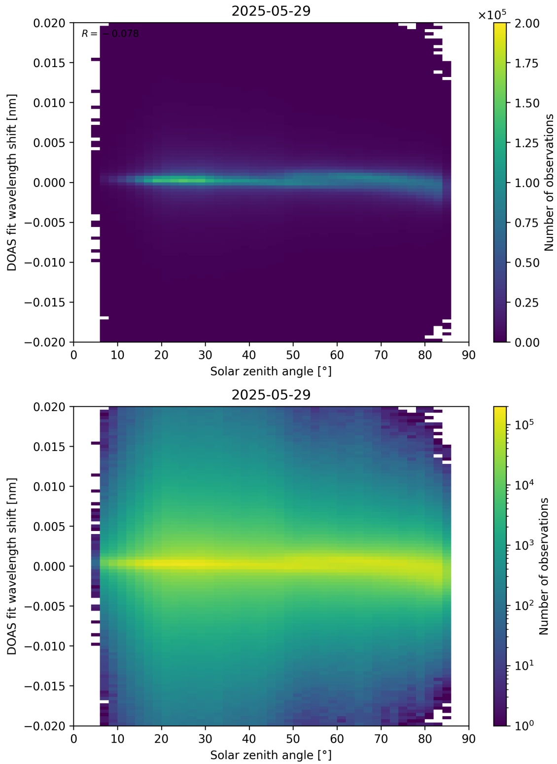
Figure 168: Scatter density plot of “Solar zenith angle” against “DOAS fit wavelength shift” for 2025-05-28 to 2025-05-30.
