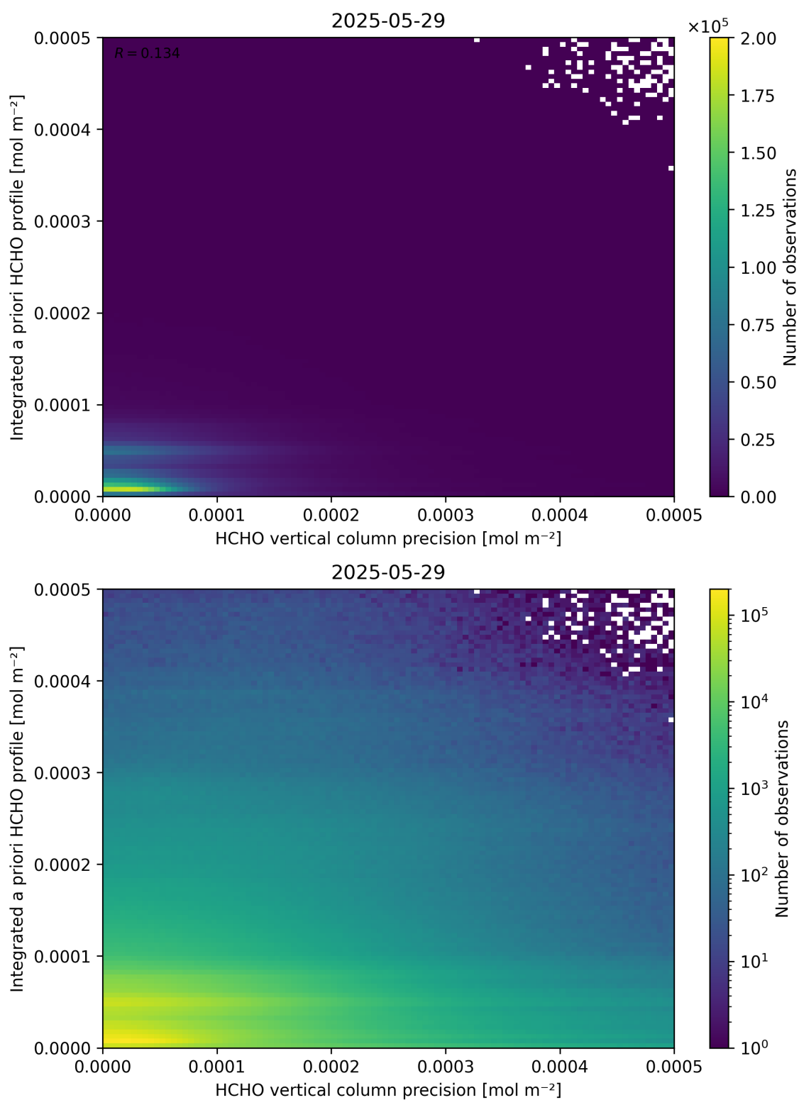
Figure 147: Scatter density plot of “HCHO vertical column precision” against “Integrated a priori HCHO profile” for 2025-05-28 to 2025-05-30.
