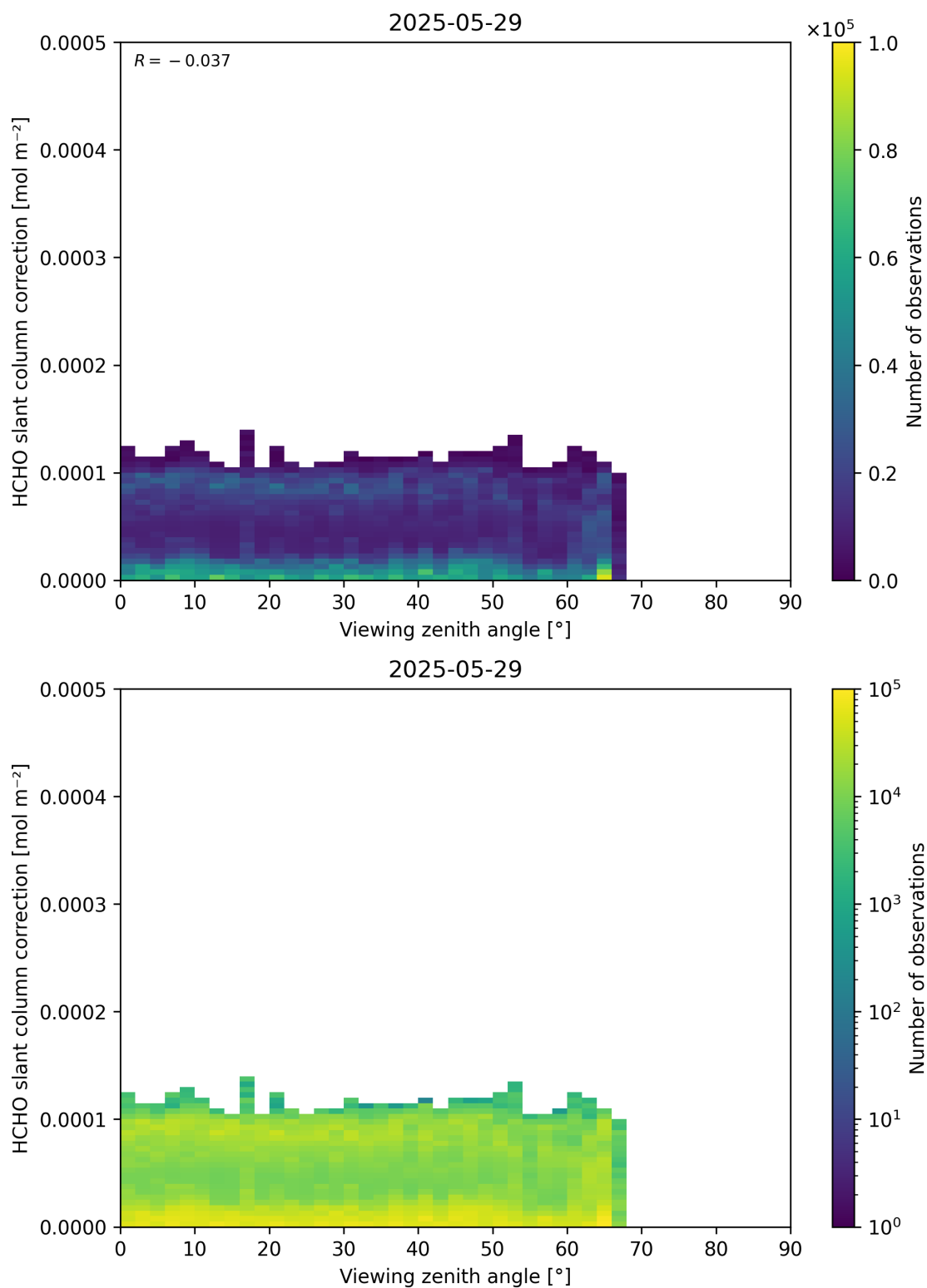
Figure 187: Scatter density plot of “Viewing zenith angle” against “HCHO slant column correction” for 2025-05-28 to 2025-05-30.
