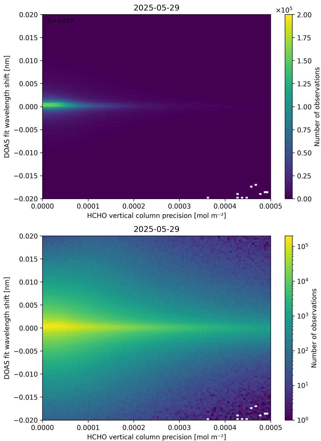
Figure 137: Scatter density plot of “HCHO vertical column precision” against “DOAS fit wavelength shift” for 2025-05-28 to 2025-05-30.
