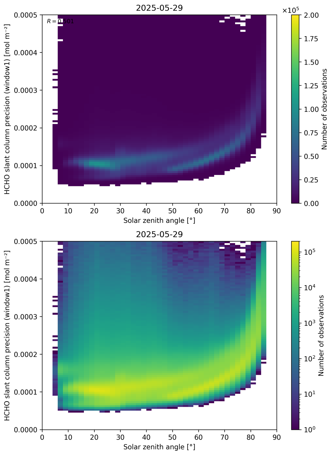
Figure 174: Scatter density plot of “Solar zenith angle” against “HCHO slant column precision (window1)” for 2025-05-28 to 2025-05-30.
