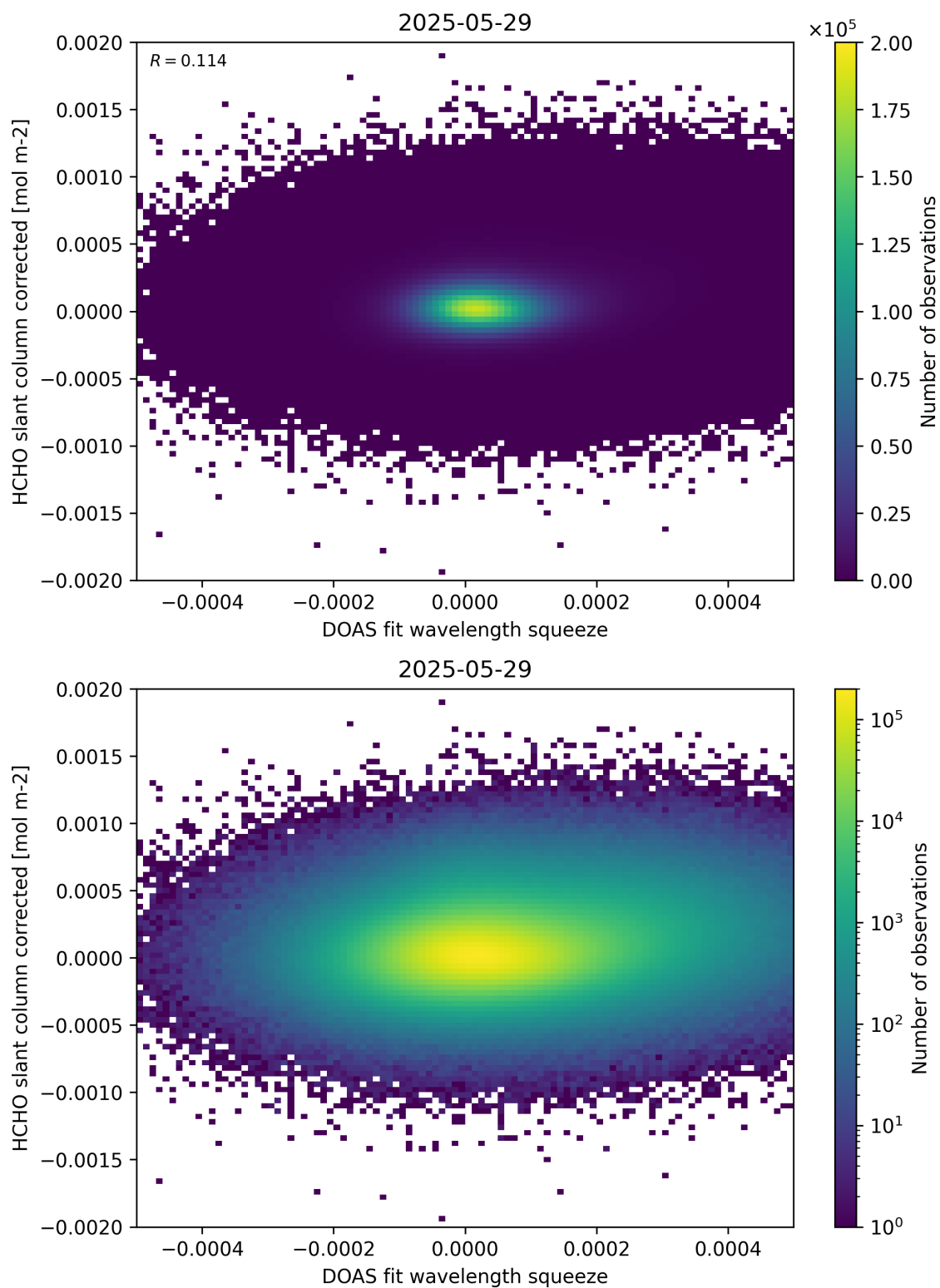
Figure 69: Scatter density plot of “DOAS fit wavelength squeeze” against “HCHO slant column corrected” for 2025-05-28 to 2025-05-30.
