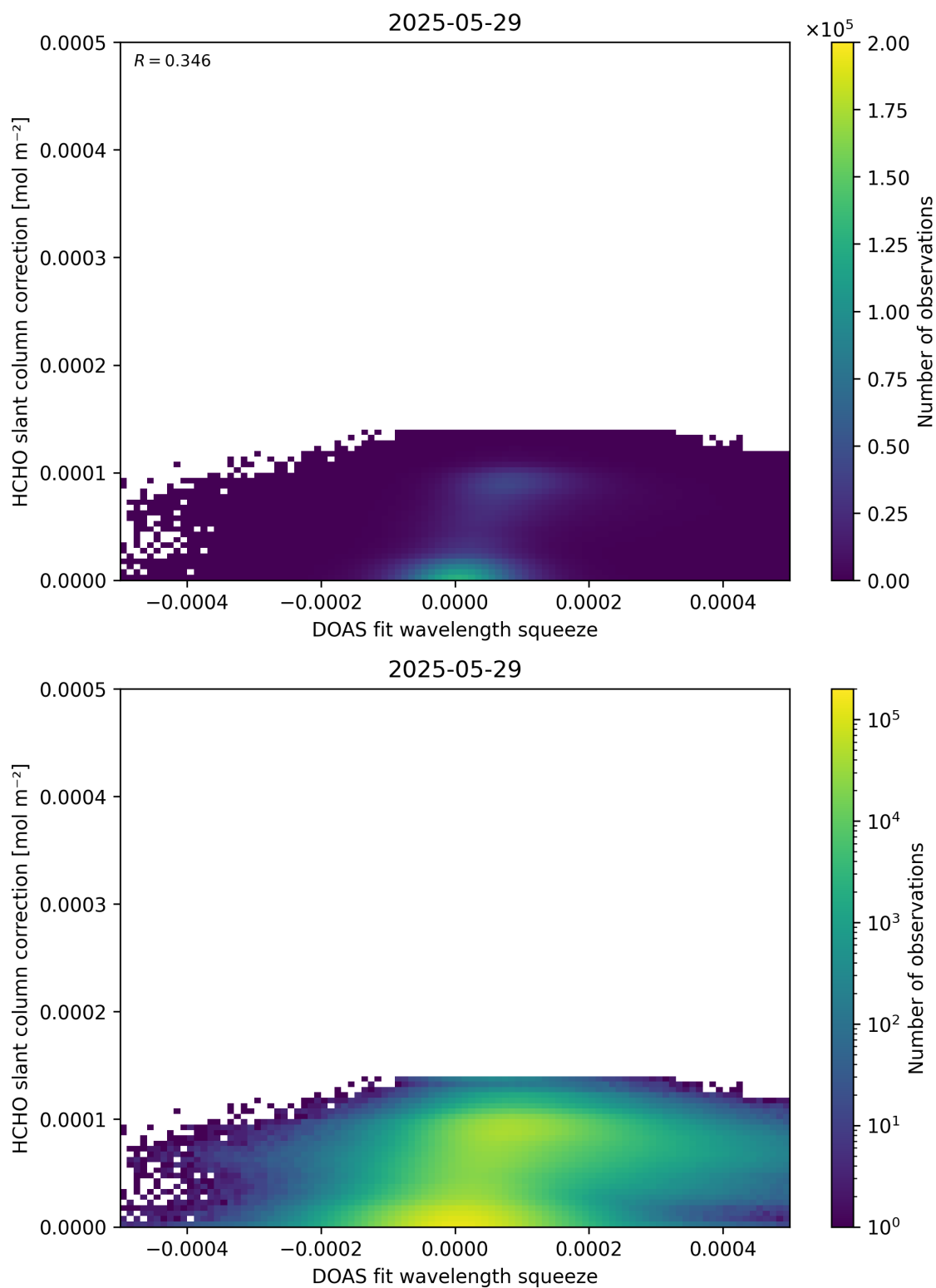
Figure 70: Scatter density plot of “DOAS fit wavelength squeeze” against “HCHO slant column correction” for 2025-05-28 to 2025-05-30.
