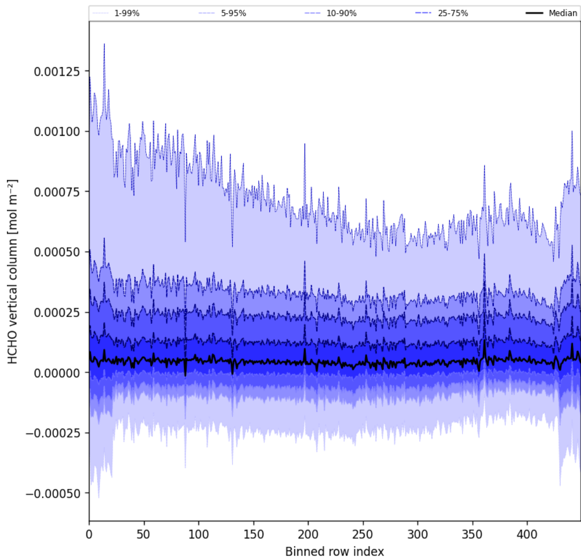
Figure 49: Along track statistics of “HCHO vertical column” for 2025-05-28 to 2025-05-30
