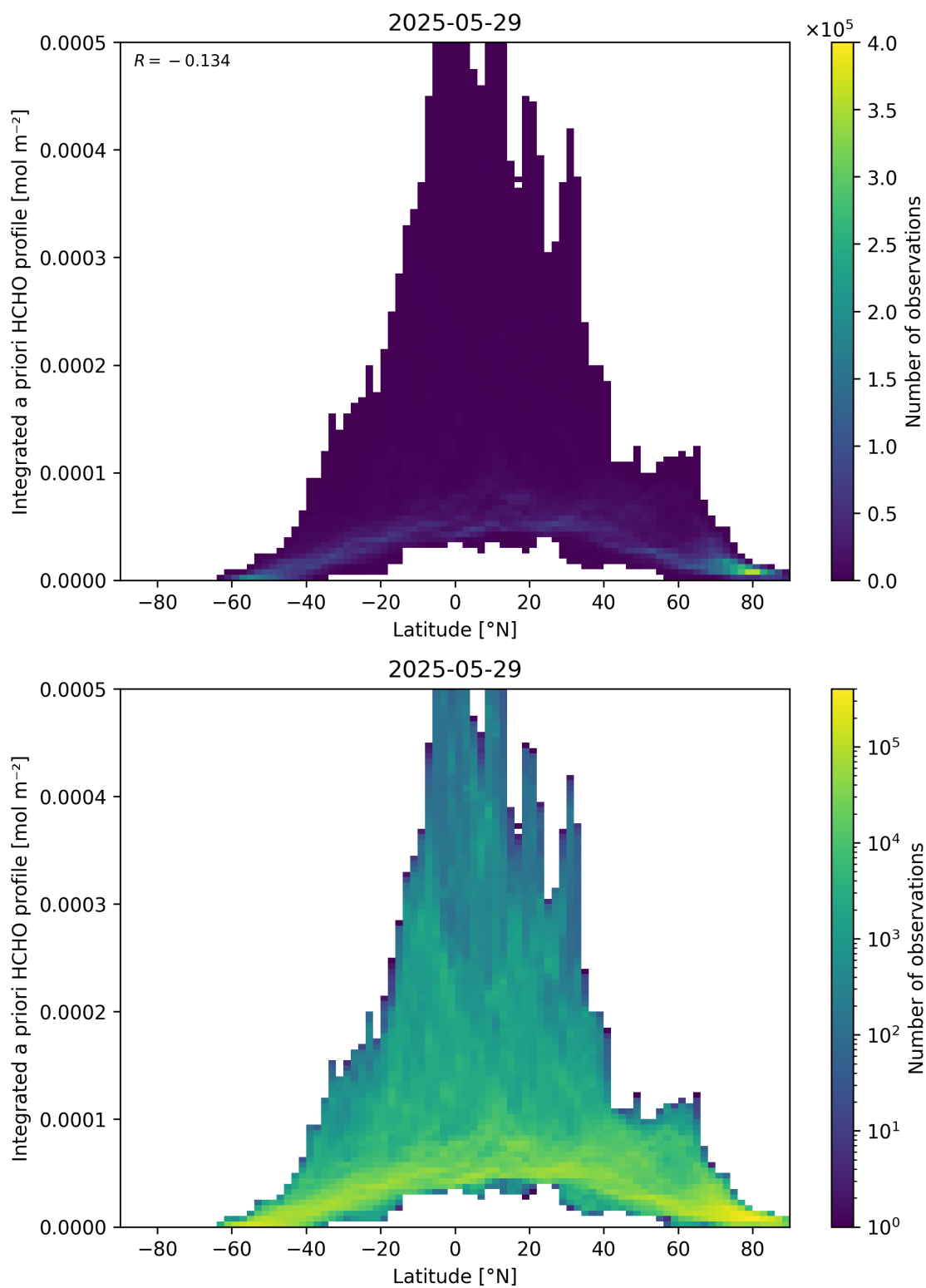
Figure 166: Scatter density plot of “Latitude” against “Integrated a priori HCHO profile” for 2025-05-28 to 2025-05-30.
