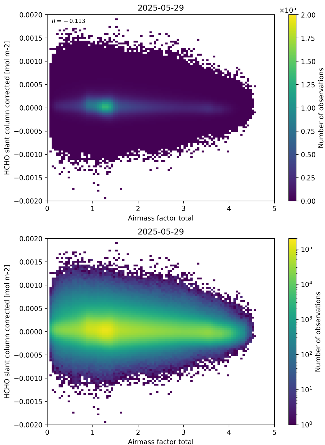
Figure 101: Scatter density plot of “Airmass factor total” against “HCHO slant column corrected” for 2025-05-28 to 2025-05-30.
