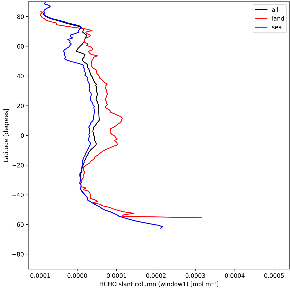
Figure 24: Zonal average of “HCHO slant column (window1)” for 2025-05-28 to 2025-05-30.
