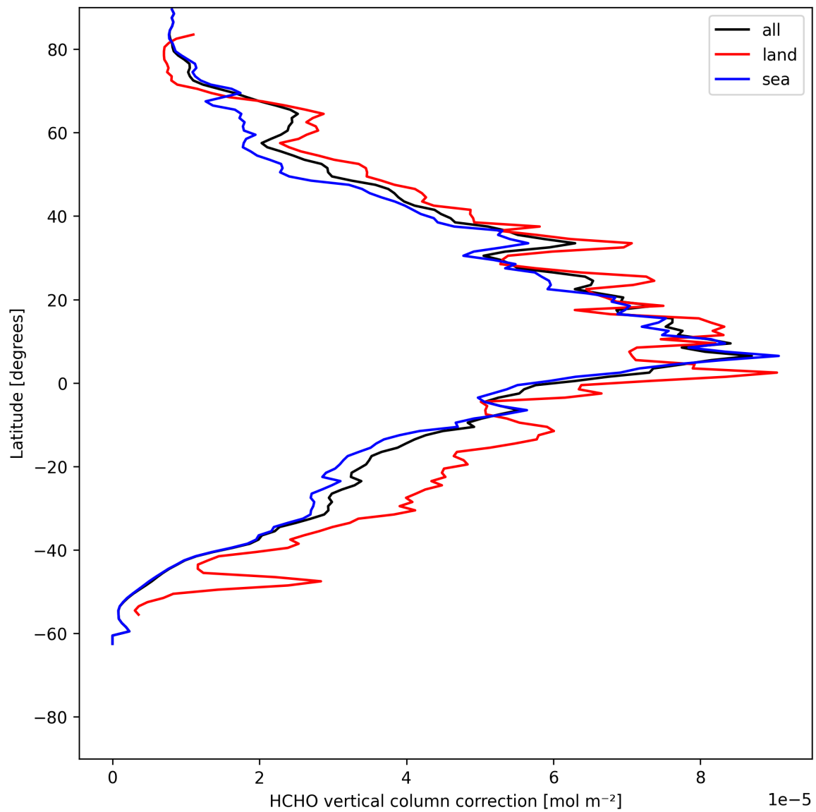
Figure 23: Zonal average of “HCHO vertical column correction” for 2025-05-28 to 2025-05-30.
