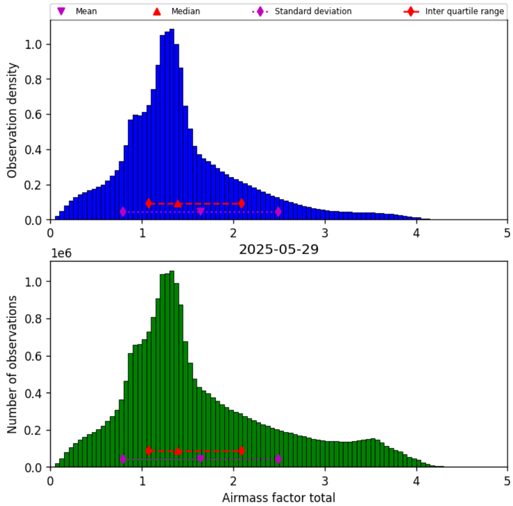
Figure 40: Histogram of “Airmass factor total” for 2025-05-28 to 2025-05-30
