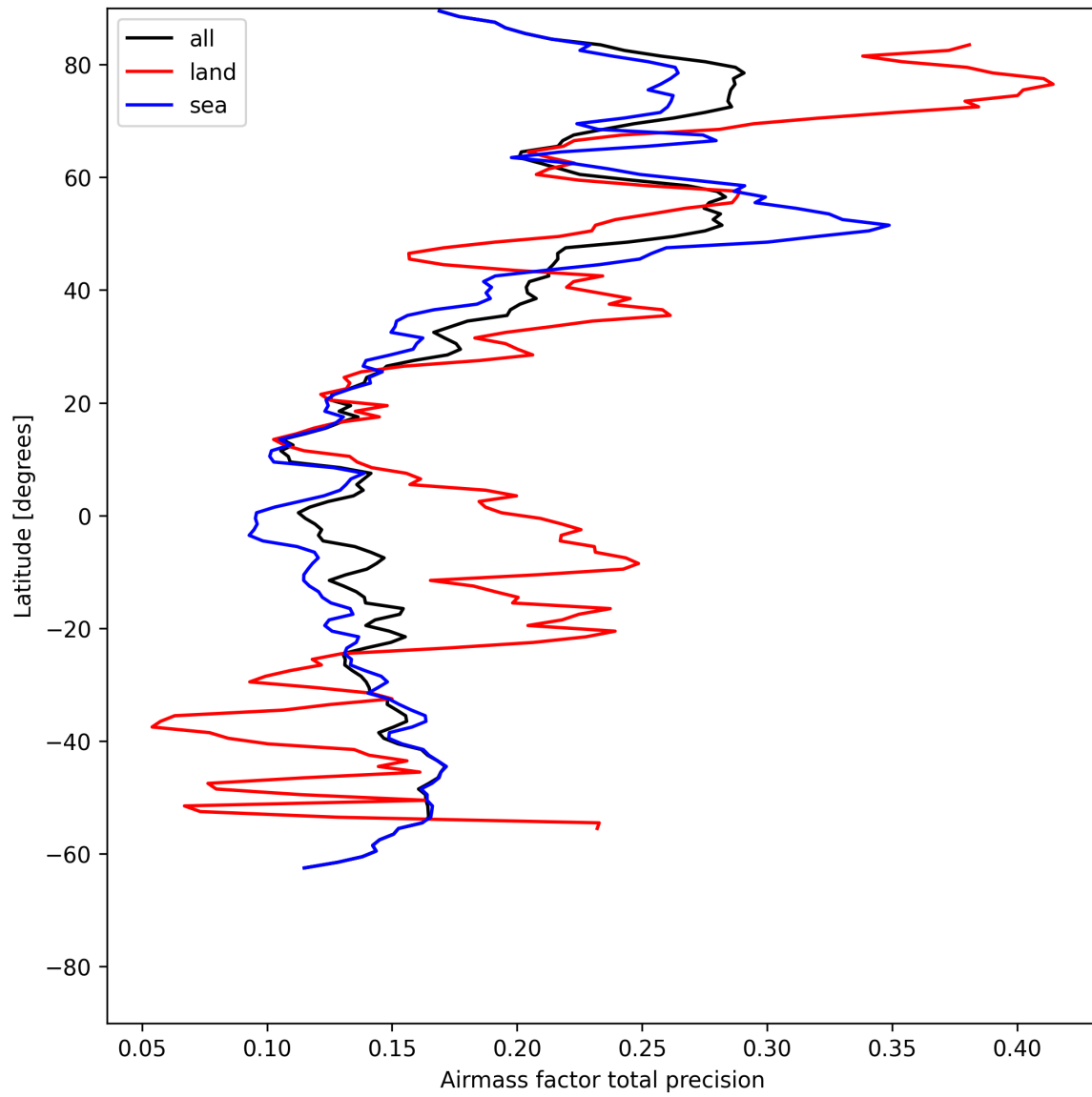
Figure 27: Zonal average of “Airmass factor total precision” for 2025-05-28 to 2025-05-30.
