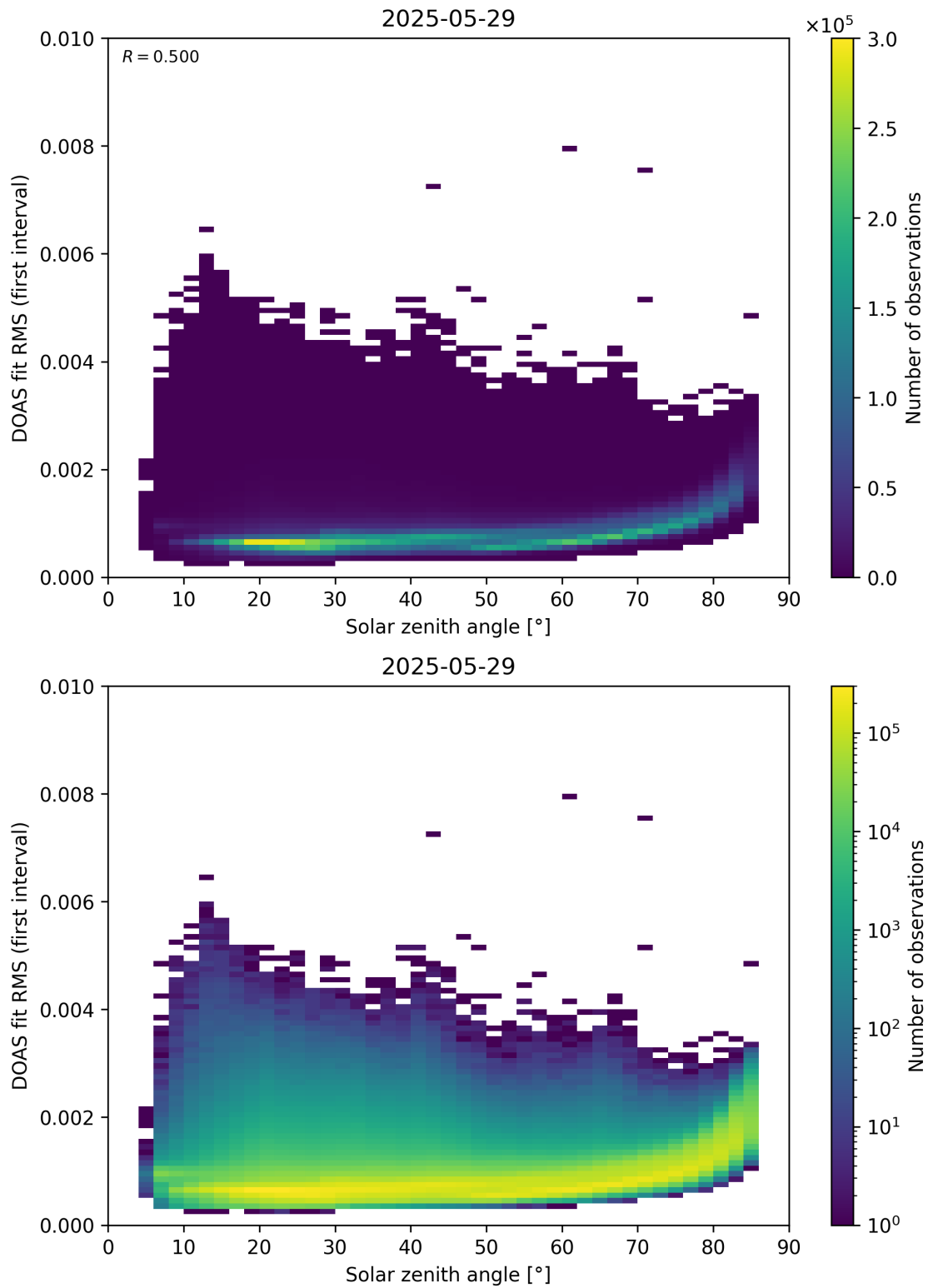
Figure 167: Scatter density plot of “Solar zenith angle” against “DOAS fit RMS (first interval)” for 2025-05-28 to 2025-05-30.
