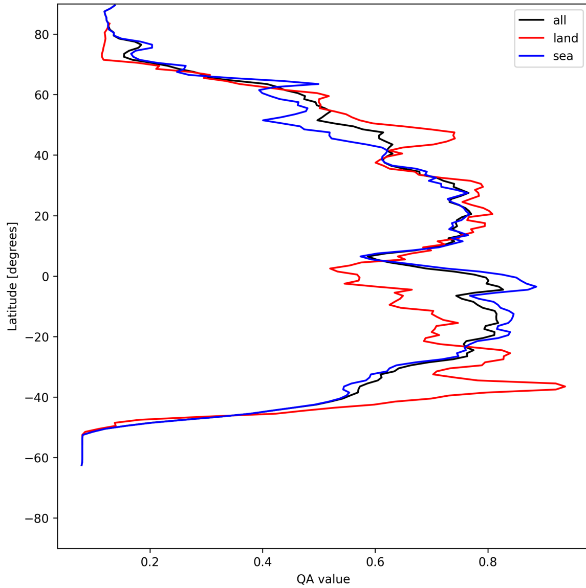
Figure 20: Zonal average of “QA value” for 2025-05-28 to 2025-05-30.
