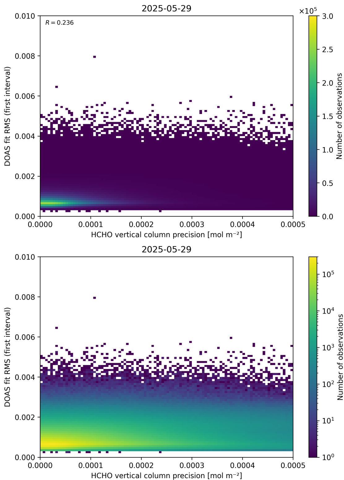
Figure 136: Scatter density plot of “HCHO vertical column precision” against “DOAS fit RMS (first interval)” for 2025-05-28 to 2025-05-30.
