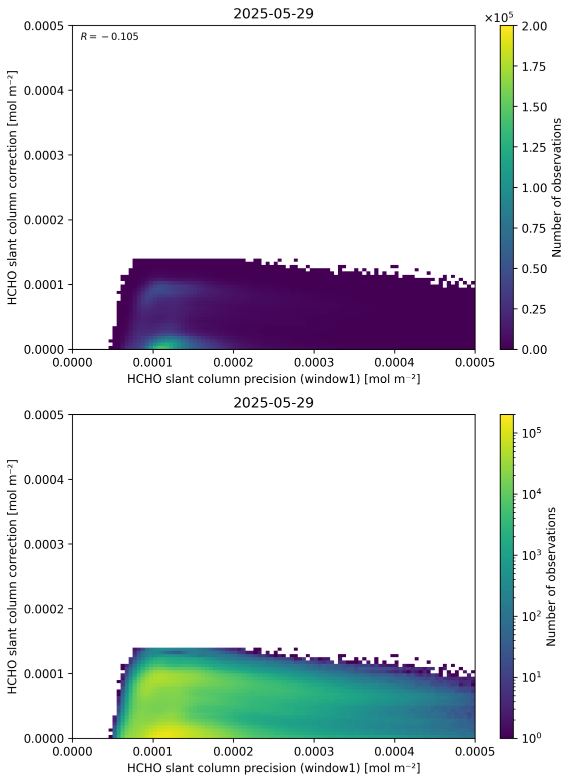
Figure 93: Scatter density plot of “HCHO slant column precision (window1)” against “HCHO slant column correction” for 2025-05-28 to 2025-05-30.
