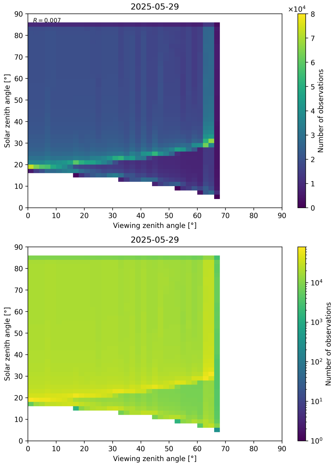
Figure 197: Scatter density plot of “Viewing zenith angle” against “Solar zenith angle” for 2025-05-28 to 2025-05-30.
