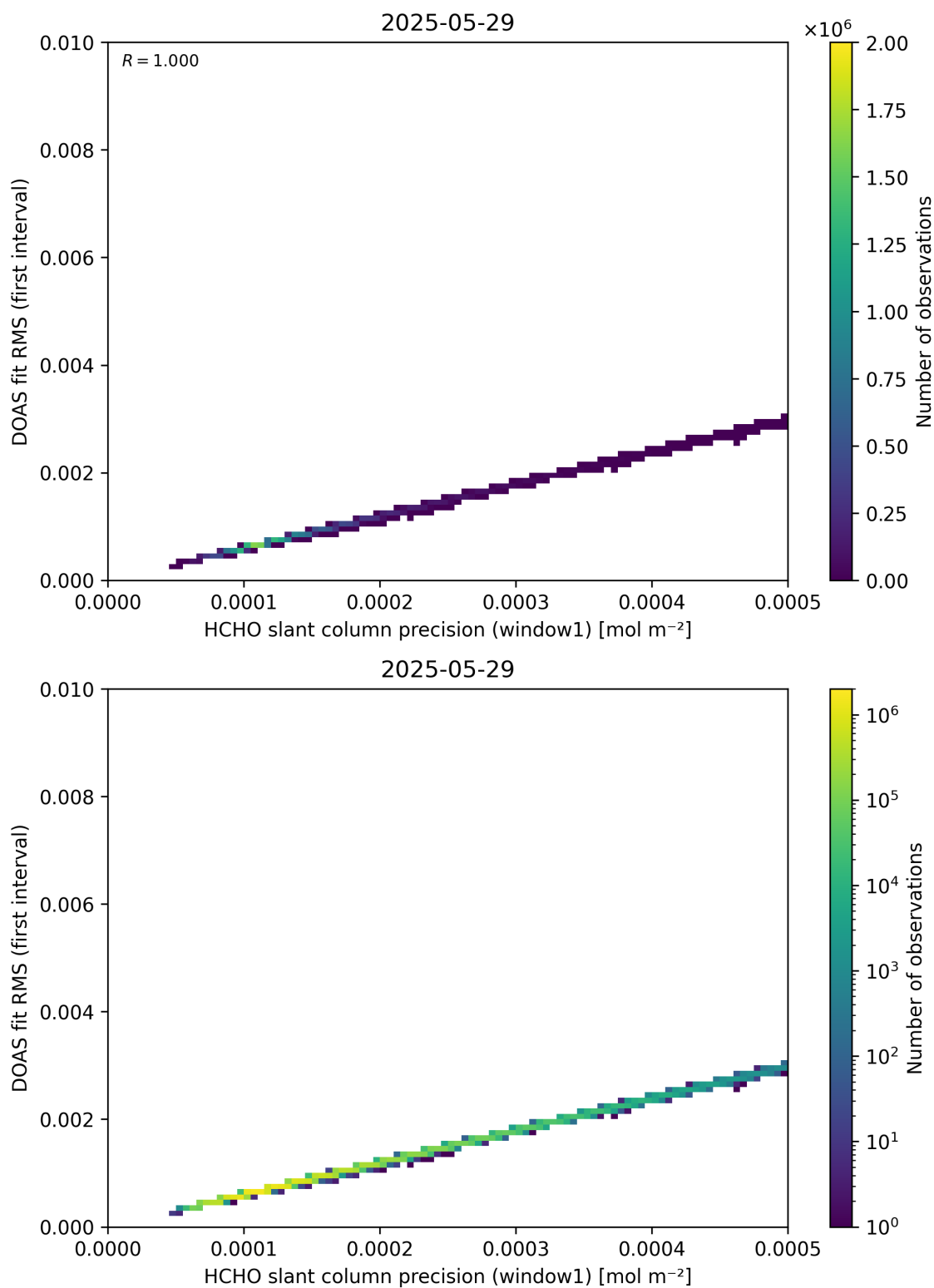
Figure 88: Scatter density plot of “HCHO slant column precision (window1)” against “DOAS fit RMS (first interval)” for 2025-05-28 to 2025-05-30.
