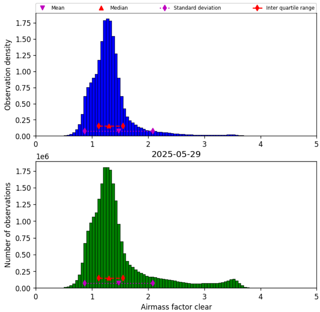
Figure 42: Histogram of “Airmass factor clear” for 2025-05-28 to 2025-05-30
