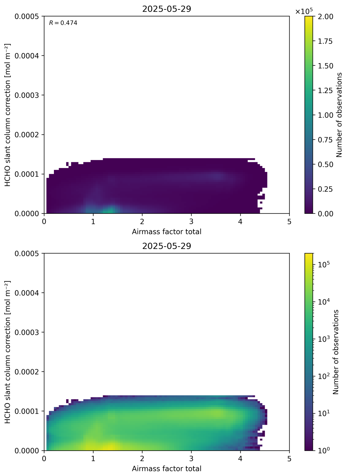
Figure 102: Scatter density plot of “Airmass factor total” against “HCHO slant column correction” for 2025-05-28 to 2025-05-30.
