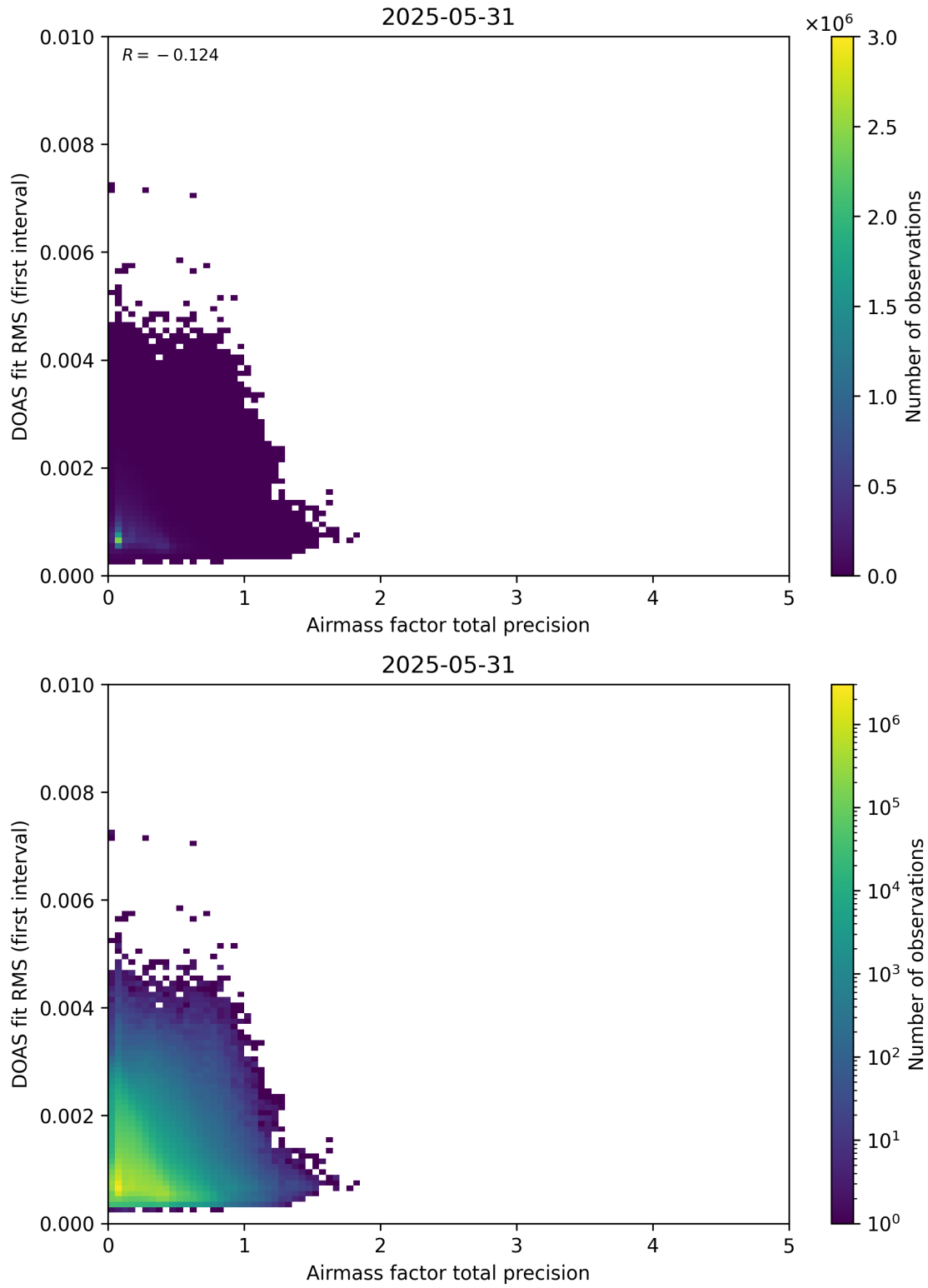
Figure 105: Scatter density plot of “Airmass factor total precision” against “DOAS fit RMS (first interval)” for 2025-05-31 to 2025-06-01.
