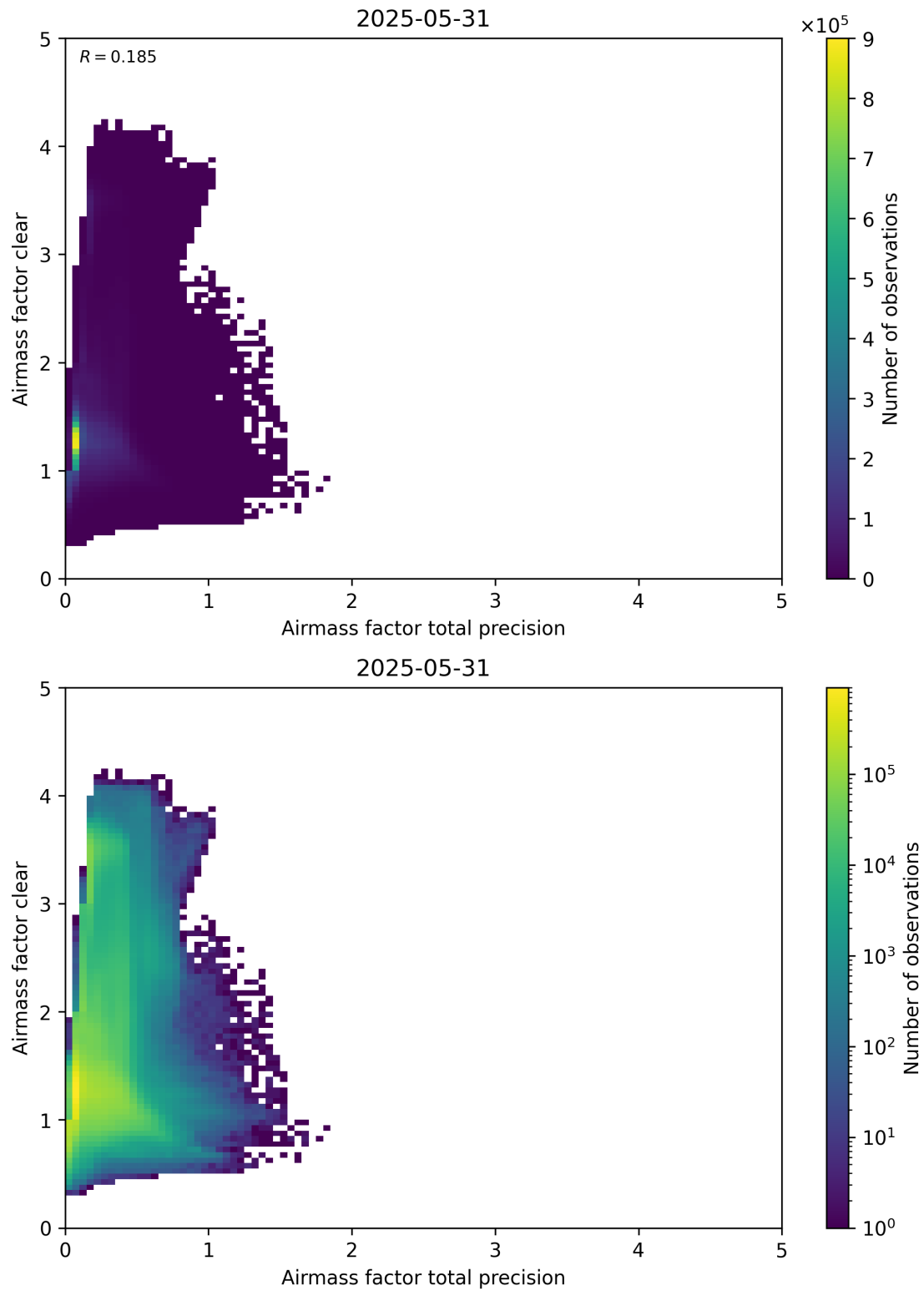
Figure 108: Scatter density plot of “Airmass factor total precision” against “Airmass factor clear” for 2025-05-31 to 2025-06-01.
