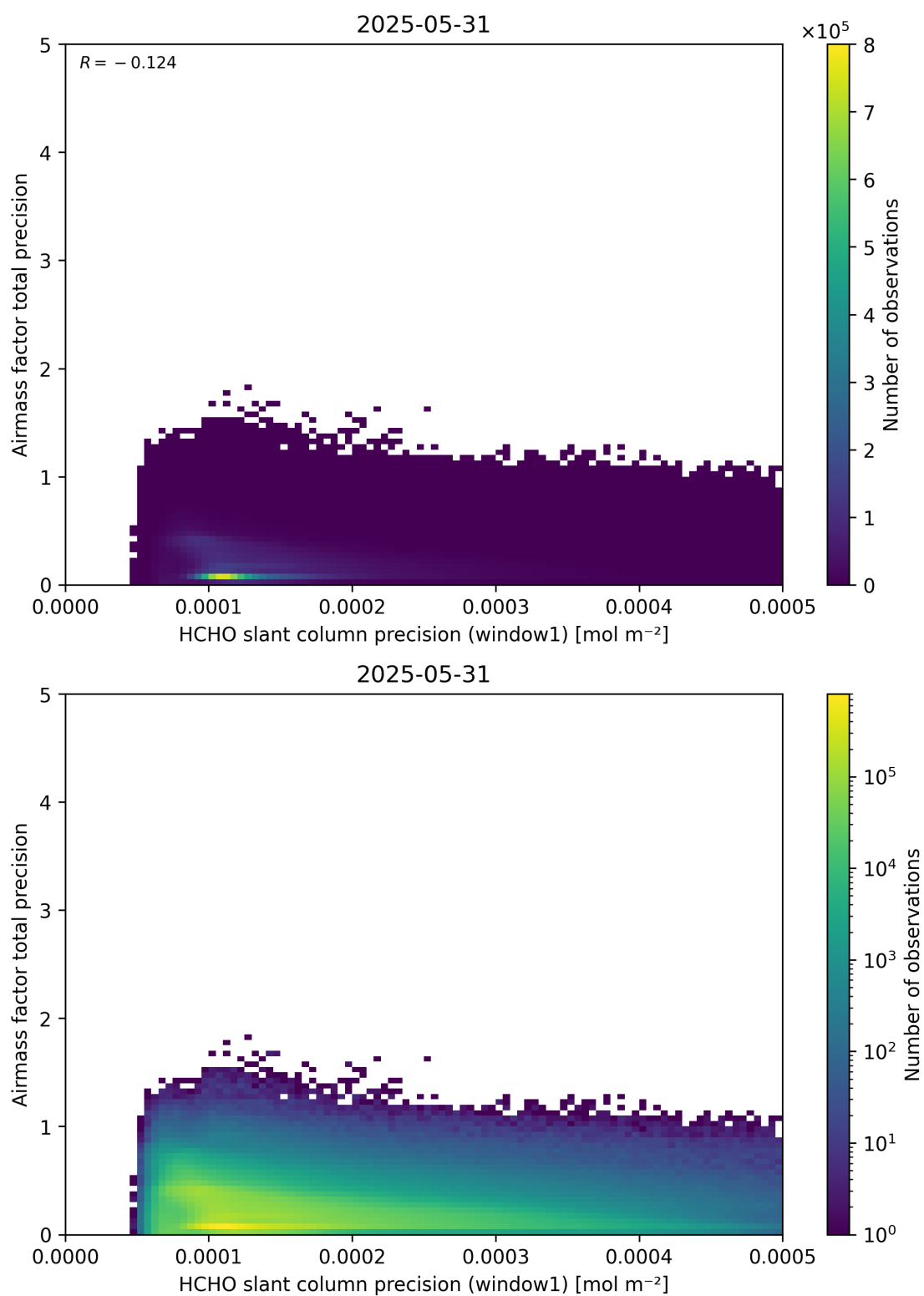
Figure 95: Scatter density plot of “HCHO slant column precision (window1)” against “Airmass factor total precision” for 2025-05-31 to 2025-06-01.
