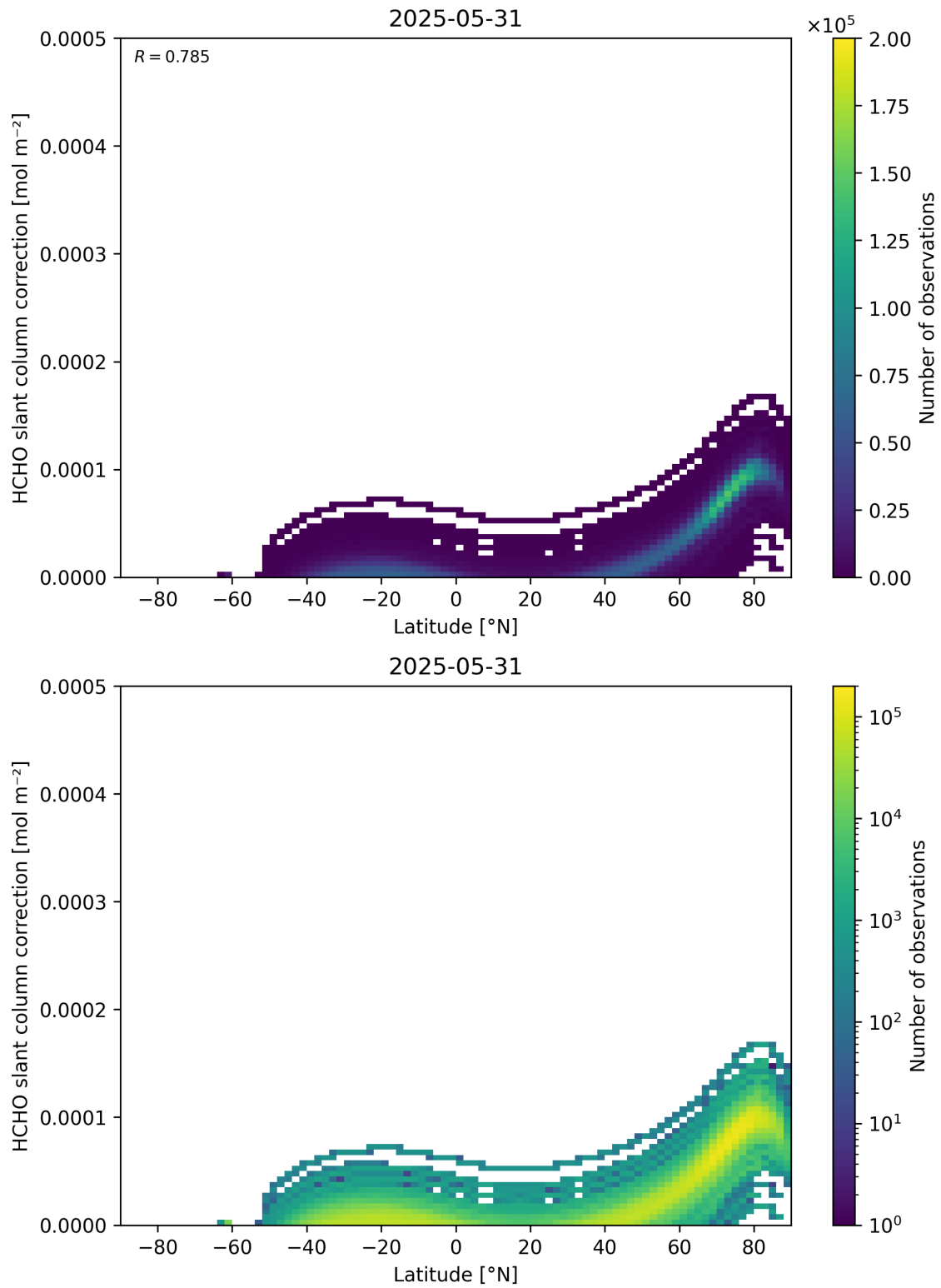
Figure 158: Scatter density plot of “Latitude” against “HCHO slant column correction” for 2025-05-31 to 2025-06-01.
