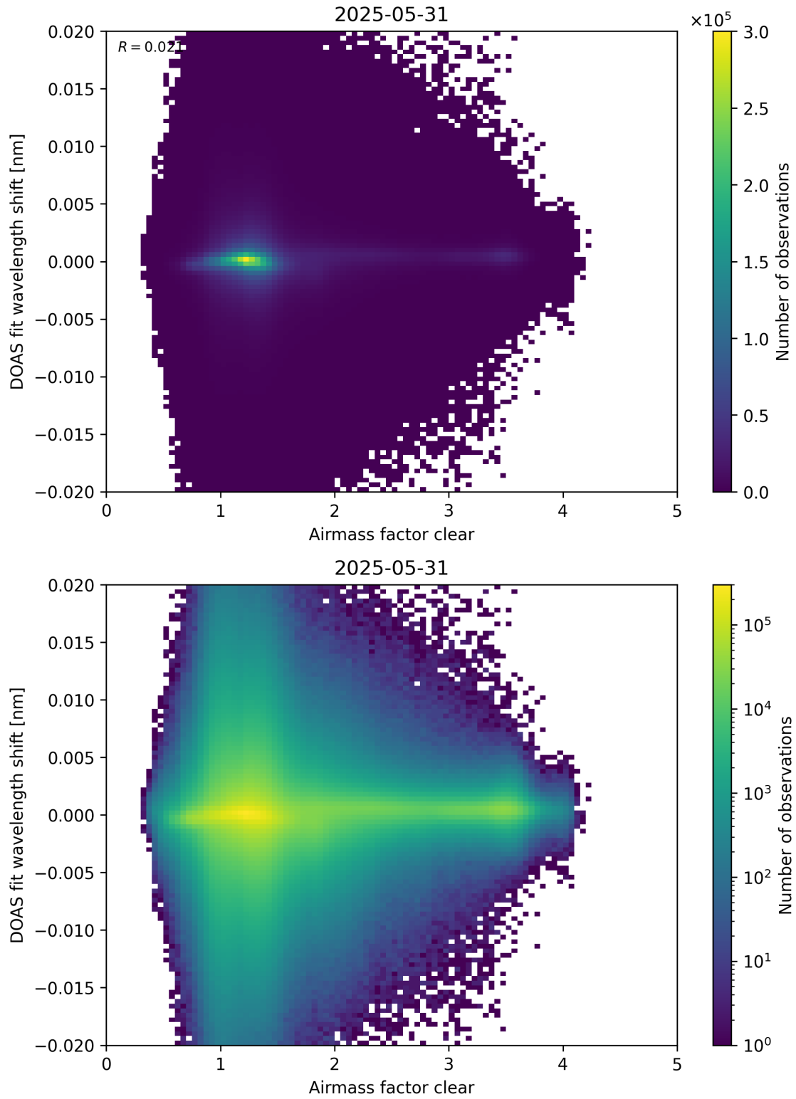
Figure 72: Scatter density plot of “Airmass factor clear” against “DOAS fit wavelength shift” for 2025-05-31 to 2025-06-01.
