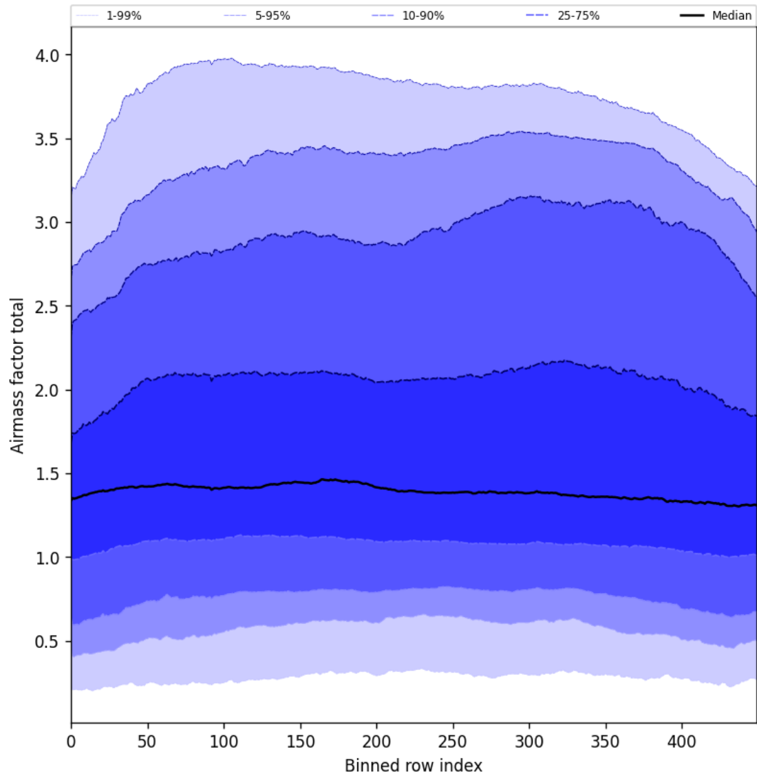
Figure 54: Along track statistics of “Airmass factor total” for 2025-05-31 to 2025-06-01
