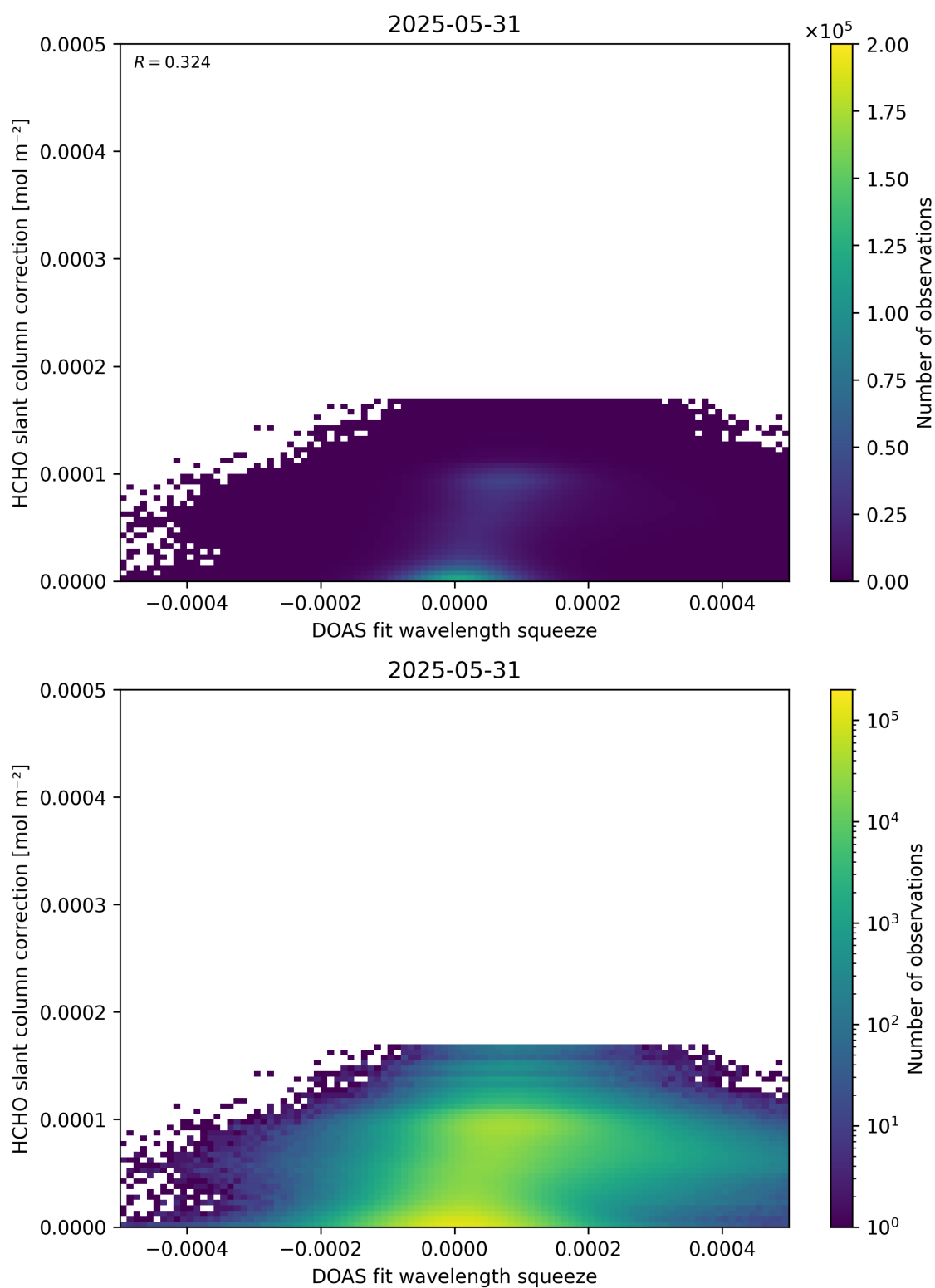
Figure 70: Scatter density plot of “DOAS fit wavelength squeeze” against “HCHO slant column correction” for 2025-05-31 to 2025-06-01.
