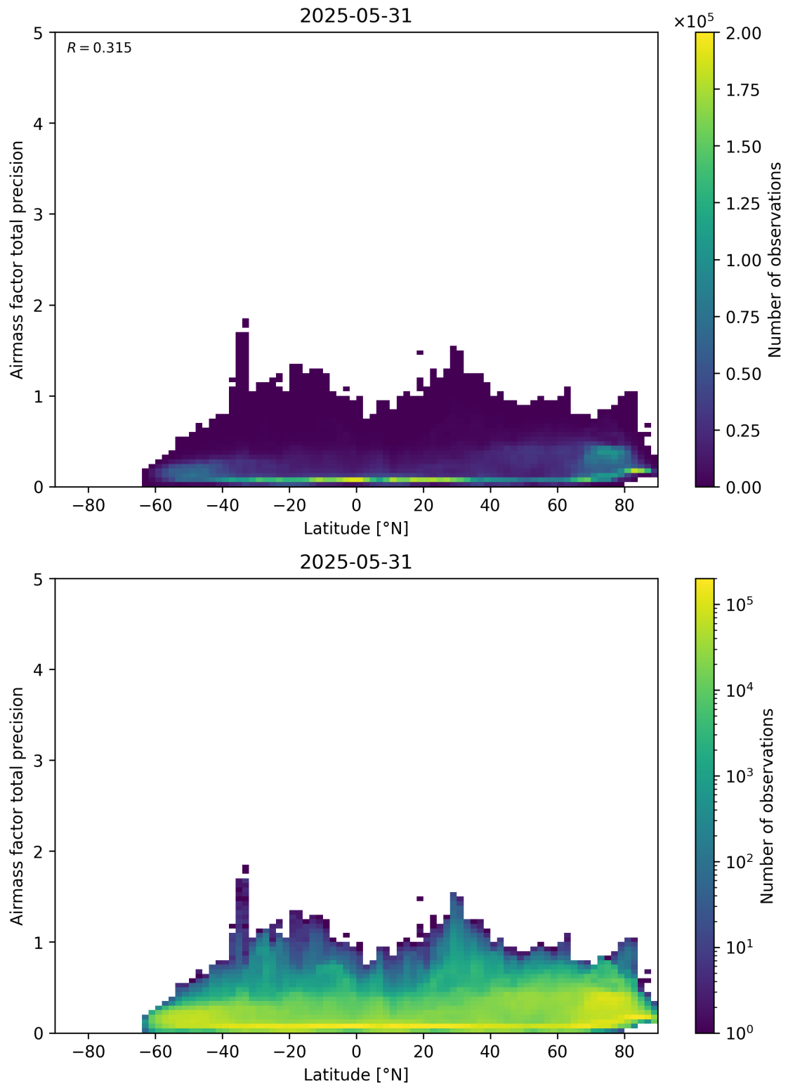
Figure 162: Scatter density plot of “Latitude” against “Airmass factor total precision” for 2025-05-31 to 2025-06-01.
