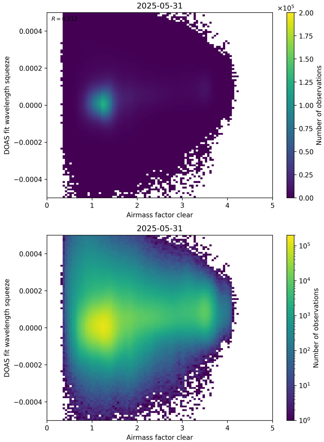
Figure 73: Scatter density plot of “Airmass factor clear” against “DOAS fit wavelength squeeze” for 2025-05-31 to 2025-06-01.
