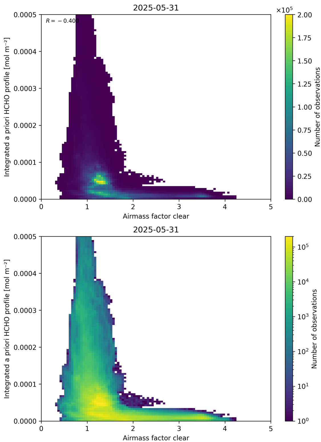
Figure 76: Scatter density plot of “Airmass factor clear” against “Integrated a priori HCHO profile” for 2025-05-31 to 2025-06-01.
