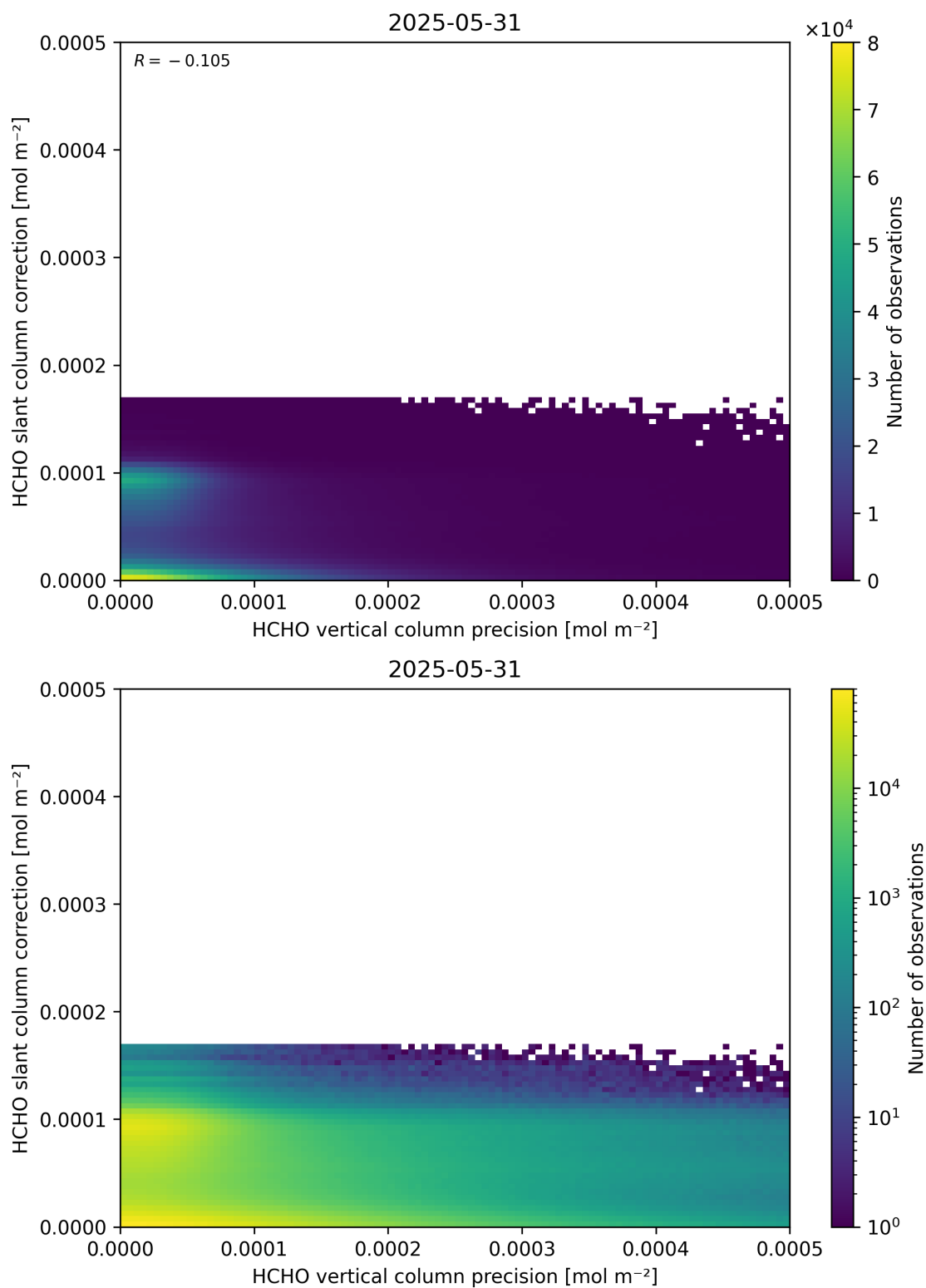
Figure 141: Scatter density plot of “HCHO vertical column precision” against “HCHO slant column correction” for 2025-05-31 to 2025-06-01.
