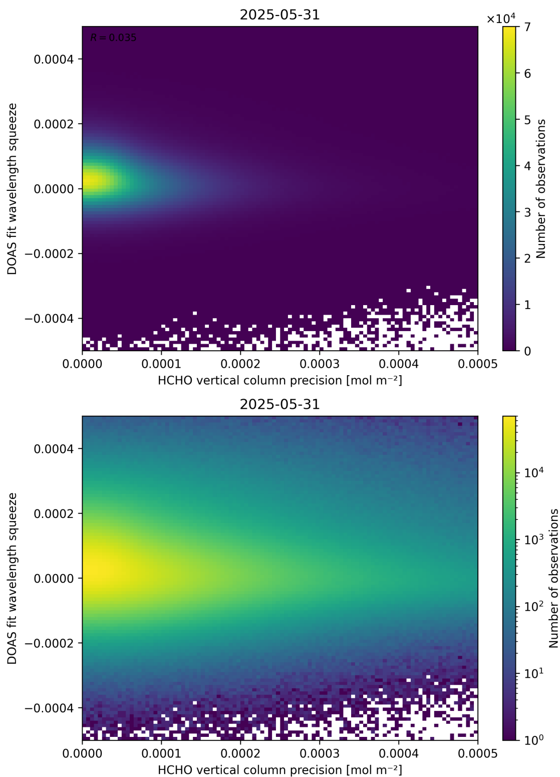
Figure 138: Scatter density plot of “HCHO vertical column precision” against “DOAS fit wavelength squeeze” for 2025-05-31 to 2025-06-01.
