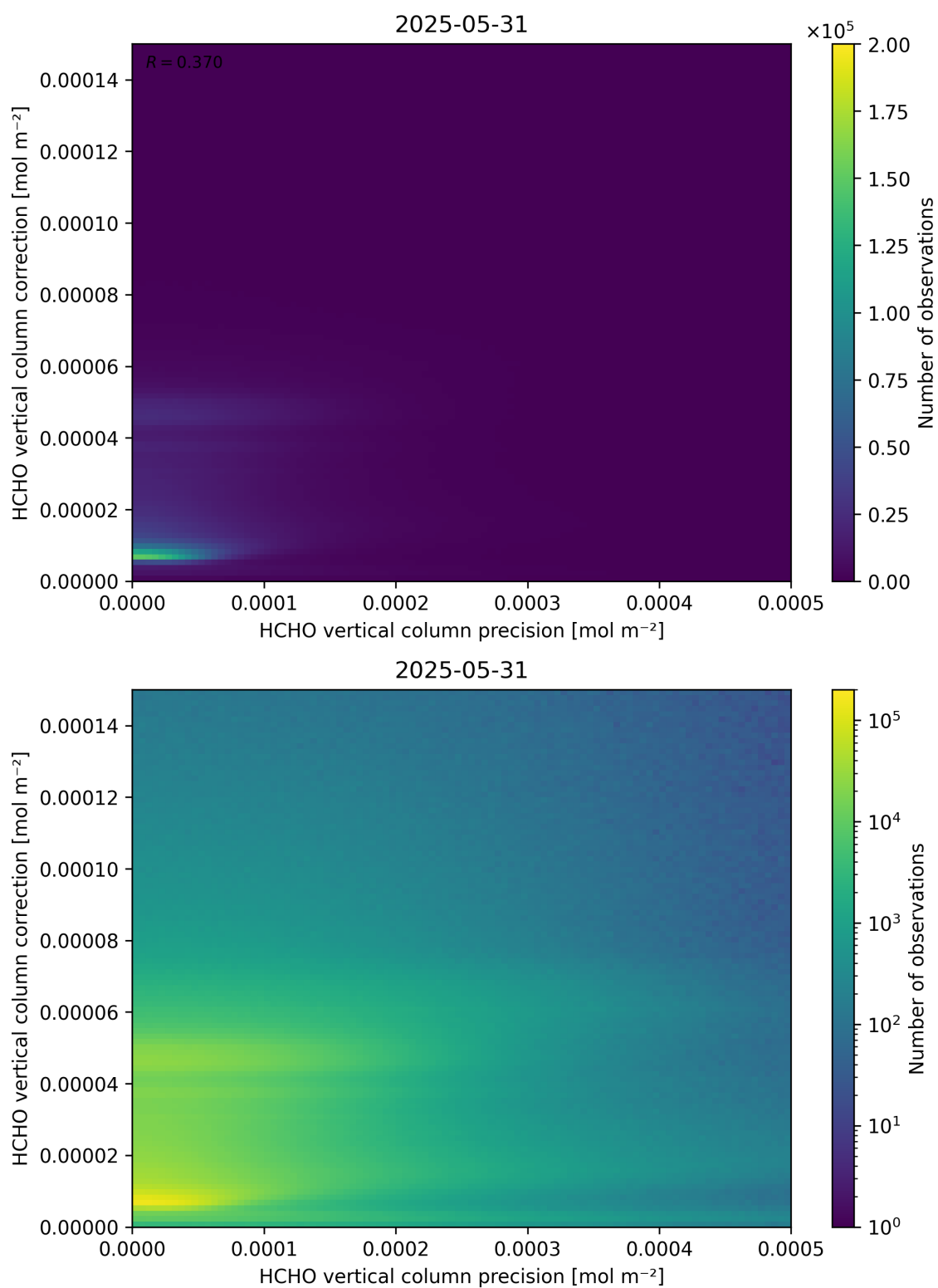
Figure 146: Scatter density plot of “HCHO vertical column precision” against “HCHO vertical column correction” for 2025-05-31 to 2025-06-01.
