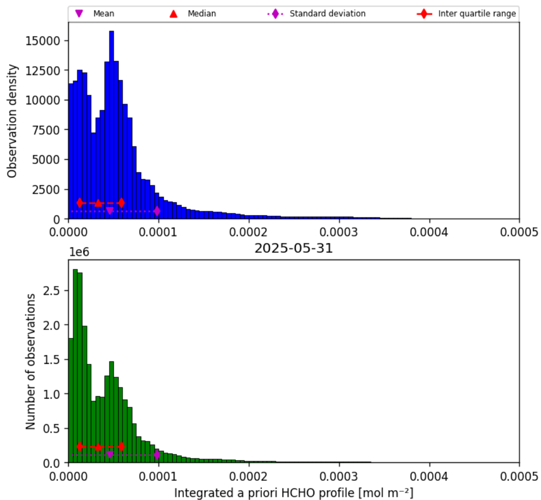
Figure 43: Histogram of “Integrated a priori HCHO profile” for 2025-05-31 to 2025-06-01
