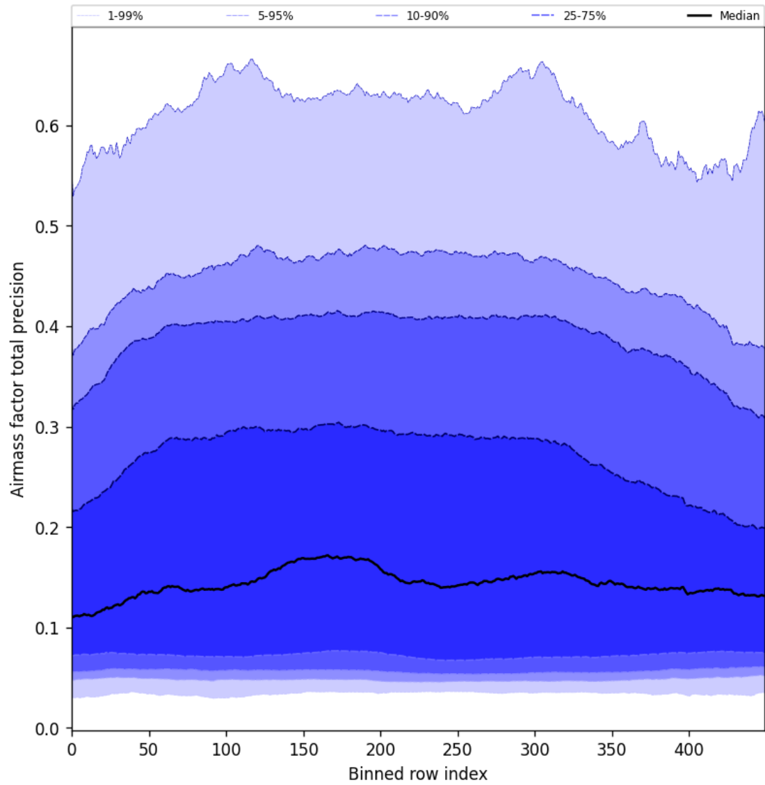
Figure 55: Along track statistics of “Airmass factor total precision” for 2025-05-31 to 2025-06-01
