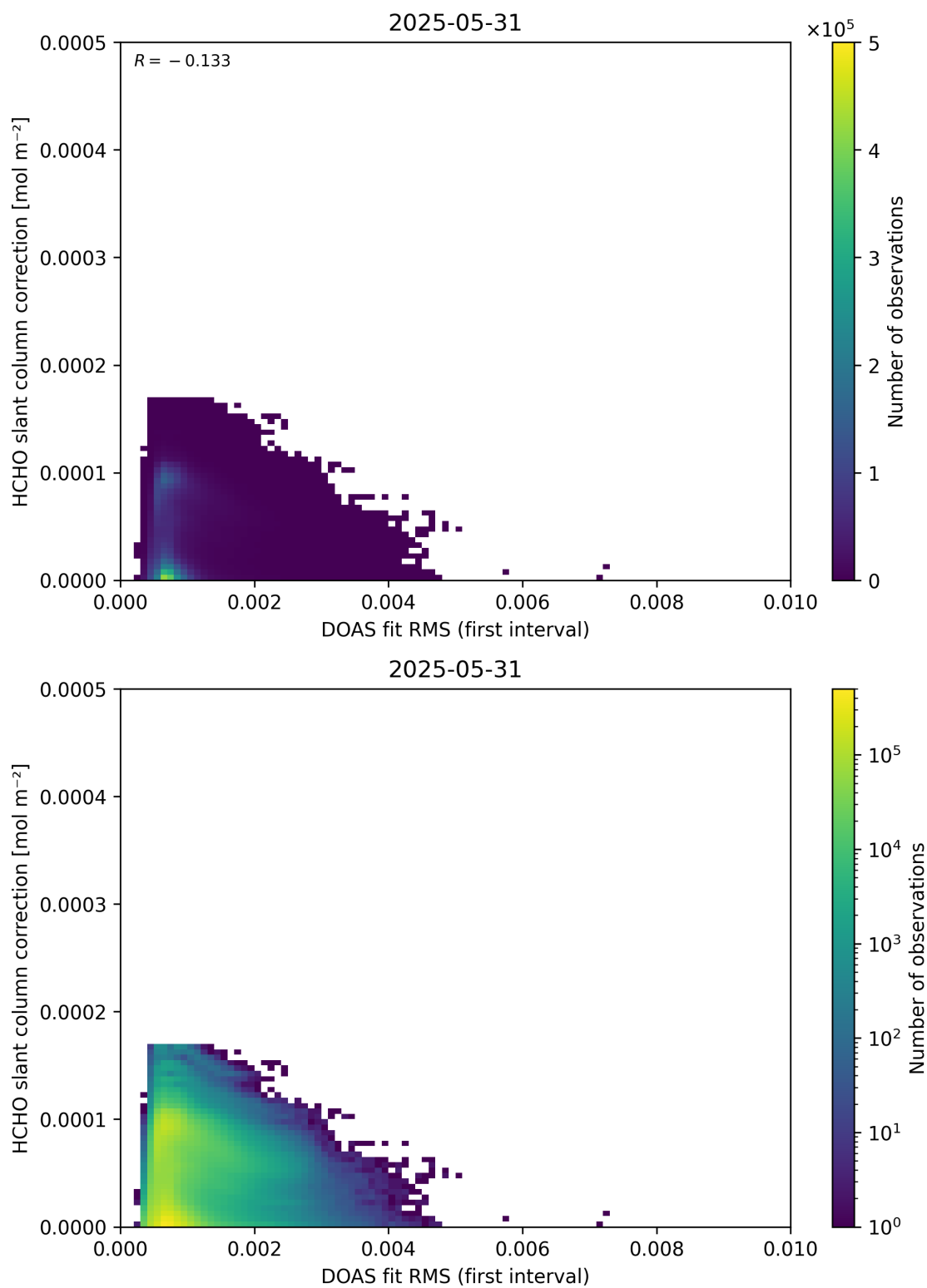
Figure 63: Scatter density plot of “DOAS fit RMS (first interval)” against “HCHO slant column correction” for 2025-05-31 to 2025-06-01.
