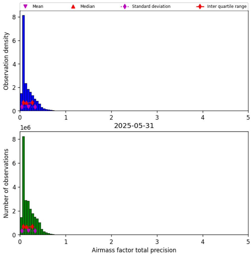
Figure 41: Histogram of “Airmass factor total precision” for 2025-05-31 to 2025-06-01
