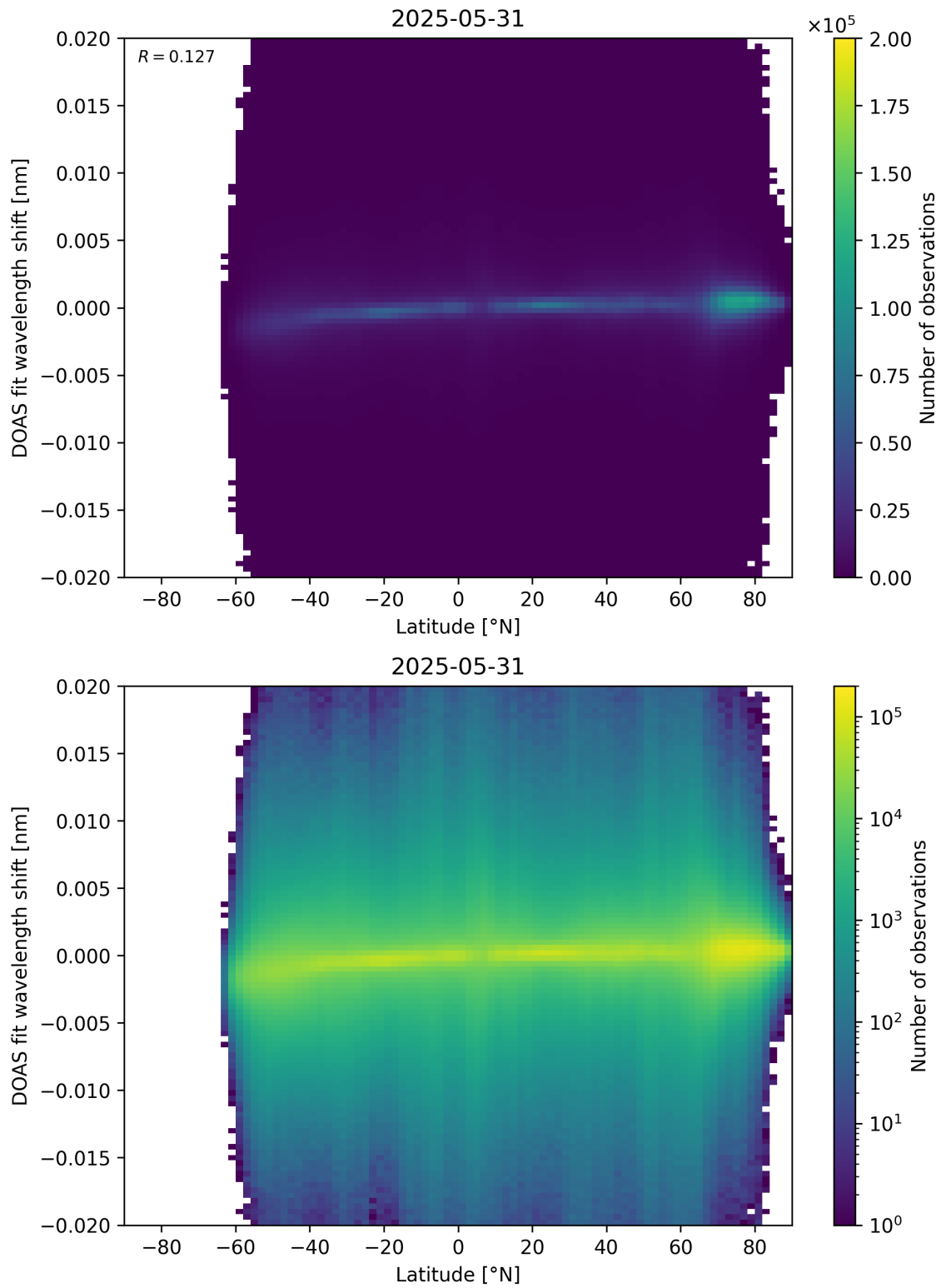
Figure 154: Scatter density plot of “Latitude” against “DOAS fit wavelength shift” for 2025-05-31 to 2025-06-01.
