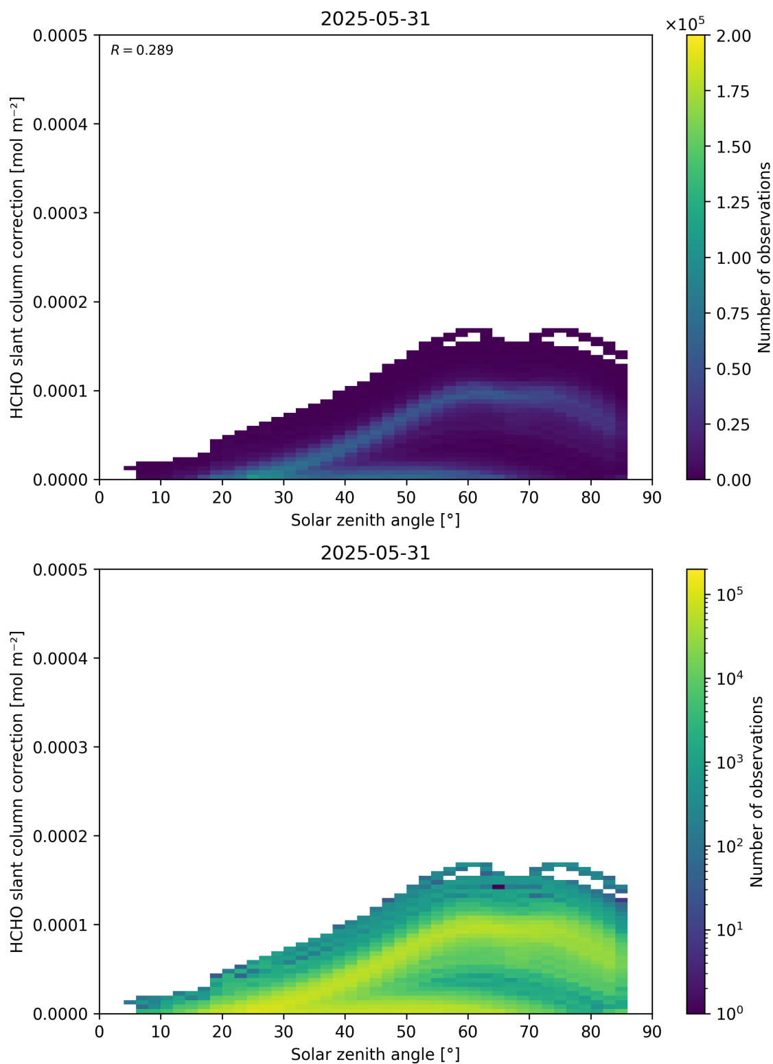
Figure 172: Scatter density plot of “Solar zenith angle” against “HCHO slant column correction” for 2025-05-31 to 2025-06-01.
