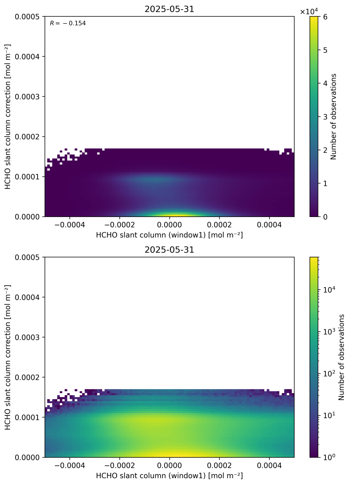
Figure 83: Scatter density plot of “HCHO slant column (window1)” against “HCHO slant column correction” for 2025-05-31 to 2025-06-01.
