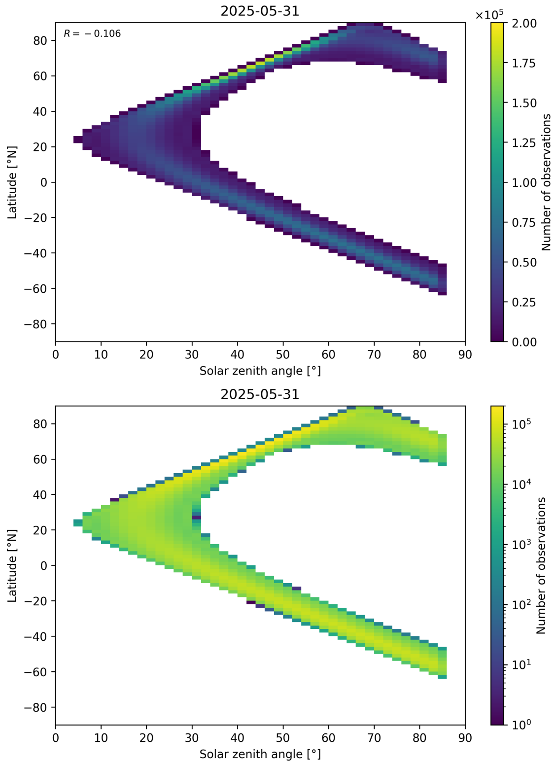
Figure 181: Scatter density plot of “Solar zenith angle” against “Latitude” for 2025-05-31 to 2025-06-01.
