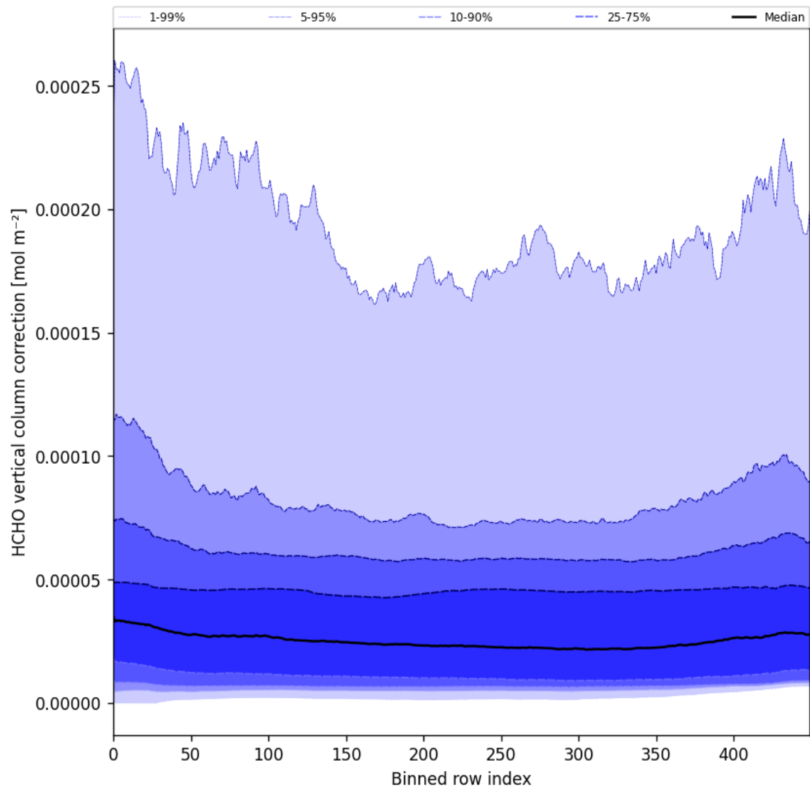
Figure 51: Along track statistics of “HCHO vertical column correction” for 2025-05-31 to 2025-06-01
