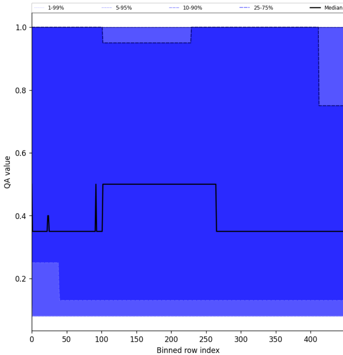
Figure 48: Along track statistics of “QA value” for 2025-05-31 to 2025-06-01
