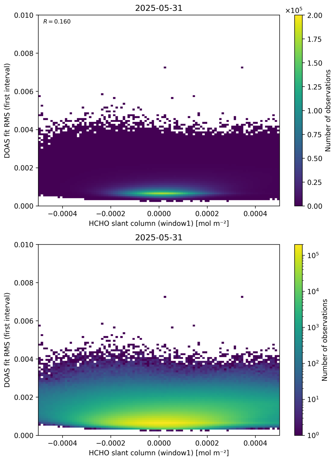
Figure 78: Scatter density plot of “HCHO slant column (window1)” against “DOAS fit RMS (first interval)” for 2025-05-31 to 2025-06-01.
