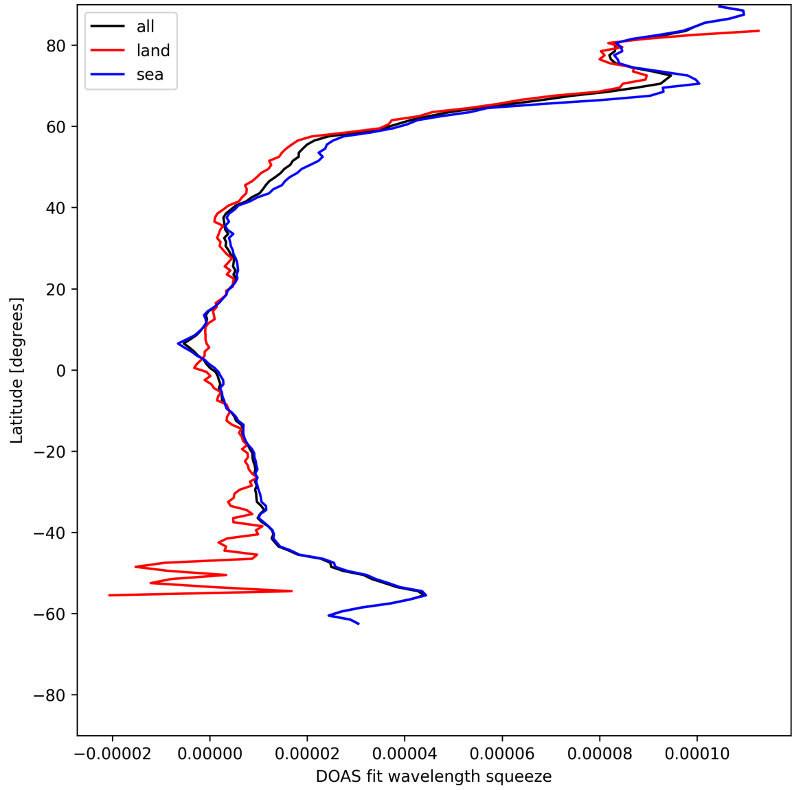
Figure 31: Zonal average of “DOAS fit wavelength squeeze” for 2025-05-31 to 2025-06-01.
