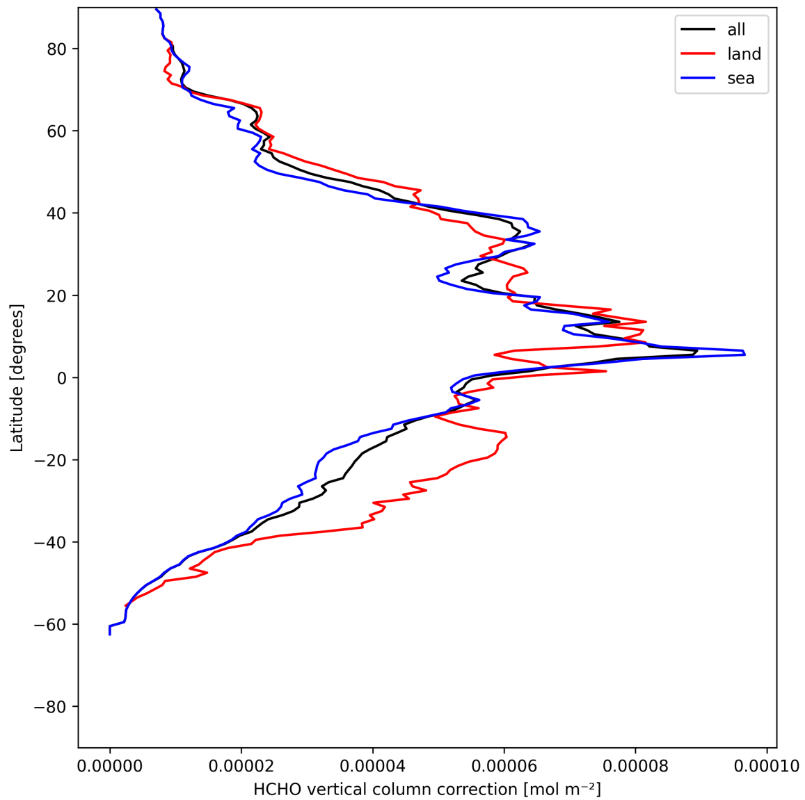
Figure 23: Zonal average of “HCHO vertical column correction” for 2025-05-31 to 2025-06-01.
