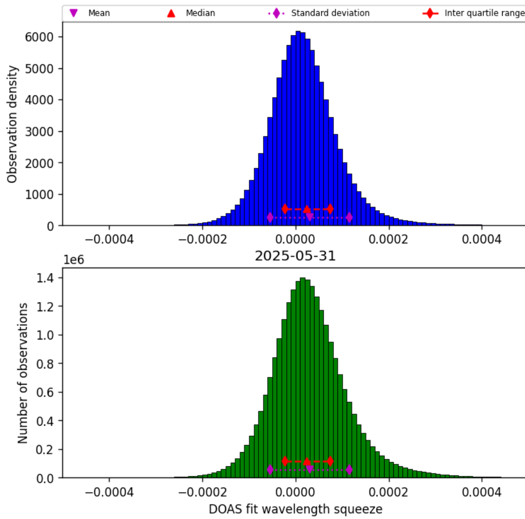
Figure 45: Histogram of “DOAS fit wavelength squeeze” for 2025-05-31 to 2025-06-01
