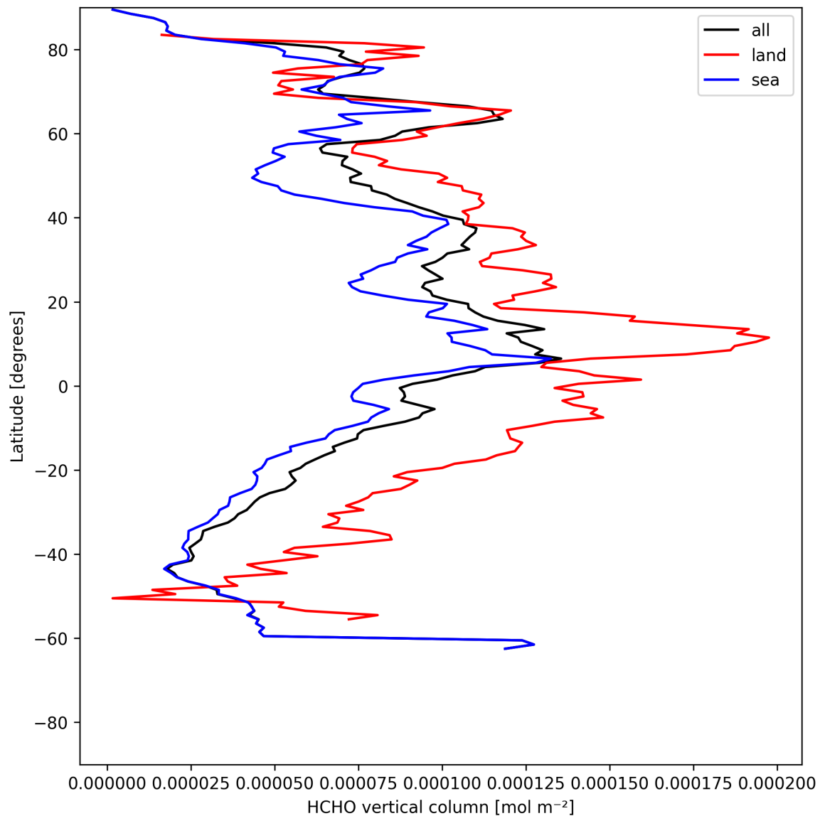
Figure 21: Zonal average of “HCHO vertical column” for 2025-05-31 to 2025-06-01.
