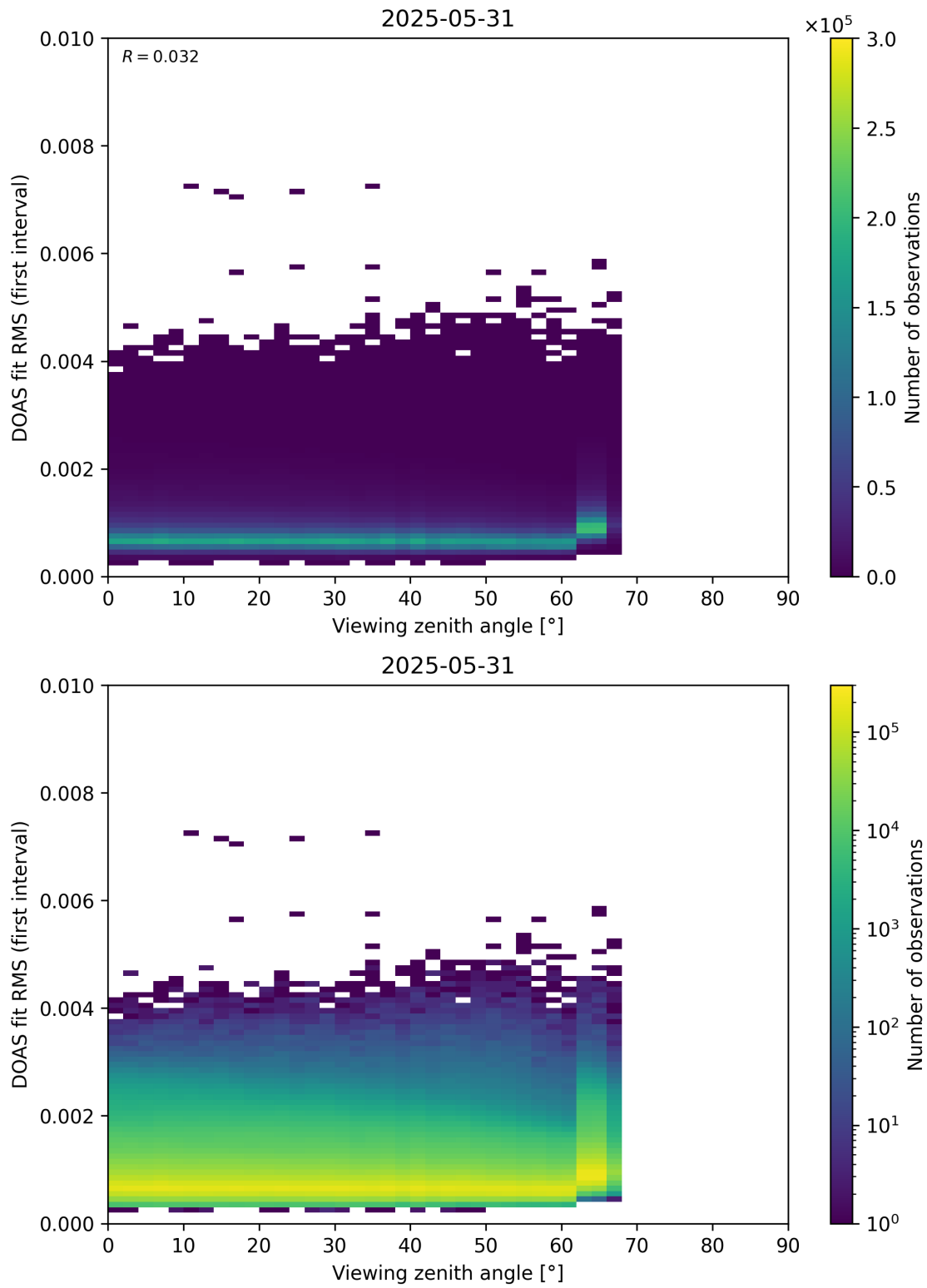
Figure 182: Scatter density plot of “Viewing zenith angle” against “DOAS fit RMS (first interval)” for 2025-05-31 to 2025-06-01.
