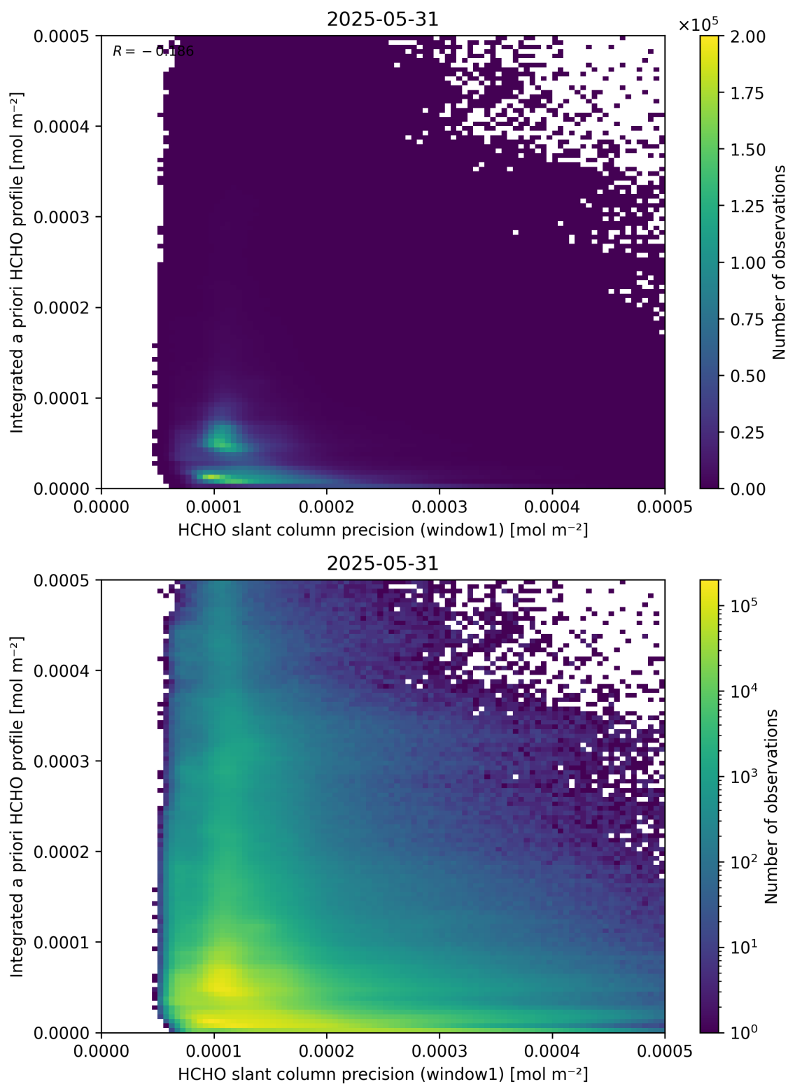
Figure 96: Scatter density plot of “HCHO slant column precision (window1)” against “Integrated a priori HCHO profile” for 2025-05-31 to 2025-06-01.
