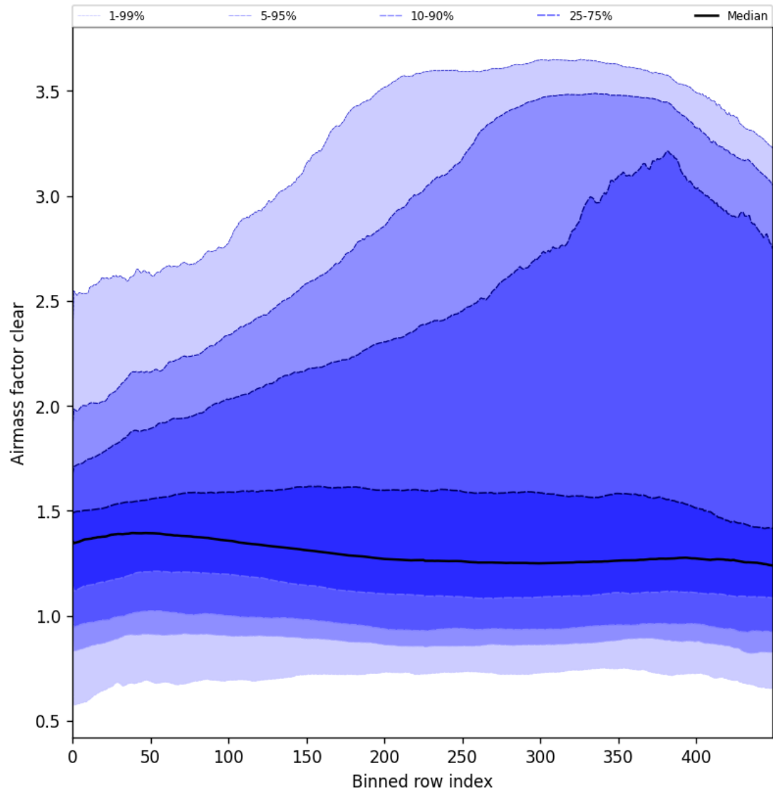
Figure 56: Along track statistics of “Airmass factor clear” for 2025-05-31 to 2025-06-01
