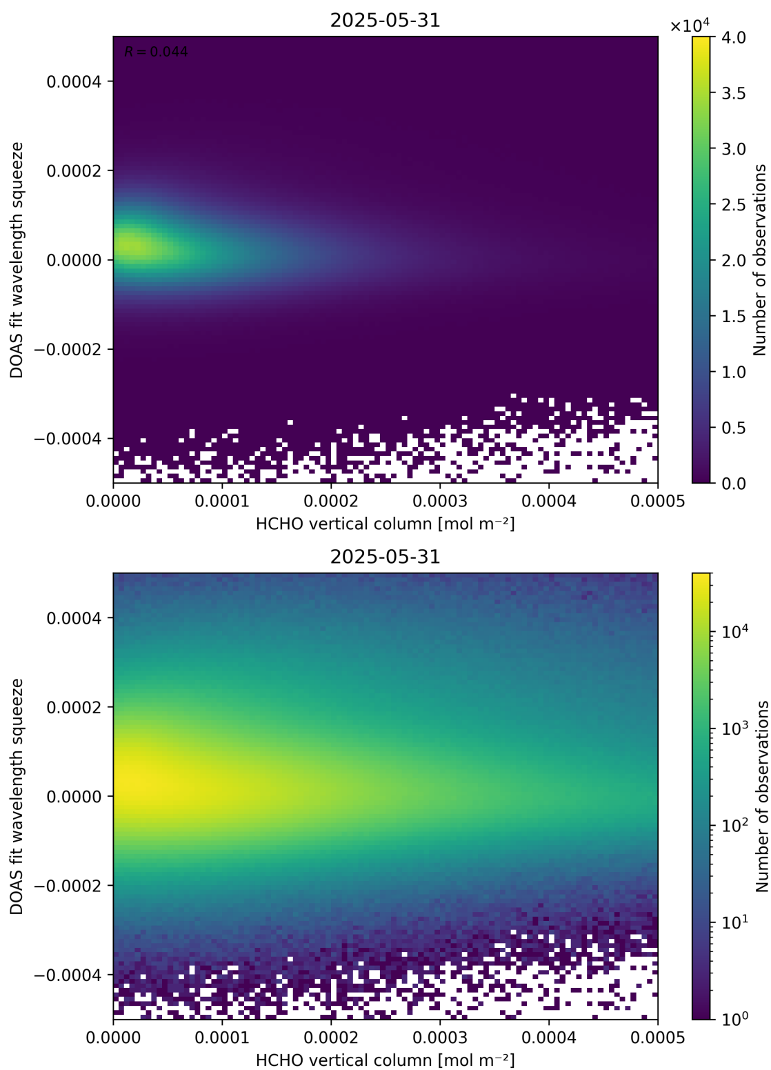
Figure 125: Scatter density plot of “HCHO vertical column” against “DOAS fit wavelength squeeze” for 2025-05-31 to 2025-06-01.
