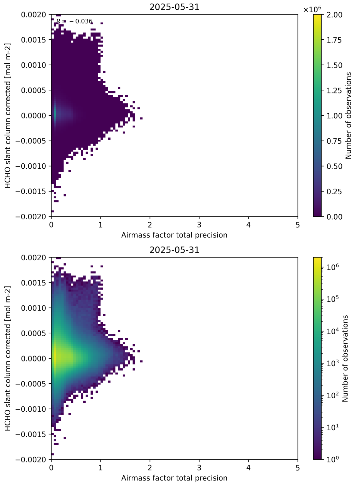
Figure 109: Scatter density plot of “Airmass factor total precision” against “HCHO slant column corrected” for 2025-05-31 to 2025-06-01.
