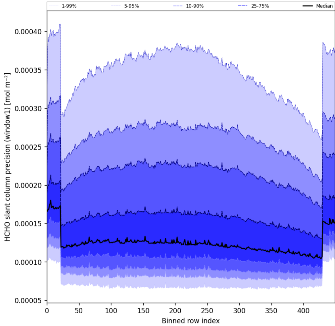
Figure 53: Along track statistics of “HCHO slant column precision (window1)” for 2025-05-31 to 2025-06-01
