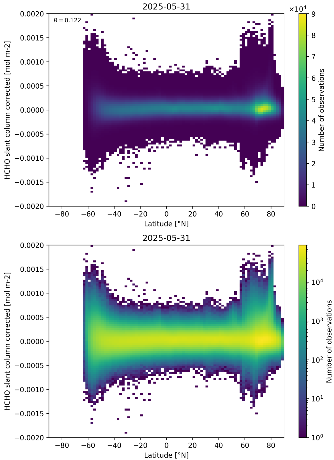
Figure 157: Scatter density plot of “Latitude” against “HCHO slant column corrected” for 2025-05-31 to 2025-06-01.
