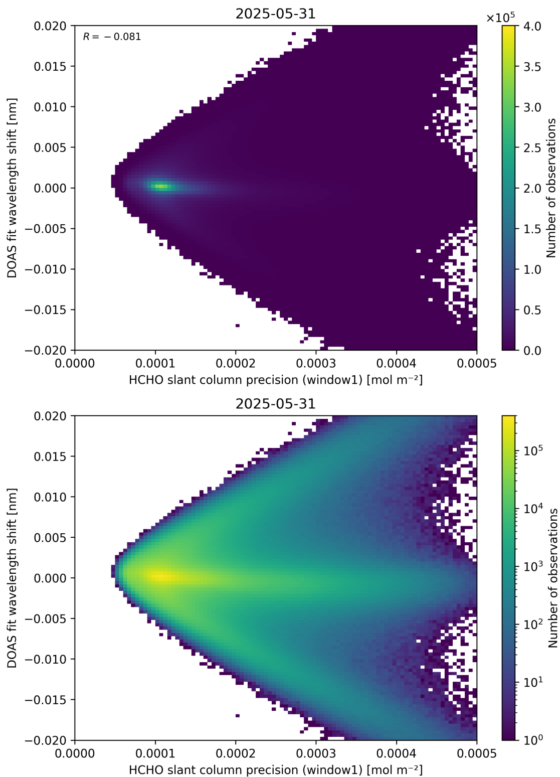
Figure 89: Scatter density plot of “HCHO slant column precision (window1)” against “DOAS fit wavelength shift” for 2025-05-31 to 2025-06-01.
