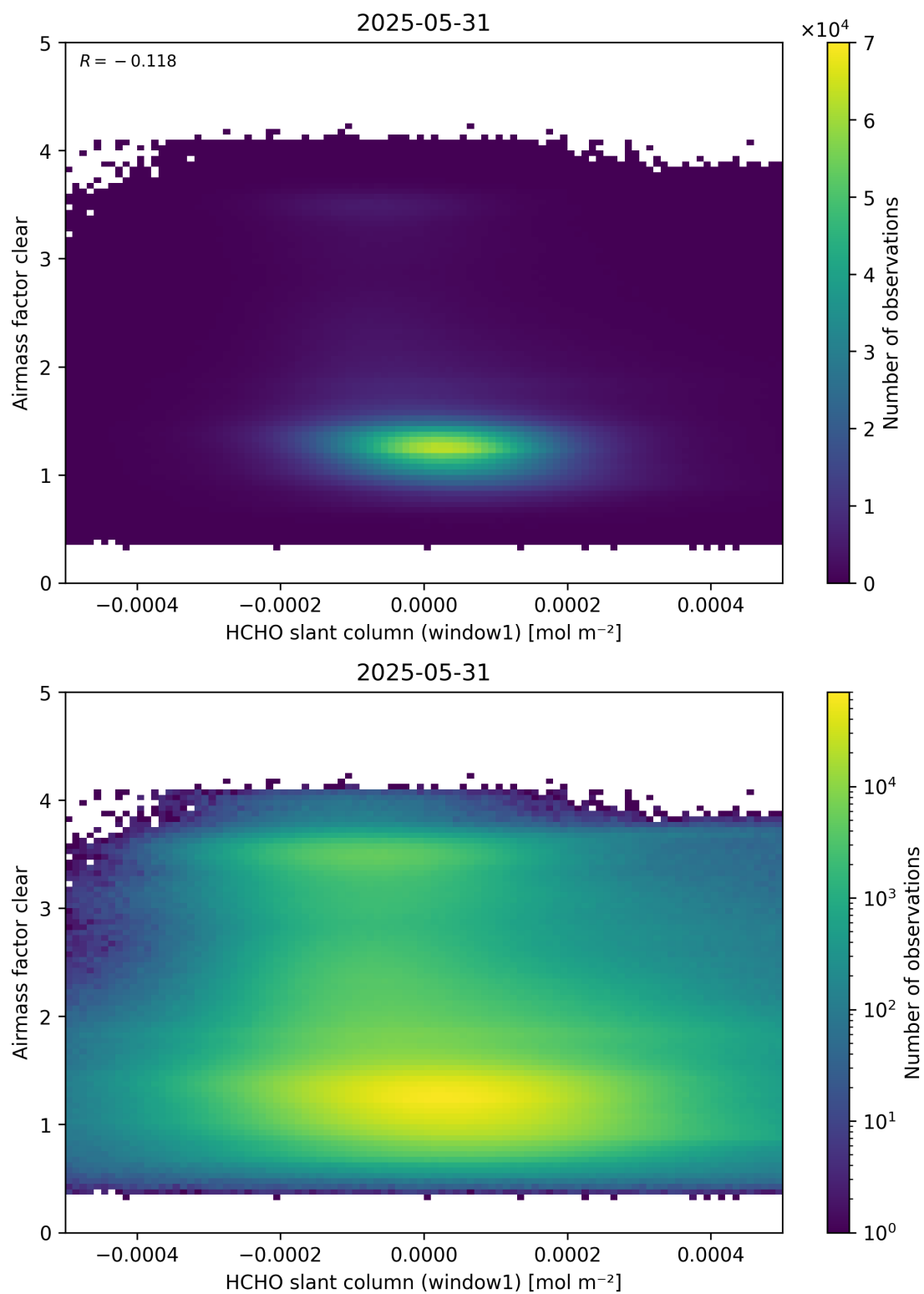
Figure 81: Scatter density plot of “HCHO slant column (window1)” against “Airmass factor clear” for 2025-05-31 to 2025-06-01.
