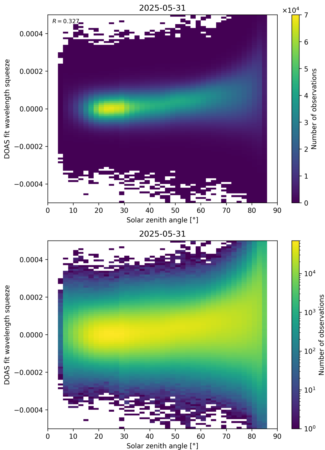
Figure 169: Scatter density plot of “Solar zenith angle” against “DOAS fit wavelength squeeze” for 2025-05-31 to 2025-06-01.
