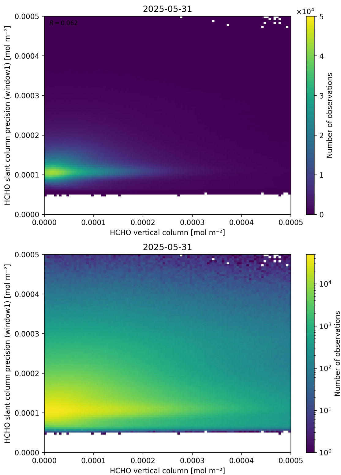
Figure 130: Scatter density plot of “HCHO vertical column” against “HCHO slant column precision (window1)” for 2025-05-31 to 2025-06-01.
