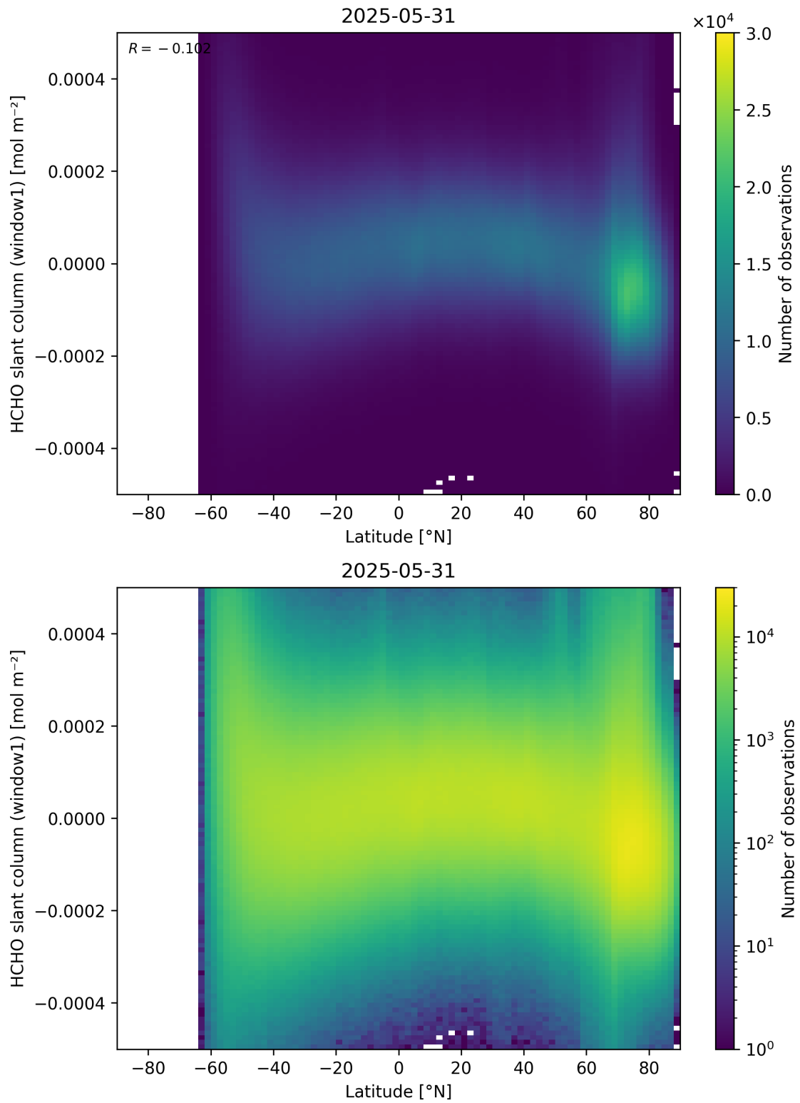
Figure 159: Scatter density plot of “Latitude” against “HCHO slant column (window1)” for 2025-05-31 to 2025-06-01.
