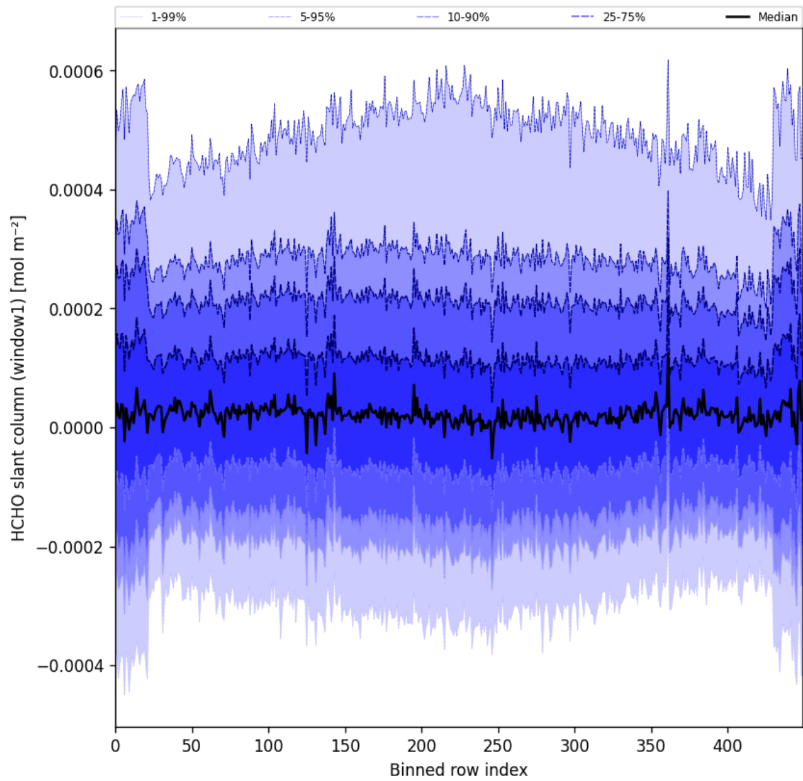
Figure 52: Along track statistics of “HCHO slant column (window1)” for 2025-05-31 to 2025-06-01
