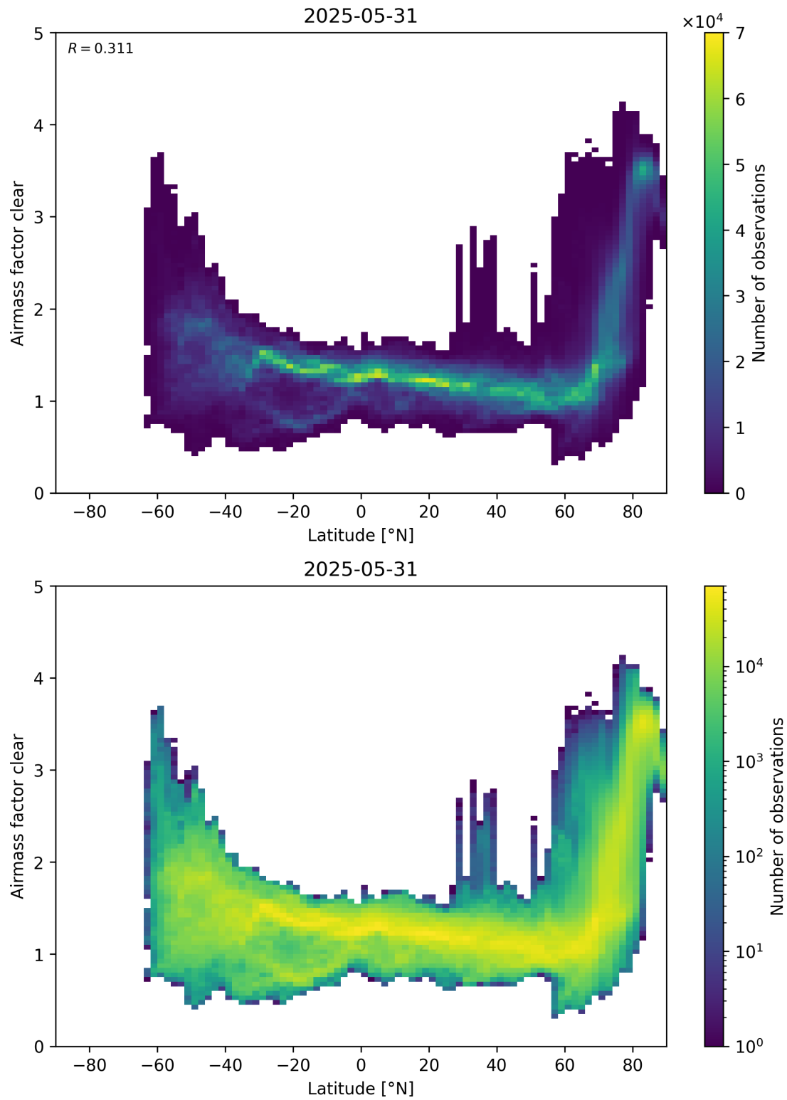
Figure 156: Scatter density plot of “Latitude” against “Airmass factor clear” for 2025-05-31 to 2025-06-01.
