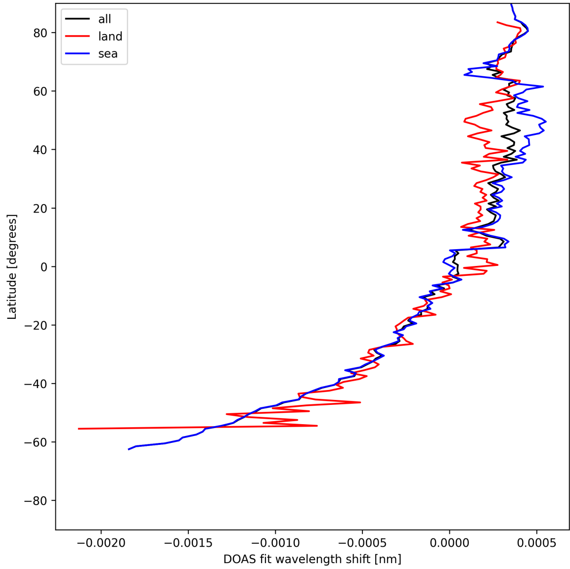
Figure 30: Zonal average of “DOAS fit wavelength shift” for 2025-05-31 to 2025-06-01.
