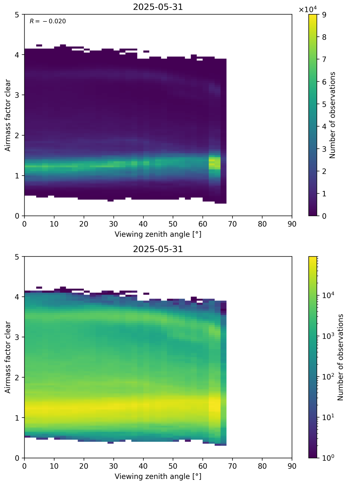
Figure 185: Scatter density plot of “Viewing zenith angle” against “Airmass factor clear” for 2025-05-31 to 2025-06-01.
