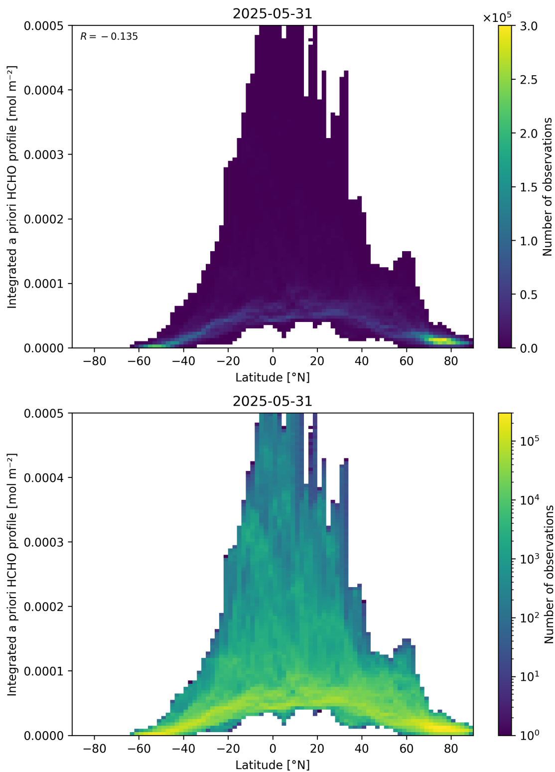
Figure 166: Scatter density plot of “Latitude” against “Integrated a priori HCHO profile” for 2025-05-31 to 2025-06-01.
