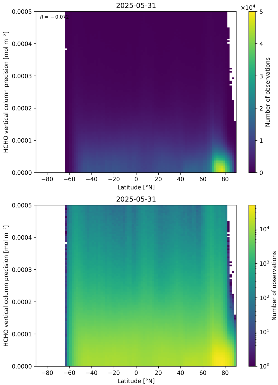
Figure 165: Scatter density plot of “Latitude” against “HCHO vertical column precision” for 2025-05-31 to 2025-06-01.
