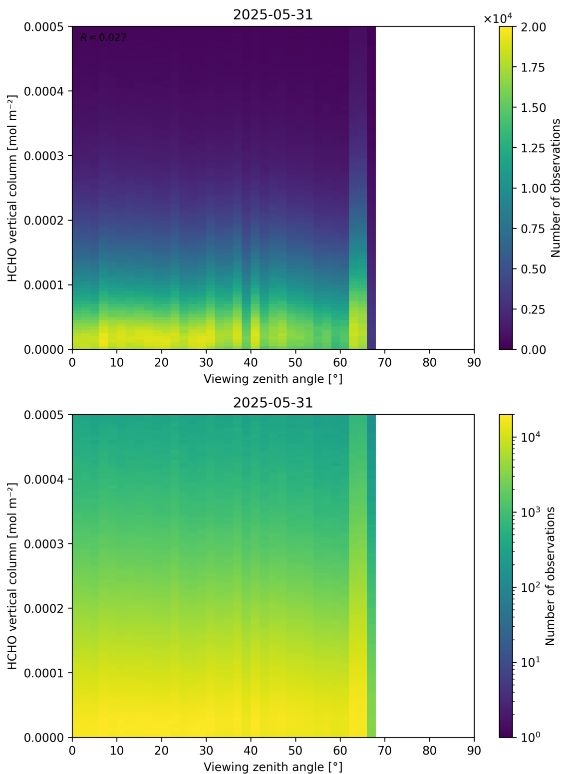
Figure 192: Scatter density plot of “Viewing zenith angle” against “HCHO vertical column” for 2025-05-31 to 2025-06-01.
