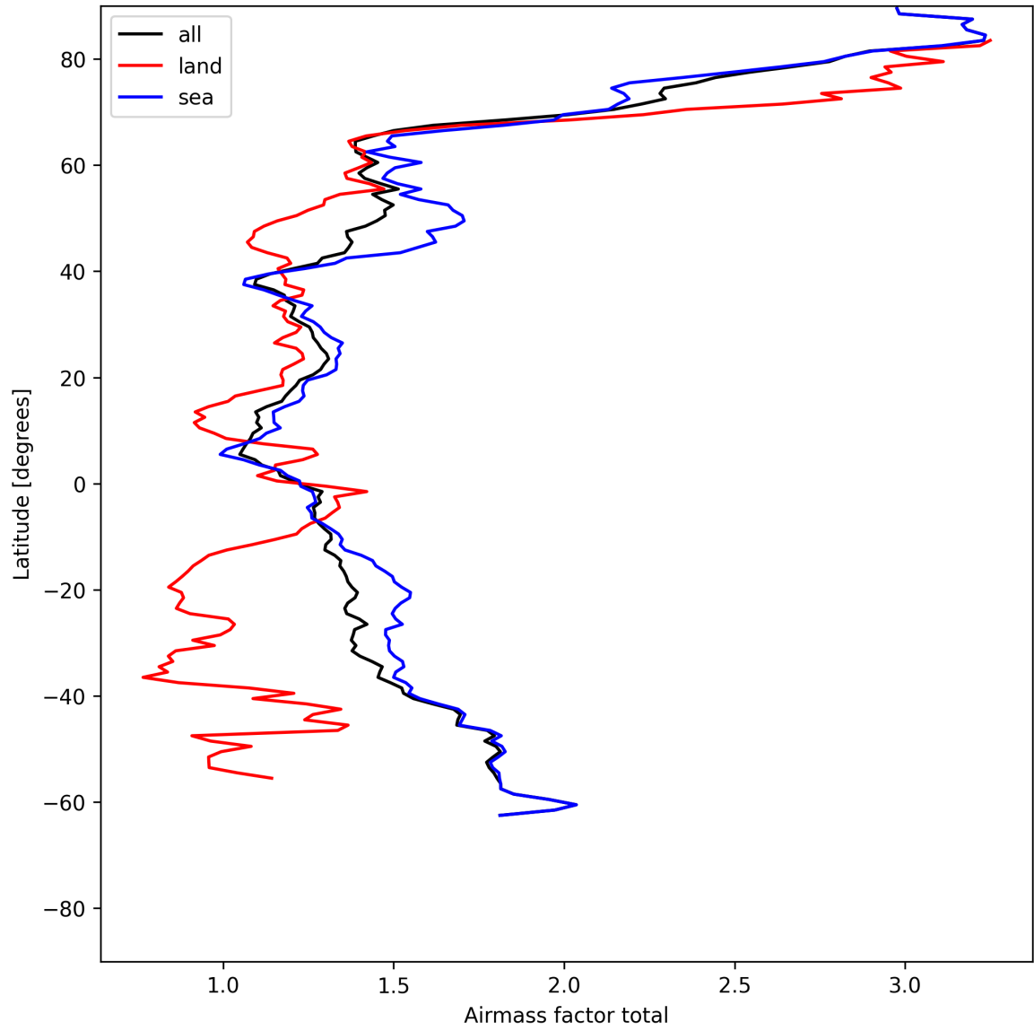
Figure 26: Zonal average of “Airmass factor total” for 2025-05-31 to 2025-06-01.
