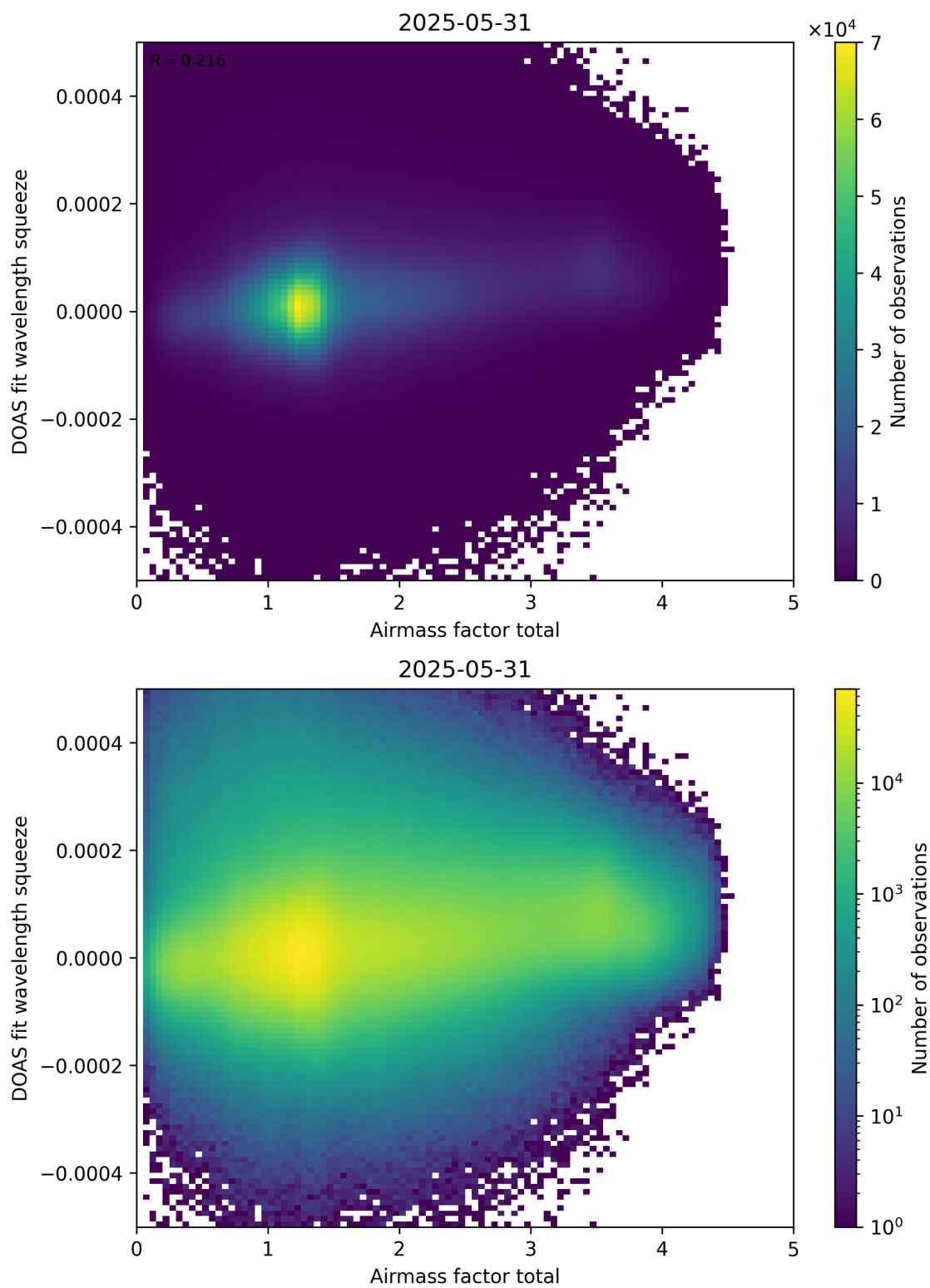
Figure 99: Scatter density plot of “Airmass factor total” against “DOAS fit wavelength squeeze” for 2025-05-31 to 2025-06-01.
