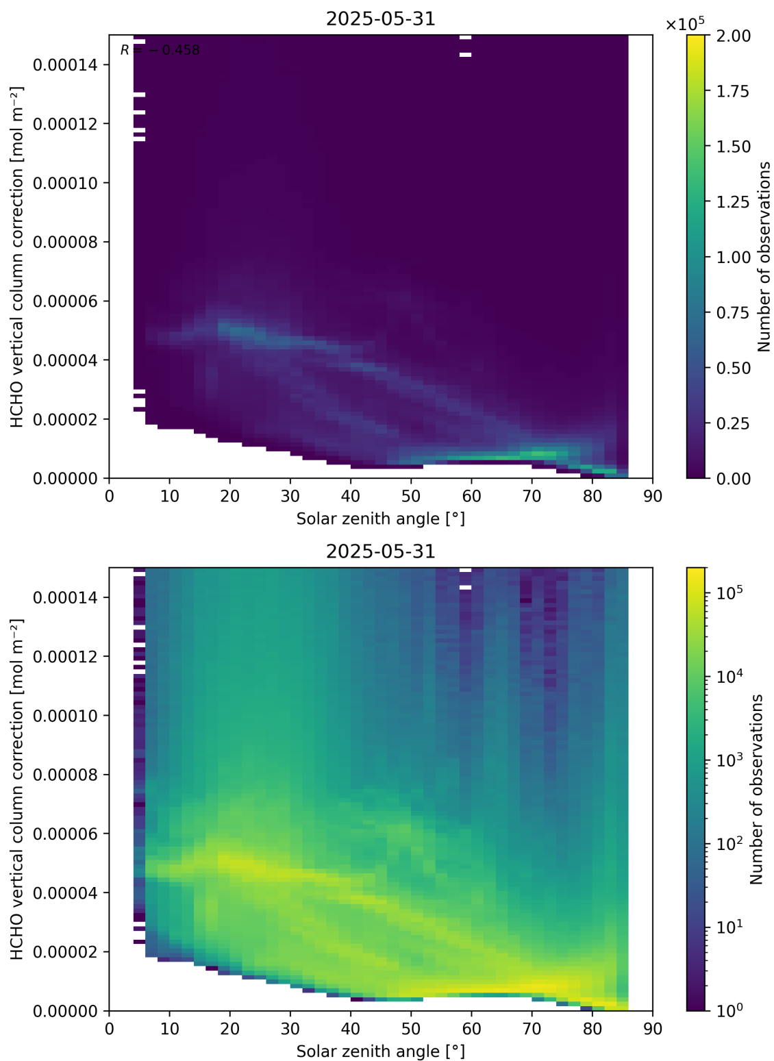
Figure 178: Scatter density plot of “Solar zenith angle” against “HCHO vertical column correction” for 2025-05-31 to 2025-06-01.
