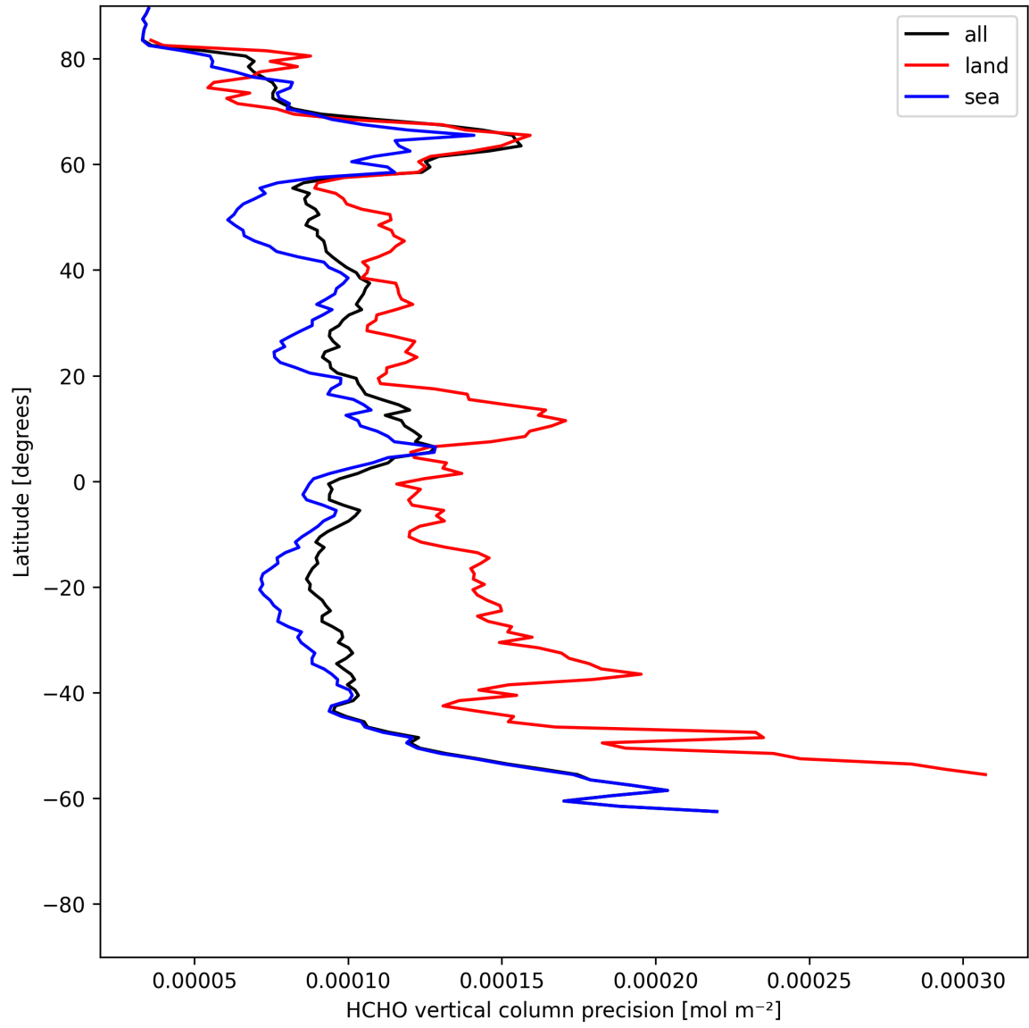
Figure 22: Zonal average of “HCHO vertical column precision” for 2025-05-31 to 2025-06-01.
