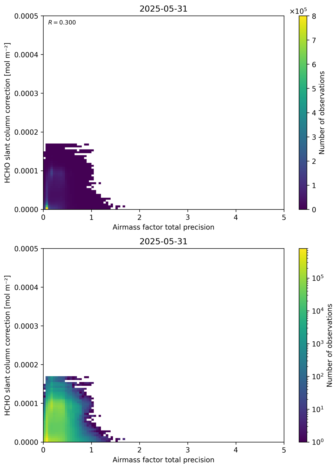
Figure 110: Scatter density plot of “Airmass factor total precision” against “HCHO slant column correction” for 2025-05-31 to 2025-06-01.
