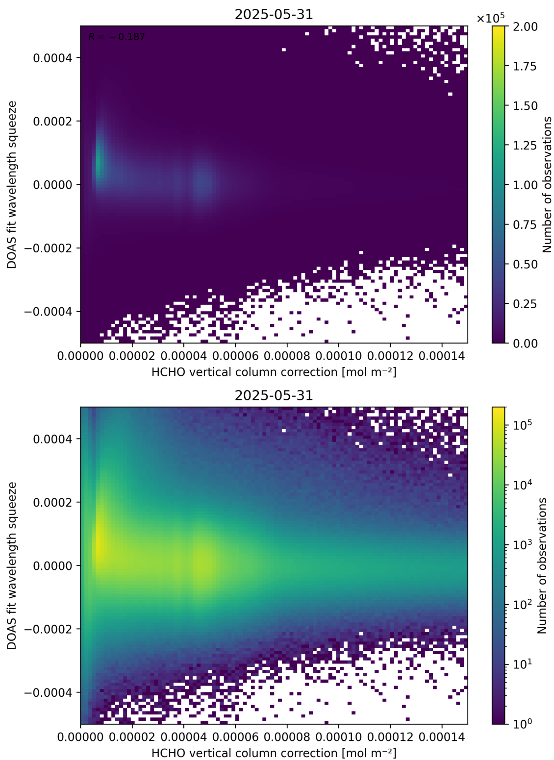
Figure 114: Scatter density plot of “HCHO vertical column correction” against “DOAS fit wavelength squeeze” for 2025-05-31 to 2025-06-01.
