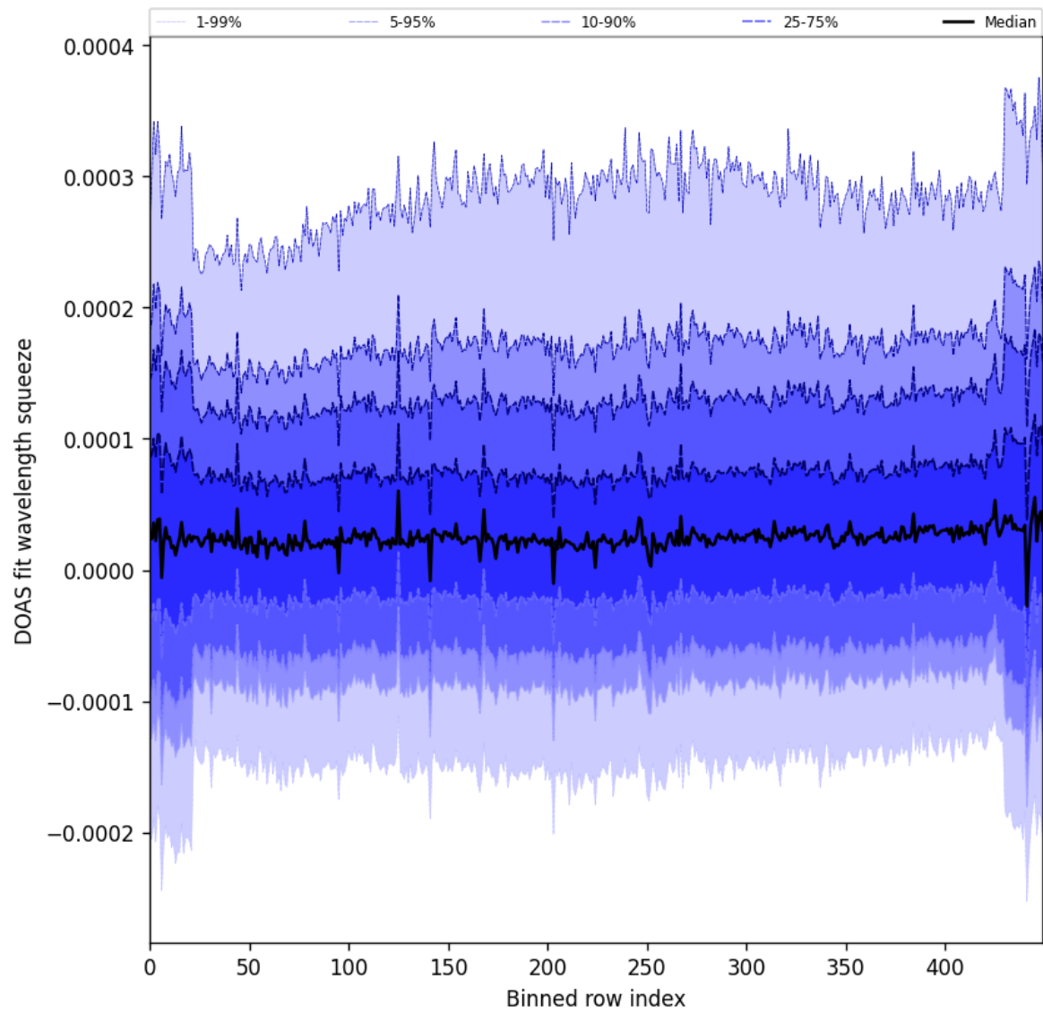
Figure 59: Along track statistics of “DOAS fit wavelength squeeze” for 2025-05-31 to 2025-06-01
