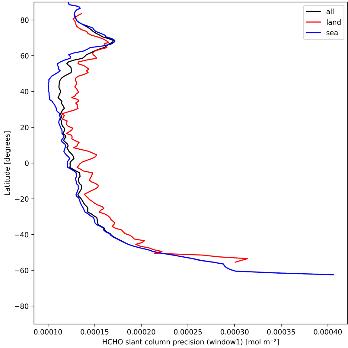
Figure 25: Zonal average of "HCHO slant column precision (window1)" for 2025-05-31 to 2025-06-01.
