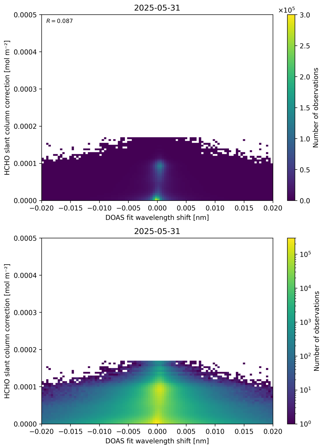
Figure 67: Scatter density plot of “DOAS fit wavelength shift” against “HCHO slant column correction” for 2025-05-31 to 2025-06-01.
