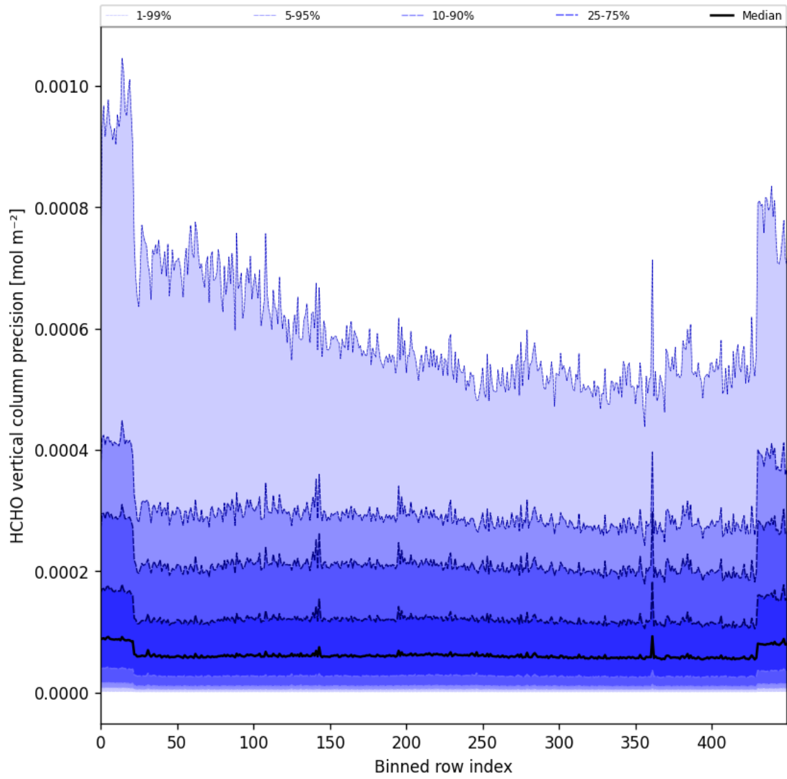
Figure 50: Along track statistics of “HCHO vertical column precision” for 2025-05-31 to 2025-06-01
