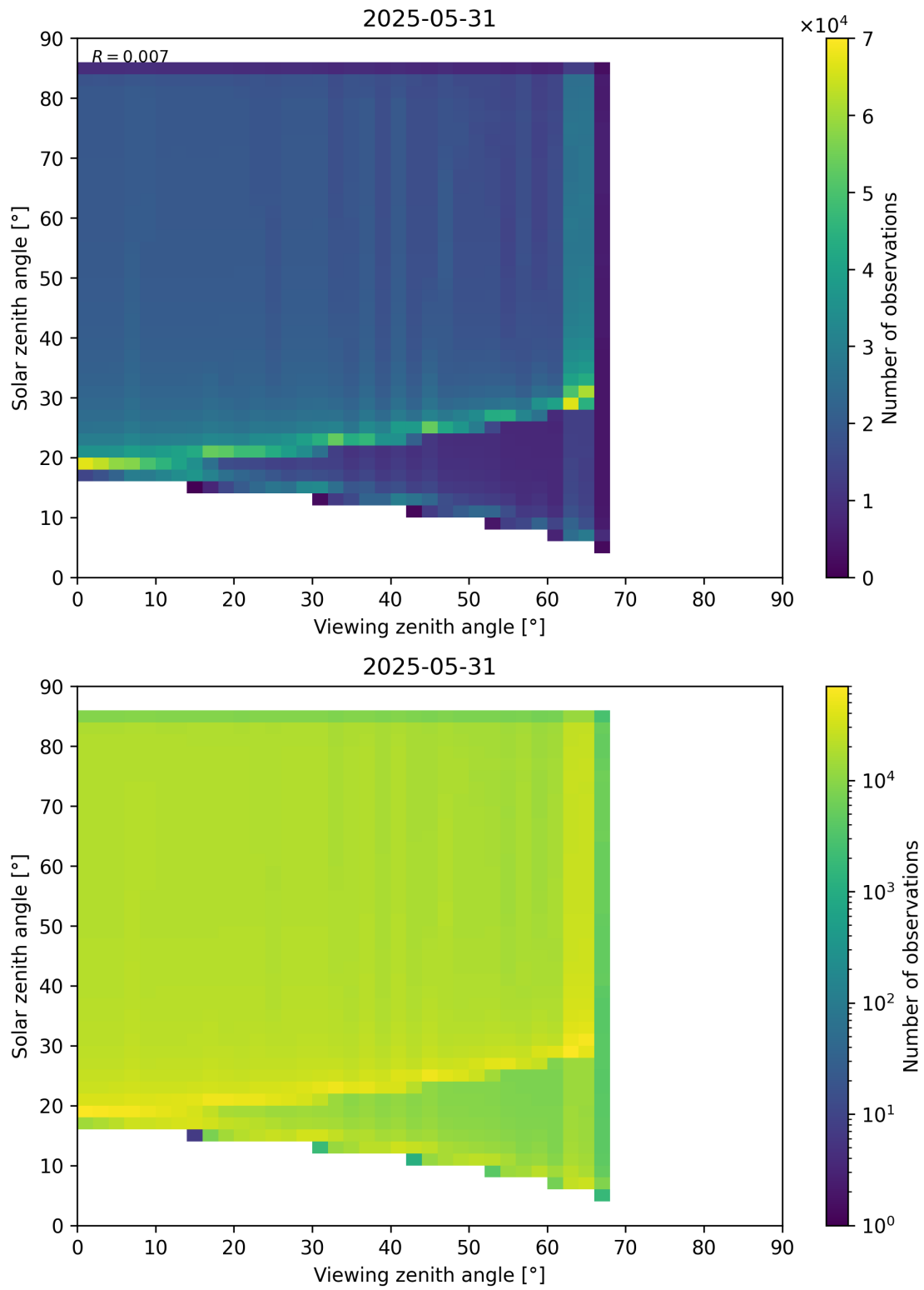
Figure 197: Scatter density plot of “Viewing zenith angle” against “Solar zenith angle” for 2025-05-31 to 2025-06-01.
