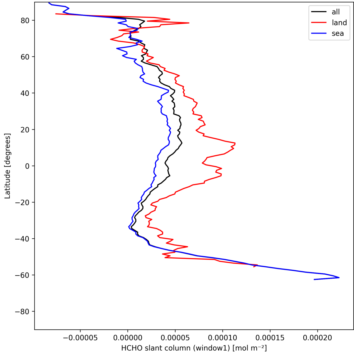
Figure 24: Zonal average of “HCHO slant column (window1)” for 2025-05-31 to 2025-06-01.
