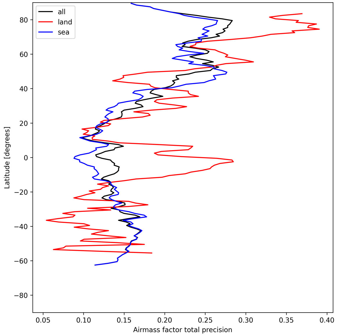
Figure 27: Zonal average of “Airmass factor total precision” for 2025-05-31 to 2025-06-01.
