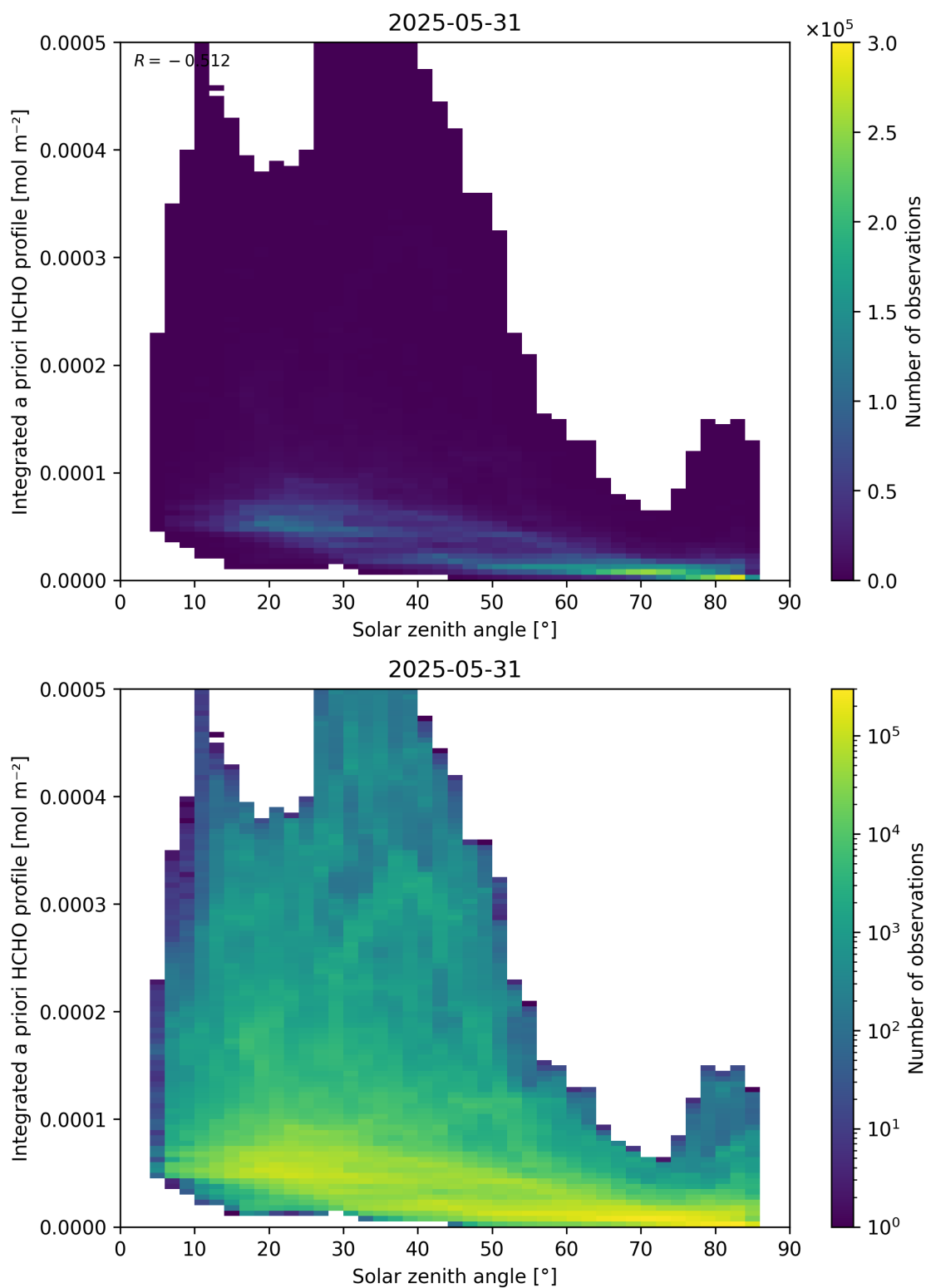
Figure 180: Scatter density plot of “Solar zenith angle” against “Integrated a priori HCHO profile” for 2025-05-31 to 2025-06-01.
