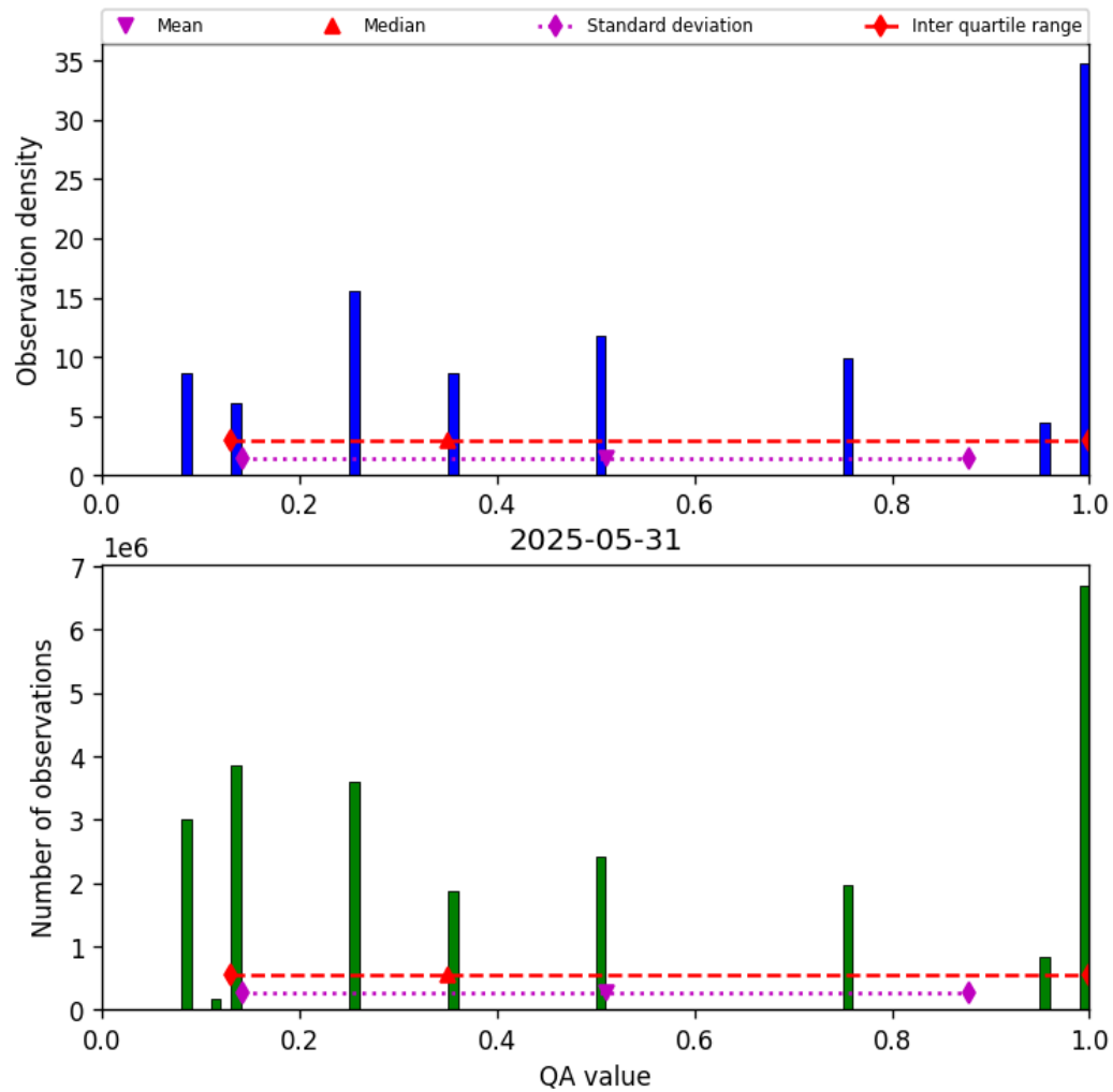
Figure 34: Histogram of “QA value” for 2025-05-31 to 2025-06-01
