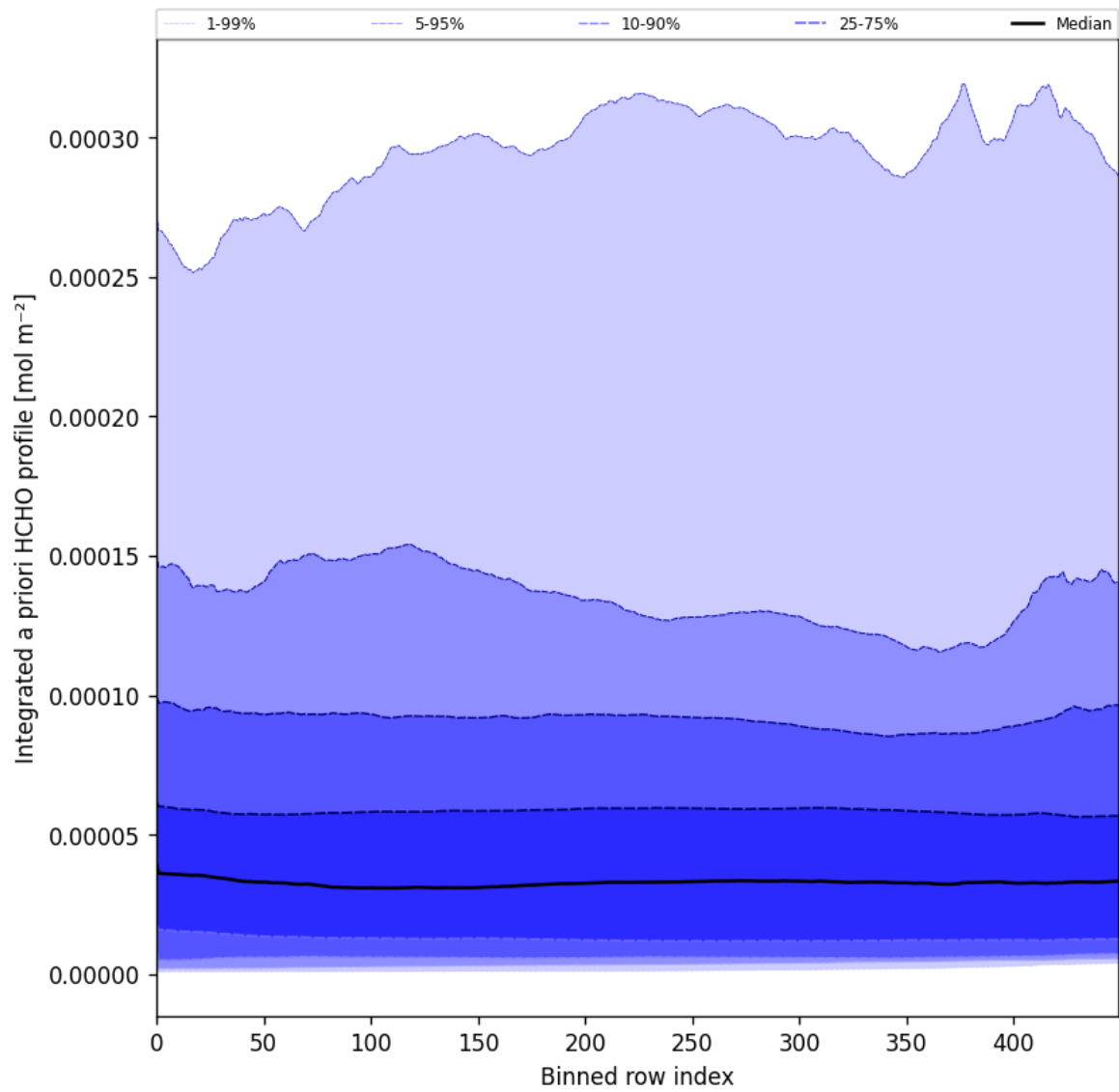
Figure 57: Along track statistics of “Integrated a priori HCHO profile” for 2025-05-31 to 2025-06-01
