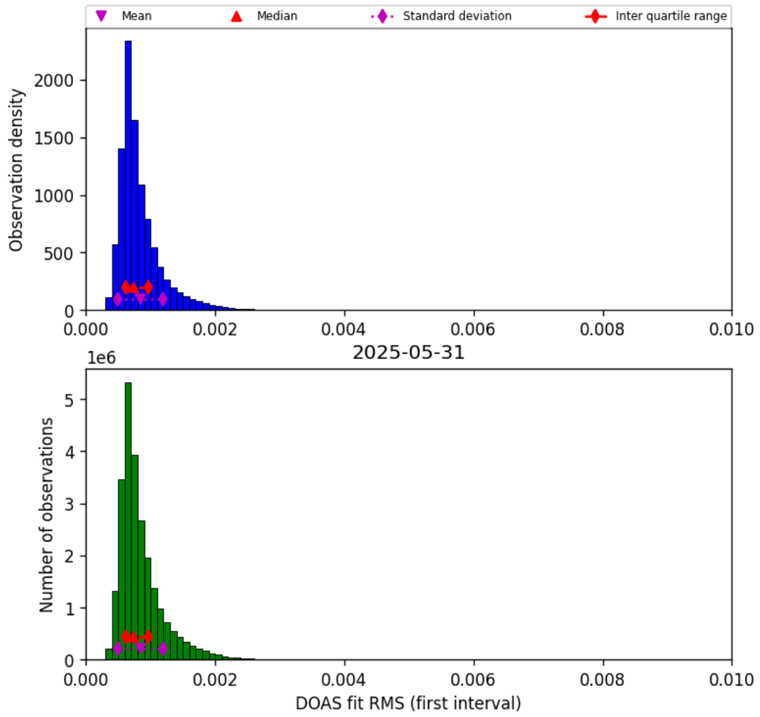
Figure 46: Histogram of “DOAS fit RMS (first interval)” for 2025-05-31 to 2025-06-01
