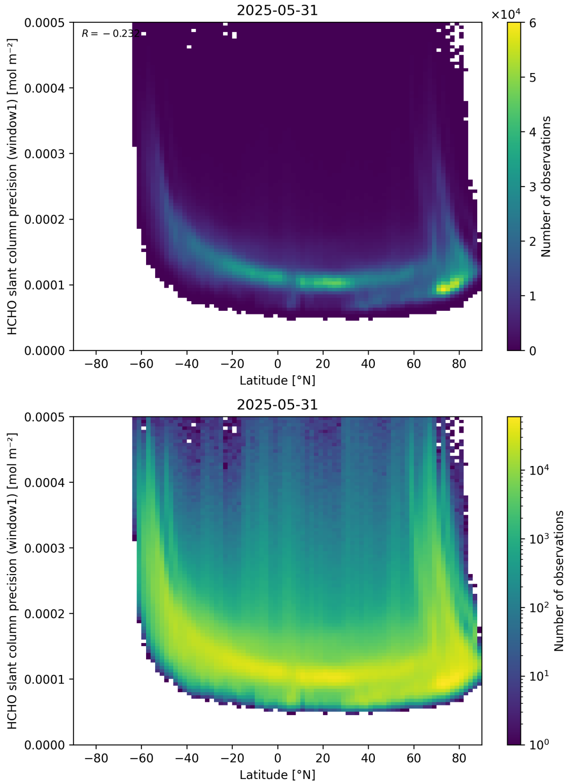
Figure 160: Scatter density plot of “Latitude” against “HCHO slant column precision (window1)” for 2025-05-31 to 2025-06-01.
