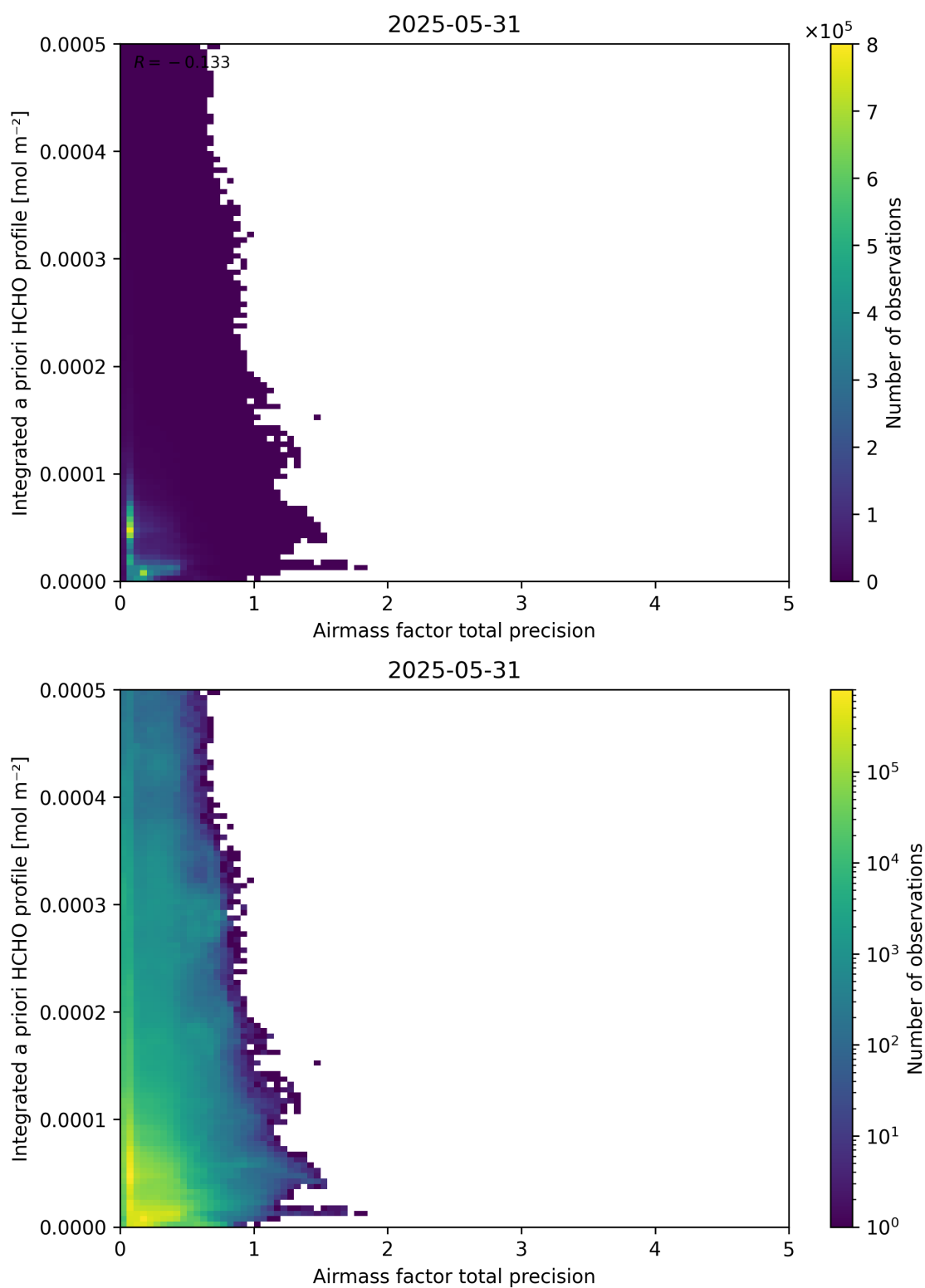
Figure 111: Scatter density plot of “Airmass factor total precision” against “Integrated a priori HCHO profile” for 2025-05-31 to 2025-06-01.
