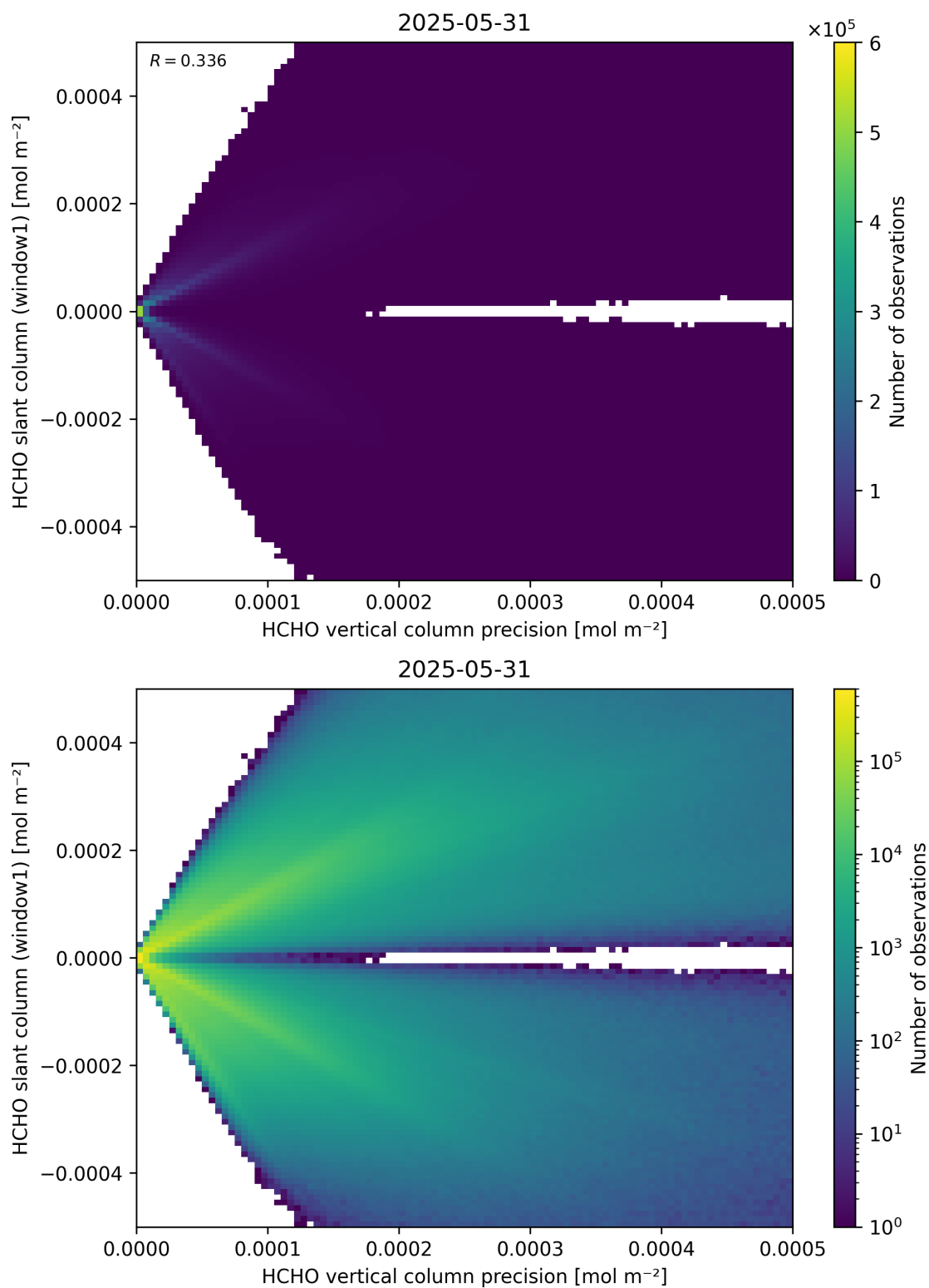
Figure 142: Scatter density plot of “HCHO vertical column precision” against “HCHO slant column (window1)” for 2025-05-31 to 2025-06-01.
