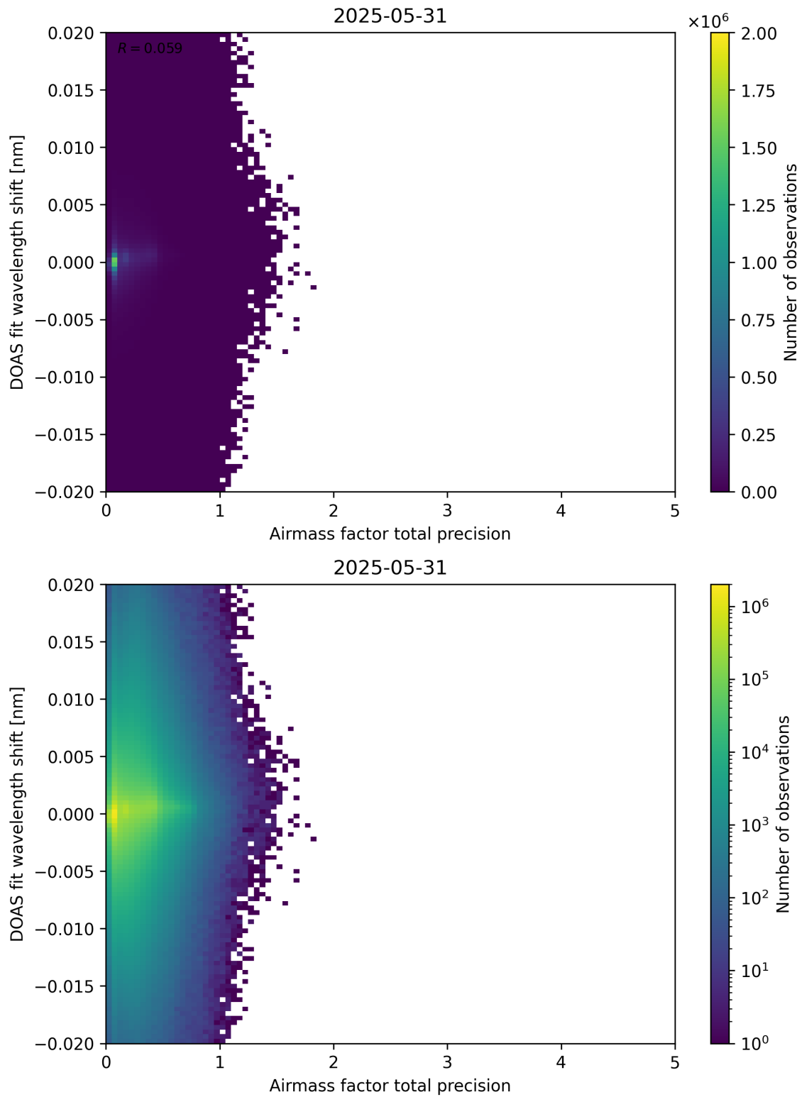
Figure 106: Scatter density plot of “Airmass factor total precision” against “DOAS fit wavelength shift” for 2025-05-31 to 2025-06-01.
