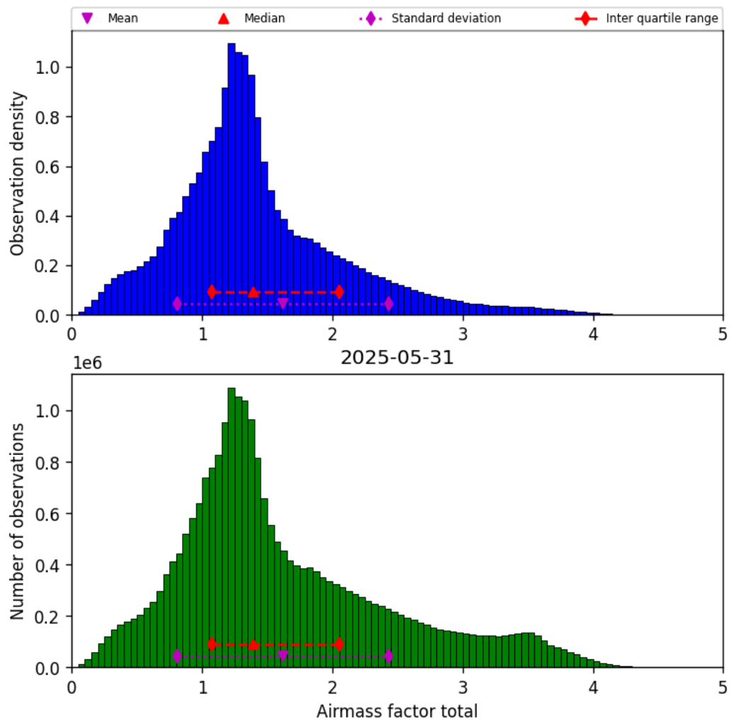
Figure 40: Histogram of “Airmass factor total” for 2025-05-31 to 2025-06-01
