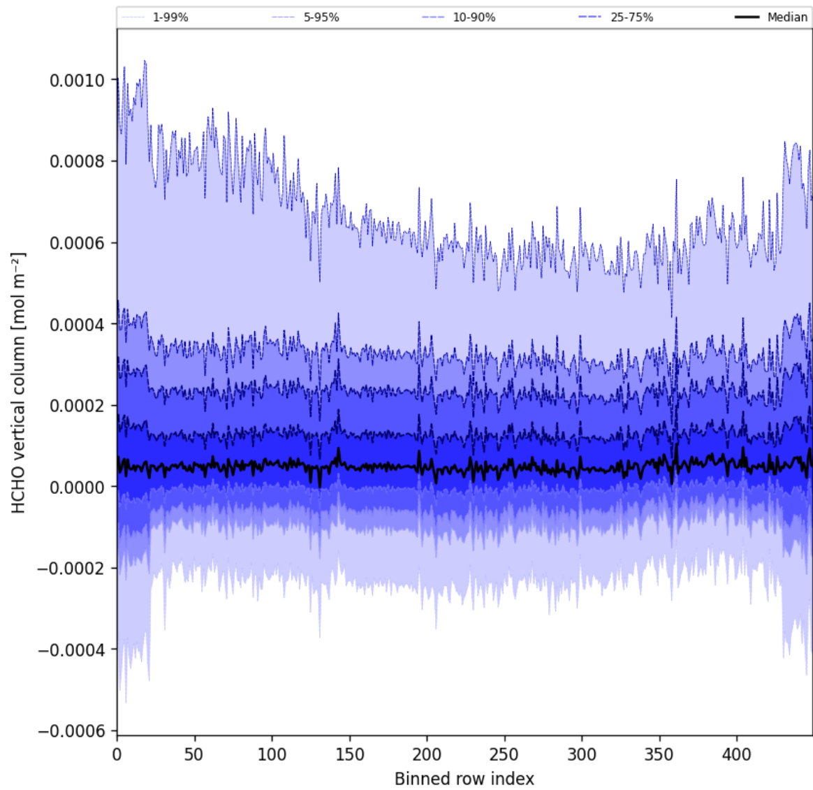
Figure 49: Along track statistics of “HCHO vertical column” for 2025-05-31 to 2025-06-01
