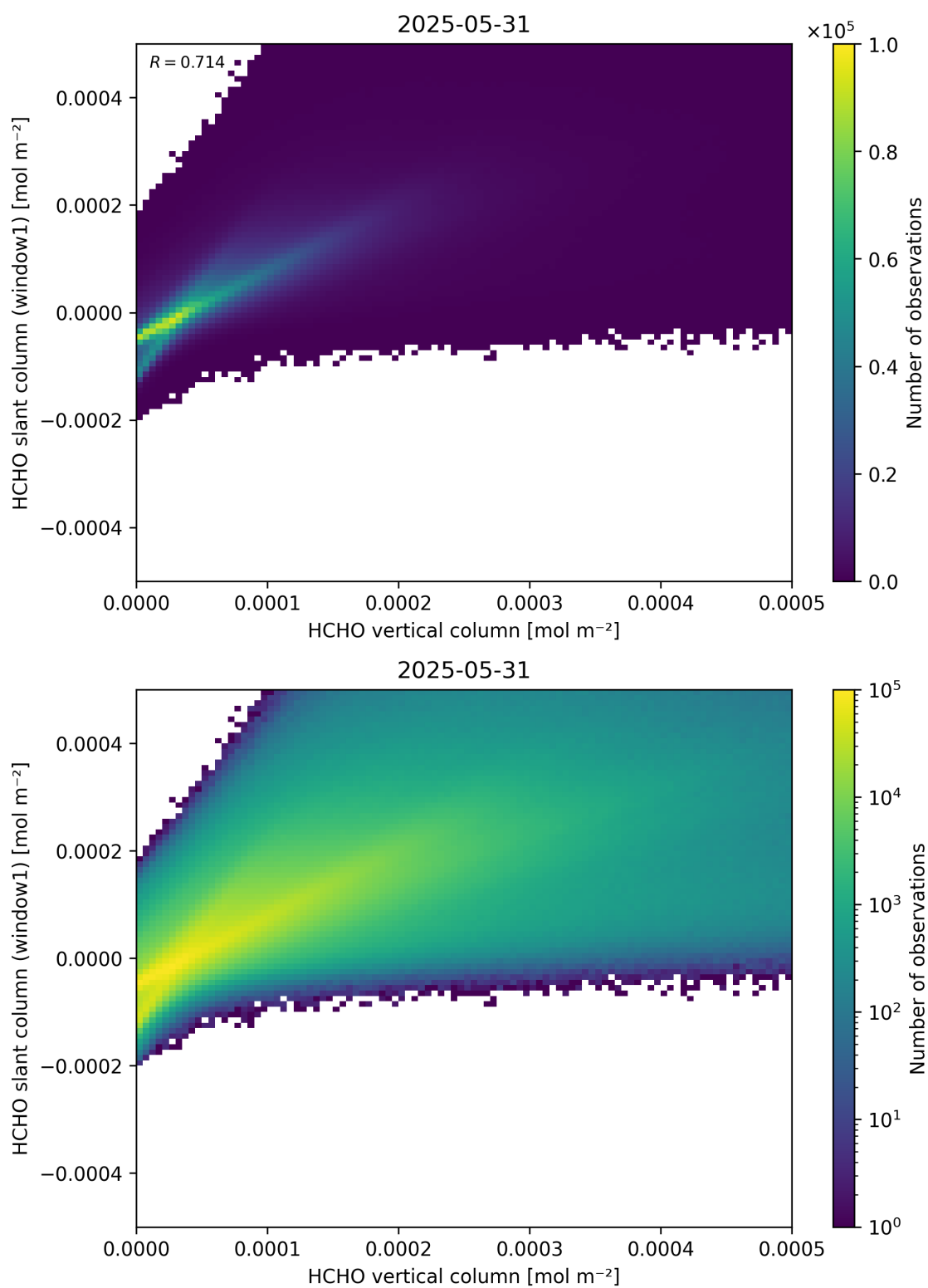
Figure 129: Scatter density plot of “HCHO vertical column” against “HCHO slant column (window1)” for 2025-05-31 to 2025-06-01.
