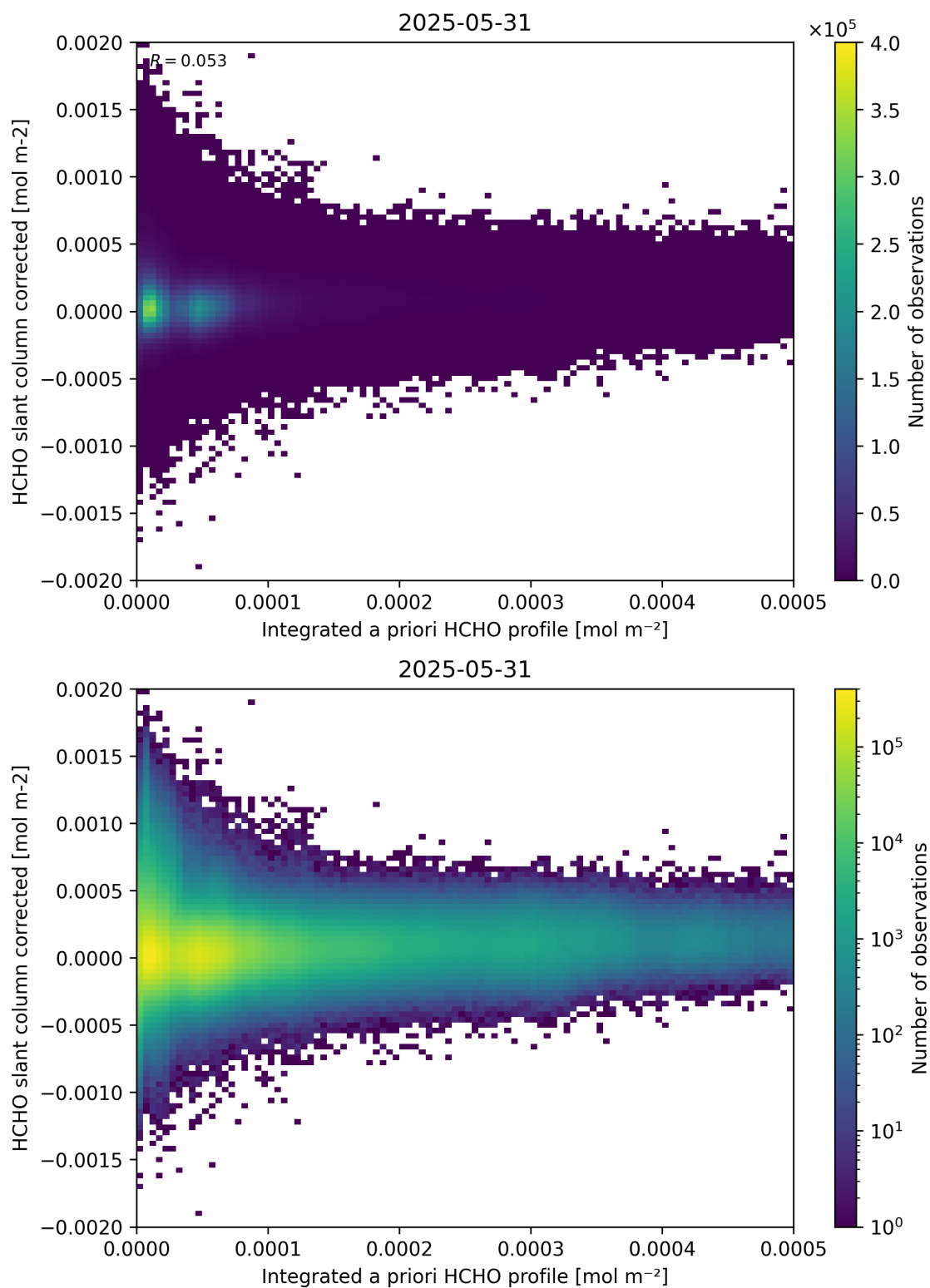
Figure 151: Scatter density plot of “Integrated a priori HCHO profile” against “HCHO slant column corrected” for 2025-05-31 to 2025-06-01.
