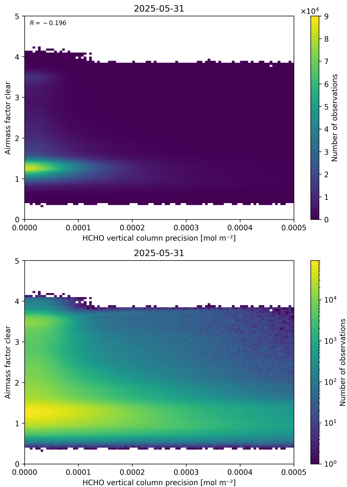
Figure 139: Scatter density plot of “HCHO vertical column precision” against “Airmass factor clear” for 2025-05-31 to 2025-06-01.
