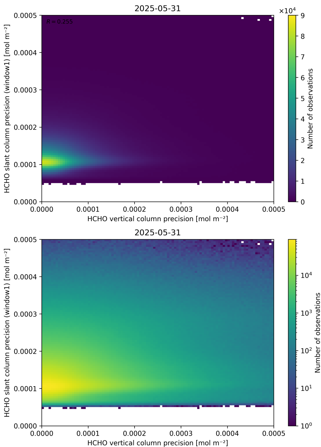
Figure 143: Scatter density plot of “HCHO vertical column precision” against “HCHO slant column precision (window1)” for 2025-05-31 to 2025-06-01.
