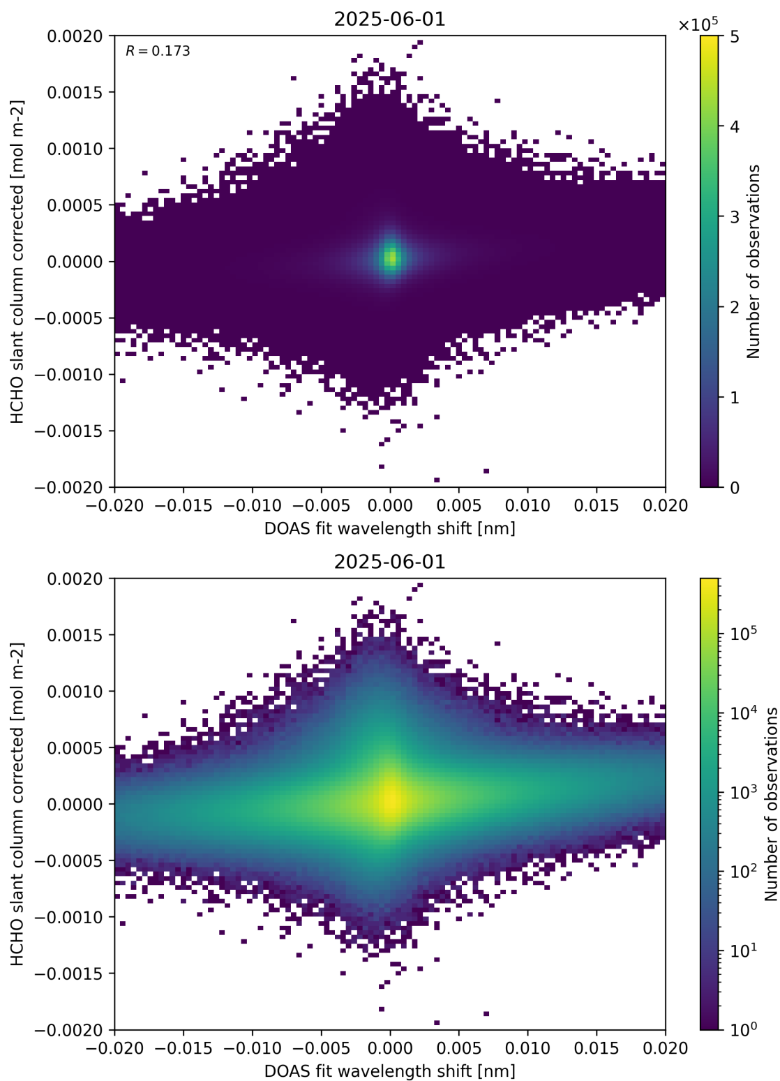
Figure 66: Scatter density plot of “DOAS fit wavelength shift” against “HCHO slant column corrected” for 2025-06-01 to 2025-06-02.
