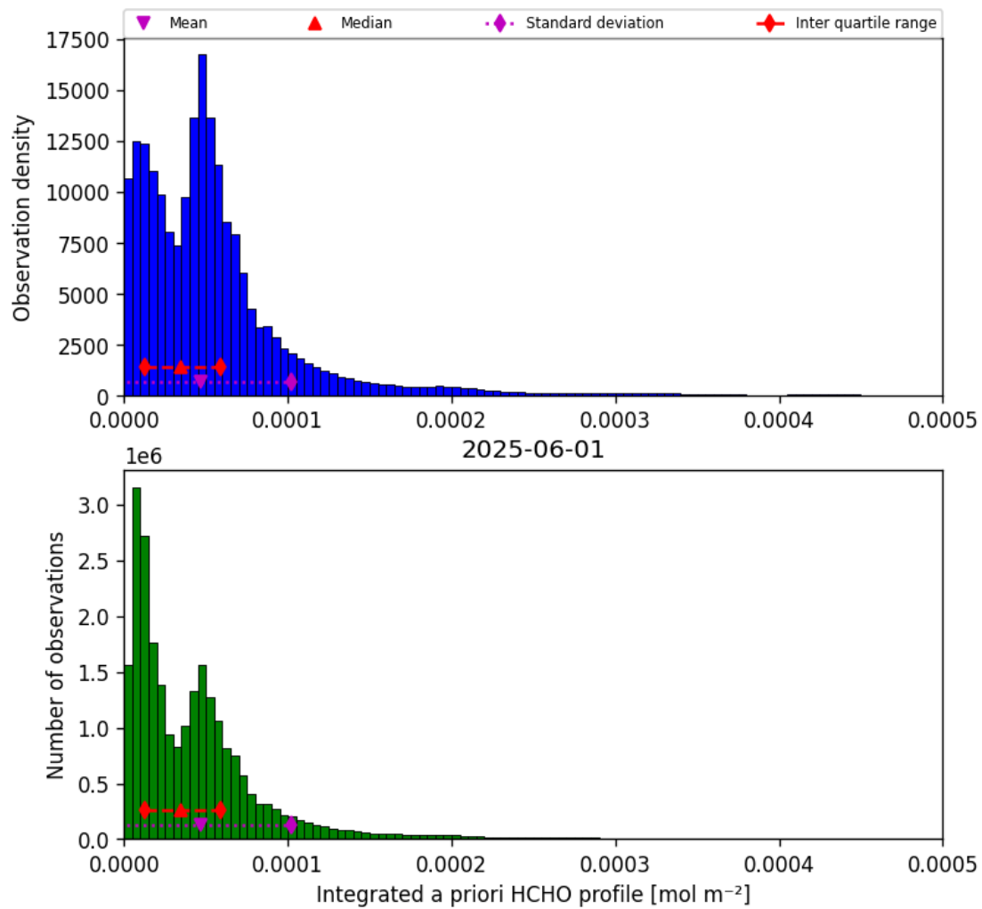
Figure 43: Histogram of “Integrated a priori HCHO profile” for 2025-06-01 to 2025-06-02
