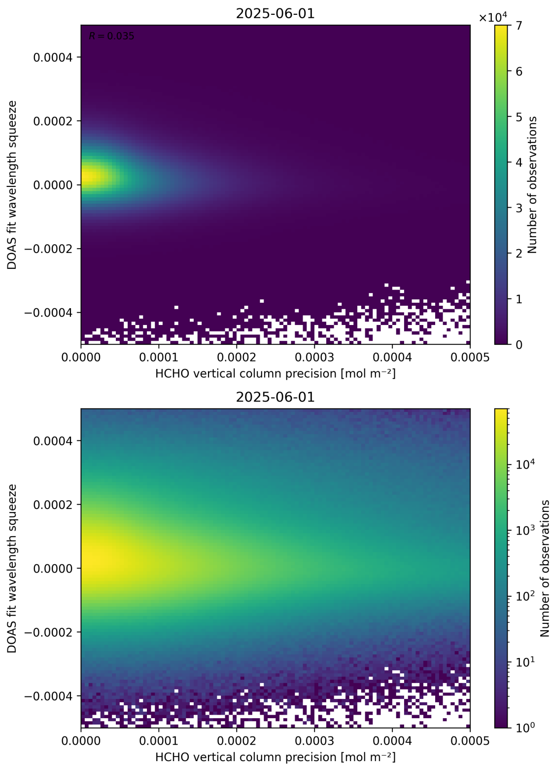
Figure 138: Scatter density plot of “HCHO vertical column precision” against “DOAS fit wavelength squeeze” for 2025-06-01 to 2025-06-02.
