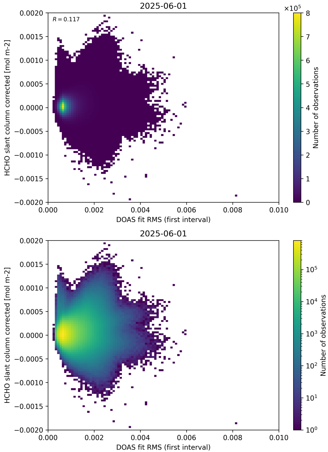
Figure 62: Scatter density plot of “DOAS fit RMS (first interval)” against “HCHO slant column corrected” for 2025-06-01 to 2025-06-02.
