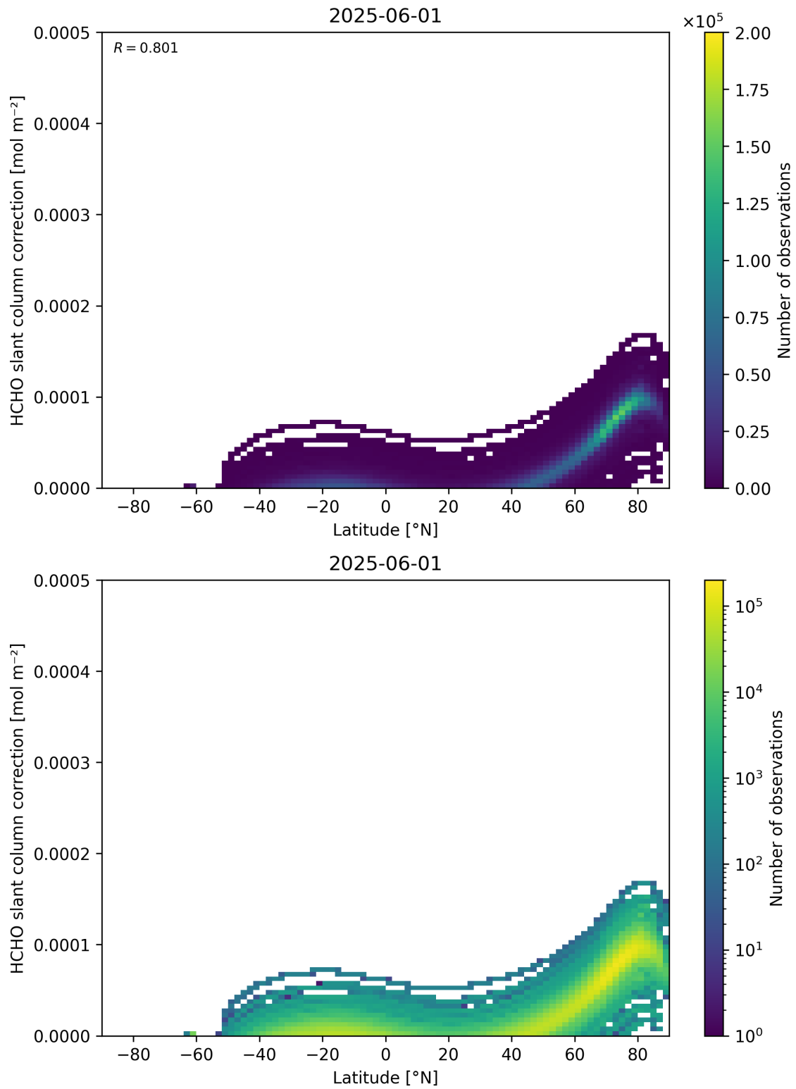
Figure 158: Scatter density plot of “Latitude” against “HCHO slant column correction” for 2025-06-01 to 2025-06-02.
