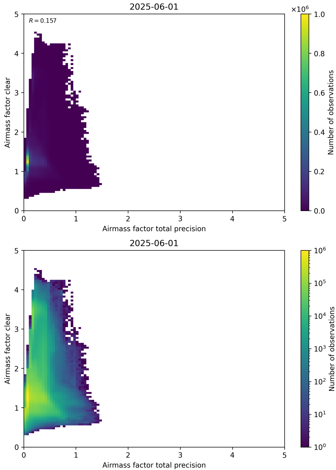
Figure 108: Scatter density plot of “Airmass factor total precision” against “Airmass factor clear” for 2025-06-01 to 2025-06-02.
