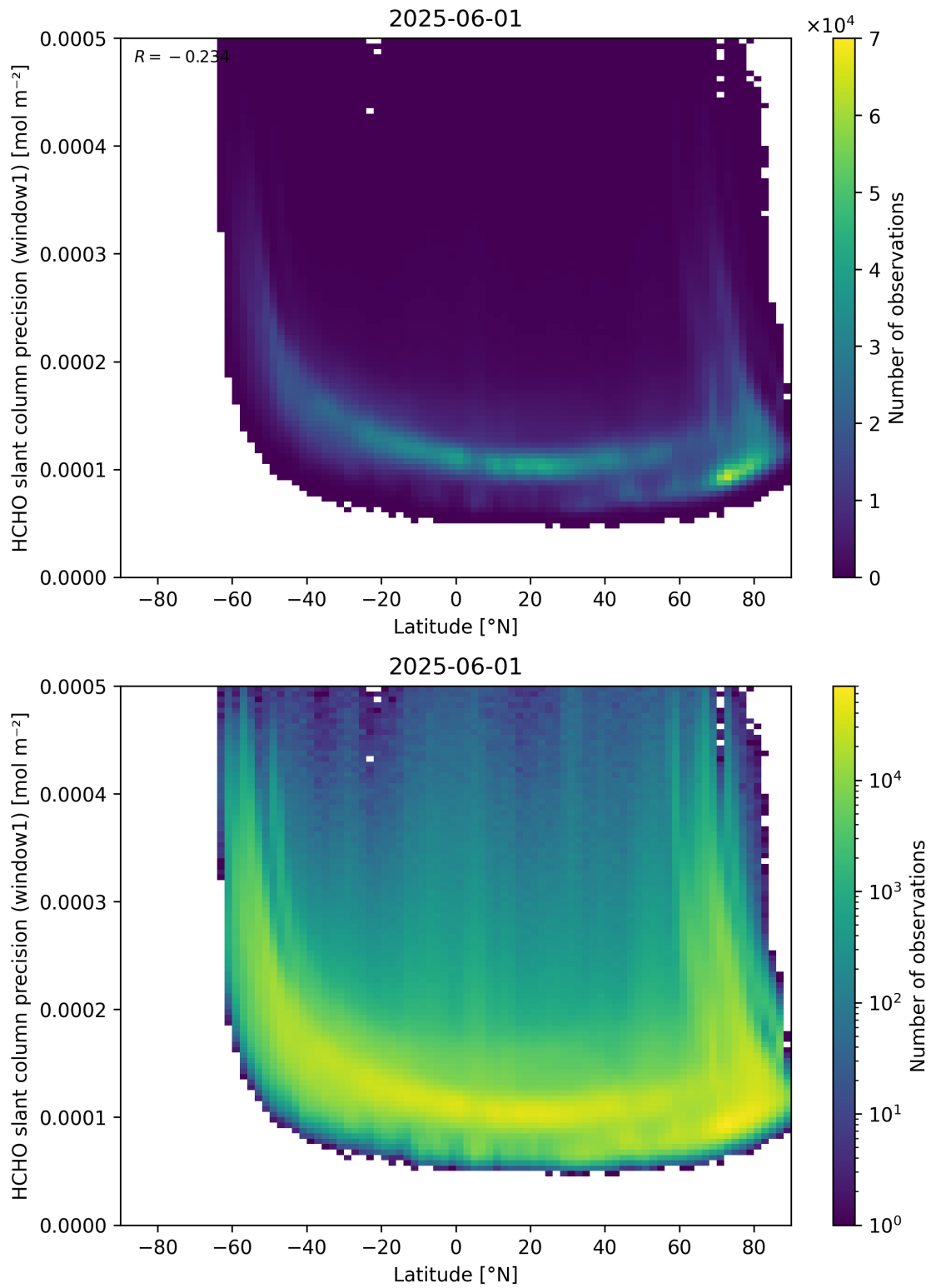
Figure 160: Scatter density plot of “Latitude” against “HCHO slant column precision (window1)” for 2025-06-01 to 2025-06-02.
