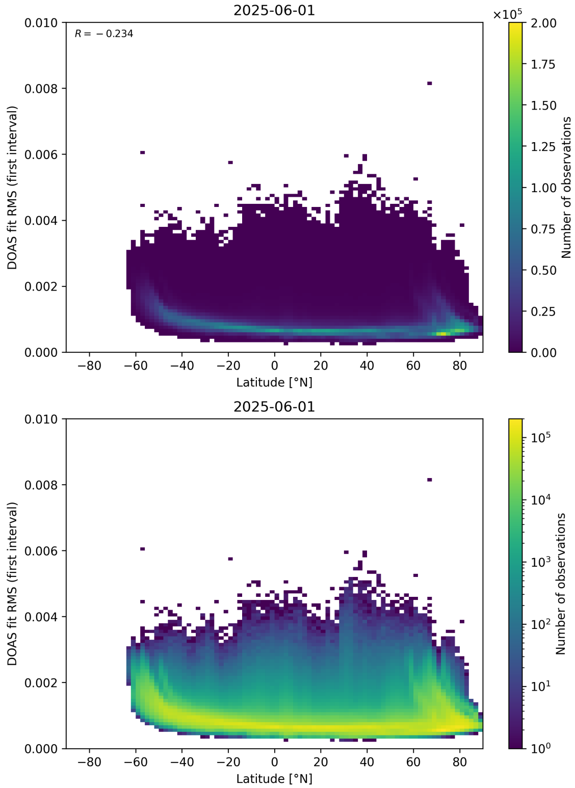
Figure 153: Scatter density plot of “Latitude” against “DOAS fit RMS (first interval)” for 2025-06-01 to 2025-06-02.
