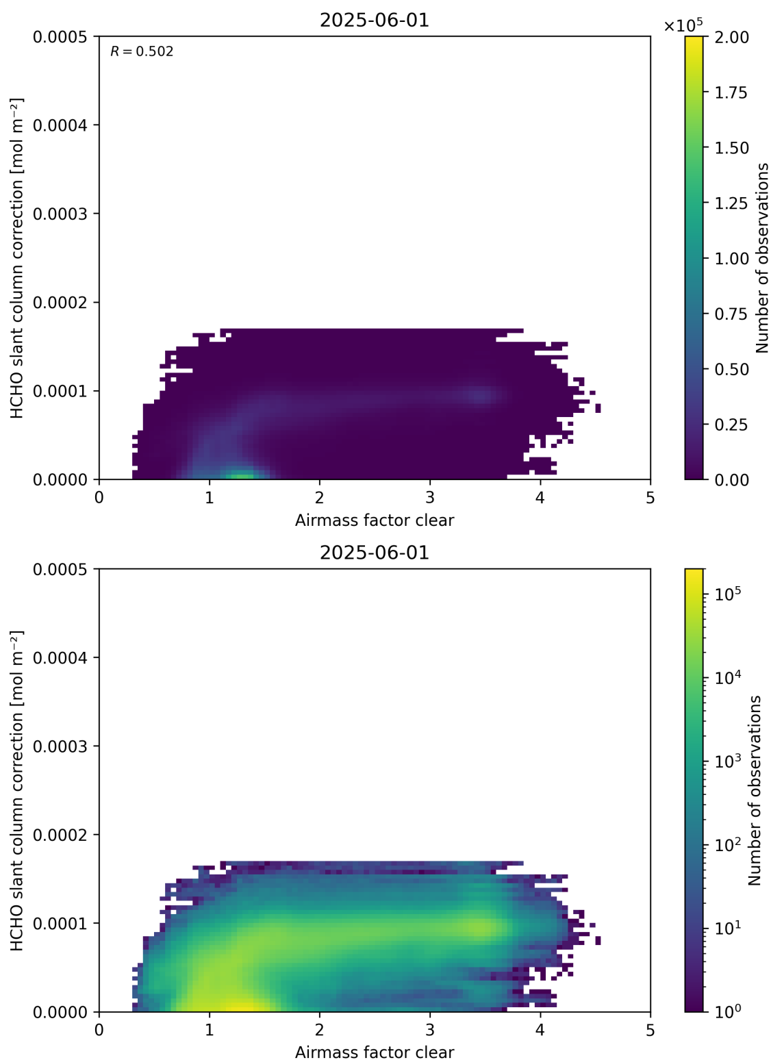
Figure 75: Scatter density plot of “Airmass factor clear” against “HCHO slant column correction” for 2025-06-01 to 2025-06-02.
