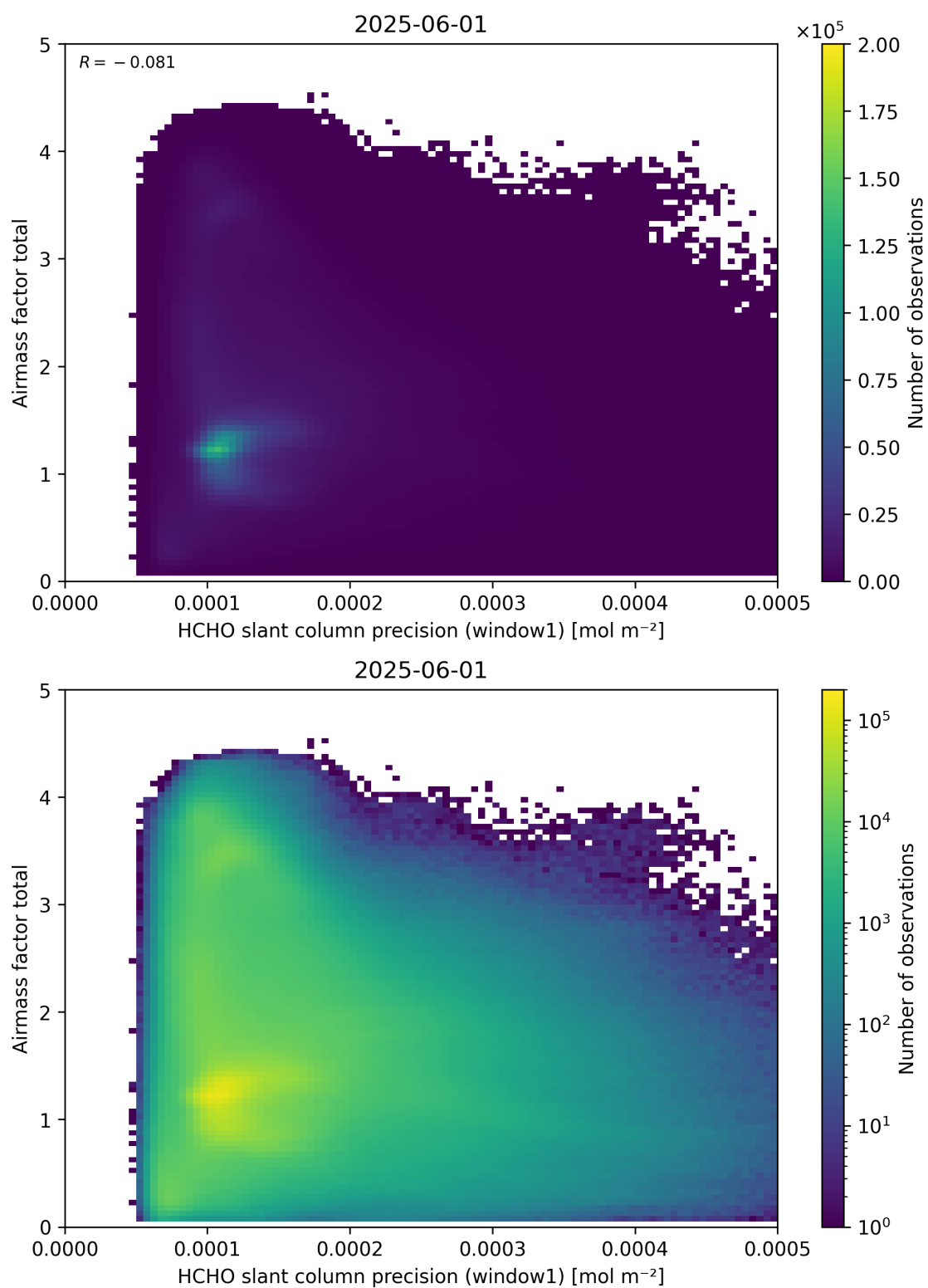
Figure 94: Scatter density plot of “HCHO slant column precision (window1)” against “Airmass factor total” for 2025-06-01 to 2025-06-02.
