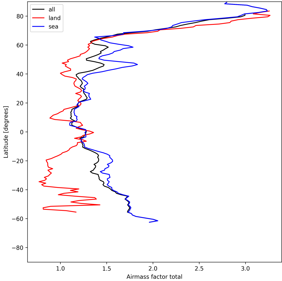
Figure 26: Zonal average of “Airmass factor total” for 2025-06-01 to 2025-06-02.
