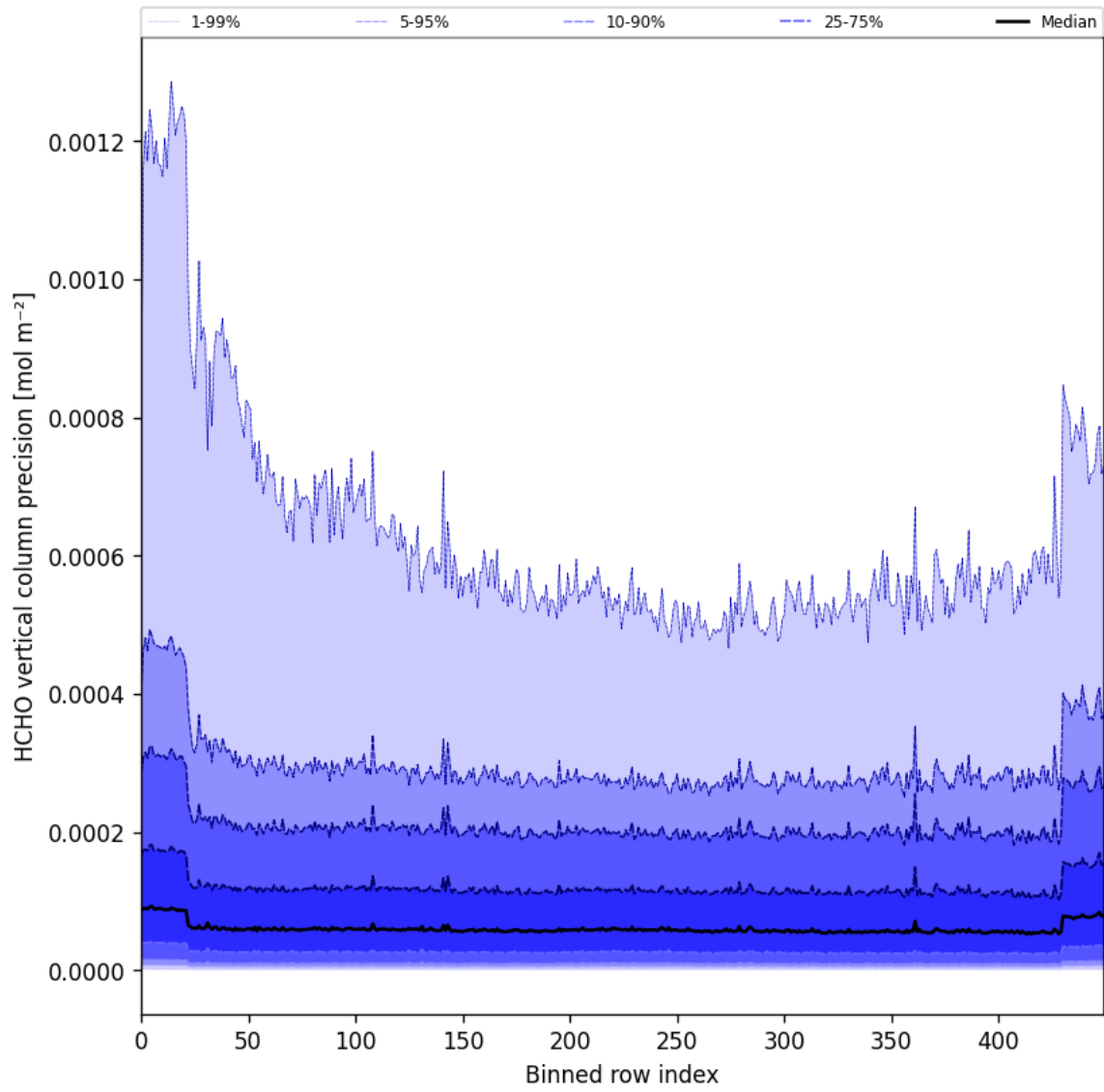
Figure 50: Along track statistics of “HCHO vertical column precision” for 2025-06-01 to 2025-06-02
