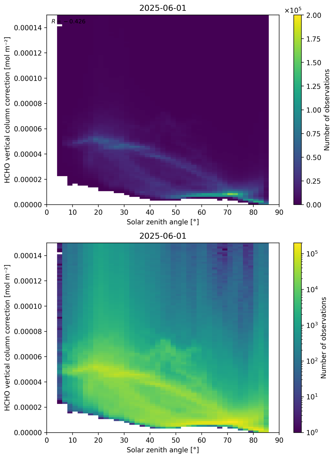
Figure 178: Scatter density plot of “Solar zenith angle” against “HCHO vertical column correction” for 2025-06-01 to 2025-06-02.
