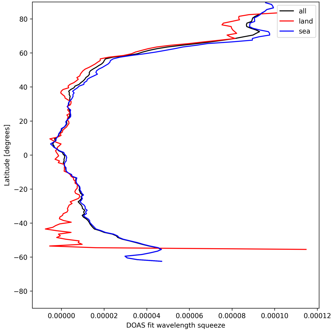
Figure 31: Zonal average of “DOAS fit wavelength squeeze” for 2025-06-01 to 2025-06-02.
