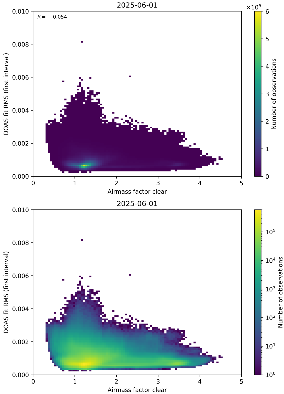
Figure 71: Scatter density plot of “Airmass factor clear” against “DOAS fit RMS (first interval)” for 2025-06-01 to 2025-06-02.
