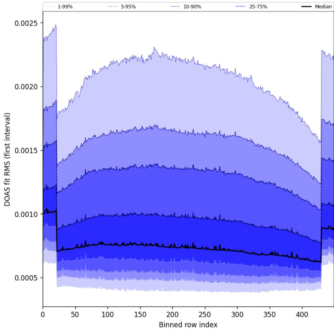
Figure 60: Along track statistics of “DOAS fit RMS (first interval)” for 2025-06-01 to 2025-06-02
