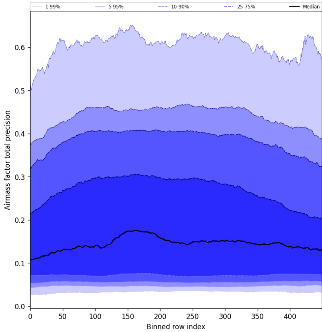
Figure 55: Along track statistics of “Airmass factor total precision” for 2025-06-01 to 2025-06-02
