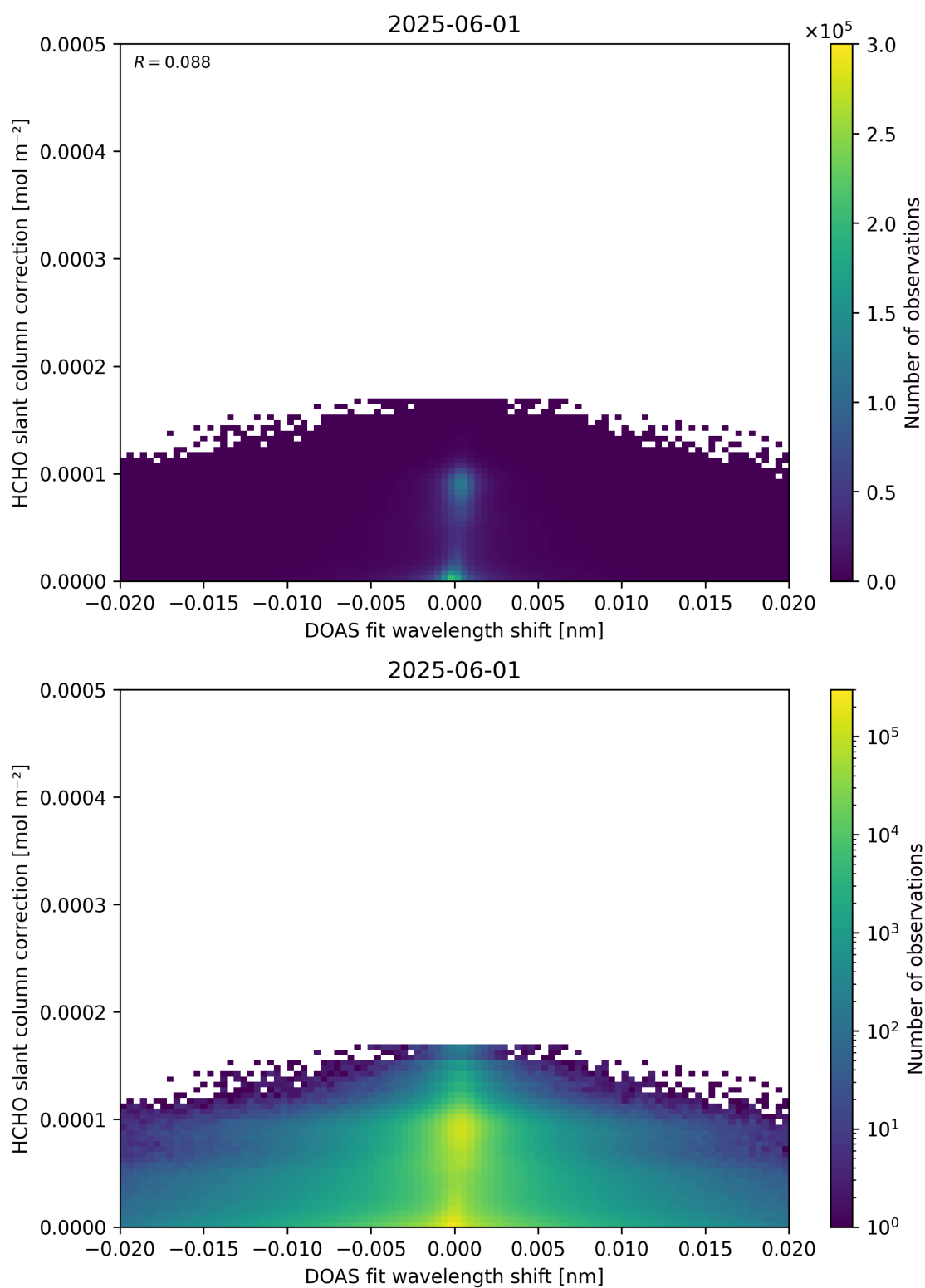
Figure 67: Scatter density plot of “DOAS fit wavelength shift” against “HCHO slant column correction” for 2025-06-01 to 2025-06-02.
