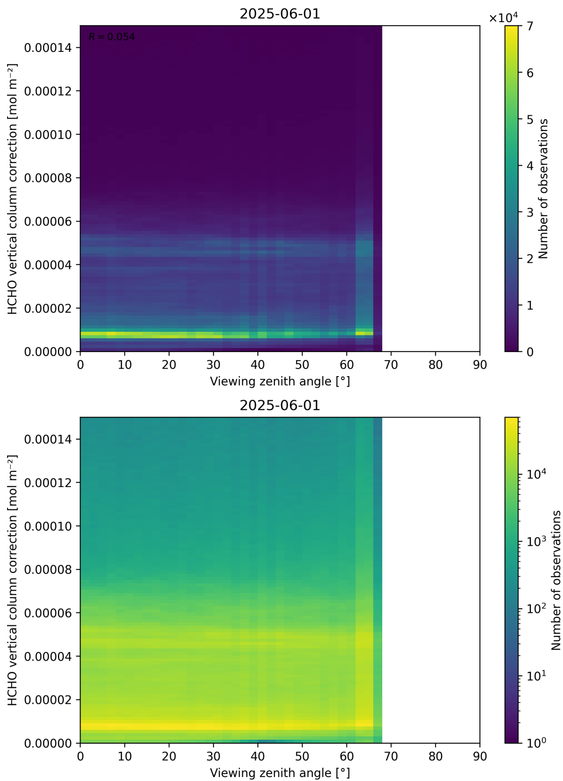
Figure 193: Scatter density plot of “Viewing zenith angle” against “HCHO vertical column correction” for 2025-06-01 to 2025-06-02.
