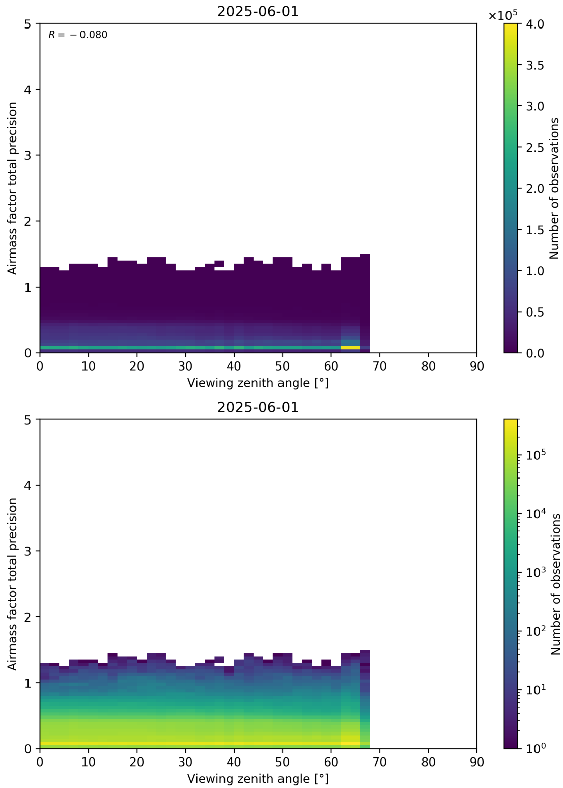
Figure 191: Scatter density plot of “Viewing zenith angle” against “Airmass factor total precision” for 2025-06-01 to 2025-06-02.
