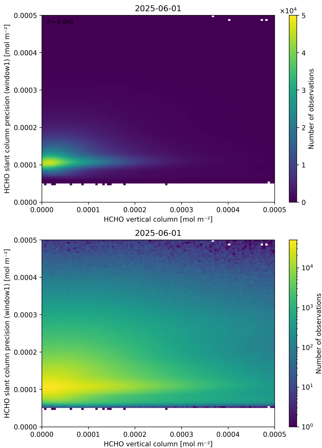
Figure 130: Scatter density plot of “HCHO vertical column” against “HCHO slant column precision (window1)” for 2025-06-01 to 2025-06-02.
