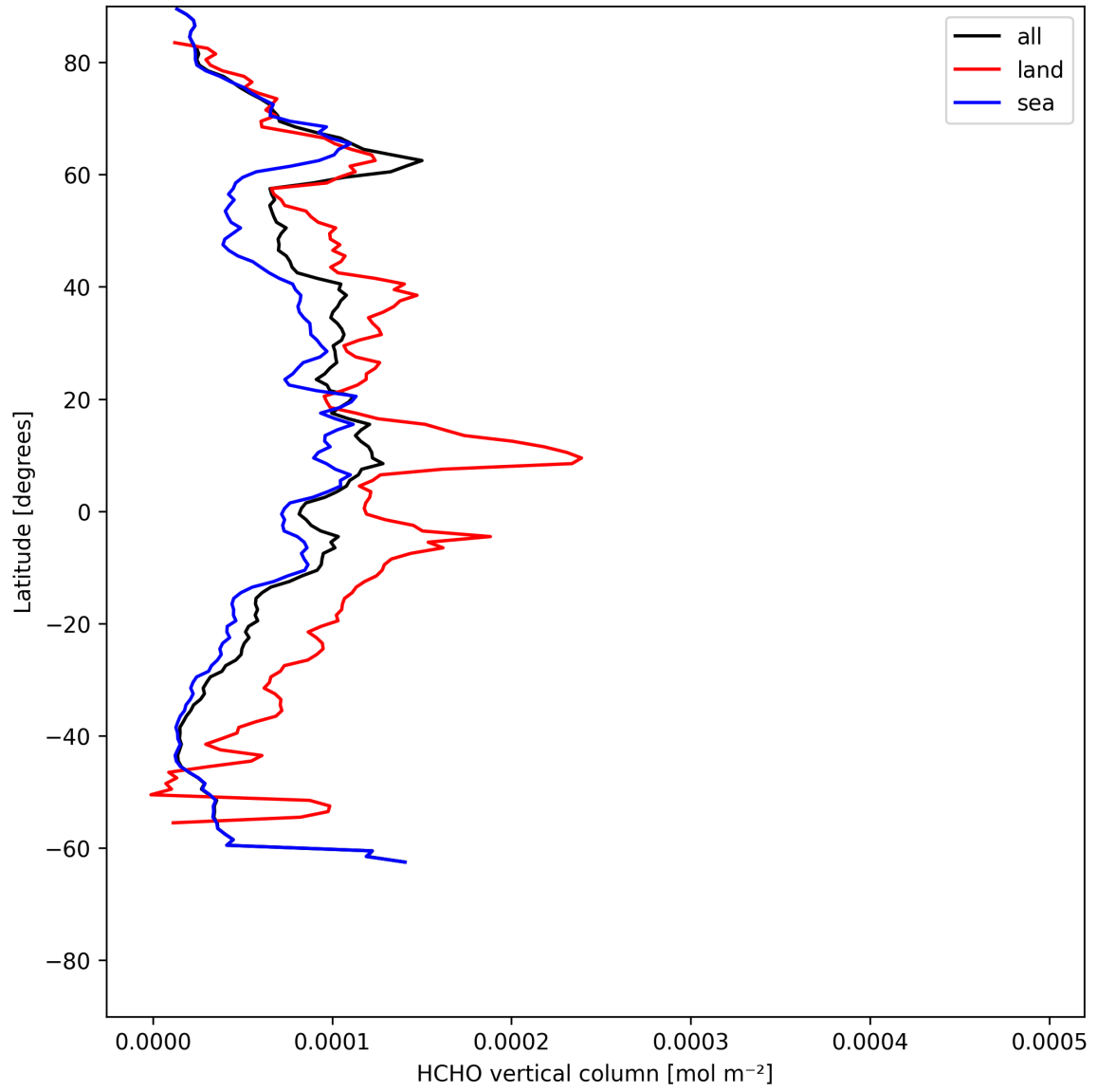
Figure 21: Zonal average of “HCHO vertical column” for 2025-06-01 to 2025-06-02.
