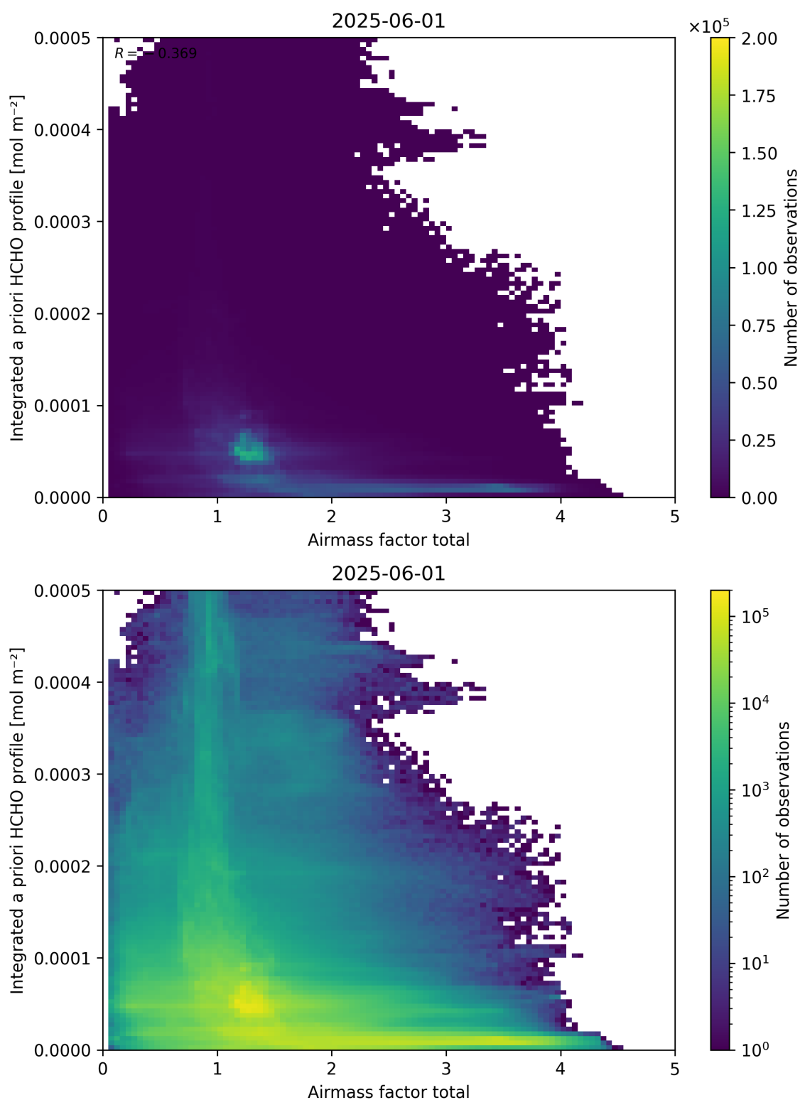
Figure 104: Scatter density plot of “Airmass factor total” against “Integrated a priori HCHO profile” for 2025-06-01 to 2025-06-02.
