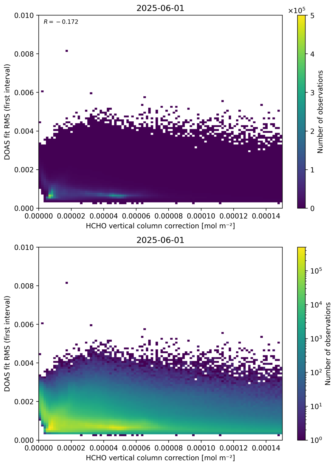
Figure 112: Scatter density plot of “HCHO vertical column correction” against “DOAS fit RMS (first interval)” for 2025-06-01 to 2025-06-02.
