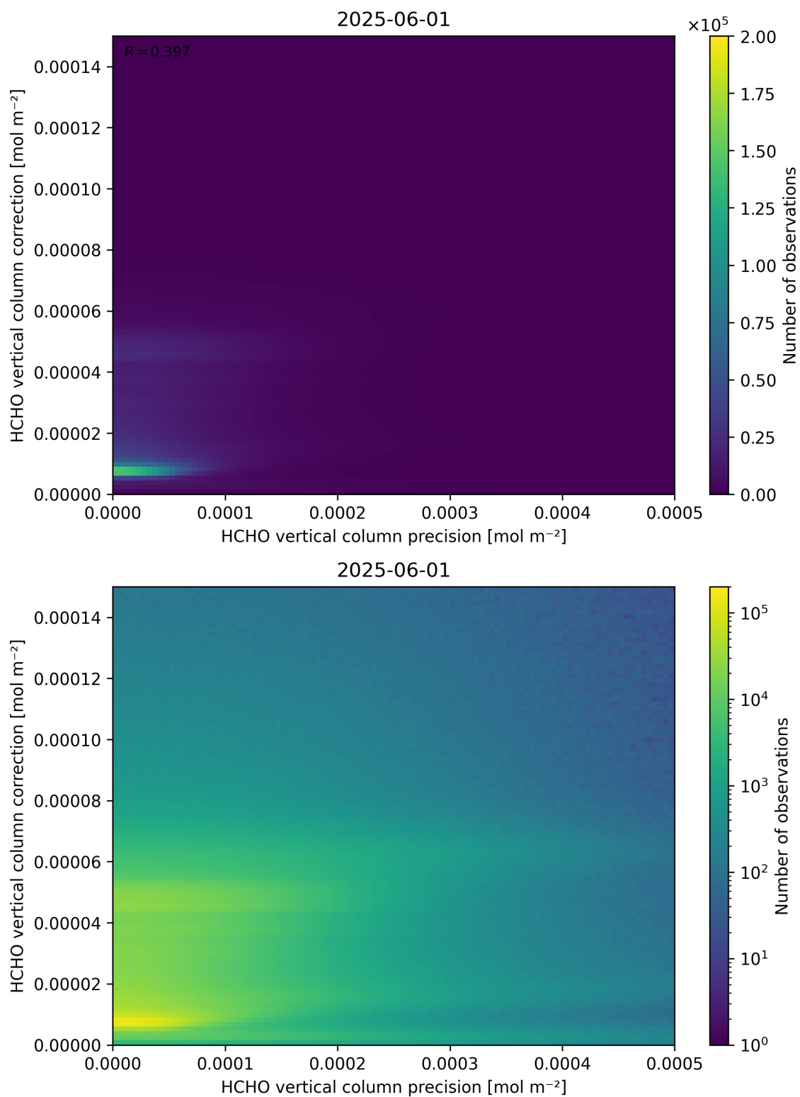
Figure 146: Scatter density plot of “HCHO vertical column precision” against “HCHO vertical column correction” for 2025-06-01 to 2025-06-02.
