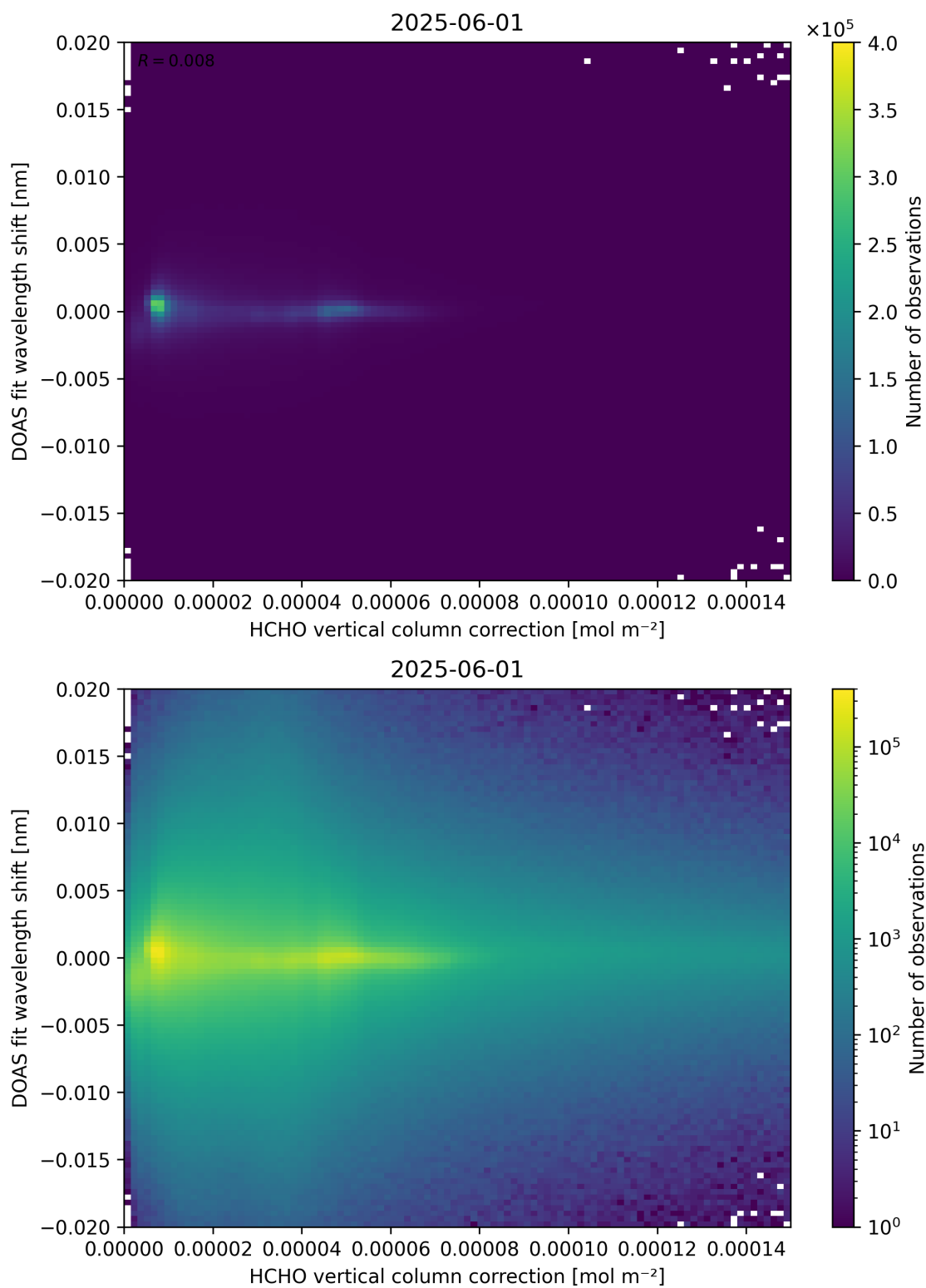
Figure 113: Scatter density plot of “HCHO vertical column correction” against “DOAS fit wavelength shift” for 2025-06-01 to 2025-06-02.
