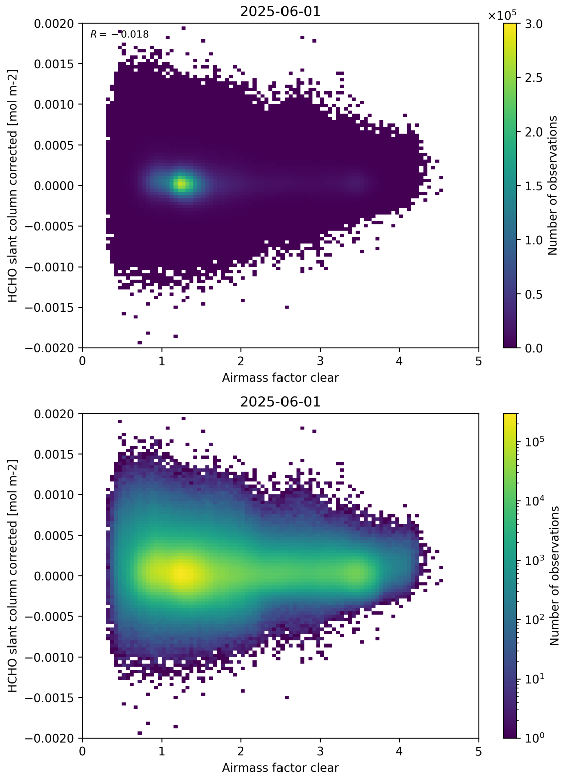
Figure 74: Scatter density plot of “Airmass factor clear” against “HCHO slant column corrected” for 2025-06-01 to 2025-06-02.
