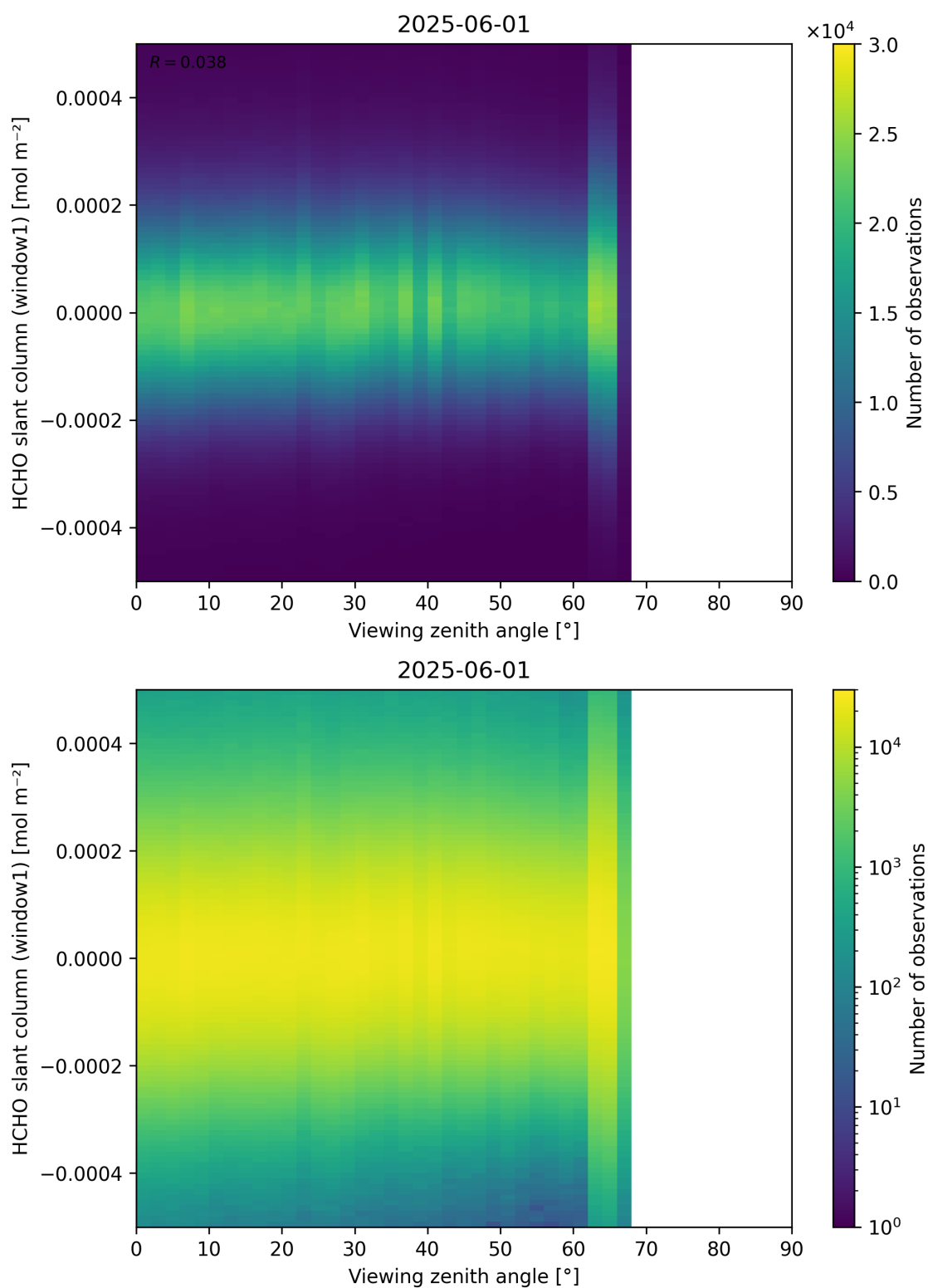
Figure 188: Scatter density plot of “Viewing zenith angle” against “HCHO slant column (window1)” for 2025-06-01 to 2025-06-02.
