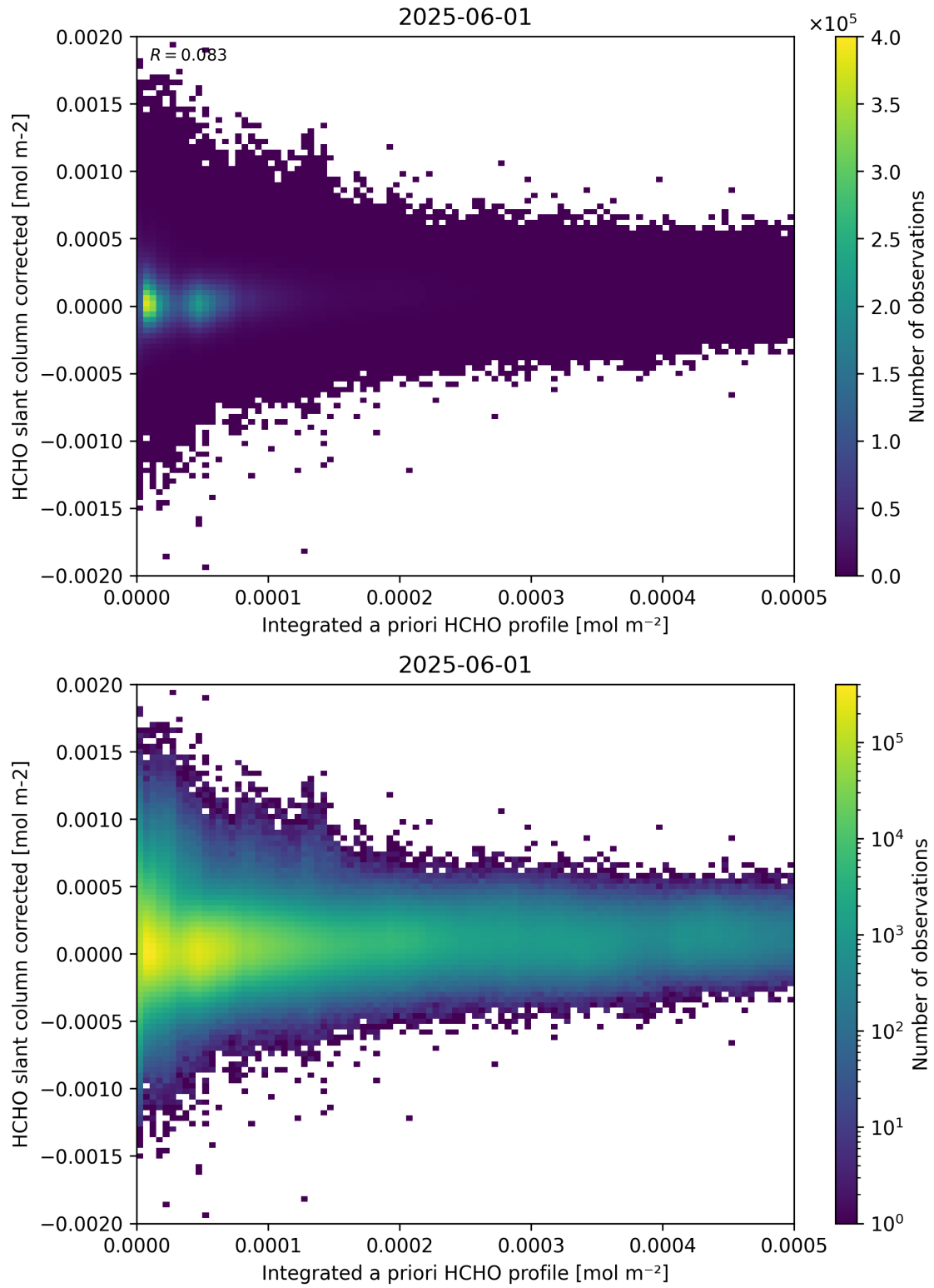
Figure 151: Scatter density plot of “Integrated a priori HCHO profile” against “HCHO slant column corrected” for 2025-06-01 to 2025-06-02.
