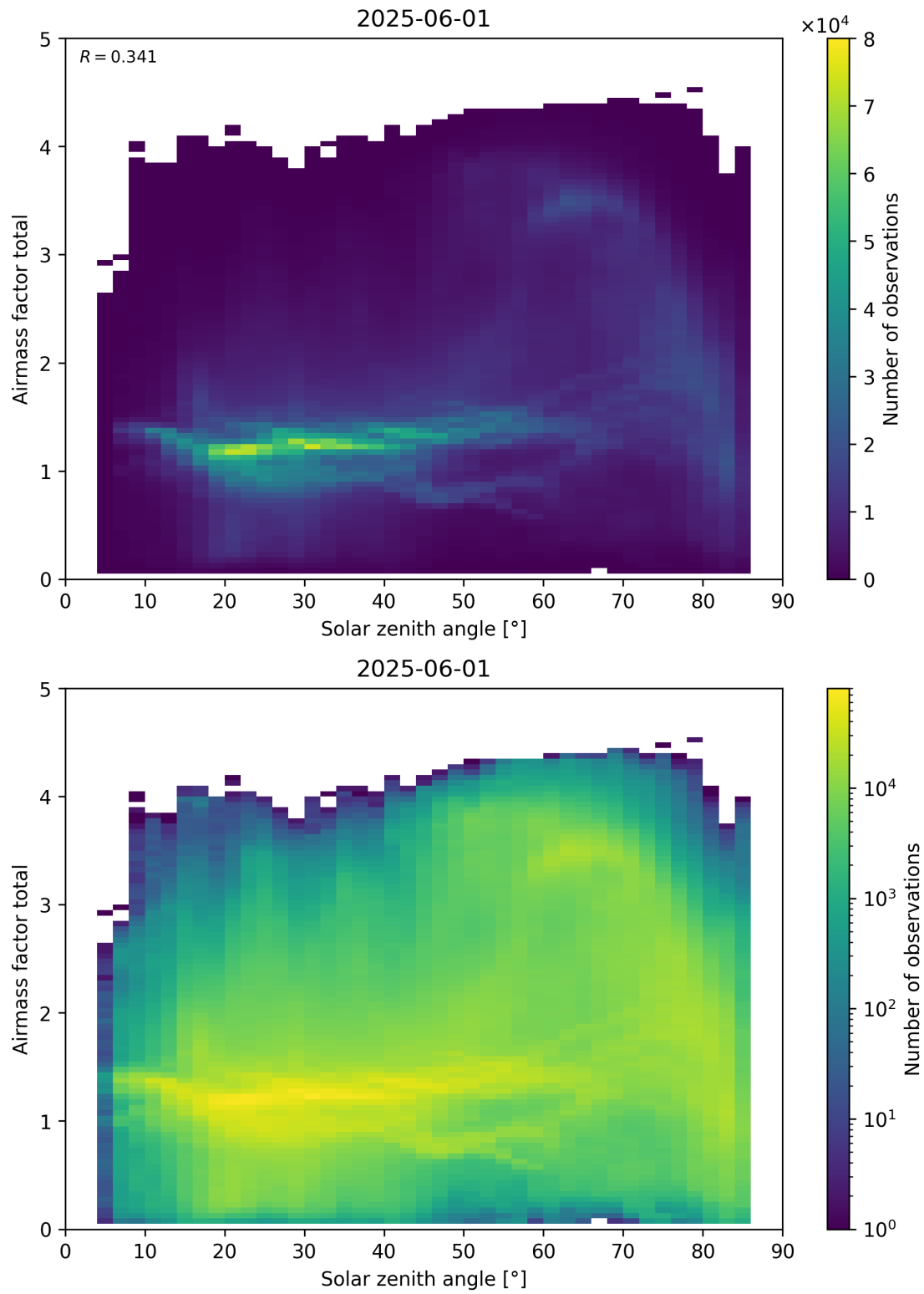
Figure 175: Scatter density plot of “Solar zenith angle” against “Airmass factor total” for 2025-06-01 to 2025-06-02.
