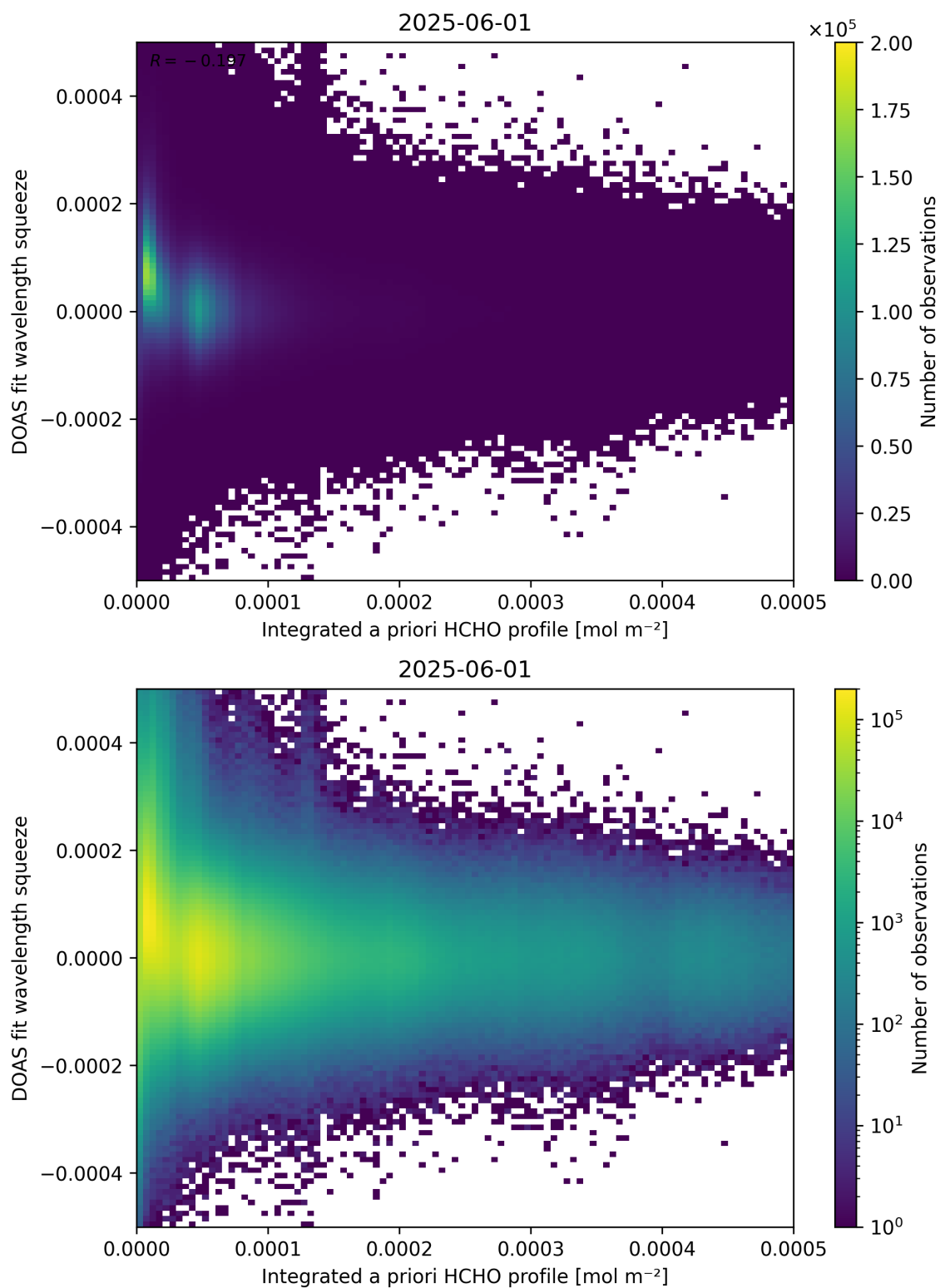
Figure 150: Scatter density plot of “Integrated a priori HCHO profile” against “DOAS fit wavelength squeeze” for 2025-06-01 to 2025-06-02.
