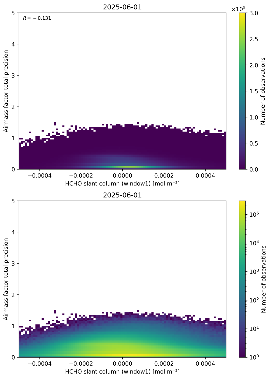
Figure 86: Scatter density plot of “HCHO slant column (window1)” against “Airmass factor total precision” for 2025-06-01 to 2025-06-02.
