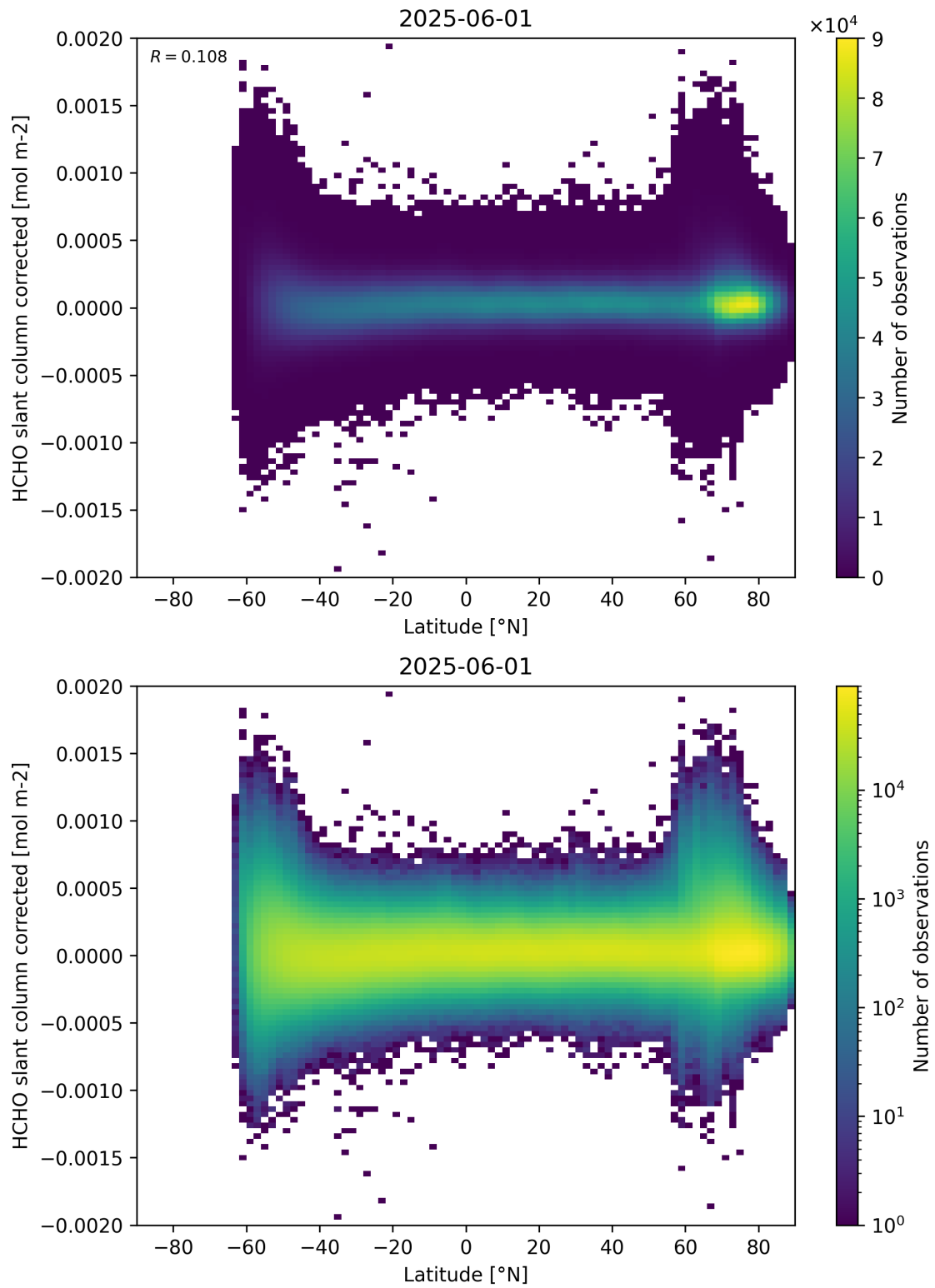
Figure 157: Scatter density plot of “Latitude” against “HCHO slant column corrected” for 2025-06-01 to 2025-06-02.
