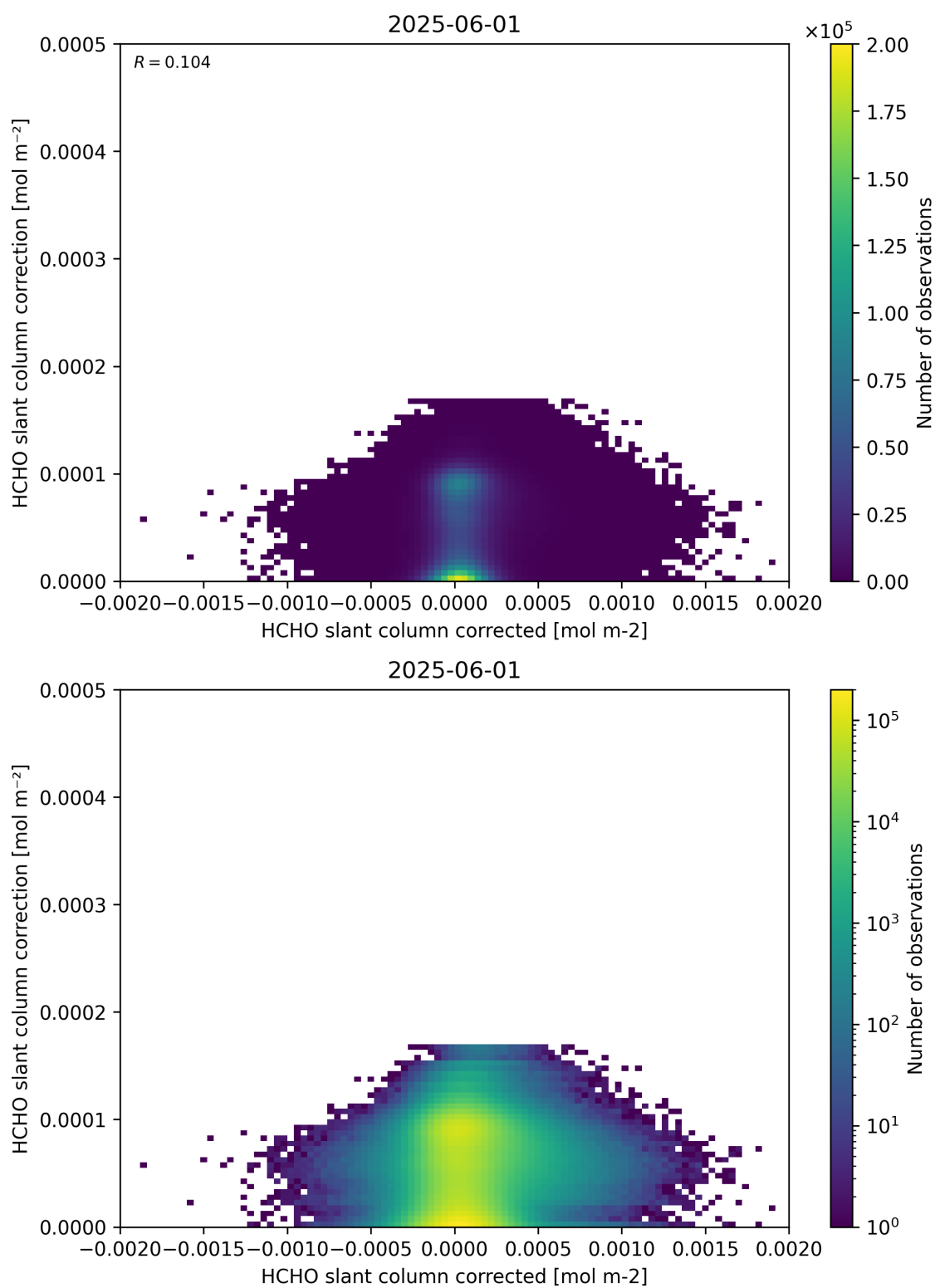
Figure 77: Scatter density plot of “HCHO slant column corrected” against “HCHO slant column correction” for 2025-06-01 to 2025-06-02.
