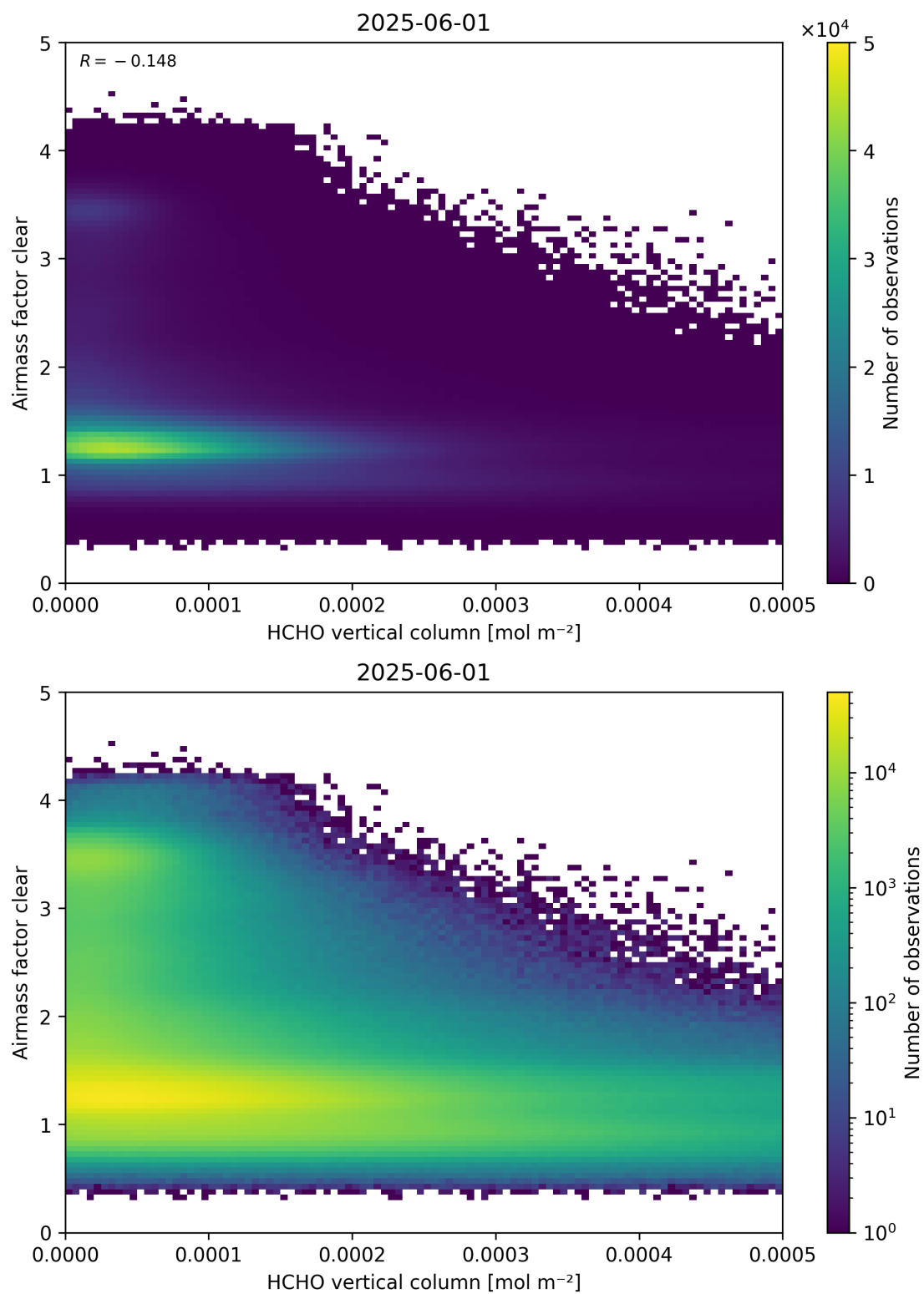
Figure 126: Scatter density plot of “HCHO vertical column” against “Airmass factor clear” for 2025-06-01 to 2025-06-02.
