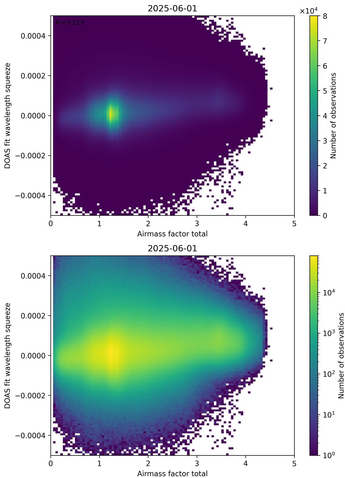
Figure 99: Scatter density plot of “Airmass factor total” against “DOAS fit wavelength squeeze” for 2025-06-01 to 2025-06-02.
