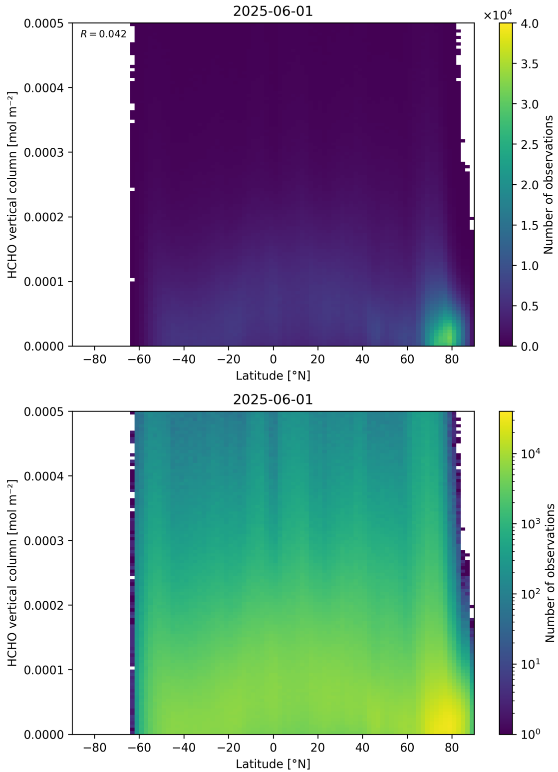
Figure 163: Scatter density plot of “Latitude” against “HCHO vertical column” for 2025-06-01 to 2025-06-02.
