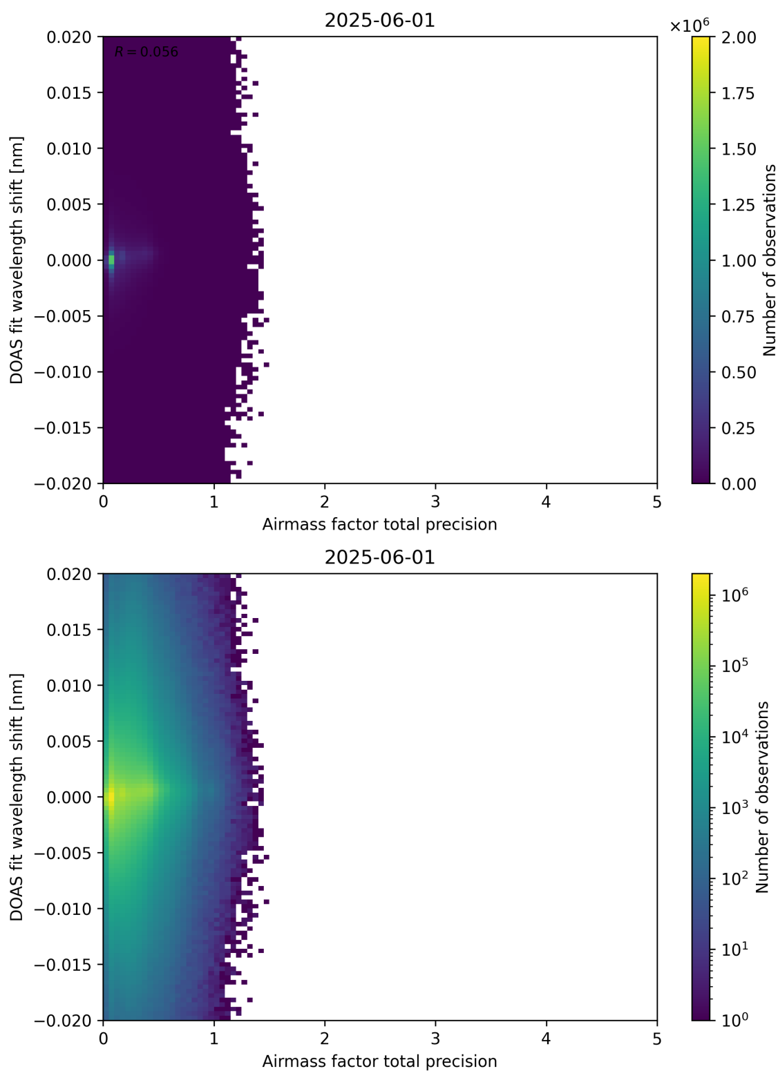
Figure 106: Scatter density plot of “Airmass factor total precision” against “DOAS fit wavelength shift” for 2025-06-01 to 2025-06-02.
