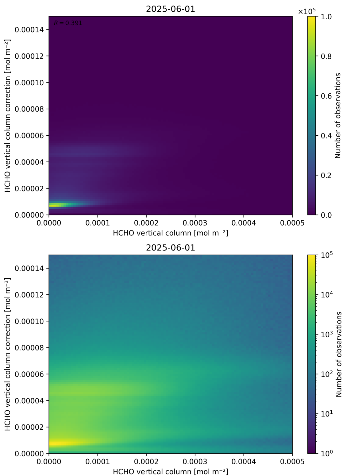
Figure 133: Scatter density plot of “HCHO vertical column” against “HCHO vertical column correction” for 2025-06-01 to 2025-06-02.
