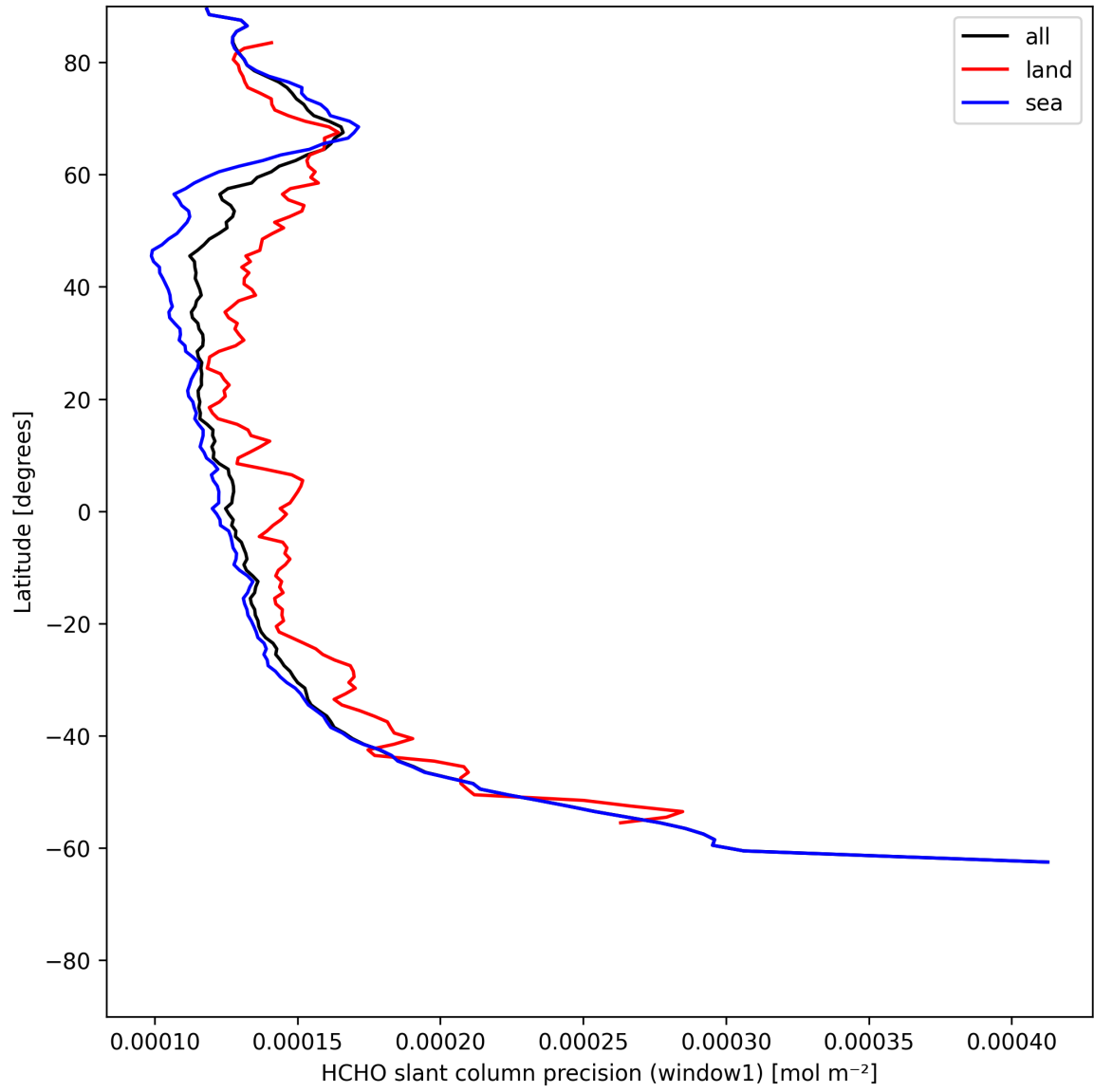
Figure 25: Zonal average of "HCHO slant column precision (window1)" for 2025-06-01 to 2025-06-02.
