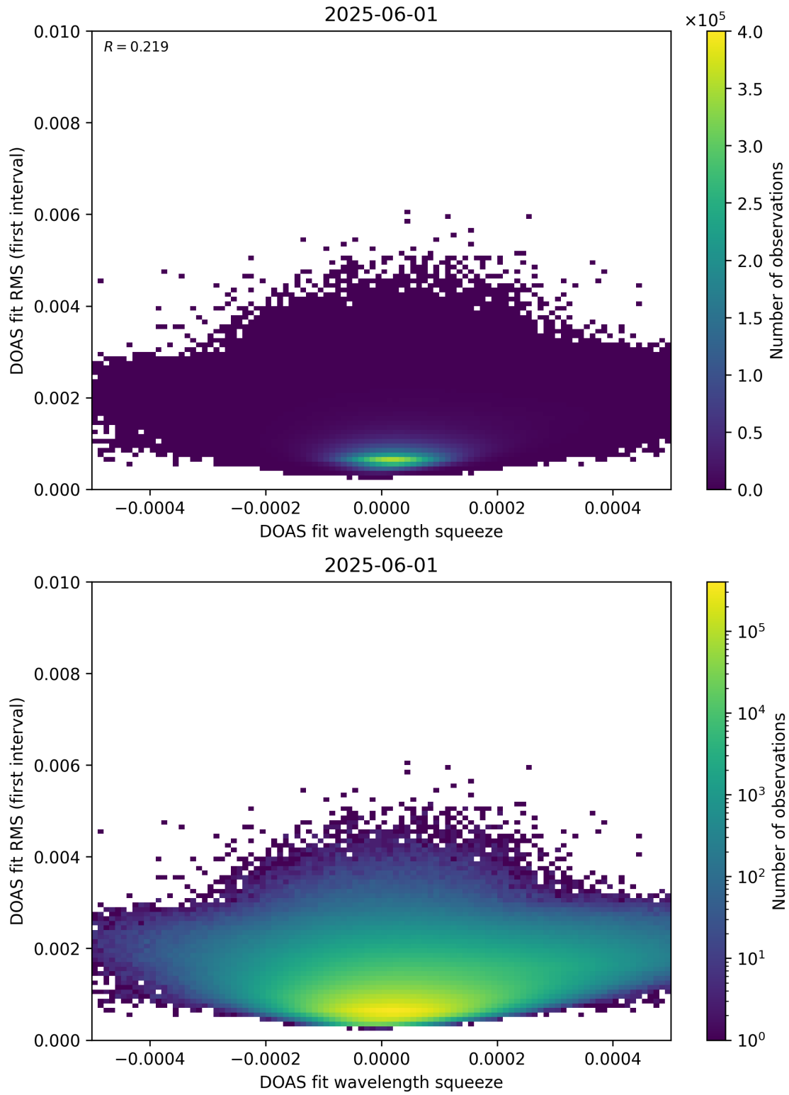
Figure 68: Scatter density plot of “DOAS fit wavelength squeeze” against “DOAS fit RMS (first interval)” for 2025-06-01 to 2025-06-02.
