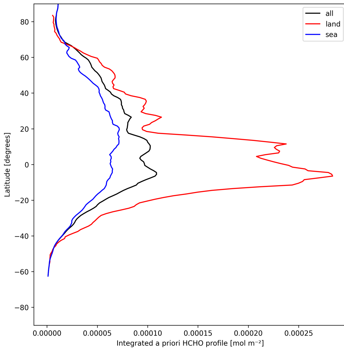
Figure 29: Zonal average of “Integrated a priori HCHO profile” for 2025-06-01 to 2025-06-02.
