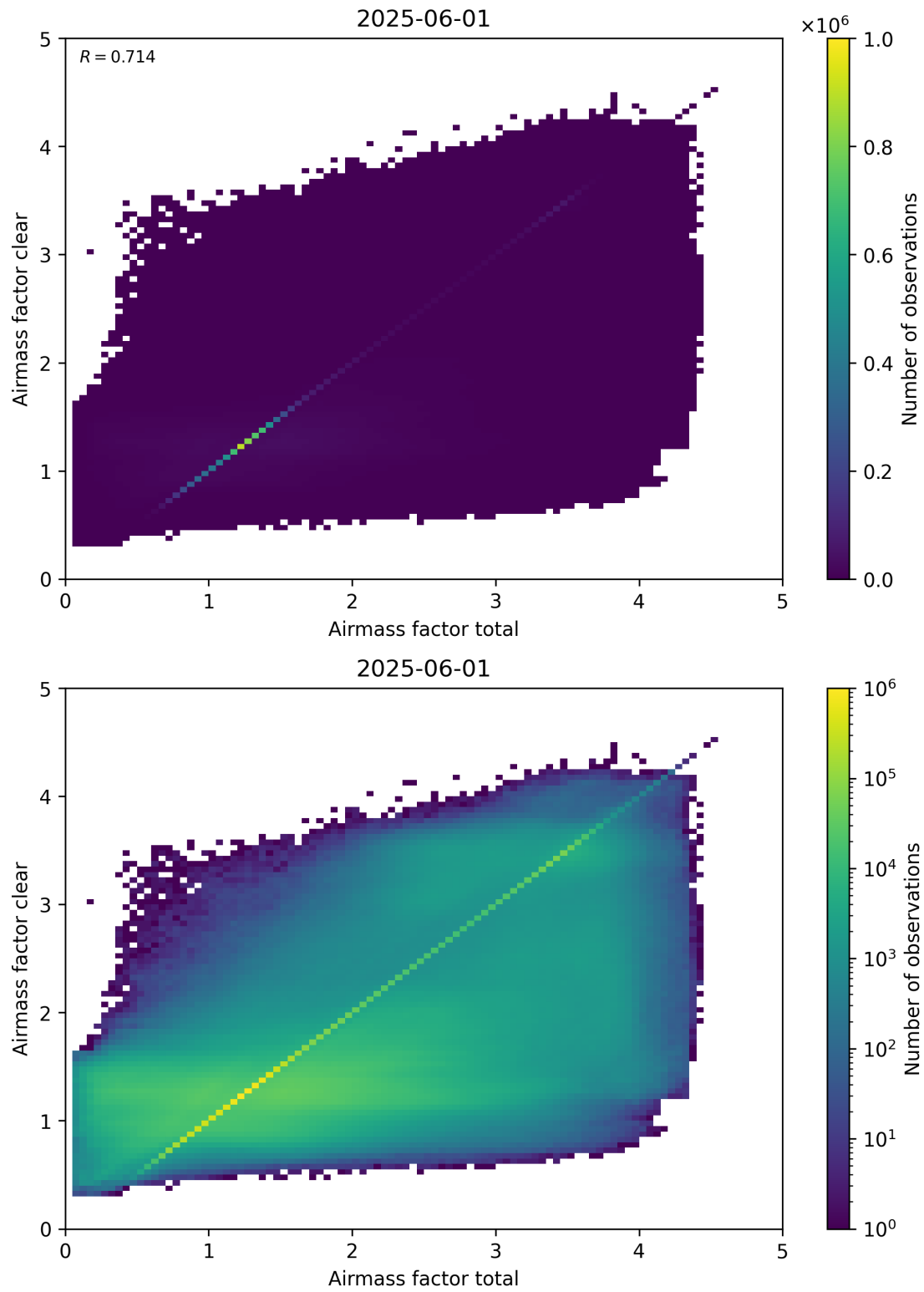
Figure 100: Scatter density plot of “Airmass factor total” against “Airmass factor clear” for 2025-06-01 to 2025-06-02.
