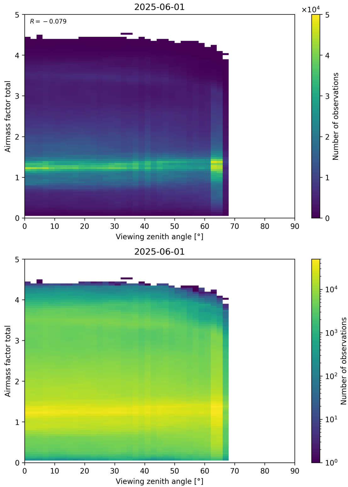
Figure 190: Scatter density plot of “Viewing zenith angle” against “Airmass factor total” for 2025-06-01 to 2025-06-02.
