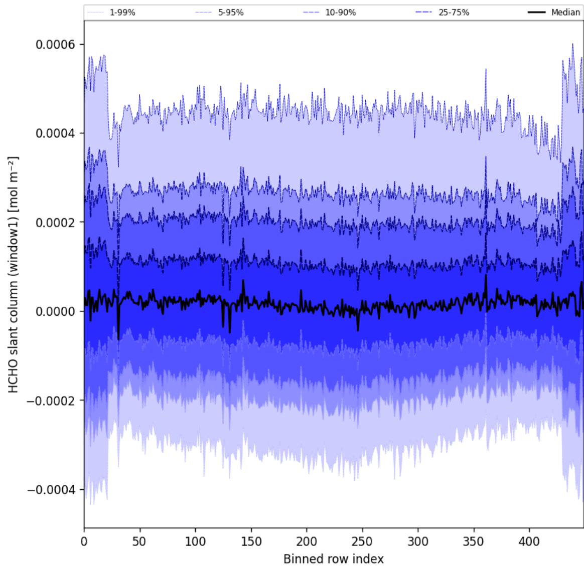
Figure 52: Along track statistics of "HCHO slant column (window1)" for 2025-06-01 to 2025-06-02
