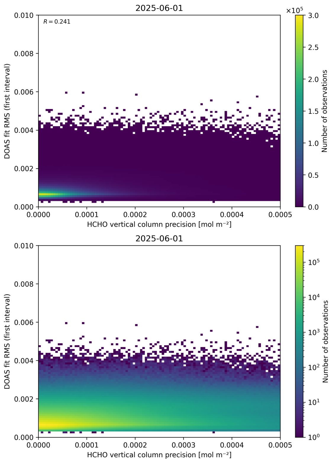
Figure 136: Scatter density plot of “HCHO vertical column precision” against “DOAS fit RMS (first interval)” for 2025-06-01 to 2025-06-02.
