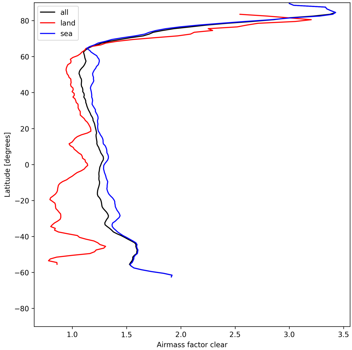
Figure 28: Zonal average of “Airmass factor clear” for 2025-06-01 to 2025-06-02.
