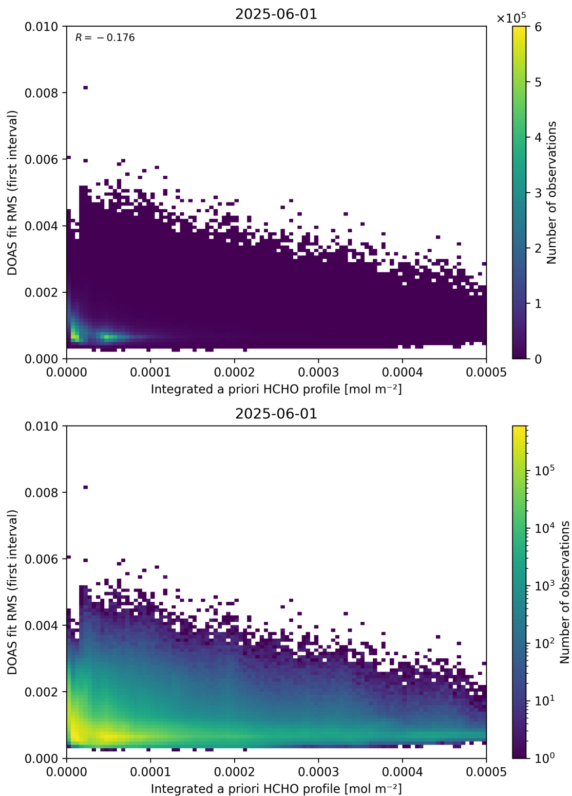
Figure 148: Scatter density plot of “Integrated a priori HCHO profile” against “DOAS fit RMS (first interval)” for 2025-06-01 to 2025-06-02.
