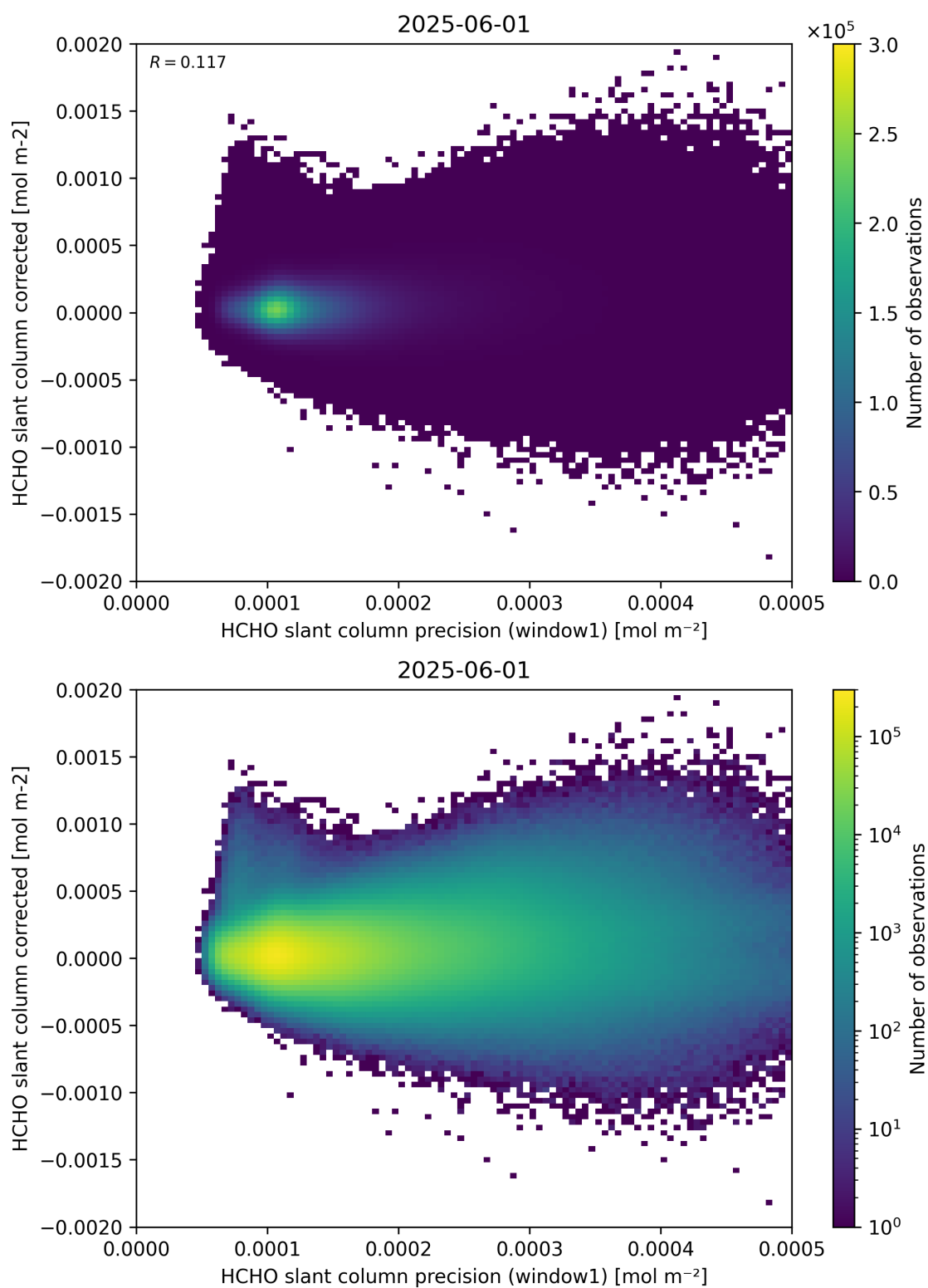
Figure 92: Scatter density plot of “HCHO slant column precision (window1)” against “HCHO slant column corrected” for 2025-06-01 to 2025-06-02.
