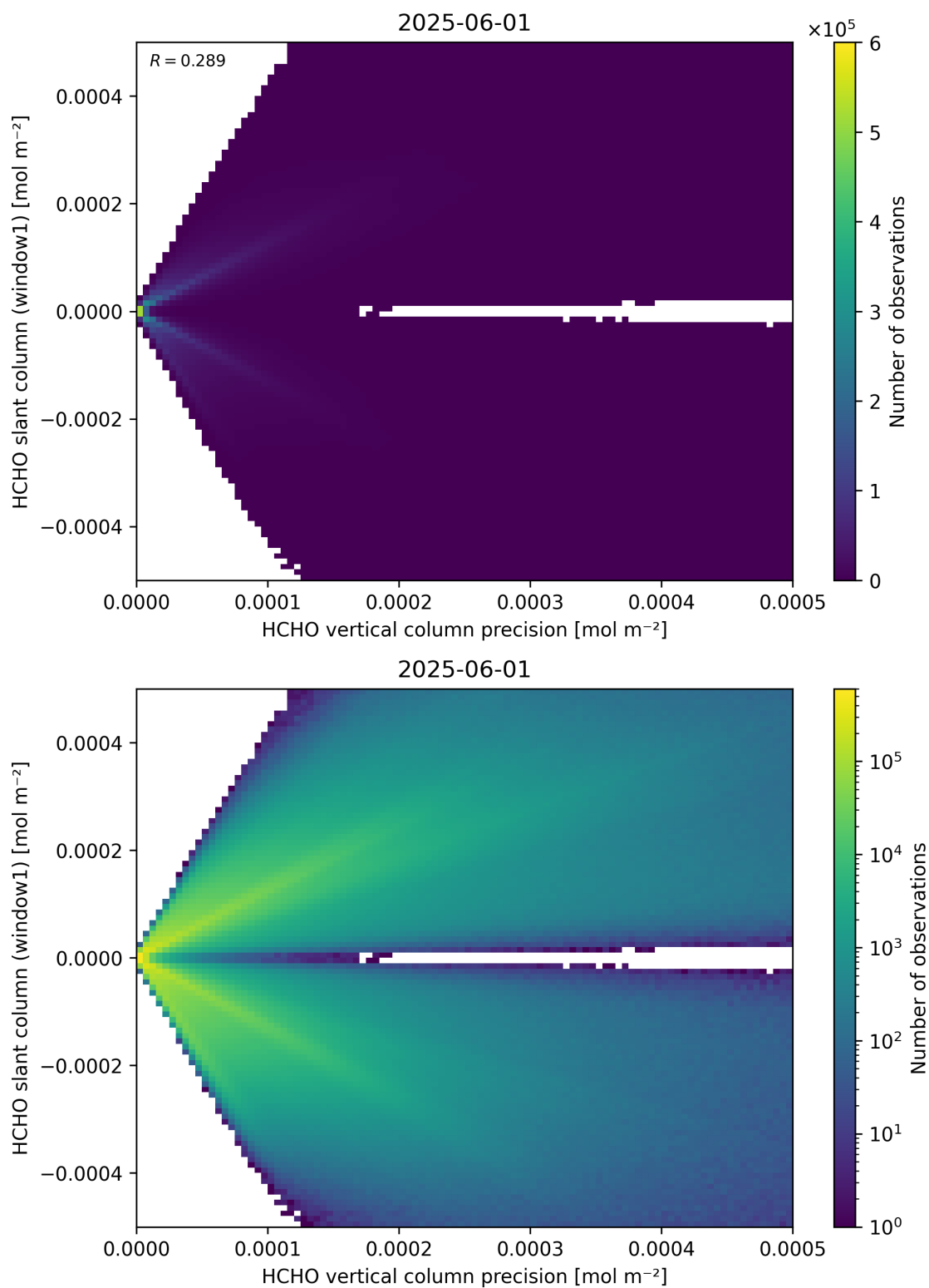
Figure 142: Scatter density plot of “HCHO vertical column precision” against “HCHO slant column (window1)” for 2025-06-01 to 2025-06-02.
