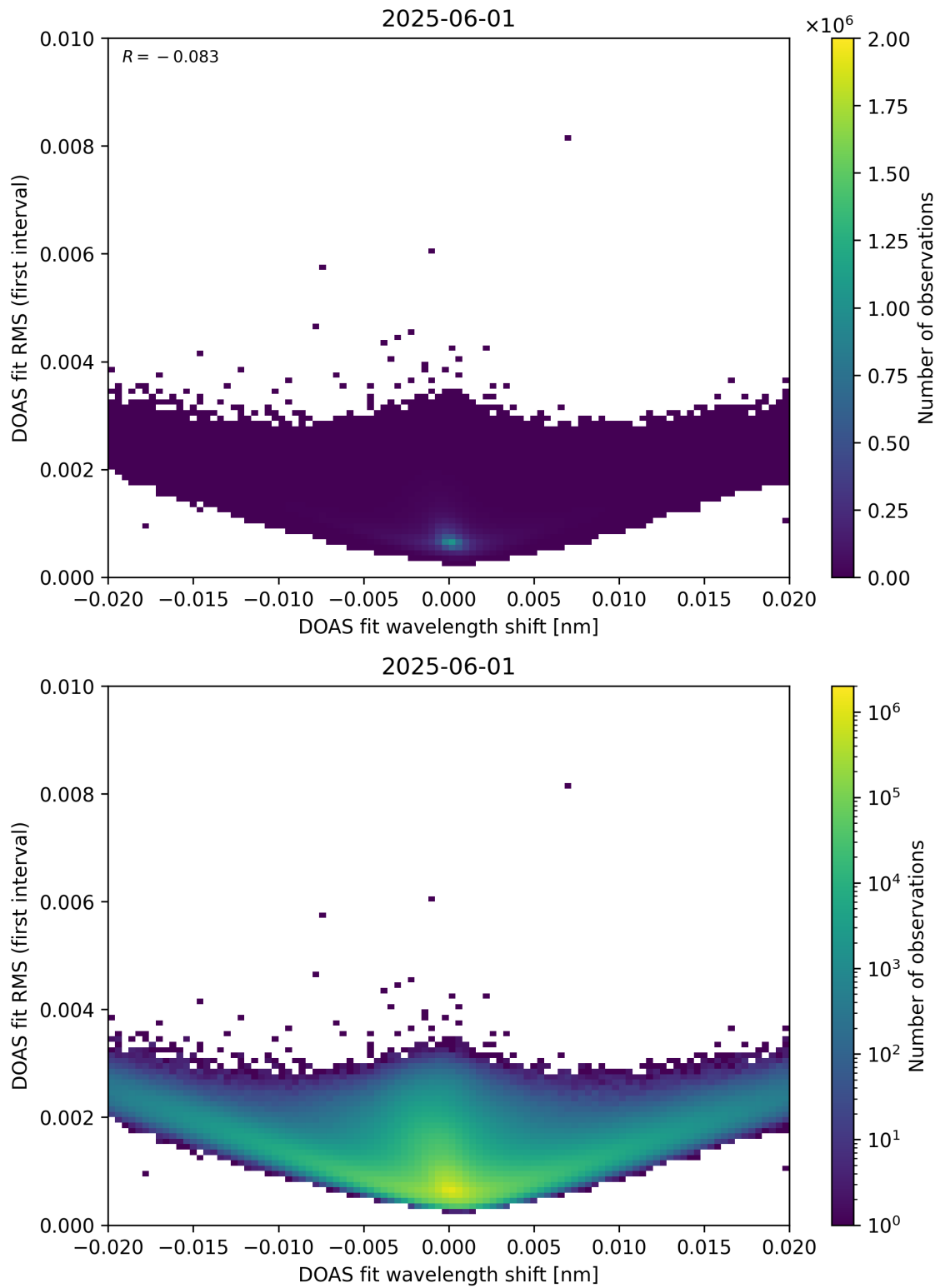
Figure 64: Scatter density plot of “DOAS fit wavelength shift” against “DOAS fit RMS (first interval)” for 2025-06-01 to 2025-06-02.
