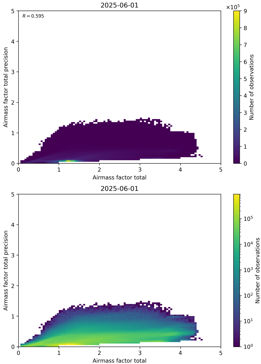
Figure 103: Scatter density plot of “Airmass factor total” against “Airmass factor total precision” for 2025-06-01 to 2025-06-02.
