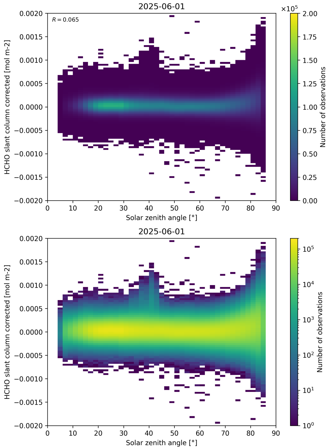
Figure 171: Scatter density plot of “Solar zenith angle” against “HCHO slant column corrected” for 2025-06-01 to 2025-06-02.
