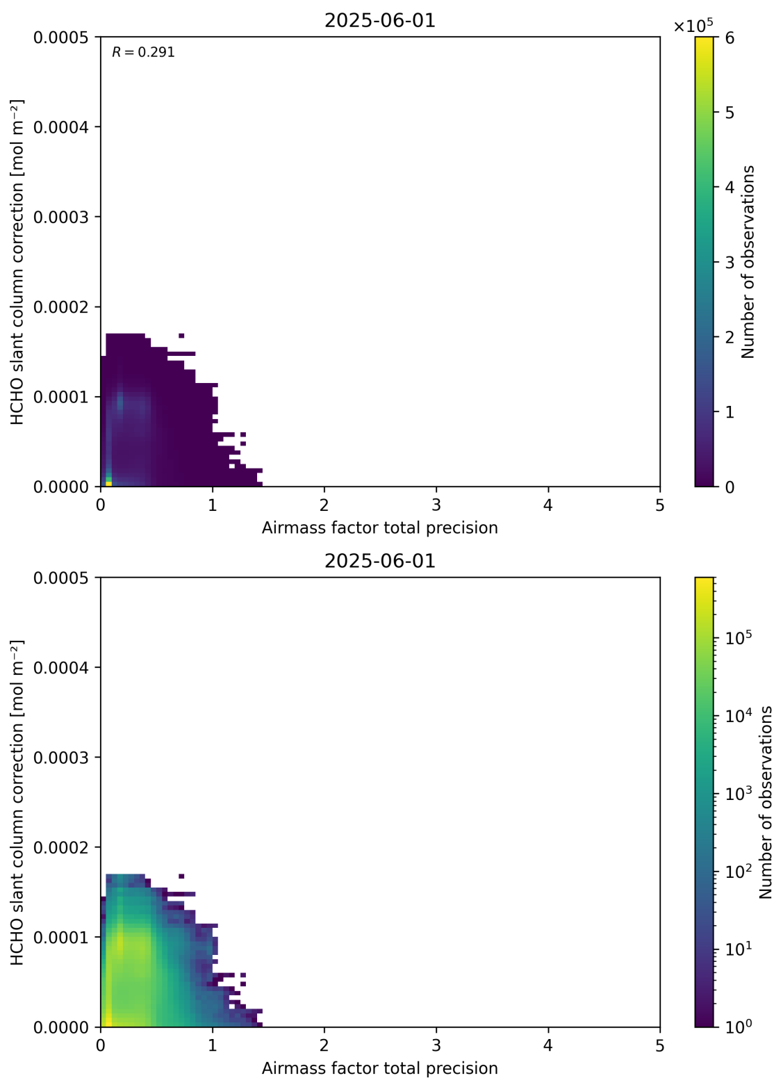
Figure 110: Scatter density plot of “Airmass factor total precision” against “HCHO slant column correction” for 2025-06-01 to 2025-06-02.
