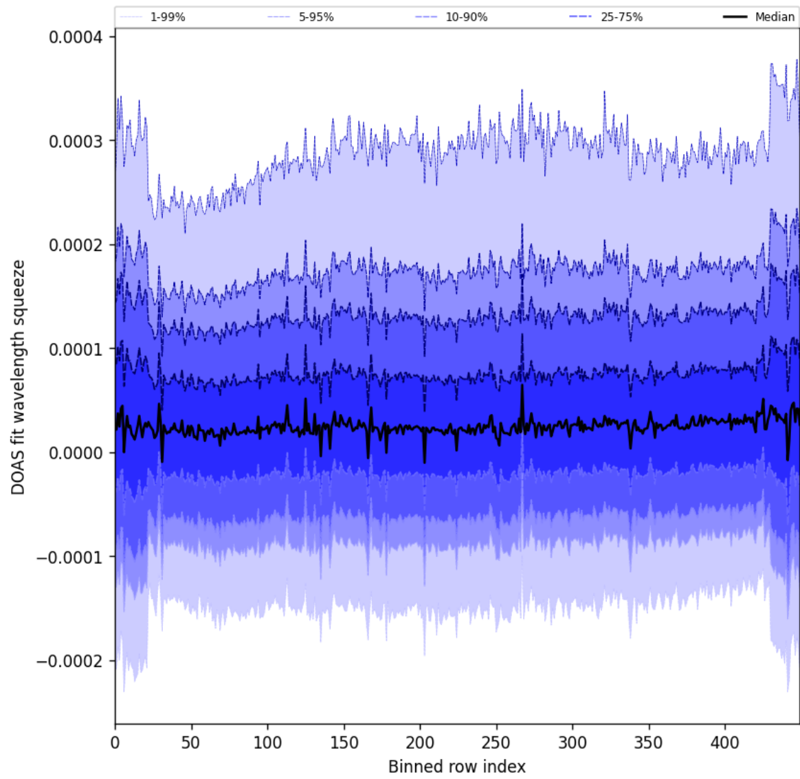
Figure 59: Along track statistics of “DOAS fit wavelength squeeze” for 2025-06-01 to 2025-06-02
