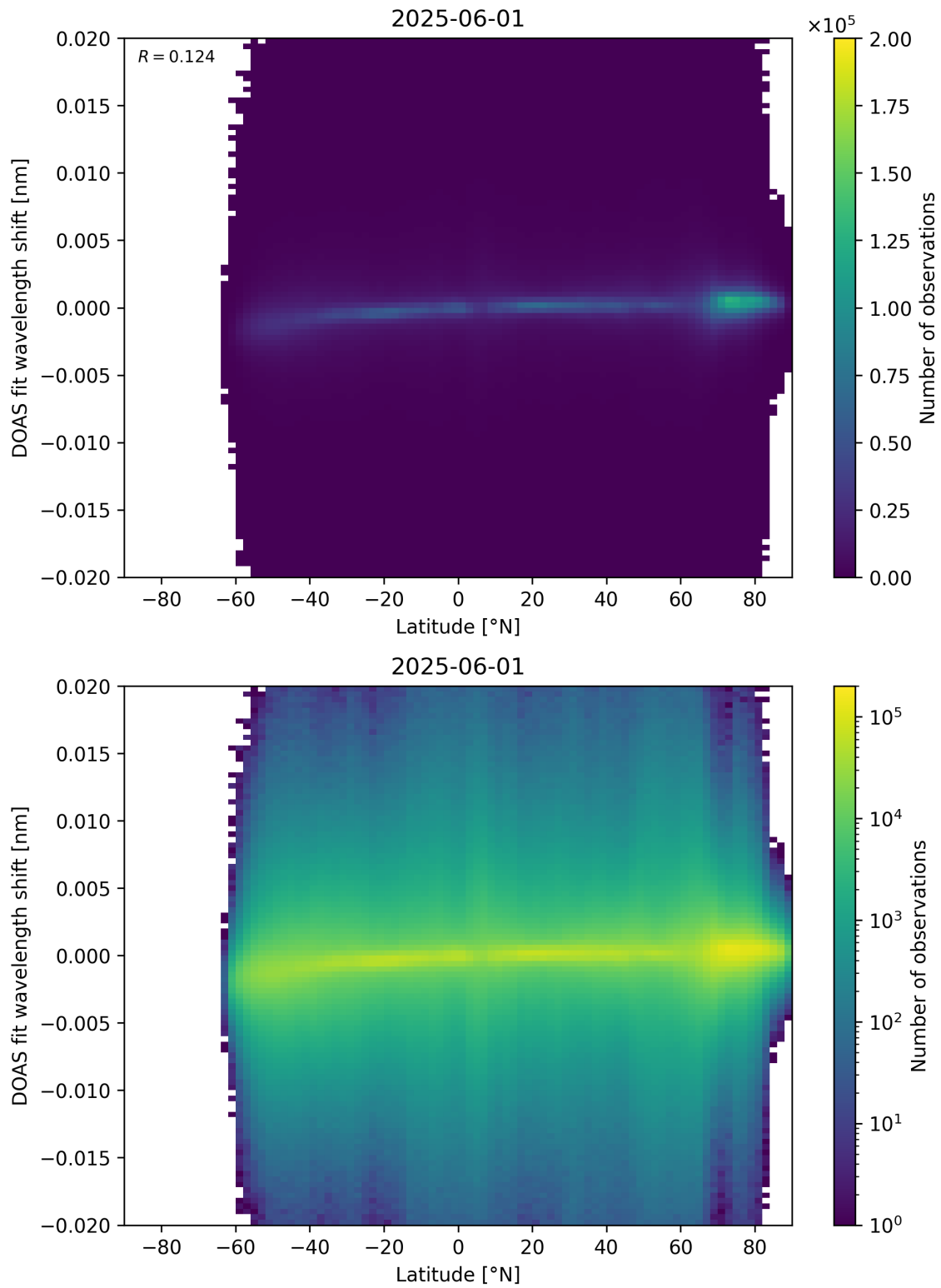
Figure 154: Scatter density plot of “Latitude” against “DOAS fit wavelength shift” for 2025-06-01 to 2025-06-02.
