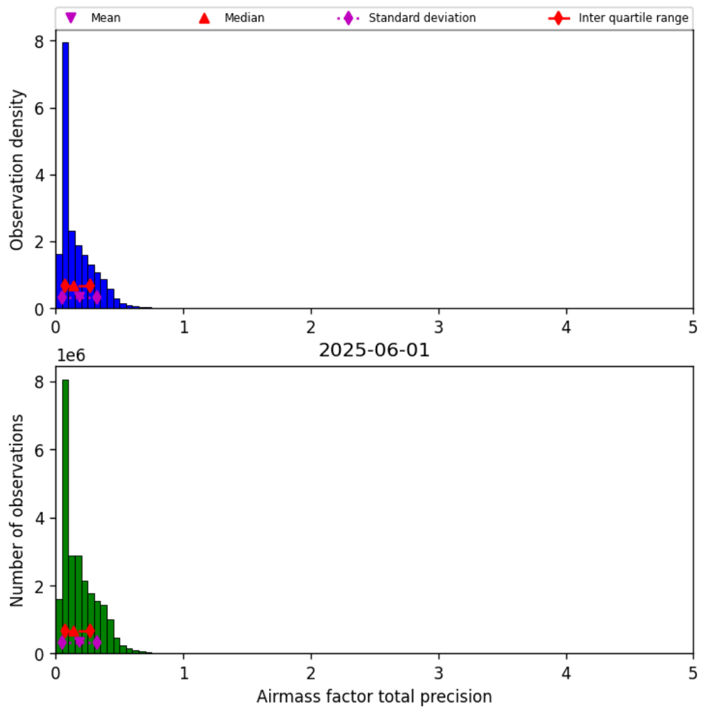
Figure 41: Histogram of “Airmass factor total precision” for 2025-06-01 to 2025-06-02
