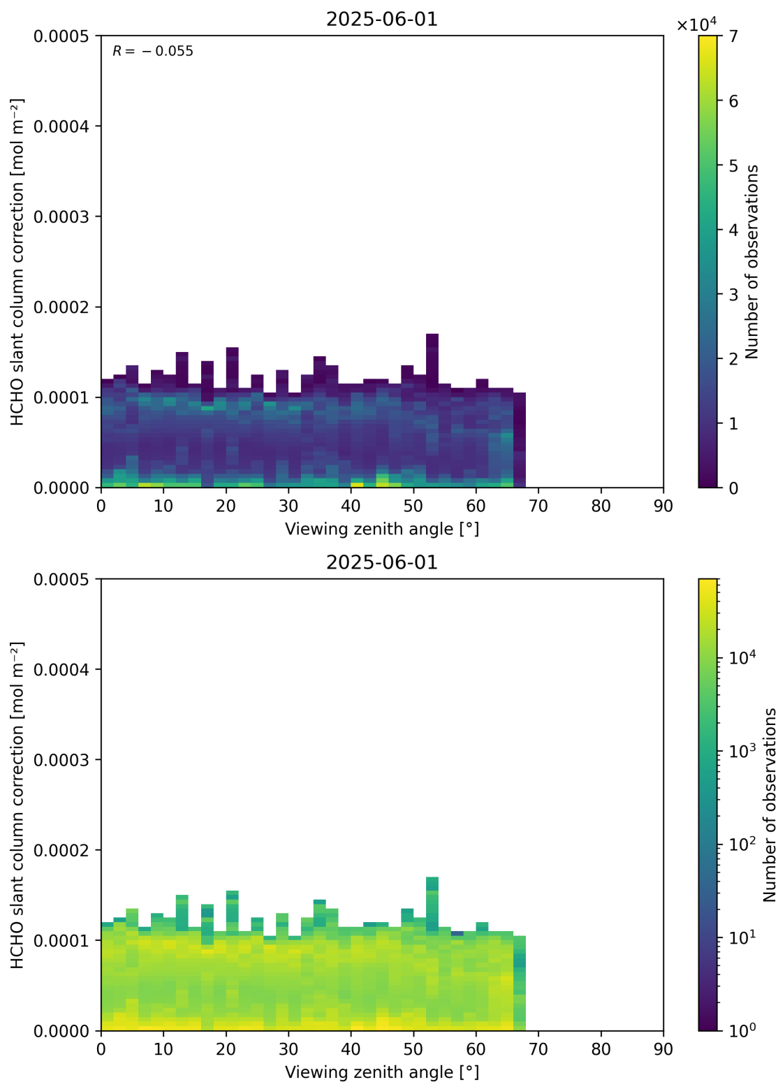
Figure 187: Scatter density plot of “Viewing zenith angle” against “HCHO slant column correction” for 2025-06-01 to 2025-06-02.
