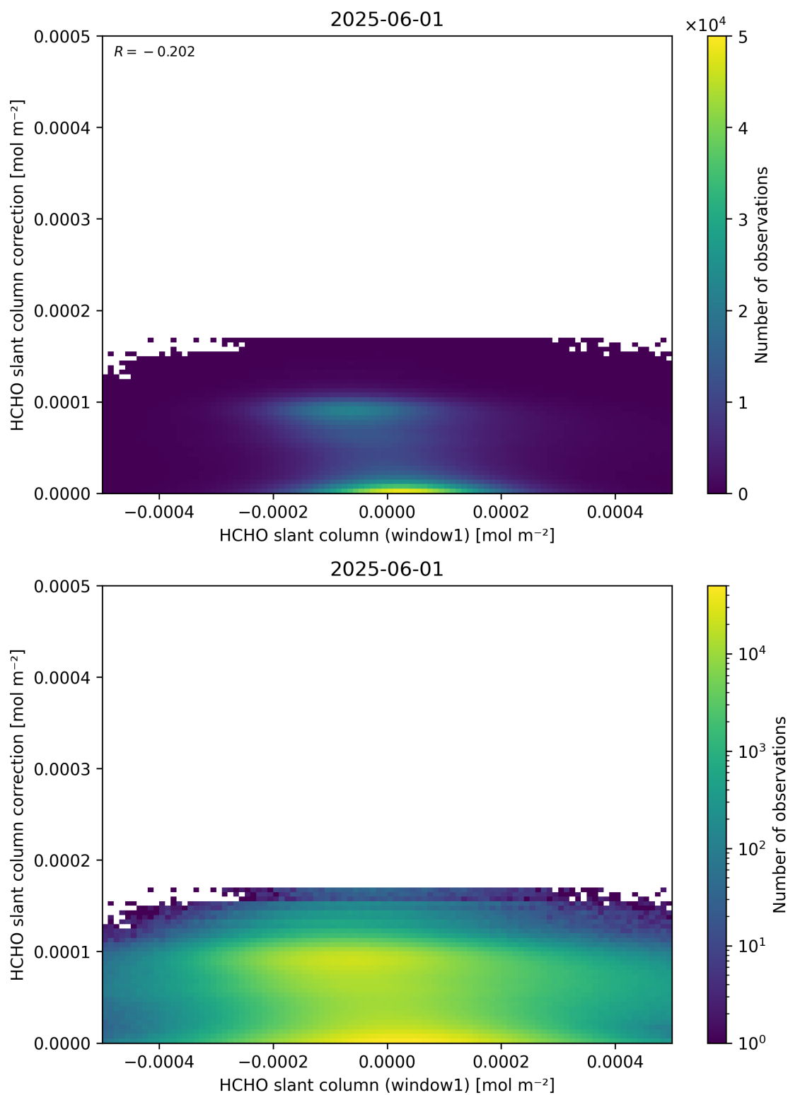
Figure 83: Scatter density plot of “HCHO slant column (window1)” against “HCHO slant column correction” for 2025-06-01 to 2025-06-02.
