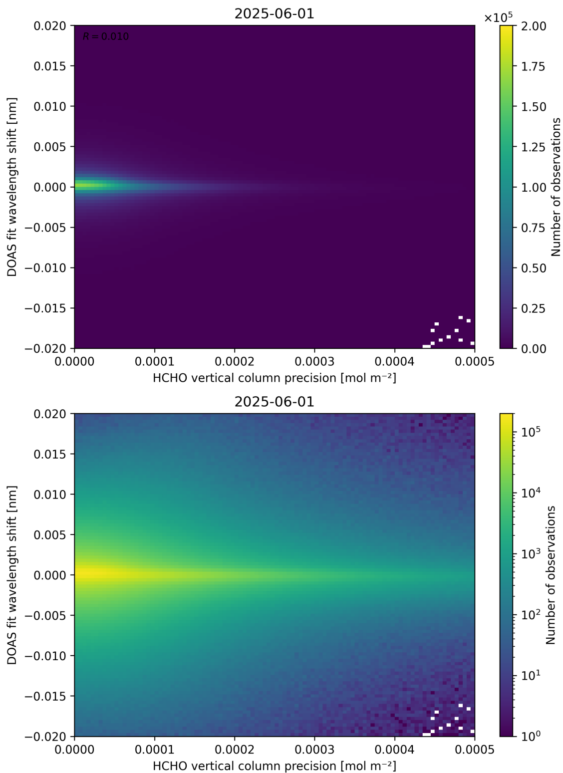
Figure 137: Scatter density plot of “HCHO vertical column precision” against “DOAS fit wavelength shift” for 2025-06-01 to 2025-06-02.
