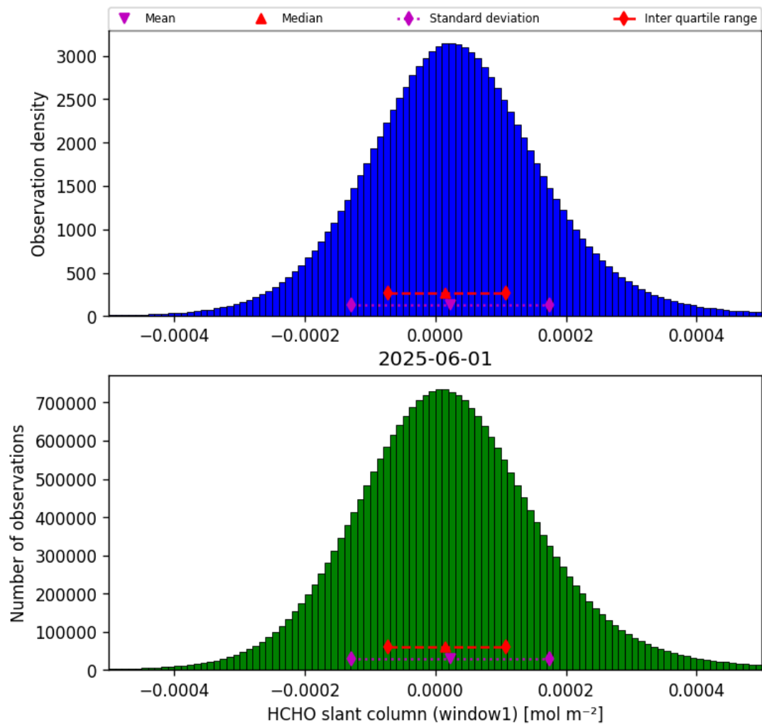
Figure 38: Histogram of “HCHO slant column (window1)” for 2025-06-01 to 2025-06-02
