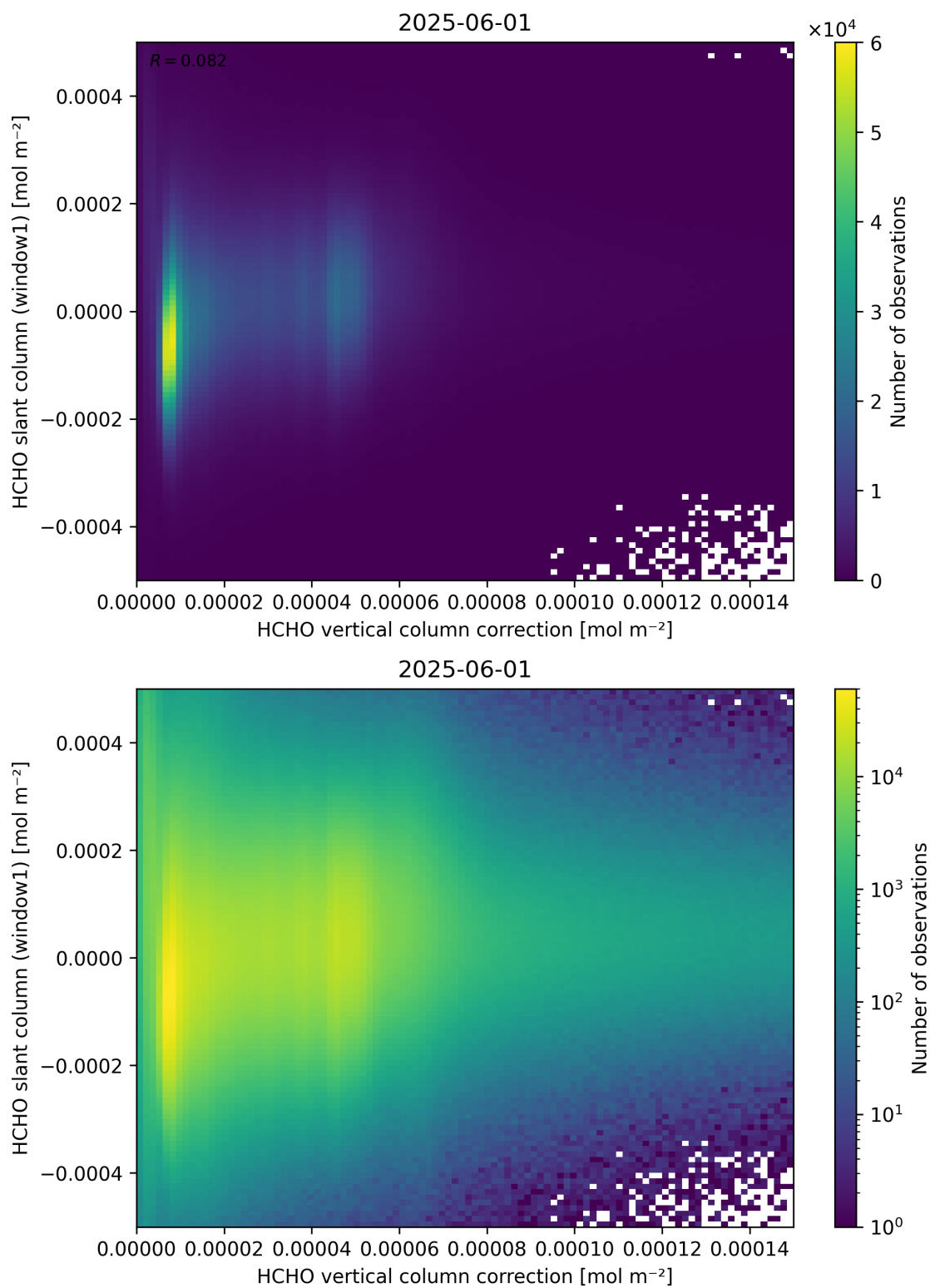
Figure 118: Scatter density plot of “HCHO vertical column correction” against “HCHO slant column (window1)” for 2025-06-01 to 2025-06-02.
