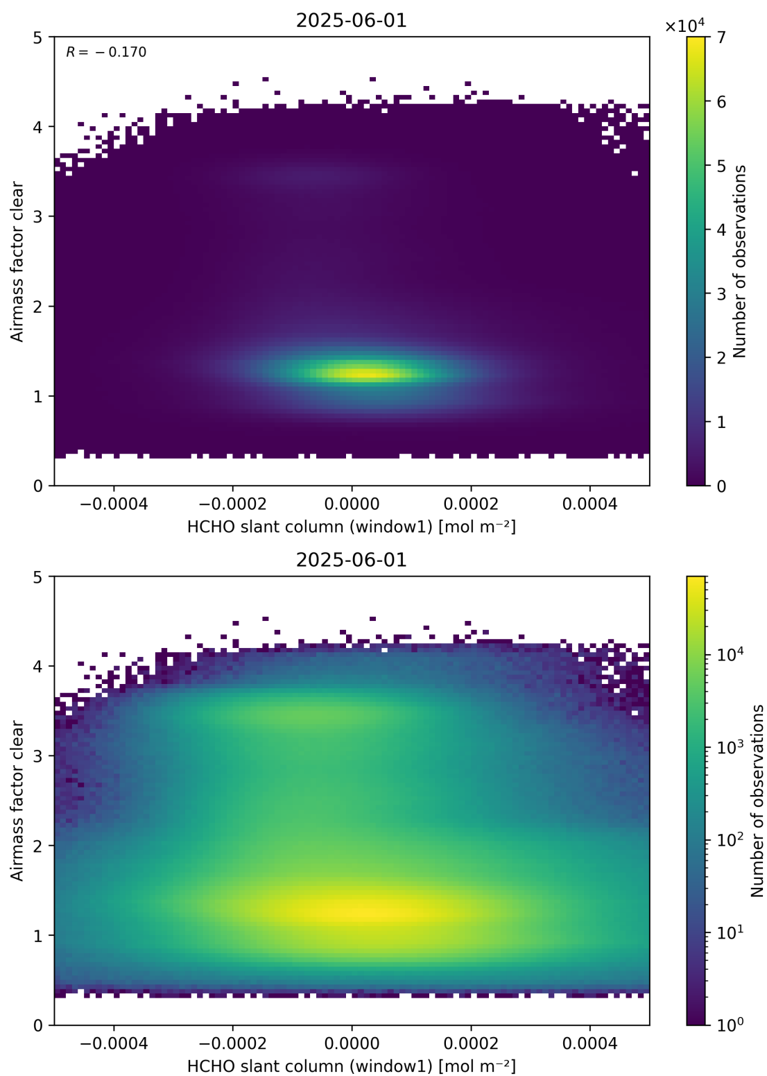
Figure 81: Scatter density plot of “HCHO slant column (window1)” against “Airmass factor clear” for 2025-06-01 to 2025-06-02.
