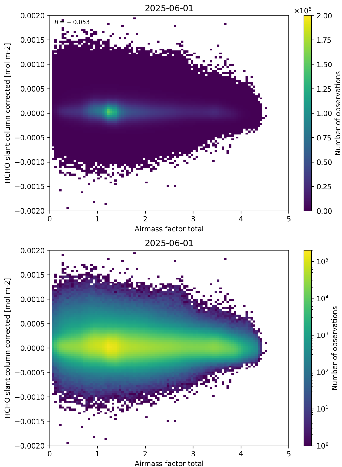
Figure 101: Scatter density plot of “Airmass factor total” against “HCHO slant column corrected” for 2025-06-01 to 2025-06-02.
