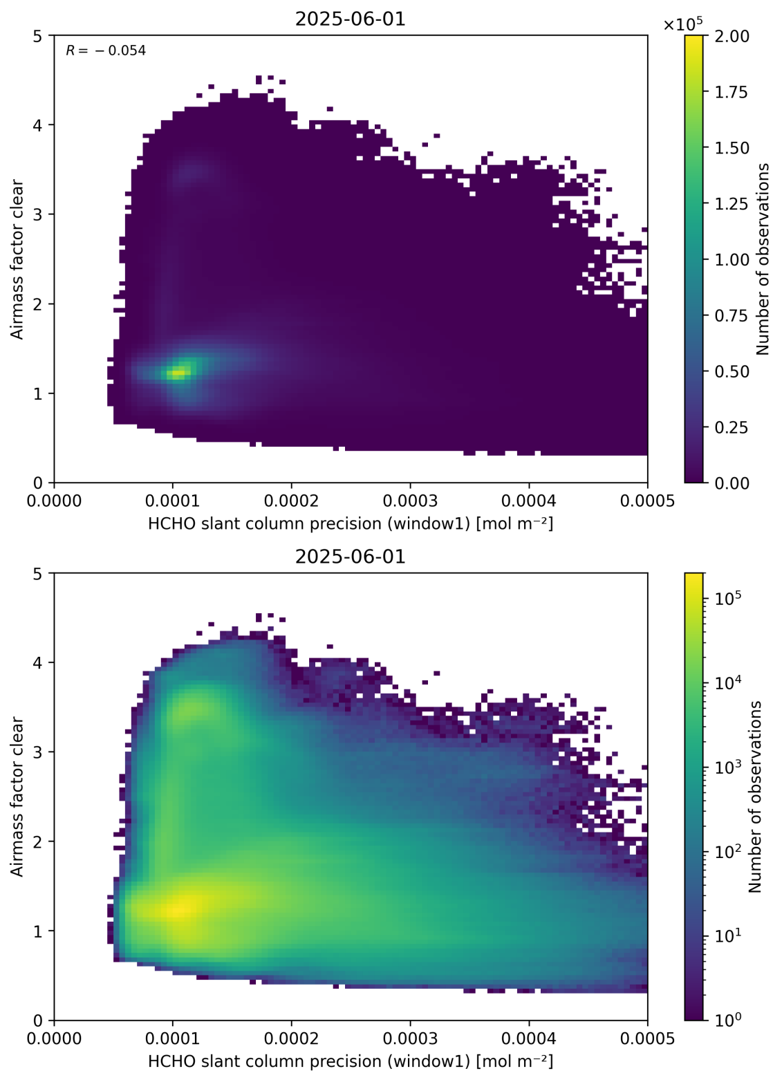
Figure 91: Scatter density plot of “HCHO slant column precision (window1)” against “Airmass factor clear” for 2025-06-01 to 2025-06-02.
