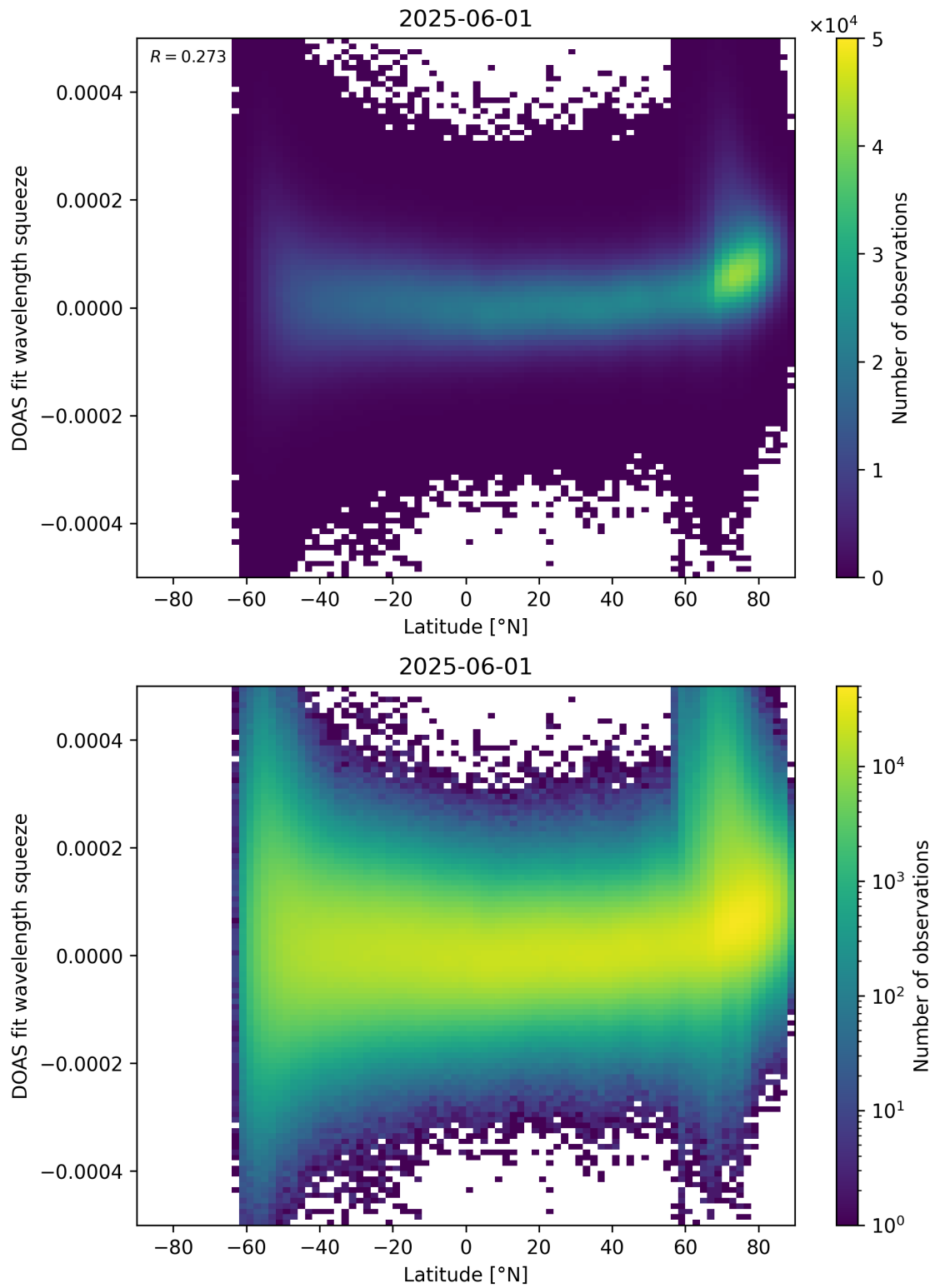
Figure 155: Scatter density plot of “Latitude” against “DOAS fit wavelength squeeze” for 2025-06-01 to 2025-06-02.
