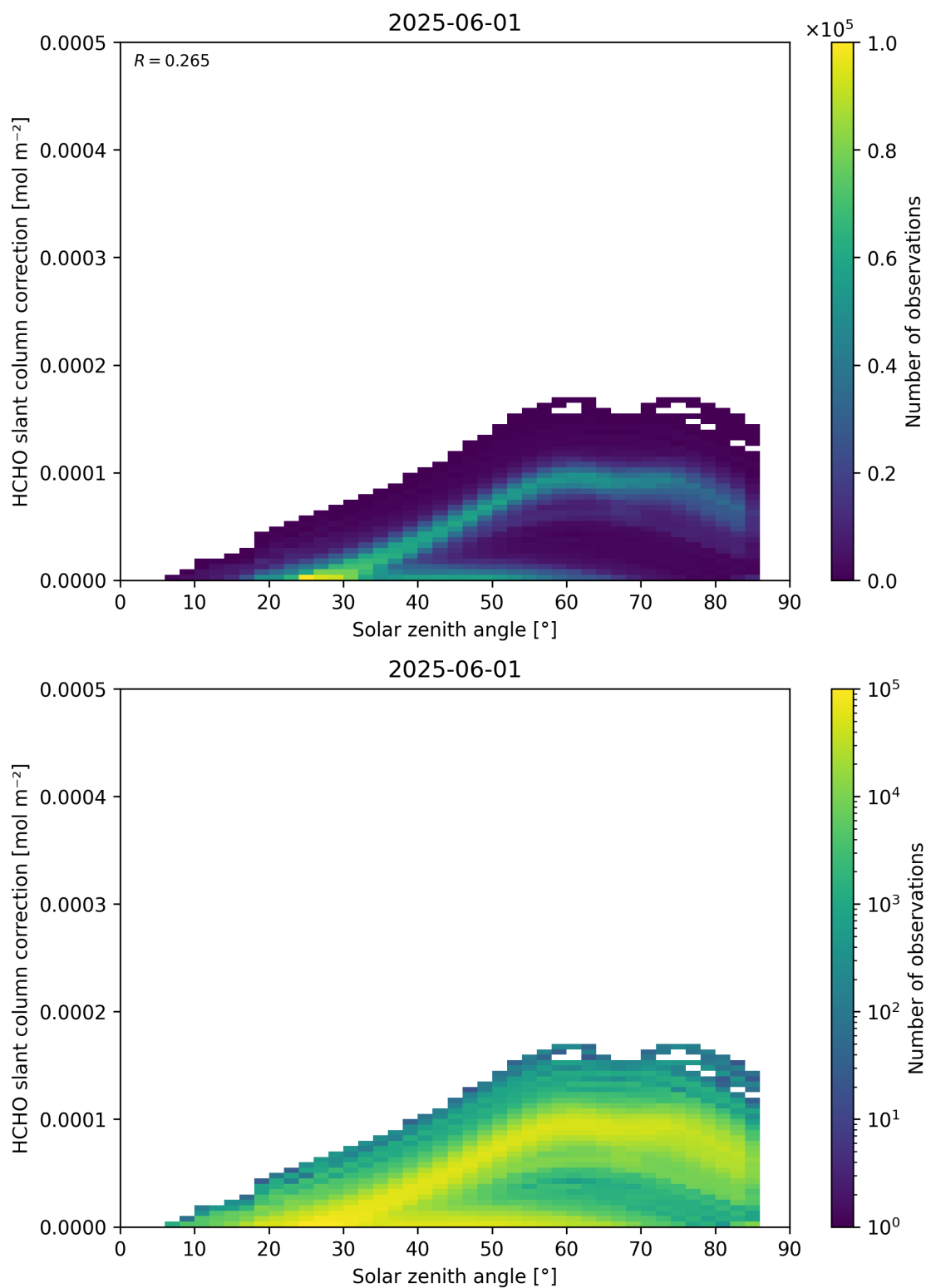
Figure 172: Scatter density plot of “Solar zenith angle” against “HCHO slant column correction” for 2025-06-01 to 2025-06-02.
