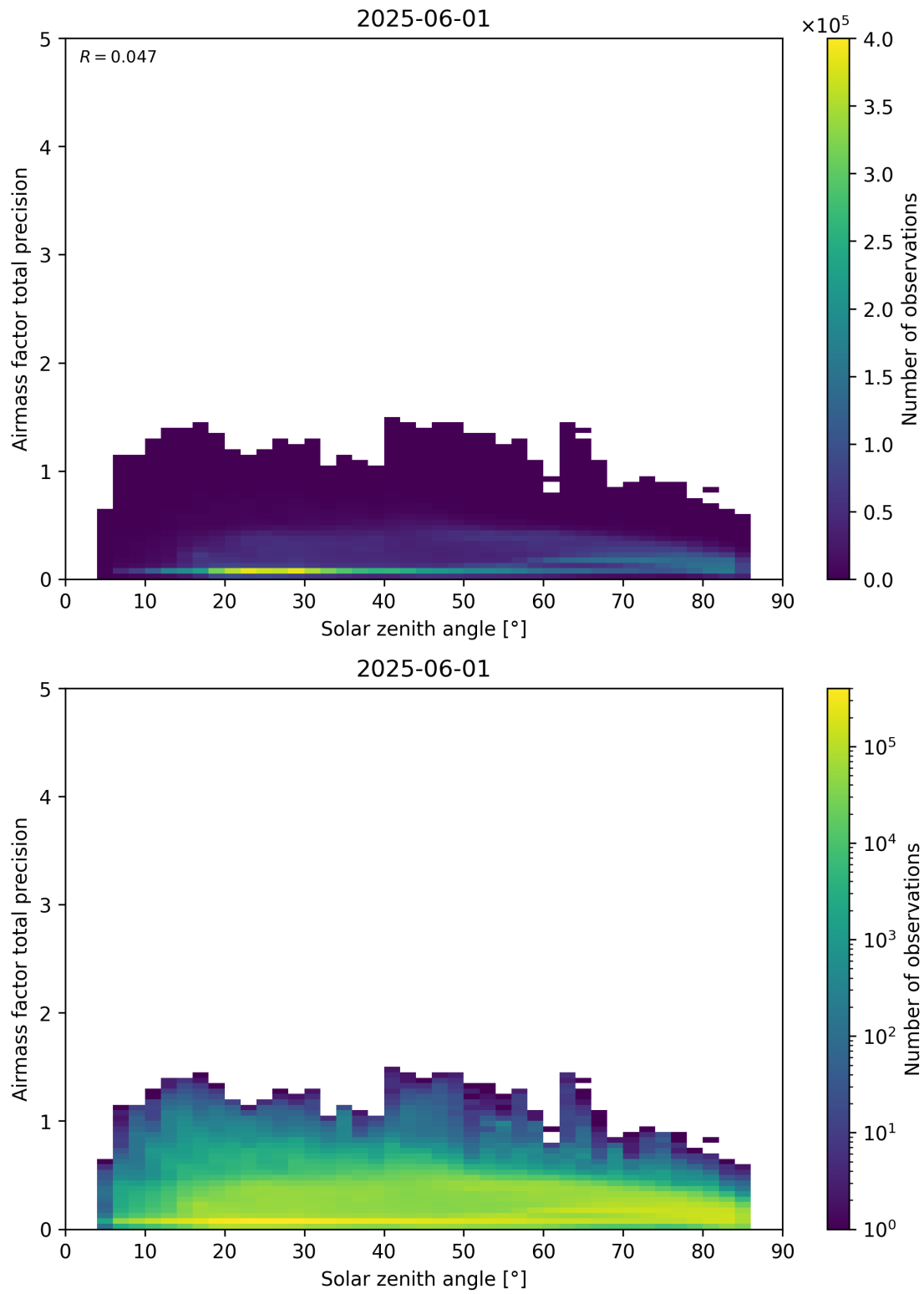
Figure 176: Scatter density plot of “Solar zenith angle” against “Airmass factor total precision” for 2025-06-01 to 2025-06-02.
