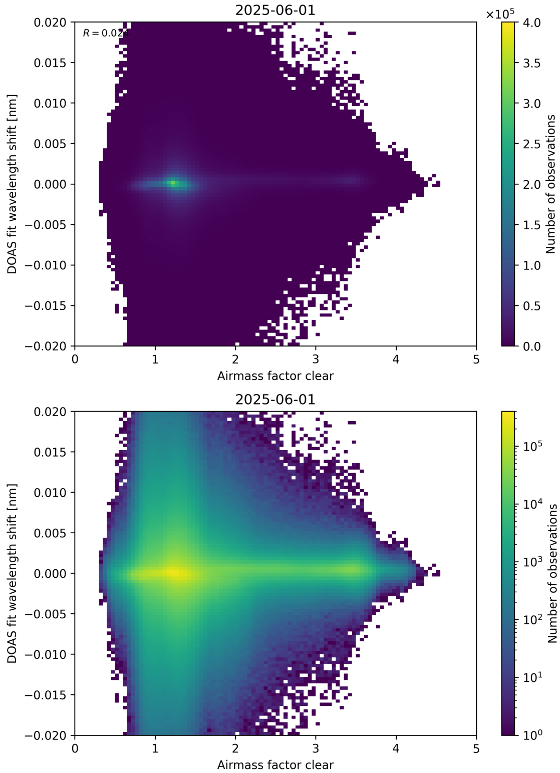
Figure 72: Scatter density plot of “Airmass factor clear” against “DOAS fit wavelength shift” for 2025-06-01 to 2025-06-02.
