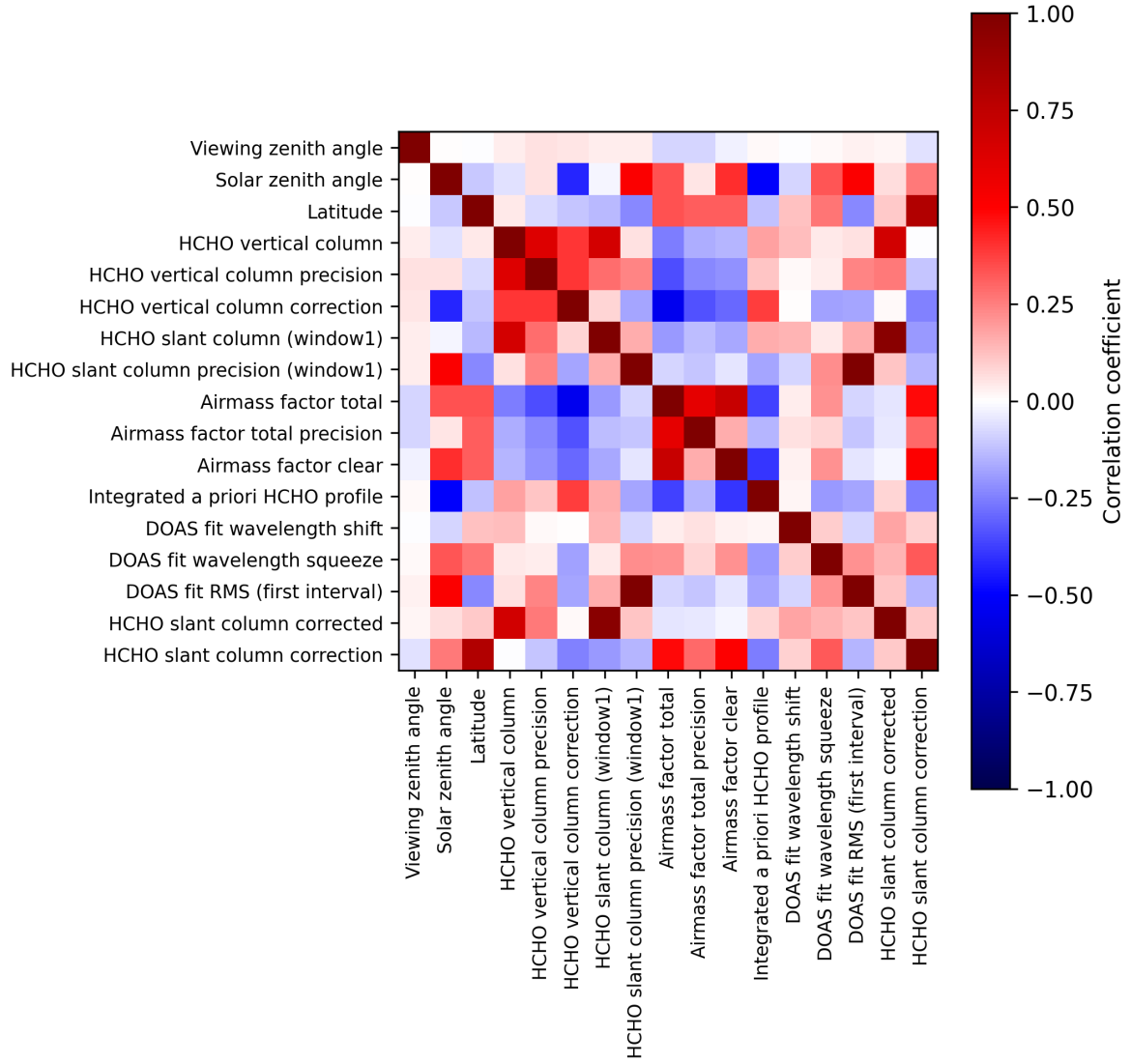
Figure 2: Map of correlation matrix for 2025-06-01 to 2025-06-02.
