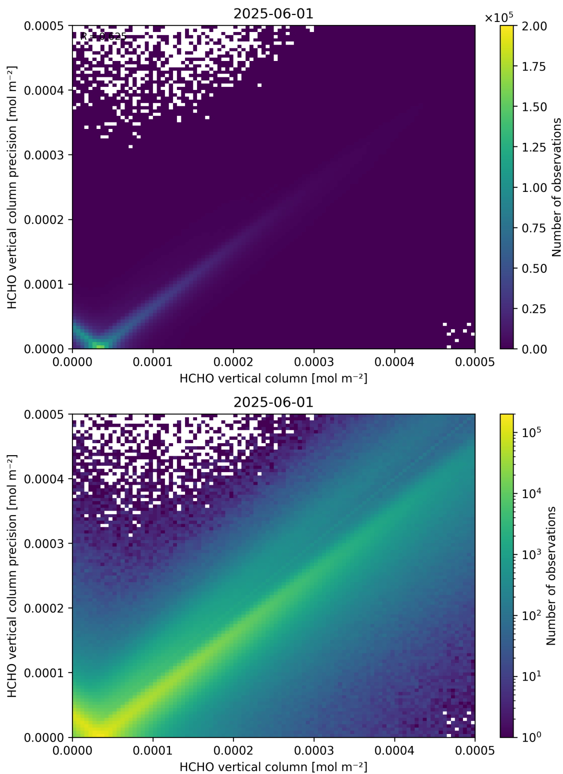
Figure 134: Scatter density plot of “HCHO vertical column” against “HCHO vertical column precision” for 2025-06-01 to 2025-06-02.
