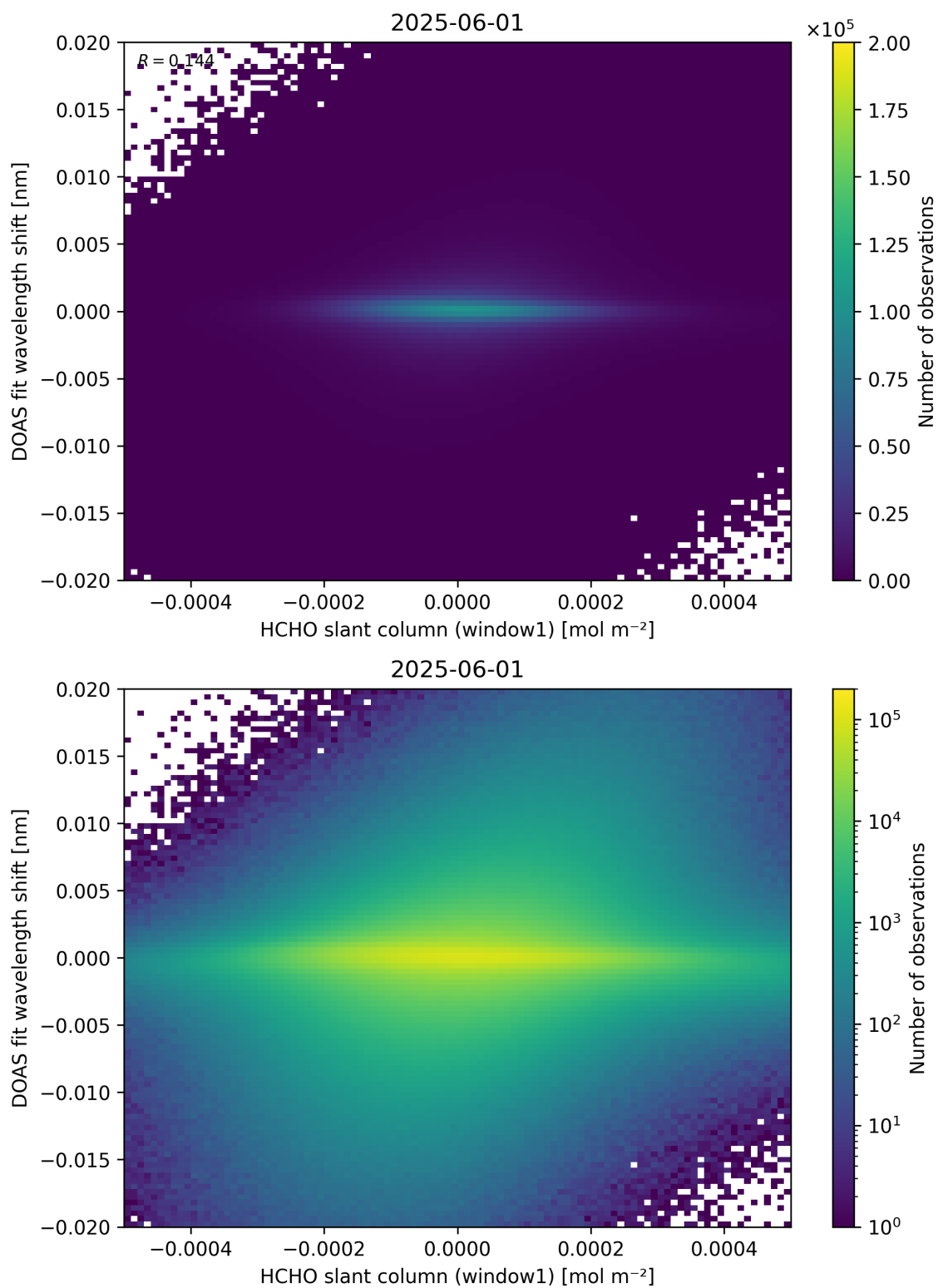
Figure 79: Scatter density plot of “HCHO slant column (window1)” against “DOAS fit wavelength shift” for 2025-06-01 to 2025-06-02.
