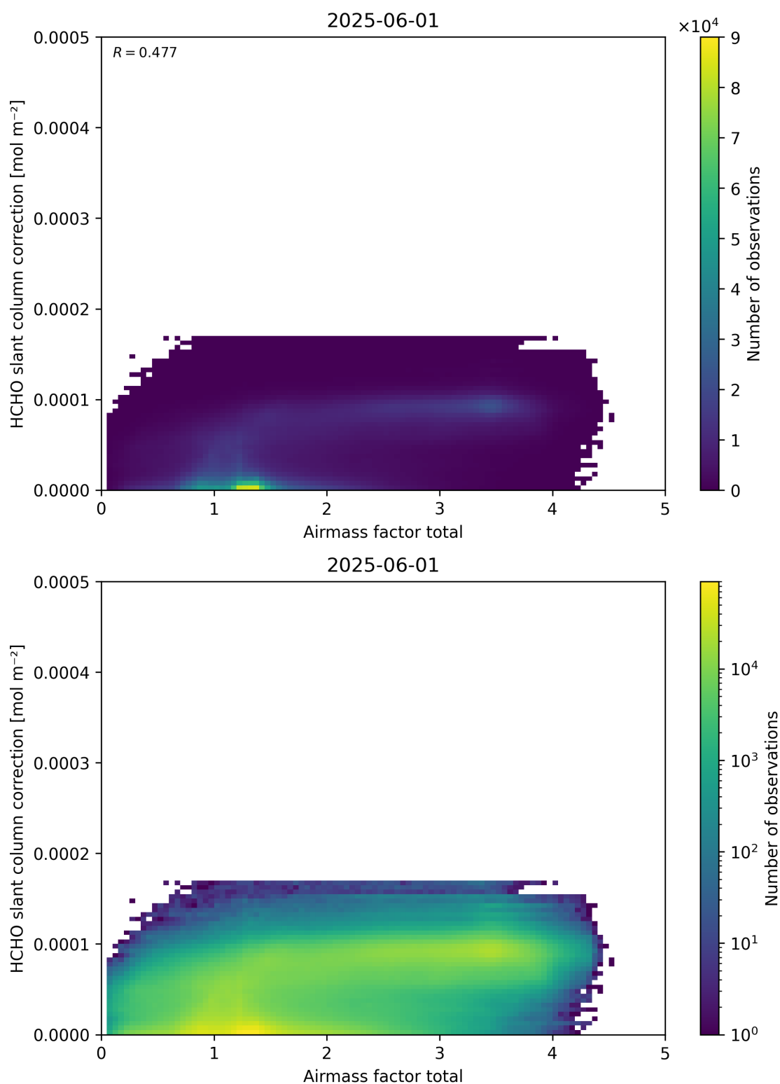
Figure 102: Scatter density plot of “Airmass factor total” against “HCHO slant column correction” for 2025-06-01 to 2025-06-02.
