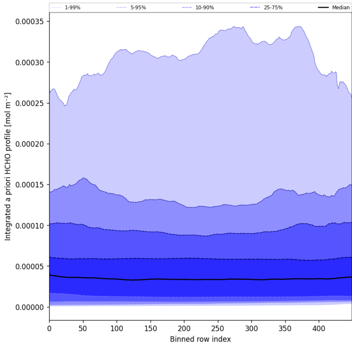
Figure 57: Along track statistics of “Integrated a priori HCHO profile” for 2025-06-01 to 2025-06-02
