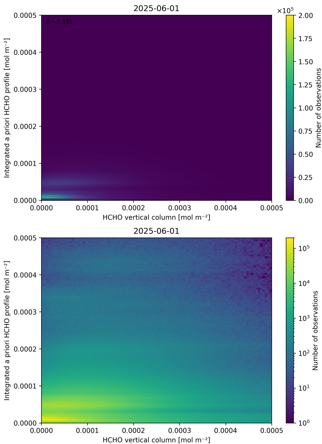
Figure 135: Scatter density plot of “HCHO vertical column” against “Integrated a priori HCHO profile” for 2025-06-01 to 2025-06-02.
