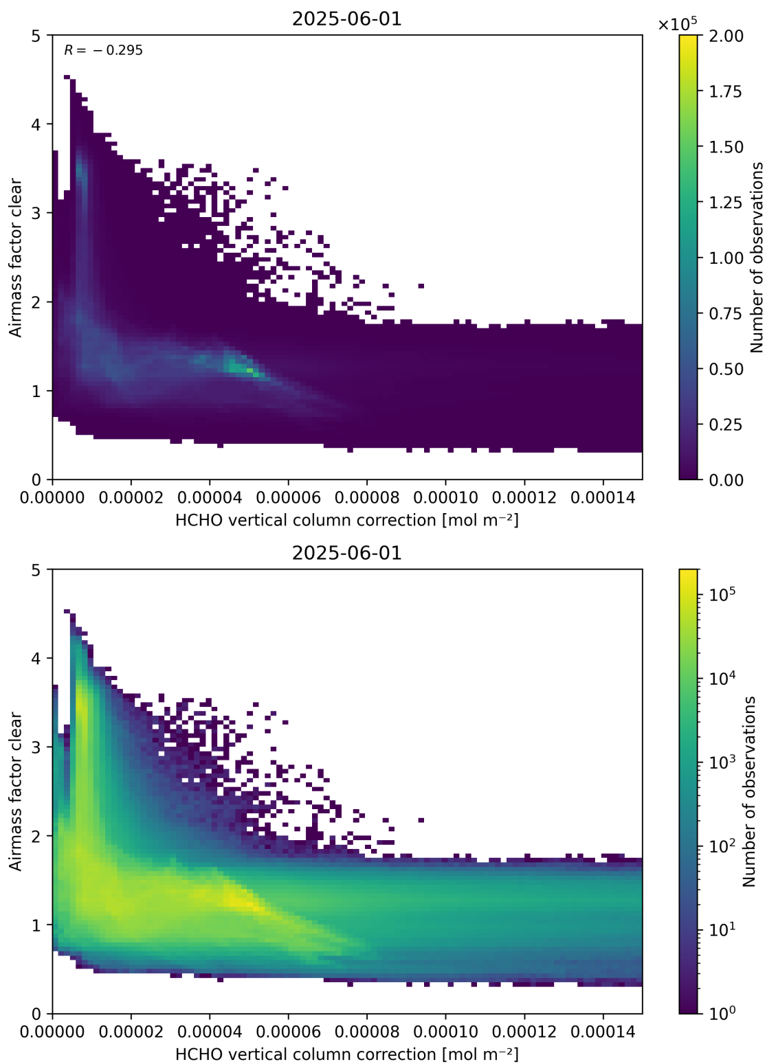
Figure 115: Scatter density plot of “HCHO vertical column correction” against “Airmass factor clear” for 2025-06-01 to 2025-06-02.
