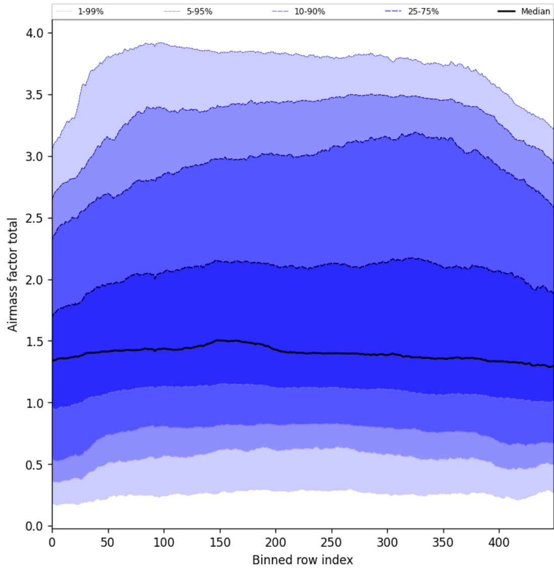
Figure 54: Along track statistics of “Airmass factor total” for 2025-06-01 to 2025-06-02
