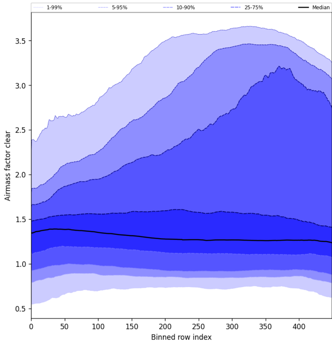
Figure 56: Along track statistics of “Airmass factor clear” for 2025-06-01 to 2025-06-02
