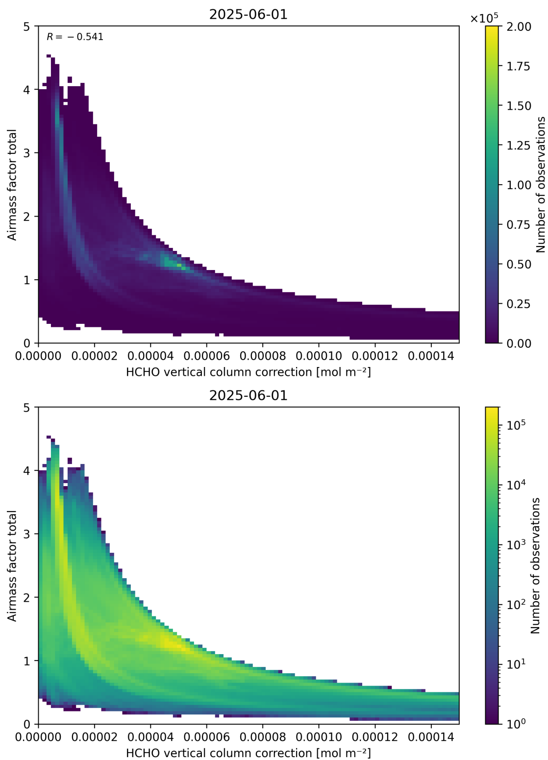
Figure 120: Scatter density plot of “HCHO vertical column correction” against “Airmass factor total” for 2025-06-01 to 2025-06-02.
