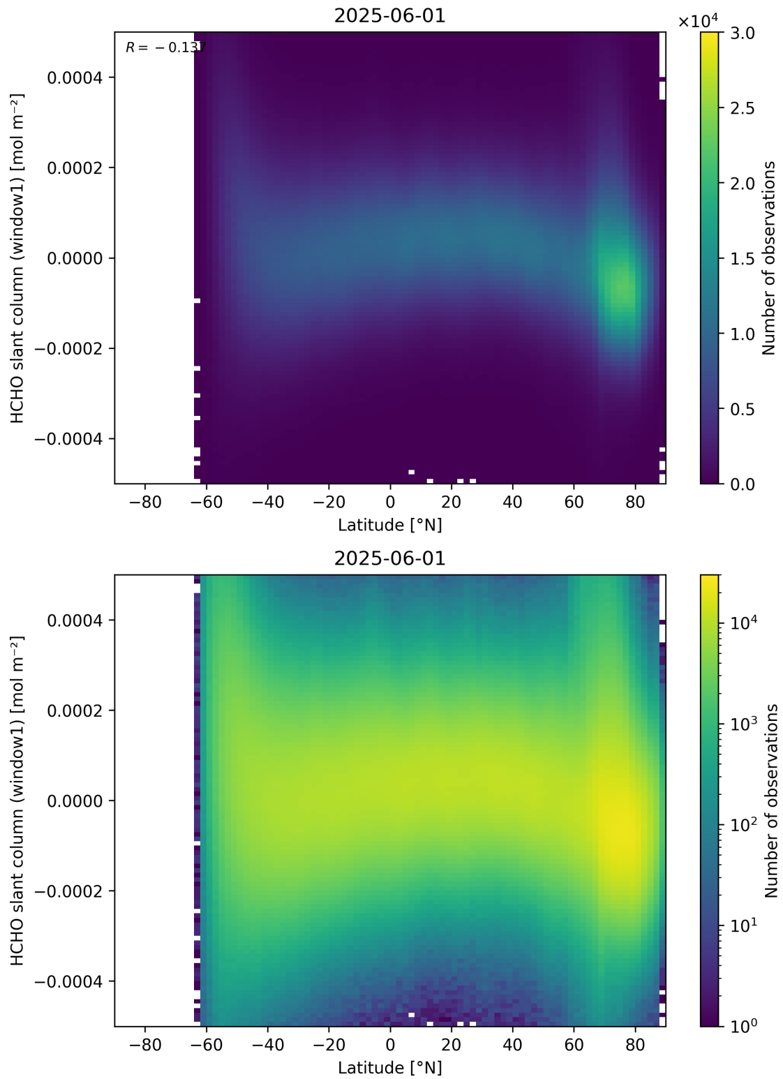
Figure 159: Scatter density plot of “Latitude” against “HCHO slant column (window1)” for 2025-06-01 to 2025-06-02.
