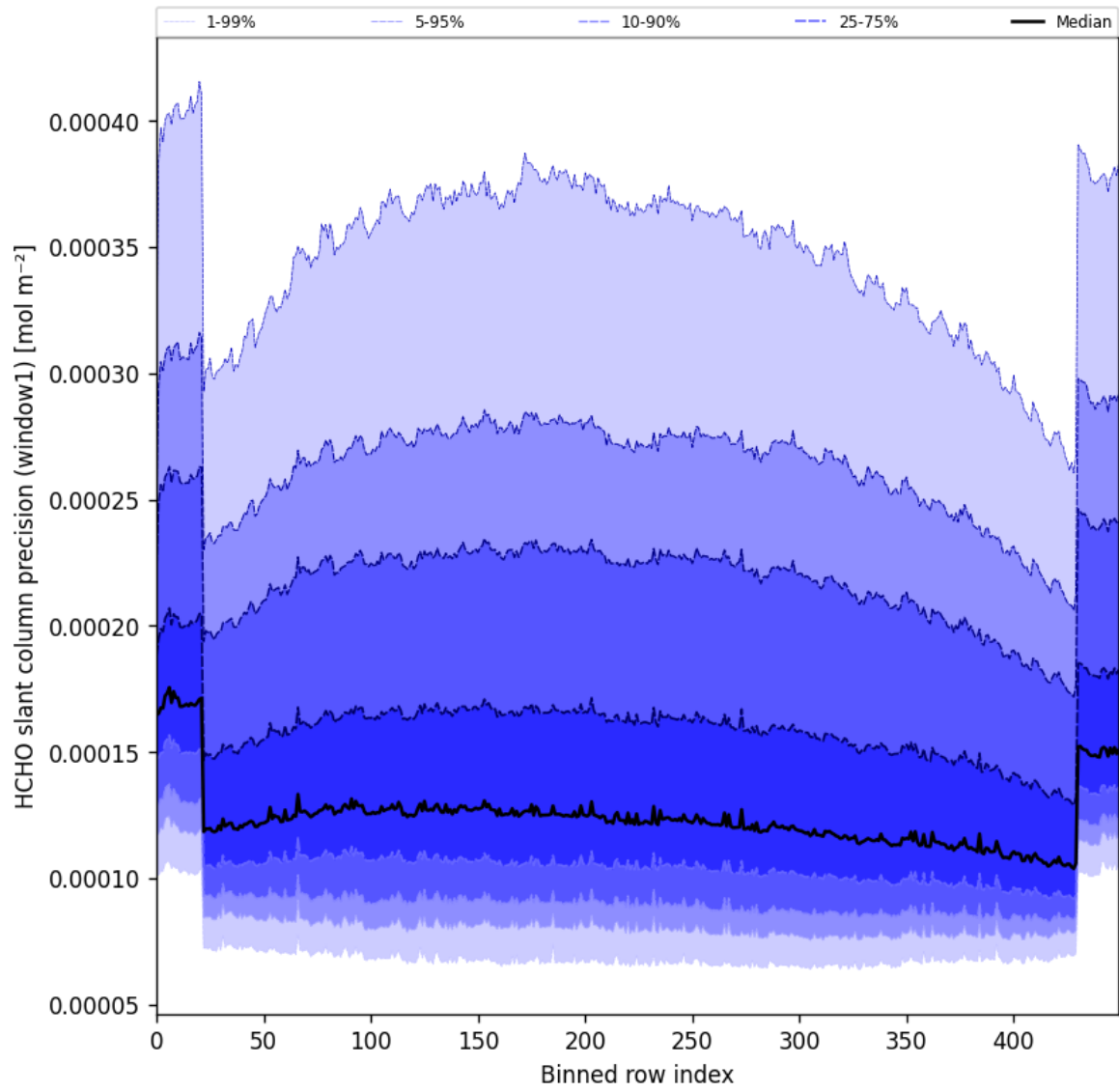
Figure 53: Along track statistics of “HCHO slant column precision (window1)” for 2025-06-01 to 2025-06-02
