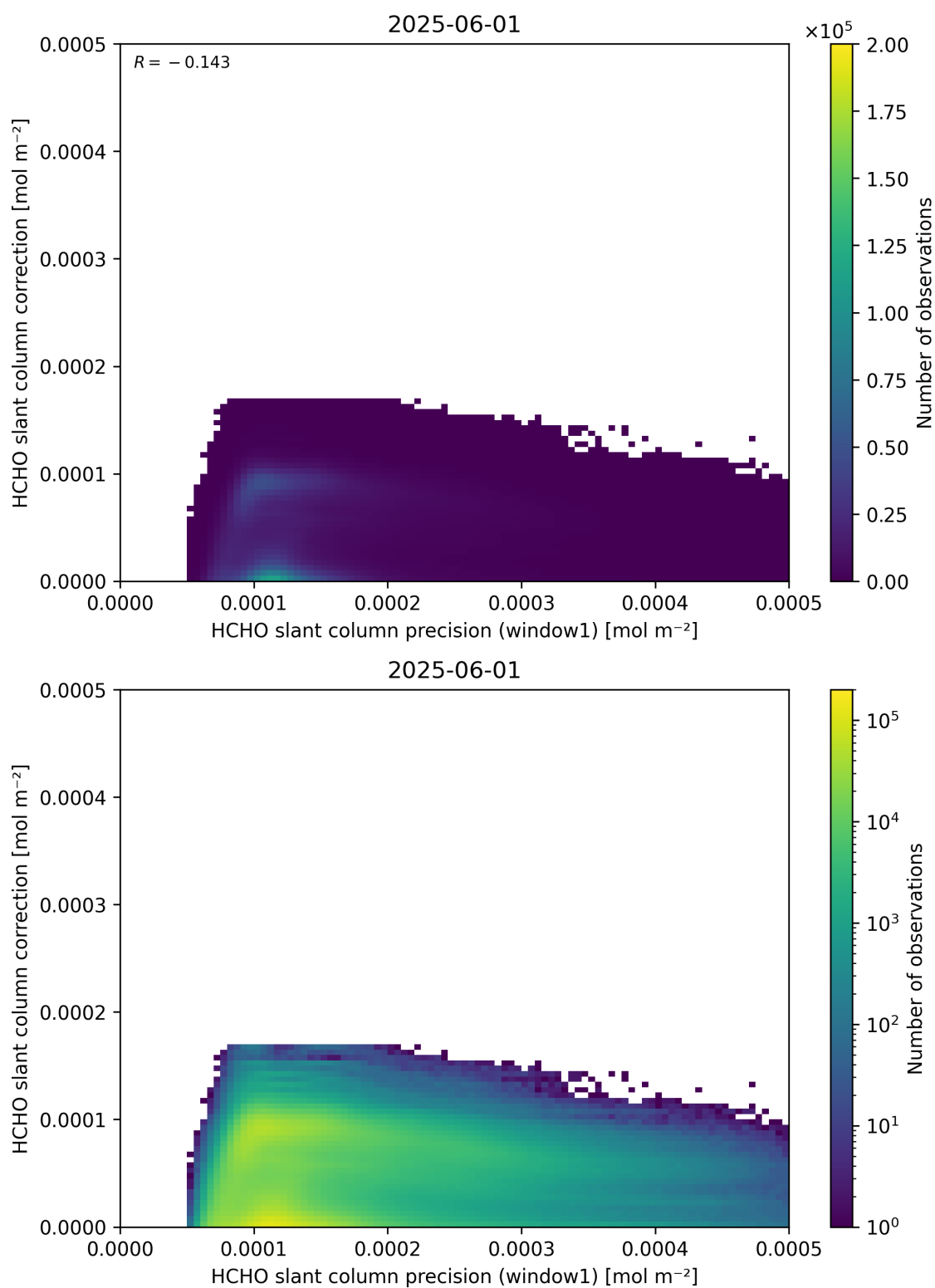
Figure 93: Scatter density plot of “HCHO slant column precision (window1)” against “HCHO slant column correction” for 2025-06-01 to 2025-06-02.
