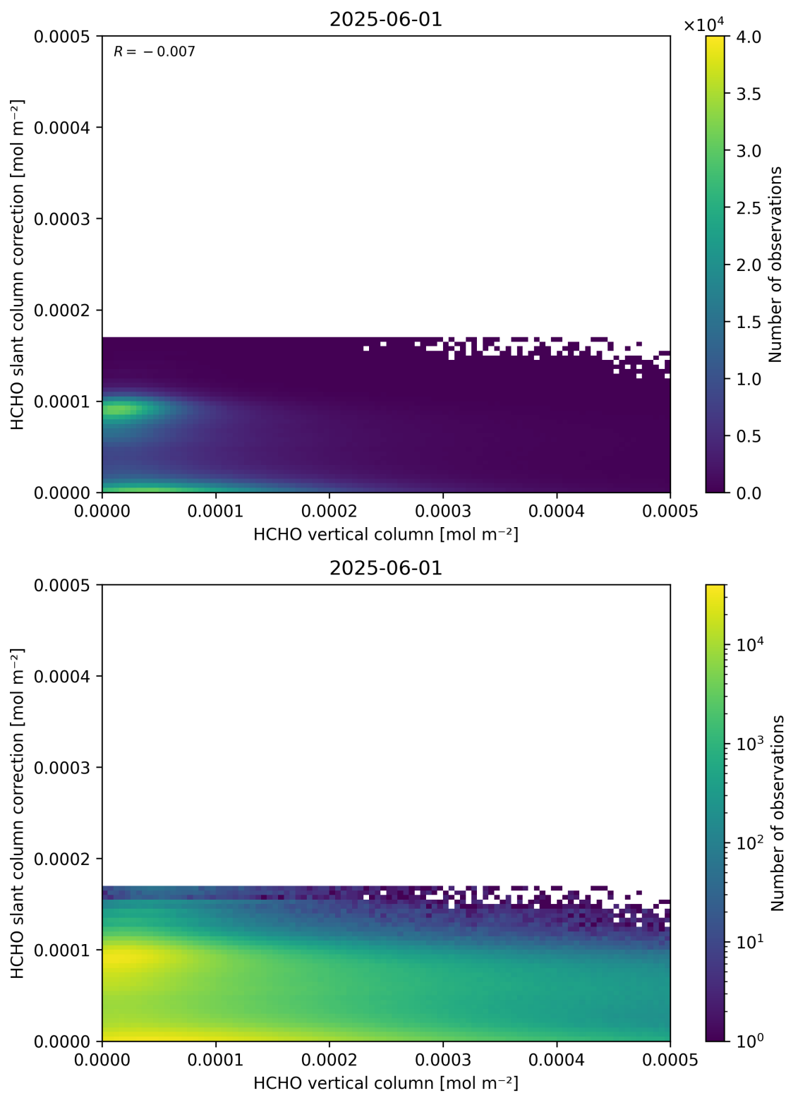
Figure 128: Scatter density plot of “HCHO vertical column” against “HCHO slant column correction” for 2025-06-01 to 2025-06-02.
