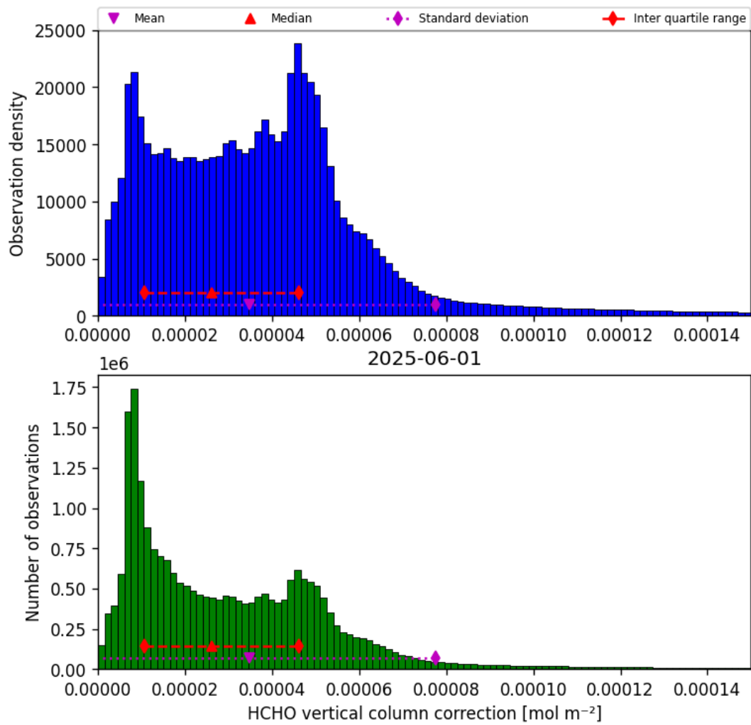
Figure 37: Histogram of “HCHO vertical column correction” for 2025-06-01 to 2025-06-02
