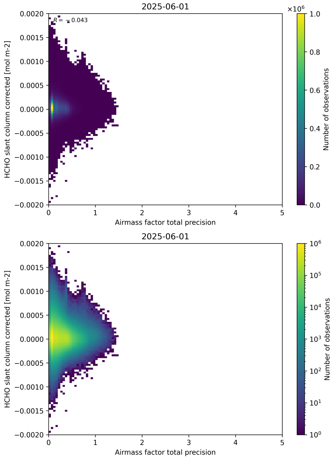
Figure 109: Scatter density plot of “Airmass factor total precision” against “HCHO slant column corrected” for 2025-06-01 to 2025-06-02.
