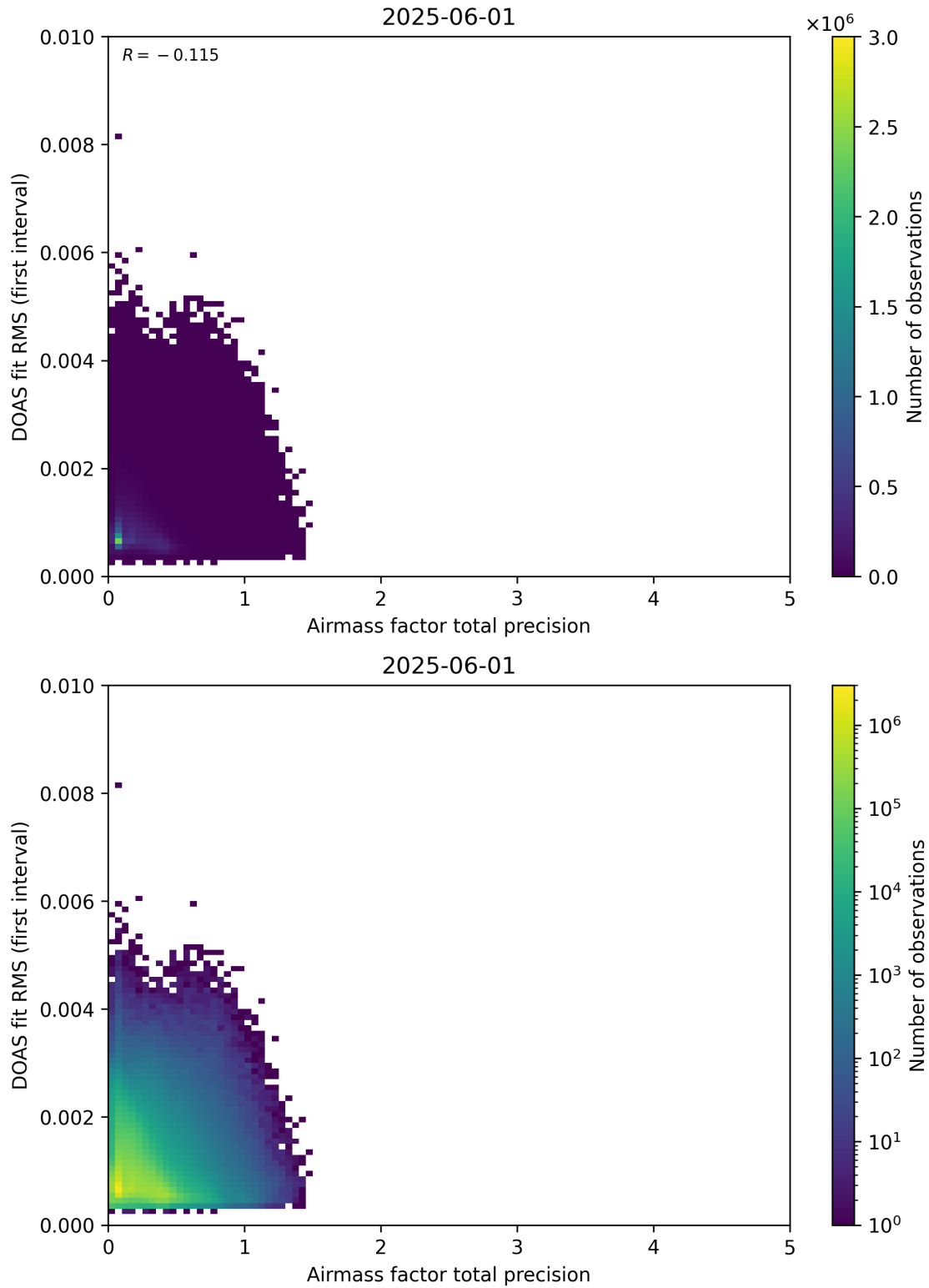
Figure 105: Scatter density plot of “Airmass factor total precision” against “DOAS fit RMS (first interval)” for 2025-06-01 to 2025-06-02.
