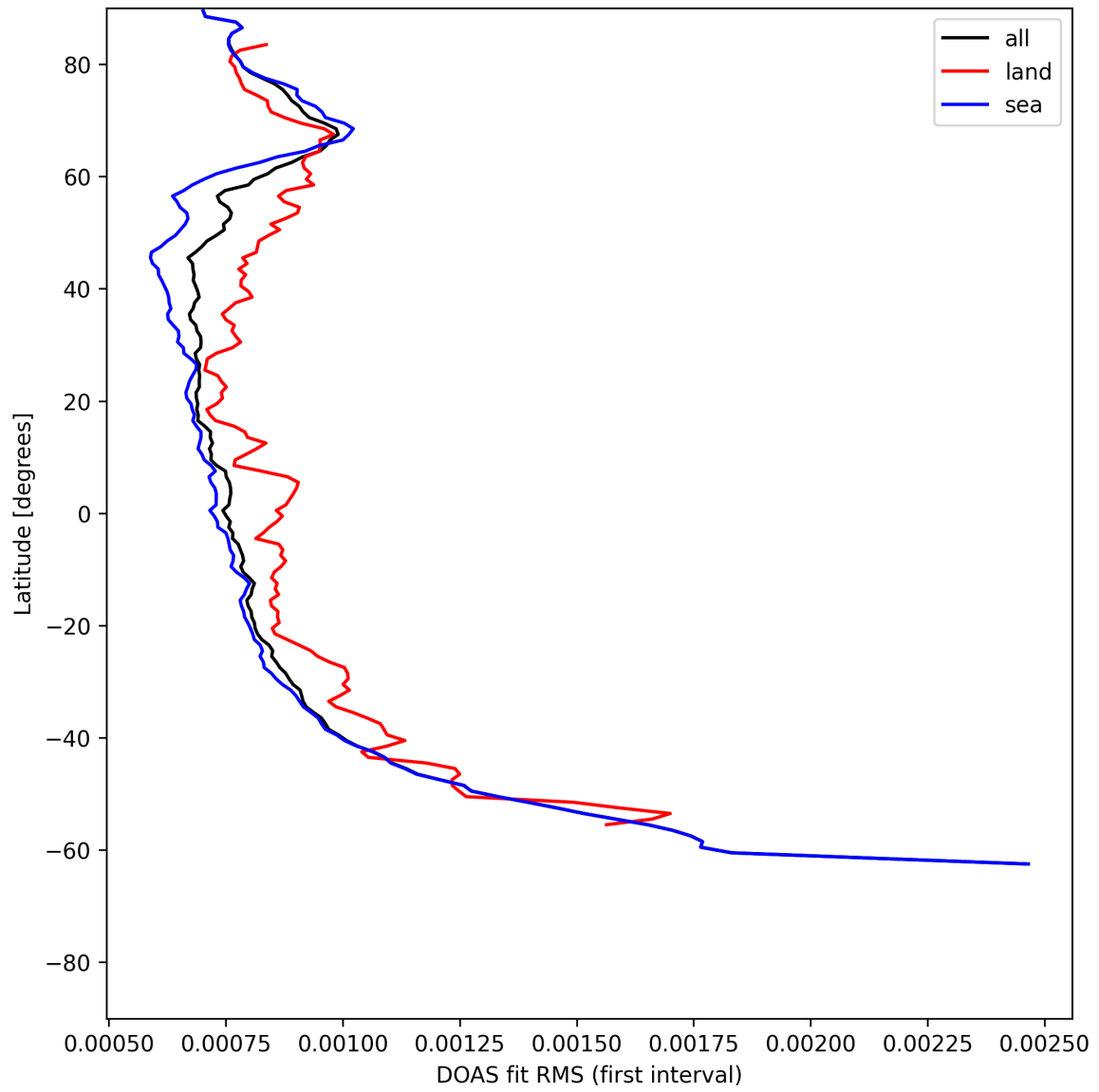
Figure 32: Zonal average of “DOAS fit RMS (first interval)” for 2025-06-01 to 2025-06-02.
