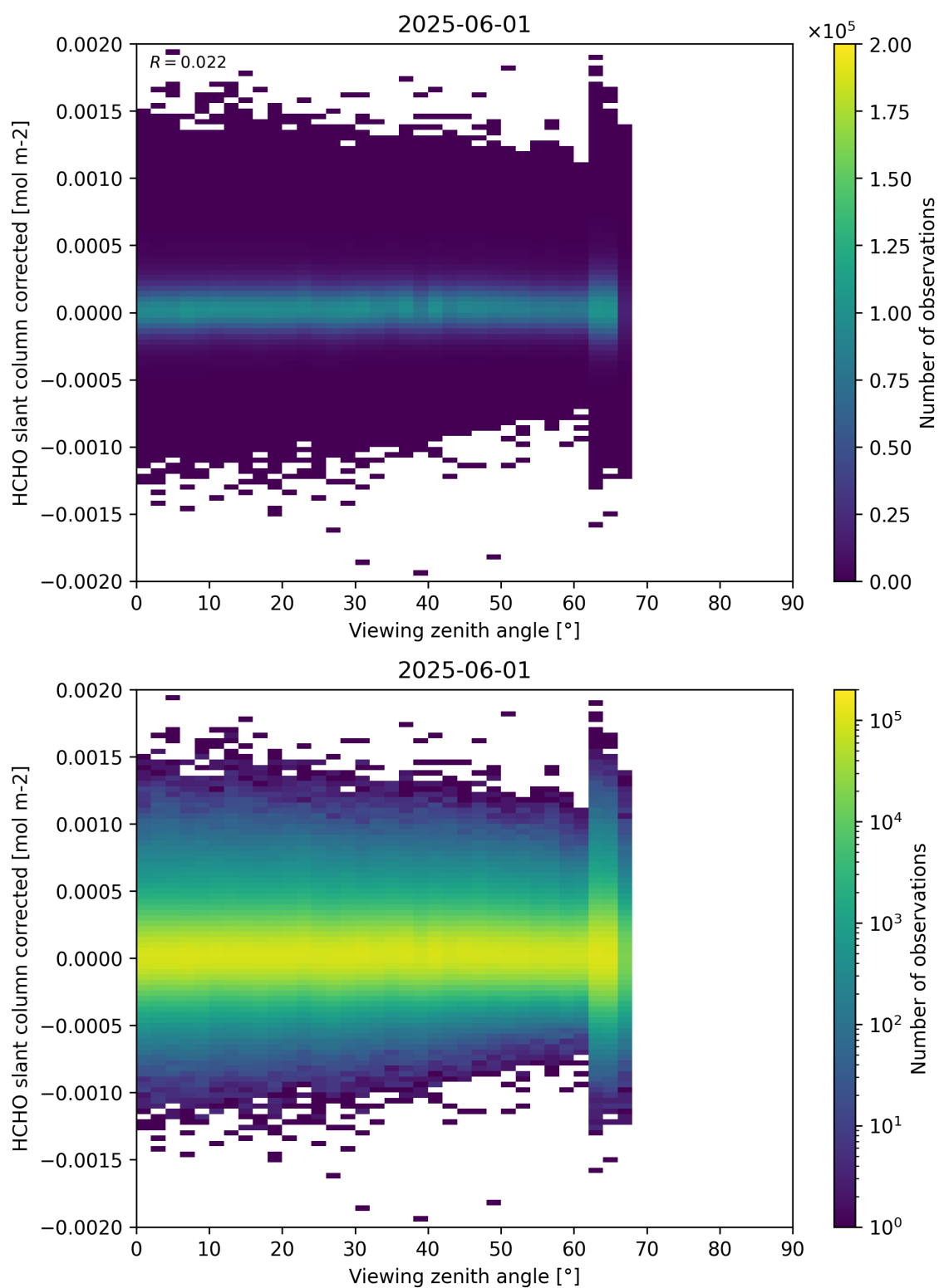
Figure 186: Scatter density plot of “Viewing zenith angle” against “HCHO slant column corrected” for 2025-06-01 to 2025-06-02.
