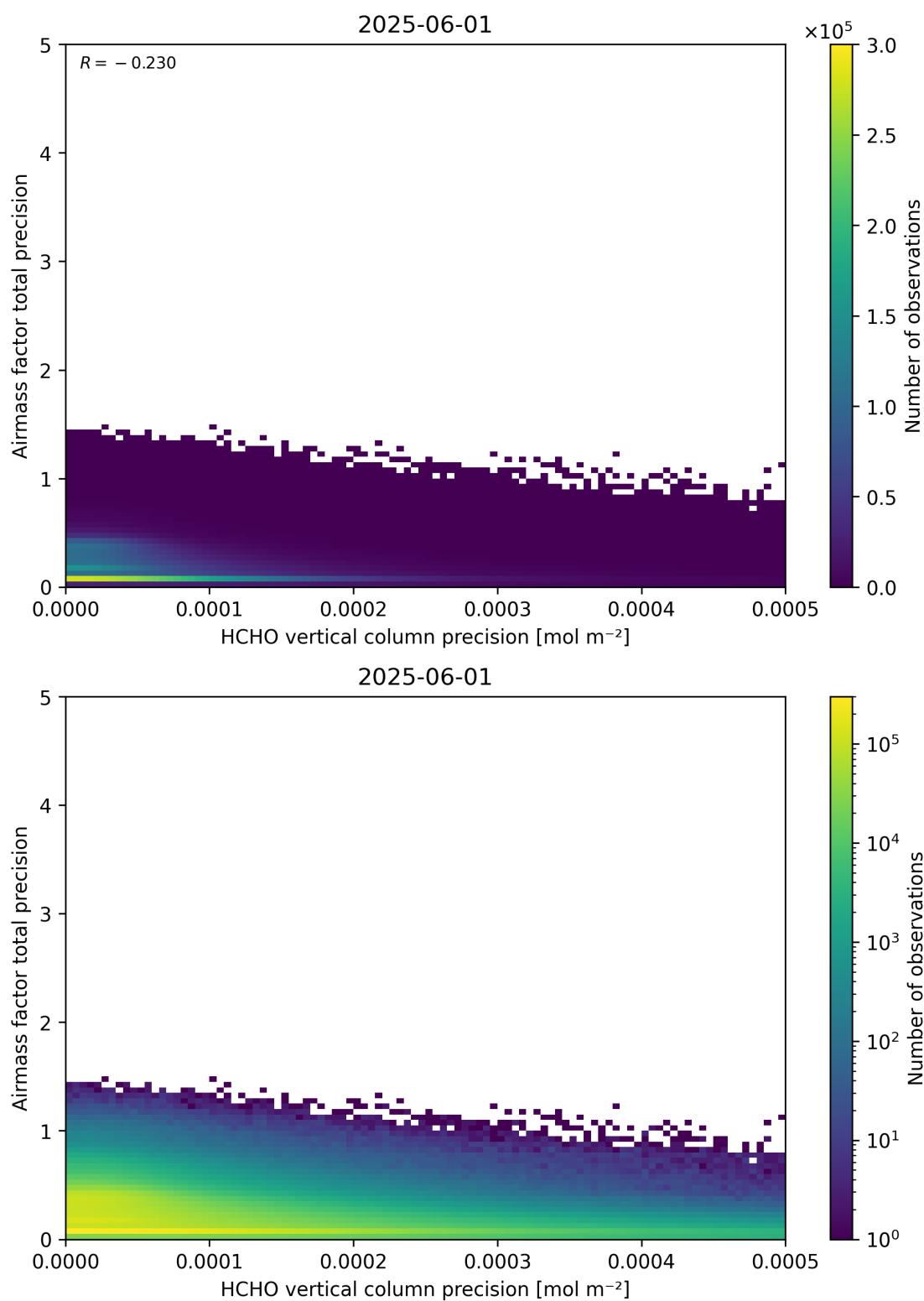
Figure 145: Scatter density plot of “HCHO vertical column precision” against “Airmass factor total precision” for 2025-06-01 to 2025-06-02.
