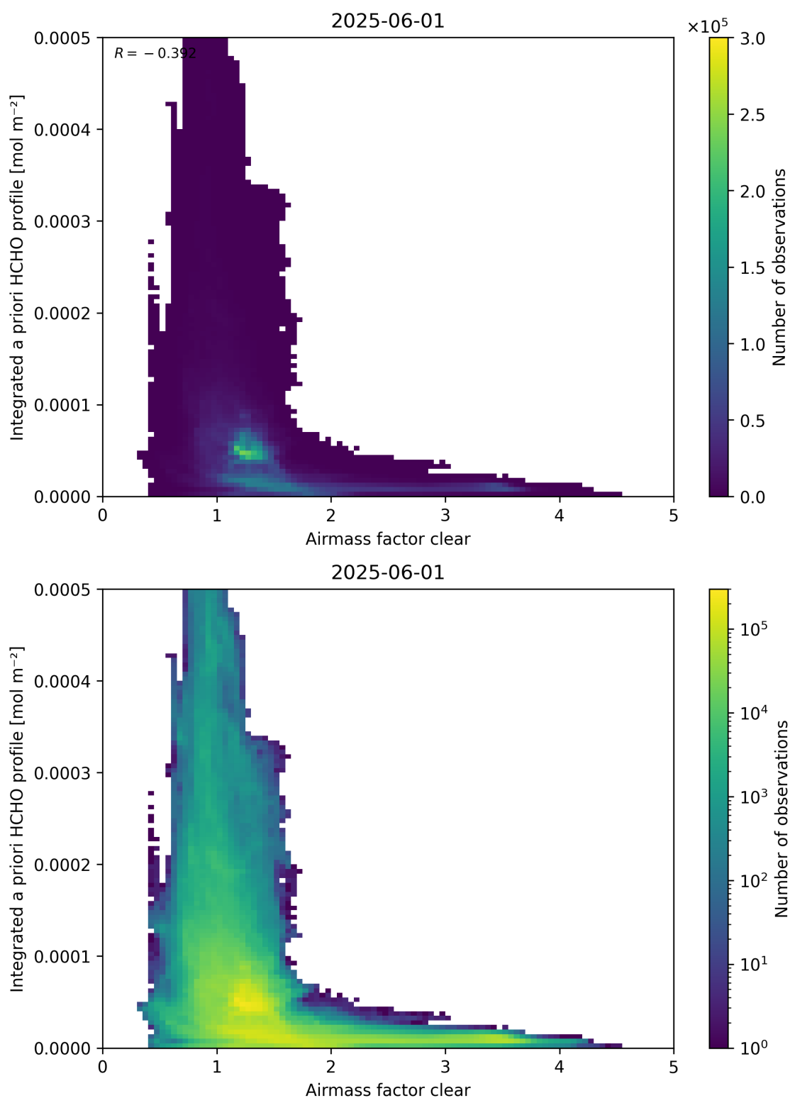
Figure 76: Scatter density plot of “Airmass factor clear” against “Integrated a priori HCHO profile” for 2025-06-01 to 2025-06-02.
