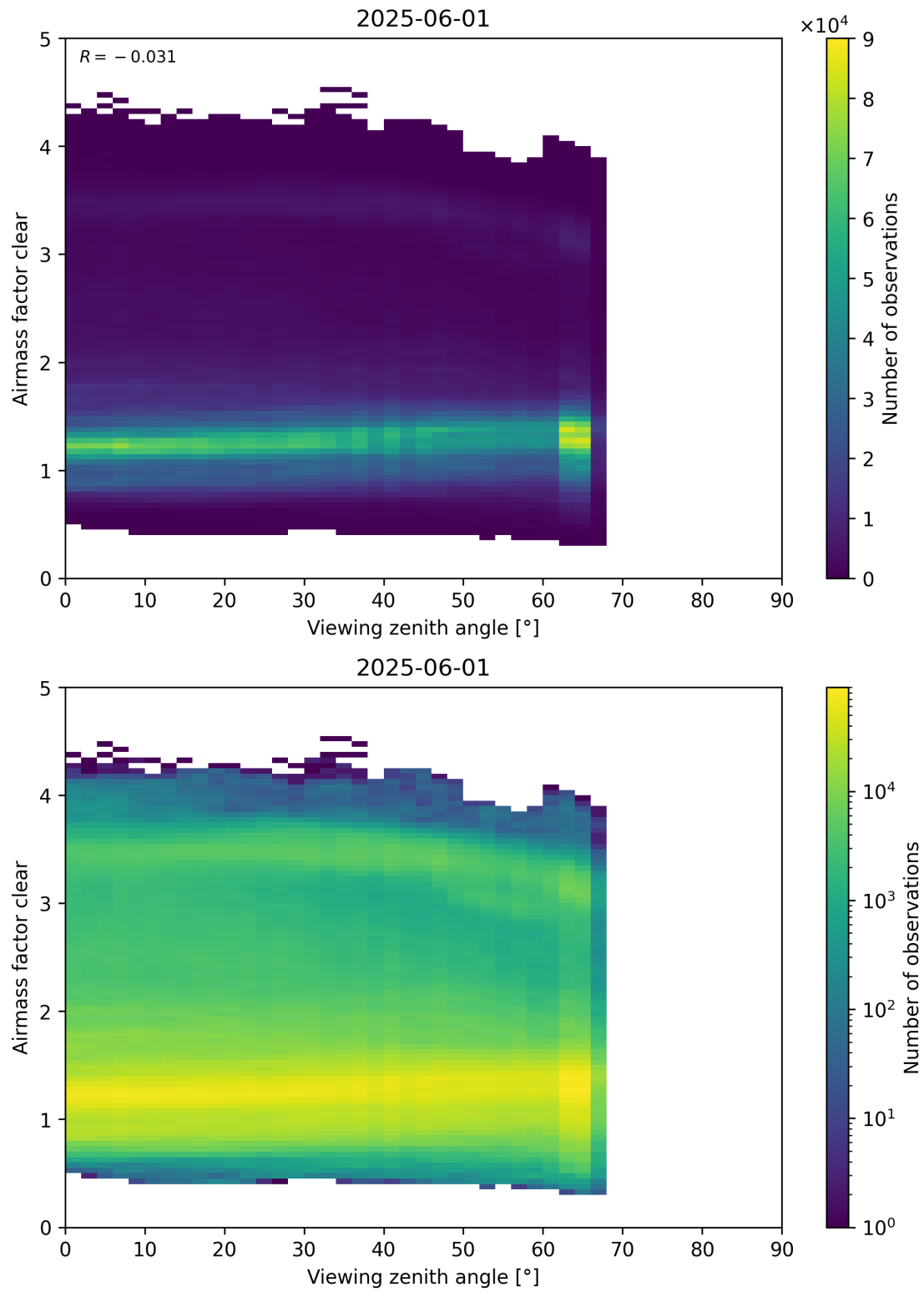
Figure 185: Scatter density plot of “Viewing zenith angle” against “Airmass factor clear” for 2025-06-01 to 2025-06-02.
