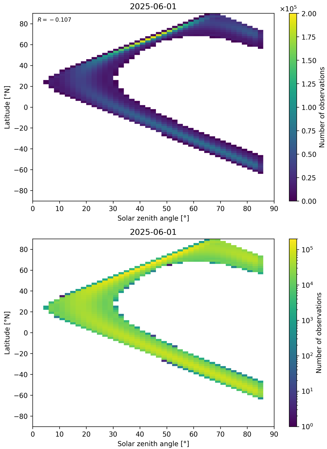
Figure 181: Scatter density plot of “Solar zenith angle” against “Latitude” for 2025-06-01 to 2025-06-02.
