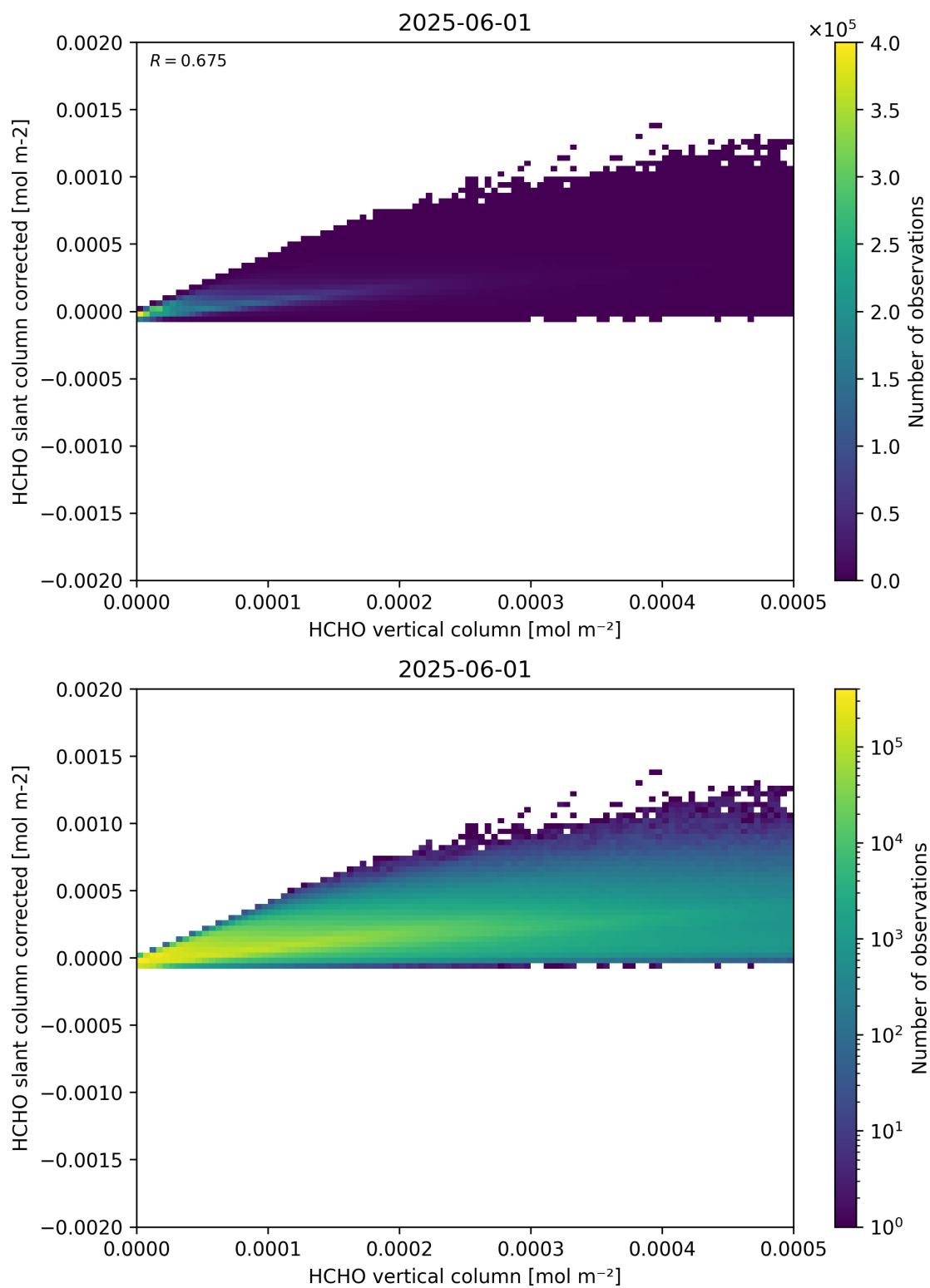
Figure 127: Scatter density plot of “HCHO vertical column” against “HCHO slant column corrected” for 2025-06-01 to 2025-06-02.
