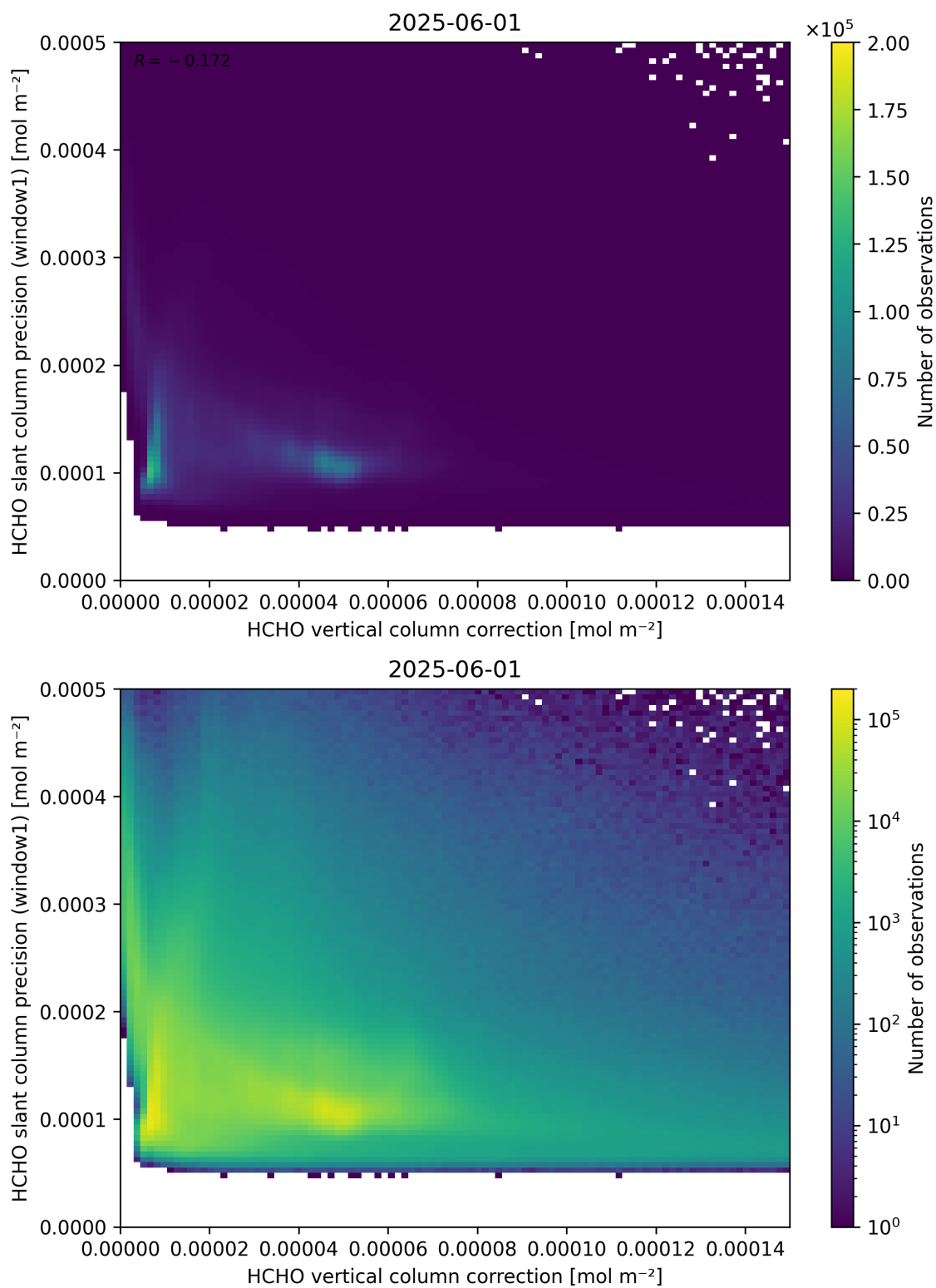
Figure 119: Scatter density plot of “HCHO vertical column correction” against “HCHO slant column precision (window1)” for 2025-06-01 to 2025-06-02.
