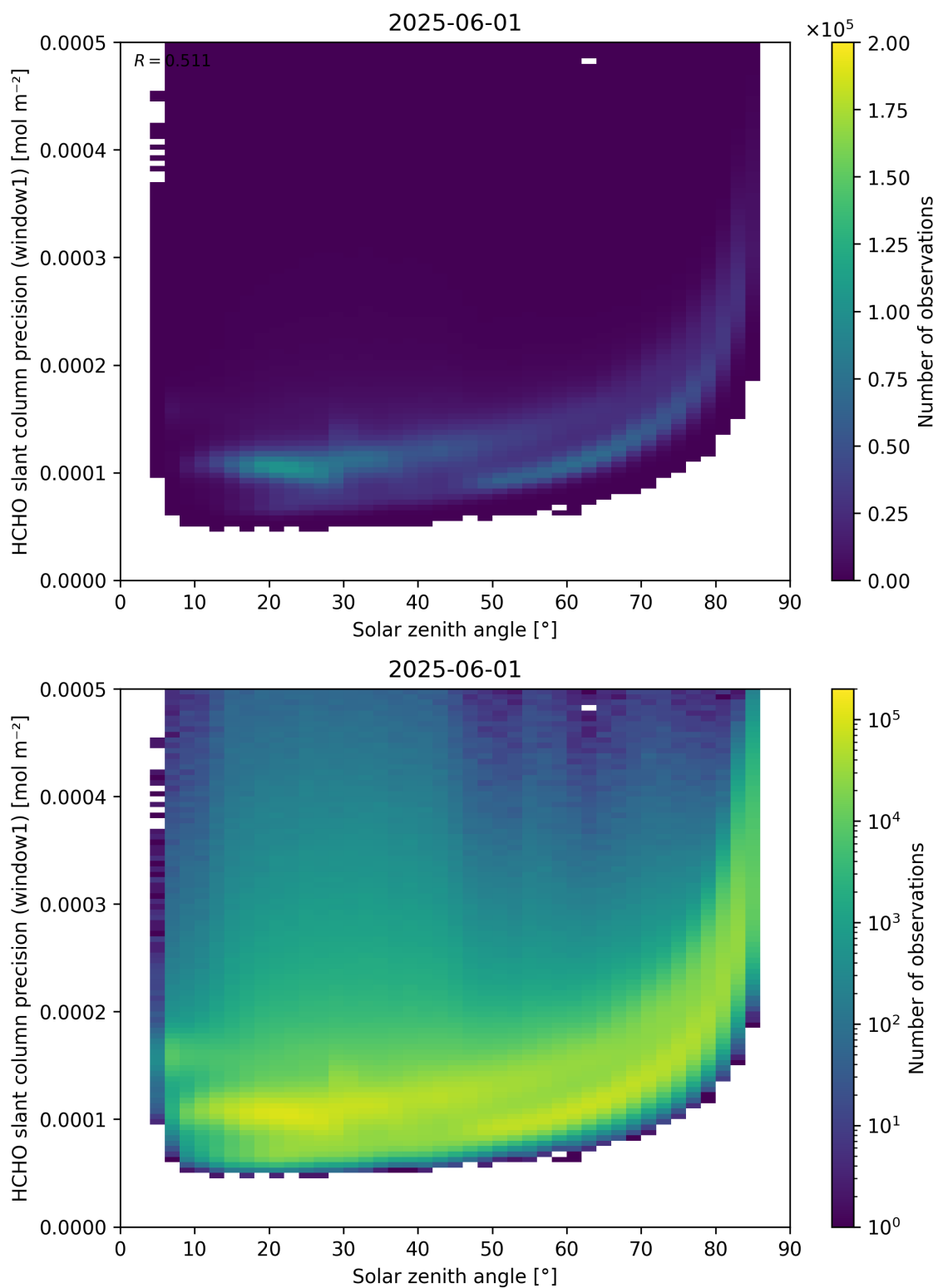
Figure 174: Scatter density plot of “Solar zenith angle” against “HCHO slant column precision (window1)” for 2025-06-01 to 2025-06-02.
