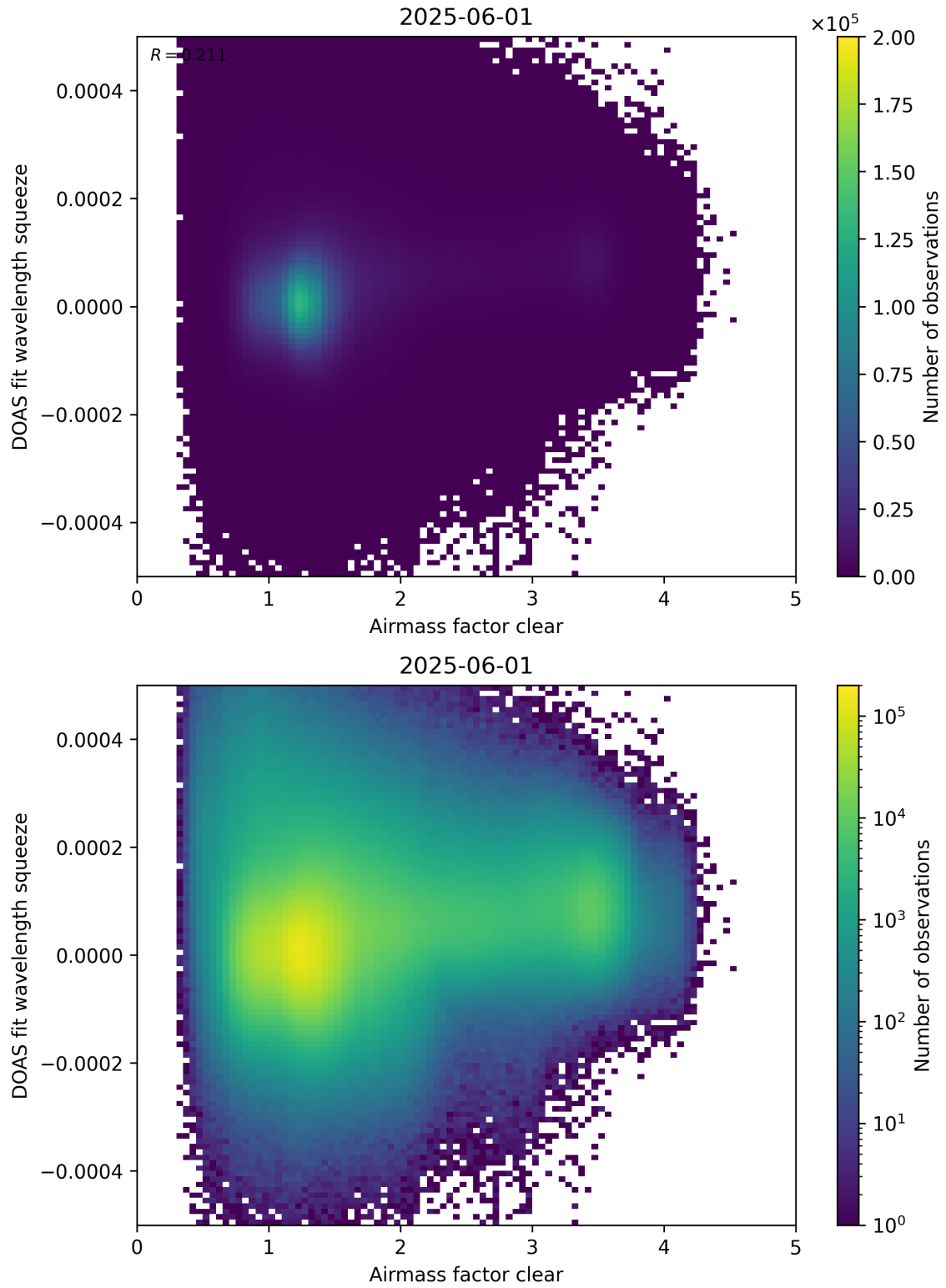
Figure 73: Scatter density plot of “Airmass factor clear” against “DOAS fit wavelength squeeze” for 2025-06-01 to 2025-06-02.
