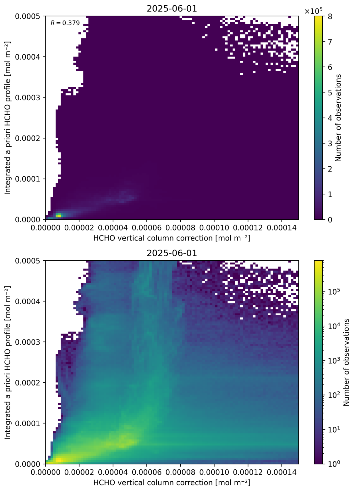
Figure 122: Scatter density plot of “HCHO vertical column correction” against “Integrated a priori HCHO profile” for 2025-06-01 to 2025-06-02.
