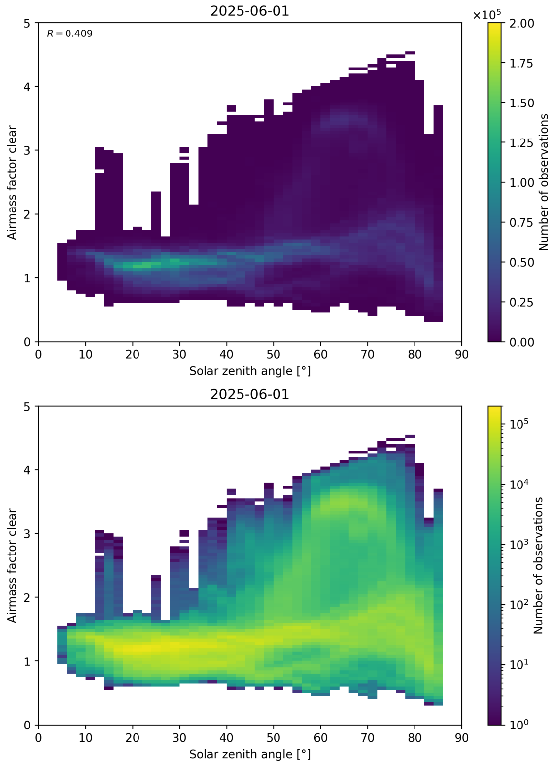
Figure 170: Scatter density plot of “Solar zenith angle” against “Airmass factor clear” for 2025-06-01 to 2025-06-02.
