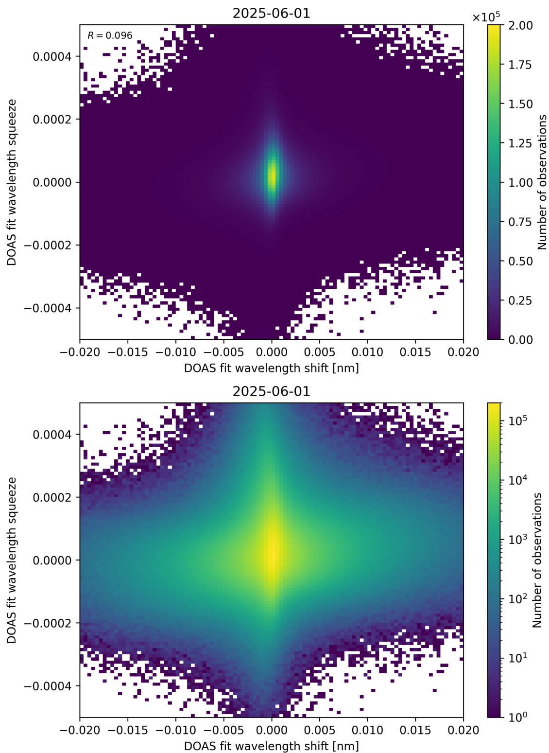
Figure 65: Scatter density plot of “DOAS fit wavelength shift” against “DOAS fit wavelength squeeze” for 2025-06-01 to 2025-06-02.
