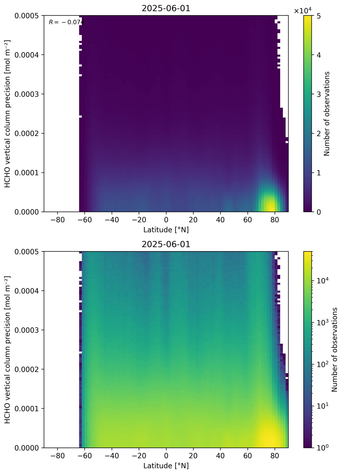
Figure 165: Scatter density plot of “Latitude” against “HCHO vertical column precision” for 2025-06-01 to 2025-06-02.
