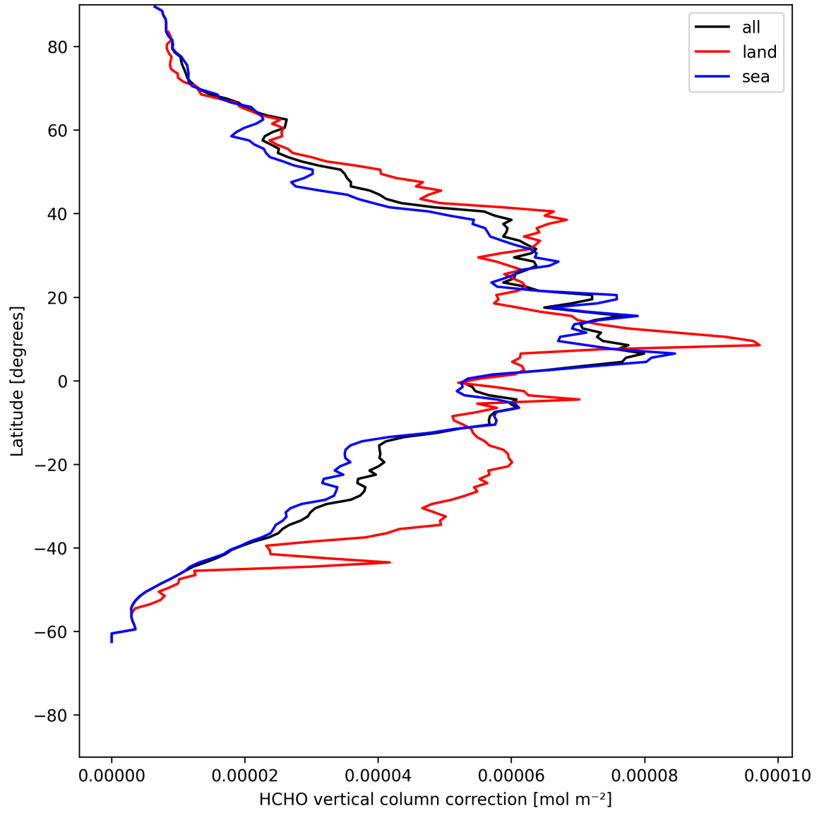
Figure 23: Zonal average of “HCHO vertical column correction” for 2025-06-01 to 2025-06-02.
