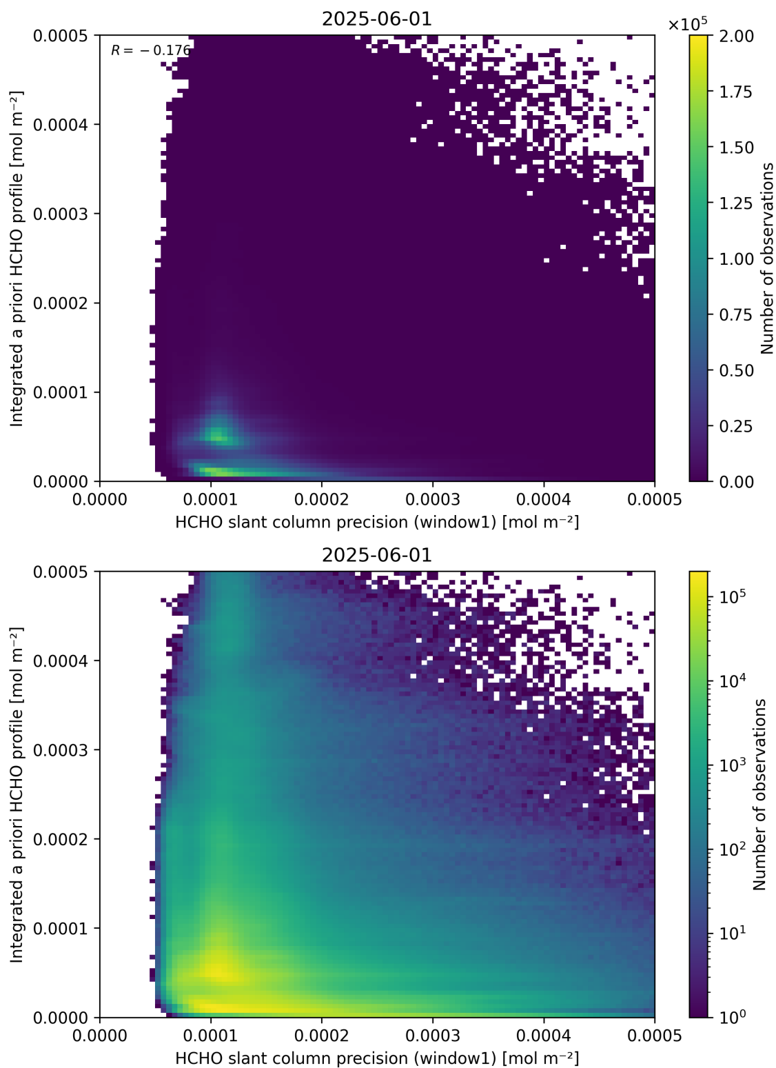
Figure 96: Scatter density plot of “HCHO slant column precision (window1)” against “Integrated a priori HCHO profile” for 2025-06-01 to 2025-06-02.
