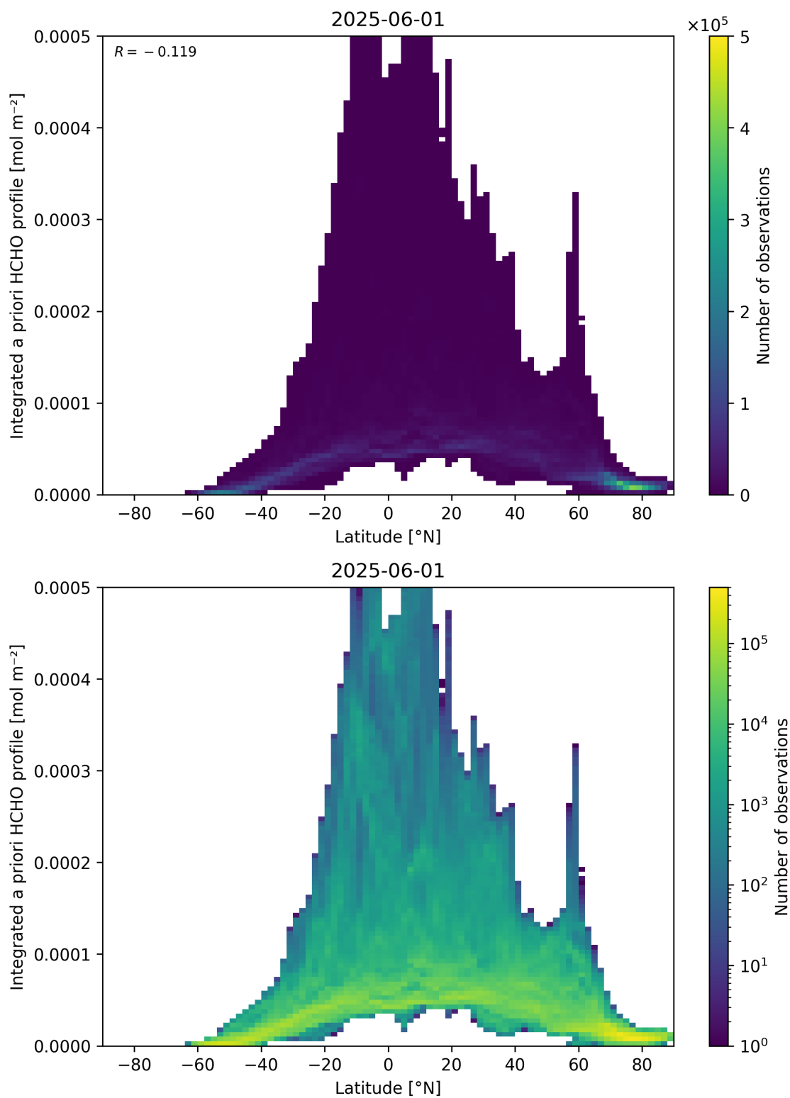
Figure 166: Scatter density plot of “Latitude” against “Integrated a priori HCHO profile” for 2025-06-01 to 2025-06-02.
