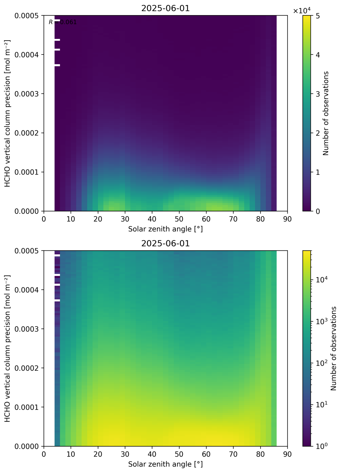
Figure 179: Scatter density plot of “Solar zenith angle” against “HCHO vertical column precision” for 2025-06-01 to 2025-06-02.
