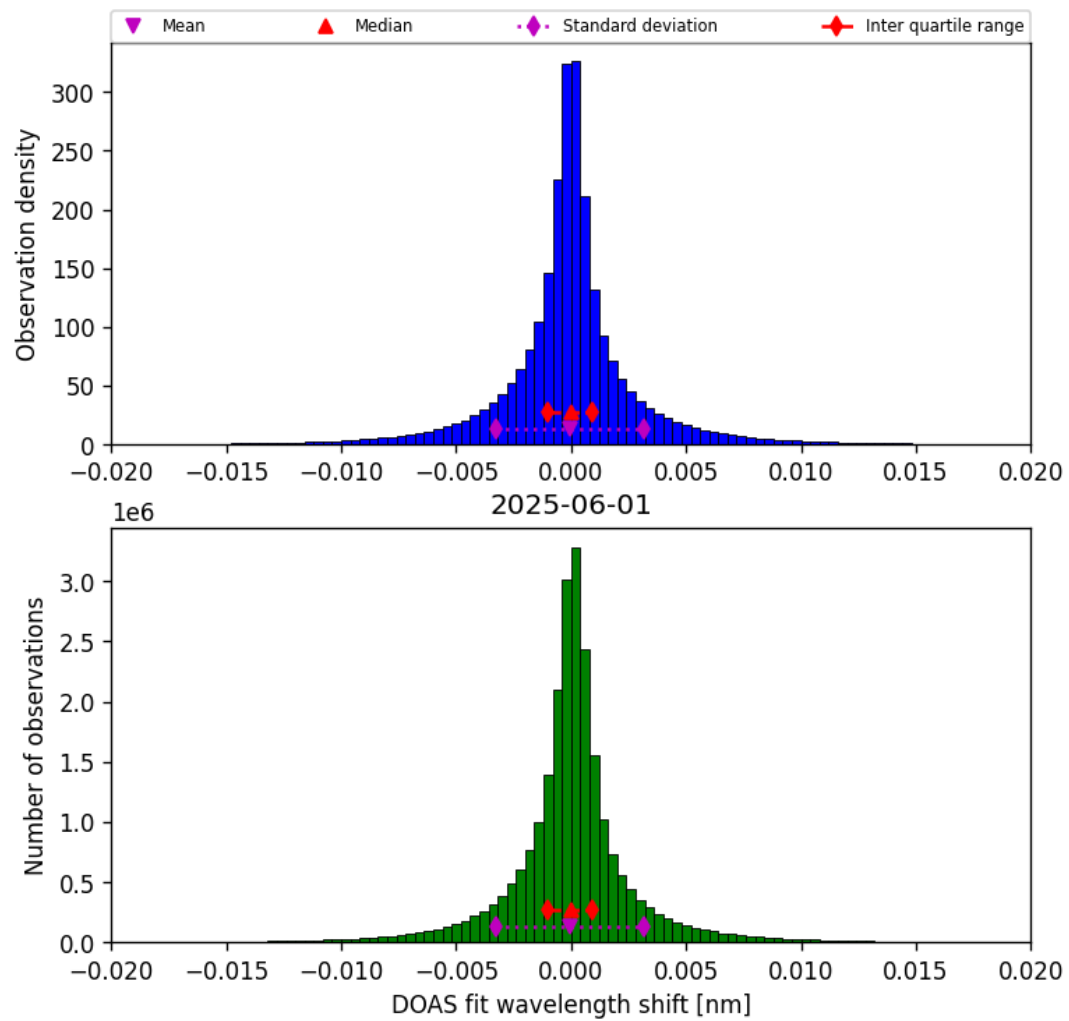
Figure 44: Histogram of “DOAS fit wavelength shift” for 2025-06-01 to 2025-06-02
