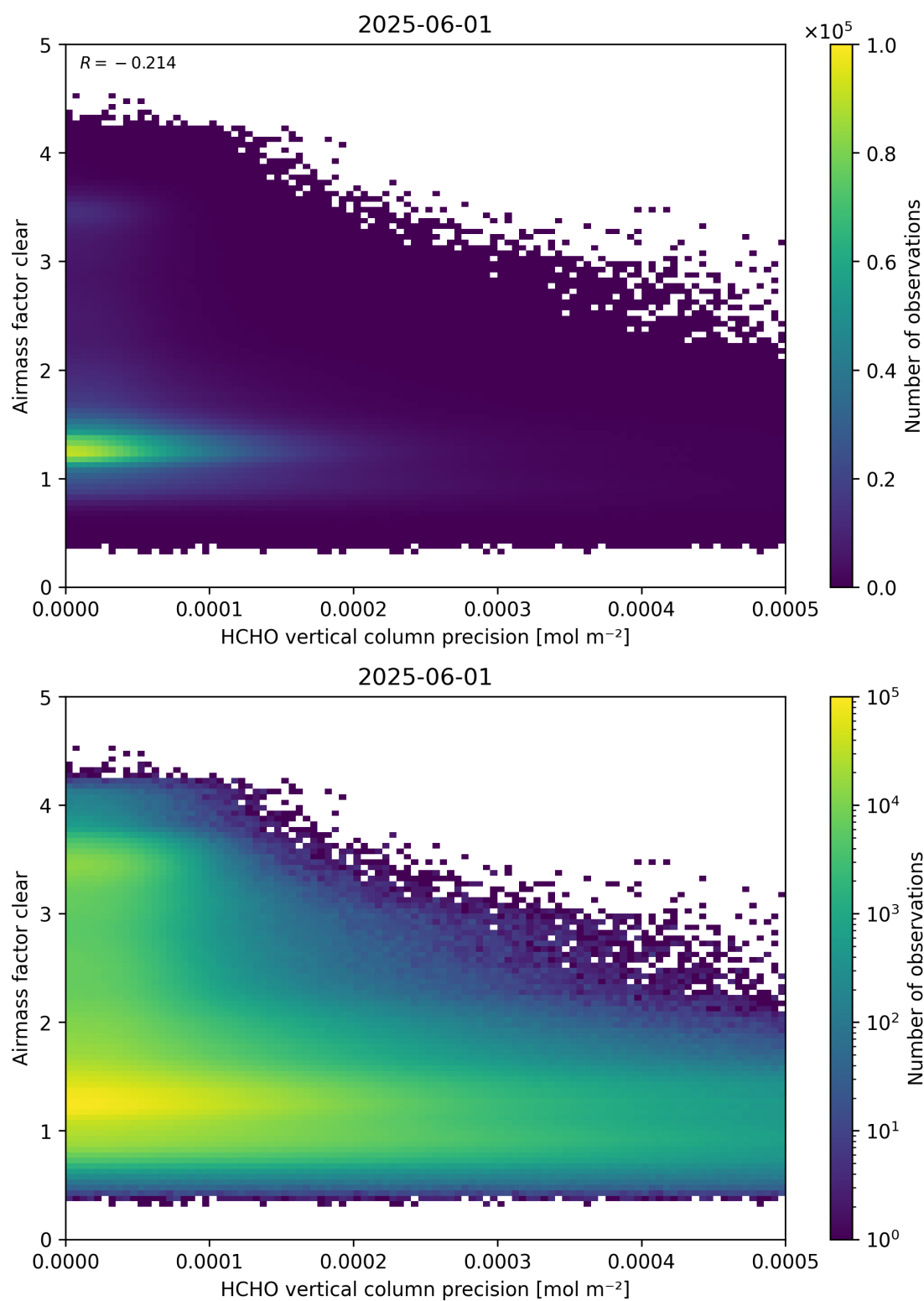
Figure 139: Scatter density plot of “HCHO vertical column precision” against “Airmass factor clear” for 2025-06-01 to 2025-06-02.
