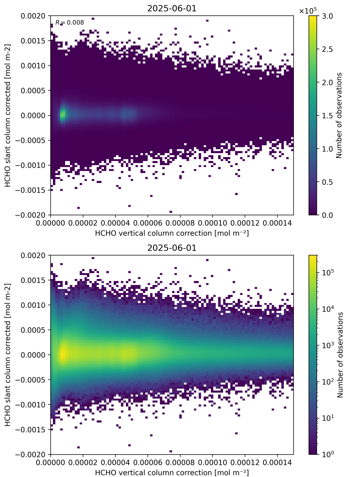
Figure 116: Scatter density plot of “HCHO vertical column correction” against “HCHO slant column corrected” for 2025-06-01 to 2025-06-02.
