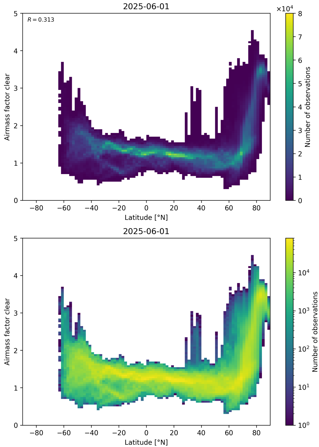
Figure 156: Scatter density plot of “Latitude” against “Airmass factor clear” for 2025-06-01 to 2025-06-02.
