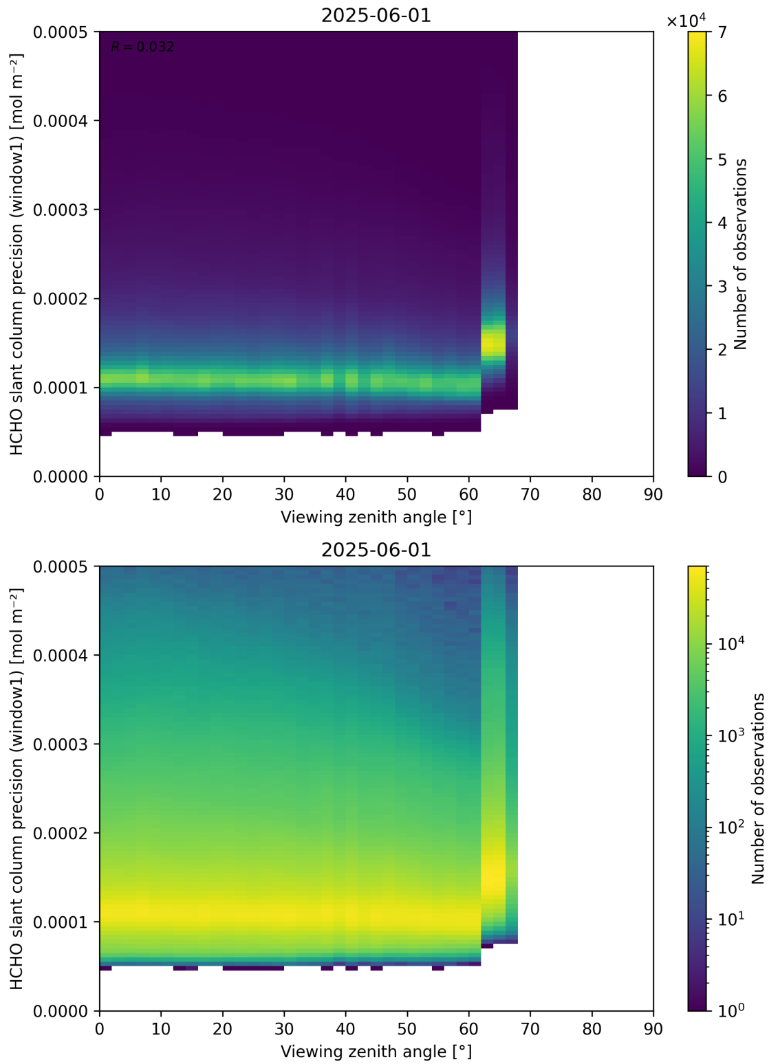
Figure 189: Scatter density plot of “Viewing zenith angle” against “HCHO slant column precision (window1)” for 2025-06-01 to 2025-06-02.
