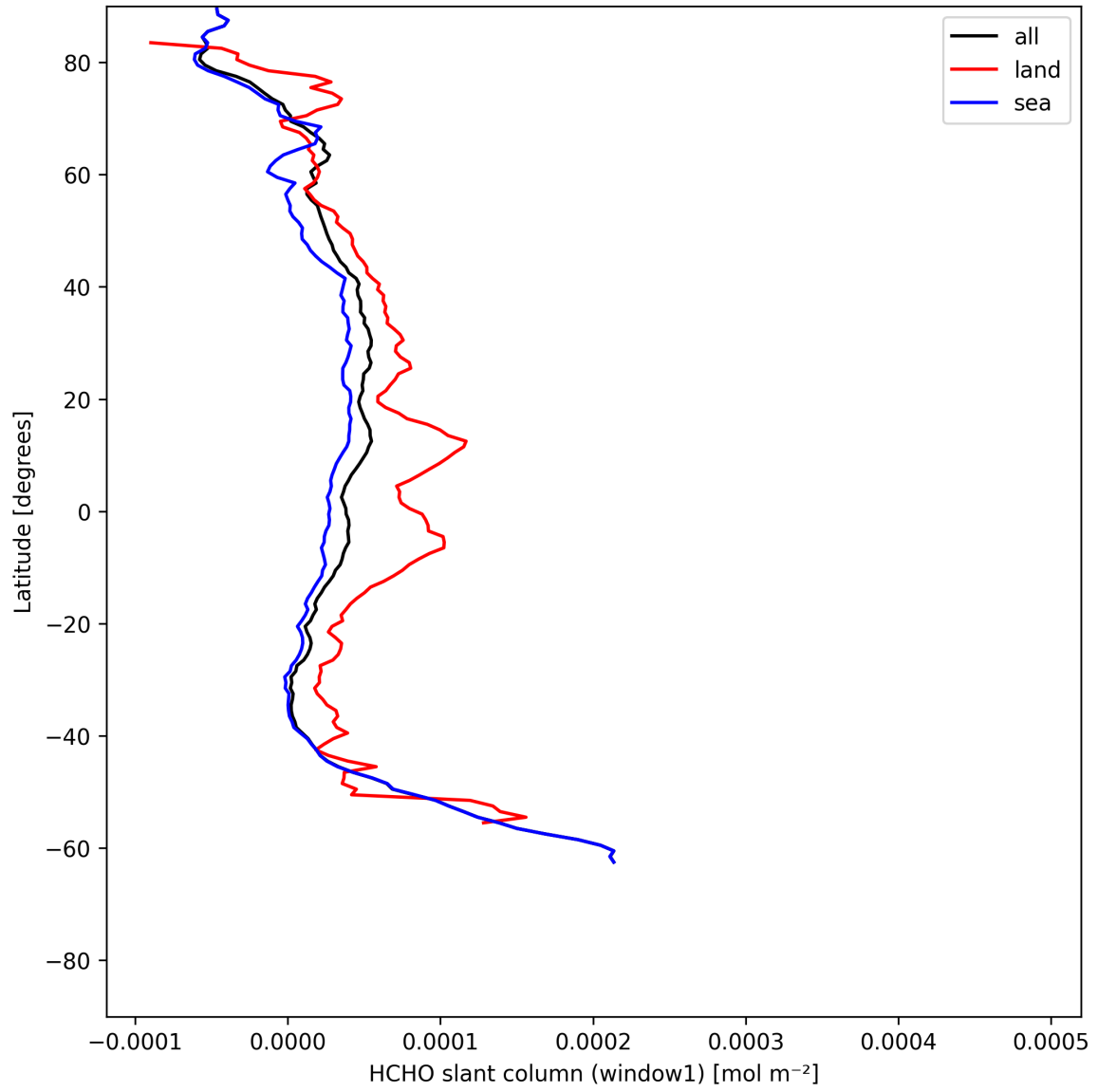
Figure 24: Zonal average of “HCHO slant column (window1)” for 2025-06-01 to 2025-06-02.
