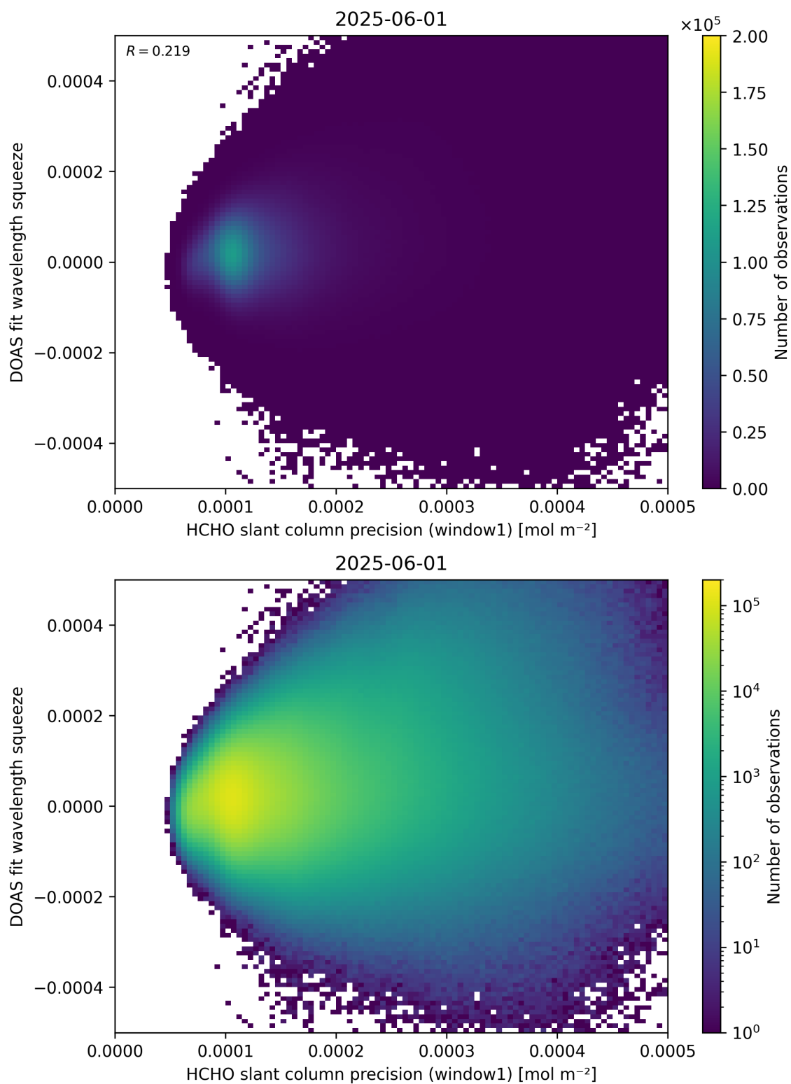
Figure 90: Scatter density plot of “HCHO slant column precision (window1)” against “DOAS fit wavelength squeeze” for 2025-06-01 to 2025-06-02.
