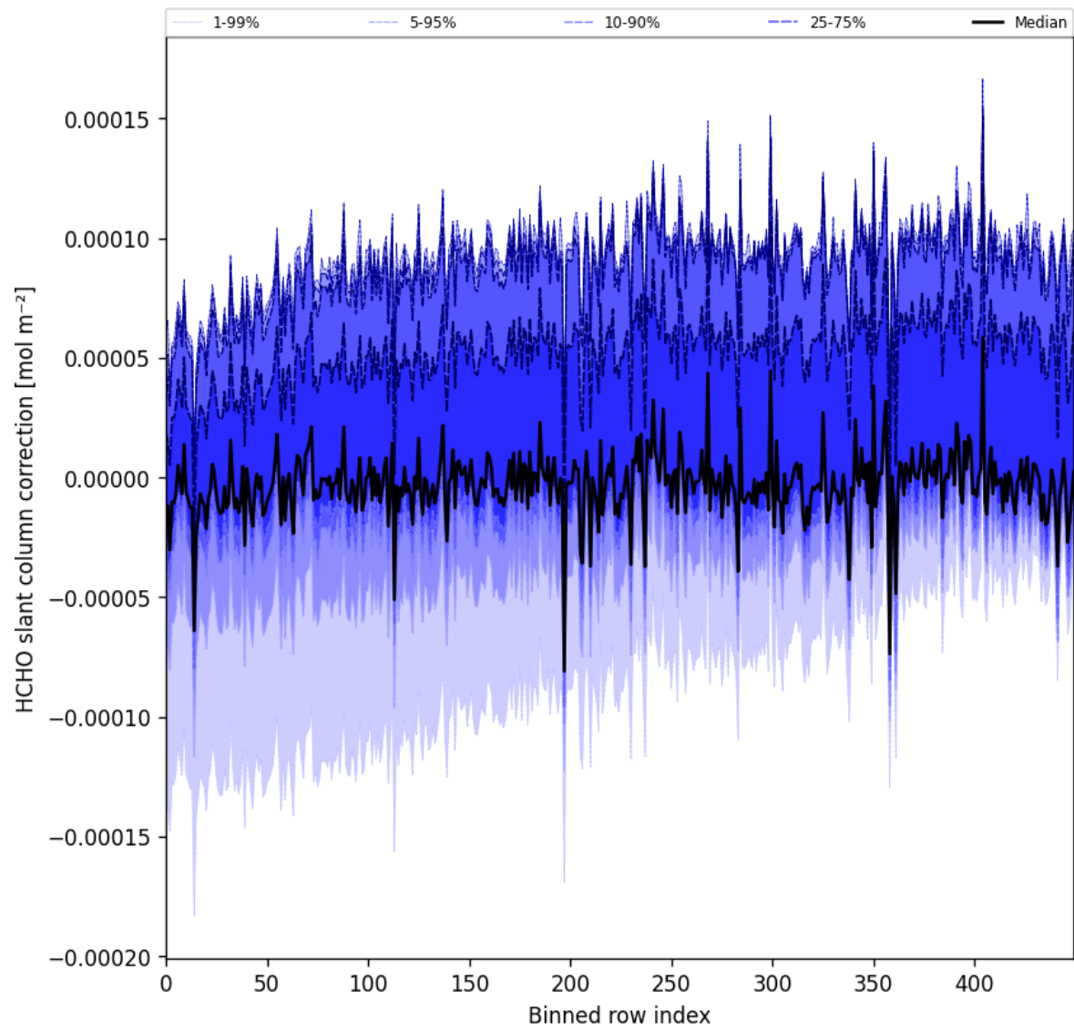
Figure 61: Along track statistics of “HCHO slant column correction” for 2025-06-01 to 2025-06-02
