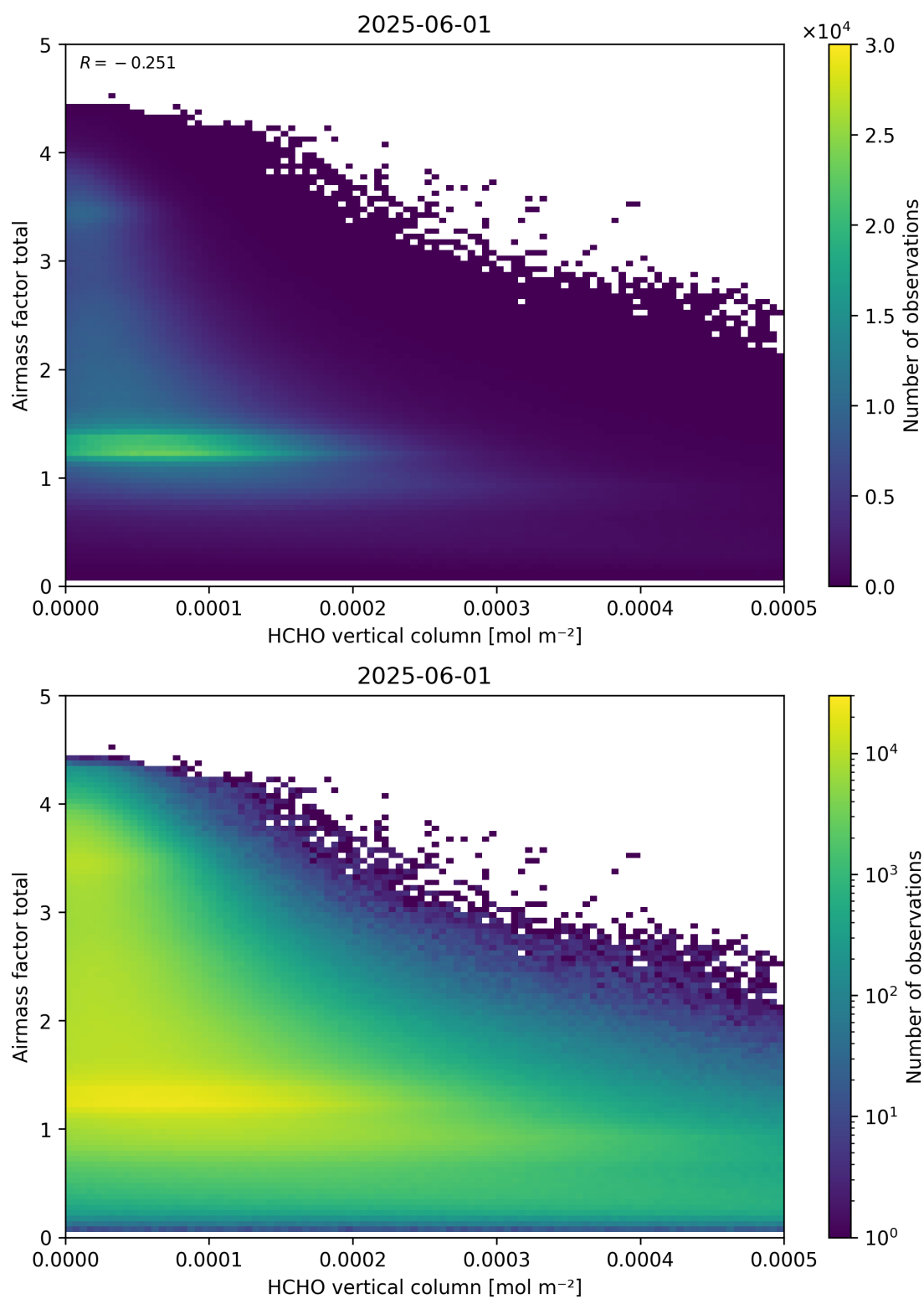
Figure 131: Scatter density plot of “HCHO vertical column” against “Airmass factor total” for 2025-06-01 to 2025-06-02.
