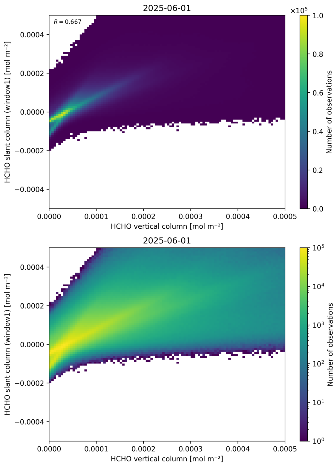
Figure 129: Scatter density plot of “HCHO vertical column” against “HCHO slant column (window1)” for 2025-06-01 to 2025-06-02.
