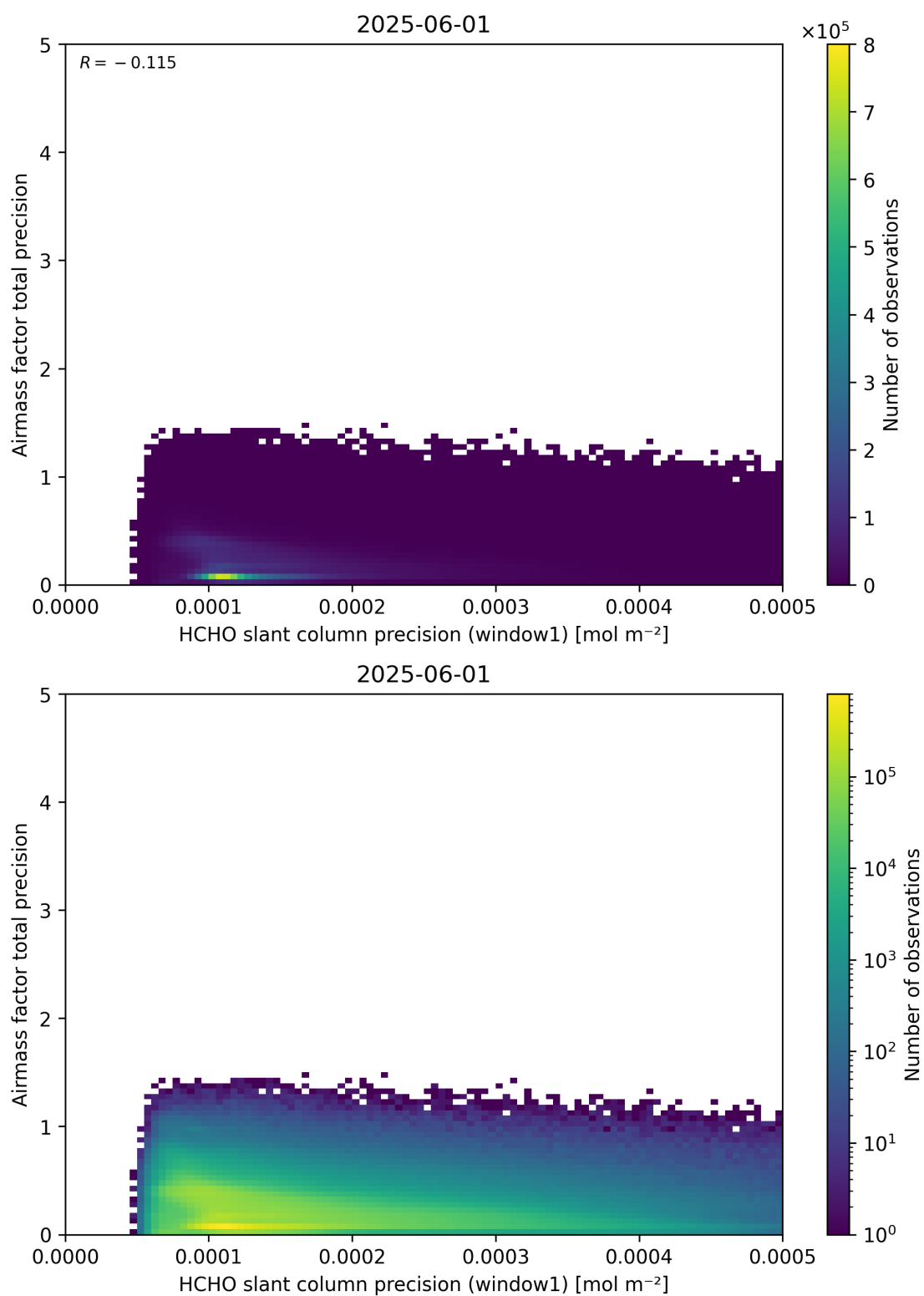
Figure 95: Scatter density plot of “HCHO slant column precision (window1)” against “Airmass factor total precision” for 2025-06-01 to 2025-06-02.
