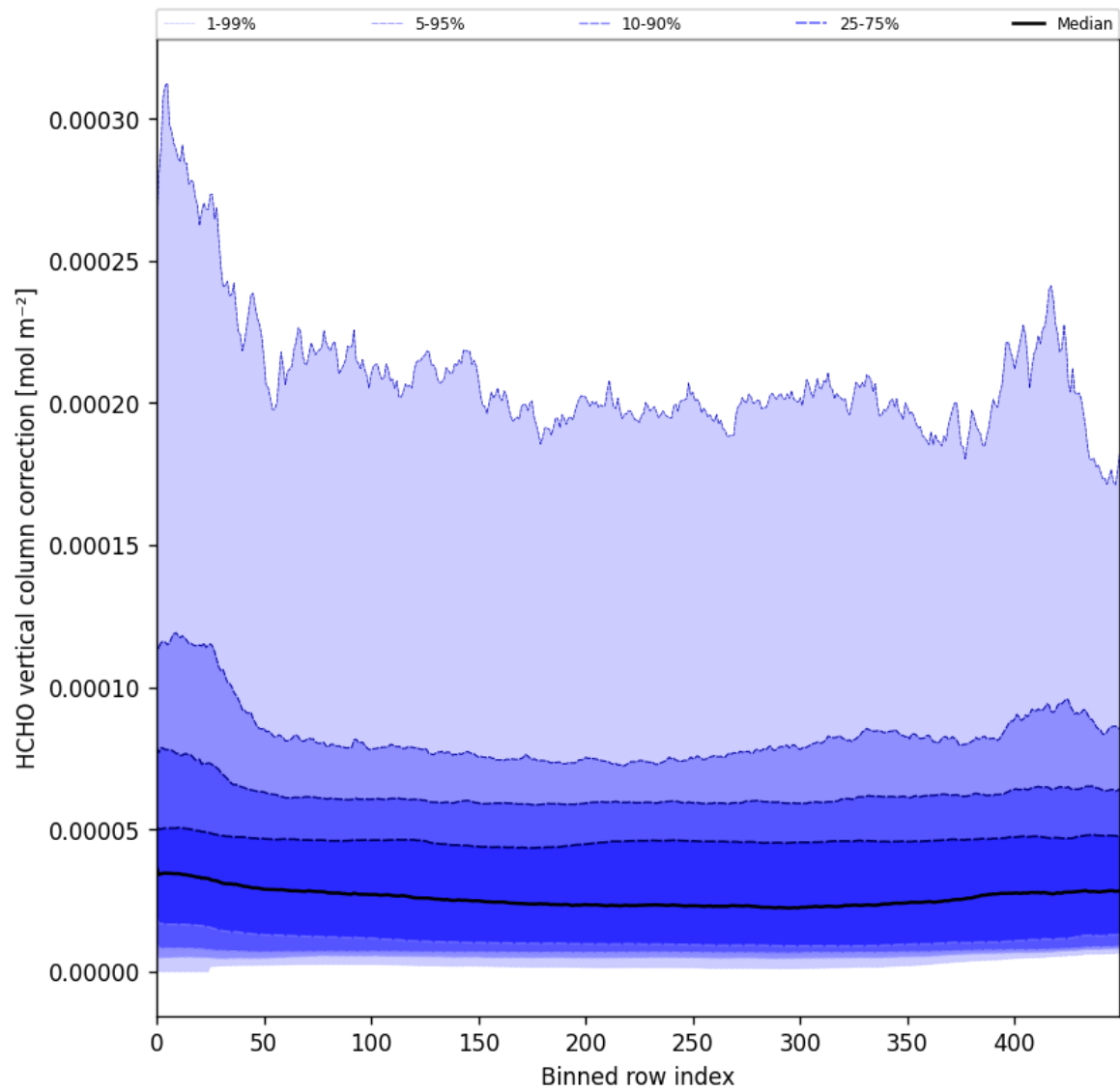
Figure 51: Along track statistics of “HCHO vertical column correction” for 2025-06-01 to 2025-06-02
