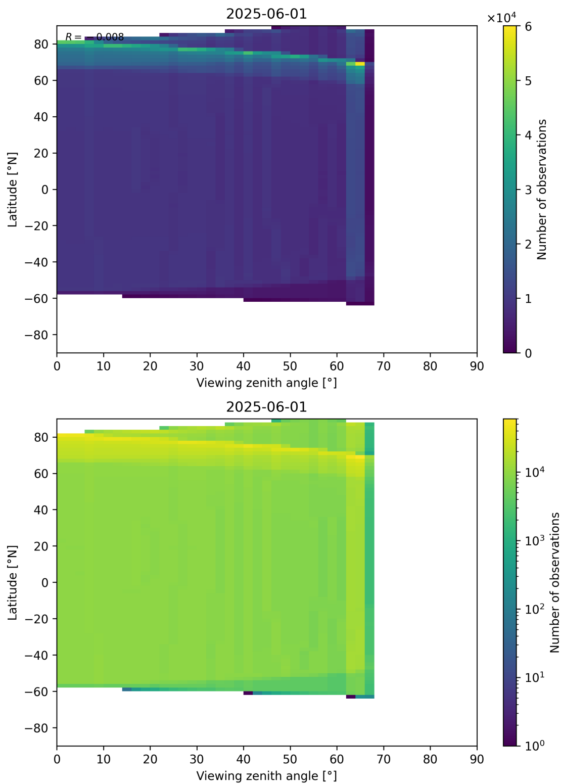
Figure 196: Scatter density plot of “Viewing zenith angle” against “Latitude” for 2025-06-01 to 2025-06-02.
