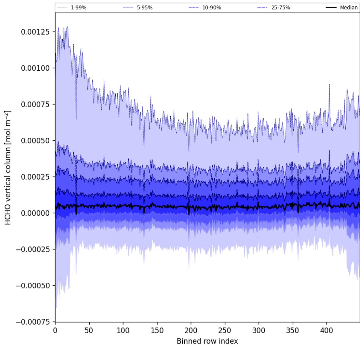
Figure 49: Along track statistics of “HCHO vertical column” for 2025-06-01 to 2025-06-02
