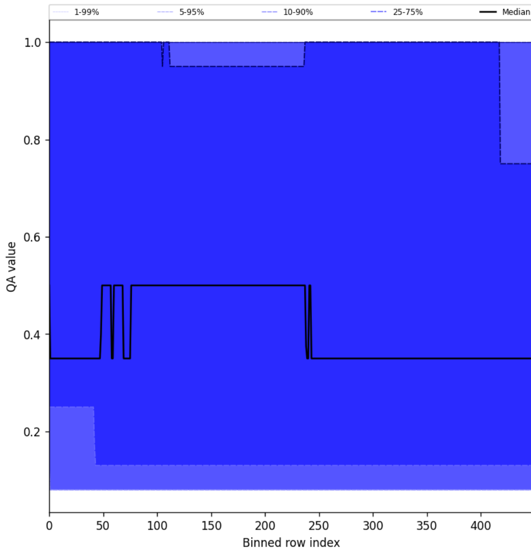
Figure 48: Along track statistics of “QA value” for 2025-06-01 to 2025-06-02
