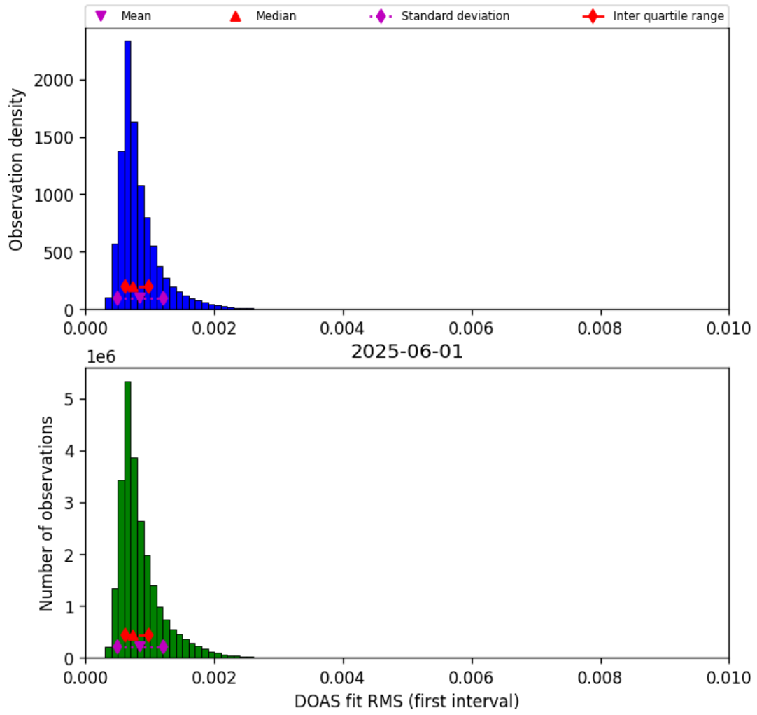
Figure 46: Histogram of "DOAS fit RMS (first interval)" for 2025-06-01 to 2025-06-02
