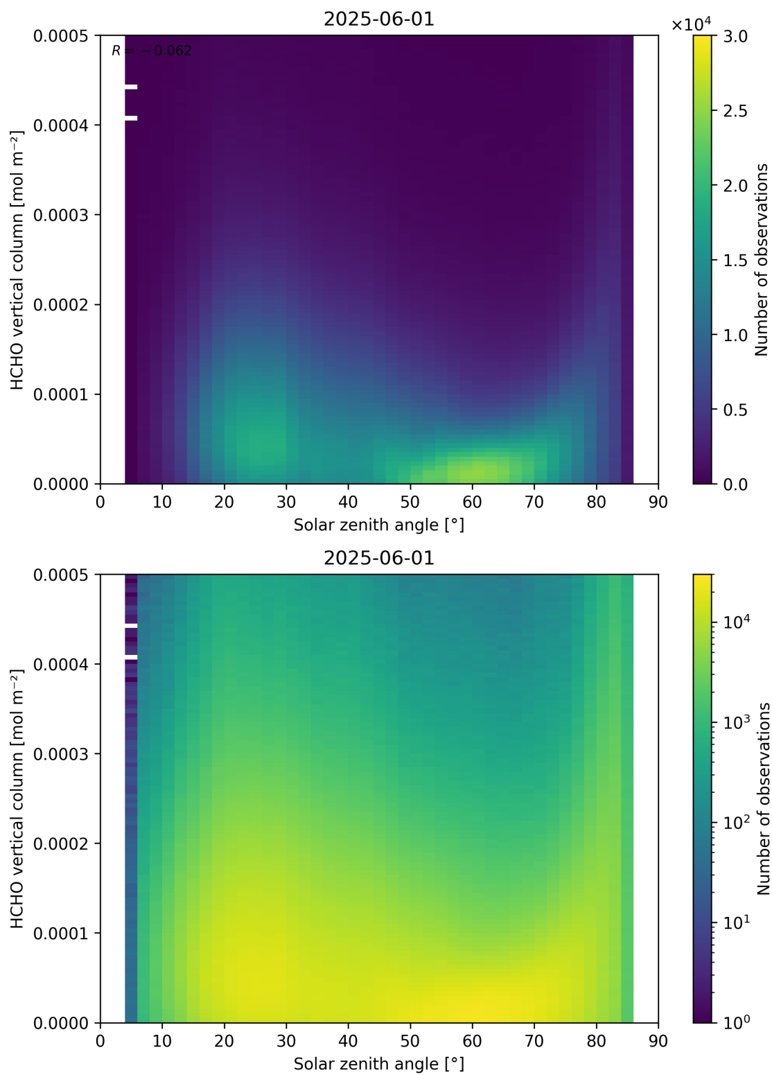
Figure 177: Scatter density plot of “Solar zenith angle” against “HCHO vertical column” for 2025-06-01 to 2025-06-02.
