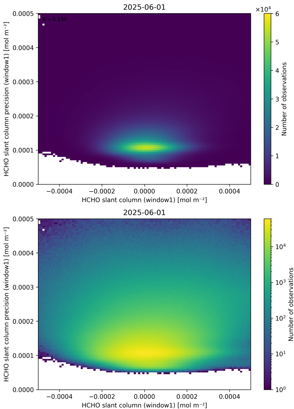
Figure 84: Scatter density plot of “HCHO slant column (window1)” against “HCHO slant column precision (window1)” for 2025-06-01 to 2025-06-02.
