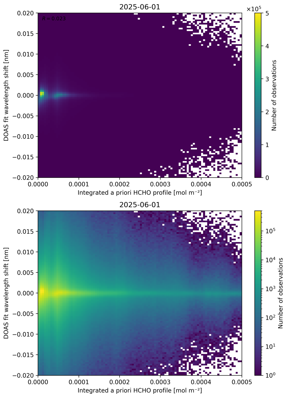
Figure 149: Scatter density plot of “Integrated a priori HCHO profile” against “DOAS fit wavelength shift” for 2025-06-01 to 2025-06-02.
