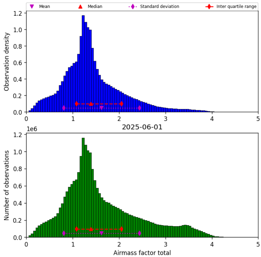
Figure 40: Histogram of “Airmass factor total” for 2025-06-01 to 2025-06-02
