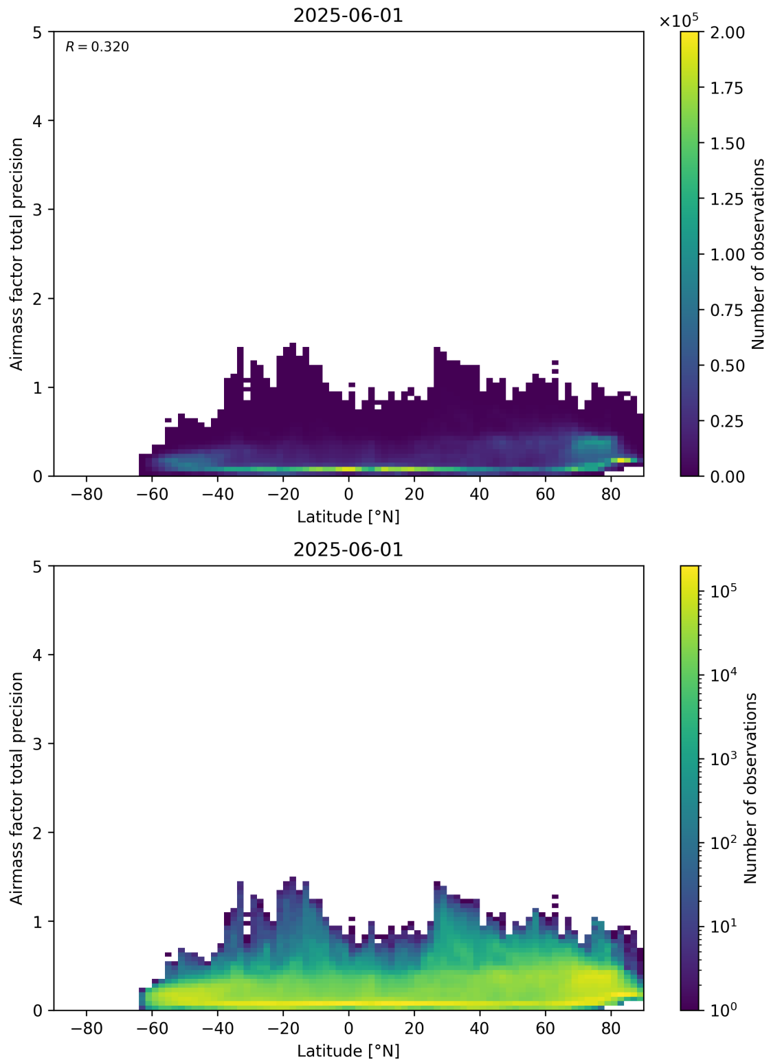
Figure 162: Scatter density plot of “Latitude” against “Airmass factor total precision” for 2025-06-01 to 2025-06-02.
