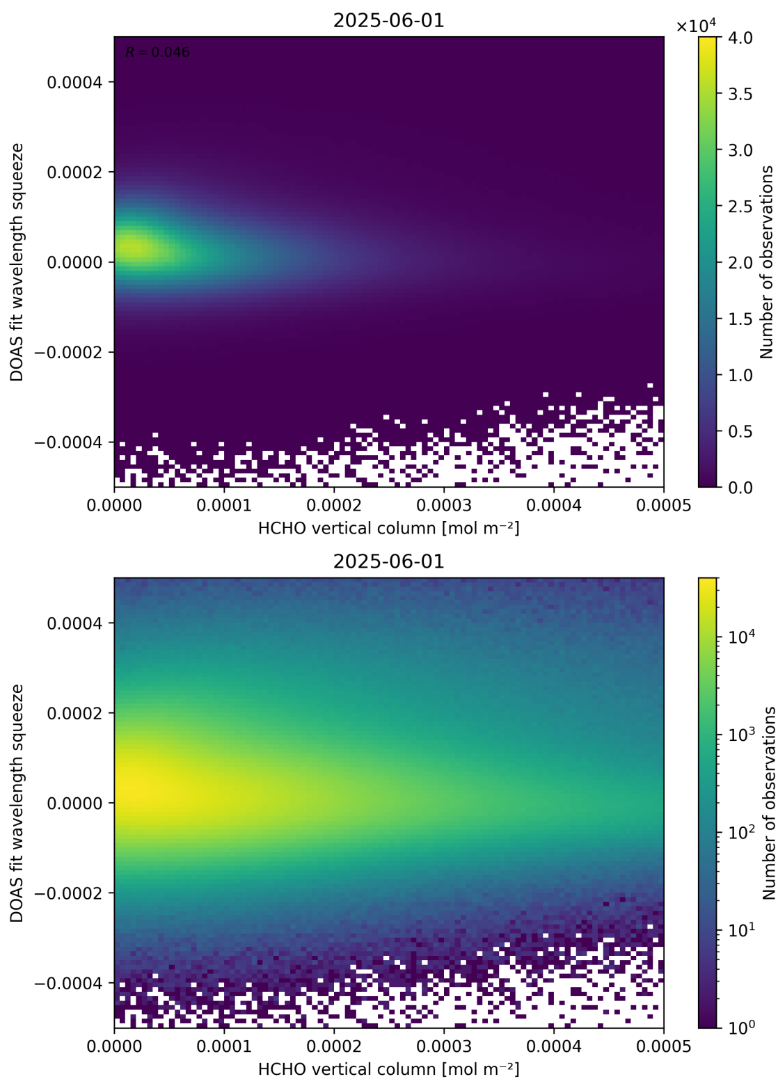
Figure 125: Scatter density plot of “HCHO vertical column” against “DOAS fit wavelength squeeze” for 2025-06-01 to 2025-06-02.
