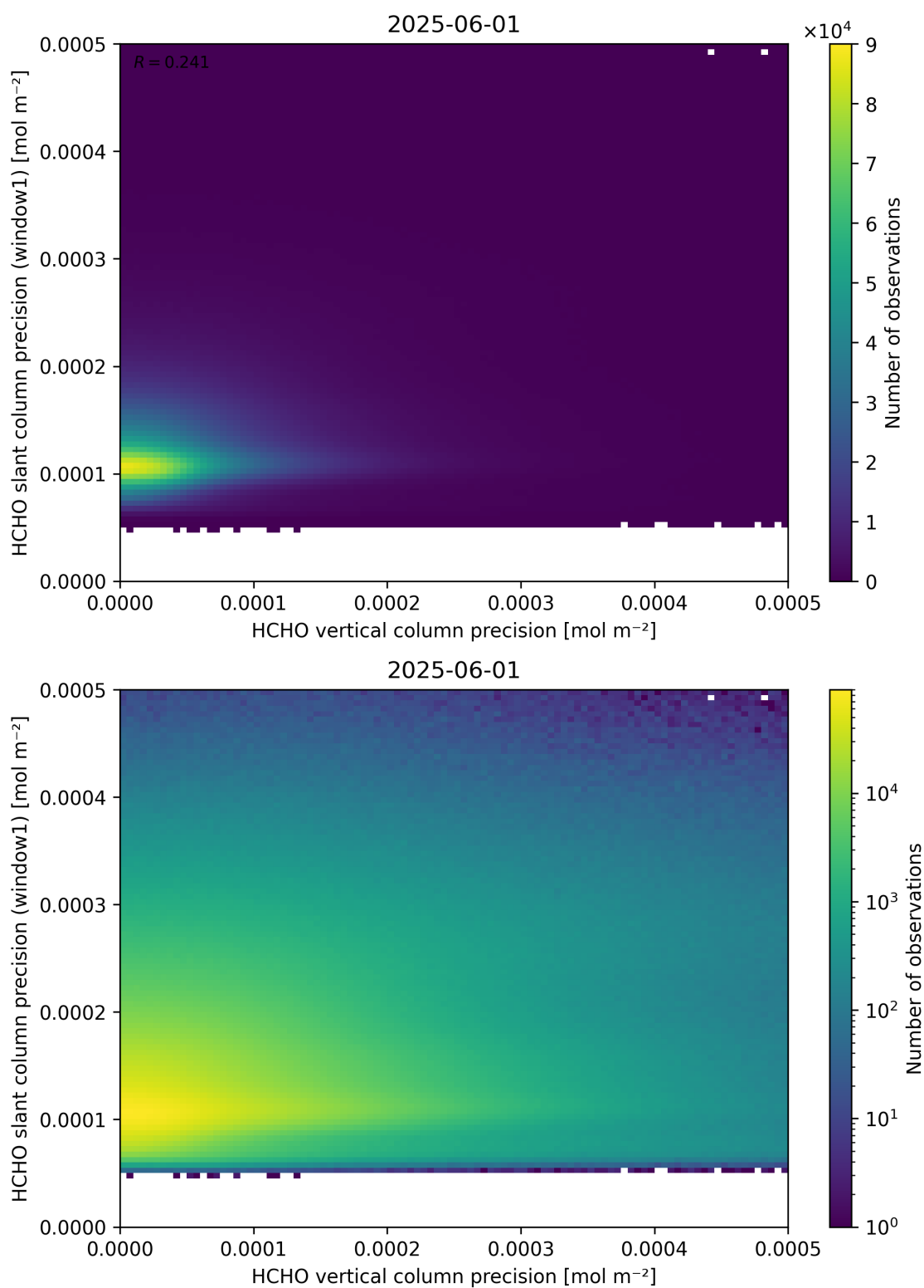
Figure 143: Scatter density plot of “HCHO vertical column precision” against “HCHO slant column precision (window1)” for 2025-06-01 to 2025-06-02.
