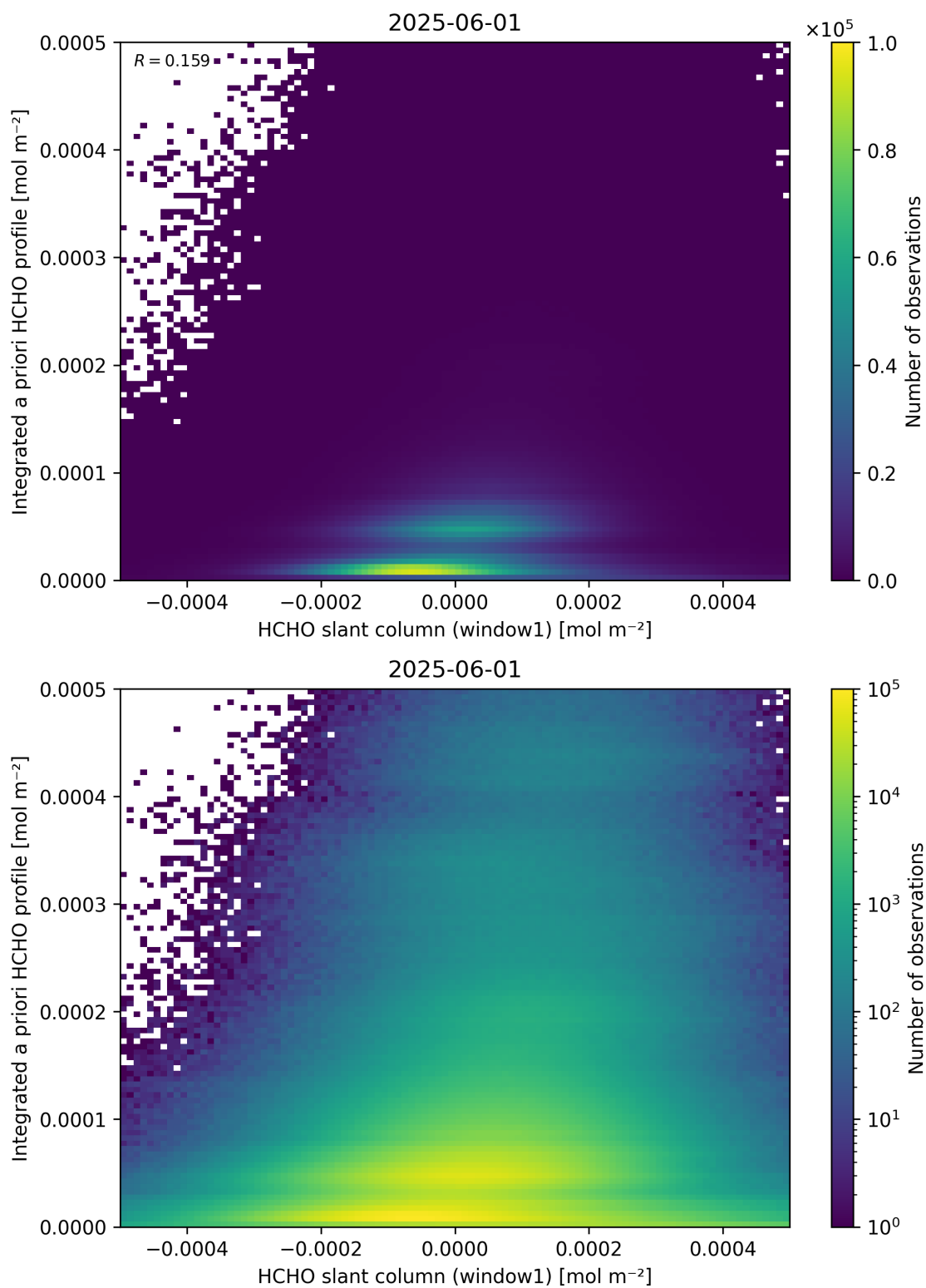
Figure 87: Scatter density plot of “HCHO slant column (window1)” against “Integrated a priori HCHO profile” for 2025-06-01 to 2025-06-02.
