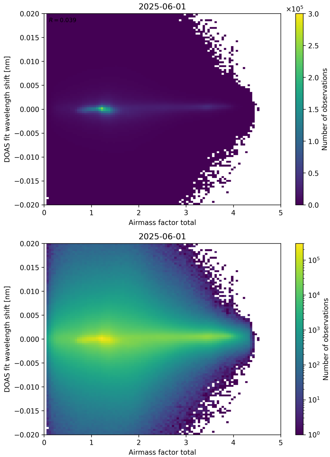
Figure 98: Scatter density plot of “Airmass factor total” against “DOAS fit wavelength shift” for 2025-06-01 to 2025-06-02.
