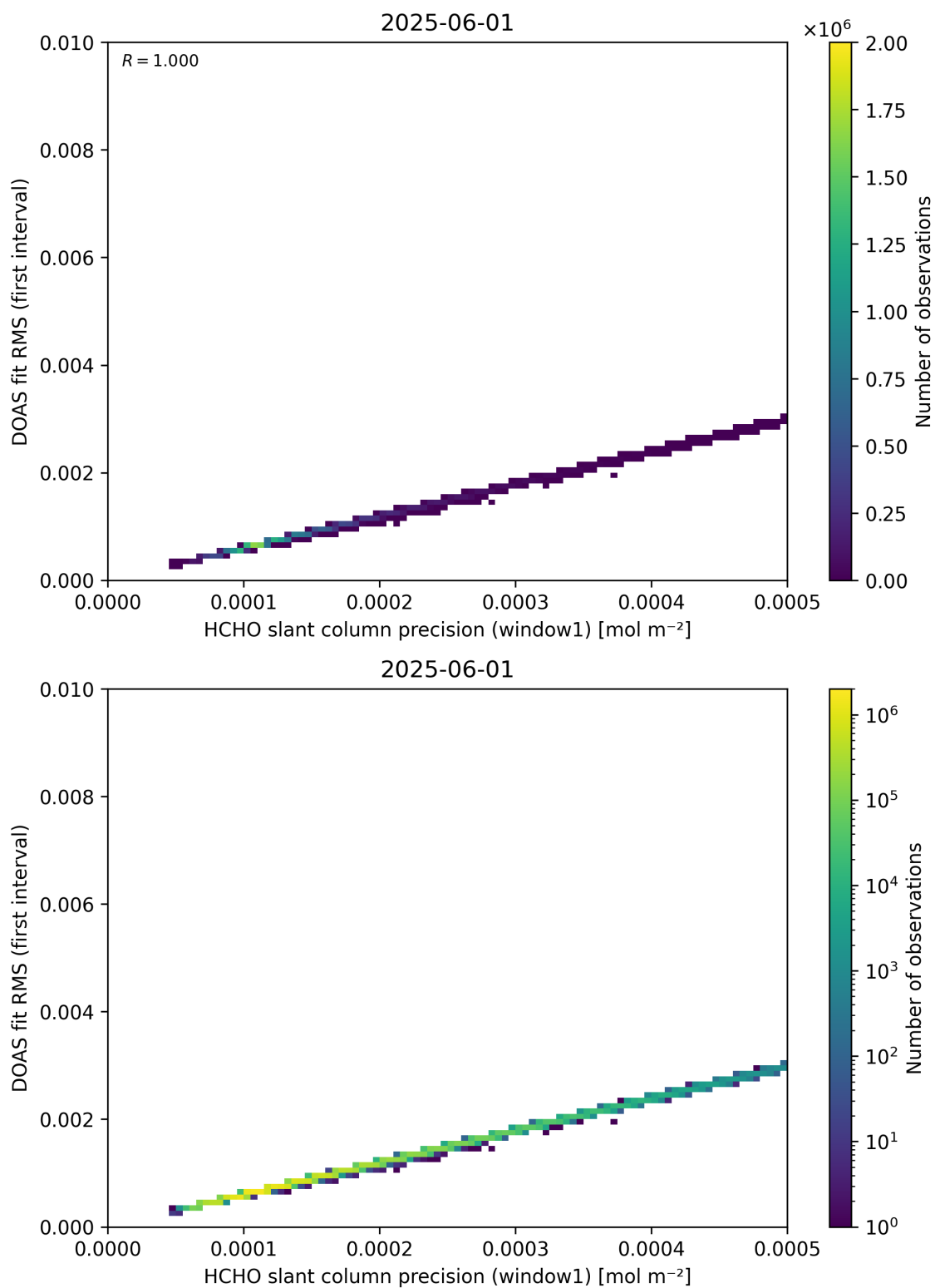
Figure 88: Scatter density plot of “HCHO slant column precision (window1)” against “DOAS fit RMS (first interval)” for 2025-06-01 to 2025-06-02.
