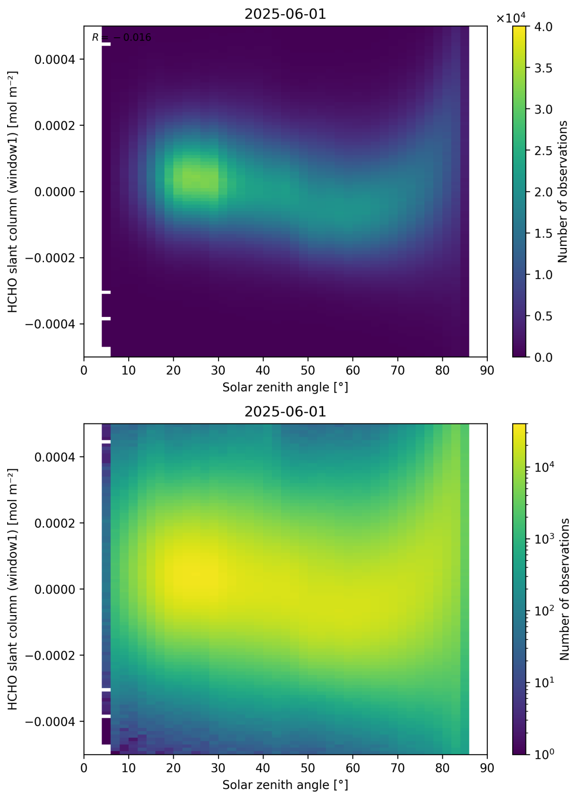
Figure 173: Scatter density plot of “Solar zenith angle” against “HCHO slant column (window1)” for 2025-06-01 to 2025-06-02.
