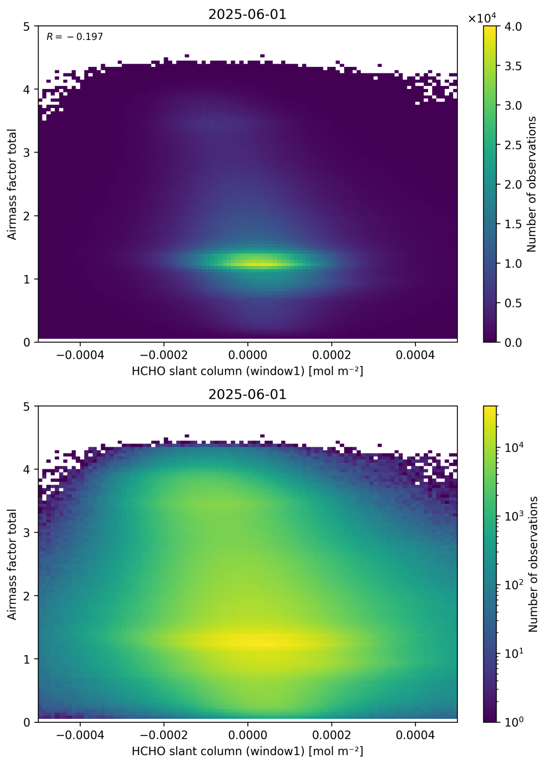
Figure 85: Scatter density plot of “HCHO slant column (window1)” against “Airmass factor total” for 2025-06-01 to 2025-06-02.
