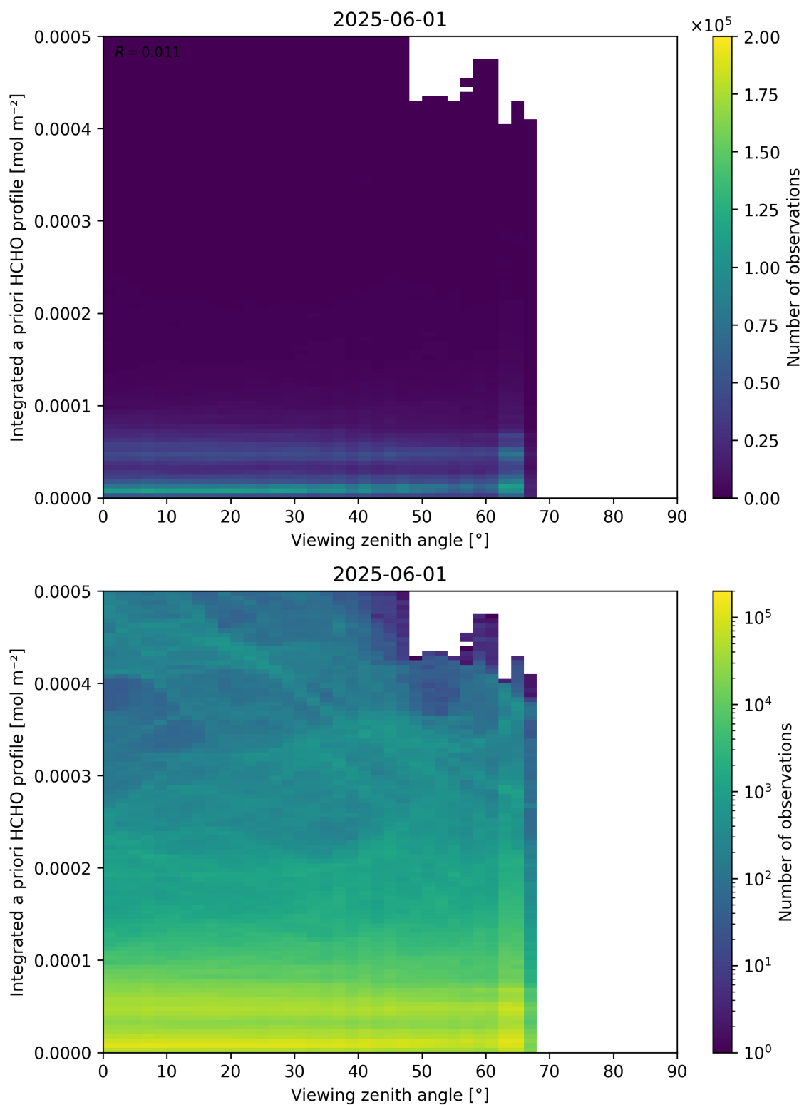
Figure 195: Scatter density plot of “Viewing zenith angle” against “Integrated a priori HCHO profile” for 2025-06-01 to 2025-06-02.
