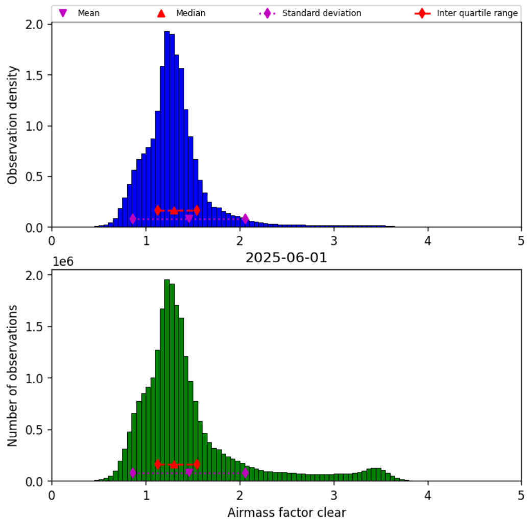
Figure 42: Histogram of “Airmass factor clear” for 2025-06-01 to 2025-06-02
