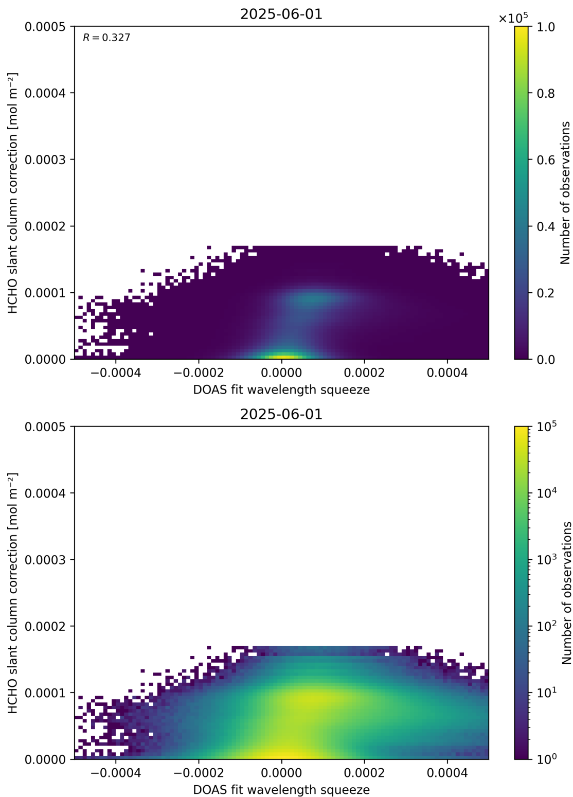
Figure 70: Scatter density plot of “DOAS fit wavelength squeeze” against “HCHO slant column correction” for 2025-06-01 to 2025-06-02.
