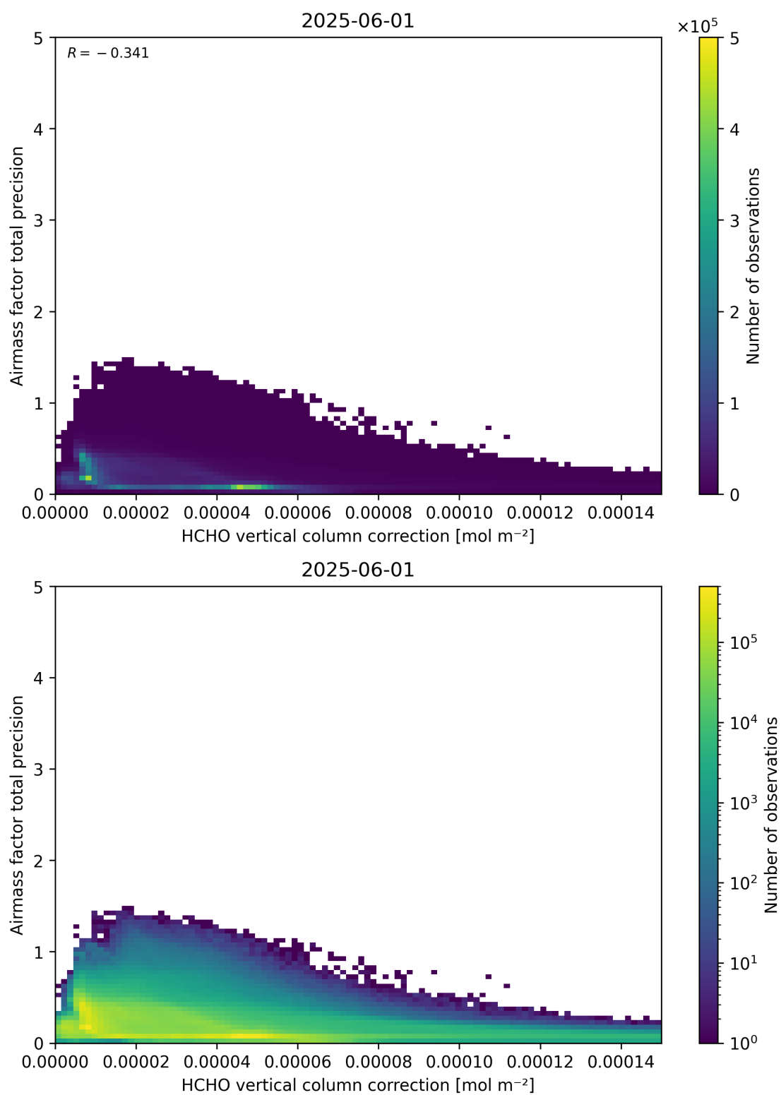
Figure 121: Scatter density plot of “HCHO vertical column correction” against “Airmass factor total precision” for 2025-06-01 to 2025-06-02.
