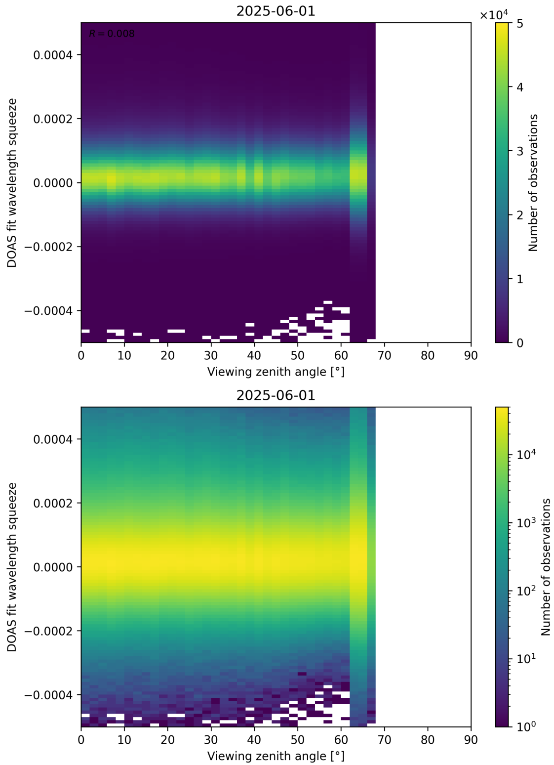
Figure 184: Scatter density plot of “Viewing zenith angle” against “DOAS fit wavelength squeeze” for 2025-06-01 to 2025-06-02.
