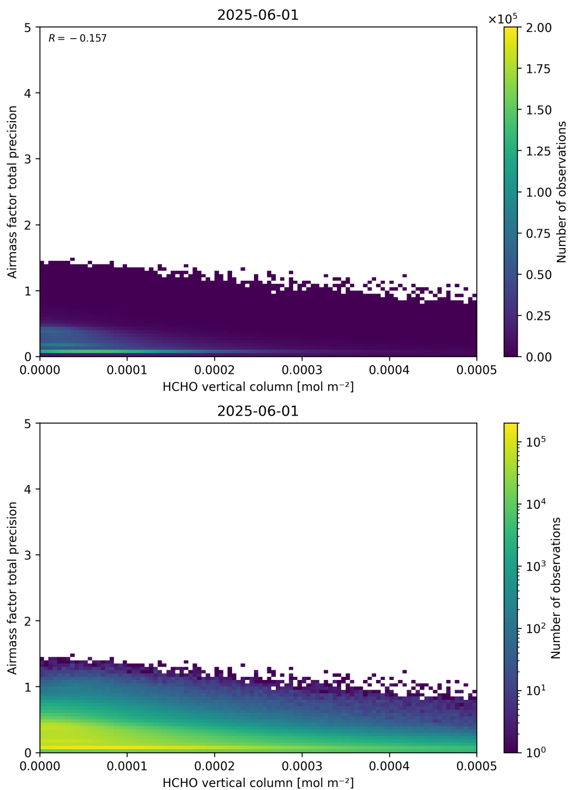
Figure 132: Scatter density plot of “HCHO vertical column” against “Airmass factor total precision” for 2025-06-01 to 2025-06-02.
