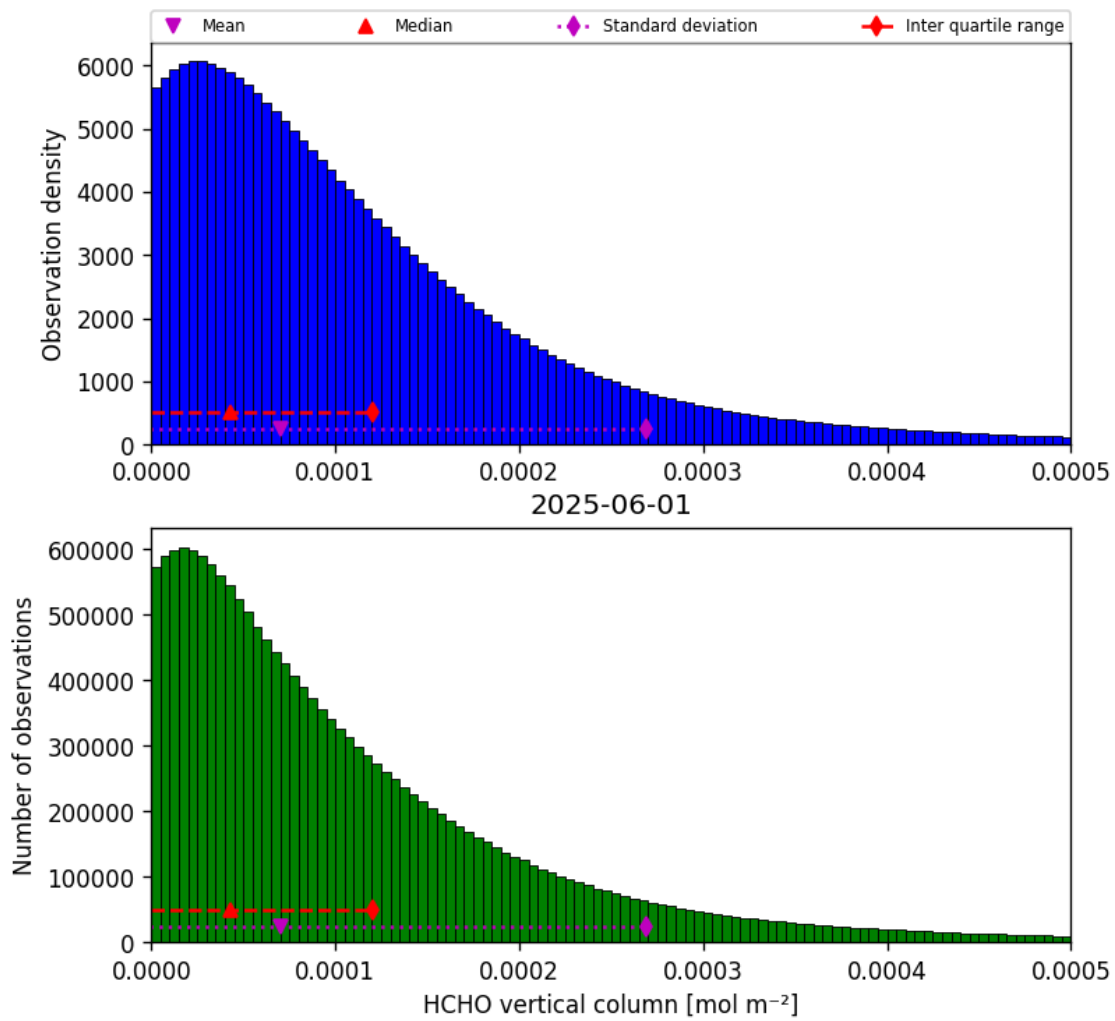
Figure 35: Histogram of “HCHO vertical column” for 2025-06-01 to 2025-06-02
