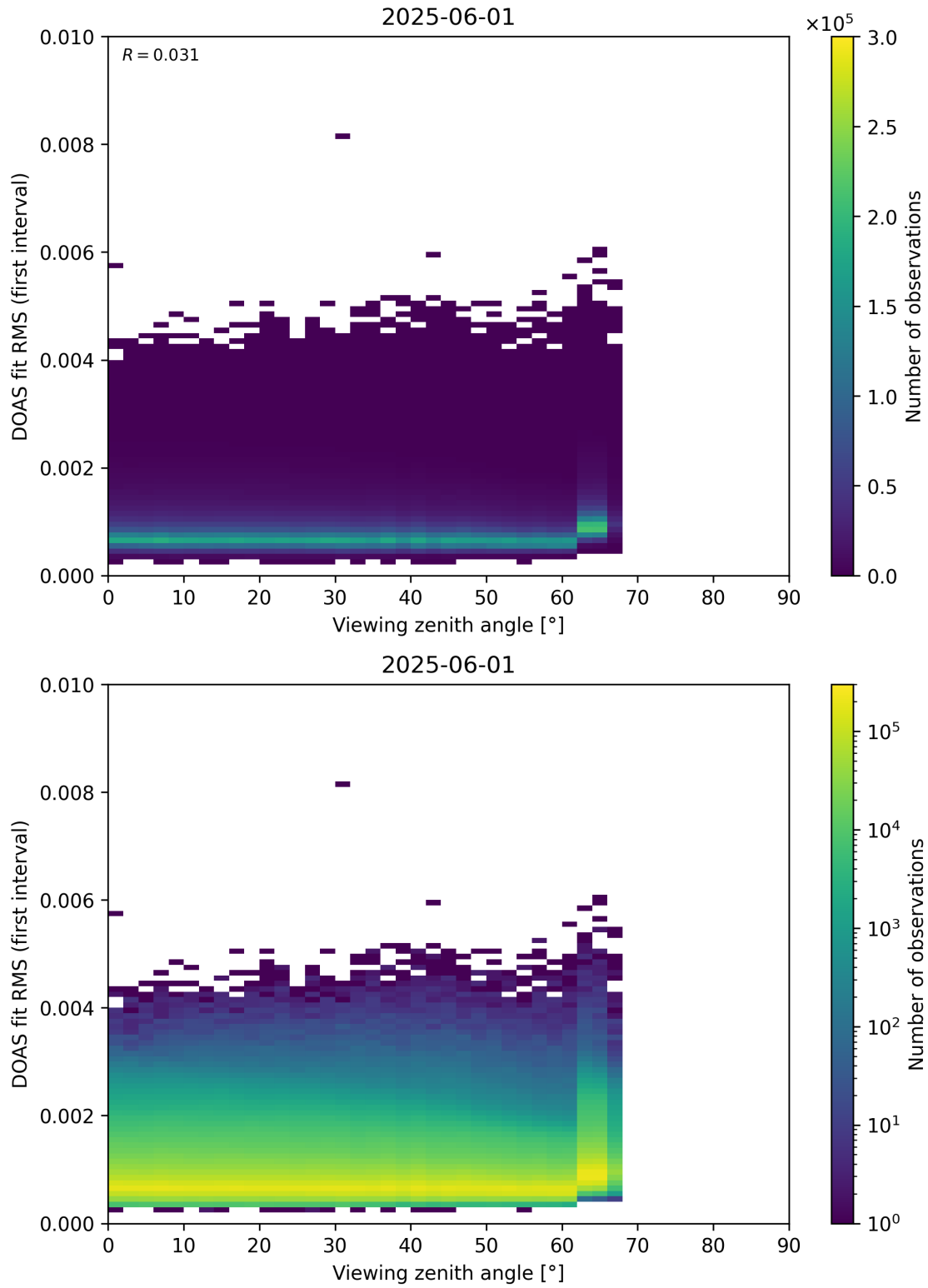
Figure 182: Scatter density plot of “Viewing zenith angle” against “DOAS fit RMS (first interval)” for 2025-06-01 to 2025-06-02.
