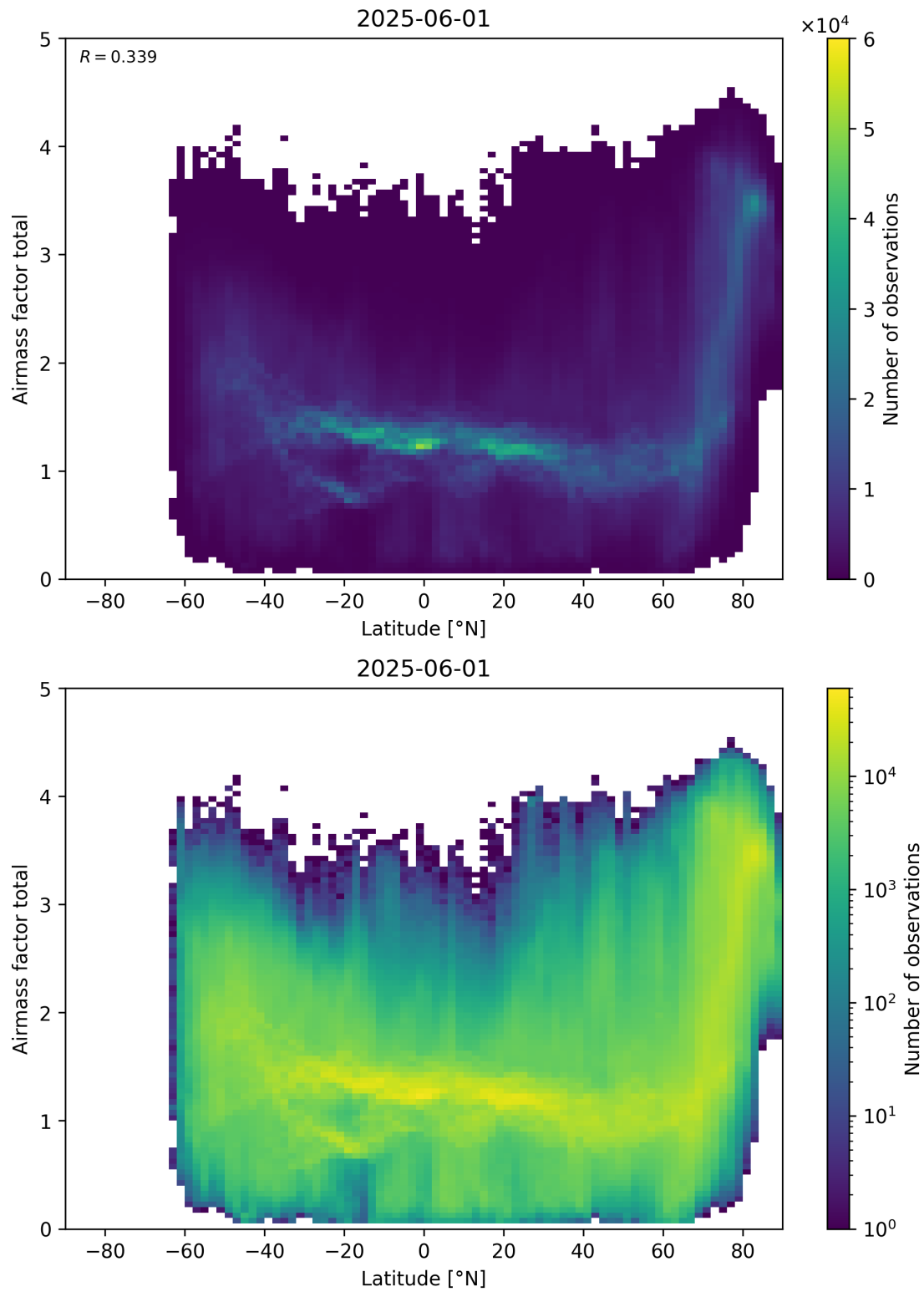
Figure 161: Scatter density plot of “Latitude” against “Airmass factor total” for 2025-06-01 to 2025-06-02.
