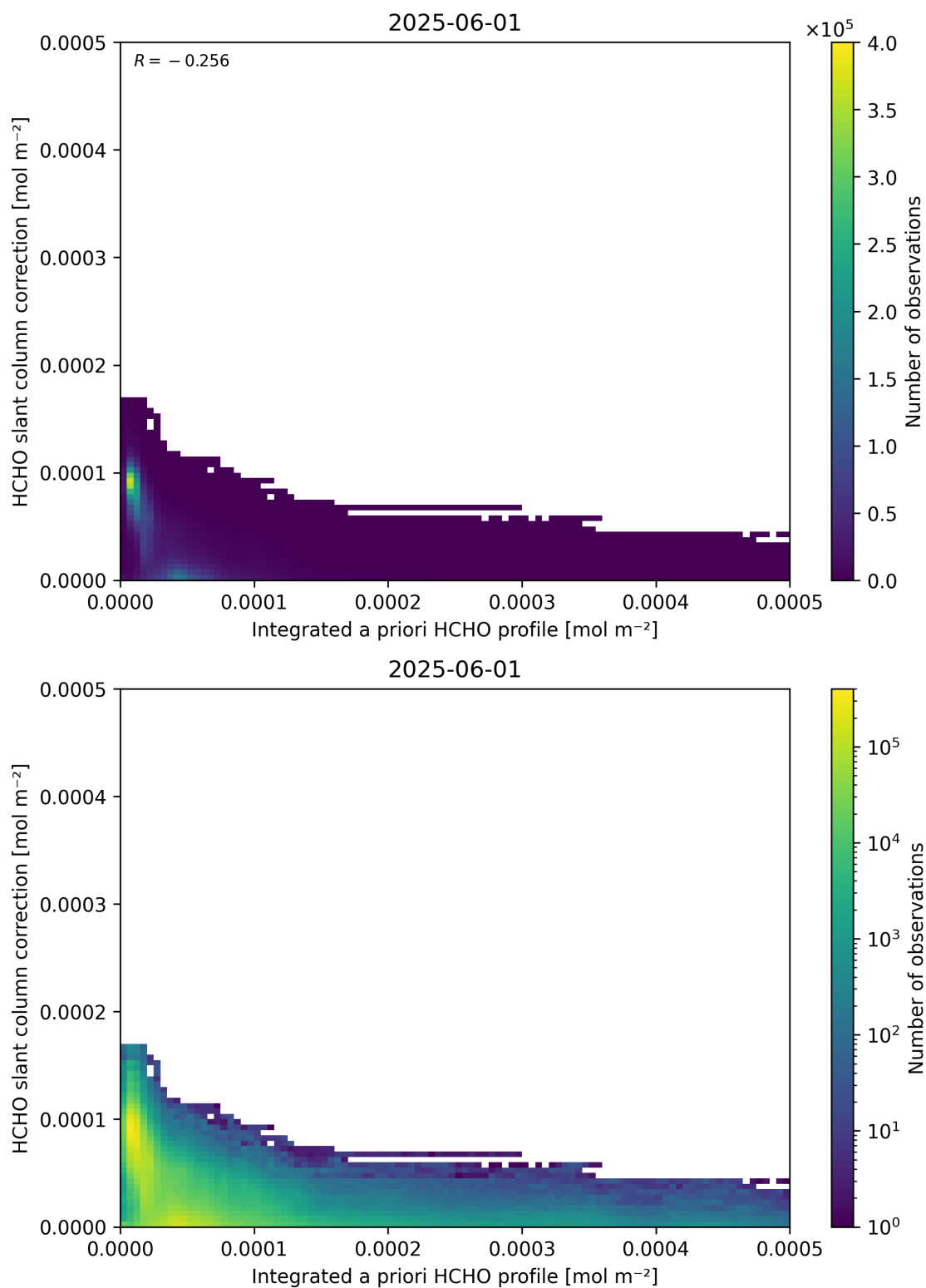
Figure 152: Scatter density plot of “Integrated a priori HCHO profile” against “HCHO slant column correction” for 2025-06-01 to 2025-06-02.
