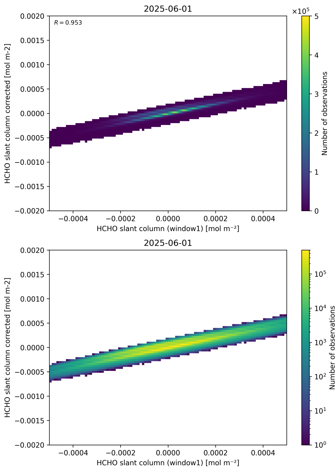
Figure 82: Scatter density plot of “HCHO slant column (window1)” against “HCHO slant column corrected” for 2025-06-01 to 2025-06-02.
