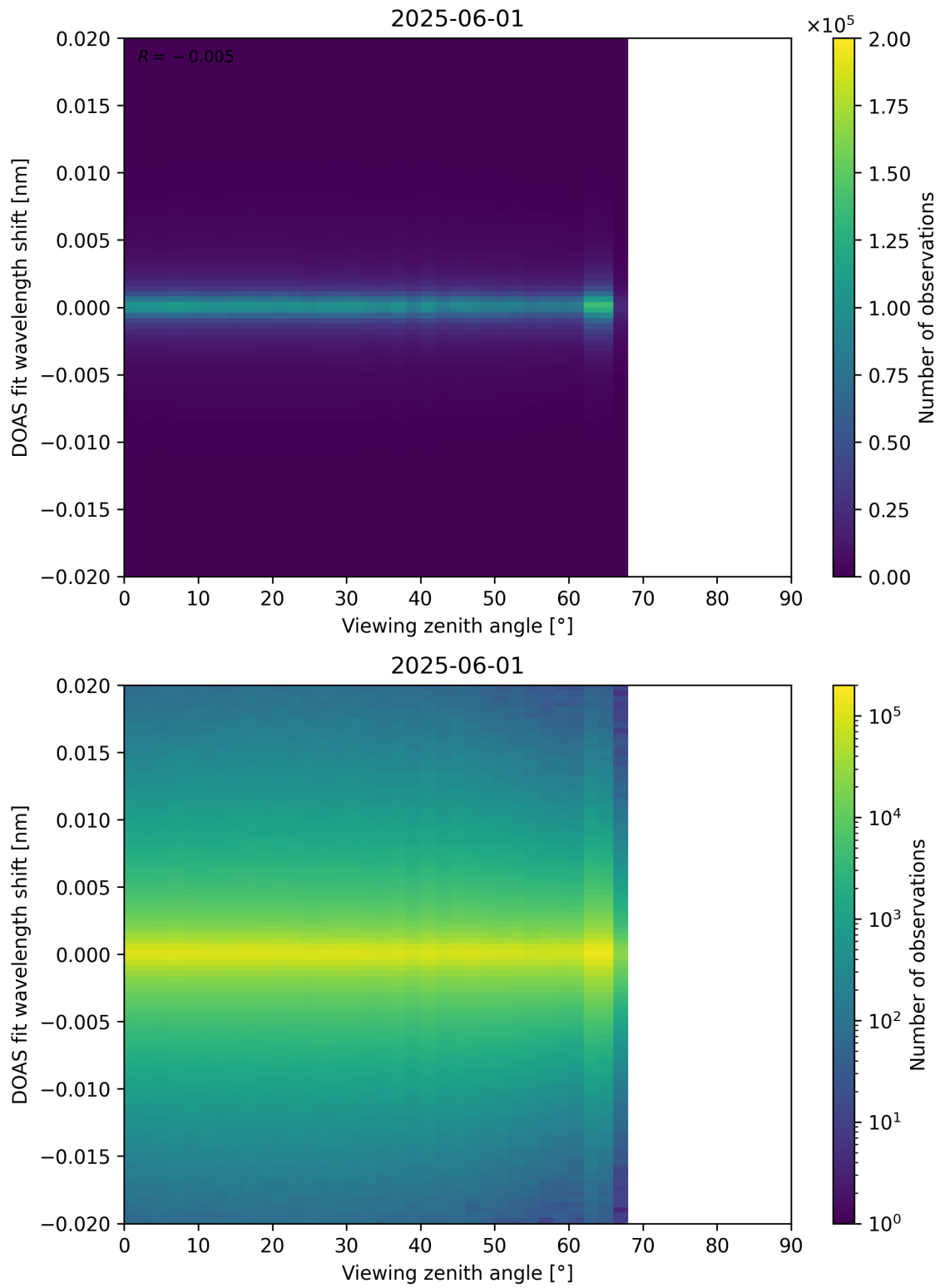
Figure 183: Scatter density plot of “Viewing zenith angle” against “DOAS fit wavelength shift” for 2025-06-01 to 2025-06-02.
