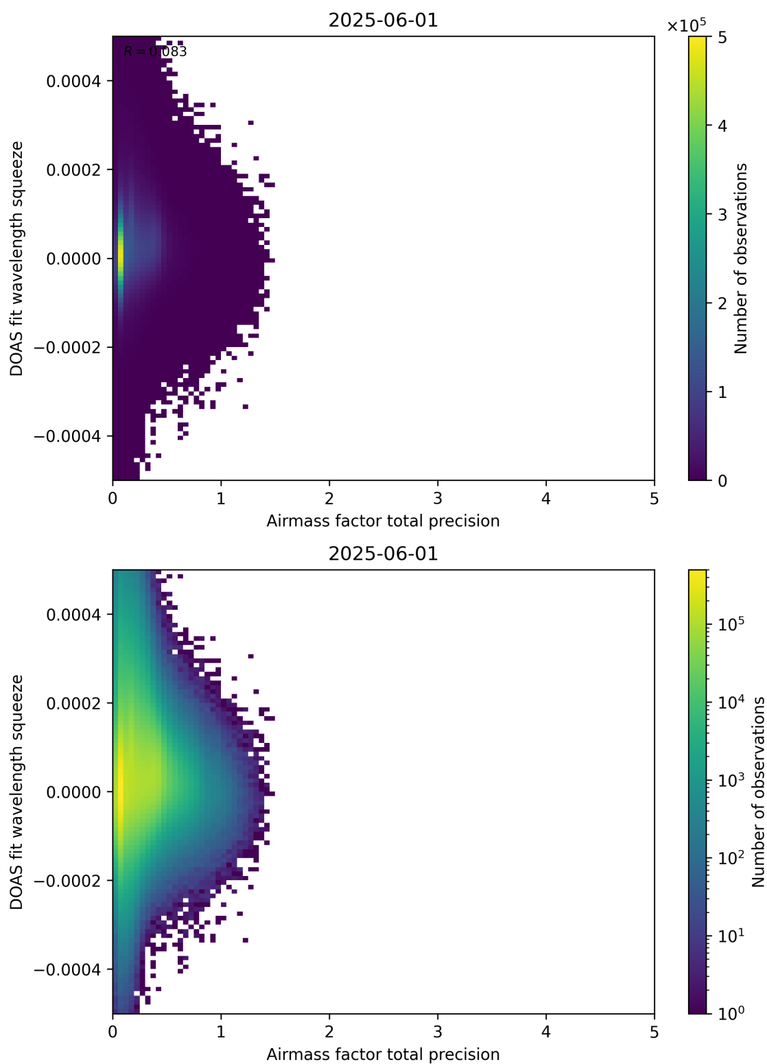
Figure 107: Scatter density plot of “Airmass factor total precision” against “DOAS fit wavelength squeeze” for 2025-06-01 to 2025-06-02.
