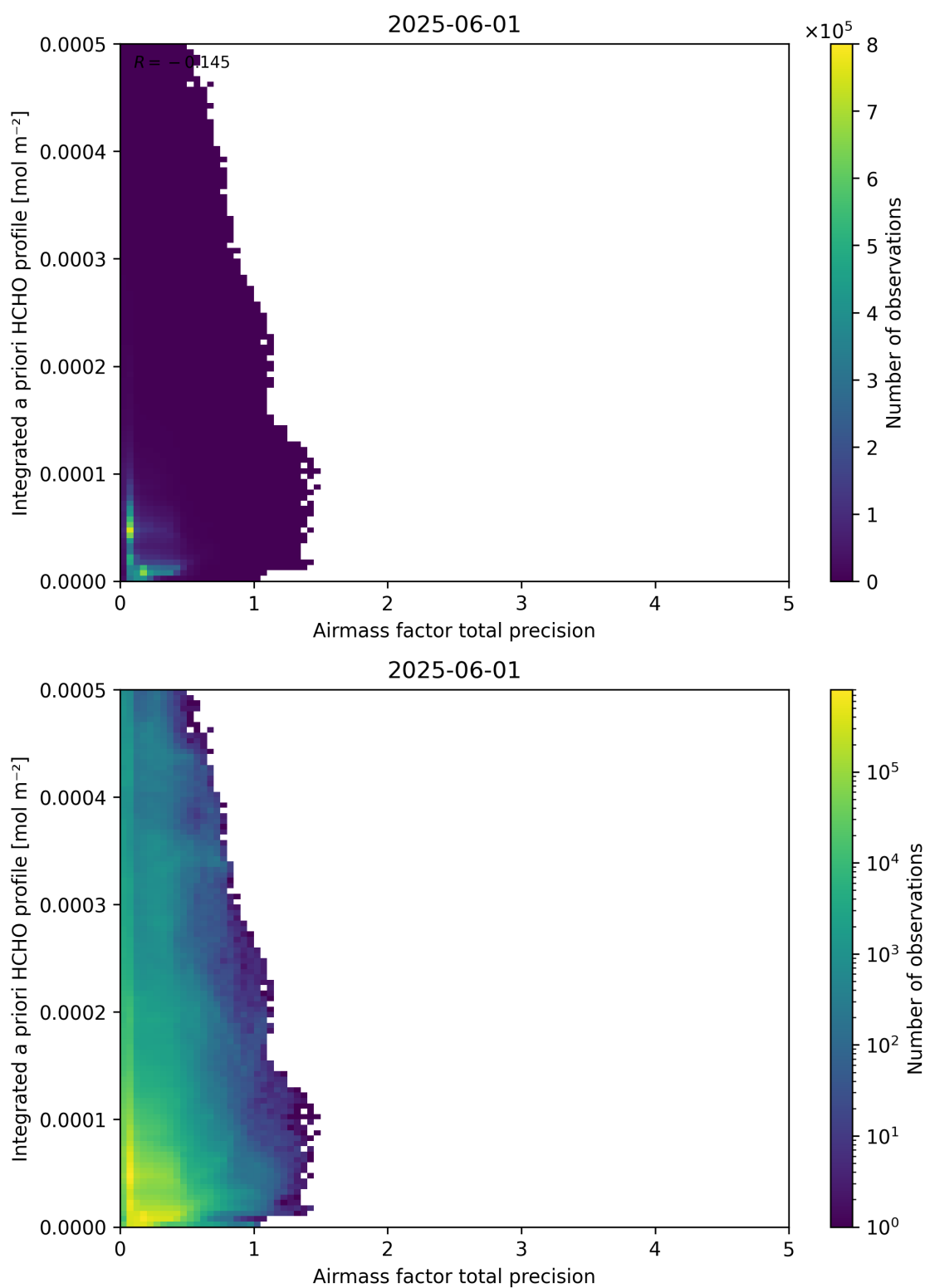
Figure 111: Scatter density plot of “Airmass factor total precision” against “Integrated a priori HCHO profile” for 2025-06-01 to 2025-06-02.
