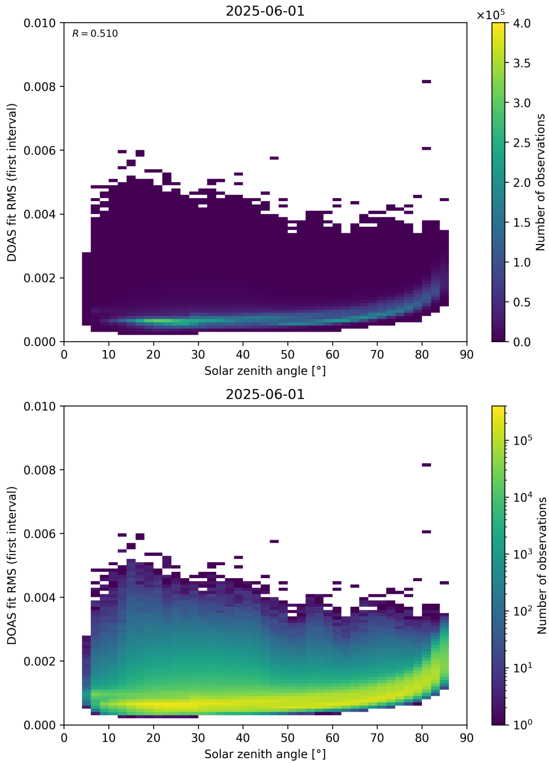
Figure 167: Scatter density plot of “Solar zenith angle” against “DOAS fit RMS (first interval)” for 2025-06-01 to 2025-06-02.
