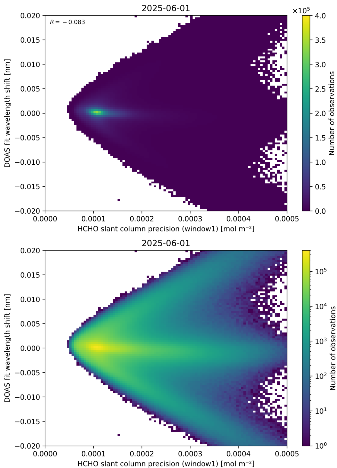
Figure 89: Scatter density plot of “HCHO slant column precision (window1)” against “DOAS fit wavelength shift” for 2025-06-01 to 2025-06-02.
