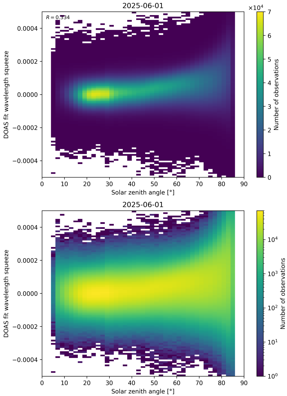
Figure 169: Scatter density plot of “Solar zenith angle” against “DOAS fit wavelength squeeze” for 2025-06-01 to 2025-06-02.
