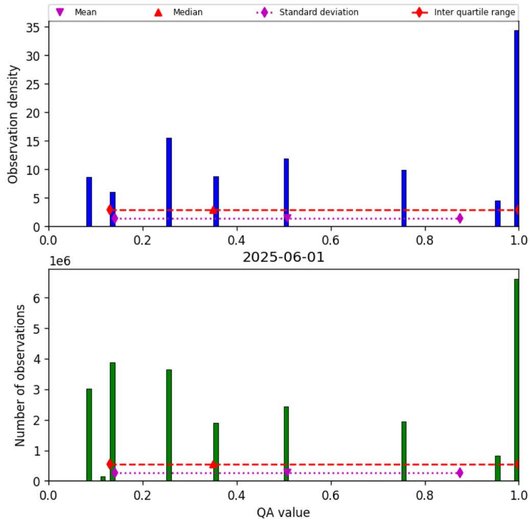
Figure 34: Histogram of “QA value” for 2025-06-01 to 2025-06-02
