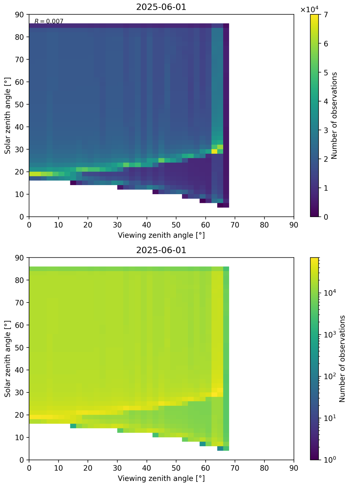
Figure 197: Scatter density plot of “Viewing zenith angle” against “Solar zenith angle” for 2025-06-01 to 2025-06-02.
