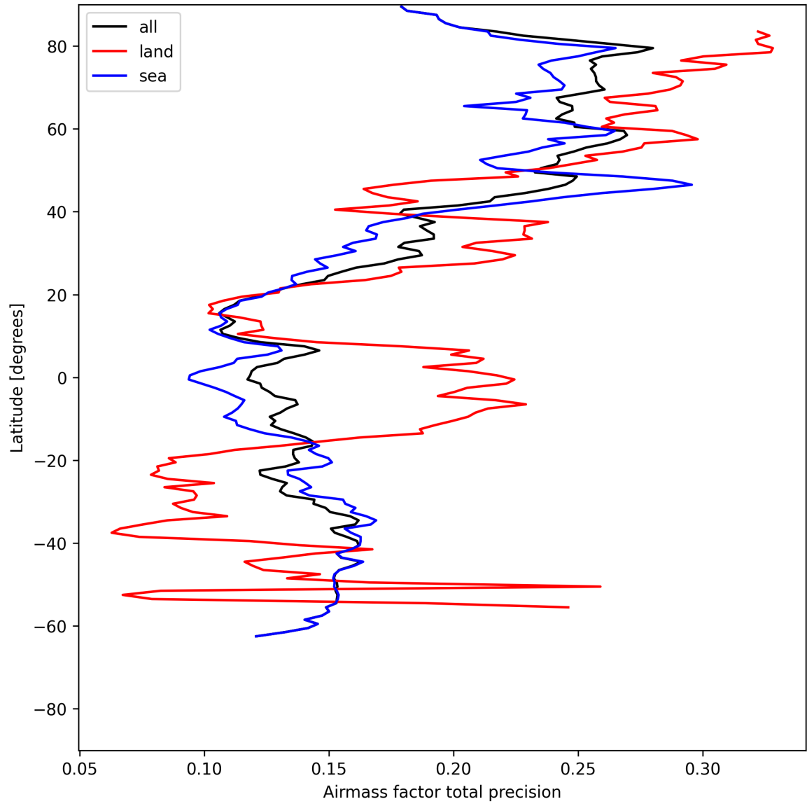
Figure 27: Zonal average of “Airmass factor total precision” for 2025-06-01 to 2025-06-02.
