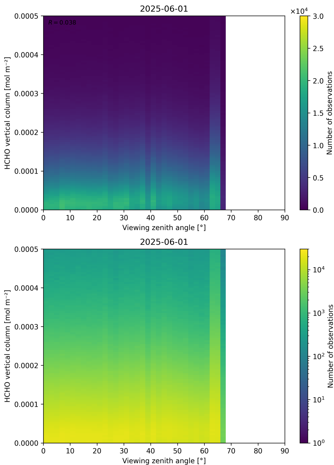
Figure 192: Scatter density plot of “Viewing zenith angle” against “HCHO vertical column” for 2025-06-01 to 2025-06-02.
