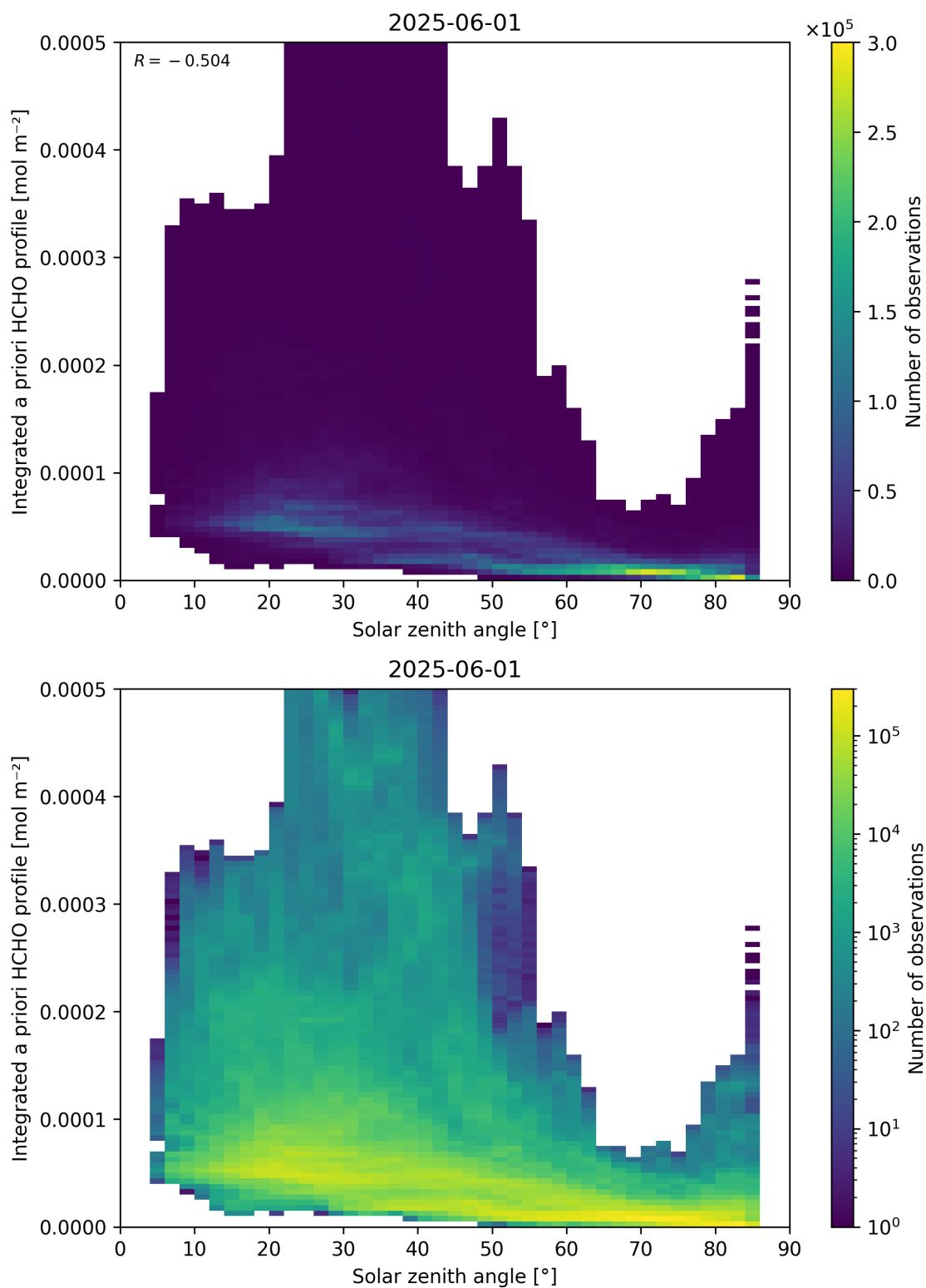
Figure 180: Scatter density plot of “Solar zenith angle” against “Integrated a priori HCHO profile” for 2025-06-01 to 2025-06-02.
