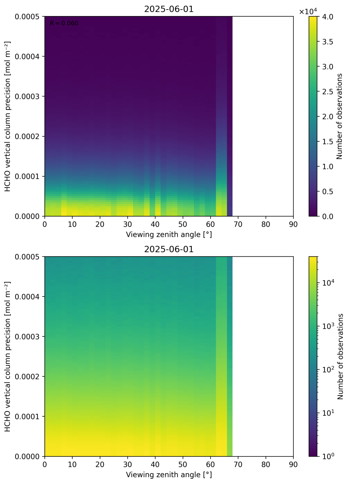
Figure 194: Scatter density plot of “Viewing zenith angle” against “HCHO vertical column precision” for 2025-06-01 to 2025-06-02.
