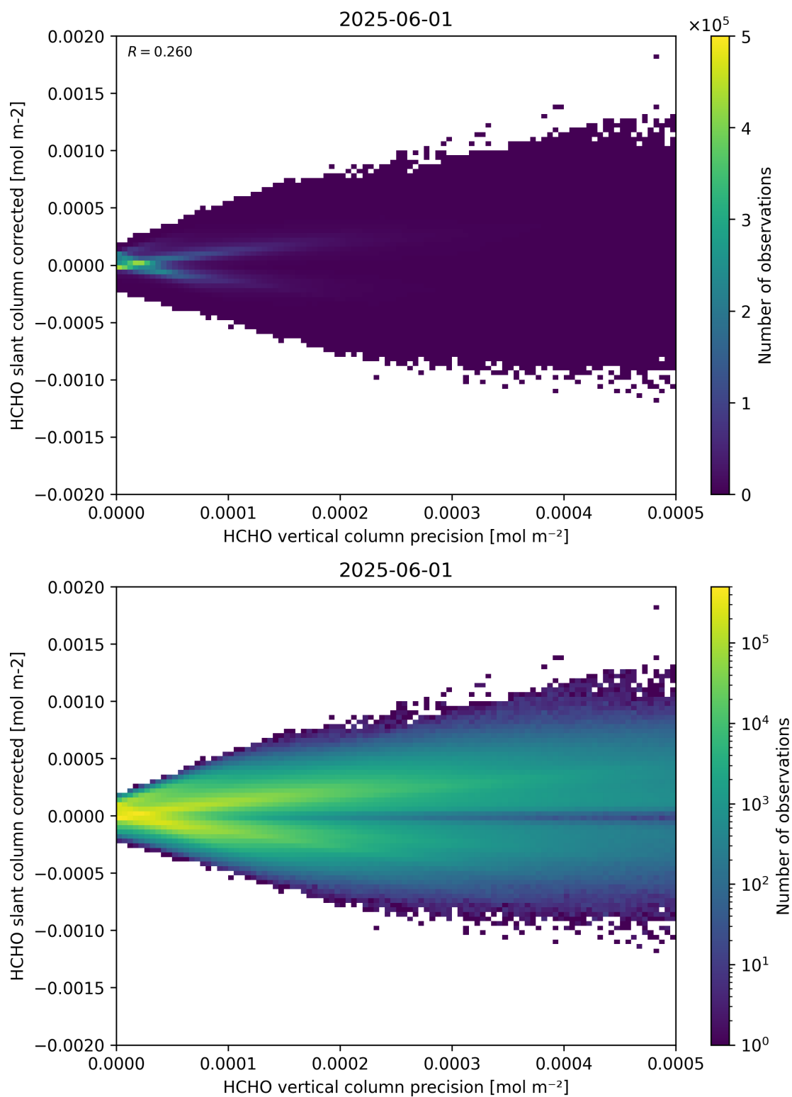
Figure 140: Scatter density plot of “HCHO vertical column precision” against “HCHO slant column corrected” for 2025-06-01 to 2025-06-02.
