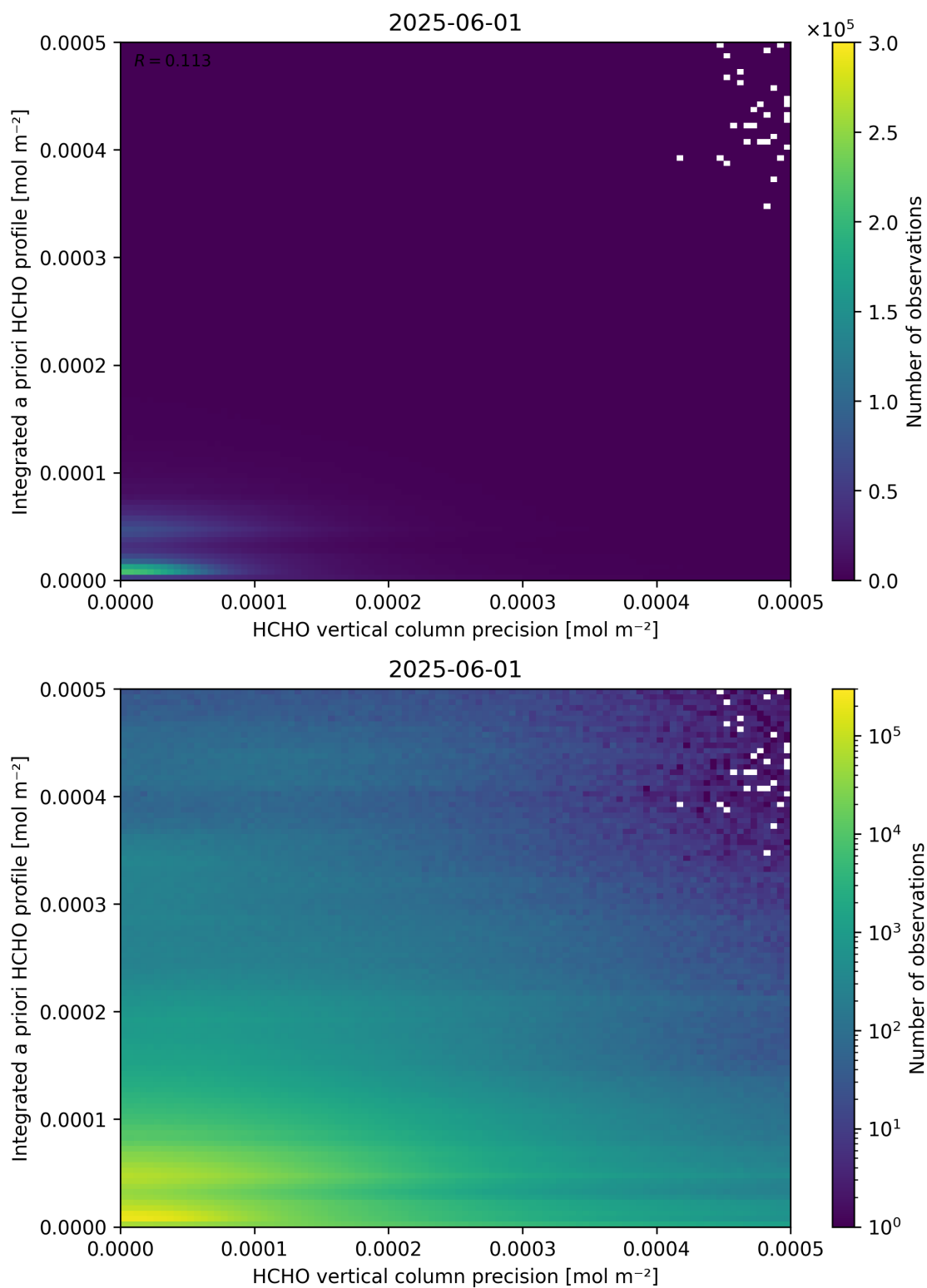
Figure 147: Scatter density plot of “HCHO vertical column precision” against “Integrated a priori HCHO profile” for 2025-06-01 to 2025-06-02.
