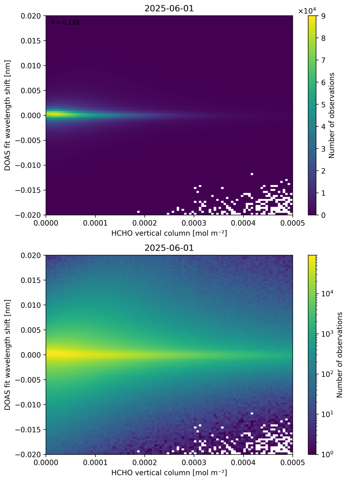
Figure 124: Scatter density plot of “HCHO vertical column” against “DOAS fit wavelength shift” for 2025-06-01 to 2025-06-02.
