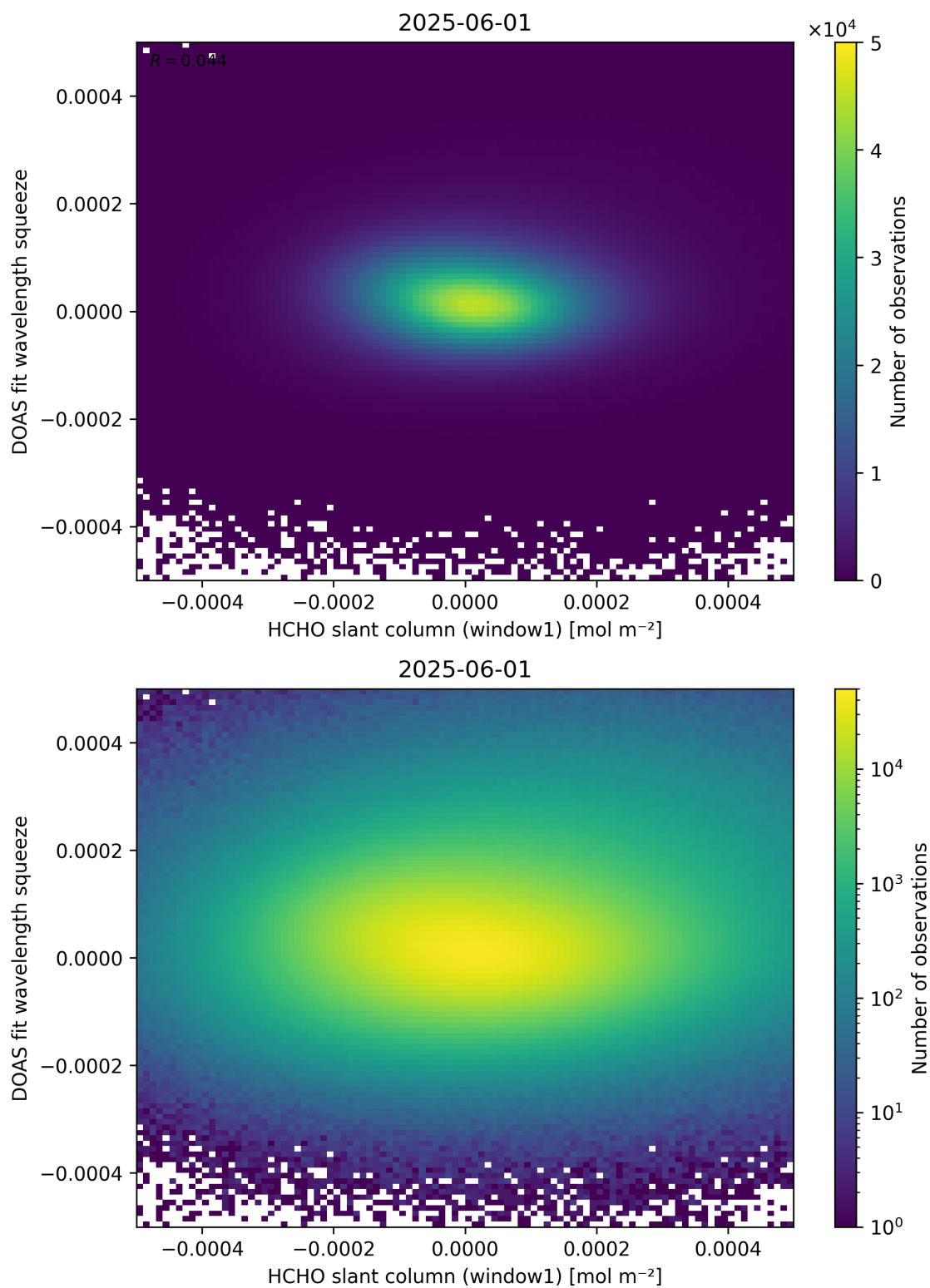
Figure 80: Scatter density plot of “HCHO slant column (window1)” against “DOAS fit wavelength squeeze” for 2025-06-01 to 2025-06-02.
