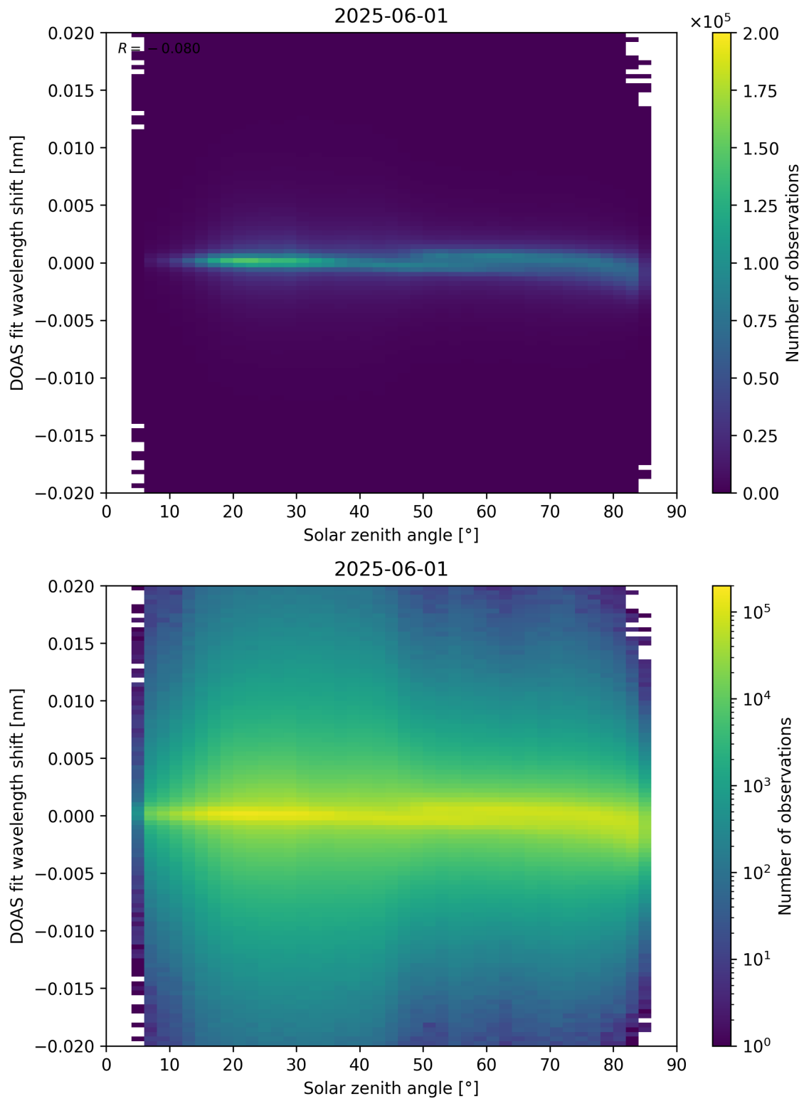
Figure 168: Scatter density plot of “Solar zenith angle” against “DOAS fit wavelength shift” for 2025-06-01 to 2025-06-02.
