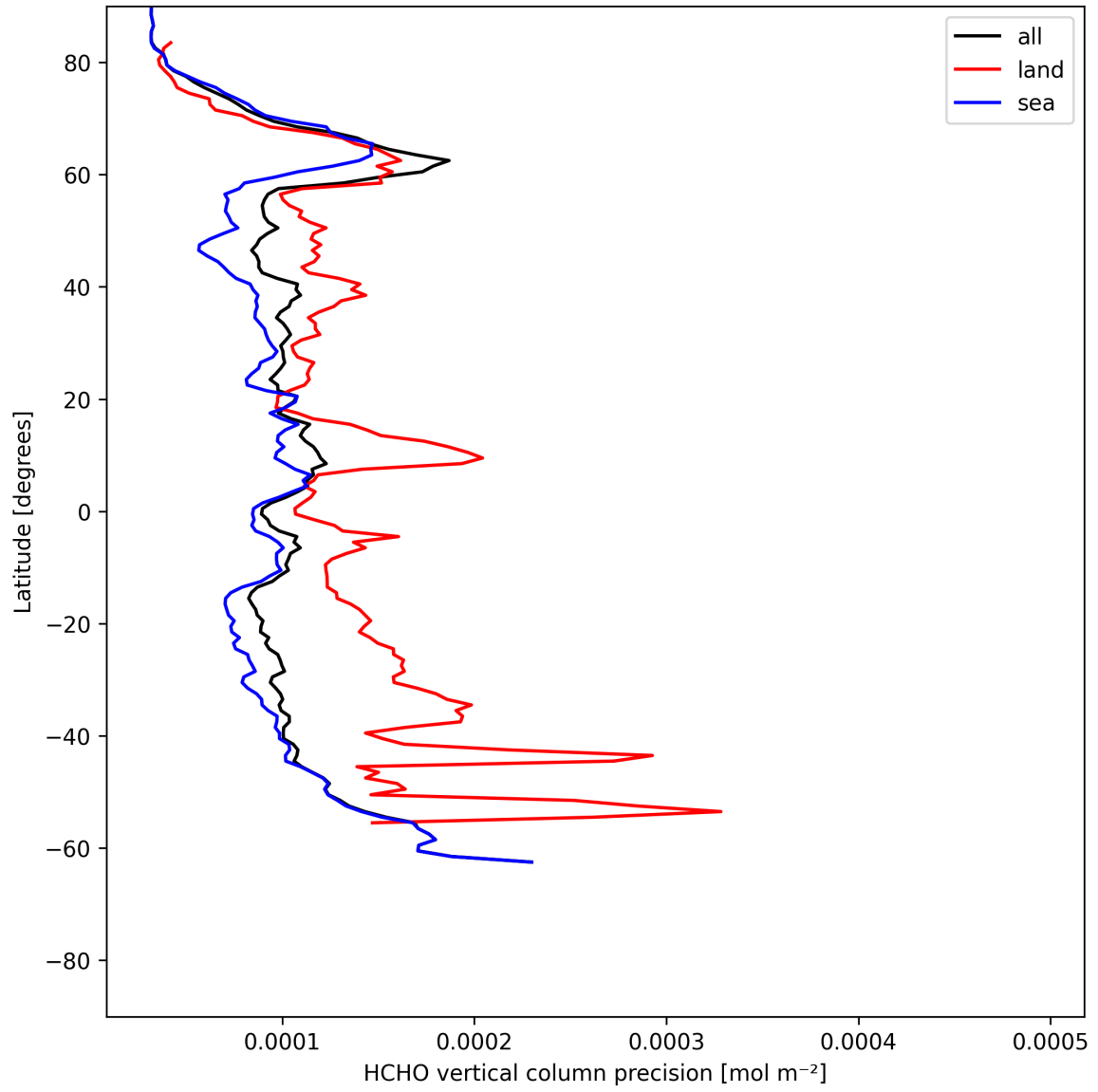
Figure 22: Zonal average of “HCHO vertical column precision” for 2025-06-01 to 2025-06-02.
