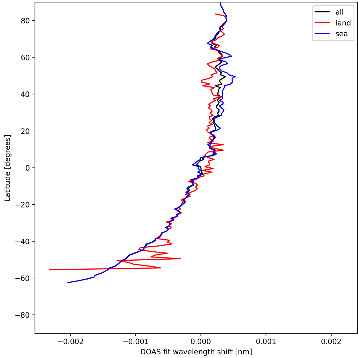
Figure 30: Zonal average of “DOAS fit wavelength shift” for 2025-06-01 to 2025-06-02.
