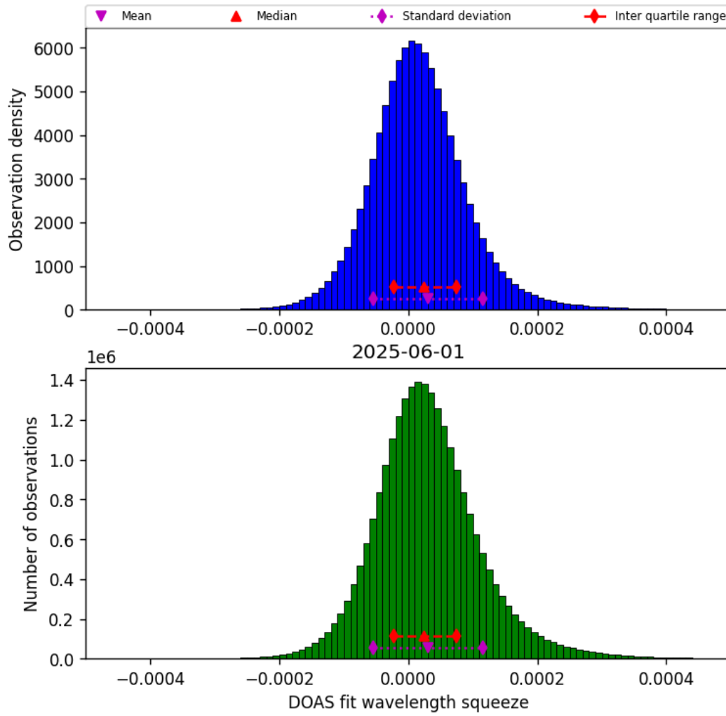
Figure 45: Histogram of “DOAS fit wavelength squeeze” for 2025-06-01 to 2025-06-02
