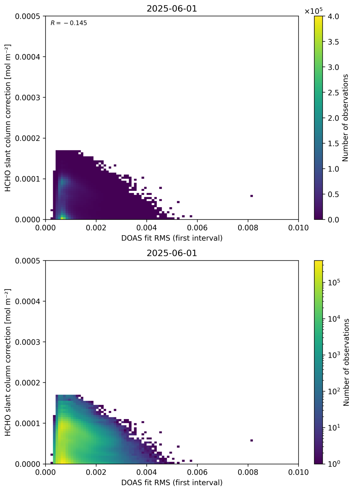
Figure 63: Scatter density plot of “DOAS fit RMS (first interval)” against “HCHO slant column correction” for 2025-06-01 to 2025-06-02.
