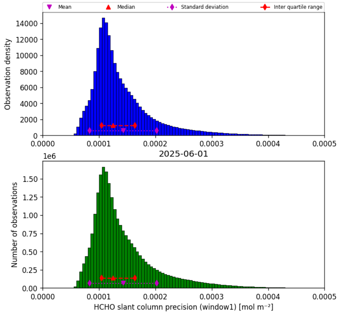
Figure 39: Histogram of “HCHO slant column precision (window1)” for 2025-06-01 to 2025-06-02
