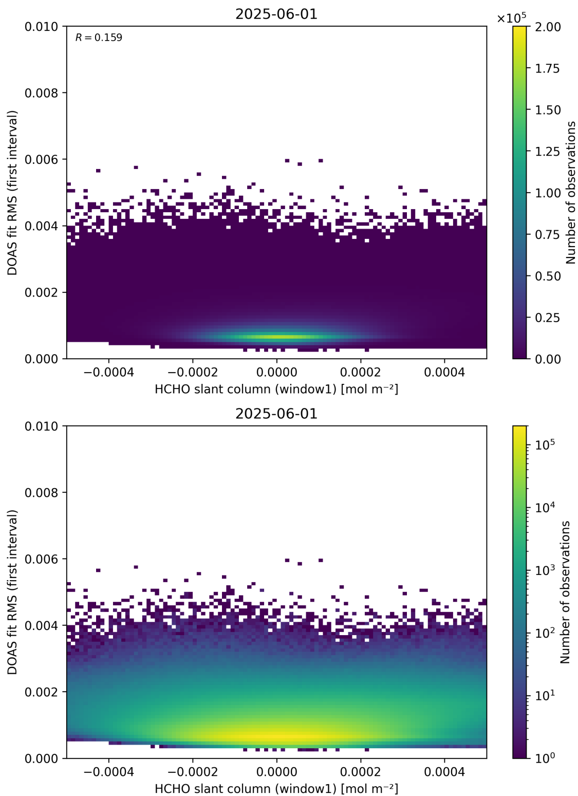
Figure 78: Scatter density plot of “HCHO slant column (window1)” against “DOAS fit RMS (first interval)” for 2025-06-01 to 2025-06-02.
