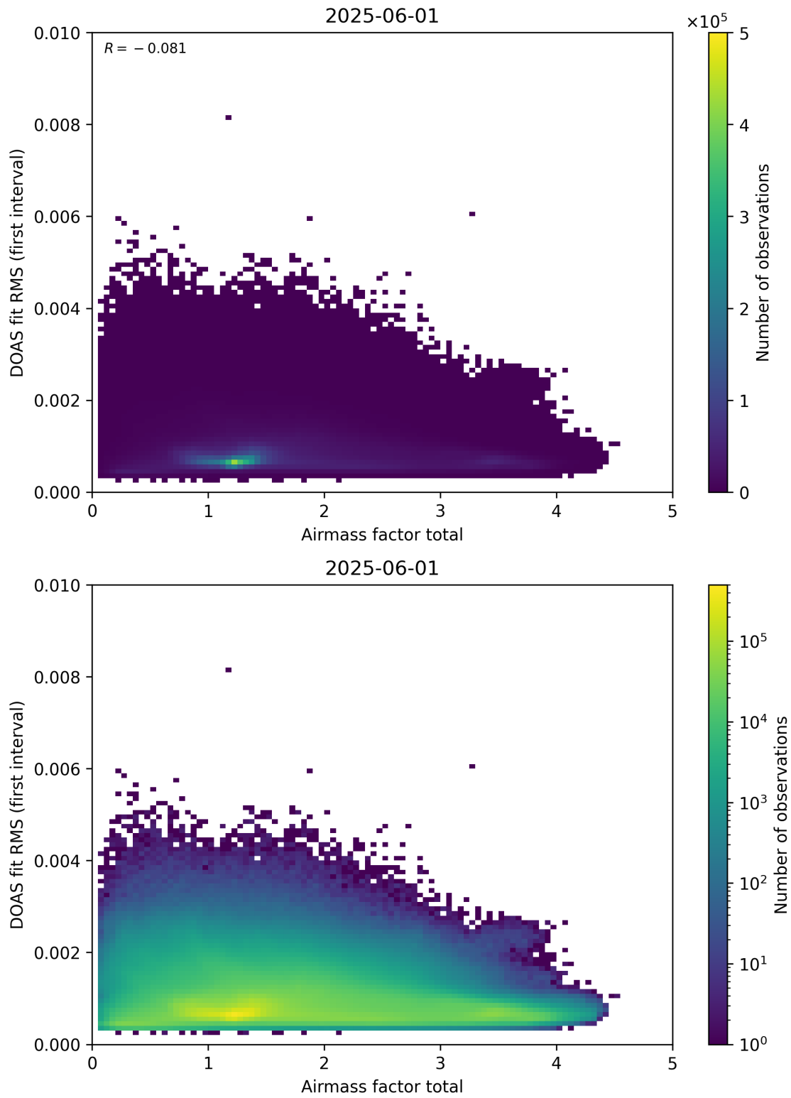
Figure 97: Scatter density plot of “Airmass factor total” against “DOAS fit RMS (first interval)” for 2025-06-01 to 2025-06-02.
