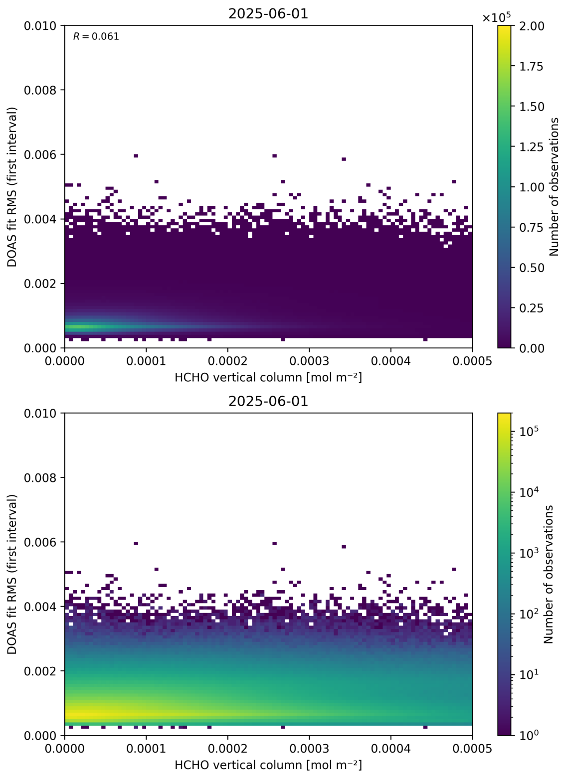
Figure 123: Scatter density plot of “HCHO vertical column” against “DOAS fit RMS (first interval)” for 2025-06-01 to 2025-06-02.
