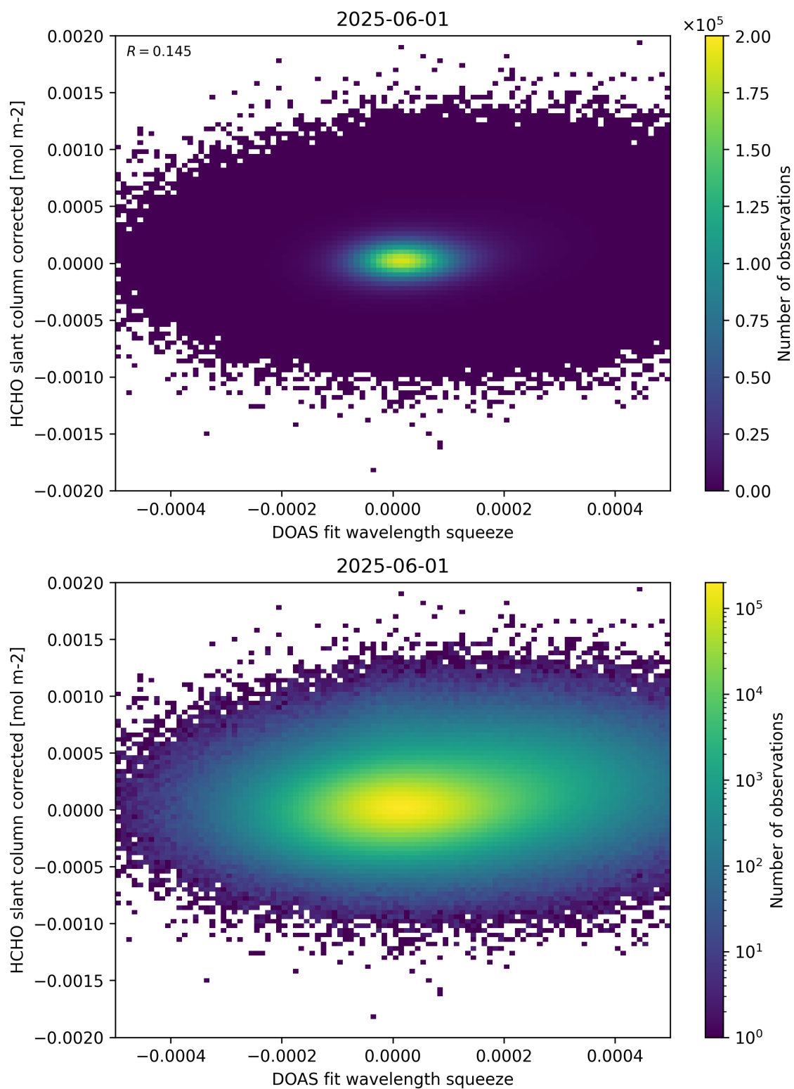
Figure 69: Scatter density plot of “DOAS fit wavelength squeeze” against “HCHO slant column corrected” for 2025-06-01 to 2025-06-02.
