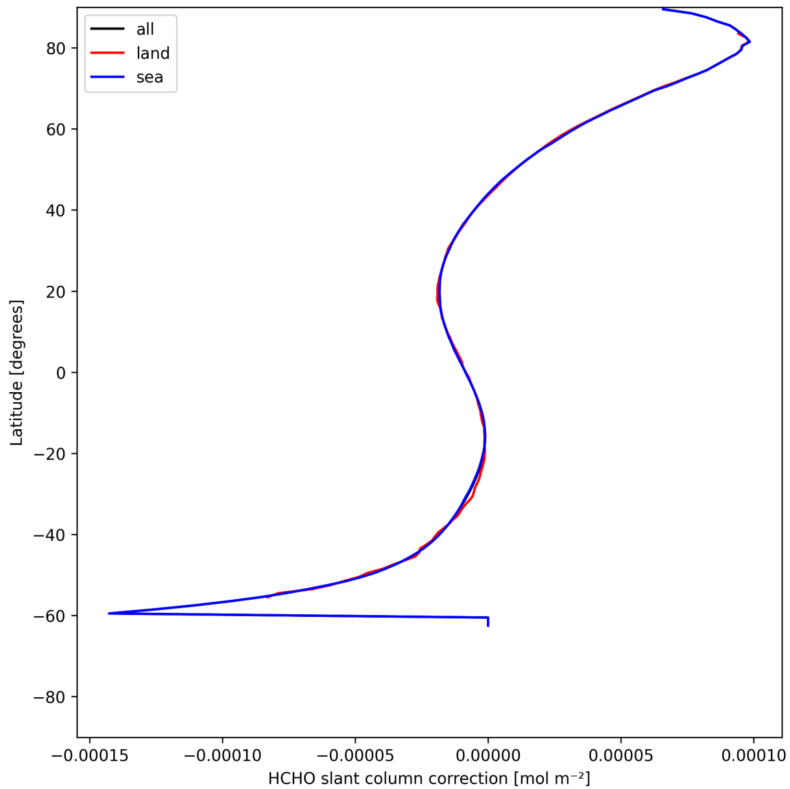
Figure 33: Zonal average of “HCHO slant column correction” for 2025-06-01 to 2025-06-02.
