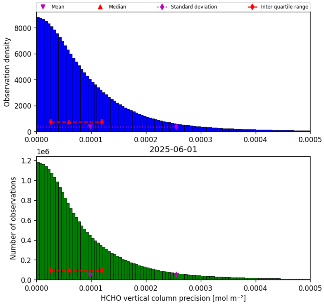
Figure 36: Histogram of “HCHO vertical column precision” for 2025-06-01 to 2025-06-02
