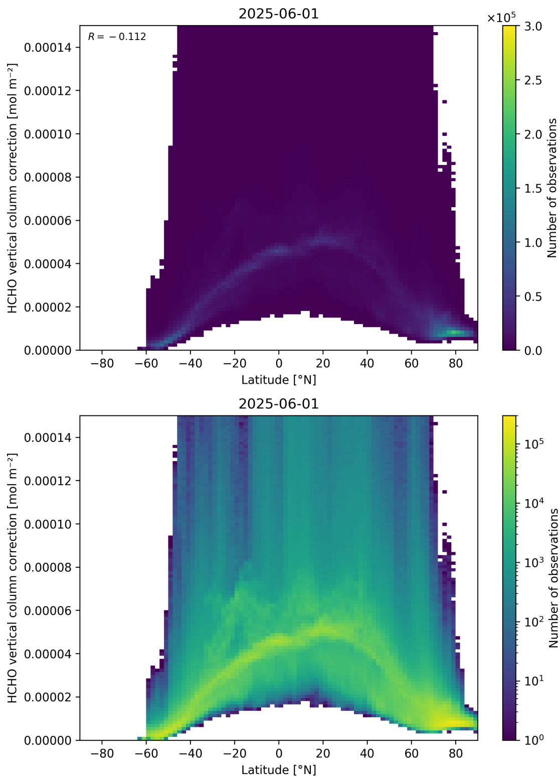
Figure 164: Scatter density plot of “Latitude” against “HCHO vertical column correction” for 2025-06-01 to 2025-06-02.
