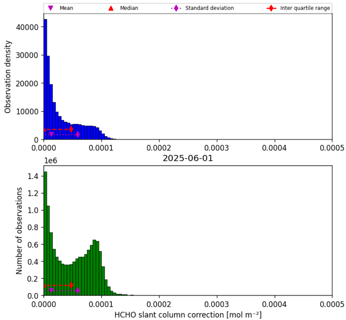
Figure 47: Histogram of “HCHO slant column correction” for 2025-06-01 to 2025-06-02
