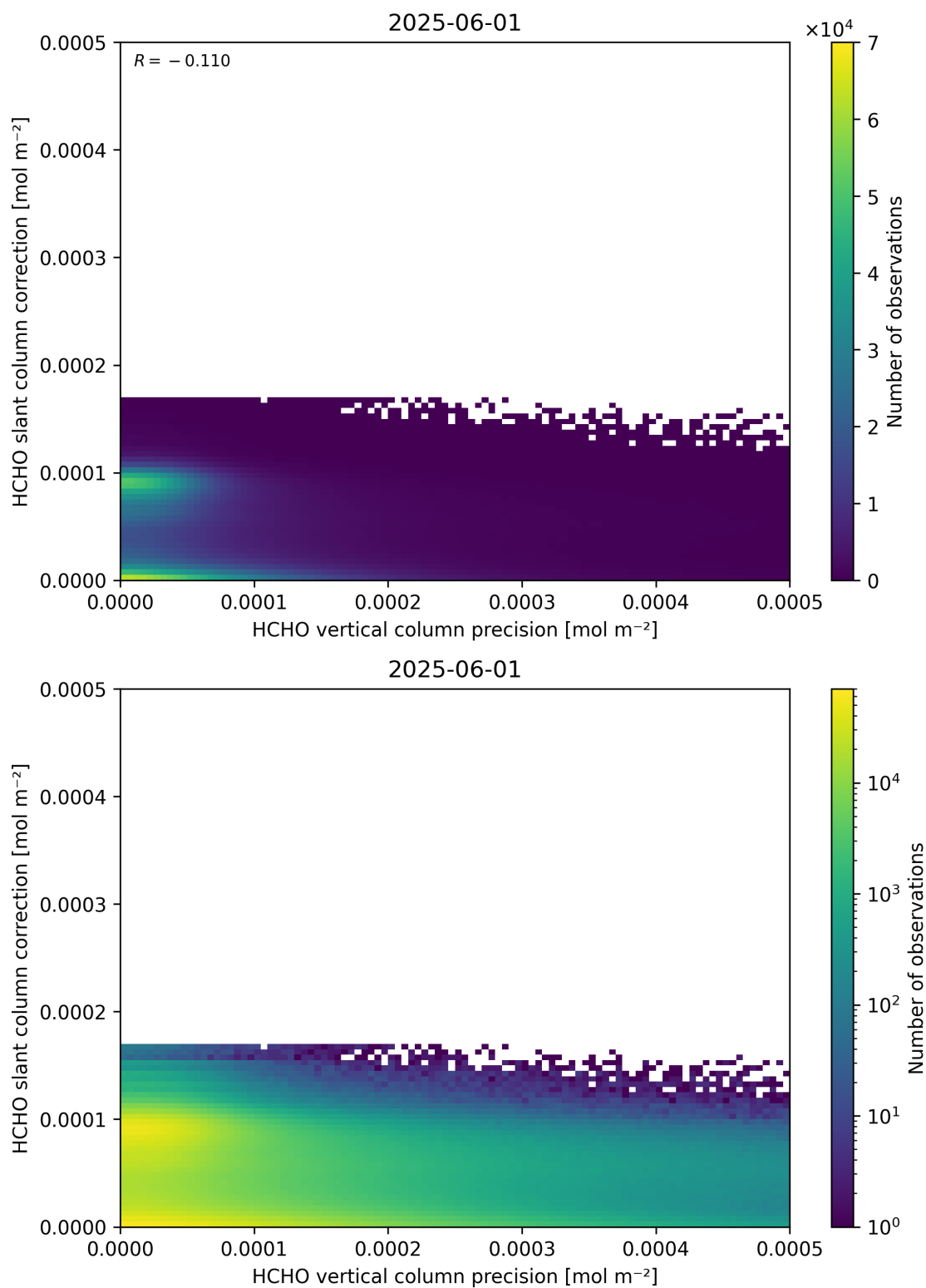
Figure 141: Scatter density plot of “HCHO vertical column precision” against “HCHO slant column correction” for 2025-06-01 to 2025-06-02.
