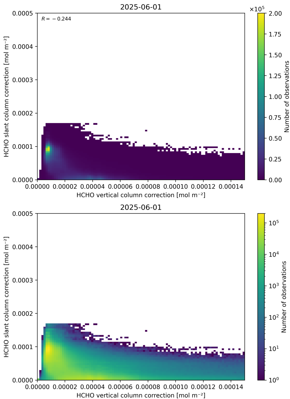
Figure 117: Scatter density plot of “HCHO vertical column correction” against “HCHO slant column correction” for 2025-06-01 to 2025-06-02.
