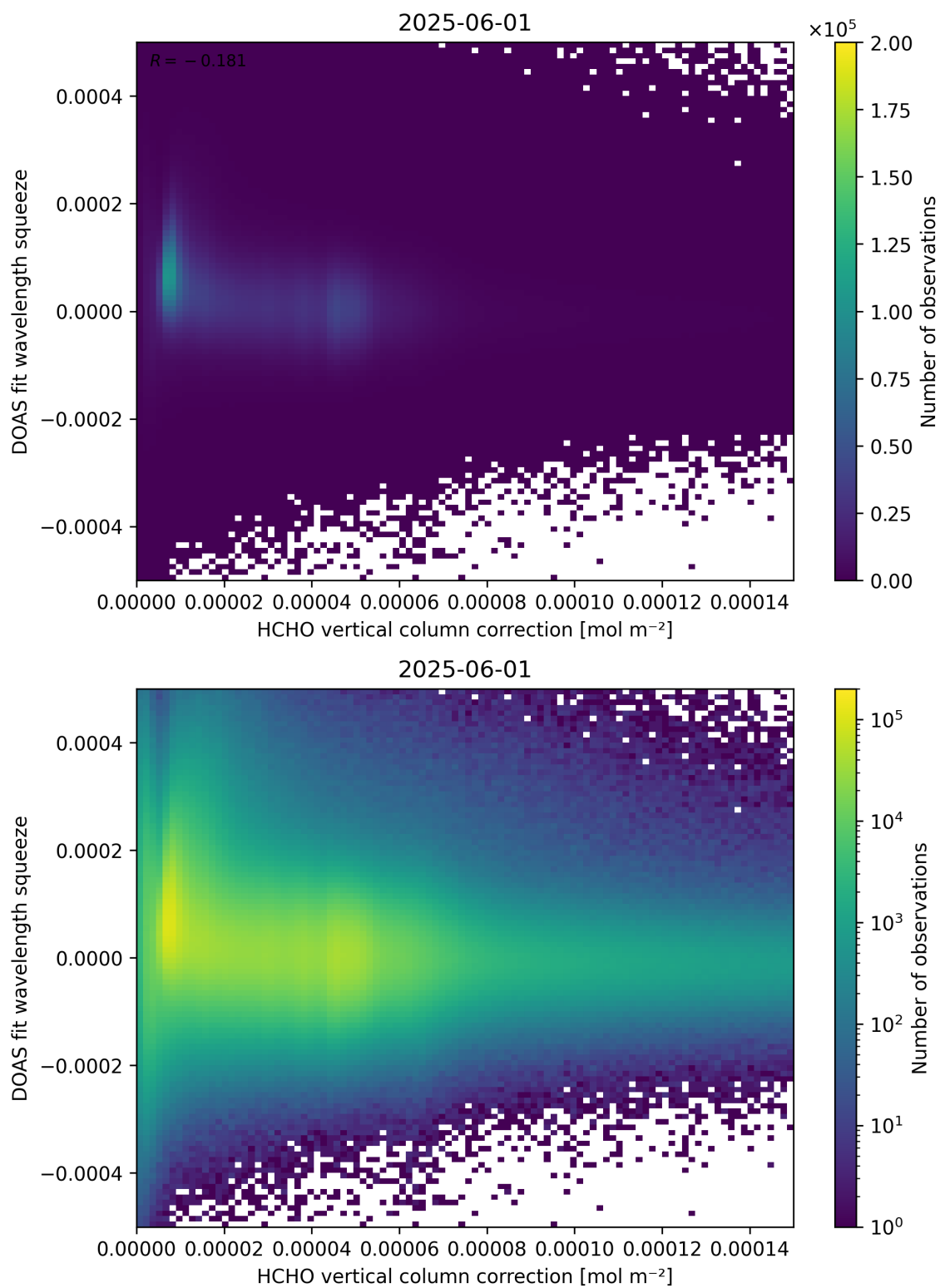
Figure 114: Scatter density plot of “HCHO vertical column correction” against “DOAS fit wavelength squeeze” for 2025-06-01 to 2025-06-02.
