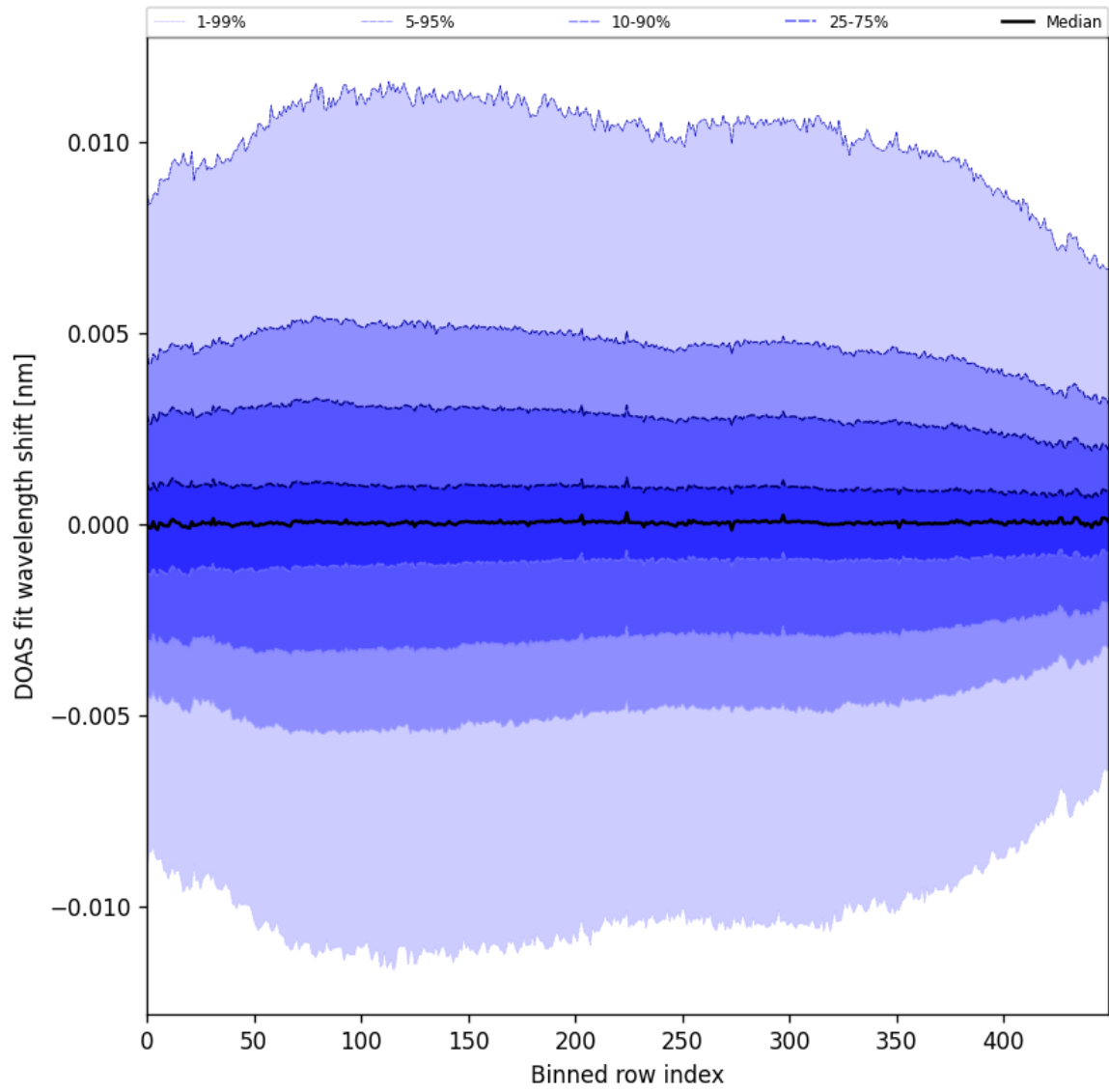
Figure 58: Along track statistics of “DOAS fit wavelength shift” for 2025-06-01 to 2025-06-02
