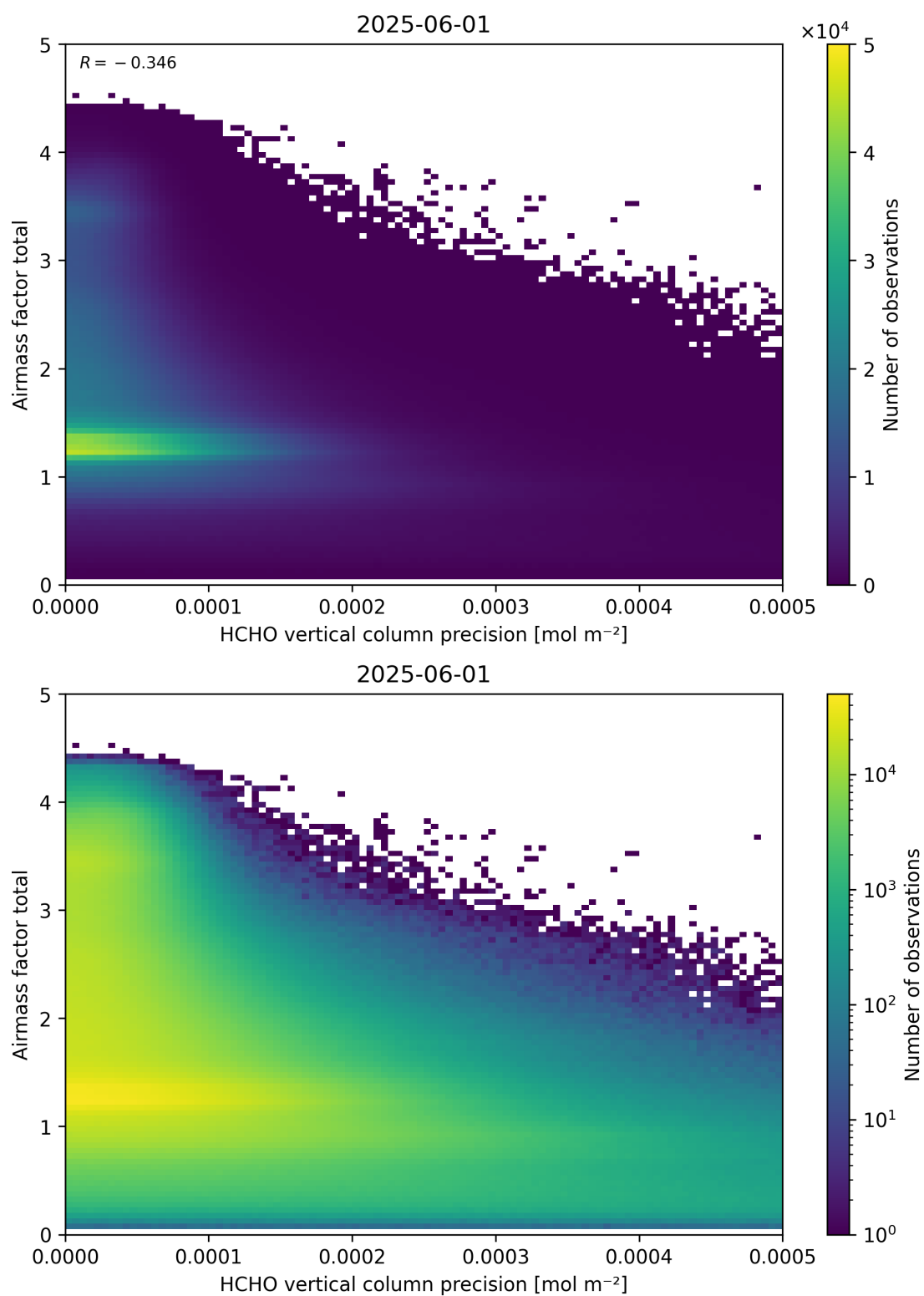
Figure 144: Scatter density plot of “HCHO vertical column precision” against “Airmass factor total” for 2025-06-01 to 2025-06-02.
