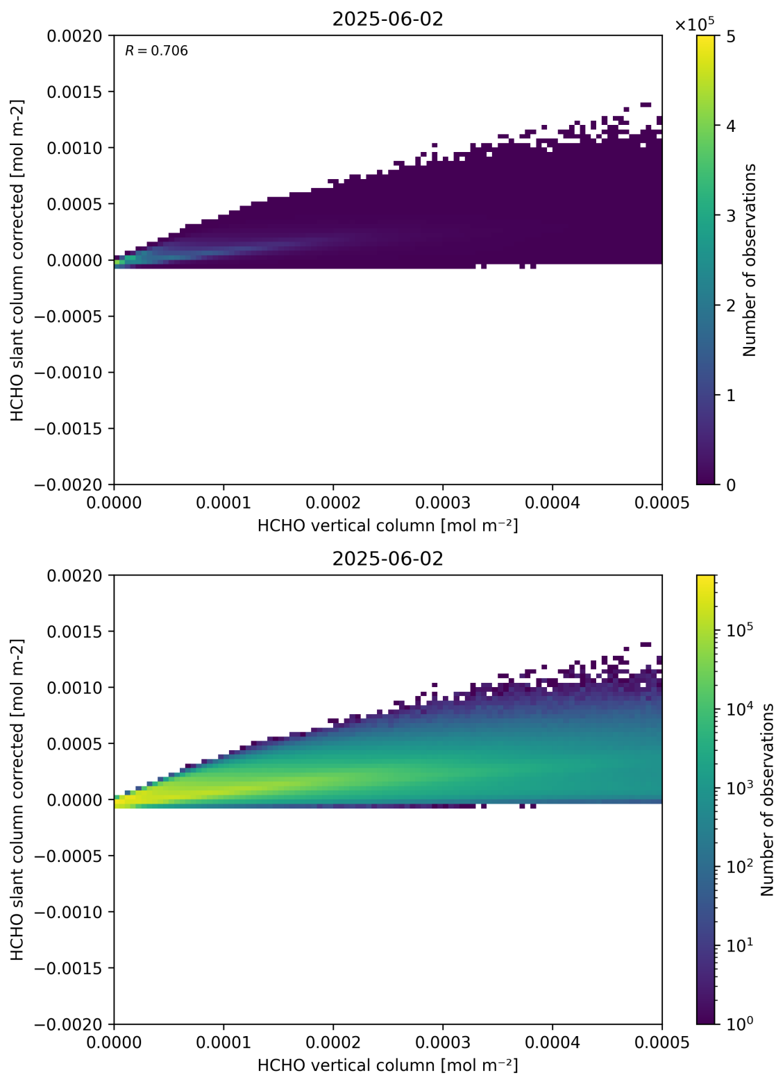
Figure 127: Scatter density plot of “HCHO vertical column” against “HCHO slant column corrected” for 2025-06-01 to 2025-06-03.
