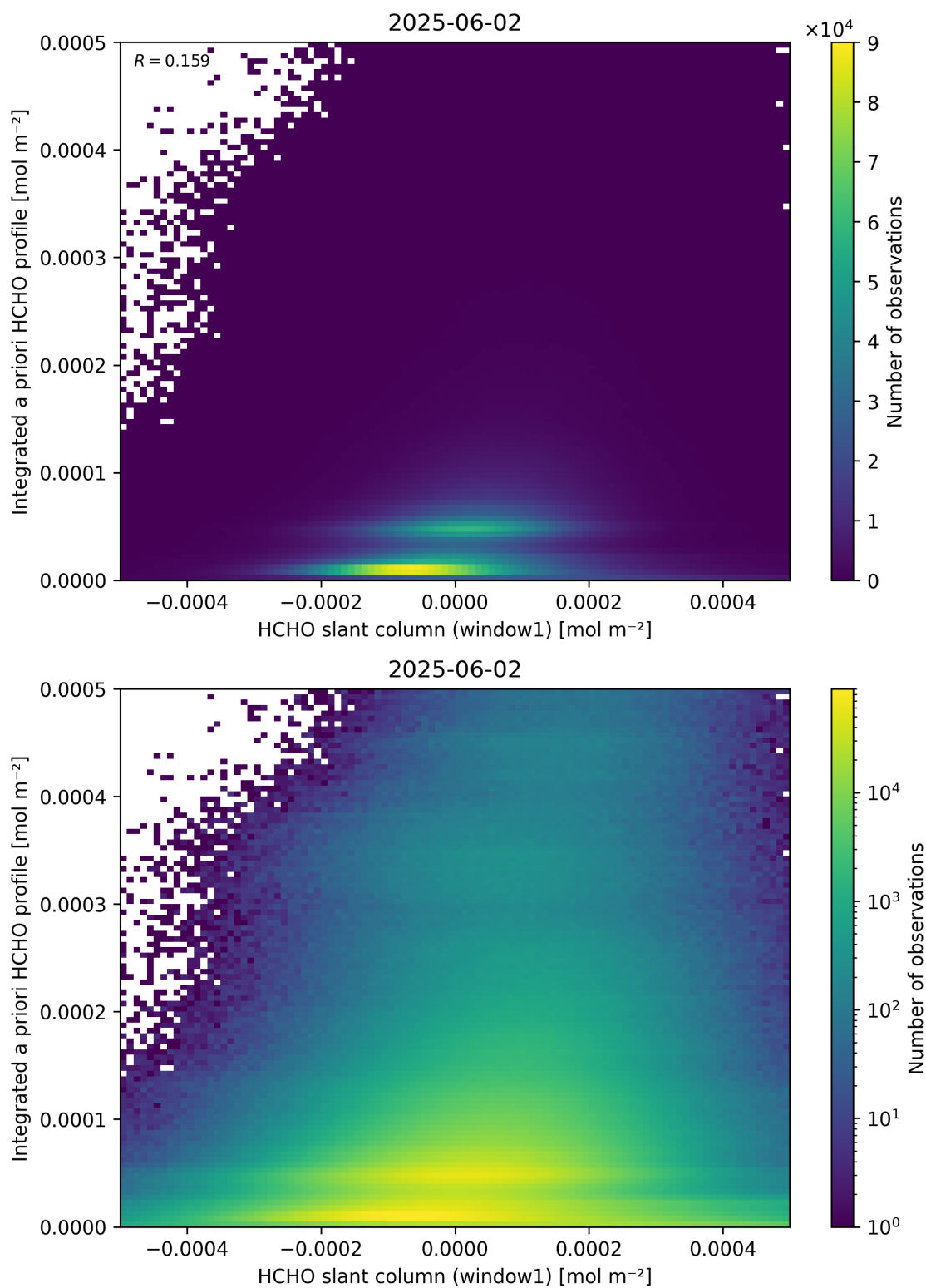
Figure 87: Scatter density plot of “HCHO slant column (window1)” against “Integrated a priori HCHO profile” for 2025-06-01 to 2025-06-03.
