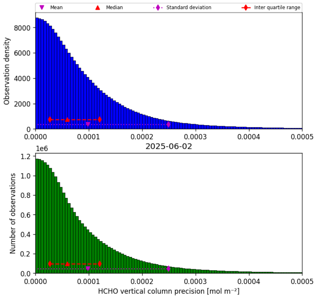
Figure 36: Histogram of “HCHO vertical column precision” for 2025-06-01 to 2025-06-03
