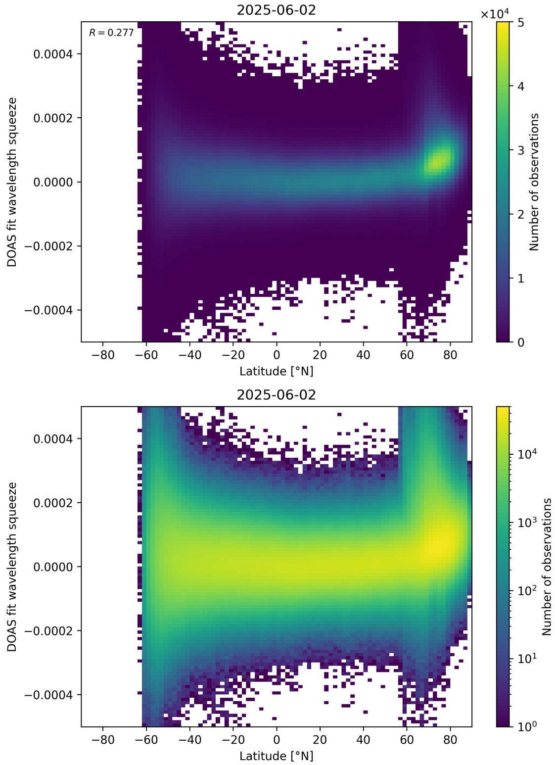
Figure 155: Scatter density plot of “Latitude” against “DOAS fit wavelength squeeze” for 2025-06-01 to 2025-06-03.
