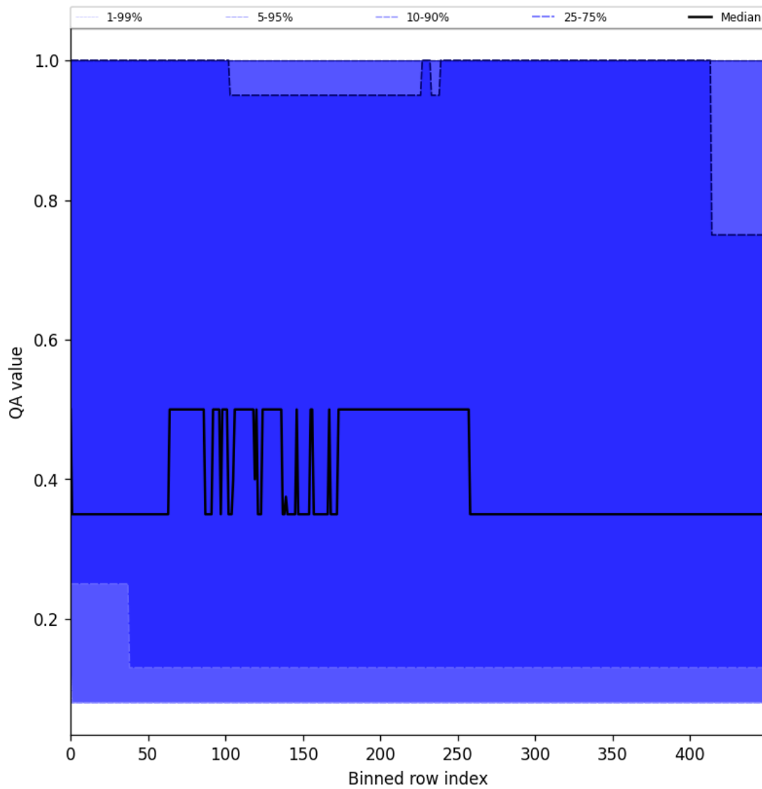
Figure 48: Along track statistics of “QA value” for 2025-06-01 to 2025-06-03
