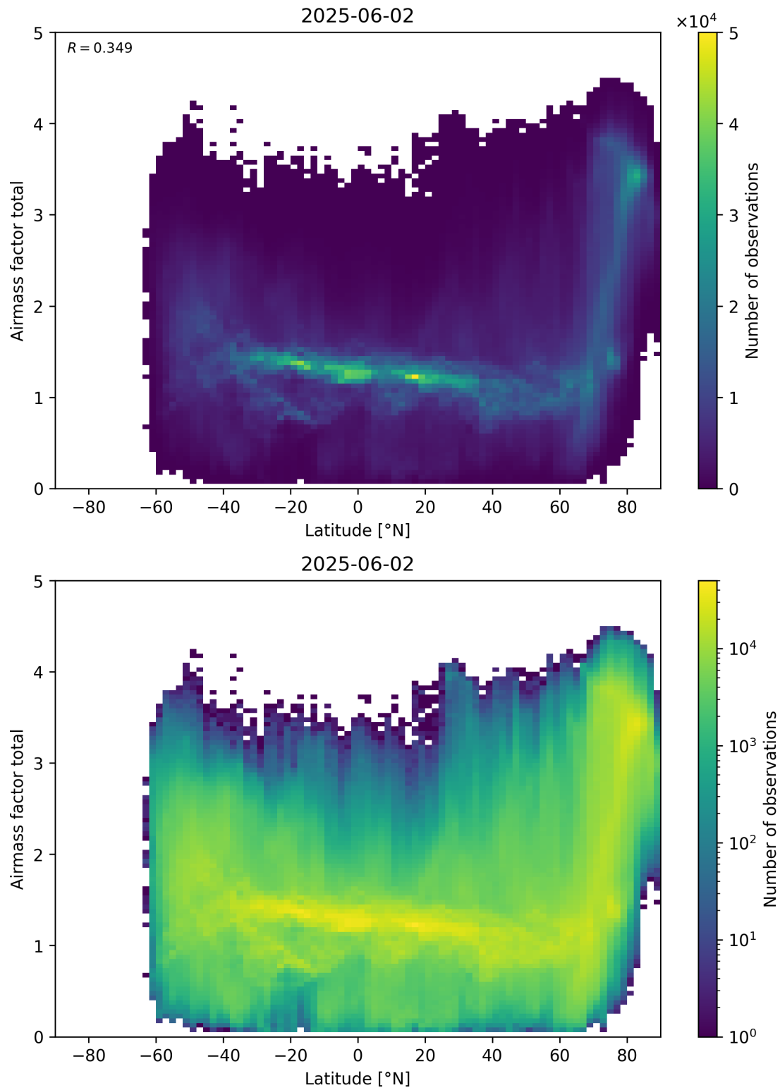
Figure 161: Scatter density plot of “Latitude” against “Airmass factor total” for 2025-06-01 to 2025-06-03.
