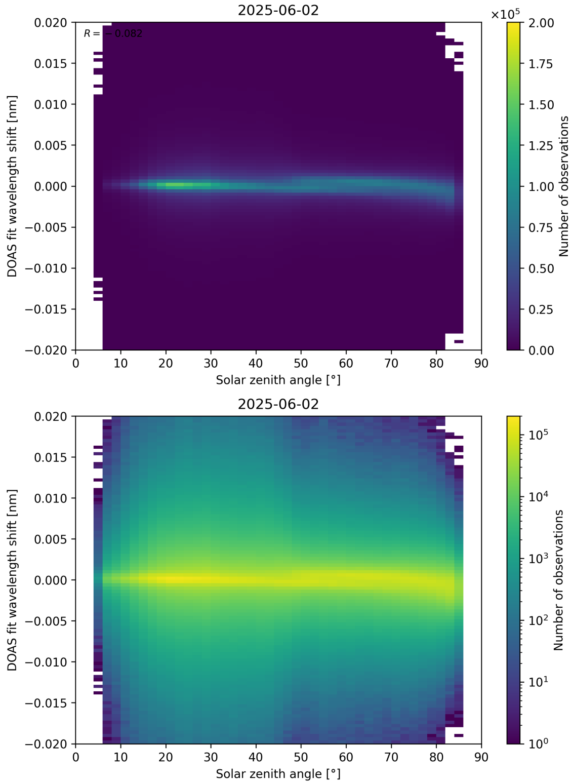
Figure 168: Scatter density plot of “Solar zenith angle” against “DOAS fit wavelength shift” for 2025-06-01 to 2025-06-03.
