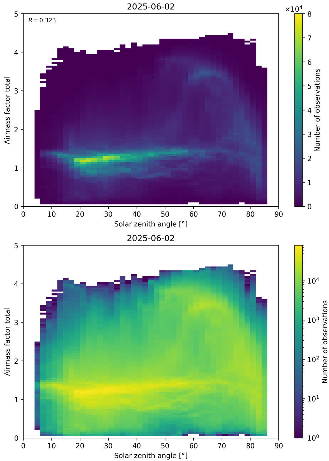
Figure 175: Scatter density plot of “Solar zenith angle” against “Airmass factor total” for 2025-06-01 to 2025-06-03.
