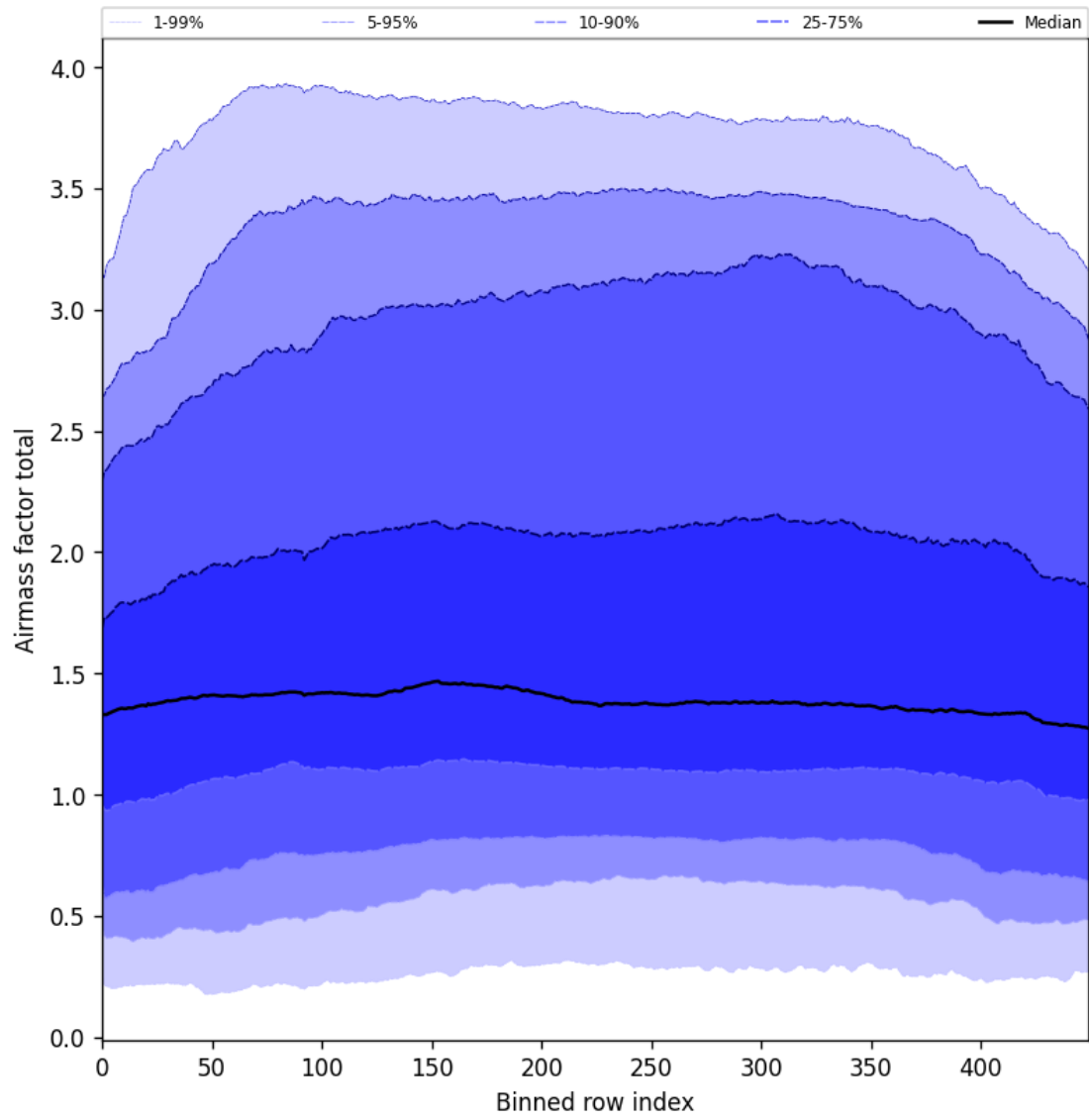
Figure 54: Along track statistics of “Airmass factor total” for 2025-06-01 to 2025-06-03
