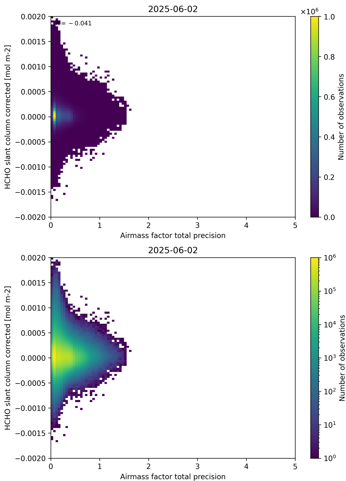
Figure 109: Scatter density plot of “Airmass factor total precision” against “HCHO slant column corrected” for 2025-06-01 to 2025-06-03.
