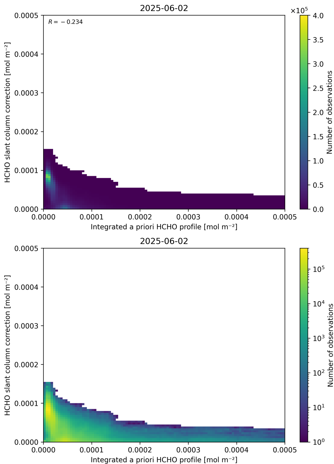
Figure 152: Scatter density plot of “Integrated a priori HCHO profile” against “HCHO slant column correction” for 2025-06-01 to 2025-06-03.
