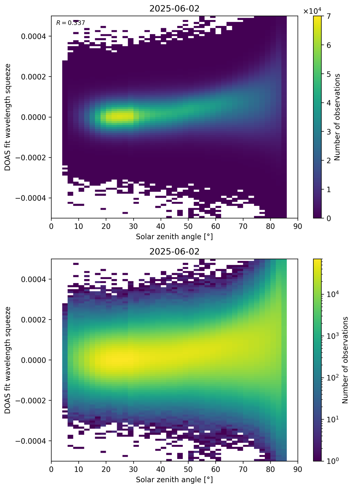
Figure 169: Scatter density plot of “Solar zenith angle” against “DOAS fit wavelength squeeze” for 2025-06-01 to 2025-06-03.
