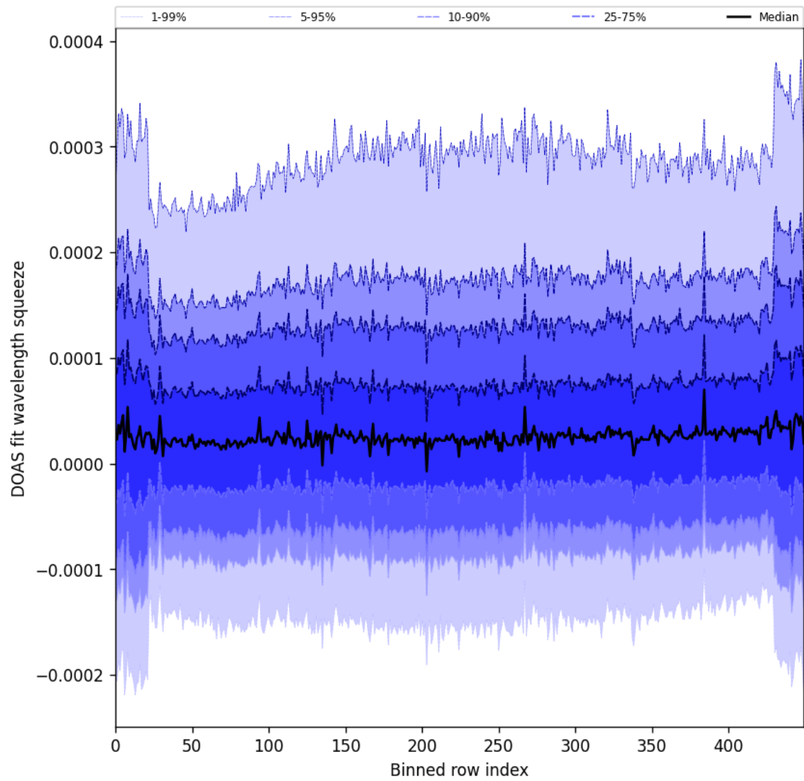
Figure 59: Along track statistics of “DOAS fit wavelength squeeze” for 2025-06-01 to 2025-06-03
