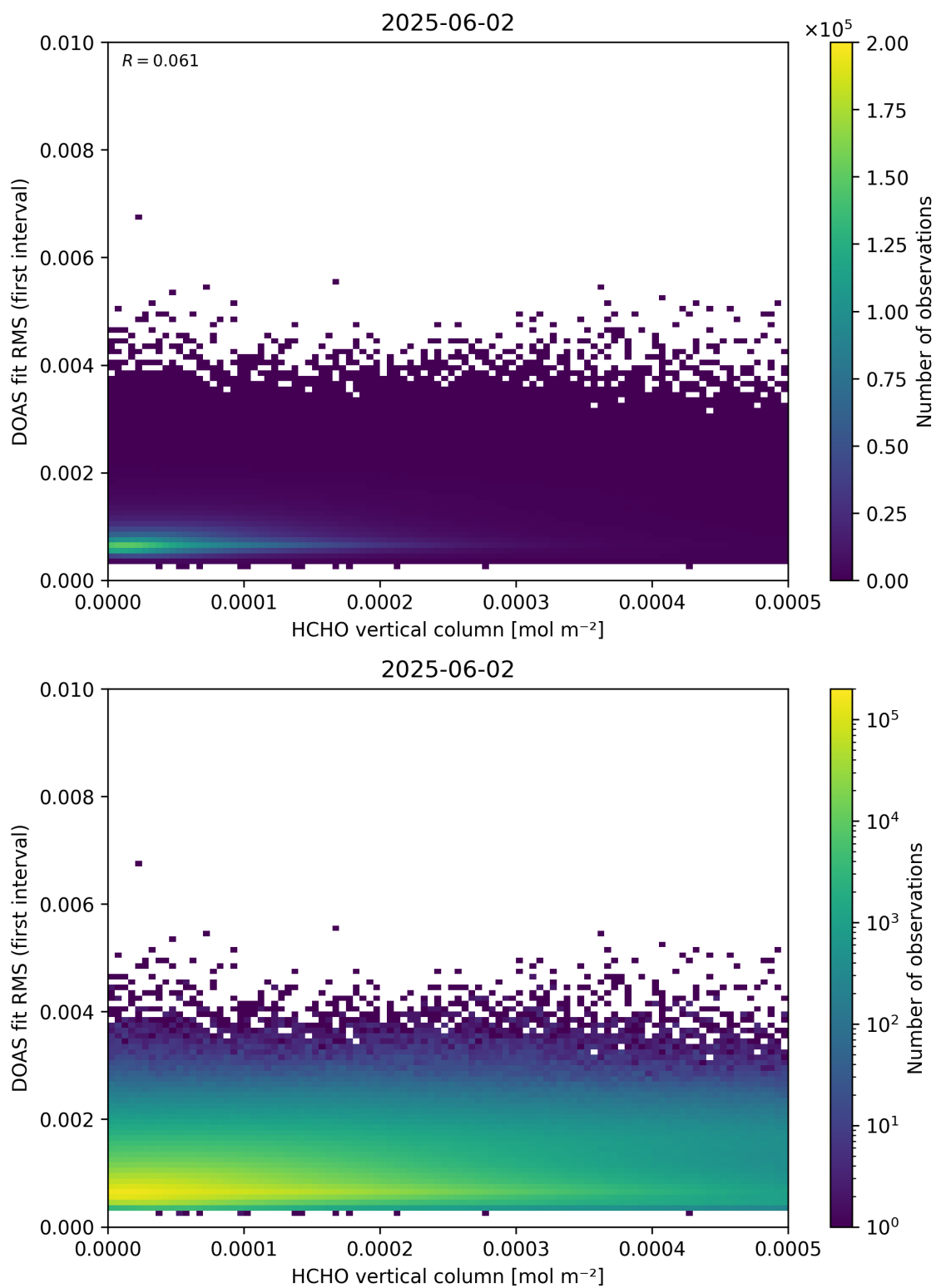
Figure 123: Scatter density plot of “HCHO vertical column” against “DOAS fit RMS (first interval)” for 2025-06-01 to 2025-06-03.
