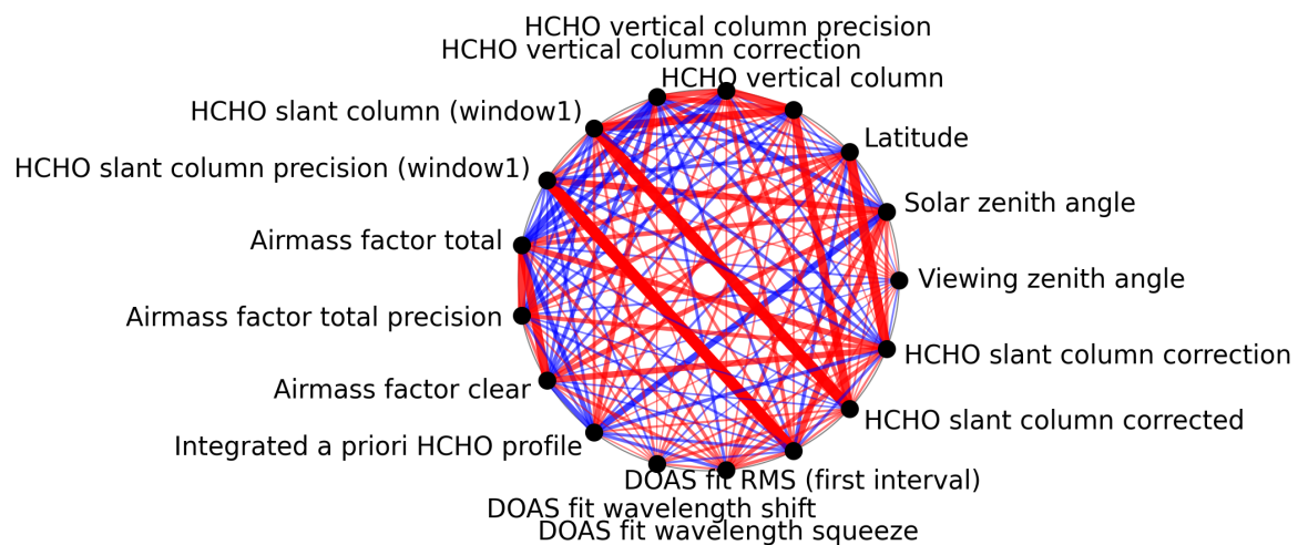
Figure 1: Map of correlation graph for 2025-06-01 to 2025-06-03.
