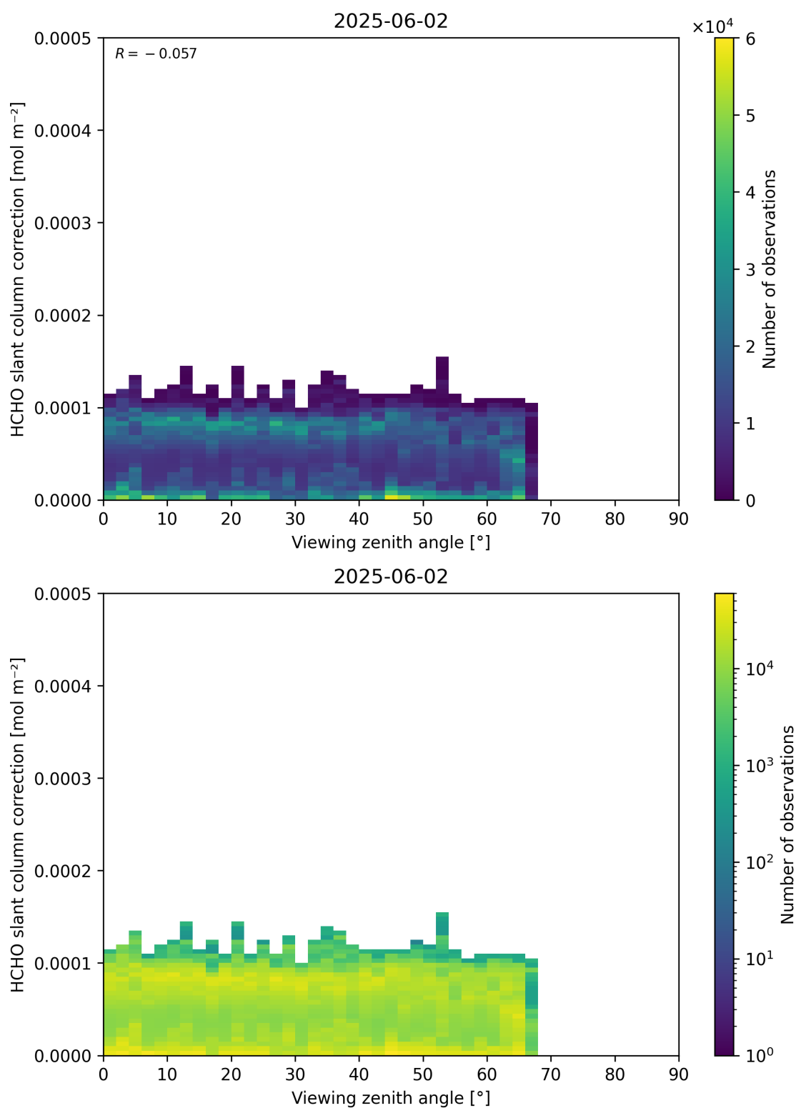
Figure 187: Scatter density plot of “Viewing zenith angle” against “HCHO slant column correction” for 2025-06-01 to 2025-06-03.
