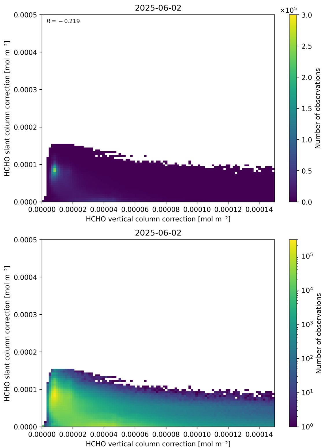
Figure 117: Scatter density plot of “HCHO vertical column correction” against “HCHO slant column correction” for 2025-06-01 to 2025-06-03.
