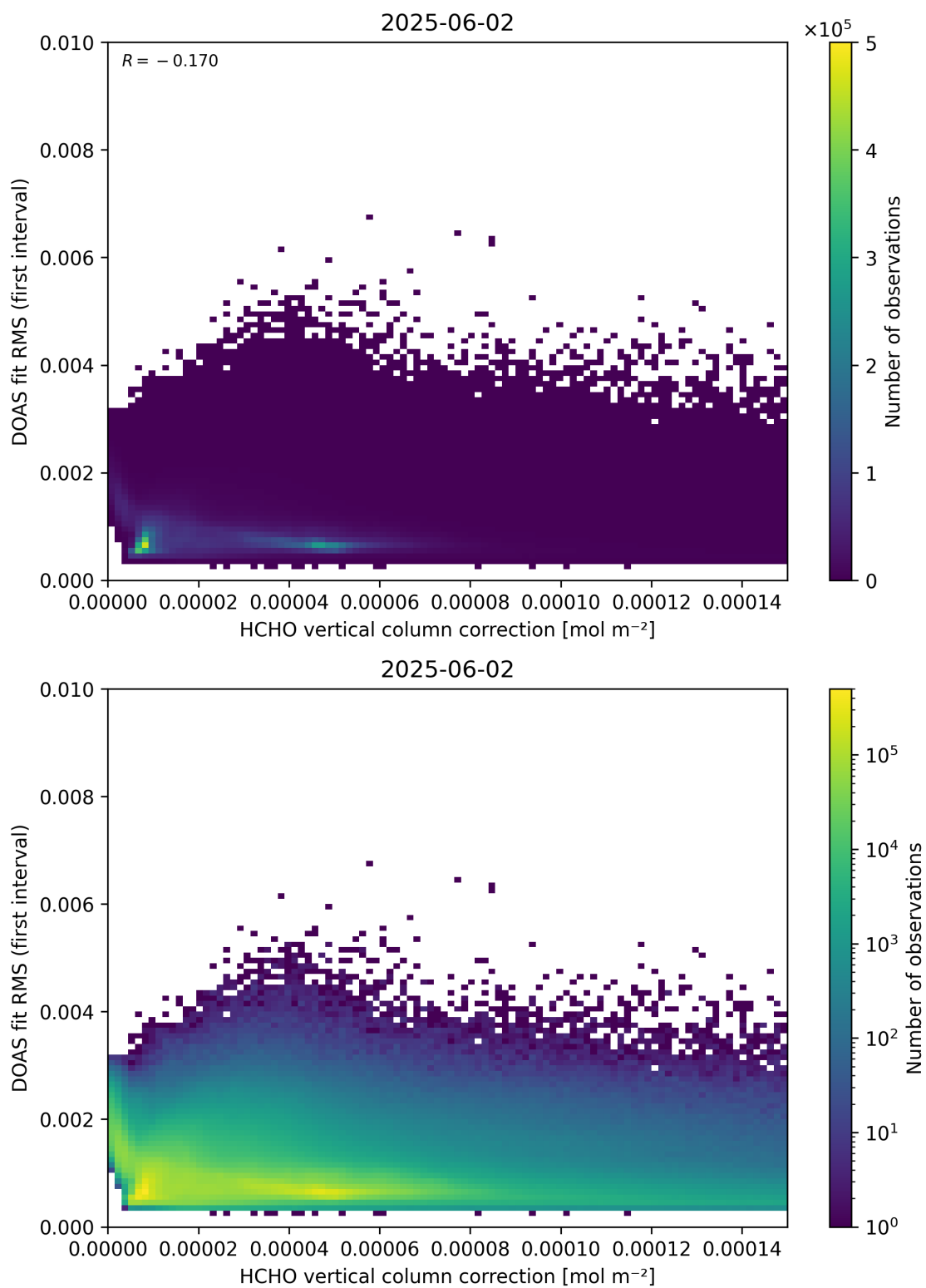
Figure 112: Scatter density plot of “HCHO vertical column correction” against “DOAS fit RMS (first interval)” for 2025-06-01 to 2025-06-03.
