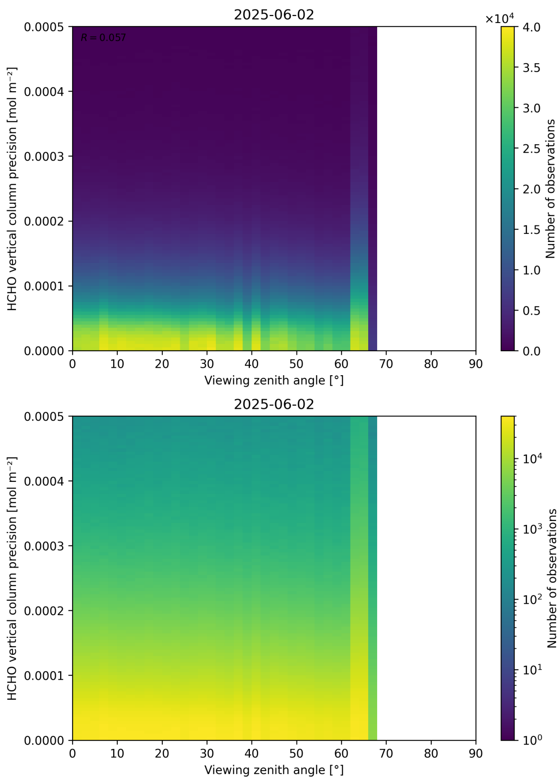
Figure 194: Scatter density plot of “Viewing zenith angle” against “HCHO vertical column precision” for 2025-06-01 to 2025-06-03.
