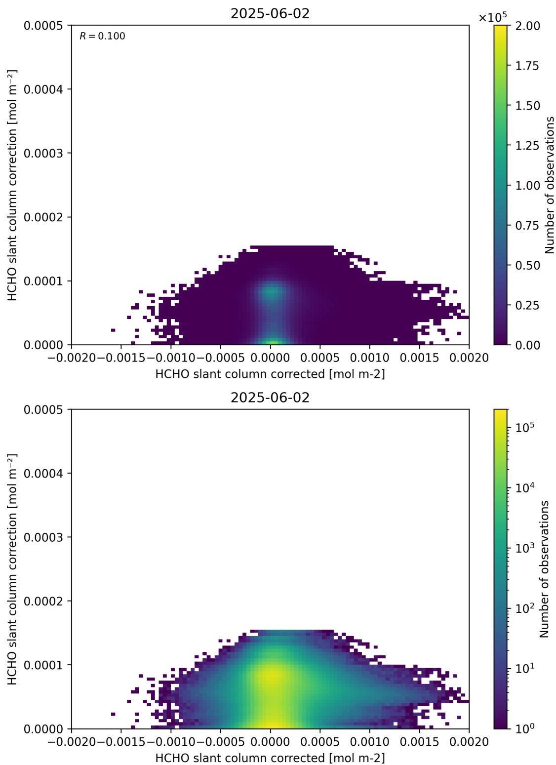
Figure 77: Scatter density plot of “HCHO slant column corrected” against “HCHO slant column correction” for 2025-06-01 to 2025-06-03.
