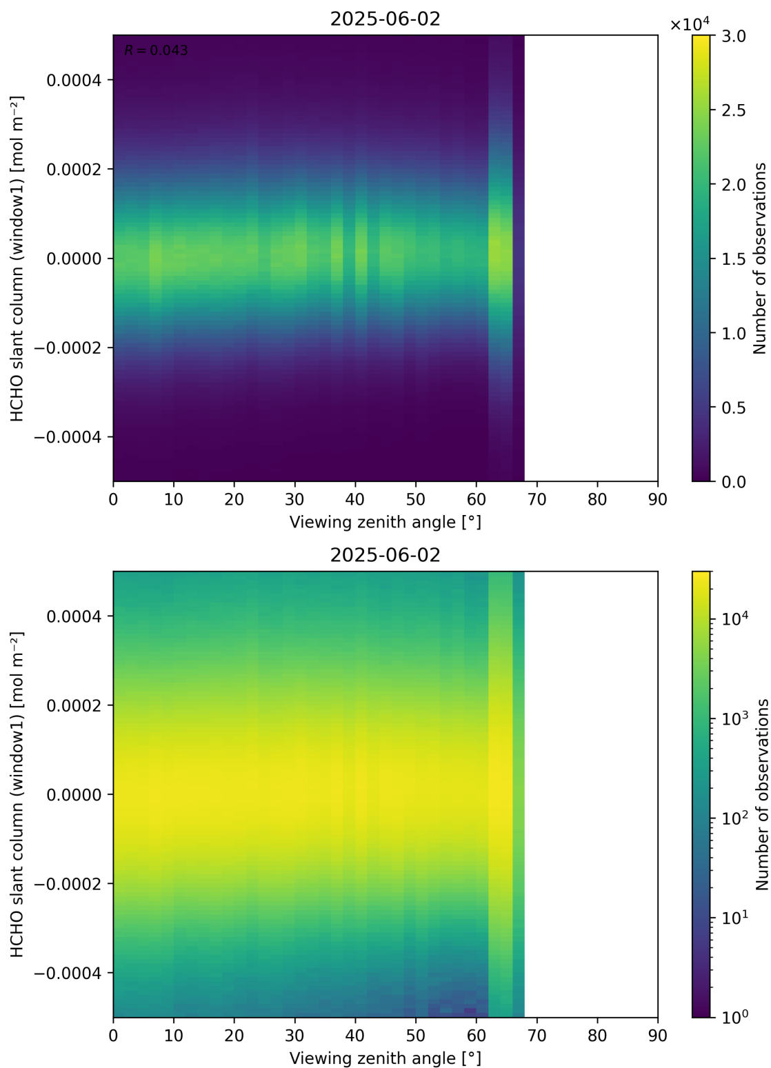
Figure 188: Scatter density plot of “Viewing zenith angle” against “HCHO slant column (window1)” for 2025-06-01 to 2025-06-03.
