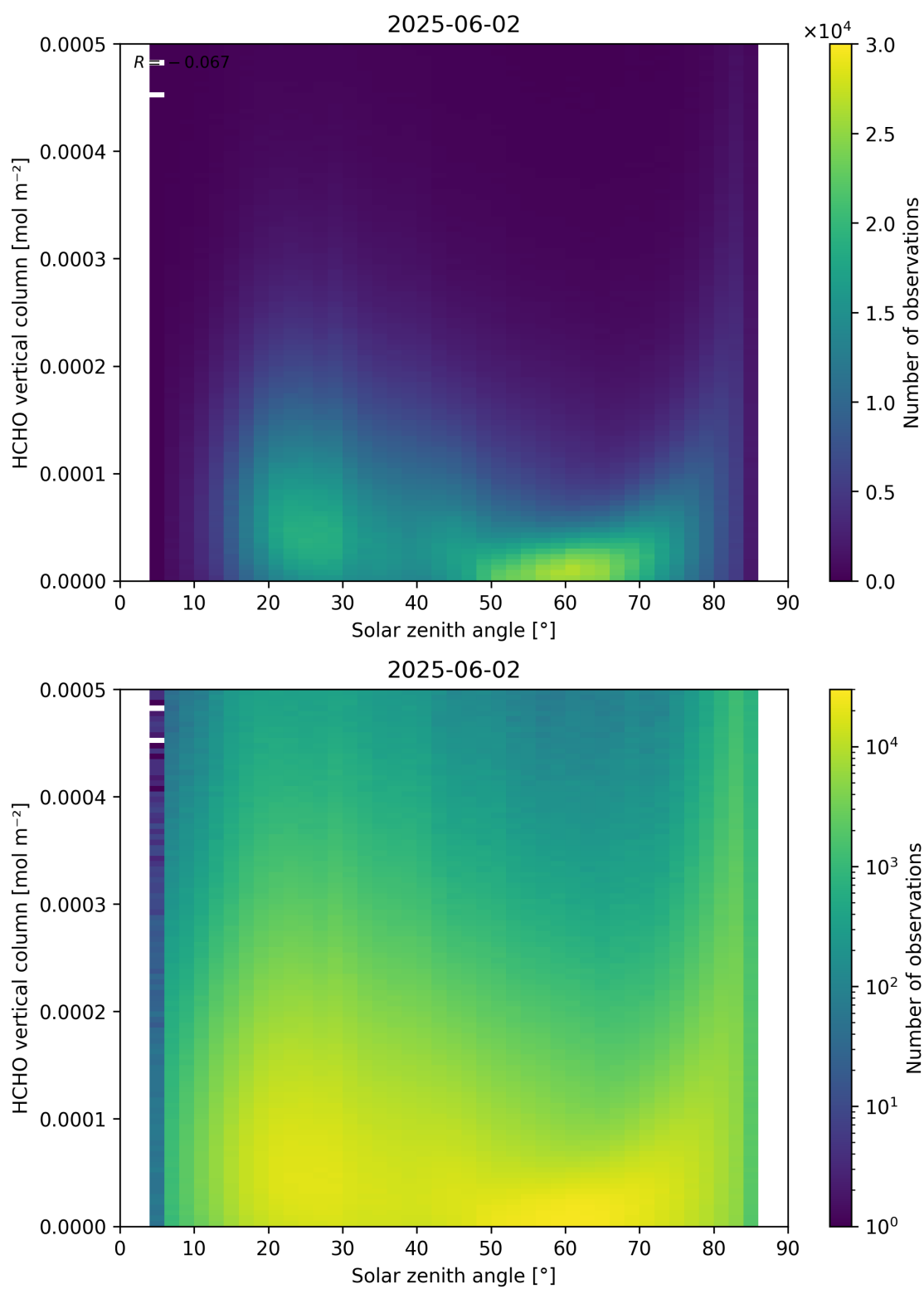
Figure 177: Scatter density plot of “Solar zenith angle” against “HCHO vertical column” for 2025-06-01 to 2025-06-03.
