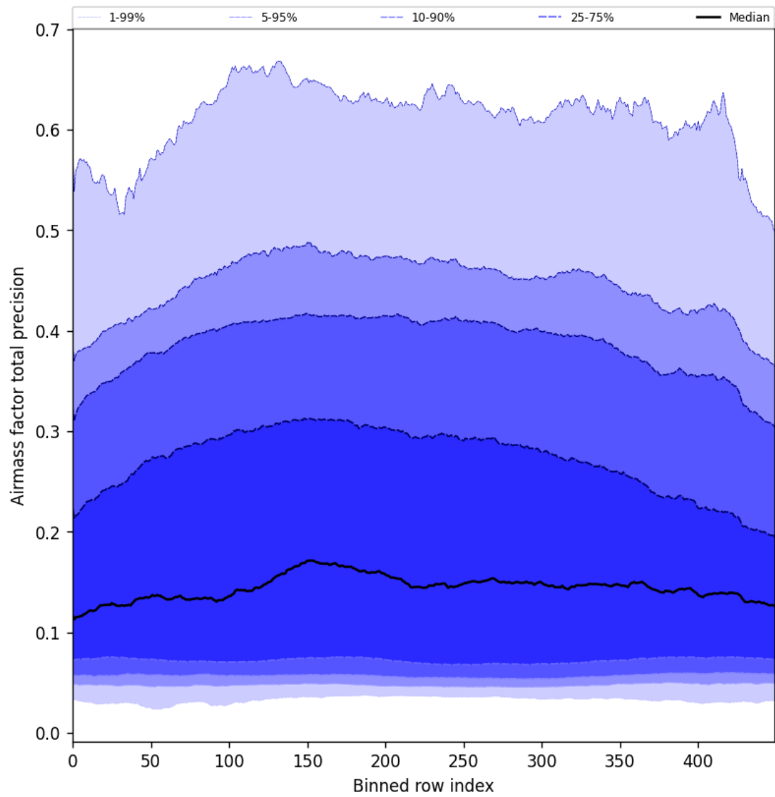
Figure 55: Along track statistics of “Airmass factor total precision” for 2025-06-01 to 2025-06-03
