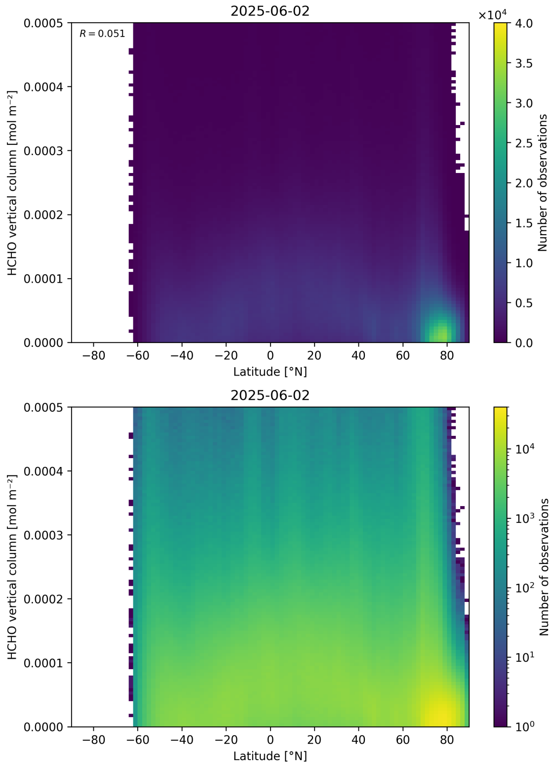
Figure 163: Scatter density plot of “Latitude” against “HCHO vertical column” for 2025-06-01 to 2025-06-03.
