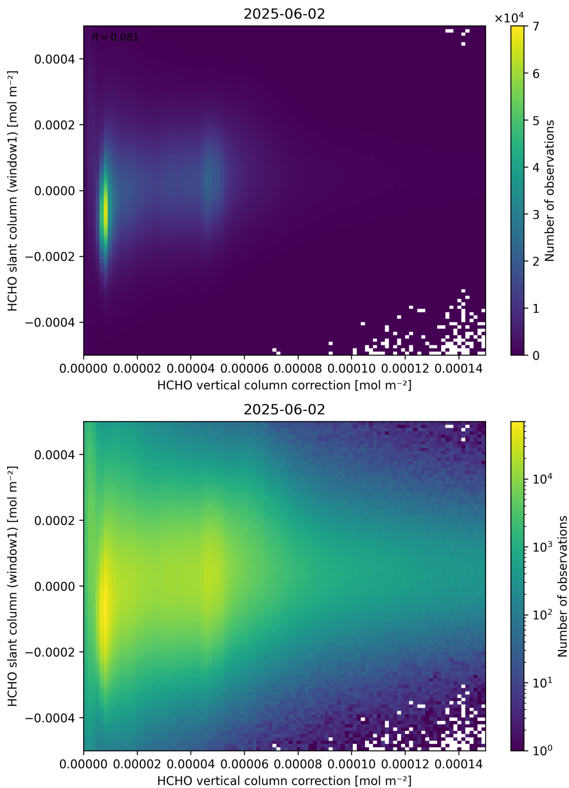
Figure 118: Scatter density plot of “HCHO vertical column correction” against “HCHO slant column (window1)” for 2025-06-01 to 2025-06-03.
