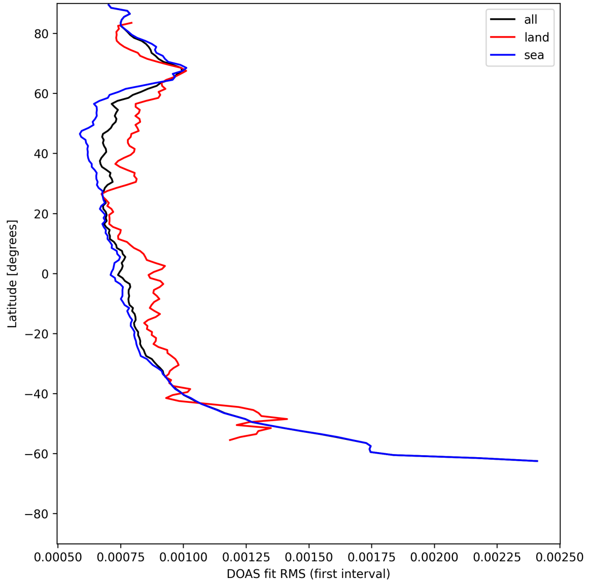
Figure 32: Zonal average of "DOAS fit RMS (first interval)" for 2025-06-01 to 2025-06-03.
