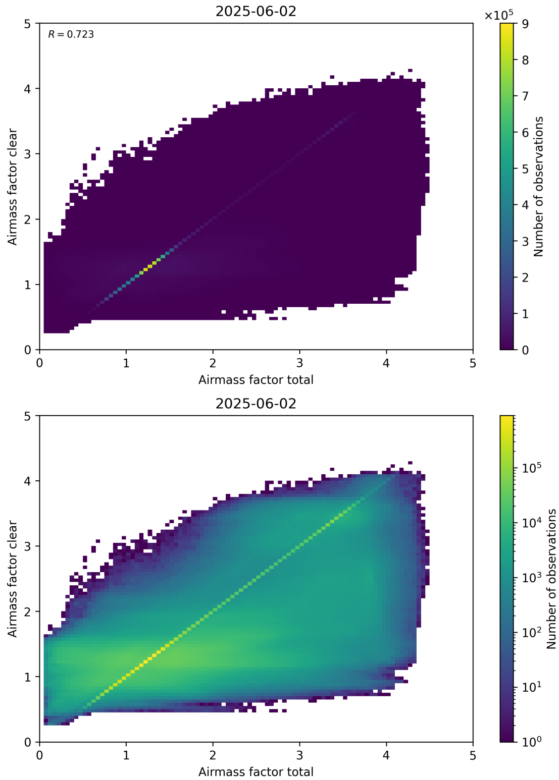
Figure 100: Scatter density plot of “Airmass factor total” against “Airmass factor clear” for 2025-06-01 to 2025-06-03.
