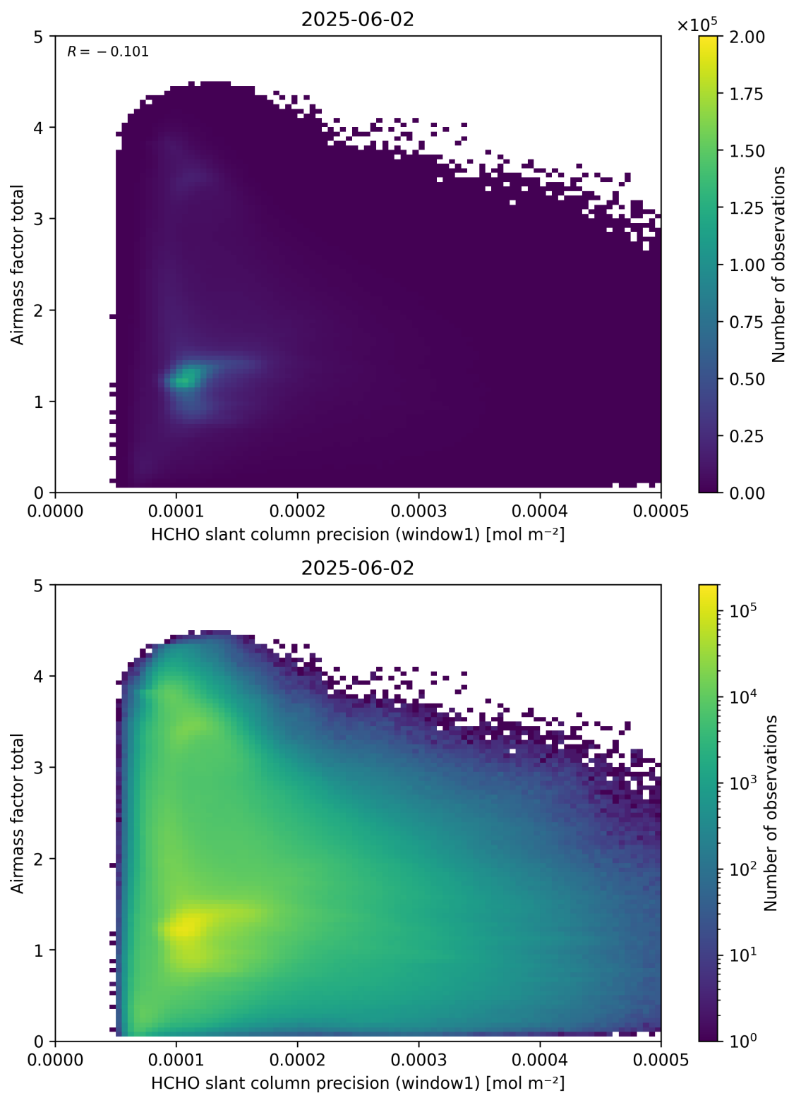
Figure 94: Scatter density plot of “HCHO slant column precision (window1)” against “Airmass factor total” for 2025-06-01 to 2025-06-03.
