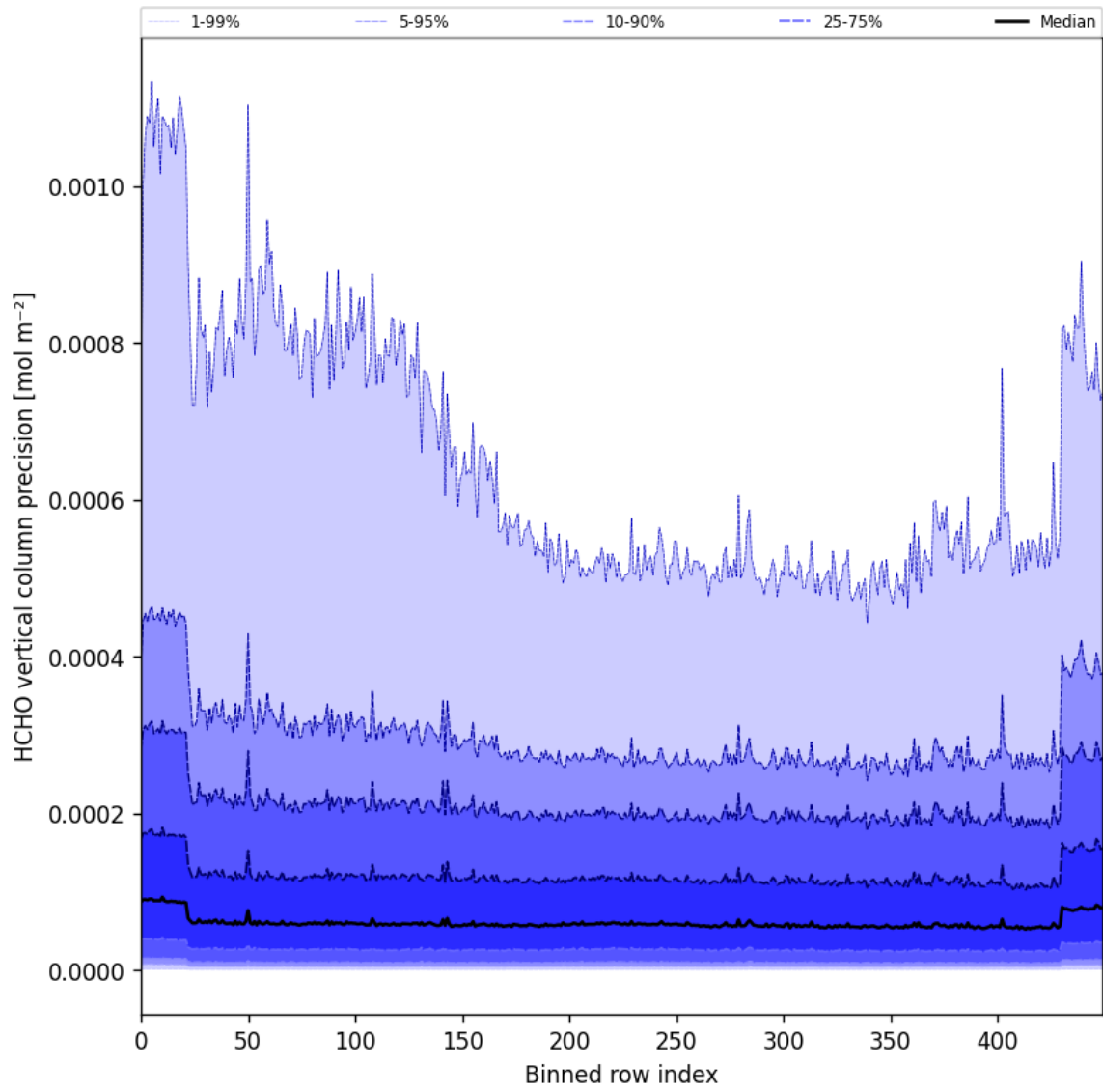
Figure 50: Along track statistics of "HCHO vertical column precision" for 2025-06-01 to 2025-06-03
