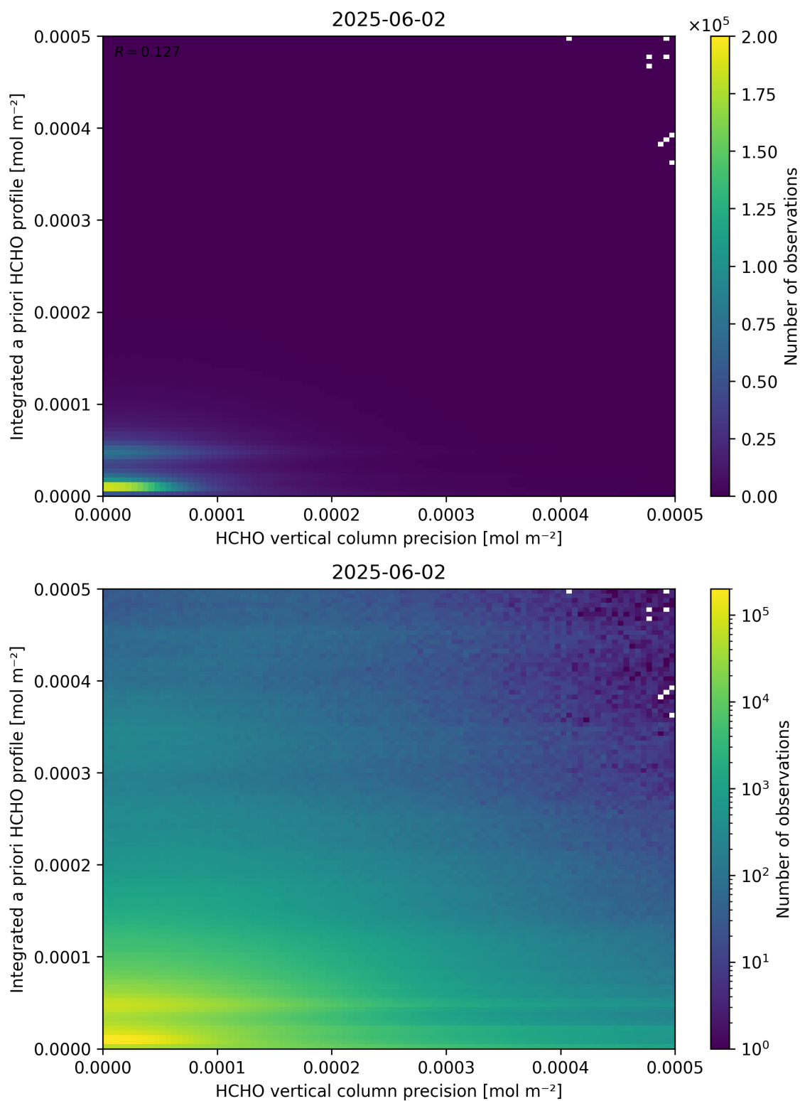
Figure 147: Scatter density plot of “HCHO vertical column precision” against “Integrated a priori HCHO profile” for 2025-06-01 to 2025-06-03.
