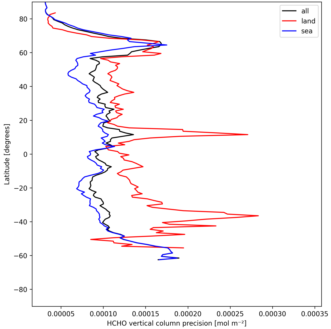
Figure 22: Zonal average of “HCHO vertical column precision” for 2025-06-01 to 2025-06-03.
