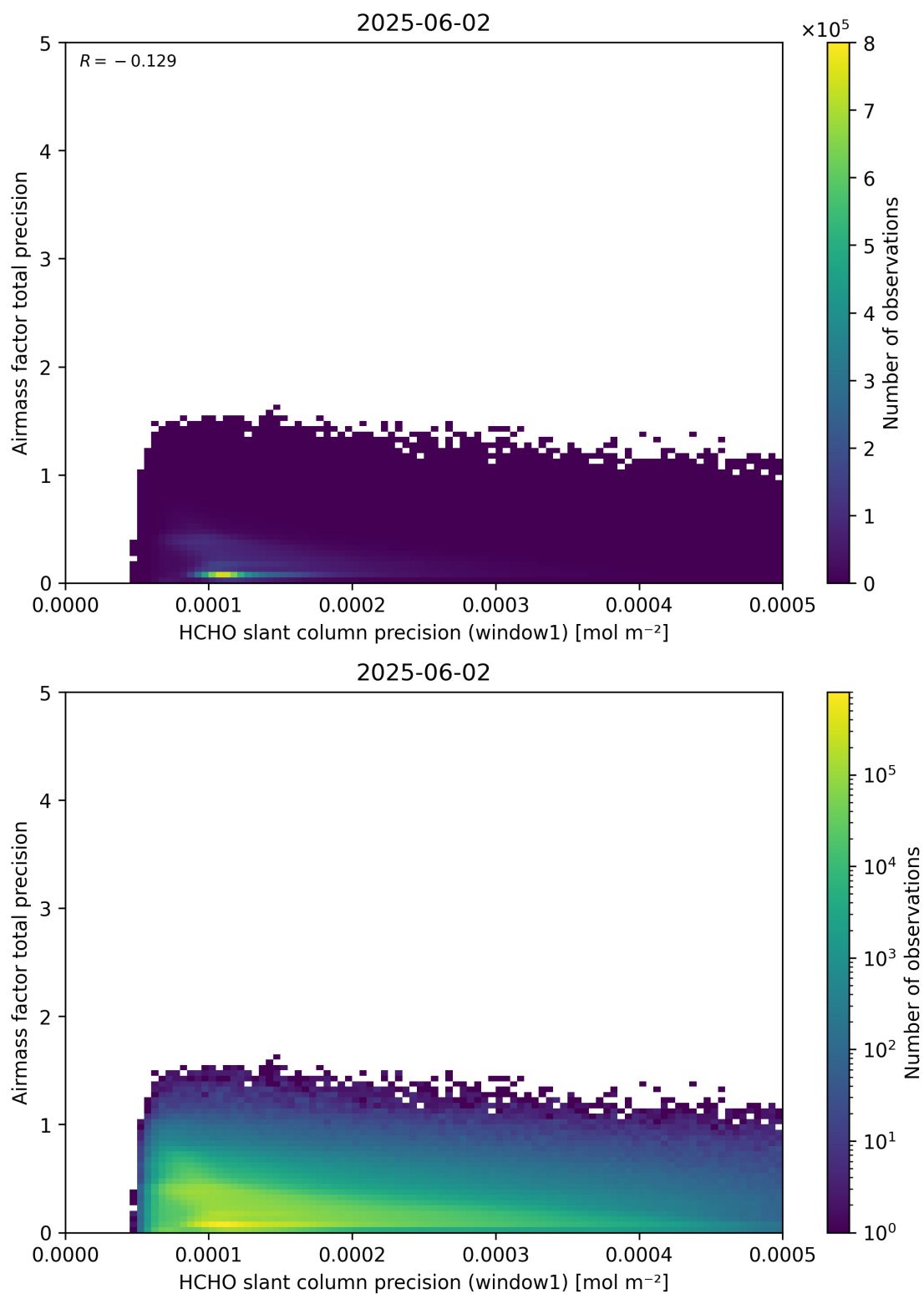
Figure 95: Scatter density plot of “HCHO slant column precision (window1)” against “Airmass factor total precision” for 2025-06-01 to 2025-06-03.
