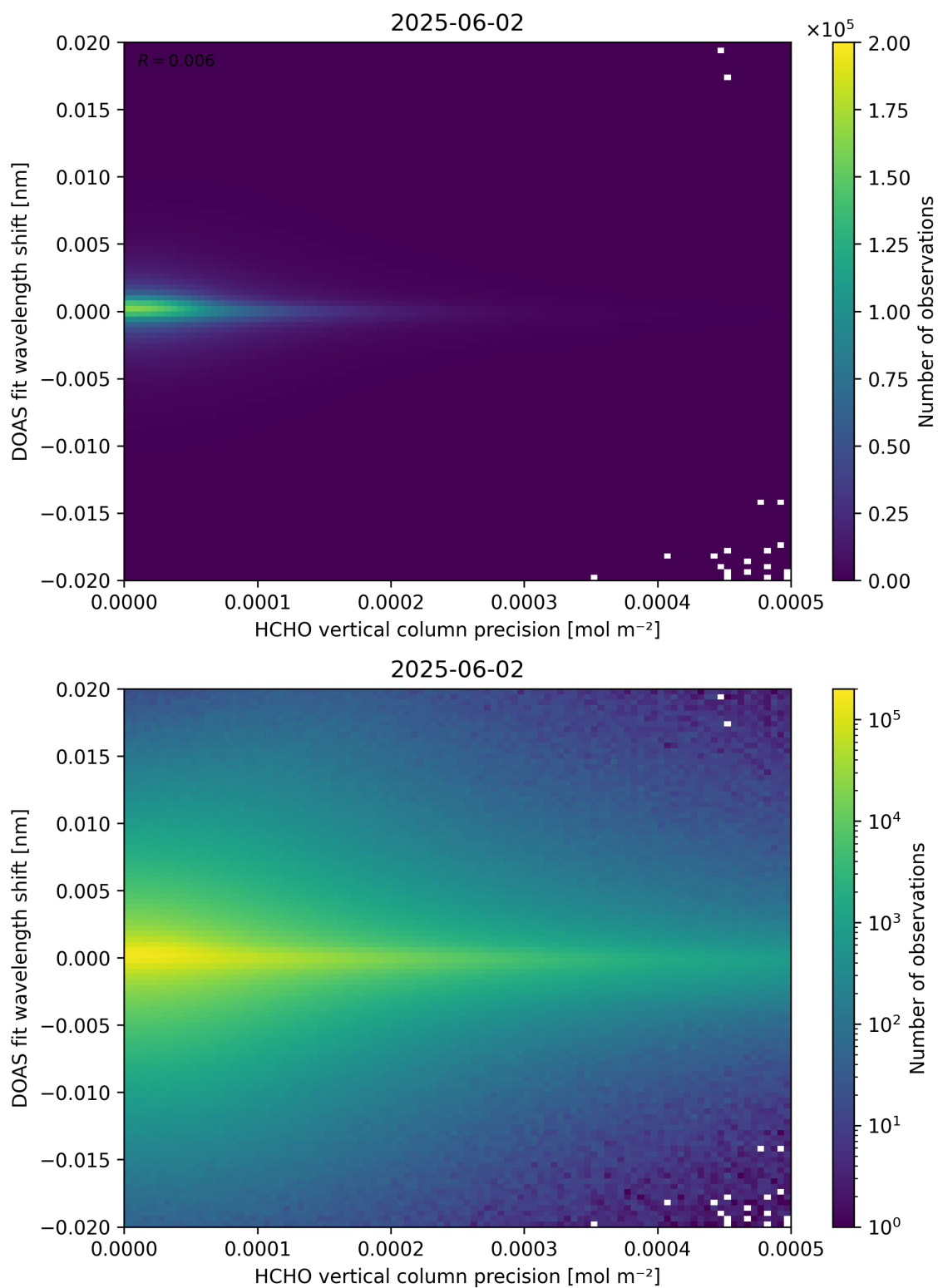
Figure 137: Scatter density plot of “HCHO vertical column precision” against “DOAS fit wavelength shift” for 2025-06-01 to 2025-06-03.
