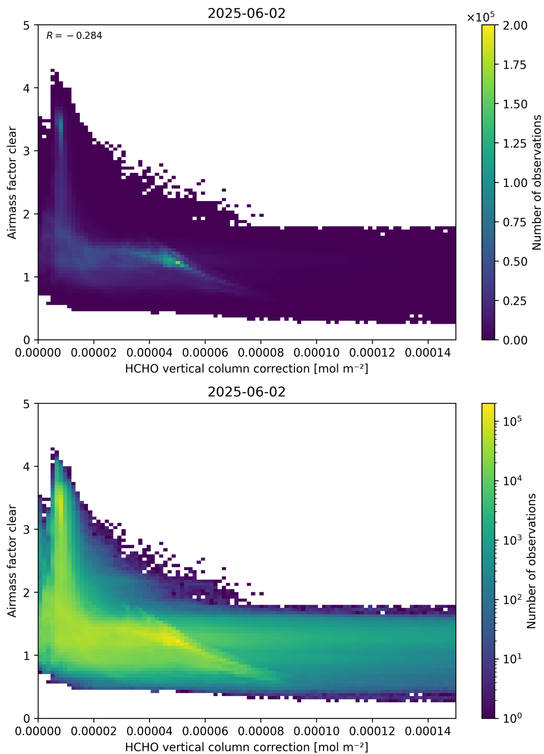
Figure 115: Scatter density plot of “HCHO vertical column correction” against “Airmass factor clear” for 2025-06-01 to 2025-06-03.
