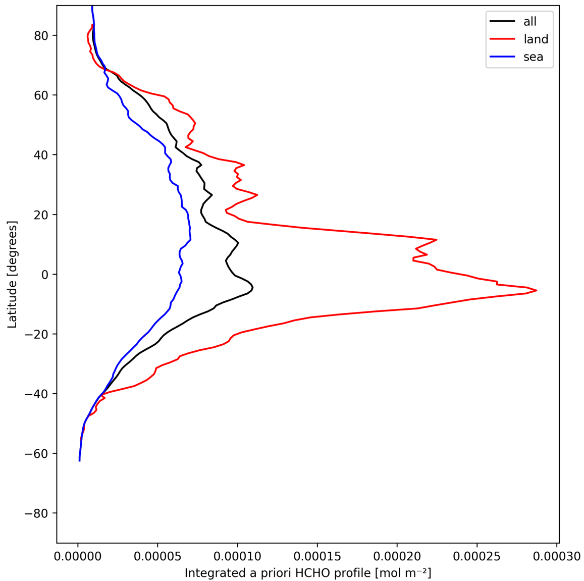
Figure 29: Zonal average of “Integrated a priori HCHO profile” for 2025-06-01 to 2025-06-03.
