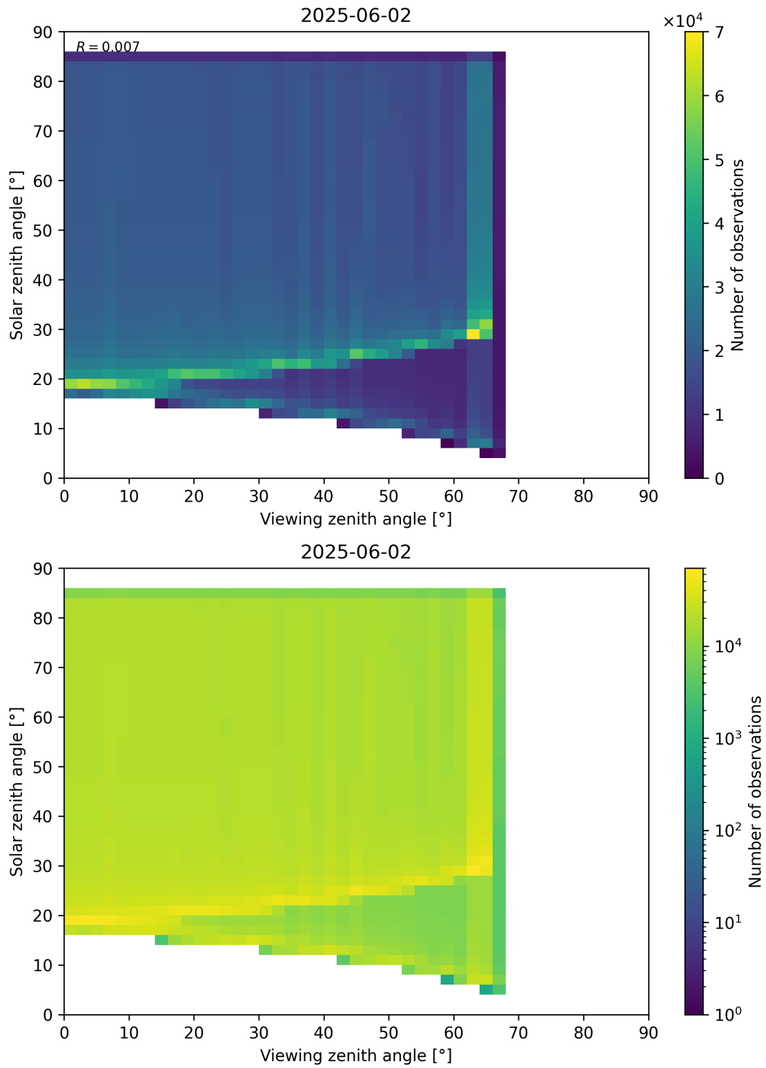
Figure 197: Scatter density plot of “Viewing zenith angle” against “Solar zenith angle” for 2025-06-01 to 2025-06-03.
