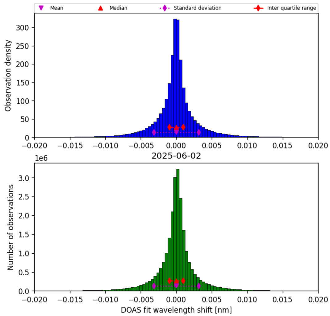
Figure 44: Histogram of “DOAS fit wavelength shift” for 2025-06-01 to 2025-06-03
