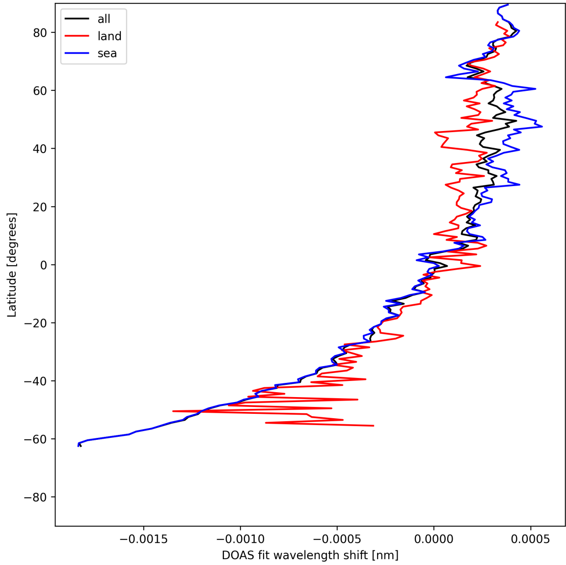
Figure 30: Zonal average of “DOAS fit wavelength shift” for 2025-06-01 to 2025-06-03.
