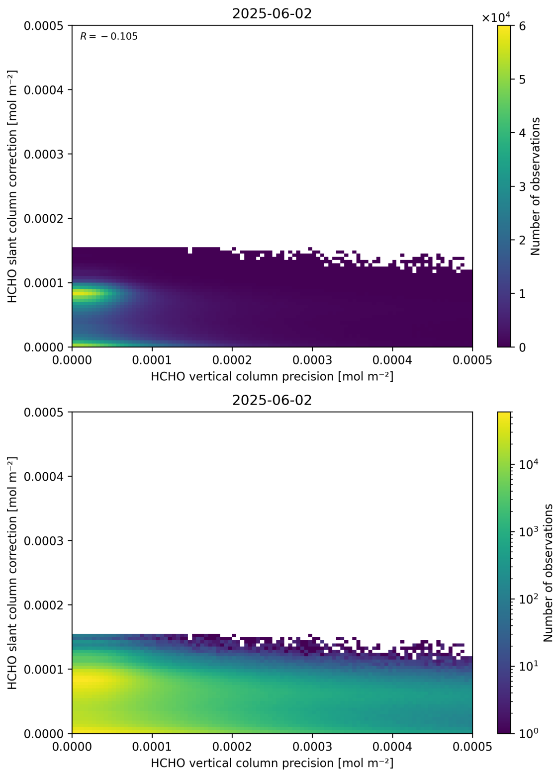
Figure 141: Scatter density plot of “HCHO vertical column precision” against “HCHO slant column correction” for 2025-06-01 to 2025-06-03.
