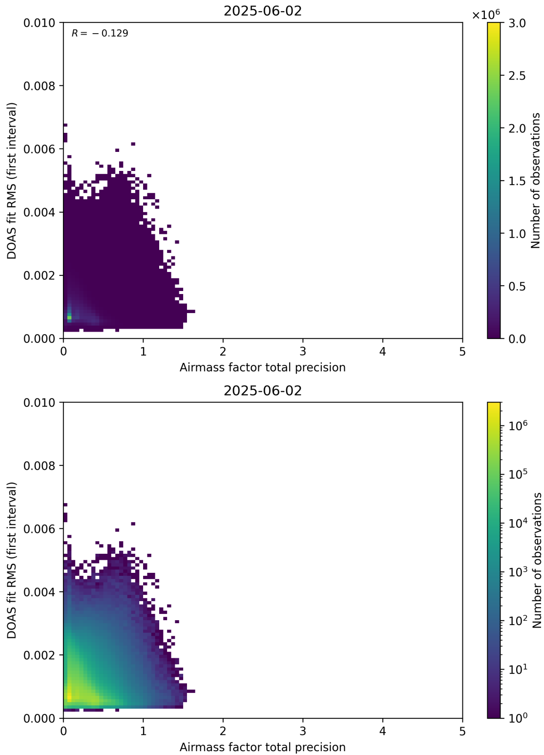
Figure 105: Scatter density plot of “Airmass factor total precision” against “DOAS fit RMS (first interval)” for 2025-06-01 to 2025-06-03.
