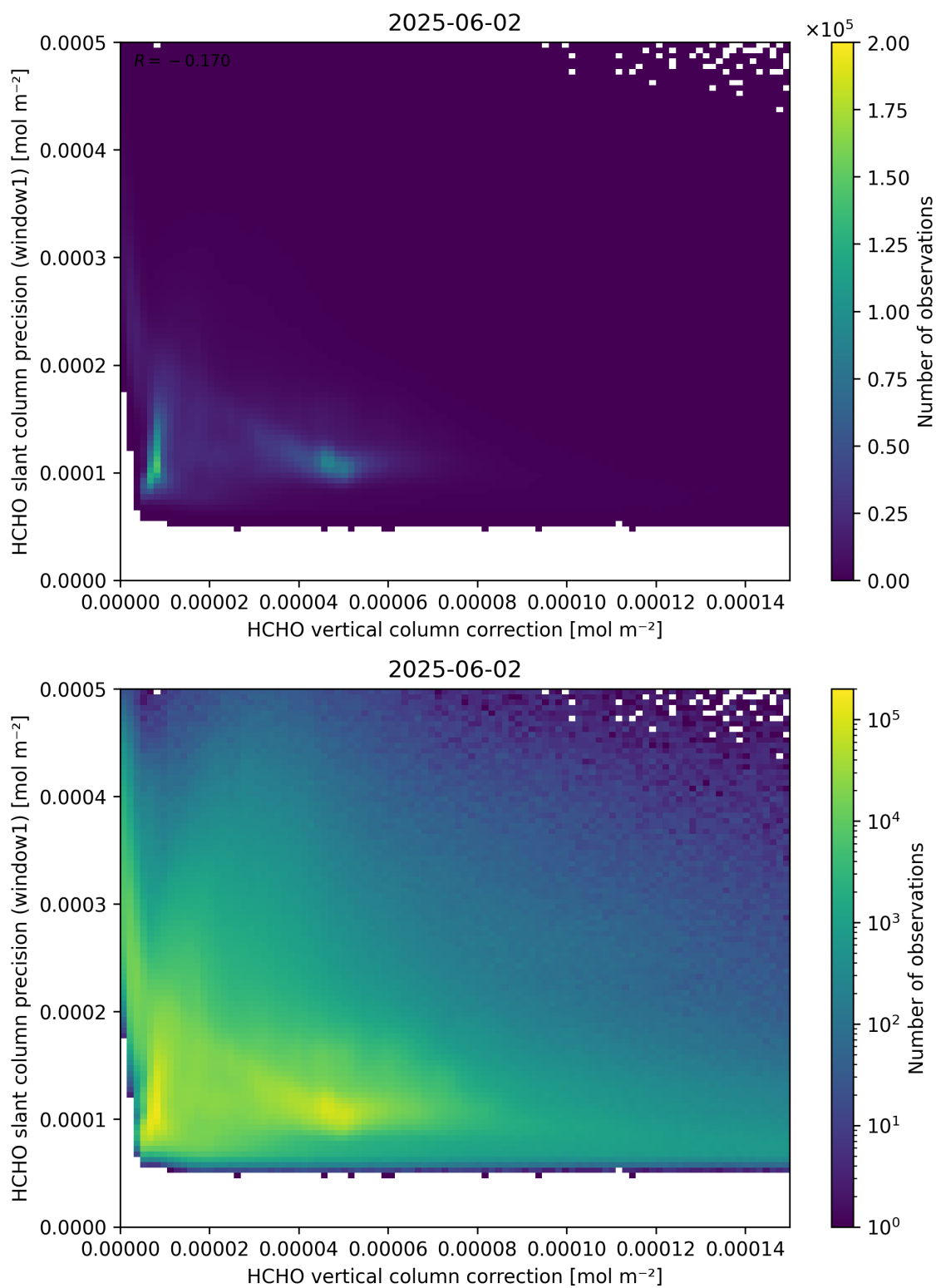
Figure 119: Scatter density plot of “HCHO vertical column correction” against “HCHO slant column precision (window1)” for 2025-06-01 to 2025-06-03.
