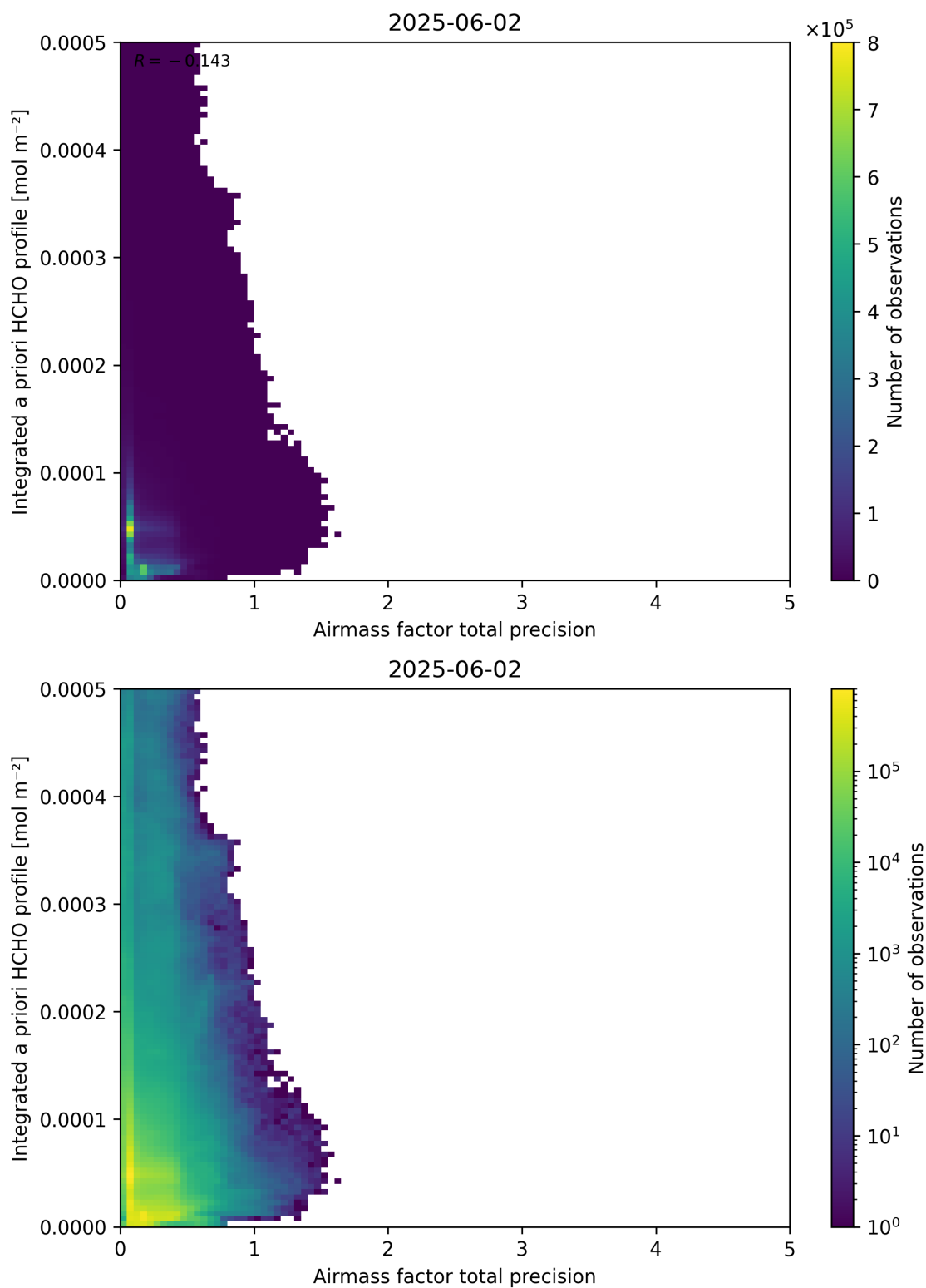
Figure 111: Scatter density plot of “Airmass factor total precision” against “Integrated a priori HCHO profile” for 2025-06-01 to 2025-06-03.
