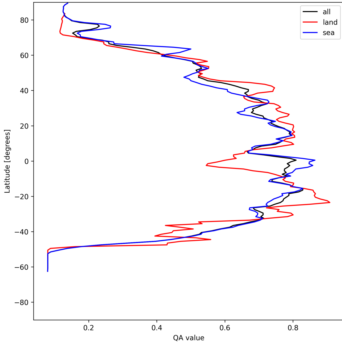
Figure 20: Zonal average of “QA value” for 2025-06-01 to 2025-06-03.
