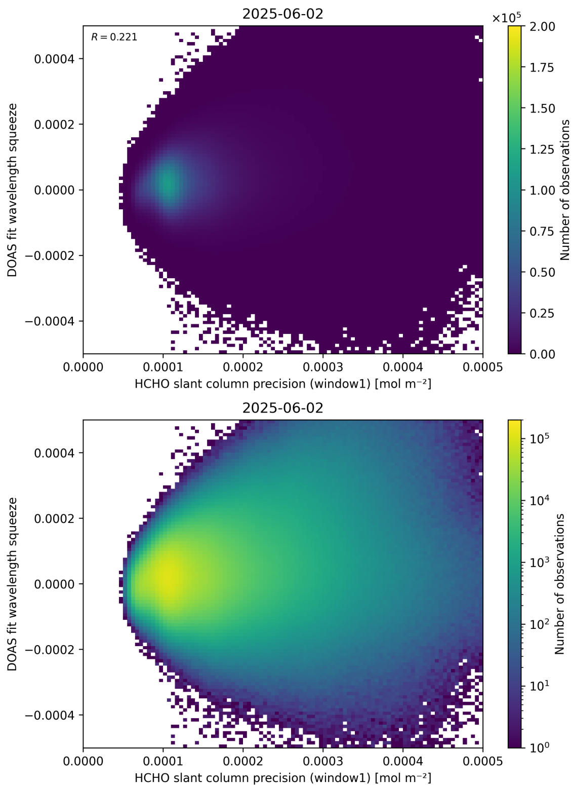
Figure 90: Scatter density plot of “HCHO slant column precision (window1)” against “DOAS fit wavelength squeeze” for 2025-06-01 to 2025-06-03.
