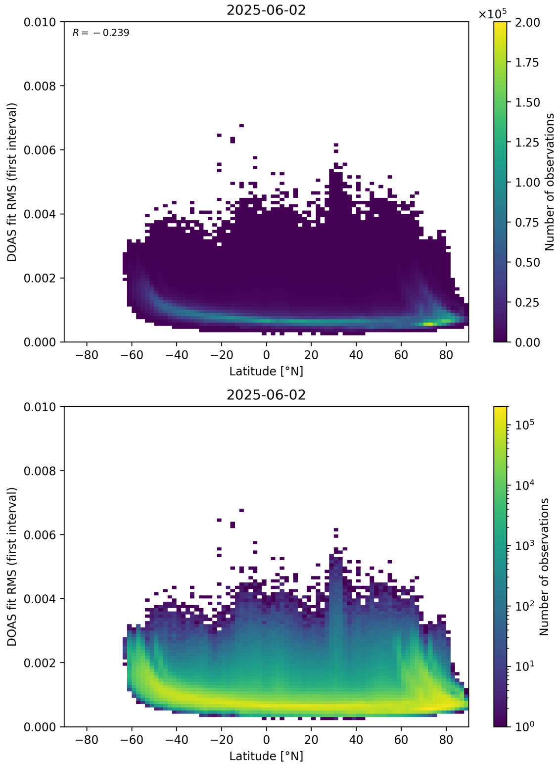
Figure 153: Scatter density plot of “Latitude” against “DOAS fit RMS (first interval)” for 2025-06-01 to 2025-06-03.
