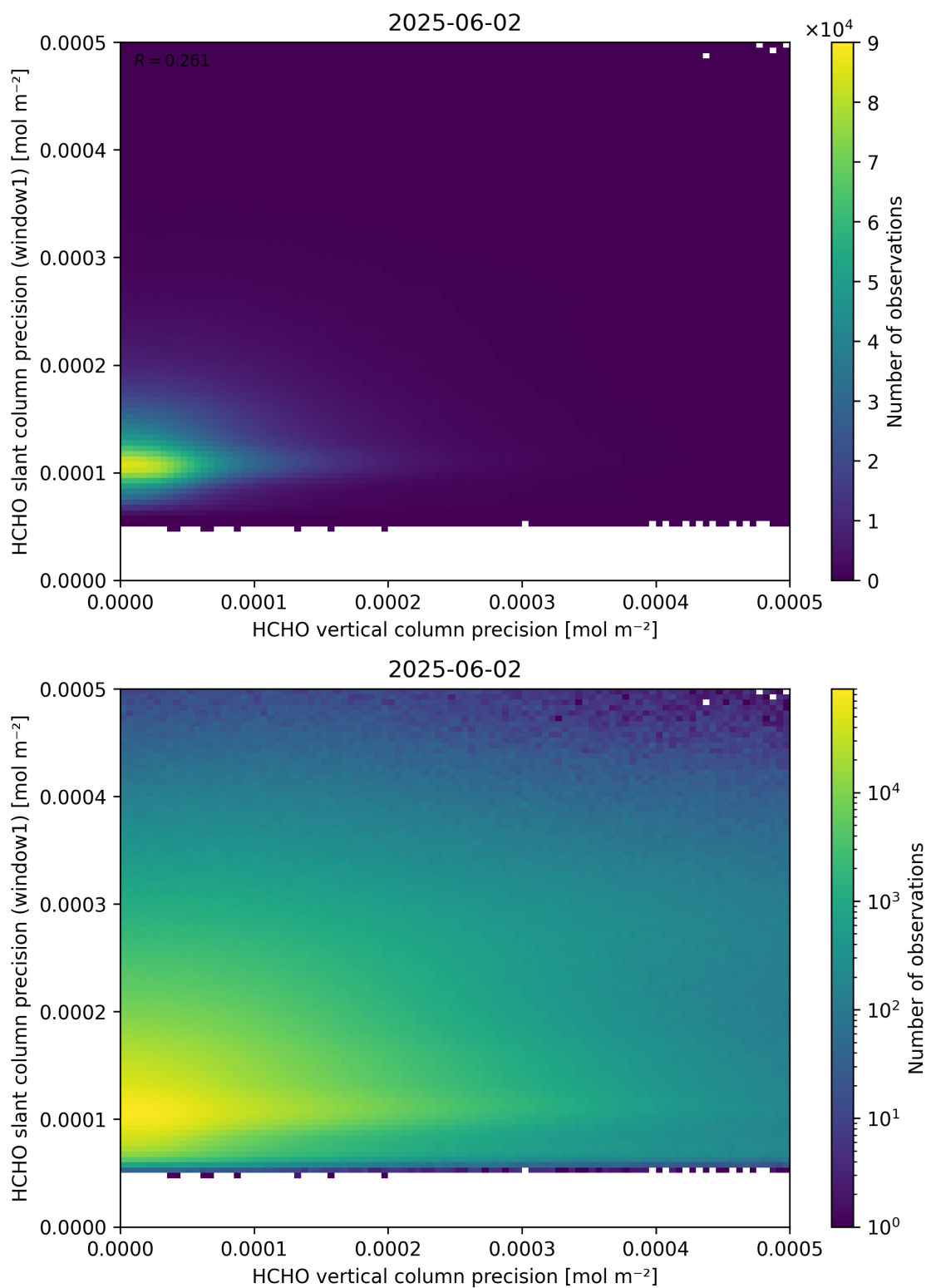
Figure 143: Scatter density plot of “HCHO vertical column precision” against “HCHO slant column precision (window1)” for 2025-06-01 to 2025-06-03.
