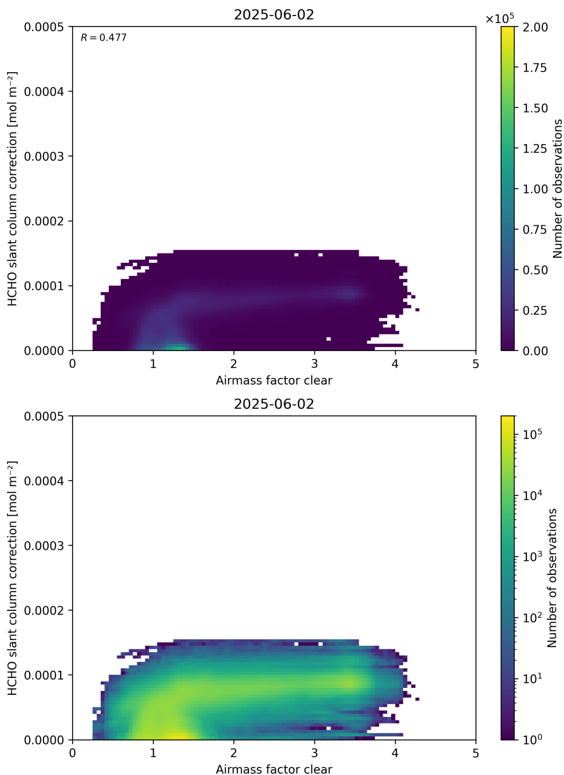
Figure 75: Scatter density plot of “Airmass factor clear” against “HCHO slant column correction” for 2025-06-01 to 2025-06-03.
