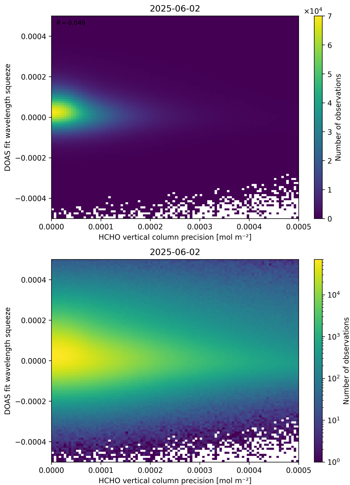
Figure 138: Scatter density plot of “HCHO vertical column precision” against “DOAS fit wavelength squeeze” for 2025-06-01 to 2025-06-03.
