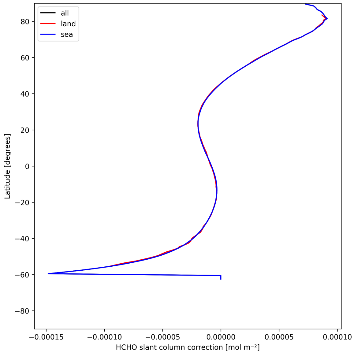
Figure 33: Zonal average of “HCHO slant column correction” for 2025-06-01 to 2025-06-03.
