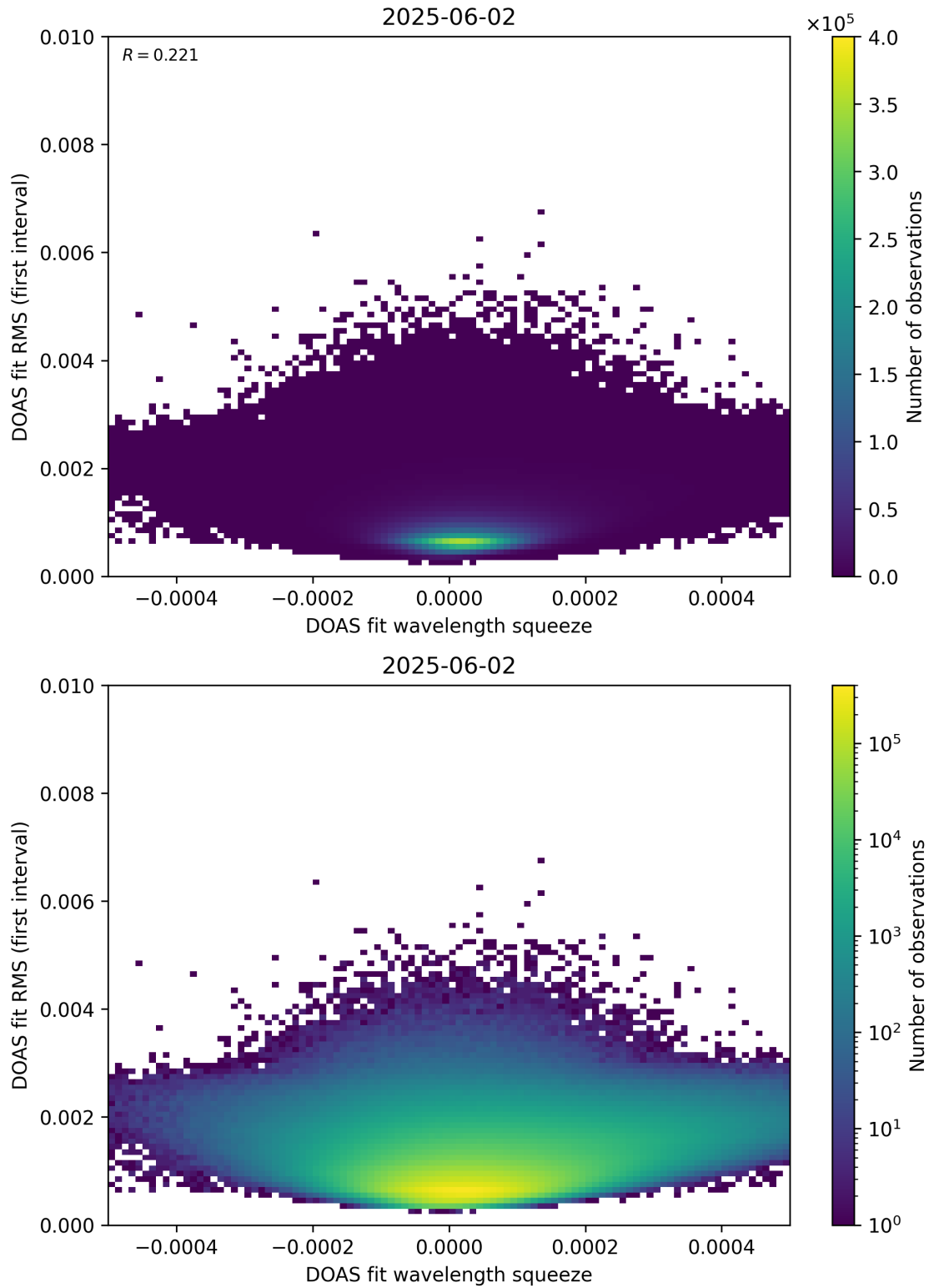
Figure 68: Scatter density plot of “DOAS fit wavelength squeeze” against “DOAS fit RMS (first interval)” for 2025-06-01 to 2025-06-03.
