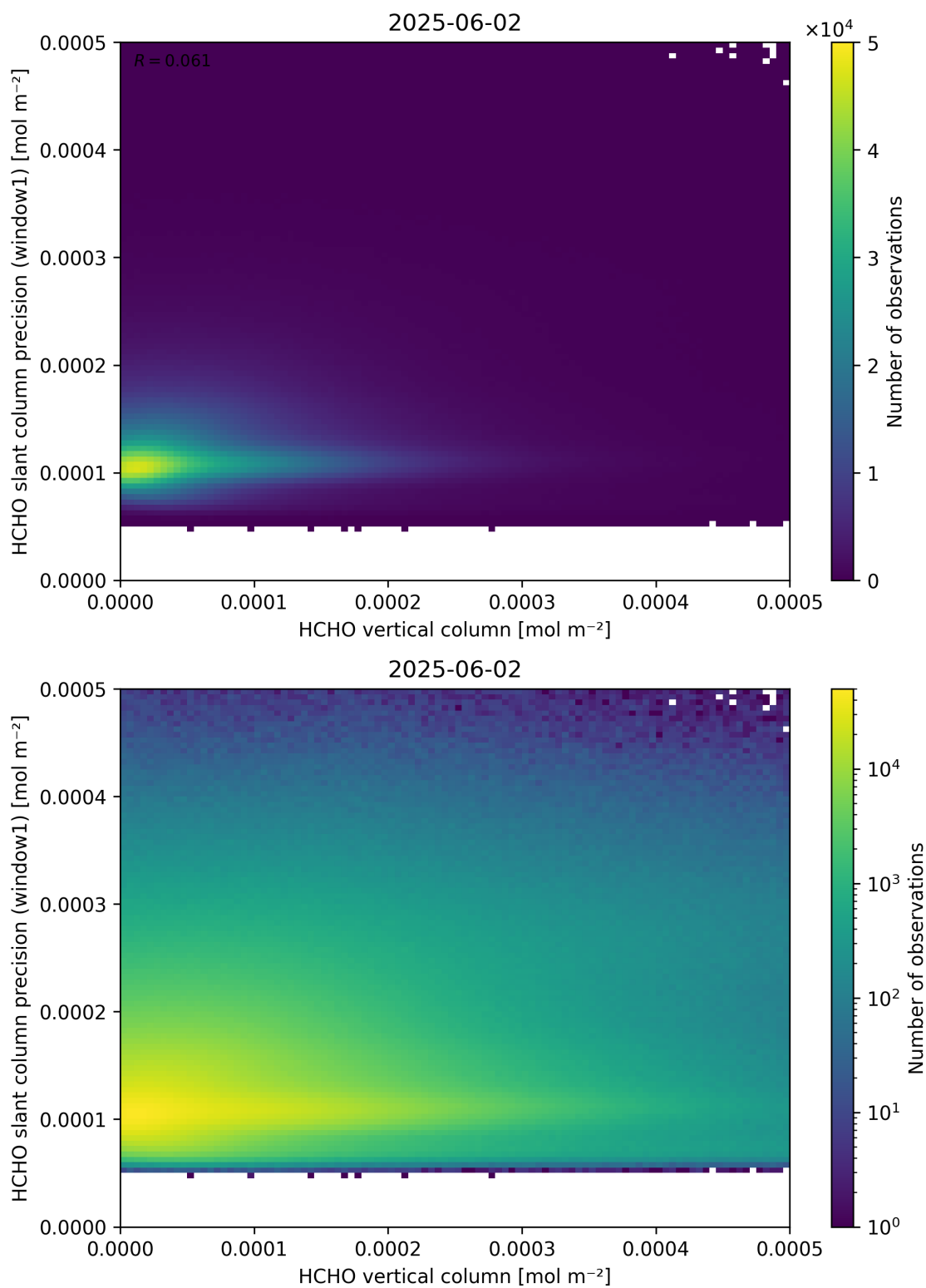
Figure 130: Scatter density plot of “HCHO vertical column” against “HCHO slant column precision (window1)” for 2025-06-01 to 2025-06-03.
