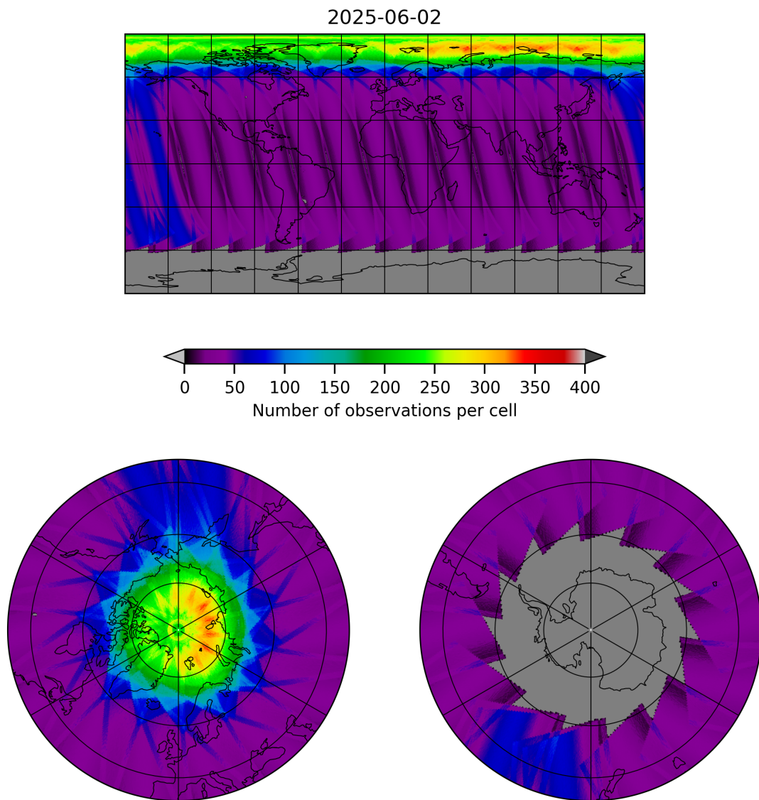
Figure 19: Map of the number of observations for 2025-06-01 to 2025-06-03
