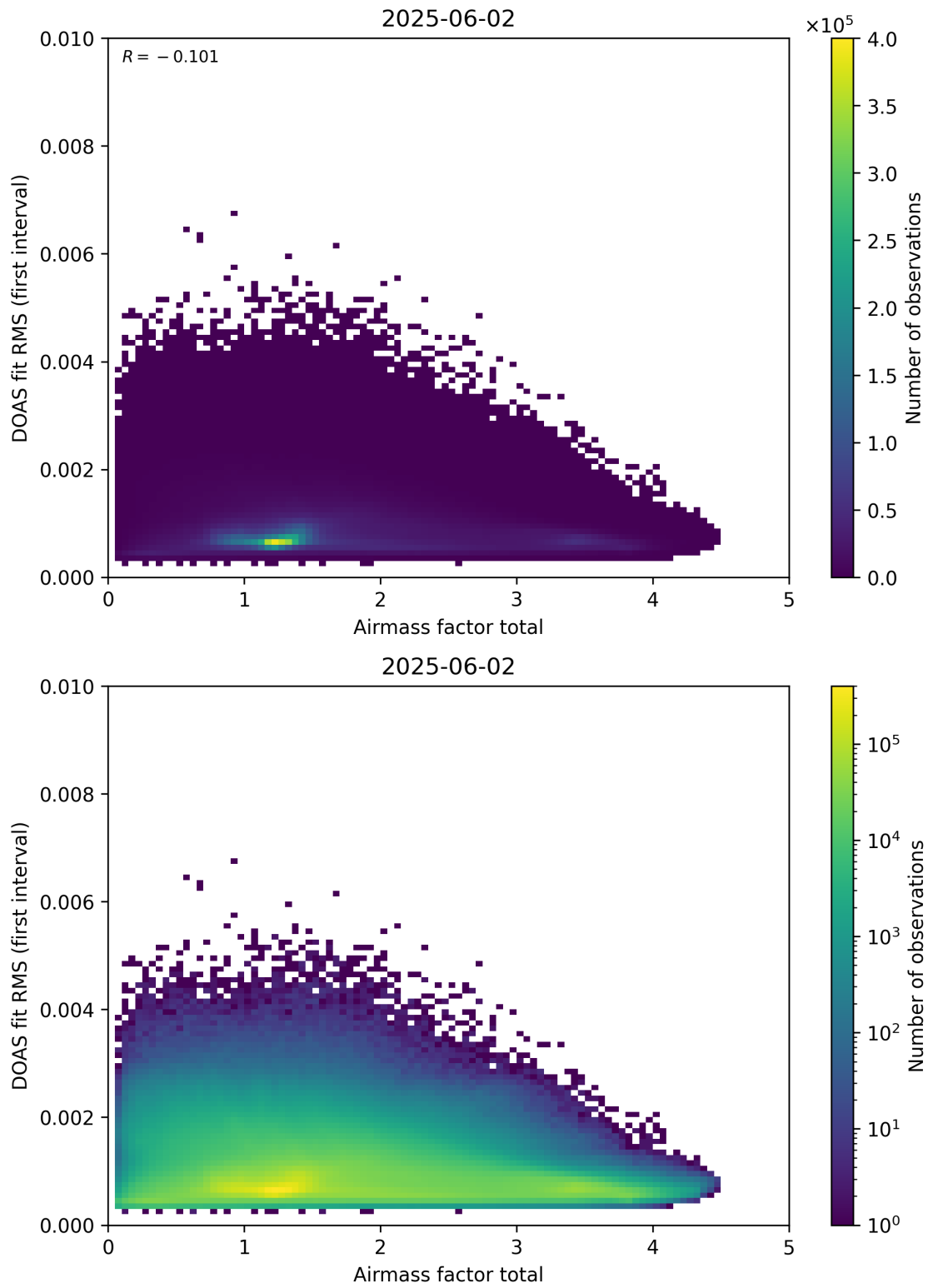
Figure 97: Scatter density plot of “Airmass factor total” against “DOAS fit RMS (first interval)” for 2025-06-01 to 2025-06-03.
