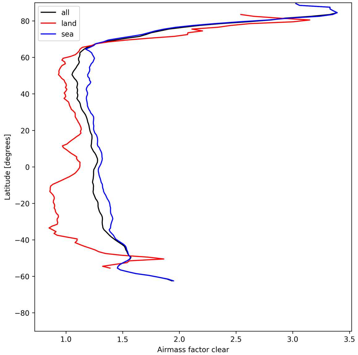
Figure 28: Zonal average of “Airmass factor clear” for 2025-06-01 to 2025-06-03.
