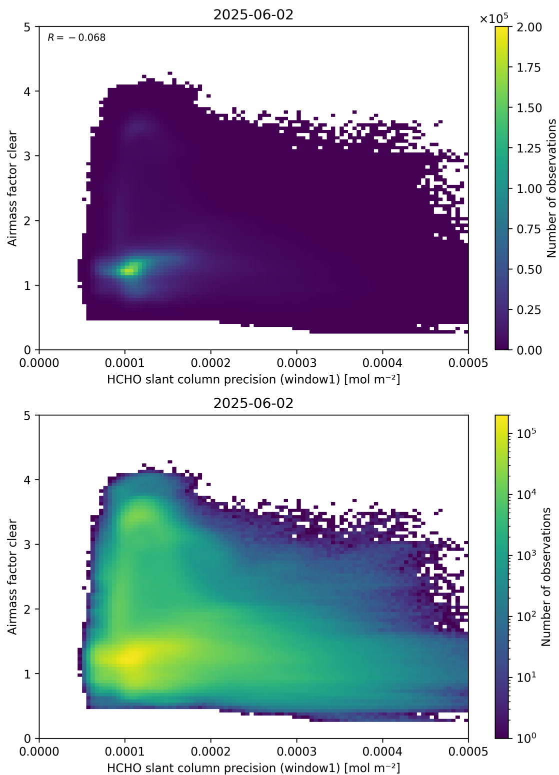
Figure 91: Scatter density plot of “HCHO slant column precision (window1)” against “Airmass factor clear” for 2025-06-01 to 2025-06-03.
