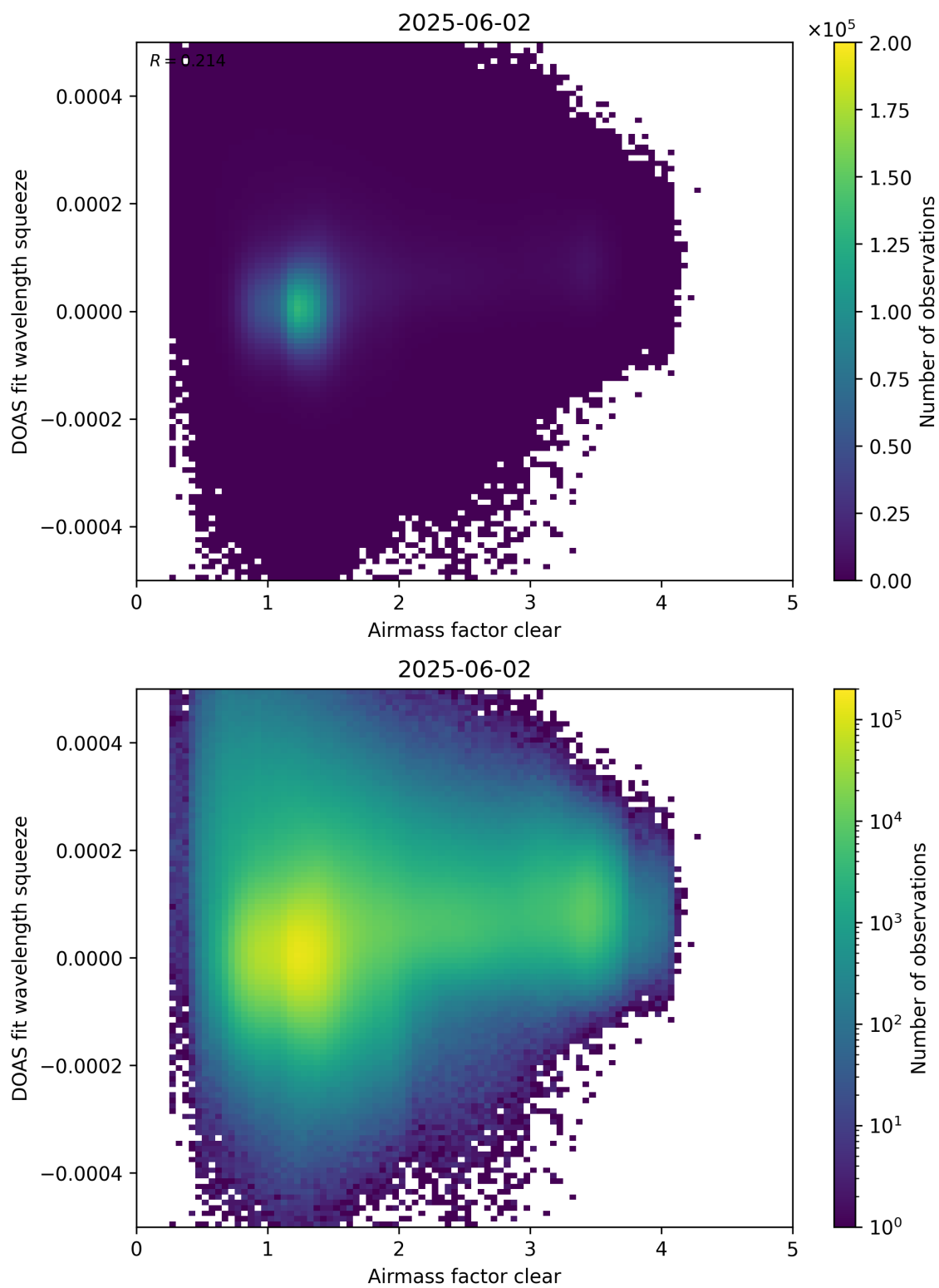
Figure 73: Scatter density plot of “Airmass factor clear” against “DOAS fit wavelength squeeze” for 2025-06-01 to 2025-06-03.
