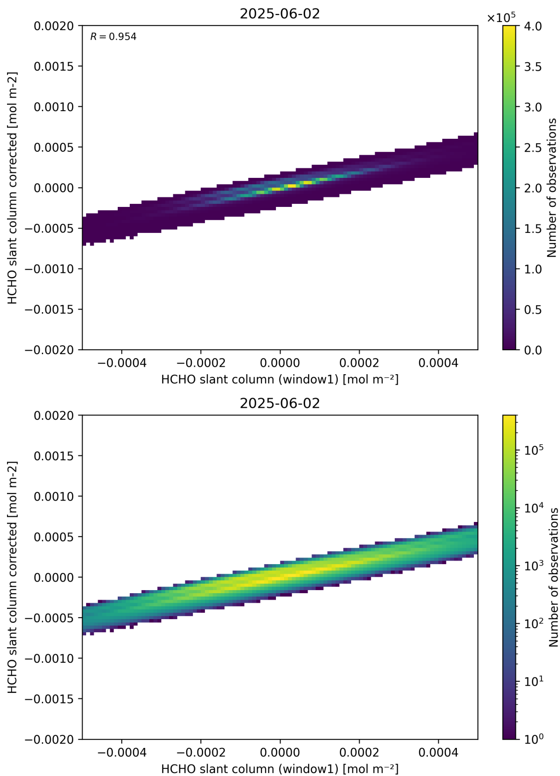
Figure 82: Scatter density plot of “HCHO slant column (window1)” against “HCHO slant column corrected” for 2025-06-01 to 2025-06-03.
