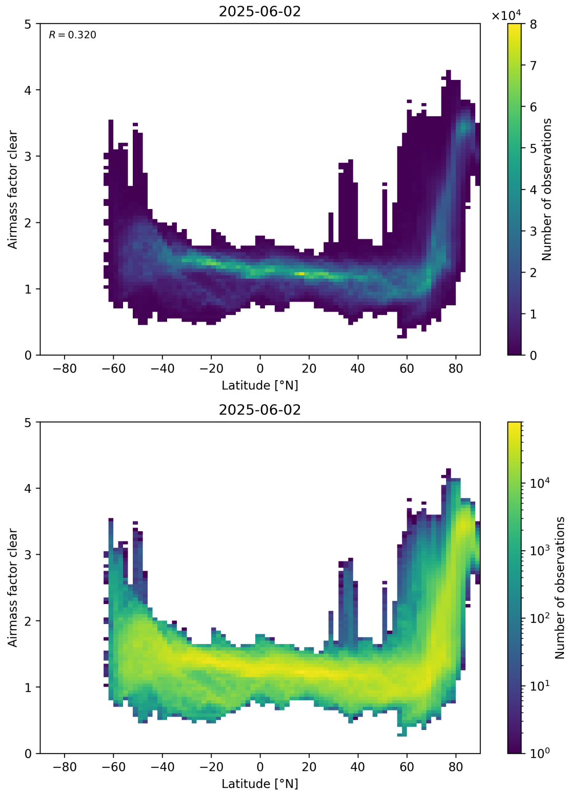
Figure 156: Scatter density plot of “Latitude” against “Airmass factor clear” for 2025-06-01 to 2025-06-03.
