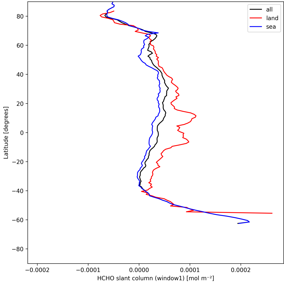
Figure 24: Zonal average of “HCHO slant column (window1)” for 2025-06-01 to 2025-06-03.
