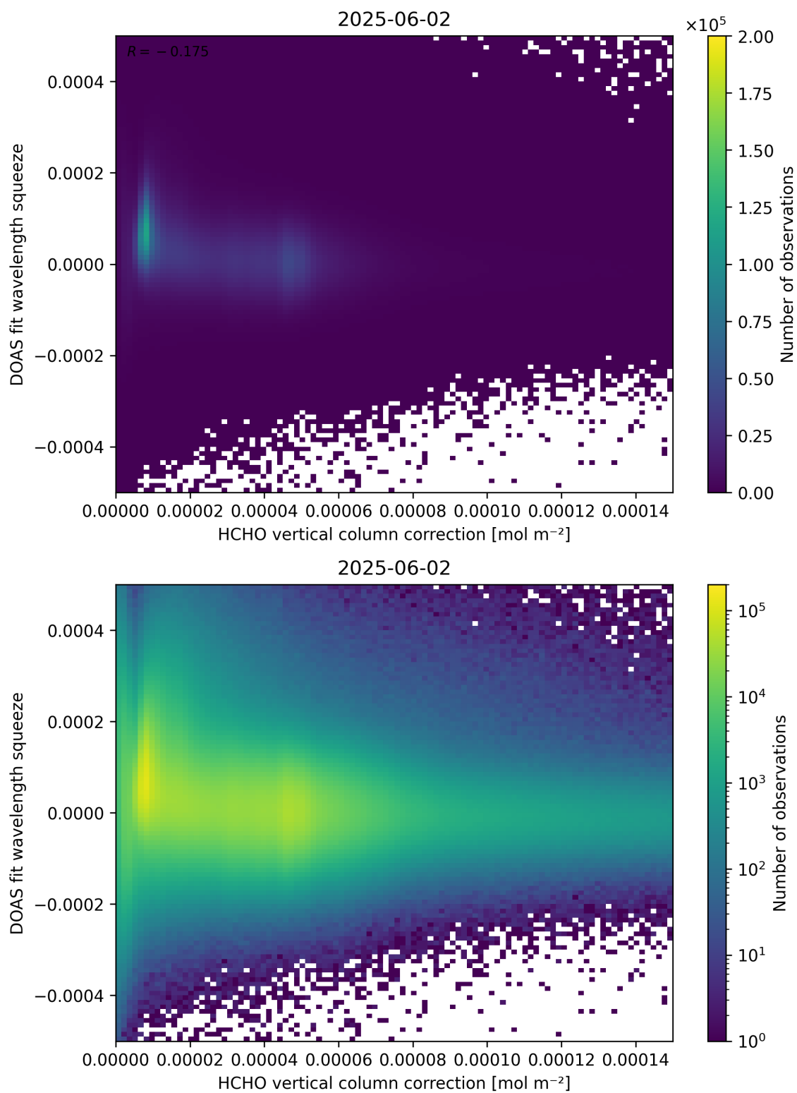
Figure 114: Scatter density plot of “HCHO vertical column correction” against “DOAS fit wavelength squeeze” for 2025-06-01 to 2025-06-03.
