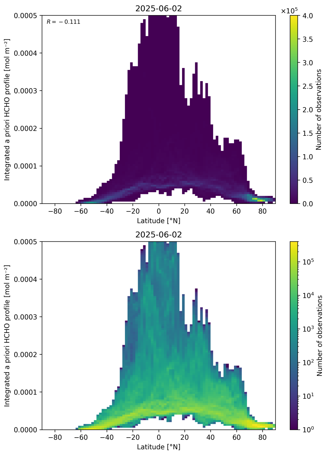
Figure 166: Scatter density plot of “Latitude” against “Integrated a priori HCHO profile” for 2025-06-01 to 2025-06-03.
