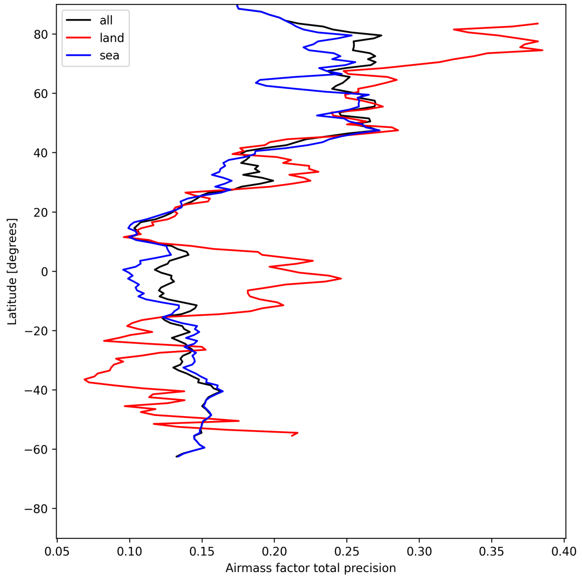
Figure 27: Zonal average of “Airmass factor total precision” for 2025-06-01 to 2025-06-03.
