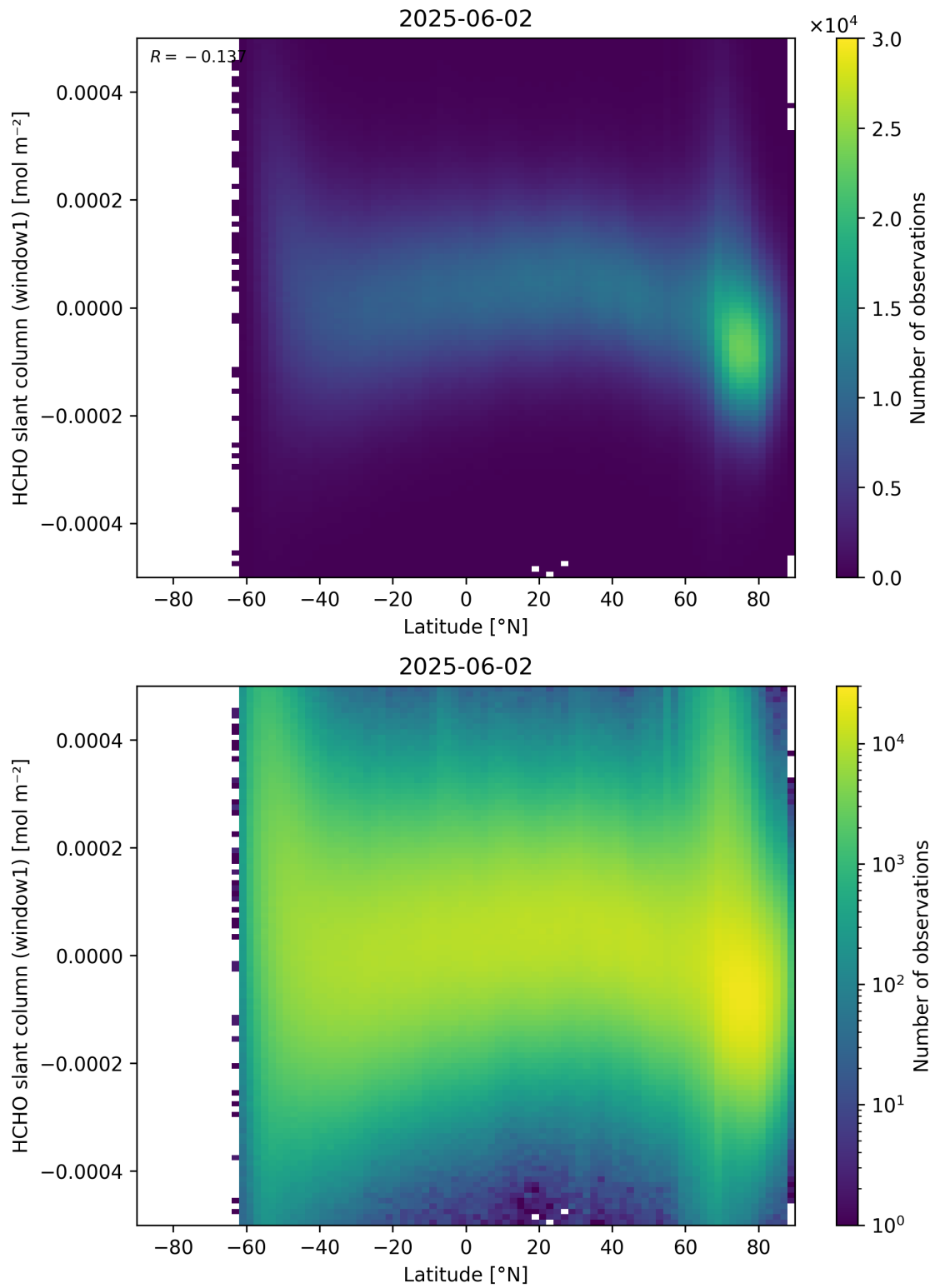
Figure 159: Scatter density plot of “Latitude” against “HCHO slant column (window1)” for 2025-06-01 to 2025-06-03.
