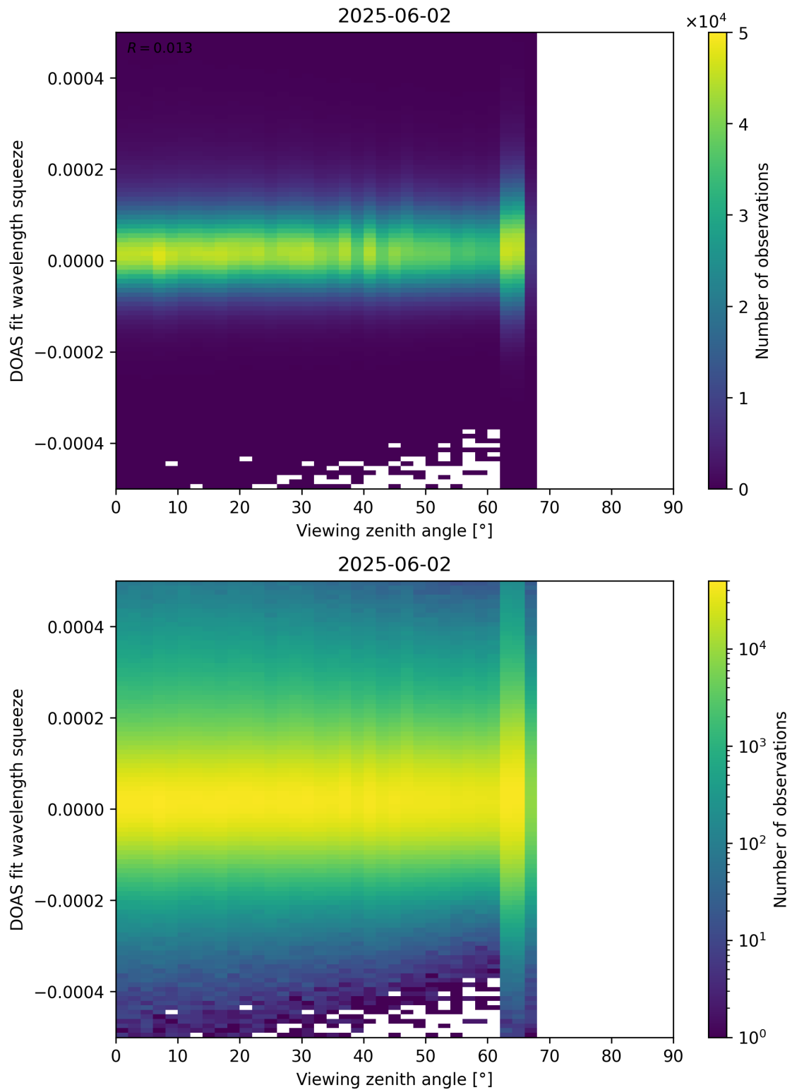
Figure 184: Scatter density plot of “Viewing zenith angle” against “DOAS fit wavelength squeeze” for 2025-06-01 to 2025-06-03.
