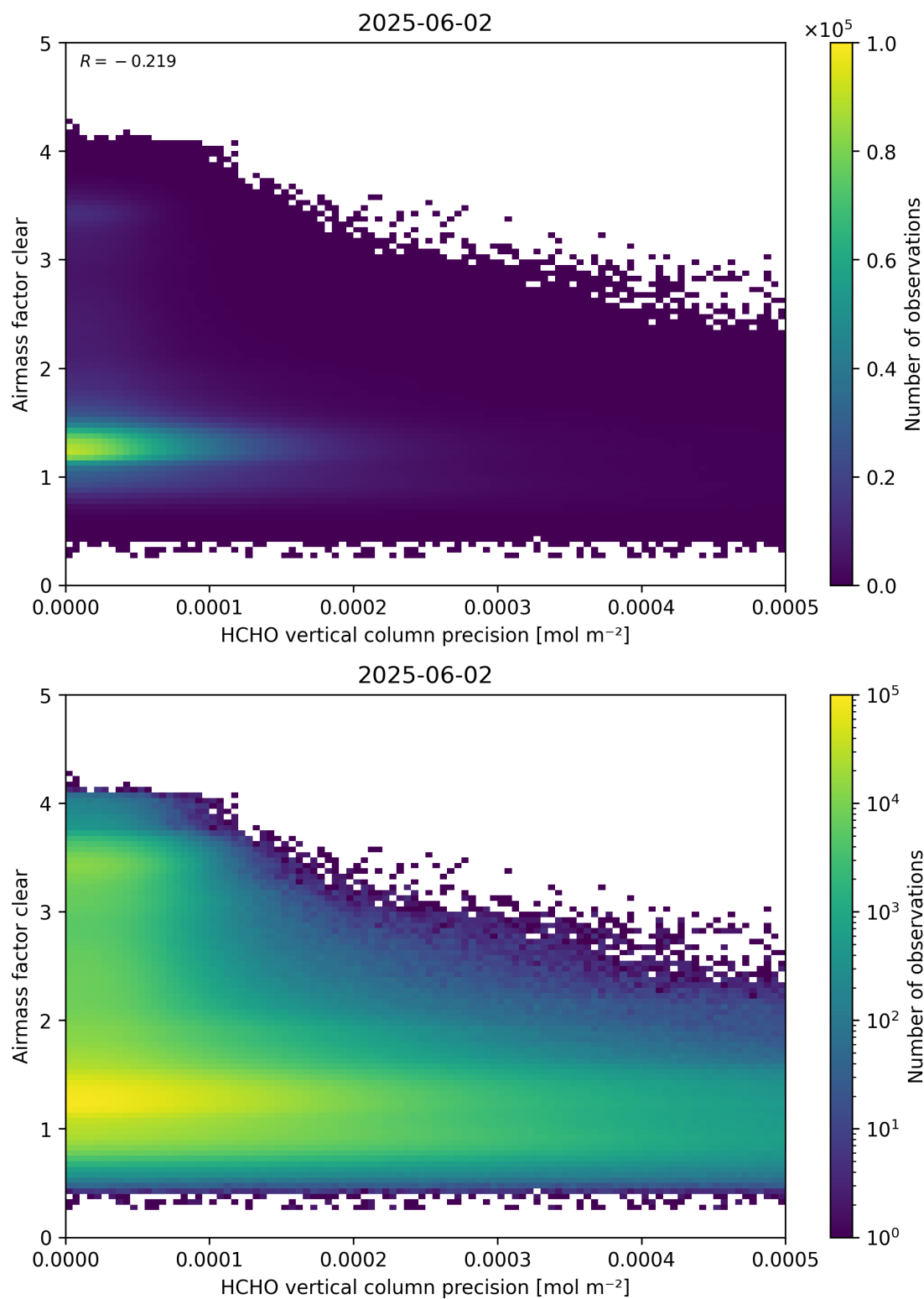
Figure 139: Scatter density plot of “HCHO vertical column precision” against “Airmass factor clear” for 2025-06-01 to 2025-06-03.
