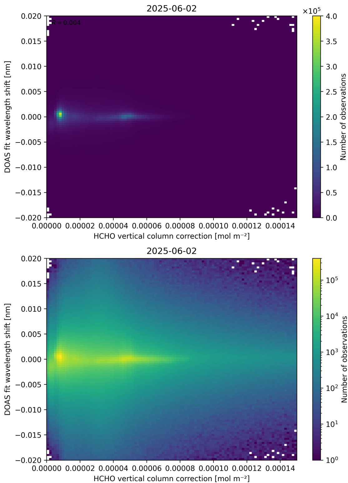
Figure 113: Scatter density plot of “HCHO vertical column correction” against “DOAS fit wavelength shift” for 2025-06-01 to 2025-06-03.
