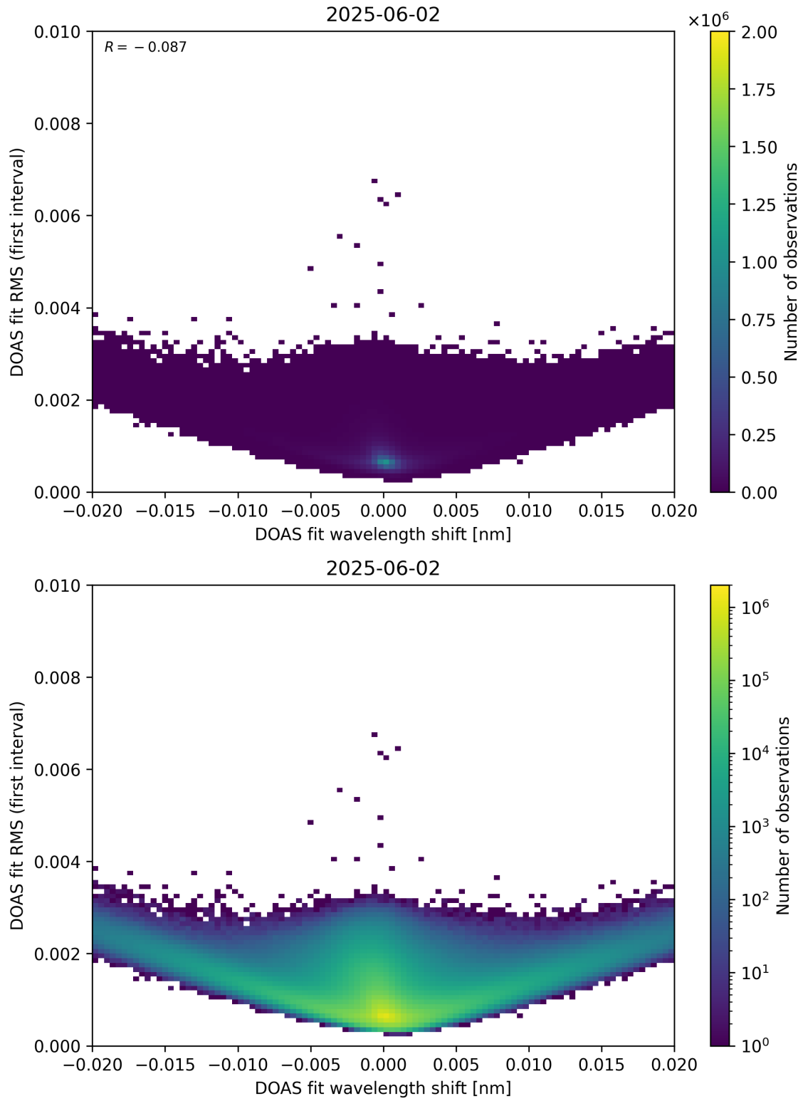
Figure 64: Scatter density plot of “DOAS fit wavelength shift” against “DOAS fit RMS (first interval)” for 2025-06-01 to 2025-06-03.
