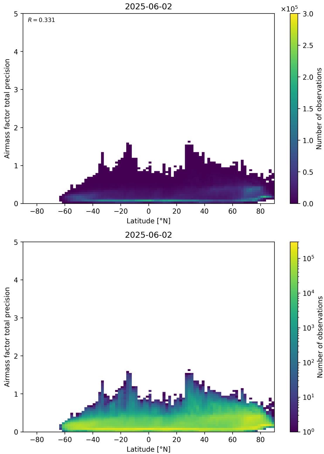
Figure 162: Scatter density plot of “Latitude” against “Airmass factor total precision” for 2025-06-01 to 2025-06-03.
