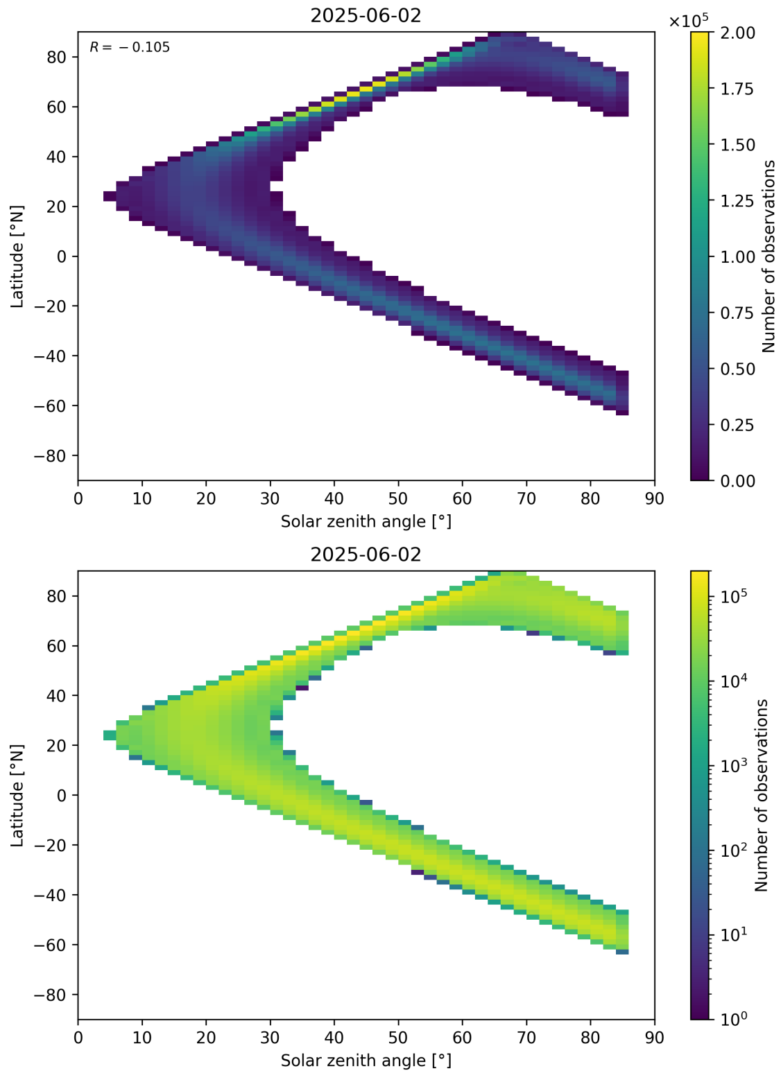
Figure 181: Scatter density plot of “Solar zenith angle” against “Latitude” for 2025-06-01 to 2025-06-03.
