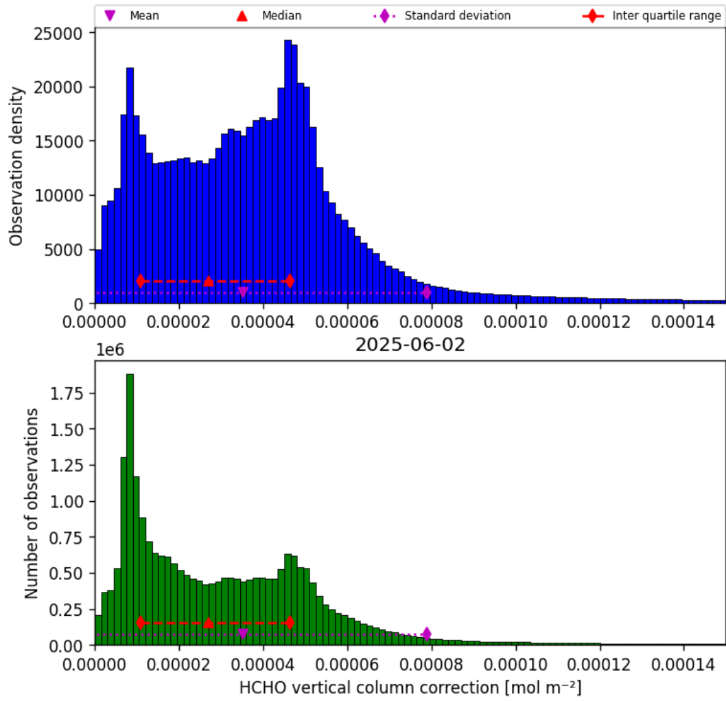
Figure 37: Histogram of “HCHO vertical column correction” for 2025-06-01 to 2025-06-03
