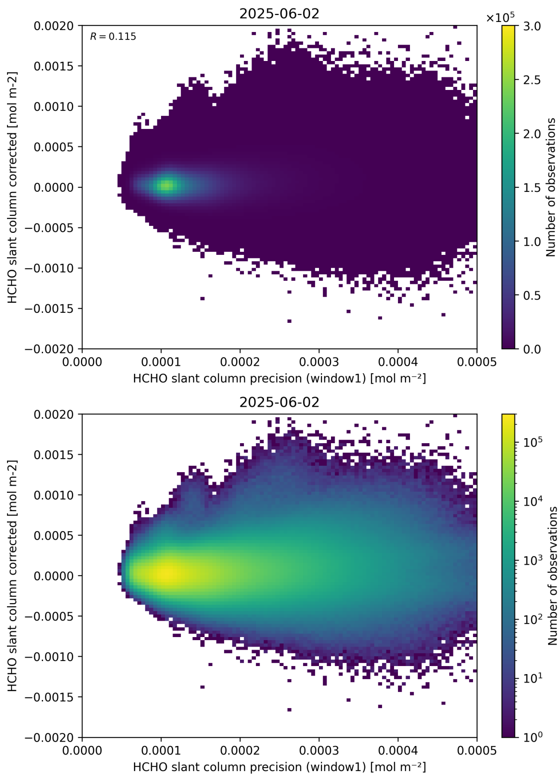
Figure 92: Scatter density plot of “HCHO slant column precision (window1)” against “HCHO slant column corrected” for 2025-06-01 to 2025-06-03.
