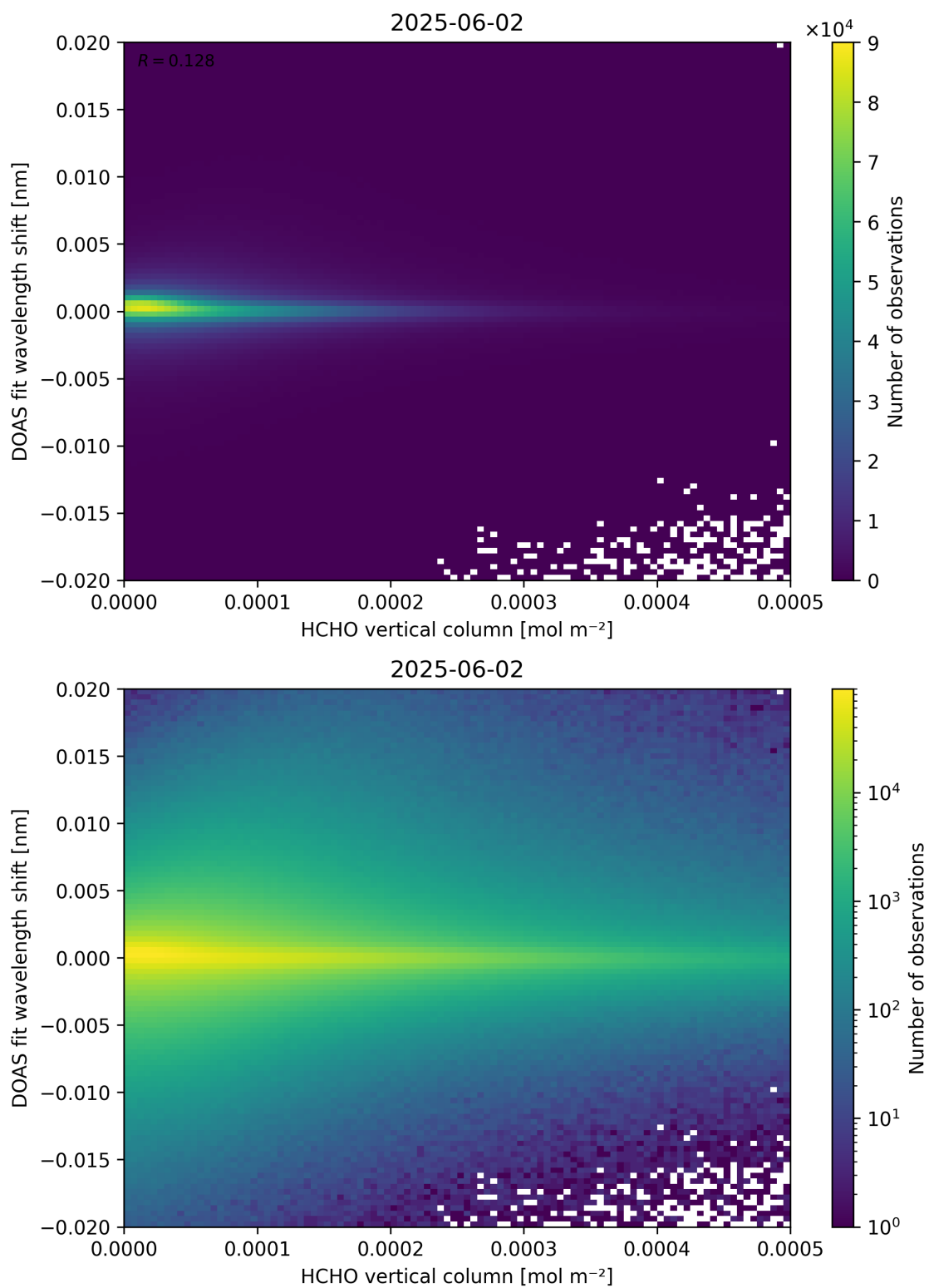
Figure 124: Scatter density plot of “HCHO vertical column” against “DOAS fit wavelength shift” for 2025-06-01 to 2025-06-03.
