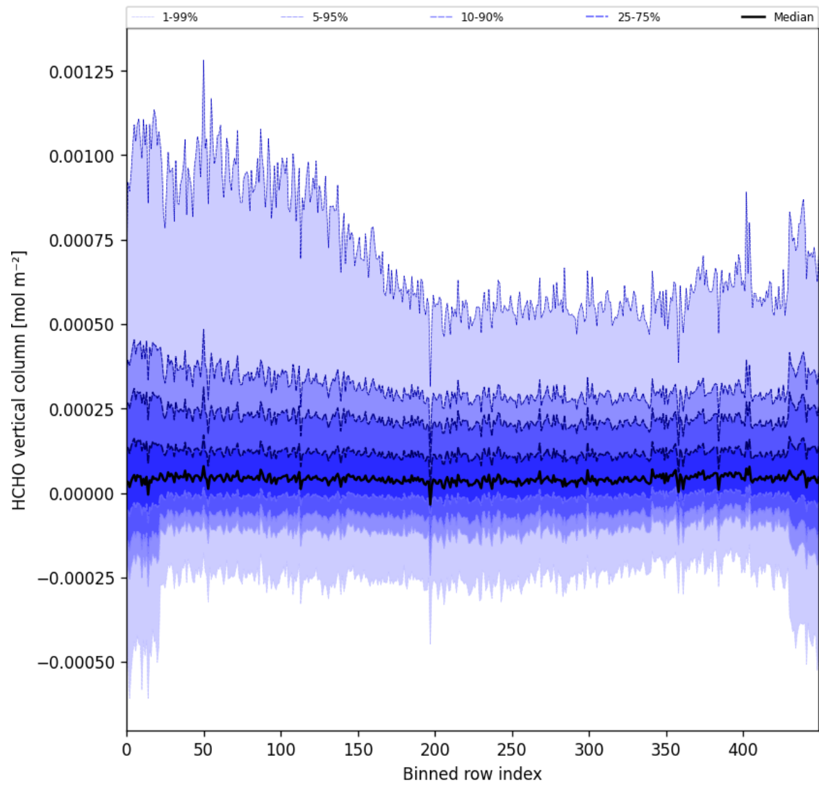
Figure 49: Along track statistics of “HCHO vertical column” for 2025-06-01 to 2025-06-03
