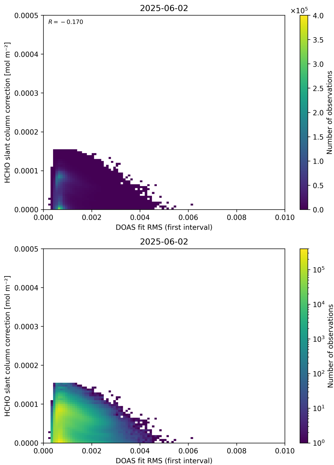
Figure 63: Scatter density plot of “DOAS fit RMS (first interval)” against “HCHO slant column correction” for 2025-06-01 to 2025-06-03.
