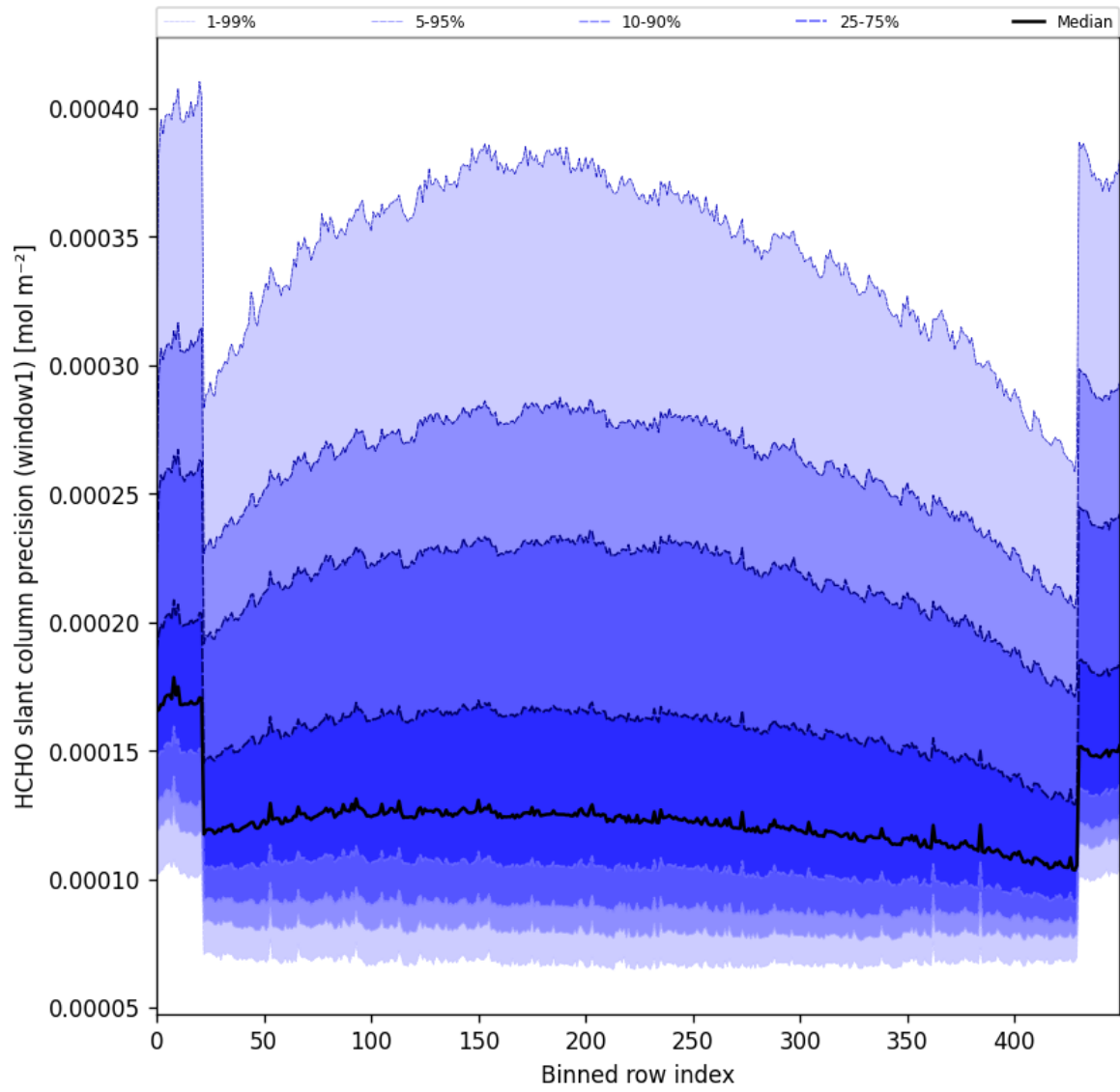
Figure 53: Along track statistics of “HCHO slant column precision (window1)” for 2025-06-01 to 2025-06-03
