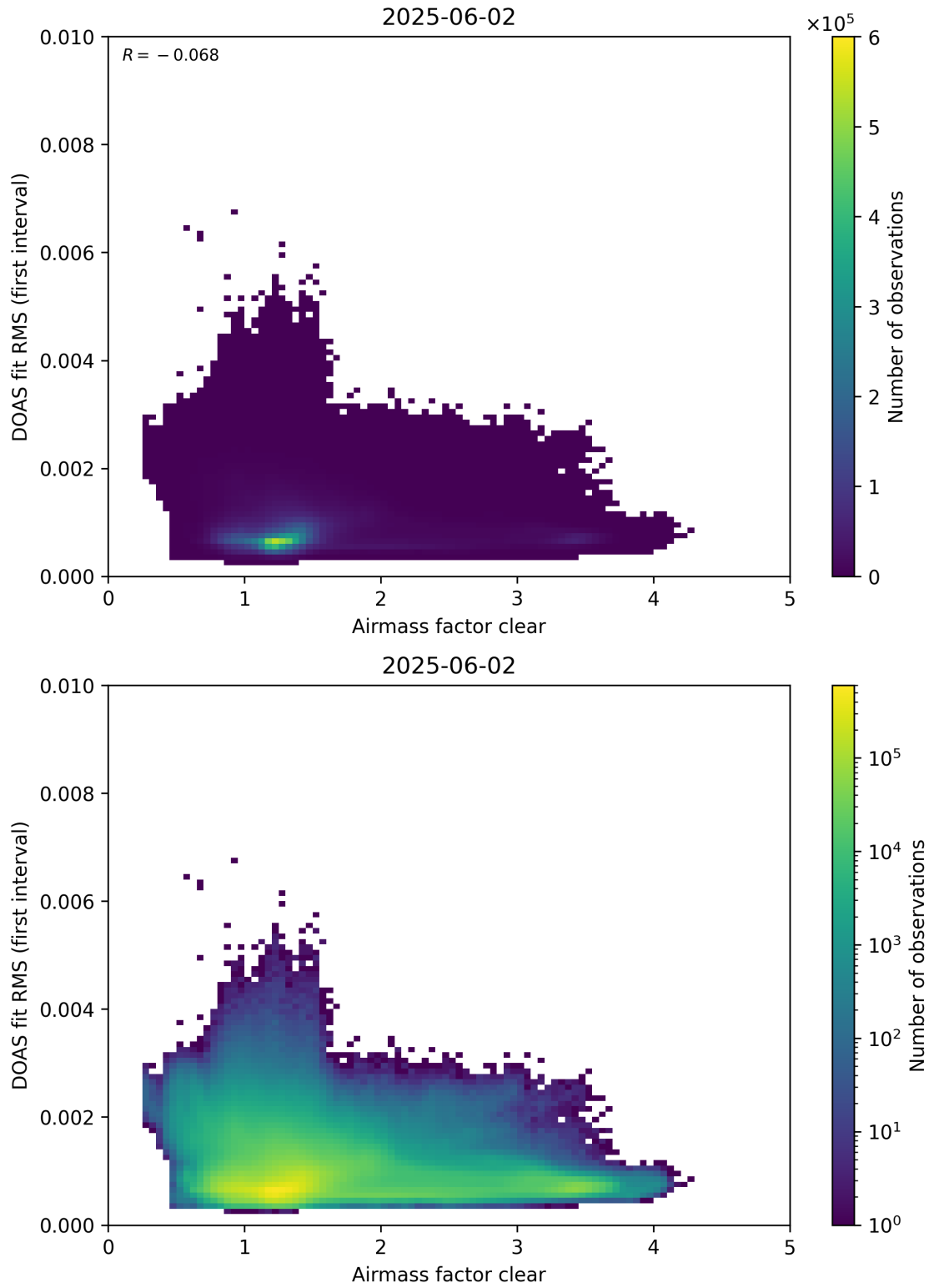
Figure 71: Scatter density plot of “Airmass factor clear” against “DOAS fit RMS (first interval)” for 2025-06-01 to 2025-06-03.
