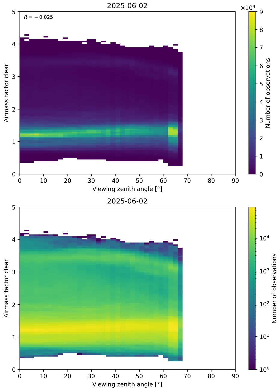
Figure 185: Scatter density plot of “Viewing zenith angle” against “Airmass factor clear” for 2025-06-01 to 2025-06-03.
