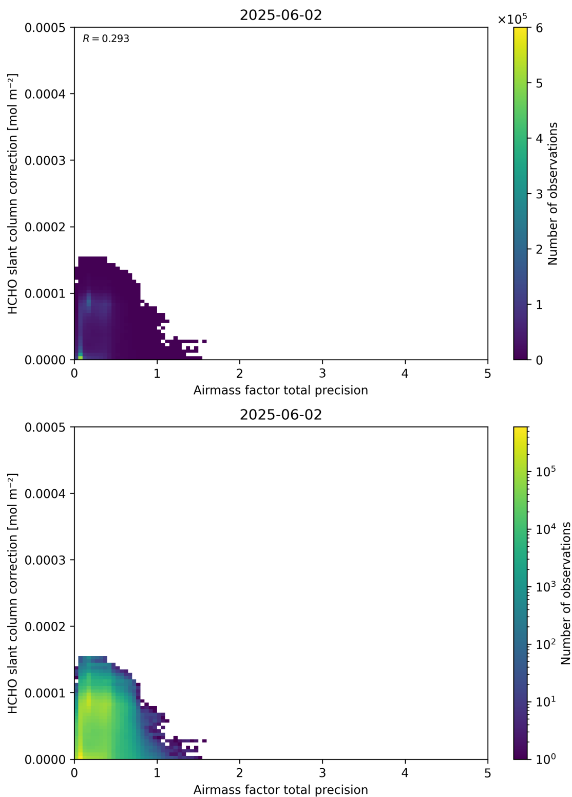
Figure 110: Scatter density plot of “Airmass factor total precision” against “HCHO slant column correction” for 2025-06-01 to 2025-06-03.
