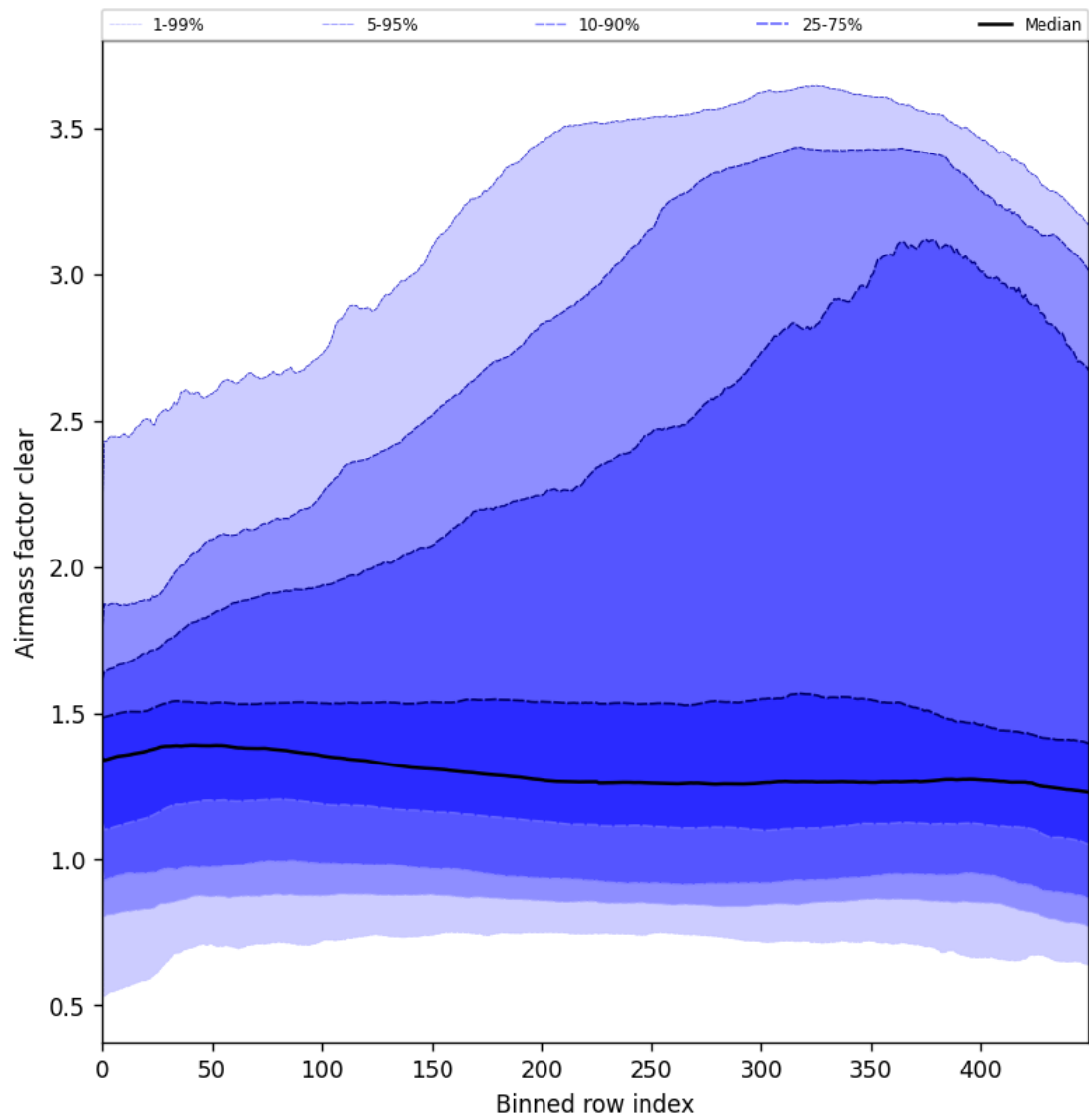
Figure 56: Along track statistics of “Air mass factor clear” for 2025-06-01 to 2025-06-03
