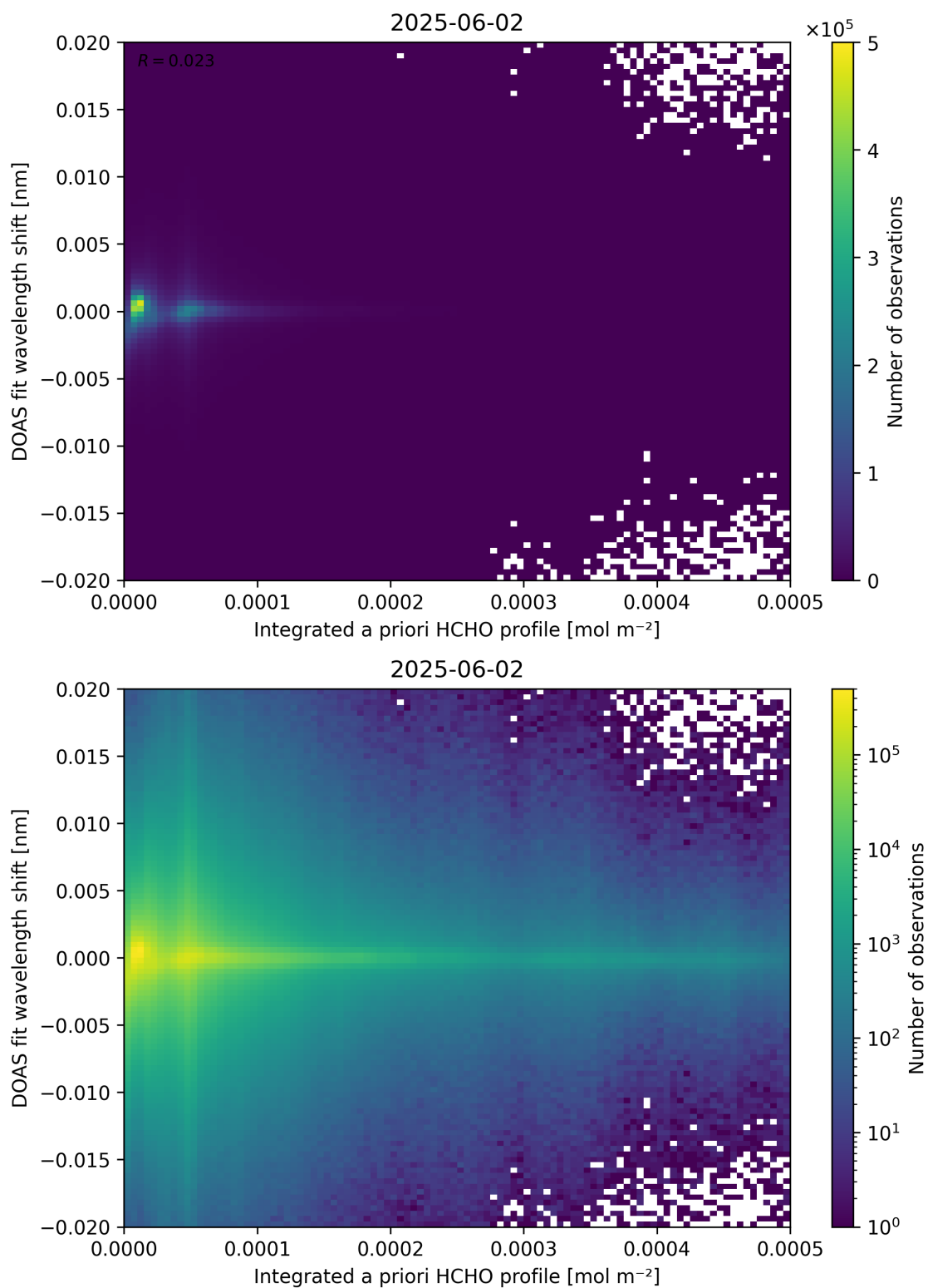
Figure 149: Scatter density plot of “Integrated a priori HCHO profile” against “DOAS fit wavelength shift” for 2025-06-01 to 2025-06-03.
