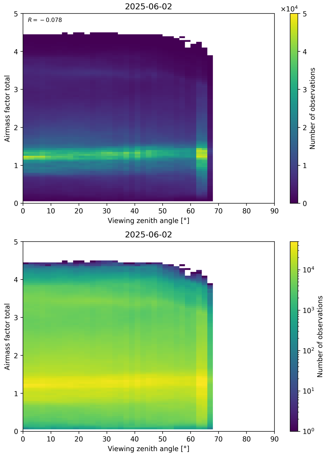
Figure 190: Scatter density plot of “Viewing zenith angle” against “Airmass factor total” for 2025-06-01 to 2025-06-03.
