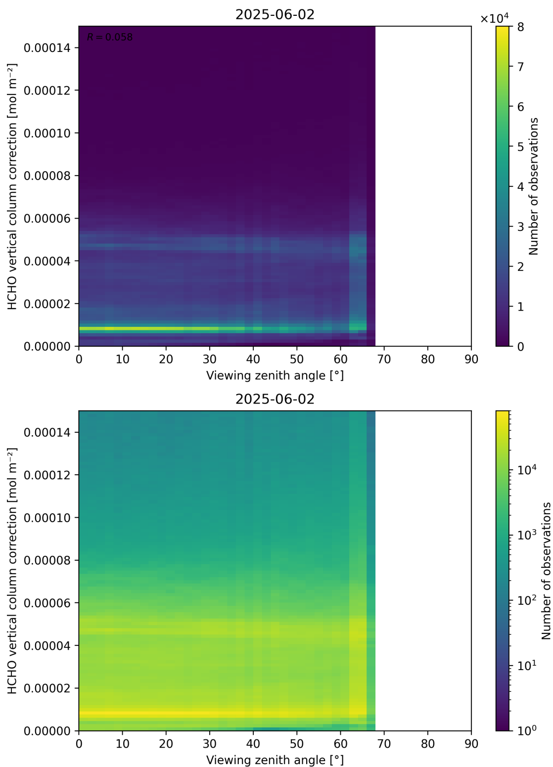
Figure 193: Scatter density plot of “Viewing zenith angle” against “HCHO vertical column correction” for 2025-06-01 to 2025-06-03.
