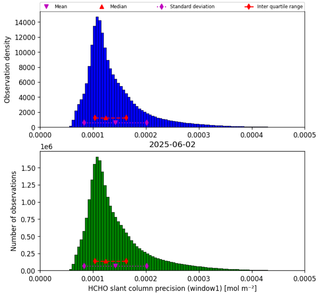
Figure 39: Histogram of “HCHO slant column precision (window1)” for 2025-06-01 to 2025-06-03
