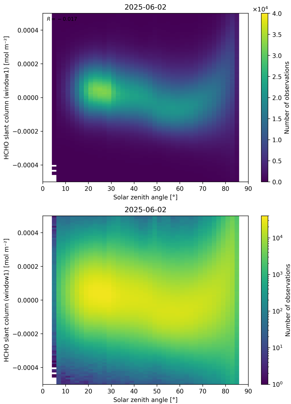
Figure 173: Scatter density plot of “Solar zenith angle” against “HCHO slant column (window1)” for 2025-06-01 to 2025-06-03.
