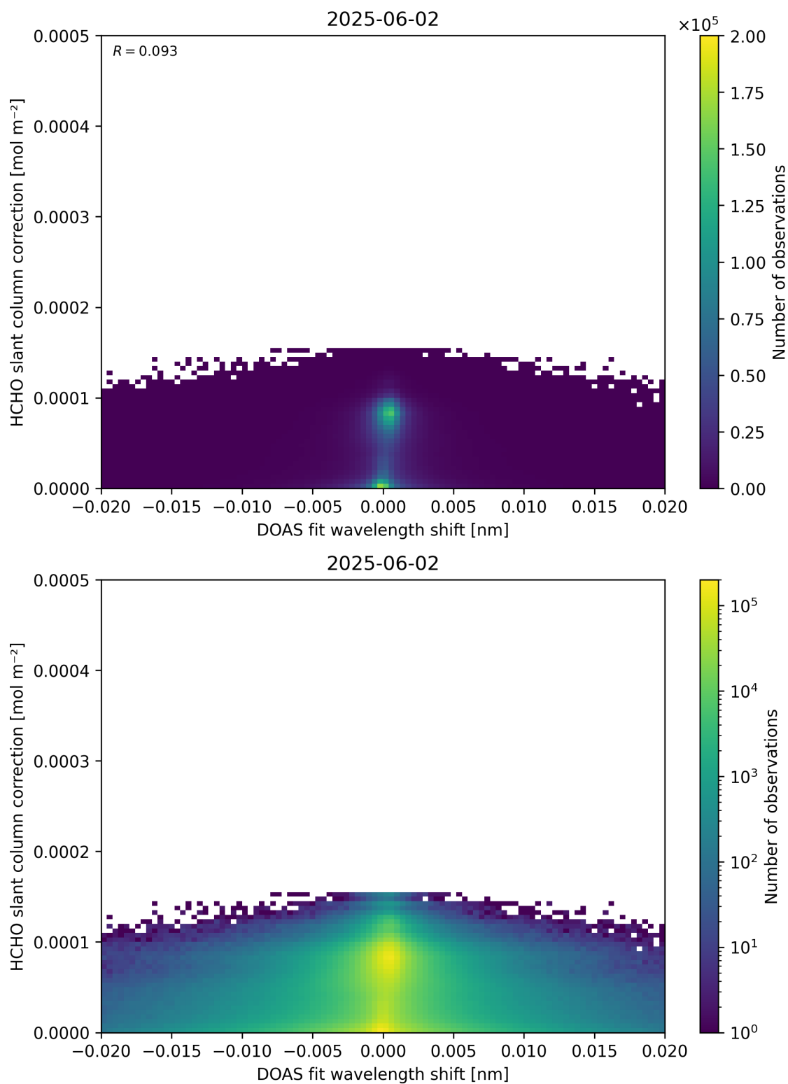
Figure 67: Scatter density plot of “DOAS fit wavelength shift” against “HCHO slant column correction” for 2025-06-01 to 2025-06-03.
