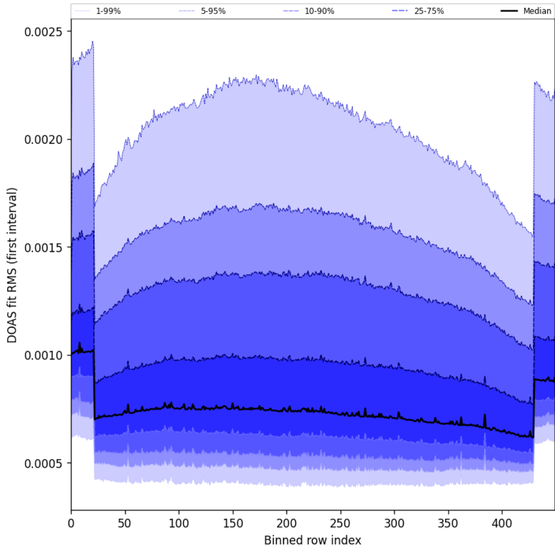
Figure 60: Along track statistics of “DOAS fit RMS (first interval)” for 2025-06-01 to 2025-06-03
