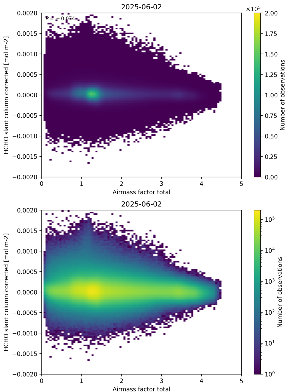
Figure 101: Scatter density plot of “Airmass factor total” against “HCHO slant column corrected” for 2025-06-01 to 2025-06-03.
