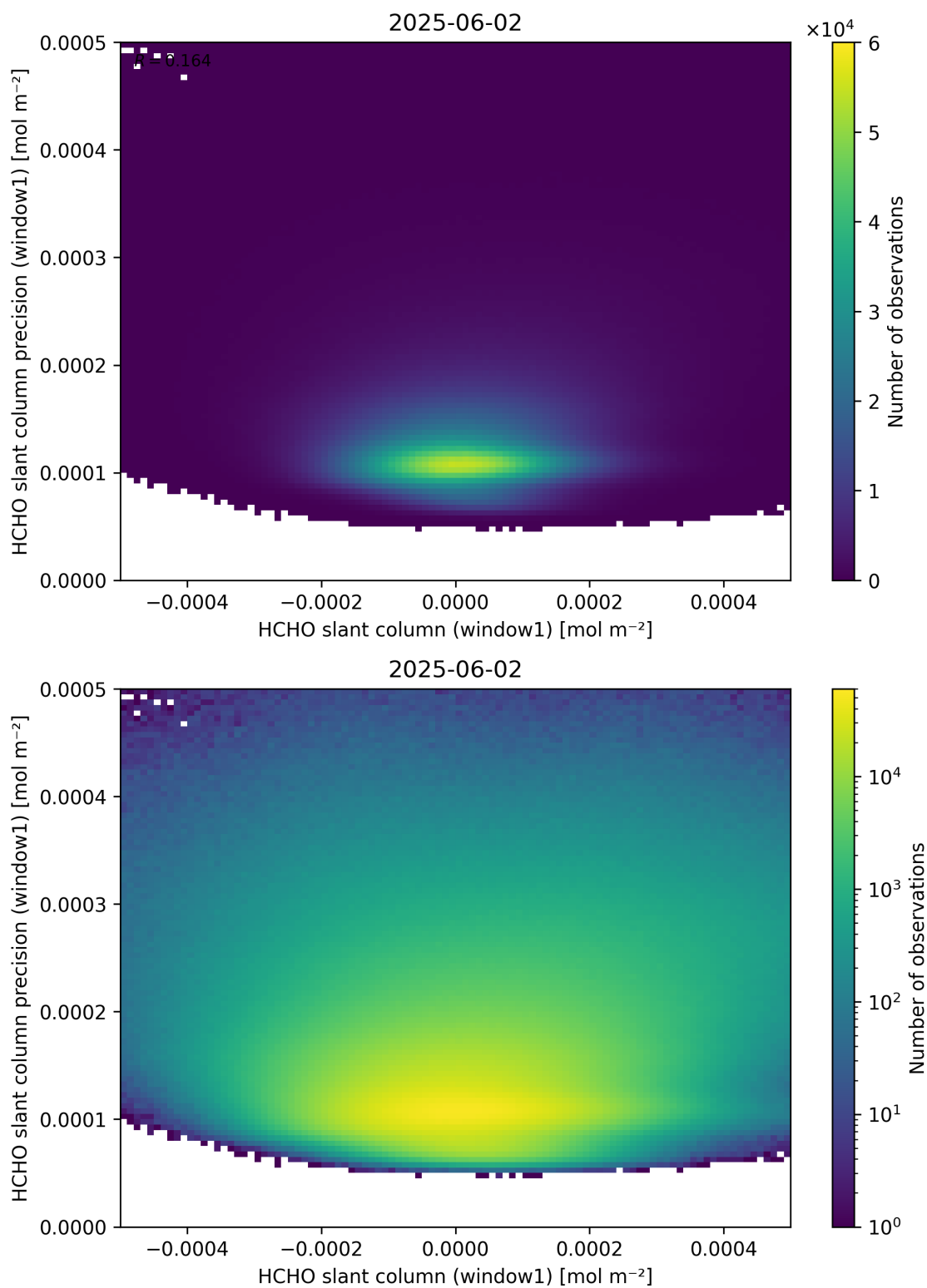
Figure 84: Scatter density plot of “HCHO slant column (window1)” against “HCHO slant column precision (window1)” for 2025-06-01 to 2025-06-03.
