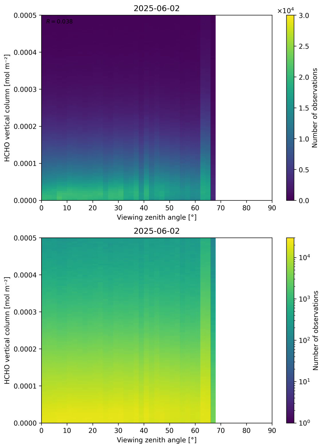
Figure 192: Scatter density plot of “Viewing zenith angle” against “HCHO vertical column” for 2025-06-01 to 2025-06-03.
