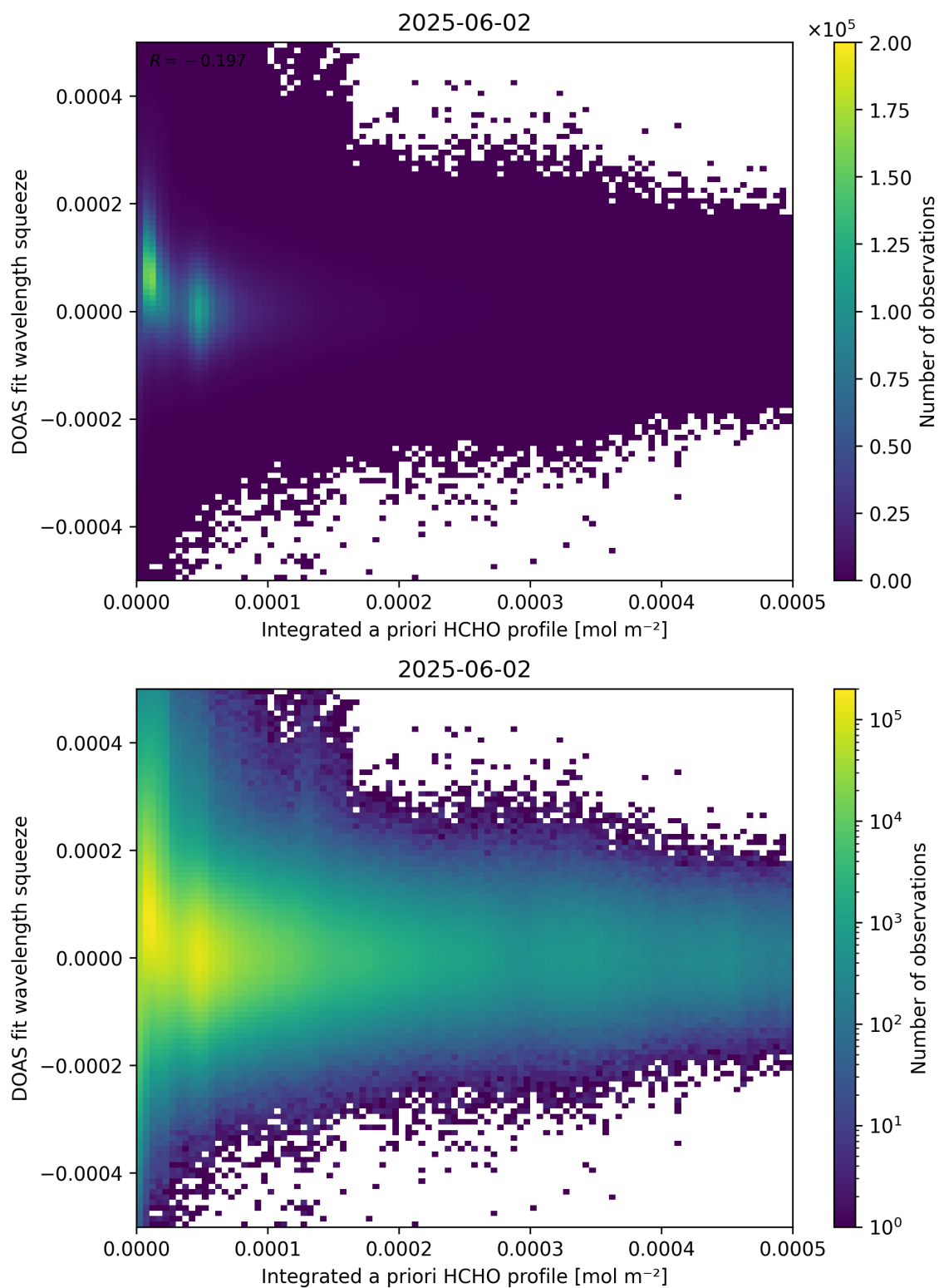
Figure 150: Scatter density plot of “Integrated a priori HCHO profile” against “DOAS fit wavelength squeeze” for 2025-06-01 to 2025-06-03.
