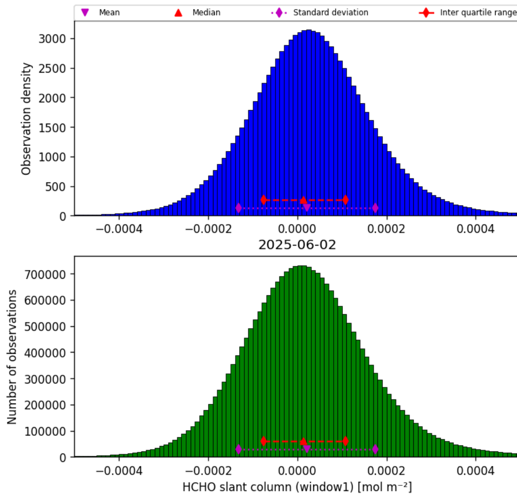
Figure 38: Histogram of “HCHO slant column (window1)” for 2025-06-01 to 2025-06-03
