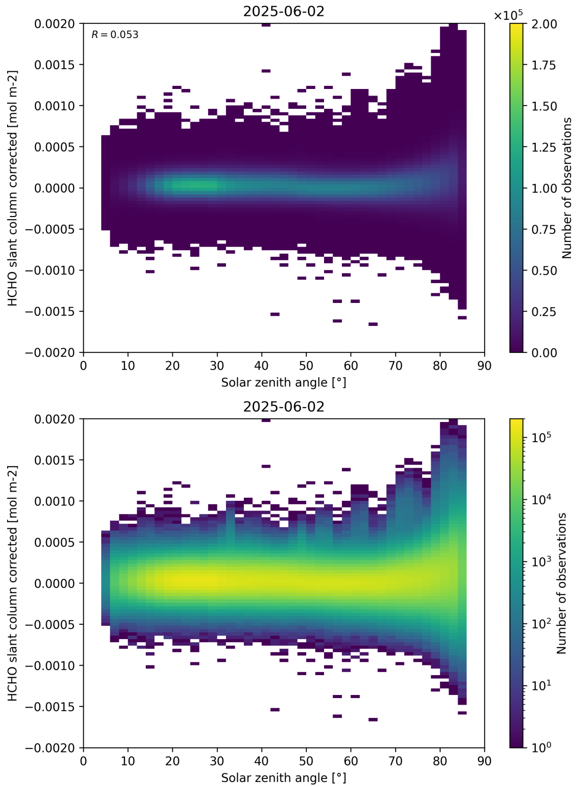
Figure 171: Scatter density plot of “Solar zenith angle” against “HCHO slant column corrected” for 2025-06-01 to 2025-06-03.
