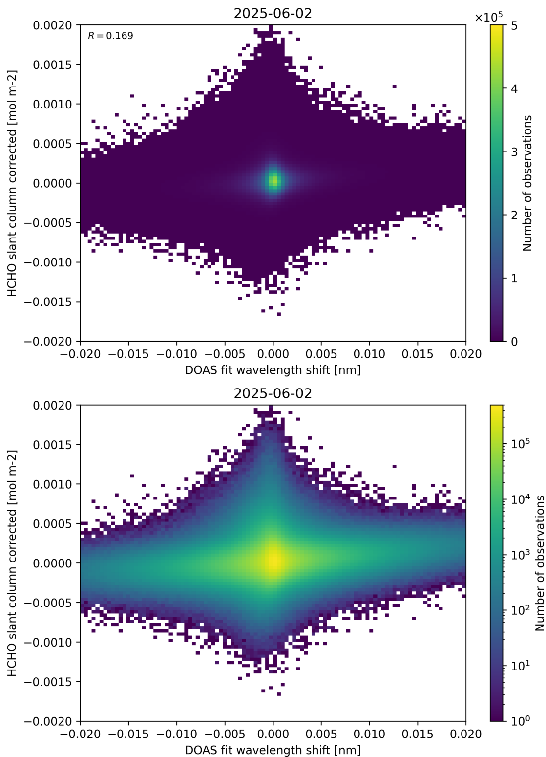
Figure 66: Scatter density plot of “DOAS fit wavelength shift” against “HCHO slant column corrected” for 2025-06-01 to 2025-06-03.
