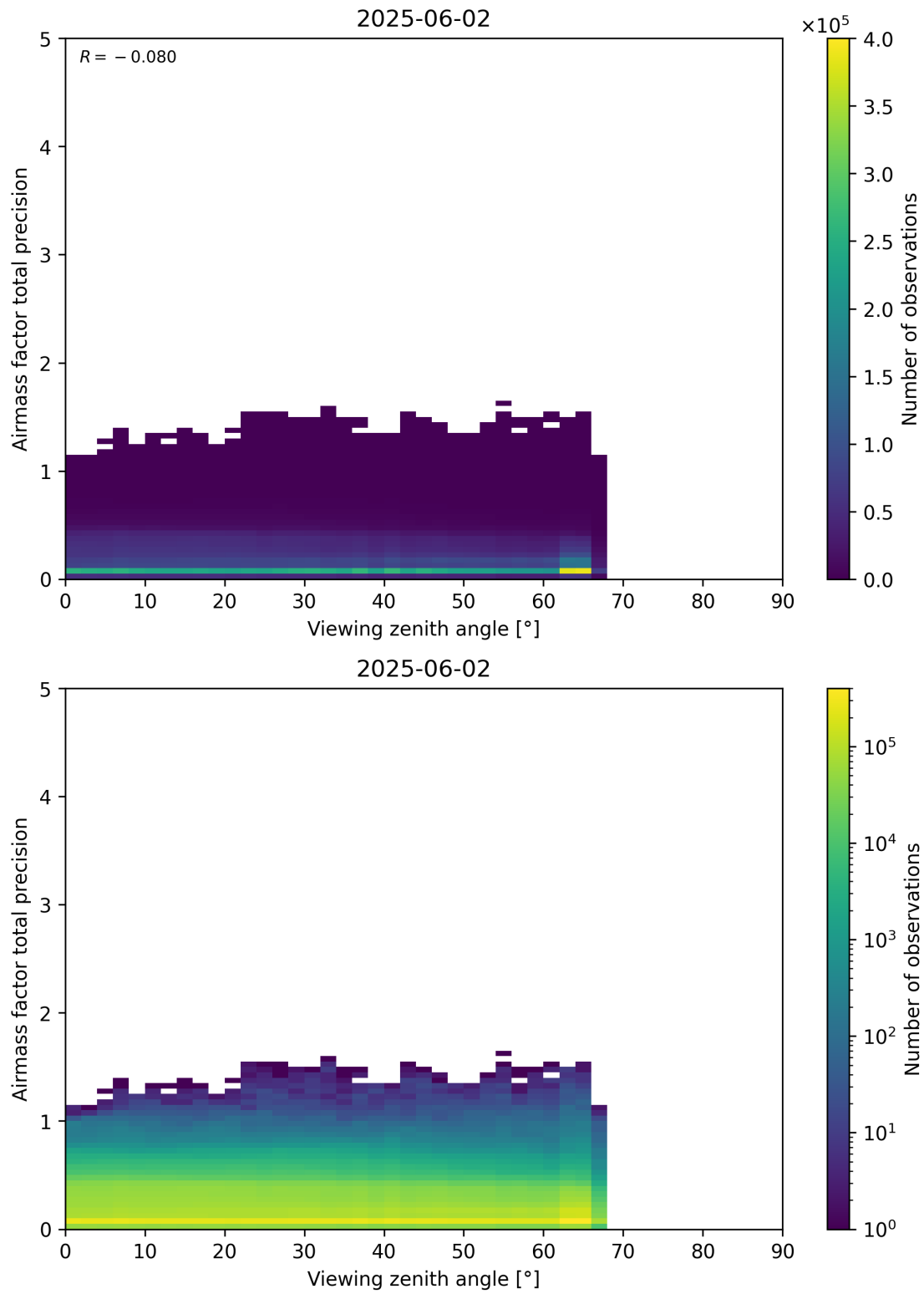
Figure 191: Scatter density plot of “Viewing zenith angle” against “Airmass factor total precision” for 2025-06-01 to 2025-06-03.
