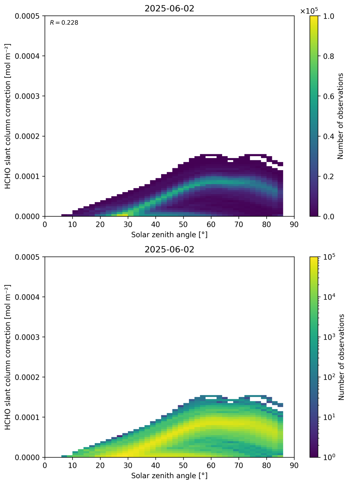
Figure 172: Scatter density plot of “Solar zenith angle” against “HCHO slant column correction” for 2025-06-01 to 2025-06-03.
