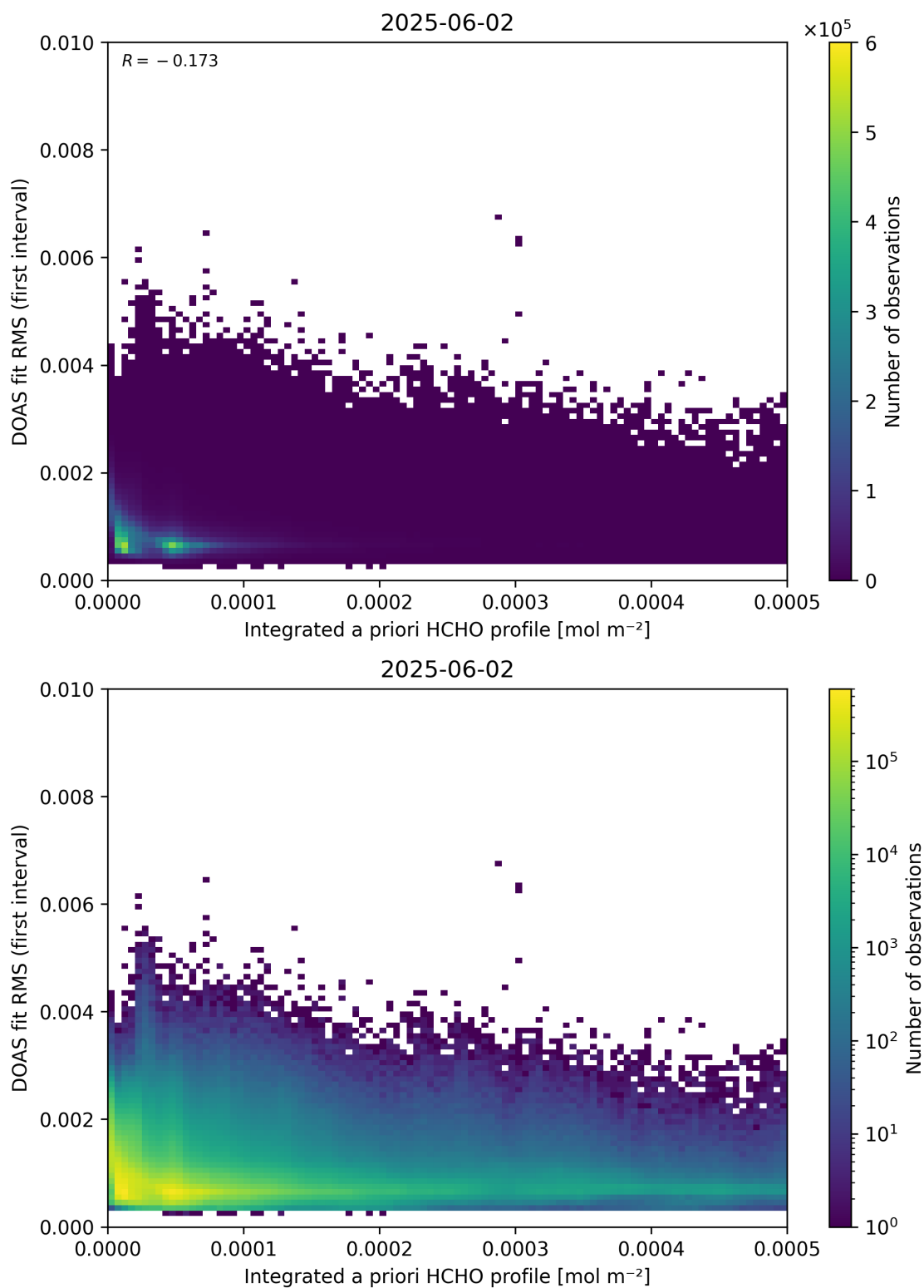
Figure 148: Scatter density plot of “Integrated a priori HCHO profile” against “DOAS fit RMS (first interval)” for 2025-06-01 to 2025-06-03.
