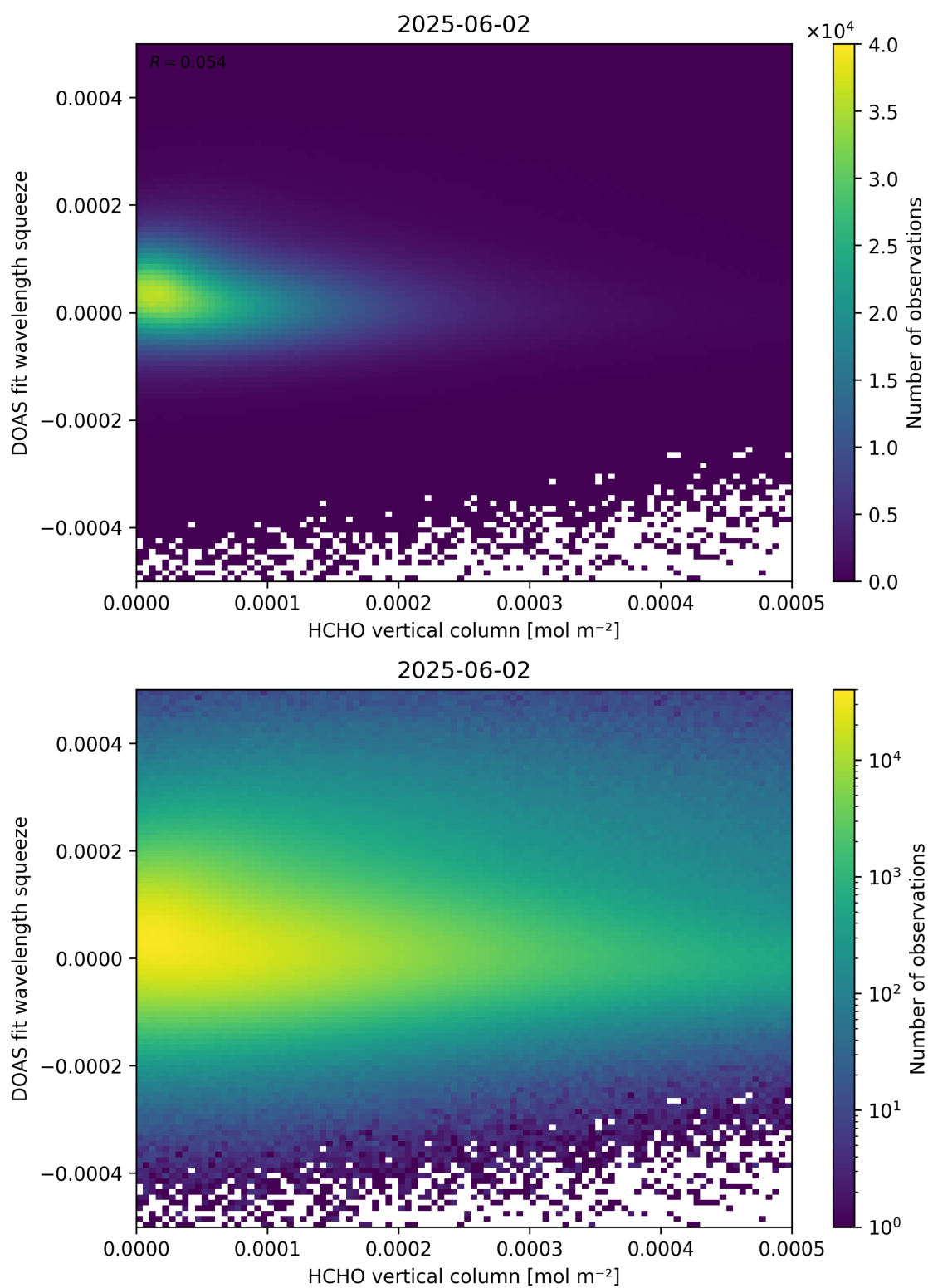
Figure 125: Scatter density plot of “HCHO vertical column” against “DOAS fit wavelength squeeze” for 2025-06-01 to 2025-06-03.
