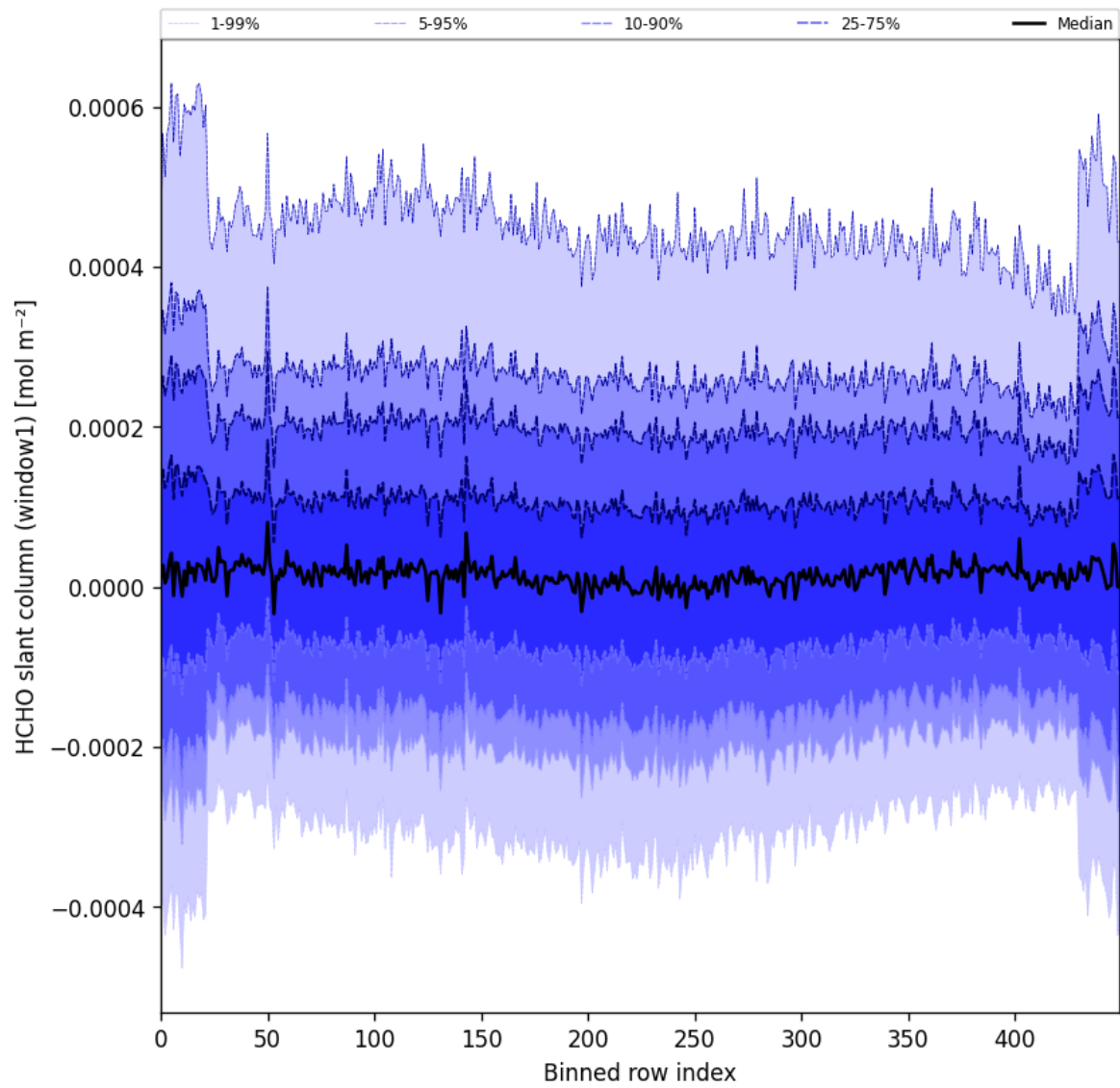
Figure 52: Along track statistics of "HCHO slant column (window1)" for 2025-06-01 to 2025-06-03
