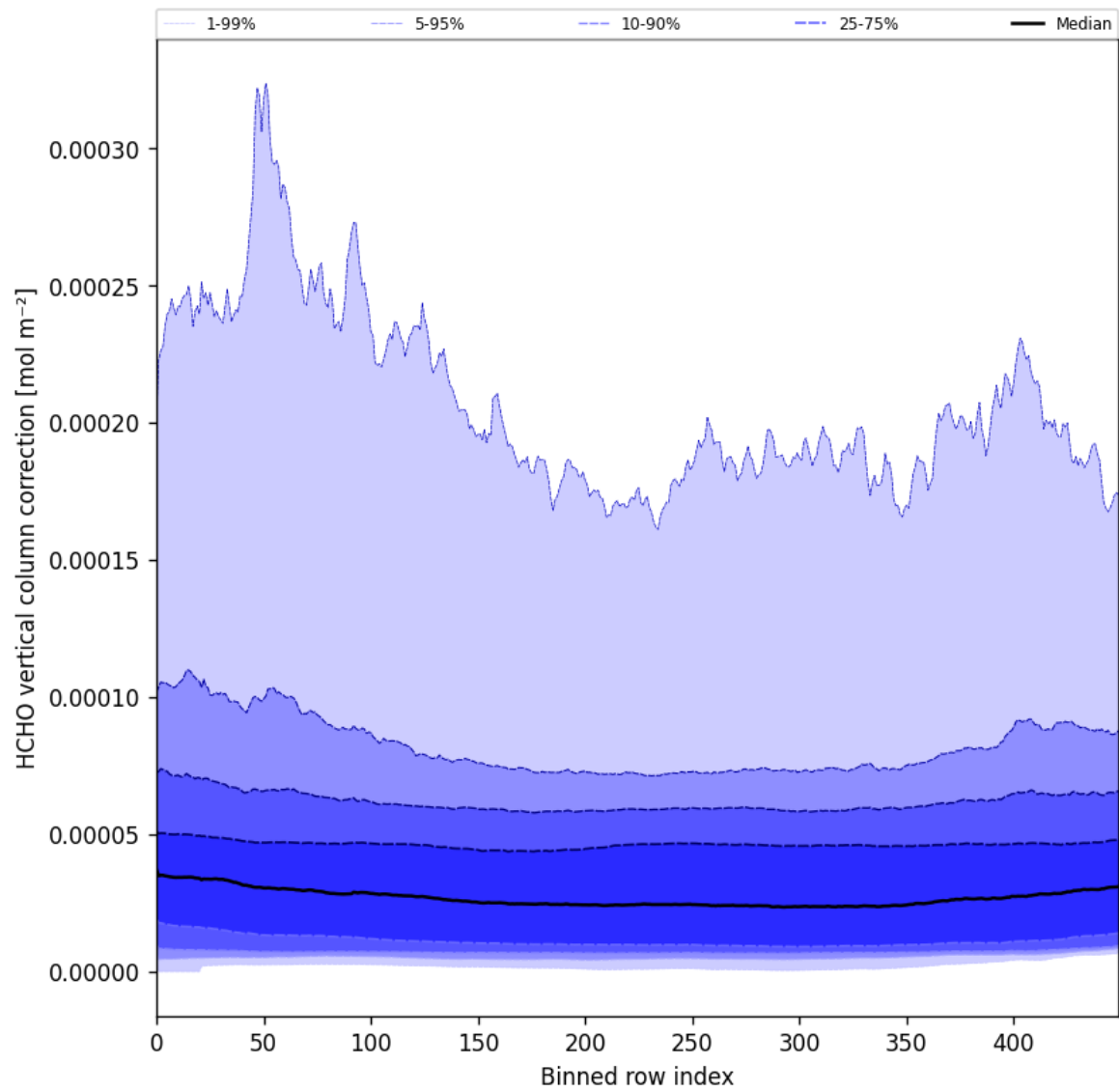
Figure 51: Along track statistics of “HCHO vertical column correction” for 2025-06-01 to 2025-06-03
