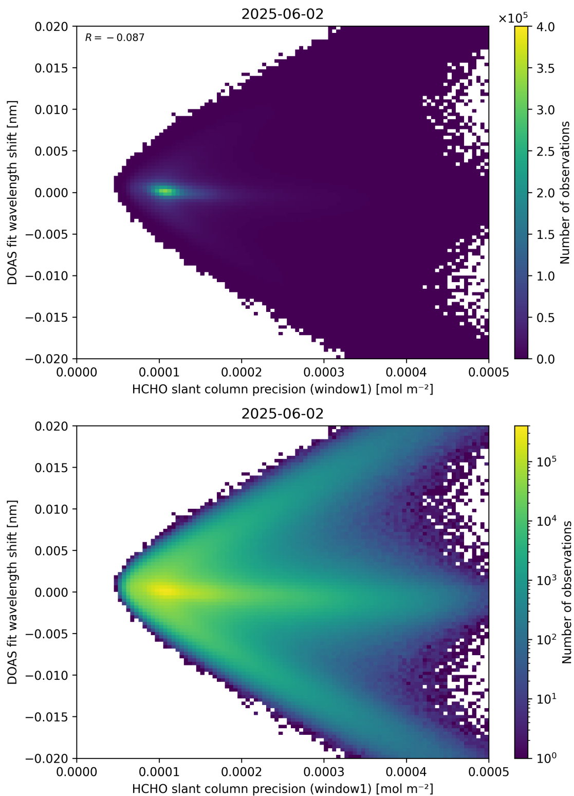
Figure 89: Scatter density plot of “HCHO slant column precision (window1)” against “DOAS fit wavelength shift” for 2025-06-01 to 2025-06-03.
