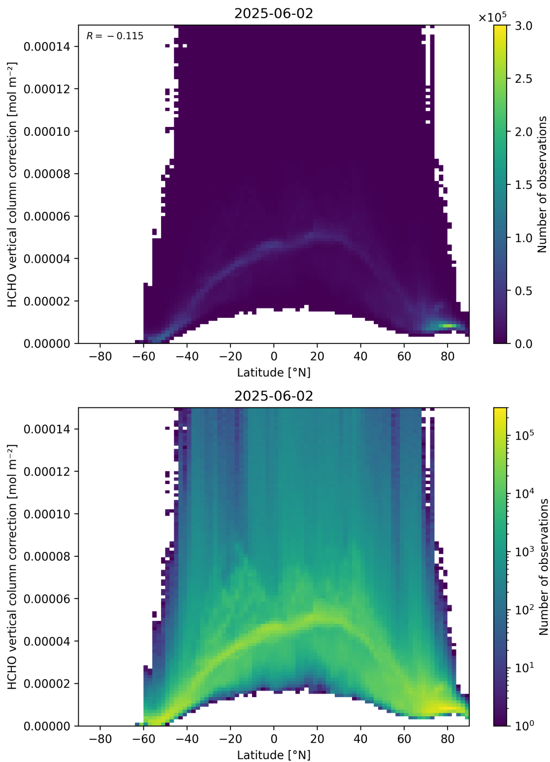
Figure 164: Scatter density plot of “Latitude” against “HCHO vertical column correction” for 2025-06-01 to 2025-06-03.
