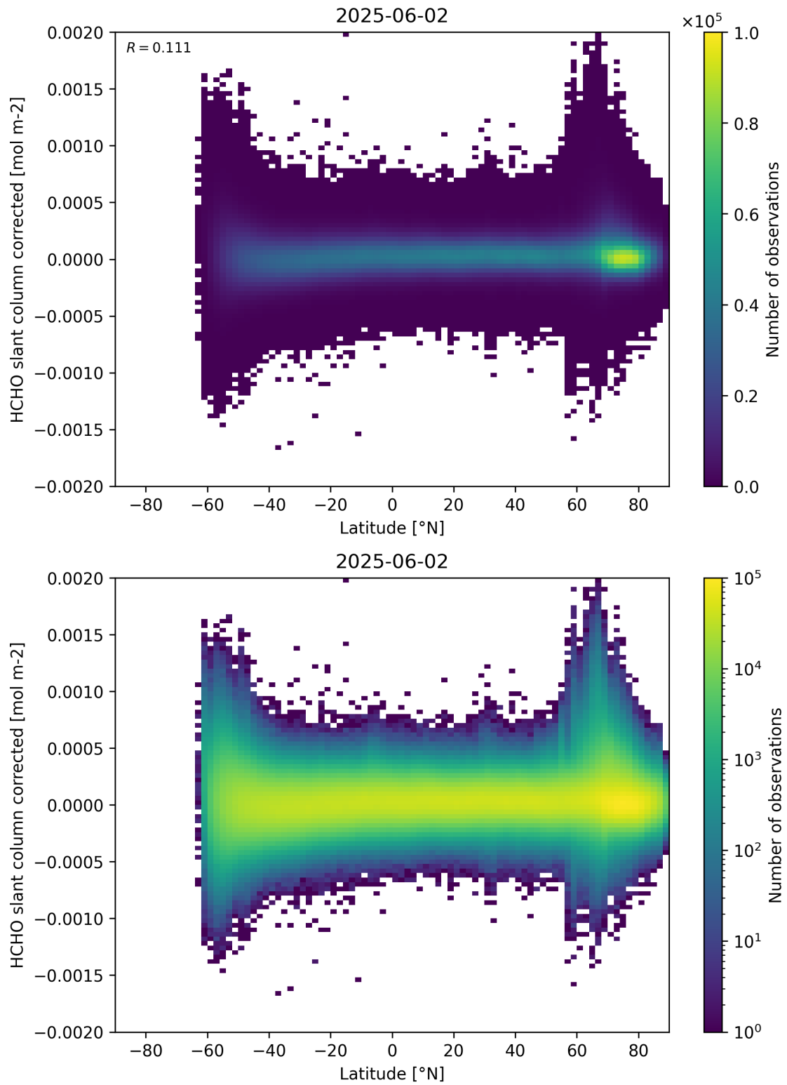
Figure 157: Scatter density plot of “Latitude” against “HCHO slant column corrected” for 2025-06-01 to 2025-06-03.
