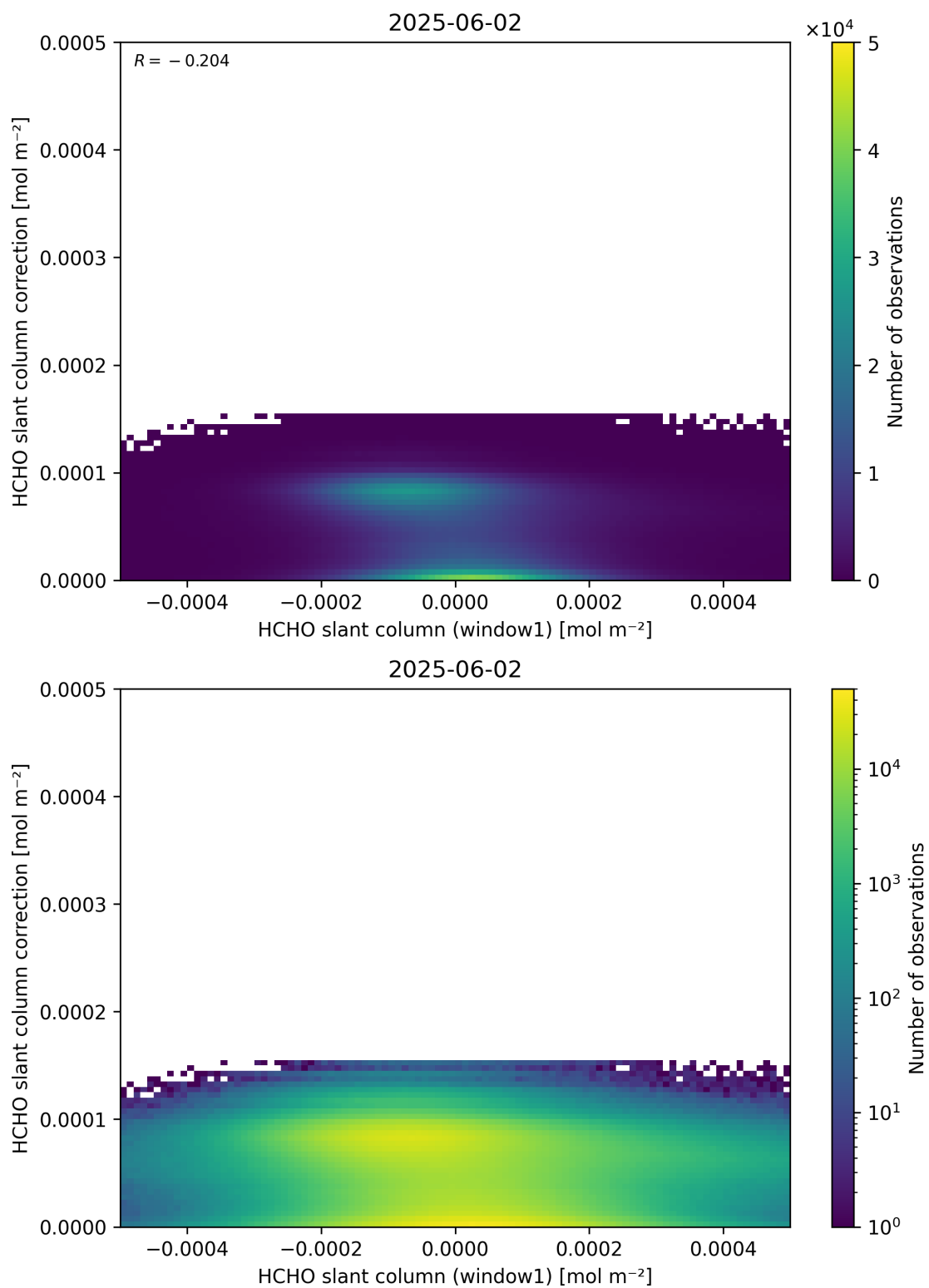
Figure 83: Scatter density plot of “HCHO slant column (window1)” against “HCHO slant column correction” for 2025-06-01 to 2025-06-03.
