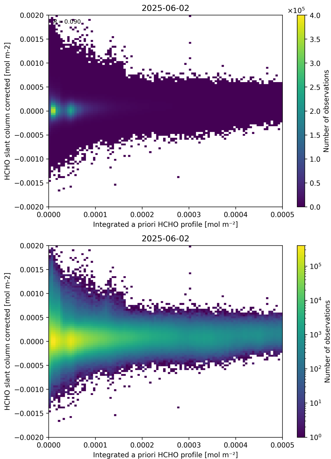
Figure 151: Scatter density plot of “Integrated a priori HCHO profile” against “HCHO slant column corrected” for 2025-06-01 to 2025-06-03.
