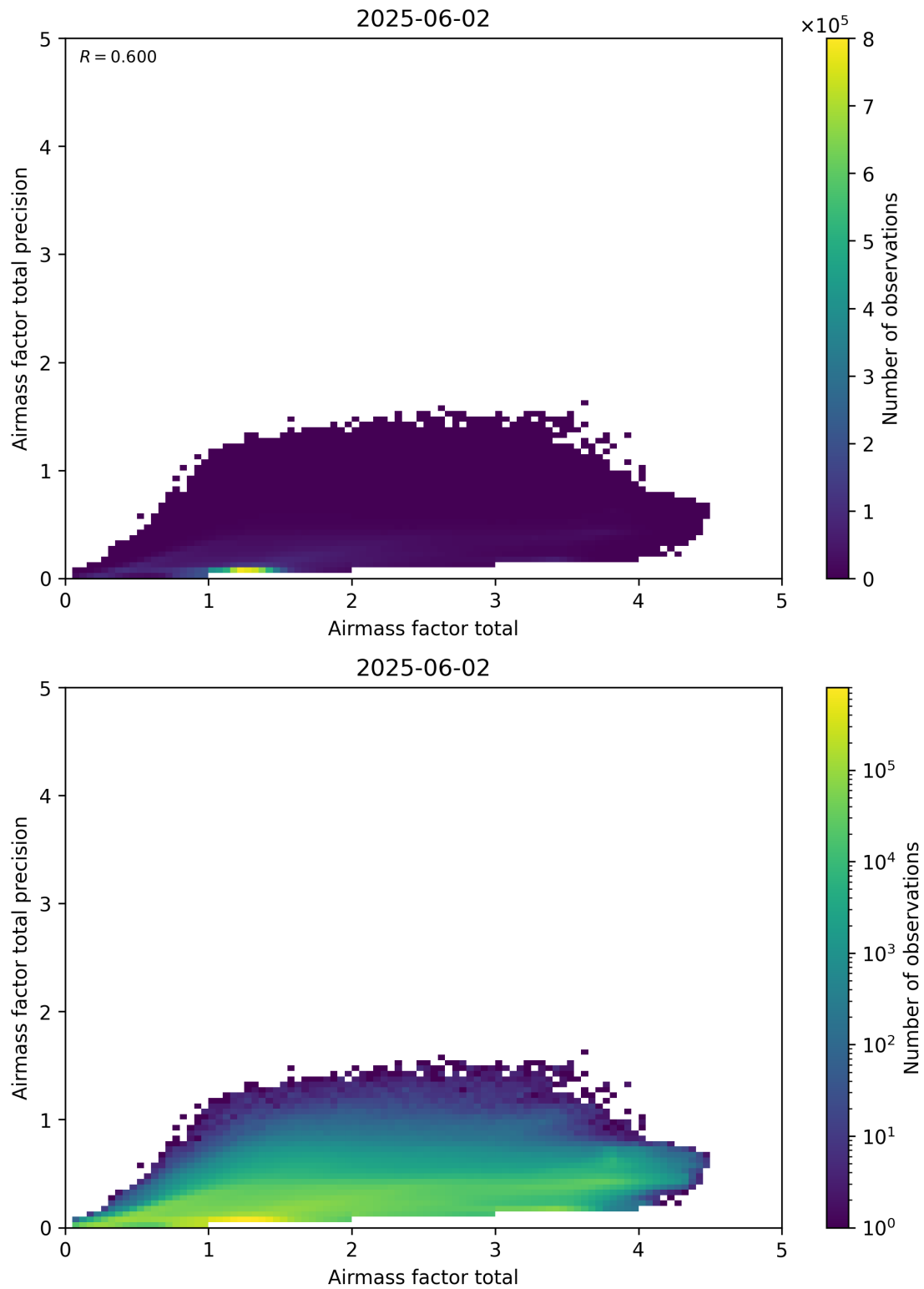
Figure 103: Scatter density plot of “Airmass factor total” against “Airmass factor total precision” for 2025-06-01 to 2025-06-03.
