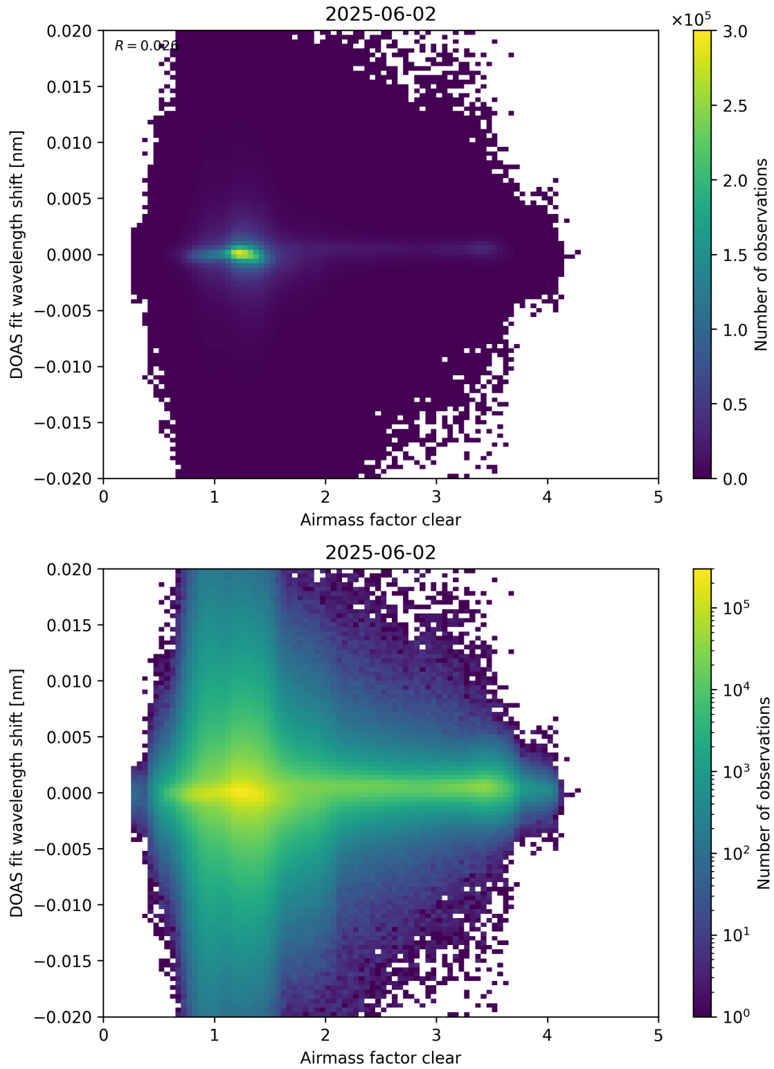
Figure 72: Scatter density plot of “Airmass factor clear” against “DOAS fit wavelength shift” for 2025-06-01 to 2025-06-03.
