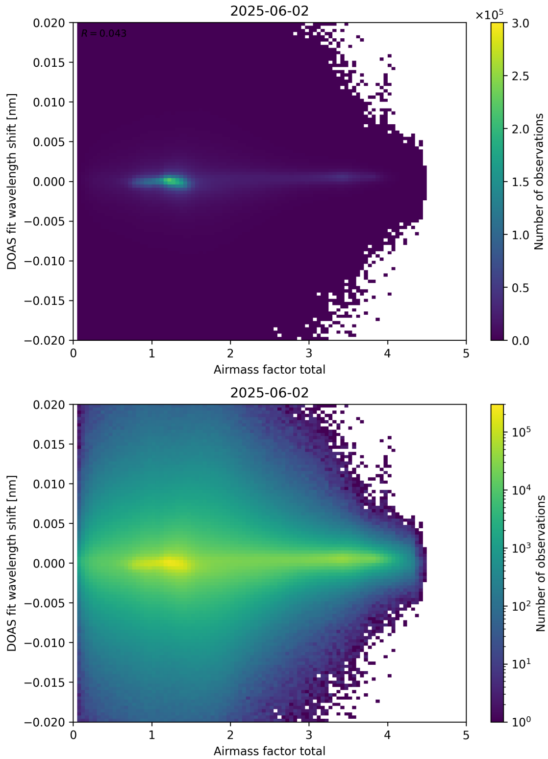
Figure 98: Scatter density plot of “Airmass factor total” against “DOAS fit wavelength shift” for 2025-06-01 to 2025-06-03.
