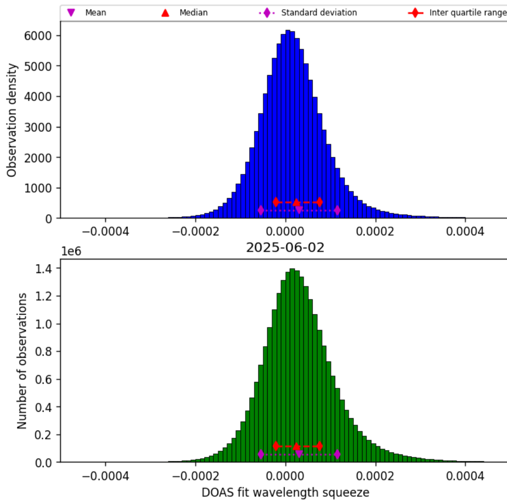
Figure 45: Histogram of “DOAS fit wavelength squeeze” for 2025-06-01 to 2025-06-03
