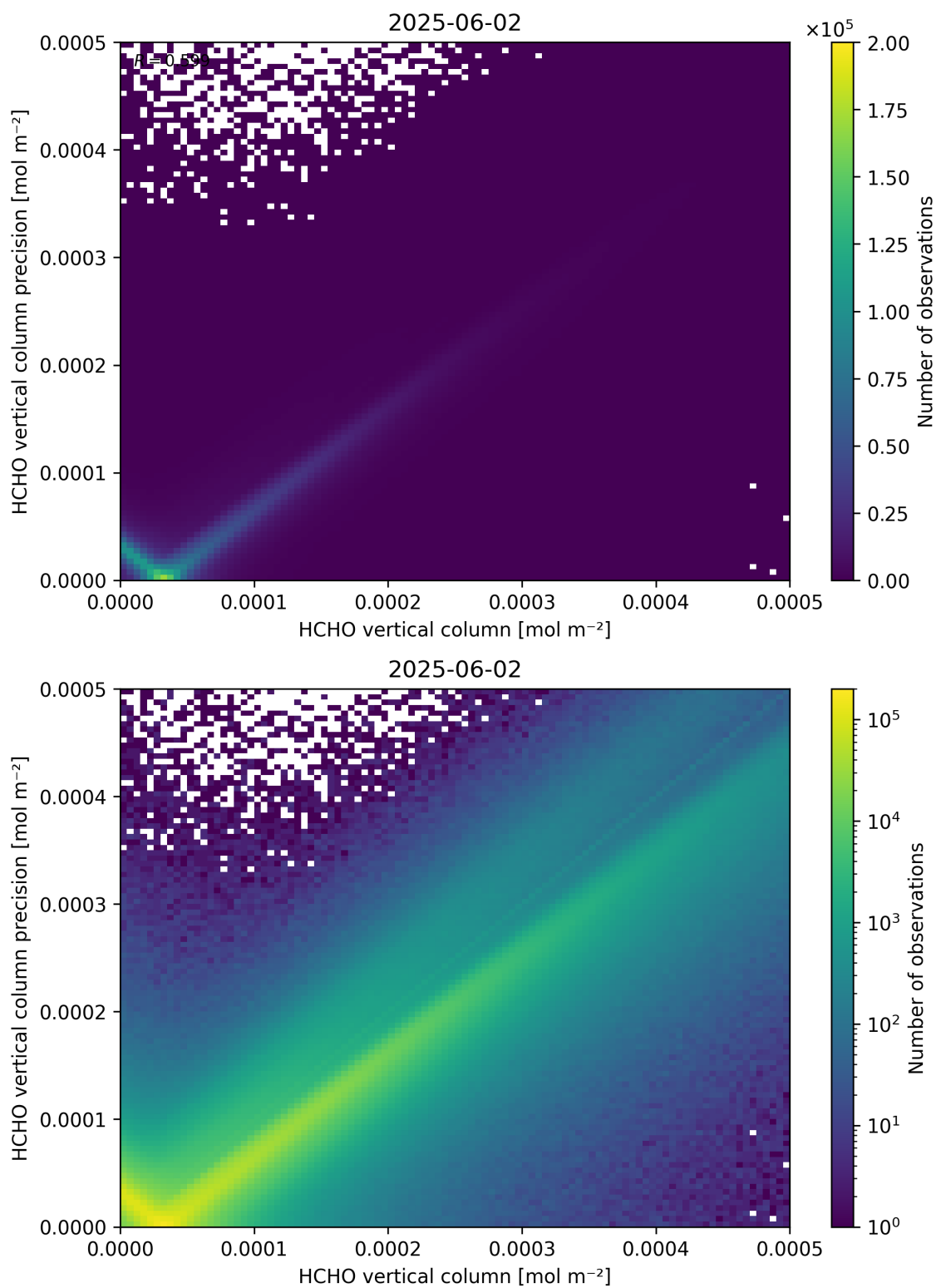
Figure 134: Scatter density plot of “HCHO vertical column” against “HCHO vertical column precision” for 2025-06-01 to 2025-06-03.
