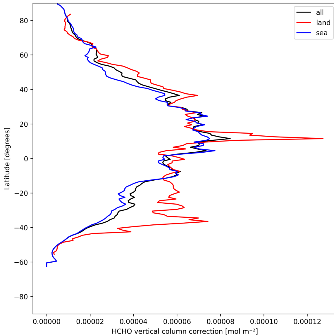
Figure 23: Zonal average of “HCHO vertical column correction” for 2025-06-01 to 2025-06-03.
