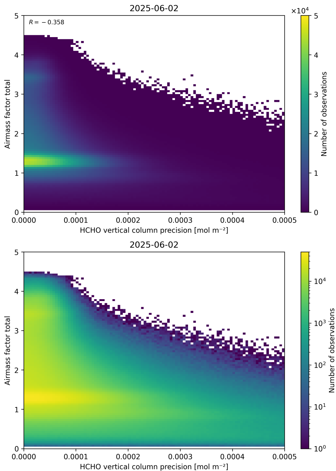
Figure 144: Scatter density plot of “HCHO vertical column precision” against “Airmass factor total” for 2025-06-01 to 2025-06-03.
