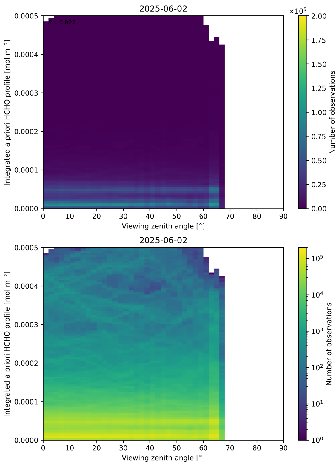
Figure 195: Scatter density plot of “Viewing zenith angle” against “Integrated a priori HCHO profile” for 2025-06-01 to 2025-06-03.
