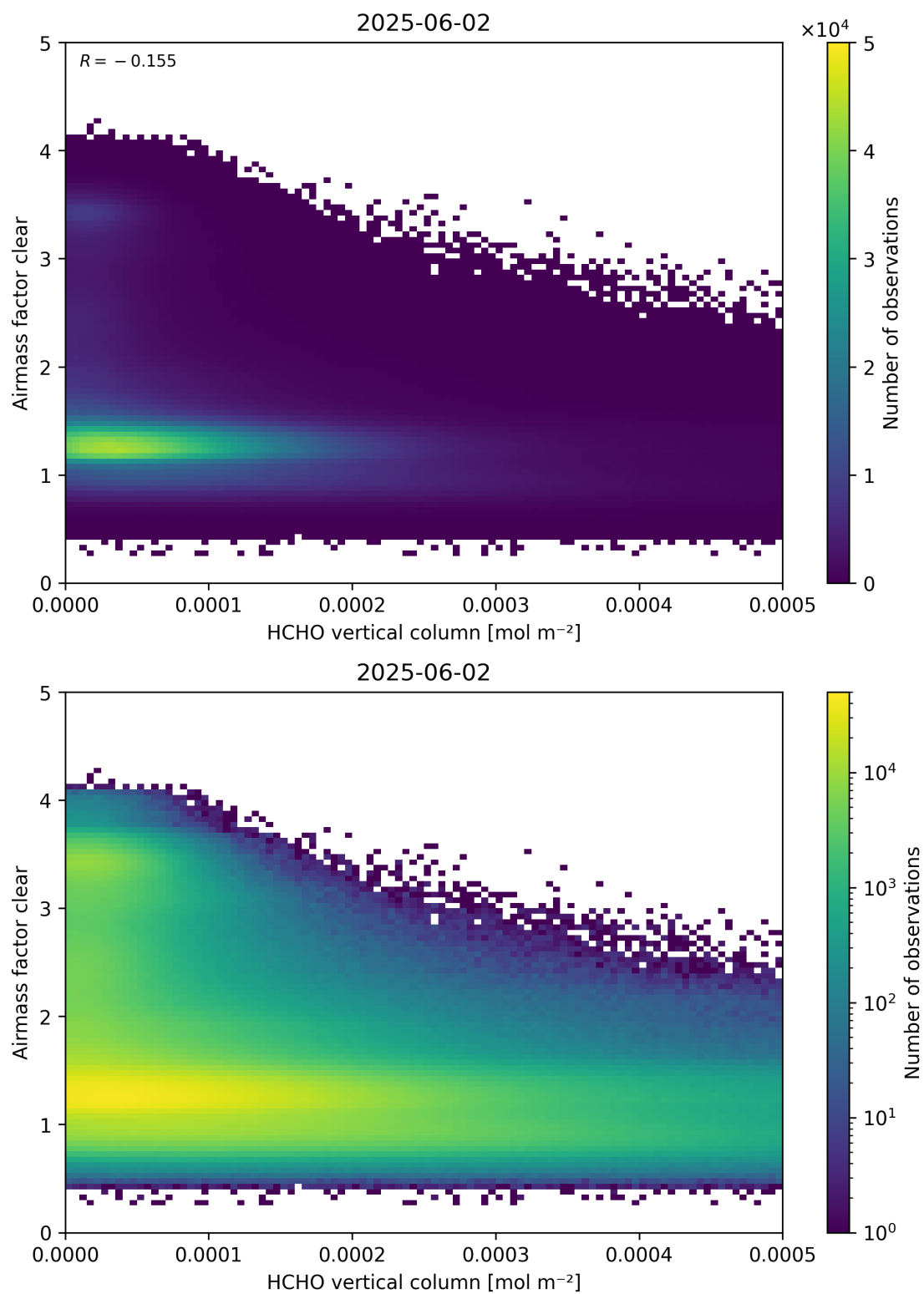
Figure 126: Scatter density plot of “HCHO vertical column” against “Airmass factor clear” for 2025-06-01 to 2025-06-03.
