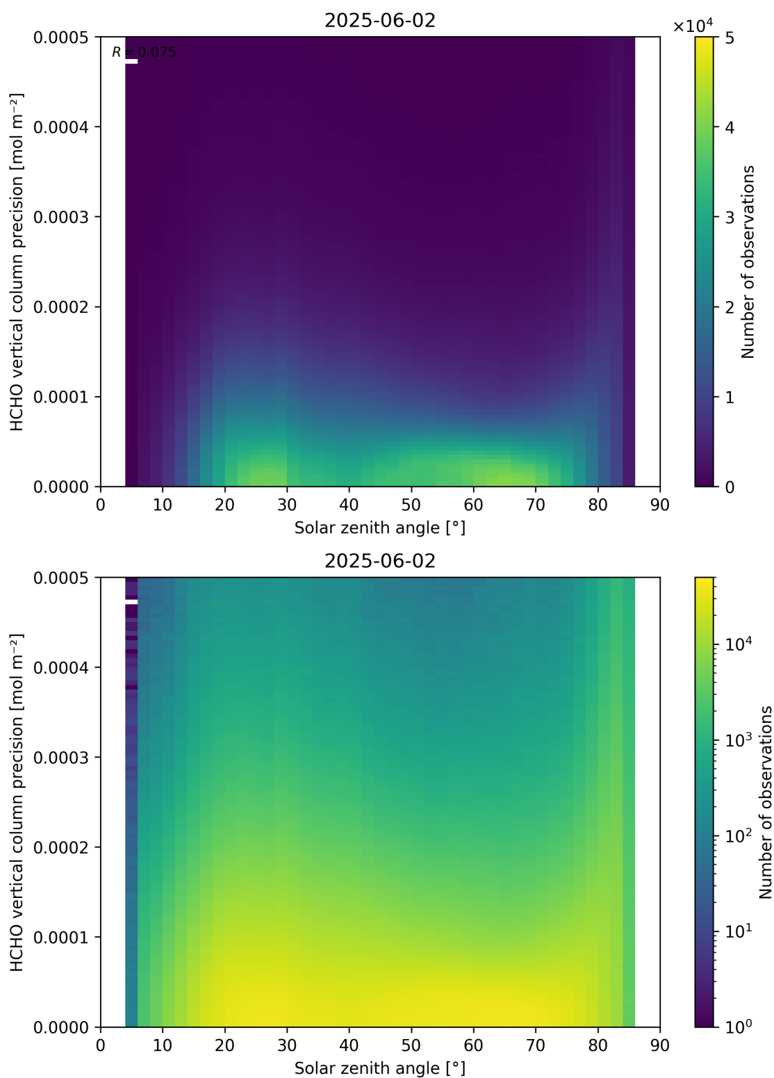
Figure 179: Scatter density plot of “Solar zenith angle” against “HCHO vertical column precision” for 2025-06-01 to 2025-06-03.
