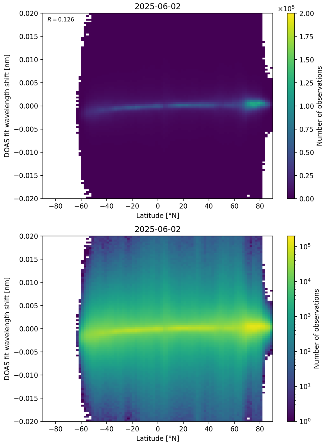
Figure 154: Scatter density plot of “Latitude” against “DOAS fit wavelength shift” for 2025-06-01 to 2025-06-03.
