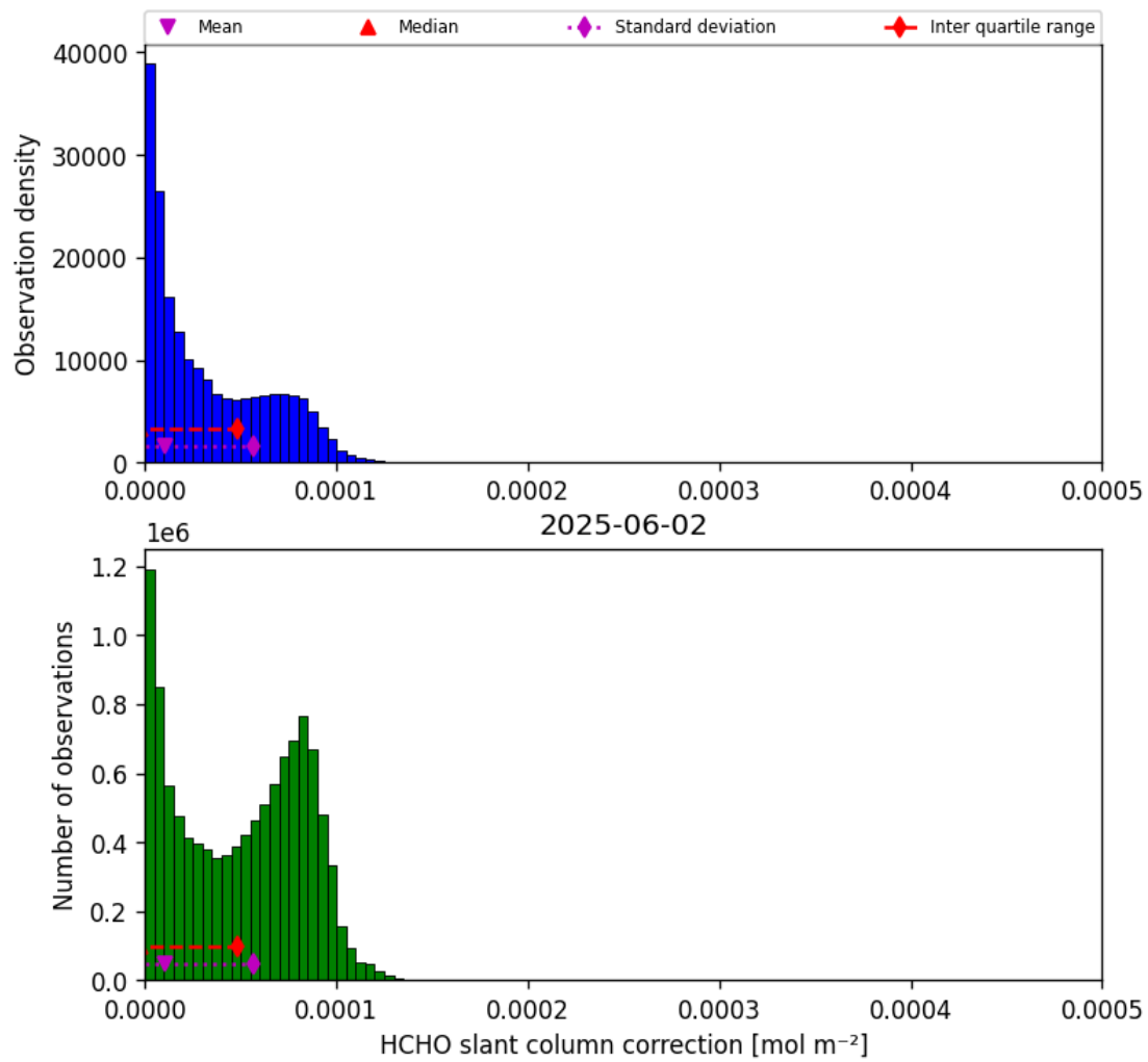
Figure 47: Histogram of “HCHO slant column correction” for 2025-06-01 to 2025-06-03
