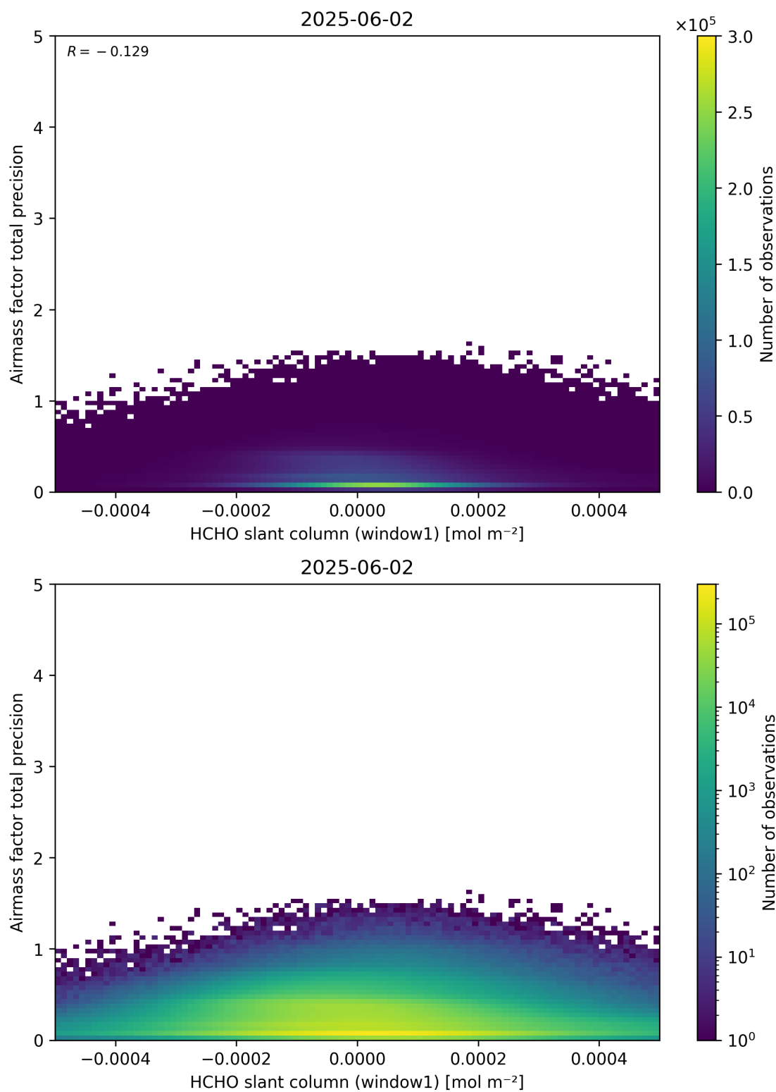
Figure 86: Scatter density plot of “HCHO slant column (window1)” against “Airmass factor total precision” for 2025-06-01 to 2025-06-03.
