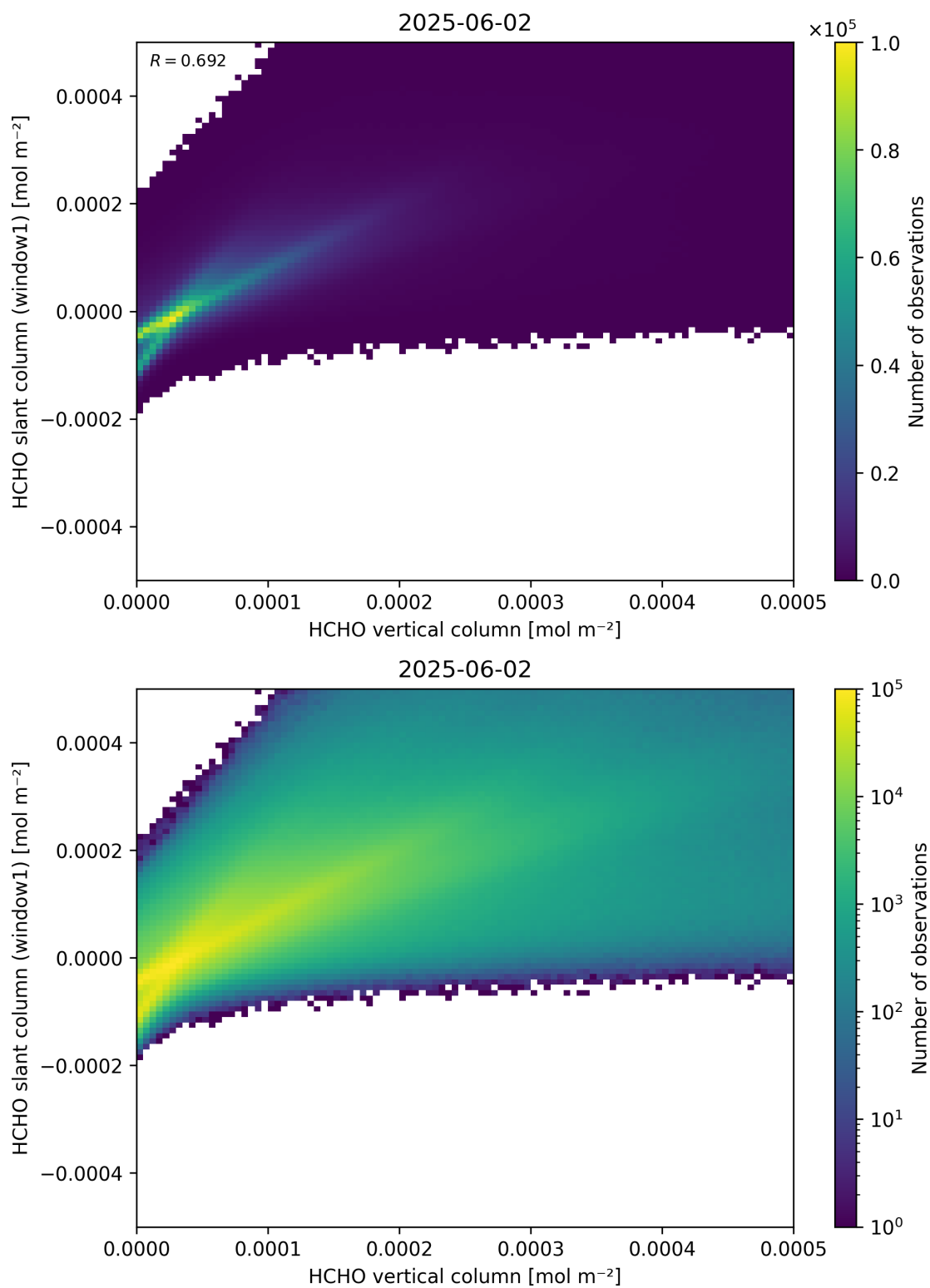
Figure 129: Scatter density plot of “HCHO vertical column” against “HCHO slant column (window1)” for 2025-06-01 to 2025-06-03.
