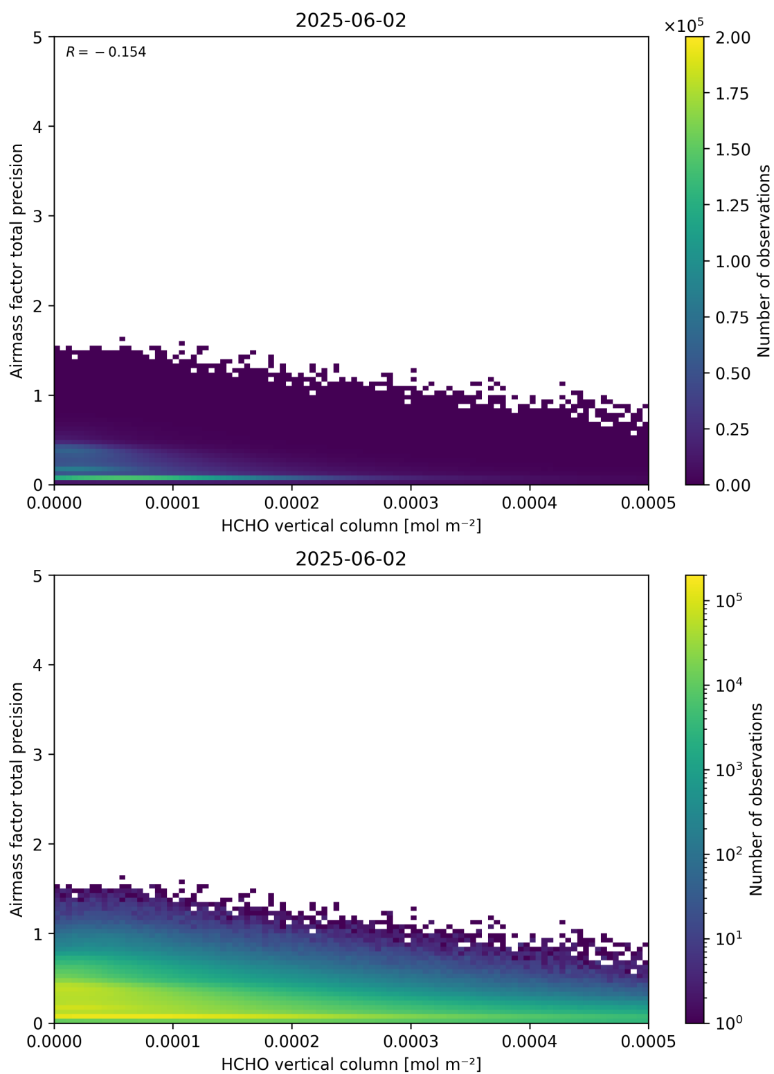
Figure 132: Scatter density plot of “HCHO vertical column” against “Airmass factor total precision” for 2025-06-01 to 2025-06-03.
