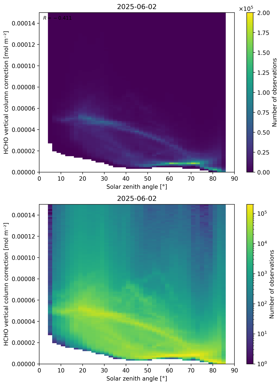
Figure 178: Scatter density plot of “Solar zenith angle” against “HCHO vertical column correction” for 2025-06-01 to 2025-06-03.
