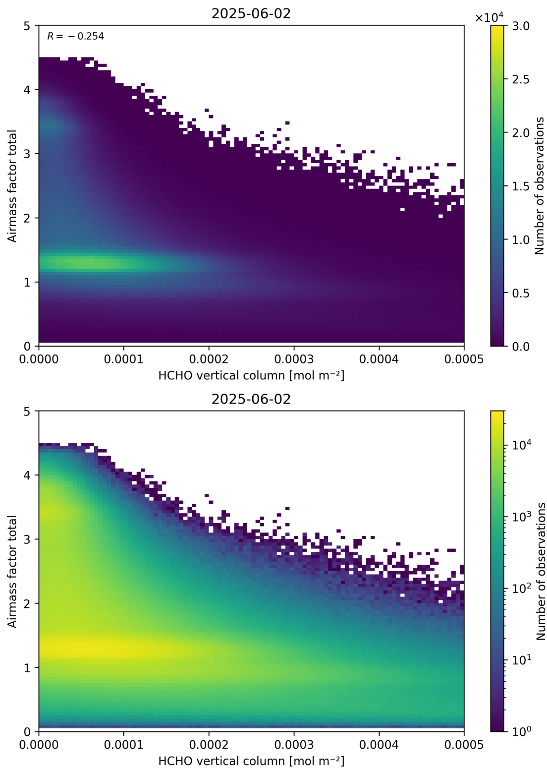
Figure 131: Scatter density plot of “HCHO vertical column” against “Airmass factor total” for 2025-06-01 to 2025-06-03.
