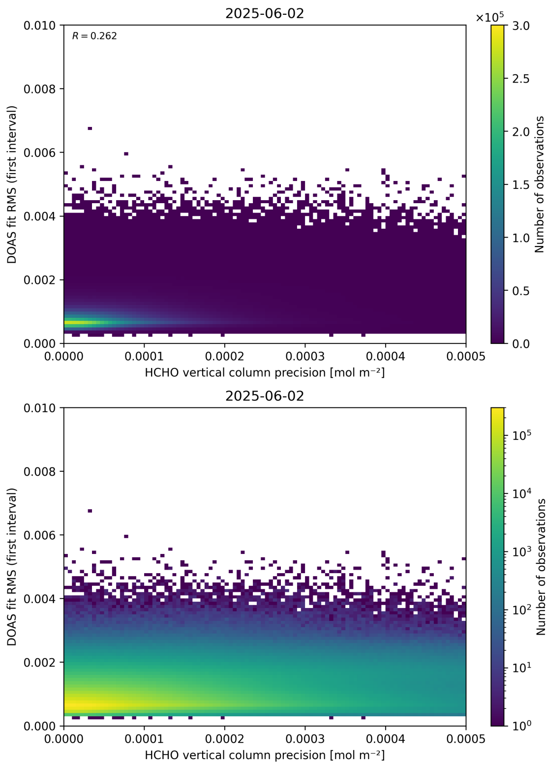
Figure 136: Scatter density plot of “HCHO vertical column precision” against “DOAS fit RMS (first interval)” for 2025-06-01 to 2025-06-03.
