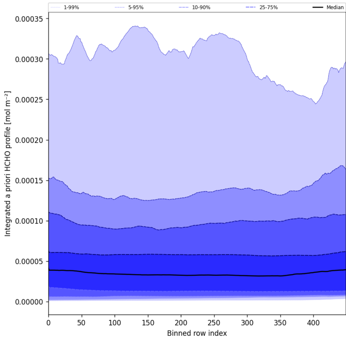
Figure 57: Along track statistics of “Integrated a priori HCHO profile” for 2025-06-01 to 2025-06-03
