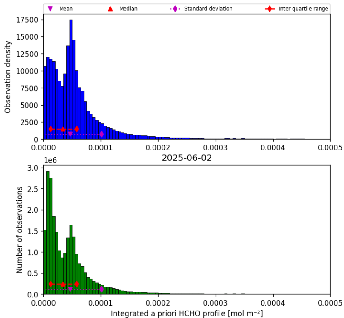
Figure 43: Histogram of “Integrated a priori HCHO profile” for 2025-06-01 to 2025-06-03
