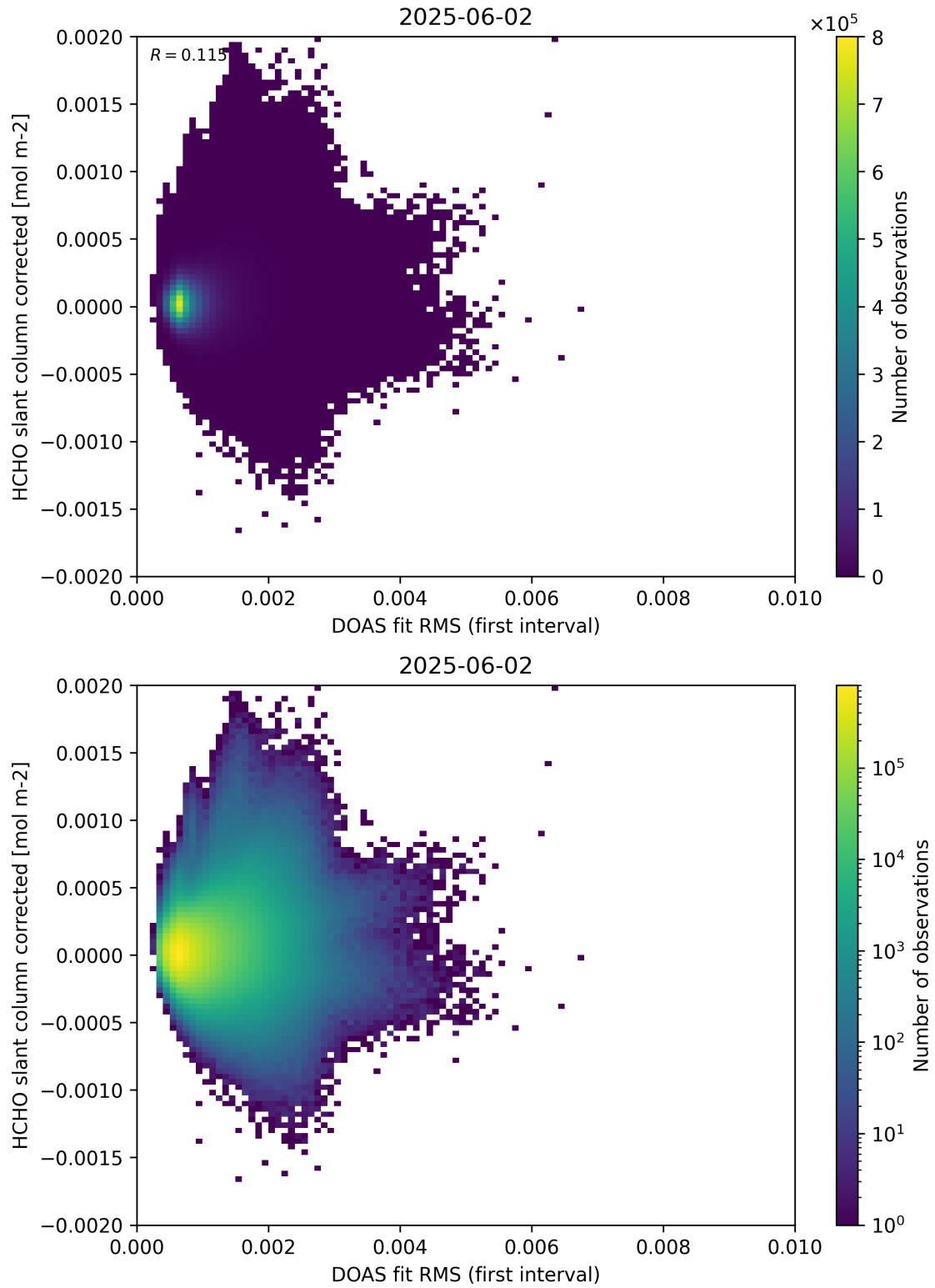
Figure 62: Scatter density plot of “DOAS fit RMS (first interval)” against “HCHO slant column corrected” for 2025-06-01 to 2025-06-03.
