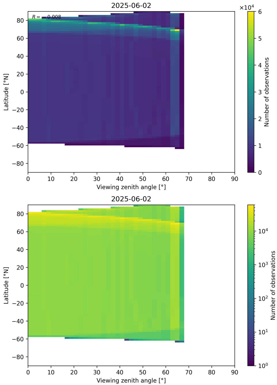
Figure 196: Scatter density plot of “Viewing zenith angle” against “Latitude” for 2025-06-01 to 2025-06-03.
