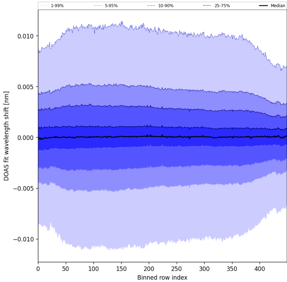
Figure 58: Along track statistics of “DOAS fit wavelength shift” for 2025-06-01 to 2025-06-03
