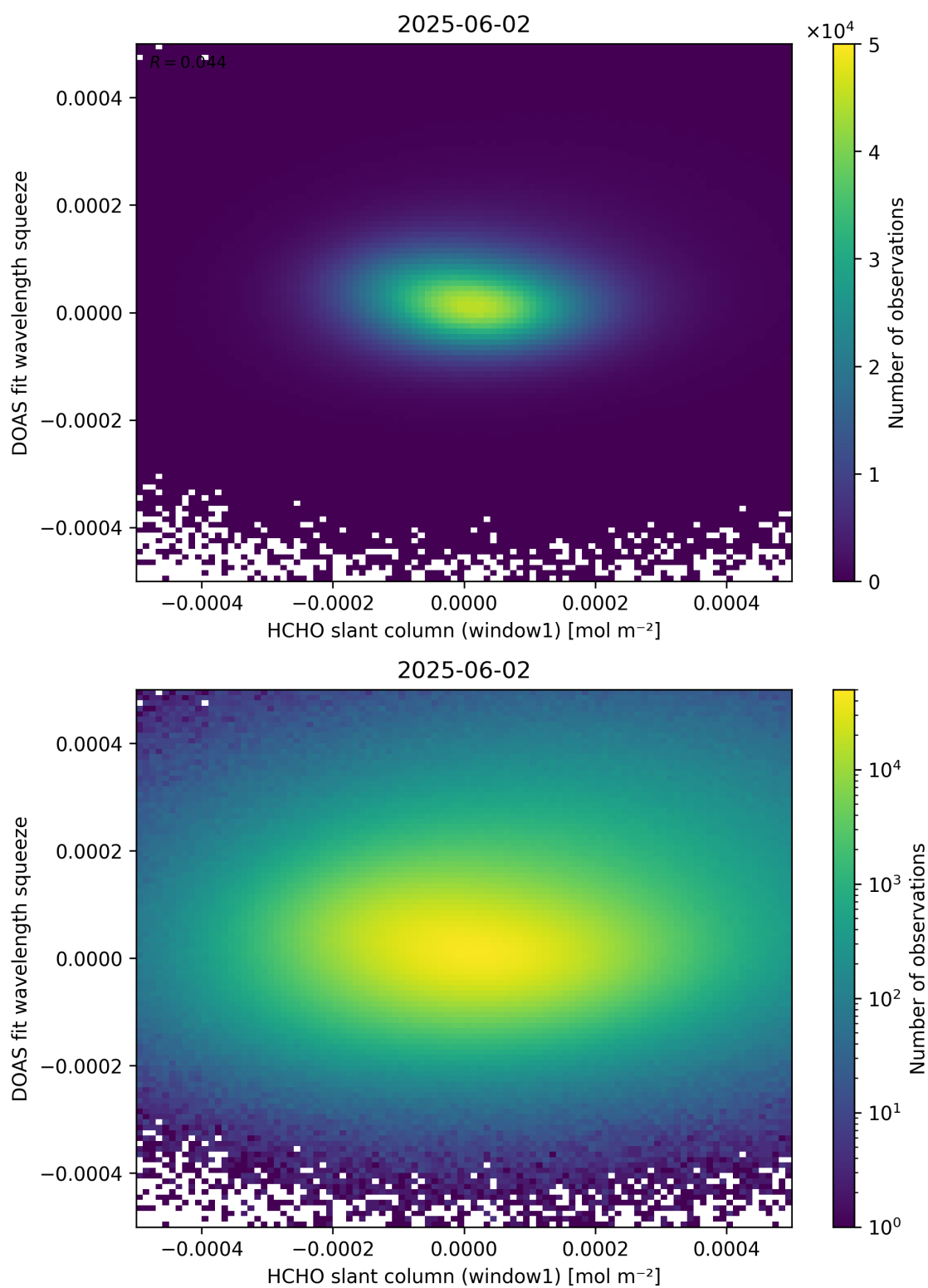
Figure 80: Scatter density plot of “HCHO slant column (window1)” against “DOAS fit wavelength squeeze” for 2025-06-01 to 2025-06-03.
