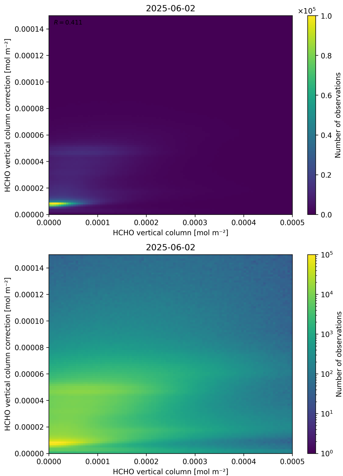
Figure 133: Scatter density plot of “HCHO vertical column” against “HCHO vertical column correction” for 2025-06-01 to 2025-06-03.
