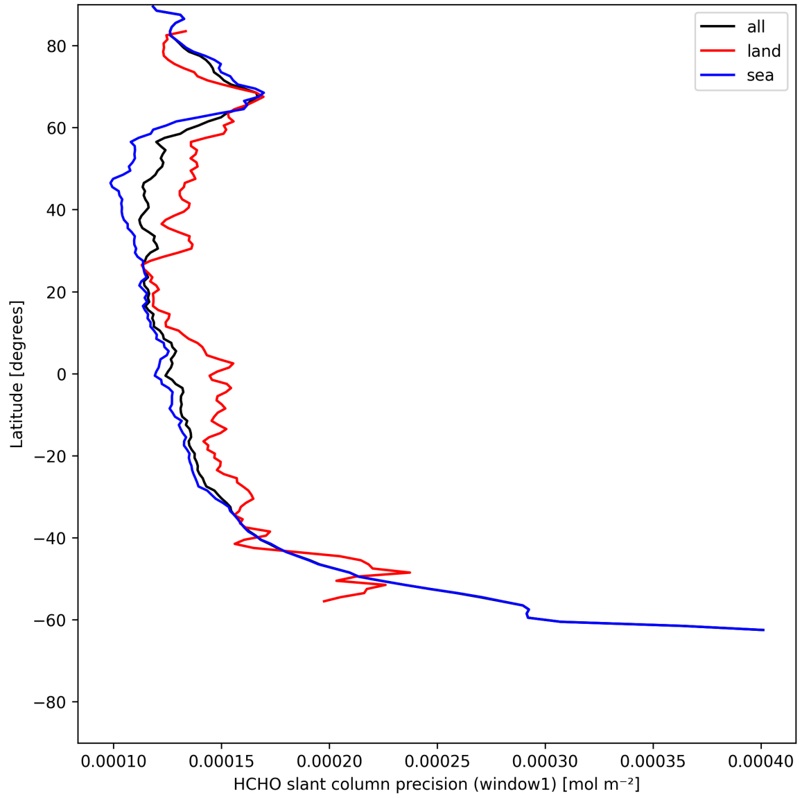
Figure 25: Zonal average of "HCHO slant column precision (window1)" for 2025-06-01 to 2025-06-03.
