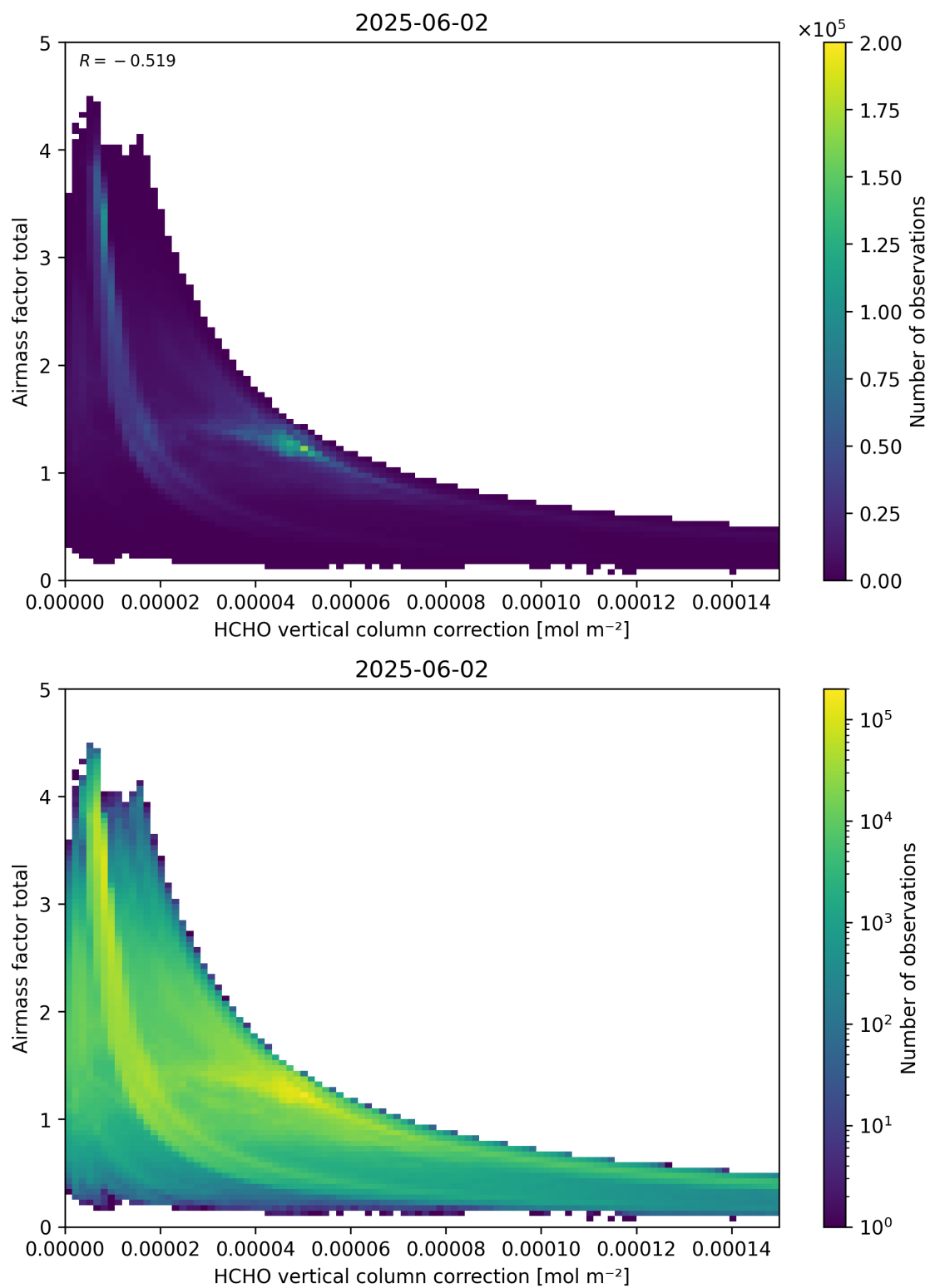
Figure 120: Scatter density plot of “HCHO vertical column correction” against “Airmass factor total” for 2025-06-01 to 2025-06-03.
