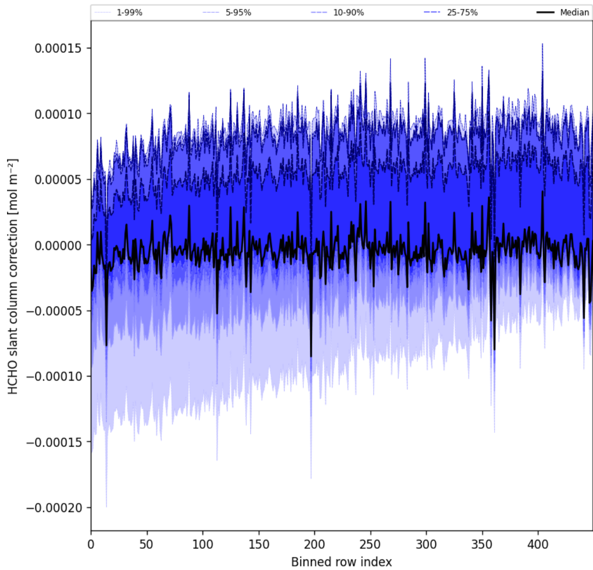
Figure 61: Along track statistics of "HCHO slant column correction" for 2025-06-01 to 2025-06-03
