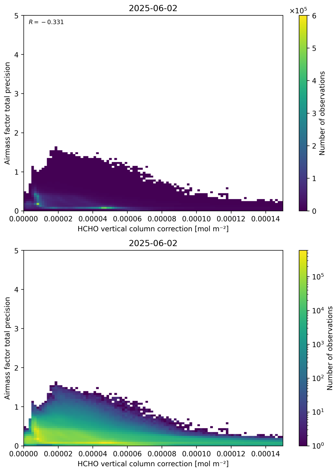
Figure 121: Scatter density plot of “HCHO vertical column correction” against “Airmass factor total precision” for 2025-06-01 to 2025-06-03.
