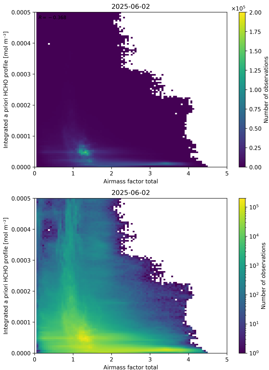
Figure 104: Scatter density plot of “Airmass factor total” against “Integrated a priori HCHO profile” for 2025-06-01 to 2025-06-03.
