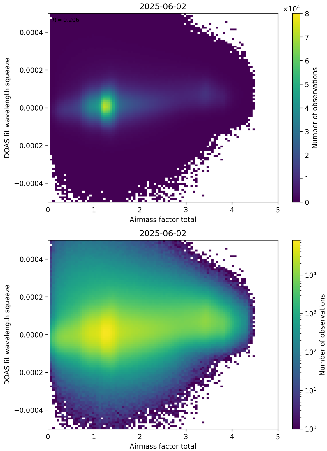
Figure 99: Scatter density plot of “Airmass factor total” against “DOAS fit wavelength squeeze” for 2025-06-01 to 2025-06-03.
