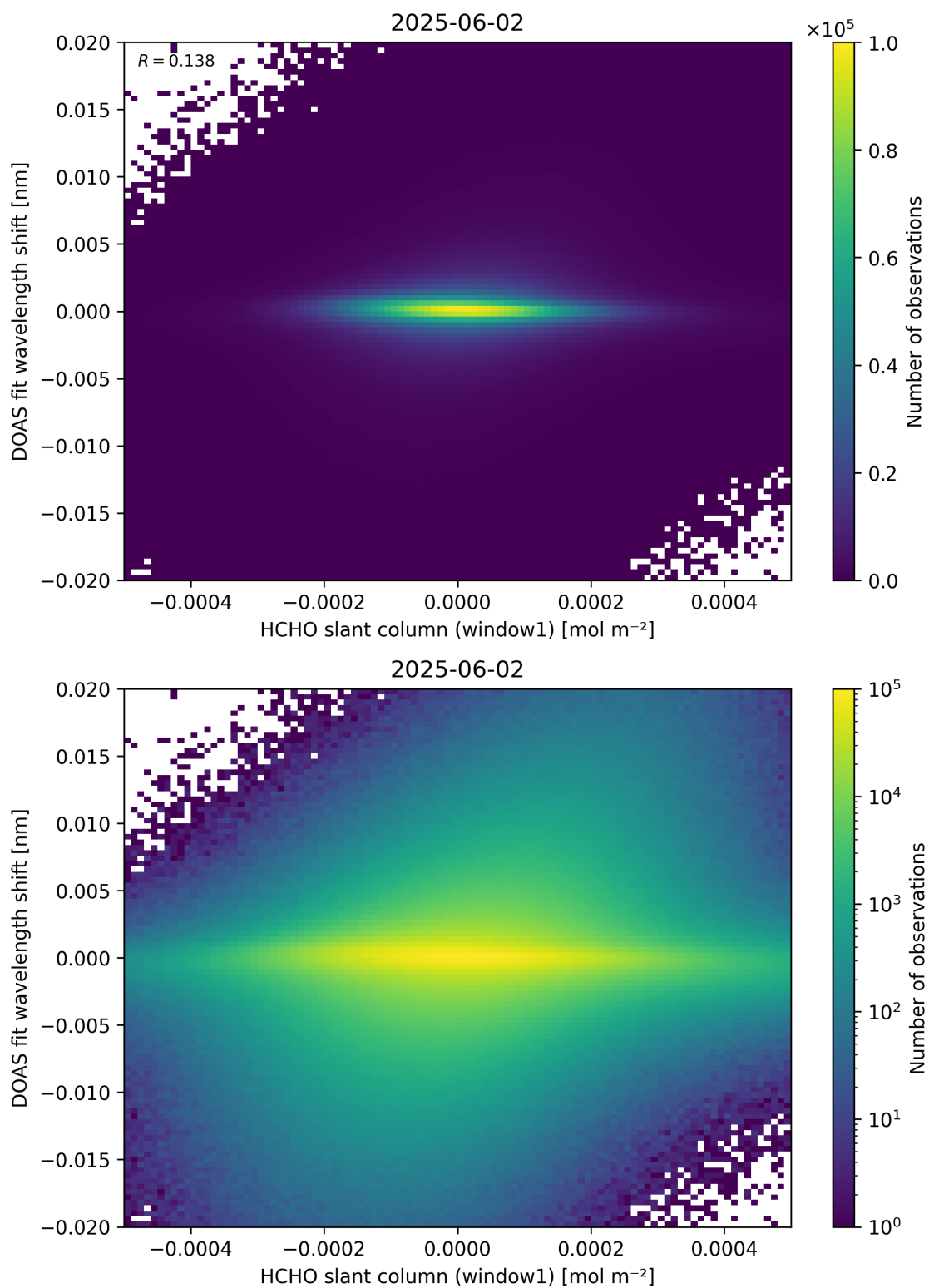
Figure 79: Scatter density plot of “HCHO slant column (window1)” against “DOAS fit wavelength shift” for 2025-06-01 to 2025-06-03.
