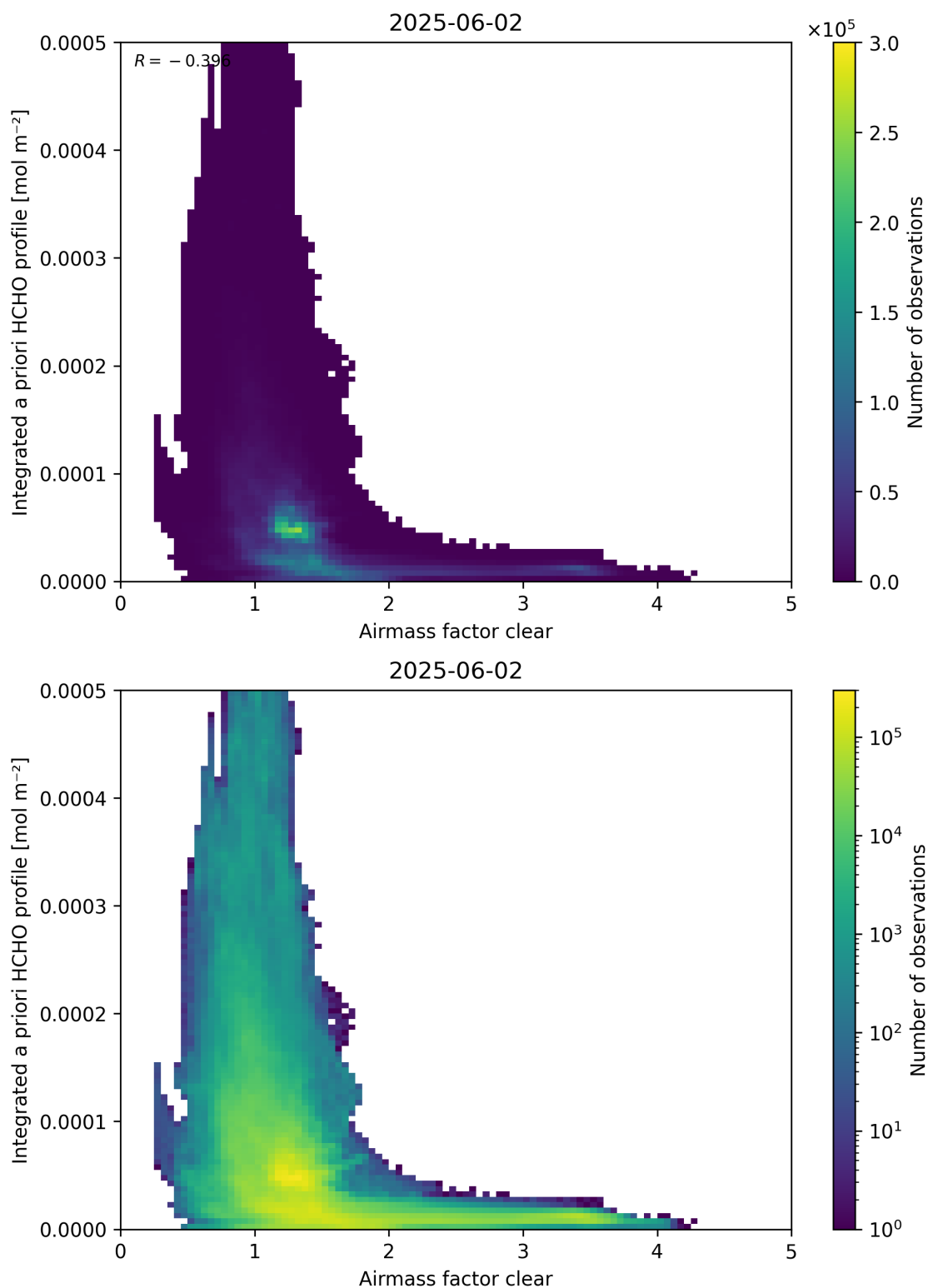
Figure 76: Scatter density plot of “Airmass factor clear” against “Integrated a priori HCHO profile” for 2025-06-01 to 2025-06-03.
