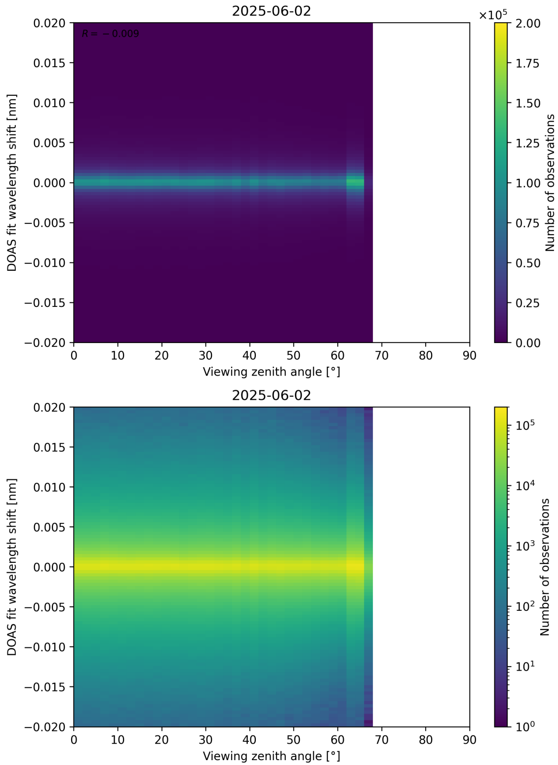
Figure 183: Scatter density plot of “Viewing zenith angle” against “DOAS fit wavelength shift” for 2025-06-01 to 2025-06-03.
