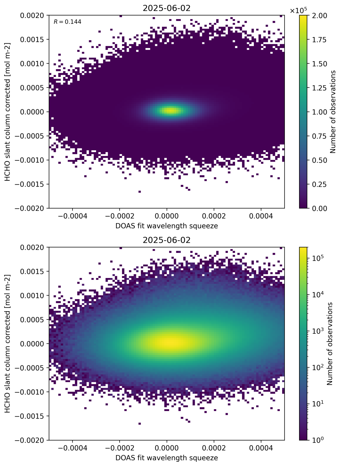
Figure 69: Scatter density plot of “DOAS fit wavelength squeeze” against “HCHO slant column corrected” for 2025-06-01 to 2025-06-03.
