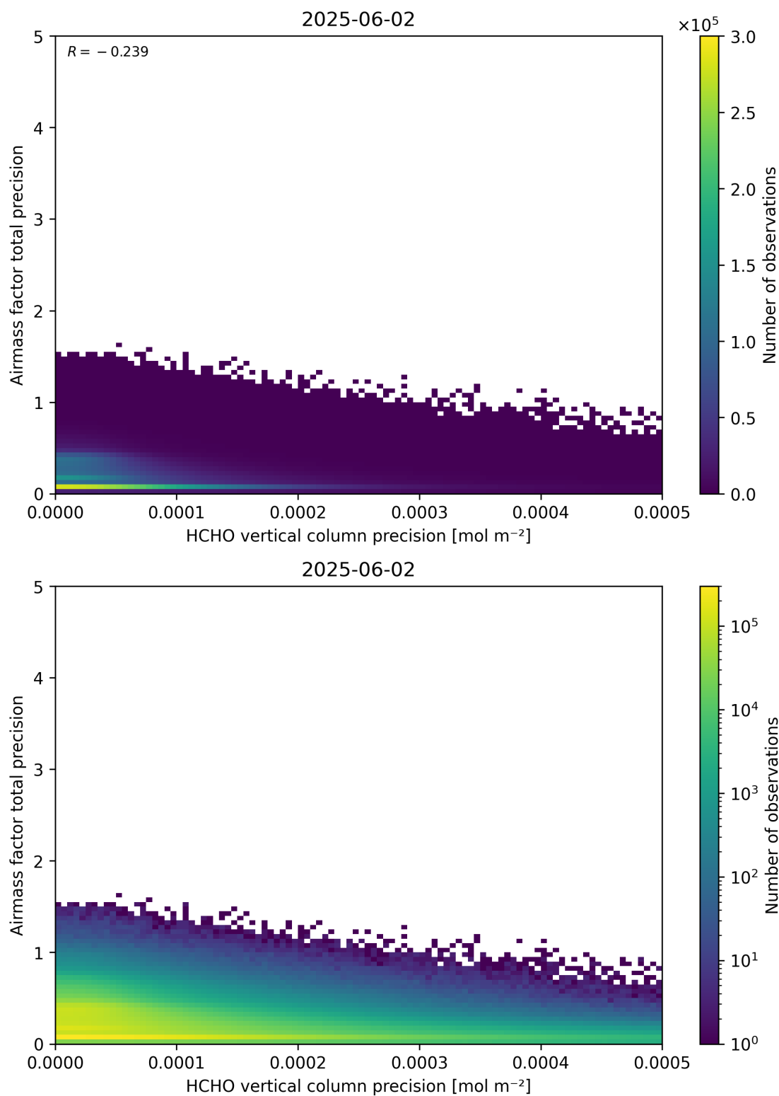
Figure 145: Scatter density plot of “HCHO vertical column precision” against “Airmass factor total precision” for 2025-06-01 to 2025-06-03.
