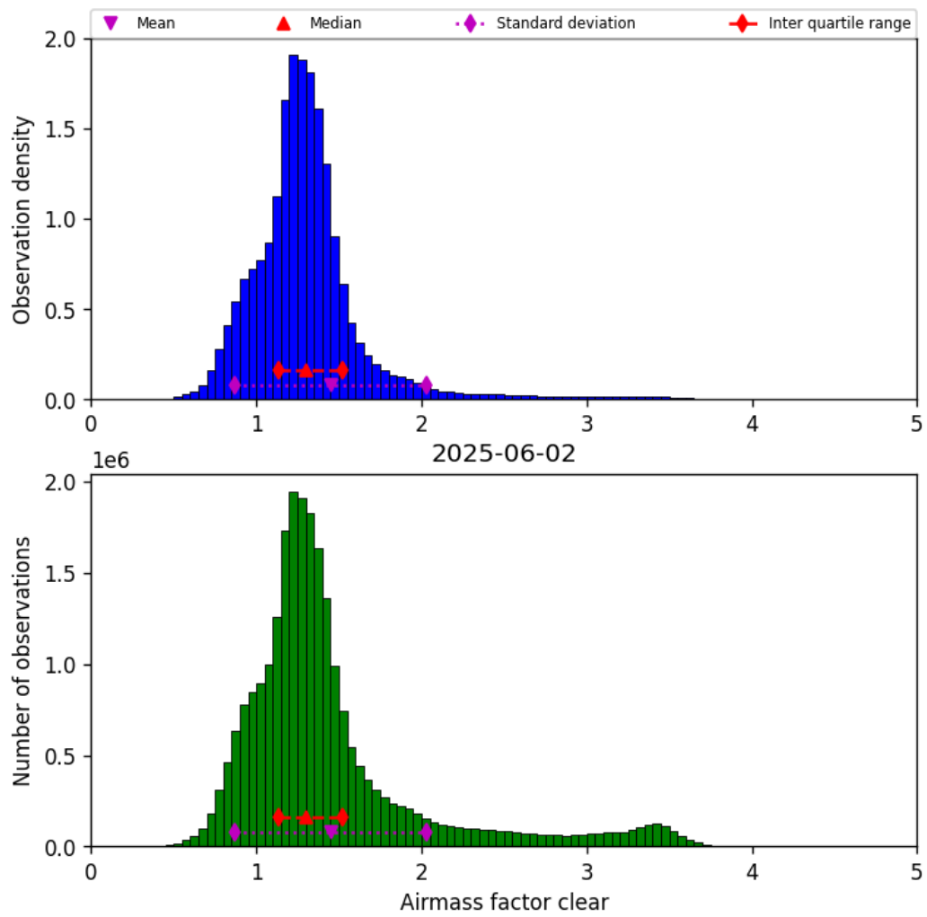
Figure 42: Histogram of “Airmass factor clear” for 2025-06-01 to 2025-06-03
