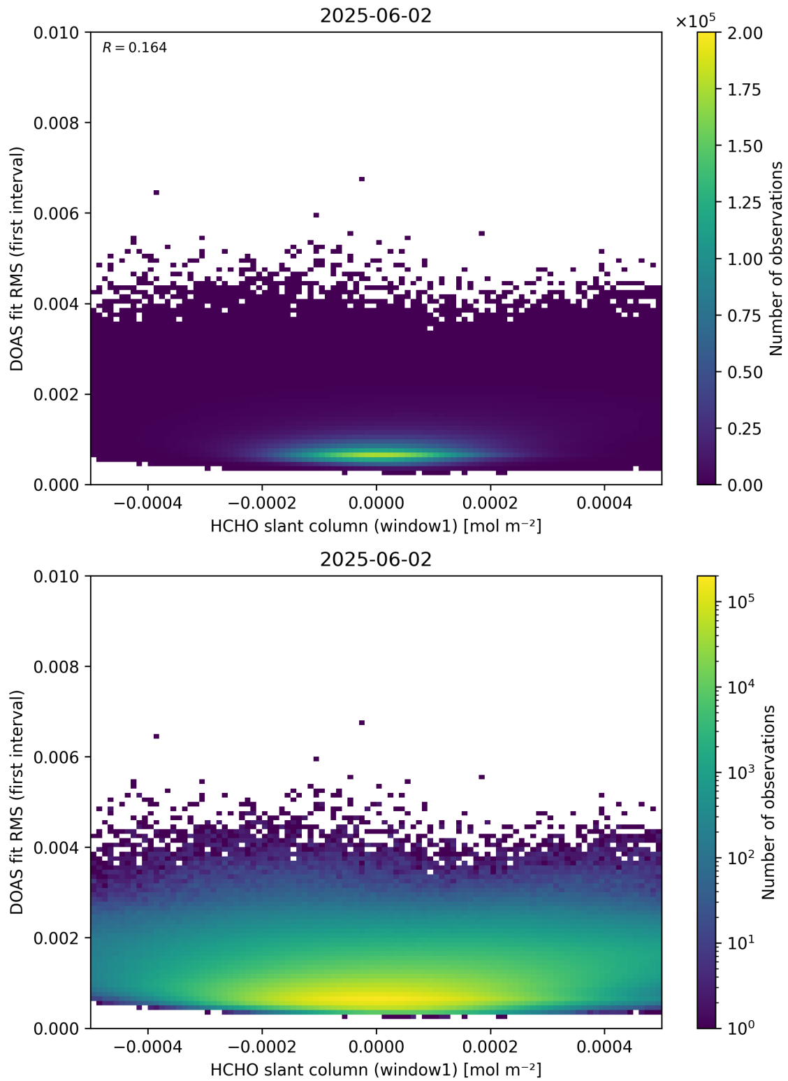
Figure 78: Scatter density plot of “HCHO slant column (window1)” against “DOAS fit RMS (first interval)” for 2025-06-01 to 2025-06-03.
