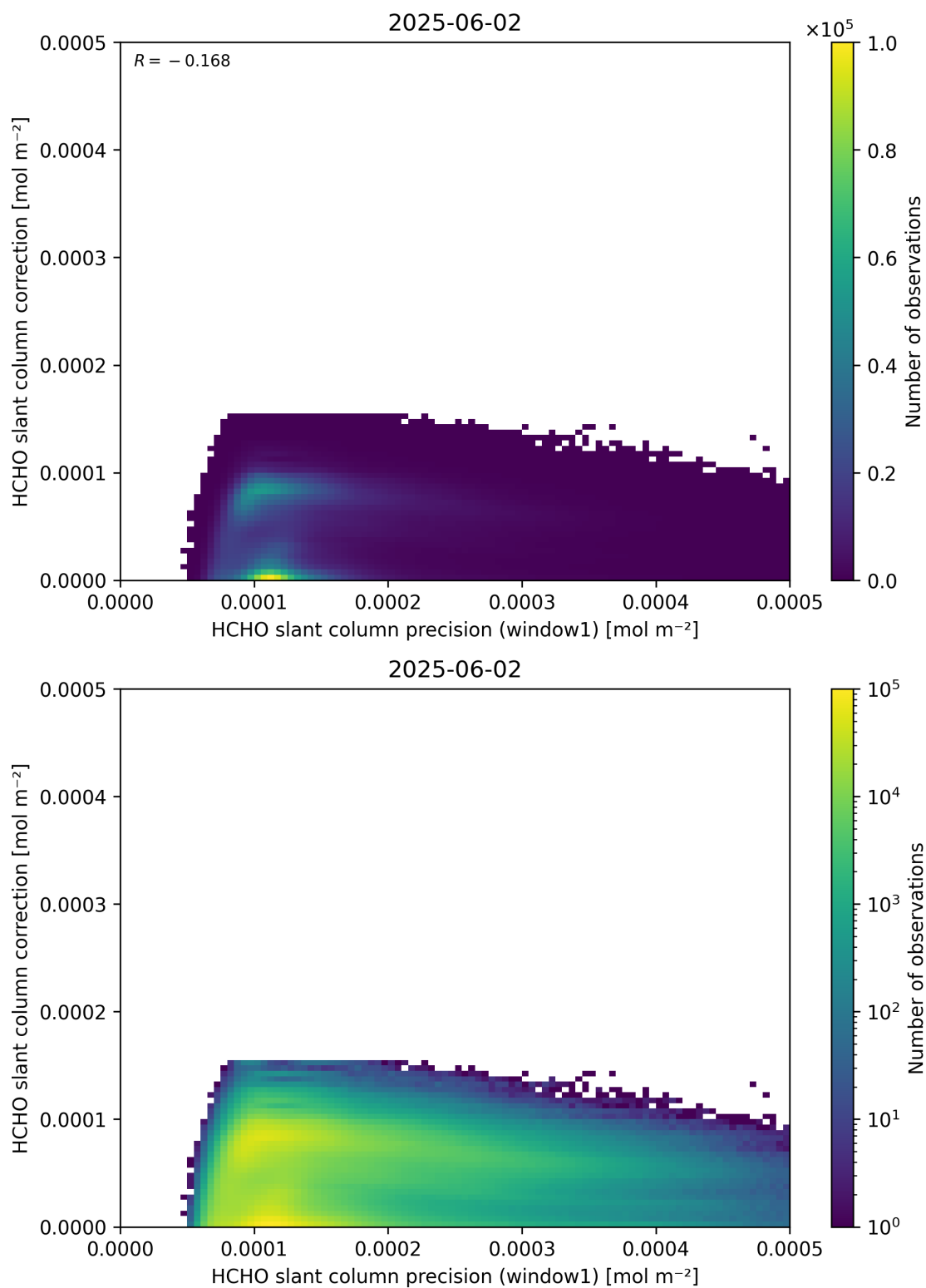
Figure 93: Scatter density plot of “HCHO slant column precision (window1)” against “HCHO slant column correction” for 2025-06-01 to 2025-06-03.
