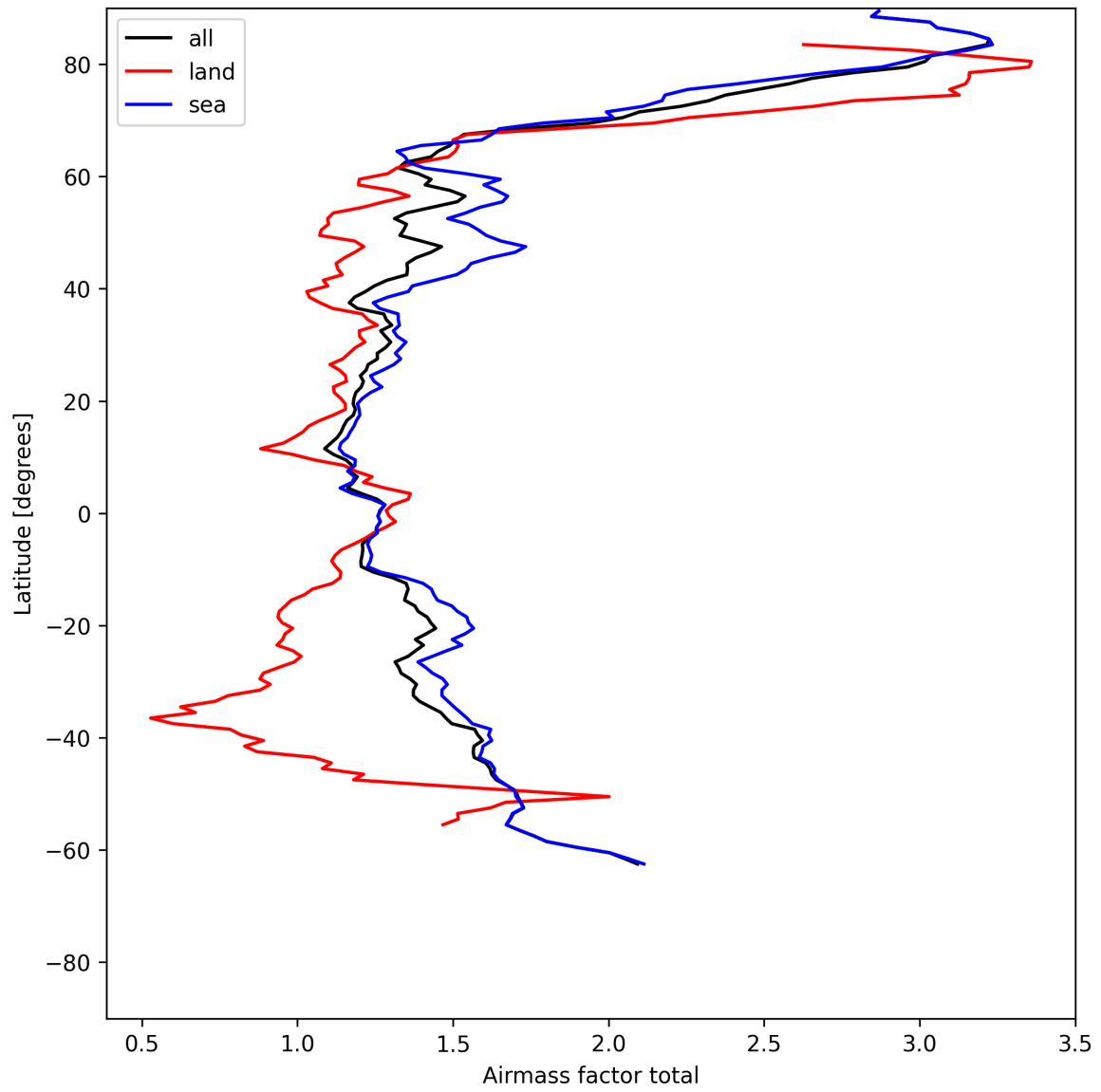
Figure 26: Zonal average of “Airmass factor total” for 2025-06-01 to 2025-06-03.
