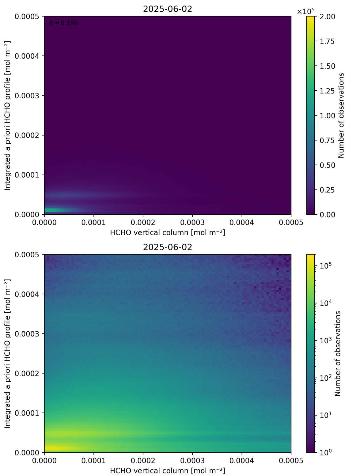
Figure 135: Scatter density plot of “HCHO vertical column” against “Integrated a priori HCHO profile” for 2025-06-01 to 2025-06-03.
