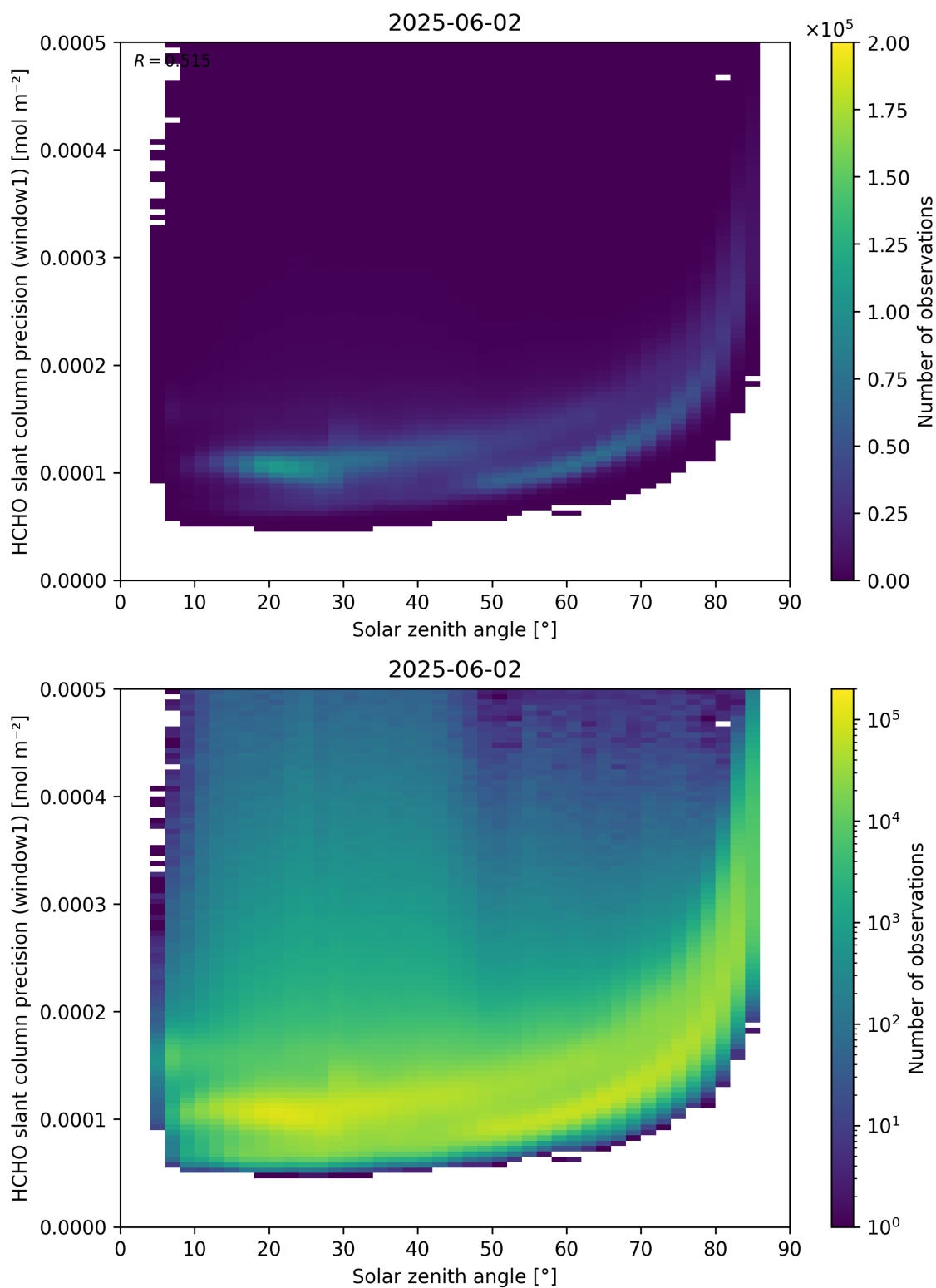
Figure 174: Scatter density plot of “Solar zenith angle” against “HCHO slant column precision (window1)” for 2025-06-01 to 2025-06-03.
