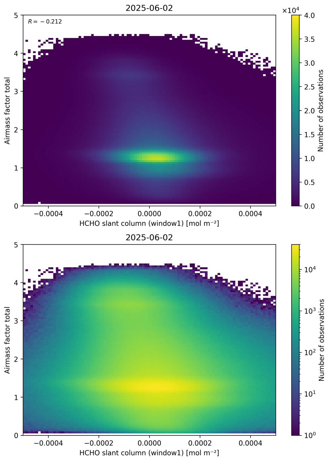
Figure 85: Scatter density plot of “HCHO slant column (window1)” against “Airmass factor total” for 2025-06-01 to 2025-06-03.
