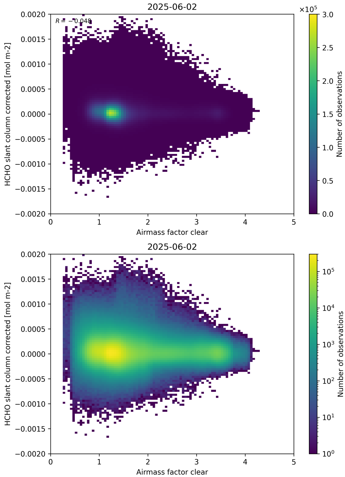
Figure 74: Scatter density plot of “Airmass factor clear” against “HCHO slant column corrected” for 2025-06-01 to 2025-06-03.
