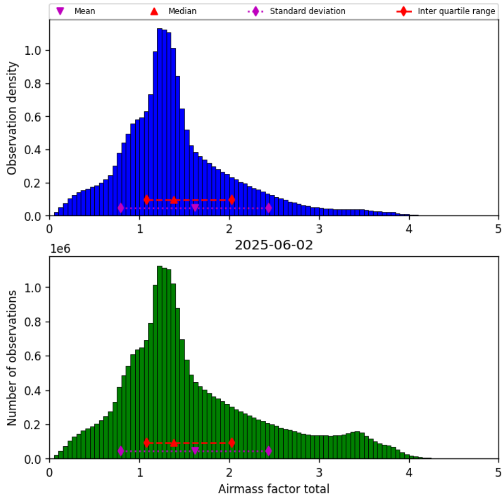
Figure 40: Histogram of “Airmass factor total” for 2025-06-01 to 2025-06-03
