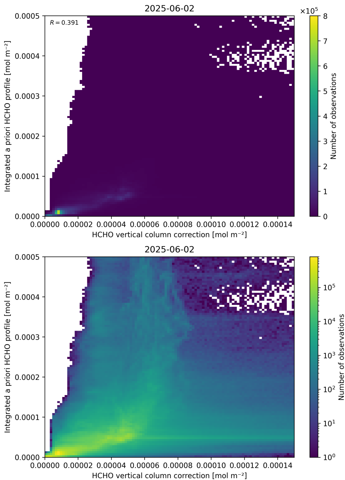
Figure 122: Scatter density plot of “HCHO vertical column correction” against “Integrated a priori HCHO profile” for 2025-06-01 to 2025-06-03.
