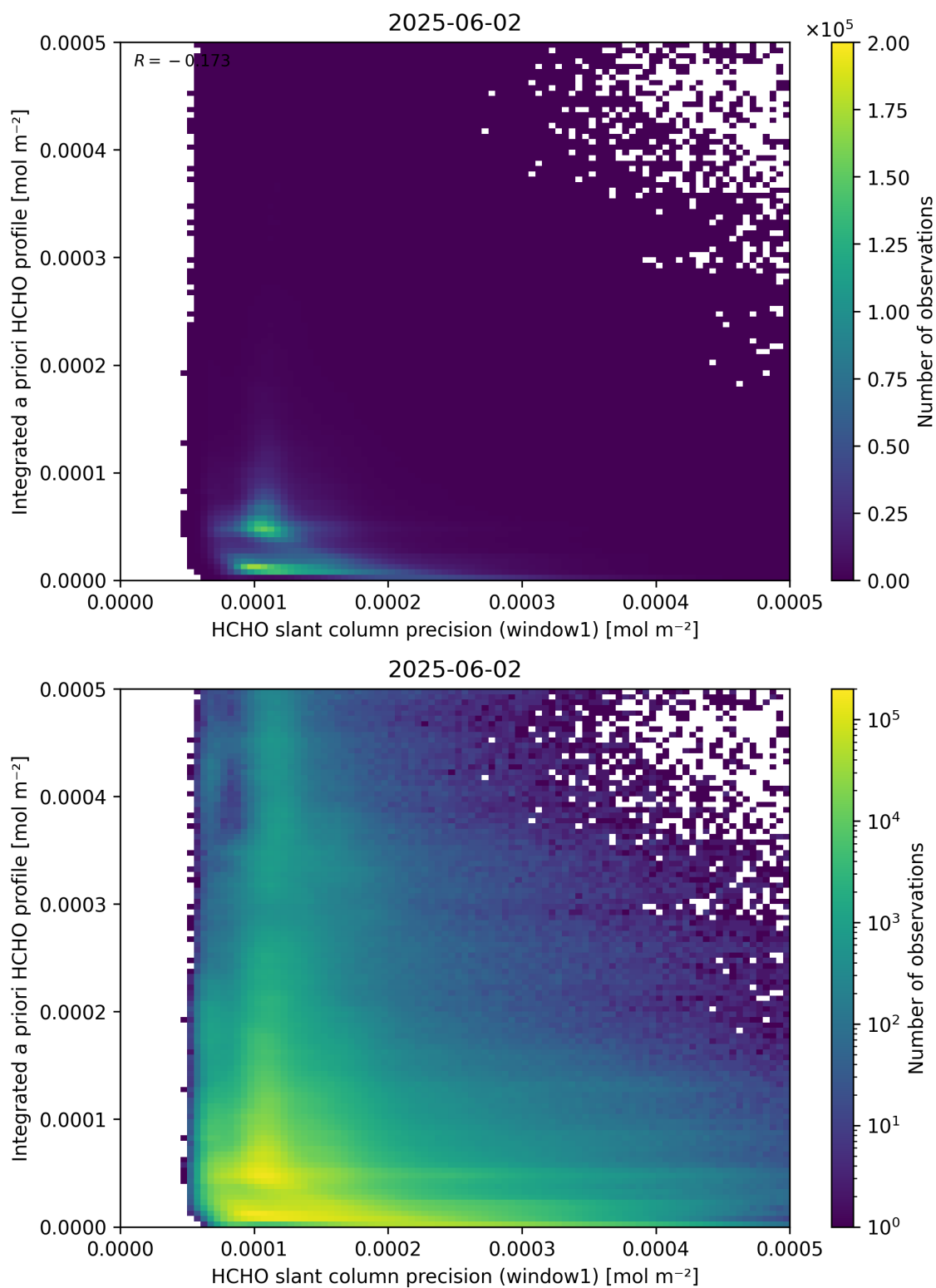
Figure 96: Scatter density plot of “HCHO slant column precision (window1)” against “Integrated a priori HCHO profile” for 2025-06-01 to 2025-06-03.
