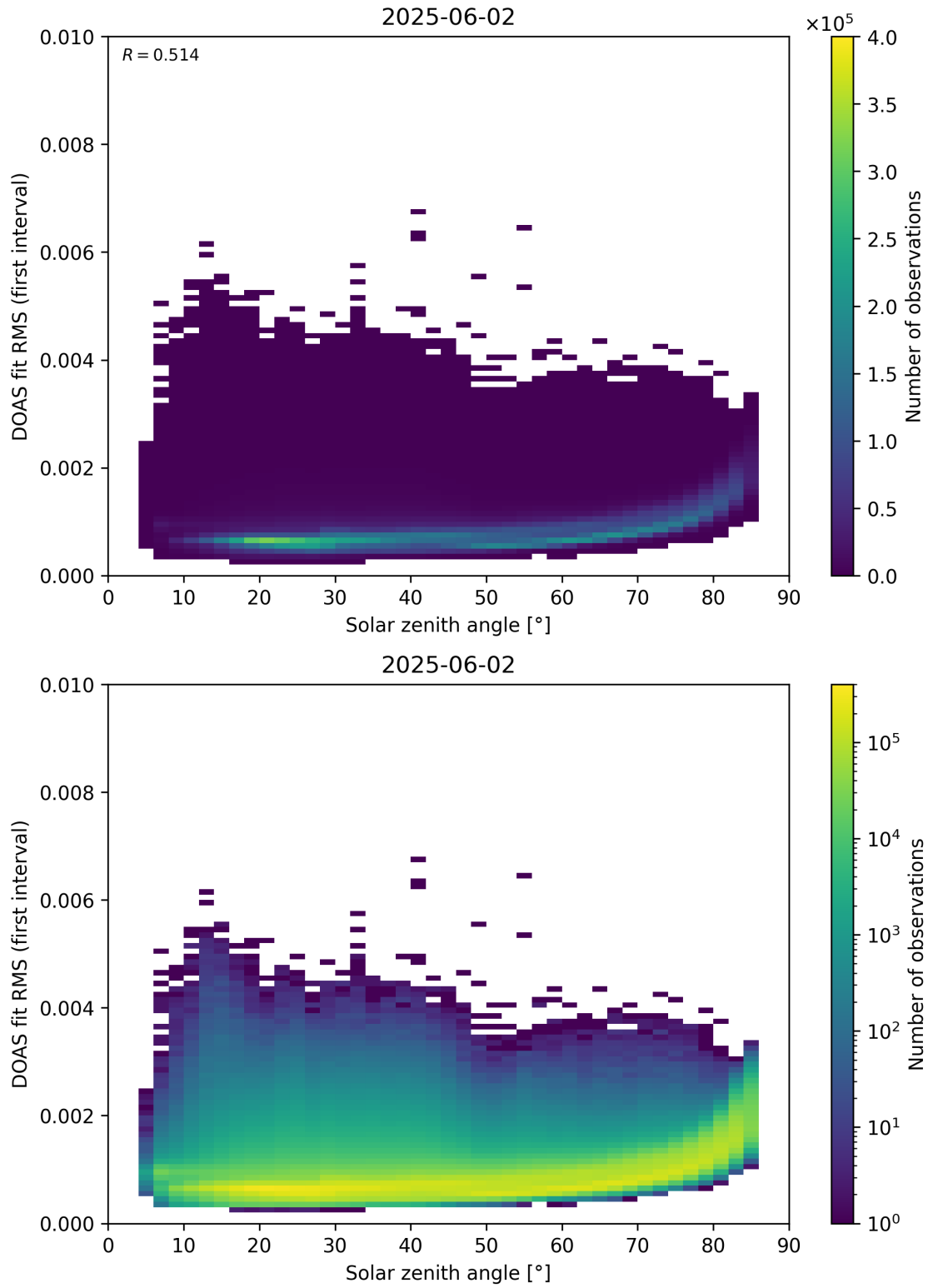
Figure 167: Scatter density plot of “Solar zenith angle” against “DOAS fit RMS (first interval)” for 2025-06-01 to 2025-06-03.
