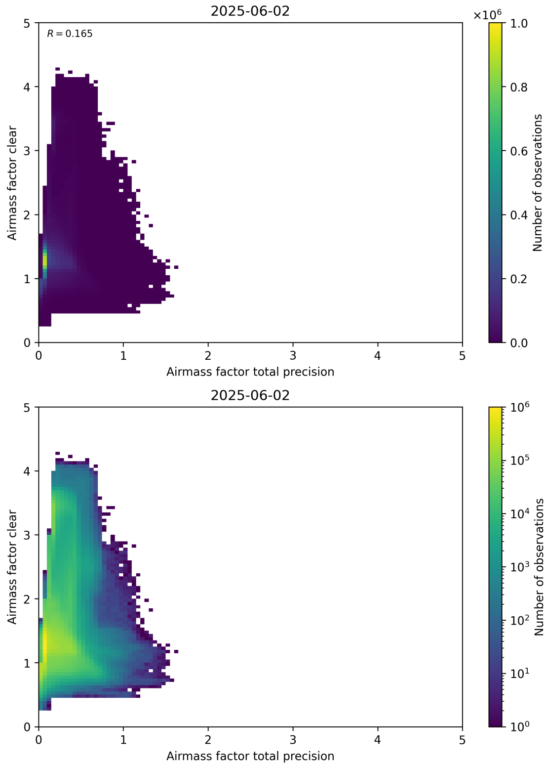
Figure 108: Scatter density plot of “Airmass factor total precision” against “Airmass factor clear” for 2025-06-01 to 2025-06-03.
