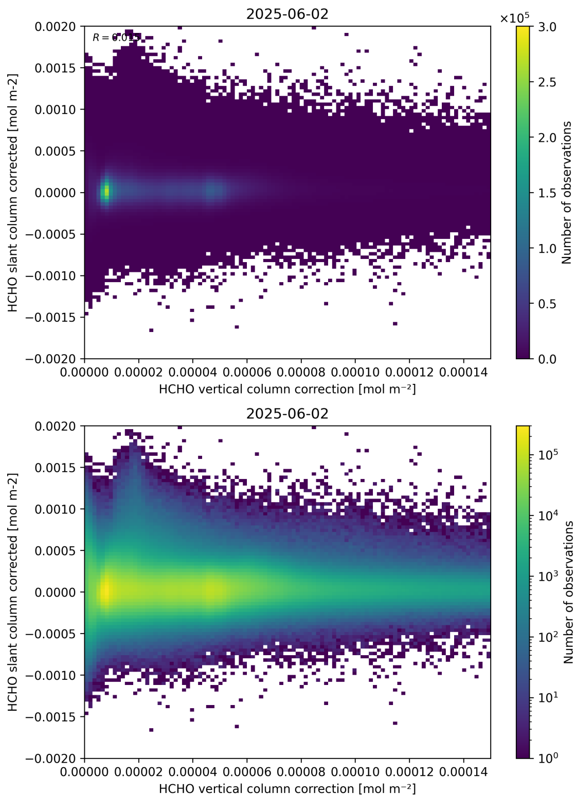
Figure 116: Scatter density plot of “HCHO vertical column correction” against “HCHO slant column corrected” for 2025-06-01 to 2025-06-03.
