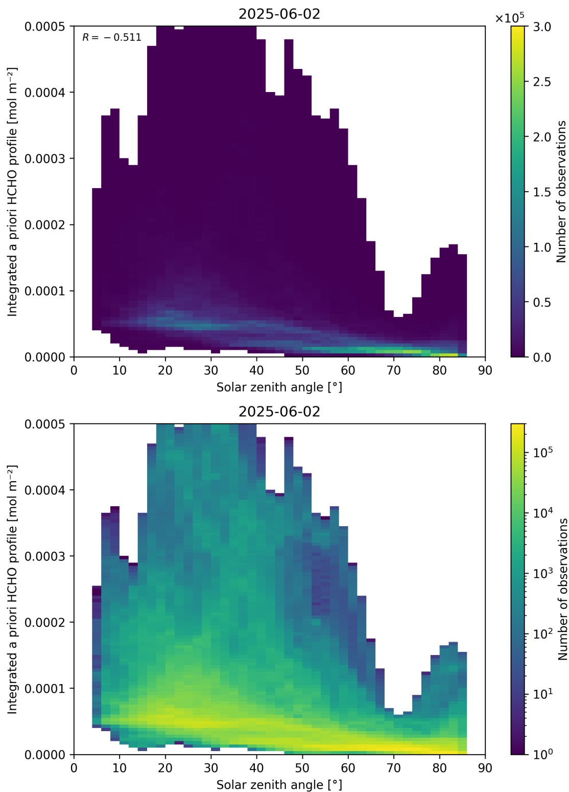
Figure 180: Scatter density plot of “Solar zenith angle” against “Integrated a priori HCHO profile” for 2025-06-01 to 2025-06-03.
