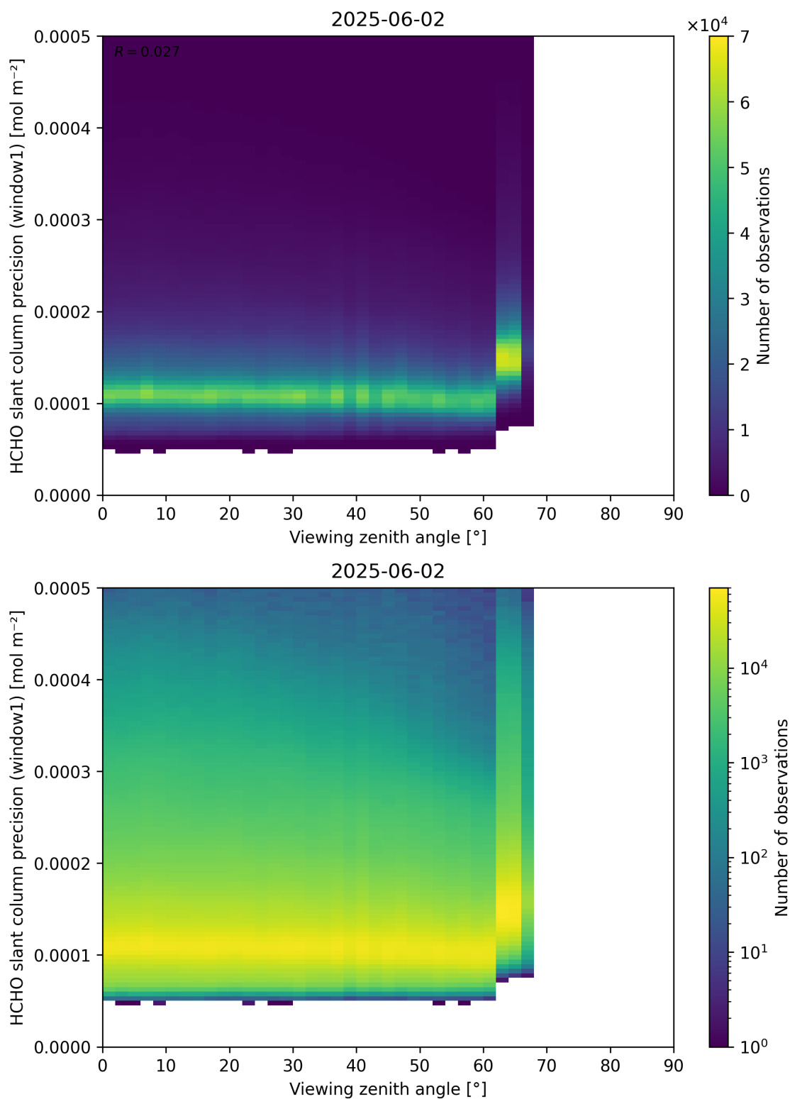
Figure 189: Scatter density plot of “Viewing zenith angle” against “HCHO slant column precision (window1)” for 2025-06-01 to 2025-06-03.
