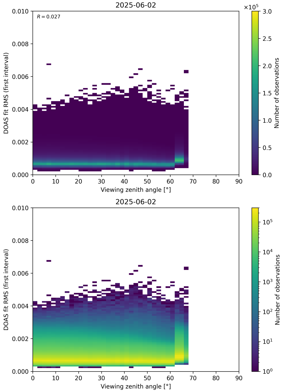
Figure 182: Scatter density plot of “Viewing zenith angle” against “DOAS fit RMS (first interval)” for 2025-06-01 to 2025-06-03.
