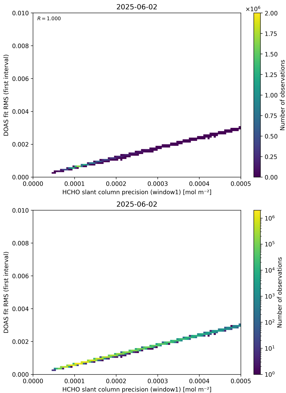
Figure 88: Scatter density plot of “HCHO slant column precision (window1)” against “DOAS fit RMS (first interval)” for 2025-06-01 to 2025-06-03.
