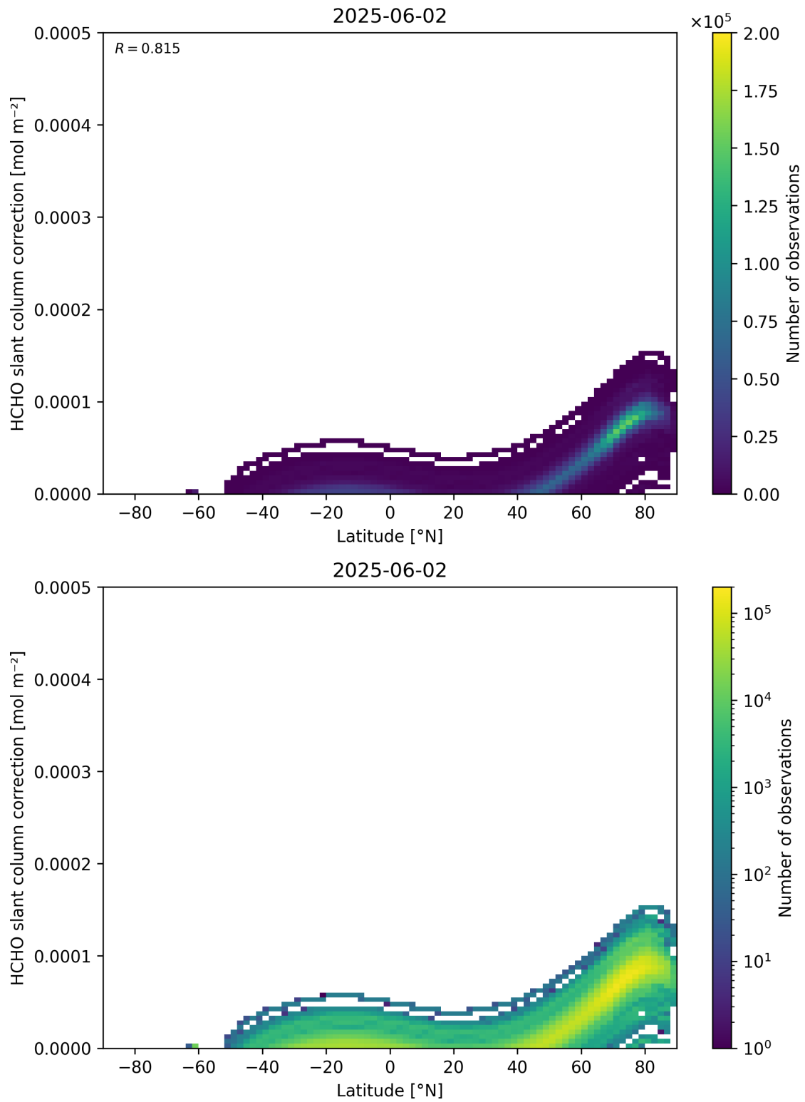
Figure 158: Scatter density plot of “Latitude” against “HCHO slant column correction” for 2025-06-01 to 2025-06-03.
