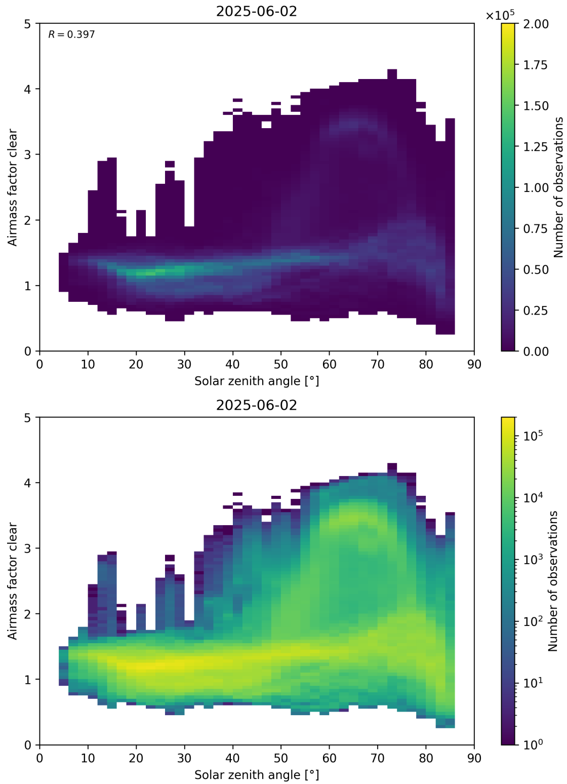
Figure 170: Scatter density plot of “Solar zenith angle” against “Airmass factor clear” for 2025-06-01 to 2025-06-03.
