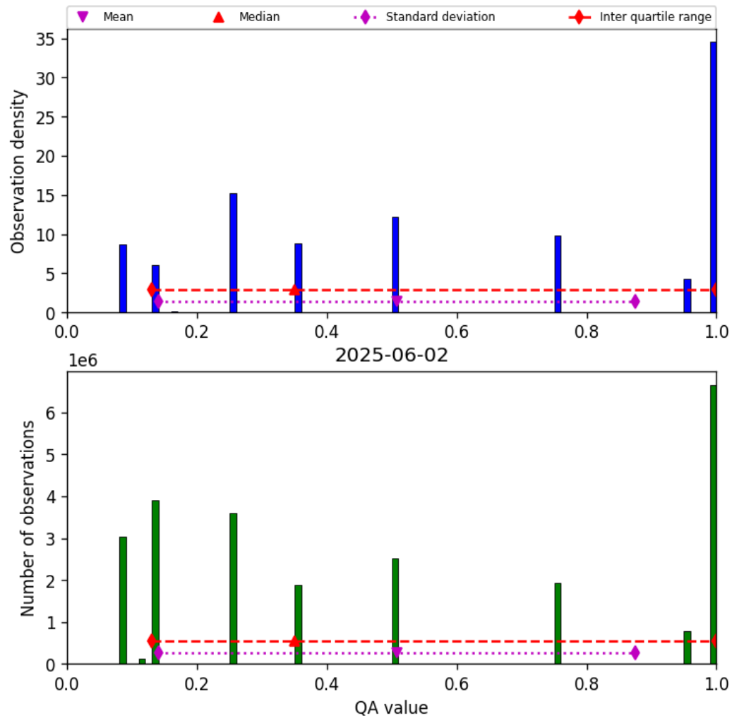
Figure 34: Histogram of “QA value” for 2025-06-01 to 2025-06-03
