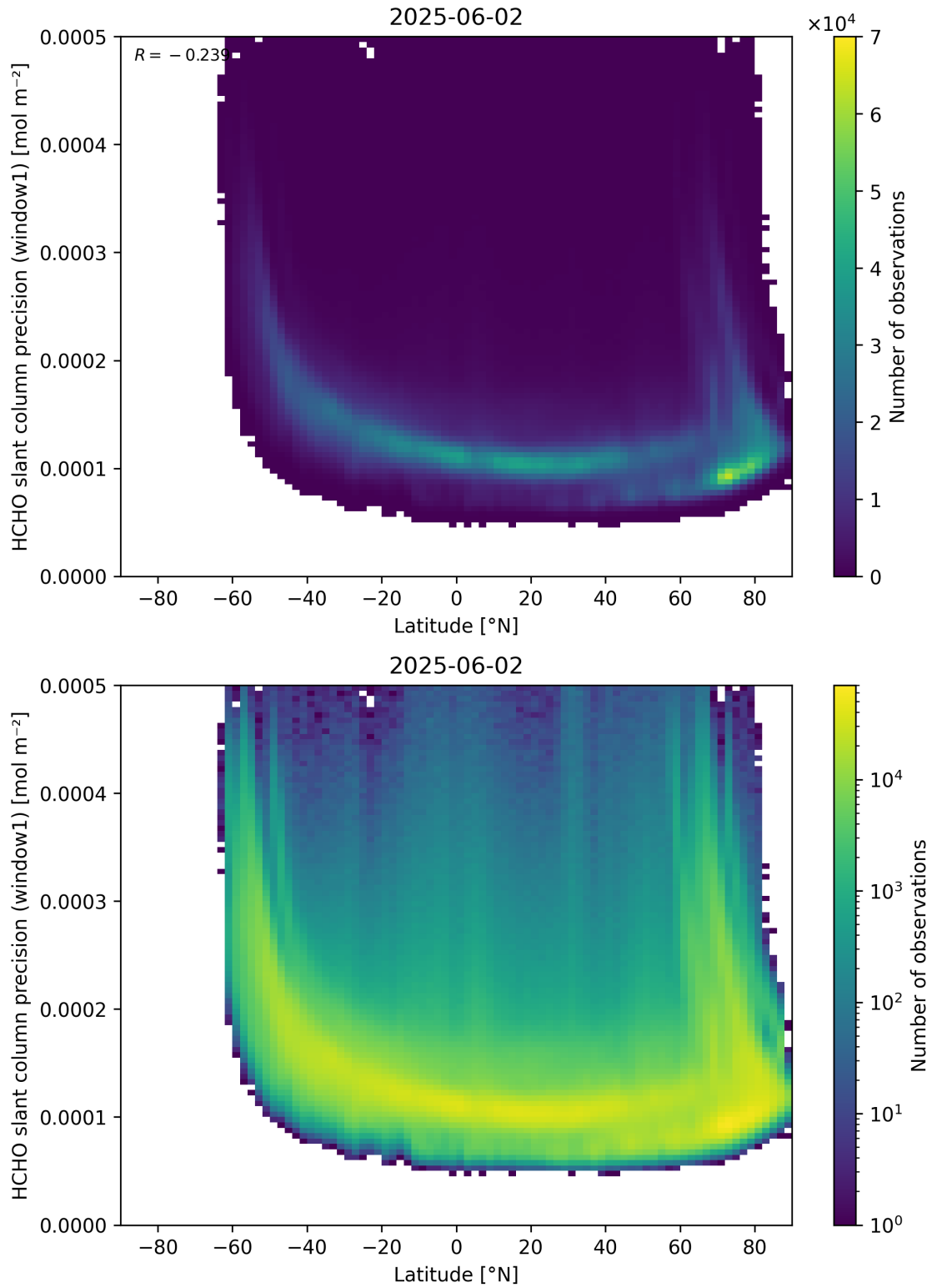
Figure 160: Scatter density plot of “Latitude” against “HCHO slant column precision (window1)” for 2025-06-01 to 2025-06-03.
