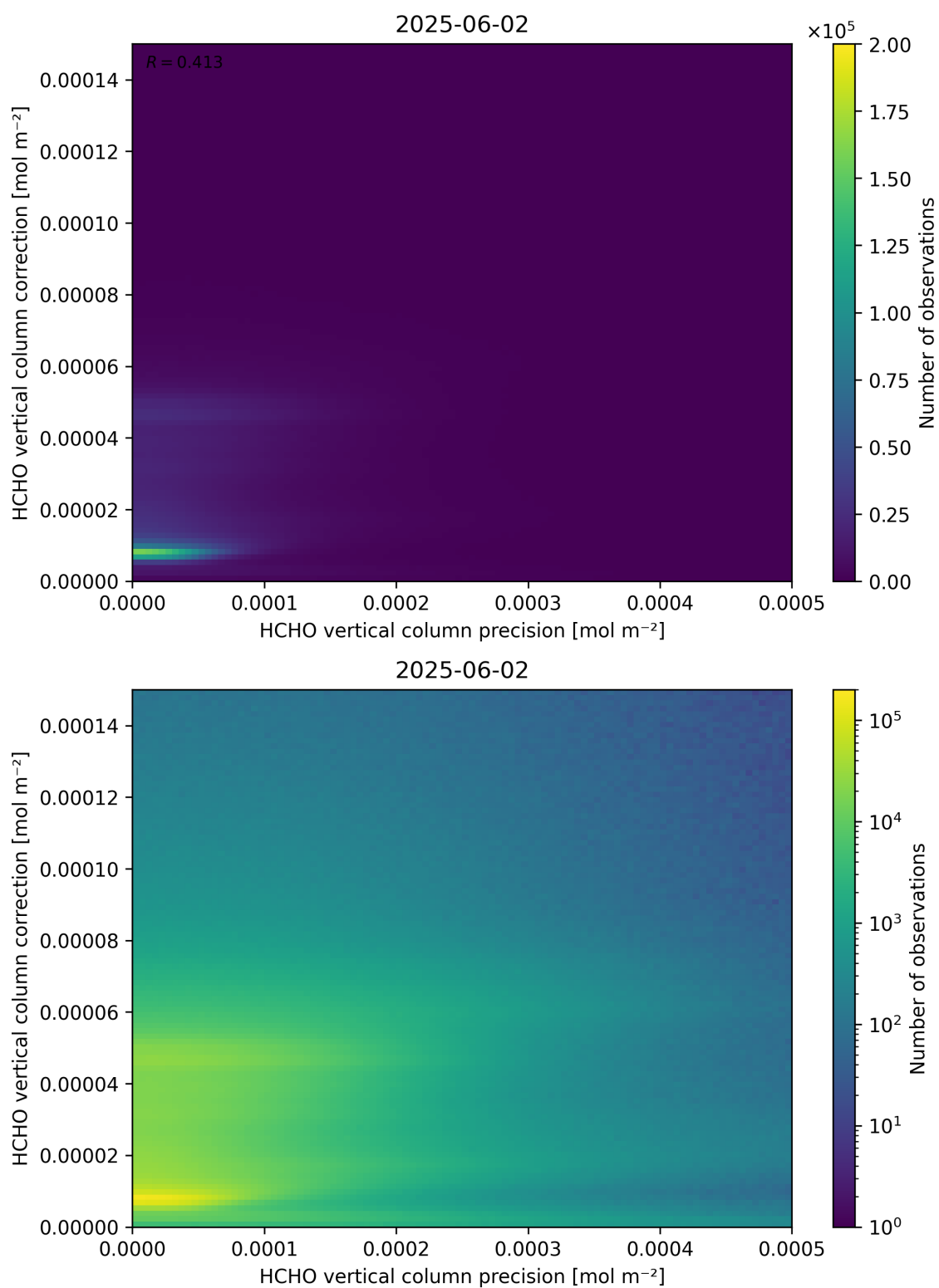
Figure 146: Scatter density plot of “HCHO vertical column precision” against “HCHO vertical column correction” for 2025-06-01 to 2025-06-03.
