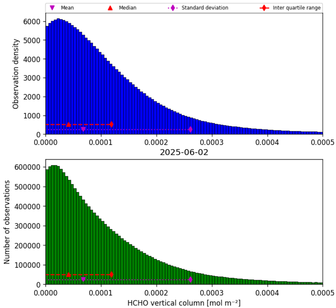
Figure 35: Histogram of “HCHO vertical column” for 2025-06-01 to 2025-06-03
