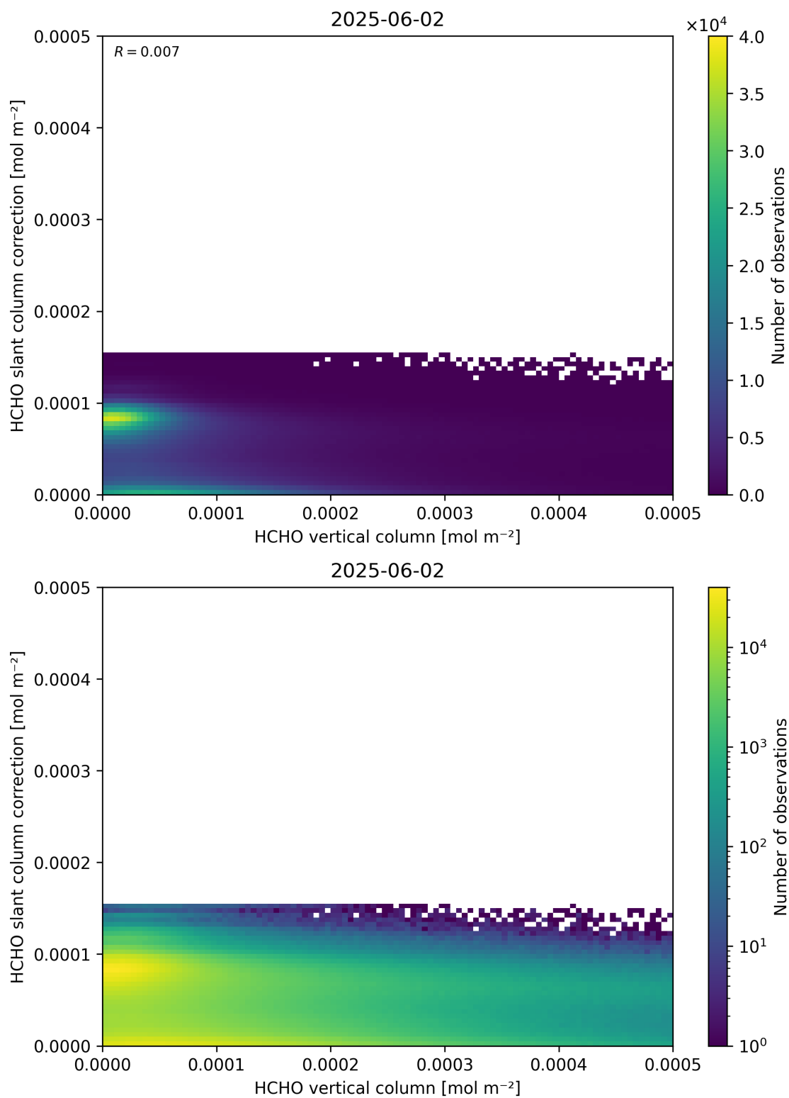
Figure 128: Scatter density plot of “HCHO vertical column” against “HCHO slant column correction” for 2025-06-01 to 2025-06-03.
