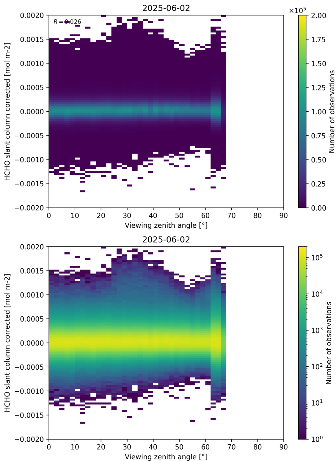
Figure 186: Scatter density plot of “Viewing zenith angle” against “HCHO slant column corrected” for 2025-06-01 to 2025-06-03.
