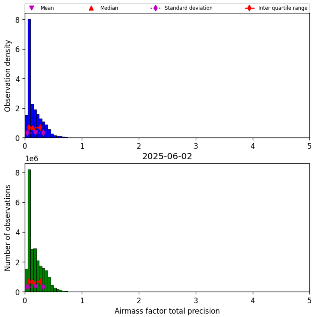
Figure 41: Histogram of “Airmass factor total precision” for 2025-06-01 to 2025-06-03
