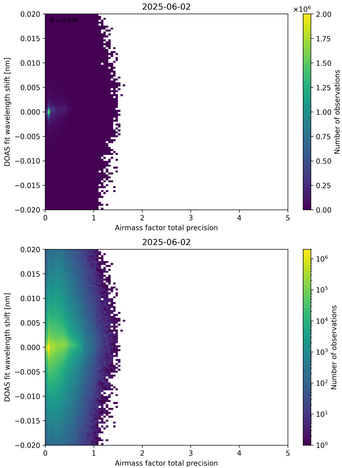
Figure 106: Scatter density plot of “Airmass factor total precision” against “DOAS fit wavelength shift” for 2025-06-01 to 2025-06-03.
