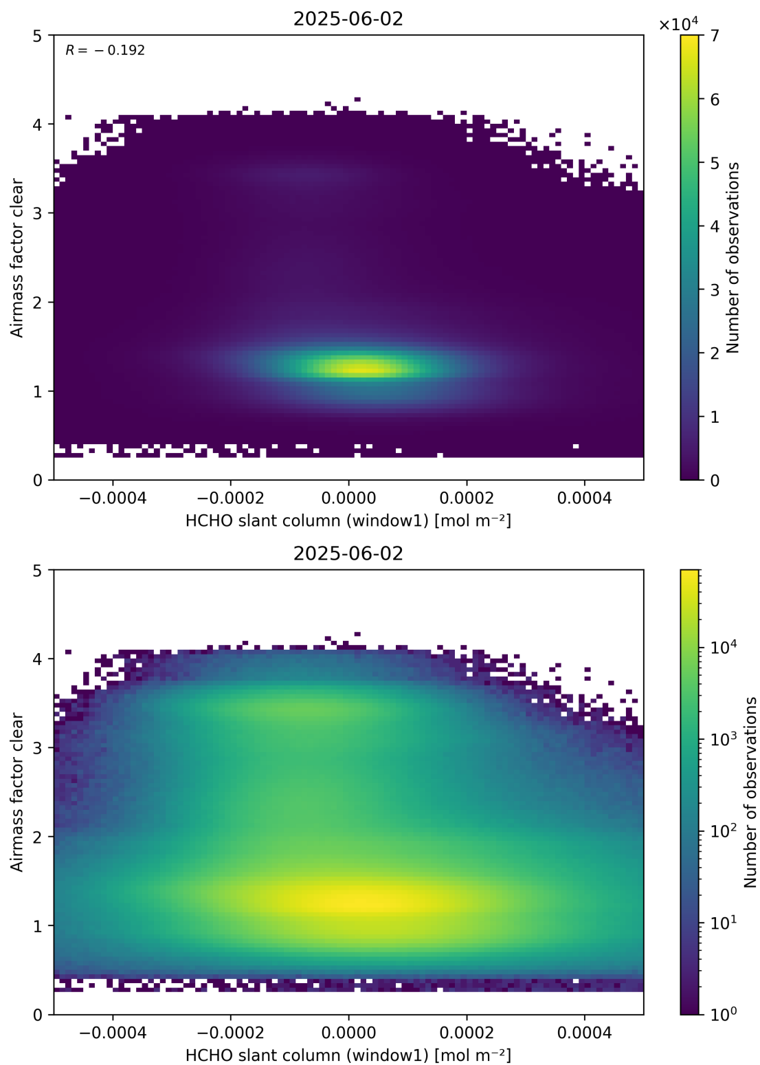
Figure 81: Scatter density plot of “HCHO slant column (window1)” against “Airmass factor clear” for 2025-06-01 to 2025-06-03.
