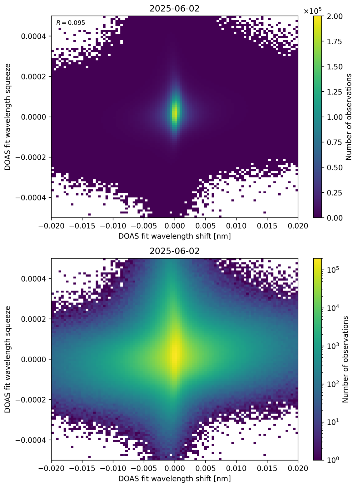
Figure 65: Scatter density plot of “DOAS fit wavelength shift” against “DOAS fit wavelength squeeze” for 2025-06-01 to 2025-06-03.
