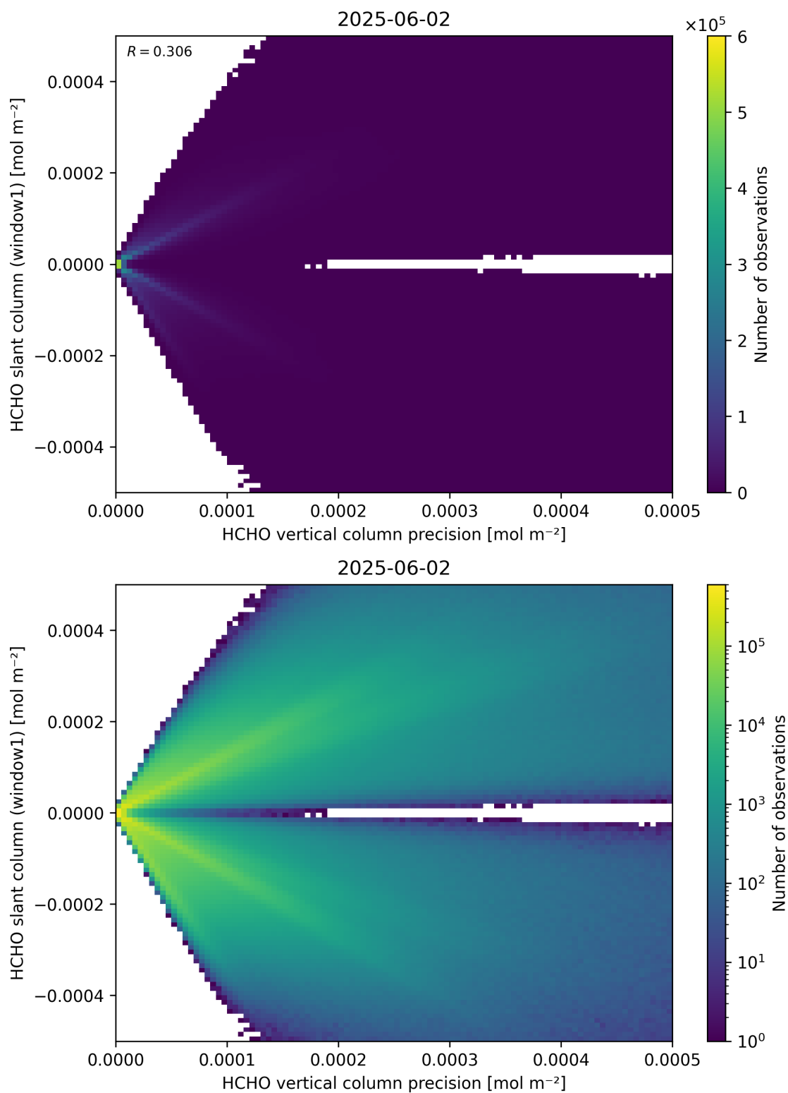
Figure 142: Scatter density plot of “HCHO vertical column precision” against “HCHO slant column (window1)” for 2025-06-01 to 2025-06-03.
