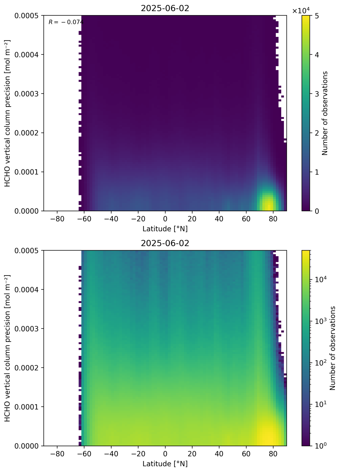
Figure 165: Scatter density plot of “Latitude” against “HCHO vertical column precision” for 2025-06-01 to 2025-06-03.
