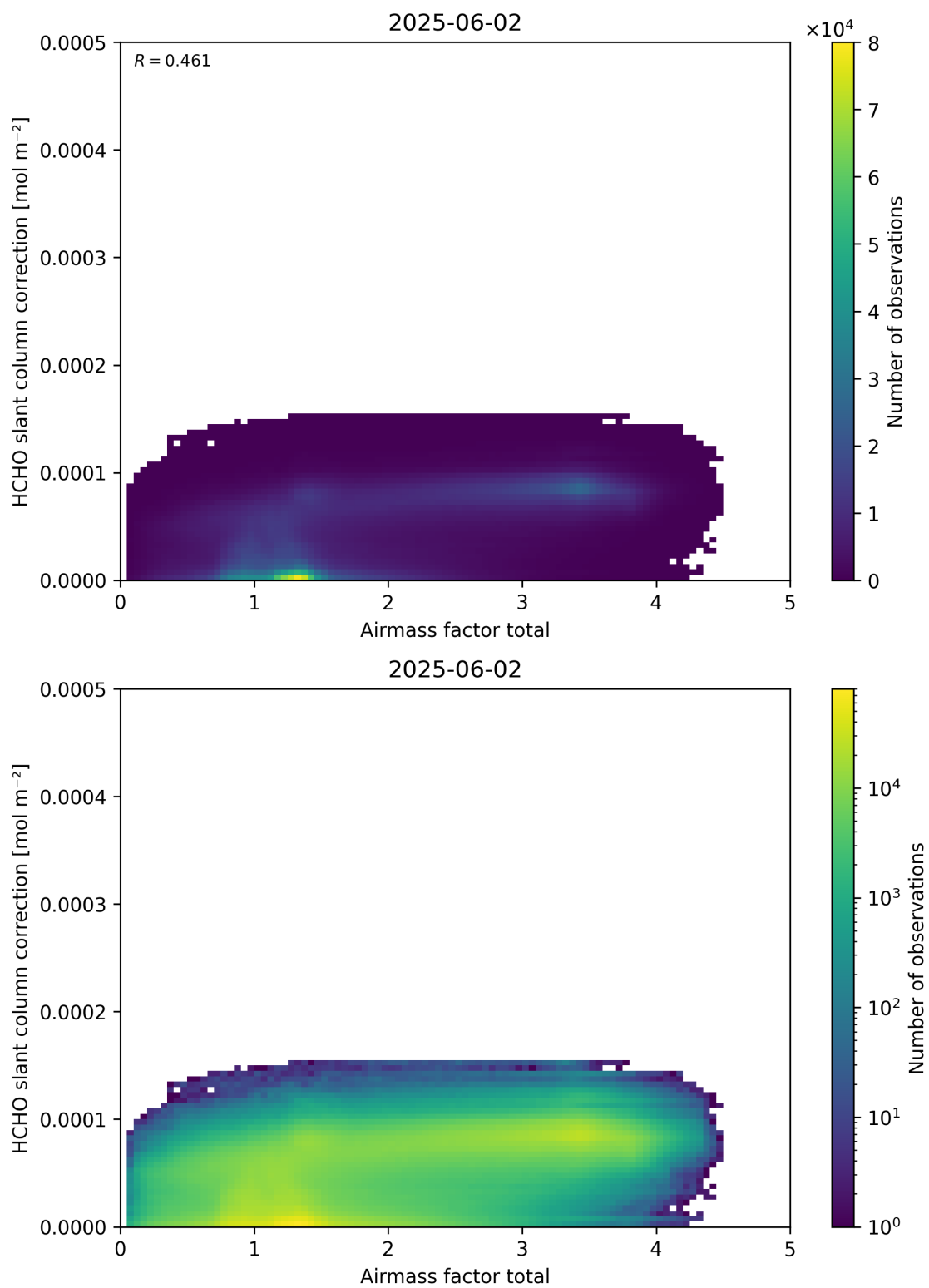
Figure 102: Scatter density plot of “Airmass factor total” against “HCHO slant column correction” for 2025-06-01 to 2025-06-03.
