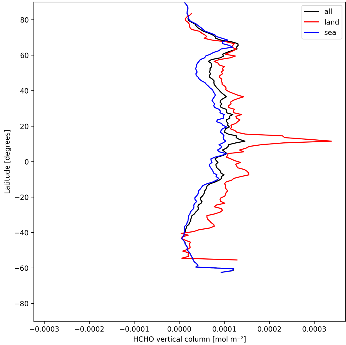
Figure 21: Zonal average of “HCHO vertical column” for 2025-06-01 to 2025-06-03.
