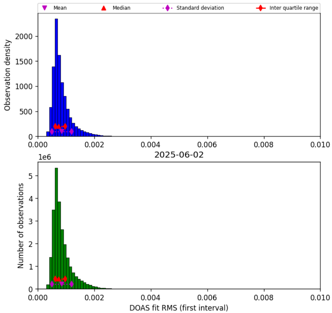
Figure 46: Histogram of “DOAS fit RMS (first interval)” for 2025-06-01 to 2025-06-03
