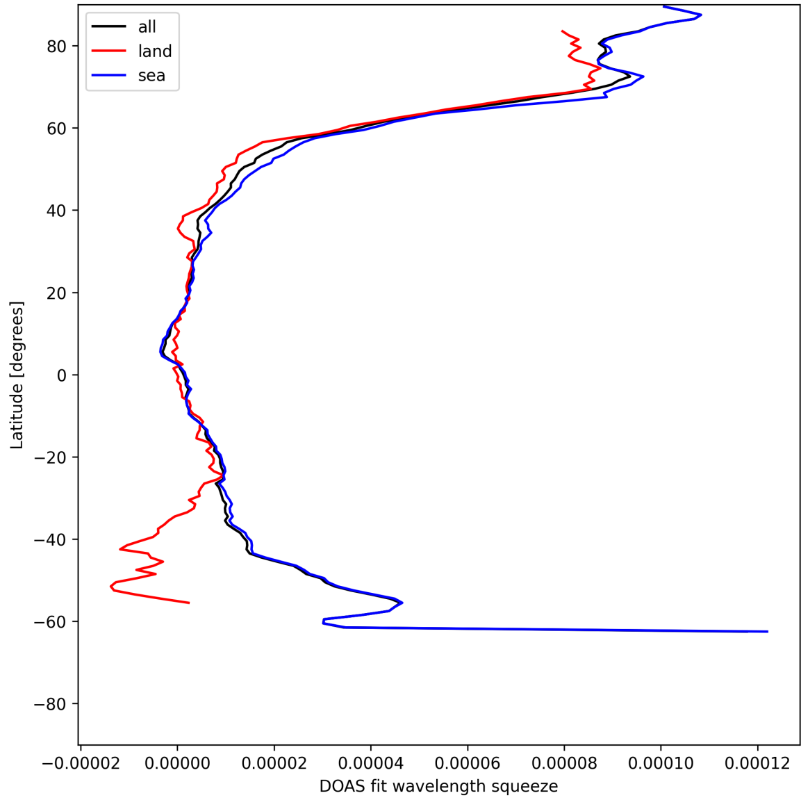
Figure 31: Zonal average of “DOAS fit wavelength squeeze” for 2025-06-01 to 2025-06-03.
