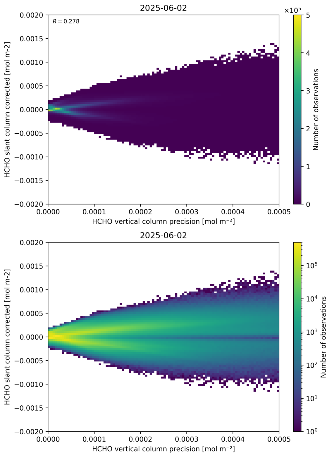
Figure 140: Scatter density plot of “HCHO vertical column precision” against “HCHO slant column corrected” for 2025-06-01 to 2025-06-03.
