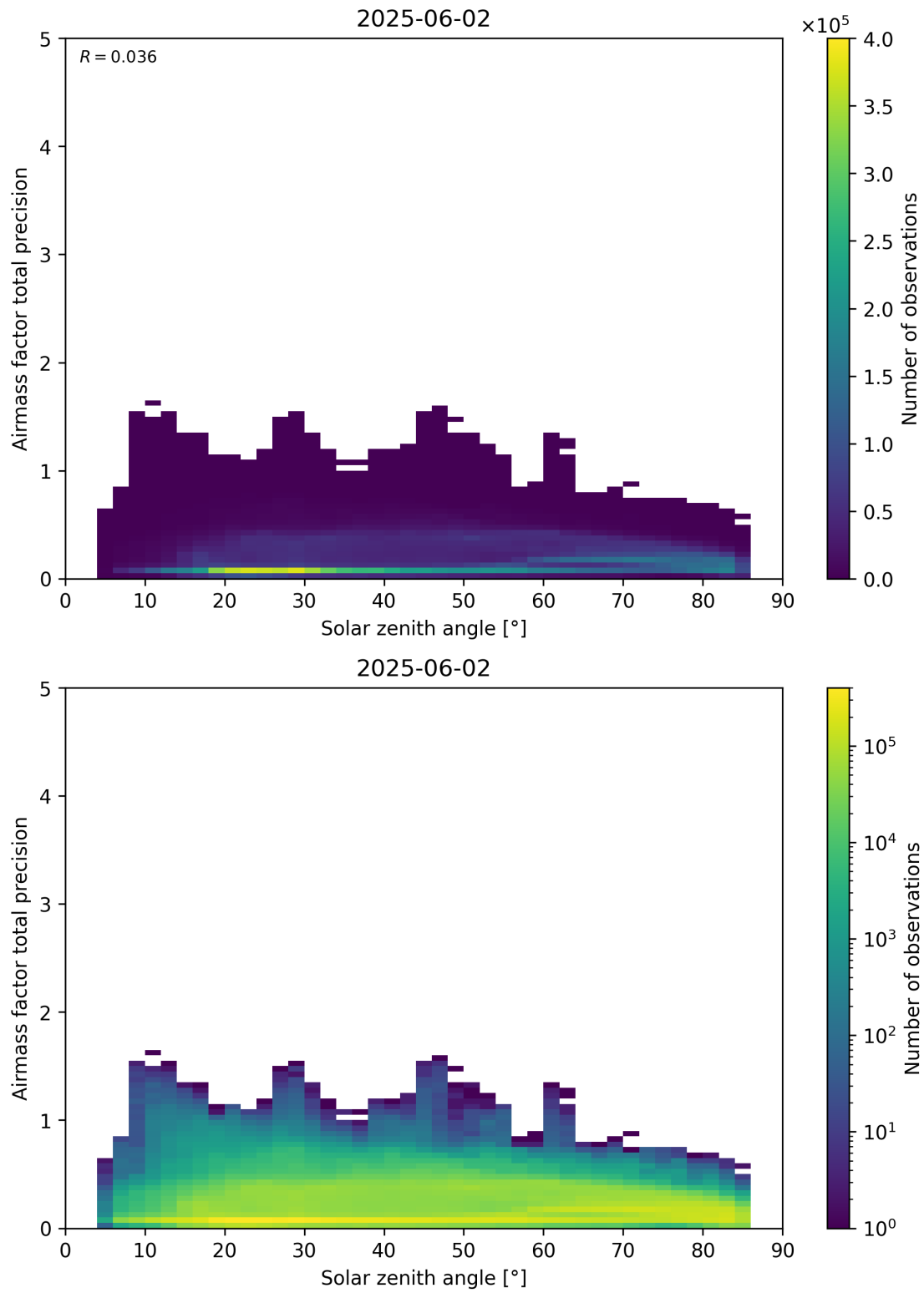
Figure 176: Scatter density plot of “Solar zenith angle” against “Airmass factor total precision” for 2025-06-01 to 2025-06-03.
