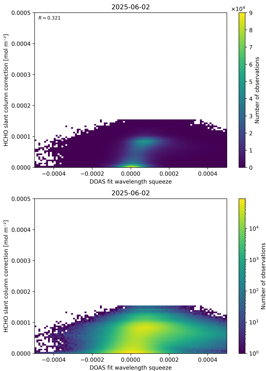
Figure 70: Scatter density plot of “DOAS fit wavelength squeeze” against “HCHO slant column correction” for 2025-06-01 to 2025-06-03.
