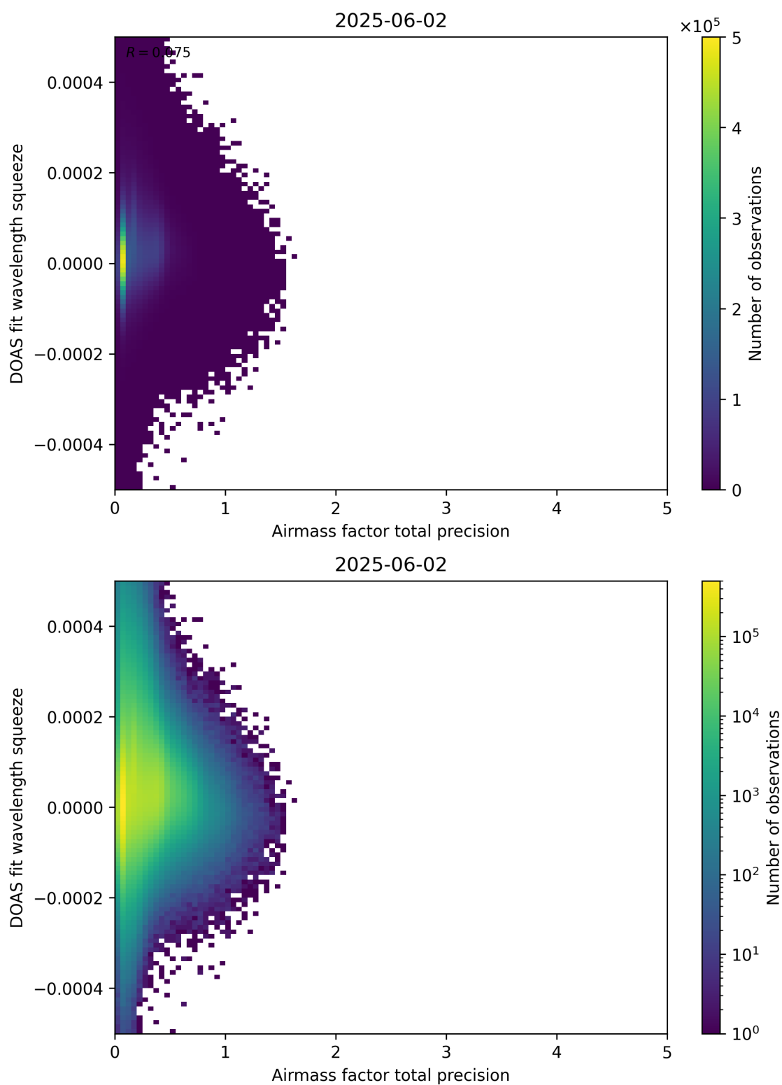
Figure 107: Scatter density plot of “Airmass factor total precision” against “DOAS fit wavelength squeeze” for 2025-06-01 to 2025-06-03.
