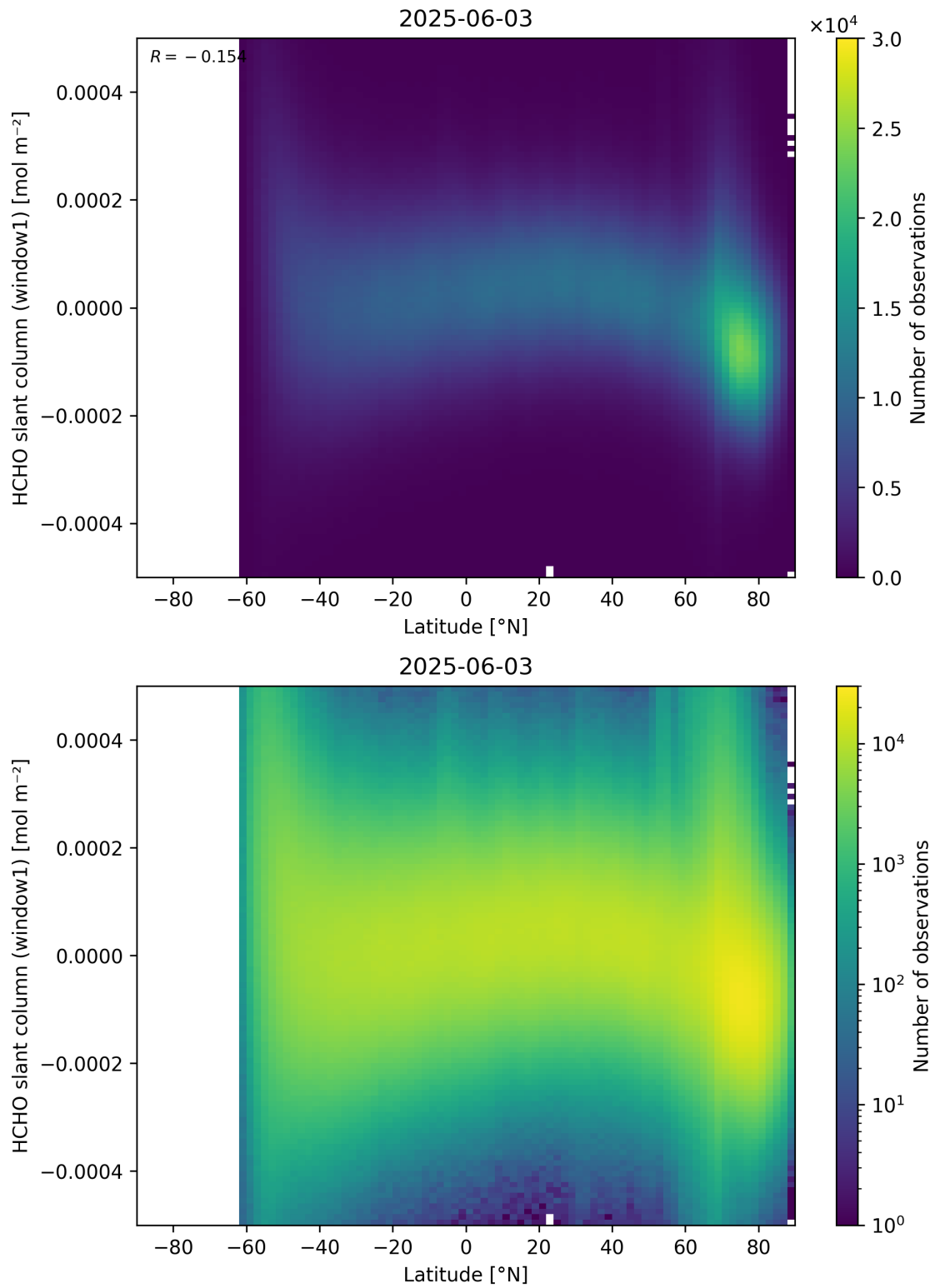
Figure 159: Scatter density plot of “Latitude” against “HCHO slant column (window1)” for 2025-06-02 to 2025-06-04.
