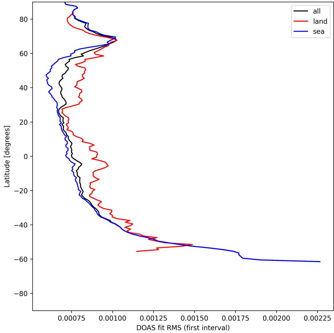
Figure 32: Zonal average of "DOAS fit RMS (first interval)" for 2025-06-02 to 2025-06-04.
