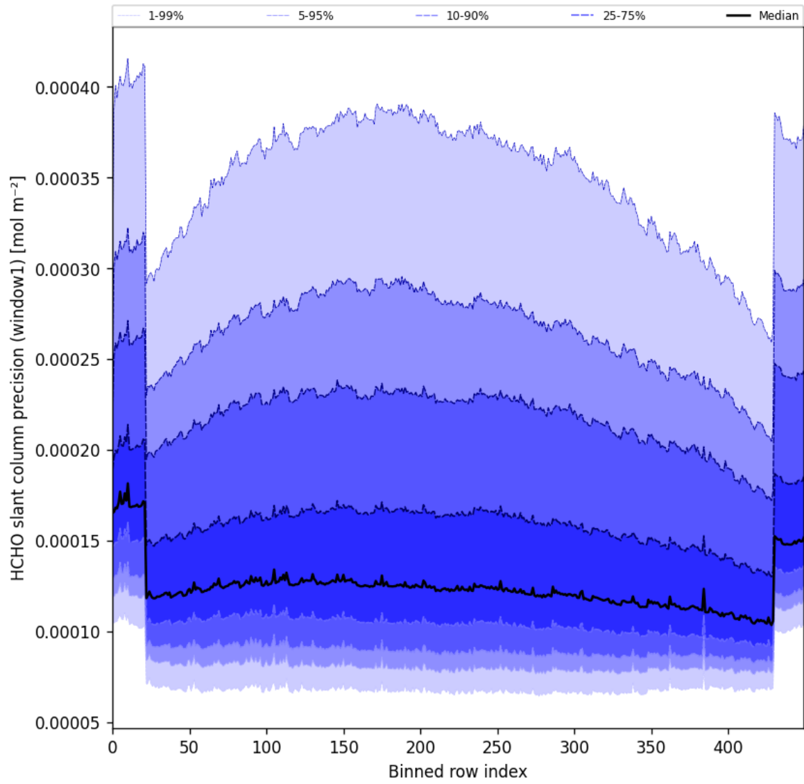
Figure 53: Along track statistics of “HCHO slant column precision (window1)” for 2025-06-02 to 2025-06-04
