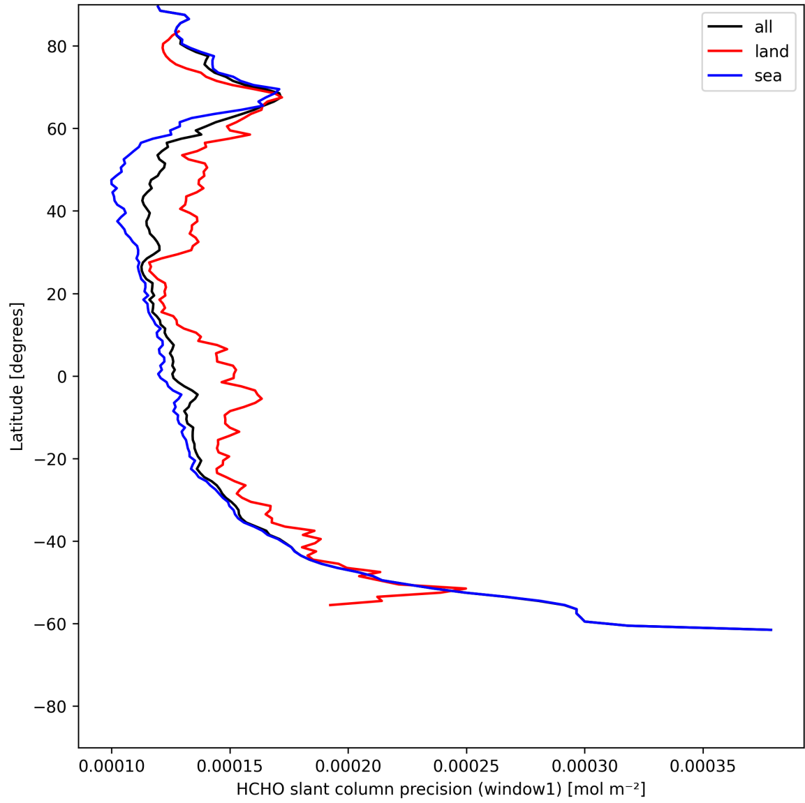
Figure 25: Zonal average of "HCHO slant column precision (window1)" for 2025-06-02 to 2025-06-04.
