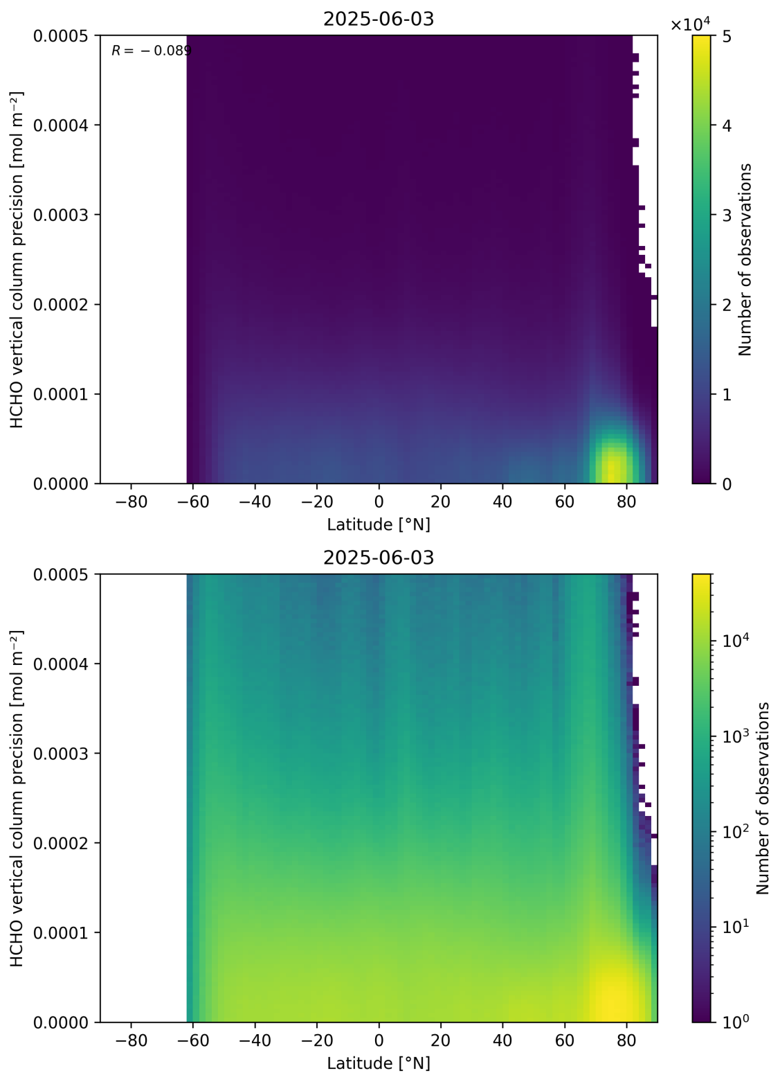
Figure 165: Scatter density plot of “Latitude” against “HCHO vertical column precision” for 2025-06-02 to 2025-06-04.
