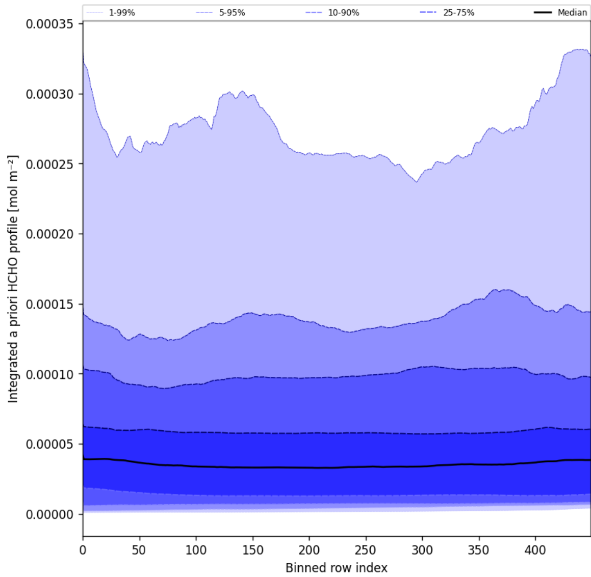
Figure 57: Along track statistics of “Integrated a priori HCHO profile” for 2025-06-02 to 2025-06-04
