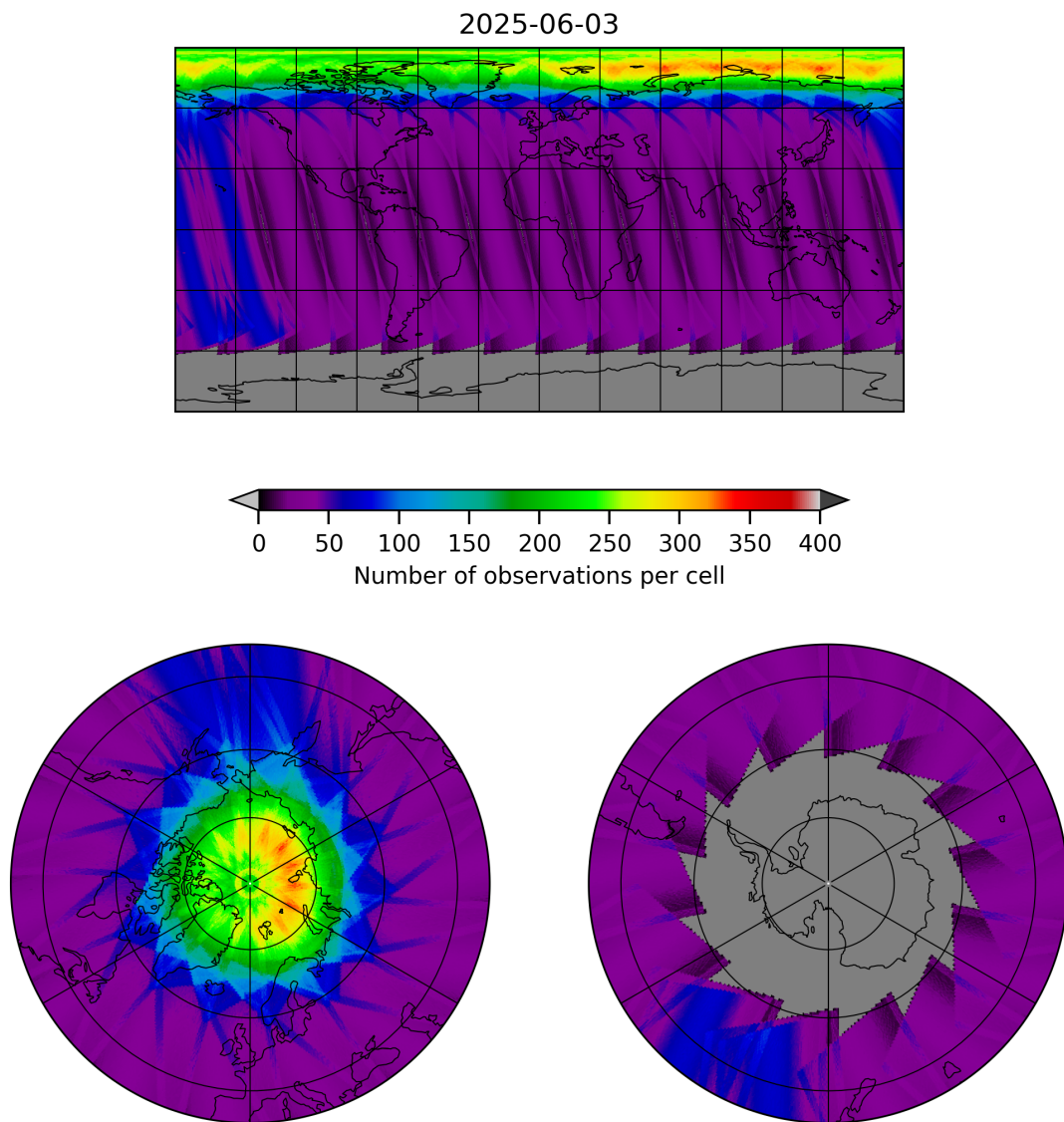
Figure 19: Map of the number of observations for 2025-06-02 to 2025-06-04
