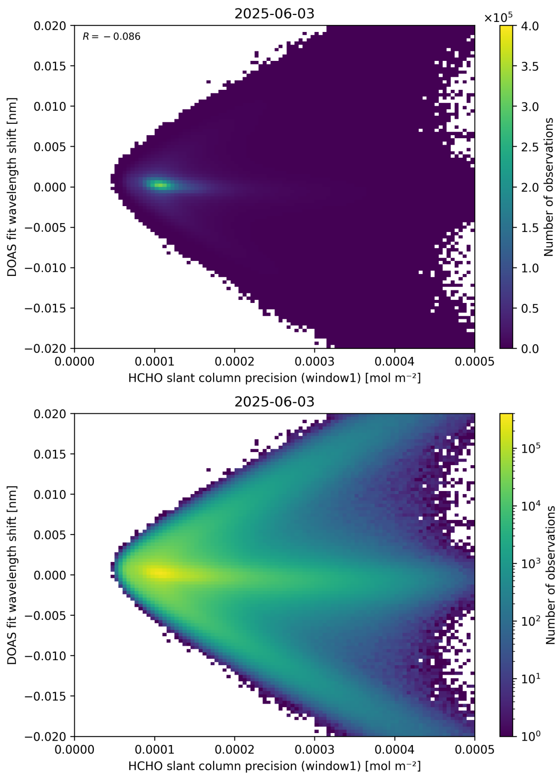
Figure 89: Scatter density plot of “HCHO slant column precision (window1)” against “DOAS fit wavelength shift” for 2025-06-02 to 2025-06-04.
