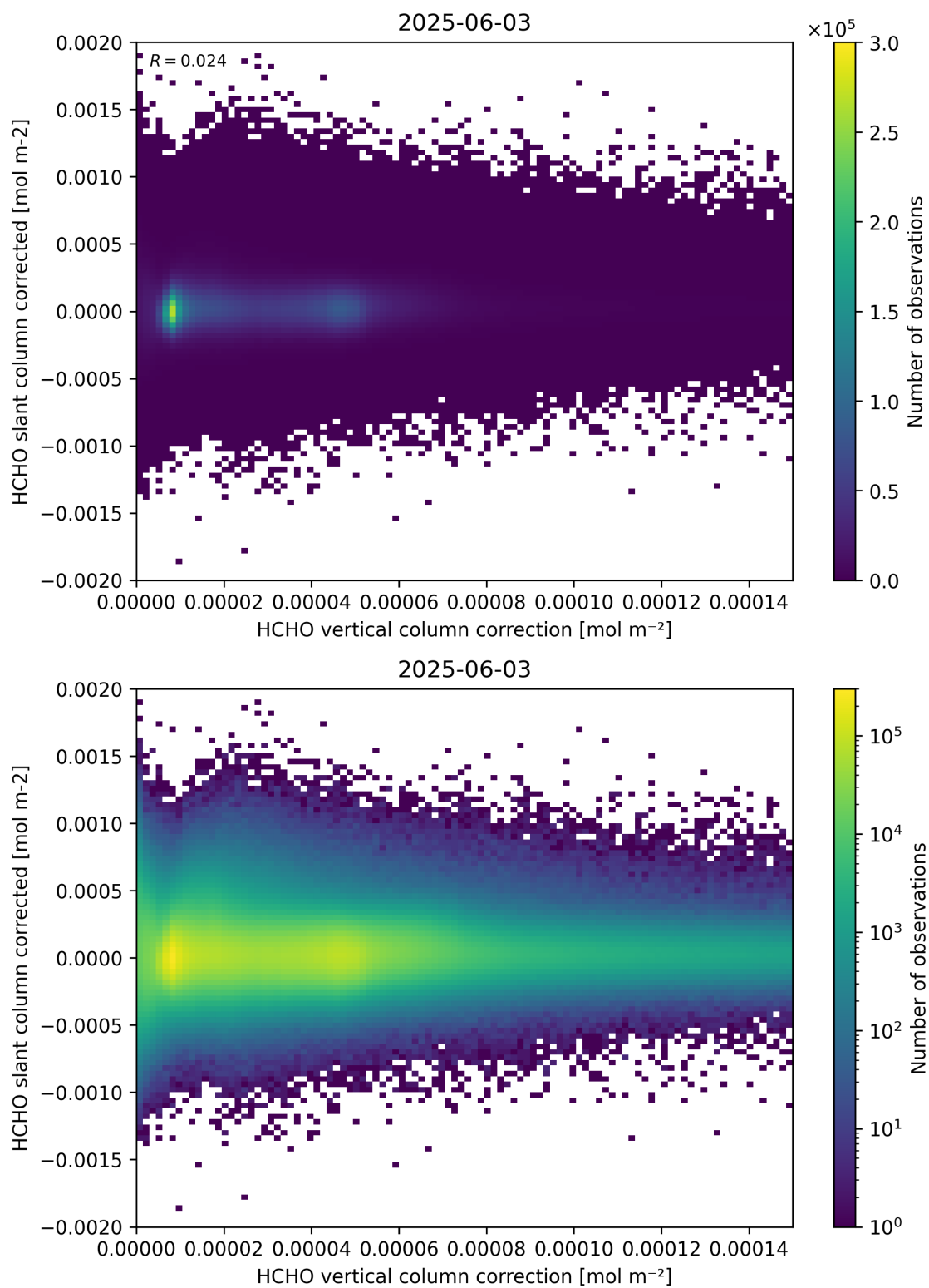
Figure 116: Scatter density plot of “HCHO vertical column correction” against “HCHO slant column corrected” for 2025-06-02 to 2025-06-04.
