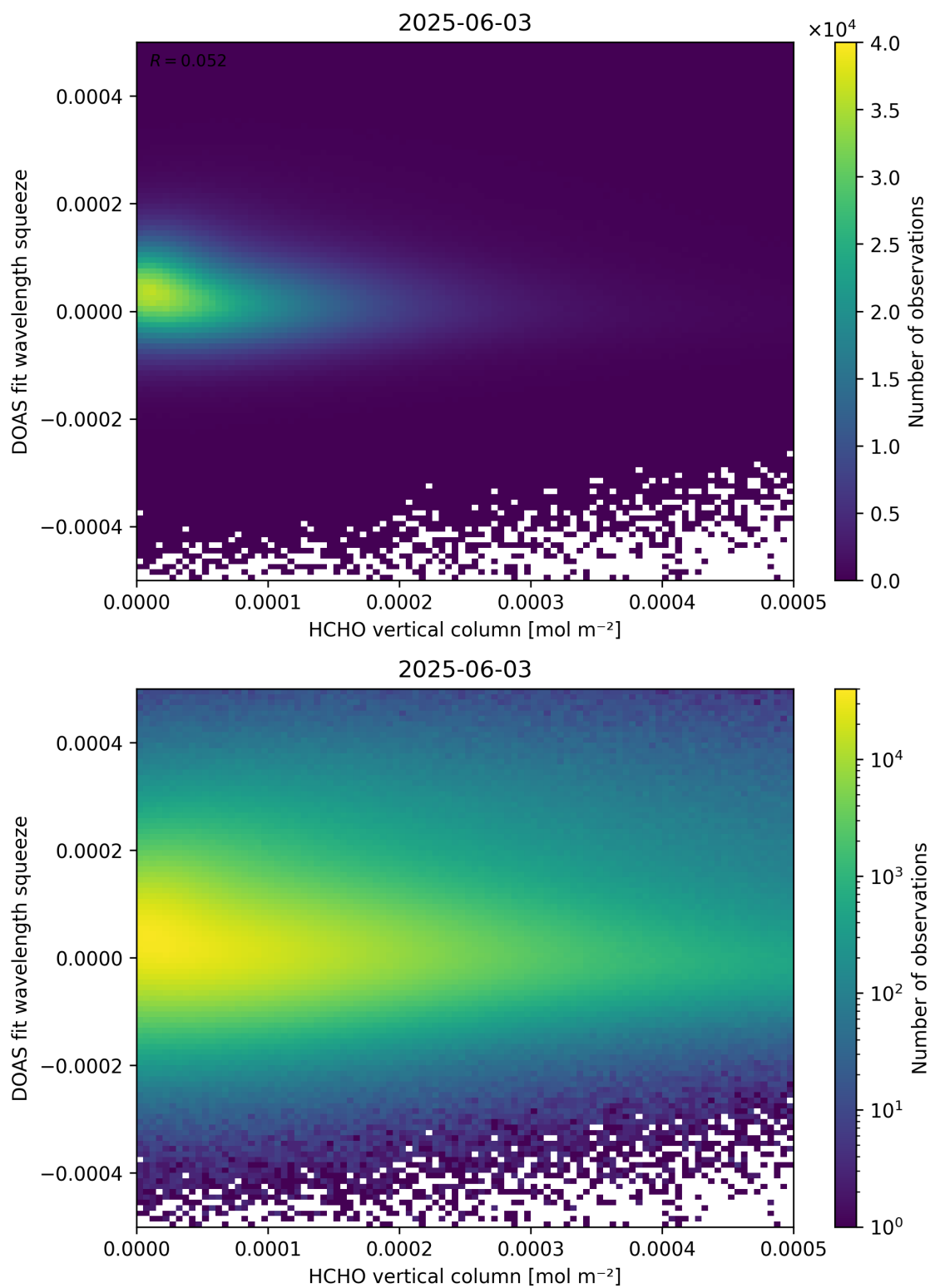
Figure 125: Scatter density plot of “HCHO vertical column” against “DOAS fit wavelength squeeze” for 2025-06-02 to 2025-06-04.
