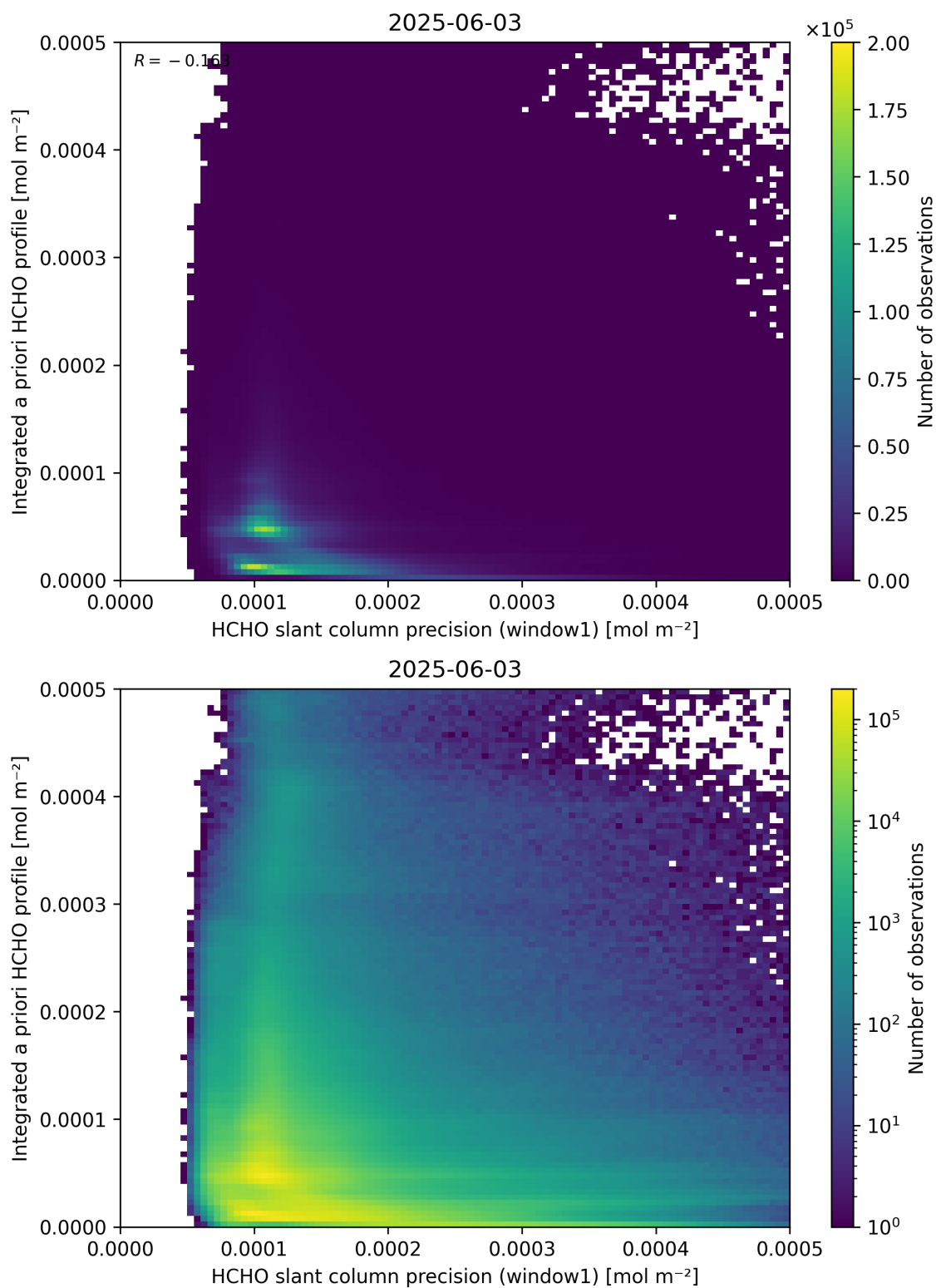
Figure 96: Scatter density plot of “HCHO slant column precision (window1)” against “Integrated a priori HCHO profile” for 2025-06-02 to 2025-06-04.
