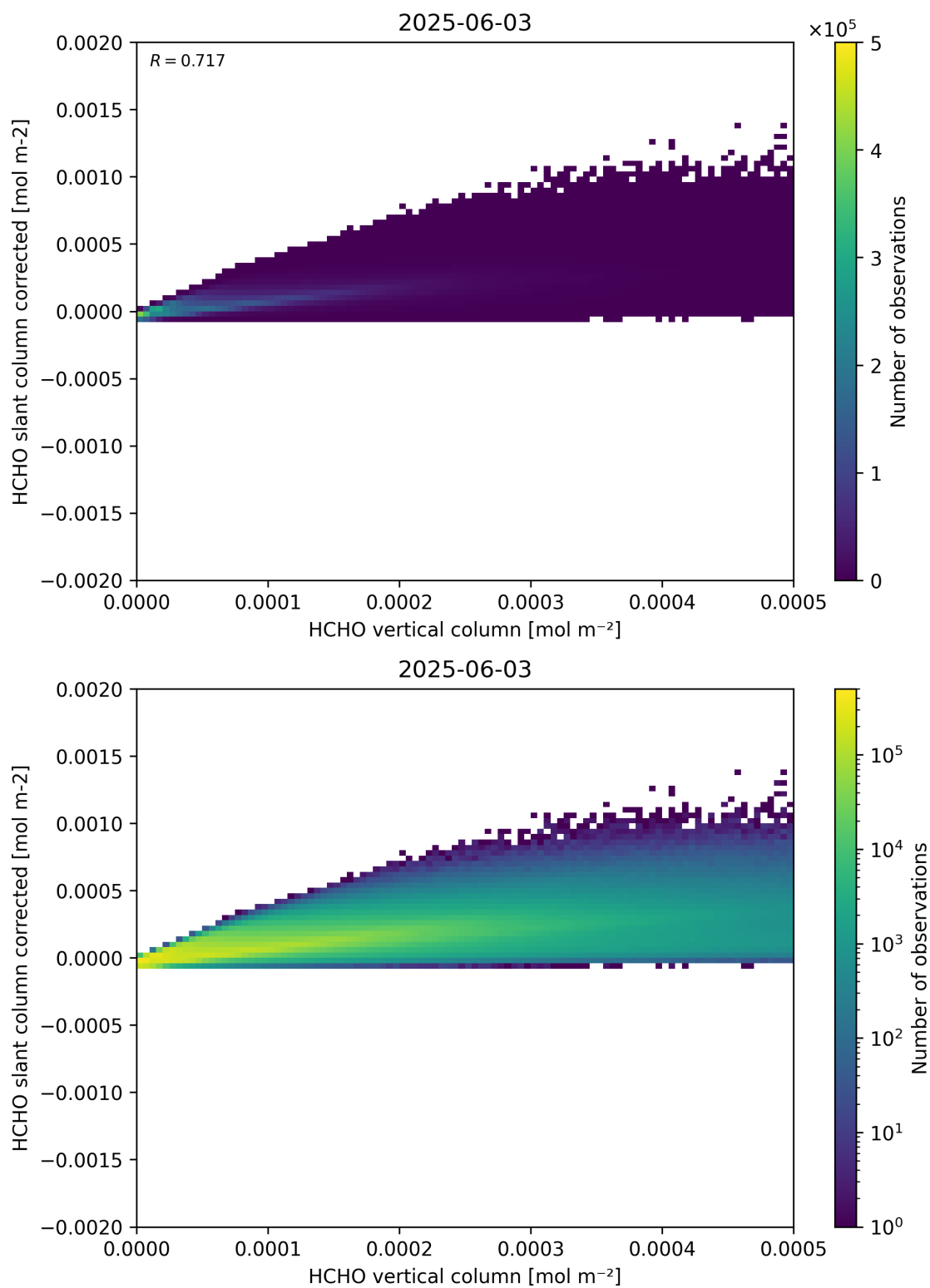
Figure 127: Scatter density plot of “HCHO vertical column” against “HCHO slant column corrected” for 2025-06-02 to 2025-06-04.
