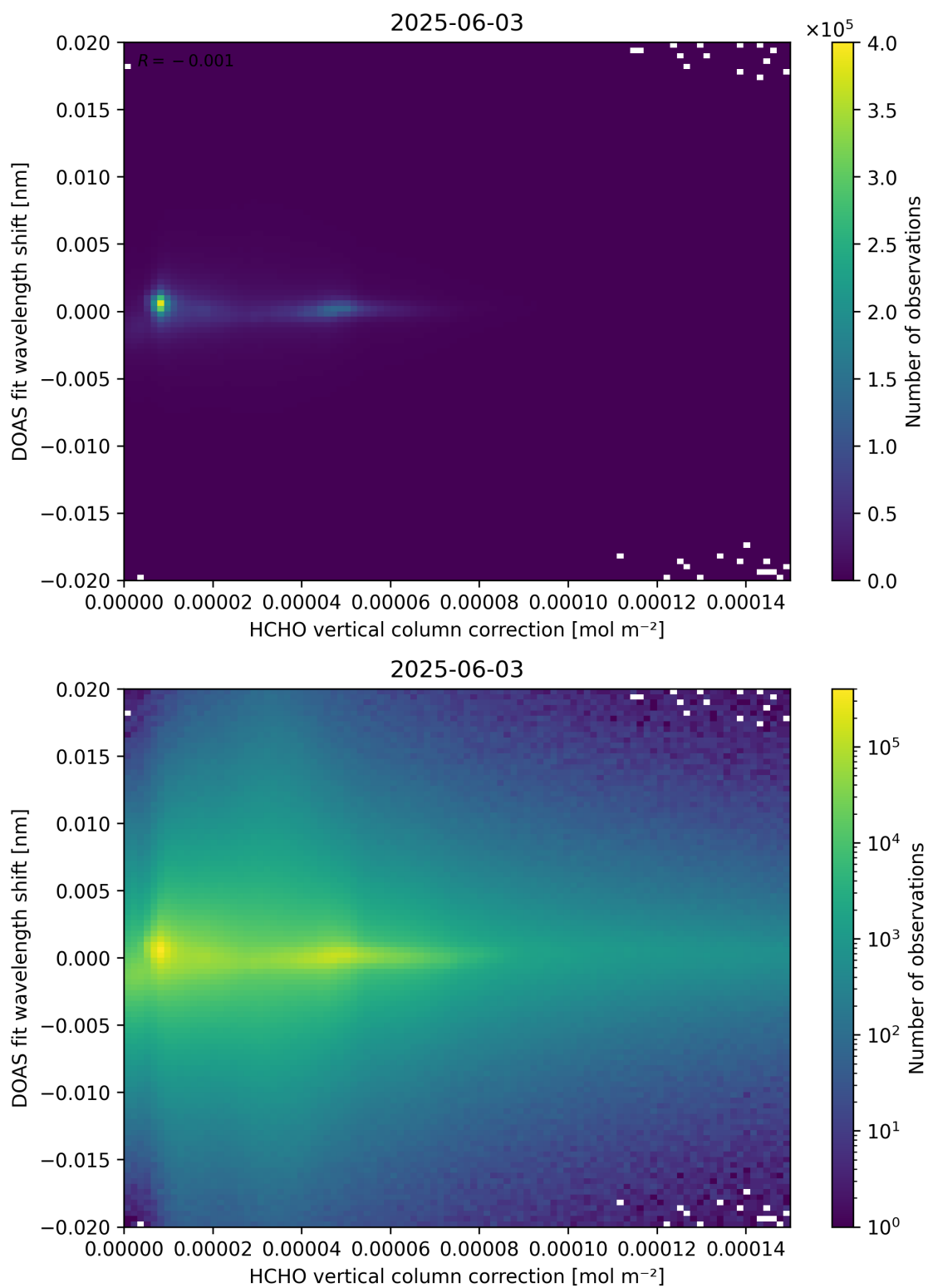
Figure 113: Scatter density plot of “HCHO vertical column correction” against “DOAS fit wavelength shift” for 2025-06-02 to 2025-06-04.
