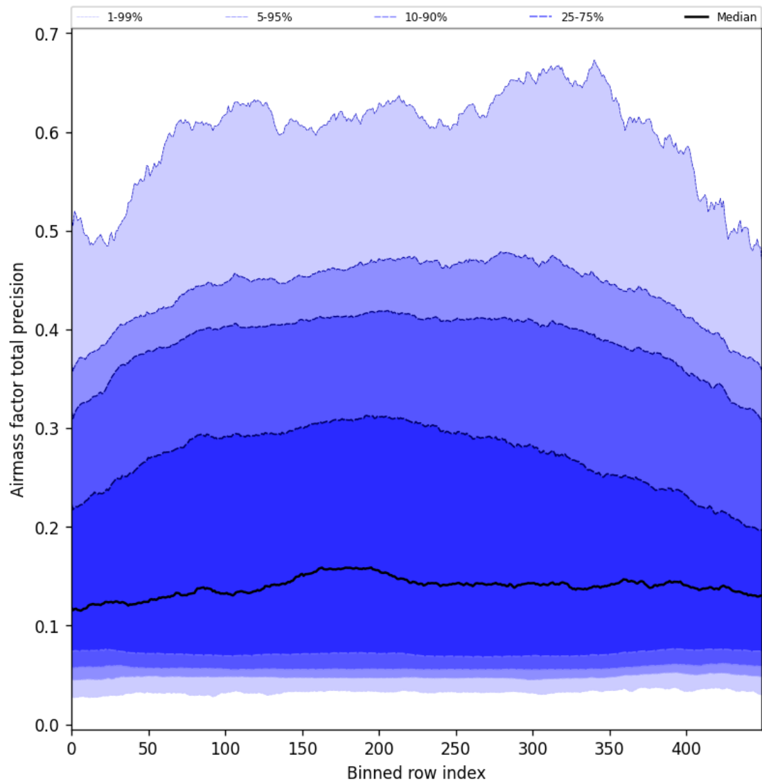
Figure 55: Along track statistics of “Airmass factor total precision” for 2025-06-02 to 2025-06-04
