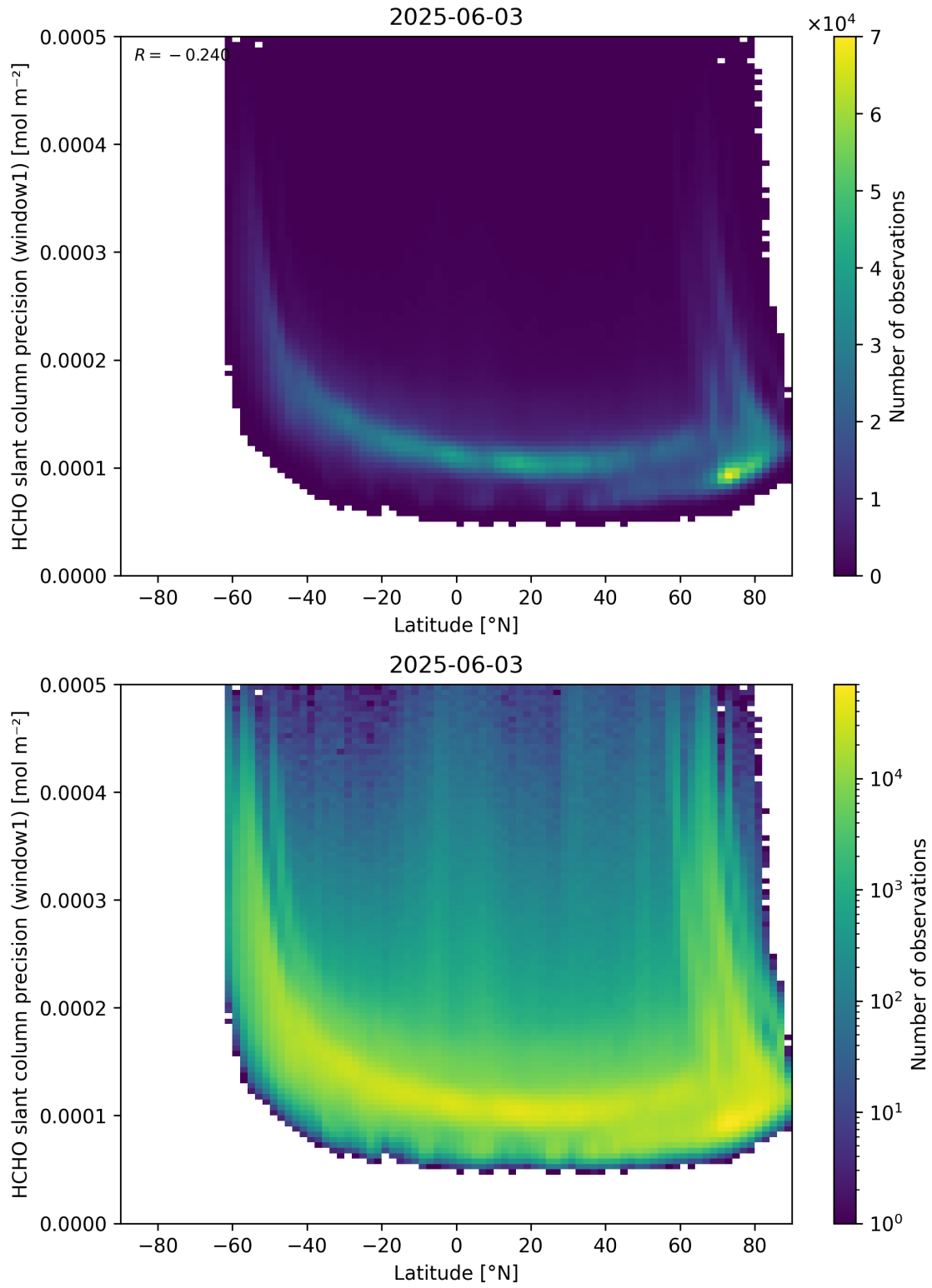
Figure 160: Scatter density plot of “Latitude” against “HCHO slant column precision (window1)” for 2025-06-02 to 2025-06-04.
