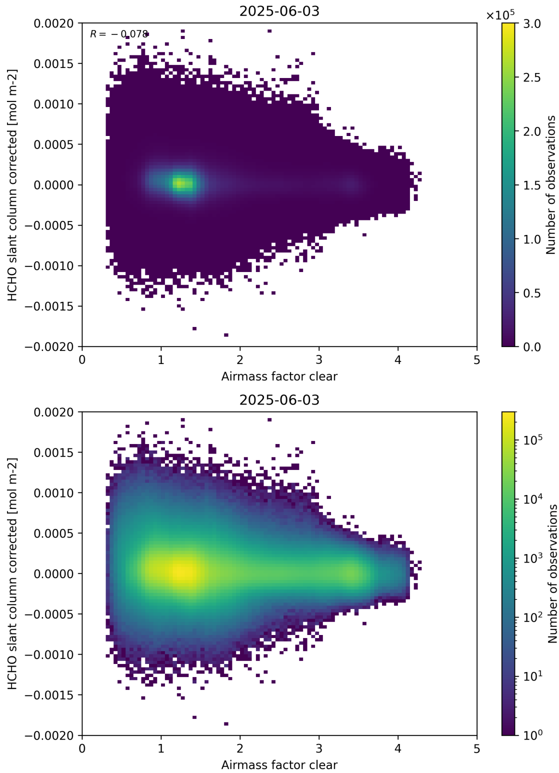
Figure 74: Scatter density plot of “Airmass factor clear” against “HCHO slant column corrected” for 2025-06-02 to 2025-06-04.
