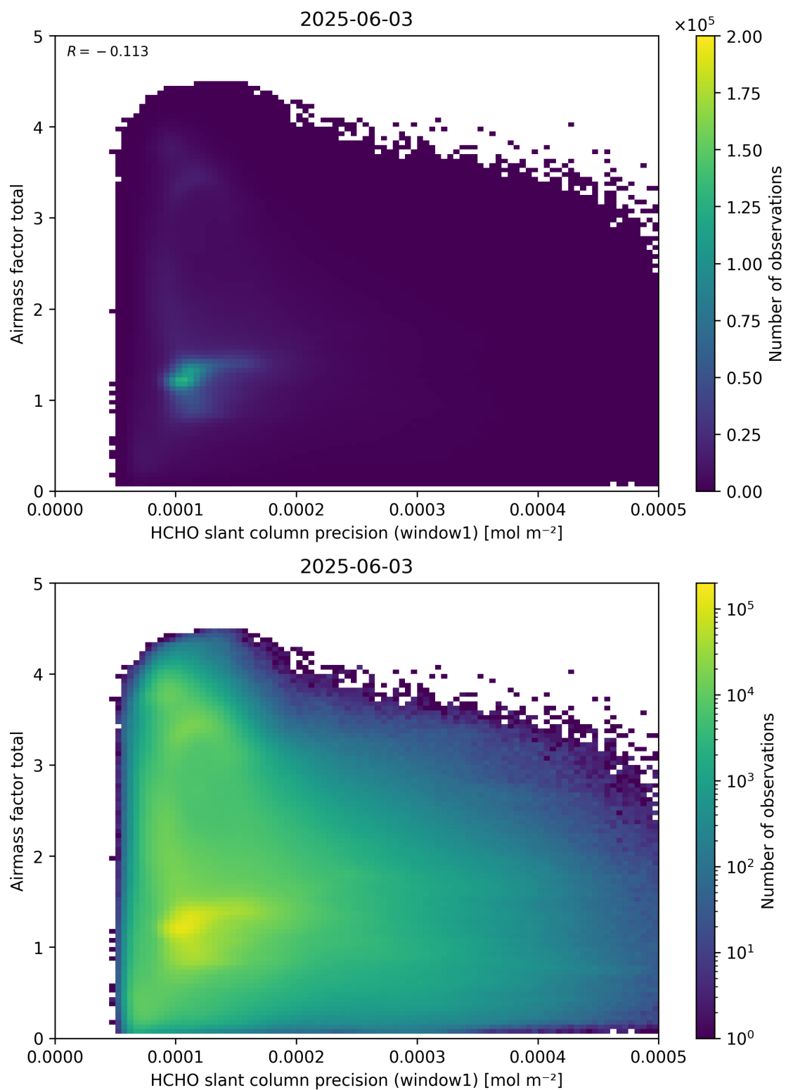
Figure 94: Scatter density plot of “HCHO slant column precision (window1)” against “Airmass factor total” for 2025-06-02 to 2025-06-04.
