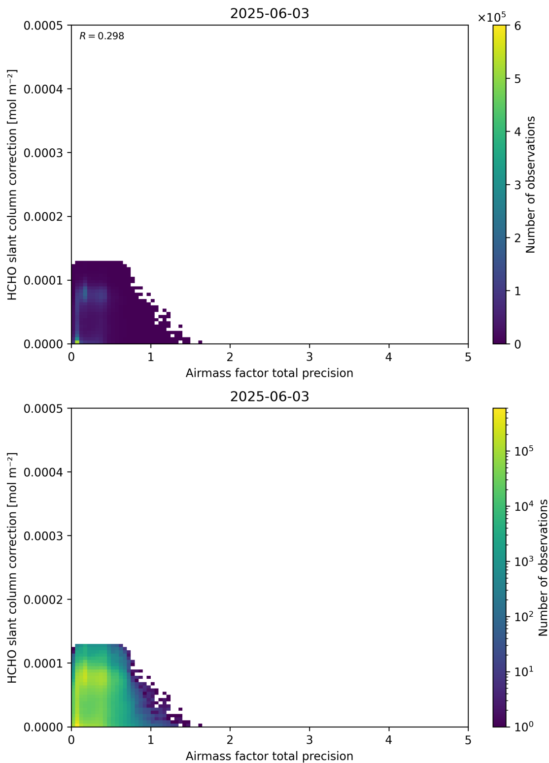
Figure 110: Scatter density plot of “Airmass factor total precision” against “HCHO slant column correction” for 2025-06-02 to 2025-06-04.
