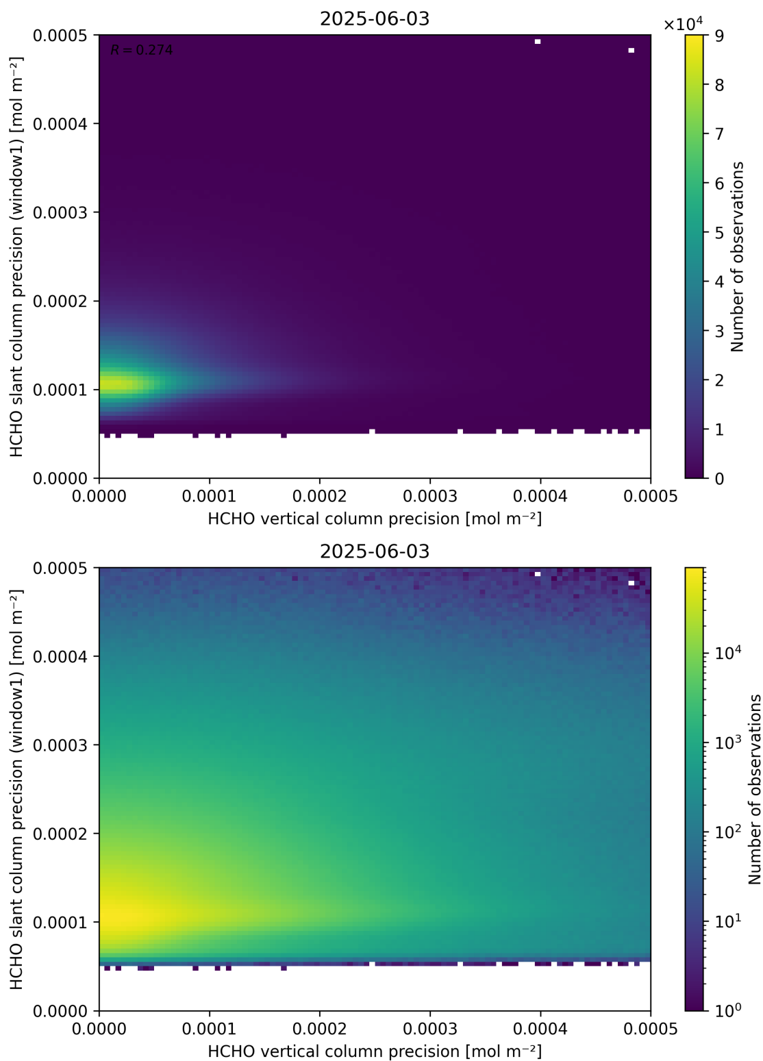
Figure 143: Scatter density plot of “HCHO vertical column precision” against “HCHO slant column precision (window1)” for 2025-06-02 to 2025-06-04.
