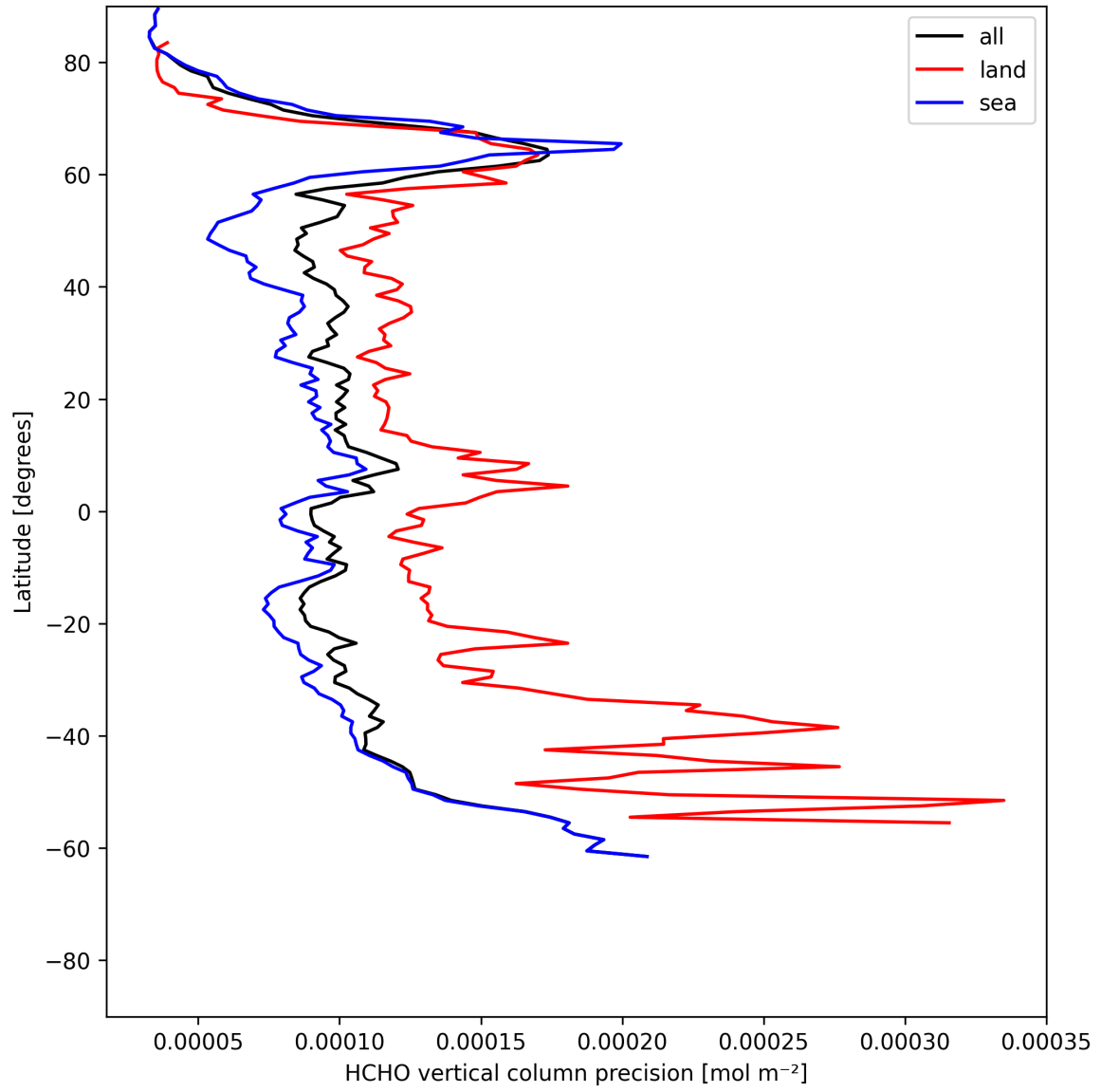
Figure 22: Zonal average of “HCHO vertical column precision” for 2025-06-02 to 2025-06-04.
