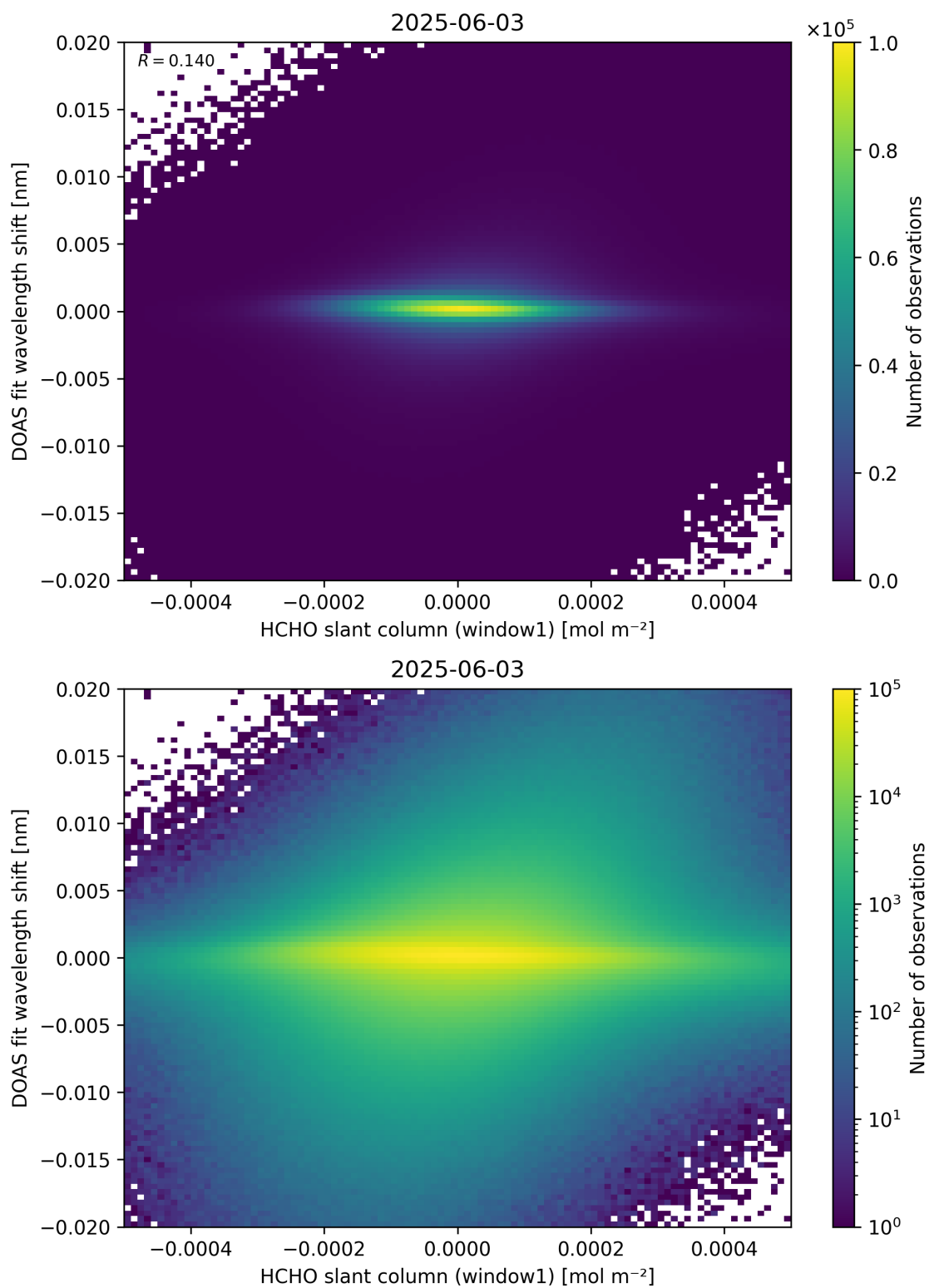
Figure 79: Scatter density plot of “HCHO slant column (window1)” against “DOAS fit wavelength shift” for 2025-06-02 to 2025-06-04.
