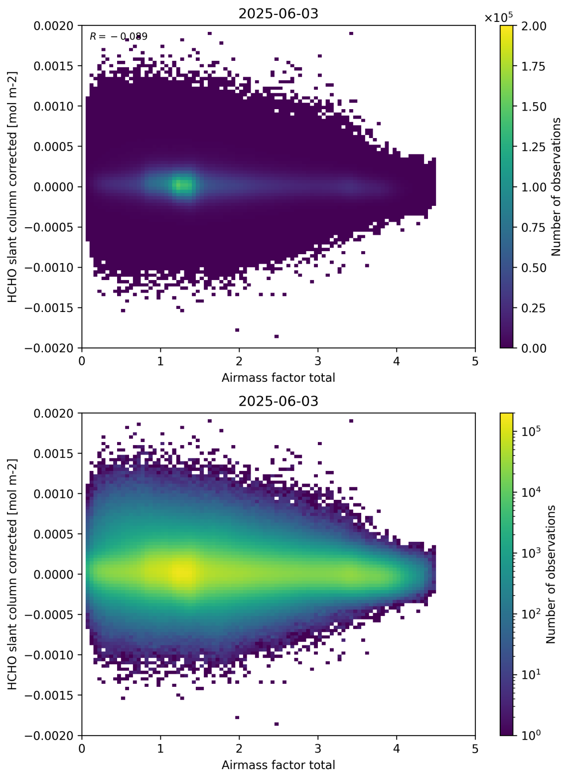
Figure 101: Scatter density plot of “Airmass factor total” against “HCHO slant column corrected” for 2025-06-02 to 2025-06-04.
