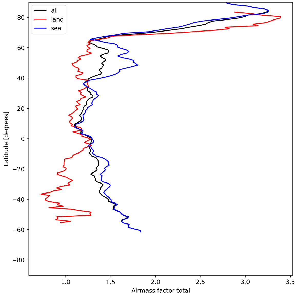
Figure 26: Zonal average of “Airmass factor total” for 2025-06-02 to 2025-06-04.
