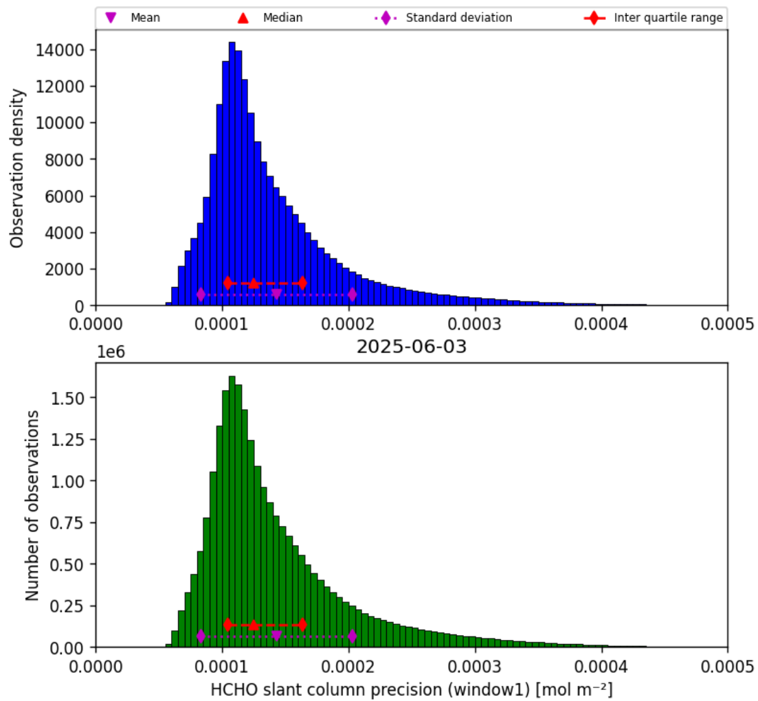
Figure 39: Histogram of “HCHO slant column precision (window1)” for 2025-06-02 to 2025-06-04
