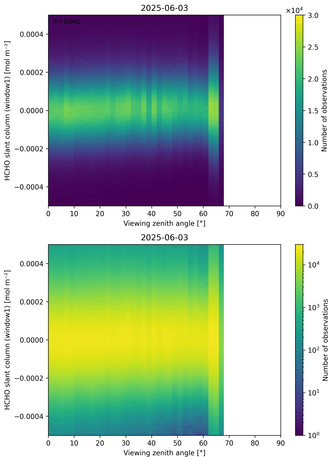
Figure 188: Scatter density plot of “Viewing zenith angle” against “HCHO slant column (window1)” for 2025-06-02 to 2025-06-04.
