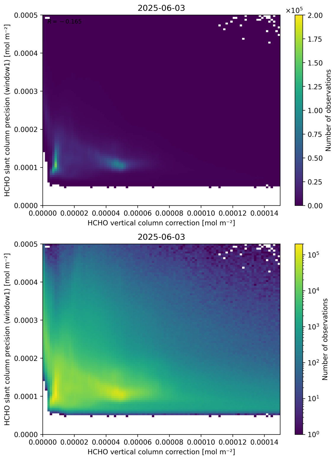
Figure 119: Scatter density plot of “HCHO vertical column correction” against “HCHO slant column precision (window1)” for 2025-06-02 to 2025-06-04.
