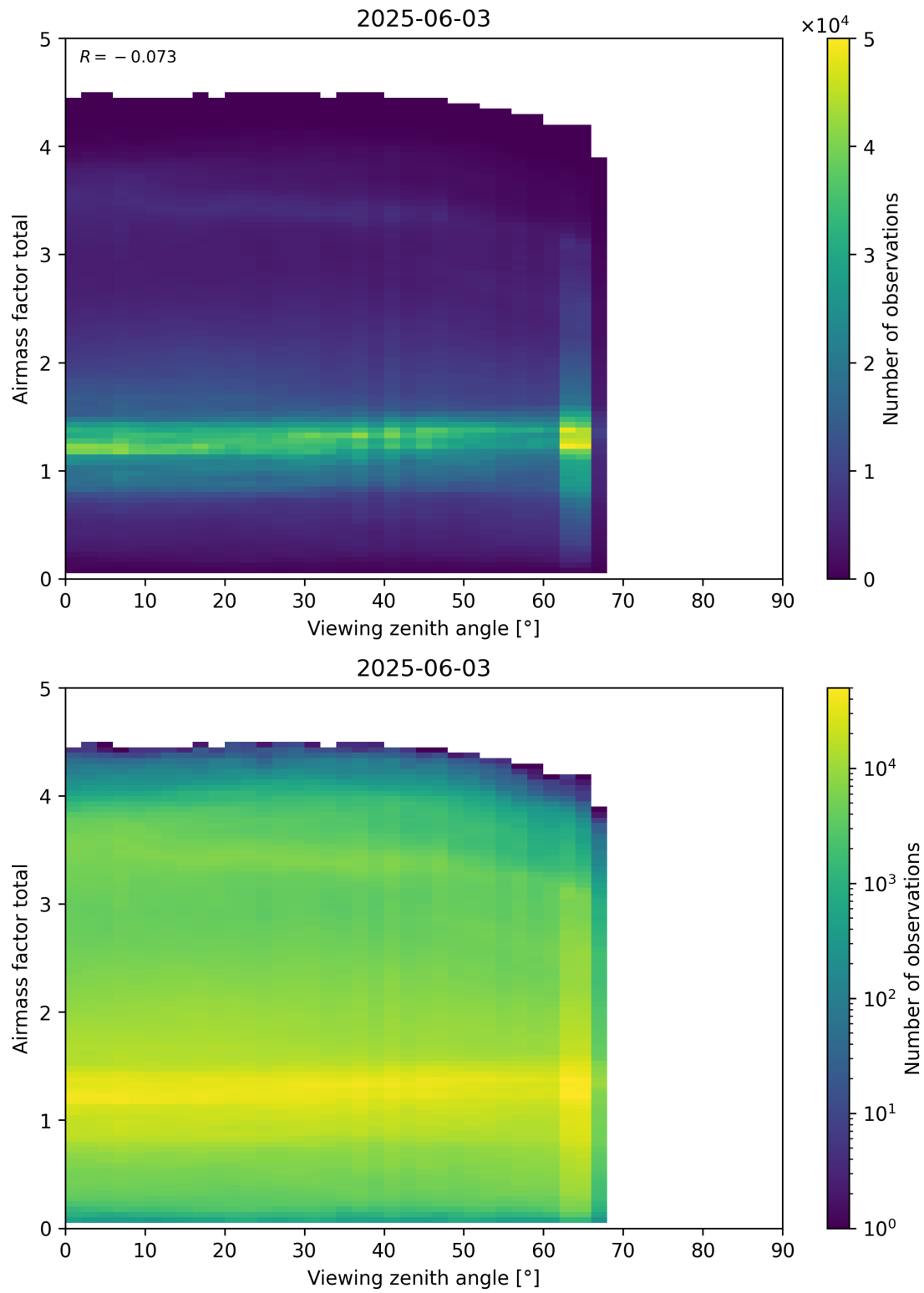
Figure 190: Scatter density plot of “Viewing zenith angle” against “Airmass factor total” for 2025-06-02 to 2025-06-04.
