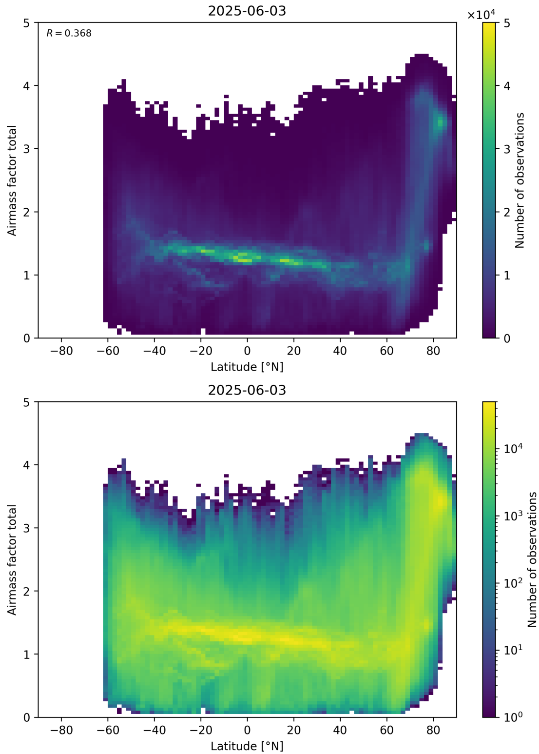
Figure 161: Scatter density plot of “Latitude” against “Airmass factor total” for 2025-06-02 to 2025-06-04.
