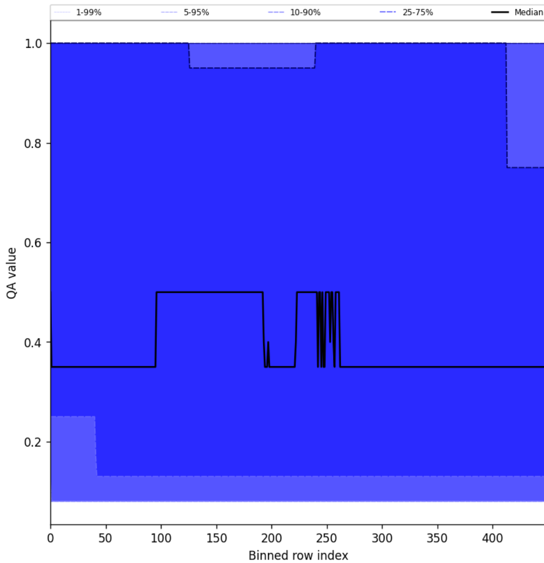
Figure 48: Along track statistics of “QA value” for 2025-06-02 to 2025-06-04
