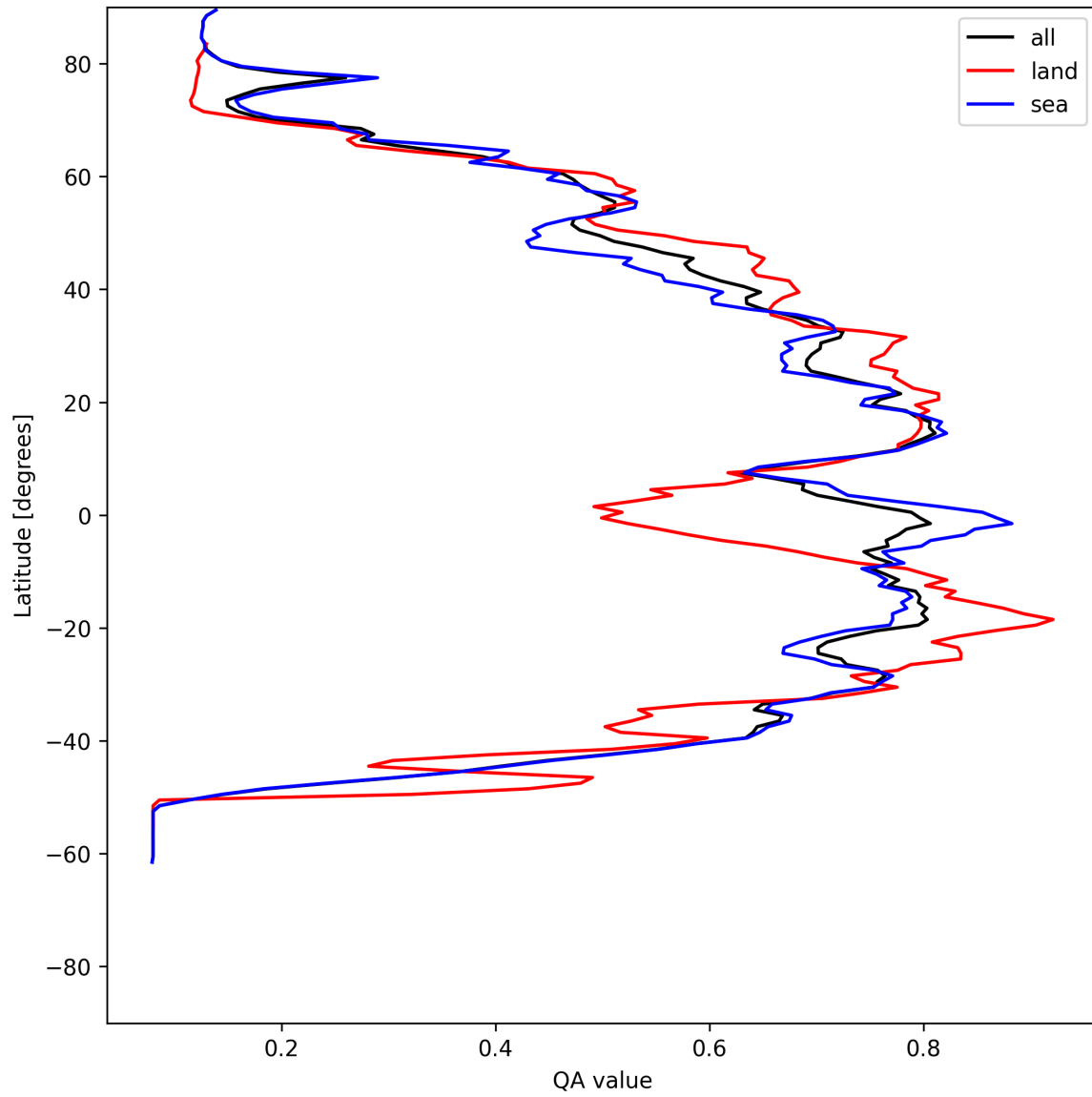
Figure 20: Zonal average of “QA value” for 2025-06-02 to 2025-06-04.
