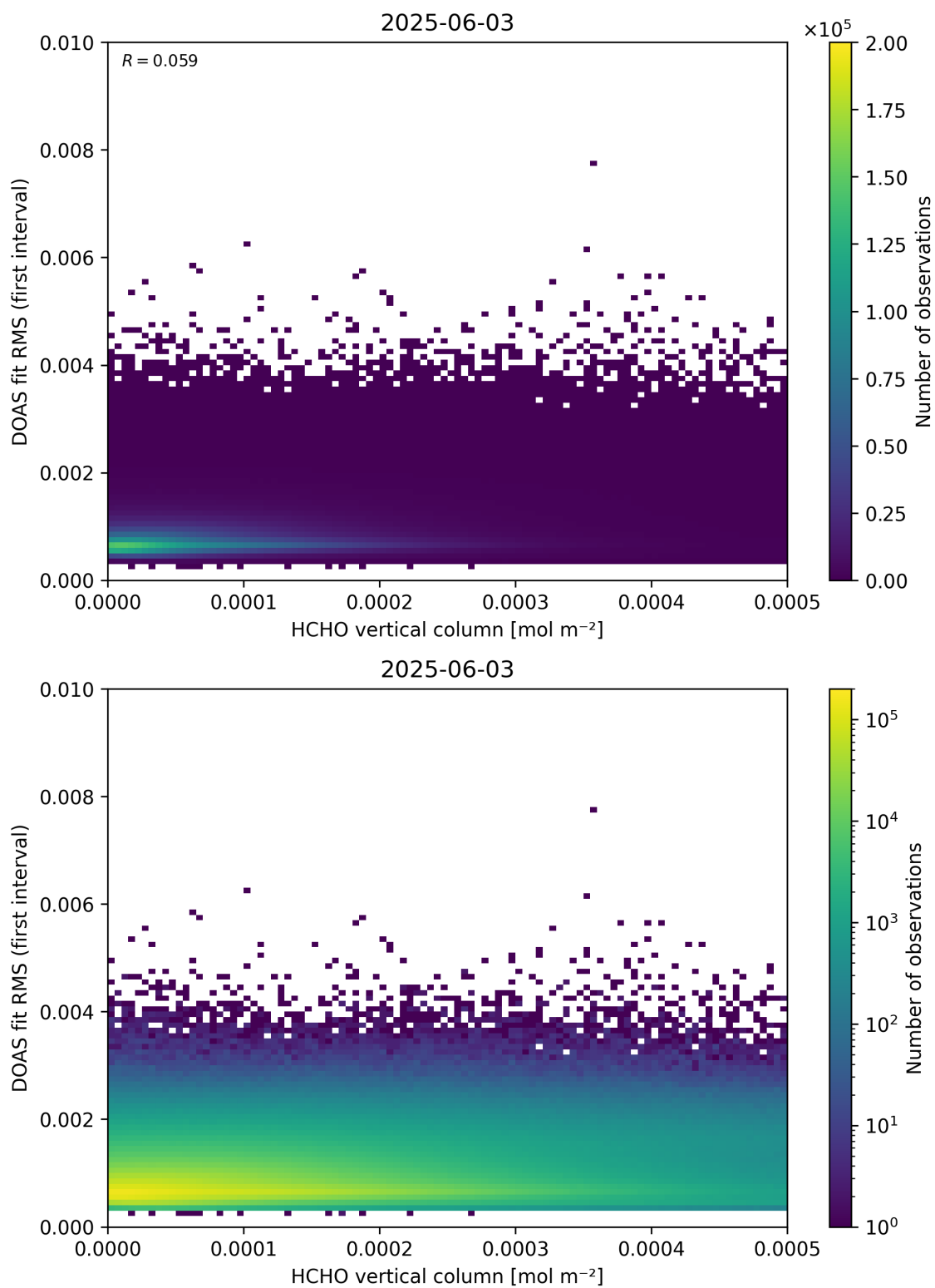
Figure 123: Scatter density plot of “HCHO vertical column” against “DOAS fit RMS (first interval)” for 2025-06-02 to 2025-06-04.
