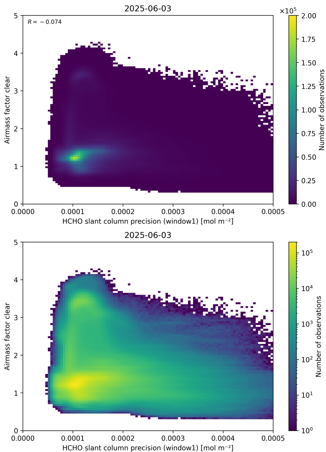
Figure 91: Scatter density plot of “HCHO slant column precision (window1)” against “Airmass factor clear” for 2025-06-02 to 2025-06-04.
