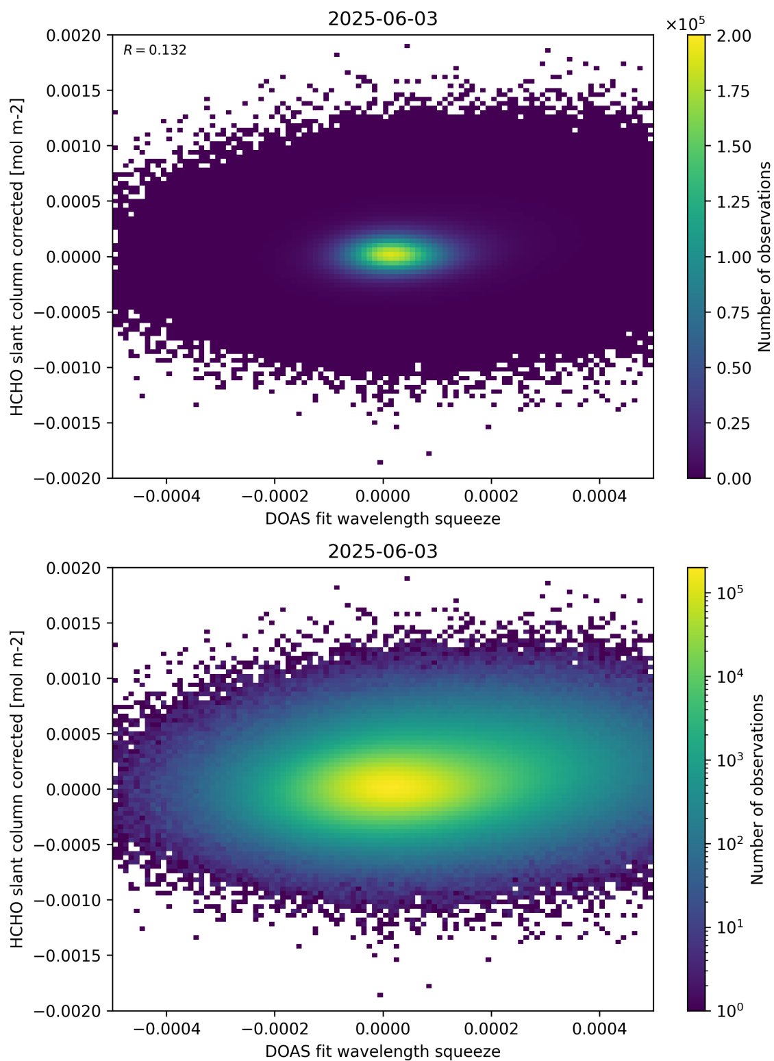
Figure 69: Scatter density plot of “DOAS fit wavelength squeeze” against “HCHO slant column corrected” for 2025-06-02 to 2025-06-04.
