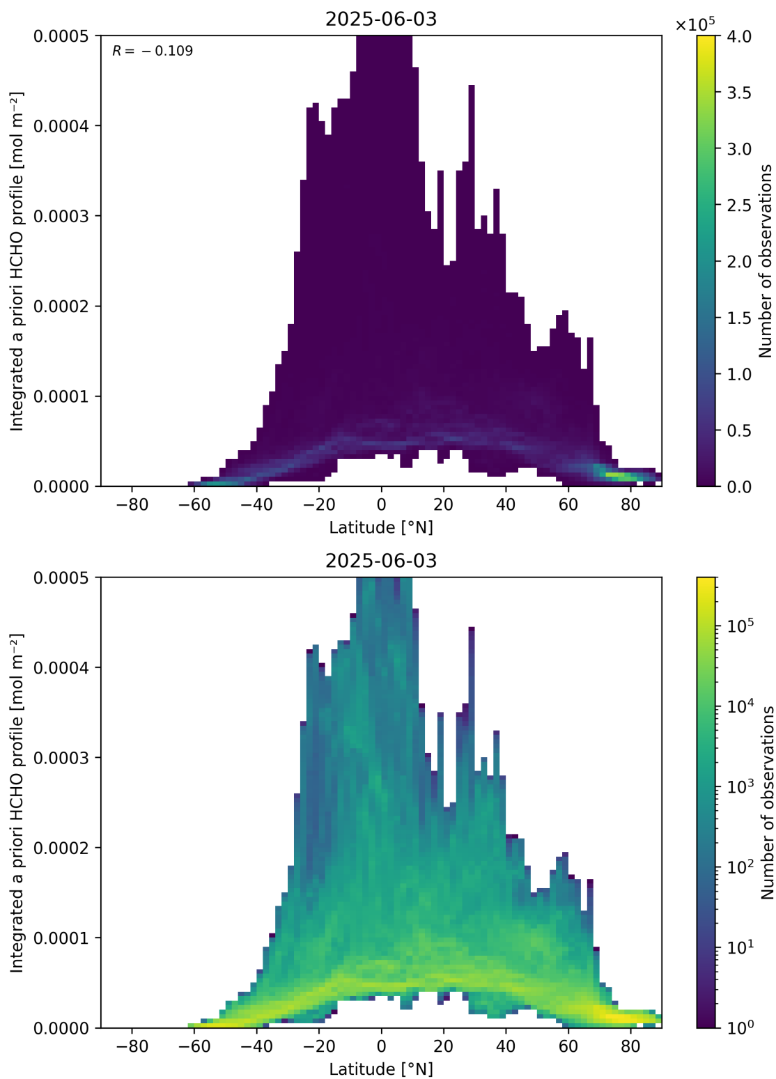
Figure 166: Scatter density plot of “Latitude” against “Integrated a priori HCHO profile” for 2025-06-02 to 2025-06-04.
