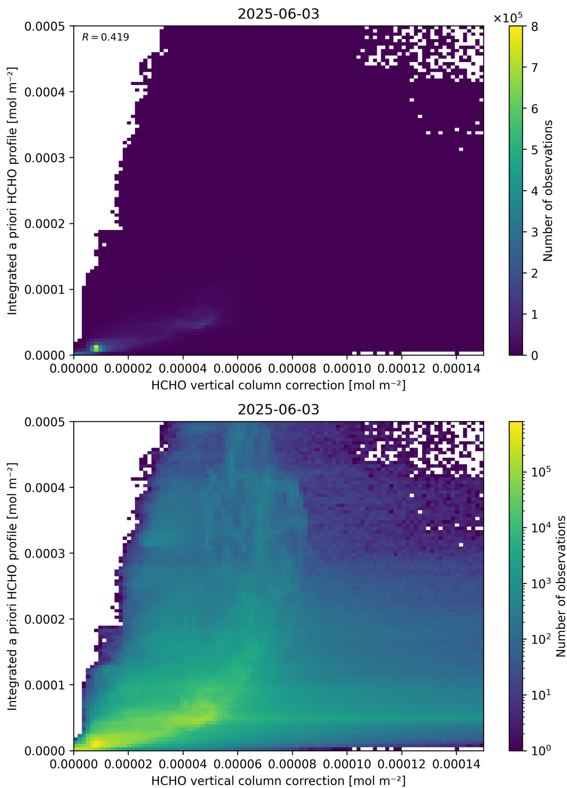
Figure 122: Scatter density plot of “HCHO vertical column correction” against “Integrated a priori HCHO profile” for 2025-06-02 to 2025-06-04.
