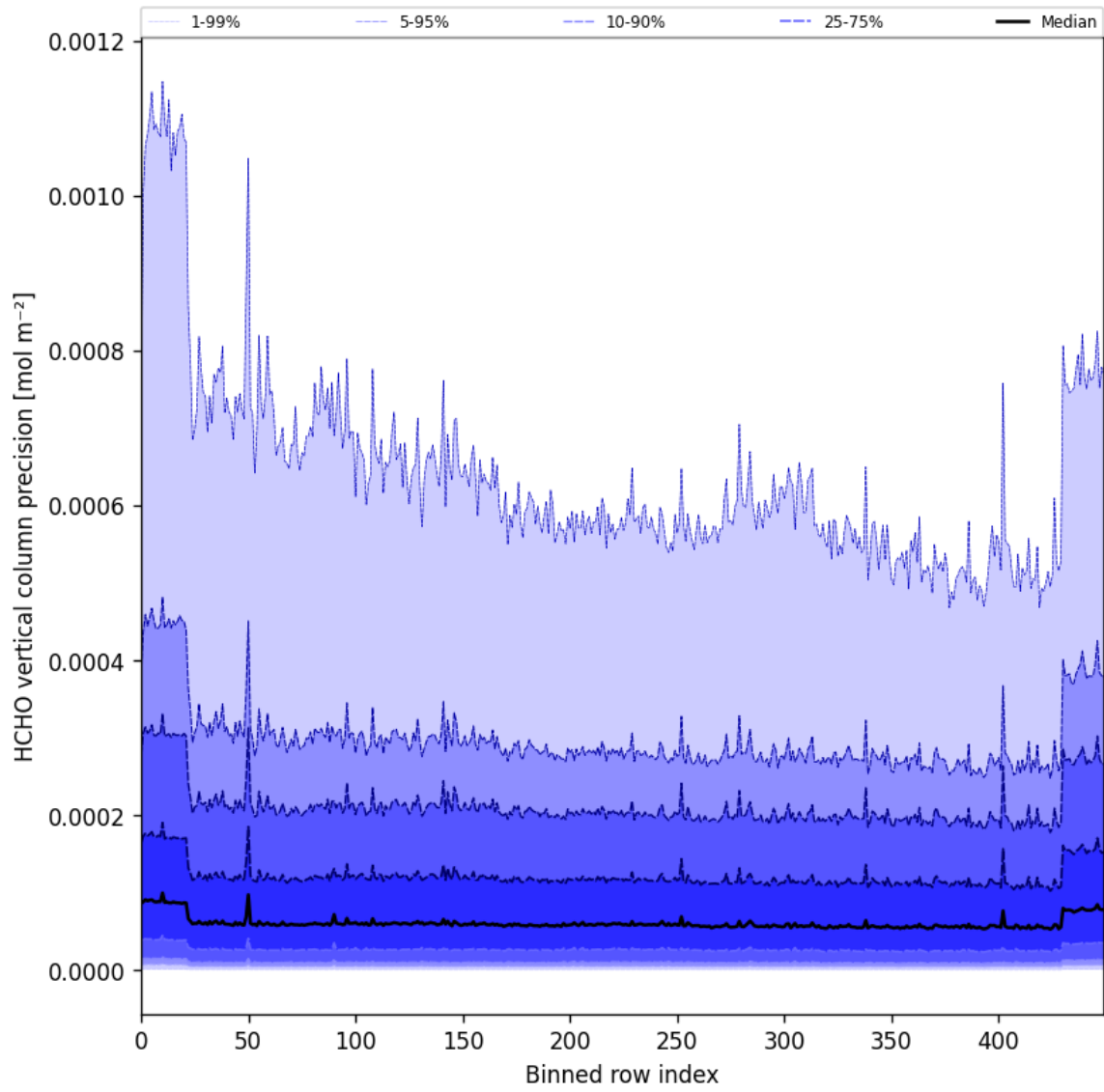
Figure 50: Along track statistics of “HCHO vertical column precision” for 2025-06-02 to 2025-06-04
