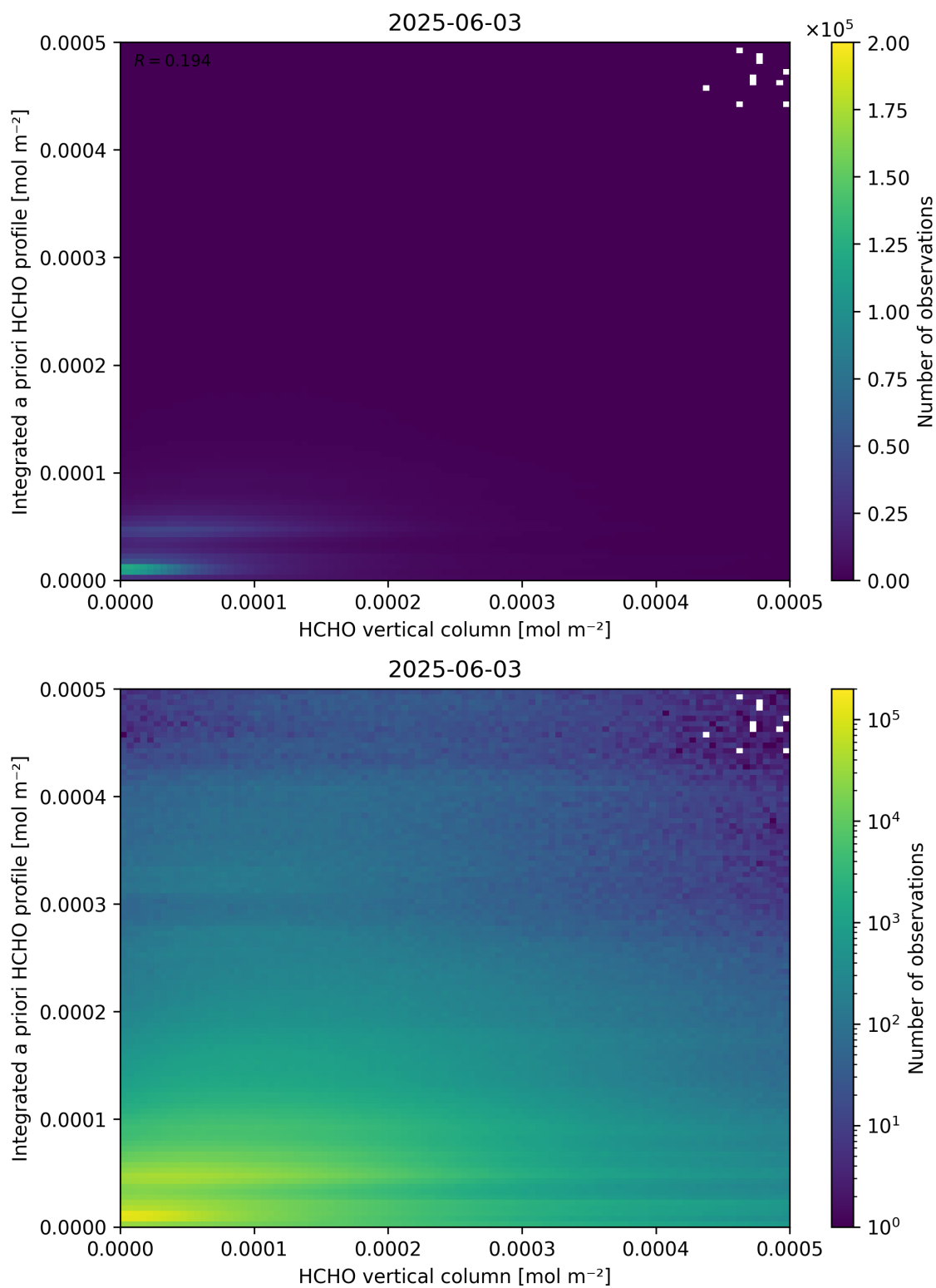
Figure 135: Scatter density plot of “HCHO vertical column” against “Integrated a priori HCHO profile” for 2025-06-02 to 2025-06-04.
