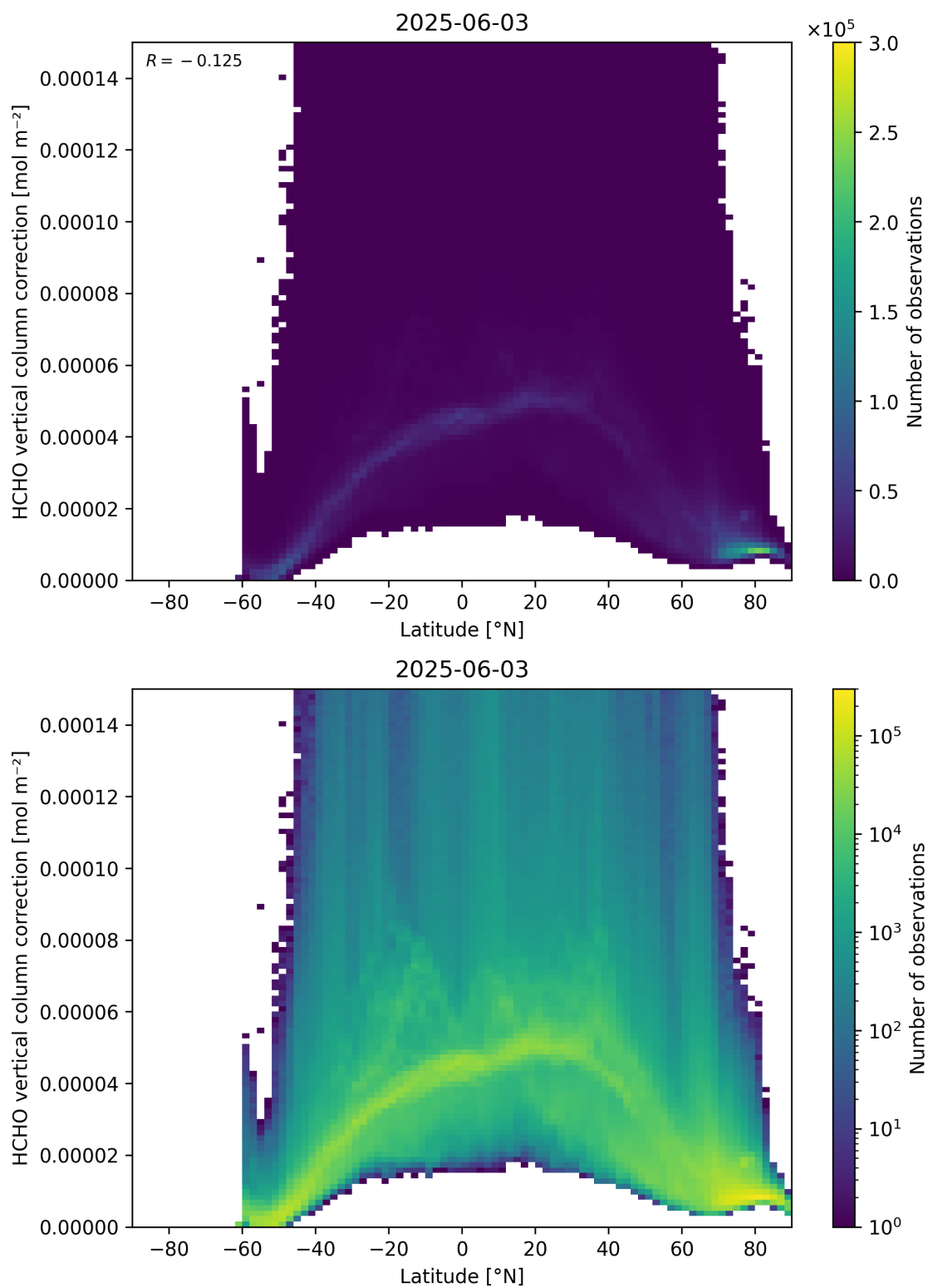
Figure 164: Scatter density plot of “Latitude” against “HCHO vertical column correction” for 2025-06-02 to 2025-06-04.
