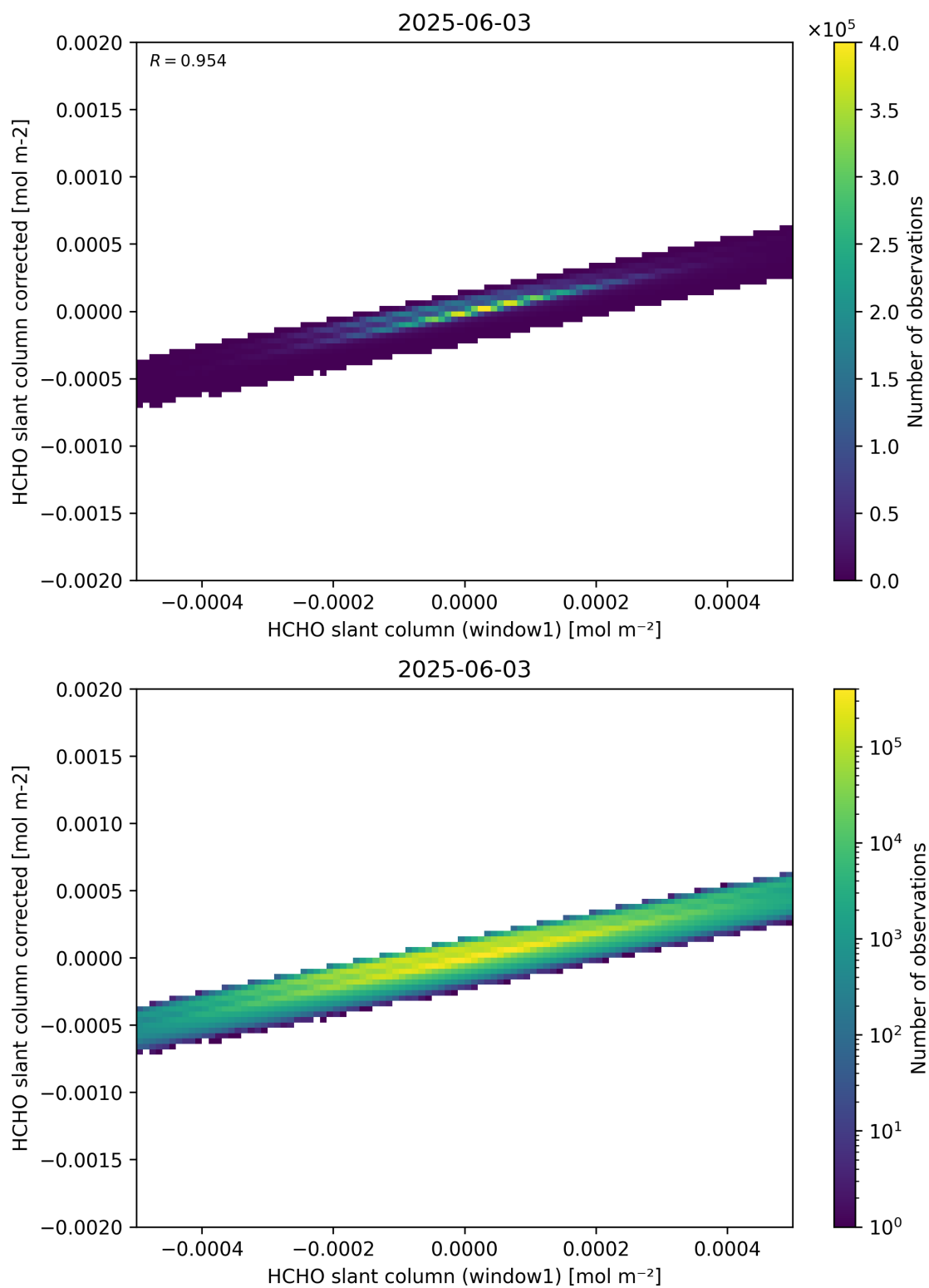
Figure 82: Scatter density plot of “HCHO slant column (window1)” against “HCHO slant column corrected” for 2025-06-02 to 2025-06-04.
