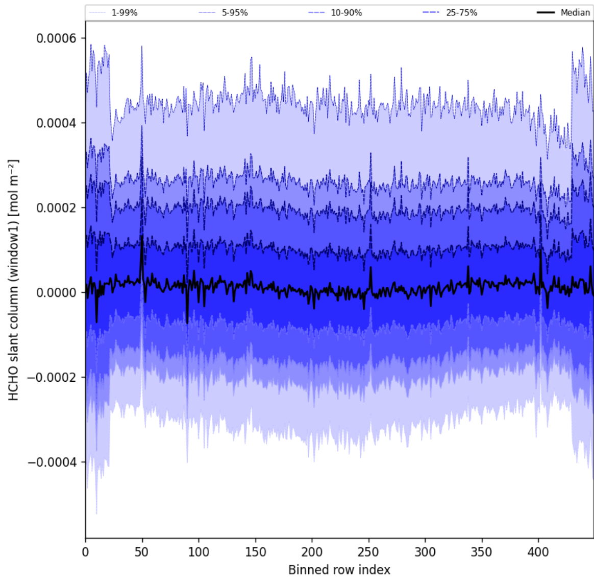
Figure 52: Along track statistics of “HCHO slant column (window1)” for 2025-06-02 to 2025-06-04
