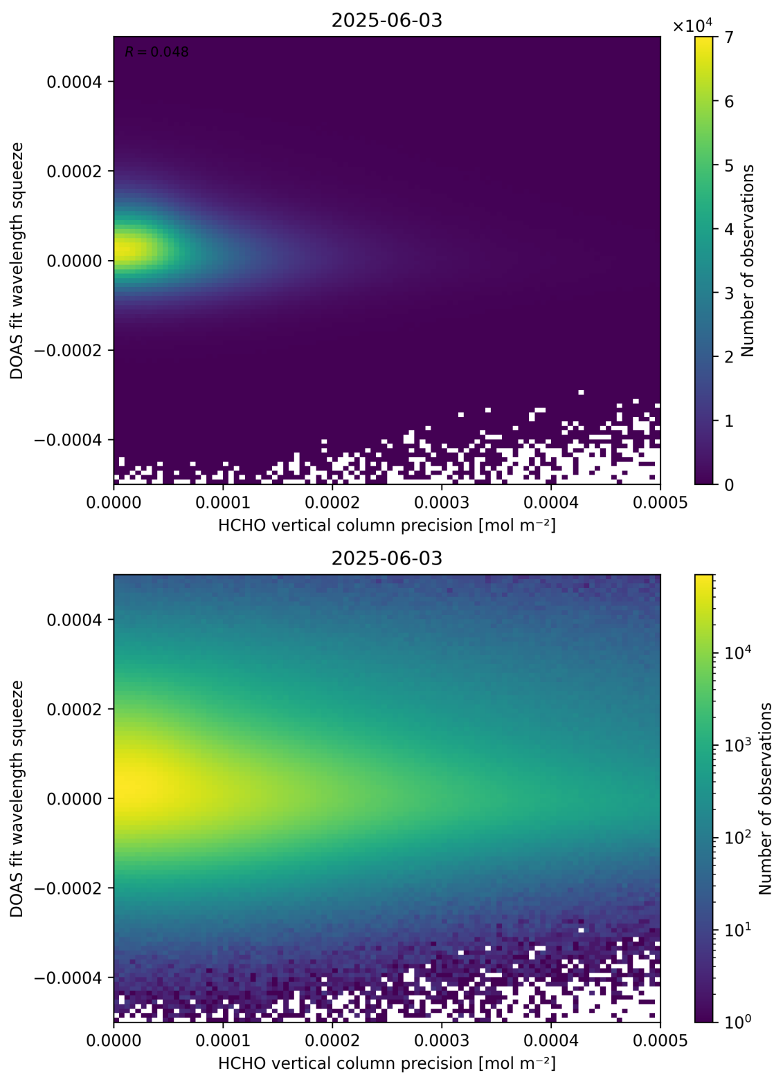
Figure 138: Scatter density plot of “HCHO vertical column precision” against “DOAS fit wavelength squeeze” for 2025-06-02 to 2025-06-04.
