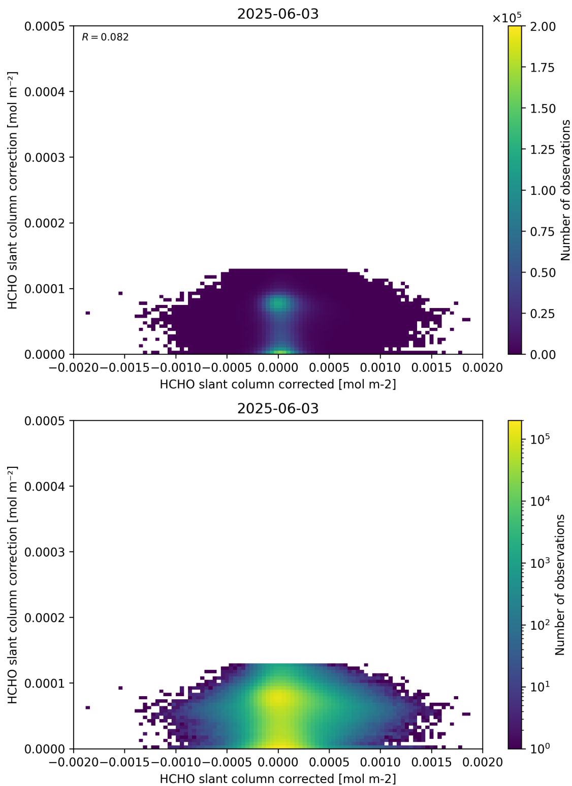
Figure 77: Scatter density plot of “HCHO slant column corrected” against “HCHO slant column correction” for 2025-06-02 to 2025-06-04.
