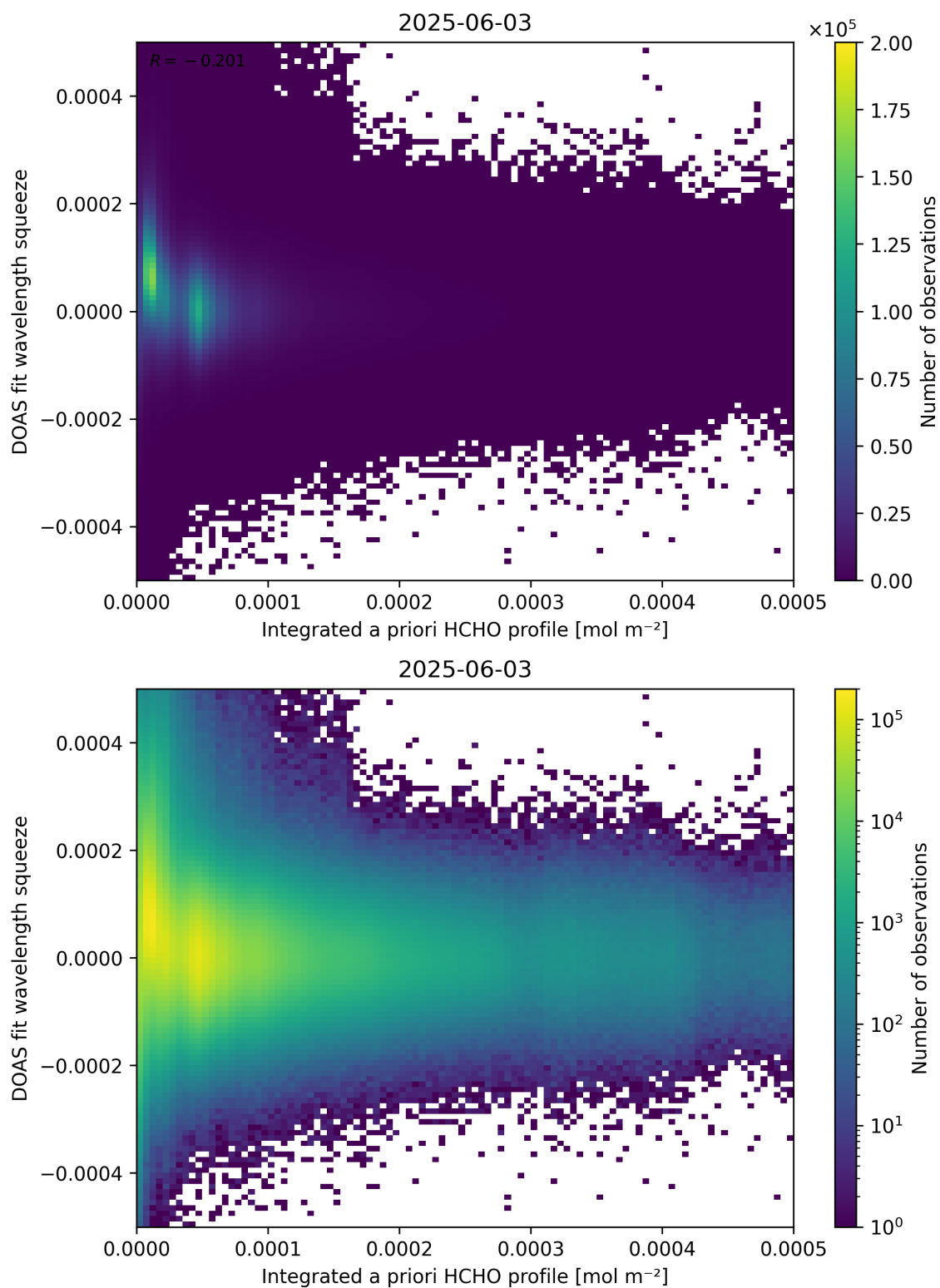
Figure 150: Scatter density plot of “Integrated a priori HCHO profile” against “DOAS fit wavelength squeeze” for 2025-06-02 to 2025-06-04.
