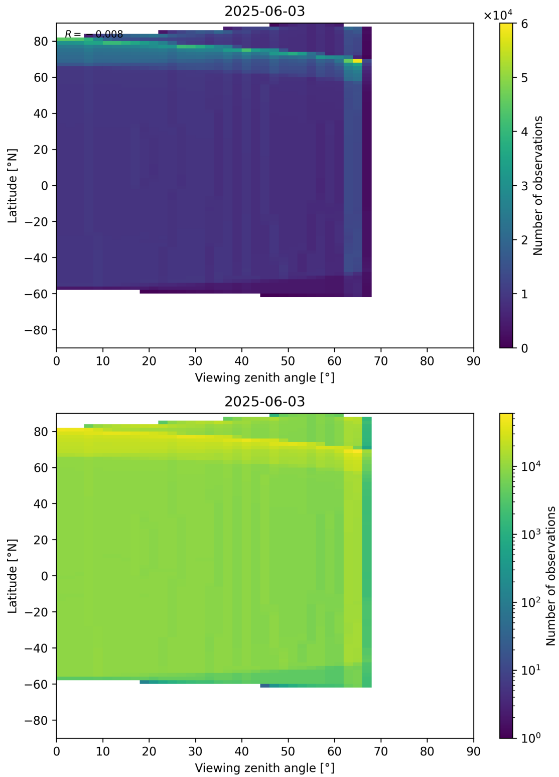
Figure 196: Scatter density plot of “Viewing zenith angle” against “Latitude” for 2025-06-02 to 2025-06-04.
