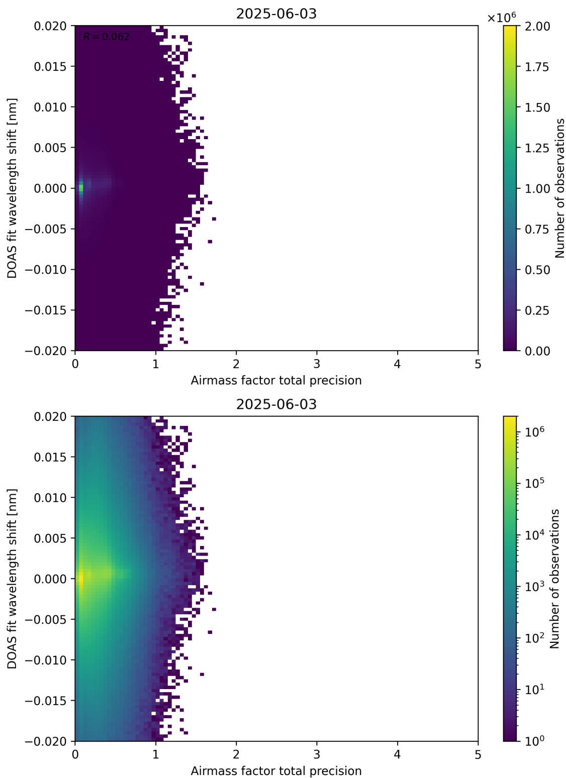
Figure 106: Scatter density plot of “Airmass factor total precision” against “DOAS fit wavelength shift” for 2025-06-02 to 2025-06-04.
