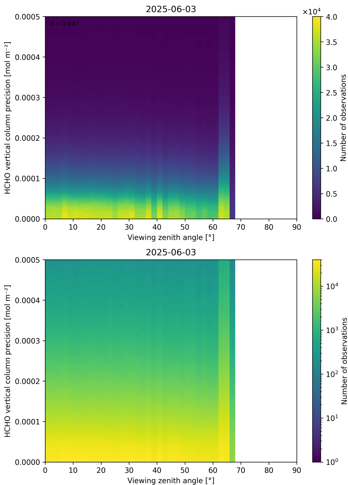
Figure 194: Scatter density plot of “Viewing zenith angle” against “HCHO vertical column precision” for 2025-06-02 to 2025-06-04.
