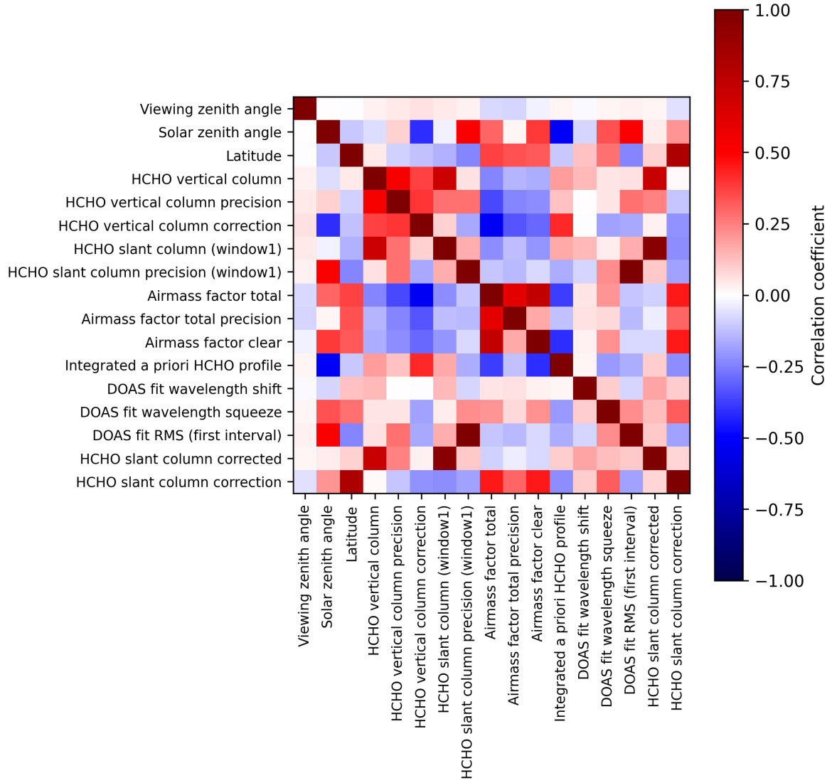
Figure 2: Map of correlation matrix for 2025-06-02 to 2025-06-04.
