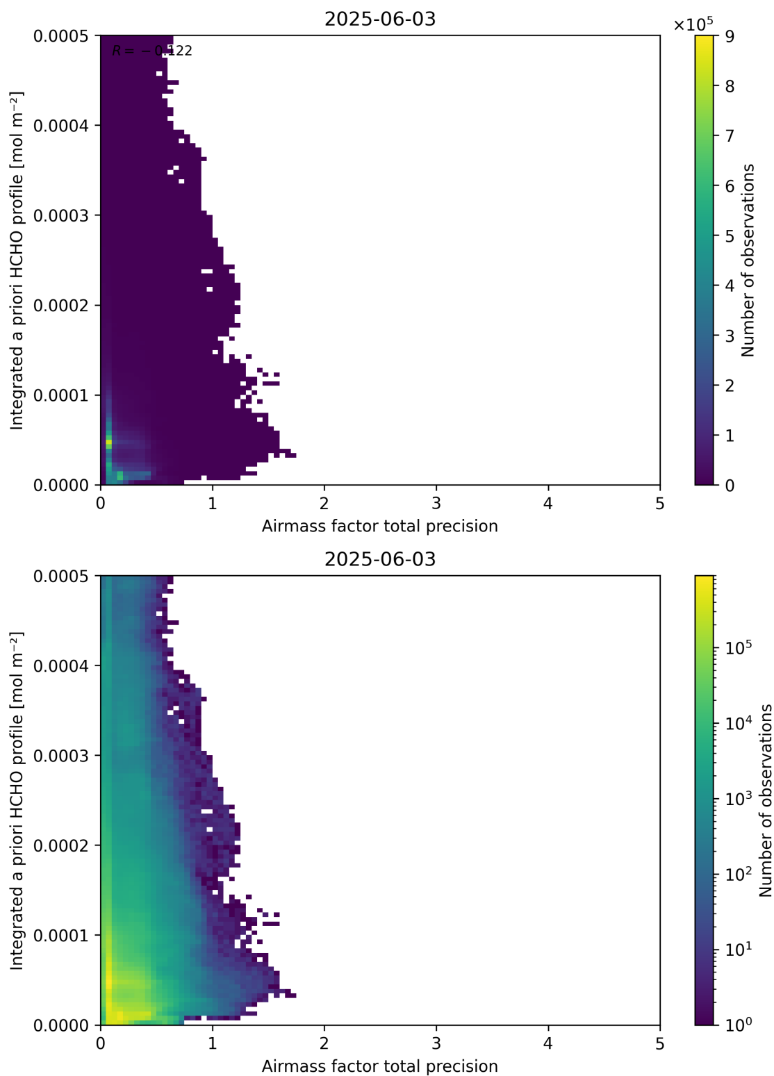
Figure 111: Scatter density plot of “Airmass factor total precision” against “Integrated a priori HCHO profile” for 2025-06-02 to 2025-06-04.
