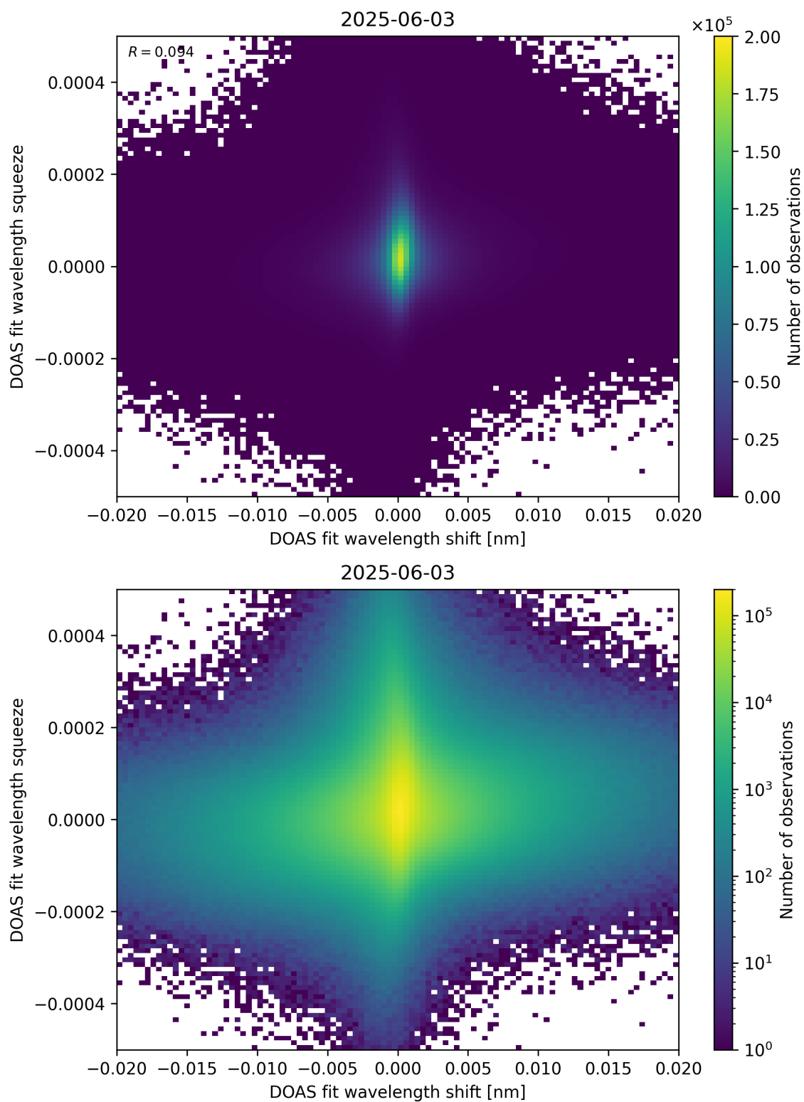
Figure 65: Scatter density plot of “DOAS fit wavelength shift” against “DOAS fit wavelength squeeze” for 2025-06-02 to 2025-06-04.
