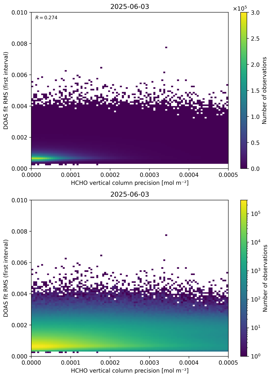
Figure 136: Scatter density plot of “HCHO vertical column precision” against “DOAS fit RMS (first interval)” for 2025-06-02 to 2025-06-04.
