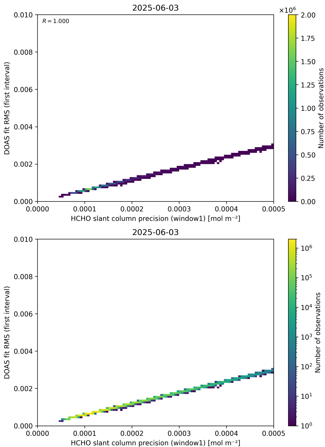
Figure 88: Scatter density plot of “HCHO slant column precision (window1)” against “DOAS fit RMS (first interval)” for 2025-06-02 to 2025-06-04.
