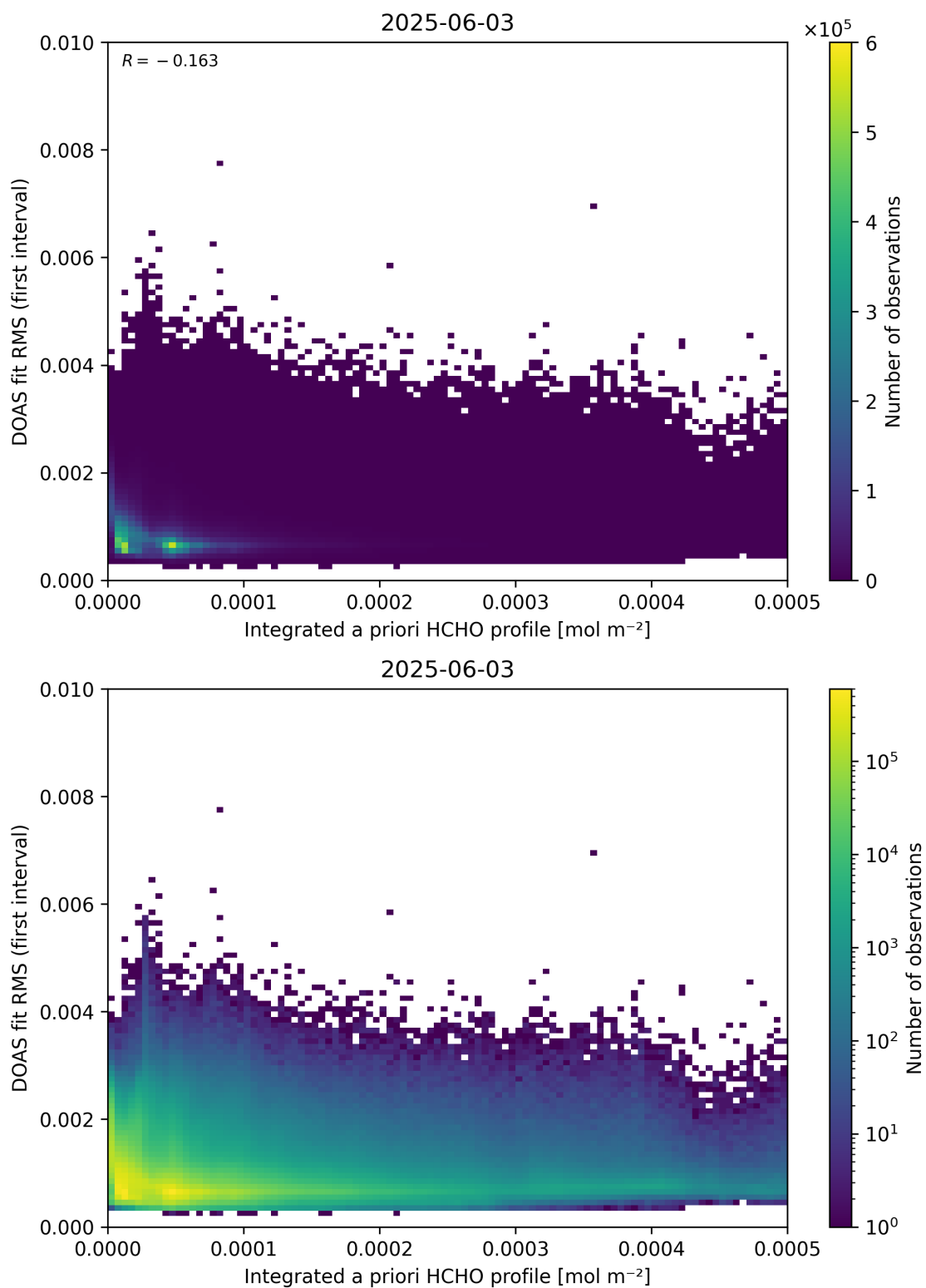
Figure 148: Scatter density plot of “Integrated a priori HCHO profile” against “DOAS fit RMS (first interval)” for 2025-06-02 to 2025-06-04.
