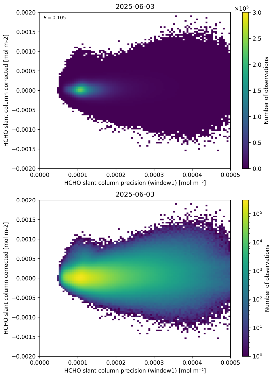
Figure 92: Scatter density plot of “HCHO slant column precision (window1)” against “HCHO slant column corrected” for 2025-06-02 to 2025-06-04.
