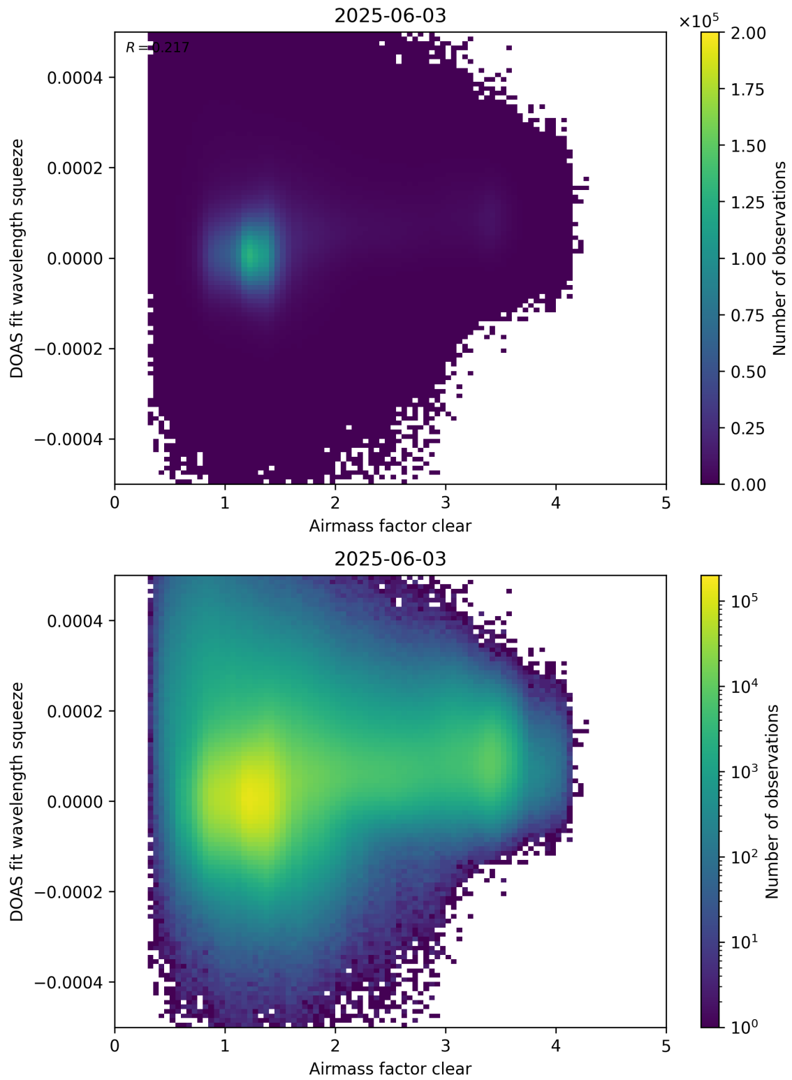
Figure 73: Scatter density plot of “Airmass factor clear” against “DOAS fit wavelength squeeze” for 2025-06-02 to 2025-06-04.
