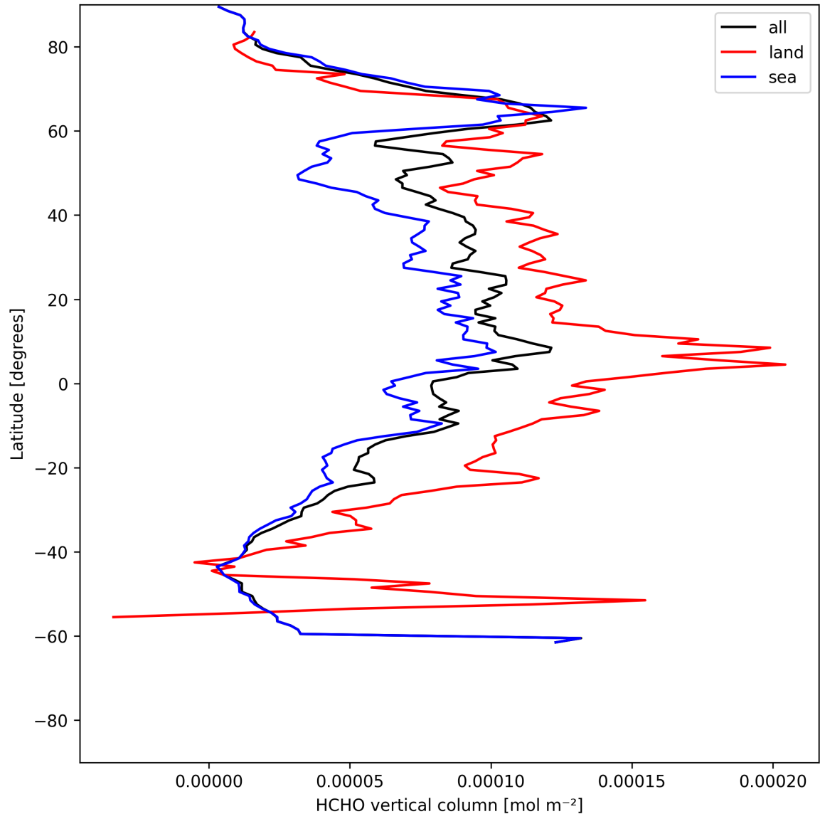
Figure 21: Zonal average of “HCHO vertical column” for 2025-06-02 to 2025-06-04.
