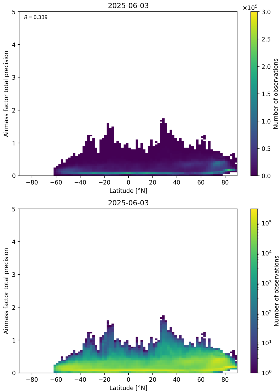
Figure 162: Scatter density plot of “Latitude” against “Airmass factor total precision” for 2025-06-02 to 2025-06-04.
