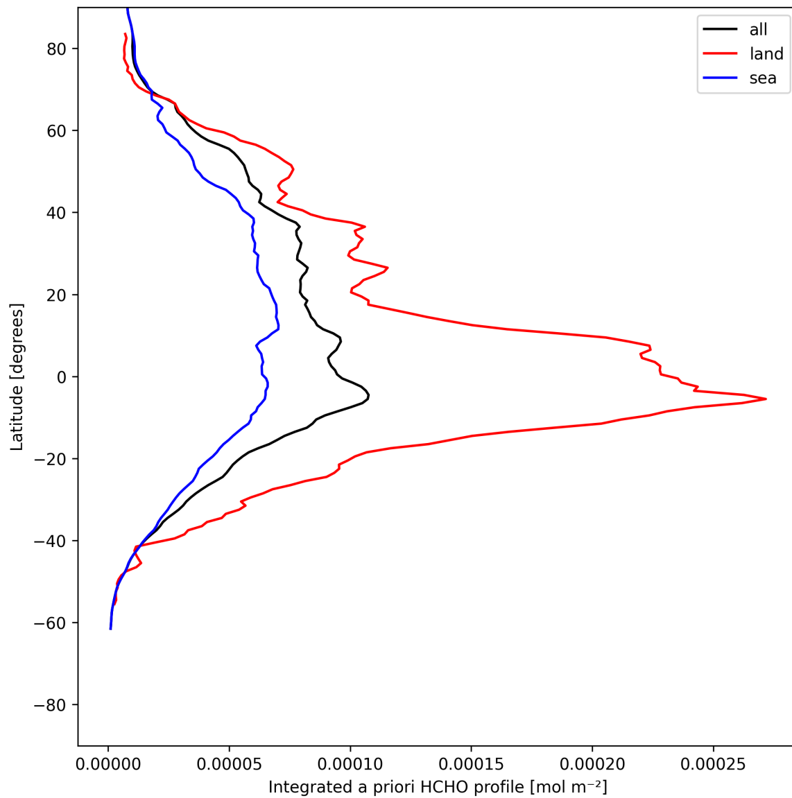
Figure 29: Zonal average of “Integrated a priori HCHO profile” for 2025-06-02 to 2025-06-04.
