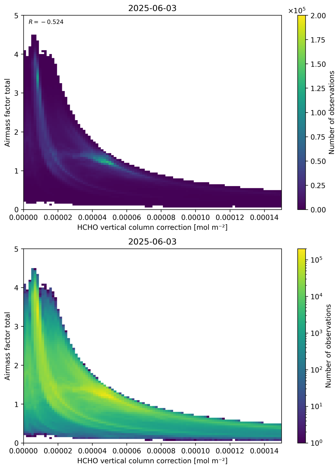
Figure 120: Scatter density plot of “HCHO vertical column correction” against “Airmass factor total” for 2025-06-02 to 2025-06-04.
