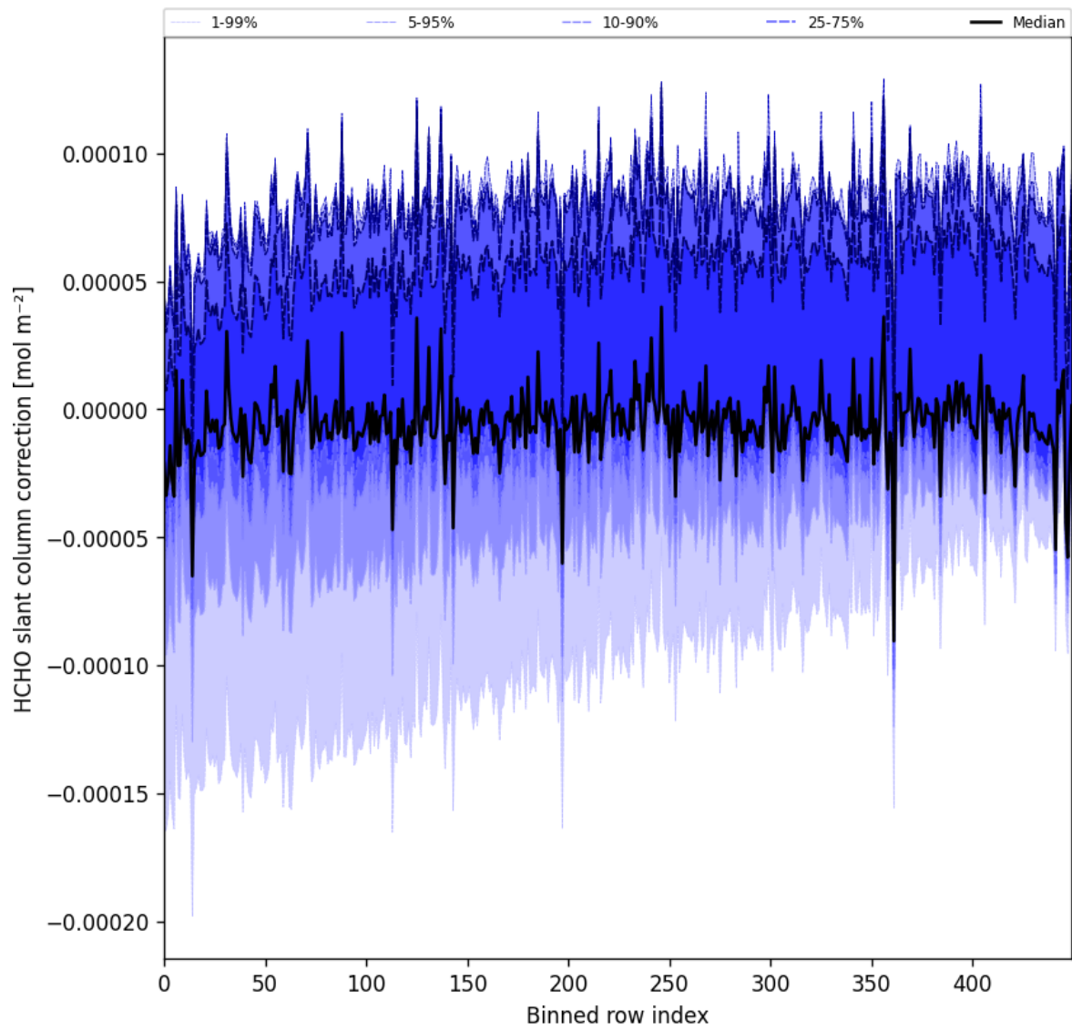
Figure 61: Along track statistics of “HCHO slant column correction” for 2025-06-02 to 2025-06-04
