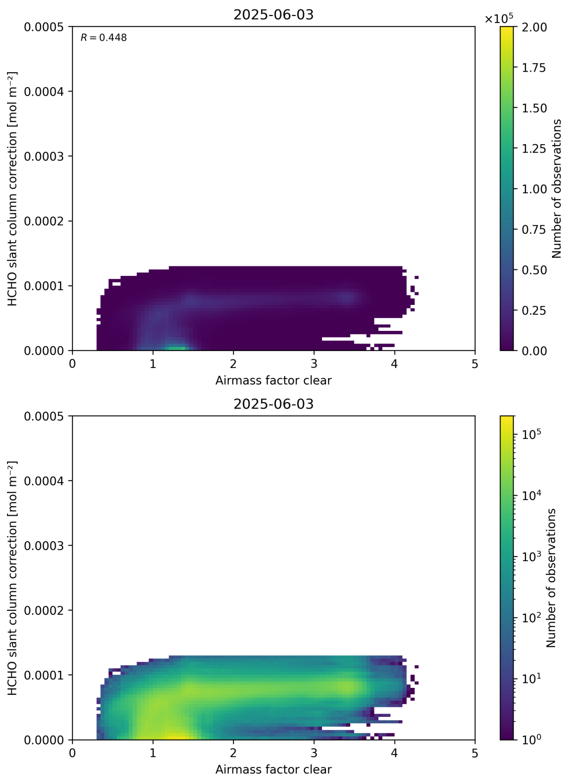
Figure 75: Scatter density plot of “Airmass factor clear” against “HCHO slant column correction” for 2025-06-02 to 2025-06-04.
