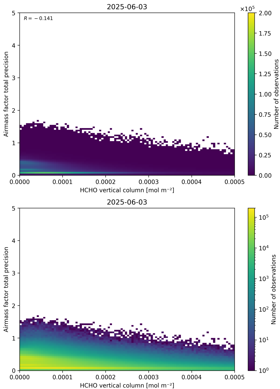
Figure 132: Scatter density plot of “HCHO vertical column” against “Airmass factor total precision” for 2025-06-02 to 2025-06-04.
