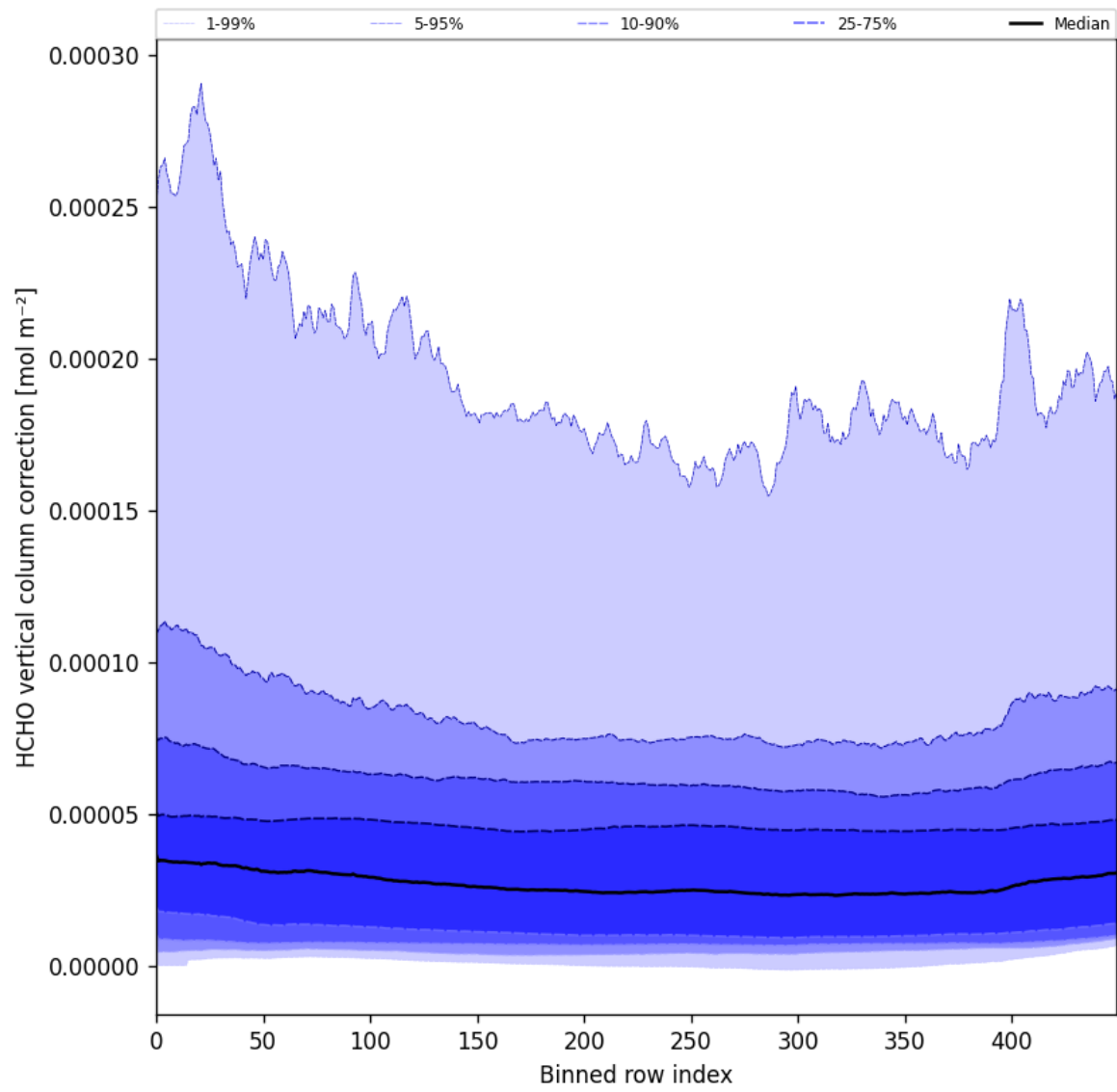
Figure 51: Along track statistics of “HCHO vertical column correction” for 2025-06-02 to 2025-06-04
