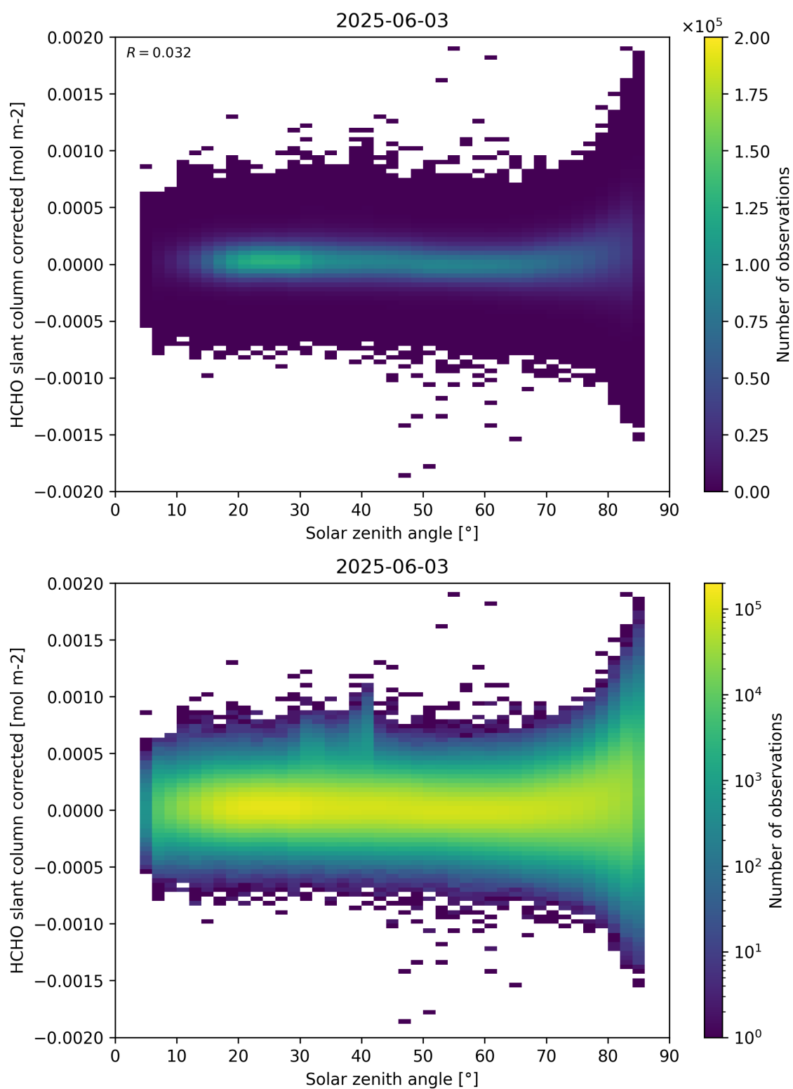
Figure 171: Scatter density plot of “Solar zenith angle” against “HCHO slant column corrected” for 2025-06-02 to 2025-06-04.
