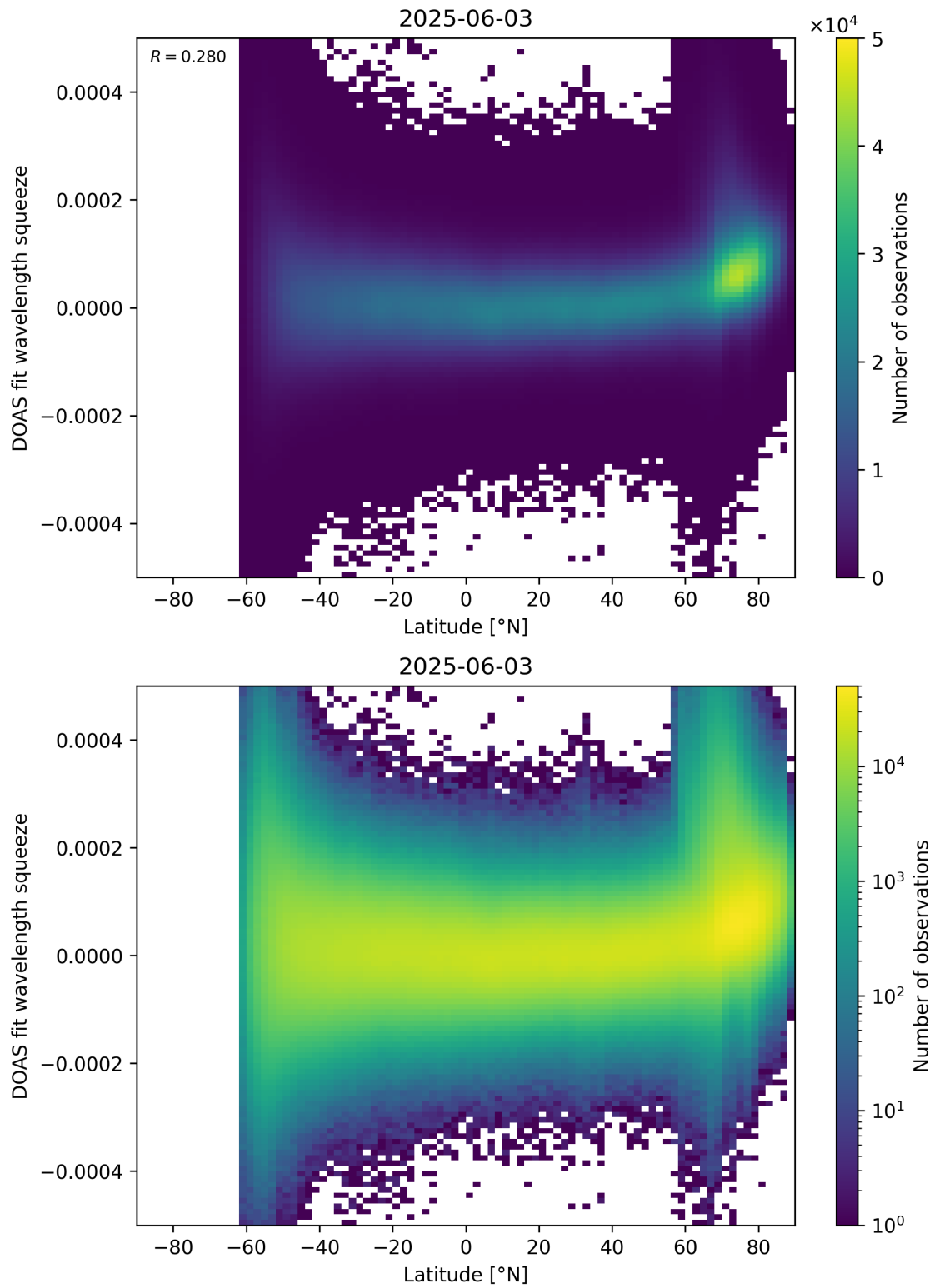
Figure 155: Scatter density plot of “Latitude” against “DOAS fit wavelength squeeze” for 2025-06-02 to 2025-06-04.
