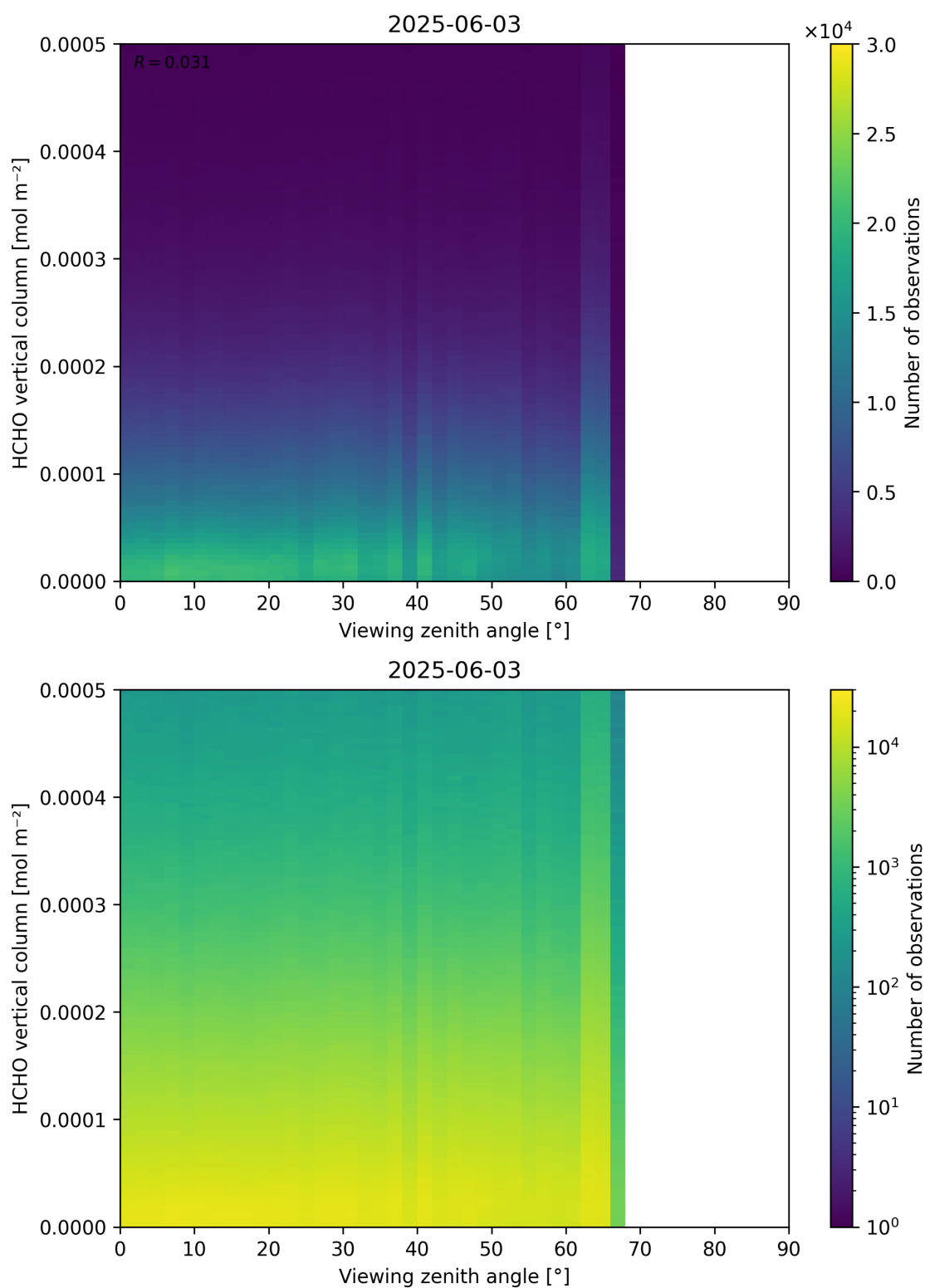
Figure 192: Scatter density plot of “Viewing zenith angle” against “HCHO vertical column” for 2025-06-02 to 2025-06-04.
