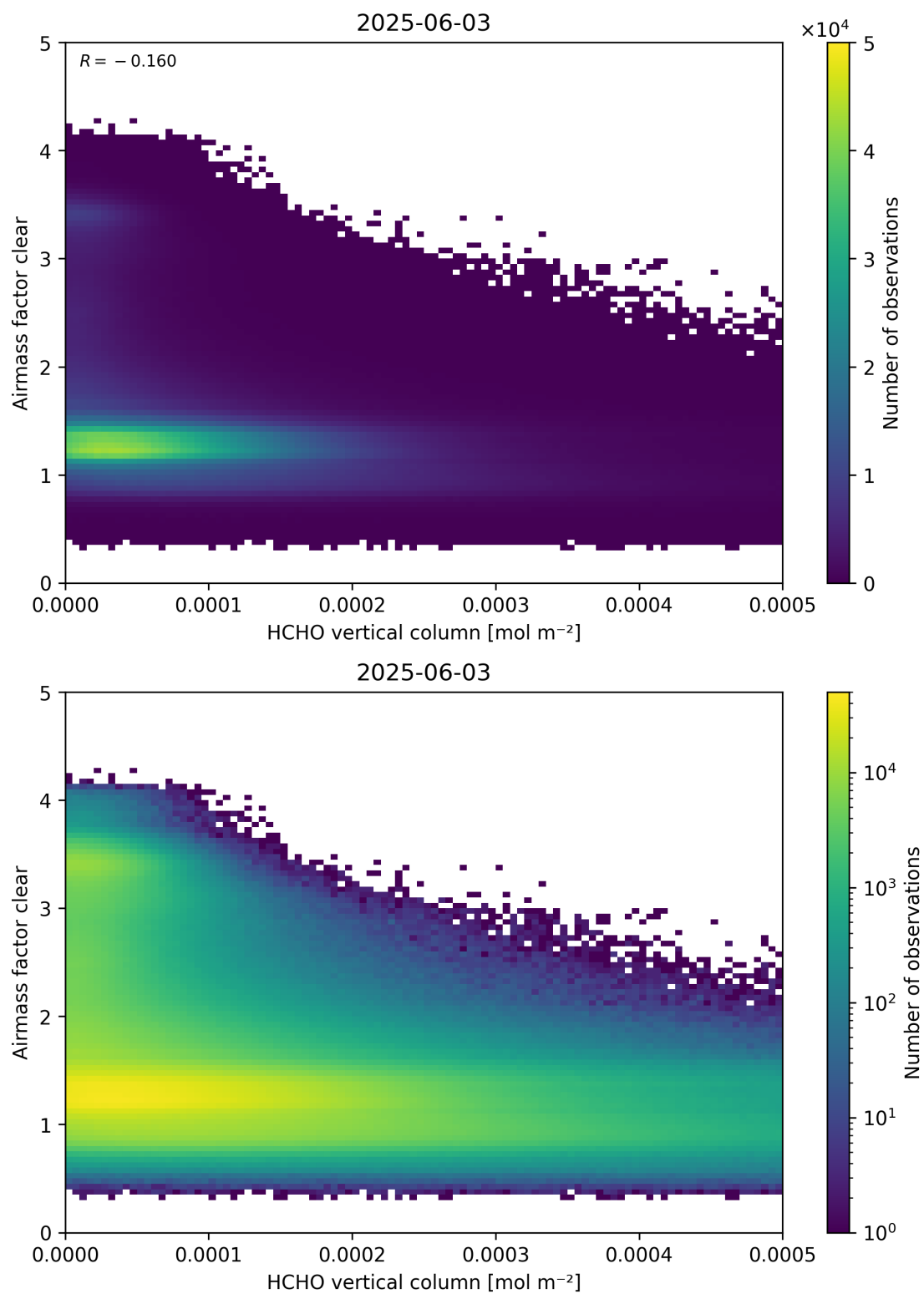
Figure 126: Scatter density plot of “HCHO vertical column” against “Airmass factor clear” for 2025-06-02 to 2025-06-04.
