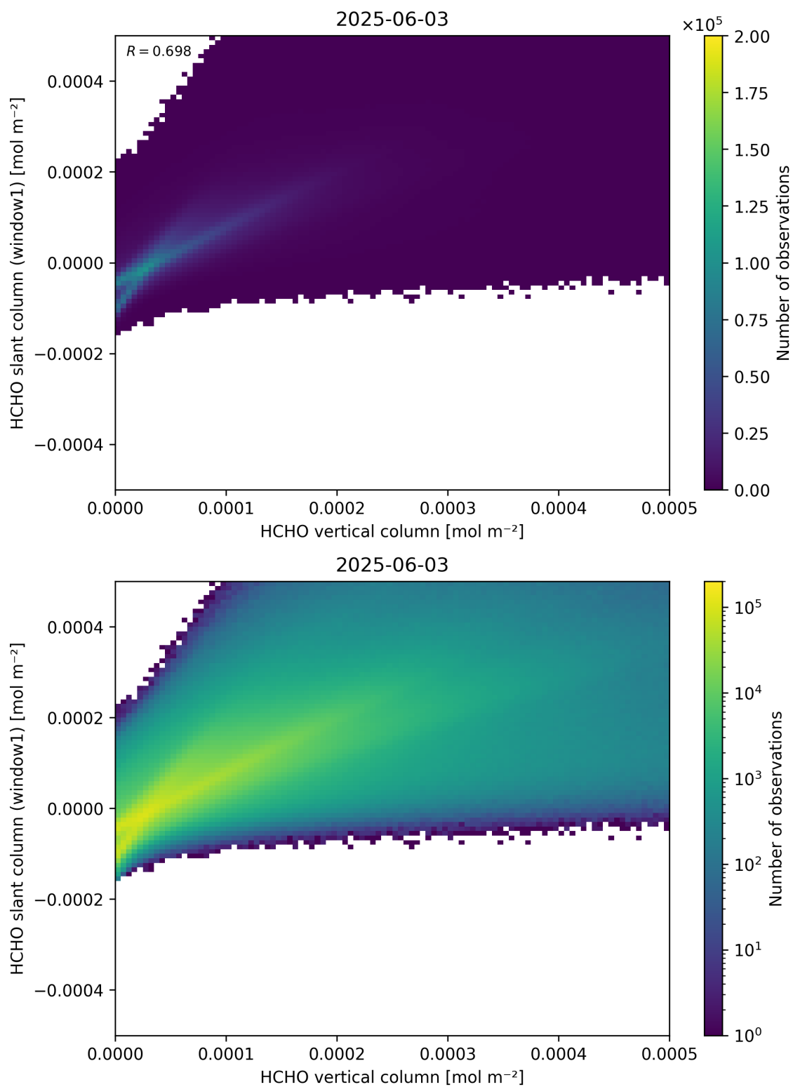
Figure 129: Scatter density plot of “HCHO vertical column” against “HCHO slant column (window1)” for 2025-06-02 to 2025-06-04.
