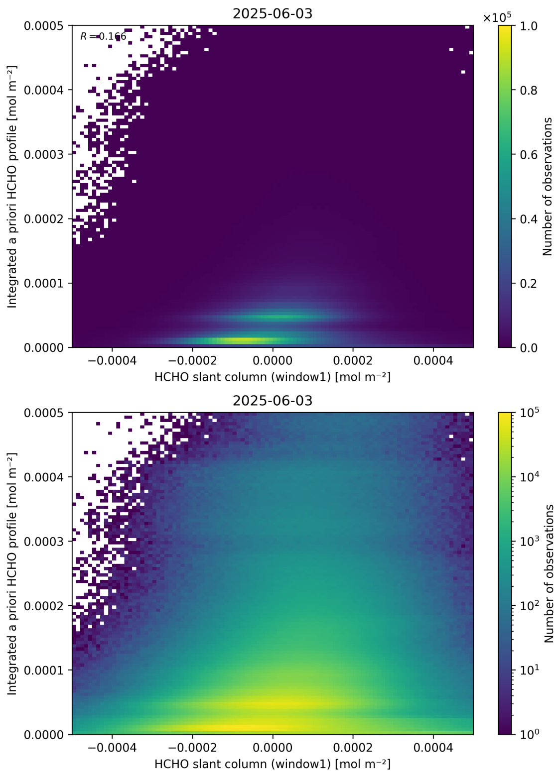
Figure 87: Scatter density plot of “HCHO slant column (window1)” against “Integrated a priori HCHO profile” for 2025-06-02 to 2025-06-04.
