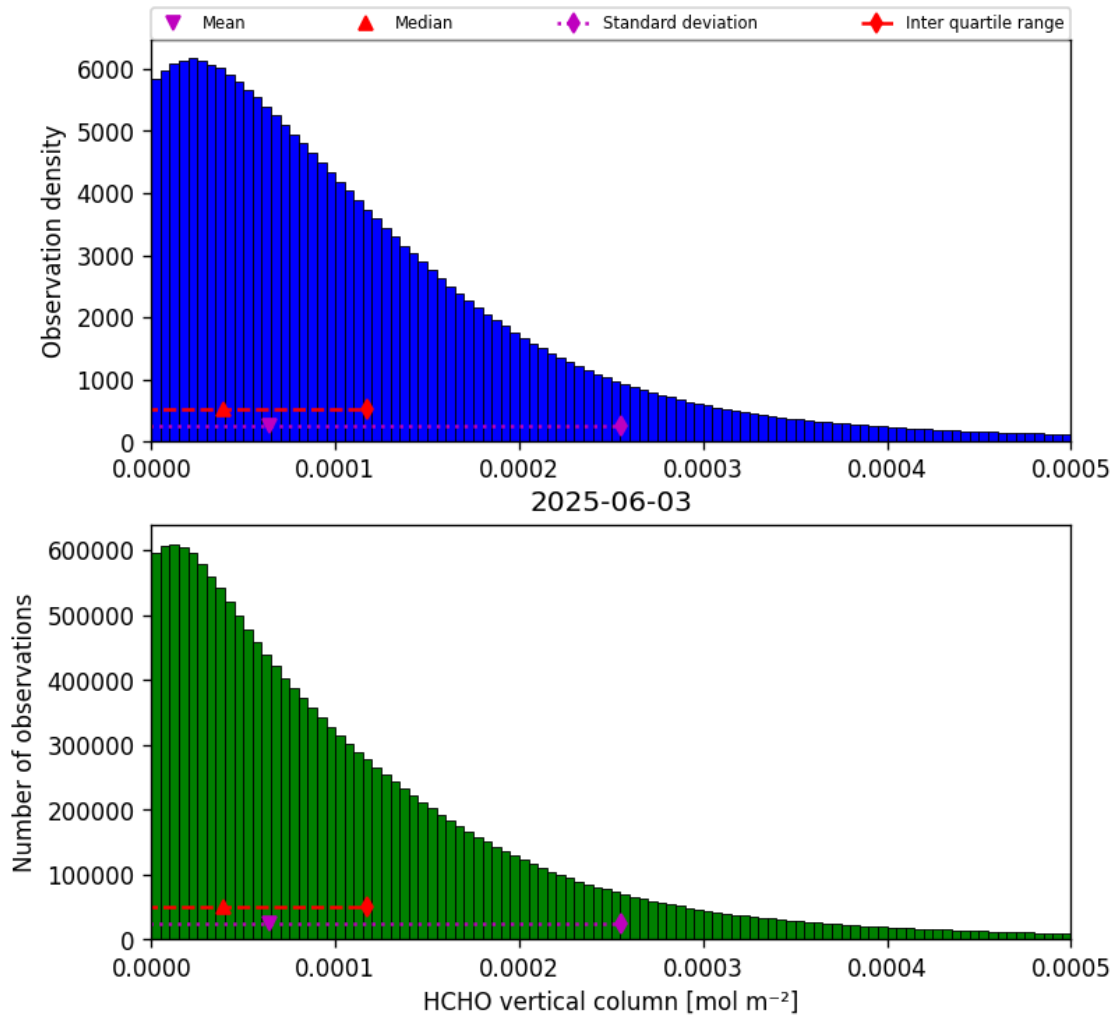
Figure 35: Histogram of “HCHO vertical column” for 2025-06-02 to 2025-06-04
