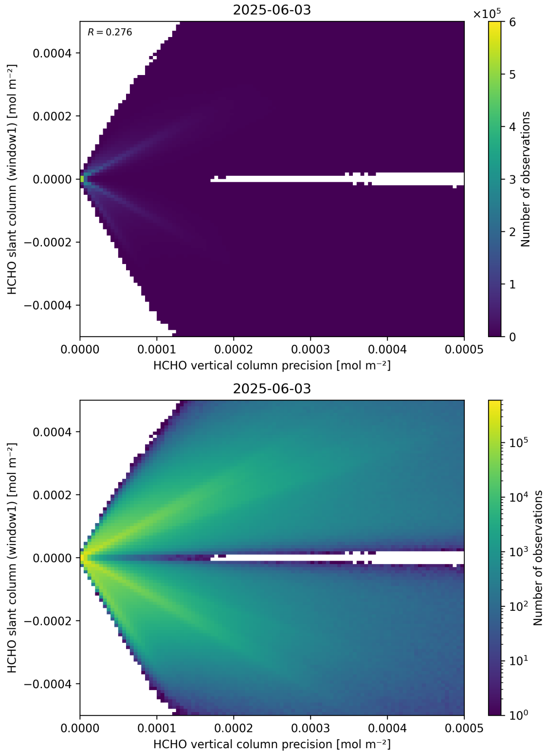
Figure 142: Scatter density plot of “HCHO vertical column precision” against “HCHO slant column (window1)” for 2025-06-02 to 2025-06-04.
