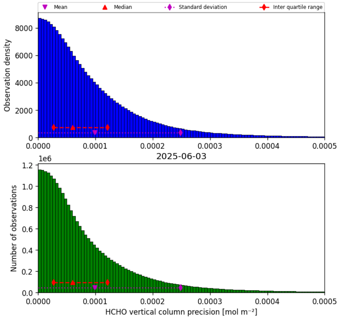
Figure 36: Histogram of “HCHO vertical column precision” for 2025-06-02 to 2025-06-04
