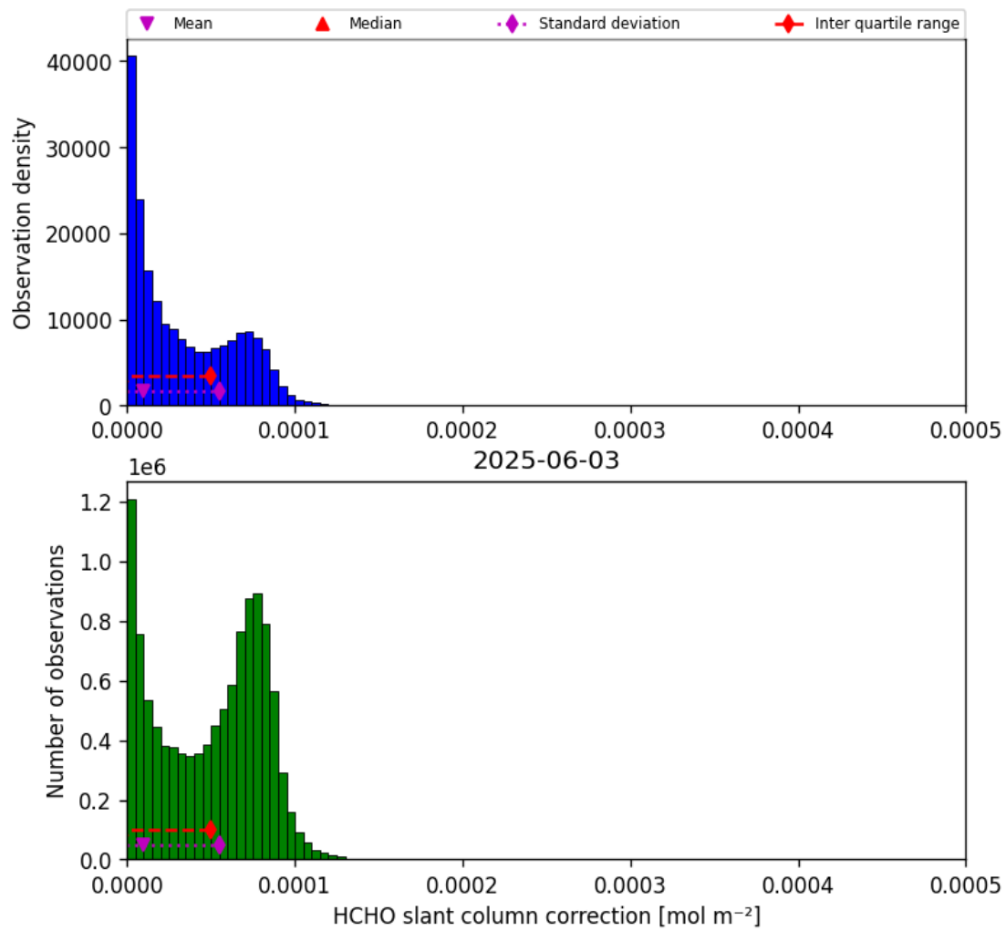
Figure 47: Histogram of “HCHO slant column correction” for 2025-06-02 to 2025-06-04
