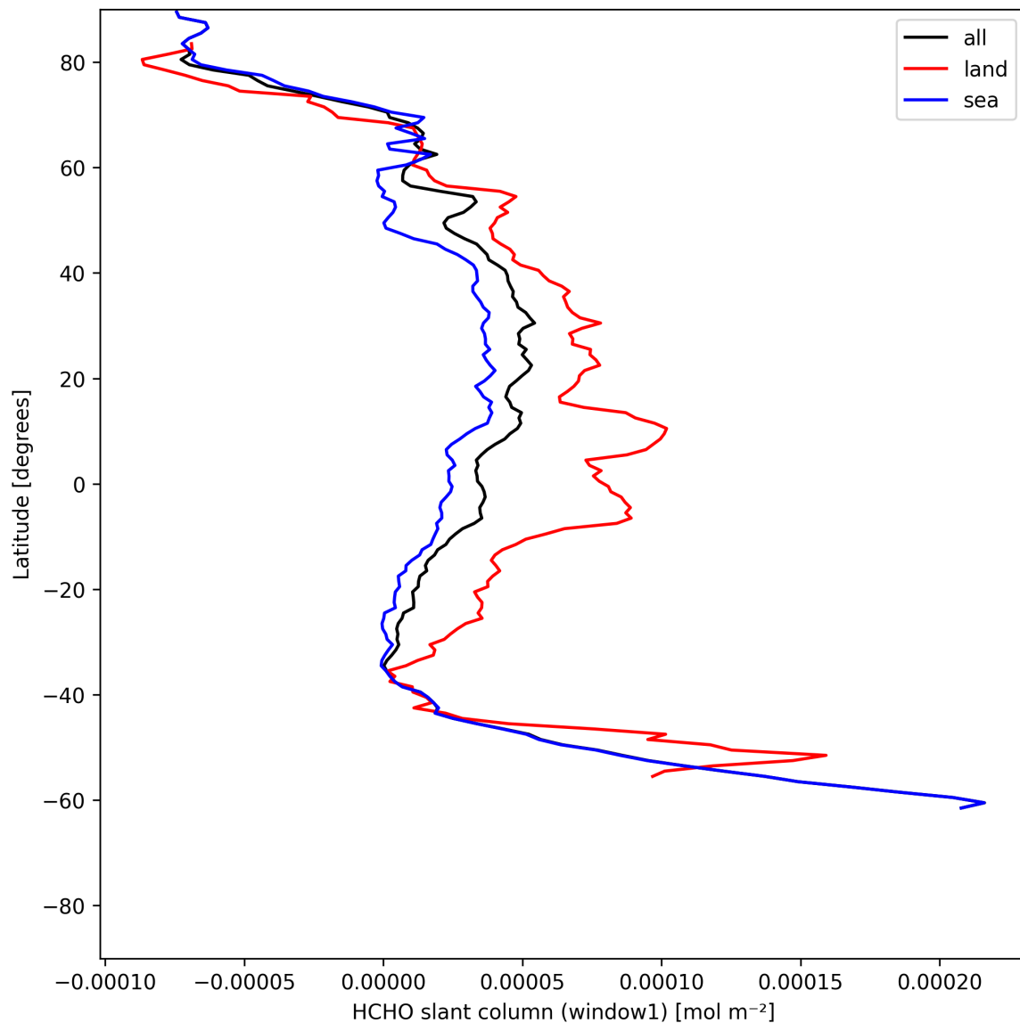
Figure 24: Zonal average of “HCHO slant column (window1)” for 2025-06-02 to 2025-06-04.
