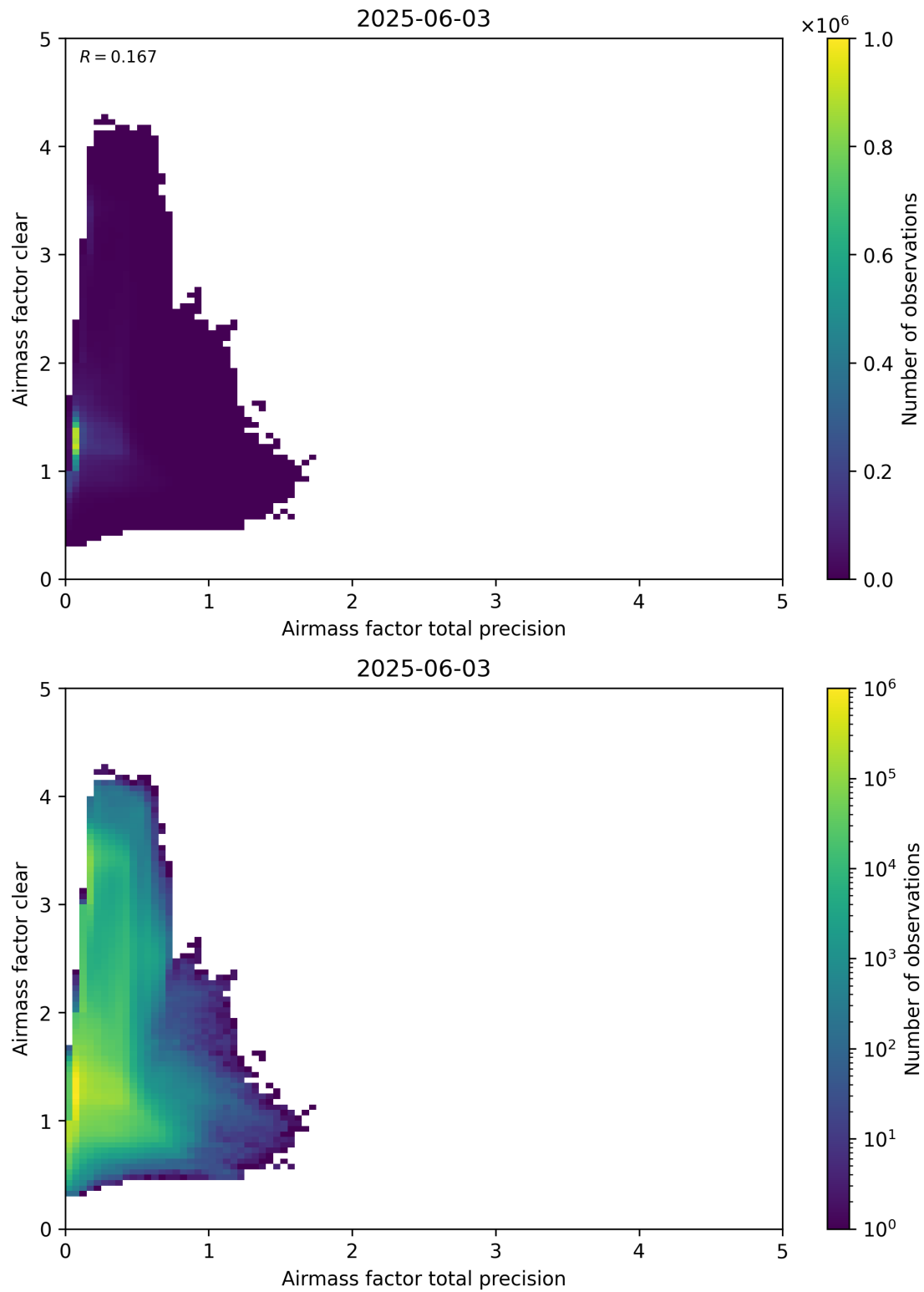
Figure 108: Scatter density plot of “Airmass factor total precision” against “Airmass factor clear” for 2025-06-02 to 2025-06-04.
