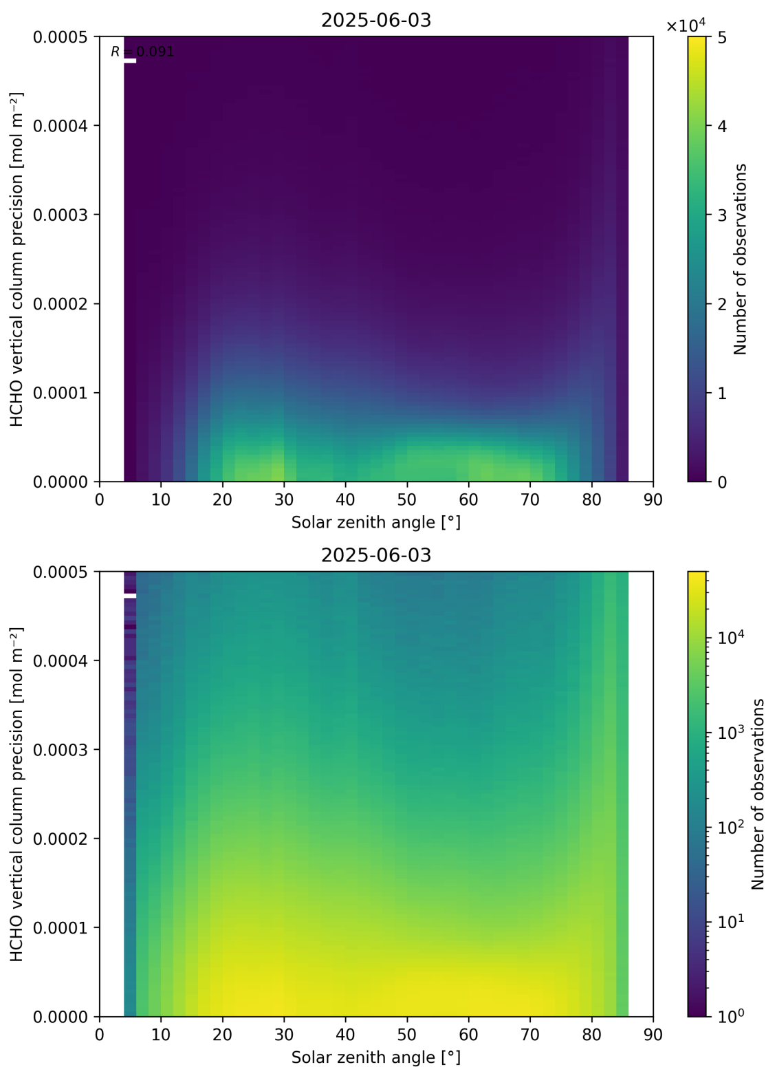
Figure 179: Scatter density plot of “Solar zenith angle” against “HCHO vertical column precision” for 2025-06-02 to 2025-06-04.
