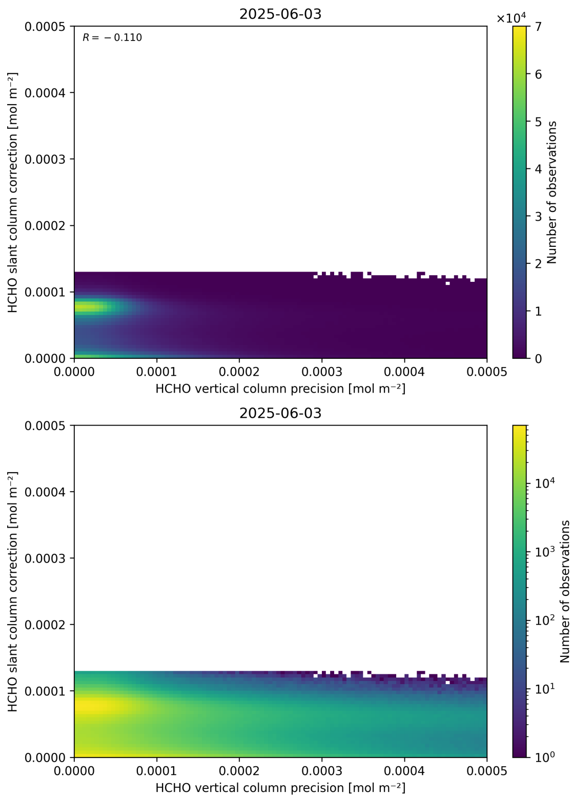
Figure 141: Scatter density plot of “HCHO vertical column precision” against “HCHO slant column correction” for 2025-06-02 to 2025-06-04.
