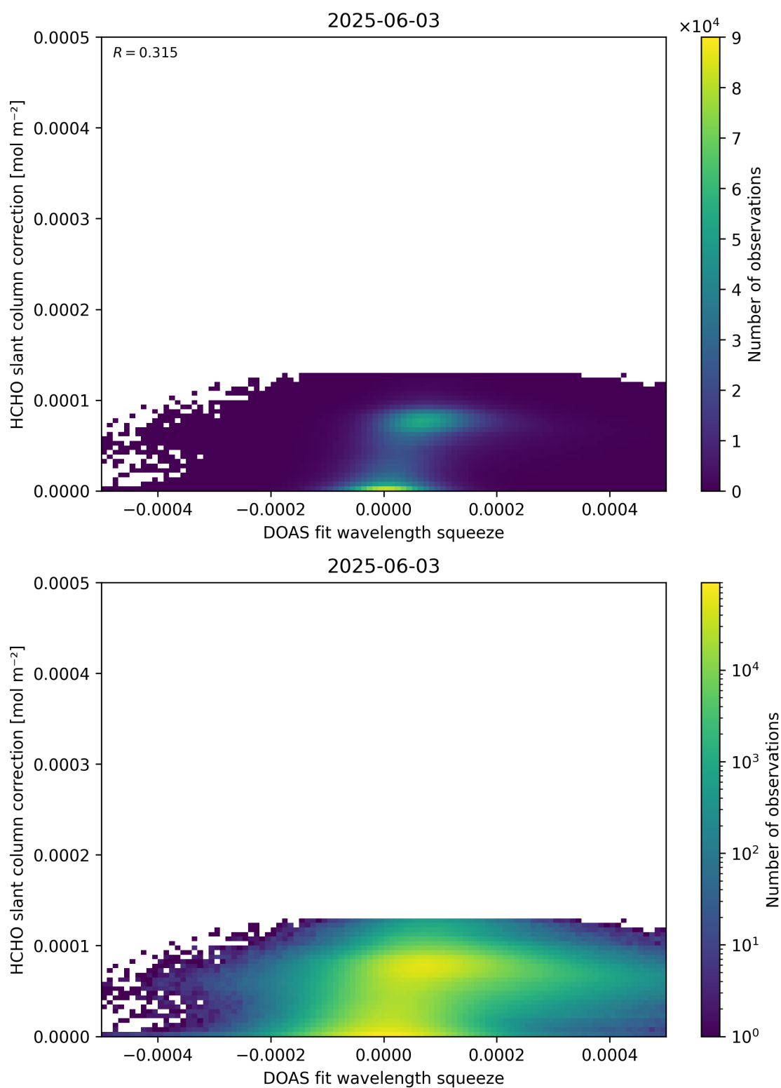
Figure 70: Scatter density plot of “DOAS fit wavelength squeeze” against “HCHO slant column correction” for 2025-06-02 to 2025-06-04.
