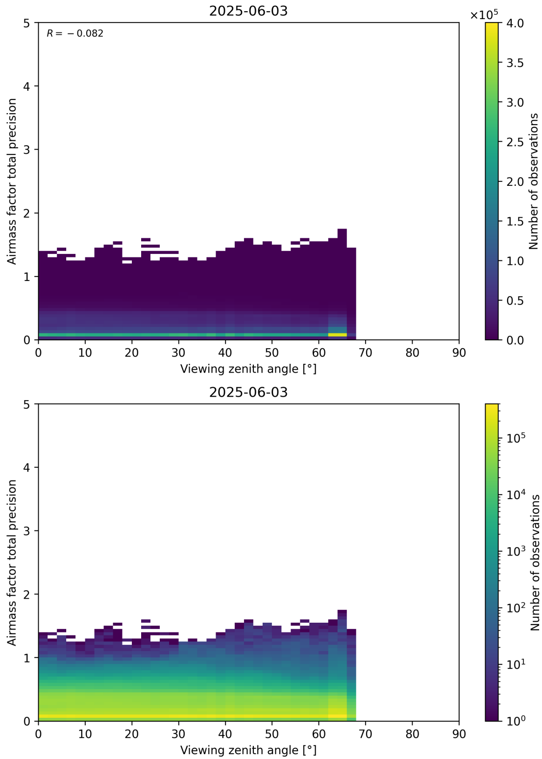
Figure 191: Scatter density plot of “Viewing zenith angle” against “Airmass factor total precision” for 2025-06-02 to 2025-06-04.
