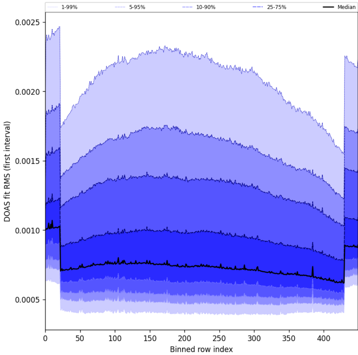
Figure 60: Along track statistics of “DOAS fit RMS (first interval)” for 2025-06-02 to 2025-06-04
