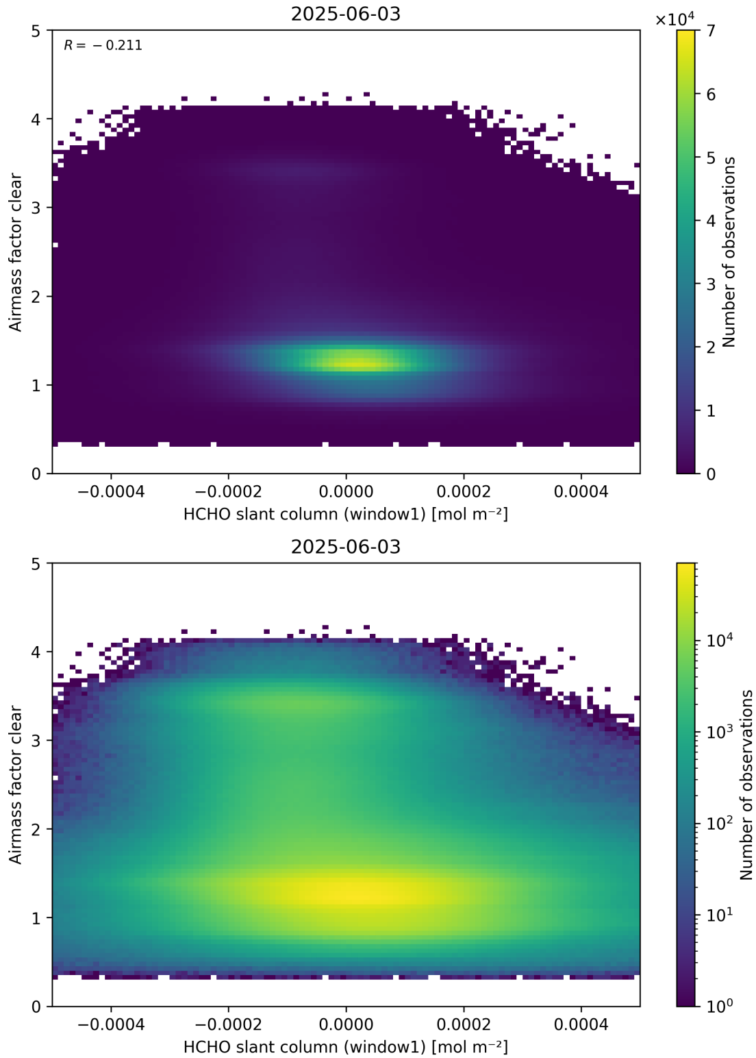
Figure 81: Scatter density plot of “HCHO slant column (window1)” against “Airmass factor clear” for 2025-06-02 to 2025-06-04.
