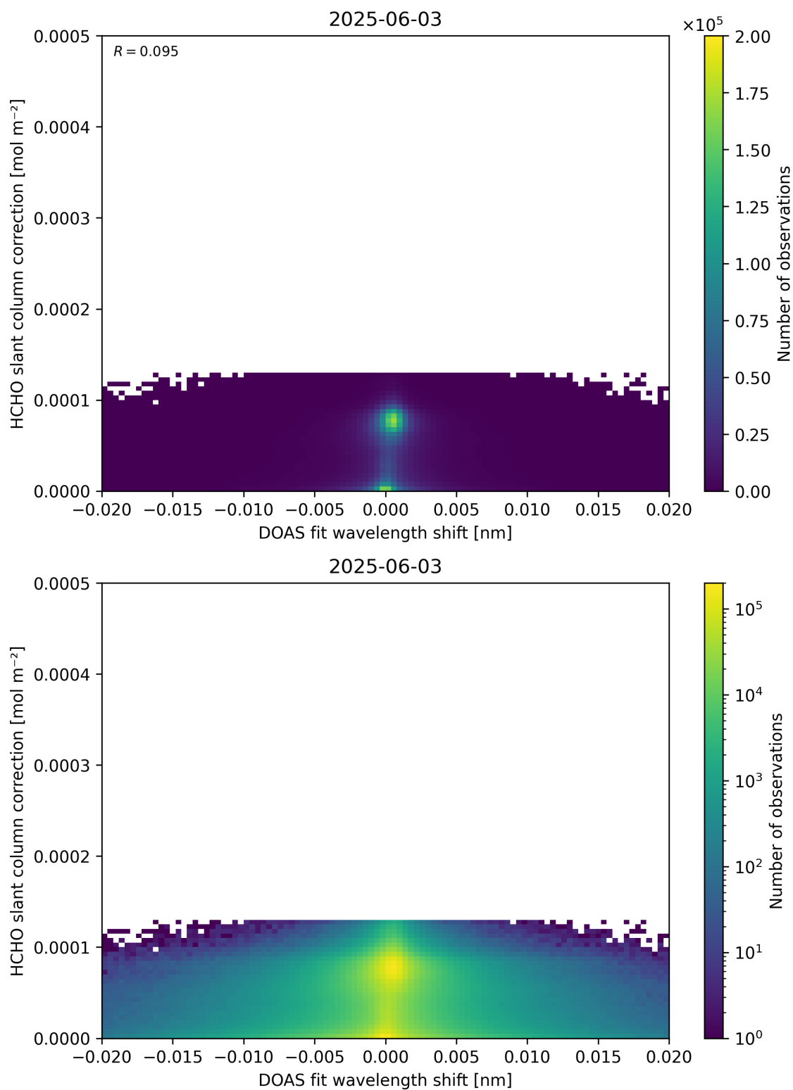
Figure 67: Scatter density plot of “DOAS fit wavelength shift” against “HCHO slant column correction” for 2025-06-02 to 2025-06-04.
