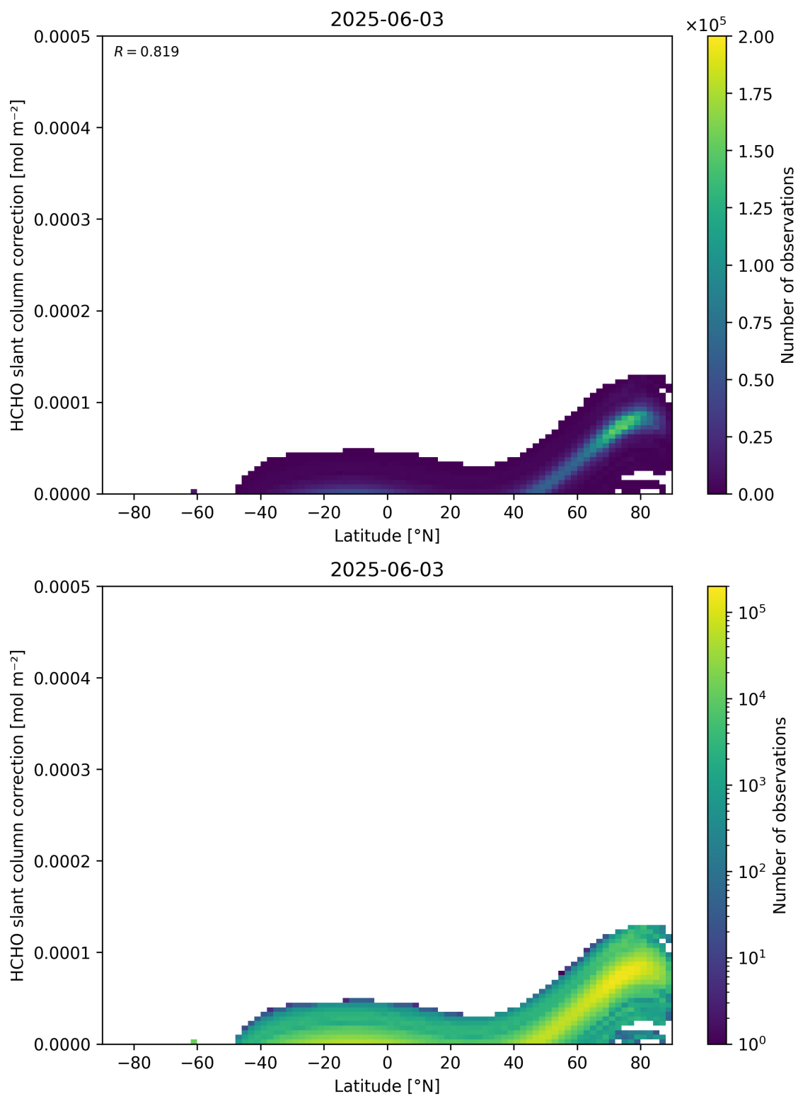
Figure 158: Scatter density plot of “Latitude” against “HCHO slant column correction” for 2025-06-02 to 2025-06-04.
