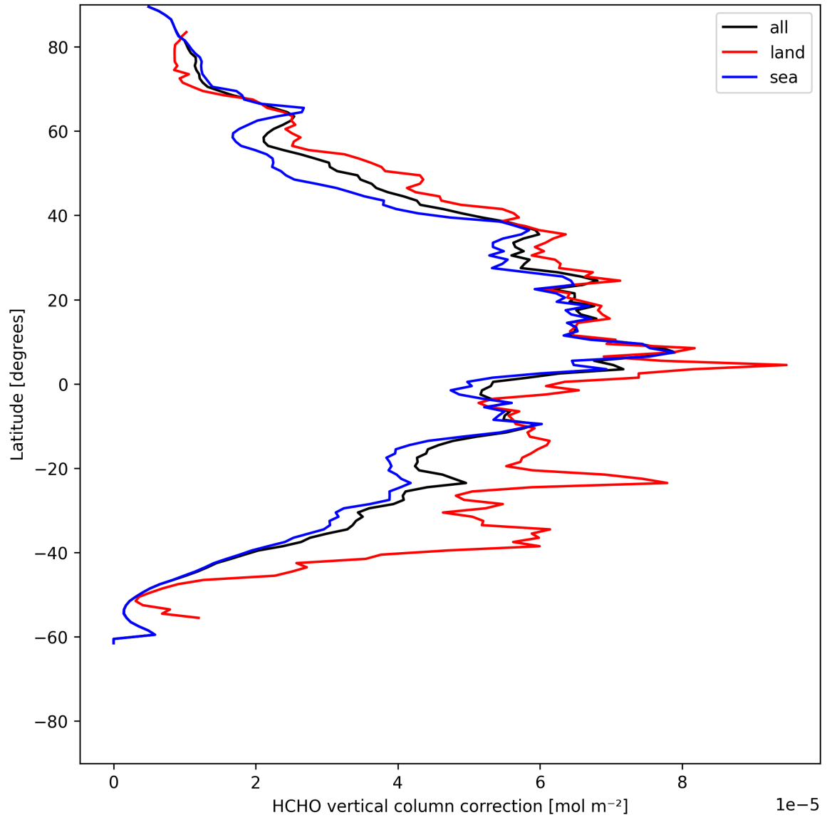
Figure 23: Zonal average of “HCHO vertical column correction” for 2025-06-02 to 2025-06-04.
