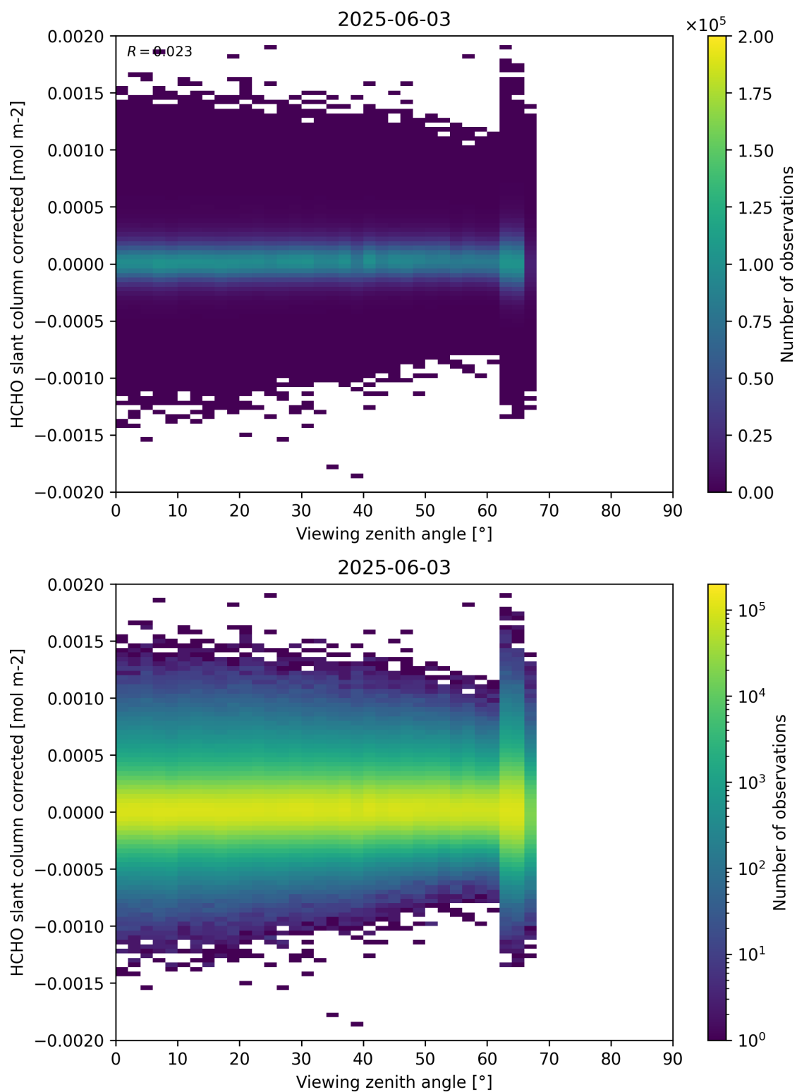
Figure 186: Scatter density plot of “Viewing zenith angle” against “HCHO slant column corrected” for 2025-06-02 to 2025-06-04.
