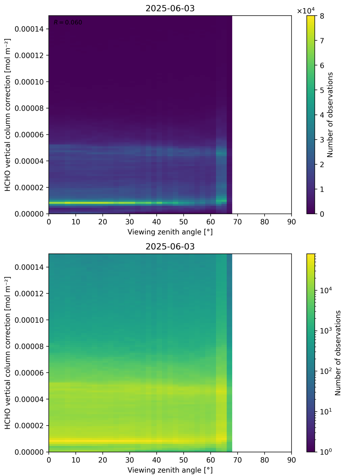
Figure 193: Scatter density plot of “Viewing zenith angle” against “HCHO vertical column correction” for 2025-06-02 to 2025-06-04.
