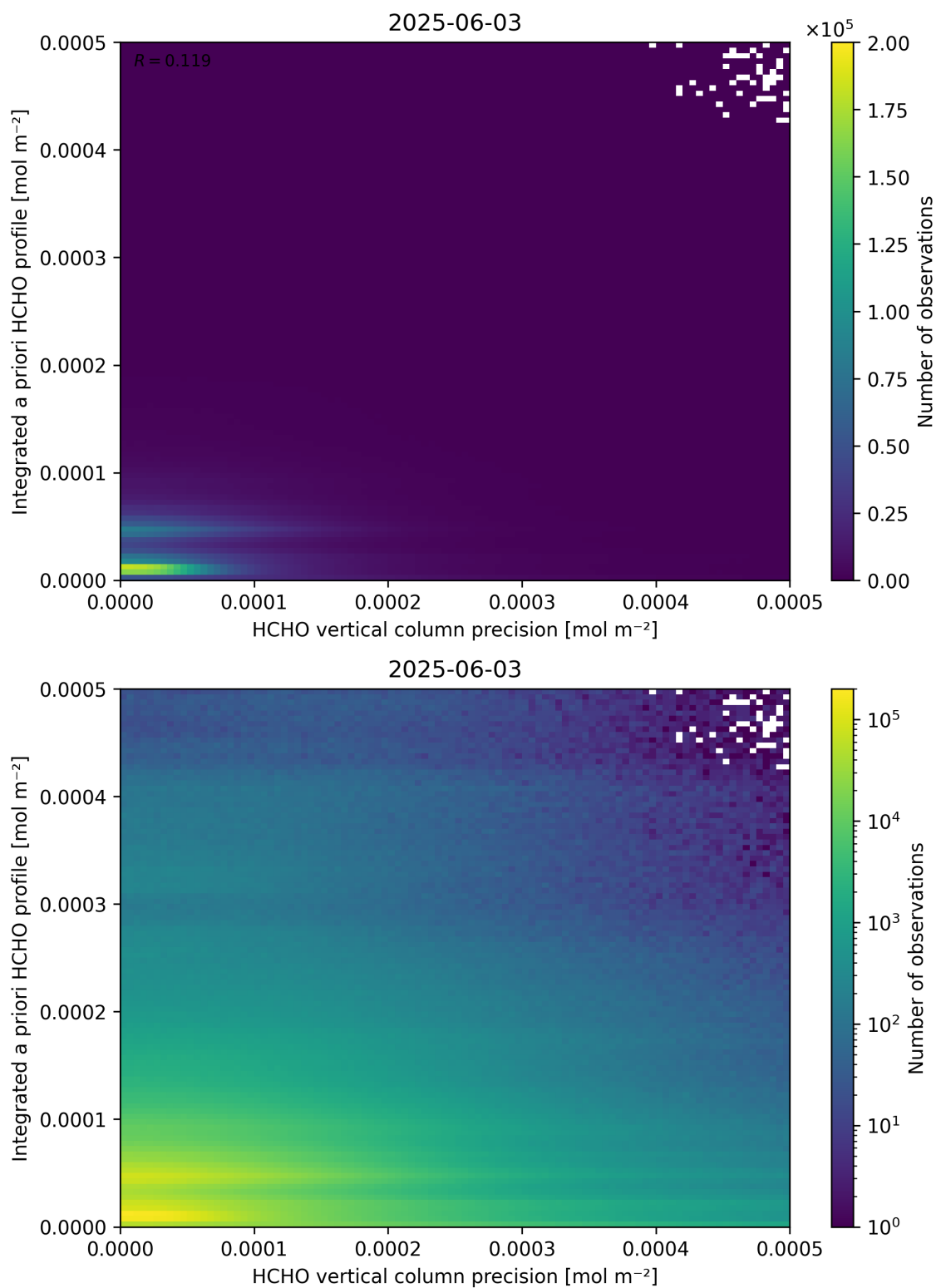
Figure 147: Scatter density plot of “HCHO vertical column precision” against “Integrated a priori HCHO profile” for 2025-06-02 to 2025-06-04.
