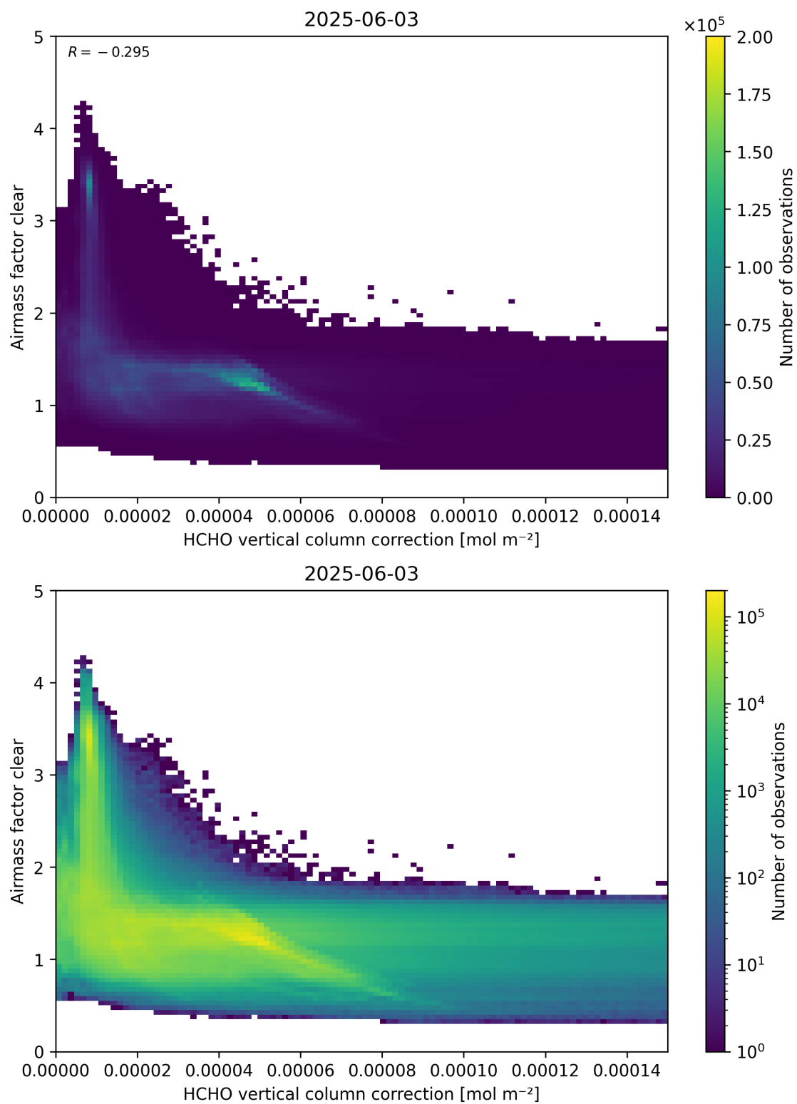
Figure 115: Scatter density plot of “HCHO vertical column correction” against “Airmass factor clear” for 2025-06-02 to 2025-06-04.
