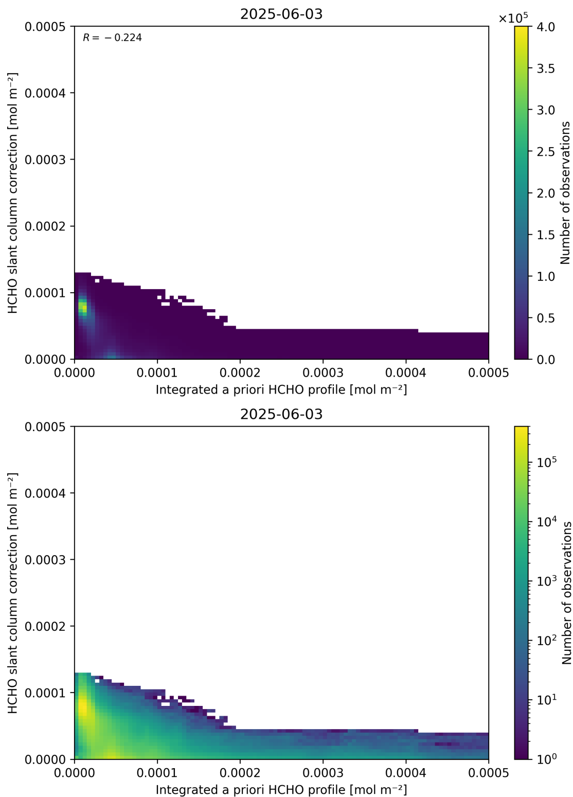
Figure 152: Scatter density plot of “Integrated a priori HCHO profile” against “HCHO slant column correction” for 2025-06-02 to 2025-06-04.
