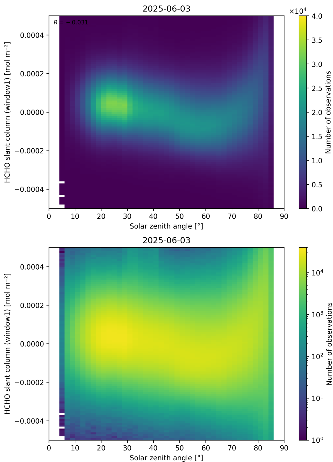
Figure 173: Scatter density plot of “Solar zenith angle” against “HCHO slant column (window1)” for 2025-06-02 to 2025-06-04.
