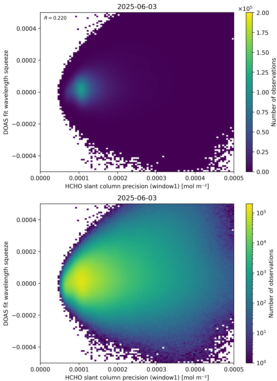
Figure 90: Scatter density plot of “HCHO slant column precision (window1)” against “DOAS fit wavelength squeeze” for 2025-06-02 to 2025-06-04.
