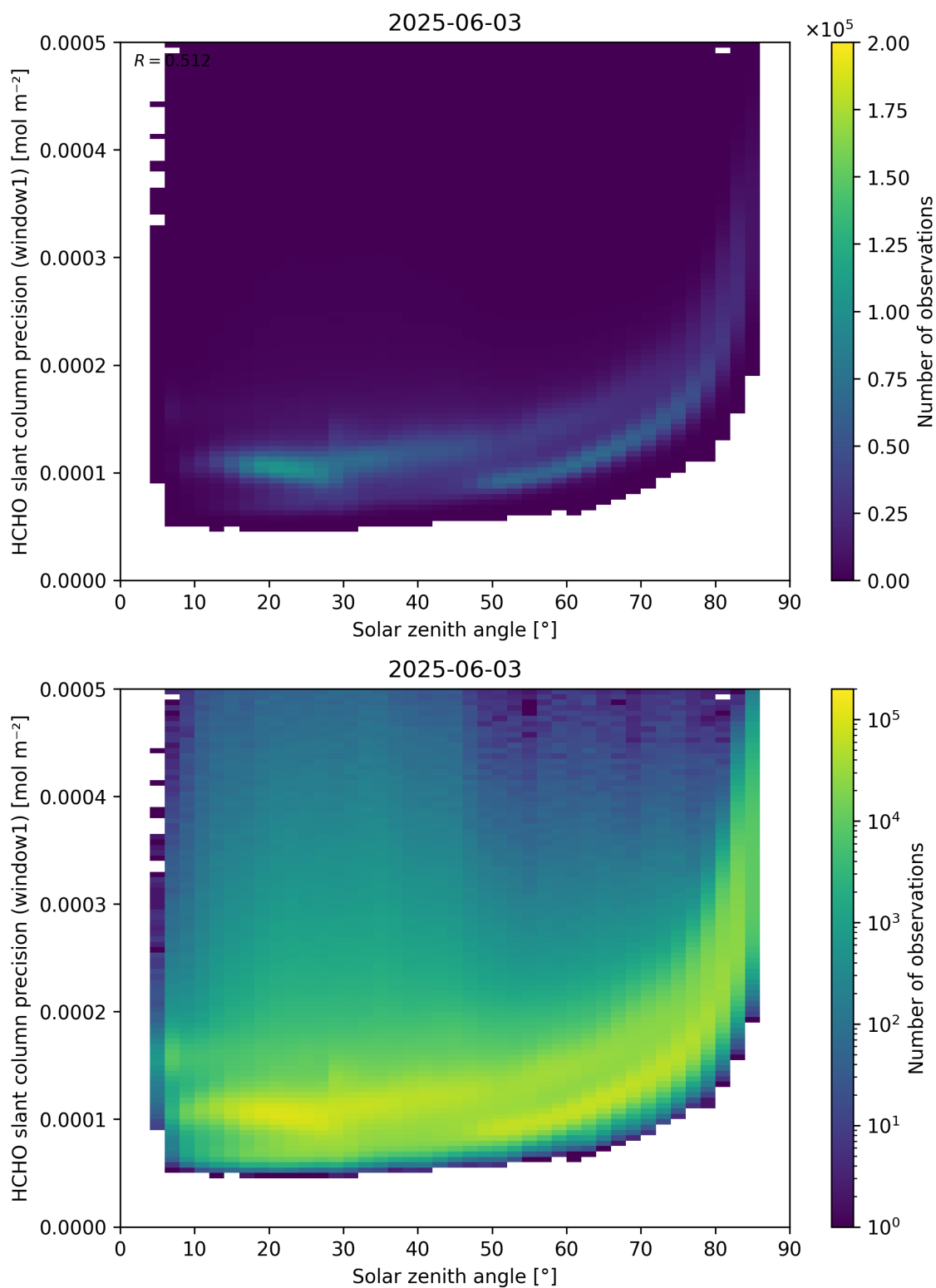
Figure 174: Scatter density plot of “Solar zenith angle” against “HCHO slant column precision (window1)” for 2025-06-02 to 2025-06-04.
