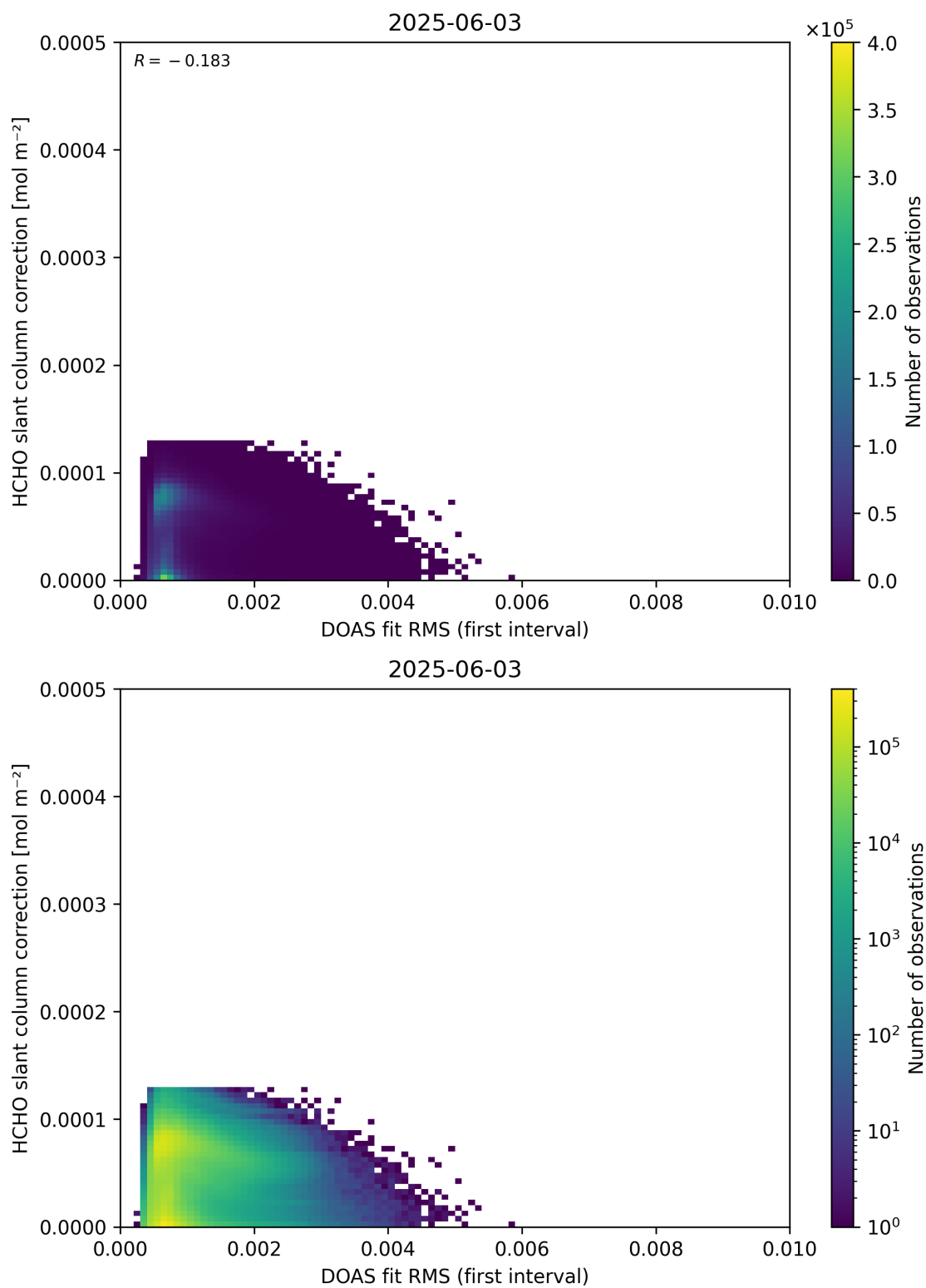
Figure 63: Scatter density plot of “DOAS fit RMS (first interval)” against “HCHO slant column correction” for 2025-06-02 to 2025-06-04.
