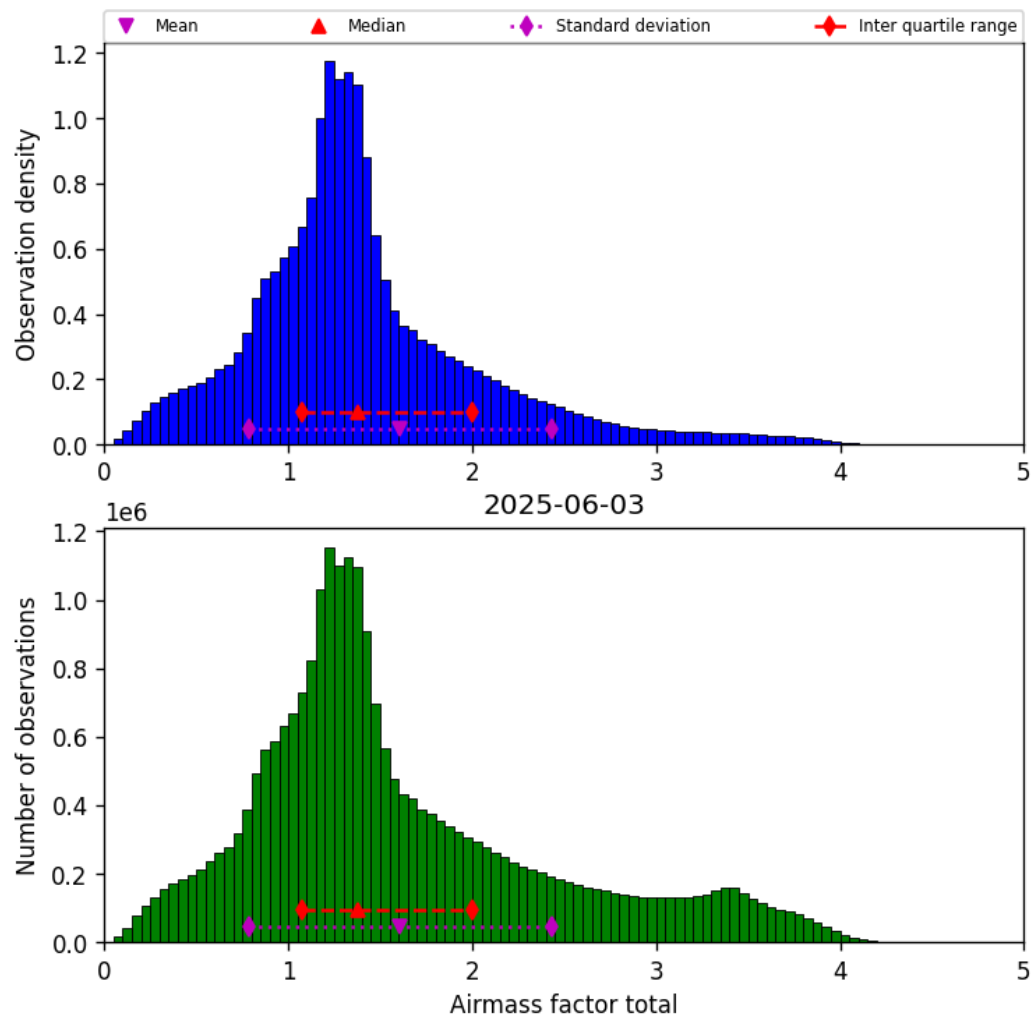
Figure 40: Histogram of “Airmass factor total” for 2025-06-02 to 2025-06-04
