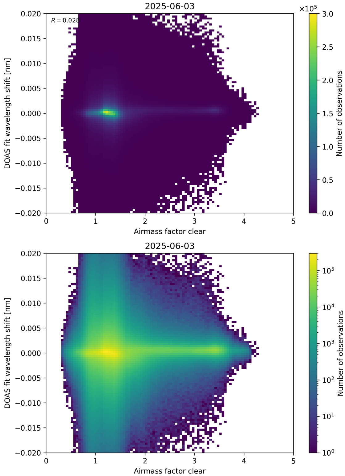
Figure 72: Scatter density plot of “Airmass factor clear” against “DOAS fit wavelength shift” for 2025-06-02 to 2025-06-04.
