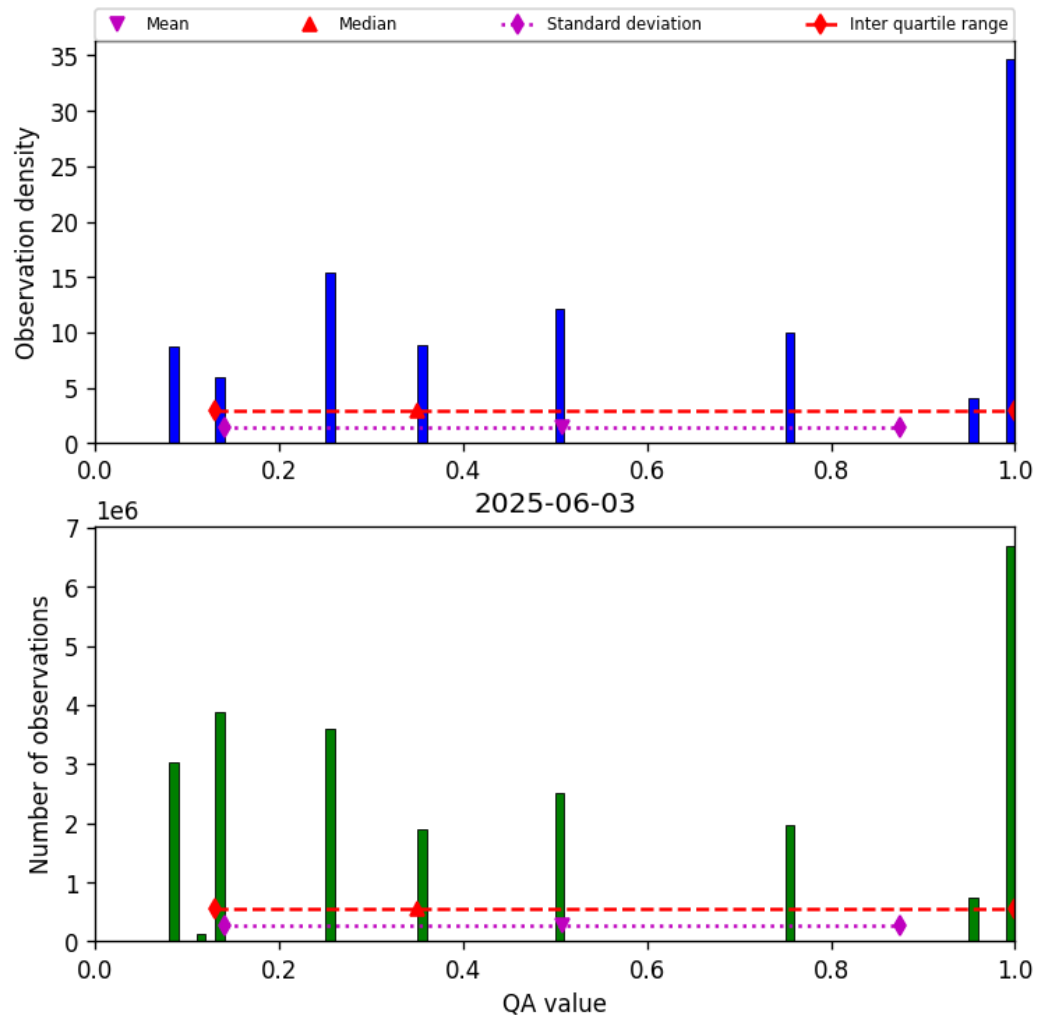
Figure 34: Histogram of “QA value” for 2025-06-02 to 2025-06-04
