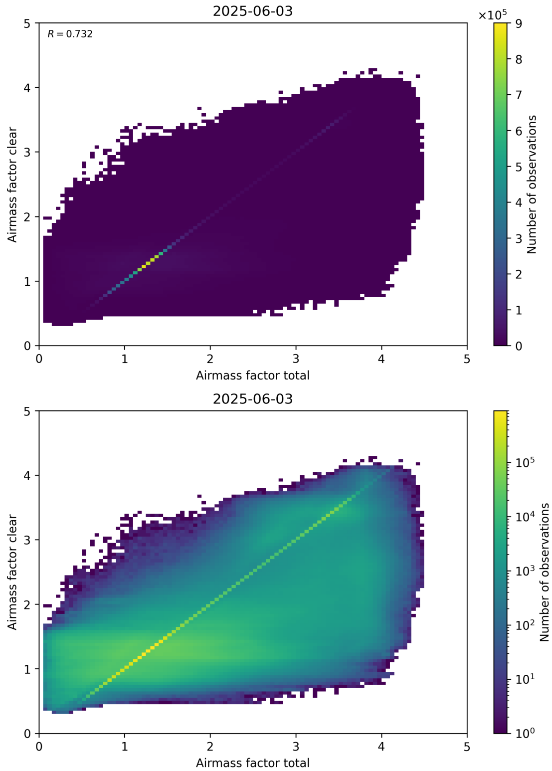
Figure 100: Scatter density plot of “Airmass factor total” against “Airmass factor clear” for 2025-06-02 to 2025-06-04.
