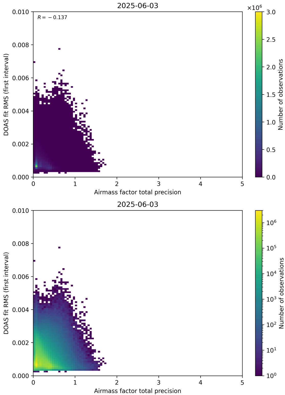
Figure 105: Scatter density plot of “Airmass factor total precision” against “DOAS fit RMS (first interval)” for 2025-06-02 to 2025-06-04.
