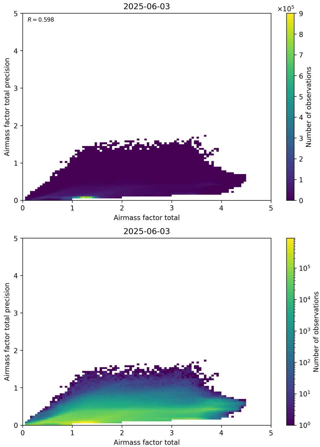
Figure 103: Scatter density plot of “Airmass factor total” against “Airmass factor total precision” for 2025-06-02 to 2025-06-04.
