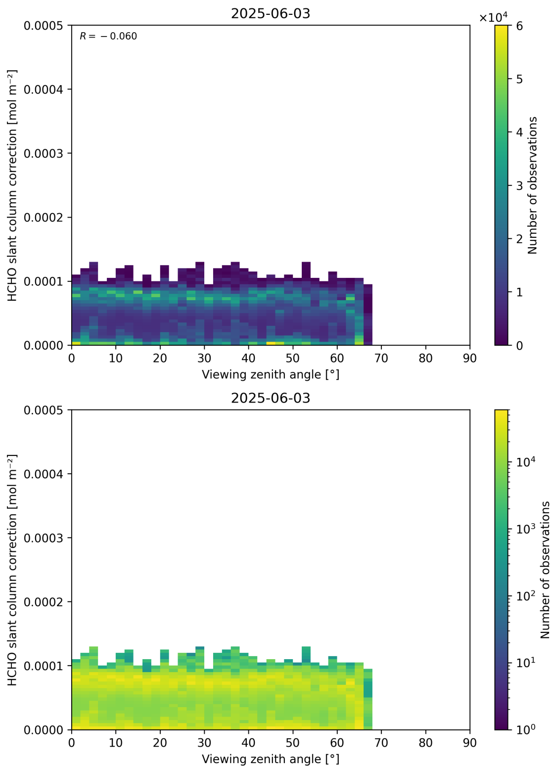
Figure 187: Scatter density plot of “Viewing zenith angle” against “HCHO slant column correction” for 2025-06-02 to 2025-06-04.
