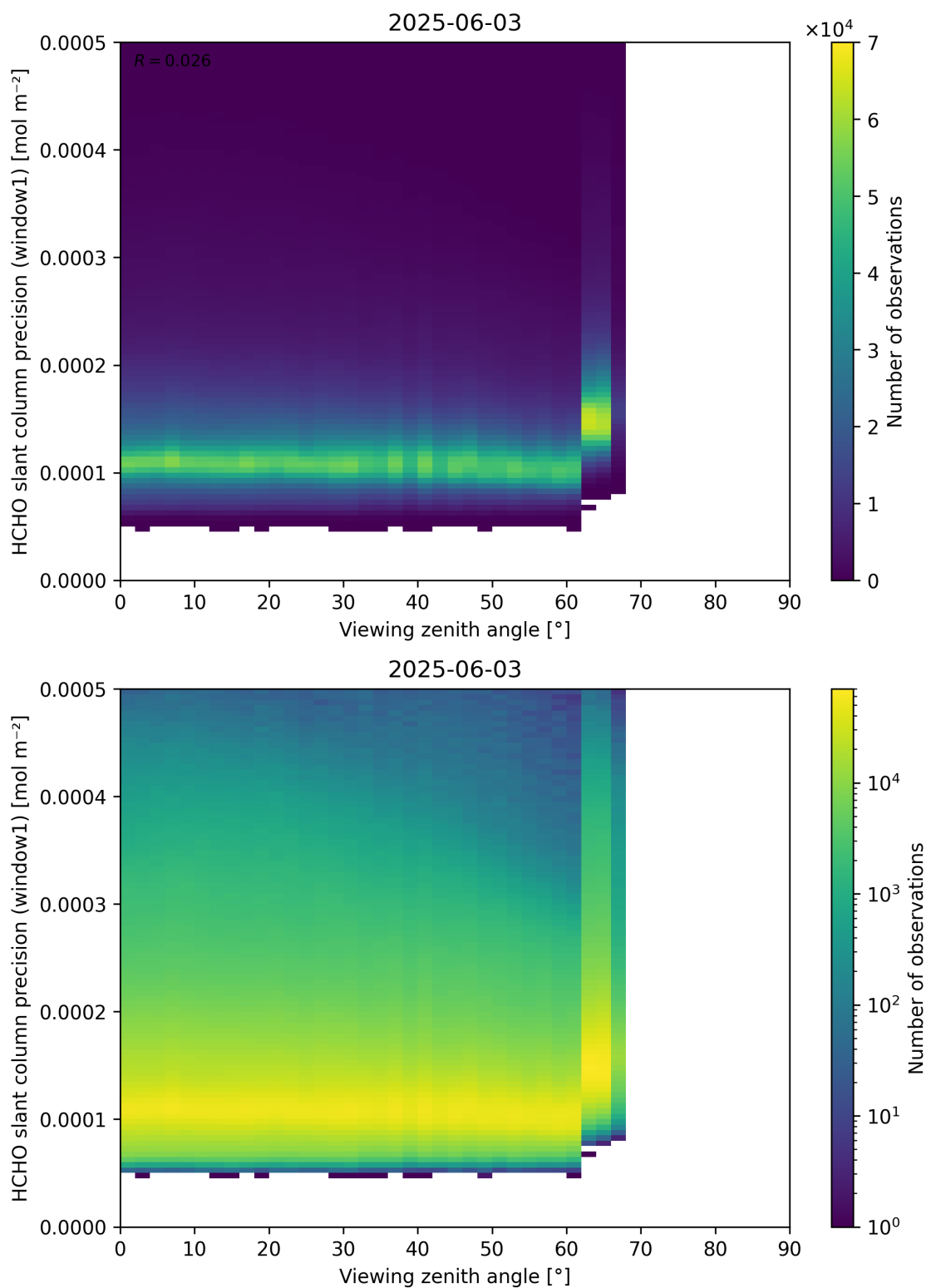
Figure 189: Scatter density plot of “Viewing zenith angle” against “HCHO slant column precision (window1)” for 2025-06-02 to 2025-06-04.
