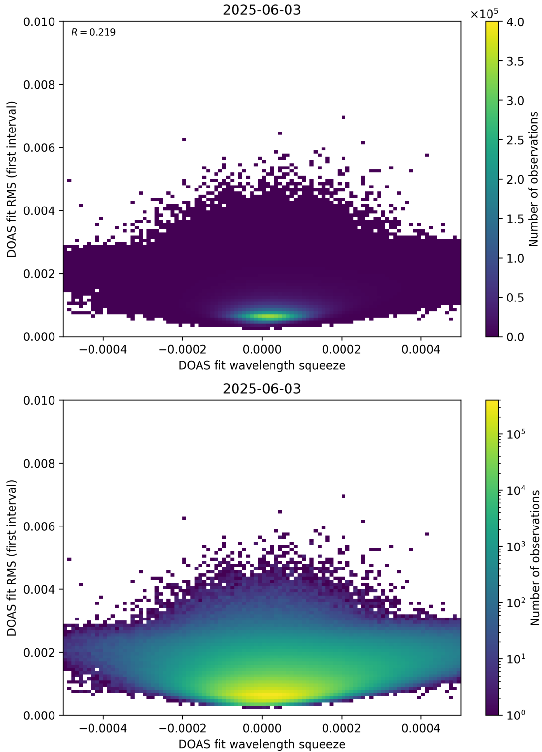
Figure 68: Scatter density plot of “DOAS fit wavelength squeeze” against “DOAS fit RMS (first interval)” for 2025-06-02 to 2025-06-04.
