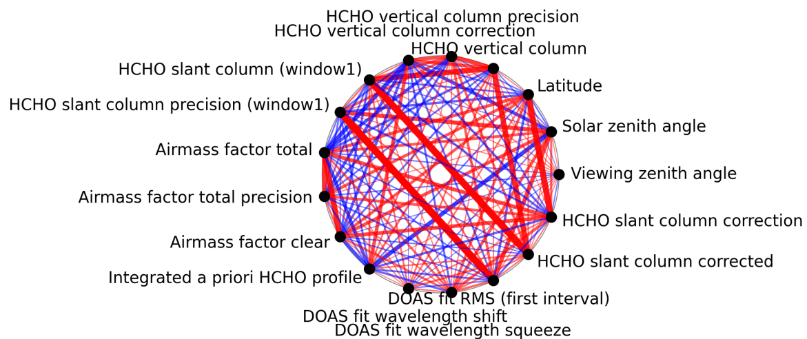
Figure 1: Map of correlation graph for 2025-06-02 to 2025-06-04.
