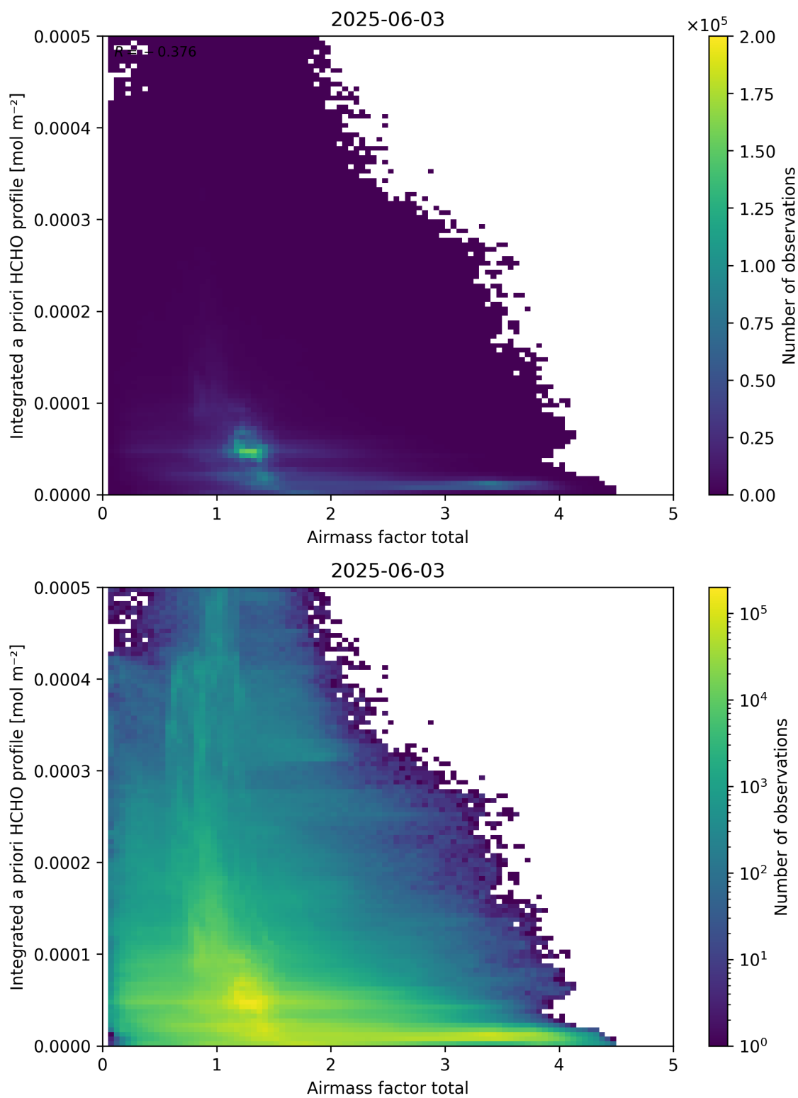
Figure 104: Scatter density plot of “Airmass factor total” against “Integrated a priori HCHO profile” for 2025-06-02 to 2025-06-04.
