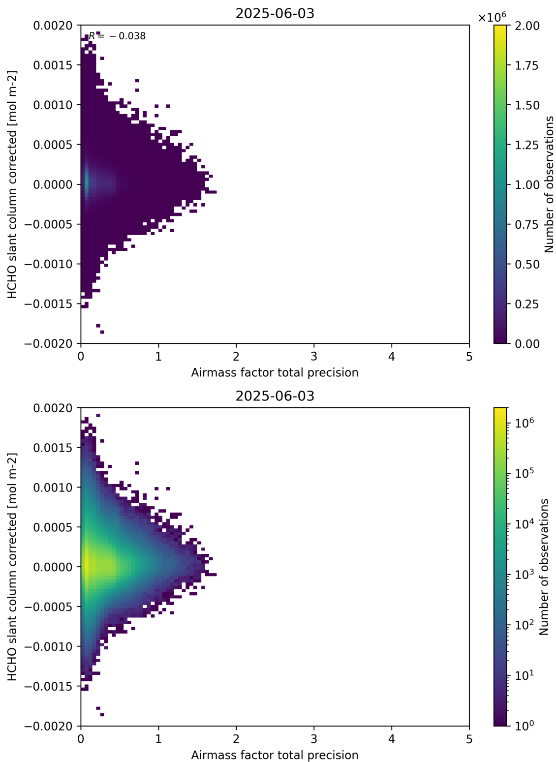
Figure 109: Scatter density plot of “Airmass factor total precision” against “HCHO slant column corrected” for 2025-06-02 to 2025-06-04.
