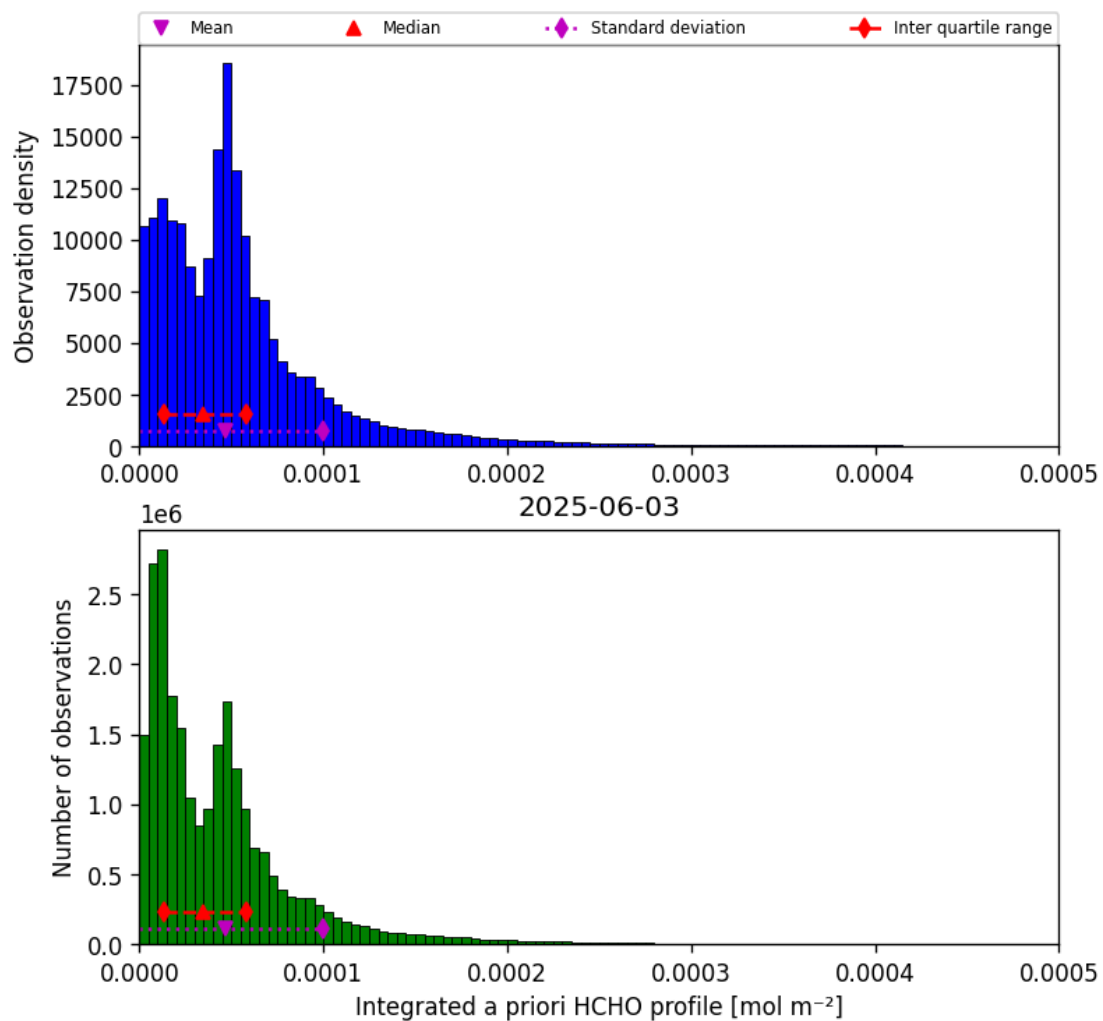
Figure 43: Histogram of “Integrated a priori HCHO profile” for 2025-06-02 to 2025-06-04
