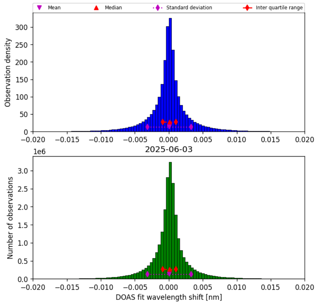
Figure 44: Histogram of “DOAS fit wavelength shift” for 2025-06-02 to 2025-06-04
