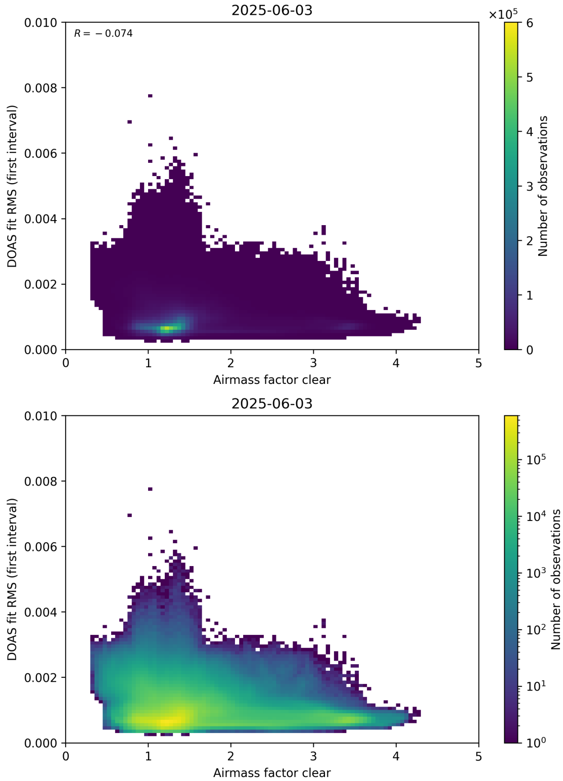
Figure 71: Scatter density plot of “Airmass factor clear” against “DOAS fit RMS (first interval)” for 2025-06-02 to 2025-06-04.
