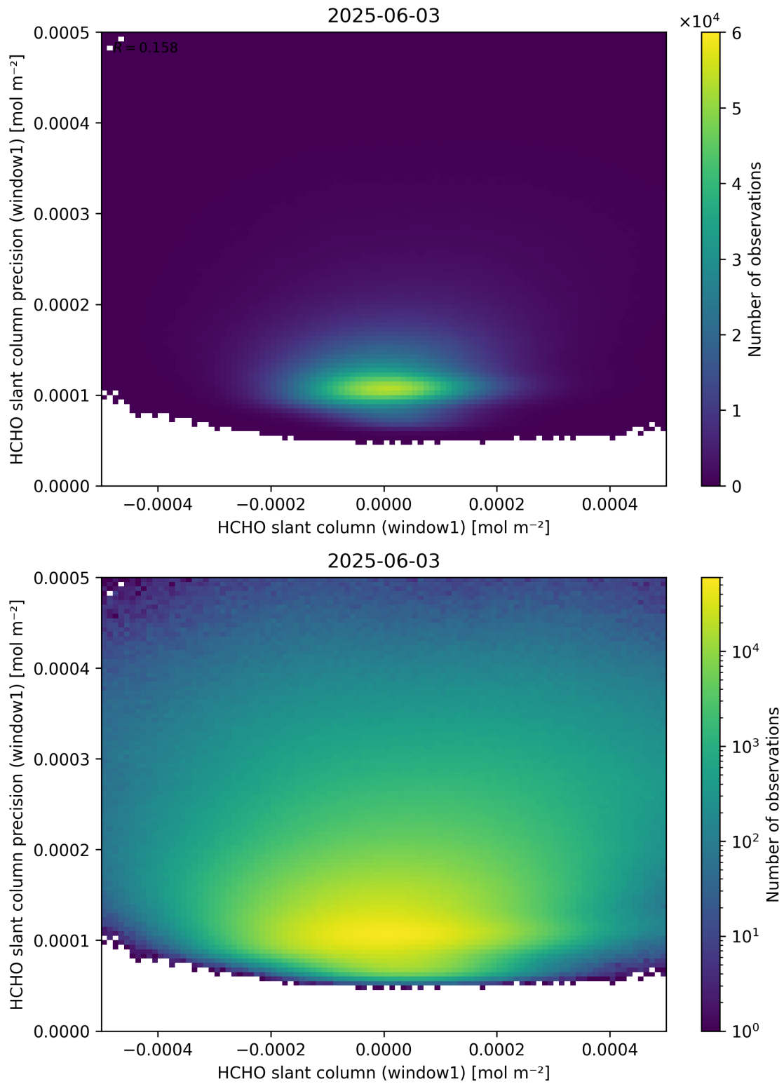
Figure 84: Scatter density plot of “HCHO slant column (window1)” against “HCHO slant column precision (window1)” for 2025-06-02 to 2025-06-04.
