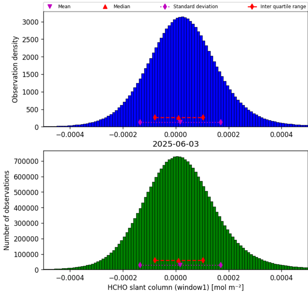
Figure 38: Histogram of “HCHO slant column (window1)” for 2025-06-02 to 2025-06-04
