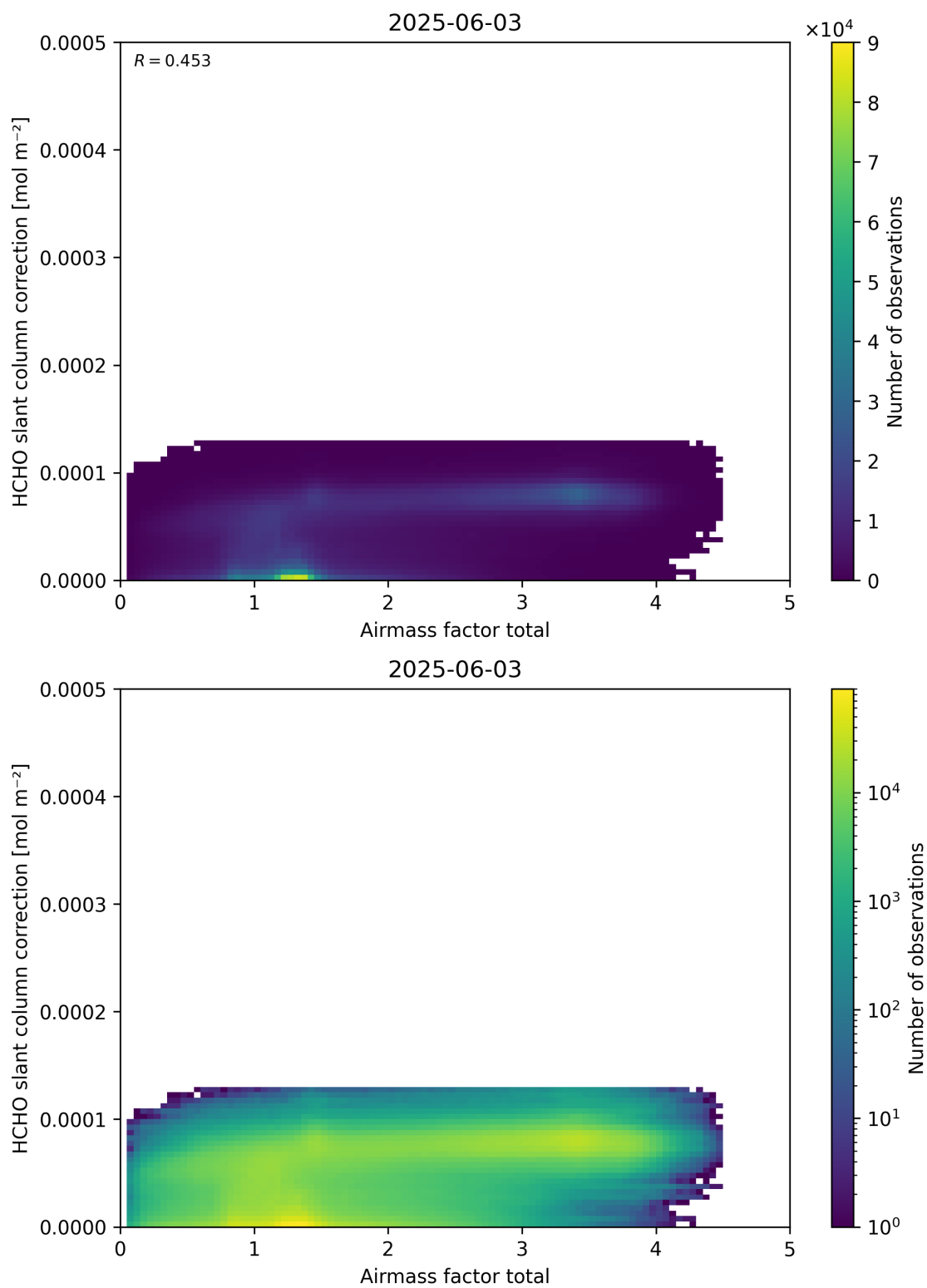
Figure 102: Scatter density plot of “Airmass factor total” against “HCHO slant column correction” for 2025-06-02 to 2025-06-04.
