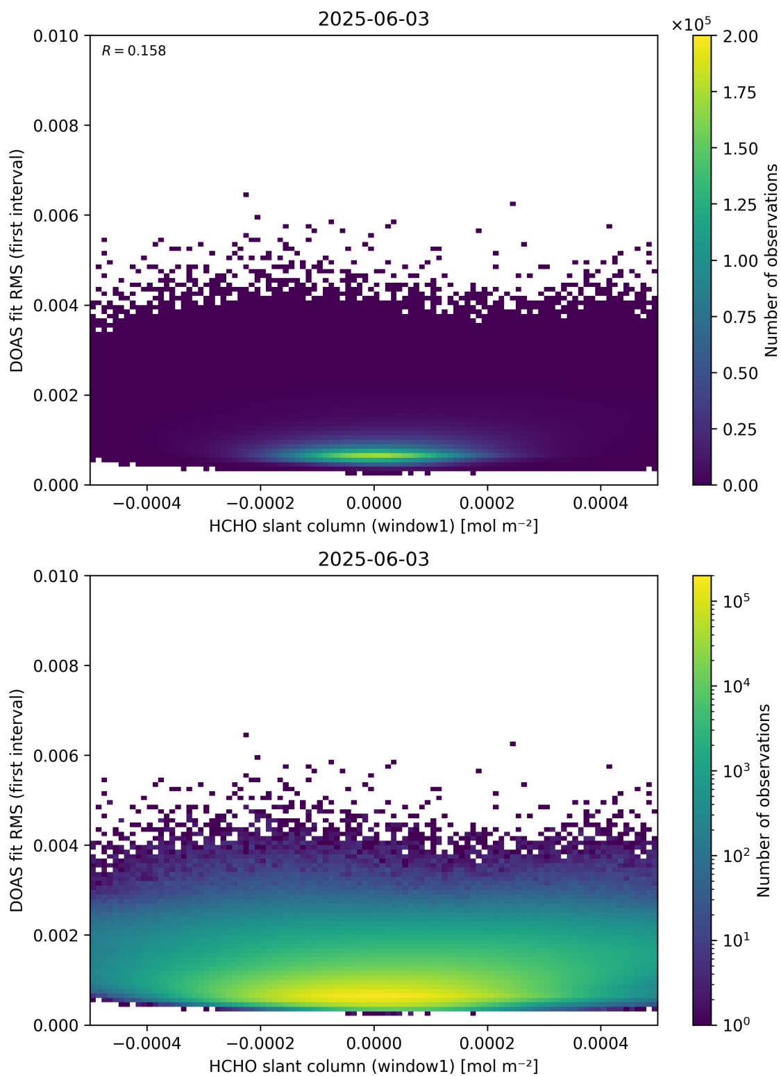
Figure 78: Scatter density plot of “HCHO slant column (window1)” against “DOAS fit RMS (first interval)” for 2025-06-02 to 2025-06-04.
