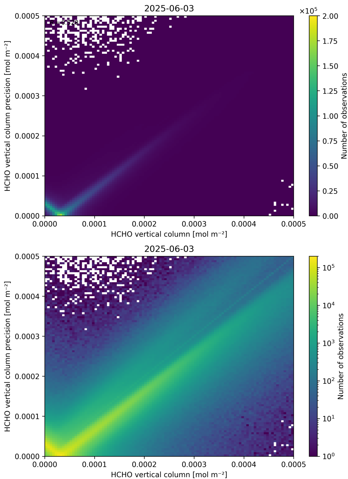
Figure 134: Scatter density plot of “HCHO vertical column” against “HCHO vertical column precision” for 2025-06-02 to 2025-06-04.
