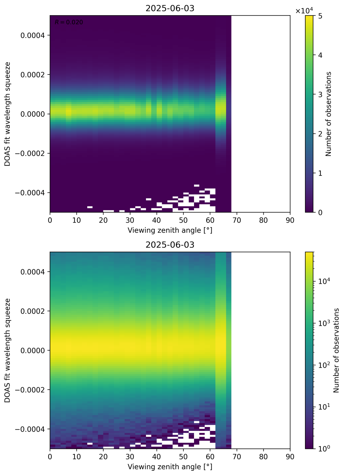
Figure 184: Scatter density plot of “Viewing zenith angle” against “DOAS fit wavelength squeeze” for 2025-06-02 to 2025-06-04.
