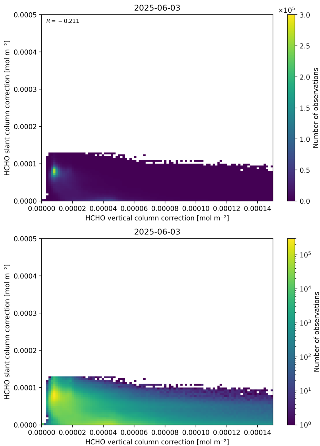
Figure 117: Scatter density plot of “HCHO vertical column correction” against “HCHO slant column correction” for 2025-06-02 to 2025-06-04.
