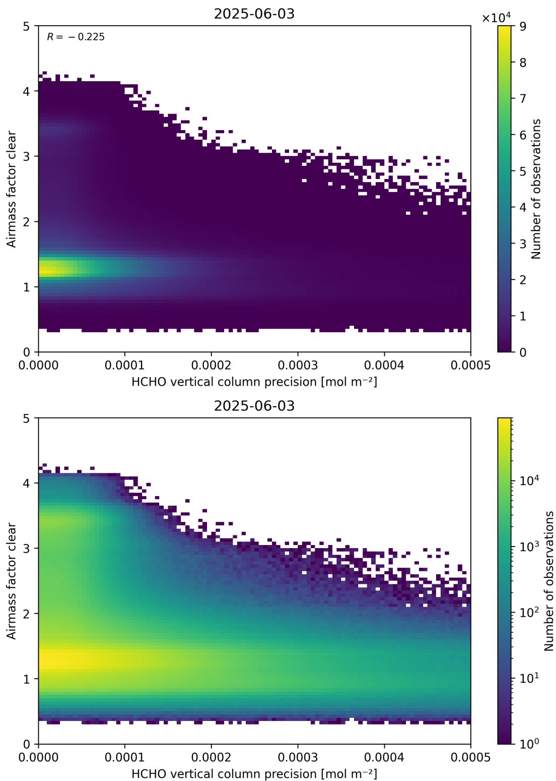
Figure 139: Scatter density plot of “HCHO vertical column precision” against “Airmass factor clear” for 2025-06-02 to 2025-06-04.
