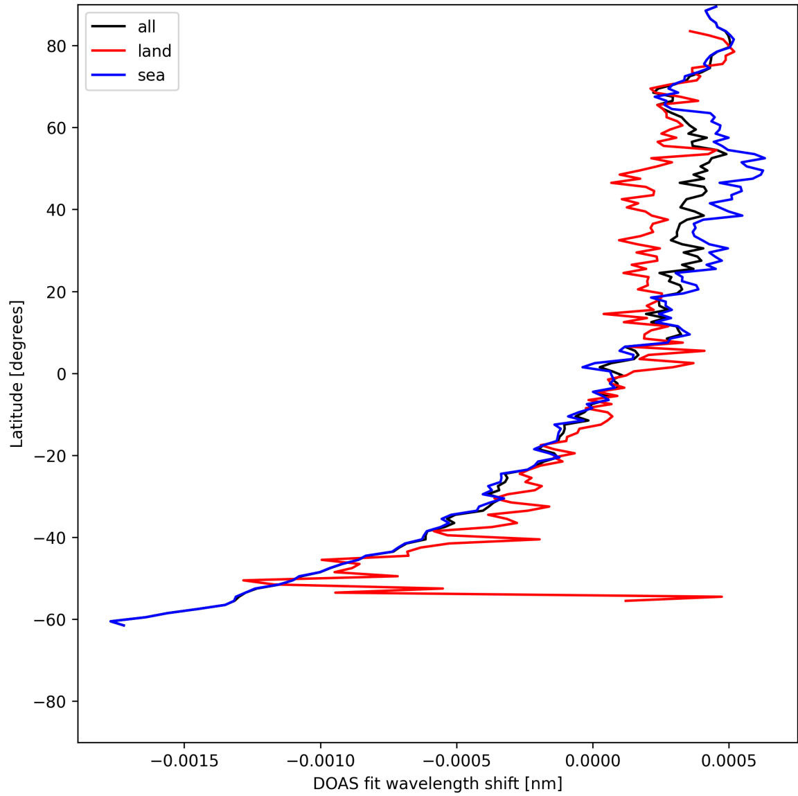
Figure 30: Zonal average of “DOAS fit wavelength shift” for 2025-06-02 to 2025-06-04.
