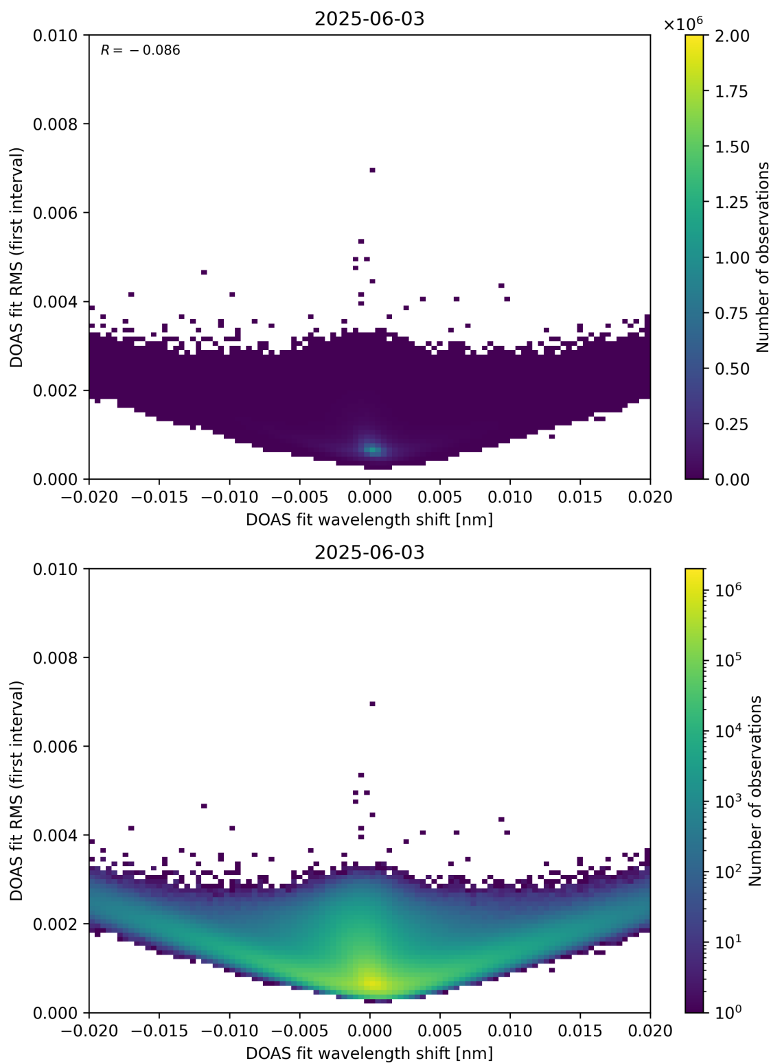
Figure 64: Scatter density plot of “DOAS fit wavelength shift” against “DOAS fit RMS (first interval)” for 2025-06-02 to 2025-06-04.
