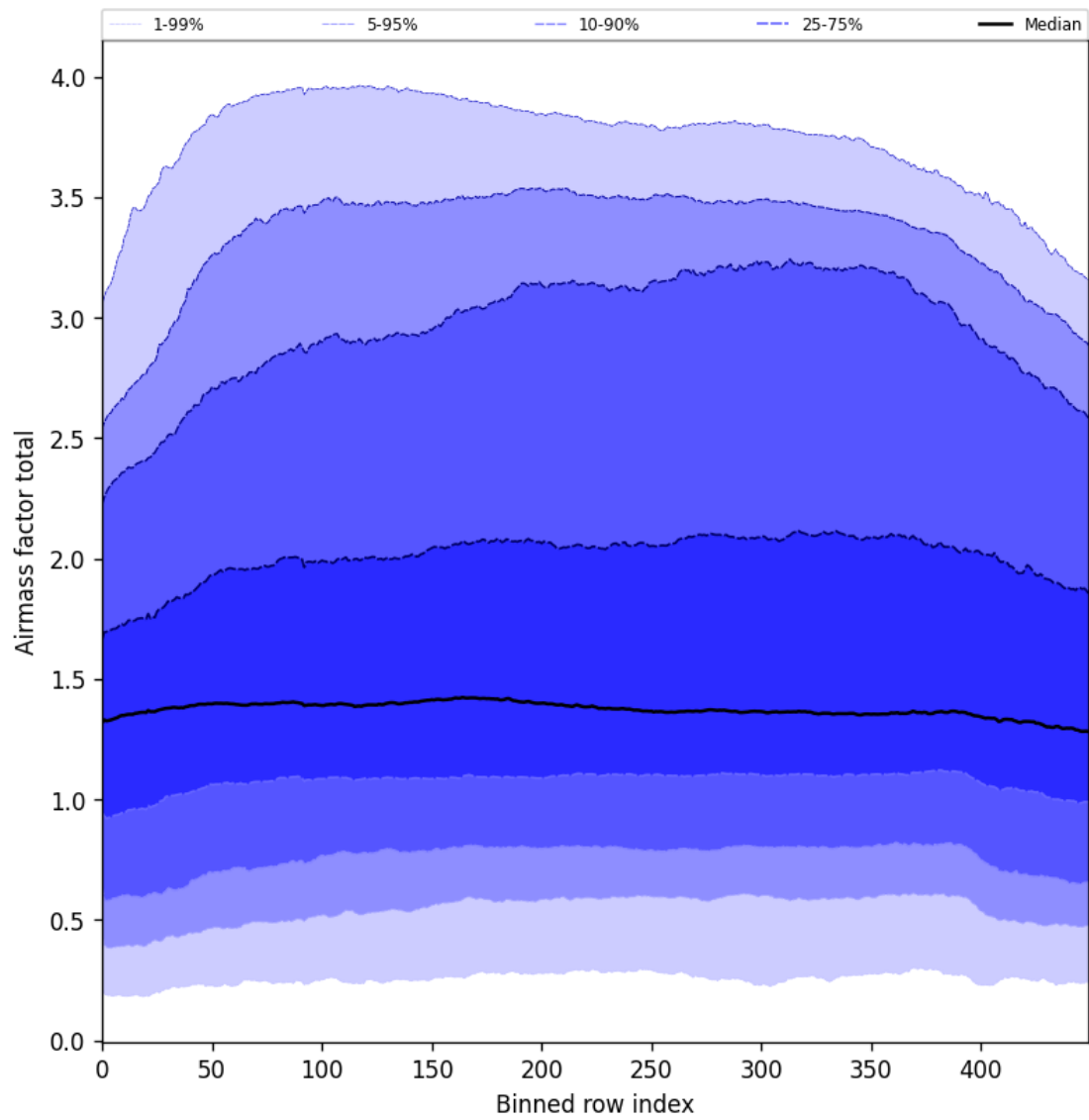
Figure 54: Along track statistics of “Airmass factor total” for 2025-06-02 to 2025-06-04
