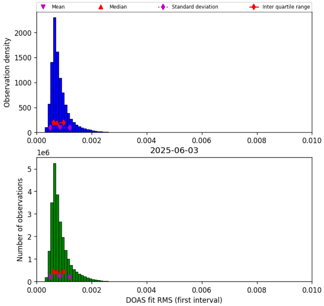
Figure 46: Histogram of “DOAS fit RMS (first interval)” for 2025-06-02 to 2025-06-04
