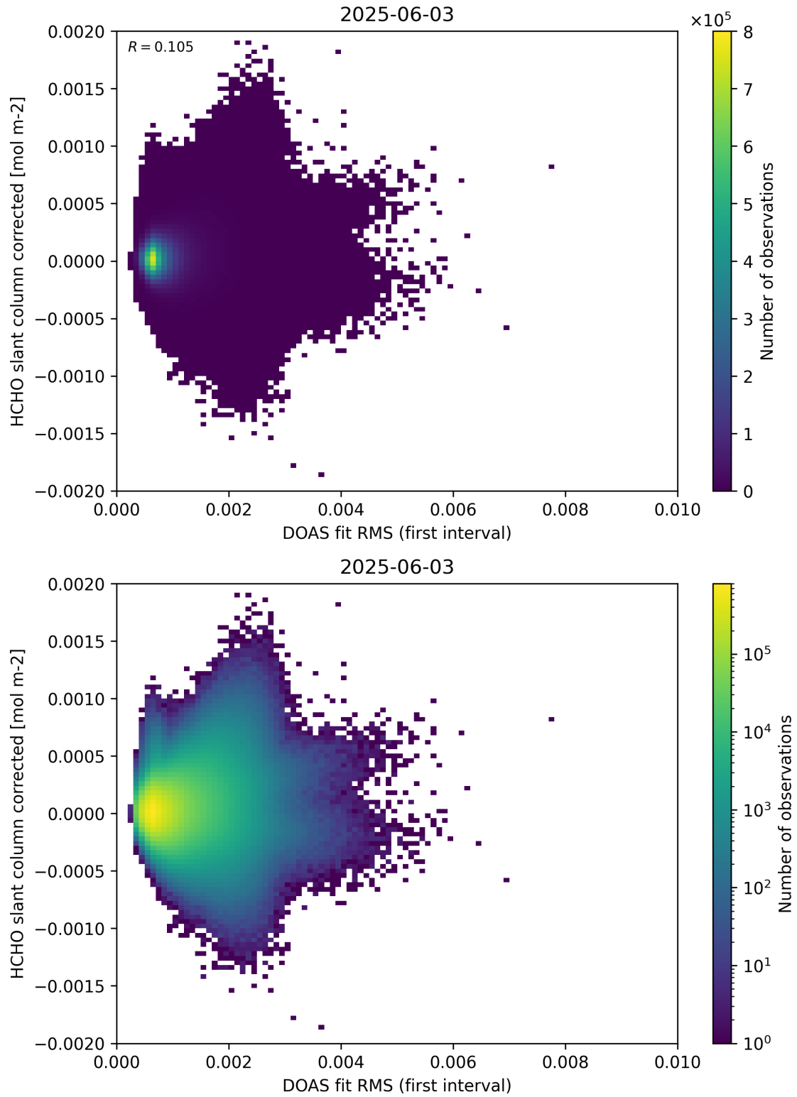
Figure 62: Scatter density plot of “DOAS fit RMS (first interval)” against “HCHO slant column corrected” for 2025-06-02 to 2025-06-04.
