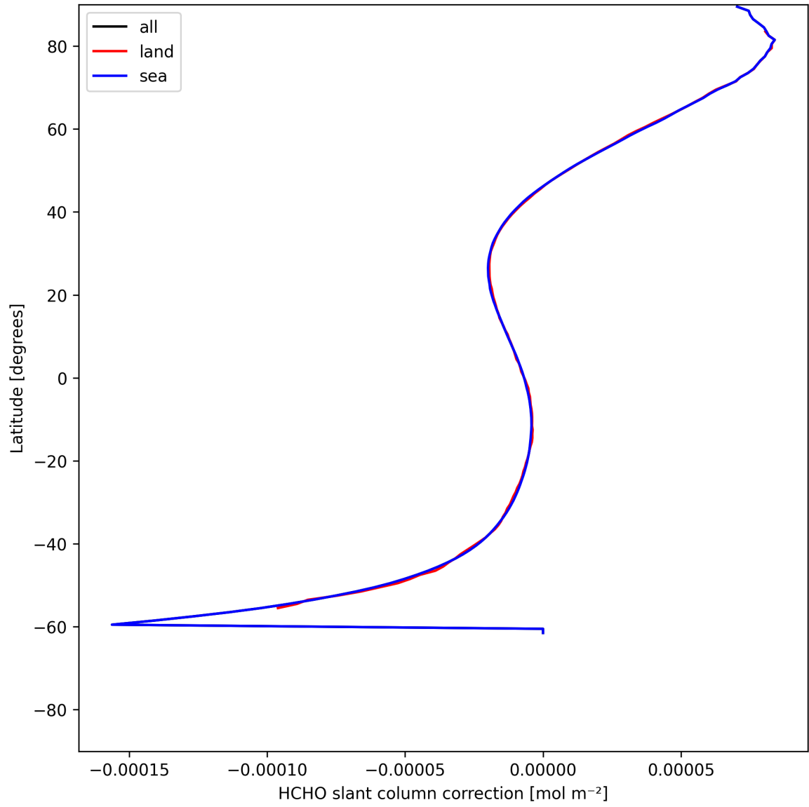
Figure 33: Zonal average of “HCHO slant column correction” for 2025-06-02 to 2025-06-04.
