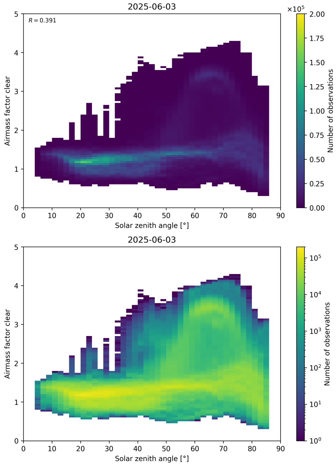
Figure 170: Scatter density plot of “Solar zenith angle” against “Airmass factor clear” for 2025-06-02 to 2025-06-04.
