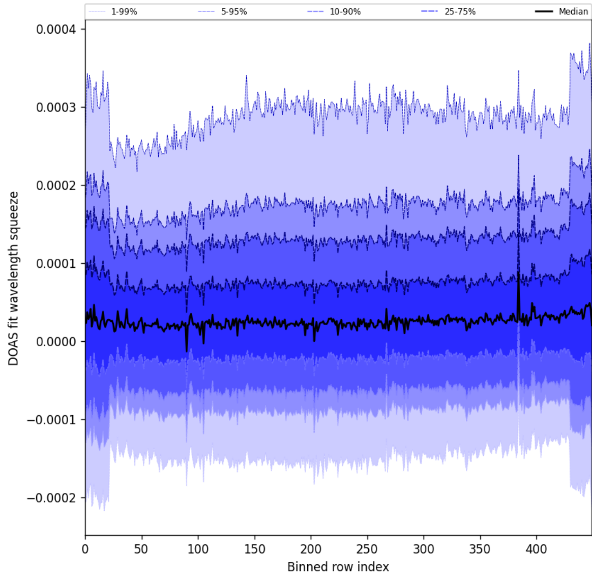
Figure 59: Along track statistics of “DOAS fit wavelength squeeze” for 2025-06-02 to 2025-06-04
