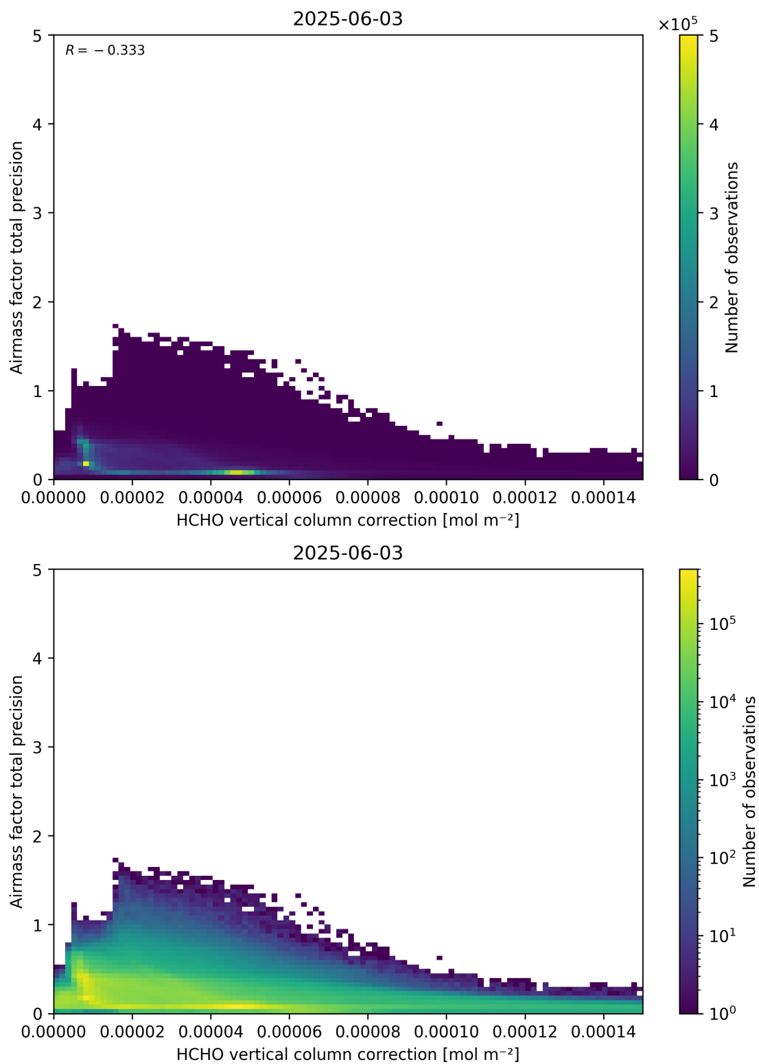
Figure 121: Scatter density plot of “HCHO vertical column correction” against “Airmass factor total precision” for 2025-06-02 to 2025-06-04.
