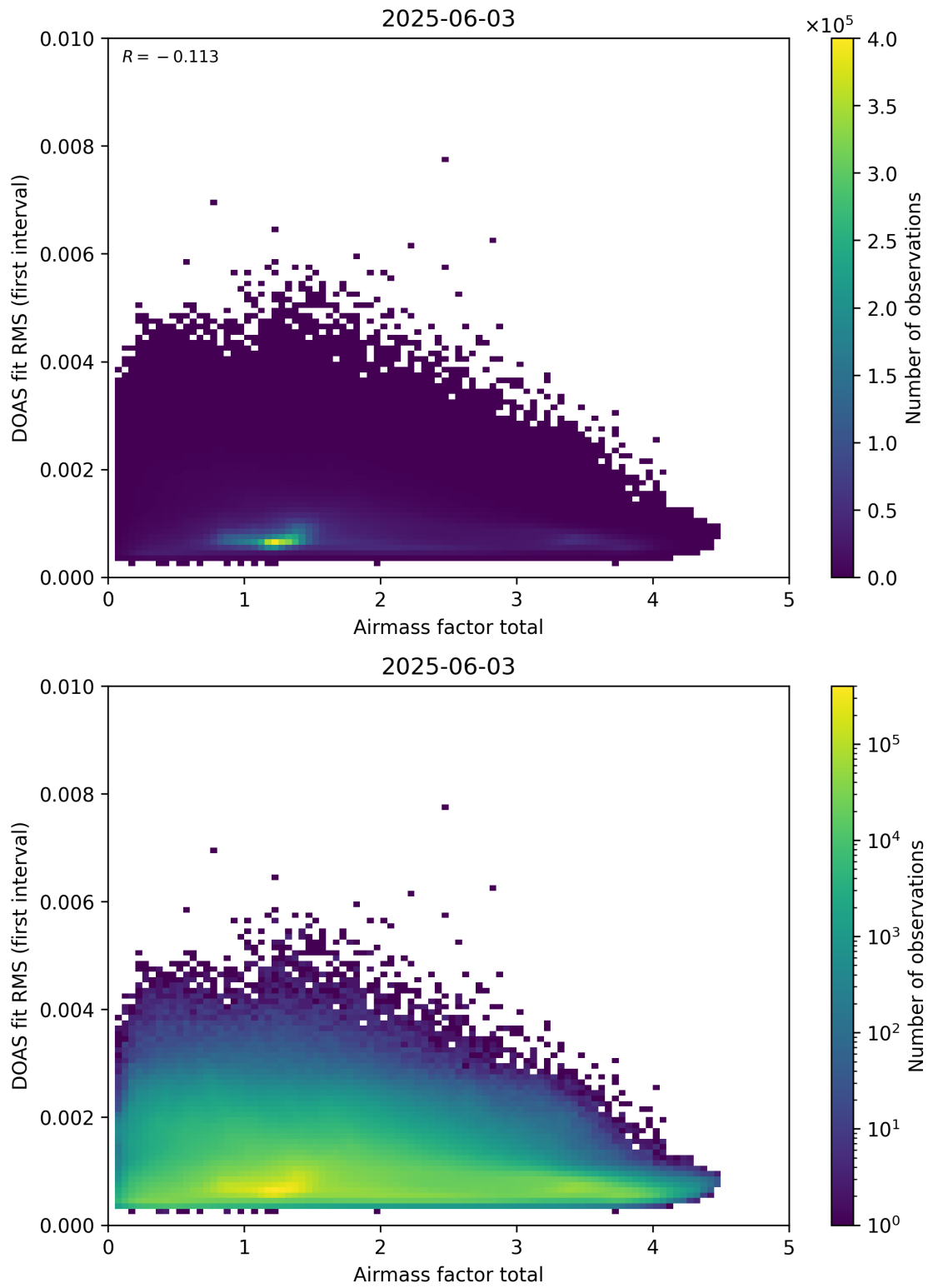
Figure 97: Scatter density plot of “Airmass factor total” against “DOAS fit RMS (first interval)” for 2025-06-02 to 2025-06-04.
