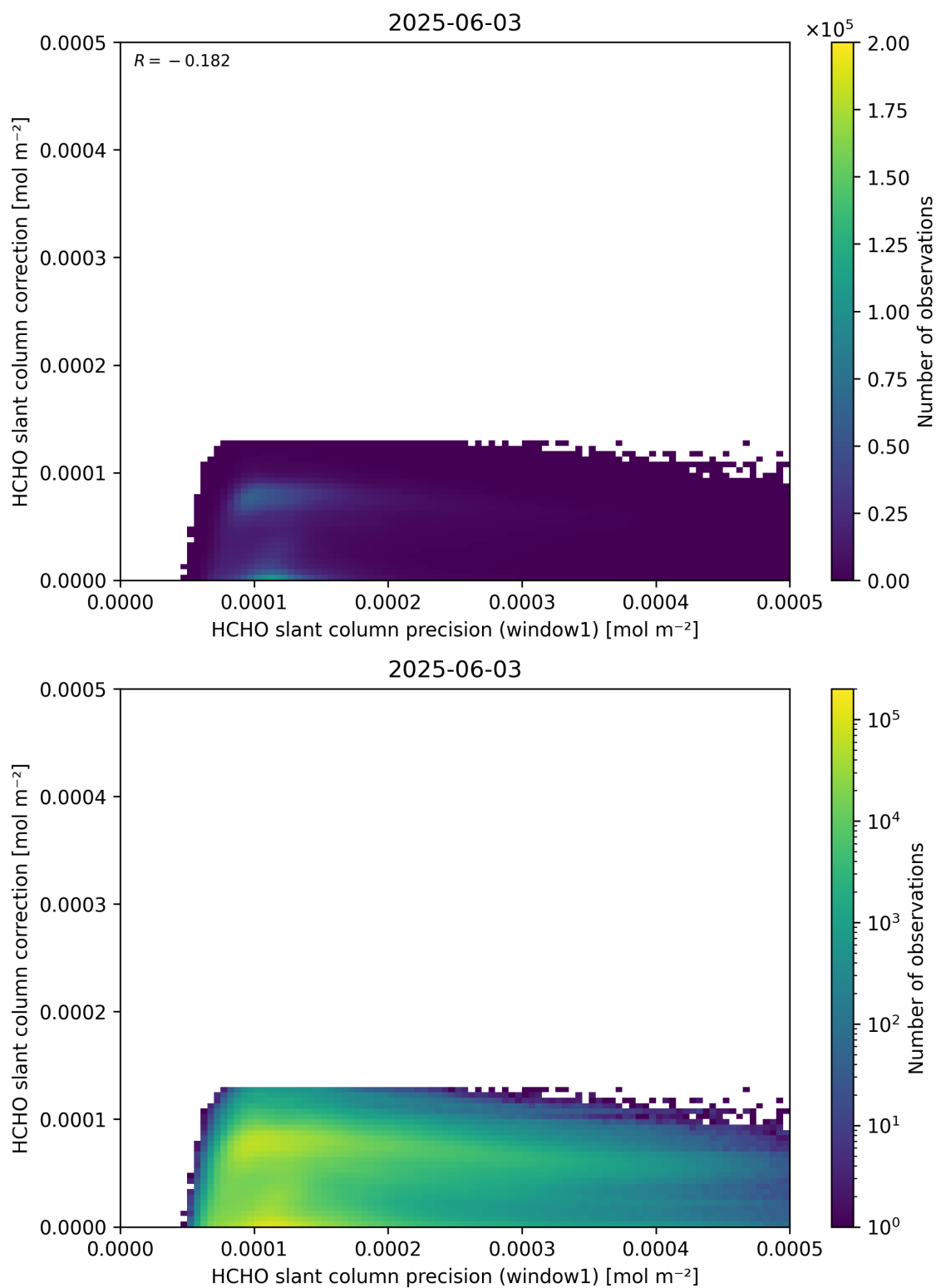
Figure 93: Scatter density plot of “HCHO slant column precision (window1)” against “HCHO slant column correction” for 2025-06-02 to 2025-06-04.
