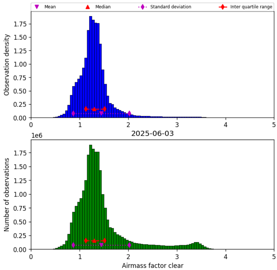
Figure 42: Histogram of “Airmass factor clear” for 2025-06-02 to 2025-06-04
