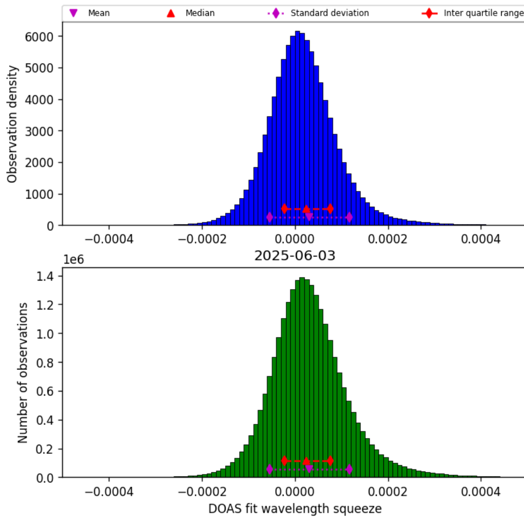
Figure 45: Histogram of “DOAS fit wavelength squeeze” for 2025-06-02 to 2025-06-04
