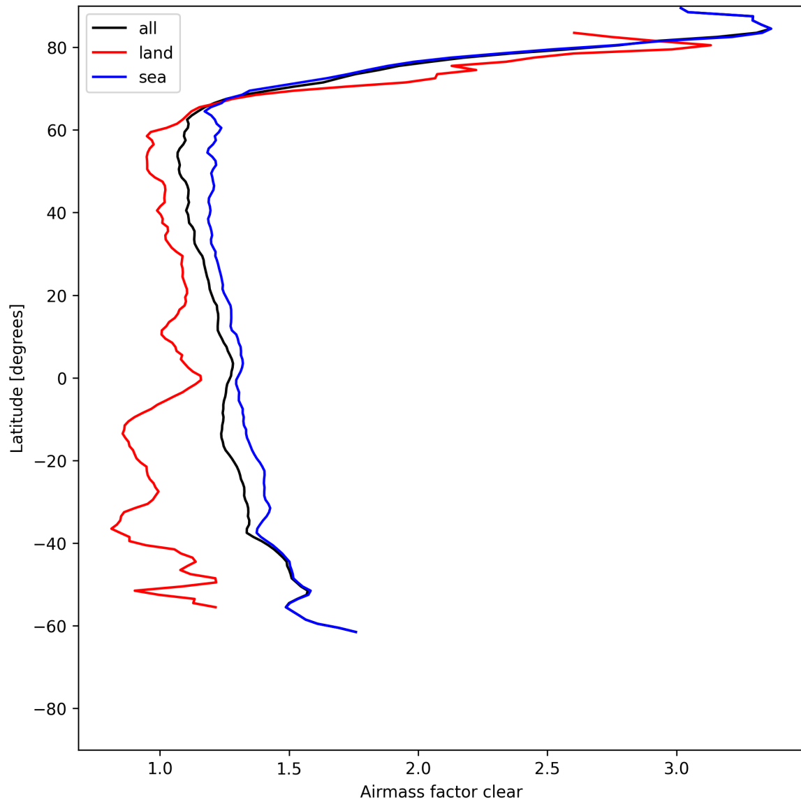
Figure 28: Zonal average of “Airmass factor clear” for 2025-06-02 to 2025-06-04.
