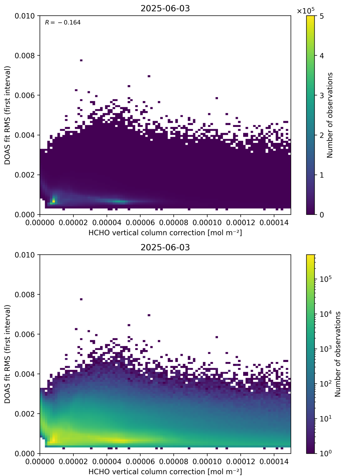
Figure 112: Scatter density plot of “HCHO vertical column correction” against “DOAS fit RMS (first interval)” for 2025-06-02 to 2025-06-04.
