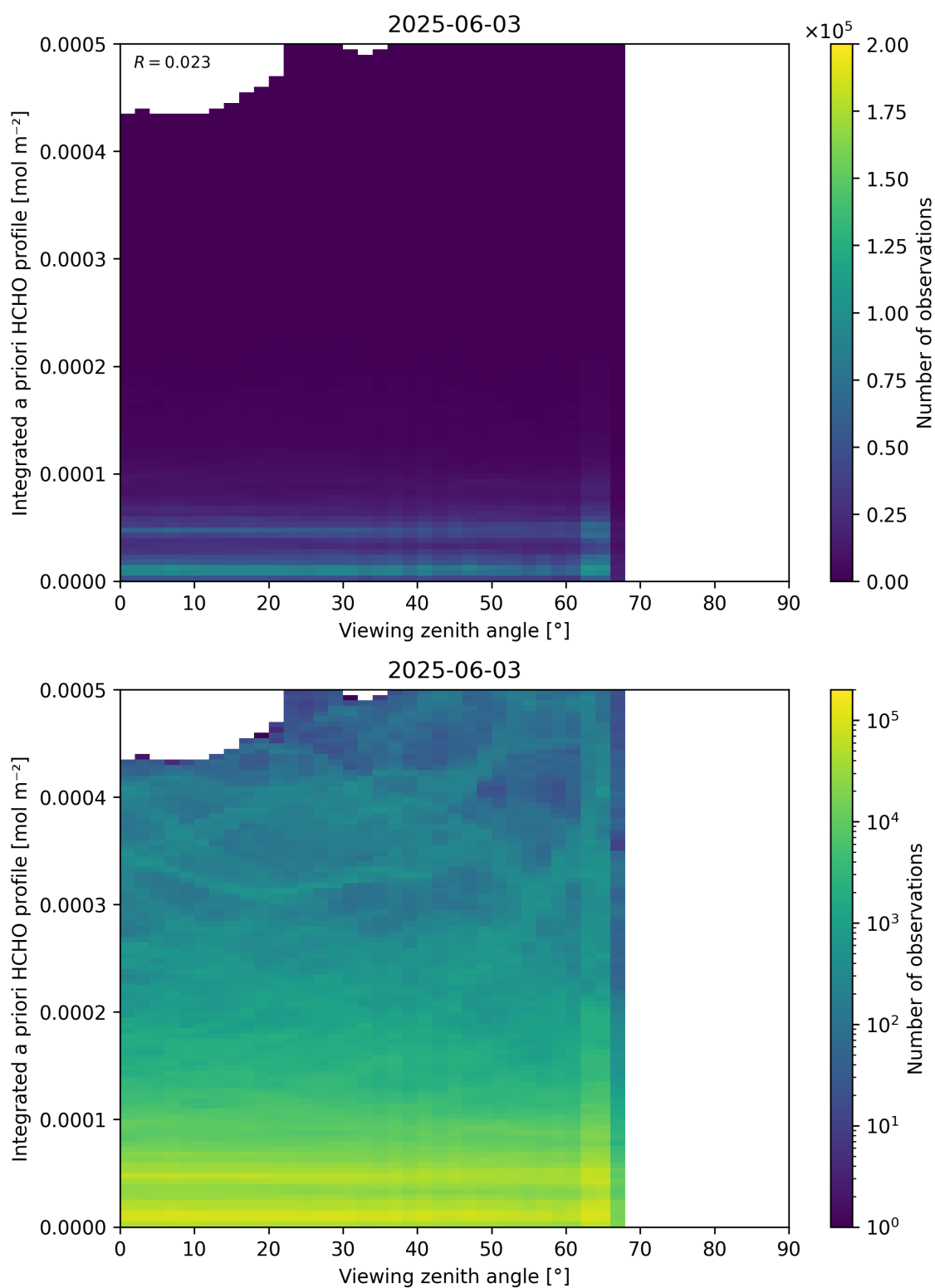
Figure 195: Scatter density plot of “Viewing zenith angle” against “Integrated a priori HCHO profile” for 2025-06-02 to 2025-06-04.
