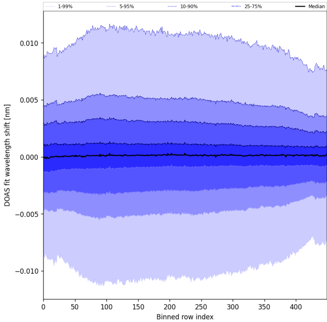
Figure 58: Along track statistics of “DOAS fit wavelength shift” for 2025-06-02 to 2025-06-04
