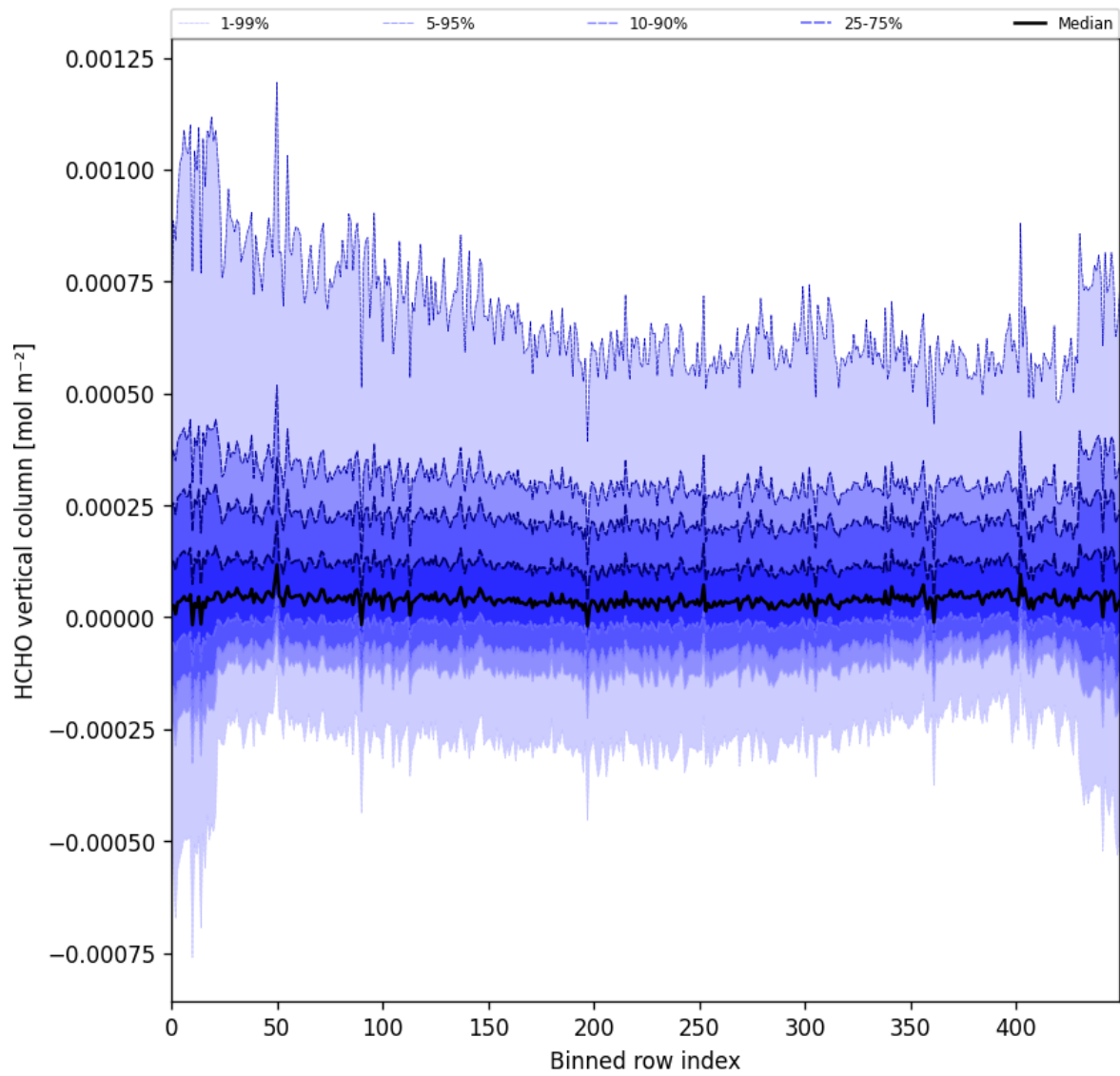
Figure 49: Along track statistics of “HCHO vertical column” for 2025-06-02 to 2025-06-04
