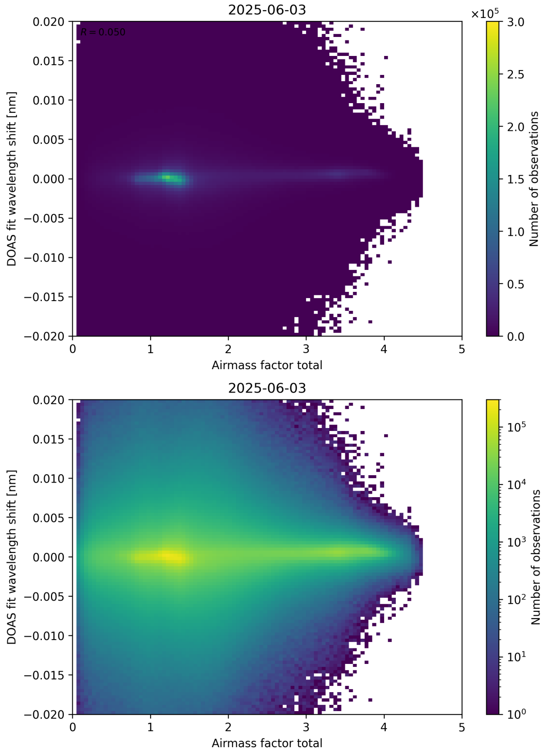
Figure 98: Scatter density plot of “Airmass factor total” against “DOAS fit wavelength shift” for 2025-06-02 to 2025-06-04.
