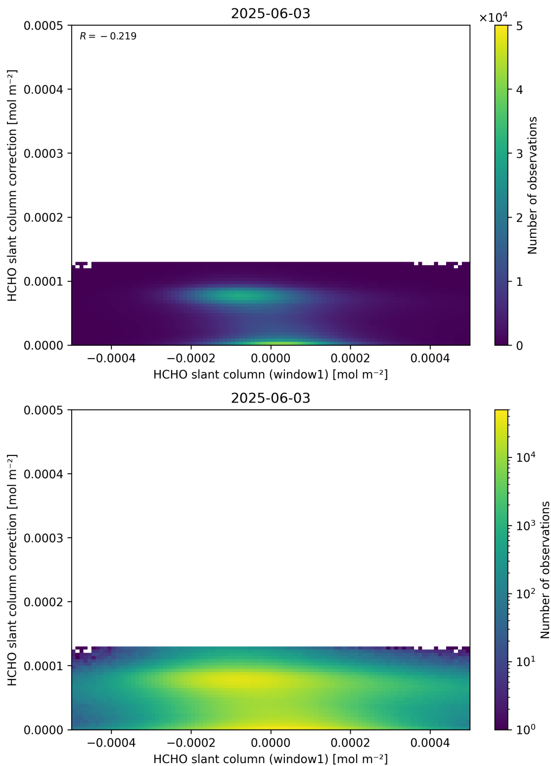
Figure 83: Scatter density plot of “HCHO slant column (window1)” against “HCHO slant column correction” for 2025-06-02 to 2025-06-04.
