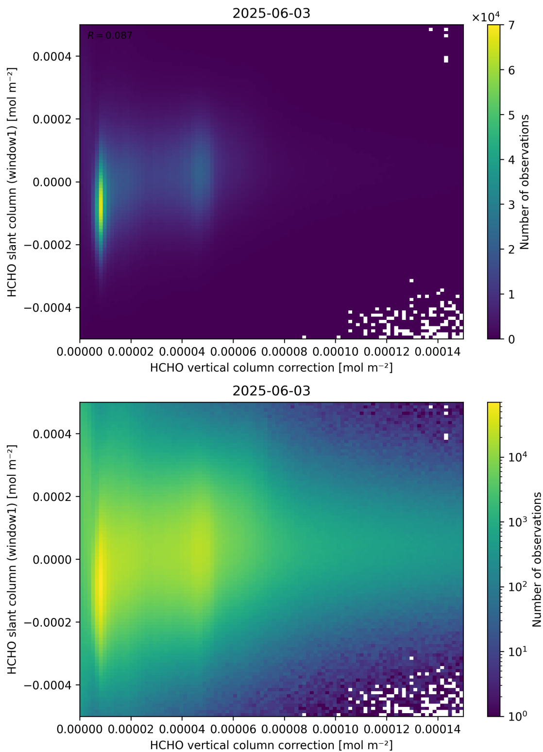
Figure 118: Scatter density plot of “HCHO vertical column correction” against “HCHO slant column (window1)” for 2025-06-02 to 2025-06-04.
