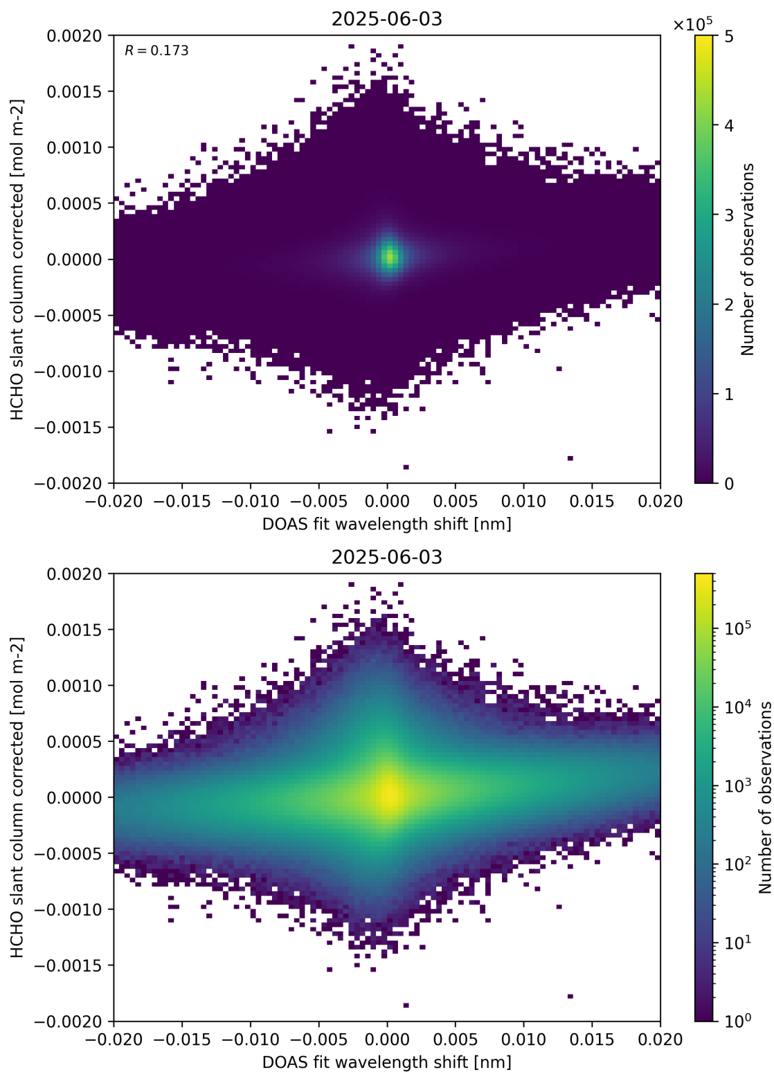
Figure 66: Scatter density plot of “DOAS fit wavelength shift” against “HCHO slant column corrected” for 2025-06-02 to 2025-06-04.
