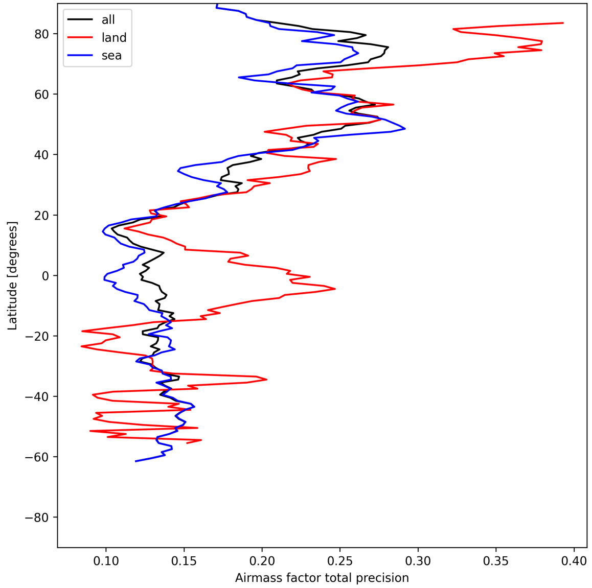
Figure 27: Zonal average of “Airmass factor total precision” for 2025-06-02 to 2025-06-04.
