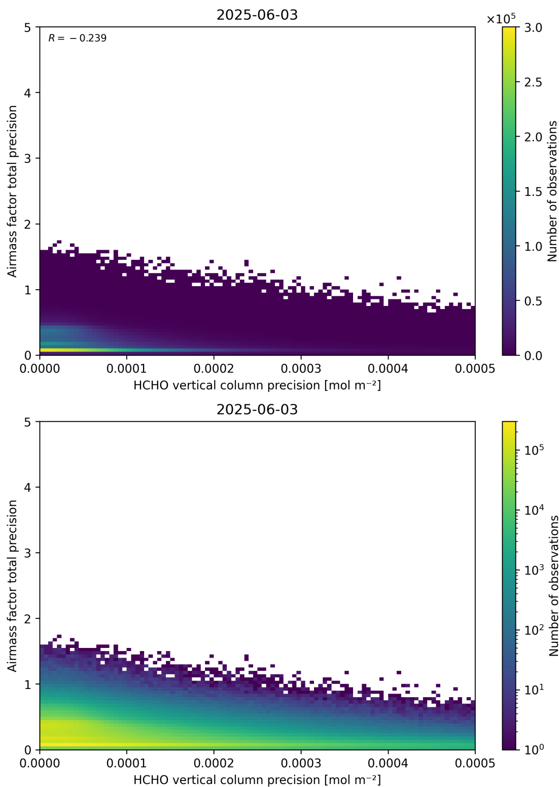
Figure 145: Scatter density plot of “HCHO vertical column precision” against “Airmass factor total precision” for 2025-06-02 to 2025-06-04.
