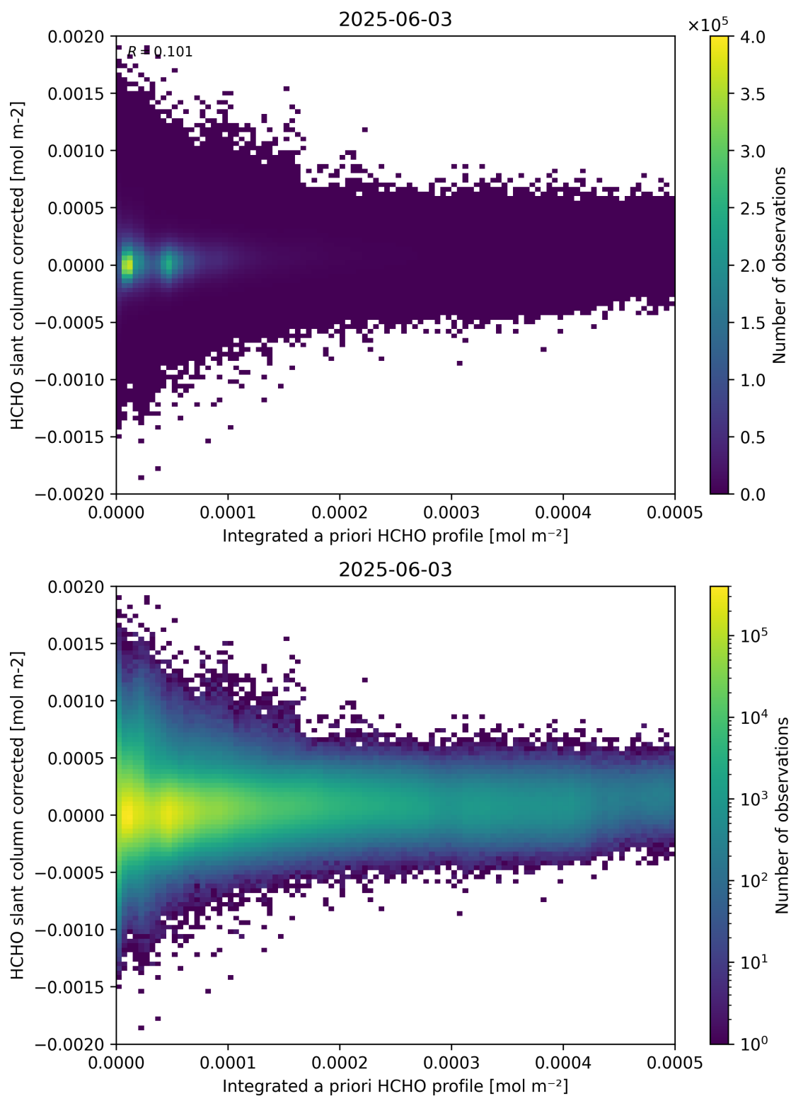
Figure 151: Scatter density plot of “Integrated a priori HCHO profile” against “HCHO slant column corrected” for 2025-06-02 to 2025-06-04.
