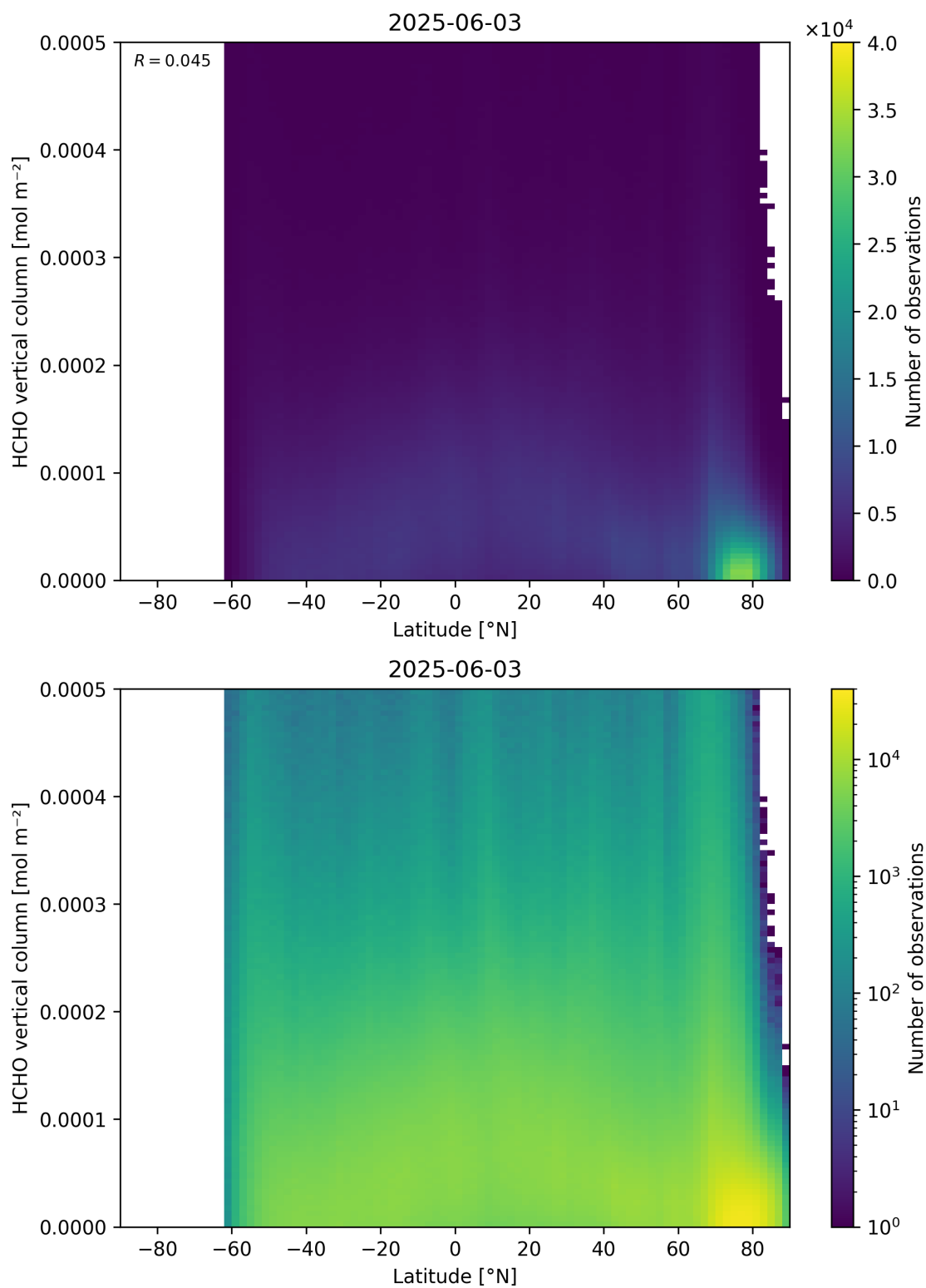
Figure 163: Scatter density plot of “Latitude” against “HCHO vertical column” for 2025-06-02 to 2025-06-04.
