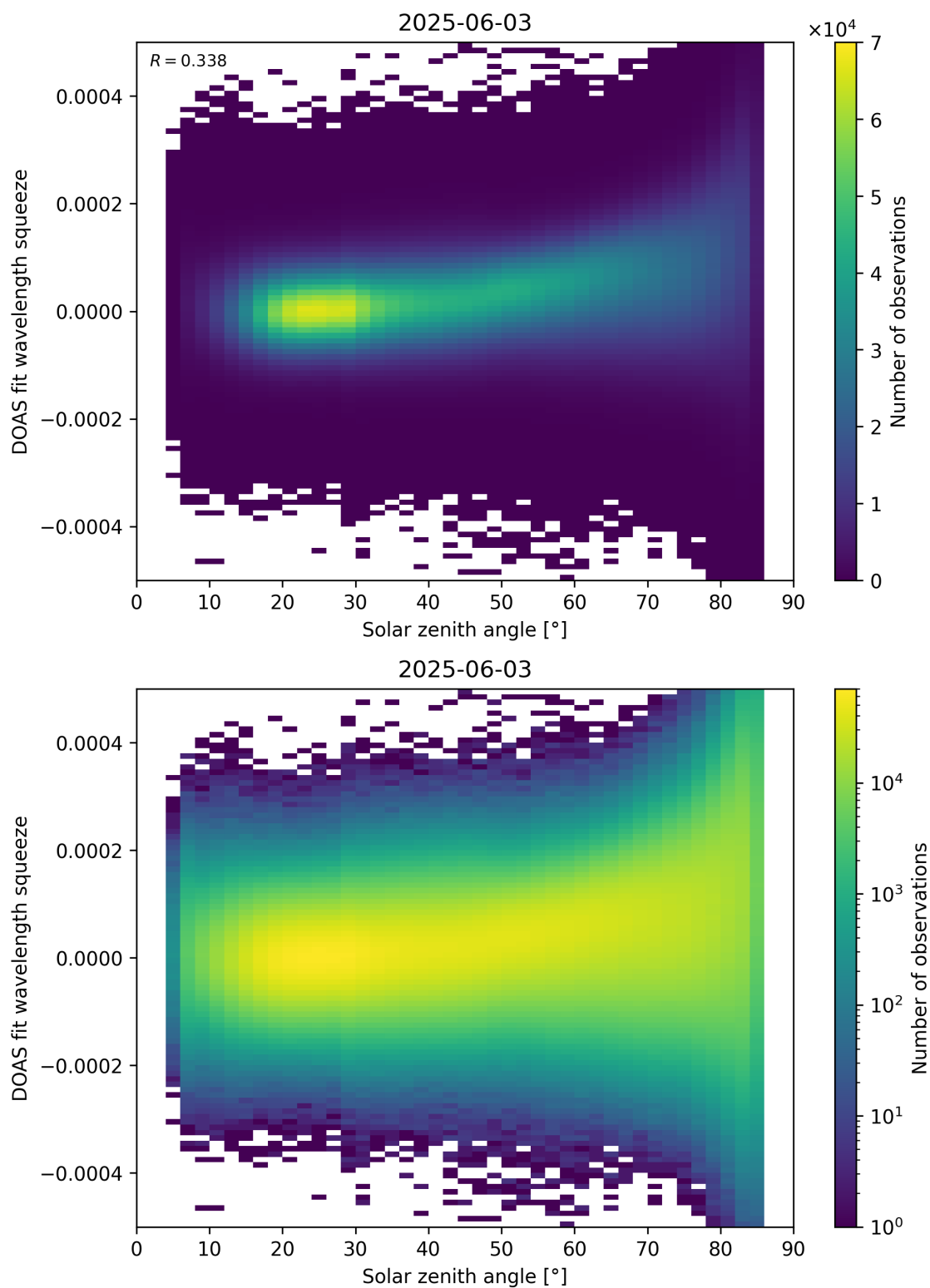
Figure 169: Scatter density plot of “Solar zenith angle” against “DOAS fit wavelength squeeze” for 2025-06-02 to 2025-06-04.
