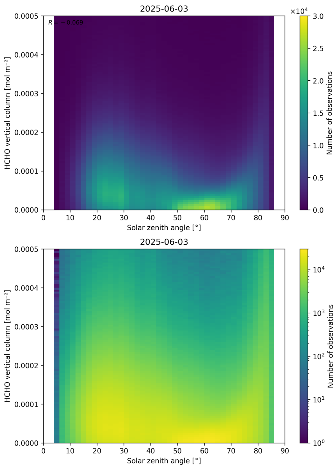
Figure 177: Scatter density plot of “Solar zenith angle” against “HCHO vertical column” for 2025-06-02 to 2025-06-04.
