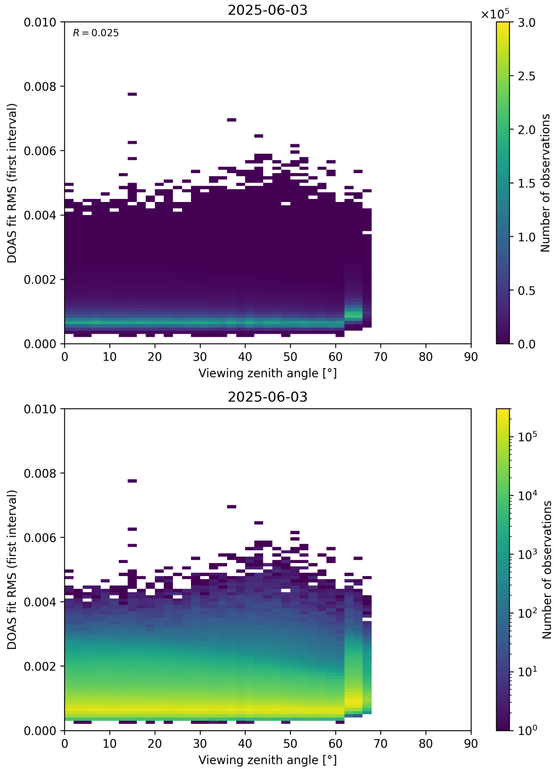
Figure 182: Scatter density plot of “Viewing zenith angle” against “DOAS fit RMS (first interval)” for 2025-06-02 to 2025-06-04.
