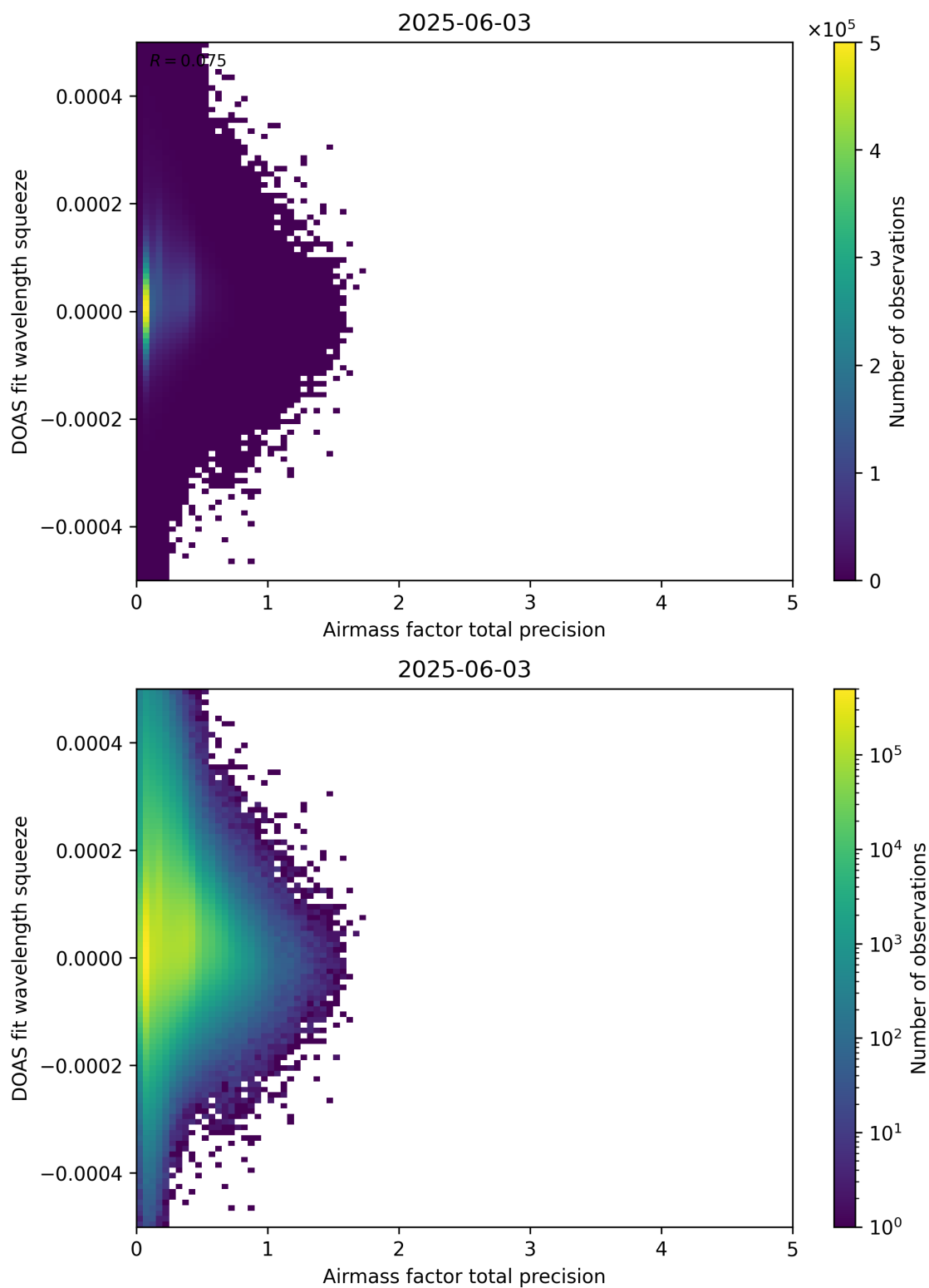
Figure 107: Scatter density plot of “Airmass factor total precision” against “DOAS fit wavelength squeeze” for 2025-06-02 to 2025-06-04.
