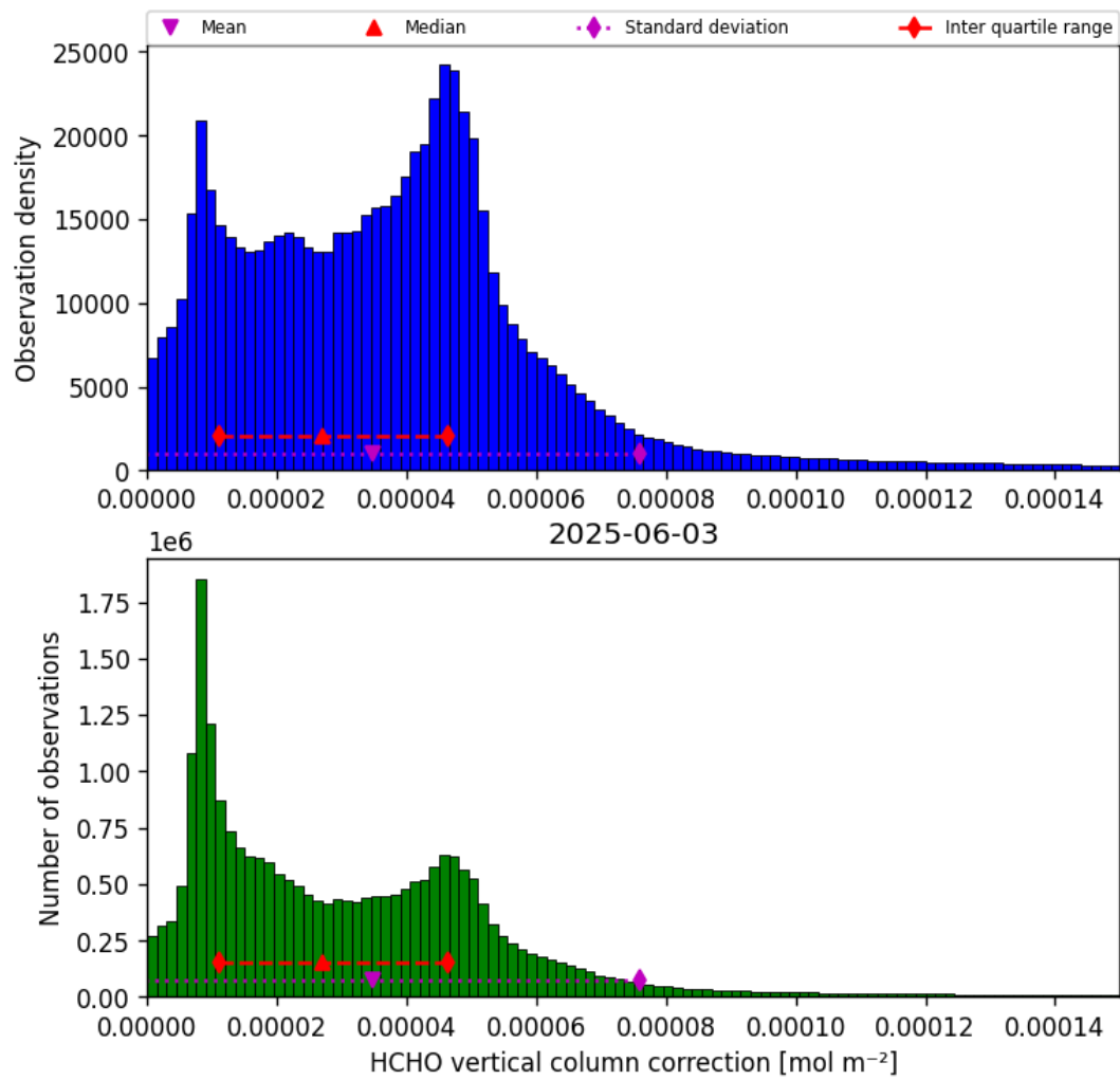
Figure 37: Histogram of “HCHO vertical column correction” for 2025-06-02 to 2025-06-04
