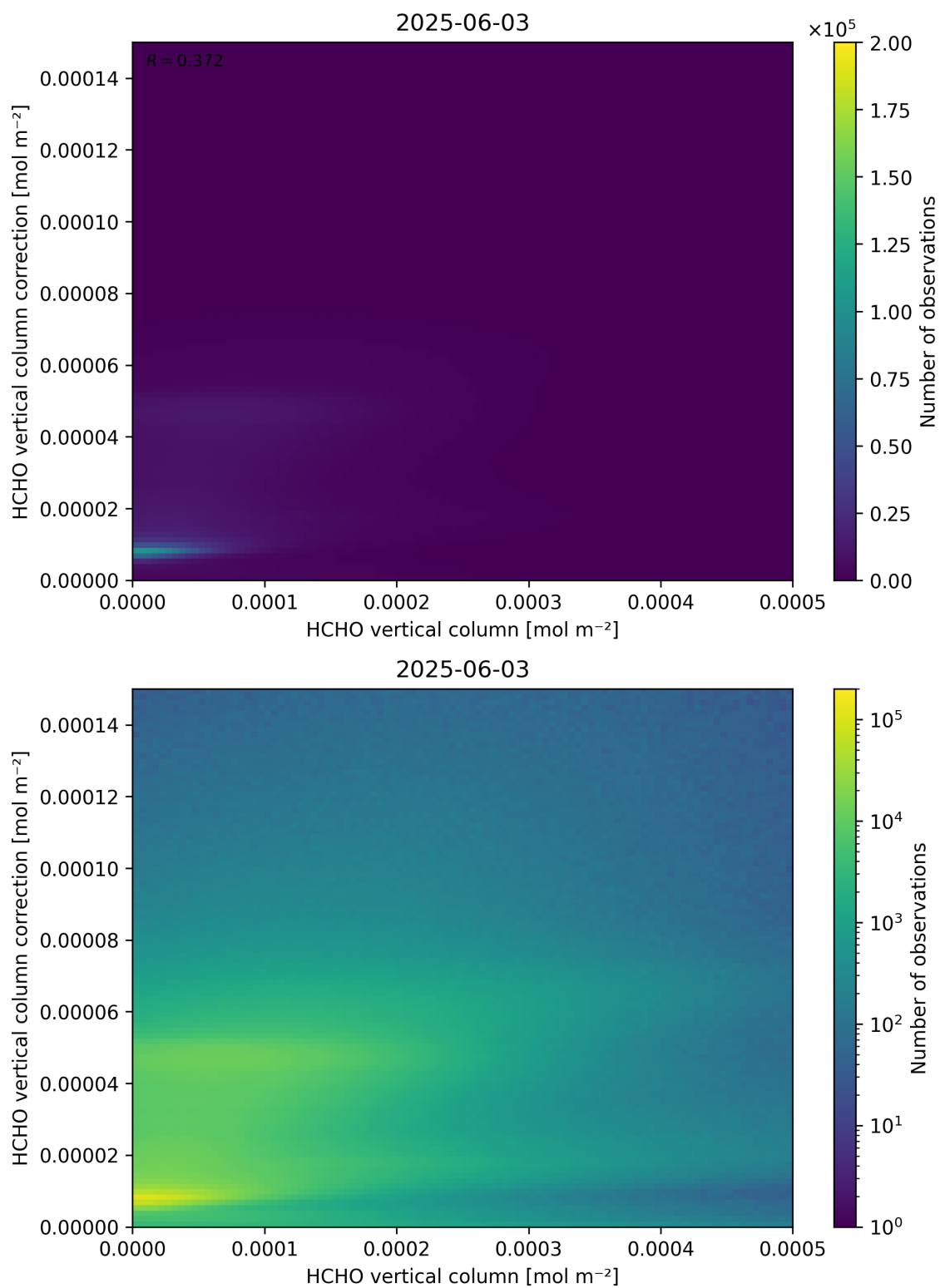
Figure 133: Scatter density plot of “HCHO vertical column” against “HCHO vertical column correction” for 2025-06-02 to 2025-06-04.
