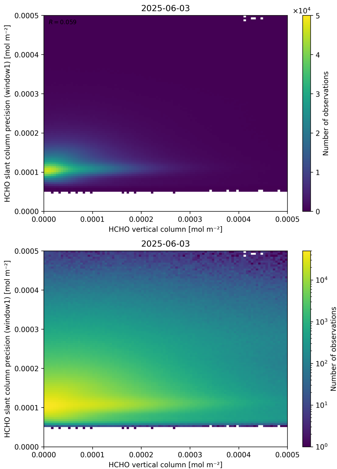
Figure 130: Scatter density plot of “HCHO vertical column” against “HCHO slant column precision (window1)” for 2025-06-02 to 2025-06-04.
