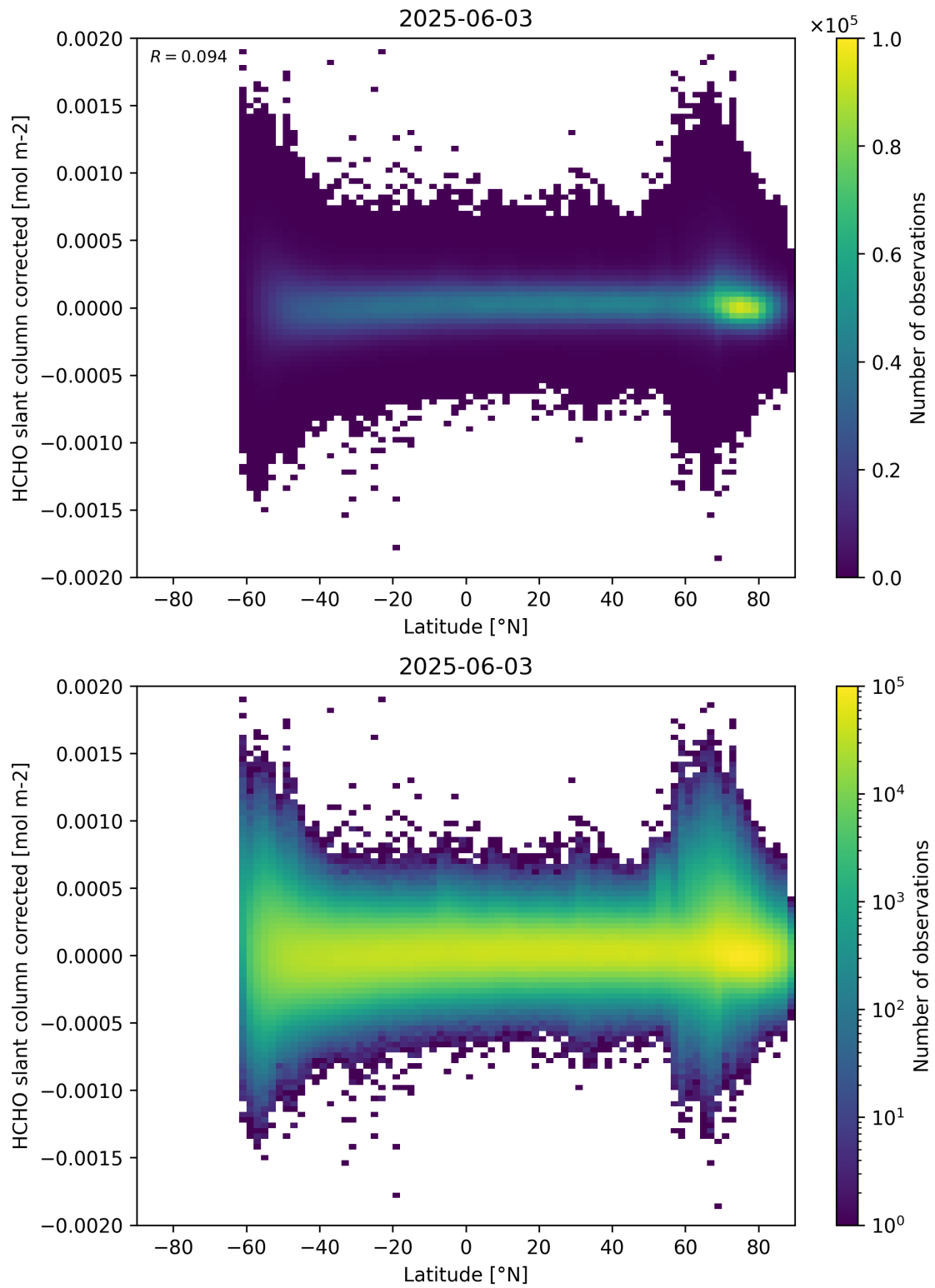
Figure 157: Scatter density plot of “Latitude” against “HCHO slant column corrected” for 2025-06-02 to 2025-06-04.
