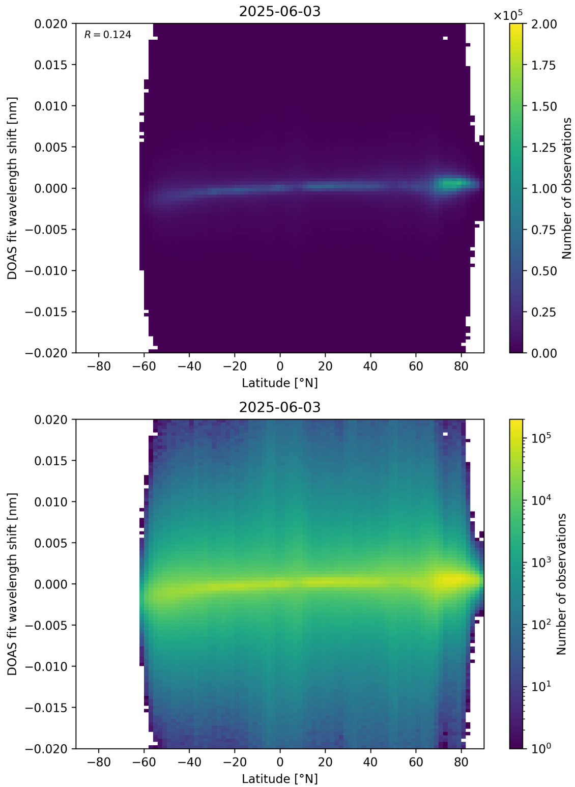
Figure 154: Scatter density plot of “Latitude” against “DOAS fit wavelength shift” for 2025-06-02 to 2025-06-04.
