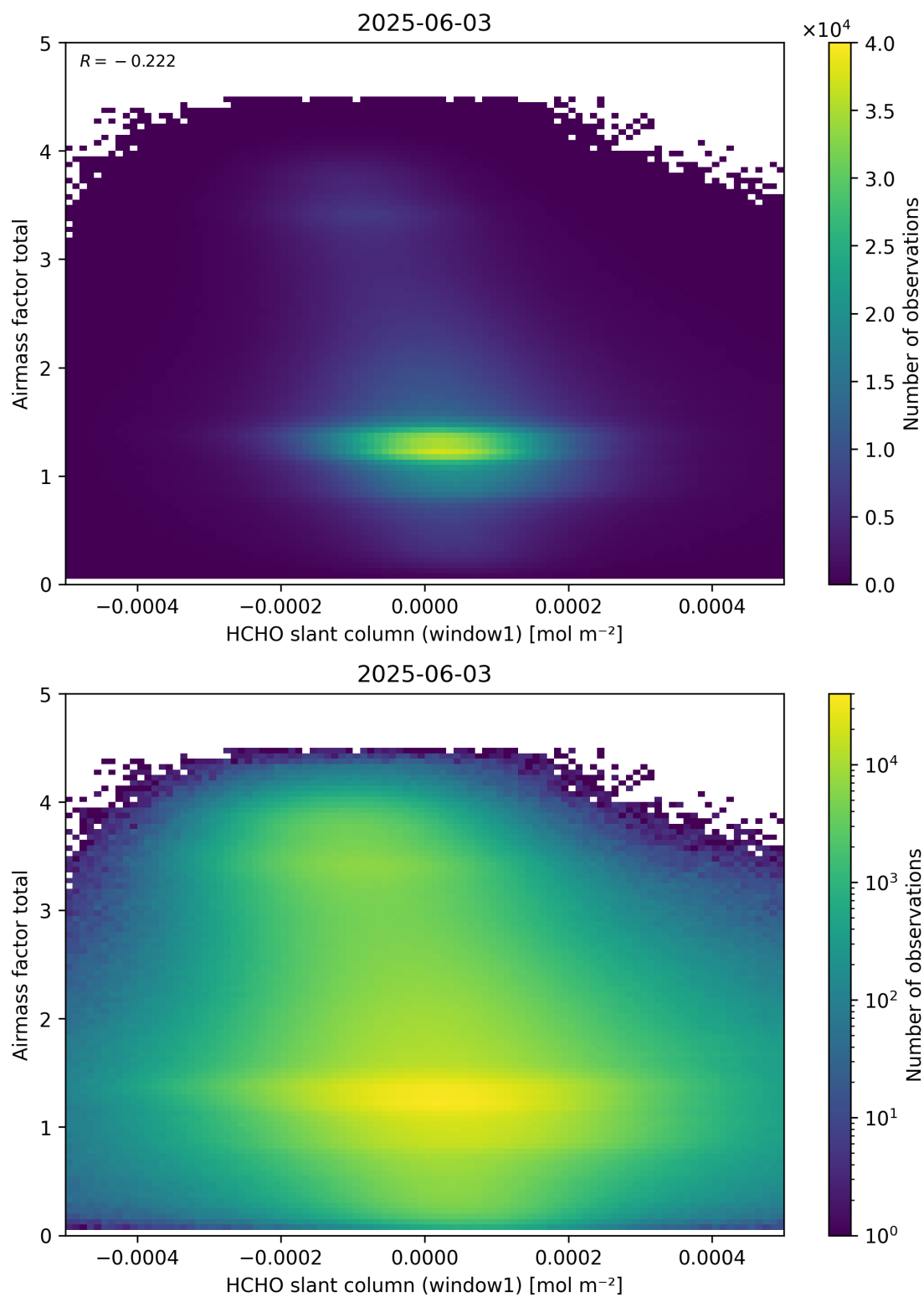
Figure 85: Scatter density plot of “HCHO slant column (window1)” against “Airmass factor total” for 2025-06-02 to 2025-06-04.
