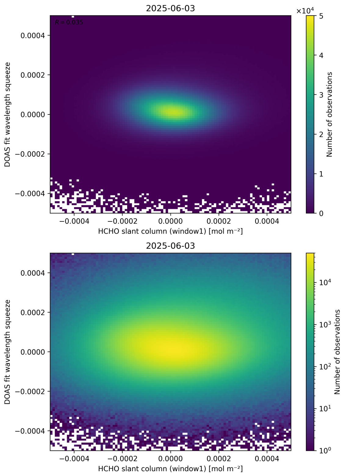
Figure 80: Scatter density plot of “HCHO slant column (window1)” against “DOAS fit wavelength squeeze” for 2025-06-02 to 2025-06-04.
