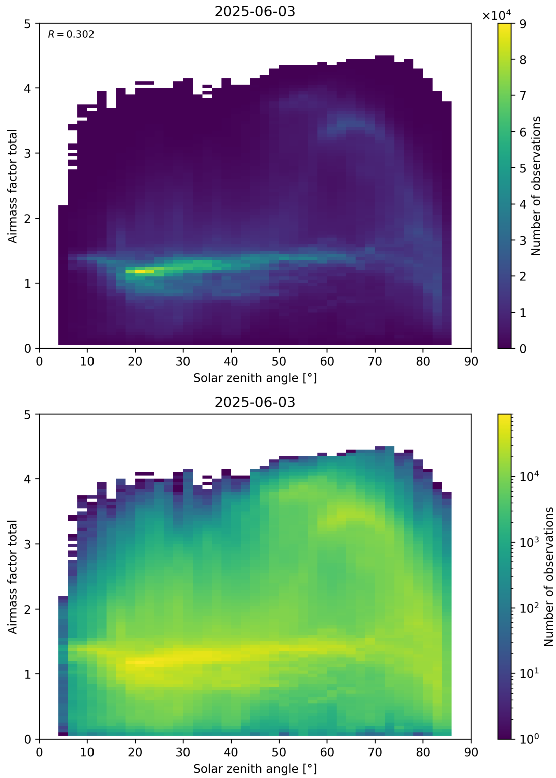
Figure 175: Scatter density plot of “Solar zenith angle” against “Airmass factor total” for 2025-06-02 to 2025-06-04.
