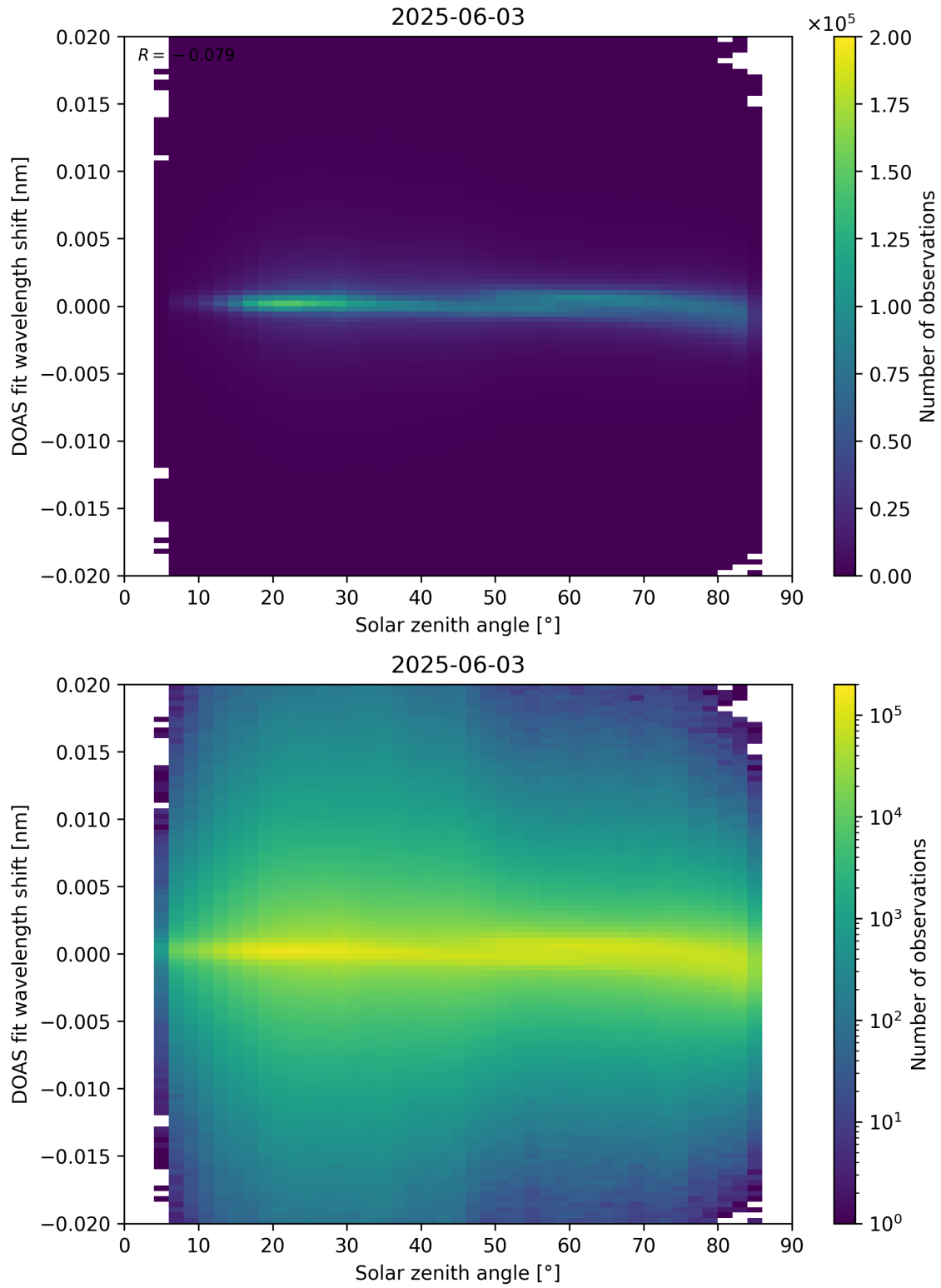
Figure 168: Scatter density plot of “Solar zenith angle” against “DOAS fit wavelength shift” for 2025-06-02 to 2025-06-04.
