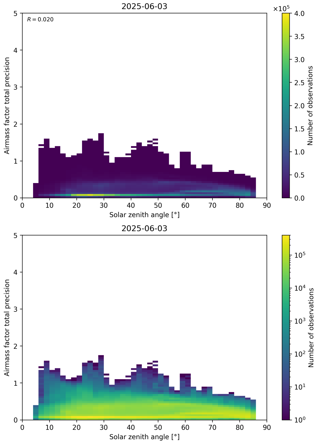
Figure 176: Scatter density plot of “Solar zenith angle” against “Airmass factor total precision” for 2025-06-02 to 2025-06-04.
