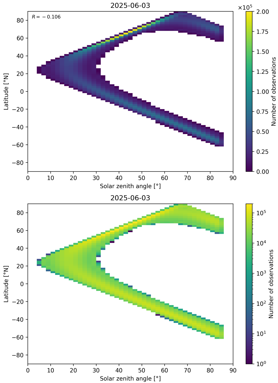
Figure 181: Scatter density plot of “Solar zenith angle” against “Latitude” for 2025-06-02 to 2025-06-04.
