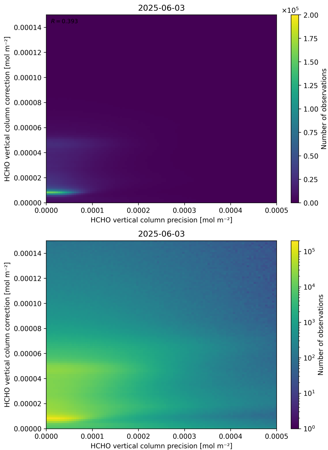
Figure 146: Scatter density plot of “HCHO vertical column precision” against “HCHO vertical column correction” for 2025-06-02 to 2025-06-04.
