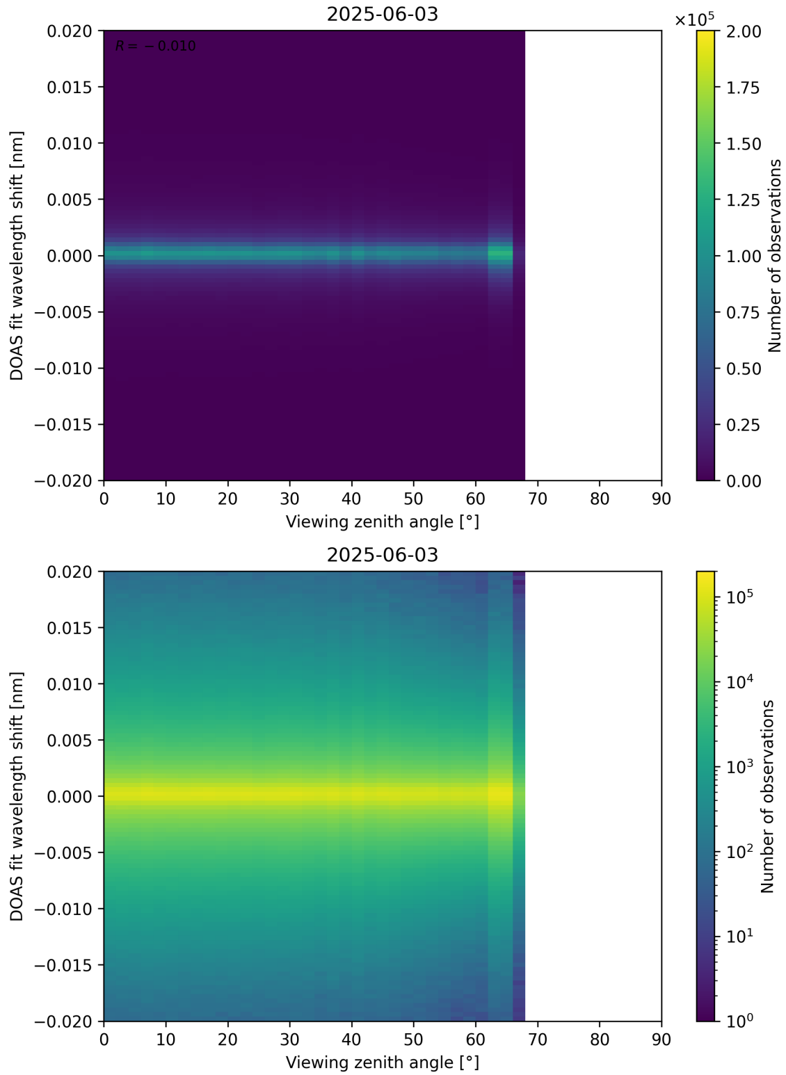
Figure 183: Scatter density plot of “Viewing zenith angle” against “DOAS fit wavelength shift” for 2025-06-02 to 2025-06-04.
