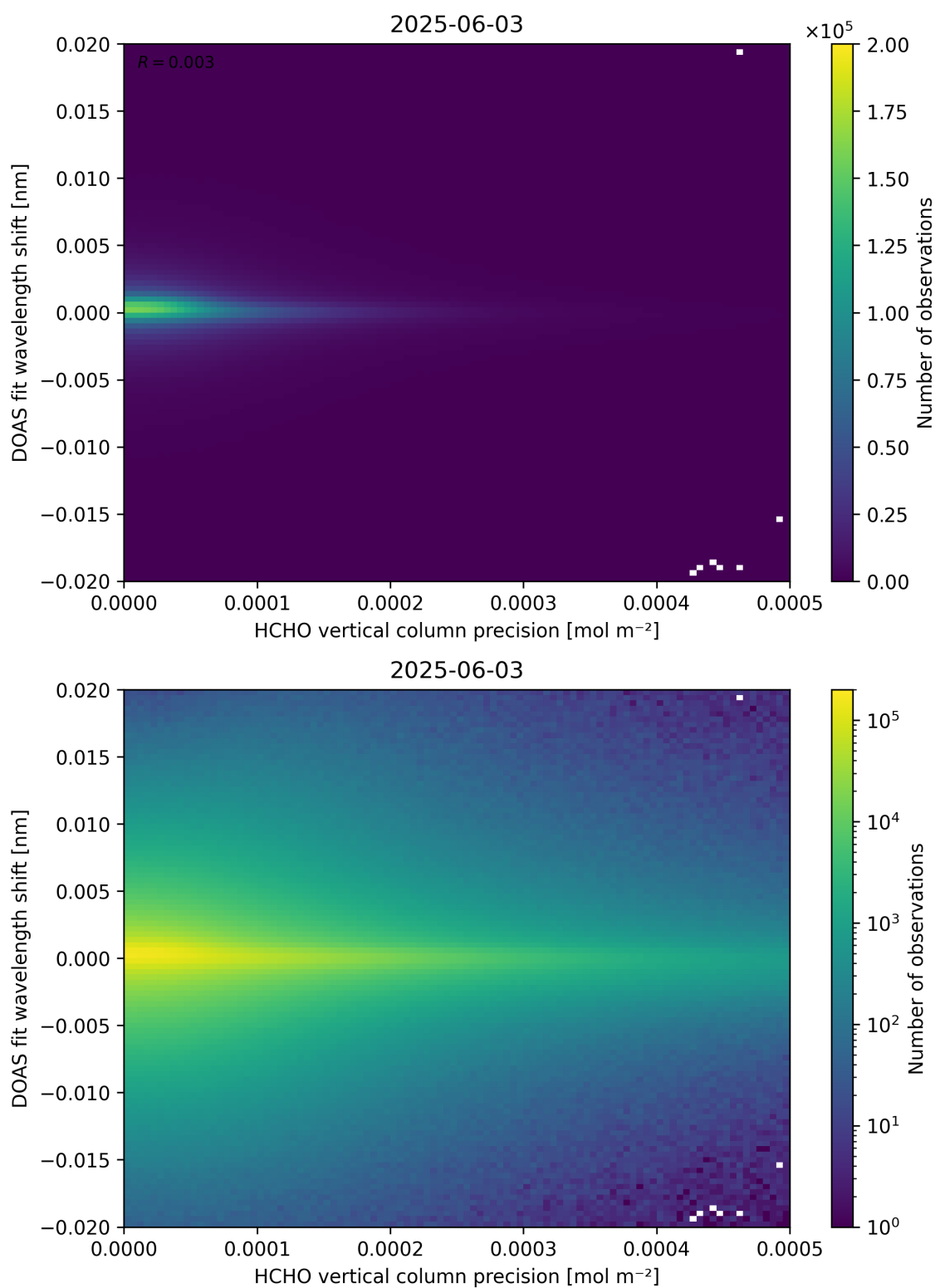
Figure 137: Scatter density plot of “HCHO vertical column precision” against “DOAS fit wavelength shift” for 2025-06-02 to 2025-06-04.
