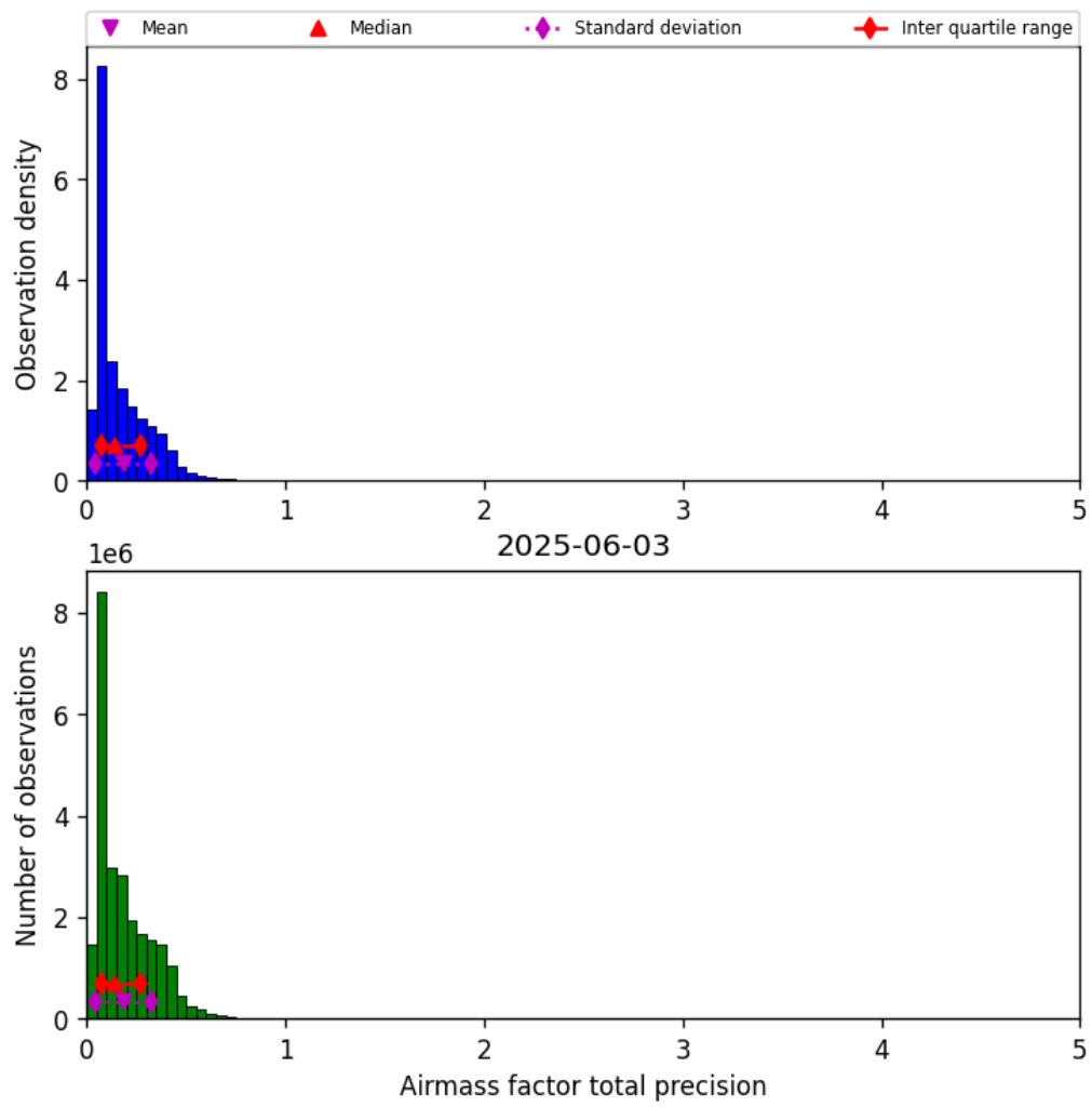
Figure 41: Histogram of “Airmass factor total precision” for 2025-06-02 to 2025-06-04
