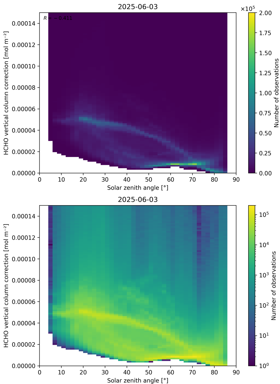
Figure 178: Scatter density plot of “Solar zenith angle” against “HCHO vertical column correction” for 2025-06-02 to 2025-06-04.
