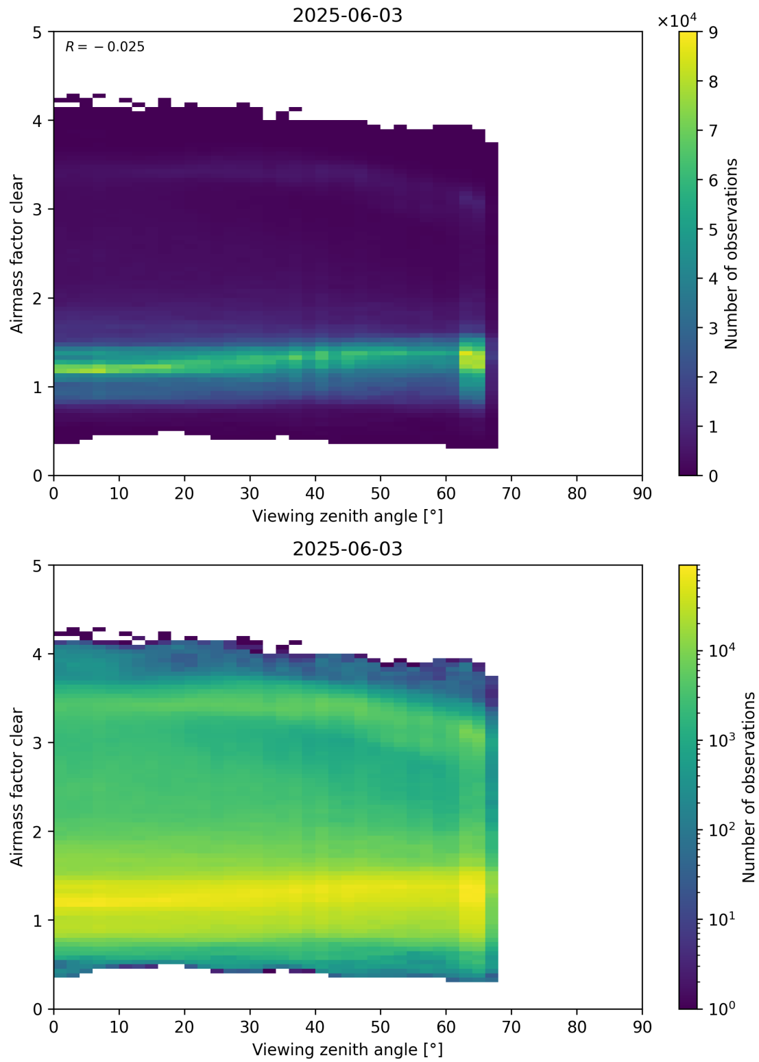
Figure 185: Scatter density plot of “Viewing zenith angle” against “Airmass factor clear” for 2025-06-02 to 2025-06-04.
