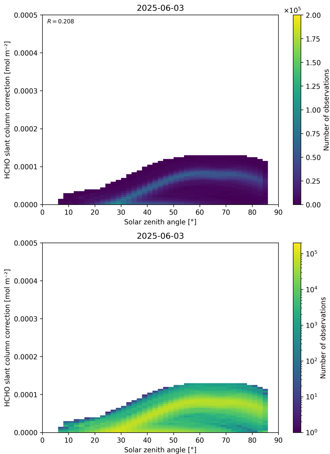
Figure 172: Scatter density plot of “Solar zenith angle” against “HCHO slant column correction” for 2025-06-02 to 2025-06-04.
