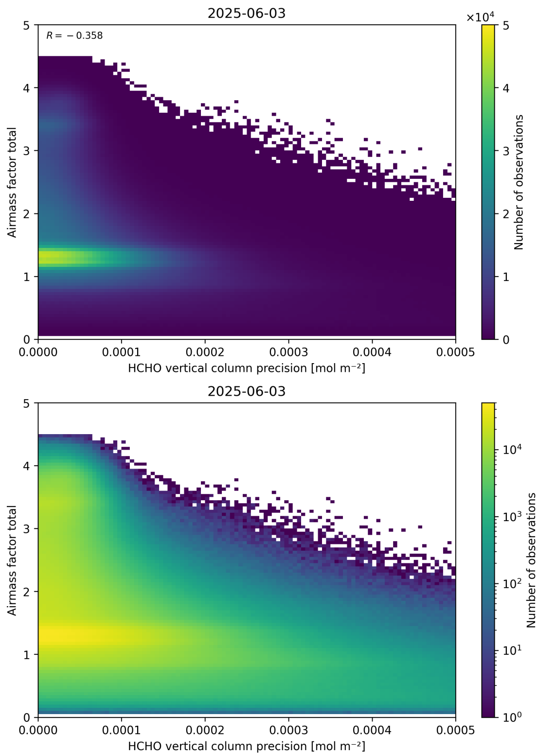
Figure 144: Scatter density plot of “HCHO vertical column precision” against “Airmass factor total” for 2025-06-02 to 2025-06-04.
