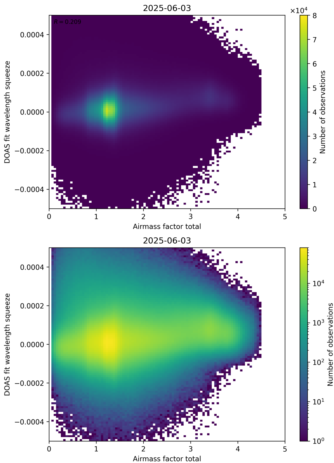
Figure 99: Scatter density plot of “Airmass factor total” against “DOAS fit wavelength squeeze” for 2025-06-02 to 2025-06-04.
