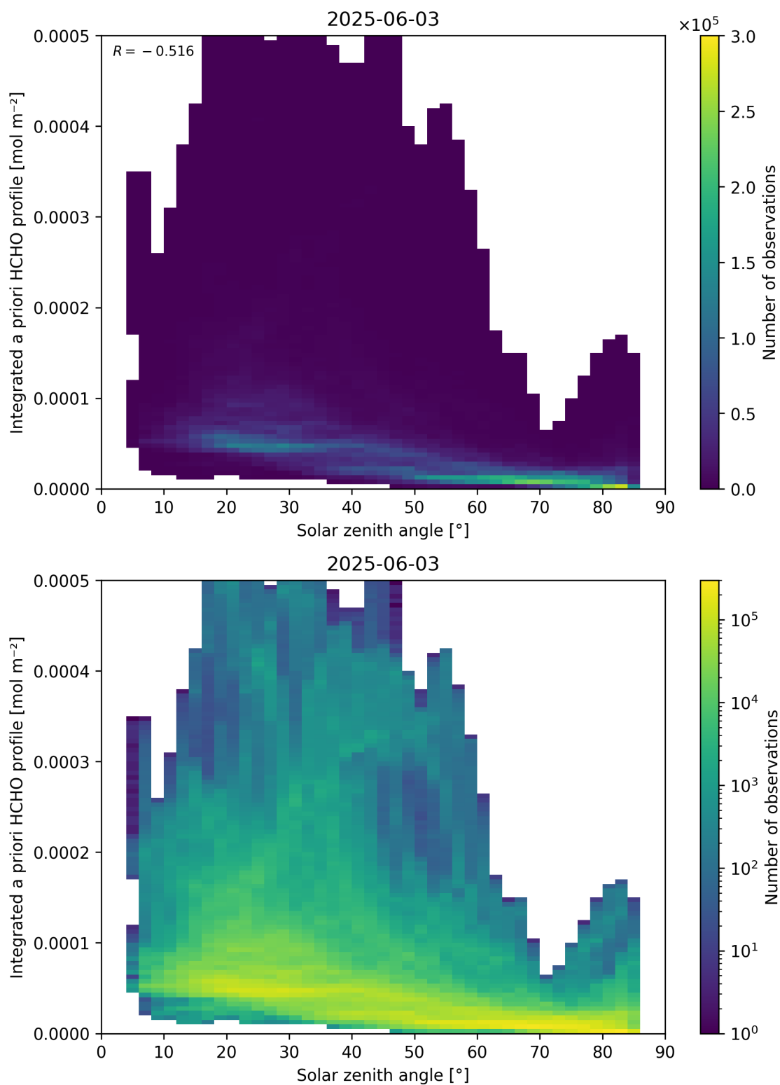
Figure 180: Scatter density plot of “Solar zenith angle” against “Integrated a priori HCHO profile” for 2025-06-02 to 2025-06-04.
