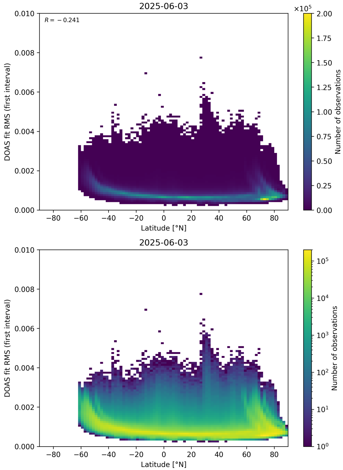
Figure 153: Scatter density plot of “Latitude” against “DOAS fit RMS (first interval)” for 2025-06-02 to 2025-06-04.
