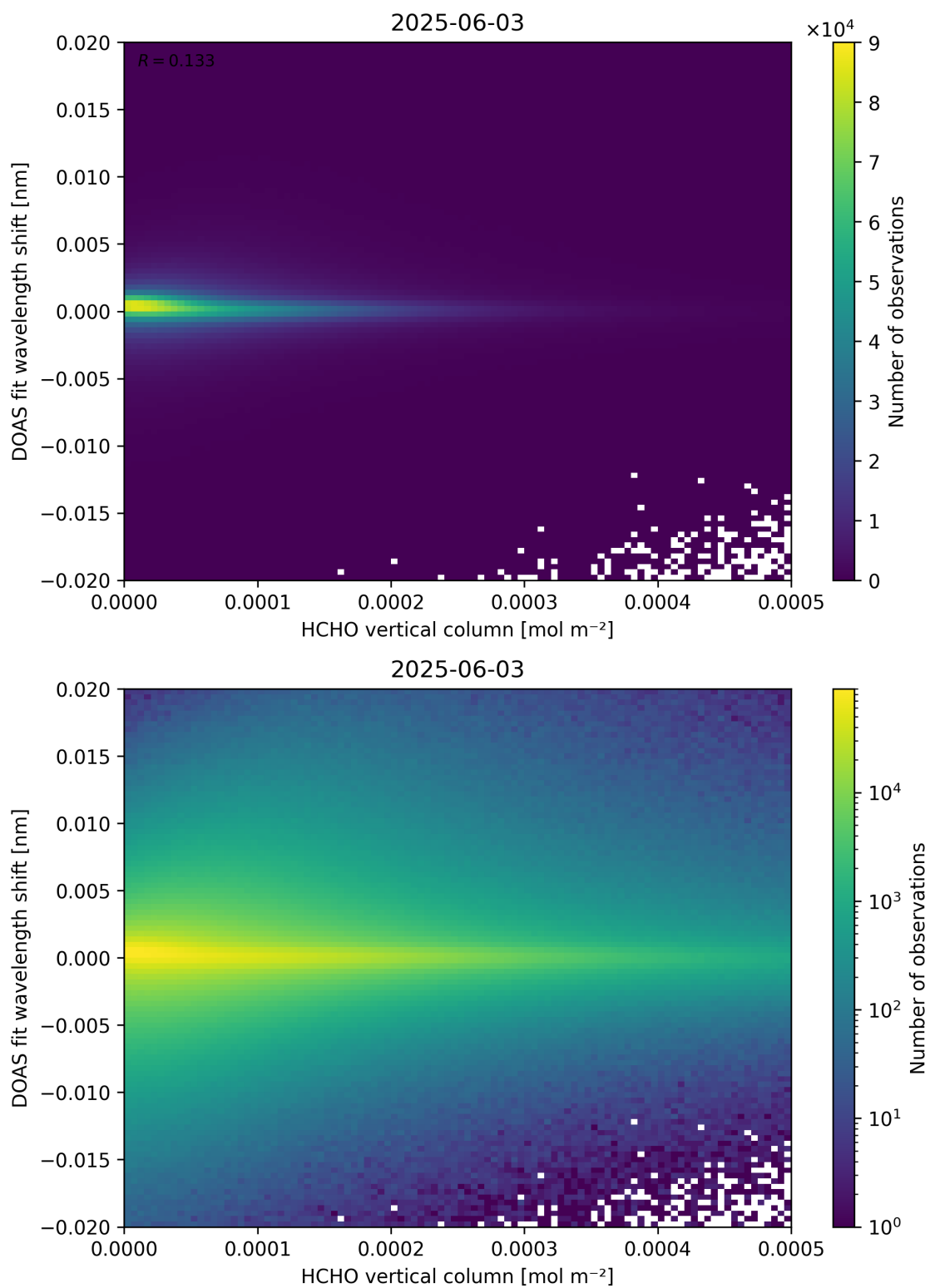
Figure 124: Scatter density plot of “HCHO vertical column” against “DOAS fit wavelength shift” for 2025-06-02 to 2025-06-04.
