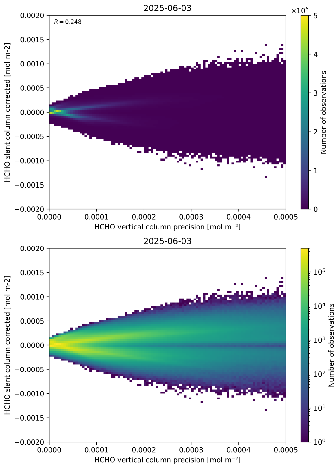
Figure 140: Scatter density plot of “HCHO vertical column precision” against “HCHO slant column corrected” for 2025-06-02 to 2025-06-04.
