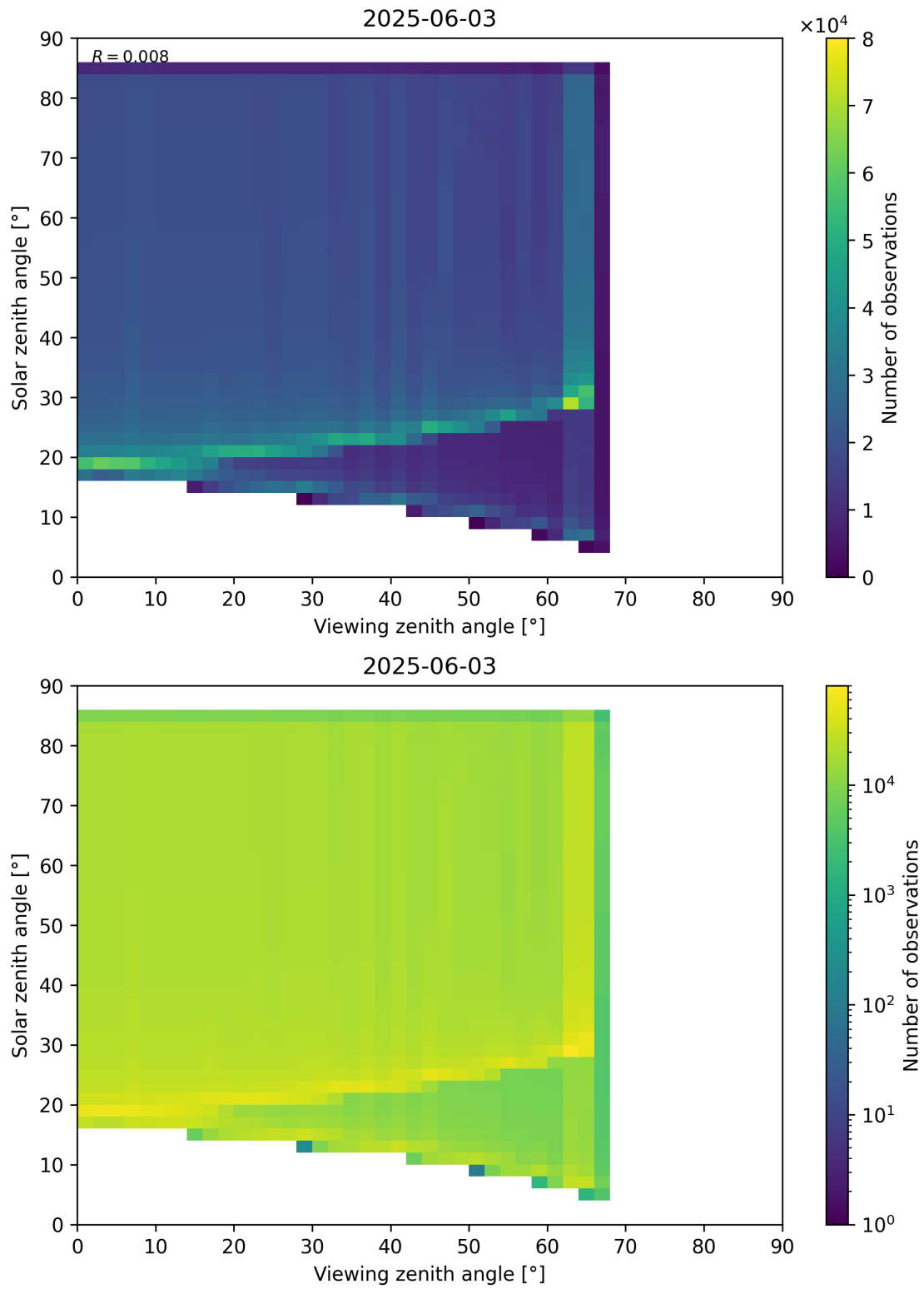
Figure 197: Scatter density plot of “Viewing zenith angle” against “Solar zenith angle” for 2025-06-02 to 2025-06-04.
