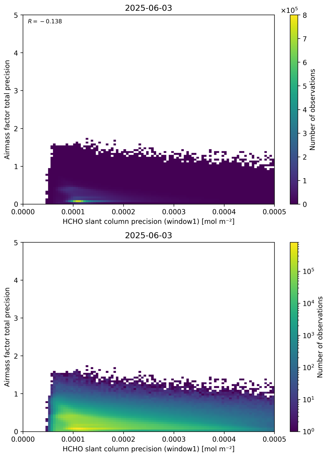
Figure 95: Scatter density plot of “HCHO slant column precision (window1)” against “Airmass factor total precision” for 2025-06-02 to 2025-06-04.
