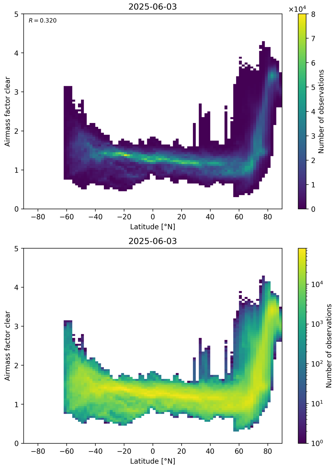
Figure 156: Scatter density plot of “Latitude” against “Airmass factor clear” for 2025-06-02 to 2025-06-04.
