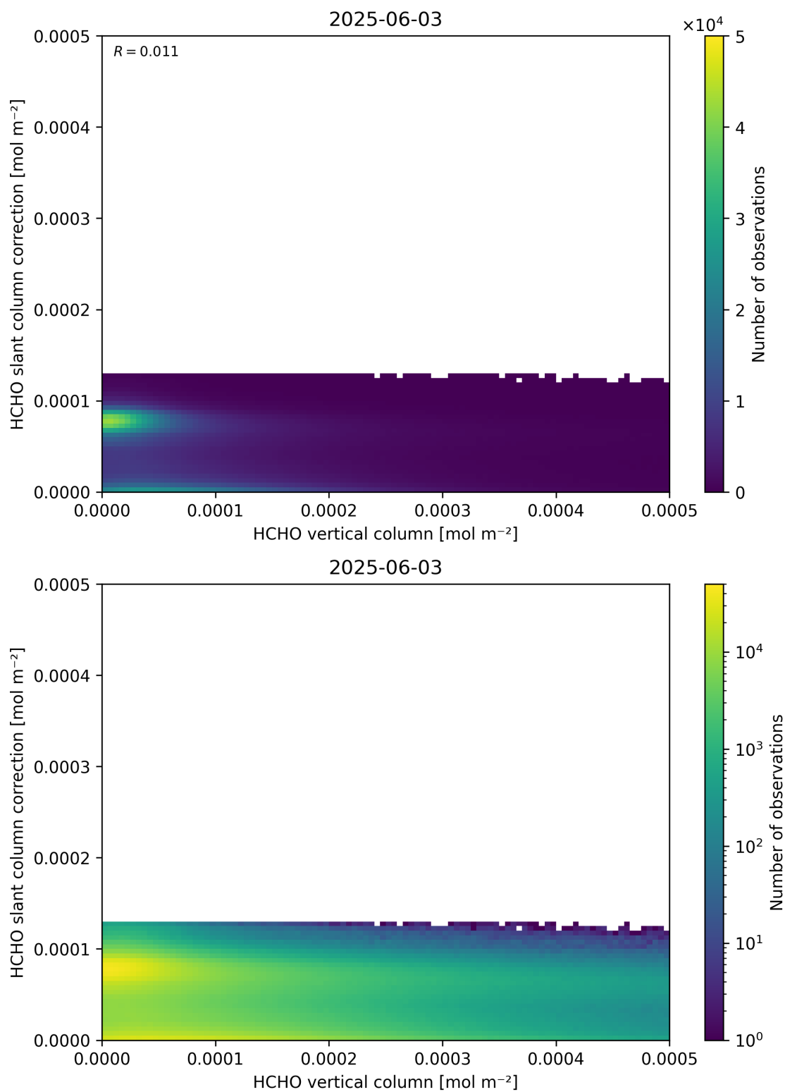
Figure 128: Scatter density plot of “HCHO vertical column” against “HCHO slant column correction” for 2025-06-02 to 2025-06-04.
