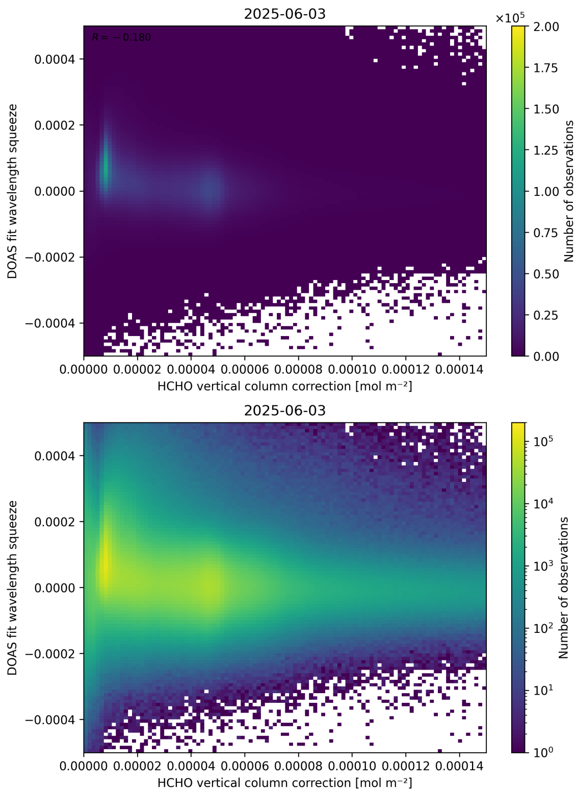
Figure 114: Scatter density plot of “HCHO vertical column correction” against “DOAS fit wavelength squeeze” for 2025-06-02 to 2025-06-04.
