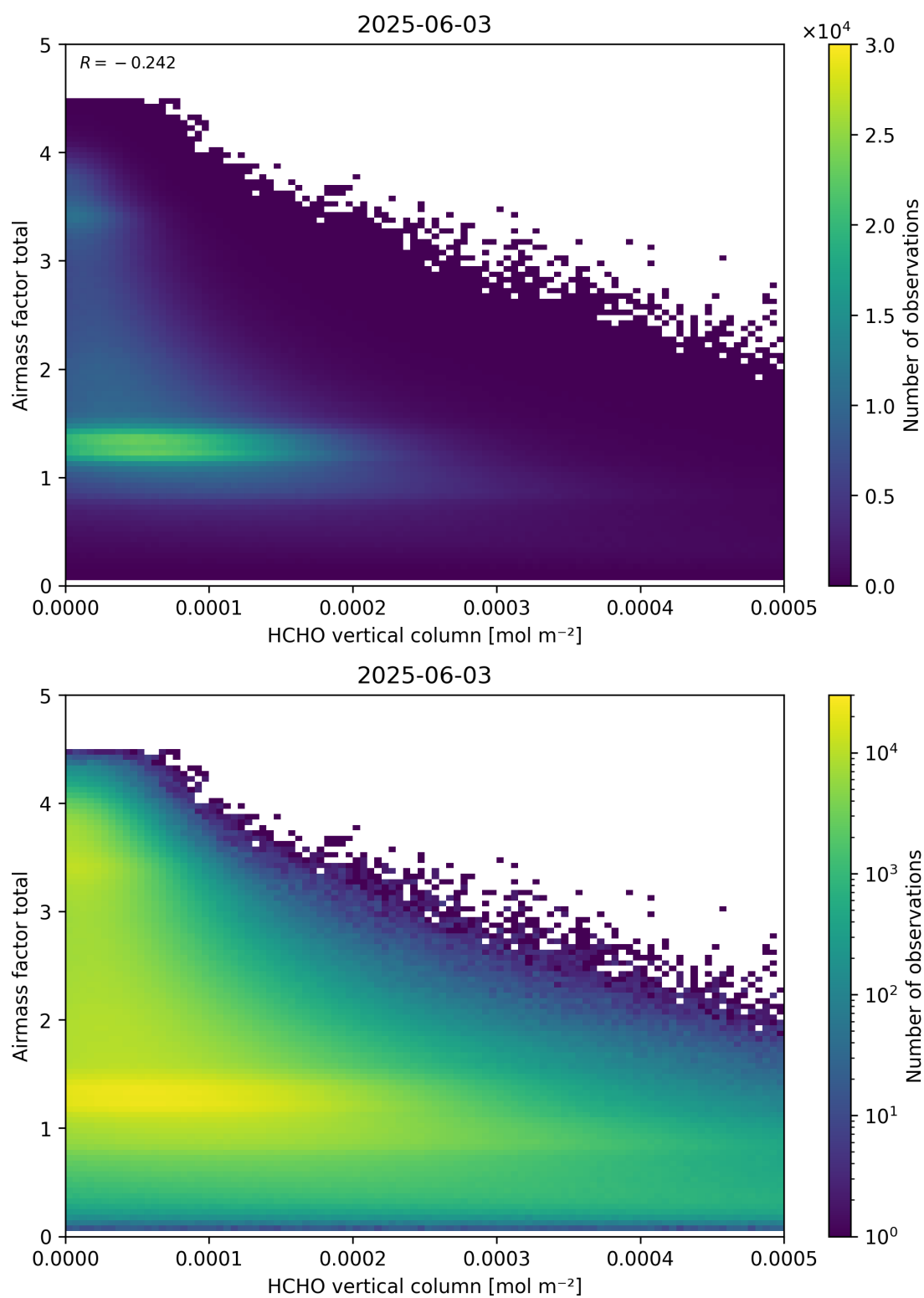
Figure 131: Scatter density plot of “HCHO vertical column” against “Airmass factor total” for 2025-06-02 to 2025-06-04.
