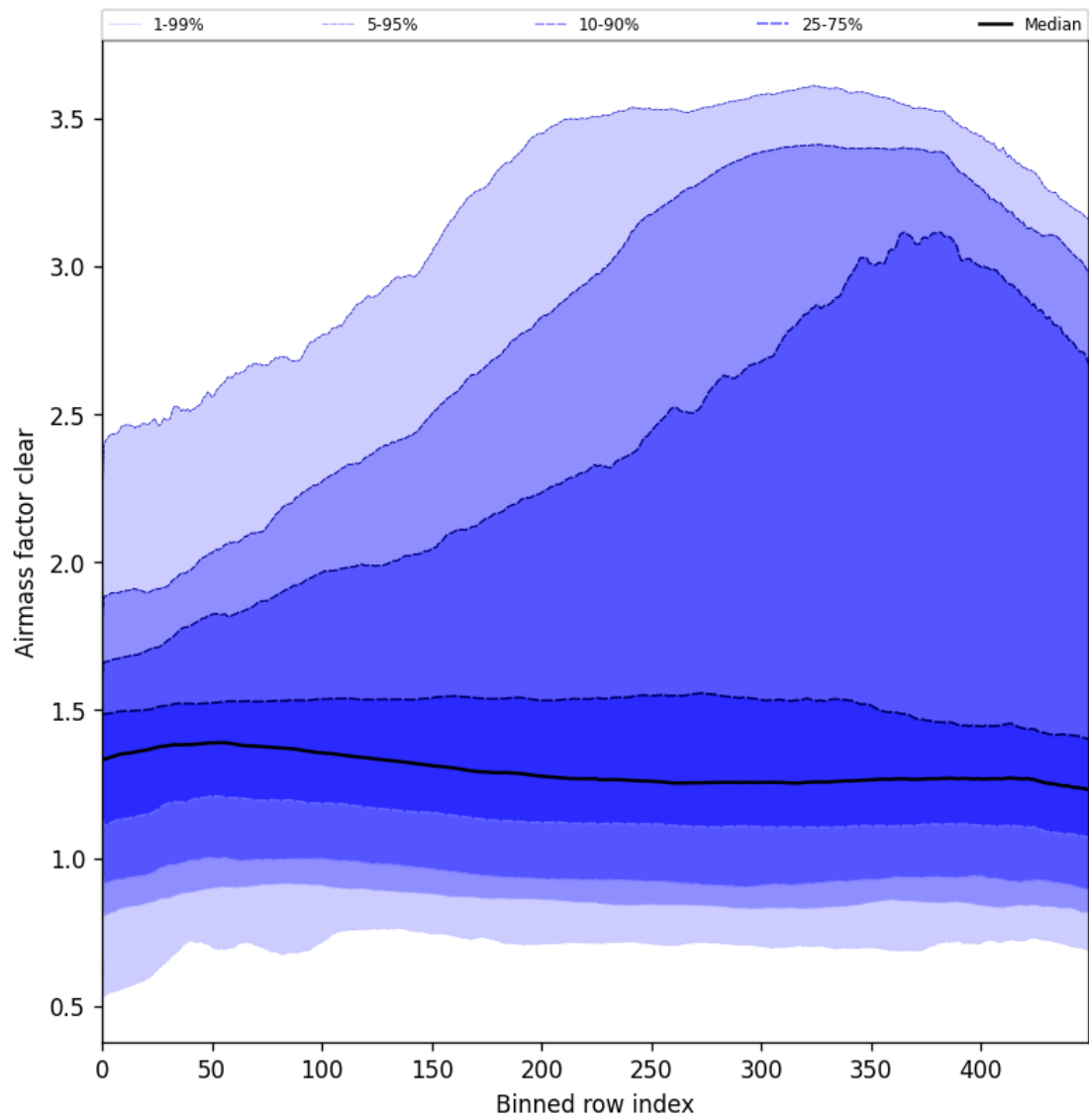
Figure 56: Along track statistics of “Airmass factor clear” for 2025-06-02 to 2025-06-04
