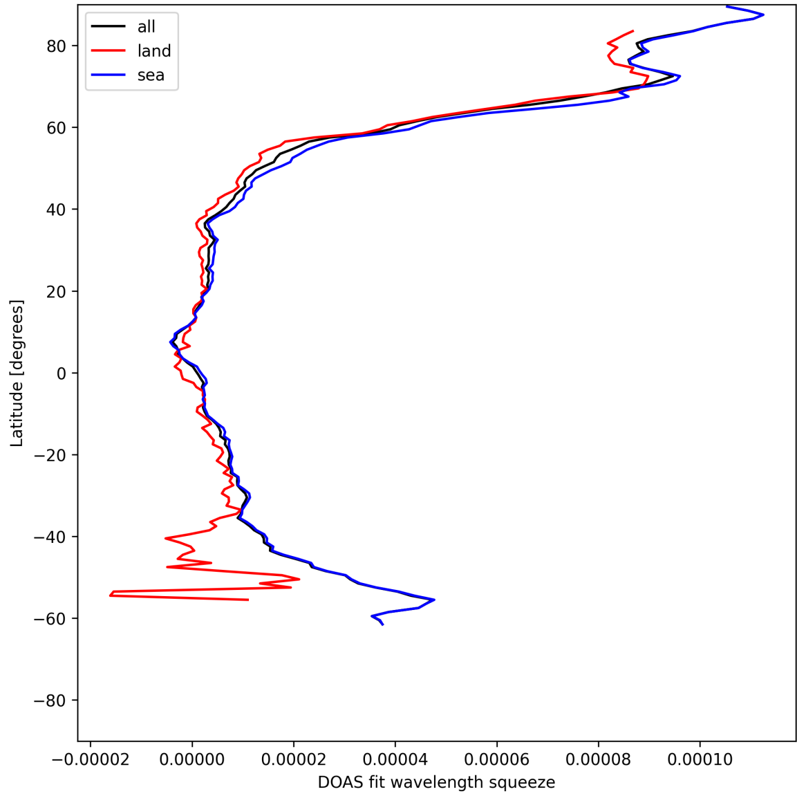
Figure 31: Zonal average of “DOAS fit wavelength squeeze” for 2025-06-02 to 2025-06-04.
