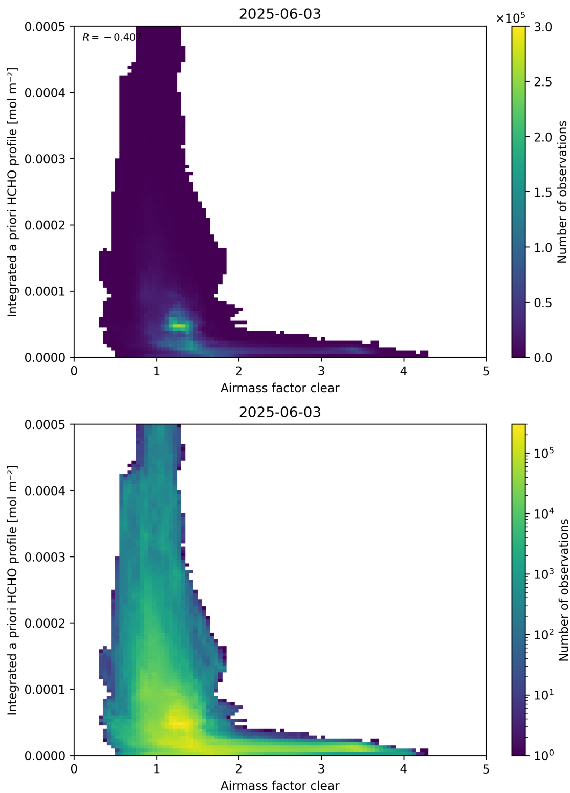
Figure 76: Scatter density plot of “Airmass factor clear” against “Integrated a priori HCHO profile” for 2025-06-02 to 2025-06-04.
