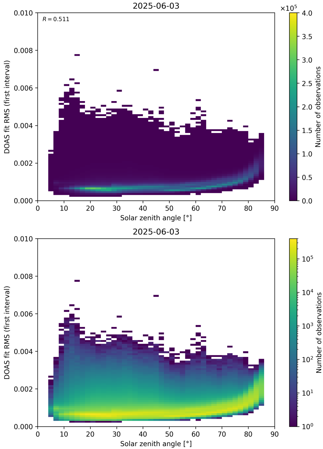
Figure 167: Scatter density plot of “Solar zenith angle” against “DOAS fit RMS (first interval)” for 2025-06-02 to 2025-06-04.
