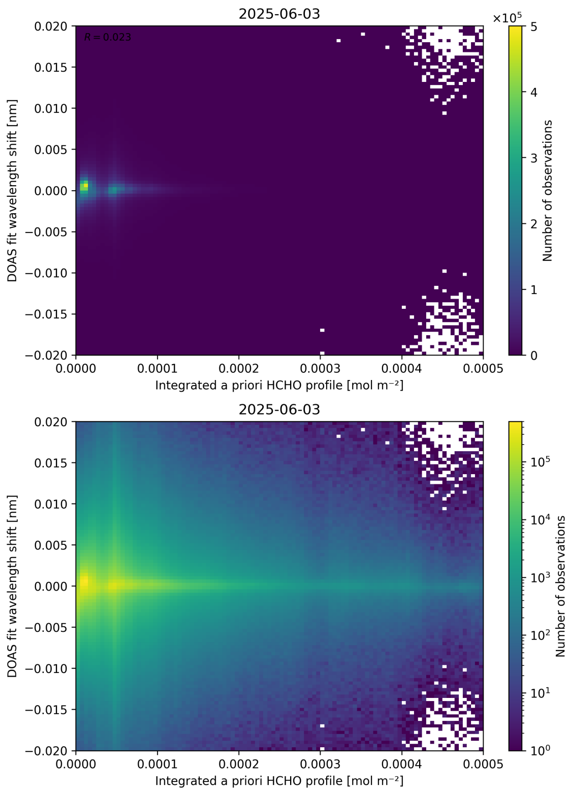
Figure 149: Scatter density plot of “Integrated a priori HCHO profile” against “DOAS fit wavelength shift” for 2025-06-02 to 2025-06-04.
