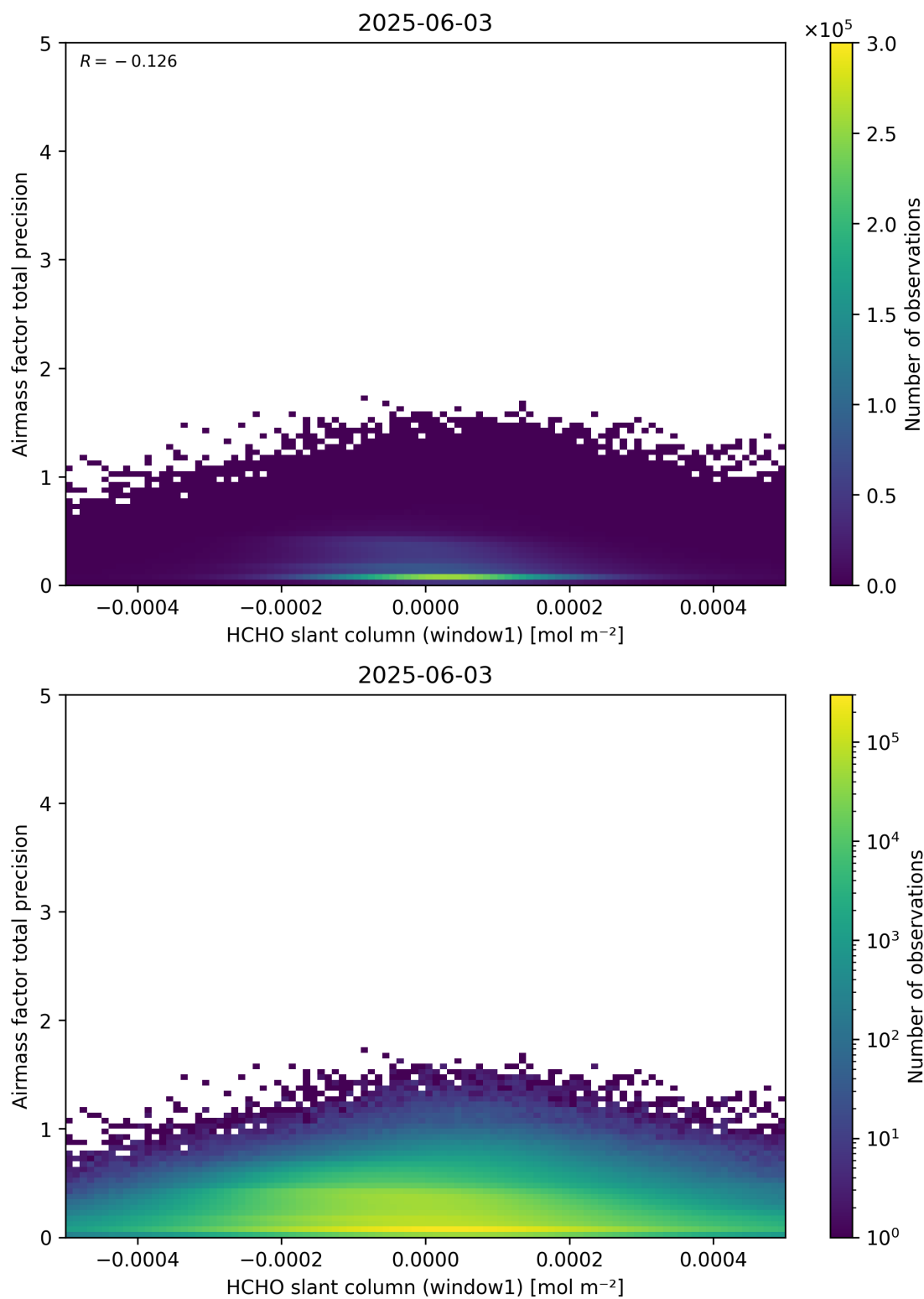
Figure 86: Scatter density plot of “HCHO slant column (window1)” against “Airmass factor total precision” for 2025-06-02 to 2025-06-04.
