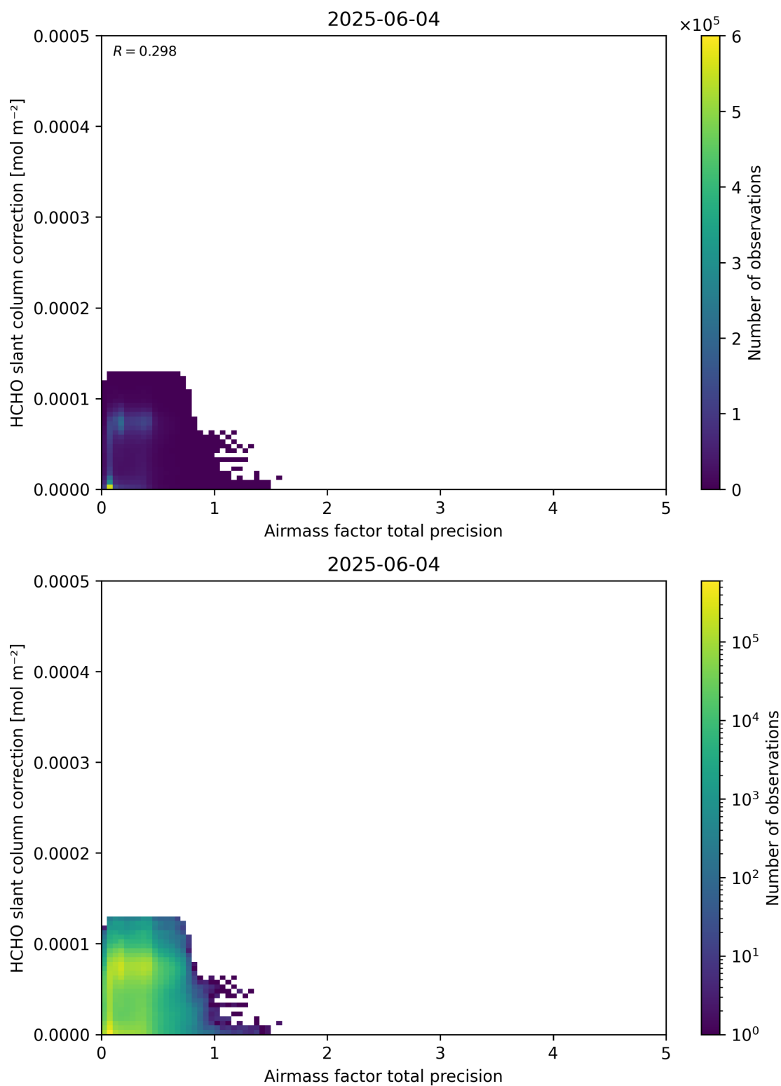
Figure 110: Scatter density plot of “Airmass factor total precision” against “HCHO slant column correction” for 2025-06-03 to 2025-06-05.
