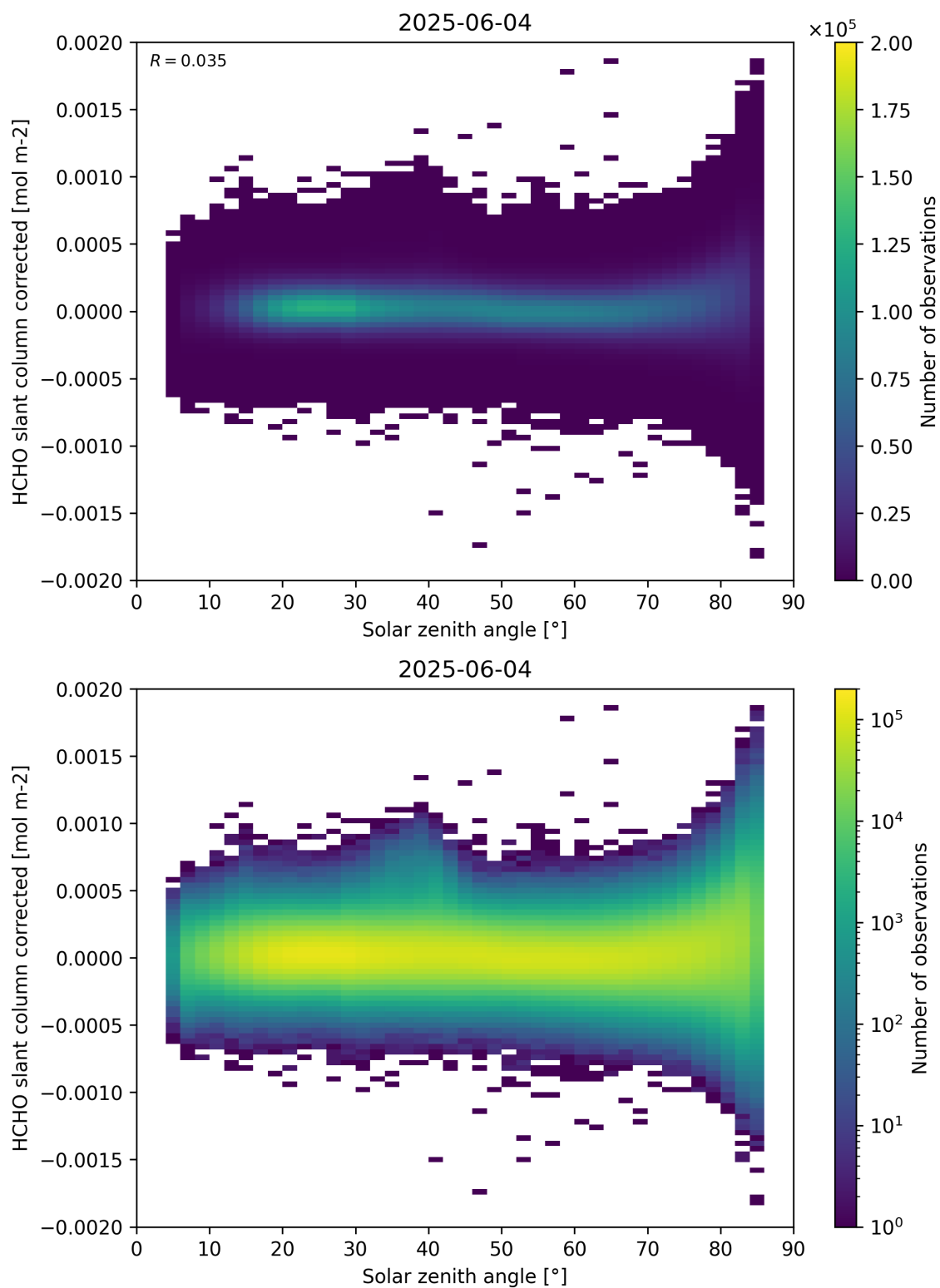
Figure 171: Scatter density plot of “Solar zenith angle” against “HCHO slant column corrected” for 2025-06-03 to 2025-06-05.
