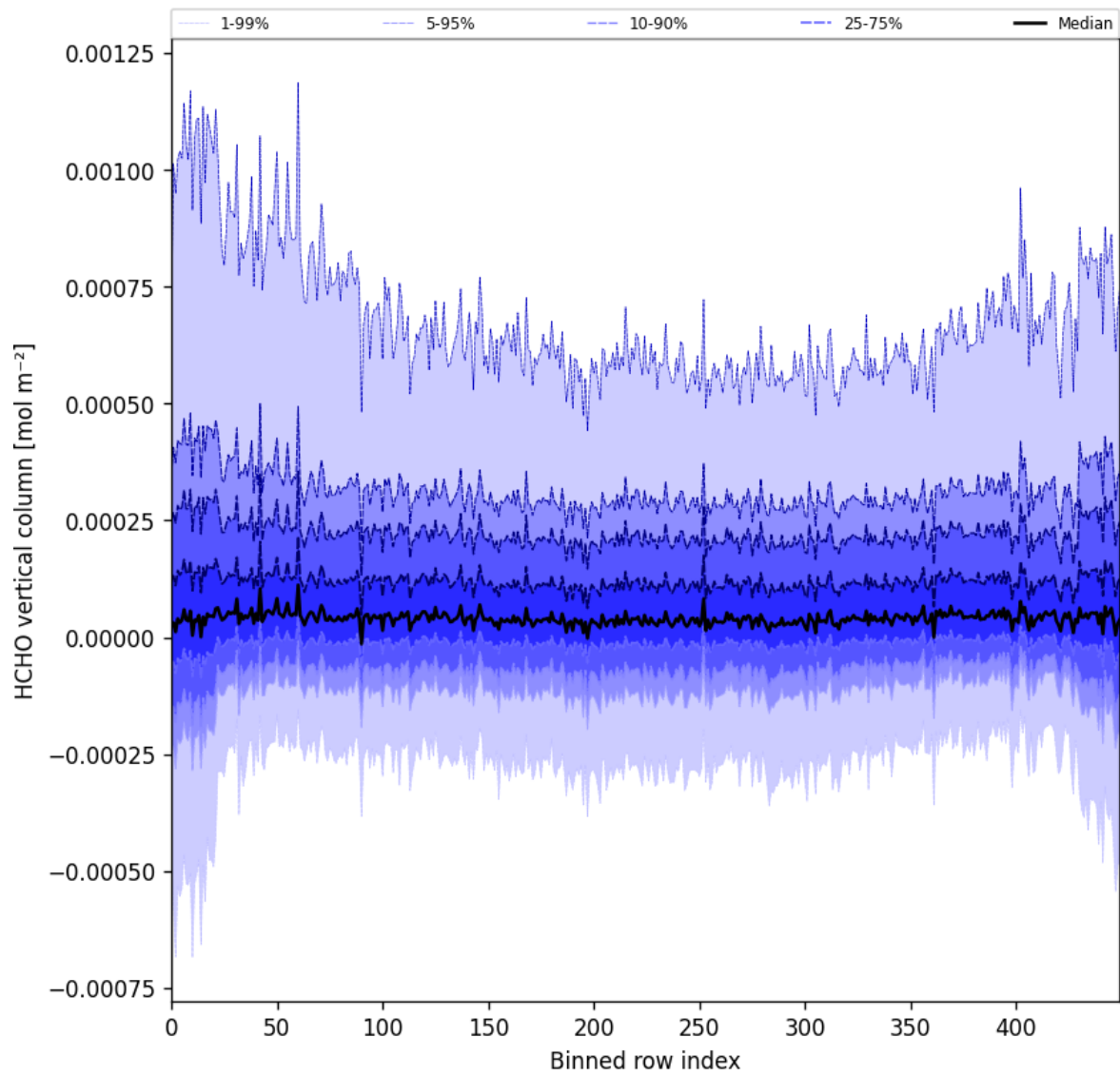
Figure 49: Along track statistics of “HCHO vertical column” for 2025-06-03 to 2025-06-05
