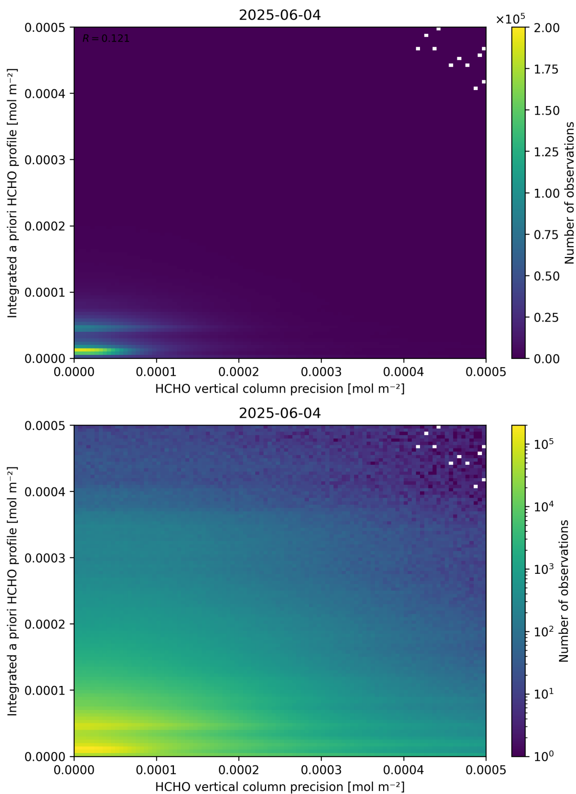
Figure 147: Scatter density plot of “HCHO vertical column precision” against “Integrated a priori HCHO profile” for 2025-06-03 to 2025-06-05.
