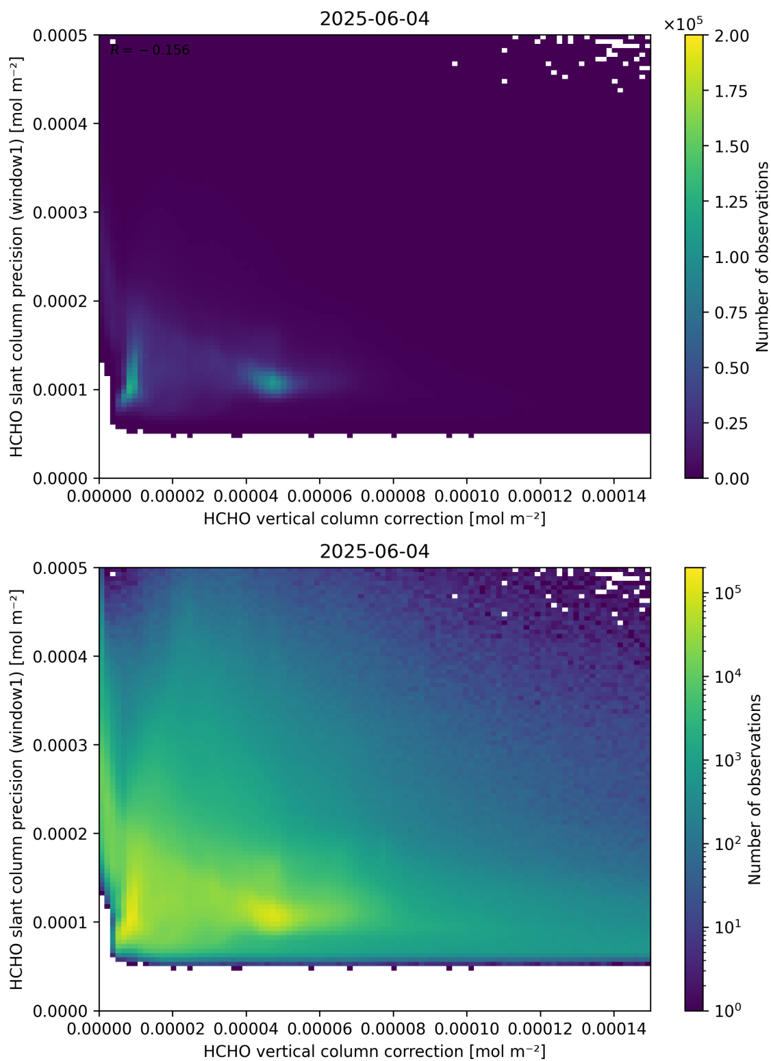
Figure 119: Scatter density plot of “HCHO vertical column correction” against “HCHO slant column precision (window1)” for 2025-06-03 to 2025-06-05.
