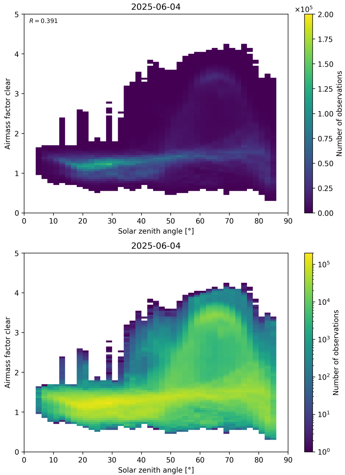
Figure 170: Scatter density plot of “Solar zenith angle” against “Airmass factor clear” for 2025-06-03 to 2025-06-05.
