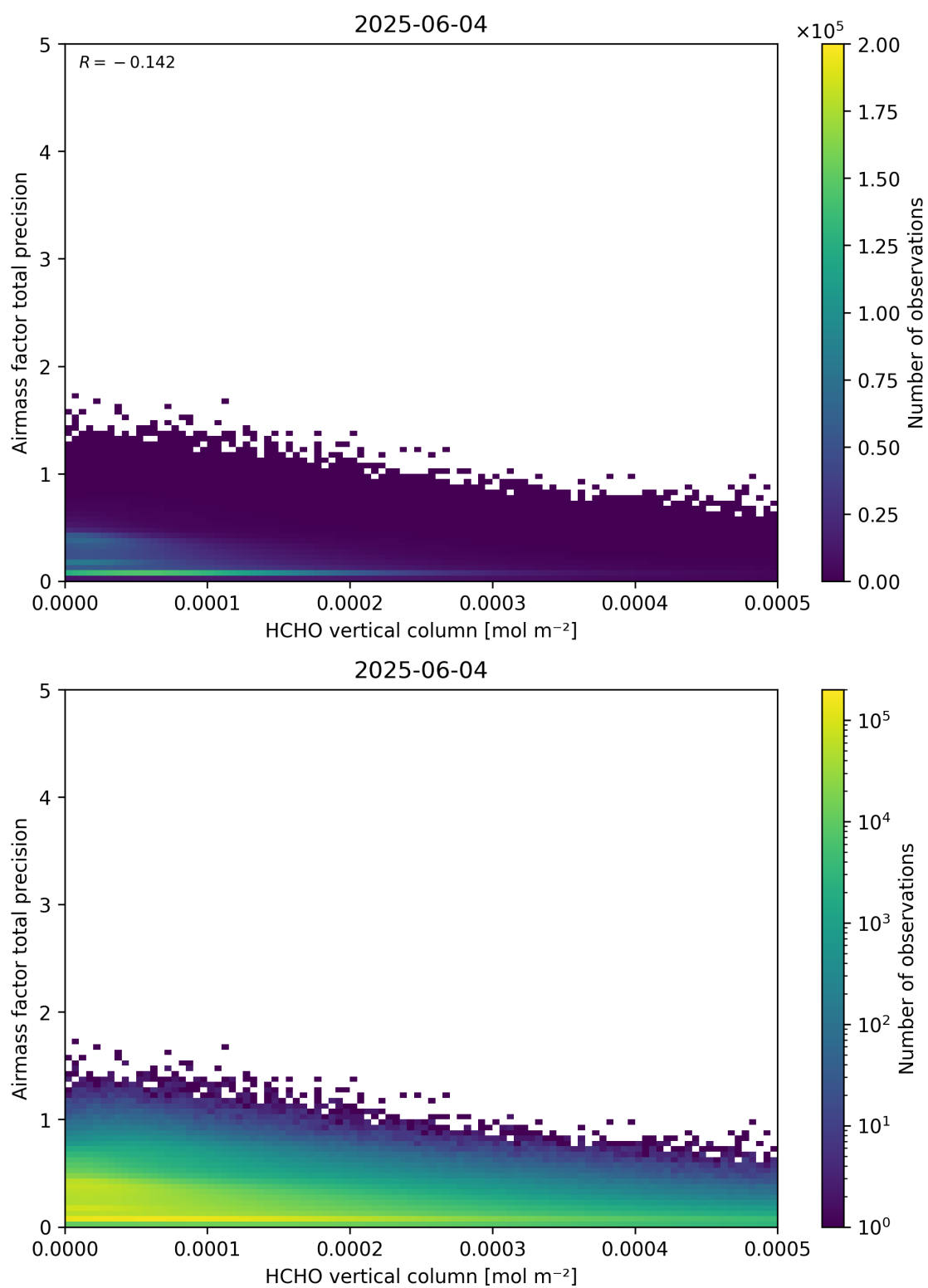
Figure 132: Scatter density plot of “HCHO vertical column” against “Airmass factor total precision” for 2025-06-03 to 2025-06-05.
