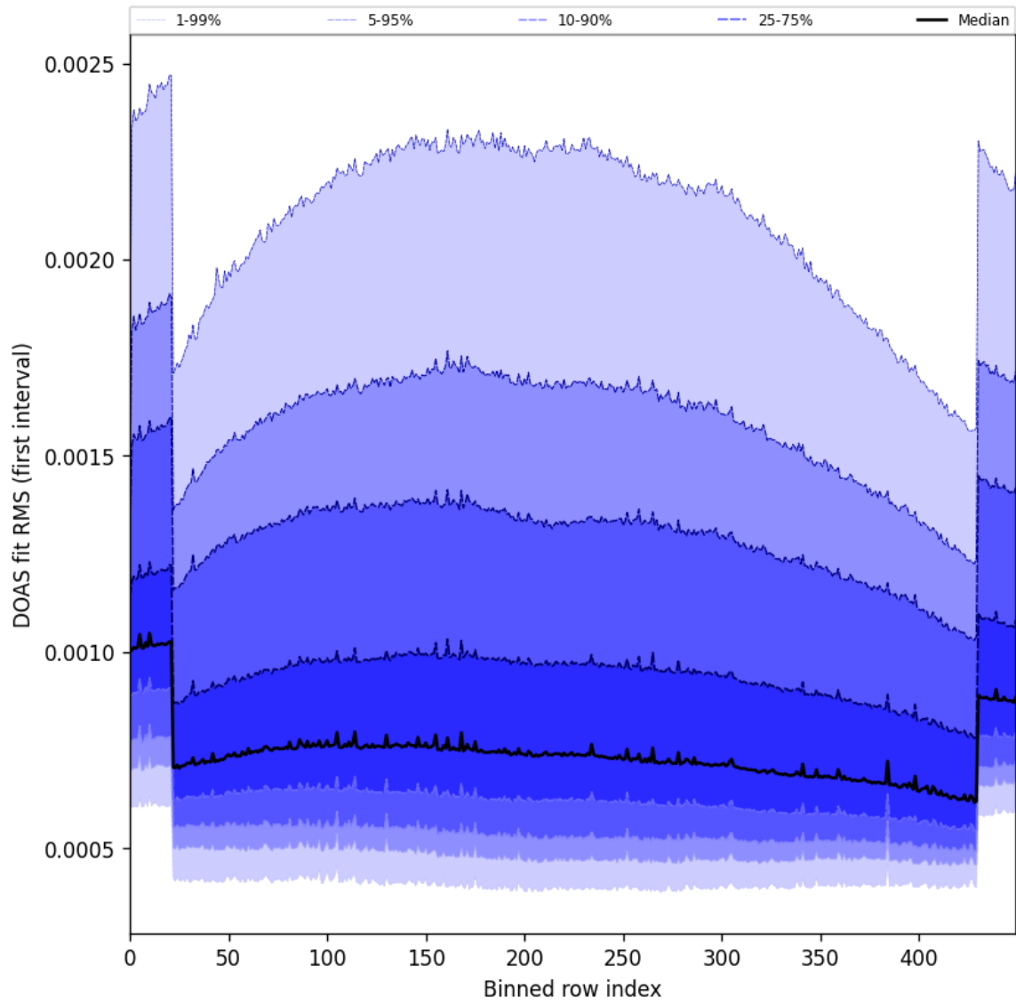
Figure 60: Along track statistics of “DOAS fit RMS (first interval)” for 2025-06-03 to 2025-06-05
