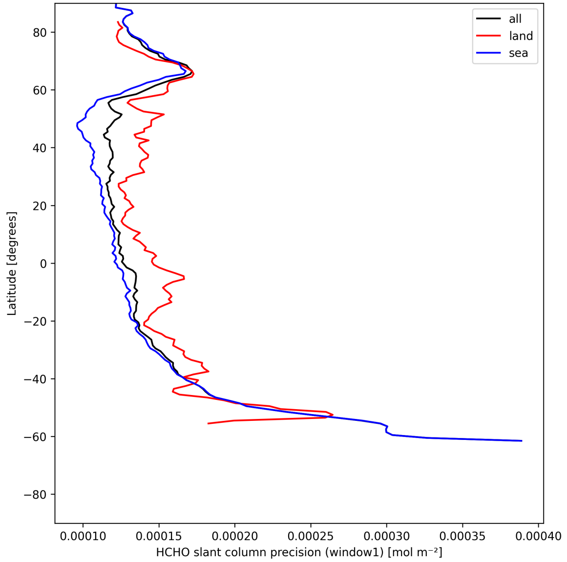
Figure 25: Zonal average of “HCHO slant column precision (window1)” for 2025-06-03 to 2025-06-05.
