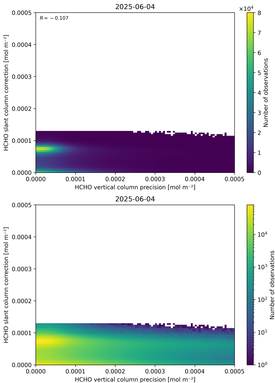
Figure 141: Scatter density plot of “HCHO vertical column precision” against “HCHO slant column correction” for 2025-06-03 to 2025-06-05.
