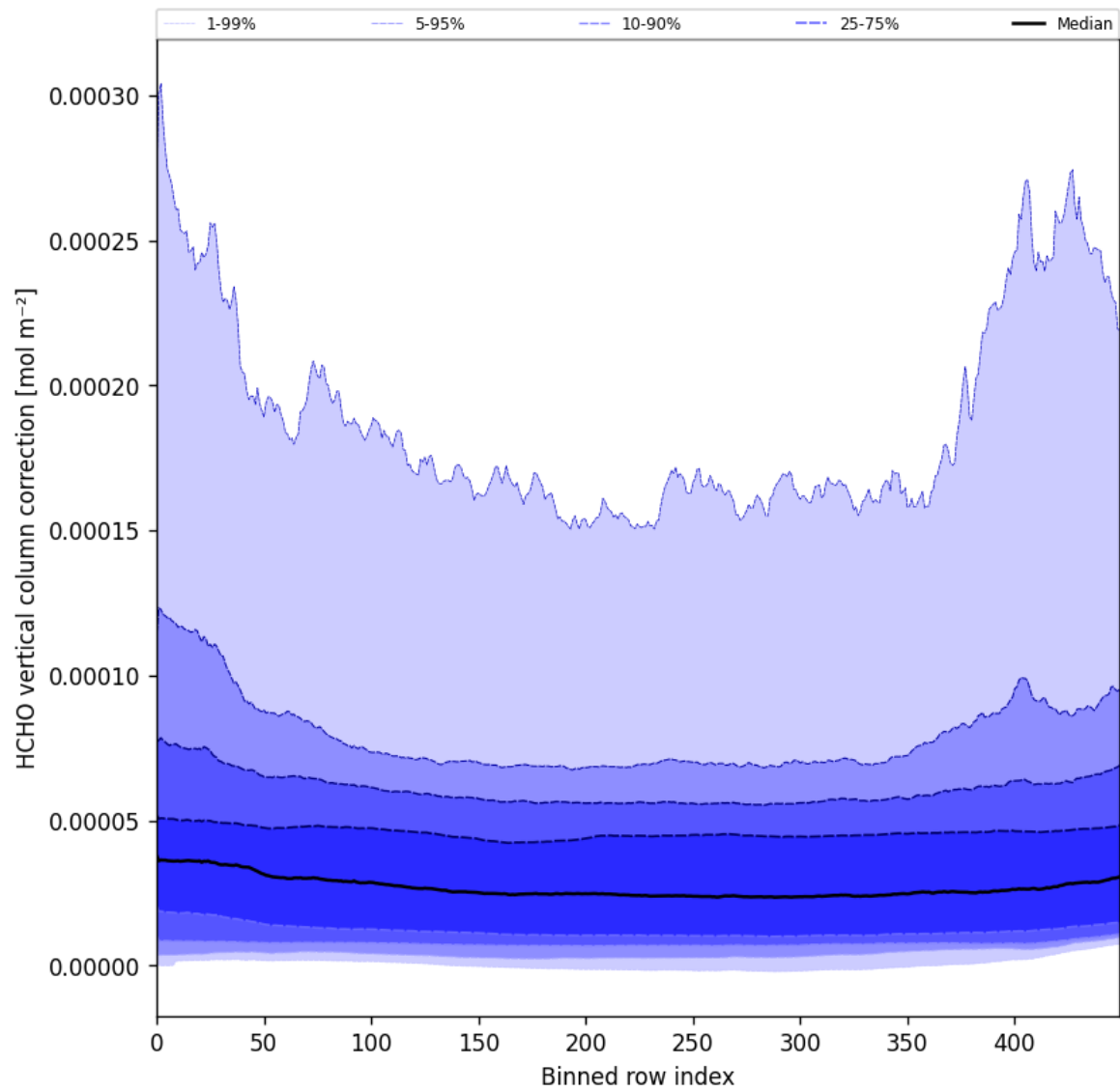
Figure 51: Along track statistics of “HCHO vertical column correction” for 2025-06-03 to 2025-06-05
