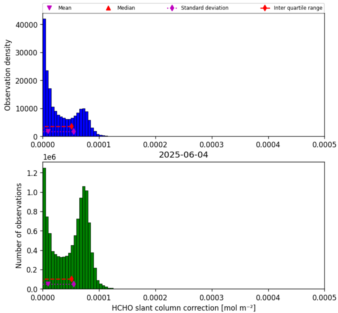
Figure 47: Histogram of "HCHO slant column correction" for 2025-06-03 to 2025-06-05
