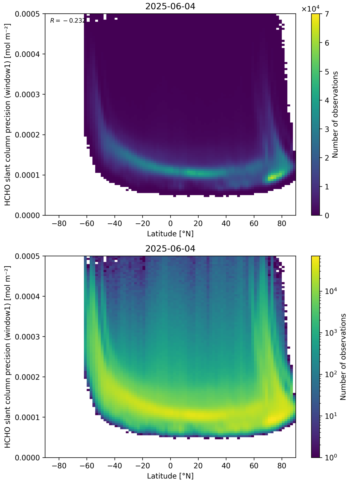
Figure 160: Scatter density plot of “Latitude” against “HCHO slant column precision (window1)” for 2025-06-03 to 2025-06-05.
