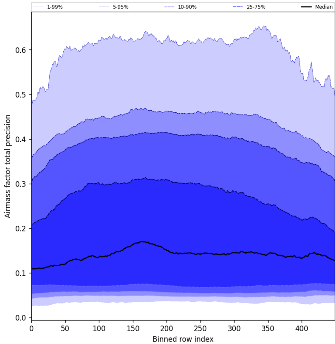
Figure 55: Along track statistics of “Airmass factor total precision” for 2025-06-03 to 2025-06-05
