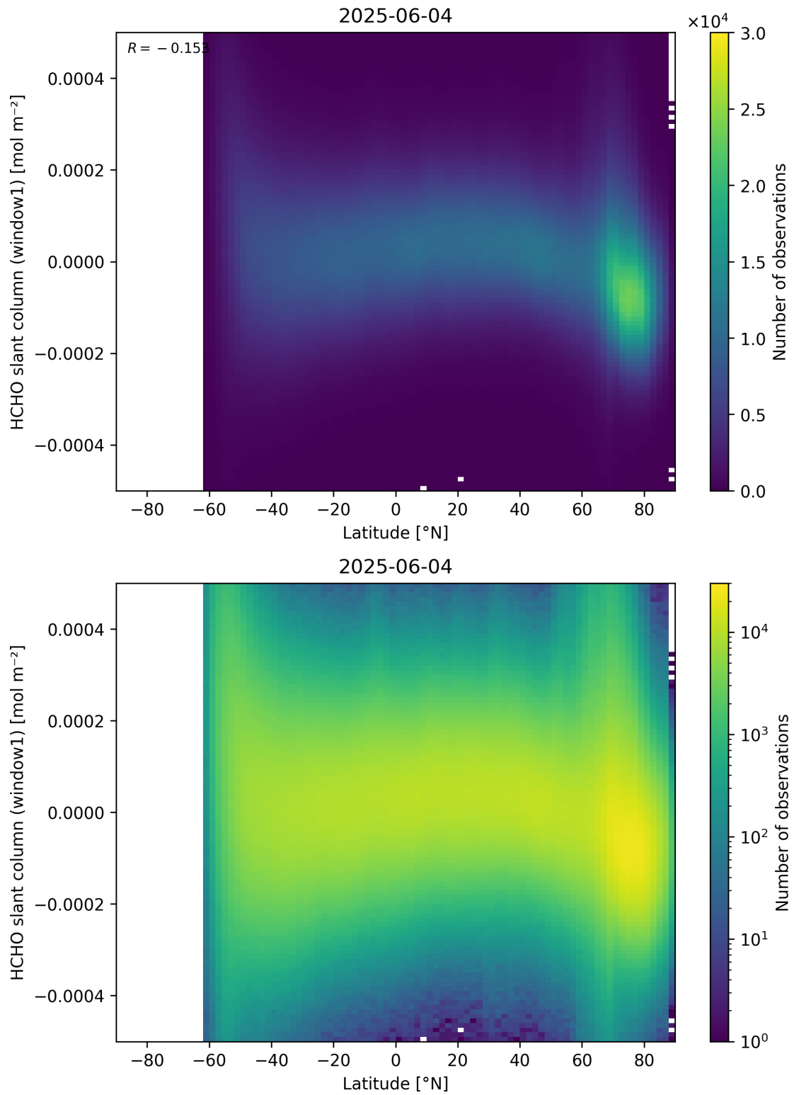
Figure 159: Scatter density plot of “Latitude” against “HCHO slant column (window1)” for 2025-06-03 to 2025-06-05.
