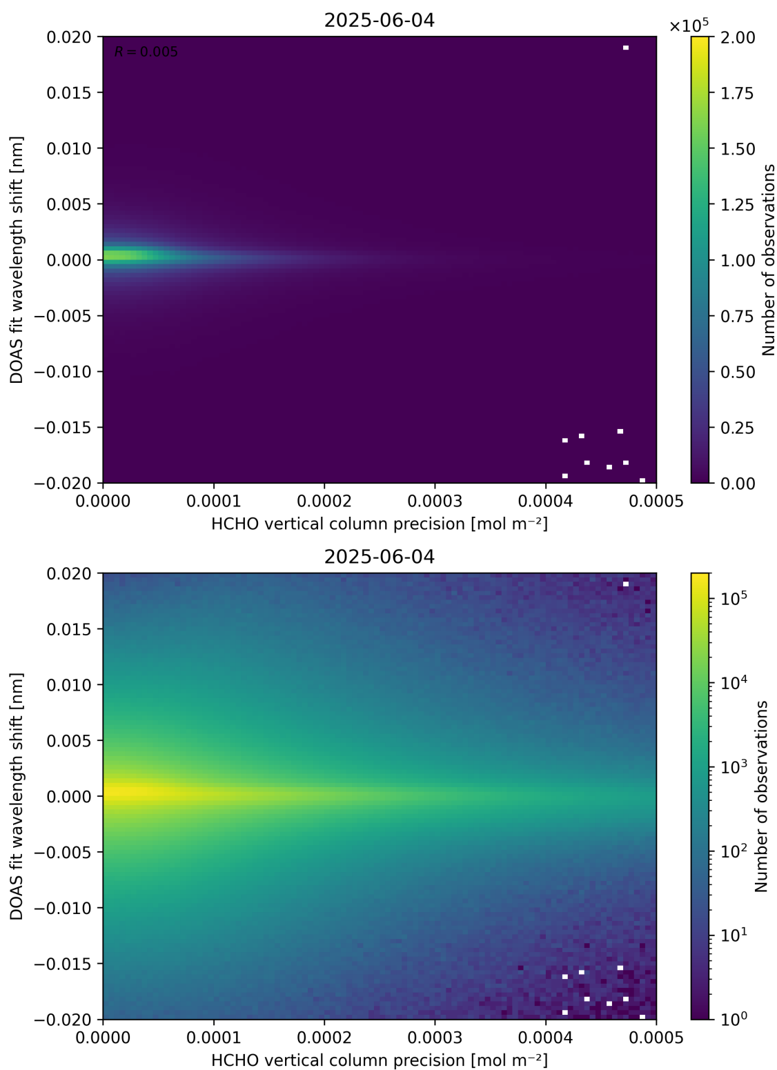
Figure 137: Scatter density plot of “HCHO vertical column precision” against “DOAS fit wavelength shift” for 2025-06-03 to 2025-06-05.
