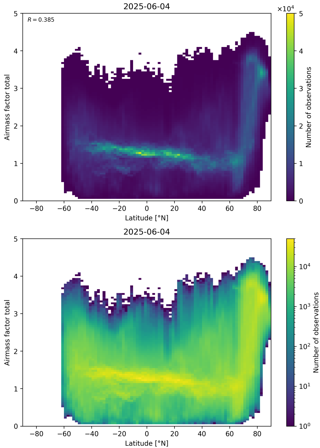
Figure 161: Scatter density plot of “Latitude” against “Airmass factor total” for 2025-06-03 to 2025-06-05.
