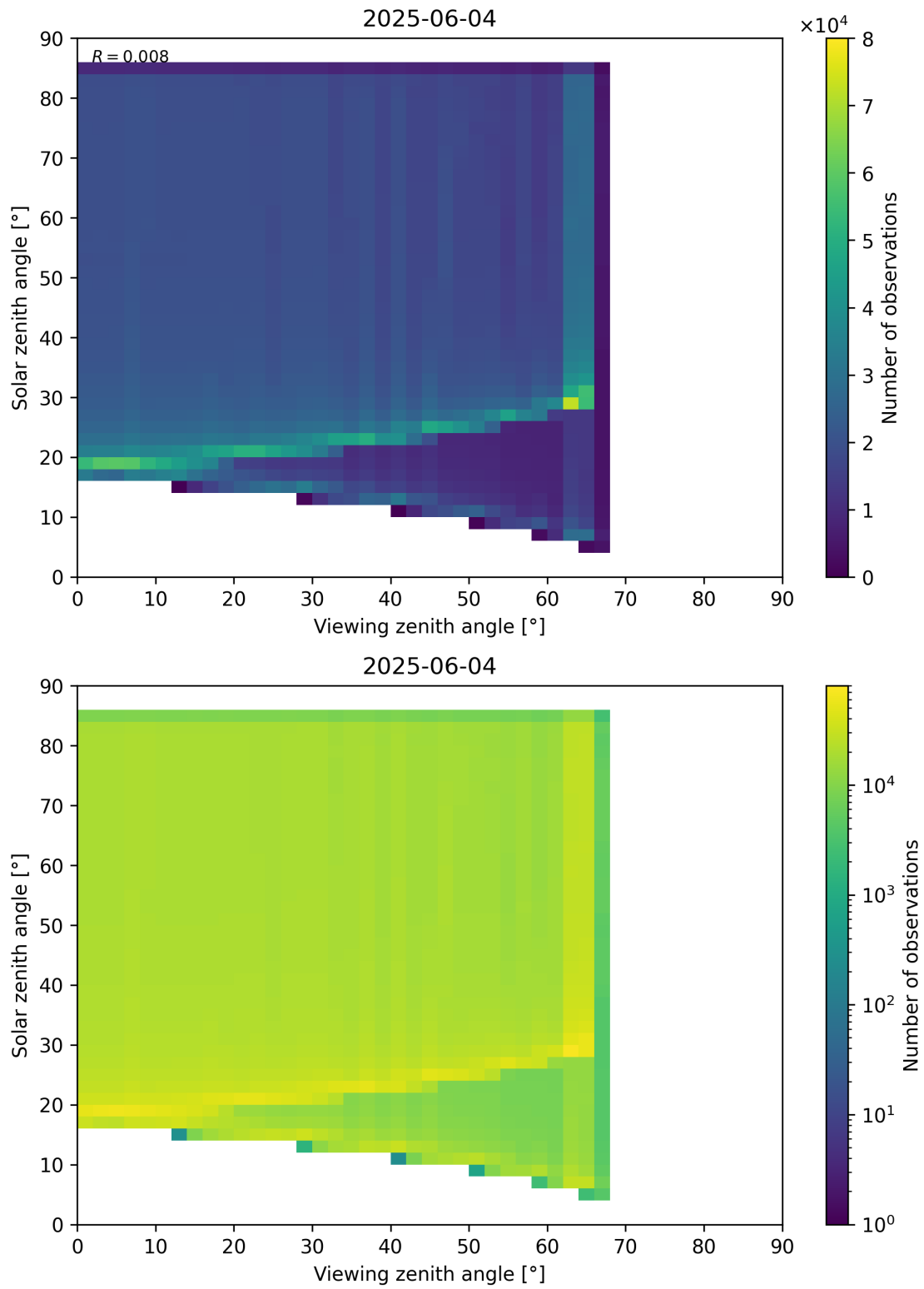
Figure 197: Scatter density plot of “Viewing zenith angle” against “Solar zenith angle” for 2025-06-03 to 2025-06-05.
