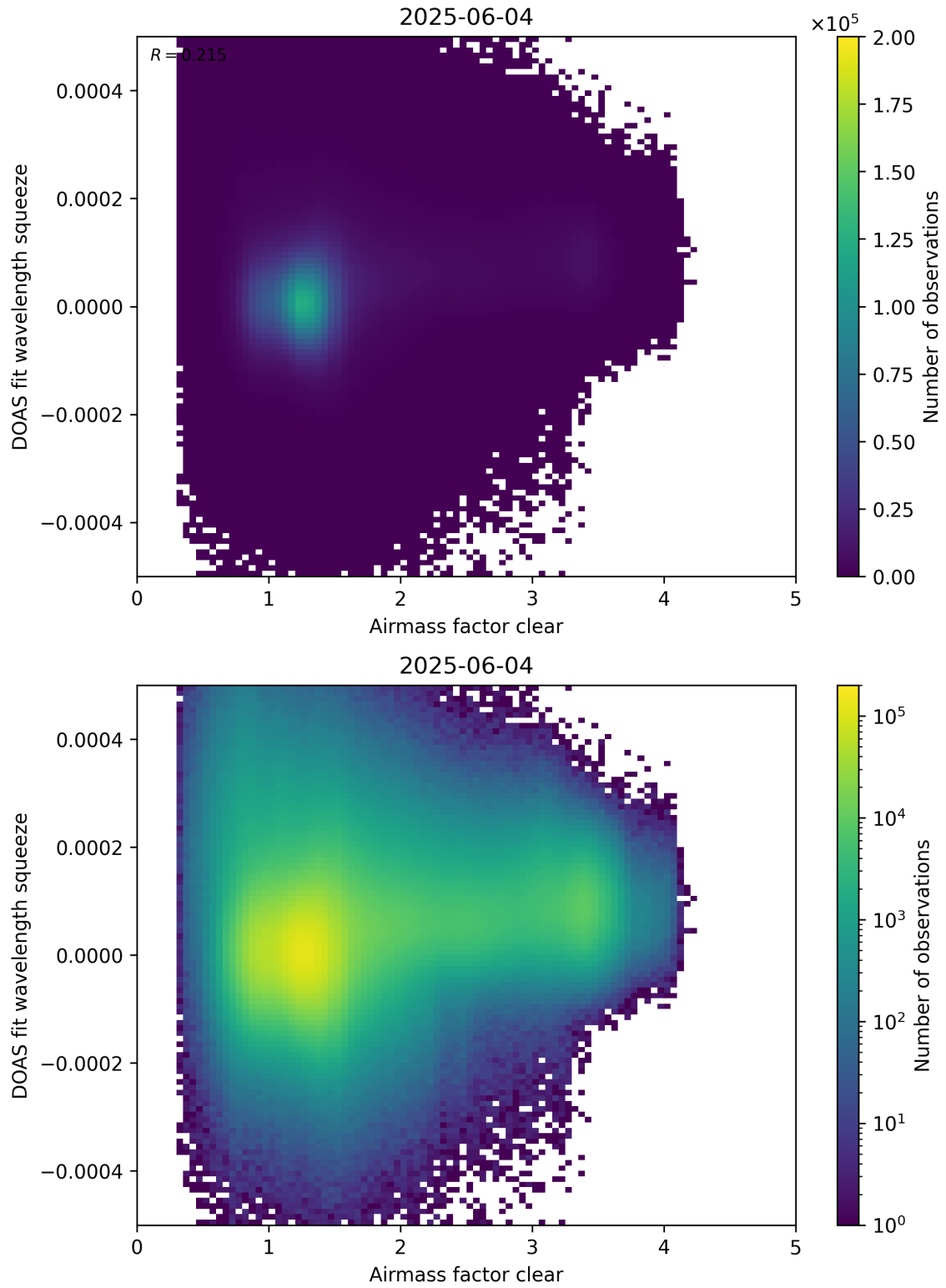
Figure 73: Scatter density plot of “Airmass factor clear” against “DOAS fit wavelength squeeze” for 2025-06-03 to 2025-06-05.
