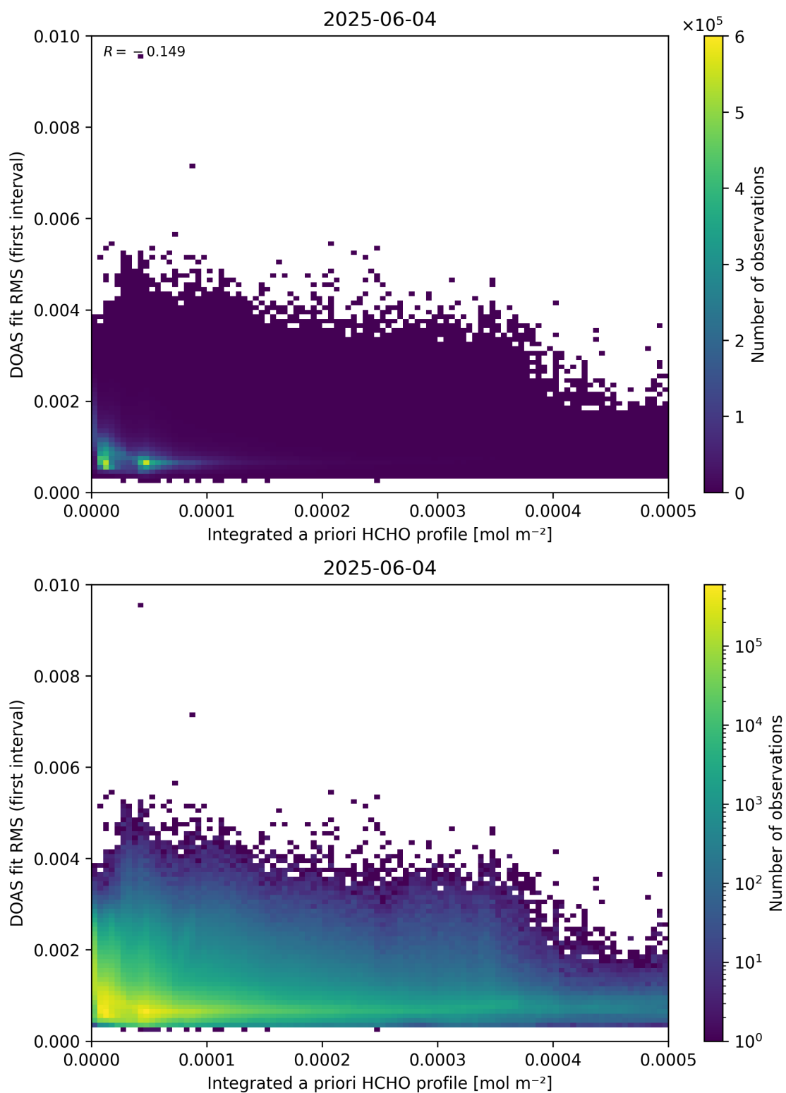
Figure 148: Scatter density plot of “Integrated a priori HCHO profile” against “DOAS fit RMS (first interval)” for 2025-06-03 to 2025-06-05.
