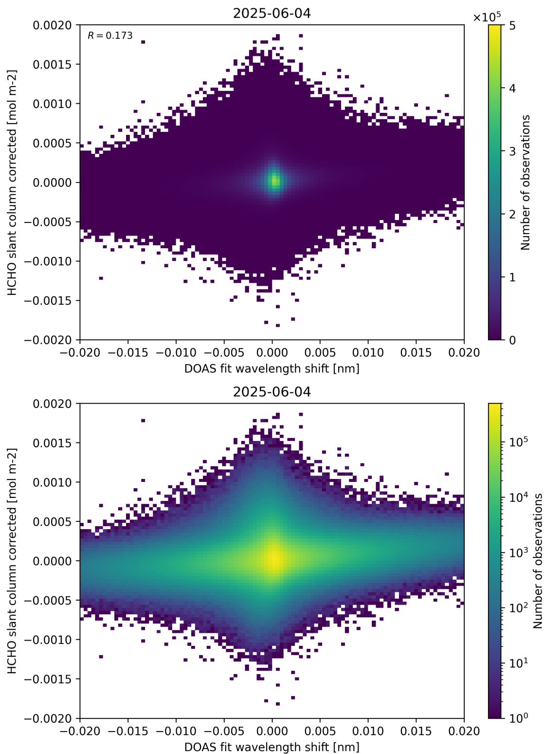
Figure 66: Scatter density plot of “DOAS fit wavelength shift” against “HCHO slant column corrected” for 2025-06-03 to 2025-06-05.
