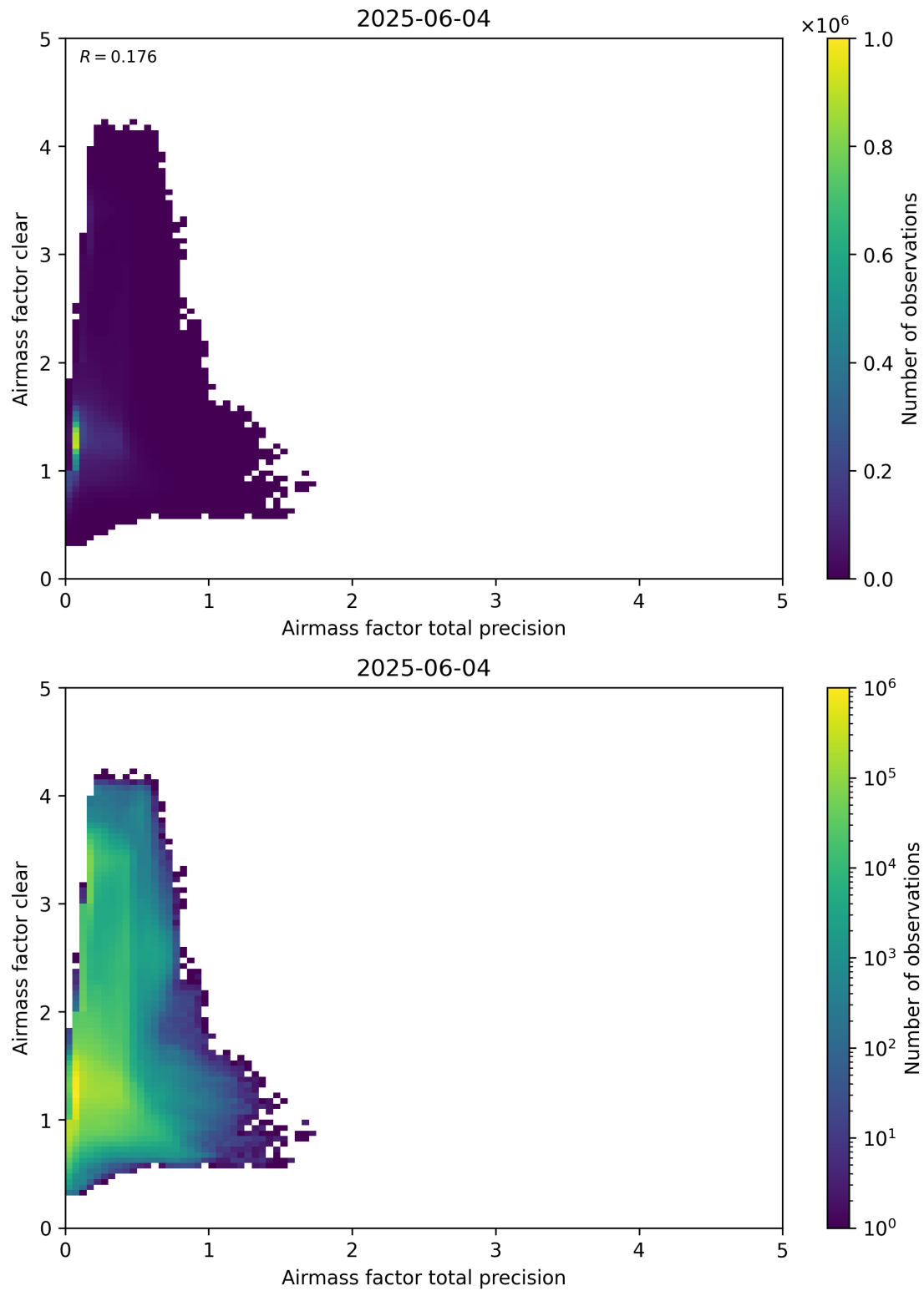
Figure 108: Scatter density plot of “Airmass factor total precision” against “Airmass factor clear” for 2025-06-03 to 2025-06-05.
