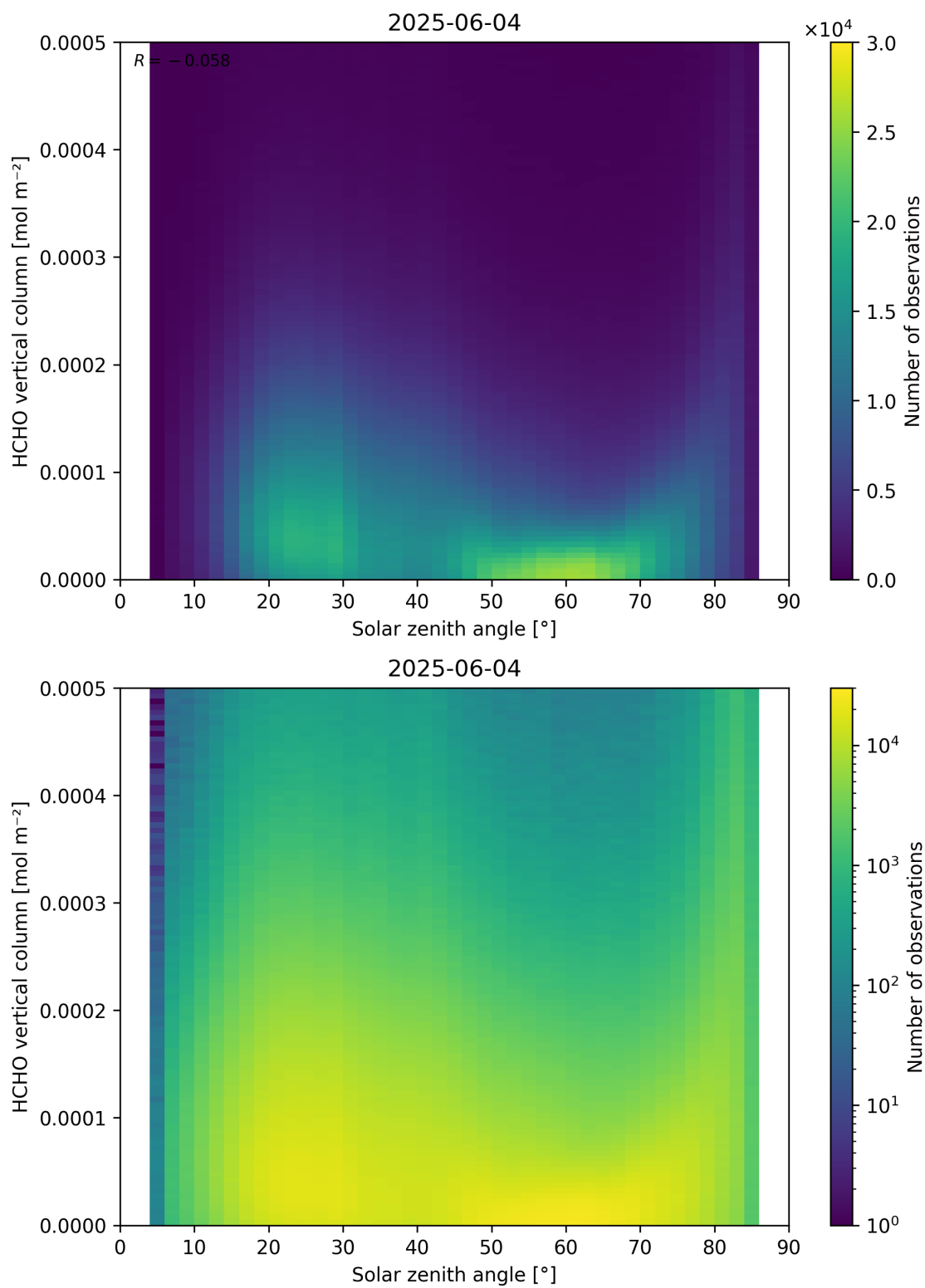
Figure 177: Scatter density plot of “Solar zenith angle” against “HCHO vertical column” for 2025-06-03 to 2025-06-05.
