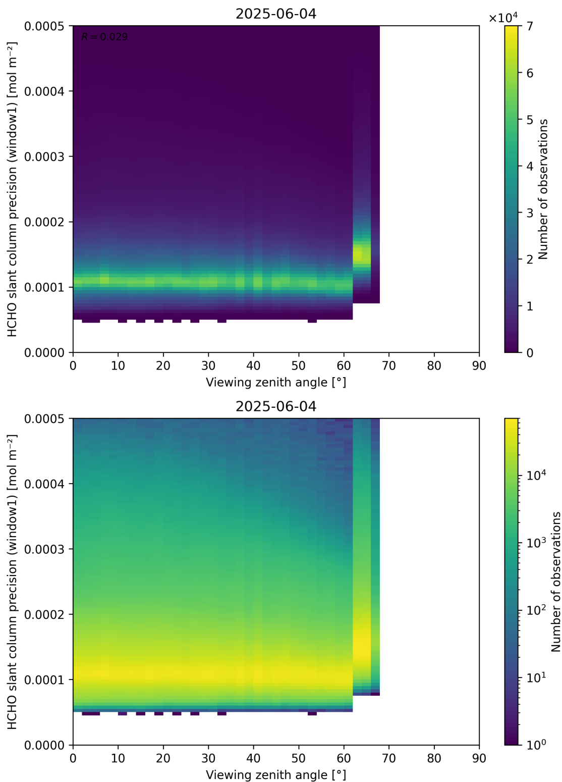
Figure 189: Scatter density plot of “Viewing zenith angle” against “HCHO slant column precision (window1)” for 2025-06-03 to 2025-06-05.
