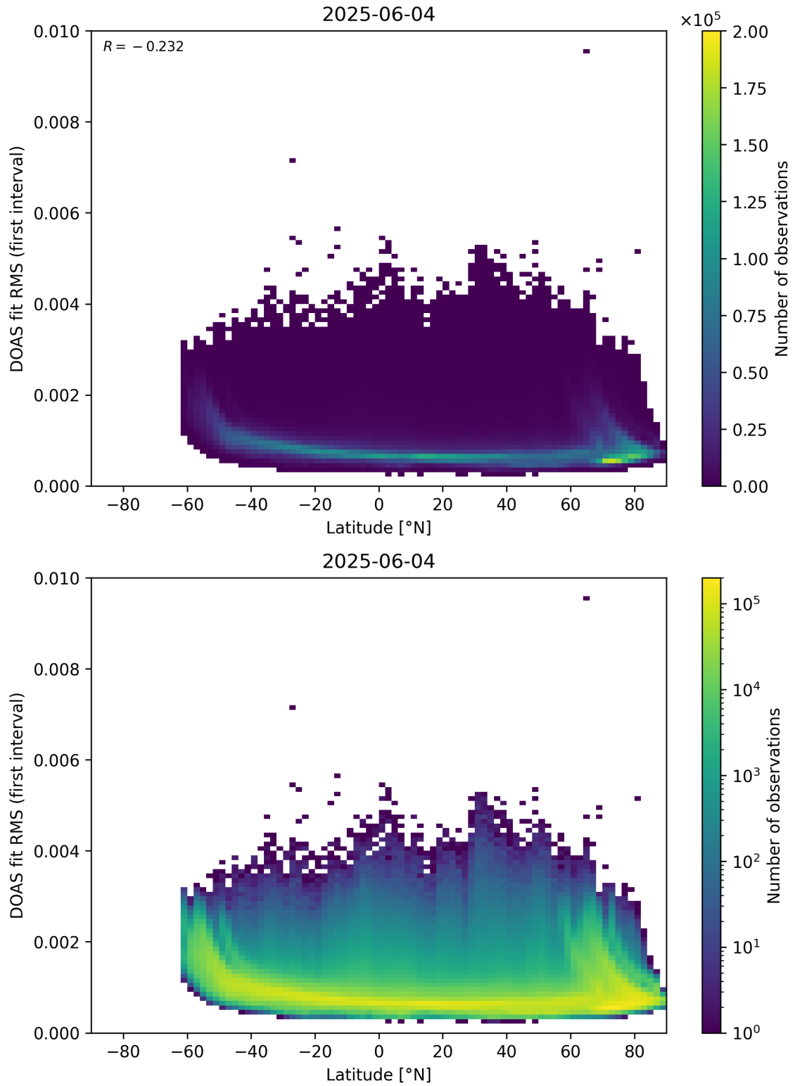
Figure 153: Scatter density plot of “Latitude” against “DOAS fit RMS (first interval)” for 2025-06-03 to 2025-06-05.
