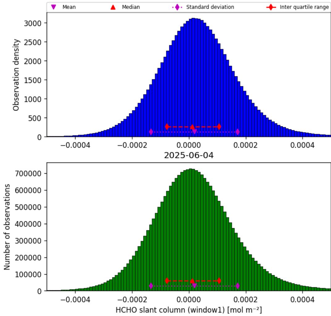
Figure 38: Histogram of “HCHO slant column (window1)” for 2025-06-03 to 2025-06-05
