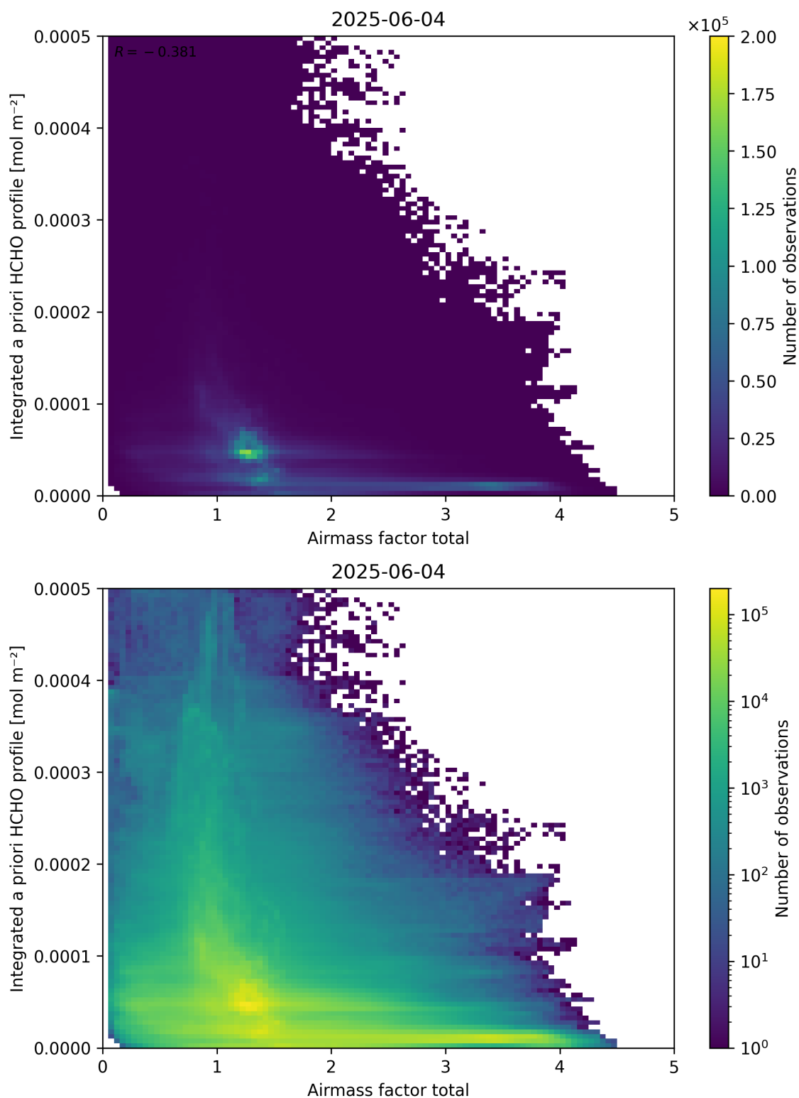
Figure 104: Scatter density plot of “Airmass factor total” against “Integrated a priori HCHO profile” for 2025-06-03 to 2025-06-05.
