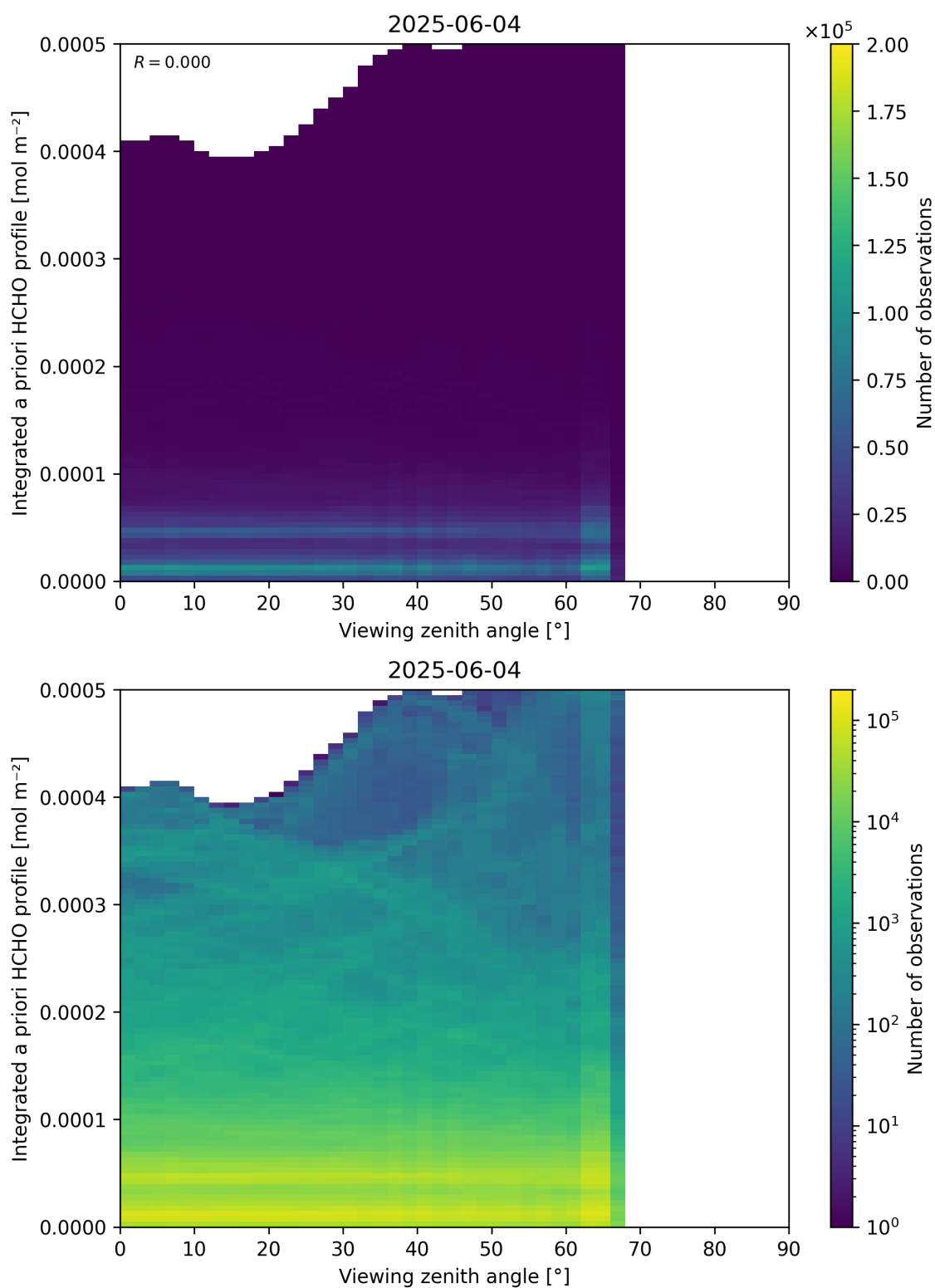
Figure 195: Scatter density plot of “Viewing zenith angle” against “Integrated a priori HCHO profile” for 2025-06-03 to 2025-06-05.
