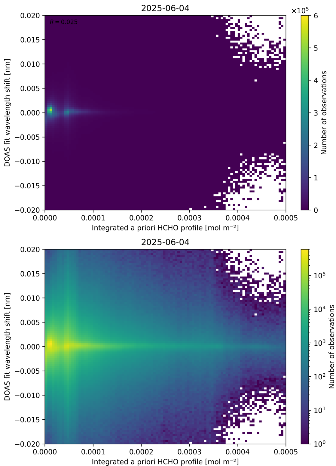
Figure 149: Scatter density plot of “Integrated a priori HCHO profile” against “DOAS fit wavelength shift” for 2025-06-03 to 2025-06-05.
