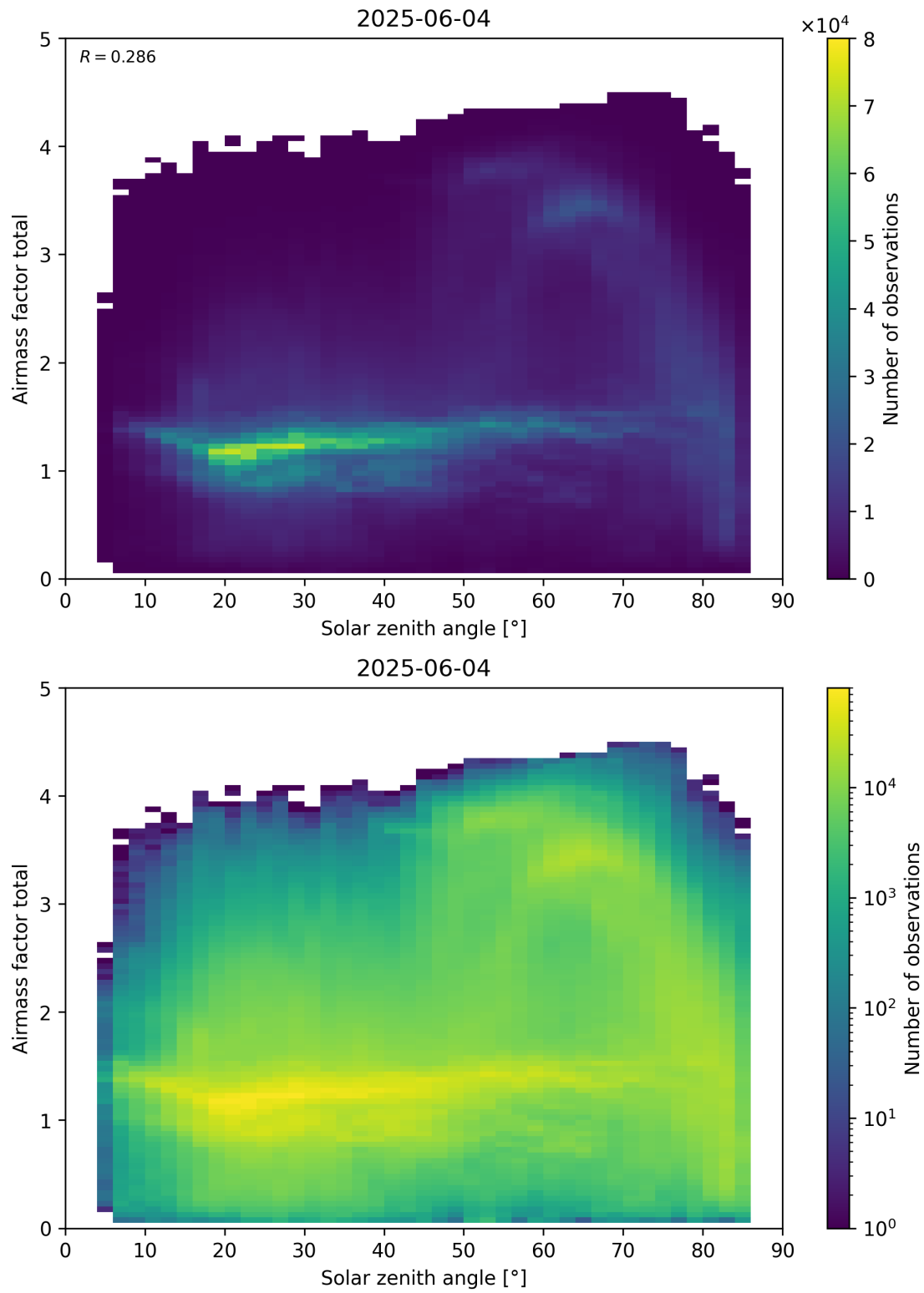
Figure 175: Scatter density plot of “Solar zenith angle” against “Airmass factor total” for 2025-06-03 to 2025-06-05.
