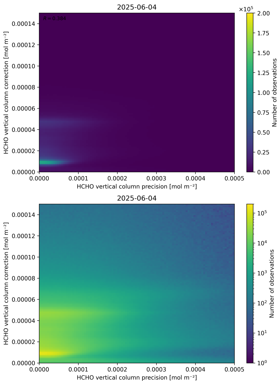
Figure 146: Scatter density plot of “HCHO vertical column precision” against “HCHO vertical column correction” for 2025-06-03 to 2025-06-05.
