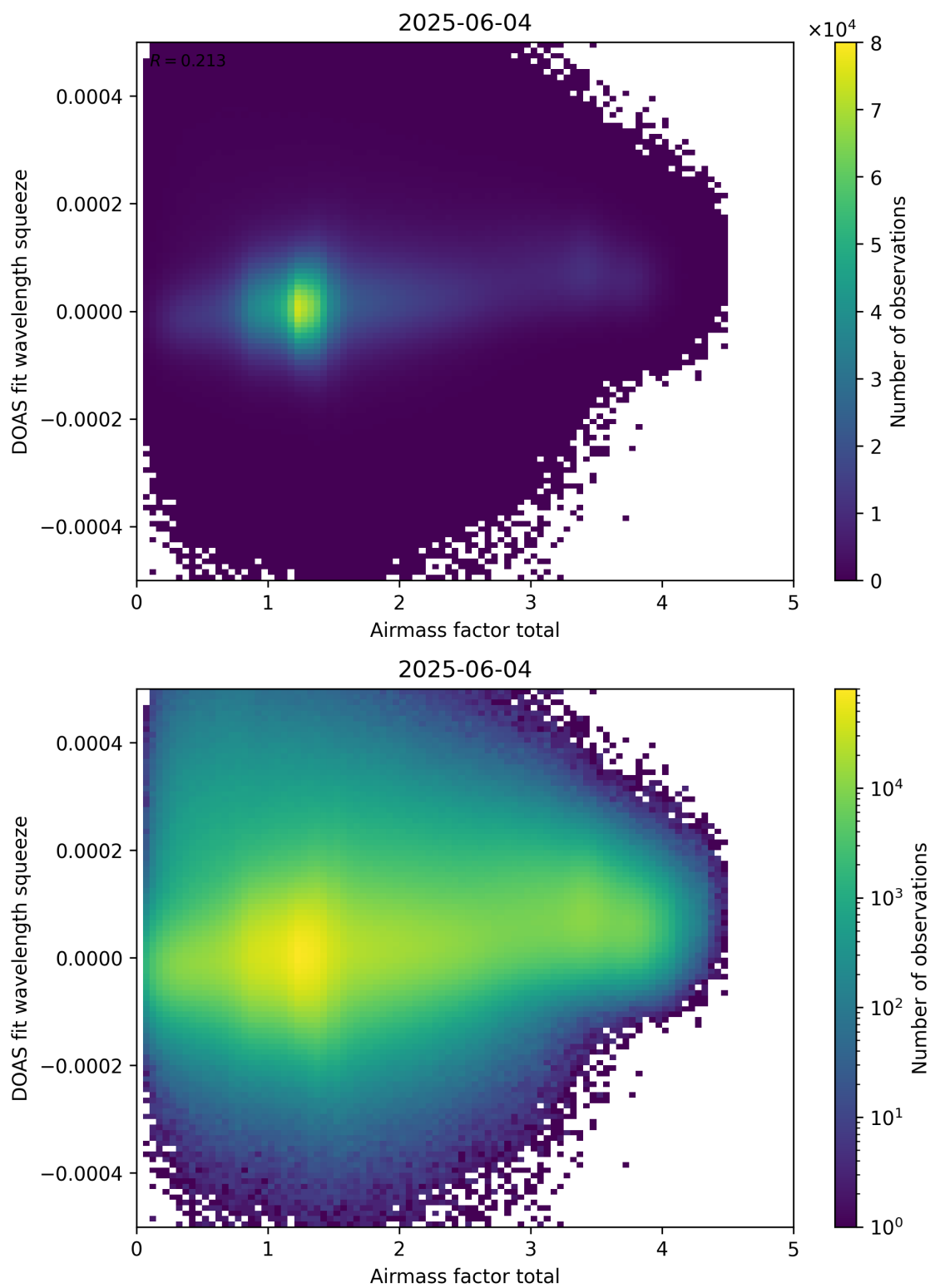
Figure 99: Scatter density plot of “Airmass factor total” against “DOAS fit wavelength squeeze” for 2025-06-03 to 2025-06-05.
