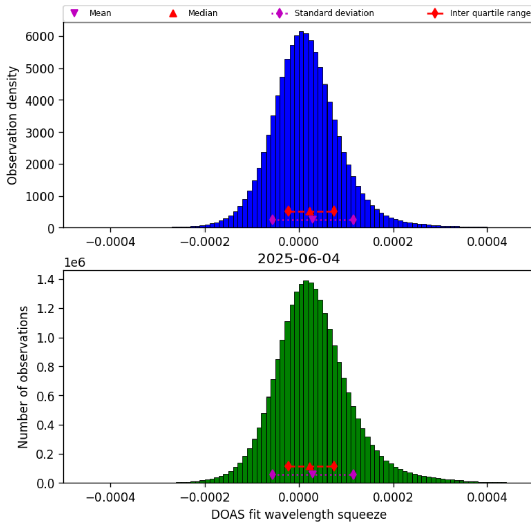
Figure 45: Histogram of “DOAS fit wavelength squeeze” for 2025-06-03 to 2025-06-05
