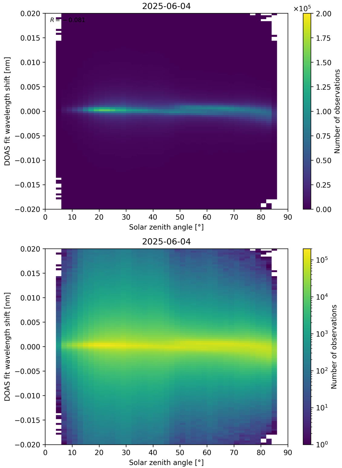
Figure 168: Scatter density plot of “Solar zenith angle” against “DOAS fit wavelength shift” for 2025-06-03 to 2025-06-05.
