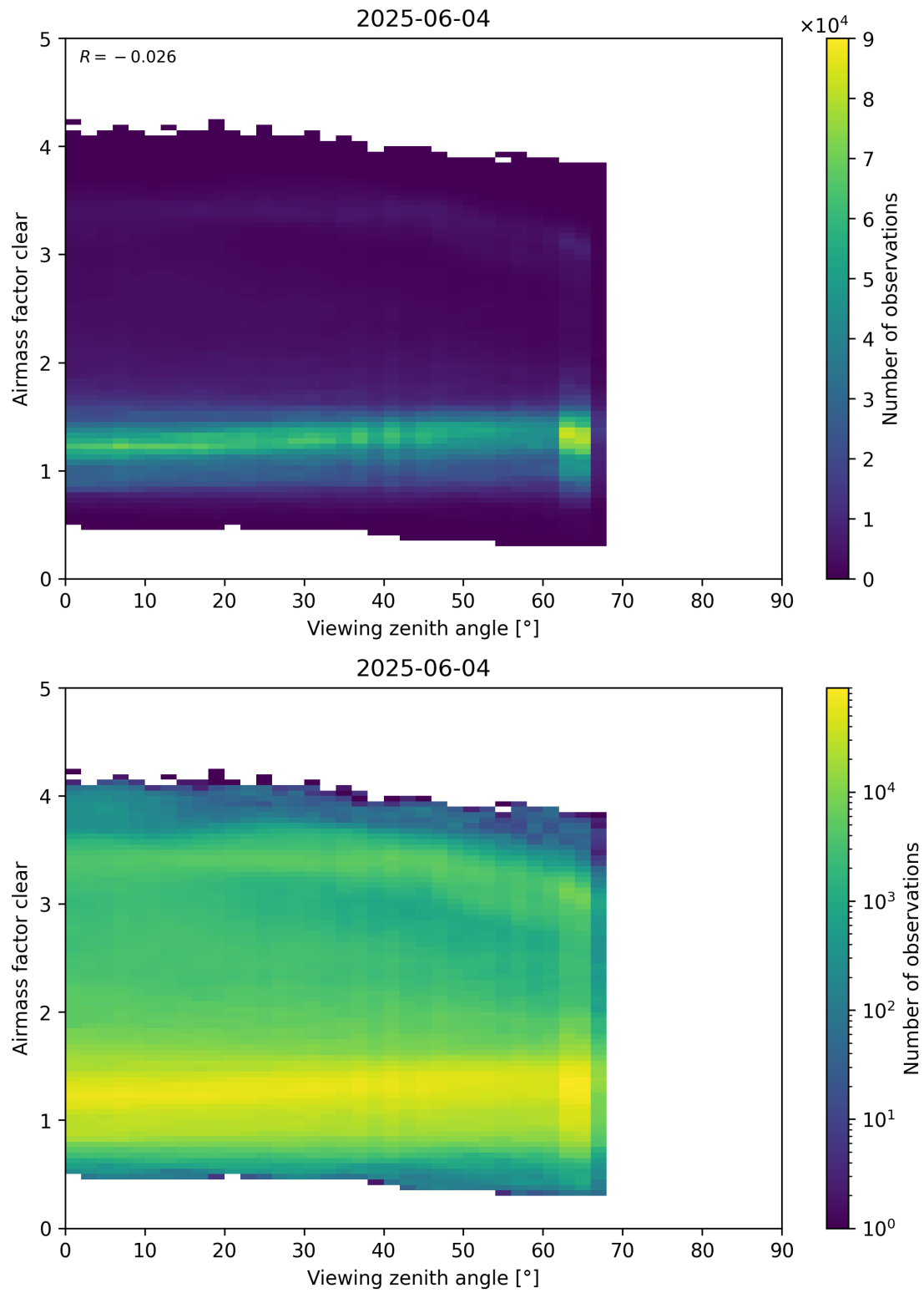
Figure 185: Scatter density plot of “Viewing zenith angle” against “Airmass factor clear” for 2025-06-03 to 2025-06-05.
