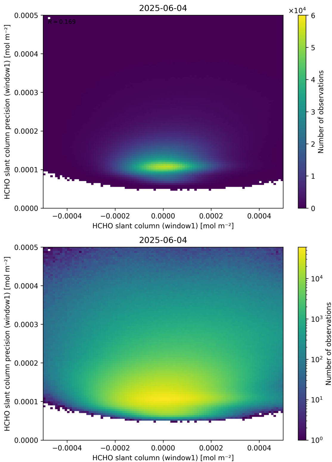
Figure 84: Scatter density plot of “HCHO slant column (window1)” against “HCHO slant column precision (window1)” for 2025-06-03 to 2025-06-05.
