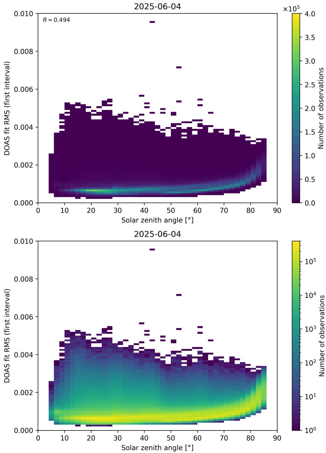
Figure 167: Scatter density plot of “Solar zenith angle” against “DOAS fit RMS (first interval)” for 2025-06-03 to 2025-06-05.
