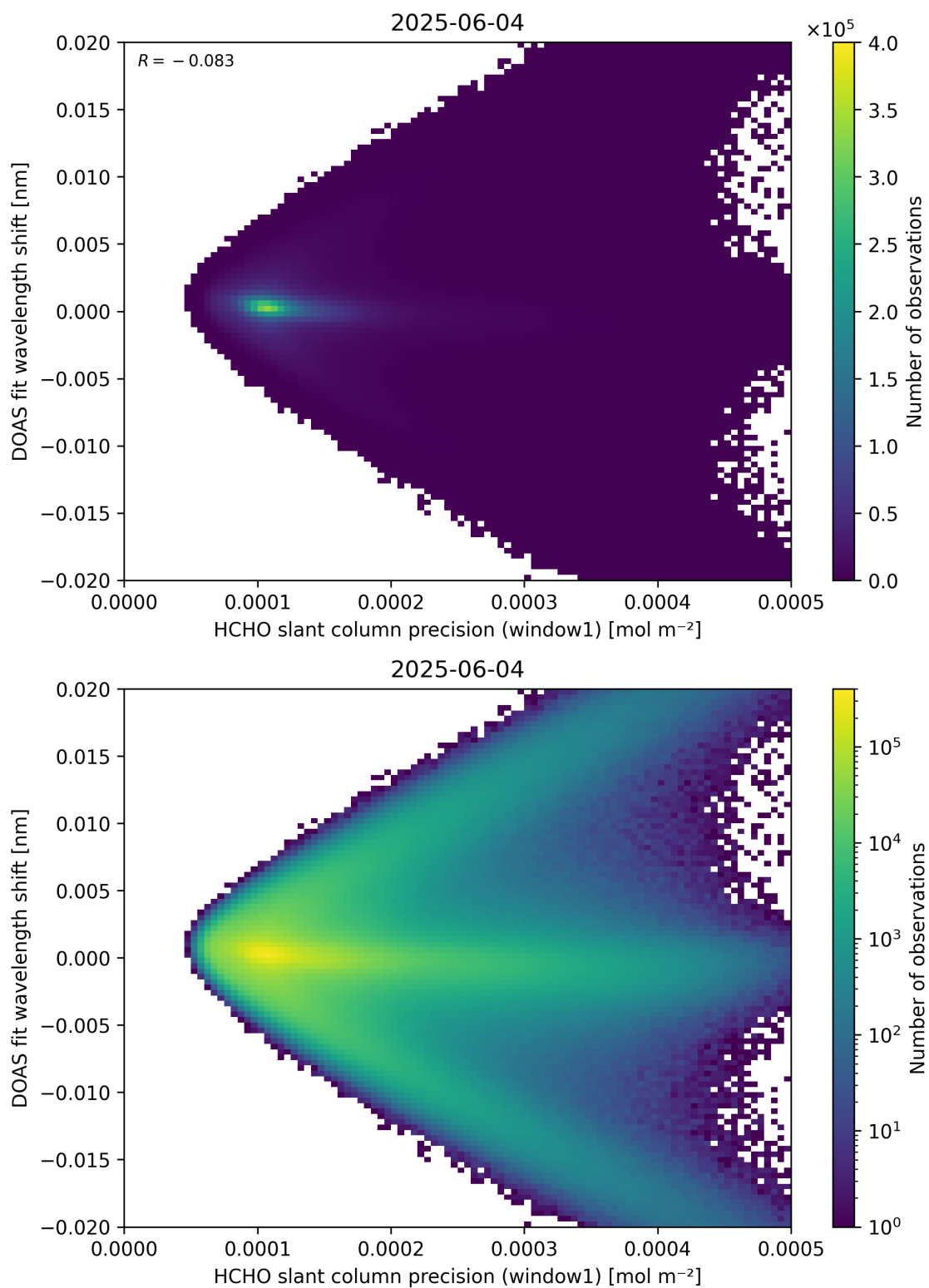
Figure 89: Scatter density plot of “HCHO slant column precision (window1)” against “DOAS fit wavelength shift” for 2025-06-03 to 2025-06-05.
