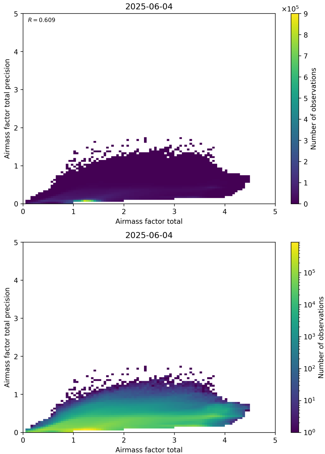
Figure 103: Scatter density plot of “Airmass factor total” against “Airmass factor total precision” for 2025-06-03 to 2025-06-05.
