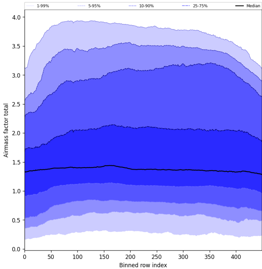
Figure 54: Along track statistics of “Airmass factor total” for 2025-06-03 to 2025-06-05
