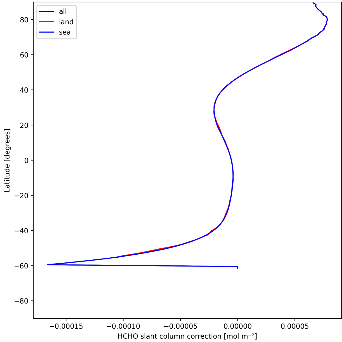
Figure 33: Zonal average of "HCHO slant column correction" for 2025-06-03 to 2025-06-05.
