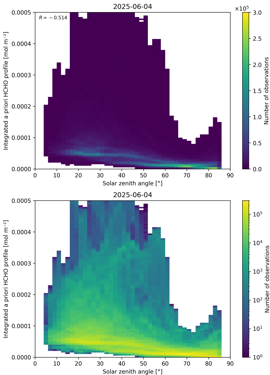
Figure 180: Scatter density plot of “Solar zenith angle” against “Integrated a priori HCHO profile” for 2025-06-03 to 2025-06-05.
