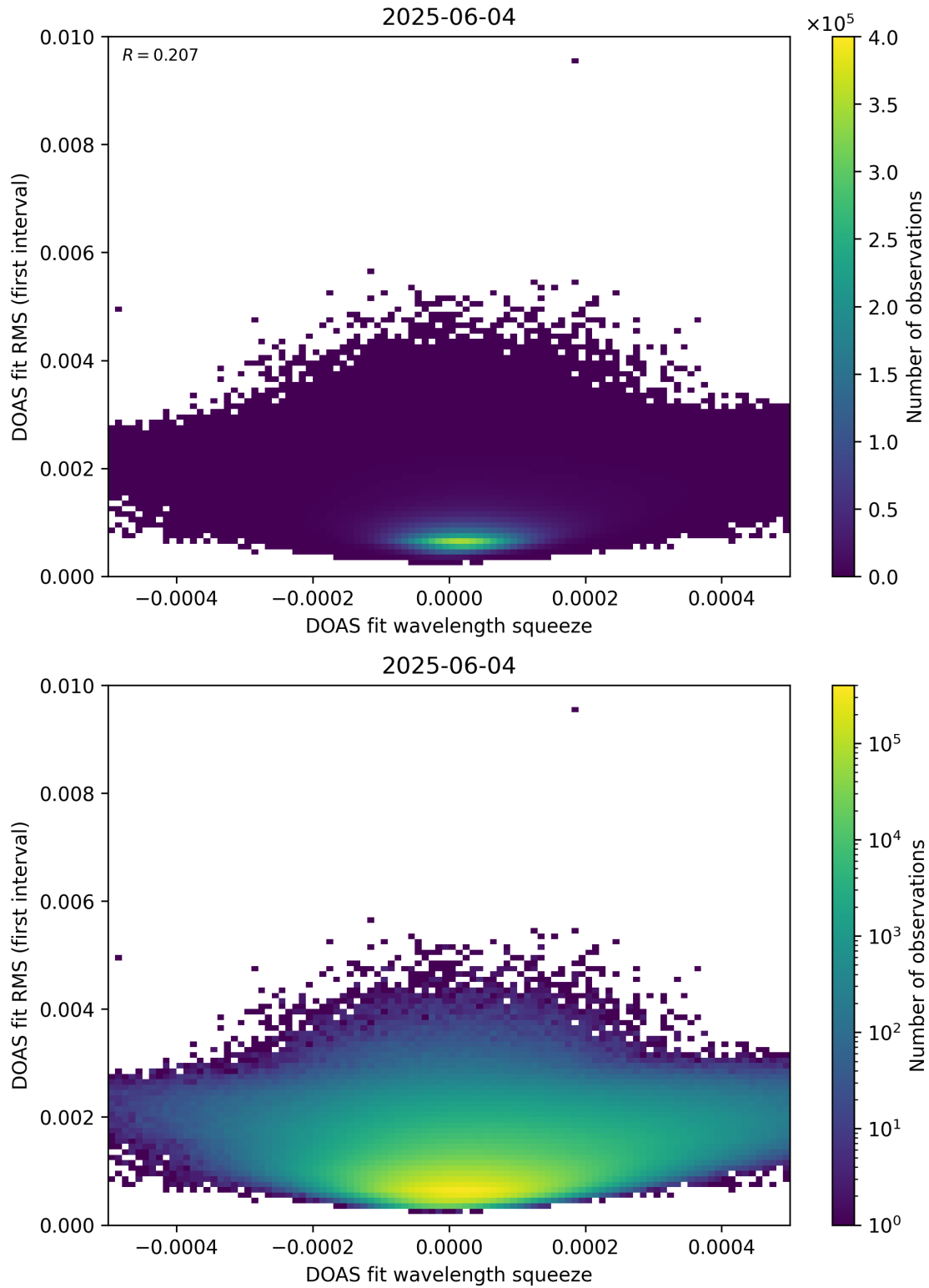
Figure 68: Scatter density plot of “DOAS fit wavelength squeeze” against “DOAS fit RMS (first interval)” for 2025-06-03 to 2025-06-05.
