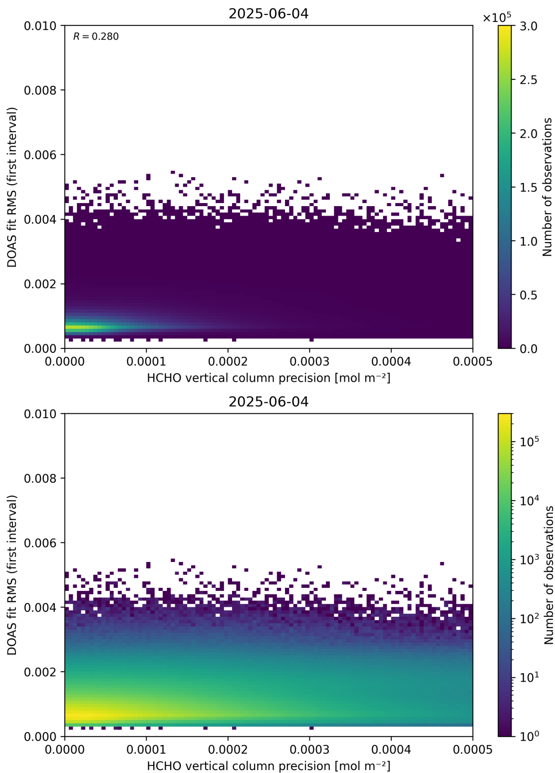
Figure 136: Scatter density plot of “HCHO vertical column precision” against “DOAS fit RMS (first interval)” for 2025-06-03 to 2025-06-05.
