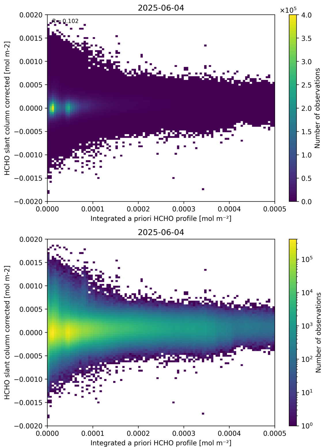
Figure 151: Scatter density plot of “Integrated a priori HCHO profile” against “HCHO slant column corrected” for 2025-06-03 to 2025-06-05.
