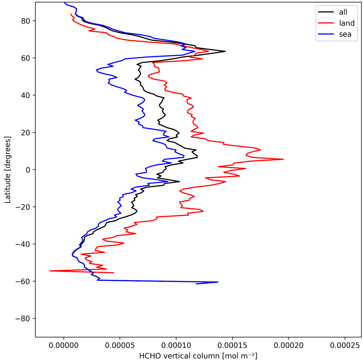
Figure 21: Zonal average of “HCHO vertical column” for 2025-06-03 to 2025-06-05.
