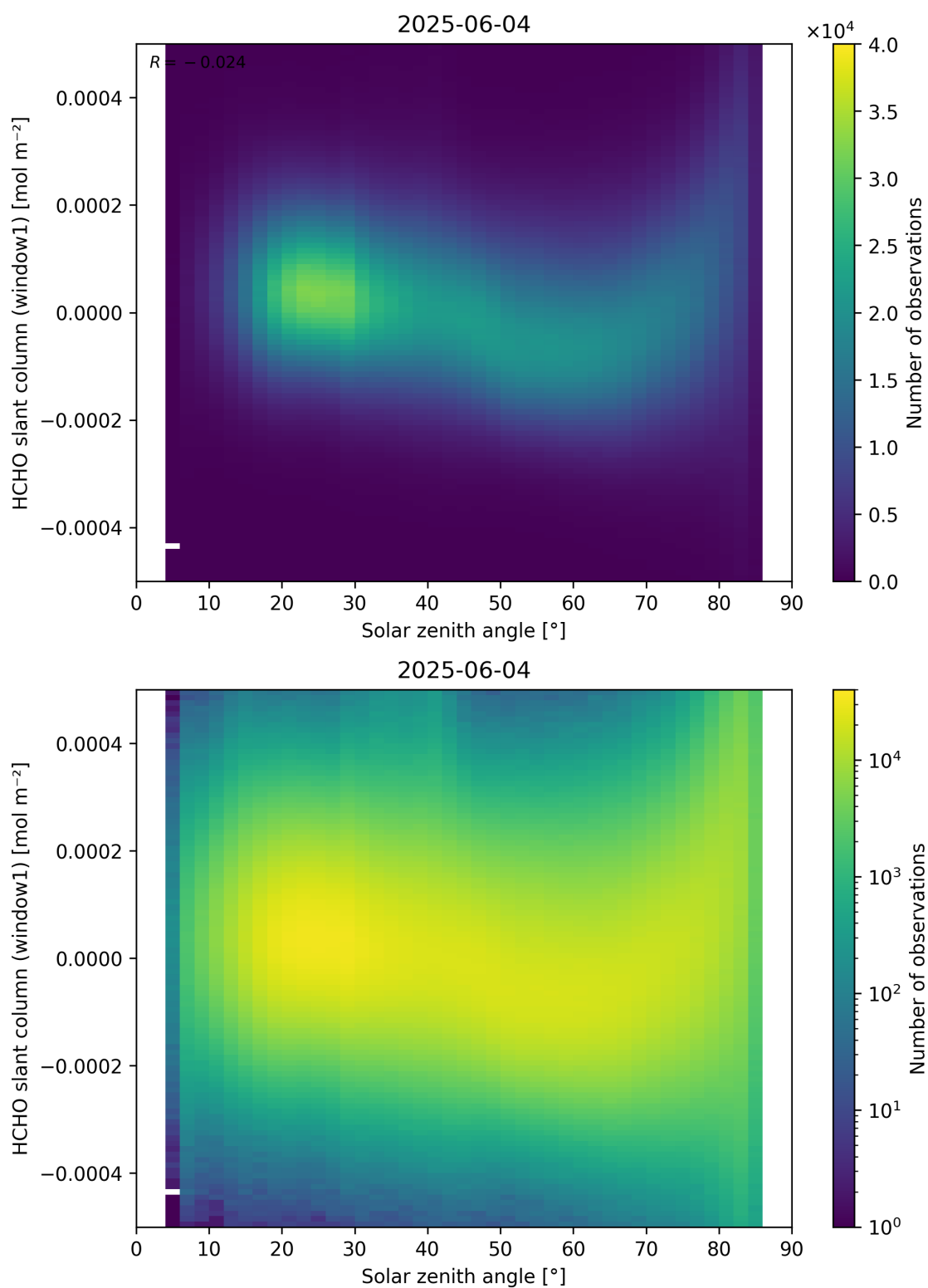
Figure 173: Scatter density plot of “Solar zenith angle” against “HCHO slant column (window1)” for 2025-06-03 to 2025-06-05.
