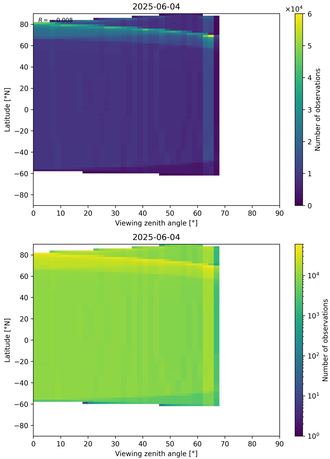
Figure 196: Scatter density plot of “Viewing zenith angle” against “Latitude” for 2025-06-03 to 2025-06-05.
