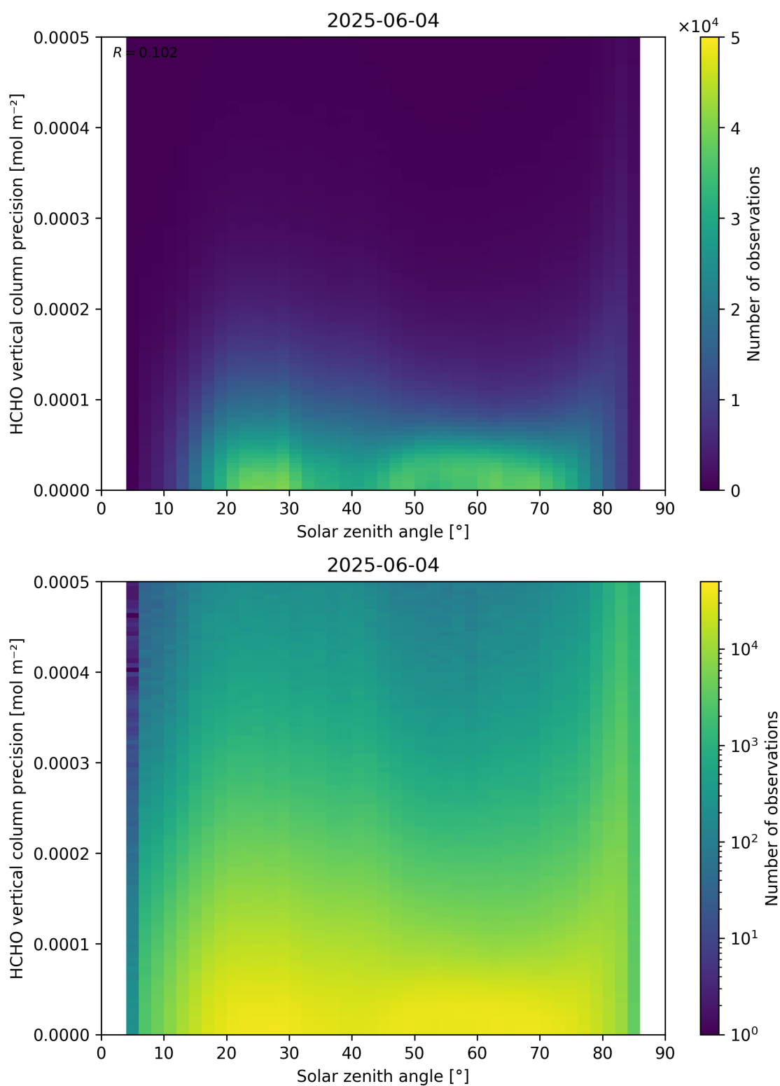
Figure 179: Scatter density plot of “Solar zenith angle” against “HCHO vertical column precision” for 2025-06-03 to 2025-06-05.
