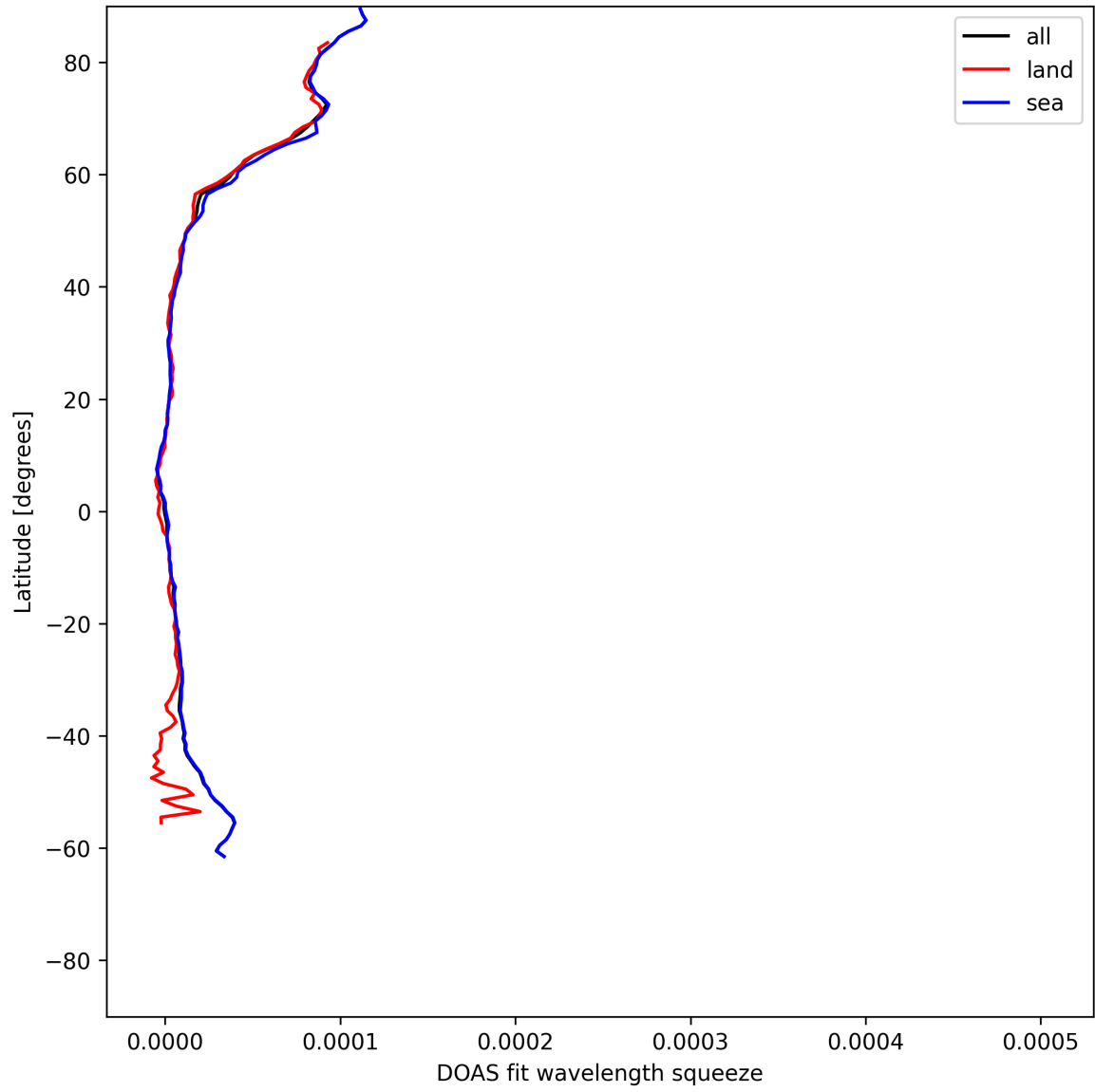
Figure 31: Zonal average of “DOAS fit wavelength squeeze” for 2025-06-03 to 2025-06-05.
