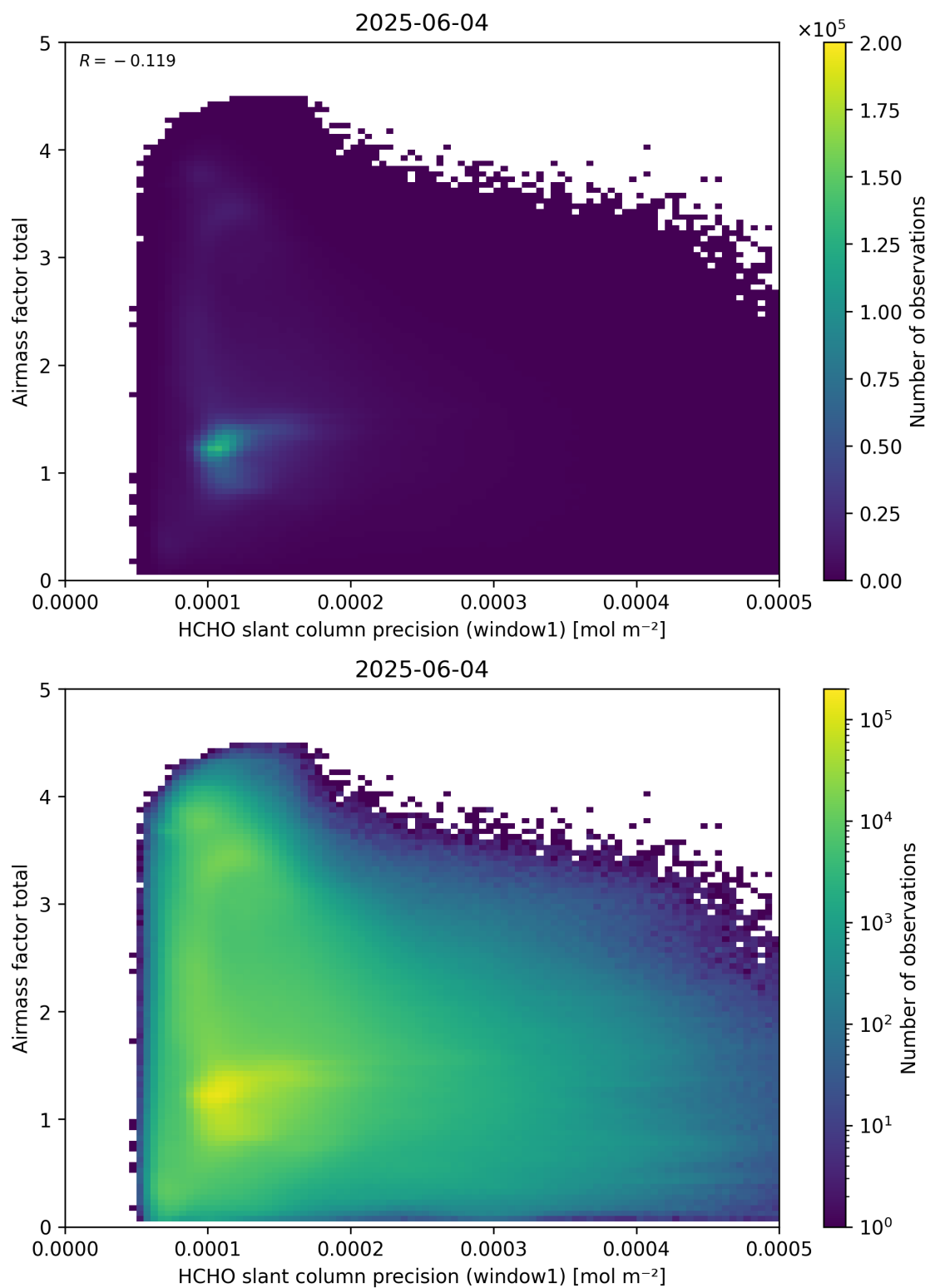
Figure 94: Scatter density plot of “HCHO slant column precision (window1)” against “Airmass factor total” for 2025-06-03 to 2025-06-05.
