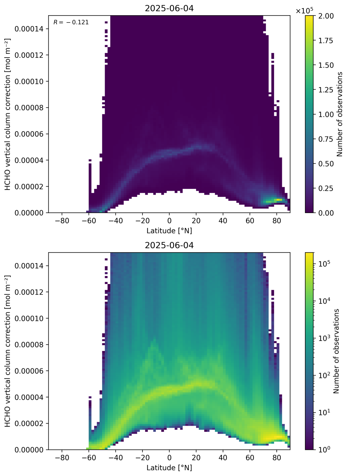
Figure 164: Scatter density plot of “Latitude” against “HCHO vertical column correction” for 2025-06-03 to 2025-06-05.
