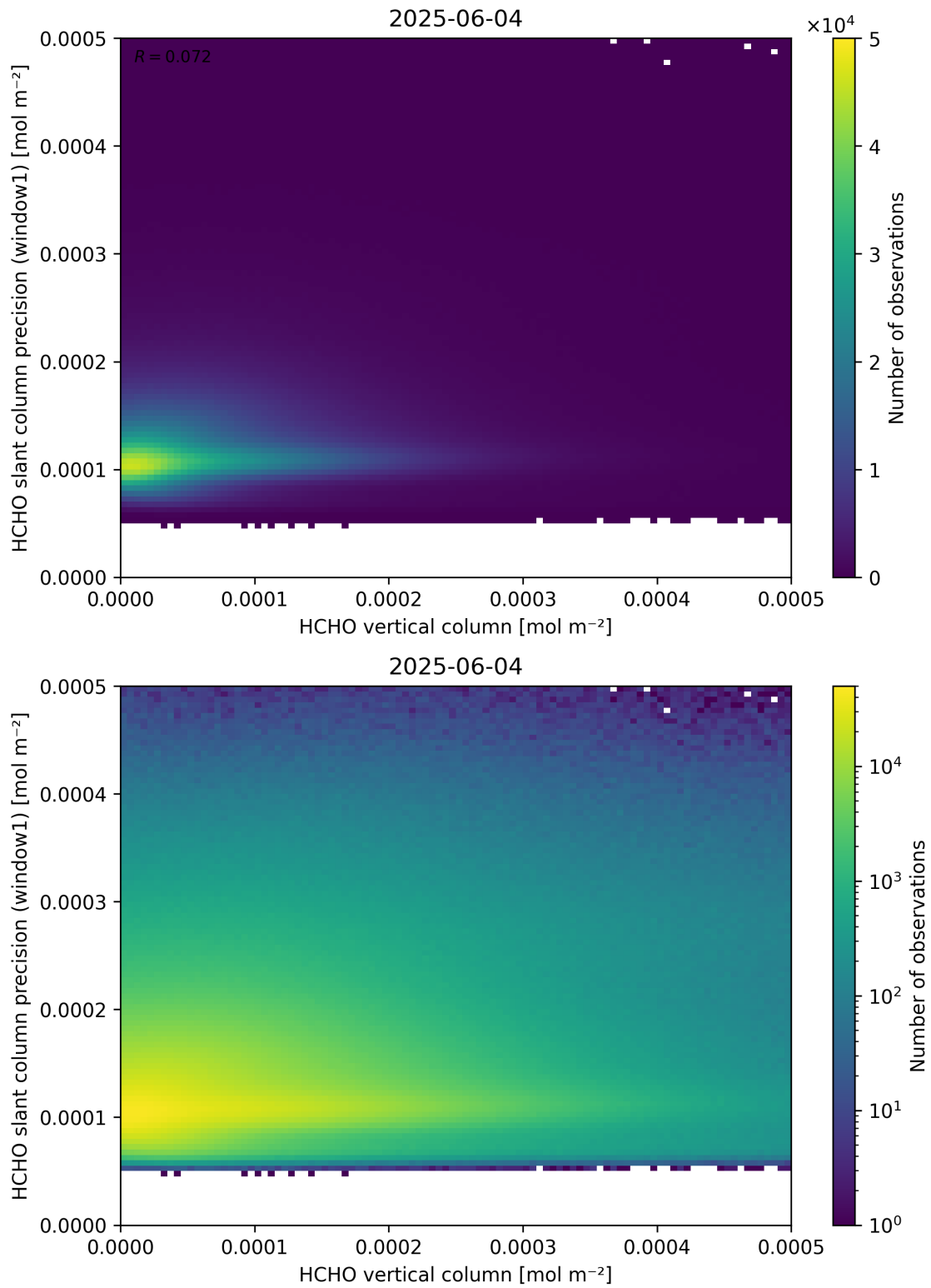
Figure 130: Scatter density plot of “HCHO vertical column” against “HCHO slant column precision (window1)” for 2025-06-03 to 2025-06-05.
