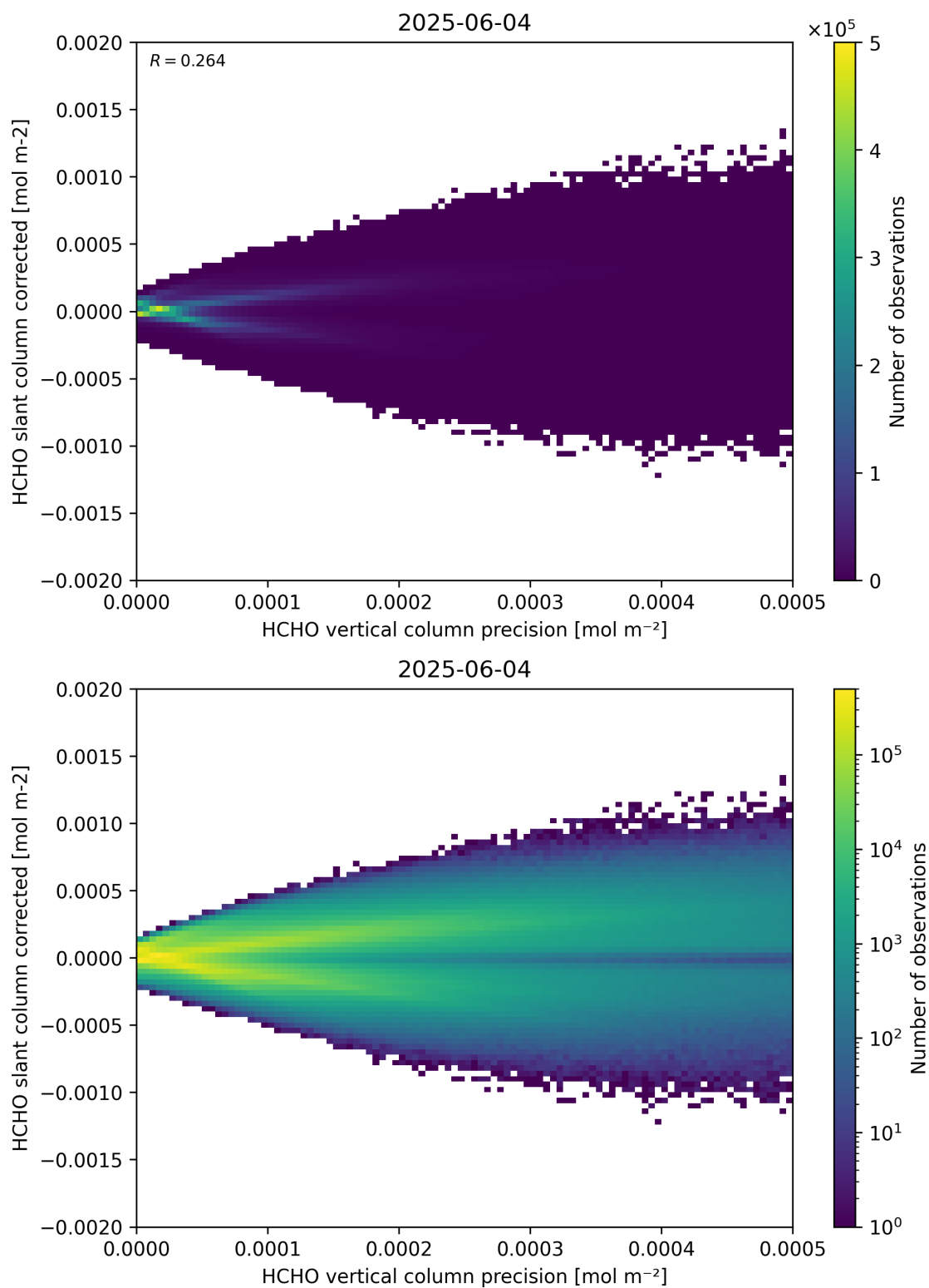
Figure 140: Scatter density plot of “HCHO vertical column precision” against “HCHO slant column corrected” for 2025-06-03 to 2025-06-05.
