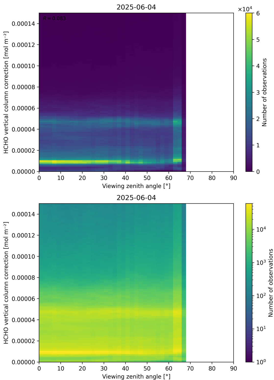
Figure 193: Scatter density plot of “Viewing zenith angle” against “HCHO vertical column correction” for 2025-06-03 to 2025-06-05.
