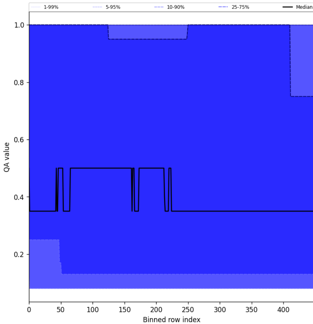
Figure 48: Along track statistics of “QA value” for 2025-06-03 to 2025-06-05
