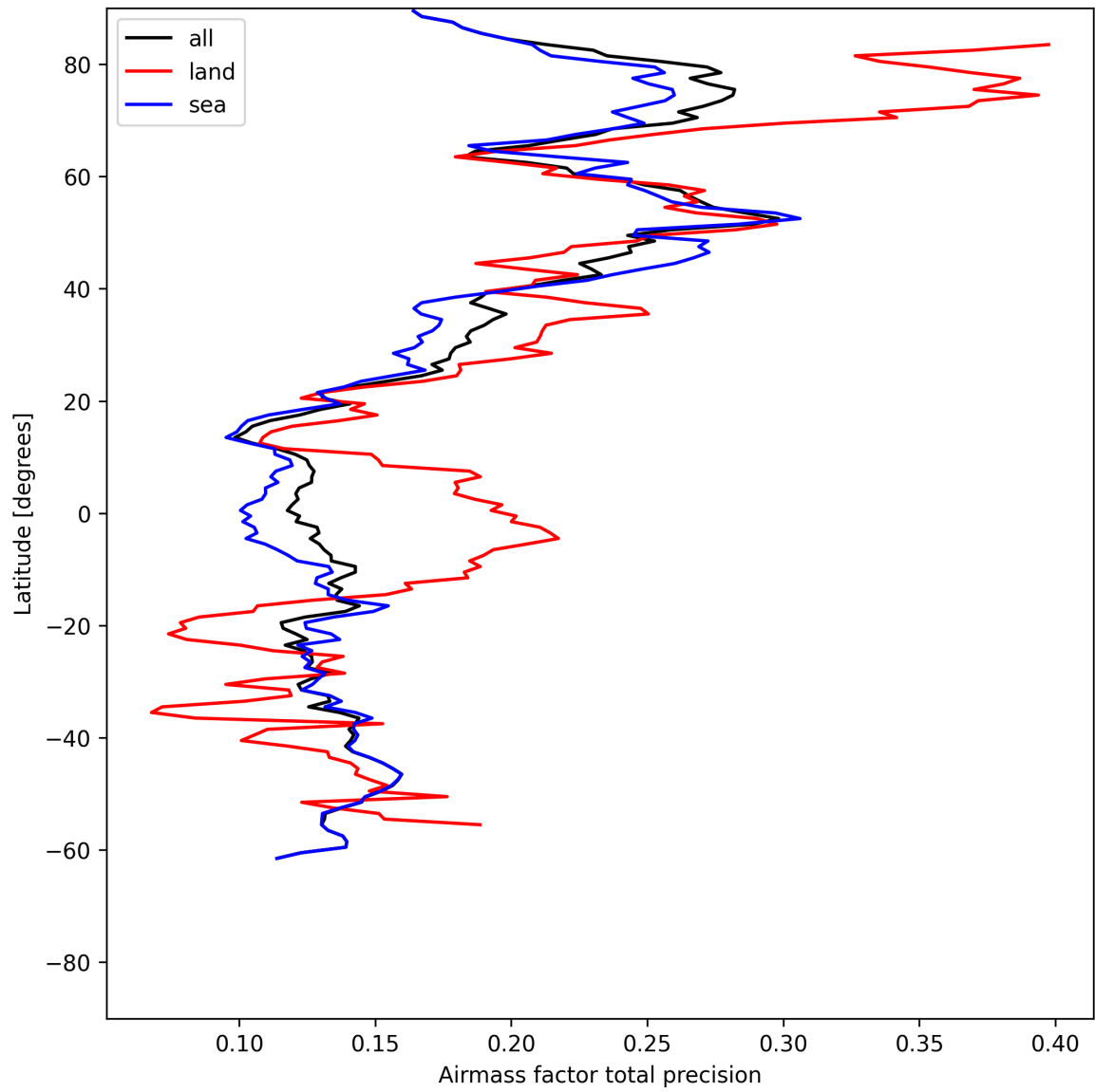
Figure 27: Zonal average of “Airmass factor total precision” for 2025-06-03 to 2025-06-05.
