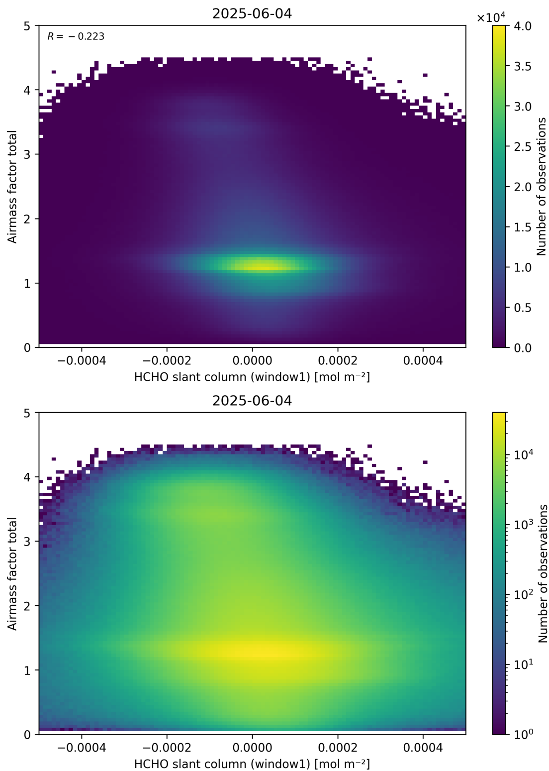
Figure 85: Scatter density plot of “HCHO slant column (window1)” against “Airmass factor total” for 2025-06-03 to 2025-06-05.
