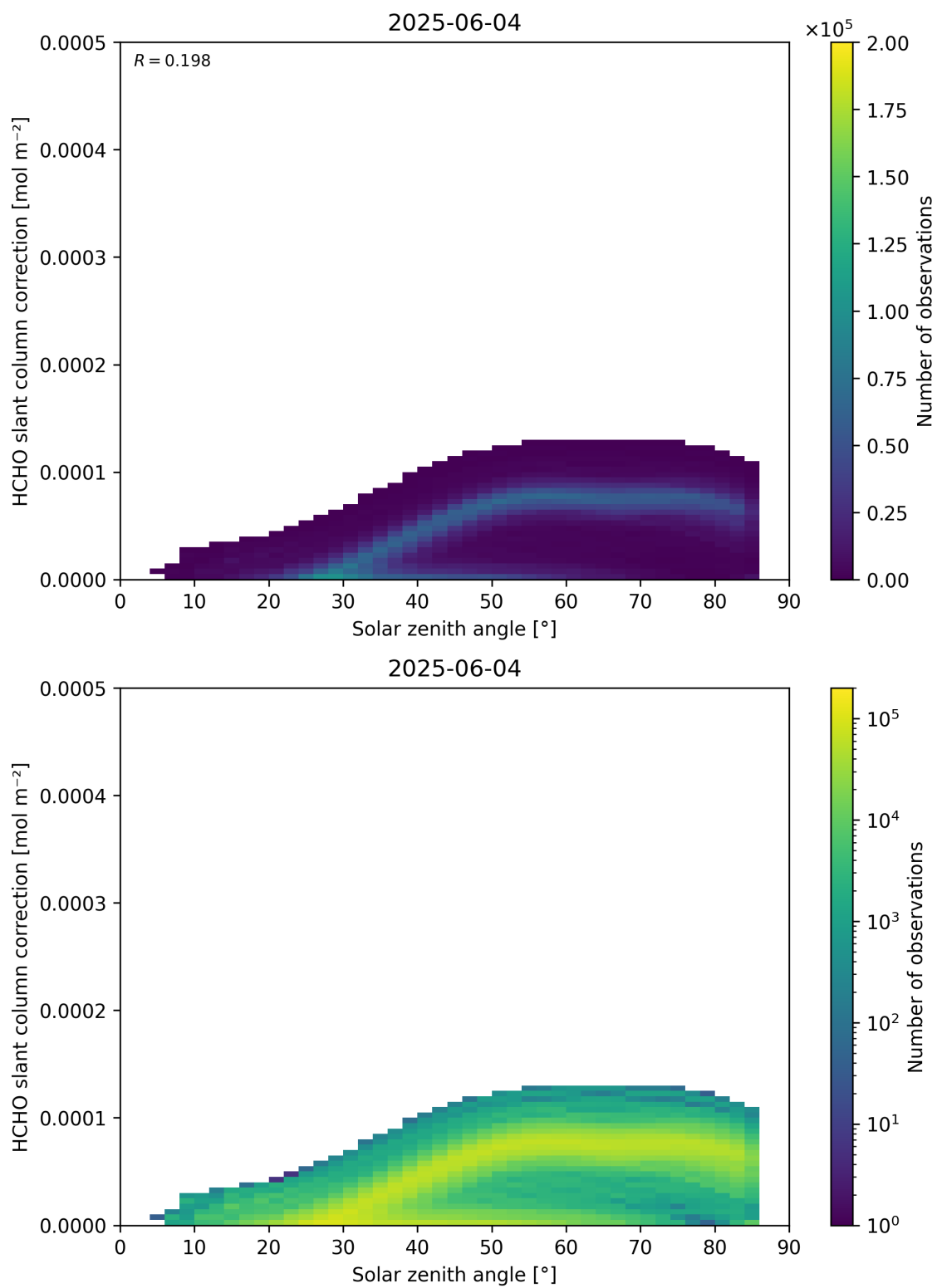
Figure 172: Scatter density plot of “Solar zenith angle” against “HCHO slant column correction” for 2025-06-03 to 2025-06-05.
