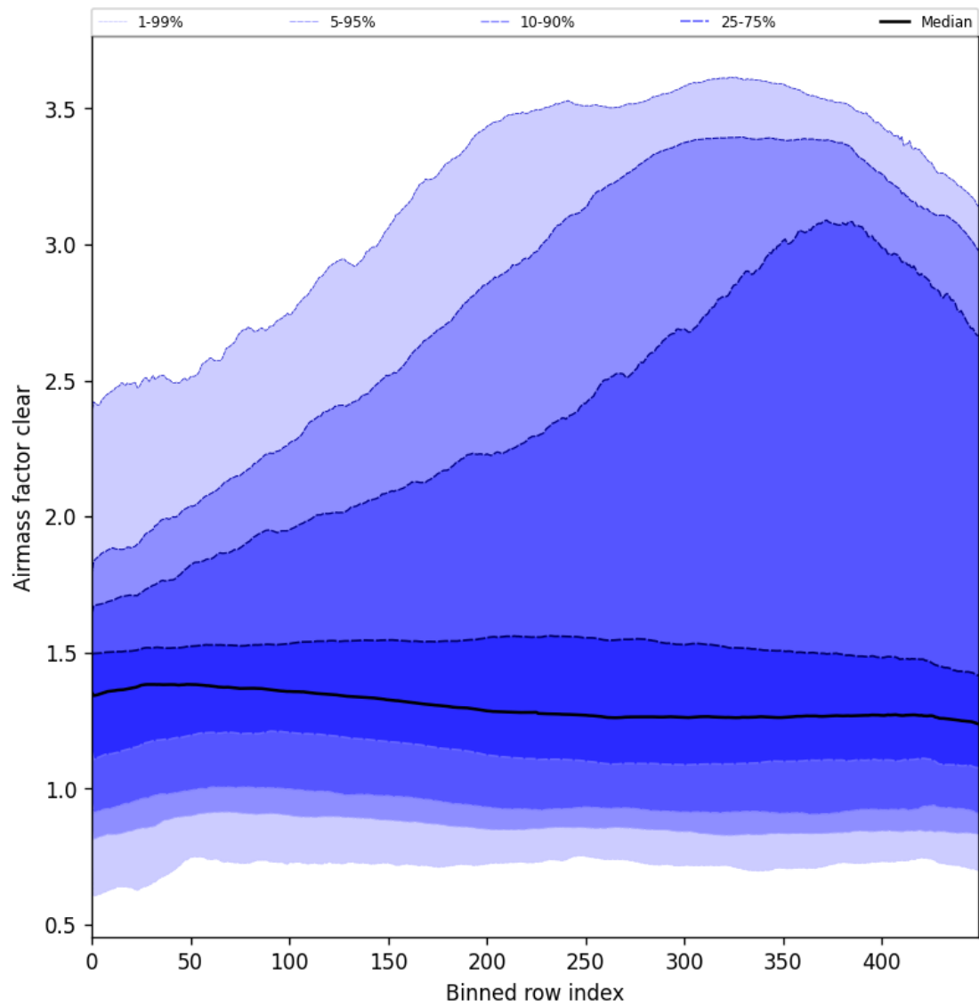
Figure 56: Along track statistics of “Air mass factor clear” for 2025-06-03 to 2025-06-05
