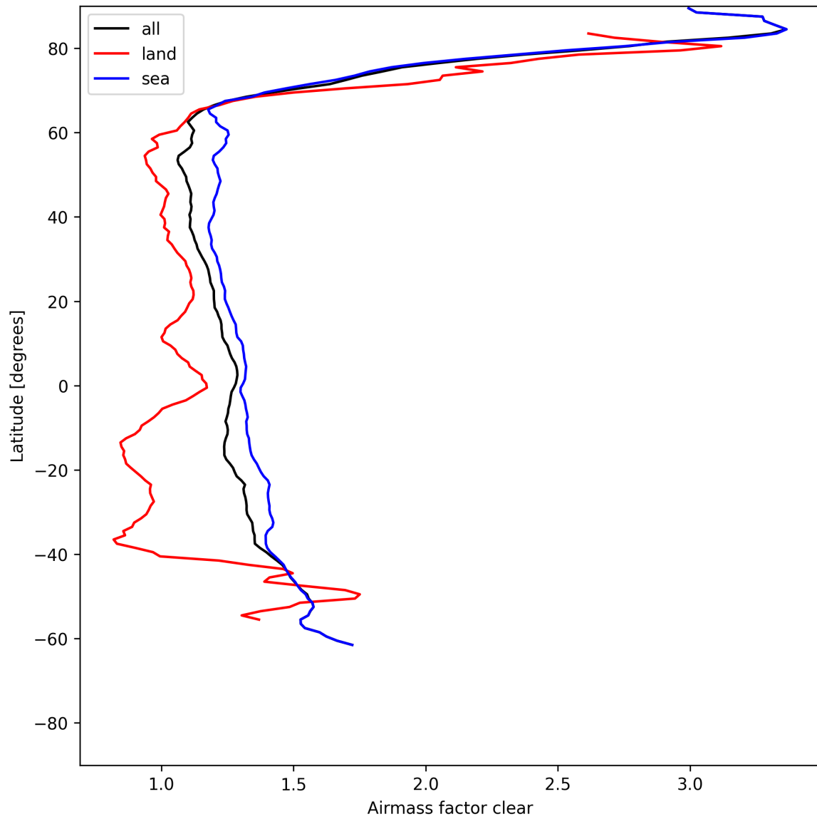
Figure 28: Zonal average of “Airmass factor clear” for 2025-06-03 to 2025-06-05.
