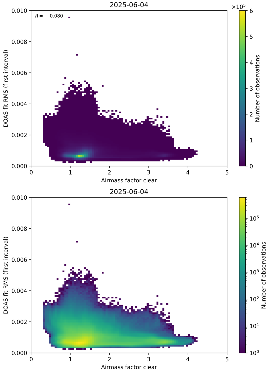
Figure 71: Scatter density plot of “Airmass factor clear” against “DOAS fit RMS (first interval)” for 2025-06-03 to 2025-06-05.
