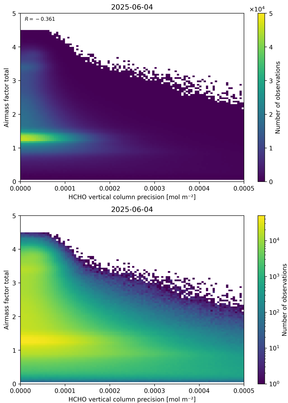
Figure 144: Scatter density plot of “HCHO vertical column precision” against “Airmass factor total” for 2025-06-03 to 2025-06-05.
