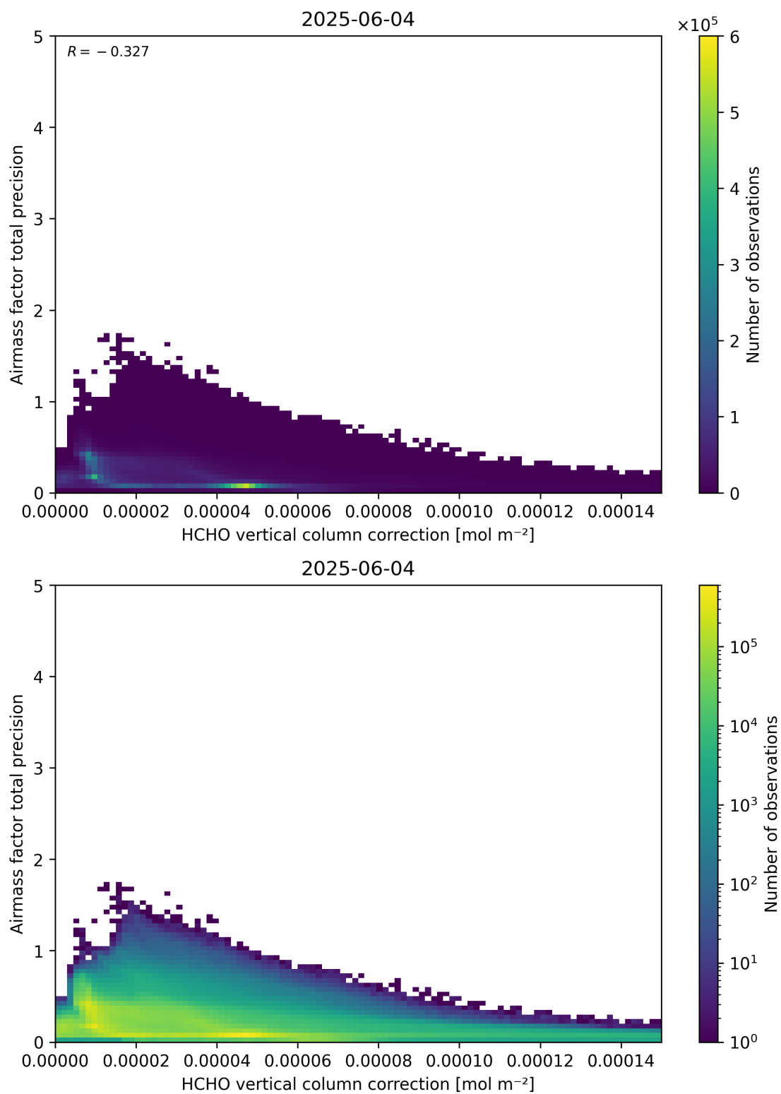
Figure 121: Scatter density plot of “HCHO vertical column correction” against “Airmass factor total precision” for 2025-06-03 to 2025-06-05.
