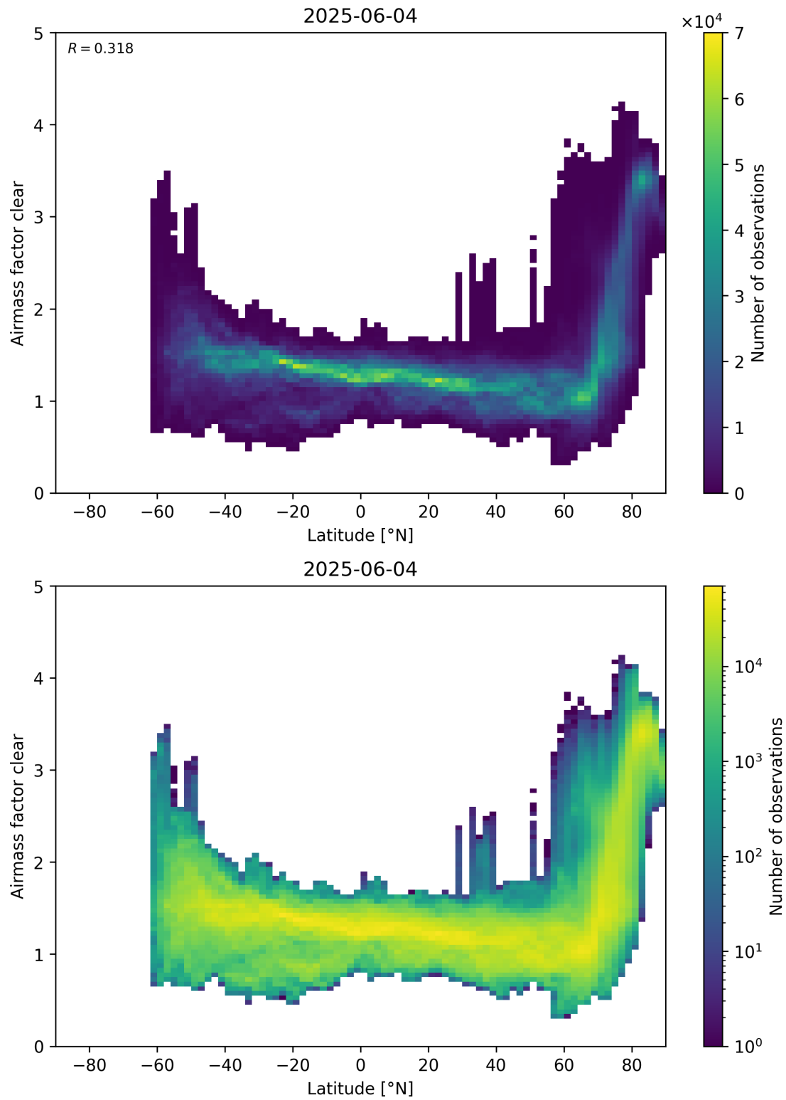
Figure 156: Scatter density plot of “Latitude” against “Airmass factor clear” for 2025-06-03 to 2025-06-05.
