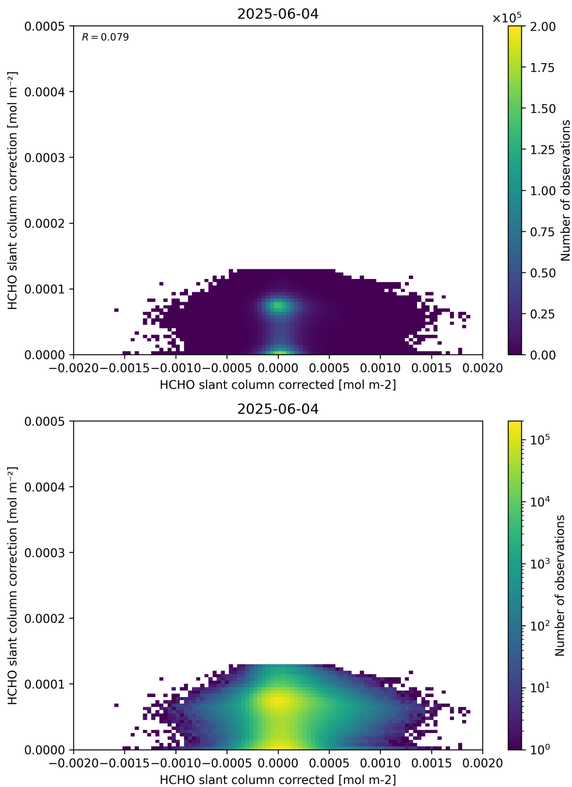
Figure 77: Scatter density plot of “HCHO slant column corrected” against “HCHO slant column correction” for 2025-06-03 to 2025-06-05.
