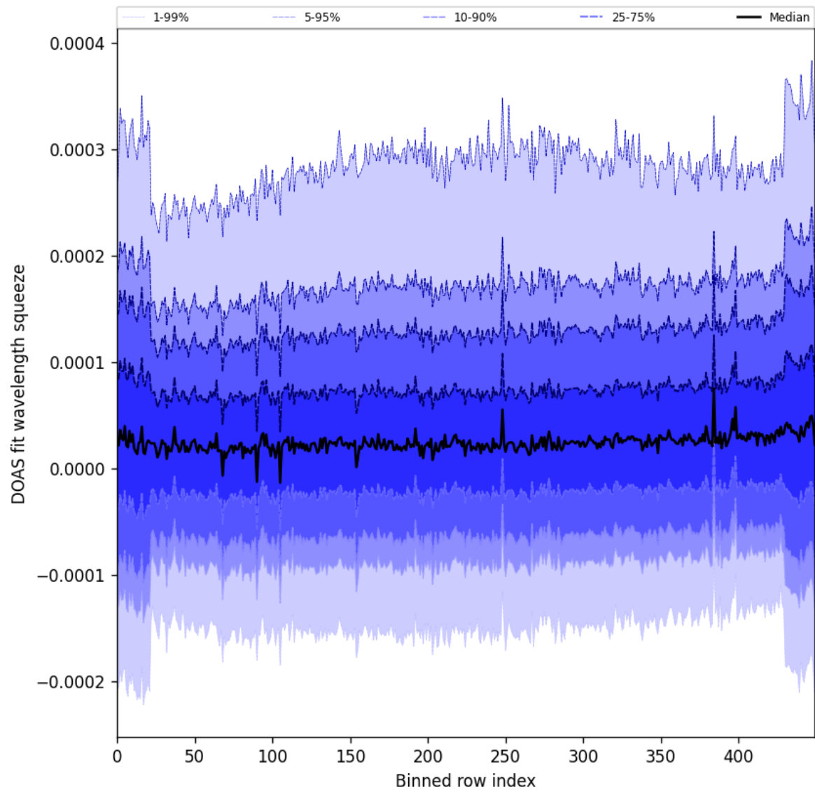
Figure 59: Along track statistics of “DOAS fit wavelength squeeze” for 2025-06-03 to 2025-06-05
