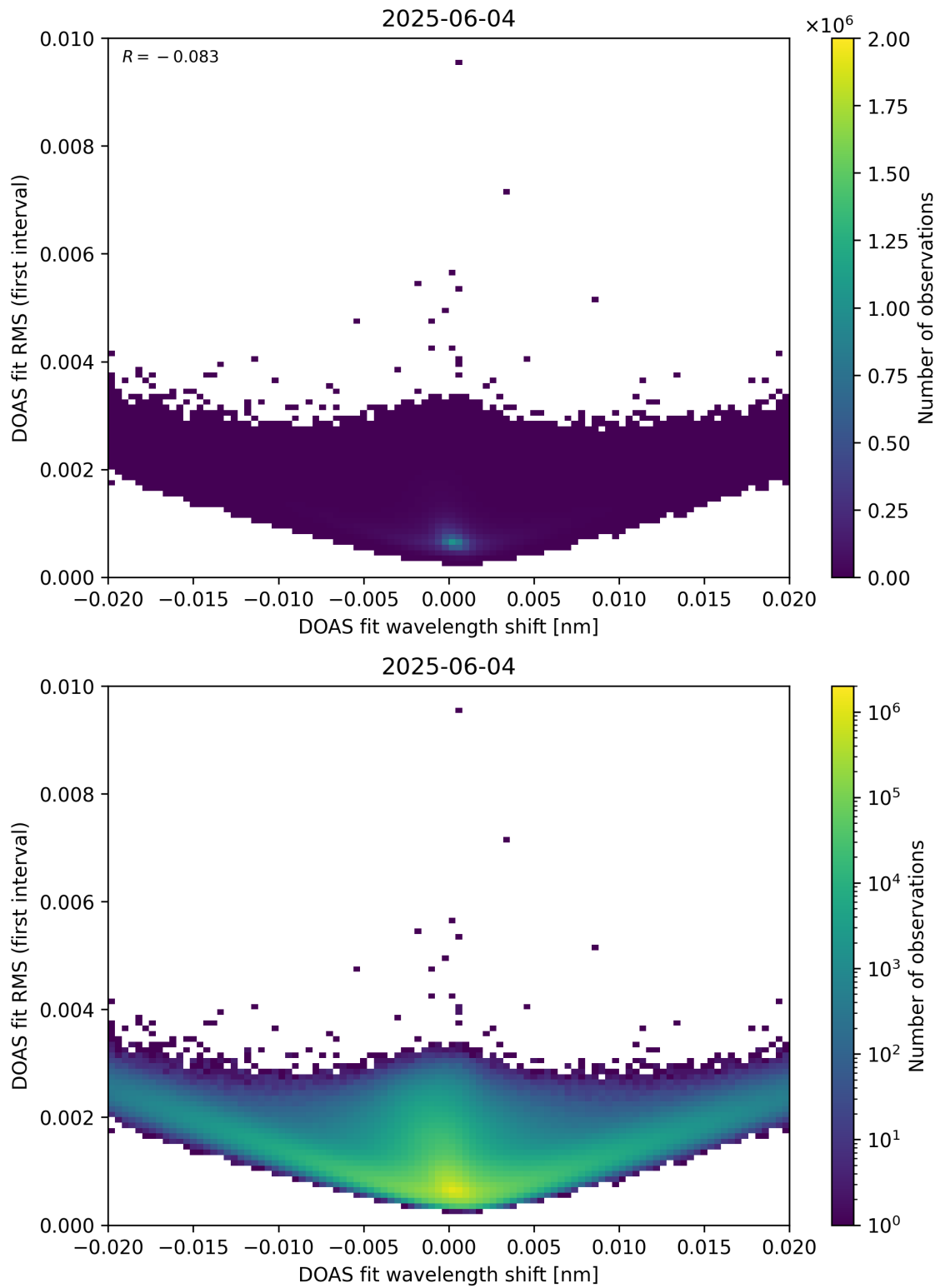
Figure 64: Scatter density plot of “DOAS fit wavelength shift” against “DOAS fit RMS (first interval)” for 2025-06-03 to 2025-06-05.
