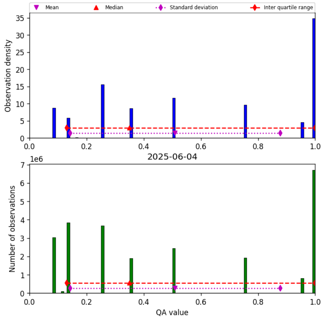
Figure 34: Histogram of “QA value” for 2025-06-03 to 2025-06-05
