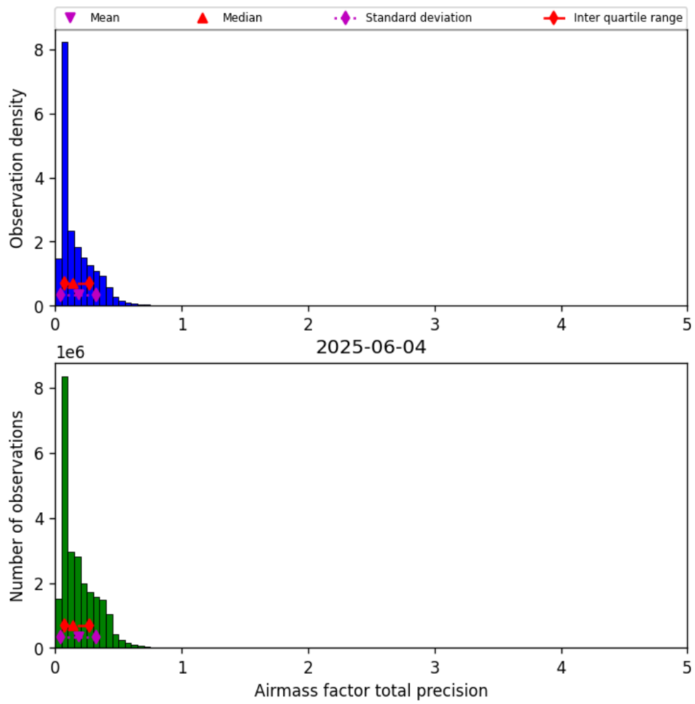
Figure 41: Histogram of “Airmass factor total precision” for 2025-06-03 to 2025-06-05
