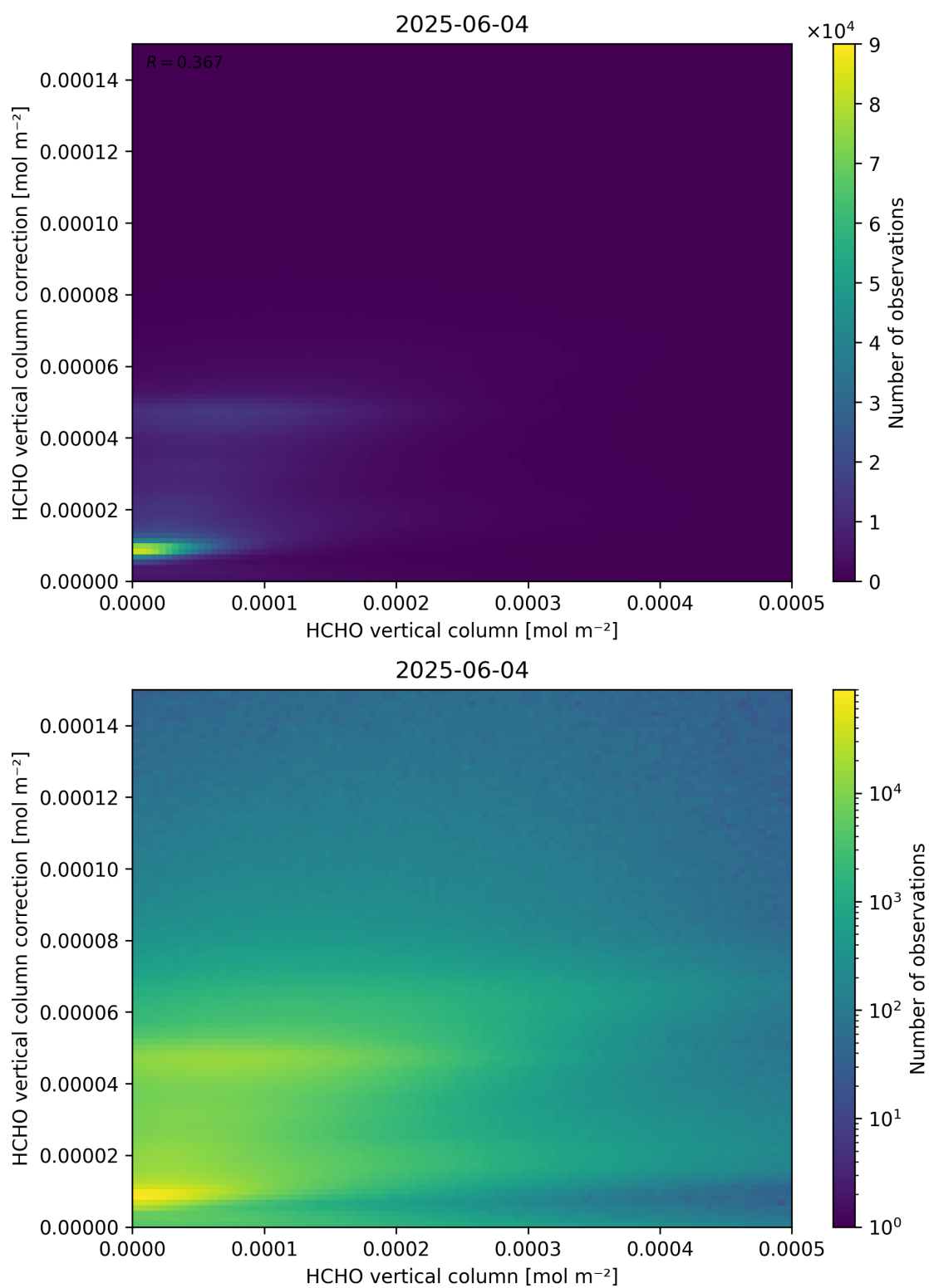
Figure 133: Scatter density plot of “HCHO vertical column” against “HCHO vertical column correction” for 2025-06-03 to 2025-06-05.
