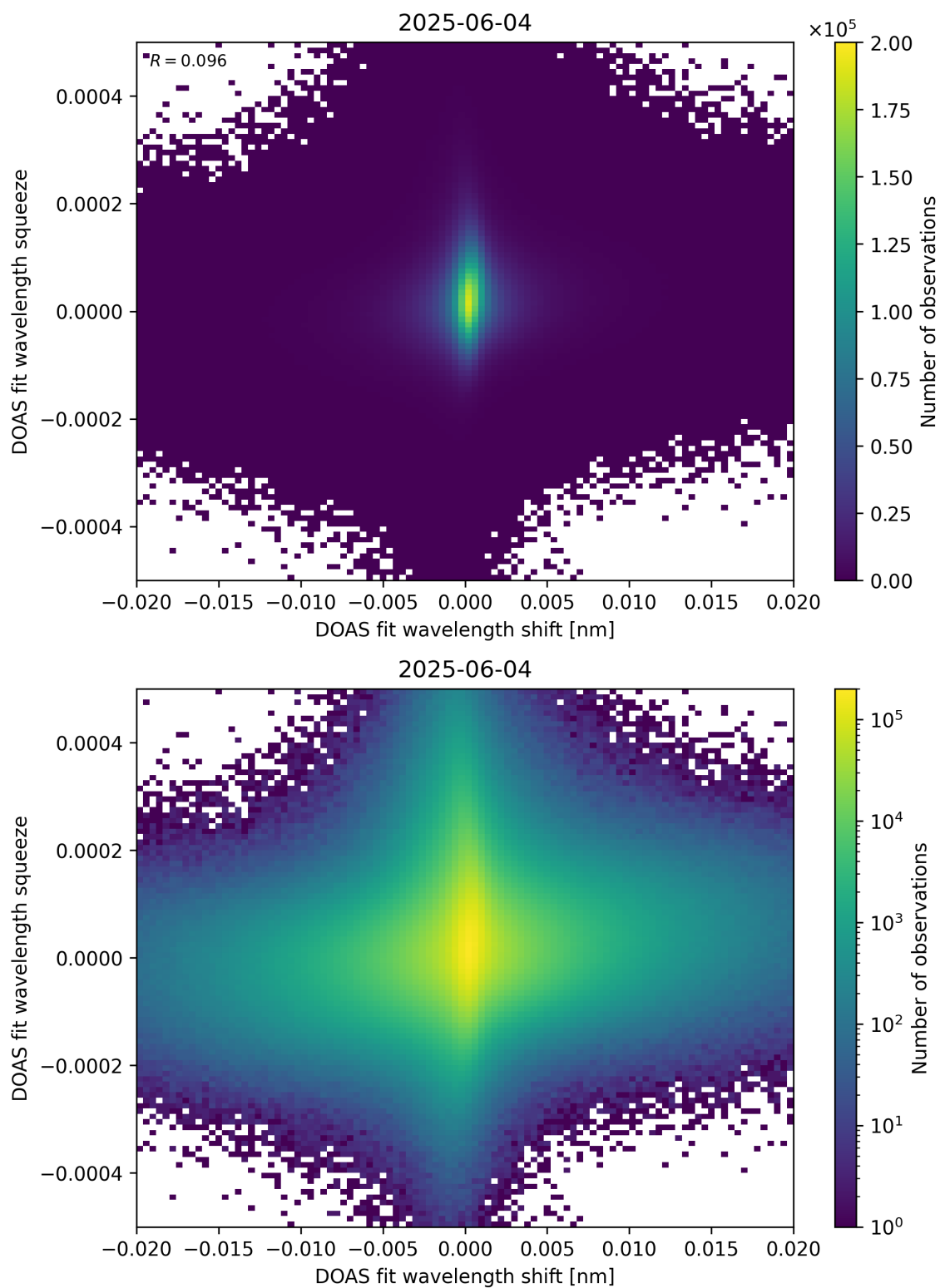
Figure 65: Scatter density plot of “DOAS fit wavelength shift” against “DOAS fit wavelength squeeze” for 2025-06-03 to 2025-06-05.
