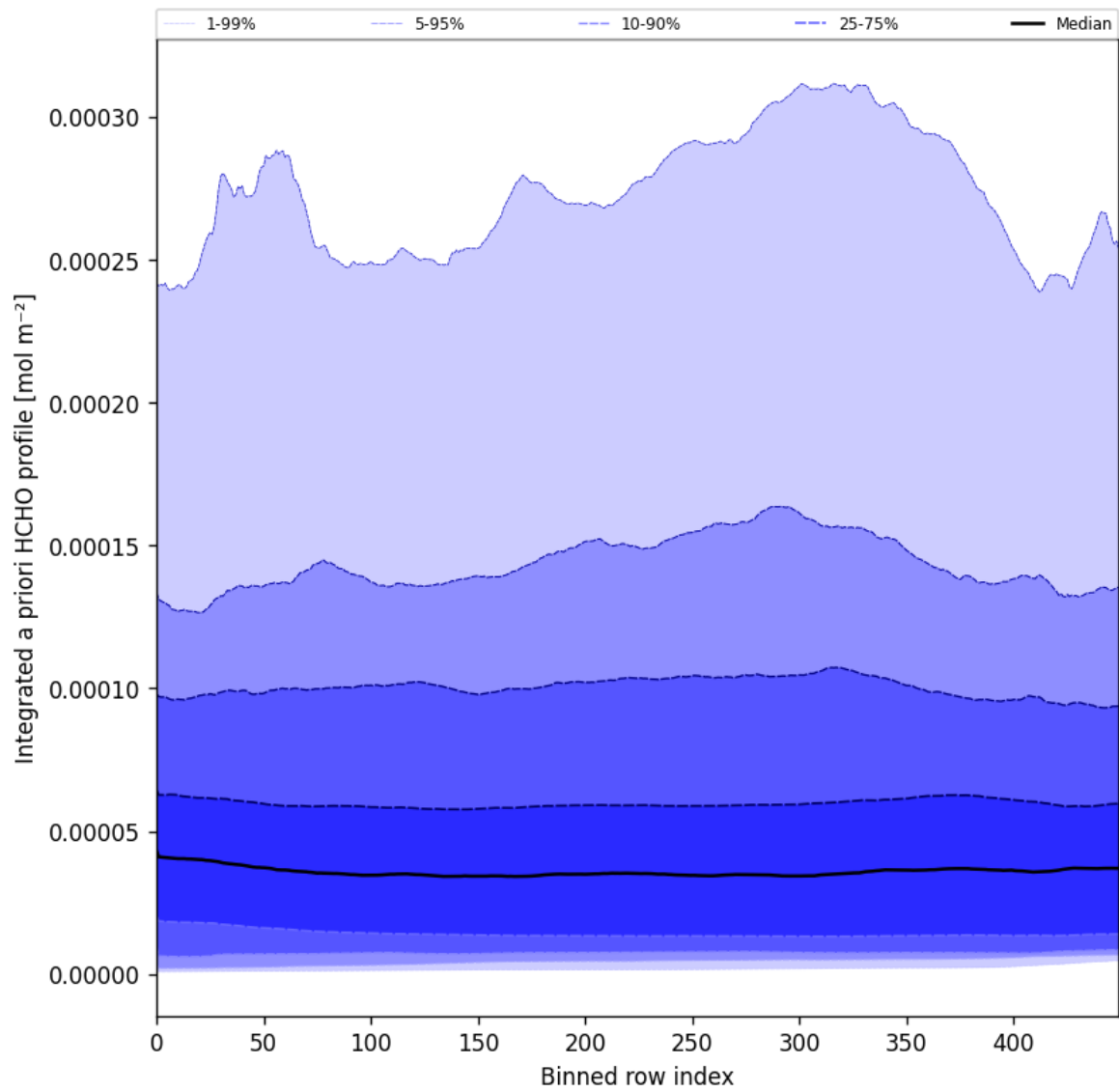
Figure 57: Along track statistics of “Integrated a priori HCHO profile” for 2025-06-03 to 2025-06-05
