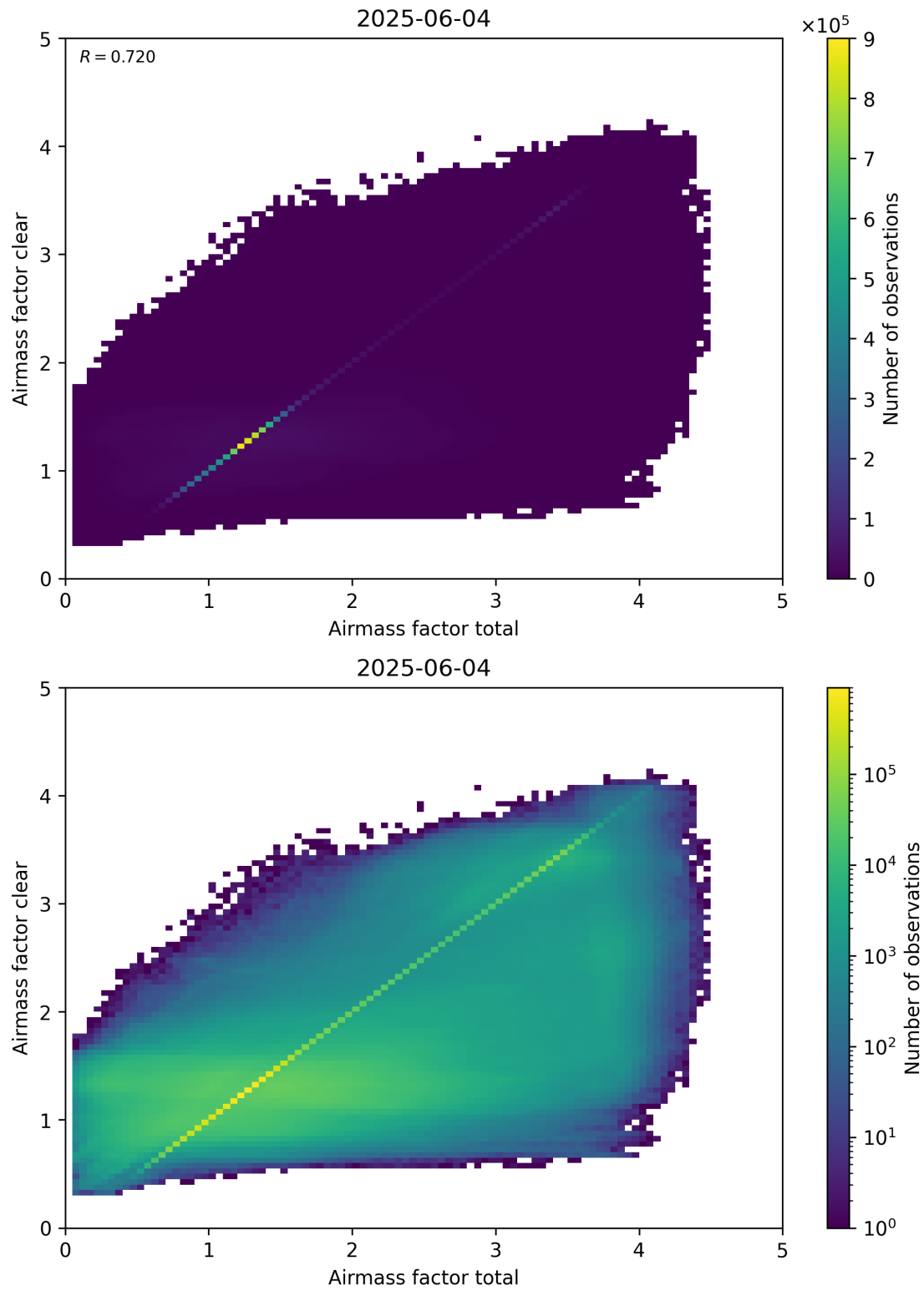
Figure 100: Scatter density plot of “Airmass factor total” against “Airmass factor clear” for 2025-06-03 to 2025-06-05.
