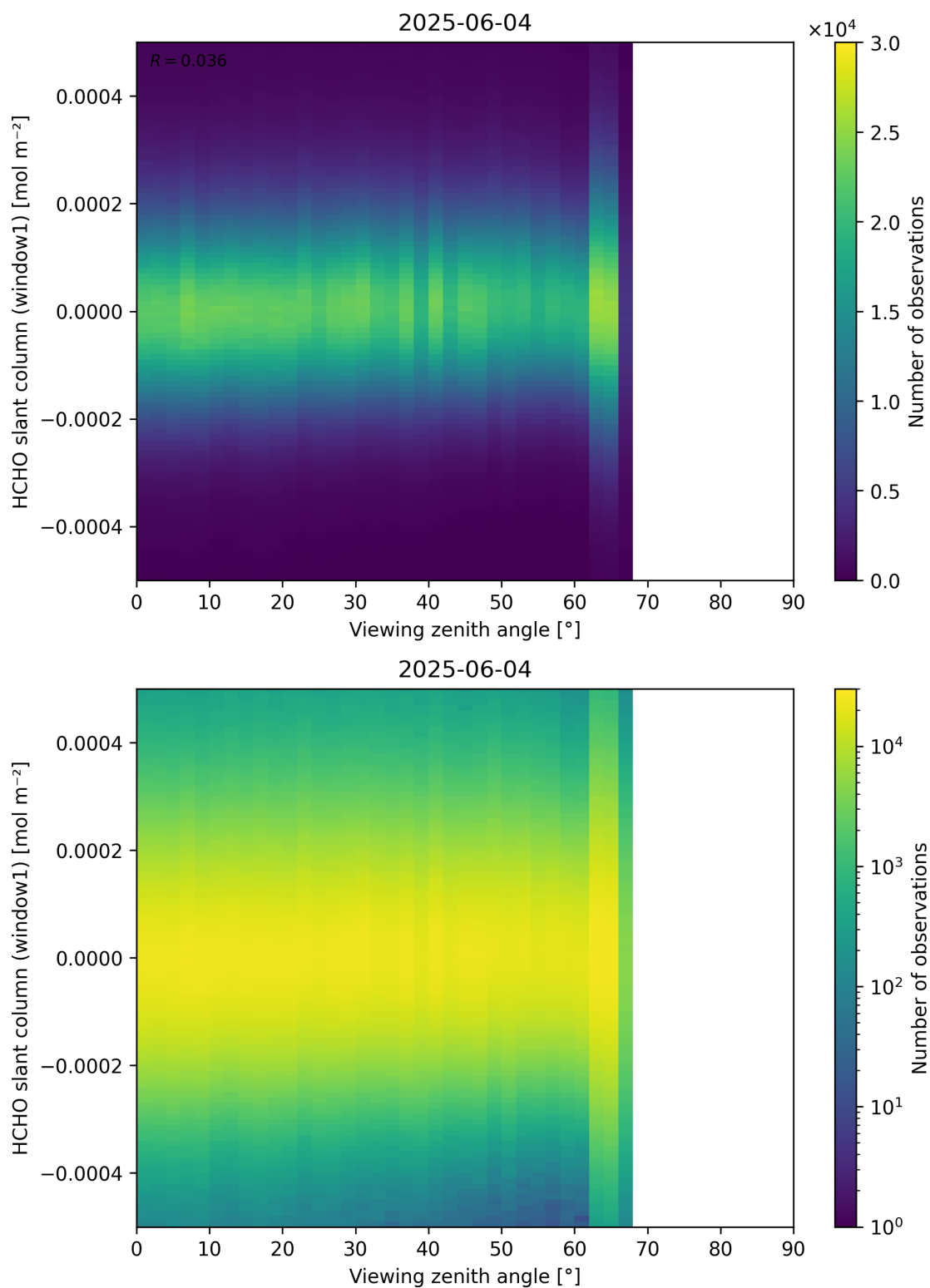
Figure 188: Scatter density plot of “Viewing zenith angle” against “HCHO slant column (window1)” for 2025-06-03 to 2025-06-05.
