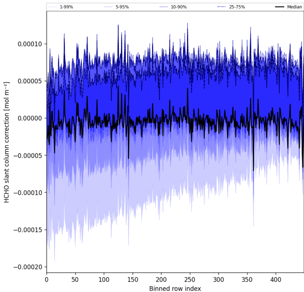
Figure 61: Along track statistics of “HCHO slant column correction” for 2025-06-03 to 2025-06-05
