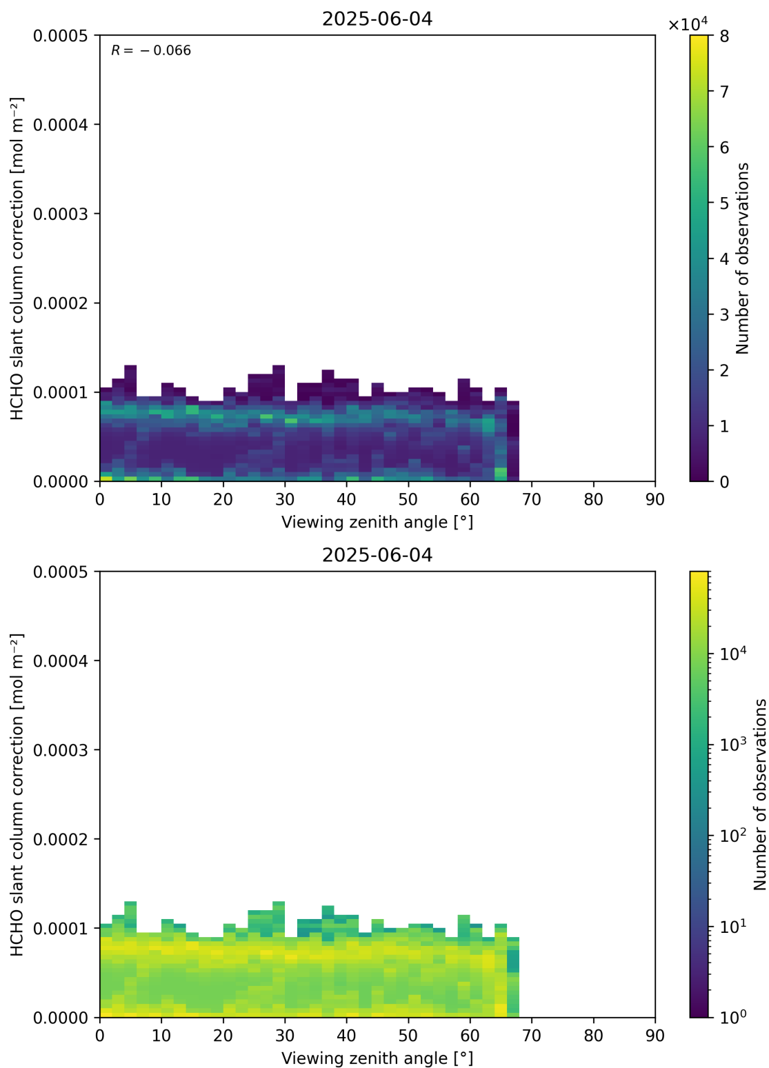
Figure 187: Scatter density plot of “Viewing zenith angle” against “HCHO slant column correction” for 2025-06-03 to 2025-06-05.
