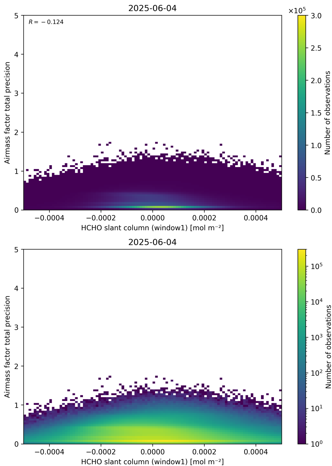
Figure 86: Scatter density plot of “HCHO slant column (window1)” against “Airmass factor total precision” for 2025-06-03 to 2025-06-05.
