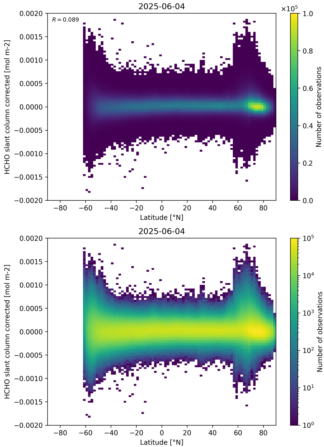
Figure 157: Scatter density plot of “Latitude” against “HCHO slant column corrected” for 2025-06-03 to 2025-06-05.
