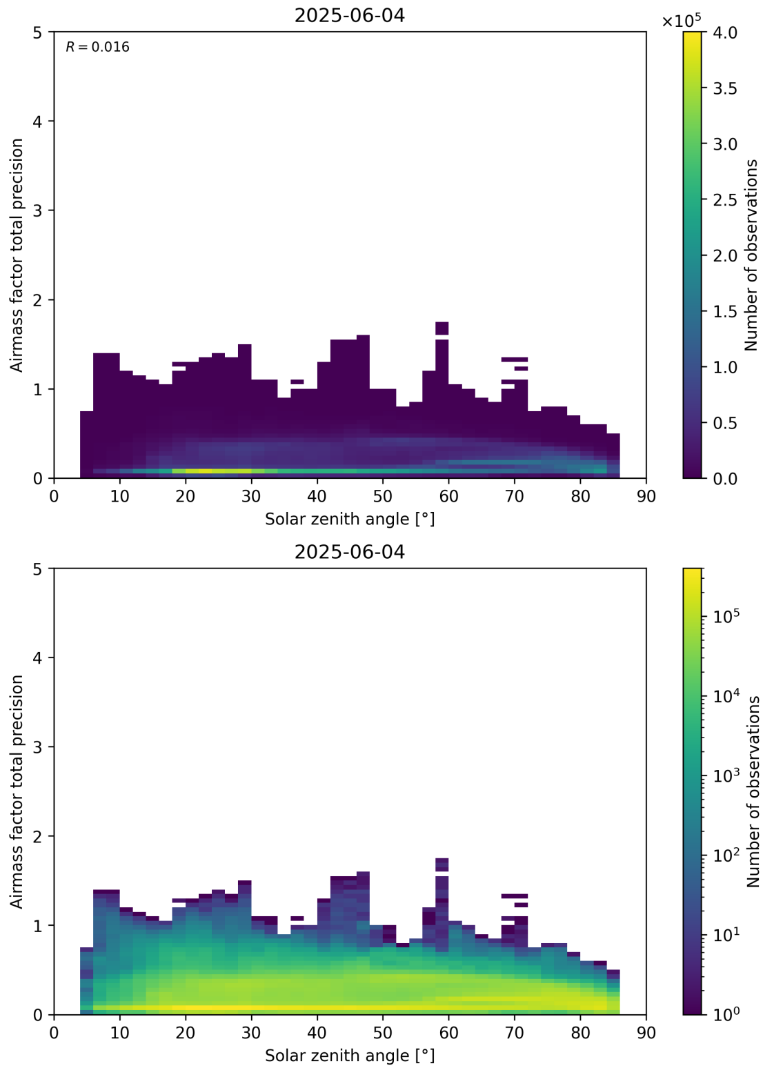
Figure 176: Scatter density plot of “Solar zenith angle” against “Airmass factor total precision” for 2025-06-03 to 2025-06-05.
