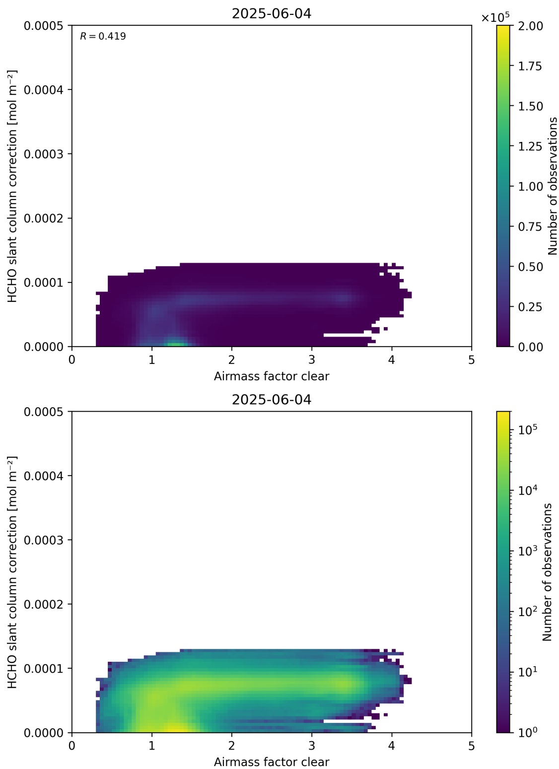
Figure 75: Scatter density plot of “Airmass factor clear” against “HCHO slant column correction” for 2025-06-03 to 2025-06-05.
