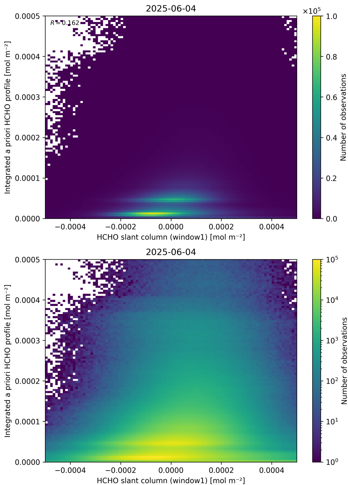
Figure 87: Scatter density plot of “HCHO slant column (window1)” against “Integrated a priori HCHO profile” for 2025-06-03 to 2025-06-05.
