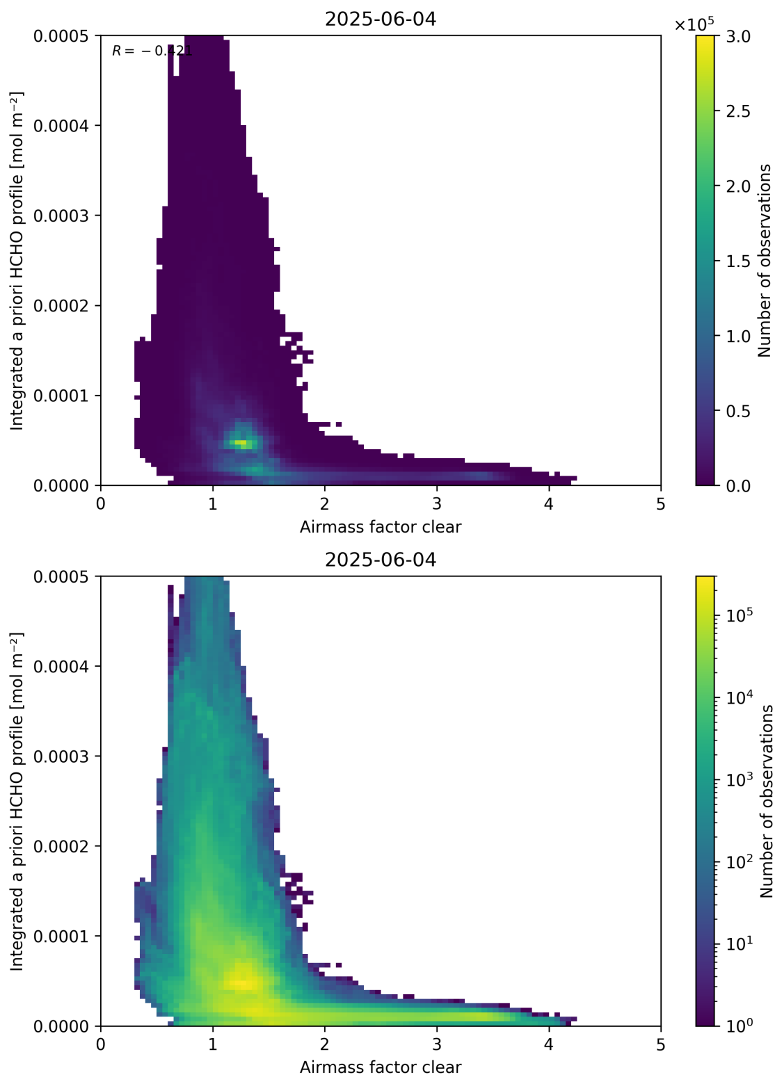
Figure 76: Scatter density plot of “Airmass factor clear” against “Integrated a priori HCHO profile” for 2025-06-03 to 2025-06-05.
