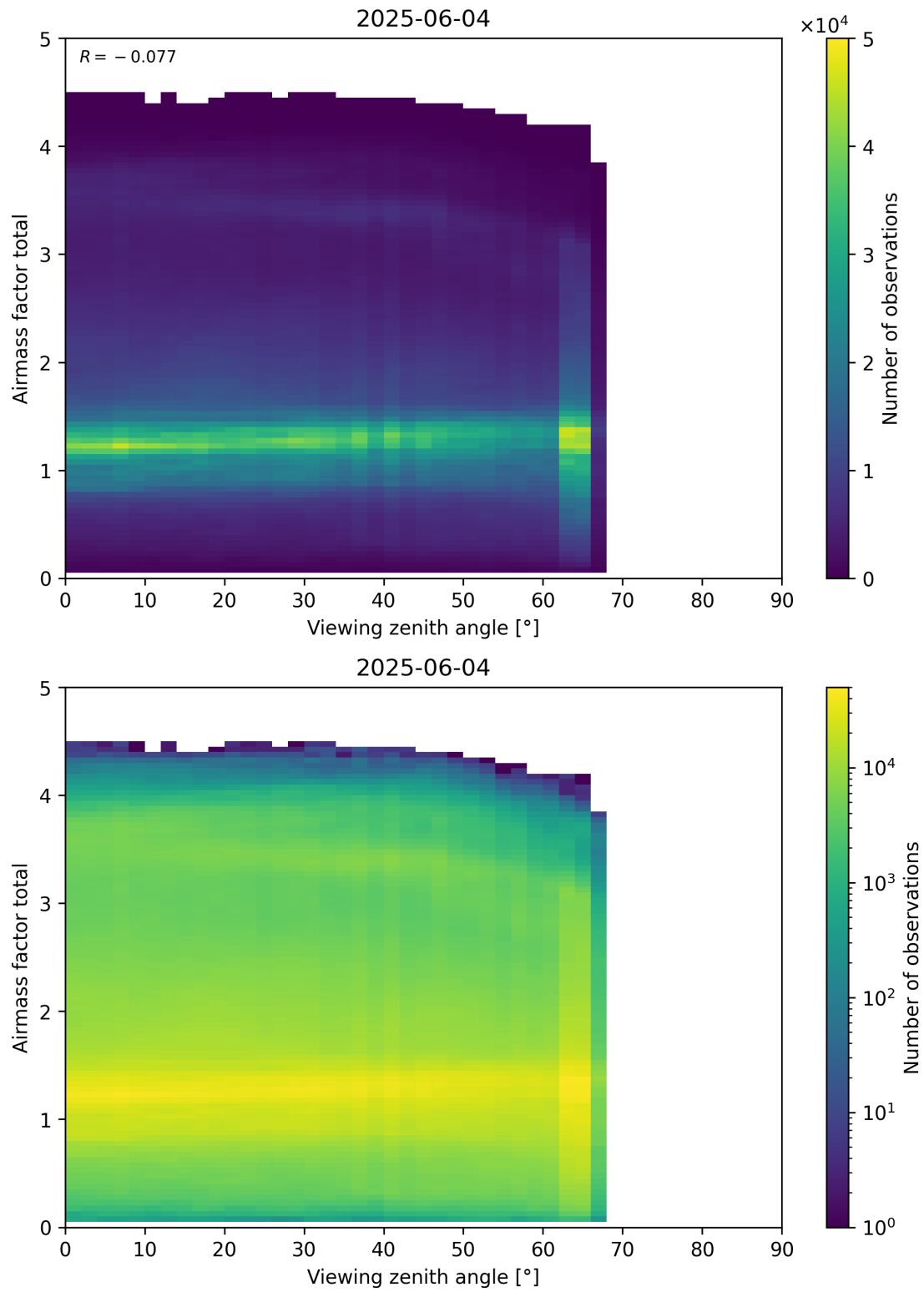
Figure 190: Scatter density plot of “Viewing zenith angle” against “Airmass factor total” for 2025-06-03 to 2025-06-05.
