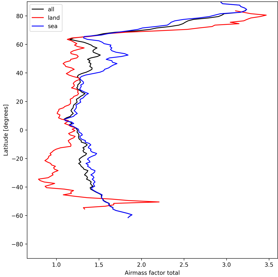
Figure 26: Zonal average of “Airmass factor total” for 2025-06-03 to 2025-06-05.
