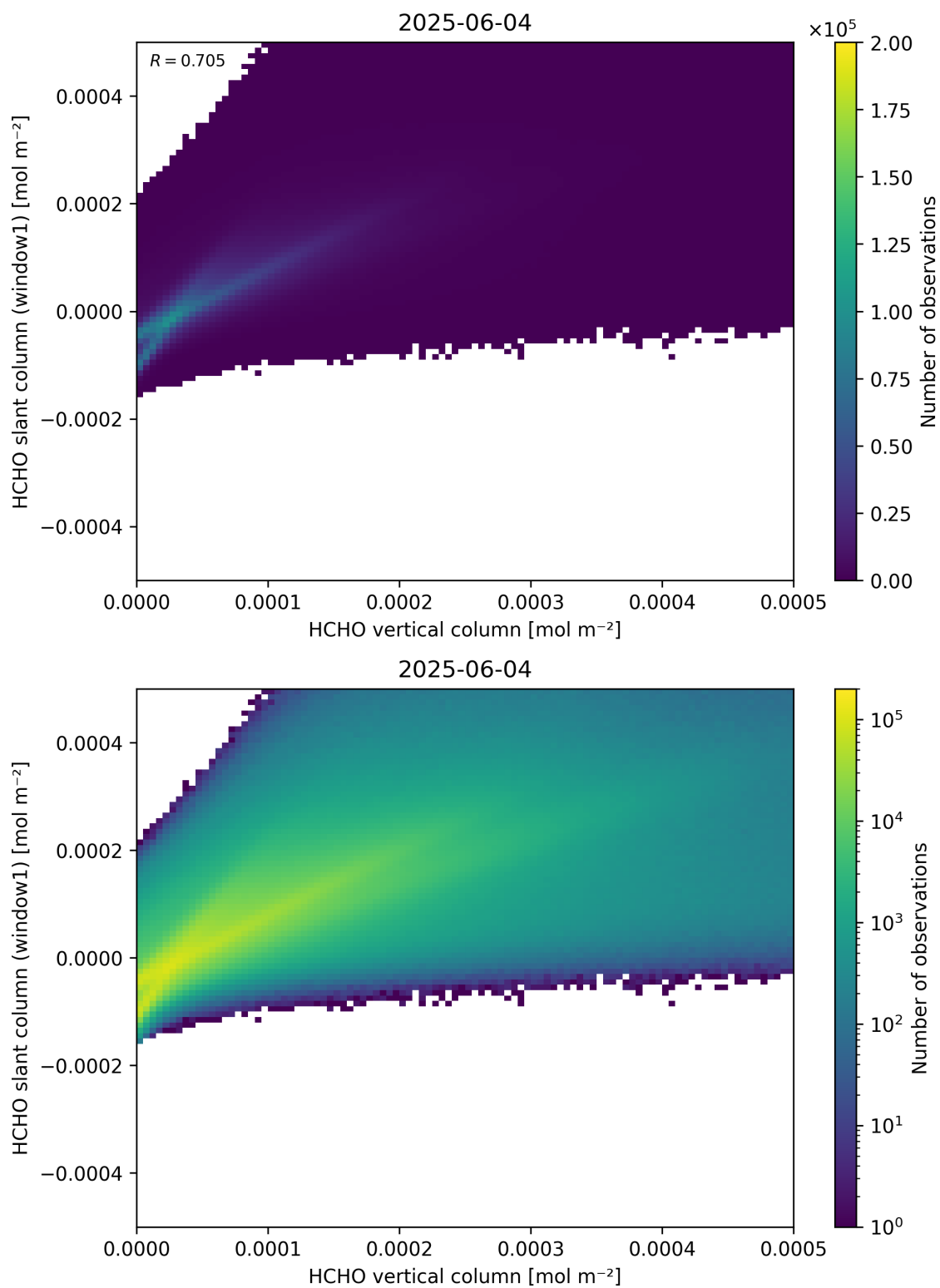
Figure 129: Scatter density plot of “HCHO vertical column” against “HCHO slant column (window1)” for 2025-06-03 to 2025-06-05.
