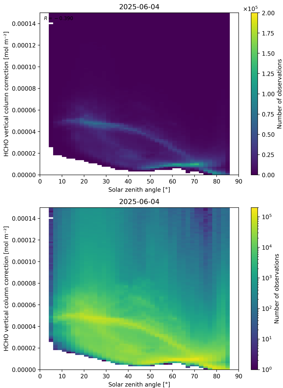
Figure 178: Scatter density plot of “Solar zenith angle” against “HCHO vertical column correction” for 2025-06-03 to 2025-06-05.
