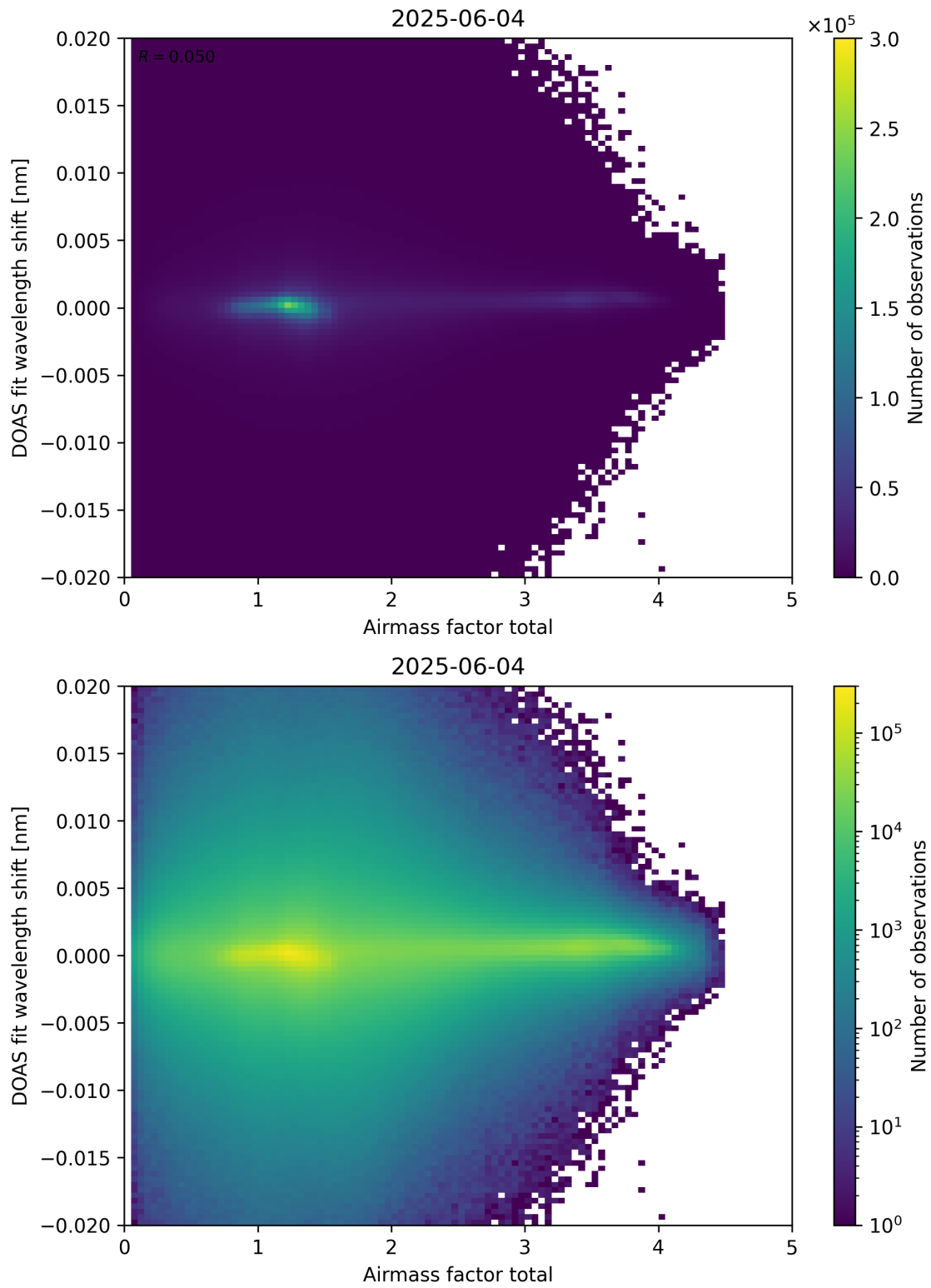
Figure 98: Scatter density plot of “Airmass factor total” against “DOAS fit wavelength shift” for 2025-06-03 to 2025-06-05.
