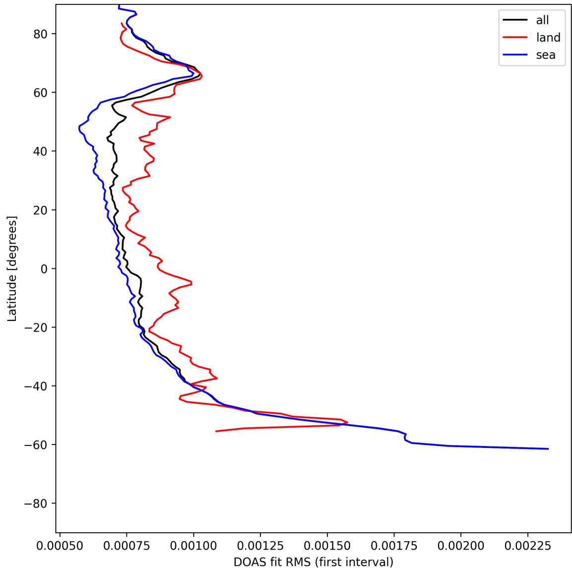
Figure 32: Zonal average of “DOAS fit RMS (first interval)” for 2025-06-03 to 2025-06-05.
