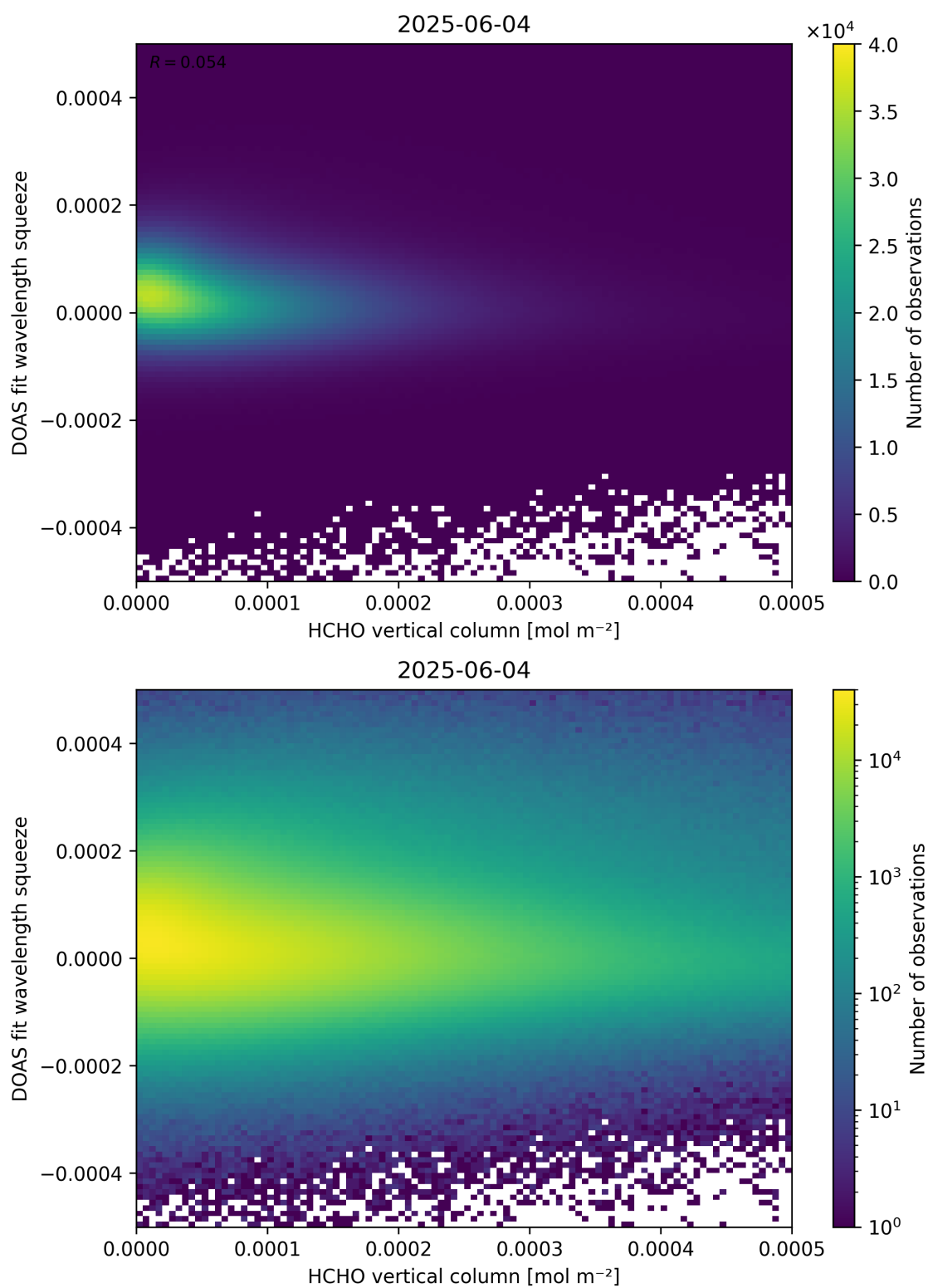
Figure 125: Scatter density plot of “HCHO vertical column” against “DOAS fit wavelength squeeze” for 2025-06-03 to 2025-06-05.
