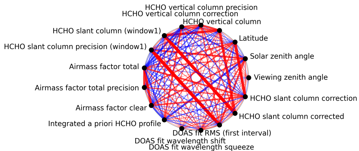
Figure 1: Map of correlation graph for 2025-06-03 to 2025-06-05.
