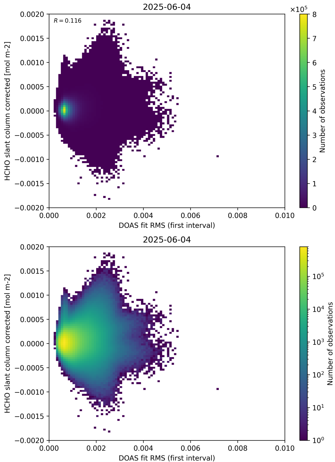
Figure 62: Scatter density plot of “DOAS fit RMS (first interval)” against “HCHO slant column corrected” for 2025-06-03 to 2025-06-05.
