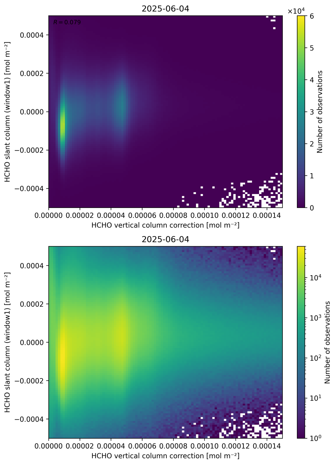
Figure 118: Scatter density plot of “HCHO vertical column correction” against “HCHO slant column (window1)” for 2025-06-03 to 2025-06-05.
