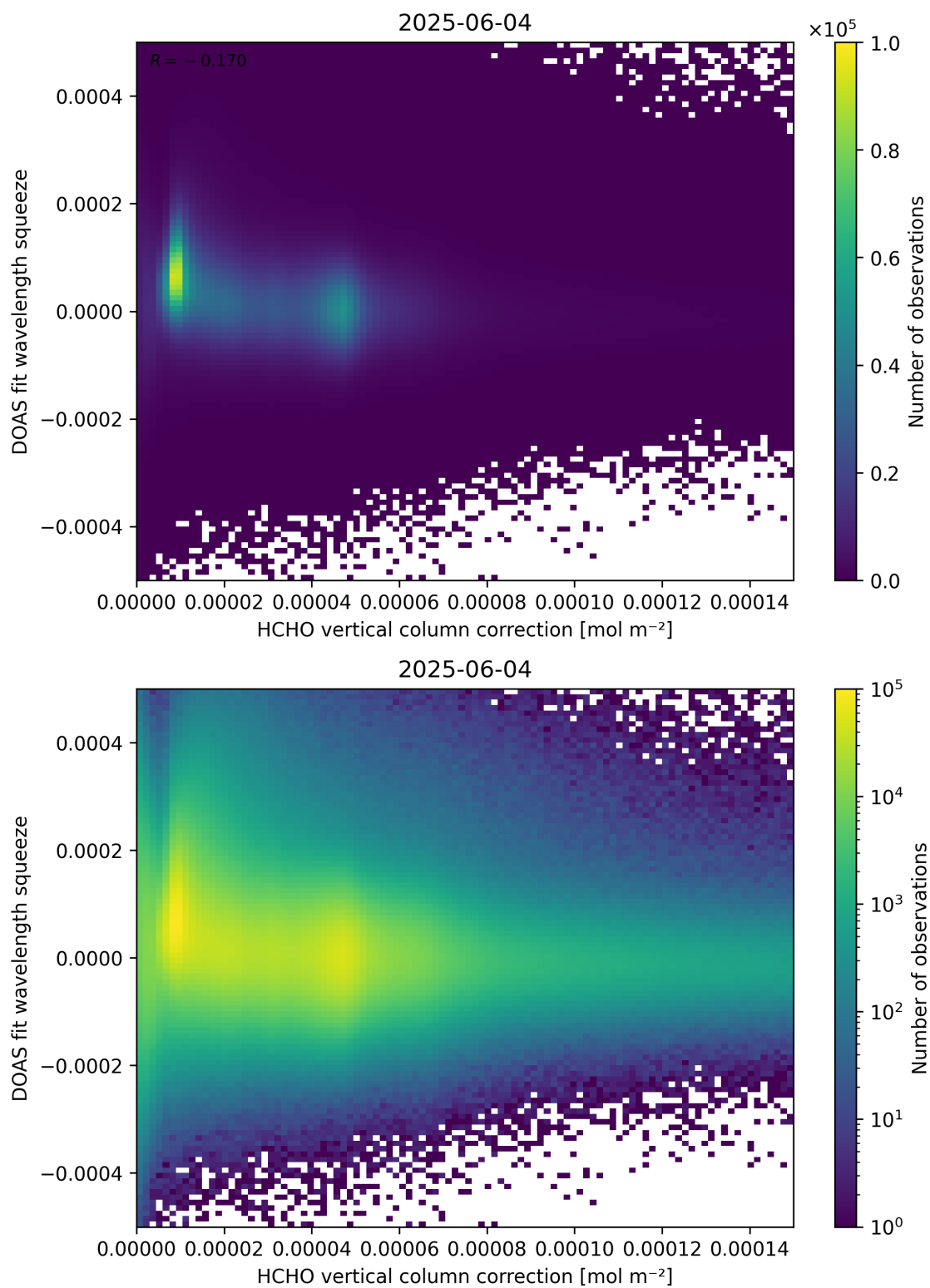
Figure 114: Scatter density plot of “HCHO vertical column correction” against “DOAS fit wavelength squeeze” for 2025-06-03 to 2025-06-05.
