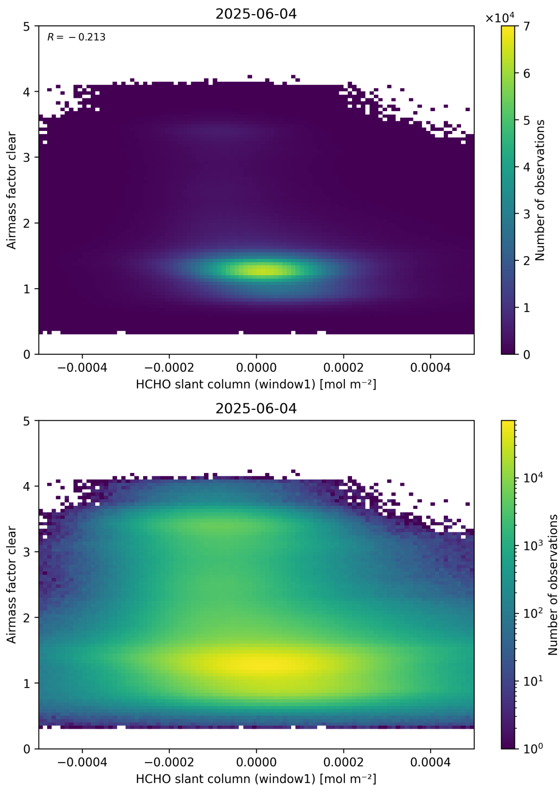
Figure 81: Scatter density plot of “HCHO slant column (window1)” against “Airmass factor clear” for 2025-06-03 to 2025-06-05.
