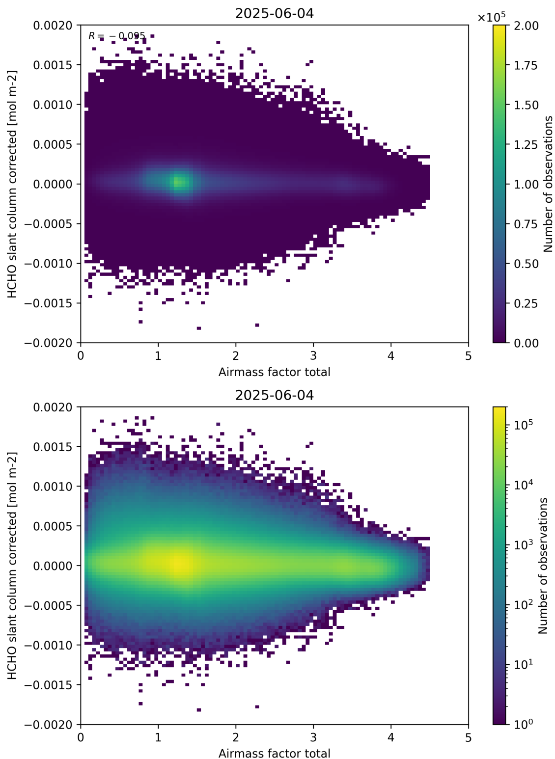
Figure 101: Scatter density plot of “Airmass factor total” against “HCHO slant column corrected” for 2025-06-03 to 2025-06-05.
