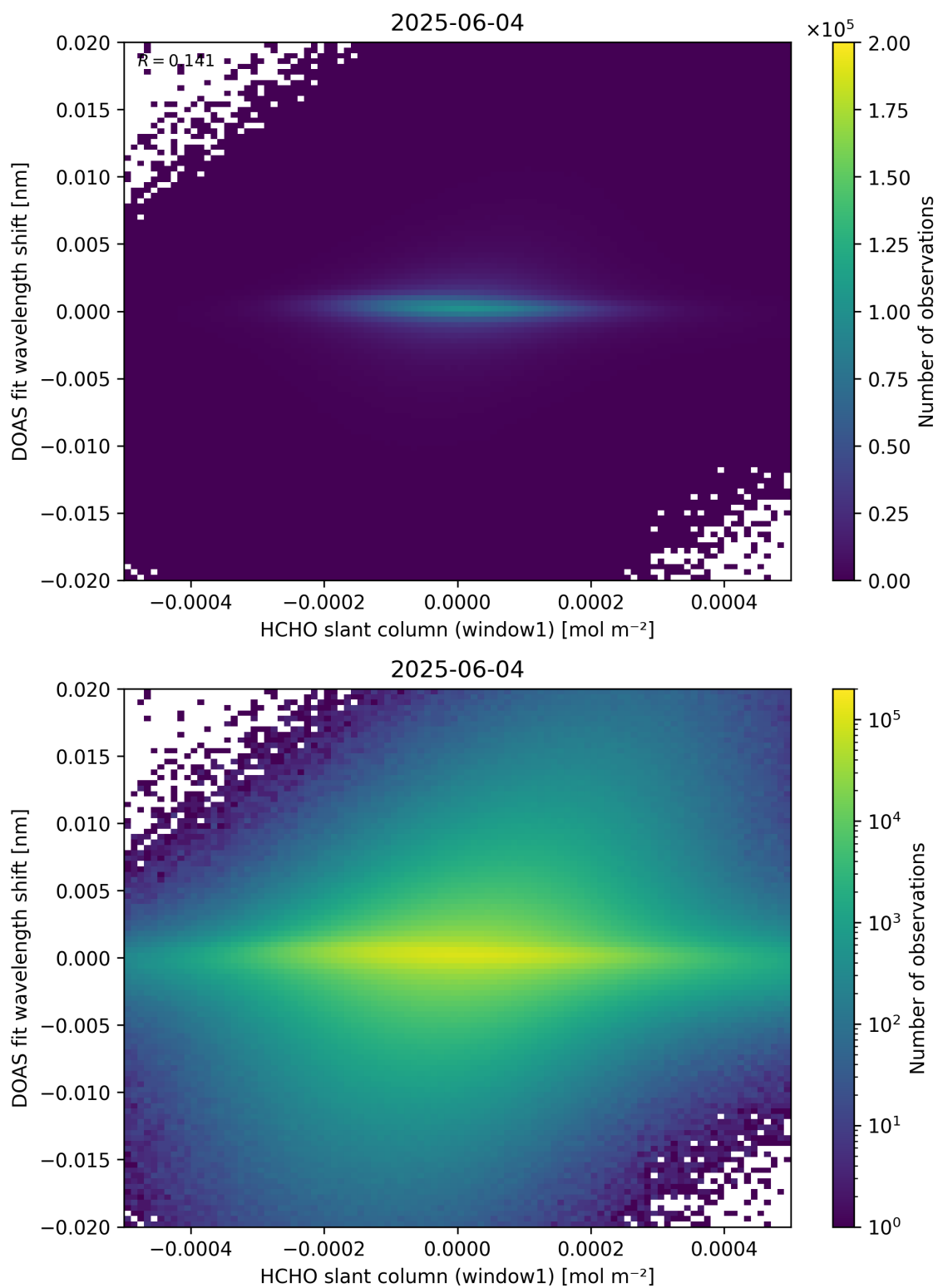
Figure 79: Scatter density plot of “HCHO slant column (window1)” against “DOAS fit wavelength shift” for 2025-06-03 to 2025-06-05.
