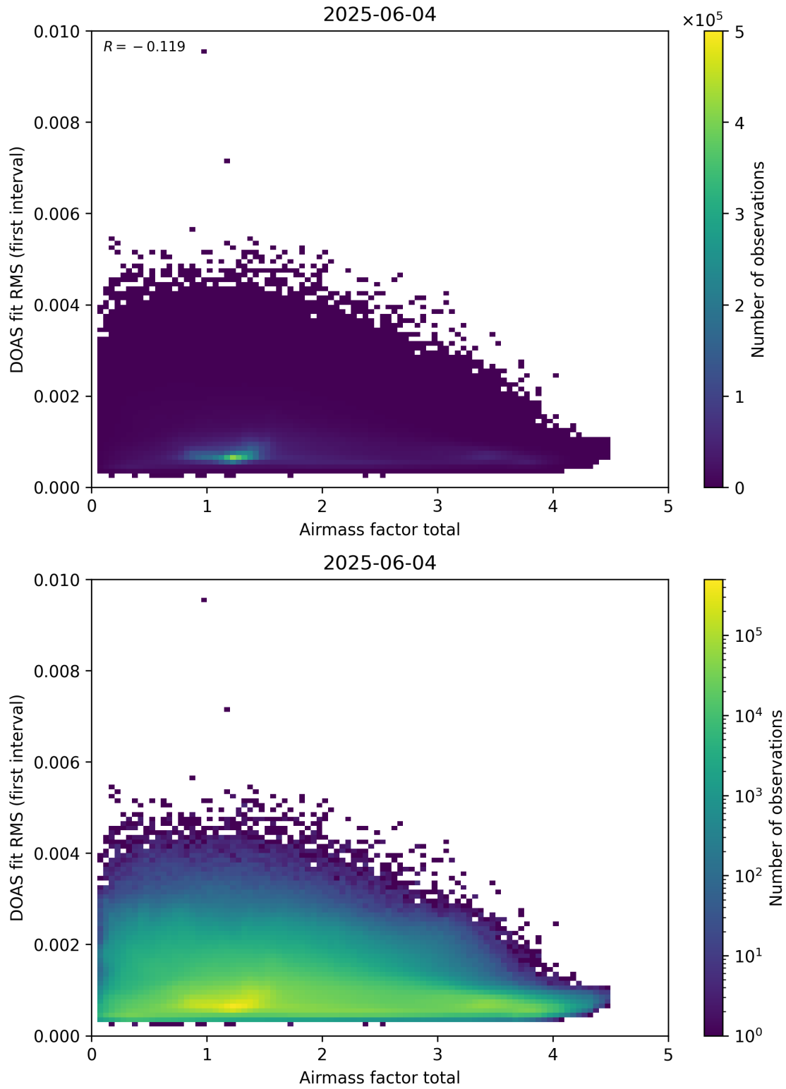
Figure 97: Scatter density plot of “Airmass factor total” against “DOAS fit RMS (first interval)” for 2025-06-03 to 2025-06-05.
