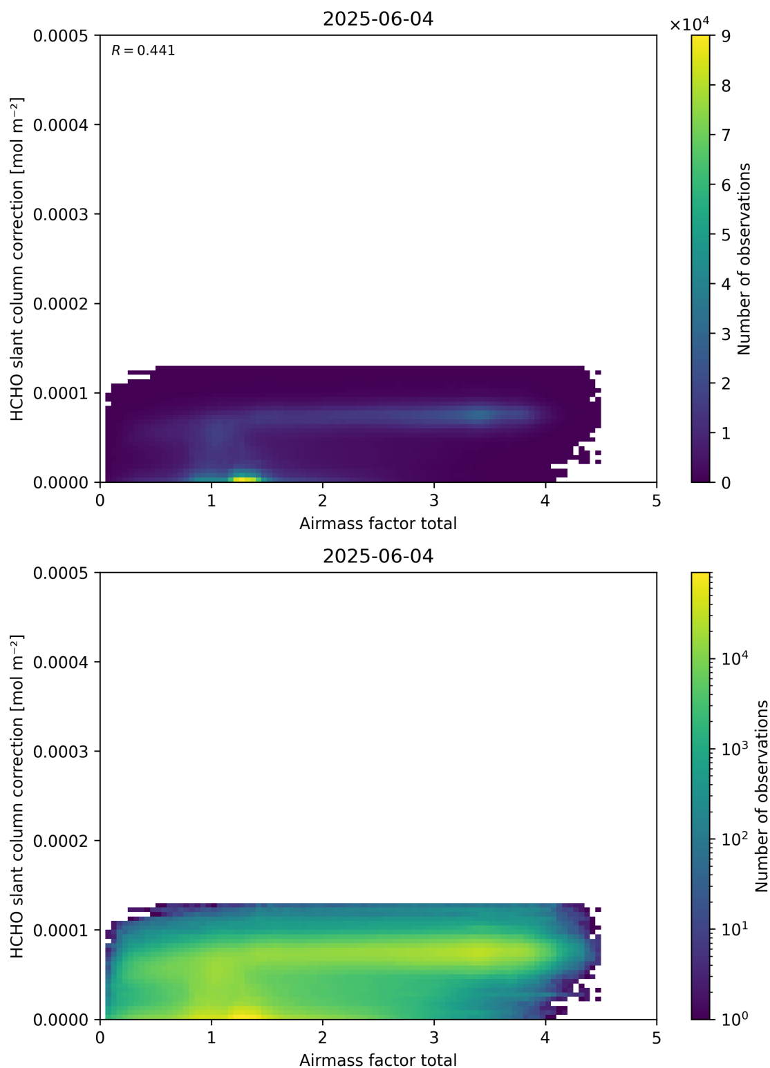
Figure 102: Scatter density plot of “Airmass factor total” against “HCHO slant column correction” for 2025-06-03 to 2025-06-05.
