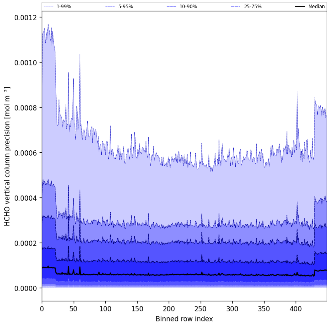
Figure 50: Along track statistics of “HCHO vertical column precision” for 2025-06-03 to 2025-06-05
