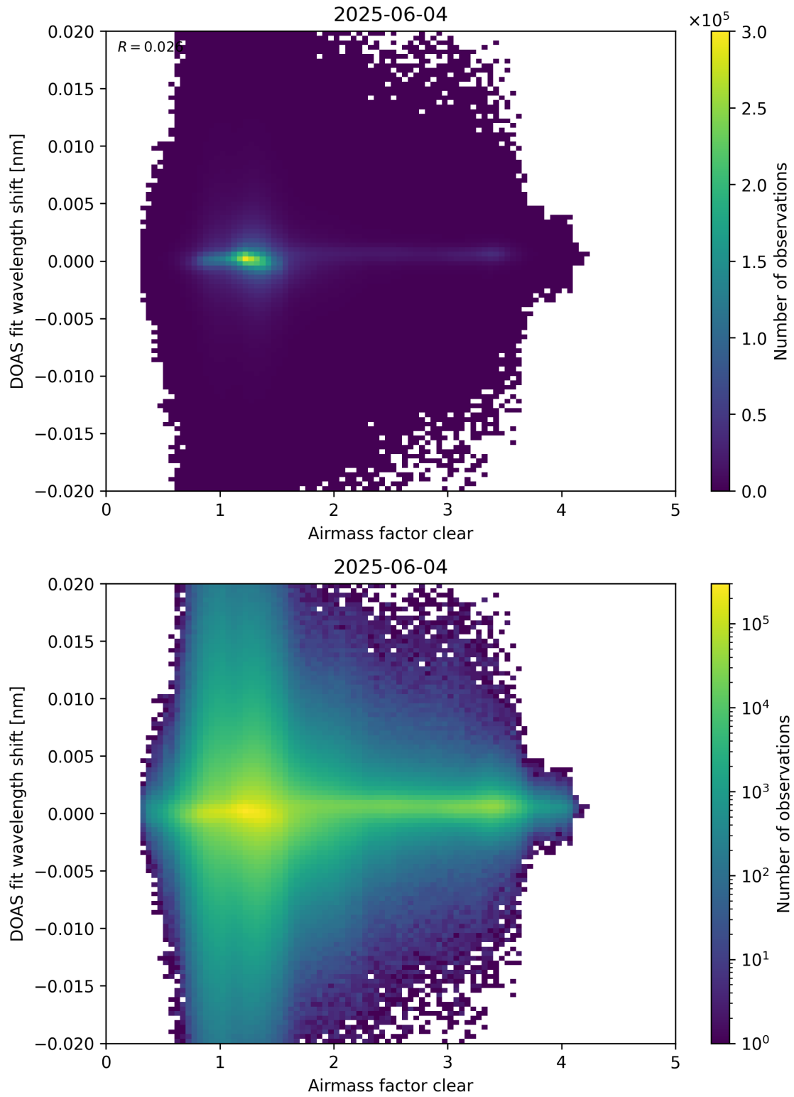
Figure 72: Scatter density plot of “Airmass factor clear” against “DOAS fit wavelength shift” for 2025-06-03 to 2025-06-05.
