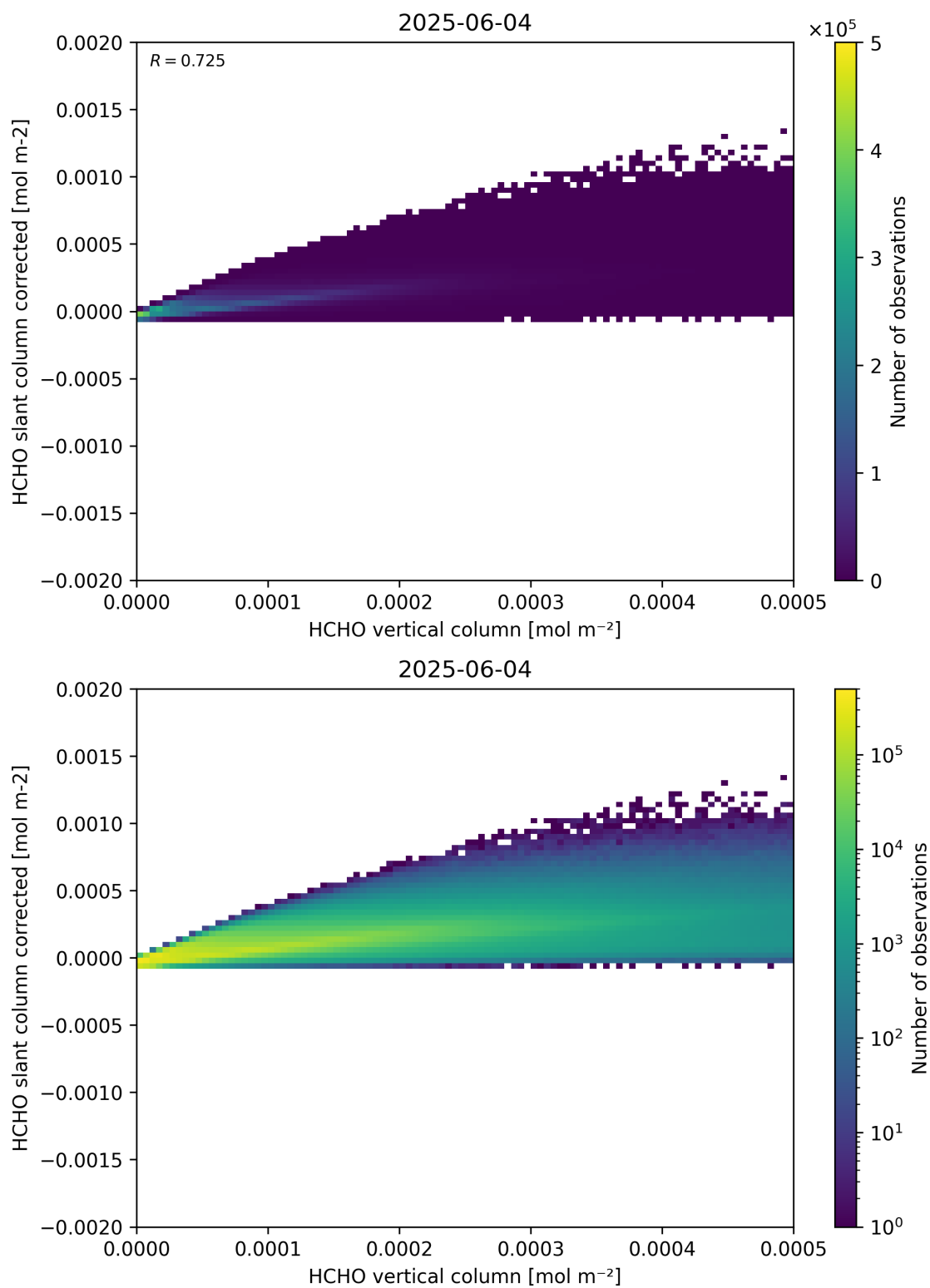
Figure 127: Scatter density plot of “HCHO vertical column” against “HCHO slant column corrected” for 2025-06-03 to 2025-06-05.
