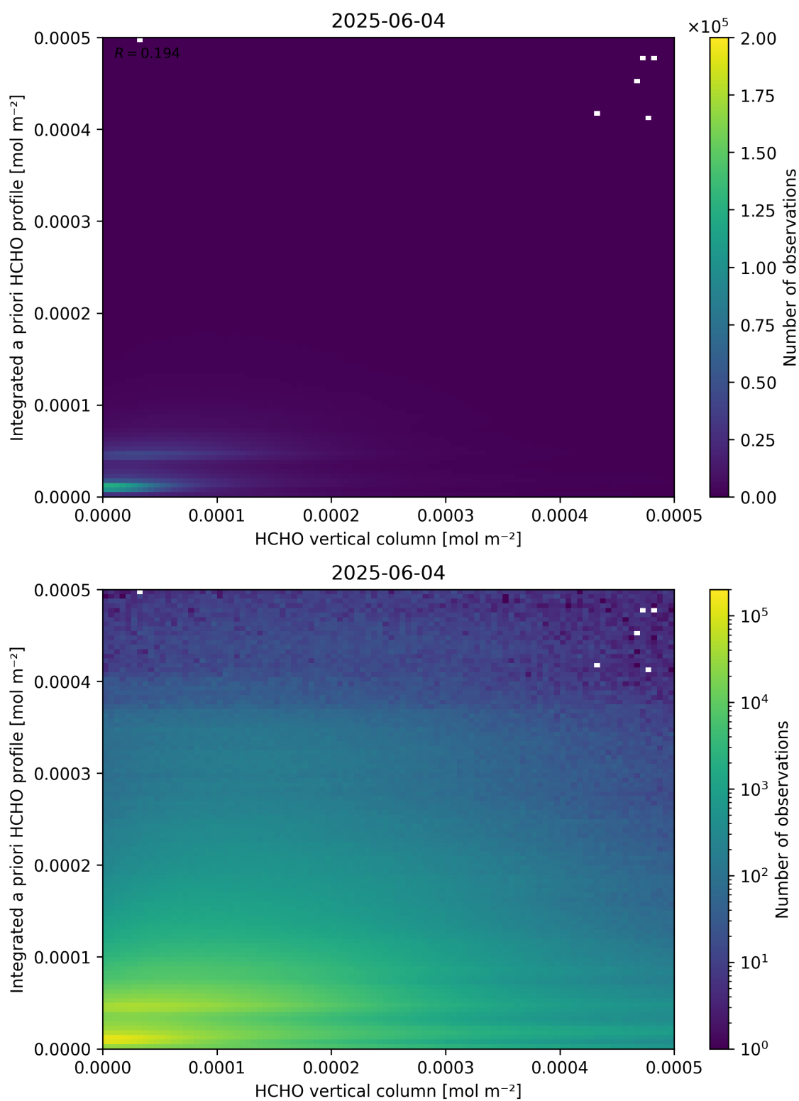
Figure 135: Scatter density plot of “HCHO vertical column” against “Integrated a priori HCHO profile” for 2025-06-03 to 2025-06-05.
