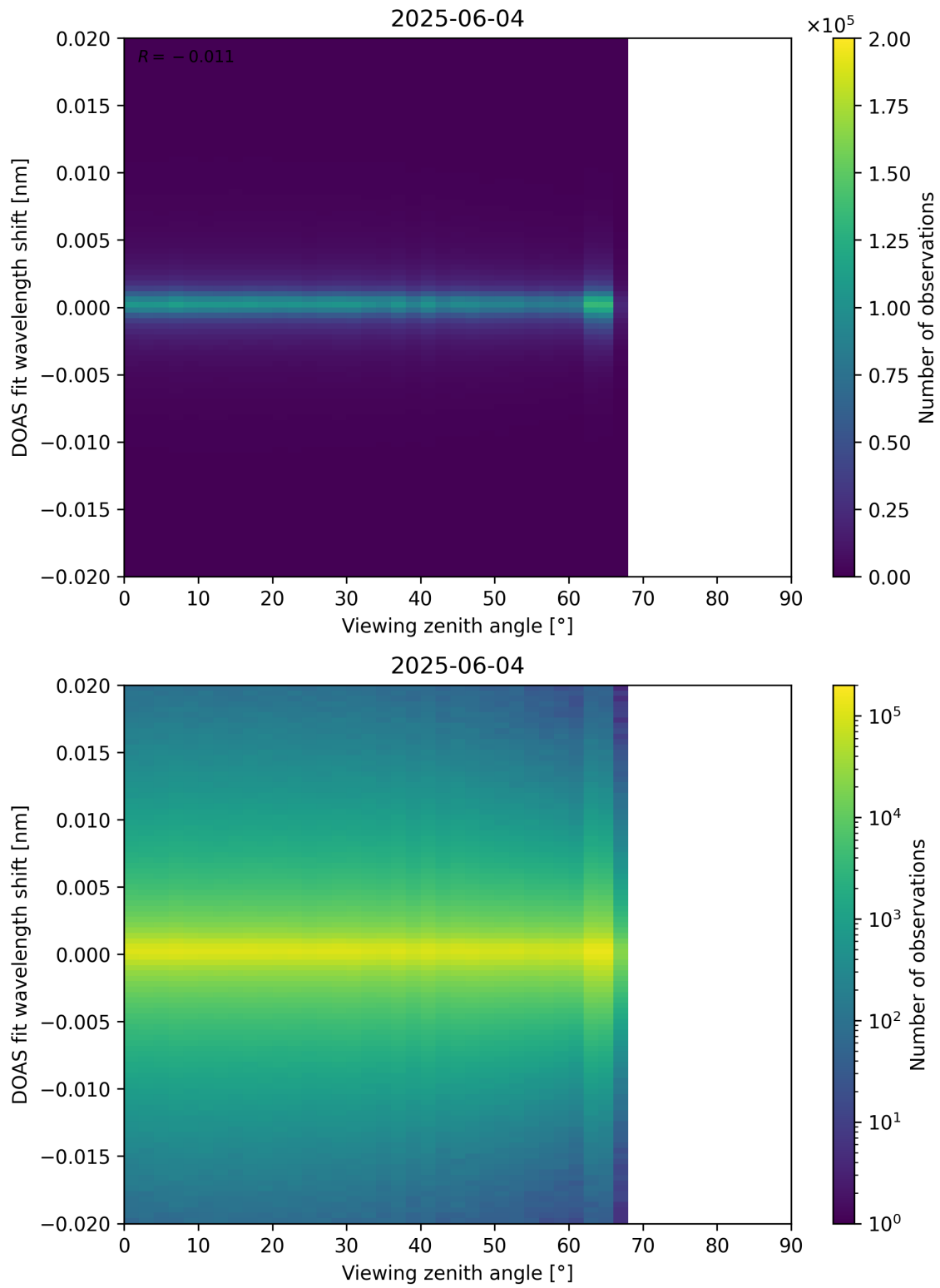
Figure 183: Scatter density plot of “Viewing zenith angle” against “DOAS fit wavelength shift” for 2025-06-03 to 2025-06-05.
