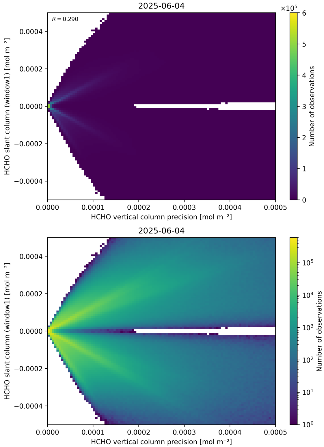
Figure 142: Scatter density plot of “HCHO vertical column precision” against “HCHO slant column (window1)” for 2025-06-03 to 2025-06-05.
