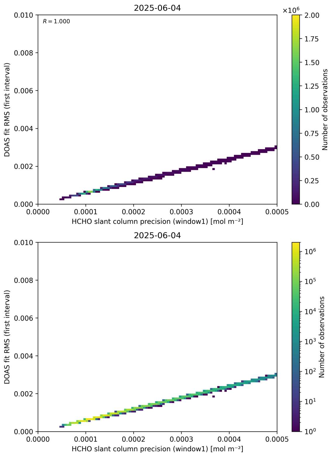
Figure 88: Scatter density plot of “HCHO slant column precision (window1)” against “DOAS fit RMS (first interval)” for 2025-06-03 to 2025-06-05.
