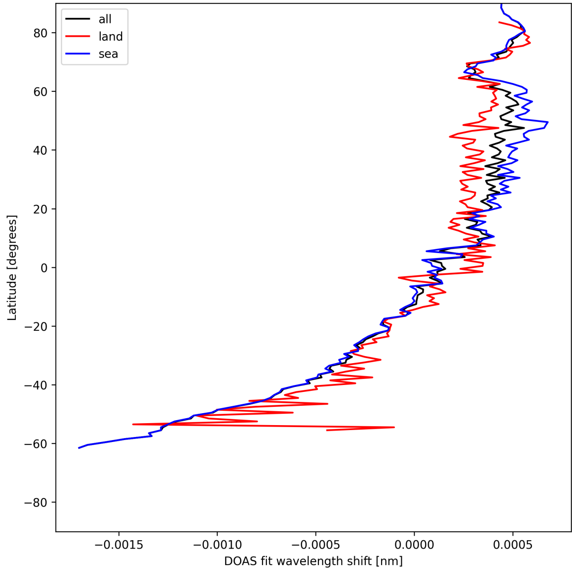
Figure 30: Zonal average of “DOAS fit wavelength shift” for 2025-06-03 to 2025-06-05.
