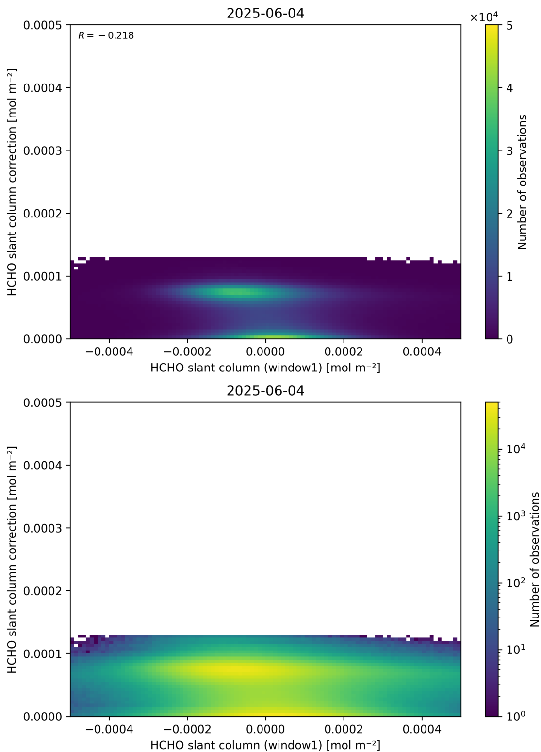
Figure 83: Scatter density plot of “HCHO slant column (window1)” against “HCHO slant column correction” for 2025-06-03 to 2025-06-05.
