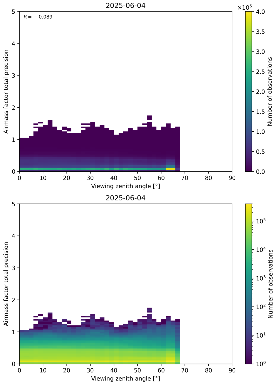
Figure 191: Scatter density plot of “Viewing zenith angle” against “Airmass factor total precision” for 2025-06-03 to 2025-06-05.
