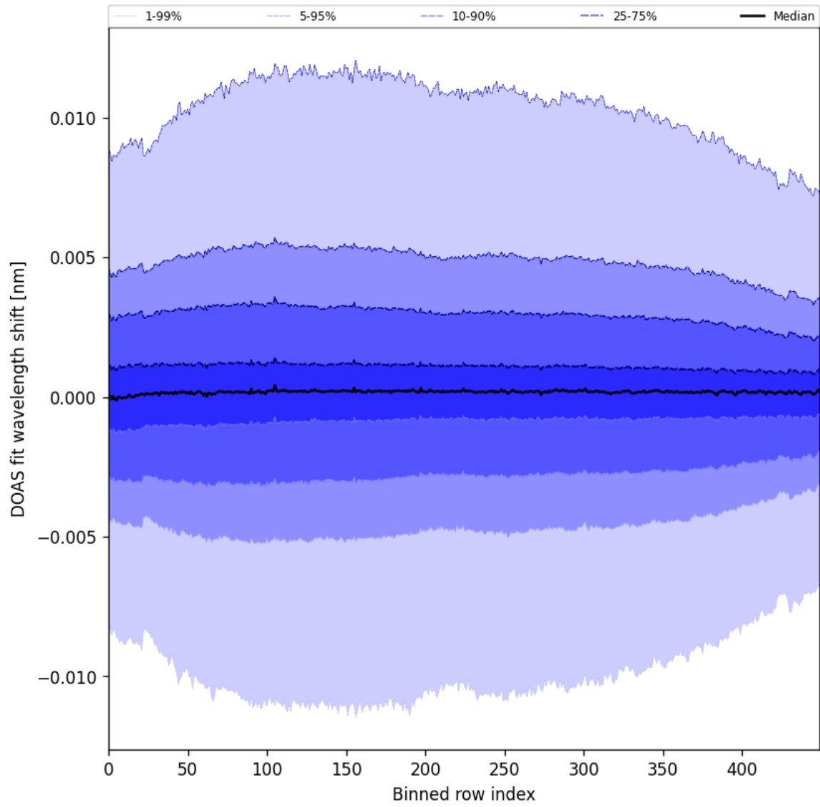
Figure 58: Along track statistics of “DOAS fit wavelength shift” for 2025-06-03 to 2025-06-05
