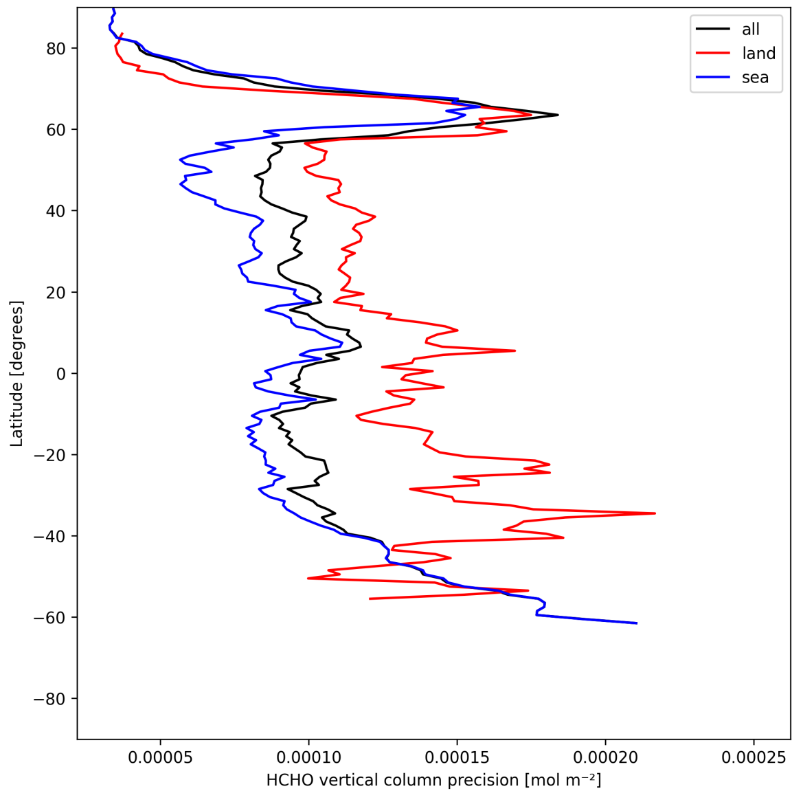
Figure 22: Zonal average of “HCHO vertical column precision” for 2025-06-03 to 2025-06-05.
