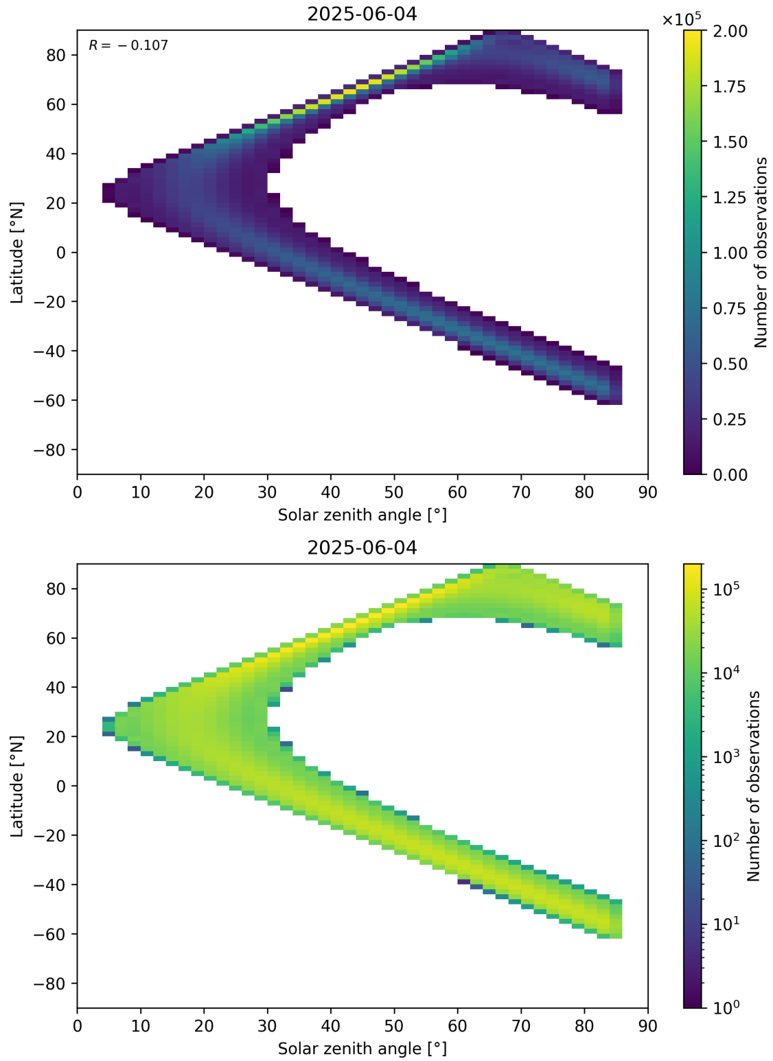
Figure 181: Scatter density plot of “Solar zenith angle” against “Latitude” for 2025-06-03 to 2025-06-05.
