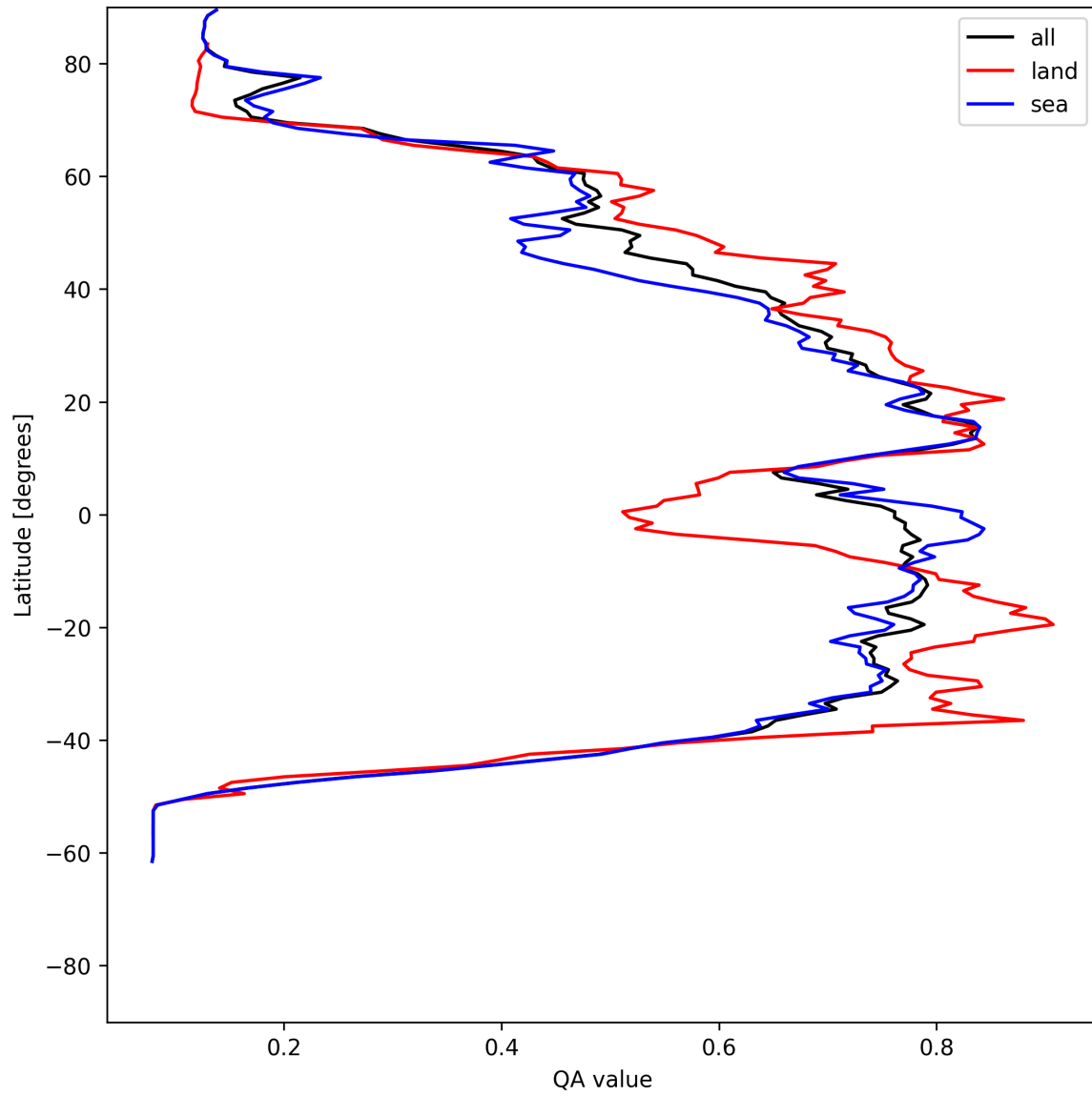
Figure 20: Zonal average of “QA value” for 2025-06-03 to 2025-06-05.
