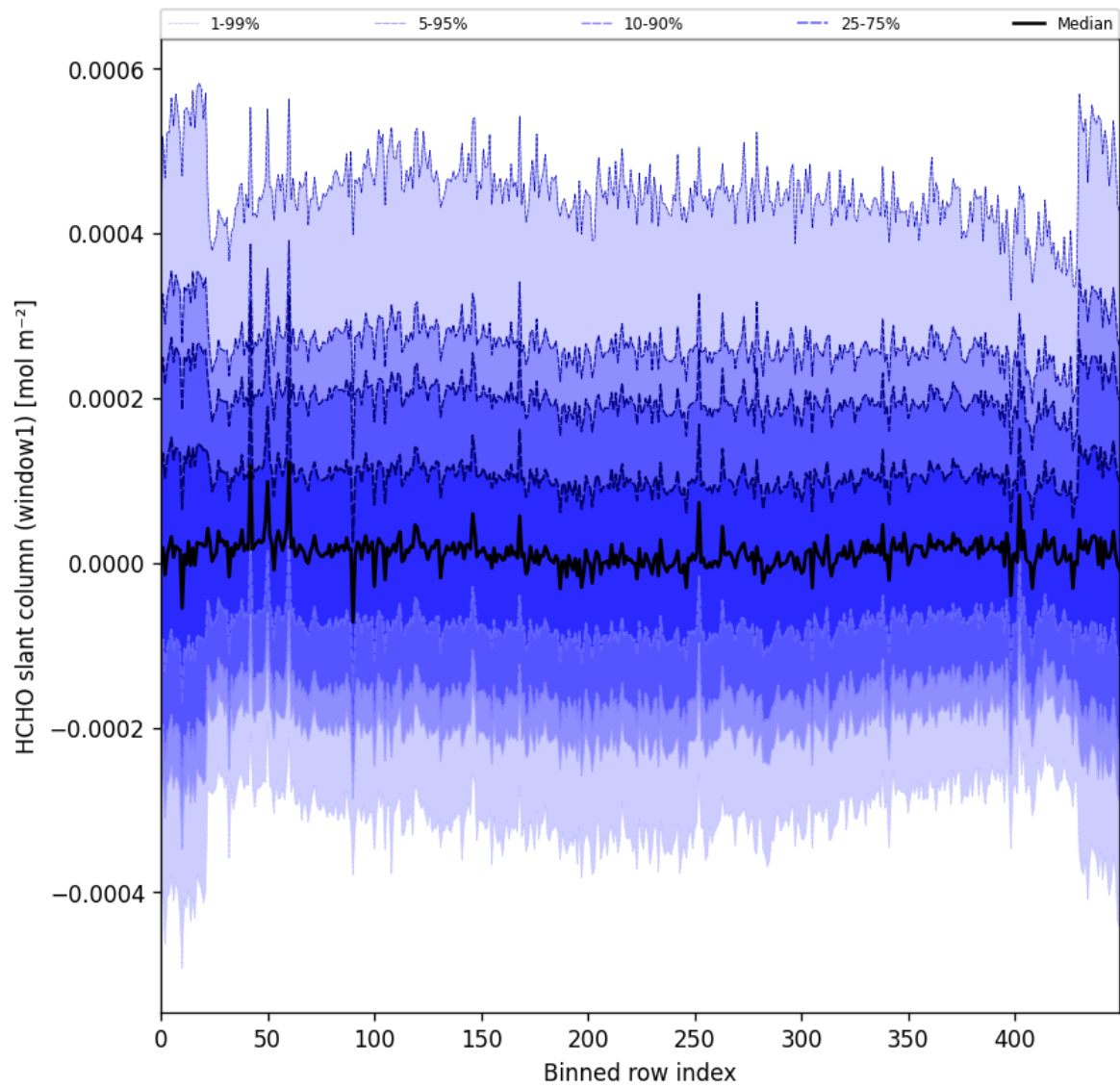
Figure 52: Along track statistics of “HCHO slant column (window1)” for 2025-06-03 to 2025-06-05
