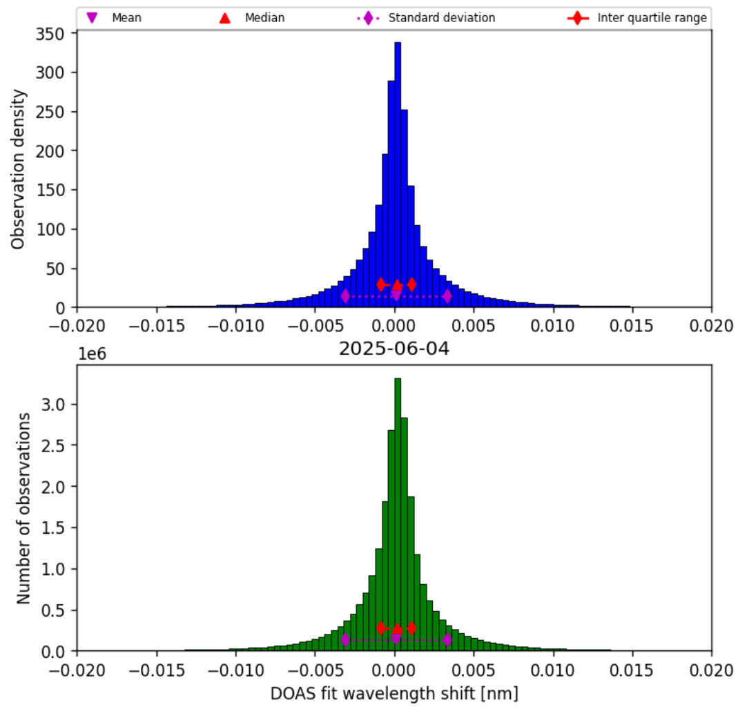
Figure 44: Histogram of “DOAS fit wavelength shift” for 2025-06-03 to 2025-06-05
