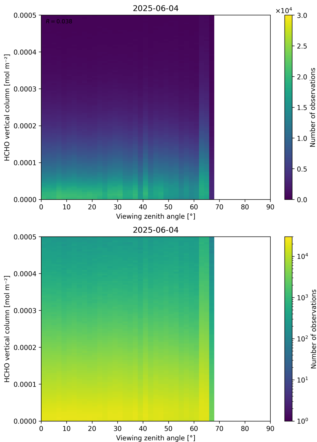
Figure 192: Scatter density plot of “Viewing zenith angle” against “HCHO vertical column” for 2025-06-03 to 2025-06-05.
