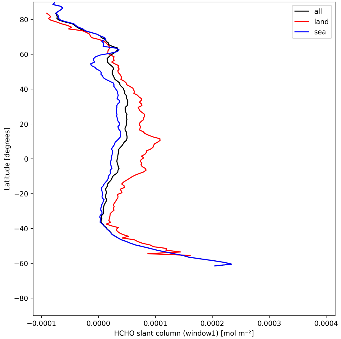
Figure 24: Zonal average of “HCHO slant column (window1)” for 2025-06-03 to 2025-06-05.
