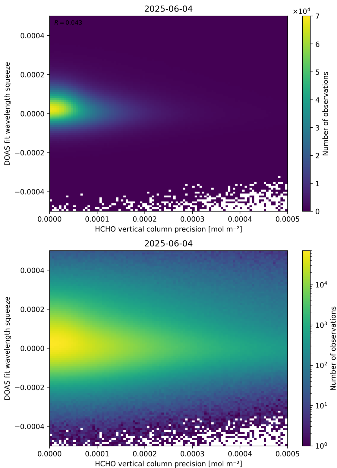
Figure 138: Scatter density plot of “HCHO vertical column precision” against “DOAS fit wavelength squeeze” for 2025-06-03 to 2025-06-05.
