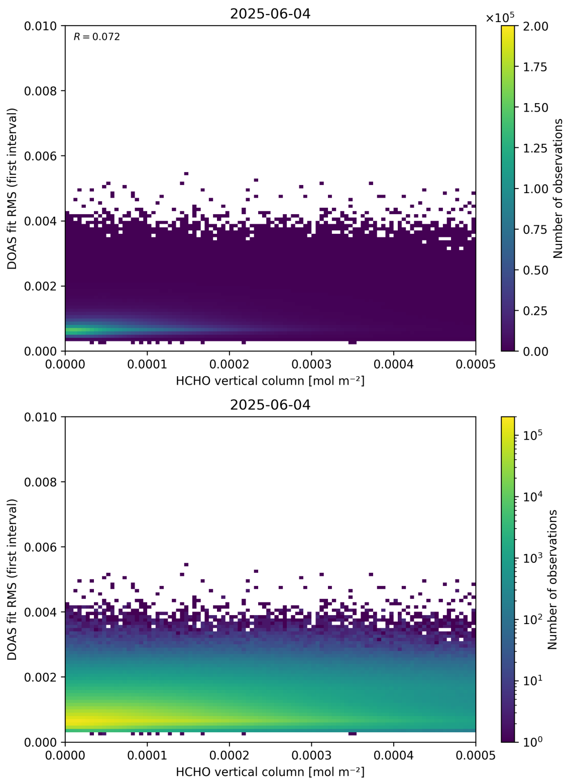
Figure 123: Scatter density plot of “HCHO vertical column” against “DOAS fit RMS (first interval)” for 2025-06-03 to 2025-06-05.
