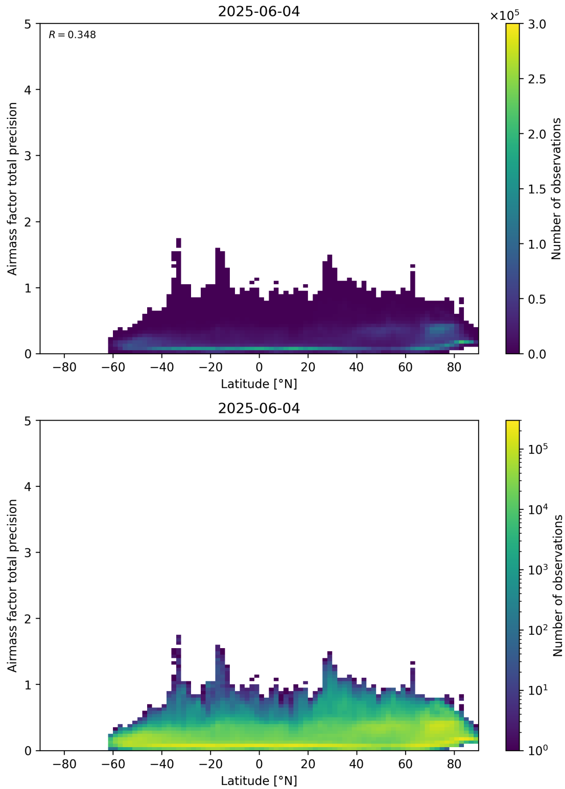
Figure 162: Scatter density plot of “Latitude” against “Airmass factor total precision” for 2025-06-03 to 2025-06-05.
