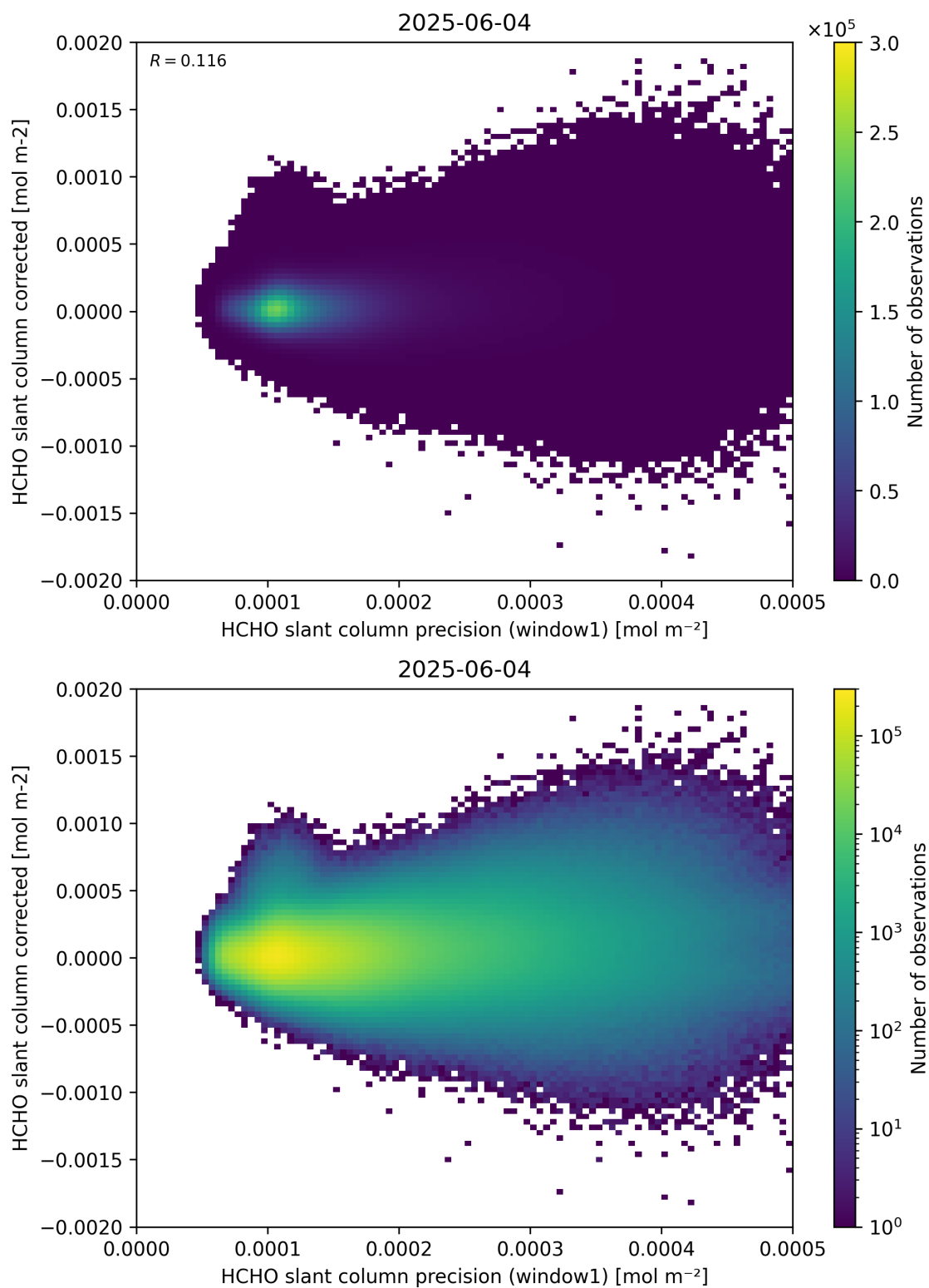
Figure 92: Scatter density plot of “HCHO slant column precision (window1)” against “HCHO slant column corrected” for 2025-06-03 to 2025-06-05.
