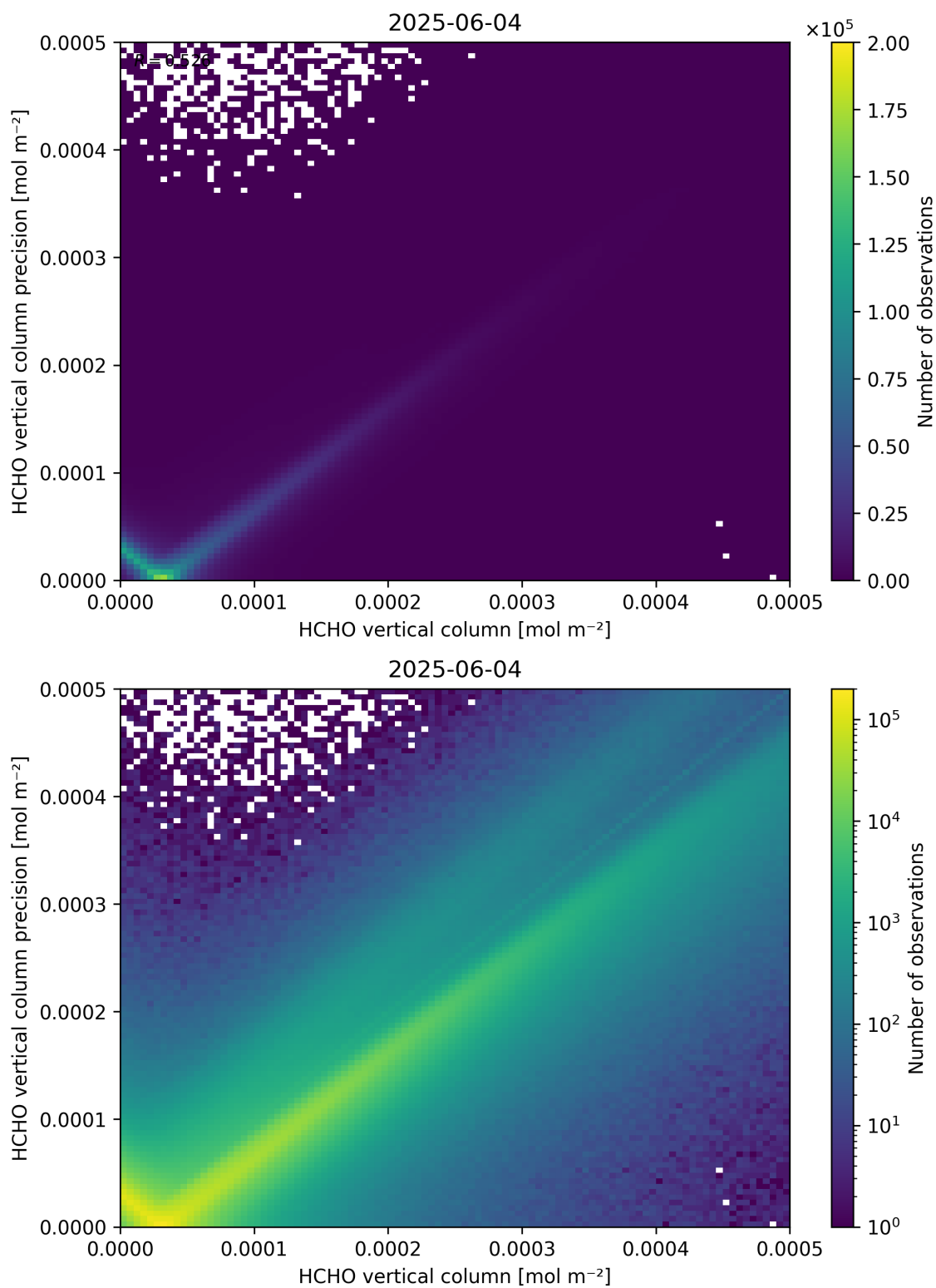
Figure 134: Scatter density plot of “HCHO vertical column” against “HCHO vertical column precision” for 2025-06-03 to 2025-06-05.
