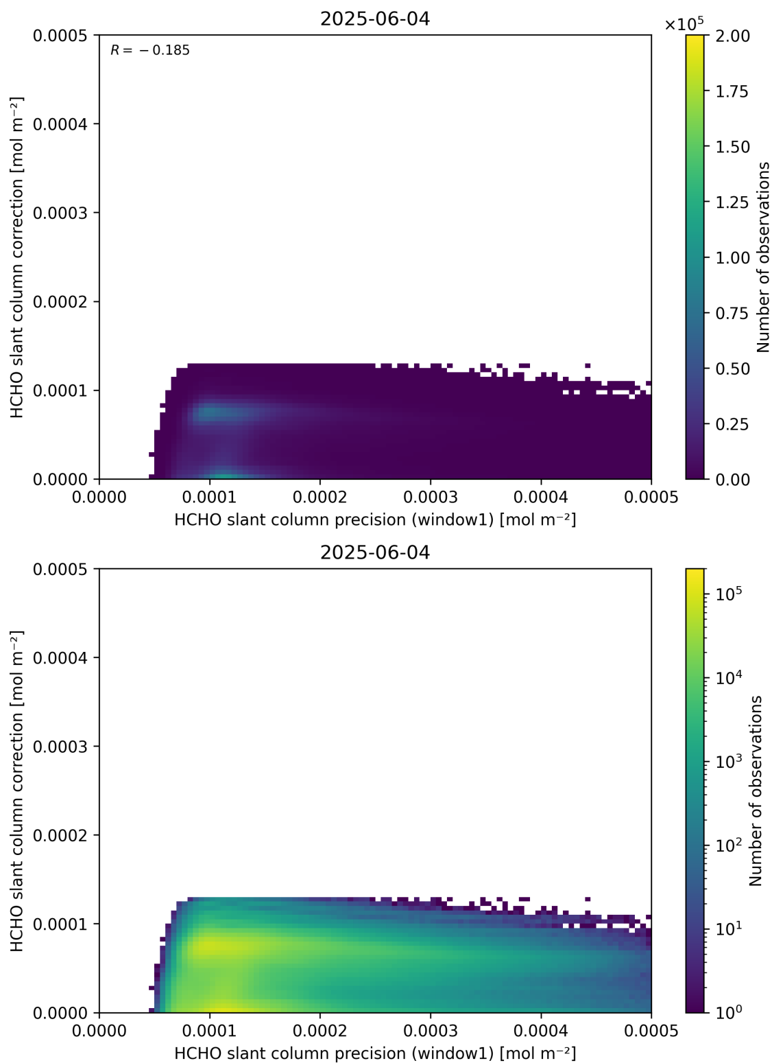
Figure 93: Scatter density plot of “HCHO slant column precision (window1)” against “HCHO slant column correction” for 2025-06-03 to 2025-06-05.
