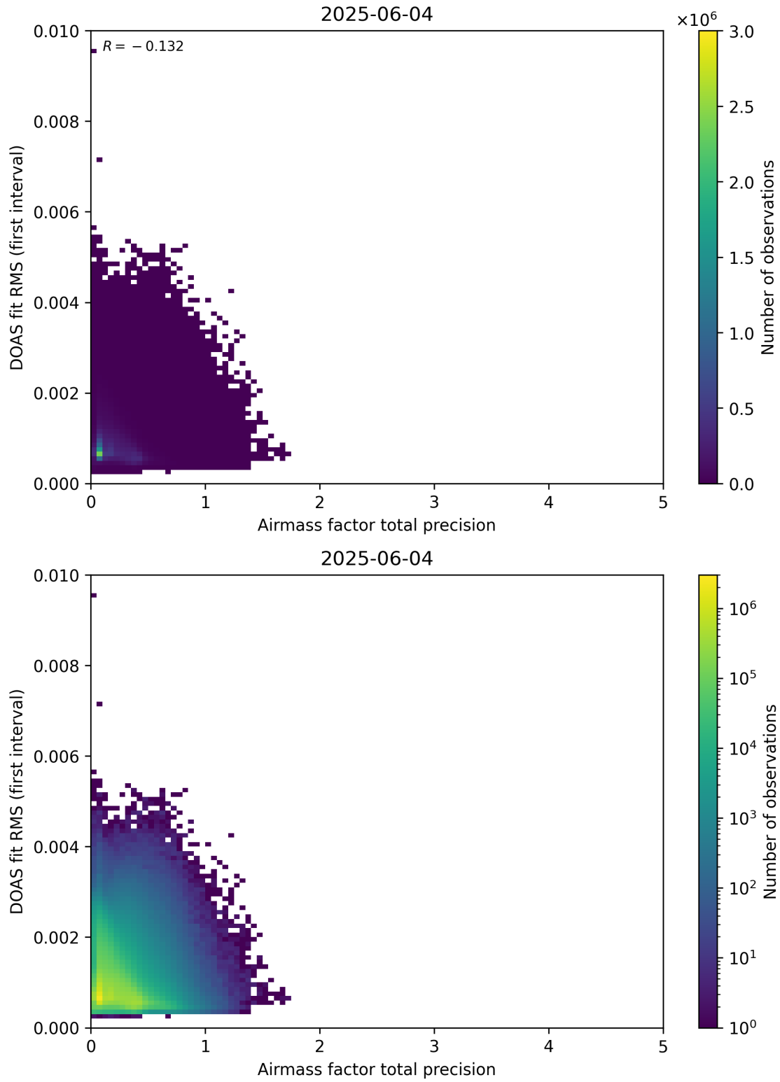
Figure 105: Scatter density plot of “Airmass factor total precision” against “DOAS fit RMS (first interval)” for 2025-06-03 to 2025-06-05.
