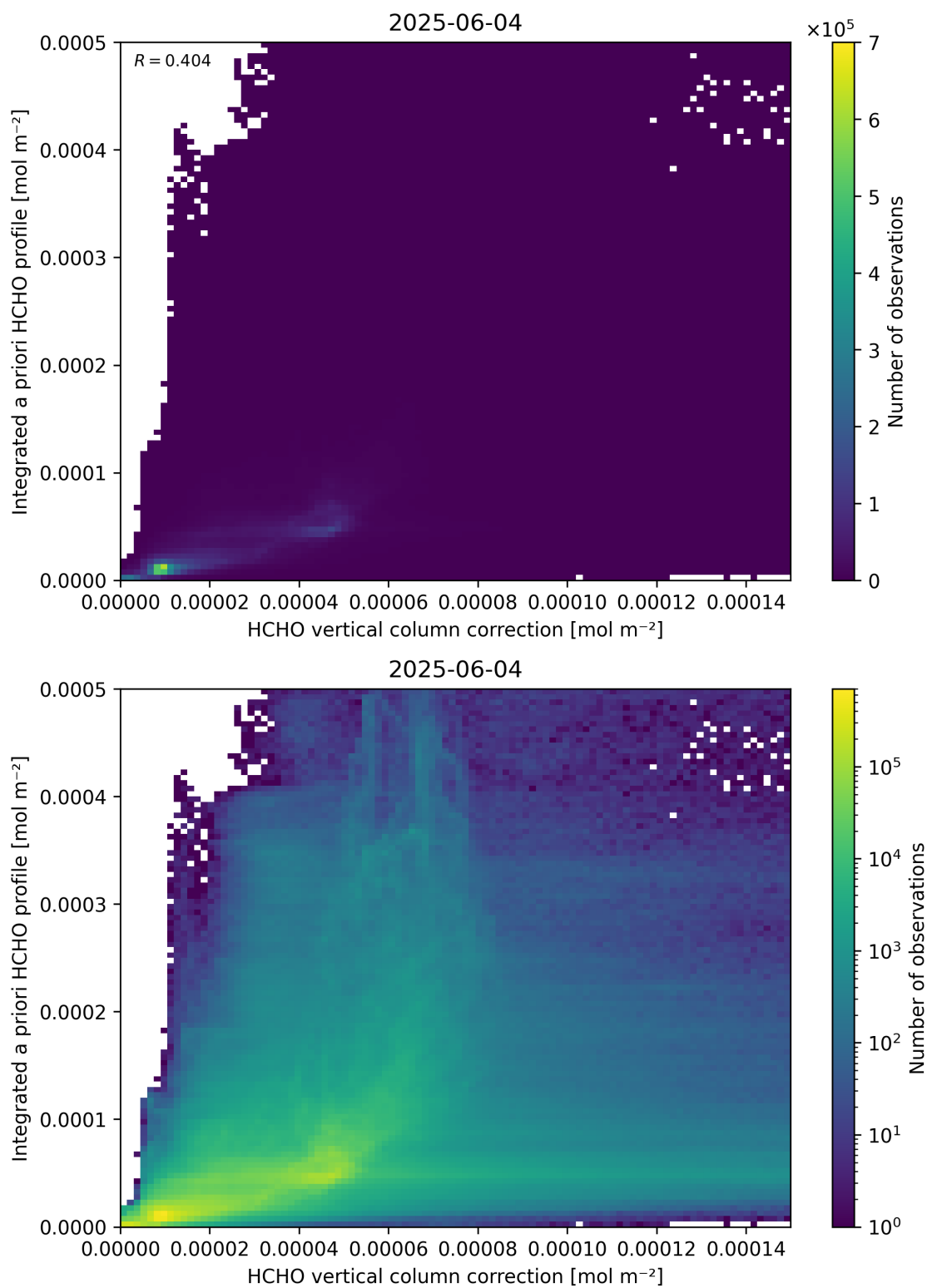
Figure 122: Scatter density plot of “HCHO vertical column correction” against “Integrated a priori HCHO profile” for 2025-06-03 to 2025-06-05.
