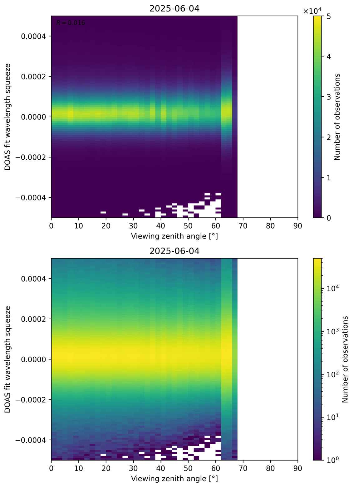
Figure 184: Scatter density plot of “Viewing zenith angle” against “DOAS fit wavelength squeeze” for 2025-06-03 to 2025-06-05.
