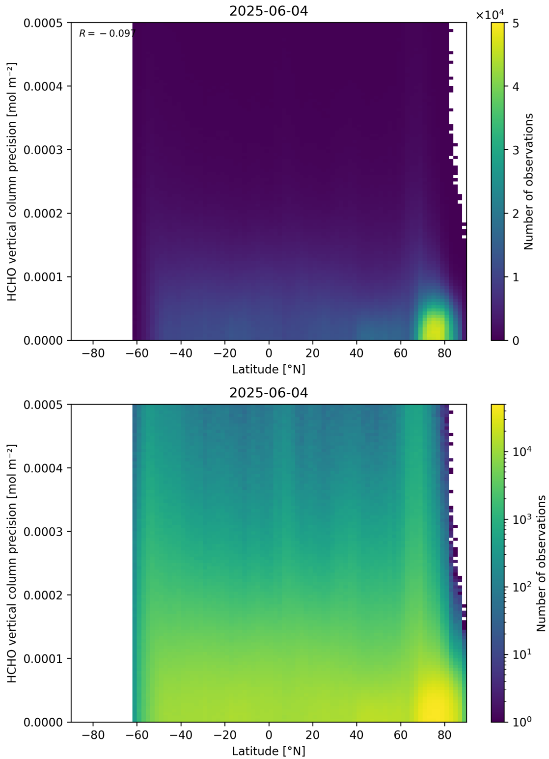
Figure 165: Scatter density plot of “Latitude” against “HCHO vertical column precision” for 2025-06-03 to 2025-06-05.
