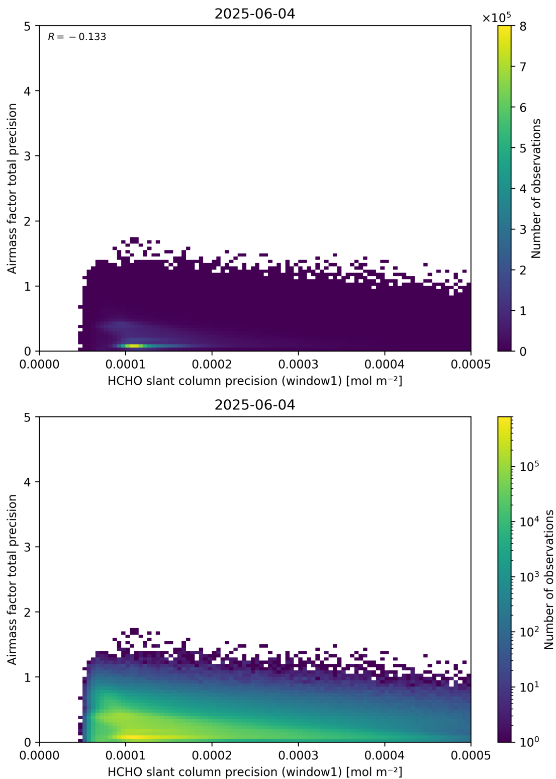
Figure 95: Scatter density plot of “HCHO slant column precision (window1)” against “Airmass factor total precision” for 2025-06-03 to 2025-06-05.
