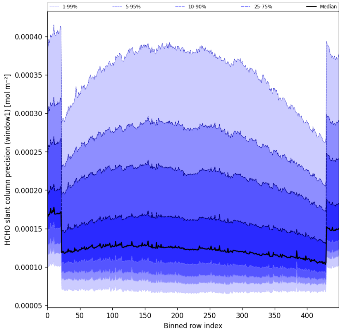
Figure 53: Along track statistics of “HCHO slant column precision (window1)” for 2025-06-03 to 2025-06-05
