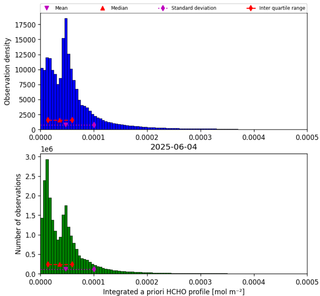
Figure 43: Histogram of “Integrated a priori HCHO profile” for 2025-06-03 to 2025-06-05
