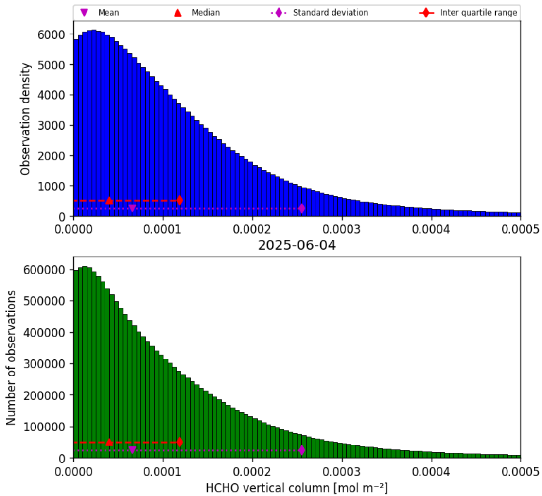
Figure 35: Histogram of “HCHO vertical column” for 2025-06-03 to 2025-06-05
