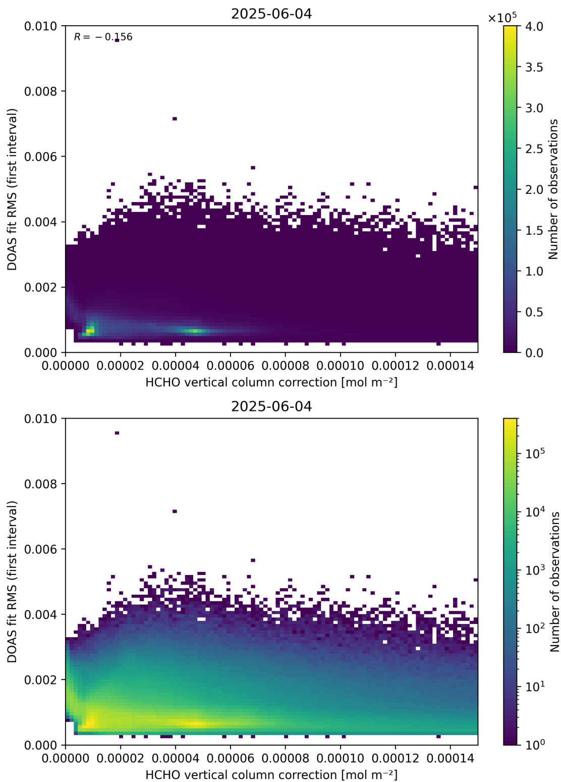
Figure 112: Scatter density plot of “HCHO vertical column correction” against “DOAS fit RMS (first interval)” for 2025-06-03 to 2025-06-05.
