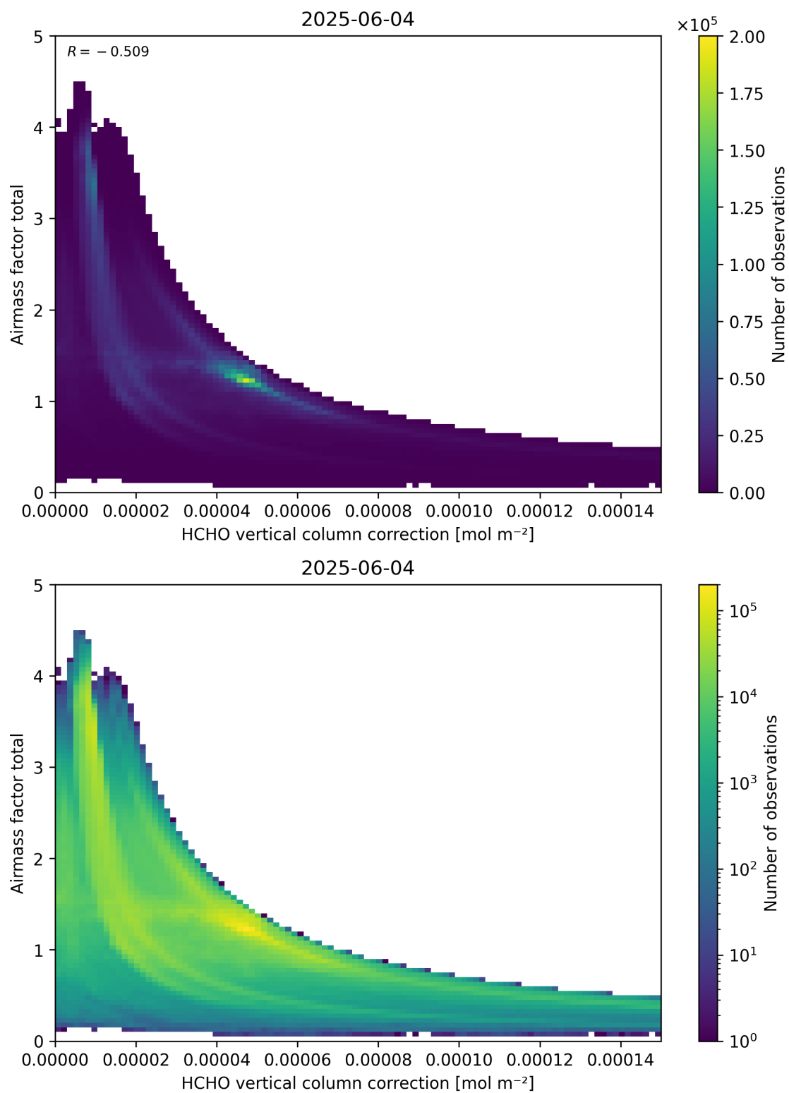
Figure 120: Scatter density plot of “HCHO vertical column correction” against “Airmass factor total” for 2025-06-03 to 2025-06-05.
