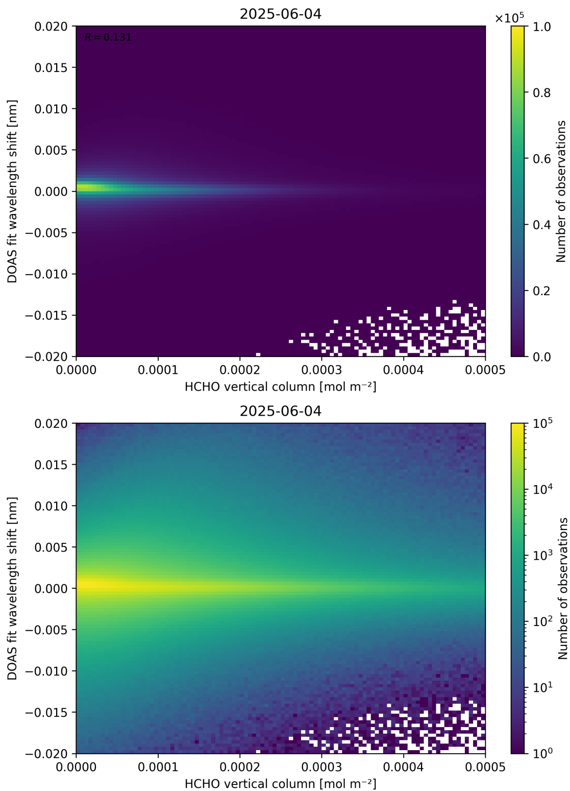
Figure 124: Scatter density plot of “HCHO vertical column” against “DOAS fit wavelength shift” for 2025-06-03 to 2025-06-05.
