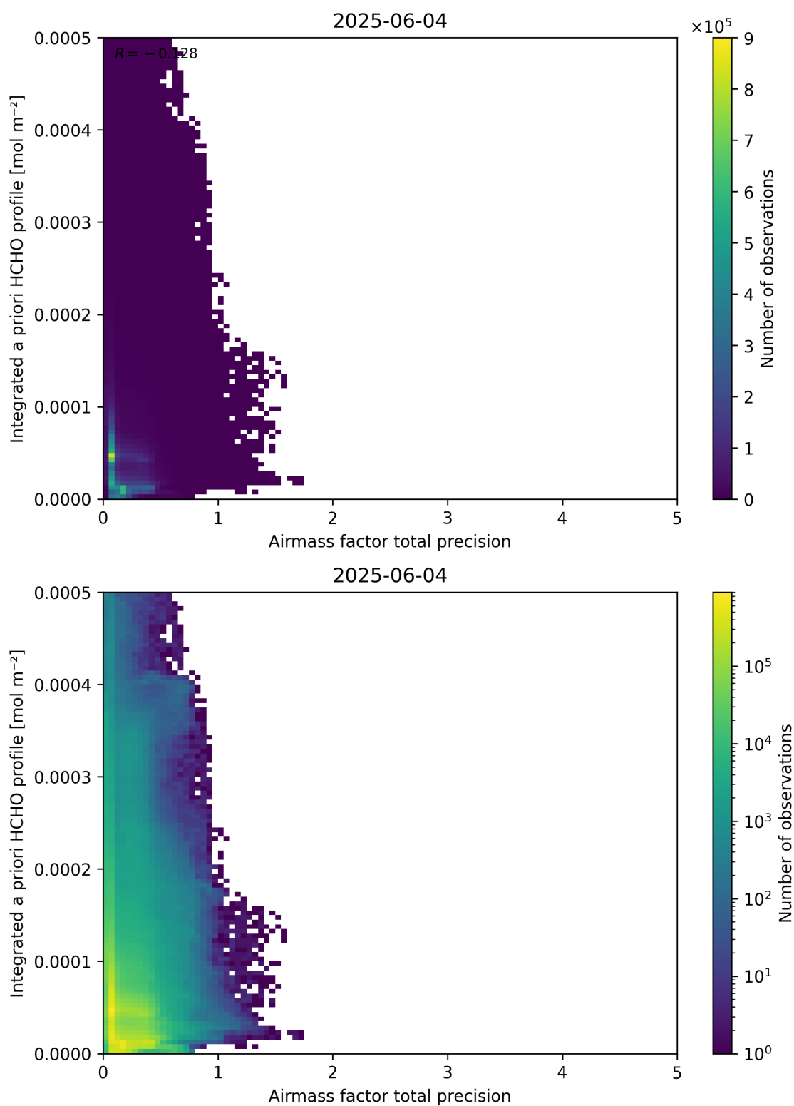
Figure 111: Scatter density plot of “Airmass factor total precision” against “Integrated a priori HCHO profile” for 2025-06-03 to 2025-06-05.
