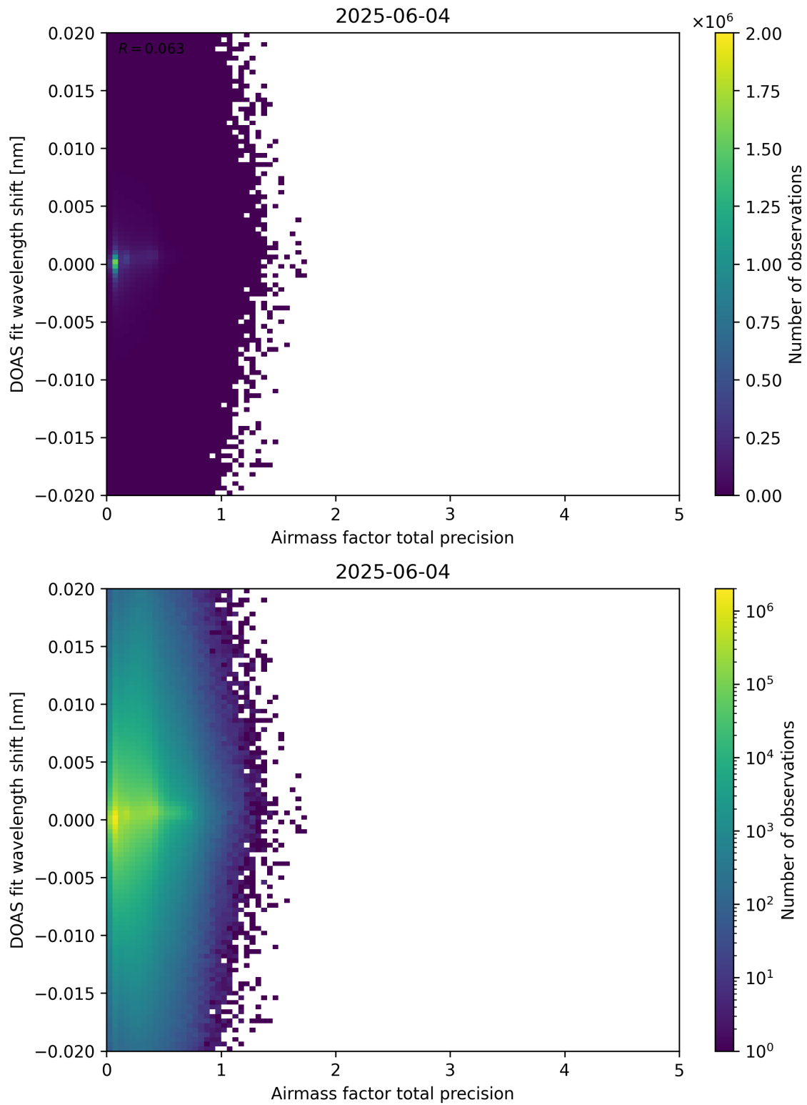
Figure 106: Scatter density plot of “Airmass factor total precision” against “DOAS fit wavelength shift” for 2025-06-03 to 2025-06-05.
