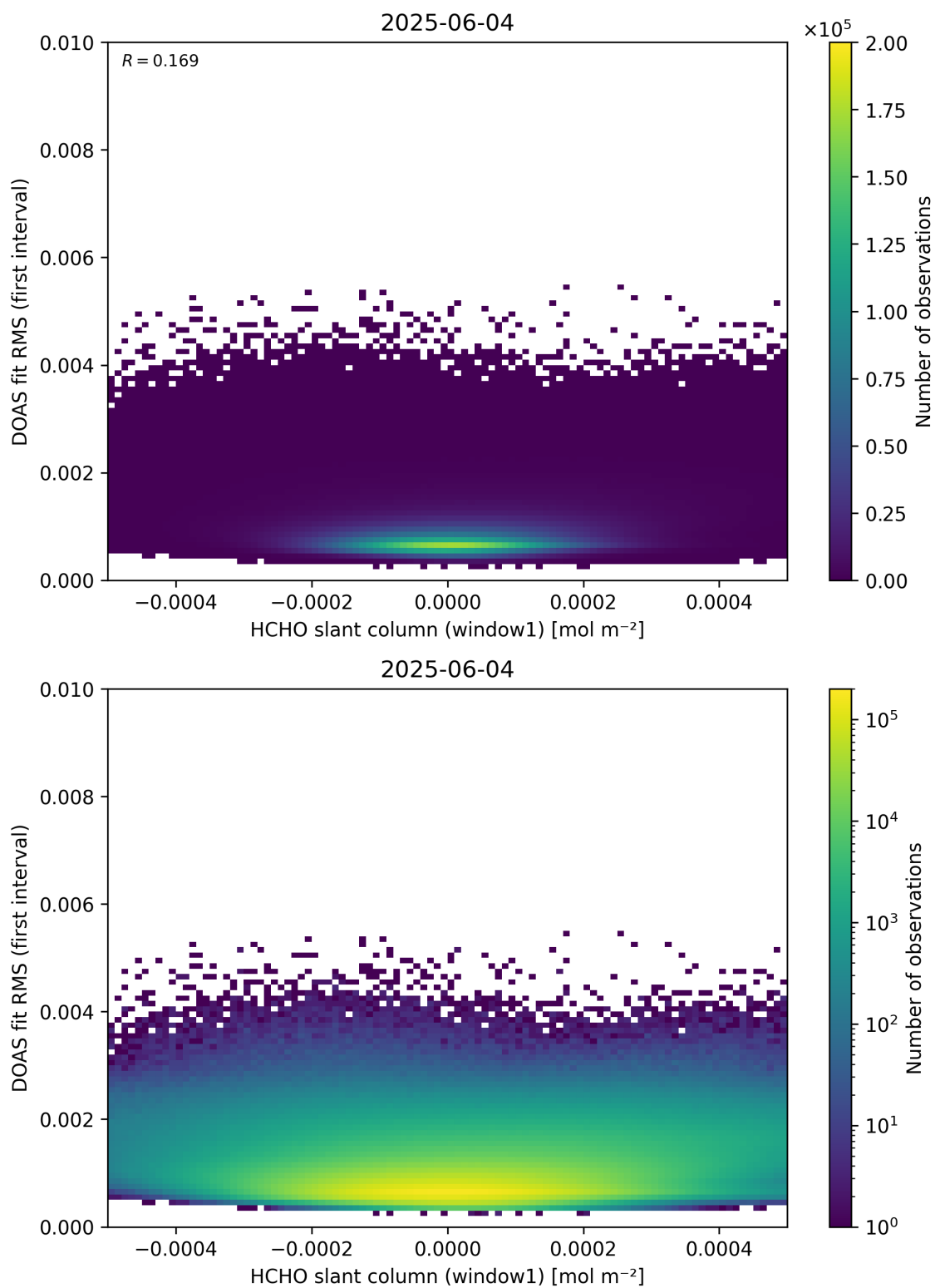
Figure 78: Scatter density plot of “HCHO slant column (window1)” against “DOAS fit RMS (first interval)” for 2025-06-03 to 2025-06-05.
