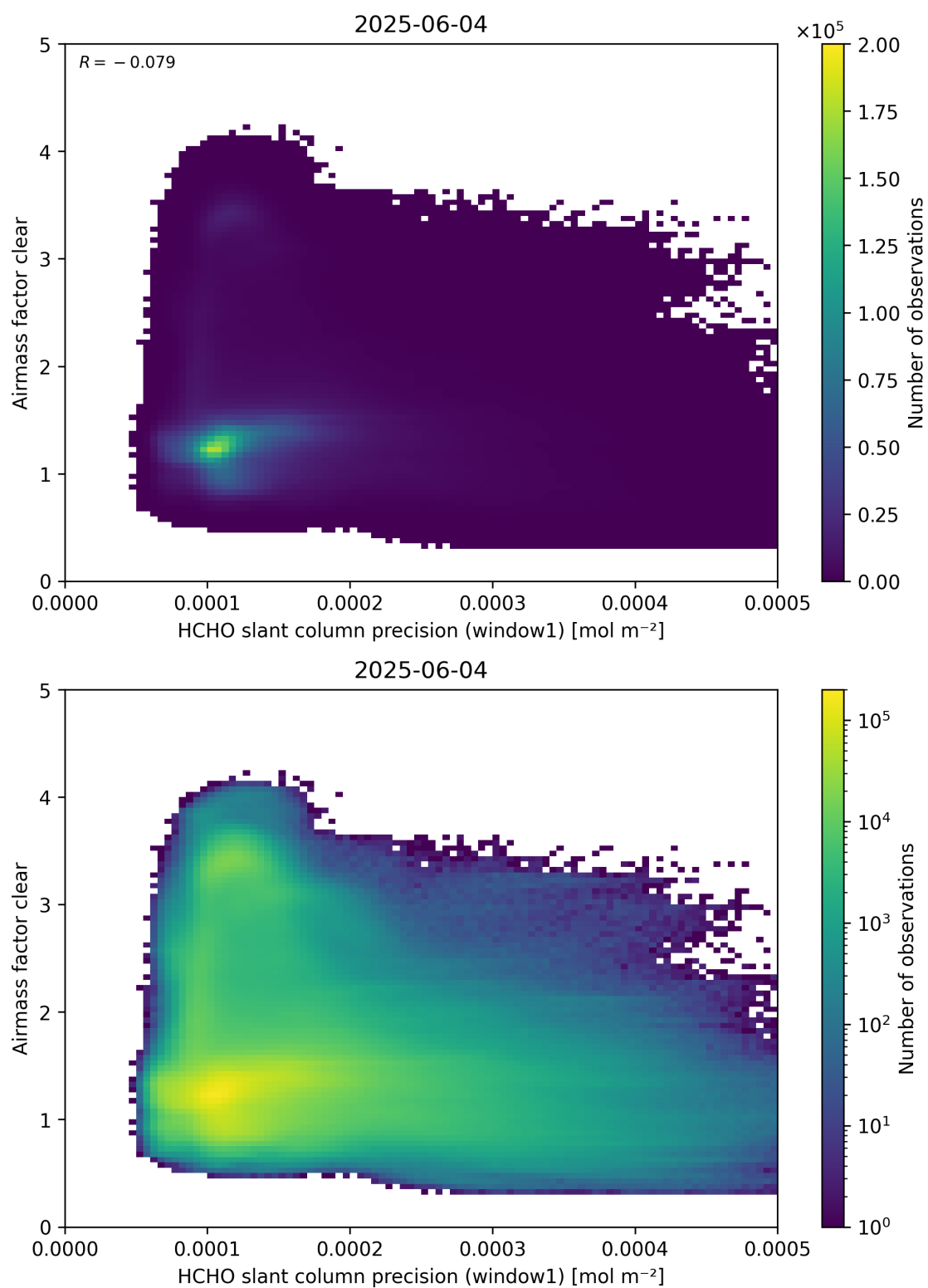
Figure 91: Scatter density plot of “HCHO slant column precision (window1)” against “Airmass factor clear” for 2025-06-03 to 2025-06-05.
