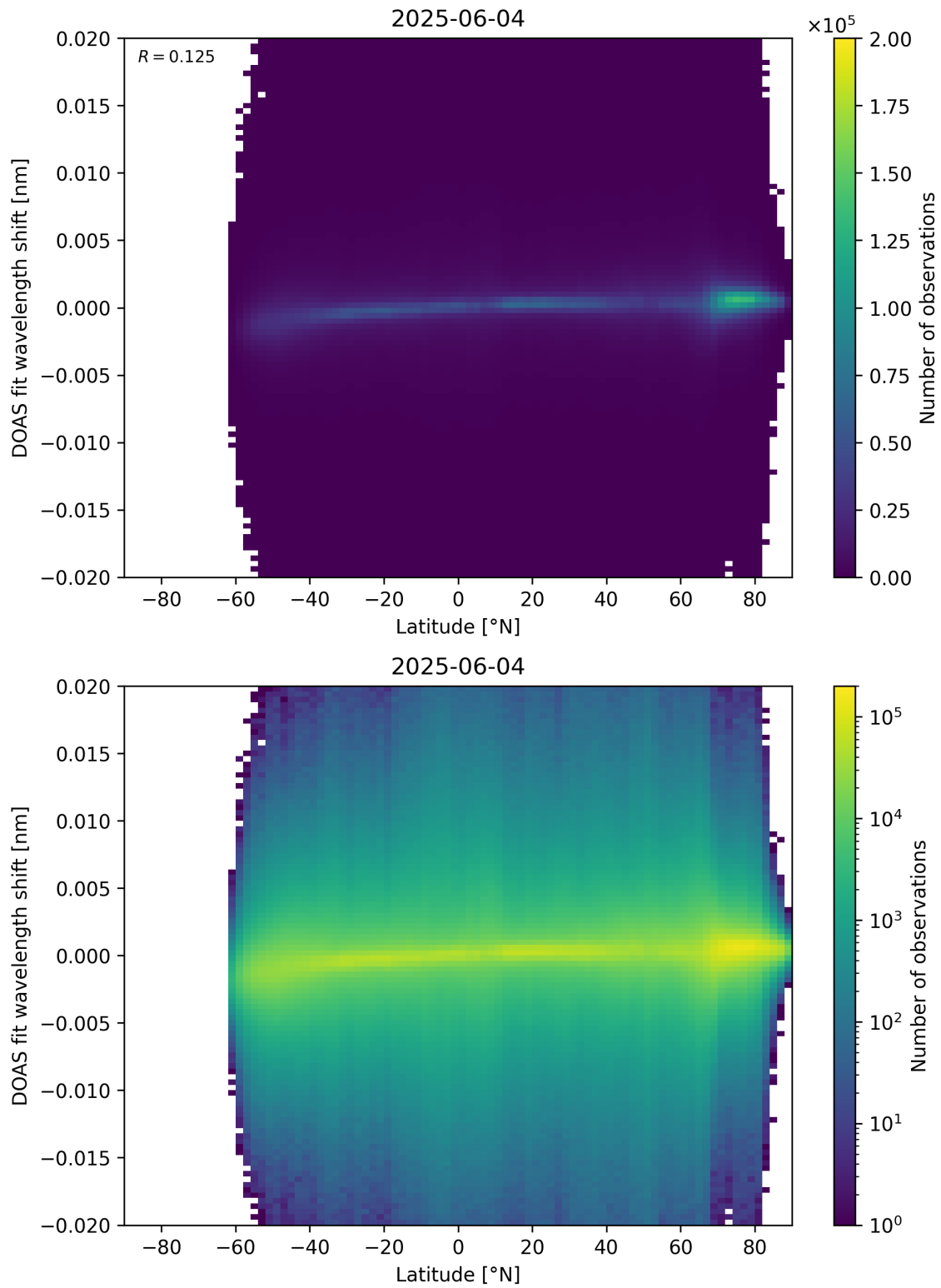
Figure 154: Scatter density plot of “Latitude” against “DOAS fit wavelength shift” for 2025-06-03 to 2025-06-05.
