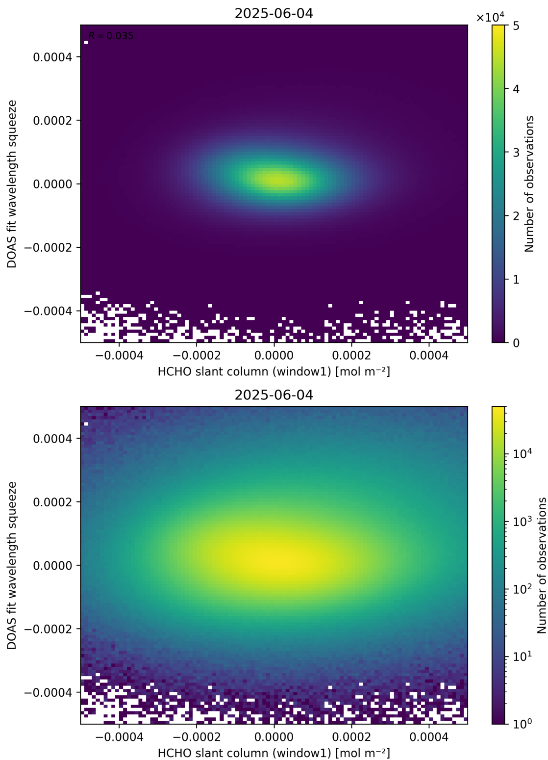
Figure 80: Scatter density plot of “HCHO slant column (window1)” against “DOAS fit wavelength squeeze” for 2025-06-03 to 2025-06-05.
