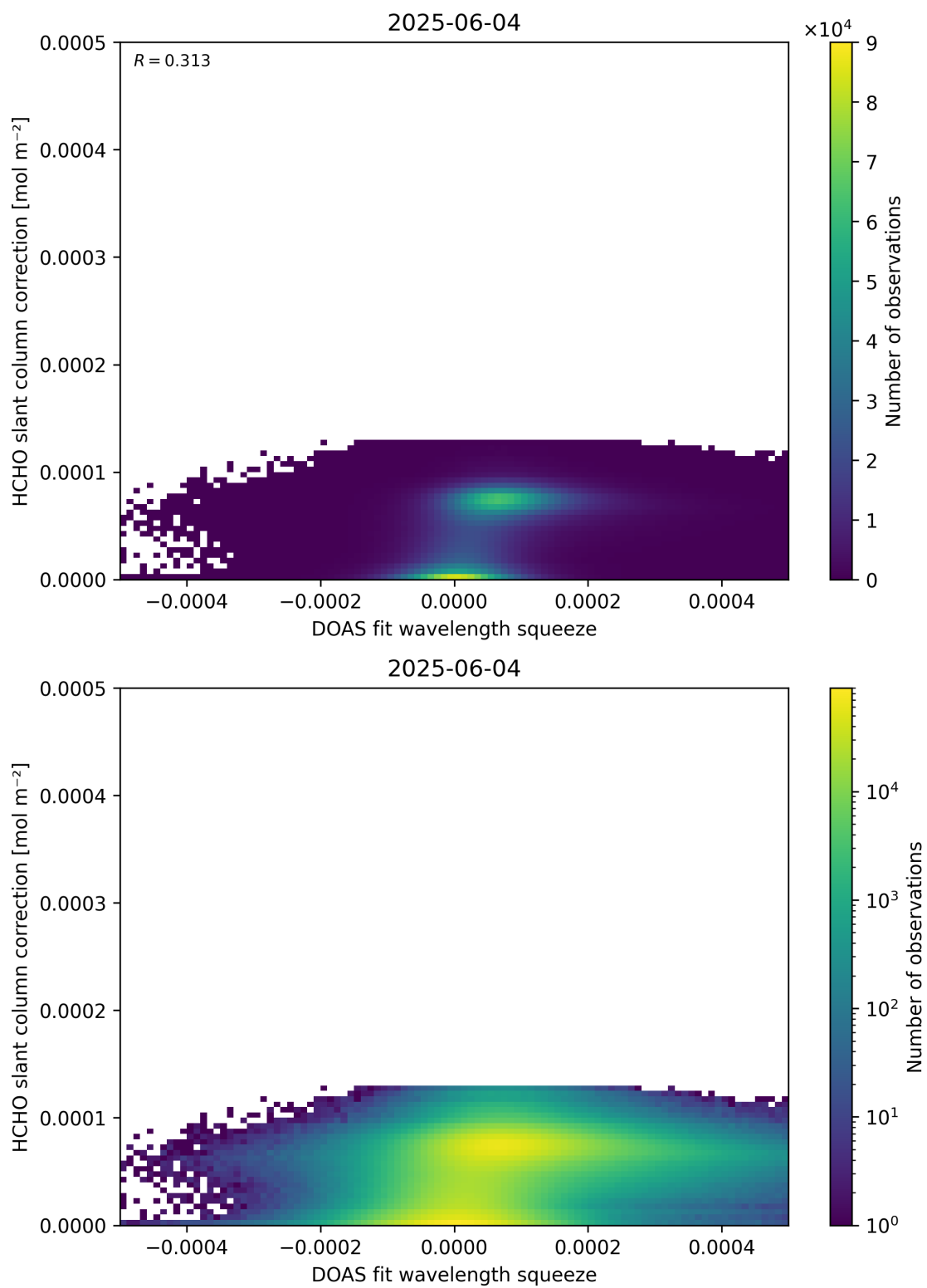
Figure 70: Scatter density plot of “DOAS fit wavelength squeeze” against “HCHO slant column correction” for 2025-06-03 to 2025-06-05.
