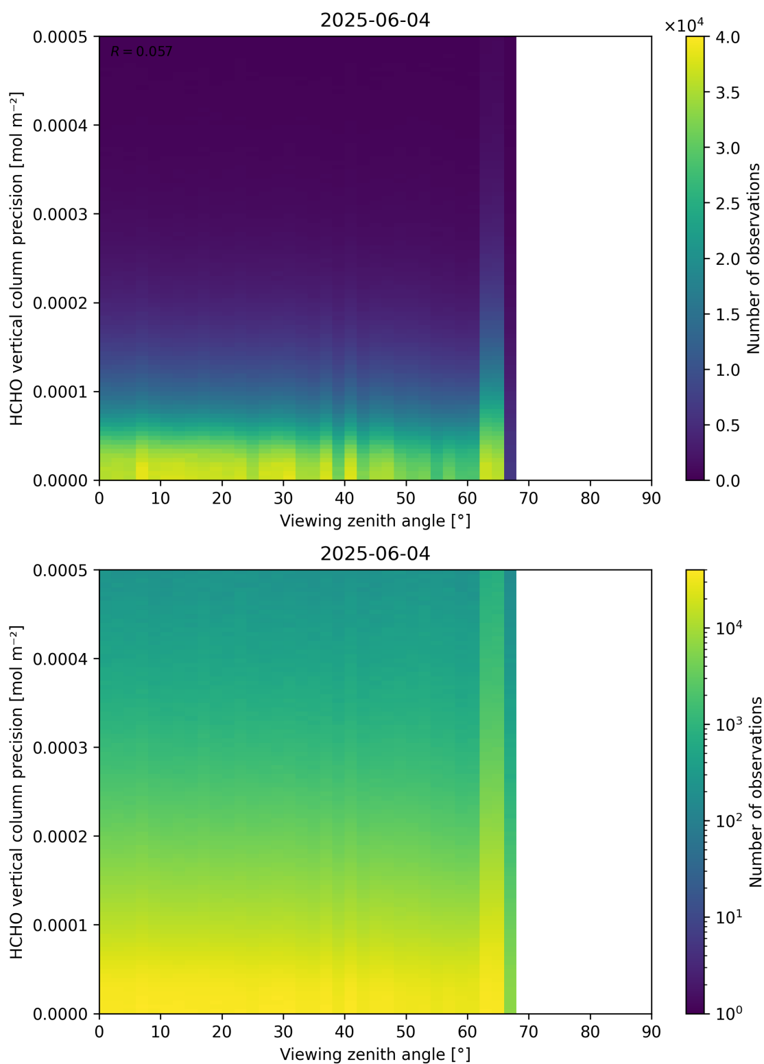
Figure 194: Scatter density plot of “Viewing zenith angle” against “HCHO vertical column precision” for 2025-06-03 to 2025-06-05.
