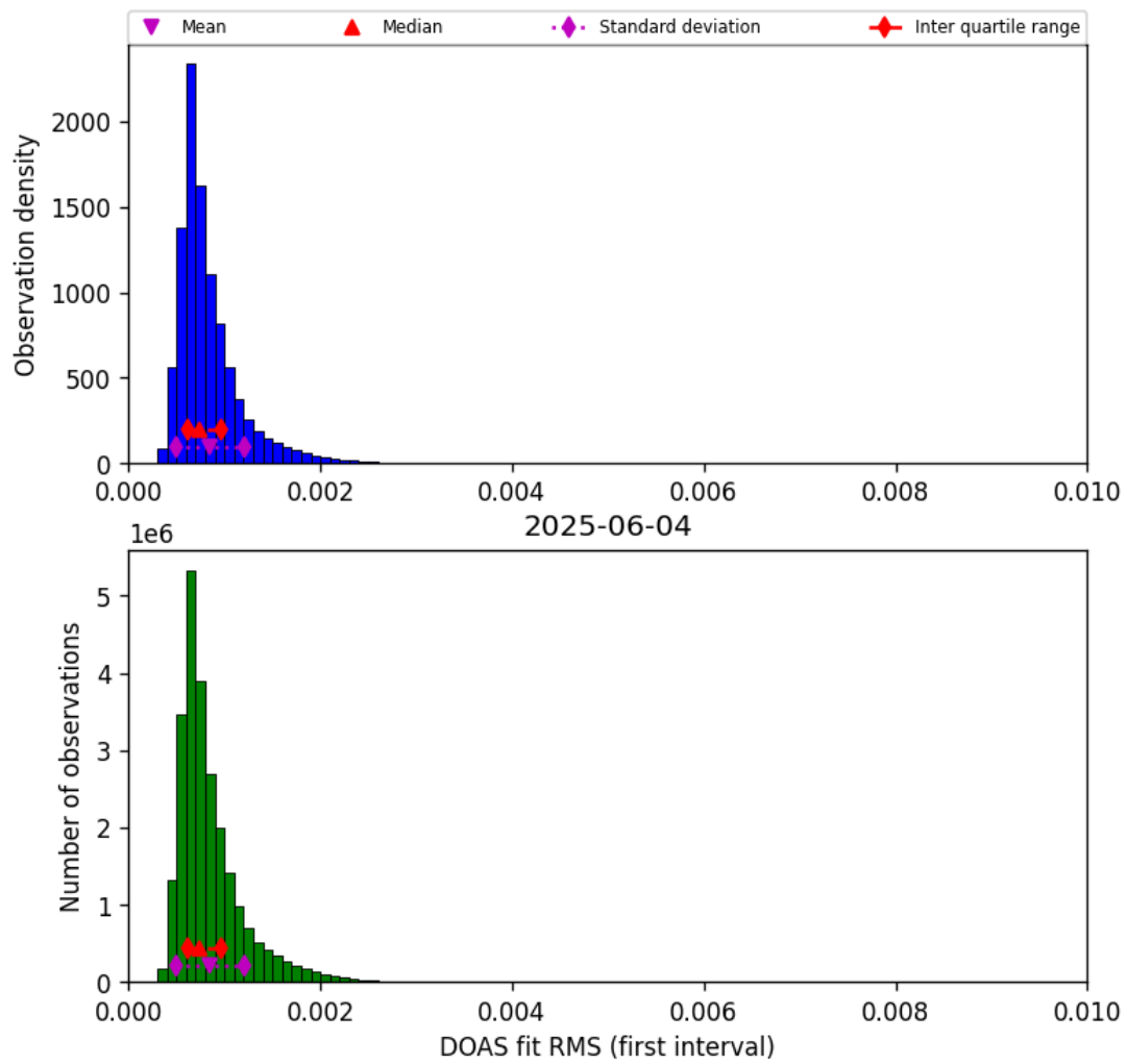
Figure 46: Histogram of “DOAS fit RMS (first interval)” for 2025-06-03 to 2025-06-05
