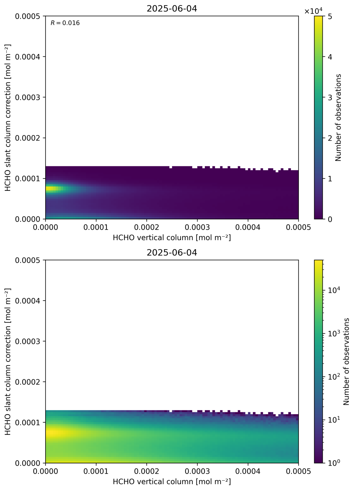
Figure 128: Scatter density plot of “HCHO vertical column” against “HCHO slant column correction” for 2025-06-03 to 2025-06-05.
