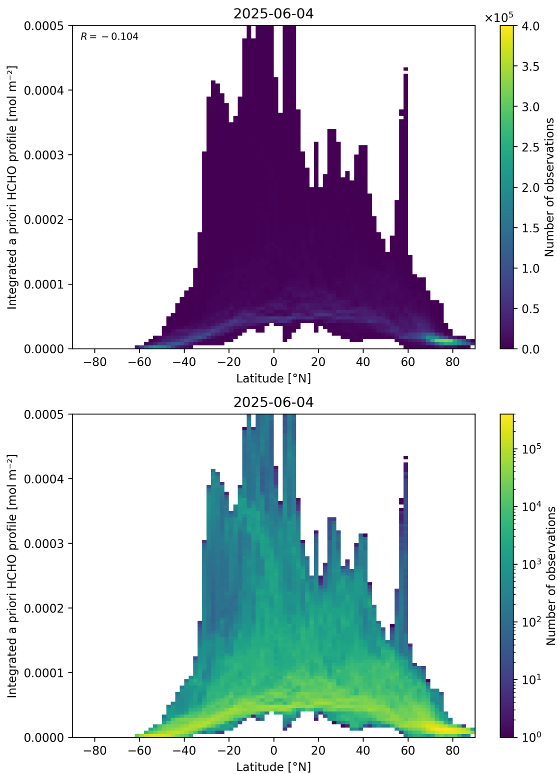
Figure 166: Scatter density plot of “Latitude” against “Integrated a priori HCHO profile” for 2025-06-03 to 2025-06-05.
