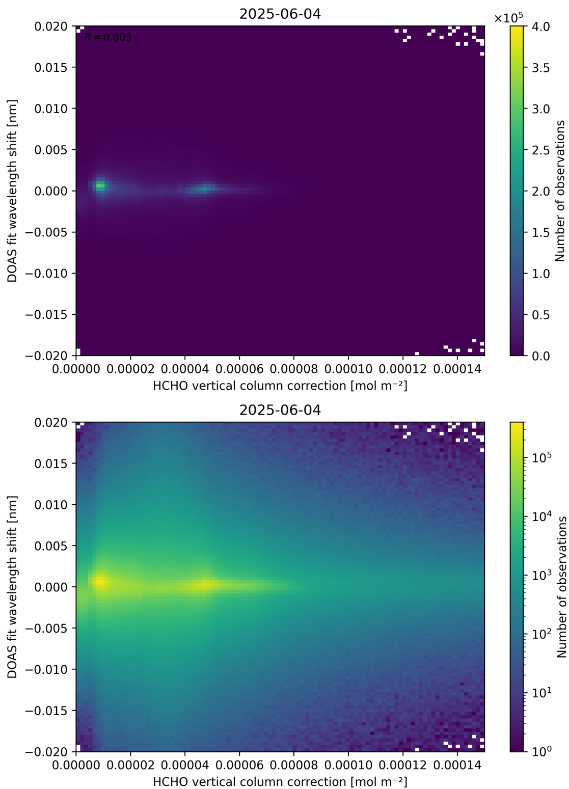
Figure 113: Scatter density plot of “HCHO vertical column correction” against “DOAS fit wavelength shift” for 2025-06-03 to 2025-06-05.
