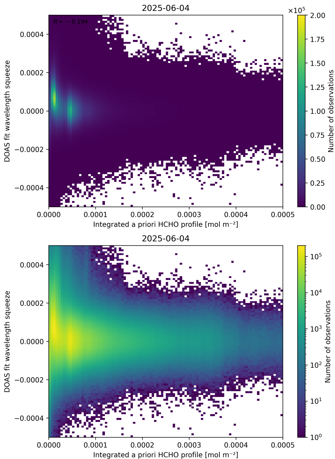
Figure 150: Scatter density plot of “Integrated a priori HCHO profile” against “DOAS fit wavelength squeeze” for 2025-06-03 to 2025-06-05.
