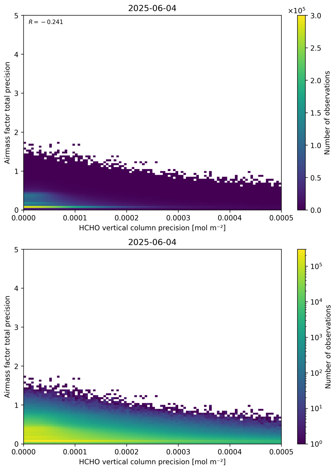
Figure 145: Scatter density plot of “HCHO vertical column precision” against “Airmass factor total precision” for 2025-06-03 to 2025-06-05.
