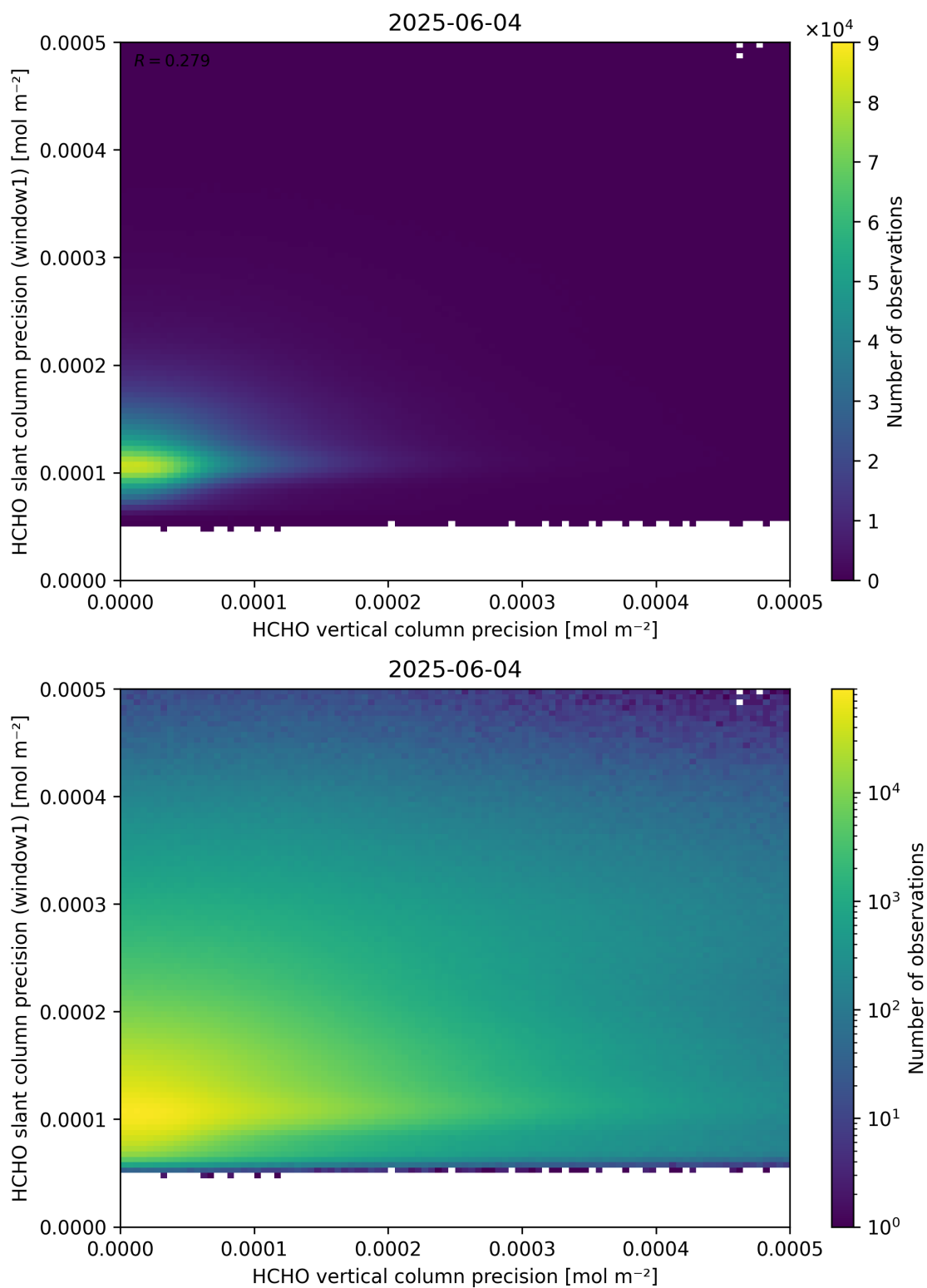
Figure 143: Scatter density plot of “HCHO vertical column precision” against “HCHO slant column precision (window1)” for 2025-06-03 to 2025-06-05.
