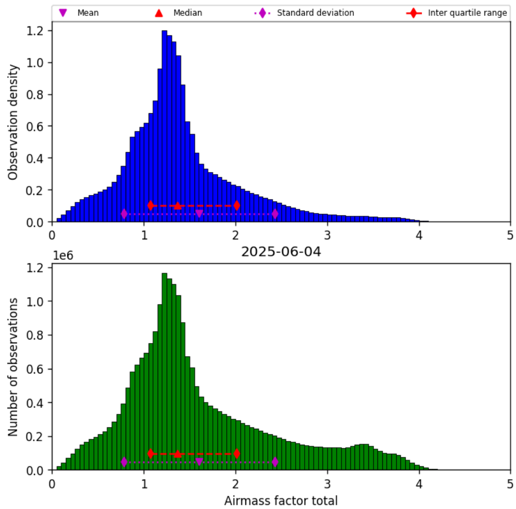
Figure 40: Histogram of “Airmass factor total” for 2025-06-03 to 2025-06-05
