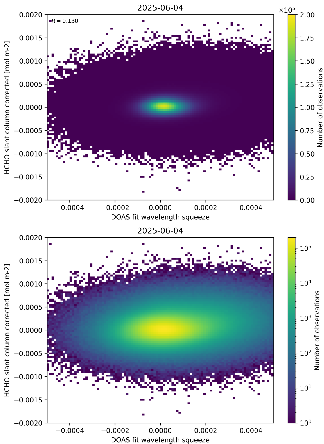
Figure 69: Scatter density plot of “DOAS fit wavelength squeeze” against “HCHO slant column corrected” for 2025-06-03 to 2025-06-05.
