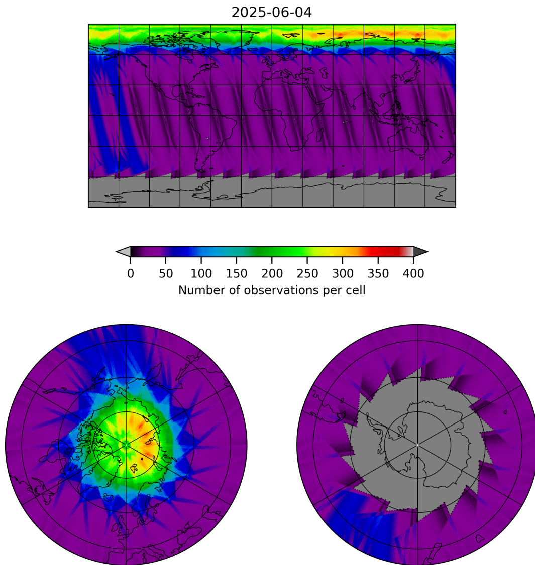
Figure 19: Map of the number of observations for 2025-06-03 to 2025-06-05
