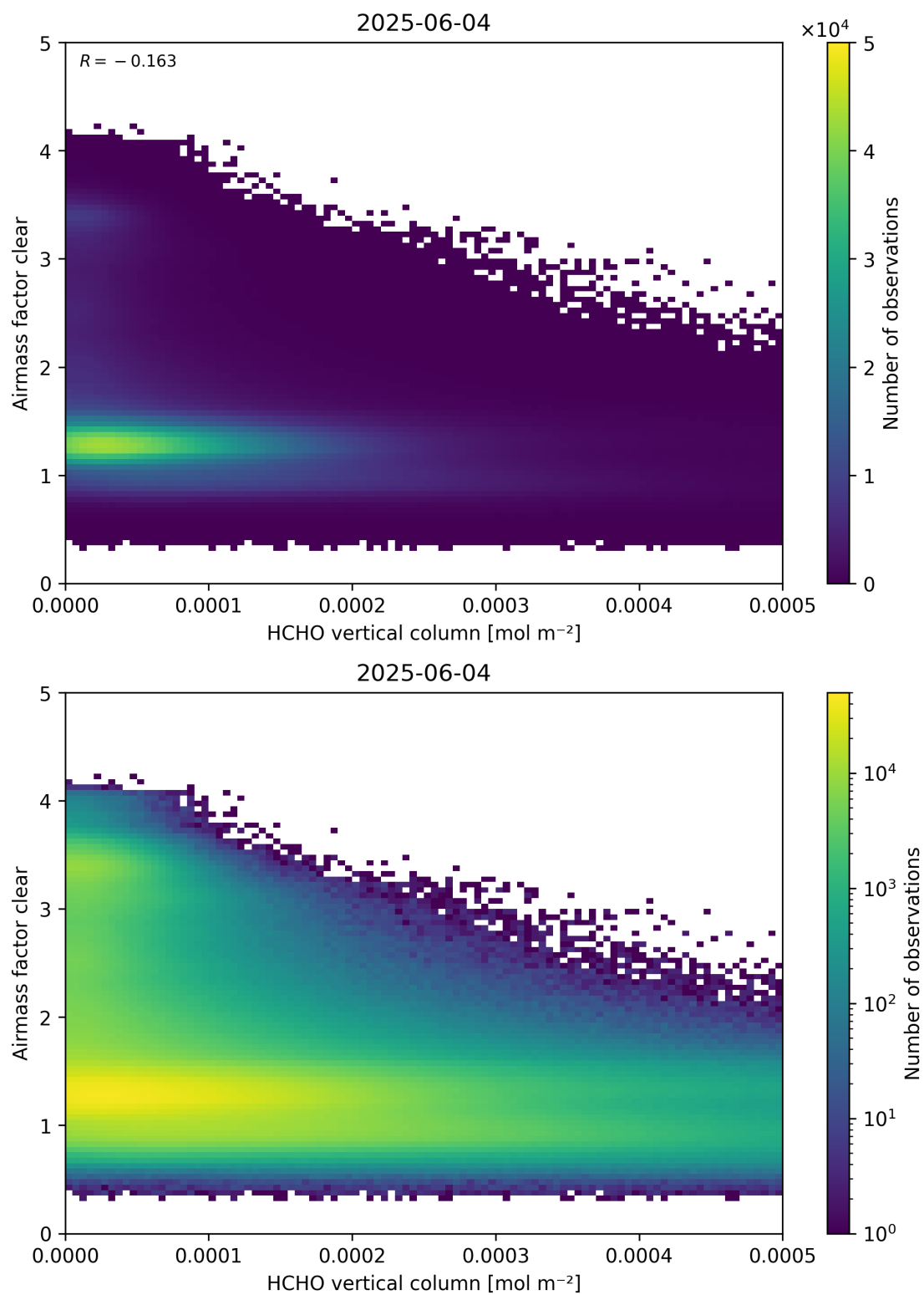
Figure 126: Scatter density plot of “HCHO vertical column” against “Airmass factor clear” for 2025-06-03 to 2025-06-05.
