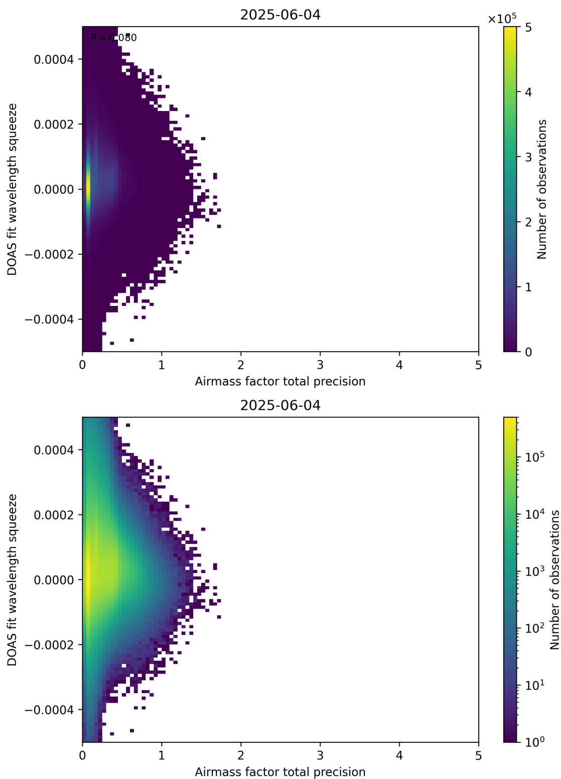
Figure 107: Scatter density plot of “Airmass factor total precision” against “DOAS fit wavelength squeeze” for 2025-06-03 to 2025-06-05.
