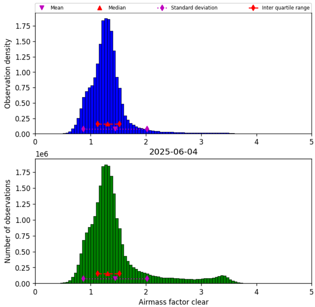
Figure 42: Histogram of “Airmass factor clear” for 2025-06-03 to 2025-06-05
