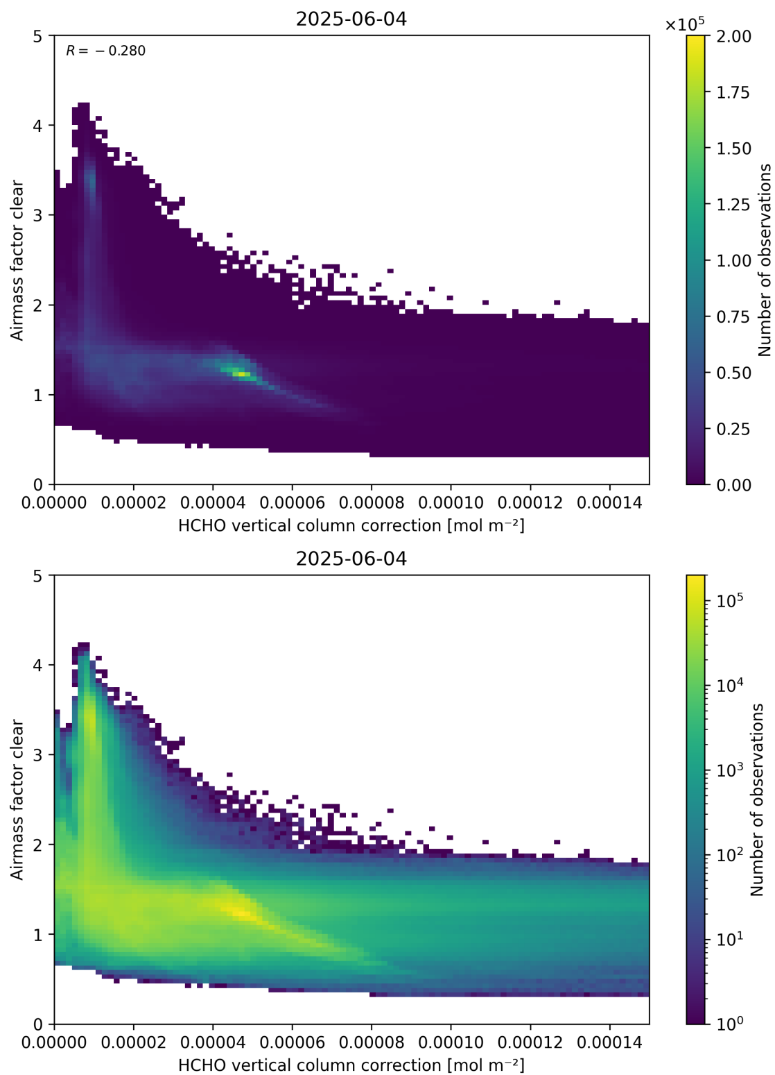
Figure 115: Scatter density plot of “HCHO vertical column correction” against “Airmass factor clear” for 2025-06-03 to 2025-06-05.
