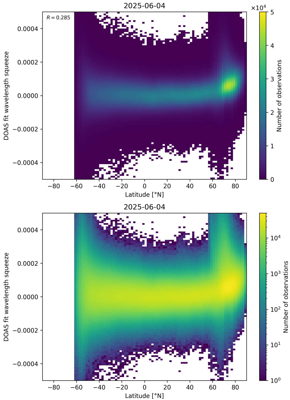
Figure 155: Scatter density plot of “Latitude” against “DOAS fit wavelength squeeze” for 2025-06-03 to 2025-06-05.
