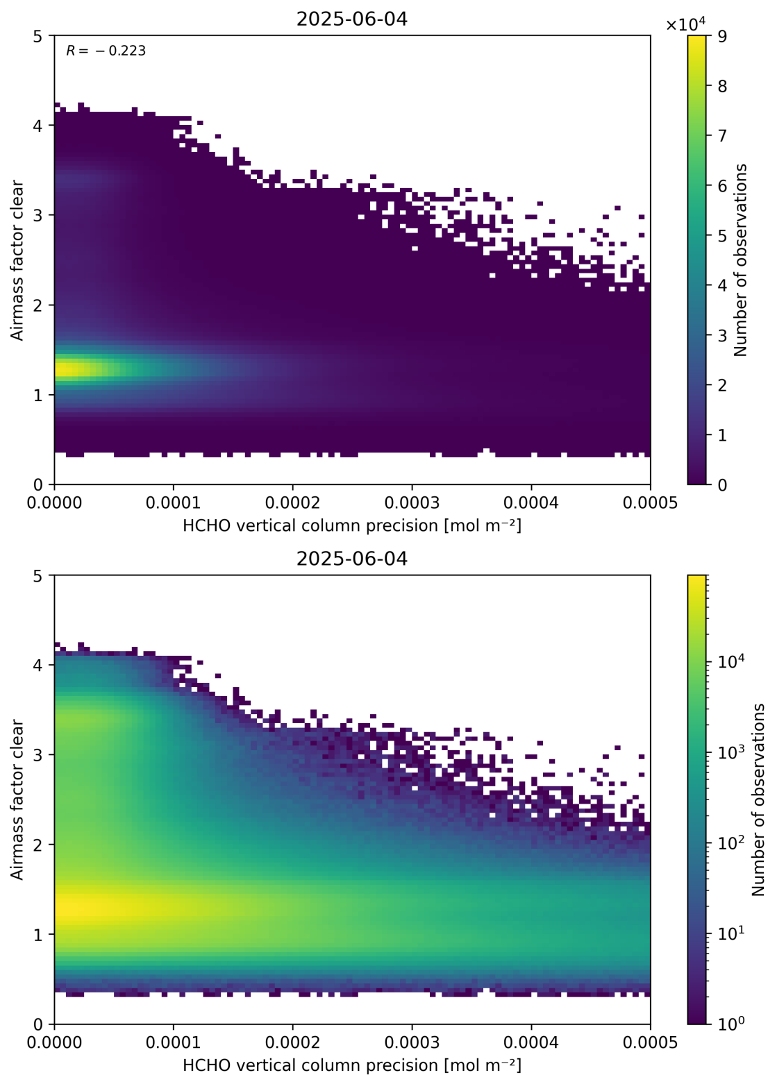
Figure 139: Scatter density plot of “HCHO vertical column precision” against “Airmass factor clear” for 2025-06-03 to 2025-06-05.
