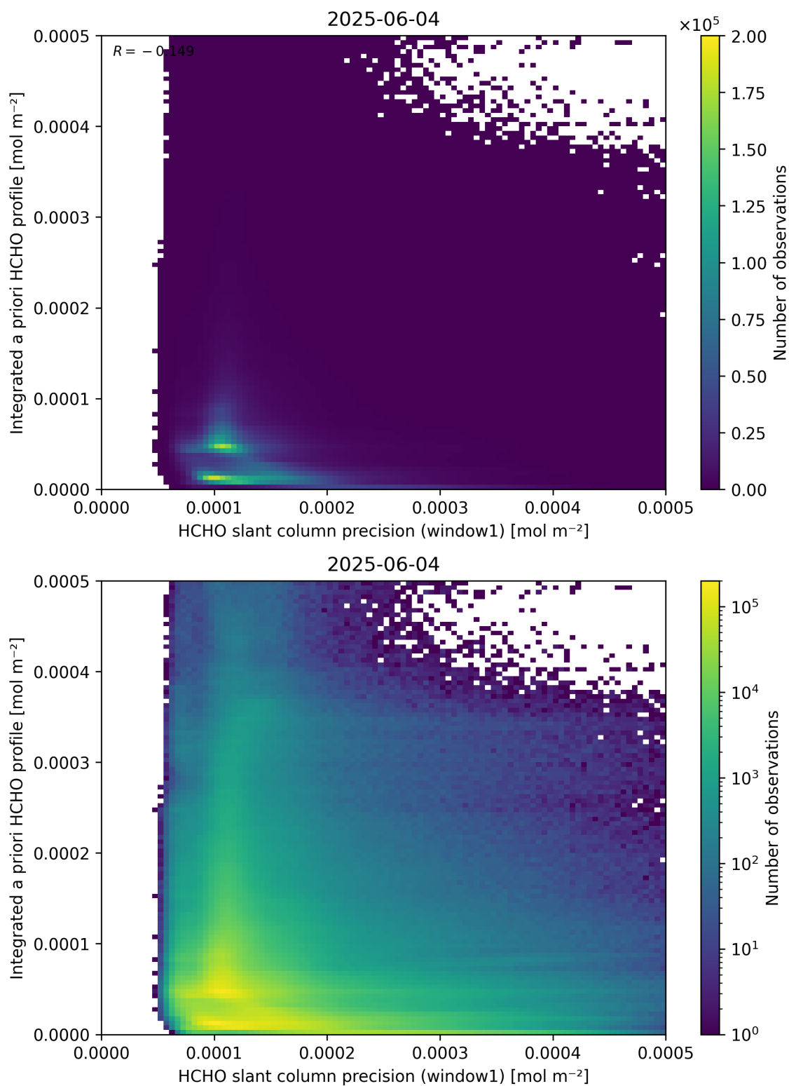
Figure 96: Scatter density plot of “HCHO slant column precision (window1)” against “Integrated a priori HCHO profile” for 2025-06-03 to 2025-06-05.
