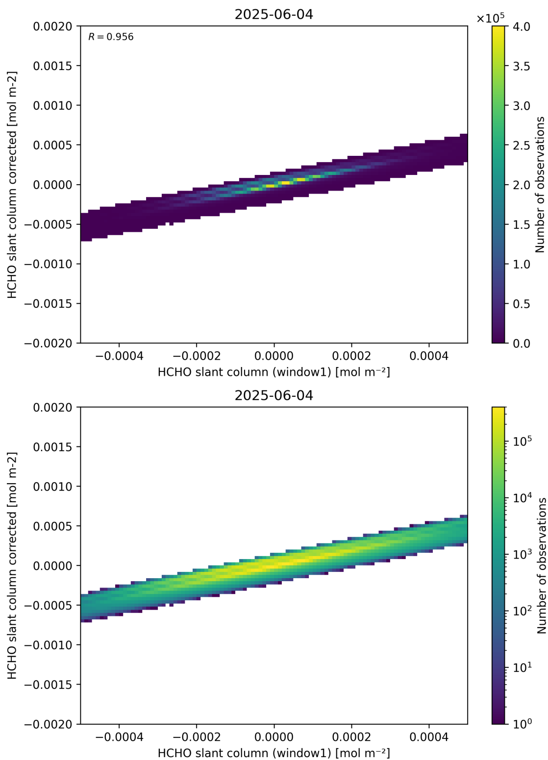
Figure 82: Scatter density plot of “HCHO slant column (window1)” against “HCHO slant column corrected” for 2025-06-03 to 2025-06-05.
