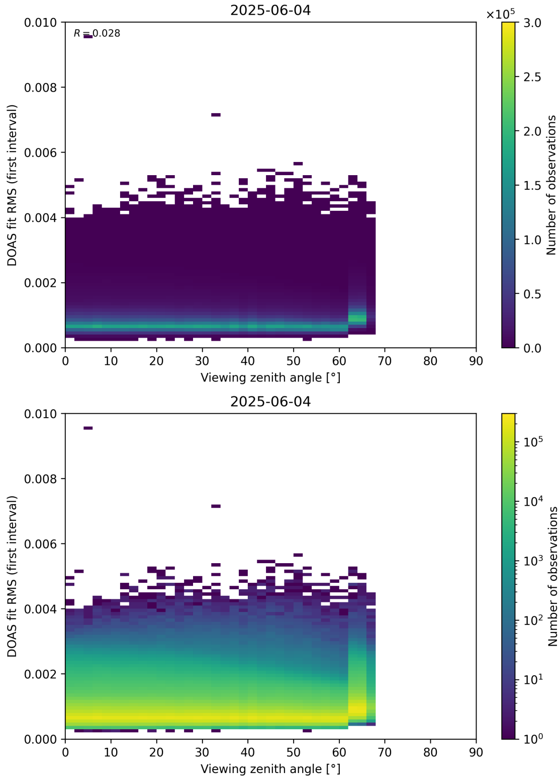
Figure 182: Scatter density plot of “Viewing zenith angle” against “DOAS fit RMS (first interval)” for 2025-06-03 to 2025-06-05.
