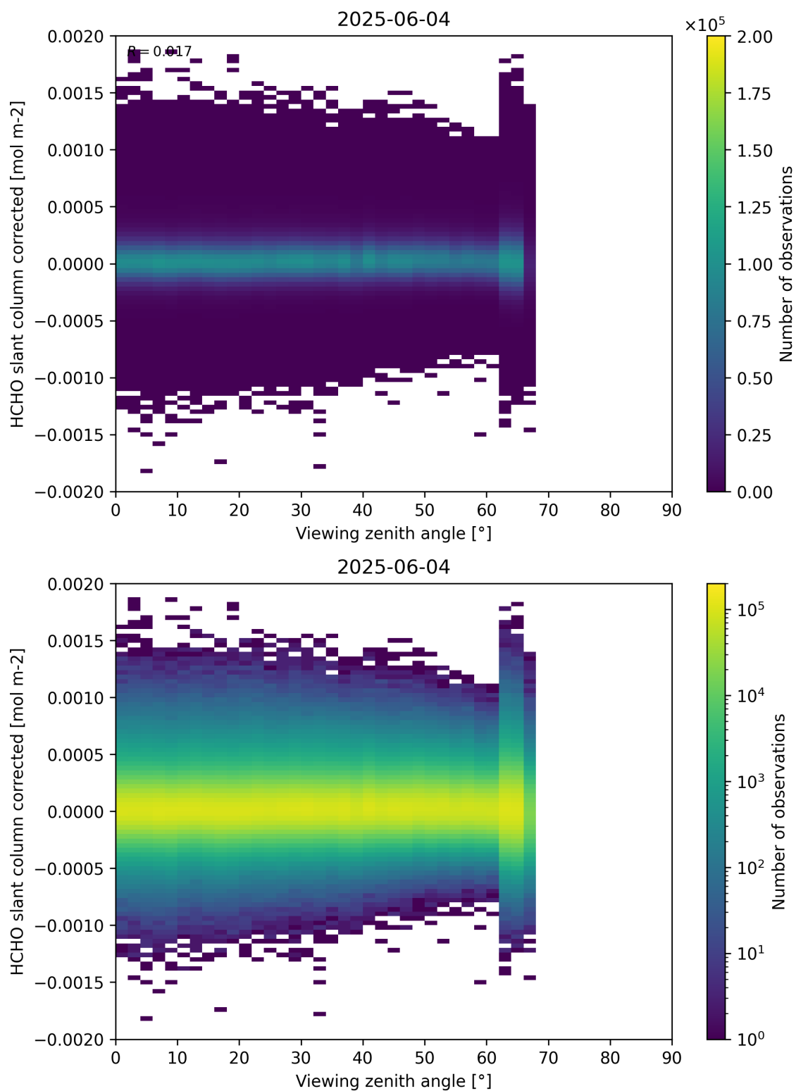
Figure 186: Scatter density plot of “Viewing zenith angle” against “HCHO slant column corrected” for 2025-06-03 to 2025-06-05.
