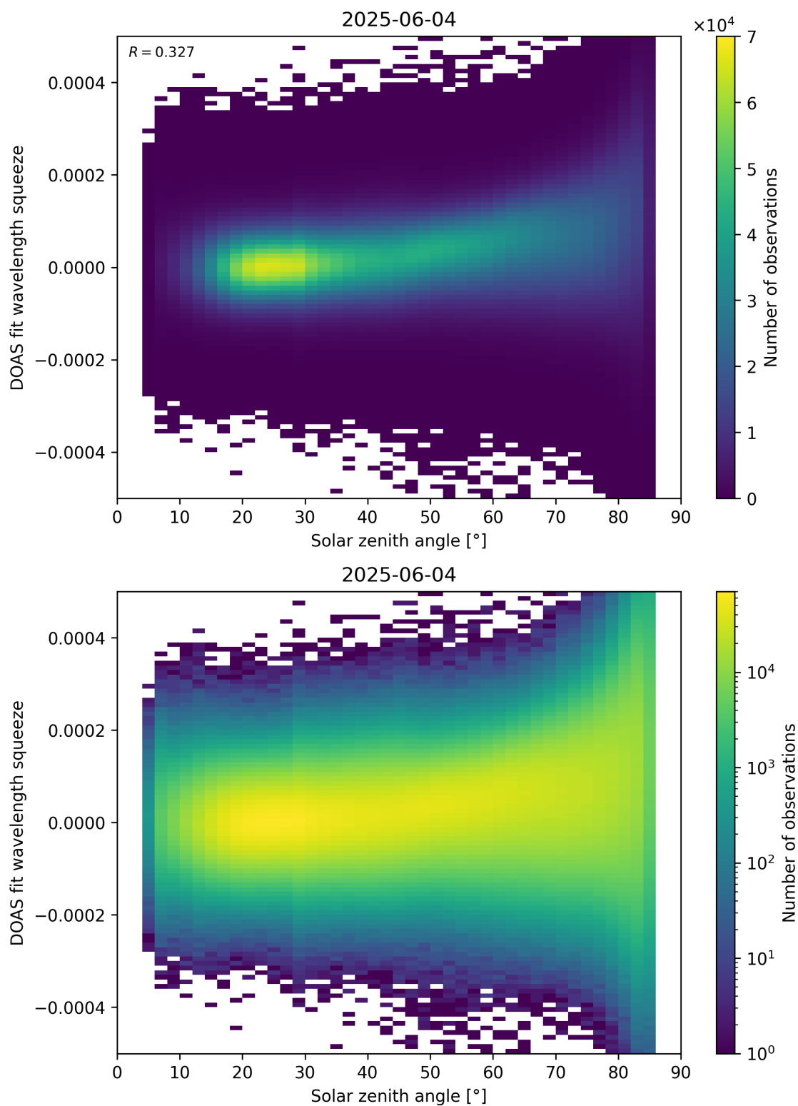
Figure 169: Scatter density plot of “Solar zenith angle” against “DOAS fit wavelength squeeze” for 2025-06-03 to 2025-06-05.
