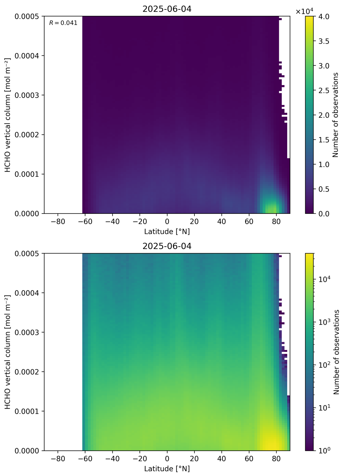
Figure 163: Scatter density plot of “Latitude” against “HCHO vertical column” for 2025-06-03 to 2025-06-05.
