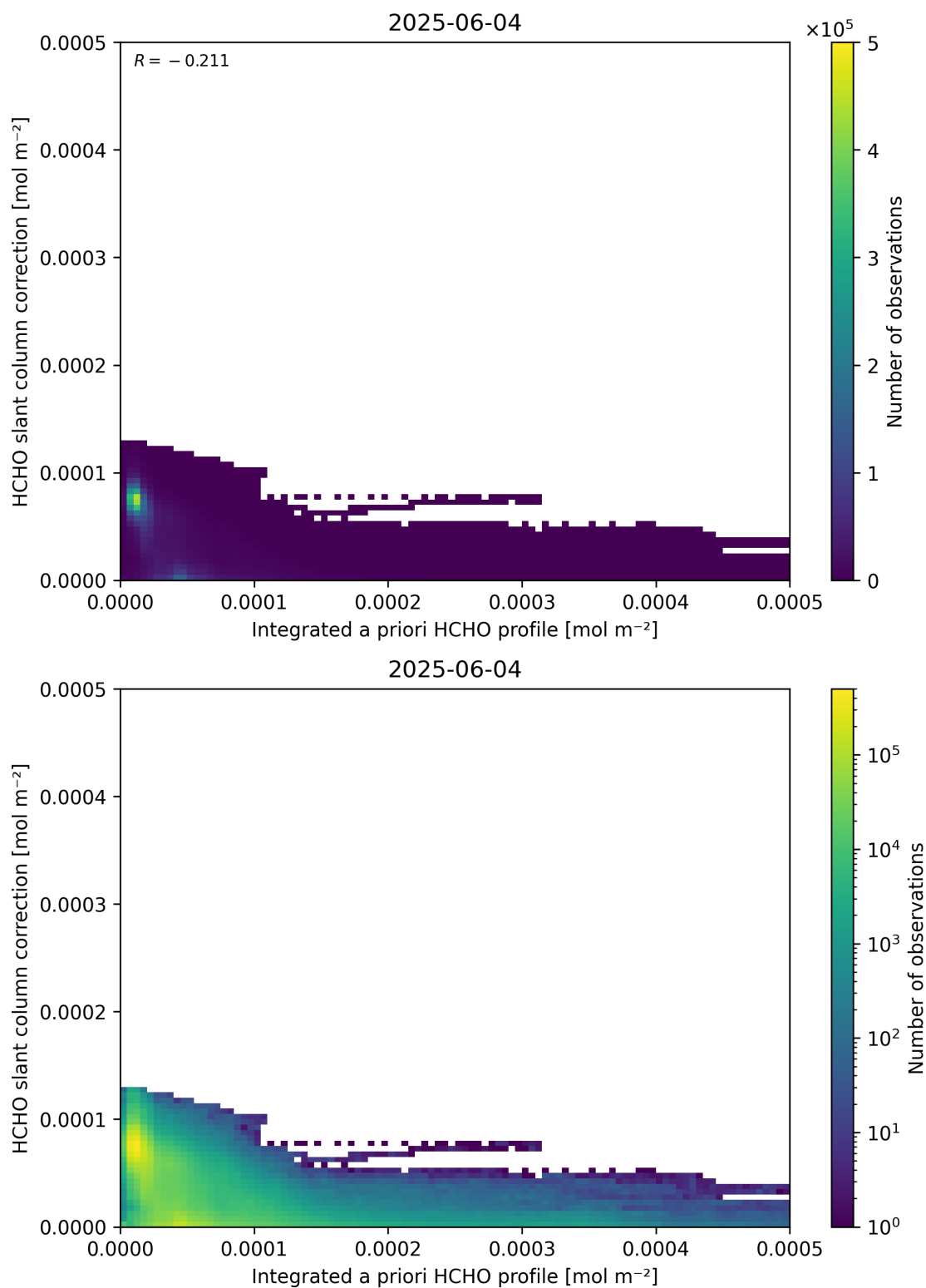
Figure 152: Scatter density plot of “Integrated a priori HCHO profile” against “HCHO slant column correction” for 2025-06-03 to 2025-06-05.
