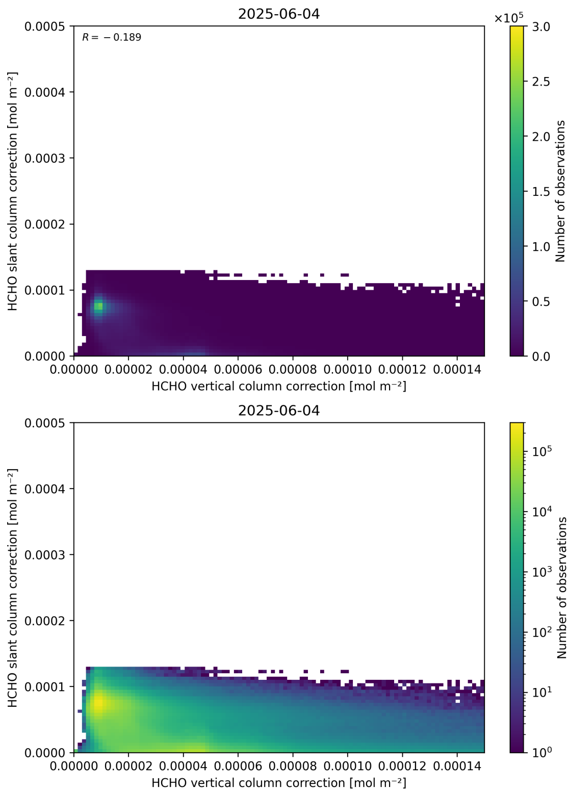
Figure 117: Scatter density plot of “HCHO vertical column correction” against “HCHO slant column correction” for 2025-06-03 to 2025-06-05.
