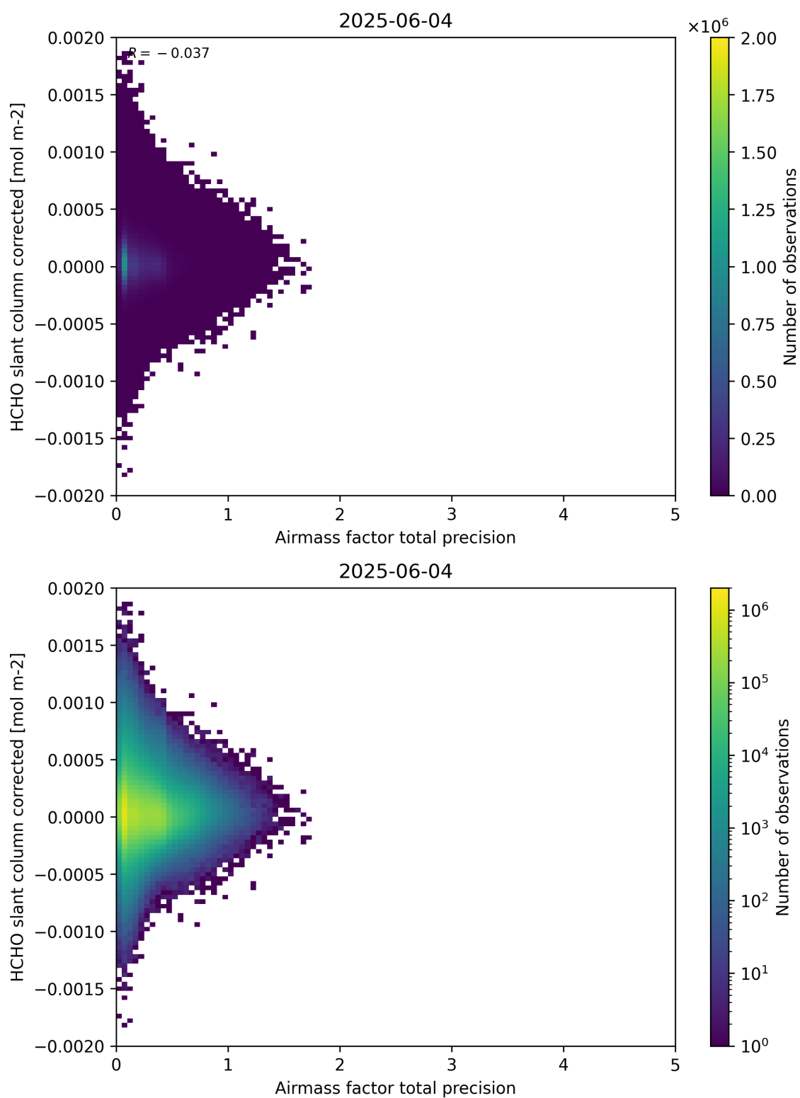
Figure 109: Scatter density plot of “Airmass factor total precision” against “HCHO slant column corrected” for 2025-06-03 to 2025-06-05.
