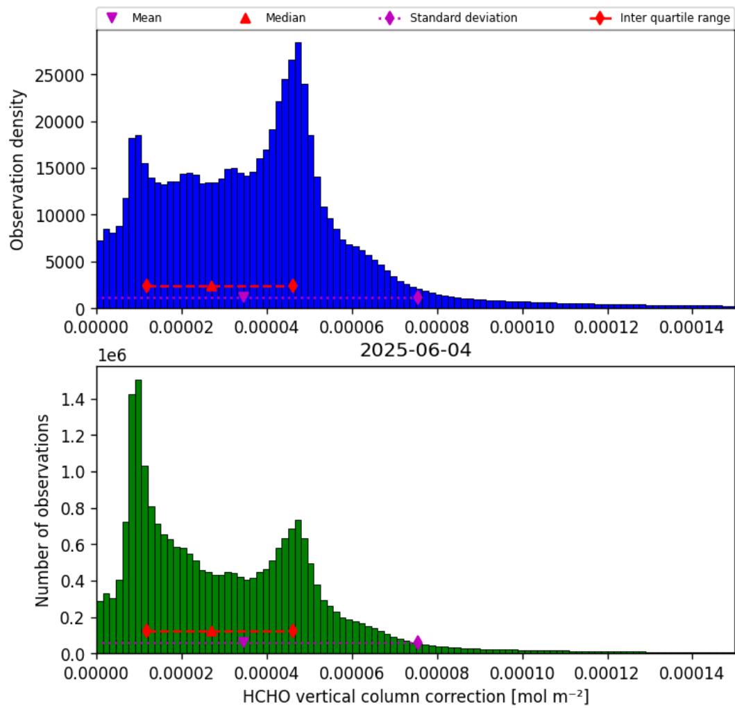
Figure 37: Histogram of “HCHO vertical column correction” for 2025-06-03 to 2025-06-05
