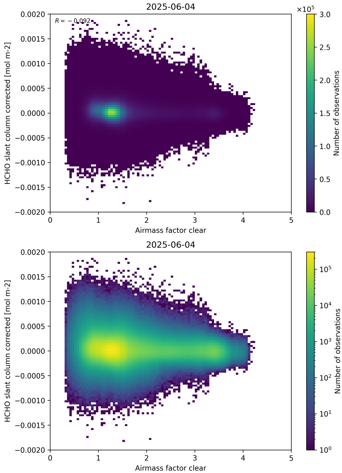
Figure 74: Scatter density plot of “Airmass factor clear” against “HCHO slant column corrected” for 2025-06-03 to 2025-06-05.
