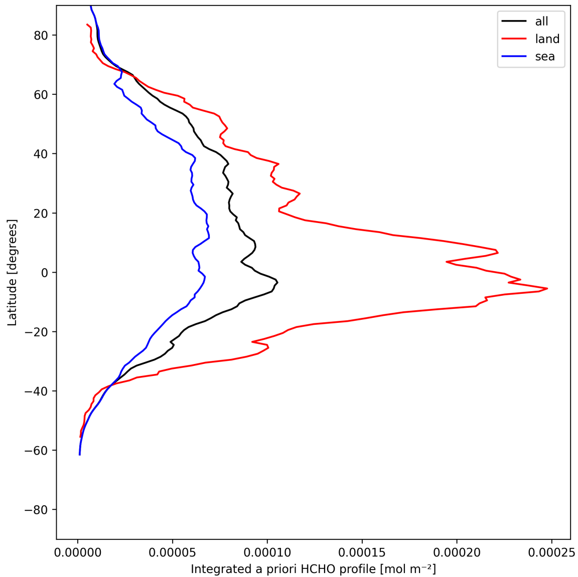
Figure 29: Zonal average of “Integrated a priori HCHO profile” for 2025-06-03 to 2025-06-05.
