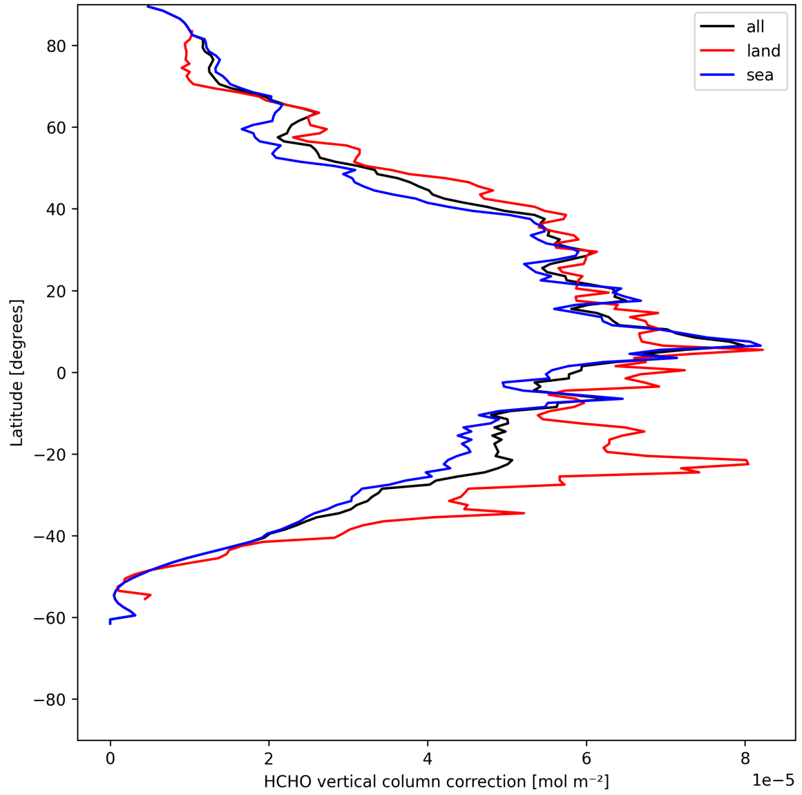
Figure 23: Zonal average of “HCHO vertical column correction” for 2025-06-03 to 2025-06-05.
