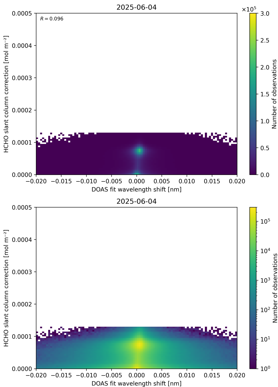
Figure 67: Scatter density plot of “DOAS fit wavelength shift” against “HCHO slant column correction” for 2025-06-03 to 2025-06-05.
