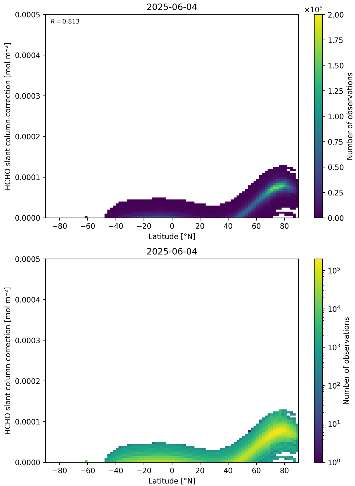
Figure 158: Scatter density plot of “Latitude” against “HCHO slant column correction” for 2025-06-03 to 2025-06-05.
