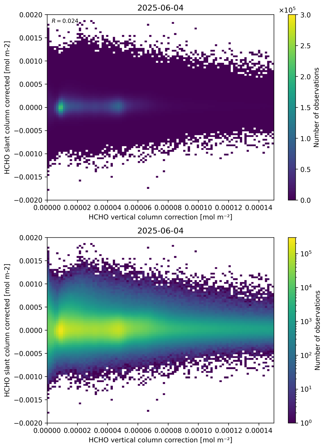
Figure 116: Scatter density plot of “HCHO vertical column correction” against “HCHO slant column corrected” for 2025-06-03 to 2025-06-05.
