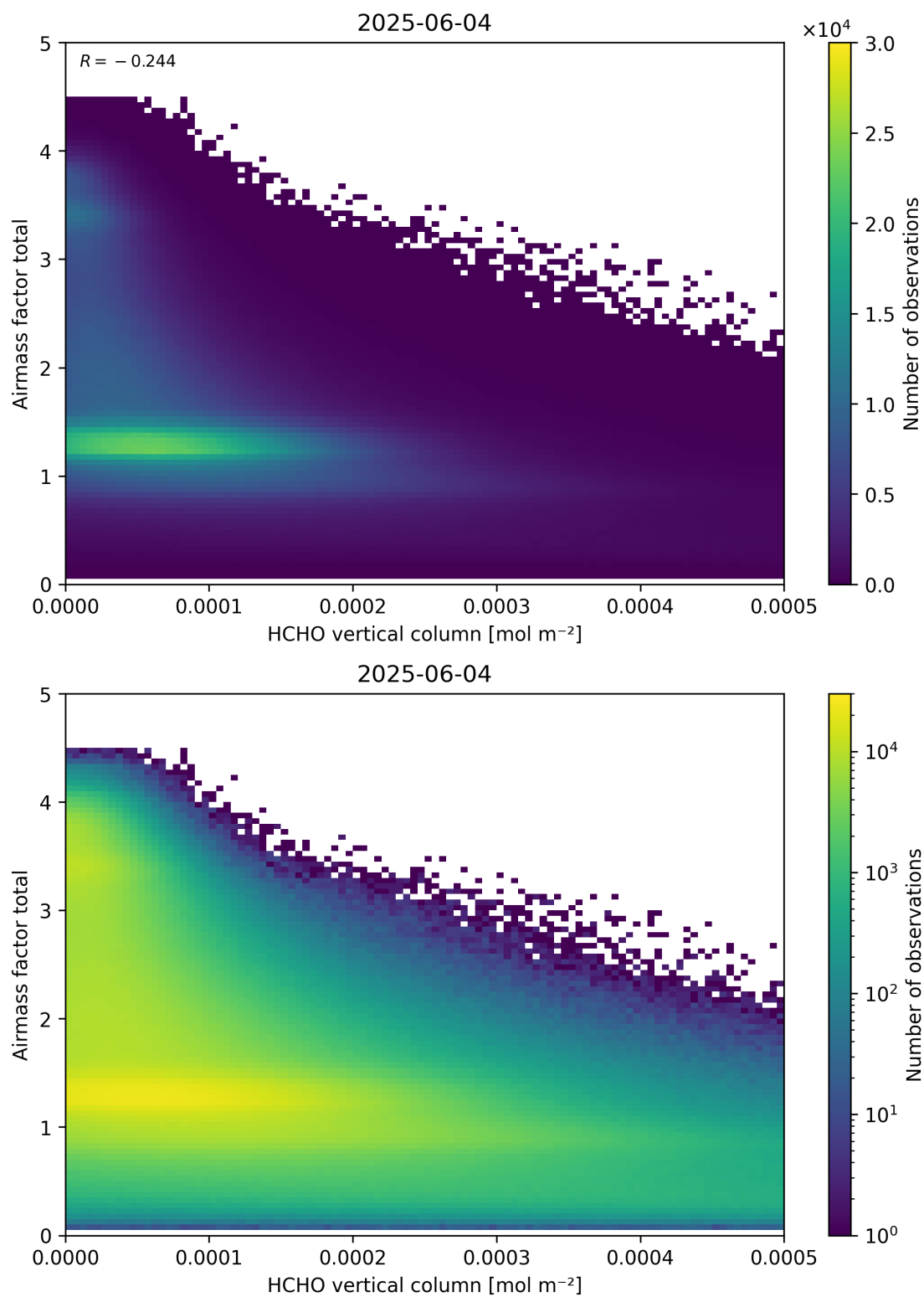
Figure 131: Scatter density plot of “HCHO vertical column” against “Airmass factor total” for 2025-06-03 to 2025-06-05.
