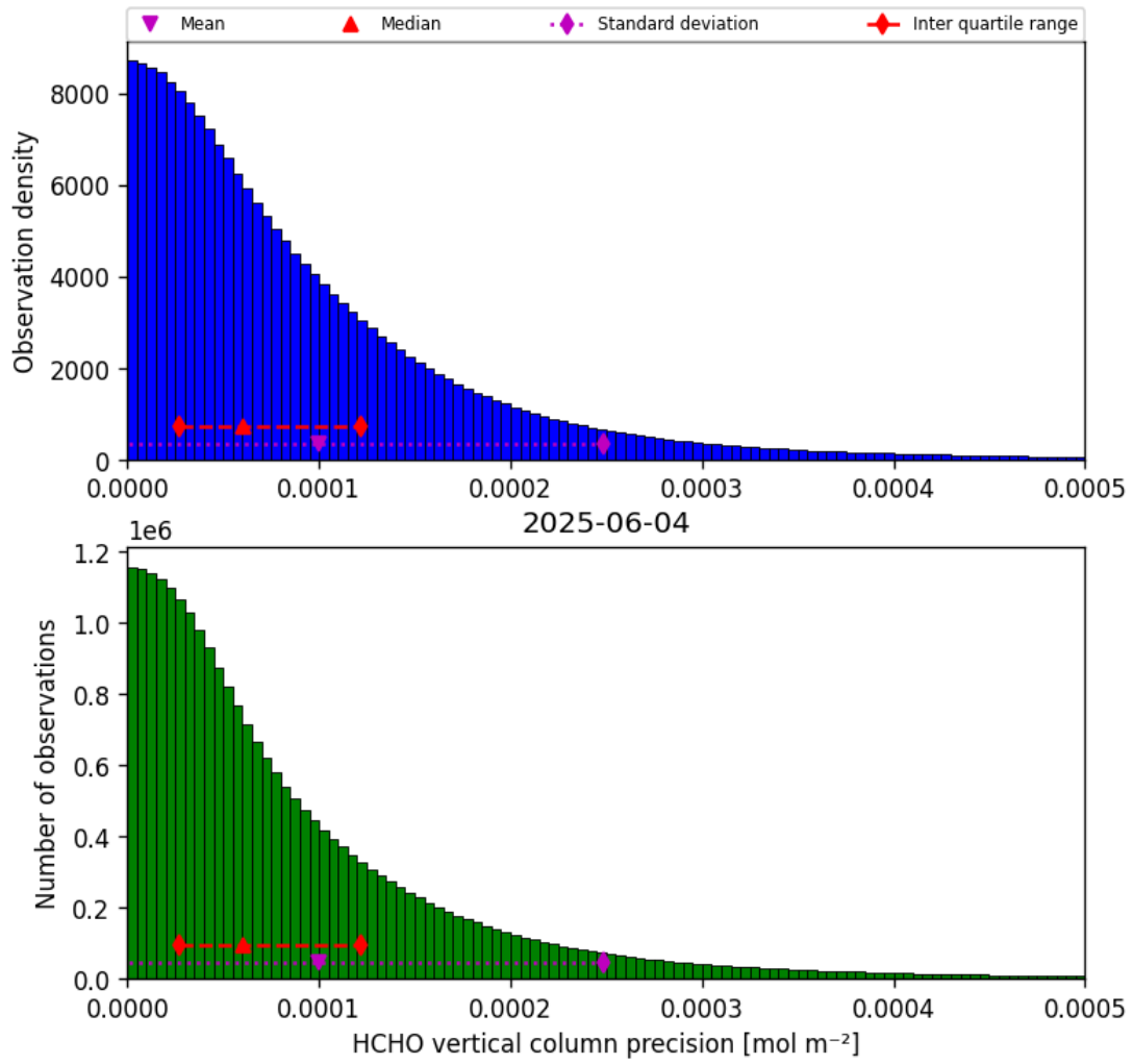
Figure 36: Histogram of “HCHO vertical column precision” for 2025-06-03 to 2025-06-05
