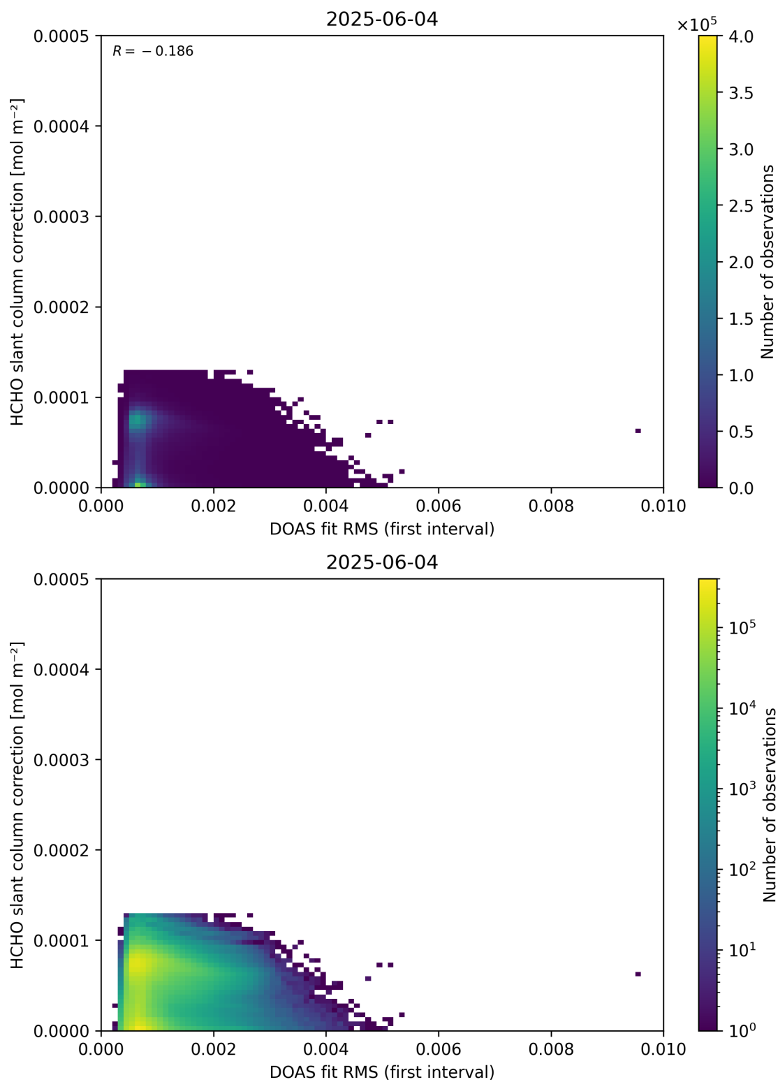
Figure 63: Scatter density plot of “DOAS fit RMS (first interval)” against “HCHO slant column correction” for 2025-06-03 to 2025-06-05.
