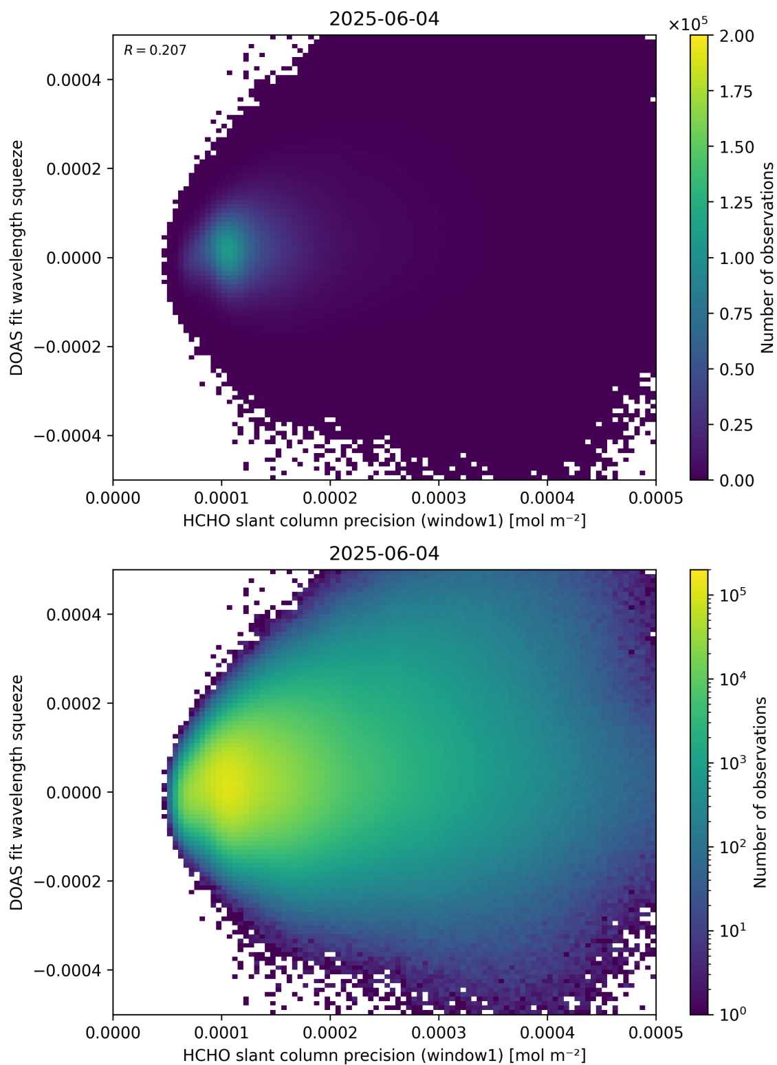
Figure 90: Scatter density plot of “HCHO slant column precision (window1)” against “DOAS fit wavelength squeeze” for 2025-06-03 to 2025-06-05.
