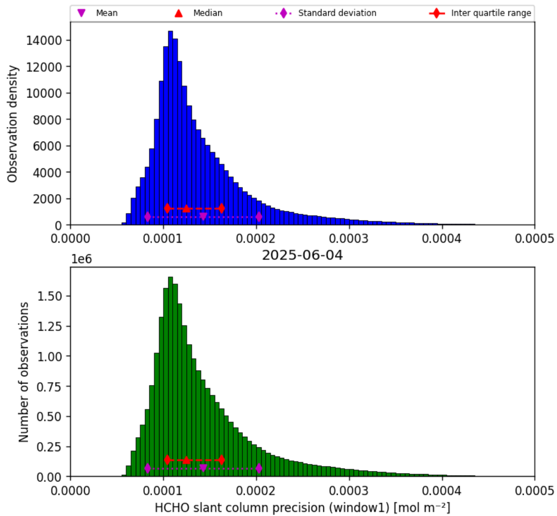
Figure 39: Histogram of “HCHO slant column precision (window1)” for 2025-06-03 to 2025-06-05
