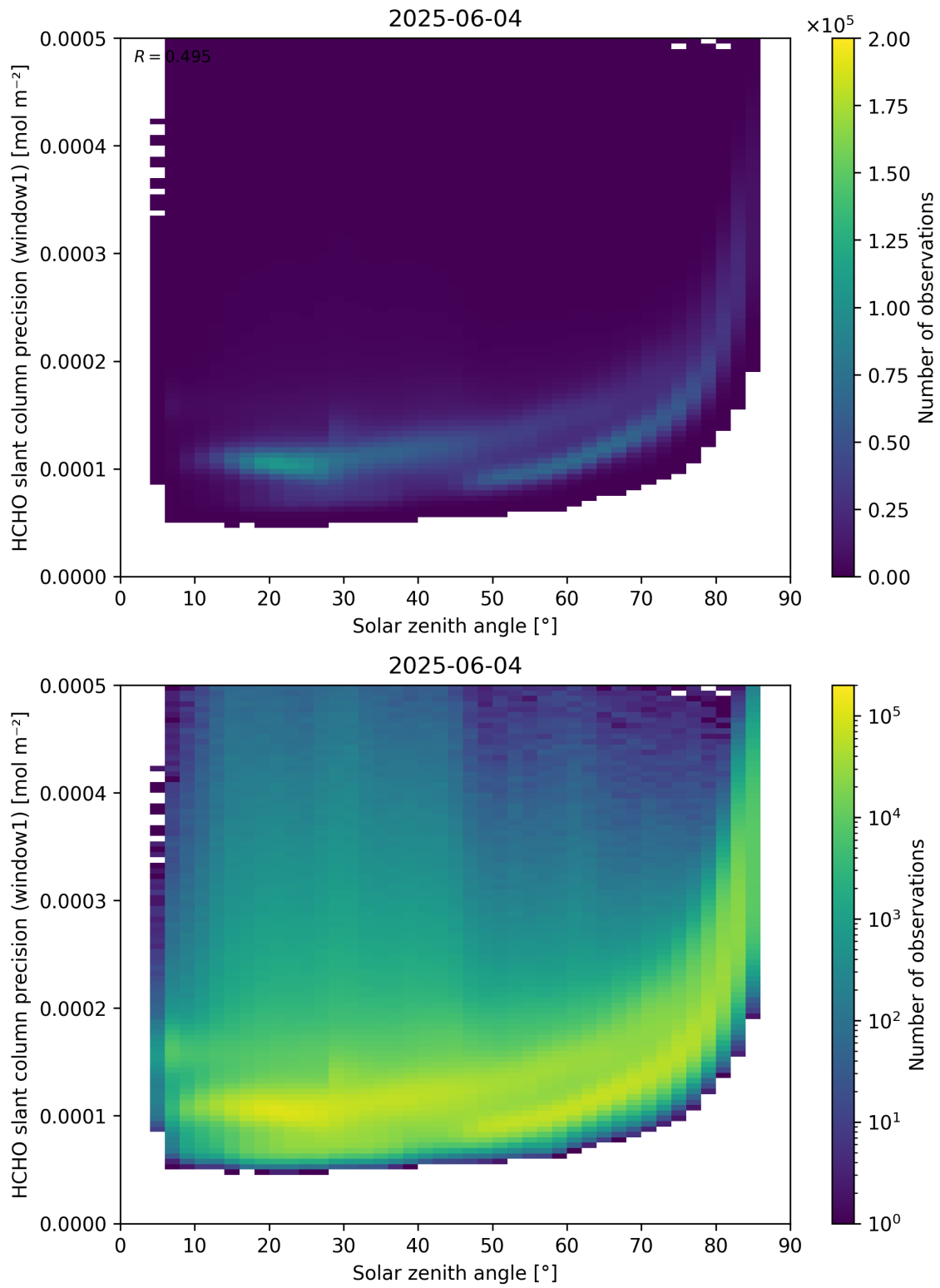
Figure 174: Scatter density plot of “Solar zenith angle” against “HCHO slant column precision (window1)” for 2025-06-03 to 2025-06-05.
