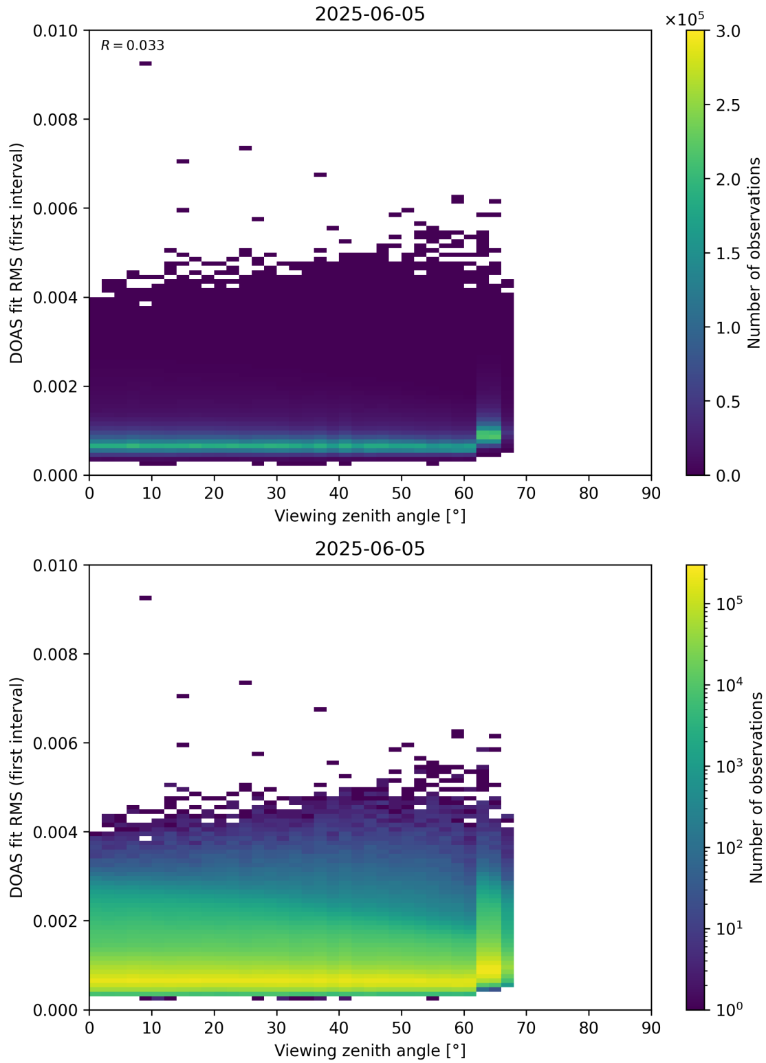
Figure 182: Scatter density plot of “Viewing zenith angle” against “DOAS fit RMS (first interval)” for 2025-06-04 to 2025-06-06.
