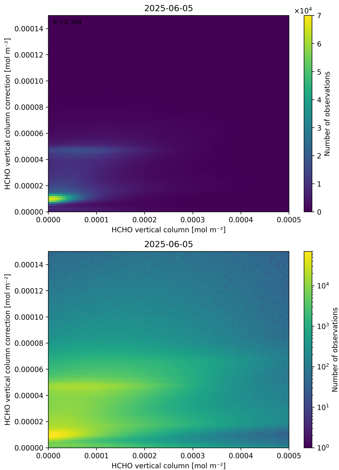
Figure 133: Scatter density plot of “HCHO vertical column” against “HCHO vertical column correction” for 2025-06-04 to 2025-06-06.
