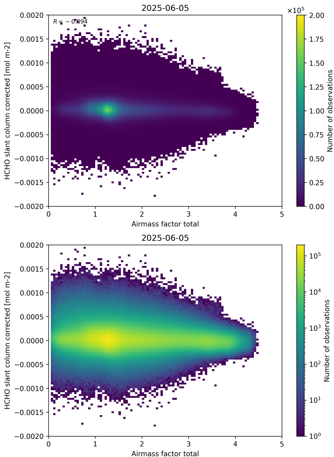
Figure 101: Scatter density plot of “Airmass factor total” against “HCHO slant column corrected” for 2025-06-04 to 2025-06-06.
