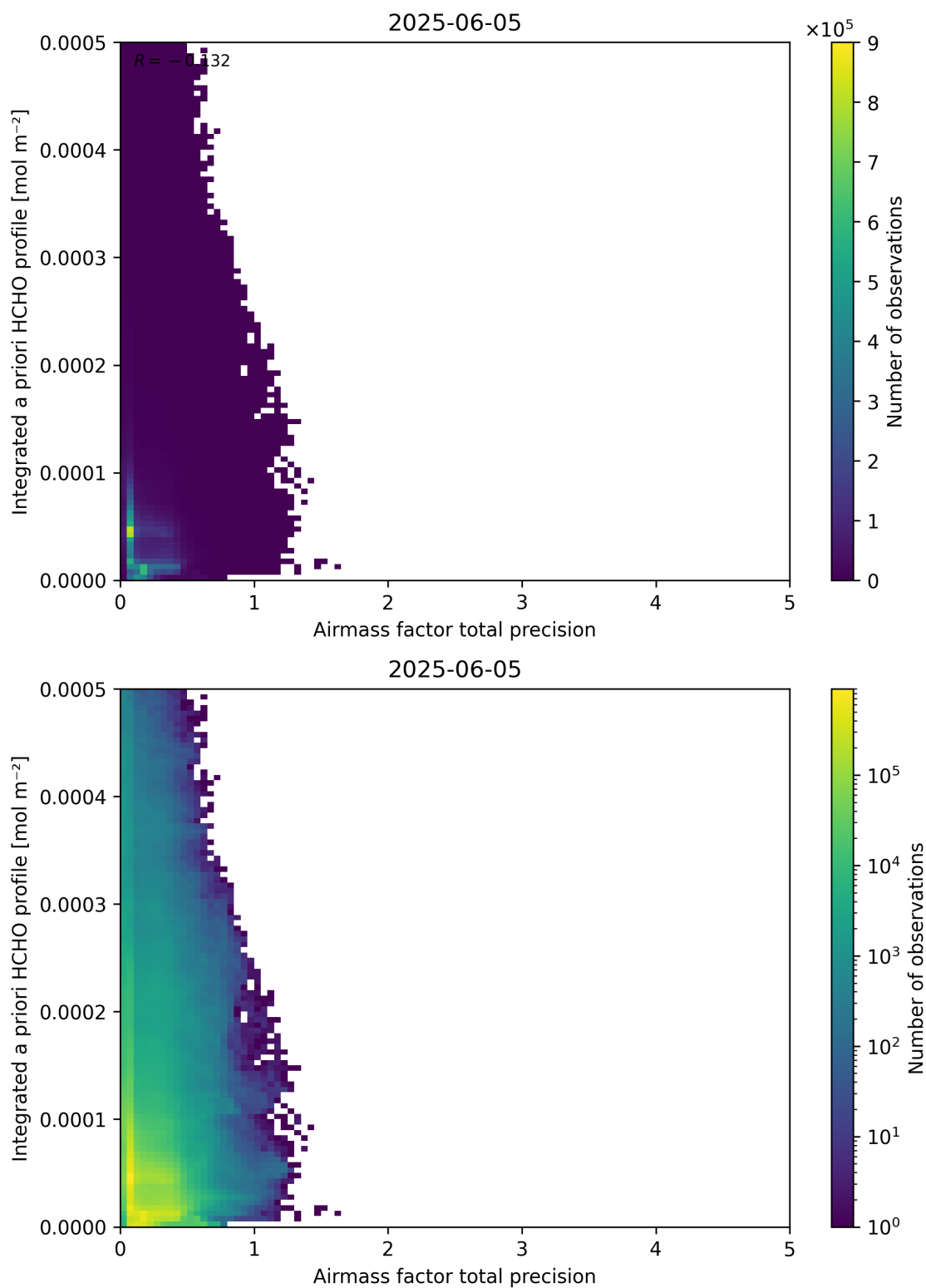
Figure 111: Scatter density plot of “Airmass factor total precision” against “Integrated a priori HCHO profile” for 2025-06-04 to 2025-06-06.
