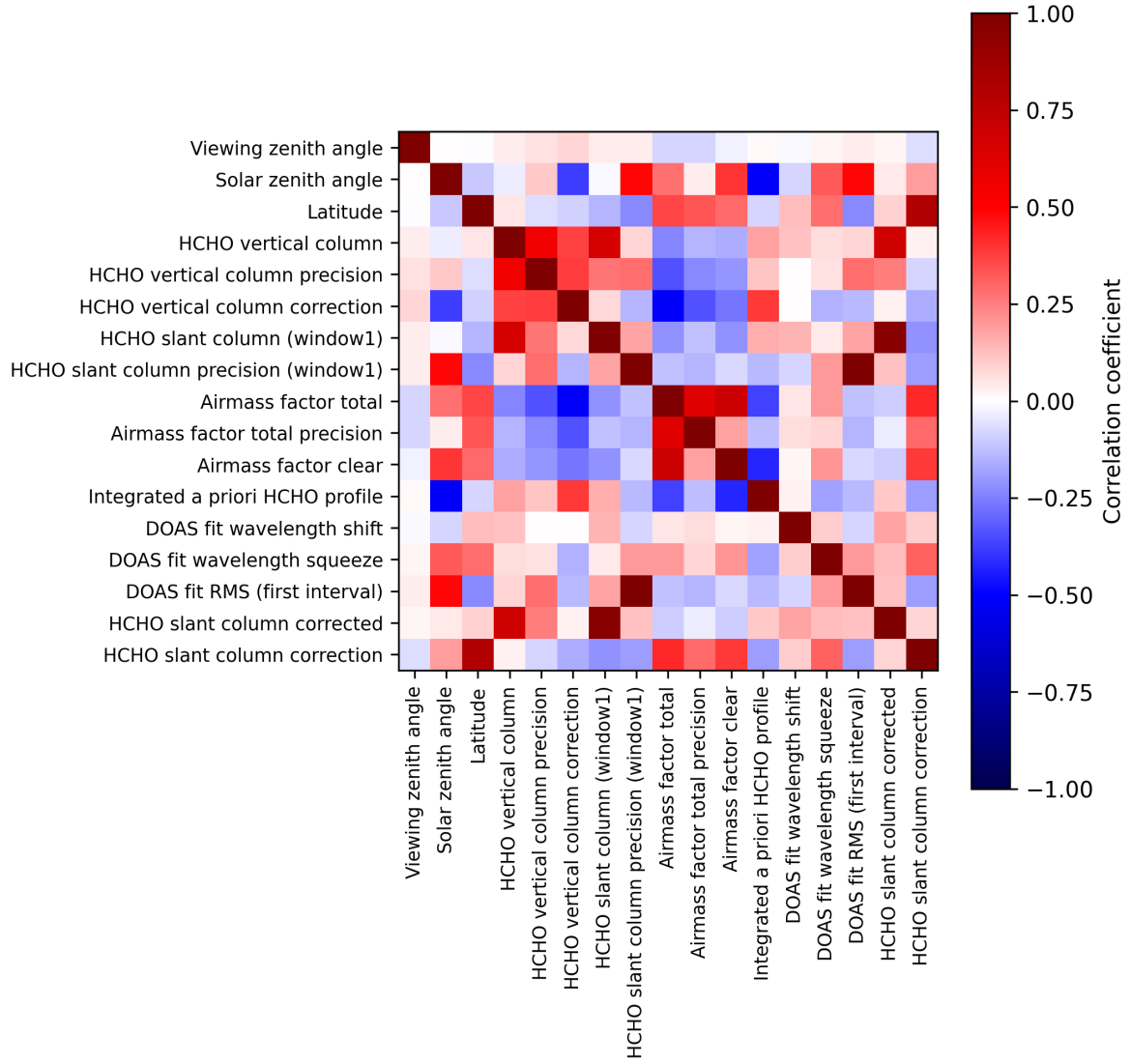
Figure 2: Map of correlation matrix for 2025-06-04 to 2025-06-06.
