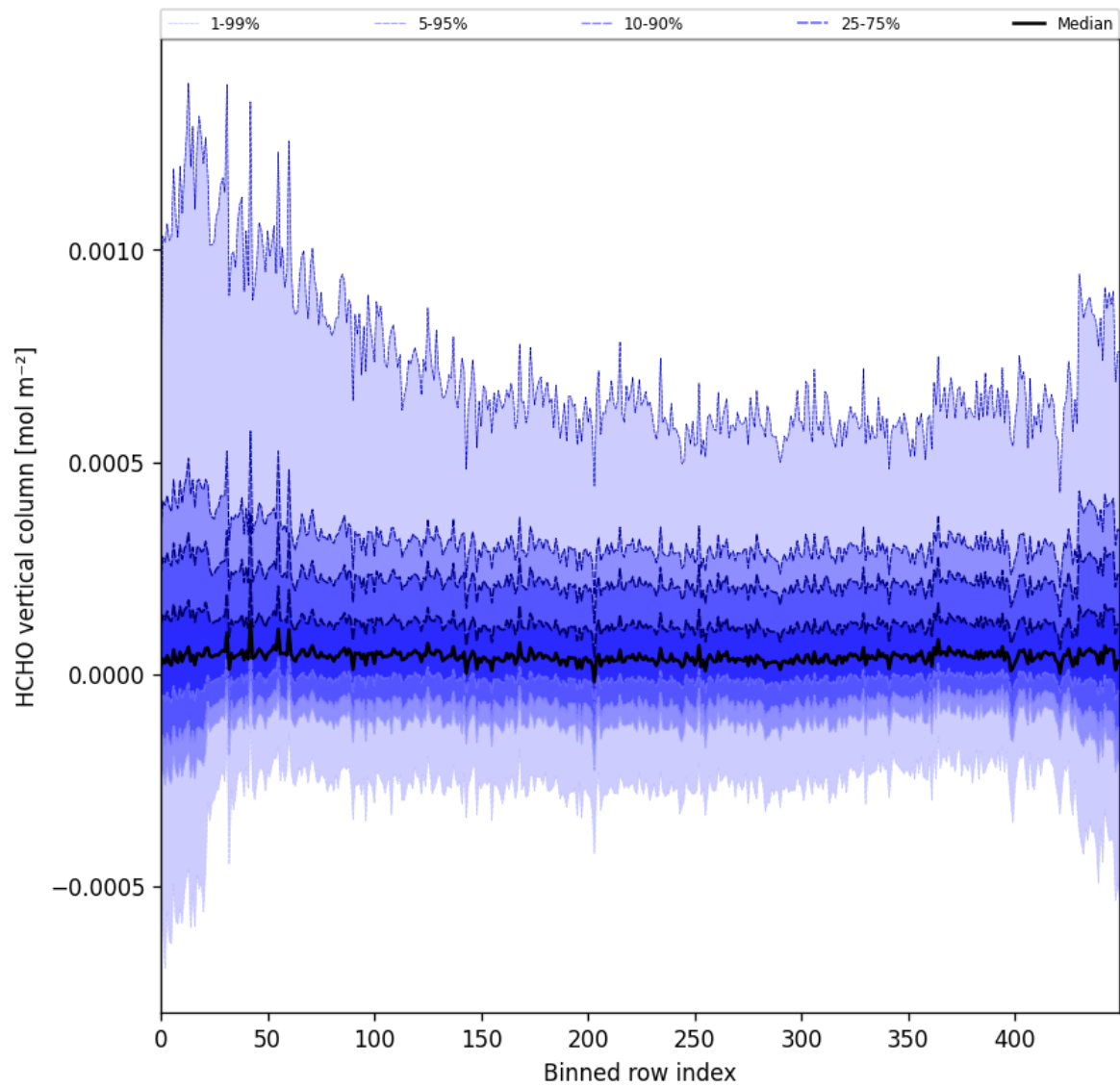
Figure 49: Along track statistics of “HCHO vertical column” for 2025-06-04 to 2025-06-06
