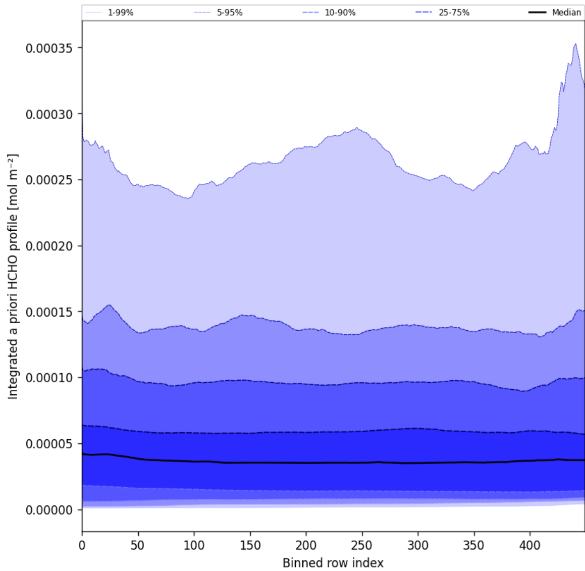
Figure 57: Along track statistics of “Integrated a priori HCHO profile” for 2025-06-04 to 2025-06-06
