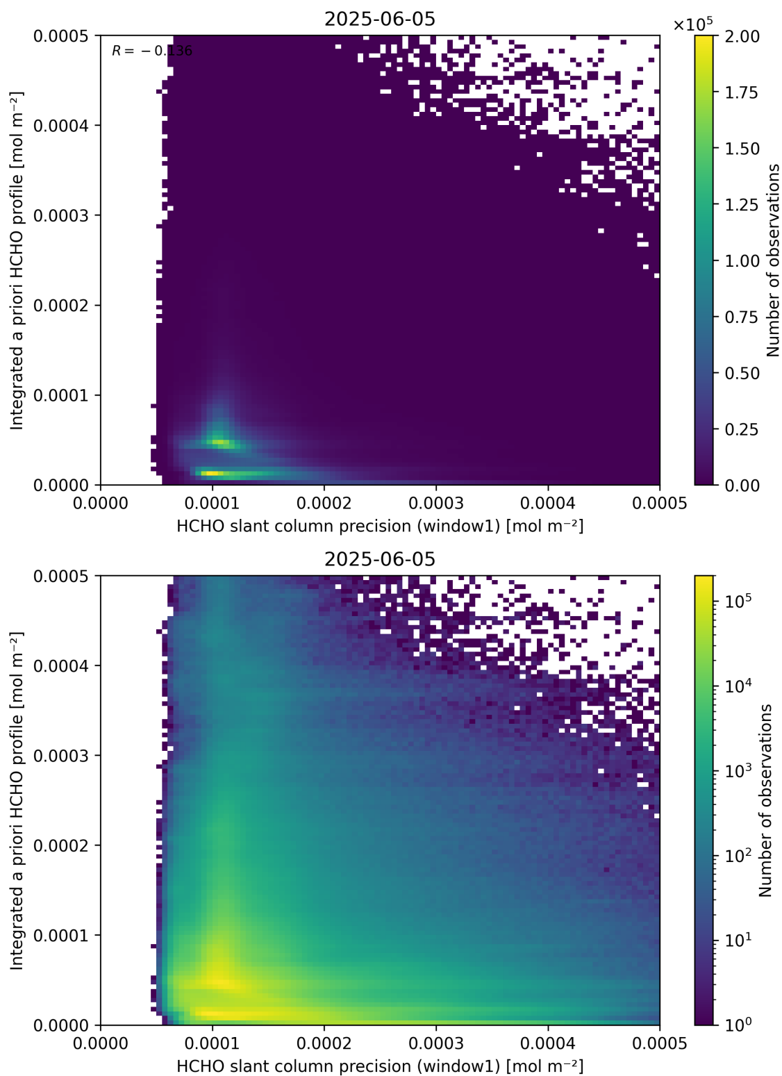
Figure 96: Scatter density plot of “HCHO slant column precision (window1)” against “Integrated a priori HCHO profile” for 2025-06-04 to 2025-06-06.
