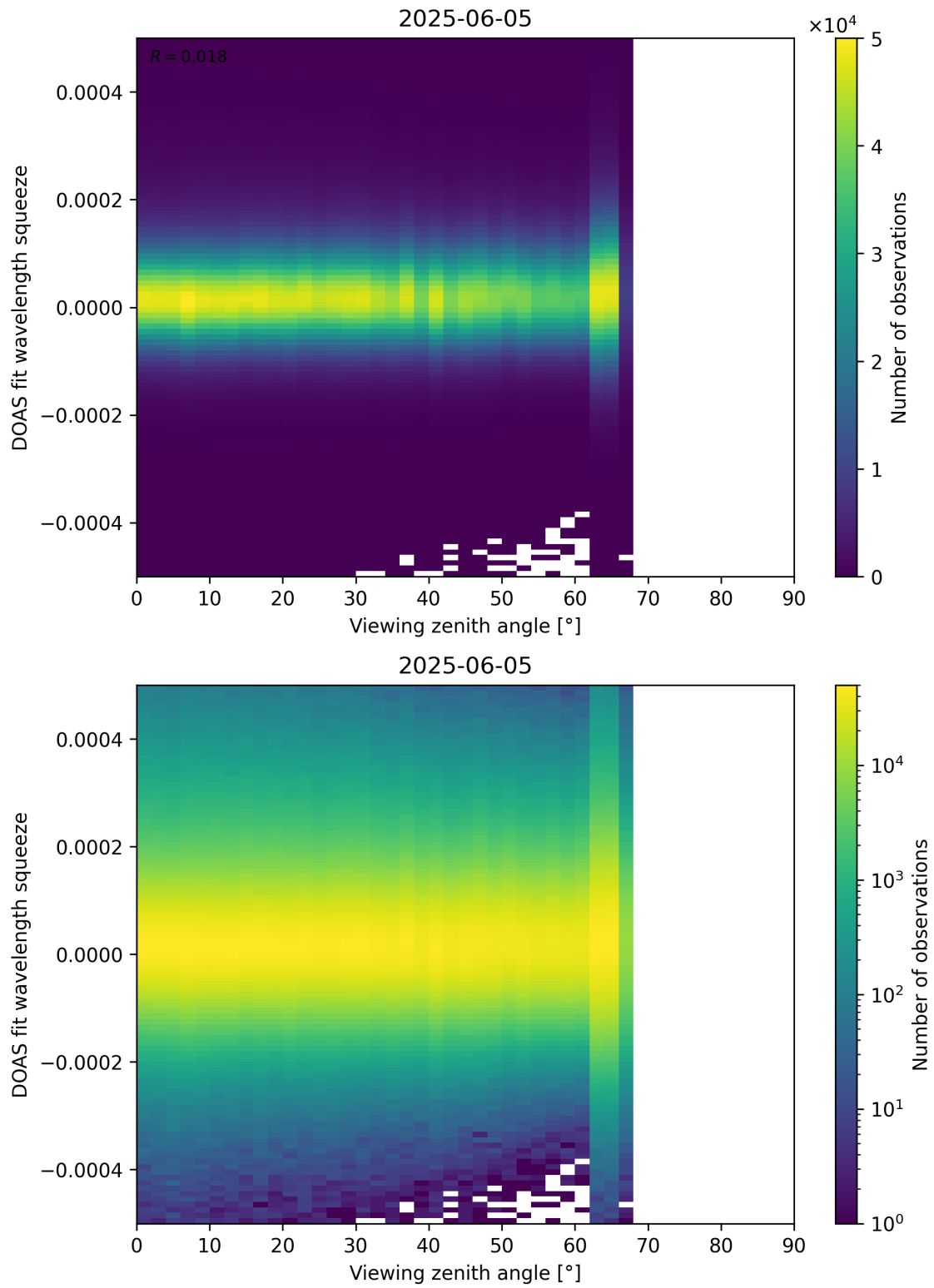
Figure 184: Scatter density plot of “Viewing zenith angle” against “DOAS fit wavelength squeeze” for 2025-06-04 to 2025-06-06.
