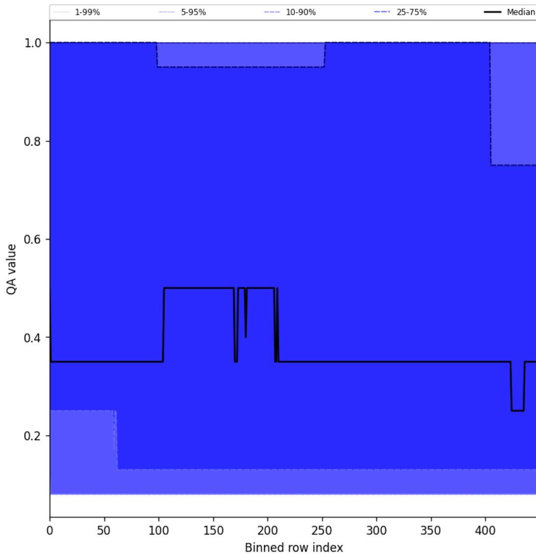
Figure 48: Along track statistics of “QA value” for 2025-06-04 to 2025-06-06
