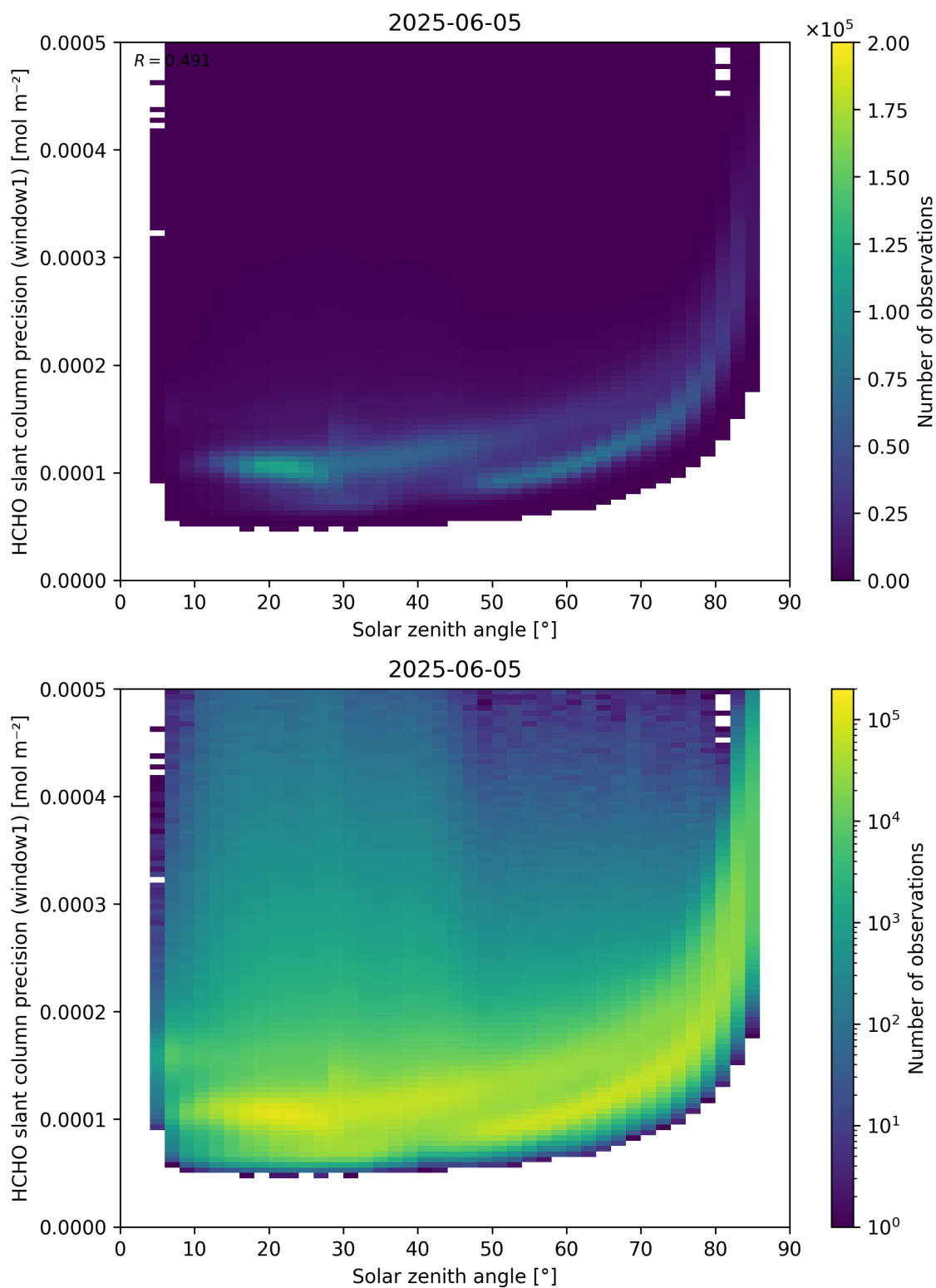
Figure 174: Scatter density plot of “Solar zenith angle” against “HCHO slant column precision (window1)” for 2025-06-04 to 2025-06-06.
