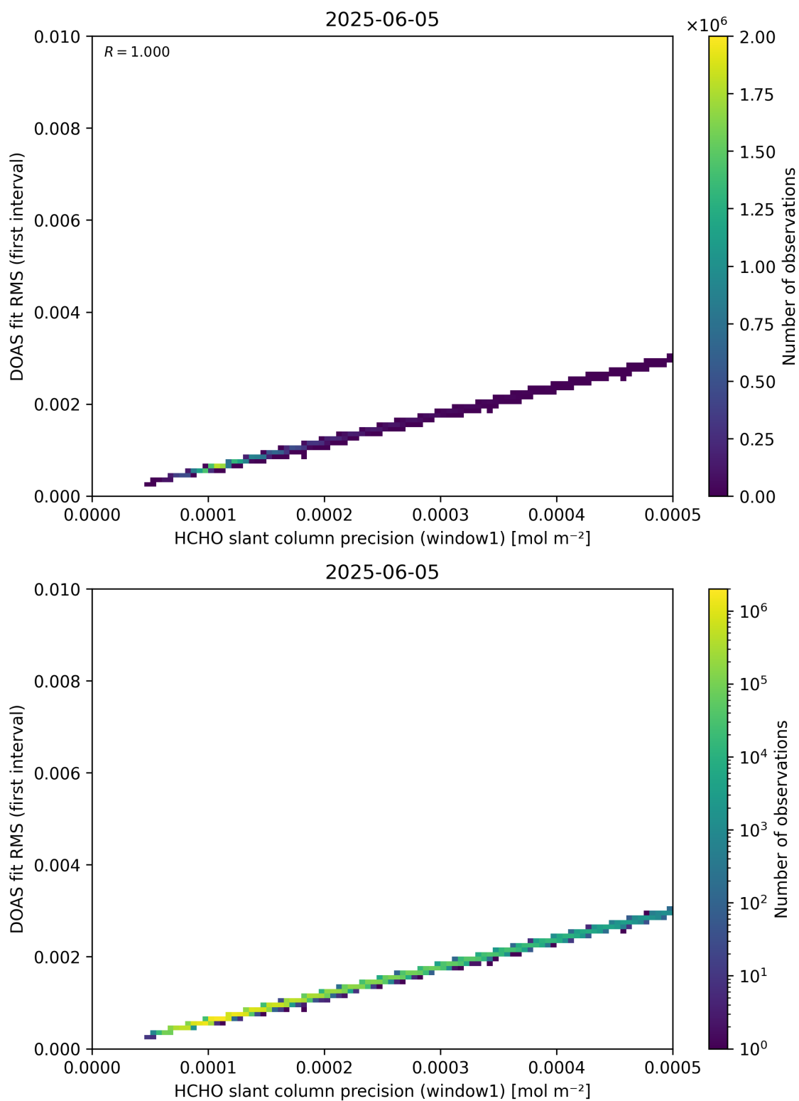
Figure 88: Scatter density plot of “HCHO slant column precision (window1)” against “DOAS fit RMS (first interval)” for 2025-06-04 to 2025-06-06.
