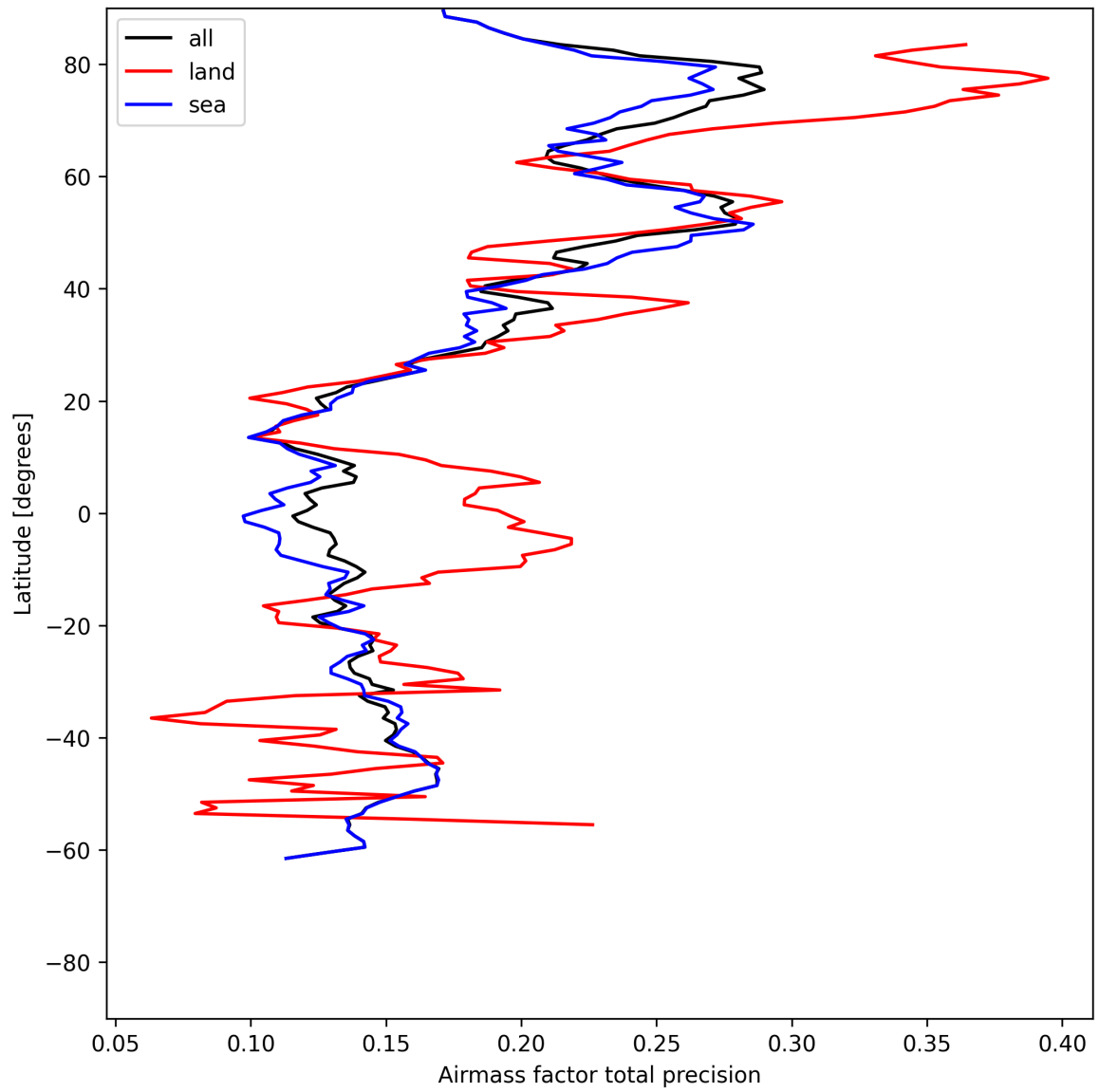
Figure 27: Zonal average of “Airmass factor total precision” for 2025-06-04 to 2025-06-06.
