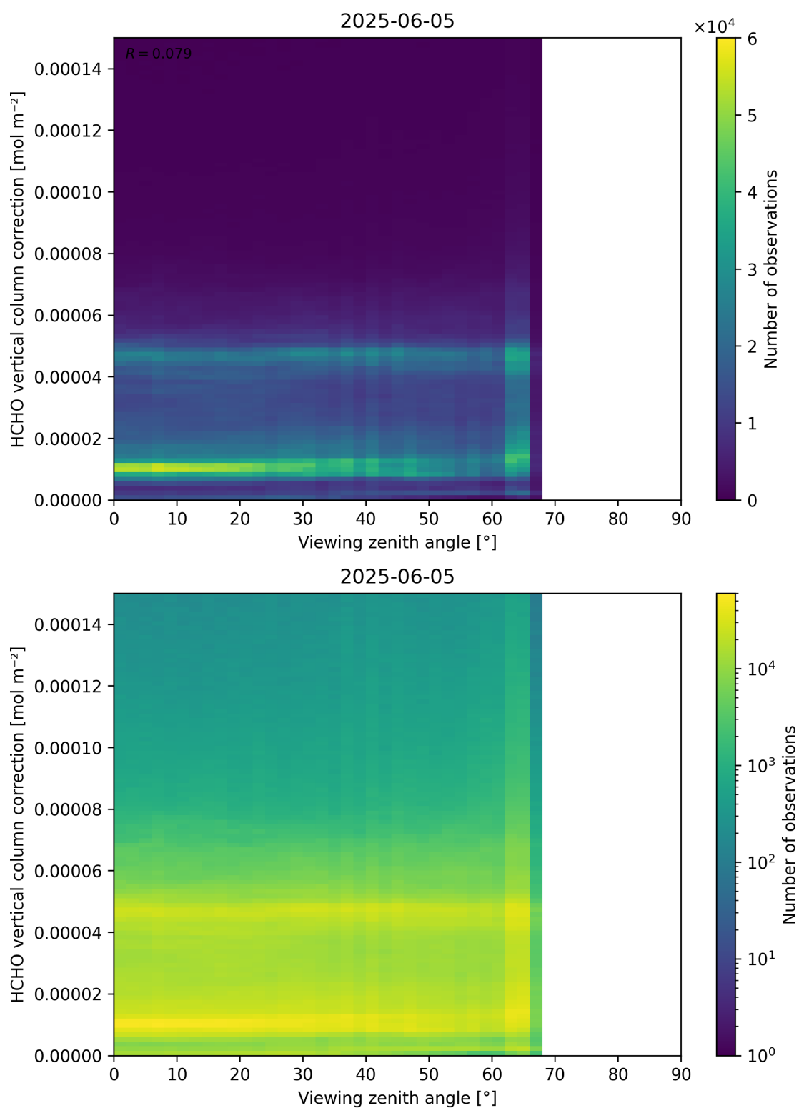
Figure 193: Scatter density plot of “Viewing zenith angle” against “HCHO vertical column correction” for 2025-06-04 to 2025-06-06.
