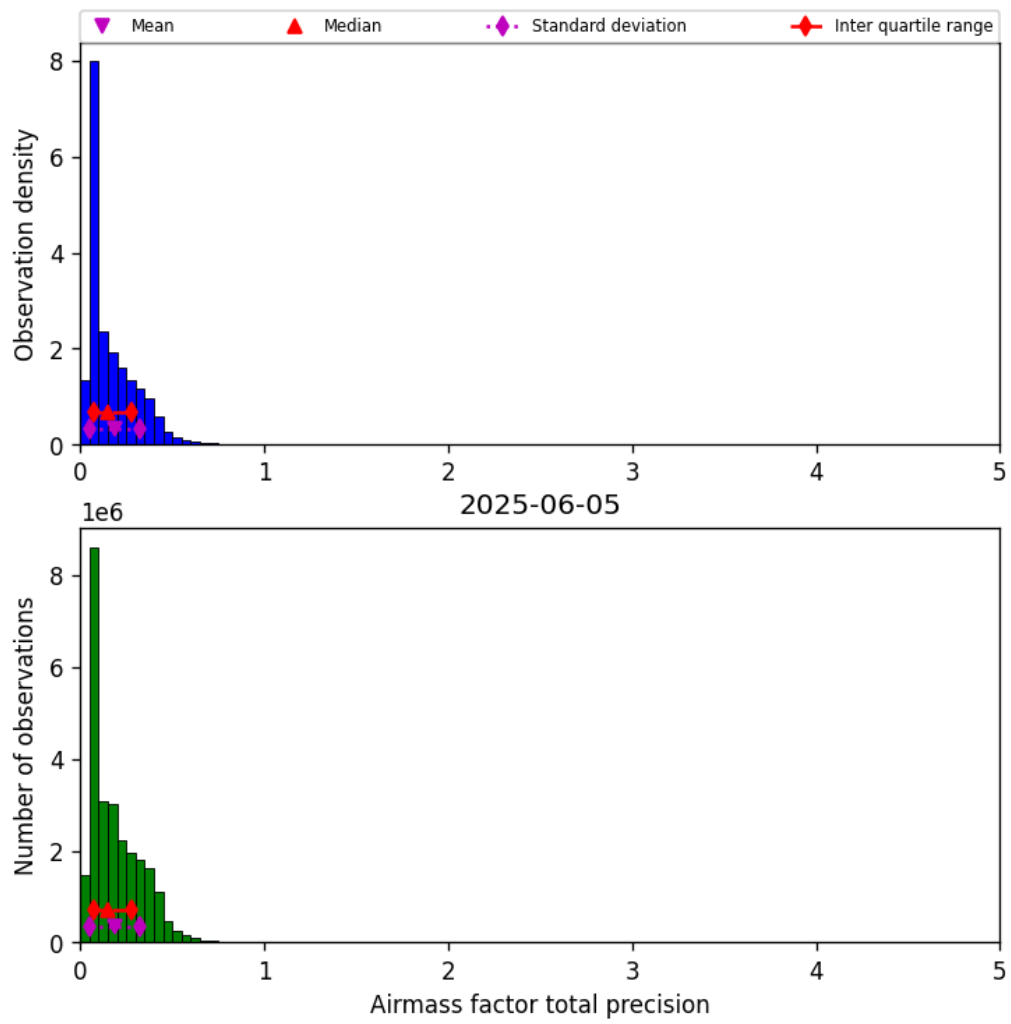
Figure 41: Histogram of “Airmass factor total precision” for 2025-06-04 to 2025-06-06
