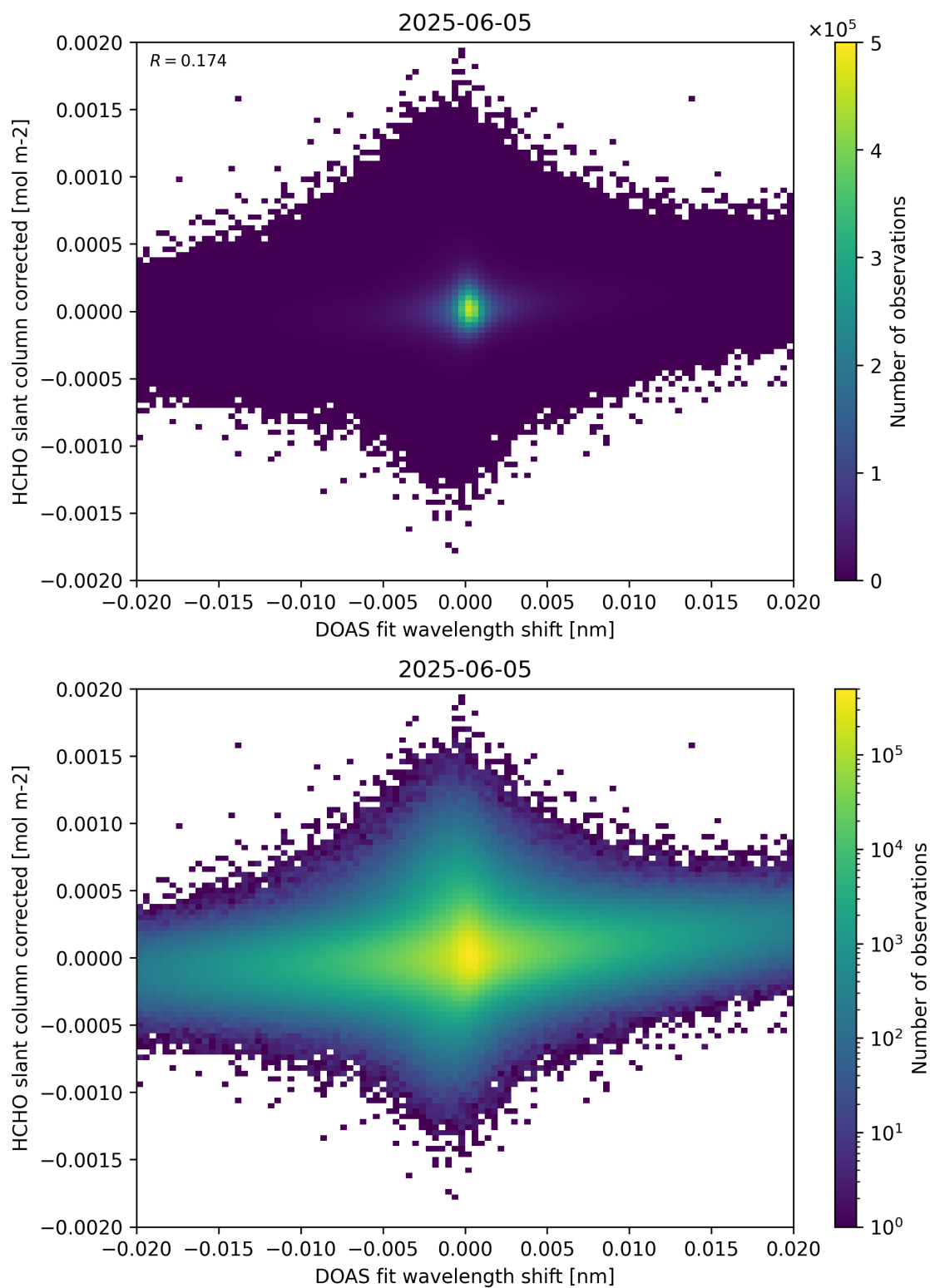
Figure 66: Scatter density plot of “DOAS fit wavelength shift” against “HCHO slant column corrected” for 2025-06-04 to 2025-06-06.
