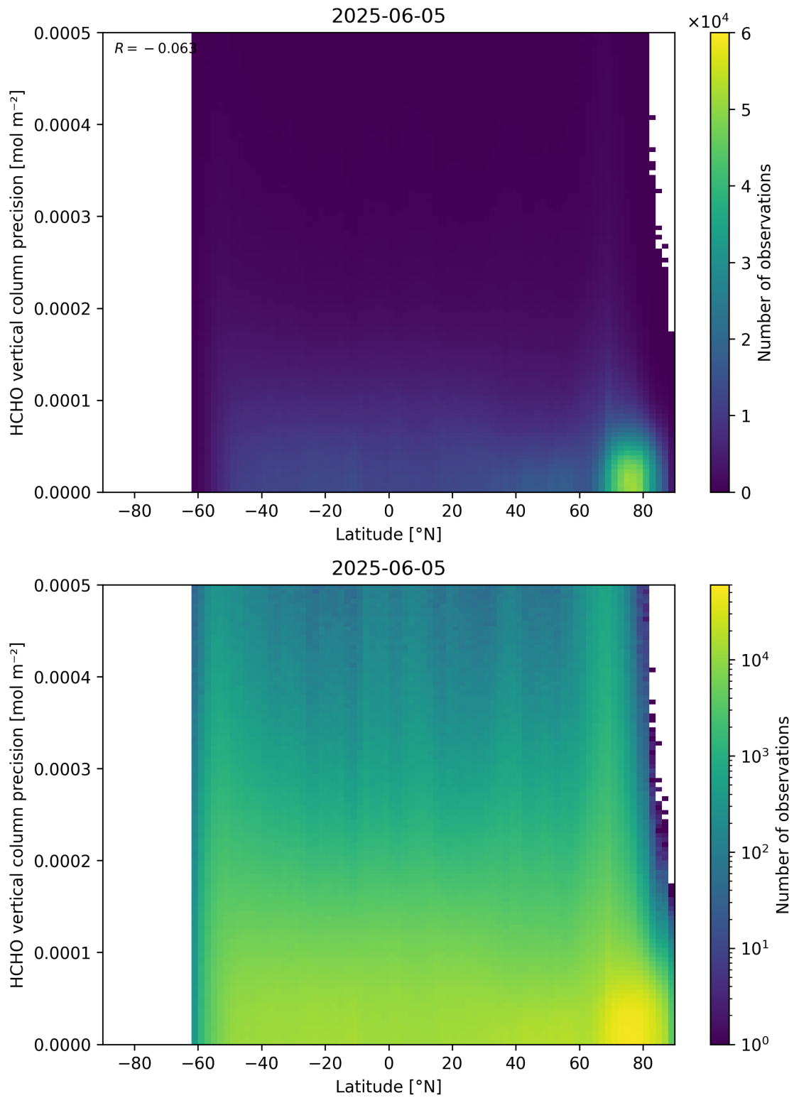
Figure 165: Scatter density plot of “Latitude” against “HCHO vertical column precision” for 2025-06-04 to 2025-06-06.
