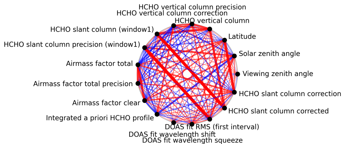
Figure 1: Map of correlation graph for 2025-06-04 to 2025-06-06.
