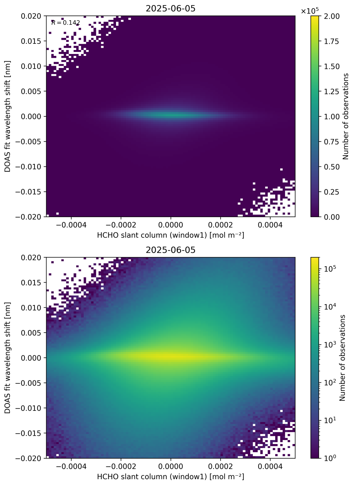
Figure 79: Scatter density plot of “HCHO slant column (window1)” against “DOAS fit wavelength shift” for 2025-06-04 to 2025-06-06.
