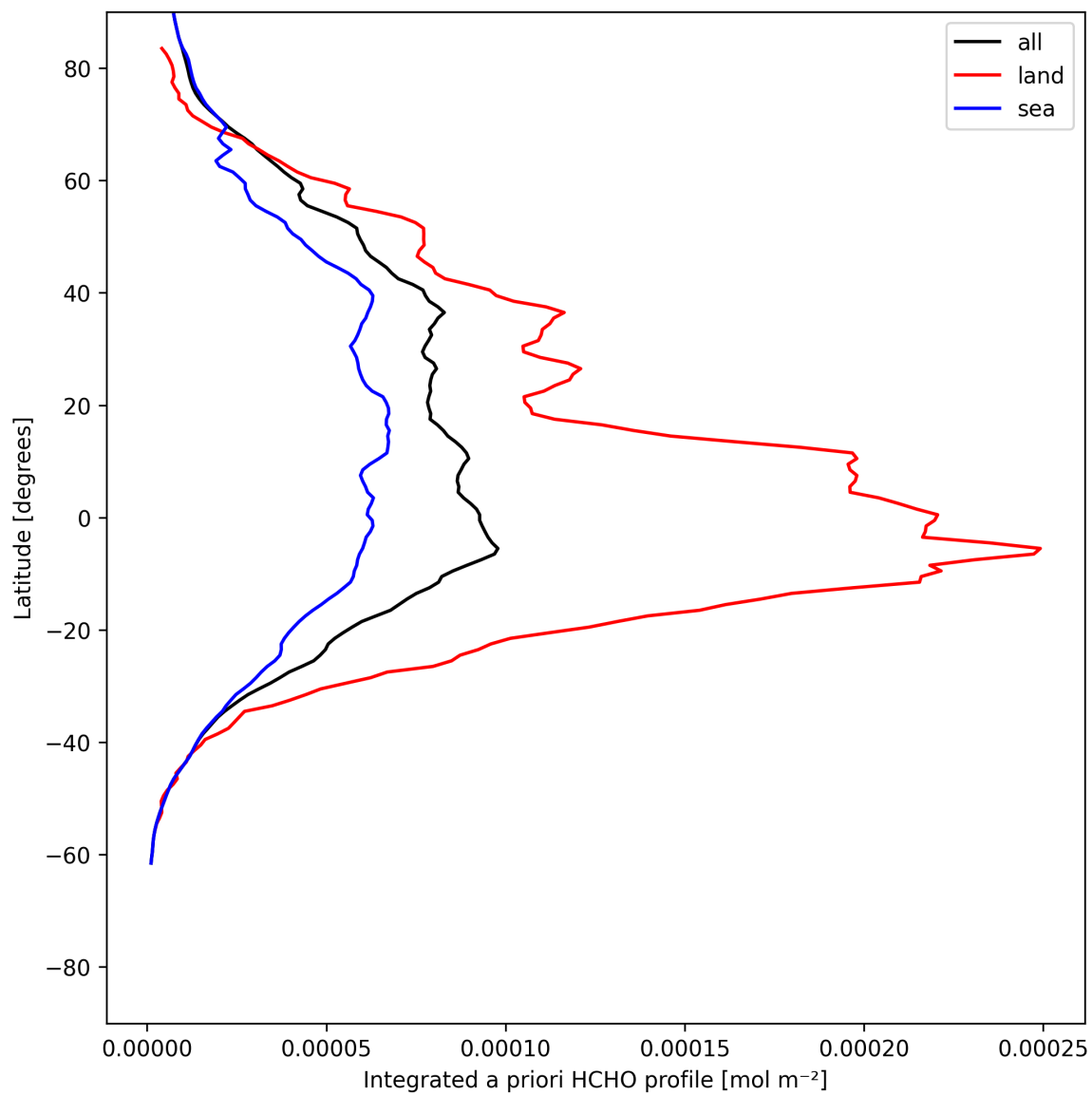
Figure 29: Zonal average of “Integrated a priori HCHO profile” for 2025-06-04 to 2025-06-06.
