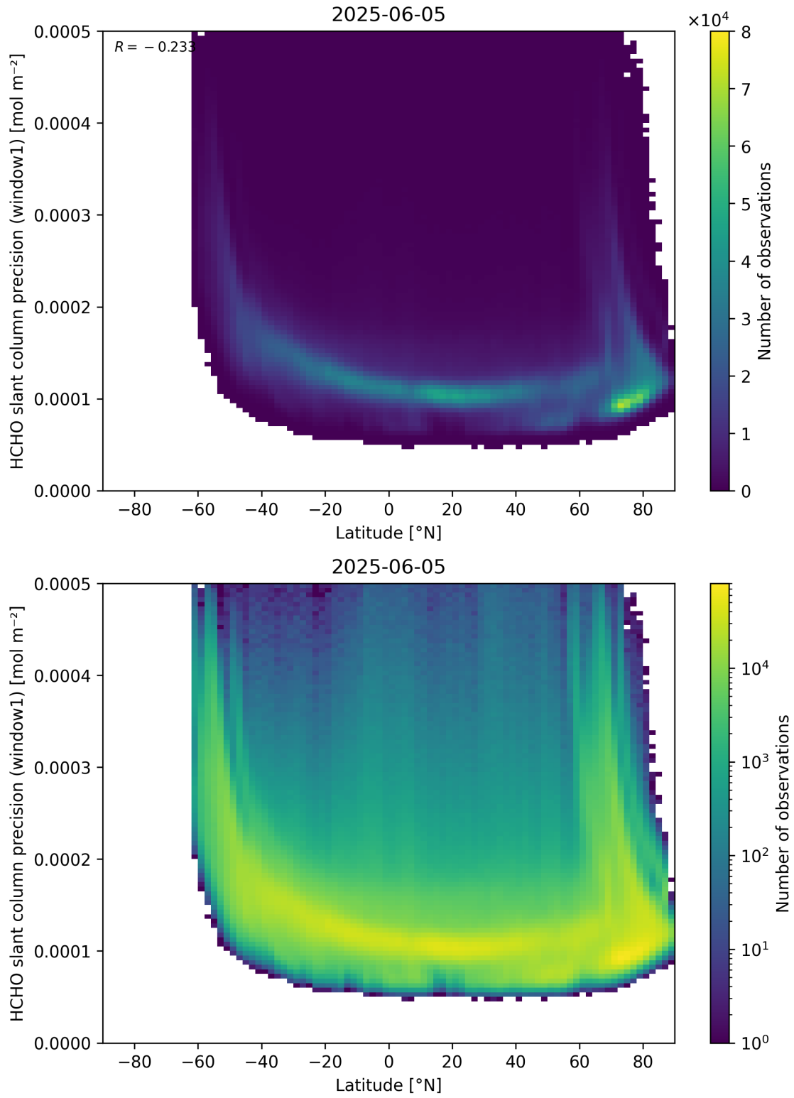
Figure 160: Scatter density plot of “Latitude” against “HCHO slant column precision (window1)” for 2025-06-04 to 2025-06-06.
