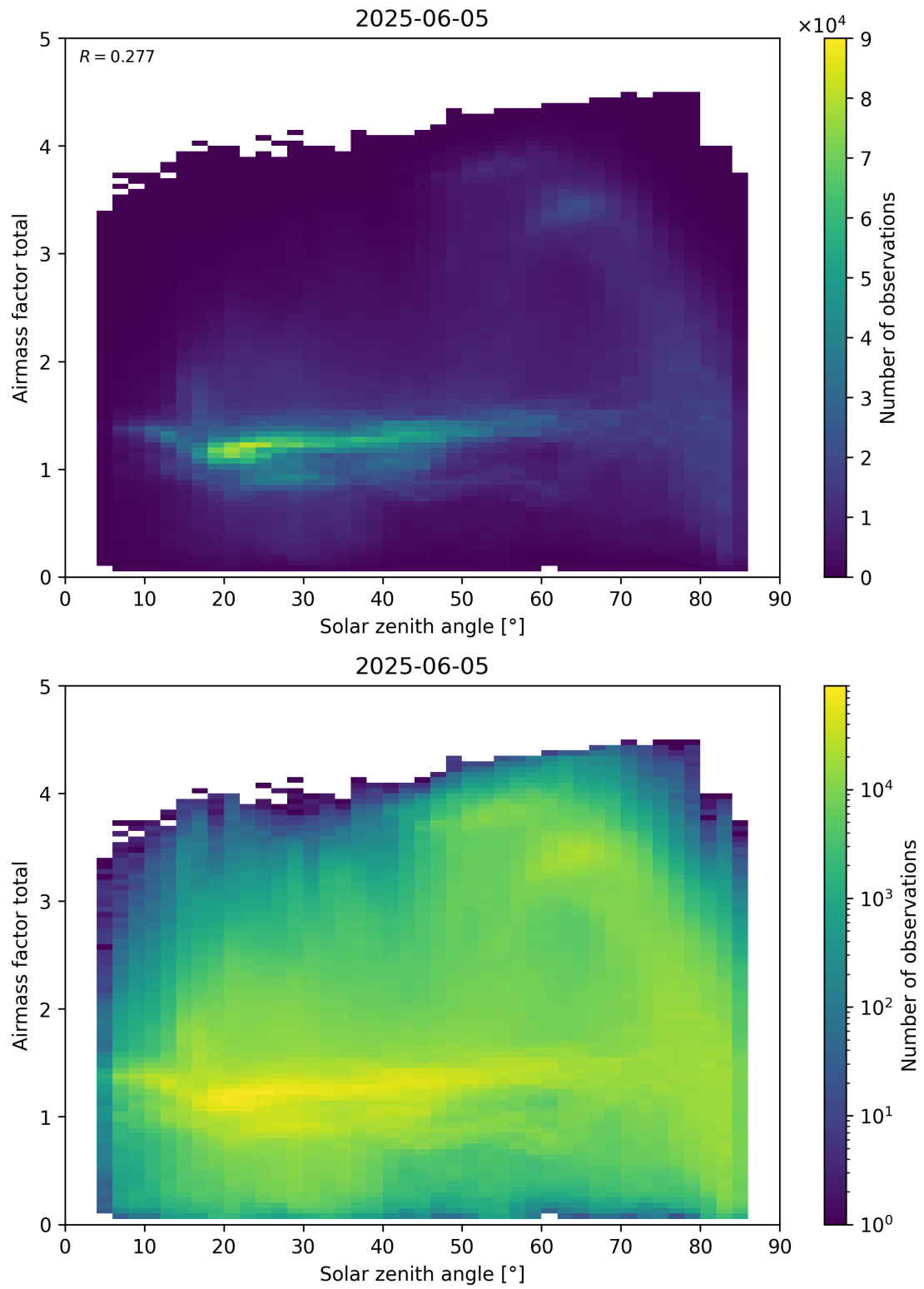
Figure 175: Scatter density plot of “Solar zenith angle” against “Airmass factor total” for 2025-06-04 to 2025-06-06.
