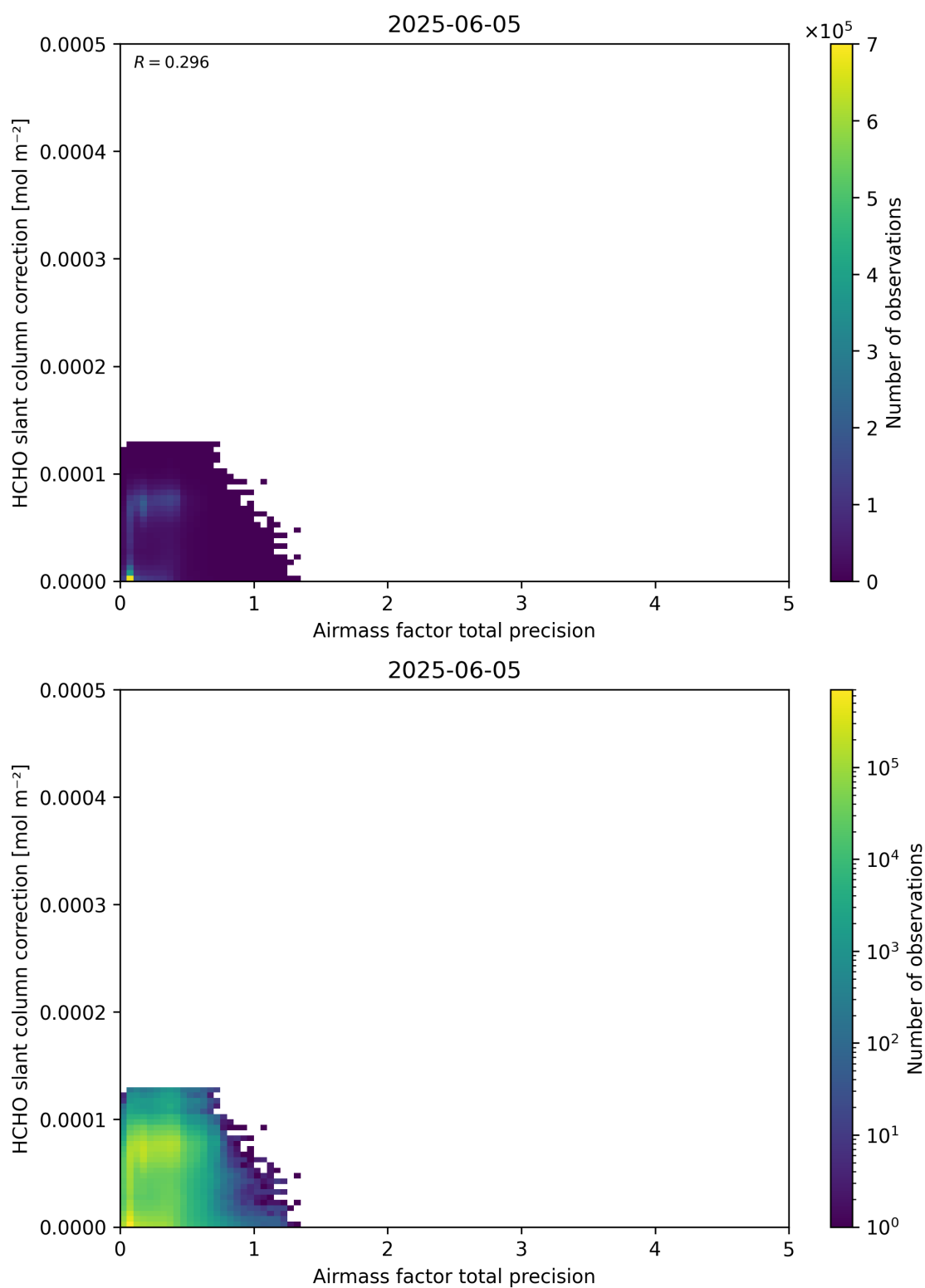
Figure 110: Scatter density plot of “Airmass factor total precision” against “HCHO slant column correction” for 2025-06-04 to 2025-06-06.
