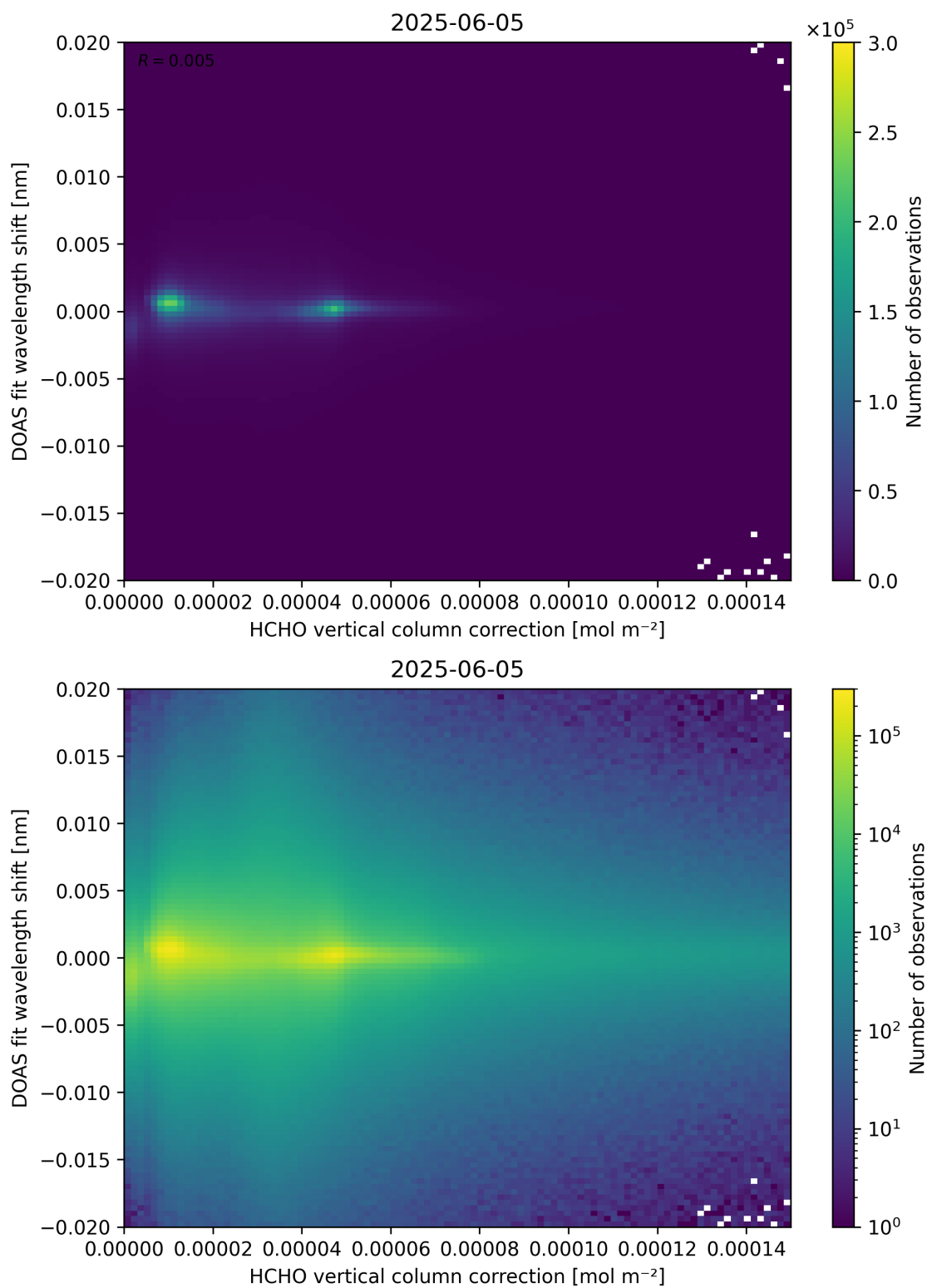
Figure 113: Scatter density plot of “HCHO vertical column correction” against “DOAS fit wavelength shift” for 2025-06-04 to 2025-06-06.
