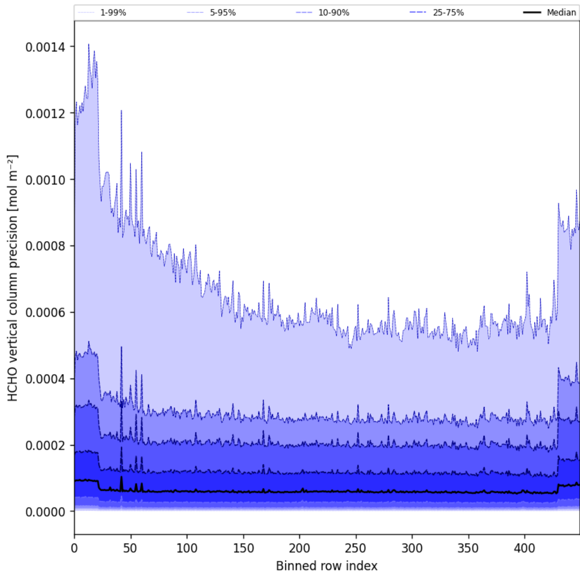
Figure 50: Along track statistics of “HCHO vertical column precision” for 2025-06-04 to 2025-06-06
