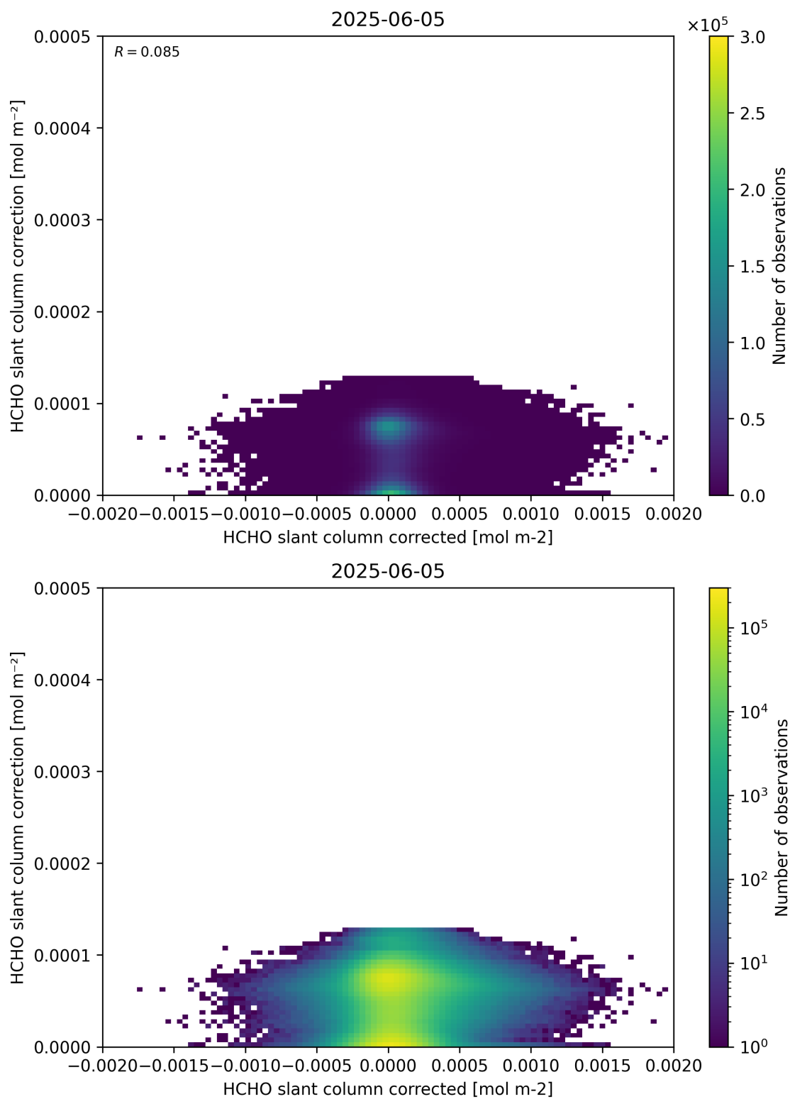
Figure 77: Scatter density plot of “HCHO slant column corrected” against “HCHO slant column correction” for 2025-06-04 to 2025-06-06.
