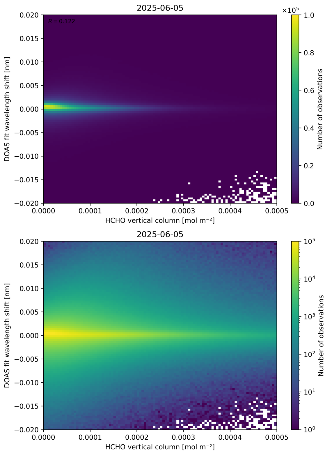
Figure 124: Scatter density plot of “HCHO vertical column” against “DOAS fit wavelength shift” for 2025-06-04 to 2025-06-06.
