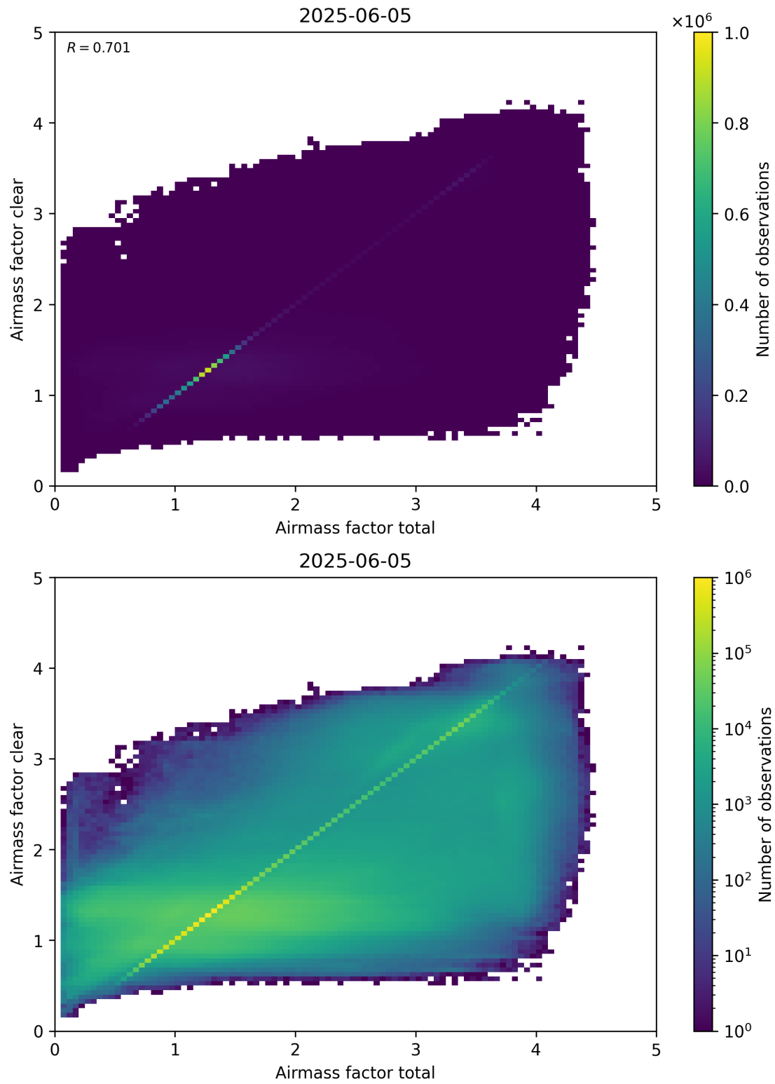
Figure 100: Scatter density plot of “Airmass factor total” against “Airmass factor clear” for 2025-06-04 to 2025-06-06.
