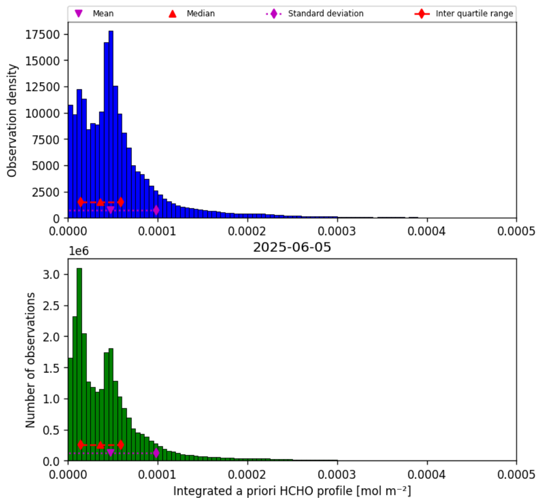
Figure 43: Histogram of “Integrated a priori HCHO profile” for 2025-06-04 to 2025-06-06
