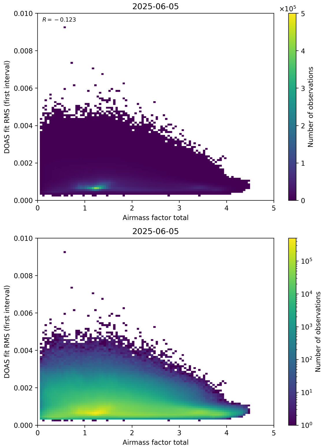
Figure 97: Scatter density plot of “Airmass factor total” against “DOAS fit RMS (first interval)” for 2025-06-04 to 2025-06-06.
