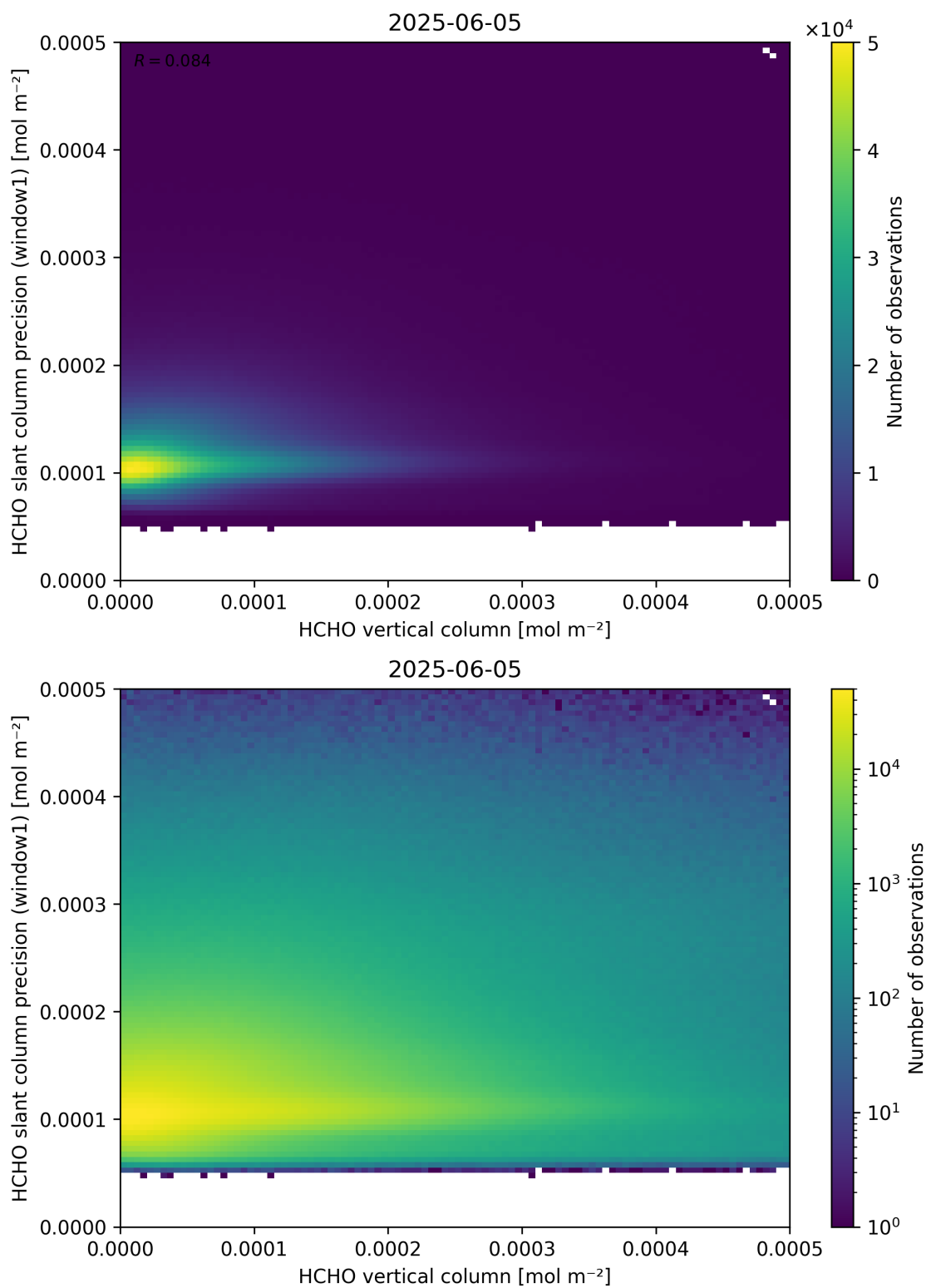
Figure 130: Scatter density plot of “HCHO vertical column” against “HCHO slant column precision (window1)” for 2025-06-04 to 2025-06-06.
