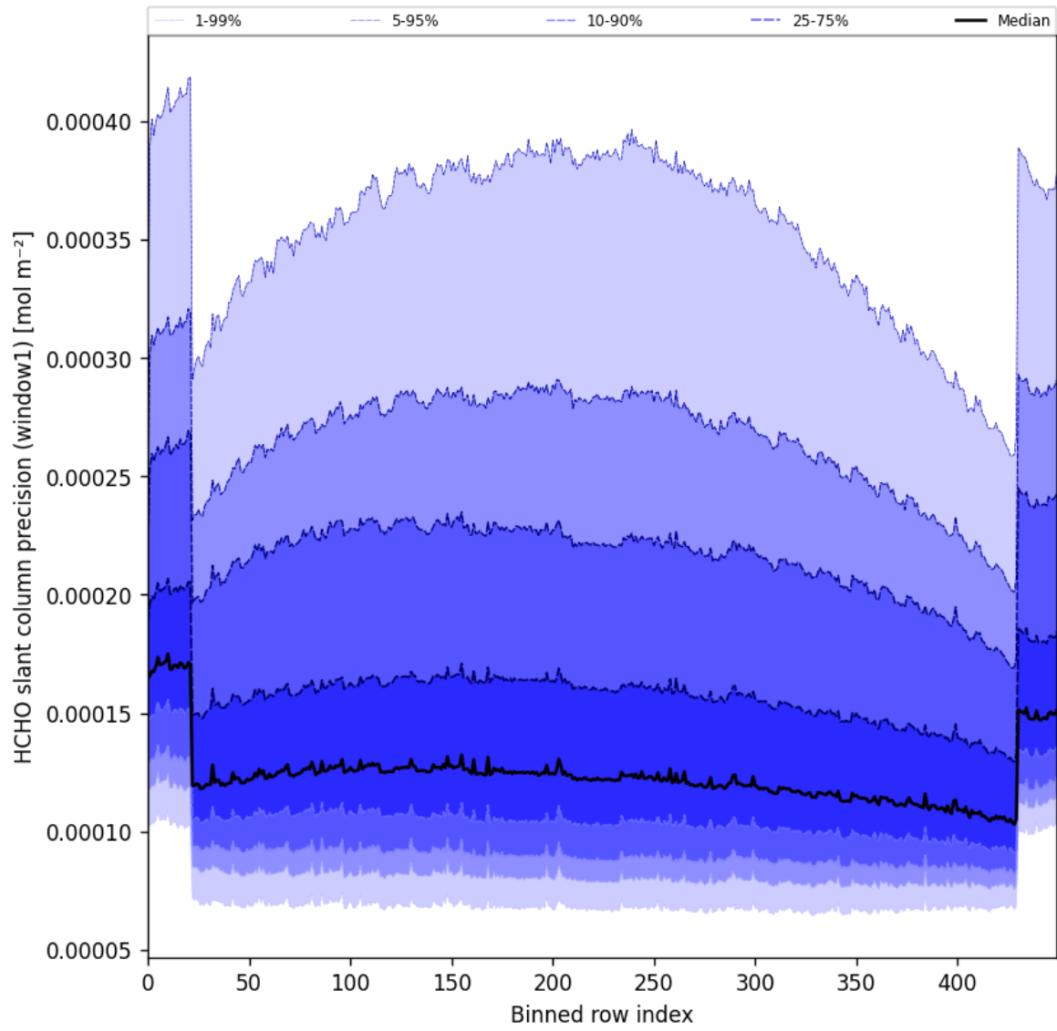
Figure 53: Along track statistics of “HCHO slant column precision (window1)” for 2025-06-04 to 2025-06-06
