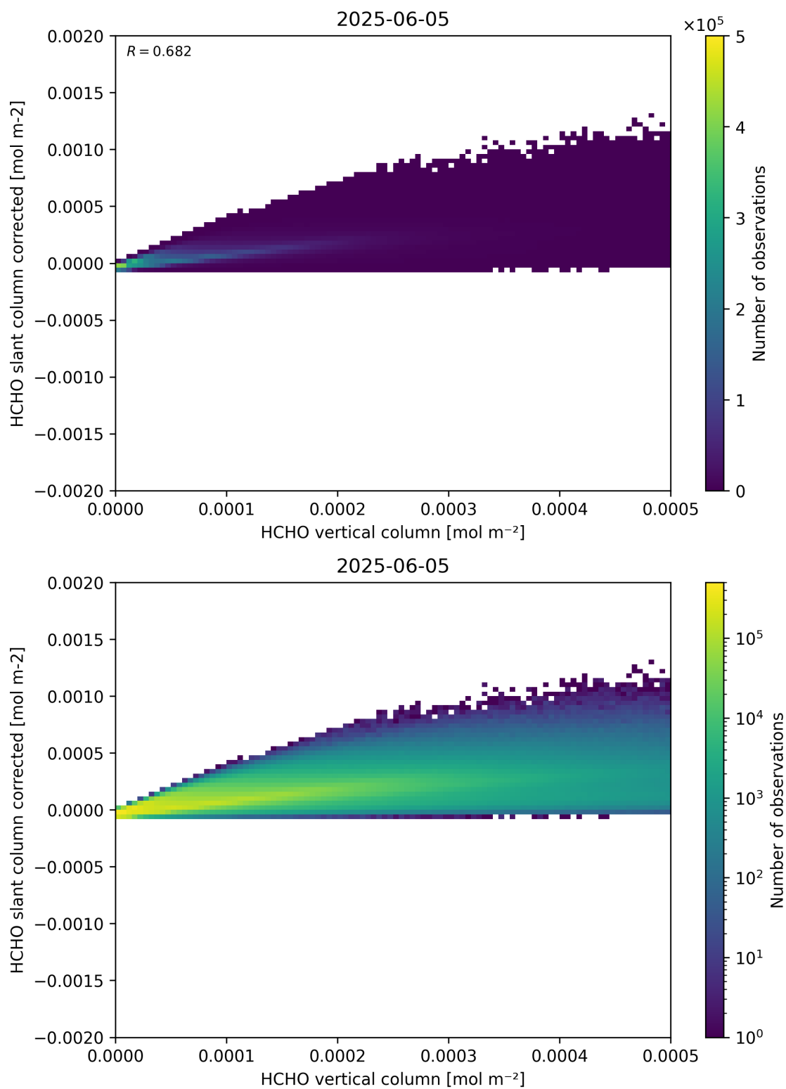
Figure 127: Scatter density plot of “HCHO vertical column” against “HCHO slant column corrected” for 2025-06-04 to 2025-06-06.
