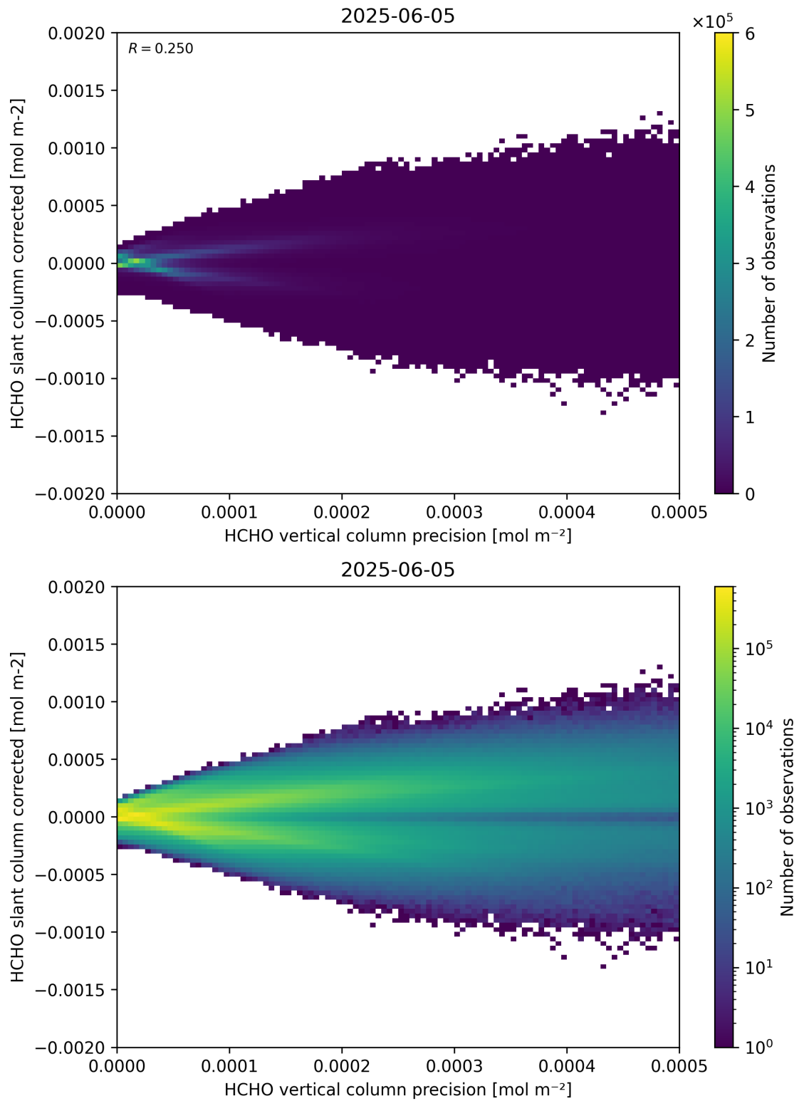
Figure 140: Scatter density plot of “HCHO vertical column precision” against “HCHO slant column corrected” for 2025-06-04 to 2025-06-06.
