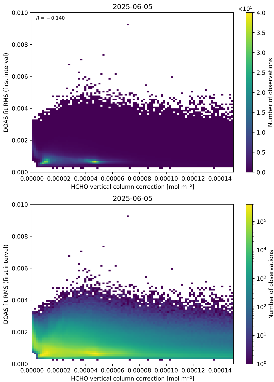
Figure 112: Scatter density plot of “HCHO vertical column correction” against “DOAS fit RMS (first interval)” for 2025-06-04 to 2025-06-06.
