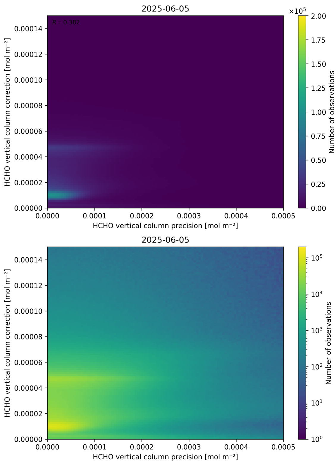
Figure 146: Scatter density plot of “HCHO vertical column precision” against “HCHO vertical column correction” for 2025-06-04 to 2025-06-06.
