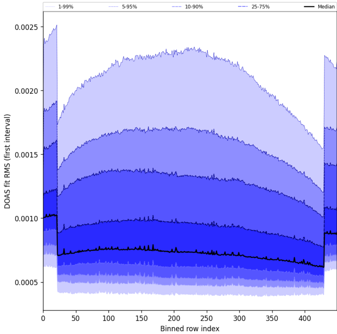
Figure 60: Along track statistics of “DOAS fit RMS (first interval)” for 2025-06-04 to 2025-06-06
