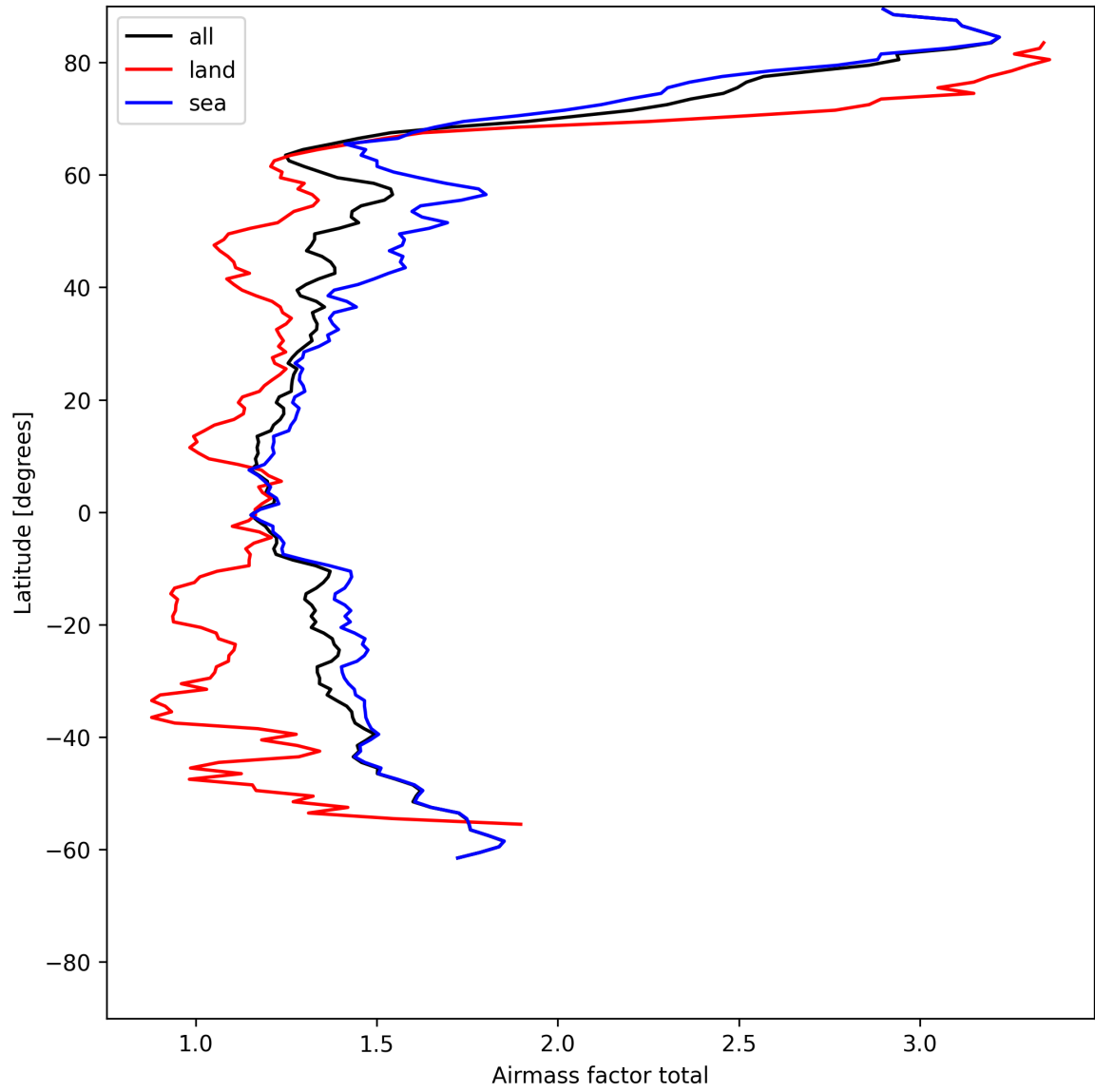
Figure 26: Zonal average of “Airmass factor total” for 2025-06-04 to 2025-06-06.
