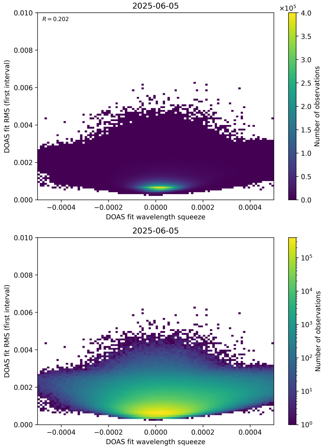
Figure 68: Scatter density plot of “DOAS fit wavelength squeeze” against “DOAS fit RMS (first interval)” for 2025-06-04 to 2025-06-06.
