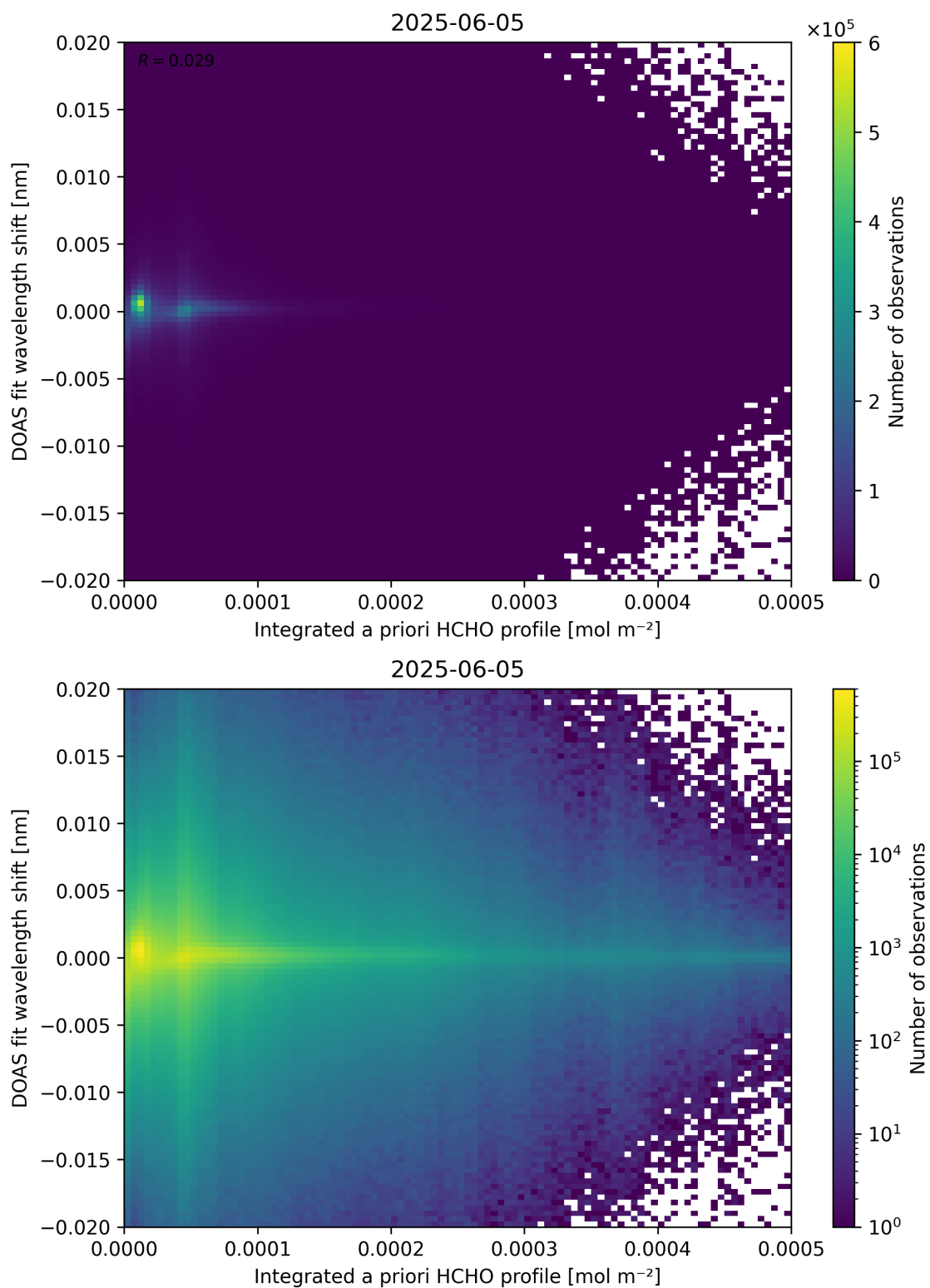
Figure 149: Scatter density plot of “Integrated a priori HCHO profile” against “DOAS fit wavelength shift” for 2025-06-04 to 2025-06-06.
