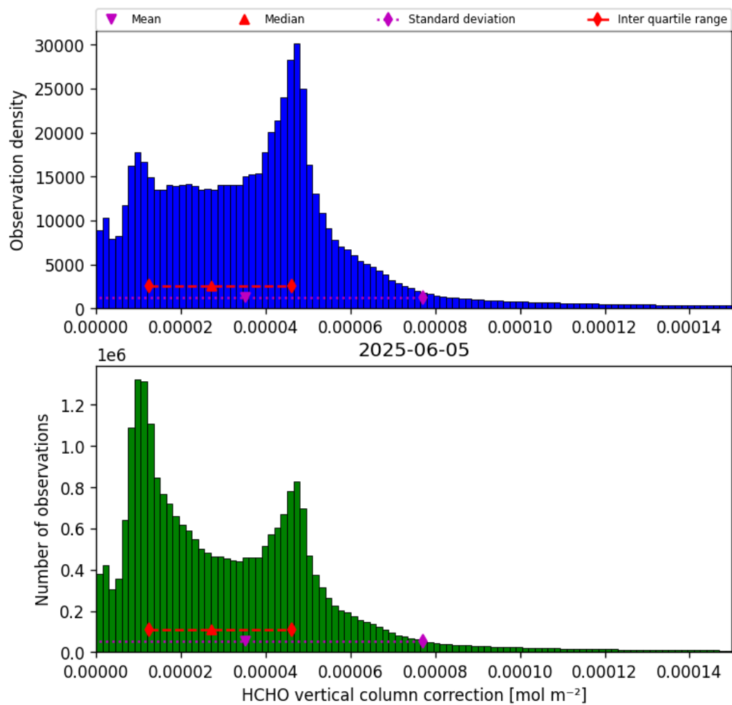
Figure 37: Histogram of “HCHO vertical column correction” for 2025-06-04 to 2025-06-06
