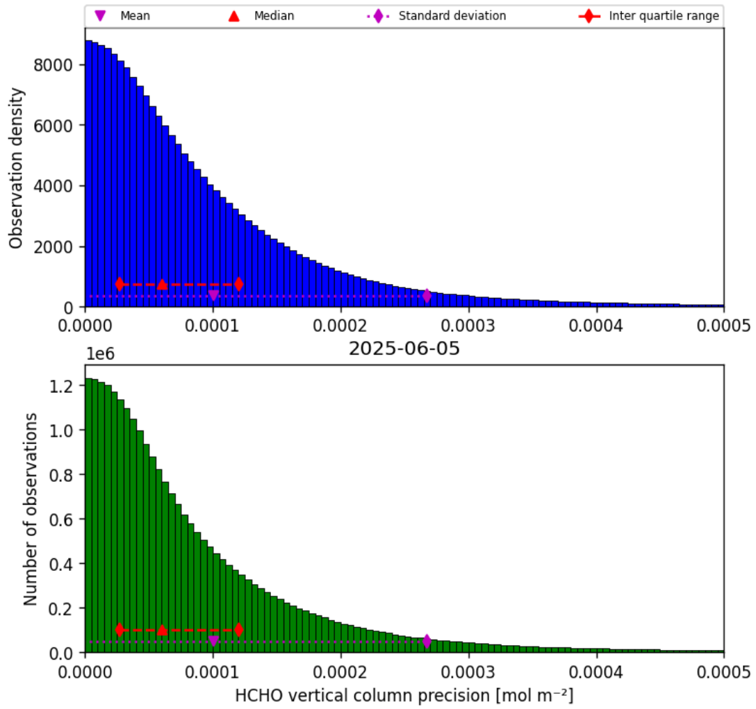
Figure 36: Histogram of “HCHO vertical column precision” for 2025-06-04 to 2025-06-06
