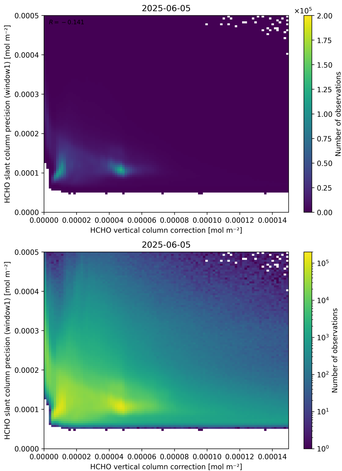
Figure 119: Scatter density plot of “HCHO vertical column correction” against “HCHO slant column precision (window1)” for 2025-06-04 to 2025-06-06.
