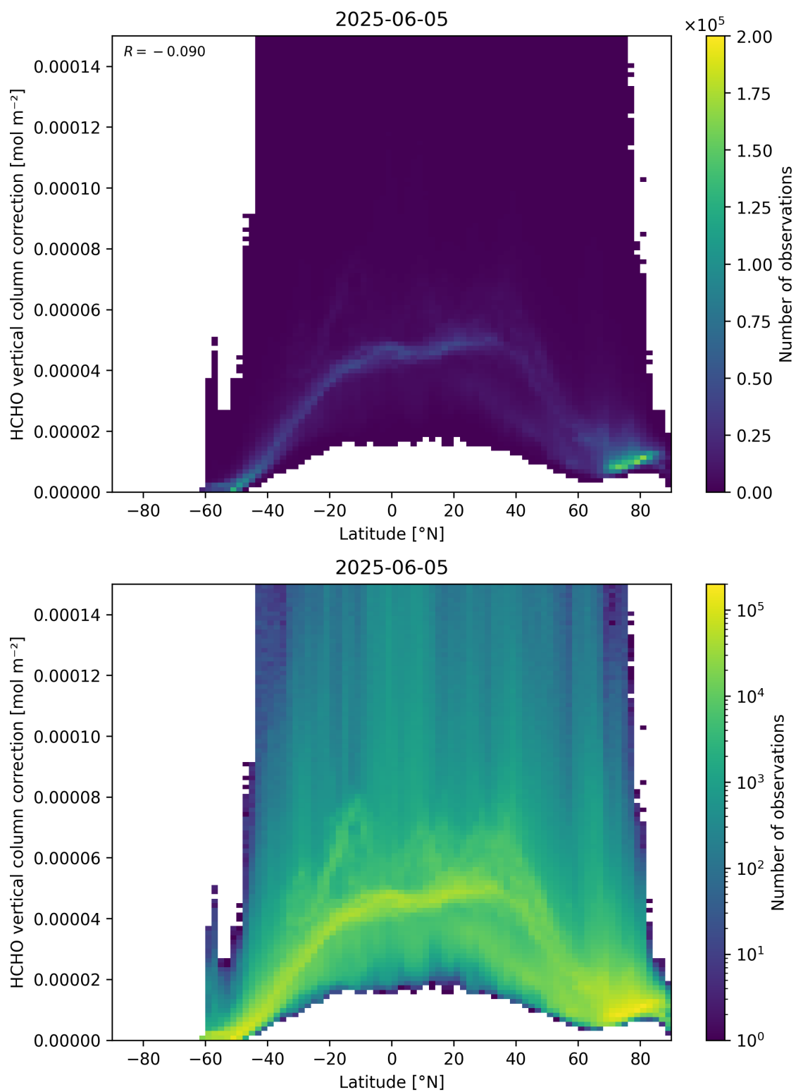
Figure 164: Scatter density plot of “Latitude” against “HCHO vertical column correction” for 2025-06-04 to 2025-06-06.
