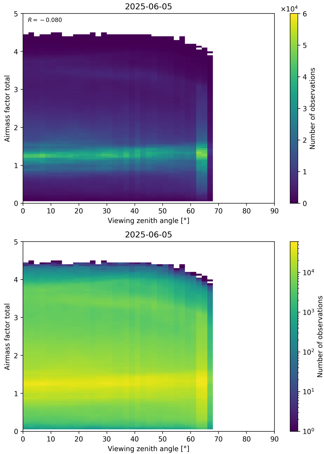
Figure 190: Scatter density plot of “Viewing zenith angle” against “Airmass factor total” for 2025-06-04 to 2025-06-06.
