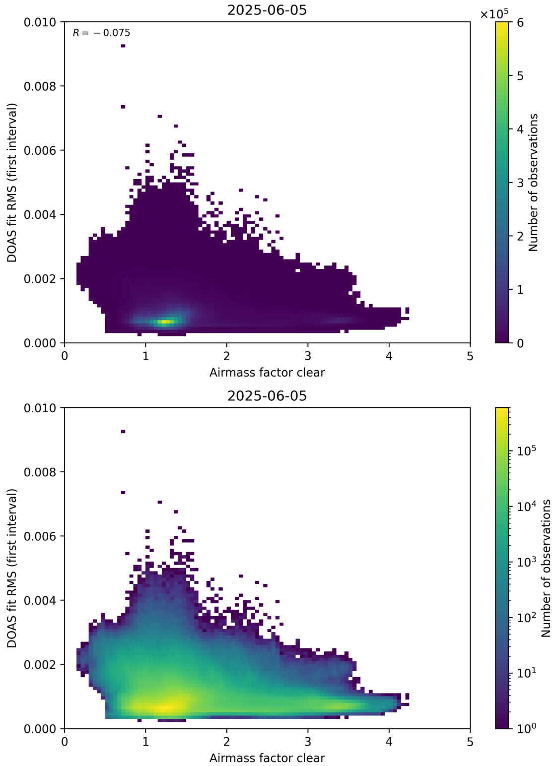
Figure 71: Scatter density plot of “Airmass factor clear” against “DOAS fit RMS (first interval)” for 2025-06-04 to 2025-06-06.
