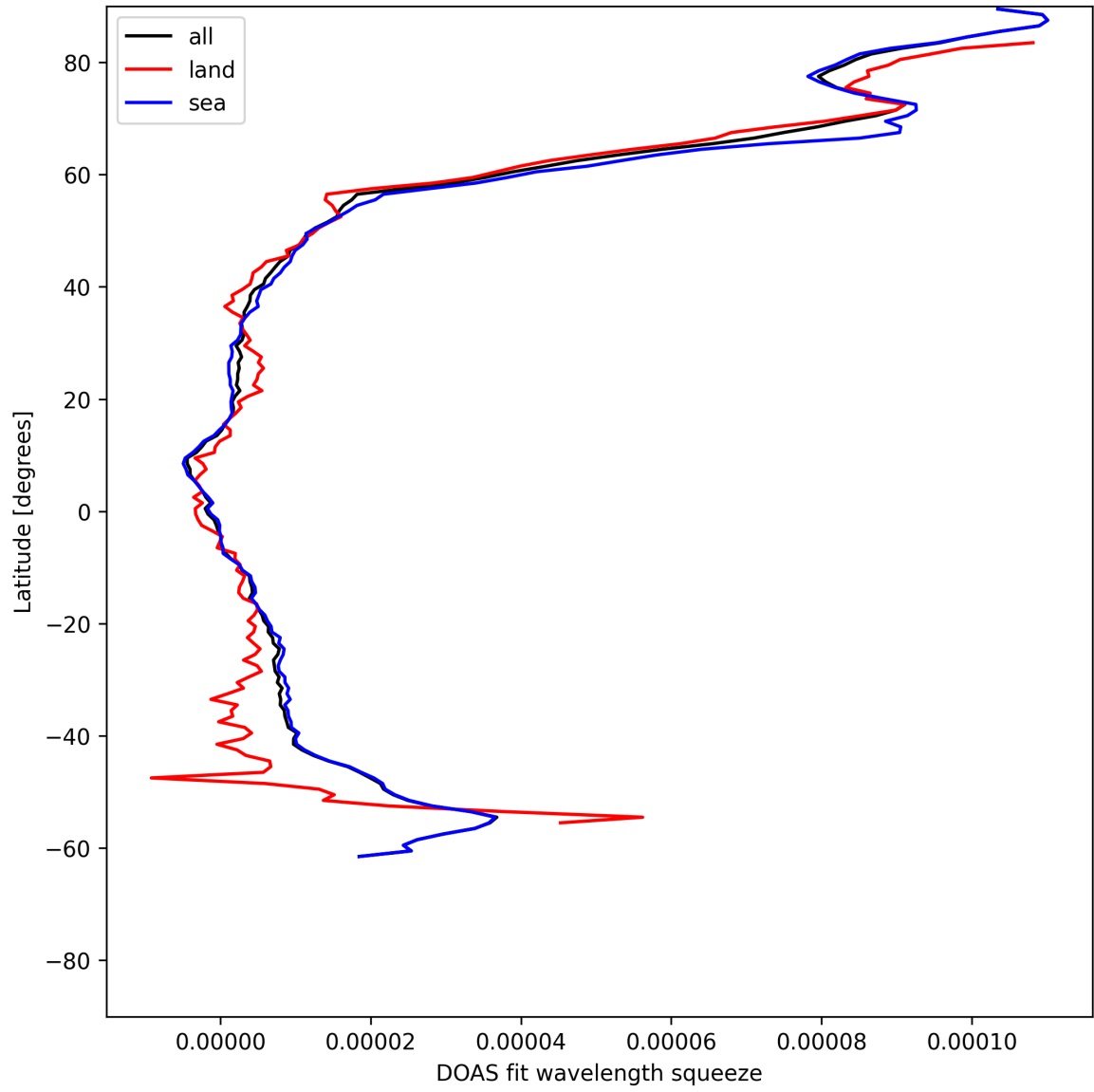
Figure 31: Zonal average of “DOAS fit wavelength squeeze” for 2025-06-04 to 2025-06-06.
