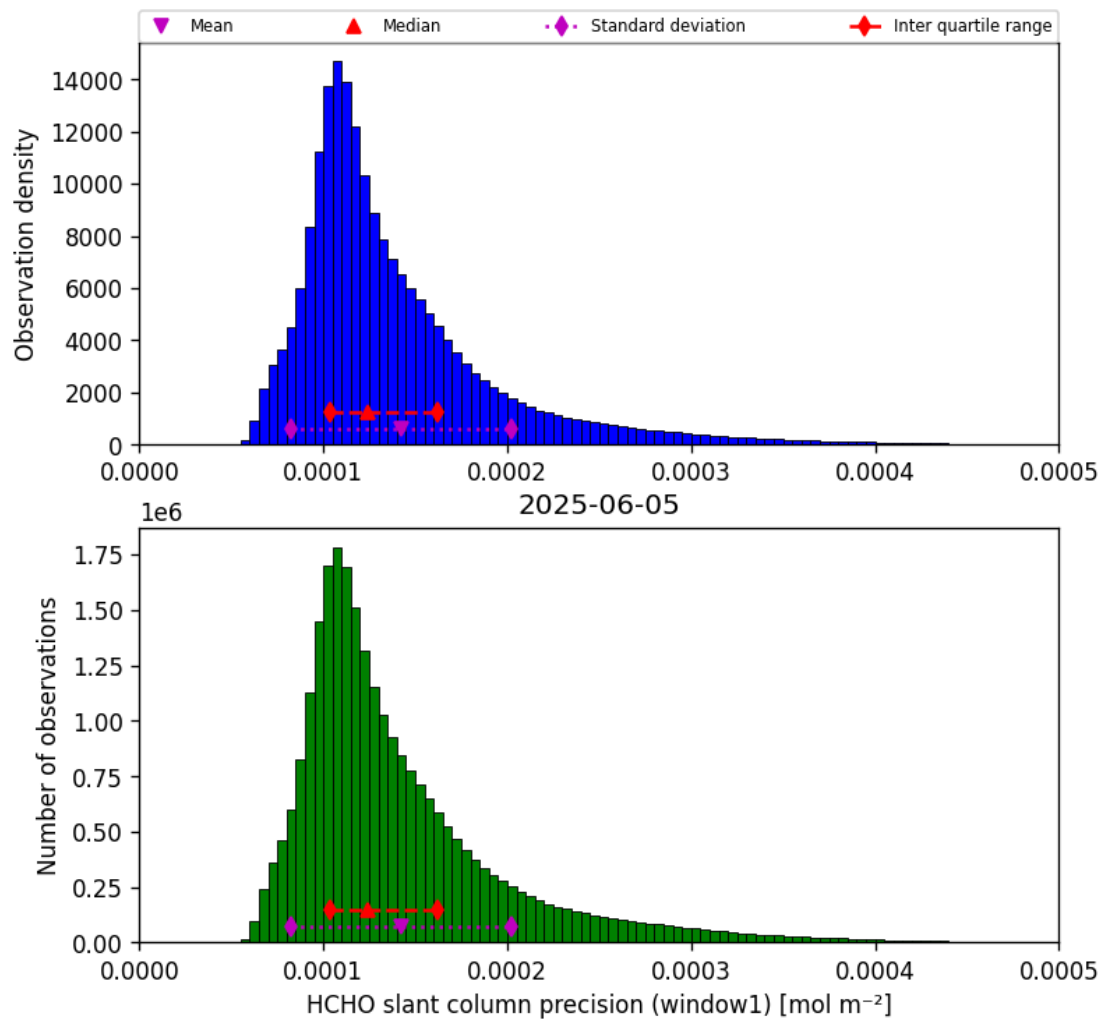
Figure 39: Histogram of “HCHO slant column precision (window1)” for 2025-06-04 to 2025-06-06
