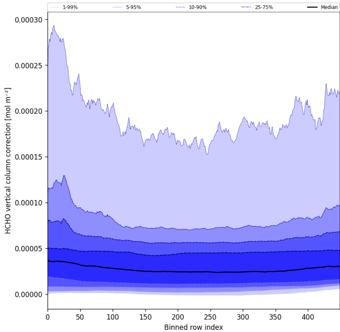
Figure 51: Along track statistics of “HCHO vertical column correction” for 2025-06-04 to 2025-06-06
