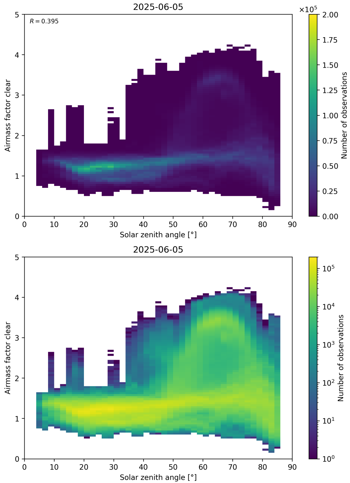
Figure 170: Scatter density plot of “Solar zenith angle” against “Airmass factor clear” for 2025-06-04 to 2025-06-06.
