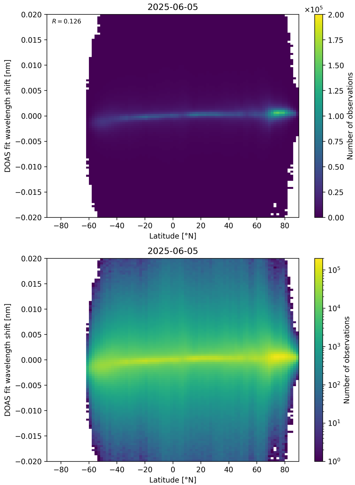
Figure 154: Scatter density plot of “Latitude” against “DOAS fit wavelength shift” for 2025-06-04 to 2025-06-06.
