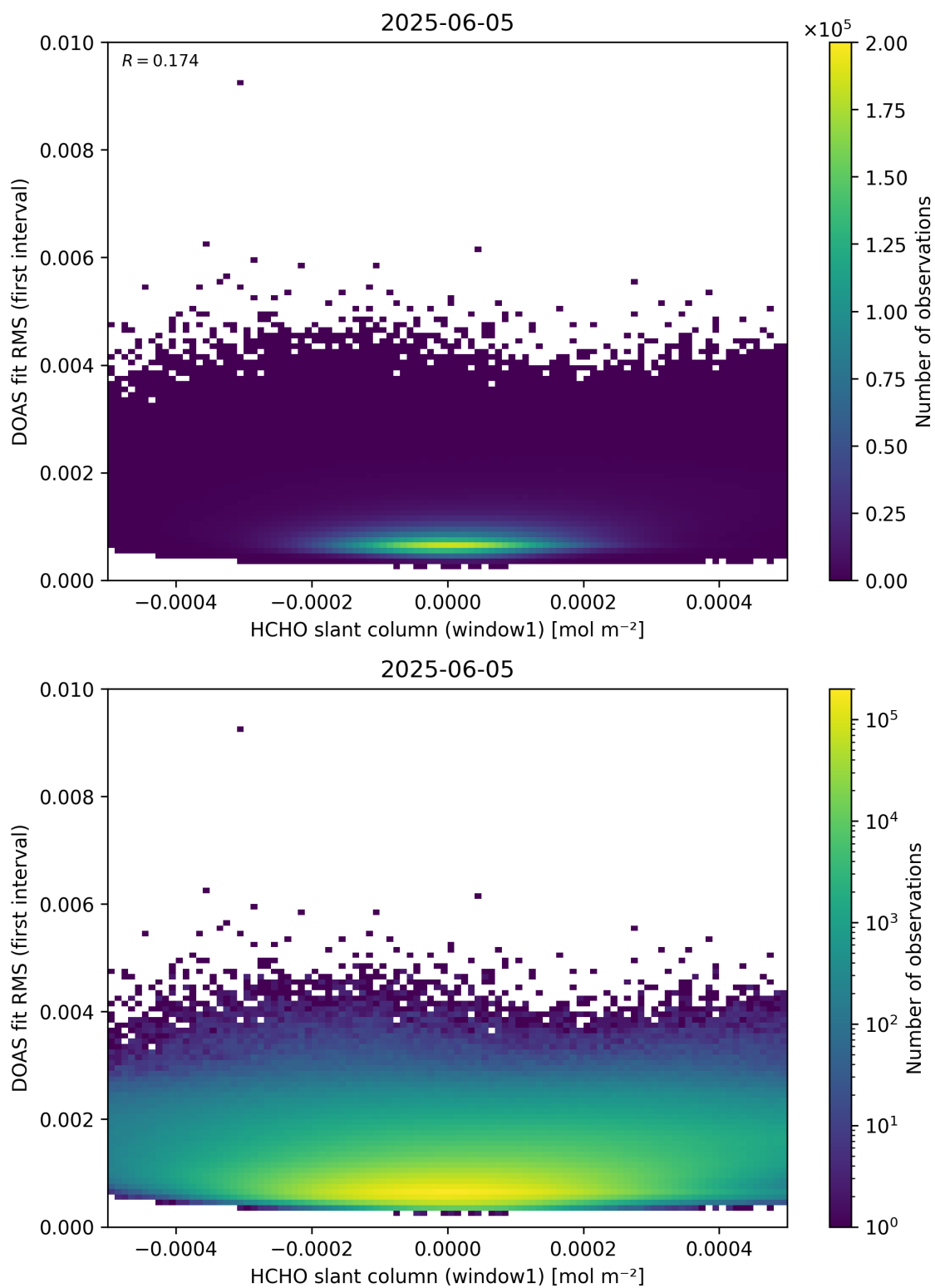
Figure 78: Scatter density plot of “HCHO slant column (window1)” against “DOAS fit RMS (first interval)” for 2025-06-04 to 2025-06-06.
