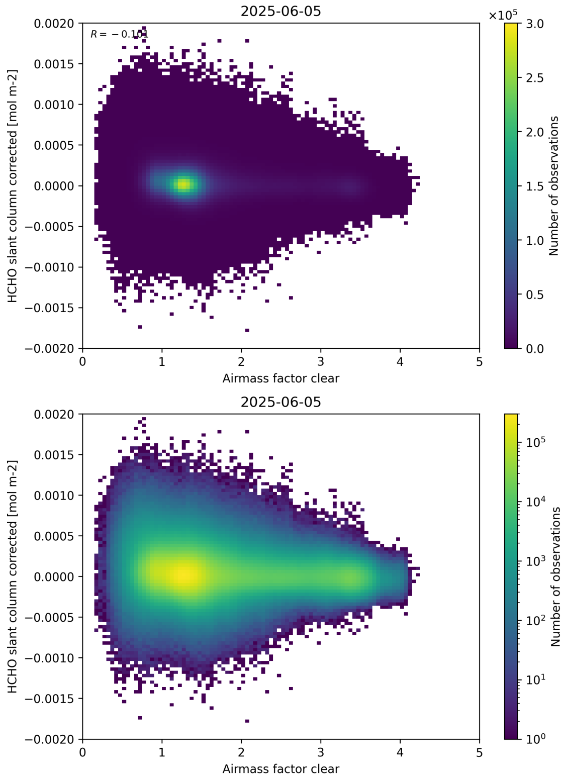
Figure 74: Scatter density plot of “Airmass factor clear” against “HCHO slant column corrected” for 2025-06-04 to 2025-06-06.
