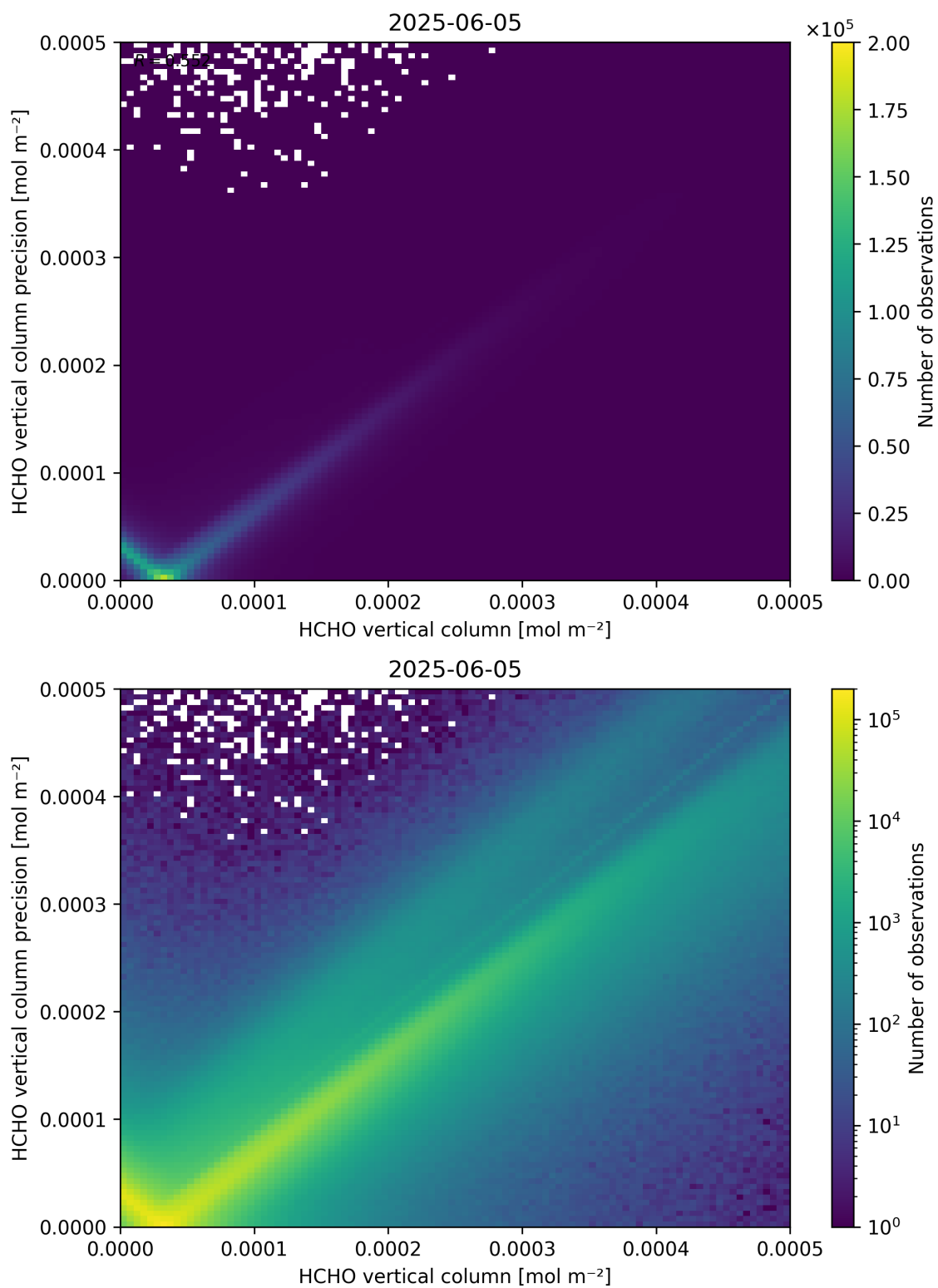
Figure 134: Scatter density plot of “HCHO vertical column” against “HCHO vertical column precision” for 2025-06-04 to 2025-06-06.
