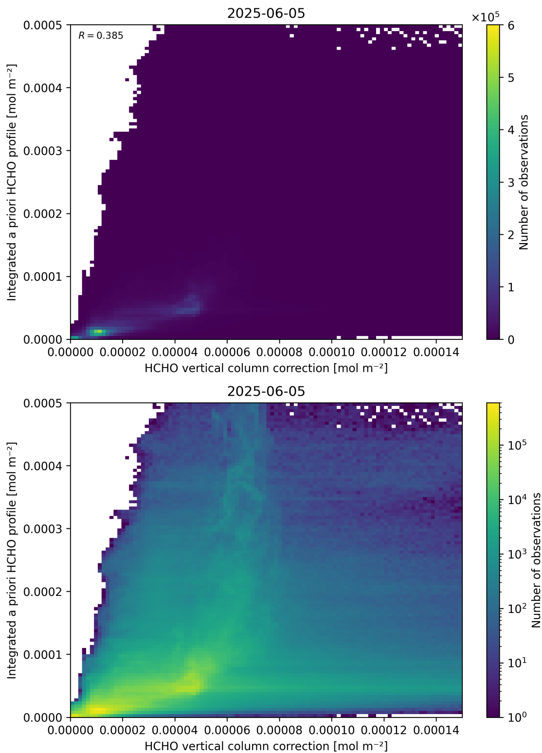
Figure 122: Scatter density plot of “HCHO vertical column correction” against “Integrated a priori HCHO profile” for 2025-06-04 to 2025-06-06.
