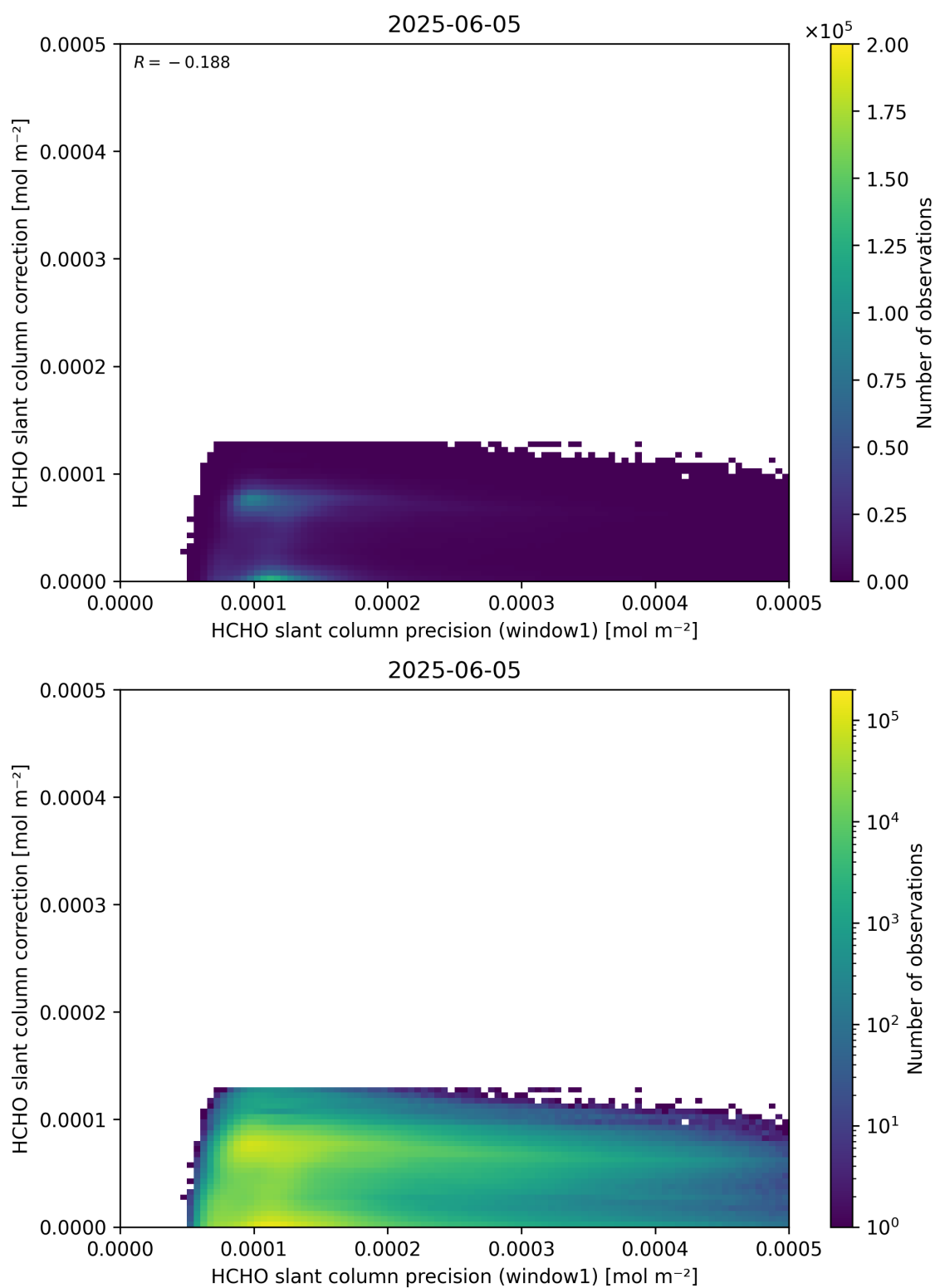
Figure 93: Scatter density plot of “HCHO slant column precision (window1)” against “HCHO slant column correction” for 2025-06-04 to 2025-06-06.
