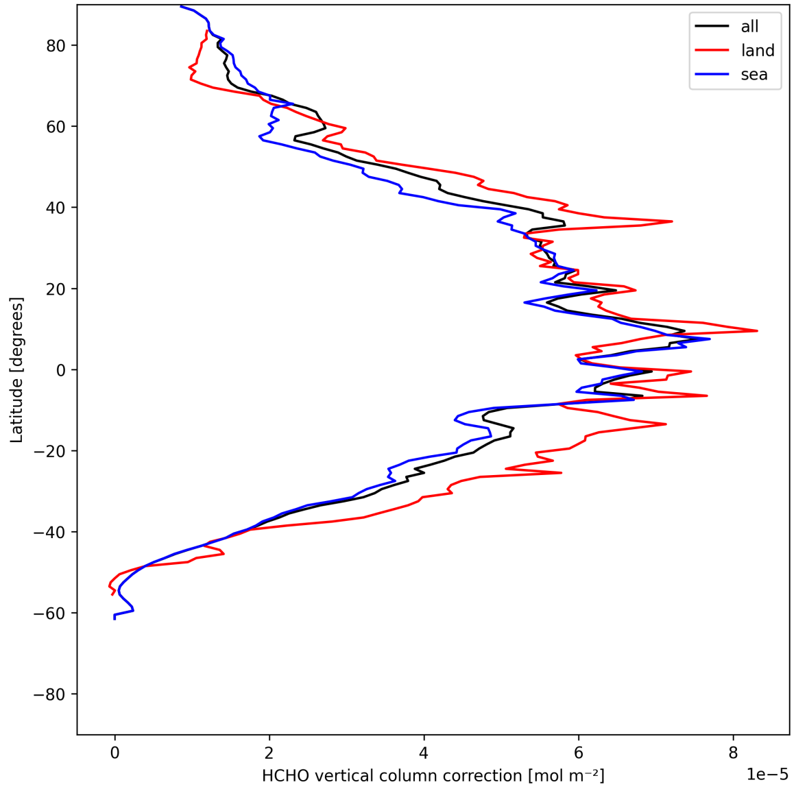
Figure 23: Zonal average of “HCHO vertical column correction” for 2025-06-04 to 2025-06-06.
