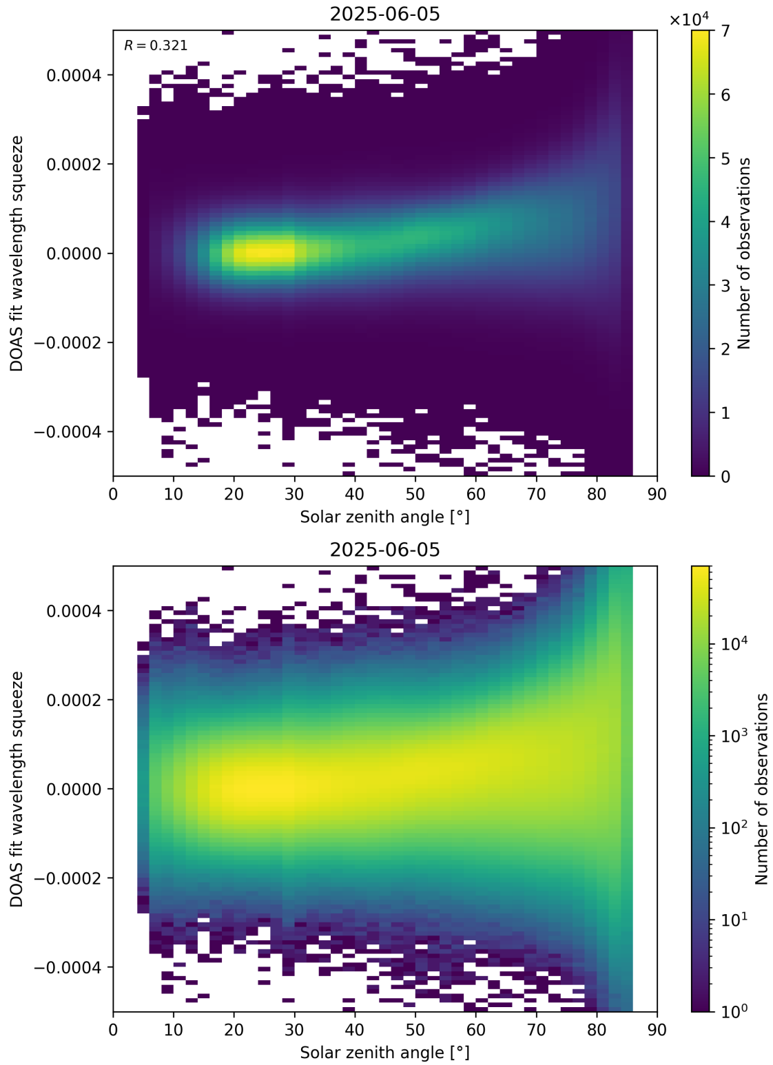
Figure 169: Scatter density plot of “Solar zenith angle” against “DOAS fit wavelength squeeze” for 2025-06-04 to 2025-06-06.
