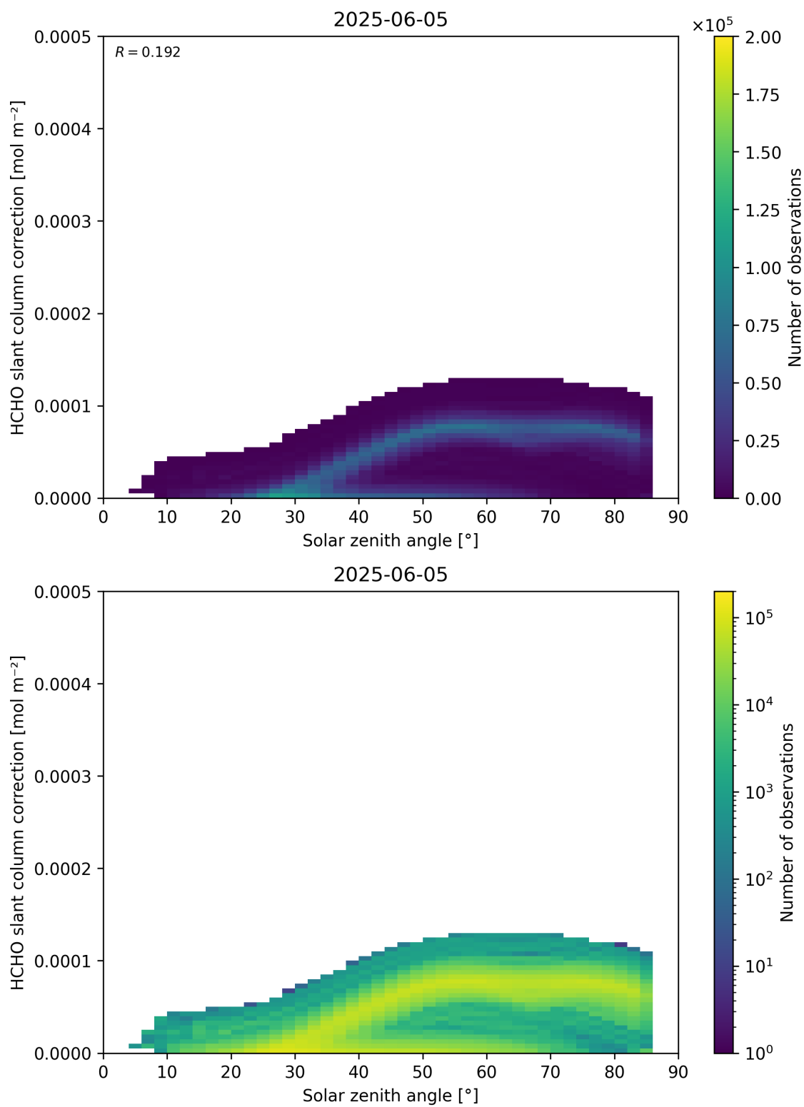
Figure 172: Scatter density plot of “Solar zenith angle” against “HCHO slant column correction” for 2025-06-04 to 2025-06-06.
