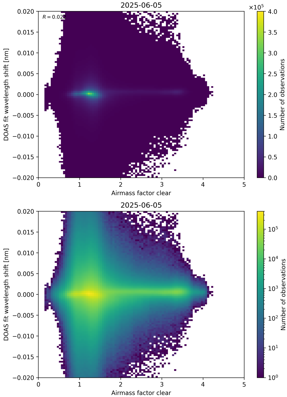
Figure 72: Scatter density plot of “Airmass factor clear” against “DOAS fit wavelength shift” for 2025-06-04 to 2025-06-06.
