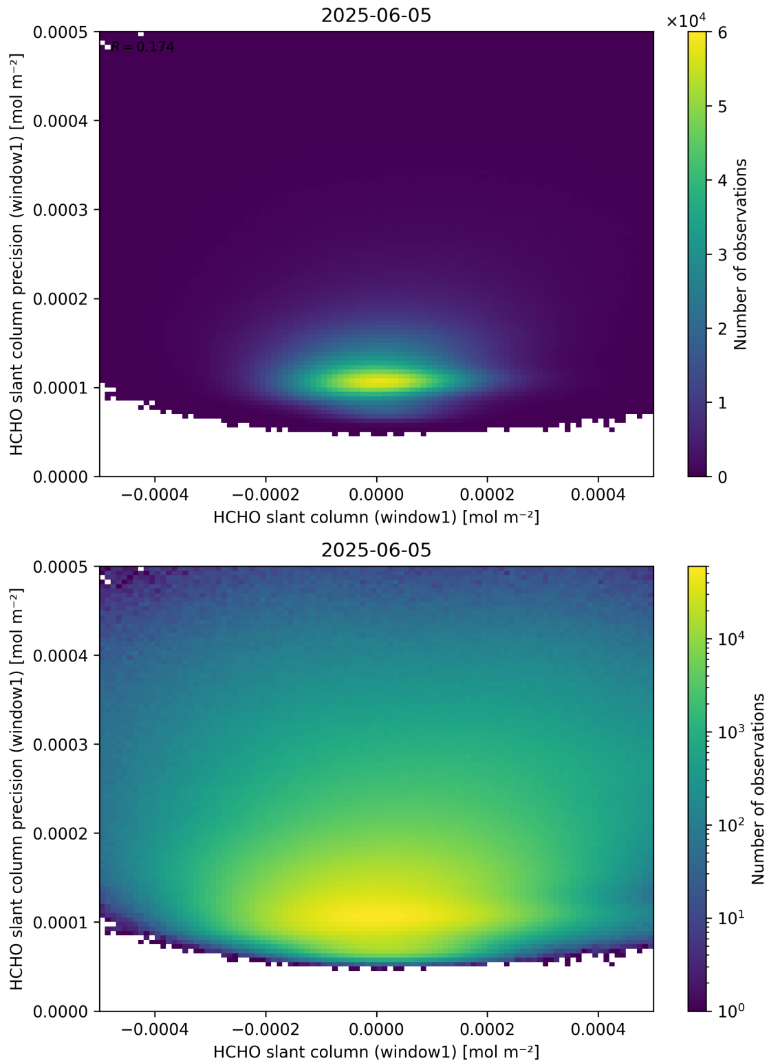
Figure 84: Scatter density plot of “HCHO slant column (window1)” against “HCHO slant column precision (window1)” for 2025-06-04 to 2025-06-06.
