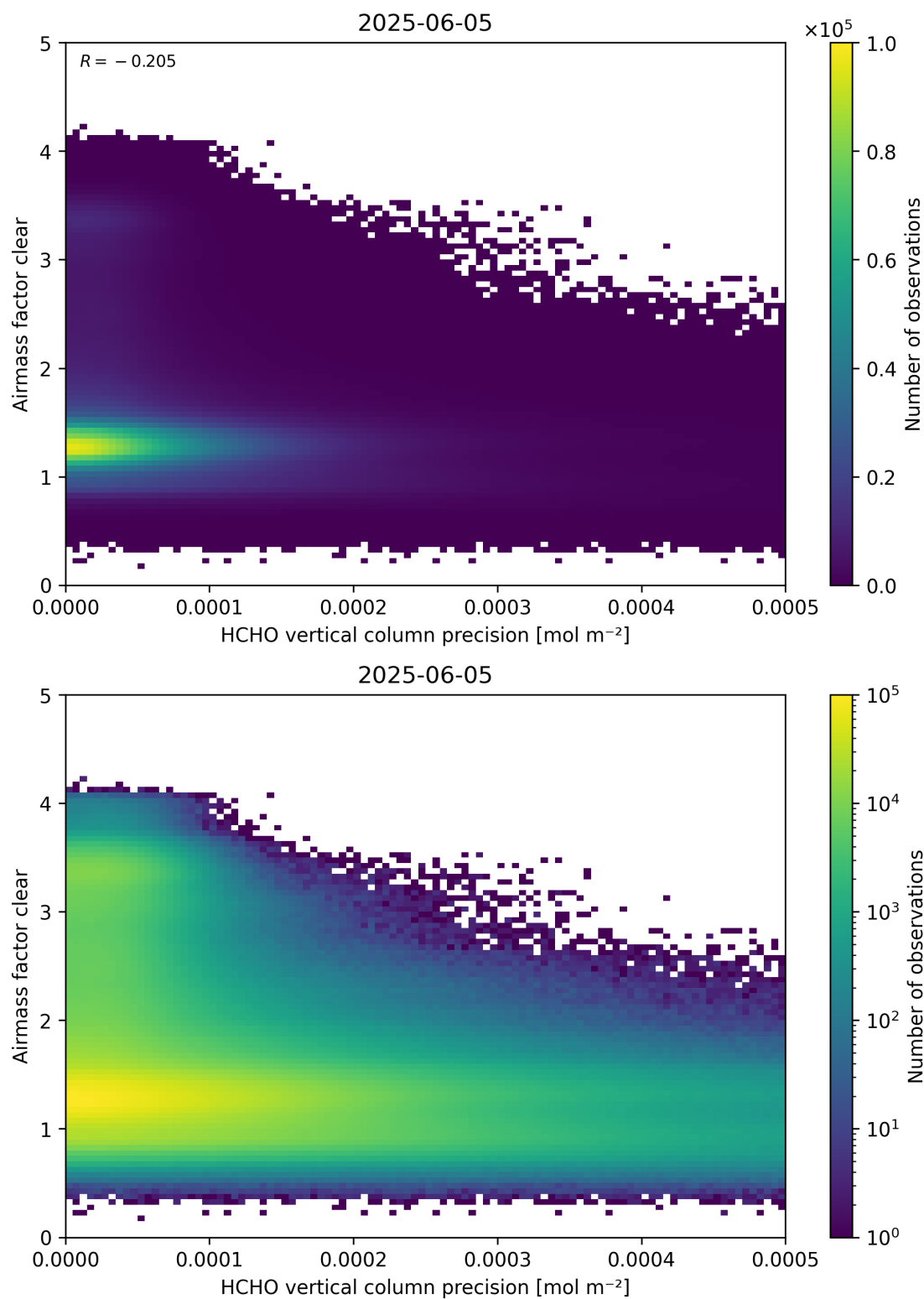
Figure 139: Scatter density plot of “HCHO vertical column precision” against “Airmass factor clear” for 2025-06-04 to 2025-06-06.
