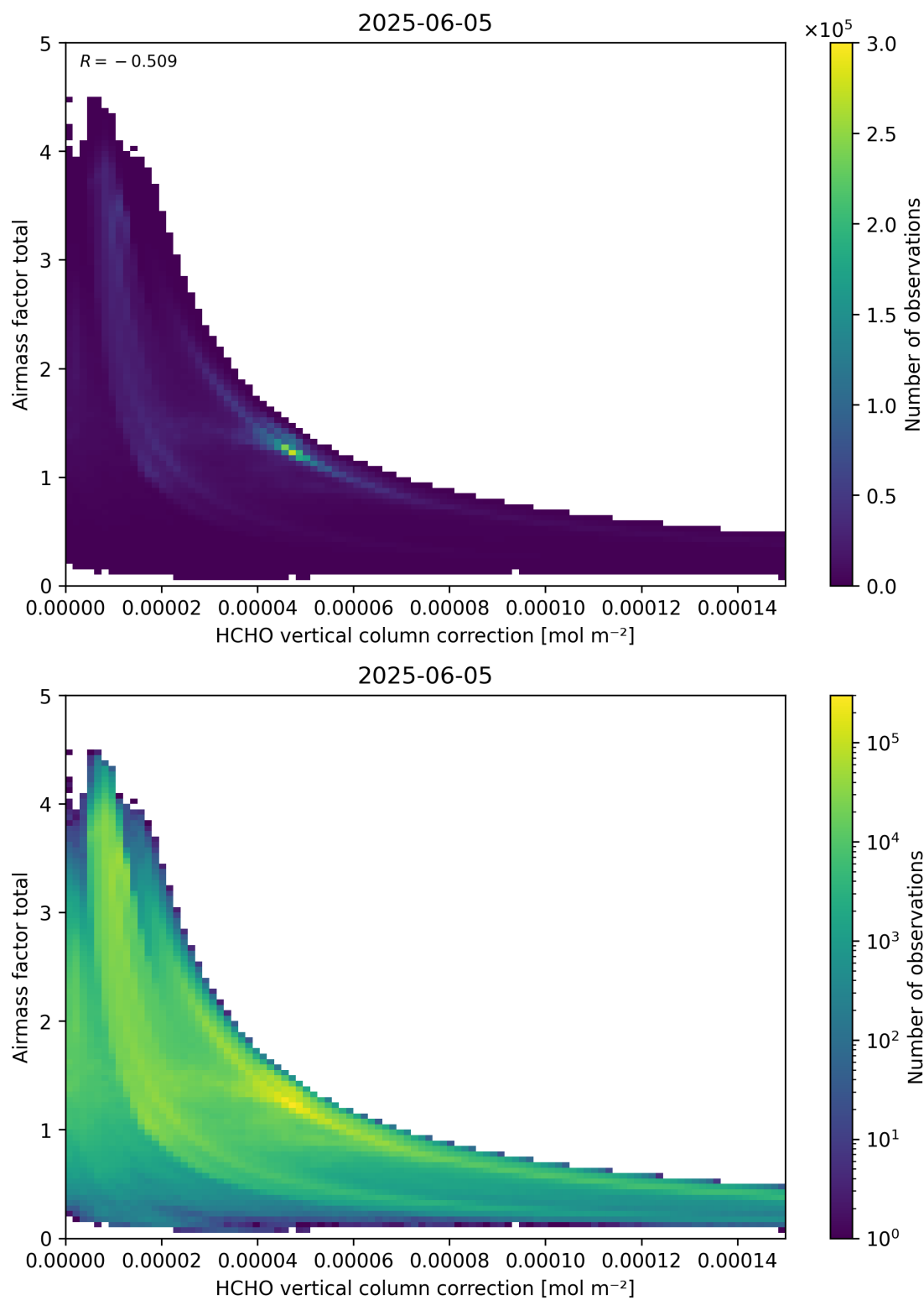
Figure 120: Scatter density plot of “HCHO vertical column correction” against “Airmass factor total” for 2025-06-04 to 2025-06-06.
