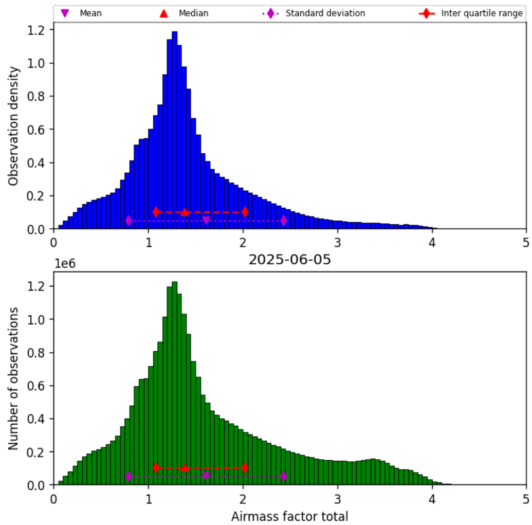
Figure 40: Histogram of “Airmass factor total” for 2025-06-04 to 2025-06-06
