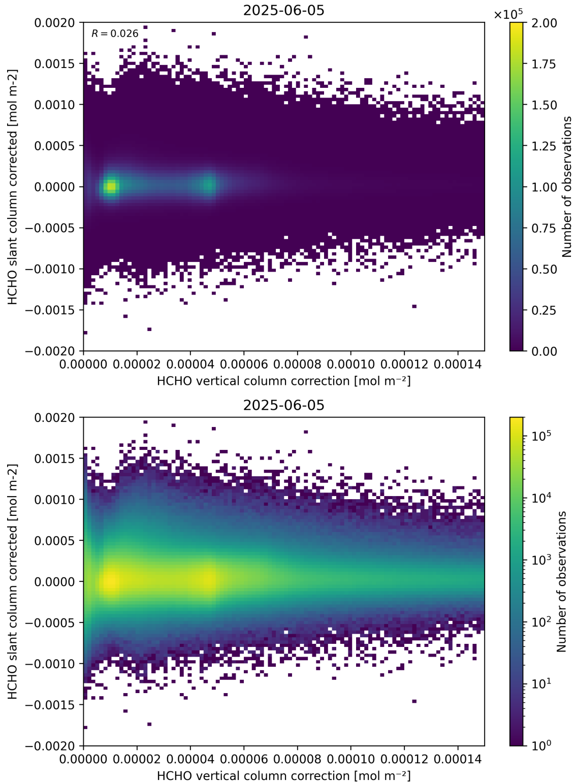
Figure 116: Scatter density plot of “HCHO vertical column correction” against “HCHO slant column corrected” for 2025-06-04 to 2025-06-06.
