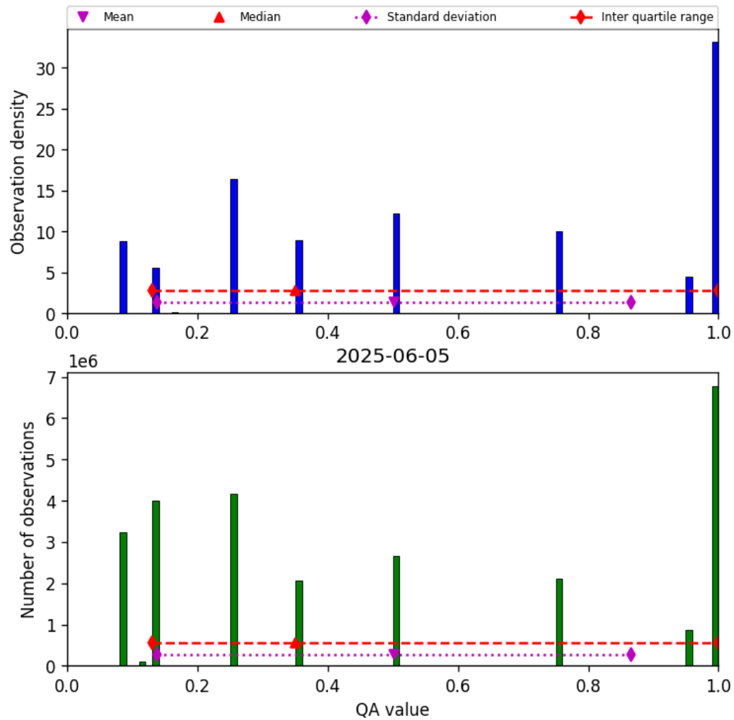
Figure 34: Histogram of “QA value” for 2025-06-04 to 2025-06-06
