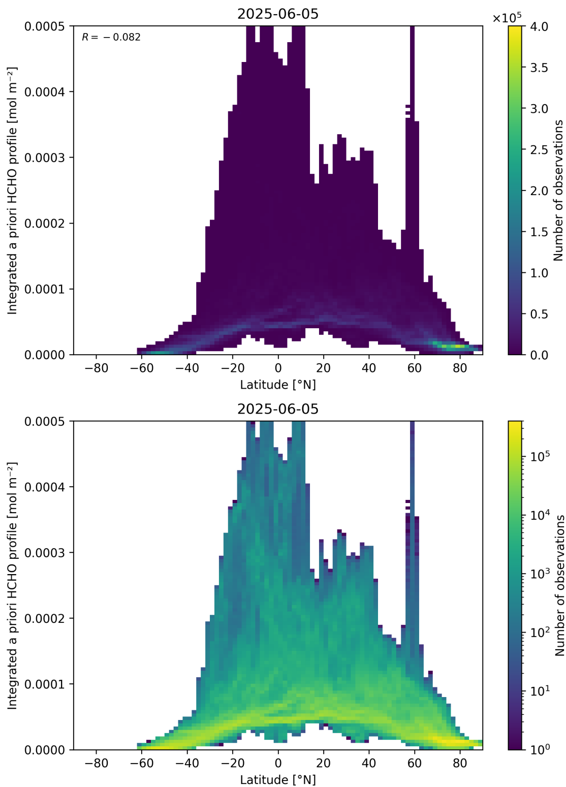
Figure 166: Scatter density plot of “Latitude” against “Integrated a priori HCHO profile” for 2025-06-04 to 2025-06-06.
