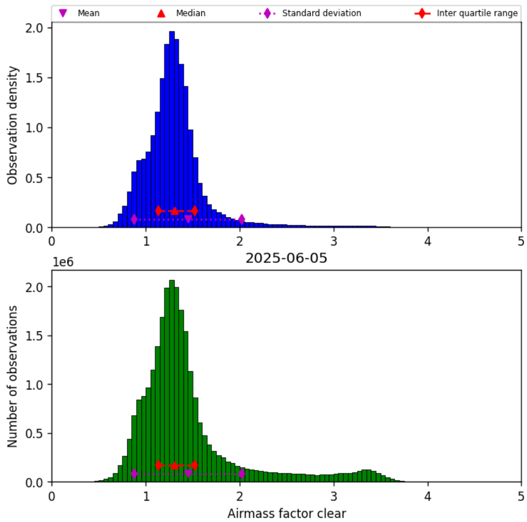
Figure 42: Histogram of “Airmass factor clear” for 2025-06-04 to 2025-06-06
