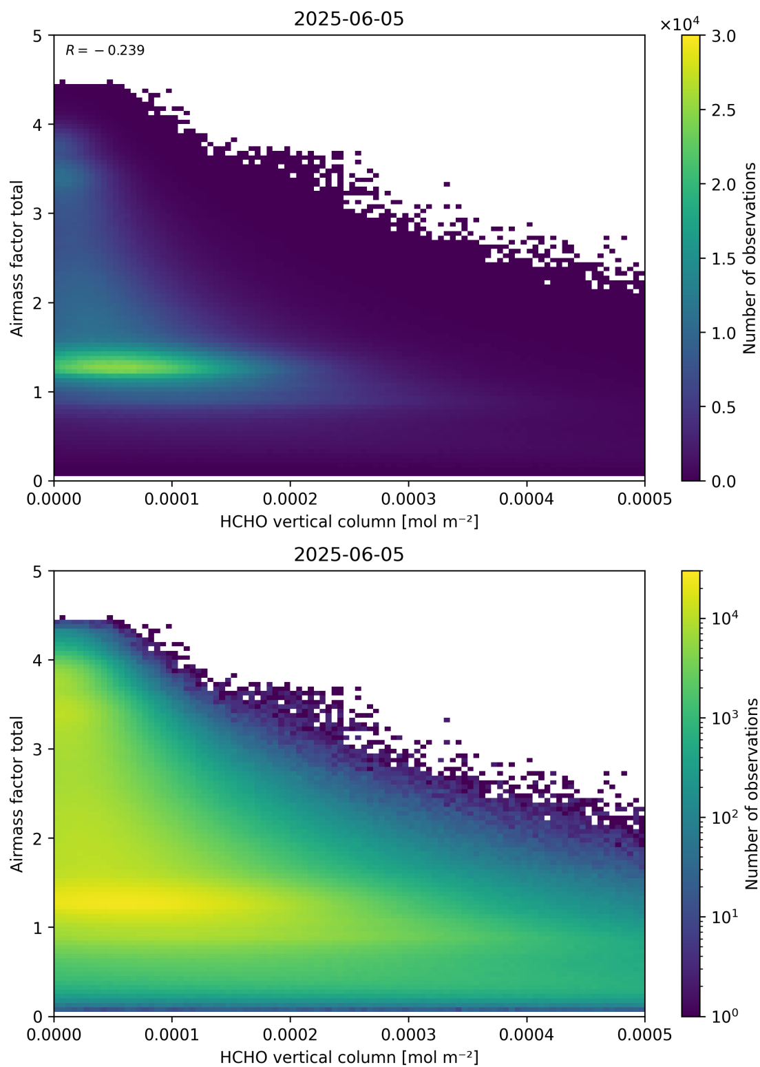
Figure 131: Scatter density plot of “HCHO vertical column” against “Airmass factor total” for 2025-06-04 to 2025-06-06.
