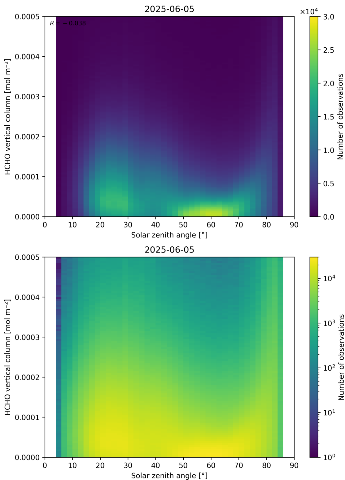
Figure 177: Scatter density plot of “Solar zenith angle” against “HCHO vertical column” for 2025-06-04 to 2025-06-06.
