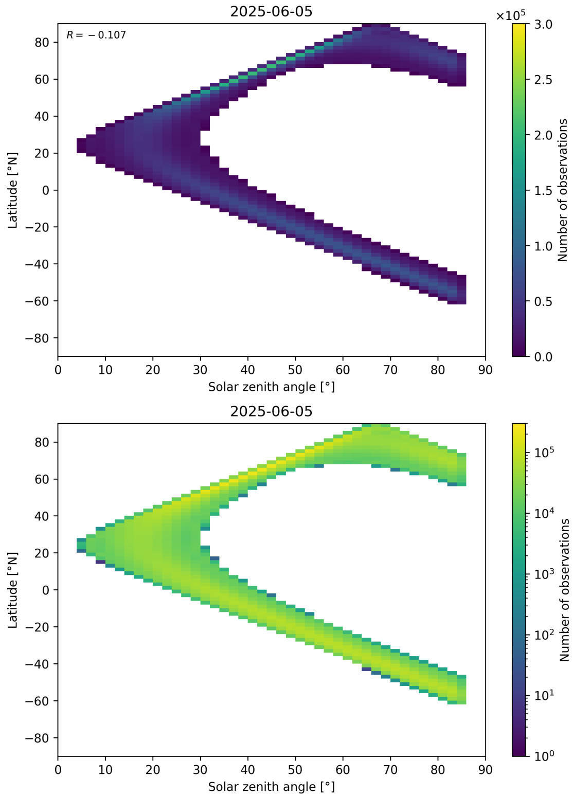
Figure 181: Scatter density plot of “Solar zenith angle” against “Latitude” for 2025-06-04 to 2025-06-06.
