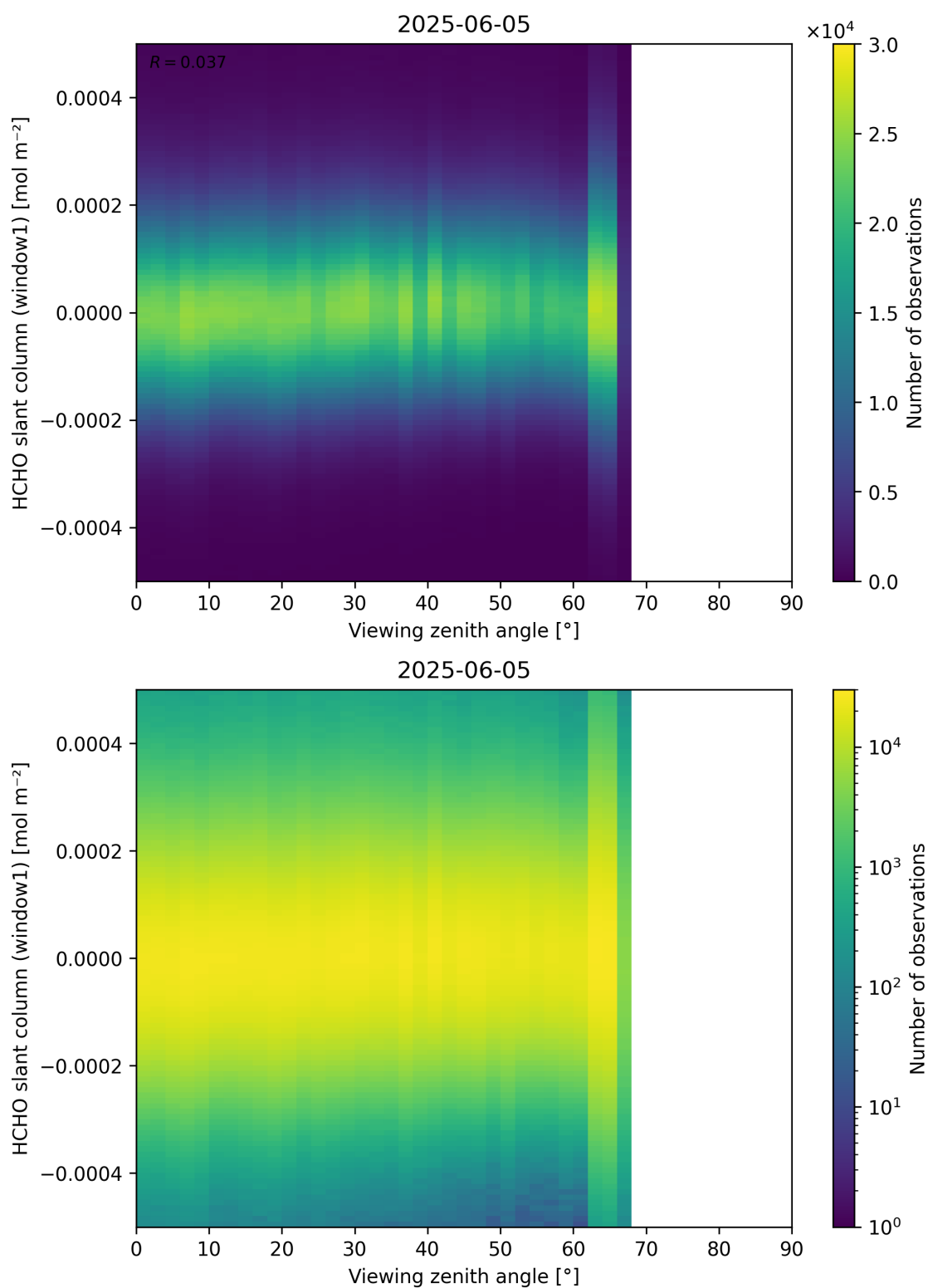
Figure 188: Scatter density plot of “Viewing zenith angle” against “HCHO slant column (window1)” for 2025-06-04 to 2025-06-06.
