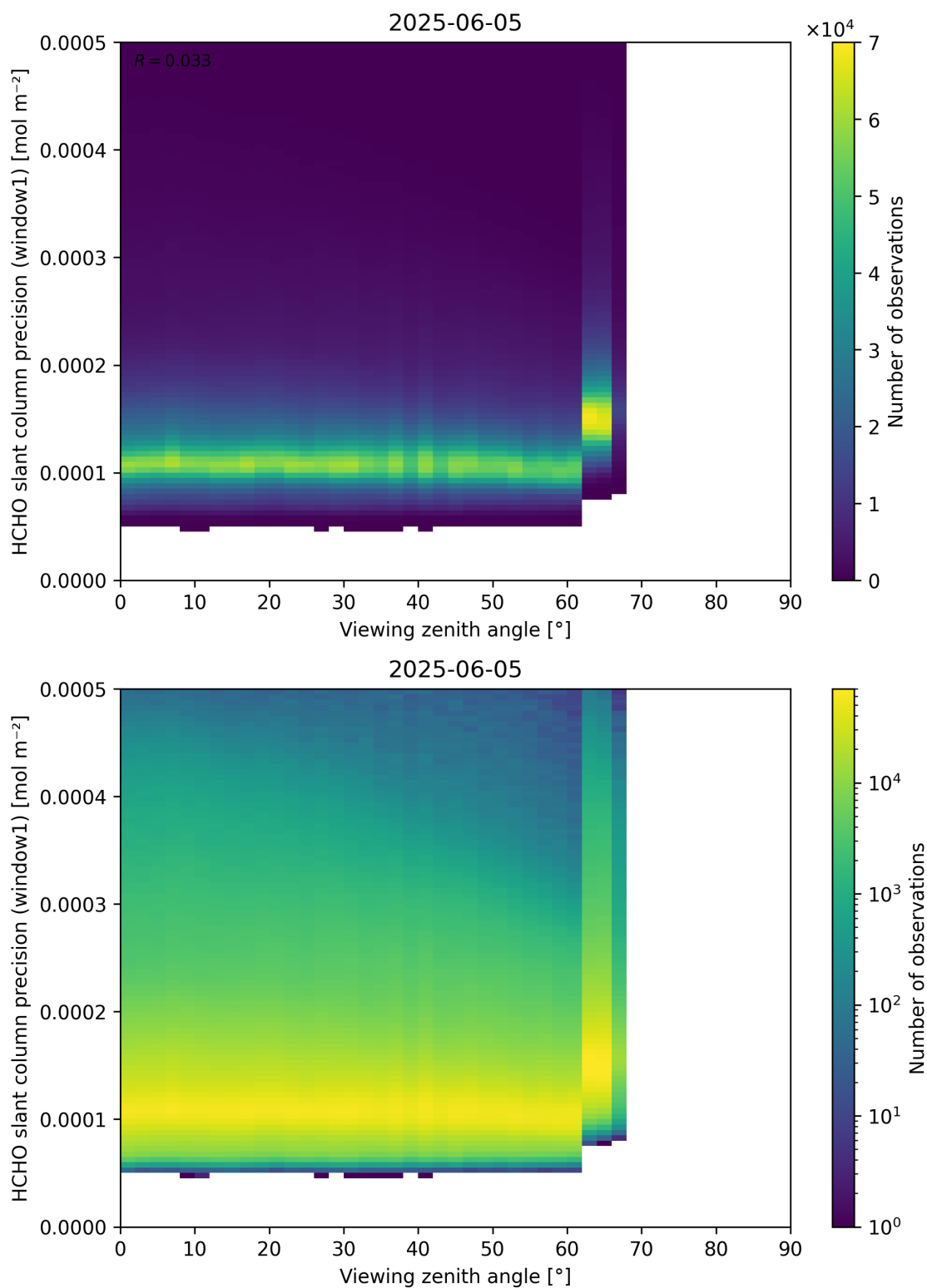
Figure 189: Scatter density plot of “Viewing zenith angle” against “HCHO slant column precision (window1)” for 2025-06-04 to 2025-06-06.
