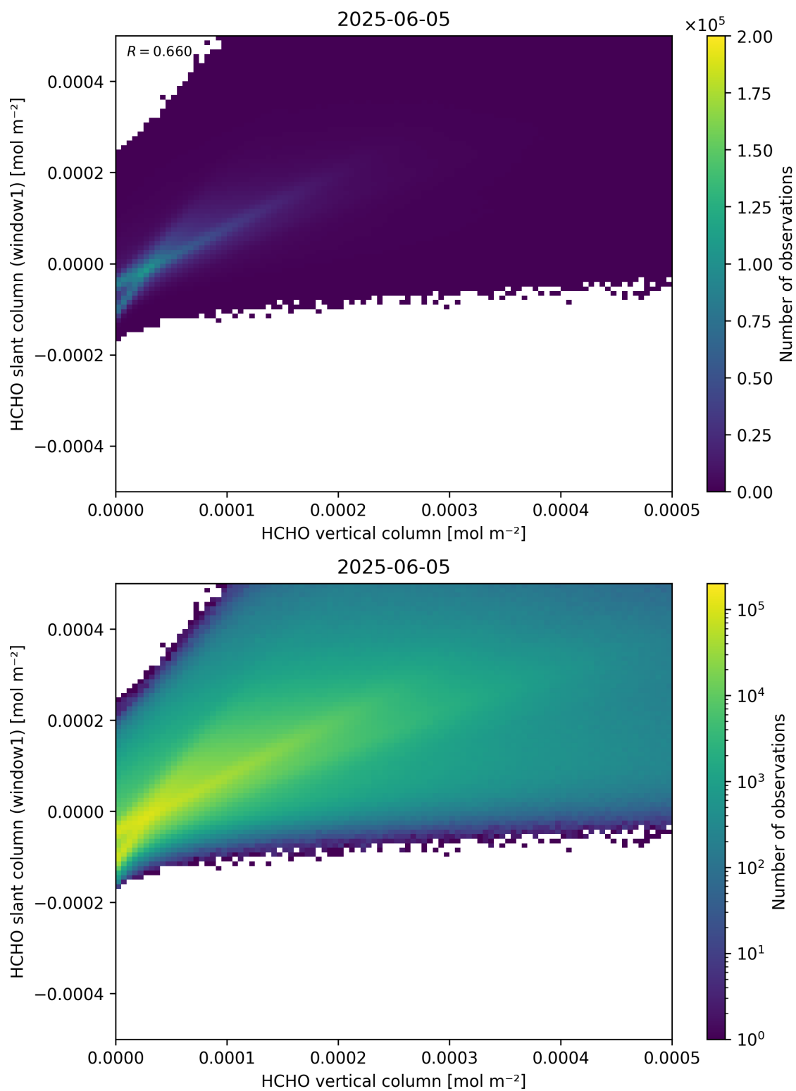
Figure 129: Scatter density plot of “HCHO vertical column” against “HCHO slant column (window1)” for 2025-06-04 to 2025-06-06.
