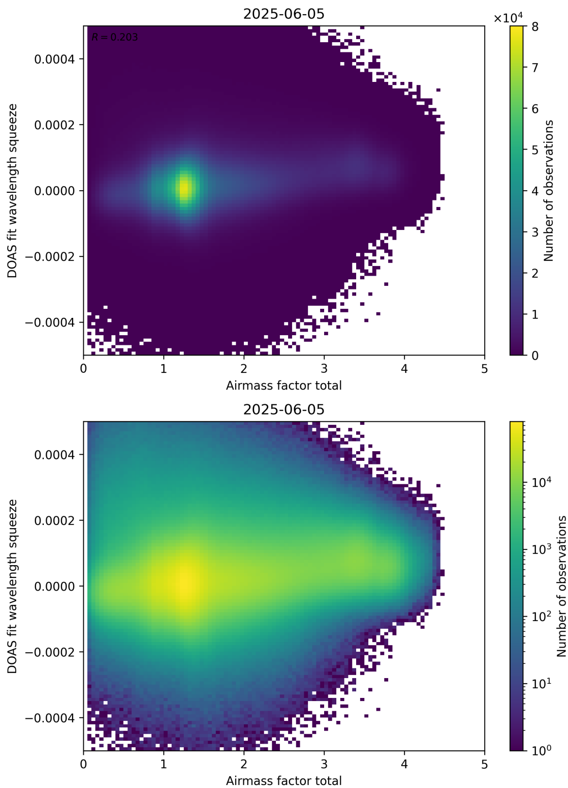
Figure 99: Scatter density plot of “Airmass factor total” against “DOAS fit wavelength squeeze” for 2025-06-04 to 2025-06-06.
