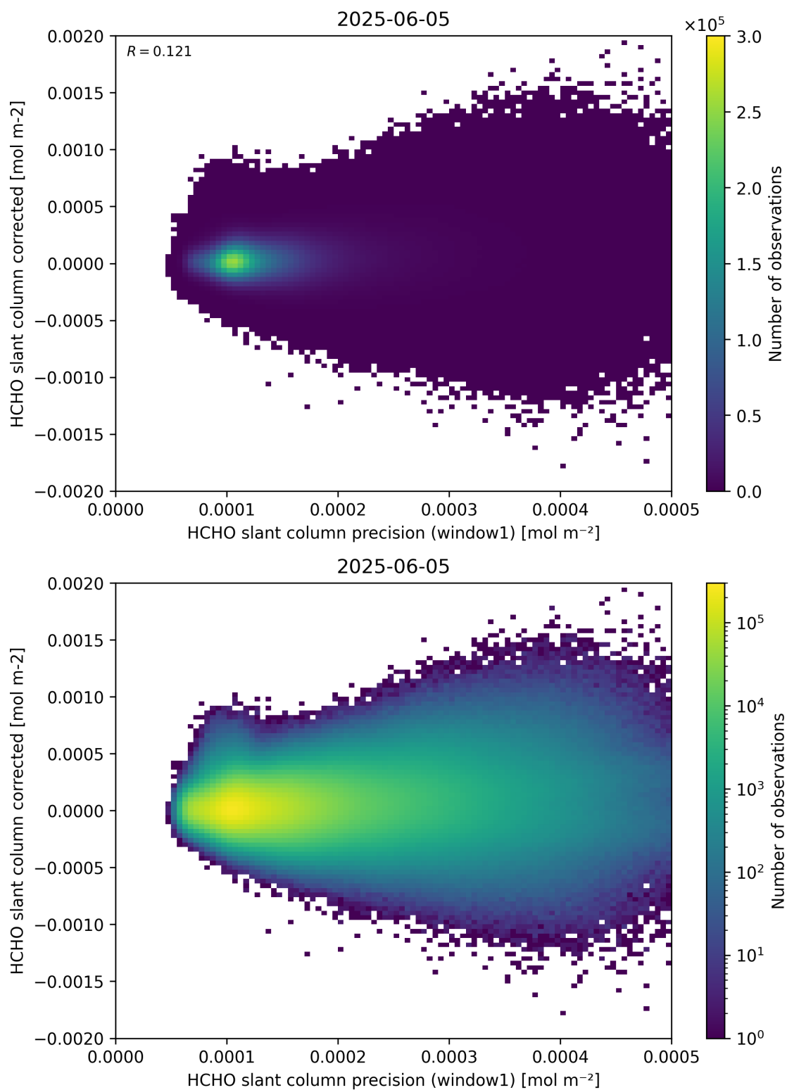
Figure 92: Scatter density plot of “HCHO slant column precision (window1)” against “HCHO slant column corrected” for 2025-06-04 to 2025-06-06.
