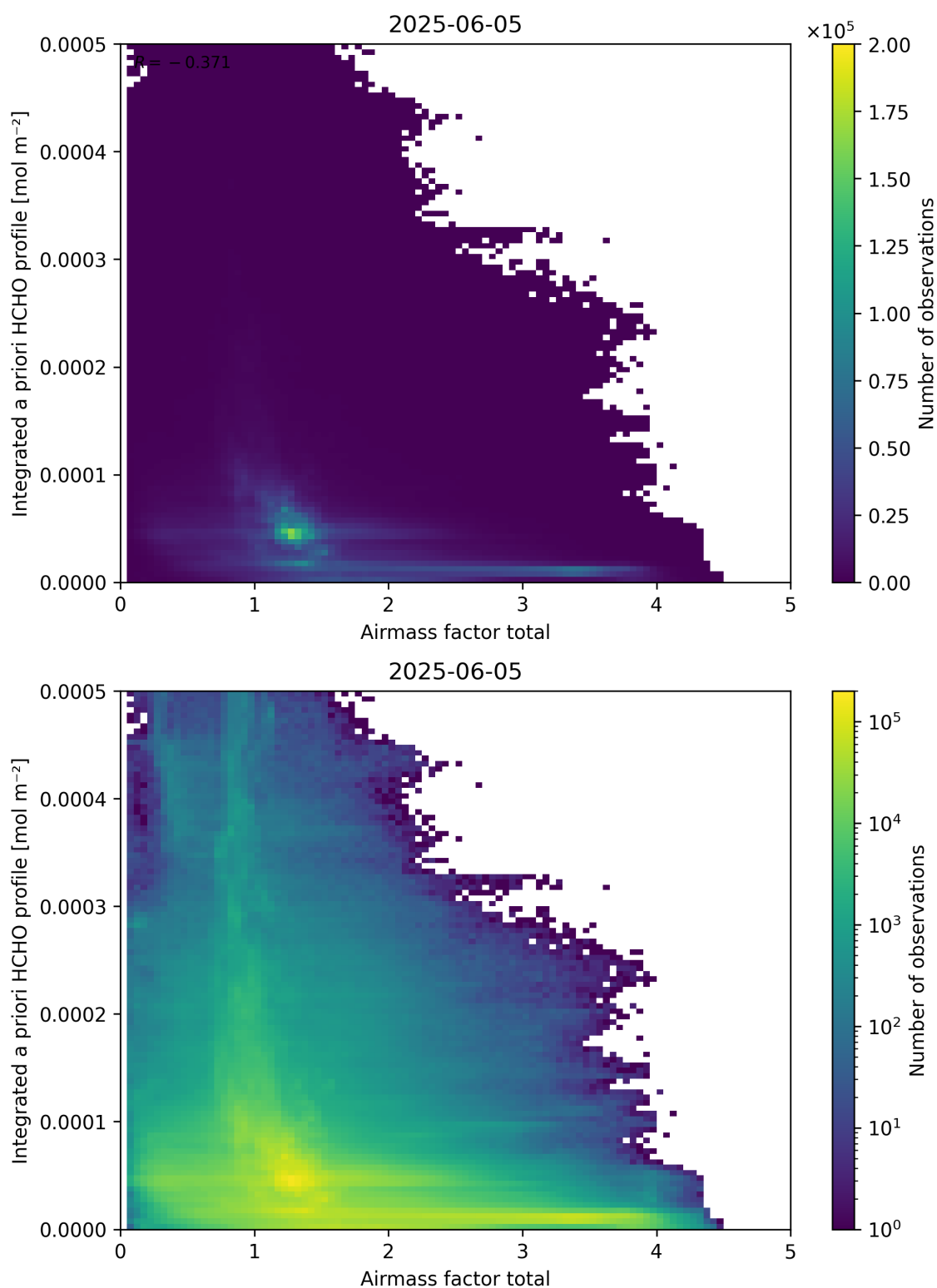
Figure 104: Scatter density plot of “Airmass factor total” against “Integrated a priori HCHO profile” for 2025-06-04 to 2025-06-06.
