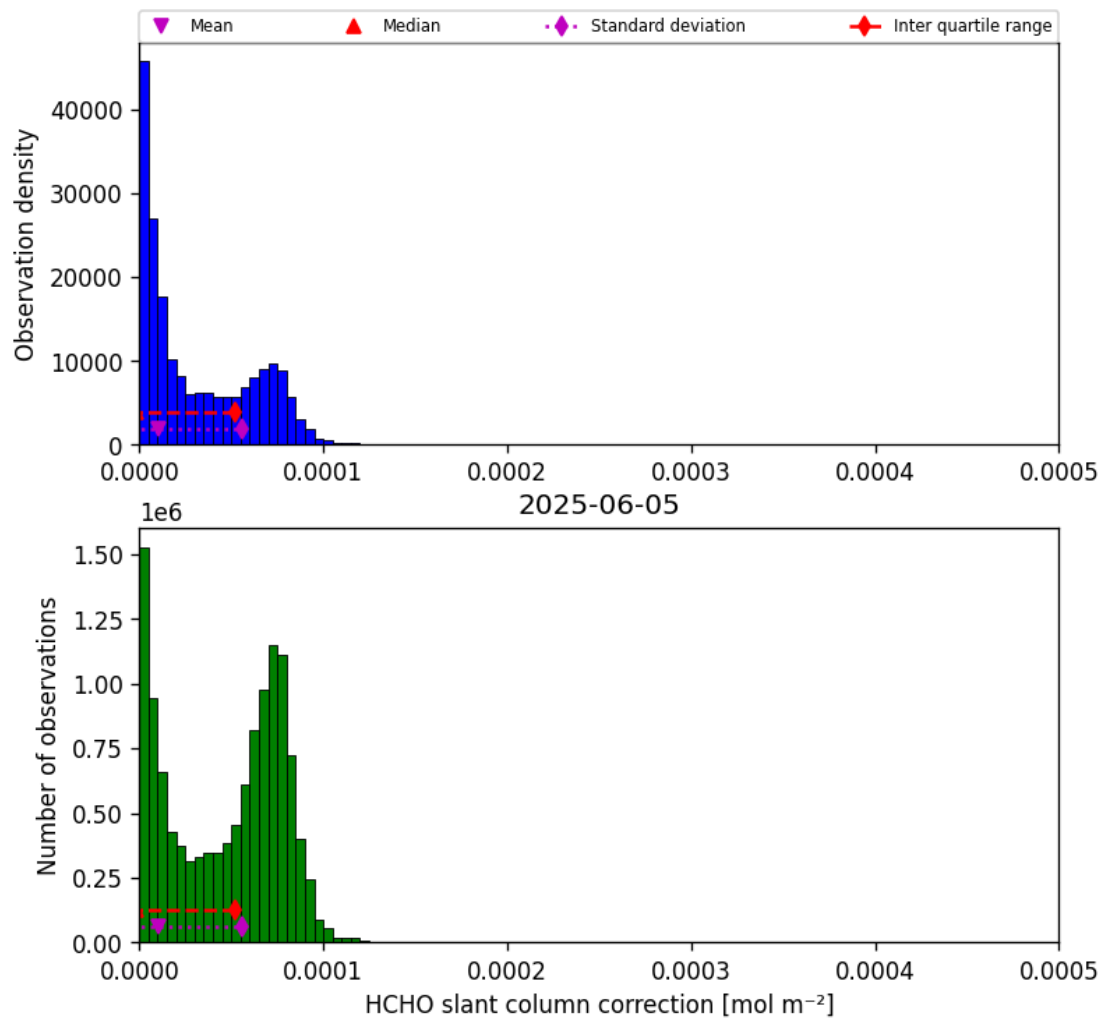
Figure 47: Histogram of “HCHO slant column correction” for 2025-06-04 to 2025-06-06
