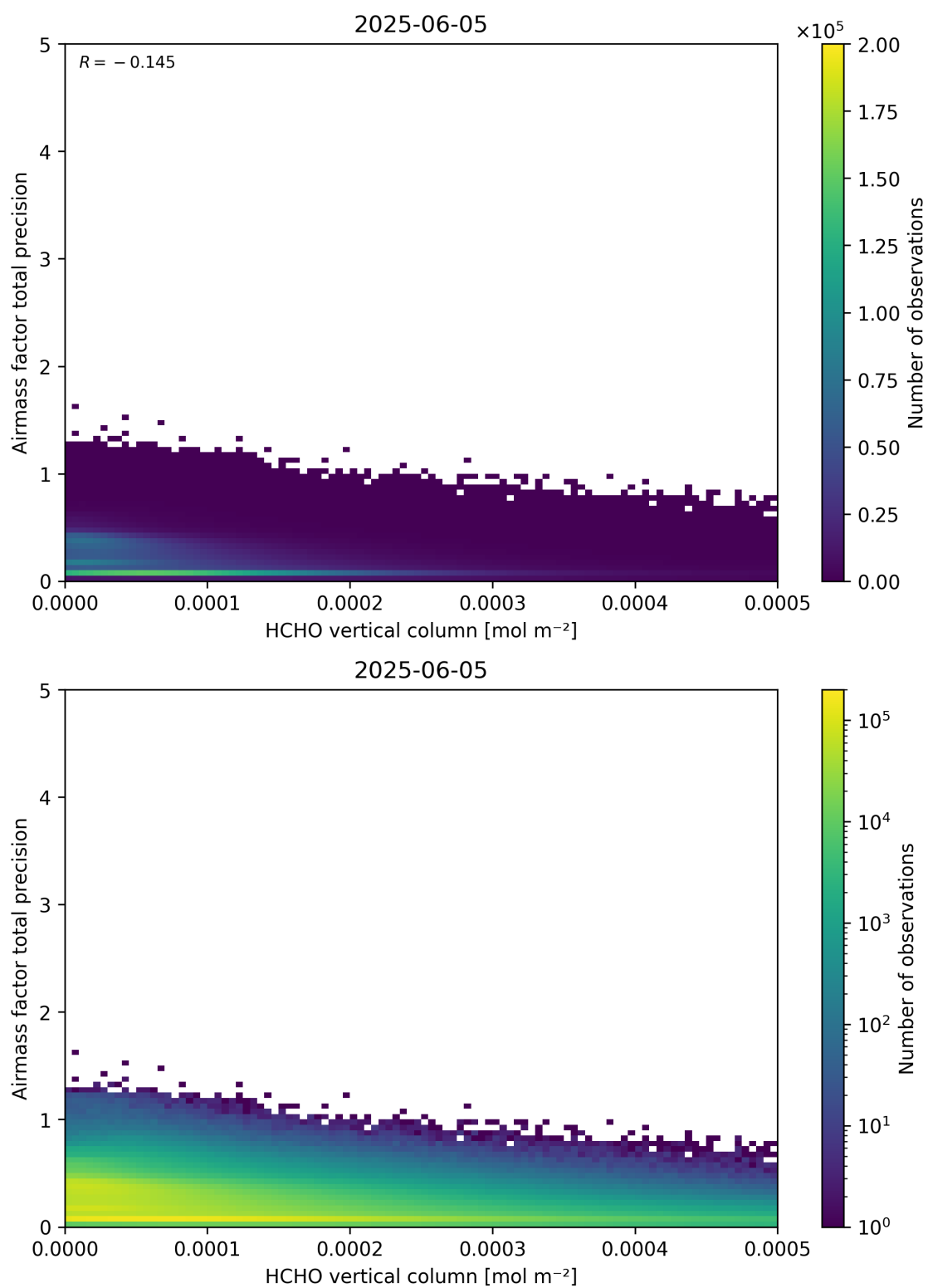
Figure 132: Scatter density plot of “HCHO vertical column” against “Airmass factor total precision” for 2025-06-04 to 2025-06-06.
