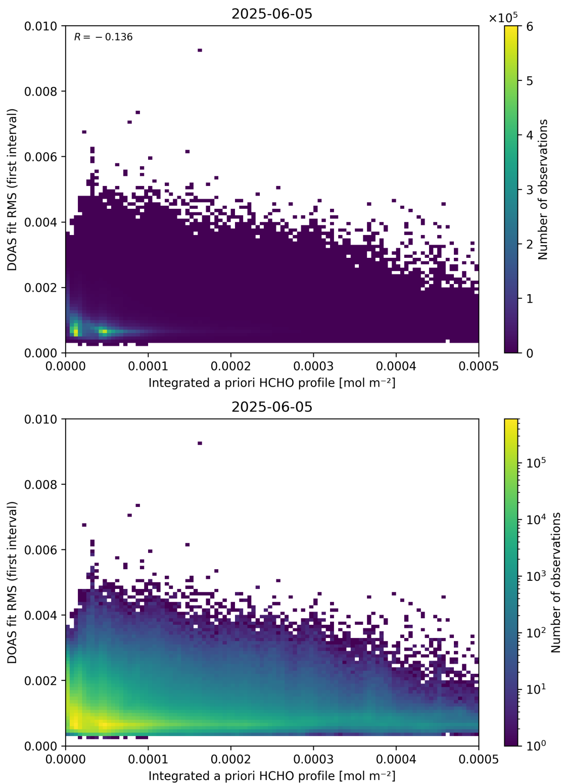
Figure 148: Scatter density plot of “Integrated a priori HCHO profile” against “DOAS fit RMS (first interval)” for 2025-06-04 to 2025-06-06.
