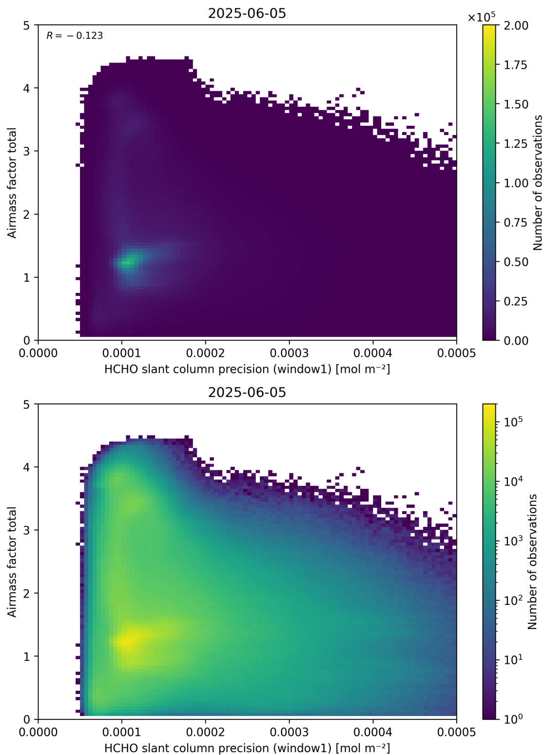
Figure 94: Scatter density plot of “HCHO slant column precision (window1)” against “Airmass factor total” for 2025-06-04 to 2025-06-06.
