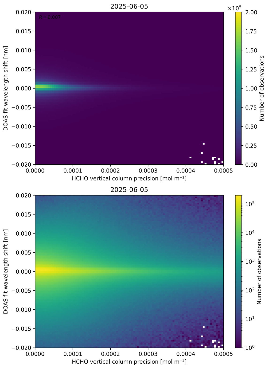
Figure 137: Scatter density plot of “HCHO vertical column precision” against “DOAS fit wavelength shift” for 2025-06-04 to 2025-06-06.
