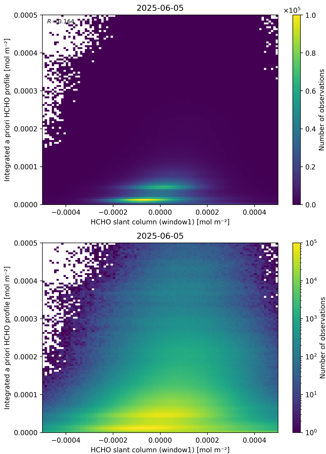
Figure 87: Scatter density plot of “HCHO slant column (window1)” against “Integrated a priori HCHO profile” for 2025-06-04 to 2025-06-06.
