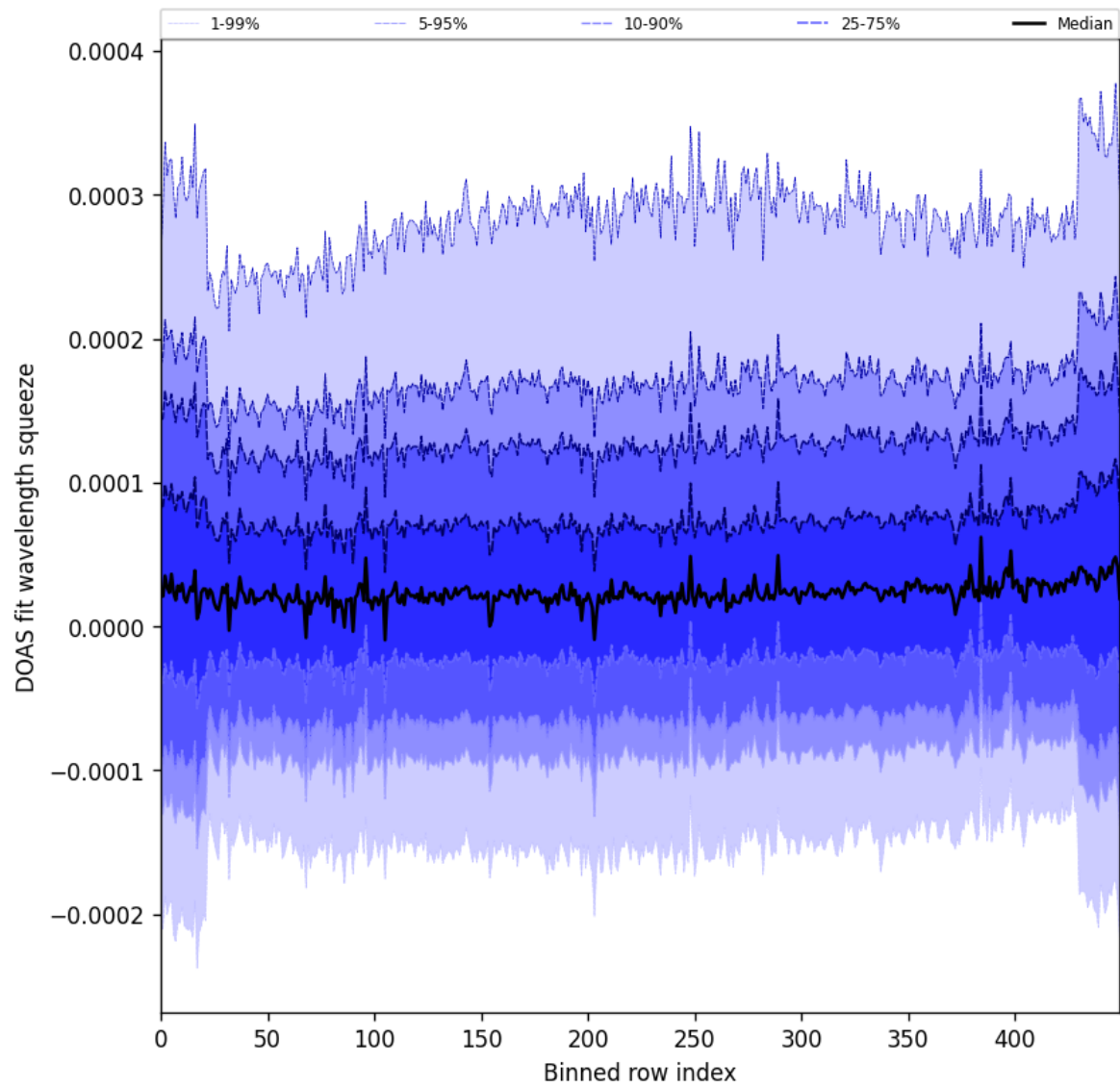
Figure 59: Along track statistics of “DOAS fit wavelength squeeze” for 2025-06-04 to 2025-06-06
