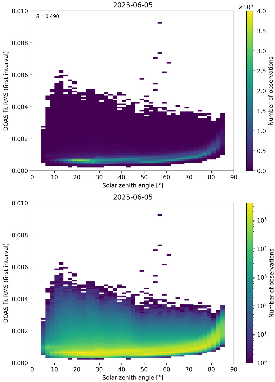
Figure 167: Scatter density plot of “Solar zenith angle” against “DOAS fit RMS (first interval)” for 2025-06-04 to 2025-06-06.
