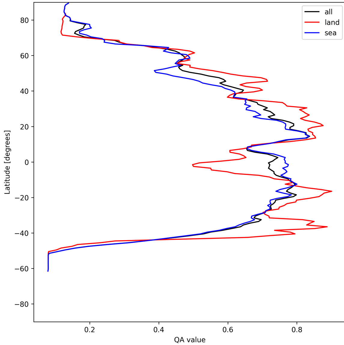
Figure 20: Zonal average of “QA value” for 2025-06-04 to 2025-06-06.
