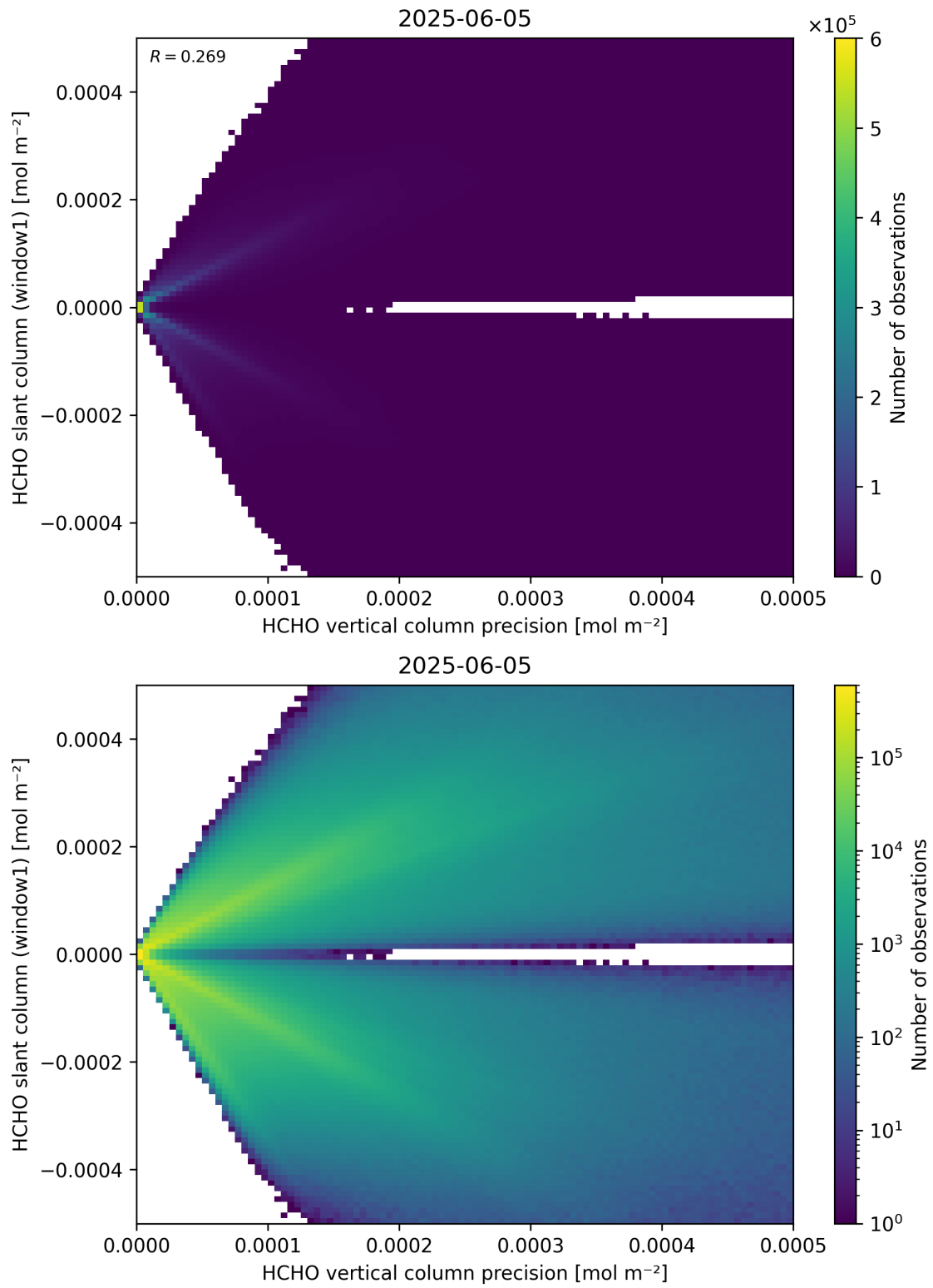
Figure 142: Scatter density plot of “HCHO vertical column precision” against “HCHO slant column (window1)” for 2025-06-04 to 2025-06-06.
