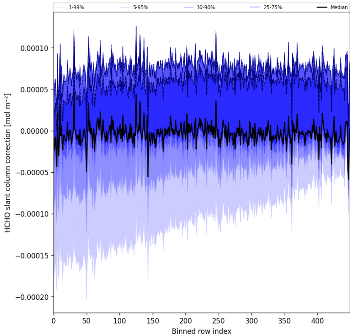
Figure 61: Along track statistics of “HCHO slant column correction” for 2025-06-04 to 2025-06-06
