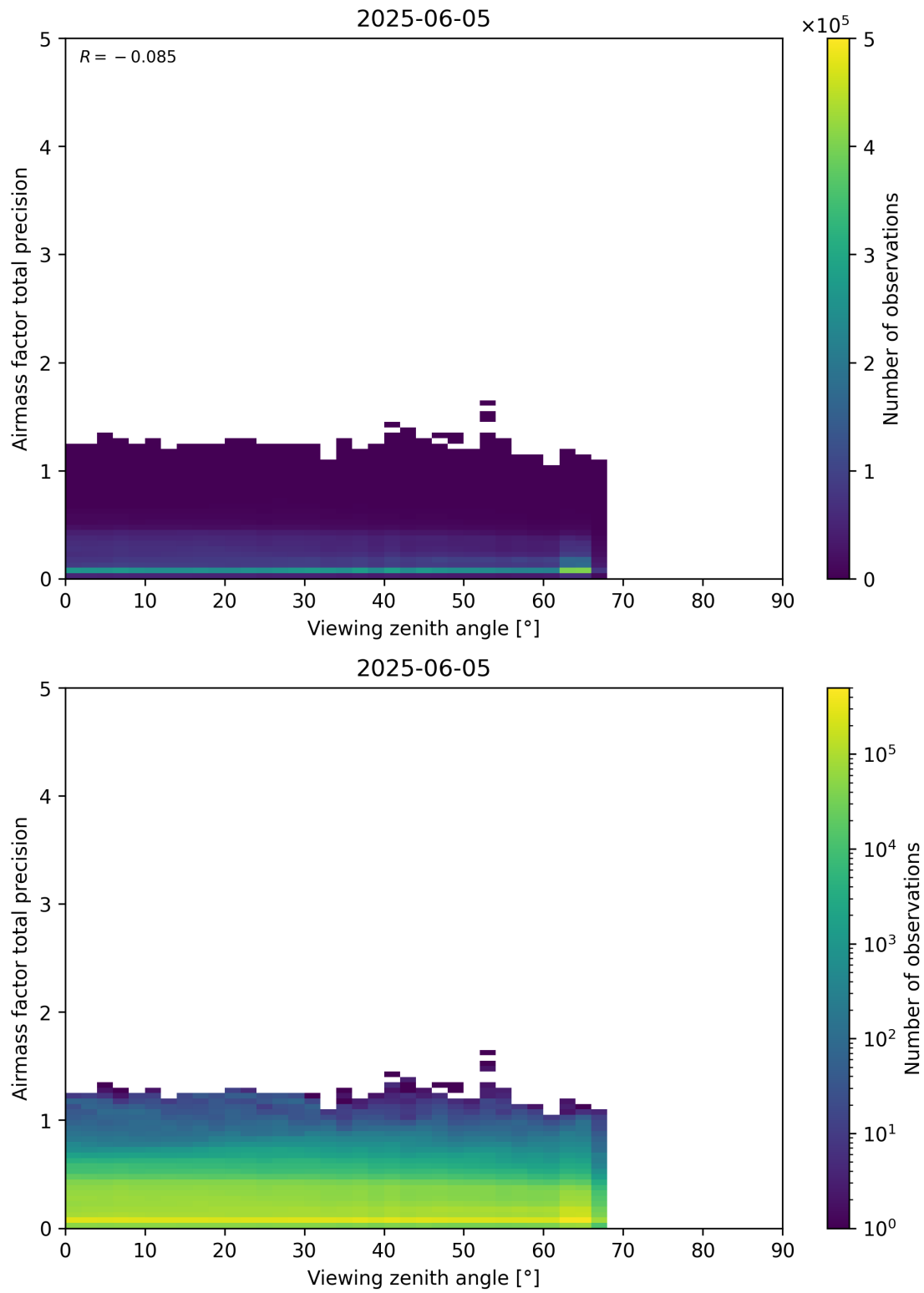
Figure 191: Scatter density plot of “Viewing zenith angle” against “Airmass factor total precision” for 2025-06-04 to 2025-06-06.
