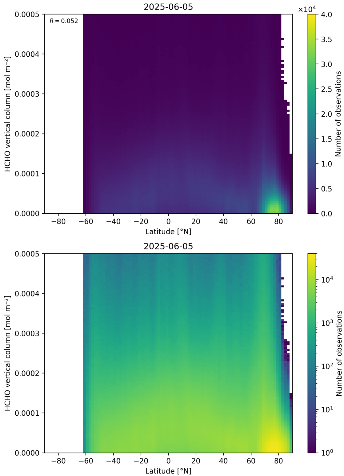
Figure 163: Scatter density plot of “Latitude” against “HCHO vertical column” for 2025-06-04 to 2025-06-06.
