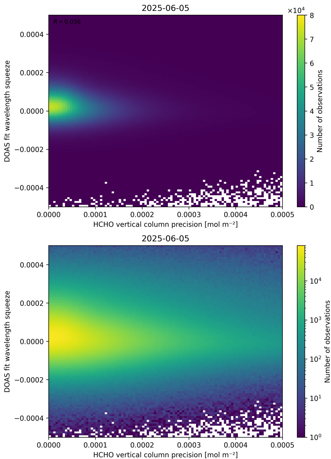
Figure 138: Scatter density plot of “HCHO vertical column precision” against “DOAS fit wavelength squeeze” for 2025-06-04 to 2025-06-06.
