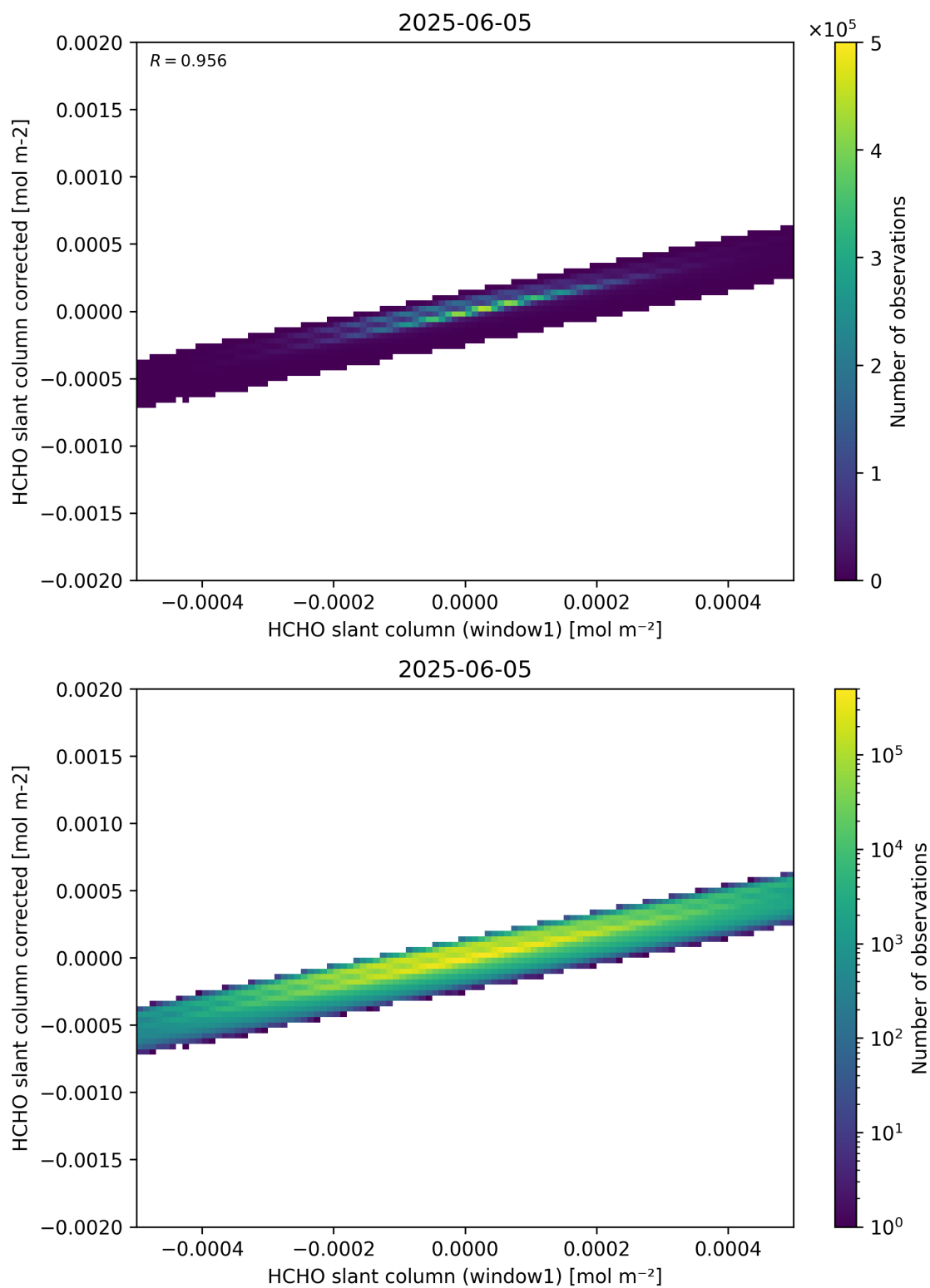
Figure 82: Scatter density plot of “HCHO slant column (window1)” against “HCHO slant column corrected” for 2025-06-04 to 2025-06-06.
