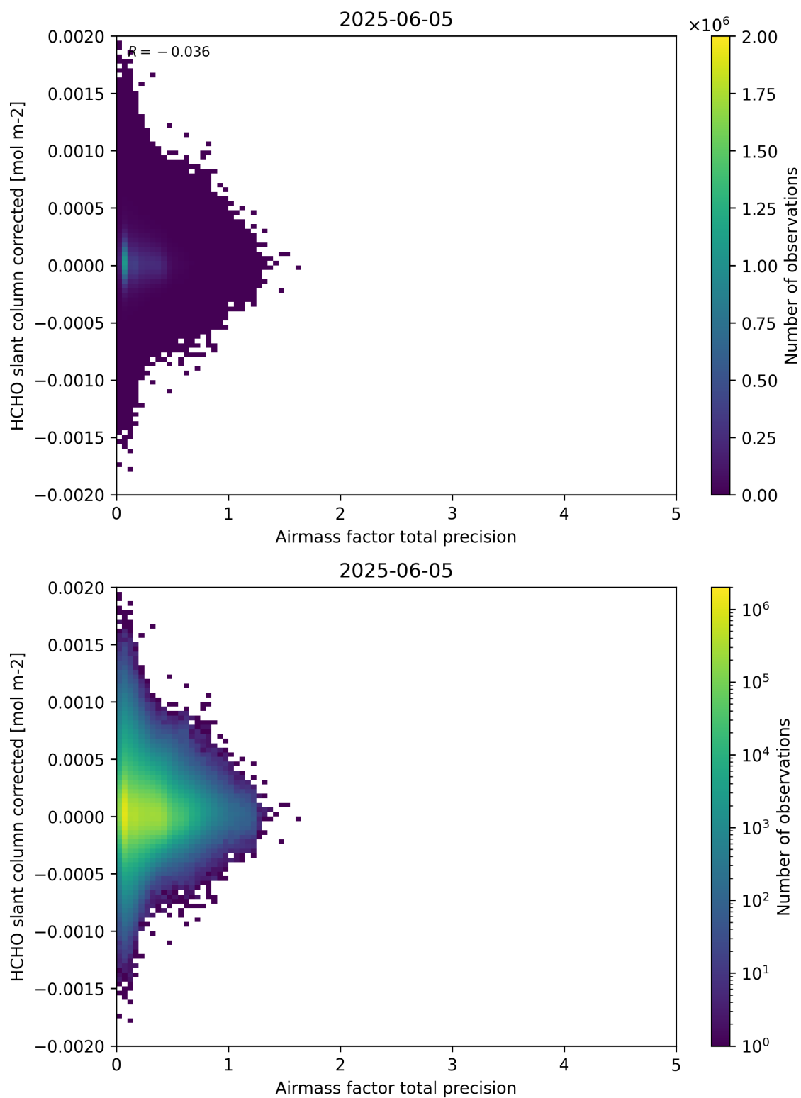
Figure 109: Scatter density plot of “Airmass factor total precision” against “HCHO slant column corrected” for 2025-06-04 to 2025-06-06.
