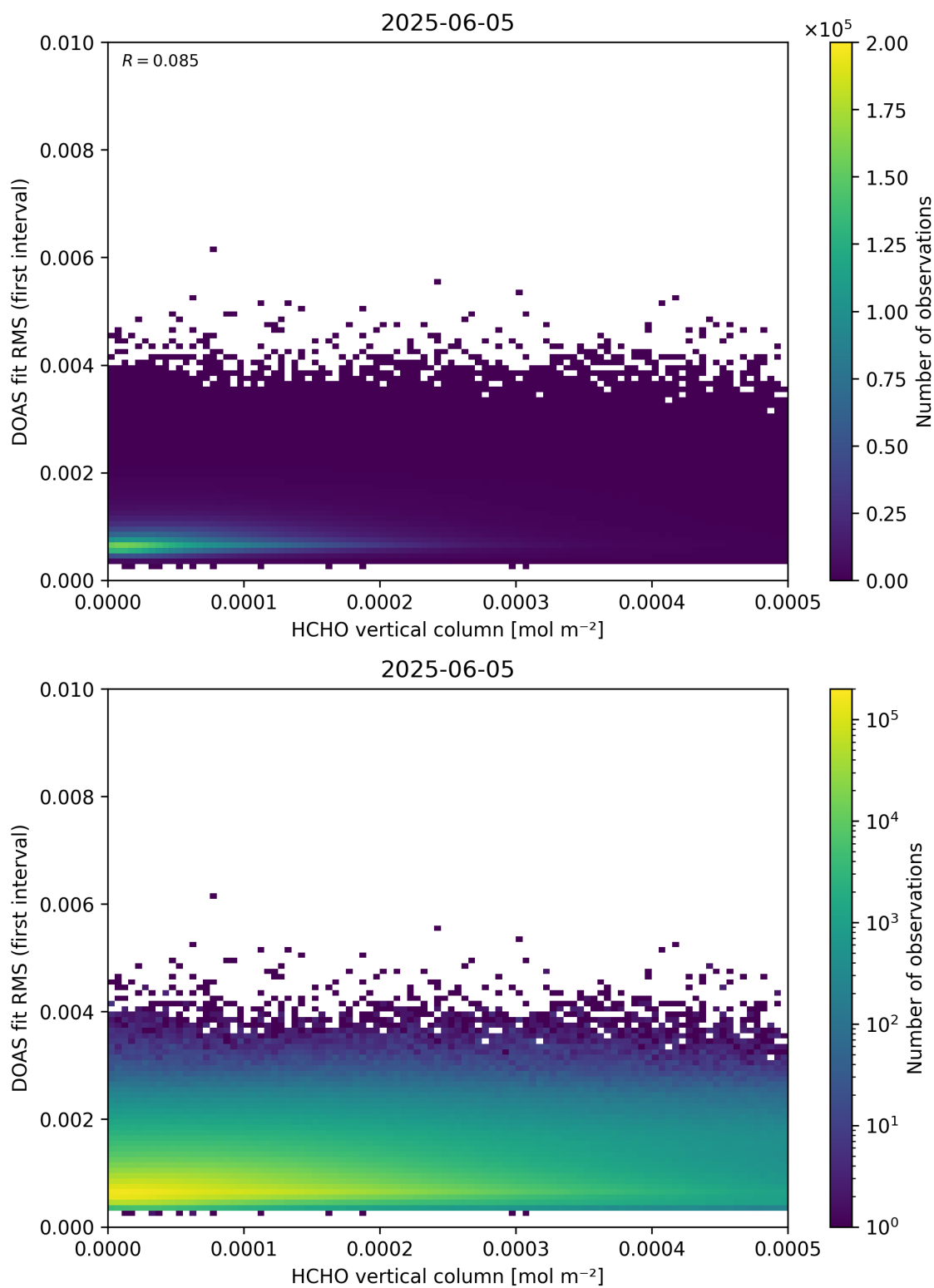
Figure 123: Scatter density plot of “HCHO vertical column” against “DOAS fit RMS (first interval)” for 2025-06-04 to 2025-06-06.
