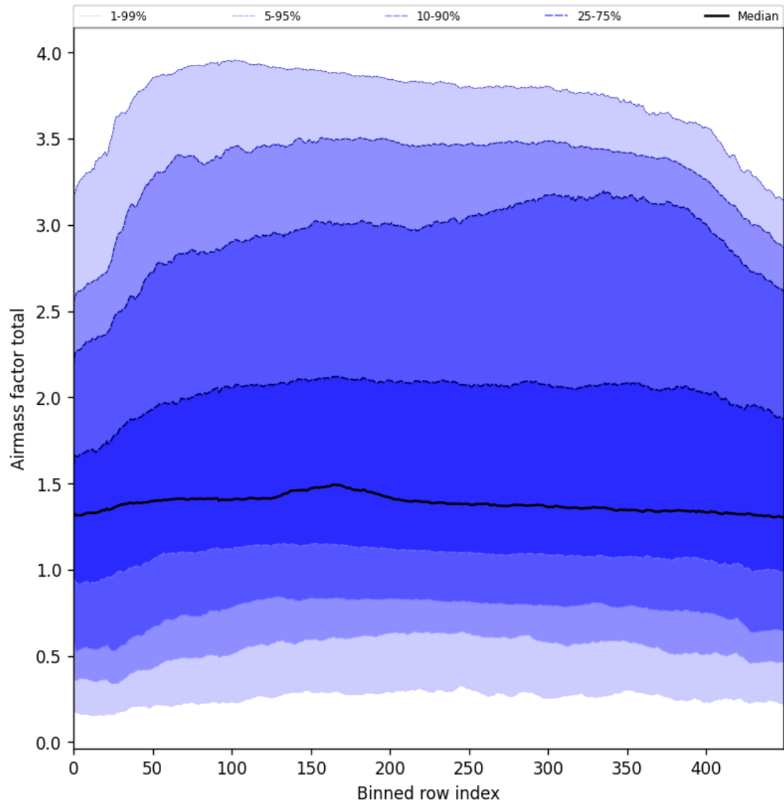
Figure 54: Along track statistics of “Airmass factor total” for 2025-06-04 to 2025-06-06
