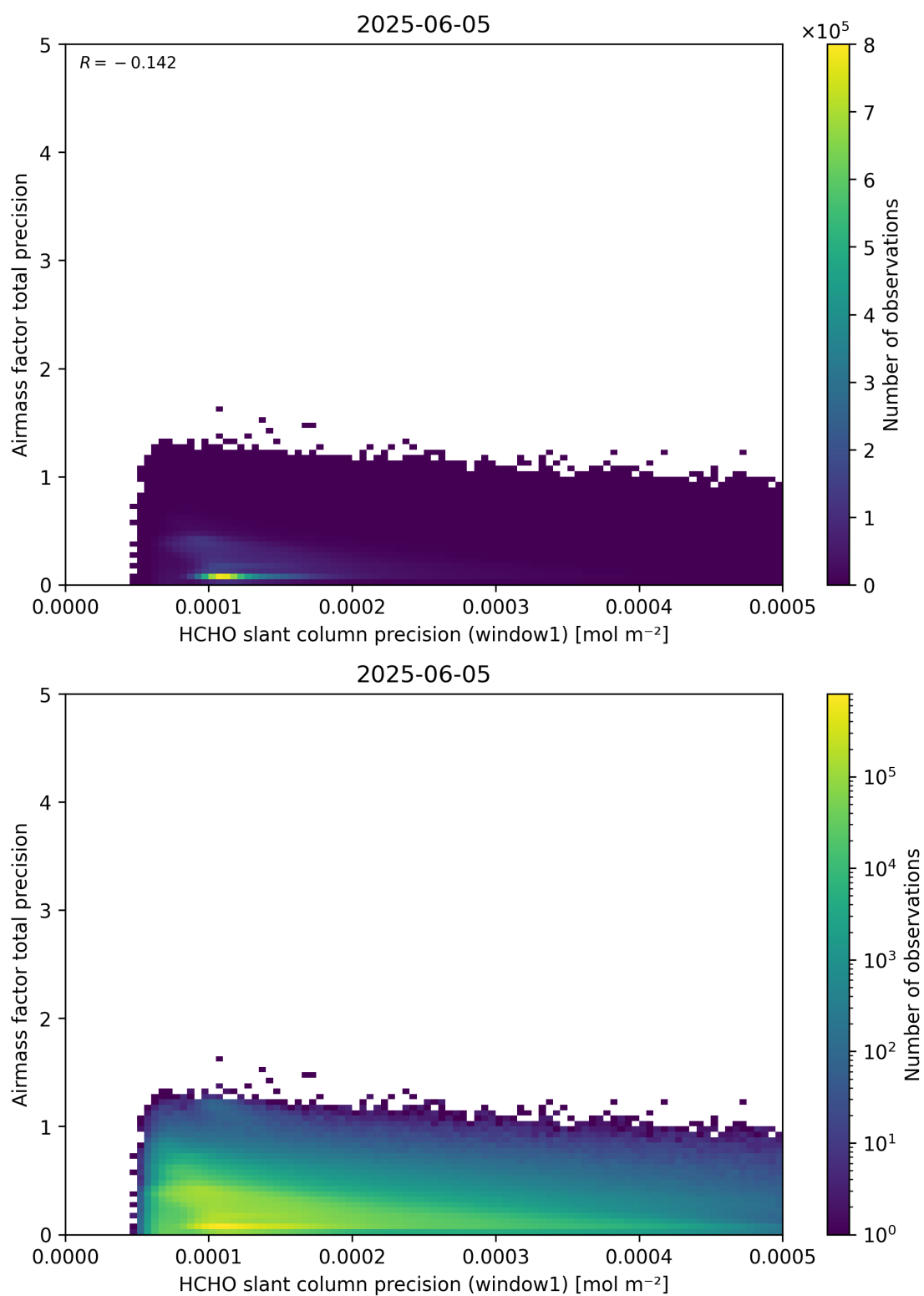
Figure 95: Scatter density plot of “HCHO slant column precision (window1)” against “Airmass factor total precision” for 2025-06-04 to 2025-06-06.
