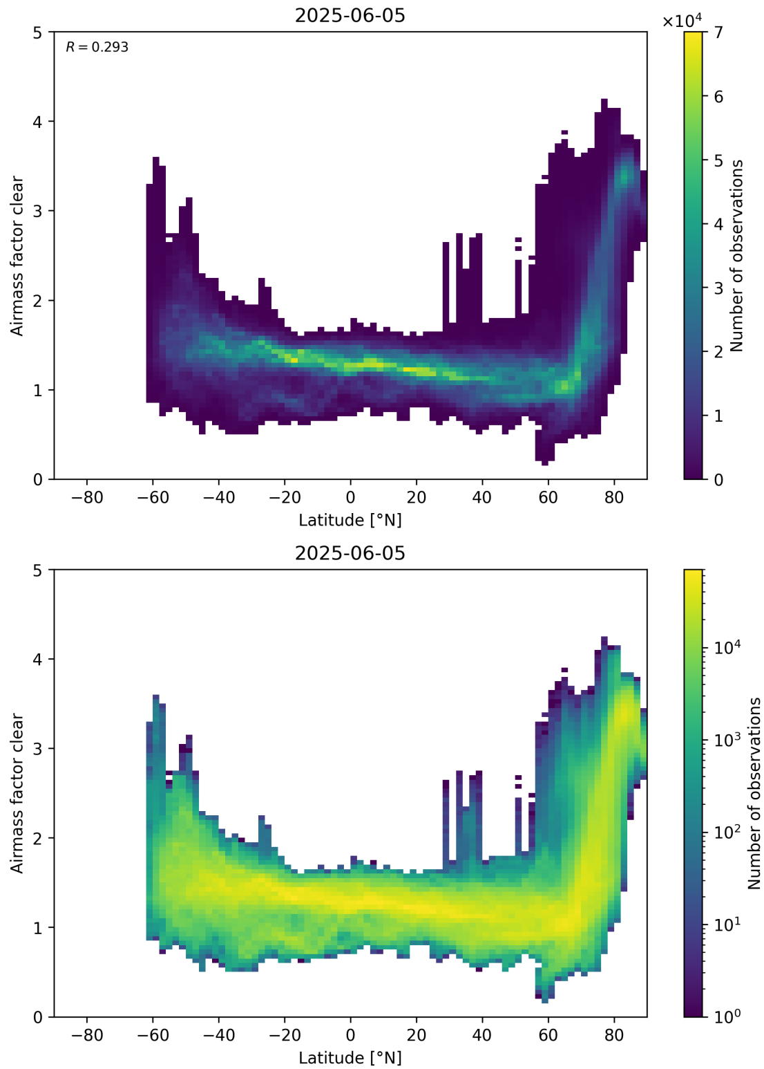
Figure 156: Scatter density plot of “Latitude” against “Airmass factor clear” for 2025-06-04 to 2025-06-06.
