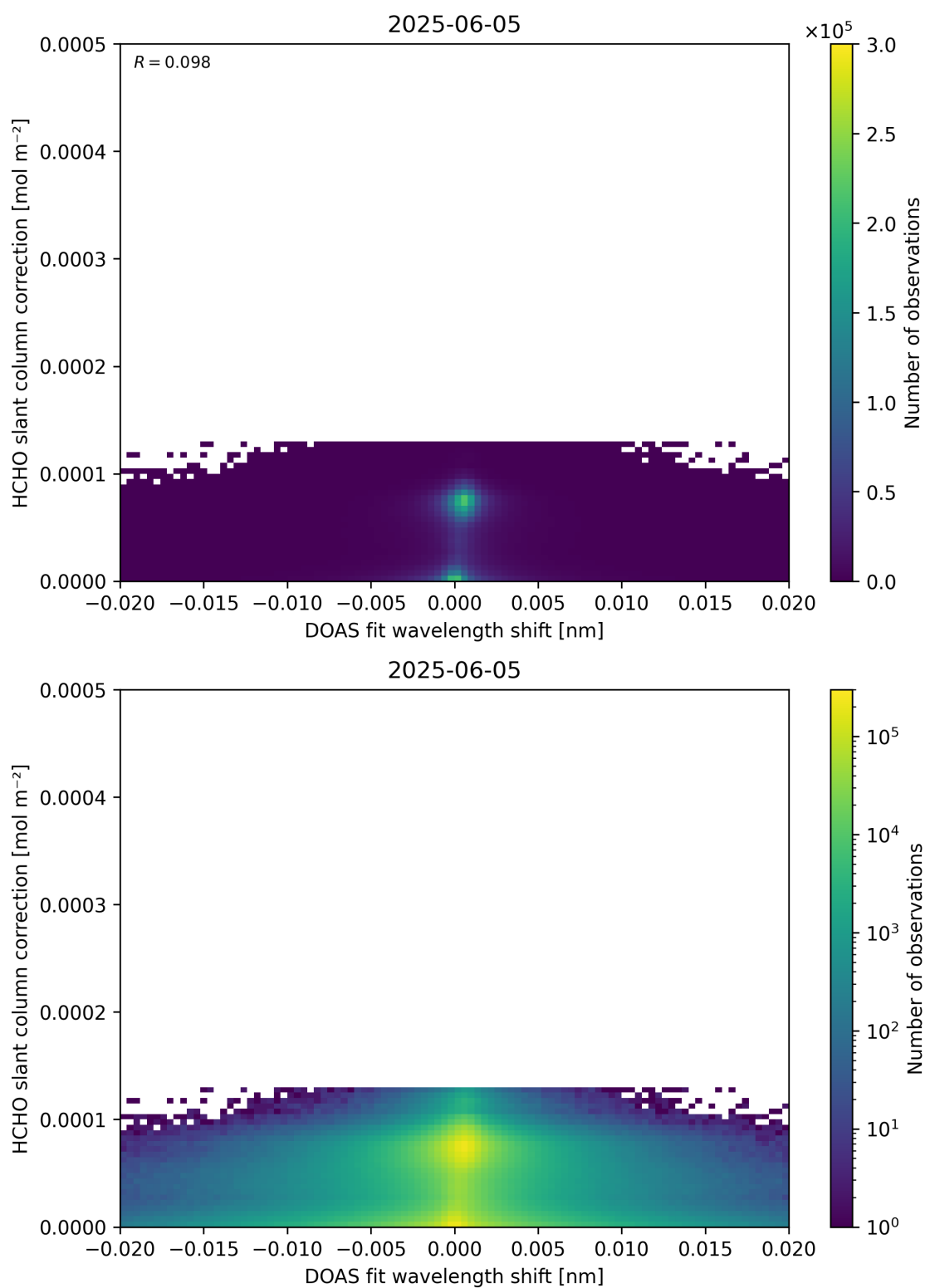
Figure 67: Scatter density plot of “DOAS fit wavelength shift” against “HCHO slant column correction” for 2025-06-04 to 2025-06-06.
