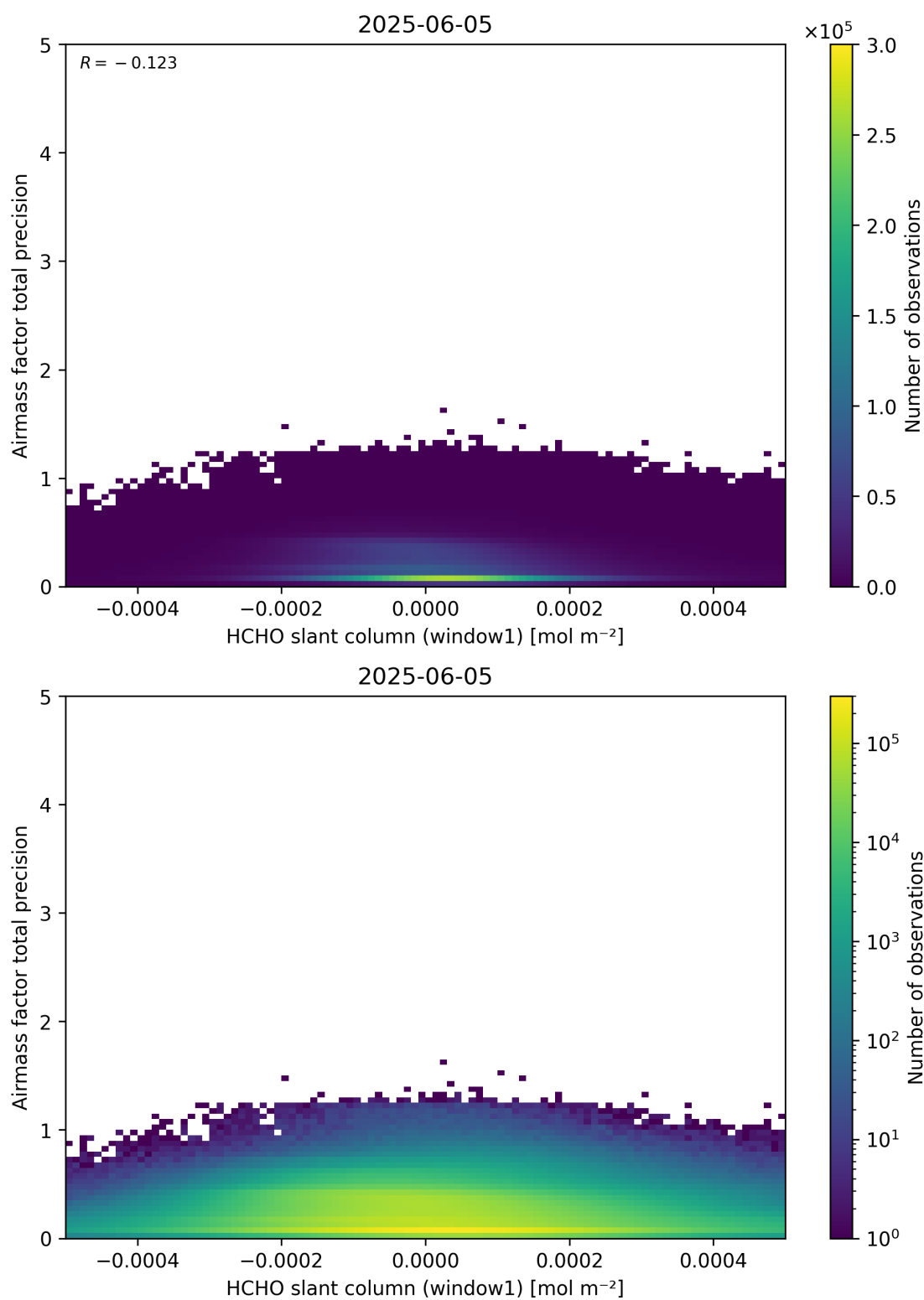
Figure 86: Scatter density plot of “HCHO slant column (window1)” against “Airmass factor total precision” for 2025-06-04 to 2025-06-06.
