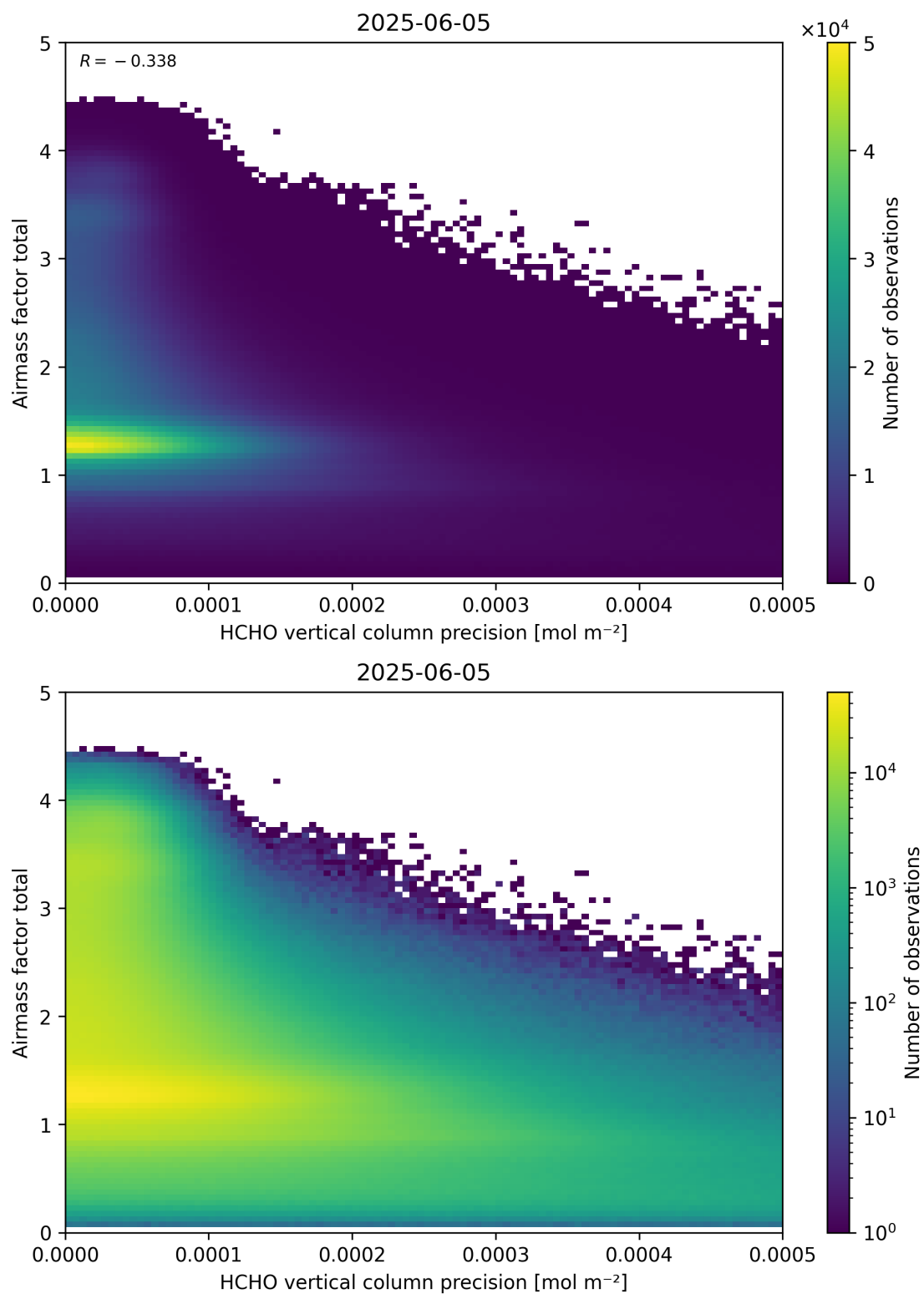
Figure 144: Scatter density plot of “HCHO vertical column precision” against “Airmass factor total” for 2025-06-04 to 2025-06-06.
