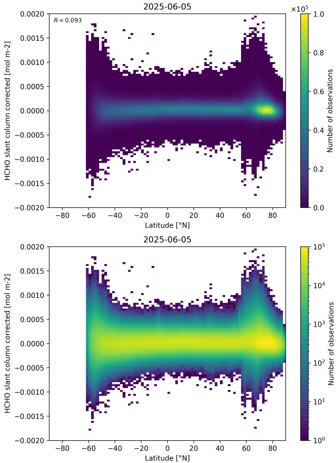
Figure 157: Scatter density plot of “Latitude” against “HCHO slant column corrected” for 2025-06-04 to 2025-06-06.
