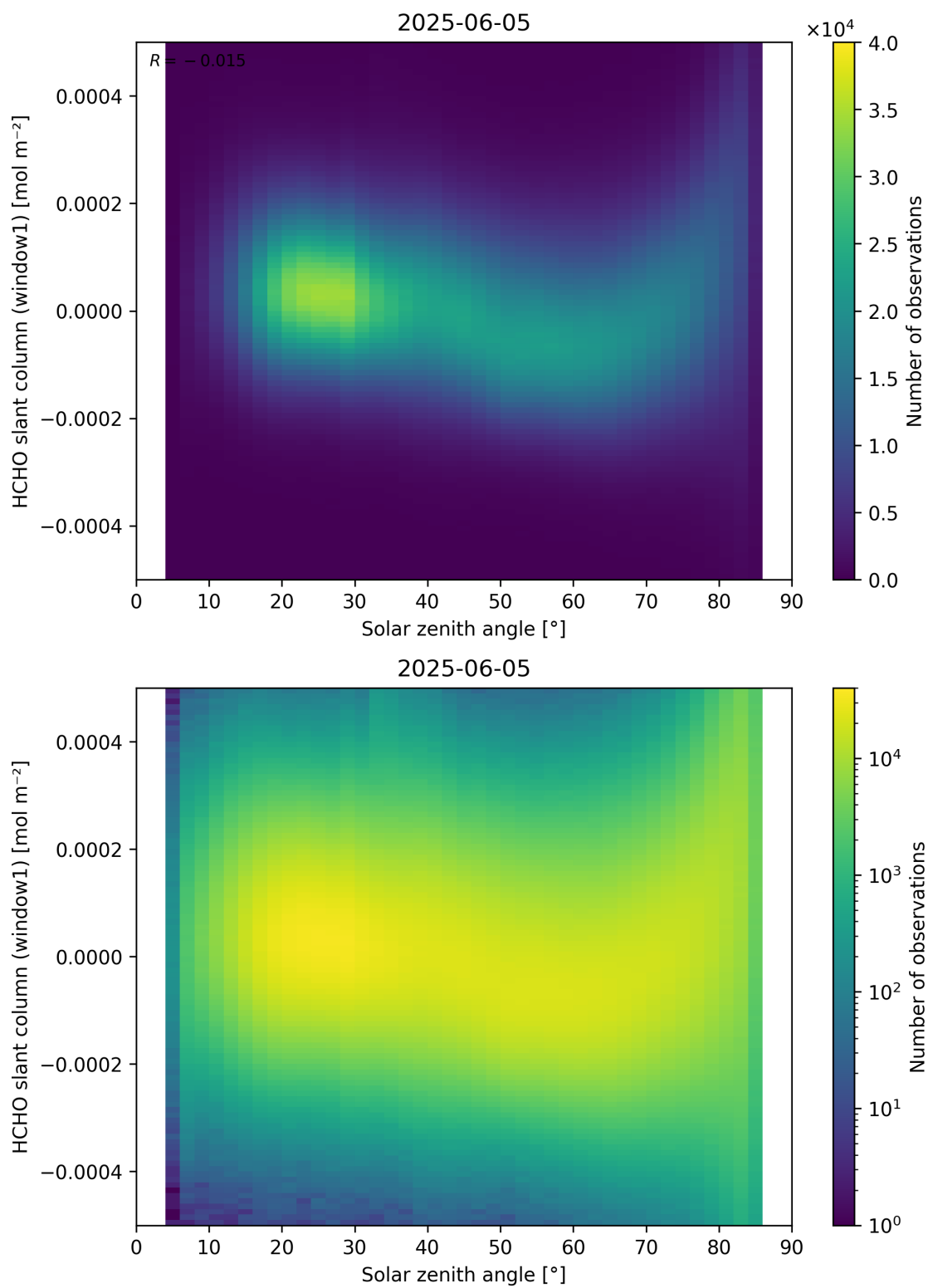
Figure 173: Scatter density plot of “Solar zenith angle” against “HCHO slant column (window1)” for 2025-06-04 to 2025-06-06.
