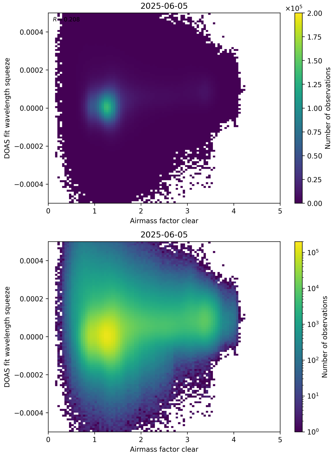
Figure 73: Scatter density plot of “Airmass factor clear” against “DOAS fit wavelength squeeze” for 2025-06-04 to 2025-06-06.
