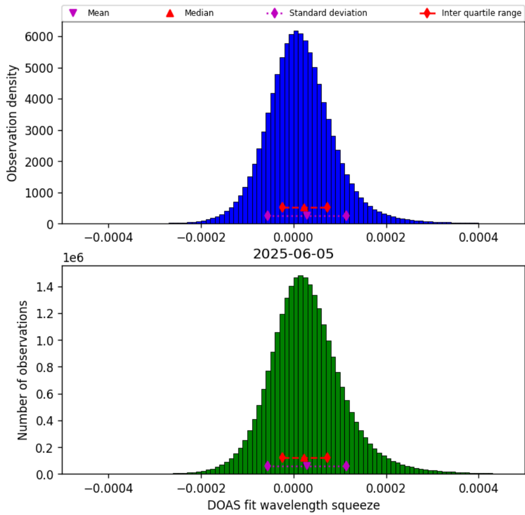
Figure 45: Histogram of “DOAS fit wavelength squeeze” for 2025-06-04 to 2025-06-06
