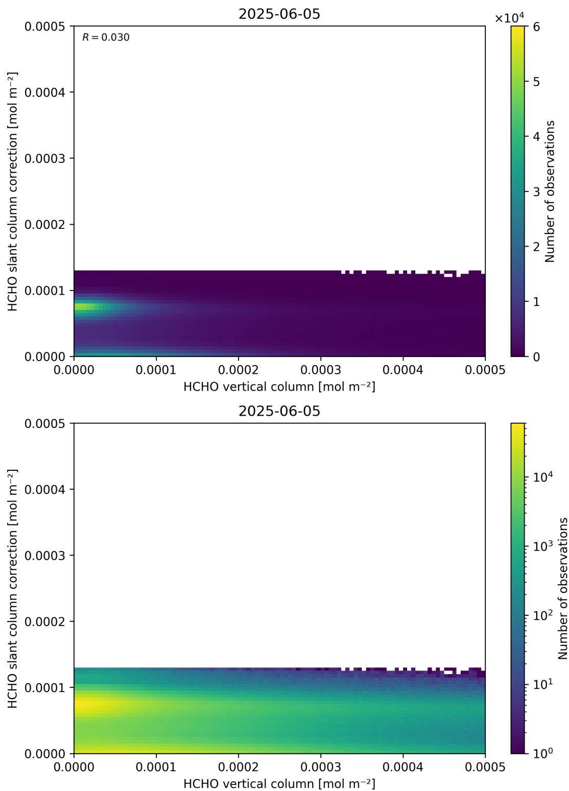
Figure 128: Scatter density plot of “HCHO vertical column” against “HCHO slant column correction” for 2025-06-04 to 2025-06-06.
