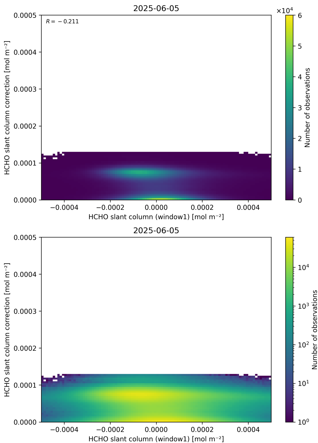
Figure 83: Scatter density plot of “HCHO slant column (window1)” against “HCHO slant column correction” for 2025-06-04 to 2025-06-06.
