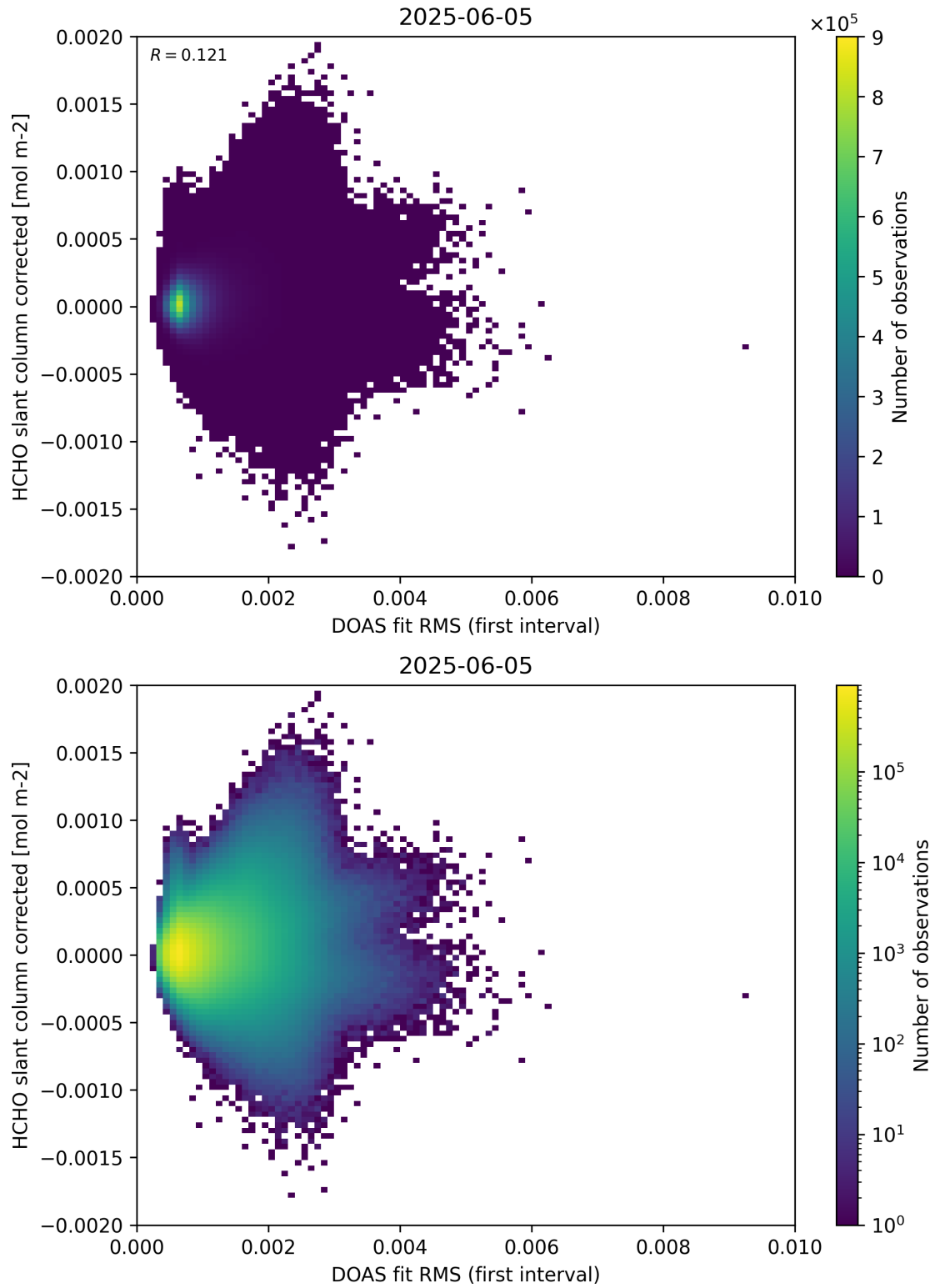
Figure 62: Scatter density plot of “DOAS fit RMS (first interval)” against “HCHO slant column corrected” for 2025-06-04 to 2025-06-06.
