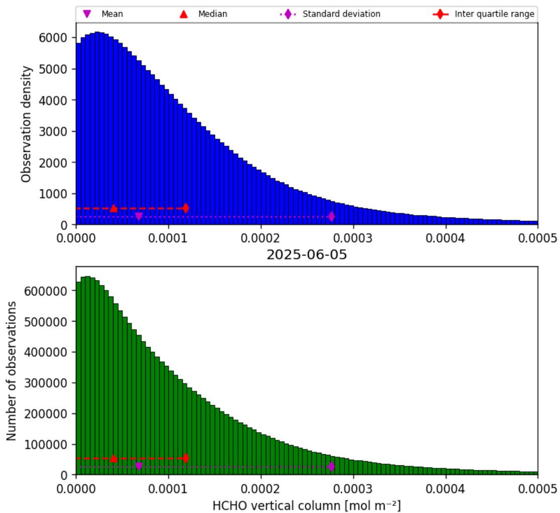
Figure 35: Histogram of “HCHO vertical column” for 2025-06-04 to 2025-06-06
