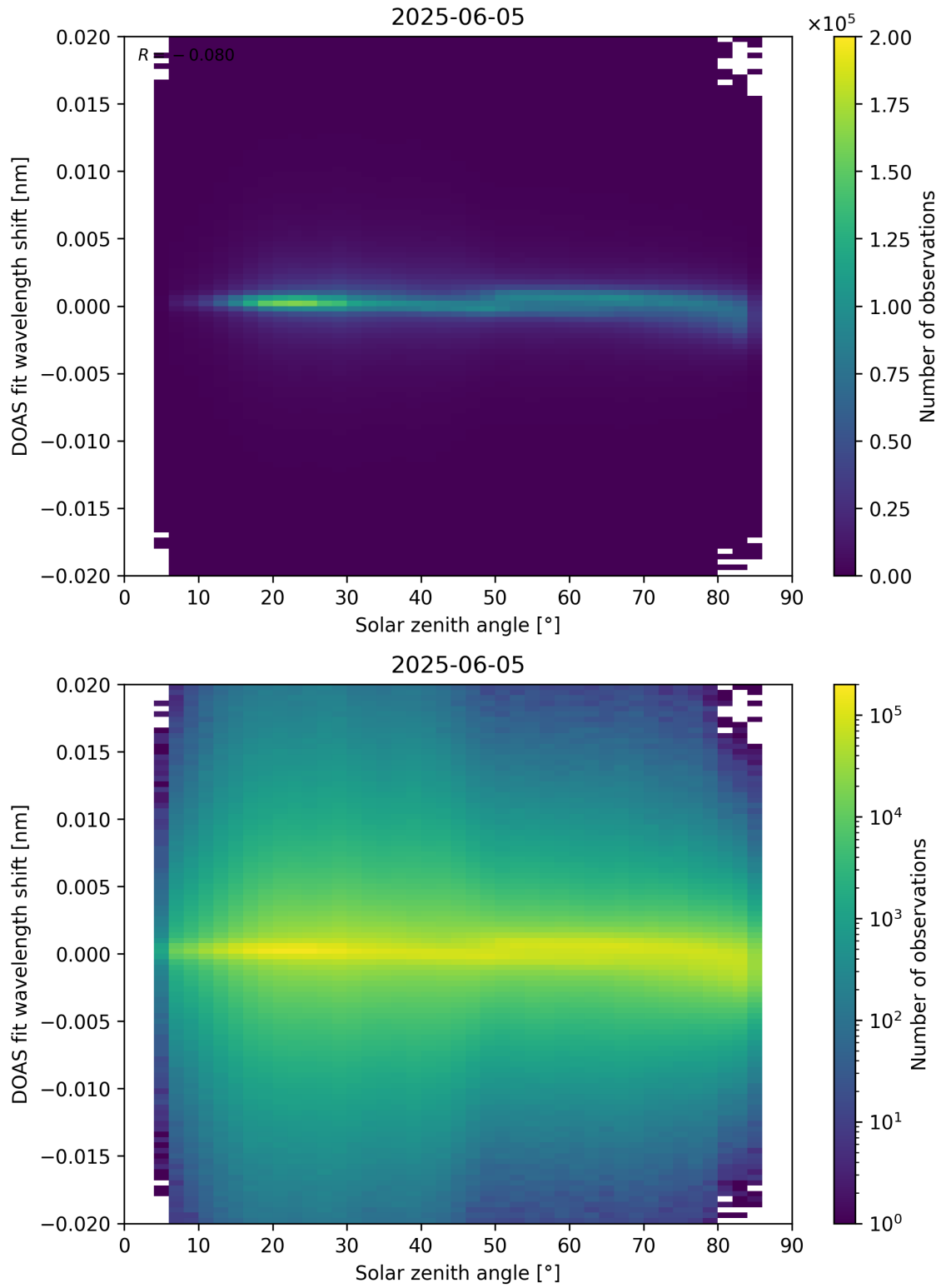
Figure 168: Scatter density plot of “Solar zenith angle” against “DOAS fit wavelength shift” for 2025-06-04 to 2025-06-06.
