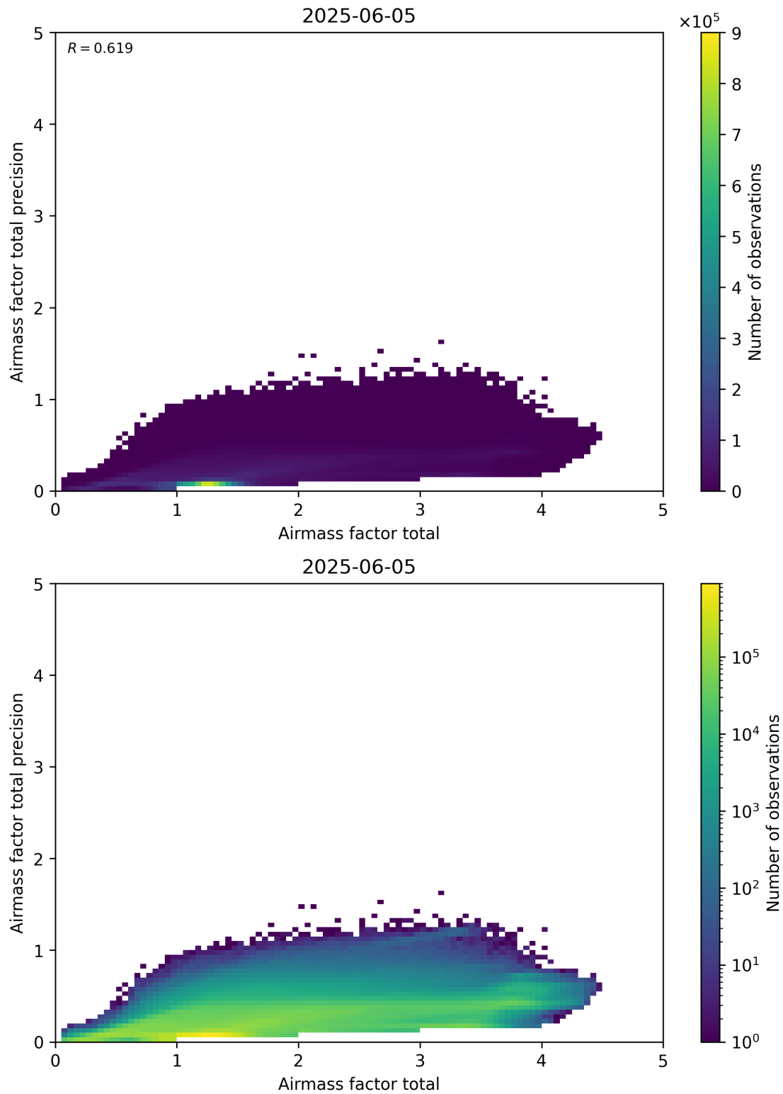
Figure 103: Scatter density plot of “Airmass factor total” against “Airmass factor total precision” for 2025-06-04 to 2025-06-06.
