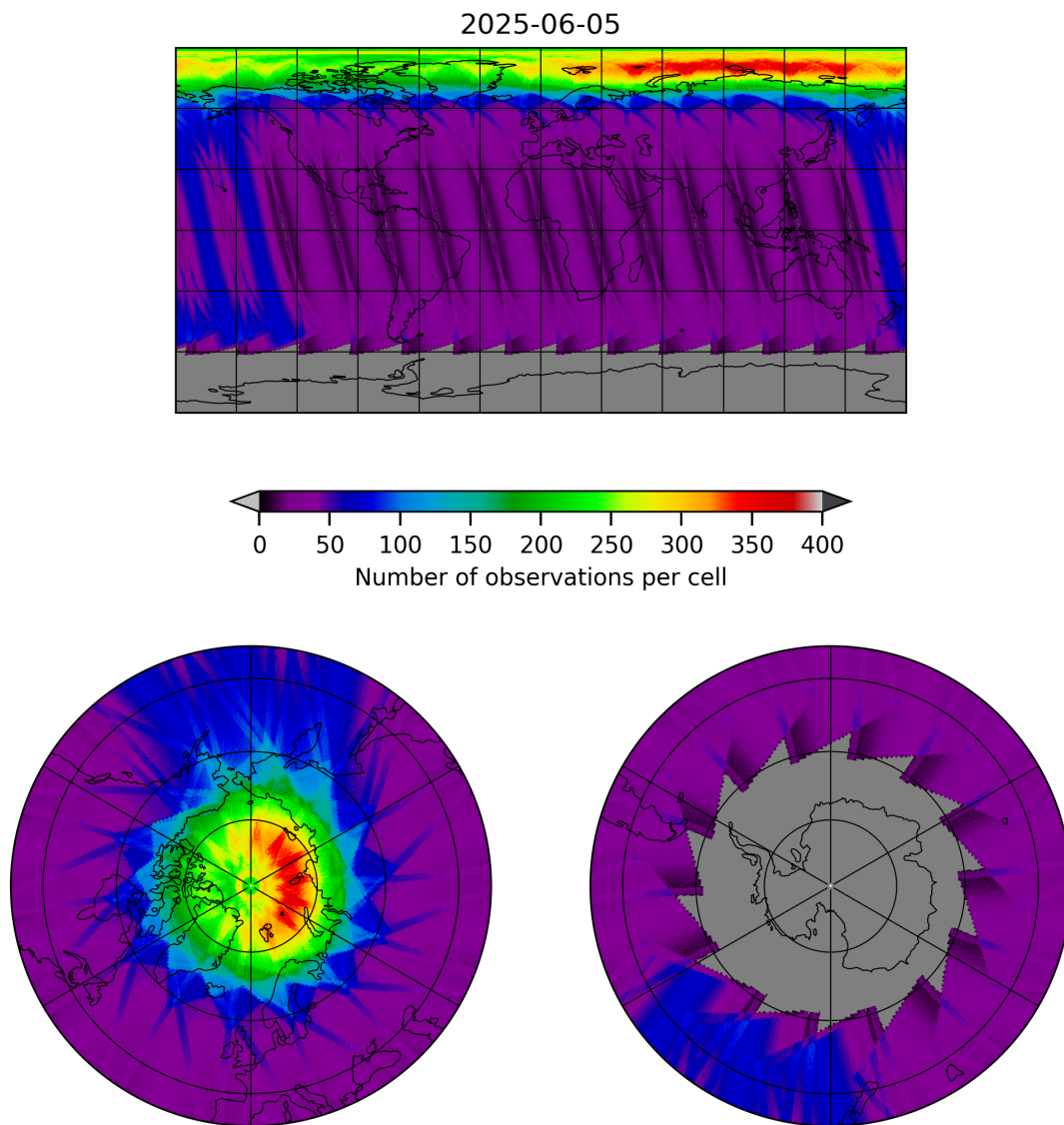
Figure 19: Map of the number of observations for 2025-06-04 to 2025-06-06
