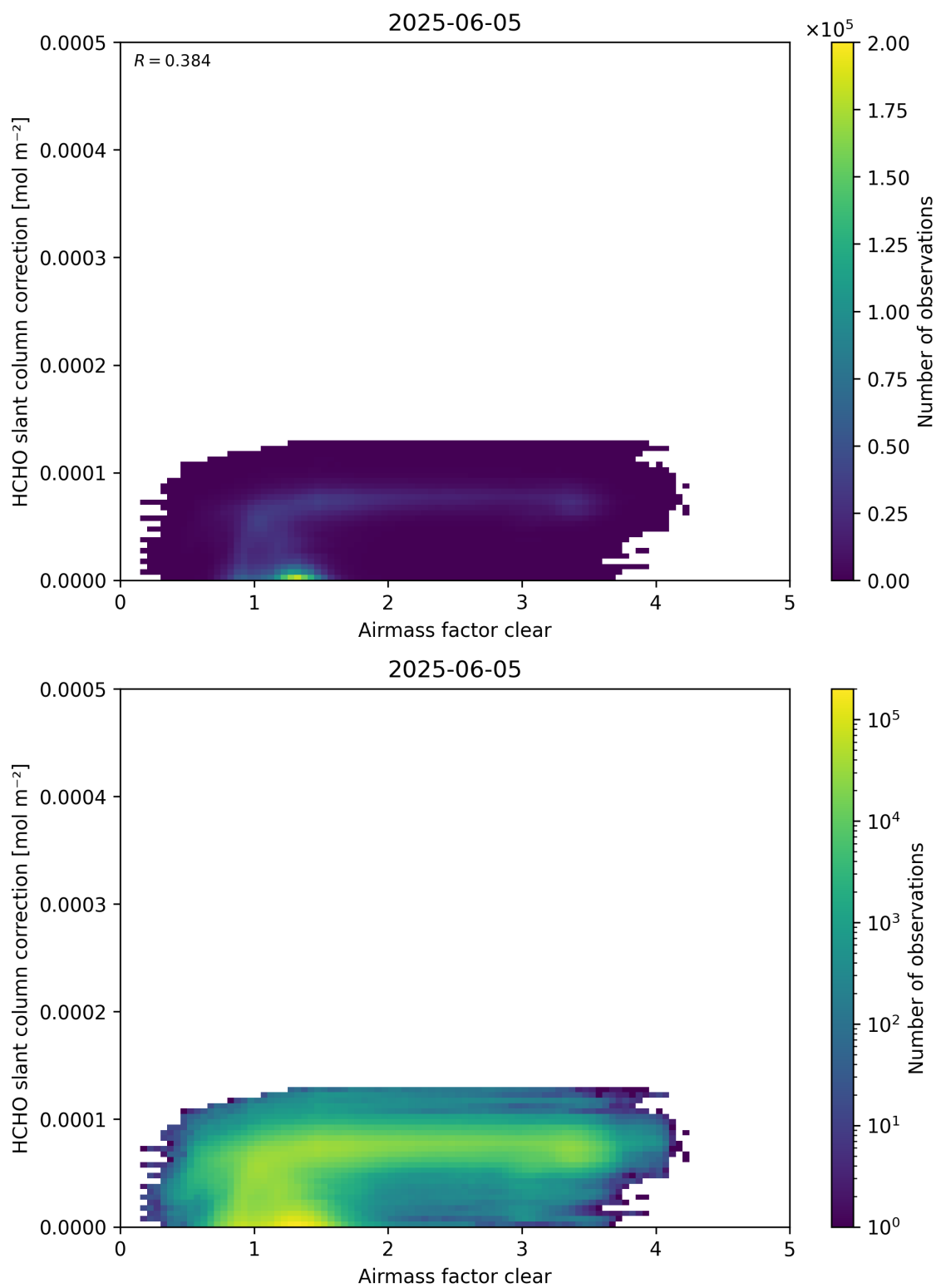
Figure 75: Scatter density plot of “Airmass factor clear” against “HCHO slant column correction” for 2025-06-04 to 2025-06-06.
