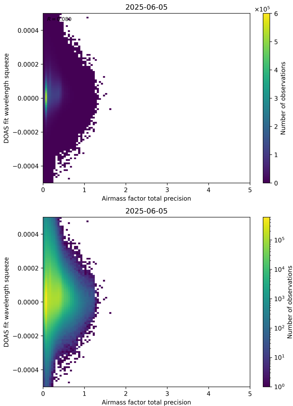
Figure 107: Scatter density plot of “Airmass factor total precision” against “DOAS fit wavelength squeeze” for 2025-06-04 to 2025-06-06.
