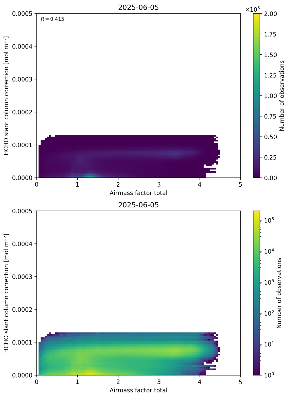
Figure 102: Scatter density plot of “Airmass factor total” against “HCHO slant column correction” for 2025-06-04 to 2025-06-06.
