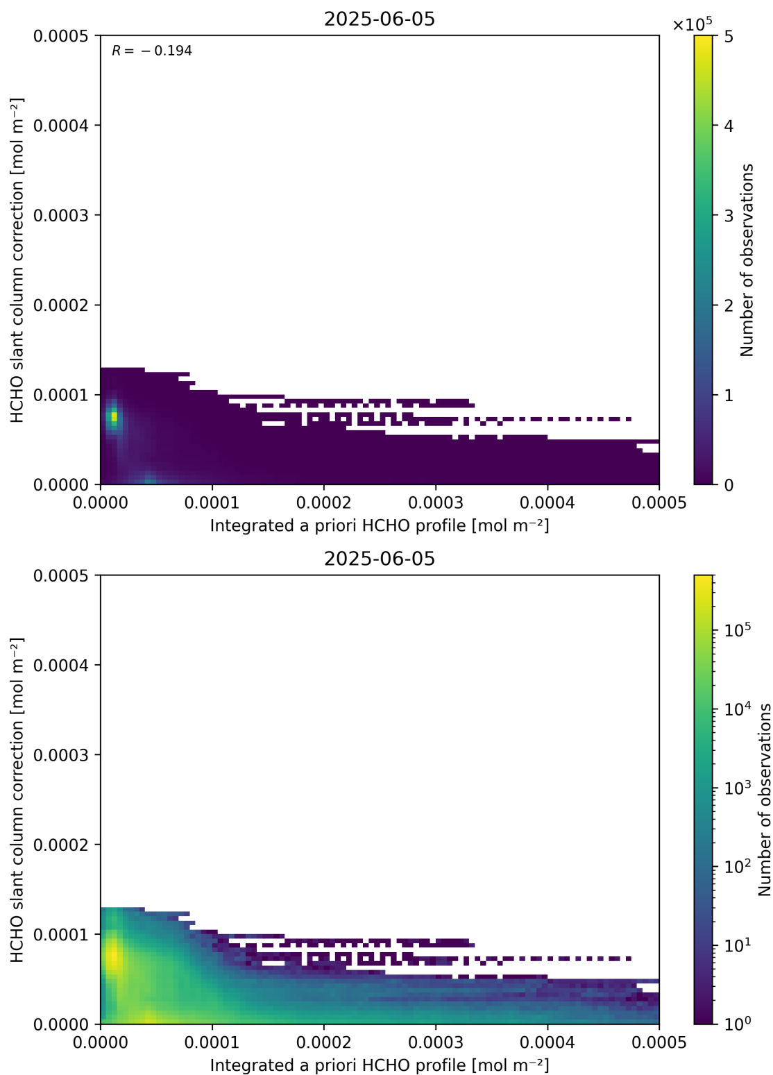
Figure 152: Scatter density plot of “Integrated a priori HCHO profile” against “HCHO slant column correction” for 2025-06-04 to 2025-06-06.
