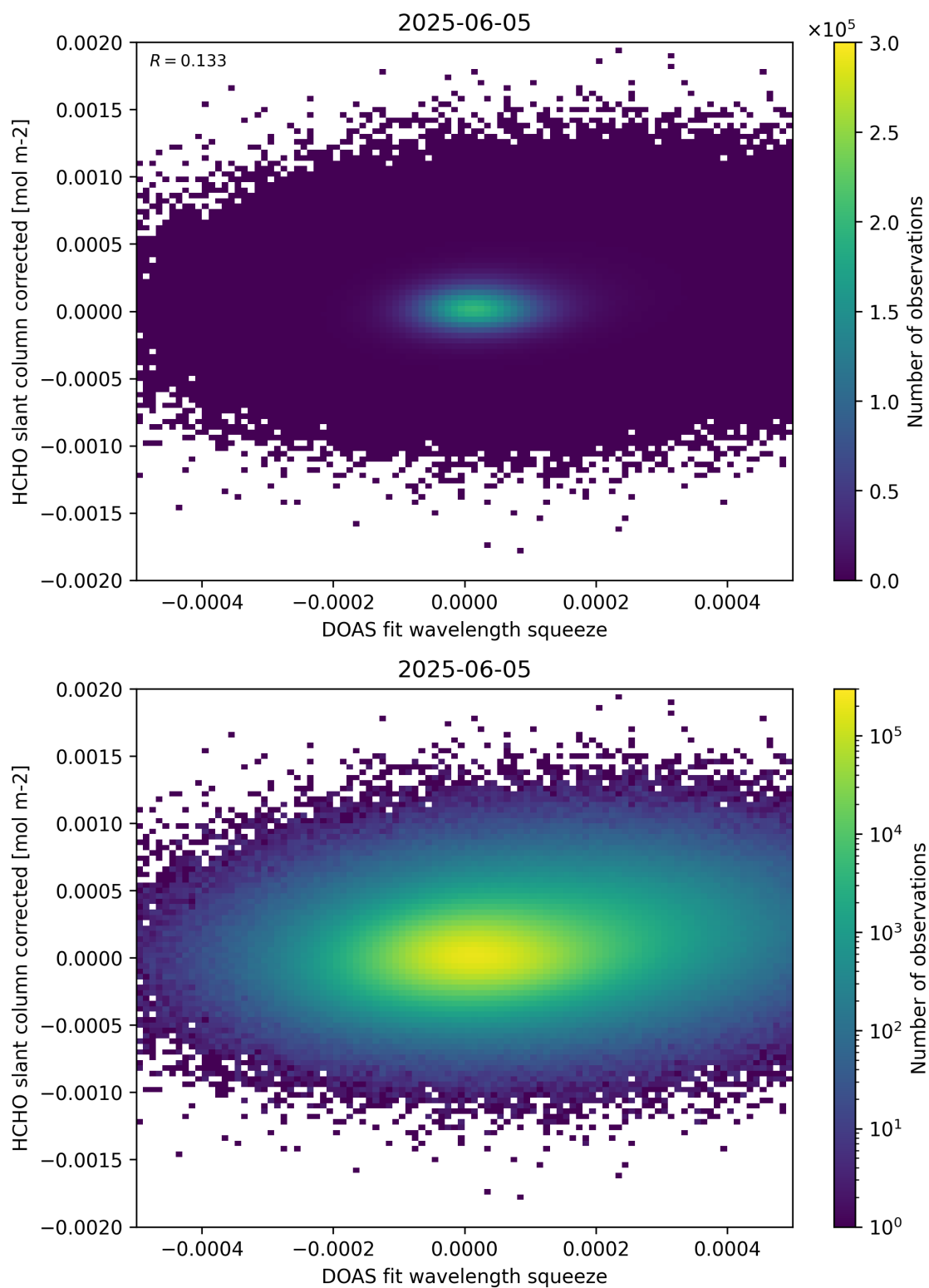
Figure 69: Scatter density plot of “DOAS fit wavelength squeeze” against “HCHO slant column corrected” for 2025-06-04 to 2025-06-06.
