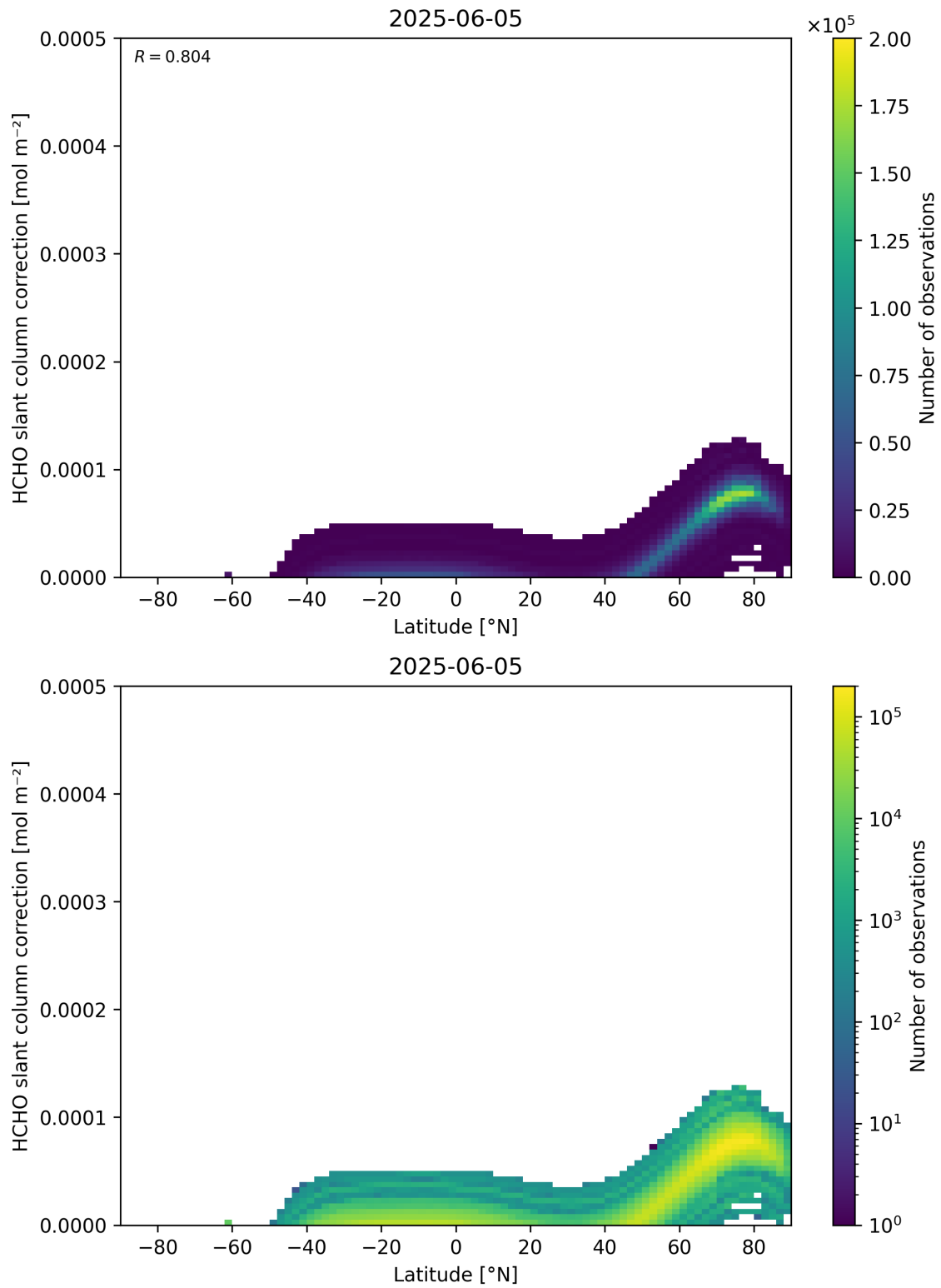
Figure 158: Scatter density plot of “Latitude” against “HCHO slant column correction” for 2025-06-04 to 2025-06-06.
