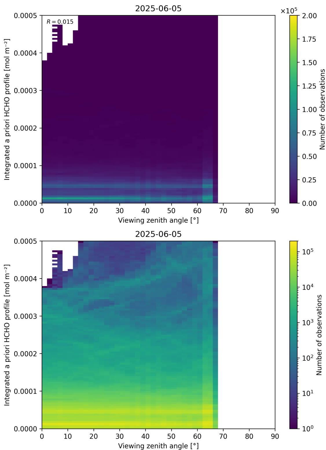
Figure 195: Scatter density plot of “Viewing zenith angle” against “Integrated a priori HCHO profile” for 2025-06-04 to 2025-06-06.
