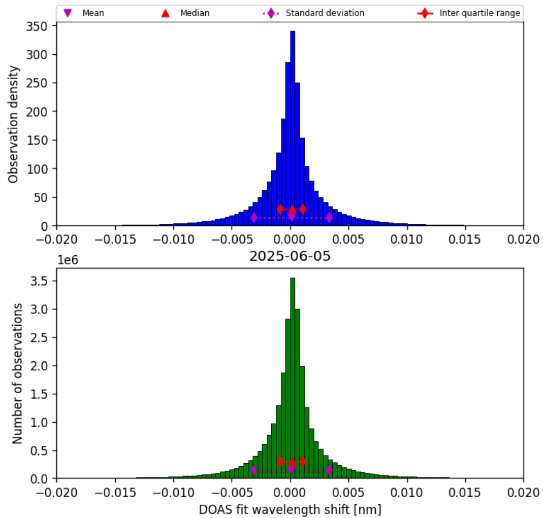
Figure 44: Histogram of “DOAS fit wavelength shift” for 2025-06-04 to 2025-06-06
