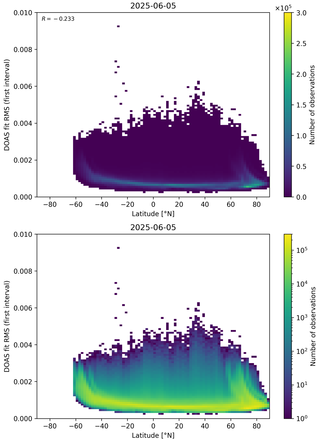
Figure 153: Scatter density plot of “Latitude” against “DOAS fit RMS (first interval)” for 2025-06-04 to 2025-06-06.
