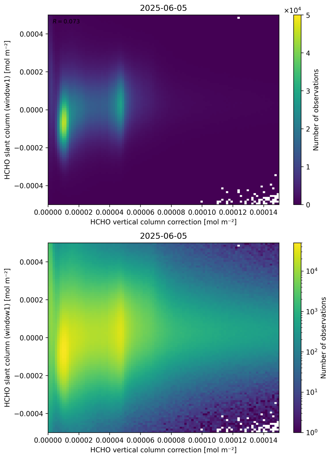
Figure 118: Scatter density plot of “HCHO vertical column correction” against “HCHO slant column (window1)” for 2025-06-04 to 2025-06-06.
