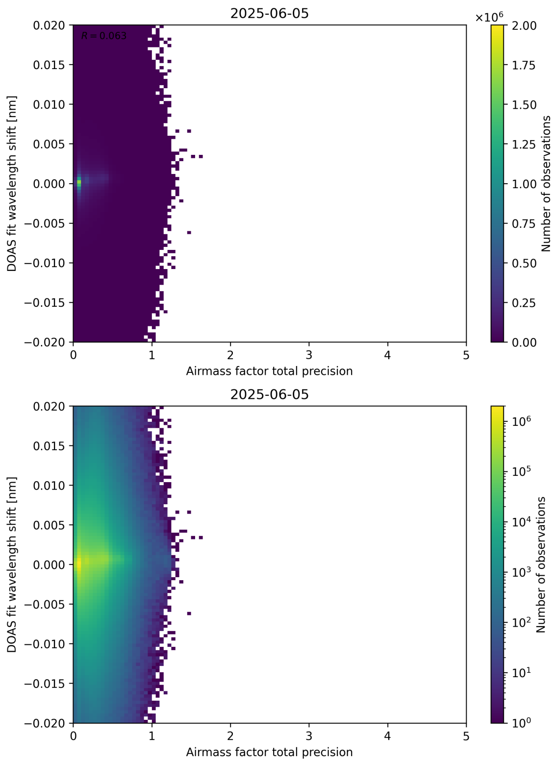
Figure 106: Scatter density plot of “Airmass factor total precision” against “DOAS fit wavelength shift” for 2025-06-04 to 2025-06-06.
