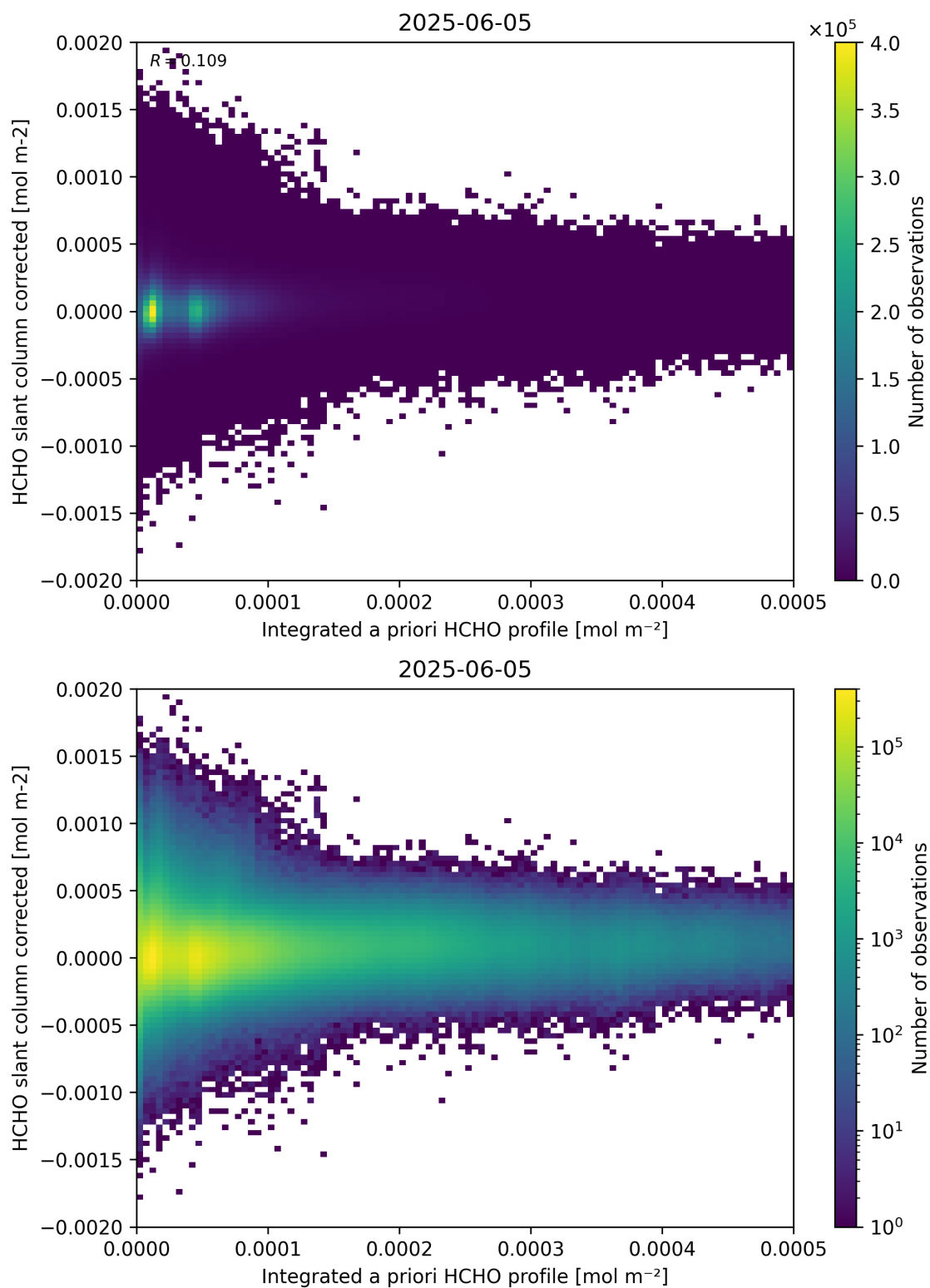
Figure 151: Scatter density plot of “Integrated a priori HCHO profile” against “HCHO slant column corrected” for 2025-06-04 to 2025-06-06.
