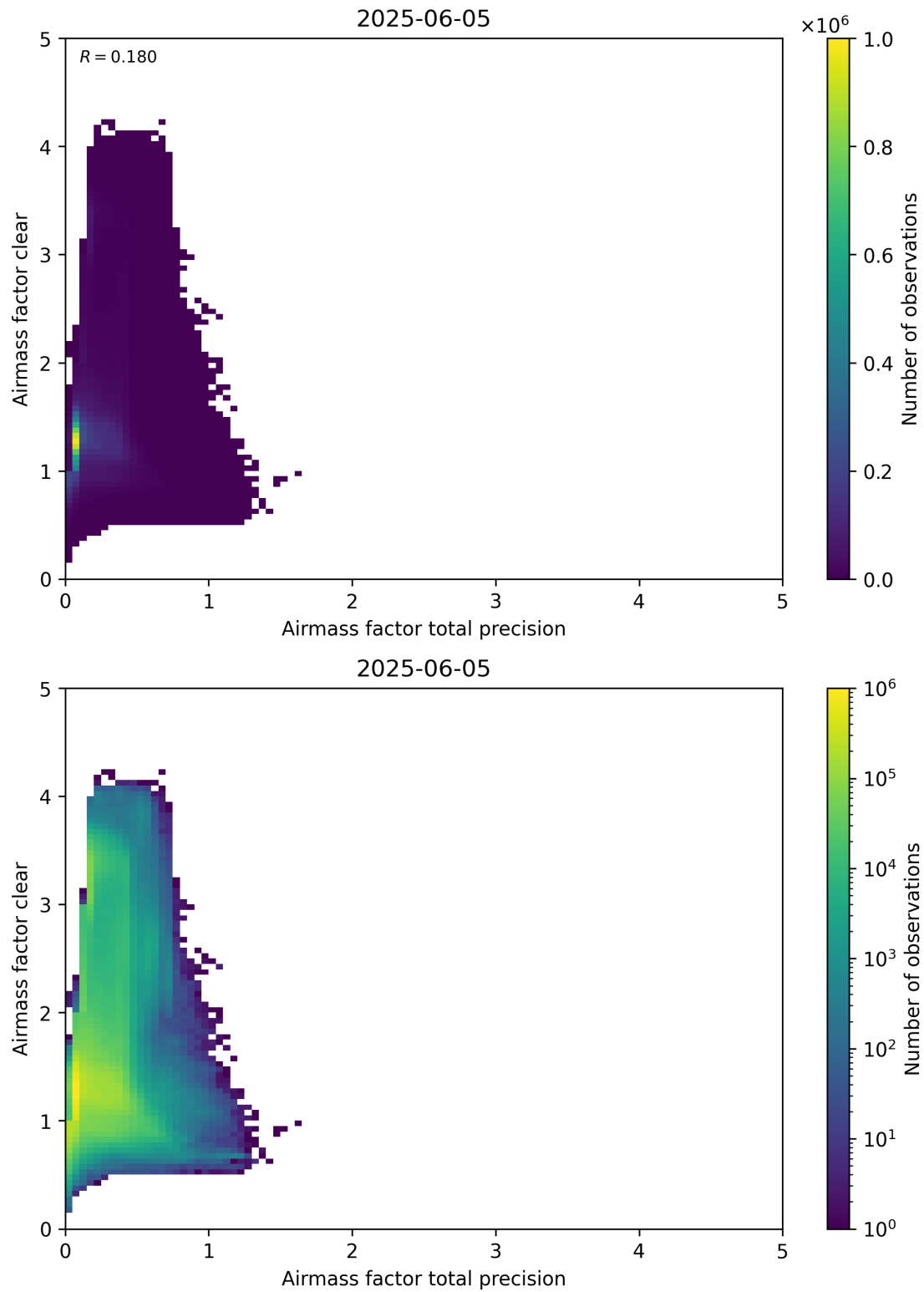
Figure 108: Scatter density plot of “Airmass factor total precision” against “Airmass factor clear” for 2025-06-04 to 2025-06-06.
