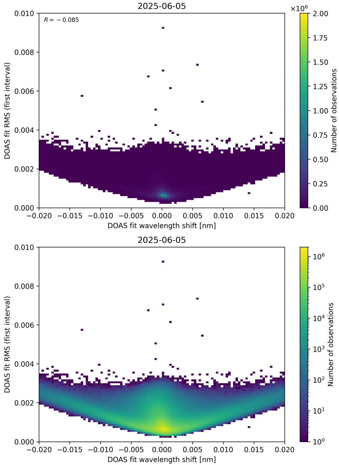
Figure 64: Scatter density plot of “DOAS fit wavelength shift” against “DOAS fit RMS (first interval)” for 2025-06-04 to 2025-06-06.
