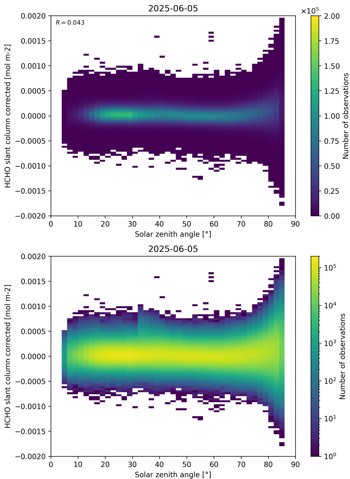
Figure 171: Scatter density plot of “Solar zenith angle” against “HCHO slant column corrected” for 2025-06-04 to 2025-06-06.
