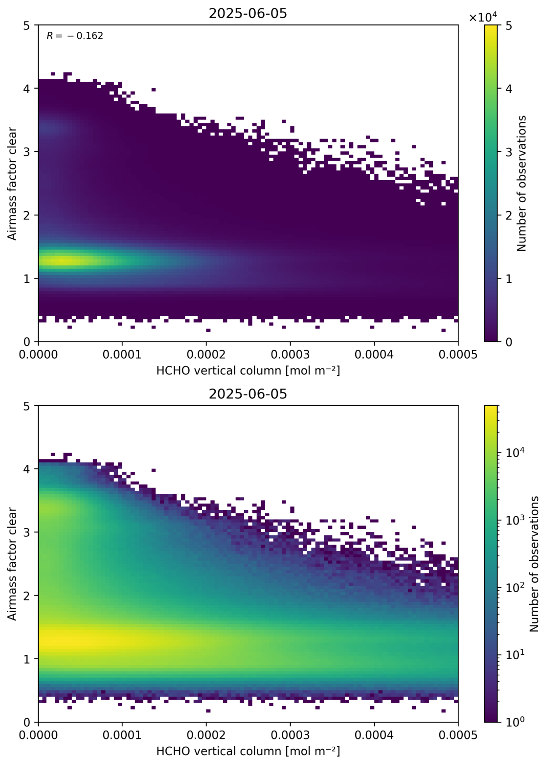
Figure 126: Scatter density plot of “HCHO vertical column” against “Airmass factor clear” for 2025-06-04 to 2025-06-06.
