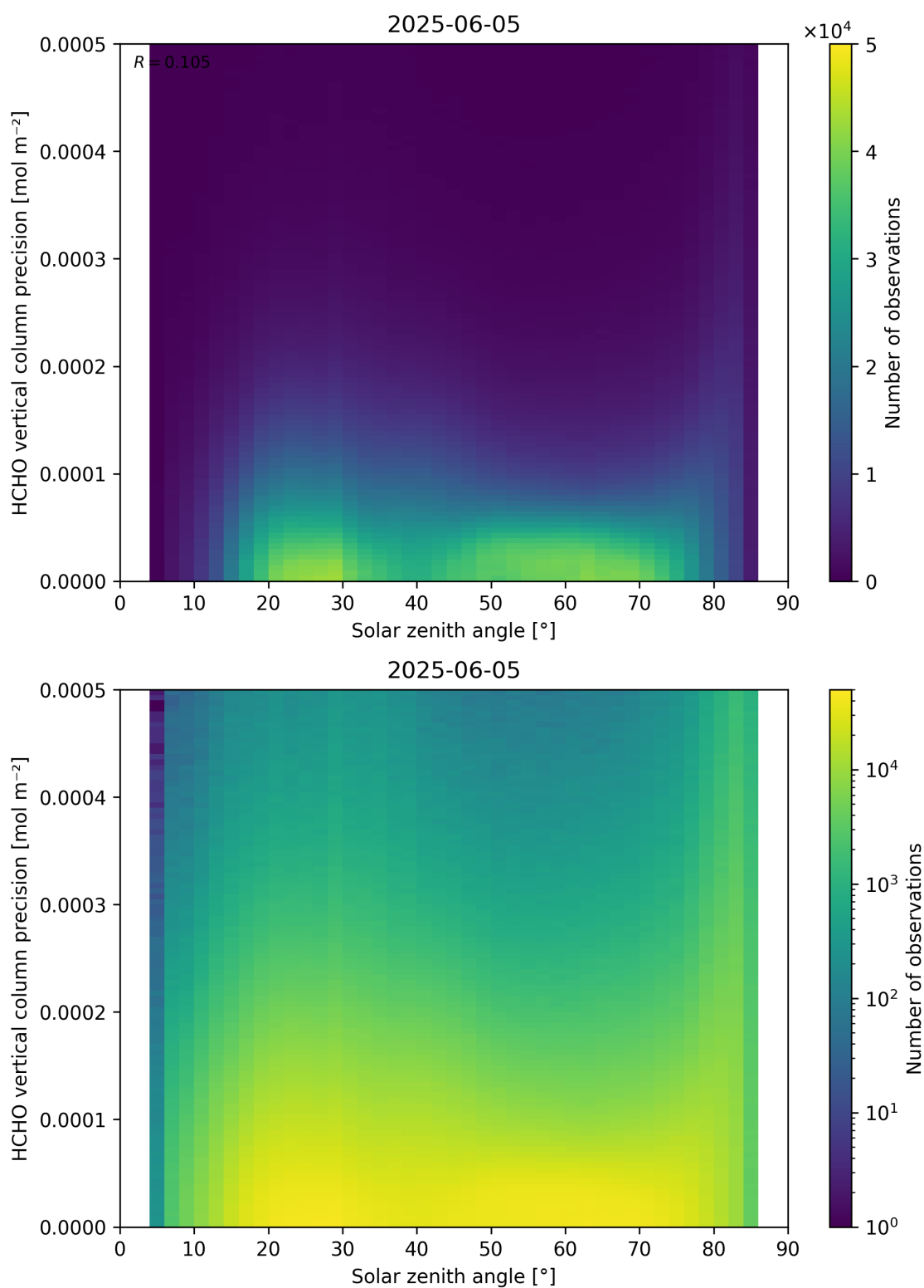
Figure 179: Scatter density plot of “Solar zenith angle” against “HCHO vertical column precision” for 2025-06-04 to 2025-06-06.
