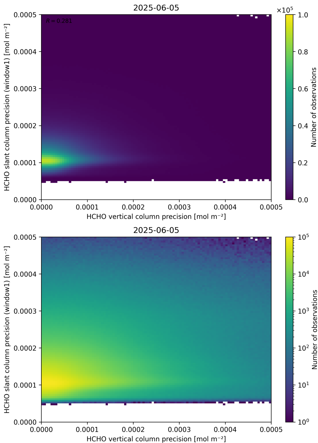
Figure 143: Scatter density plot of “HCHO vertical column precision” against “HCHO slant column precision (window1)” for 2025-06-04 to 2025-06-06.
