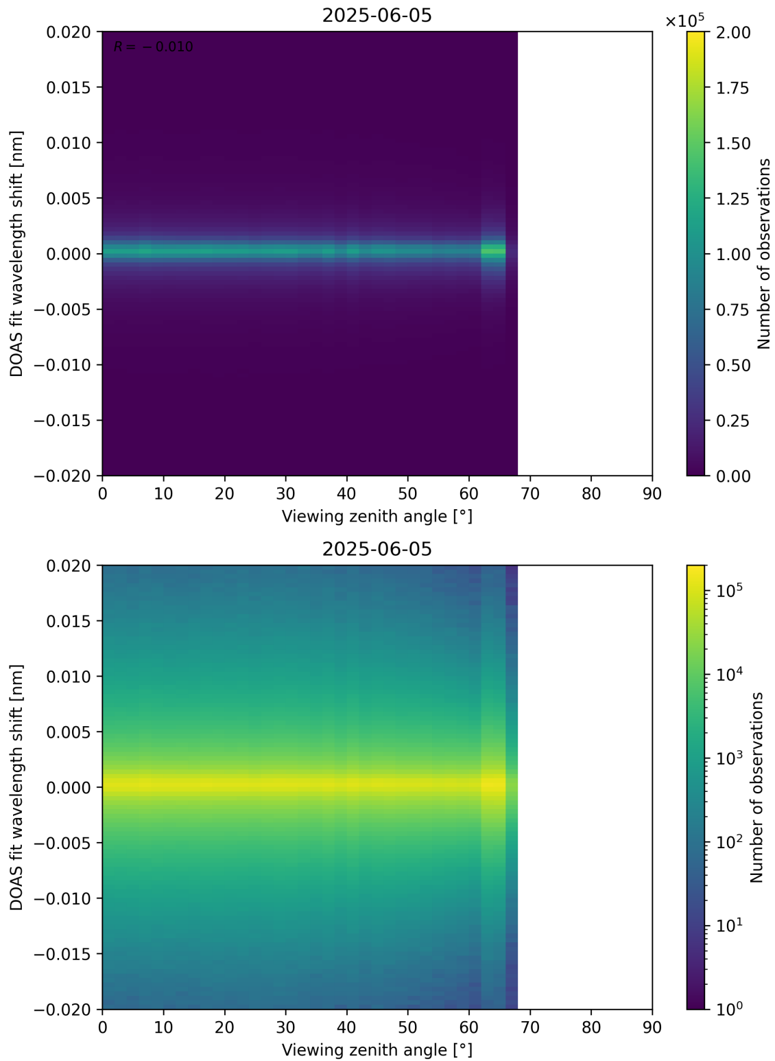
Figure 183: Scatter density plot of “Viewing zenith angle” against “DOAS fit wavelength shift” for 2025-06-04 to 2025-06-06.
