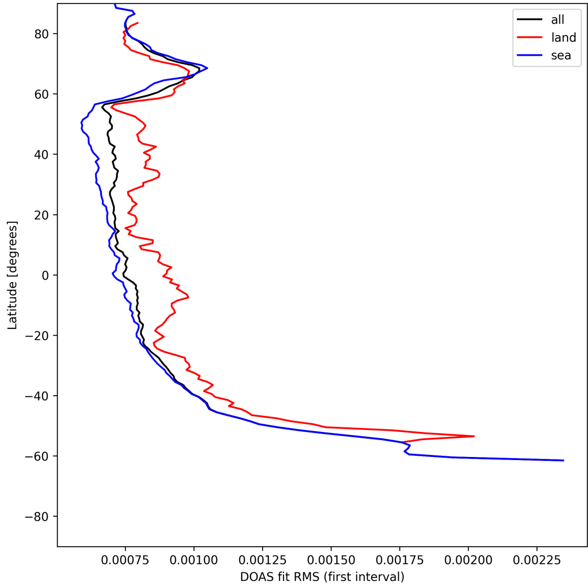
Figure 32: Zonal average of “DOAS fit RMS (first interval)” for 2025-06-04 to 2025-06-06.
