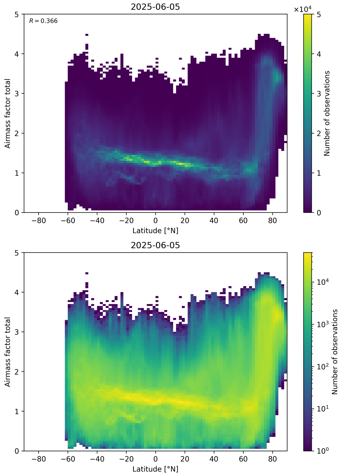
Figure 161: Scatter density plot of “Latitude” against “Airmass factor total” for 2025-06-04 to 2025-06-06.
