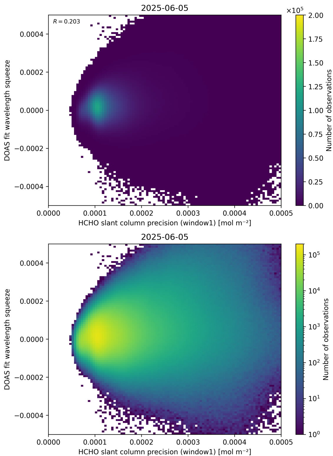
Figure 90: Scatter density plot of “HCHO slant column precision (window1)” against “DOAS fit wavelength squeeze” for 2025-06-04 to 2025-06-06.
