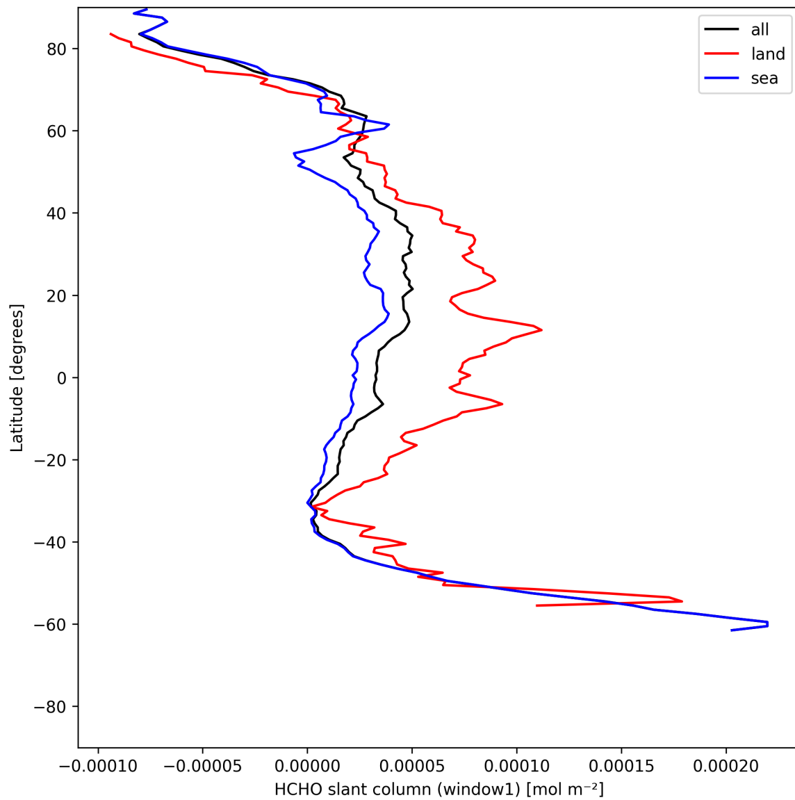
Figure 24: Zonal average of “HCHO slant column (window1)” for 2025-06-04 to 2025-06-06.
