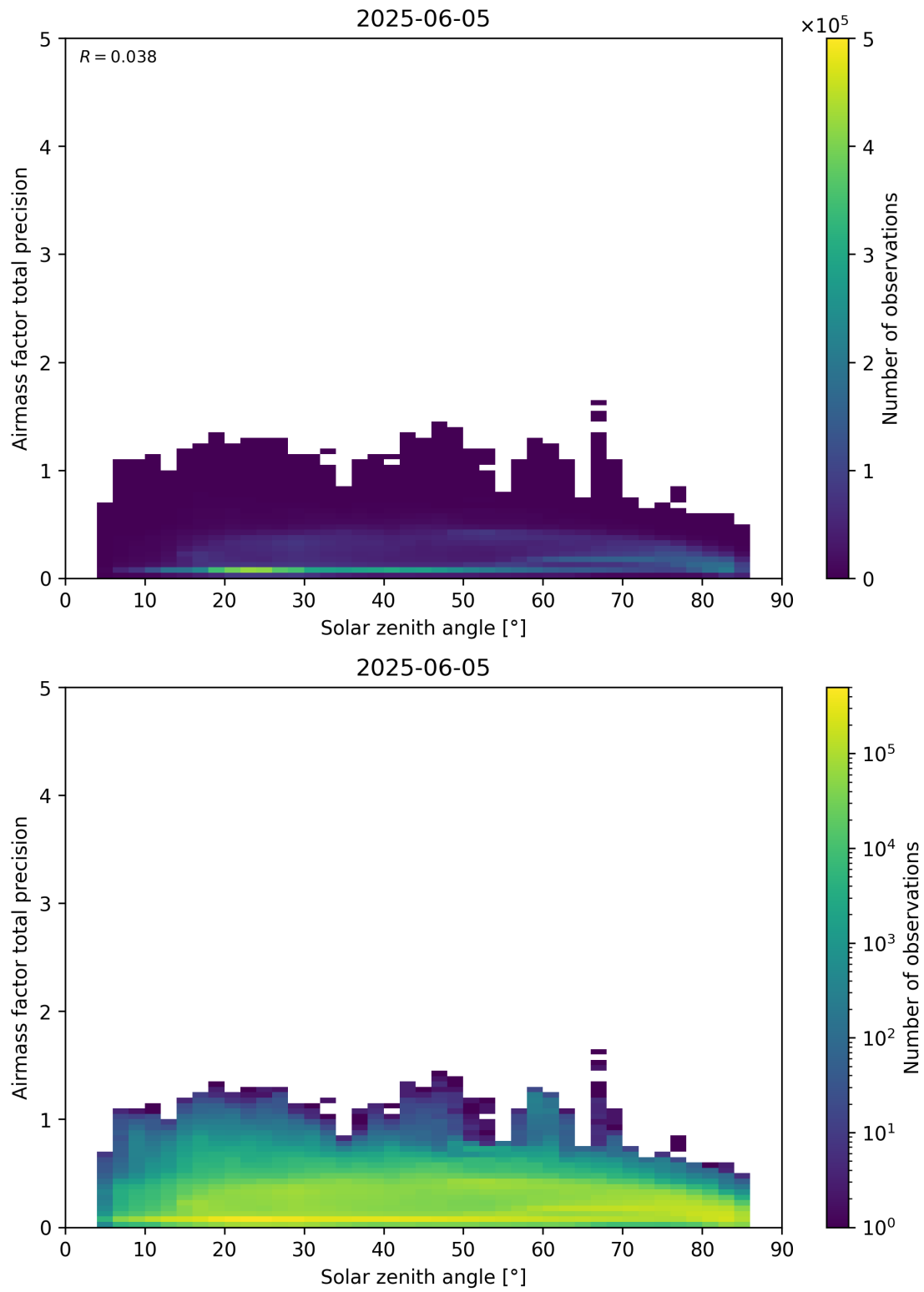
Figure 176: Scatter density plot of “Solar zenith angle” against “Airmass factor total precision” for 2025-06-04 to 2025-06-06.
