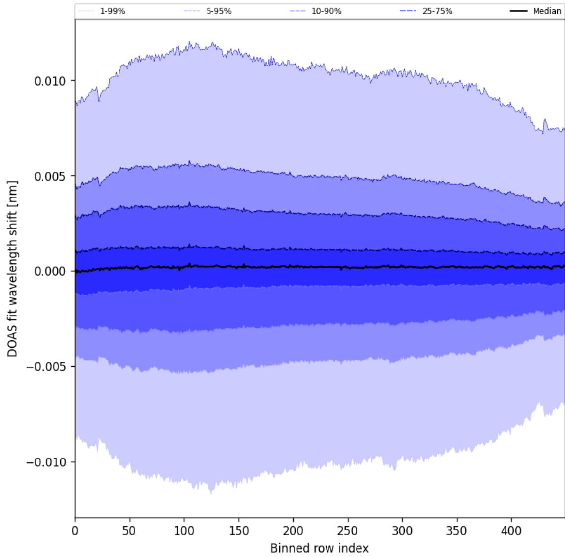
Figure 58: Along track statistics of “DOAS fit wavelength shift” for 2025-06-04 to 2025-06-06
