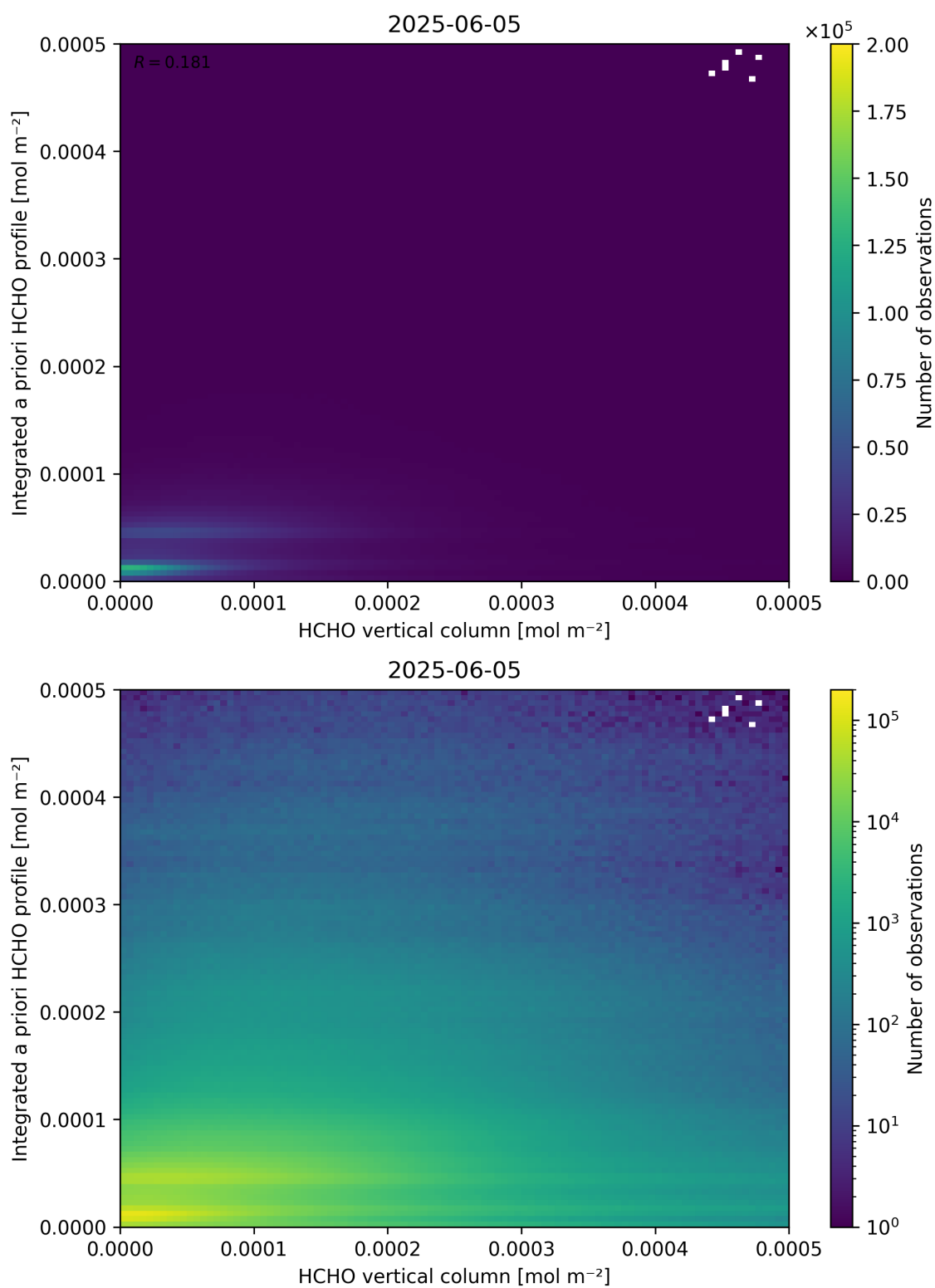
Figure 135: Scatter density plot of “HCHO vertical column” against “Integrated a priori HCHO profile” for 2025-06-04 to 2025-06-06.
