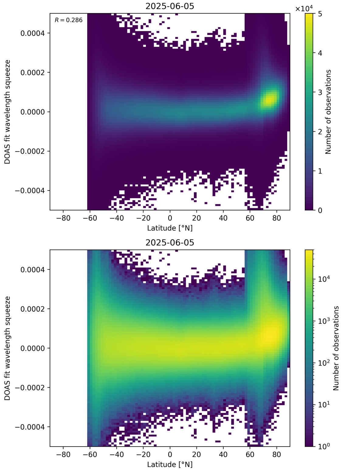
Figure 155: Scatter density plot of “Latitude” against “DOAS fit wavelength squeeze” for 2025-06-04 to 2025-06-06.
