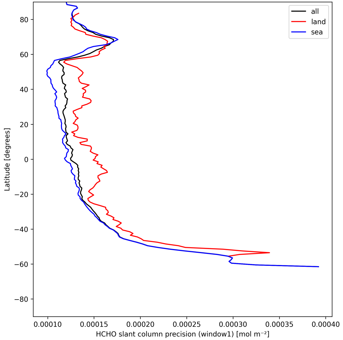
Figure 25: Zonal average of “HCHO slant column precision (window1)” for 2025-06-04 to 2025-06-06.
