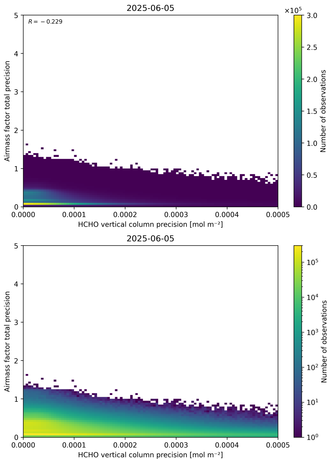
Figure 145: Scatter density plot of “HCHO vertical column precision” against “Airmass factor total precision” for 2025-06-04 to 2025-06-06.
