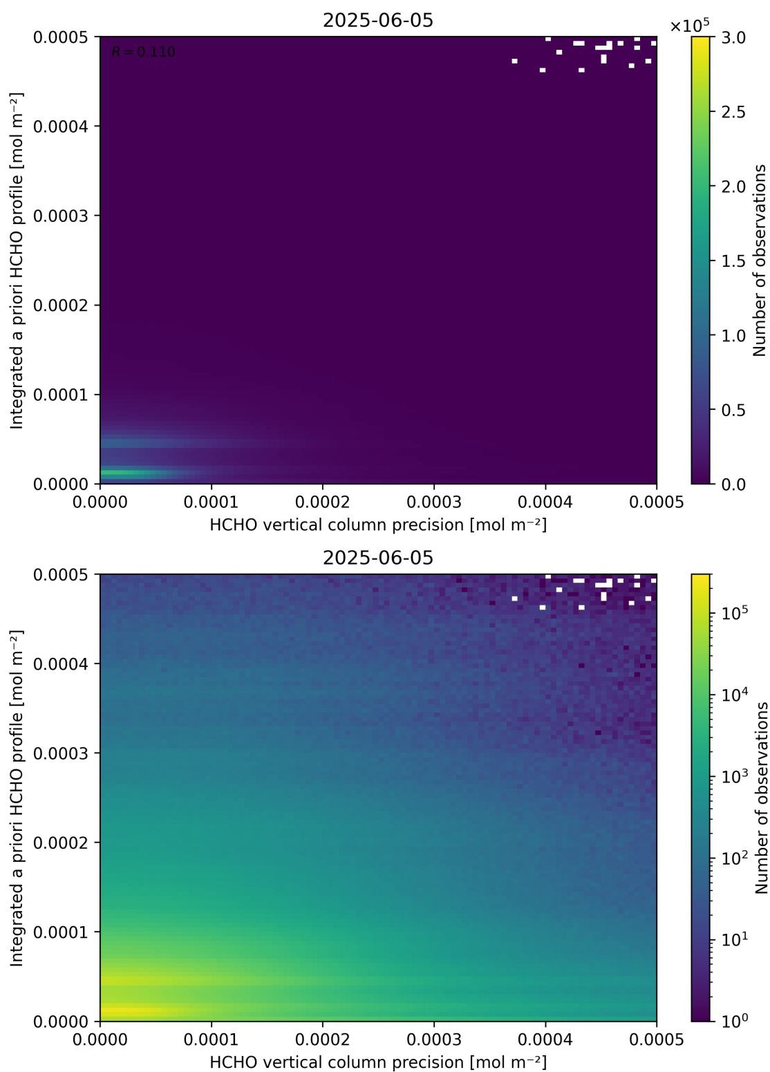
Figure 147: Scatter density plot of “HCHO vertical column precision” against “Integrated a priori HCHO profile” for 2025-06-04 to 2025-06-06.
