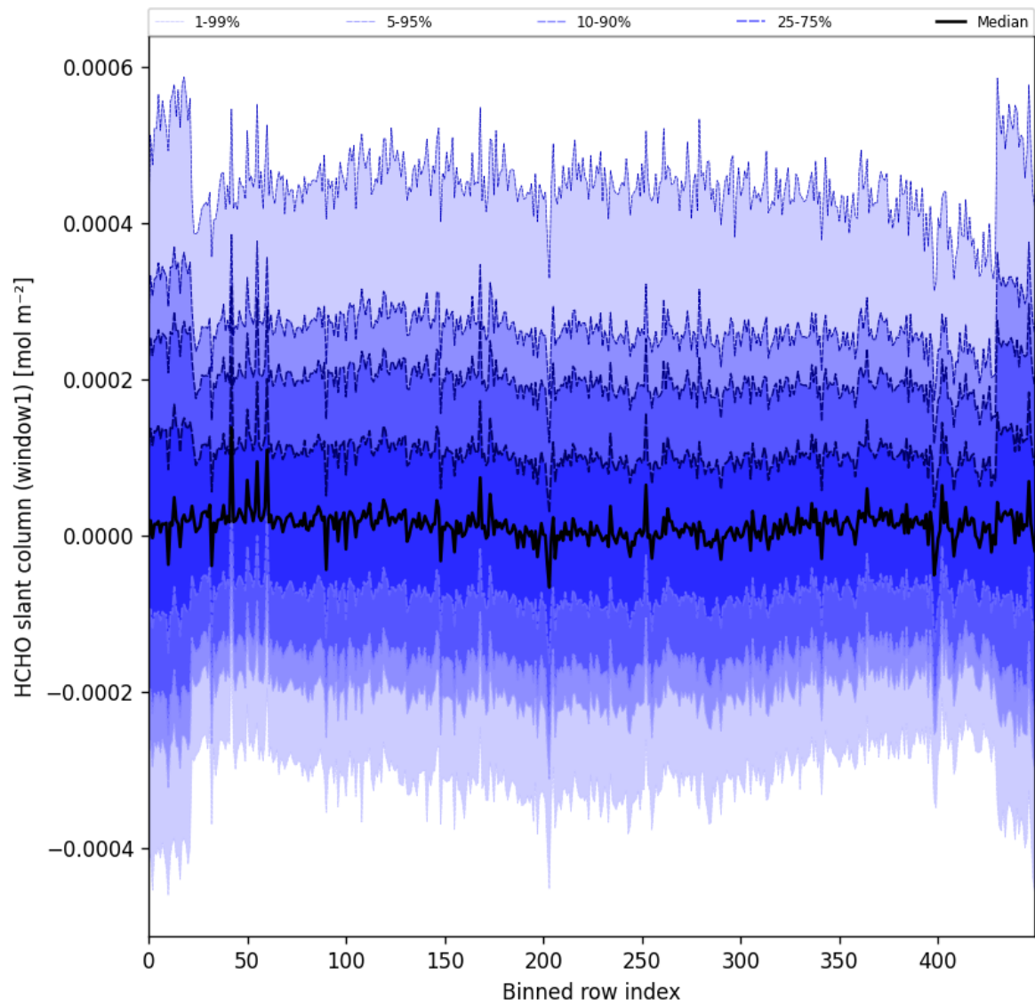
Figure 52: Along track statistics of “HCHO slant column (window1)” for 2025-06-04 to 2025-06-06
