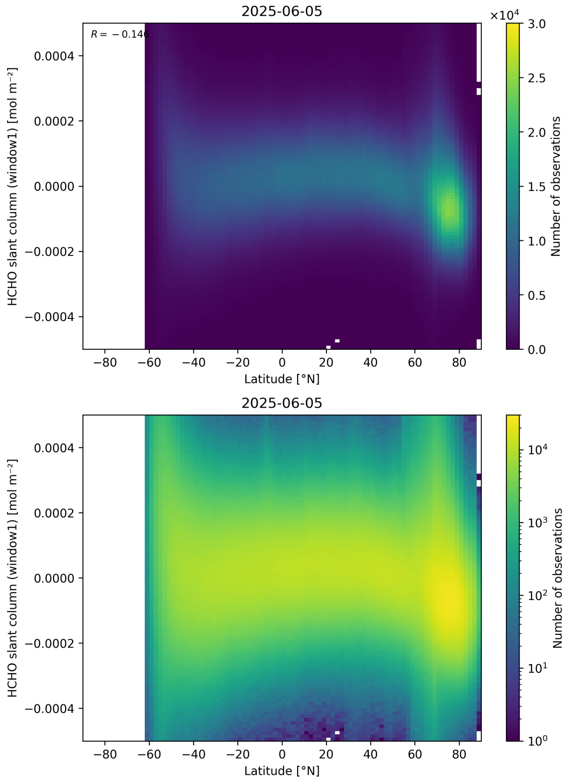
Figure 159: Scatter density plot of “Latitude” against “HCHO slant column (window1)” for 2025-06-04 to 2025-06-06.
