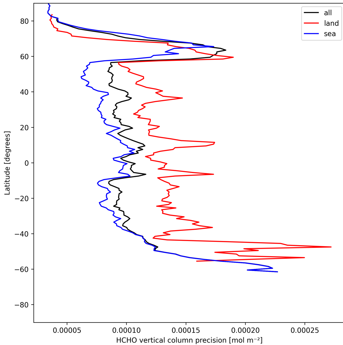
Figure 22: Zonal average of “HCHO vertical column precision” for 2025-06-04 to 2025-06-06.
