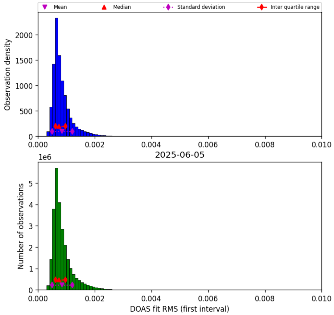
Figure 46: Histogram of “DOAS fit RMS (first interval)” for 2025-06-04 to 2025-06-06
