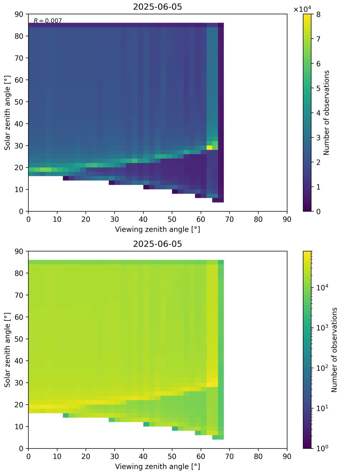
Figure 197: Scatter density plot of “Viewing zenith angle” against “Solar zenith angle” for 2025-06-04 to 2025-06-06.
