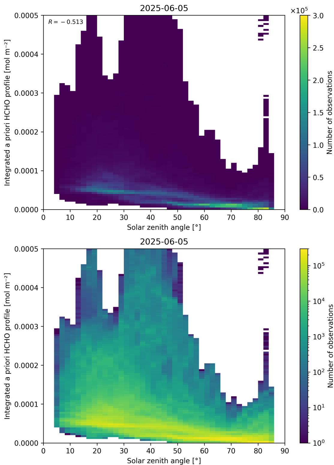
Figure 180: Scatter density plot of “Solar zenith angle” against “Integrated a priori HCHO profile” for 2025-06-04 to 2025-06-06.
