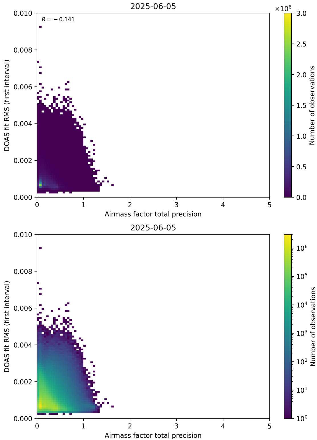
Figure 105: Scatter density plot of “Airmass factor total precision” against “DOAS fit RMS (first interval)” for 2025-06-04 to 2025-06-06.
