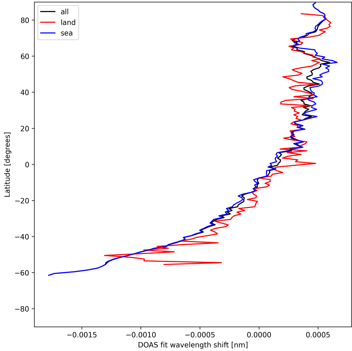
Figure 30: Zonal average of “DOAS fit wavelength shift” for 2025-06-04 to 2025-06-06.
