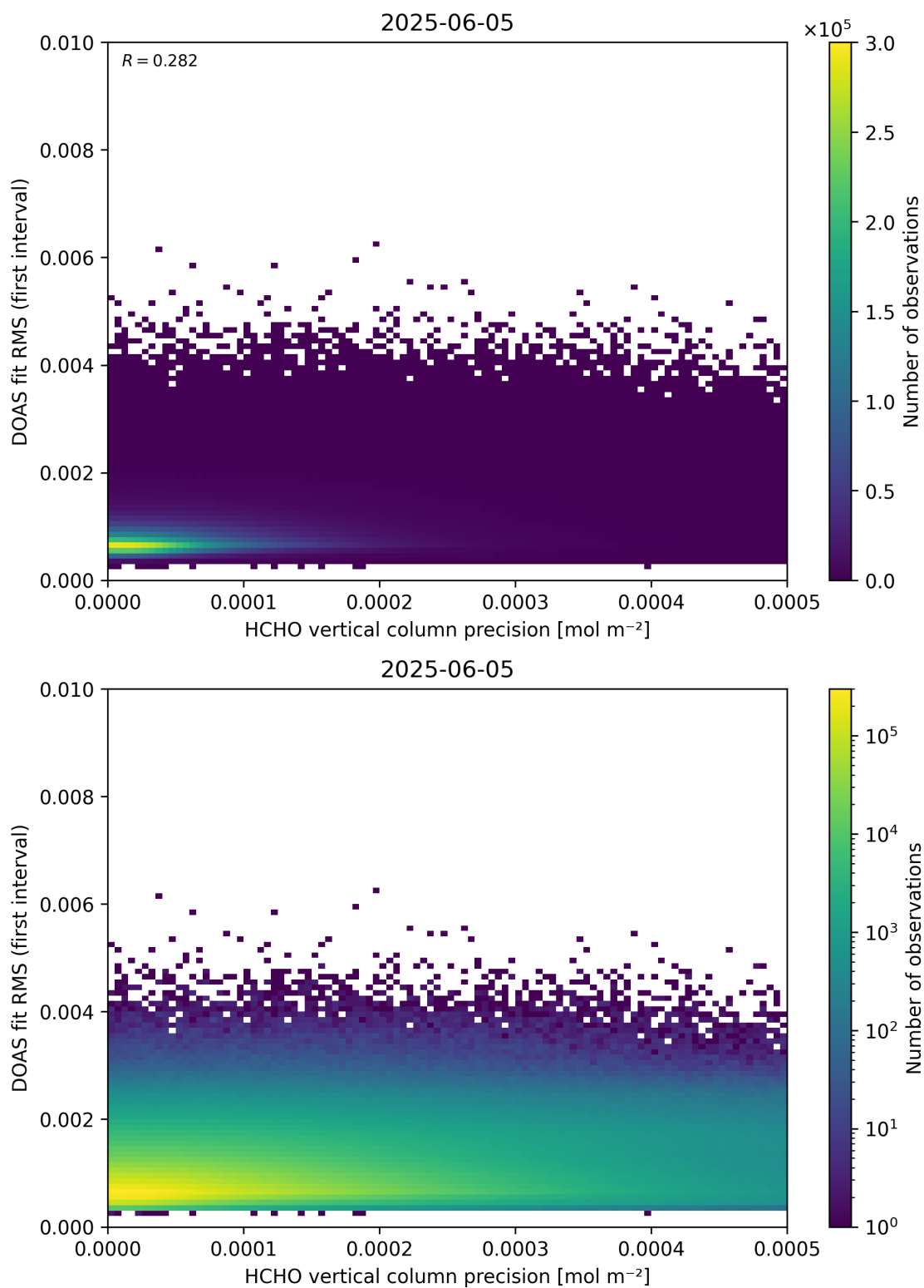
Figure 136: Scatter density plot of “HCHO vertical column precision” against “DOAS fit RMS (first interval)” for 2025-06-04 to 2025-06-06.
