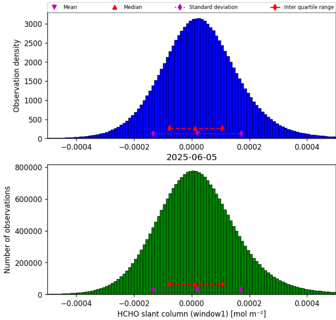
Figure 38: Histogram of “HCHO slant column (window1)” for 2025-06-04 to 2025-06-06
