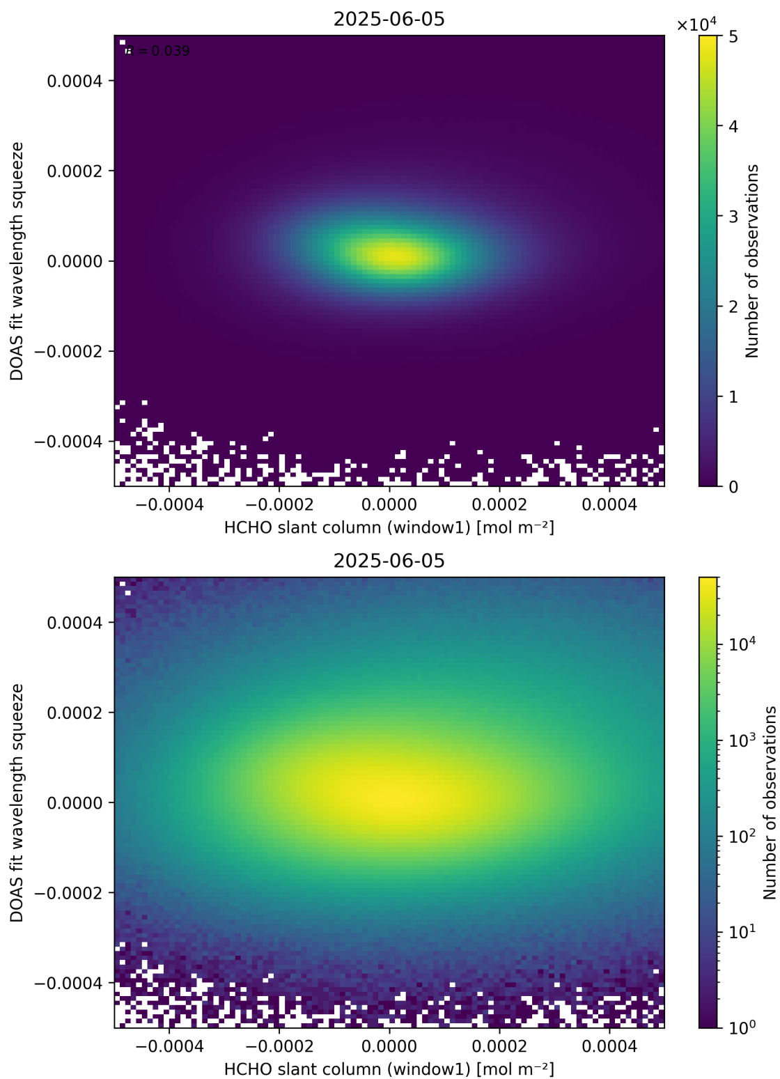
Figure 80: Scatter density plot of “HCHO slant column (window1)” against “DOAS fit wavelength squeeze” for 2025-06-04 to 2025-06-06.
