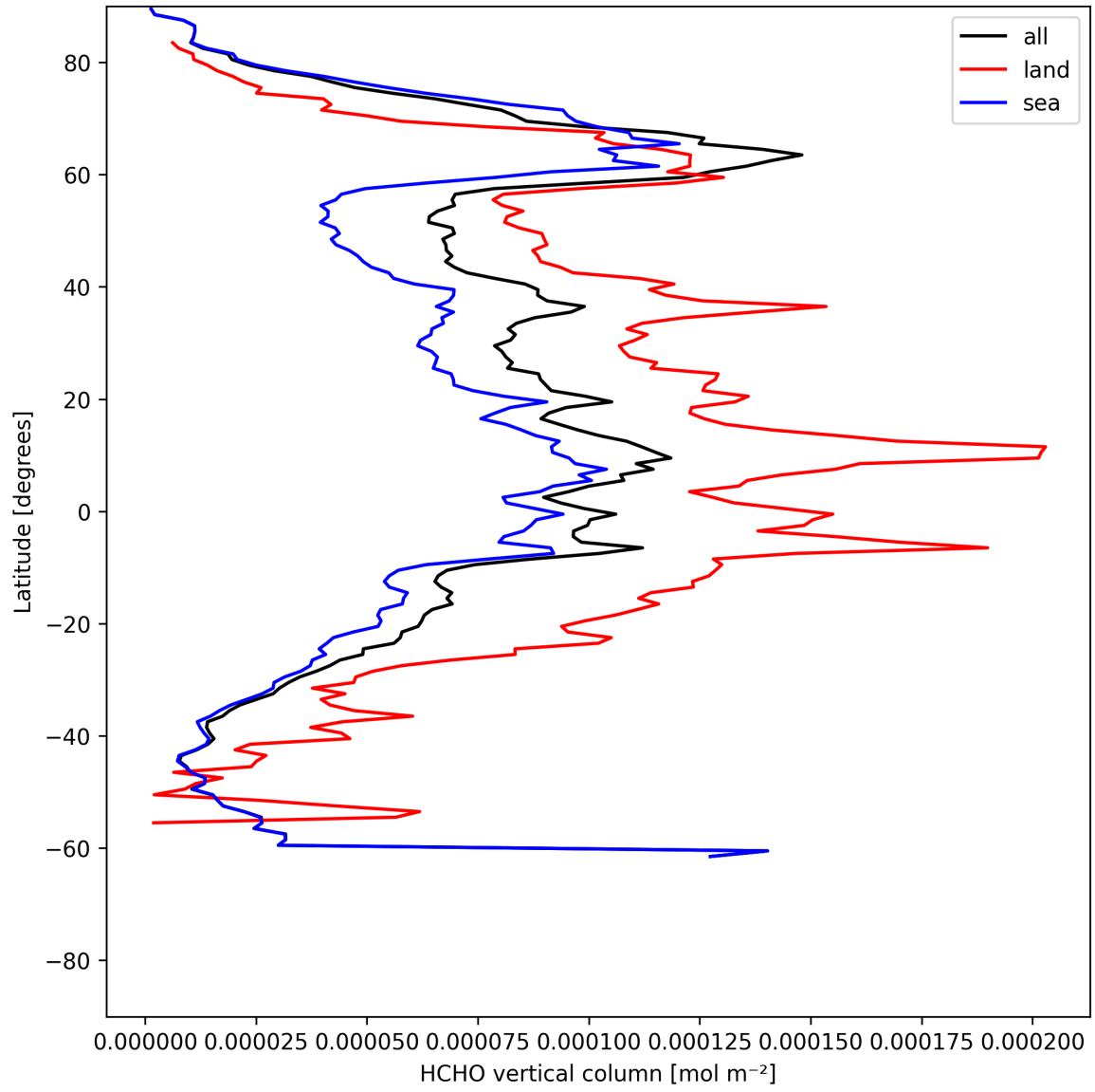
Figure 21: Zonal average of “HCHO vertical column” for 2025-06-04 to 2025-06-06.
