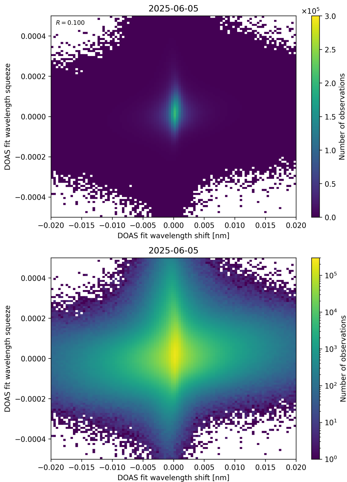
Figure 65: Scatter density plot of “DOAS fit wavelength shift” against “DOAS fit wavelength squeeze” for 2025-06-04 to 2025-06-06.
