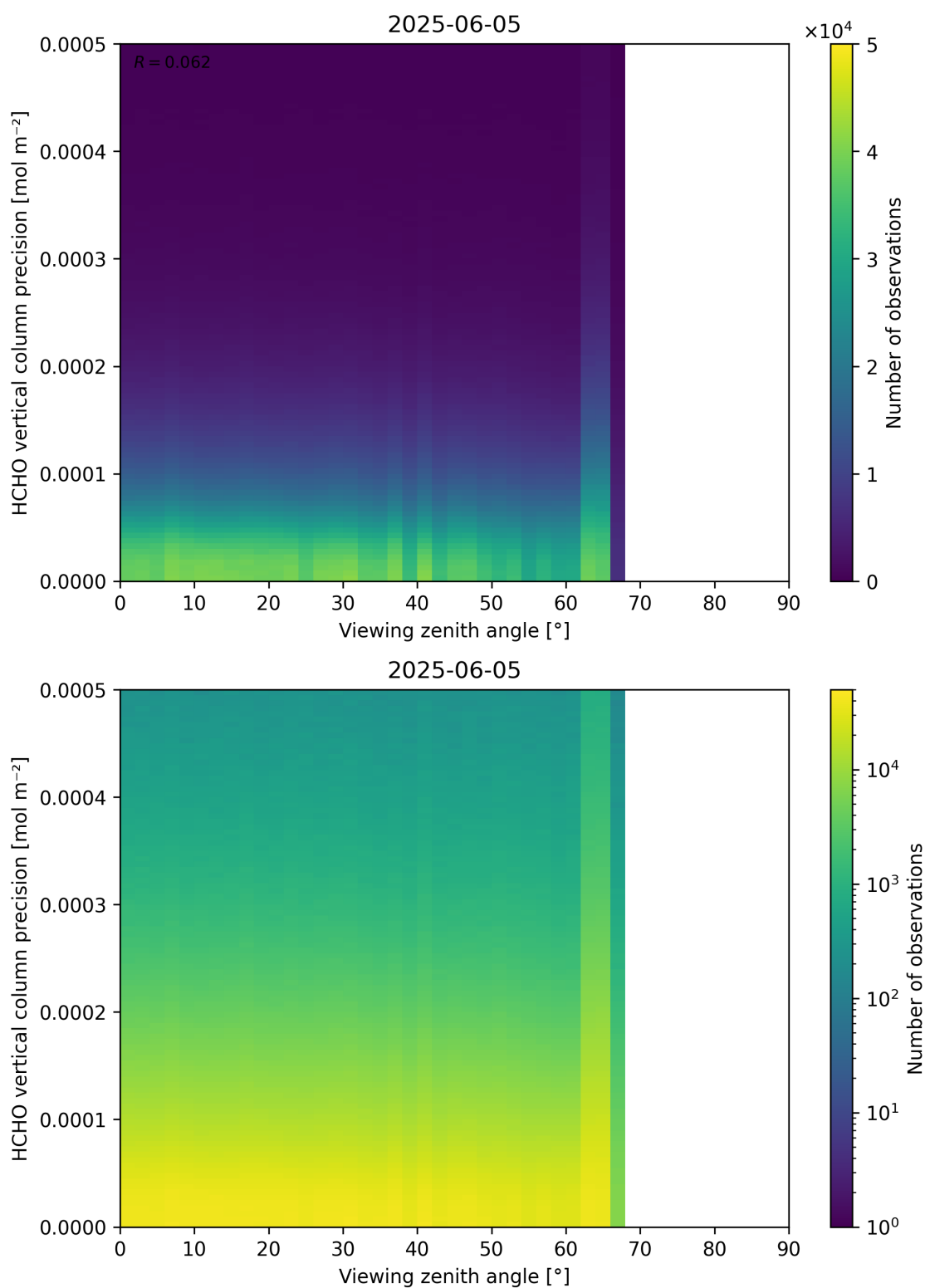
Figure 194: Scatter density plot of “Viewing zenith angle” against “HCHO vertical column precision” for 2025-06-04 to 2025-06-06.
