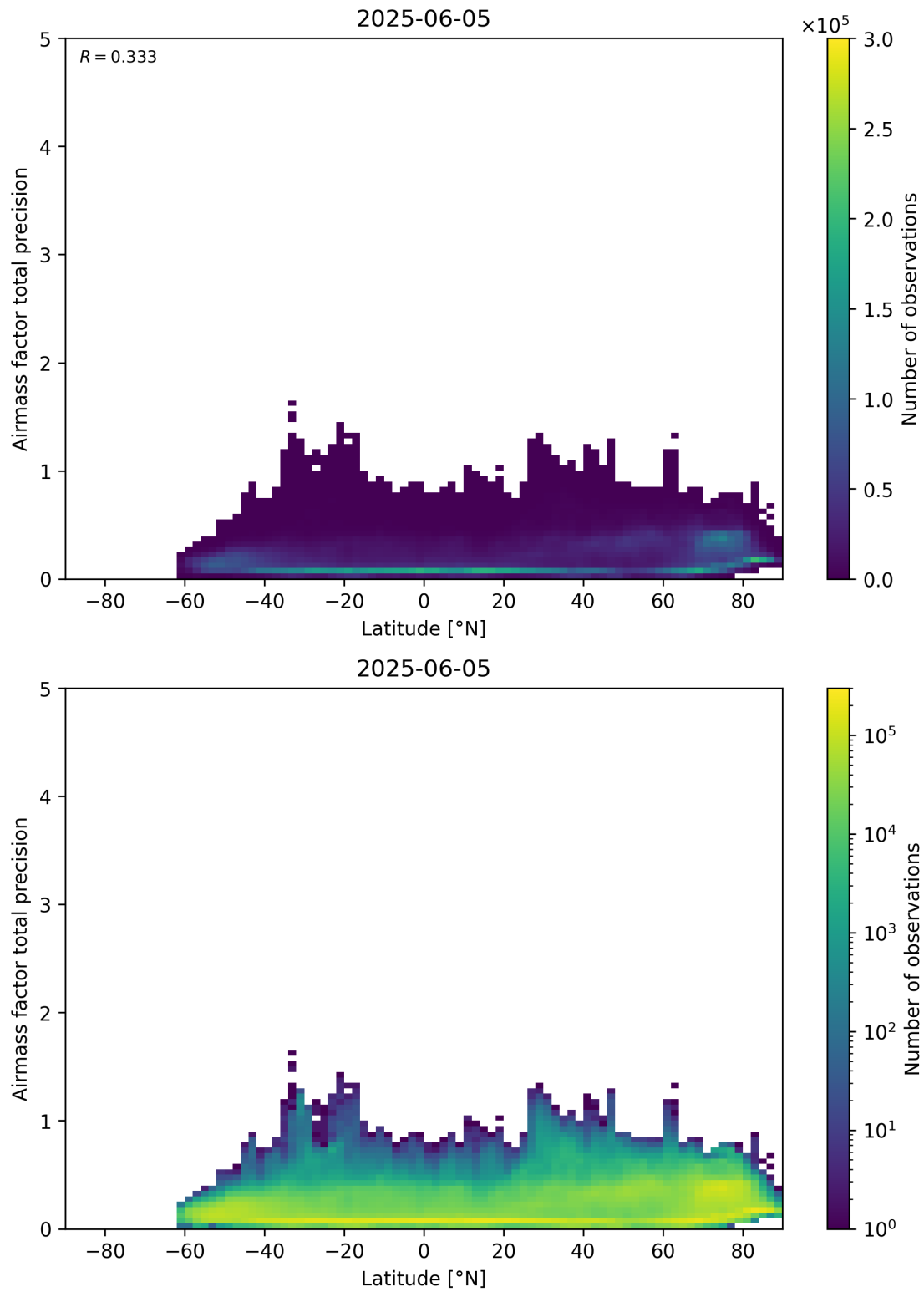
Figure 162: Scatter density plot of “Latitude” against “Airmass factor total precision” for 2025-06-04 to 2025-06-06.
