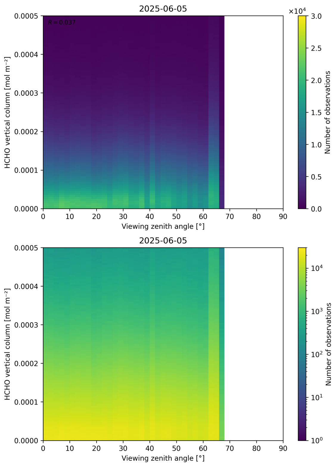
Figure 192: Scatter density plot of “Viewing zenith angle” against “HCHO vertical column” for 2025-06-04 to 2025-06-06.
