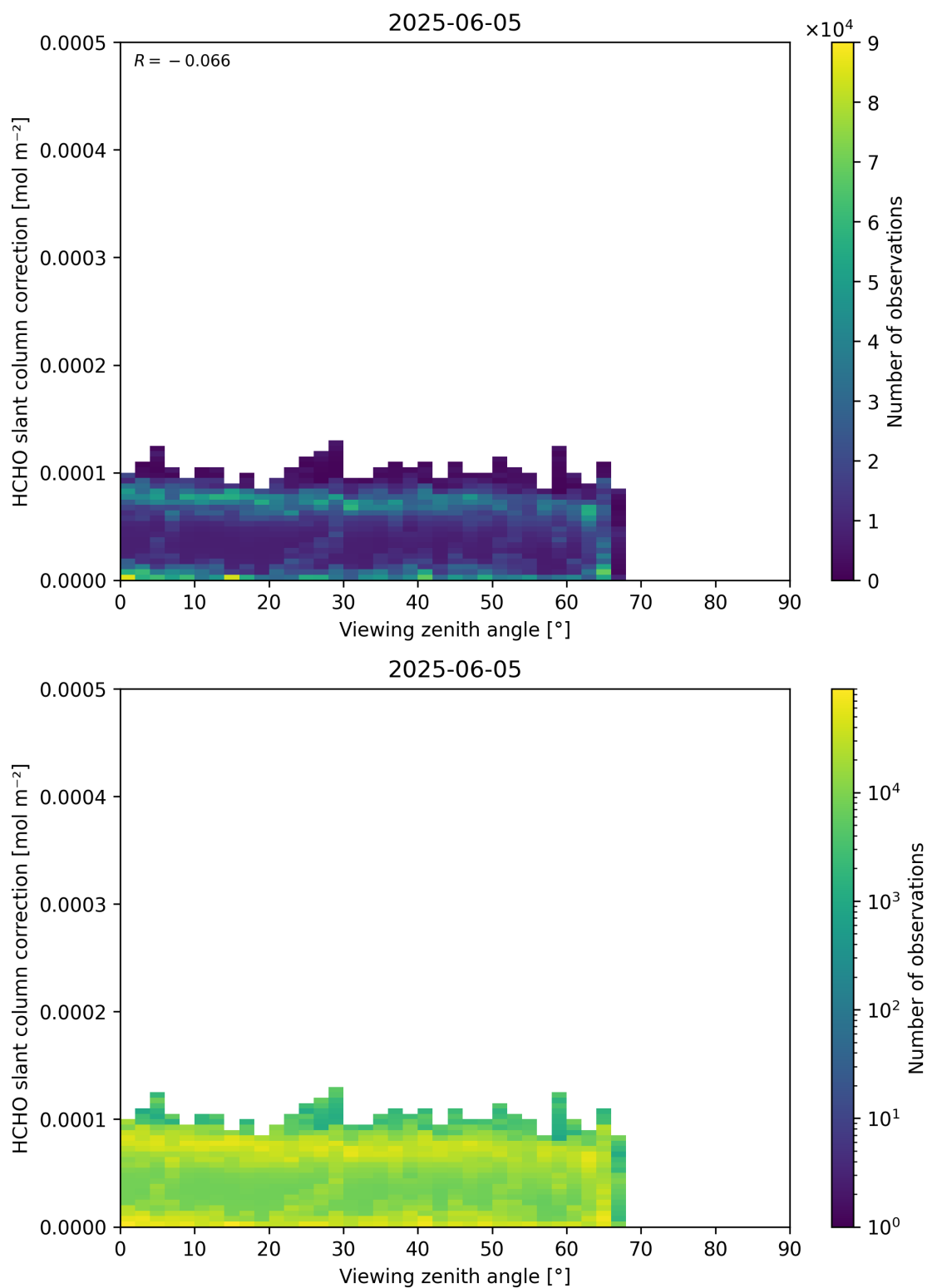
Figure 187: Scatter density plot of “Viewing zenith angle” against “HCHO slant column correction” for 2025-06-04 to 2025-06-06.
