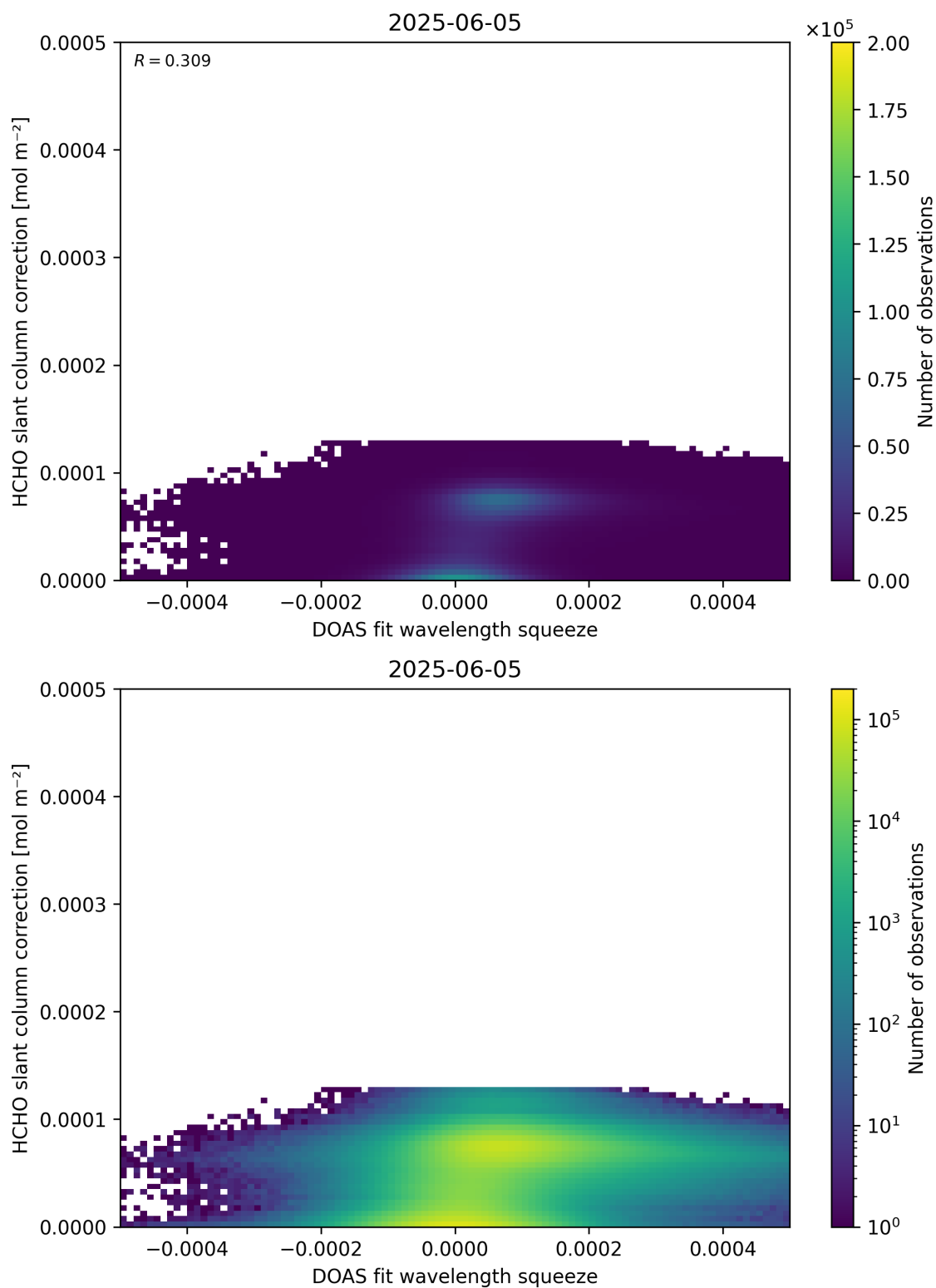
Figure 70: Scatter density plot of “DOAS fit wavelength squeeze” against “HCHO slant column correction” for 2025-06-04 to 2025-06-06.
