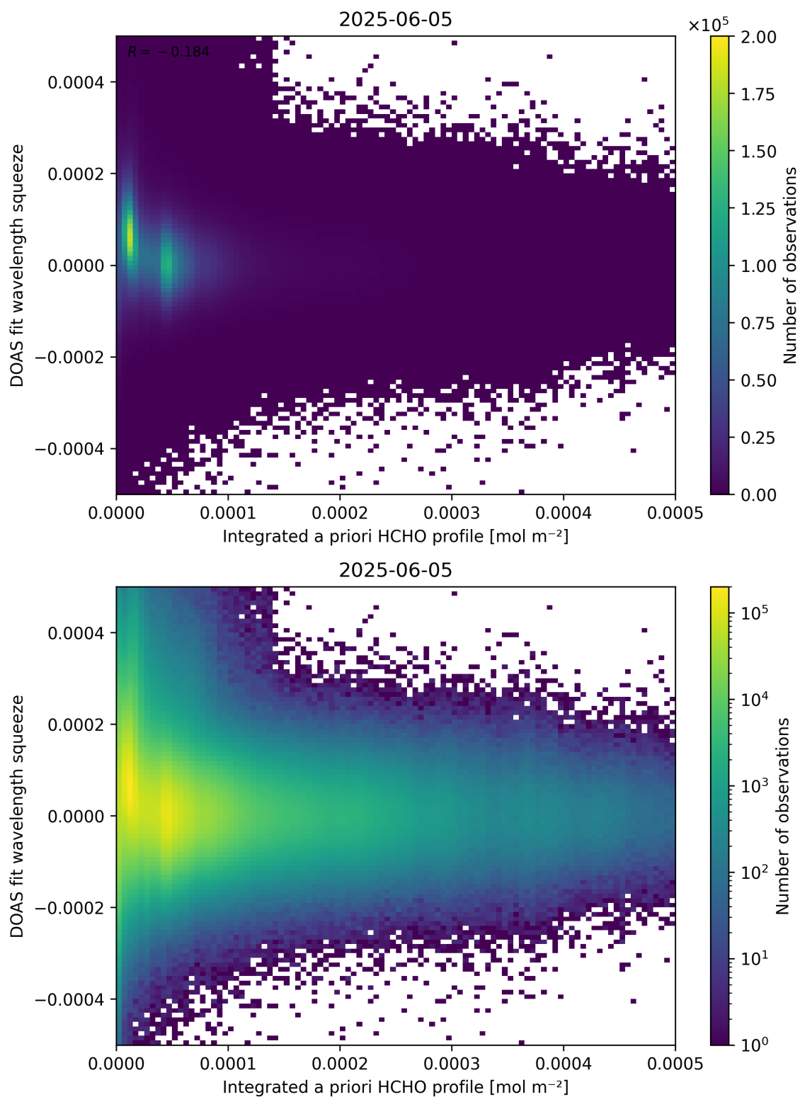
Figure 150: Scatter density plot of “Integrated a priori HCHO profile” against “DOAS fit wavelength squeeze” for 2025-06-04 to 2025-06-06.
