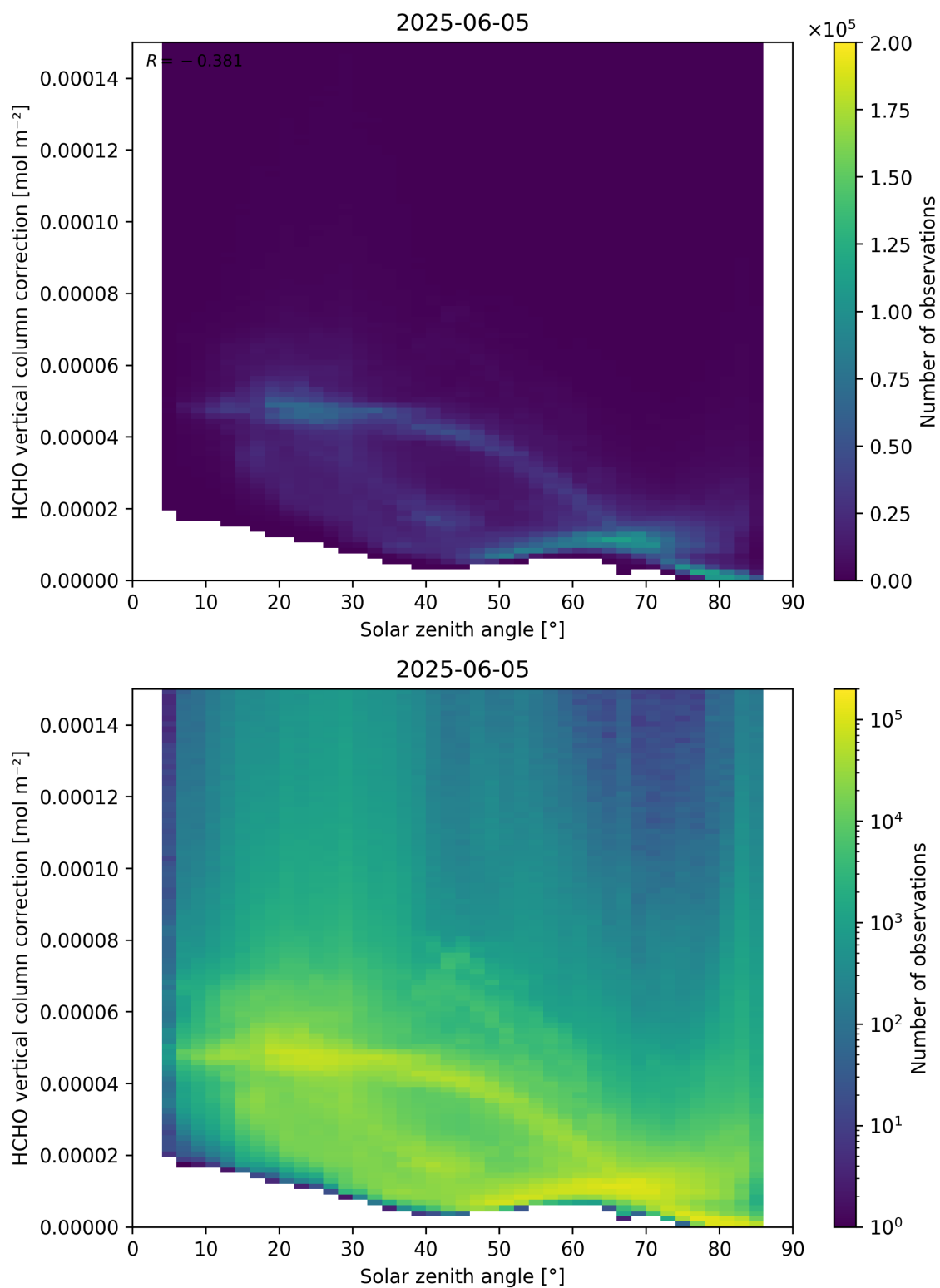
Figure 178: Scatter density plot of “Solar zenith angle” against “HCHO vertical column correction” for 2025-06-04 to 2025-06-06.
