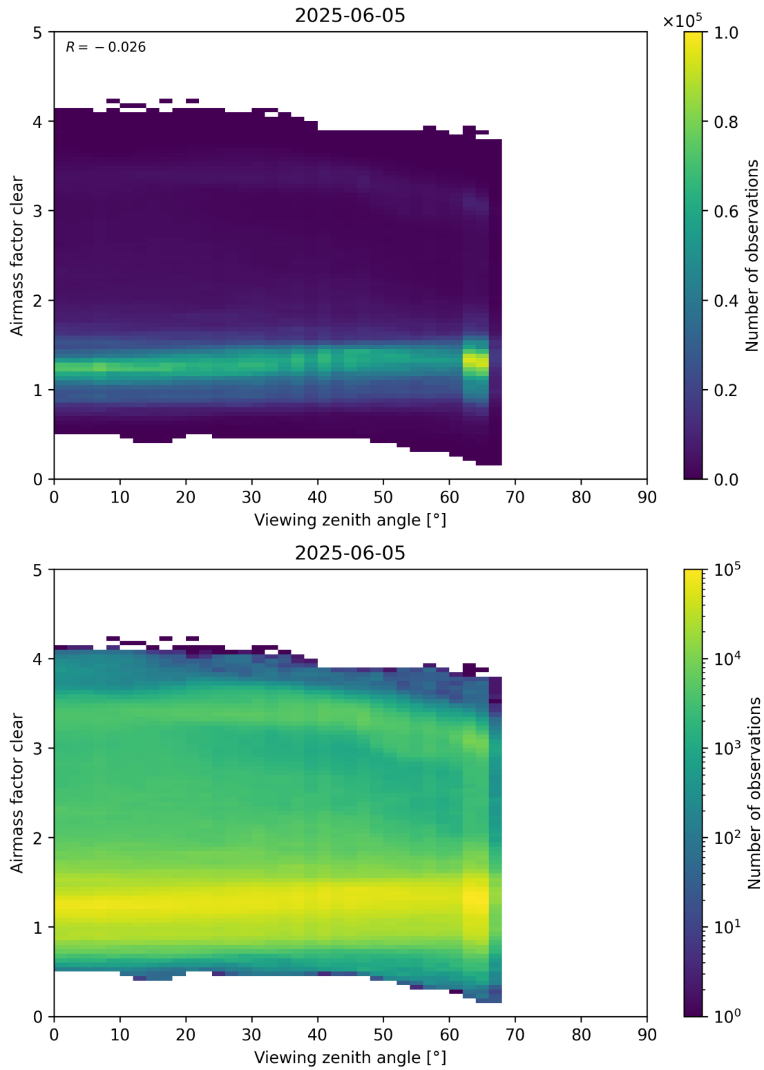
Figure 185: Scatter density plot of “Viewing zenith angle” against “Airmass factor clear” for 2025-06-04 to 2025-06-06.
