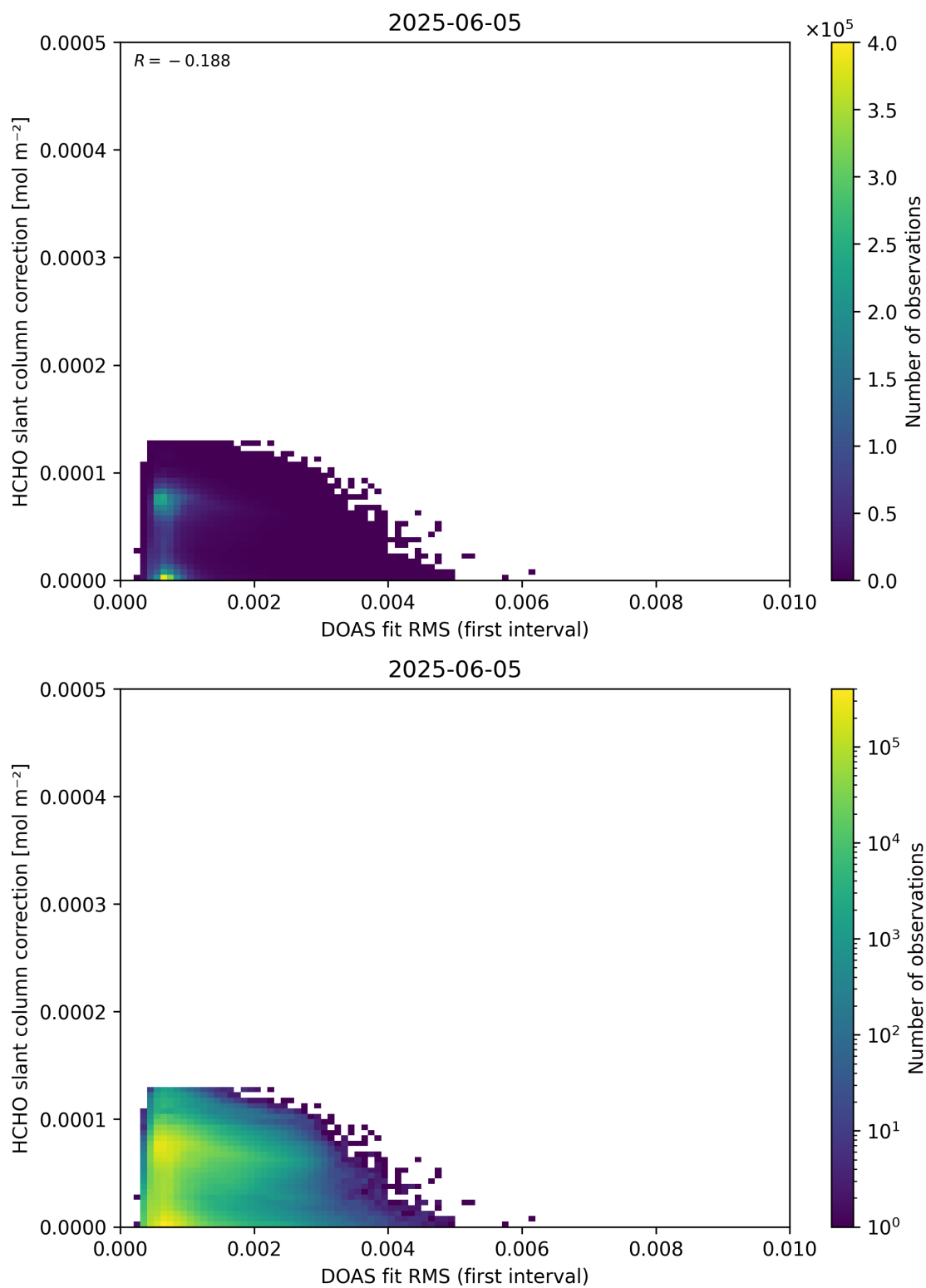
Figure 63: Scatter density plot of “DOAS fit RMS (first interval)” against “HCHO slant column correction” for 2025-06-04 to 2025-06-06.
