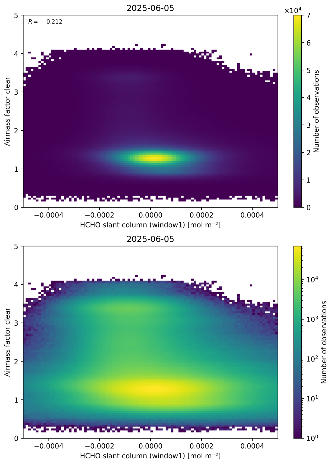
Figure 81: Scatter density plot of “HCHO slant column (window1)” against “Airmass factor clear” for 2025-06-04 to 2025-06-06.
