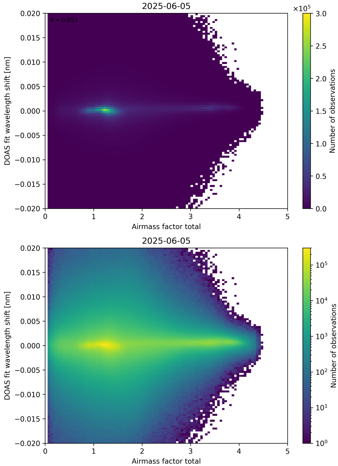
Figure 98: Scatter density plot of “Airmass factor total” against “DOAS fit wavelength shift” for 2025-06-04 to 2025-06-06.
