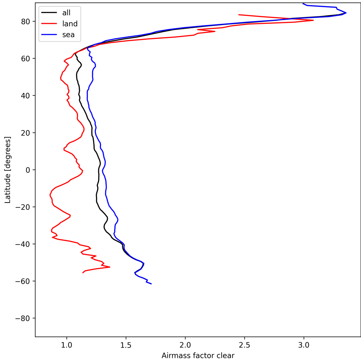
Figure 28: Zonal average of “Airmass factor clear” for 2025-06-04 to 2025-06-06.
