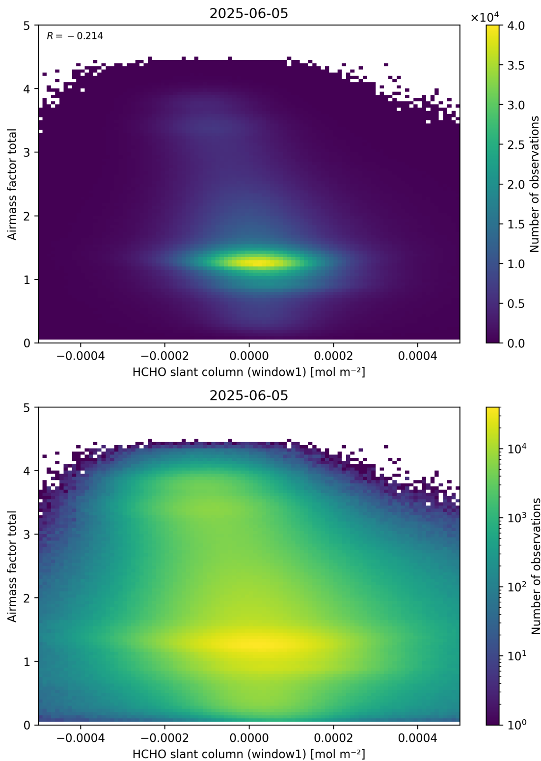
Figure 85: Scatter density plot of “HCHO slant column (window1)” against “Airmass factor total” for 2025-06-04 to 2025-06-06.
