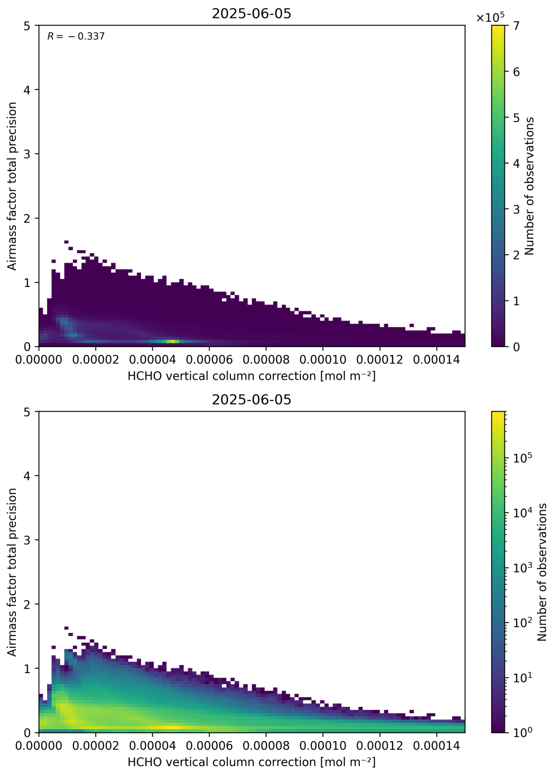
Figure 121: Scatter density plot of “HCHO vertical column correction” against “Airmass factor total precision” for 2025-06-04 to 2025-06-06.
