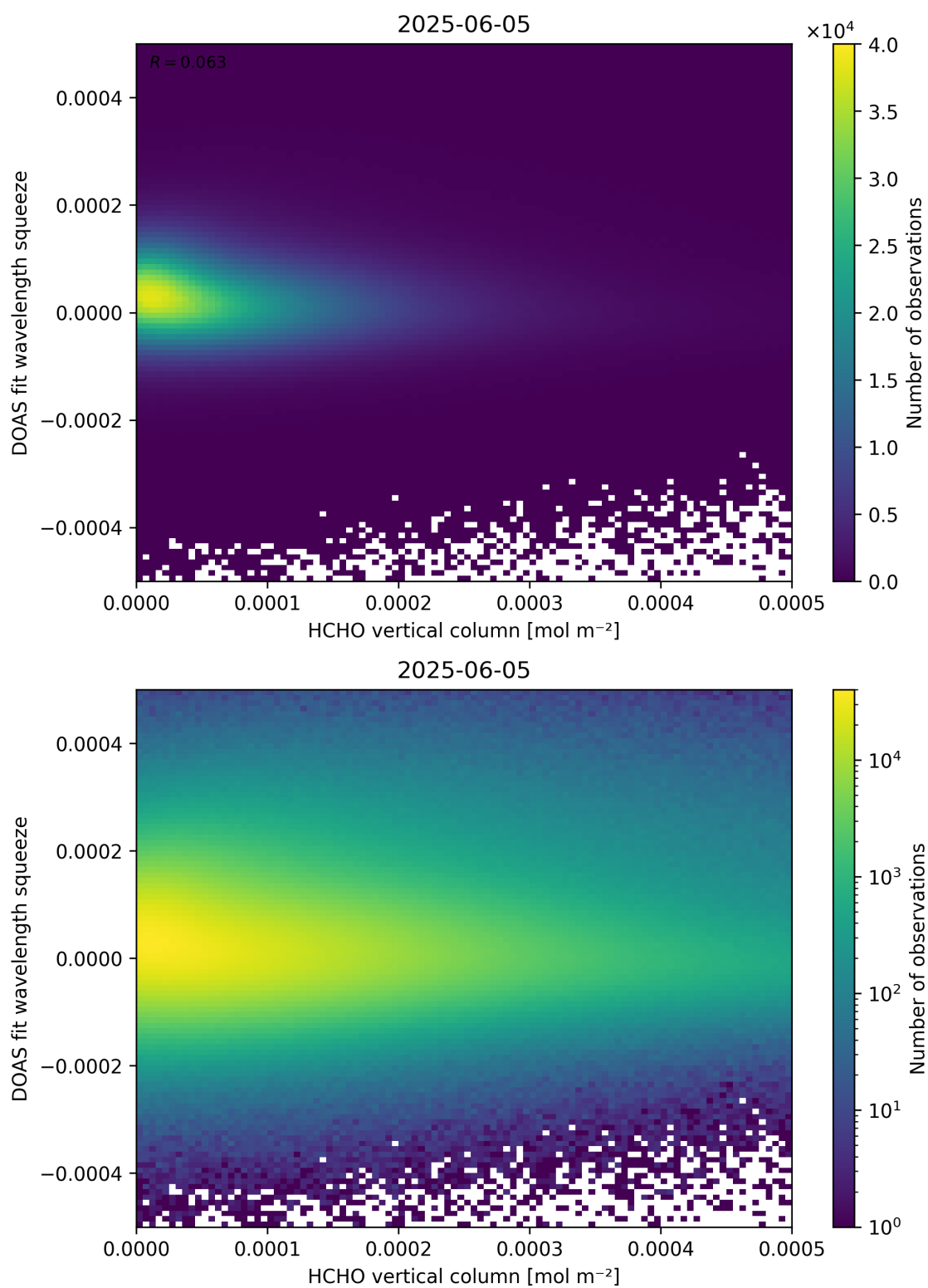
Figure 125: Scatter density plot of “HCHO vertical column” against “DOAS fit wavelength squeeze” for 2025-06-04 to 2025-06-06.
