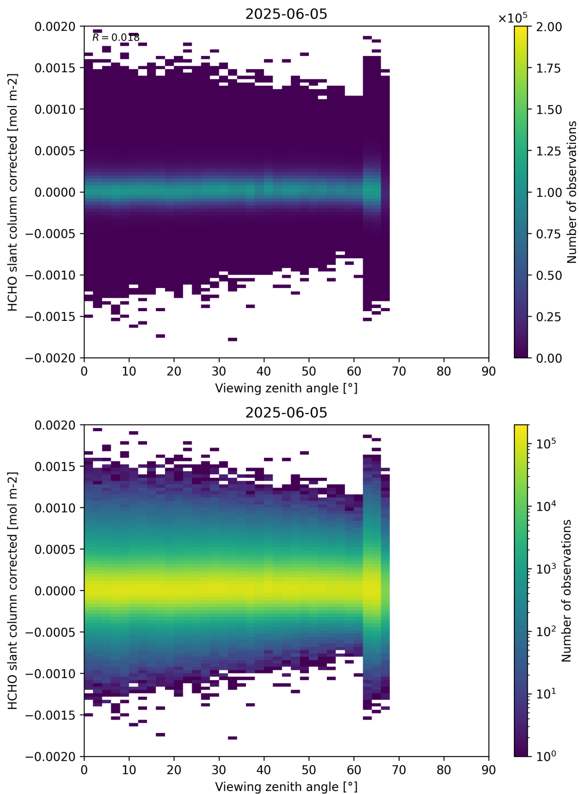
Figure 186: Scatter density plot of “Viewing zenith angle” against “HCHO slant column corrected” for 2025-06-04 to 2025-06-06.
