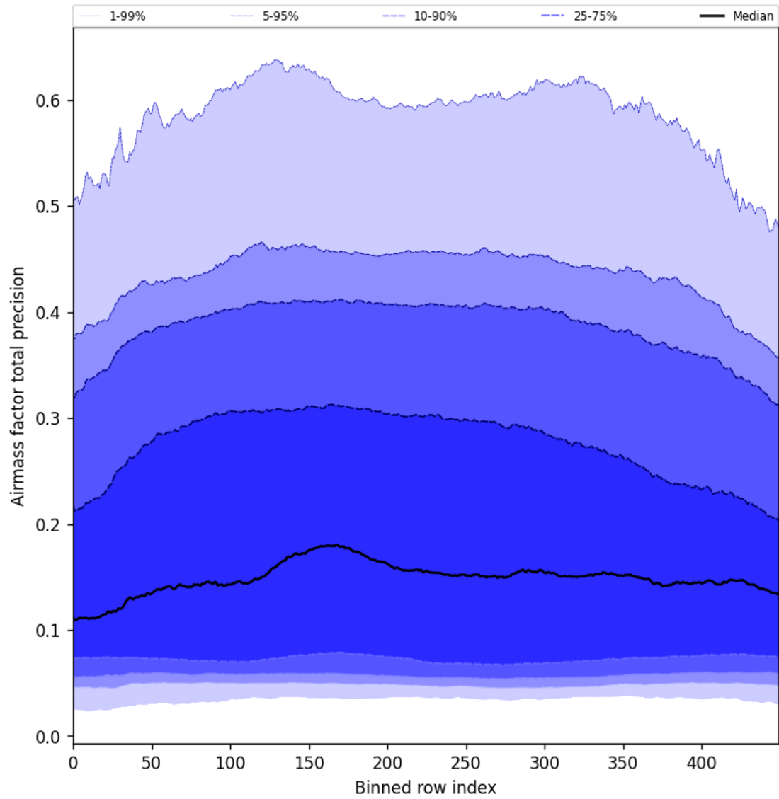
Figure 55: Along track statistics of “Airmass factor total precision” for 2025-06-04 to 2025-06-06
