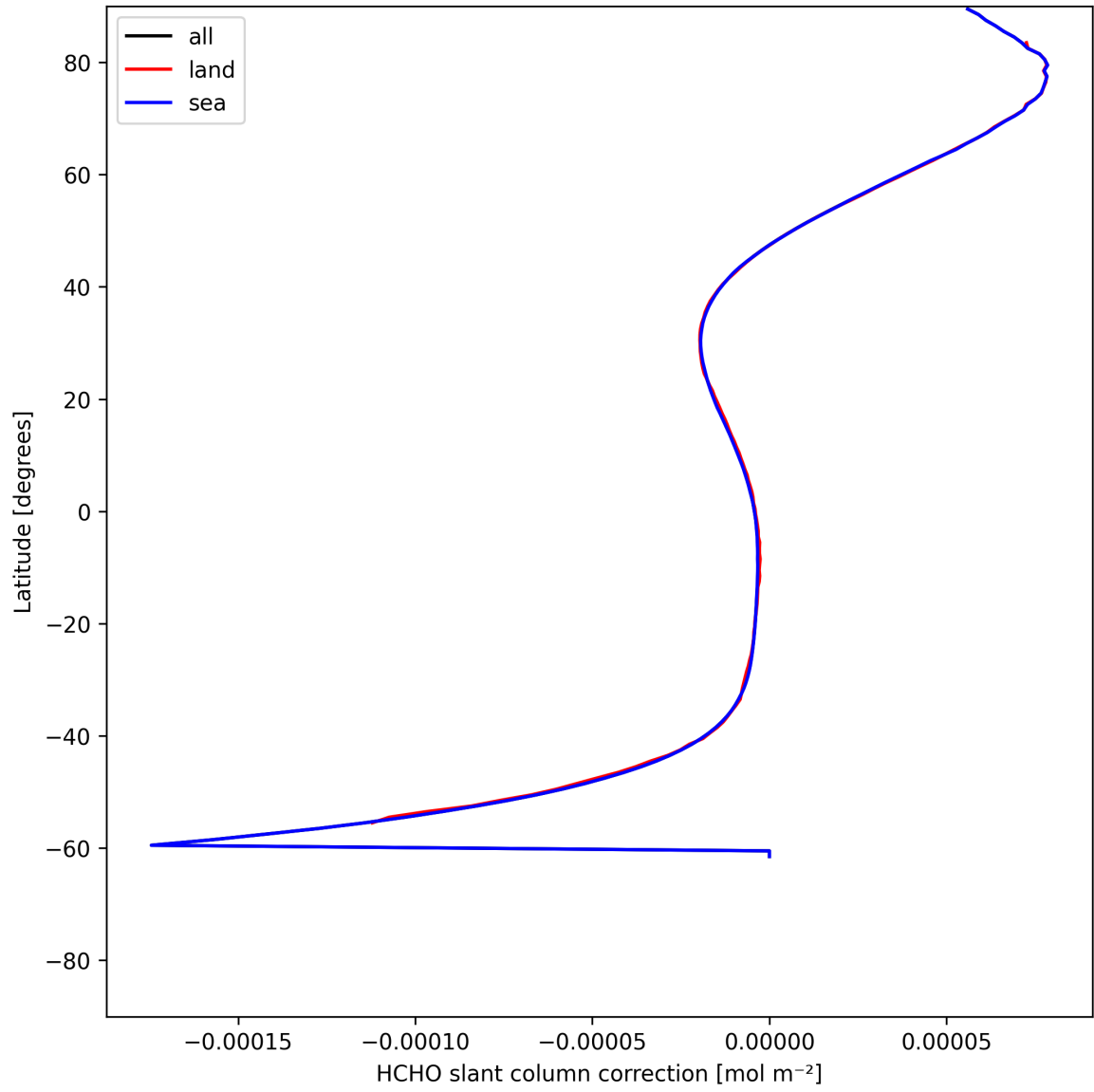
Figure 33: Zonal average of “HCHO slant column correction” for 2025-06-04 to 2025-06-06.
