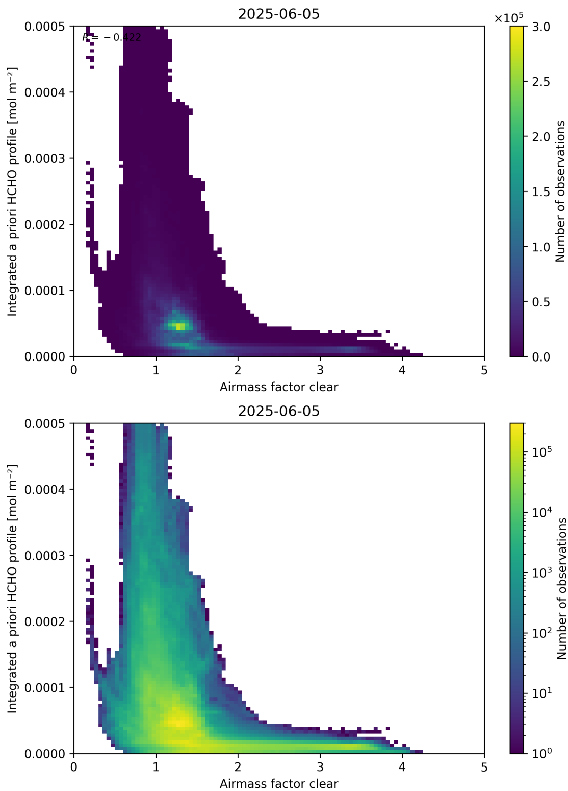
Figure 76: Scatter density plot of “Airmass factor clear” against “Integrated a priori HCHO profile” for 2025-06-04 to 2025-06-06.
