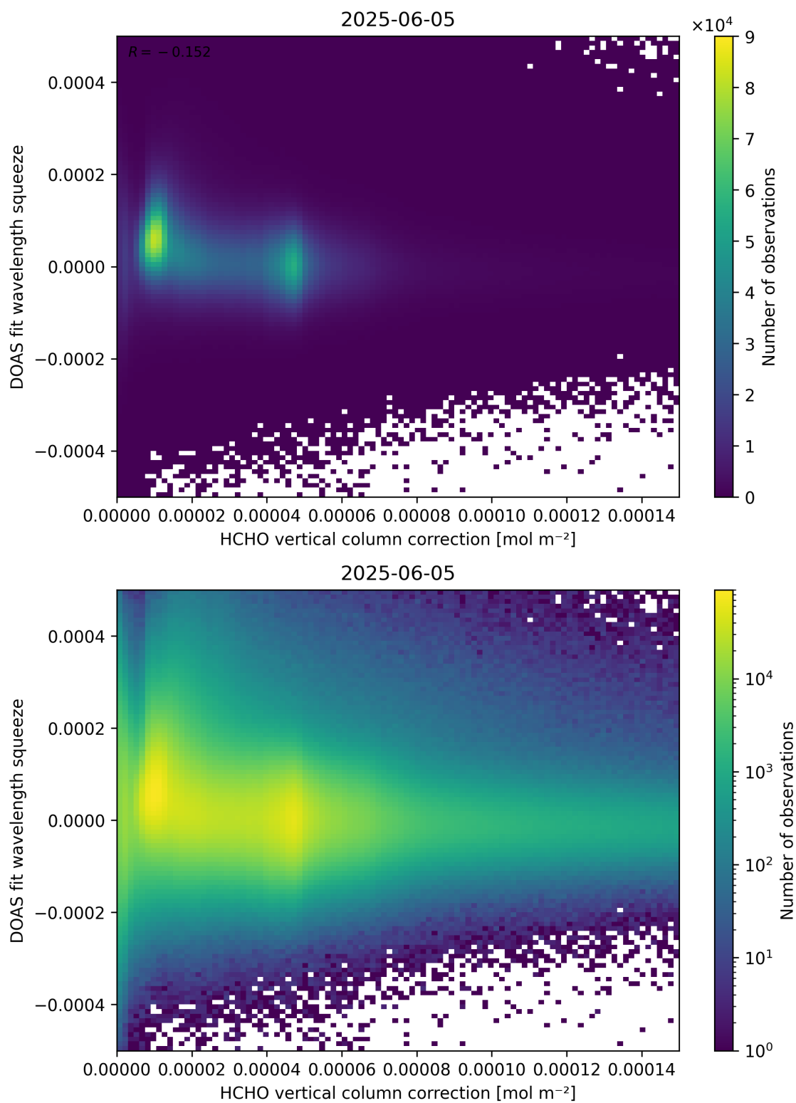
Figure 114: Scatter density plot of “HCHO vertical column correction” against “DOAS fit wavelength squeeze” for 2025-06-04 to 2025-06-06.
