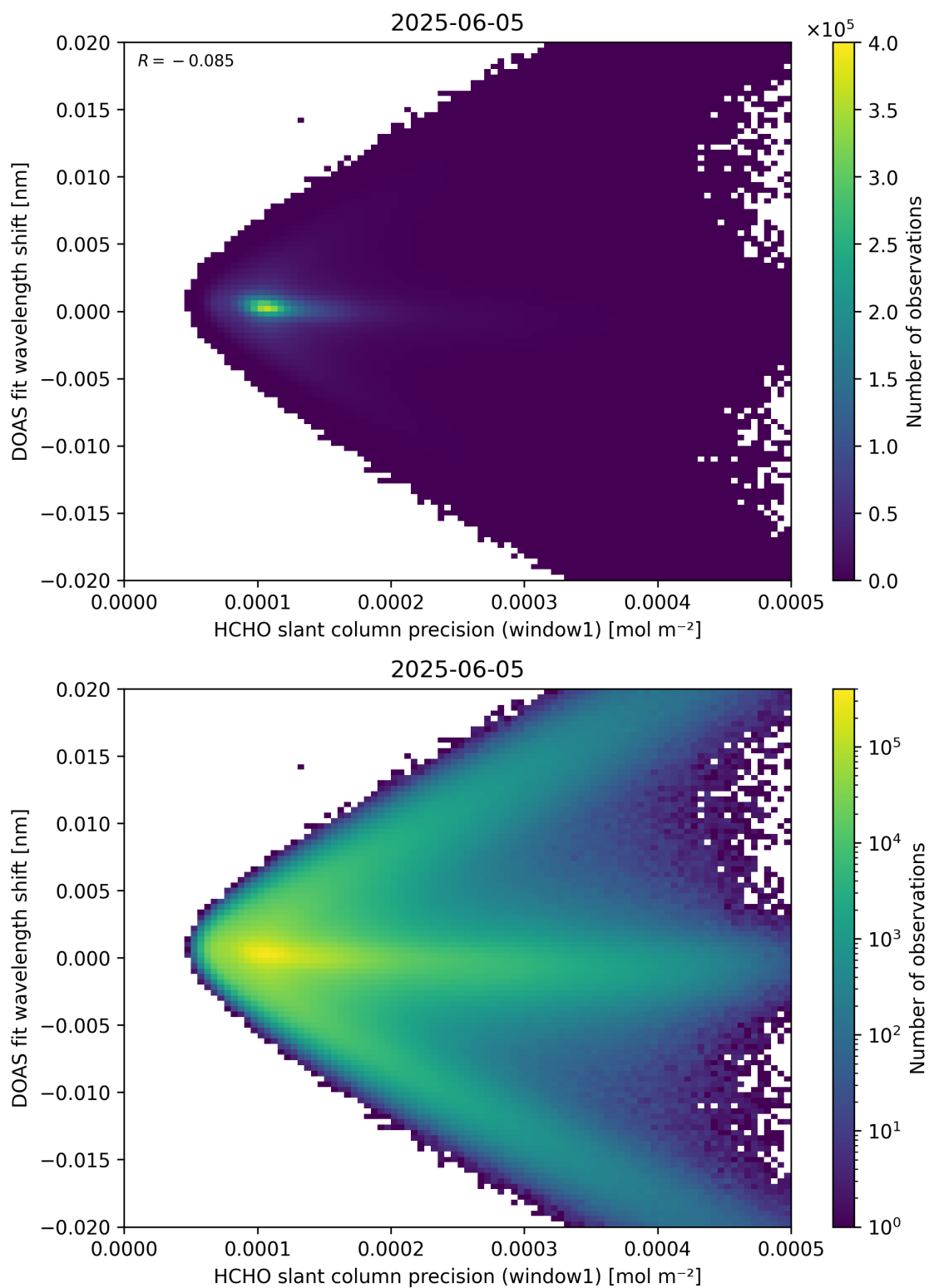
Figure 89: Scatter density plot of “HCHO slant column precision (window1)” against “DOAS fit wavelength shift” for 2025-06-04 to 2025-06-06.
