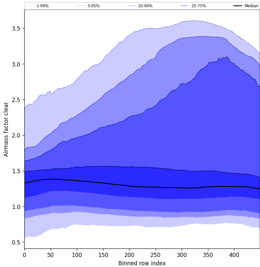
Figure 56: Along track statistics of “Air mass factor clear” for 2025-06-04 to 2025-06-06
