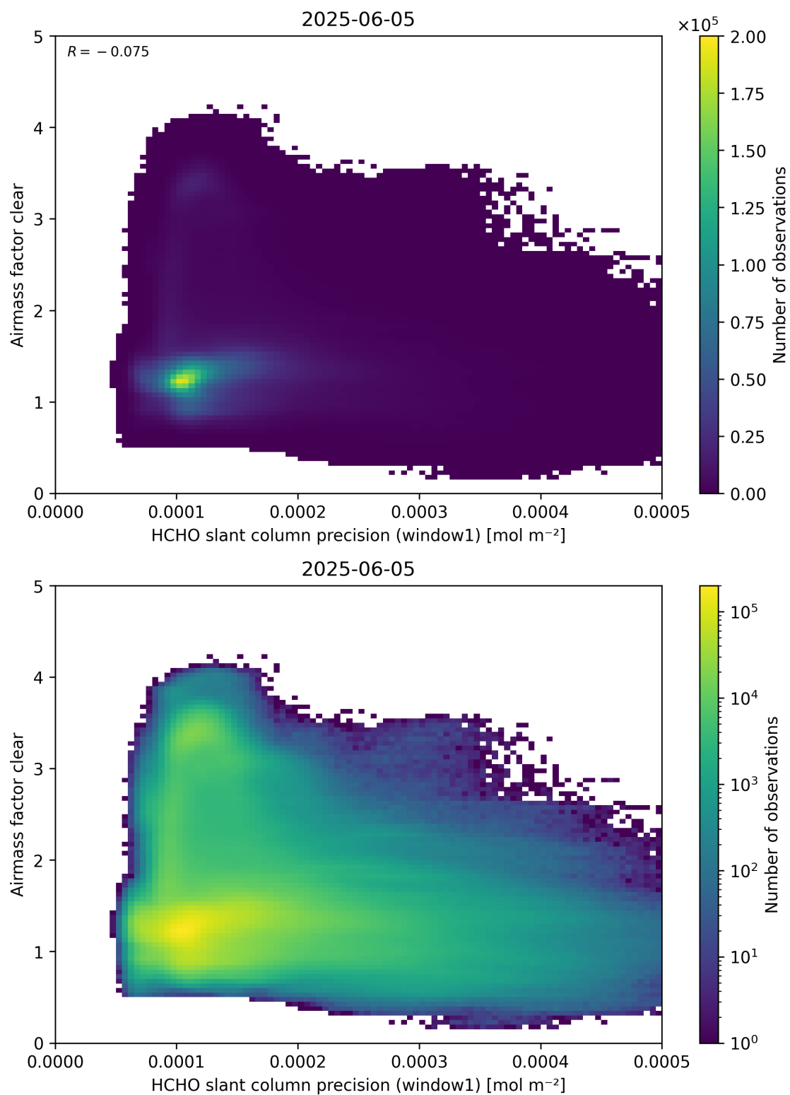
Figure 91: Scatter density plot of “HCHO slant column precision (window1)” against “Airmass factor clear” for 2025-06-04 to 2025-06-06.
