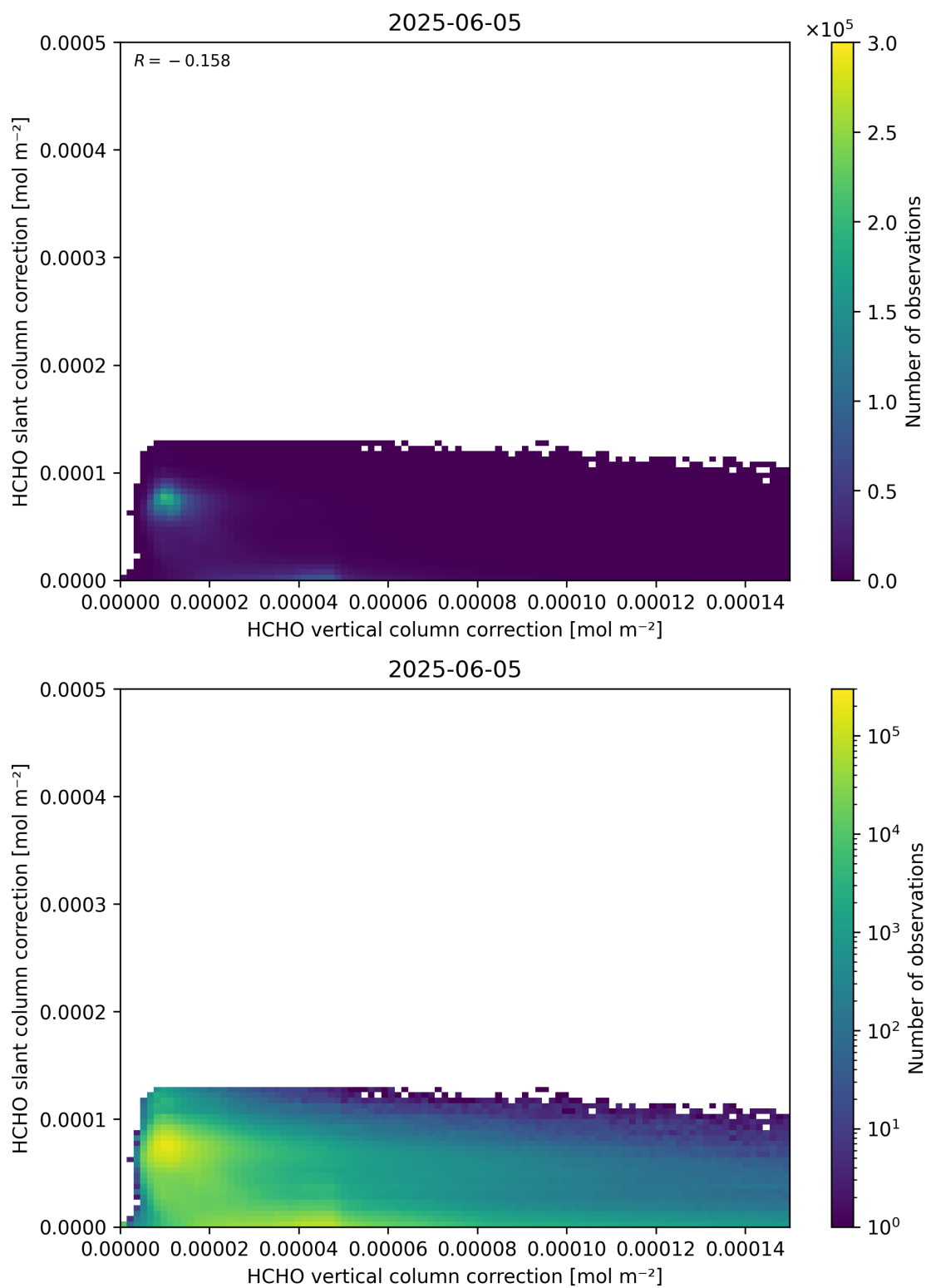
Figure 117: Scatter density plot of “HCHO vertical column correction” against “HCHO slant column correction” for 2025-06-04 to 2025-06-06.
