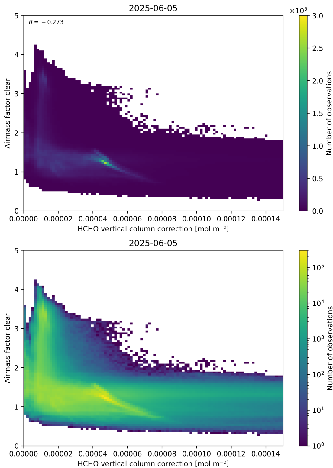
Figure 115: Scatter density plot of “HCHO vertical column correction” against “Airmass factor clear” for 2025-06-04 to 2025-06-06.
