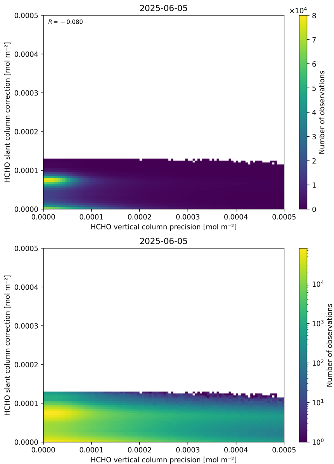
Figure 141: Scatter density plot of “HCHO vertical column precision” against “HCHO slant column correction” for 2025-06-04 to 2025-06-06.
