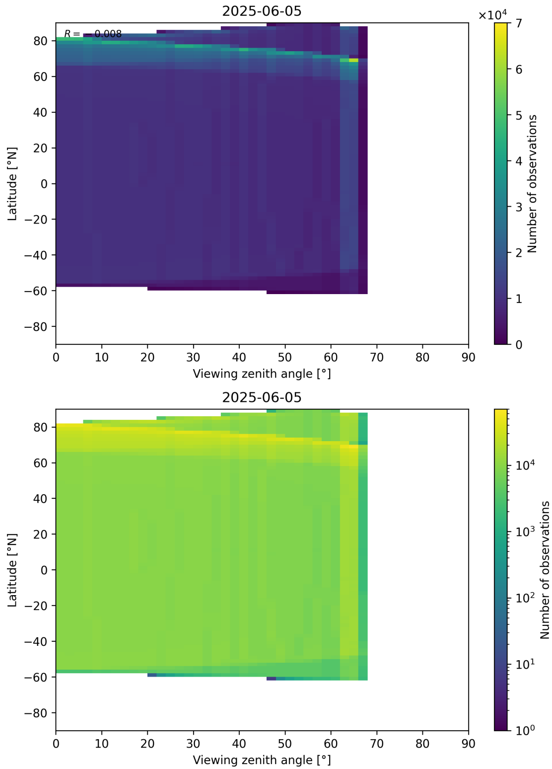
Figure 196: Scatter density plot of “Viewing zenith angle” against “Latitude” for 2025-06-04 to 2025-06-06.
