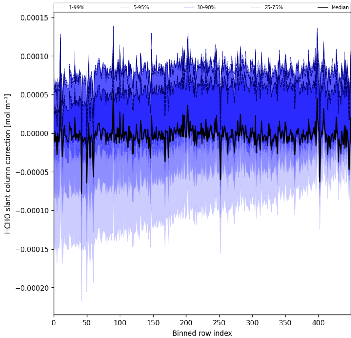
Figure 61: Along track statistics of “HCHO slant column correction” for 2025-06-07 to 2025-06-09
