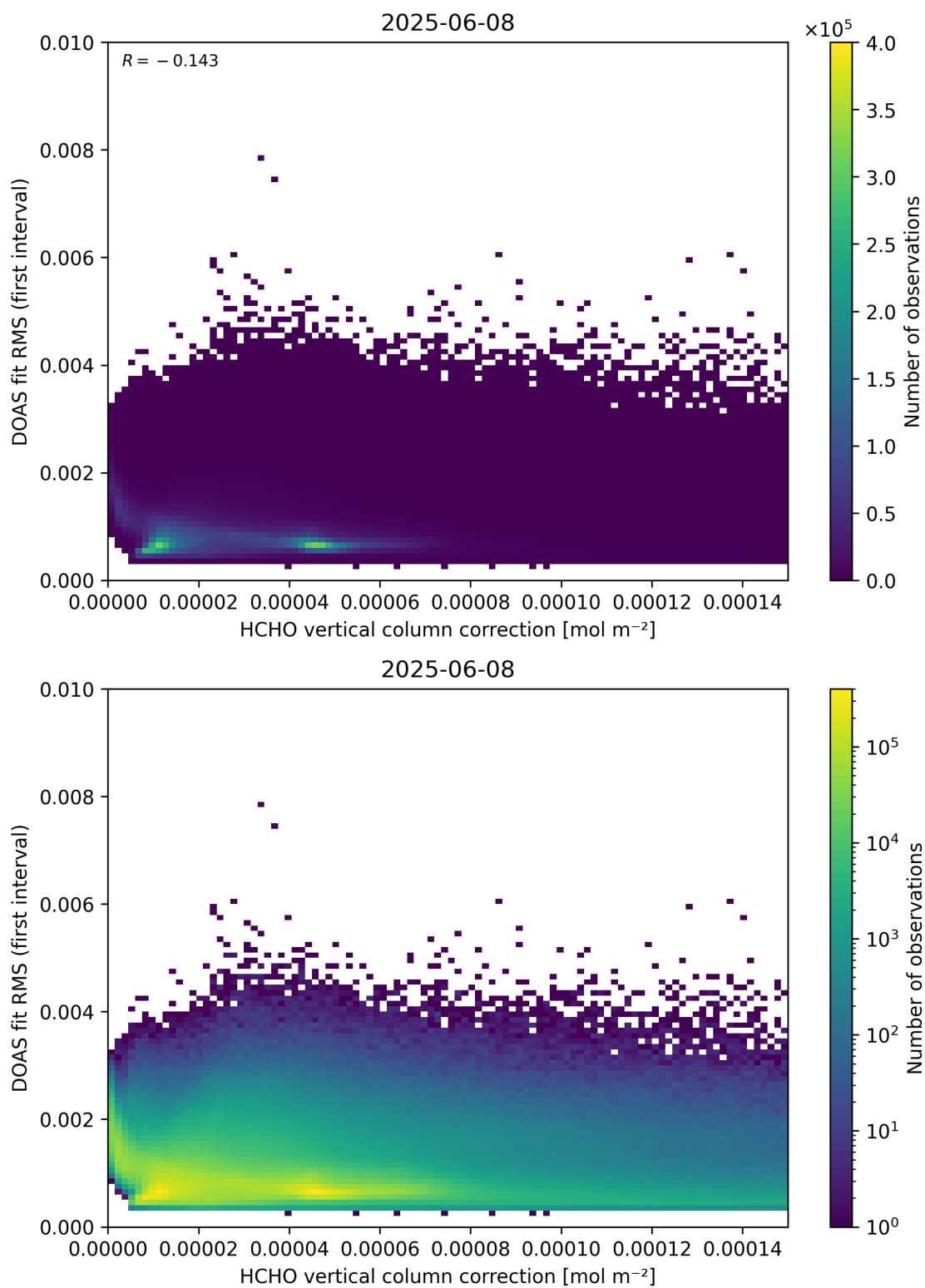
Figure 112: Scatter density plot of “HCHO vertical column correction” against “DOAS fit RMS (first interval)” for 2025-06-07 to 2025-06-09.
