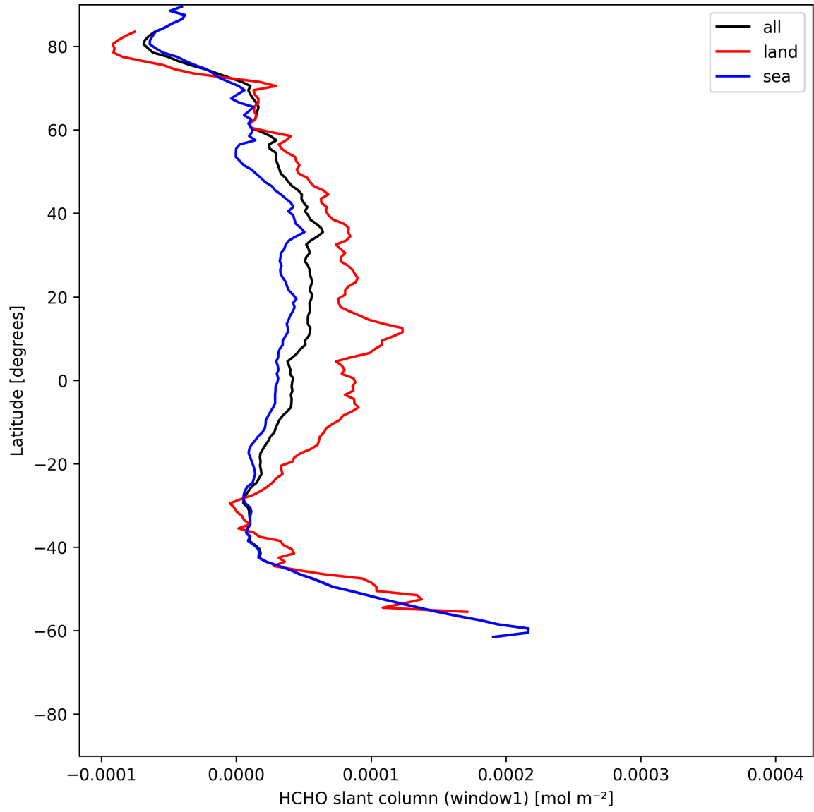
Figure 24: Zonal average of “HCHO slant column (window1)” for 2025-06-07 to 2025-06-09.
