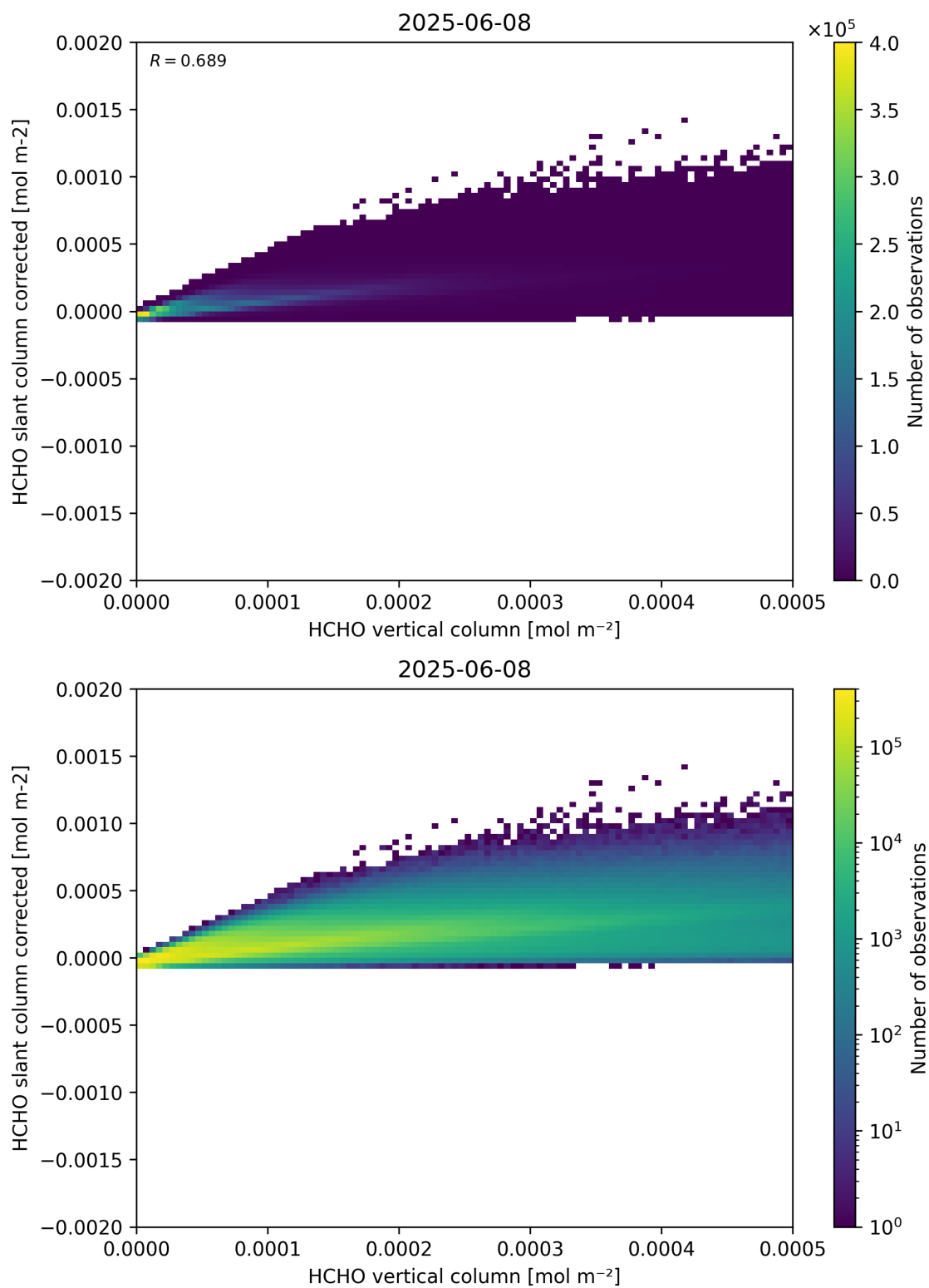
Figure 127: Scatter density plot of “HCHO vertical column” against “HCHO slant column corrected” for 2025-06-07 to 2025-06-09.
