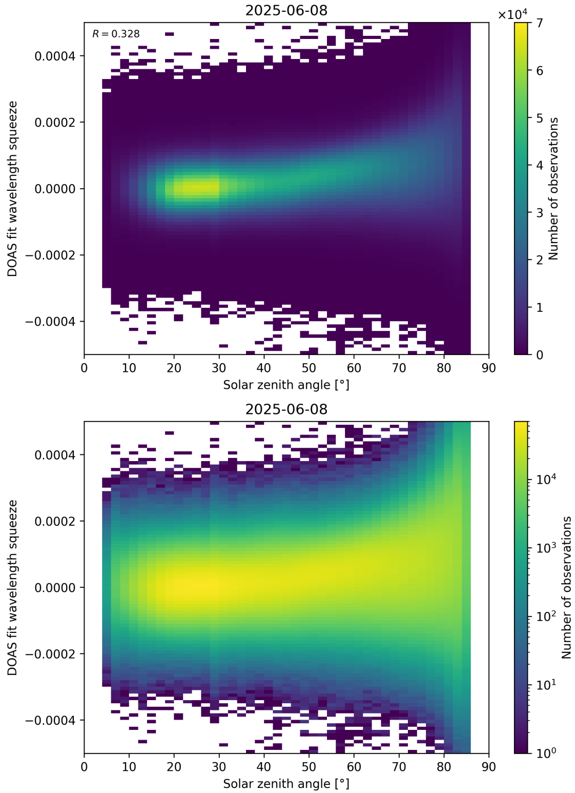
Figure 169: Scatter density plot of “Solar zenith angle” against “DOAS fit wavelength squeeze” for 2025-06-07 to 2025-06-09.
