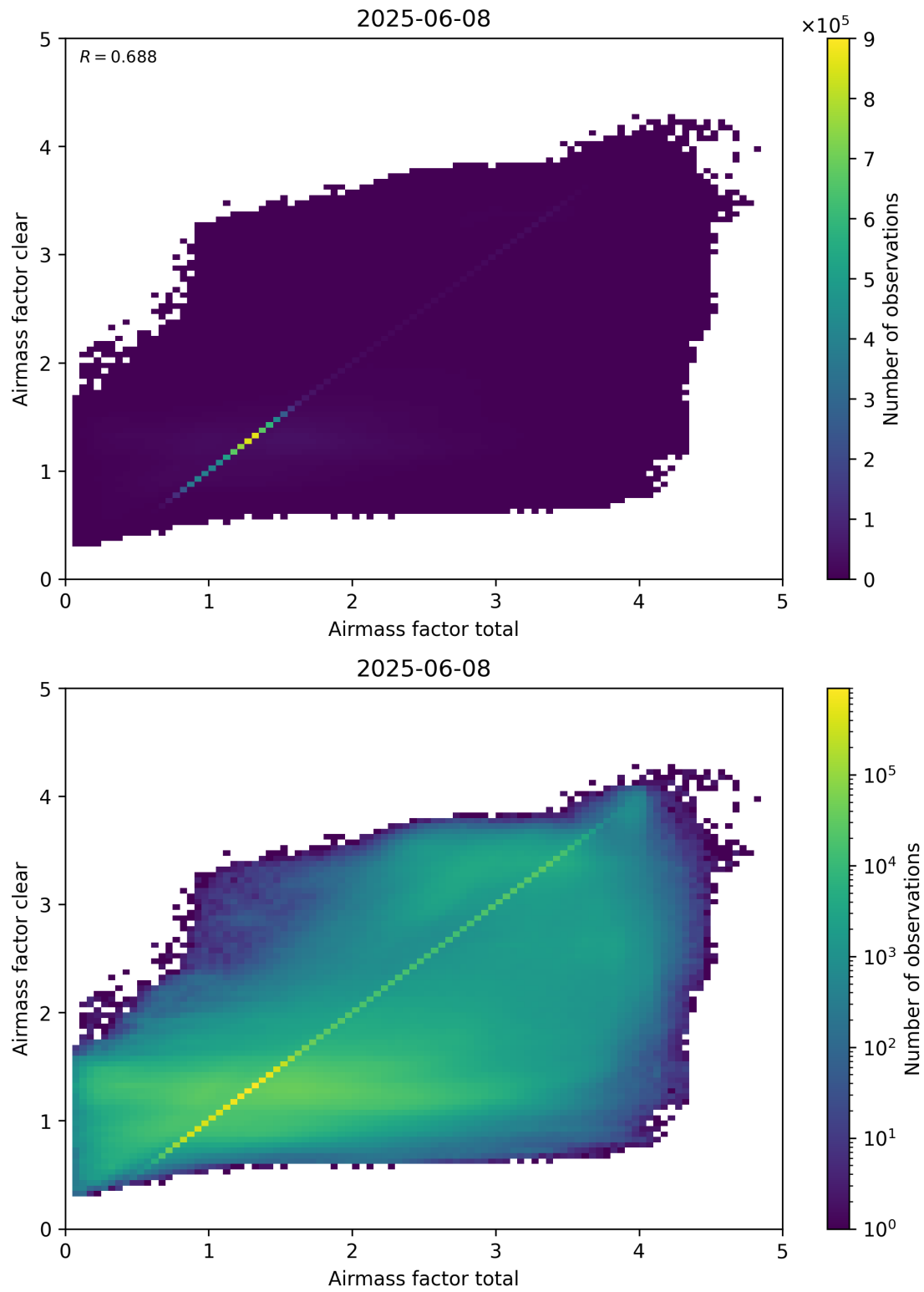
Figure 100: Scatter density plot of “Airmass factor total” against “Airmass factor clear” for 2025-06-07 to 2025-06-09.
