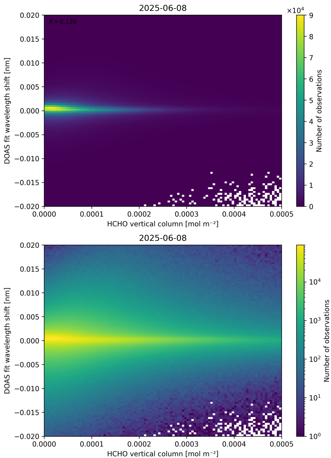
Figure 124: Scatter density plot of “HCHO vertical column” against “DOAS fit wavelength shift” for 2025-06-07 to 2025-06-09.
