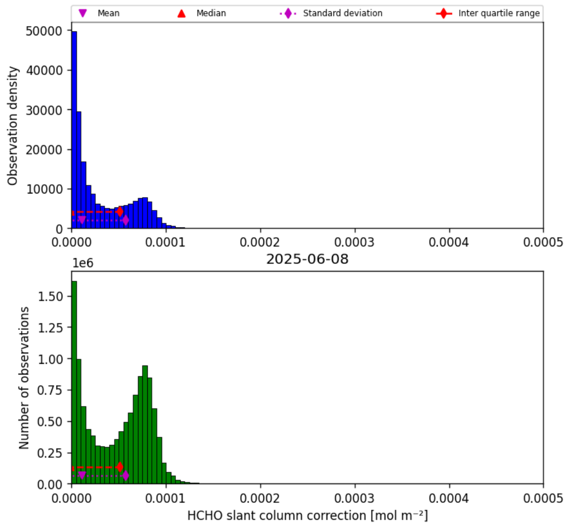
Figure 47: Histogram of “HCHO slant column correction” for 2025-06-07 to 2025-06-09
