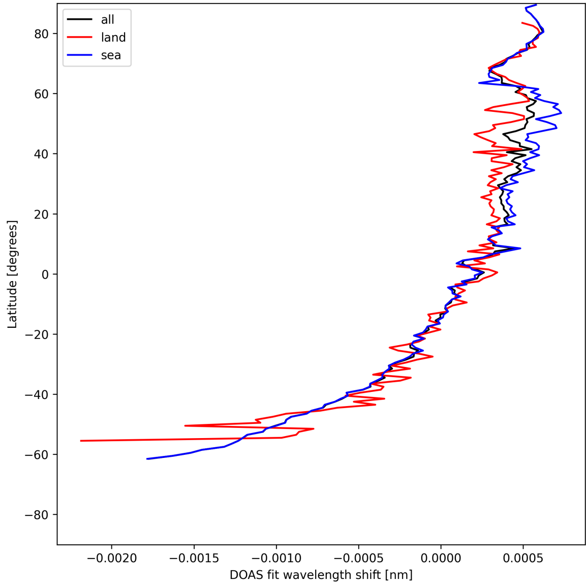
Figure 30: Zonal average of “DOAS fit wavelength shift” for 2025-06-07 to 2025-06-09.
