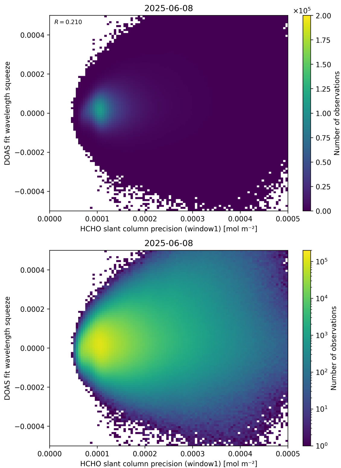
Figure 90: Scatter density plot of “HCHO slant column precision (window1)” against “DOAS fit wavelength squeeze” for 2025-06-07 to 2025-06-09.
