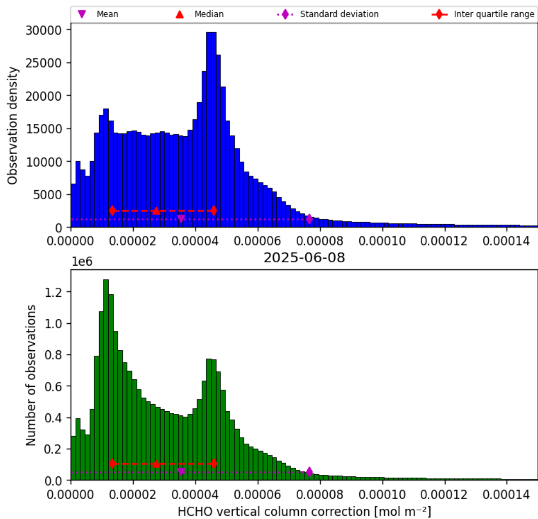
Figure 37: Histogram of “HCHO vertical column correction” for 2025-06-07 to 2025-06-09
