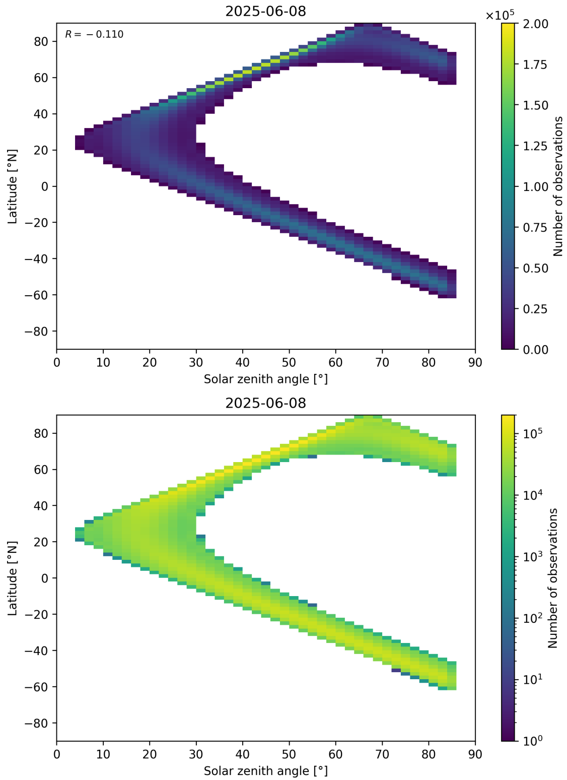
Figure 181: Scatter density plot of “Solar zenith angle” against “Latitude” for 2025-06-07 to 2025-06-09.
