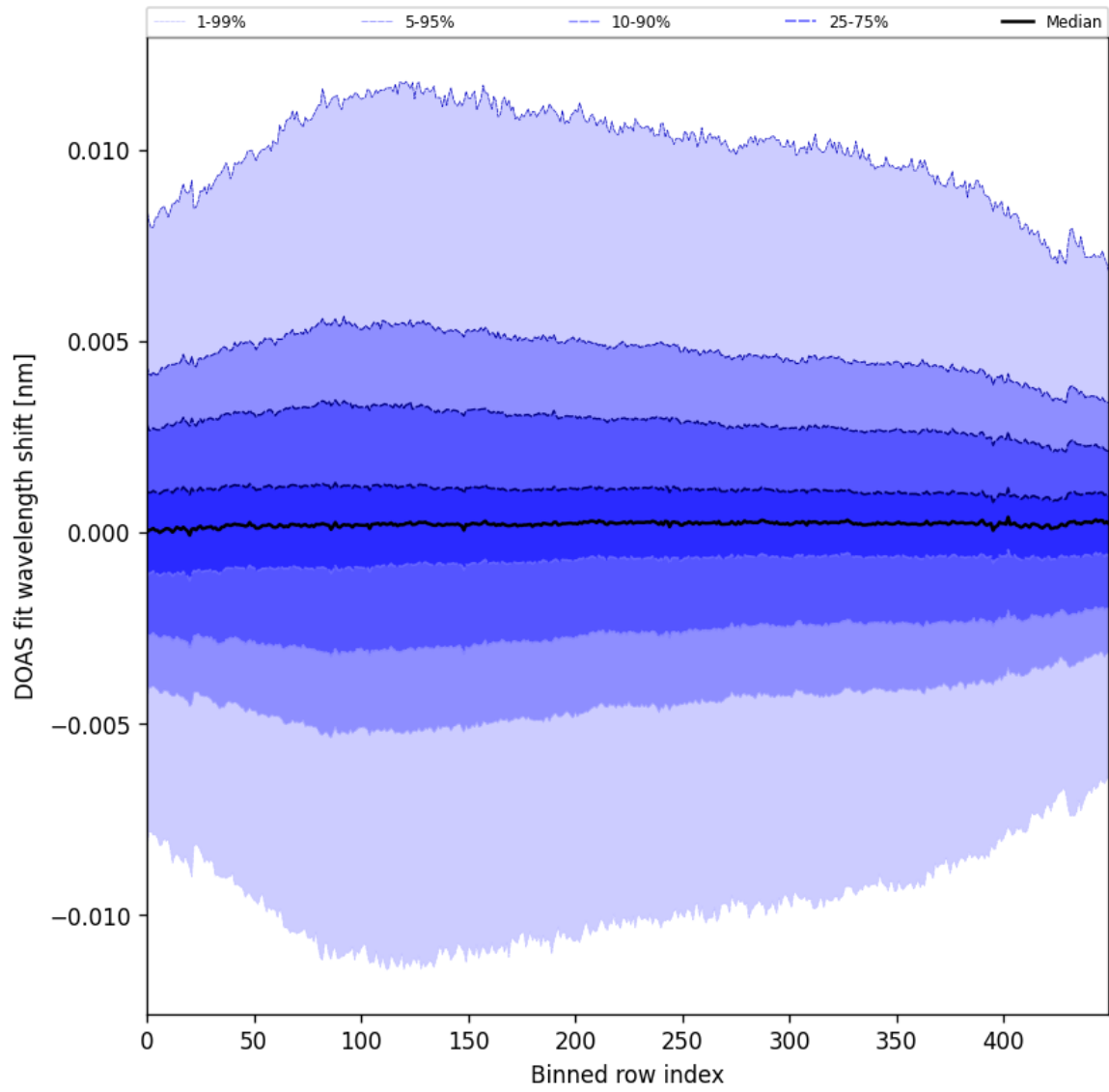
Figure 58: Along track statistics of “DOAS fit wavelength shift” for 2025-06-07 to 2025-06-09
