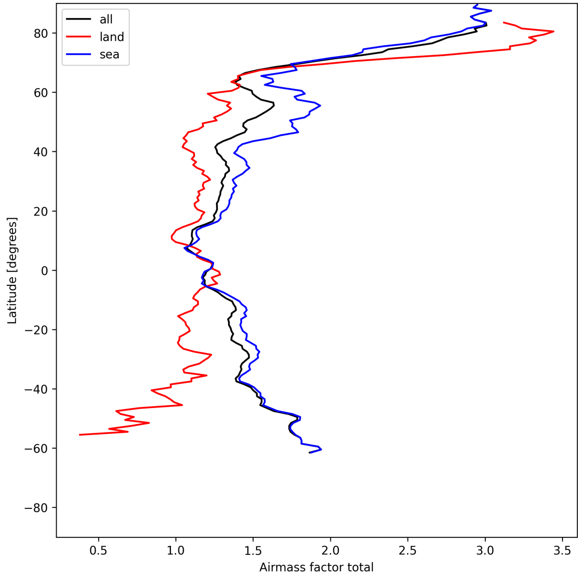
Figure 26: Zonal average of “Airmass factor total” for 2025-06-07 to 2025-06-09.
