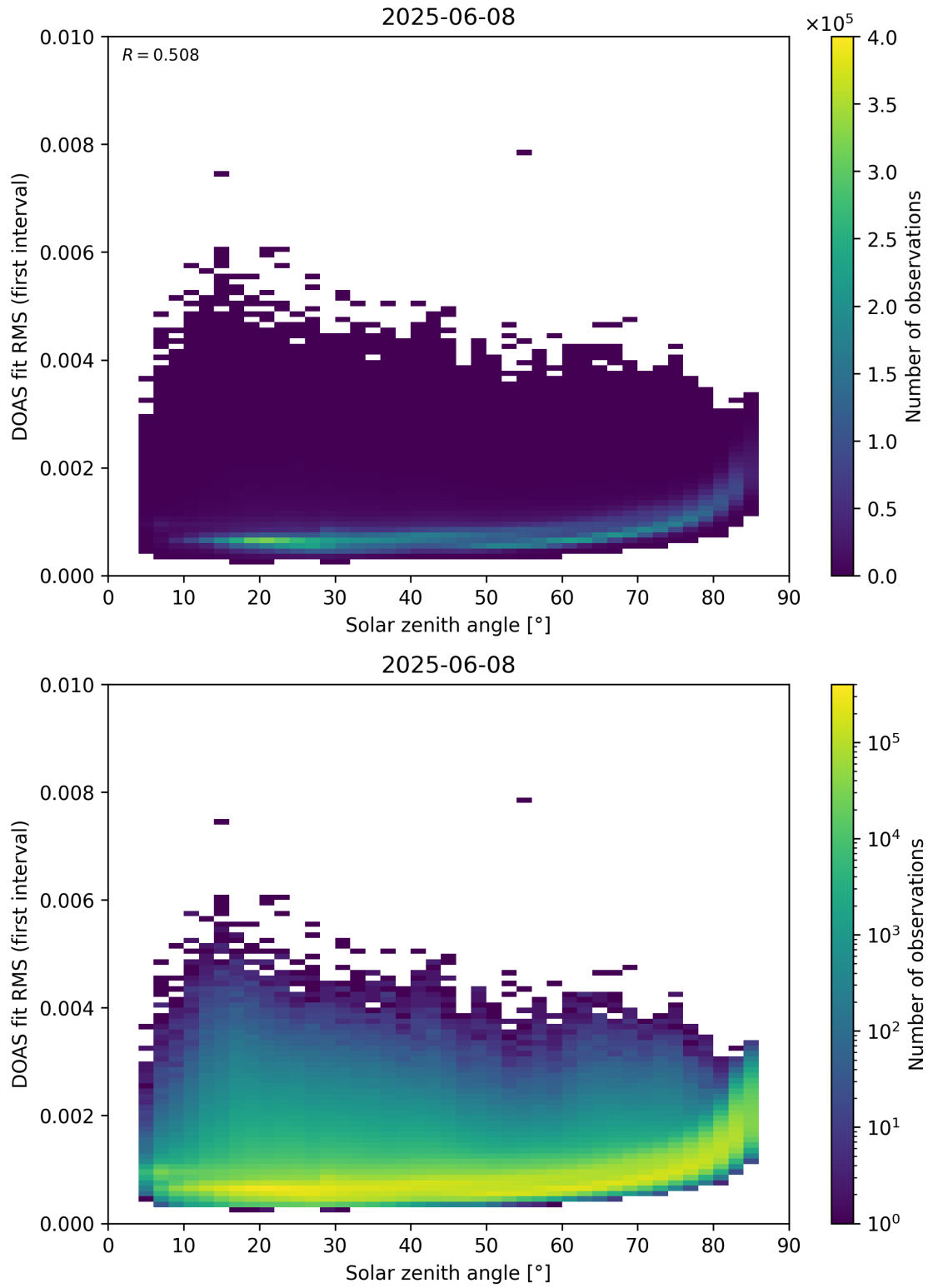
Figure 167: Scatter density plot of “Solar zenith angle” against “DOAS fit RMS (first interval)” for 2025-06-07 to 2025-06-09.
