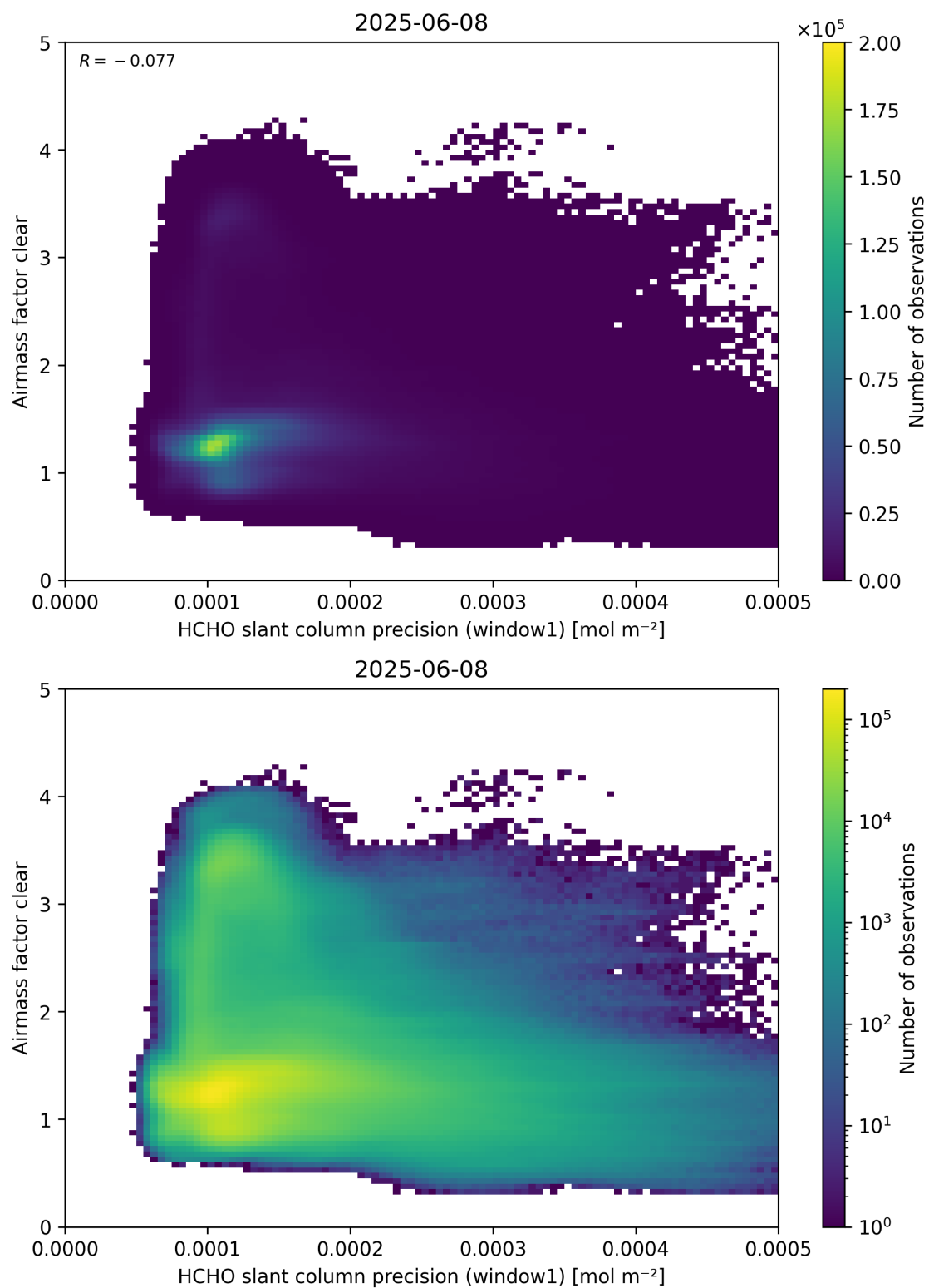
Figure 91: Scatter density plot of “HCHO slant column precision (window1)” against “Airmass factor clear” for 2025-06-07 to 2025-06-09.
