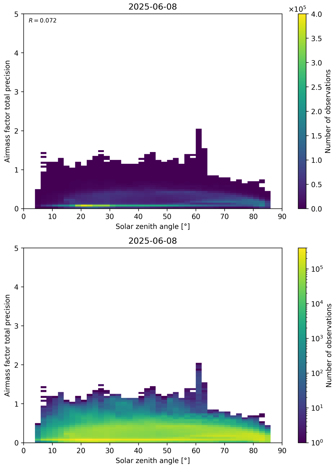
Figure 176: Scatter density plot of “Solar zenith angle” against “Airmass factor total precision” for 2025-06-07 to 2025-06-09.
