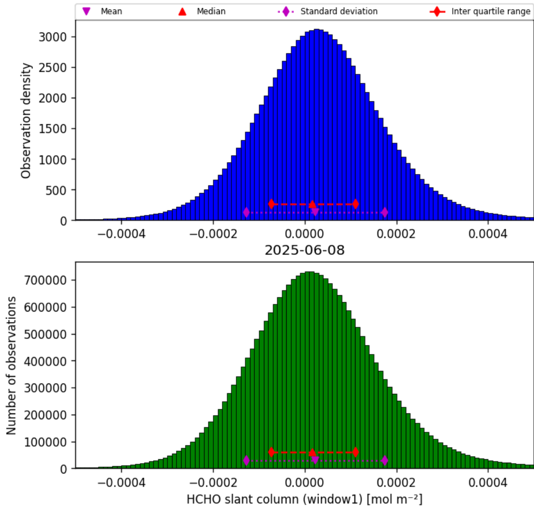
Figure 38: Histogram of “HCHO slant column (window1)” for 2025-06-07 to 2025-06-09
