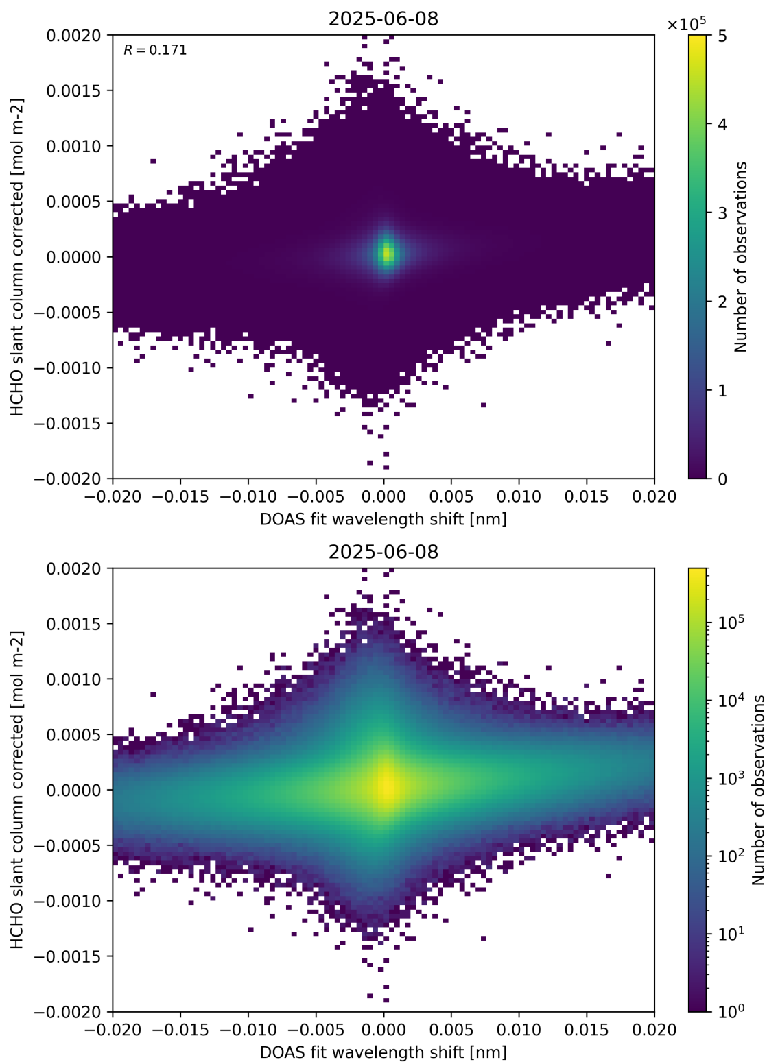
Figure 66: Scatter density plot of “DOAS fit wavelength shift” against “HCHO slant column corrected” for 2025-06-07 to 2025-06-09.
