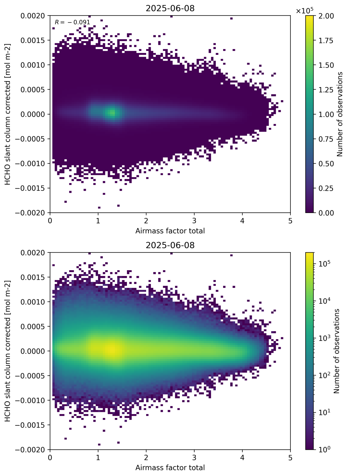
Figure 101: Scatter density plot of “Airmass factor total” against “HCHO slant column corrected” for 2025-06-07 to 2025-06-09.
