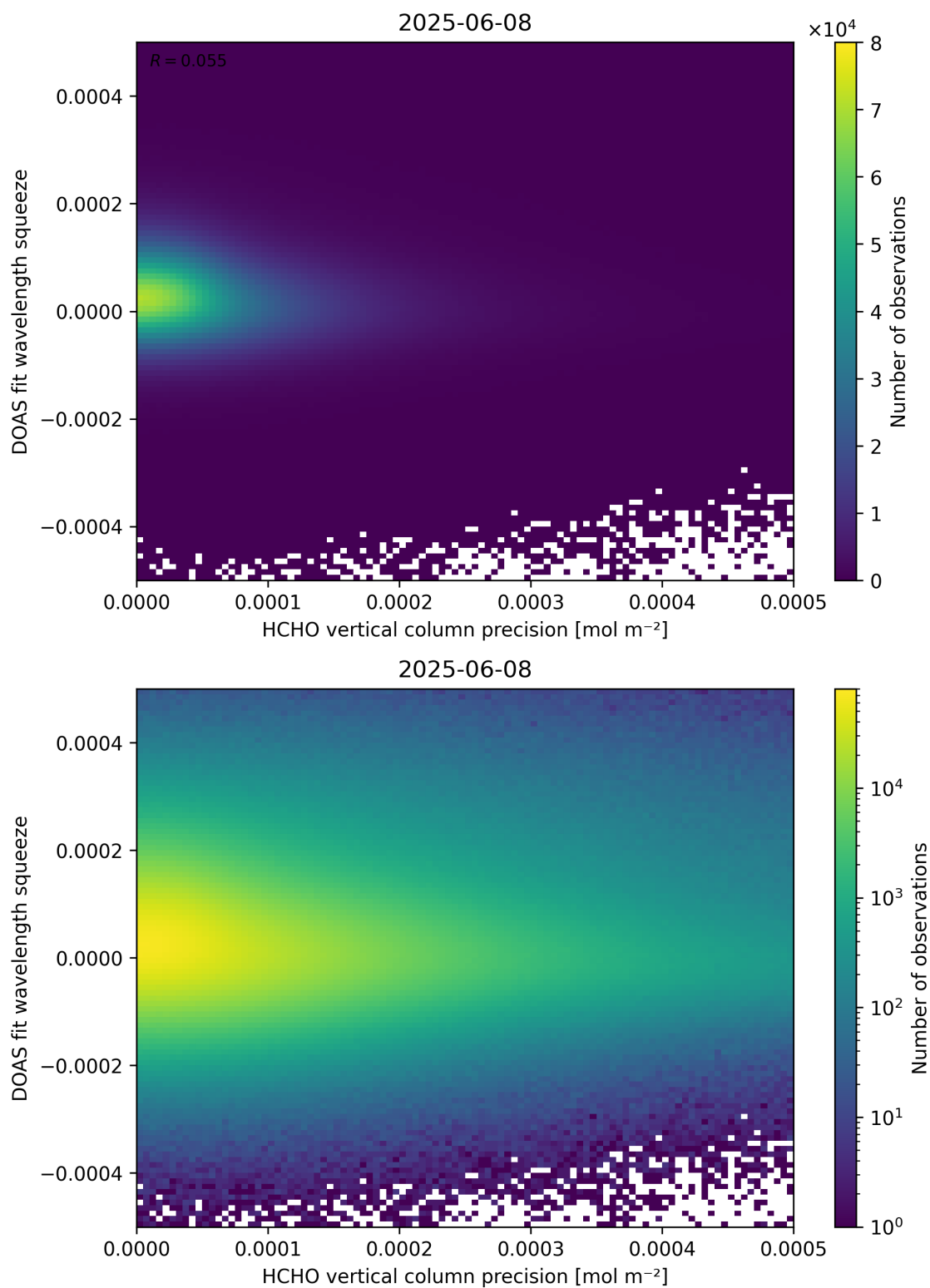
Figure 138: Scatter density plot of “HCHO vertical column precision” against “DOAS fit wavelength squeeze” for 2025-06-07 to 2025-06-09.
