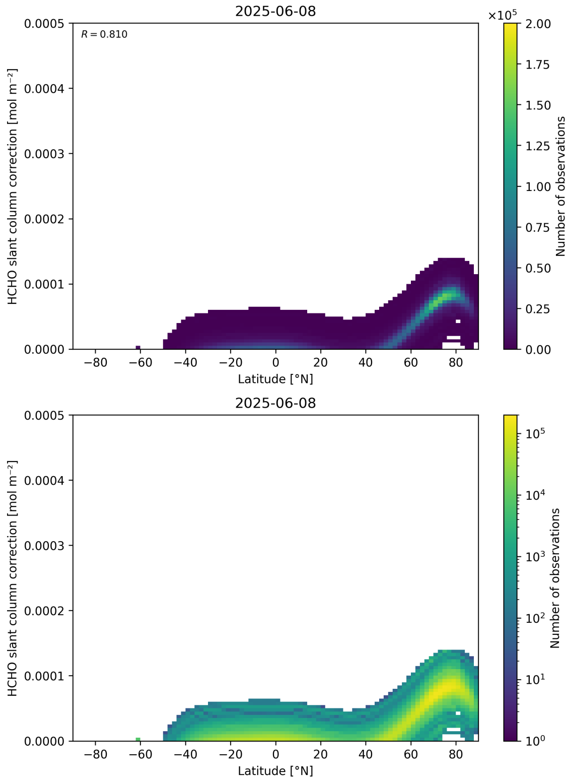
Figure 158: Scatter density plot of “Latitude” against “HCHO slant column correction” for 2025-06-07 to 2025-06-09.
