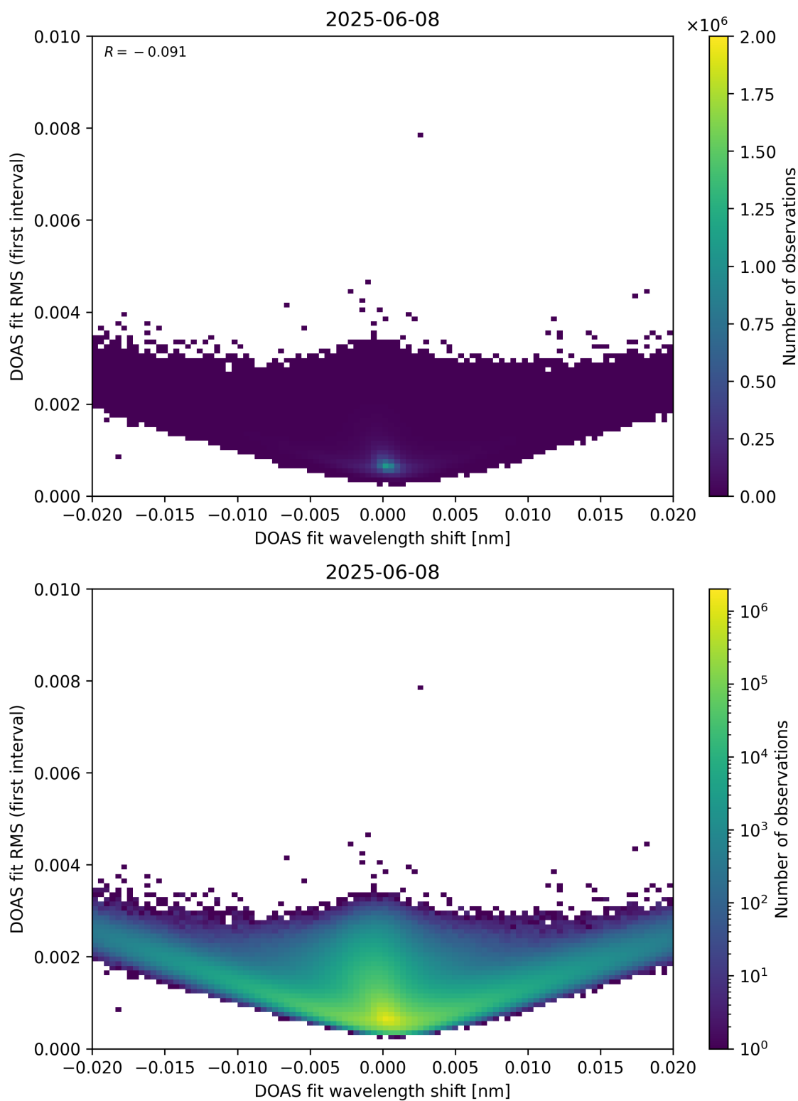
Figure 64: Scatter density plot of “DOAS fit wavelength shift” against “DOAS fit RMS (first interval)” for 2025-06-07 to 2025-06-09.
