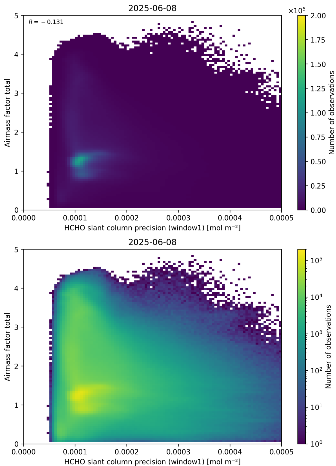
Figure 94: Scatter density plot of “HCHO slant column precision (window1)” against “Airmass factor total” for 2025-06-07 to 2025-06-09.
