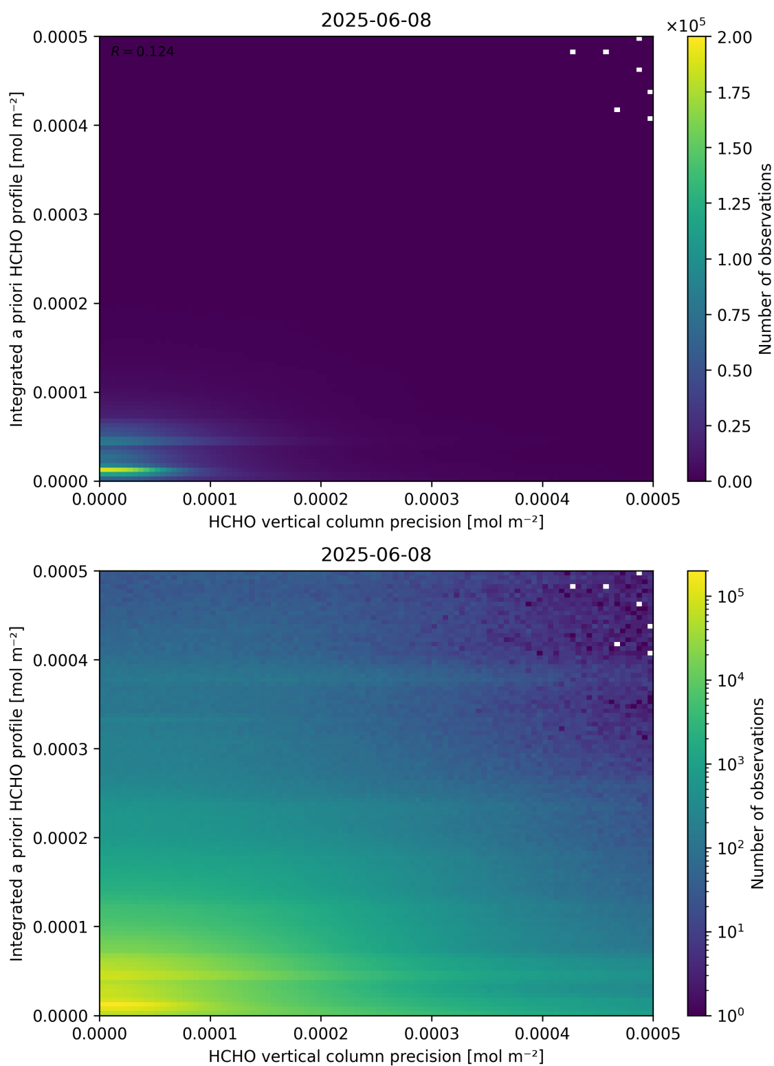
Figure 147: Scatter density plot of “HCHO vertical column precision” against “Integrated a priori HCHO profile” for 2025-06-07 to 2025-06-09.
