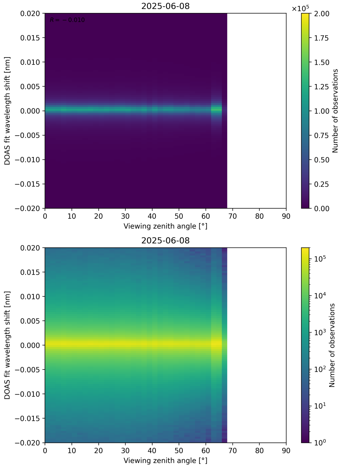
Figure 183: Scatter density plot of “Viewing zenith angle” against “DOAS fit wavelength shift” for 2025-06-07 to 2025-06-09.
