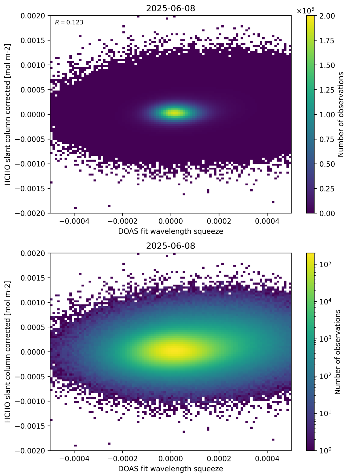
Figure 69: Scatter density plot of “DOAS fit wavelength squeeze” against “HCHO slant column corrected” for 2025-06-07 to 2025-06-09.
