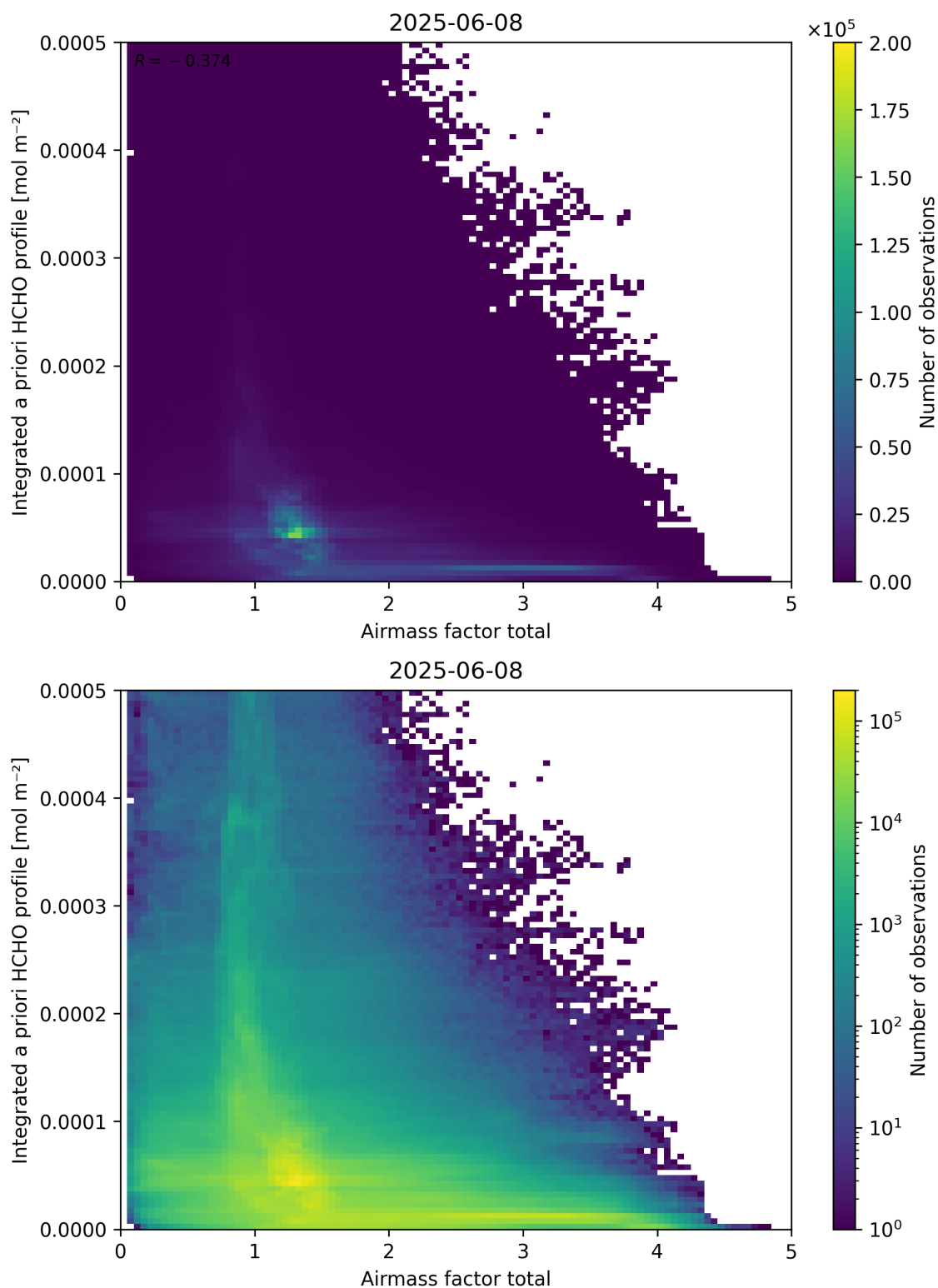
Figure 104: Scatter density plot of “Airmass factor total” against “Integrated a priori HCHO profile” for 2025-06-07 to 2025-06-09.
