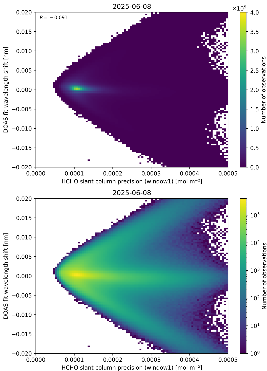
Figure 89: Scatter density plot of “HCHO slant column precision (window1)” against “DOAS fit wavelength shift” for 2025-06-07 to 2025-06-09.
