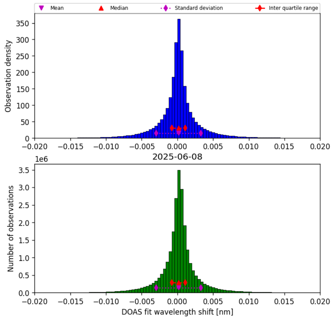
Figure 44: Histogram of “DOAS fit wavelength shift” for 2025-06-07 to 2025-06-09
