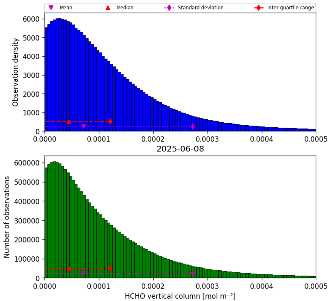
Figure 35: Histogram of “HCHO vertical column” for 2025-06-07 to 2025-06-09
