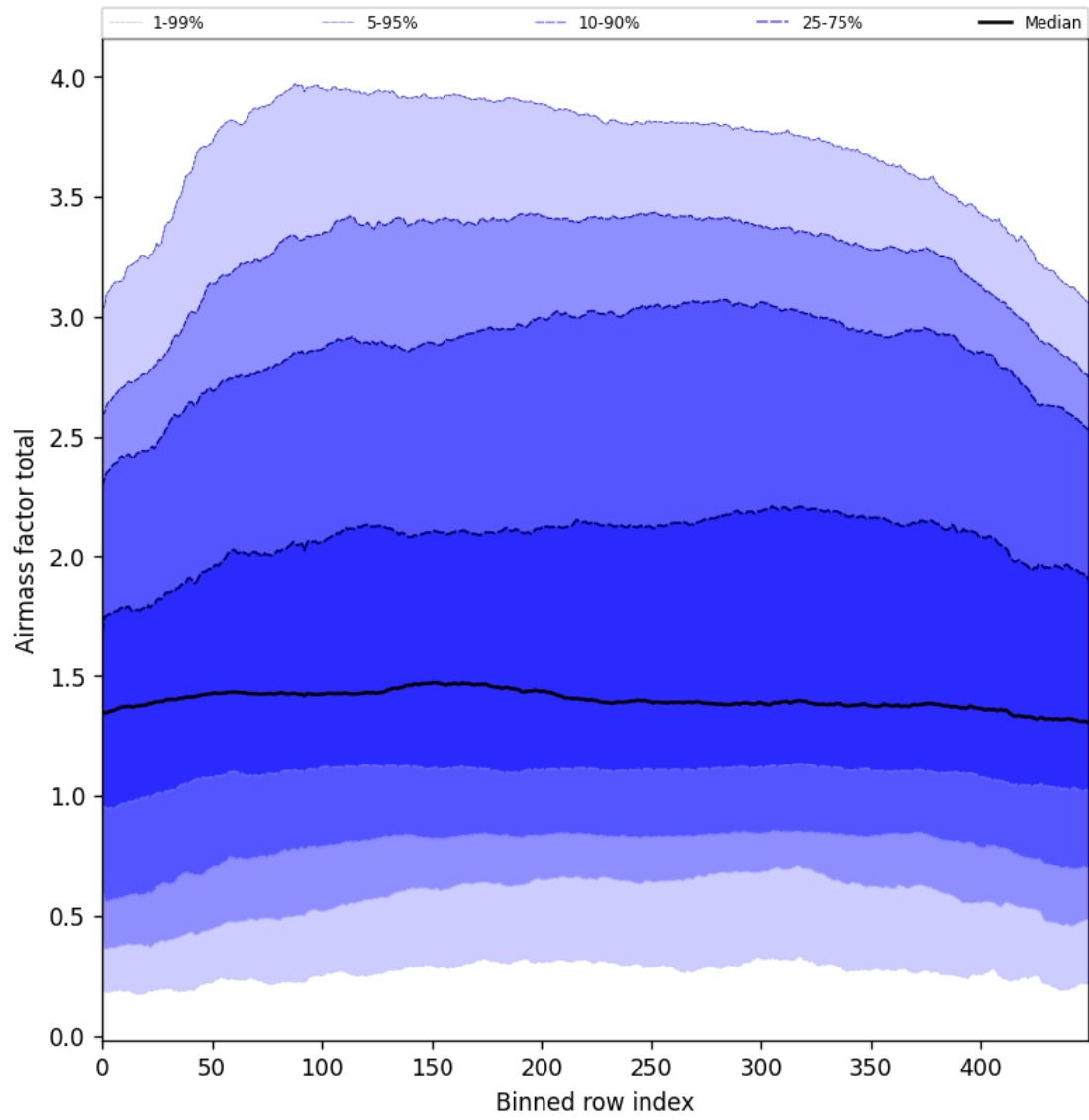
Figure 54: Along track statistics of “Airmass factor total” for 2025-06-07 to 2025-06-09
