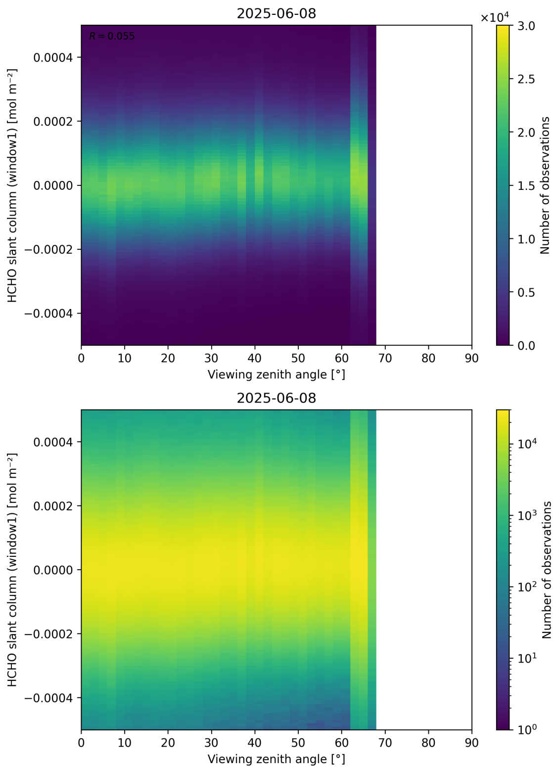
Figure 188: Scatter density plot of “Viewing zenith angle” against “HCHO slant column (window1)” for 2025-06-07 to 2025-06-09.
