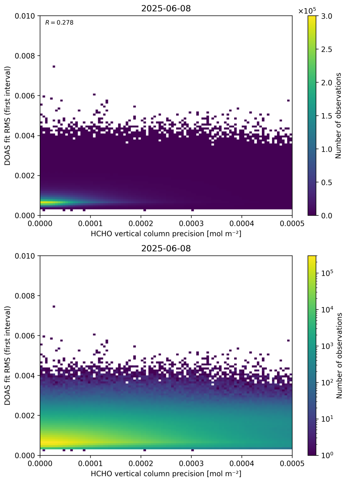
Figure 136: Scatter density plot of “HCHO vertical column precision” against “DOAS fit RMS (first interval)” for 2025-06-07 to 2025-06-09.
