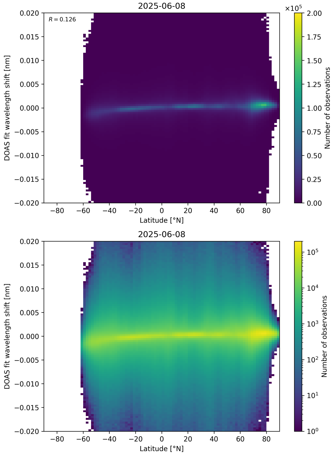
Figure 154: Scatter density plot of “Latitude” against “DOAS fit wavelength shift” for 2025-06-07 to 2025-06-09.
