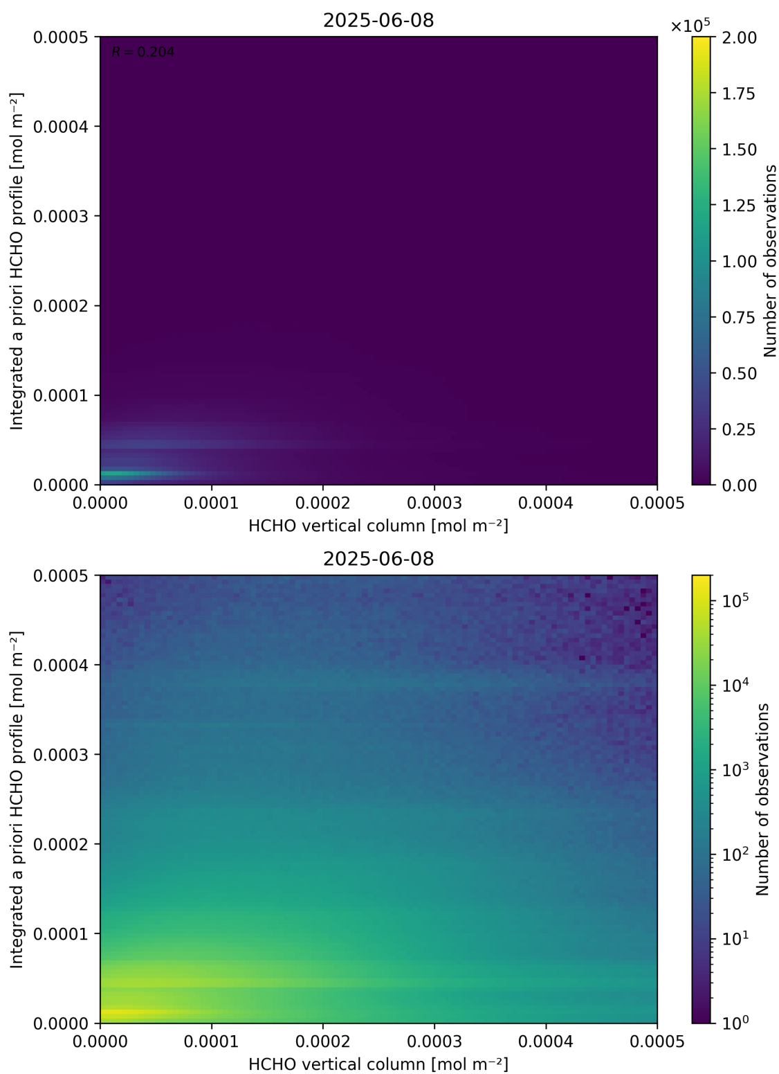
Figure 135: Scatter density plot of “HCHO vertical column” against “Integrated a priori HCHO profile” for 2025-06-07 to 2025-06-09.
