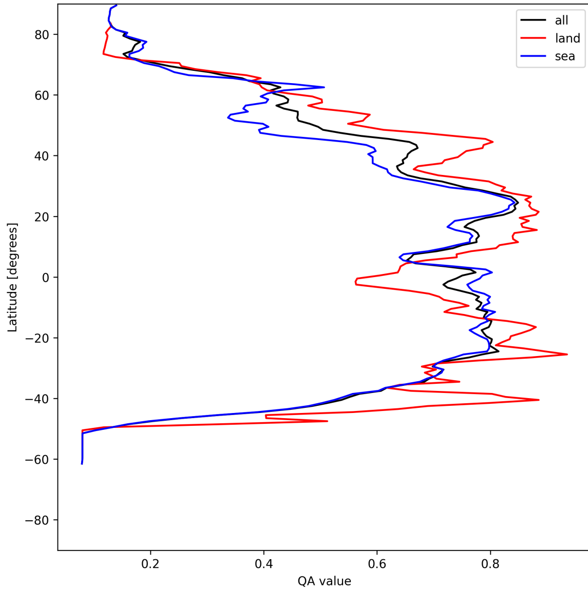
Figure 20: Zonal average of “QA value” for 2025-06-07 to 2025-06-09.
