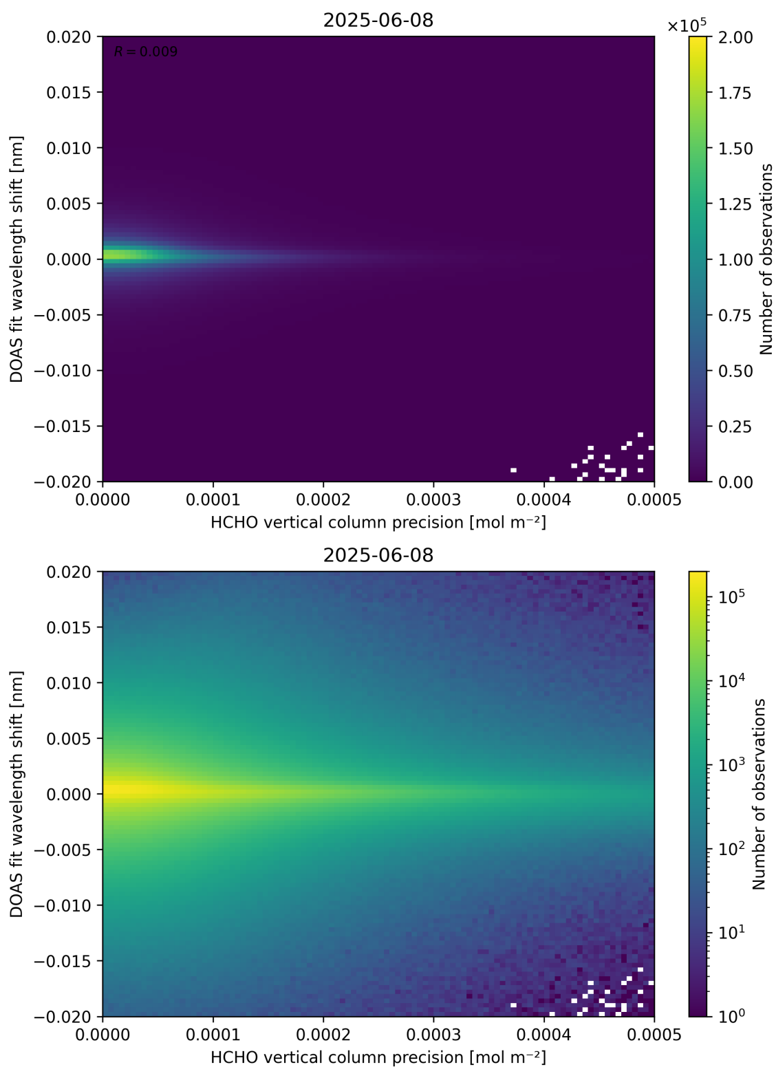
Figure 137: Scatter density plot of “HCHO vertical column precision” against “DOAS fit wavelength shift” for 2025-06-07 to 2025-06-09.
