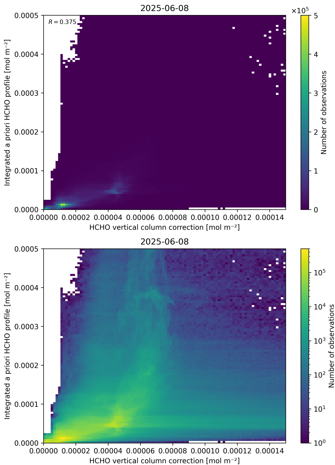
Figure 122: Scatter density plot of “HCHO vertical column correction” against “Integrated a priori HCHO profile” for 2025-06-07 to 2025-06-09.
