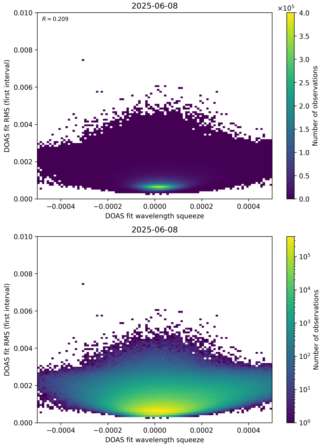
Figure 68: Scatter density plot of “DOAS fit wavelength squeeze” against “DOAS fit RMS (first interval)” for 2025-06-07 to 2025-06-09.
