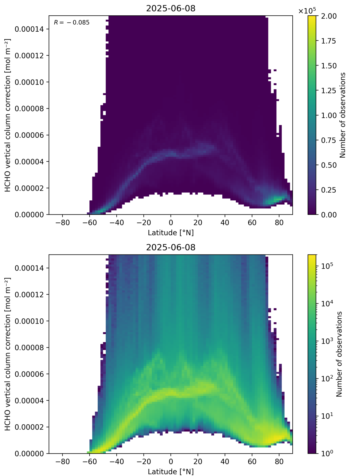
Figure 164: Scatter density plot of “Latitude” against “HCHO vertical column correction” for 2025-06-07 to 2025-06-09.
