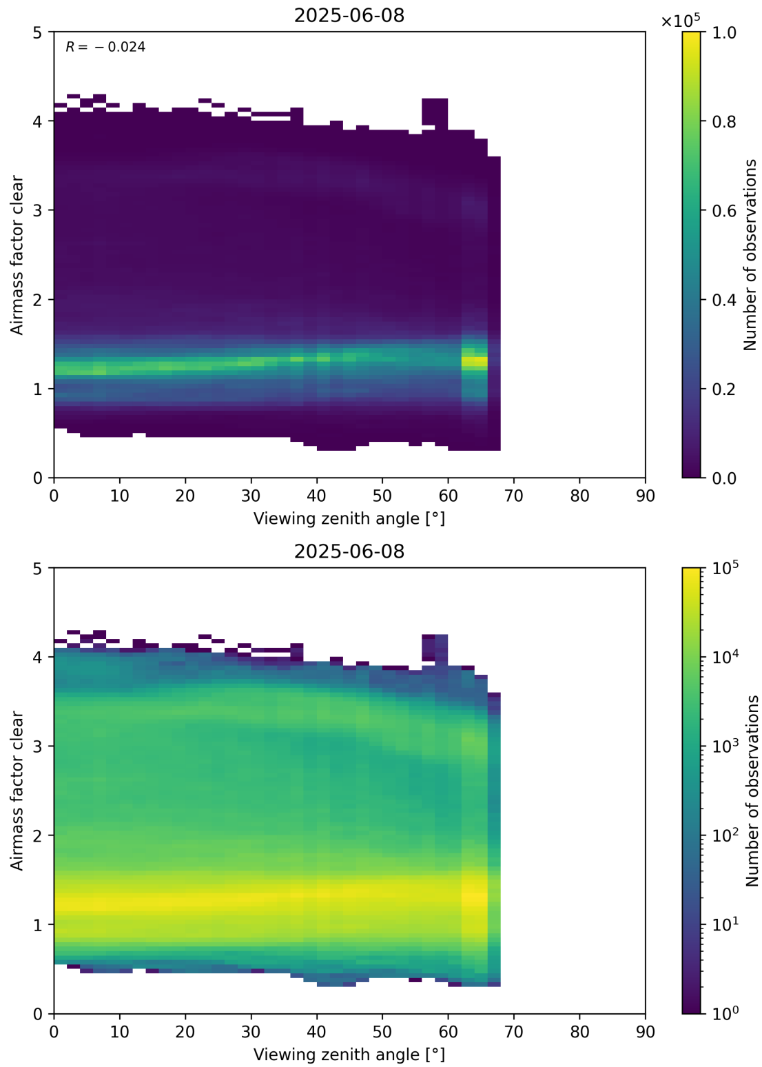
Figure 185: Scatter density plot of “Viewing zenith angle” against “Airmass factor clear” for 2025-06-07 to 2025-06-09.
