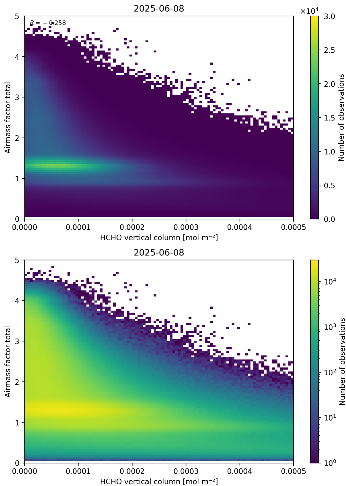
Figure 131: Scatter density plot of “HCHO vertical column” against “Airmass factor total” for 2025-06-07 to 2025-06-09.
