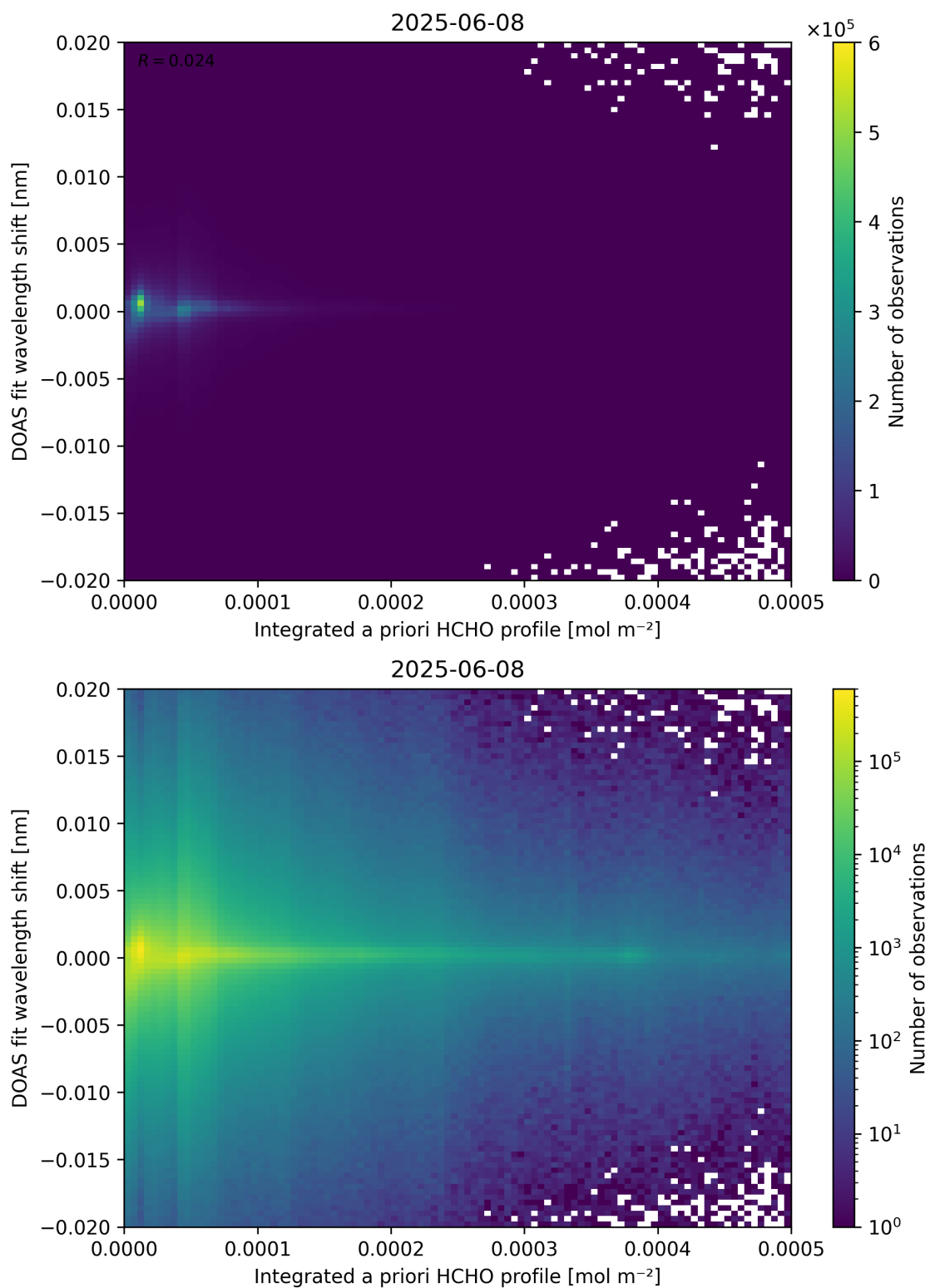
Figure 149: Scatter density plot of “Integrated a priori HCHO profile” against “DOAS fit wavelength shift” for 2025-06-07 to 2025-06-09.
