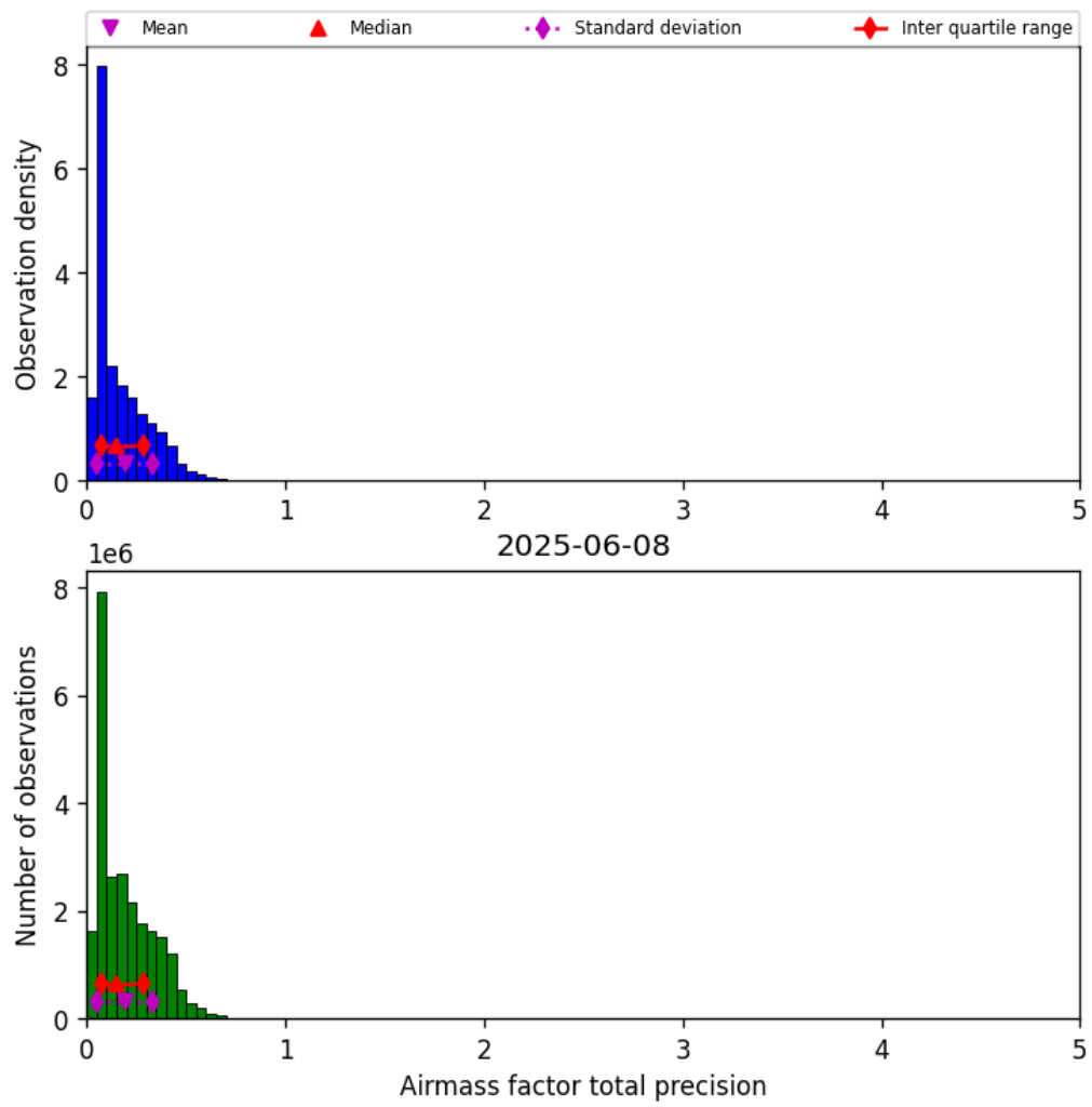
Figure 41: Histogram of “Airmass factor total precision” for 2025-06-07 to 2025-06-09
