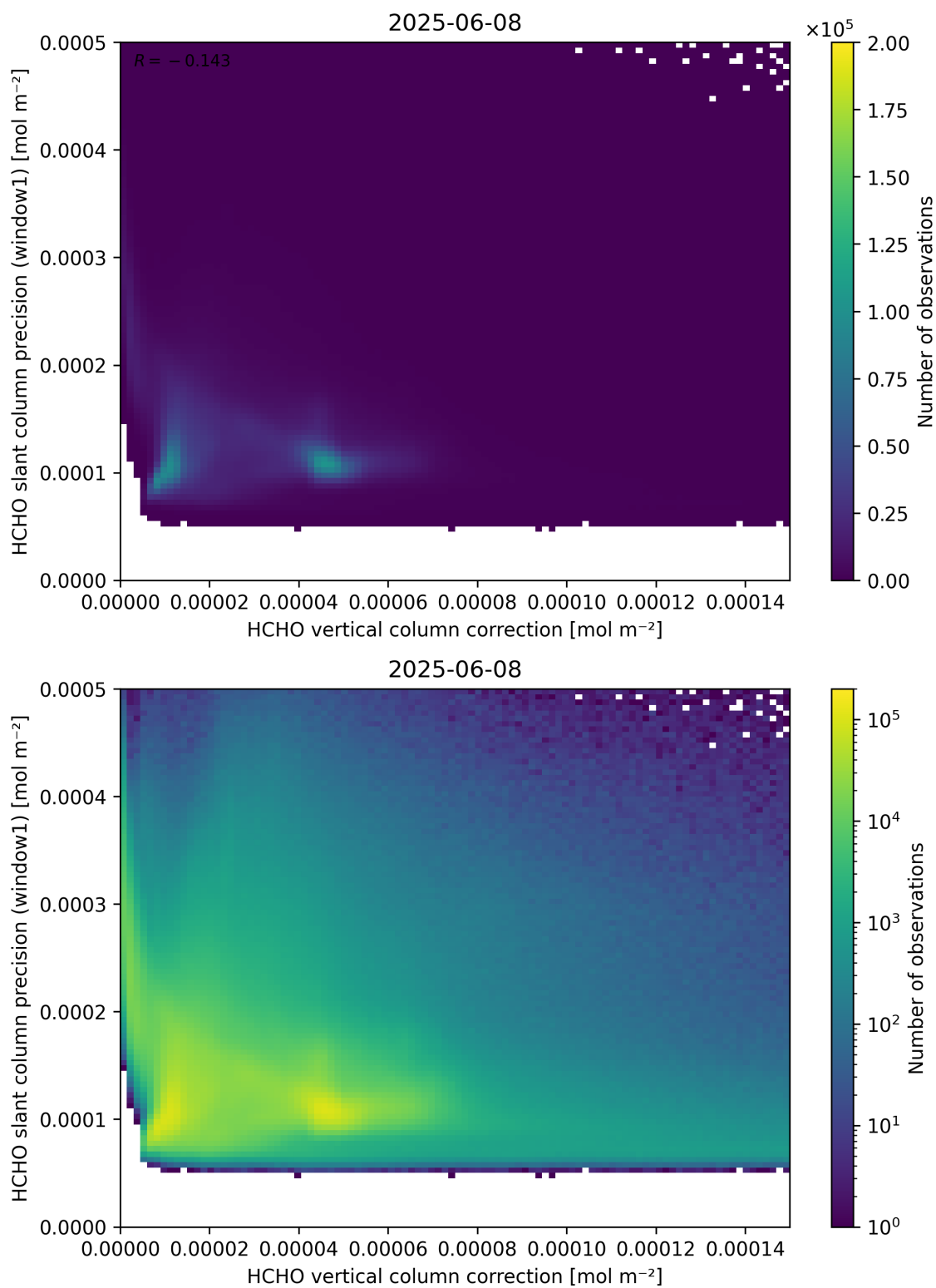
Figure 119: Scatter density plot of “HCHO vertical column correction” against “HCHO slant column precision (window1)” for 2025-06-07 to 2025-06-09.
