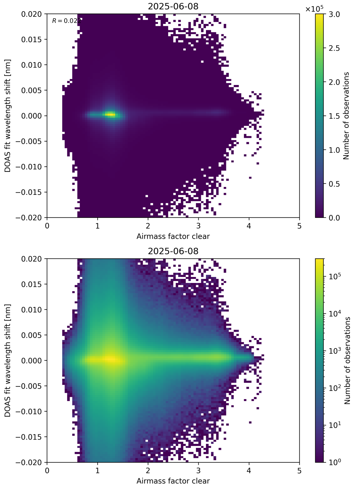
Figure 72: Scatter density plot of “Airmass factor clear” against “DOAS fit wavelength shift” for 2025-06-07 to 2025-06-09.
