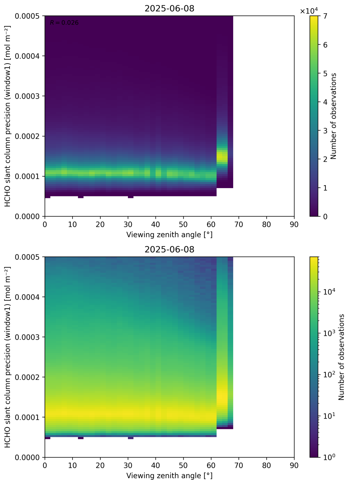
Figure 189: Scatter density plot of “Viewing zenith angle” against “HCHO slant column precision (window1)” for 2025-06-07 to 2025-06-09.
