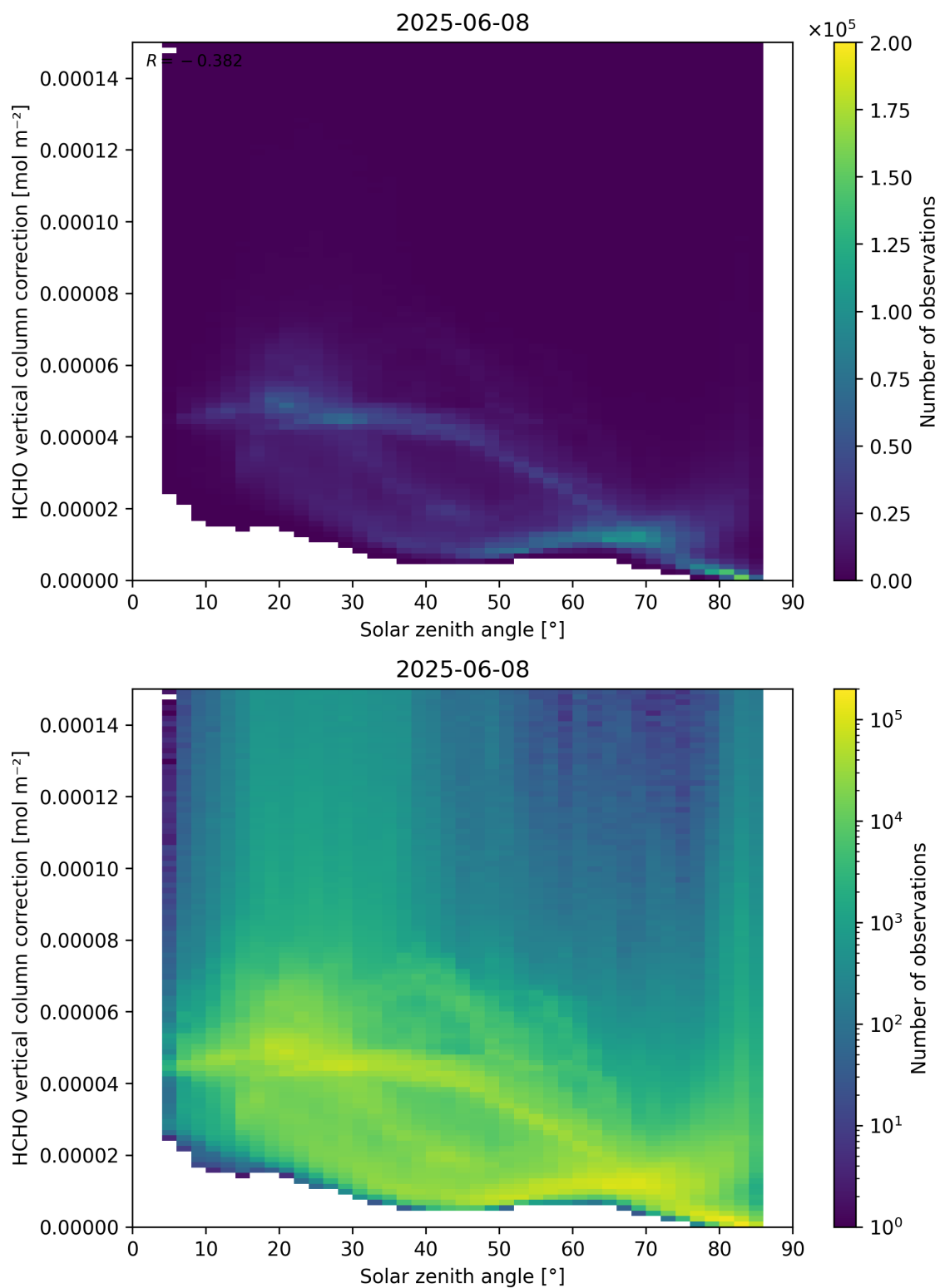
Figure 178: Scatter density plot of “Solar zenith angle” against “HCHO vertical column correction” for 2025-06-07 to 2025-06-09.
