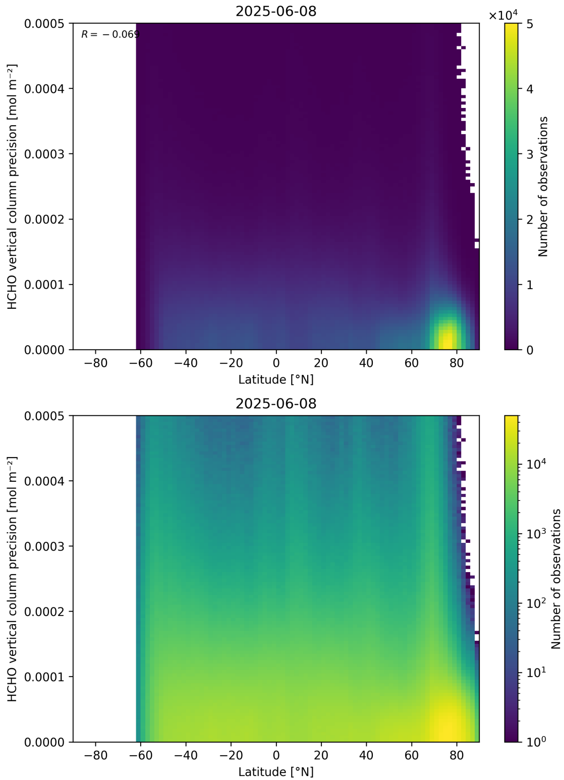
Figure 165: Scatter density plot of “Latitude” against “HCHO vertical column precision” for 2025-06-07 to 2025-06-09.
