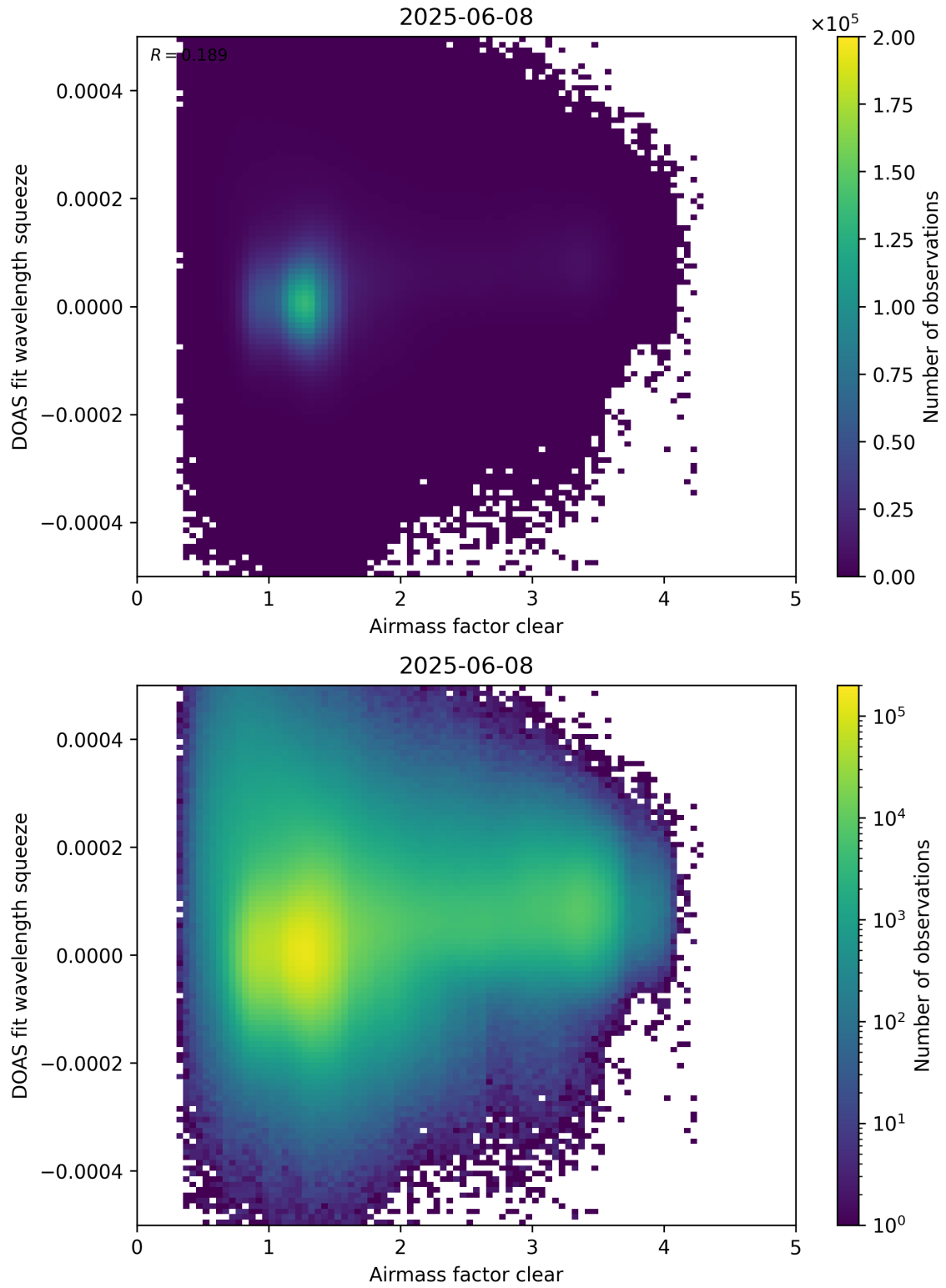
Figure 73: Scatter density plot of “Airmass factor clear” against “DOAS fit wavelength squeeze” for 2025-06-07 to 2025-06-09.
