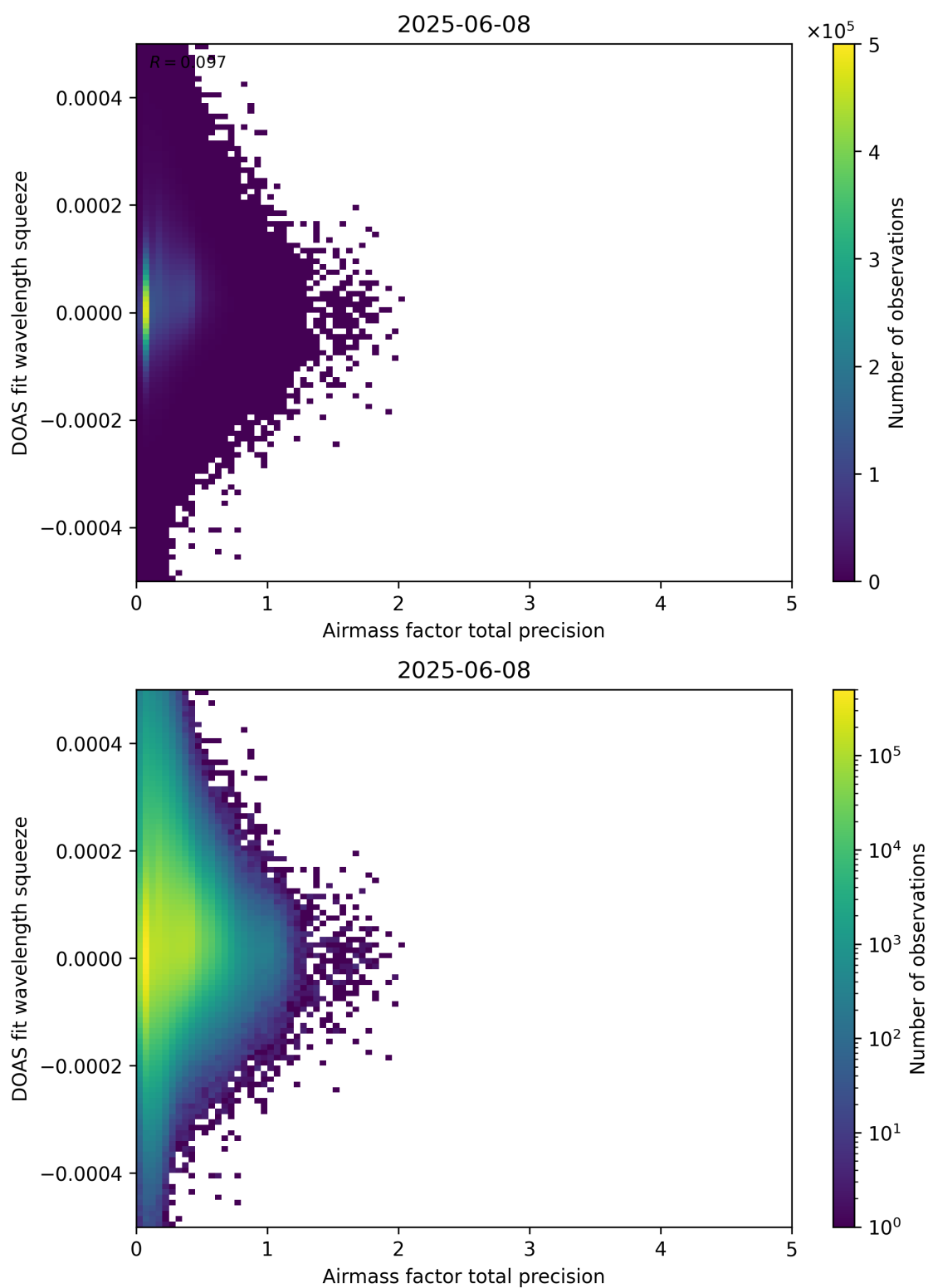
Figure 107: Scatter density plot of “Airmass factor total precision” against “DOAS fit wavelength squeeze” for 2025-06-07 to 2025-06-09.
