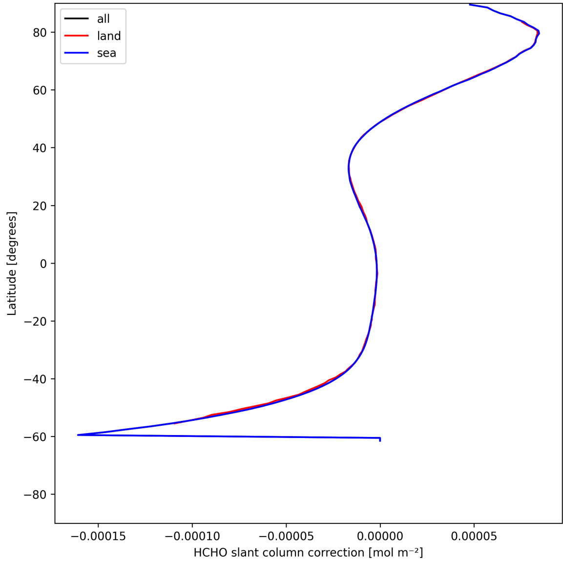
Figure 33: Zonal average of “HCHO slant column correction” for 2025-06-07 to 2025-06-09.
