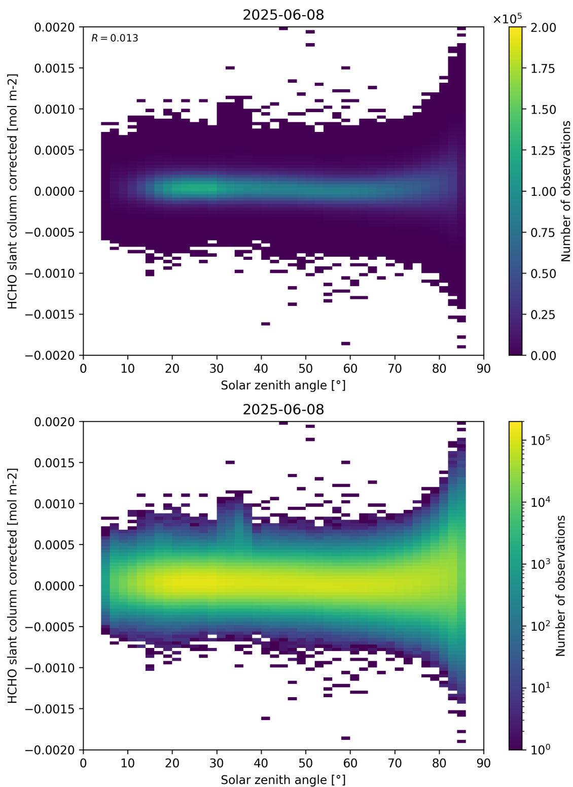
Figure 171: Scatter density plot of “Solar zenith angle” against “HCHO slant column corrected” for 2025-06-07 to 2025-06-09.
