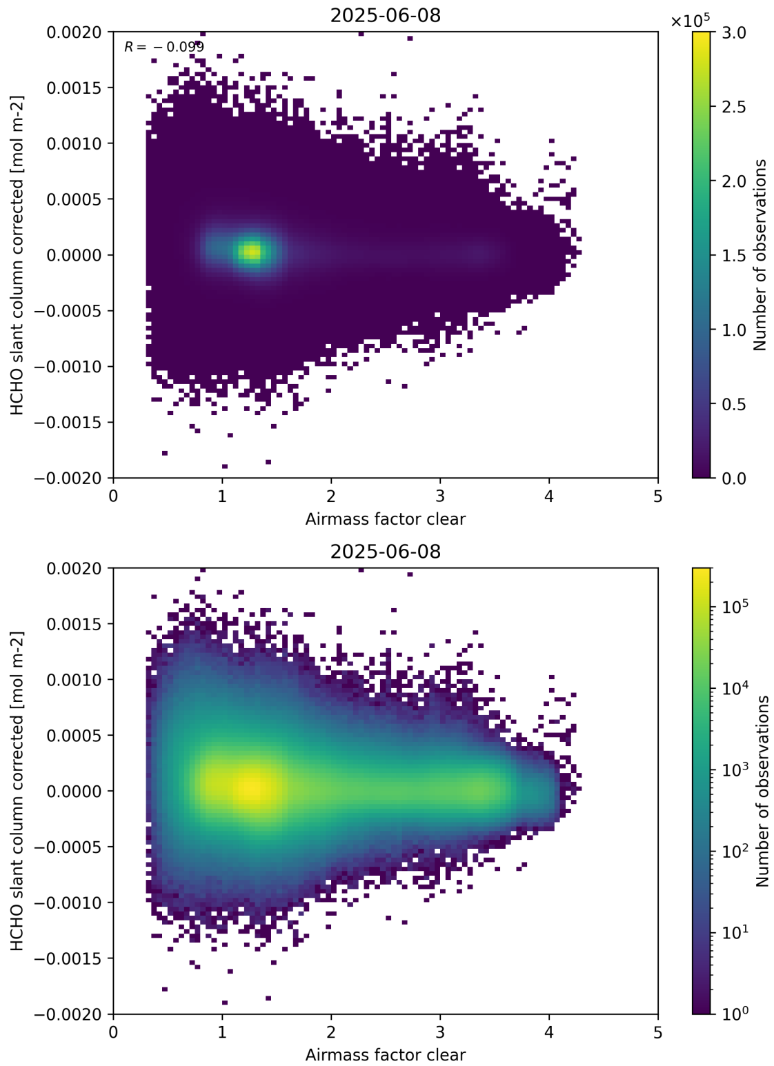
Figure 74: Scatter density plot of “Airmass factor clear” against “HCHO slant column corrected” for 2025-06-07 to 2025-06-09.
