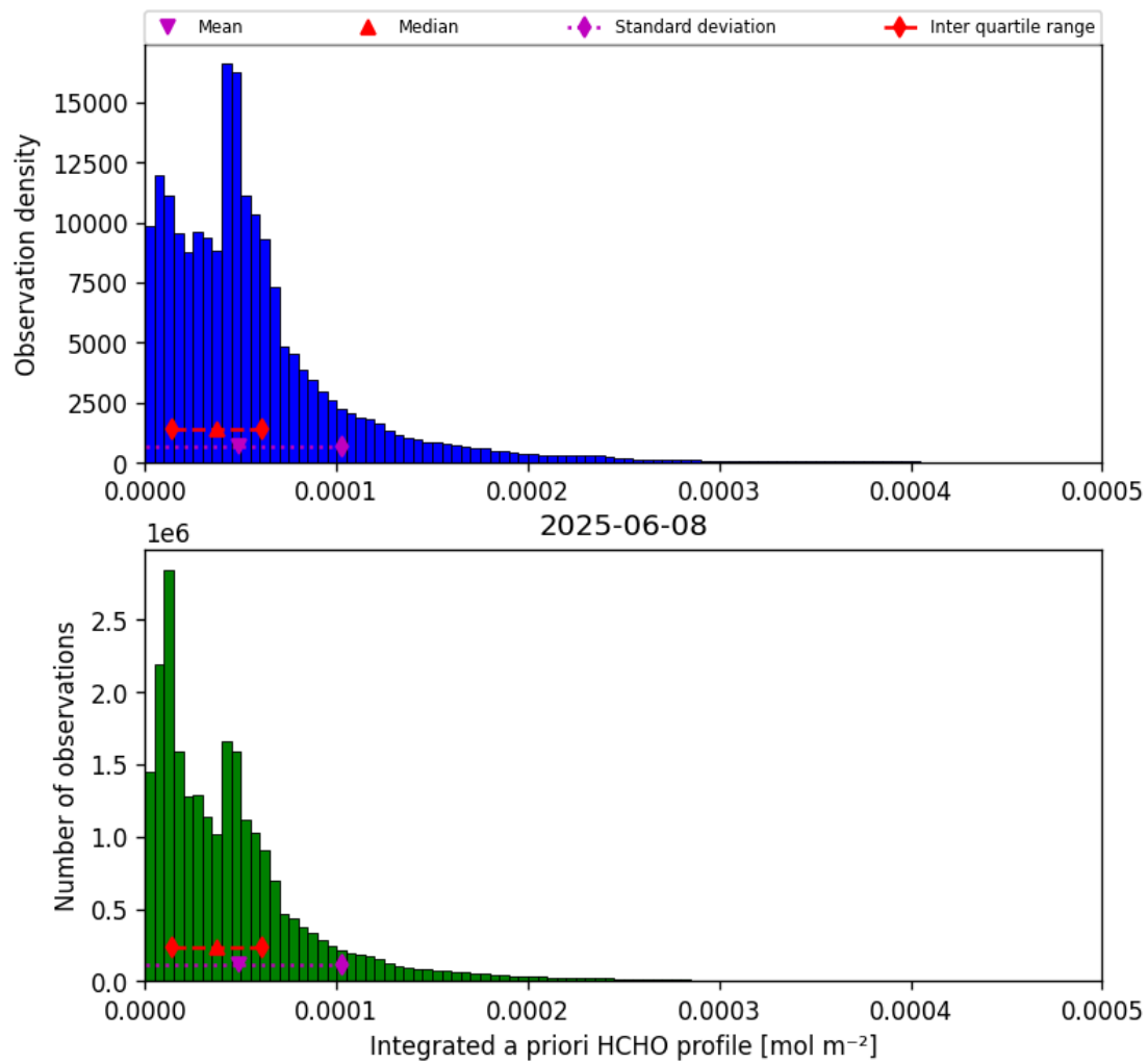
Figure 43: Histogram of “Integrated a priori HCHO profile” for 2025-06-07 to 2025-06-09
