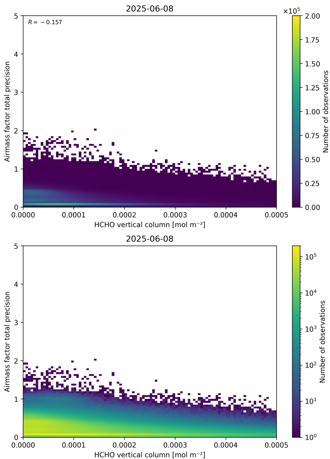
Figure 132: Scatter density plot of “HCHO vertical column” against “Airmass factor total precision” for 2025-06-07 to 2025-06-09.
