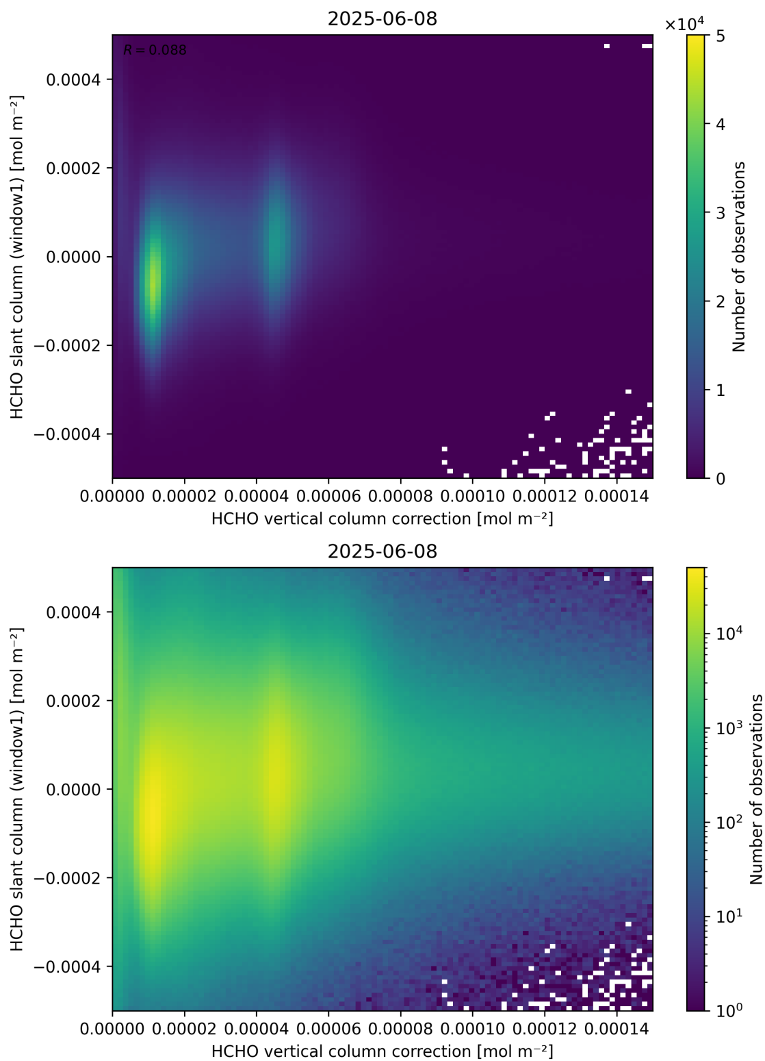
Figure 118: Scatter density plot of “HCHO vertical column correction” against “HCHO slant column (window1)” for 2025-06-07 to 2025-06-09.
