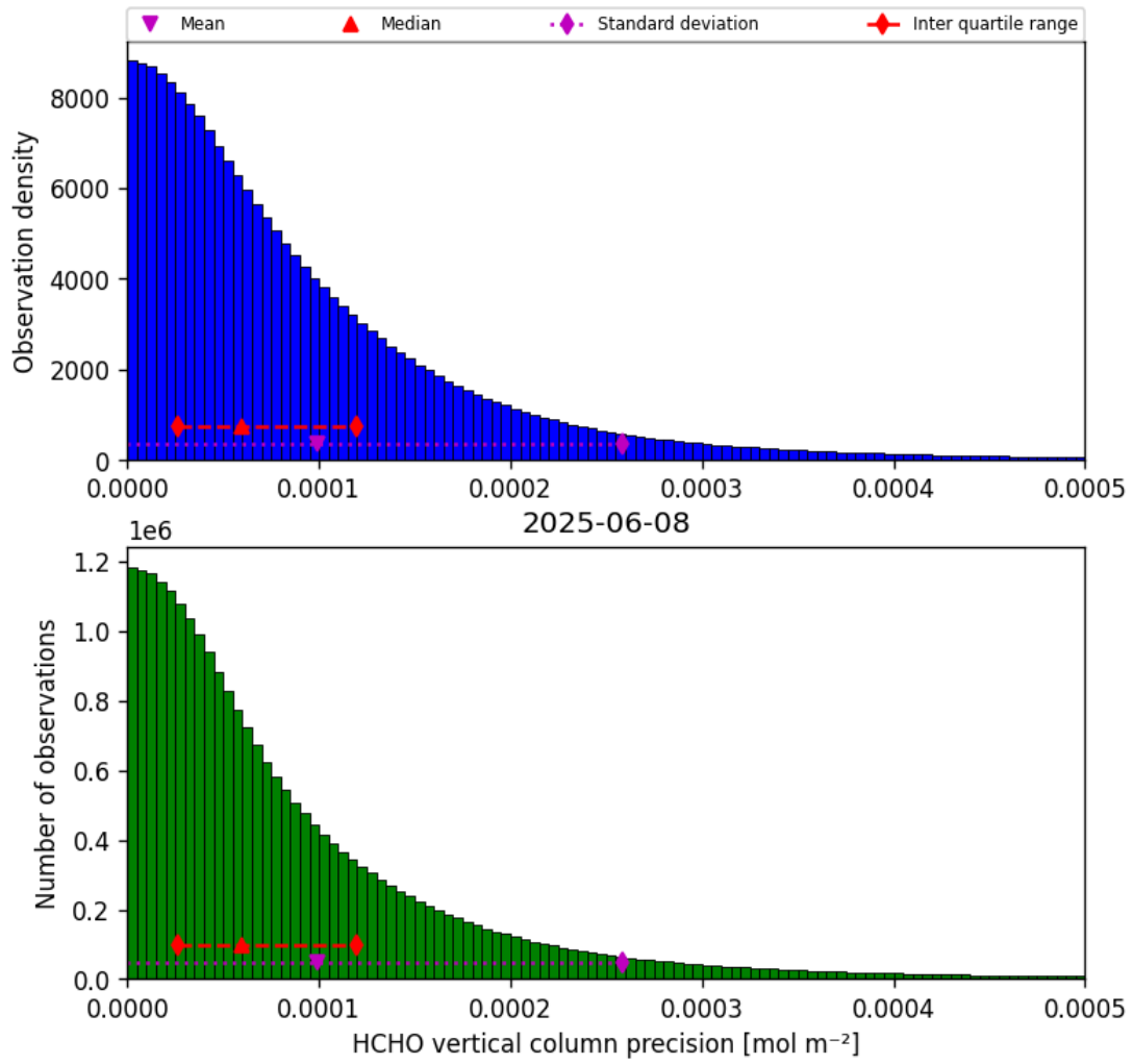
Figure 36: Histogram of “HCHO vertical column precision” for 2025-06-07 to 2025-06-09
