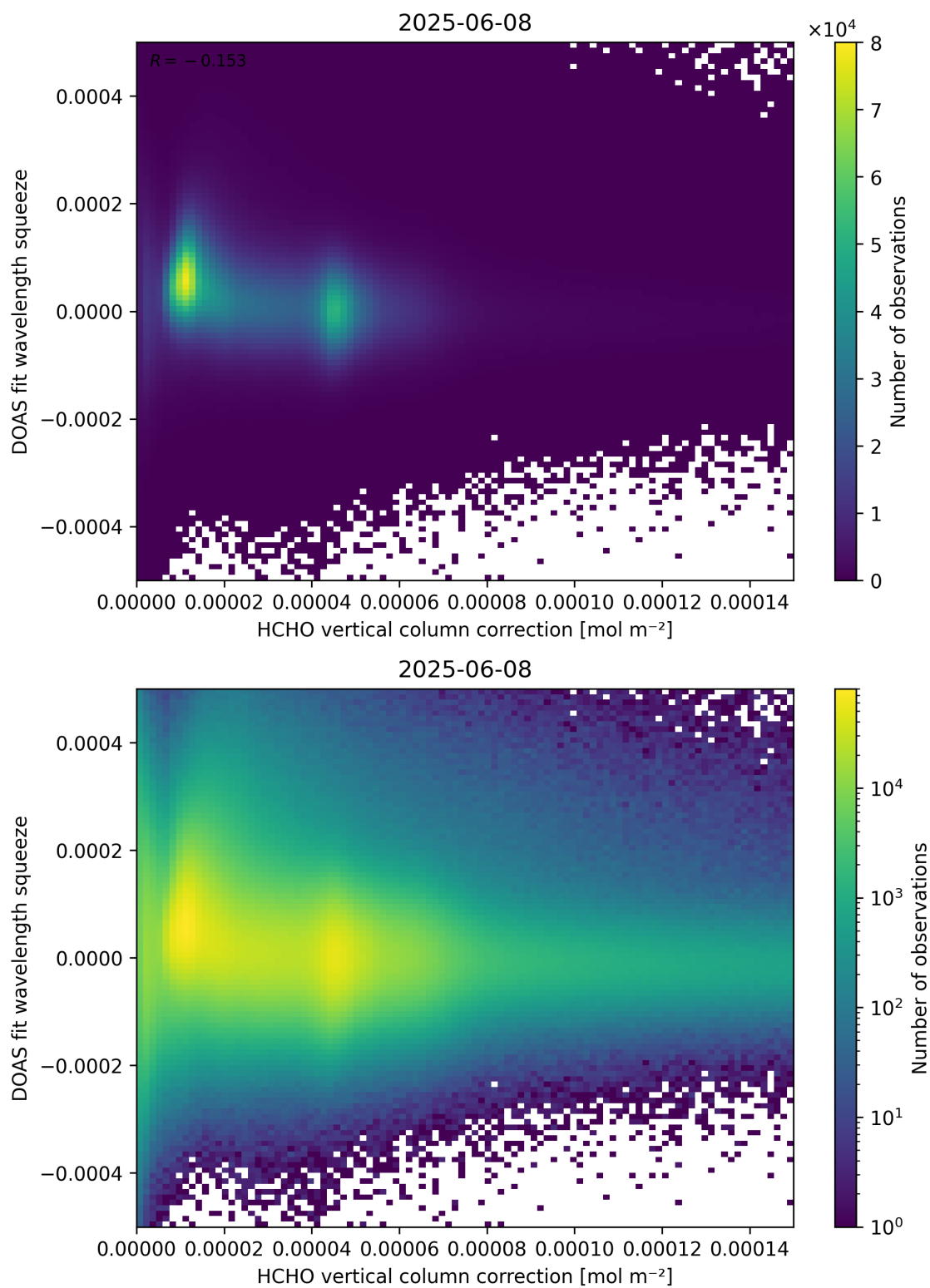
Figure 114: Scatter density plot of “HCHO vertical column correction” against “DOAS fit wavelength squeeze” for 2025-06-07 to 2025-06-09.
