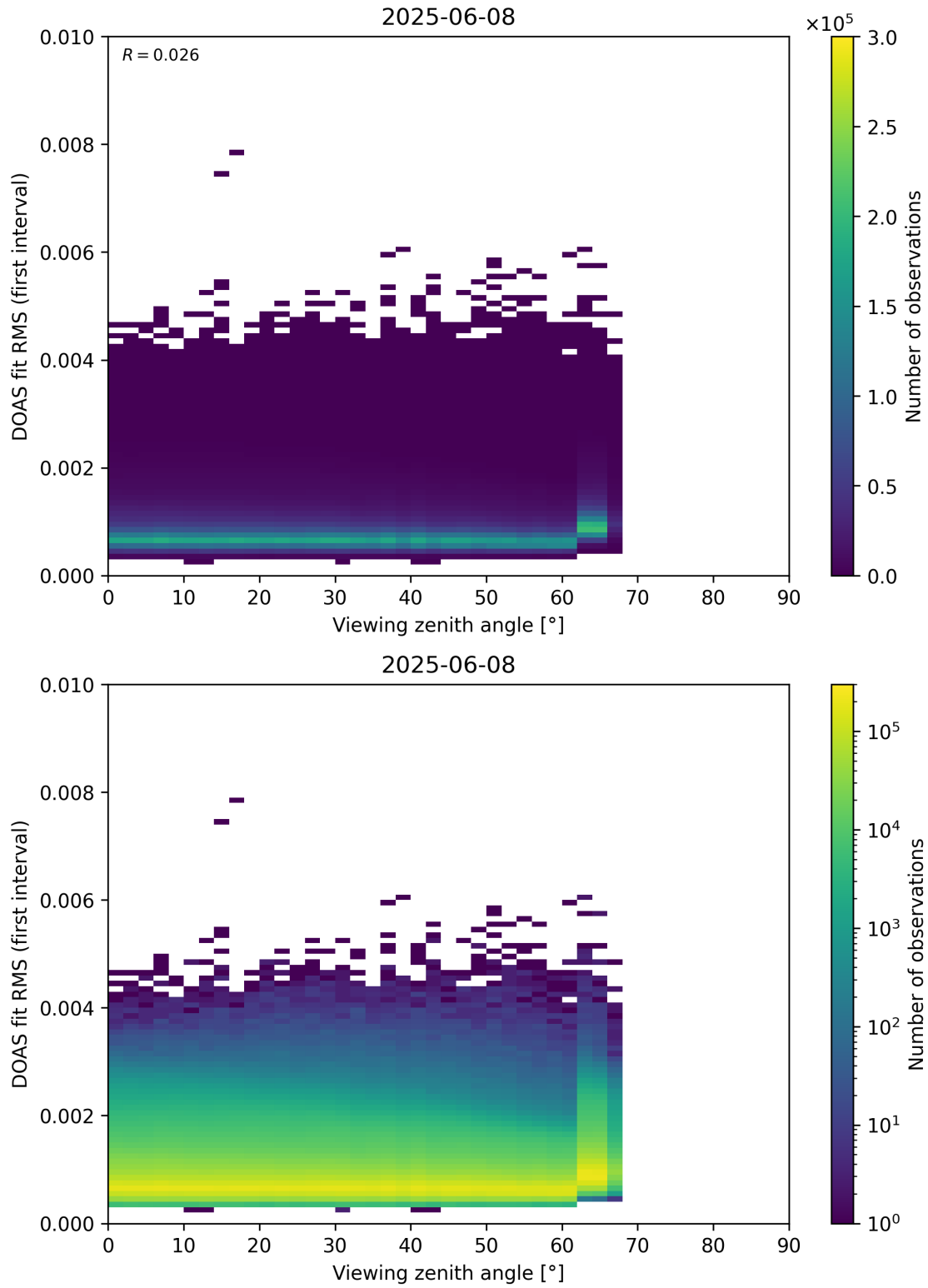
Figure 182: Scatter density plot of “Viewing zenith angle” against “DOAS fit RMS (first interval)” for 2025-06-07 to 2025-06-09.
