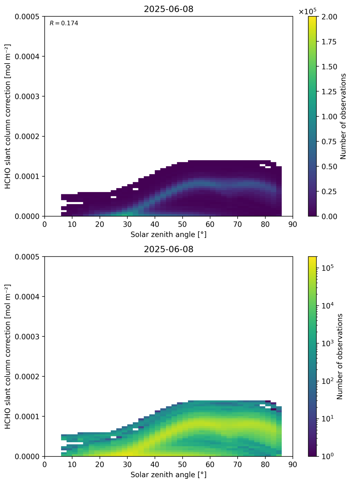
Figure 172: Scatter density plot of “Solar zenith angle” against “HCHO slant column correction” for 2025-06-07 to 2025-06-09.
