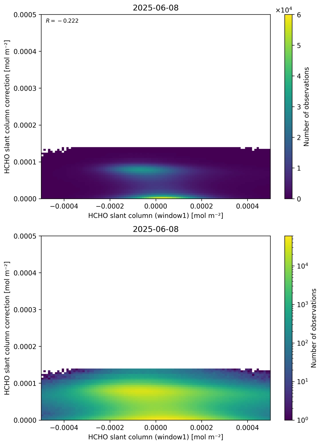
Figure 83: Scatter density plot of “HCHO slant column (window1)” against “HCHO slant column correction” for 2025-06-07 to 2025-06-09.
