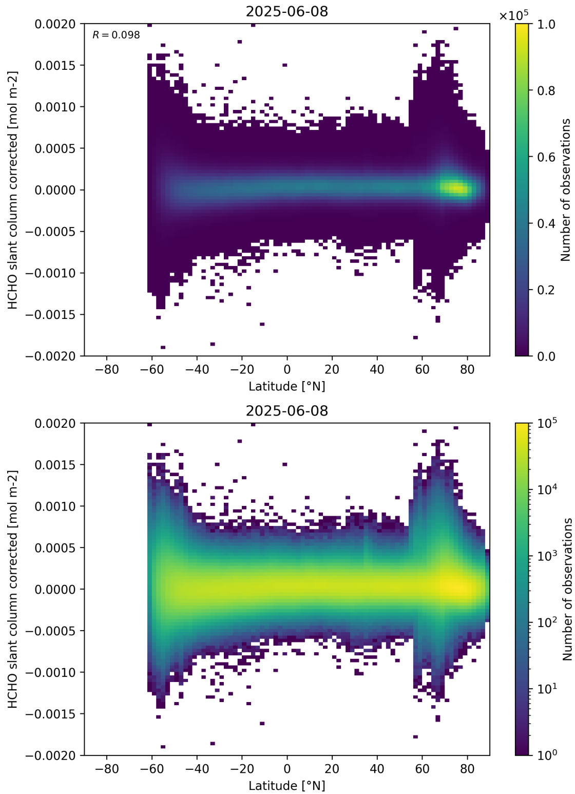
Figure 157: Scatter density plot of “Latitude” against “HCHO slant column corrected” for 2025-06-07 to 2025-06-09.
