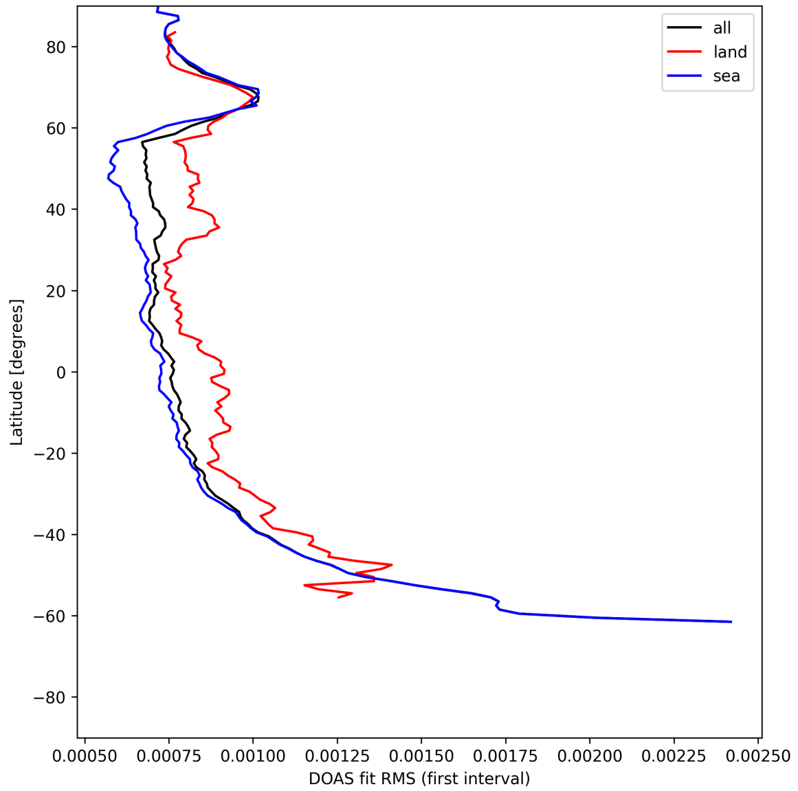
Figure 32: Zonal average of “DOAS fit RMS (first interval)” for 2025-06-07 to 2025-06-09.
