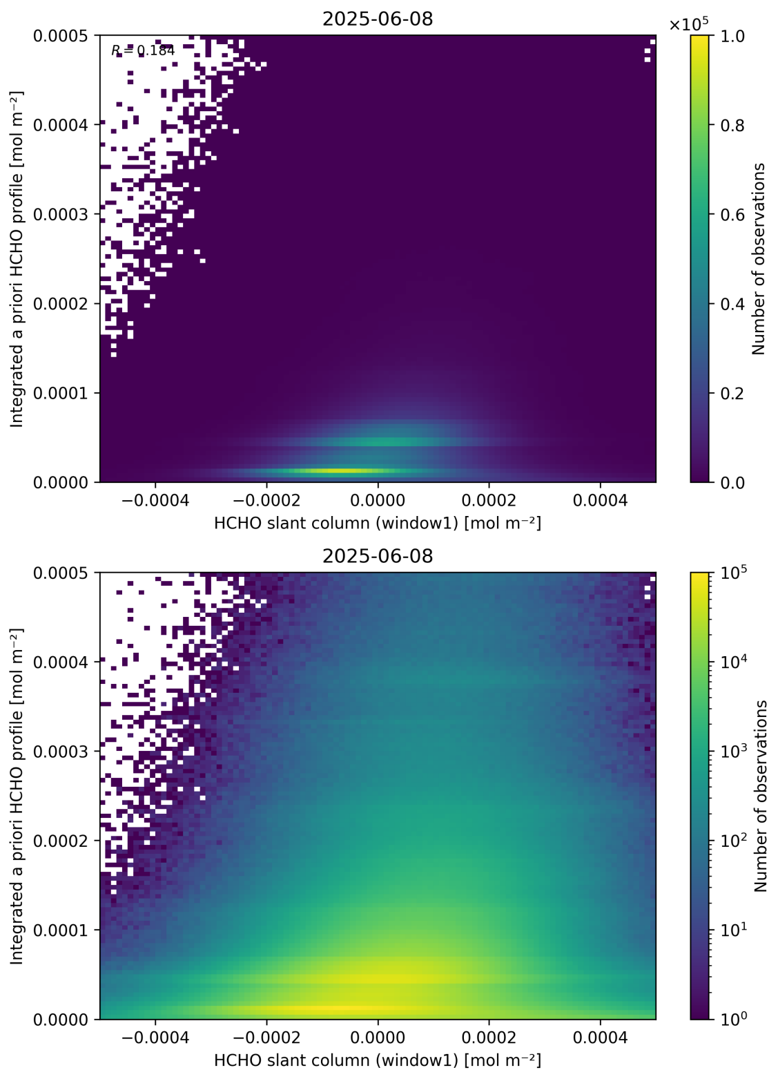
Figure 87: Scatter density plot of “HCHO slant column (window1)” against “Integrated a priori HCHO profile” for 2025-06-07 to 2025-06-09.
