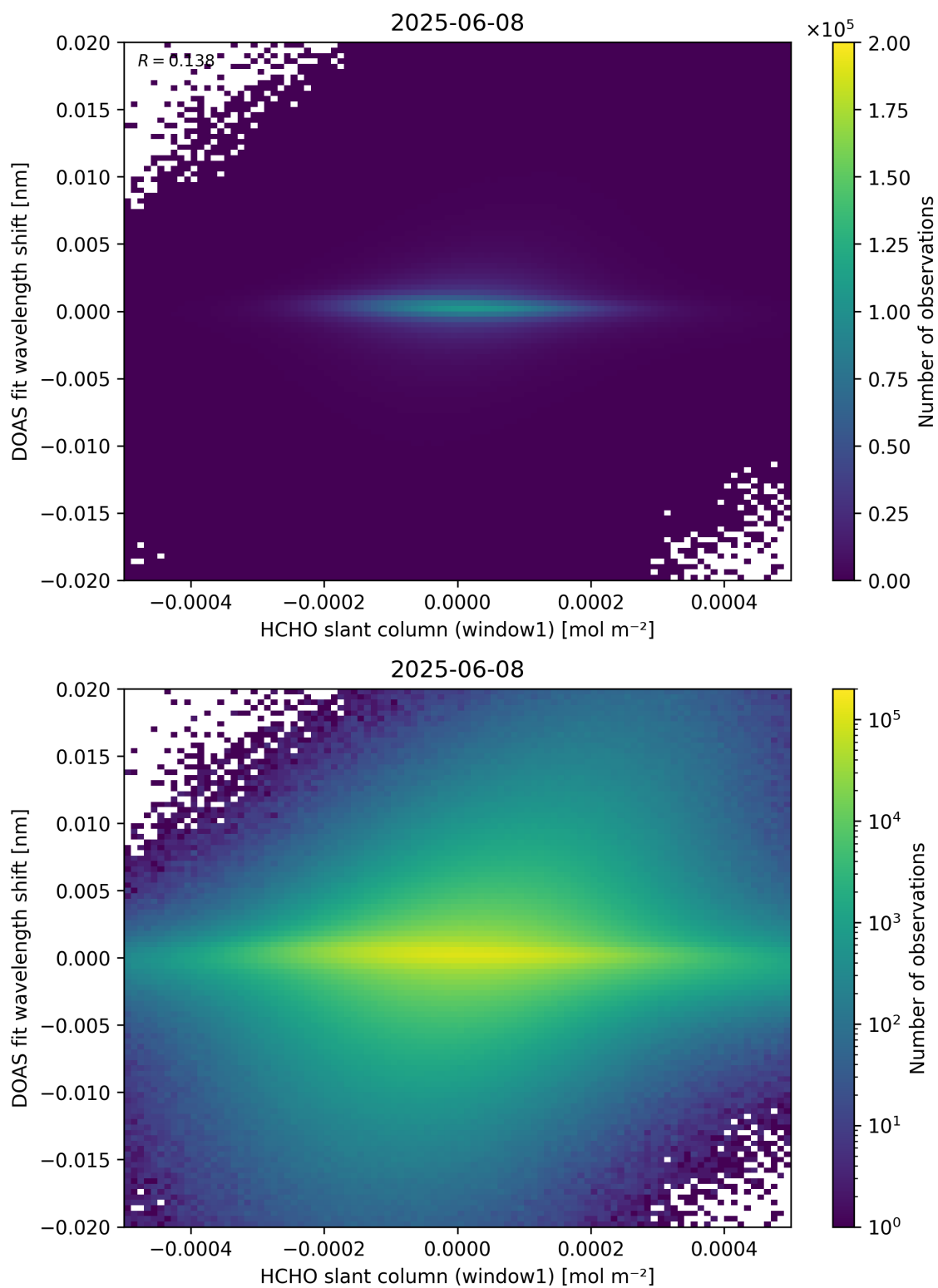
Figure 79: Scatter density plot of “HCHO slant column (window1)” against “DOAS fit wavelength shift” for 2025-06-07 to 2025-06-09.
