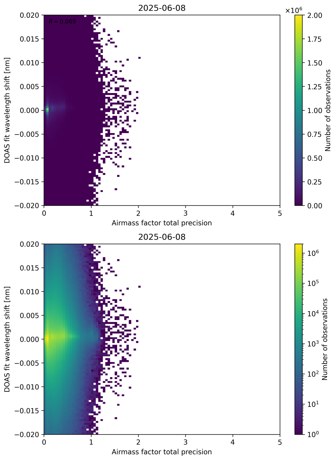
Figure 106: Scatter density plot of “Airmass factor total precision” against “DOAS fit wavelength shift” for 2025-06-07 to 2025-06-09.
