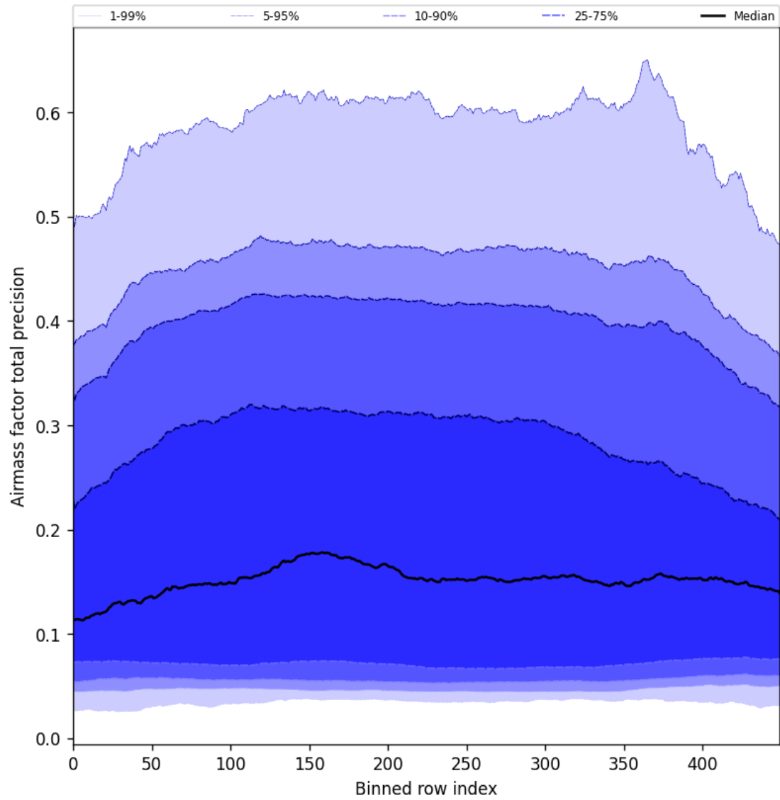
Figure 55: Along track statistics of “Airmass factor total precision” for 2025-06-07 to 2025-06-09
