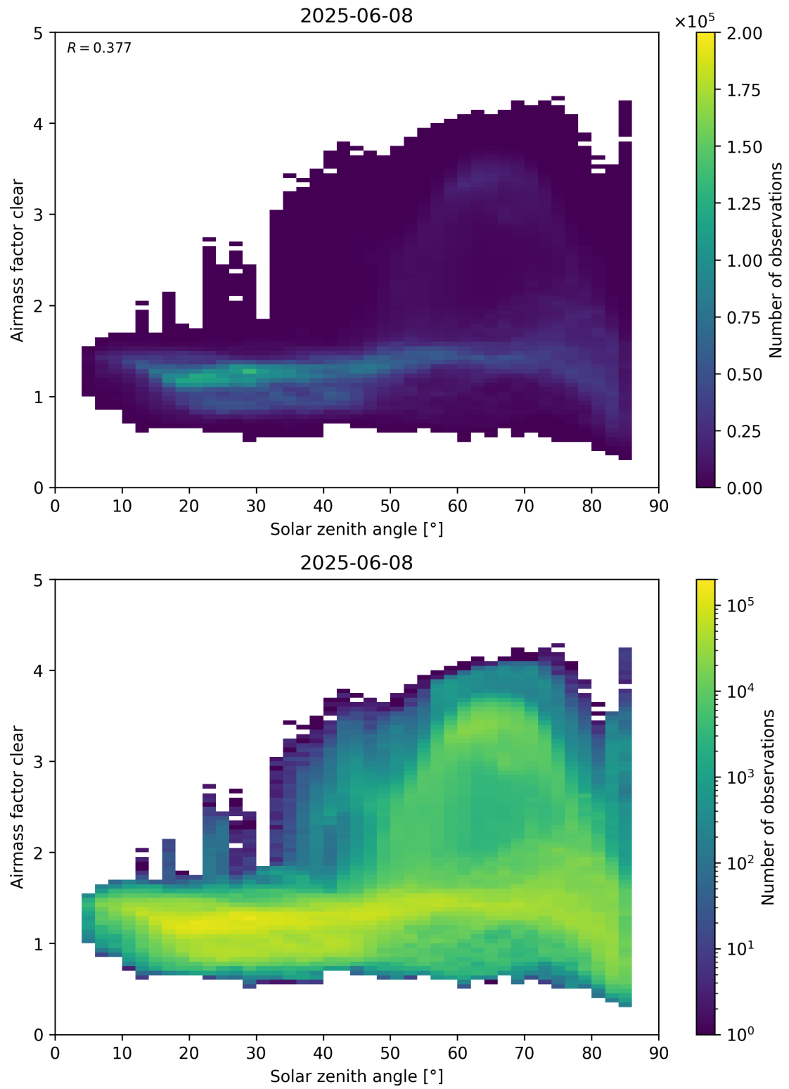
Figure 170: Scatter density plot of “Solar zenith angle” against “Airmass factor clear” for 2025-06-07 to 2025-06-09.
