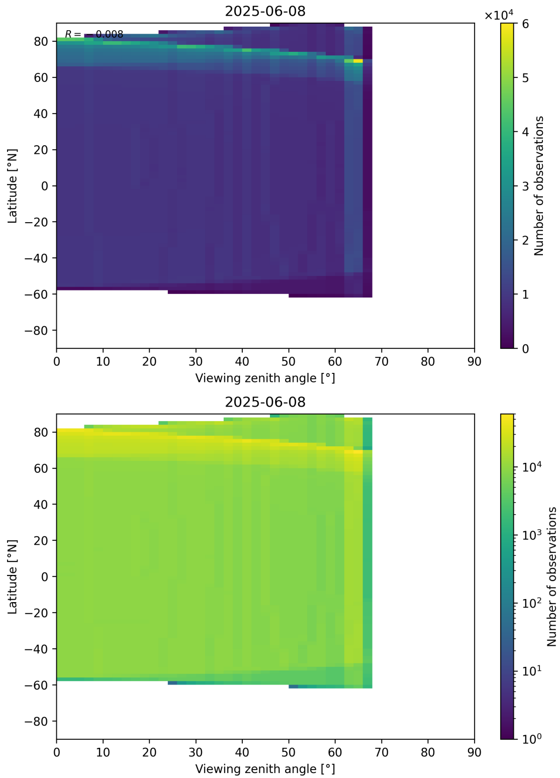
Figure 196: Scatter density plot of “Viewing zenith angle” against “Latitude” for 2025-06-07 to 2025-06-09.
