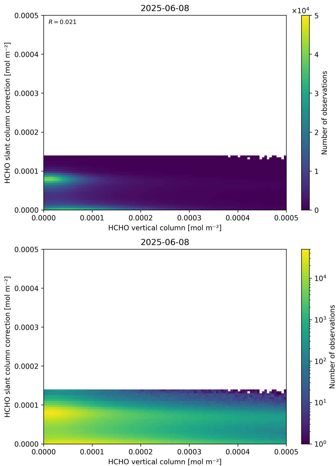
Figure 128: Scatter density plot of “HCHO vertical column” against “HCHO slant column correction” for 2025-06-07 to 2025-06-09.
