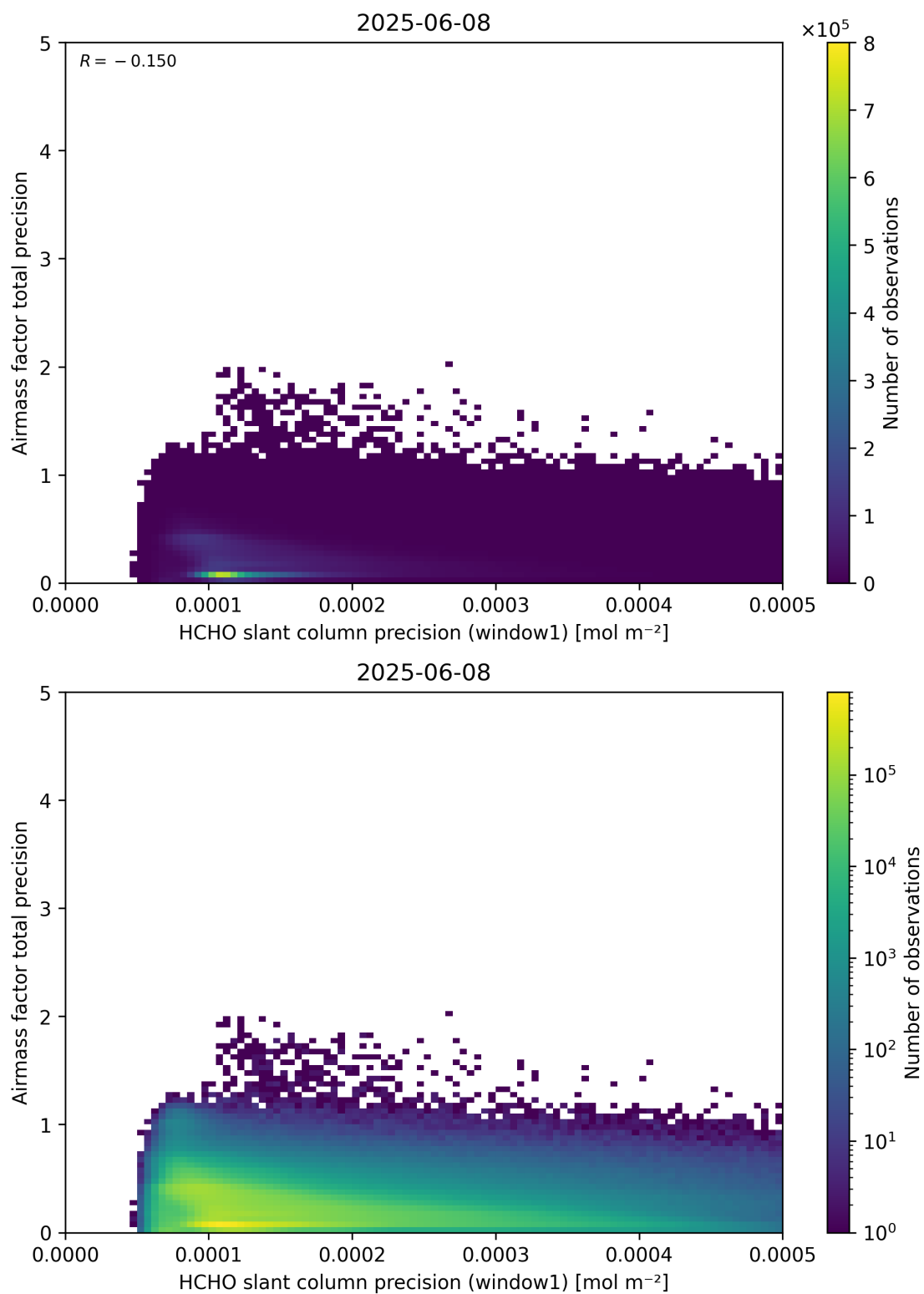
Figure 95: Scatter density plot of “HCHO slant column precision (window1)” against “Airmass factor total precision” for 2025-06-07 to 2025-06-09.
