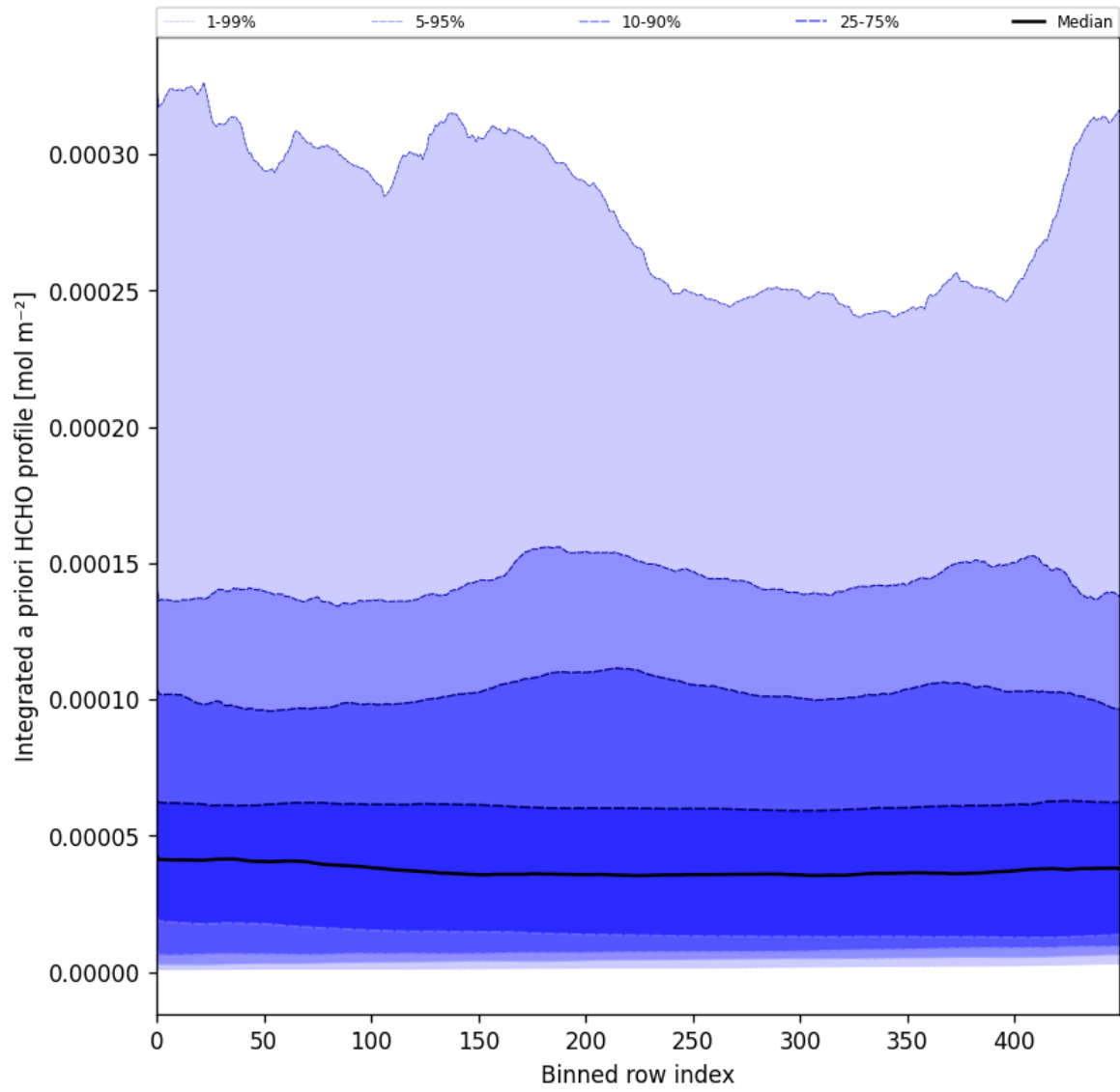
Figure 57: Along track statistics of “Integrated a priori HCHO profile” for 2025-06-07 to 2025-06-09
