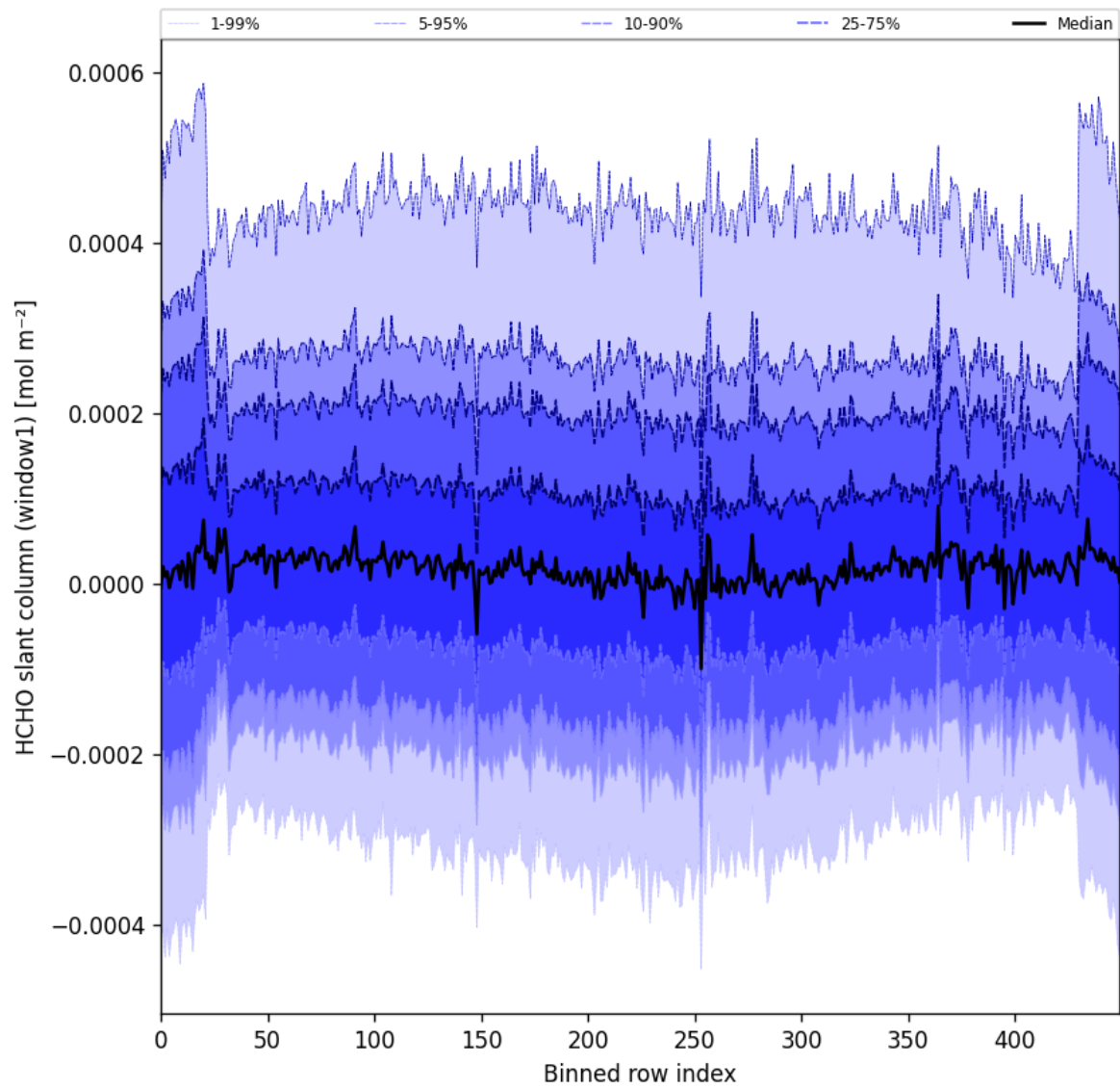
Figure 52: Along track statistics of “HCHO slant column (window1)” for 2025-06-07 to 2025-06-09
