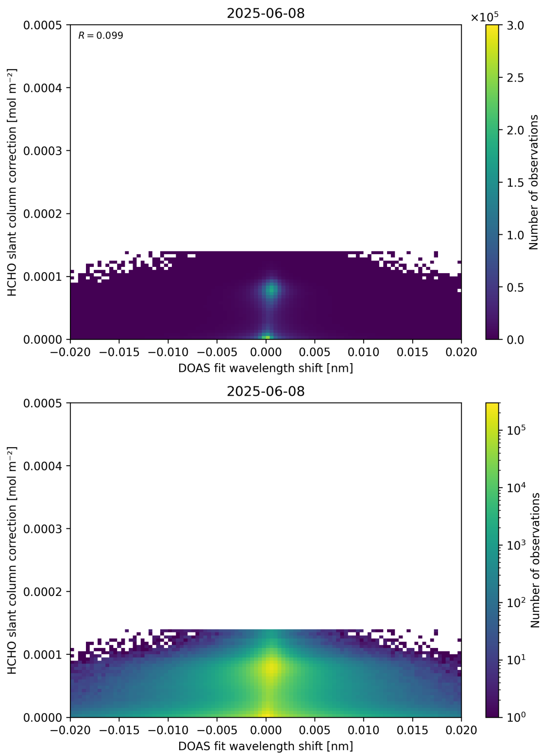
Figure 67: Scatter density plot of “DOAS fit wavelength shift” against “HCHO slant column correction” for 2025-06-07 to 2025-06-09.
