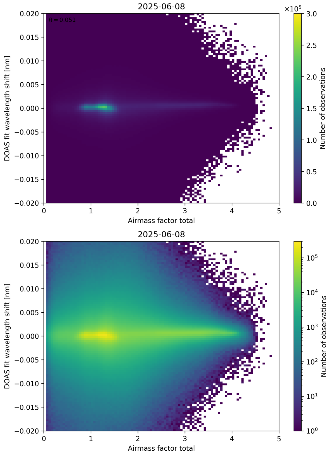
Figure 98: Scatter density plot of “Airmass factor total” against “DOAS fit wavelength shift” for 2025-06-07 to 2025-06-09.
