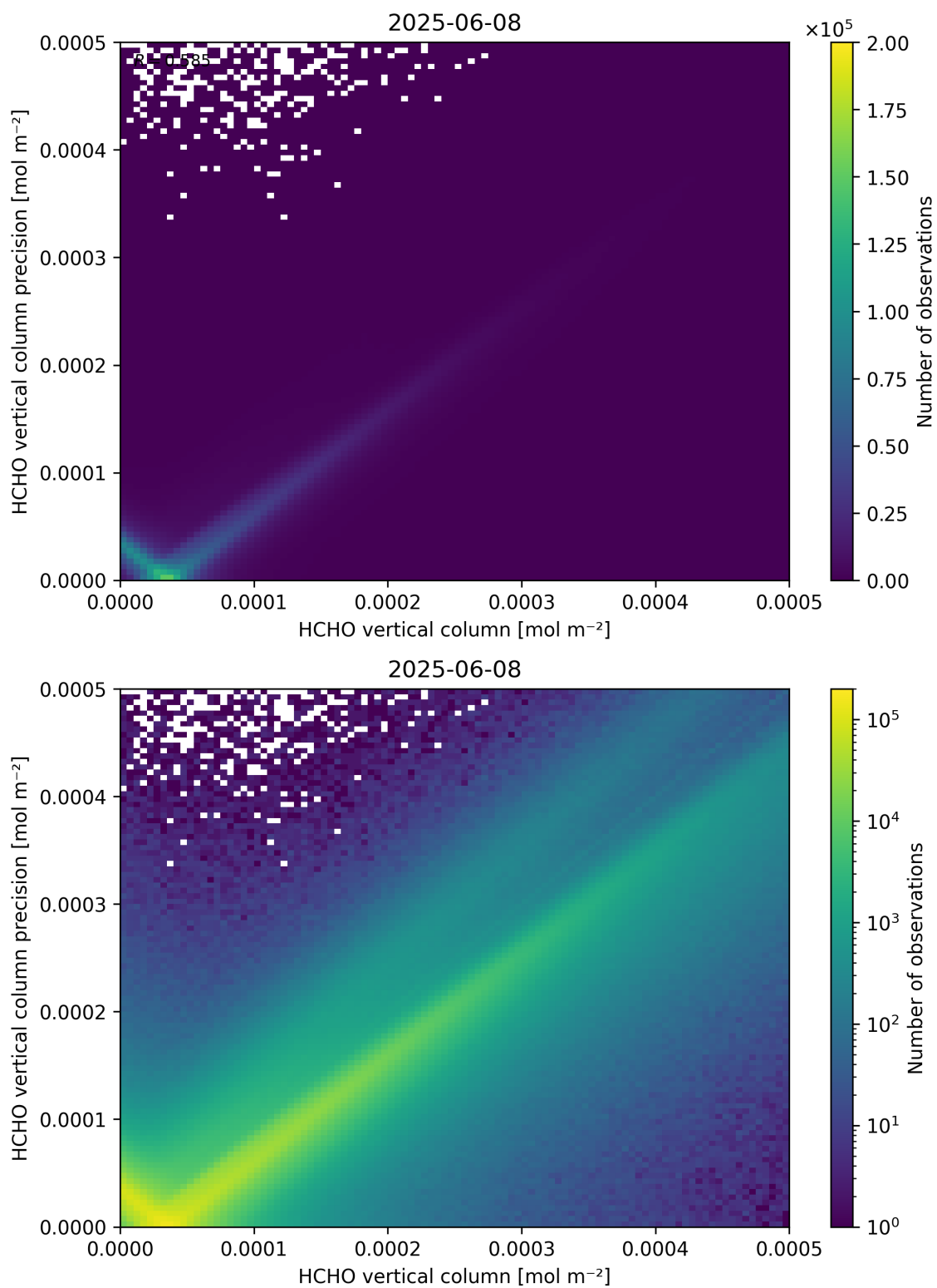
Figure 134: Scatter density plot of “HCHO vertical column” against “HCHO vertical column precision” for 2025-06-07 to 2025-06-09.
