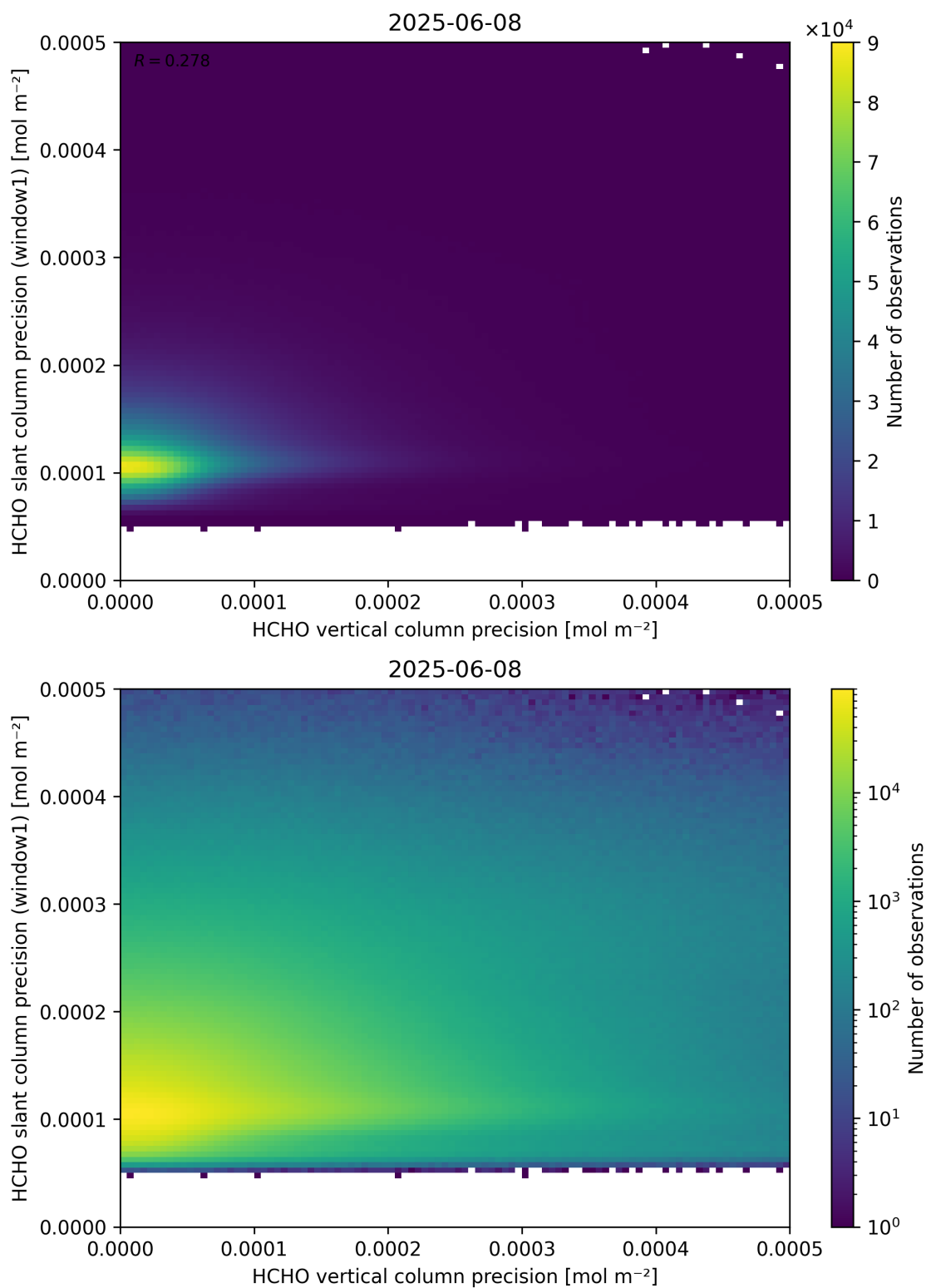
Figure 143: Scatter density plot of “HCHO vertical column precision” against “HCHO slant column precision (window1)” for 2025-06-07 to 2025-06-09.
