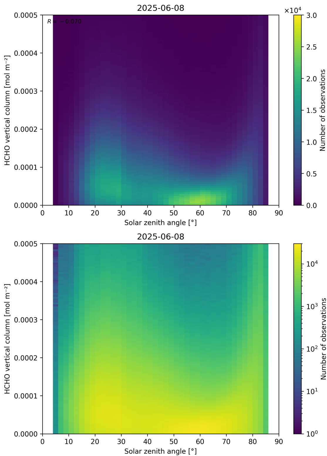
Figure 177: Scatter density plot of “Solar zenith angle” against “HCHO vertical column” for 2025-06-07 to 2025-06-09.
