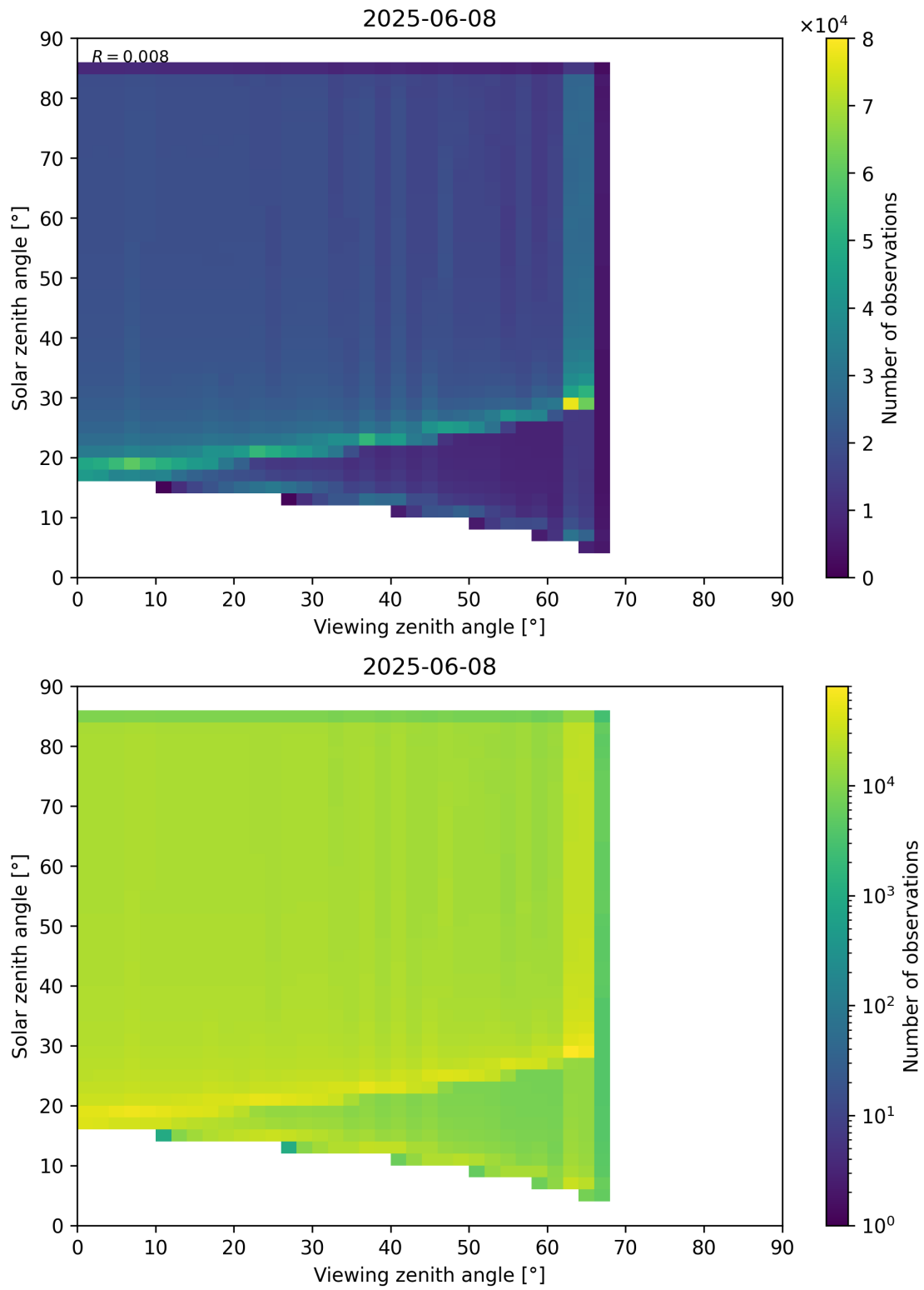
Figure 197: Scatter density plot of “Viewing zenith angle” against “Solar zenith angle” for 2025-06-07 to 2025-06-09.
