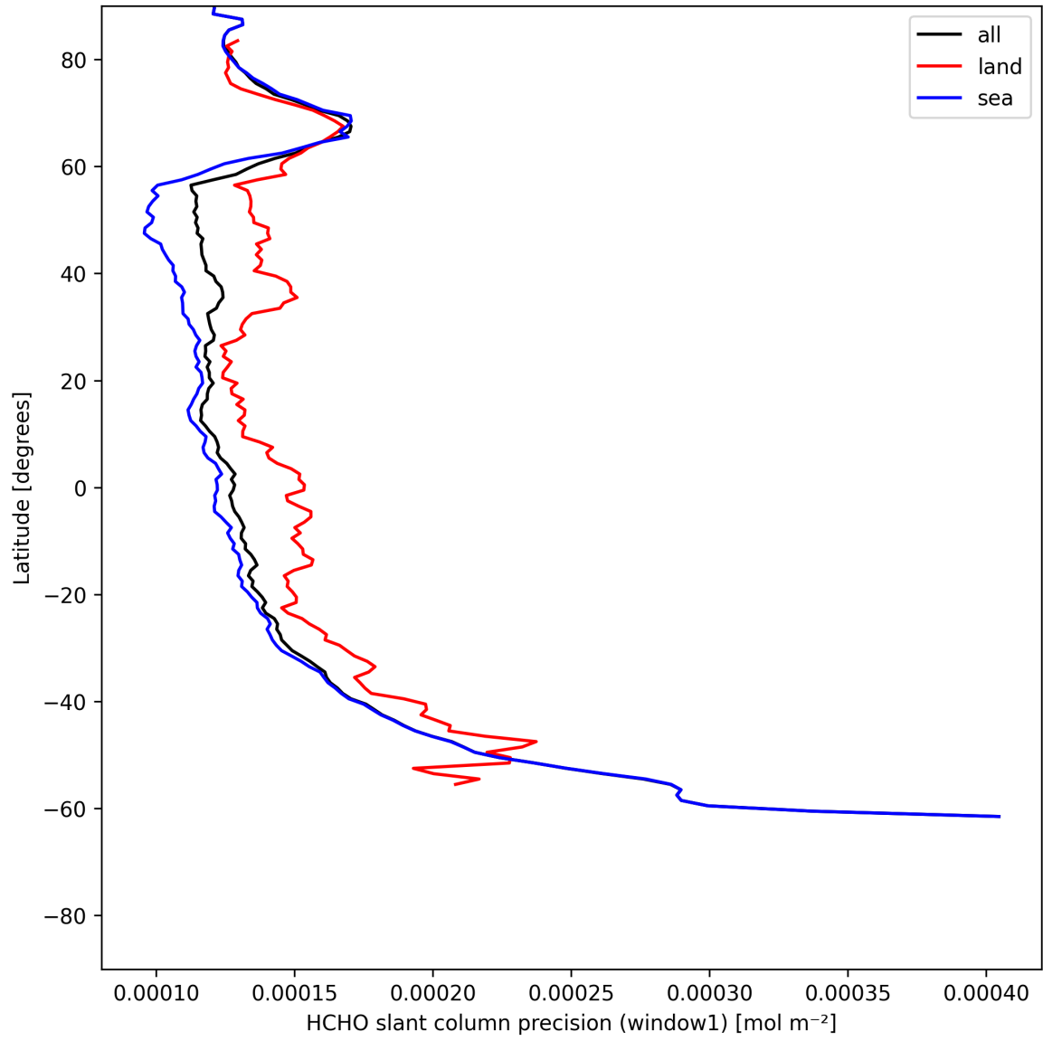
Figure 25: Zonal average of "HCHO slant column precision (window1)" for 2025-06-07 to 2025-06-09.
