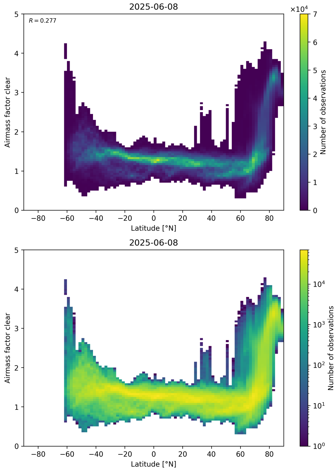
Figure 156: Scatter density plot of “Latitude” against “Airmass factor clear” for 2025-06-07 to 2025-06-09.
