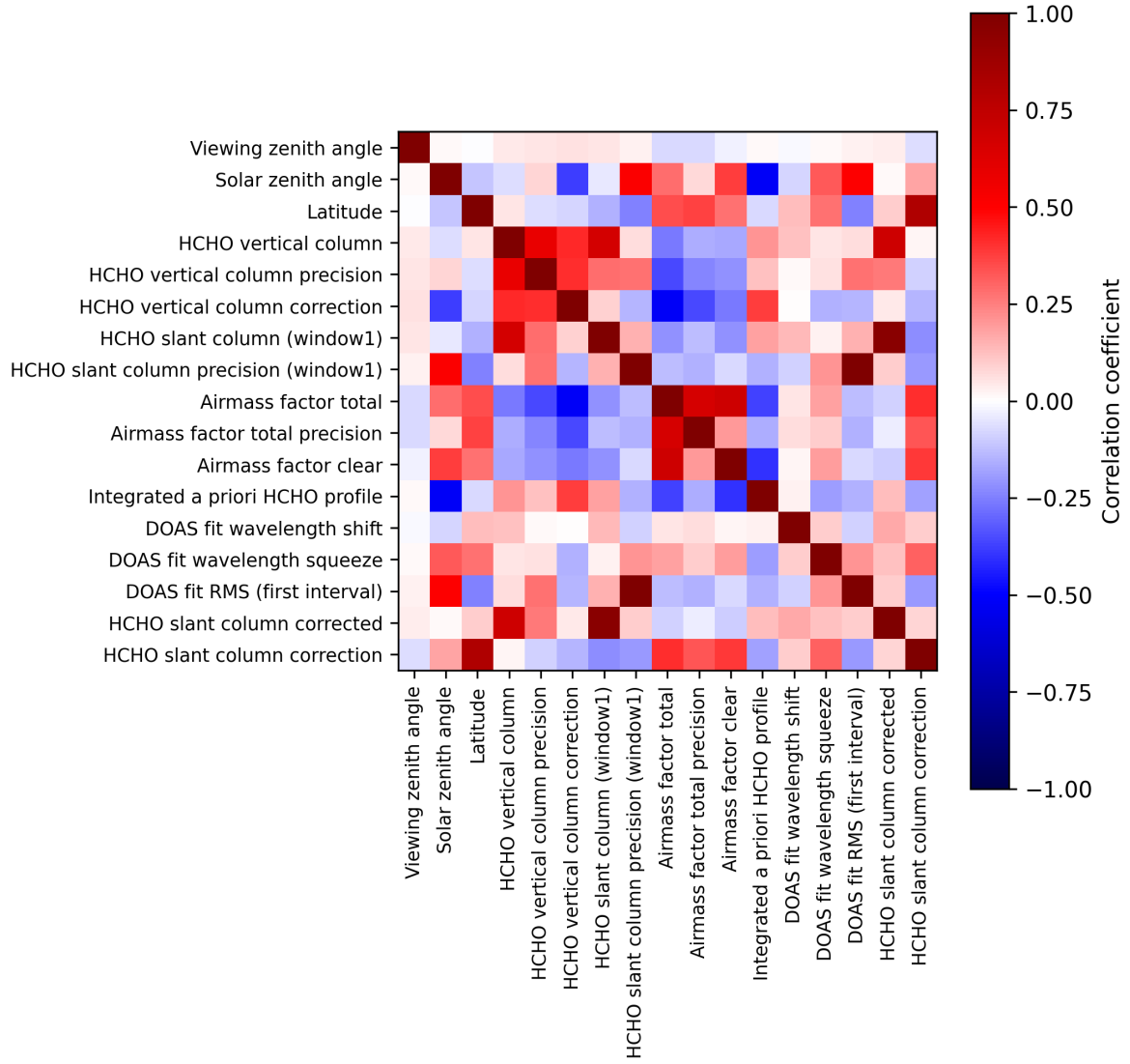
Figure 2: Map of correlation matrix for 2025-06-07 to 2025-06-09.
