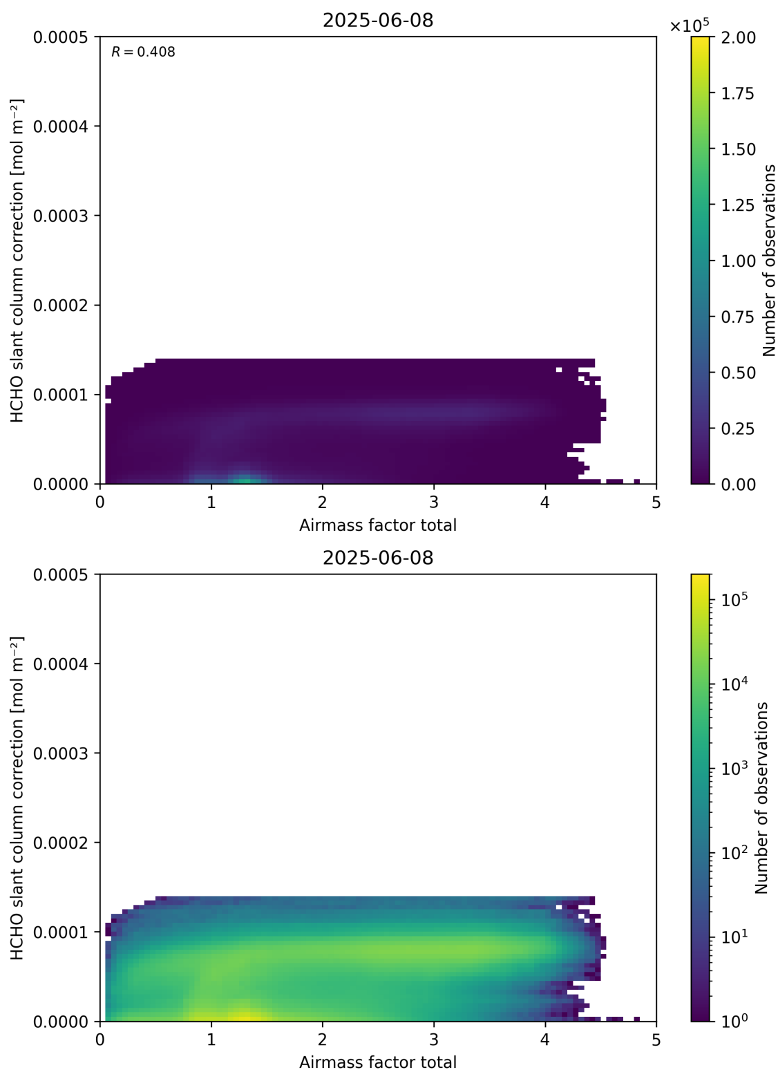
Figure 102: Scatter density plot of “Airmass factor total” against “HCHO slant column correction” for 2025-06-07 to 2025-06-09.
