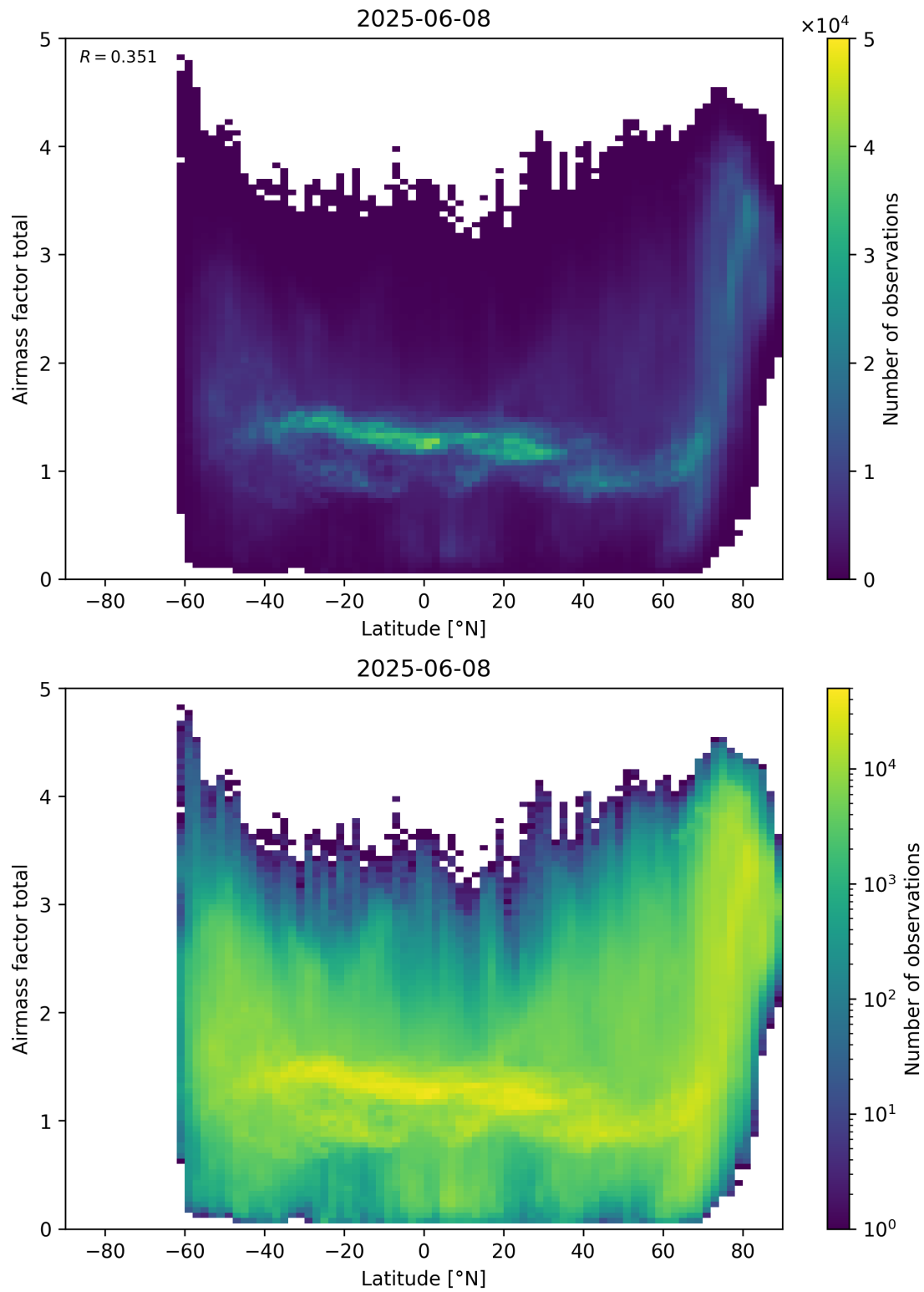
Figure 161: Scatter density plot of “Latitude” against “Airmass factor total” for 2025-06-07 to 2025-06-09.
