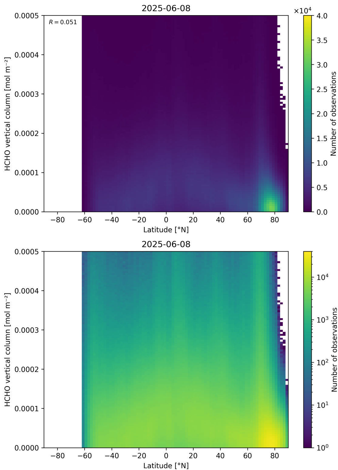
Figure 163: Scatter density plot of “Latitude” against “HCHO vertical column” for 2025-06-07 to 2025-06-09.
