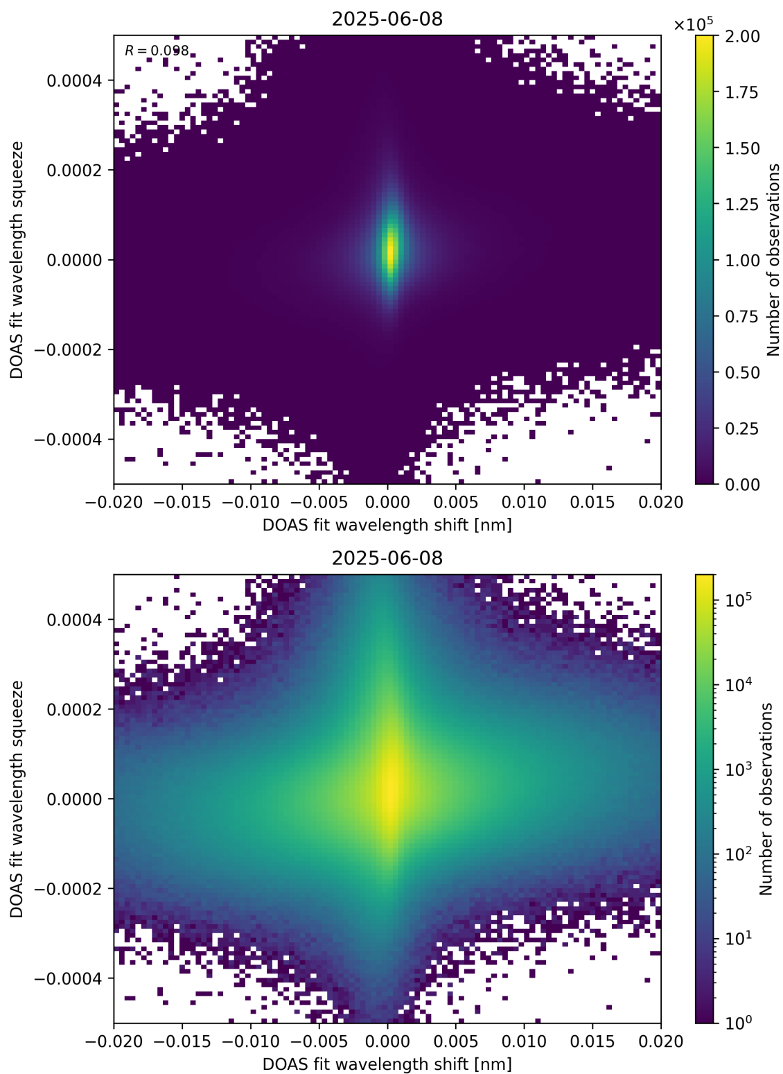
Figure 65: Scatter density plot of “DOAS fit wavelength shift” against “DOAS fit wavelength squeeze” for 2025-06-07 to 2025-06-09.
