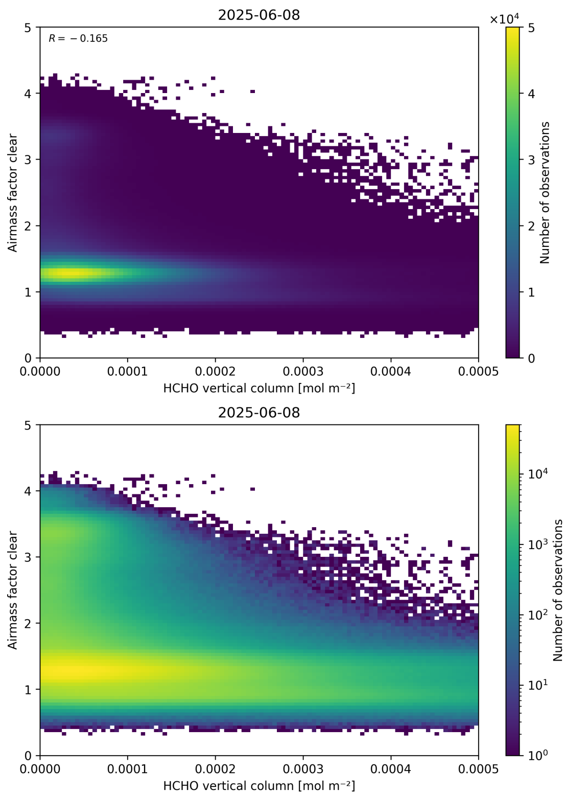
Figure 126: Scatter density plot of “HCHO vertical column” against “Airmass factor clear” for 2025-06-07 to 2025-06-09.
