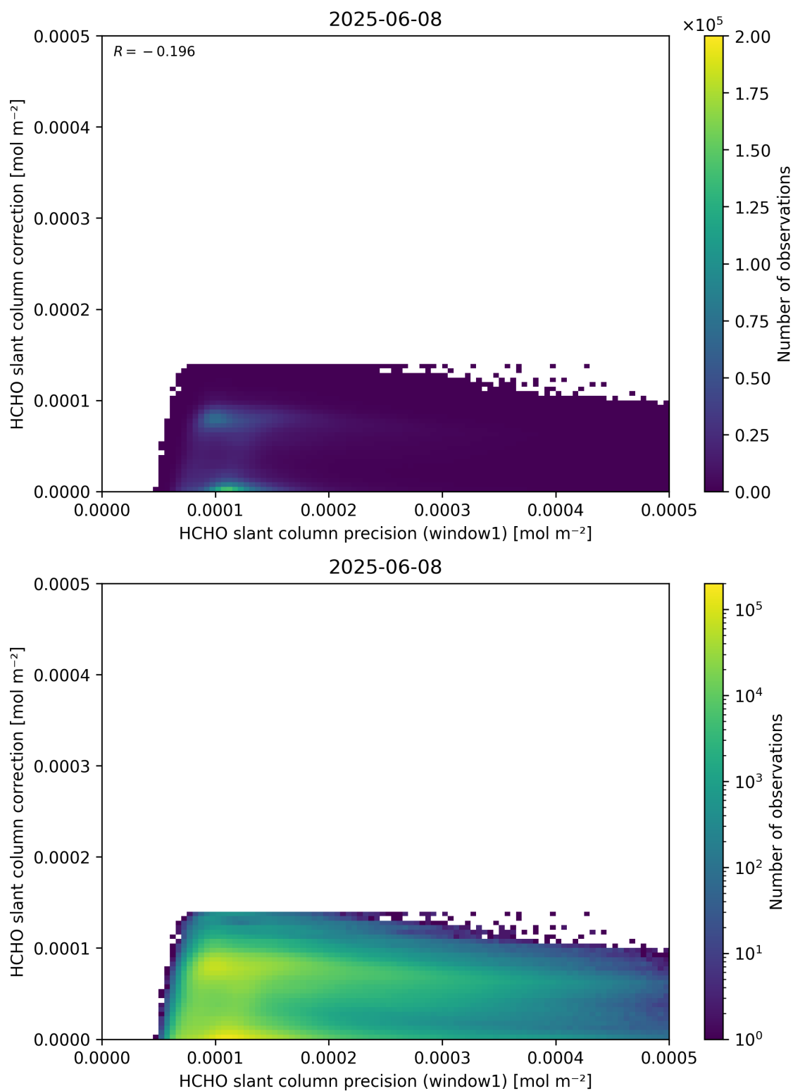
Figure 93: Scatter density plot of “HCHO slant column precision (window1)” against “HCHO slant column correction” for 2025-06-07 to 2025-06-09.
