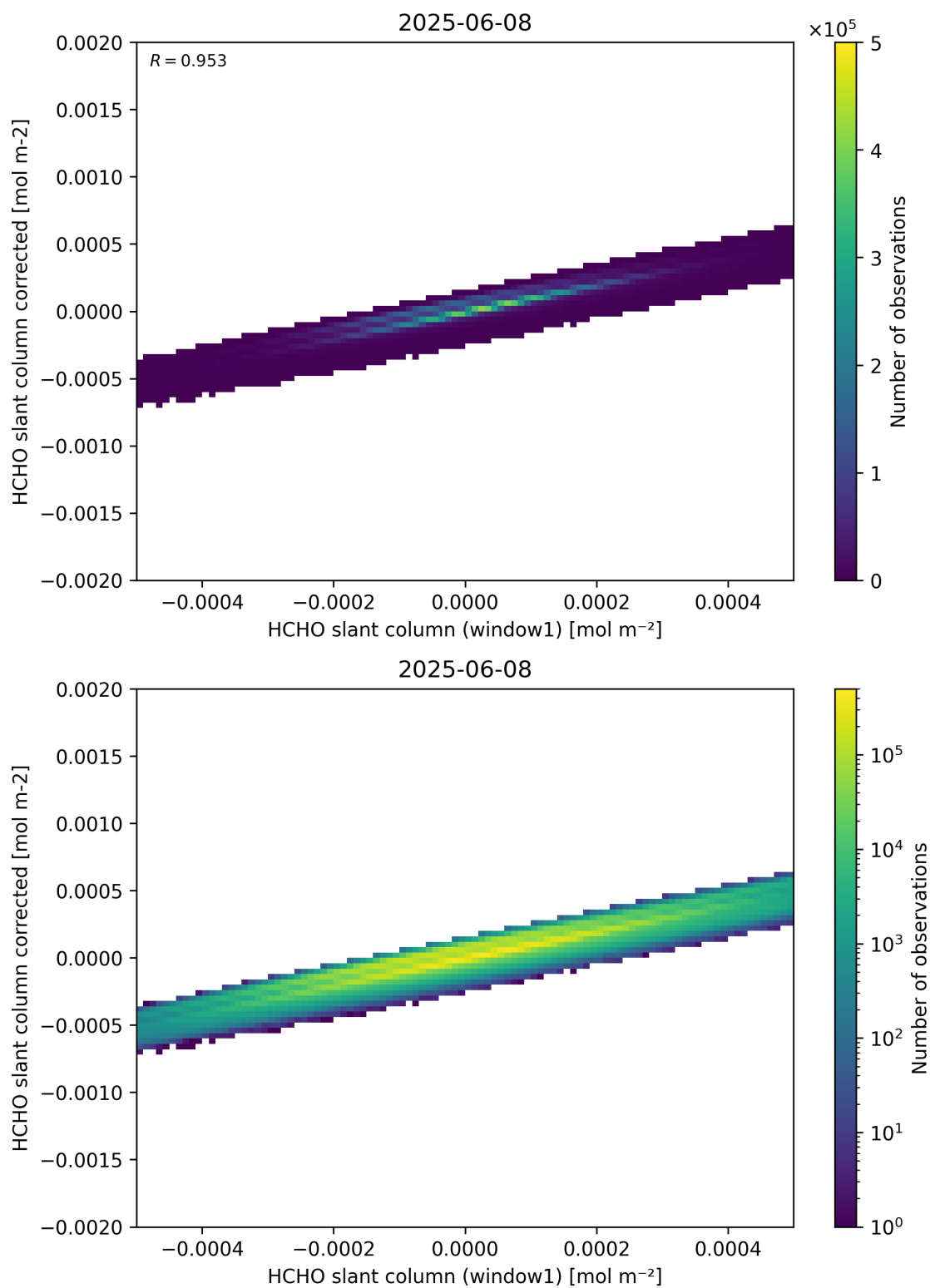
Figure 82: Scatter density plot of “HCHO slant column (window1)” against “HCHO slant column corrected” for 2025-06-07 to 2025-06-09.
