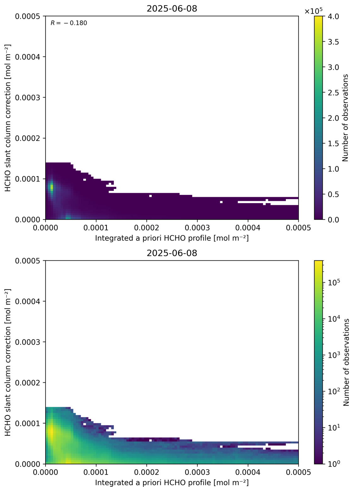
Figure 152: Scatter density plot of “Integrated a priori HCHO profile” against “HCHO slant column correction” for 2025-06-07 to 2025-06-09.
