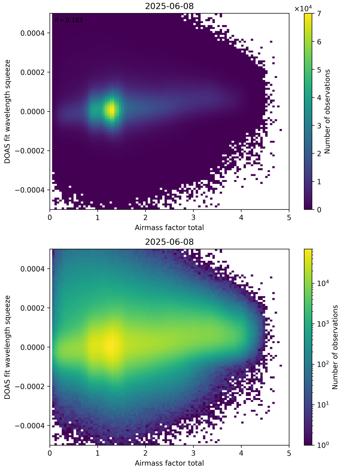
Figure 99: Scatter density plot of “Airmass factor total” against “DOAS fit wavelength squeeze” for 2025-06-07 to 2025-06-09.
