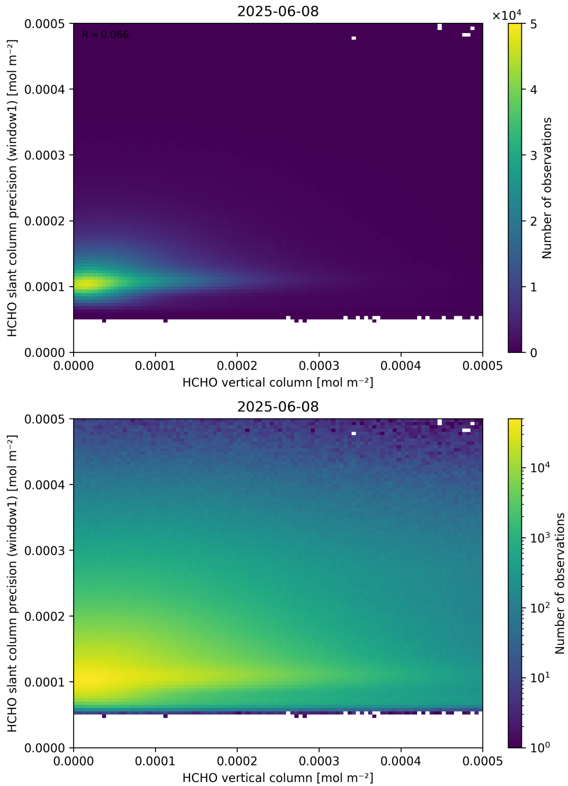
Figure 130: Scatter density plot of “HCHO vertical column” against “HCHO slant column precision (window1)” for 2025-06-07 to 2025-06-09.
