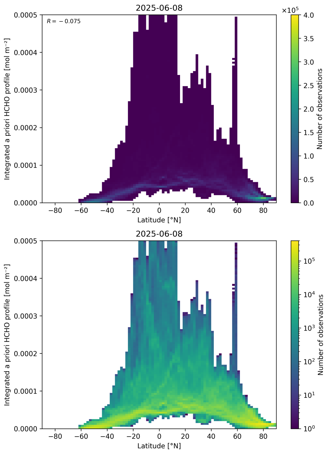
Figure 166: Scatter density plot of “Latitude” against “Integrated a priori HCHO profile” for 2025-06-07 to 2025-06-09.
