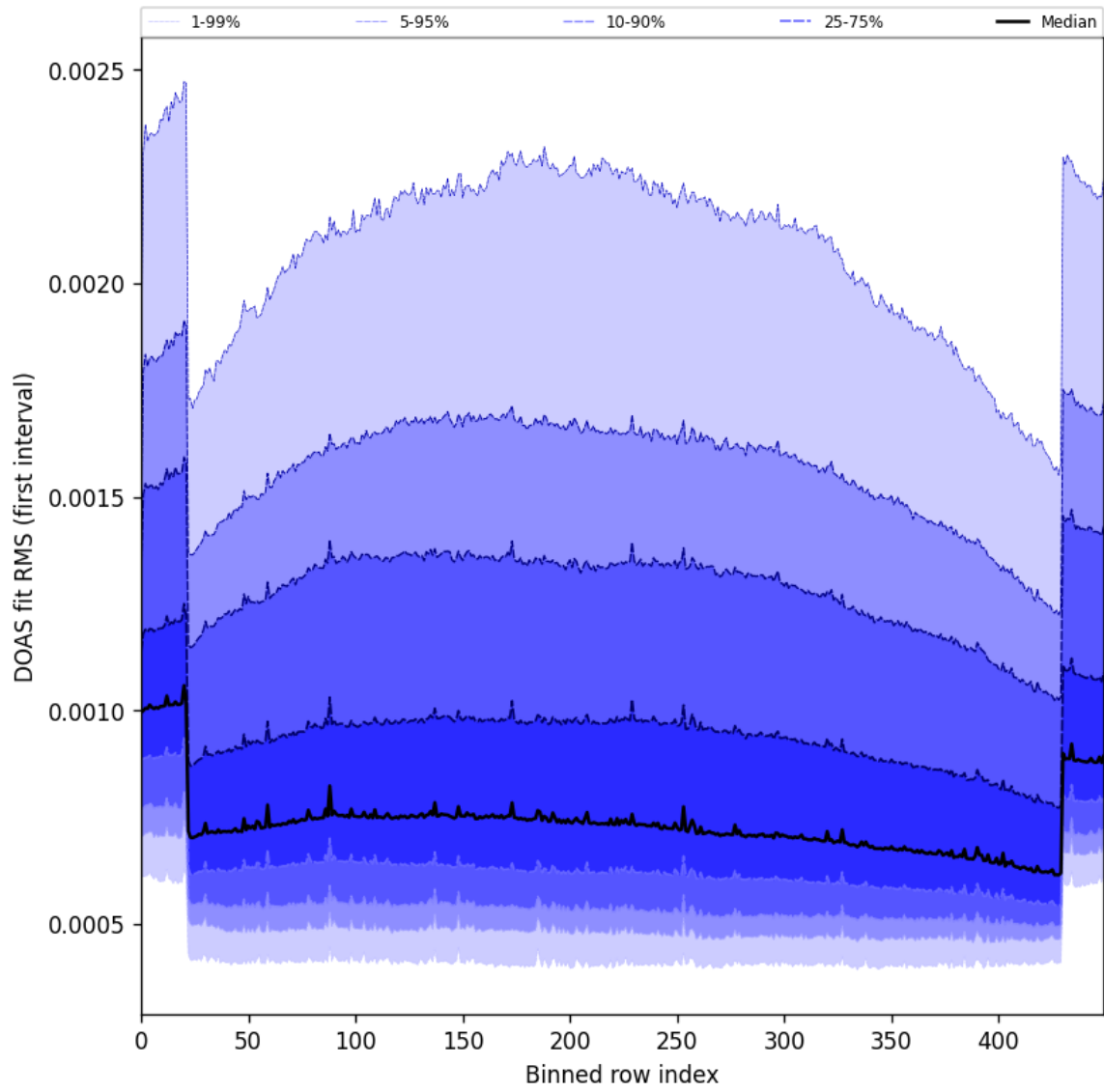
Figure 60: Along track statistics of “DOAS fit RMS (first interval)” for 2025-06-07 to 2025-06-09
