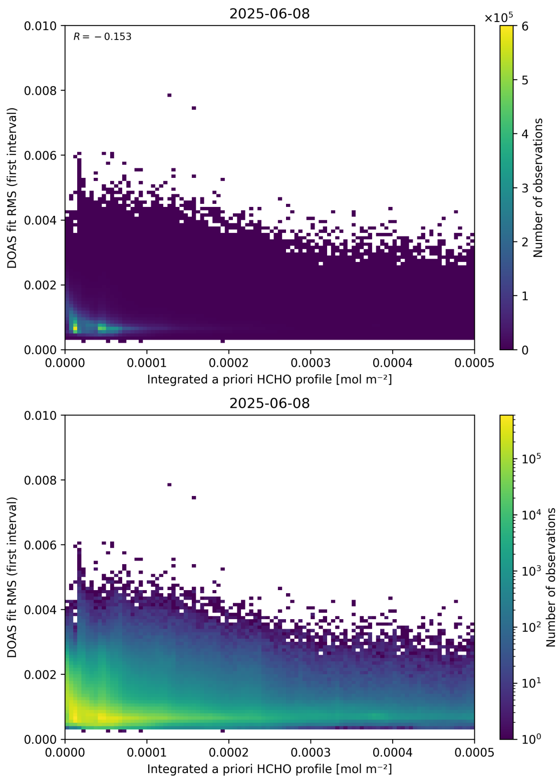
Figure 148: Scatter density plot of “Integrated a priori HCHO profile” against “DOAS fit RMS (first interval)” for 2025-06-07 to 2025-06-09.
