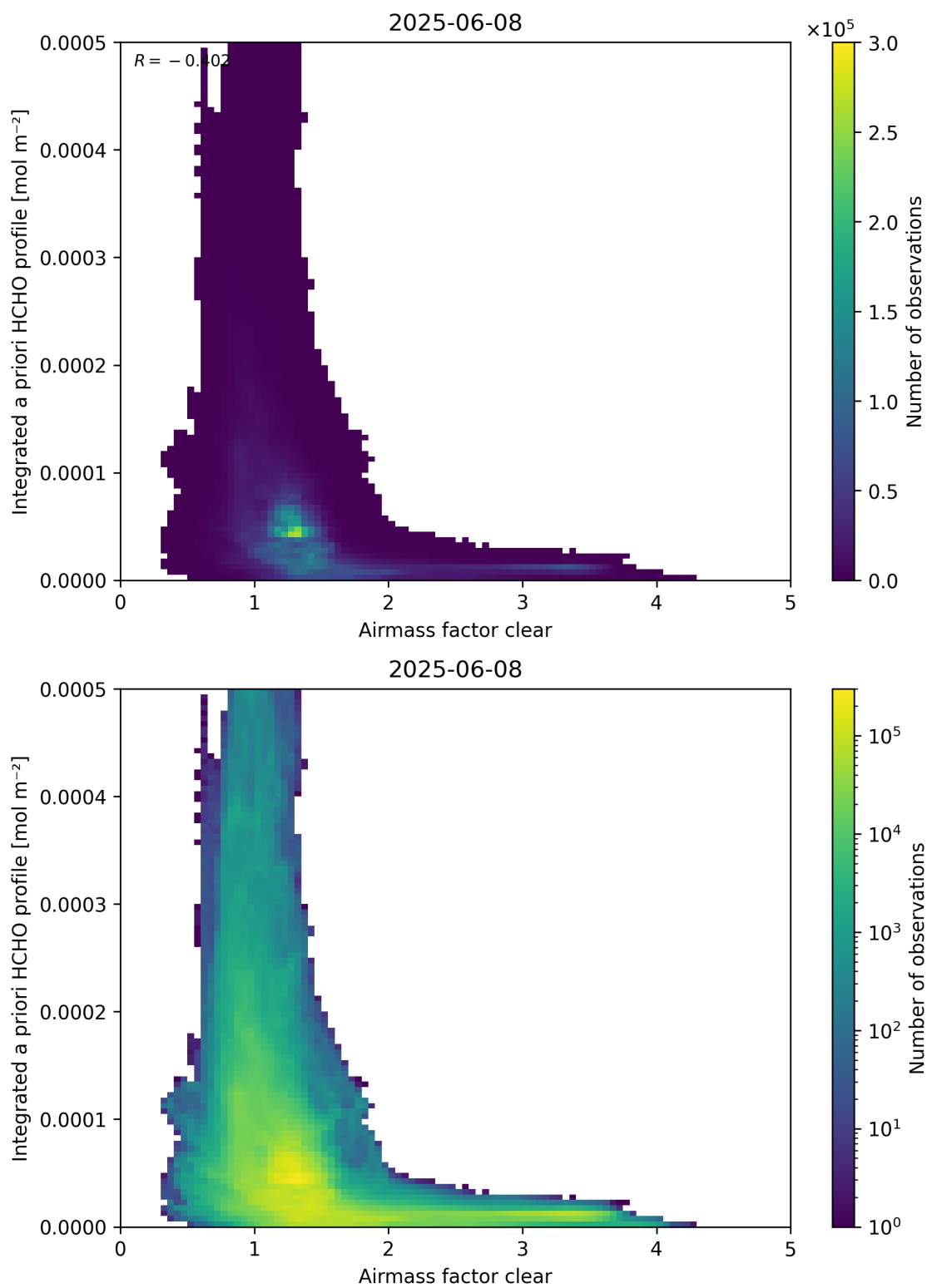
Figure 76: Scatter density plot of “Airmass factor clear” against “Integrated a priori HCHO profile” for 2025-06-07 to 2025-06-09.
