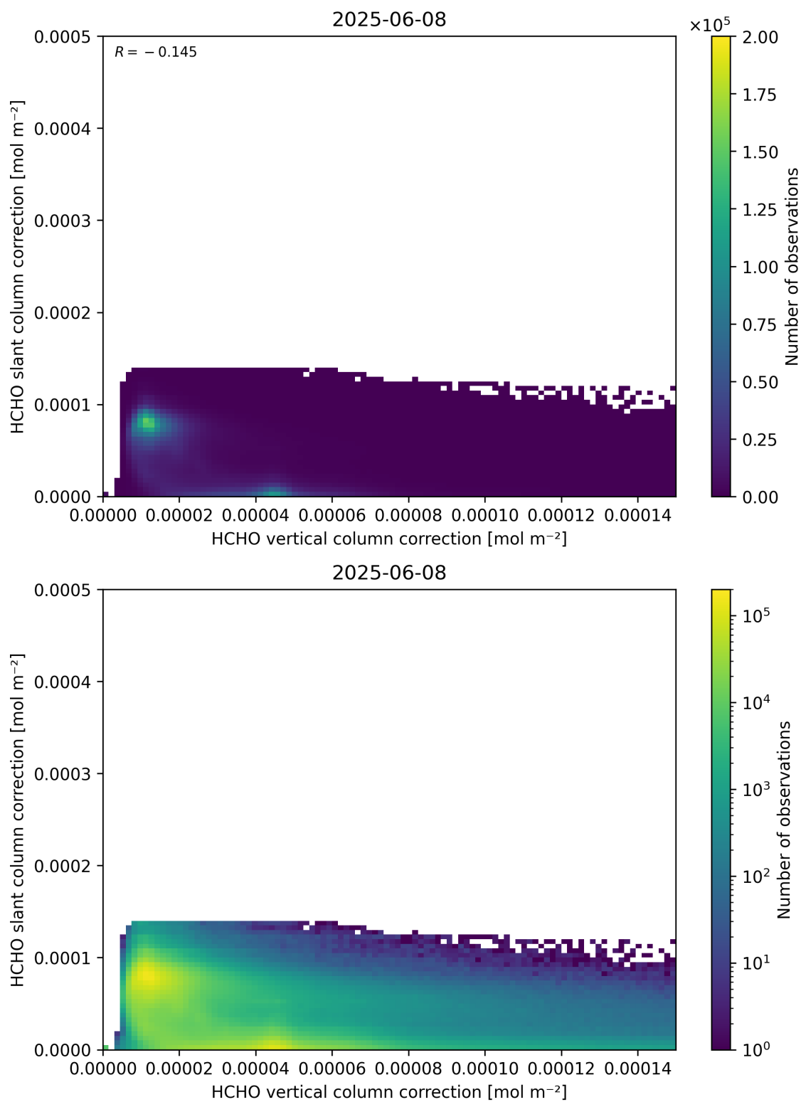
Figure 117: Scatter density plot of “HCHO vertical column correction” against “HCHO slant column correction” for 2025-06-07 to 2025-06-09.
