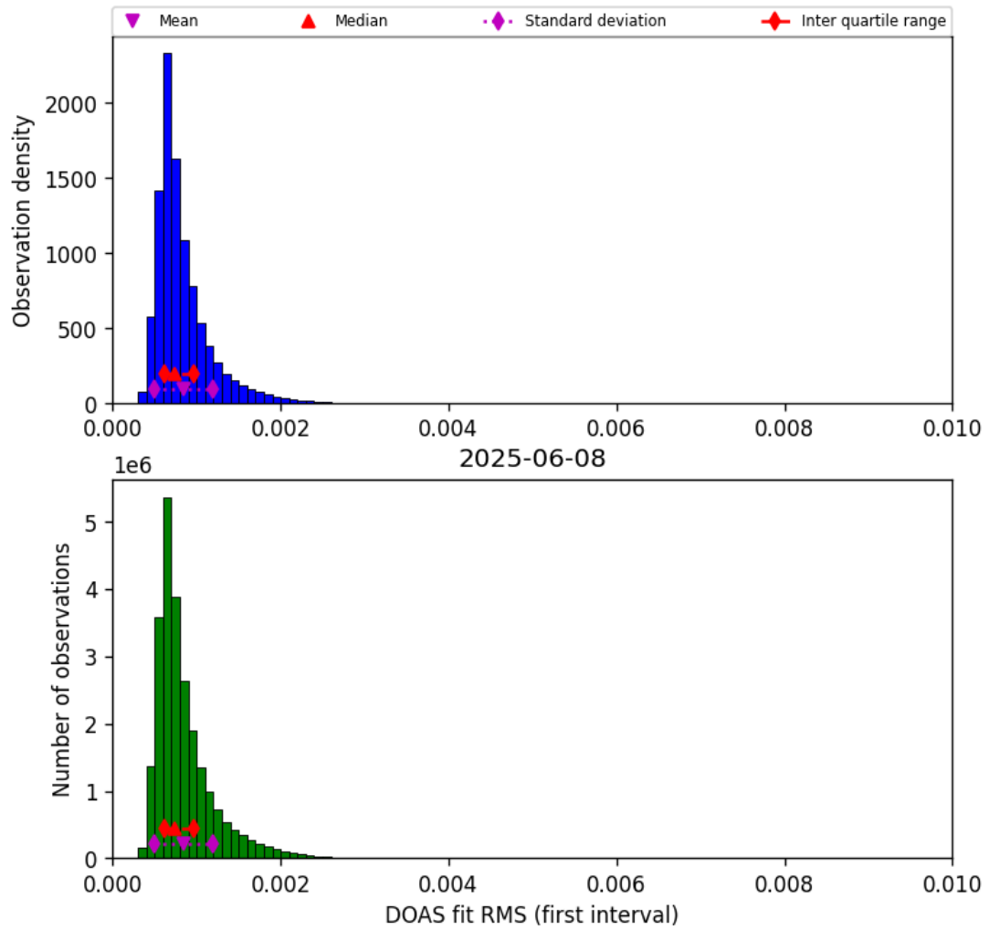
Figure 46: Histogram of “DOAS fit RMS (first interval)” for 2025-06-07 to 2025-06-09
