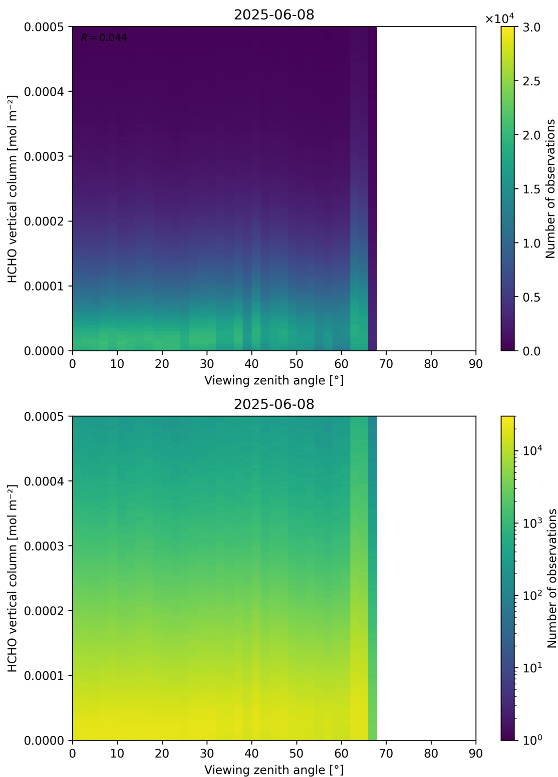
Figure 192: Scatter density plot of “Viewing zenith angle” against “HCHO vertical column” for 2025-06-07 to 2025-06-09.
