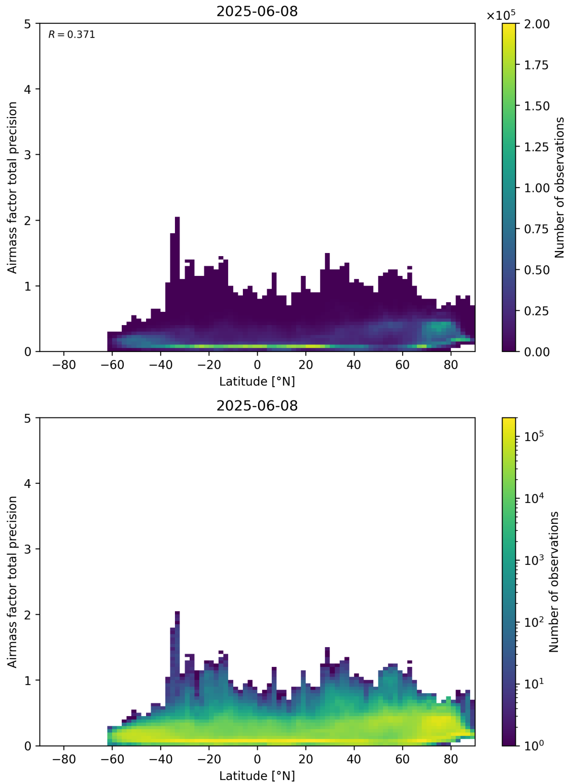
Figure 162: Scatter density plot of “Latitude” against “Airmass factor total precision” for 2025-06-07 to 2025-06-09.
