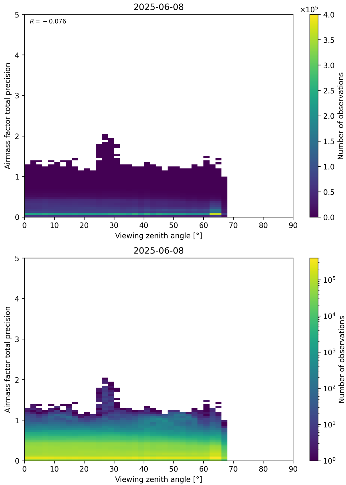
Figure 191: Scatter density plot of “Viewing zenith angle” against “Airmass factor total precision” for 2025-06-07 to 2025-06-09.
