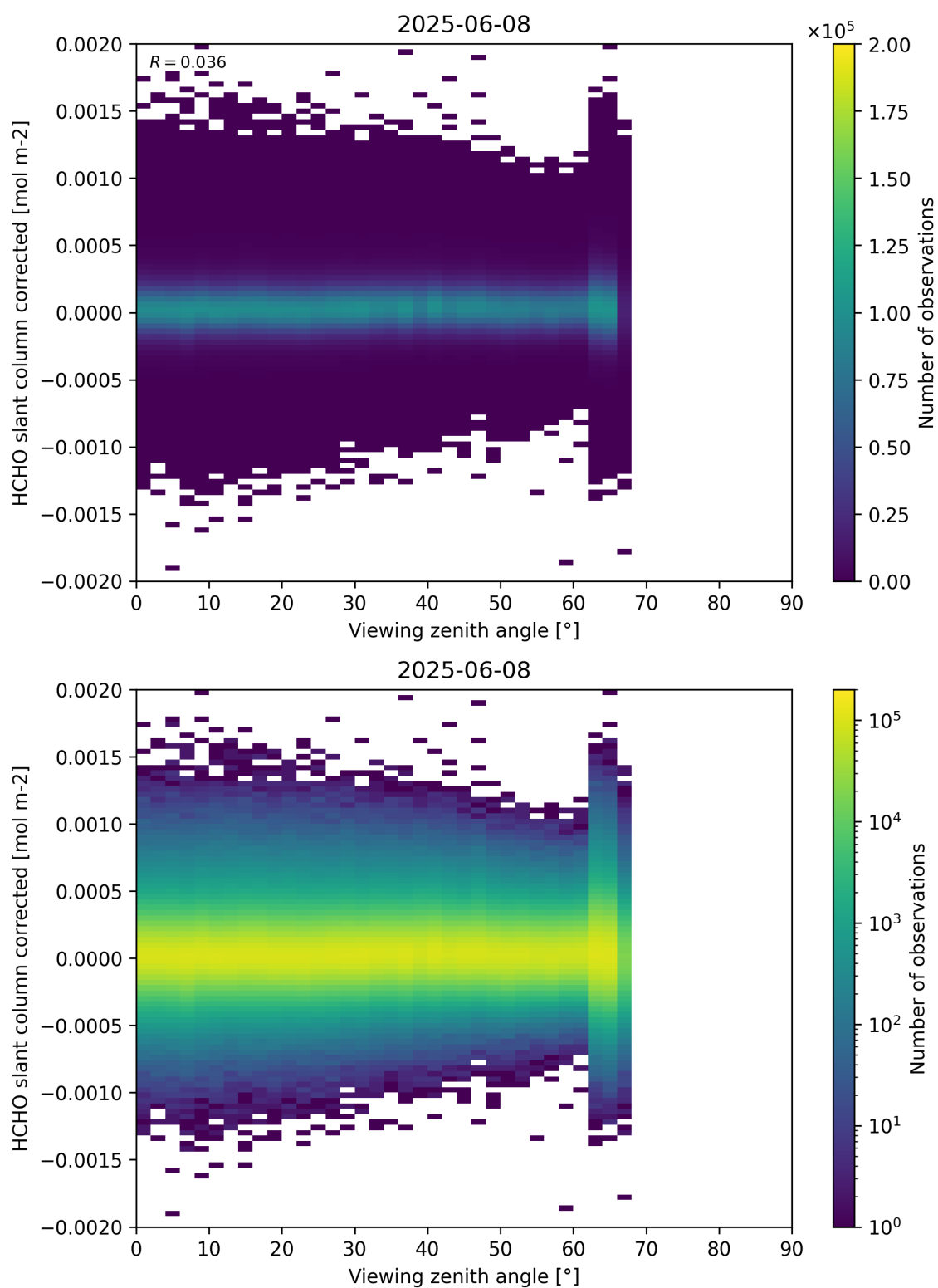
Figure 186: Scatter density plot of “Viewing zenith angle” against “HCHO slant column corrected” for 2025-06-07 to 2025-06-09.
