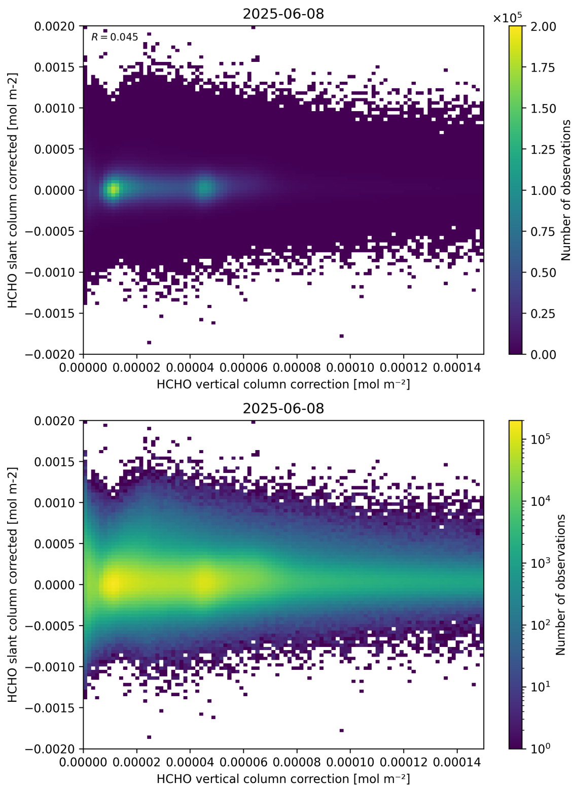
Figure 116: Scatter density plot of “HCHO vertical column correction” against “HCHO slant column corrected” for 2025-06-07 to 2025-06-09.
