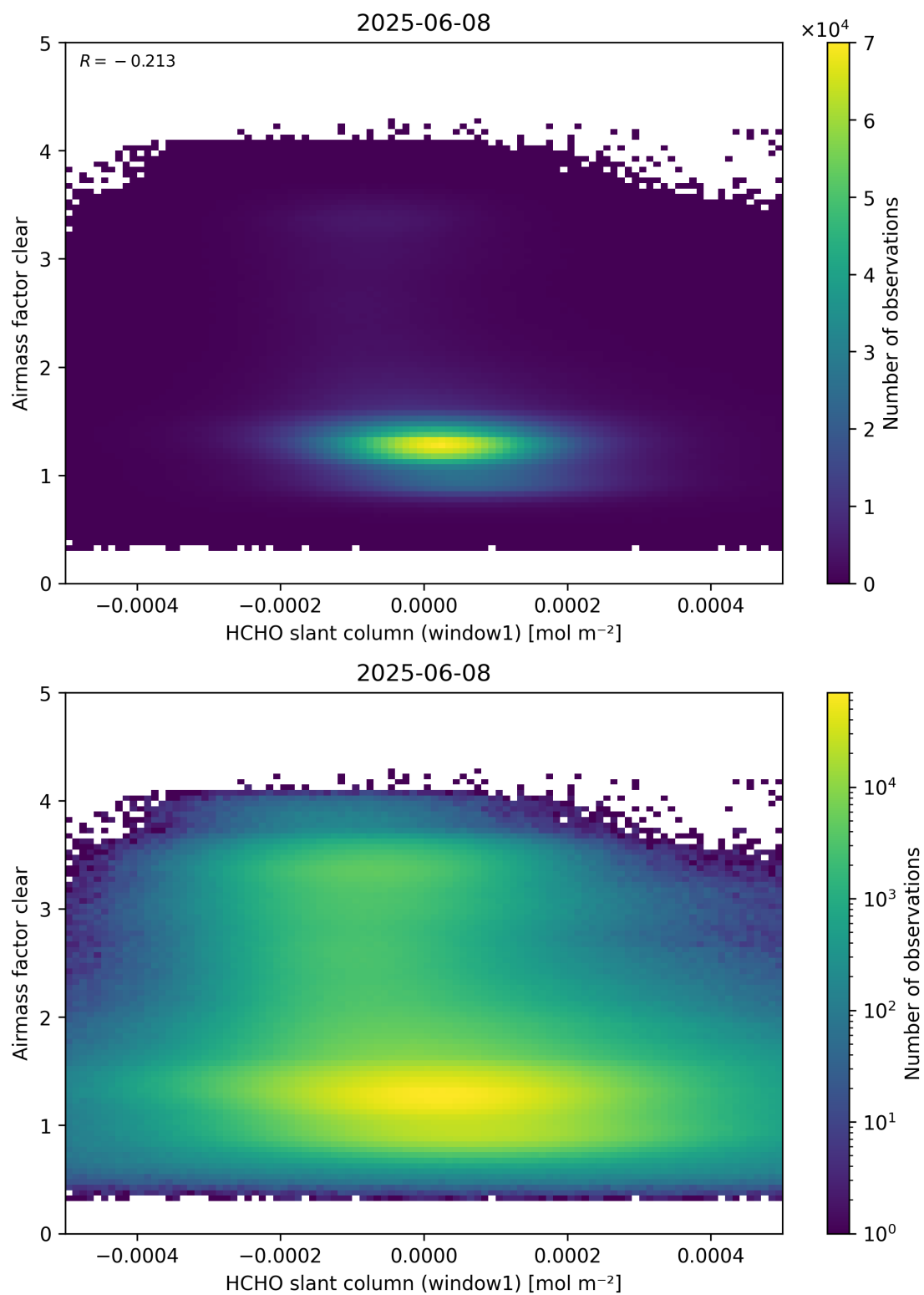
Figure 81: Scatter density plot of “HCHO slant column (window1)” against “Airmass factor clear” for 2025-06-07 to 2025-06-09.
