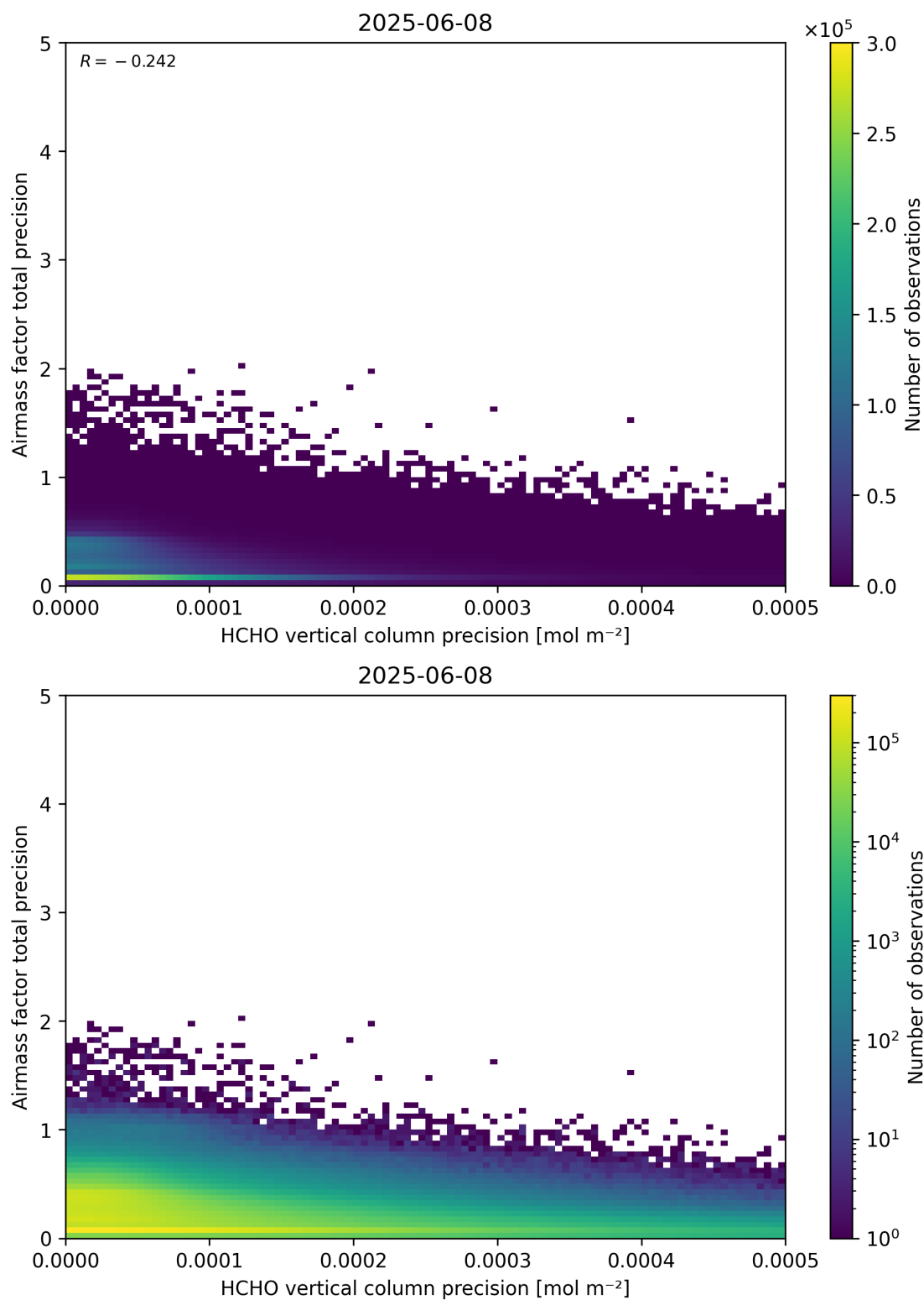
Figure 145: Scatter density plot of “HCHO vertical column precision” against “Airmass factor total precision” for 2025-06-07 to 2025-06-09.
