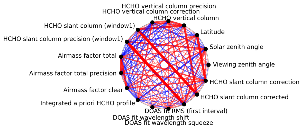
Figure 1: Map of correlation graph for 2025-06-07 to 2025-06-09.
