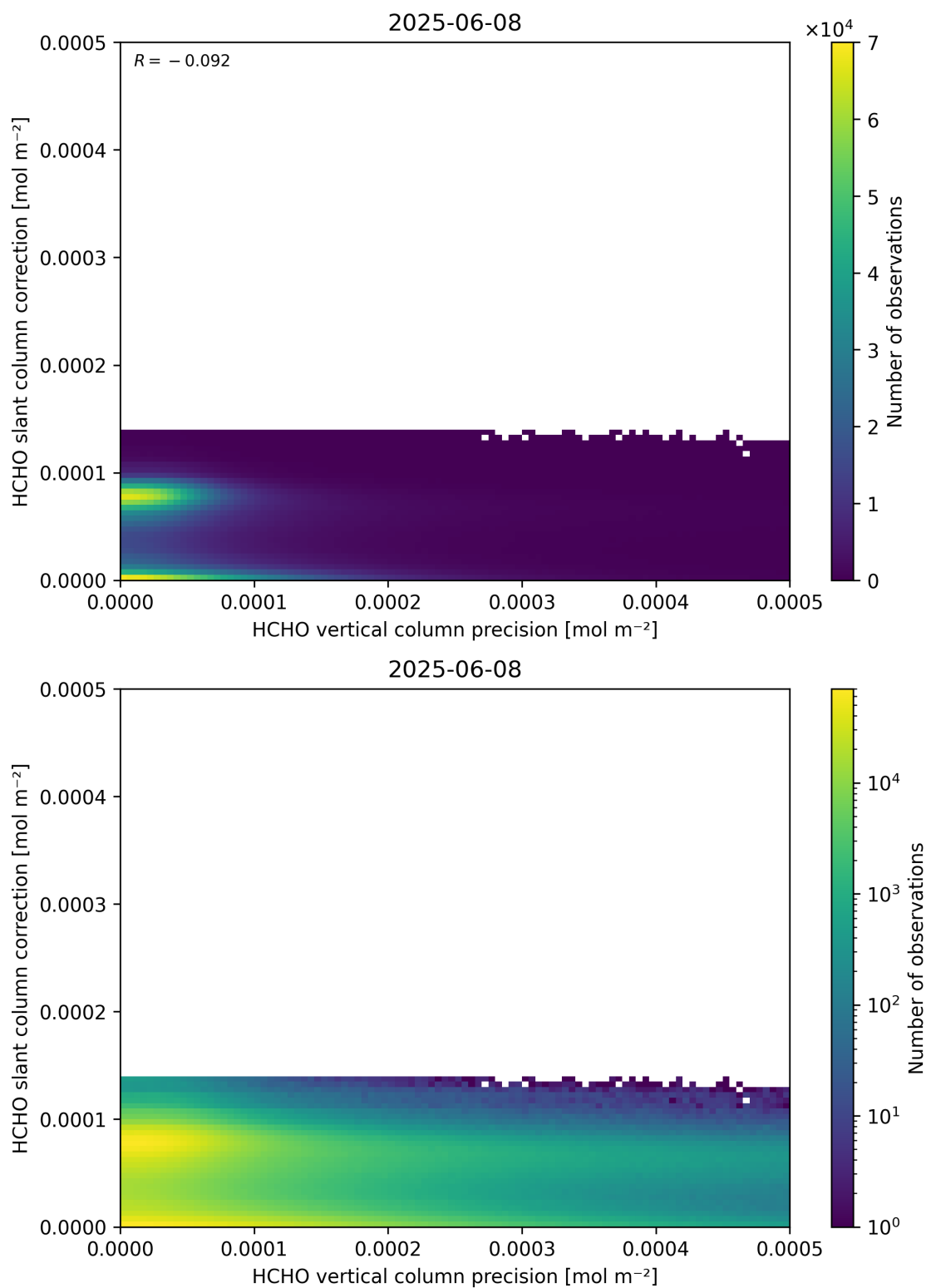
Figure 141: Scatter density plot of “HCHO vertical column precision” against “HCHO slant column correction” for 2025-06-07 to 2025-06-09.
