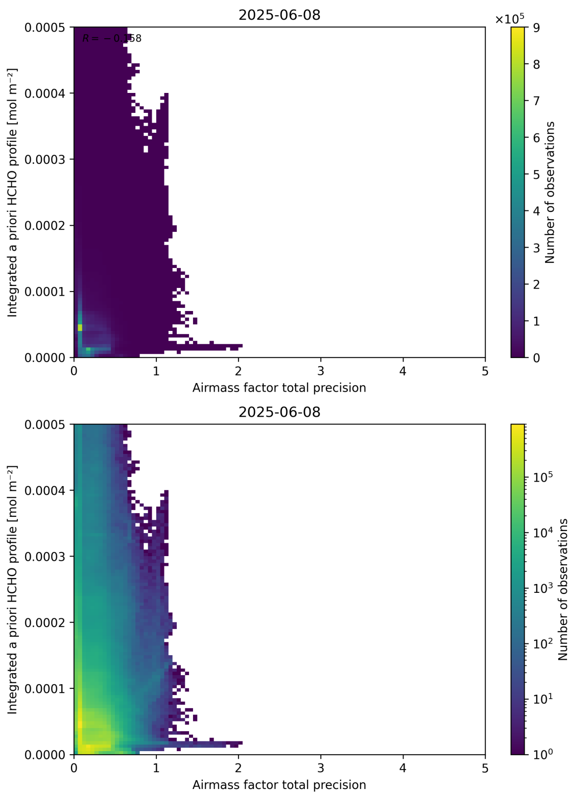
Figure 111: Scatter density plot of “Airmass factor total precision” against “Integrated a priori HCHO profile” for 2025-06-07 to 2025-06-09.
