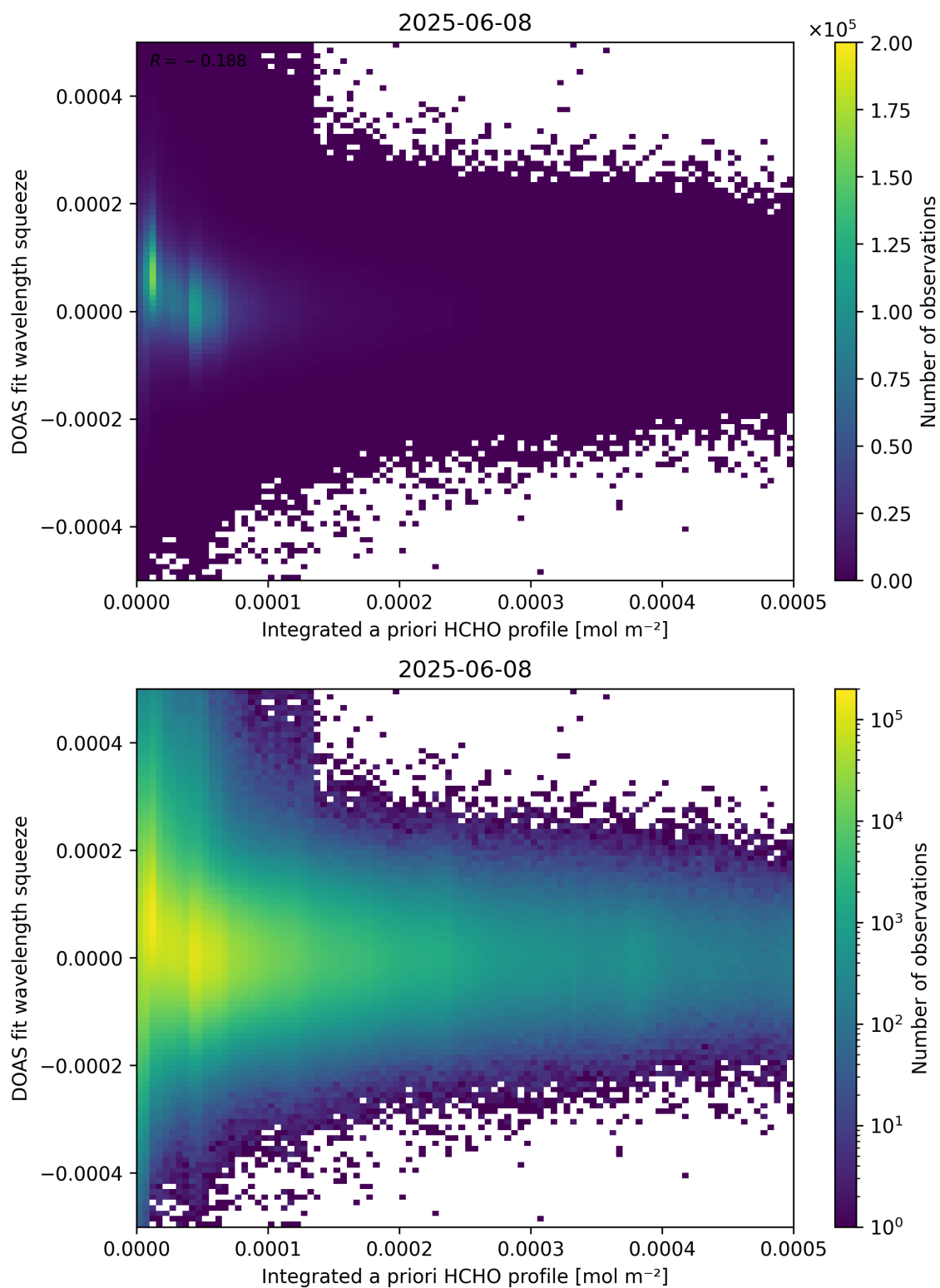
Figure 150: Scatter density plot of “Integrated a priori HCHO profile” against “DOAS fit wavelength squeeze” for 2025-06-07 to 2025-06-09.
