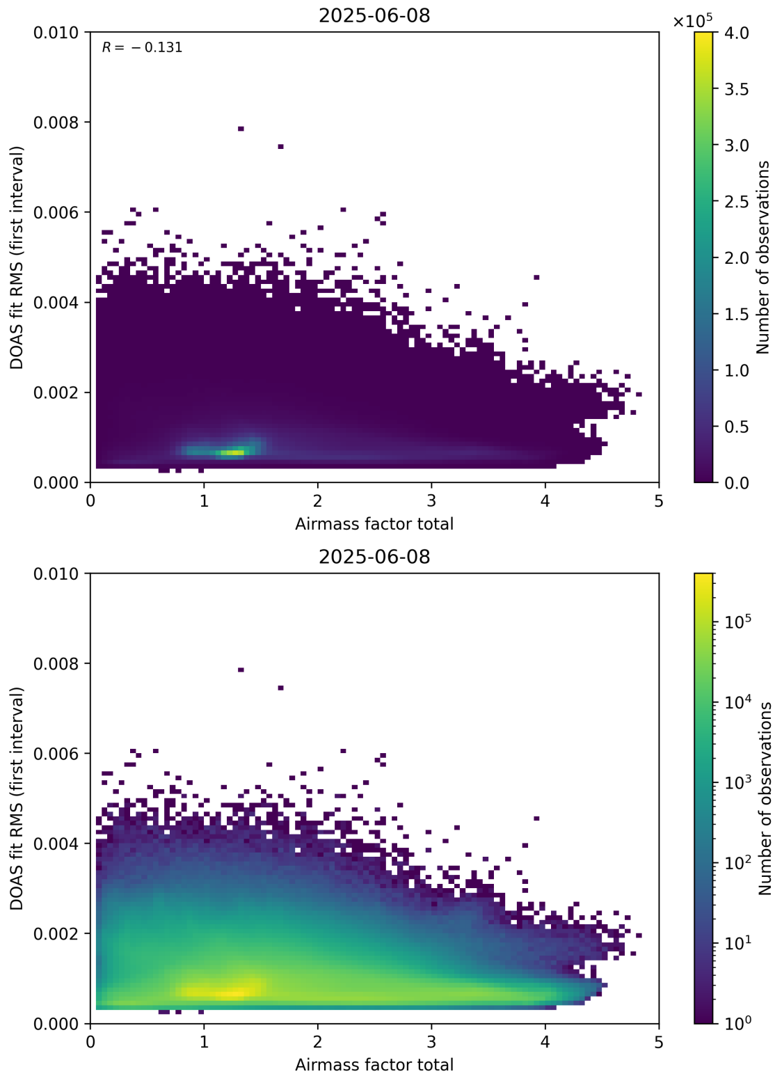
Figure 97: Scatter density plot of “Airmass factor total” against “DOAS fit RMS (first interval)” for 2025-06-07 to 2025-06-09.
