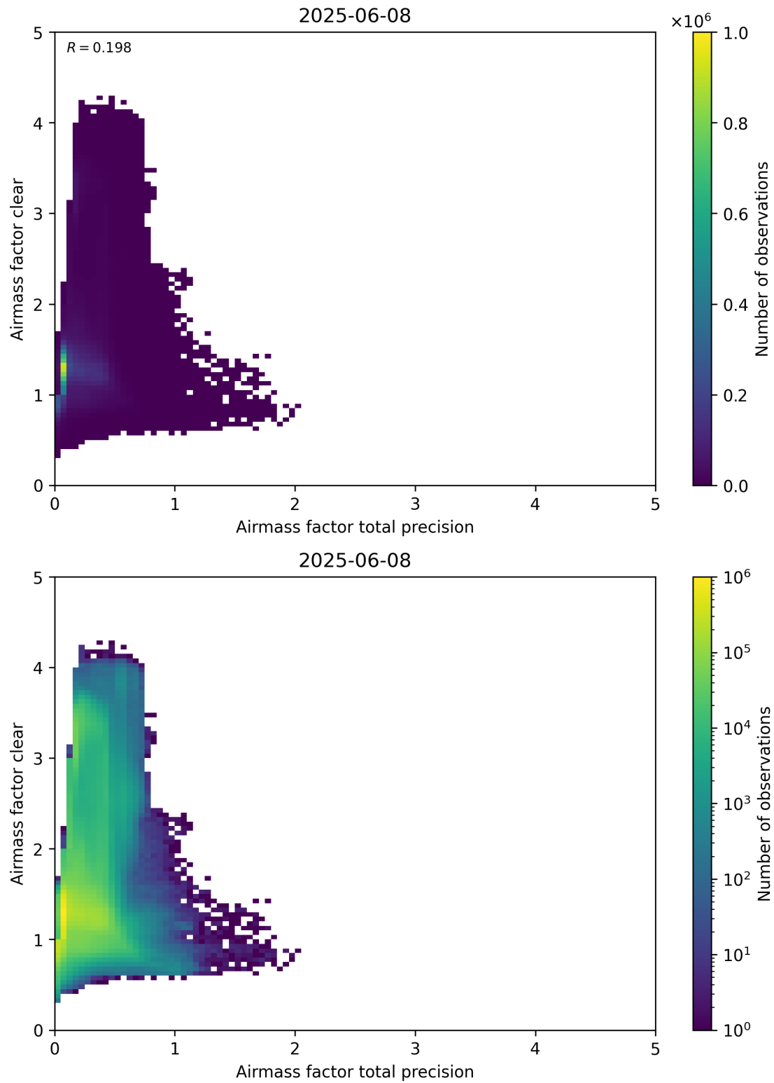
Figure 108: Scatter density plot of “Airmass factor total precision” against “Airmass factor clear” for 2025-06-07 to 2025-06-09.
