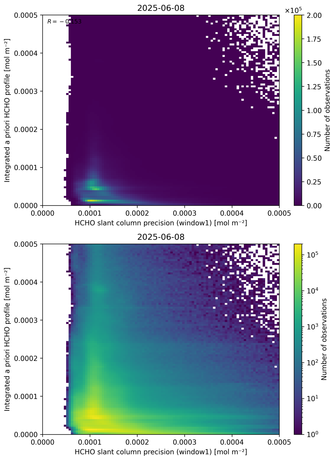
Figure 96: Scatter density plot of “HCHO slant column precision (window1)” against “Integrated a priori HCHO profile” for 2025-06-07 to 2025-06-09.
