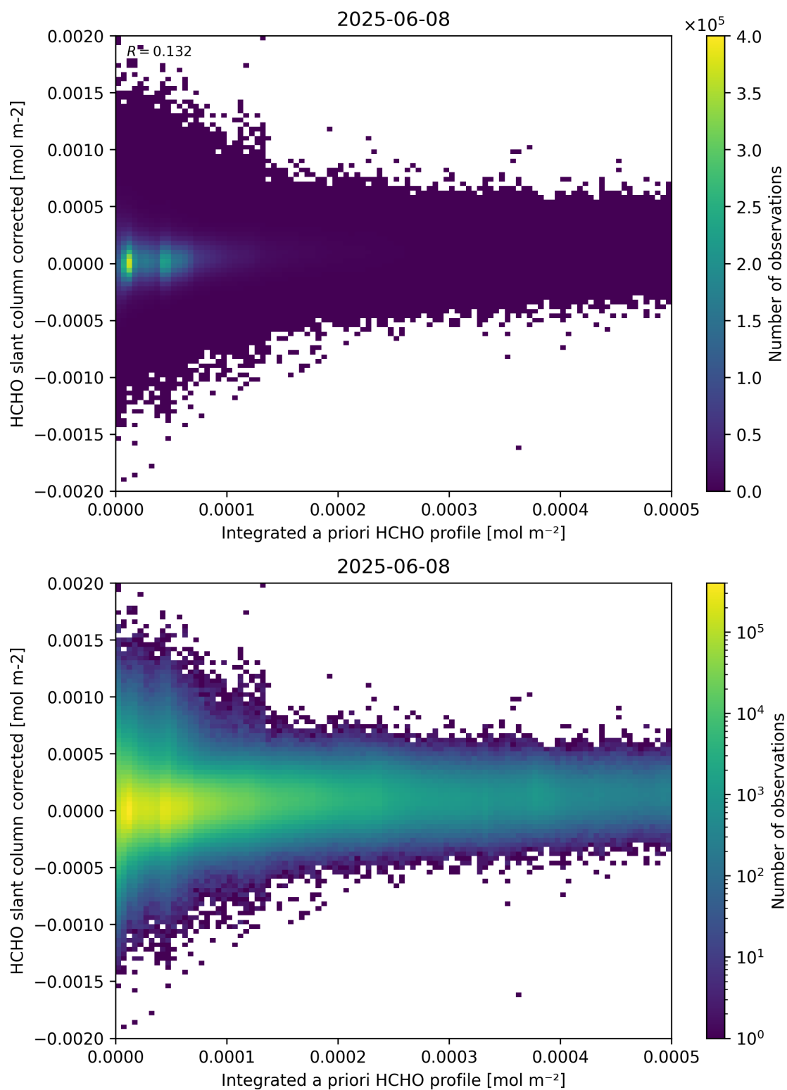
Figure 151: Scatter density plot of “Integrated a priori HCHO profile” against “HCHO slant column corrected” for 2025-06-07 to 2025-06-09.
