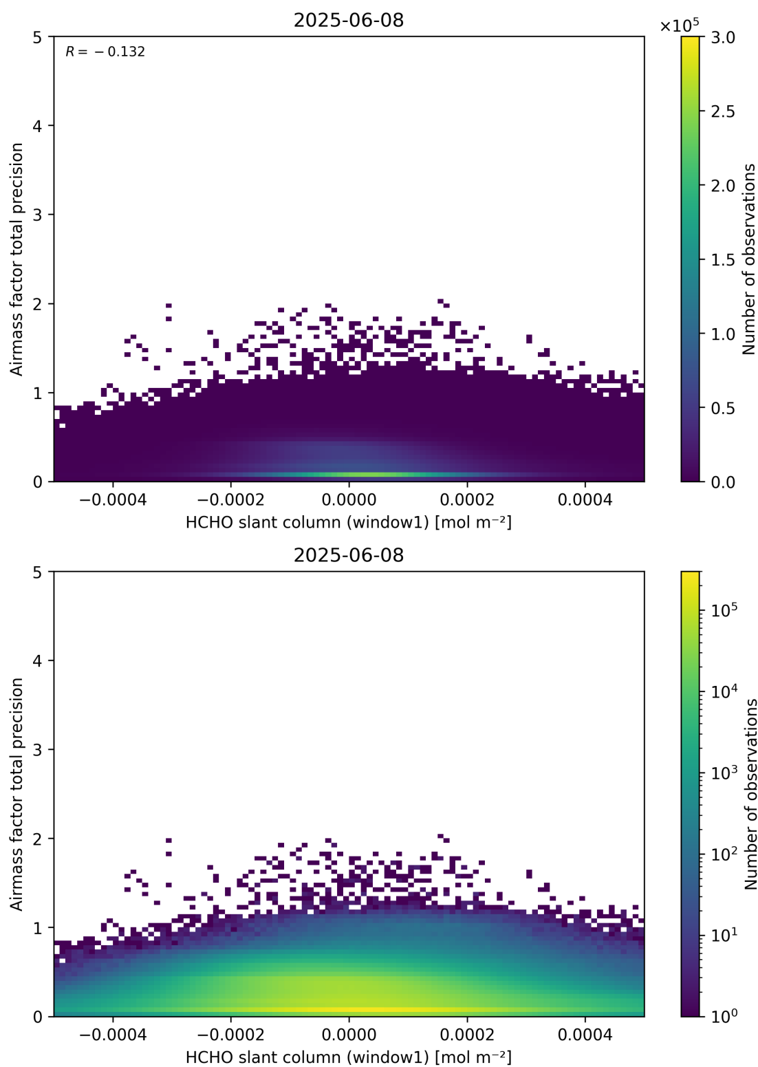
Figure 86: Scatter density plot of “HCHO slant column (window1)” against “Airmass factor total precision” for 2025-06-07 to 2025-06-09.
