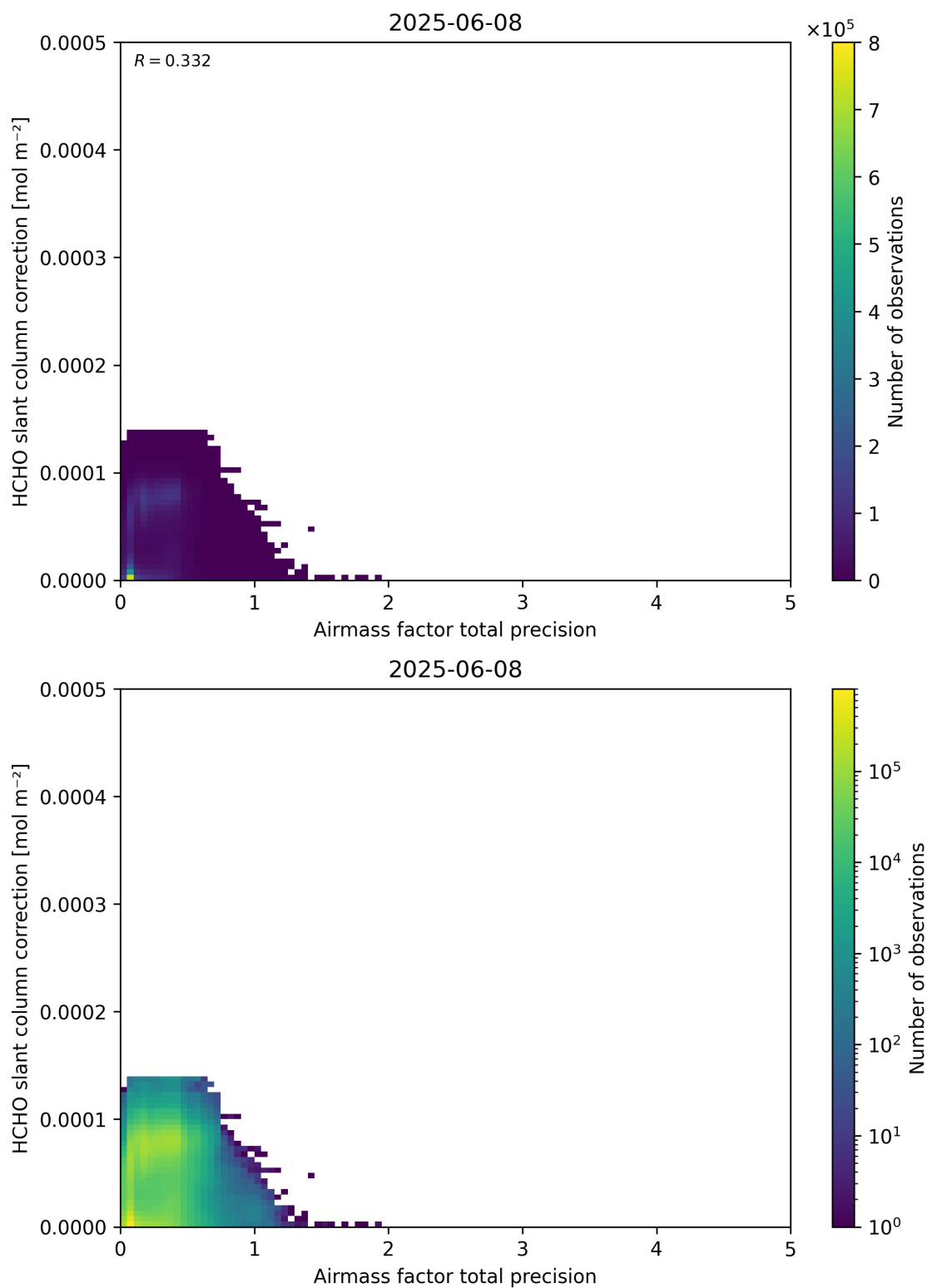
Figure 110: Scatter density plot of “Airmass factor total precision” against “HCHO slant column correction” for 2025-06-07 to 2025-06-09.
