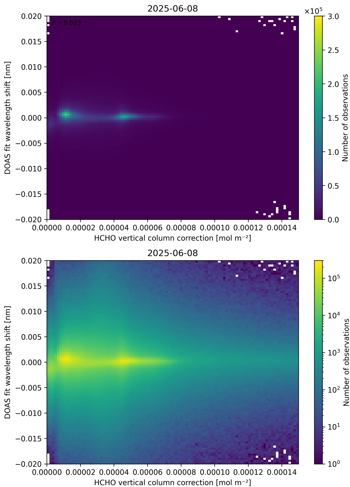
Figure 113: Scatter density plot of “HCHO vertical column correction” against “DOAS fit wavelength shift” for 2025-06-07 to 2025-06-09.
