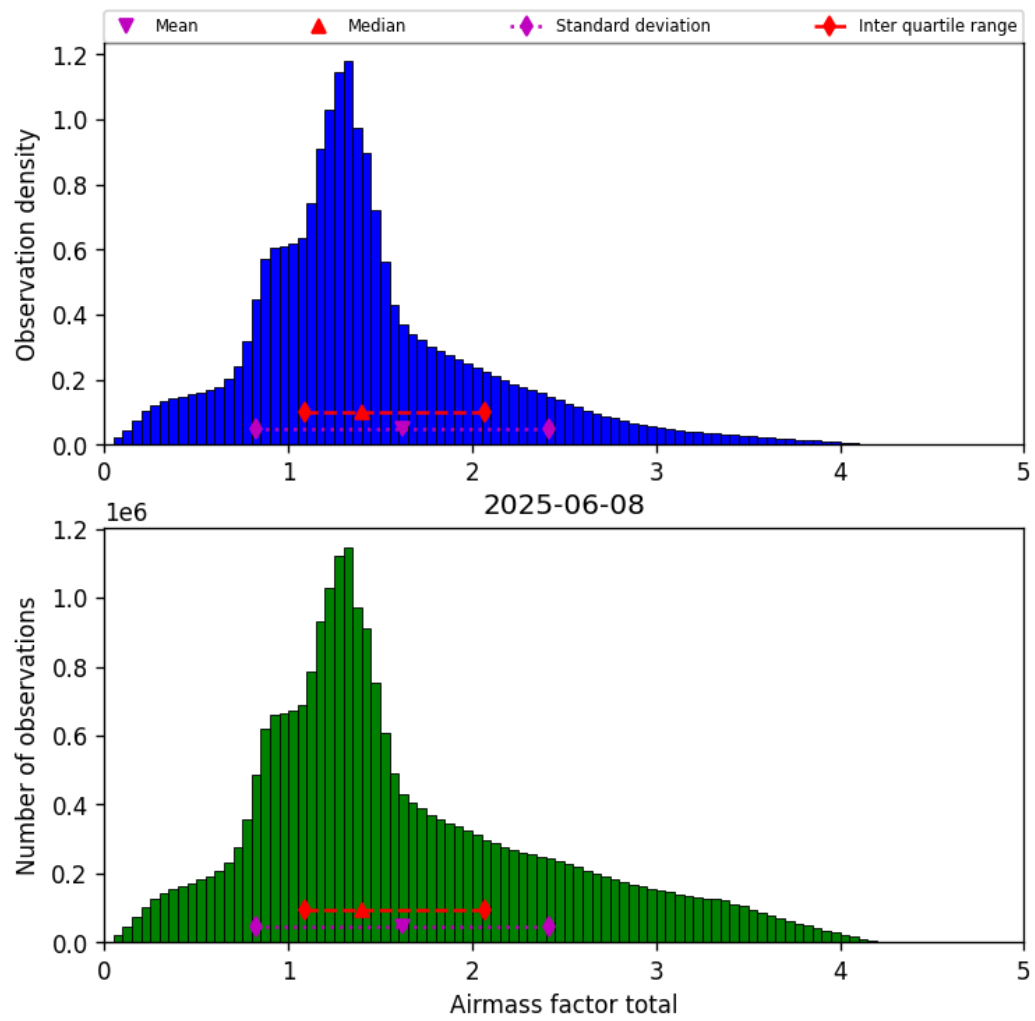
Figure 40: Histogram of “Airmass factor total” for 2025-06-07 to 2025-06-09
