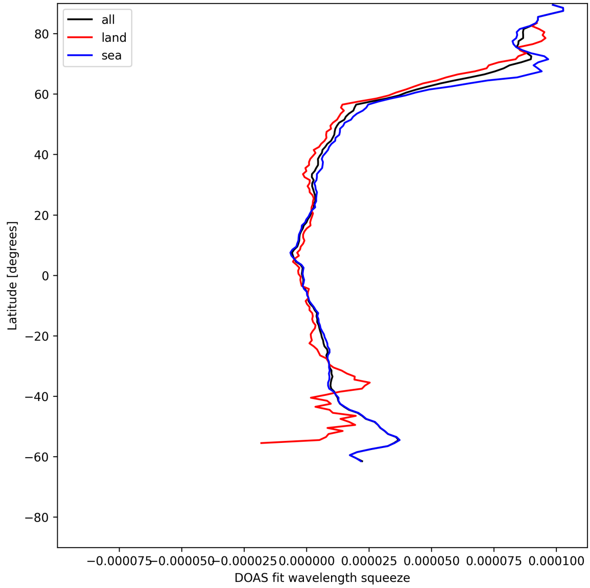
Figure 31: Zonal average of “DOAS fit wavelength squeeze” for 2025-06-07 to 2025-06-09.
