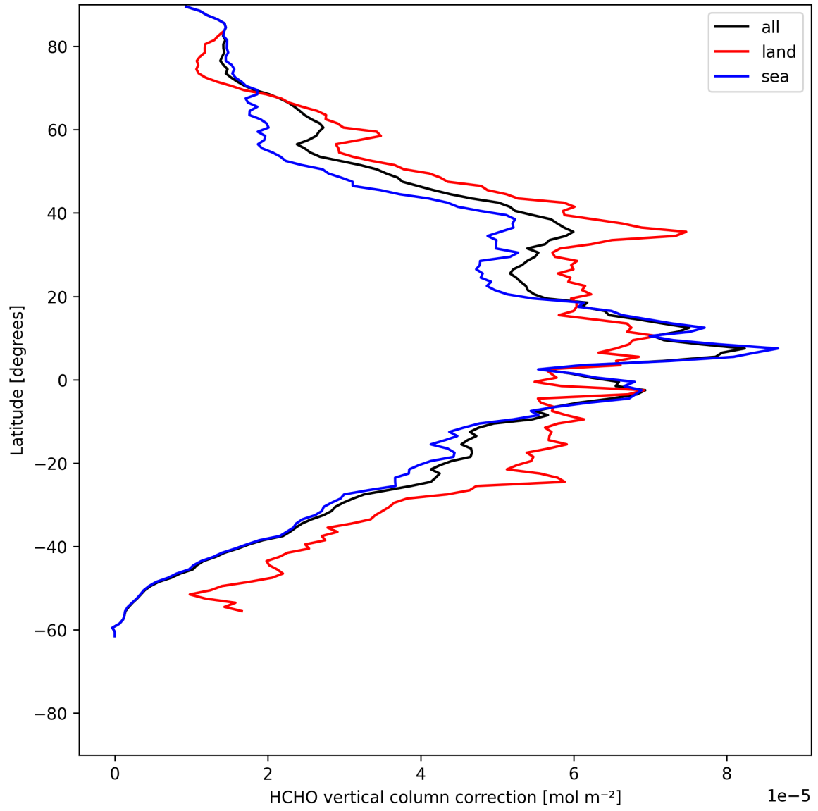
Figure 23: Zonal average of "HCHO vertical column correction" for 2025-06-07 to 2025-06-09.
