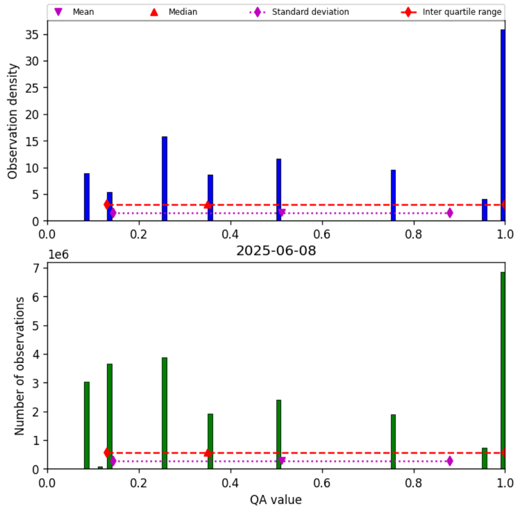
Figure 34: Histogram of “QA value” for 2025-06-07 to 2025-06-09
