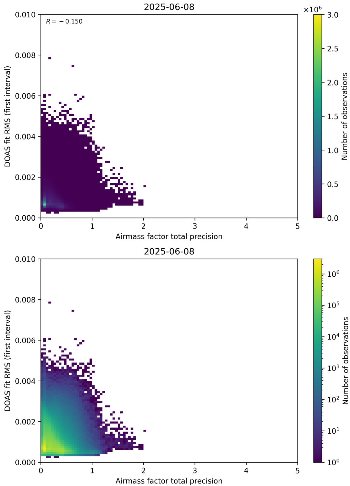
Figure 105: Scatter density plot of “Airmass factor total precision” against “DOAS fit RMS (first interval)” for 2025-06-07 to 2025-06-09.
