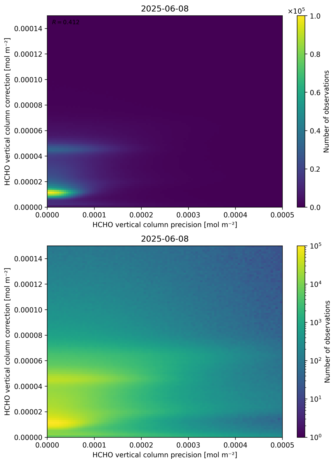
Figure 146: Scatter density plot of “HCHO vertical column precision” against “HCHO vertical column correction” for 2025-06-07 to 2025-06-09.
