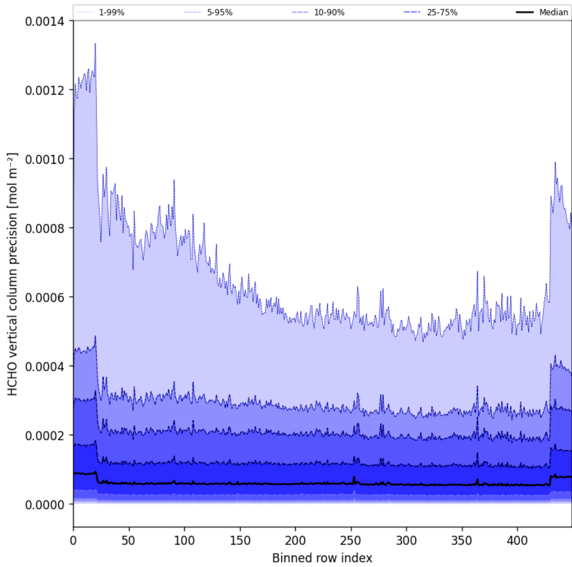
Figure 50: Along track statistics of “HCHO vertical column precision” for 2025-06-07 to 2025-06-09
