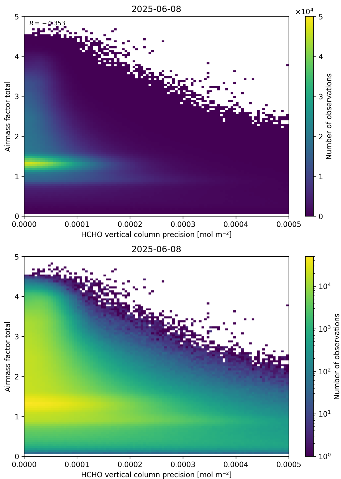
Figure 144: Scatter density plot of “HCHO vertical column precision” against “Airmass factor total” for 2025-06-07 to 2025-06-09.
