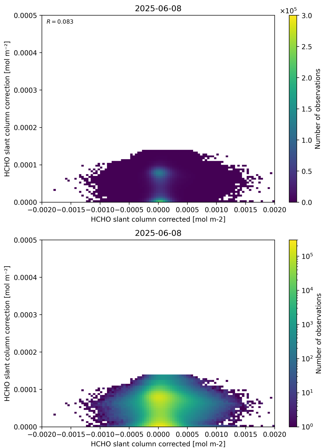
Figure 77: Scatter density plot of “HCHO slant column corrected” against “HCHO slant column correction” for 2025-06-07 to 2025-06-09.
