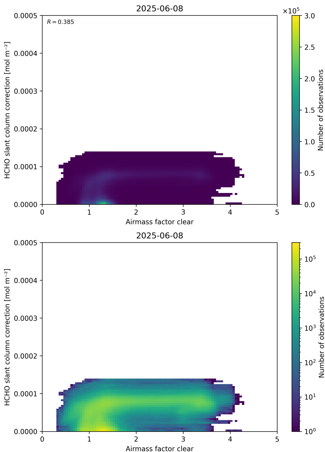
Figure 75: Scatter density plot of “Airmass factor clear” against “HCHO slant column correction” for 2025-06-07 to 2025-06-09.
