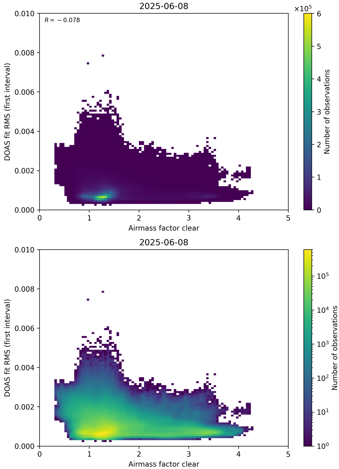
Figure 71: Scatter density plot of “Airmass factor clear” against “DOAS fit RMS (first interval)” for 2025-06-07 to 2025-06-09.
