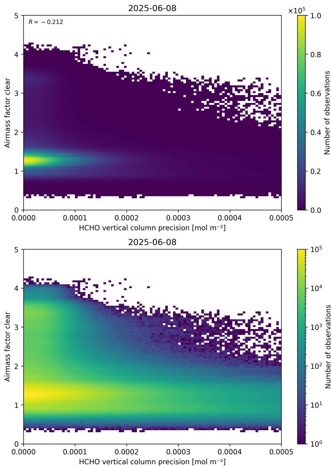
Figure 139: Scatter density plot of “HCHO vertical column precision” against “Airmass factor clear” for 2025-06-07 to 2025-06-09.
