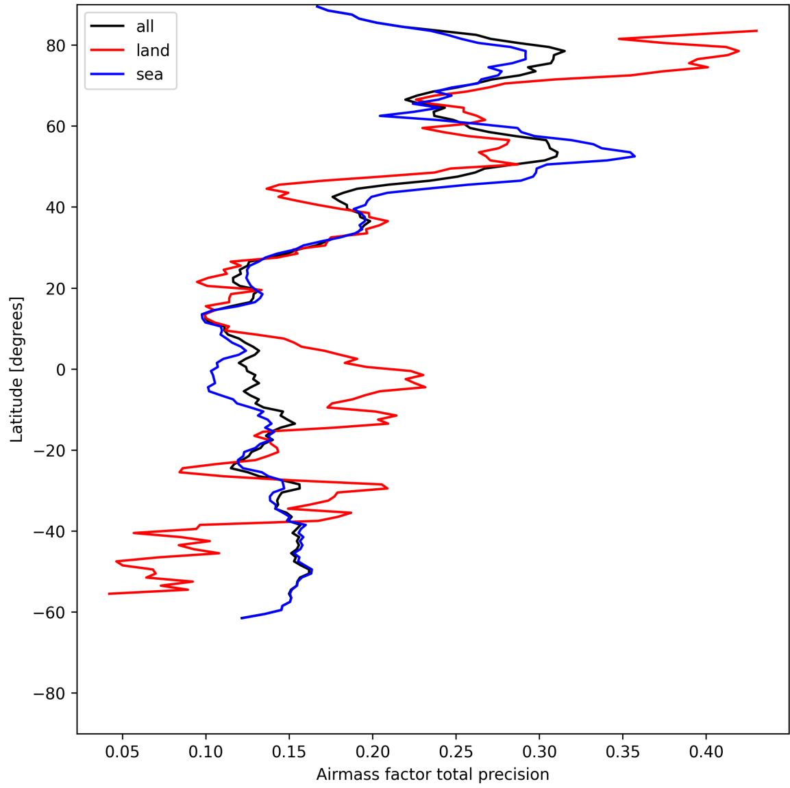
Figure 27: Zonal average of “Airmass factor total precision” for 2025-06-07 to 2025-06-09.
