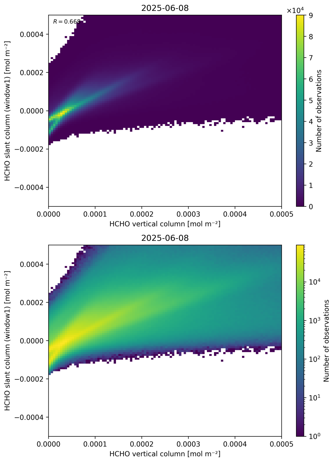
Figure 129: Scatter density plot of “HCHO vertical column” against “HCHO slant column (window1)” for 2025-06-07 to 2025-06-09.
