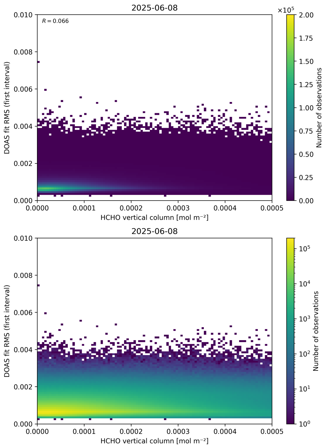
Figure 123: Scatter density plot of “HCHO vertical column” against “DOAS fit RMS (first interval)” for 2025-06-07 to 2025-06-09.
