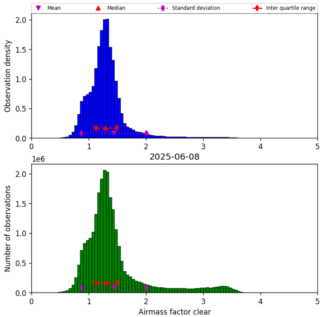
Figure 42: Histogram of “Airmass factor clear” for 2025-06-07 to 2025-06-09
