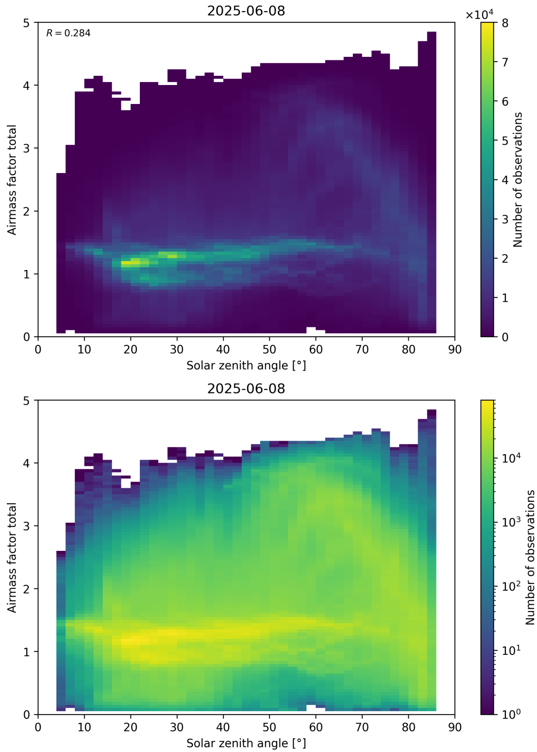
Figure 175: Scatter density plot of “Solar zenith angle” against “Airmass factor total” for 2025-06-07 to 2025-06-09.
