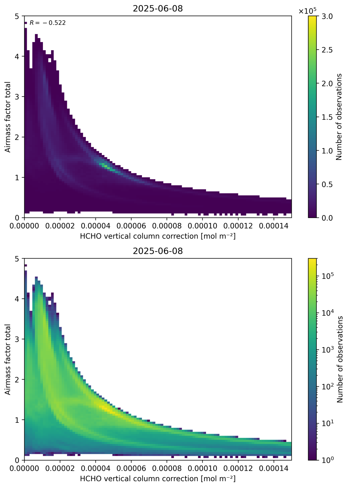
Figure 120: Scatter density plot of “HCHO vertical column correction” against “Airmass factor total” for 2025-06-07 to 2025-06-09.
