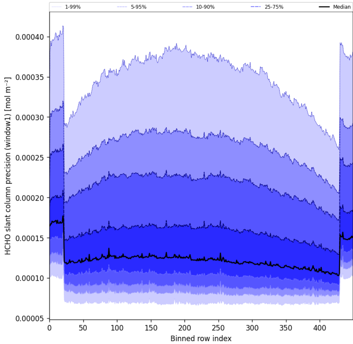
Figure 53: Along track statistics of “HCHO slant column precision (window1)” for 2025-06-07 to 2025-06-09
