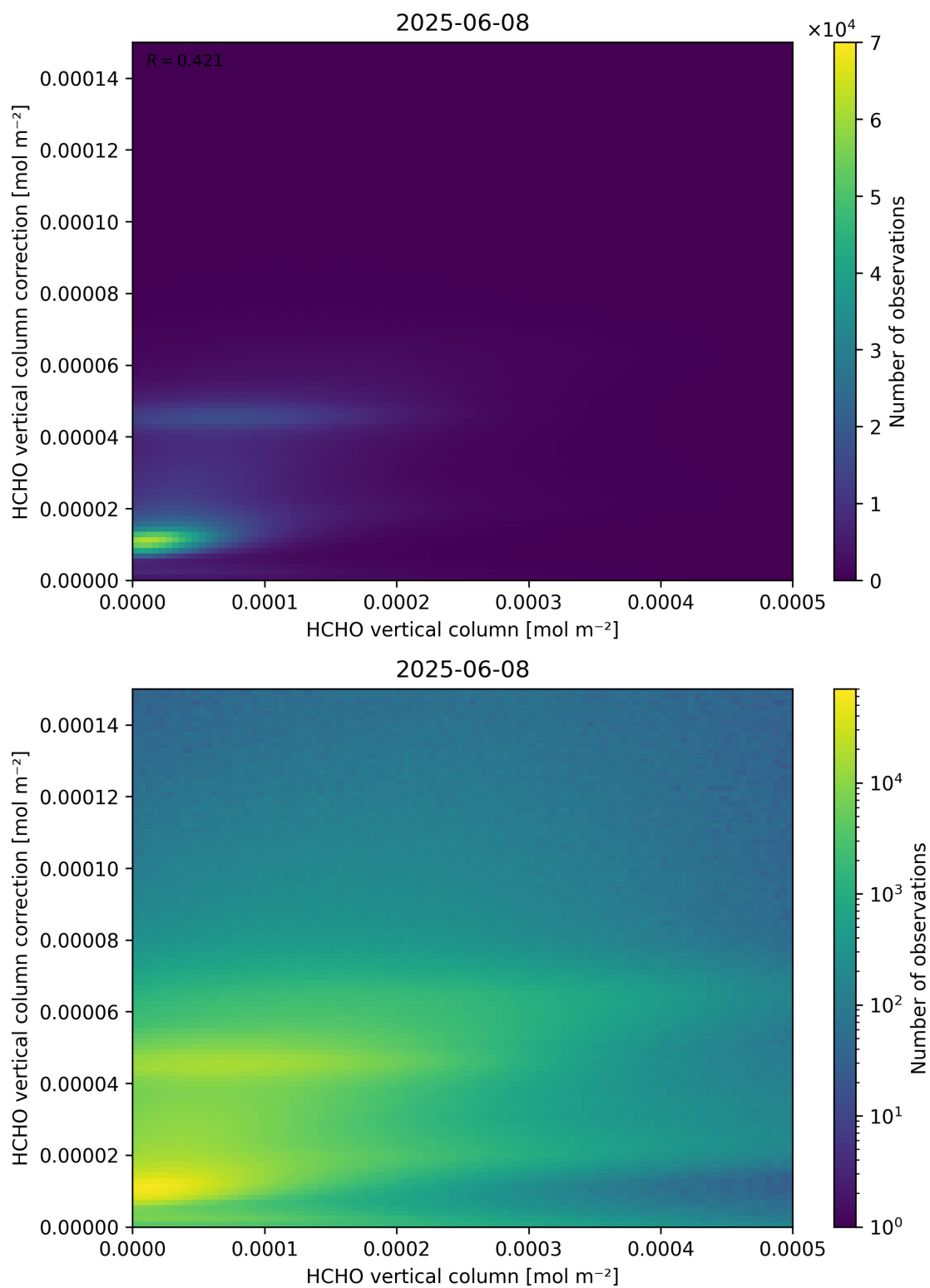
Figure 133: Scatter density plot of “HCHO vertical column” against “HCHO vertical column correction” for 2025-06-07 to 2025-06-09.
