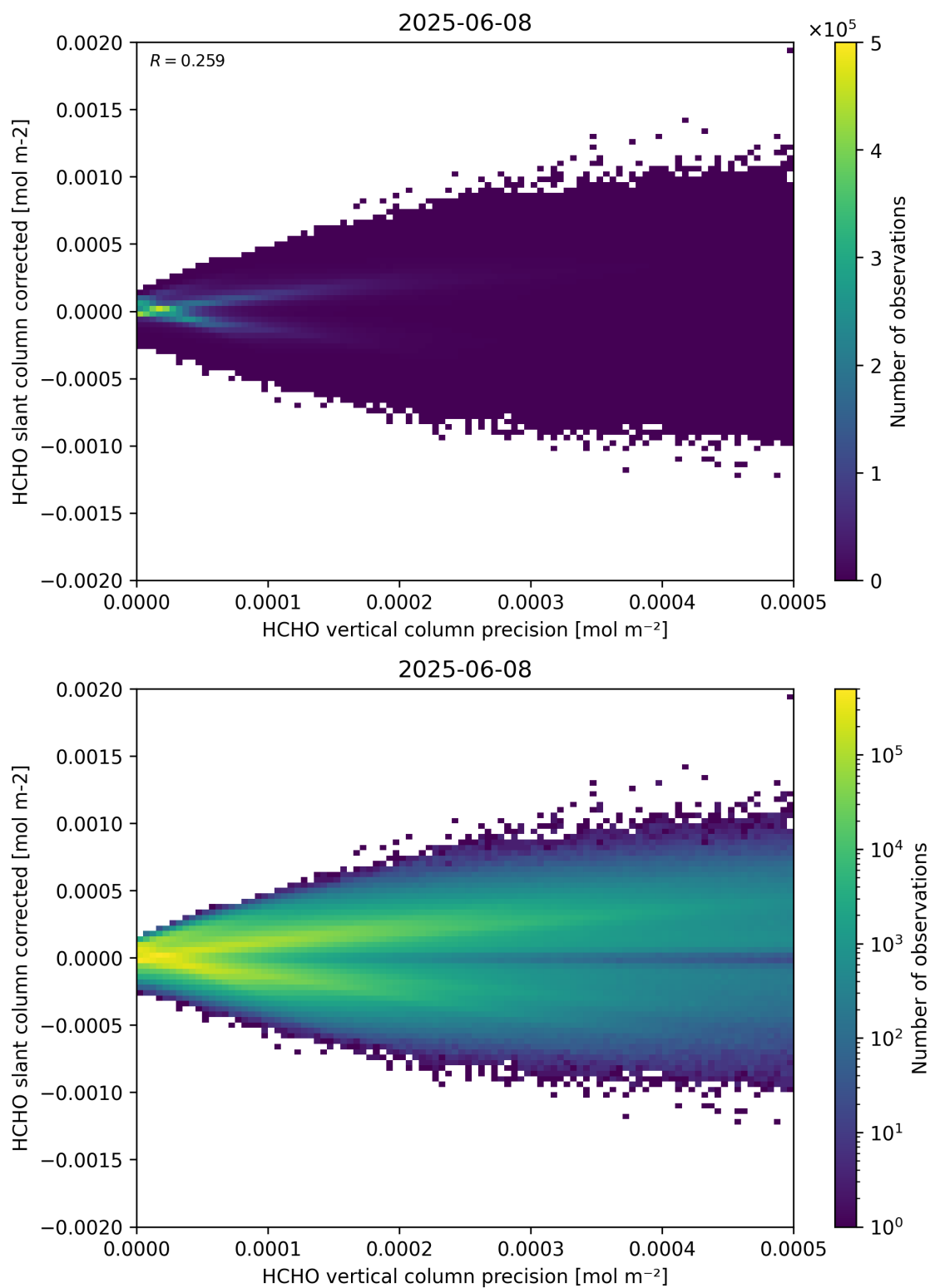
Figure 140: Scatter density plot of “HCHO vertical column precision” against “HCHO slant column corrected” for 2025-06-07 to 2025-06-09.
