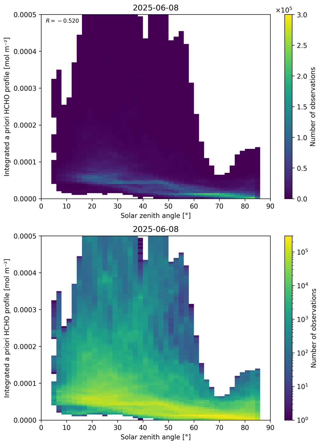
Figure 180: Scatter density plot of “Solar zenith angle” against “Integrated a priori HCHO profile” for 2025-06-07 to 2025-06-09.
