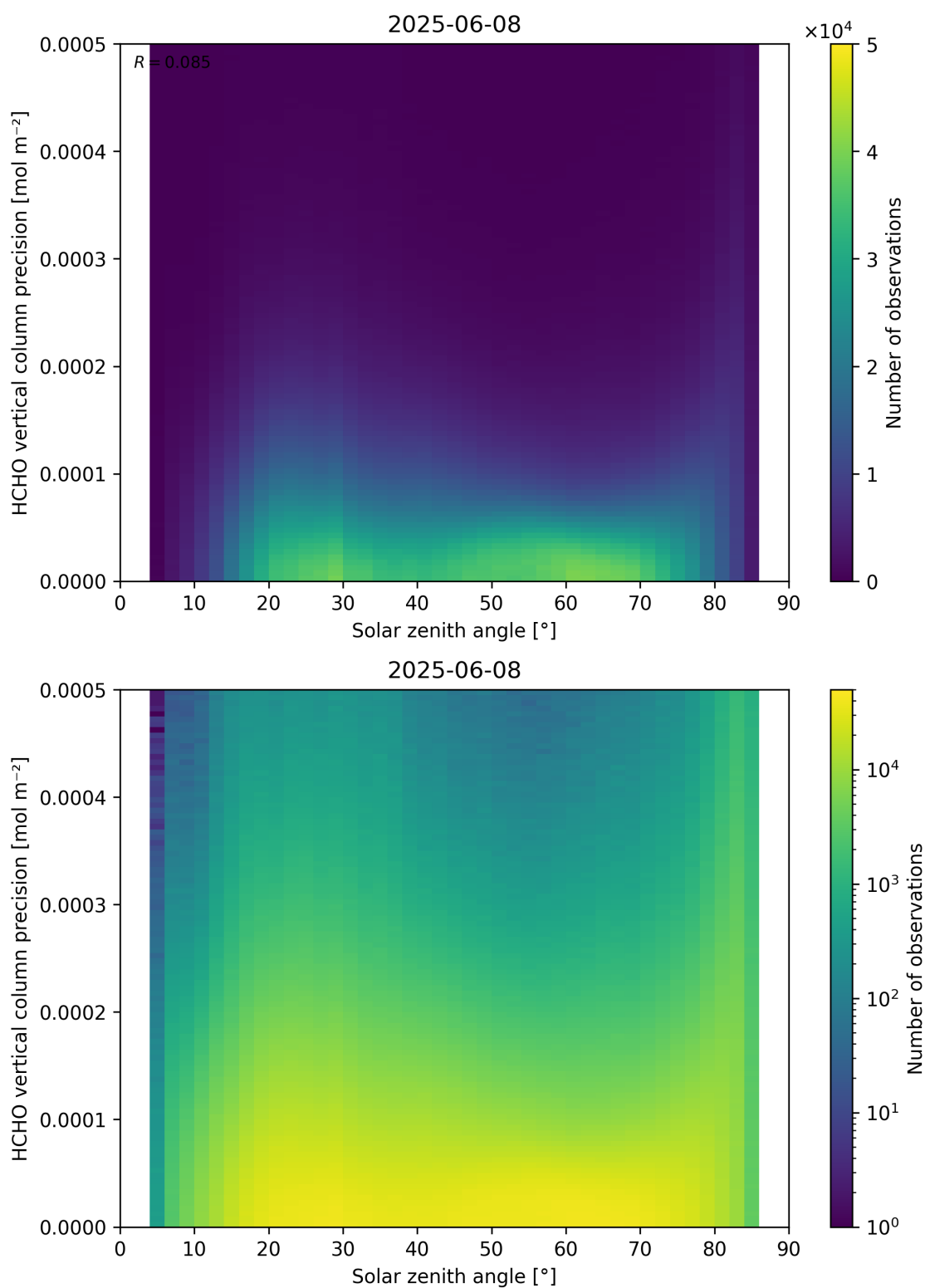
Figure 179: Scatter density plot of “Solar zenith angle” against “HCHO vertical column precision” for 2025-06-07 to 2025-06-09.
