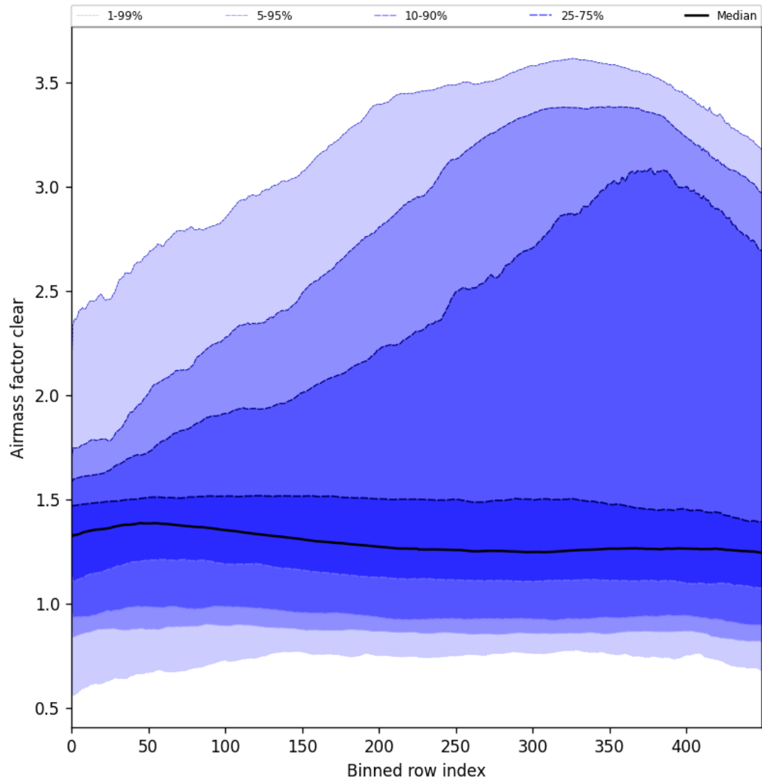
Figure 56: Along track statistics of “Airmass factor clear” for 2025-06-07 to 2025-06-09
