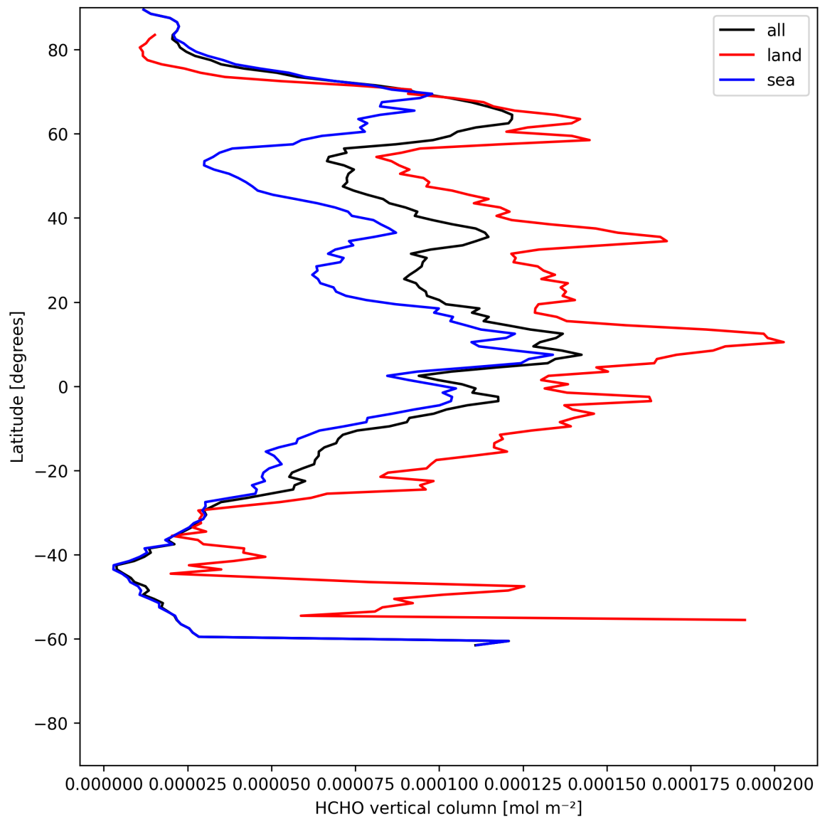
Figure 21: Zonal average of “HCHO vertical column” for 2025-06-07 to 2025-06-09.
