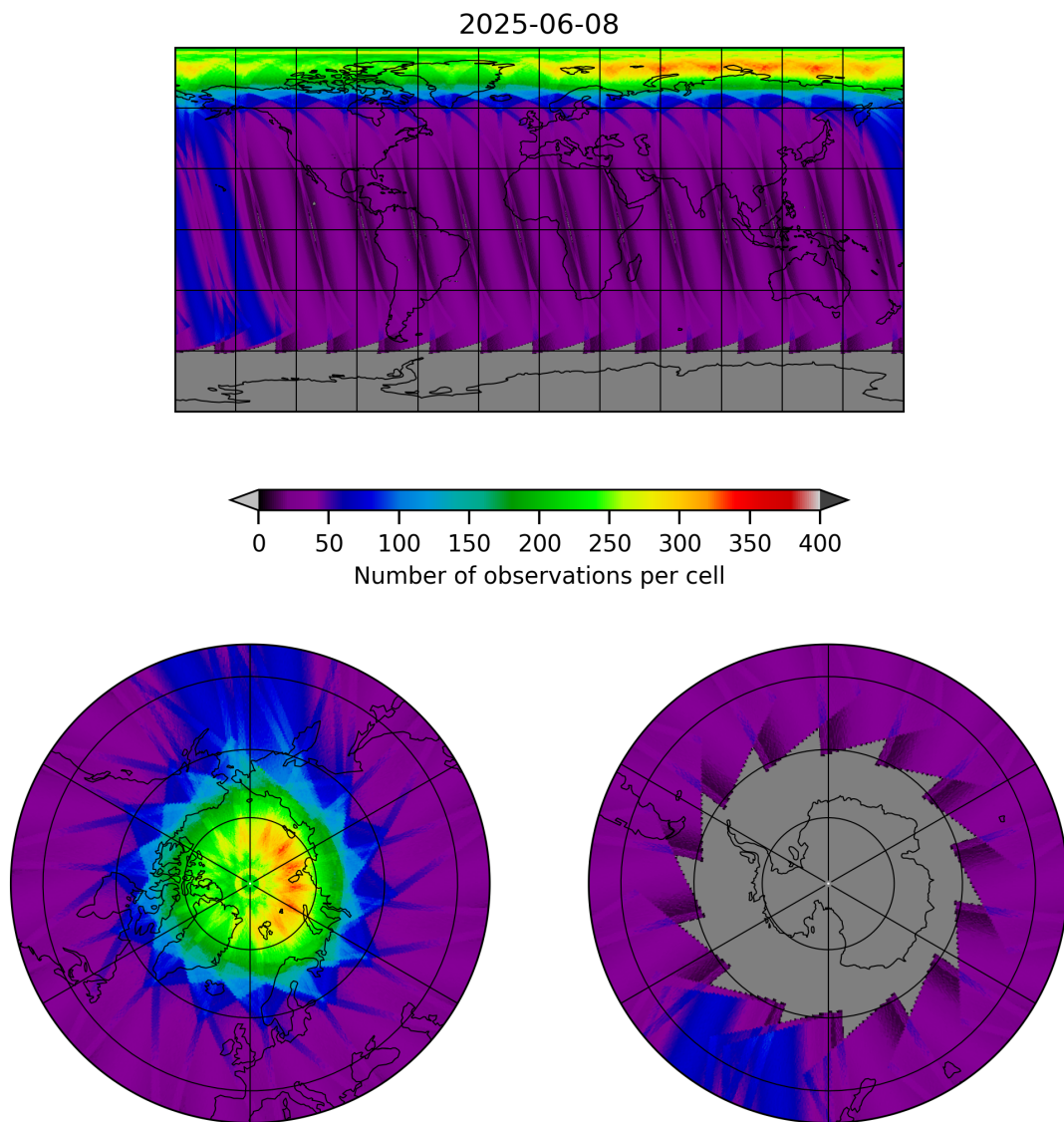
Figure 19: Map of the number of observations for 2025-06-07 to 2025-06-09
