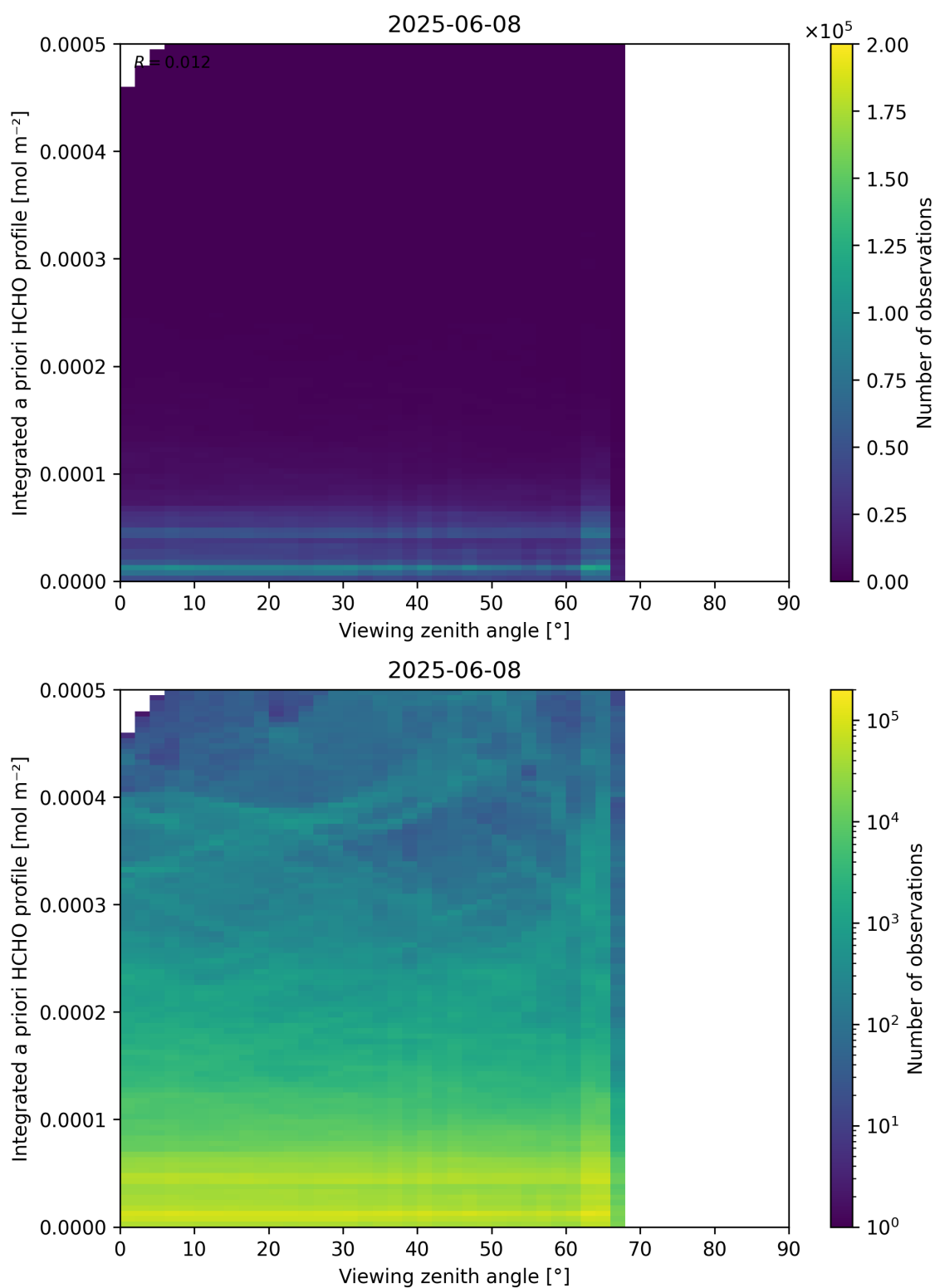
Figure 195: Scatter density plot of “Viewing zenith angle” against “Integrated a priori HCHO profile” for 2025-06-07 to 2025-06-09.
