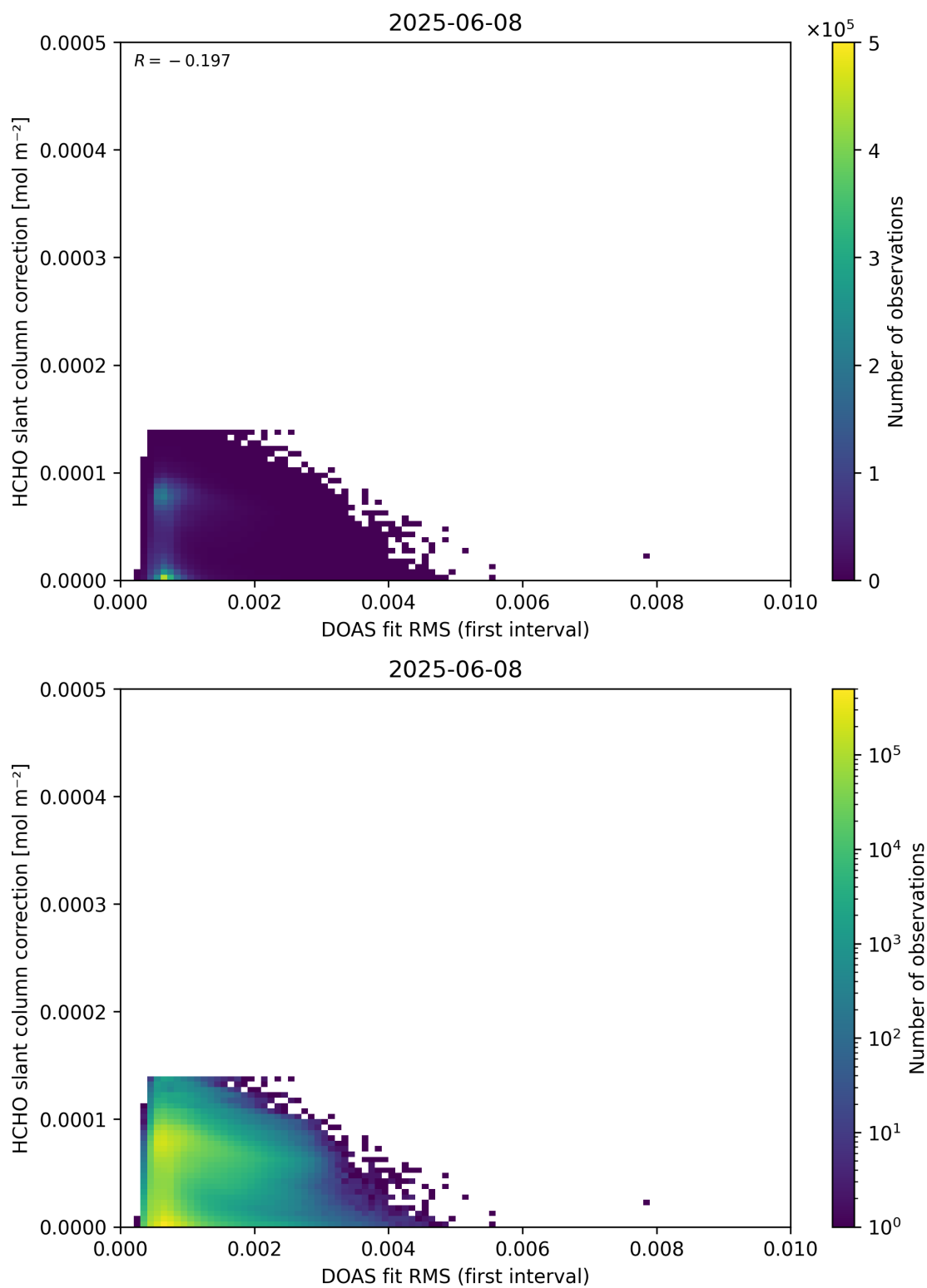
Figure 63: Scatter density plot of “DOAS fit RMS (first interval)” against “HCHO slant column correction” for 2025-06-07 to 2025-06-09.
