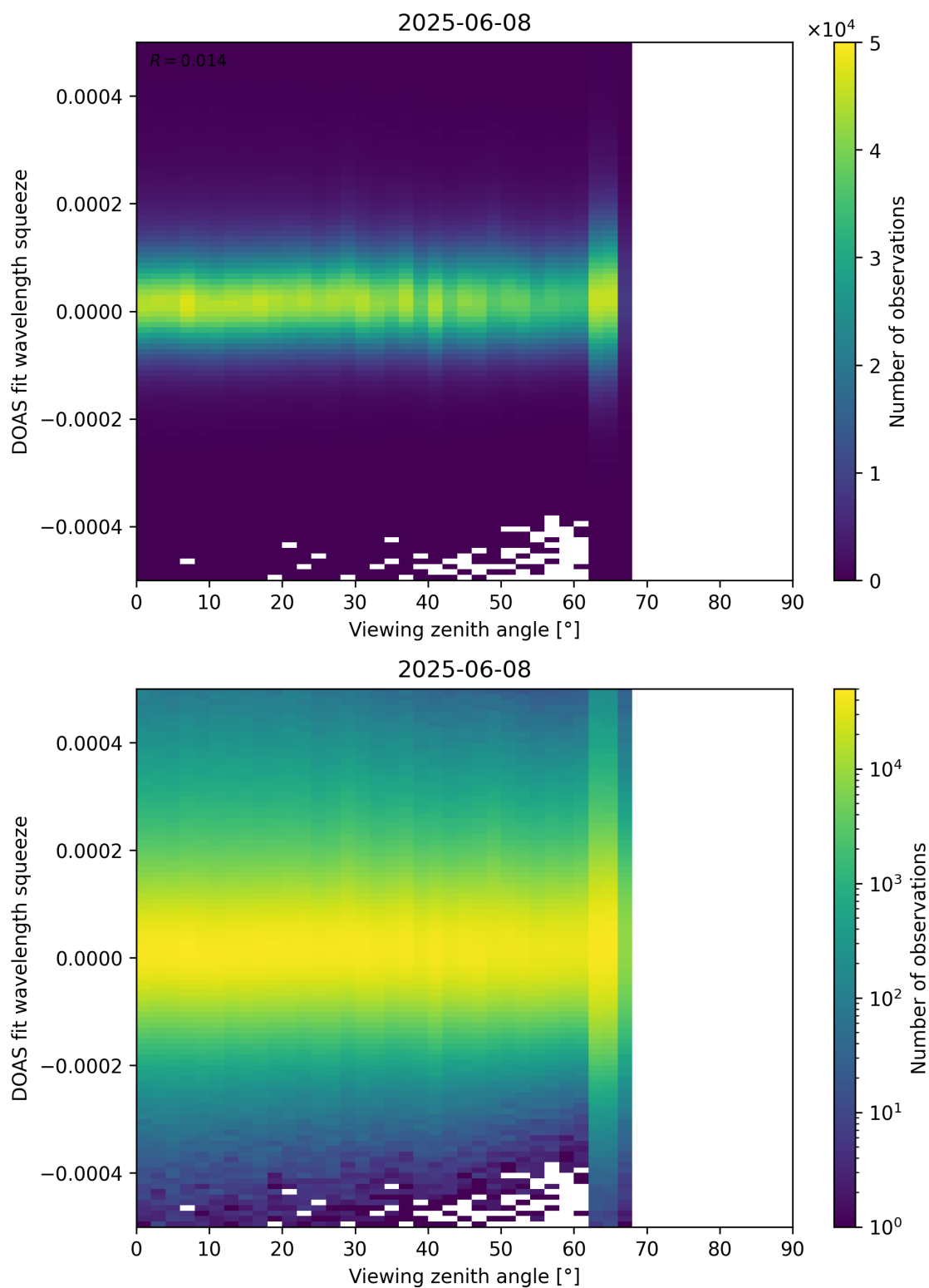
Figure 184: Scatter density plot of “Viewing zenith angle” against “DOAS fit wavelength squeeze” for 2025-06-07 to 2025-06-09.
