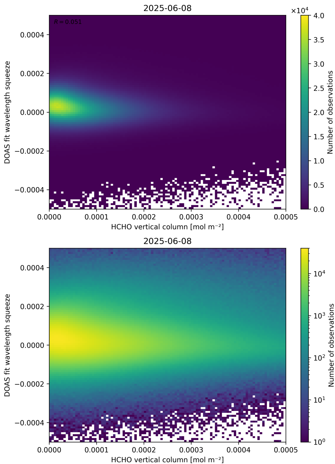
Figure 125: Scatter density plot of “HCHO vertical column” against “DOAS fit wavelength squeeze” for 2025-06-07 to 2025-06-09.
