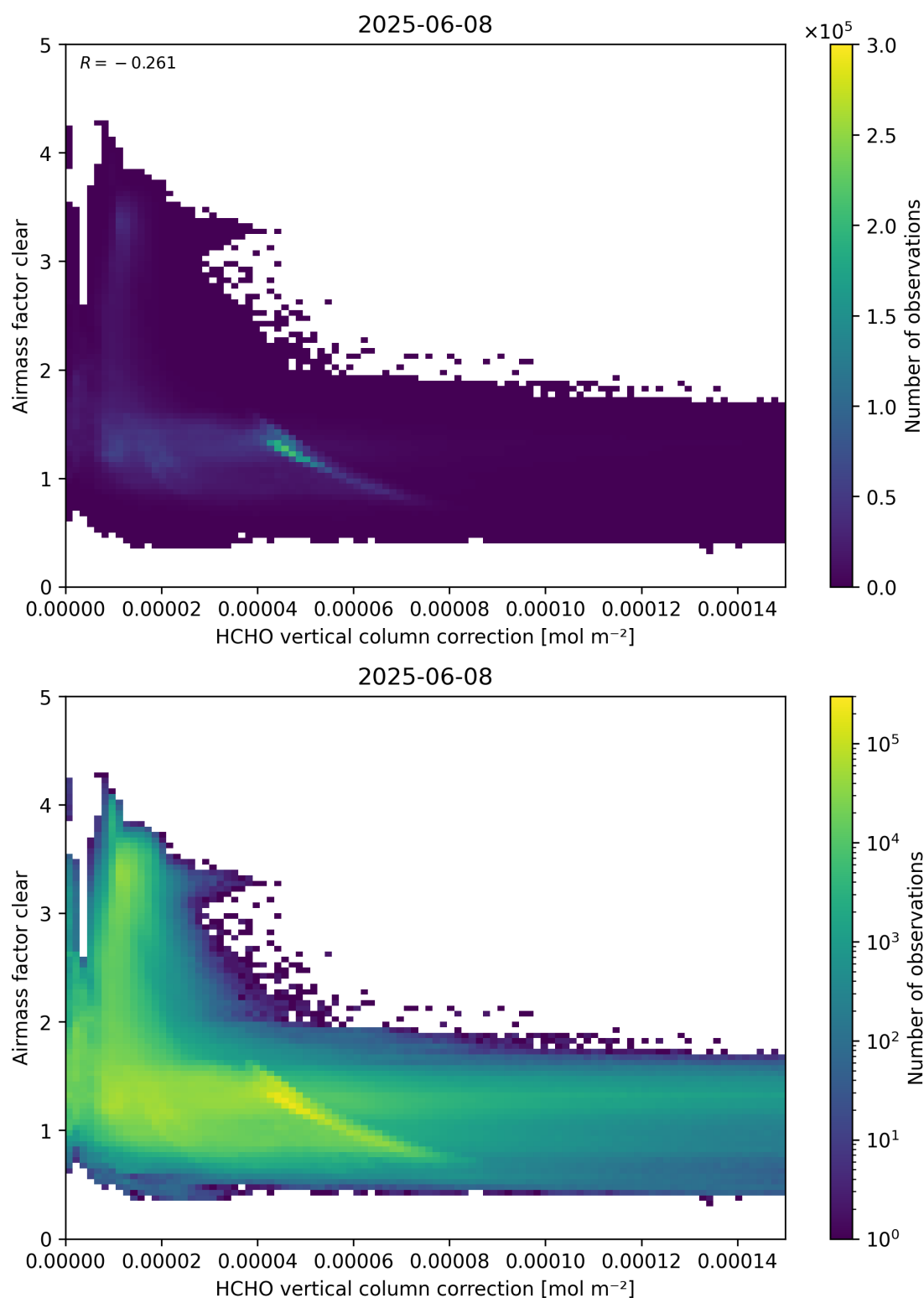
Figure 115: Scatter density plot of “HCHO vertical column correction” against “Airmass factor clear” for 2025-06-07 to 2025-06-09.
