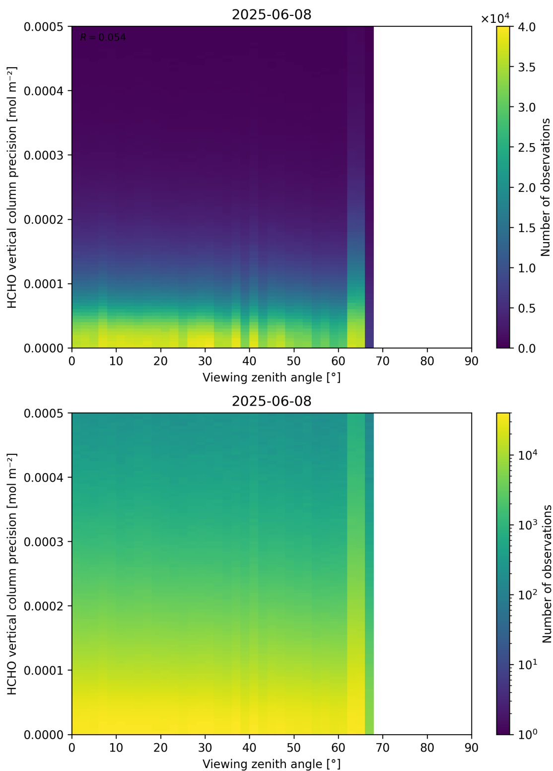
Figure 194: Scatter density plot of “Viewing zenith angle” against “HCHO vertical column precision” for 2025-06-07 to 2025-06-09.
