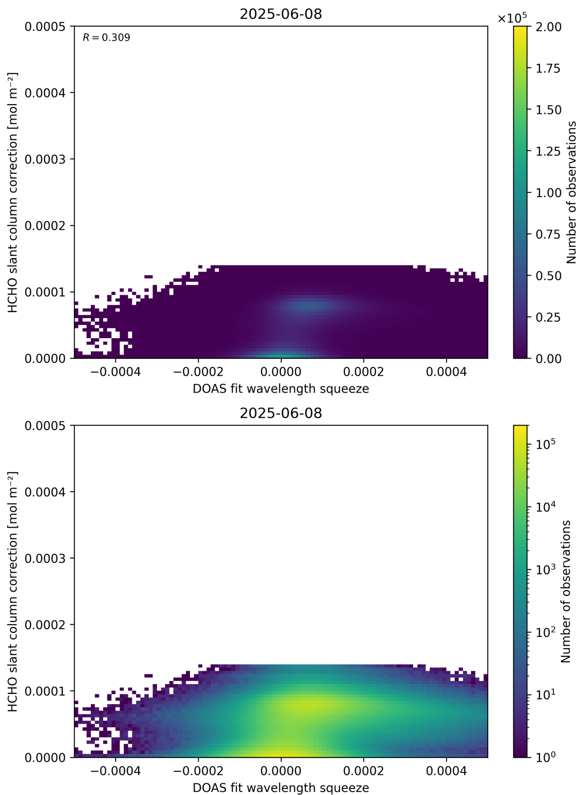
Figure 70: Scatter density plot of “DOAS fit wavelength squeeze” against “HCHO slant column correction” for 2025-06-07 to 2025-06-09.
