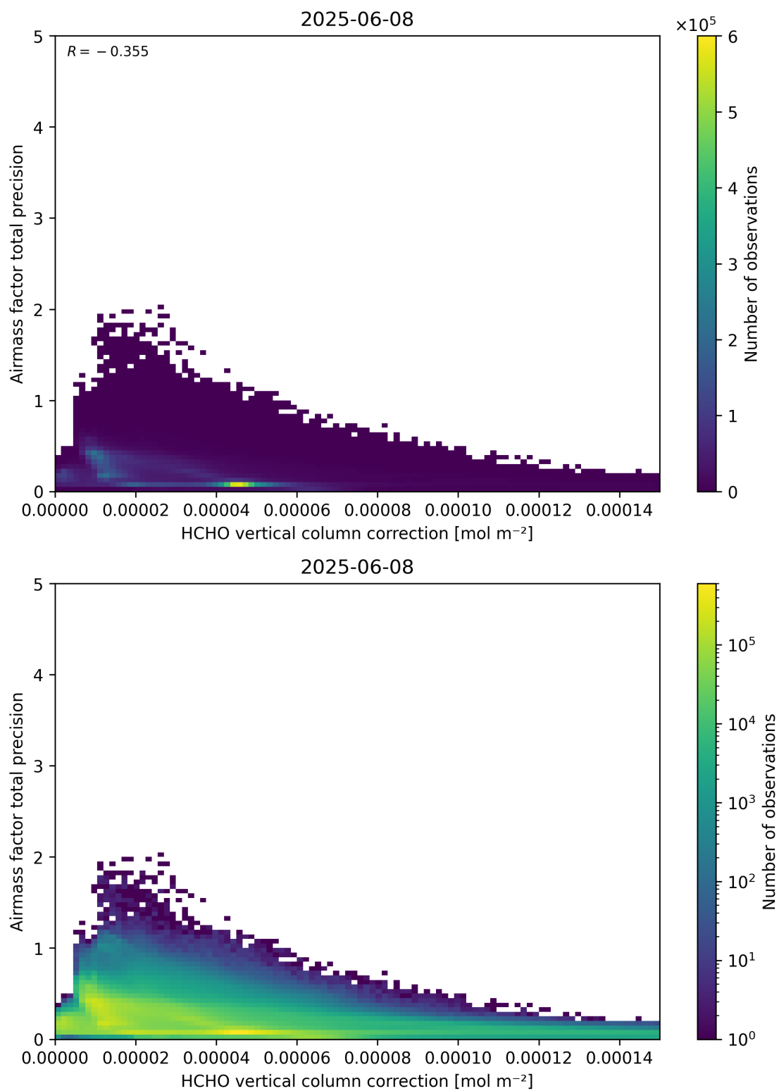
Figure 121: Scatter density plot of “HCHO vertical column correction” against “Airmass factor total precision” for 2025-06-07 to 2025-06-09.
