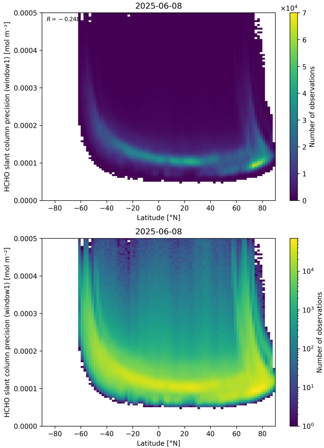
Figure 160: Scatter density plot of “Latitude” against “HCHO slant column precision (window1)” for 2025-06-07 to 2025-06-09.
