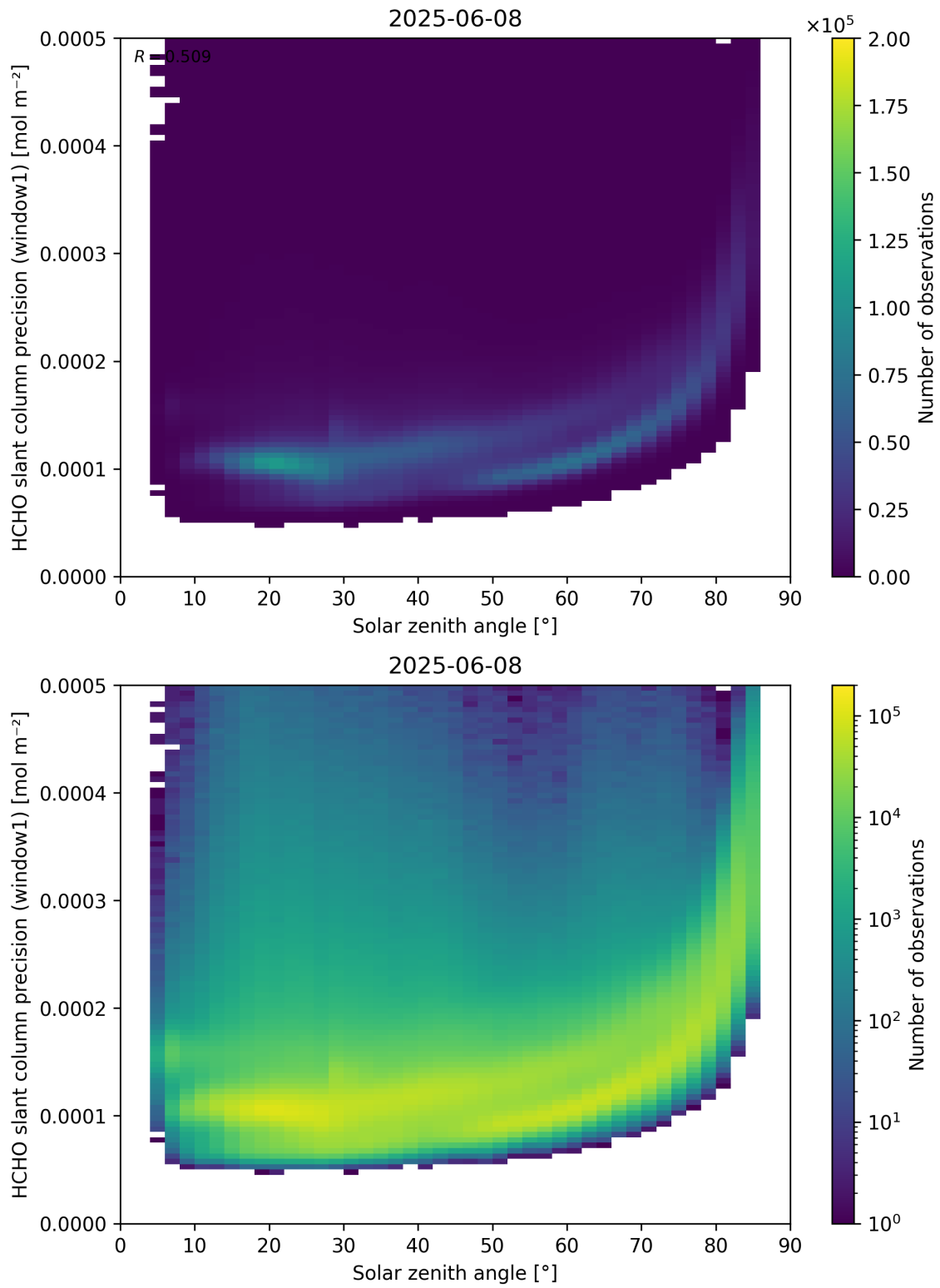
Figure 174: Scatter density plot of “Solar zenith angle” against “HCHO slant column precision (window1)” for 2025-06-07 to 2025-06-09.
