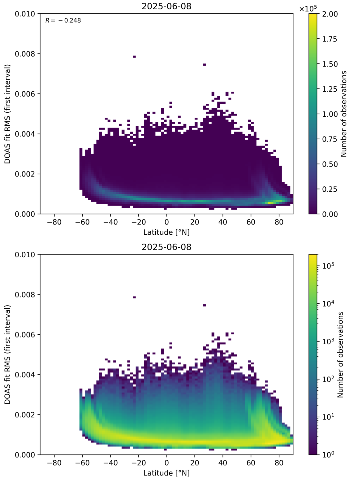
Figure 153: Scatter density plot of “Latitude” against “DOAS fit RMS (first interval)” for 2025-06-07 to 2025-06-09.
