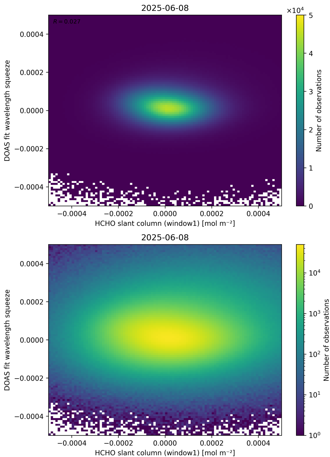
Figure 80: Scatter density plot of “HCHO slant column (window1)” against “DOAS fit wavelength squeeze” for 2025-06-07 to 2025-06-09.
