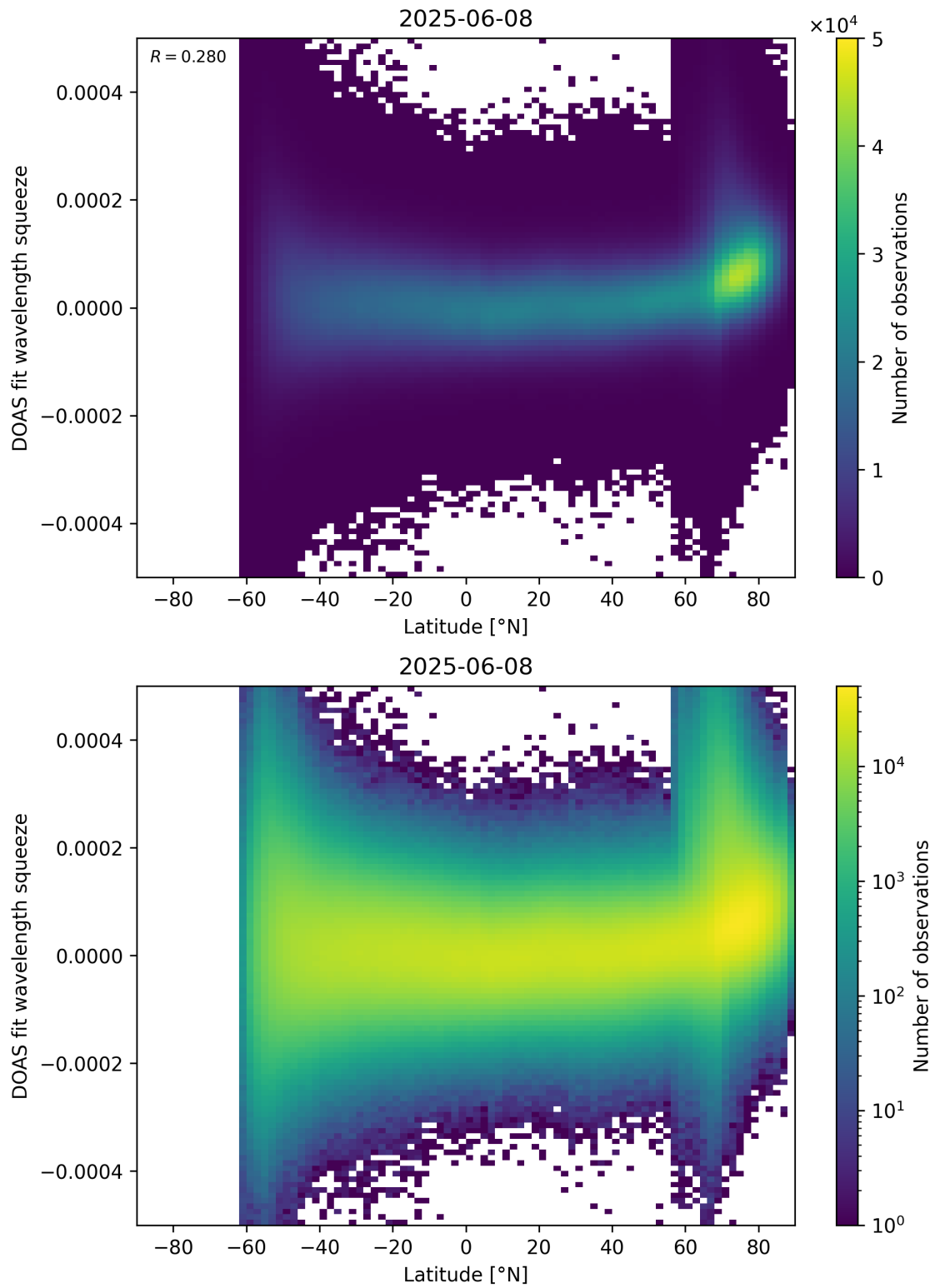
Figure 155: Scatter density plot of “Latitude” against “DOAS fit wavelength squeeze” for 2025-06-07 to 2025-06-09.
