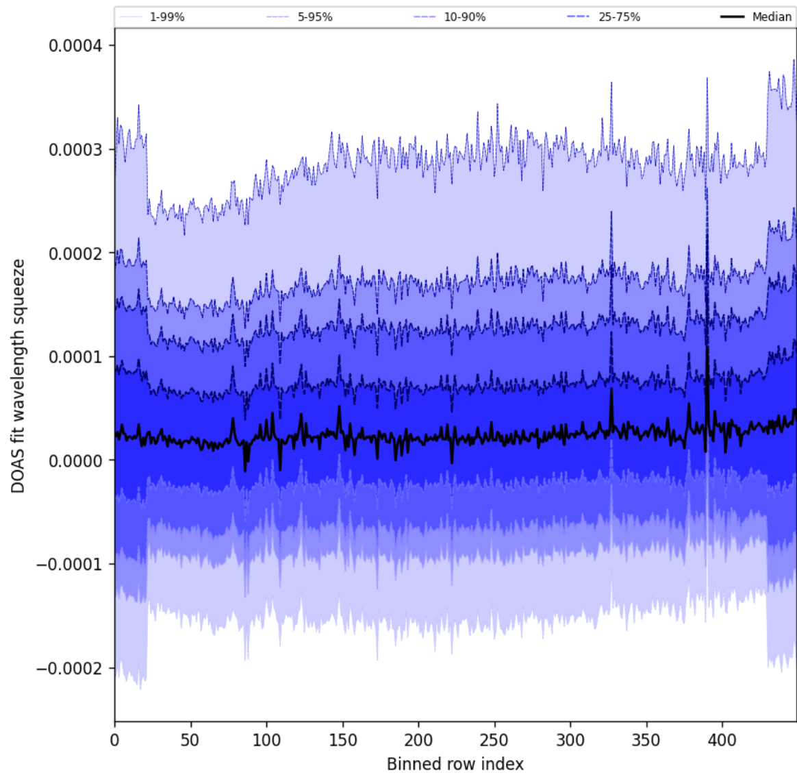
Figure 59: Along track statistics of “DOAS fit wavelength squeeze” for 2025-06-07 to 2025-06-09
