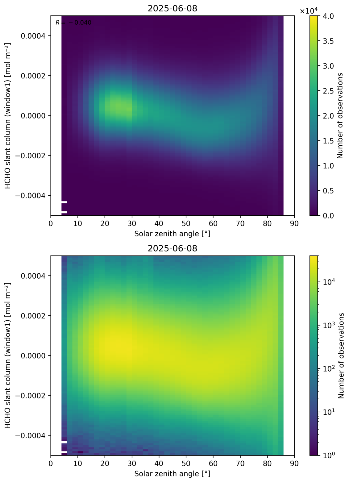
Figure 173: Scatter density plot of “Solar zenith angle” against “HCHO slant column (window1)” for 2025-06-07 to 2025-06-09.
