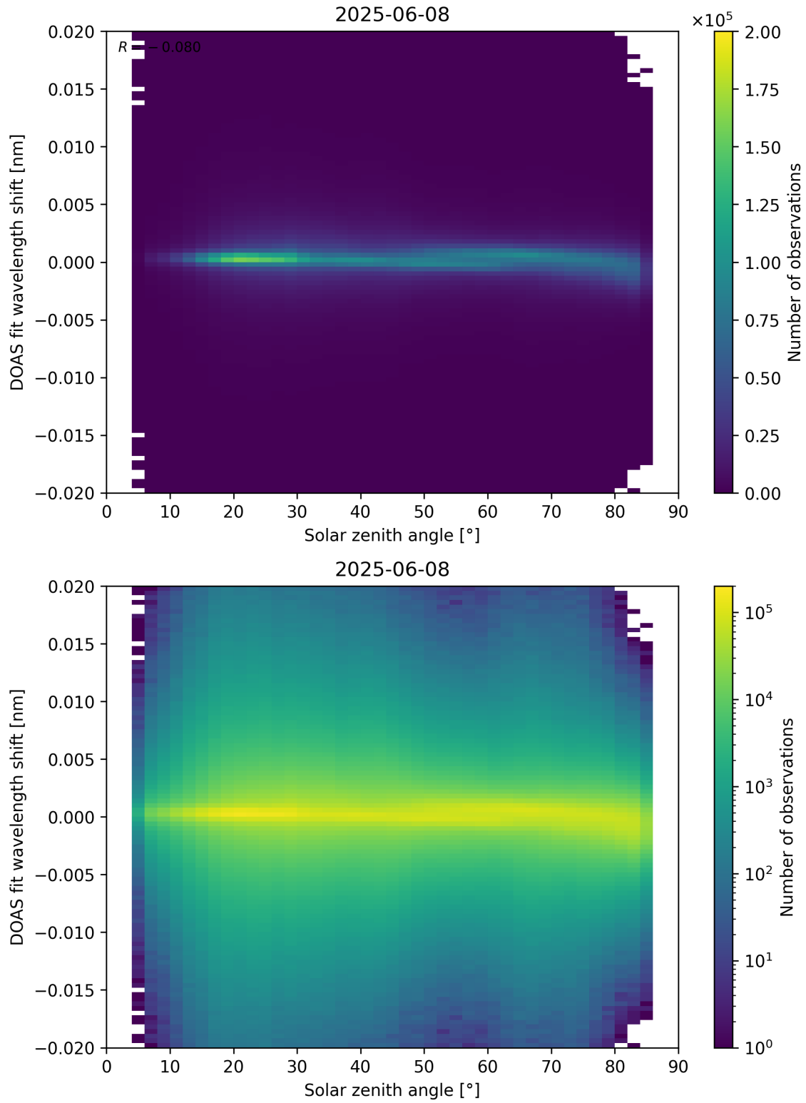
Figure 168: Scatter density plot of “Solar zenith angle” against “DOAS fit wavelength shift” for 2025-06-07 to 2025-06-09.
