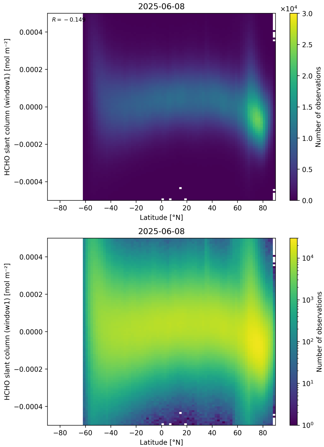
Figure 159: Scatter density plot of “Latitude” against “HCHO slant column (window1)” for 2025-06-07 to 2025-06-09.
