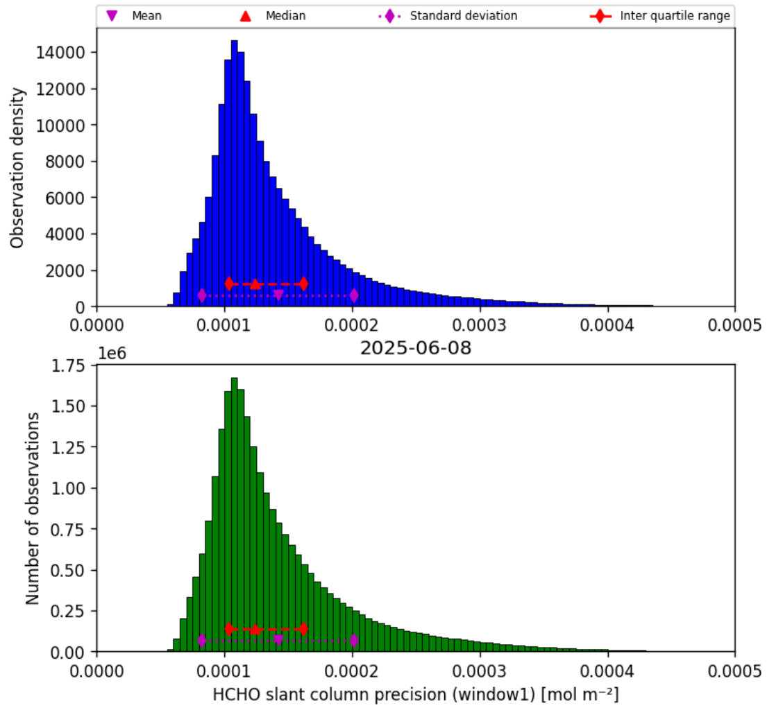
Figure 39: Histogram of “HCHO slant column precision (window1)” for 2025-06-07 to 2025-06-09
