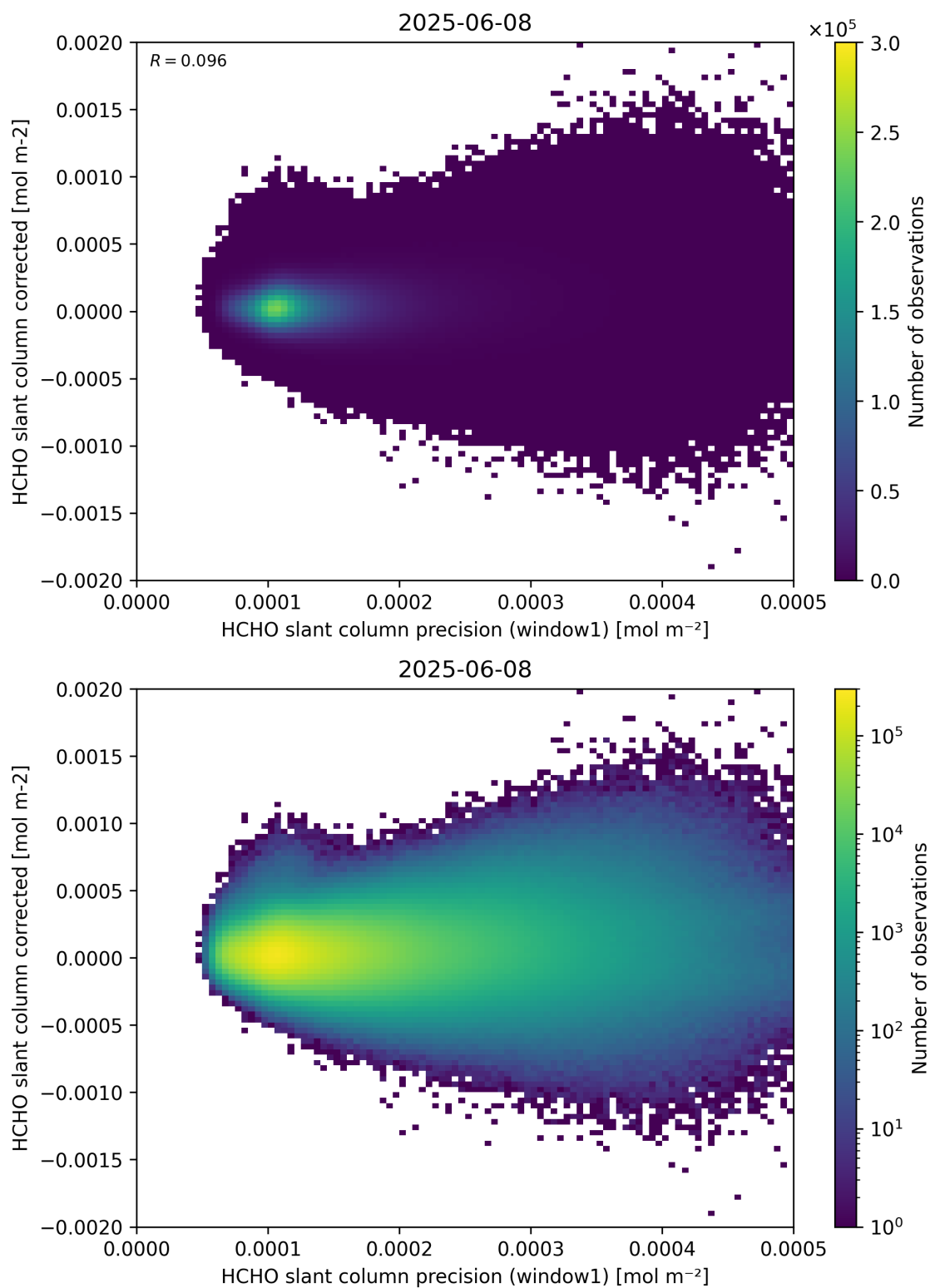
Figure 92: Scatter density plot of “HCHO slant column precision (window1)” against “HCHO slant column corrected” for 2025-06-07 to 2025-06-09.
