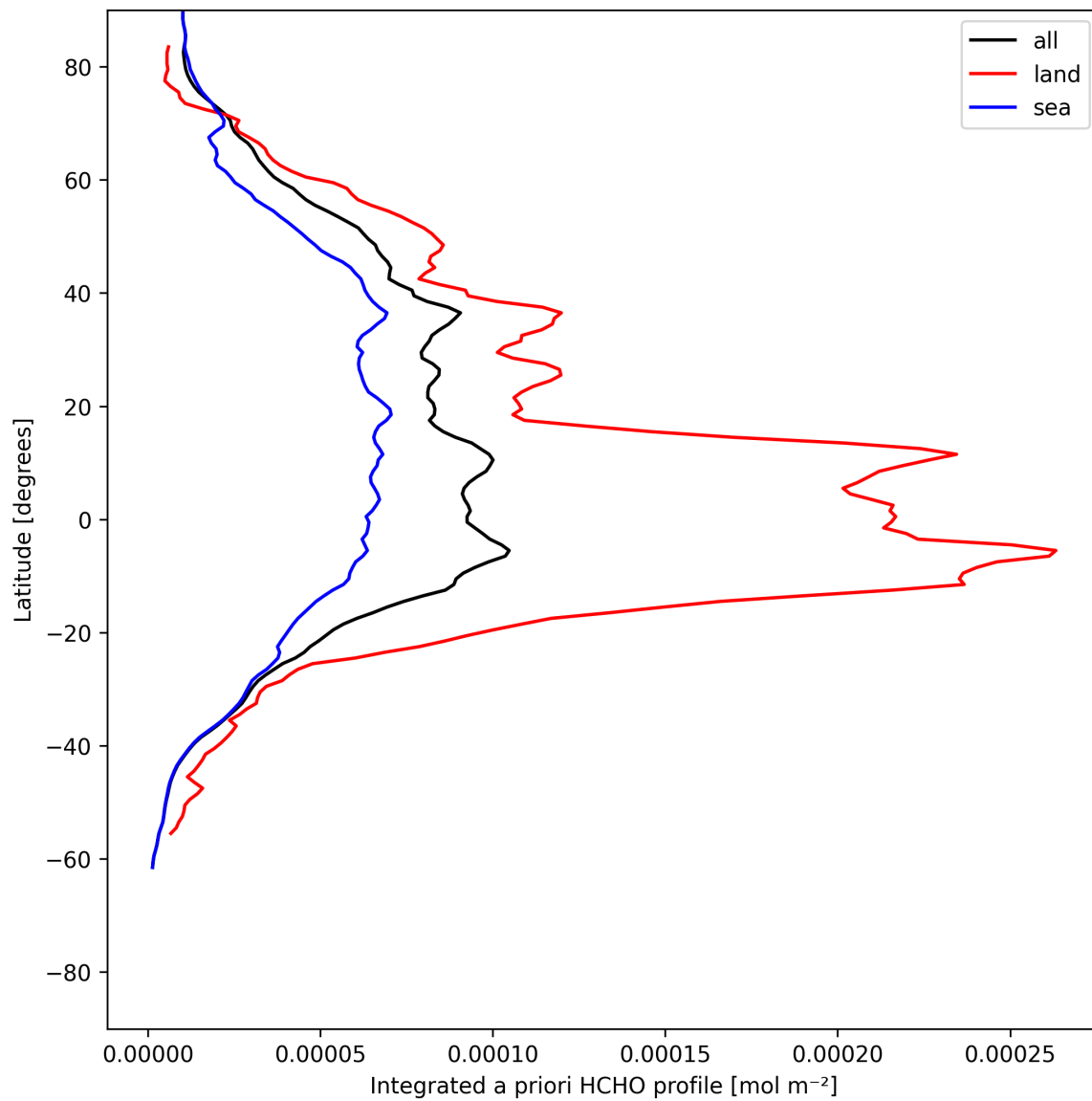
Figure 29: Zonal average of “Integrated a priori HCHO profile” for 2025-06-07 to 2025-06-09.
