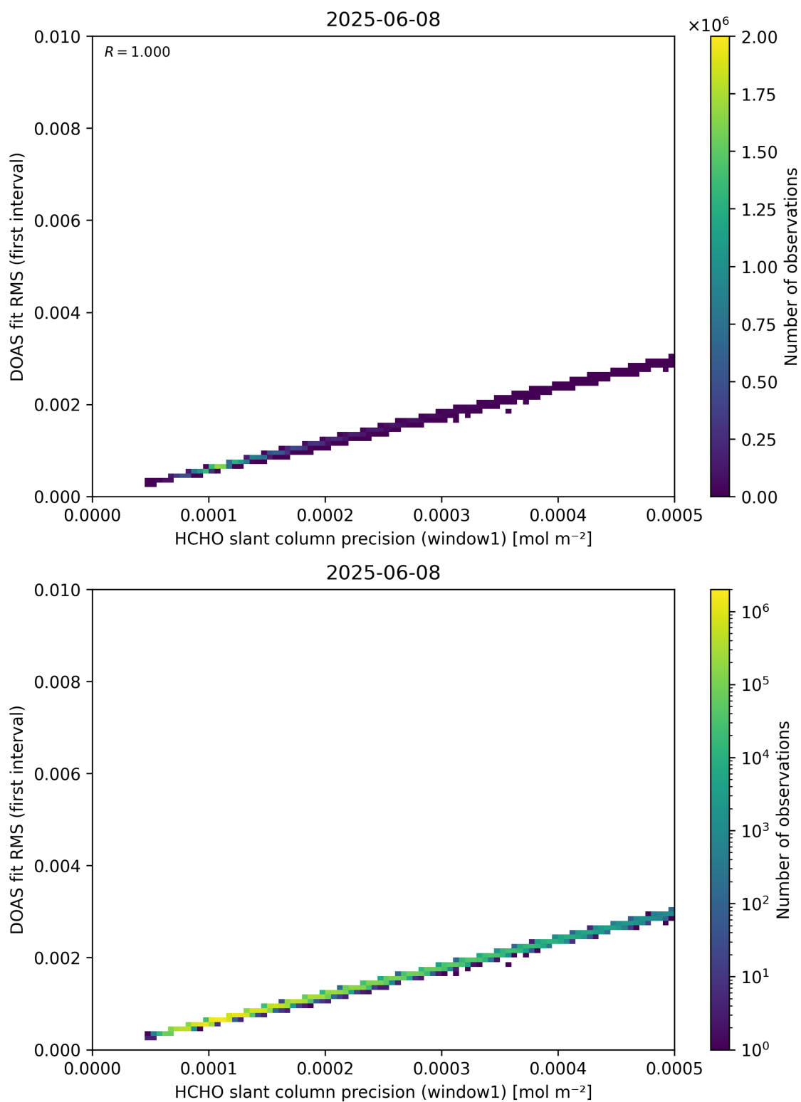
Figure 88: Scatter density plot of “HCHO slant column precision (window1)” against “DOAS fit RMS (first interval)” for 2025-06-07 to 2025-06-09.
