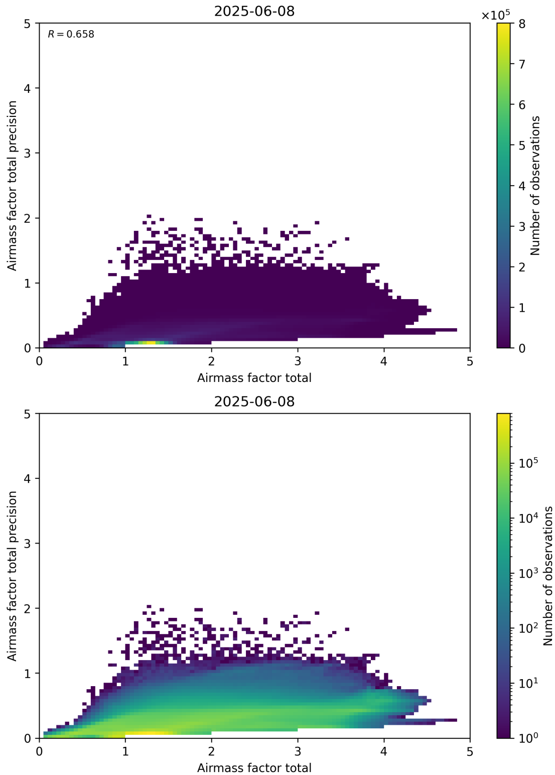
Figure 103: Scatter density plot of “Airmass factor total” against “Airmass factor total precision” for 2025-06-07 to 2025-06-09.
