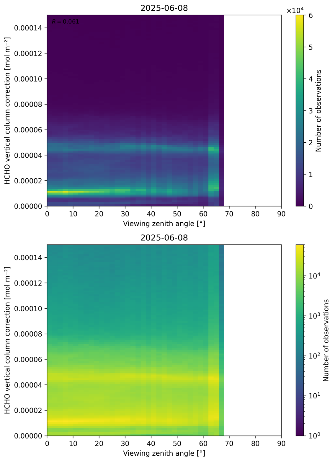
Figure 193: Scatter density plot of “Viewing zenith angle” against “HCHO vertical column correction” for 2025-06-07 to 2025-06-09.
