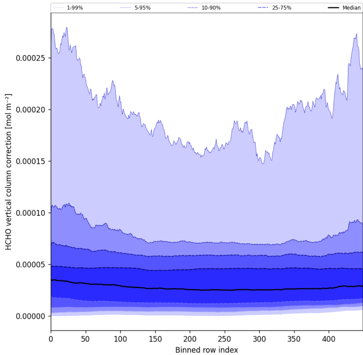
Figure 51: Along track statistics of “HCHO vertical column correction” for 2025-06-07 to 2025-06-09
