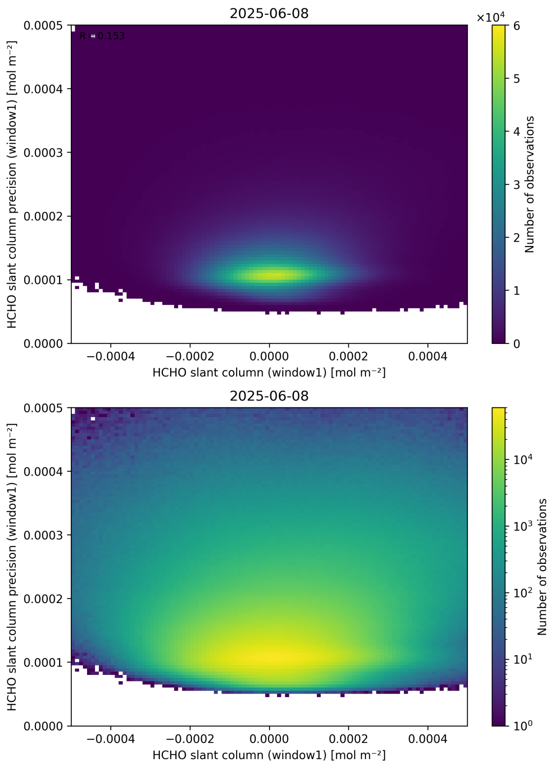
Figure 84: Scatter density plot of “HCHO slant column (window1)” against “HCHO slant column precision (window1)” for 2025-06-07 to 2025-06-09.
