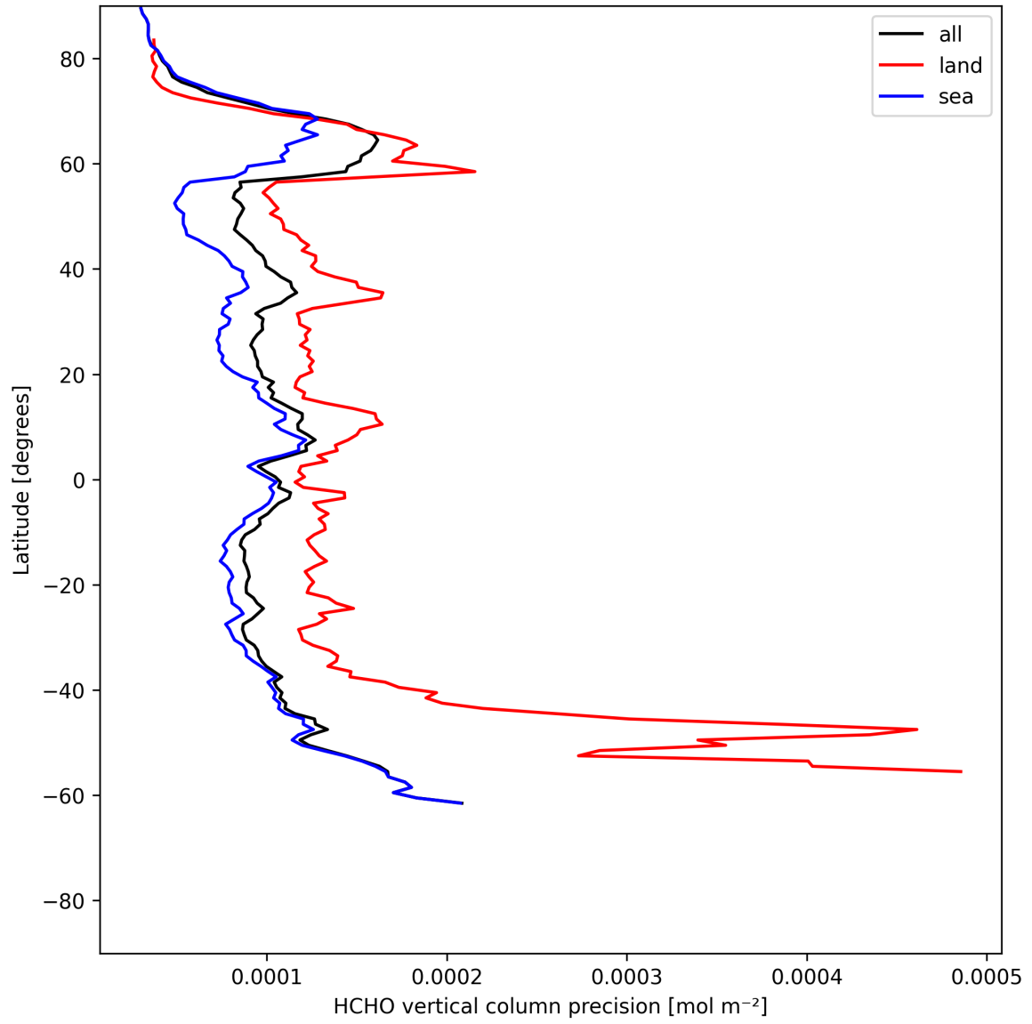
Figure 22: Zonal average of “HCHO vertical column precision” for 2025-06-07 to 2025-06-09.
