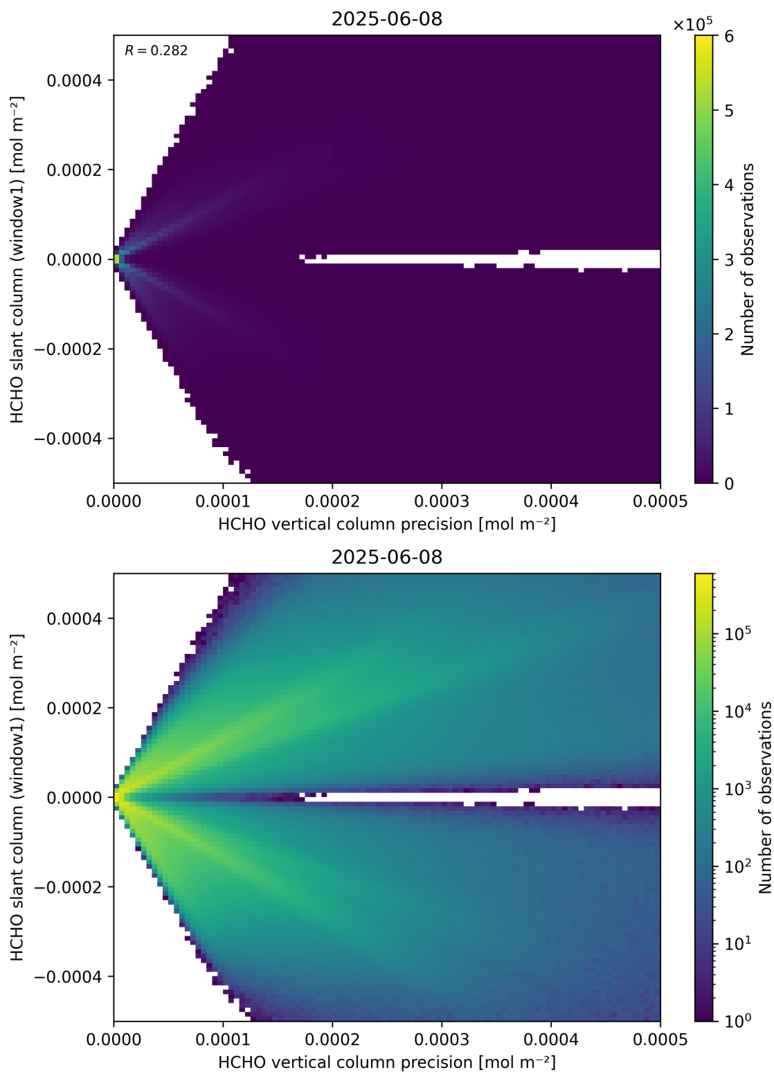
Figure 142: Scatter density plot of “HCHO vertical column precision” against “HCHO slant column (window1)” for 2025-06-07 to 2025-06-09.
