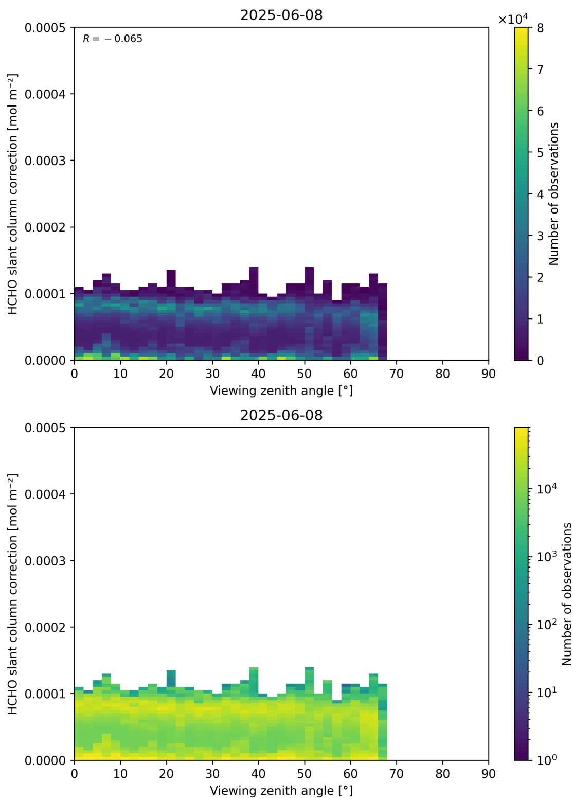
Figure 187: Scatter density plot of “Viewing zenith angle” against “HCHO slant column correction” for 2025-06-07 to 2025-06-09.
