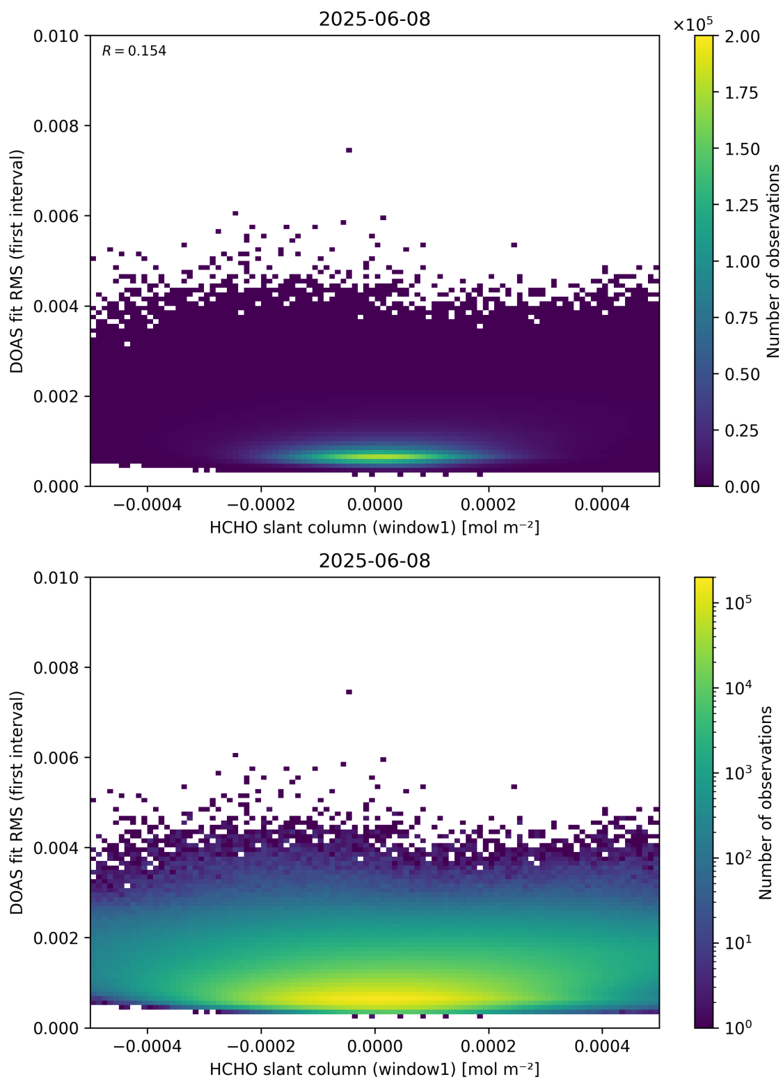
Figure 78: Scatter density plot of “HCHO slant column (window1)” against “DOAS fit RMS (first interval)” for 2025-06-07 to 2025-06-09.
