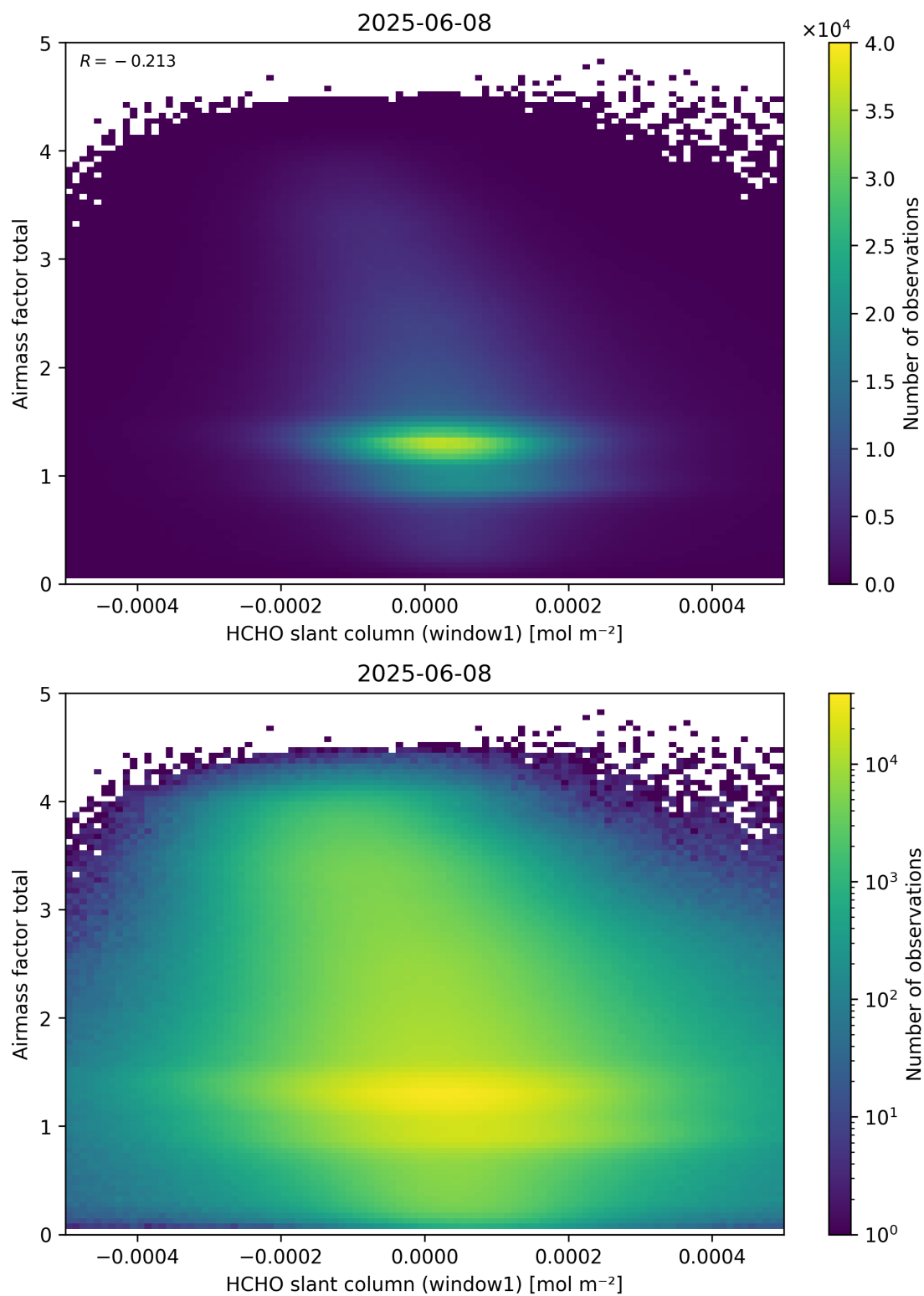
Figure 85: Scatter density plot of “HCHO slant column (window1)” against “Airmass factor total” for 2025-06-07 to 2025-06-09.
