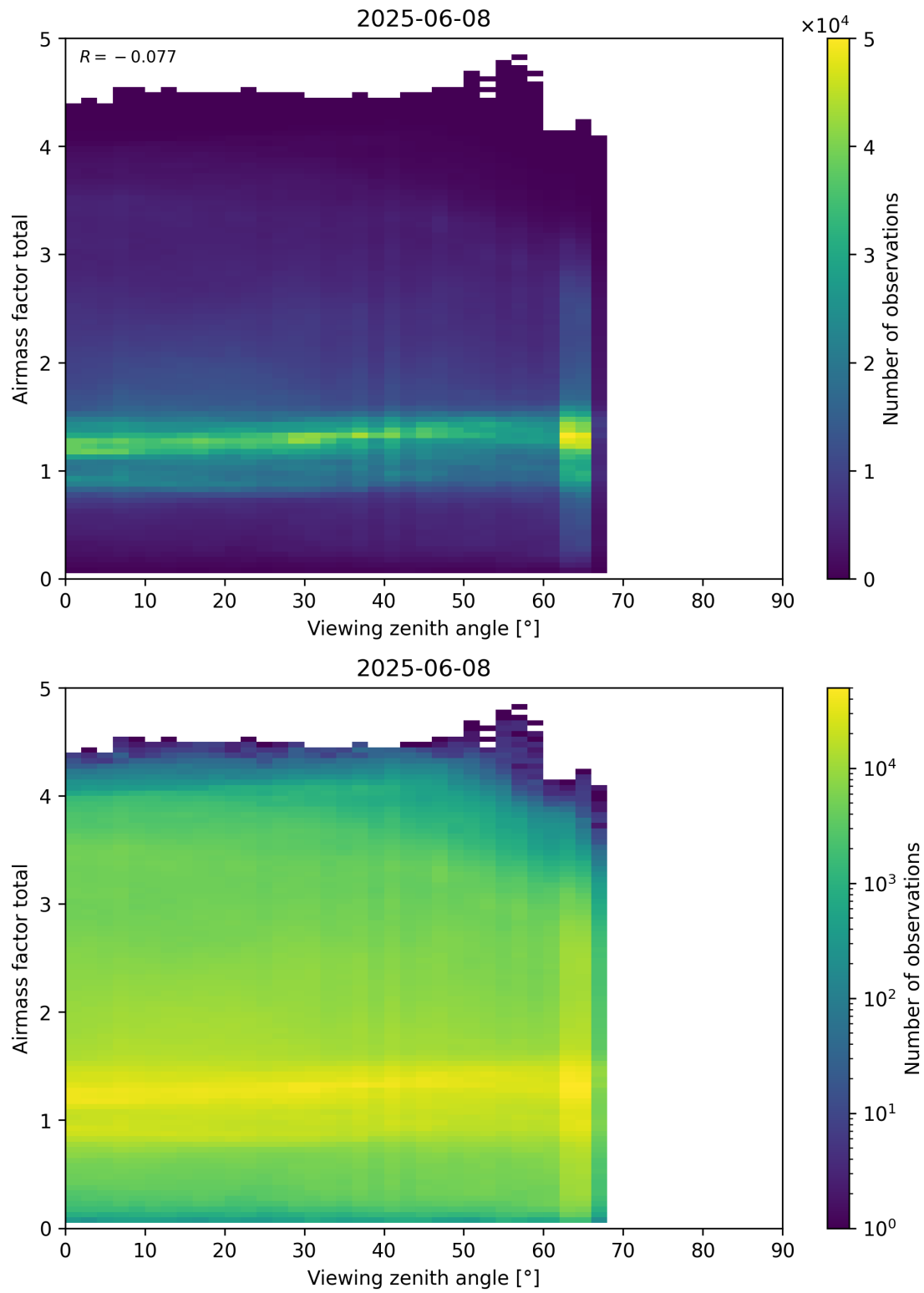
Figure 190: Scatter density plot of “Viewing zenith angle” against “Airmass factor total” for 2025-06-07 to 2025-06-09.
