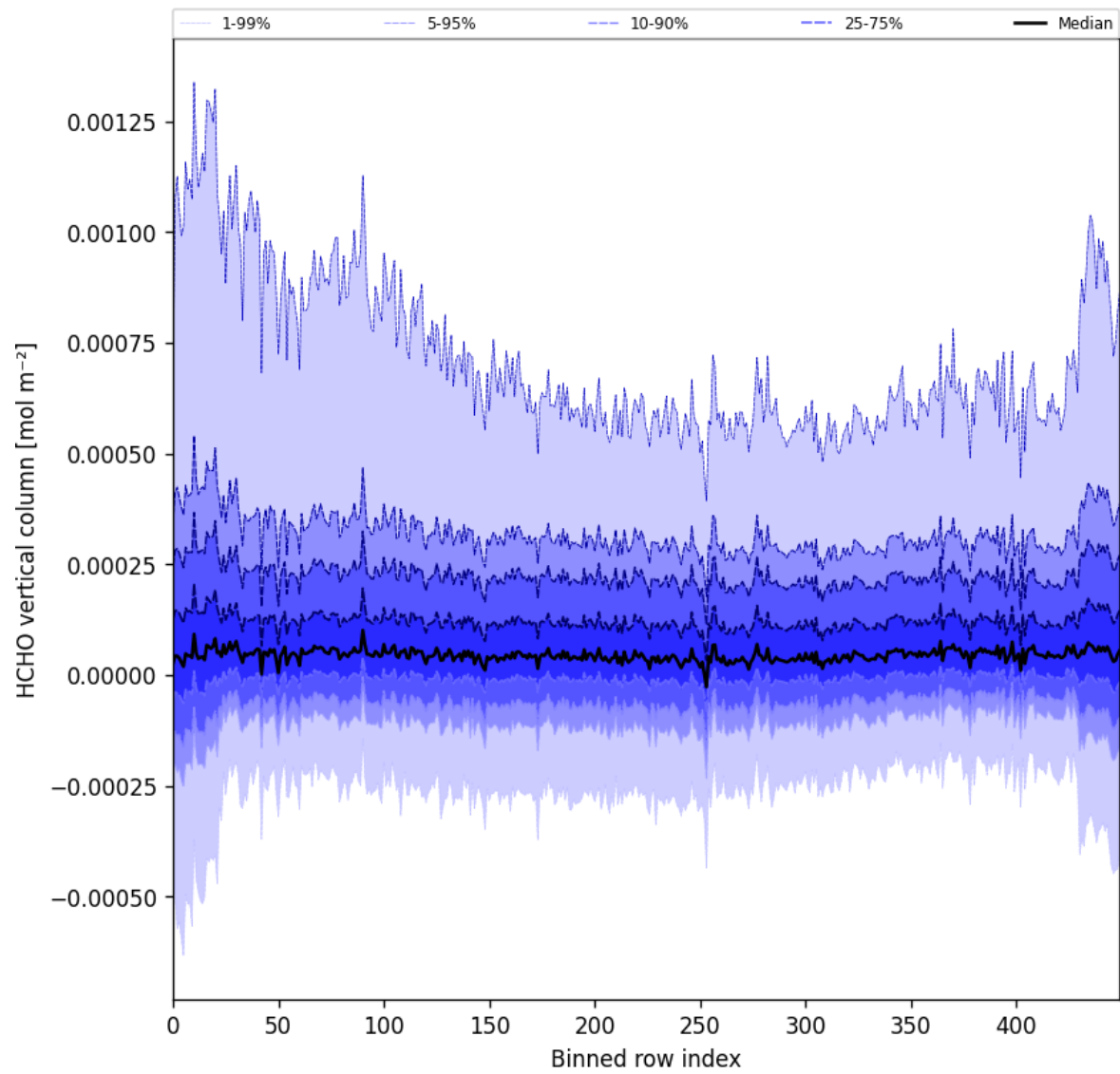
Figure 49: Along track statistics of “HCHO vertical column” for 2025-06-07 to 2025-06-09
