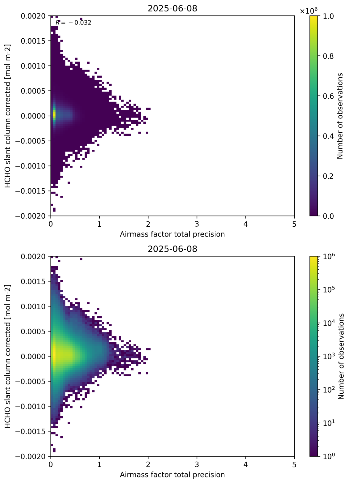
Figure 109: Scatter density plot of “Airmass factor total precision” against “HCHO slant column corrected” for 2025-06-07 to 2025-06-09.
