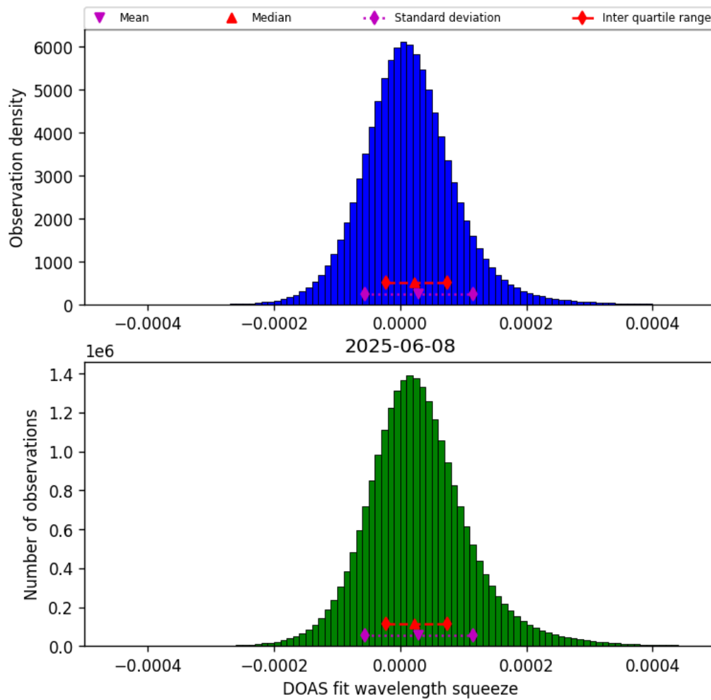
Figure 45: Histogram of “DOAS fit wavelength squeeze” for 2025-06-07 to 2025-06-09
