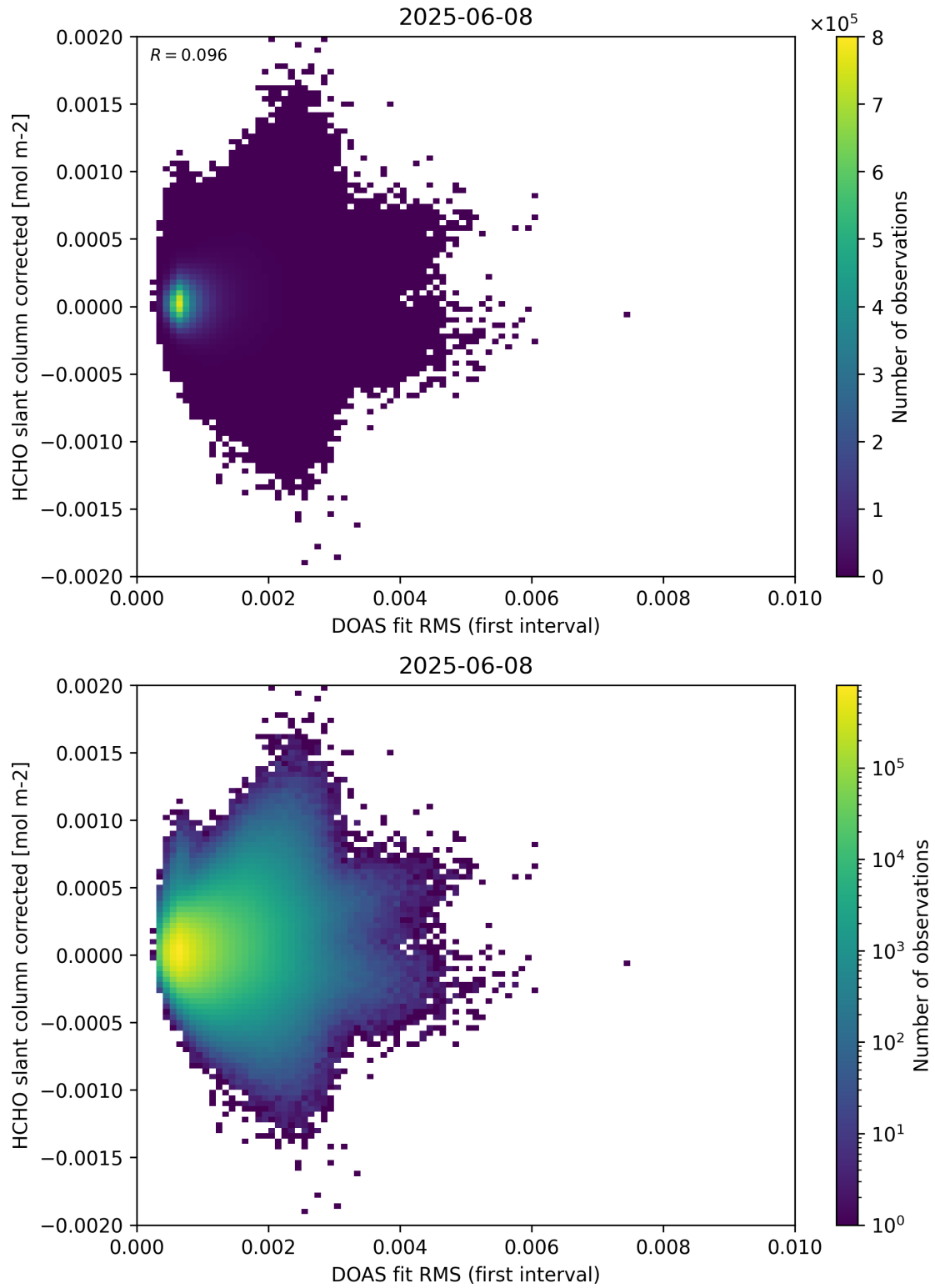
Figure 62: Scatter density plot of “DOAS fit RMS (first interval)” against “HCHO slant column corrected” for 2025-06-07 to 2025-06-09.
