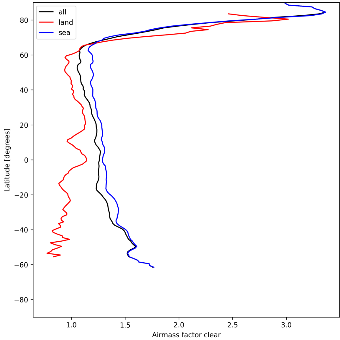
Figure 28: Zonal average of “Airmass factor clear” for 2025-06-07 to 2025-06-09.
