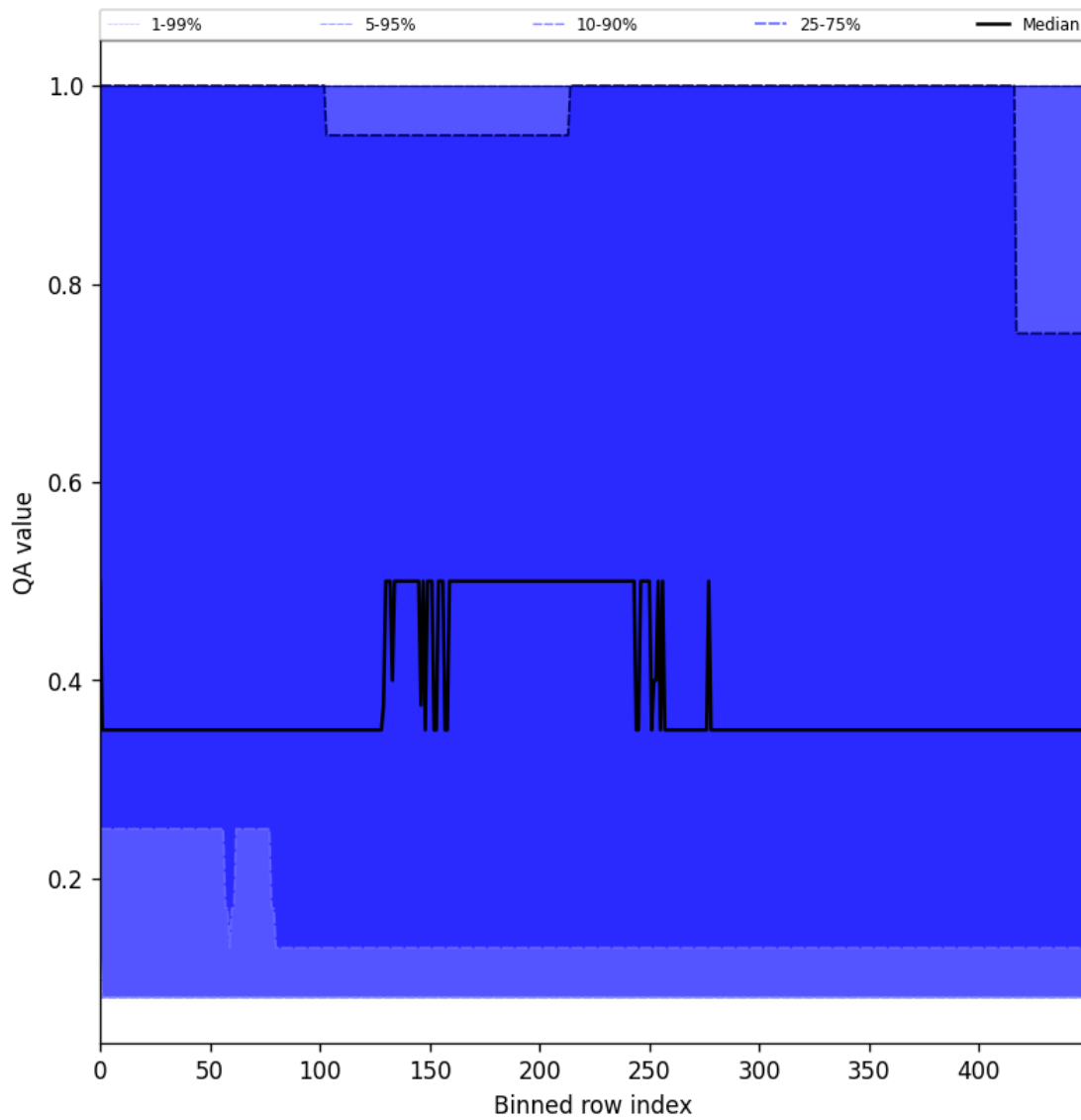
Figure 48: Along track statistics of “QA value” for 2025-06-07 to 2025-06-09
