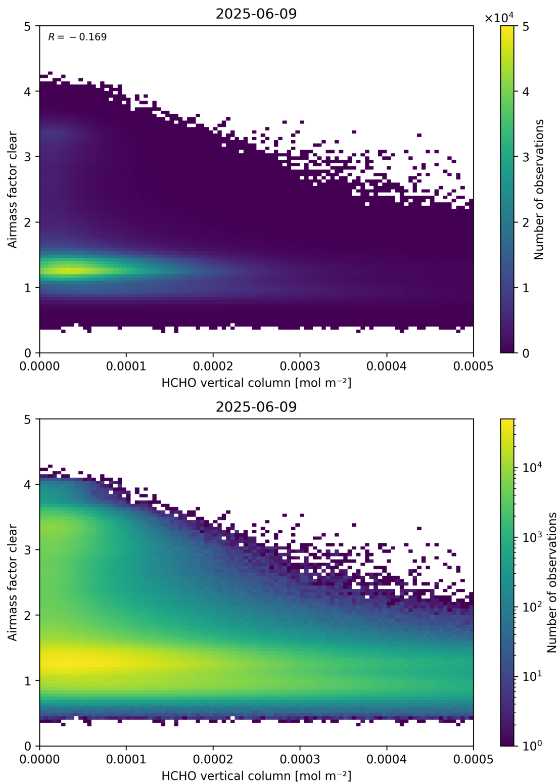
Figure 126: Scatter density plot of “HCHO vertical column” against “Airmass factor clear” for 2025-06-08 to 2025-06-10.
