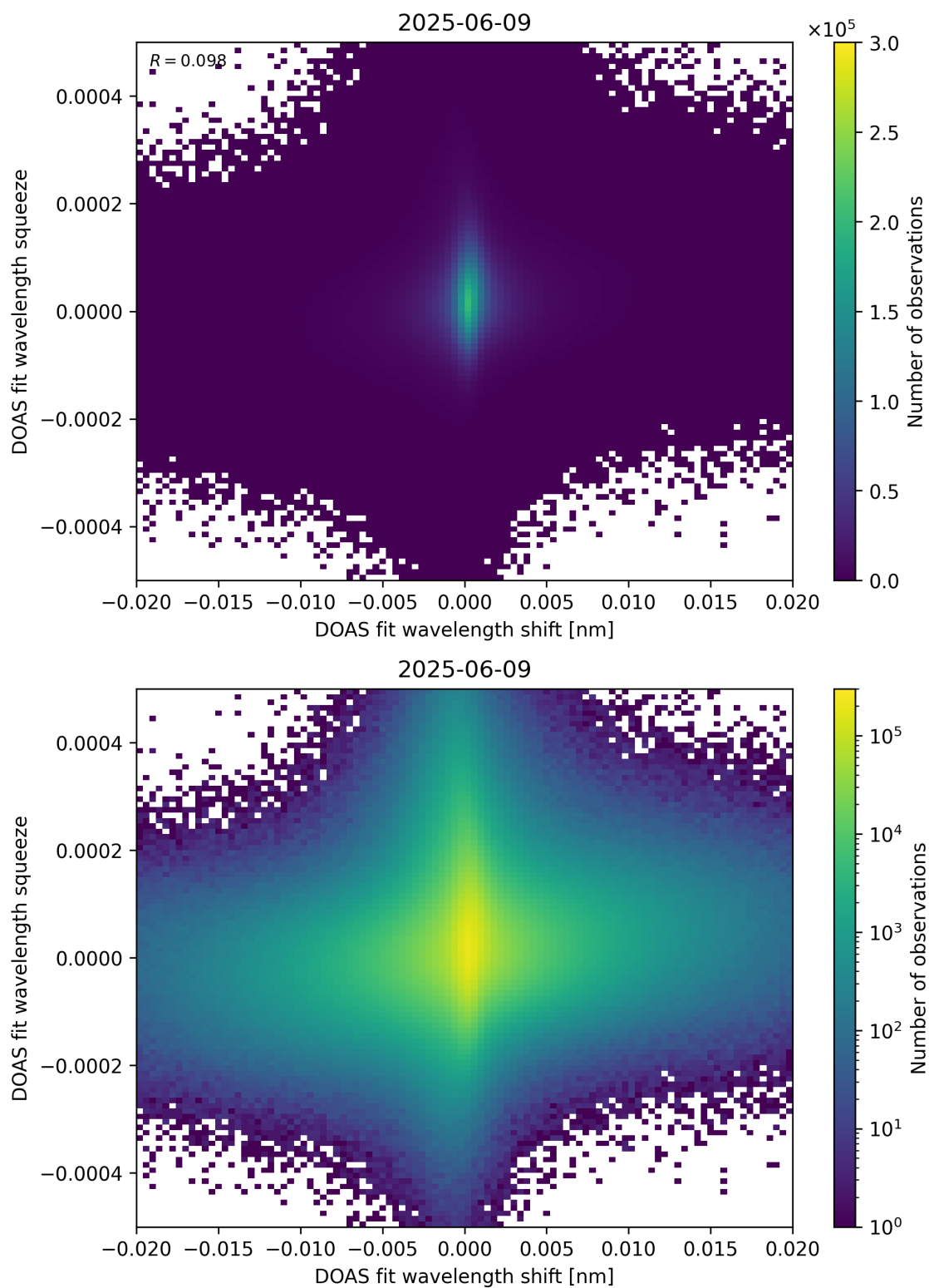
Figure 65: Scatter density plot of “DOAS fit wavelength shift” against “DOAS fit wavelength squeeze” for 2025-06-08 to 2025-06-10.
