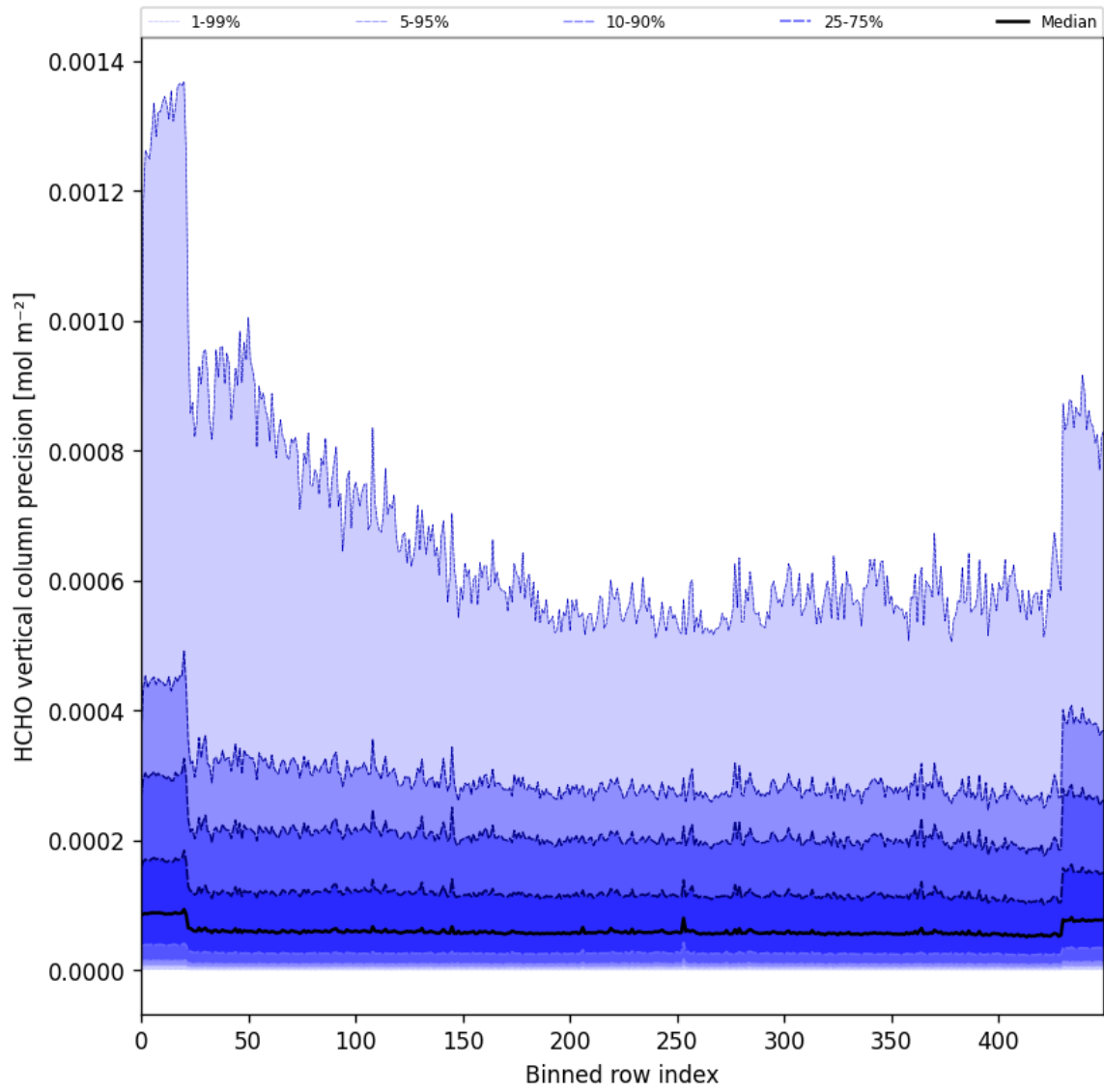
Figure 50: Along track statistics of “HCHO vertical column precision” for 2025-06-08 to 2025-06-10
