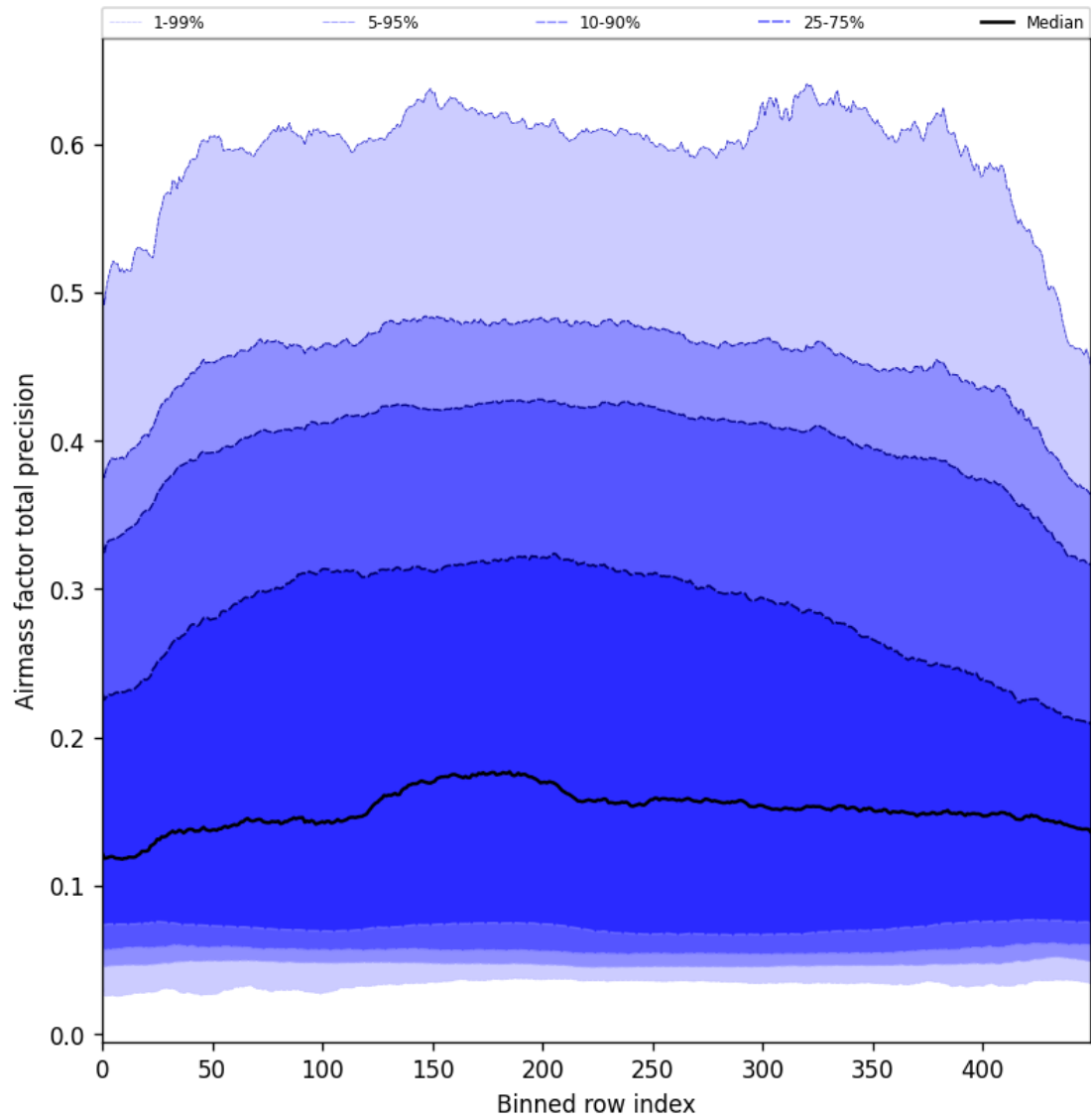
Figure 55: Along track statistics of “Airmass factor total precision” for 2025-06-08 to 2025-06-10
