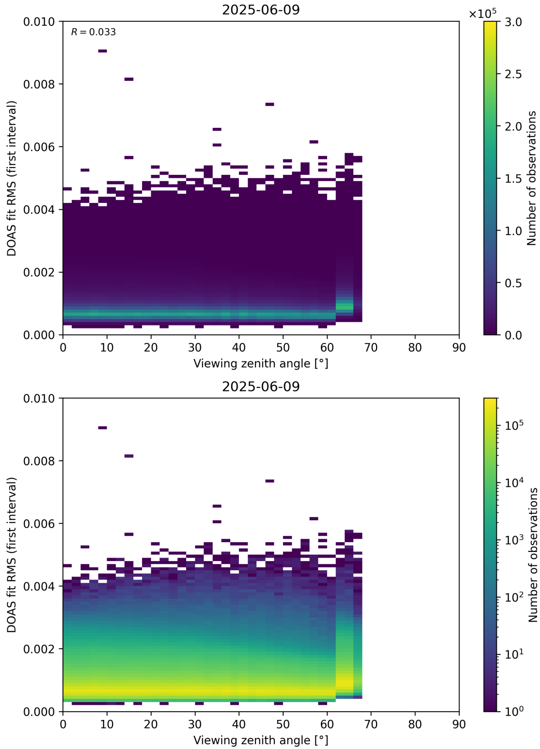
Figure 182: Scatter density plot of “Viewing zenith angle” against “DOAS fit RMS (first interval)” for 2025-06-08 to 2025-06-10.
