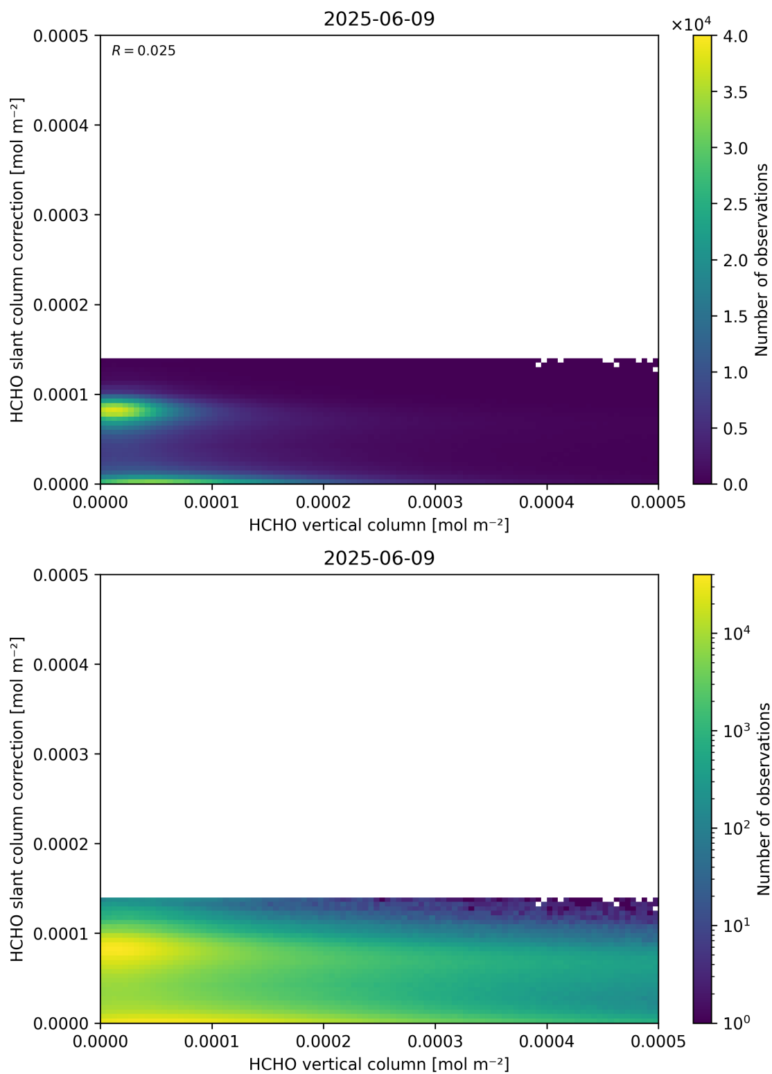
Figure 128: Scatter density plot of “HCHO vertical column” against “HCHO slant column correction” for 2025-06-08 to 2025-06-10.
