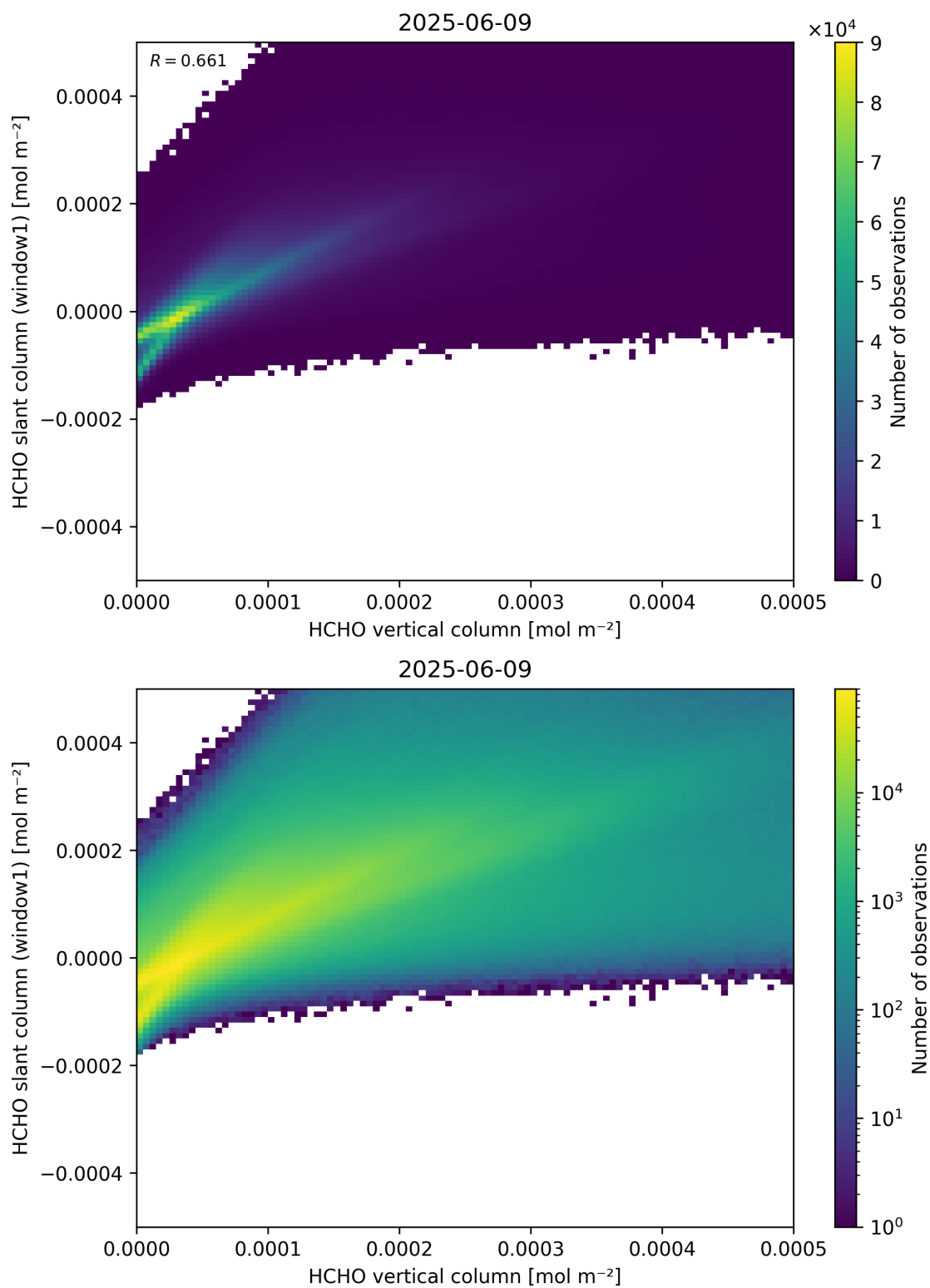
Figure 129: Scatter density plot of “HCHO vertical column” against “HCHO slant column (window1)” for 2025-06-08 to 2025-06-10.
