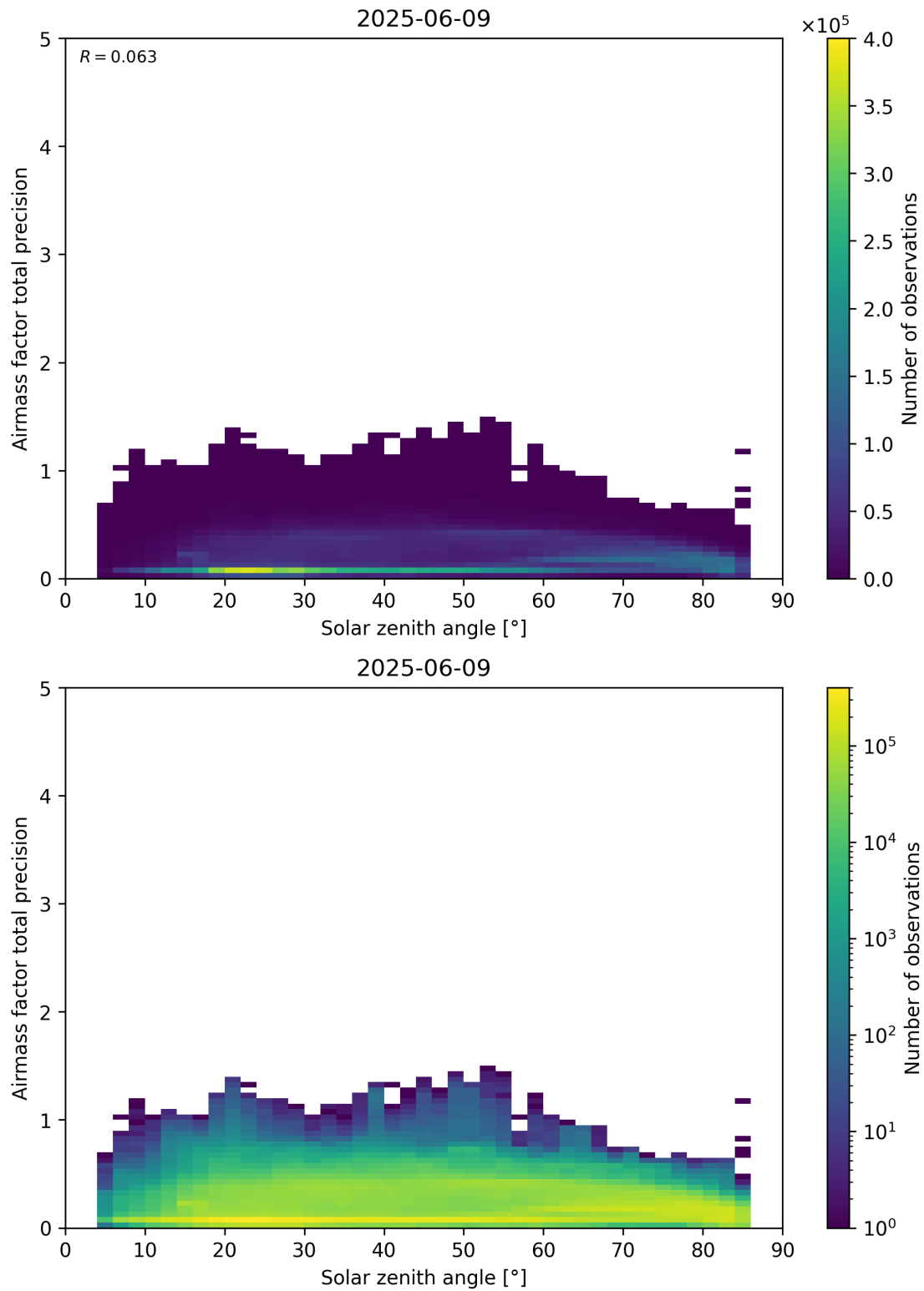
Figure 176: Scatter density plot of “Solar zenith angle” against “Airmass factor total precision” for 2025-06-08 to 2025-06-10.
