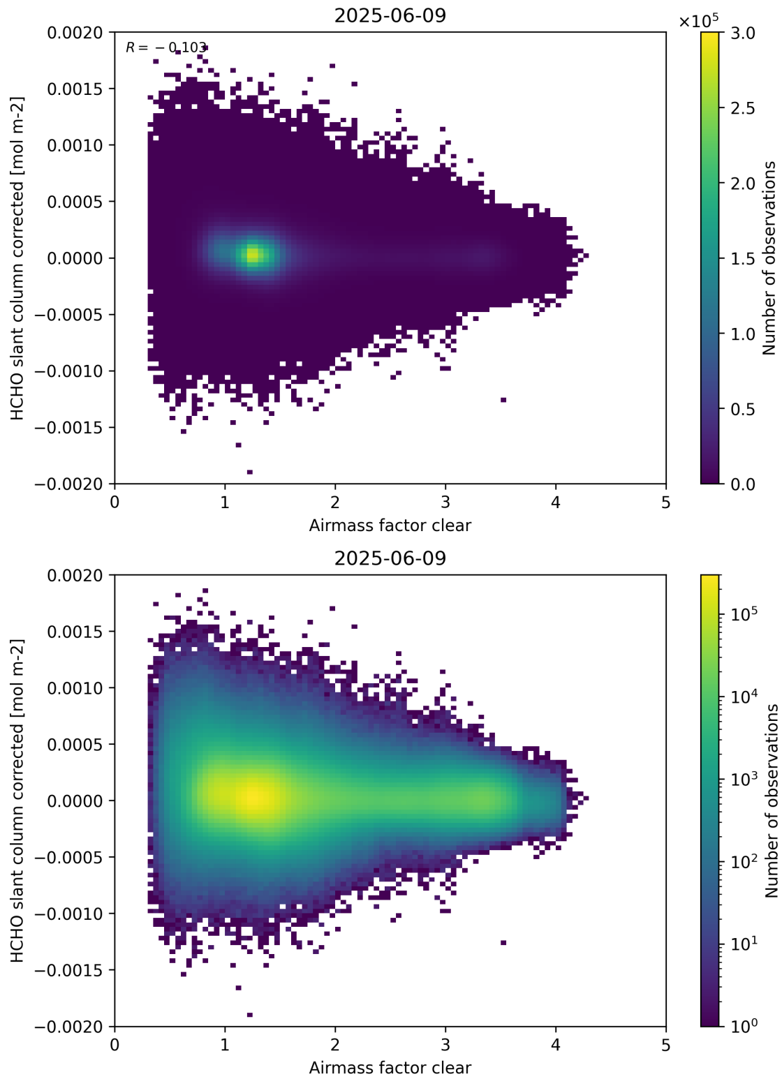
Figure 74: Scatter density plot of “Airmass factor clear” against “HCHO slant column corrected” for 2025-06-08 to 2025-06-10.
