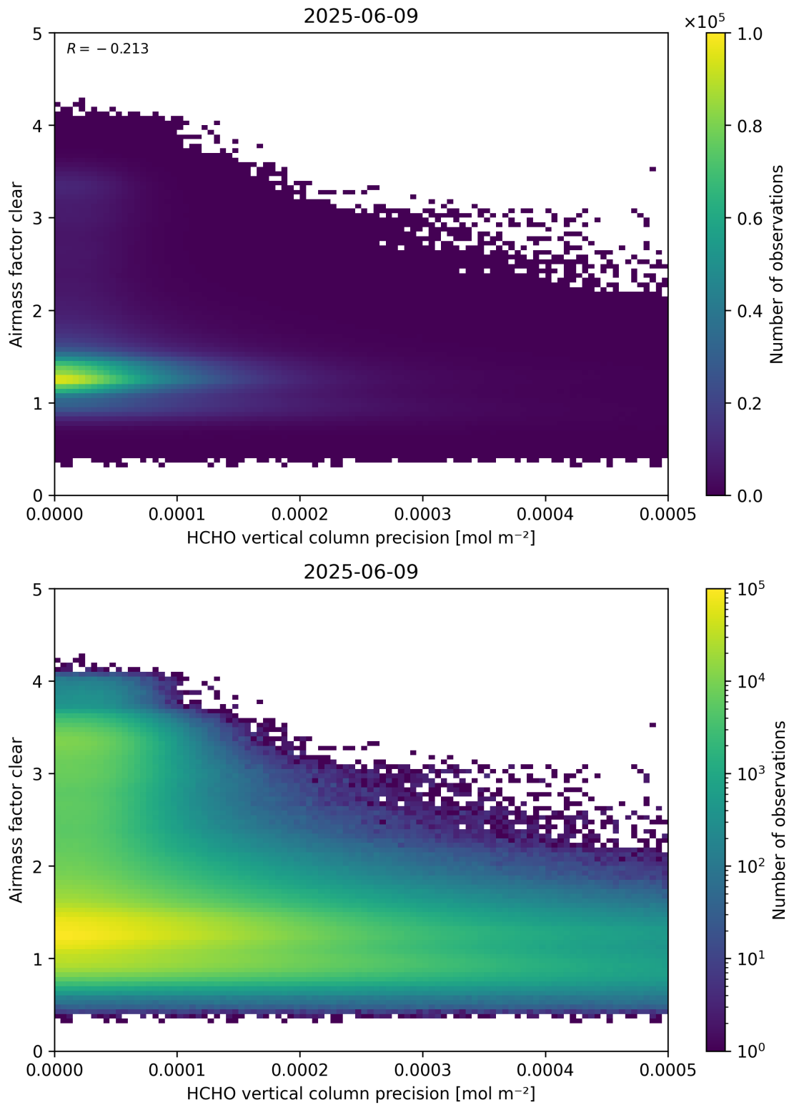
Figure 139: Scatter density plot of “HCHO vertical column precision” against “Airmass factor clear” for 2025-06-08 to 2025-06-10.
