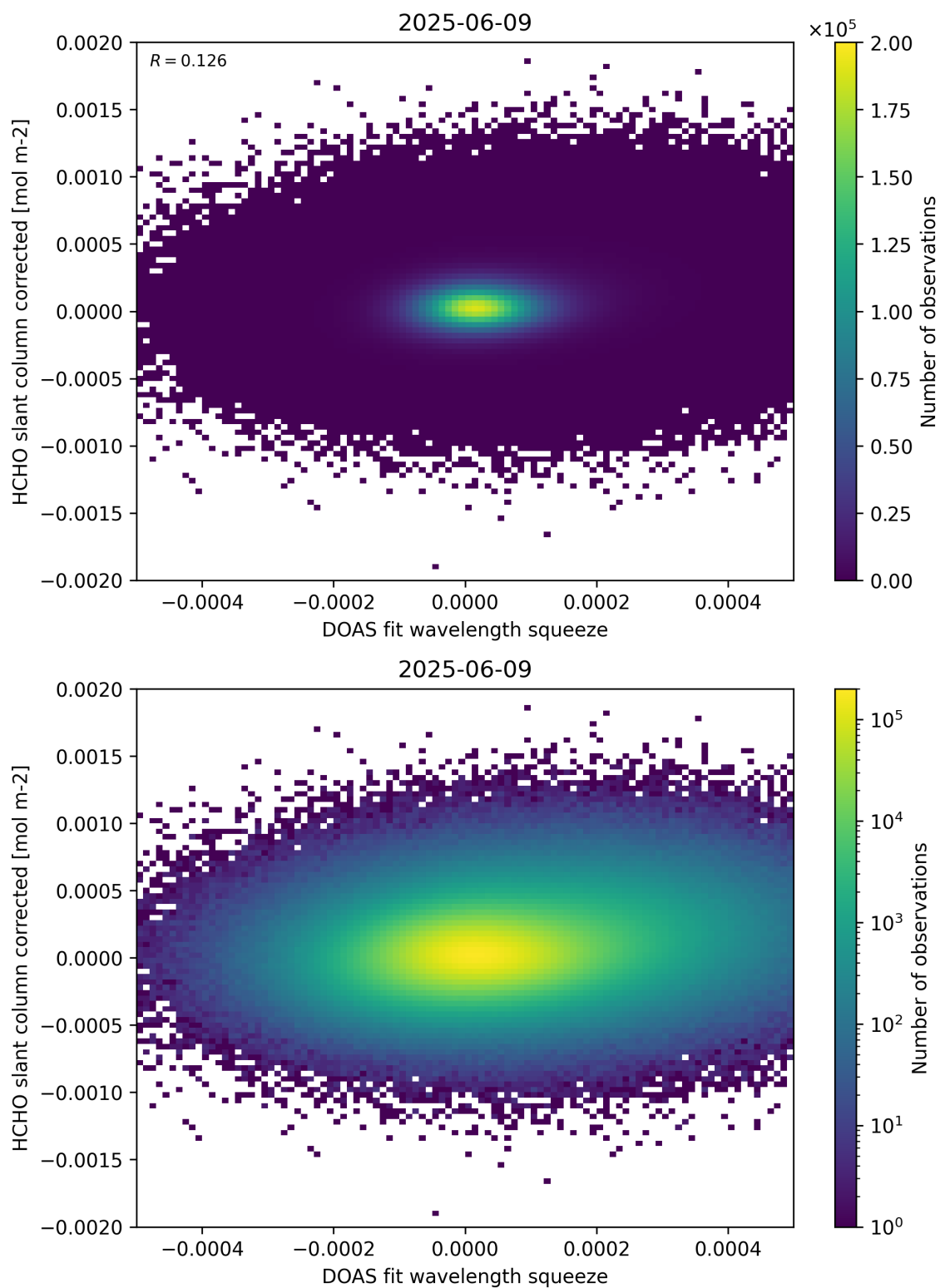
Figure 69: Scatter density plot of “DOAS fit wavelength squeeze” against “HCHO slant column corrected” for 2025-06-08 to 2025-06-10.
