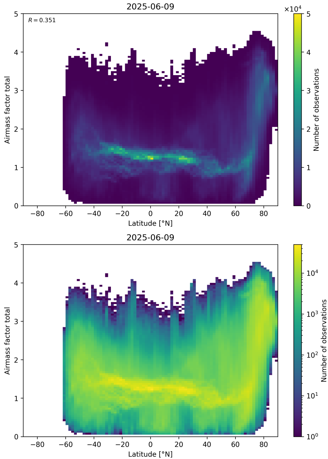
Figure 161: Scatter density plot of “Latitude” against “Airmass factor total” for 2025-06-08 to 2025-06-10.
