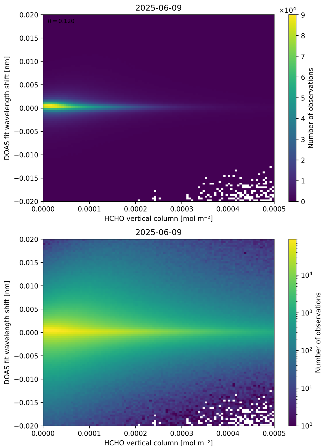
Figure 124: Scatter density plot of “HCHO vertical column” against “DOAS fit wavelength shift” for 2025-06-08 to 2025-06-10.
