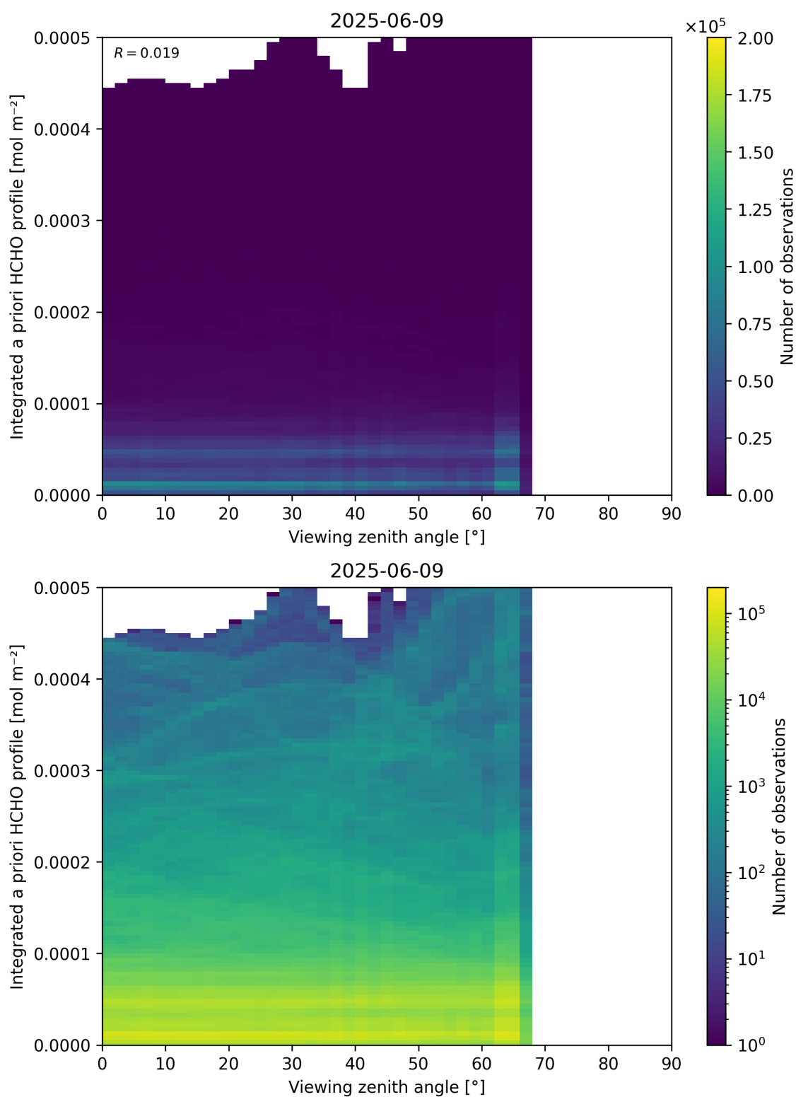
Figure 195: Scatter density plot of “Viewing zenith angle” against “Integrated a priori HCHO profile” for 2025-06-08 to 2025-06-10.
