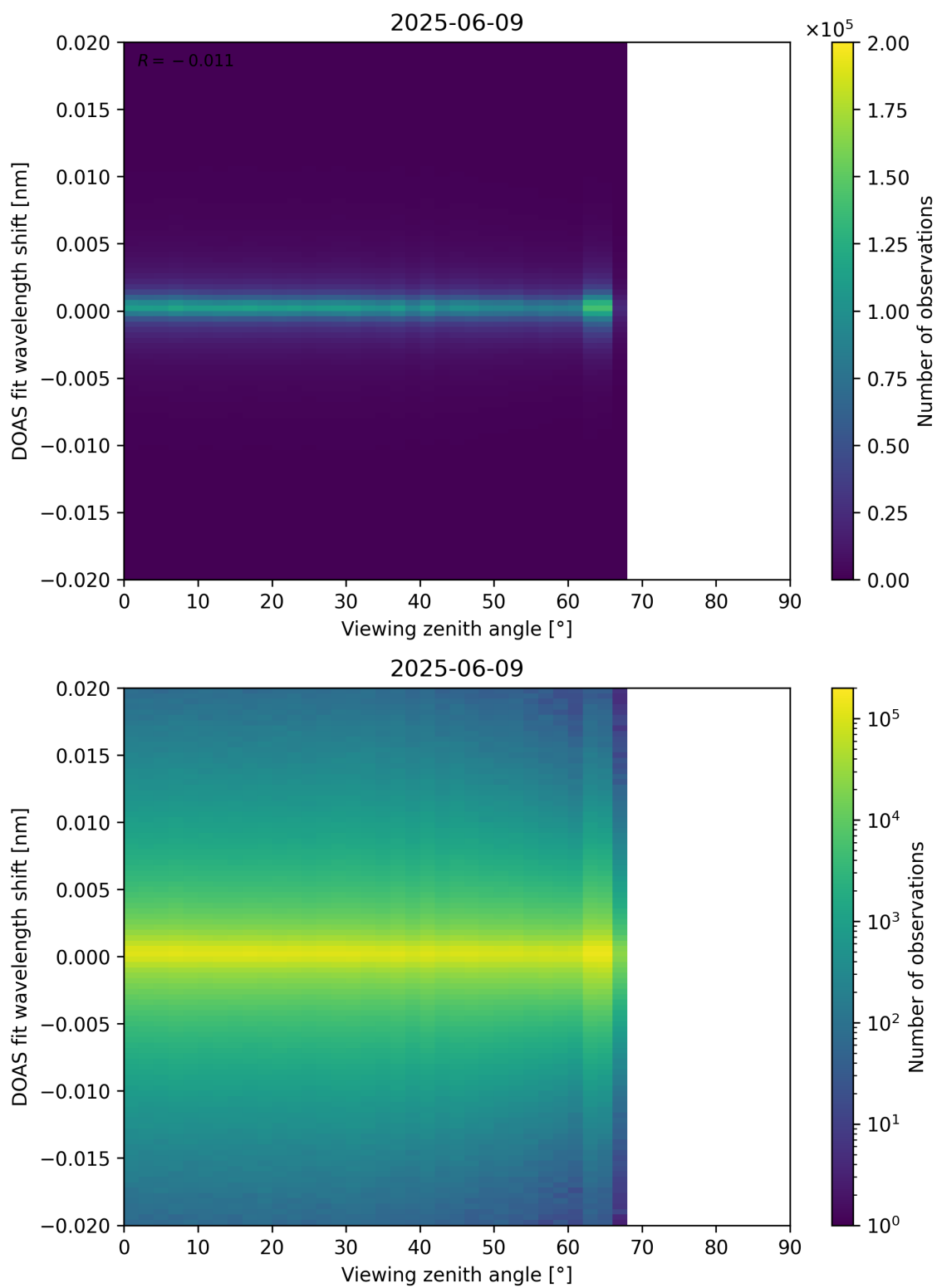
Figure 183: Scatter density plot of “Viewing zenith angle” against “DOAS fit wavelength shift” for 2025-06-08 to 2025-06-10.
