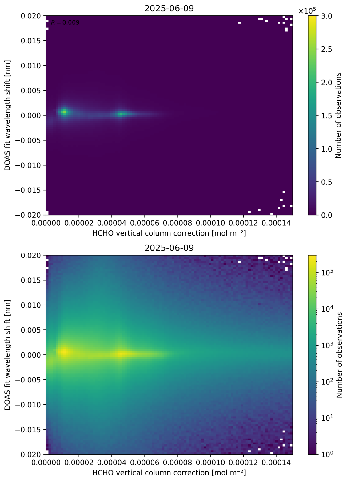
Figure 113: Scatter density plot of “HCHO vertical column correction” against “DOAS fit wavelength shift” for 2025-06-08 to 2025-06-10.
