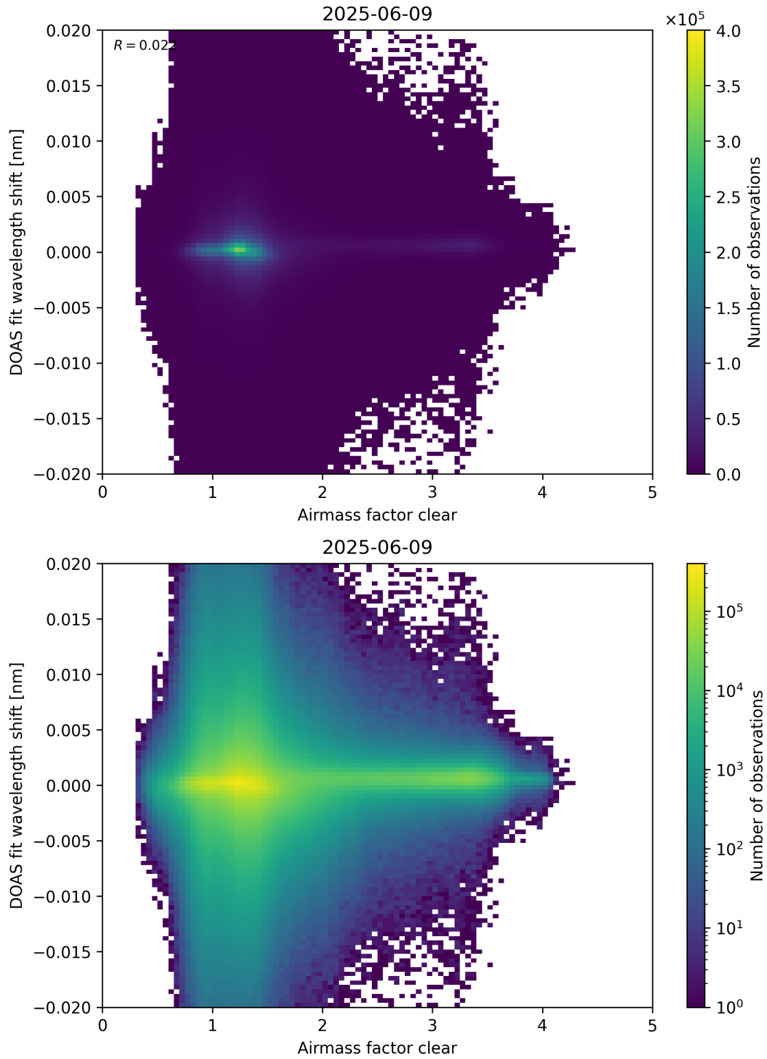
Figure 72: Scatter density plot of “Airmass factor clear” against “DOAS fit wavelength shift” for 2025-06-08 to 2025-06-10.
