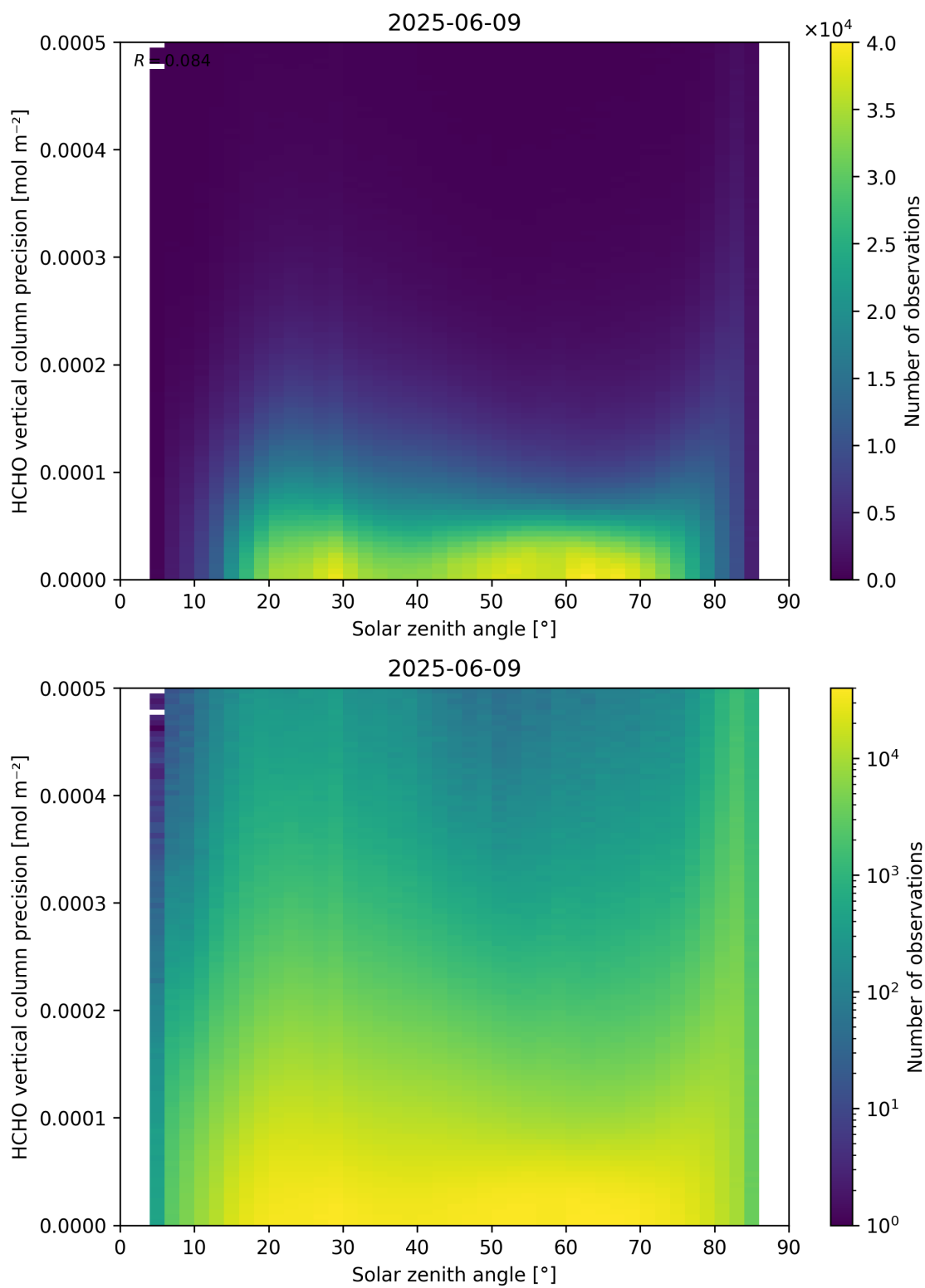
Figure 179: Scatter density plot of “Solar zenith angle” against “HCHO vertical column precision” for 2025-06-08 to 2025-06-10.
