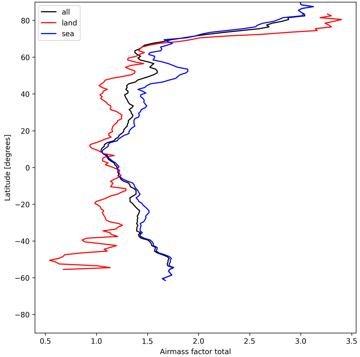
Figure 26: Zonal average of “Airmass factor total” for 2025-06-08 to 2025-06-10.
