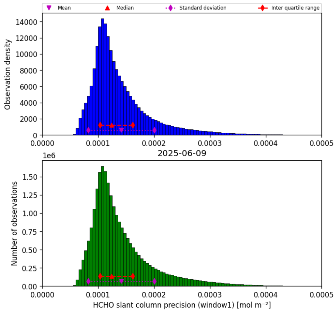
Figure 39: Histogram of “HCHO slant column precision (window1)” for 2025-06-08 to 2025-06-10
