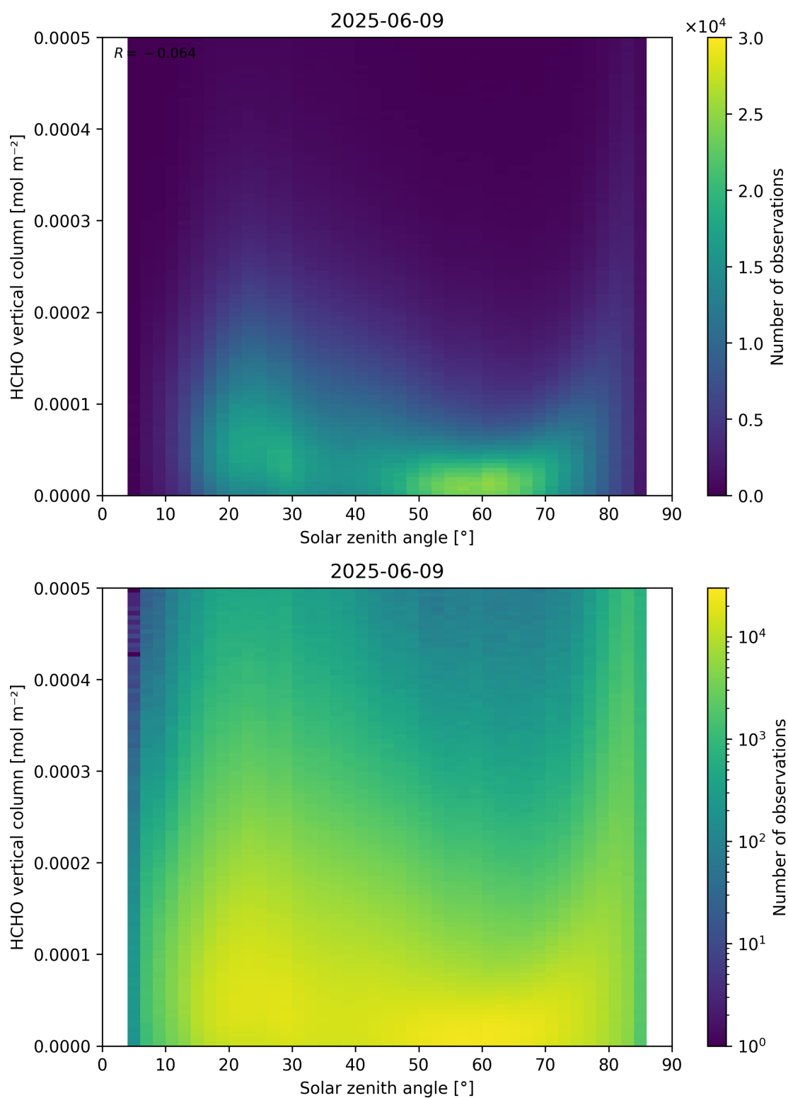
Figure 177: Scatter density plot of “Solar zenith angle” against “HCHO vertical column” for 2025-06-08 to 2025-06-10.
