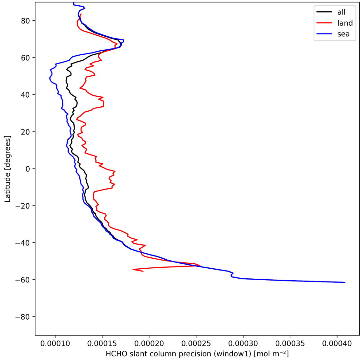
Figure 25: Zonal average of "HCHO slant column precision (window1)" for 2025-06-08 to 2025-06-10.
