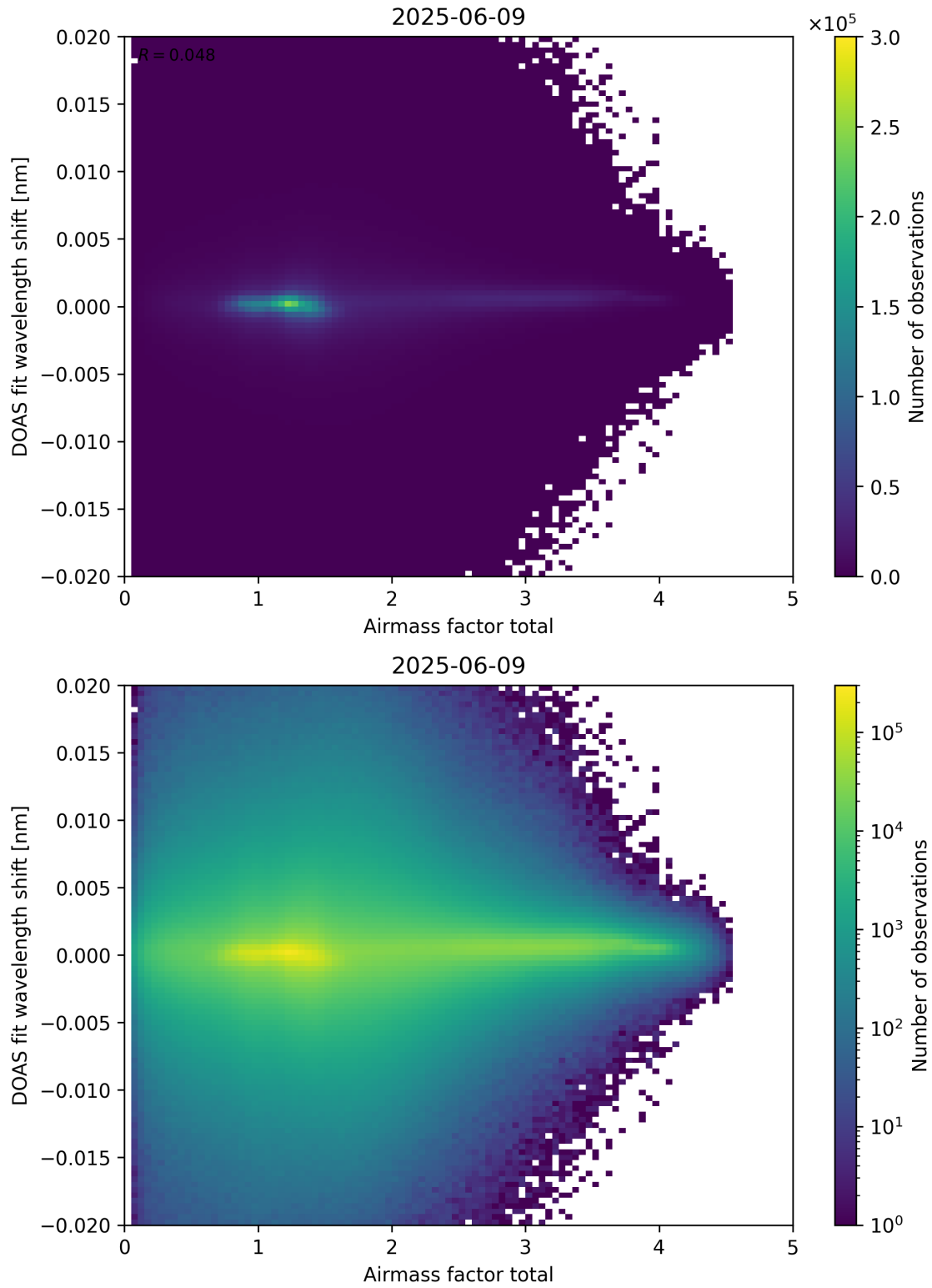
Figure 98: Scatter density plot of “Airmass factor total” against “DOAS fit wavelength shift” for 2025-06-08 to 2025-06-10.
