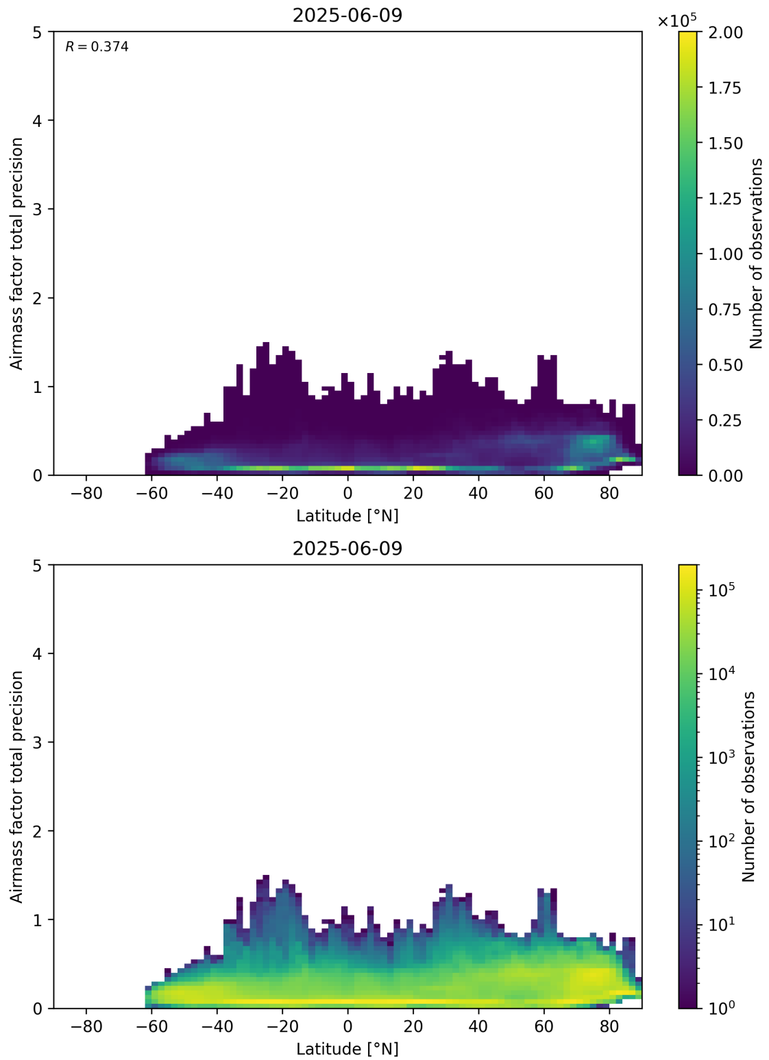
Figure 162: Scatter density plot of “Latitude” against “Airmass factor total precision” for 2025-06-08 to 2025-06-10.
