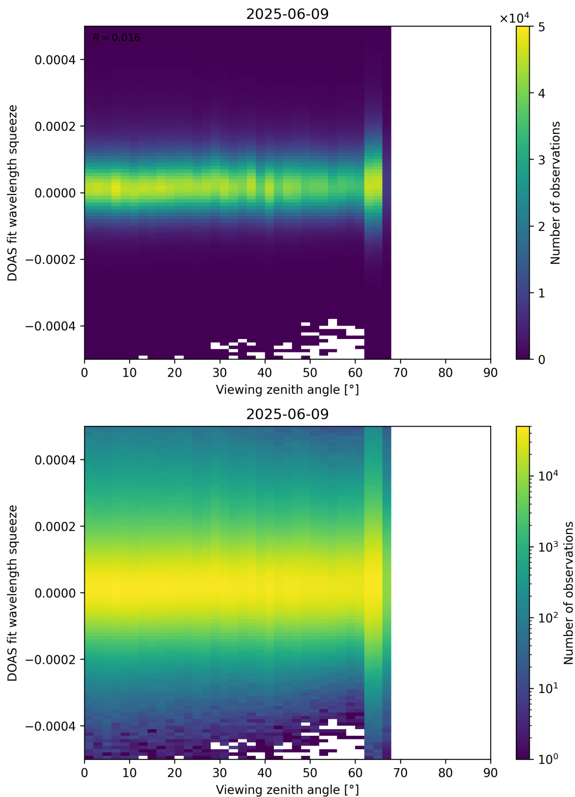
Figure 184: Scatter density plot of “Viewing zenith angle” against “DOAS fit wavelength squeeze” for 2025-06-08 to 2025-06-10.
