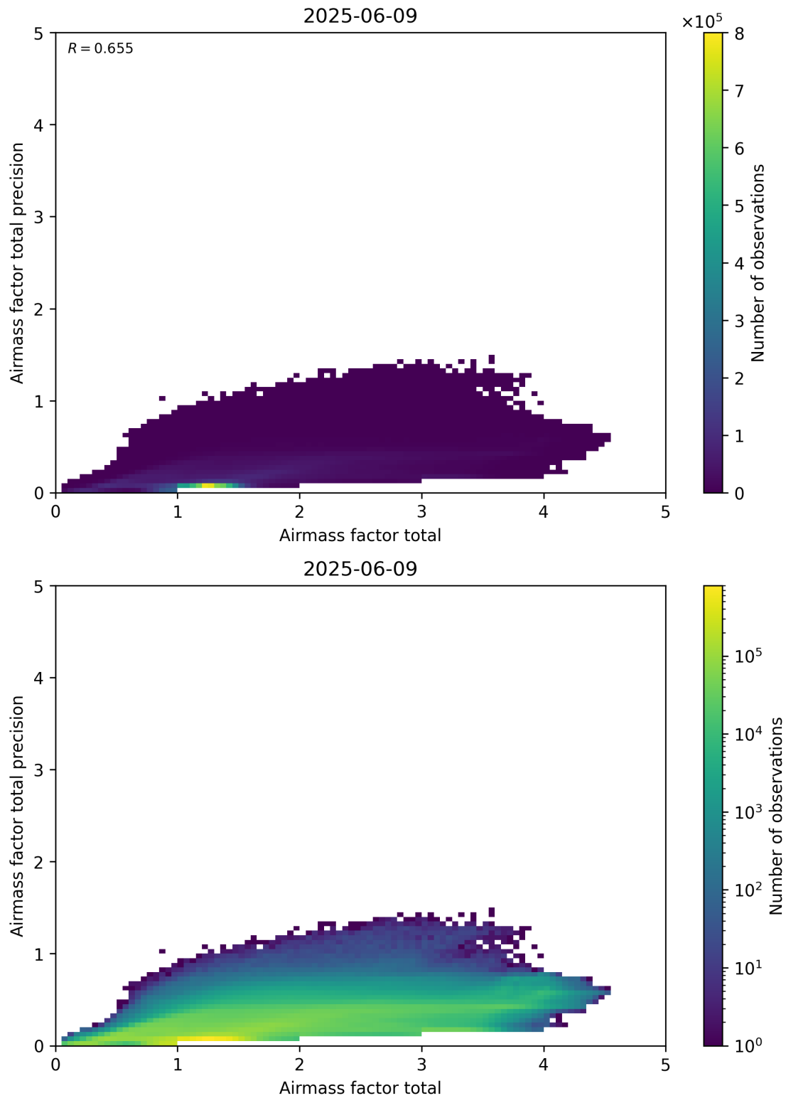
Figure 103: Scatter density plot of “Airmass factor total” against “Airmass factor total precision” for 2025-06-08 to 2025-06-10.
