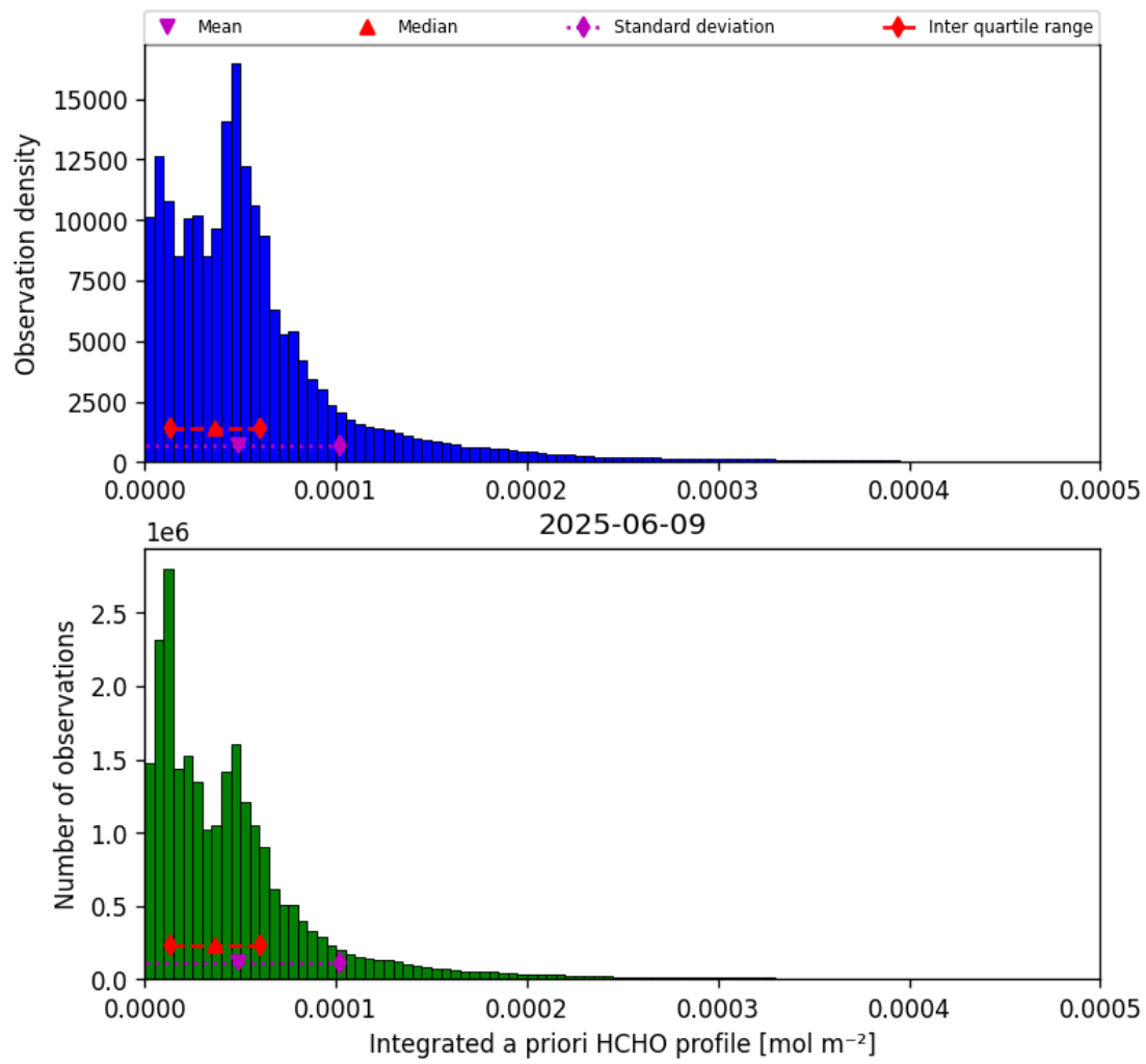
Figure 43: Histogram of “Integrated a priori HCHO profile” for 2025-06-08 to 2025-06-10
