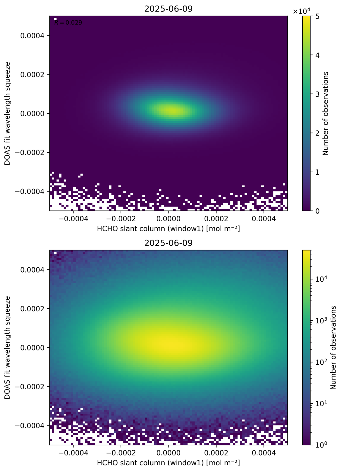
Figure 80: Scatter density plot of “HCHO slant column (window1)” against “DOAS fit wavelength squeeze” for 2025-06-08 to 2025-06-10.
