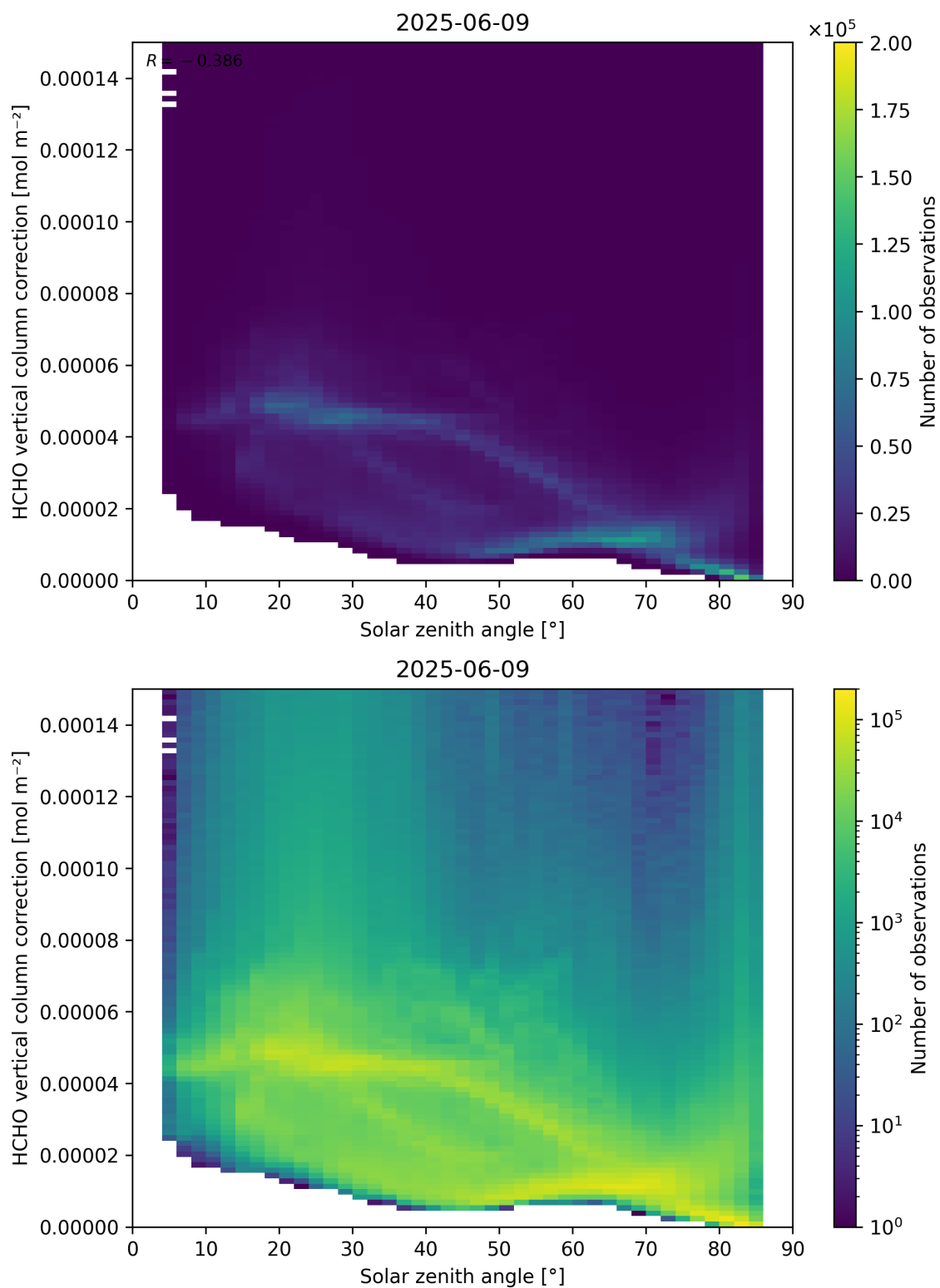
Figure 178: Scatter density plot of “Solar zenith angle” against “HCHO vertical column correction” for 2025-06-08 to 2025-06-10.
