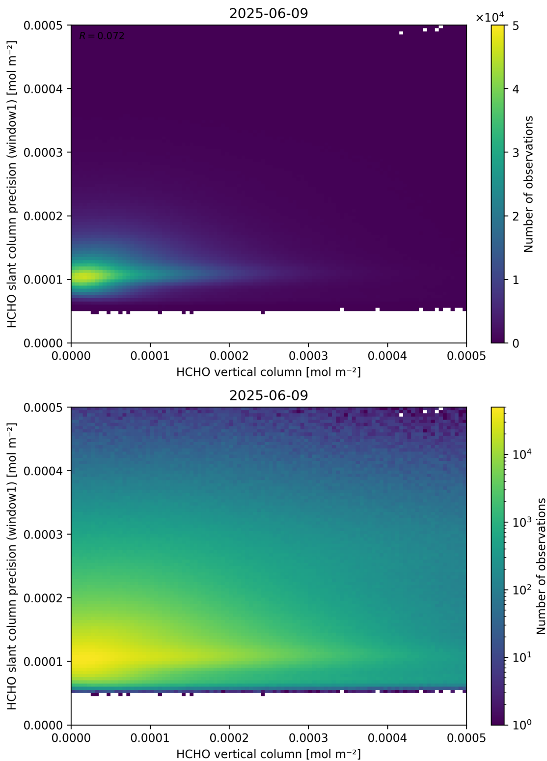
Figure 130: Scatter density plot of “HCHO vertical column” against “HCHO slant column precision (window1)” for 2025-06-08 to 2025-06-10.
