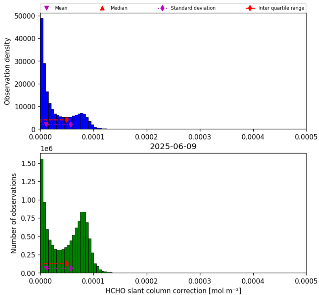
Figure 47: Histogram of “HCHO slant column correction” for 2025-06-08 to 2025-06-10
