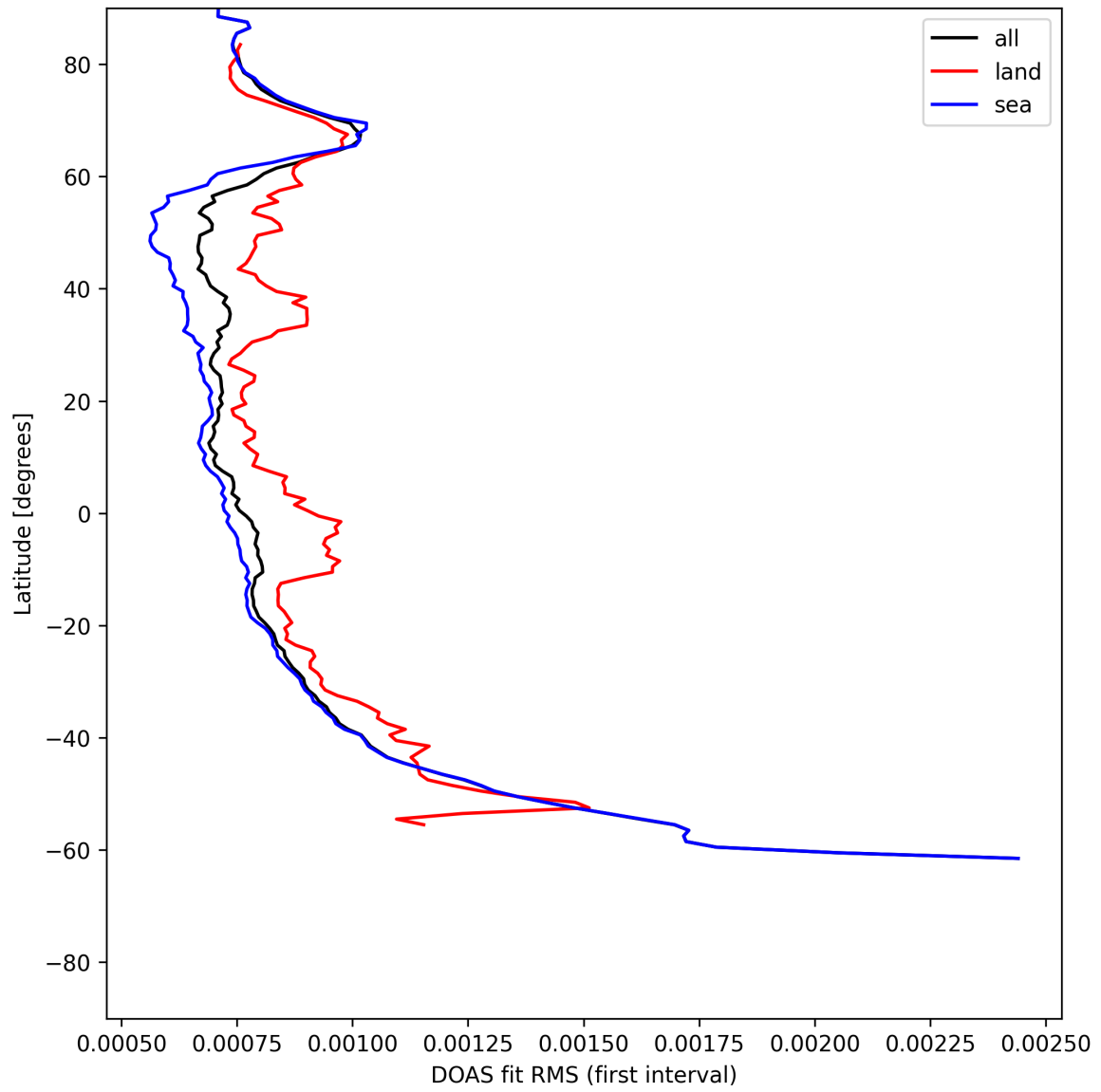
Figure 32: Zonal average of “DOAS fit RMS (first interval)” for 2025-06-08 to 2025-06-10.
