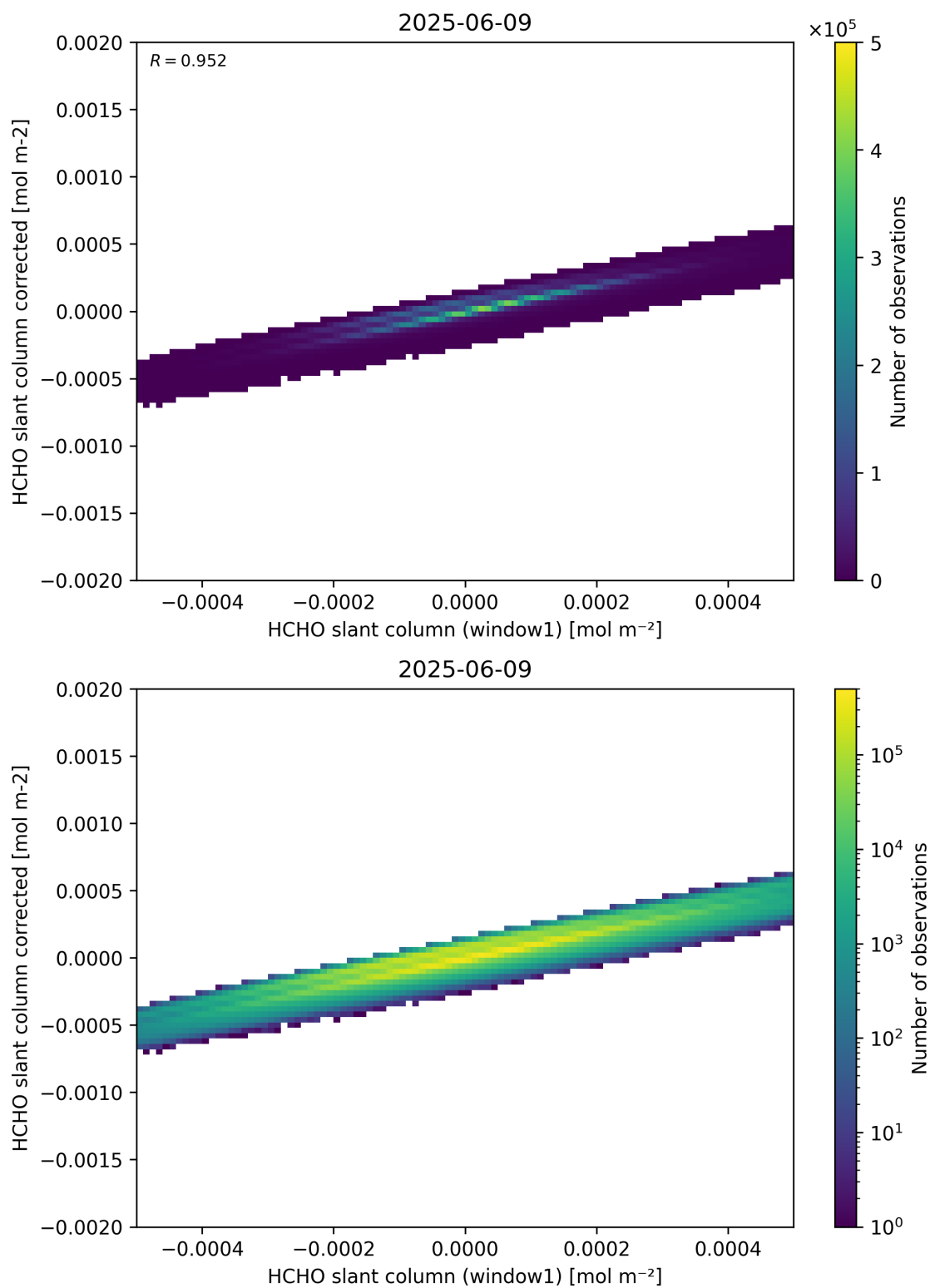
Figure 82: Scatter density plot of “HCHO slant column (window1)” against “HCHO slant column corrected” for 2025-06-08 to 2025-06-10.
