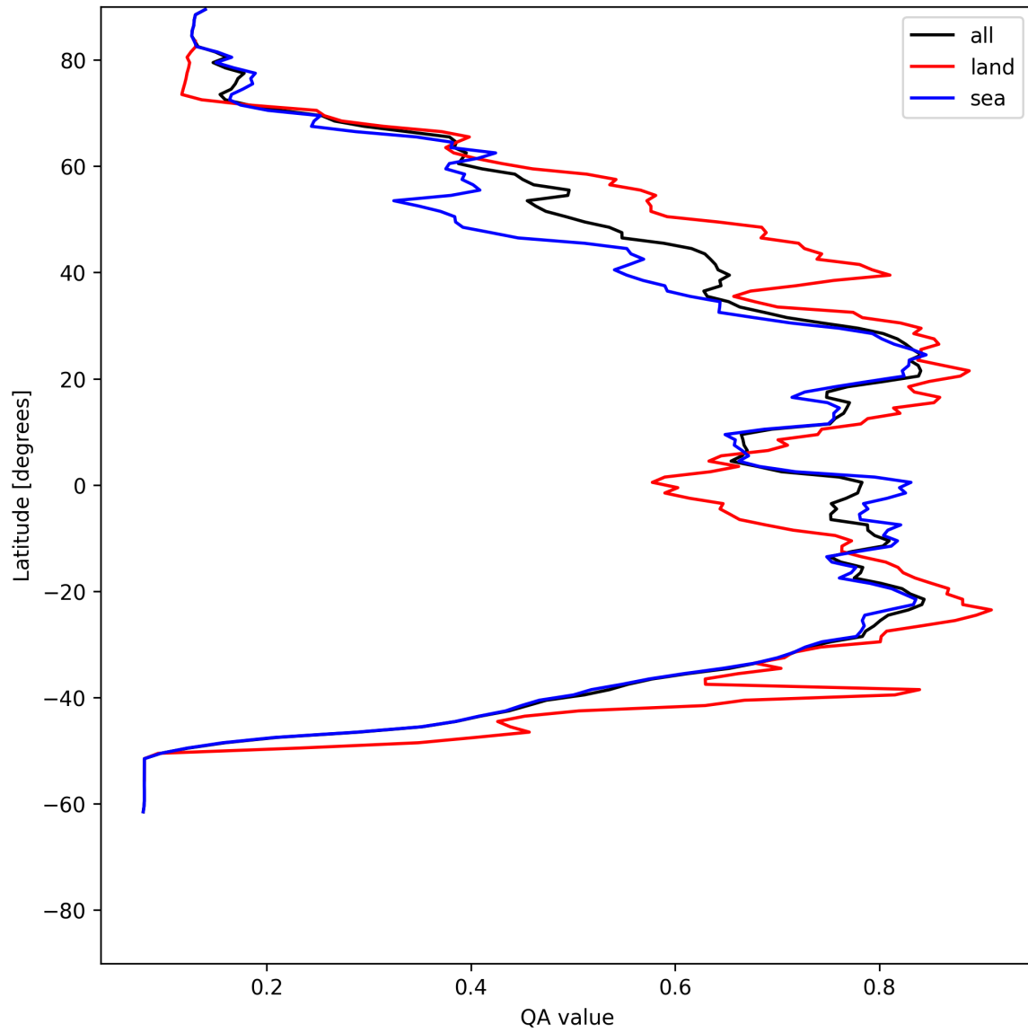
Figure 20: Zonal average of “QA value” for 2025-06-08 to 2025-06-10.
