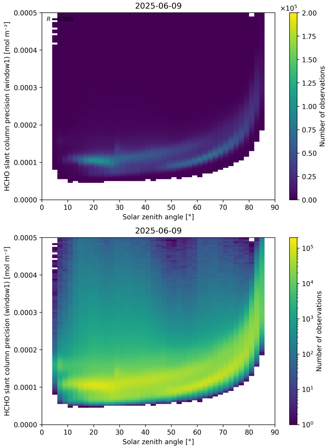
Figure 174: Scatter density plot of “Solar zenith angle” against “HCHO slant column precision (window1)” for 2025-06-08 to 2025-06-10.
