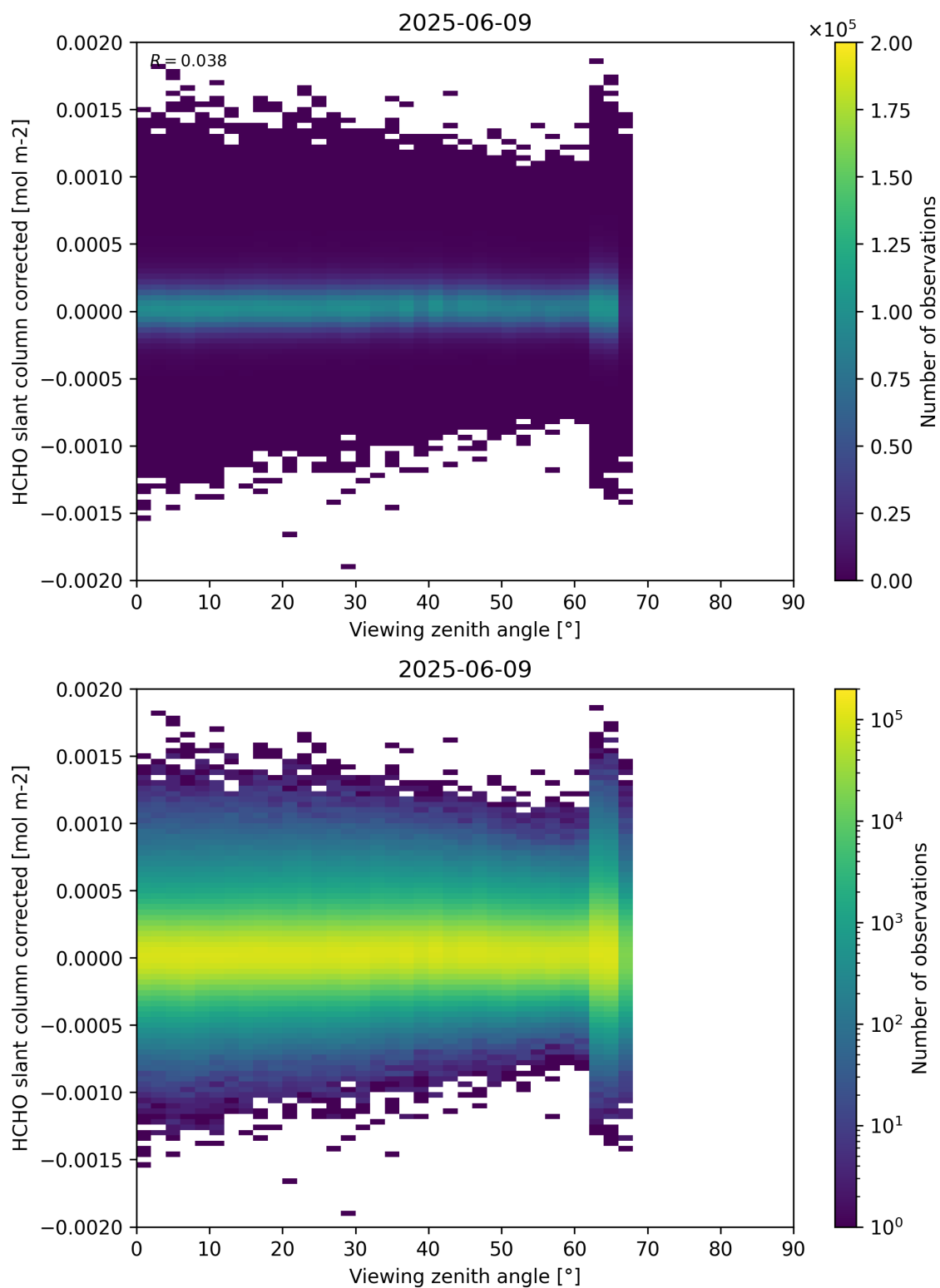
Figure 186: Scatter density plot of “Viewing zenith angle” against “HCHO slant column corrected” for 2025-06-08 to 2025-06-10.
