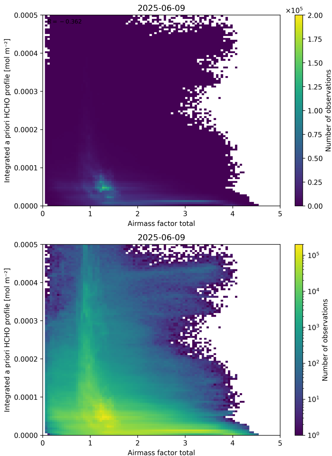
Figure 104: Scatter density plot of “Airmass factor total” against “Integrated a priori HCHO profile” for 2025-06-08 to 2025-06-10.
