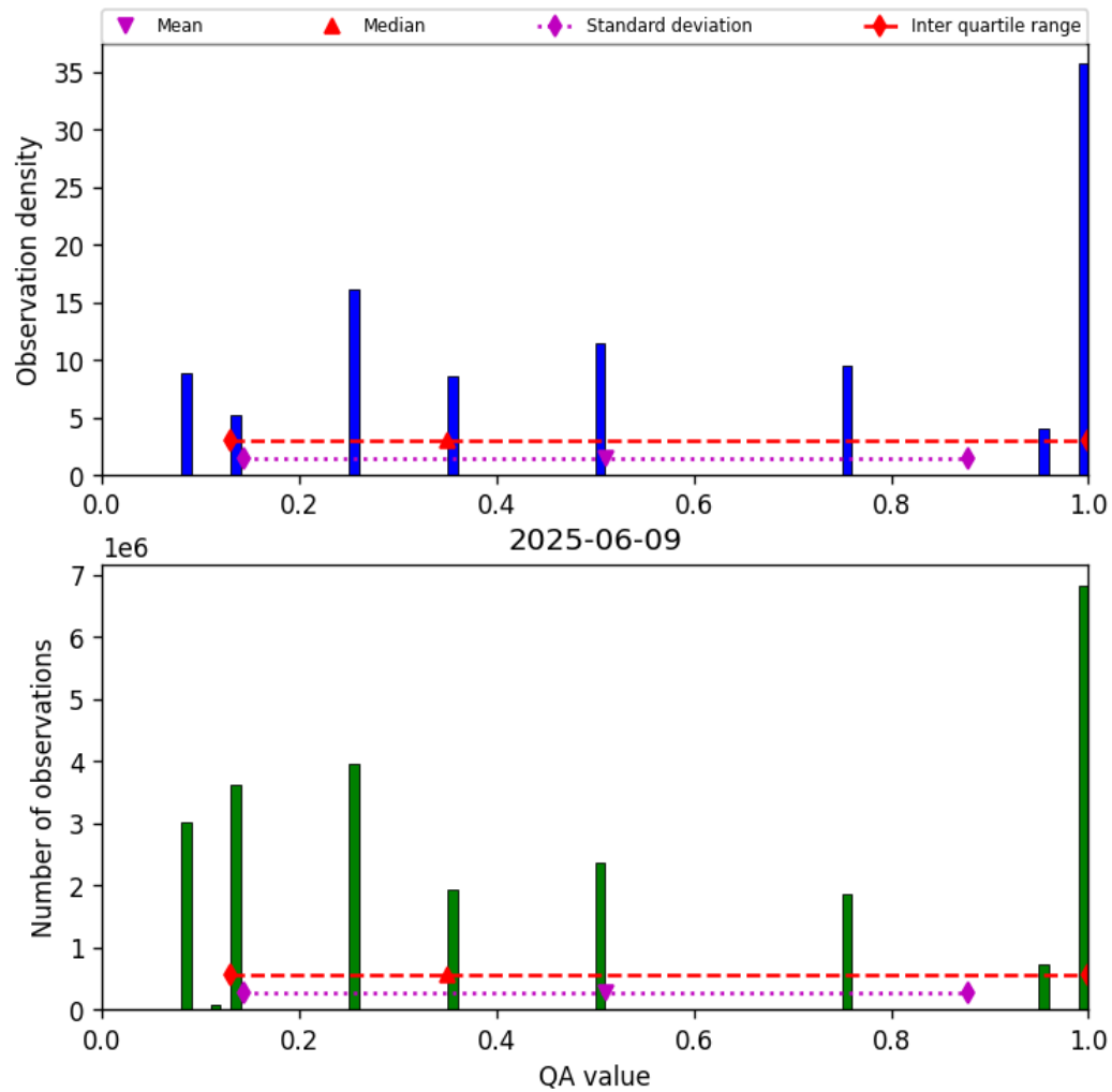
Figure 34: Histogram of “QA value” for 2025-06-08 to 2025-06-10
