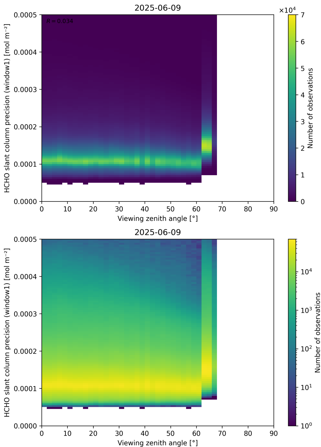
Figure 189: Scatter density plot of “Viewing zenith angle” against “HCHO slant column precision (window1)” for 2025-06-08 to 2025-06-10.
