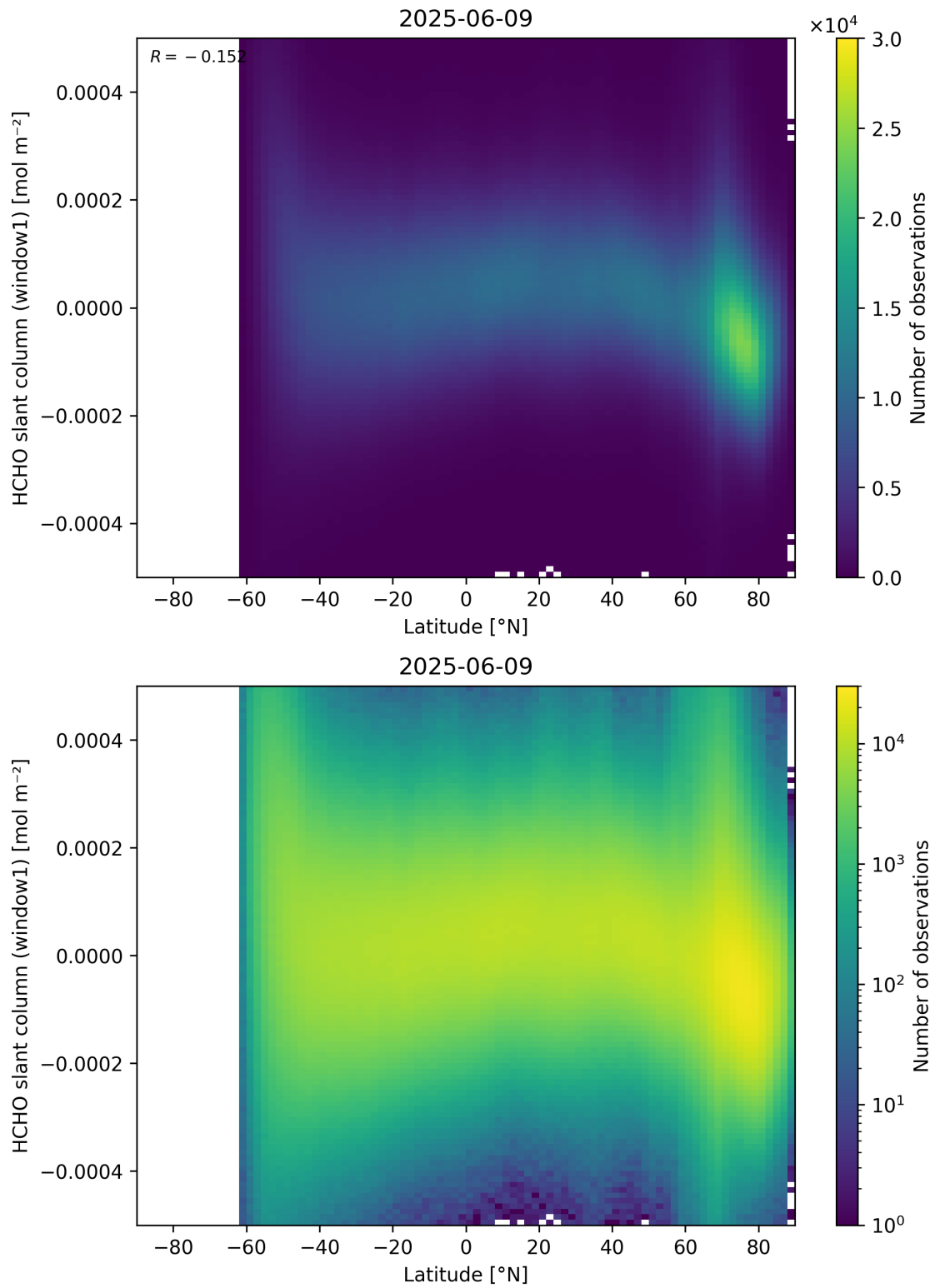
Figure 159: Scatter density plot of “Latitude” against “HCHO slant column (window1)” for 2025-06-08 to 2025-06-10.
