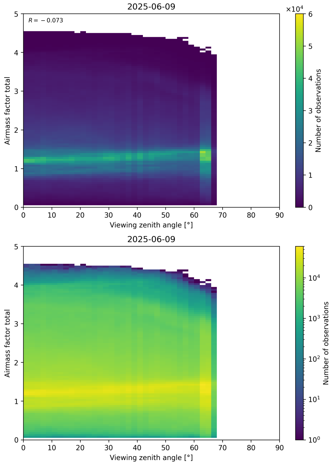
Figure 190: Scatter density plot of “Viewing zenith angle” against “Airmass factor total” for 2025-06-08 to 2025-06-10.
