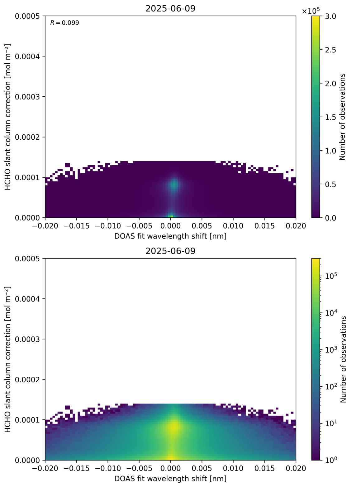
Figure 67: Scatter density plot of “DOAS fit wavelength shift” against “HCHO slant column correction” for 2025-06-08 to 2025-06-10.
