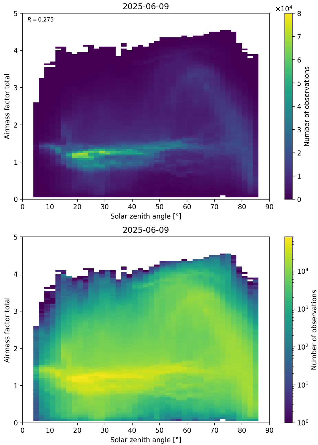
Figure 175: Scatter density plot of “Solar zenith angle” against “Airmass factor total” for 2025-06-08 to 2025-06-10.
