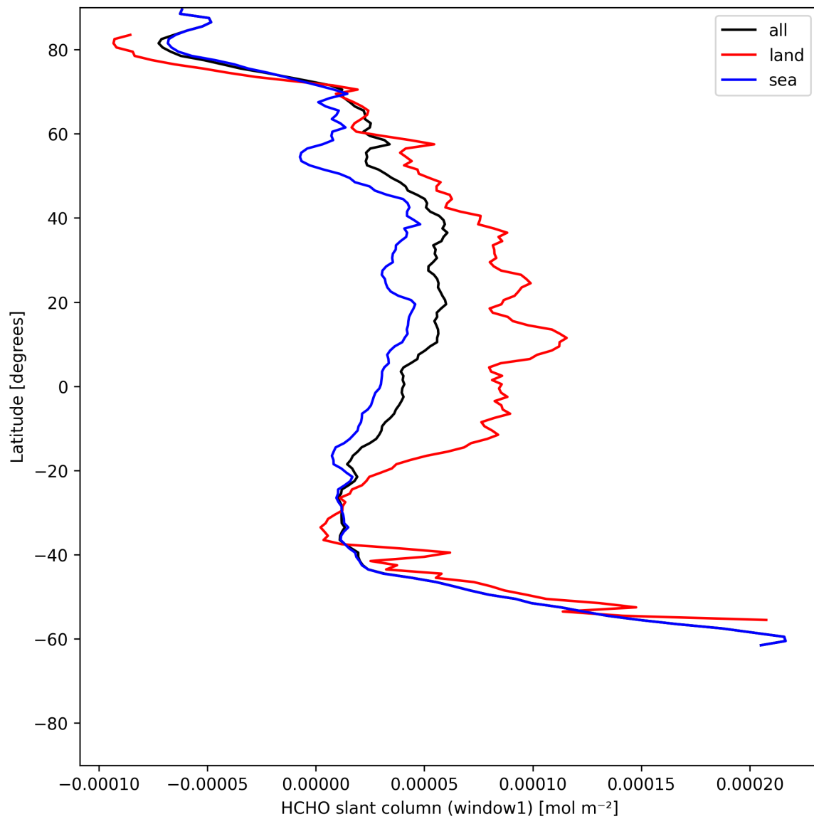
Figure 24: Zonal average of “HCHO slant column (window1)” for 2025-06-08 to 2025-06-10.
