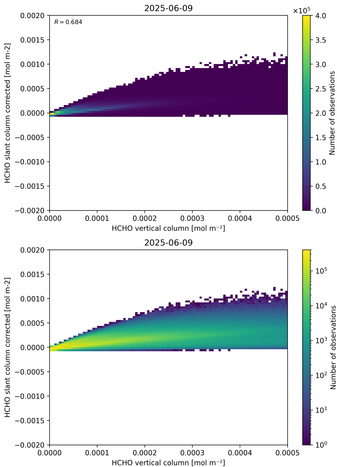
Figure 127: Scatter density plot of “HCHO vertical column” against “HCHO slant column corrected” for 2025-06-08 to 2025-06-10.
