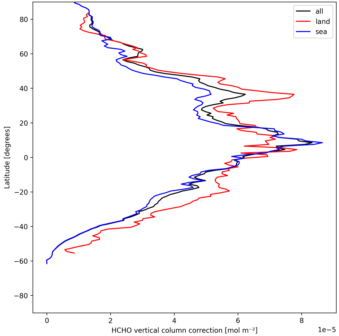
Figure 23: Zonal average of “HCHO vertical column correction” for 2025-06-08 to 2025-06-10.
