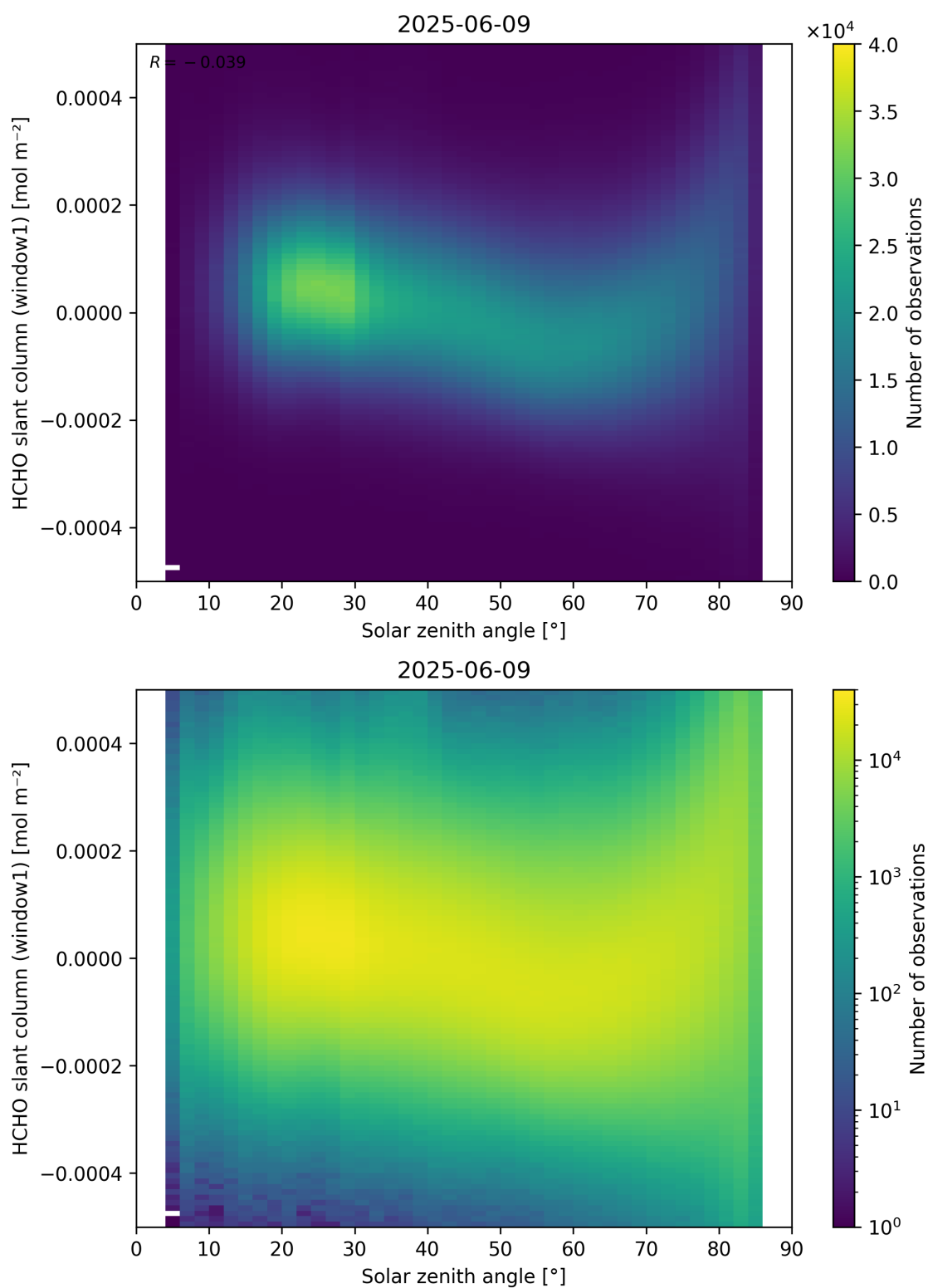
Figure 173: Scatter density plot of “Solar zenith angle” against “HCHO slant column (window1)” for 2025-06-08 to 2025-06-10.
