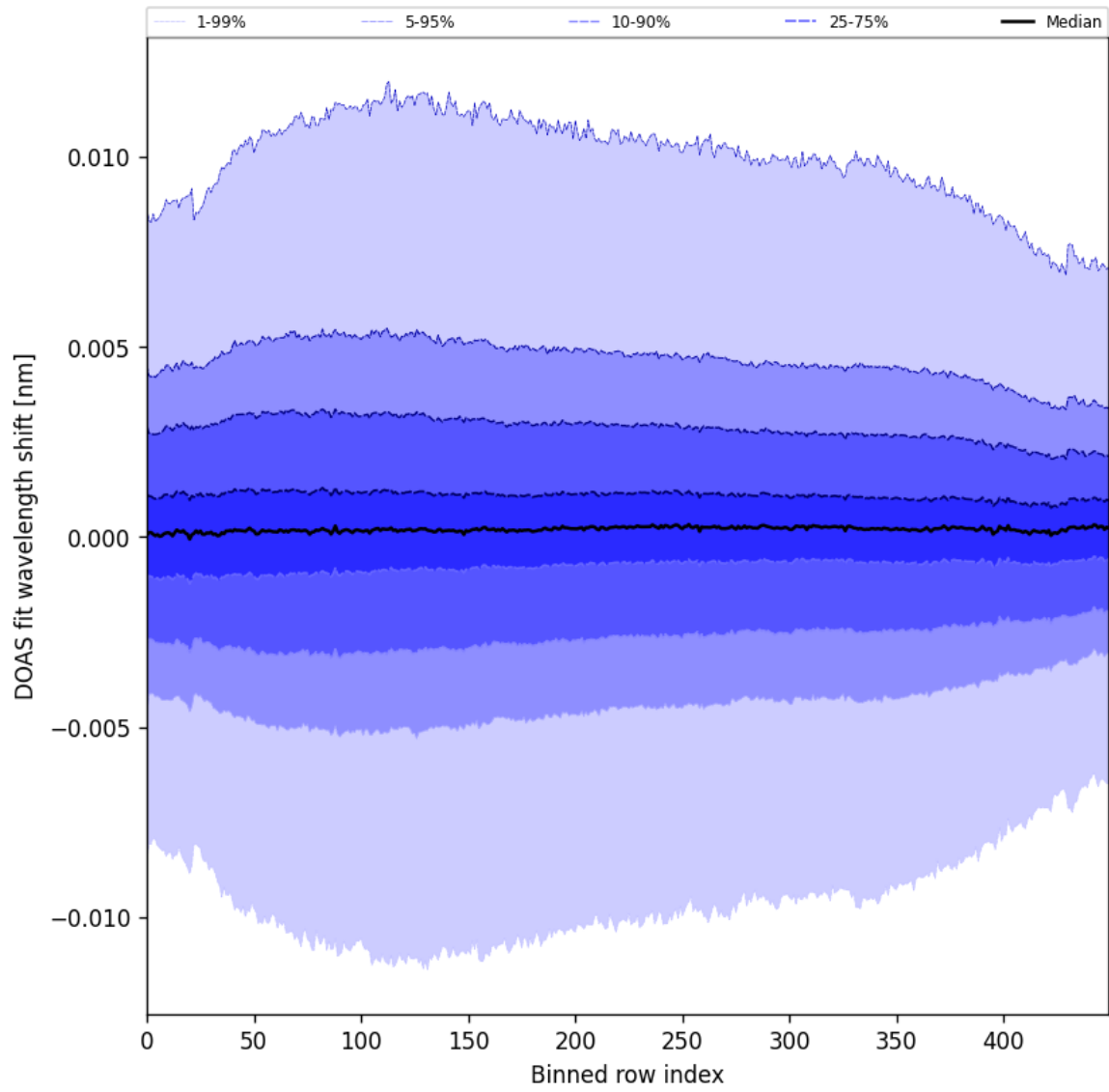
Figure 58: Along track statistics of “DOAS fit wavelength shift” for 2025-06-08 to 2025-06-10
