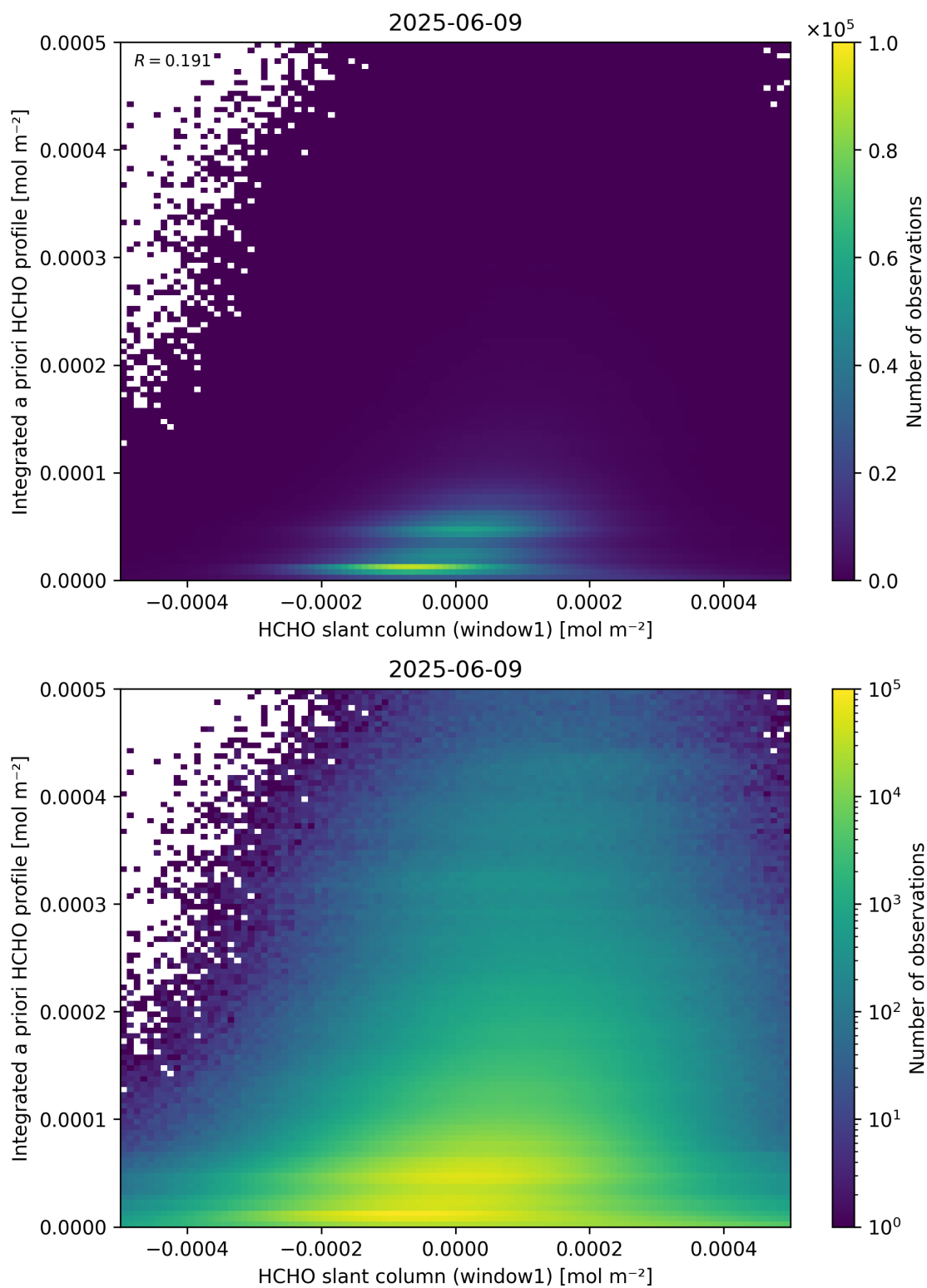
Figure 87: Scatter density plot of “HCHO slant column (window1)” against “Integrated a priori HCHO profile” for 2025-06-08 to 2025-06-10.
