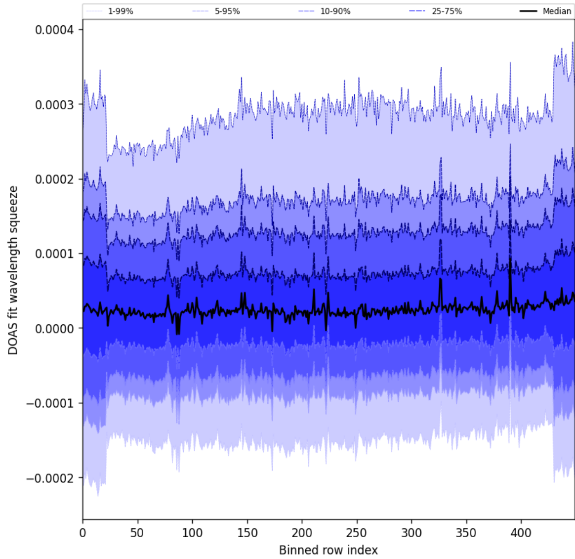
Figure 59: Along track statistics of “DOAS fit wavelength squeeze” for 2025-06-08 to 2025-06-10
