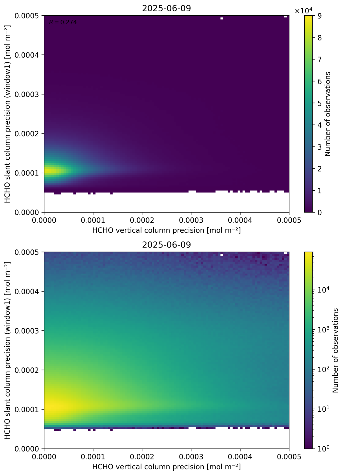
Figure 143: Scatter density plot of “HCHO vertical column precision” against “HCHO slant column precision (window1)” for 2025-06-08 to 2025-06-10.
