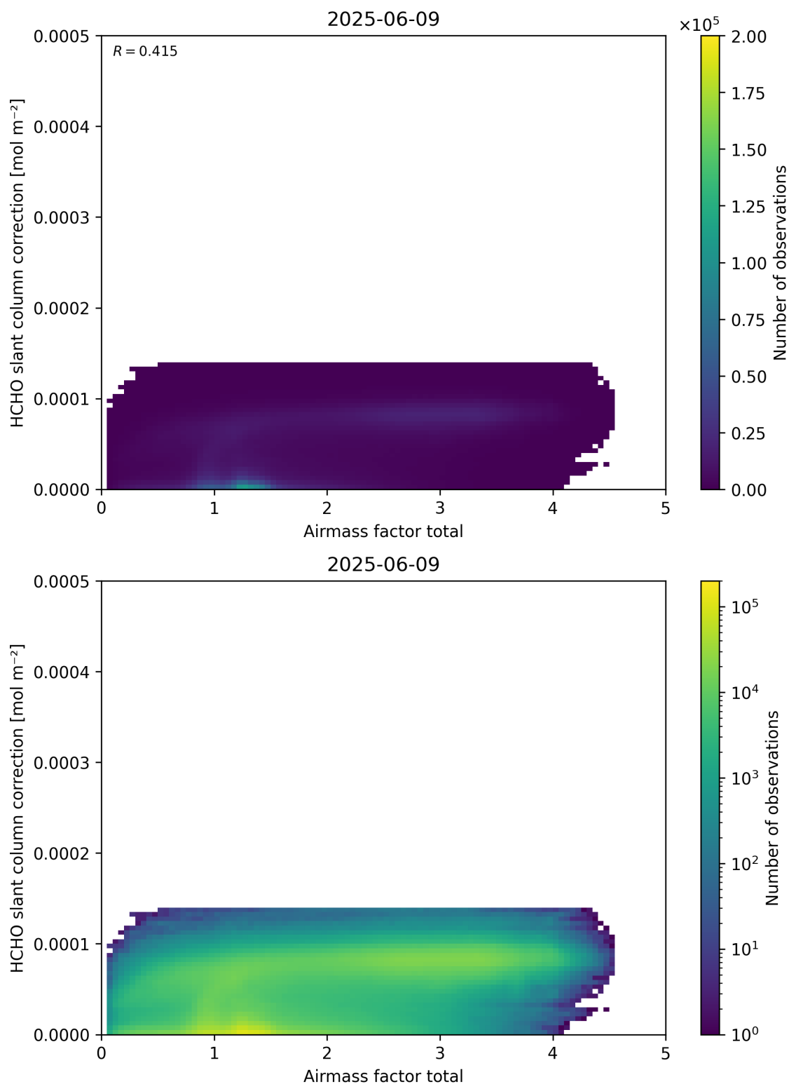
Figure 102: Scatter density plot of “Airmass factor total” against “HCHO slant column correction” for 2025-06-08 to 2025-06-10.
