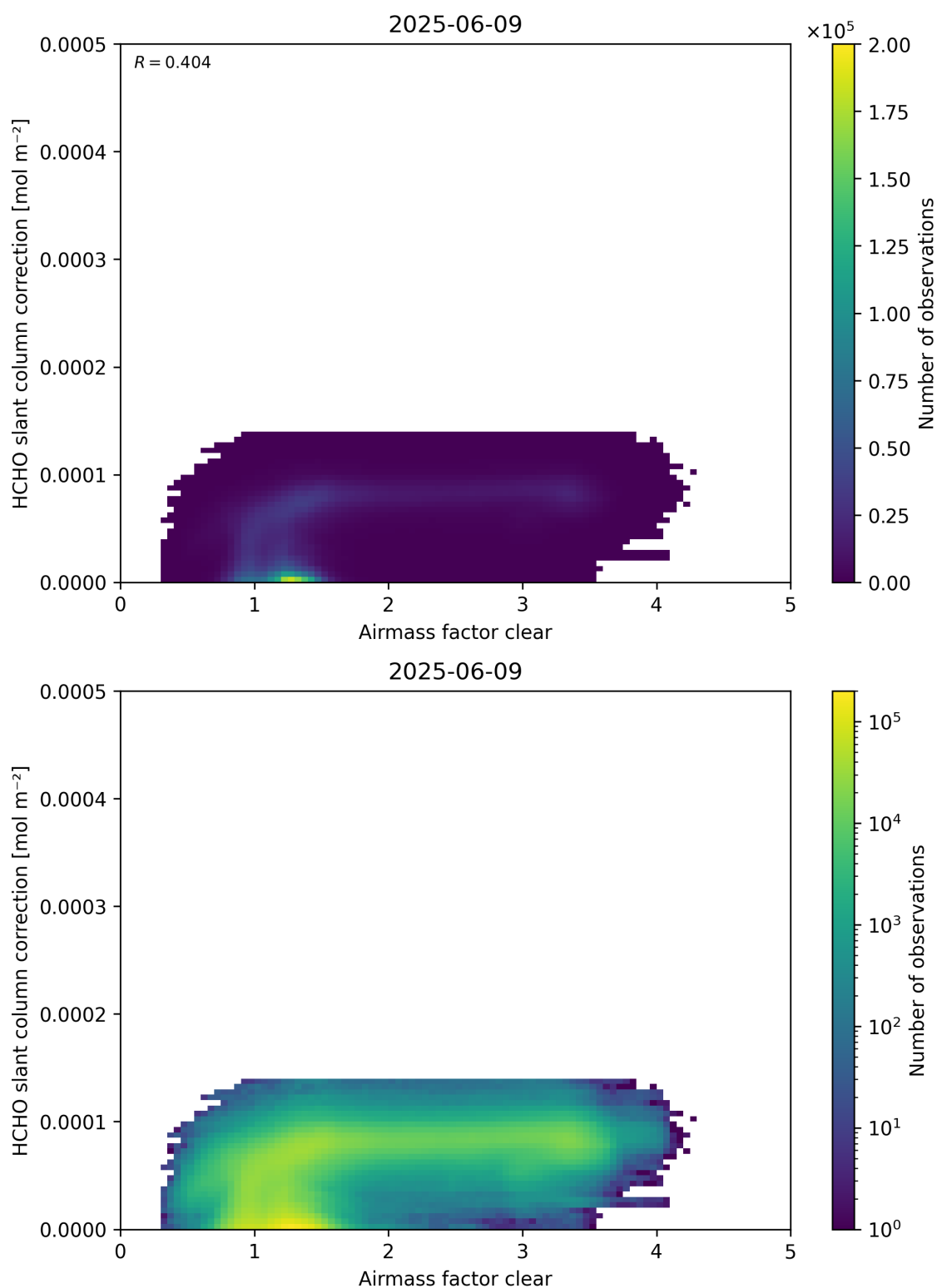
Figure 75: Scatter density plot of “Airmass factor clear” against “HCHO slant column correction” for 2025-06-08 to 2025-06-10.
