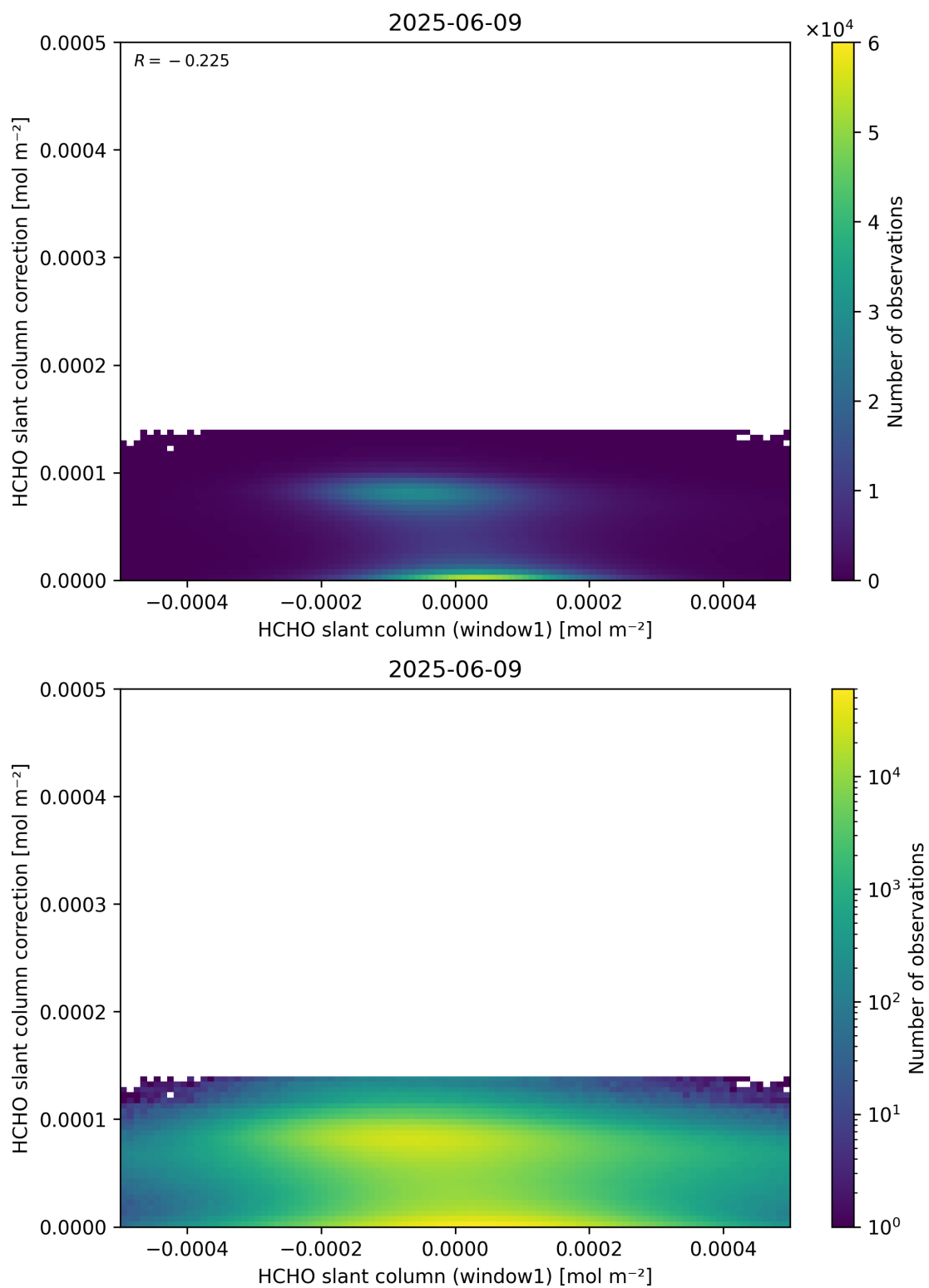
Figure 83: Scatter density plot of “HCHO slant column (window1)” against “HCHO slant column correction” for 2025-06-08 to 2025-06-10.
