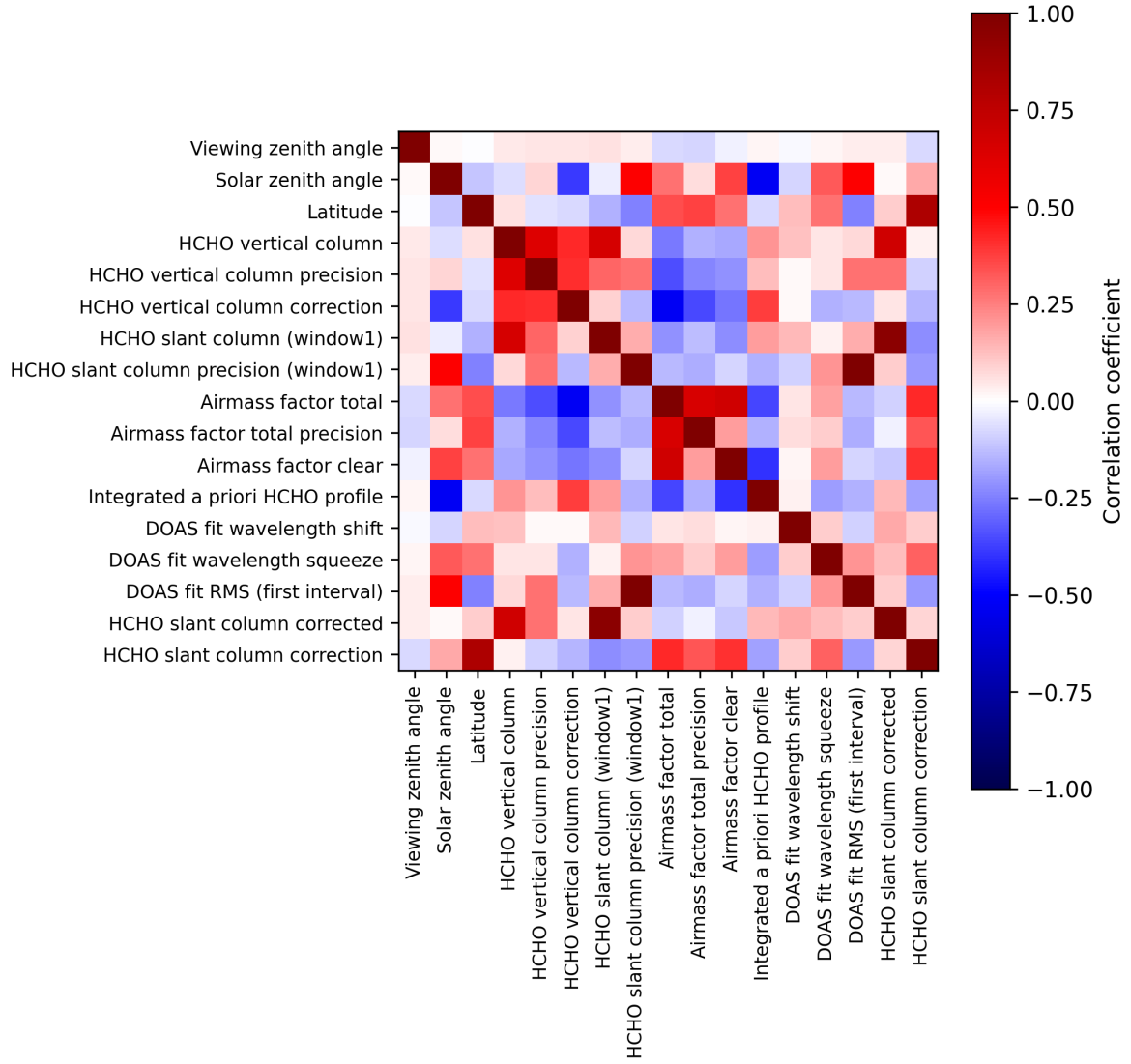
Figure 2: Map of correlation matrix for 2025-06-08 to 2025-06-10.
