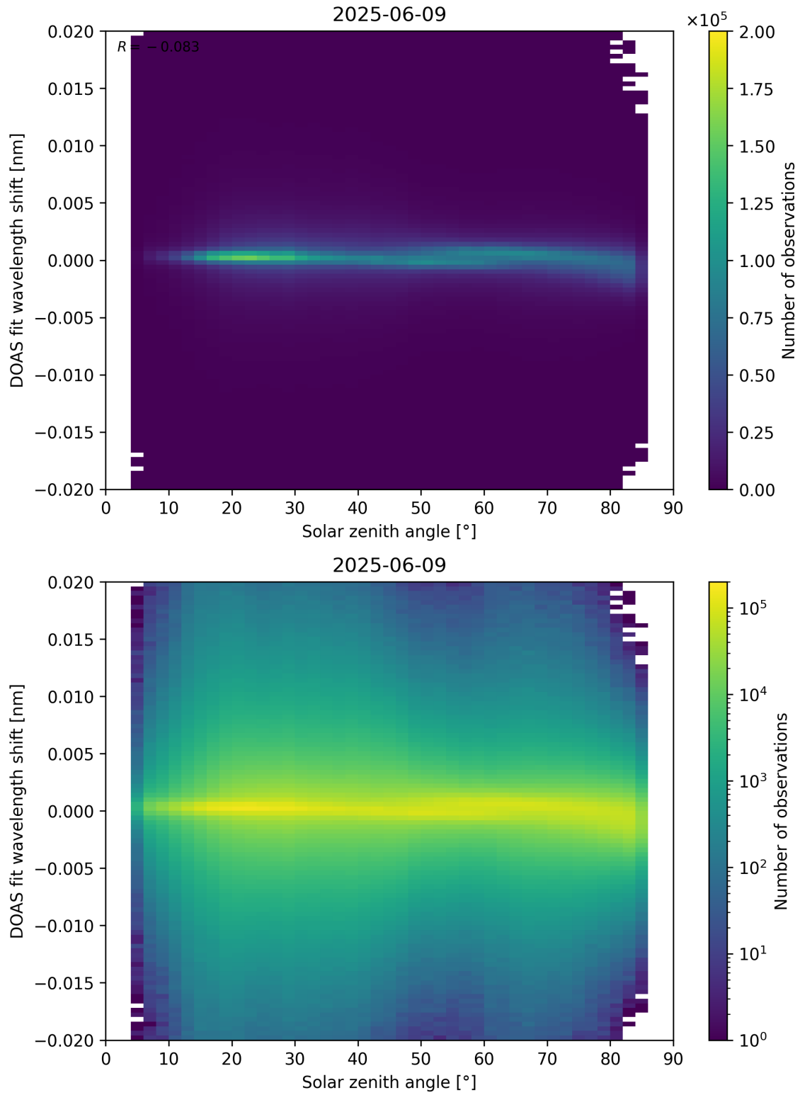
Figure 168: Scatter density plot of “Solar zenith angle” against “DOAS fit wavelength shift” for 2025-06-08 to 2025-06-10.
