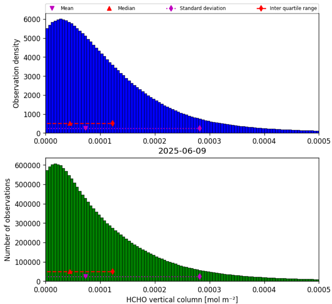
Figure 35: Histogram of “HCHO vertical column” for 2025-06-08 to 2025-06-10
