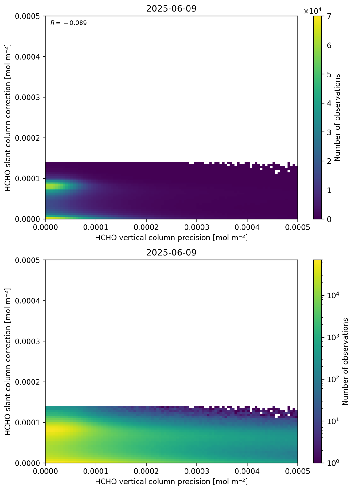
Figure 141: Scatter density plot of “HCHO vertical column precision” against “HCHO slant column correction” for 2025-06-08 to 2025-06-10.
