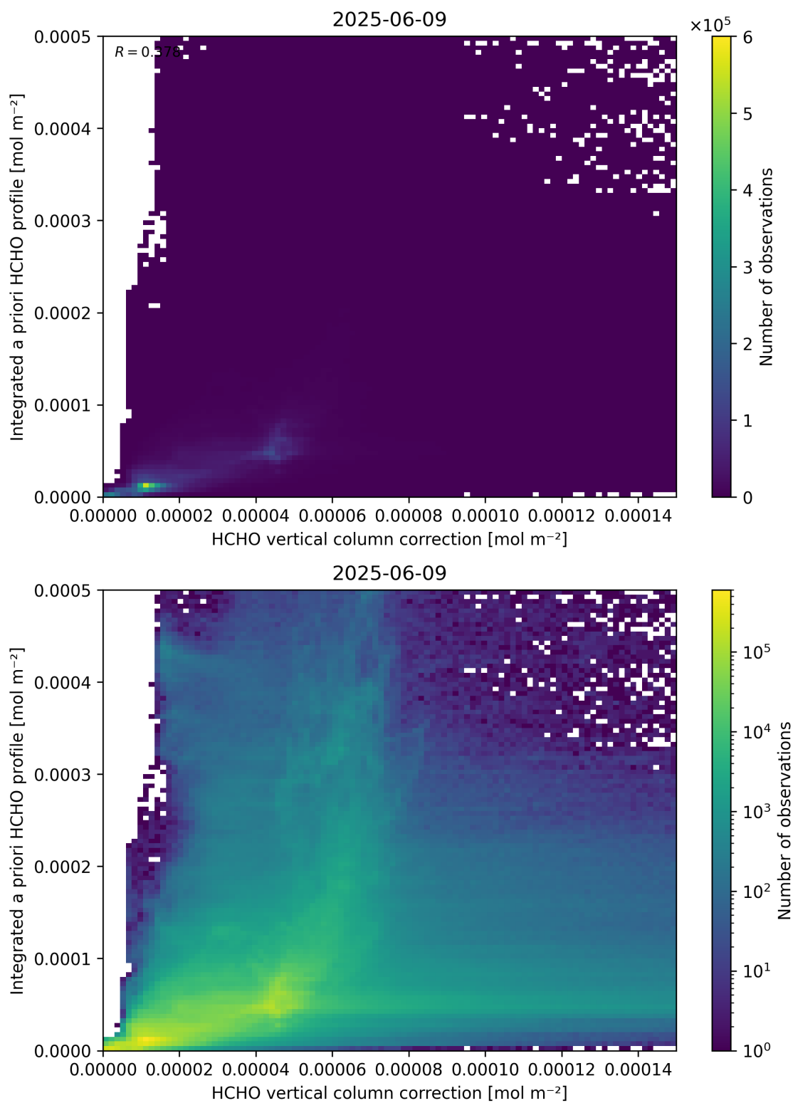
Figure 122: Scatter density plot of “HCHO vertical column correction” against “Integrated a priori HCHO profile” for 2025-06-08 to 2025-06-10.
