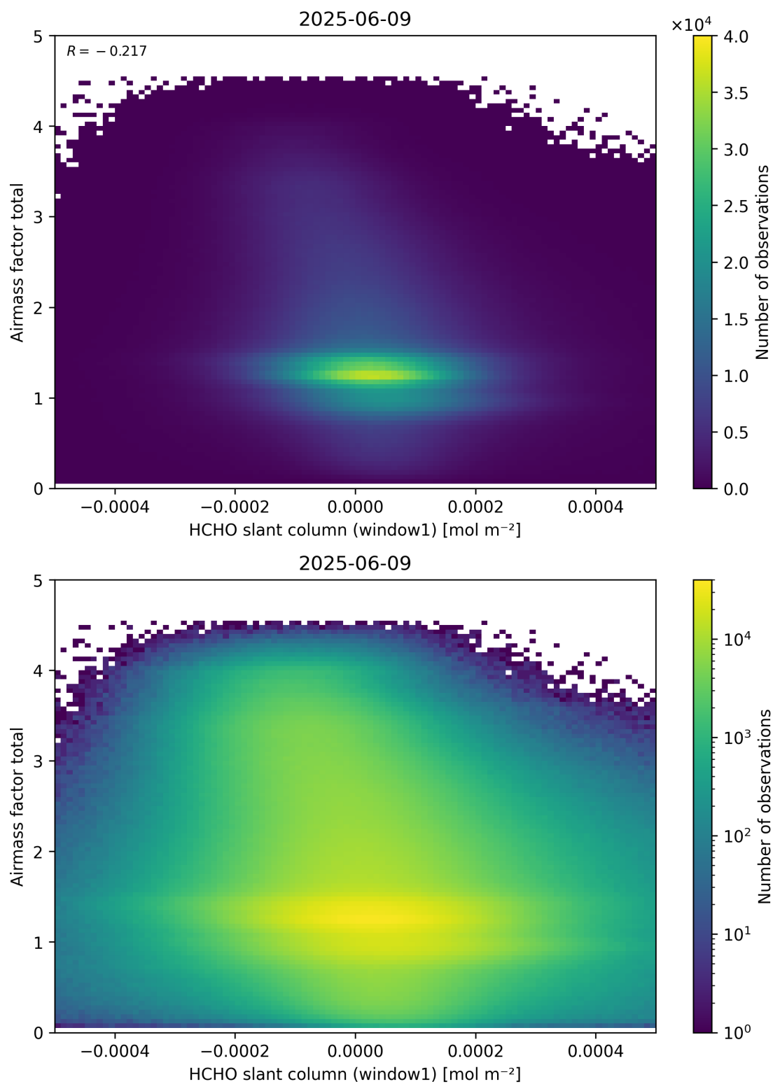
Figure 85: Scatter density plot of “HCHO slant column (window1)” against “Airmass factor total” for 2025-06-08 to 2025-06-10.
