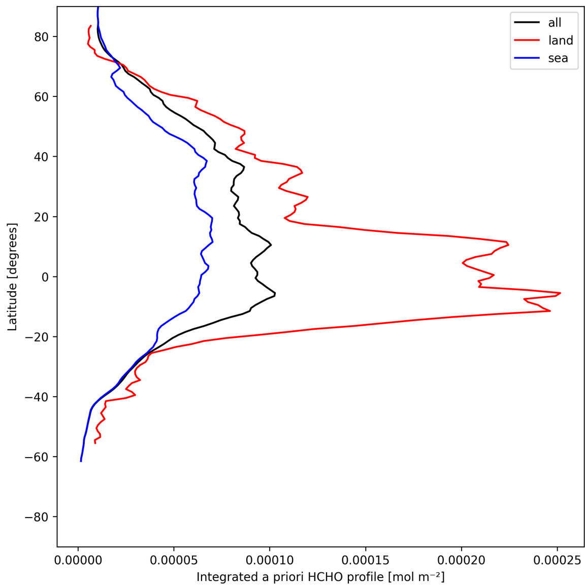
Figure 29: Zonal average of “Integrated a priori HCHO profile” for 2025-06-08 to 2025-06-10.
