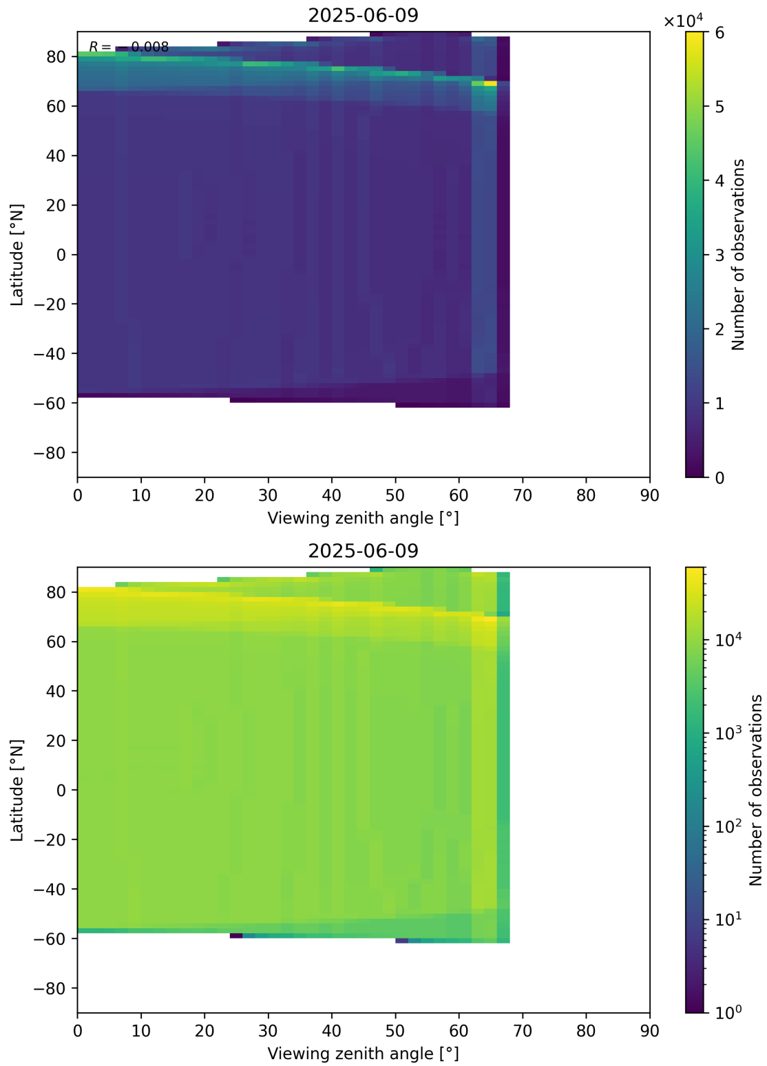
Figure 196: Scatter density plot of “Viewing zenith angle” against “Latitude” for 2025-06-08 to 2025-06-10.
