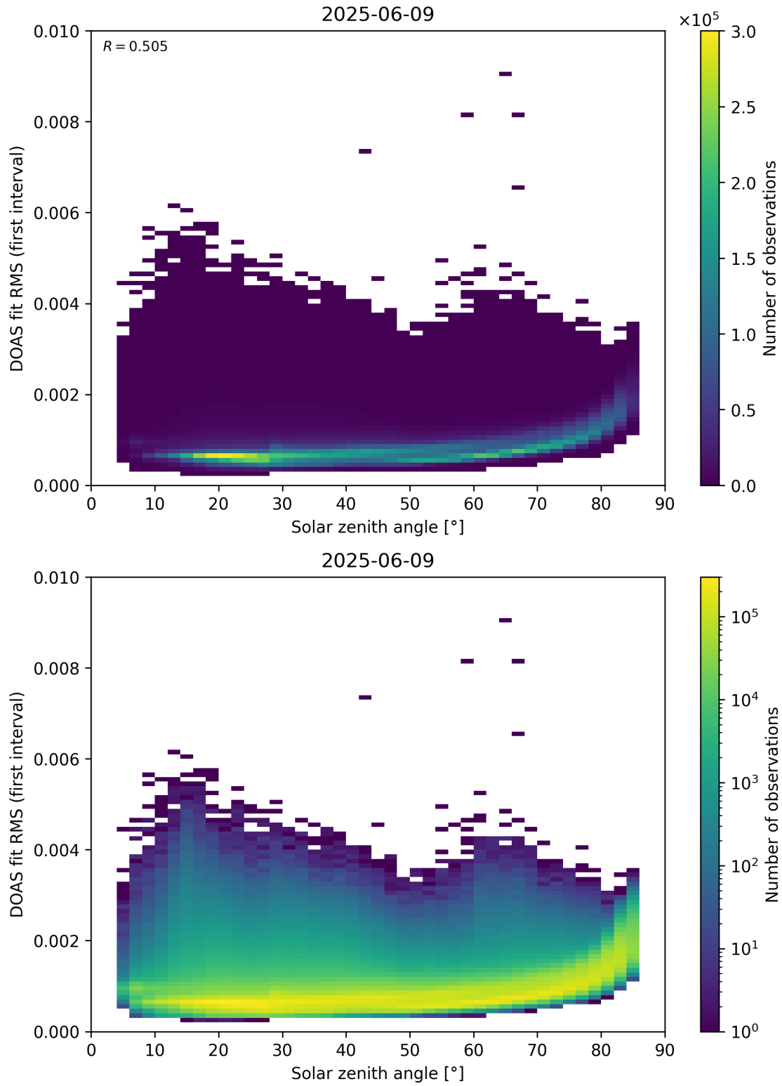
Figure 167: Scatter density plot of “Solar zenith angle” against “DOAS fit RMS (first interval)” for 2025-06-08 to 2025-06-10.
