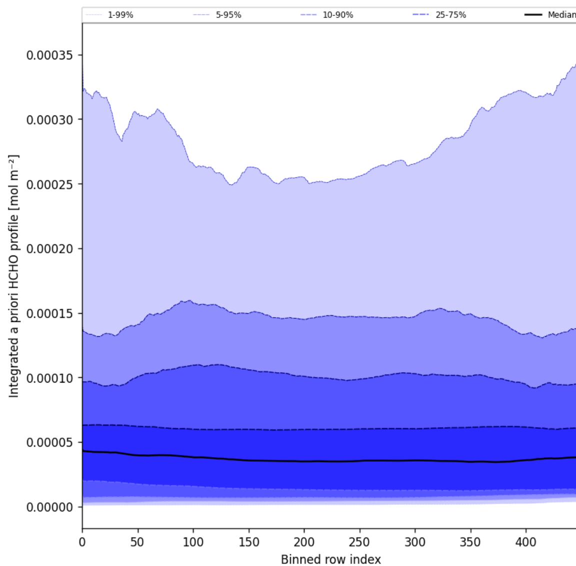
Figure 57: Along track statistics of “Integrated a priori HCHO profile” for 2025-06-08 to 2025-06-10
