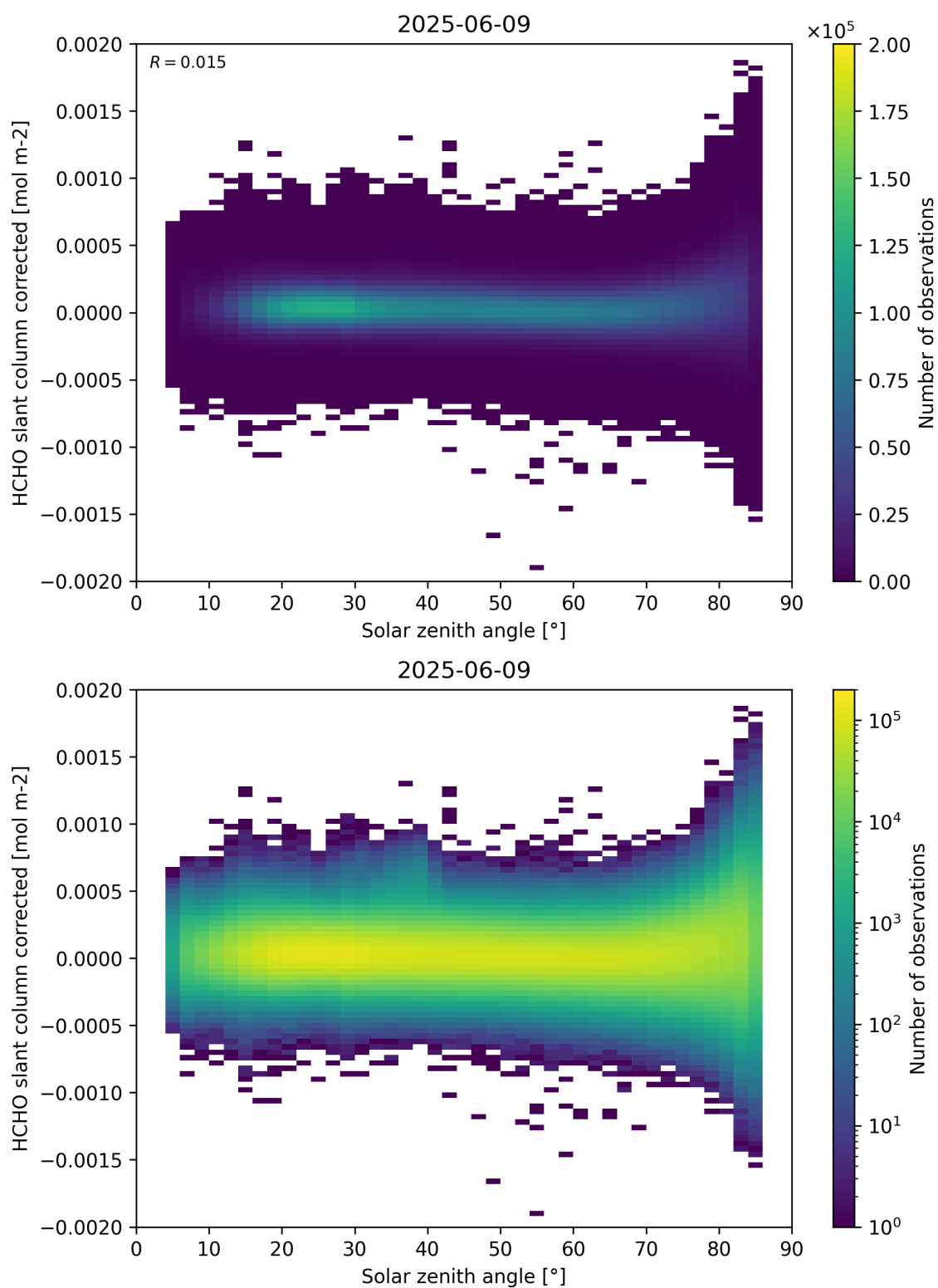
Figure 171: Scatter density plot of “Solar zenith angle” against “HCHO slant column corrected” for 2025-06-08 to 2025-06-10.
