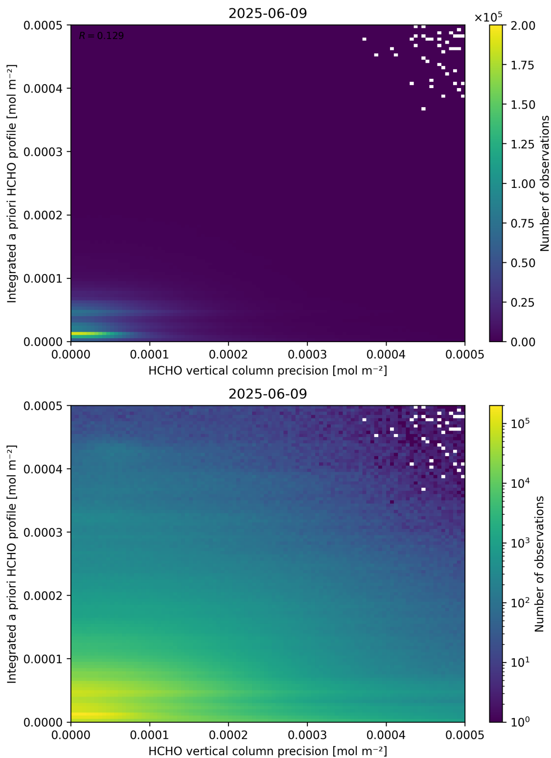
Figure 147: Scatter density plot of “HCHO vertical column precision” against “Integrated a priori HCHO profile” for 2025-06-08 to 2025-06-10.
