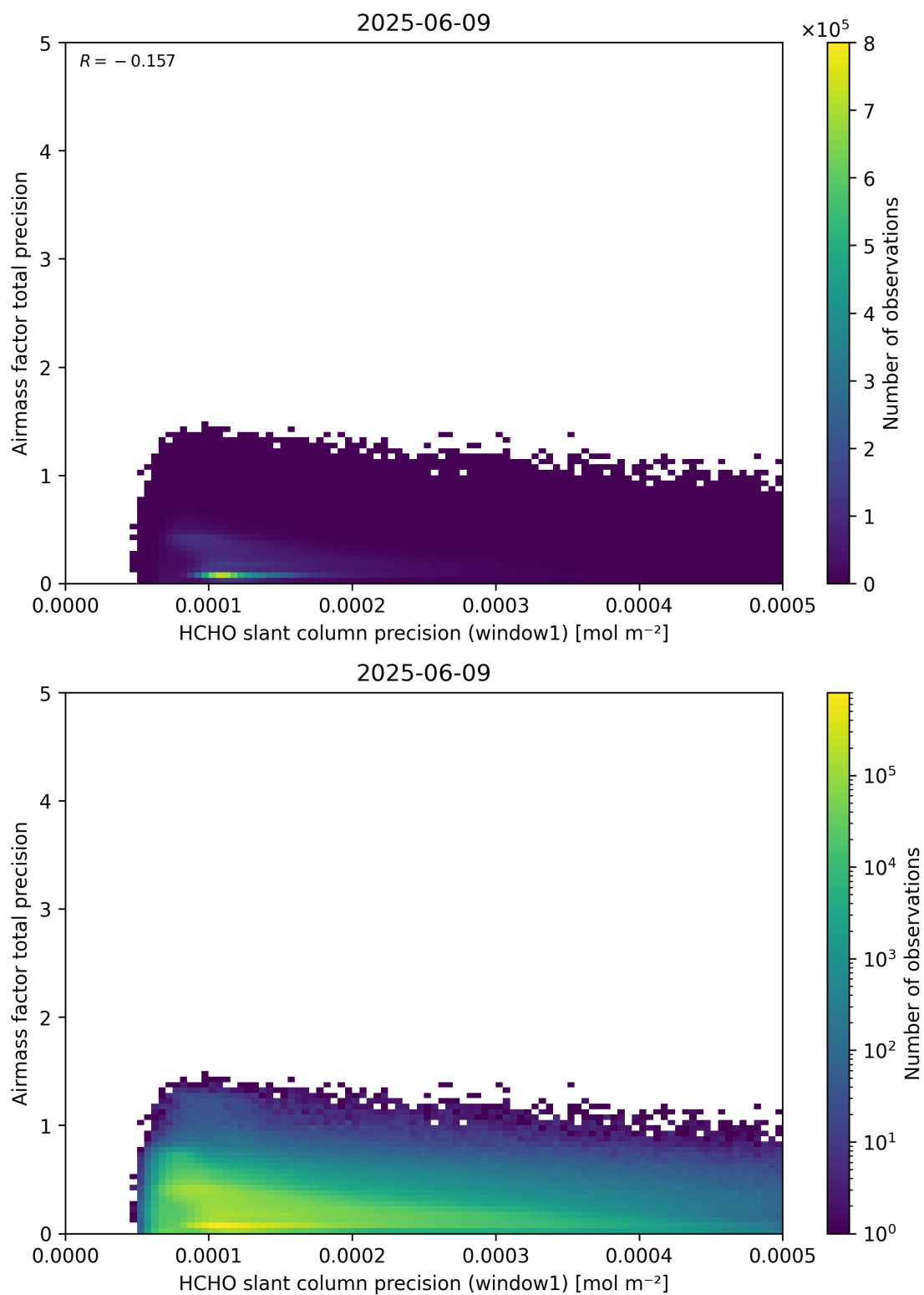
Figure 95: Scatter density plot of “HCHO slant column precision (window1)” against “Airmass factor total precision” for 2025-06-08 to 2025-06-10.
