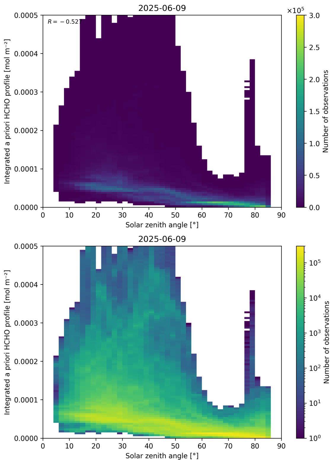
Figure 180: Scatter density plot of “Solar zenith angle” against “Integrated a priori HCHO profile” for 2025-06-08 to 2025-06-10.
