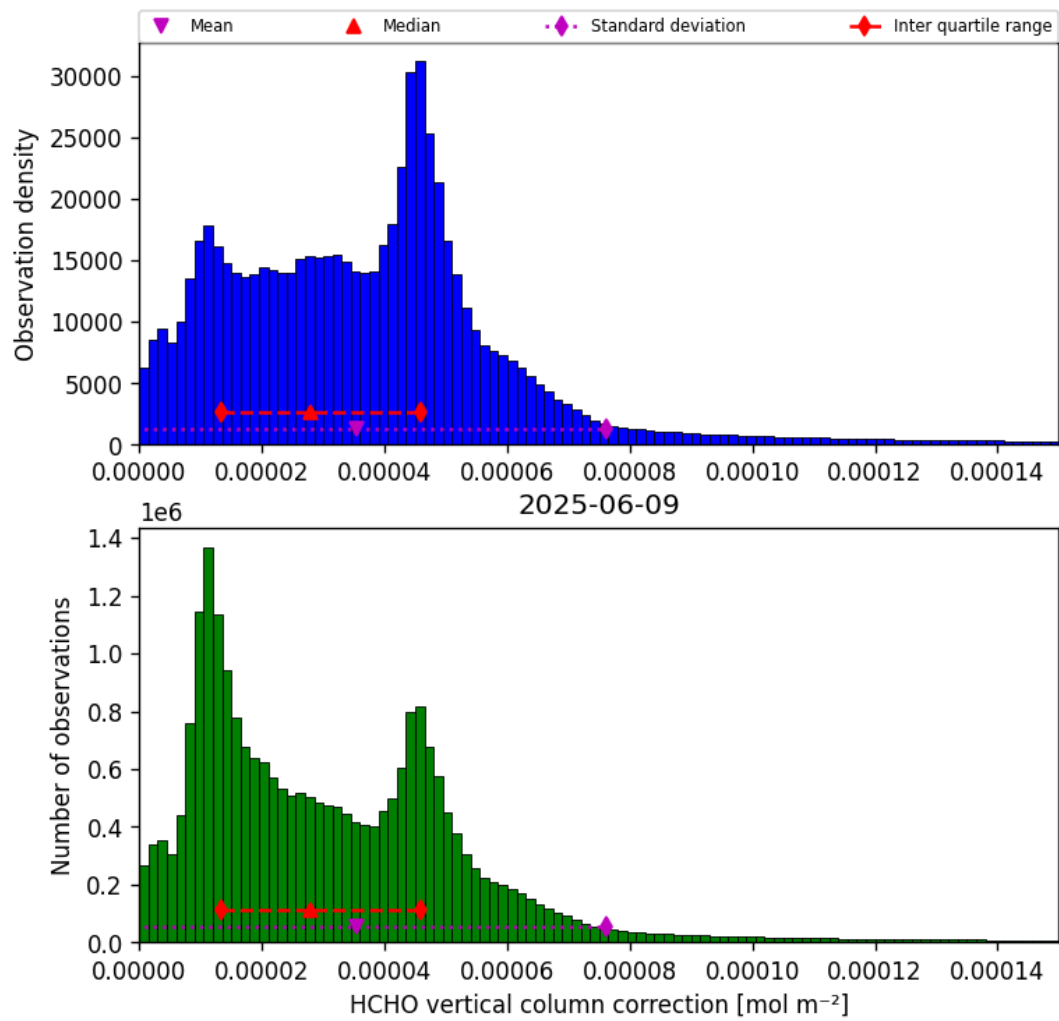
Figure 37: Histogram of “HCHO vertical column correction” for 2025-06-08 to 2025-06-10
