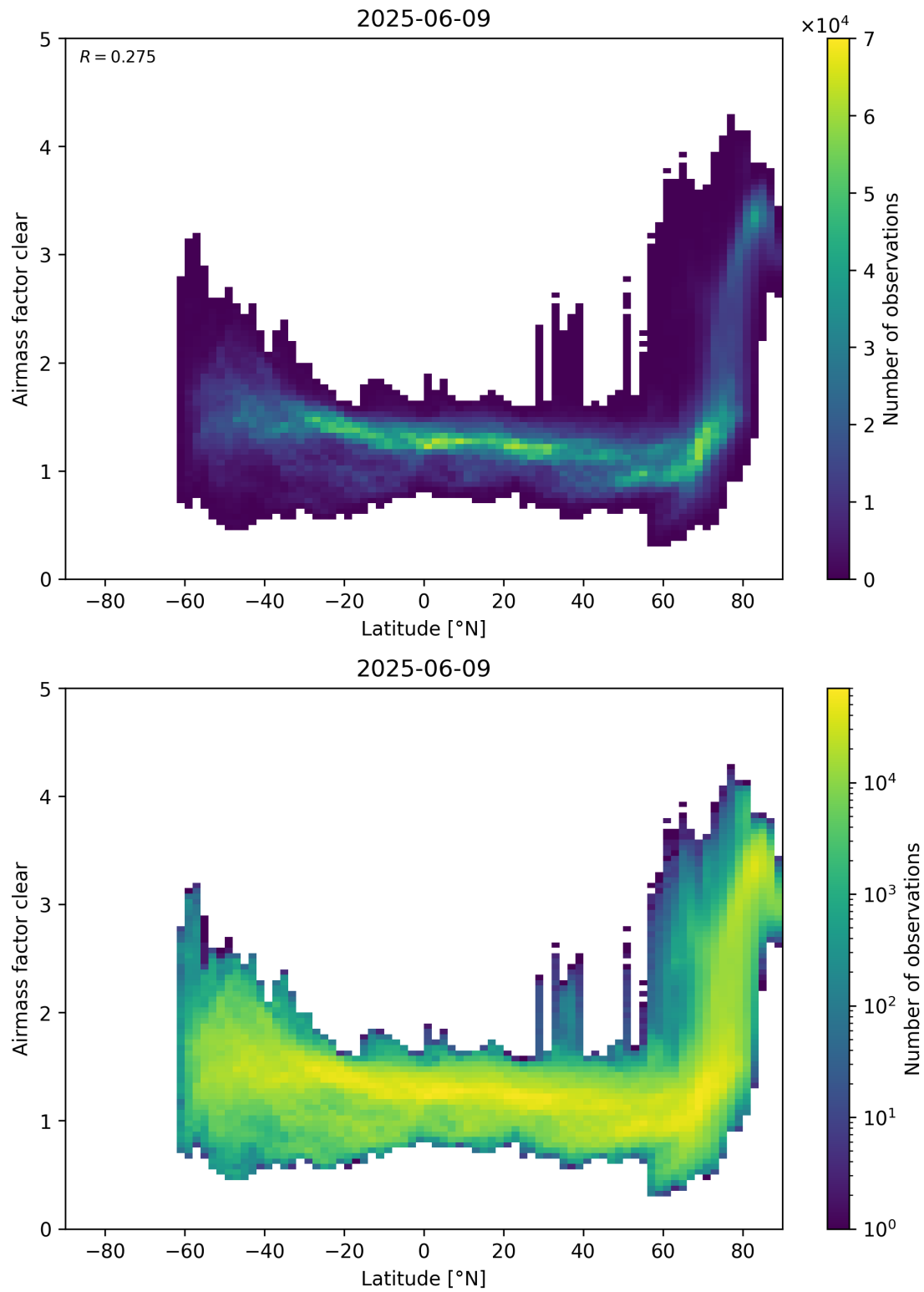
Figure 156: Scatter density plot of “Latitude” against “Airmass factor clear” for 2025-06-08 to 2025-06-10.
