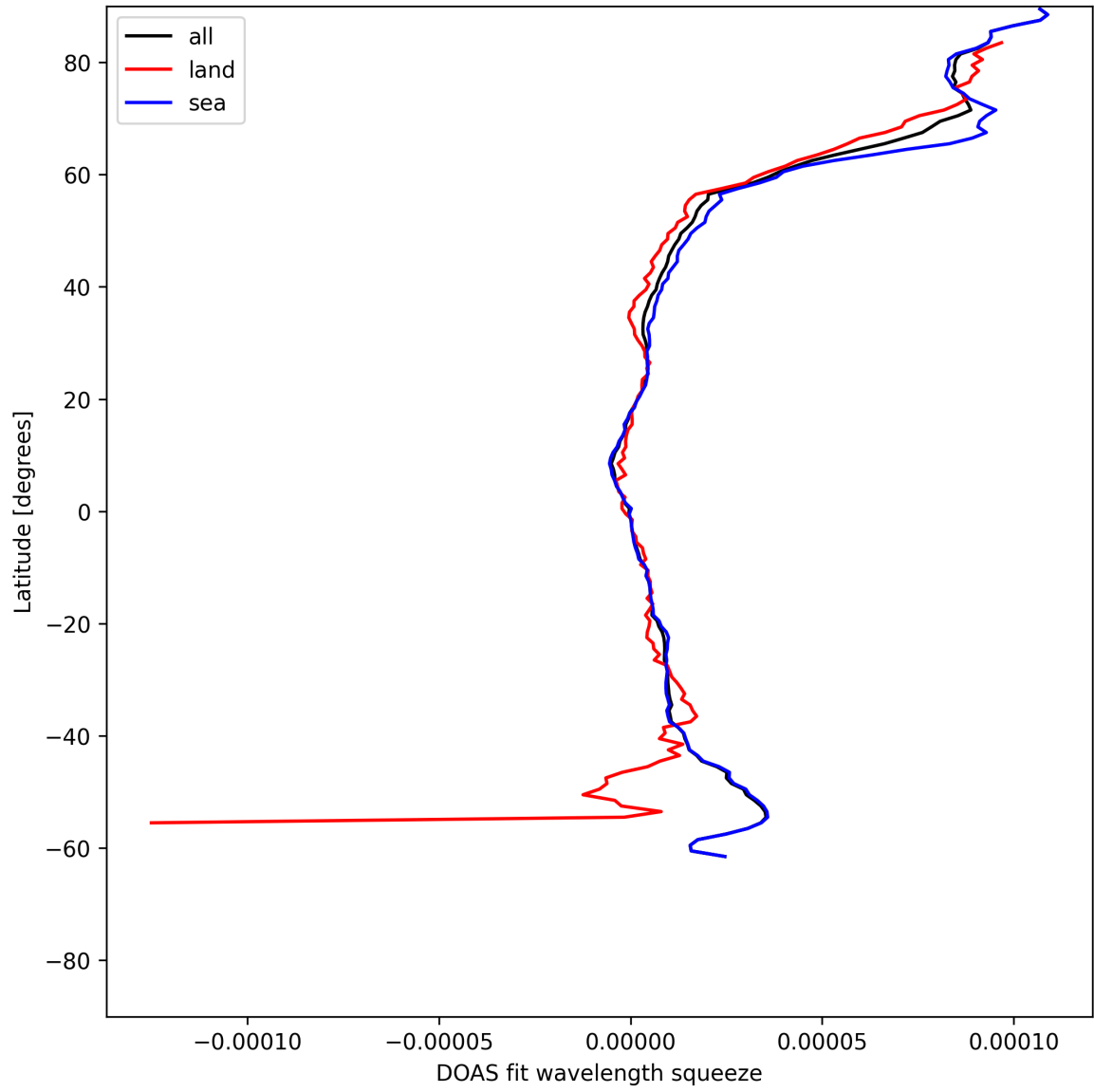
Figure 31: Zonal average of “DOAS fit wavelength squeeze” for 2025-06-08 to 2025-06-10.
