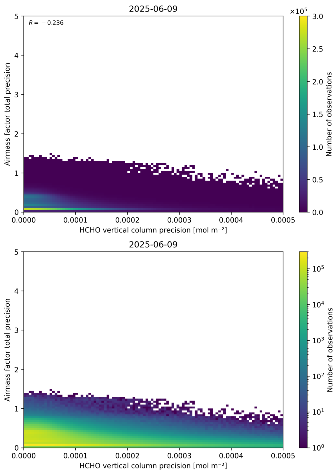
Figure 145: Scatter density plot of “HCHO vertical column precision” against “Airmass factor total precision” for 2025-06-08 to 2025-06-10.
