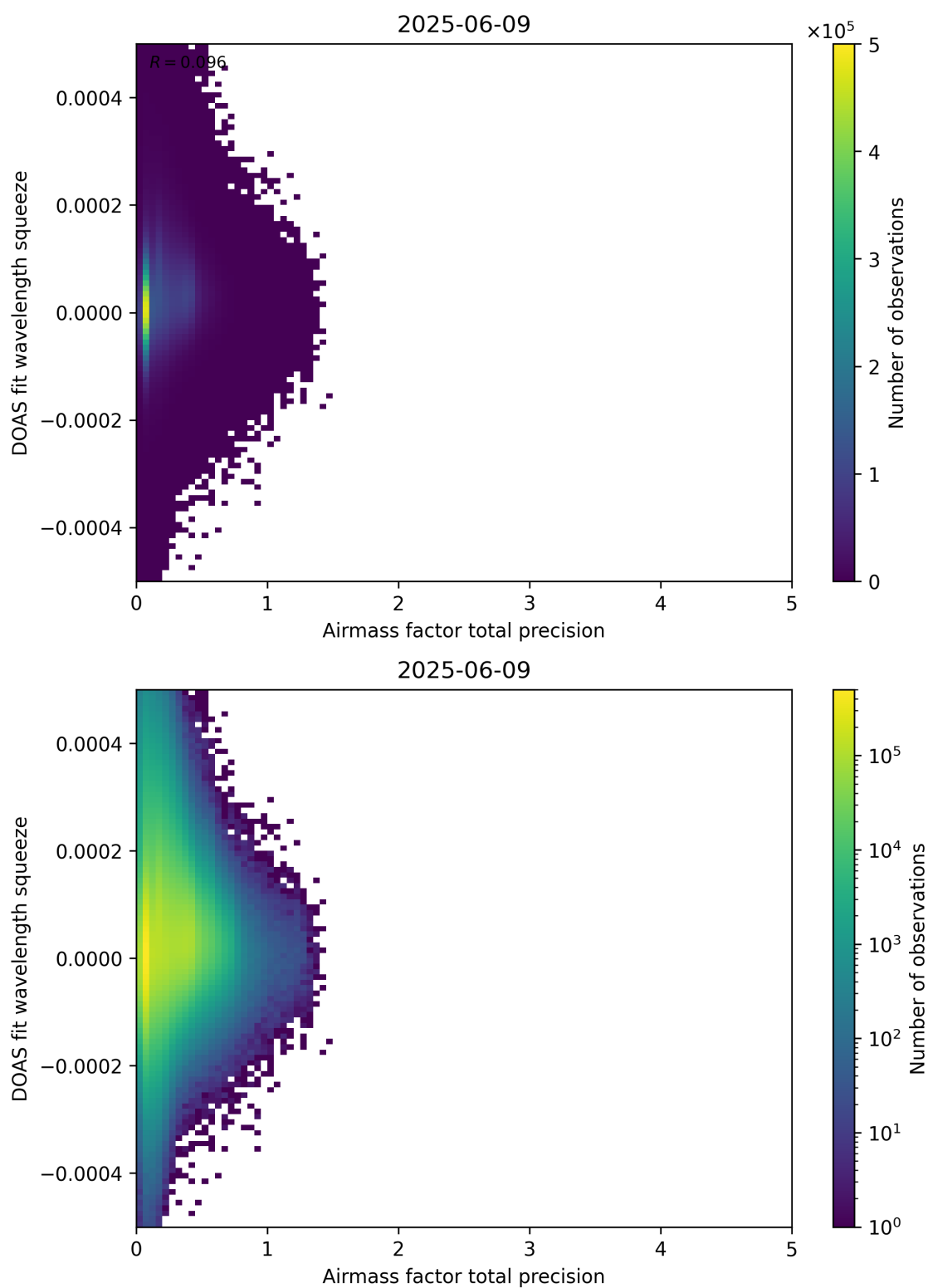
Figure 107: Scatter density plot of “Airmass factor total precision” against “DOAS fit wavelength squeeze” for 2025-06-08 to 2025-06-10.
