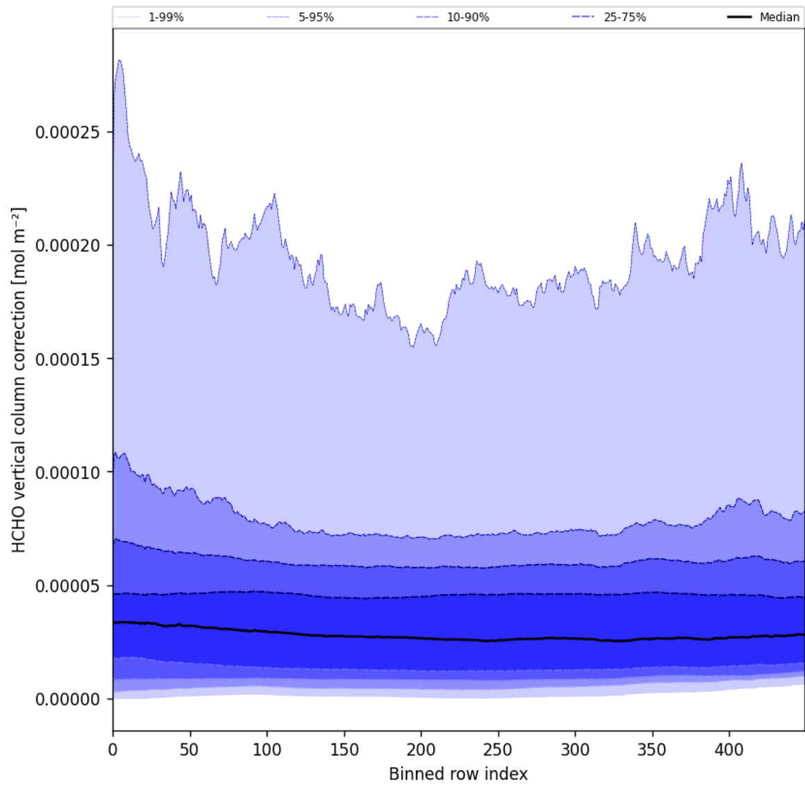
Figure 51: Along track statistics of “HCHO vertical column correction” for 2025-06-08 to 2025-06-10
