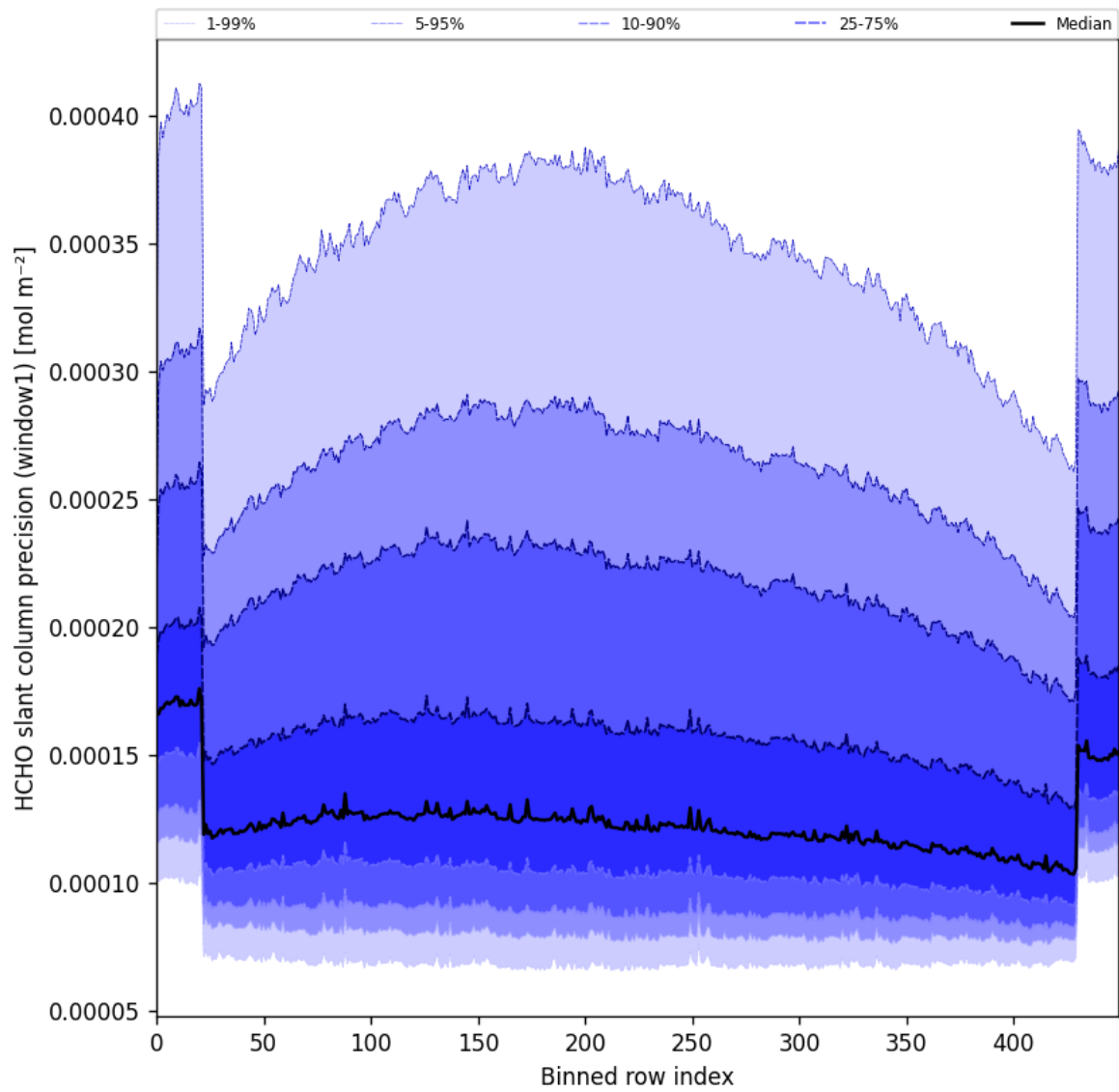
Figure 53: Along track statistics of “HCHO slant column precision (window1)” for 2025-06-08 to 2025-06-10
