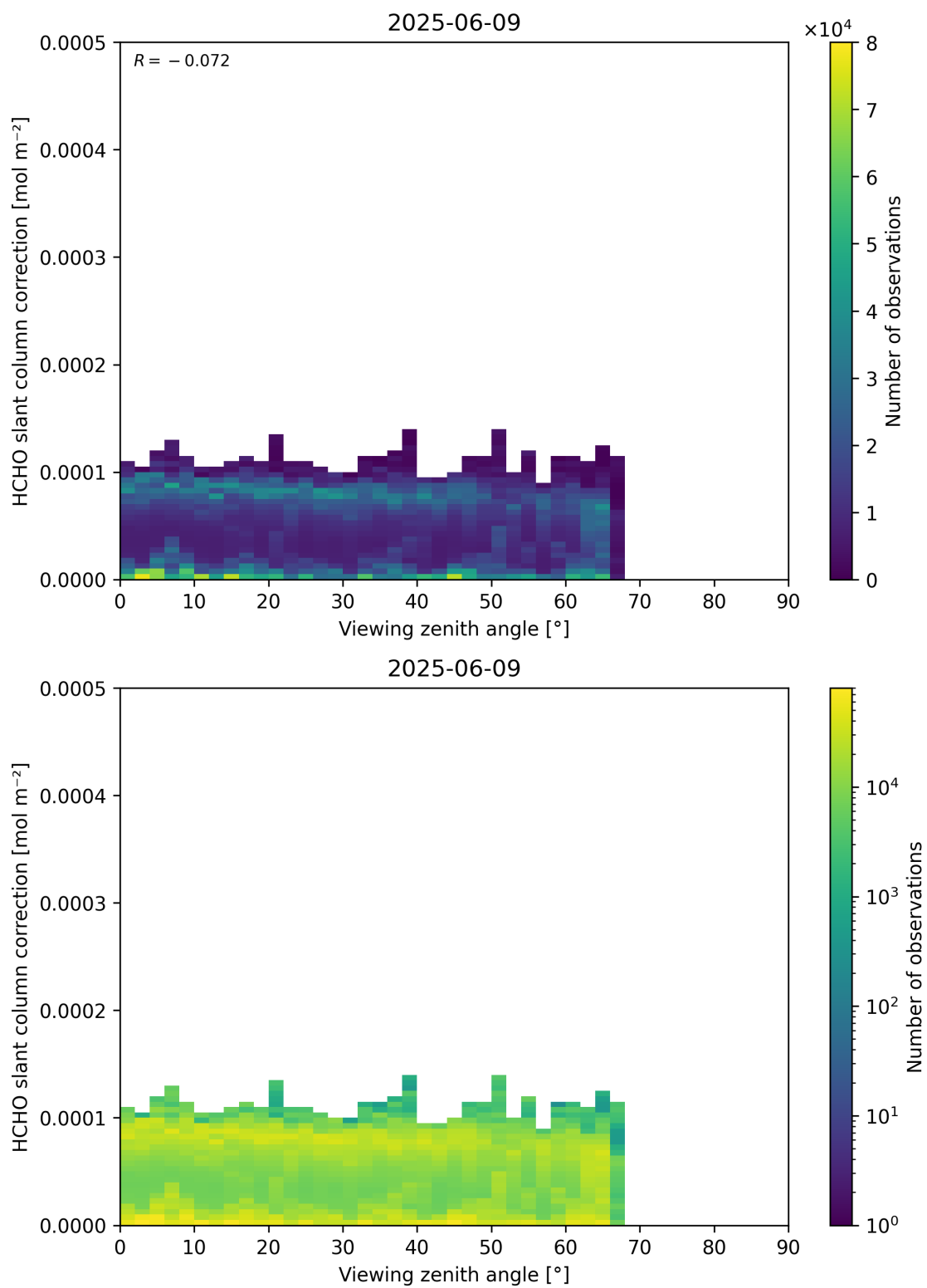
Figure 187: Scatter density plot of “Viewing zenith angle” against “HCHO slant column correction” for 2025-06-08 to 2025-06-10.
