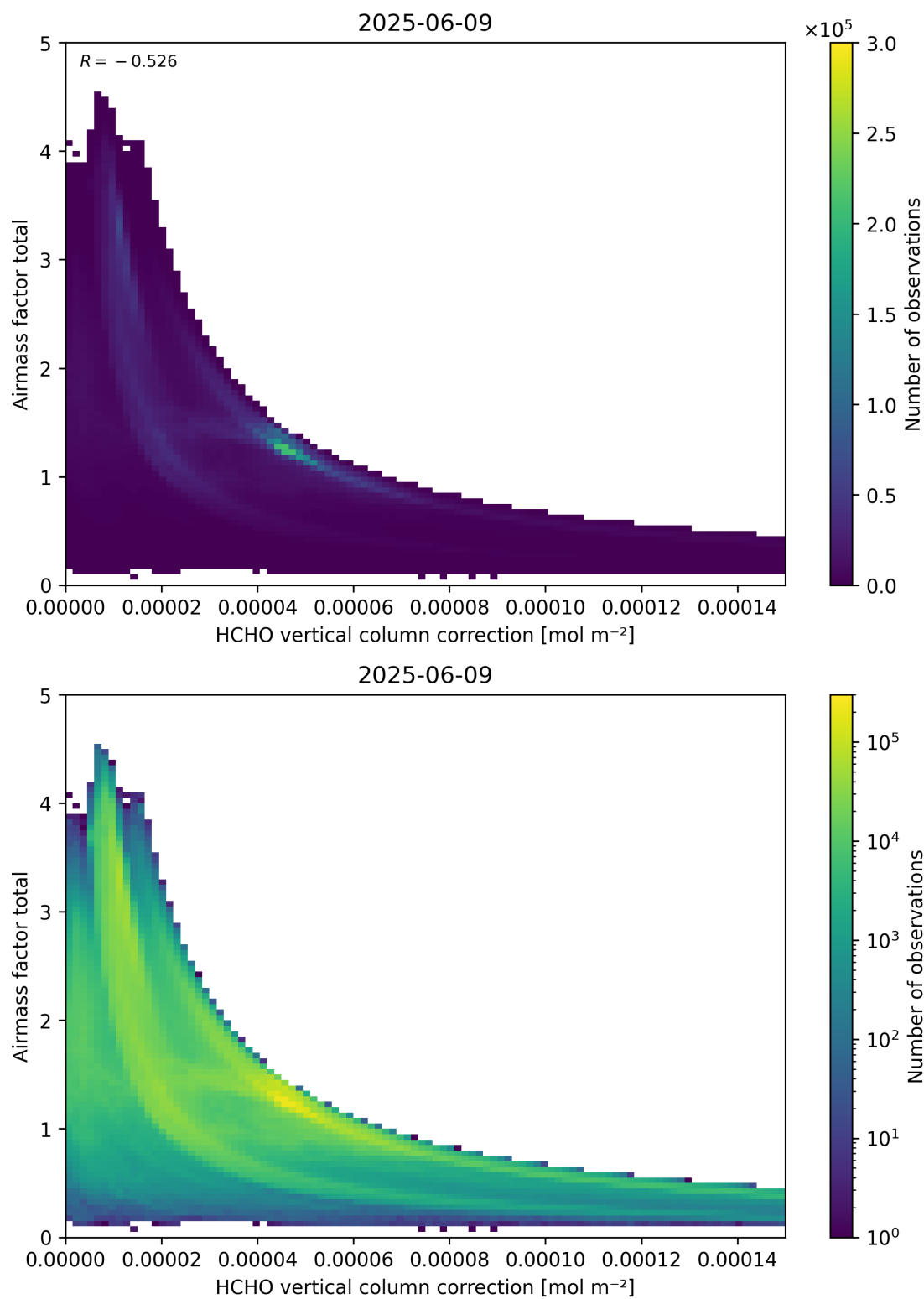
Figure 120: Scatter density plot of “HCHO vertical column correction” against “Airmass factor total” for 2025-06-08 to 2025-06-10.
