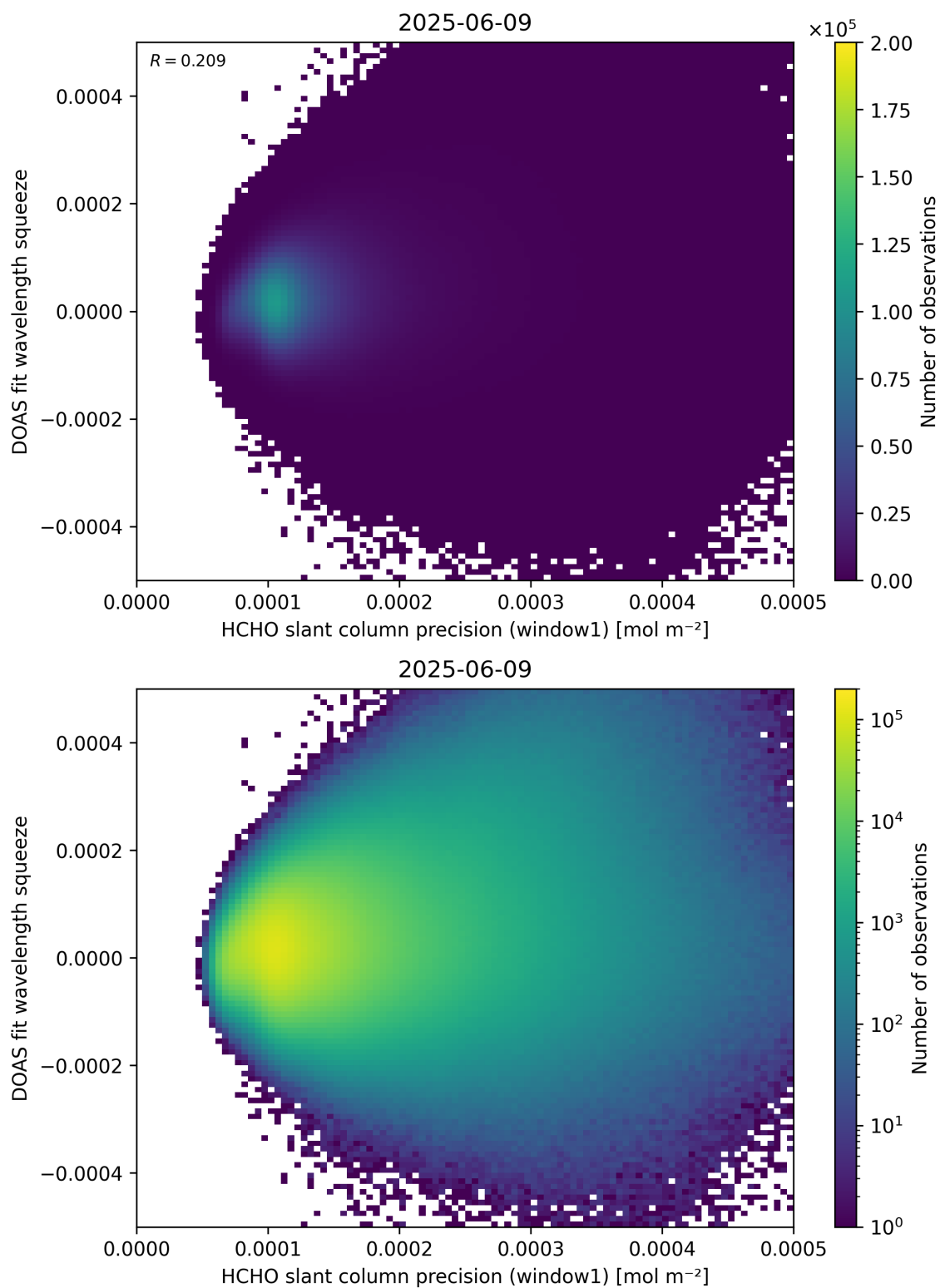
Figure 90: Scatter density plot of “HCHO slant column precision (window1)” against “DOAS fit wavelength squeeze” for 2025-06-08 to 2025-06-10.
