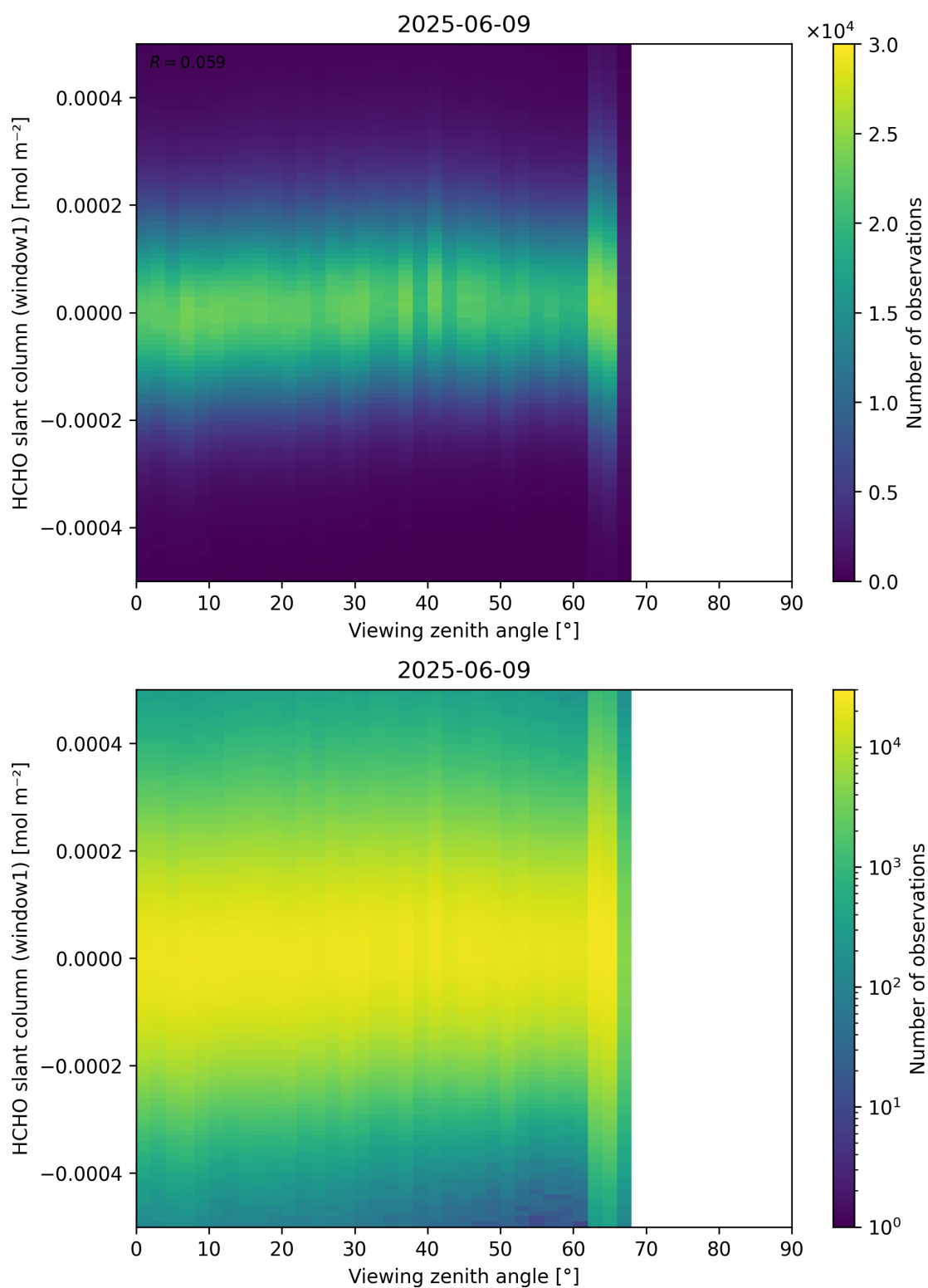
Figure 188: Scatter density plot of “Viewing zenith angle” against “HCHO slant column (window1)” for 2025-06-08 to 2025-06-10.
