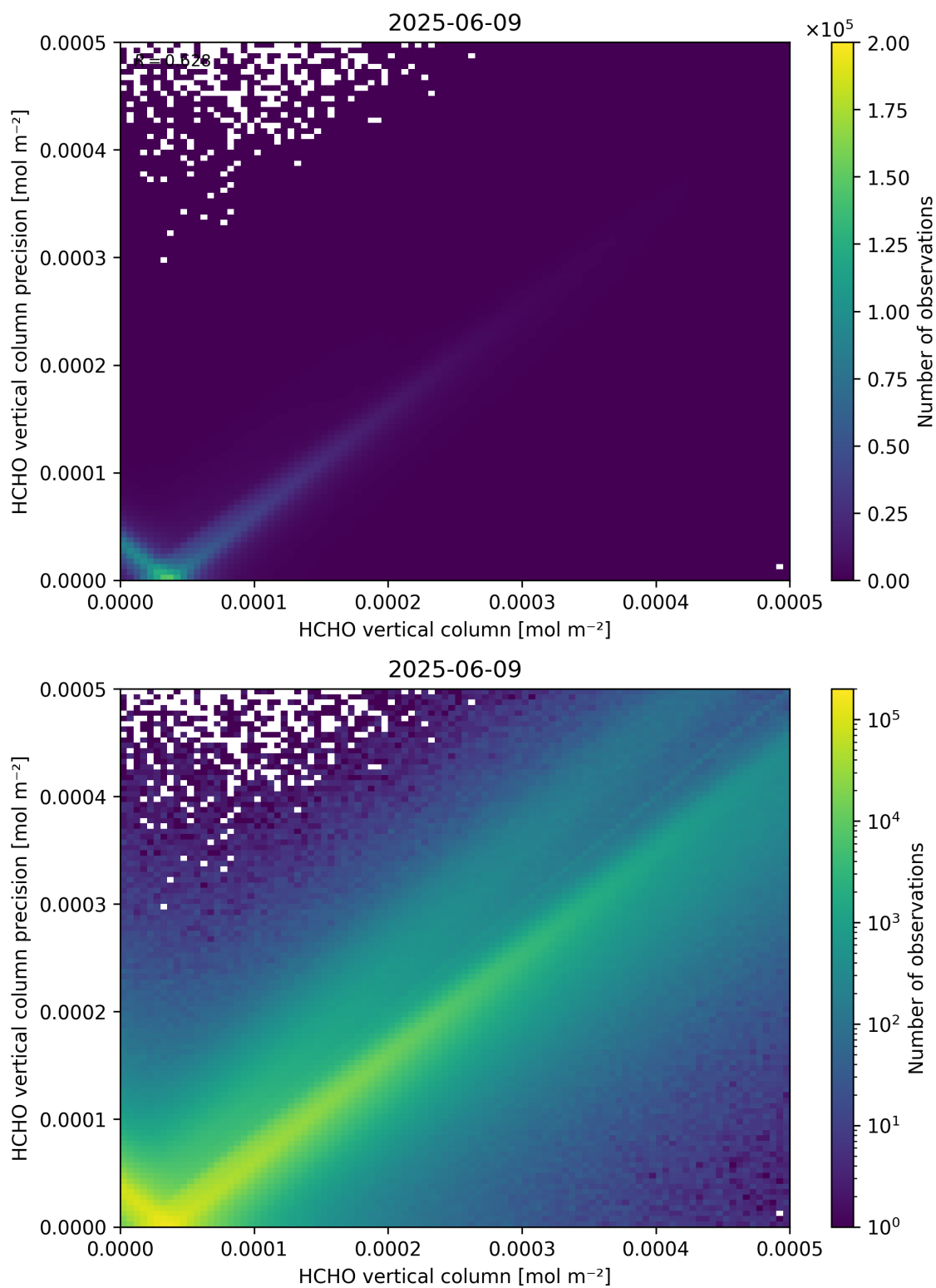
Figure 134: Scatter density plot of “HCHO vertical column” against “HCHO vertical column precision” for 2025-06-08 to 2025-06-10.
