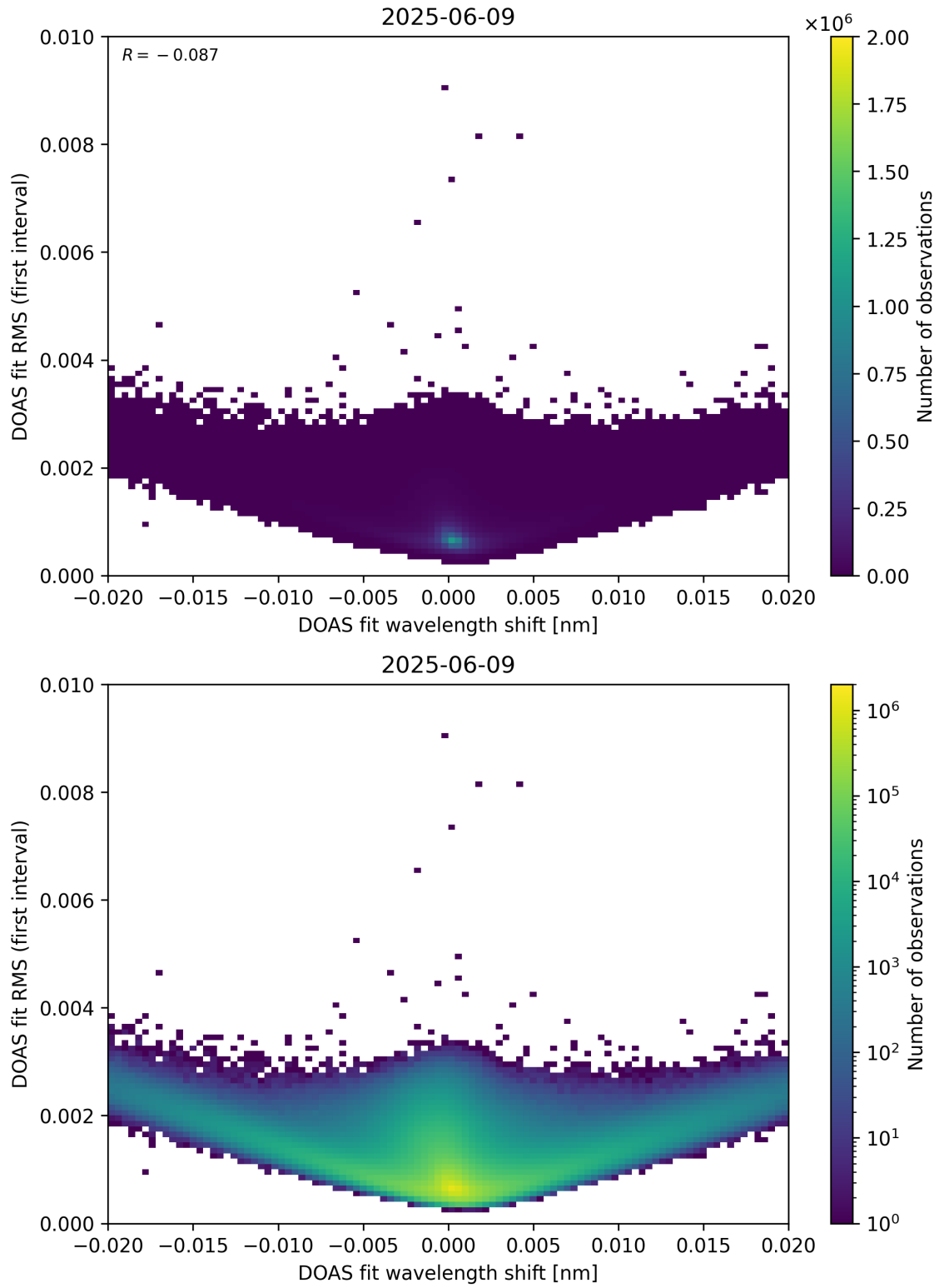
Figure 64: Scatter density plot of “DOAS fit wavelength shift” against “DOAS fit RMS (first interval)” for 2025-06-08 to 2025-06-10.
