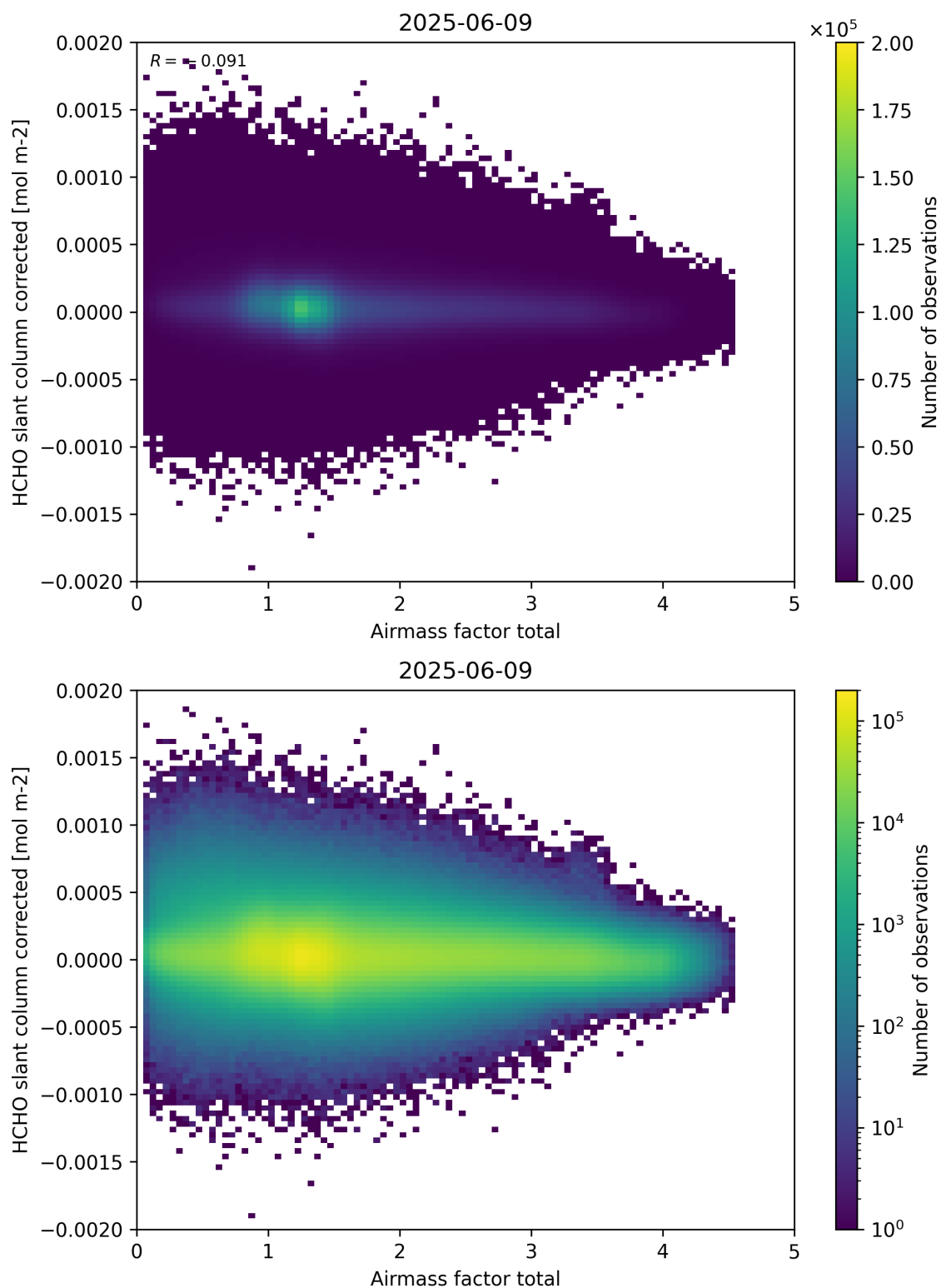
Figure 101: Scatter density plot of “Airmass factor total” against “HCHO slant column corrected” for 2025-06-08 to 2025-06-10.
