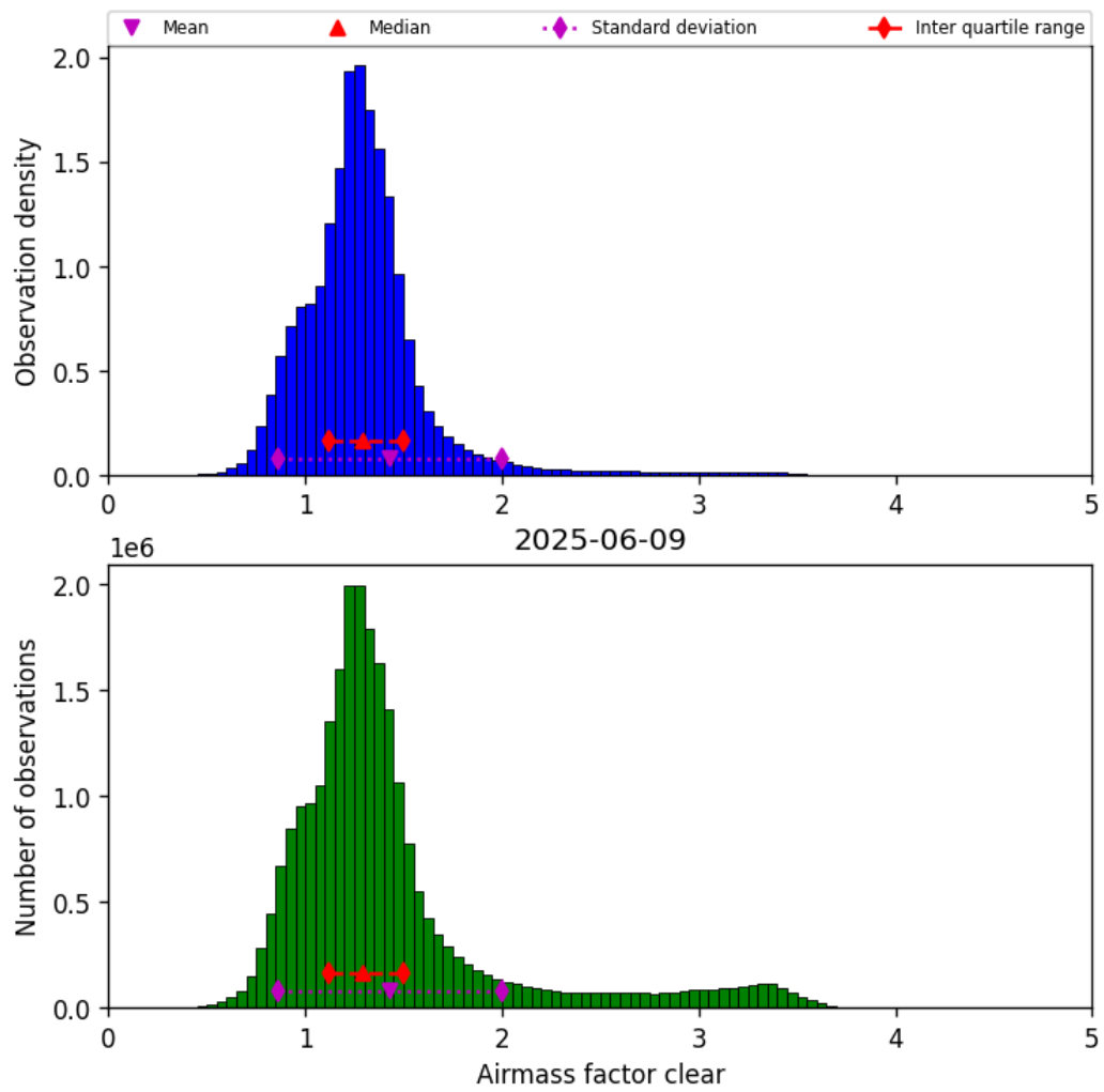
Figure 42: Histogram of “Airmass factor clear” for 2025-06-08 to 2025-06-10
