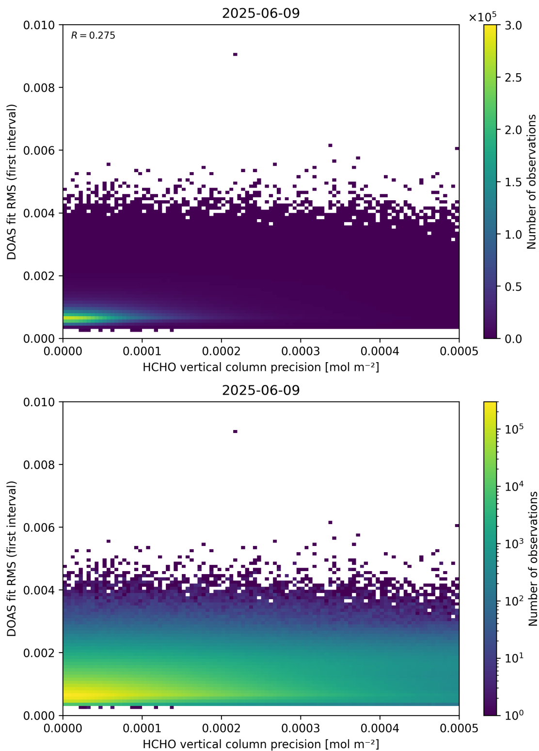
Figure 136: Scatter density plot of “HCHO vertical column precision” against “DOAS fit RMS (first interval)” for 2025-06-08 to 2025-06-10.
