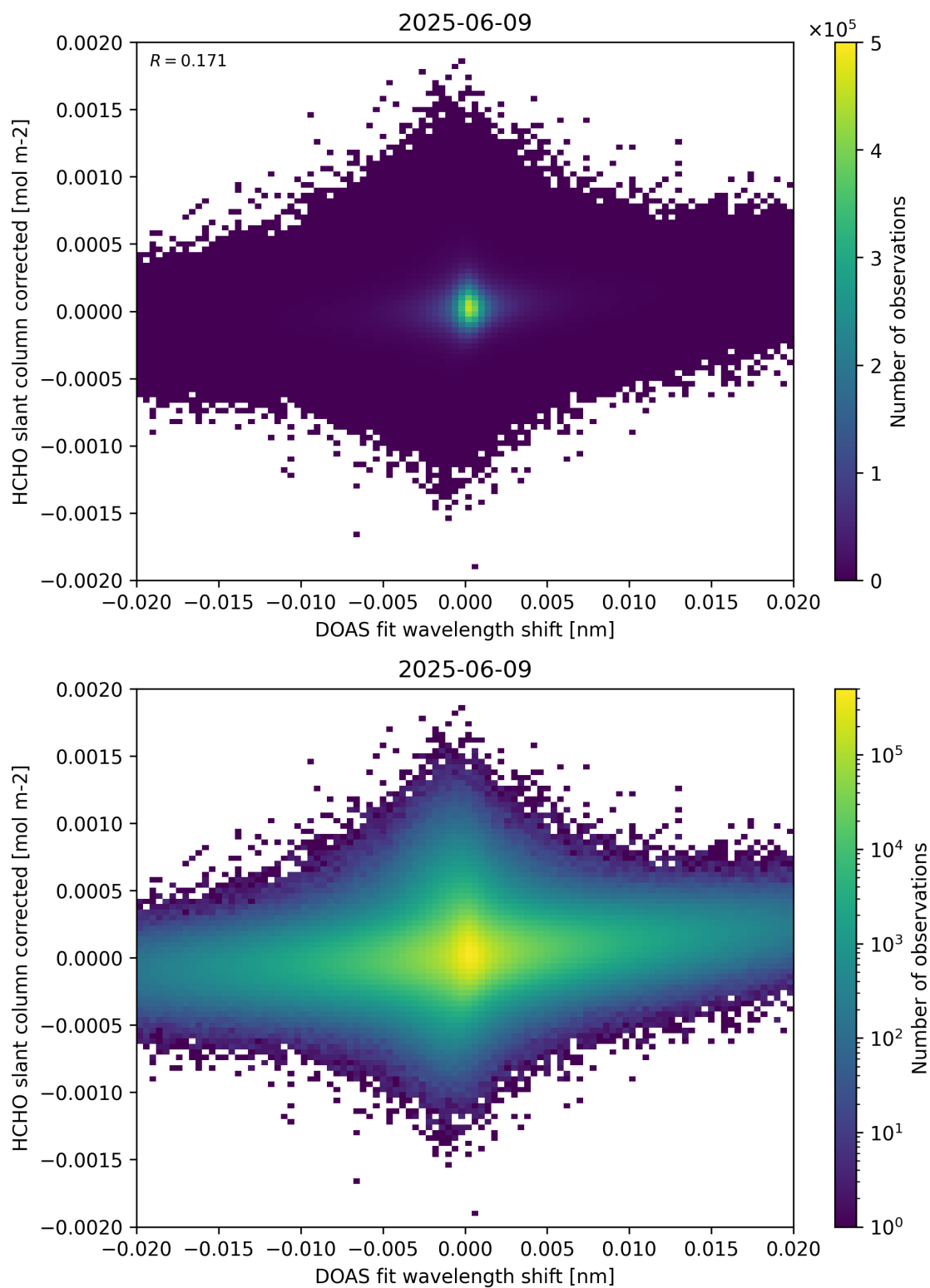
Figure 66: Scatter density plot of “DOAS fit wavelength shift” against “HCHO slant column corrected” for 2025-06-08 to 2025-06-10.
