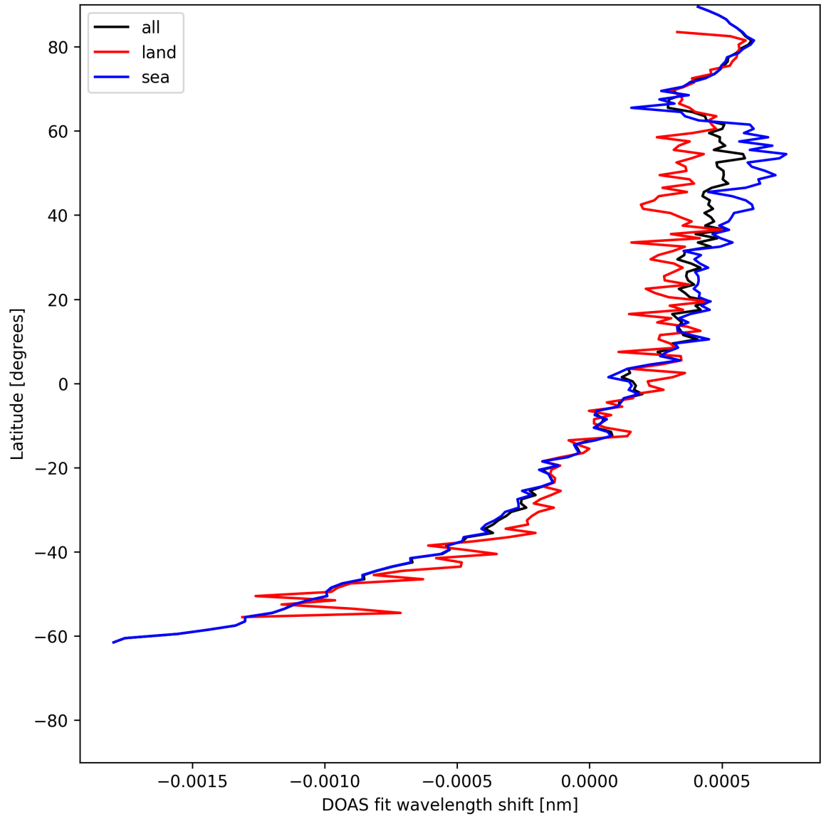
Figure 30: Zonal average of “DOAS fit wavelength shift” for 2025-06-08 to 2025-06-10.
