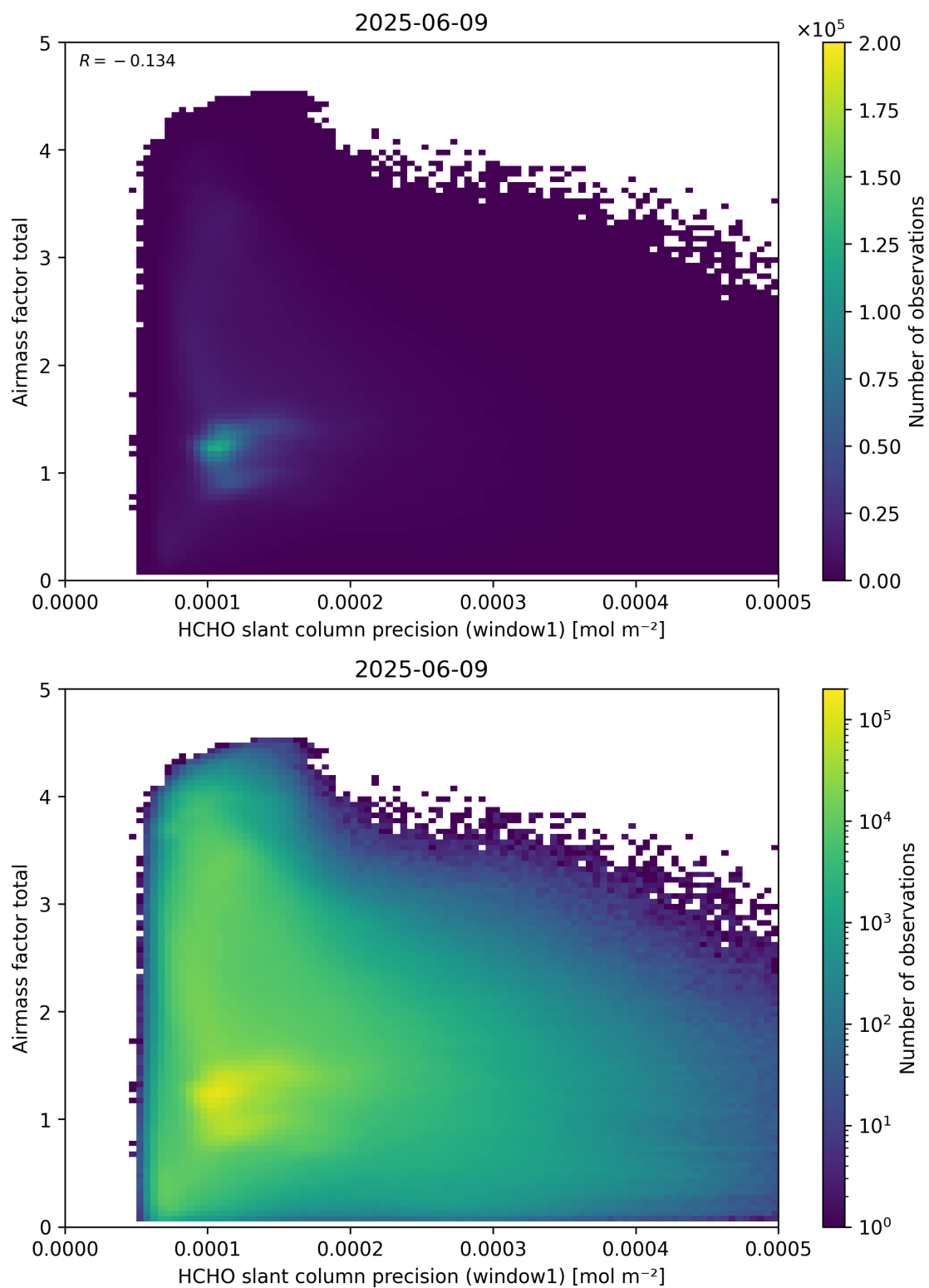
Figure 94: Scatter density plot of “HCHO slant column precision (window1)” against “Airmass factor total” for 2025-06-08 to 2025-06-10.
