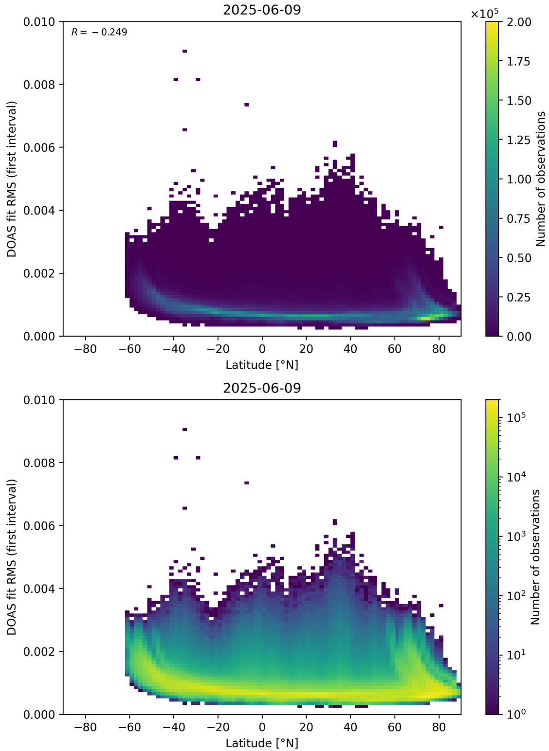
Figure 153: Scatter density plot of “Latitude” against “DOAS fit RMS (first interval)” for 2025-06-08 to 2025-06-10.
