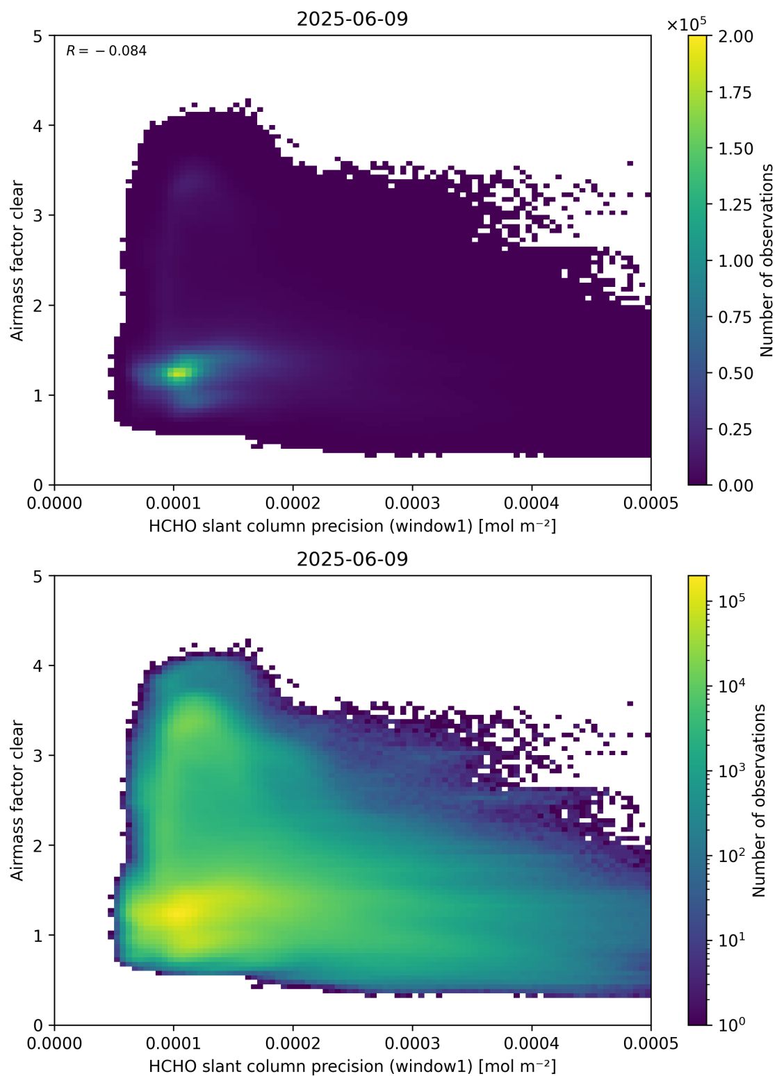
Figure 91: Scatter density plot of “HCHO slant column precision (window1)” against “Airmass factor clear” for 2025-06-08 to 2025-06-10.
