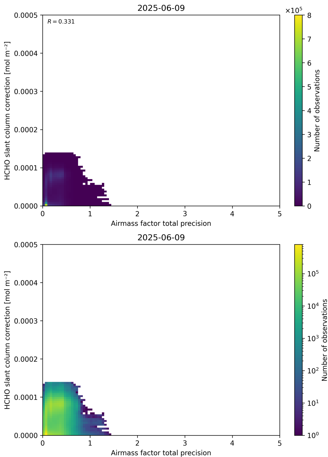
Figure 110: Scatter density plot of “Airmass factor total precision” against “HCHO slant column correction” for 2025-06-08 to 2025-06-10.
