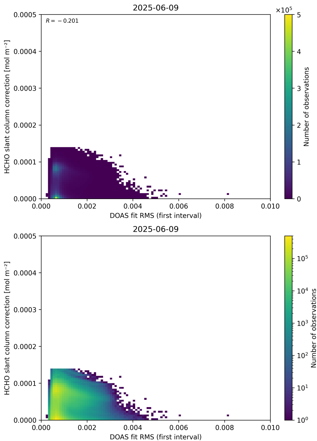
Figure 63: Scatter density plot of “DOAS fit RMS (first interval)” against “HCHO slant column correction” for 2025-06-08 to 2025-06-10.
