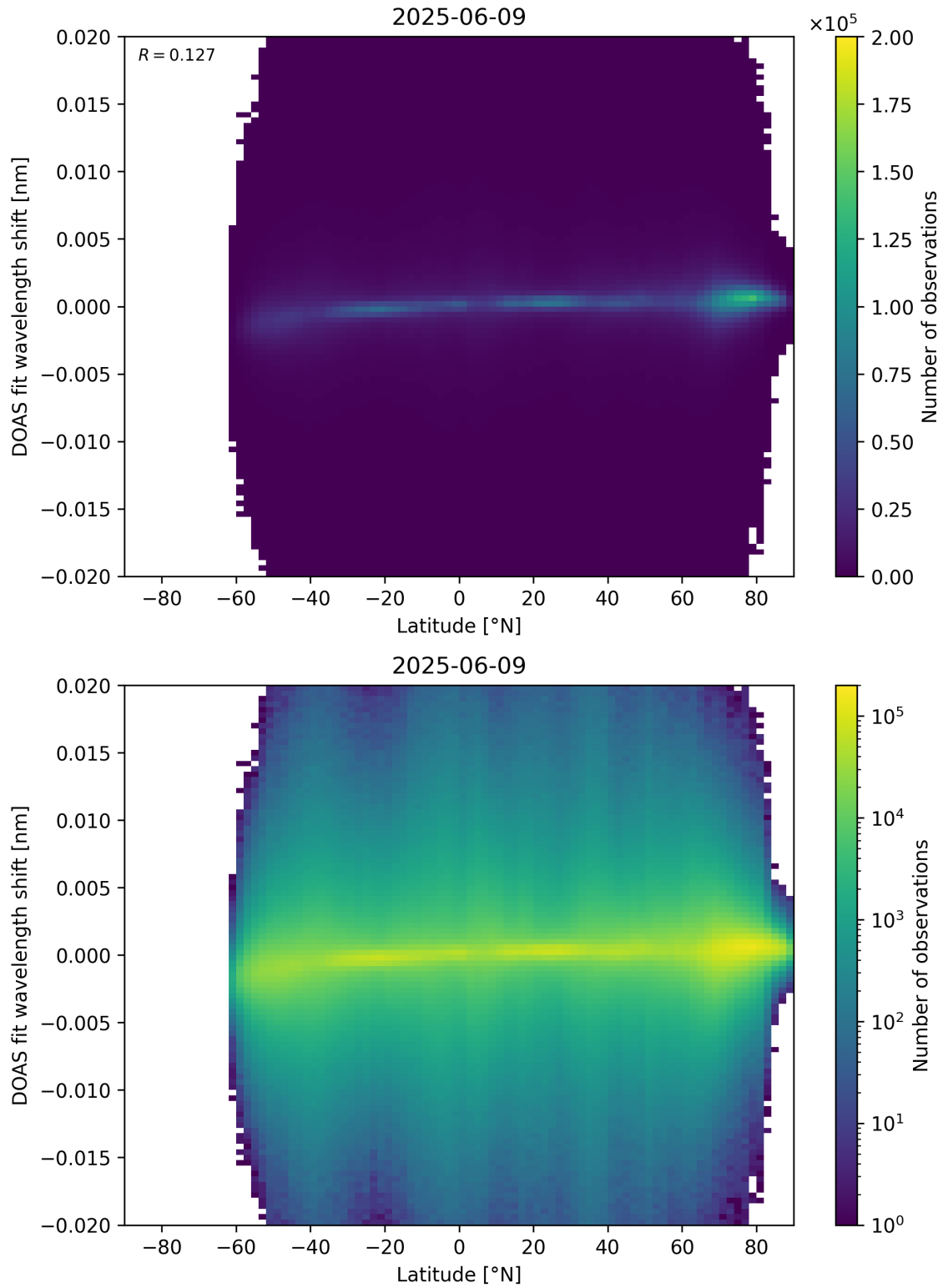
Figure 154: Scatter density plot of “Latitude” against “DOAS fit wavelength shift” for 2025-06-08 to 2025-06-10.
