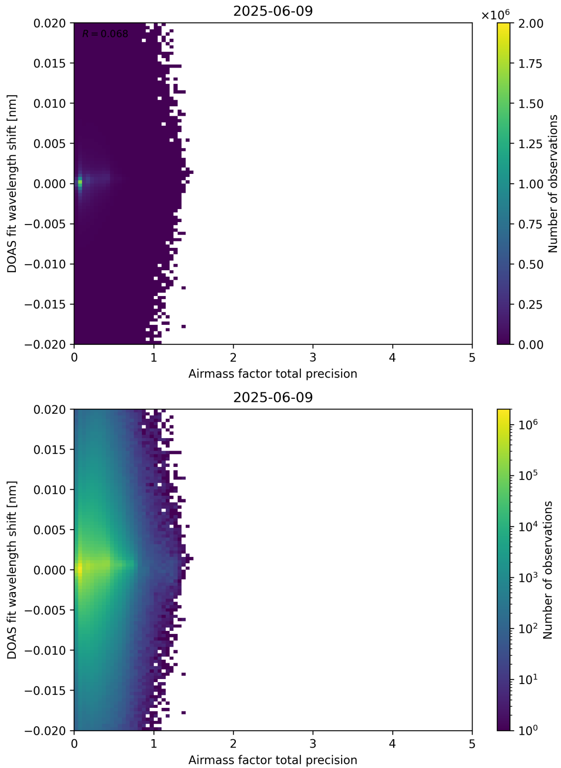
Figure 106: Scatter density plot of “Airmass factor total precision” against “DOAS fit wavelength shift” for 2025-06-08 to 2025-06-10.
