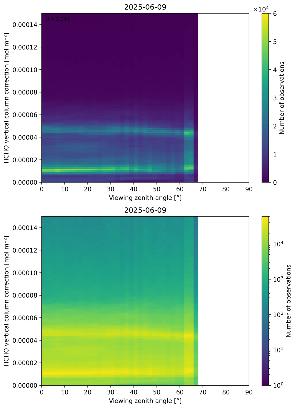
Figure 193: Scatter density plot of “Viewing zenith angle” against “HCHO vertical column correction” for 2025-06-08 to 2025-06-10.
