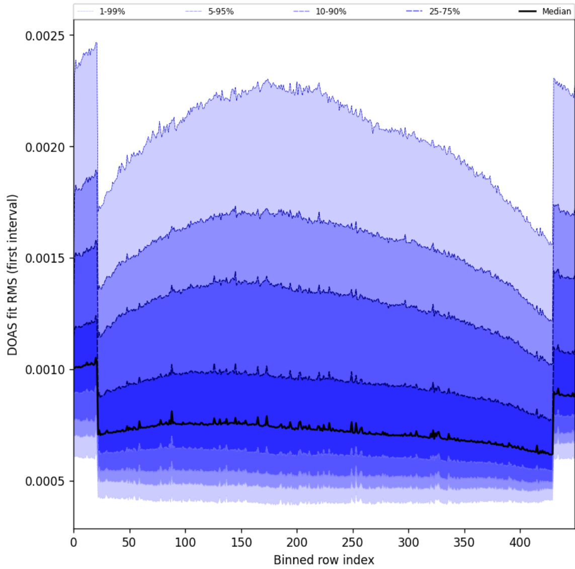
Figure 60: Along track statistics of “DOAS fit RMS (first interval)” for 2025-06-08 to 2025-06-10
