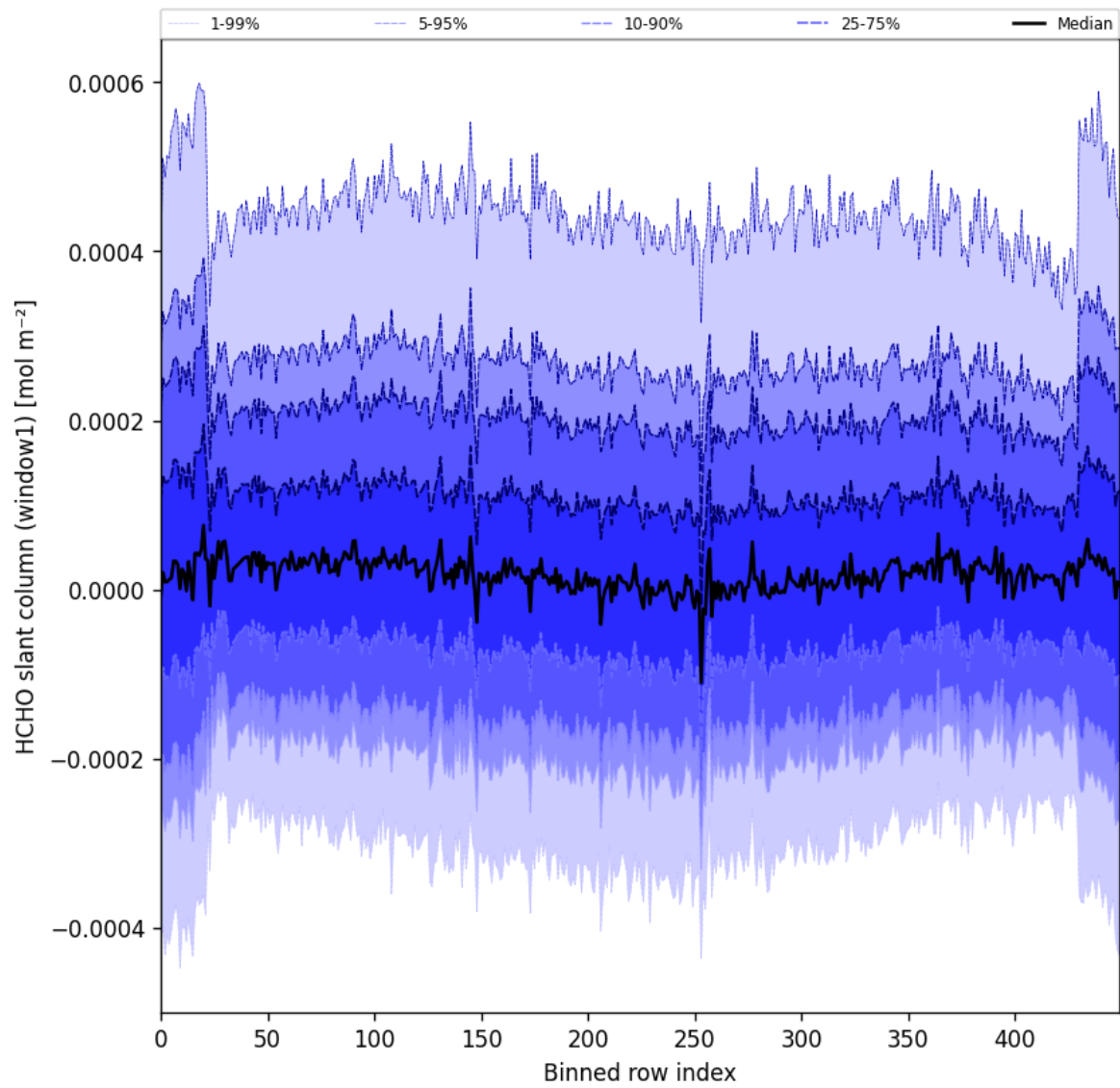
Figure 52: Along track statistics of “HCHO slant column (window1)” for 2025-06-08 to 2025-06-10
