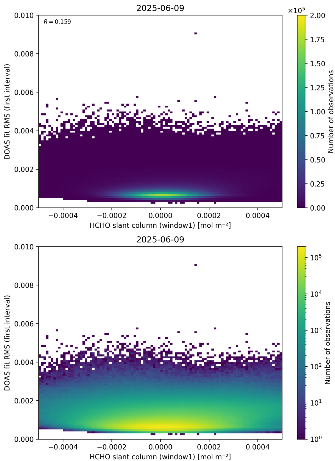
Figure 78: Scatter density plot of “HCHO slant column (window1)” against “DOAS fit RMS (first interval)” for 2025-06-08 to 2025-06-10.
