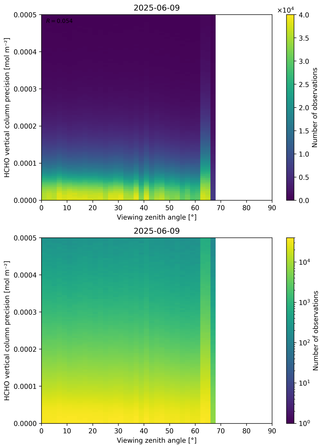
Figure 194: Scatter density plot of “Viewing zenith angle” against “HCHO vertical column precision” for 2025-06-08 to 2025-06-10.
