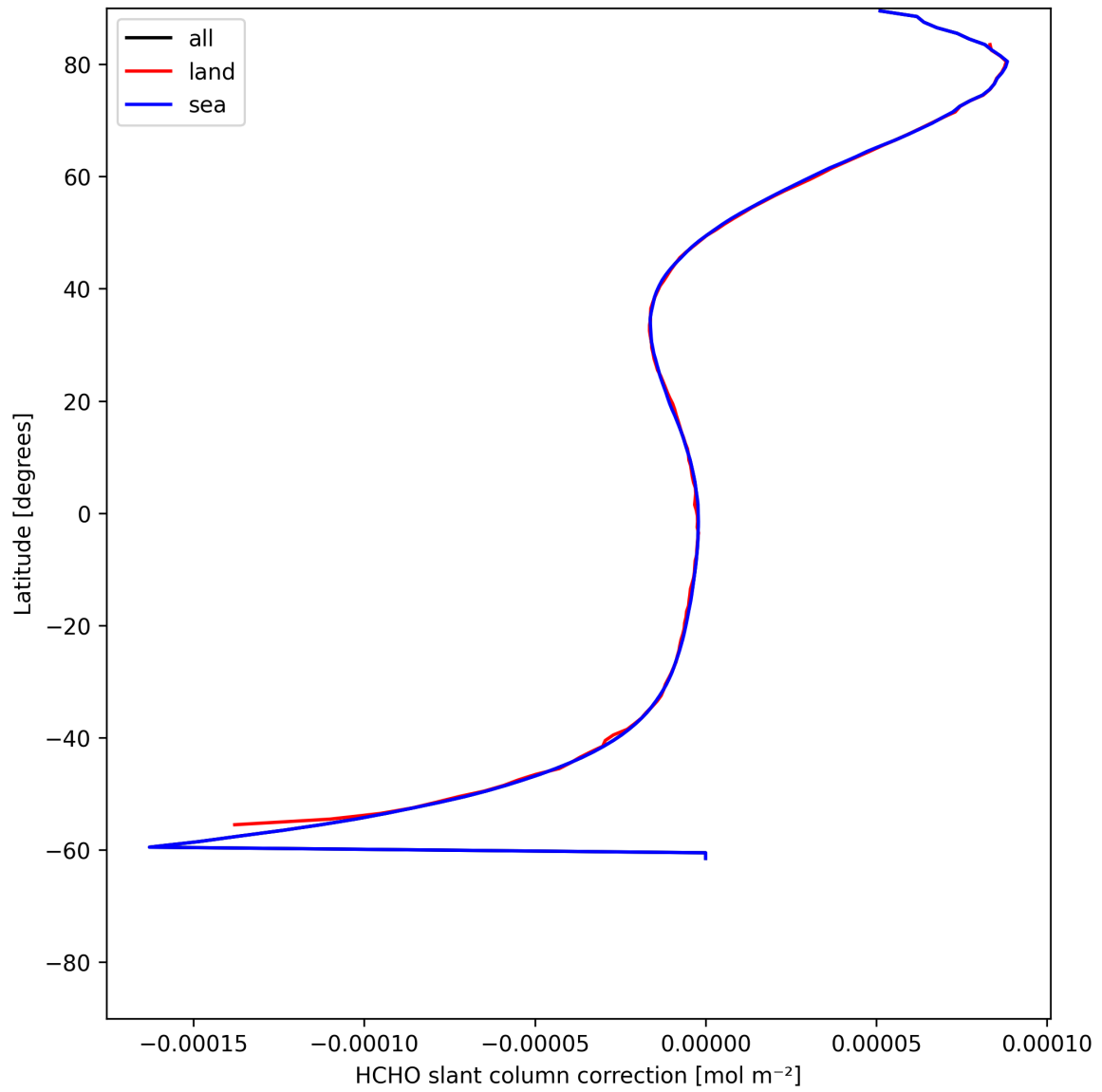
Figure 33: Zonal average of “HCHO slant column correction” for 2025-06-08 to 2025-06-10.
