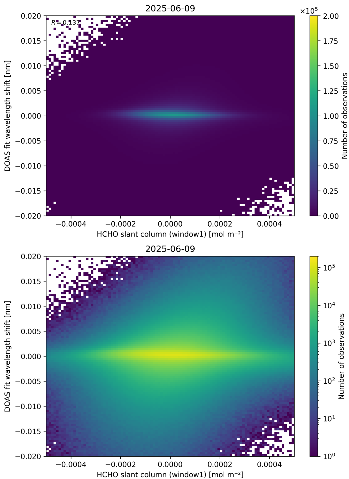
Figure 79: Scatter density plot of “HCHO slant column (window1)” against “DOAS fit wavelength shift” for 2025-06-08 to 2025-06-10.
