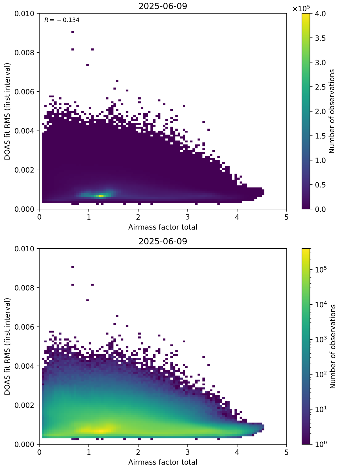
Figure 97: Scatter density plot of “Airmass factor total” against “DOAS fit RMS (first interval)” for 2025-06-08 to 2025-06-10.
