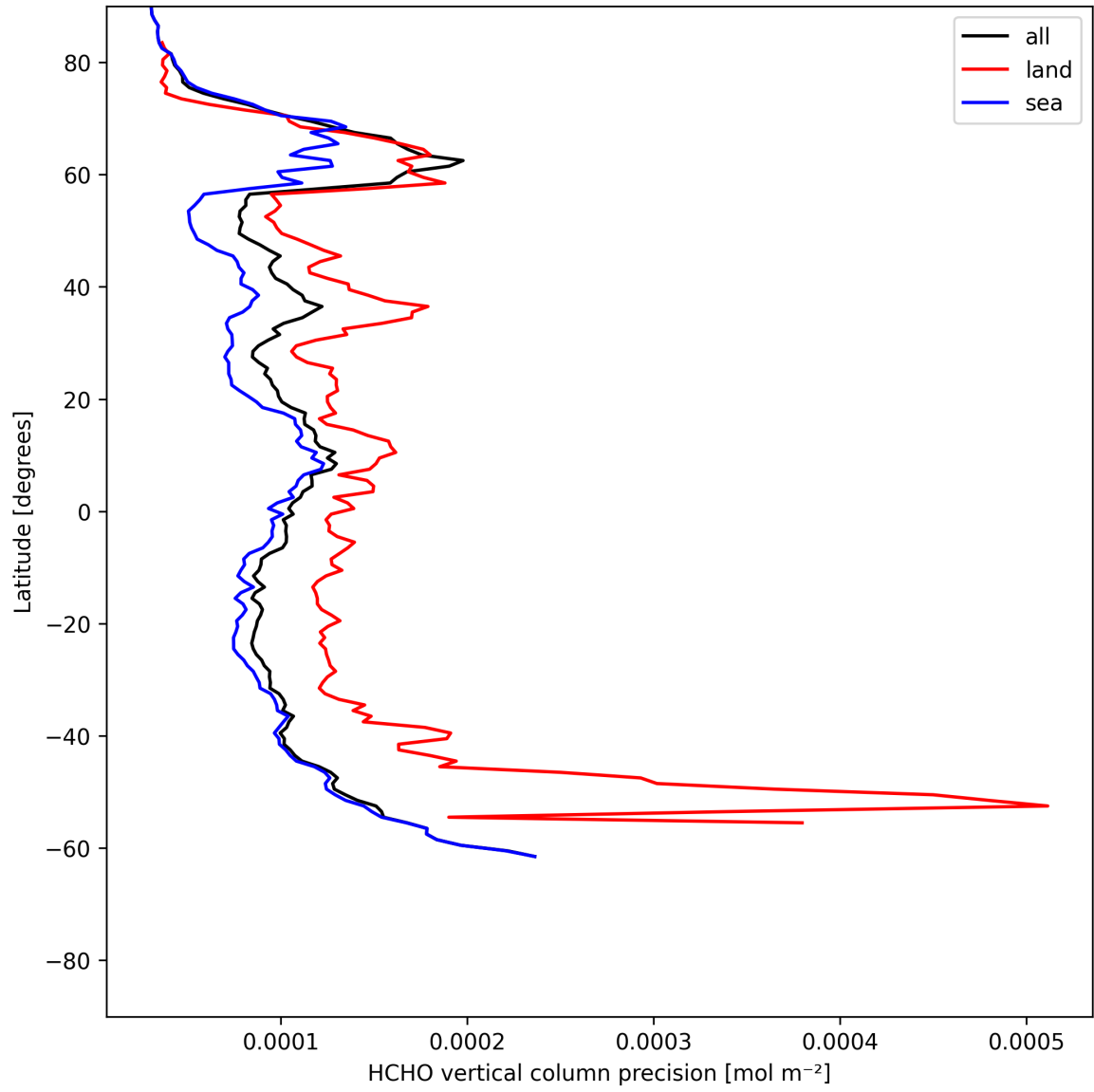
Figure 22: Zonal average of “HCHO vertical column precision” for 2025-06-08 to 2025-06-10.
