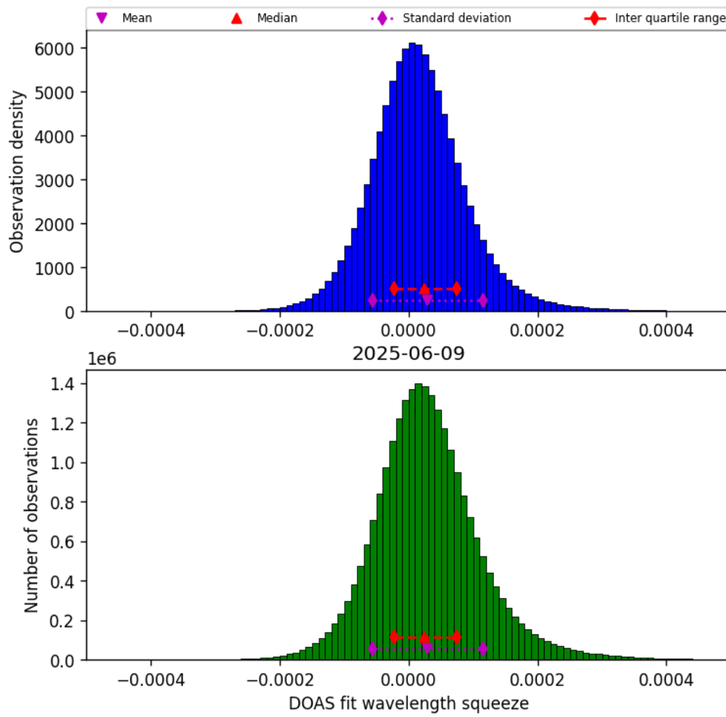
Figure 45: Histogram of “DOAS fit wavelength squeeze” for 2025-06-08 to 2025-06-10
