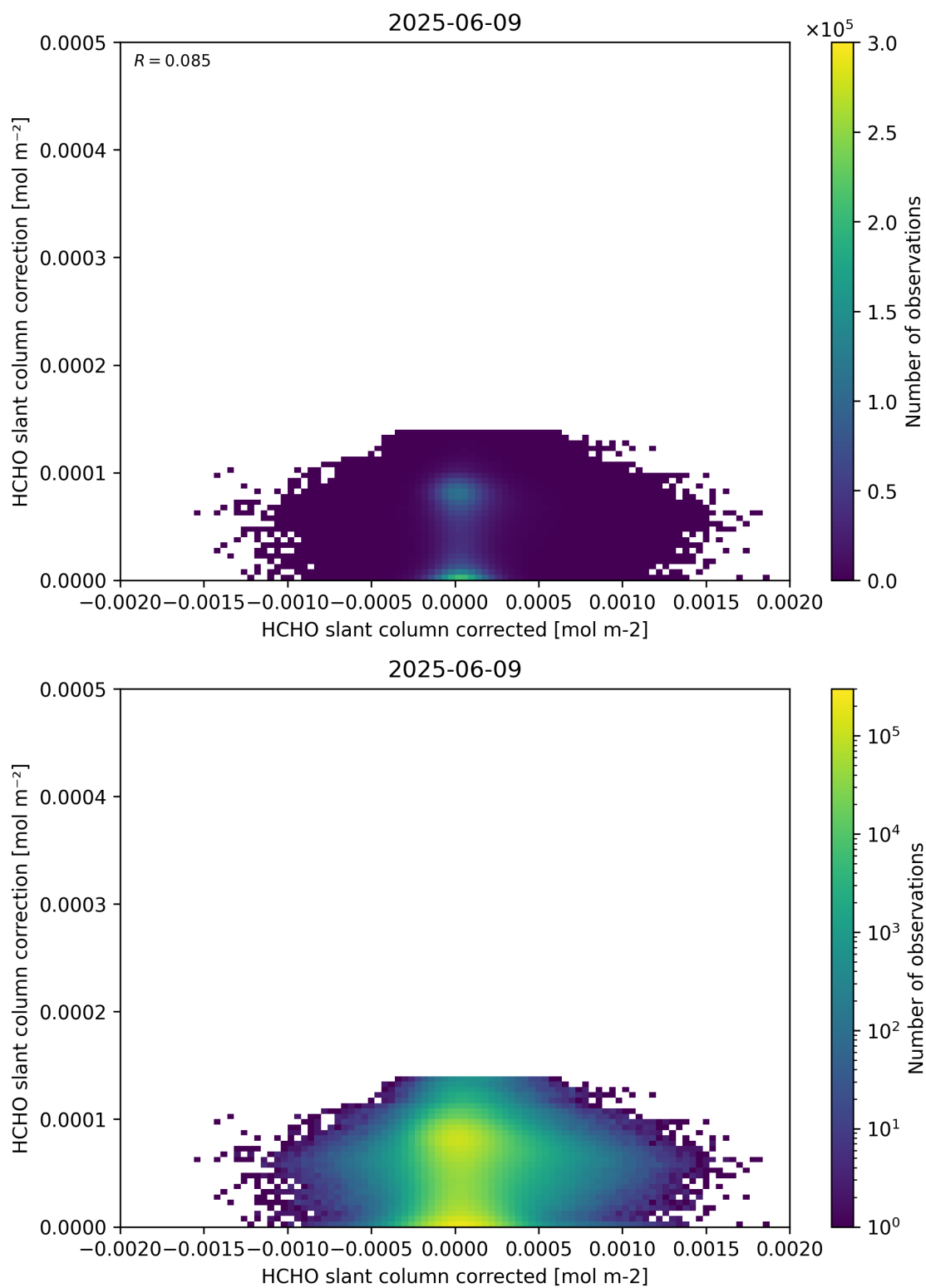
Figure 77: Scatter density plot of “HCHO slant column corrected” against “HCHO slant column correction” for 2025-06-08 to 2025-06-10.
