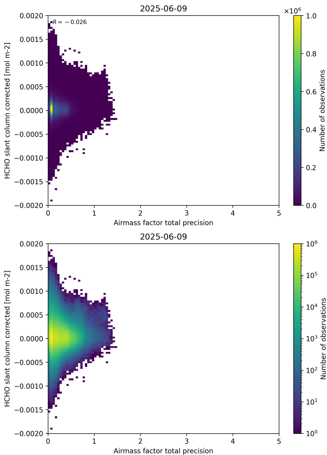
Figure 109: Scatter density plot of “Airmass factor total precision” against “HCHO slant column corrected” for 2025-06-08 to 2025-06-10.
