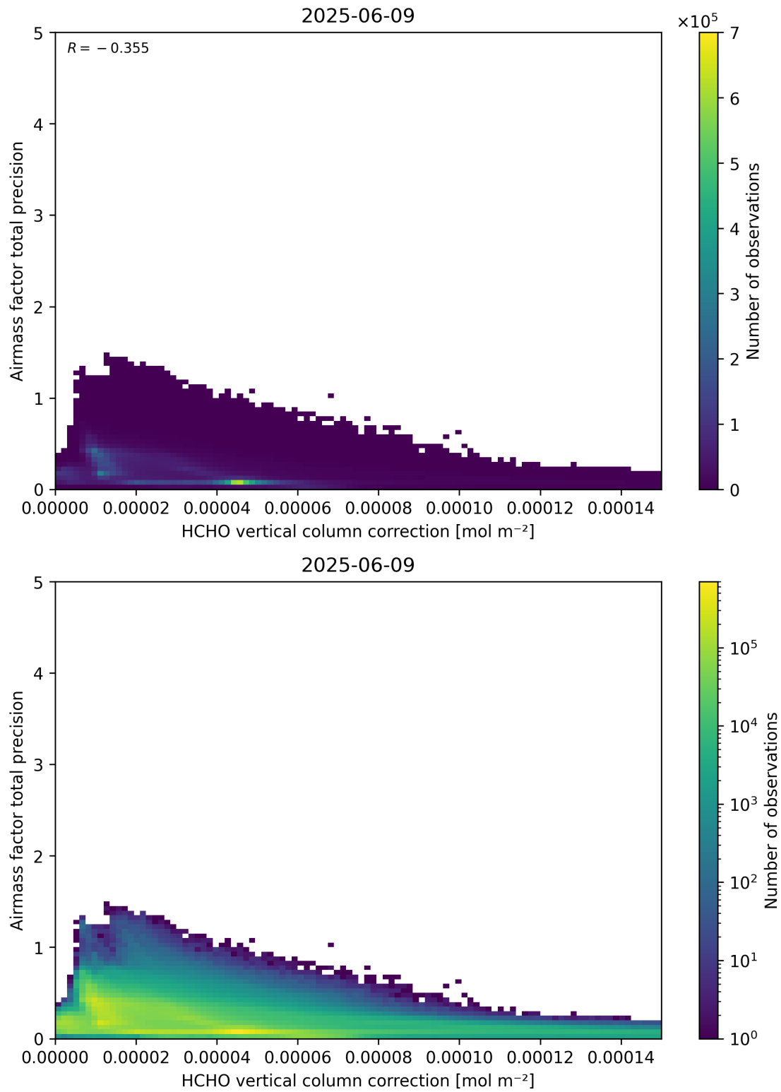
Figure 121: Scatter density plot of “HCHO vertical column correction” against “Airmass factor total precision” for 2025-06-08 to 2025-06-10.
