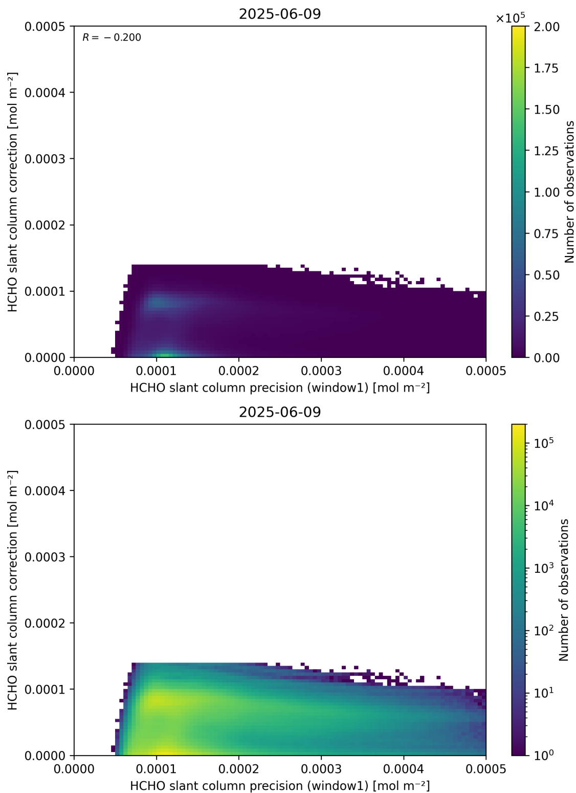
Figure 93: Scatter density plot of “HCHO slant column precision (window1)” against “HCHO slant column correction” for 2025-06-08 to 2025-06-10.
