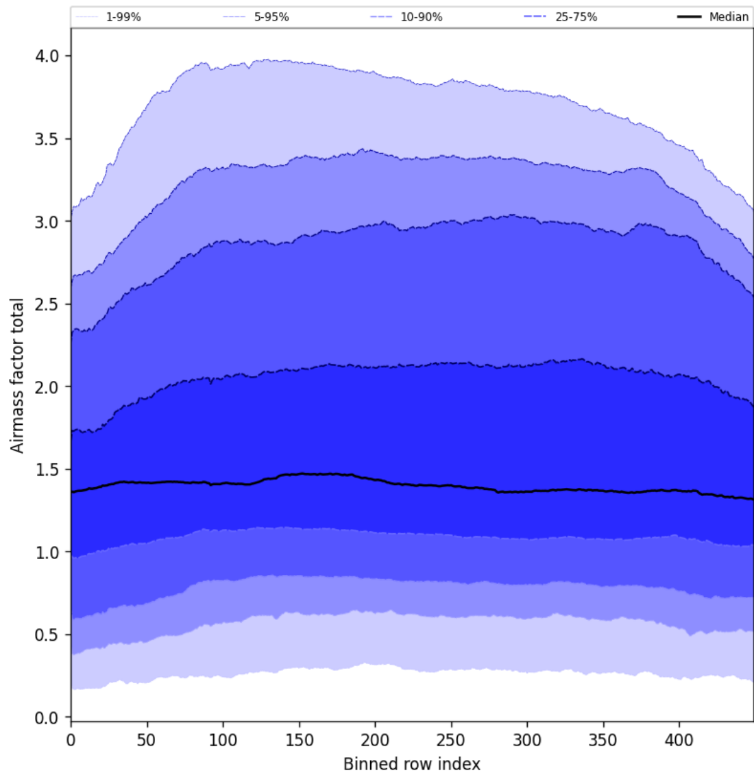
Figure 54: Along track statistics of “Airmass factor total” for 2025-06-08 to 2025-06-10
