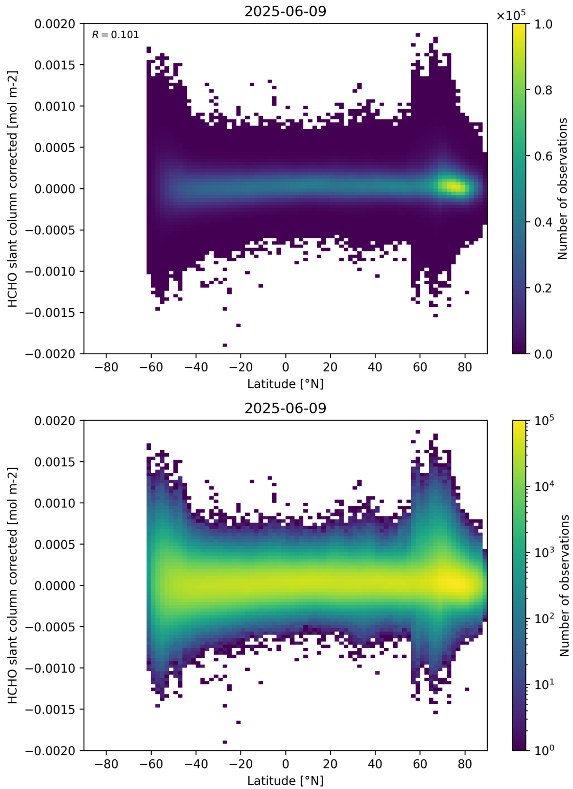
Figure 157: Scatter density plot of “Latitude” against “HCHO slant column corrected” for 2025-06-08 to 2025-06-10.
