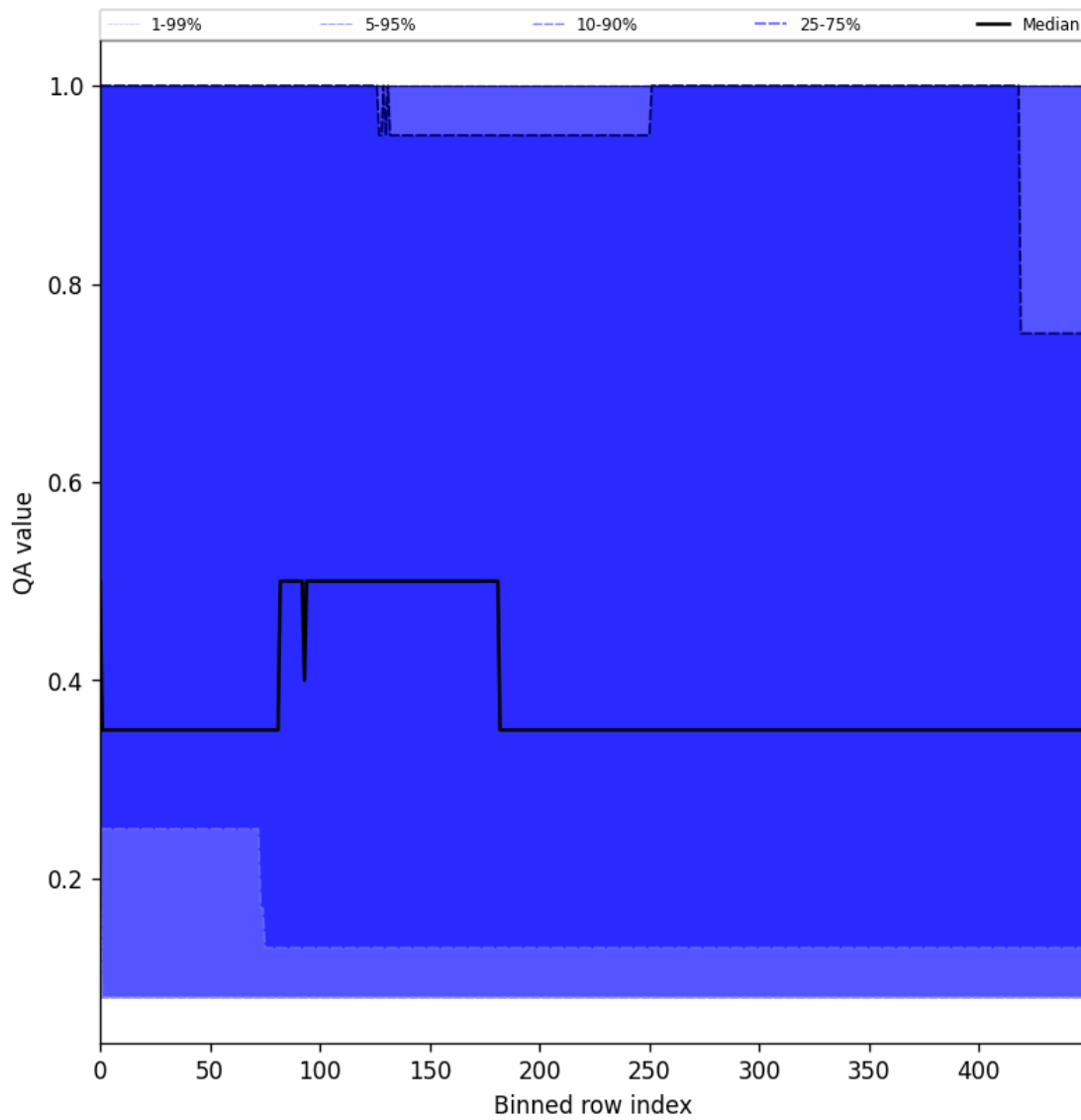
Figure 48: Along track statistics of “QA value” for 2025-06-08 to 2025-06-10
