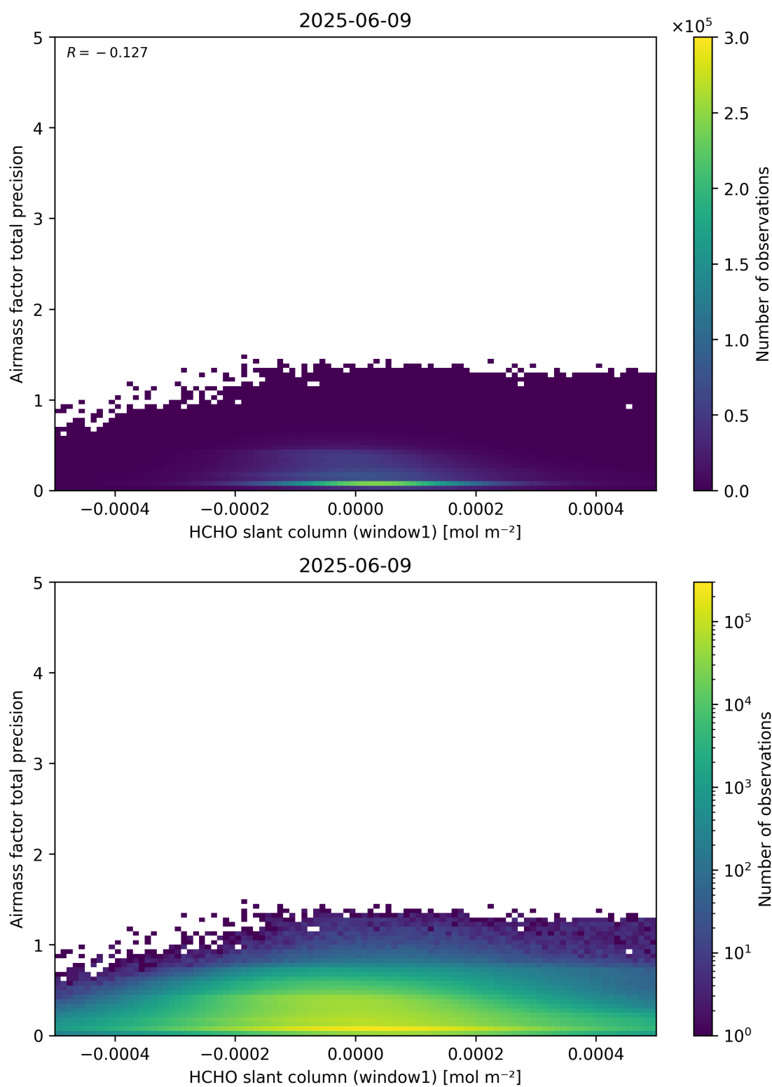
Figure 86: Scatter density plot of “HCHO slant column (window1)” against “Airmass factor total precision” for 2025-06-08 to 2025-06-10.
