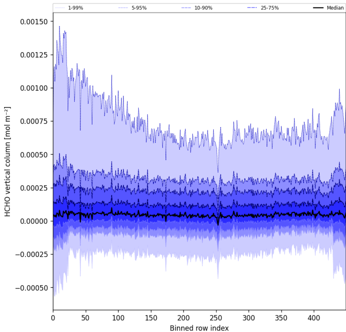
Figure 49: Along track statistics of “HCHO vertical column” for 2025-06-08 to 2025-06-10
