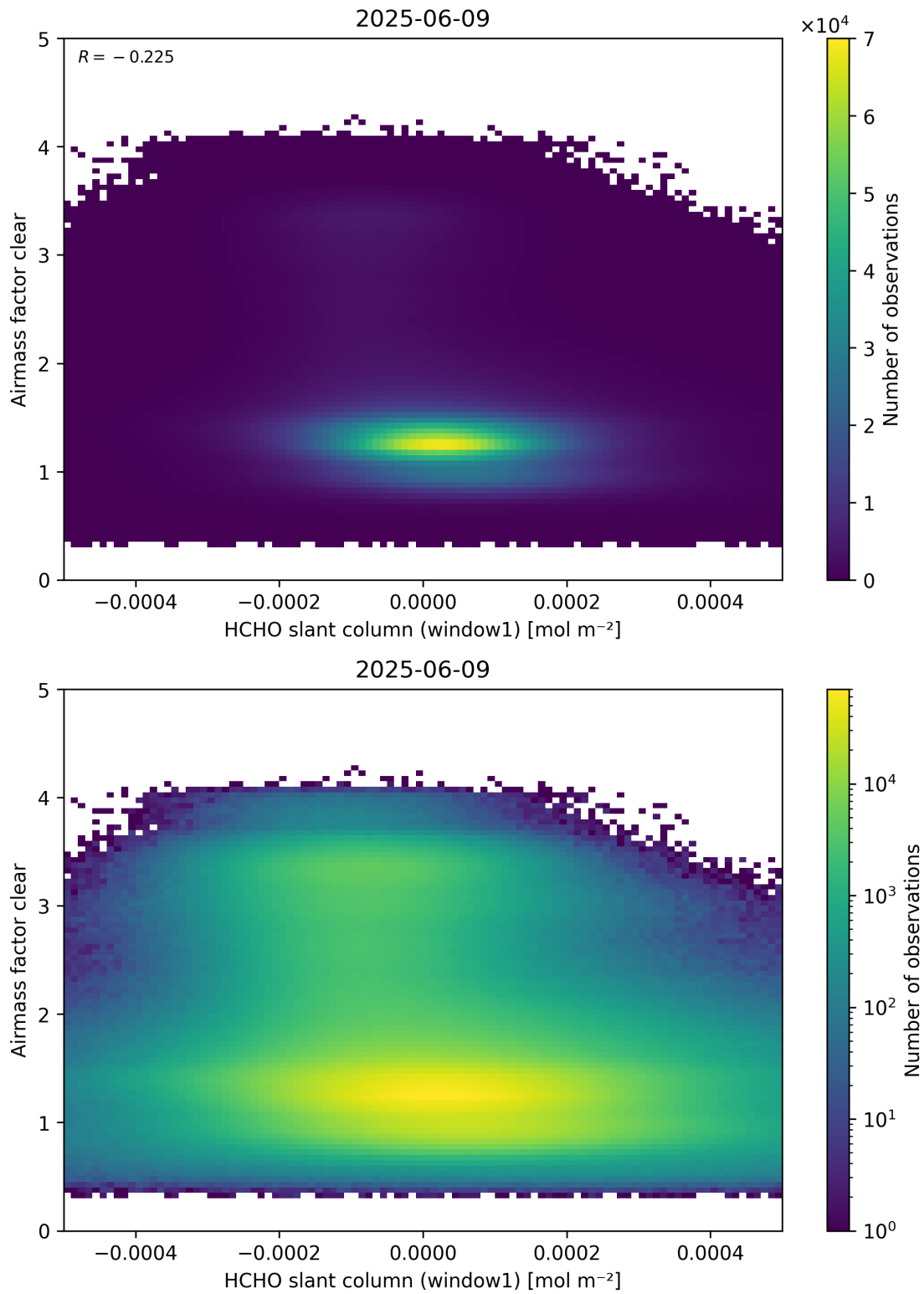
Figure 81: Scatter density plot of “HCHO slant column (window1)” against “Airmass factor clear” for 2025-06-08 to 2025-06-10.
