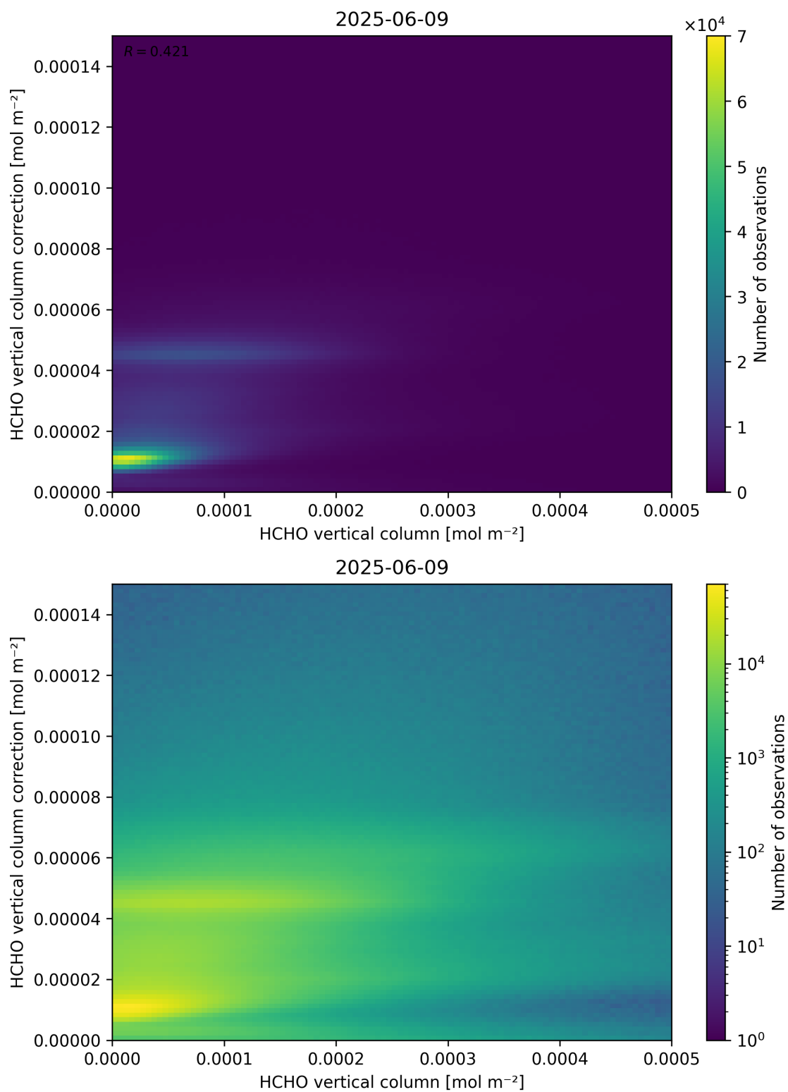
Figure 133: Scatter density plot of “HCHO vertical column” against “HCHO vertical column correction” for 2025-06-08 to 2025-06-10.
