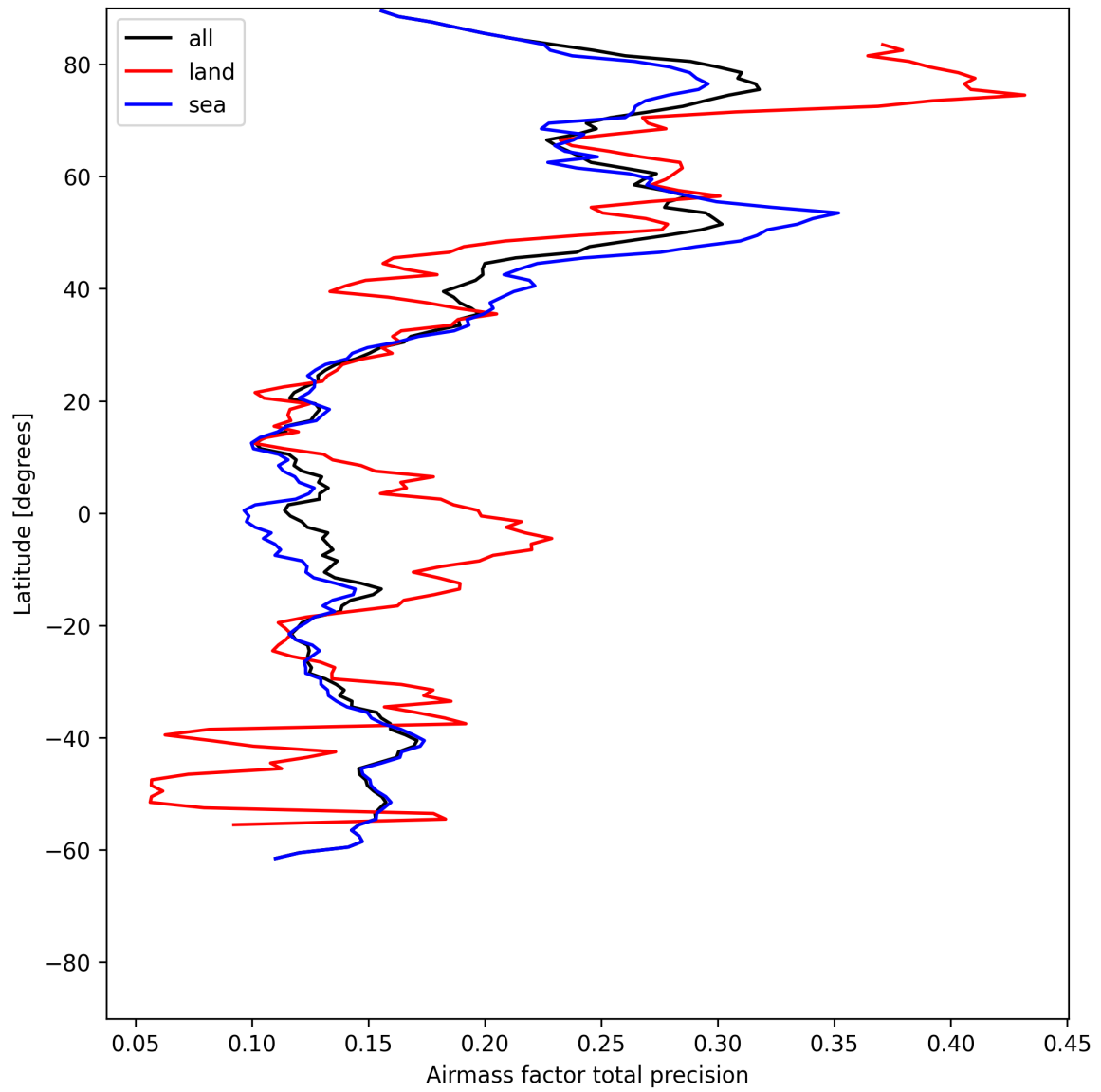
Figure 27: Zonal average of “Airmass factor total precision” for 2025-06-08 to 2025-06-10.
