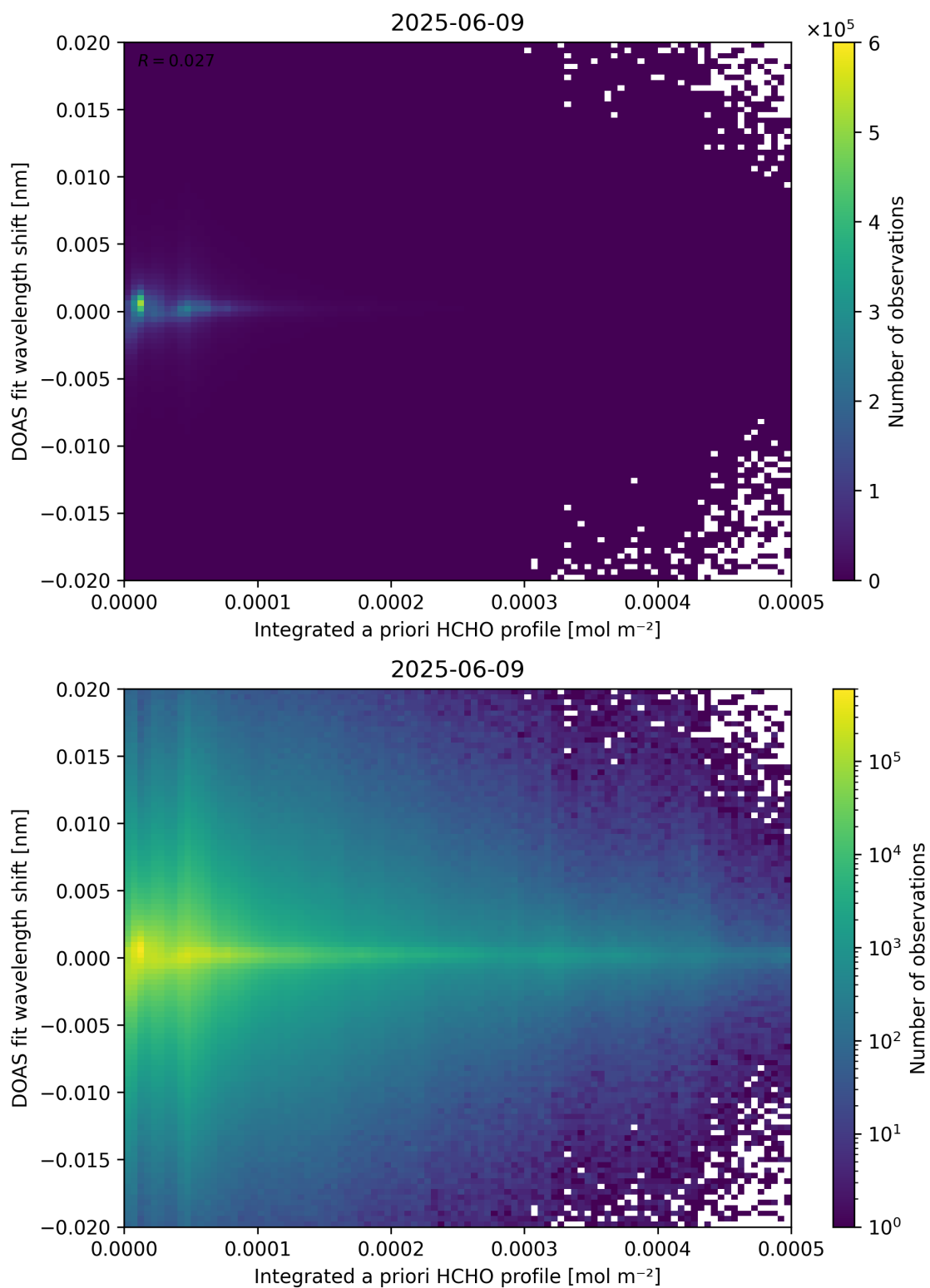
Figure 149: Scatter density plot of “Integrated a priori HCHO profile” against “DOAS fit wavelength shift” for 2025-06-08 to 2025-06-10.
