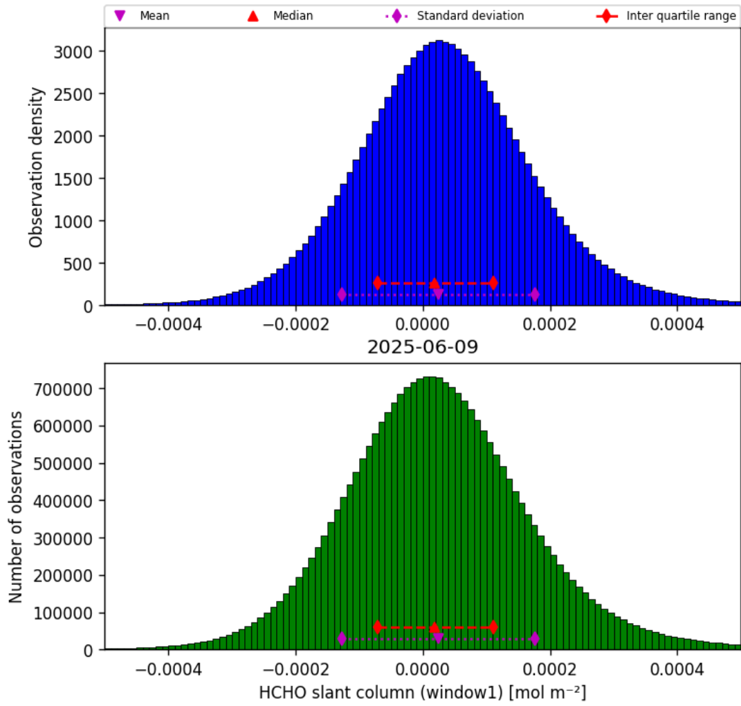
Figure 38: Histogram of “HCHO slant column (window1)” for 2025-06-08 to 2025-06-10
