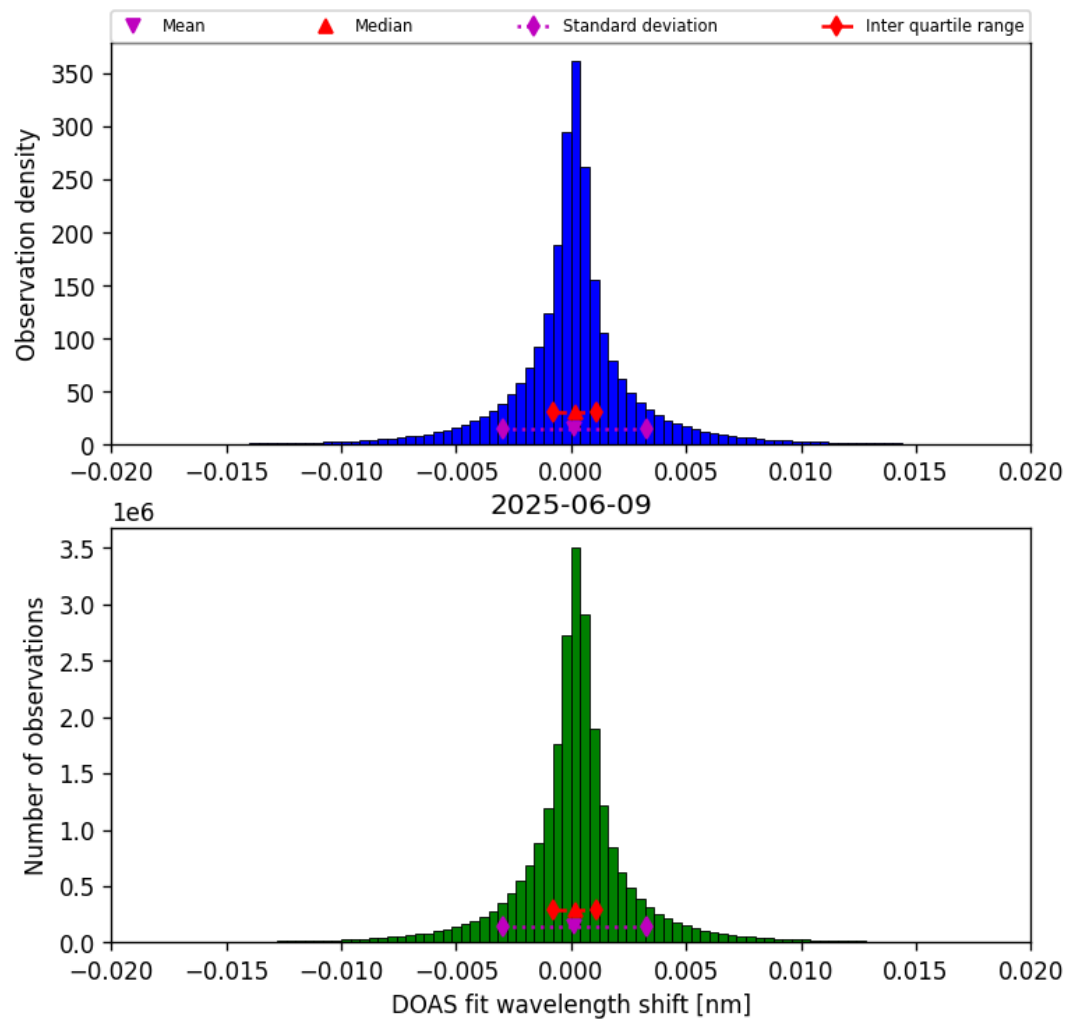
Figure 44: Histogram of “DOAS fit wavelength shift” for 2025-06-08 to 2025-06-10
