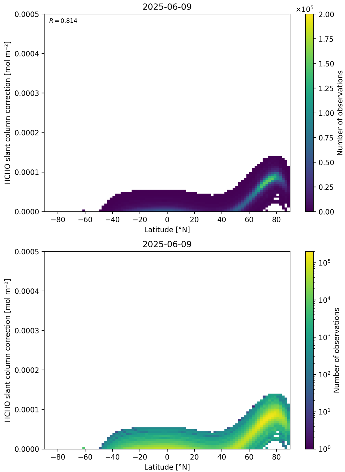
Figure 158: Scatter density plot of “Latitude” against “HCHO slant column correction” for 2025-06-08 to 2025-06-10.
