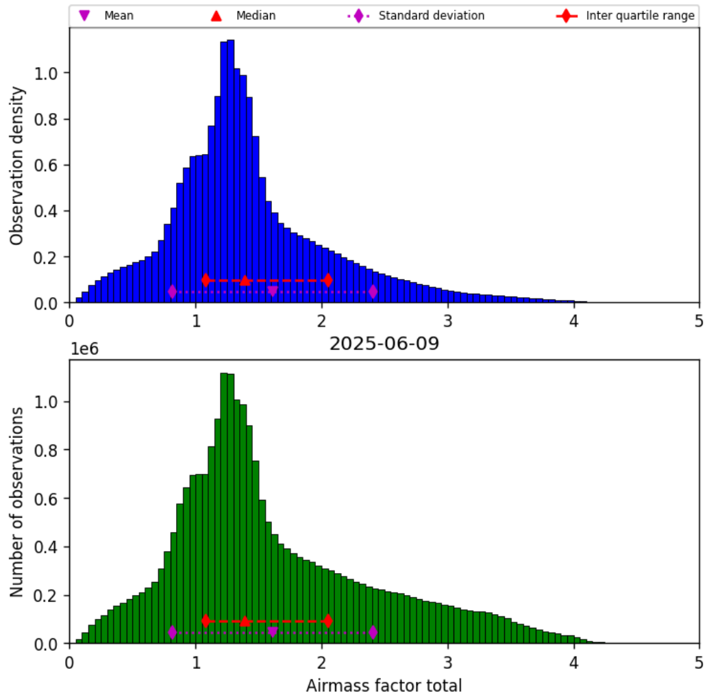
Figure 40: Histogram of “Airmass factor total” for 2025-06-08 to 2025-06-10
