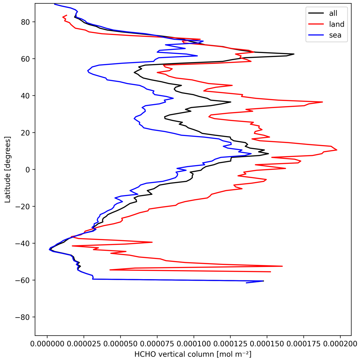
Figure 21: Zonal average of “HCHO vertical column” for 2025-06-08 to 2025-06-10.
