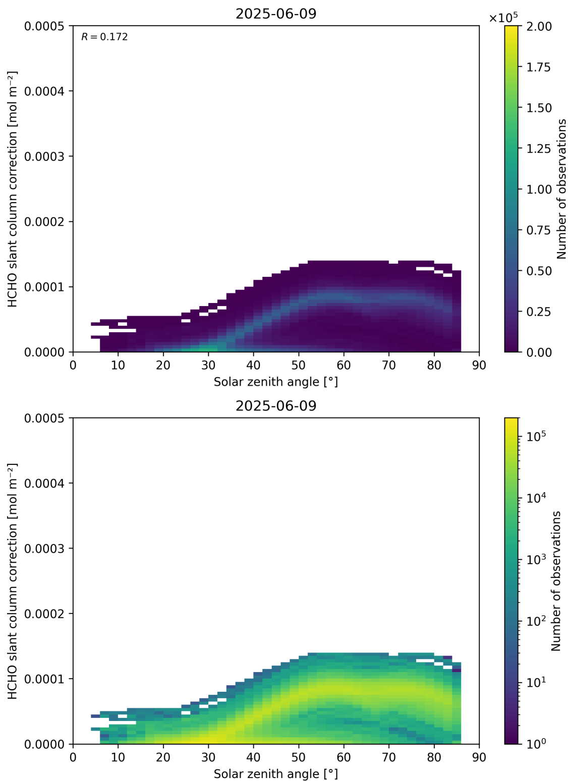
Figure 172: Scatter density plot of “Solar zenith angle” against “HCHO slant column correction” for 2025-06-08 to 2025-06-10.
