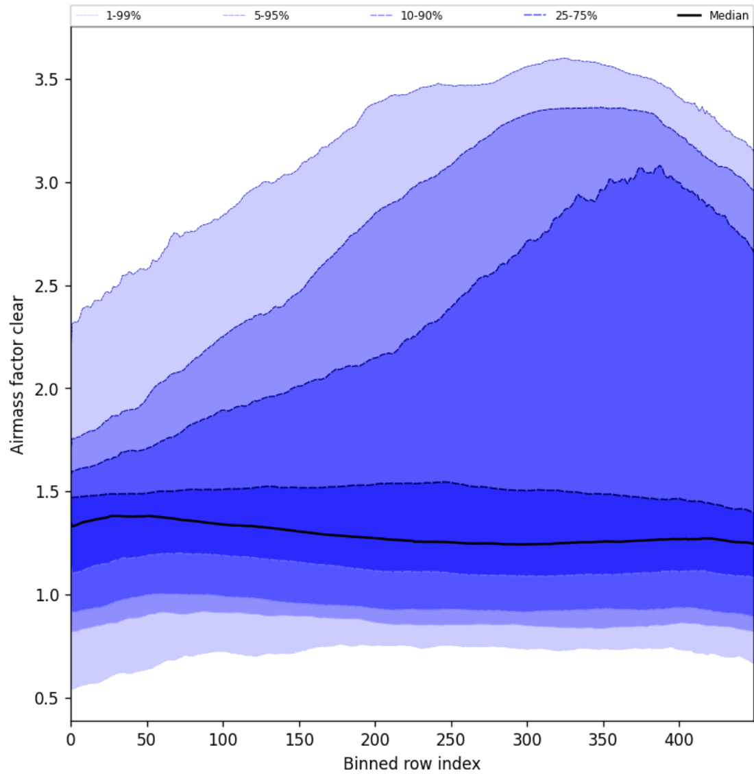
Figure 56: Along track statistics of “Air mass factor clear” for 2025-06-08 to 2025-06-10
