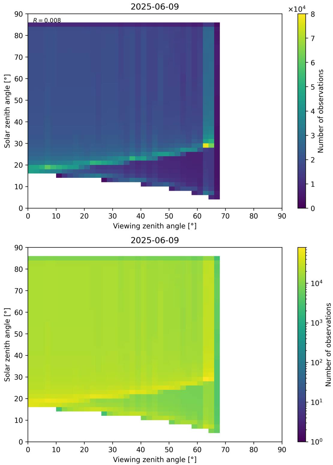
Figure 197: Scatter density plot of “Viewing zenith angle” against “Solar zenith angle” for 2025-06-08 to 2025-06-10.
