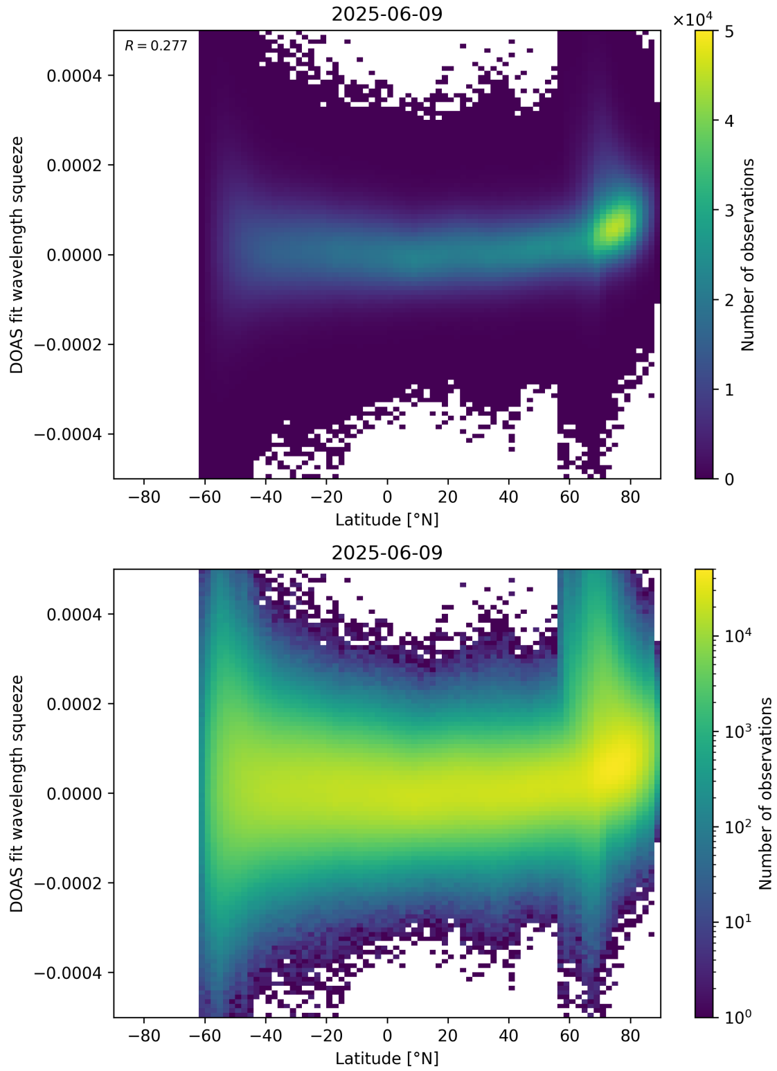
Figure 155: Scatter density plot of “Latitude” against “DOAS fit wavelength squeeze” for 2025-06-08 to 2025-06-10.
