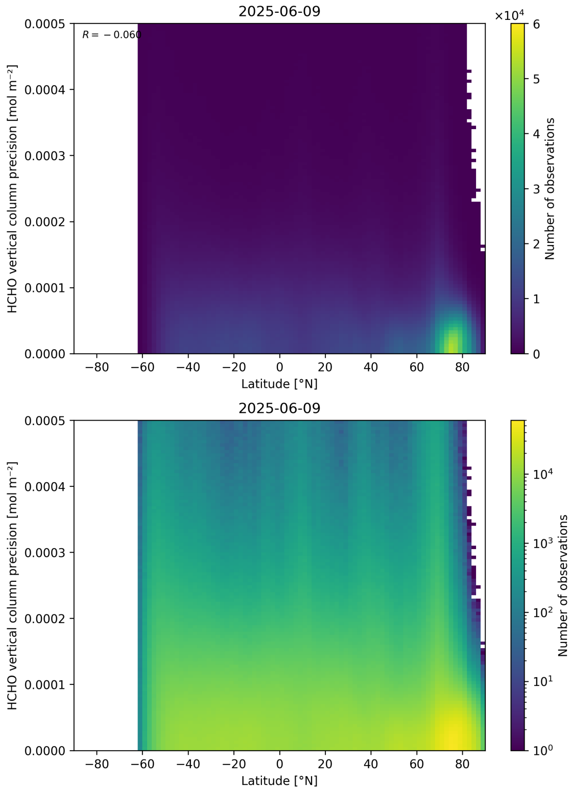
Figure 165: Scatter density plot of “Latitude” against “HCHO vertical column precision” for 2025-06-08 to 2025-06-10.
