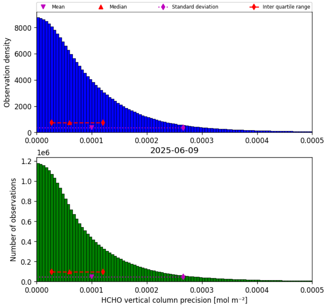
Figure 36: Histogram of “HCHO vertical column precision” for 2025-06-08 to 2025-06-10
