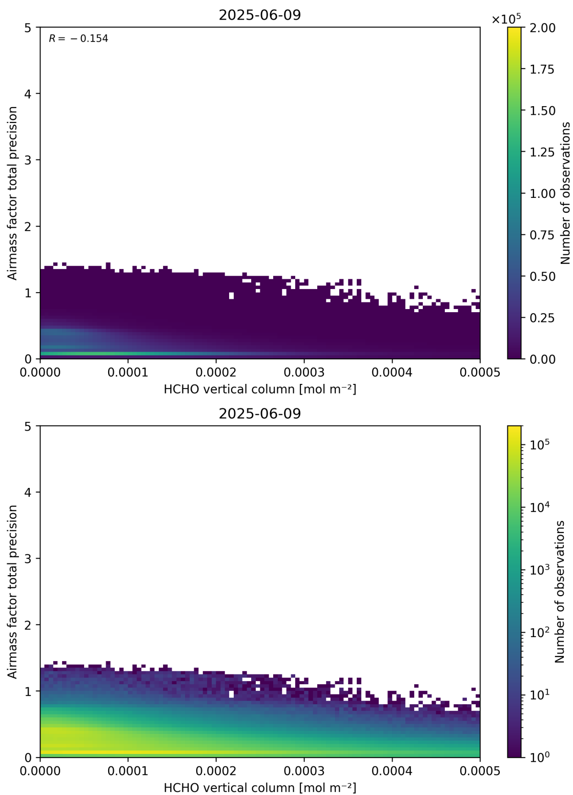
Figure 132: Scatter density plot of “HCHO vertical column” against “Airmass factor total precision” for 2025-06-08 to 2025-06-10.
