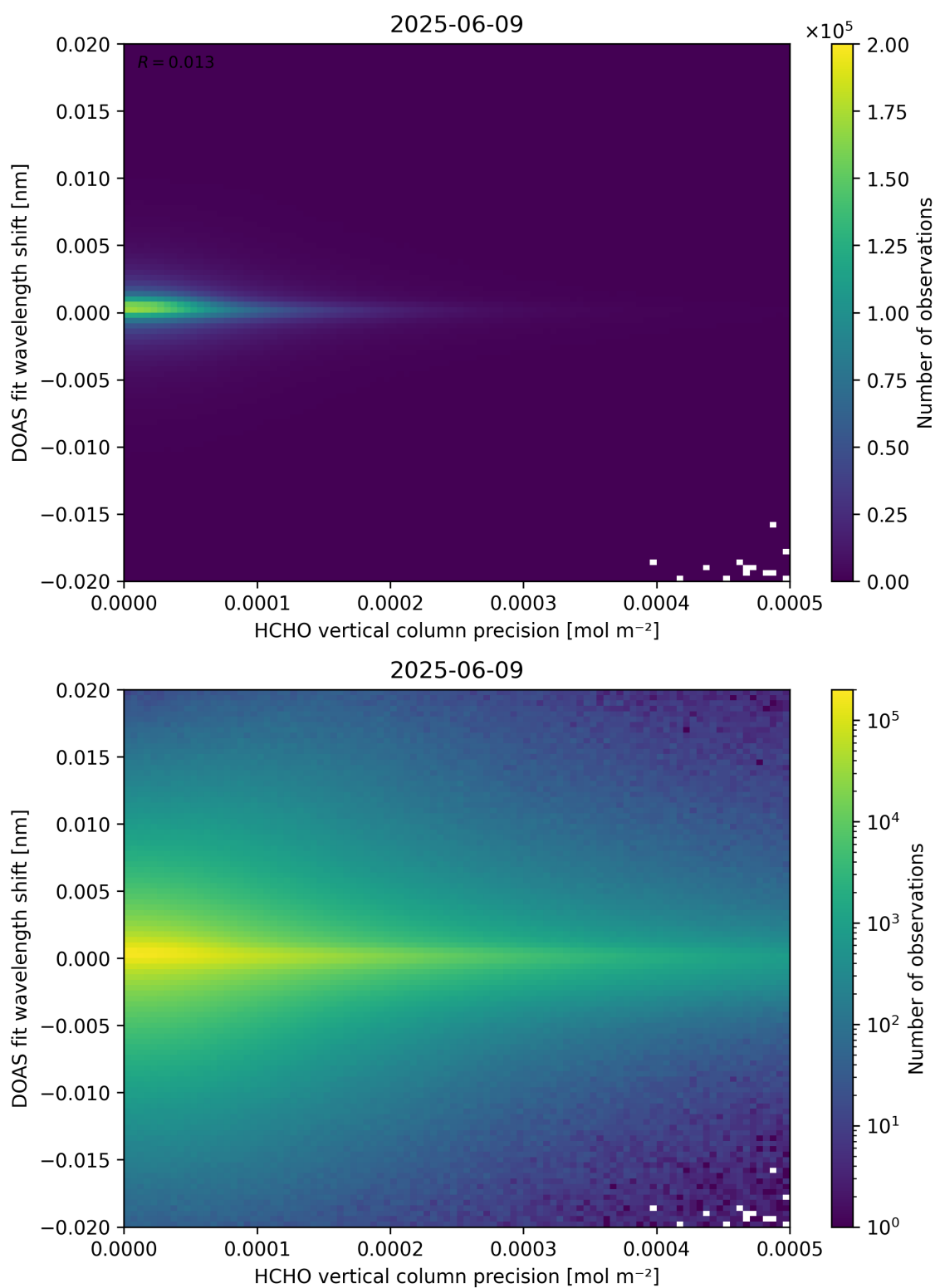
Figure 137: Scatter density plot of “HCHO vertical column precision” against “DOAS fit wavelength shift” for 2025-06-08 to 2025-06-10.
