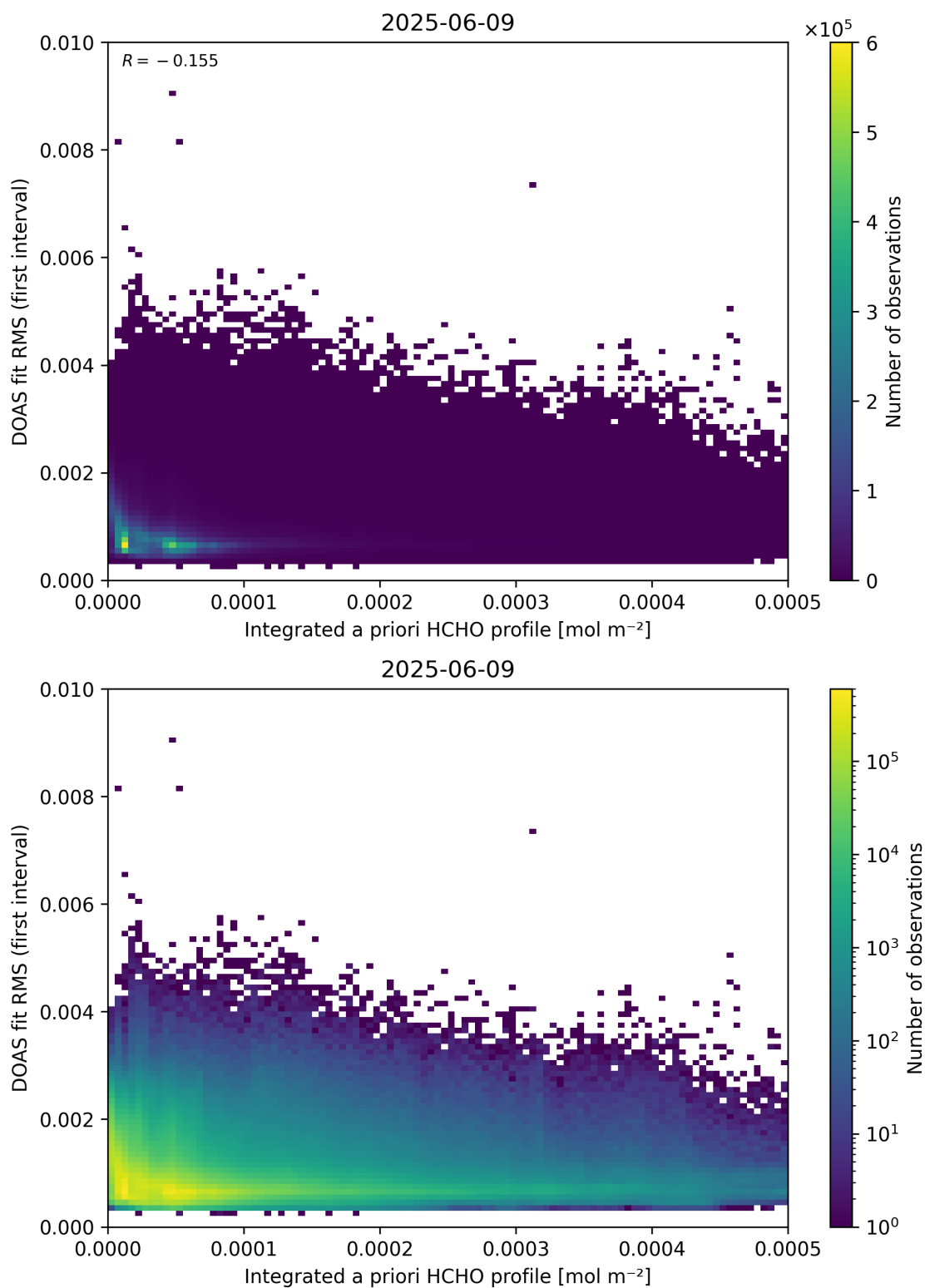
Figure 148: Scatter density plot of “Integrated a priori HCHO profile” against “DOAS fit RMS (first interval)” for 2025-06-08 to 2025-06-10.
