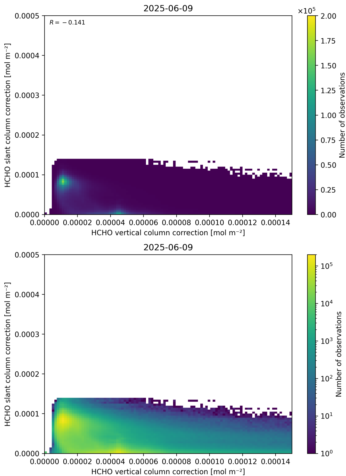
Figure 117: Scatter density plot of “HCHO vertical column correction” against “HCHO slant column correction” for 2025-06-08 to 2025-06-10.
