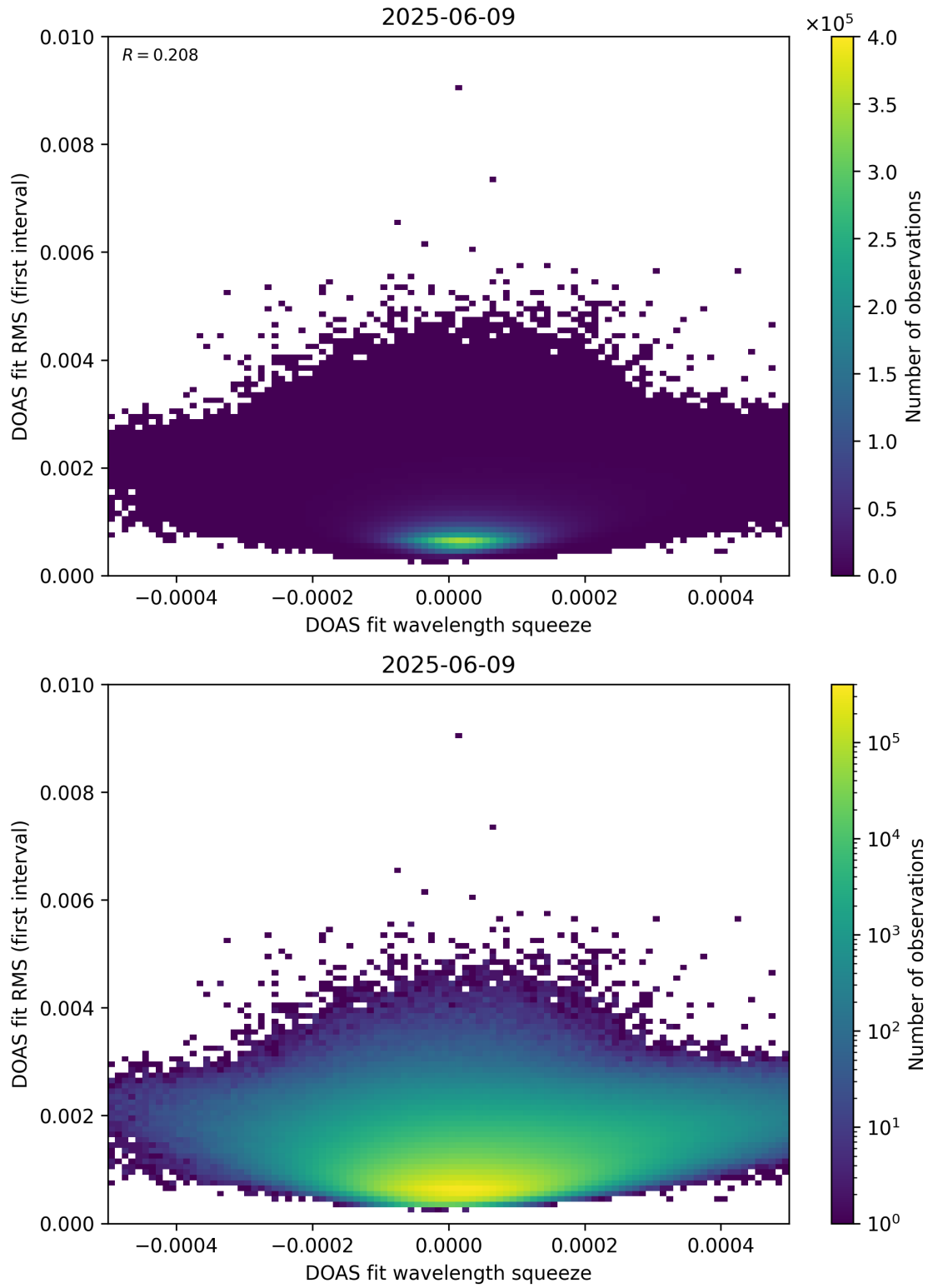
Figure 68: Scatter density plot of “DOAS fit wavelength squeeze” against “DOAS fit RMS (first interval)” for 2025-06-08 to 2025-06-10.
