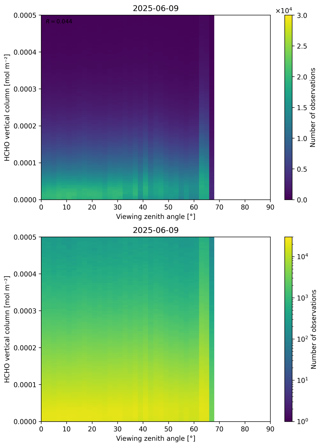
Figure 192: Scatter density plot of “Viewing zenith angle” against “HCHO vertical column” for 2025-06-08 to 2025-06-10.
