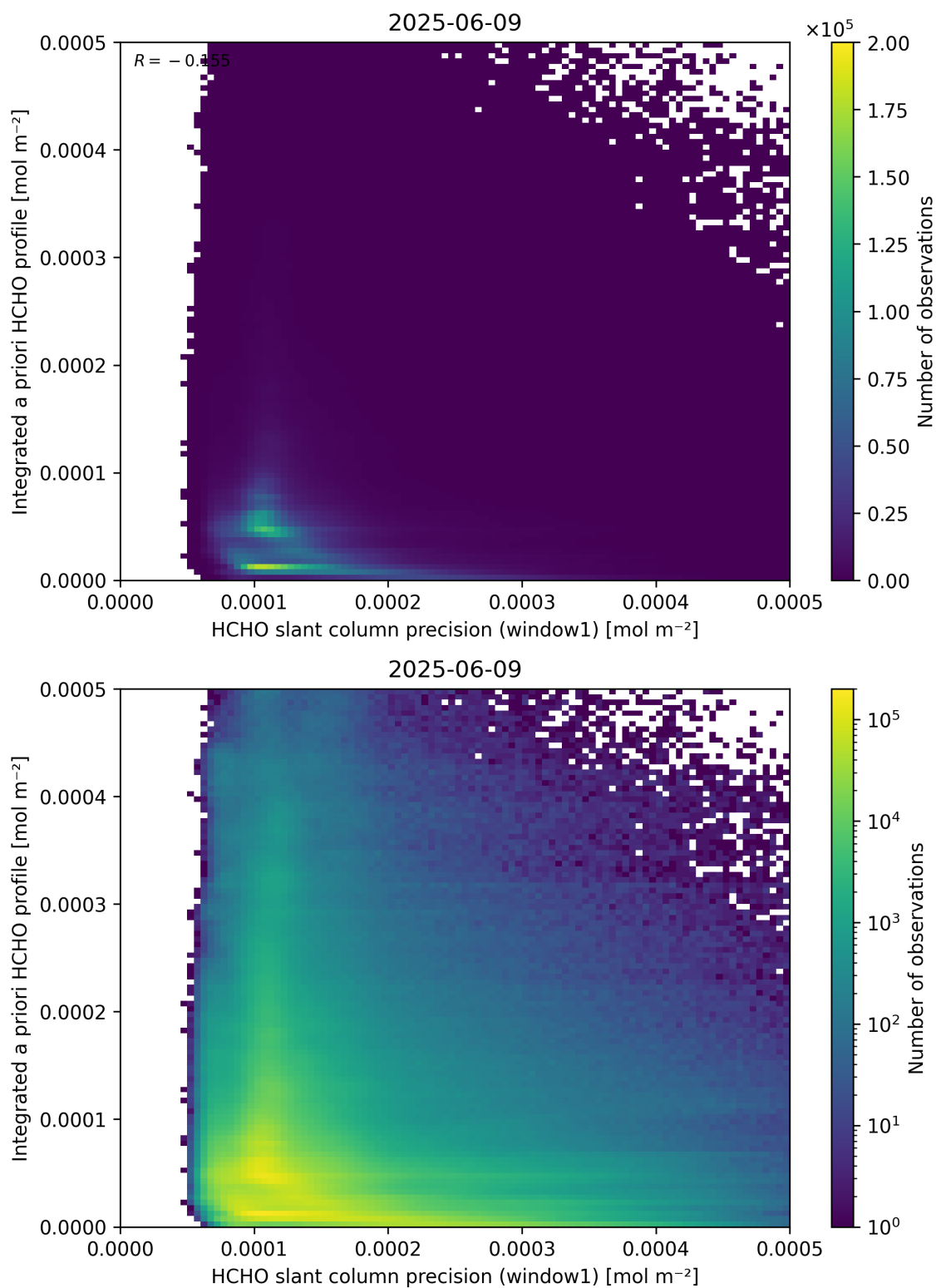
Figure 96: Scatter density plot of “HCHO slant column precision (window1)” against “Integrated a priori HCHO profile” for 2025-06-08 to 2025-06-10.
