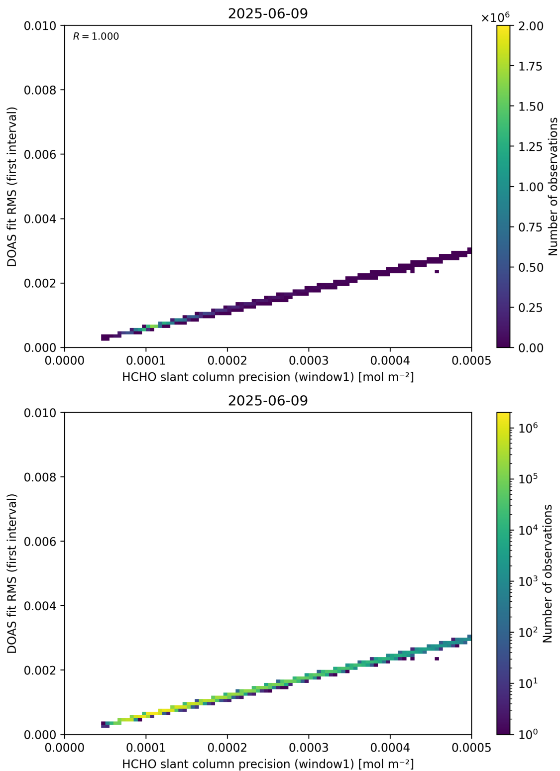
Figure 88: Scatter density plot of “HCHO slant column precision (window1)” against “DOAS fit RMS (first interval)” for 2025-06-08 to 2025-06-10.
