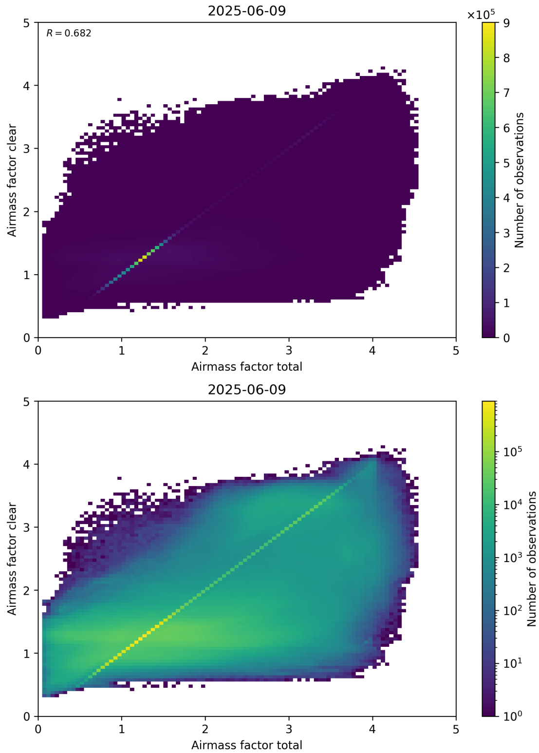
Figure 100: Scatter density plot of “Airmass factor total” against “Airmass factor clear” for 2025-06-08 to 2025-06-10.
