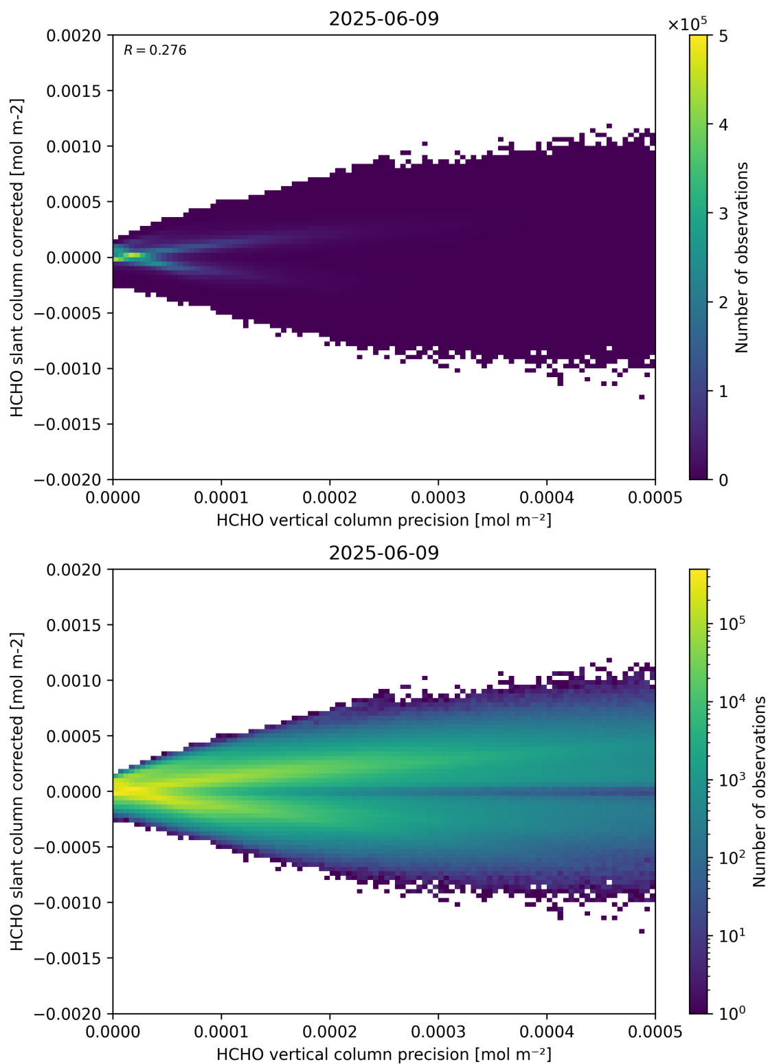
Figure 140: Scatter density plot of “HCHO vertical column precision” against “HCHO slant column corrected” for 2025-06-08 to 2025-06-10.
