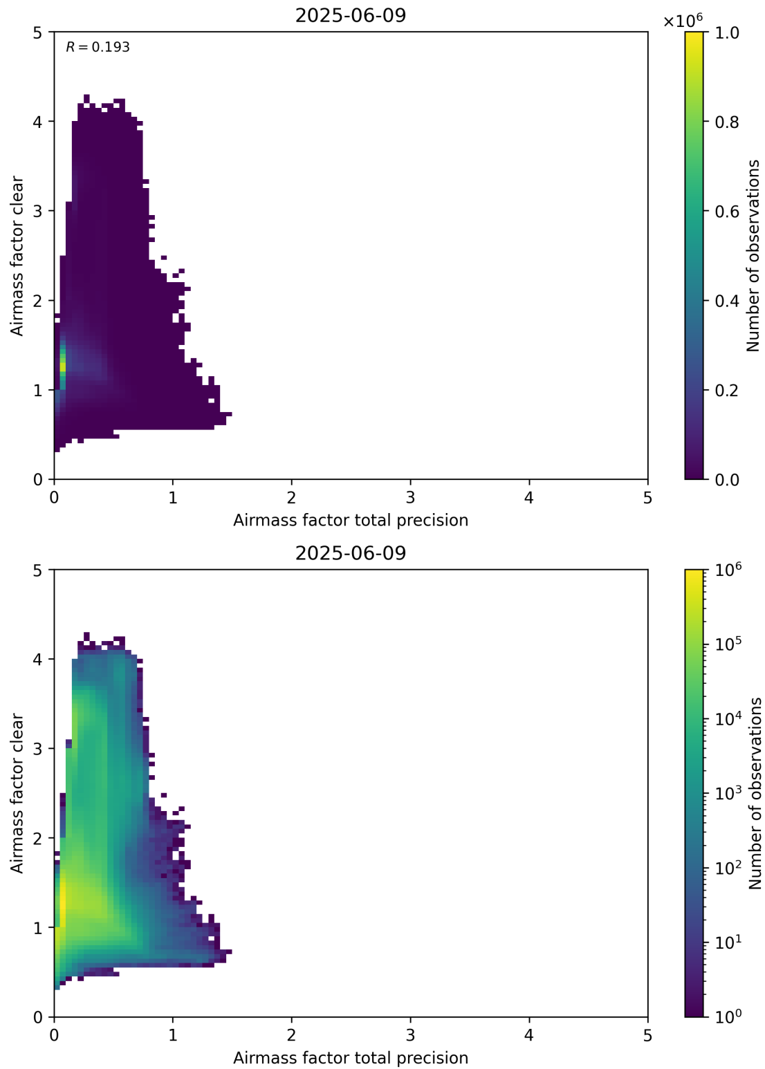
Figure 108: Scatter density plot of “Airmass factor total precision” against “Airmass factor clear” for 2025-06-08 to 2025-06-10.
