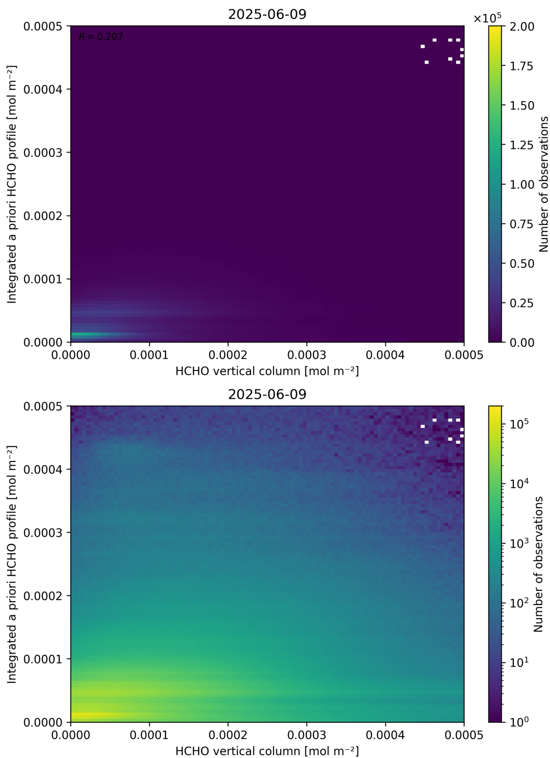
Figure 135: Scatter density plot of “HCHO vertical column” against “Integrated a priori HCHO profile” for 2025-06-08 to 2025-06-10.
