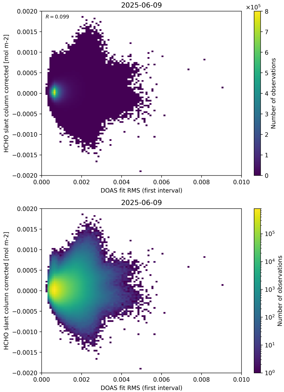
Figure 62: Scatter density plot of “DOAS fit RMS (first interval)” against “HCHO slant column corrected” for 2025-06-08 to 2025-06-10.
