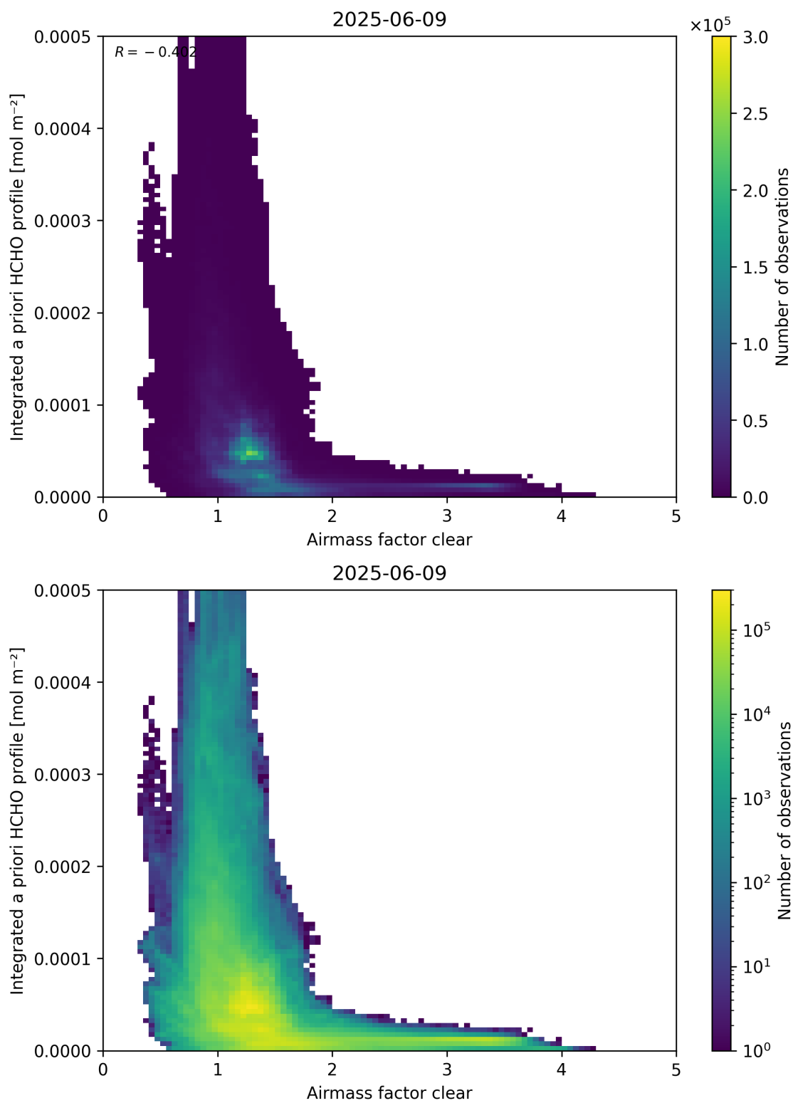
Figure 76: Scatter density plot of “Airmass factor clear” against “Integrated a priori HCHO profile” for 2025-06-08 to 2025-06-10.
