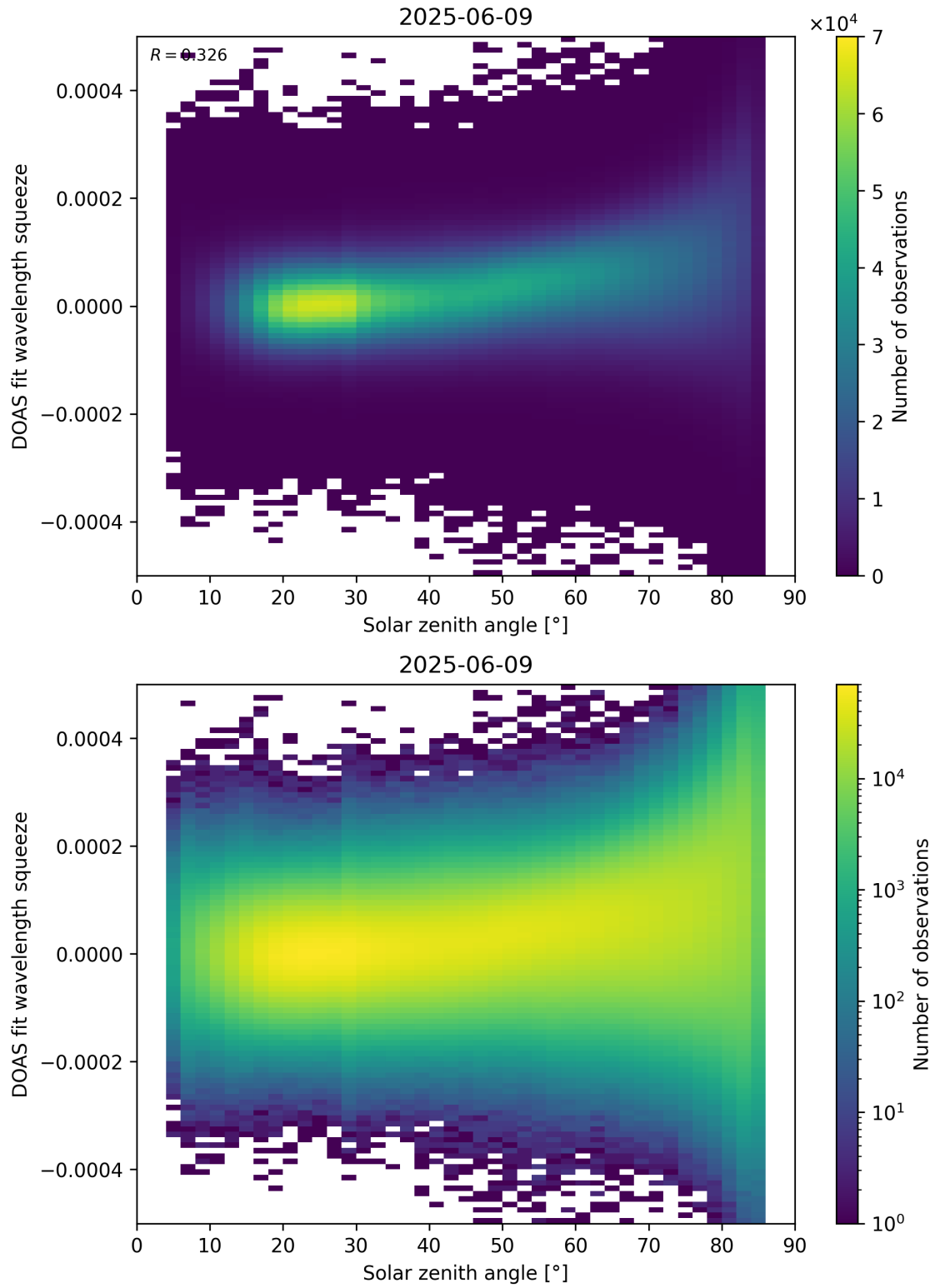
Figure 169: Scatter density plot of “Solar zenith angle” against “DOAS fit wavelength squeeze” for 2025-06-08 to 2025-06-10.
