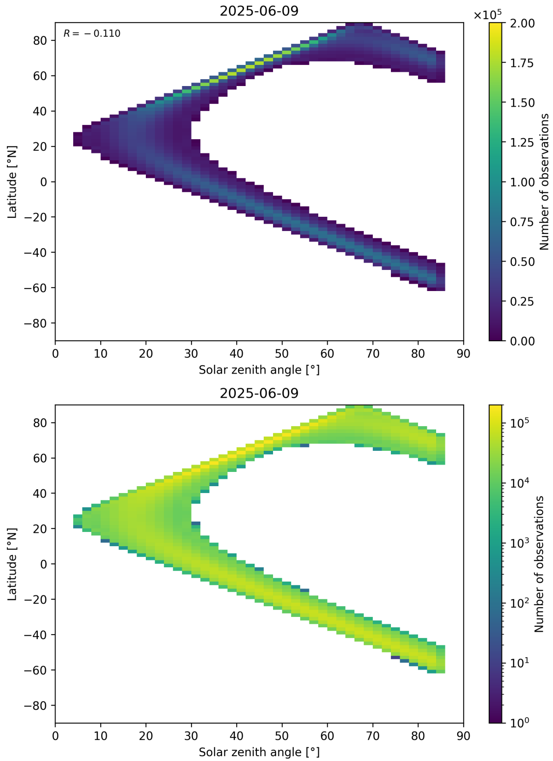
Figure 181: Scatter density plot of “Solar zenith angle” against “Latitude” for 2025-06-08 to 2025-06-10.
