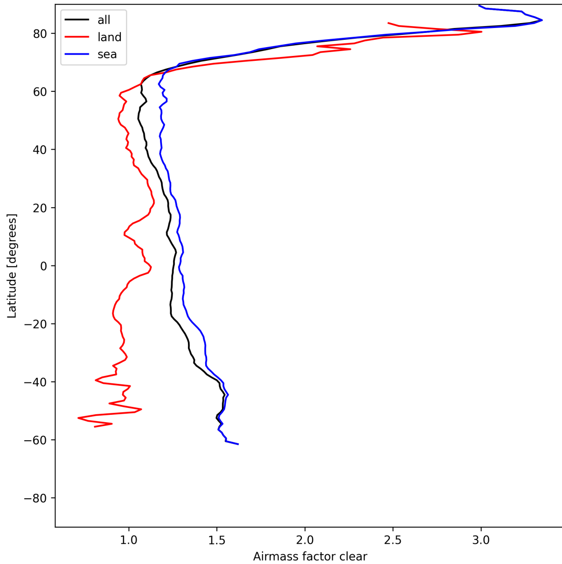
Figure 28: Zonal average of “Airmass factor clear” for 2025-06-08 to 2025-06-10.
