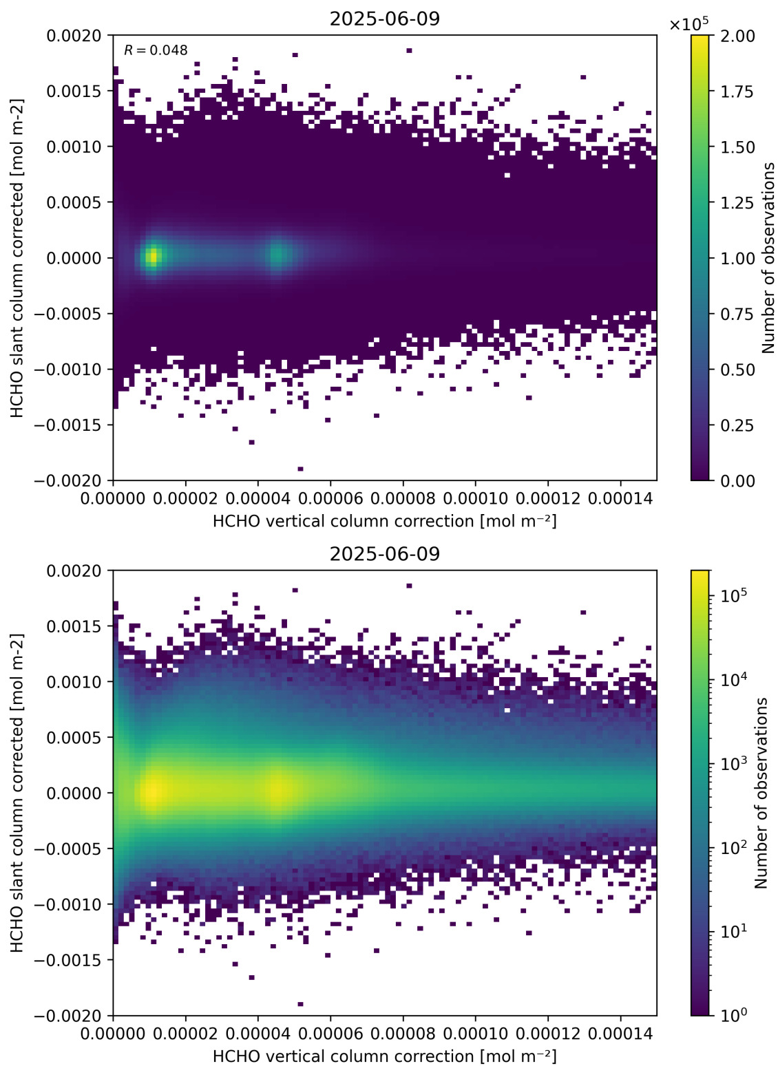
Figure 116: Scatter density plot of “HCHO vertical column correction” against “HCHO slant column corrected” for 2025-06-08 to 2025-06-10.
