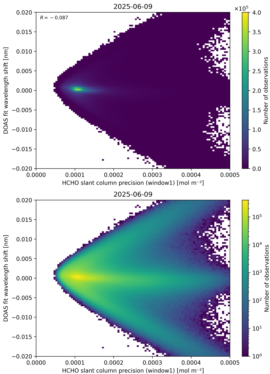
Figure 89: Scatter density plot of “HCHO slant column precision (window1)” against “DOAS fit wavelength shift” for 2025-06-08 to 2025-06-10.
