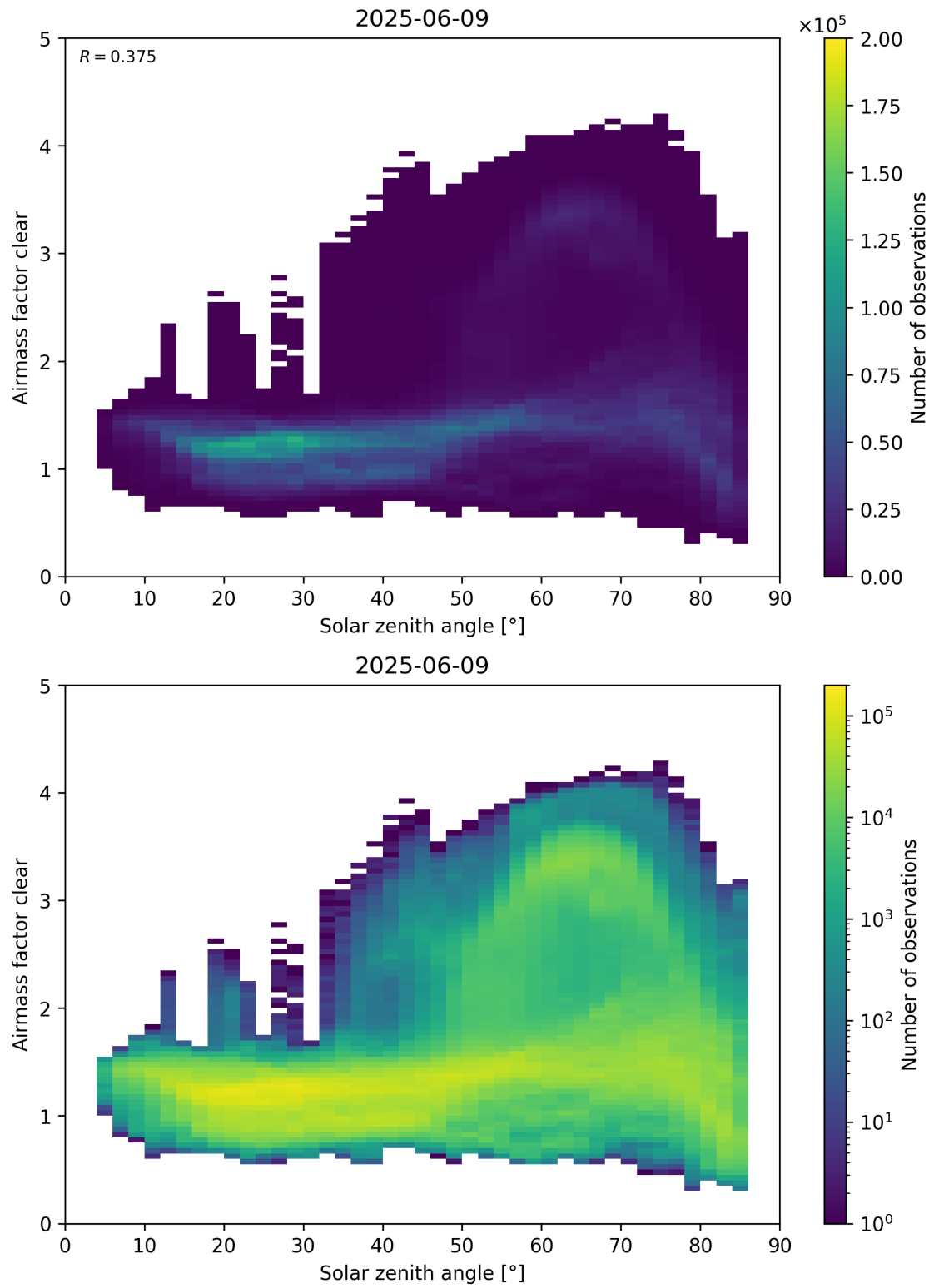
Figure 170: Scatter density plot of “Solar zenith angle” against “Airmass factor clear” for 2025-06-08 to 2025-06-10.
