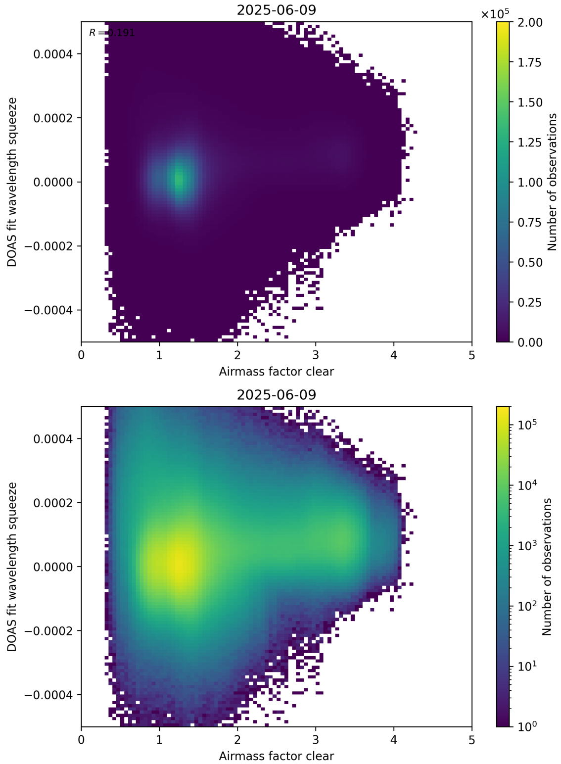
Figure 73: Scatter density plot of “Airmass factor clear” against “DOAS fit wavelength squeeze” for 2025-06-08 to 2025-06-10.
