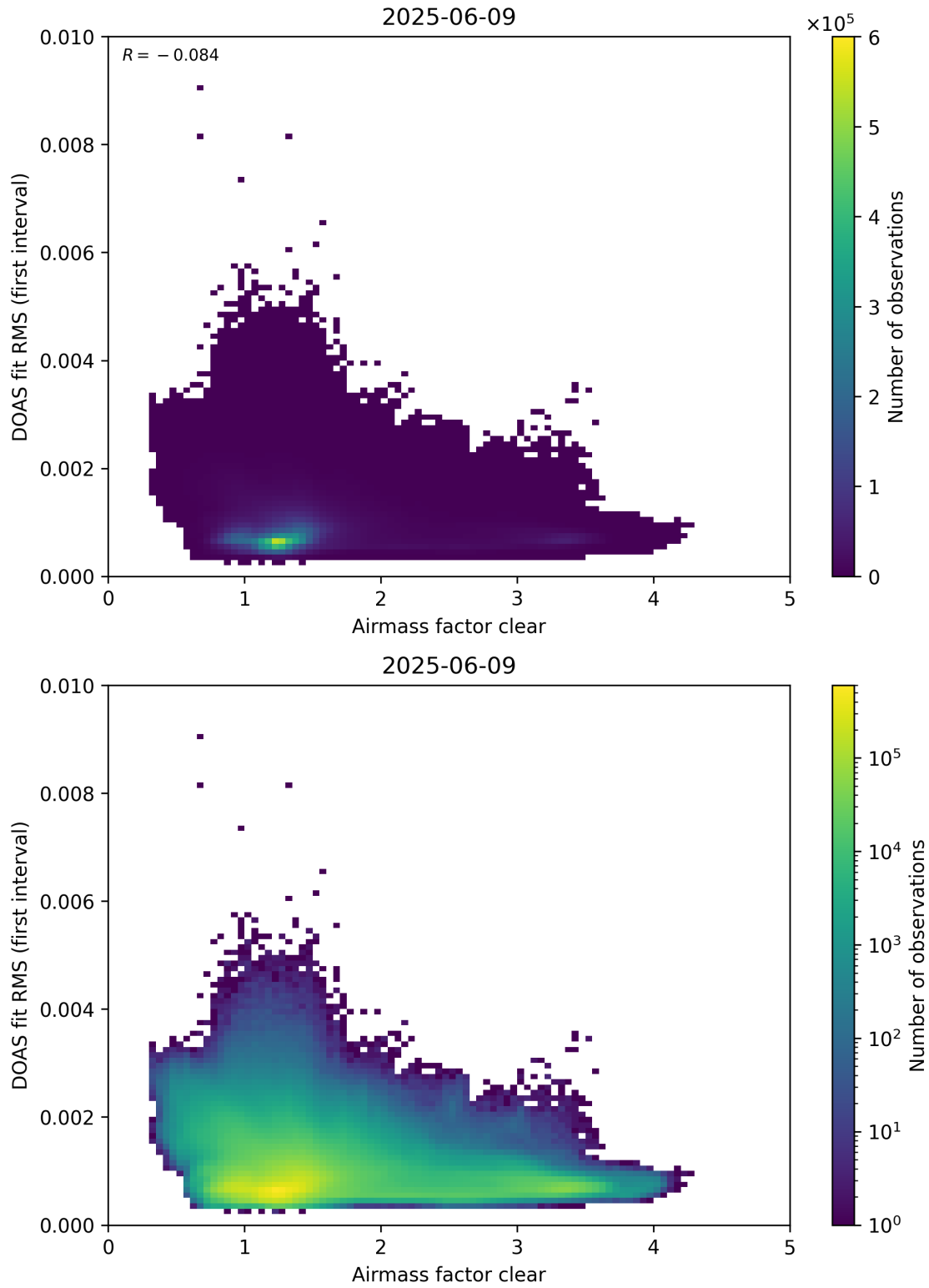
Figure 71: Scatter density plot of “Airmass factor clear” against “DOAS fit RMS (first interval)” for 2025-06-08 to 2025-06-10.
