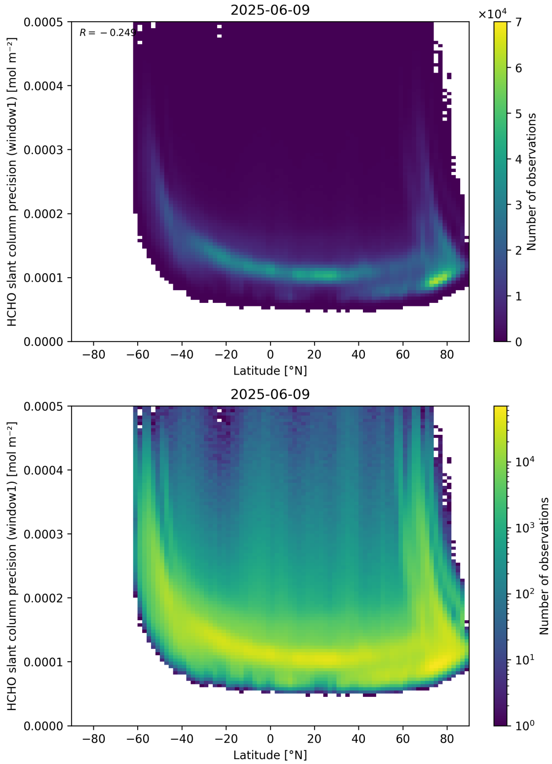
Figure 160: Scatter density plot of “Latitude” against “HCHO slant column precision (window1)” for 2025-06-08 to 2025-06-10.
