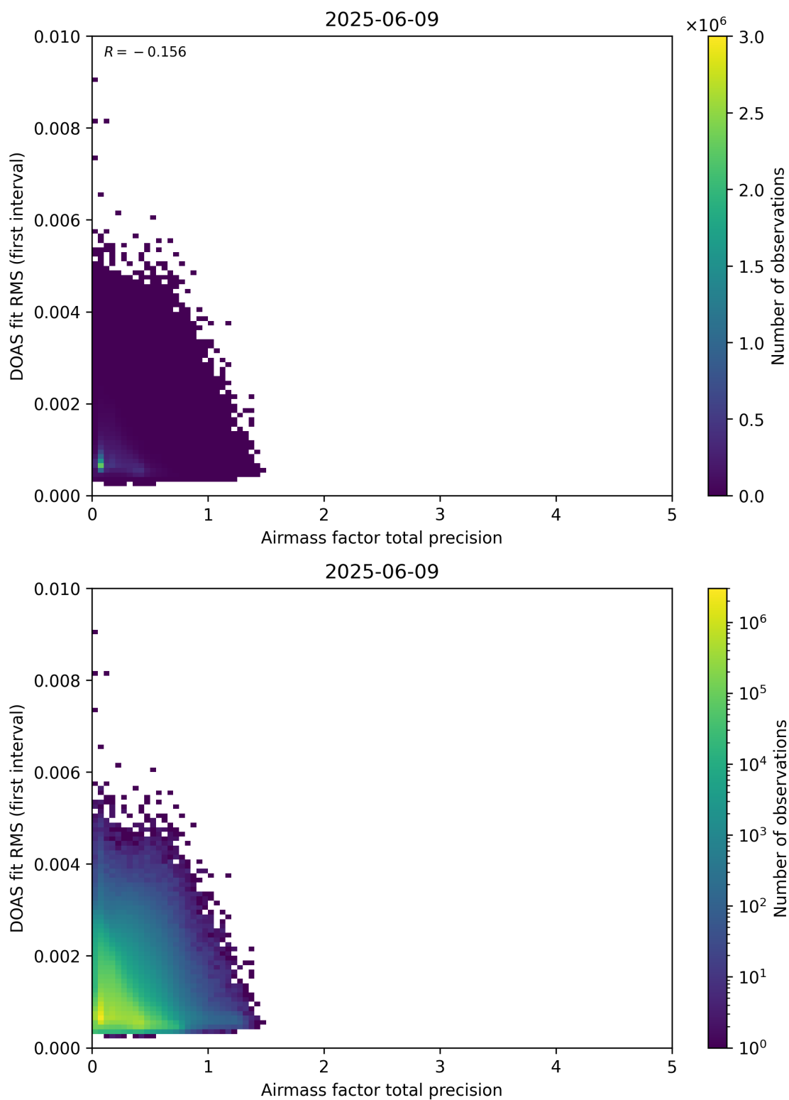
Figure 105: Scatter density plot of “Airmass factor total precision” against “DOAS fit RMS (first interval)” for 2025-06-08 to 2025-06-10.
