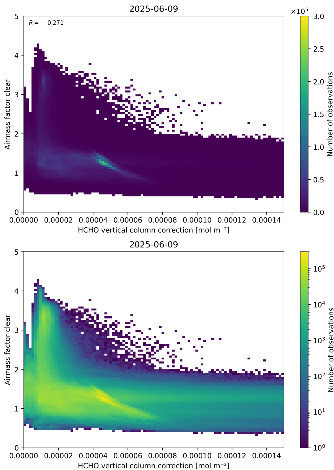
Figure 115: Scatter density plot of “HCHO vertical column correction” against “Airmass factor clear” for 2025-06-08 to 2025-06-10.
