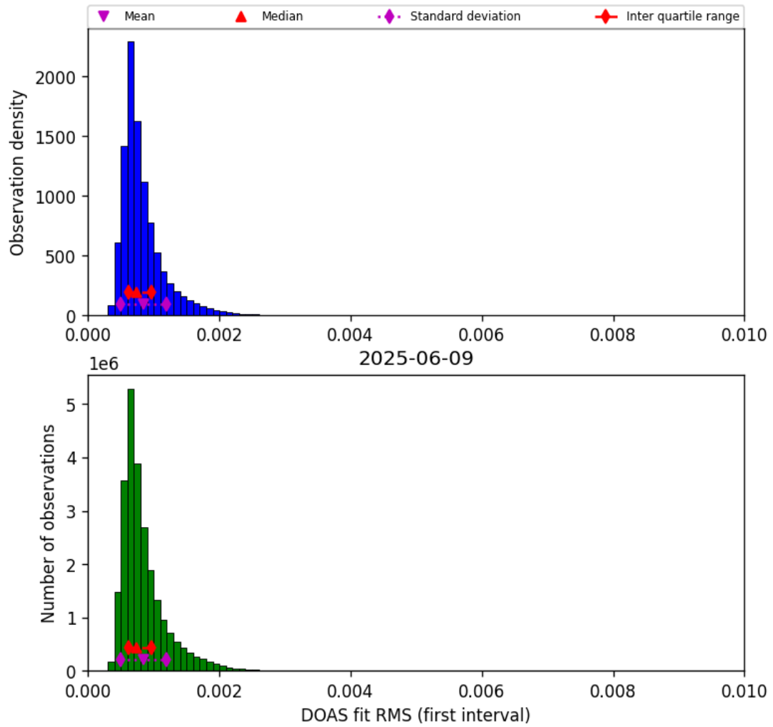
Figure 46: Histogram of “DOAS fit RMS (first interval)” for 2025-06-08 to 2025-06-10
