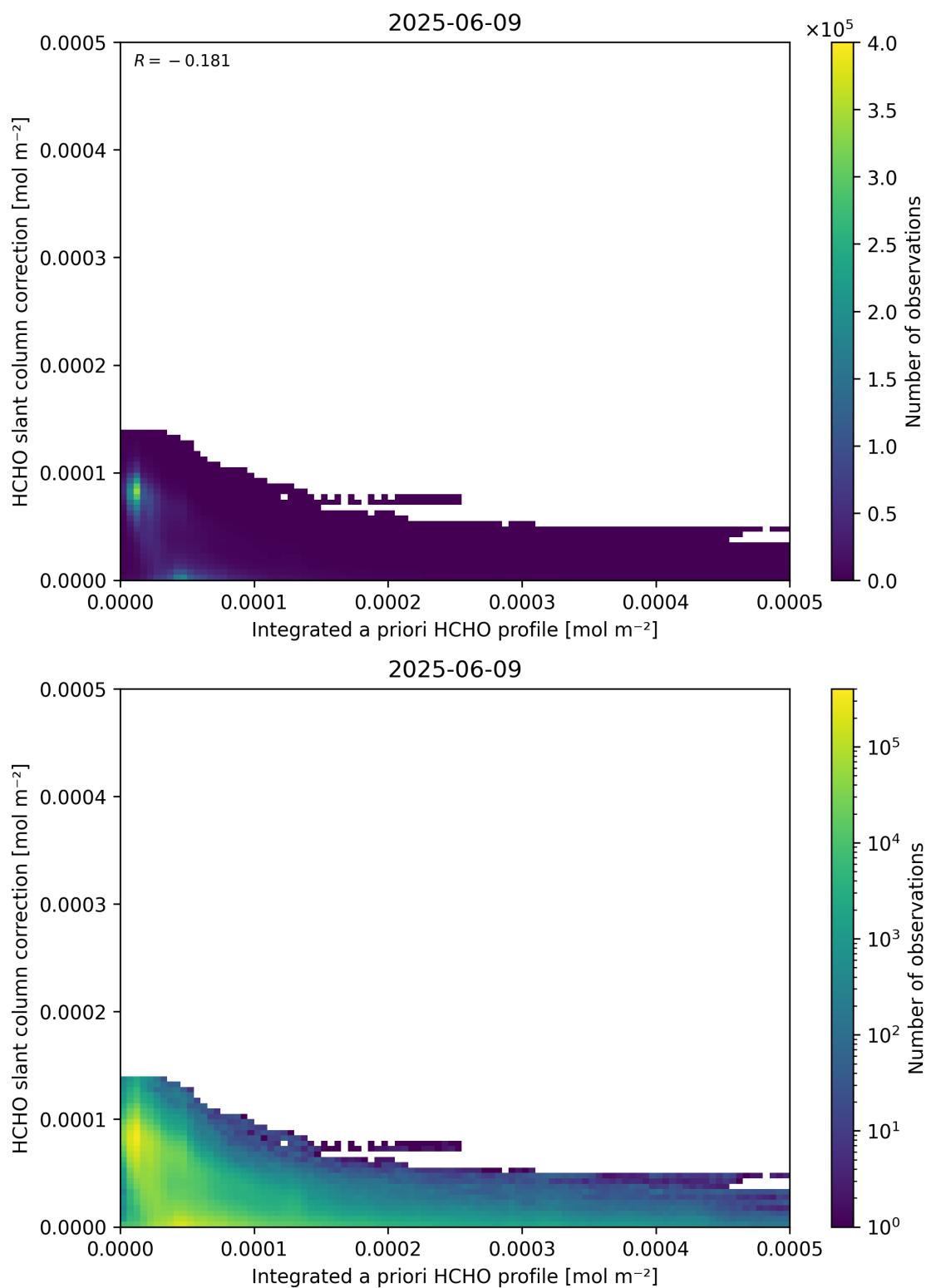
Figure 152: Scatter density plot of “Integrated a priori HCHO profile” against “HCHO slant column correction” for 2025-06-08 to 2025-06-10.
