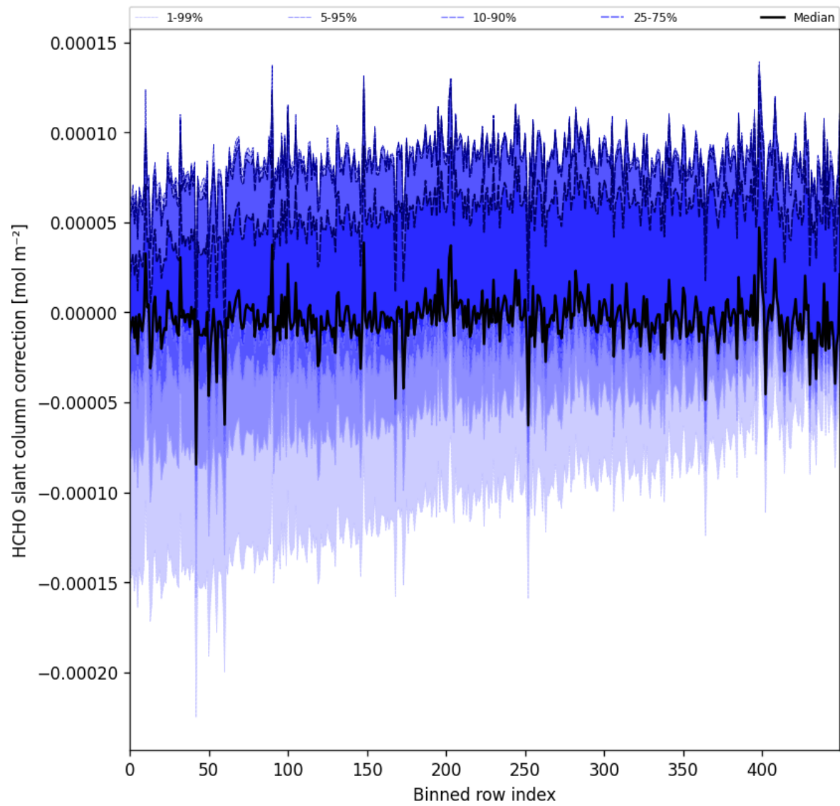
Figure 61: Along track statistics of “HCHO slant column correction” for 2025-06-08 to 2025-06-10
