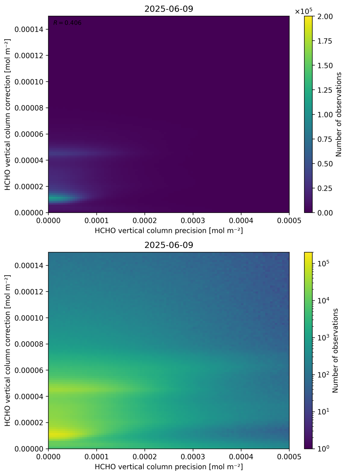
Figure 146: Scatter density plot of “HCHO vertical column precision” against “HCHO vertical column correction” for 2025-06-08 to 2025-06-10.
