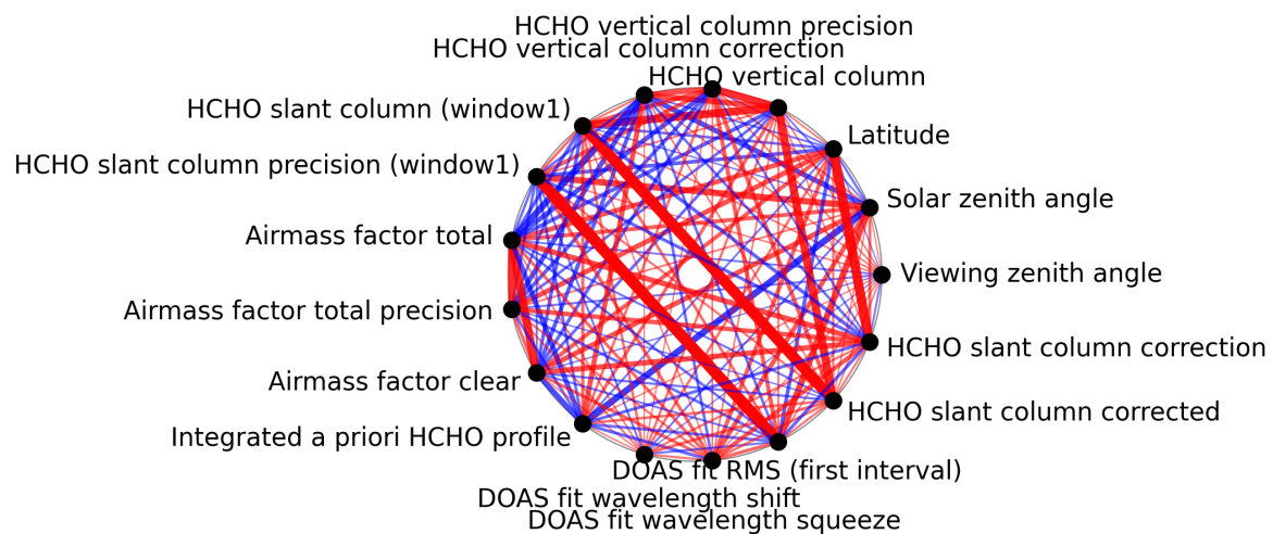
Figure 1: Map of correlation graph for 2025-06-08 to 2025-06-10.
