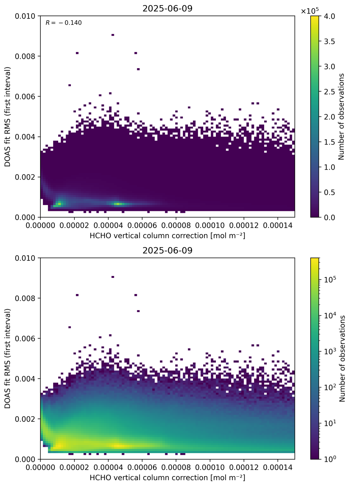
Figure 112: Scatter density plot of “HCHO vertical column correction” against “DOAS fit RMS (first interval)” for 2025-06-08 to 2025-06-10.
