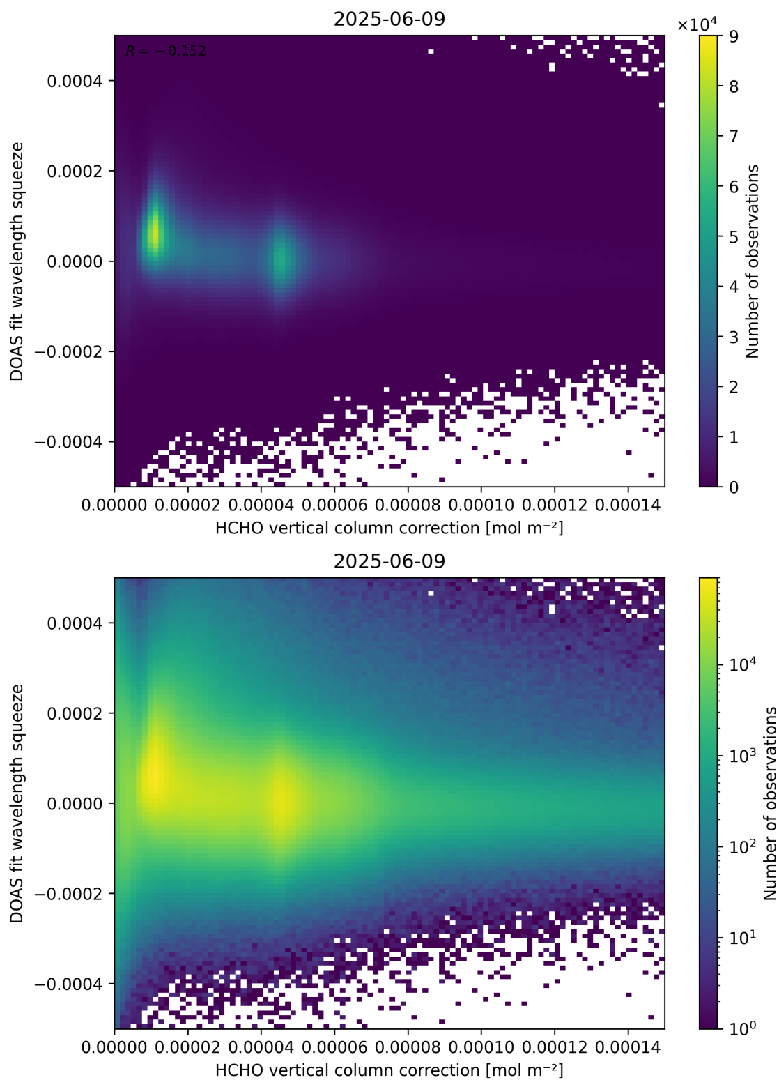
Figure 114: Scatter density plot of “HCHO vertical column correction” against “DOAS fit wavelength squeeze” for 2025-06-08 to 2025-06-10.
