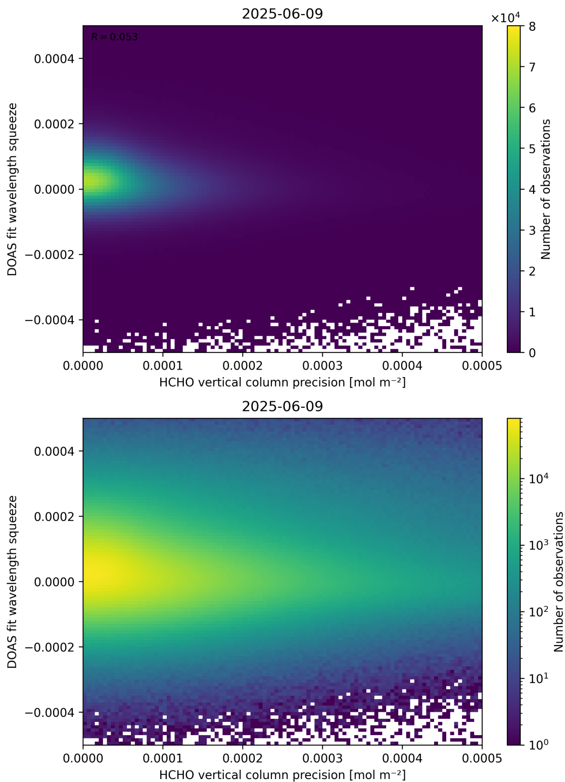
Figure 138: Scatter density plot of “HCHO vertical column precision” against “DOAS fit wavelength squeeze” for 2025-06-08 to 2025-06-10.
