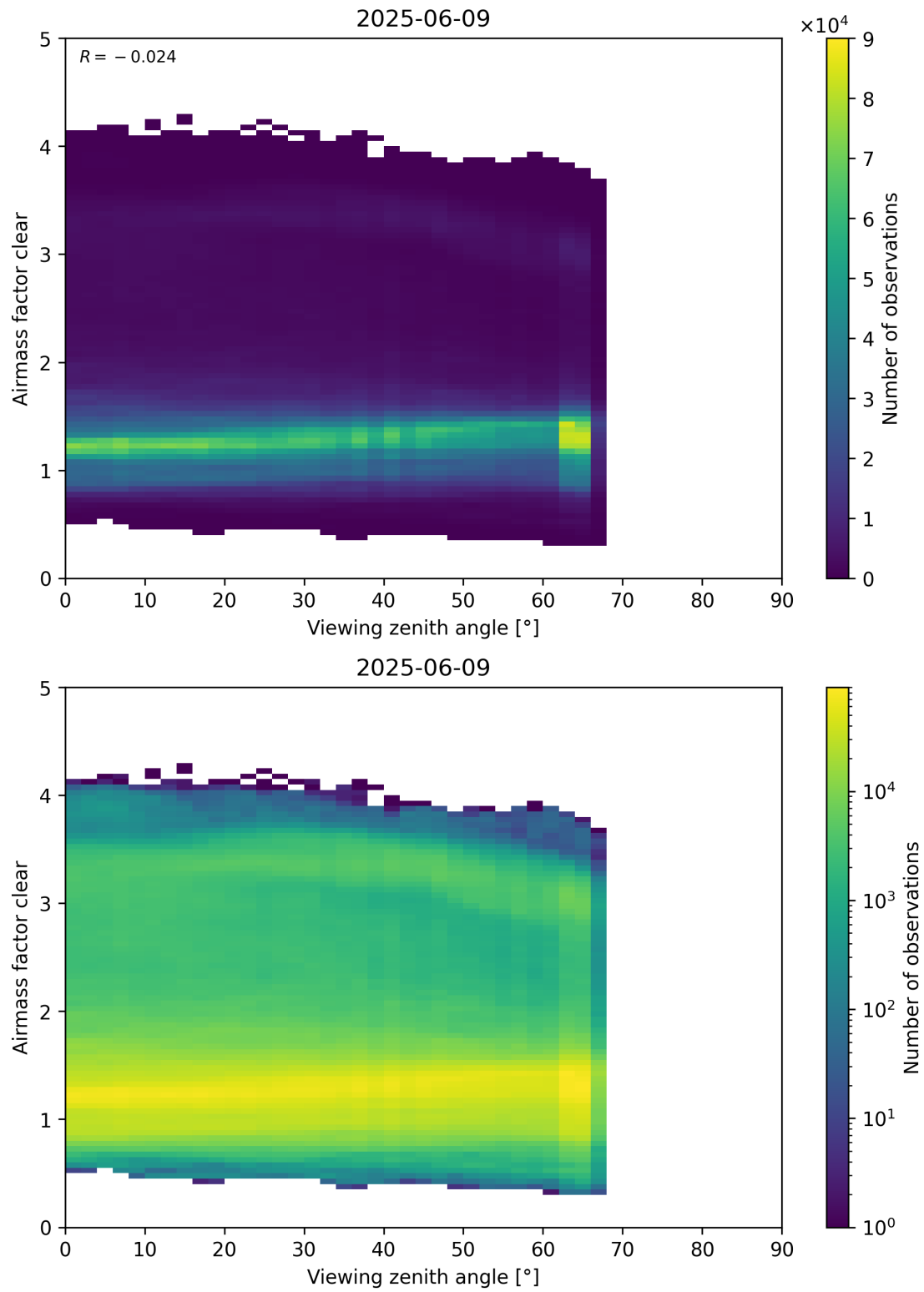
Figure 185: Scatter density plot of “Viewing zenith angle” against “Airmass factor clear” for 2025-06-08 to 2025-06-10.
