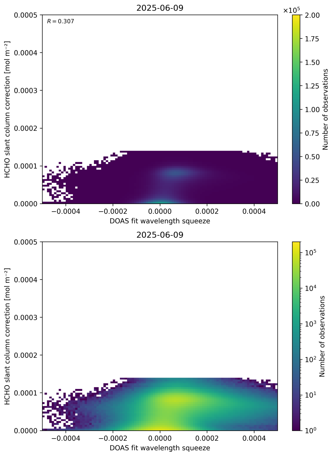
Figure 70: Scatter density plot of “DOAS fit wavelength squeeze” against “HCHO slant column correction” for 2025-06-08 to 2025-06-10.
