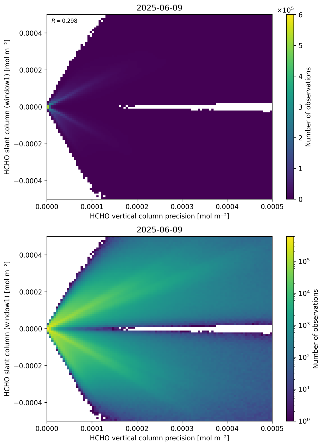
Figure 142: Scatter density plot of “HCHO vertical column precision” against “HCHO slant column (window1)” for 2025-06-08 to 2025-06-10.
