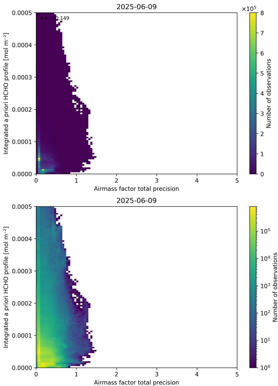
Figure 111: Scatter density plot of “Airmass factor total precision” against “Integrated a priori HCHO profile” for 2025-06-08 to 2025-06-10.
