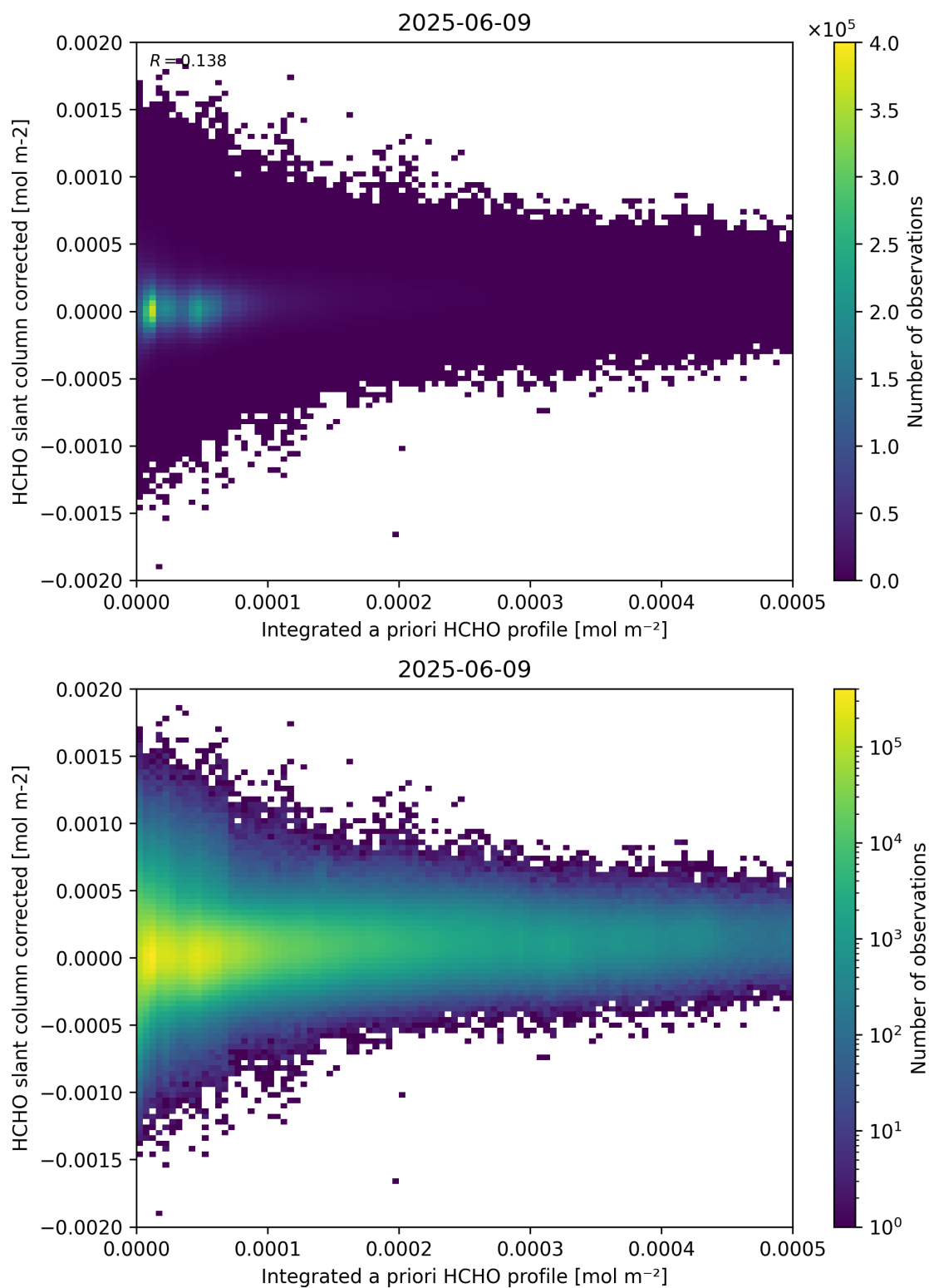
Figure 151: Scatter density plot of “Integrated a priori HCHO profile” against “HCHO slant column corrected” for 2025-06-08 to 2025-06-10.
