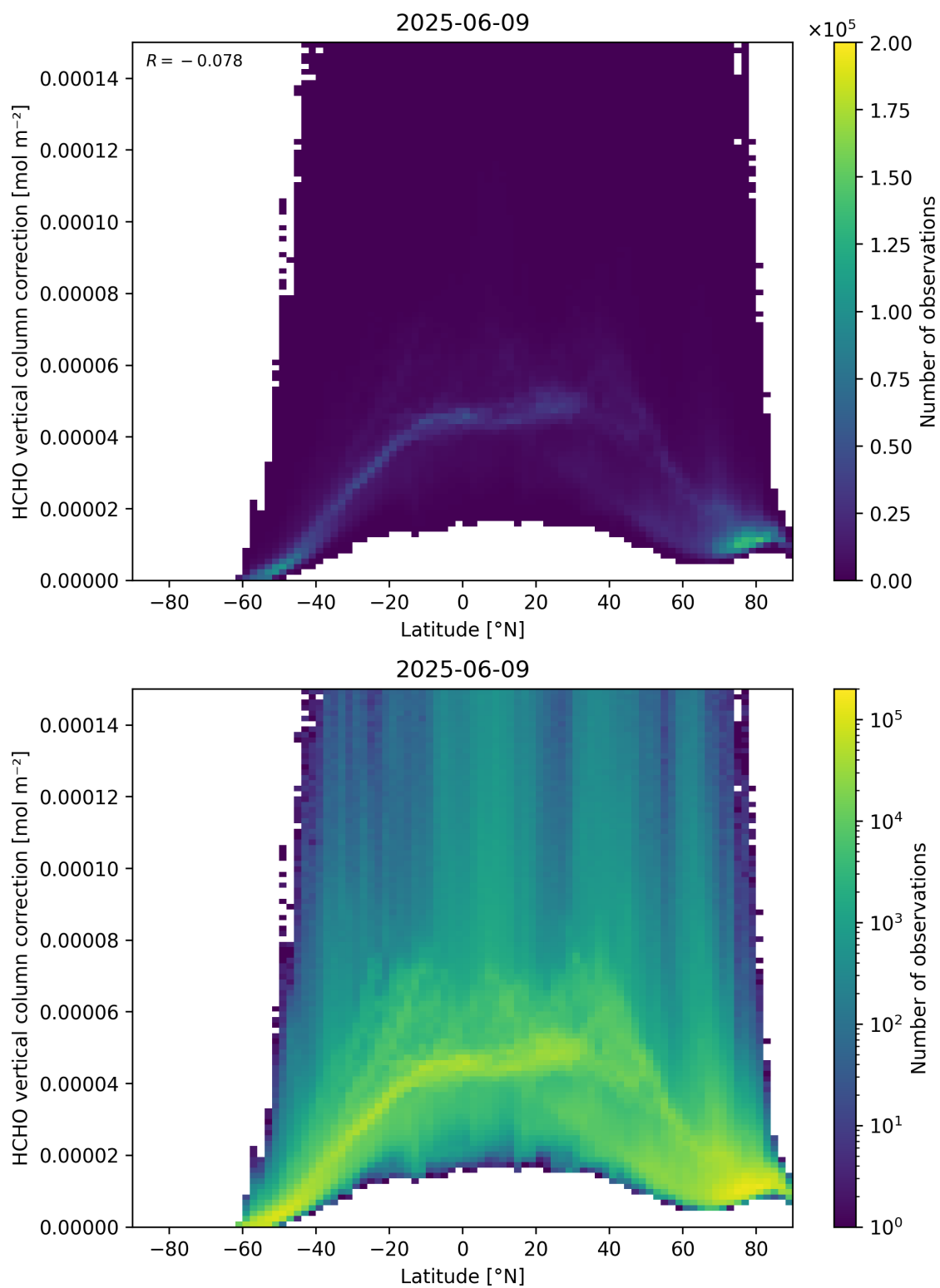
Figure 164: Scatter density plot of “Latitude” against “HCHO vertical column correction” for 2025-06-08 to 2025-06-10.
