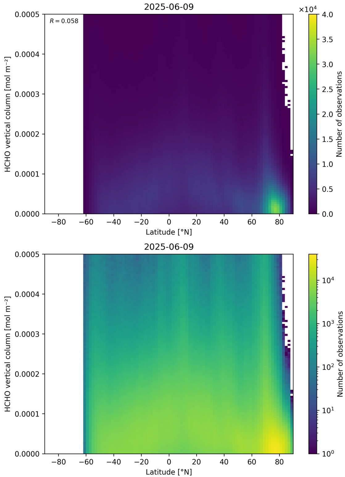
Figure 163: Scatter density plot of “Latitude” against “HCHO vertical column” for 2025-06-08 to 2025-06-10.
