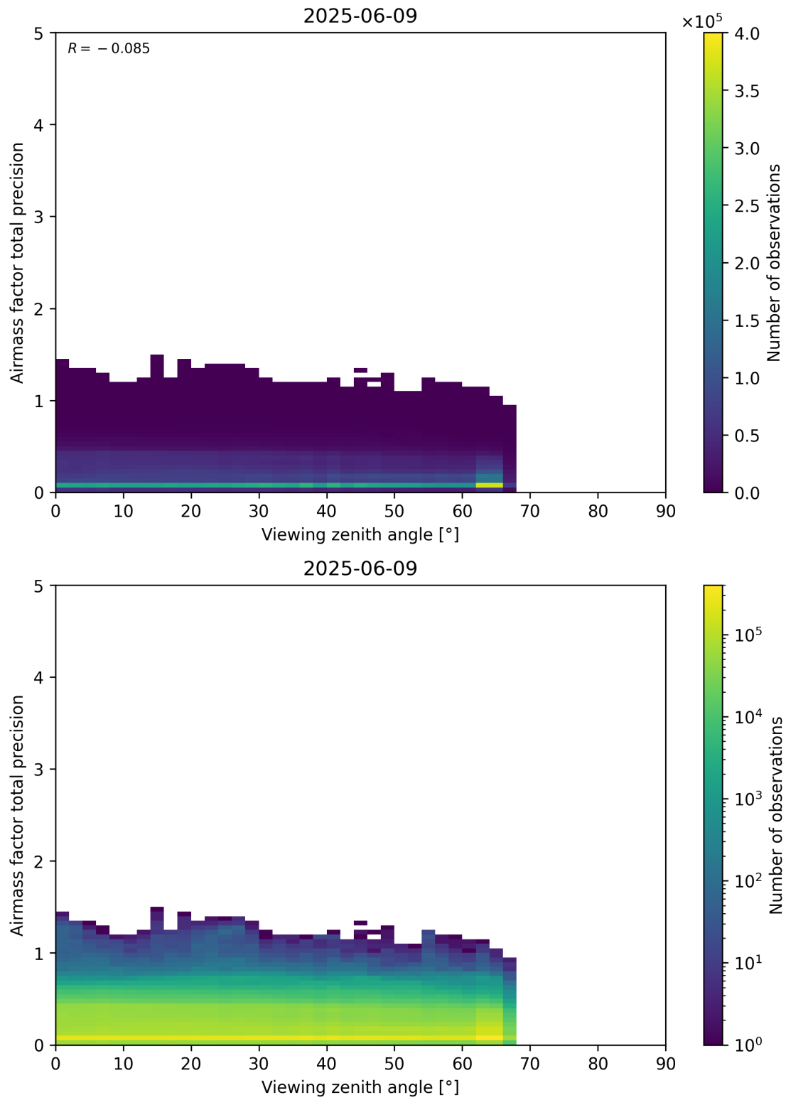
Figure 191: Scatter density plot of “Viewing zenith angle” against “Airmass factor total precision” for 2025-06-08 to 2025-06-10.
