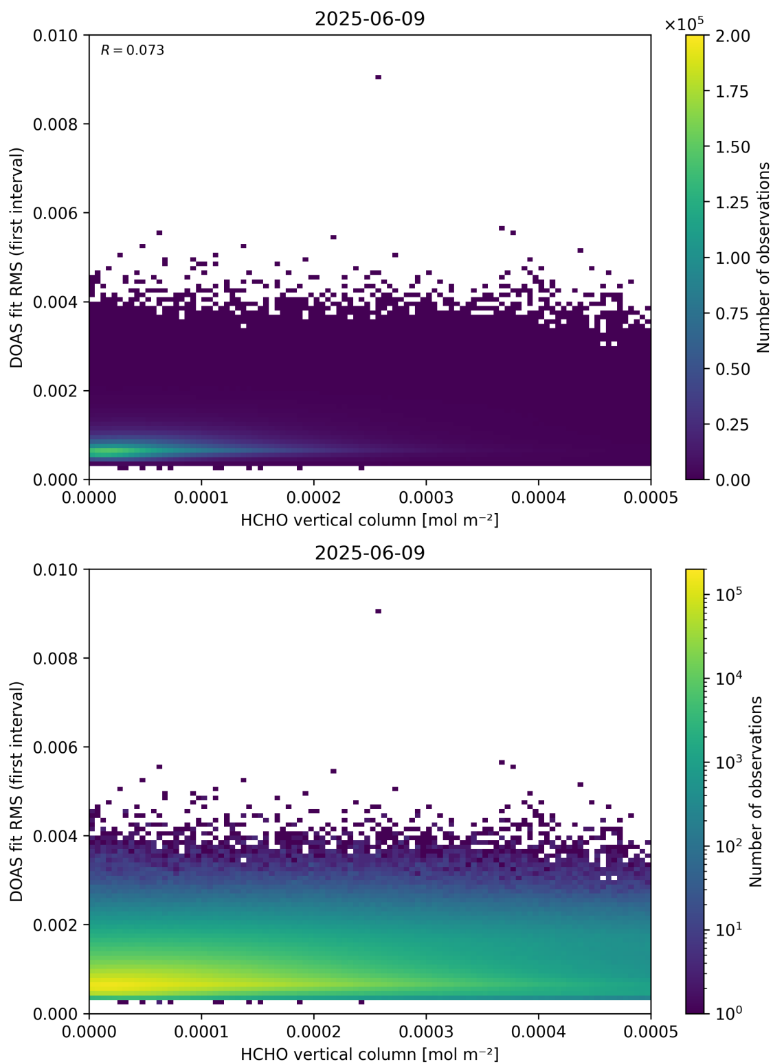
Figure 123: Scatter density plot of “HCHO vertical column” against “DOAS fit RMS (first interval)” for 2025-06-08 to 2025-06-10.
