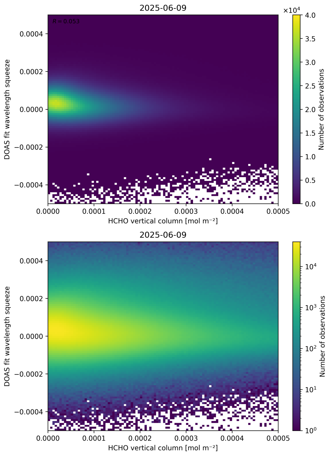
Figure 125: Scatter density plot of “HCHO vertical column” against “DOAS fit wavelength squeeze” for 2025-06-08 to 2025-06-10.
