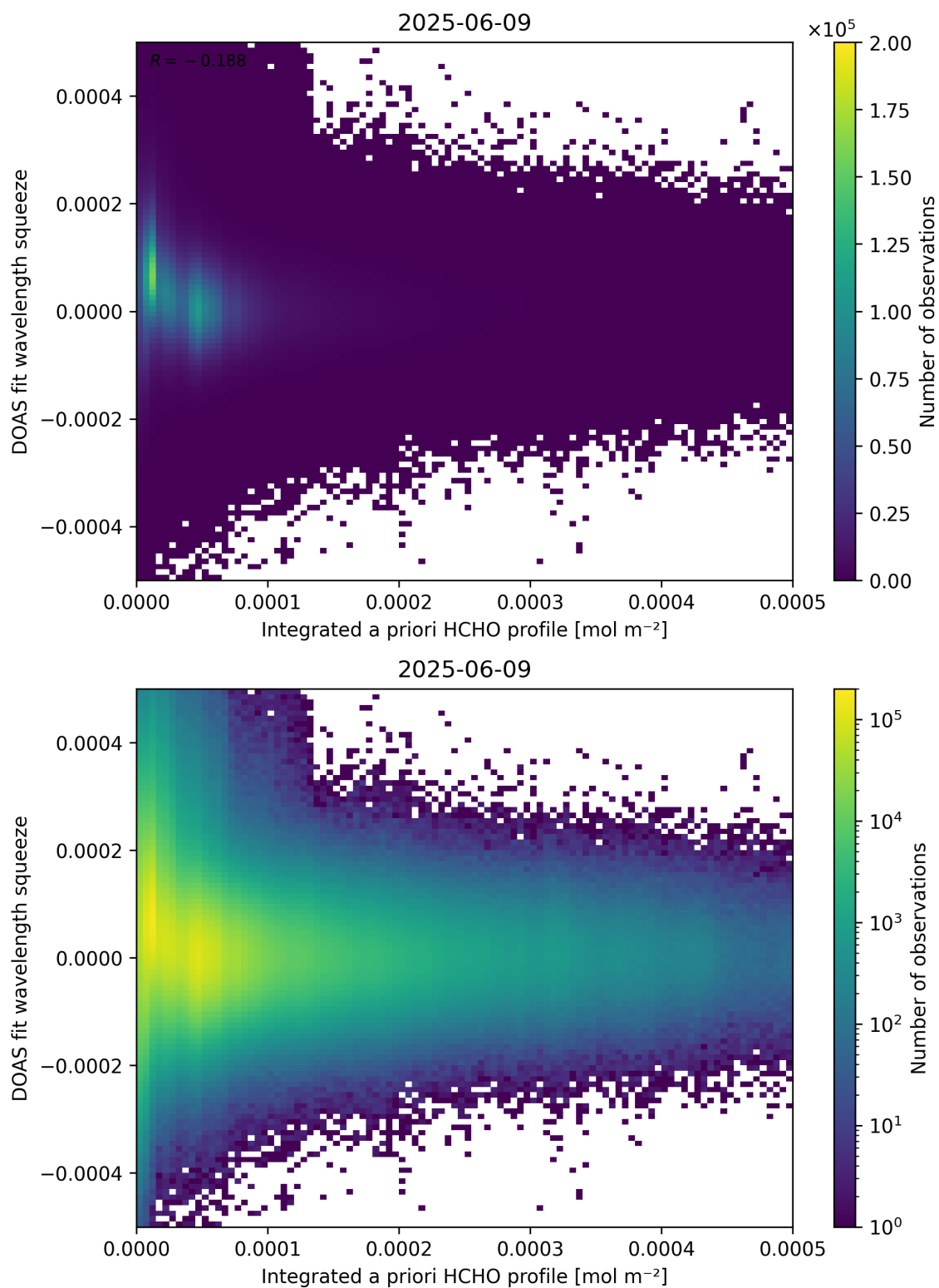
Figure 150: Scatter density plot of “Integrated a priori HCHO profile” against “DOAS fit wavelength squeeze” for 2025-06-08 to 2025-06-10.
