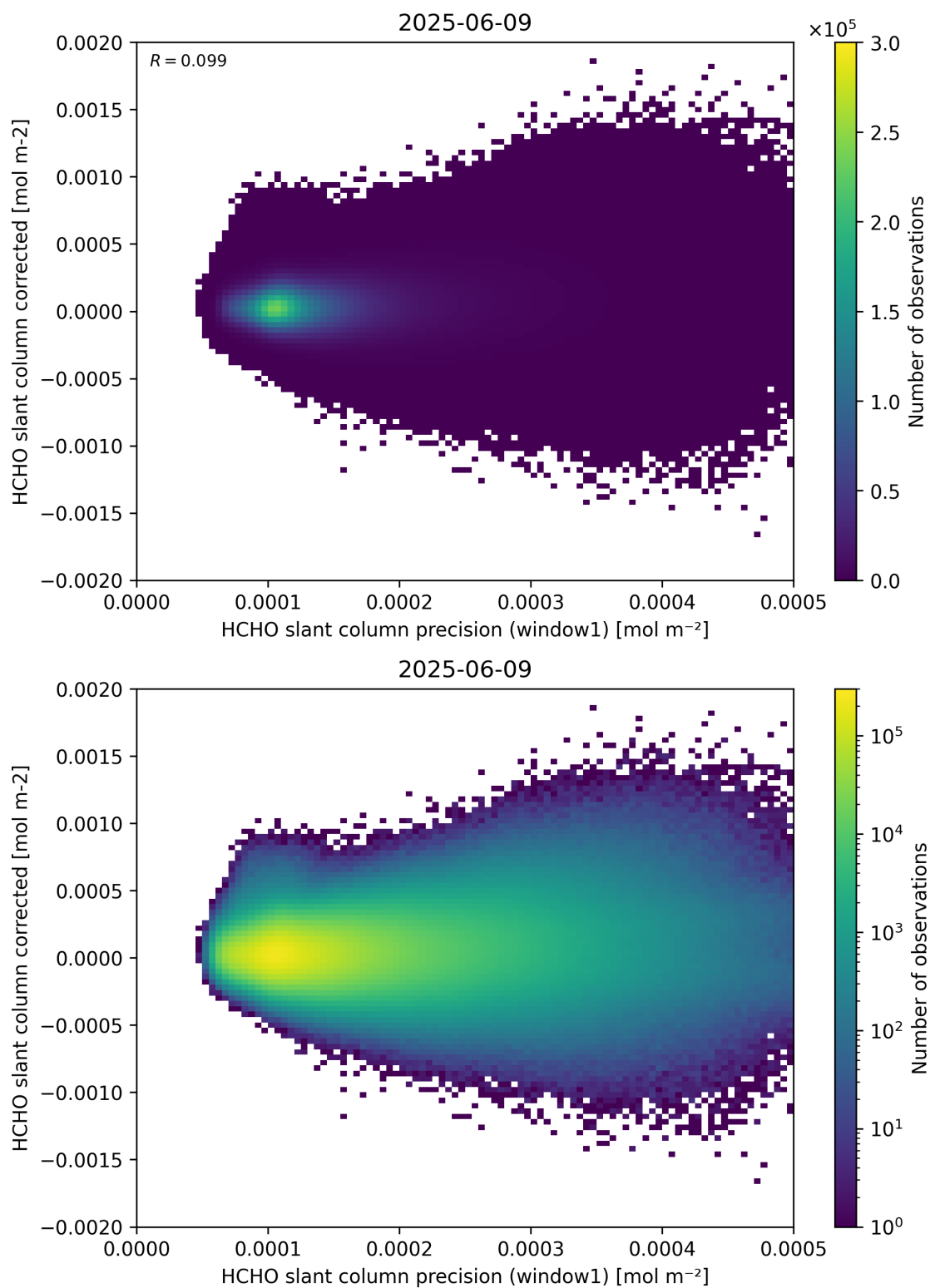
Figure 92: Scatter density plot of “HCHO slant column precision (window1)” against “HCHO slant column corrected” for 2025-06-08 to 2025-06-10.
