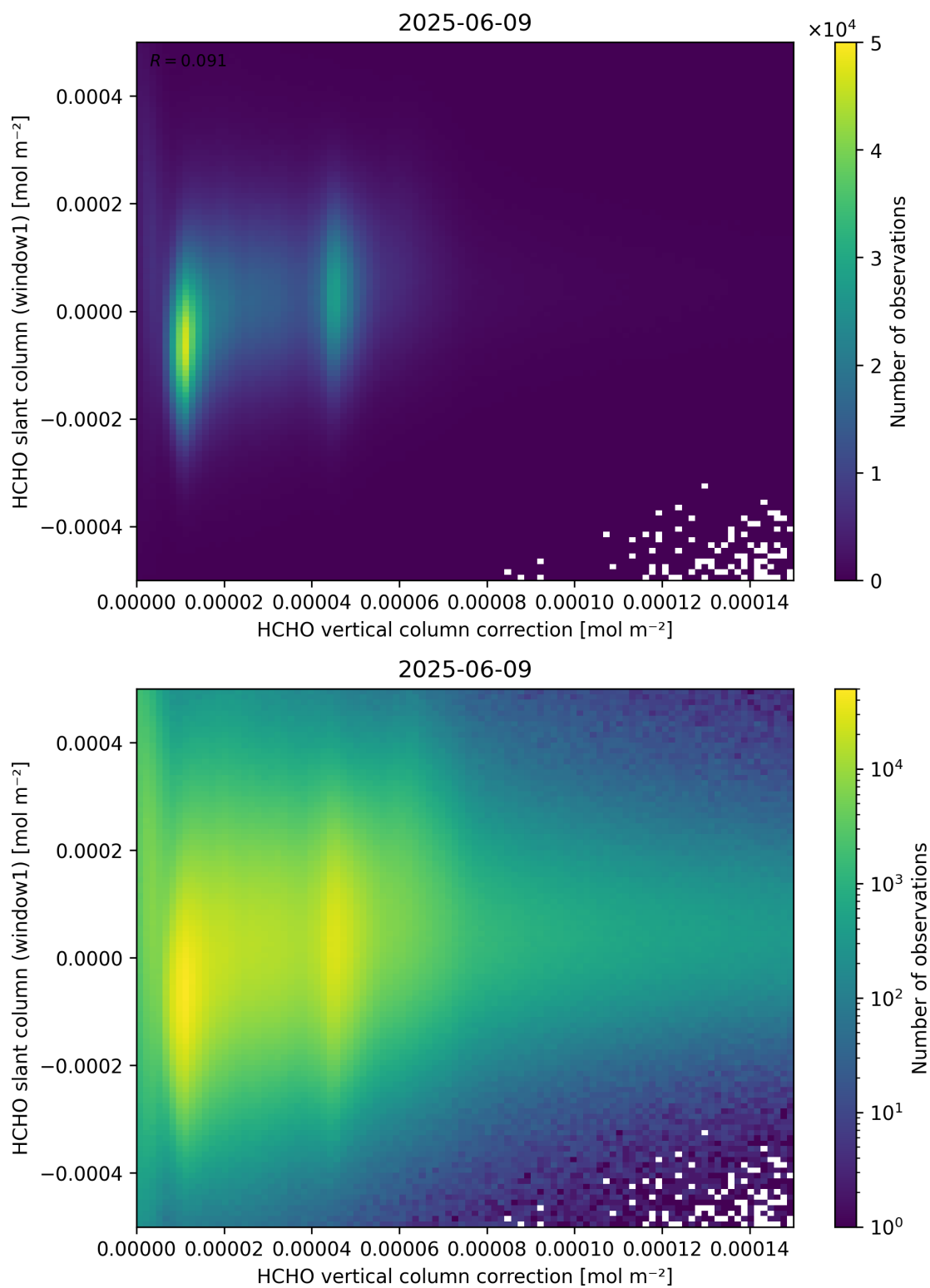
Figure 118: Scatter density plot of “HCHO vertical column correction” against “HCHO slant column (window1)” for 2025-06-08 to 2025-06-10.
