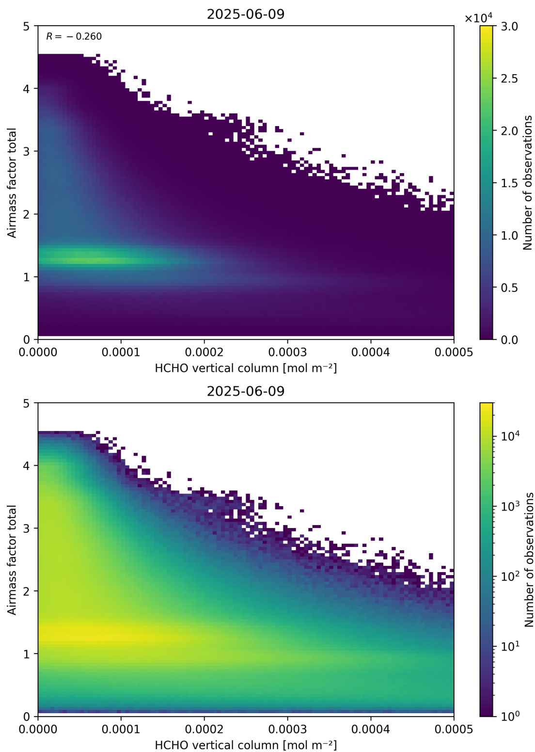
Figure 131: Scatter density plot of “HCHO vertical column” against “Airmass factor total” for 2025-06-08 to 2025-06-10.
