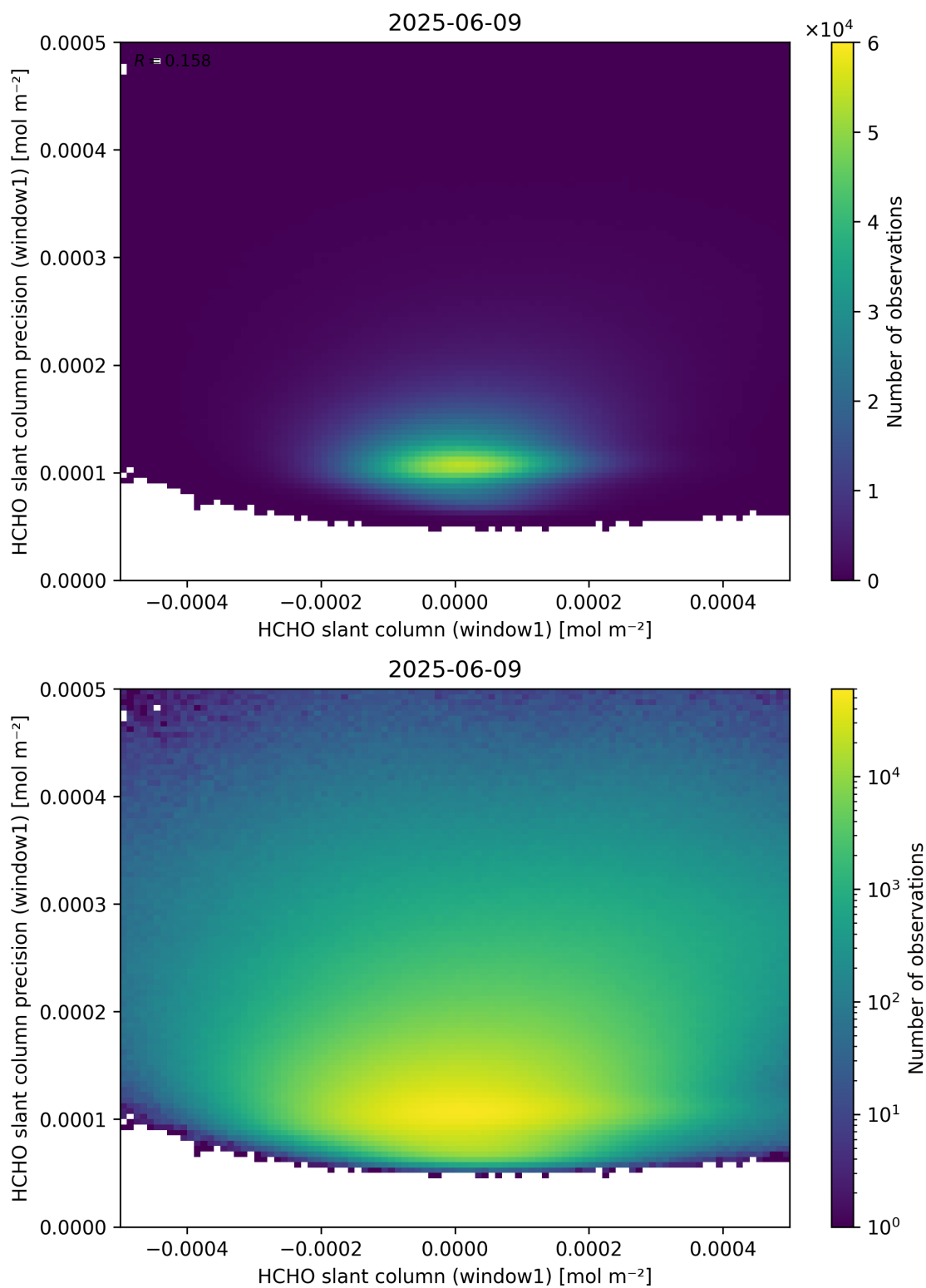
Figure 84: Scatter density plot of “HCHO slant column (window1)” against “HCHO slant column precision (window1)” for 2025-06-08 to 2025-06-10.
