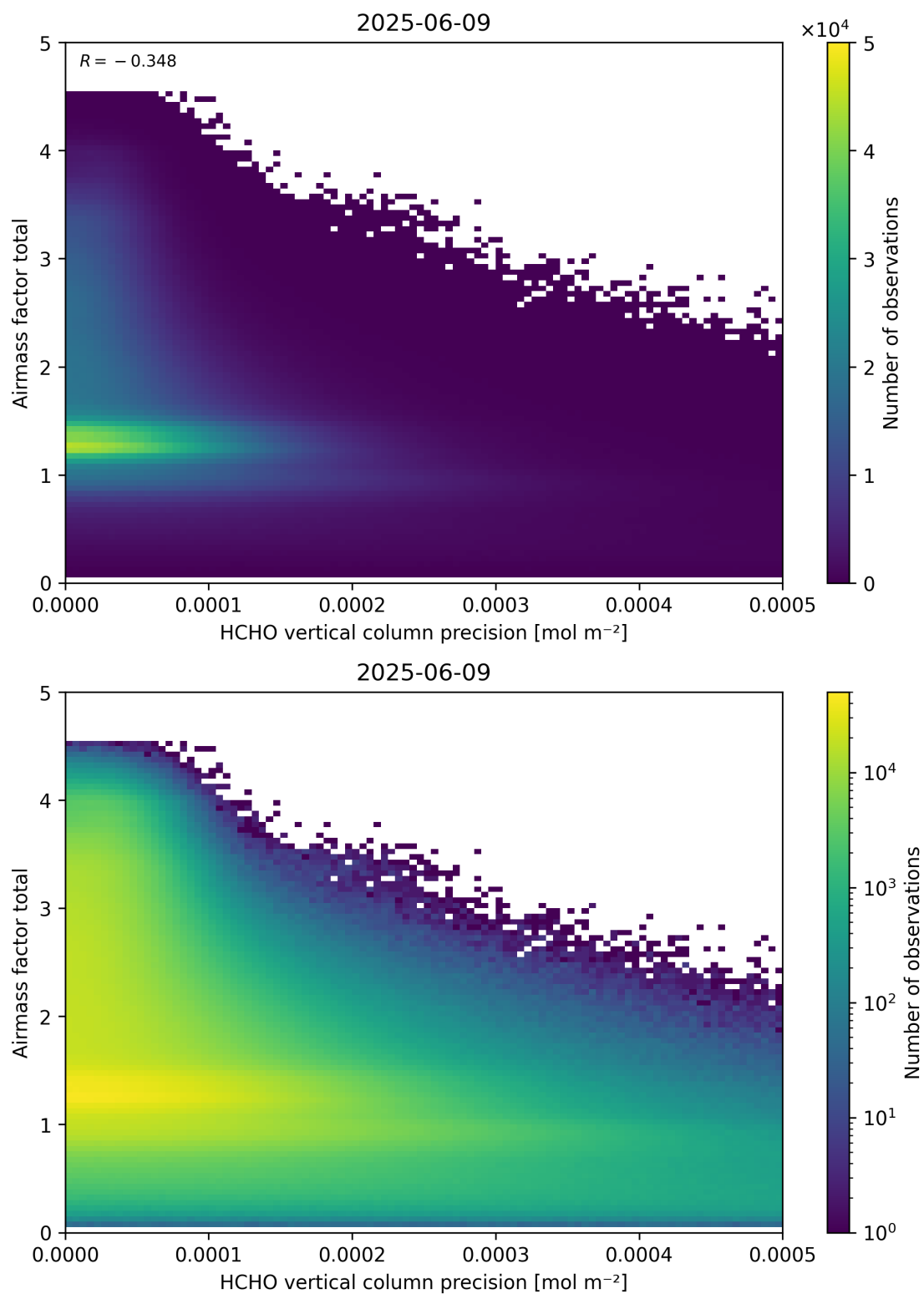
Figure 144: Scatter density plot of “HCHO vertical column precision” against “Airmass factor total” for 2025-06-08 to 2025-06-10.
