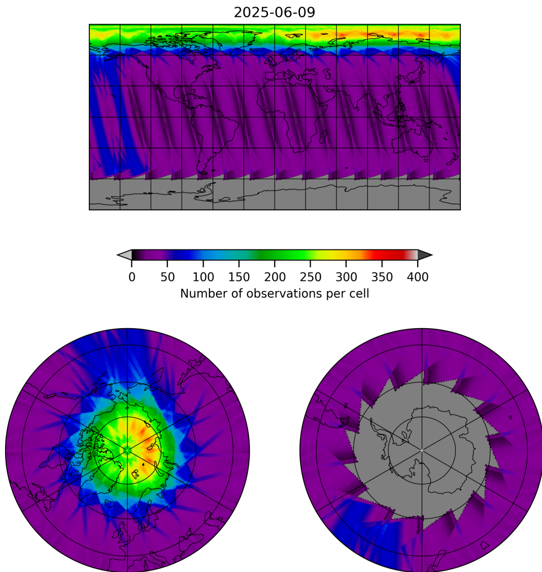
Figure 19: Map of the number of observations for 2025-06-08 to 2025-06-10
