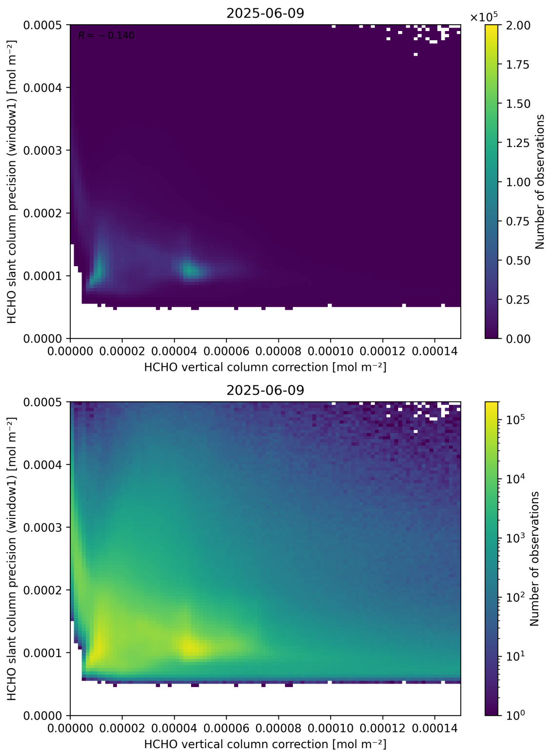
Figure 119: Scatter density plot of “HCHO vertical column correction” against “HCHO slant column precision (window1)” for 2025-06-08 to 2025-06-10.
