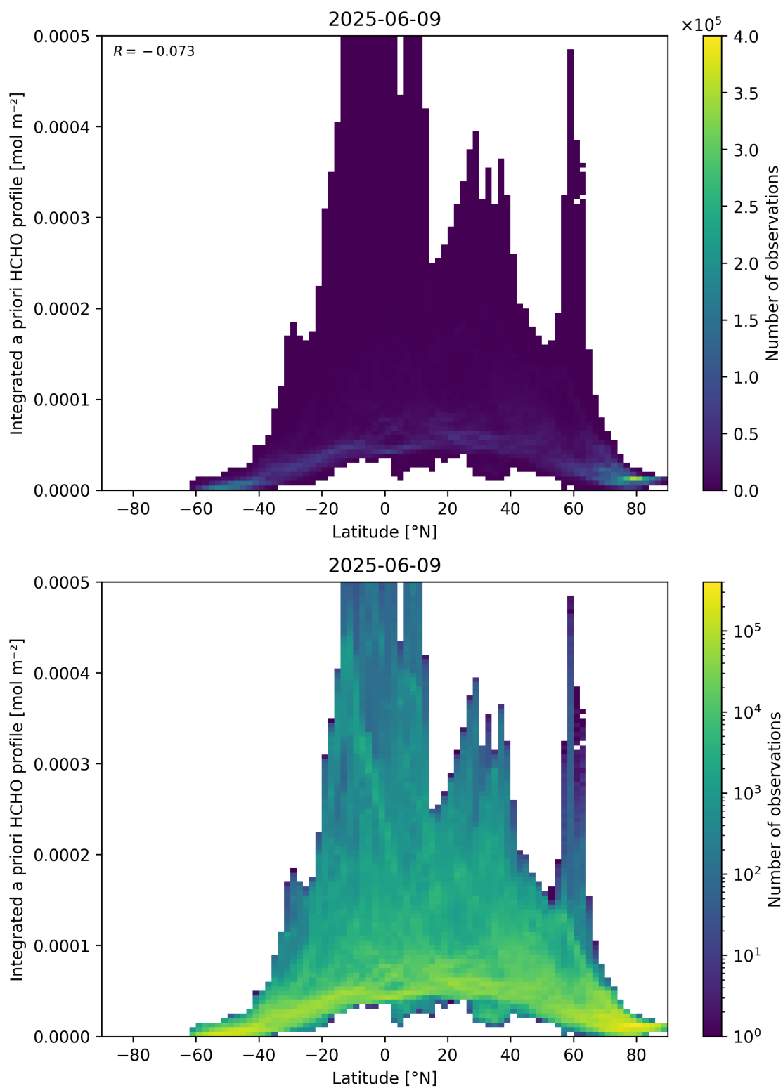
Figure 166: Scatter density plot of “Latitude” against “Integrated a priori HCHO profile” for 2025-06-08 to 2025-06-10.
