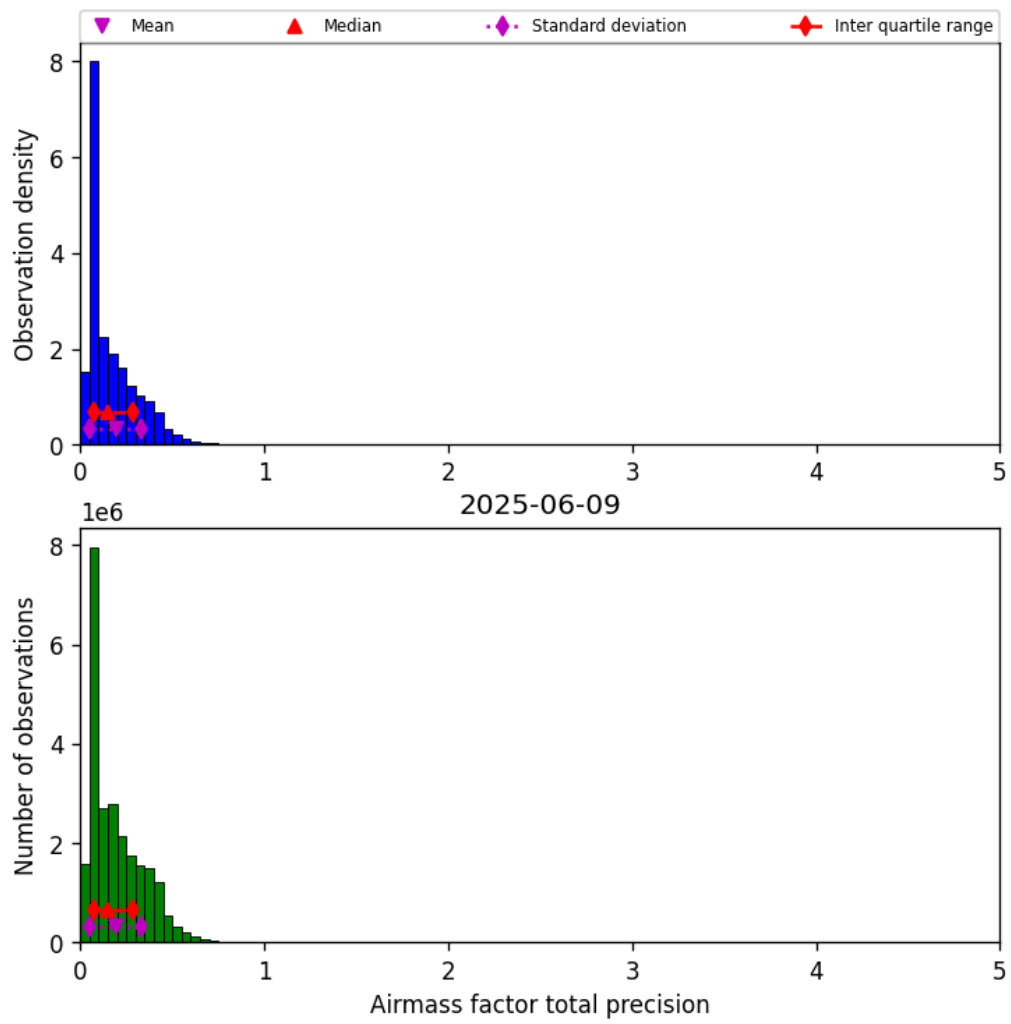
Figure 41: Histogram of “Airmass factor total precision” for 2025-06-08 to 2025-06-10
