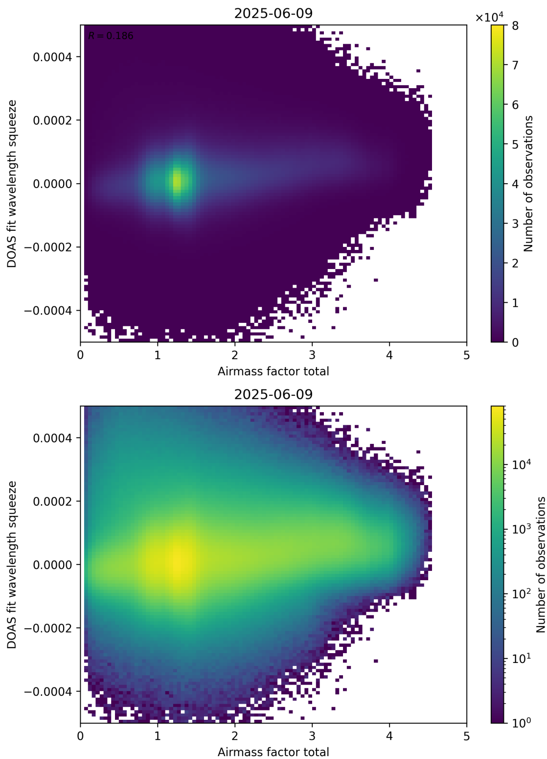
Figure 99: Scatter density plot of “Airmass factor total” against “DOAS fit wavelength squeeze” for 2025-06-08 to 2025-06-10.
