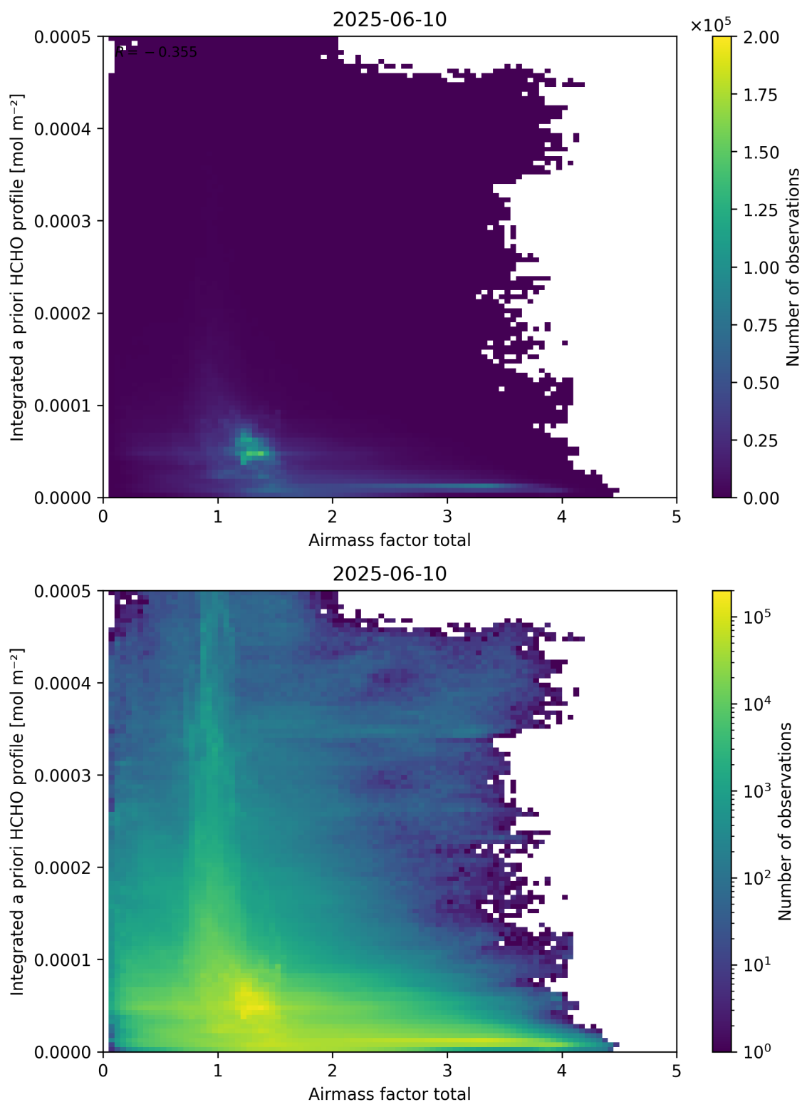
Figure 104: Scatter density plot of “Airmass factor total” against “Integrated a priori HCHO profile” for 2025-06-09 to 2025-06-11.
