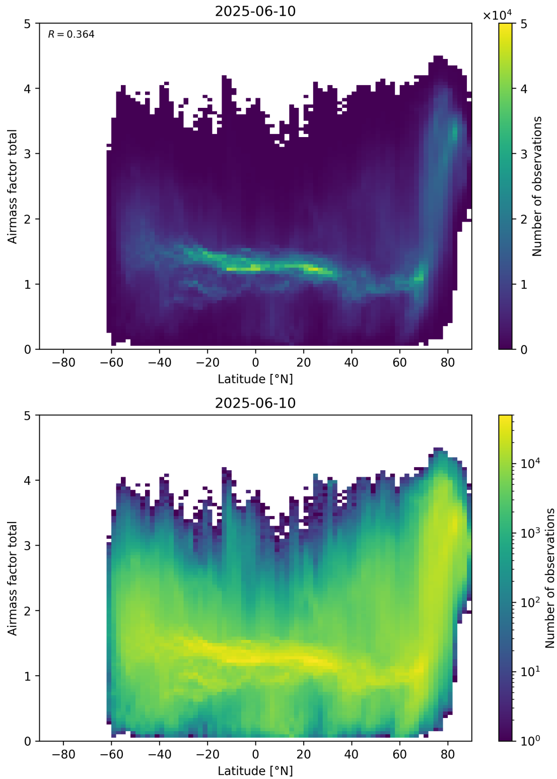
Figure 161: Scatter density plot of “Latitude” against “Airmass factor total” for 2025-06-09 to 2025-06-11.
