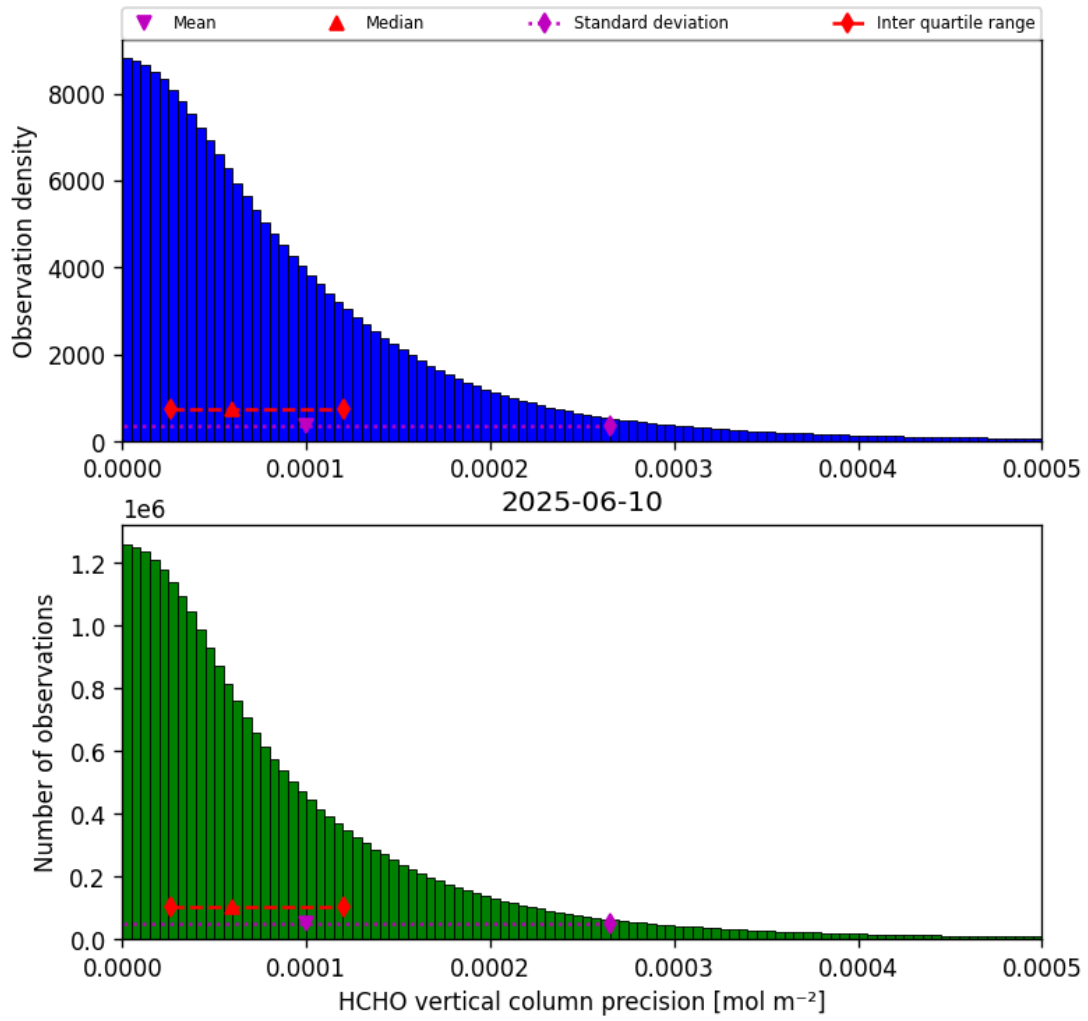
Figure 36: Histogram of “HCHO vertical column precision” for 2025-06-09 to 2025-06-11
