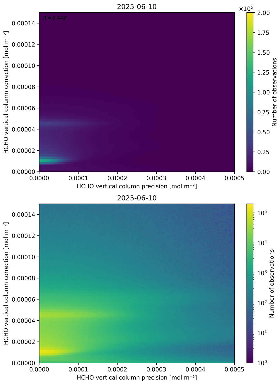
Figure 146: Scatter density plot of “HCHO vertical column precision” against “HCHO vertical column correction” for 2025-06-09 to 2025-06-11.
