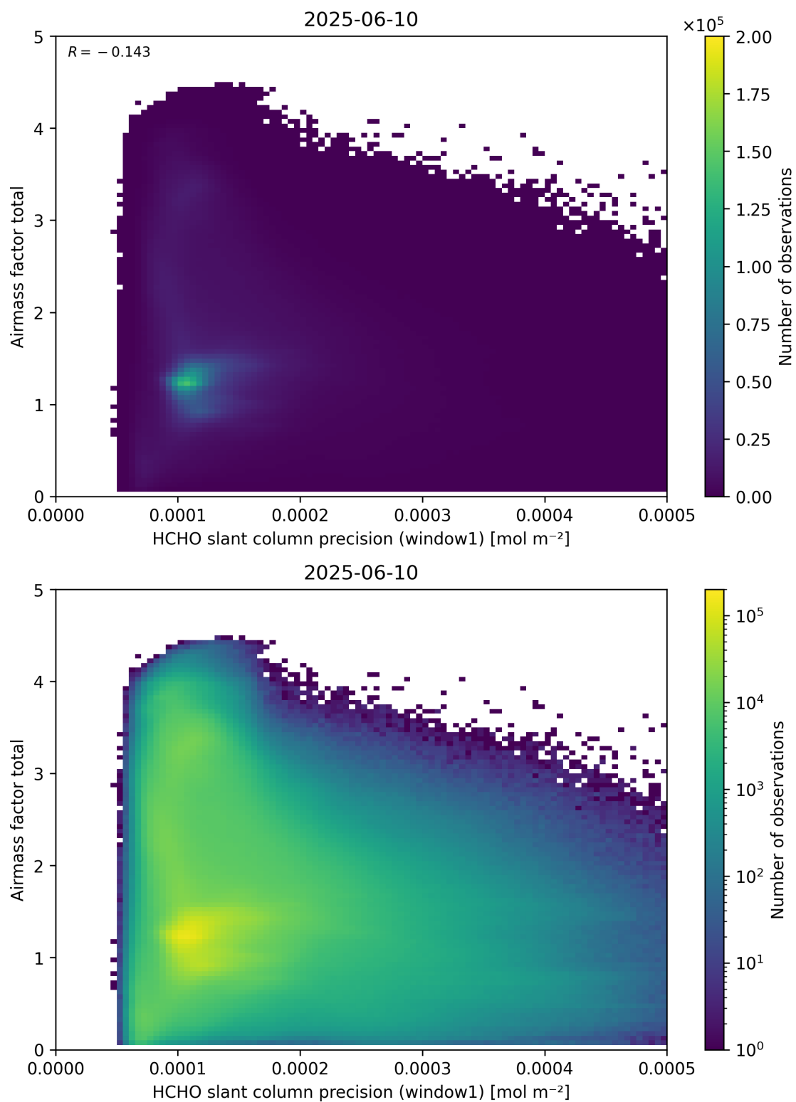
Figure 94: Scatter density plot of “HCHO slant column precision (window1)” against “Airmass factor total” for 2025-06-09 to 2025-06-11.
