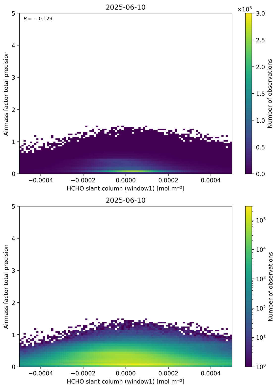
Figure 86: Scatter density plot of “HCHO slant column (window1)” against “Airmass factor total precision” for 2025-06-09 to 2025-06-11.
