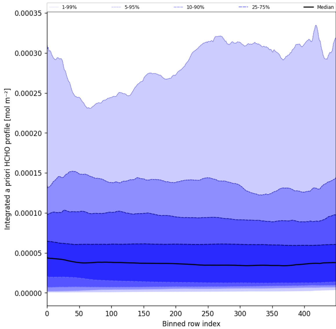
Figure 57: Along track statistics of “Integrated a priori HCHO profile” for 2025-06-09 to 2025-06-11
