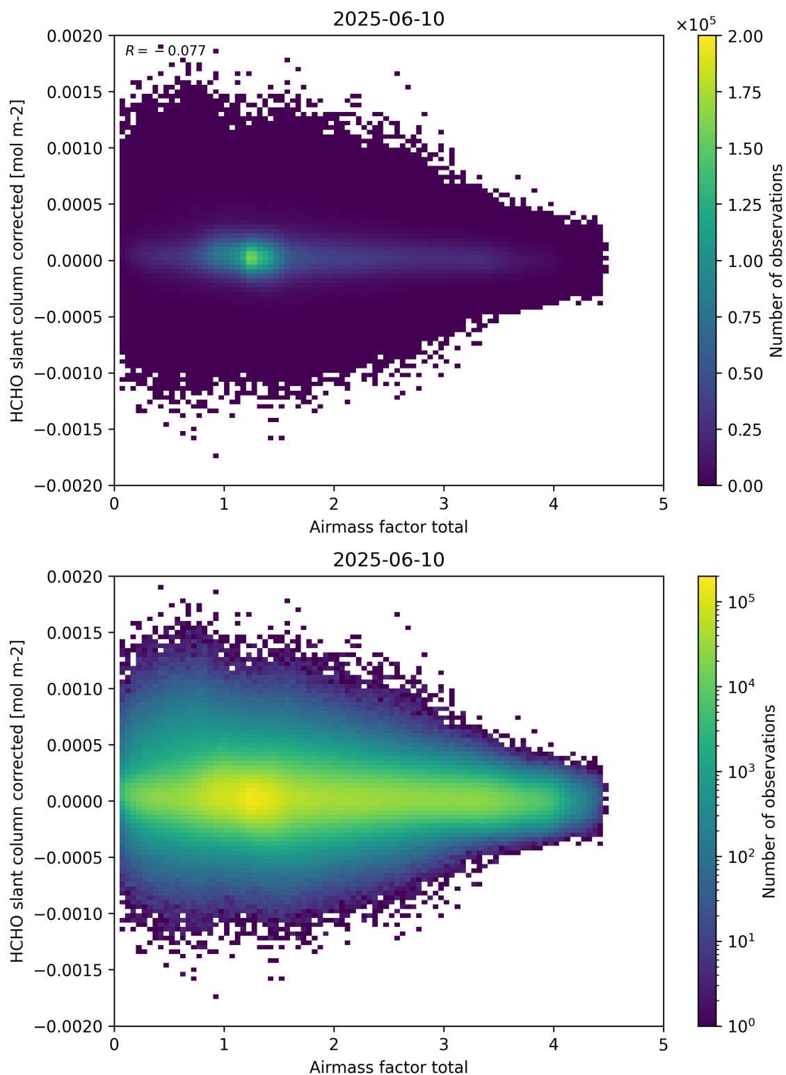
Figure 101: Scatter density plot of “Airmass factor total” against “HCHO slant column corrected” for 2025-06-09 to 2025-06-11.
