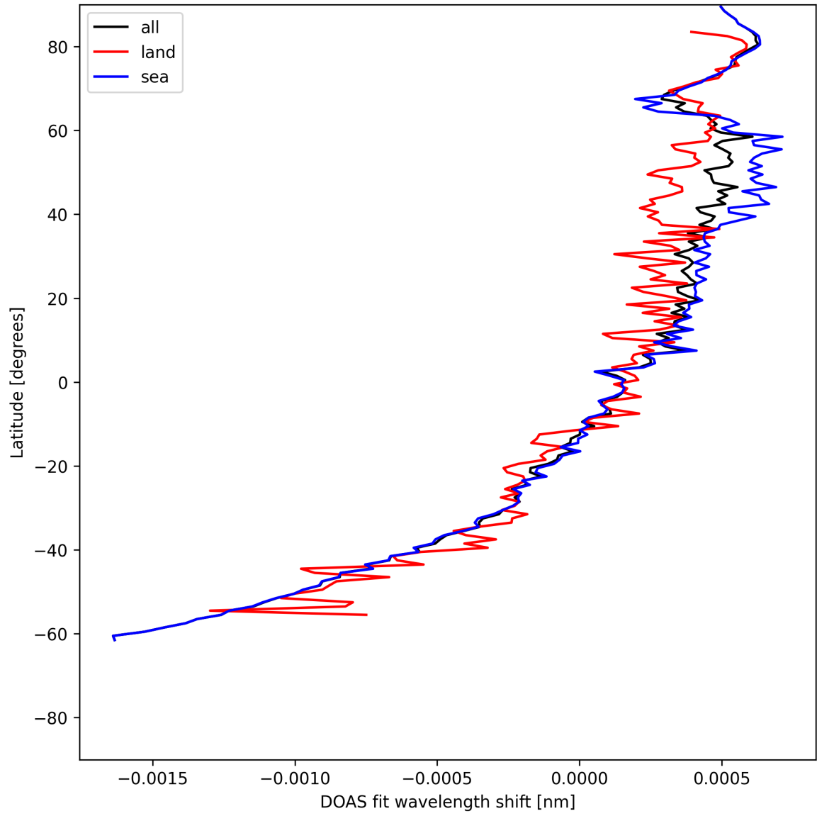
Figure 30: Zonal average of “DOAS fit wavelength shift” for 2025-06-09 to 2025-06-11.
