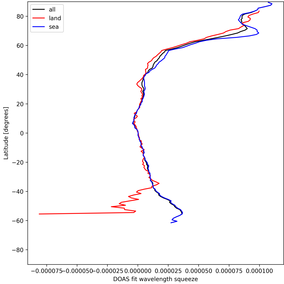
Figure 31: Zonal average of “DOAS fit wavelength squeeze” for 2025-06-09 to 2025-06-11.
