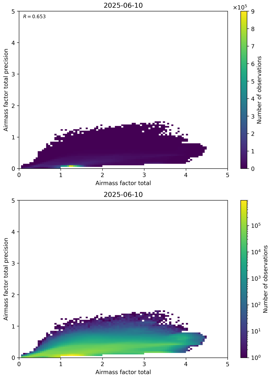
Figure 103: Scatter density plot of “Airmass factor total” against “Airmass factor total precision” for 2025-06-09 to 2025-06-11.
