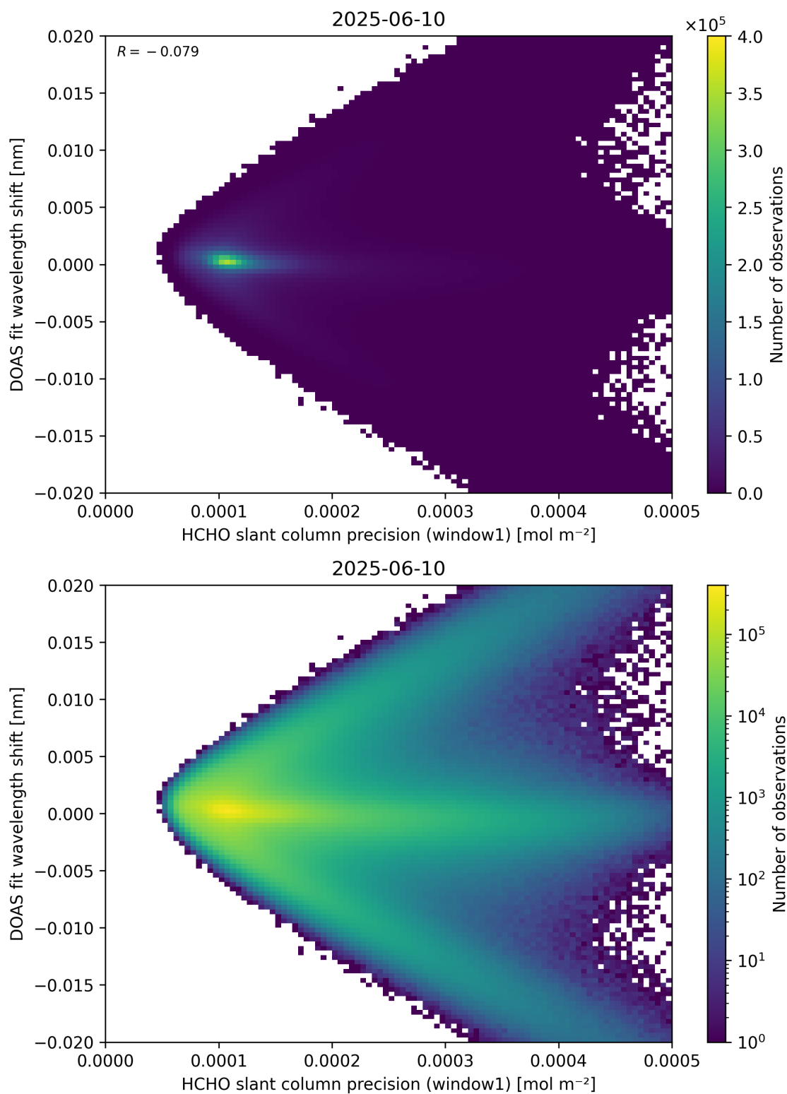
Figure 89: Scatter density plot of “HCHO slant column precision (window1)” against “DOAS fit wavelength shift” for 2025-06-09 to 2025-06-11.
