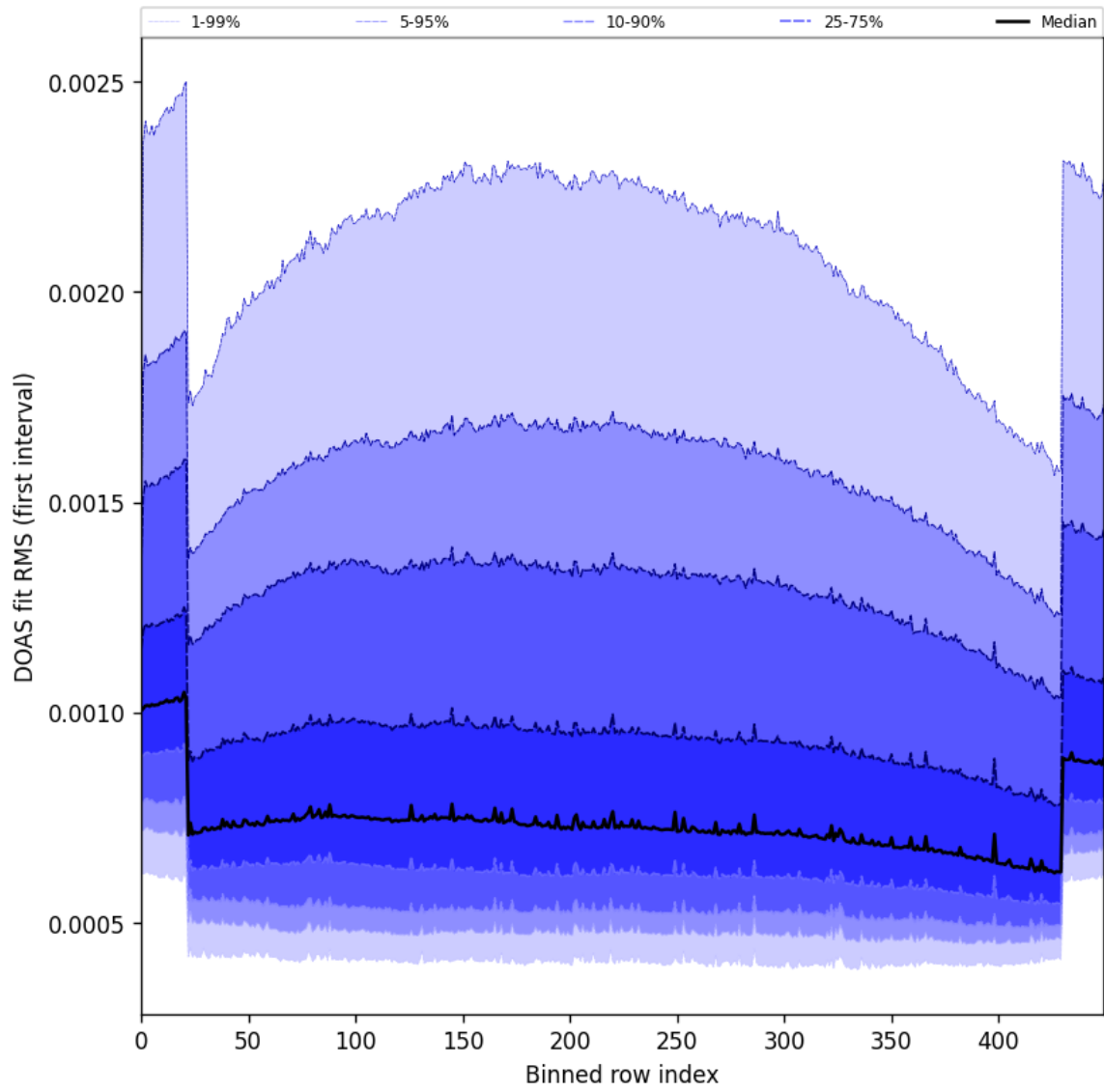
Figure 60: Along track statistics of “DOAS fit RMS (first interval)” for 2025-06-09 to 2025-06-11
