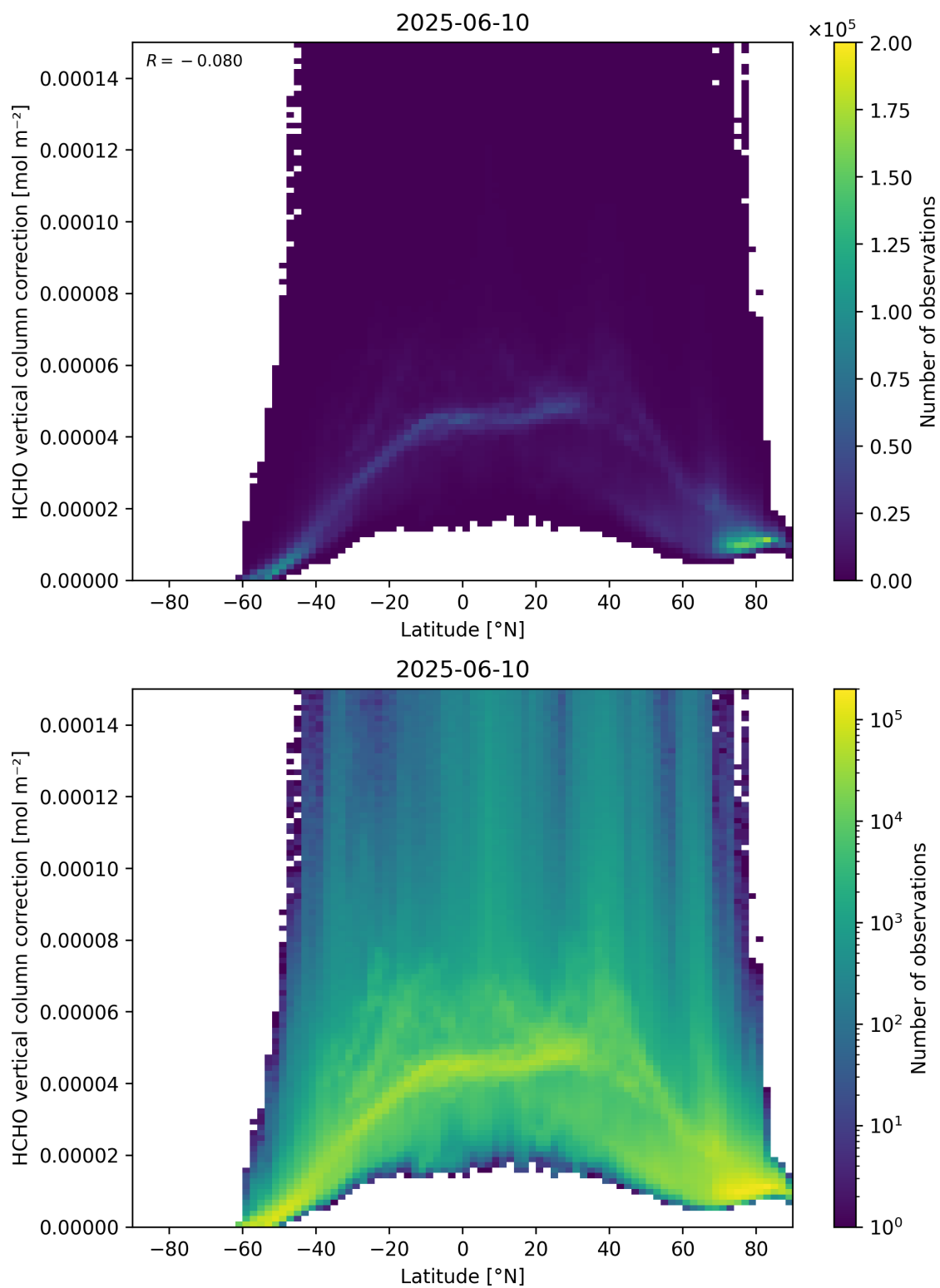
Figure 164: Scatter density plot of “Latitude” against “HCHO vertical column correction” for 2025-06-09 to 2025-06-11.
