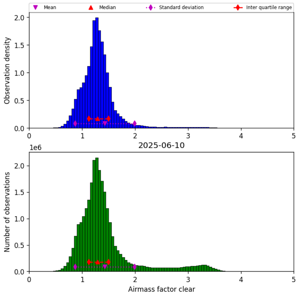
Figure 42: Histogram of “Airmass factor clear” for 2025-06-09 to 2025-06-11
