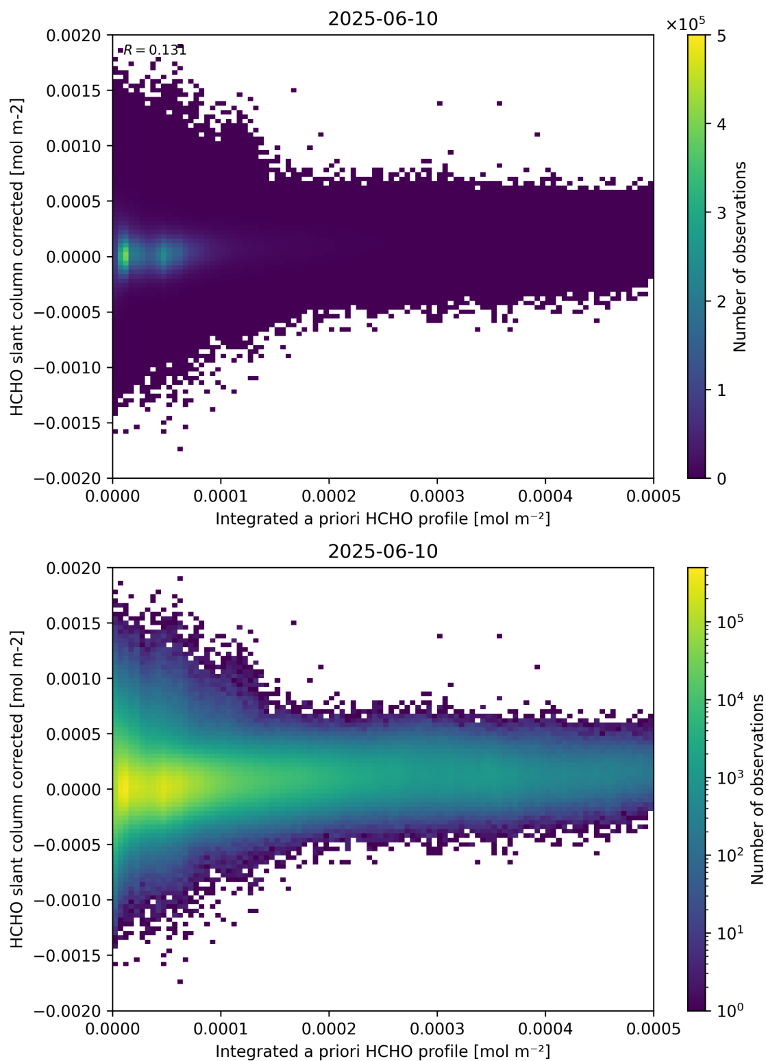
Figure 151: Scatter density plot of “Integrated a priori HCHO profile” against “HCHO slant column corrected” for 2025-06-09 to 2025-06-11.
