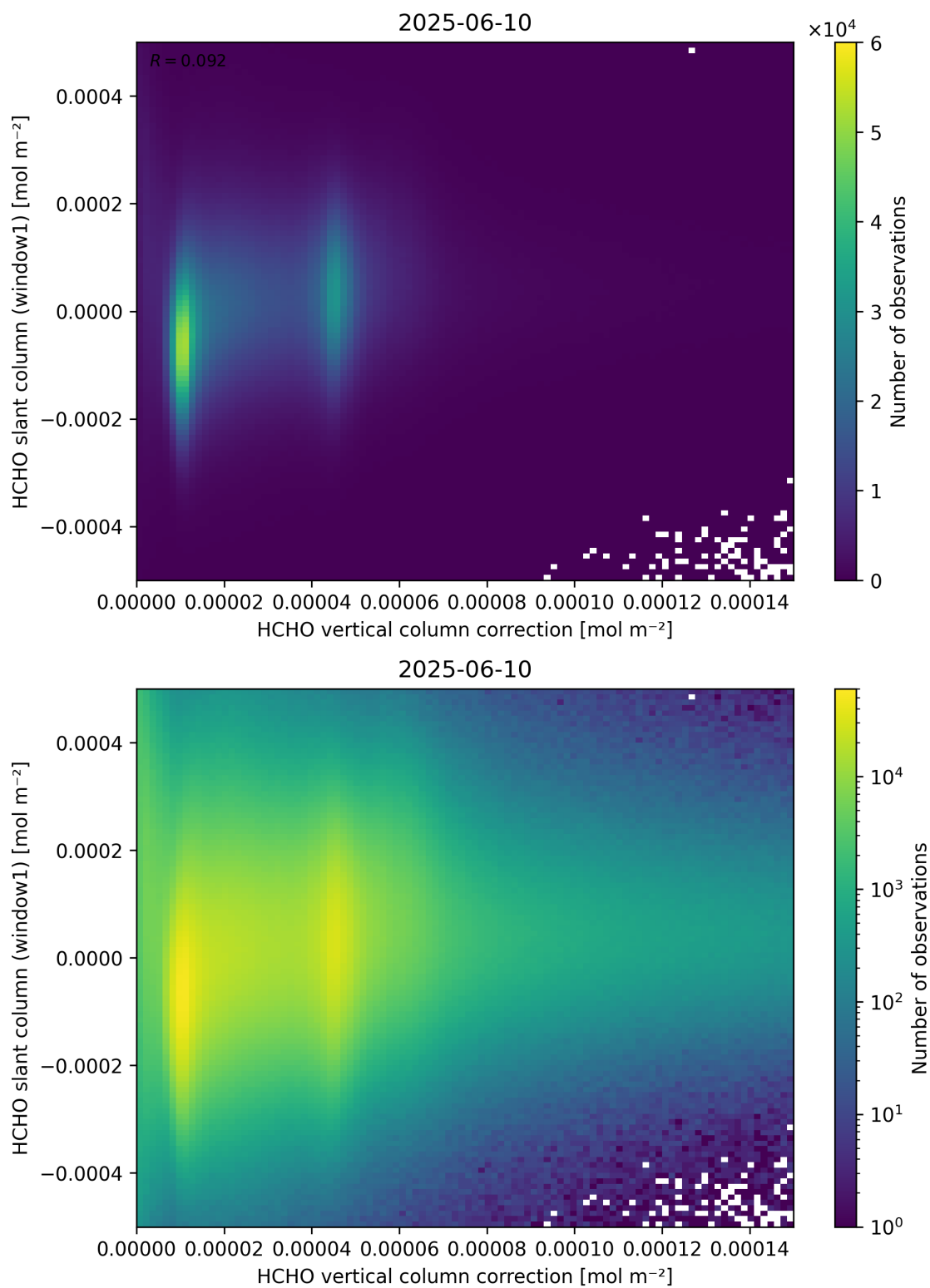
Figure 118: Scatter density plot of “HCHO vertical column correction” against “HCHO slant column (window1)” for 2025-06-09 to 2025-06-11.
