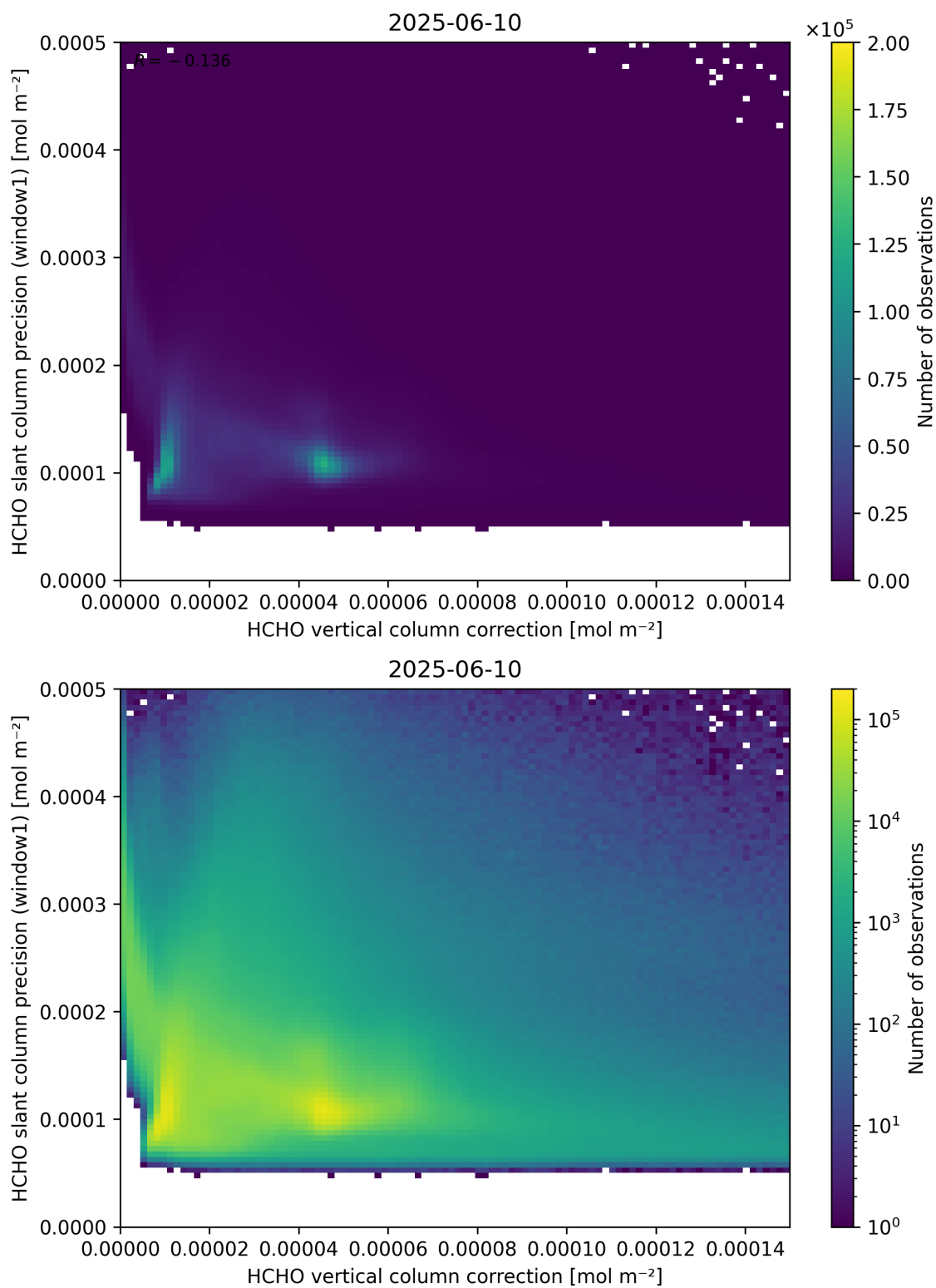
Figure 119: Scatter density plot of “HCHO vertical column correction” against “HCHO slant column precision (window1)” for 2025-06-09 to 2025-06-11.
