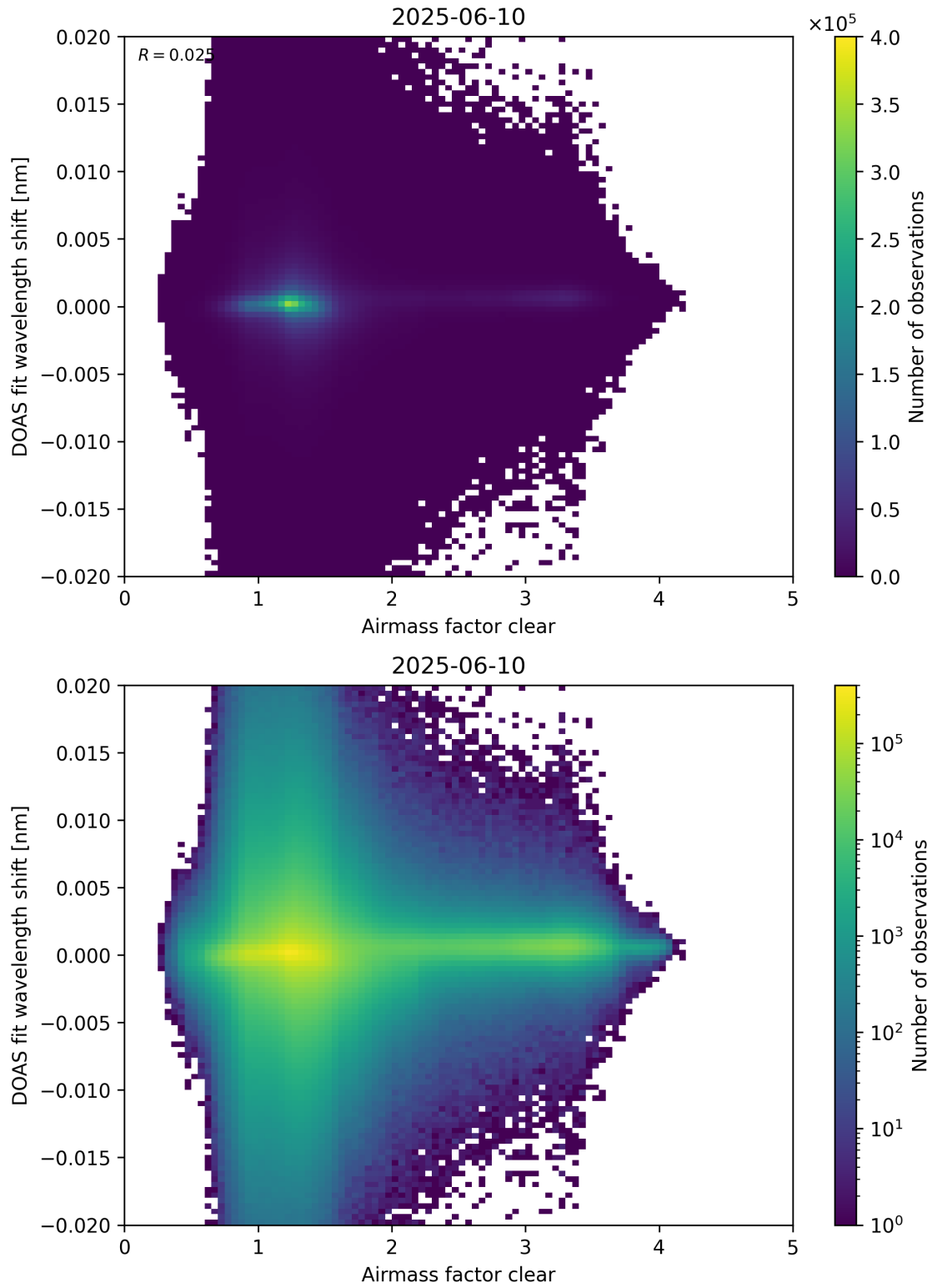
Figure 72: Scatter density plot of “Airmass factor clear” against “DOAS fit wavelength shift” for 2025-06-09 to 2025-06-11.
