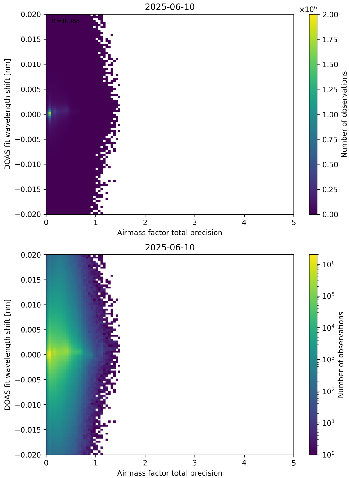
Figure 106: Scatter density plot of “Airmass factor total precision” against “DOAS fit wavelength shift” for 2025-06-09 to 2025-06-11.
