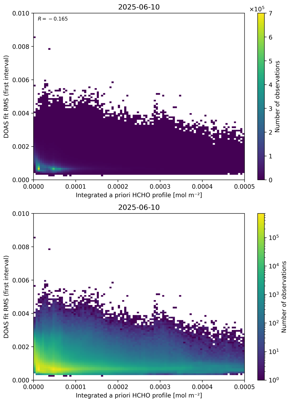
Figure 148: Scatter density plot of “Integrated a priori HCHO profile” against “DOAS fit RMS (first interval)” for 2025-06-09 to 2025-06-11.
