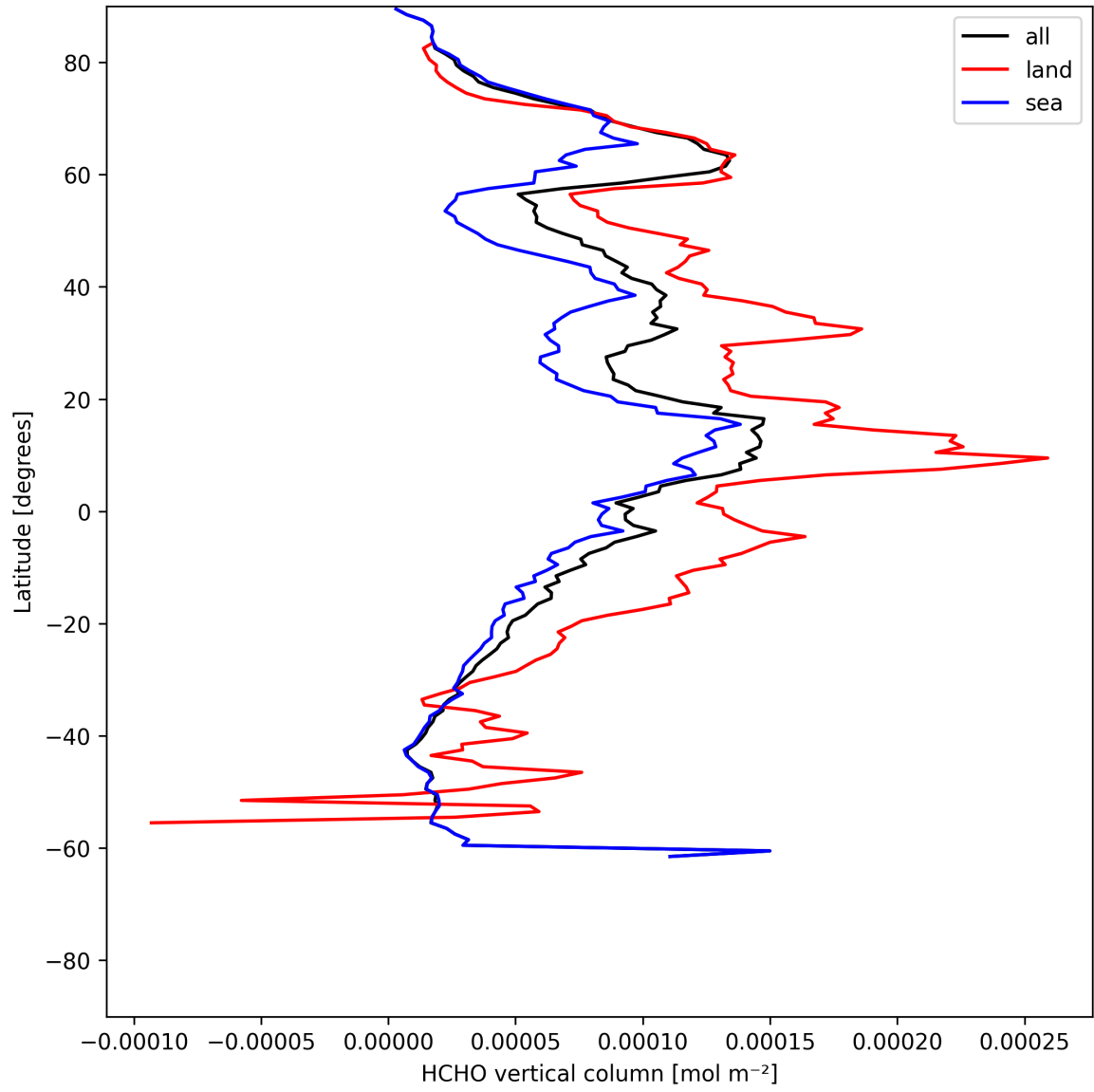
Figure 21: Zonal average of “HCHO vertical column” for 2025-06-09 to 2025-06-11.
