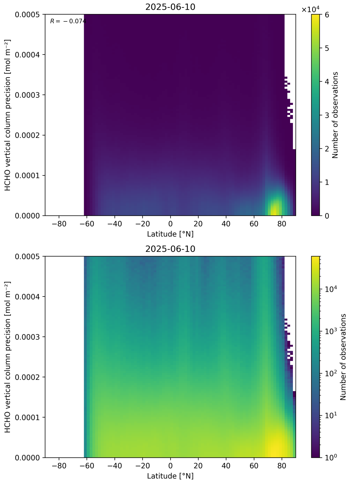
Figure 165: Scatter density plot of “Latitude” against “HCHO vertical column precision” for 2025-06-09 to 2025-06-11.
