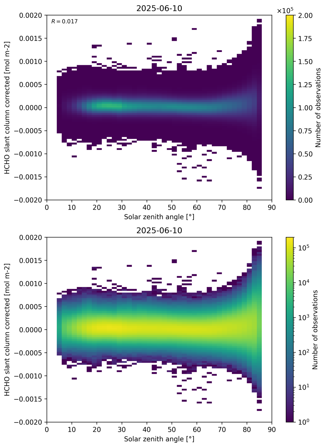
Figure 171: Scatter density plot of “Solar zenith angle” against “HCHO slant column corrected” for 2025-06-09 to 2025-06-11.
