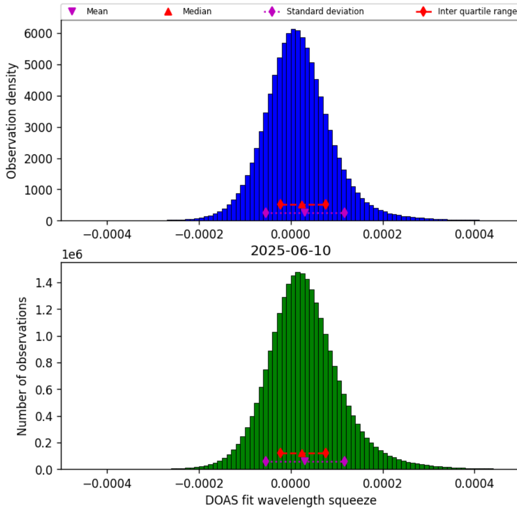
Figure 45: Histogram of “DOAS fit wavelength squeeze” for 2025-06-09 to 2025-06-11
