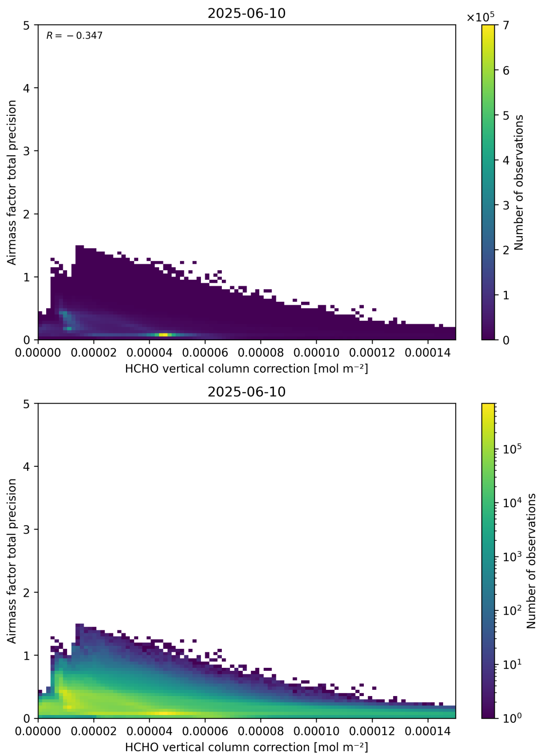
Figure 121: Scatter density plot of “HCHO vertical column correction” against “Airmass factor total precision” for 2025-06-09 to 2025-06-11.
