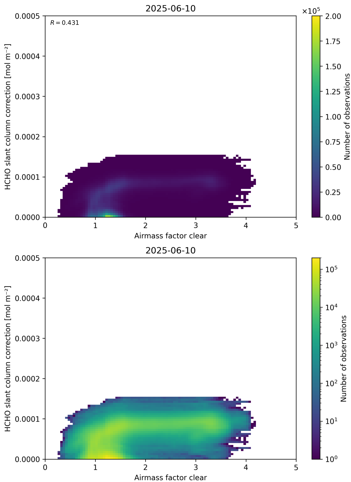
Figure 75: Scatter density plot of “Air mass factor clear” against “HCHO slant column correction” for 2025-06-09 to 2025-06-11.
