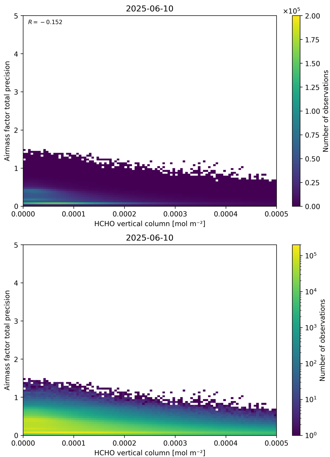
Figure 132: Scatter density plot of “HCHO vertical column” against “Airmass factor total precision” for 2025-06-09 to 2025-06-11.
