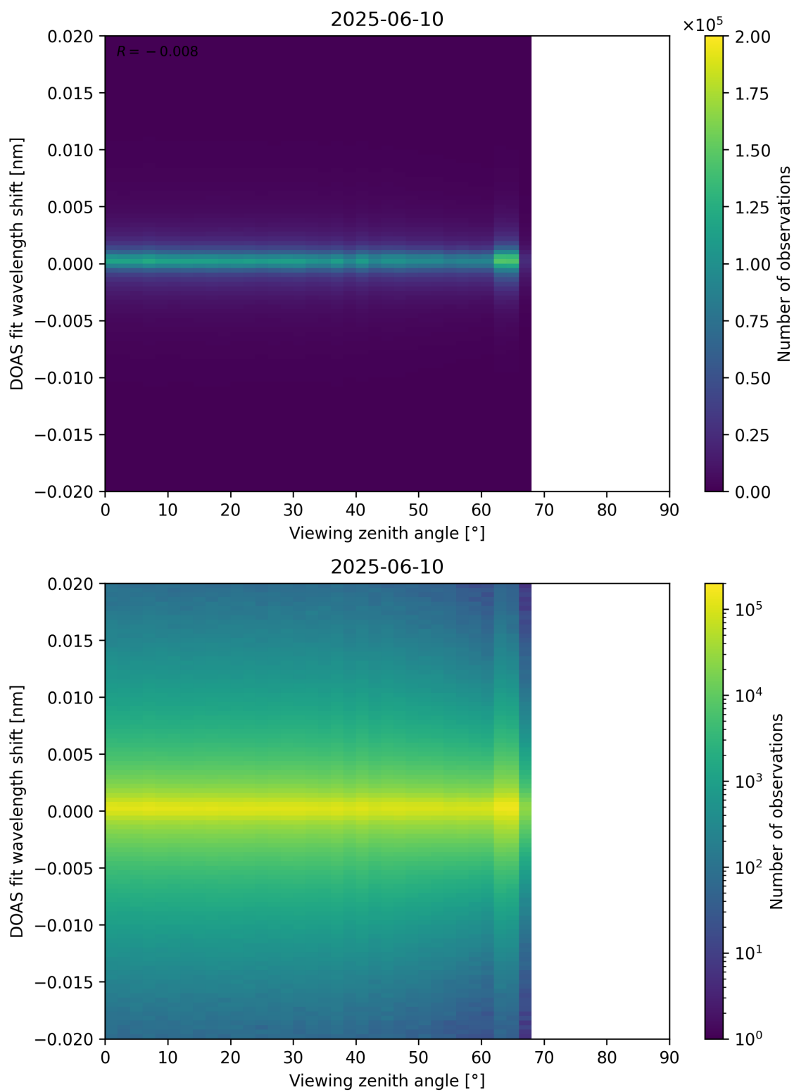
Figure 183: Scatter density plot of “Viewing zenith angle” against “DOAS fit wavelength shift” for 2025-06-09 to 2025-06-11.
