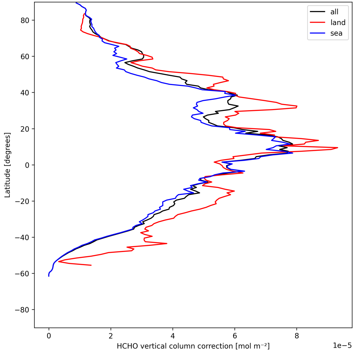
Figure 23: Zonal average of “HCHO vertical column correction” for 2025-06-09 to 2025-06-11.
