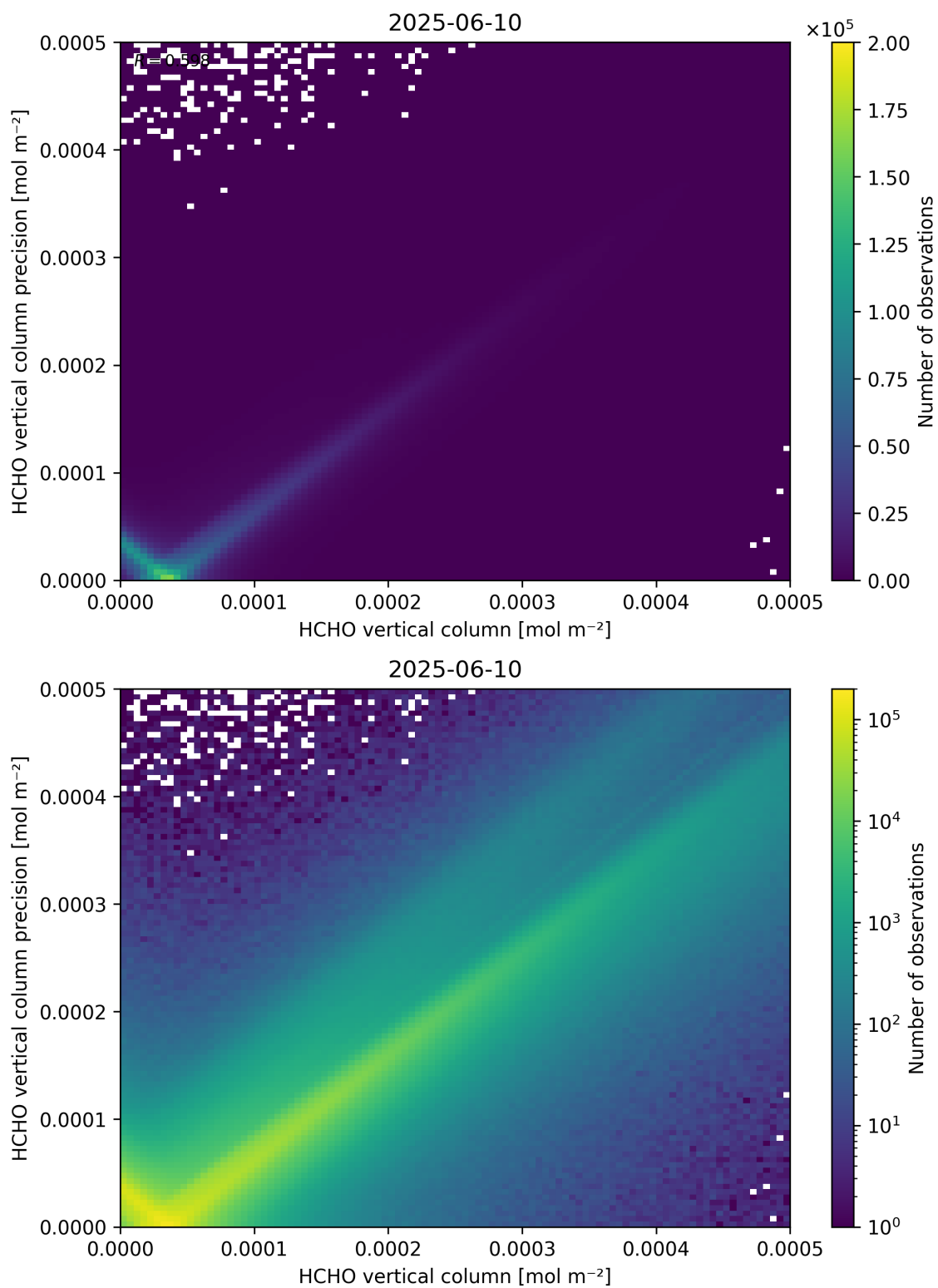
Figure 134: Scatter density plot of “HCHO vertical column” against “HCHO vertical column precision” for 2025-06-09 to 2025-06-11.
