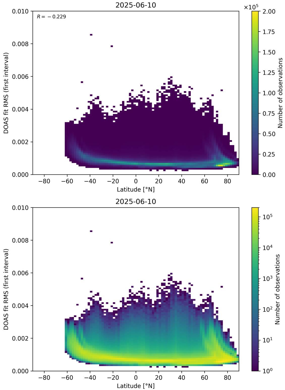
Figure 153: Scatter density plot of “Latitude” against “DOAS fit RMS (first interval)” for 2025-06-09 to 2025-06-11.
