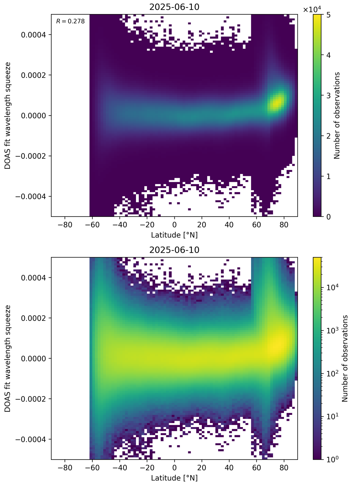
Figure 155: Scatter density plot of “Latitude” against “DOAS fit wavelength squeeze” for 2025-06-09 to 2025-06-11.
