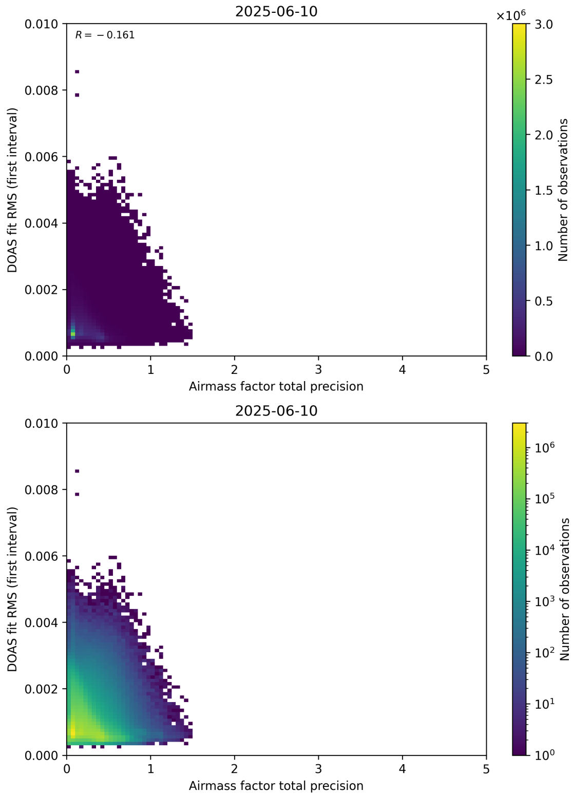
Figure 105: Scatter density plot of “Airmass factor total precision” against “DOAS fit RMS (first interval)” for 2025-06-09 to 2025-06-11.
