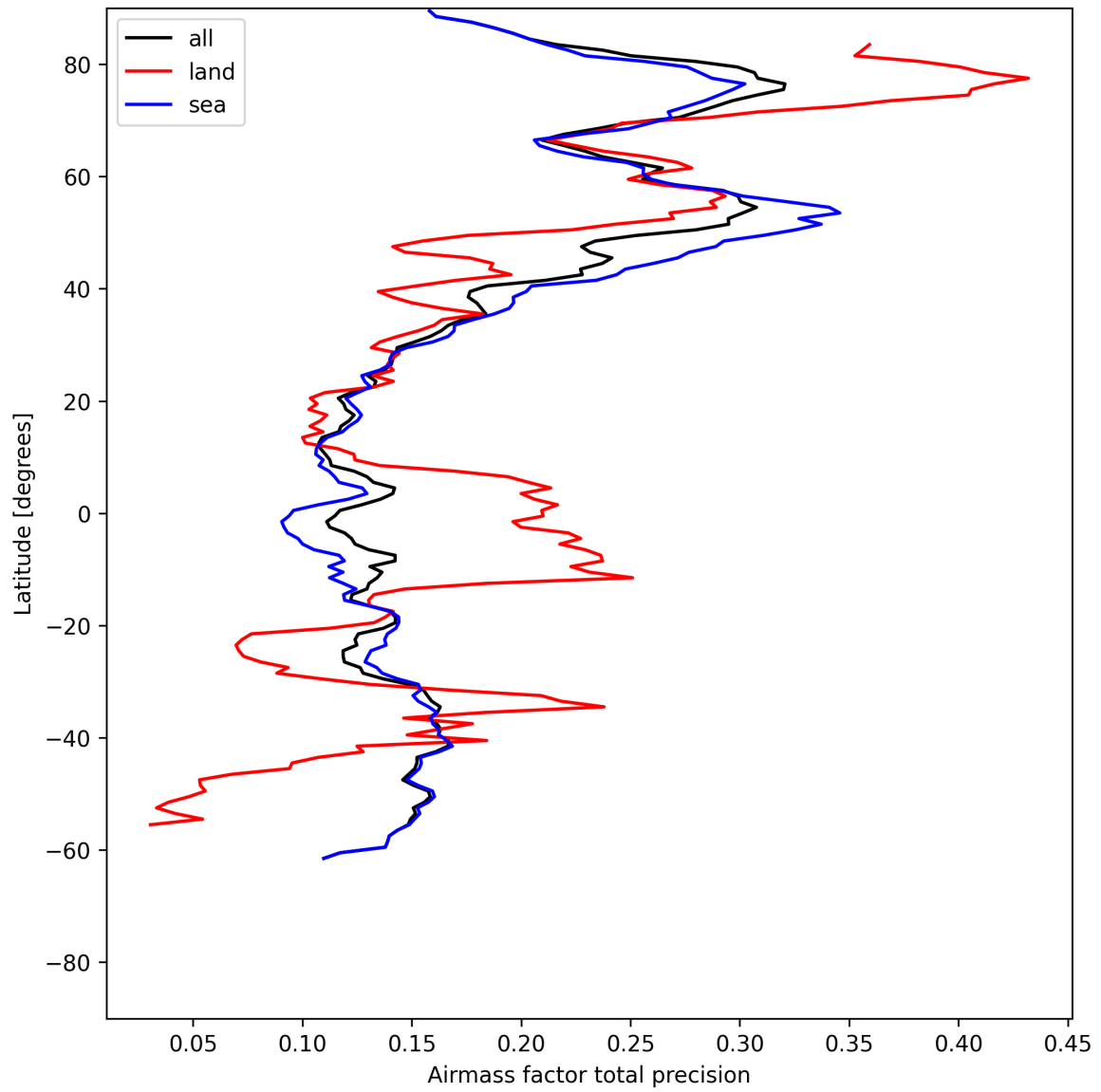
Figure 27: Zonal average of “Airmass factor total precision” for 2025-06-09 to 2025-06-11.
