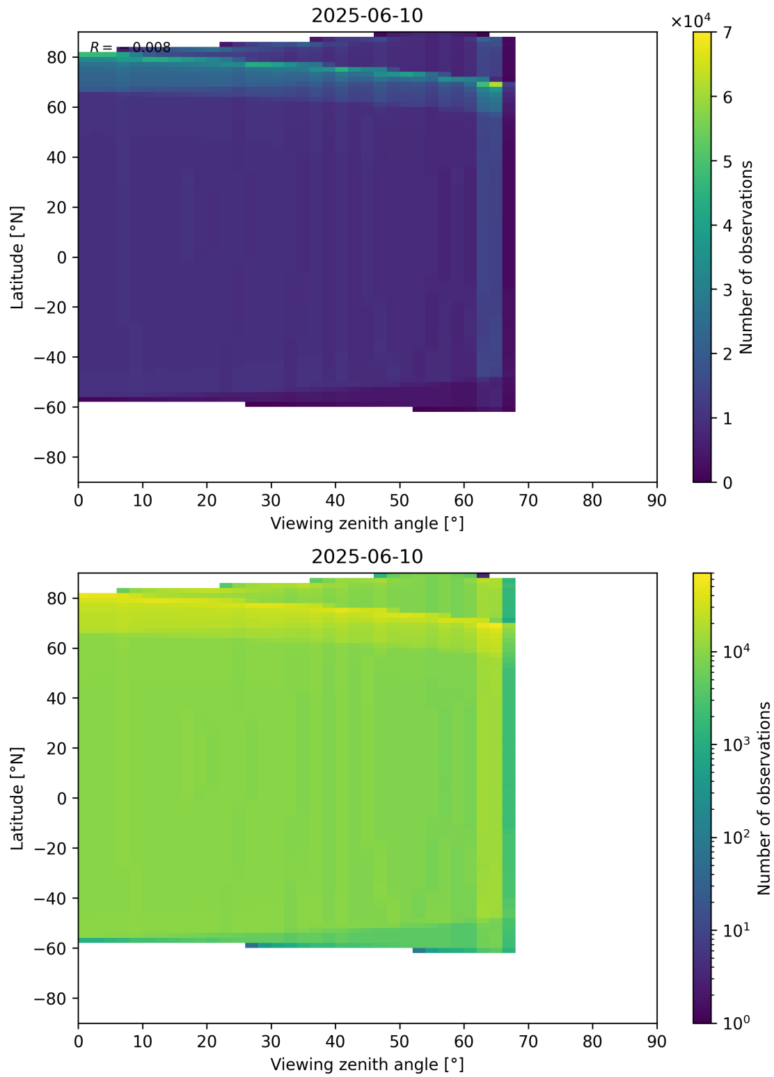
Figure 196: Scatter density plot of “Viewing zenith angle” against “Latitude” for 2025-06-09 to 2025-06-11.
