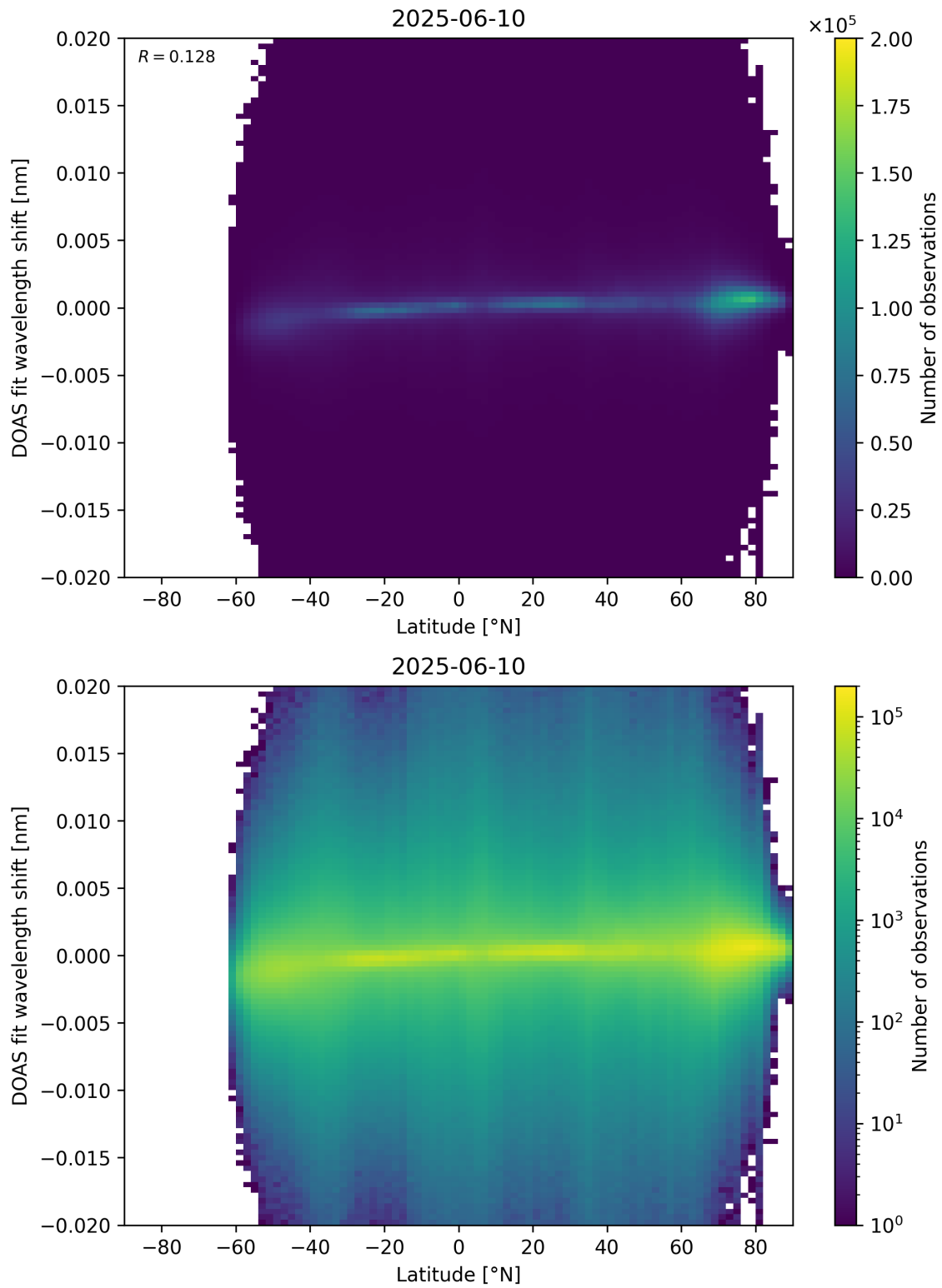
Figure 154: Scatter density plot of “Latitude” against “DOAS fit wavelength shift” for 2025-06-09 to 2025-06-11.
