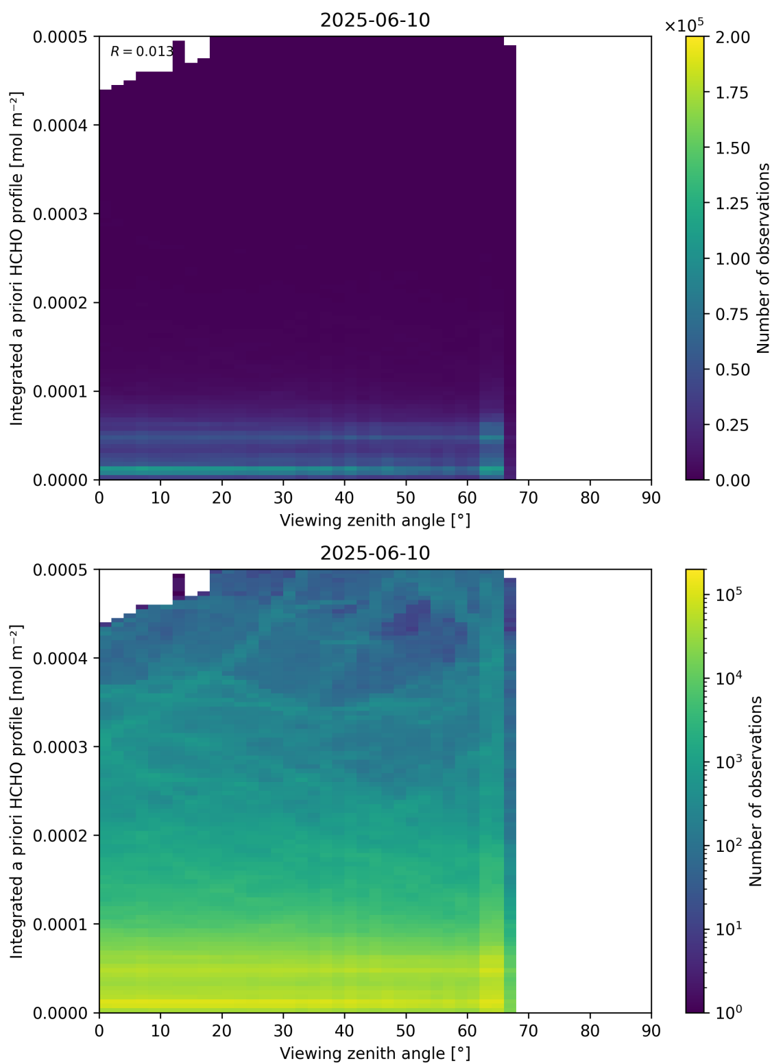
Figure 195: Scatter density plot of “Viewing zenith angle” against “Integrated a priori HCHO profile” for 2025-06-09 to 2025-06-11.
