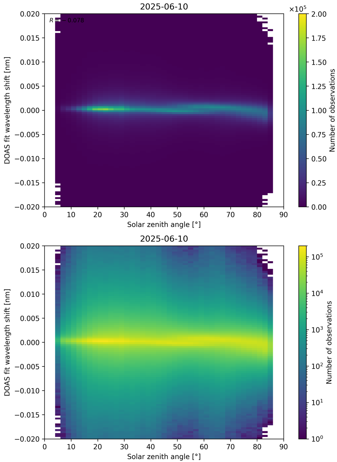
Figure 168: Scatter density plot of “Solar zenith angle” against “DOAS fit wavelength shift” for 2025-06-09 to 2025-06-11.
