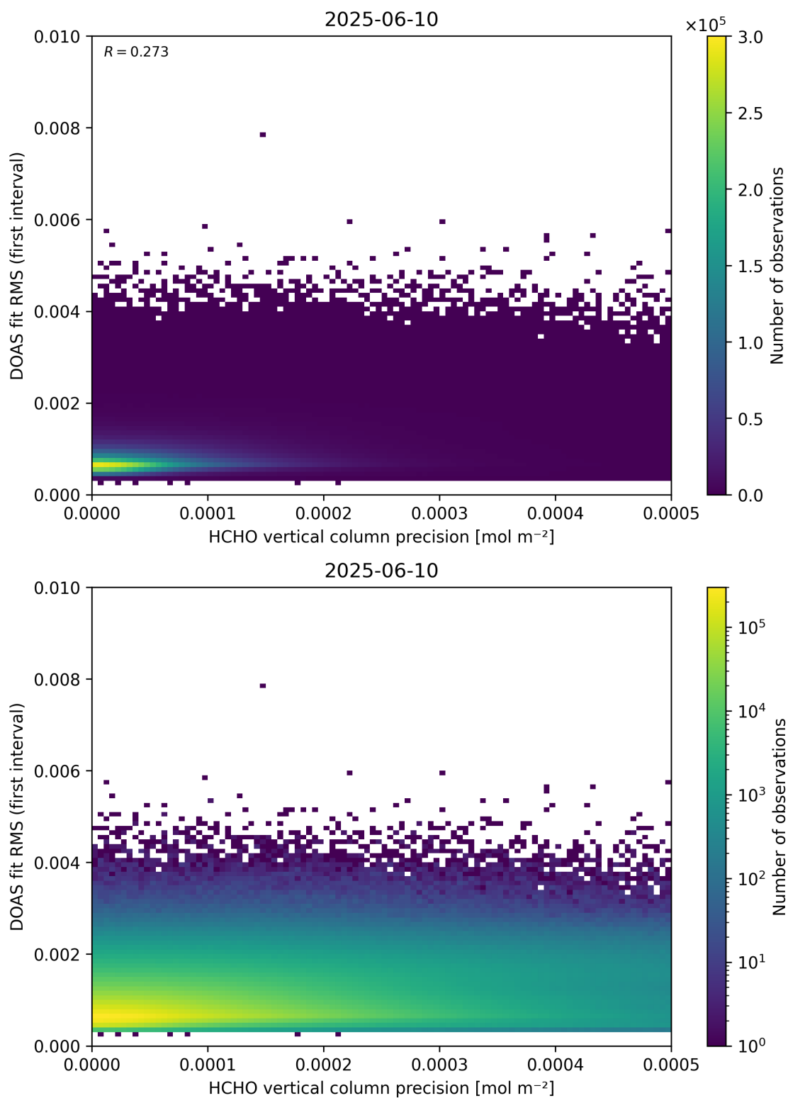
Figure 136: Scatter density plot of “HCHO vertical column precision” against “DOAS fit RMS (first interval)” for 2025-06-09 to 2025-06-11.
