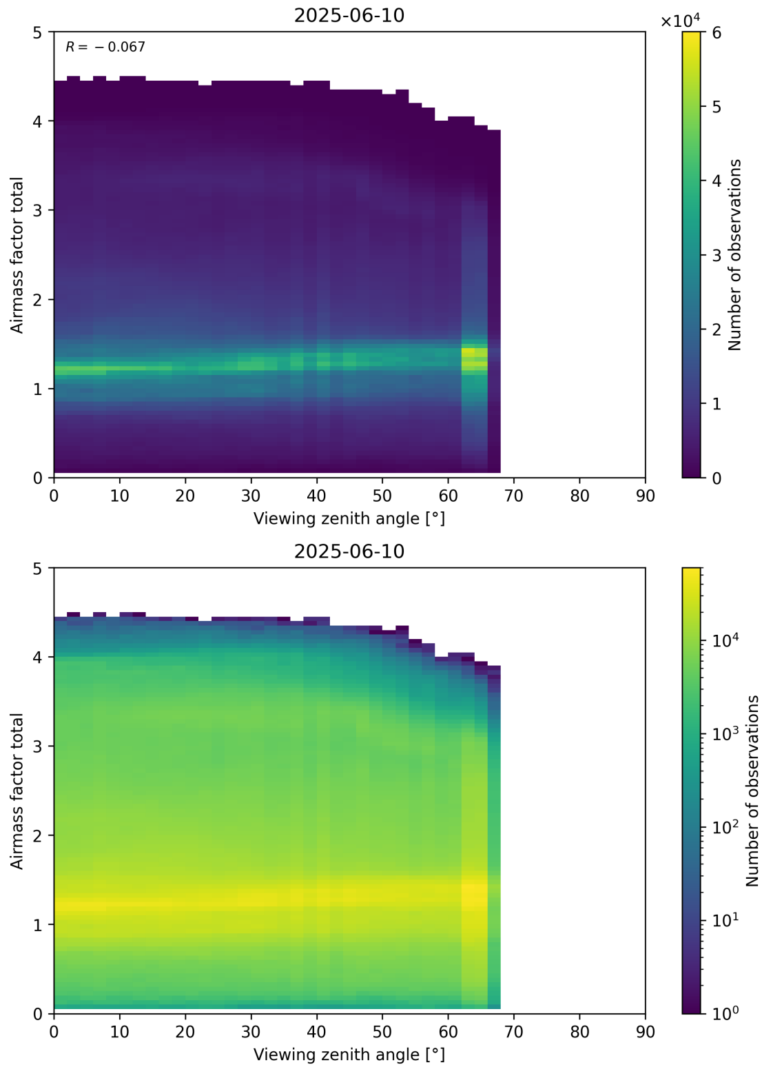
Figure 190: Scatter density plot of “Viewing zenith angle” against “Airmass factor total” for 2025-06-09 to 2025-06-11.
