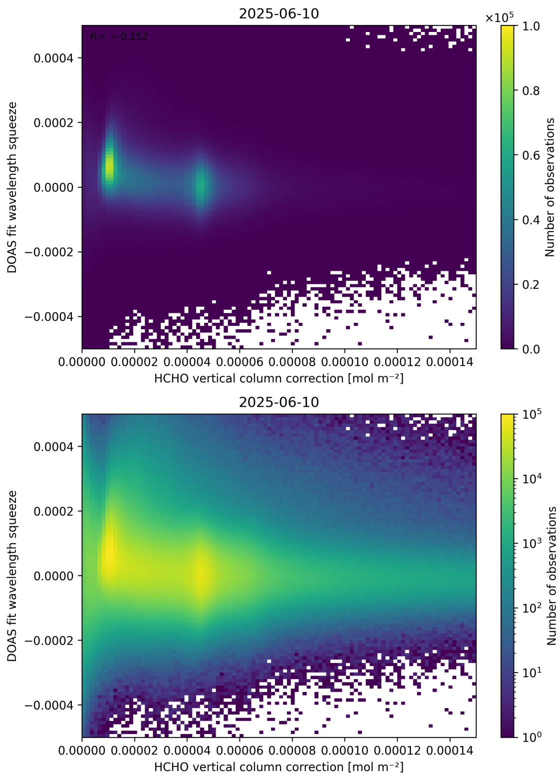
Figure 114: Scatter density plot of “HCHO vertical column correction” against “DOAS fit wavelength squeeze” for 2025-06-09 to 2025-06-11.
