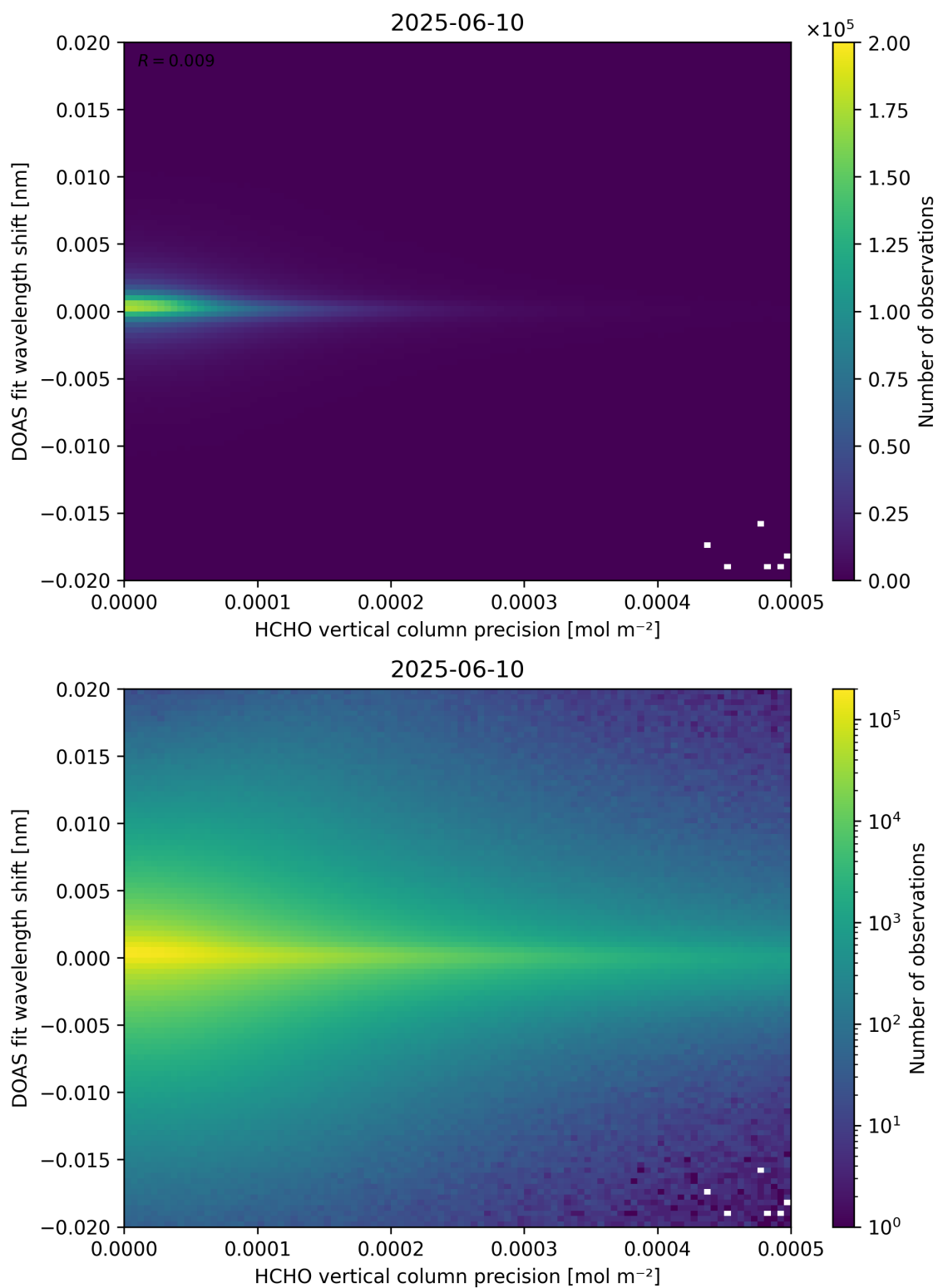
Figure 137: Scatter density plot of “HCHO vertical column precision” against “DOAS fit wavelength shift” for 2025-06-09 to 2025-06-11.
