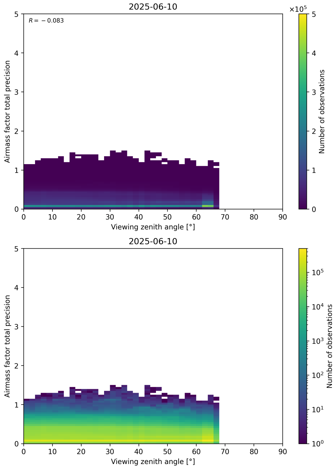
Figure 191: Scatter density plot of “Viewing zenith angle” against “Airmass factor total precision” for 2025-06-09 to 2025-06-11.
