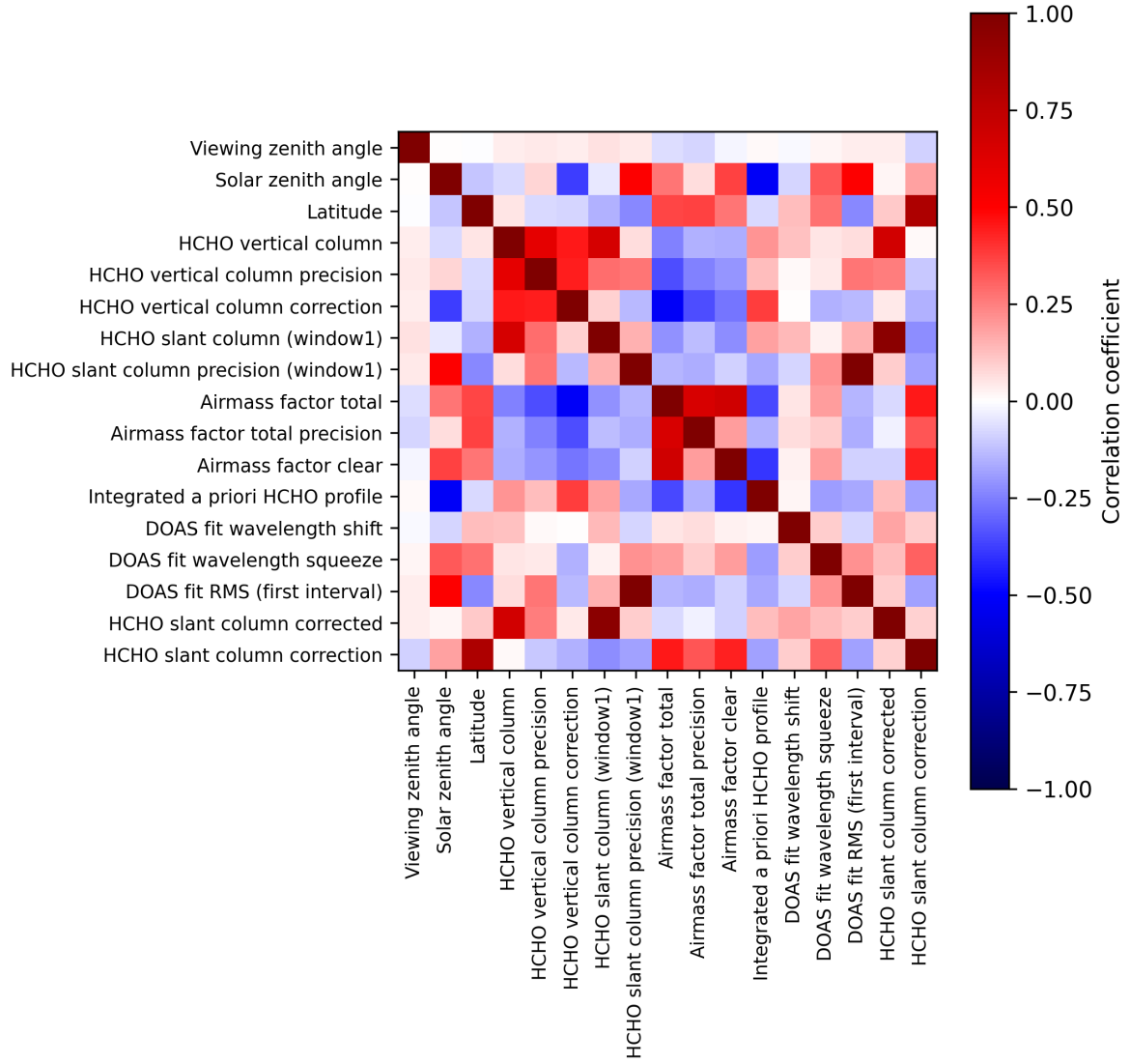
Figure 2: Map of correlation matrix for 2025-06-09 to 2025-06-11.
