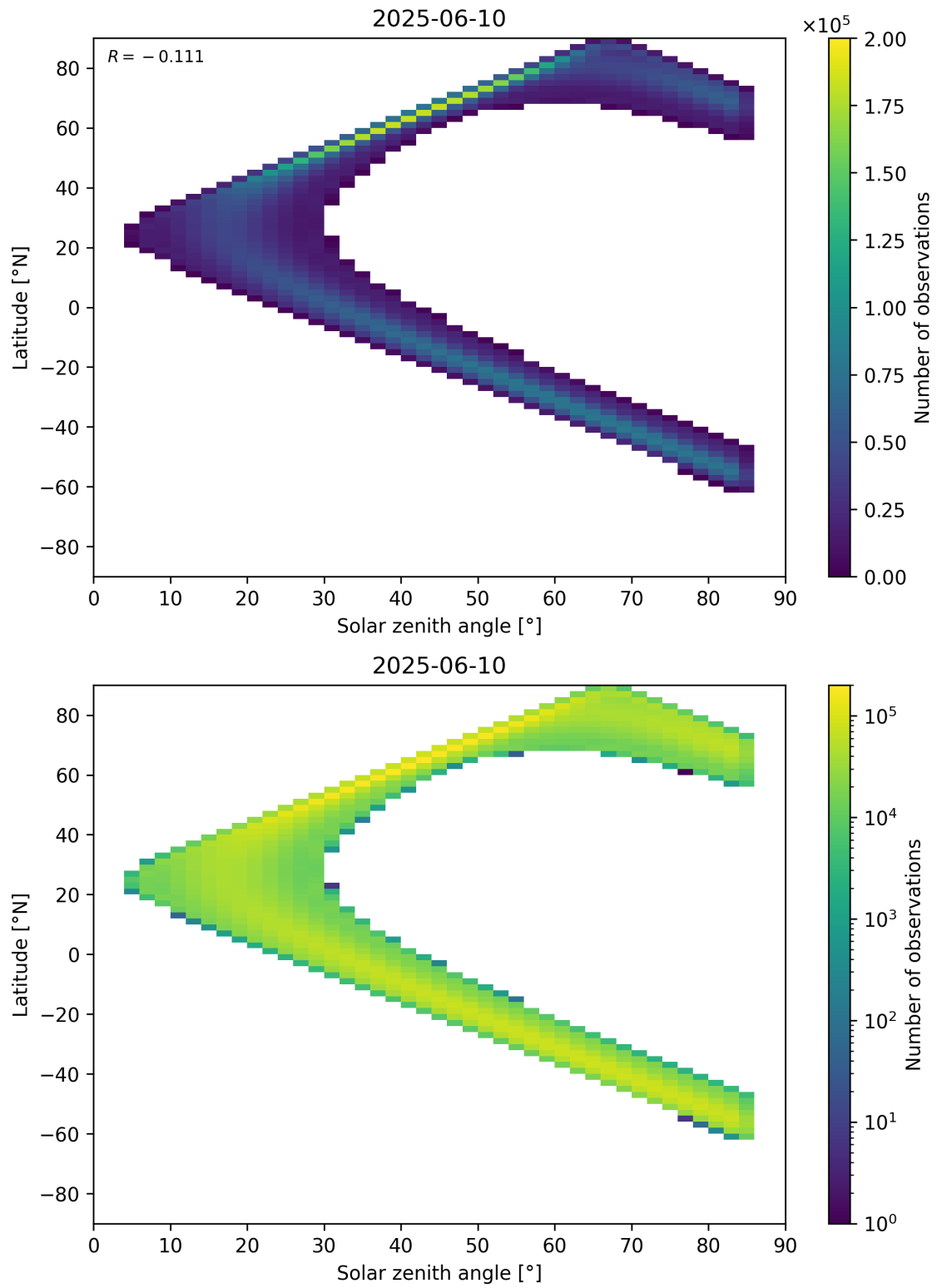
Figure 181: Scatter density plot of “Solar zenith angle” against “Latitude” for 2025-06-09 to 2025-06-11.
