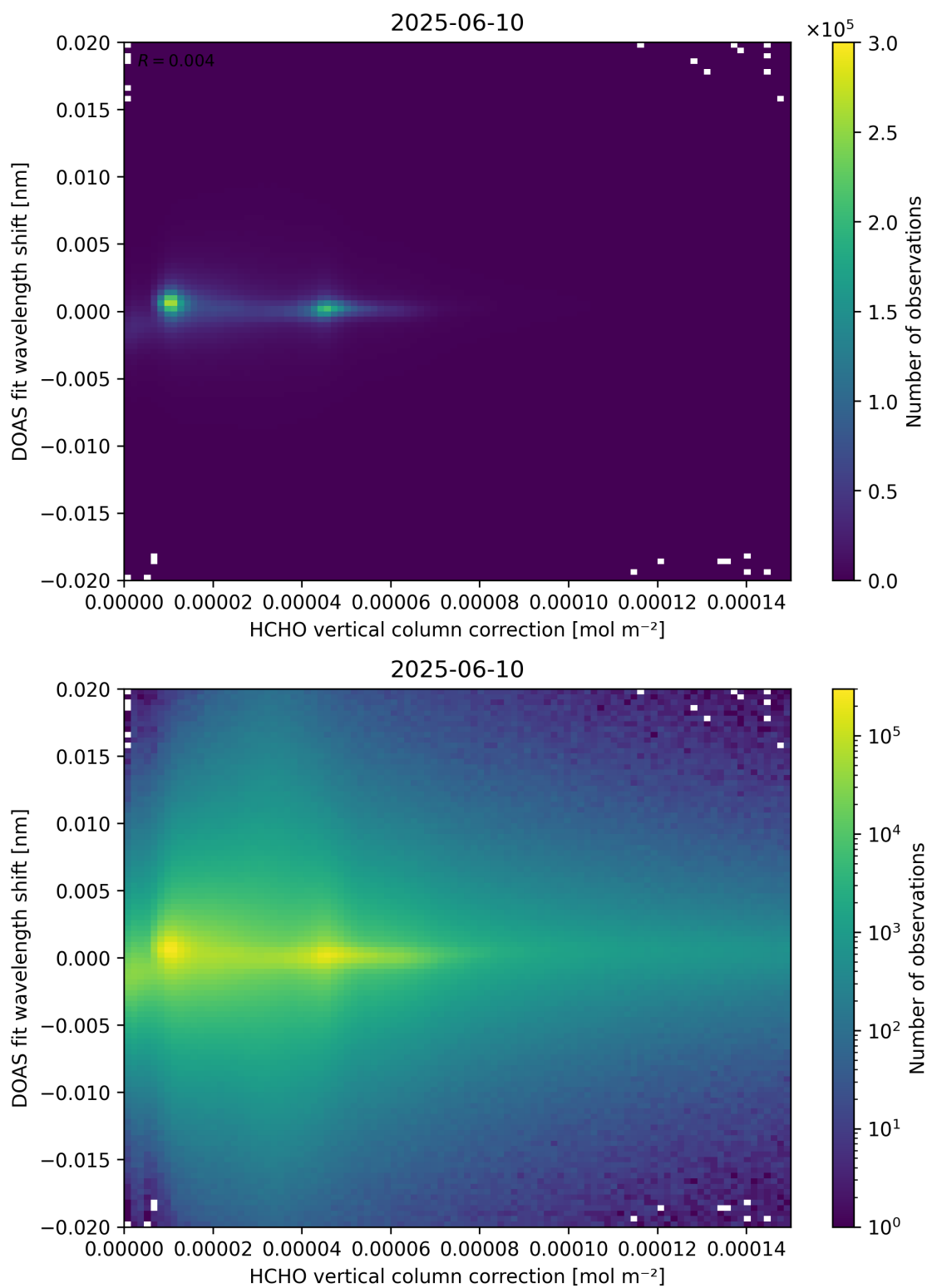
Figure 113: Scatter density plot of “HCHO vertical column correction” against “DOAS fit wavelength shift” for 2025-06-09 to 2025-06-11.
