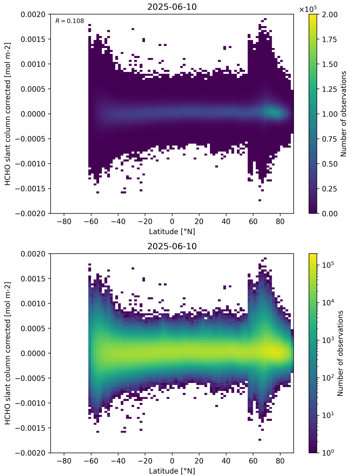
Figure 157: Scatter density plot of “Latitude” against “HCHO slant column corrected” for 2025-06-09 to 2025-06-11.
