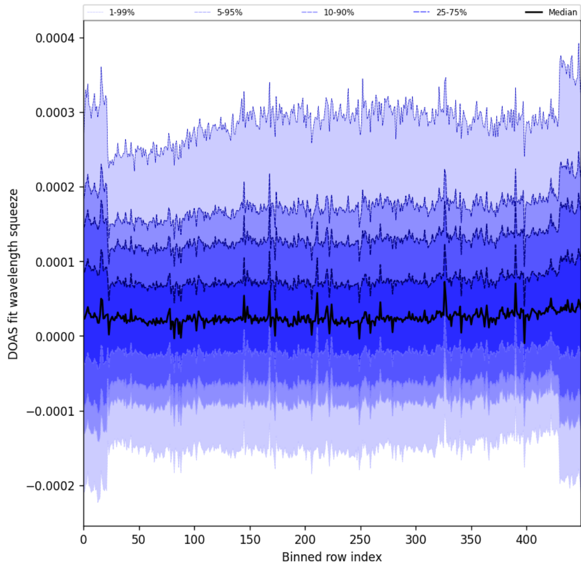
Figure 59: Along track statistics of “DOAS fit wavelength squeeze” for 2025-06-09 to 2025-06-11
