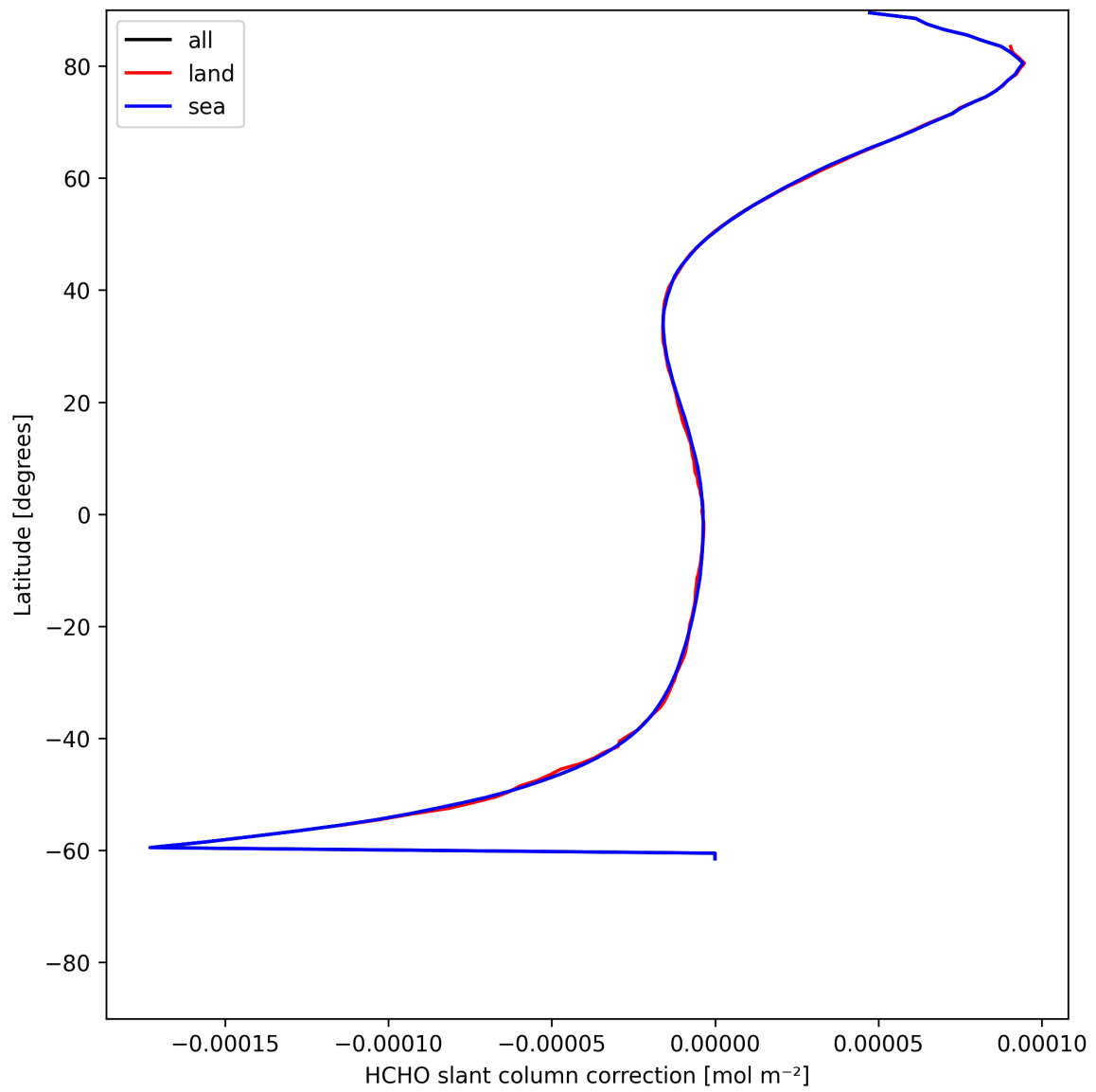
Figure 33: Zonal average of “HCHO slant column correction” for 2025-06-09 to 2025-06-11.
