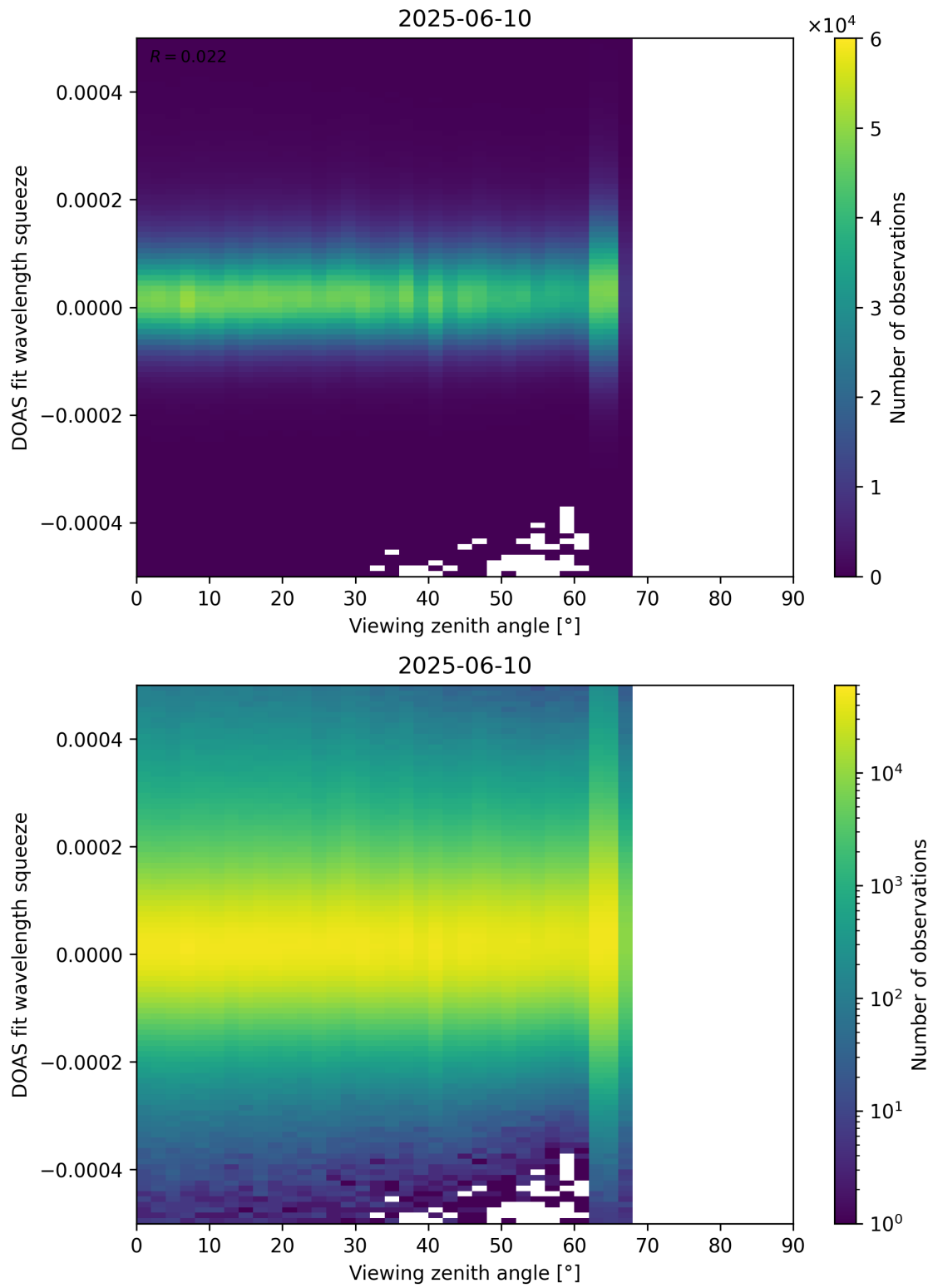
Figure 184: Scatter density plot of “Viewing zenith angle” against “DOAS fit wavelength squeeze” for 2025-06-09 to 2025-06-11.
