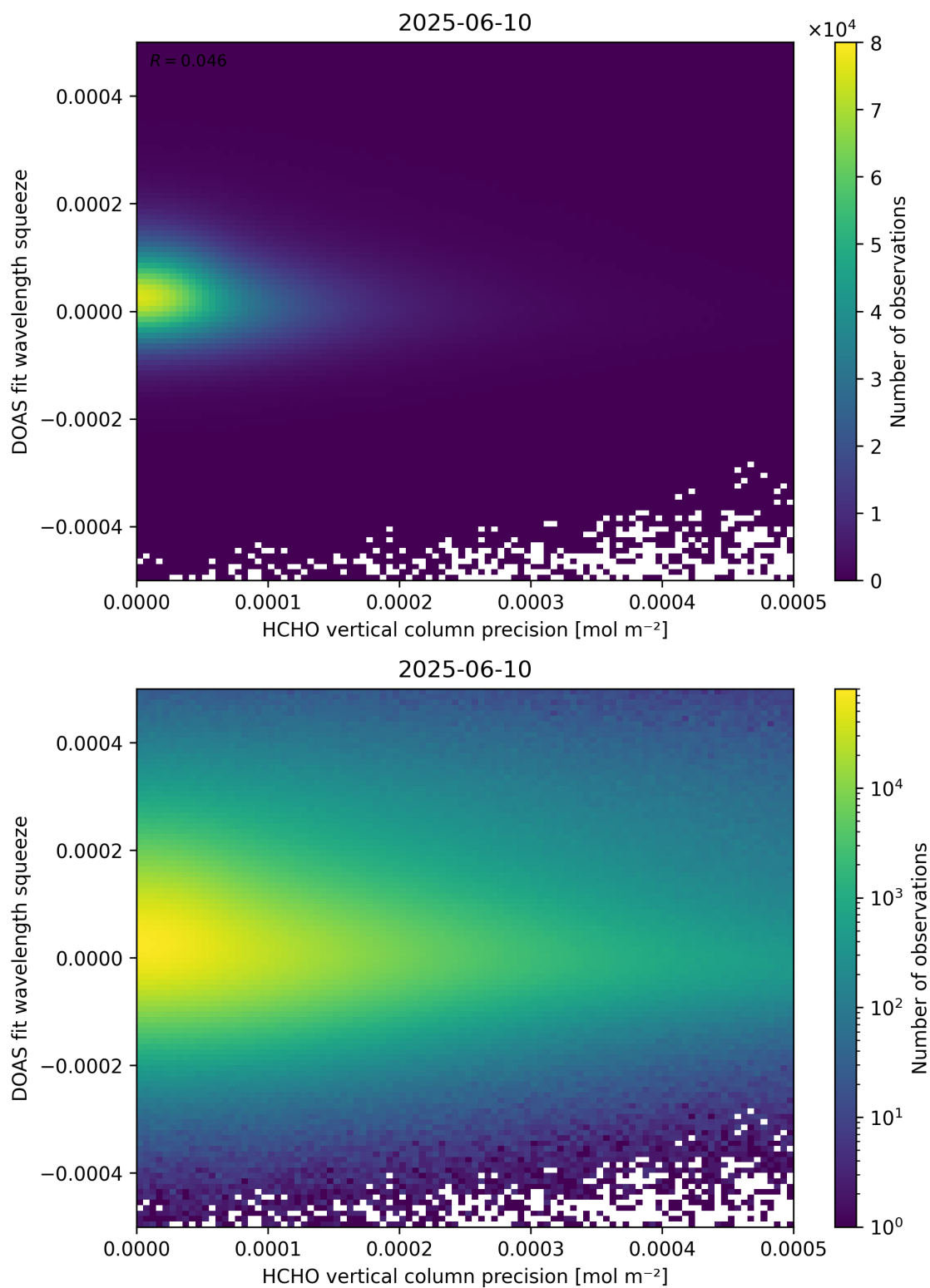
Figure 138: Scatter density plot of “HCHO vertical column precision” against “DOAS fit wavelength squeeze” for 2025-06-09 to 2025-06-11.
