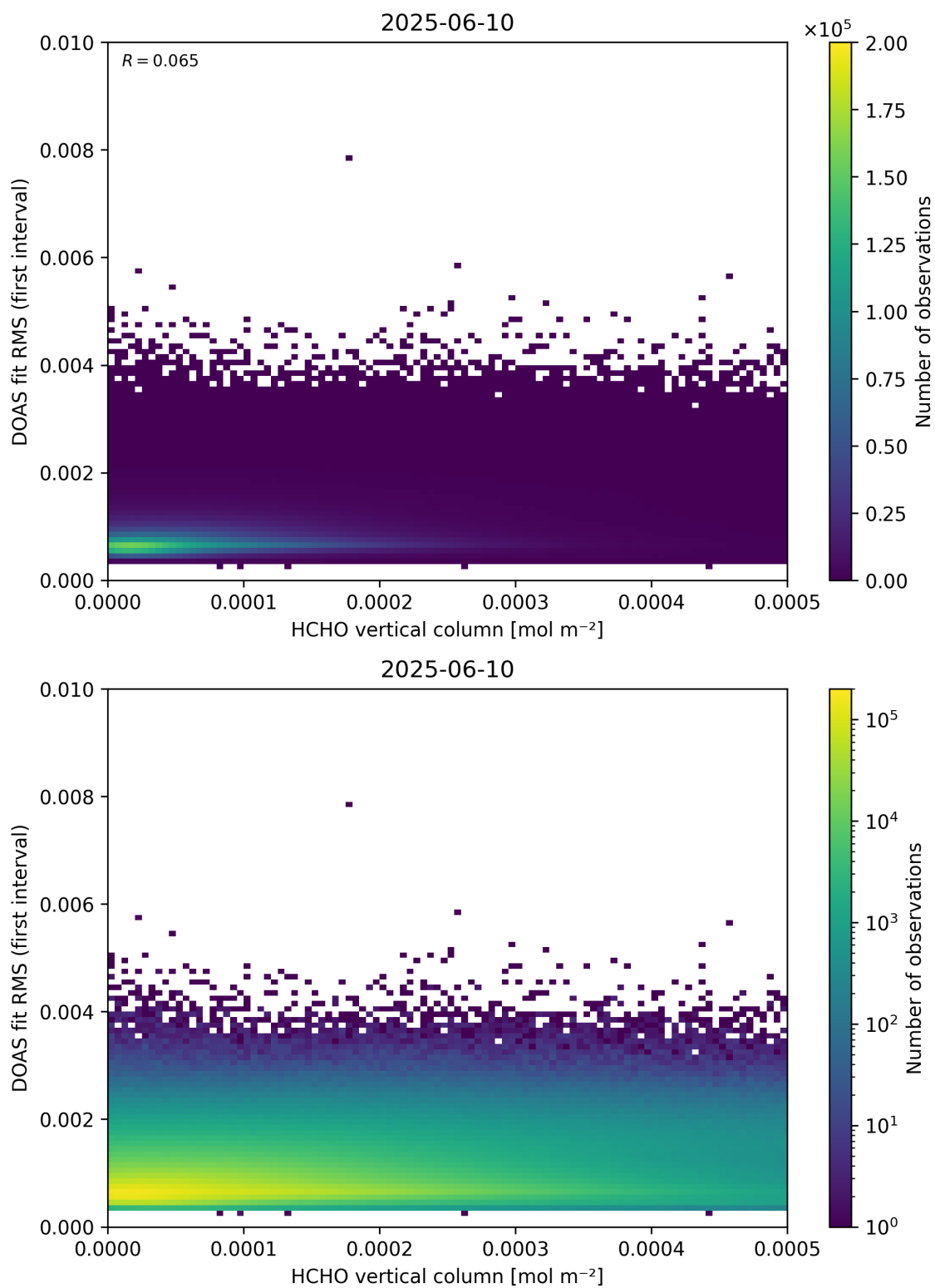
Figure 123: Scatter density plot of “HCHO vertical column” against “DOAS fit RMS (first interval)” for 2025-06-09 to 2025-06-11.
