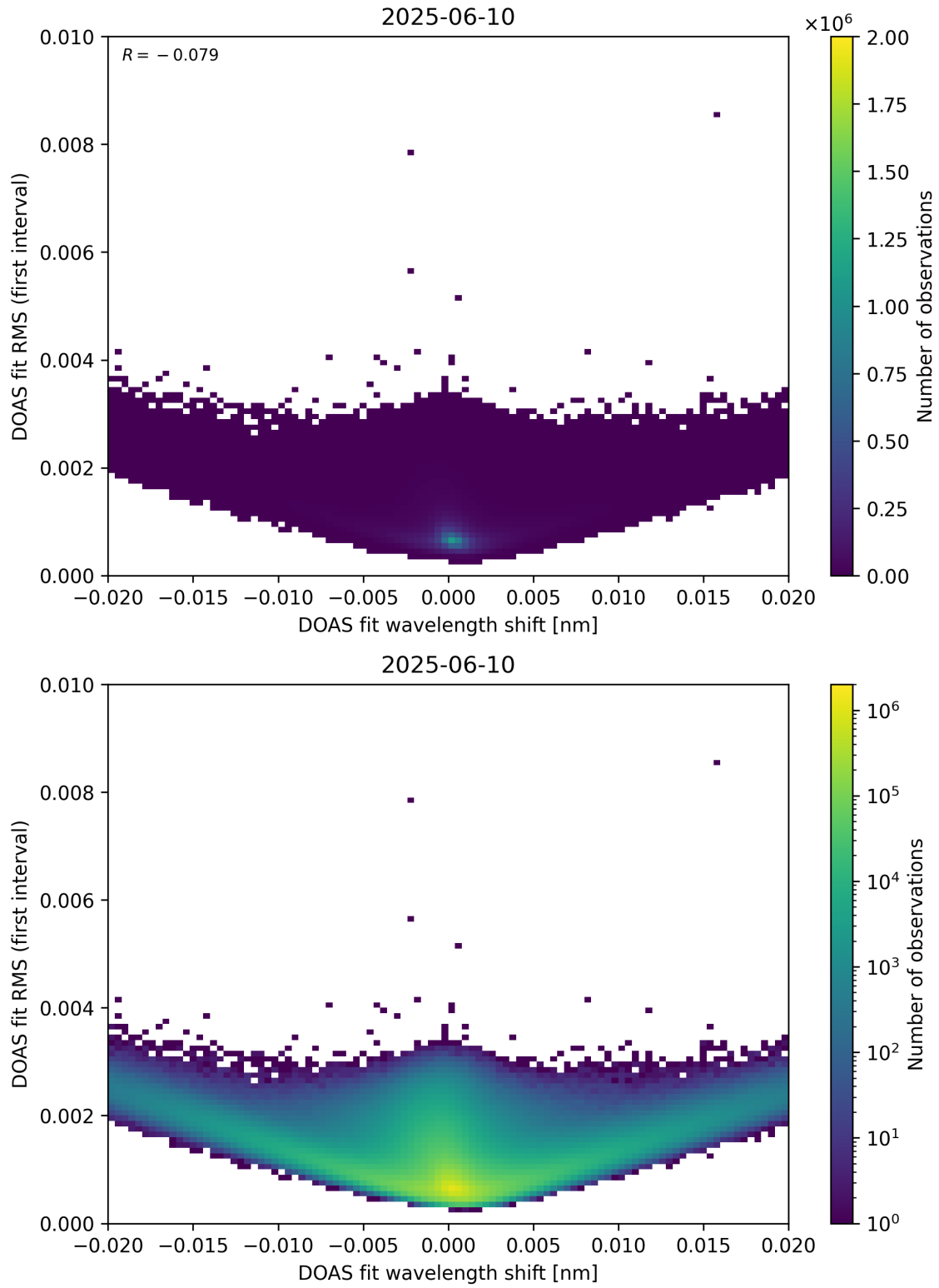
Figure 64: Scatter density plot of “DOAS fit wavelength shift” against “DOAS fit RMS (first interval)” for 2025-06-09 to 2025-06-11.
