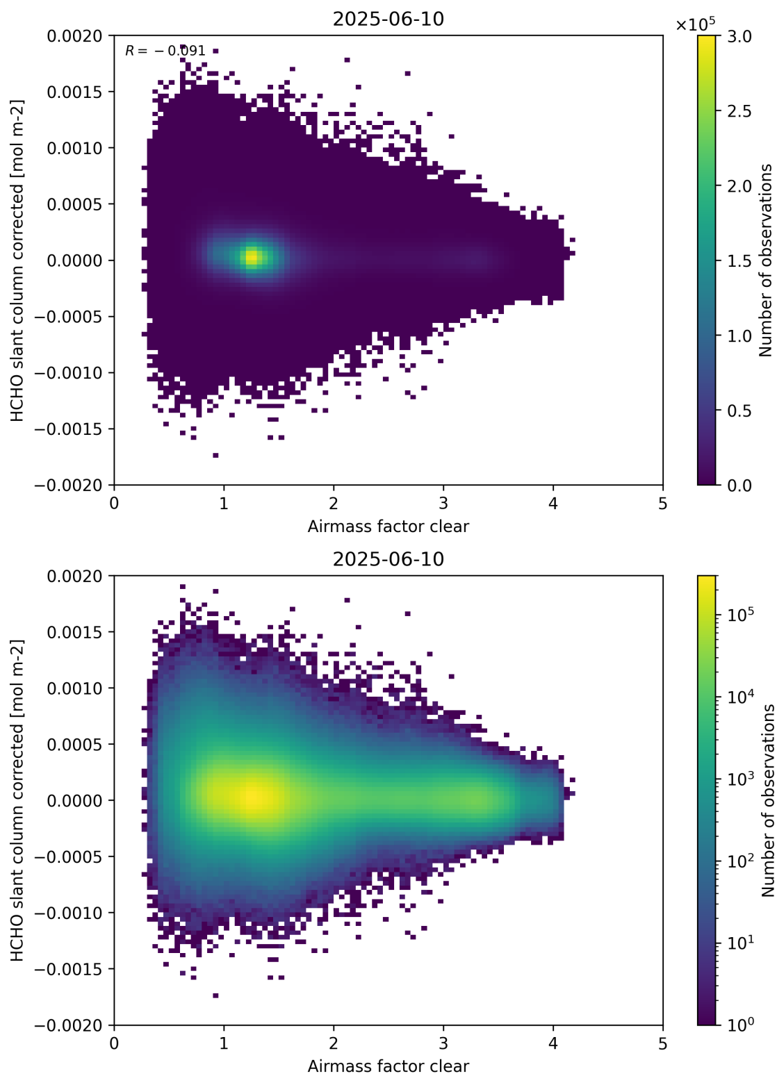
Figure 74: Scatter density plot of “Airmass factor clear” against “HCHO slant column corrected” for 2025-06-09 to 2025-06-11.
