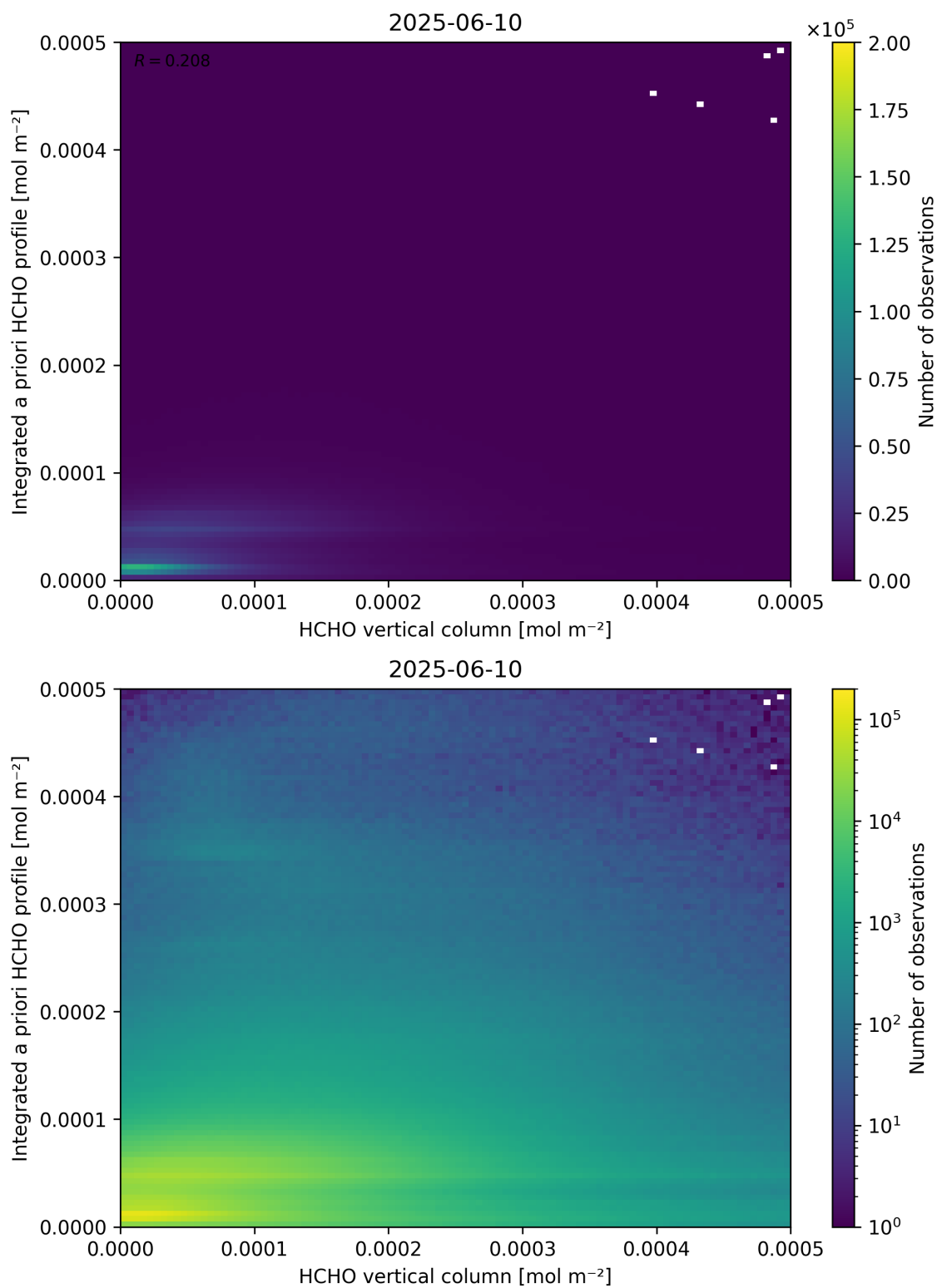
Figure 135: Scatter density plot of “HCHO vertical column” against “Integrated a priori HCHO profile” for 2025-06-09 to 2025-06-11.
