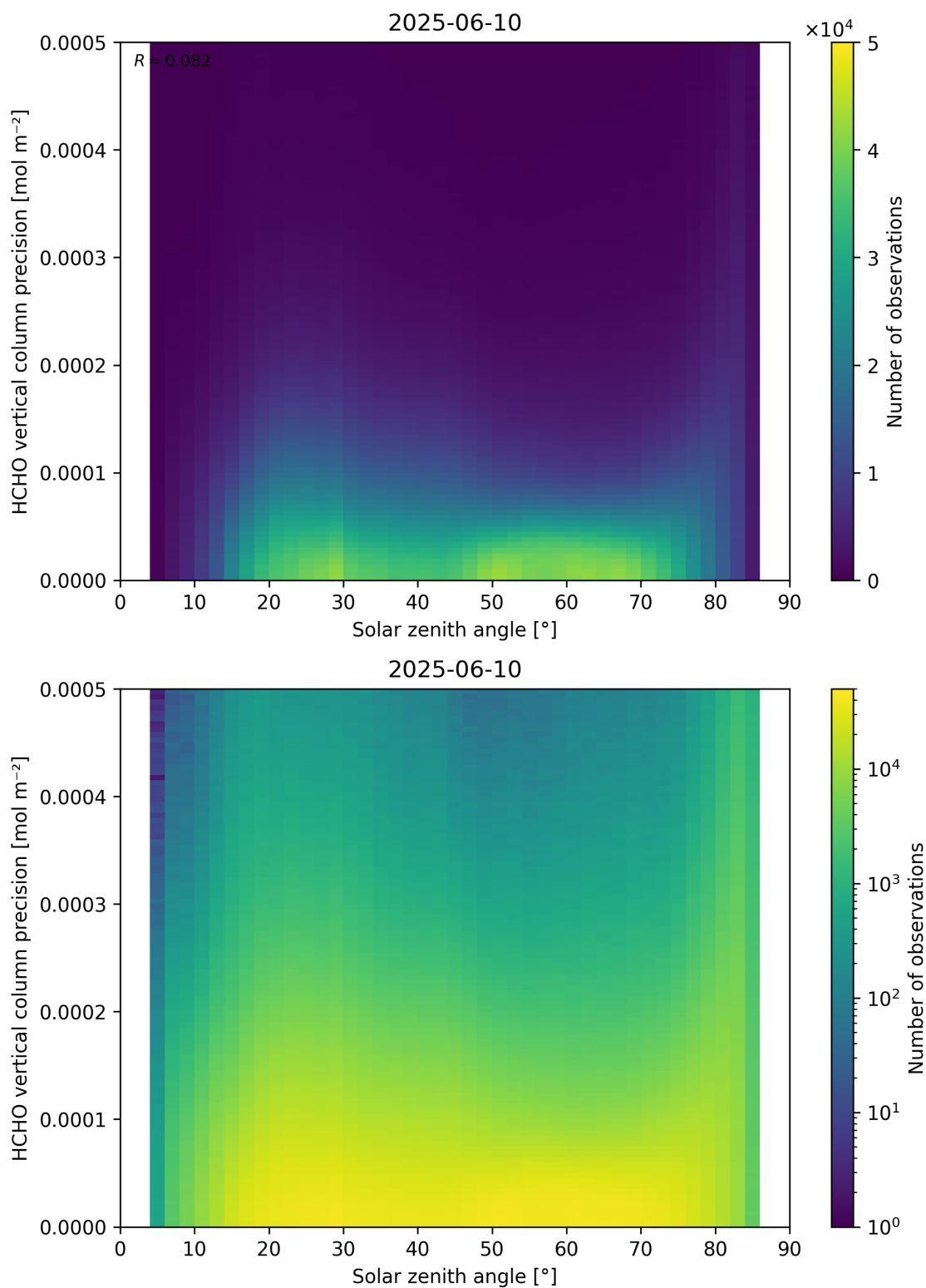
Figure 179: Scatter density plot of “Solar zenith angle” against “HCHO vertical column precision” for 2025-06-09 to 2025-06-11.
