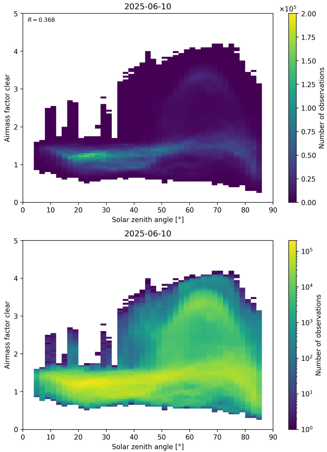
Figure 170: Scatter density plot of “Solar zenith angle” against “Airmass factor clear” for 2025-06-09 to 2025-06-11.
