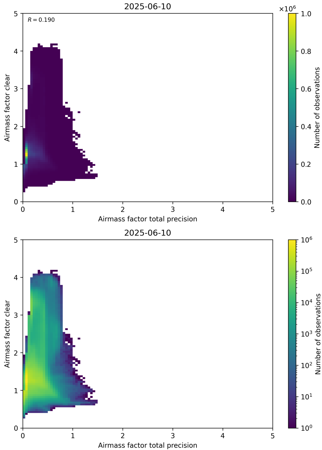
Figure 108: Scatter density plot of “Airmass factor total precision” against “Airmass factor clear” for 2025-06-09 to 2025-06-11.
