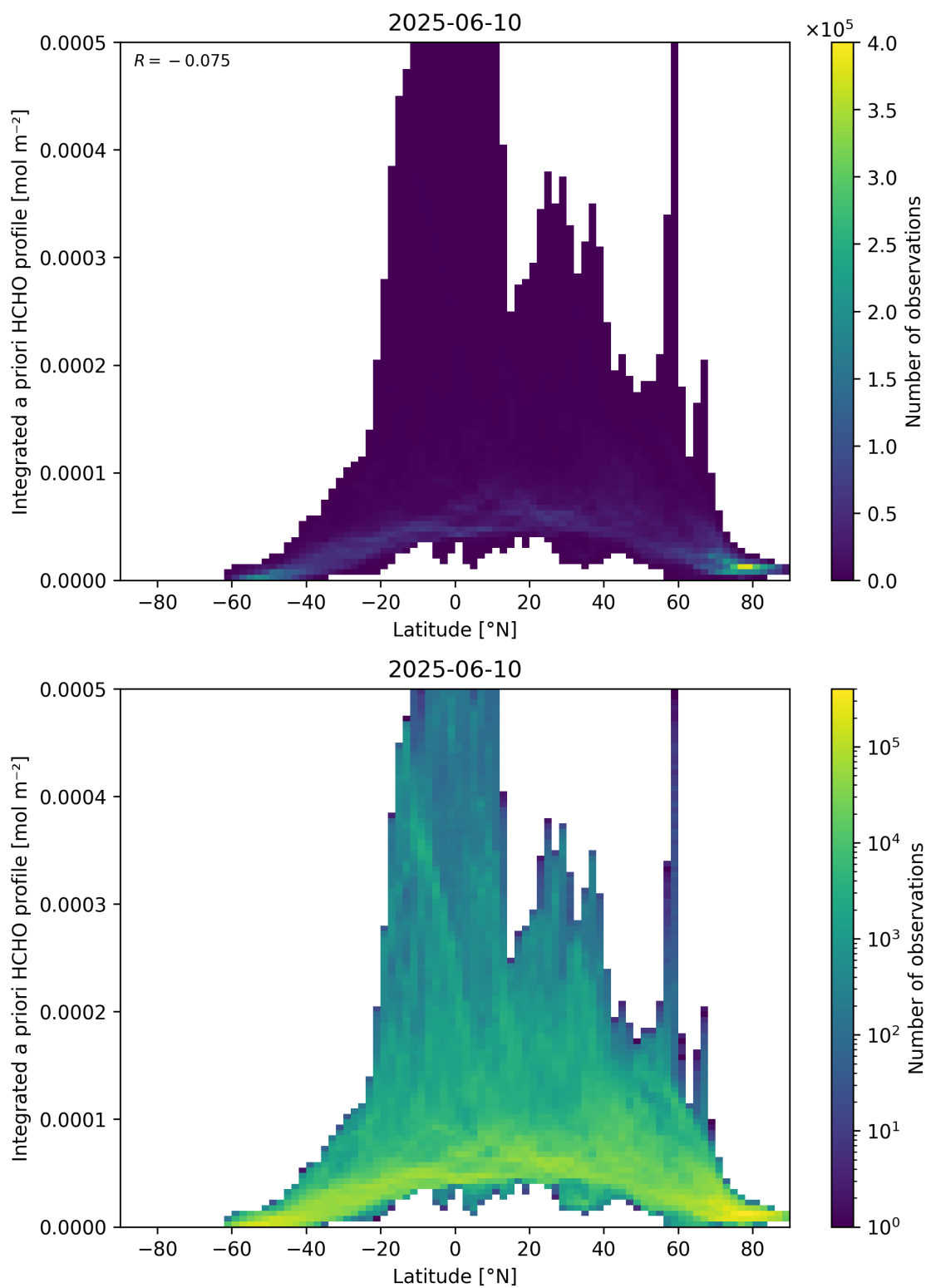
Figure 166: Scatter density plot of “Latitude” against “Integrated a priori HCHO profile” for 2025-06-09 to 2025-06-11.
