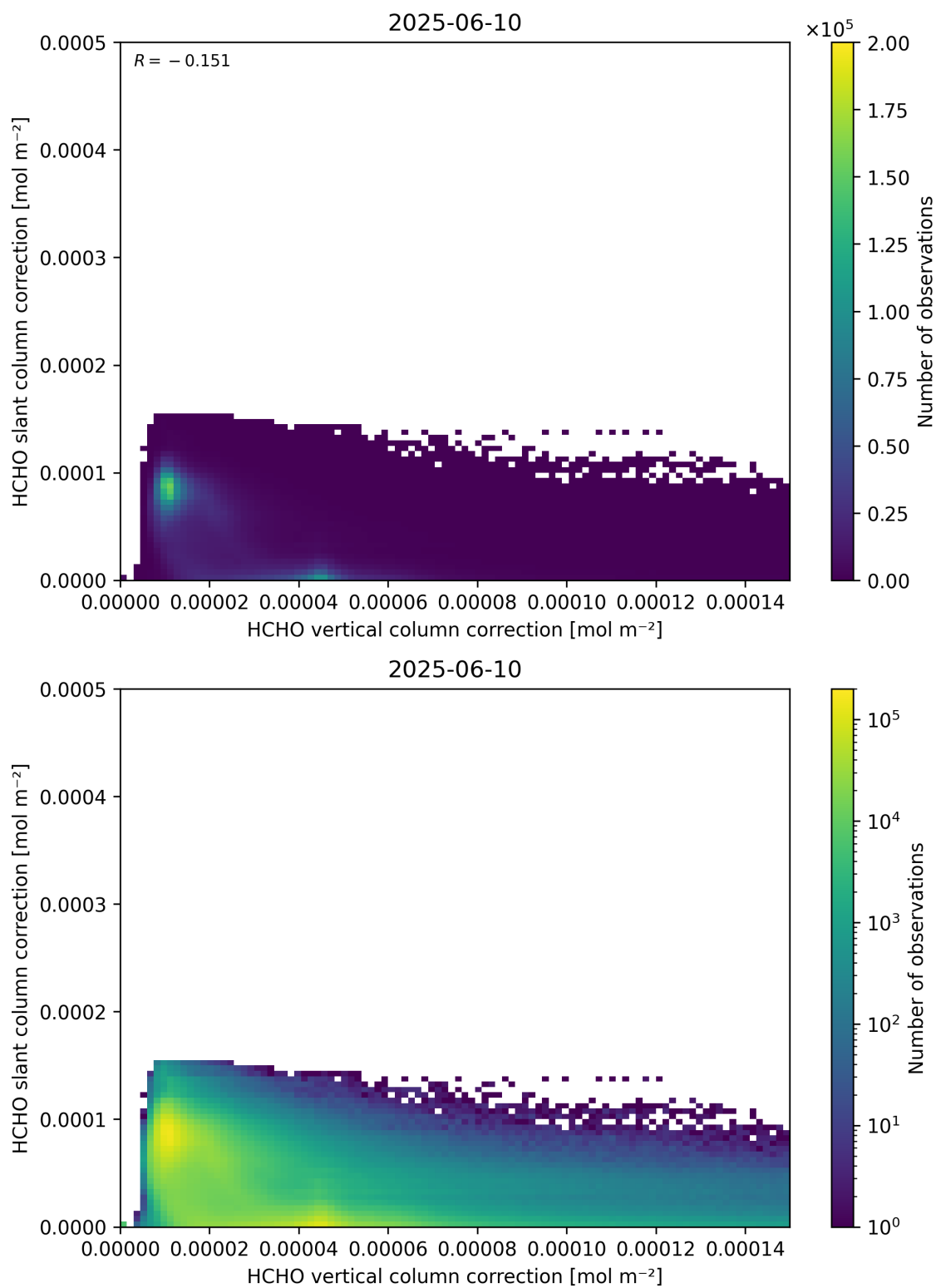
Figure 117: Scatter density plot of “HCHO vertical column correction” against “HCHO slant column correction” for 2025-06-09 to 2025-06-11.
