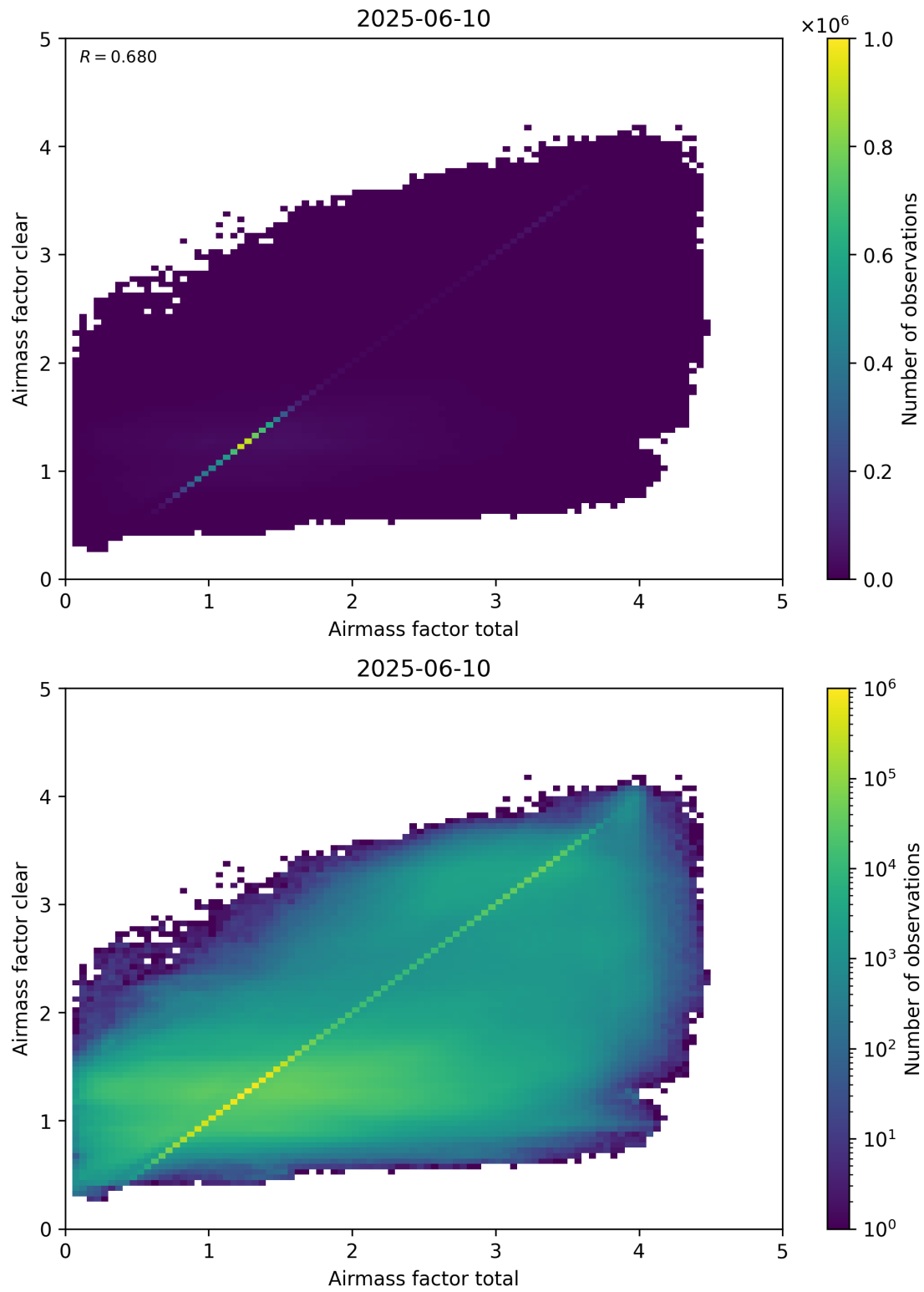
Figure 100: Scatter density plot of “Airmass factor total” against “Airmass factor clear” for 2025-06-09 to 2025-06-11.
