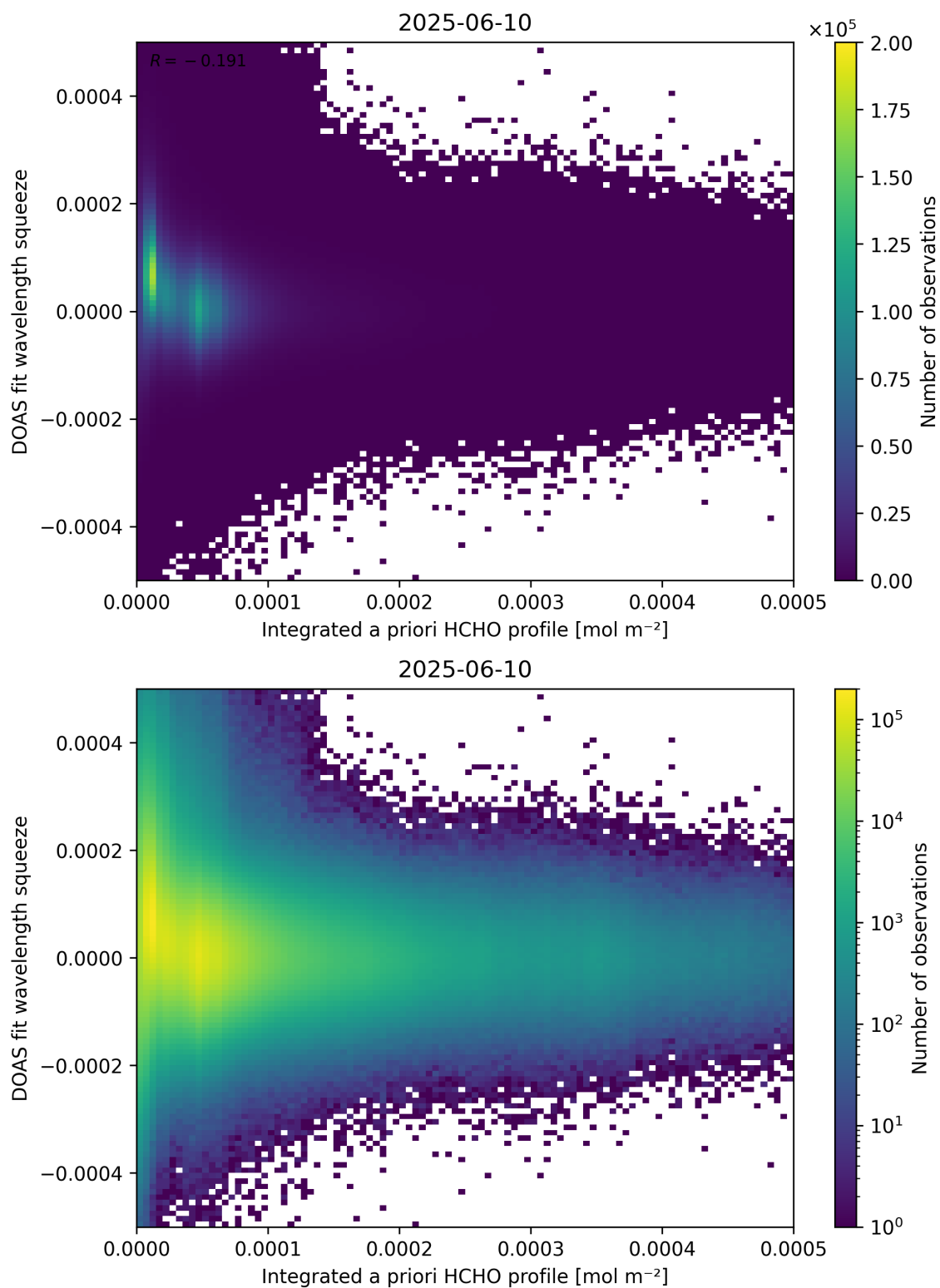
Figure 150: Scatter density plot of “Integrated a priori HCHO profile” against “DOAS fit wavelength squeeze” for 2025-06-09 to 2025-06-11.
