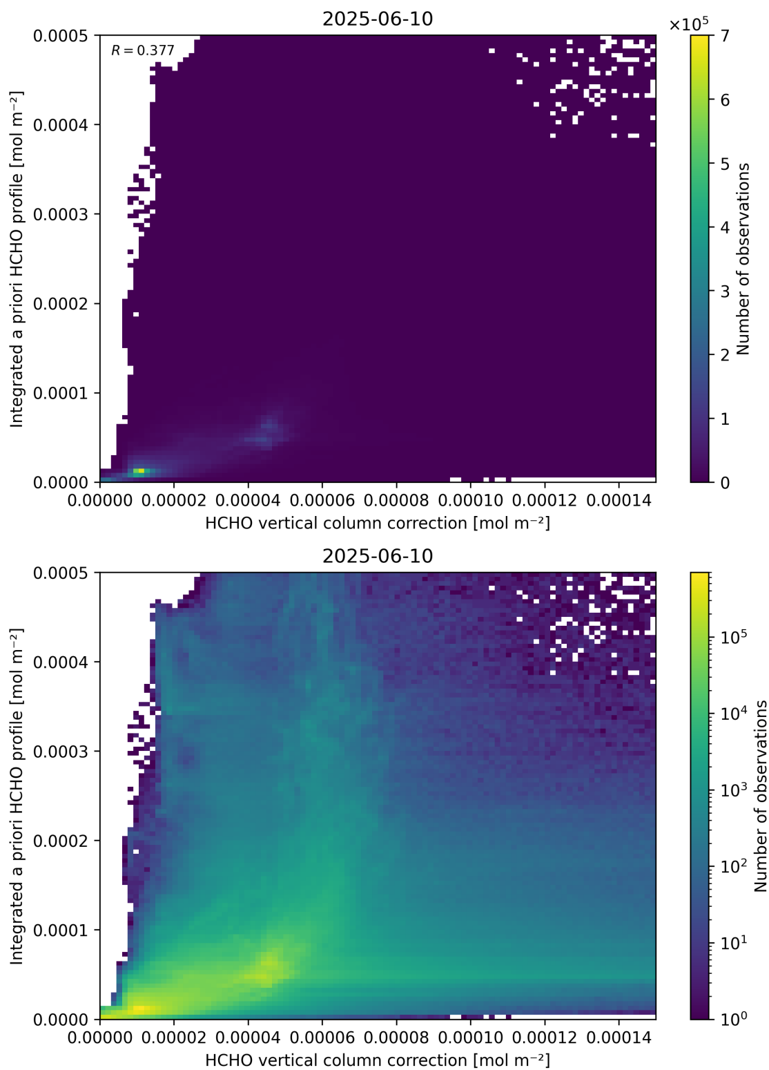
Figure 122: Scatter density plot of “HCHO vertical column correction” against “Integrated a priori HCHO profile” for 2025-06-09 to 2025-06-11.
