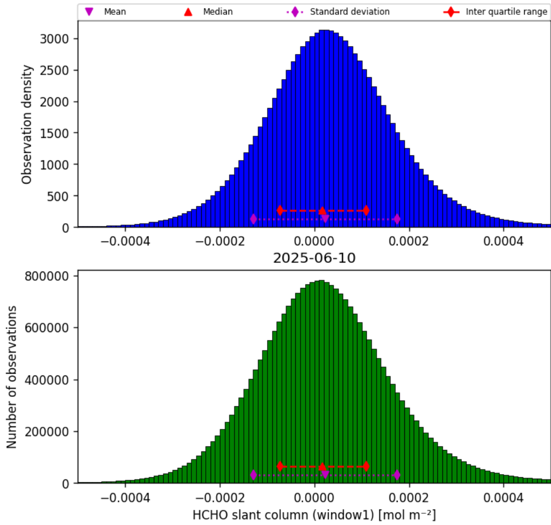
Figure 38: Histogram of “HCHO slant column (window1)” for 2025-06-09 to 2025-06-11
