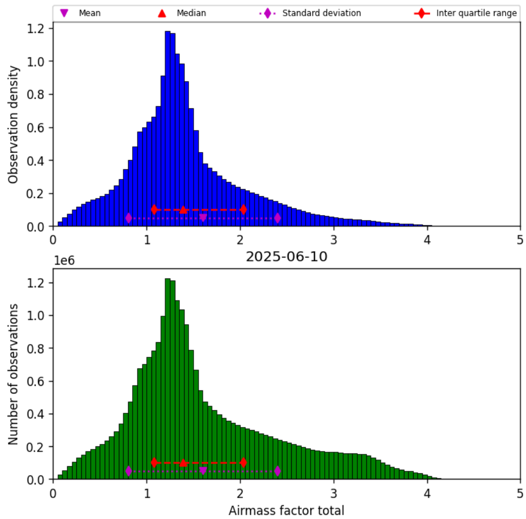
Figure 40: Histogram of “Airmass factor total” for 2025-06-09 to 2025-06-11
