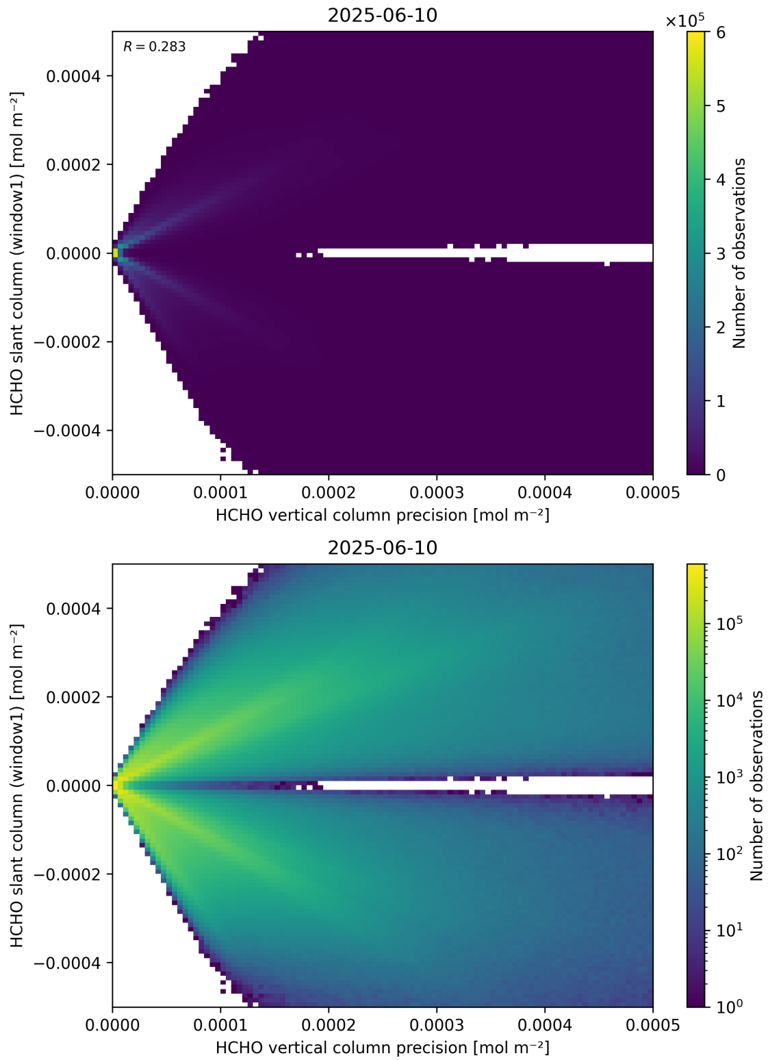
Figure 142: Scatter density plot of “HCHO vertical column precision” against “HCHO slant column (window1)” for 2025-06-09 to 2025-06-11.
