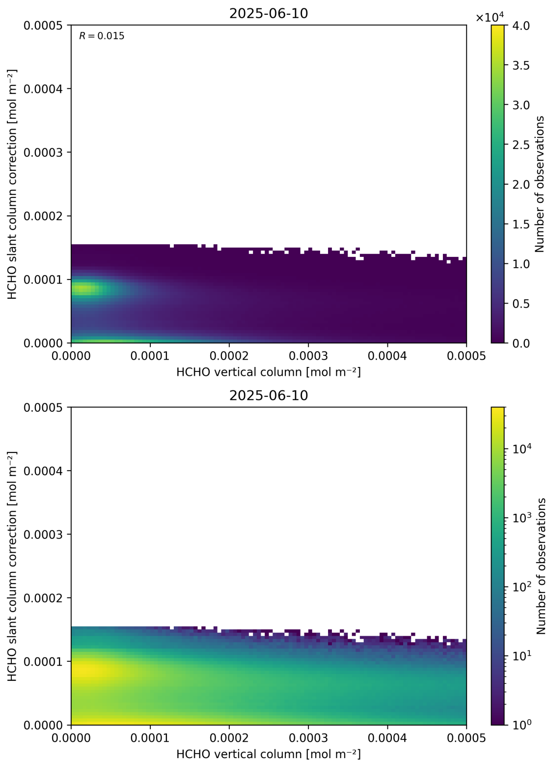
Figure 128: Scatter density plot of “HCHO vertical column” against “HCHO slant column correction” for 2025-06-09 to 2025-06-11.
