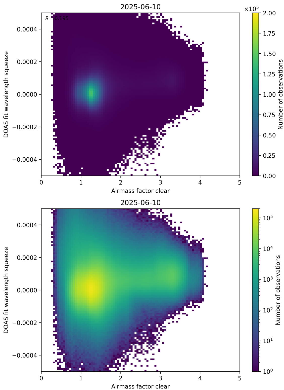
Figure 73: Scatter density plot of “Airmass factor clear” against “DOAS fit wavelength squeeze” for 2025-06-09 to 2025-06-11.
