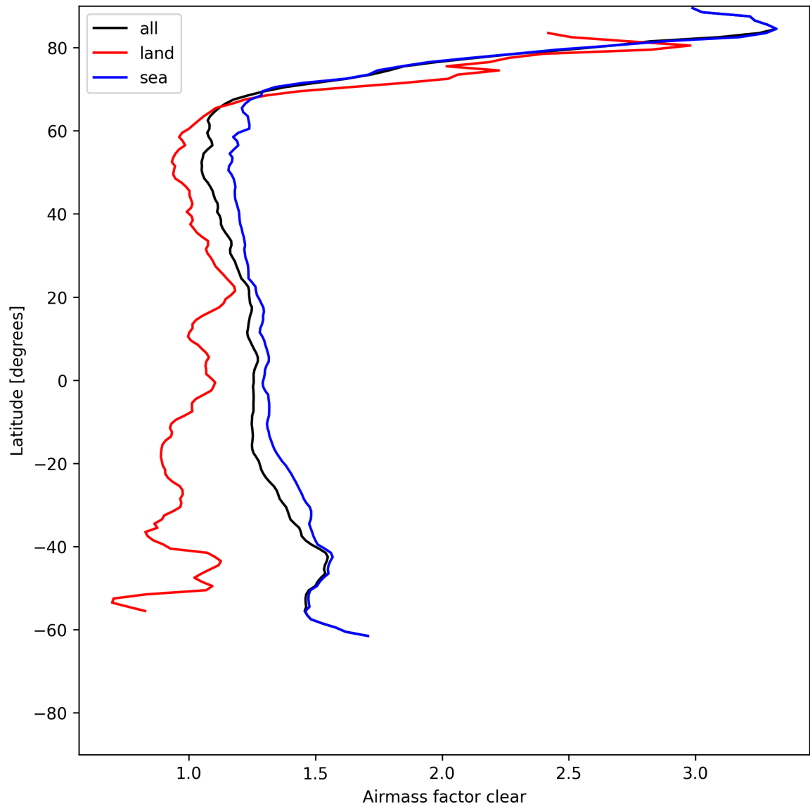
Figure 28: Zonal average of “Airmass factor clear” for 2025-06-09 to 2025-06-11.
