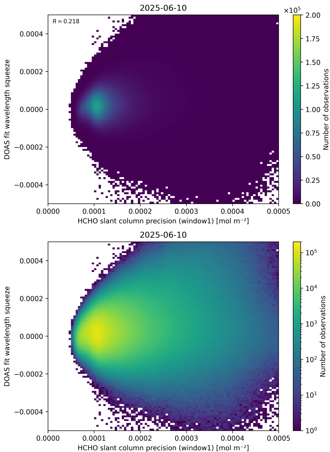
Figure 90: Scatter density plot of “HCHO slant column precision (window1)” against “DOAS fit wavelength squeeze” for 2025-06-09 to 2025-06-11.
