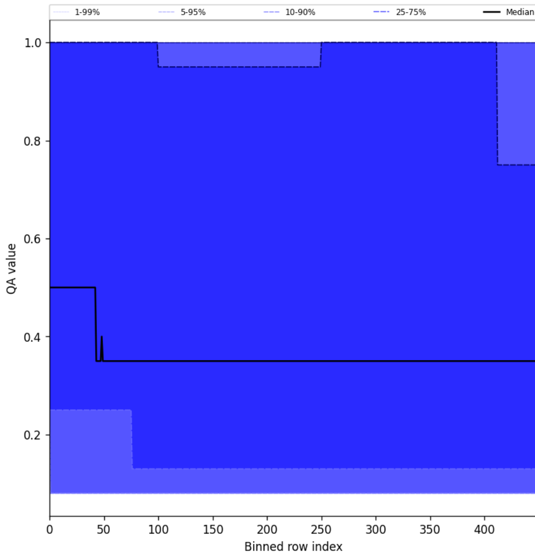
Figure 48: Along track statistics of "QA value" for 2025-06-09 to 2025-06-11
