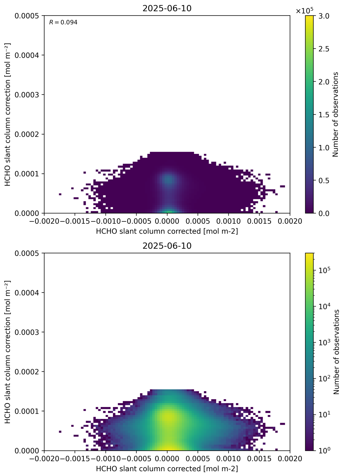
Figure 77: Scatter density plot of “HCHO slant column corrected” against “HCHO slant column correction” for 2025-06-09 to 2025-06-11.
