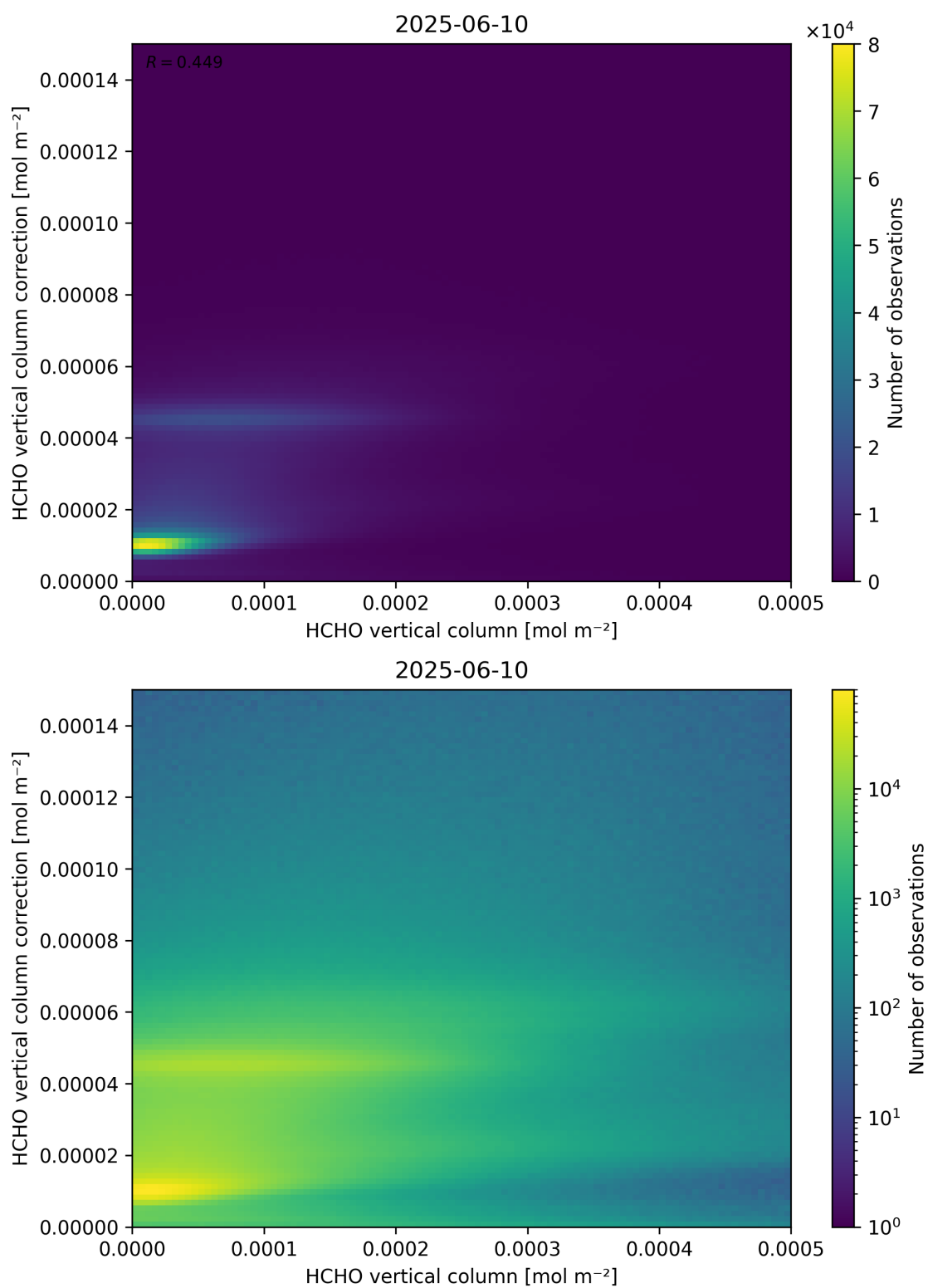
Figure 133: Scatter density plot of “HCHO vertical column” against “HCHO vertical column correction” for 2025-06-09 to 2025-06-11.
