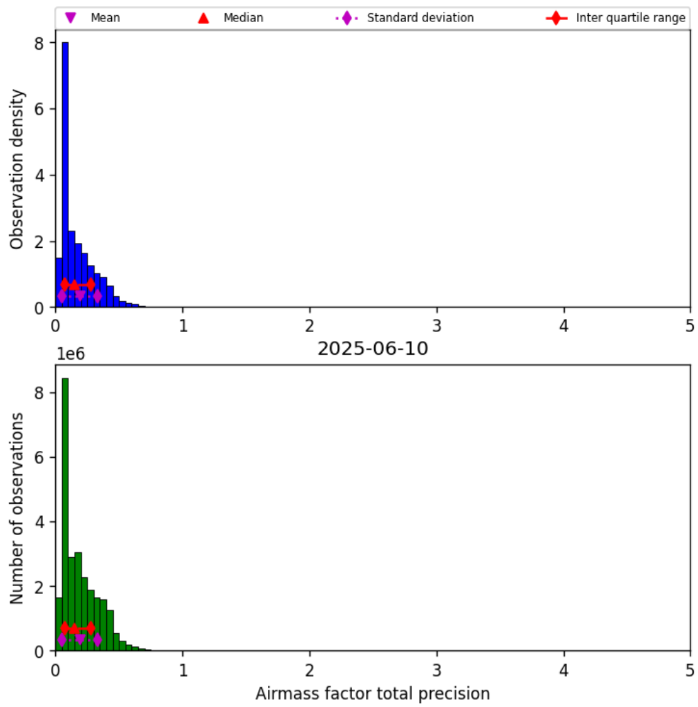
Figure 41: Histogram of “Airmass factor total precision” for 2025-06-09 to 2025-06-11
