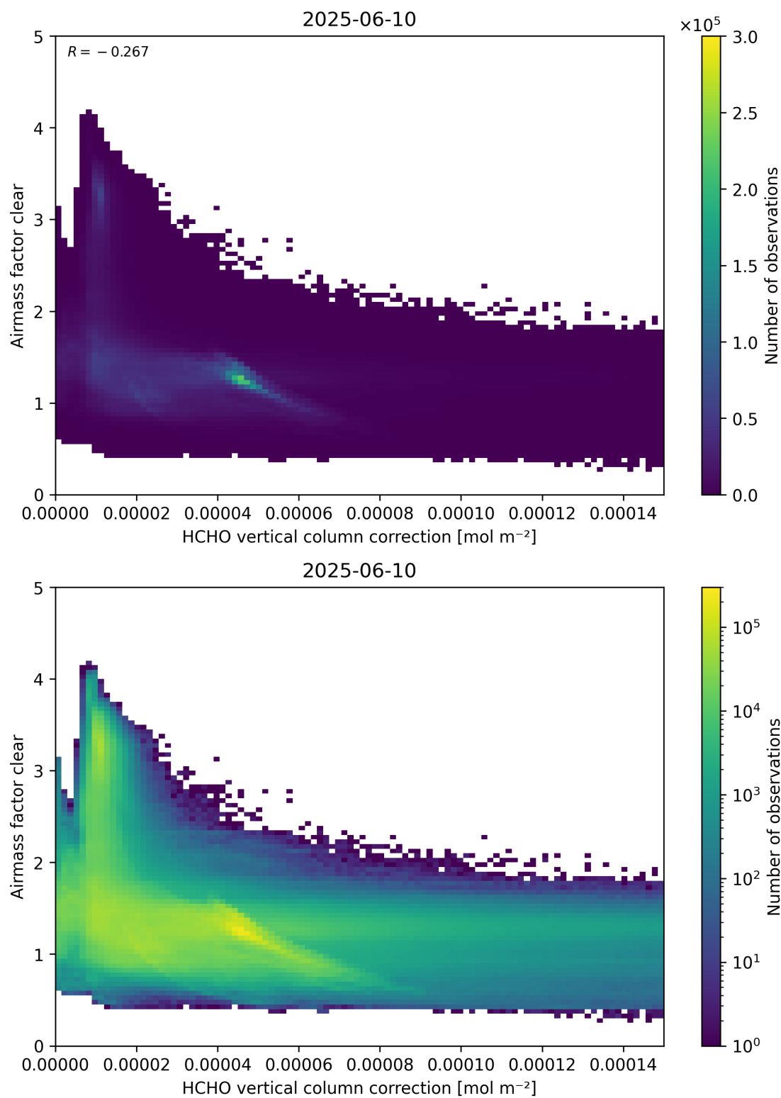
Figure 115: Scatter density plot of “HCHO vertical column correction” against “Airmass factor clear” for 2025-06-09 to 2025-06-11.
