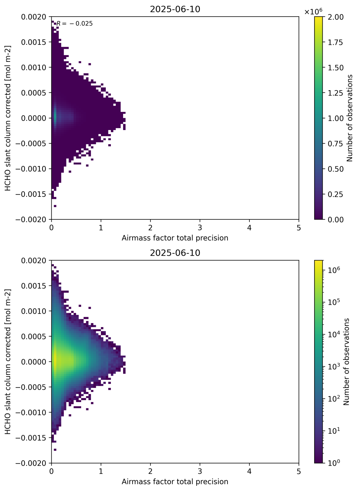
Figure 109: Scatter density plot of “Airmass factor total precision” against “HCHO slant column corrected” for 2025-06-09 to 2025-06-11.
