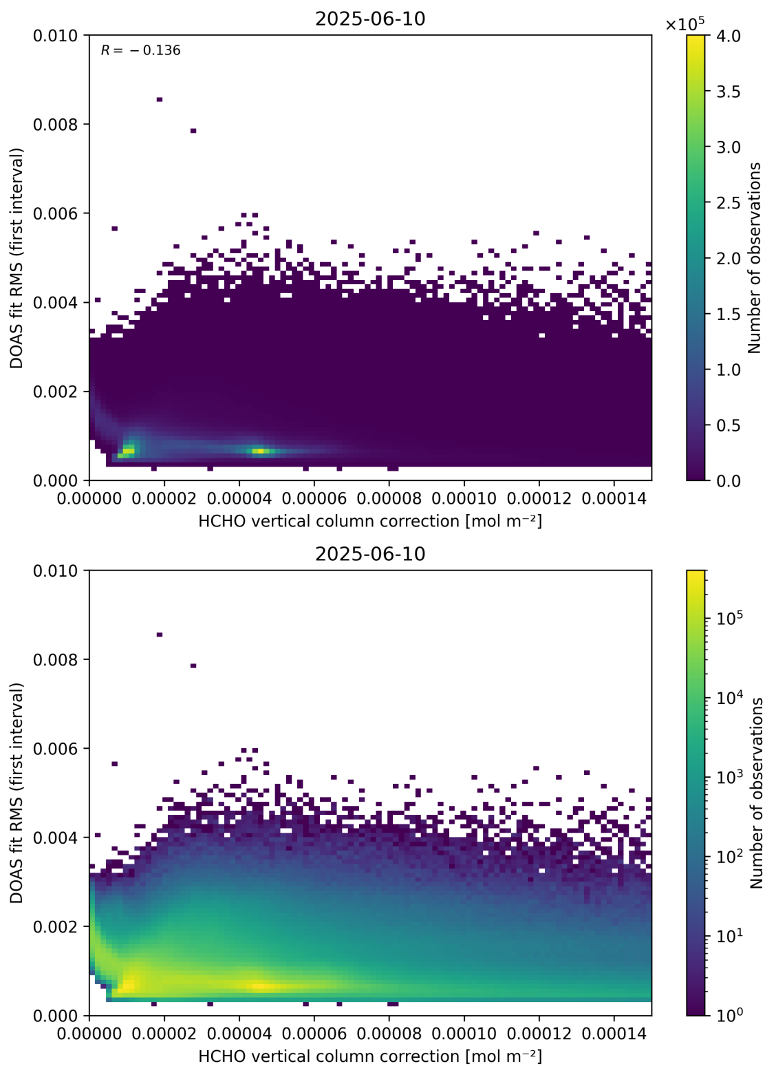
Figure 112: Scatter density plot of “HCHO vertical column correction” against “DOAS fit RMS (first interval)” for 2025-06-09 to 2025-06-11.
