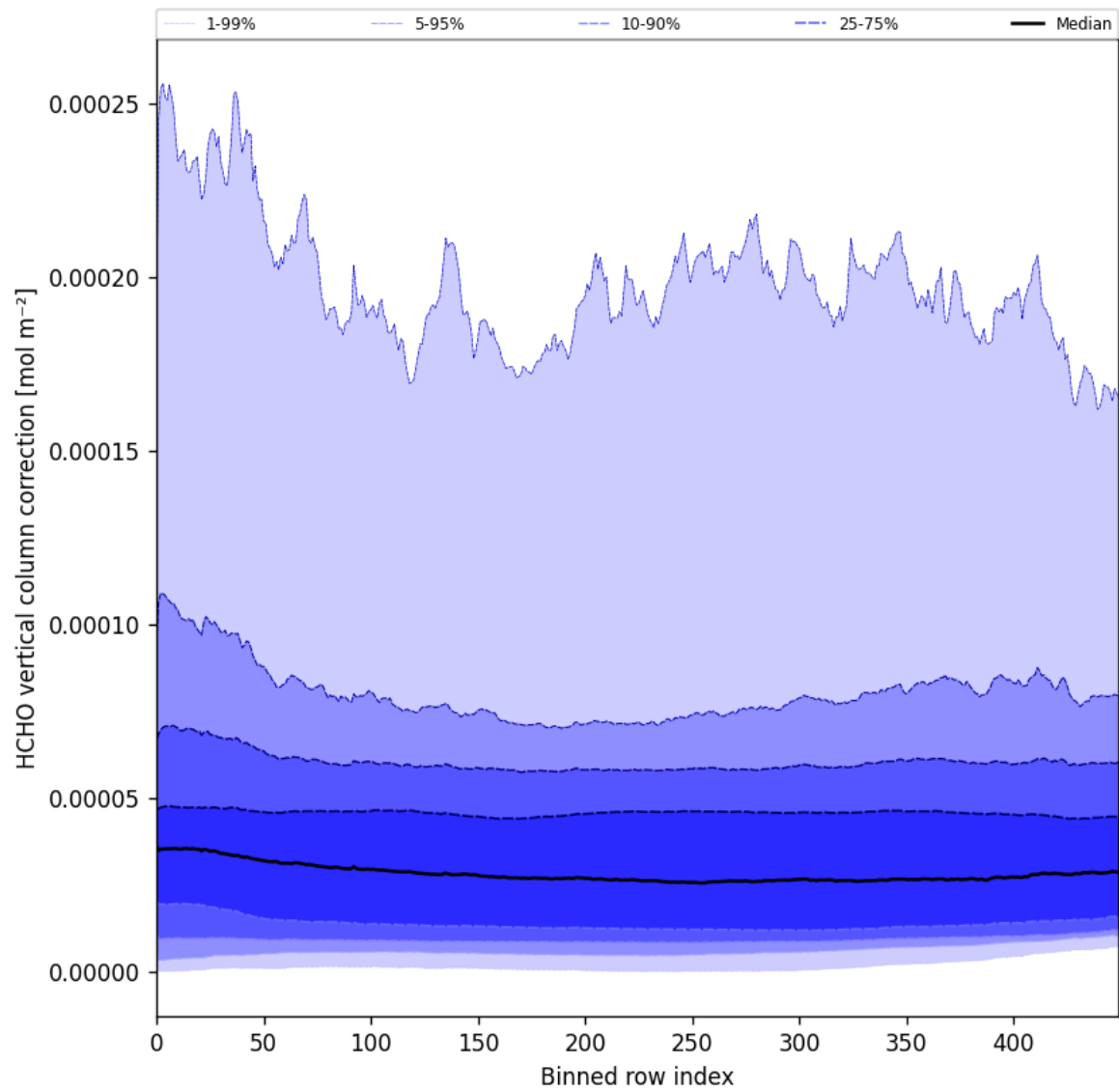
Figure 51: Along track statistics of “HCHO vertical column correction” for 2025-06-09 to 2025-06-11
