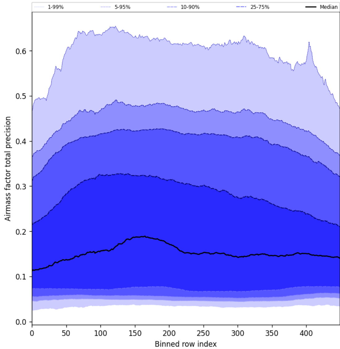
Figure 55: Along track statistics of “Airmass factor total precision” for 2025-06-09 to 2025-06-11
