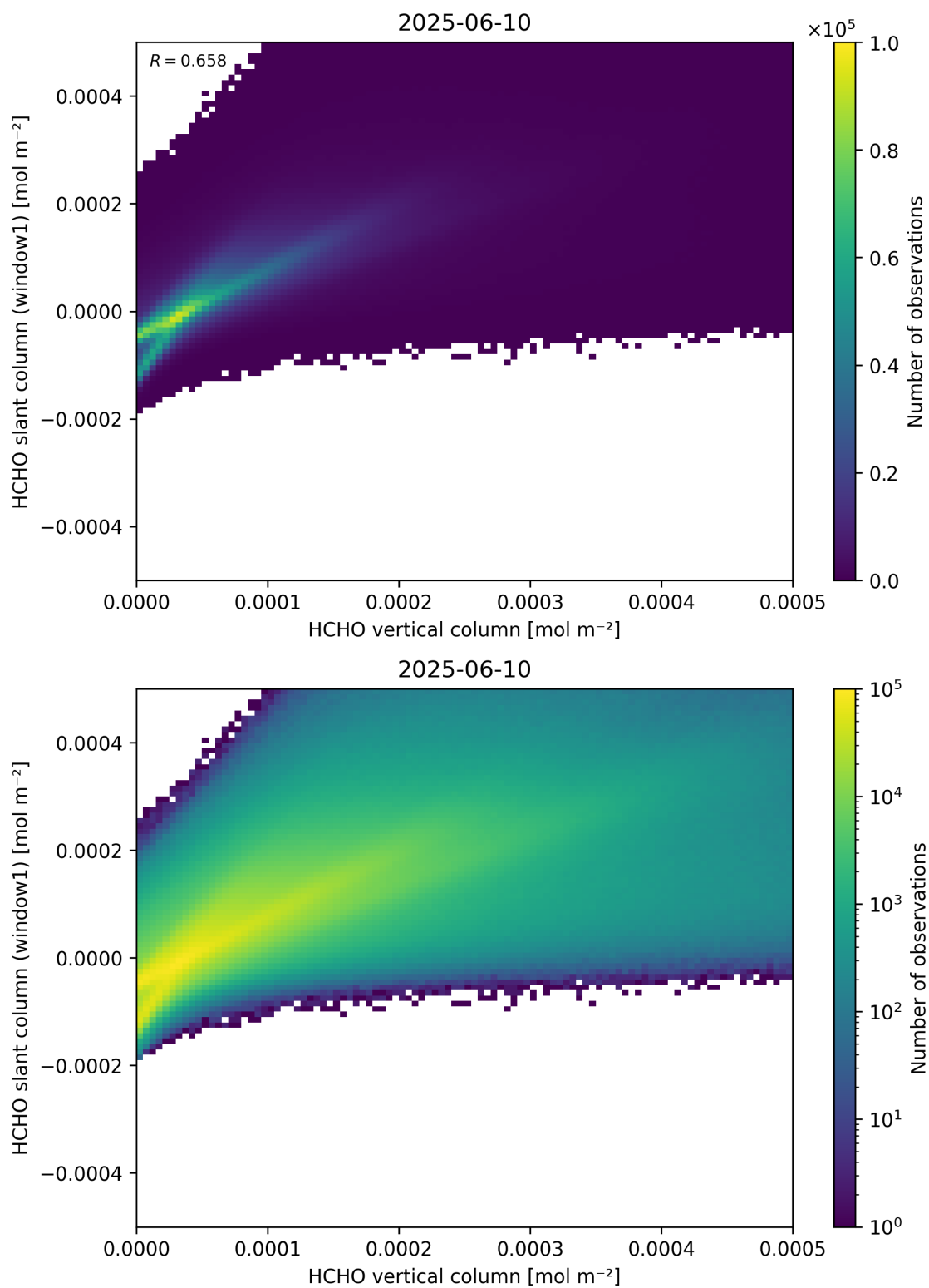
Figure 129: Scatter density plot of “HCHO vertical column” against “HCHO slant column (window1)” for 2025-06-09 to 2025-06-11.
