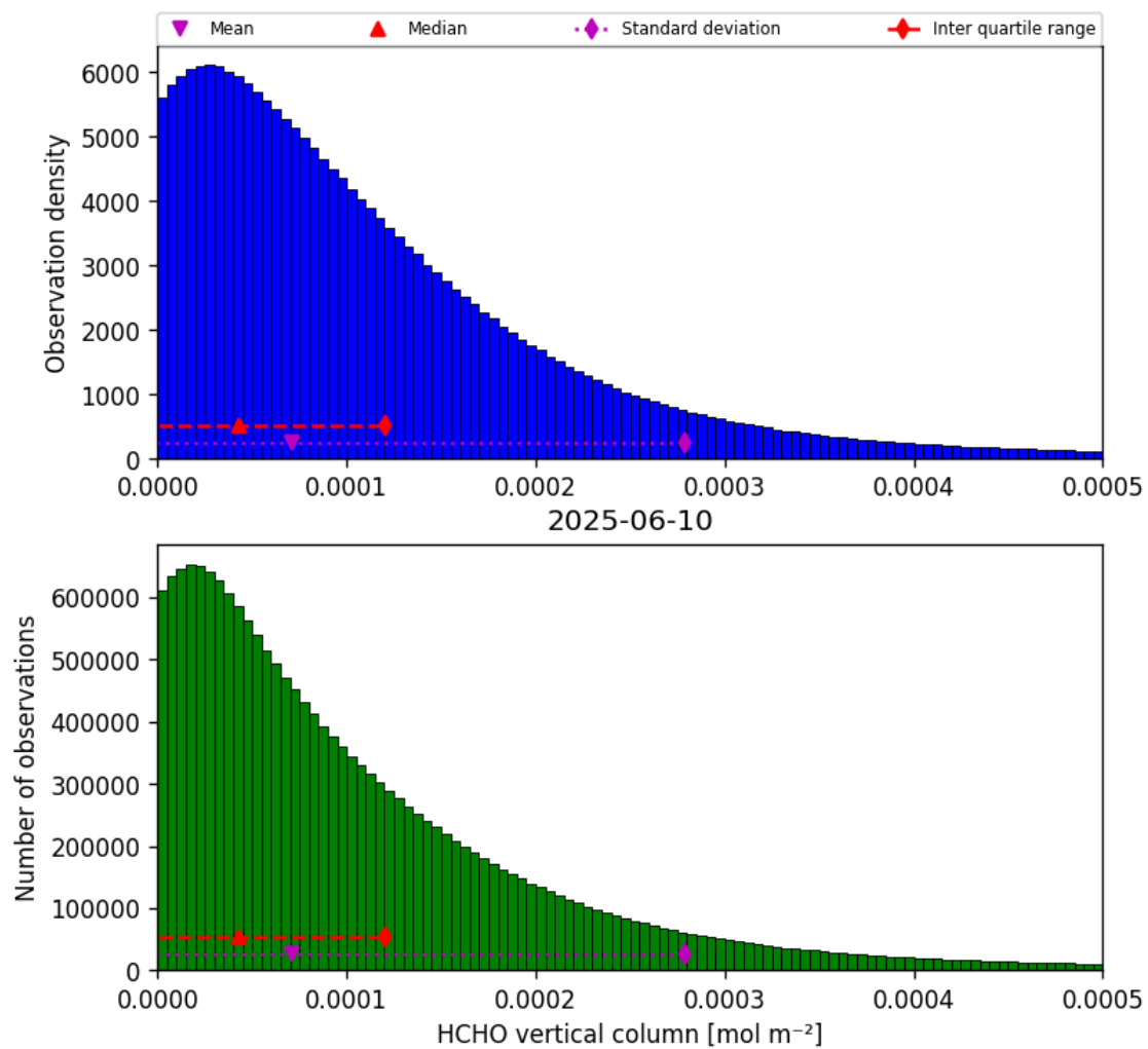
Figure 35: Histogram of “HCHO vertical column” for 2025-06-09 to 2025-06-11
