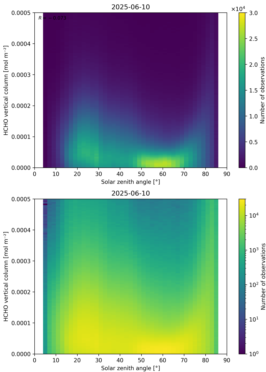
Figure 177: Scatter density plot of “Solar zenith angle” against “HCHO vertical column” for 2025-06-09 to 2025-06-11.
