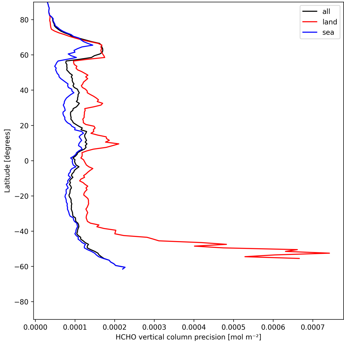
Figure 22: Zonal average of “HCHO vertical column precision” for 2025-06-09 to 2025-06-11.
