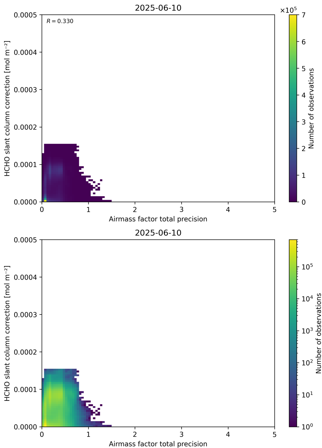
Figure 110: Scatter density plot of “Airmass factor total precision” against “HCHO slant column correction” for 2025-06-09 to 2025-06-11.
