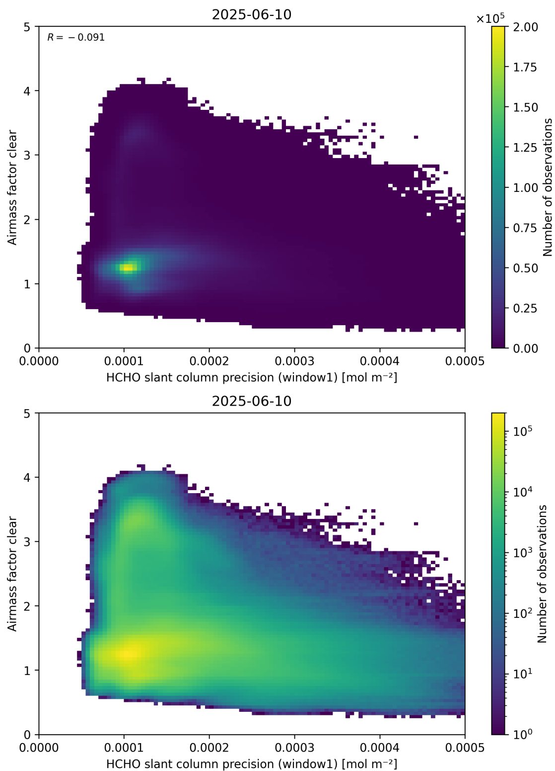
Figure 91: Scatter density plot of “HCHO slant column precision (window1)” against “Airmass factor clear” for 2025-06-09 to 2025-06-11.
