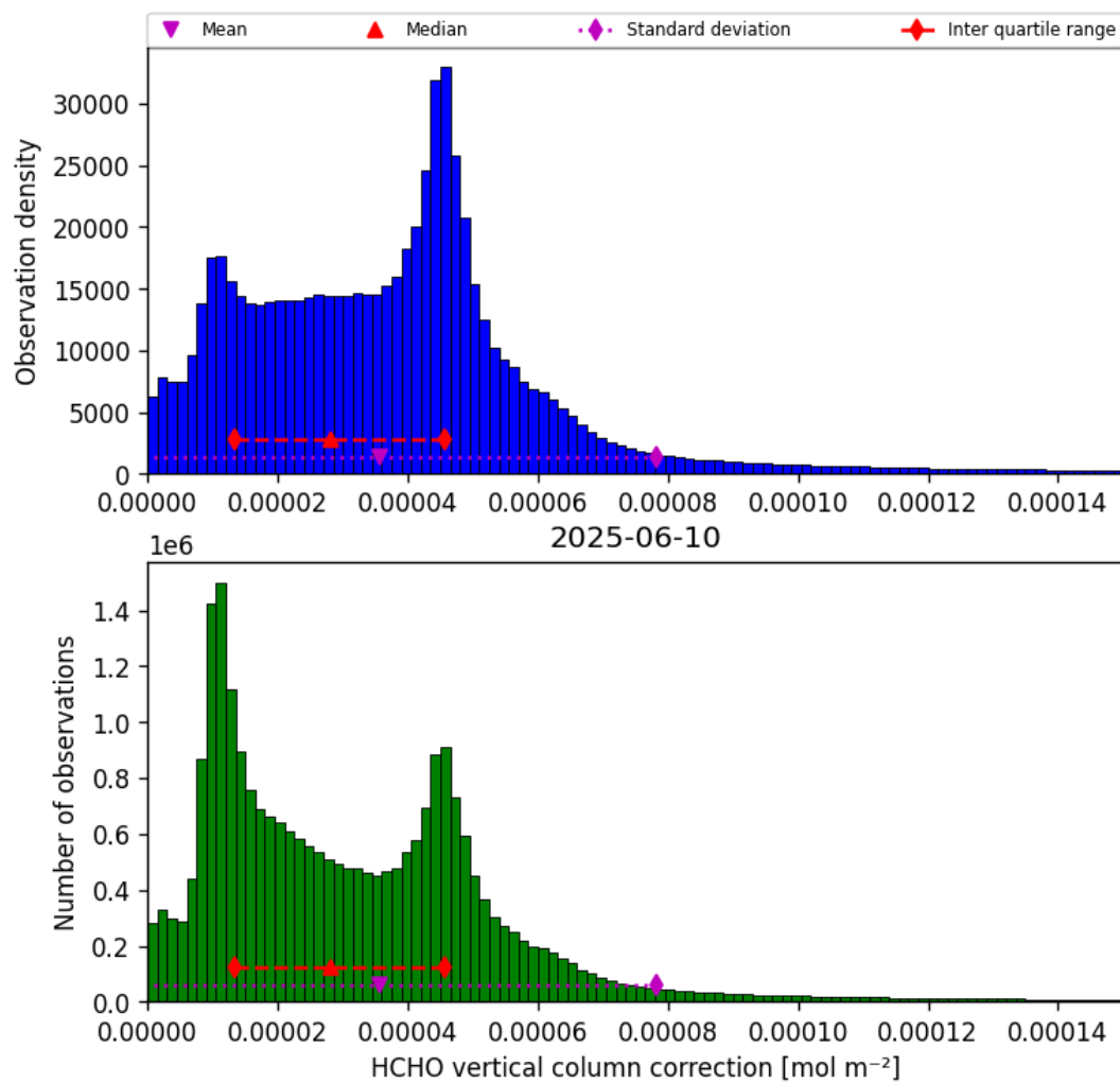
Figure 37: Histogram of “HCHO vertical column correction” for 2025-06-09 to 2025-06-11
