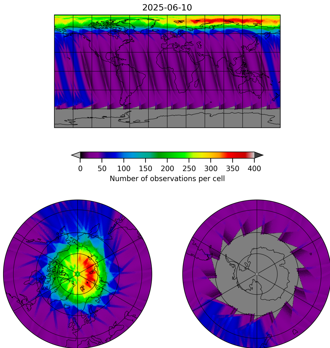
Figure 19: Map of the number of observations for 2025-06-09 to 2025-06-11
