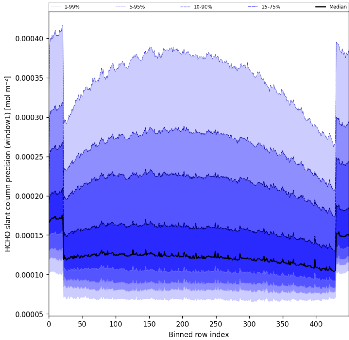
Figure 53: Along track statistics of “HCHO slant column precision (window1)” for 2025-06-09 to 2025-06-11
