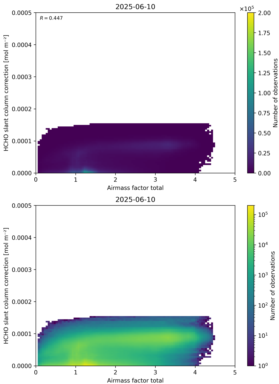
Figure 102: Scatter density plot of “Airmass factor total” against “HCHO slant column correction” for 2025-06-09 to 2025-06-11.
