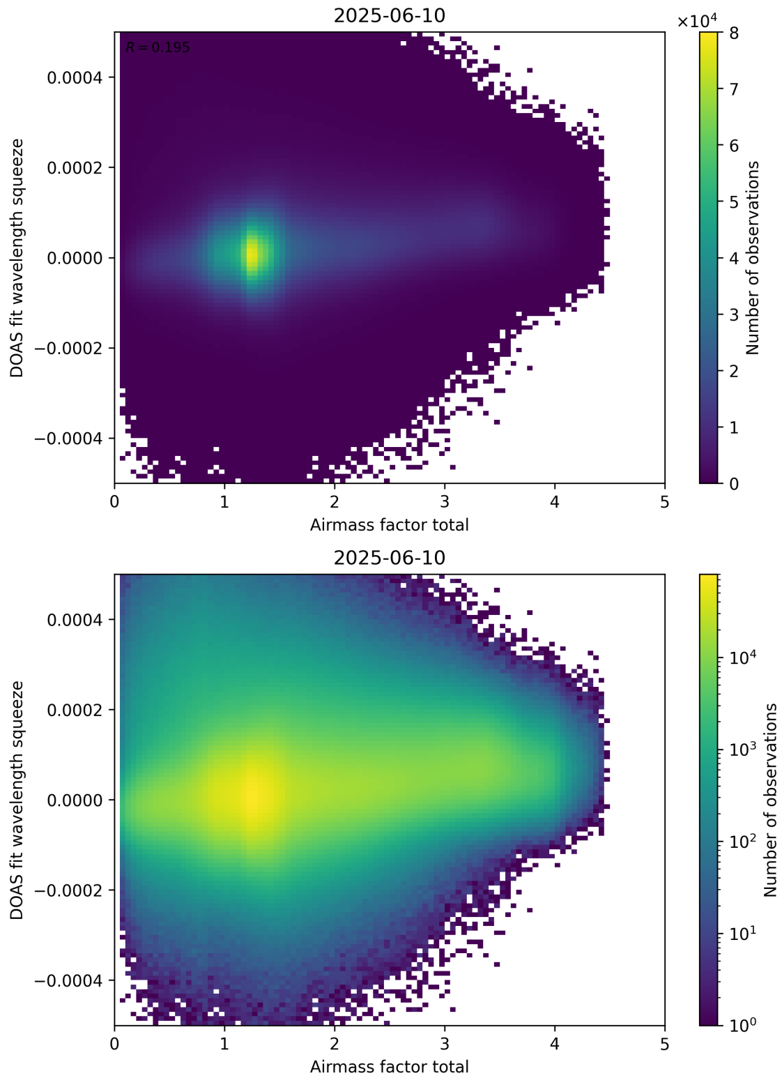
Figure 99: Scatter density plot of “Airmass factor total” against “DOAS fit wavelength squeeze” for 2025-06-09 to 2025-06-11.
