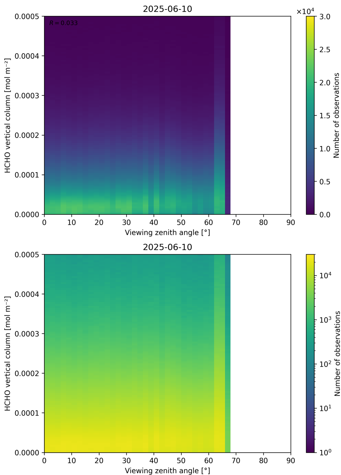
Figure 192: Scatter density plot of “Viewing zenith angle” against “HCHO vertical column” for 2025-06-09 to 2025-06-11.
