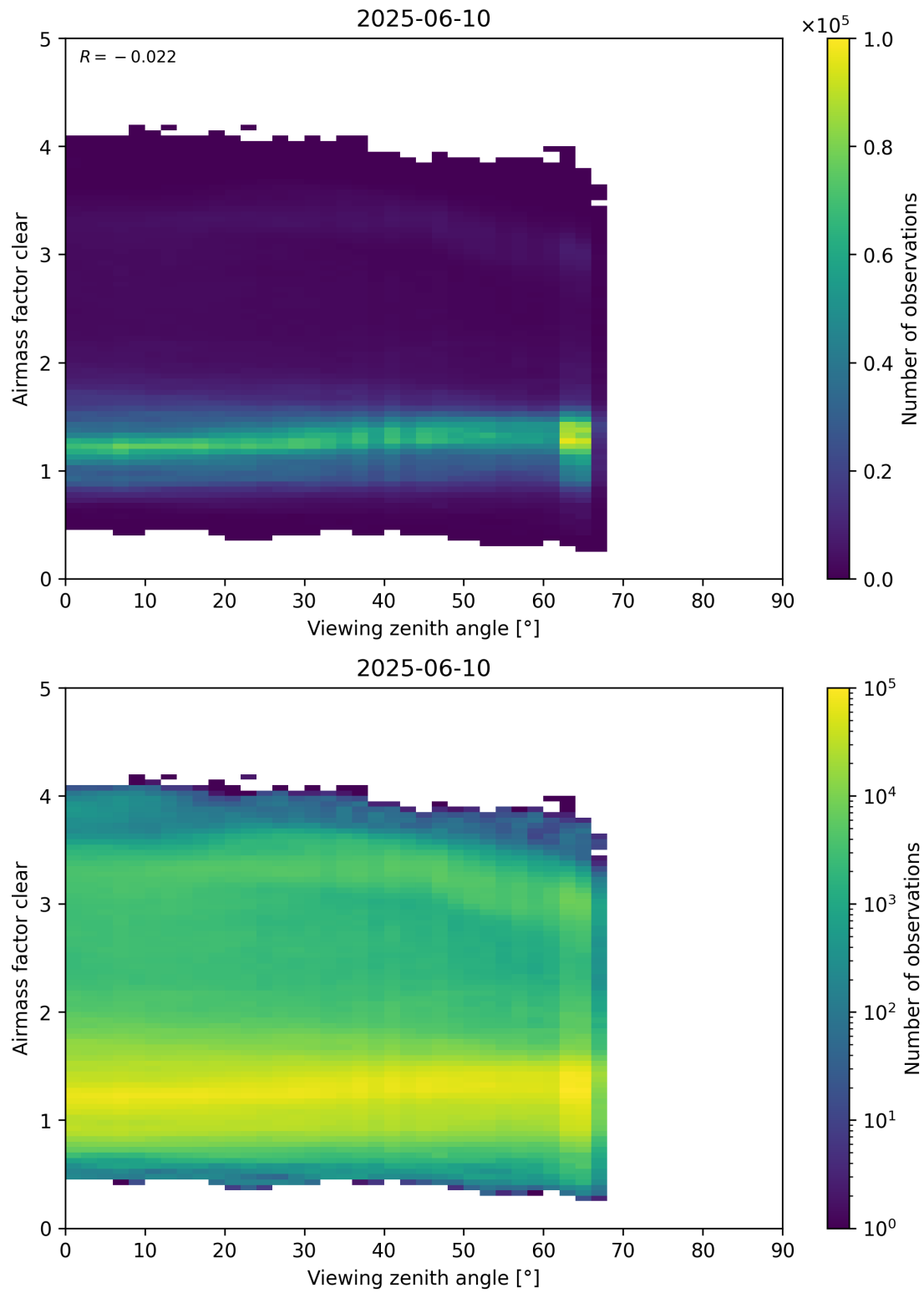
Figure 185: Scatter density plot of “Viewing zenith angle” against “Airmass factor clear” for 2025-06-09 to 2025-06-11.
