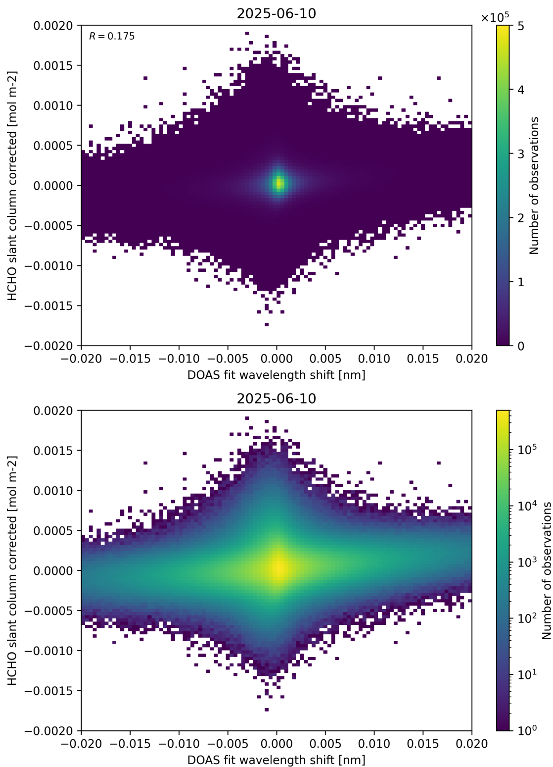
Figure 66: Scatter density plot of “DOAS fit wavelength shift” against “HCHO slant column corrected” for 2025-06-09 to 2025-06-11.
