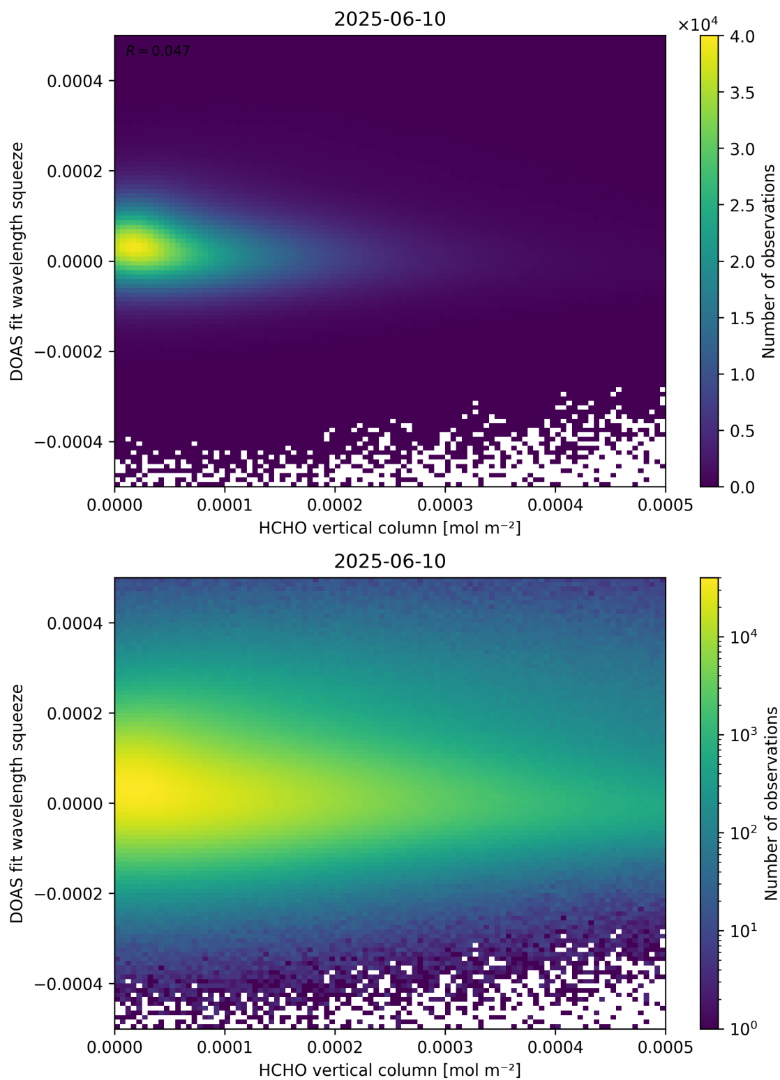
Figure 125: Scatter density plot of “HCHO vertical column” against “DOAS fit wavelength squeeze” for 2025-06-09 to 2025-06-11.
