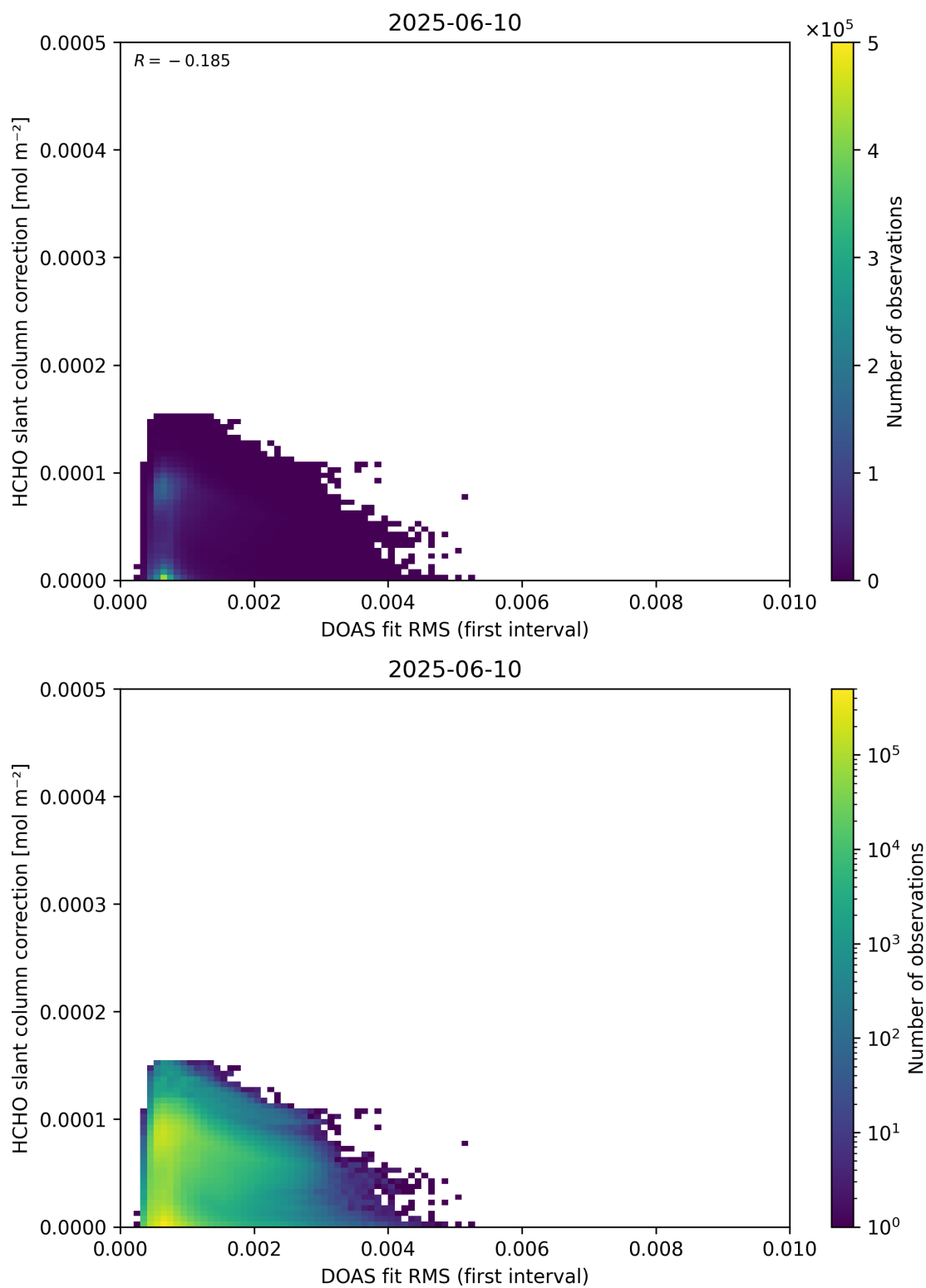
Figure 63: Scatter density plot of “DOAS fit RMS (first interval)” against “HCHO slant column correction” for 2025-06-09 to 2025-06-11.
