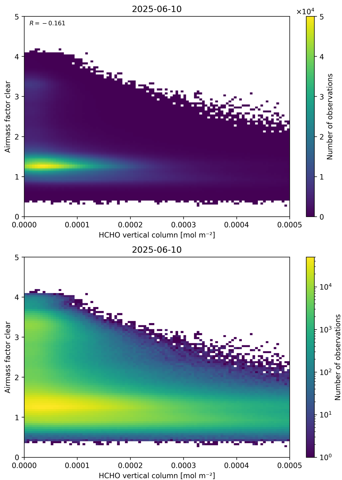
Figure 126: Scatter density plot of “HCHO vertical column” against “Airmass factor clear” for 2025-06-09 to 2025-06-11.
