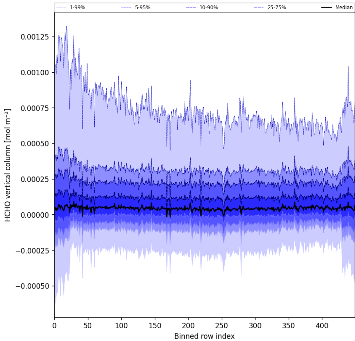
Figure 49: Along track statistics of “HCHO vertical column” for 2025-06-09 to 2025-06-11
