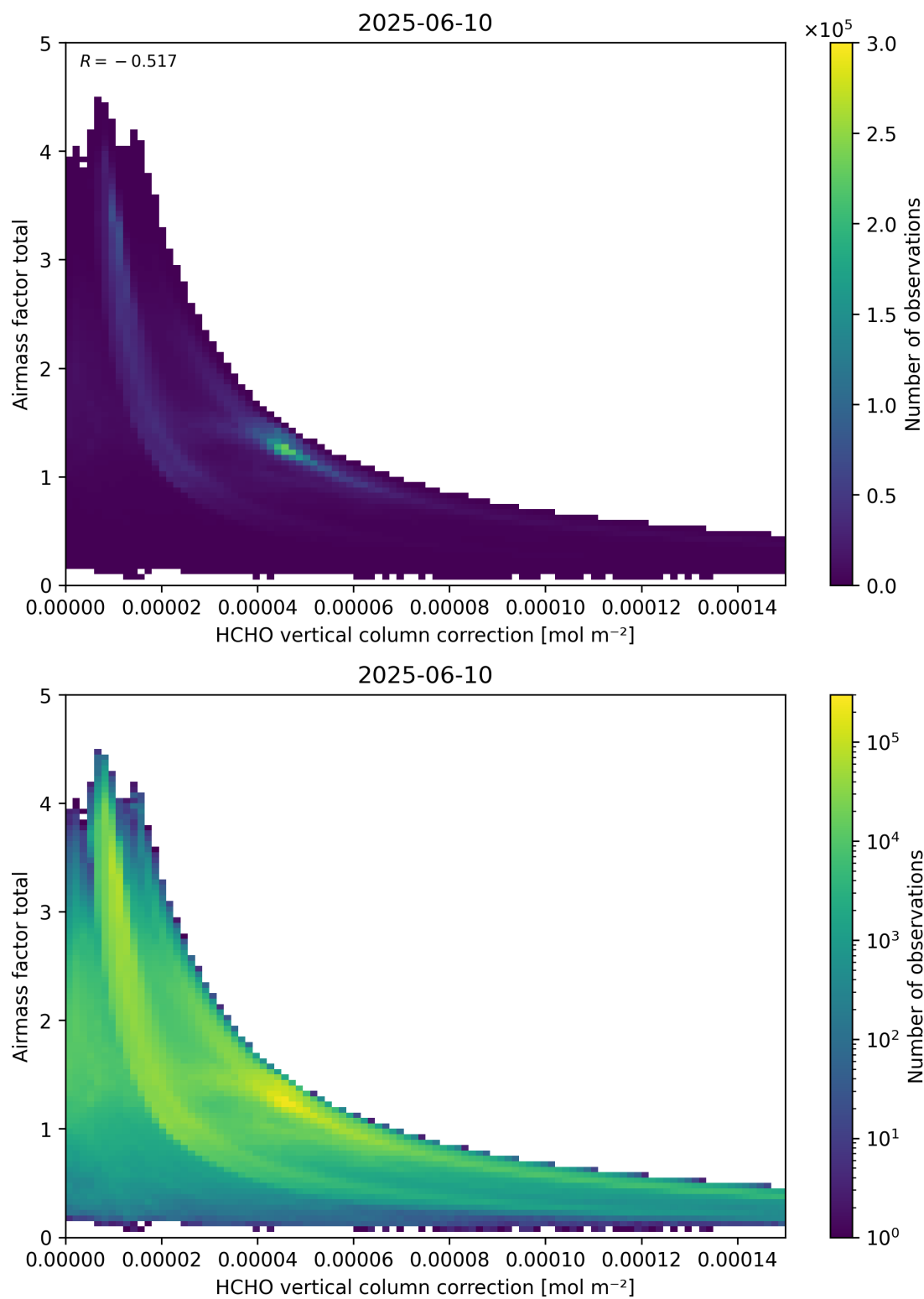
Figure 120: Scatter density plot of “HCHO vertical column correction” against “Airmass factor total” for 2025-06-09 to 2025-06-11.
