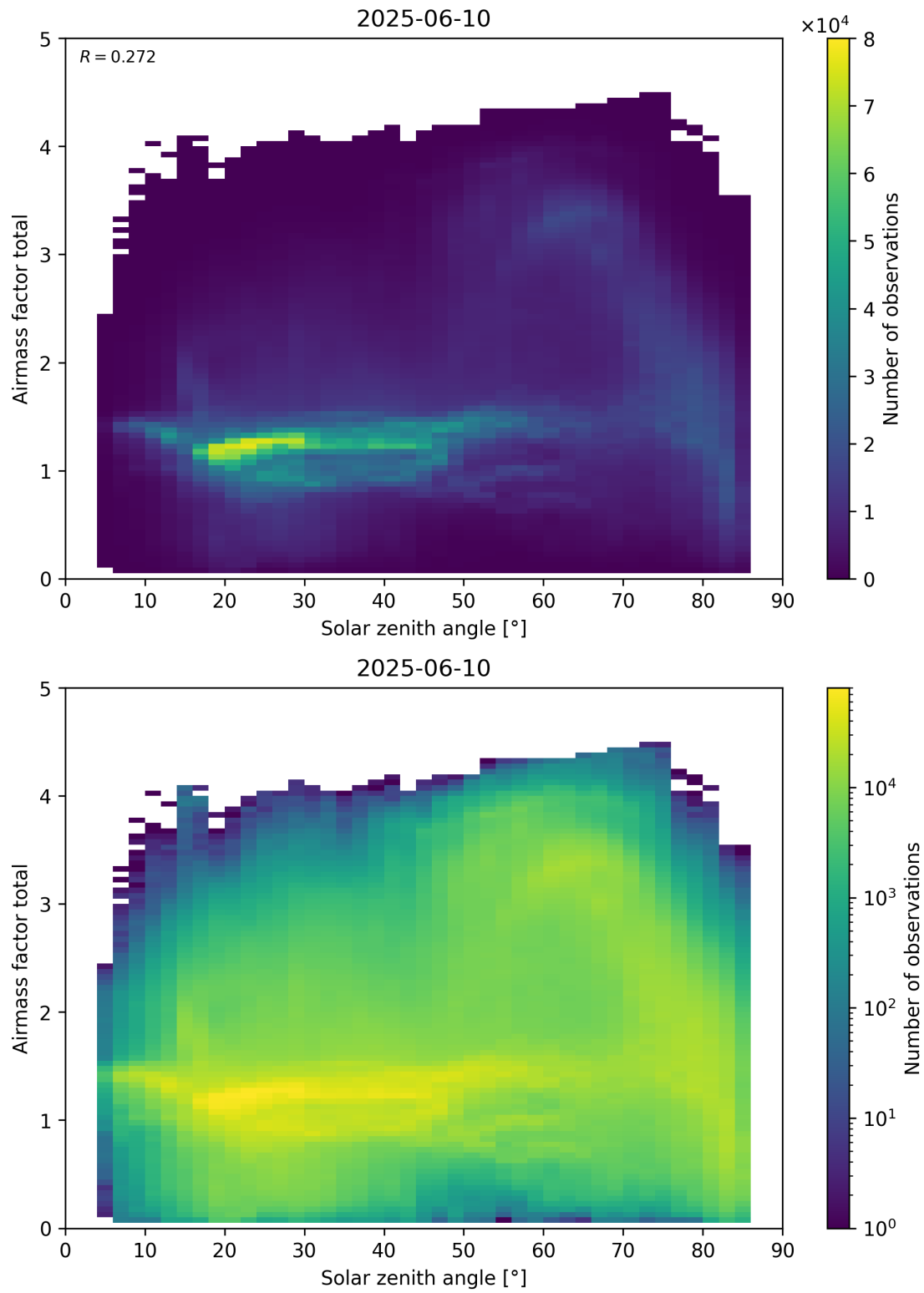
Figure 175: Scatter density plot of “Solar zenith angle” against “Airmass factor total” for 2025-06-09 to 2025-06-11.
