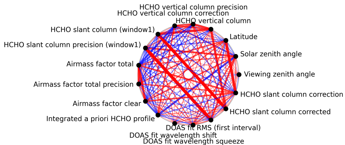
Figure 1: Map of correlation graph for 2025-06-09 to 2025-06-11.
