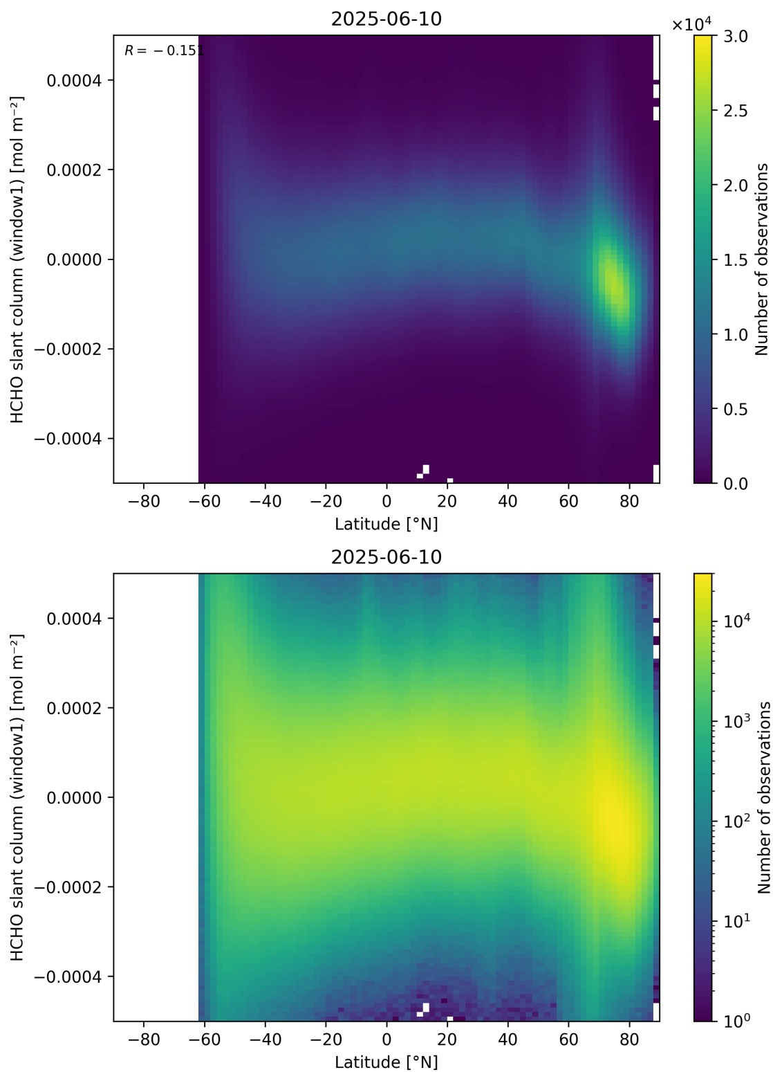
Figure 159: Scatter density plot of “Latitude” against “HCHO slant column (window1)” for 2025-06-09 to 2025-06-11.
