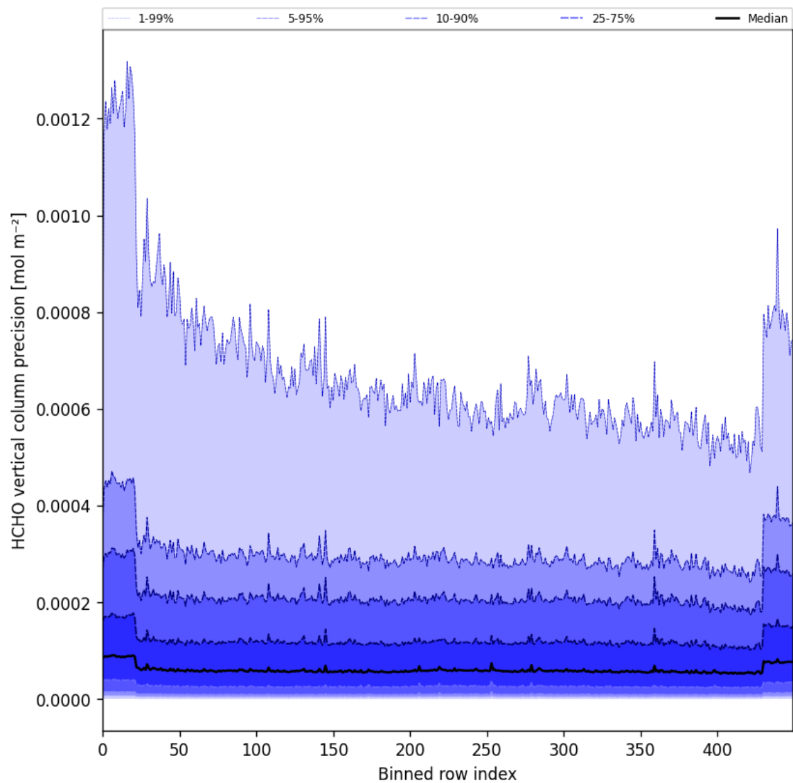
Figure 50: Along track statistics of “HCHO vertical column precision” for 2025-06-09 to 2025-06-11
