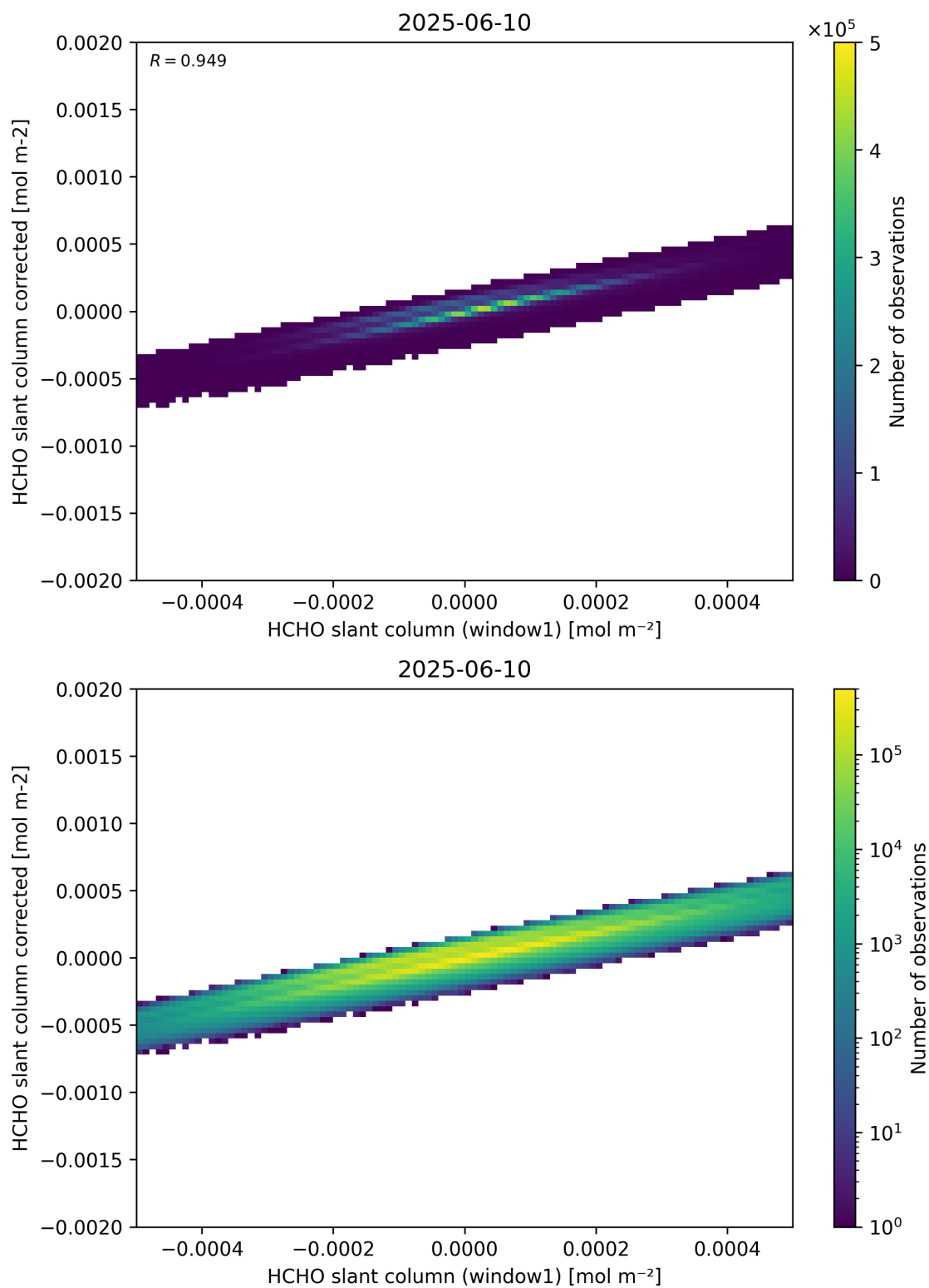
Figure 82: Scatter density plot of “HCHO slant column (window1)” against “HCHO slant column corrected” for 2025-06-09 to 2025-06-11.
