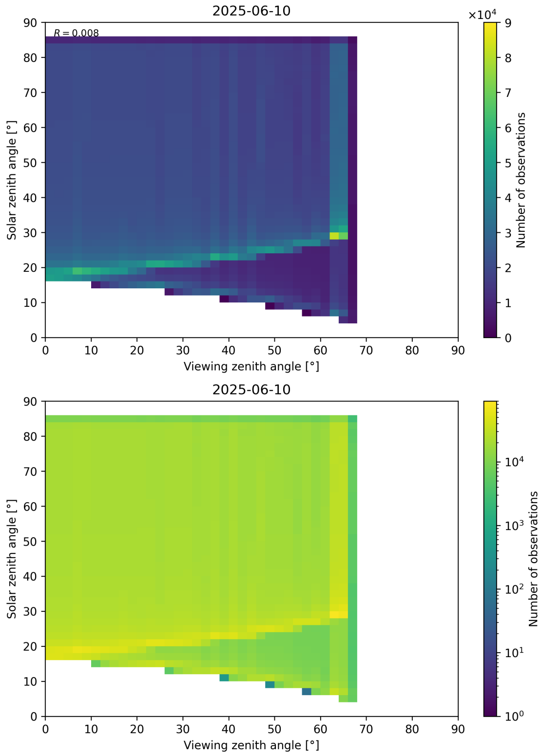
Figure 197: Scatter density plot of “Viewing zenith angle” against “Solar zenith angle” for 2025-06-09 to 2025-06-11.
