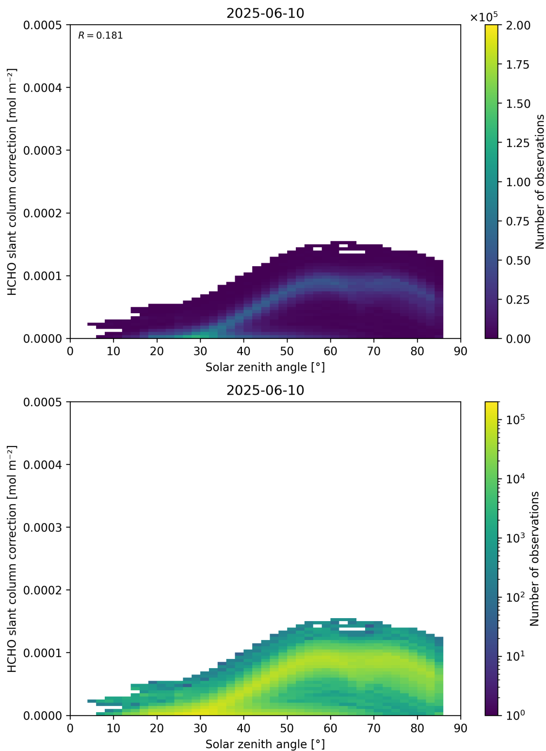
Figure 172: Scatter density plot of “Solar zenith angle” against “HCHO slant column correction” for 2025-06-09 to 2025-06-11.
