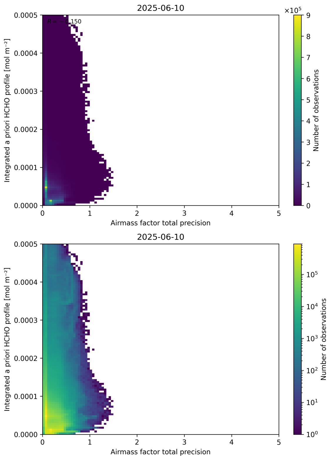
Figure 111: Scatter density plot of “Airmass factor total precision” against “Integrated a priori HCHO profile” for 2025-06-09 to 2025-06-11.
