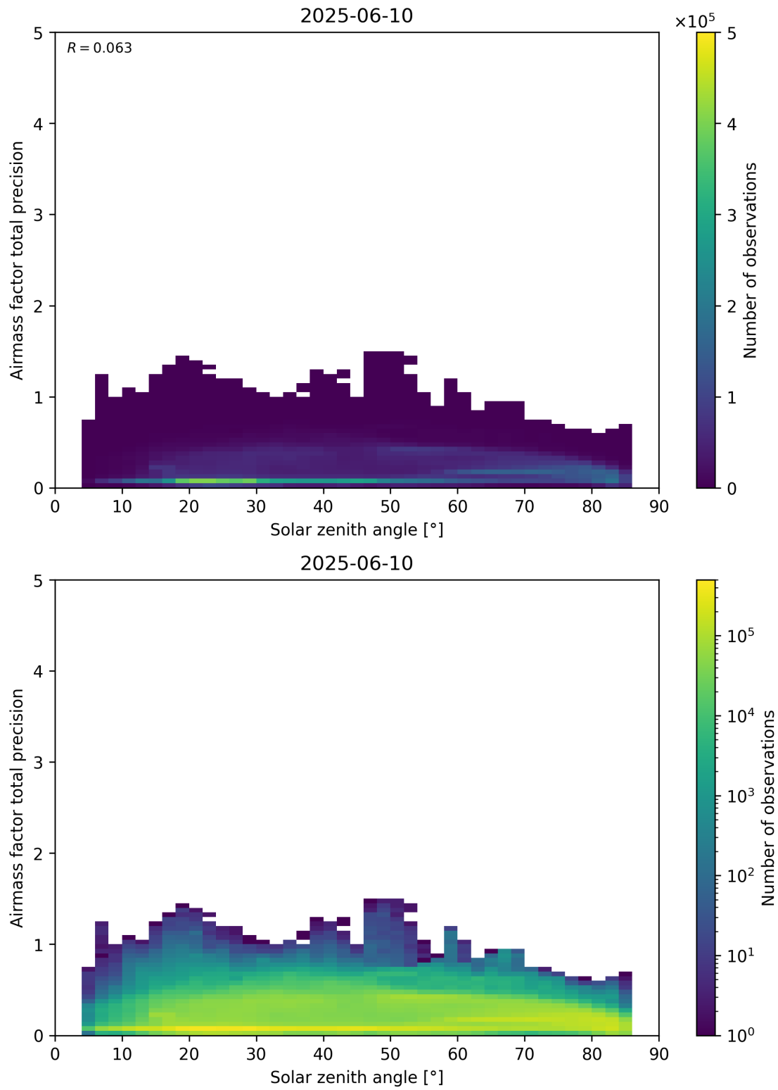
Figure 176: Scatter density plot of “Solar zenith angle” against “Airmass factor total precision” for 2025-06-09 to 2025-06-11.
