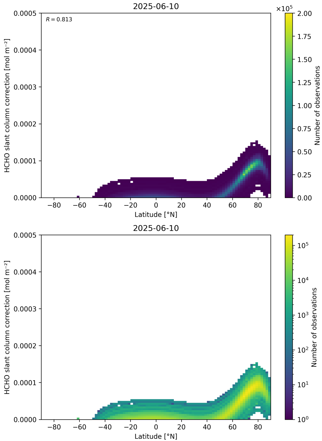
Figure 158: Scatter density plot of “Latitude” against “HCHO slant column correction” for 2025-06-09 to 2025-06-11.
