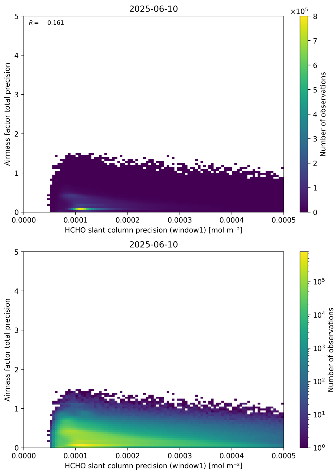
Figure 95: Scatter density plot of “HCHO slant column precision (window1)” against “Airmass factor total precision” for 2025-06-09 to 2025-06-11.
