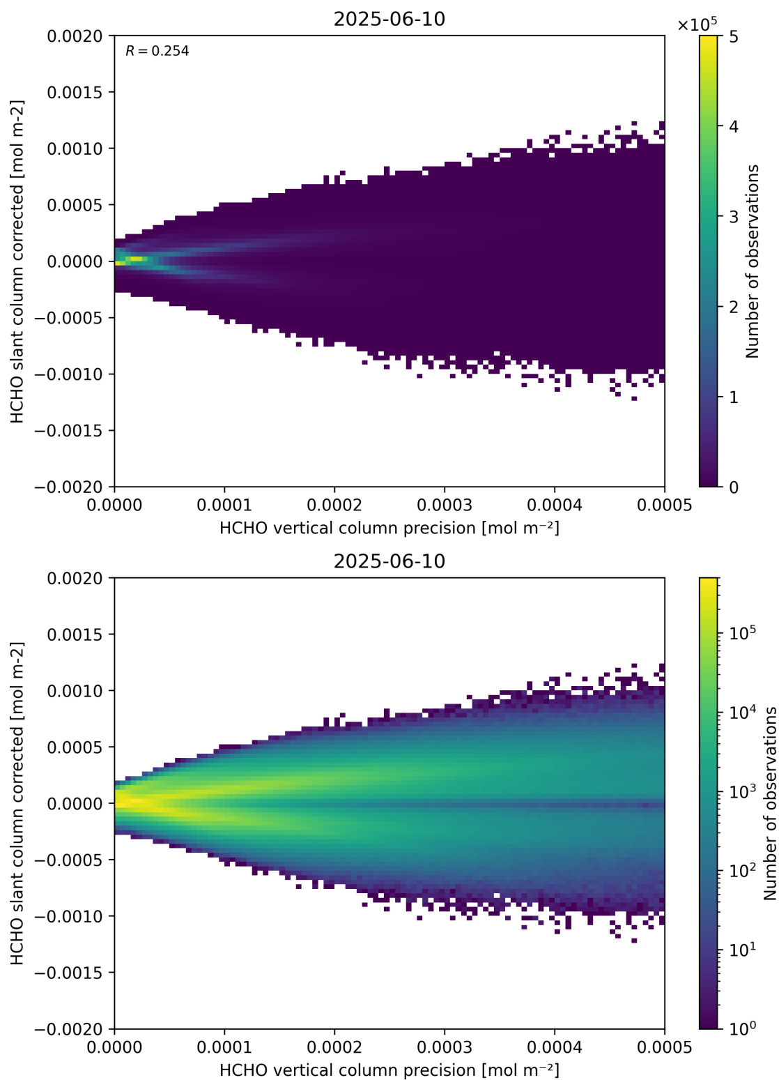
Figure 140: Scatter density plot of “HCHO vertical column precision” against “HCHO slant column corrected” for 2025-06-09 to 2025-06-11.
