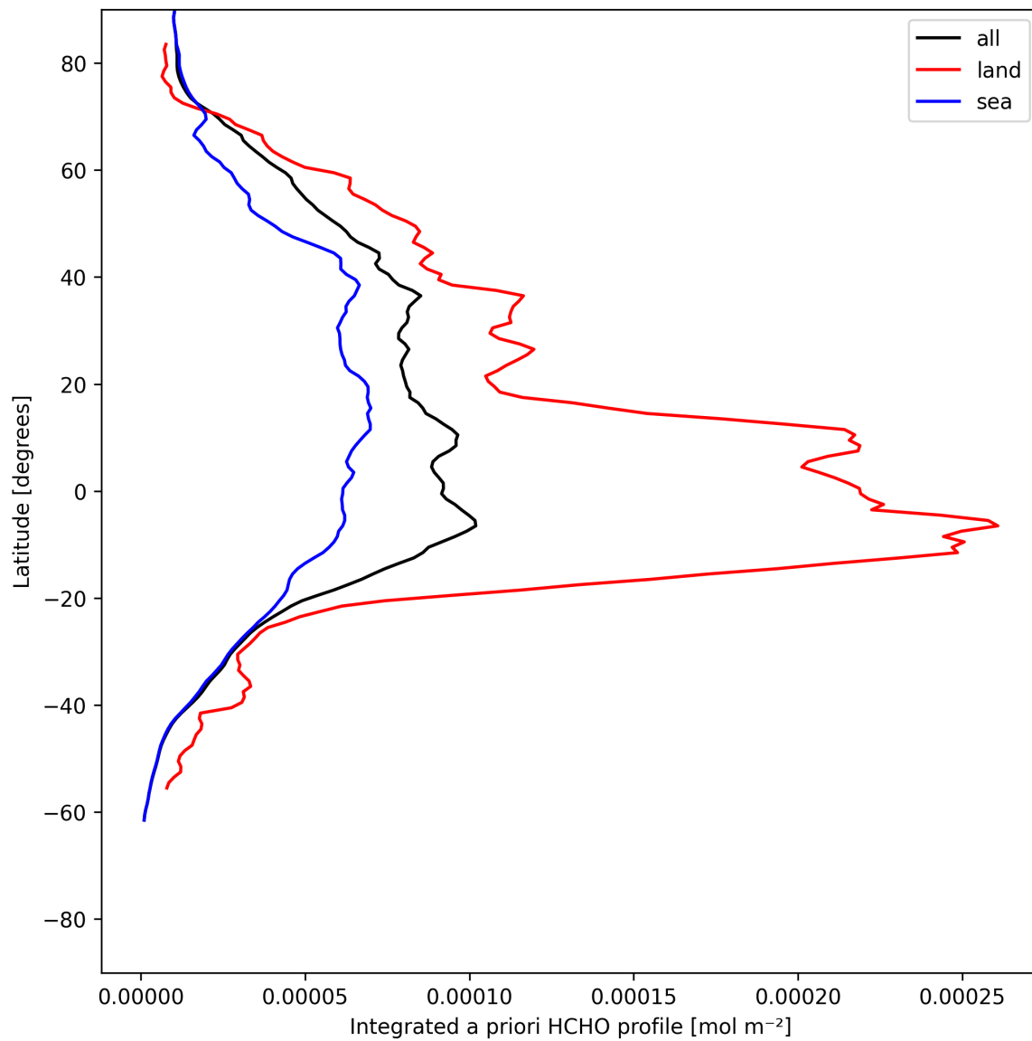
Figure 29: Zonal average of “Integrated a priori HCHO profile” for 2025-06-09 to 2025-06-11.
