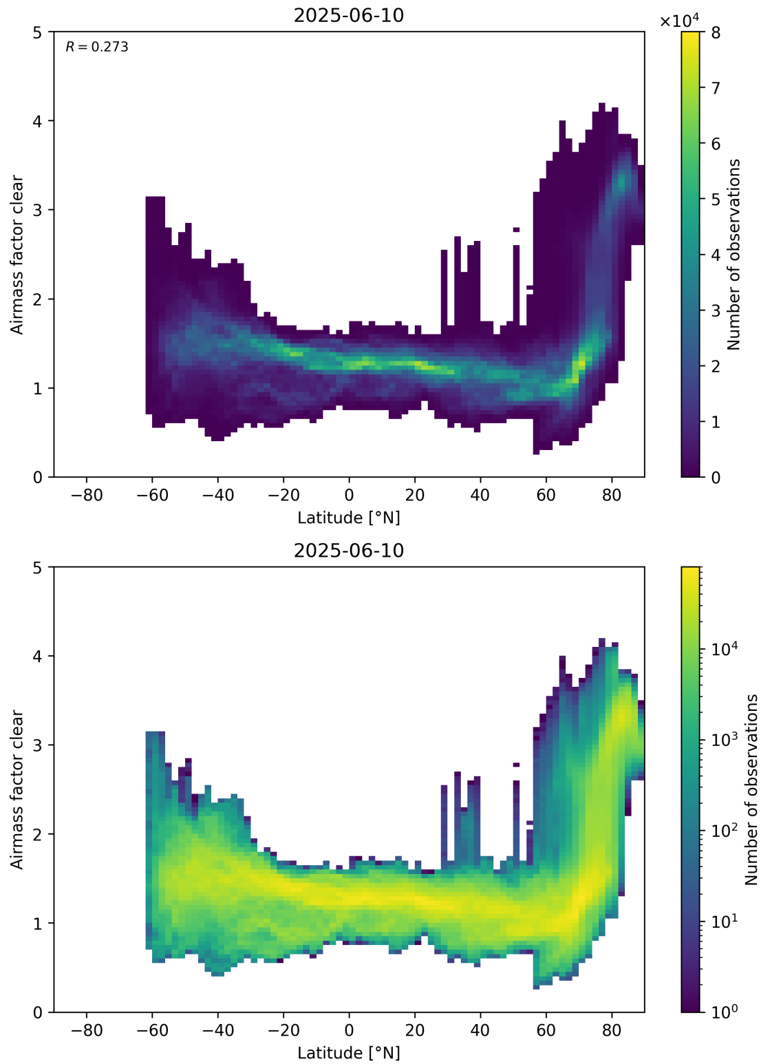
Figure 156: Scatter density plot of “Latitude” against “Airmass factor clear” for 2025-06-09 to 2025-06-11.
