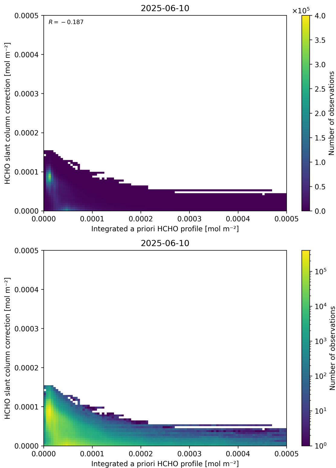
Figure 152: Scatter density plot of “Integrated a priori HCHO profile” against “HCHO slant column correction” for 2025-06-09 to 2025-06-11.
