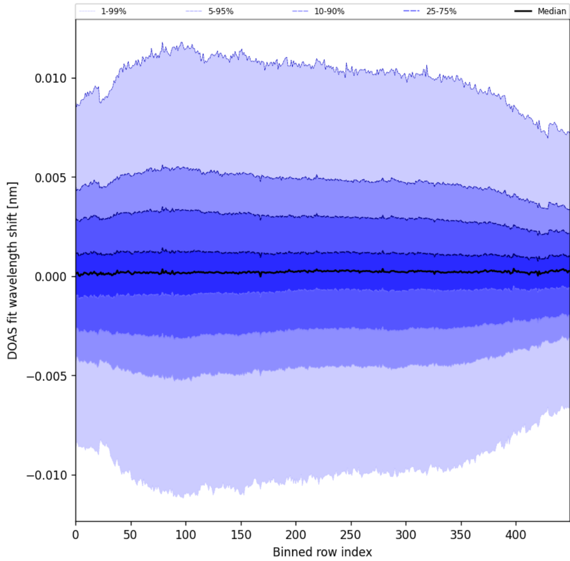
Figure 58: Along track statistics of “DOAS fit wavelength shift” for 2025-06-09 to 2025-06-11
