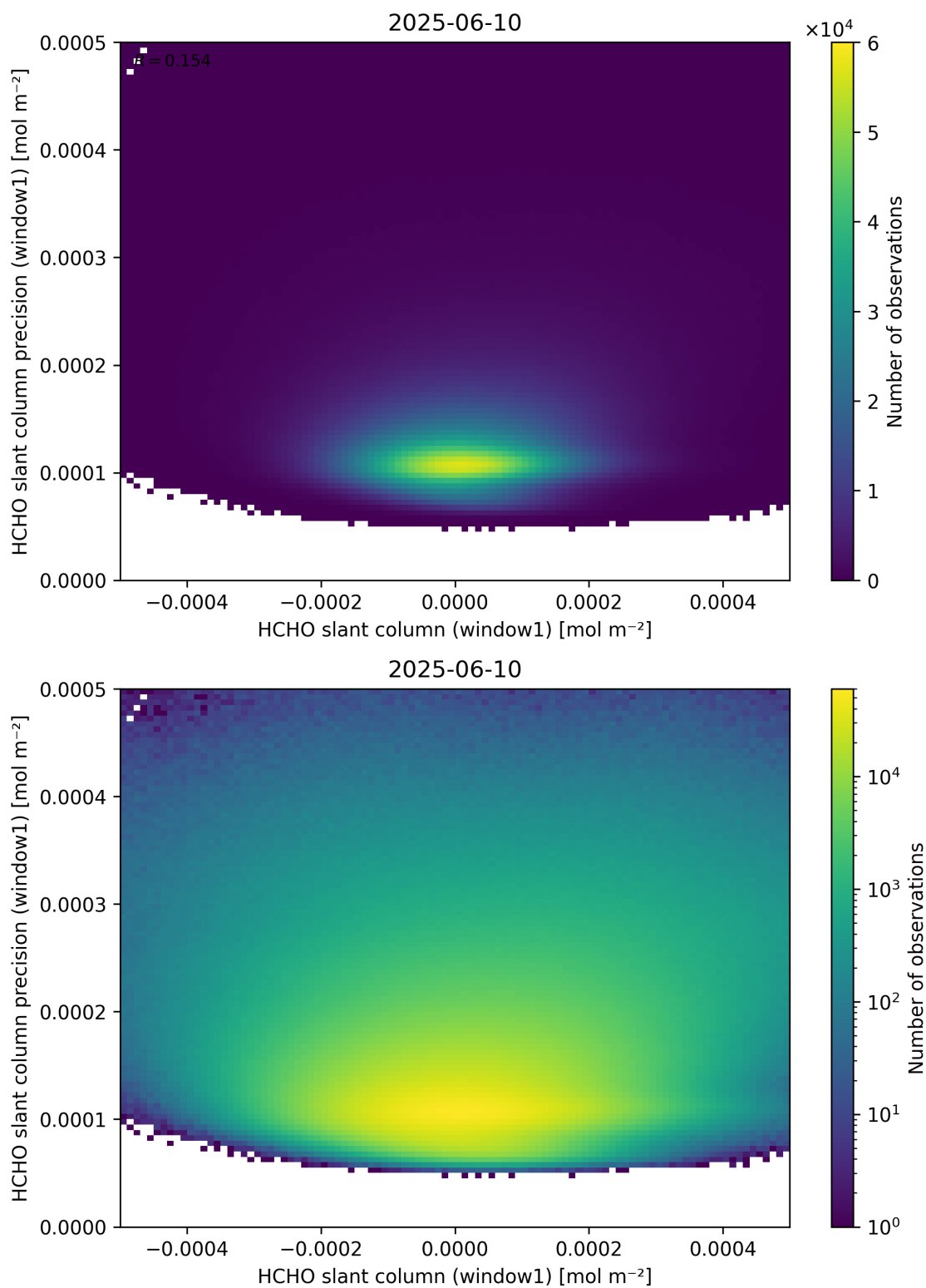
Figure 84: Scatter density plot of “HCHO slant column (window1)” against “HCHO slant column precision (window1)” for 2025-06-09 to 2025-06-11.
