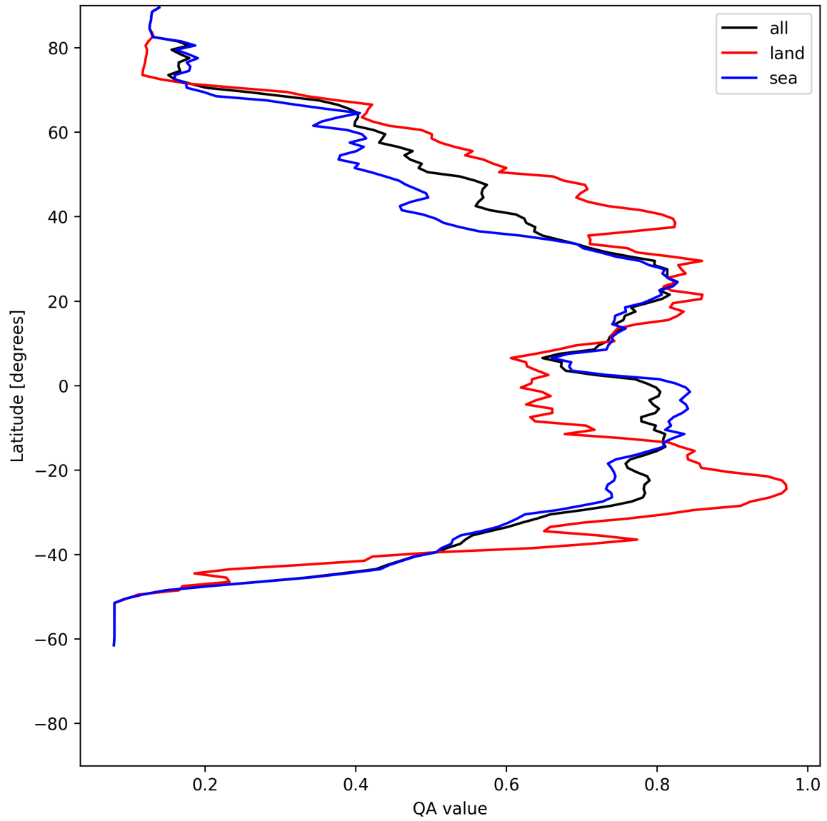
Figure 20: Zonal average of “QA value” for 2025-06-09 to 2025-06-11.
