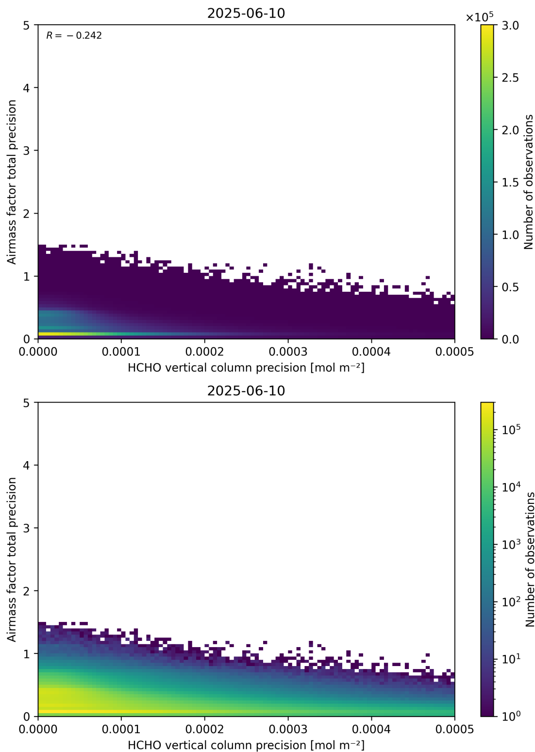
Figure 145: Scatter density plot of “HCHO vertical column precision” against “Airmass factor total precision” for 2025-06-09 to 2025-06-11.
