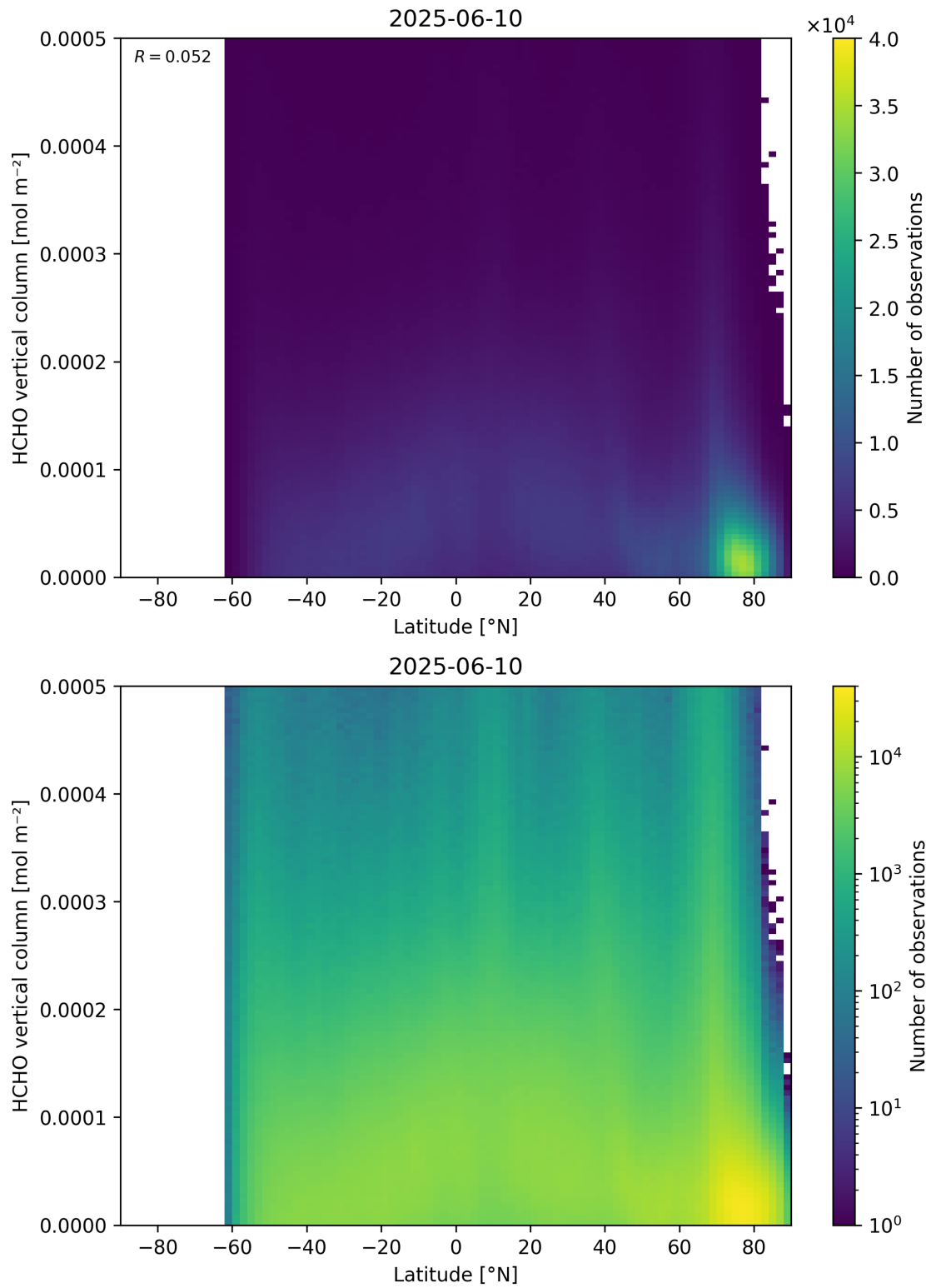
Figure 163: Scatter density plot of “Latitude” against “HCHO vertical column” for 2025-06-09 to 2025-06-11.
