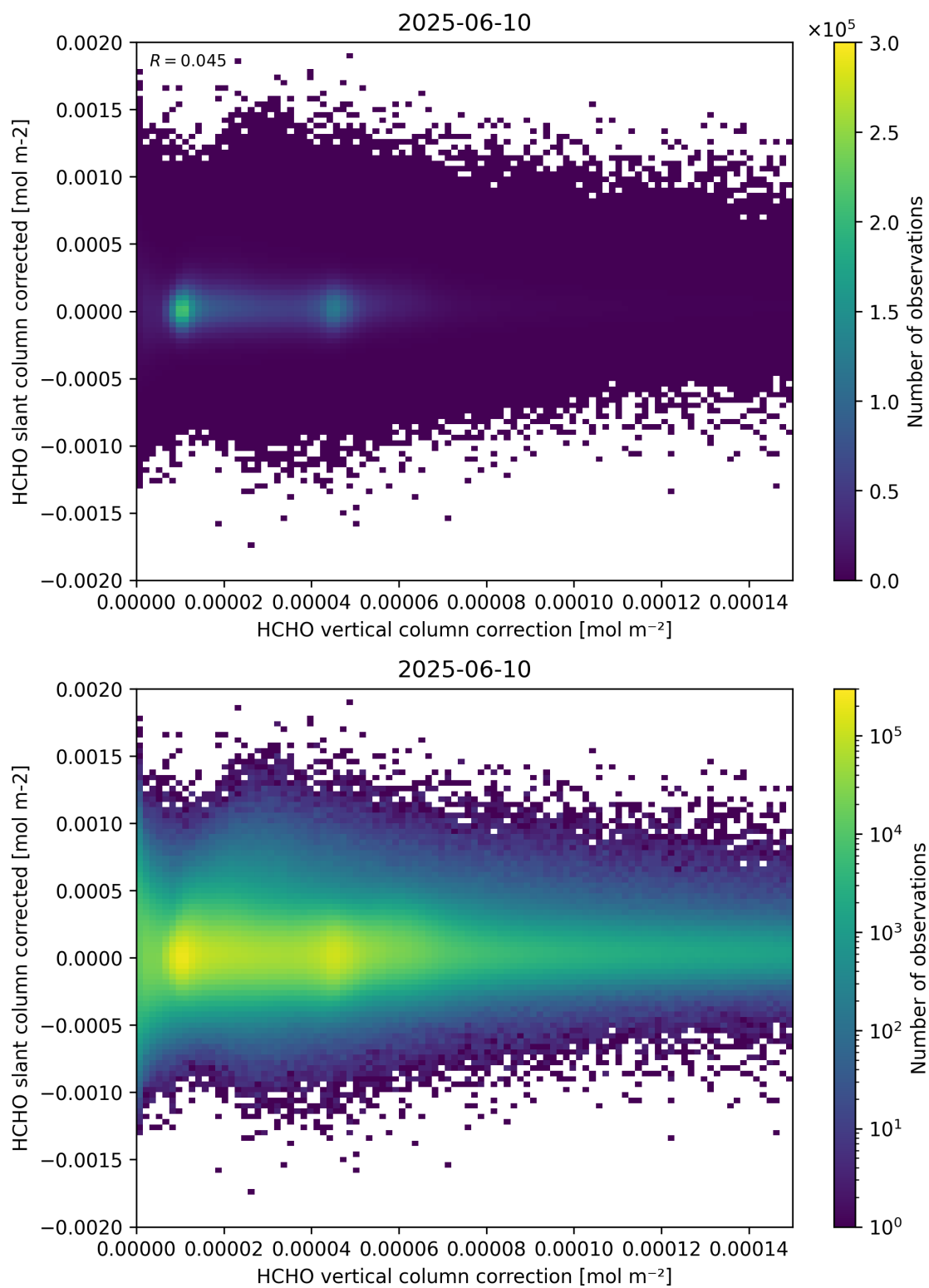
Figure 116: Scatter density plot of “HCHO vertical column correction” against “HCHO slant column corrected” for 2025-06-09 to 2025-06-11.
