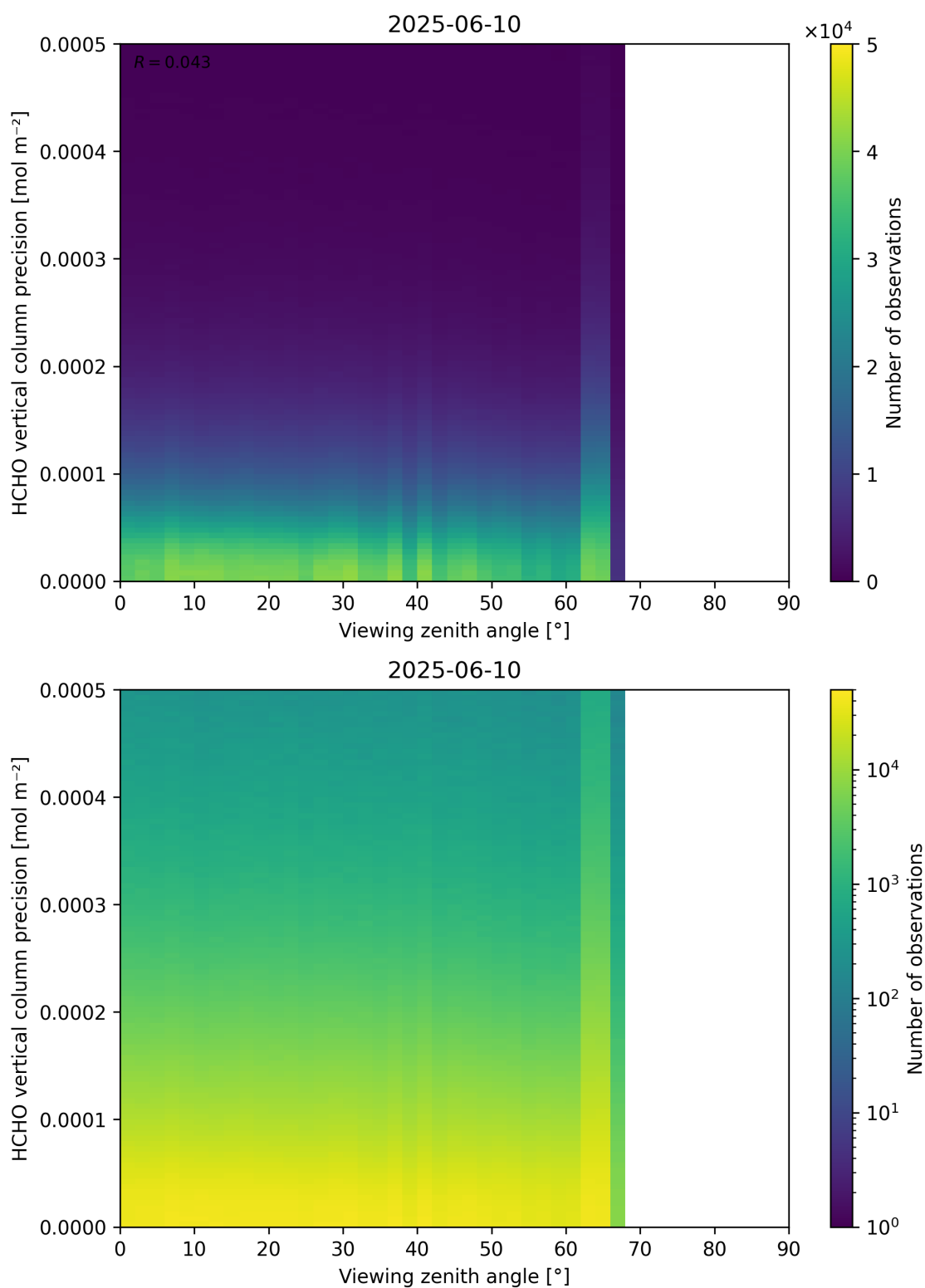
Figure 194: Scatter density plot of “Viewing zenith angle” against “HCHO vertical column precision” for 2025-06-09 to 2025-06-11.
