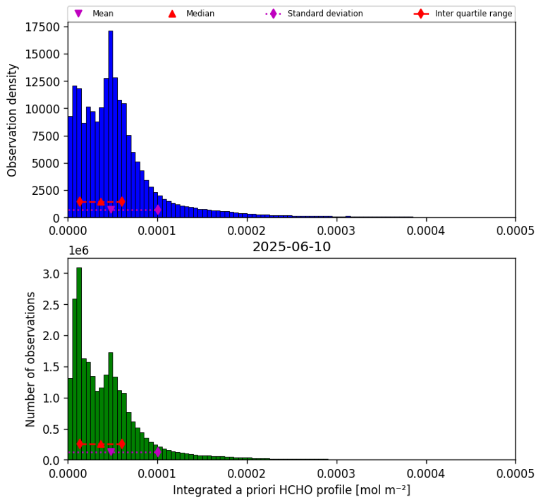
Figure 43: Histogram of “Integrated a priori HCHO profile” for 2025-06-09 to 2025-06-11
