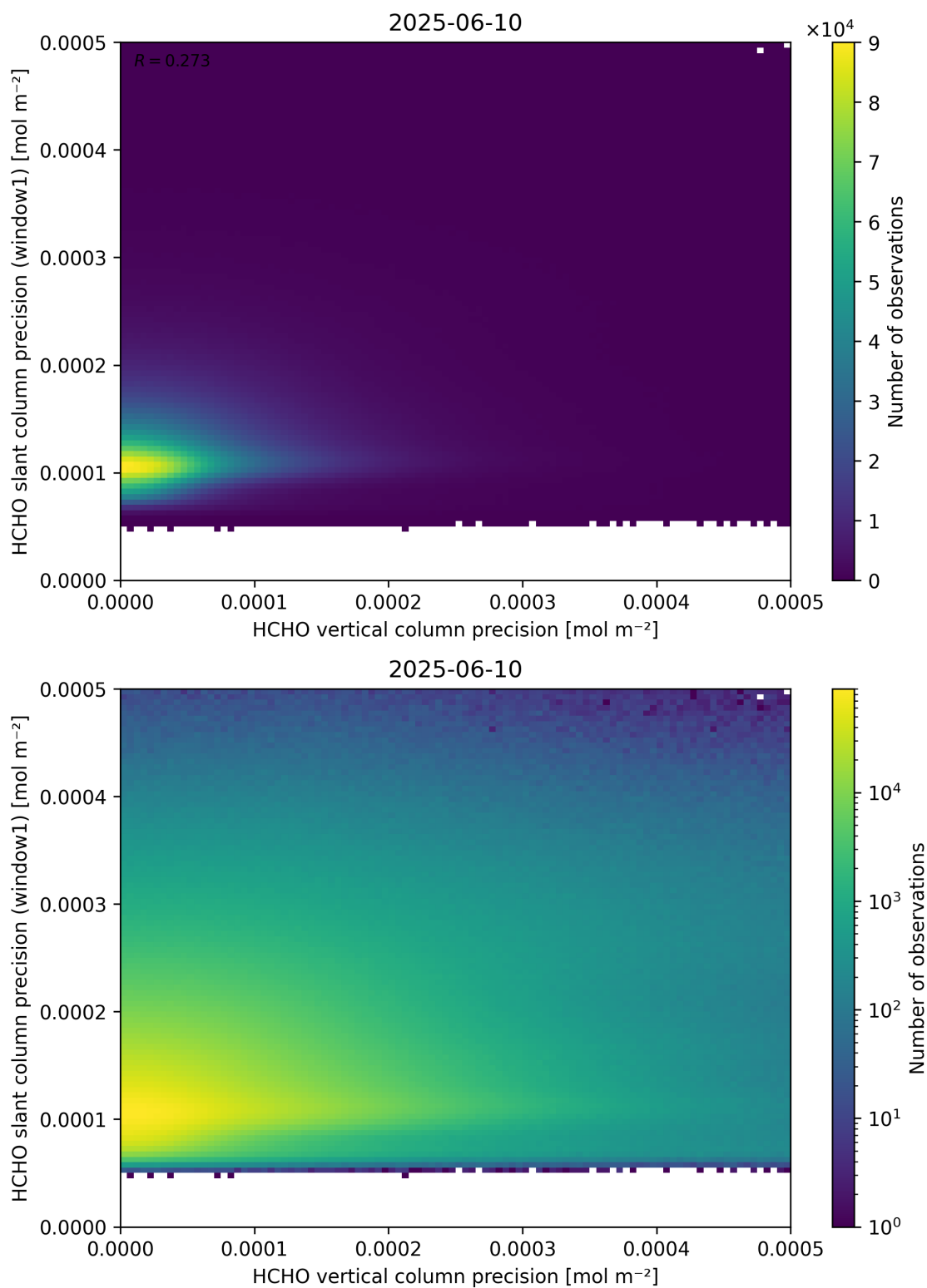
Figure 143: Scatter density plot of “HCHO vertical column precision” against “HCHO slant column precision (window1)” for 2025-06-09 to 2025-06-11.
