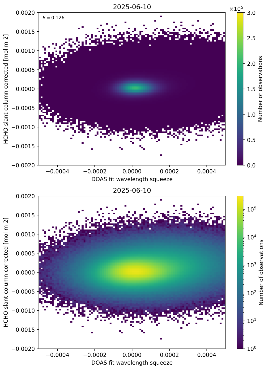
Figure 69: Scatter density plot of “DOAS fit wavelength squeeze” against “HCHO slant column corrected” for 2025-06-09 to 2025-06-11.
