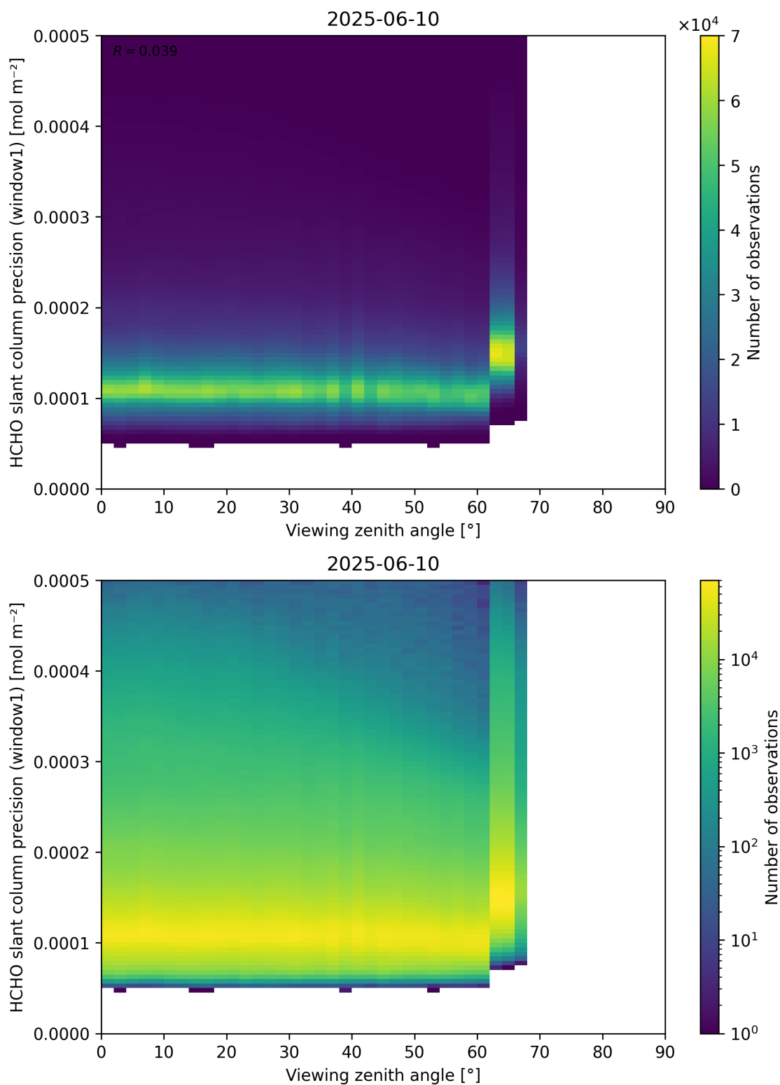
Figure 189: Scatter density plot of “Viewing zenith angle” against “HCHO slant column precision (window1)” for 2025-06-09 to 2025-06-11.
