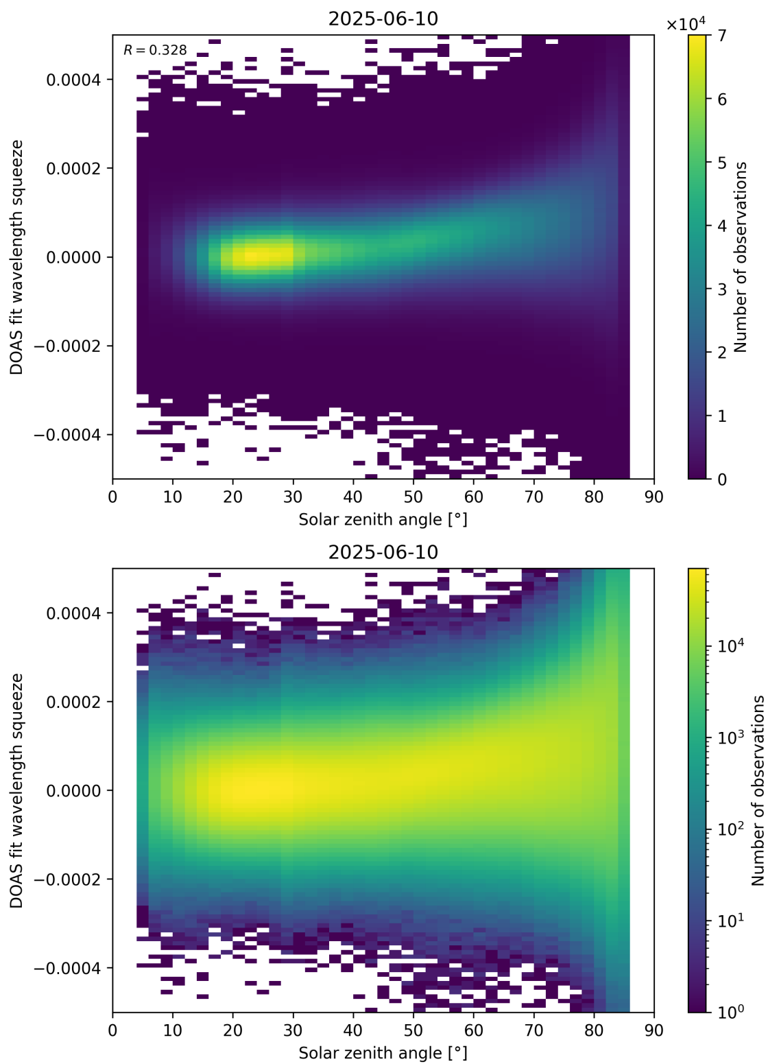
Figure 169: Scatter density plot of “Solar zenith angle” against “DOAS fit wavelength squeeze” for 2025-06-09 to 2025-06-11.
