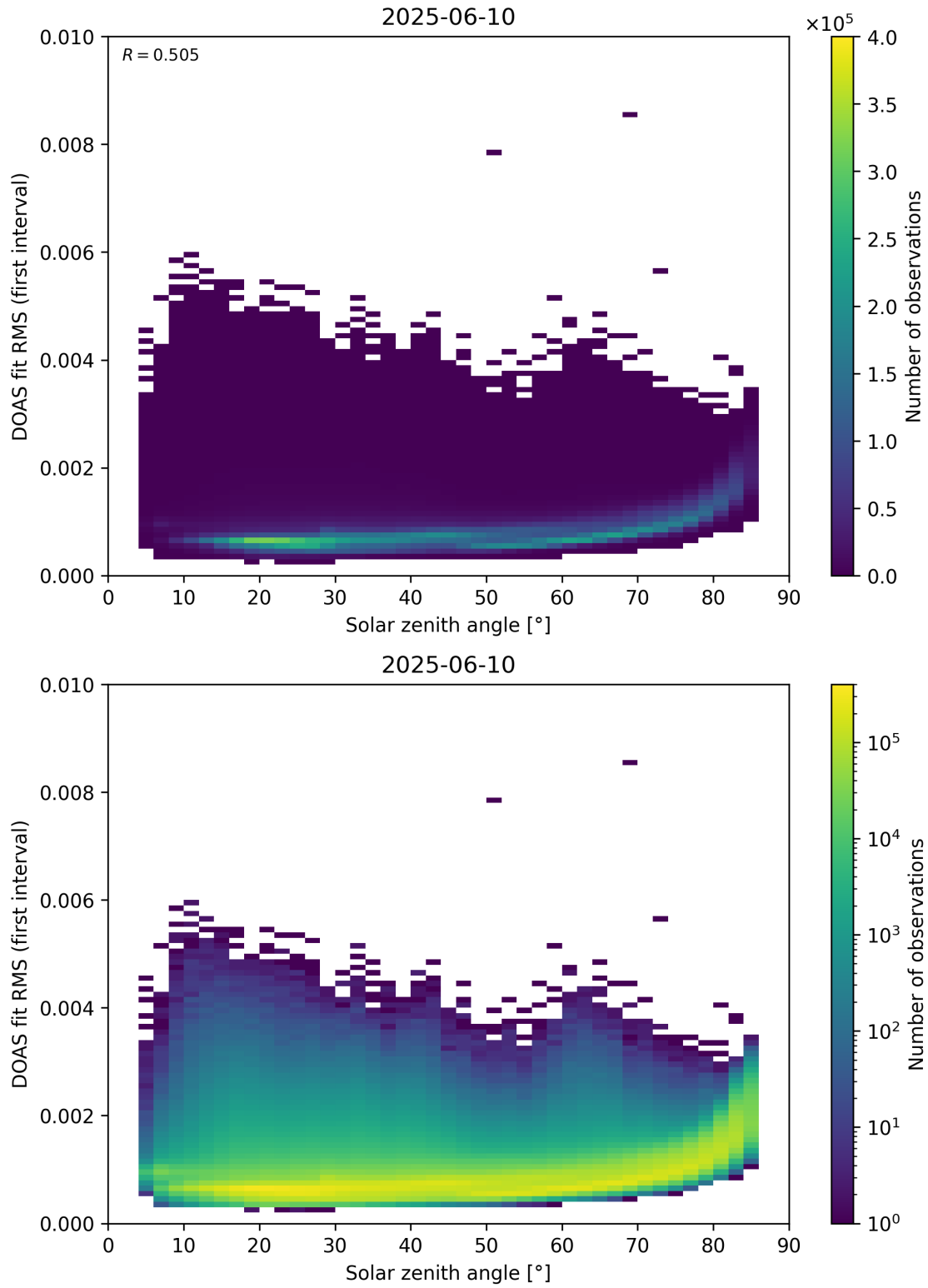
Figure 167: Scatter density plot of “Solar zenith angle” against “DOAS fit RMS (first interval)” for 2025-06-09 to 2025-06-11.
