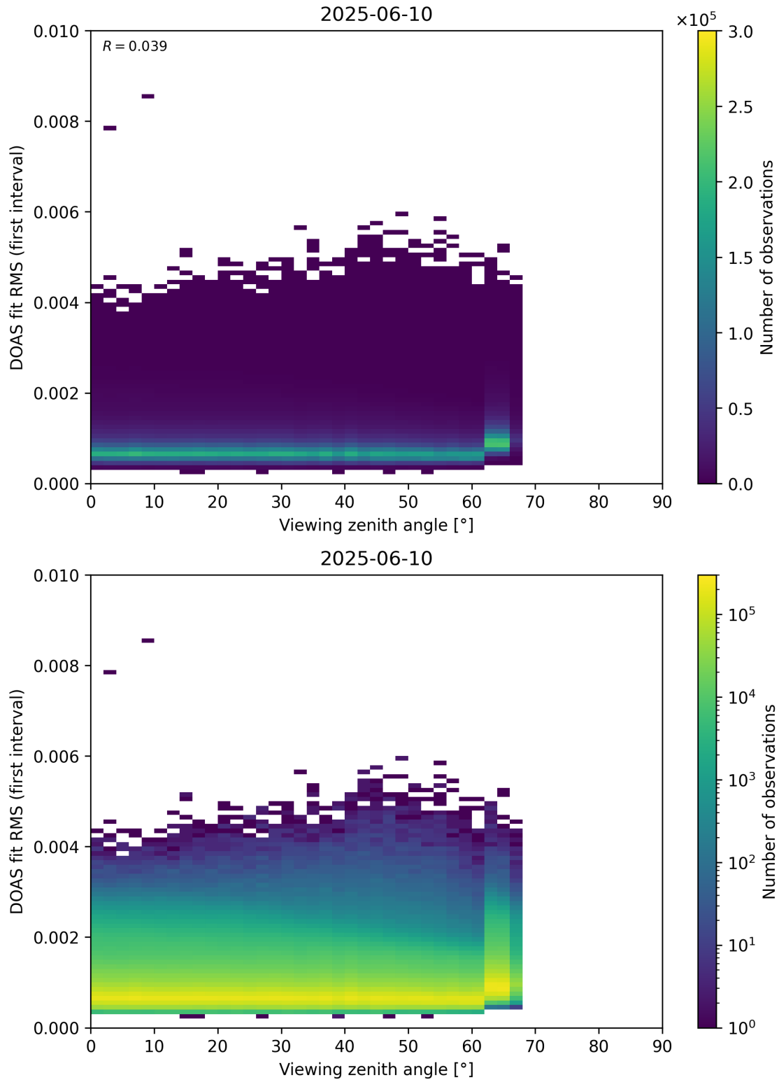
Figure 182: Scatter density plot of “Viewing zenith angle” against “DOAS fit RMS (first interval)” for 2025-06-09 to 2025-06-11.
