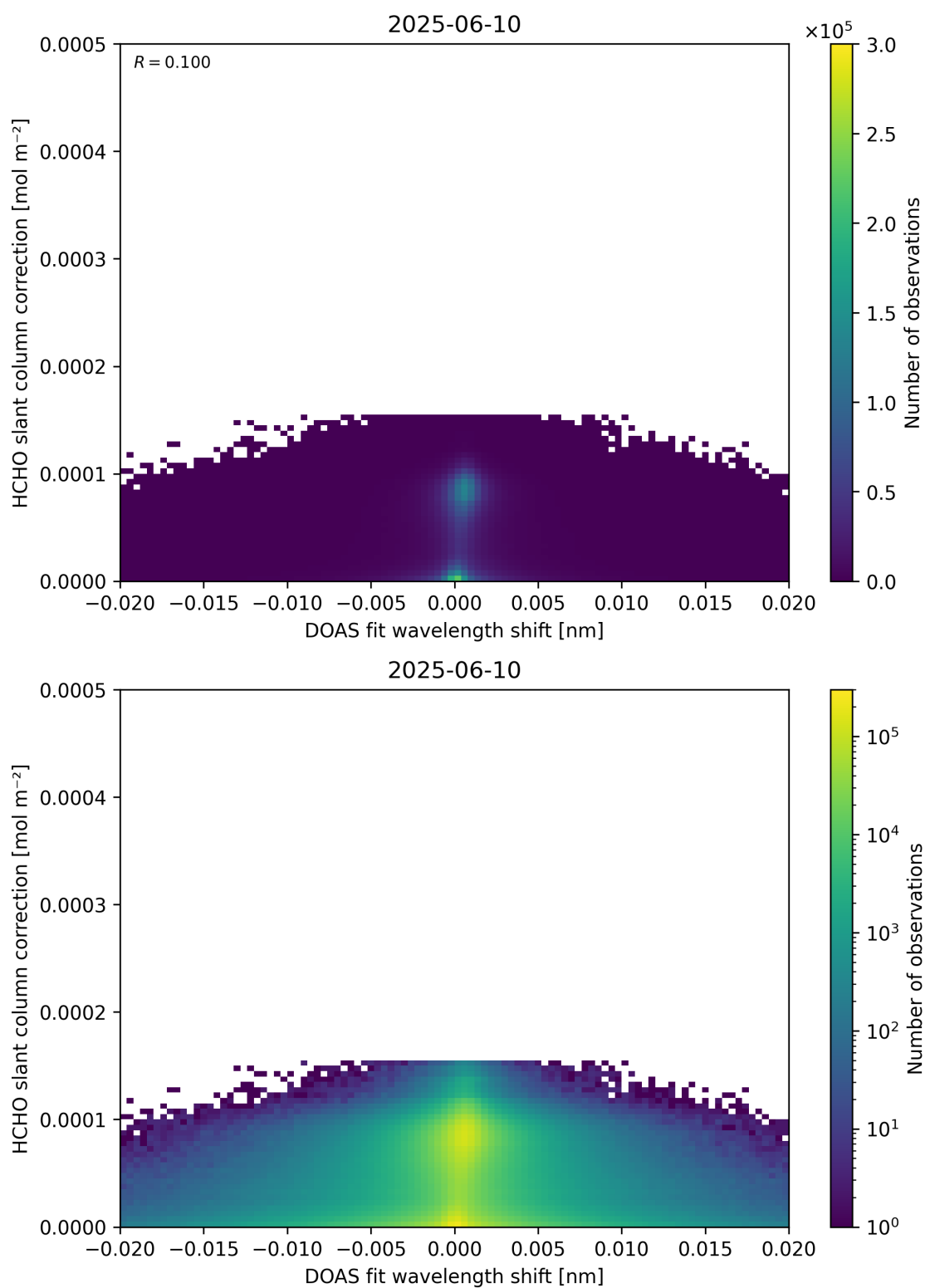
Figure 67: Scatter density plot of “DOAS fit wavelength shift” against “HCHO slant column correction” for 2025-06-09 to 2025-06-11.
