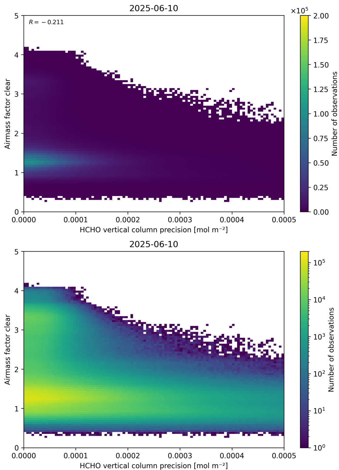
Figure 139: Scatter density plot of “HCHO vertical column precision” against “Airmass factor clear” for 2025-06-09 to 2025-06-11.
