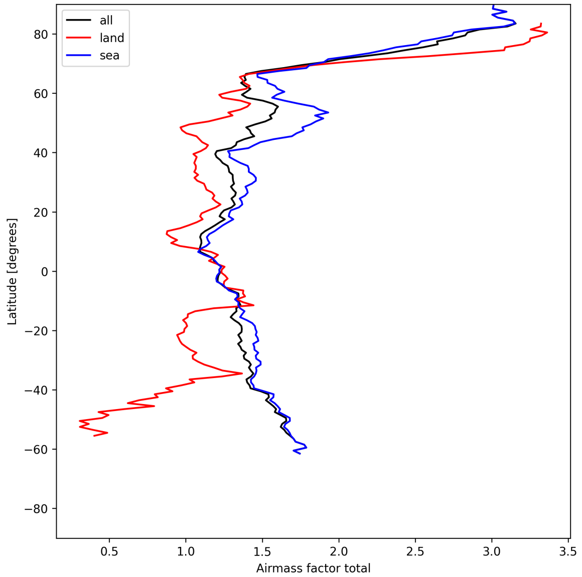
Figure 26: Zonal average of “Airmass factor total” for 2025-06-09 to 2025-06-11.
