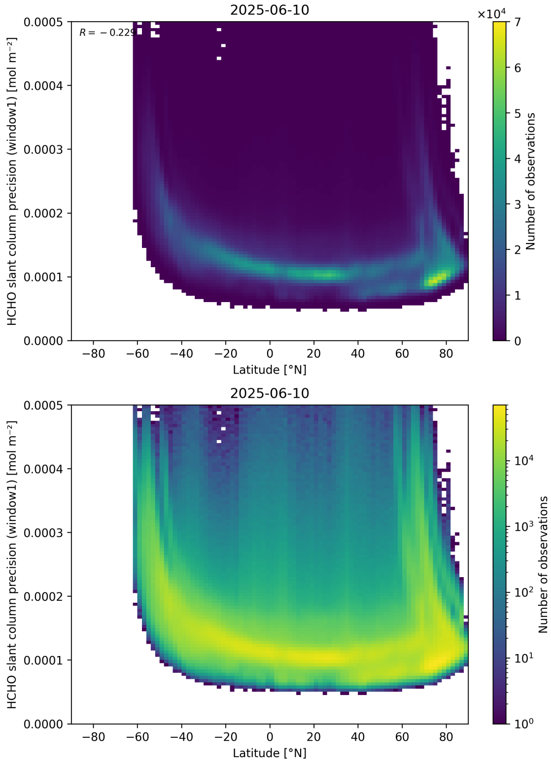
Figure 160: Scatter density plot of “Latitude” against “HCHO slant column precision (window1)” for 2025-06-09 to 2025-06-11.
