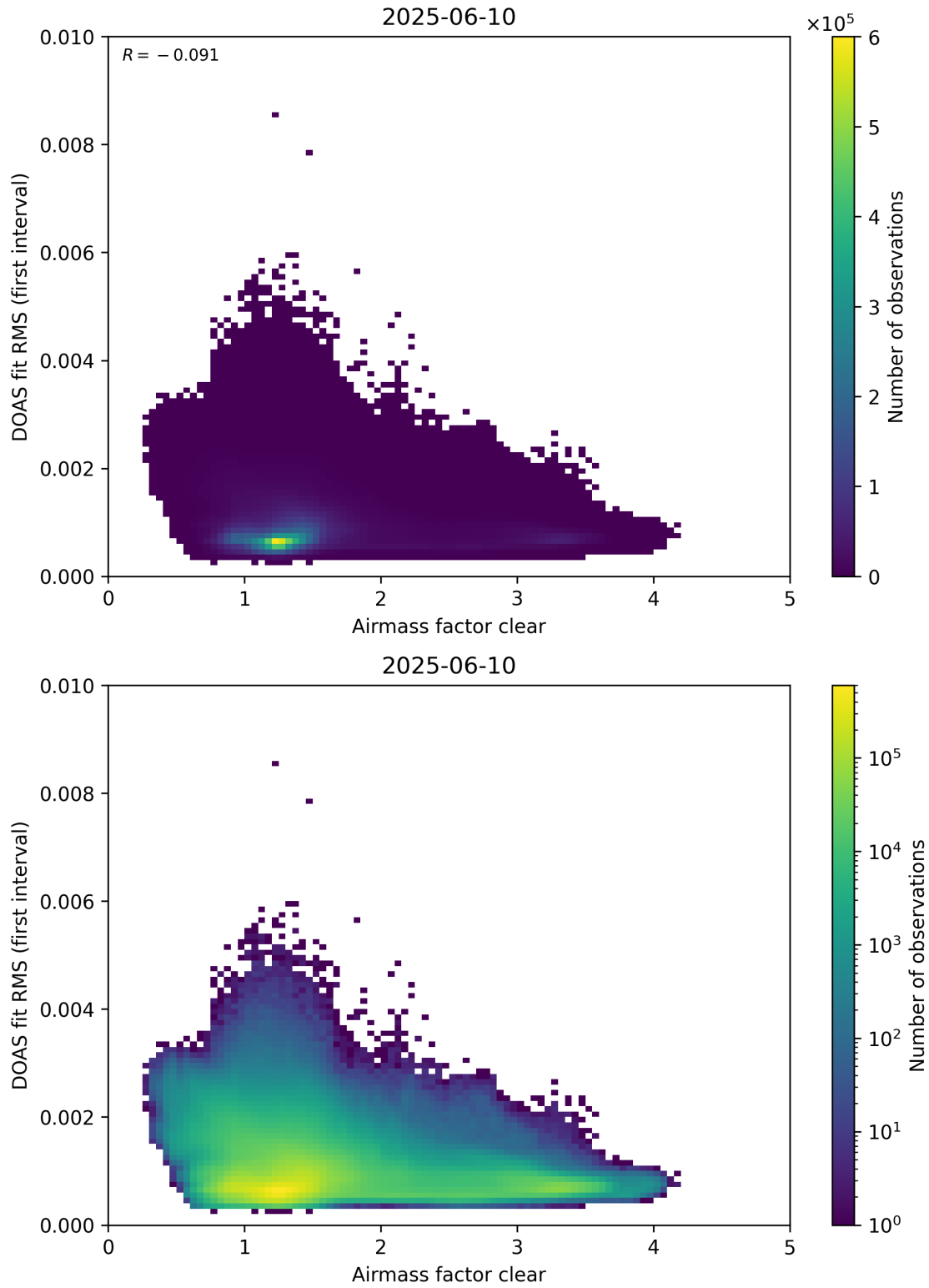
Figure 71: Scatter density plot of “Airmass factor clear” against “DOAS fit RMS (first interval)” for 2025-06-09 to 2025-06-11.
