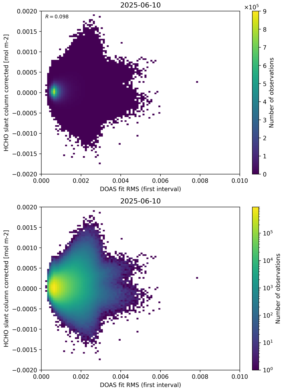
Figure 62: Scatter density plot of “DOAS fit RMS (first interval)” against “HCHO slant column corrected” for 2025-06-09 to 2025-06-11.
