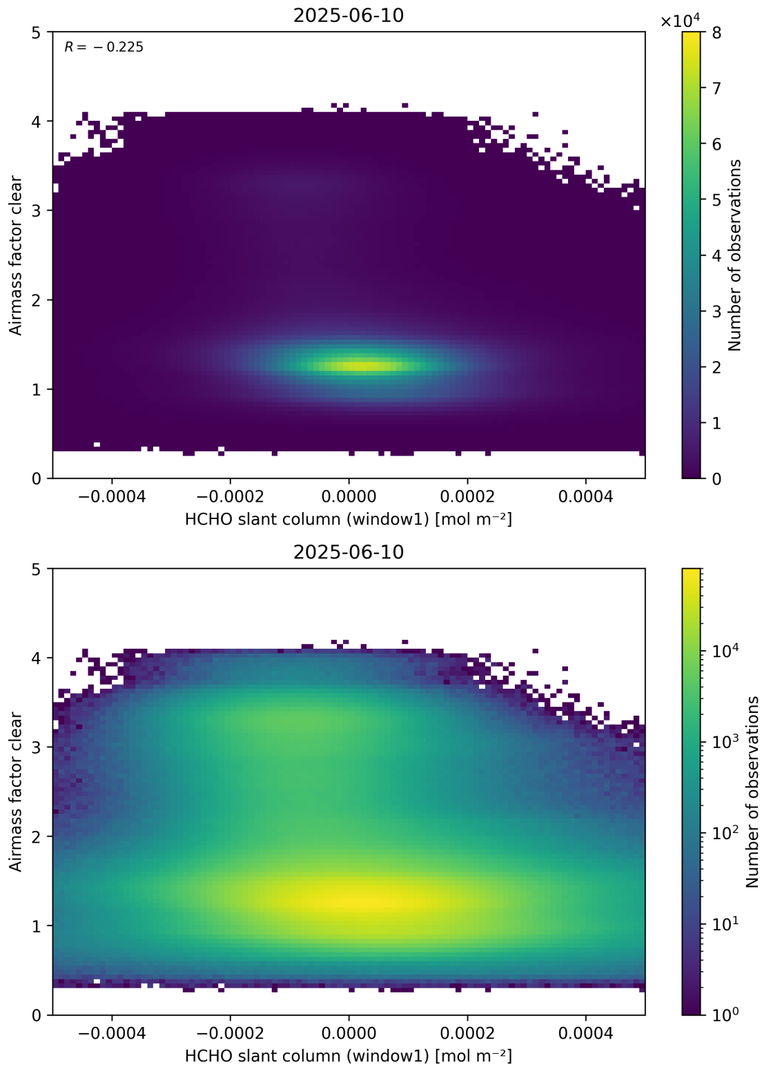
Figure 81: Scatter density plot of “HCHO slant column (window1)” against “Airmass factor clear” for 2025-06-09 to 2025-06-11.
