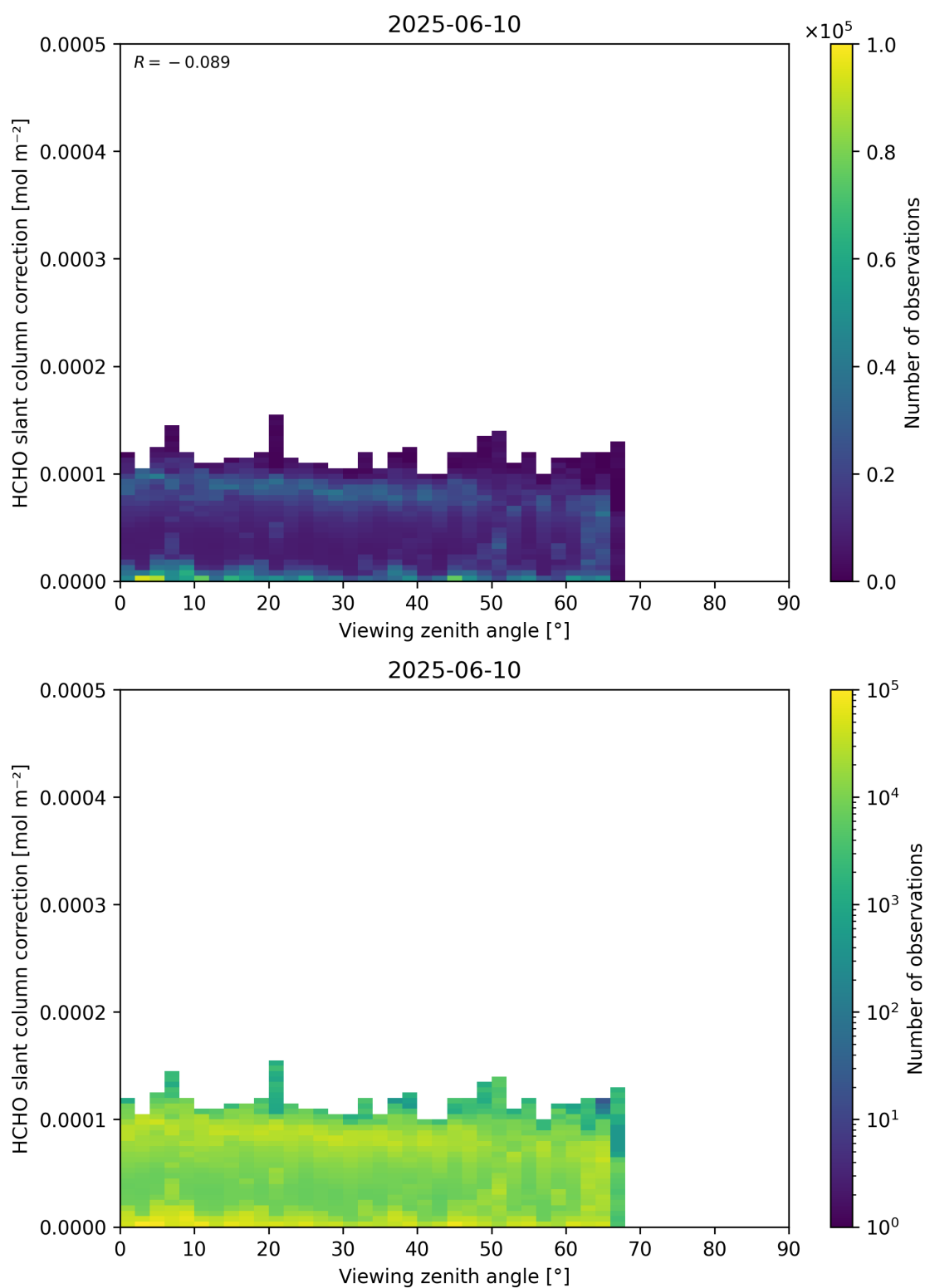
Figure 187: Scatter density plot of “Viewing zenith angle” against “HCHO slant column correction” for 2025-06-09 to 2025-06-11.
