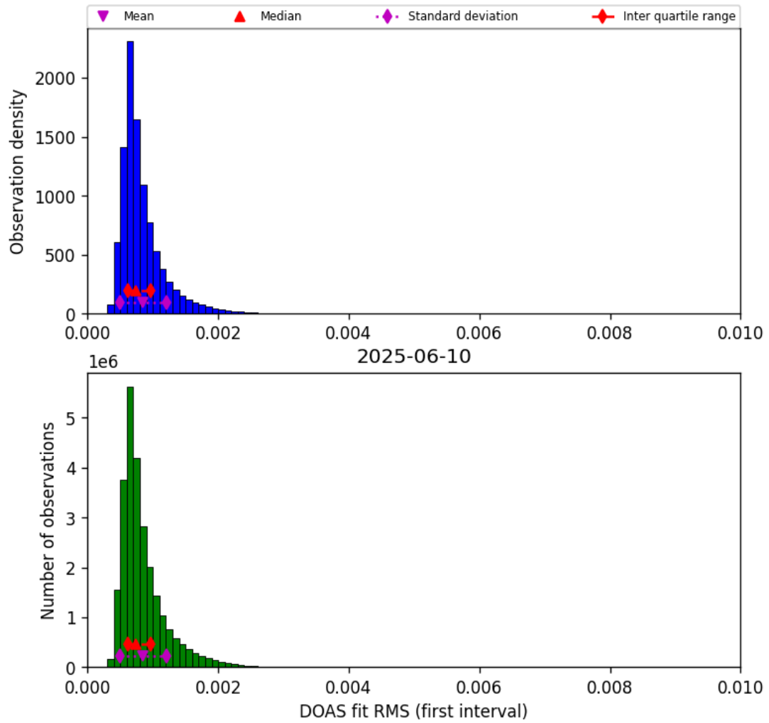
Figure 46: Histogram of “DOAS fit RMS (first interval)” for 2025-06-09 to 2025-06-11
