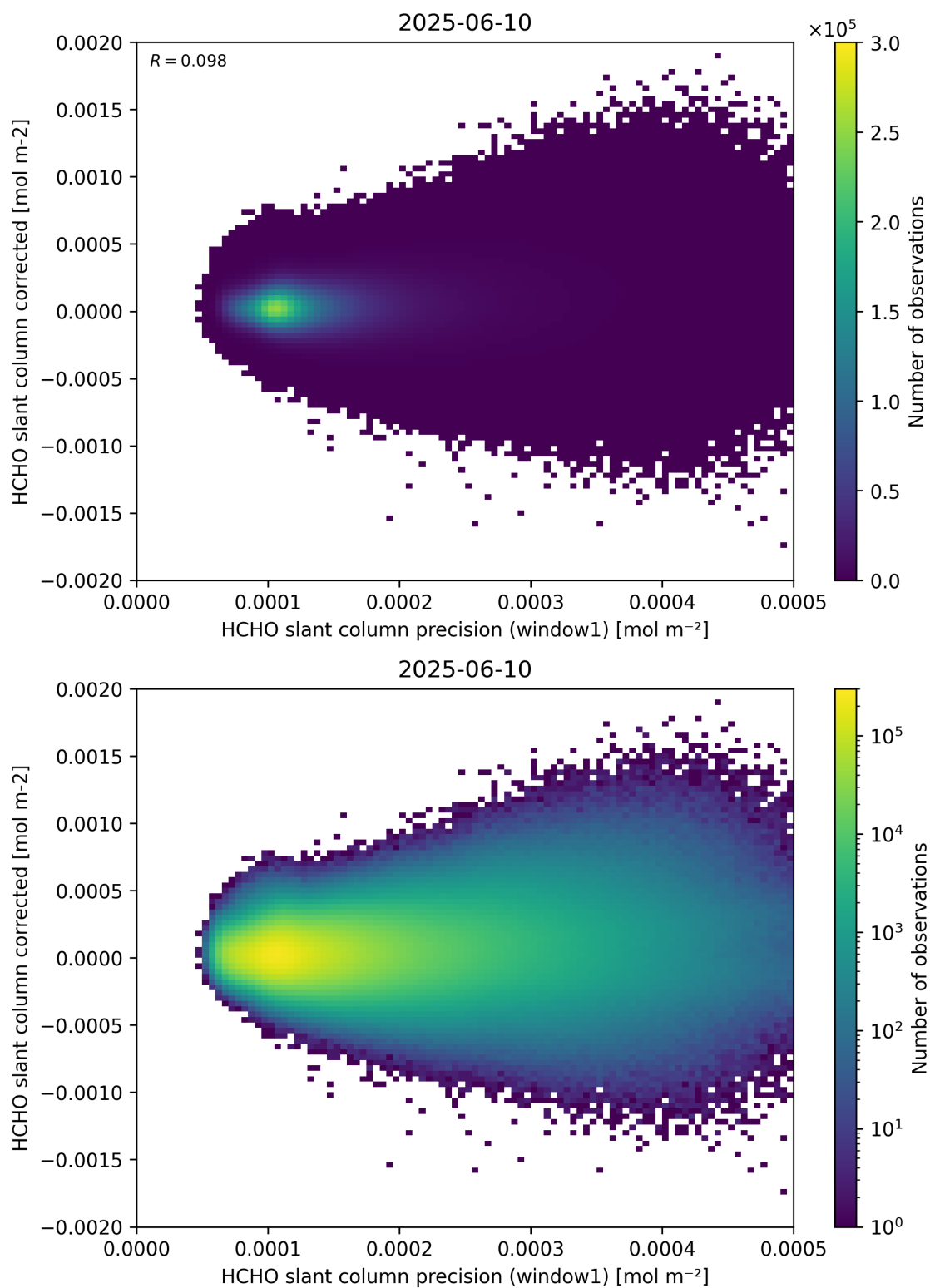
Figure 92: Scatter density plot of “HCHO slant column precision (window1)” against “HCHO slant column corrected” for 2025-06-09 to 2025-06-11.
