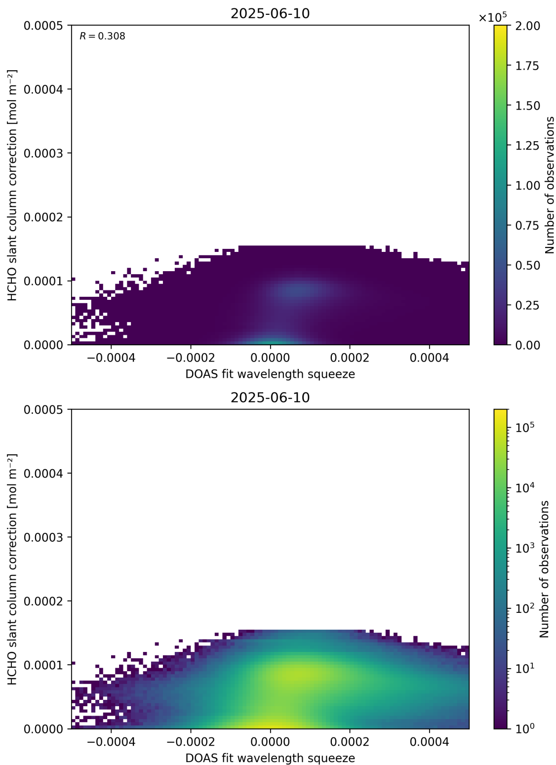
Figure 70: Scatter density plot of “DOAS fit wavelength squeeze” against “HCHO slant column correction” for 2025-06-09 to 2025-06-11.
