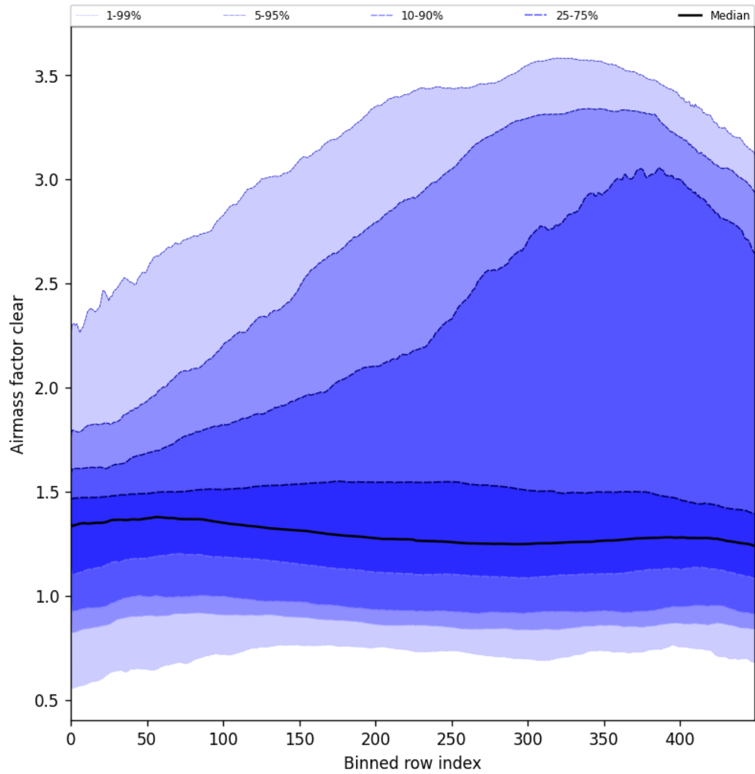
Figure 56: Along track statistics of “Air mass factor clear” for 2025-06-09 to 2025-06-11
