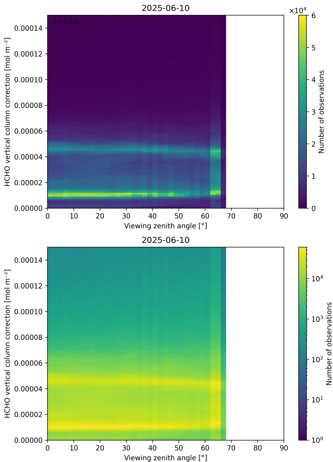
Figure 193: Scatter density plot of “Viewing zenith angle” against “HCHO vertical column correction” for 2025-06-09 to 2025-06-11.
