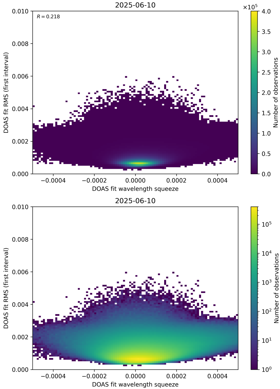
Figure 68: Scatter density plot of “DOAS fit wavelength squeeze” against “DOAS fit RMS (first interval)” for 2025-06-09 to 2025-06-11.
