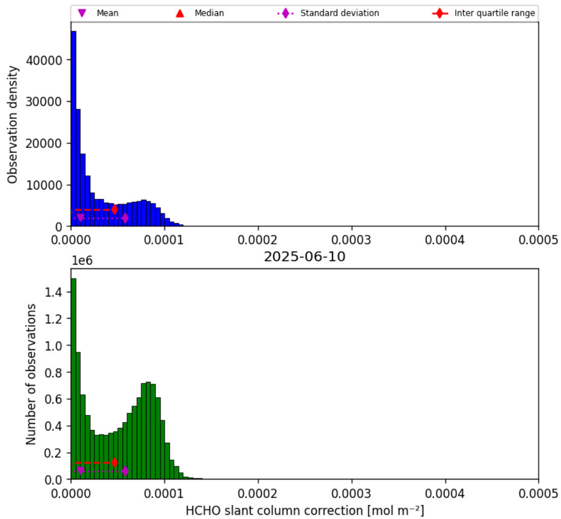
Figure 47: Histogram of “HCHO slant column correction” for 2025-06-09 to 2025-06-11
