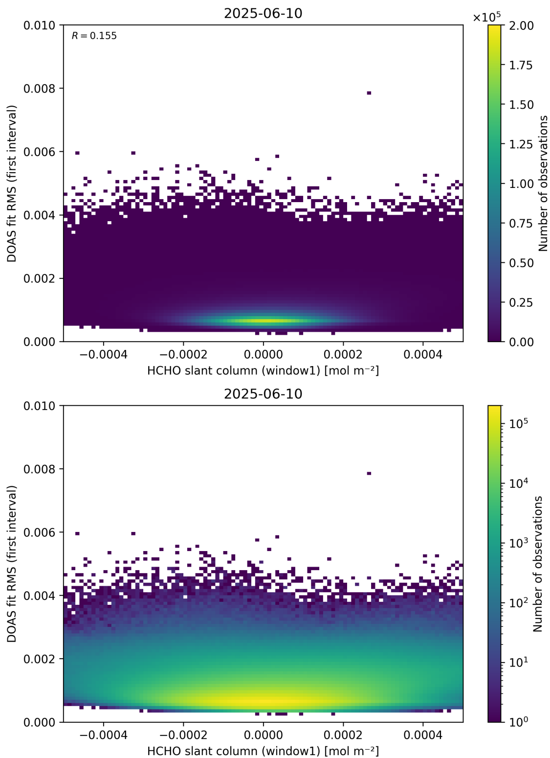
Figure 78: Scatter density plot of “HCHO slant column (window1)” against “DOAS fit RMS (first interval)” for 2025-06-09 to 2025-06-11.
