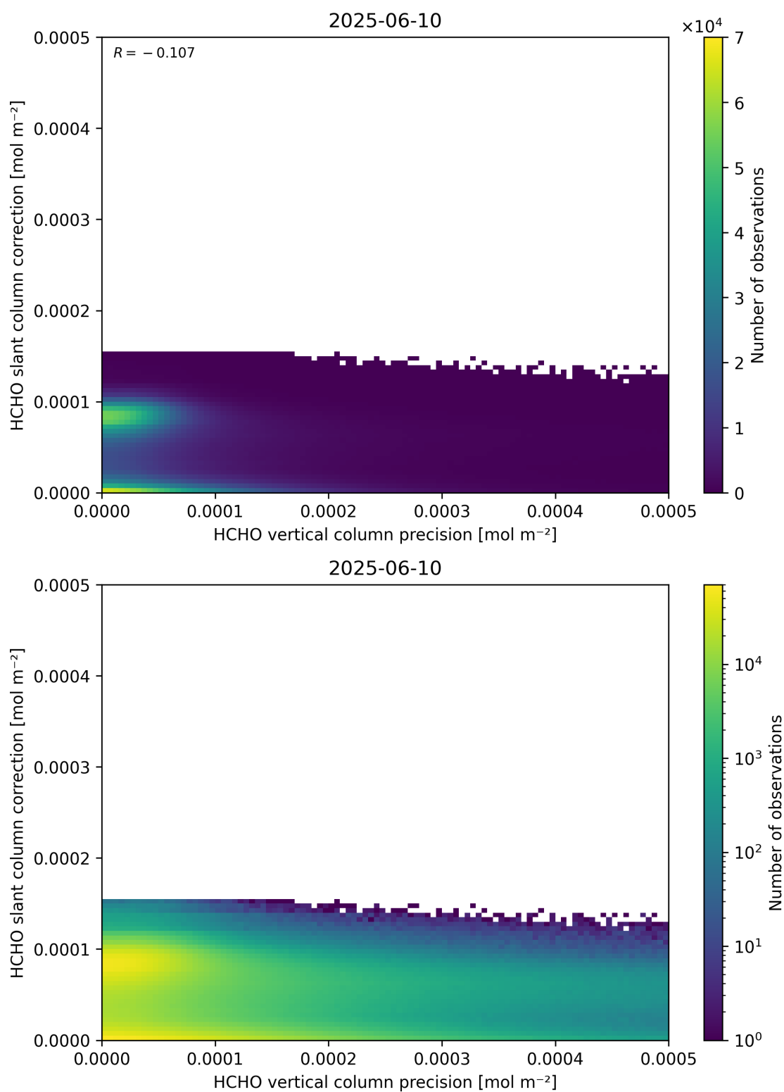
Figure 141: Scatter density plot of “HCHO vertical column precision” against “HCHO slant column correction” for 2025-06-09 to 2025-06-11.
