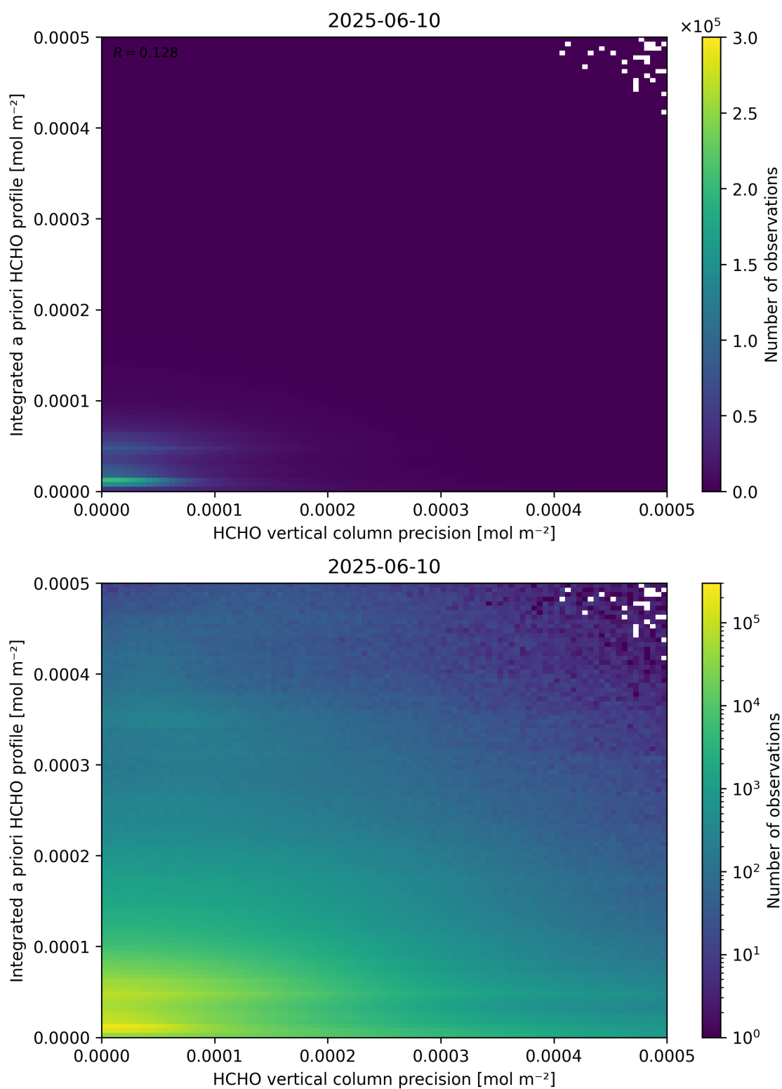
Figure 147: Scatter density plot of “HCHO vertical column precision” against “Integrated a priori HCHO profile” for 2025-06-09 to 2025-06-11.
