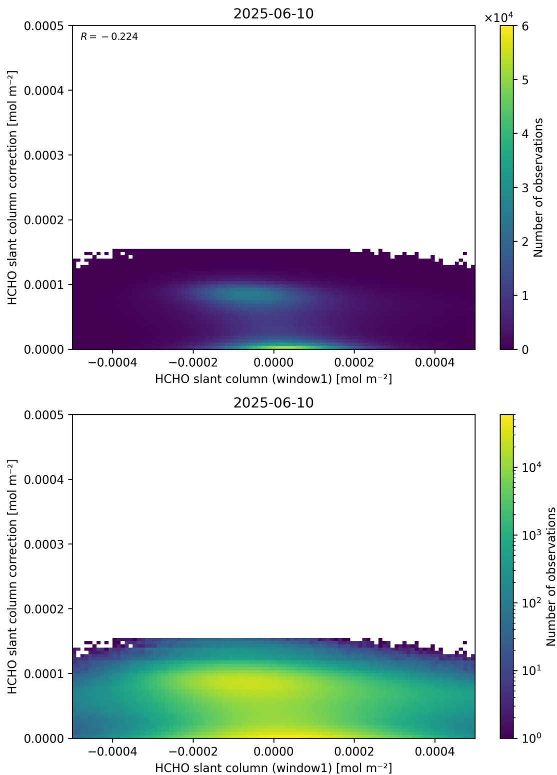
Figure 83: Scatter density plot of “HCHO slant column (window1)” against “HCHO slant column correction” for 2025-06-09 to 2025-06-11.
