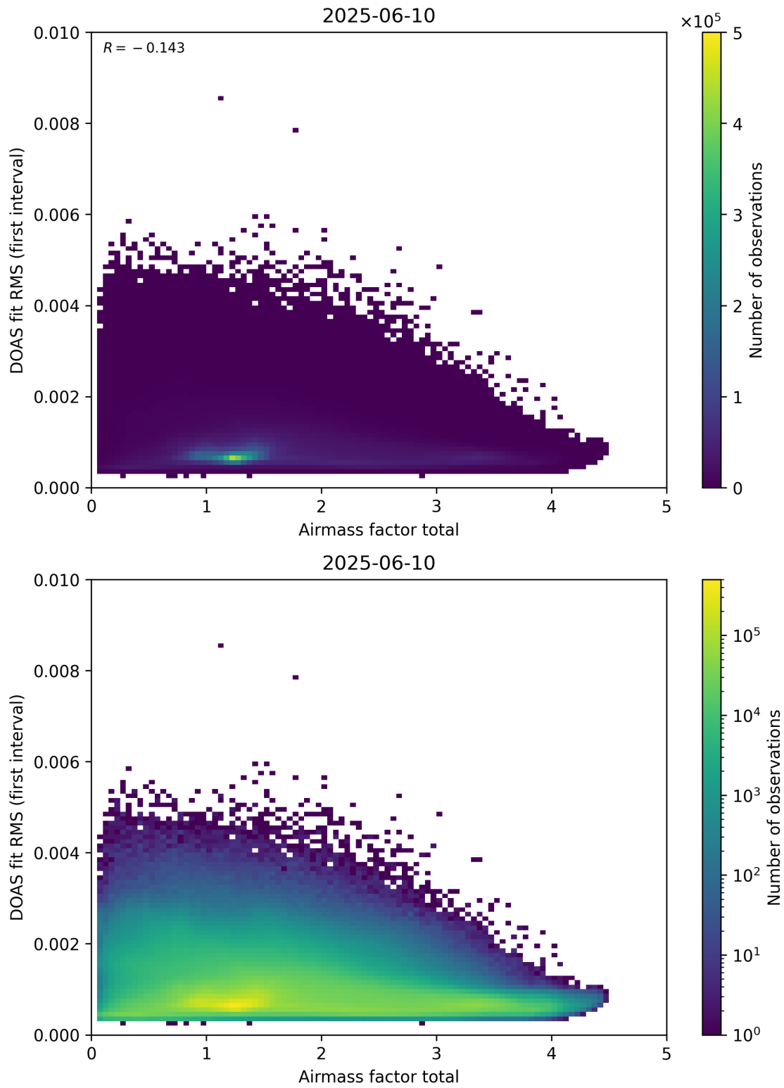
Figure 97: Scatter density plot of “Airmass factor total” against “DOAS fit RMS (first interval)” for 2025-06-09 to 2025-06-11.
