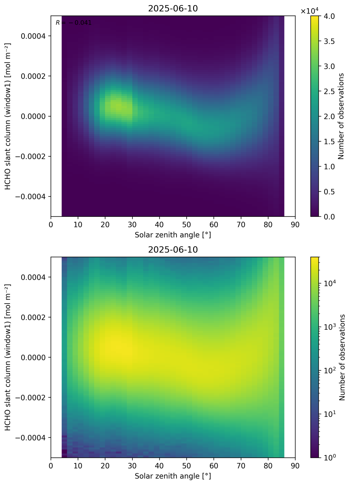
Figure 173: Scatter density plot of “Solar zenith angle” against “HCHO slant column (window1)” for 2025-06-09 to 2025-06-11.
