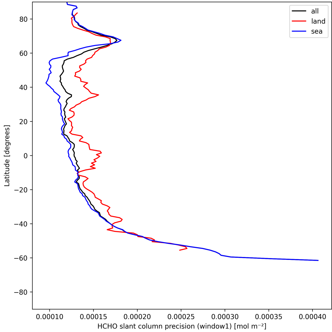
Figure 25: Zonal average of “HCHO slant column precision (window1)” for 2025-06-09 to 2025-06-11.
