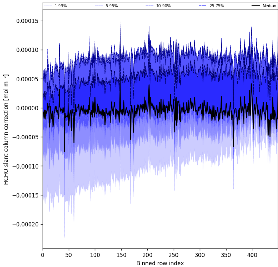
Figure 61: Along track statistics of "HCHO slant column correction" for 2025-06-09 to 2025-06-11
