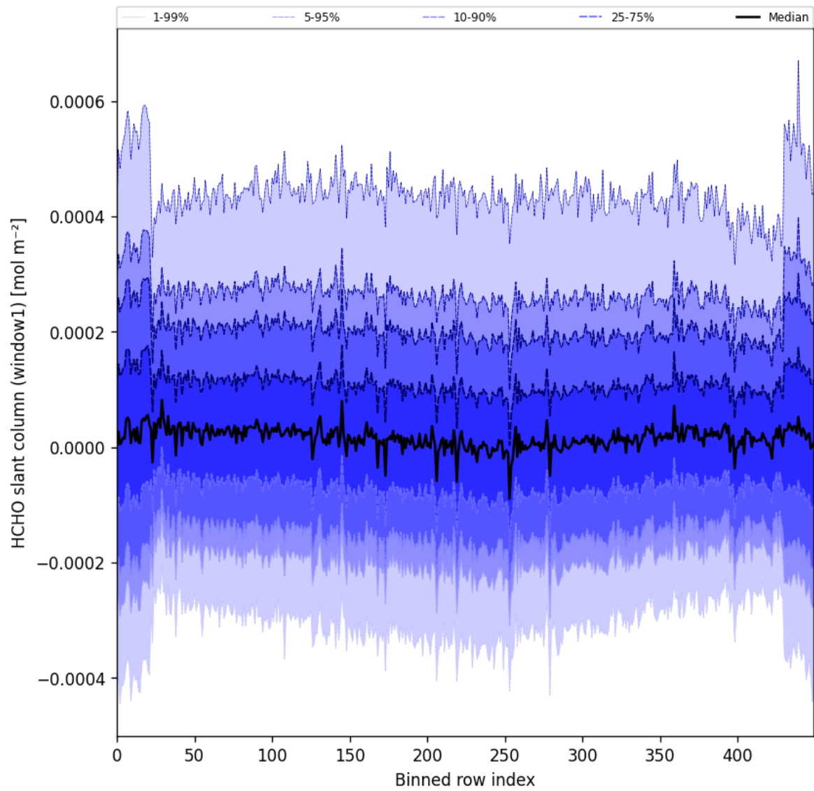
Figure 52: Along track statistics of “HCHO slant column (window1)” for 2025-06-09 to 2025-06-11
