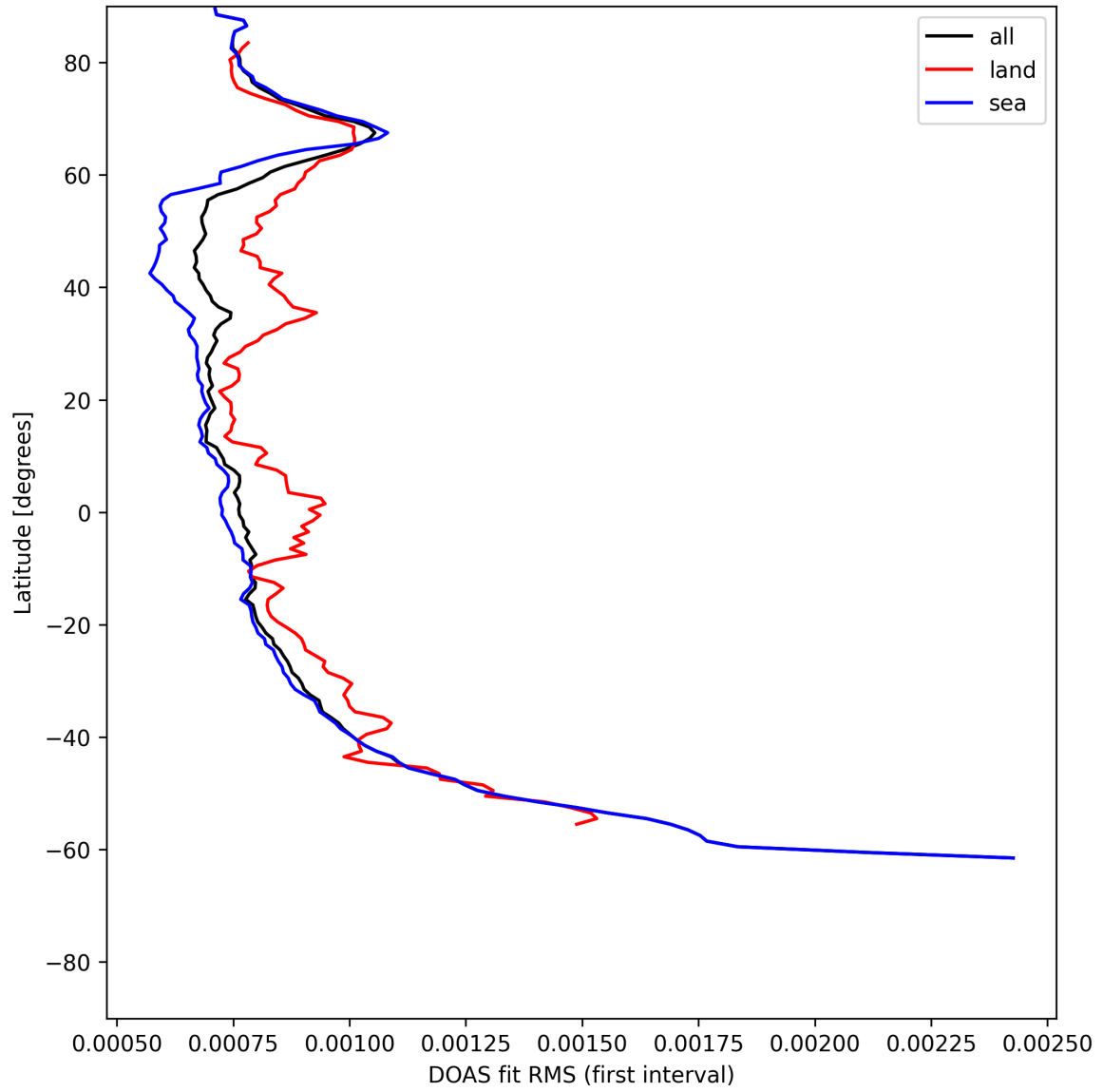
Figure 32: Zonal average of “DOAS fit RMS (first interval)” for 2025-06-09 to 2025-06-11.
