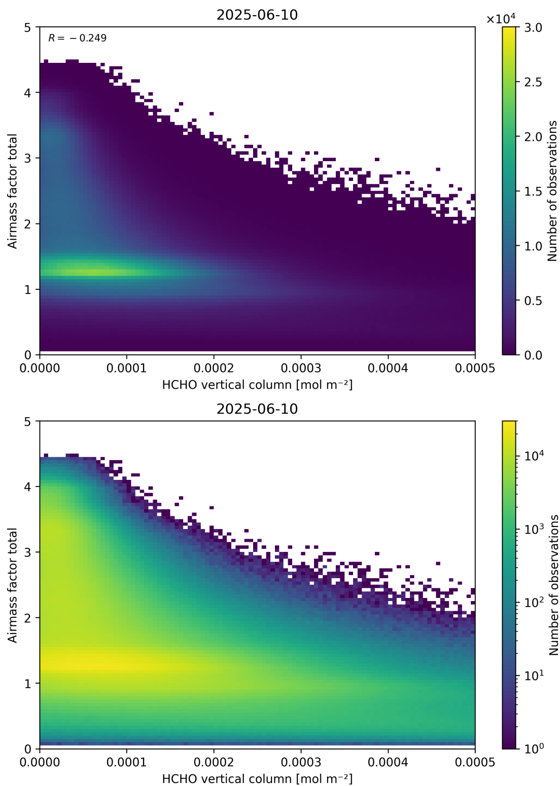
Figure 131: Scatter density plot of “HCHO vertical column” against “Airmass factor total” for 2025-06-09 to 2025-06-11.
