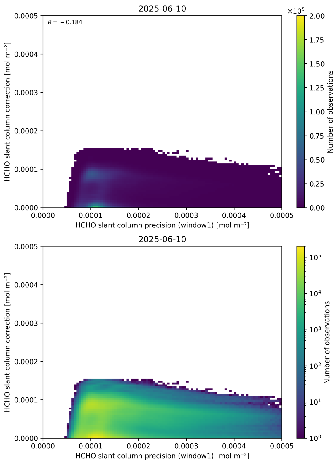
Figure 93: Scatter density plot of “HCHO slant column precision (window1)” against “HCHO slant column correction” for 2025-06-09 to 2025-06-11.
