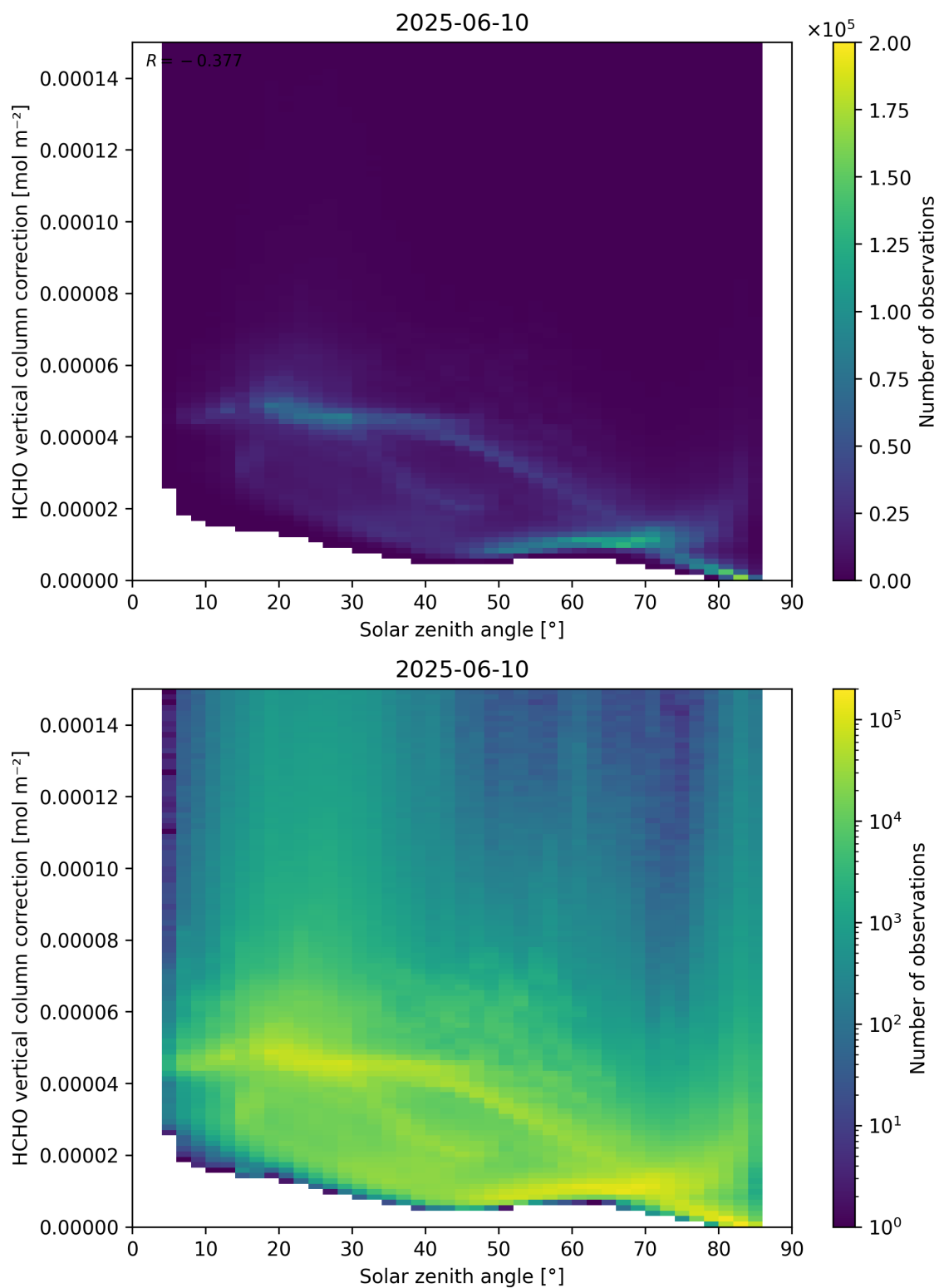
Figure 178: Scatter density plot of “Solar zenith angle” against “HCHO vertical column correction” for 2025-06-09 to 2025-06-11.
