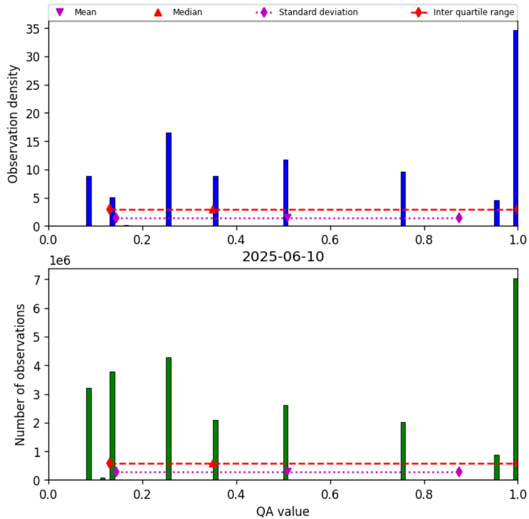
Figure 34: Histogram of “QA value” for 2025-06-09 to 2025-06-11
