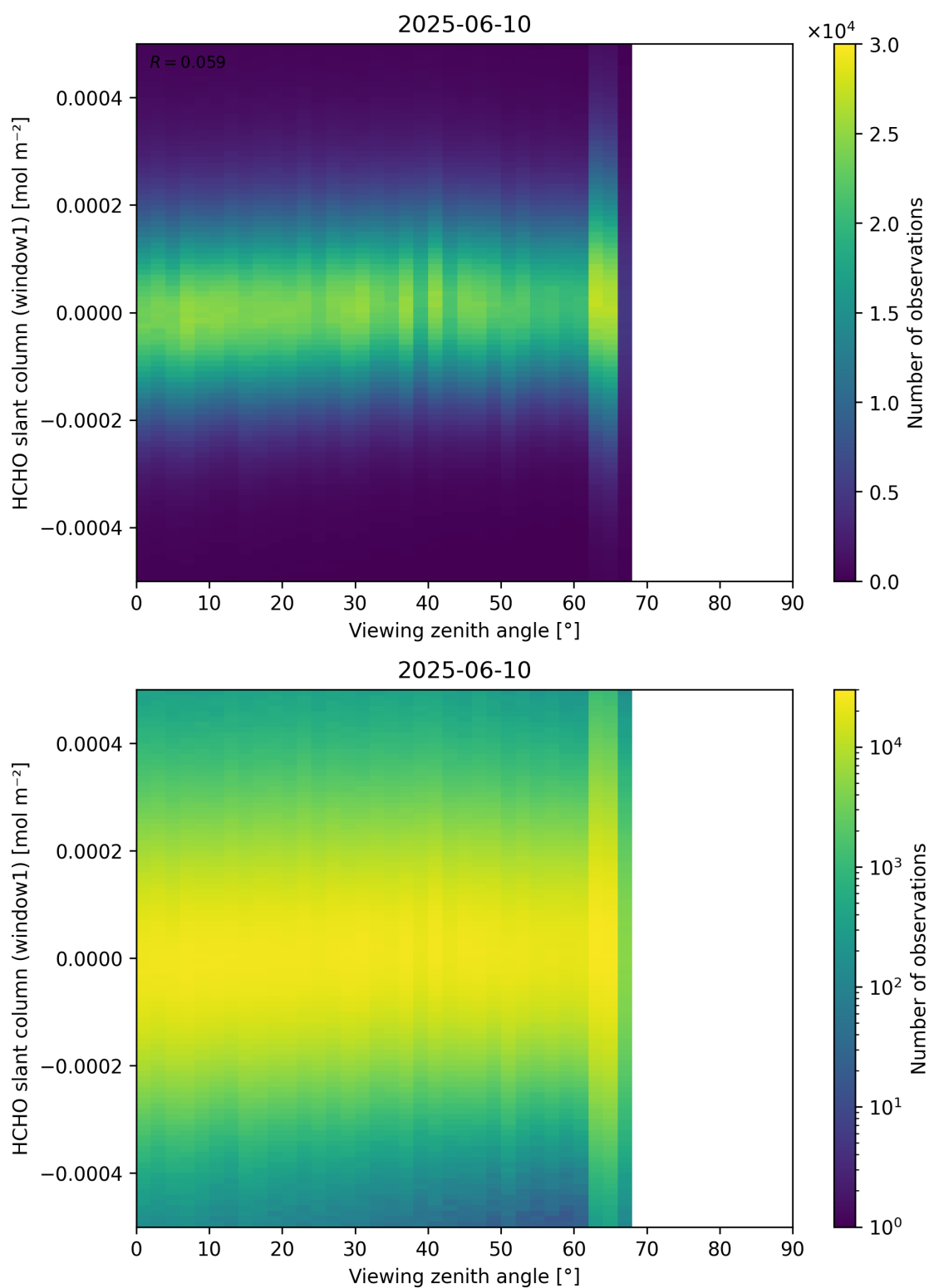
Figure 188: Scatter density plot of “Viewing zenith angle” against “HCHO slant column (window1)” for 2025-06-09 to 2025-06-11.
