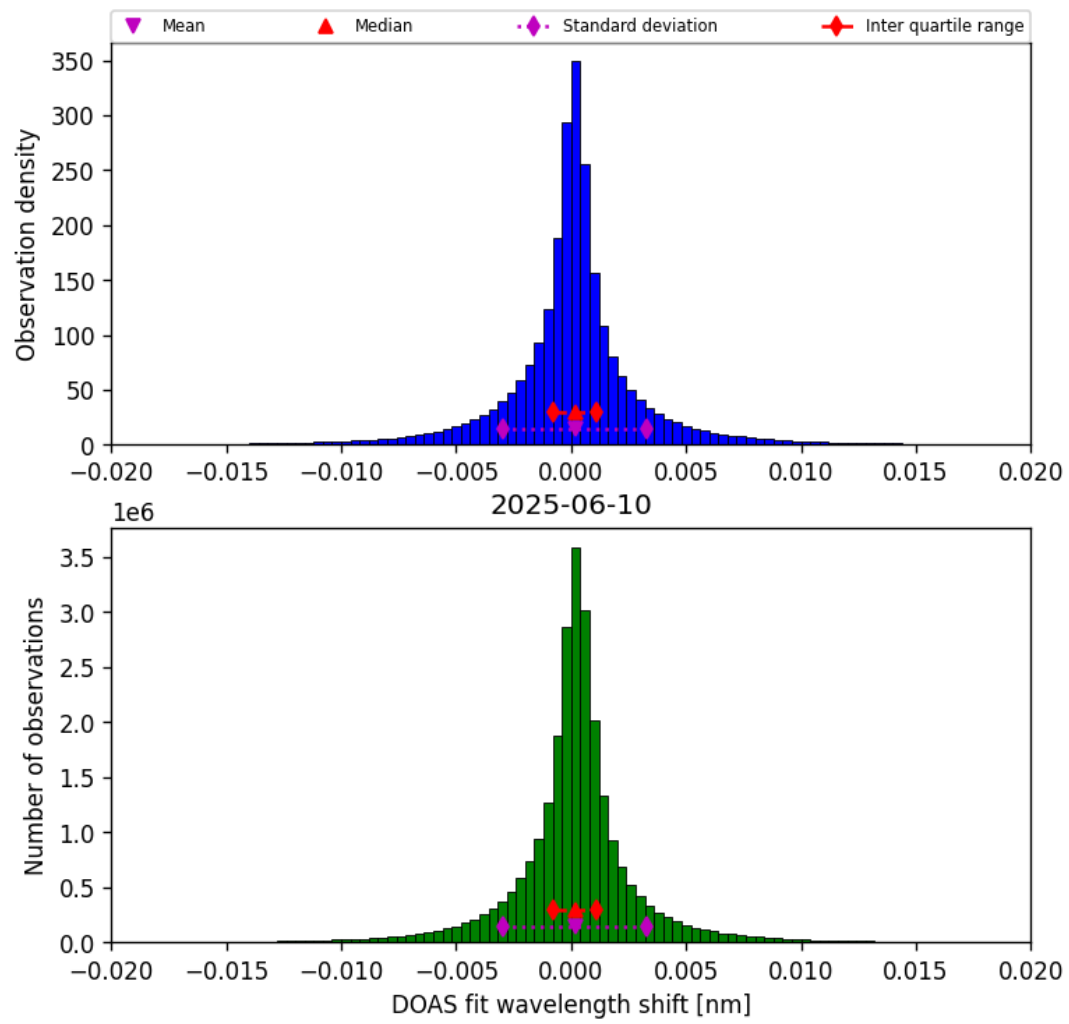
Figure 44: Histogram of “DOAS fit wavelength shift” for 2025-06-09 to 2025-06-11
