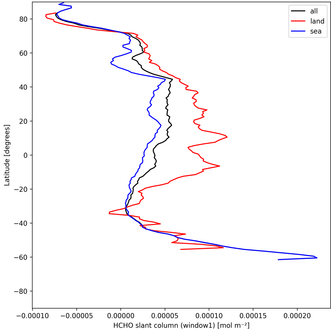
Figure 24: Zonal average of “HCHO slant column (window1)” for 2025-06-09 to 2025-06-11.
