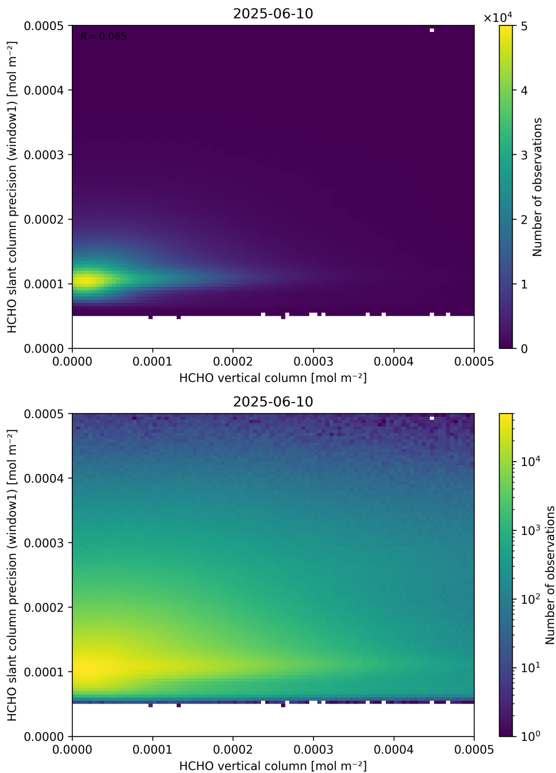
Figure 130: Scatter density plot of “HCHO vertical column” against “HCHO slant column precision (window1)” for 2025-06-09 to 2025-06-11.
