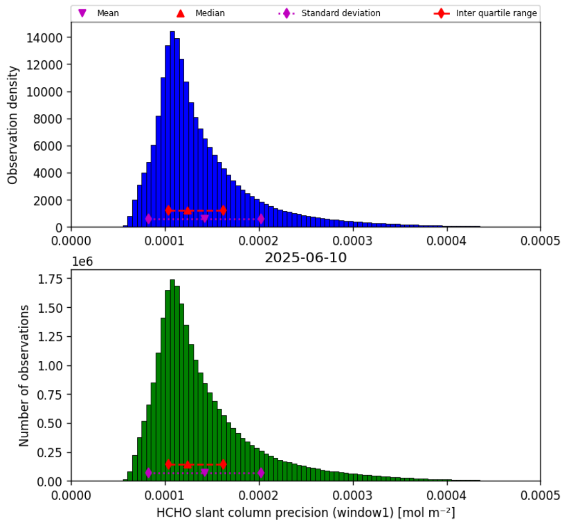
Figure 39: Histogram of “HCHO slant column precision (window1)” for 2025-06-09 to 2025-06-11
