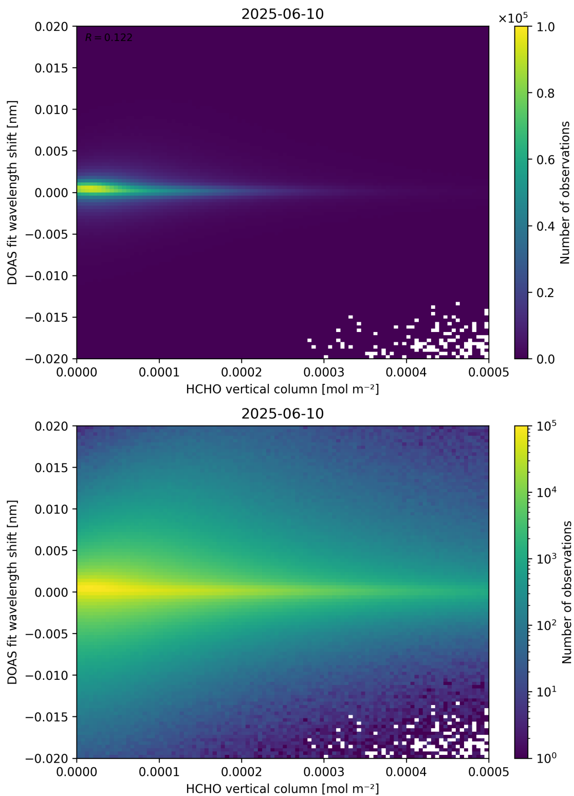
Figure 124: Scatter density plot of “HCHO vertical column” against “DOAS fit wavelength shift” for 2025-06-09 to 2025-06-11.
