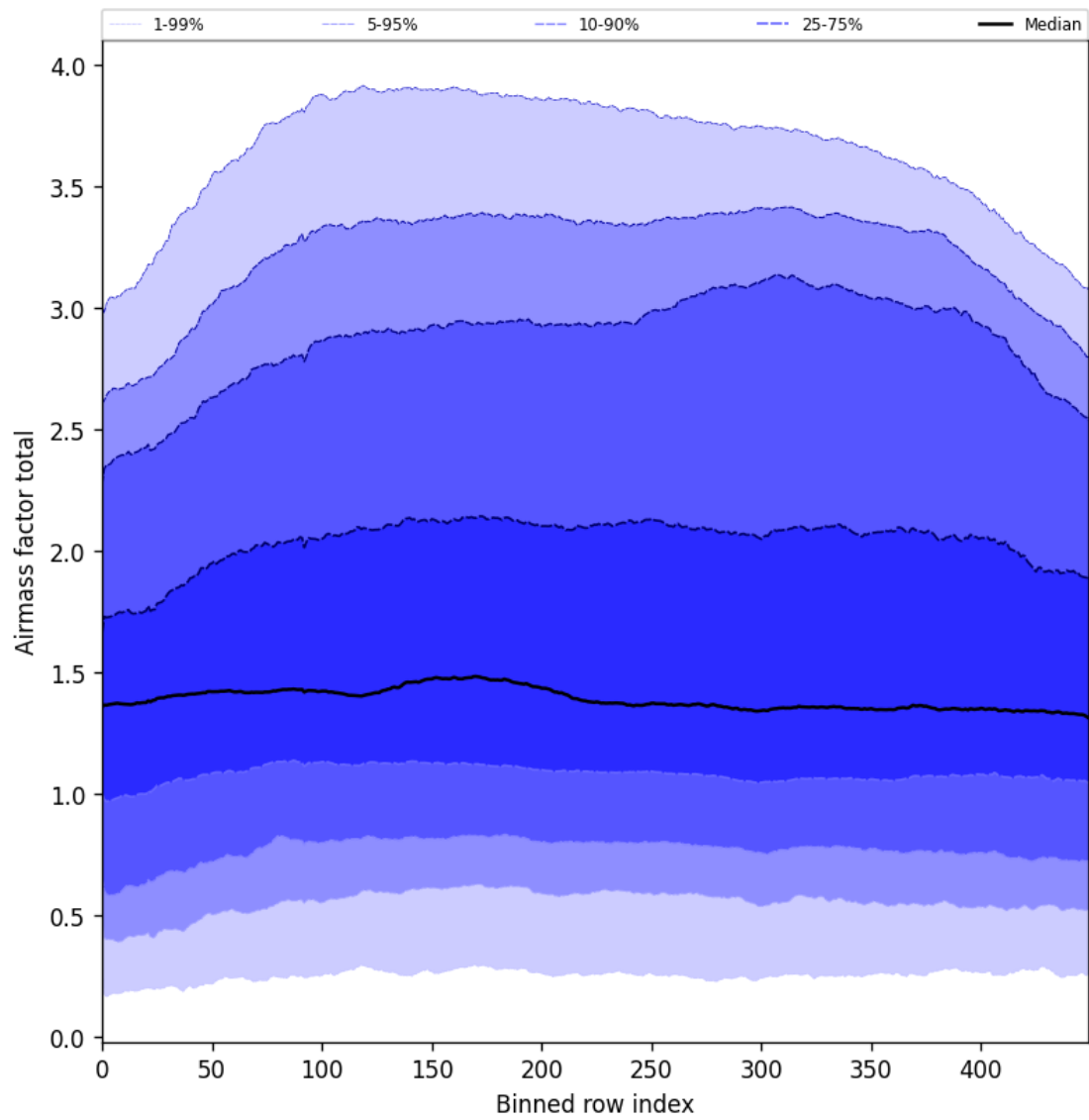
Figure 54: Along track statistics of “Airmass factor total” for 2025-06-09 to 2025-06-11
