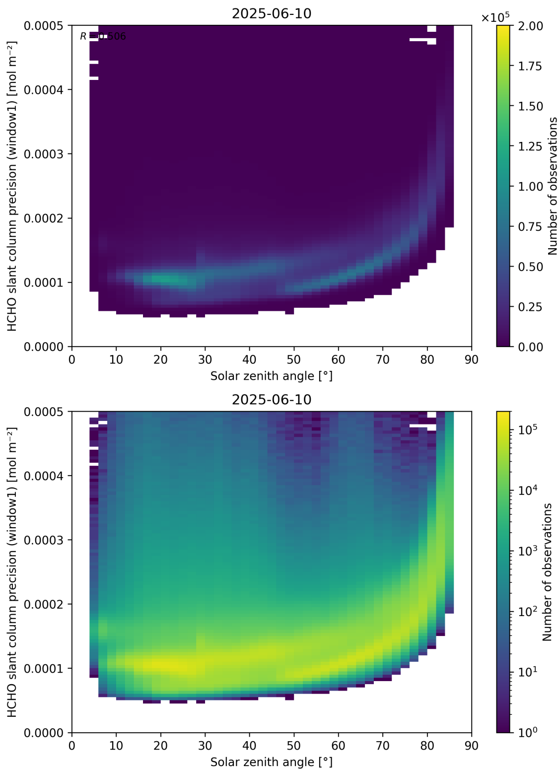
Figure 174: Scatter density plot of “Solar zenith angle” against “HCHO slant column precision (window1)” for 2025-06-09 to 2025-06-11.
