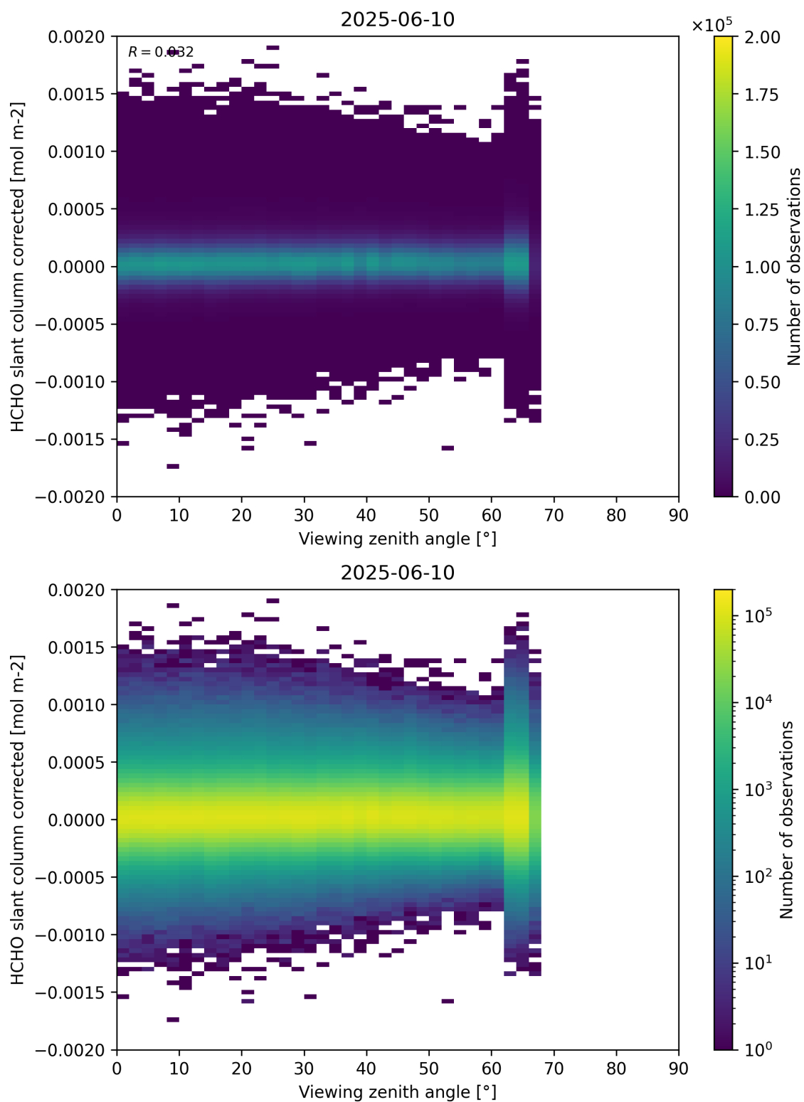
Figure 186: Scatter density plot of “Viewing zenith angle” against “HCHO slant column corrected” for 2025-06-09 to 2025-06-11.
