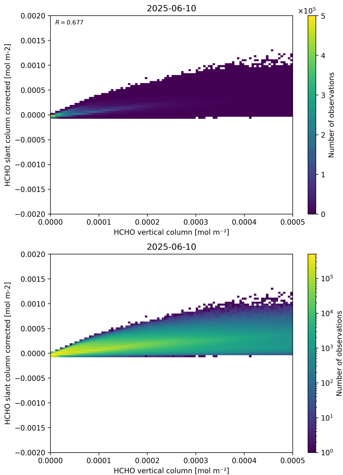
Figure 127: Scatter density plot of “HCHO vertical column” against “HCHO slant column corrected” for 2025-06-09 to 2025-06-11.
