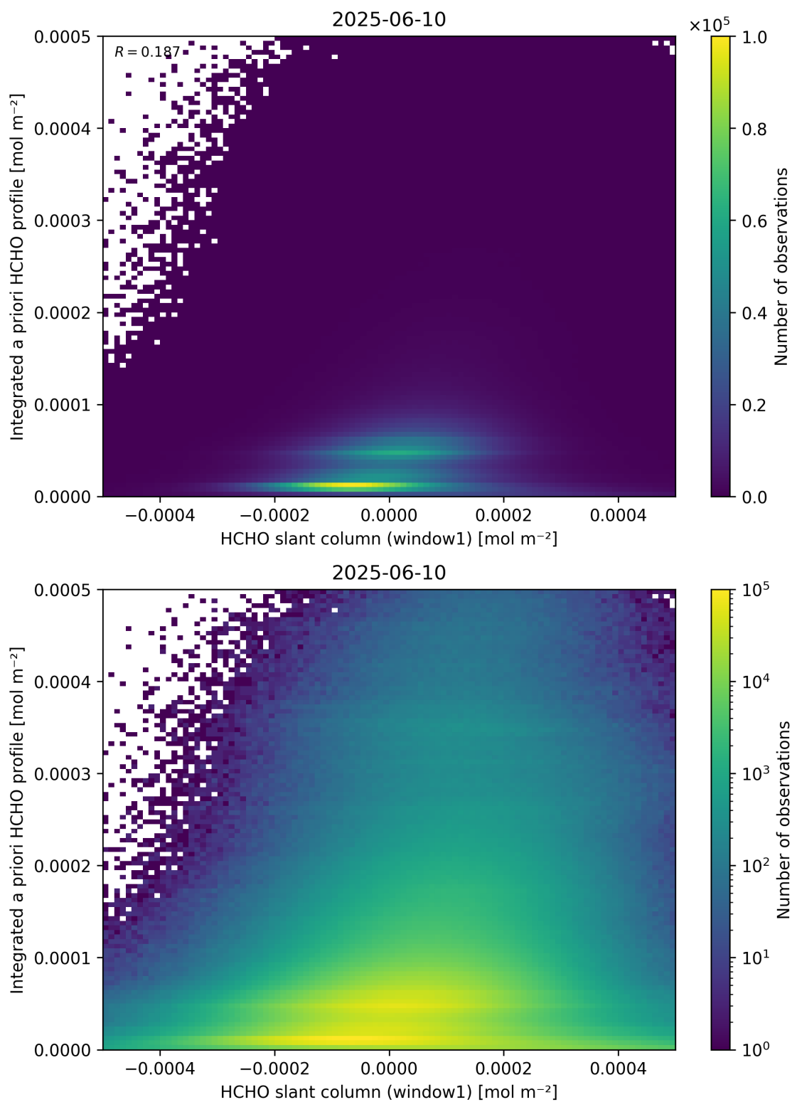
Figure 87: Scatter density plot of “HCHO slant column (window1)” against “Integrated a priori HCHO profile” for 2025-06-09 to 2025-06-11.
