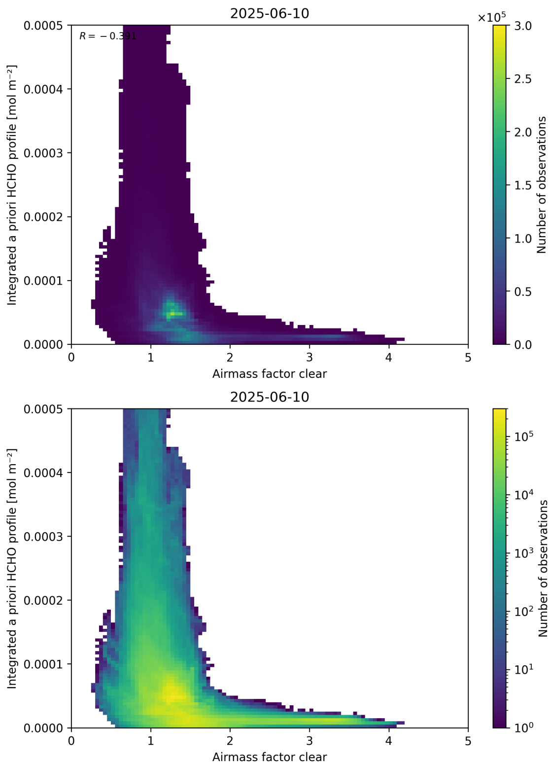
Figure 76: Scatter density plot of “Airmass factor clear” against “Integrated a priori HCHO profile” for 2025-06-09 to 2025-06-11.
