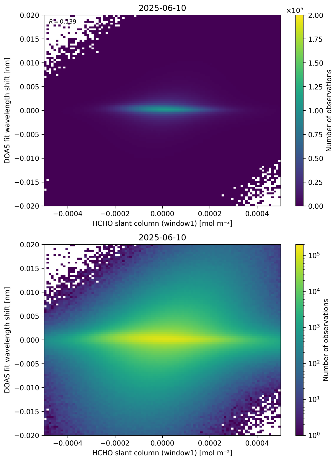
Figure 79: Scatter density plot of “HCHO slant column (window1)” against “DOAS fit wavelength shift” for 2025-06-09 to 2025-06-11.
