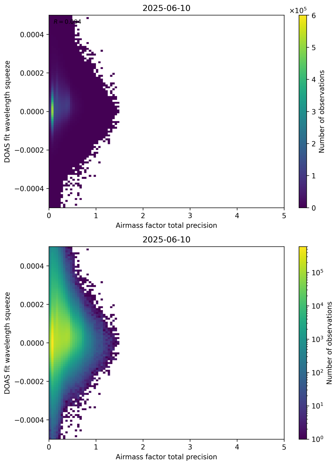
Figure 107: Scatter density plot of “Airmass factor total precision” against “DOAS fit wavelength squeeze” for 2025-06-09 to 2025-06-11.
