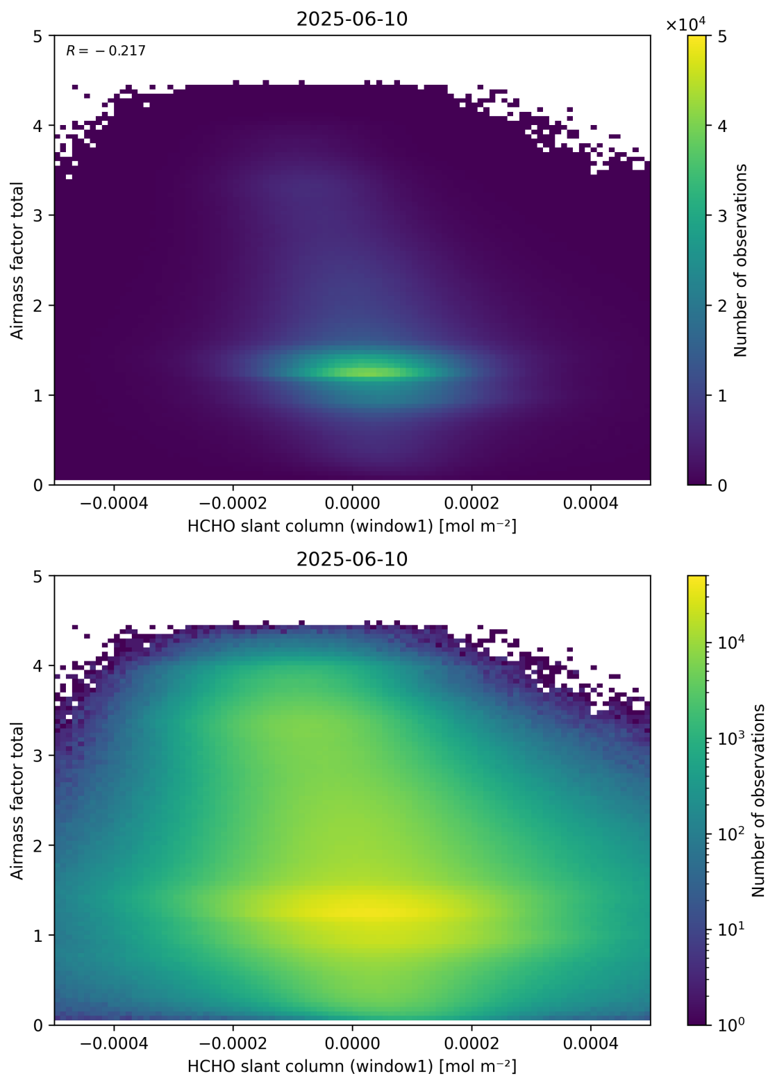
Figure 85: Scatter density plot of “HCHO slant column (window1)” against “Airmass factor total” for 2025-06-09 to 2025-06-11.
