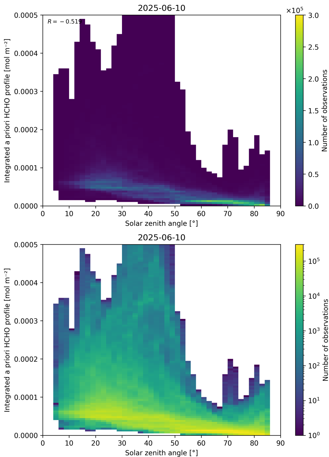
Figure 180: Scatter density plot of “Solar zenith angle” against “Integrated a priori HCHO profile” for 2025-06-09 to 2025-06-11.
