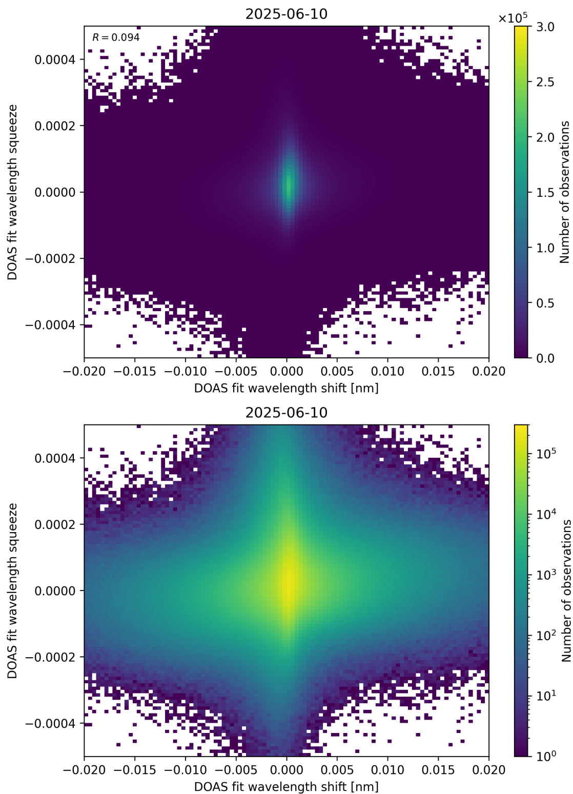
Figure 65: Scatter density plot of “DOAS fit wavelength shift” against “DOAS fit wavelength squeeze” for 2025-06-09 to 2025-06-11.
