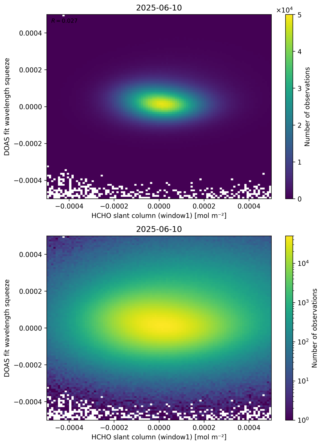
Figure 80: Scatter density plot of “HCHO slant column (window1)” against “DOAS fit wavelength squeeze” for 2025-06-09 to 2025-06-11.
