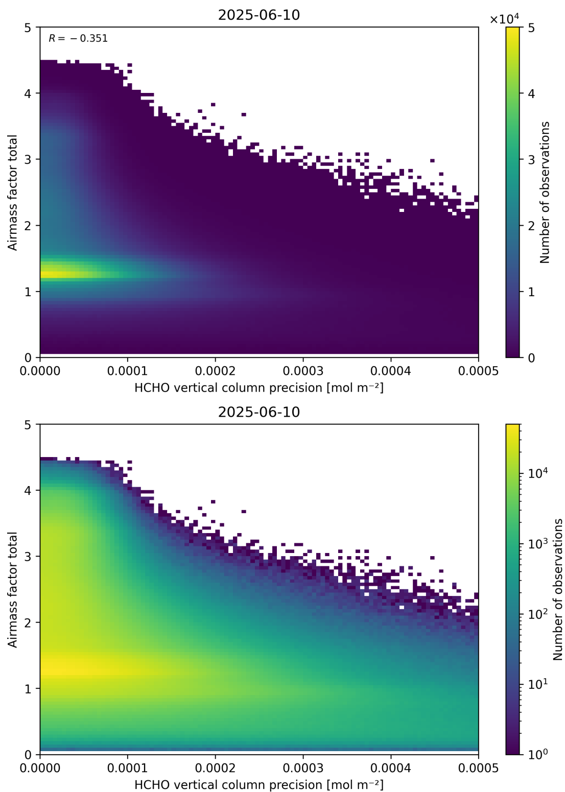
Figure 144: Scatter density plot of “HCHO vertical column precision” against “Airmass factor total” for 2025-06-09 to 2025-06-11.
