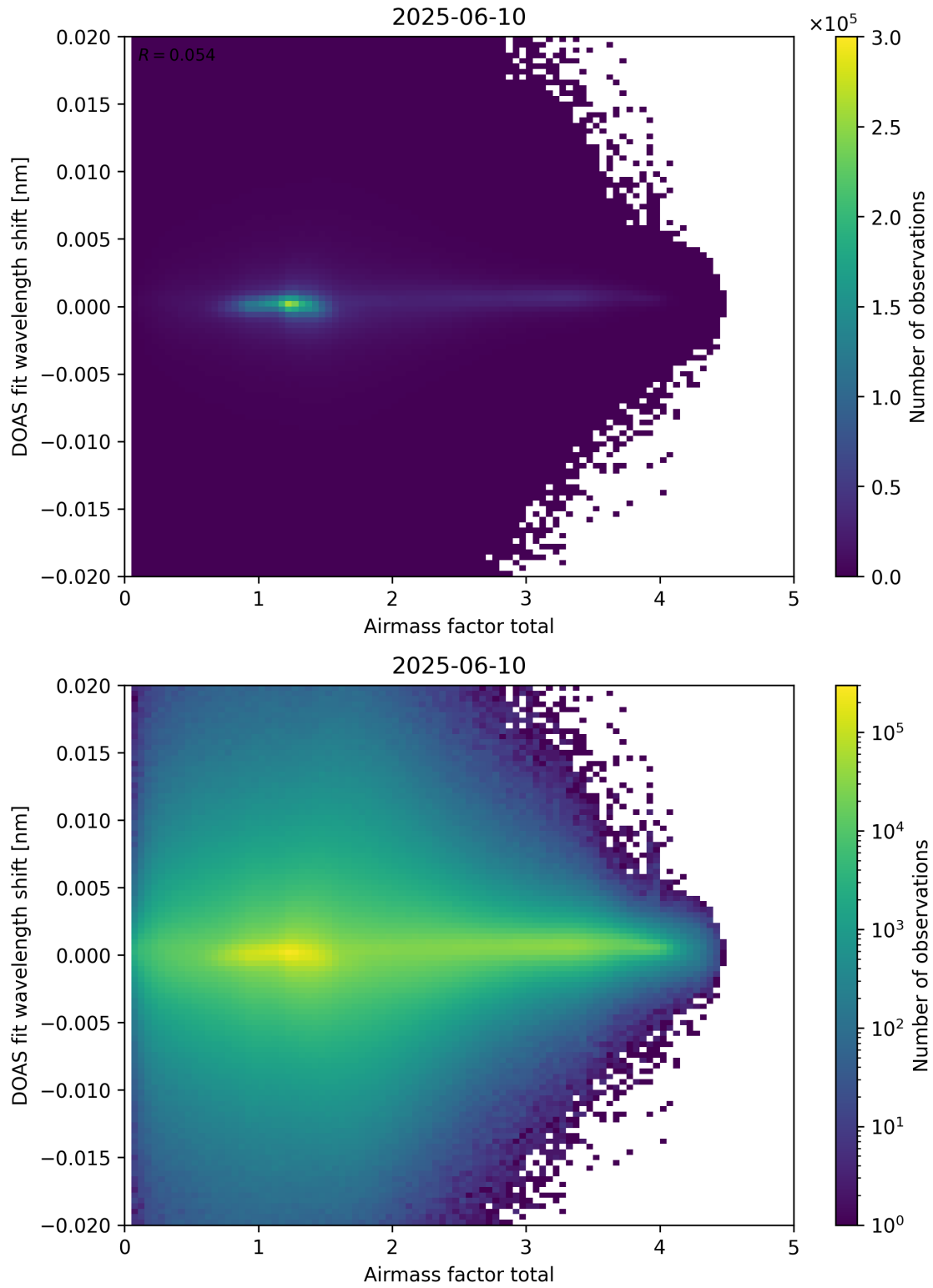
Figure 98: Scatter density plot of “Airmass factor total” against “DOAS fit wavelength shift” for 2025-06-09 to 2025-06-11.
