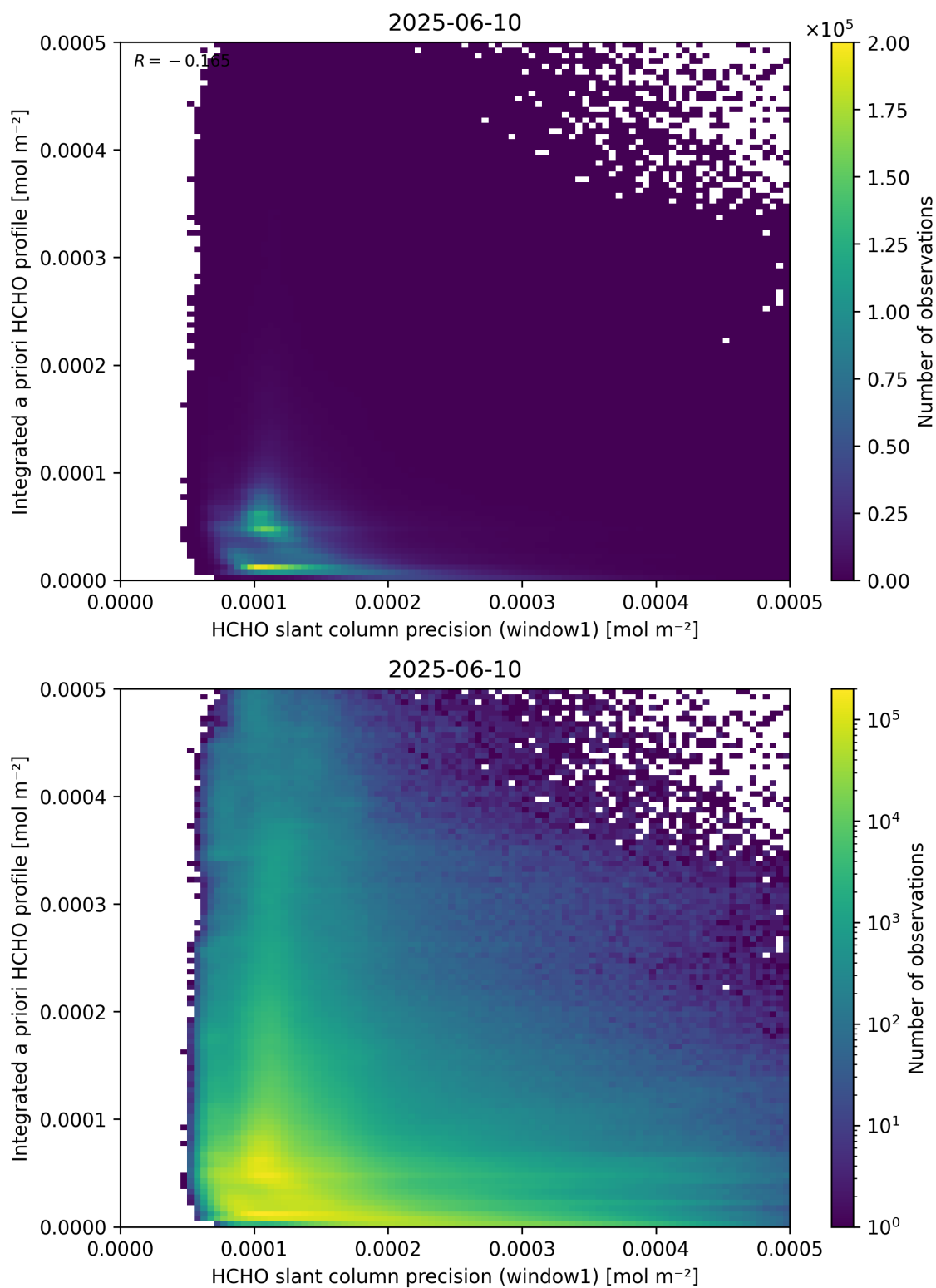
Figure 96: Scatter density plot of “HCHO slant column precision (window1)” against “Integrated a priori HCHO profile” for 2025-06-09 to 2025-06-11.
