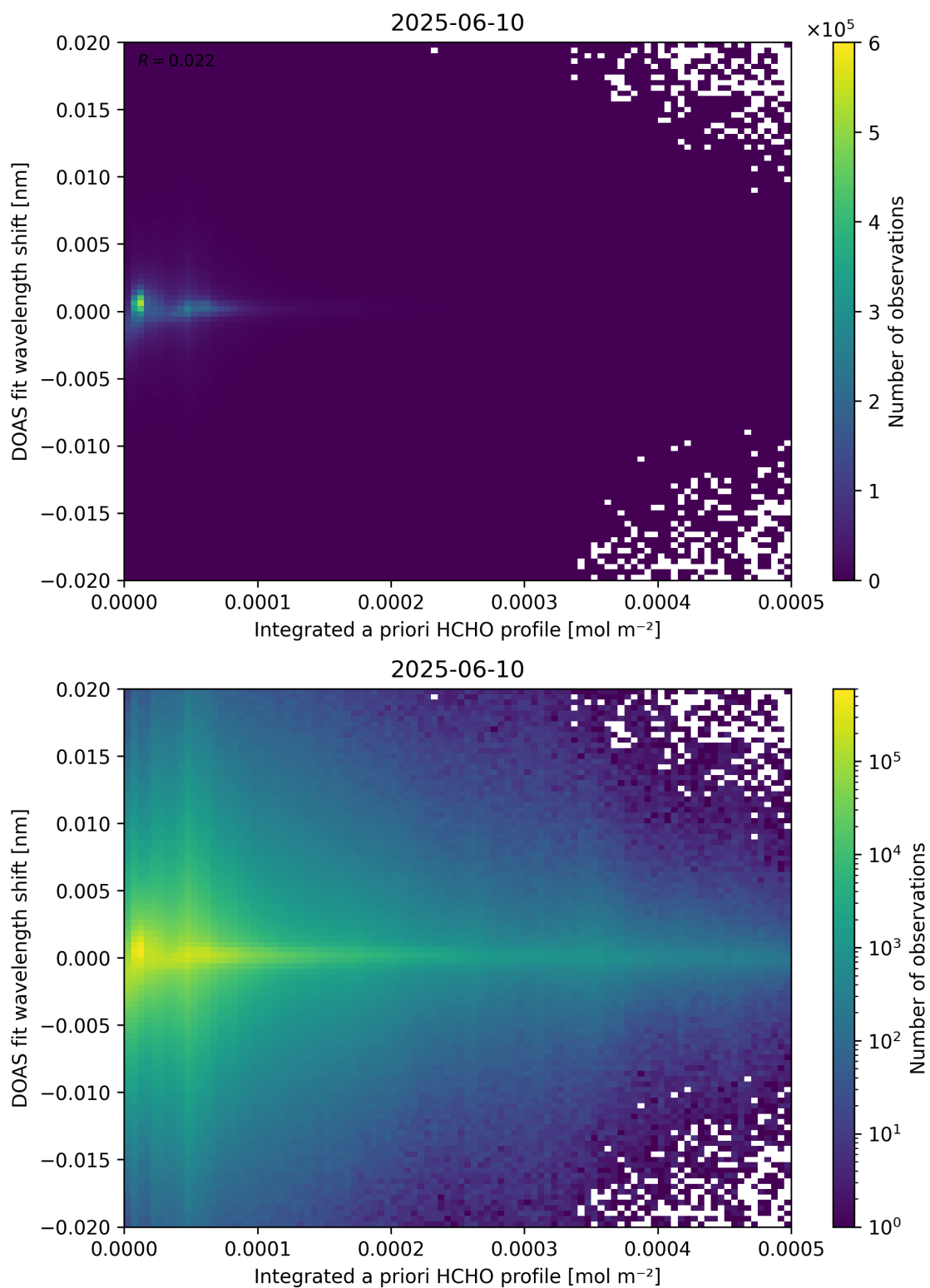
Figure 149: Scatter density plot of “Integrated a priori HCHO profile” against “DOAS fit wavelength shift” for 2025-06-09 to 2025-06-11.
