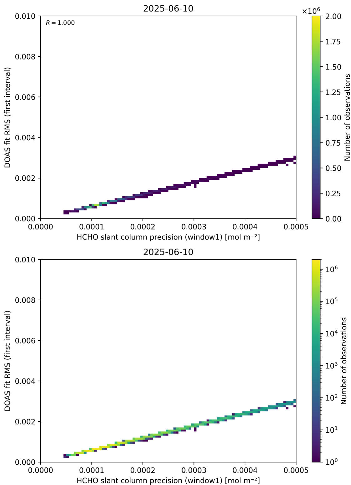
Figure 88: Scatter density plot of “HCHO slant column precision (window1)” against “DOAS fit RMS (first interval)” for 2025-06-09 to 2025-06-11.
