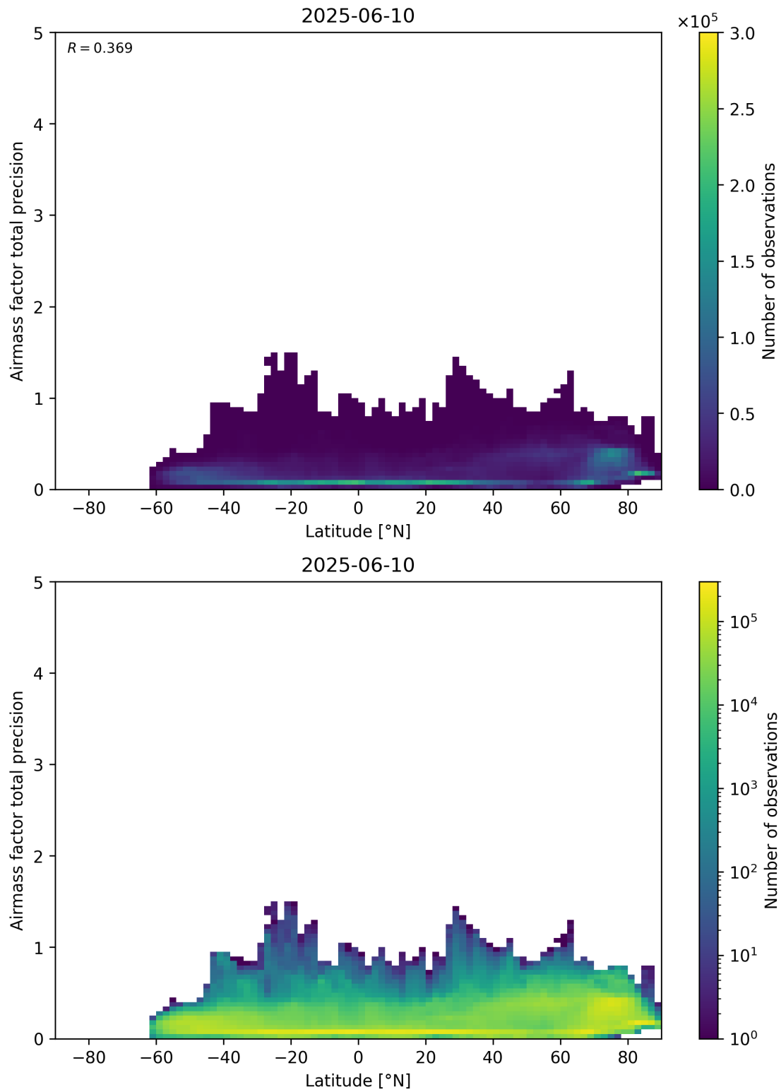
Figure 162: Scatter density plot of “Latitude” against “Airmass factor total precision” for 2025-06-09 to 2025-06-11.
