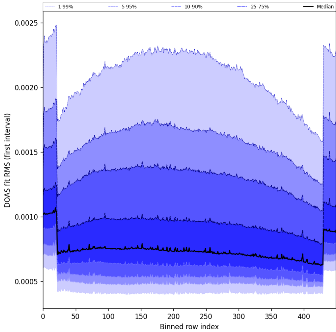
Figure 60: Along track statistics of “DOAS fit RMS (first interval)” for 2025-06-11 to 2025-06-12
