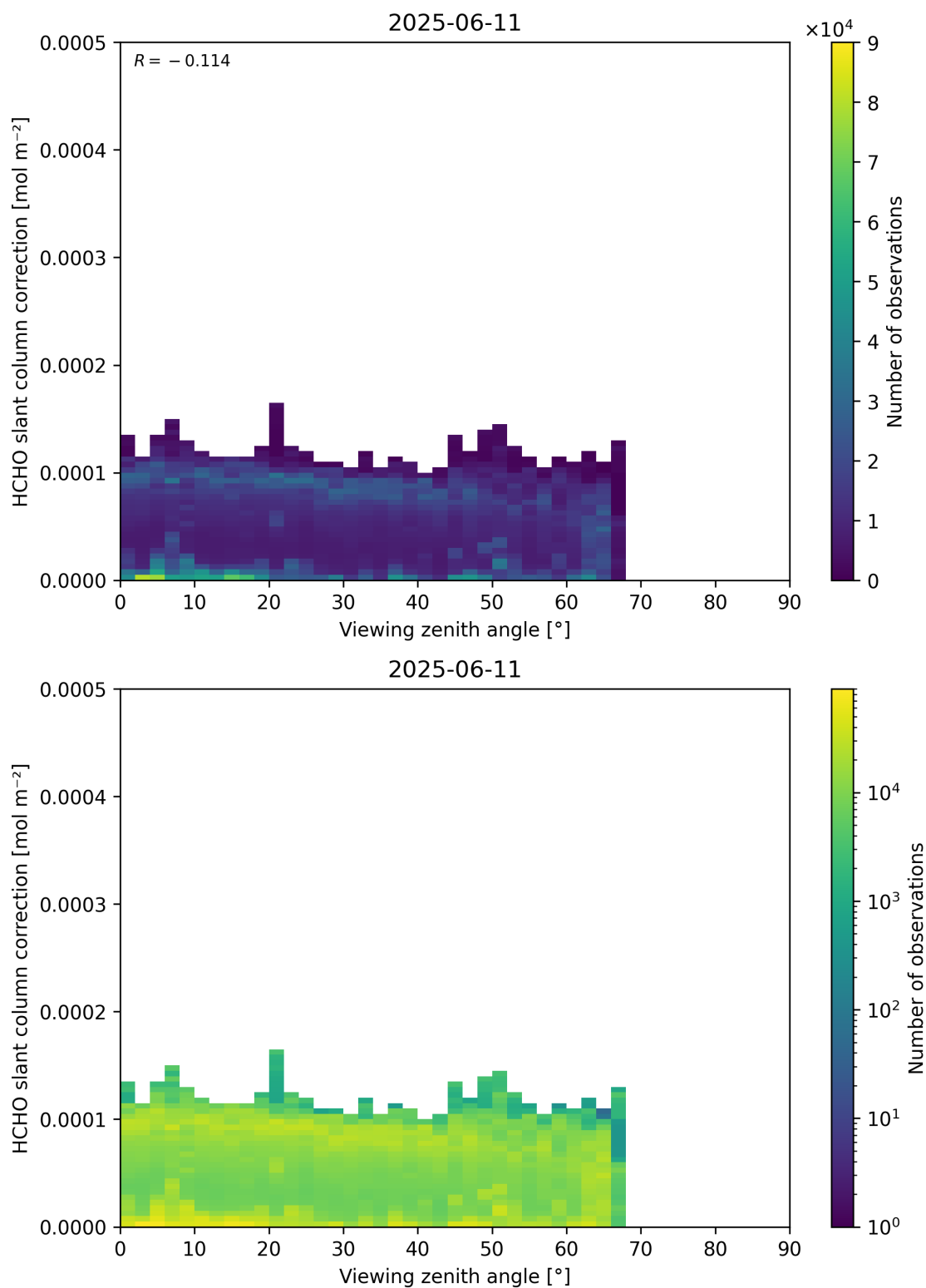
Figure 187: Scatter density plot of “Viewing zenith angle” against “HCHO slant column correction” for 2025-06-11 to 2025-06-12.
