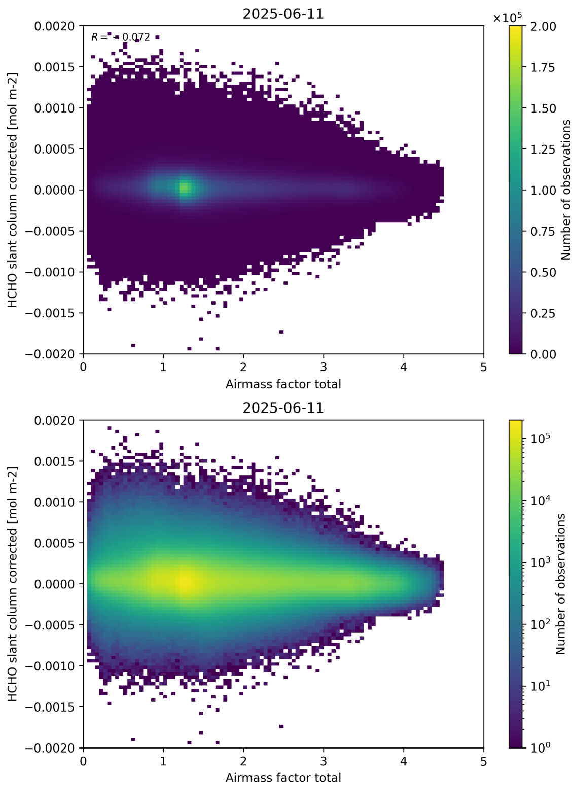
Figure 101: Scatter density plot of “Airmass factor total” against “HCHO slant column corrected” for 2025-06-11 to 2025-06-12.
