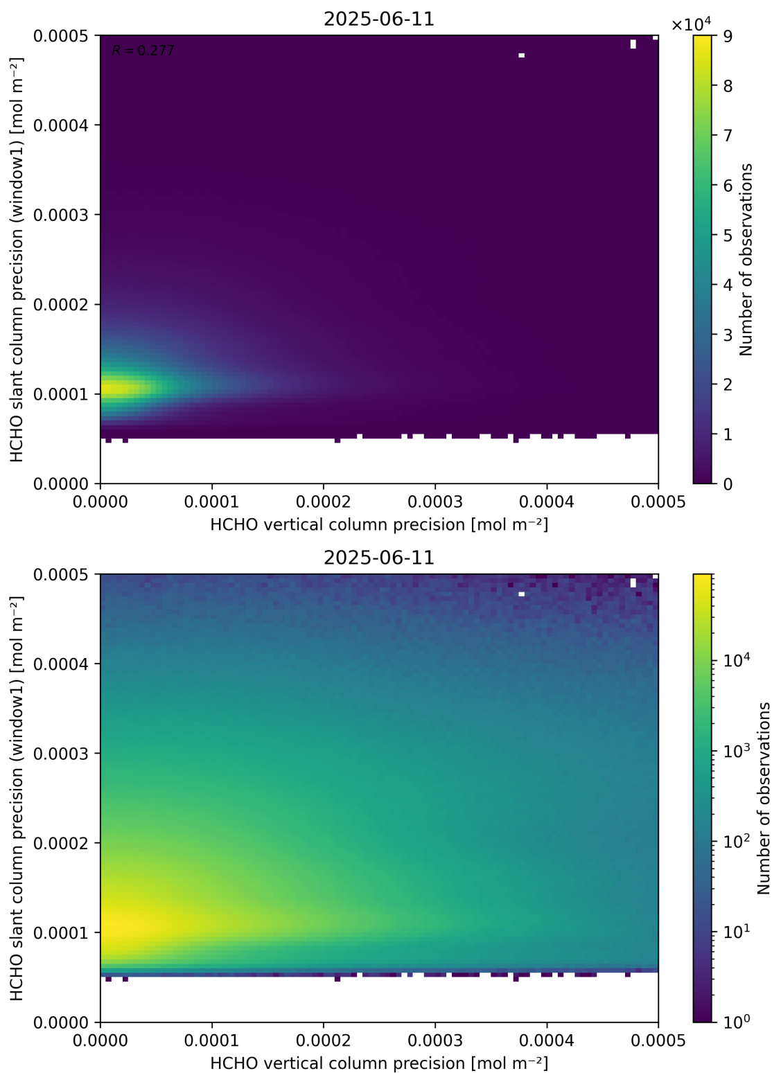
Figure 143: Scatter density plot of “HCHO vertical column precision” against “HCHO slant column precision (window1)” for 2025-06-11 to 2025-06-12.
