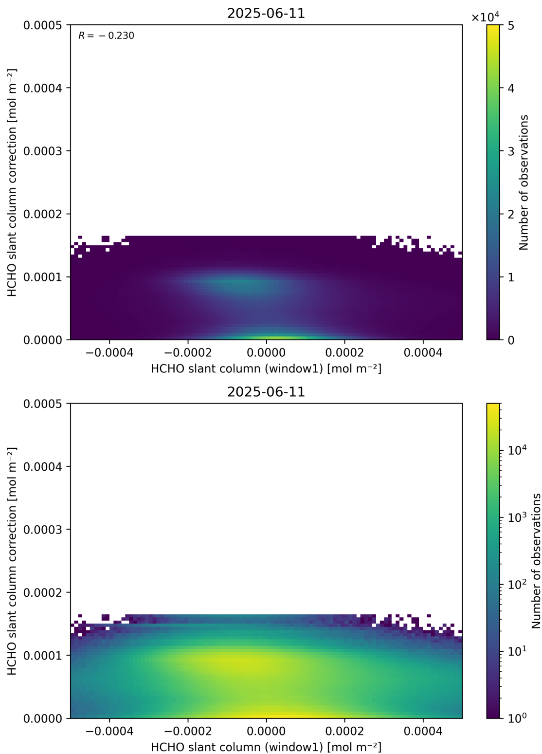
Figure 83: Scatter density plot of “HCHO slant column (window1)” against “HCHO slant column correction” for 2025-06-11 to 2025-06-12.
