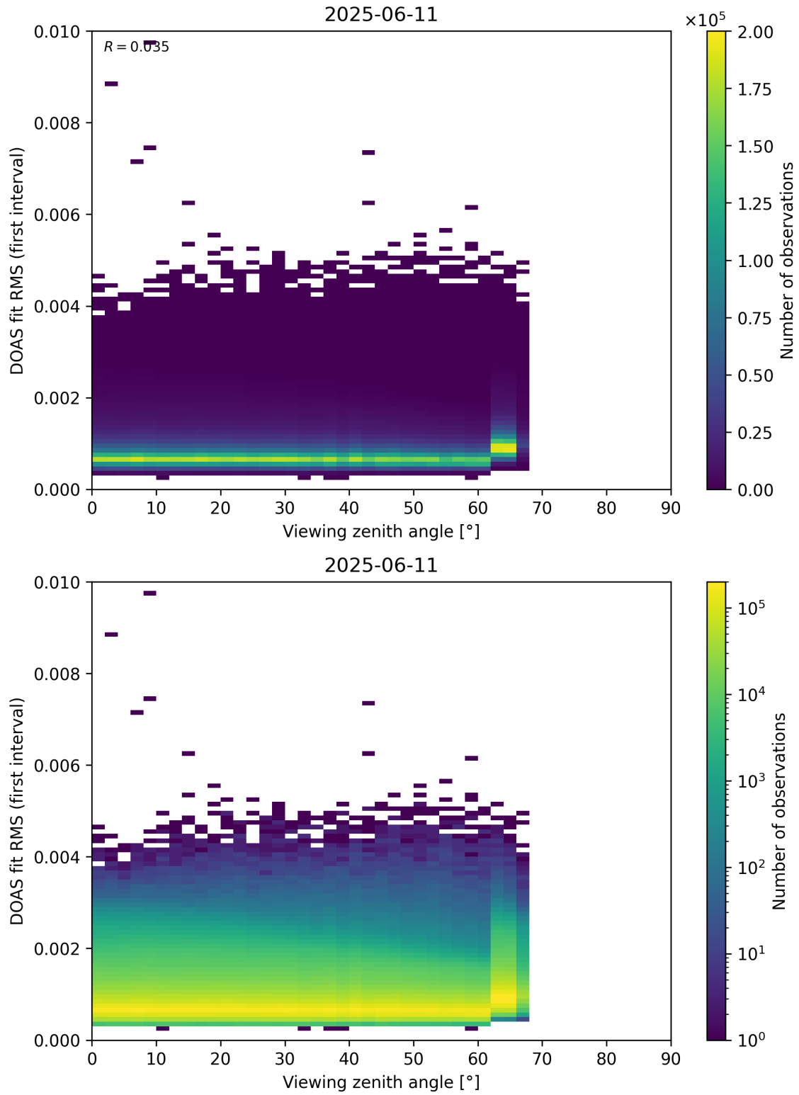
Figure 182: Scatter density plot of “Viewing zenith angle” against “DOAS fit RMS (first interval)” for 2025-06-11 to 2025-06-12.
