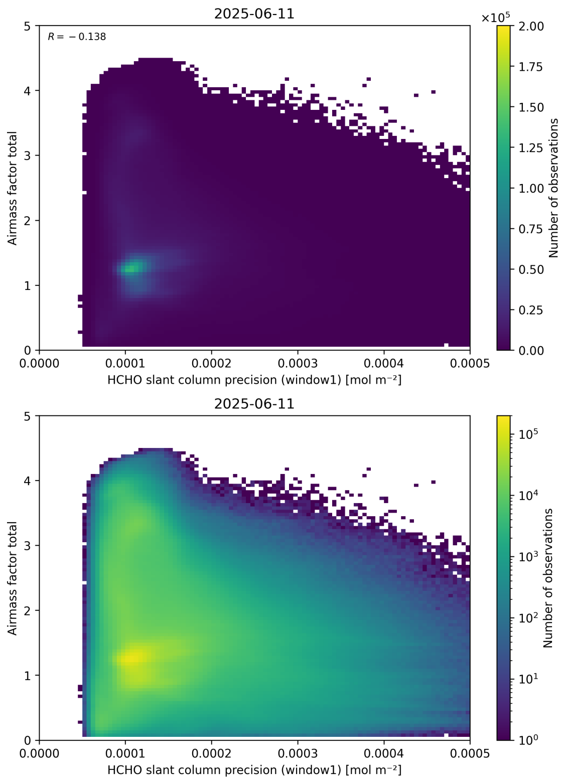
Figure 94: Scatter density plot of “HCHO slant column precision (window1)” against “Airmass factor total” for 2025-06-11 to 2025-06-12.
