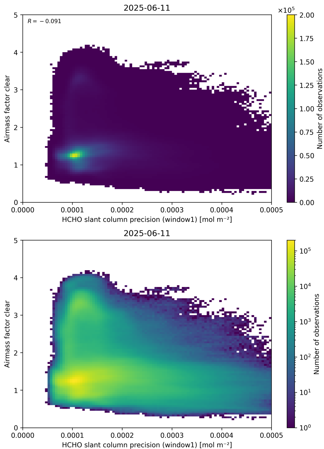
Figure 91: Scatter density plot of “HCHO slant column precision (window1)” against “Airmass factor clear” for 2025-06-11 to 2025-06-12.
