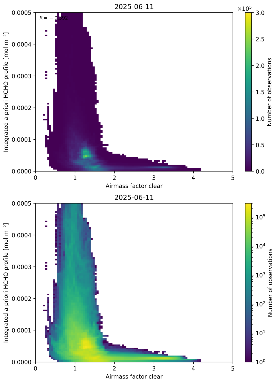
Figure 76: Scatter density plot of “Airmass factor clear” against “Integrated a priori HCHO profile” for 2025-06-11 to 2025-06-12.
