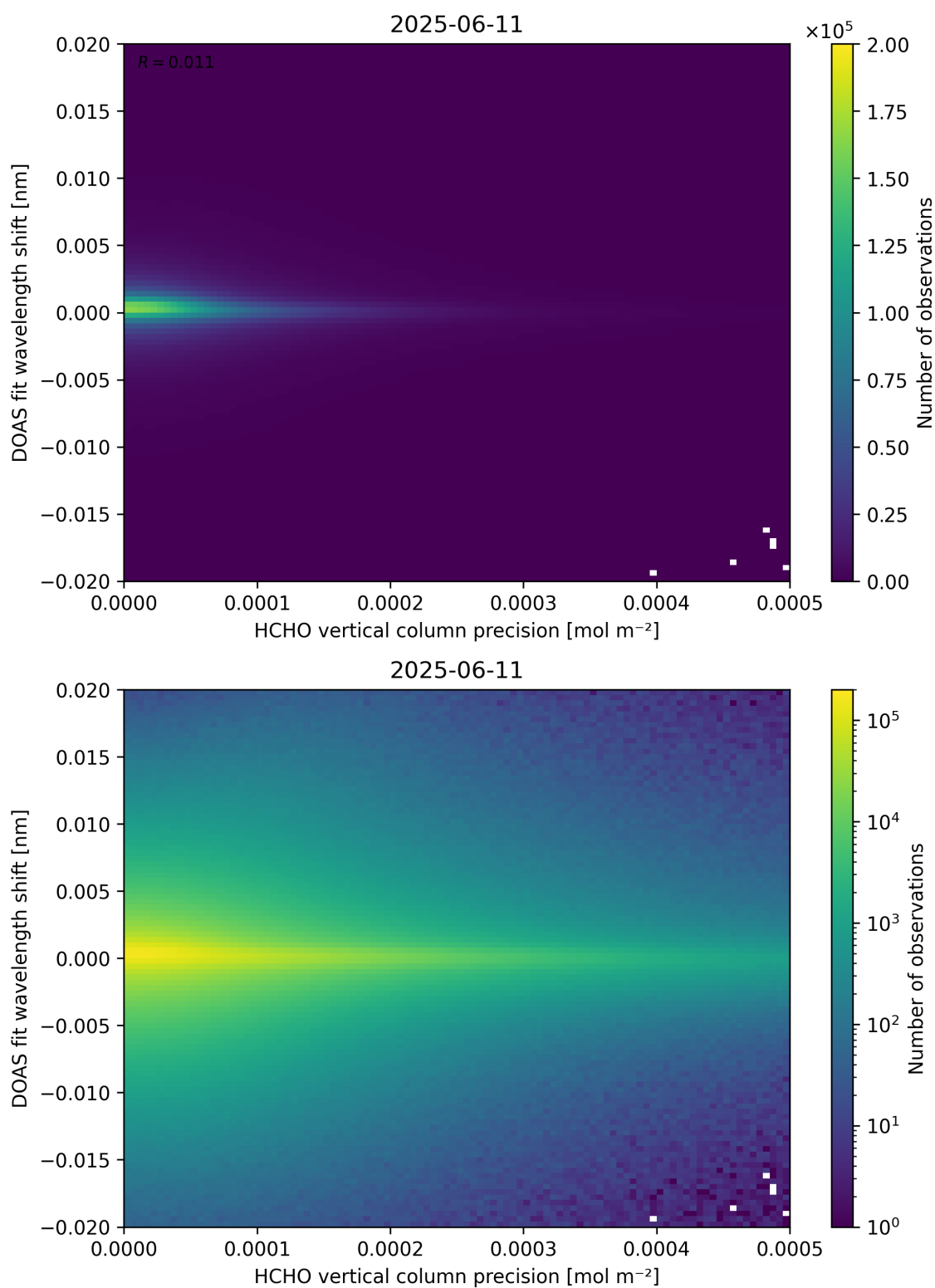
Figure 137: Scatter density plot of “HCHO vertical column precision” against “DOAS fit wavelength shift” for 2025-06-11 to 2025-06-12.
