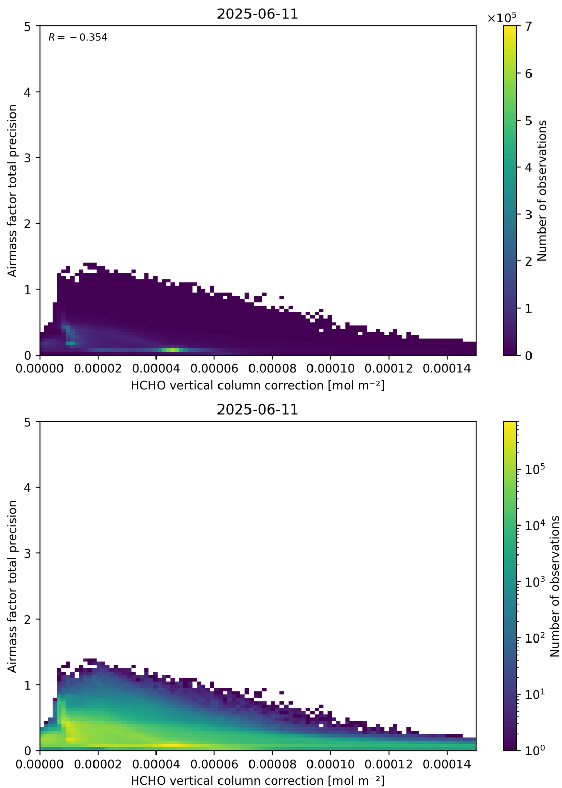
Figure 121: Scatter density plot of “HCHO vertical column correction” against “Airmass factor total precision” for 2025-06-11 to 2025-06-12.
