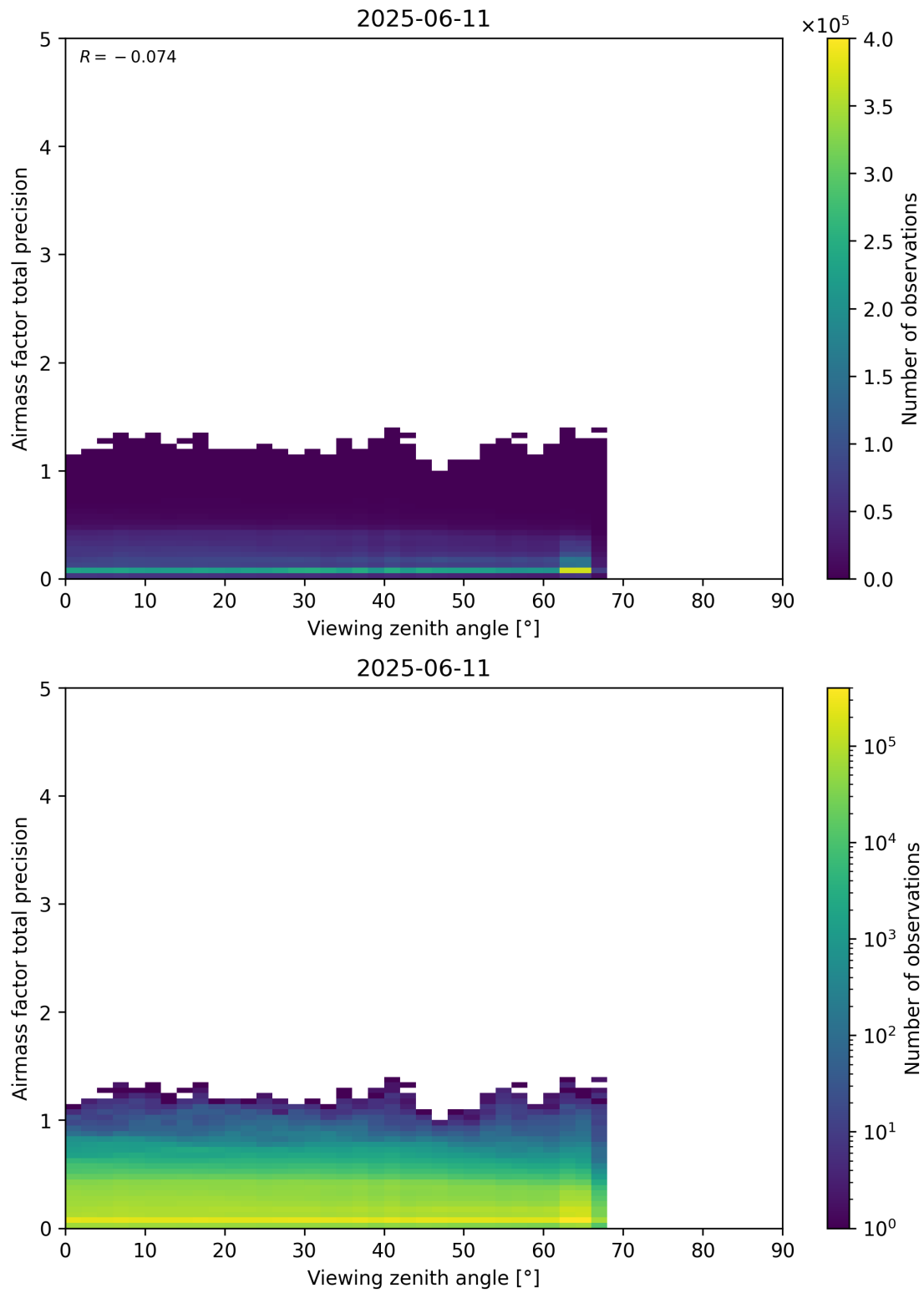
Figure 191: Scatter density plot of “Viewing zenith angle” against “Airmass factor total precision” for 2025-06-11 to 2025-06-12.
