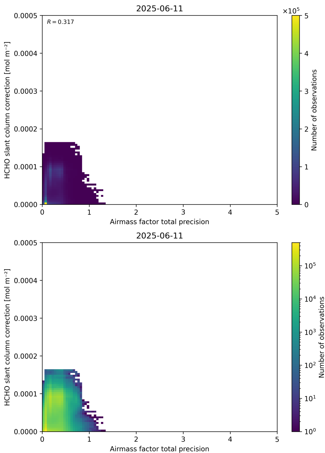
Figure 110: Scatter density plot of “Airmass factor total precision” against “HCHO slant column correction” for 2025-06-11 to 2025-06-12.
