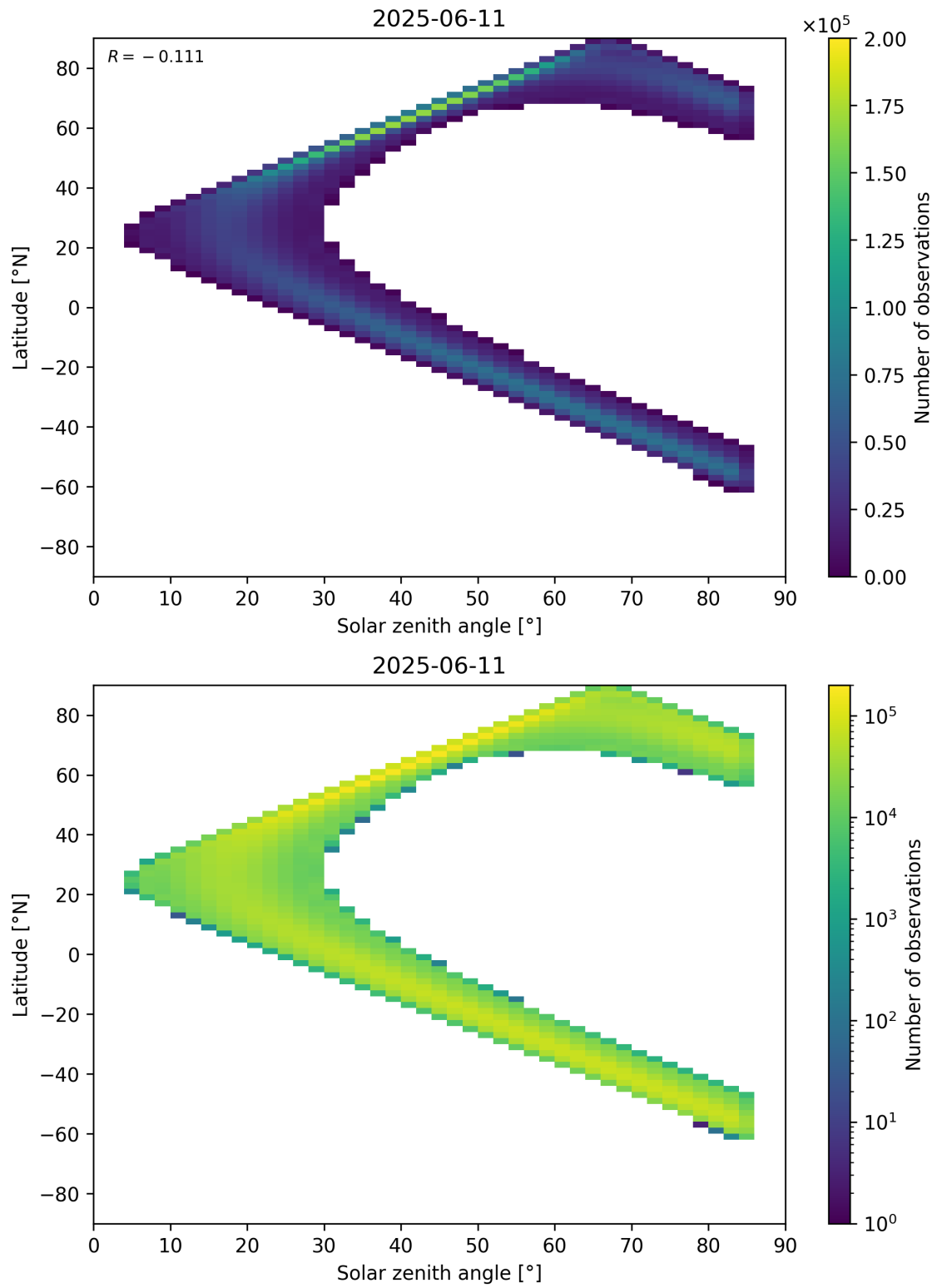
Figure 181: Scatter density plot of “Solar zenith angle” against “Latitude” for 2025-06-11 to 2025-06-12.
