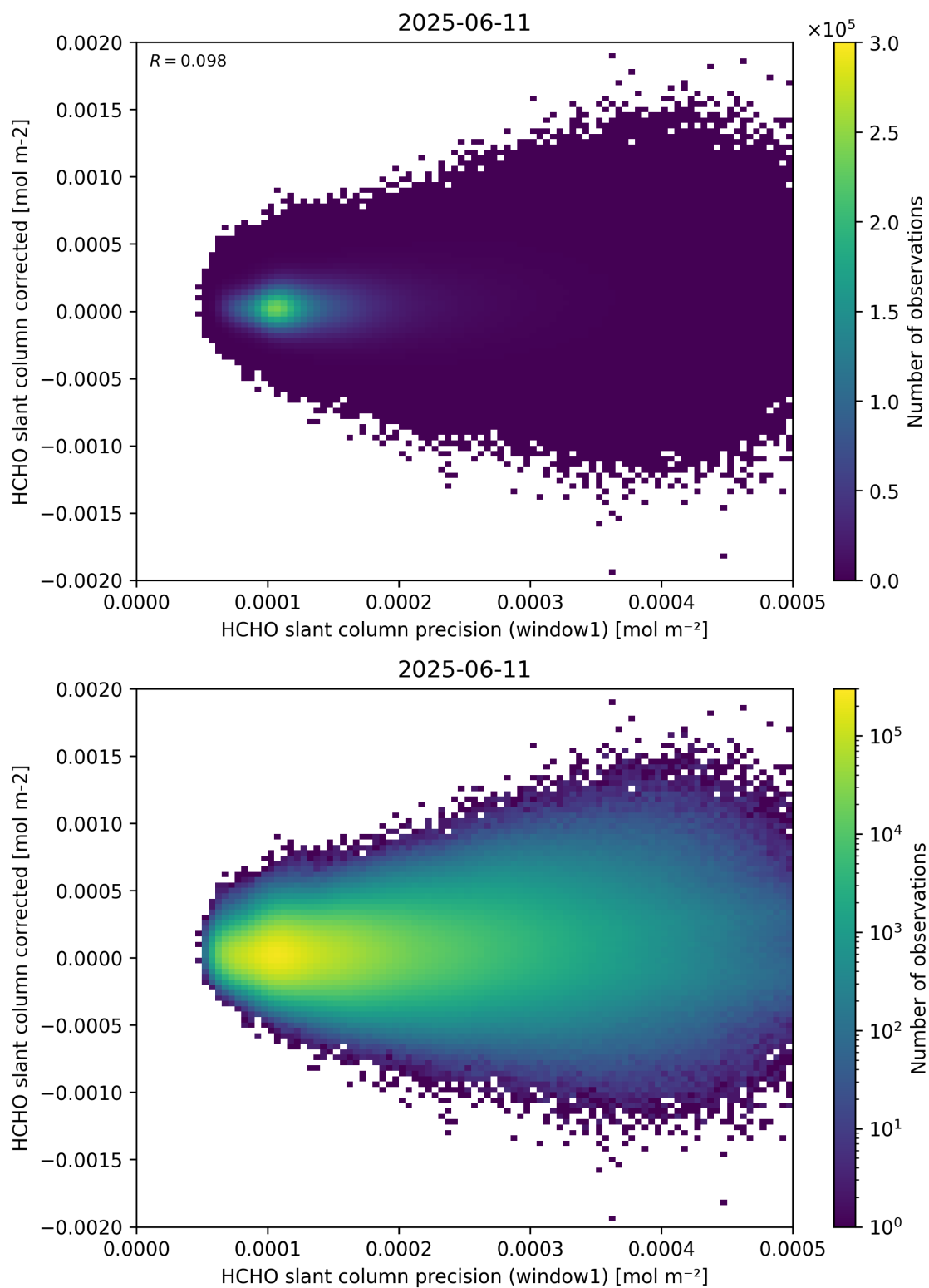
Figure 92: Scatter density plot of “HCHO slant column precision (window1)” against “HCHO slant column corrected” for 2025-06-11 to 2025-06-12.
