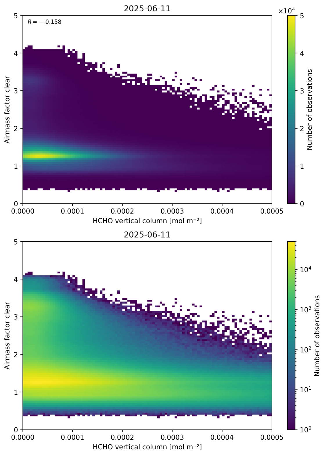
Figure 126: Scatter density plot of “HCHO vertical column” against “Airmass factor clear” for 2025-06-11 to 2025-06-12.
