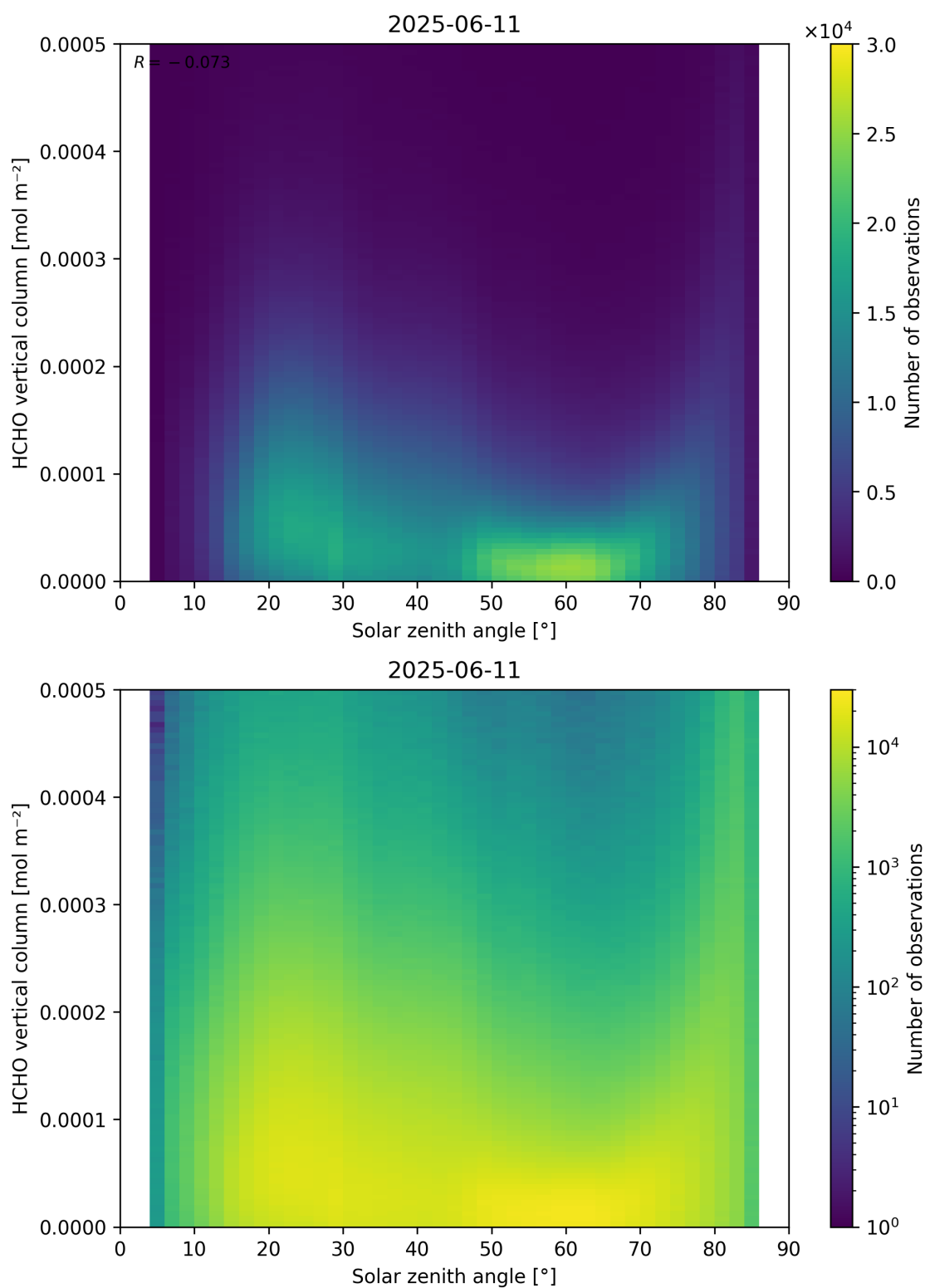
Figure 177: Scatter density plot of “Solar zenith angle” against “HCHO vertical column” for 2025-06-11 to 2025-06-12.
