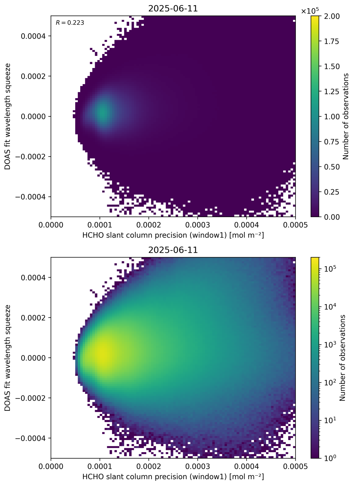
Figure 90: Scatter density plot of “HCHO slant column precision (window1)” against “DOAS fit wavelength squeeze” for 2025-06-11 to 2025-06-12.
