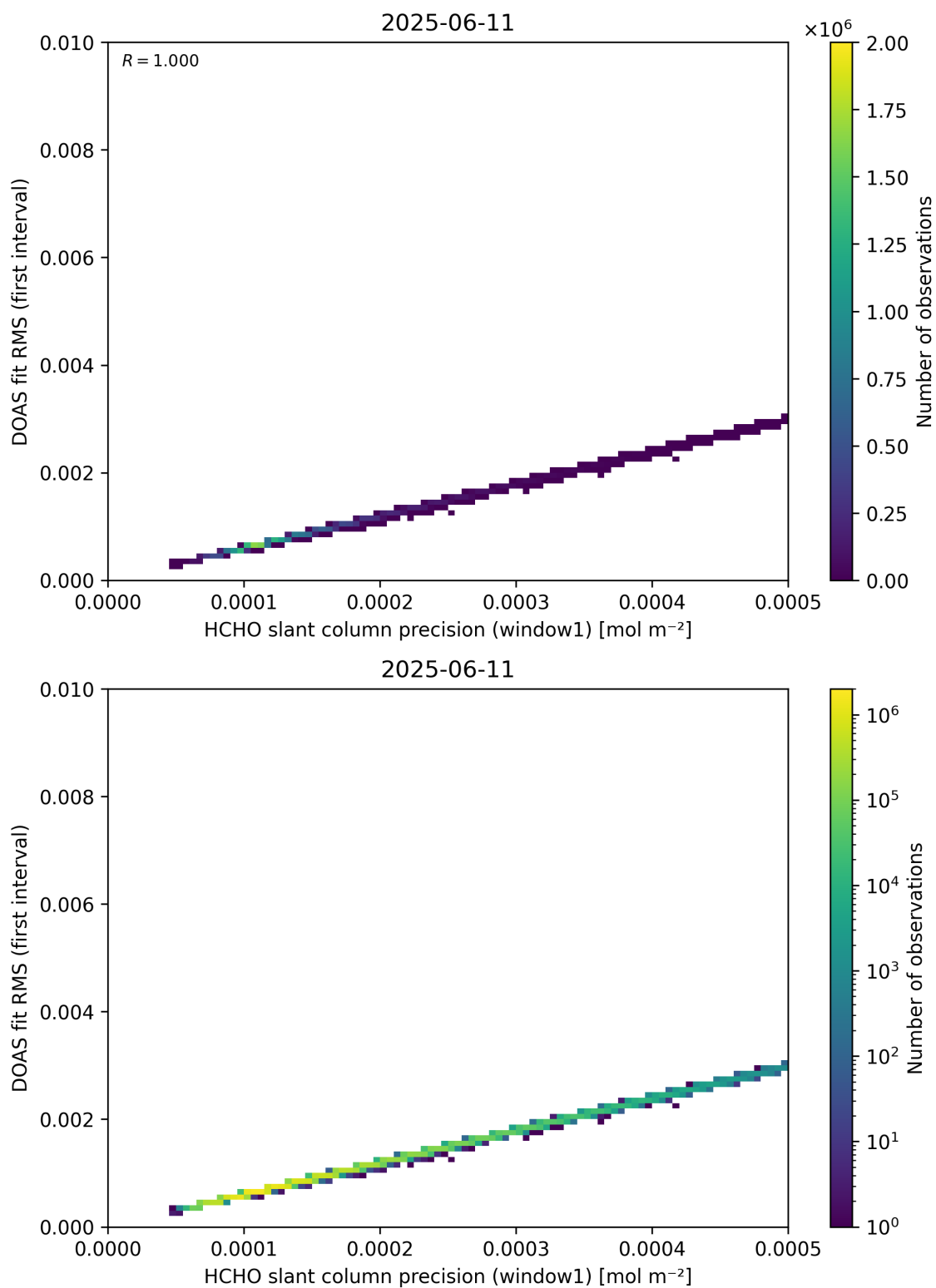
Figure 88: Scatter density plot of “HCHO slant column precision (window1)” against “DOAS fit RMS (first interval)” for 2025-06-11 to 2025-06-12.
