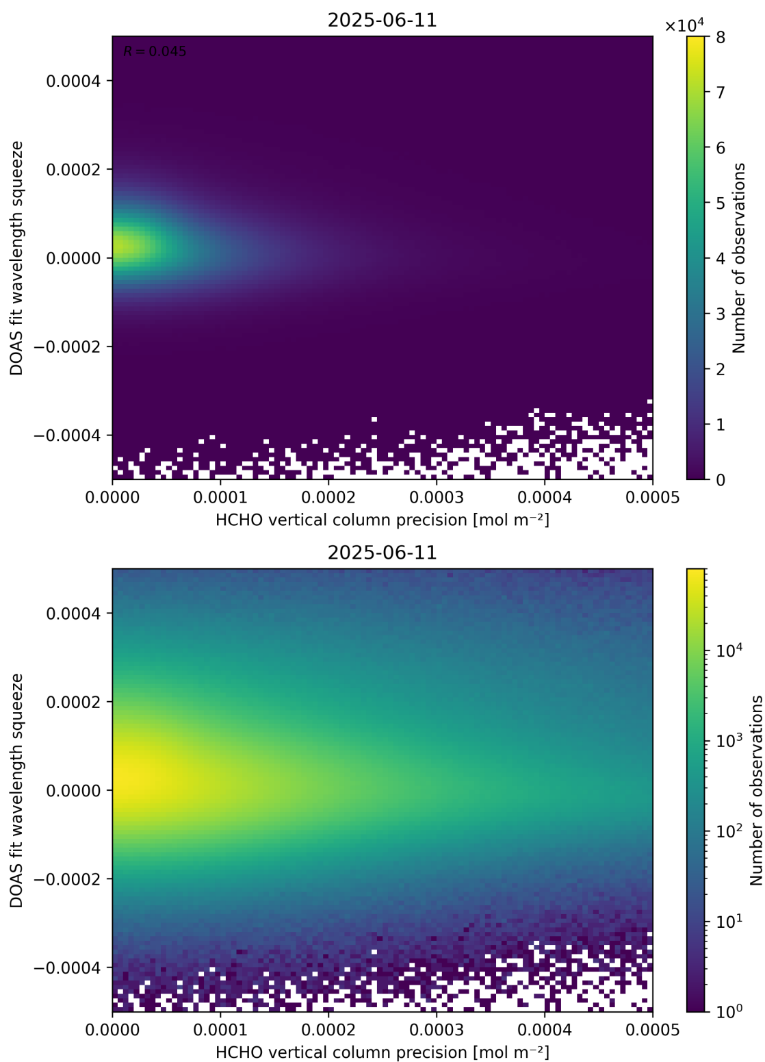
Figure 138: Scatter density plot of “HCHO vertical column precision” against “DOAS fit wavelength squeeze” for 2025-06-11 to 2025-06-12.
