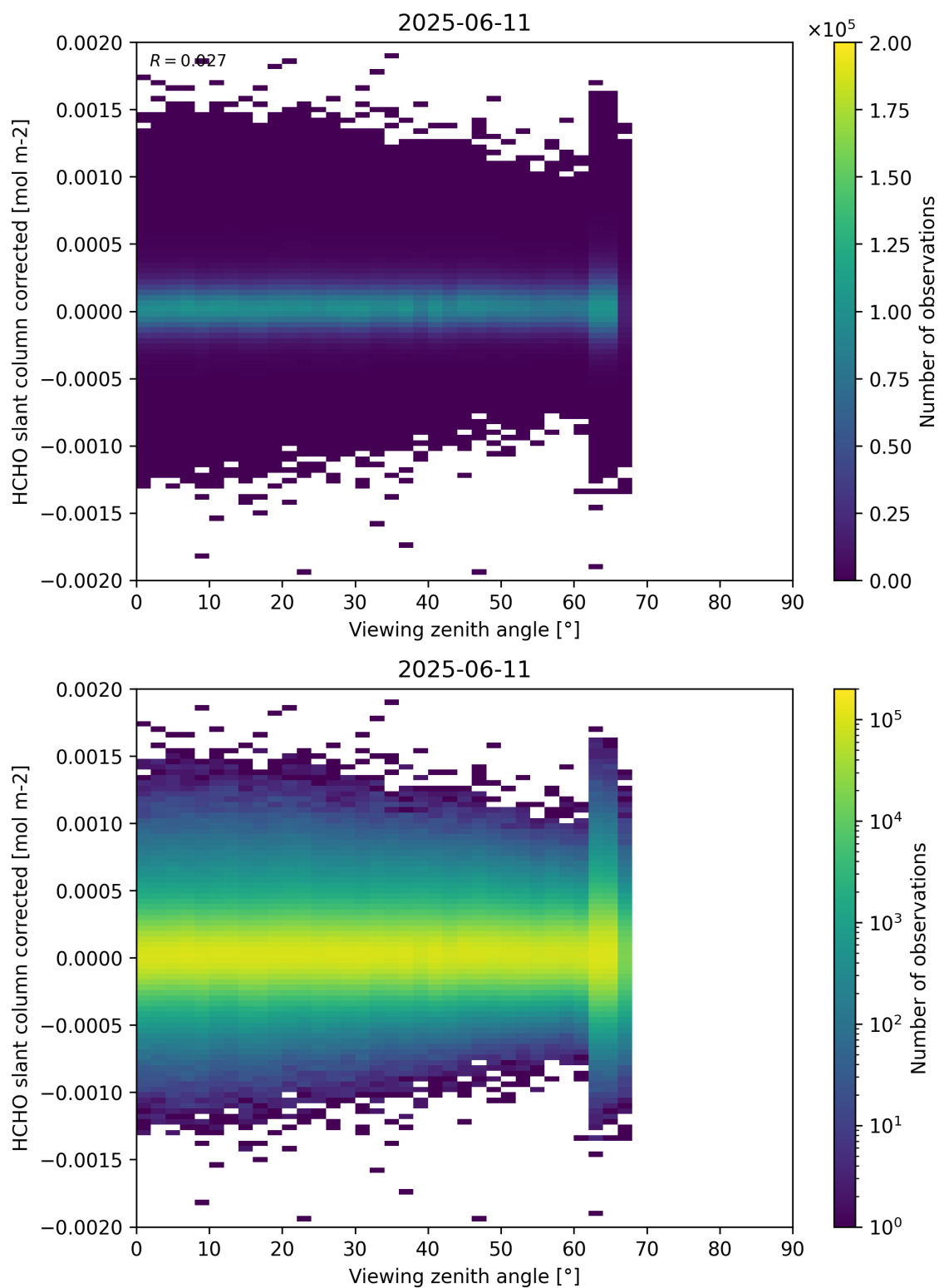
Figure 186: Scatter density plot of “Viewing zenith angle” against “HCHO slant column corrected” for 2025-06-11 to 2025-06-12.
