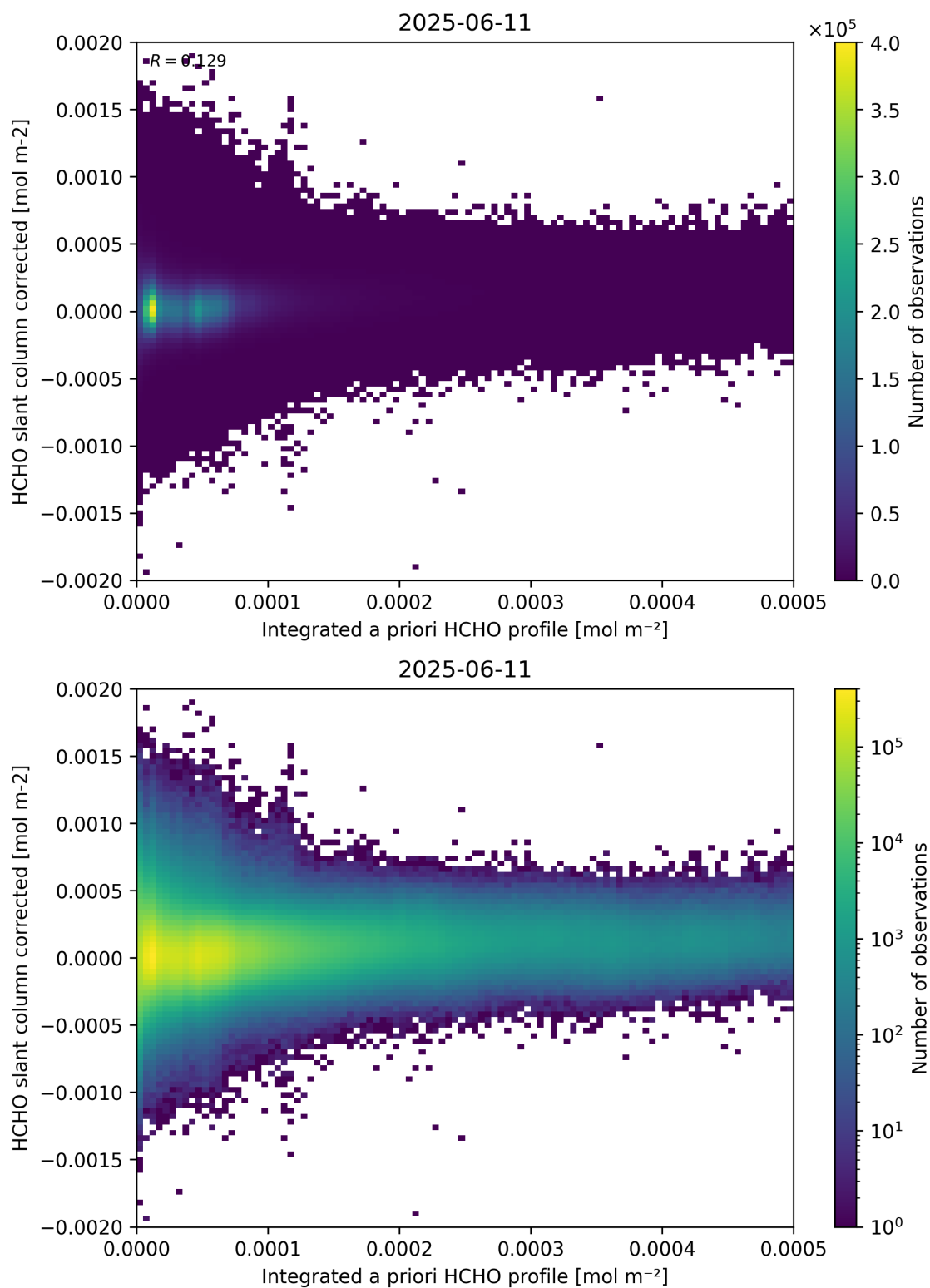
Figure 151: Scatter density plot of “Integrated a priori HCHO profile” against “HCHO slant column corrected” for 2025-06-11 to 2025-06-12.
