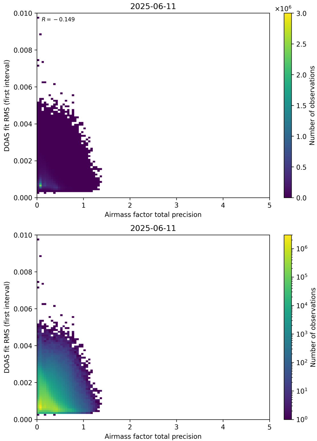
Figure 105: Scatter density plot of “Airmass factor total precision” against “DOAS fit RMS (first interval)” for 2025-06-11 to 2025-06-12.
