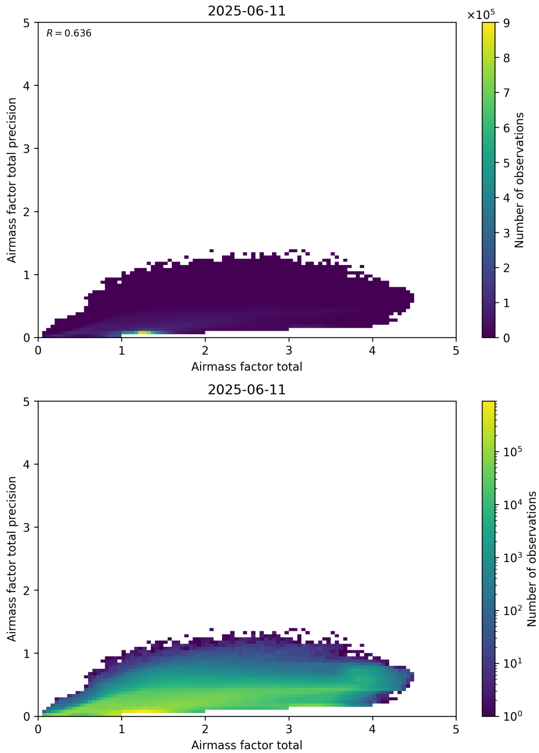
Figure 103: Scatter density plot of “Airmass factor total” against “Airmass factor total precision” for 2025-06-11 to 2025-06-12.
