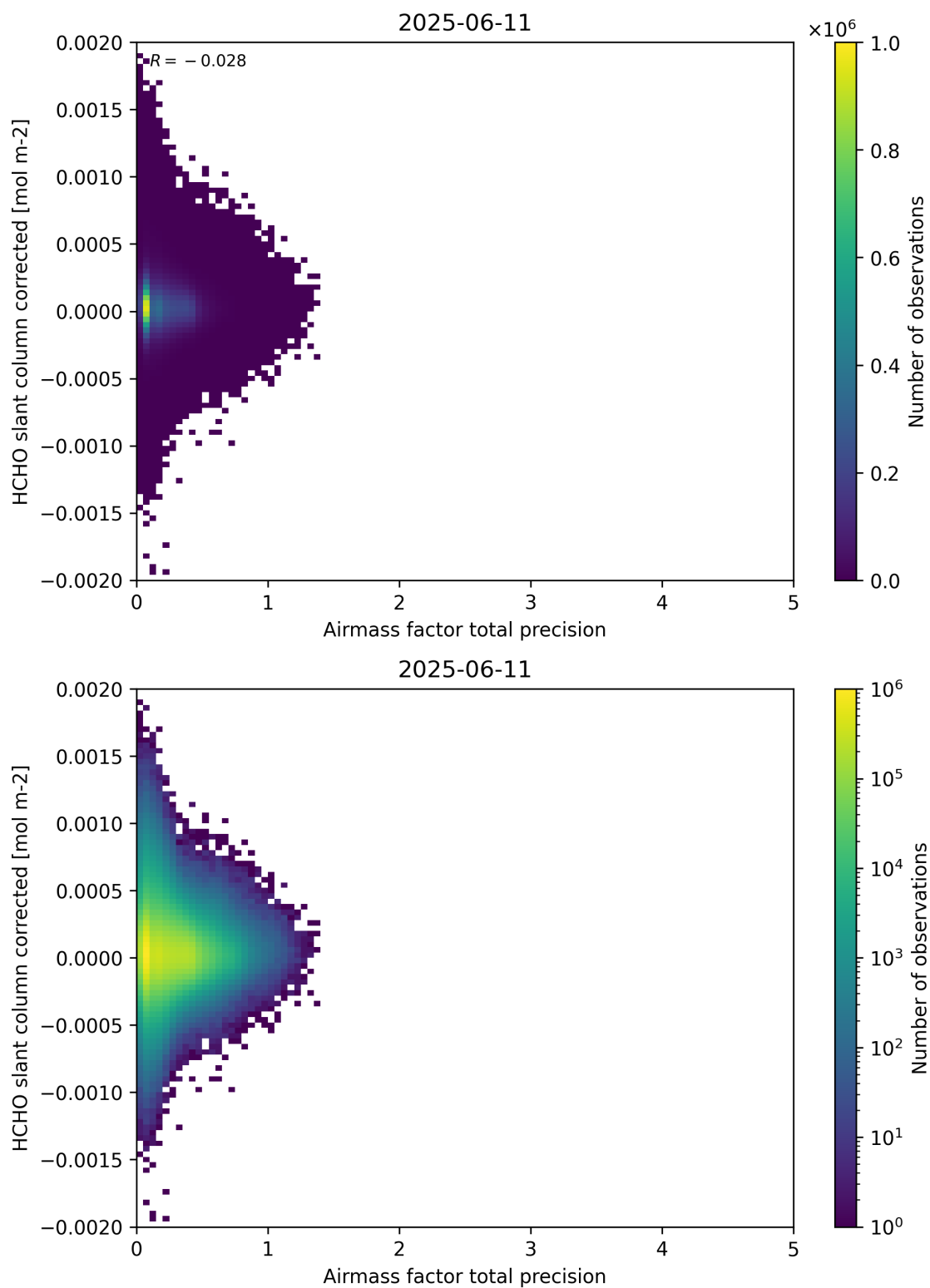
Figure 109: Scatter density plot of “Airmass factor total precision” against “HCHO slant column corrected” for 2025-06-11 to 2025-06-12.
