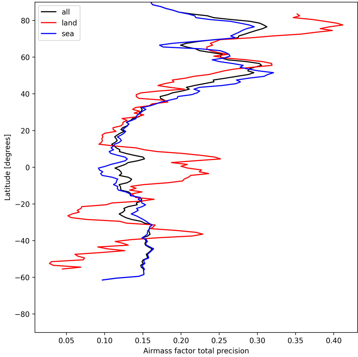
Figure 27: Zonal average of “Airmass factor total precision” for 2025-06-11 to 2025-06-12.
