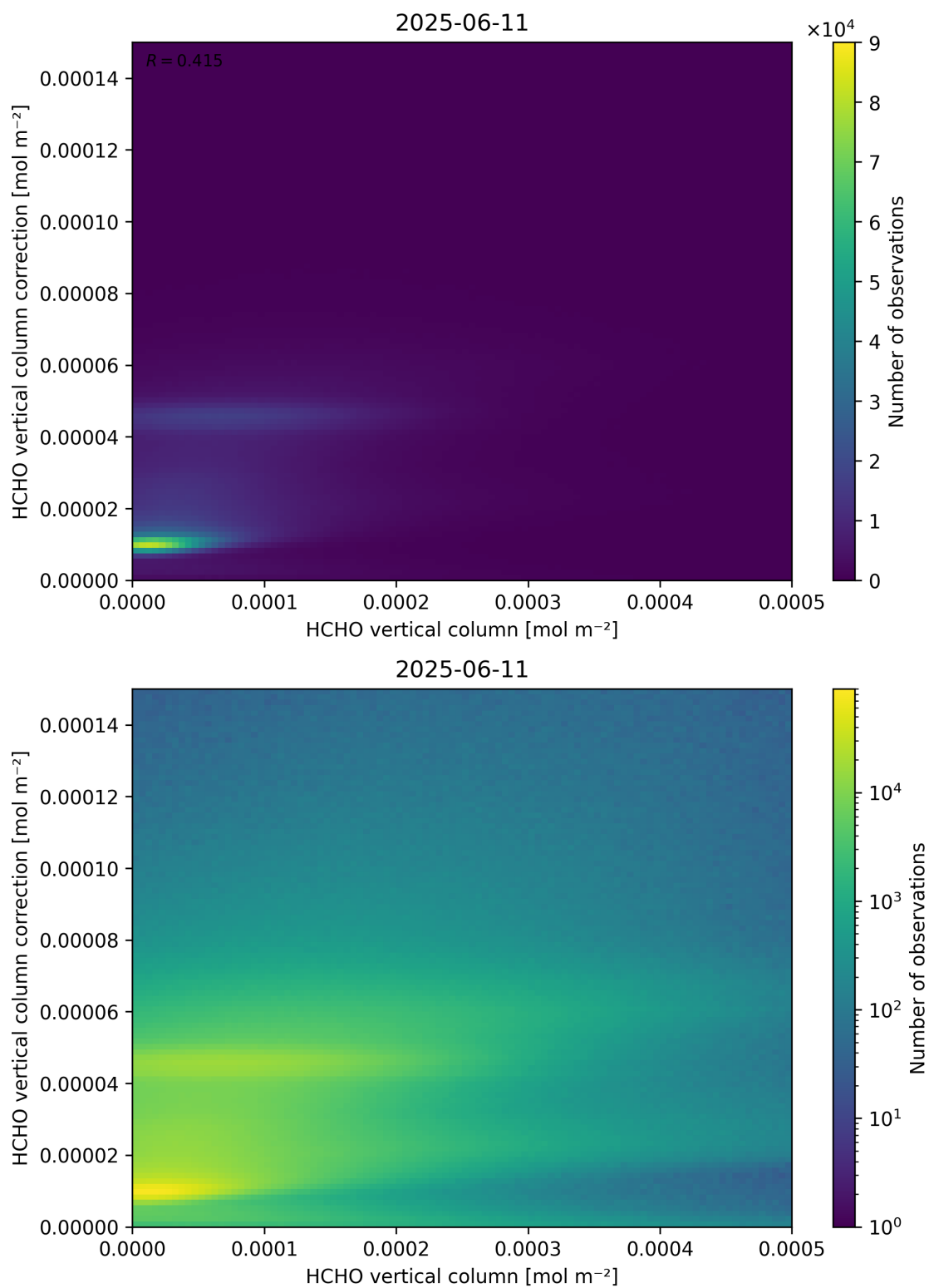
Figure 133: Scatter density plot of “HCHO vertical column” against “HCHO vertical column correction” for 2025-06-11 to 2025-06-12.
