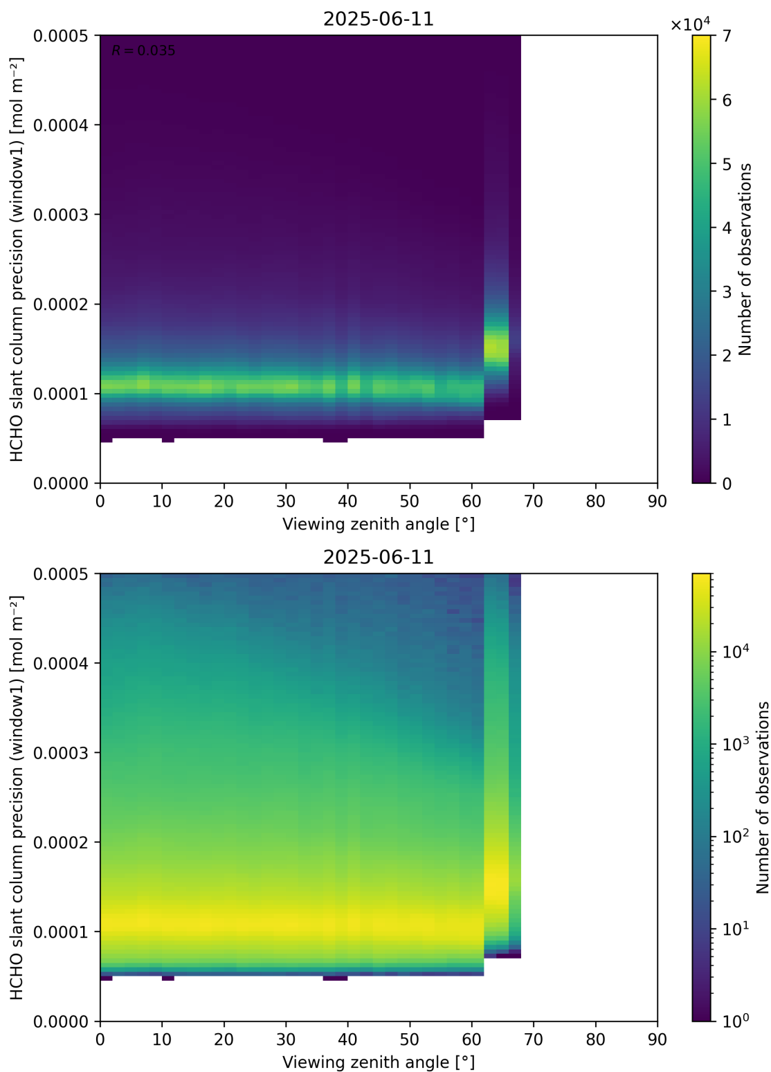
Figure 189: Scatter density plot of “Viewing zenith angle” against “HCHO slant column precision (window1)” for 2025-06-11 to 2025-06-12.
