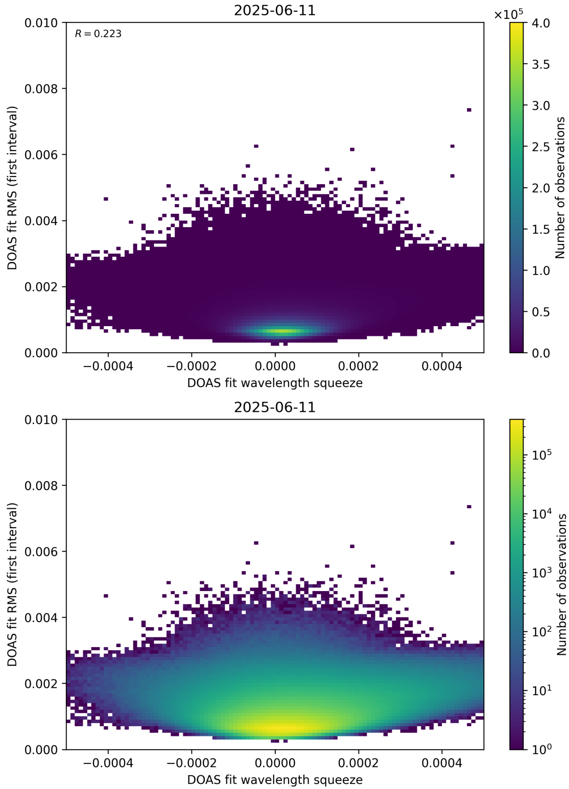
Figure 68: Scatter density plot of “DOAS fit wavelength squeeze” against “DOAS fit RMS (first interval)” for 2025-06-11 to 2025-06-12.
