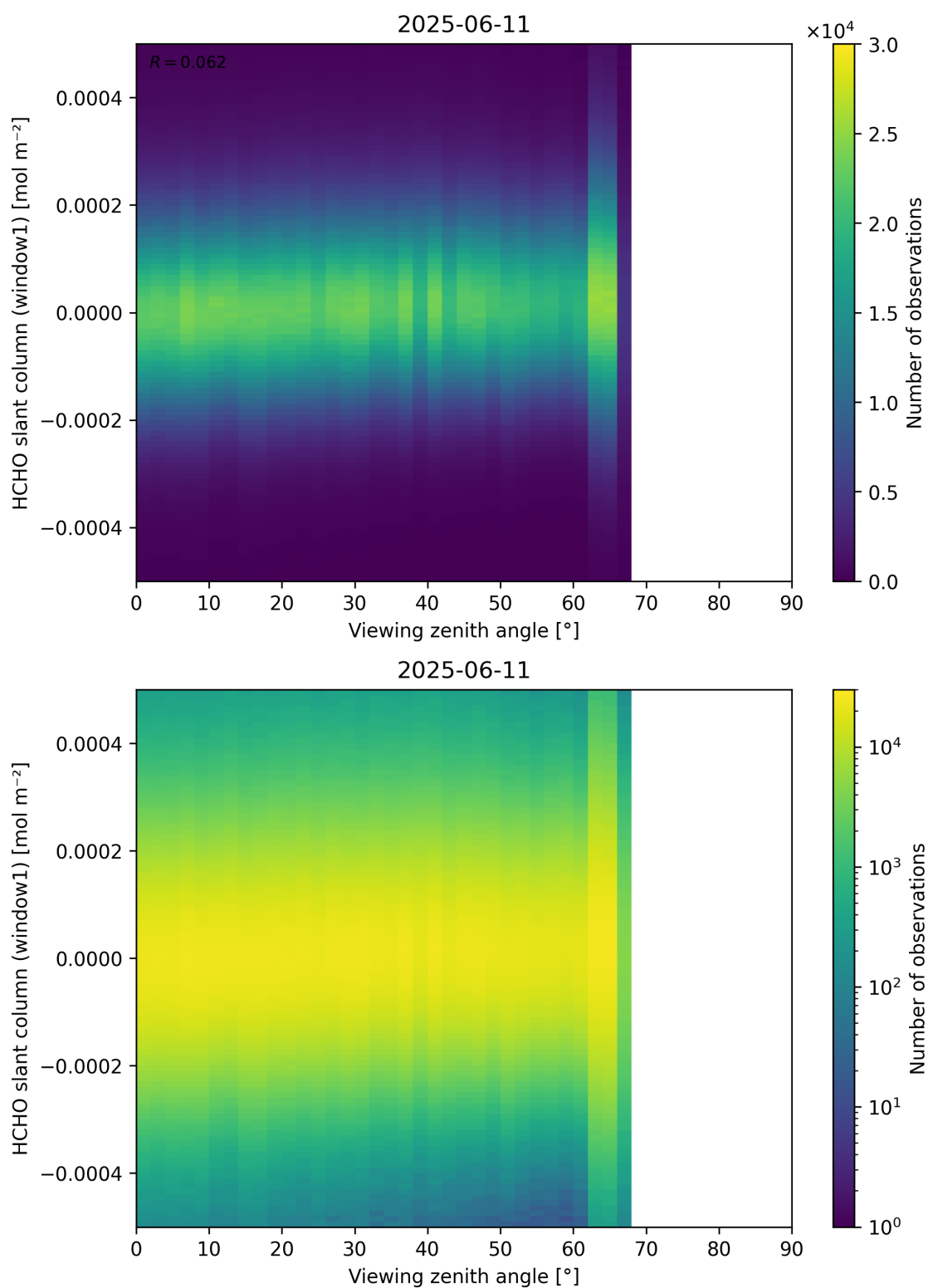
Figure 188: Scatter density plot of “Viewing zenith angle” against “HCHO slant column (window1)” for 2025-06-11 to 2025-06-12.
