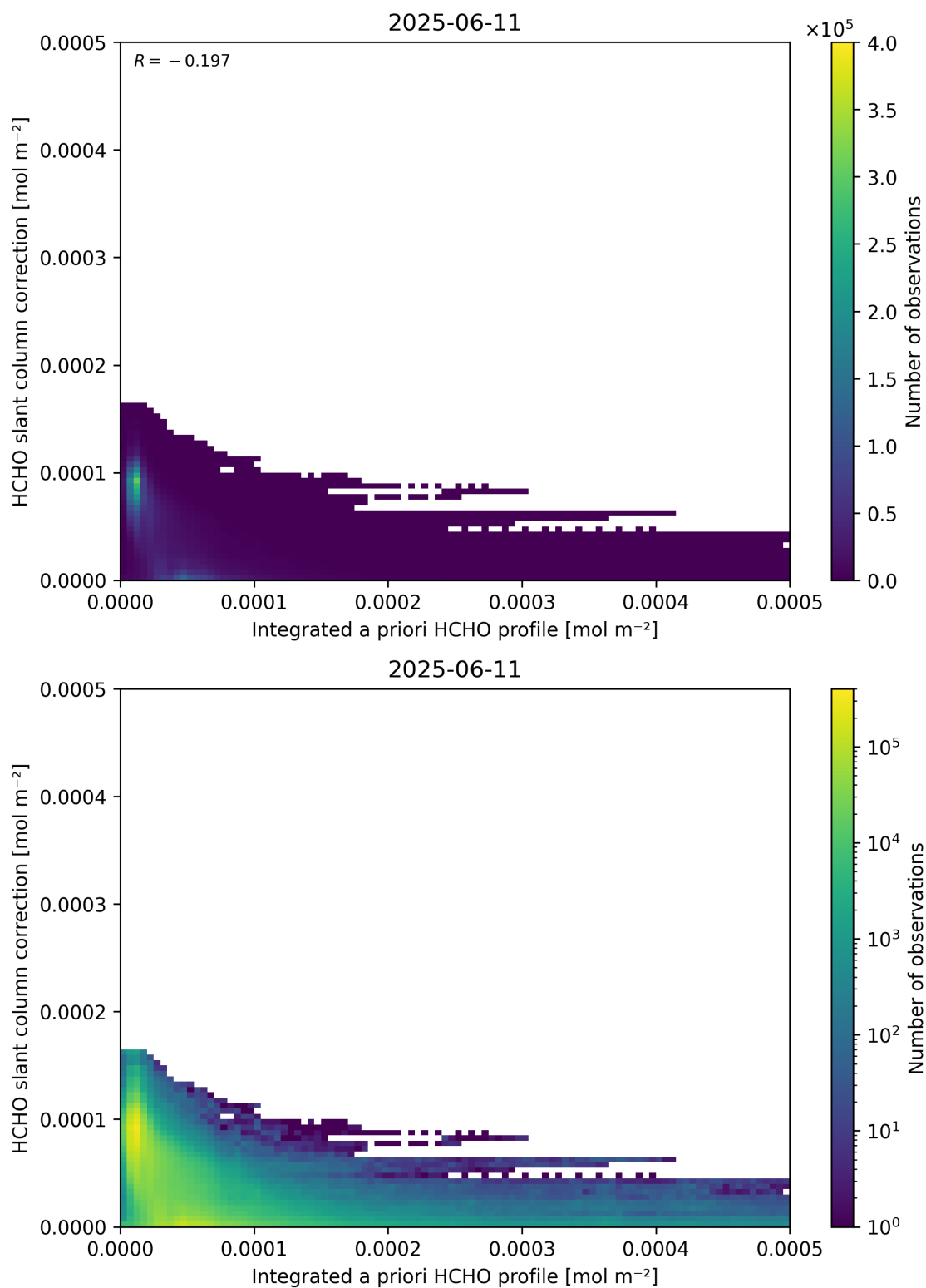
Figure 152: Scatter density plot of “Integrated a priori HCHO profile” against “HCHO slant column correction” for 2025-06-11 to 2025-06-12.
