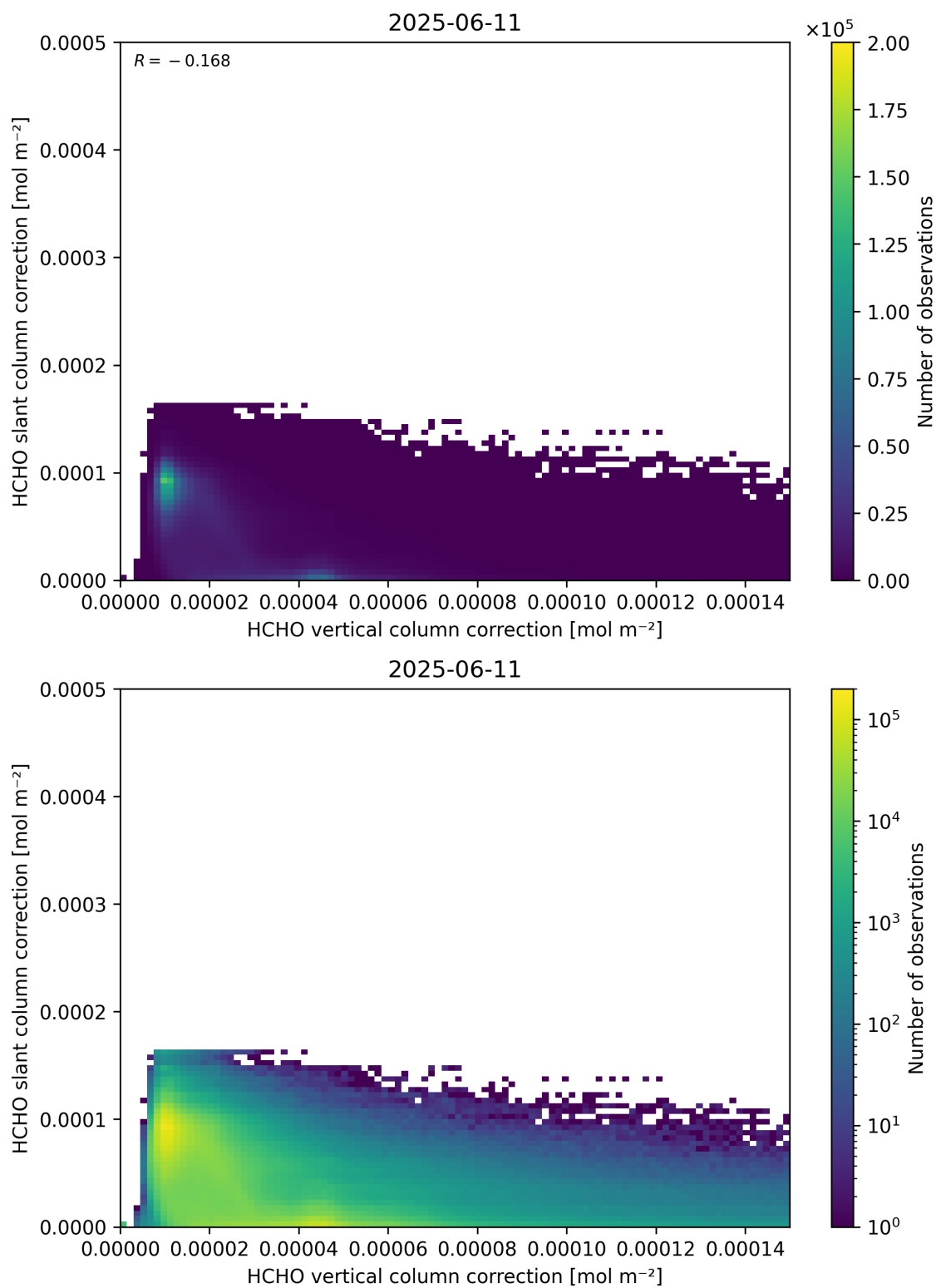
Figure 117: Scatter density plot of “HCHO vertical column correction” against “HCHO slant column correction” for 2025-06-11 to 2025-06-12.
