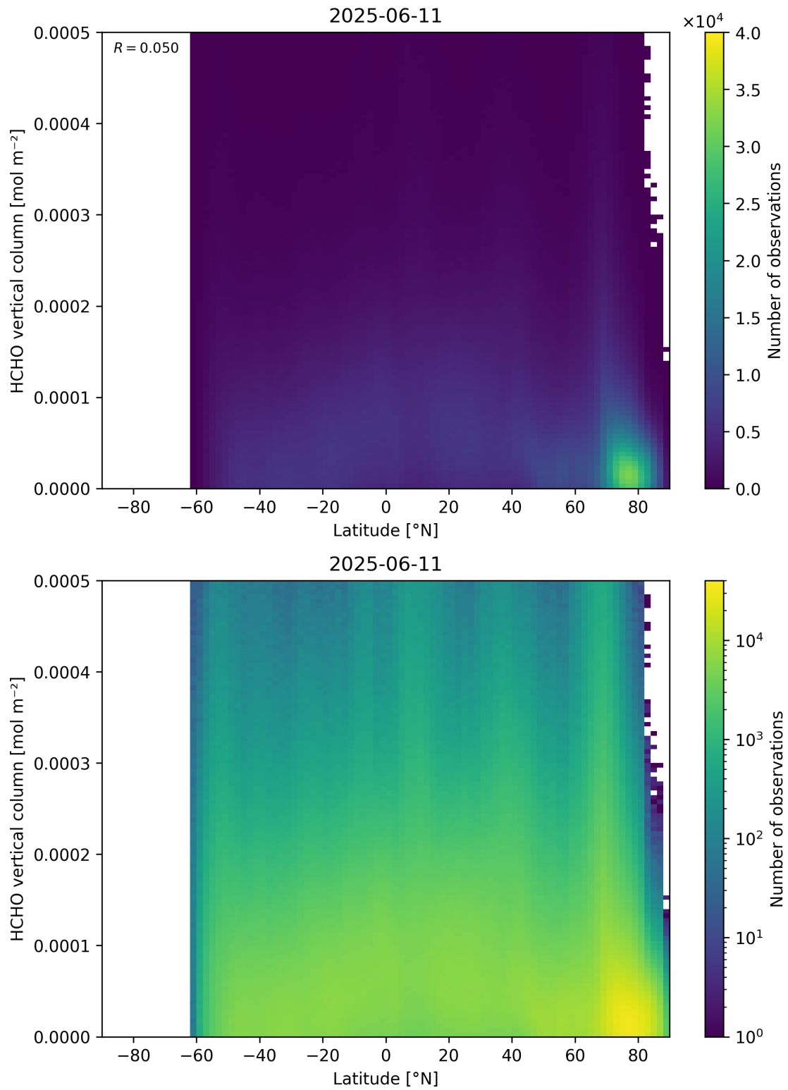
Figure 163: Scatter density plot of “Latitude” against “HCHO vertical column” for 2025-06-11 to 2025-06-12.
