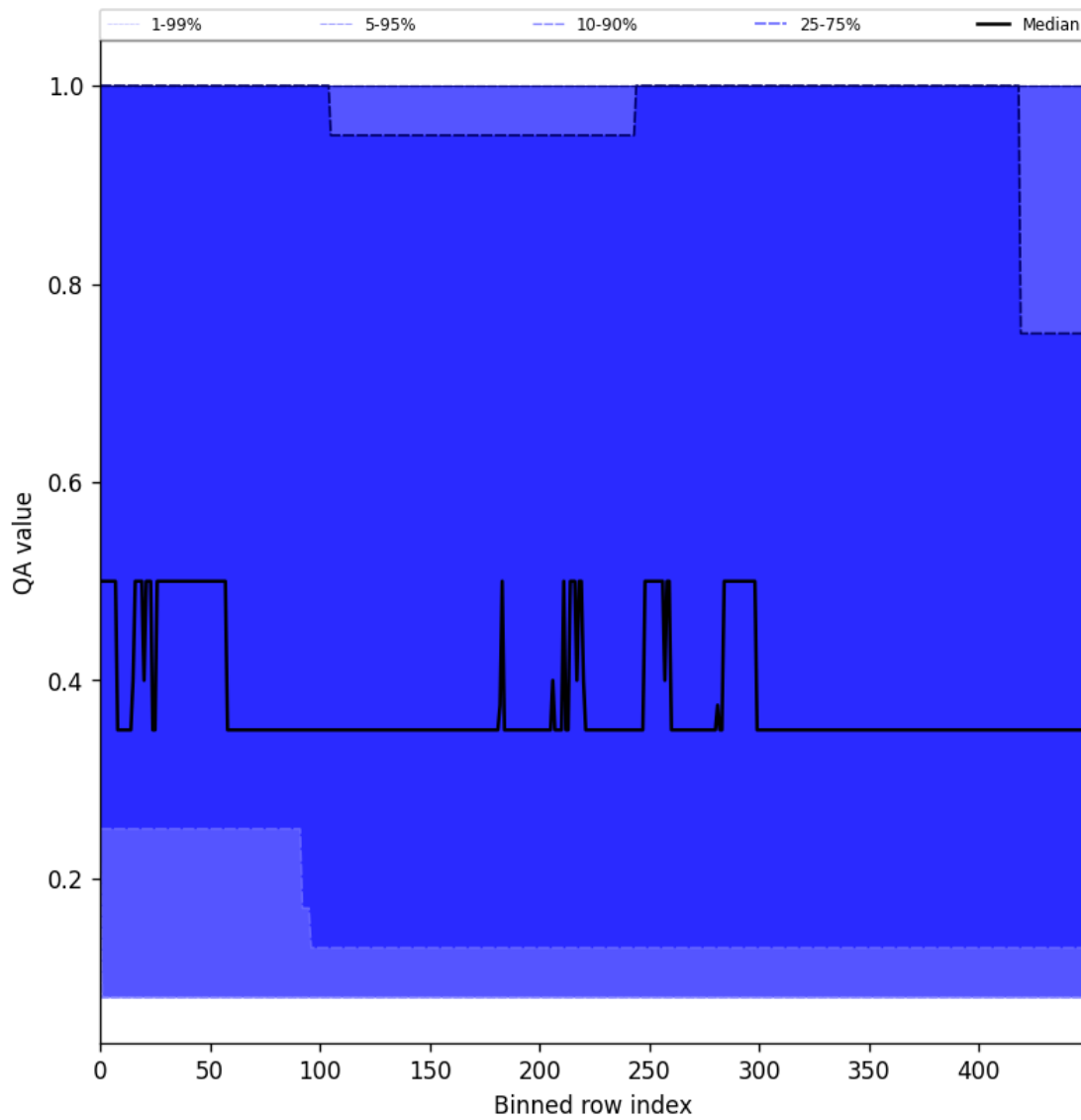
Figure 48: Along track statistics of “QA value” for 2025-06-11 to 2025-06-12
