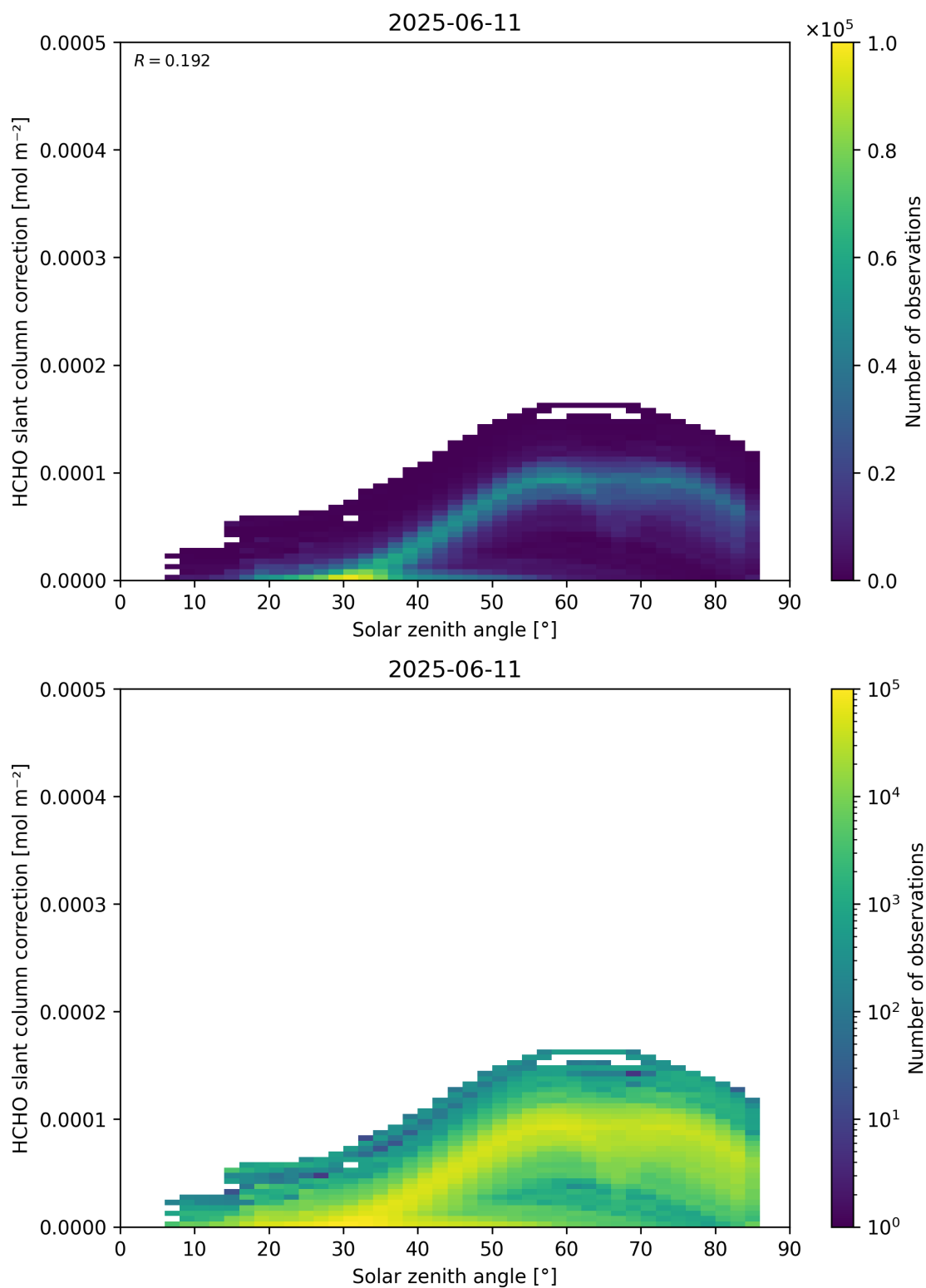
Figure 172: Scatter density plot of “Solar zenith angle” against “HCHO slant column correction” for 2025-06-11 to 2025-06-12.
