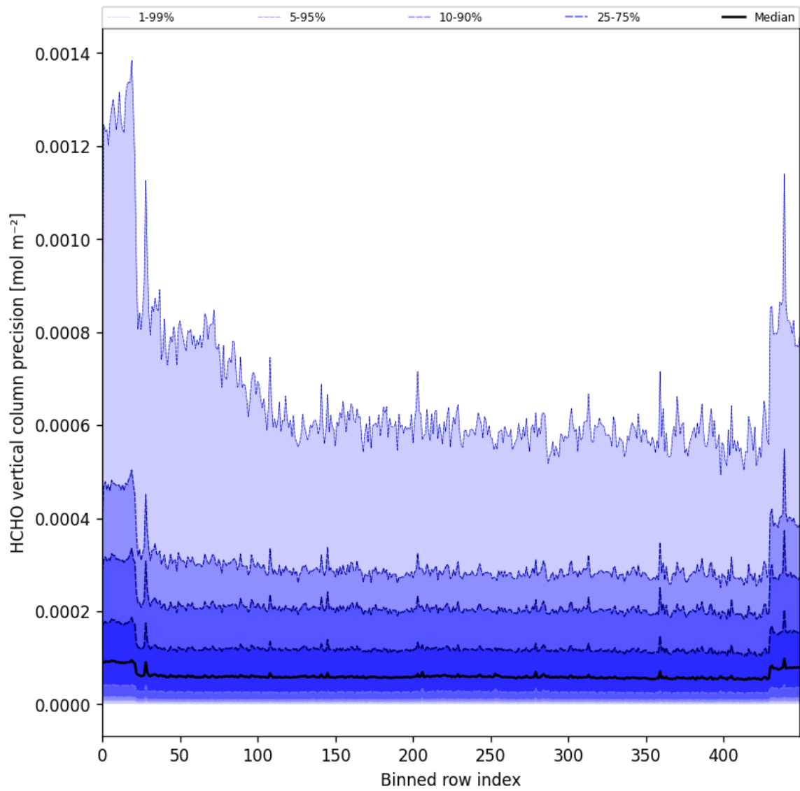
Figure 50: Along track statistics of “HCHO vertical column precision” for 2025-06-11 to 2025-06-12
