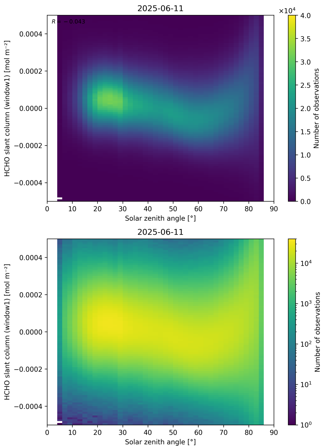
Figure 173: Scatter density plot of “Solar zenith angle” against “HCHO slant column (window1)” for 2025-06-11 to 2025-06-12.
