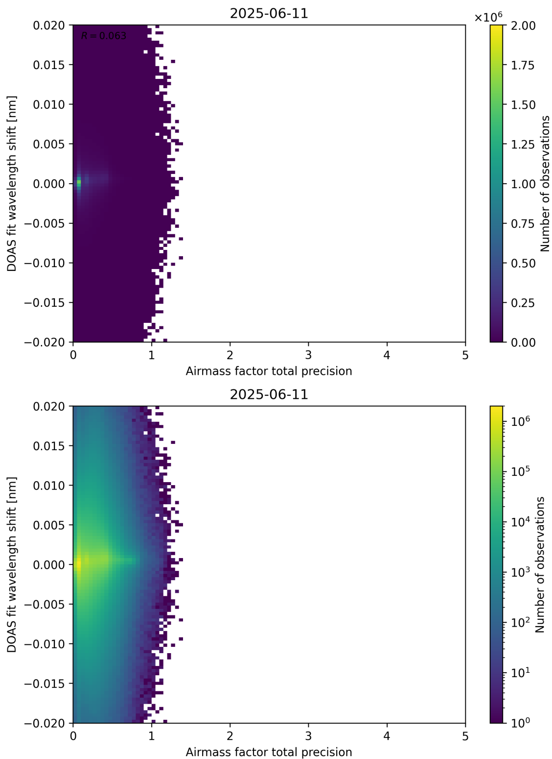
Figure 106: Scatter density plot of “Airmass factor total precision” against “DOAS fit wavelength shift” for 2025-06-11 to 2025-06-12.
