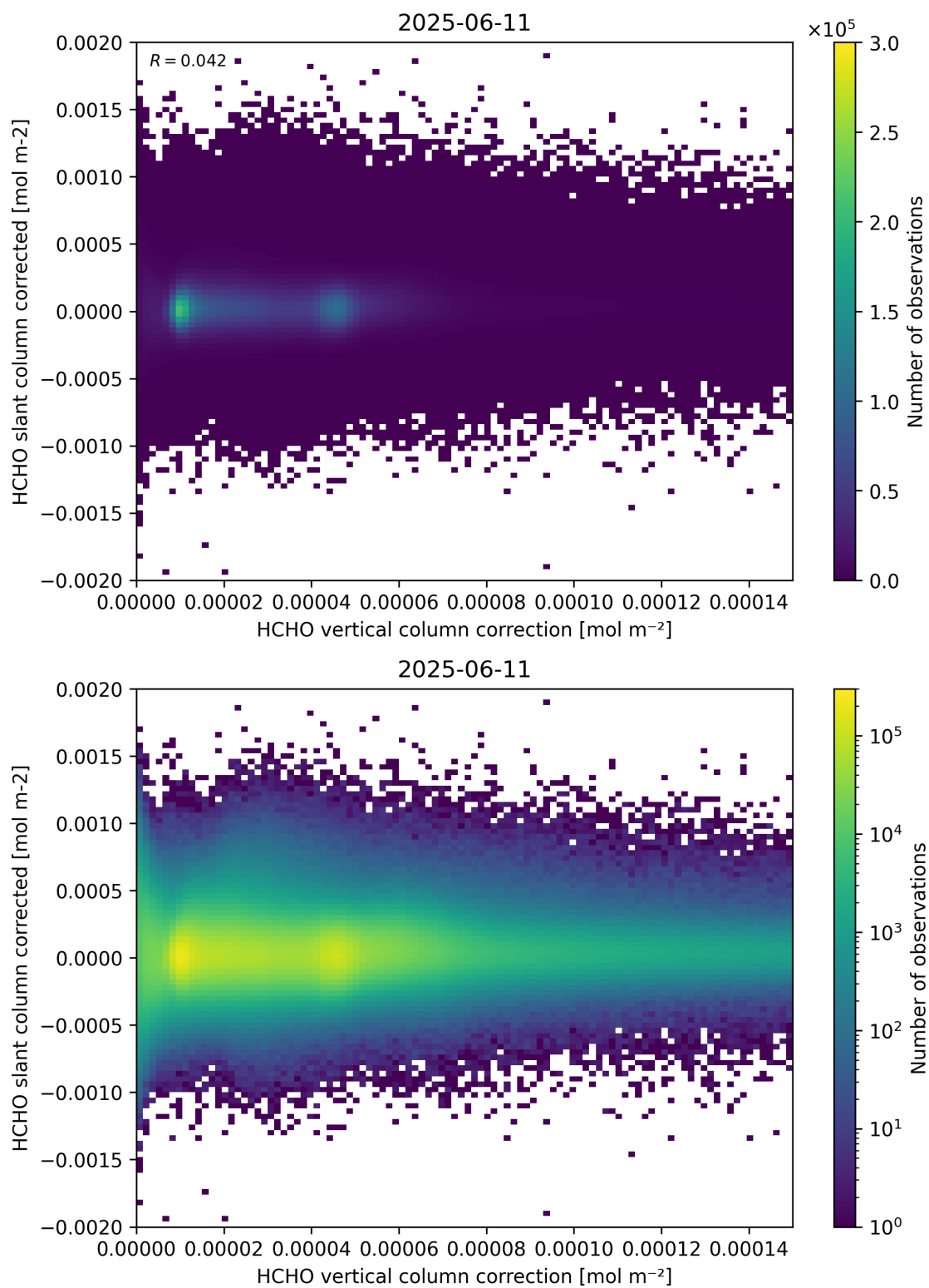
Figure 116: Scatter density plot of “HCHO vertical column correction” against “HCHO slant column corrected” for 2025-06-11 to 2025-06-12.
