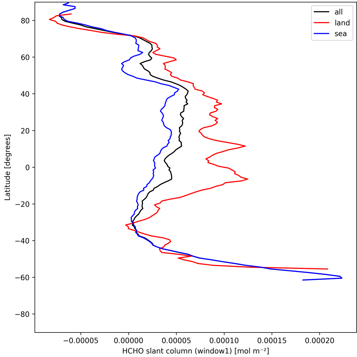
Figure 24: Zonal average of “HCHO slant column (window1)” for 2025-06-11 to 2025-06-12.
