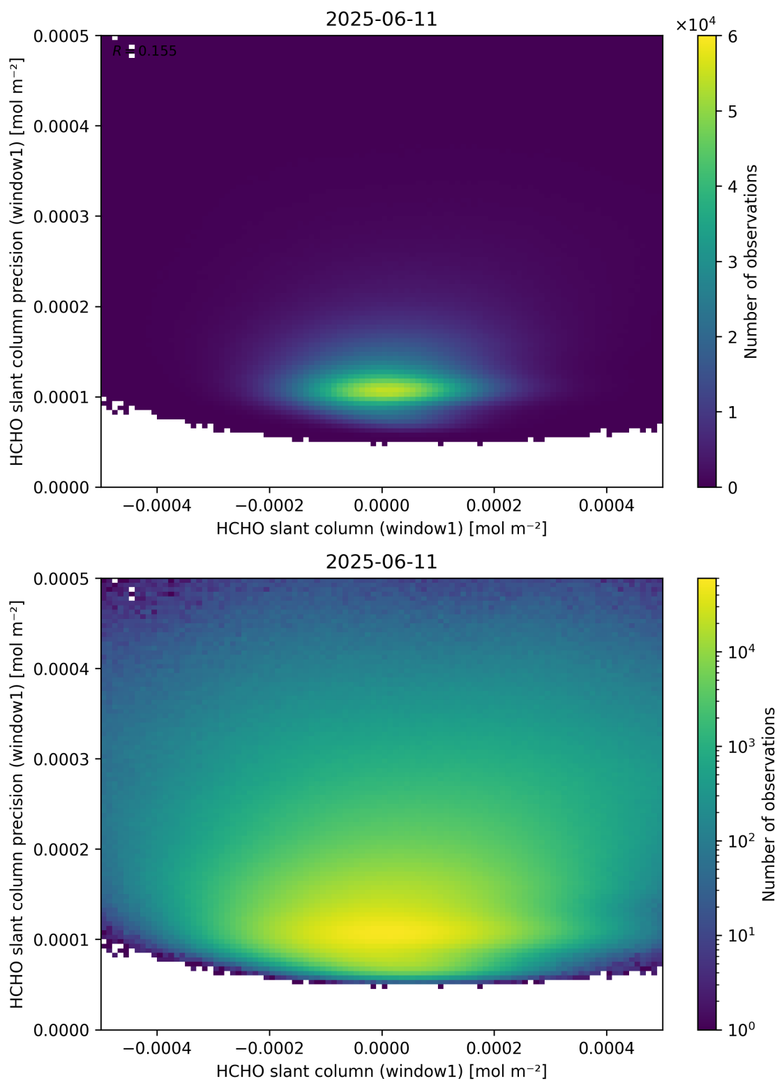
Figure 84: Scatter density plot of “HCHO slant column (window1)” against “HCHO slant column precision (window1)” for 2025-06-11 to 2025-06-12.
