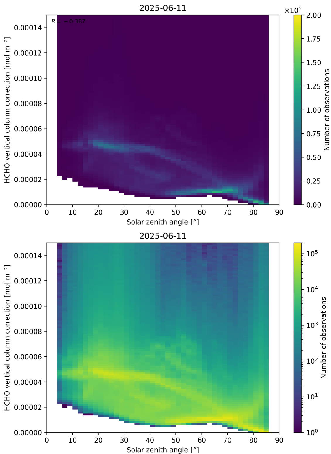
Figure 178: Scatter density plot of “Solar zenith angle” against “HCHO vertical column correction” for 2025-06-11 to 2025-06-12.
