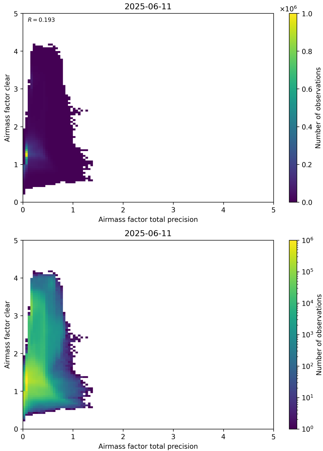
Figure 108: Scatter density plot of “Airmass factor total precision” against “Airmass factor clear” for 2025-06-11 to 2025-06-12.
