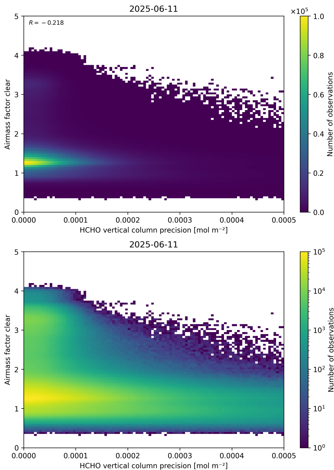
Figure 139: Scatter density plot of “HCHO vertical column precision” against “Airmass factor clear” for 2025-06-11 to 2025-06-12.
