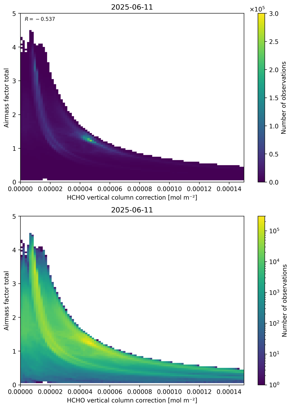
Figure 120: Scatter density plot of “HCHO vertical column correction” against “Airmass factor total” for 2025-06-11 to 2025-06-12.
