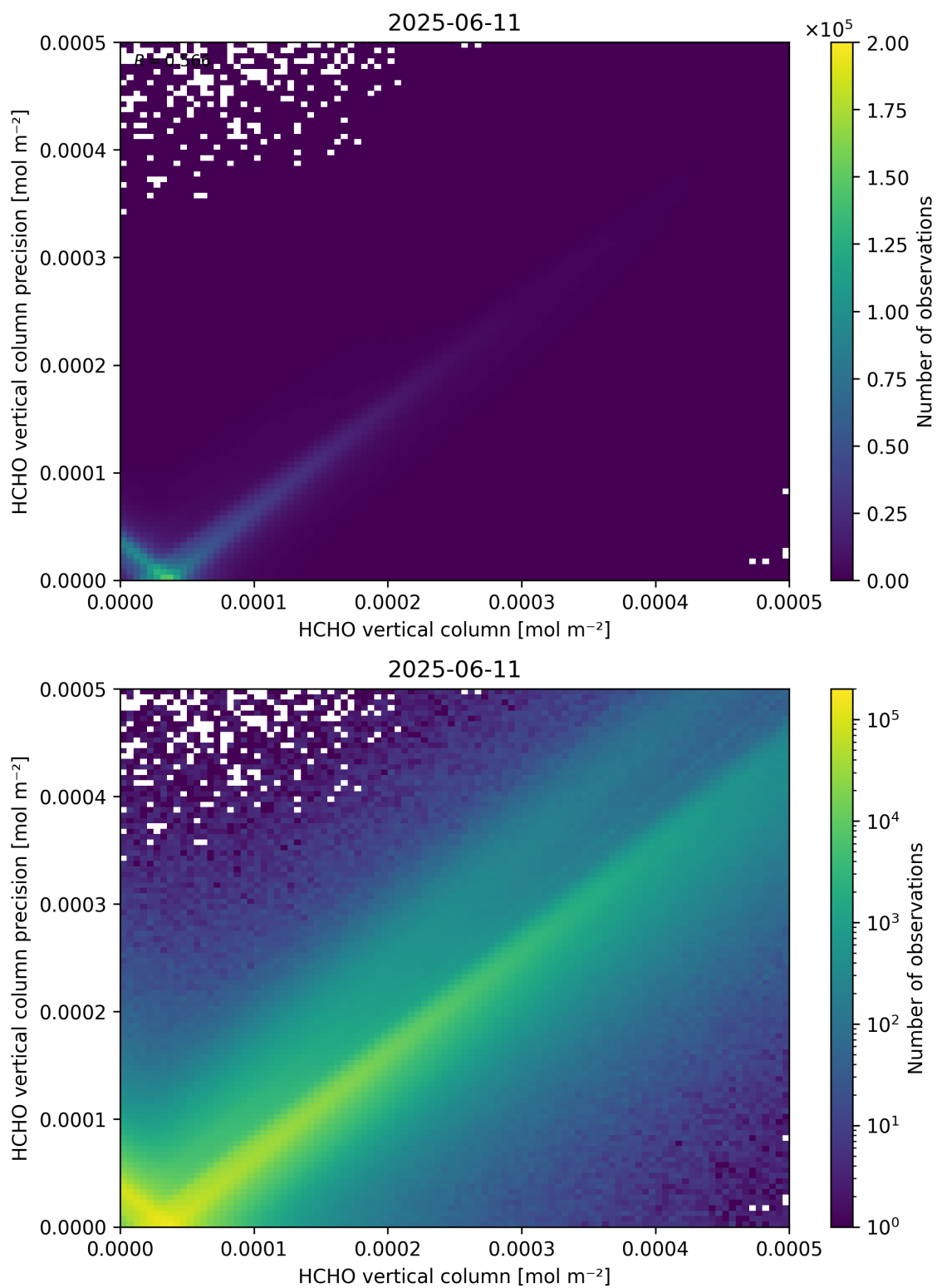
Figure 134: Scatter density plot of “HCHO vertical column” against “HCHO vertical column precision” for 2025-06-11 to 2025-06-12.
