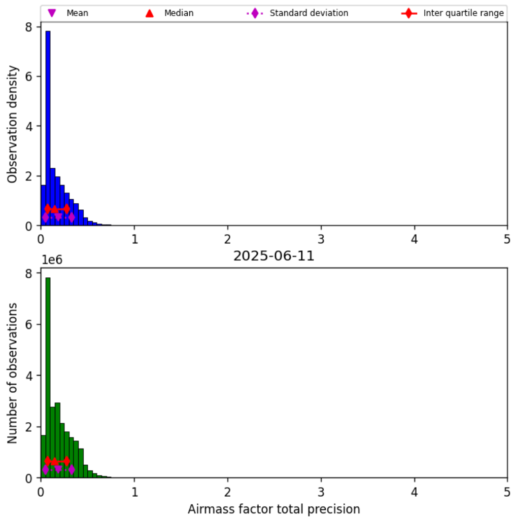
Figure 41: Histogram of “Airmass factor total precision” for 2025-06-11 to 2025-06-12
