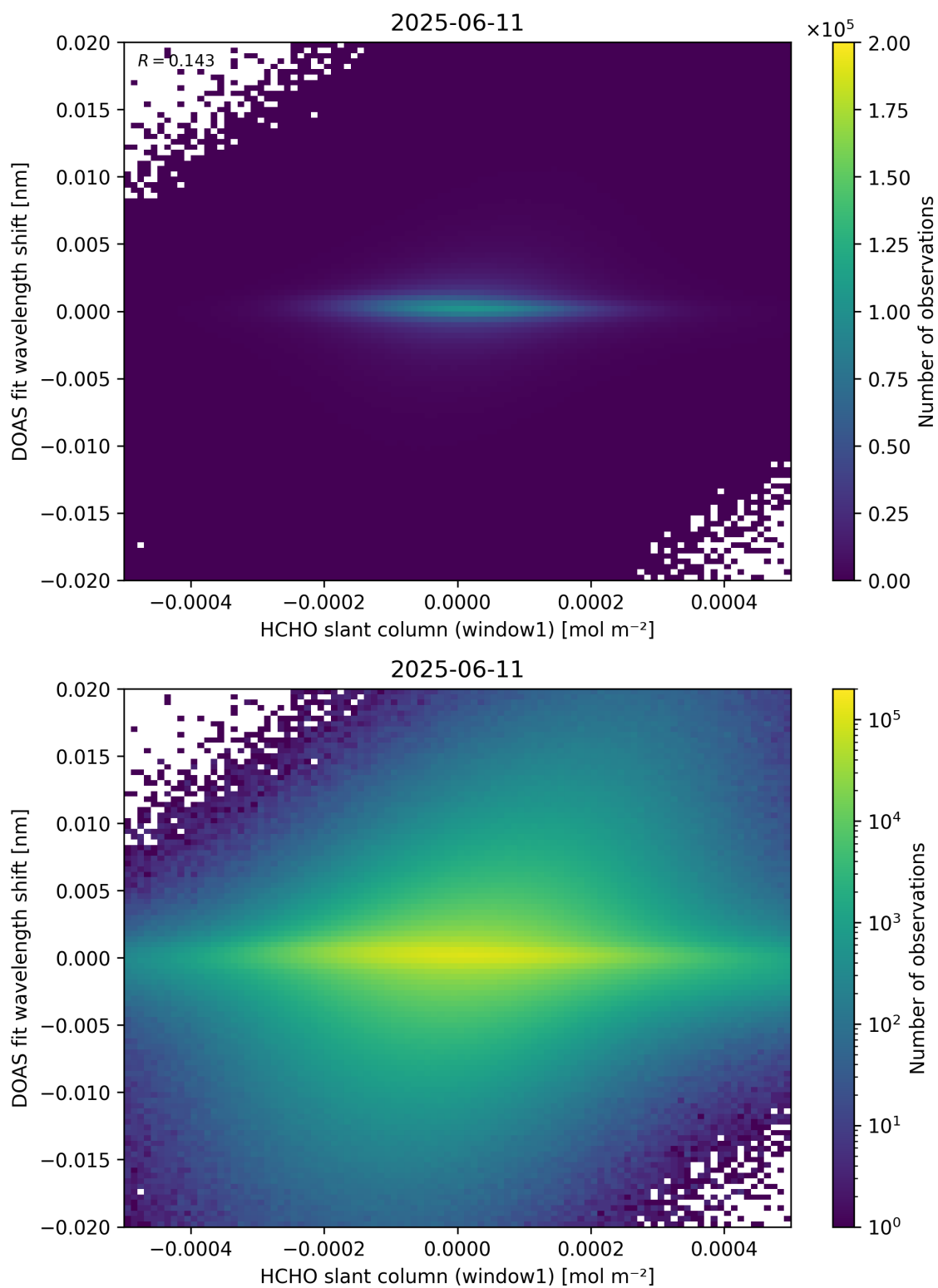
Figure 79: Scatter density plot of “HCHO slant column (window1)” against “DOAS fit wavelength shift” for 2025-06-11 to 2025-06-12.
