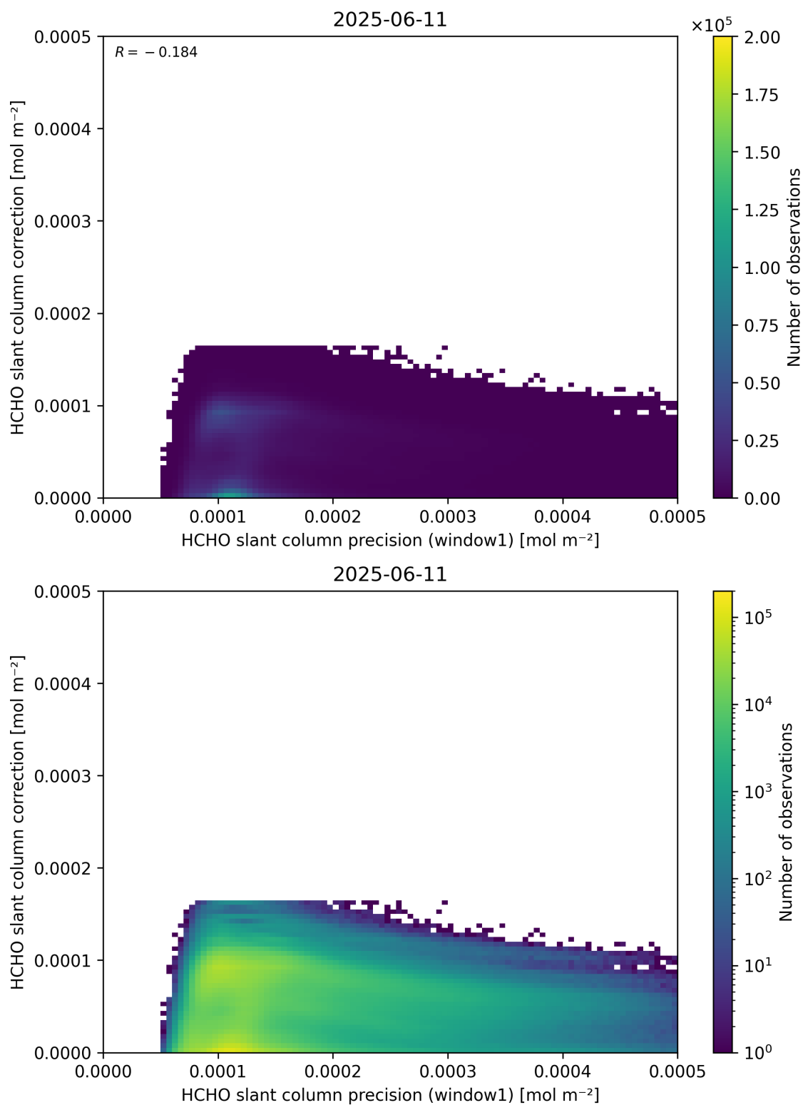
Figure 93: Scatter density plot of “HCHO slant column precision (window1)” against “HCHO slant column correction” for 2025-06-11 to 2025-06-12.
