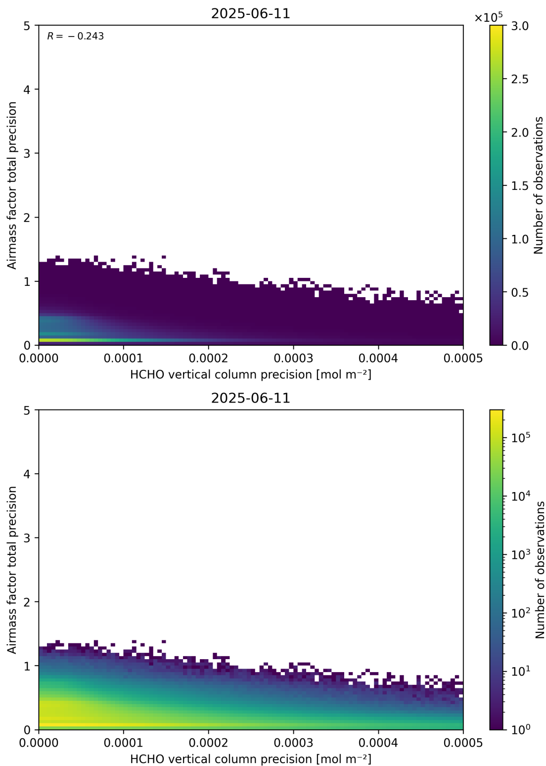
Figure 145: Scatter density plot of “HCHO vertical column precision” against “Airmass factor total precision” for 2025-06-11 to 2025-06-12.
