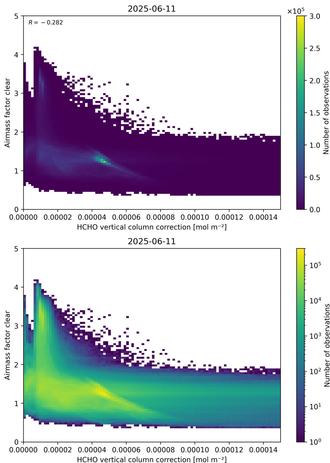
Figure 115: Scatter density plot of “HCHO vertical column correction” against “Airmass factor clear” for 2025-06-11 to 2025-06-12.
