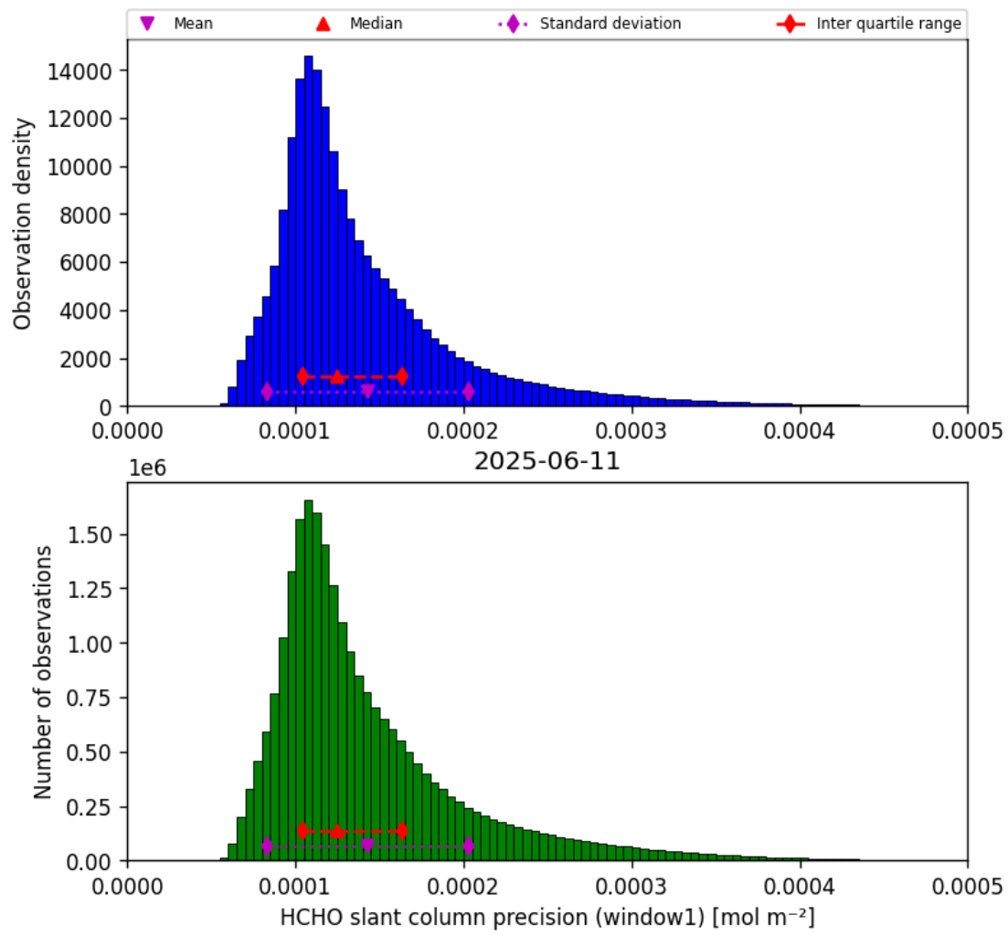
Figure 39: Histogram of “HCHO slant column precision (window1)” for 2025-06-11 to 2025-06-12
