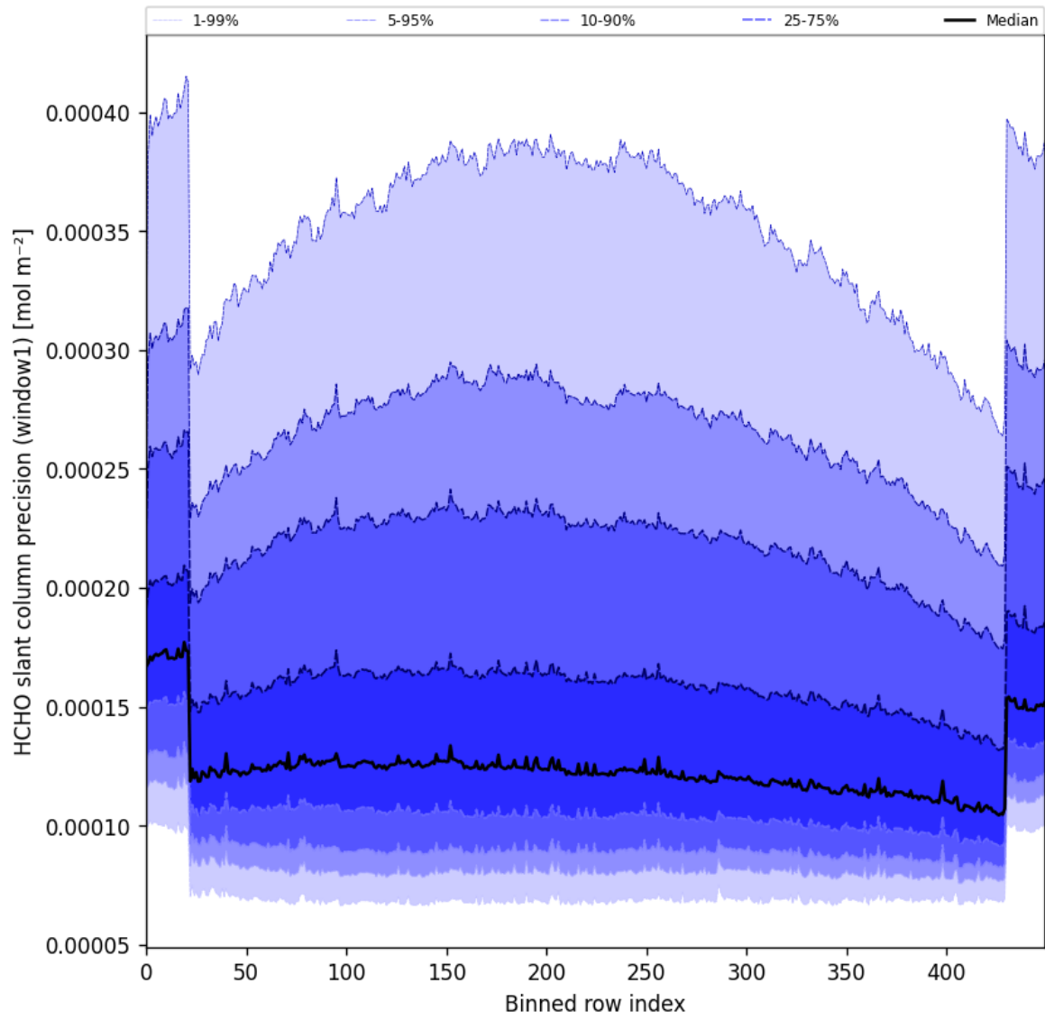
Figure 53: Along track statistics of “HCHO slant column precision (window1)” for 2025-06-11 to 2025-06-12
