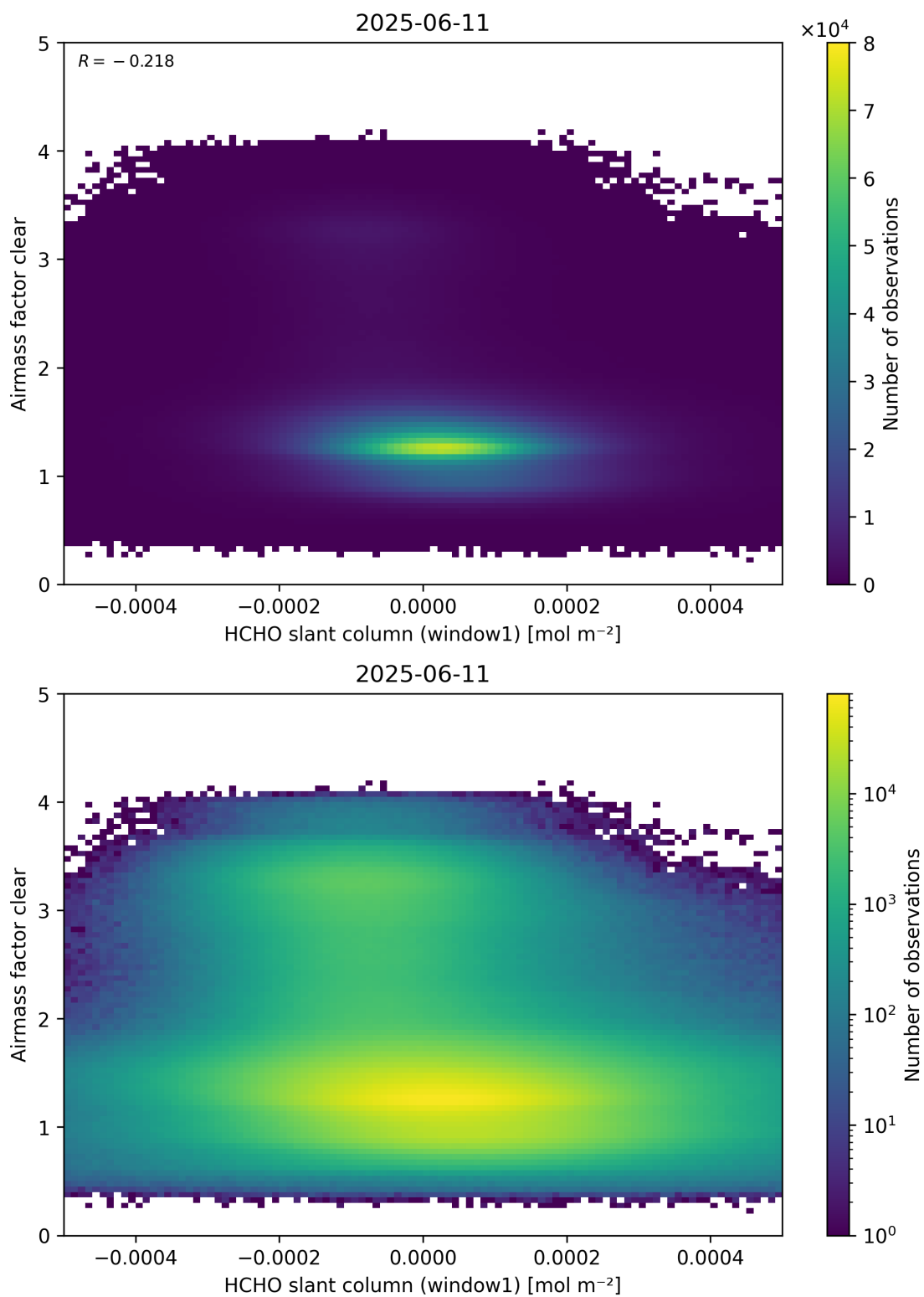
Figure 81: Scatter density plot of “HCHO slant column (window1)” against “Airmass factor clear” for 2025-06-11 to 2025-06-12.
