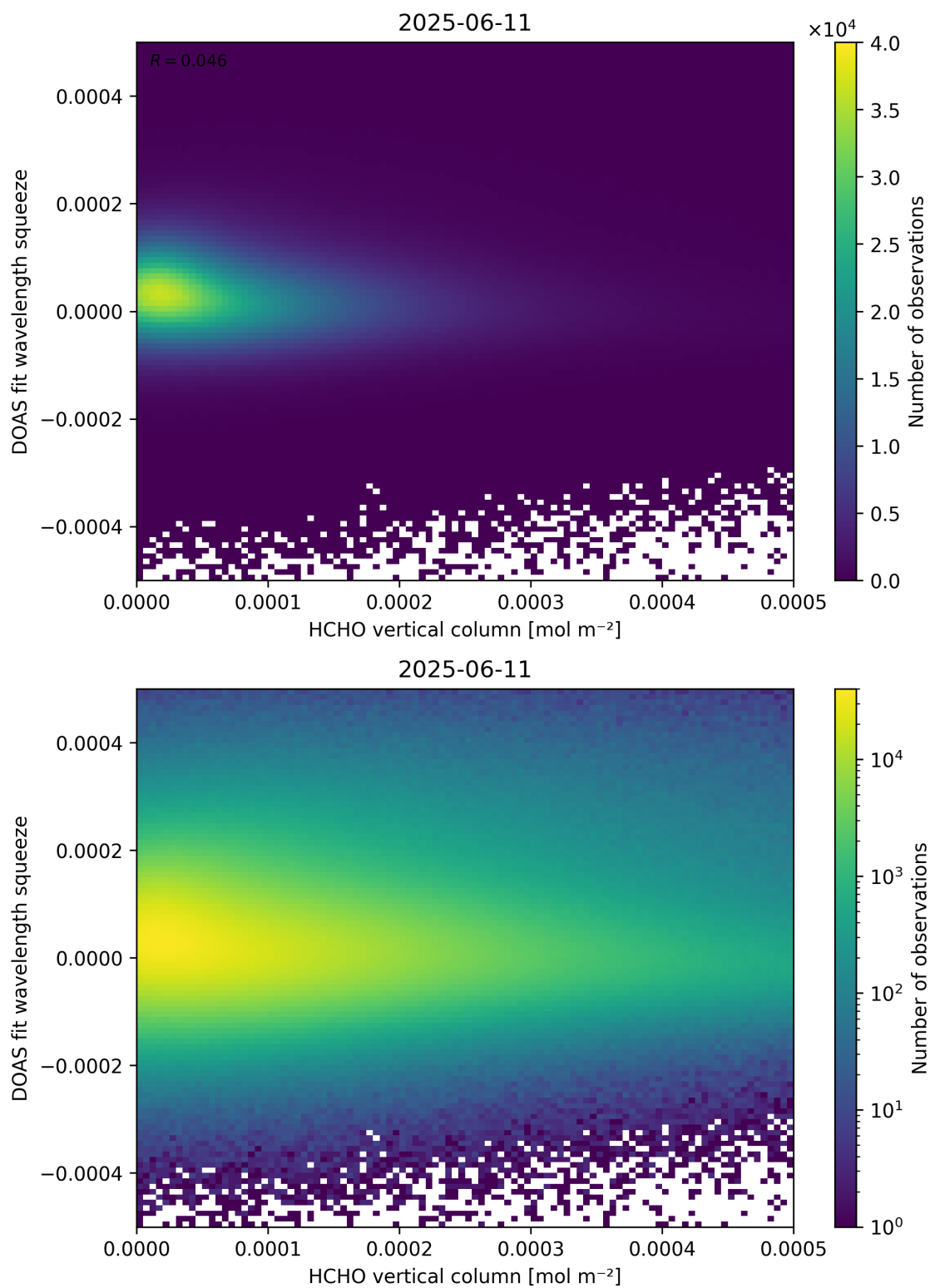
Figure 125: Scatter density plot of “HCHO vertical column” against “DOAS fit wavelength squeeze” for 2025-06-11 to 2025-06-12.
