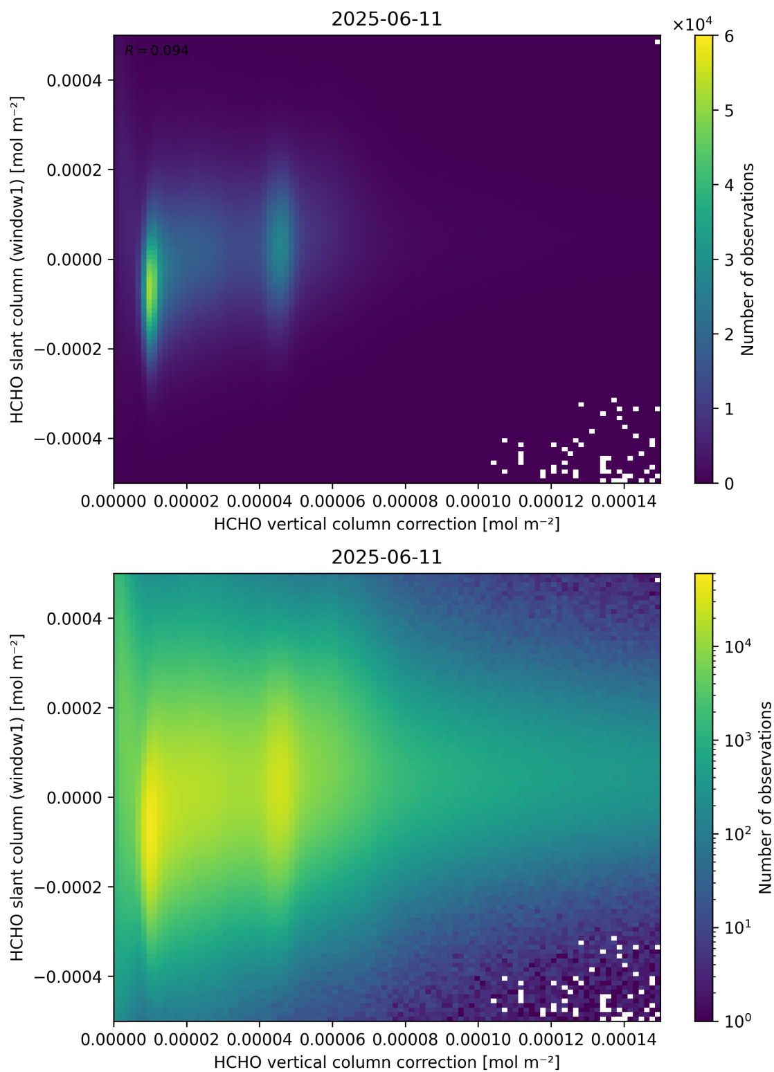
Figure 118: Scatter density plot of “HCHO vertical column correction” against “HCHO slant column (window1)” for 2025-06-11 to 2025-06-12.
