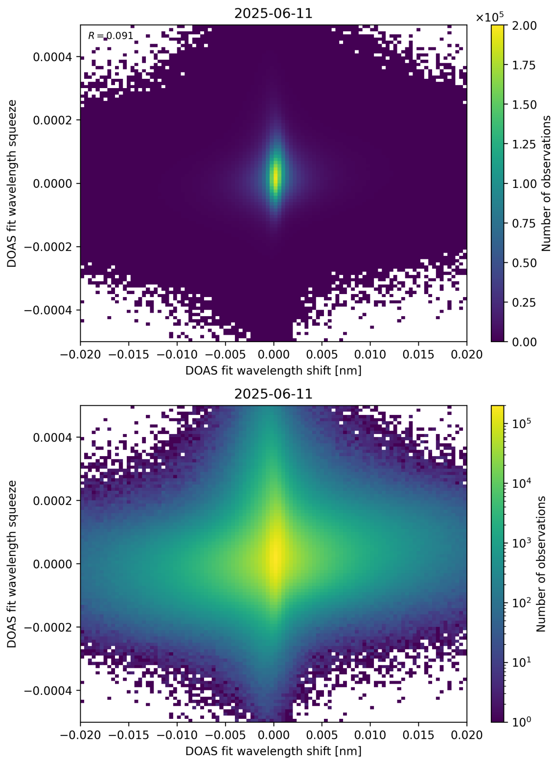
Figure 65: Scatter density plot of “DOAS fit wavelength shift” against “DOAS fit wavelength squeeze” for 2025-06-11 to 2025-06-12.
