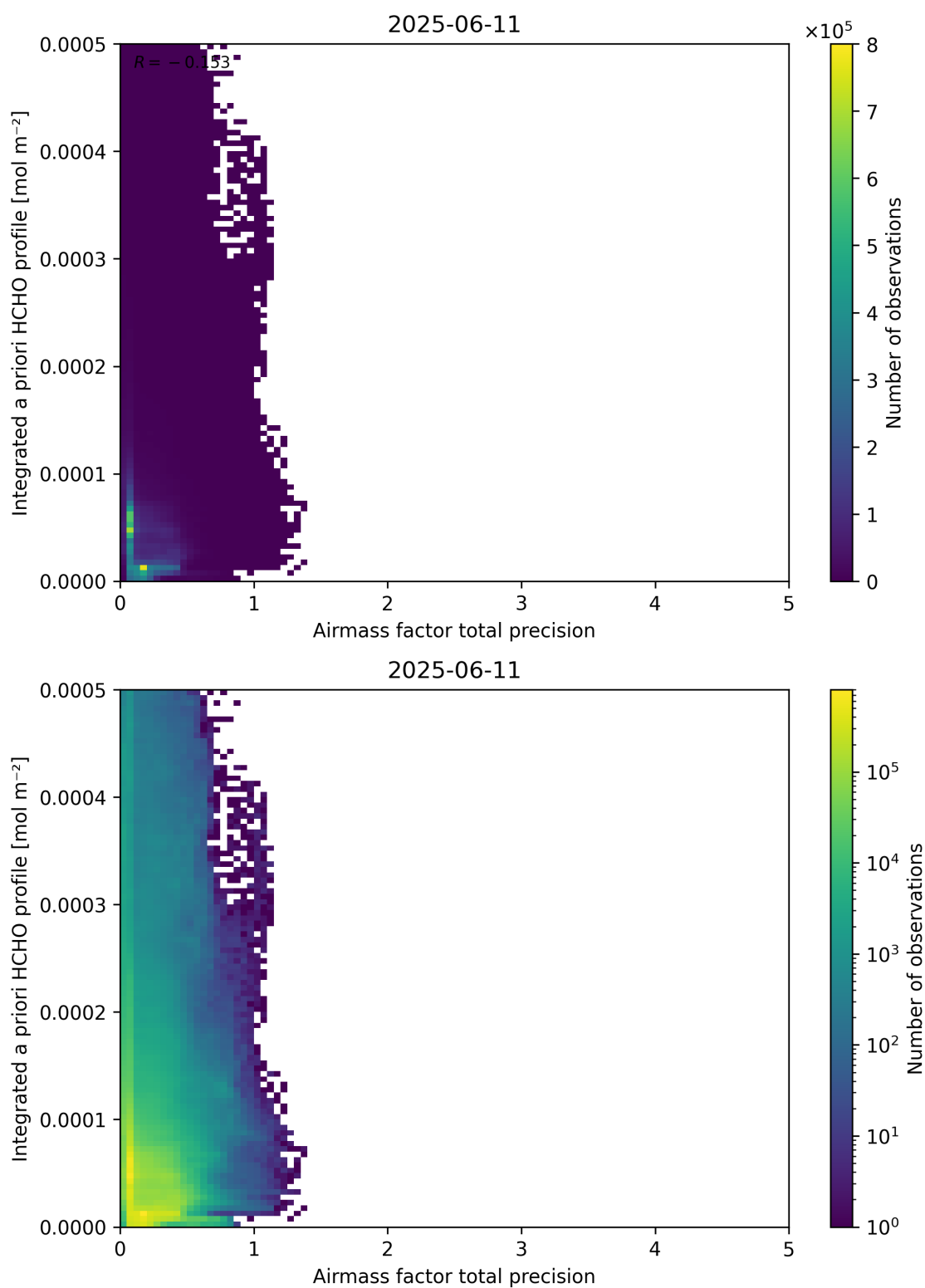
Figure 111: Scatter density plot of “Airmass factor total precision” against “Integrated a priori HCHO profile” for 2025-06-11 to 2025-06-12.
