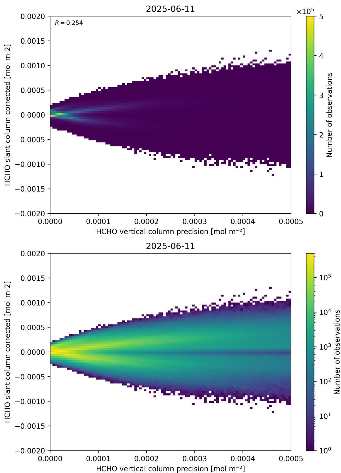
Figure 140: Scatter density plot of “HCHO vertical column precision” against “HCHO slant column corrected” for 2025-06-11 to 2025-06-12.
