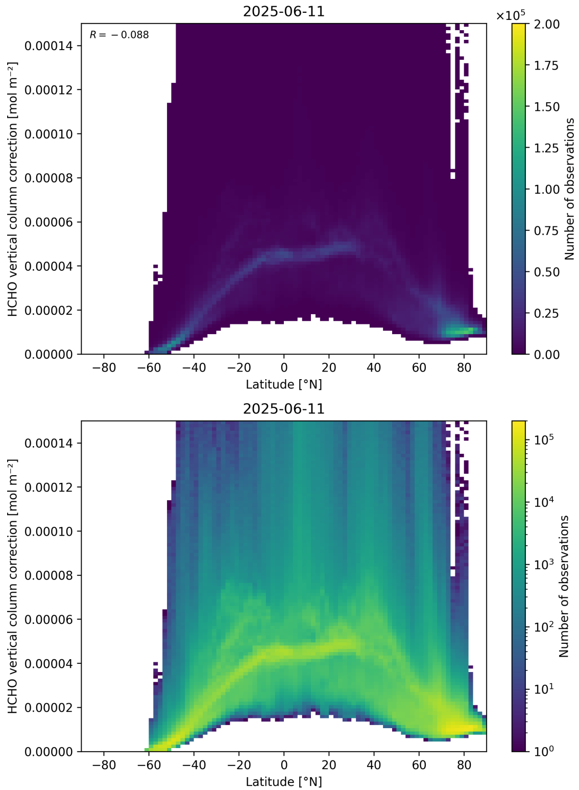
Figure 164: Scatter density plot of “Latitude” against “HCHO vertical column correction” for 2025-06-11 to 2025-06-12.
