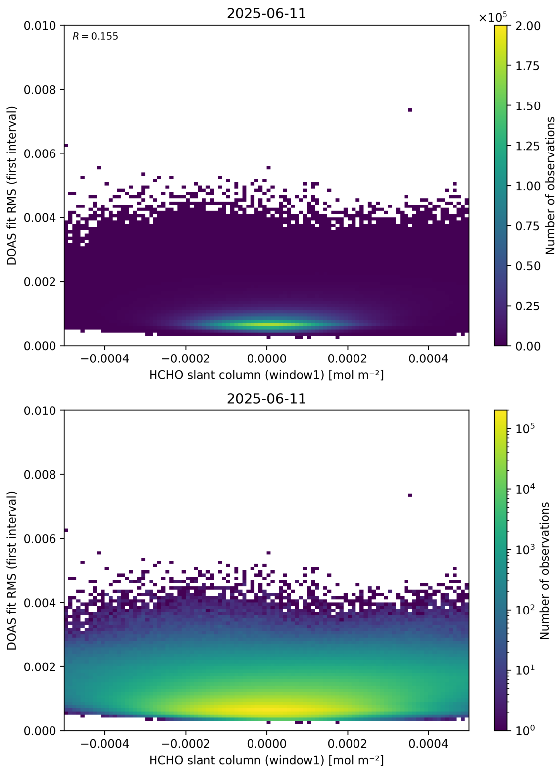
Figure 78: Scatter density plot of “HCHO slant column (window1)” against “DOAS fit RMS (first interval)” for 2025-06-11 to 2025-06-12.
