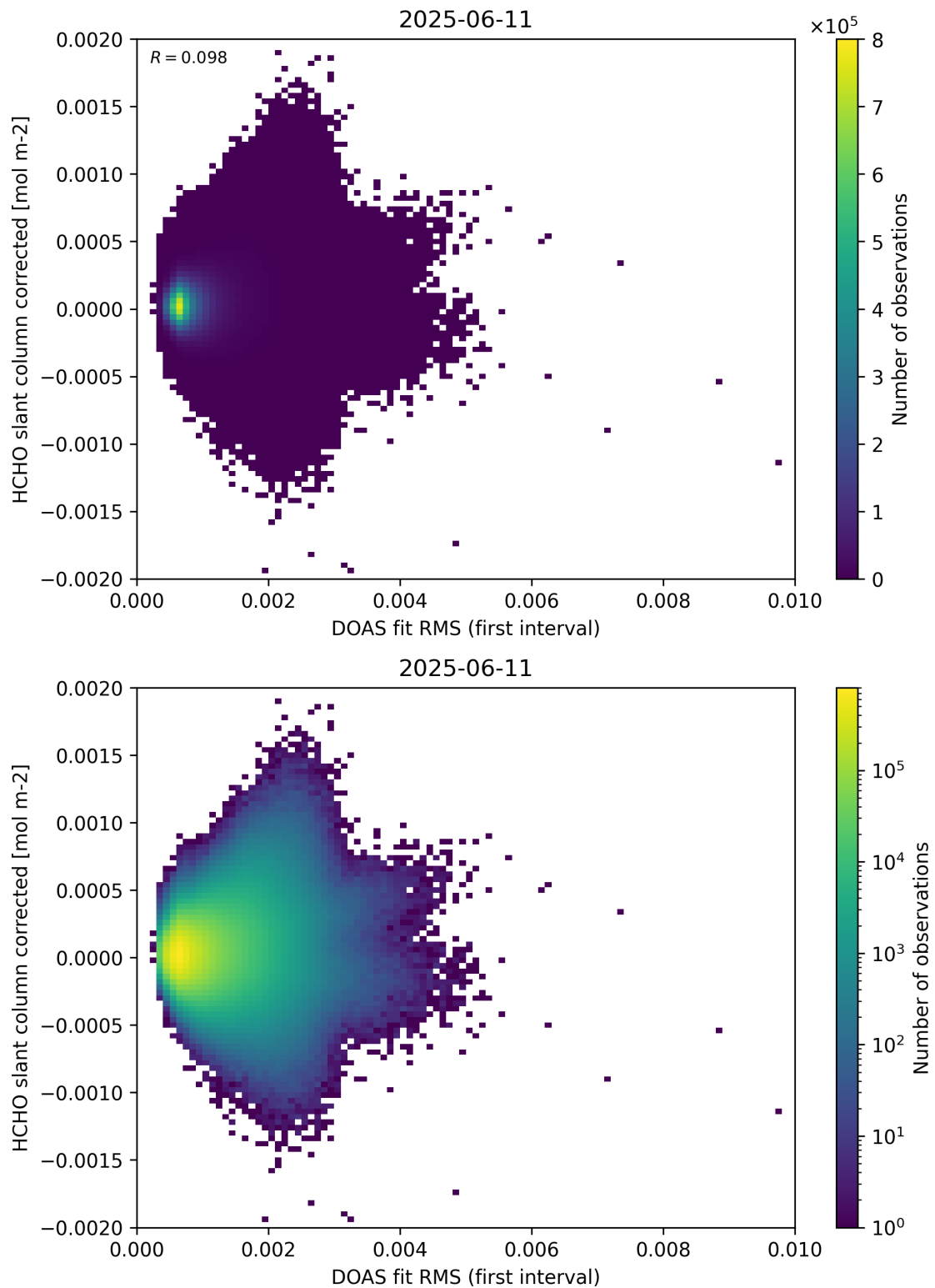
Figure 62: Scatter density plot of “DOAS fit RMS (first interval)” against “HCHO slant column corrected” for 2025-06-11 to 2025-06-12.
