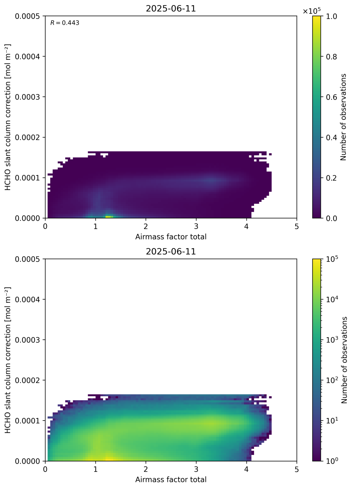
Figure 102: Scatter density plot of “Airmass factor total” against “HCHO slant column correction” for 2025-06-11 to 2025-06-12.
