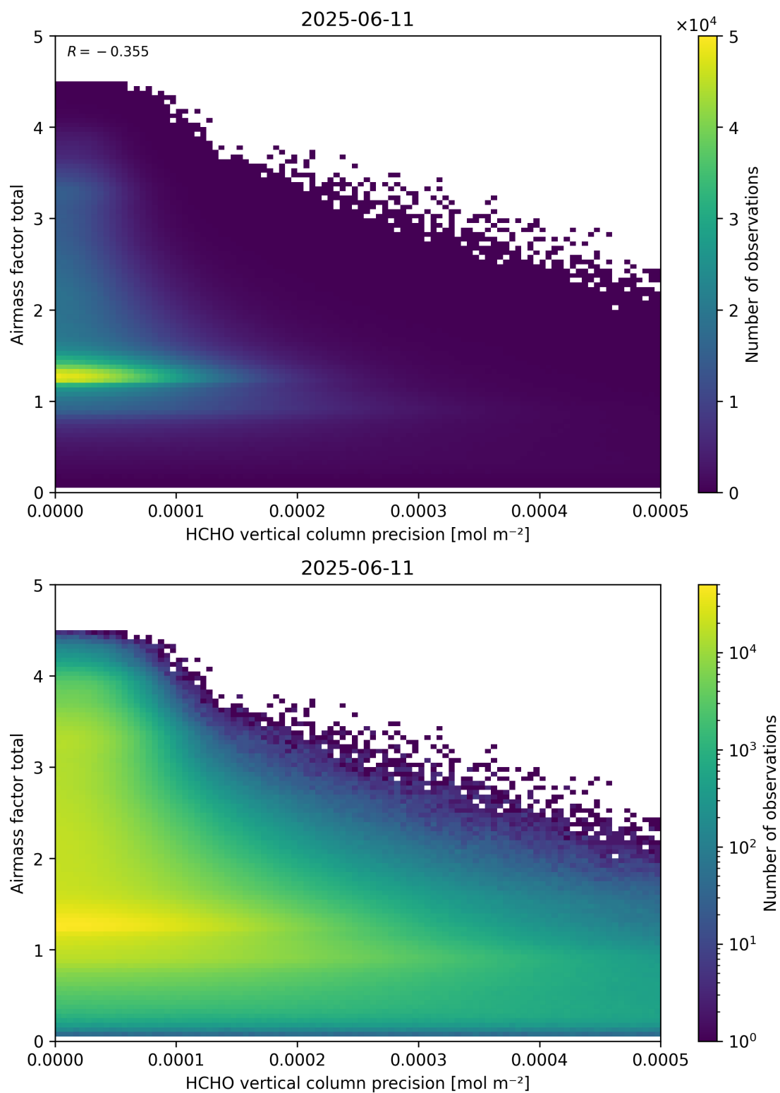
Figure 144: Scatter density plot of “HCHO vertical column precision” against “Airmass factor total” for 2025-06-11 to 2025-06-12.
