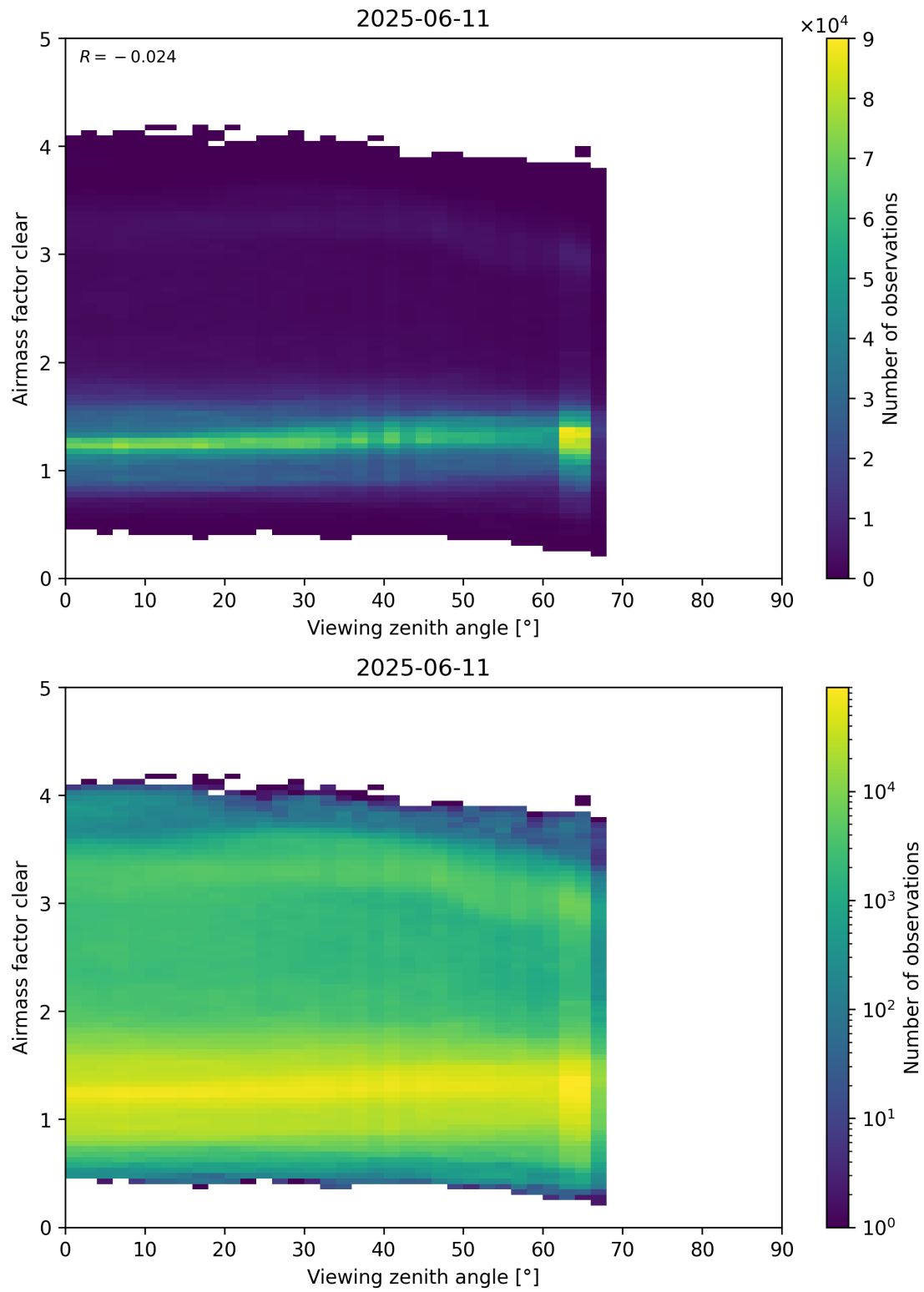
Figure 185: Scatter density plot of “Viewing zenith angle” against “Airmass factor clear” for 2025-06-11 to 2025-06-12.
