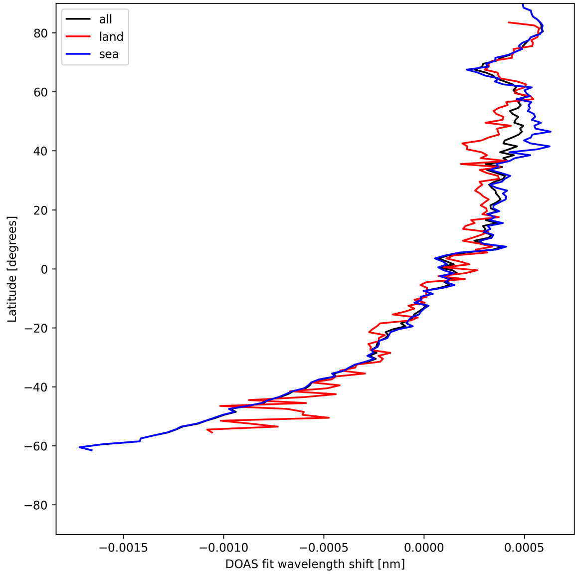
Figure 30: Zonal average of “DOAS fit wavelength shift” for 2025-06-11 to 2025-06-12.
