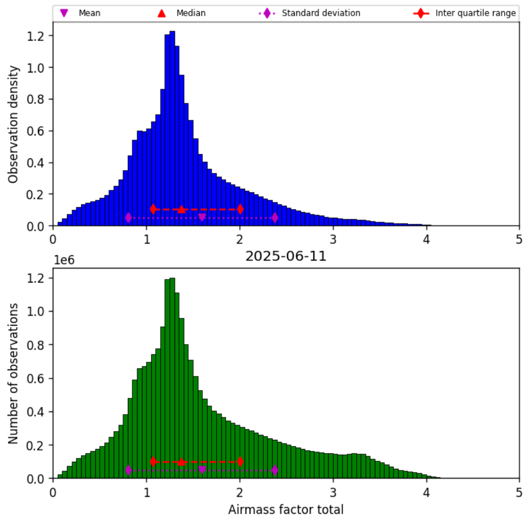
Figure 40: Histogram of “Airmass factor total” for 2025-06-11 to 2025-06-12
