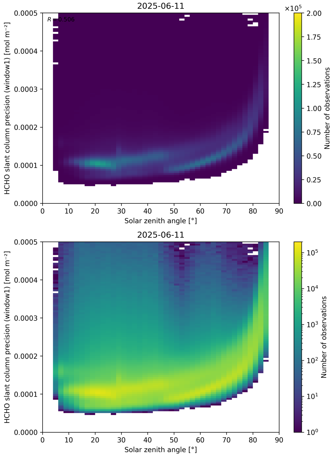
Figure 174: Scatter density plot of “Solar zenith angle” against “HCHO slant column precision (window1)” for 2025-06-11 to 2025-06-12.
