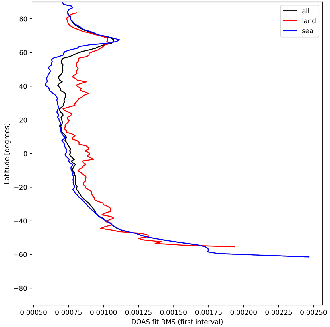
Figure 32: Zonal average of “DOAS fit RMS (first interval)” for 2025-06-11 to 2025-06-12.
