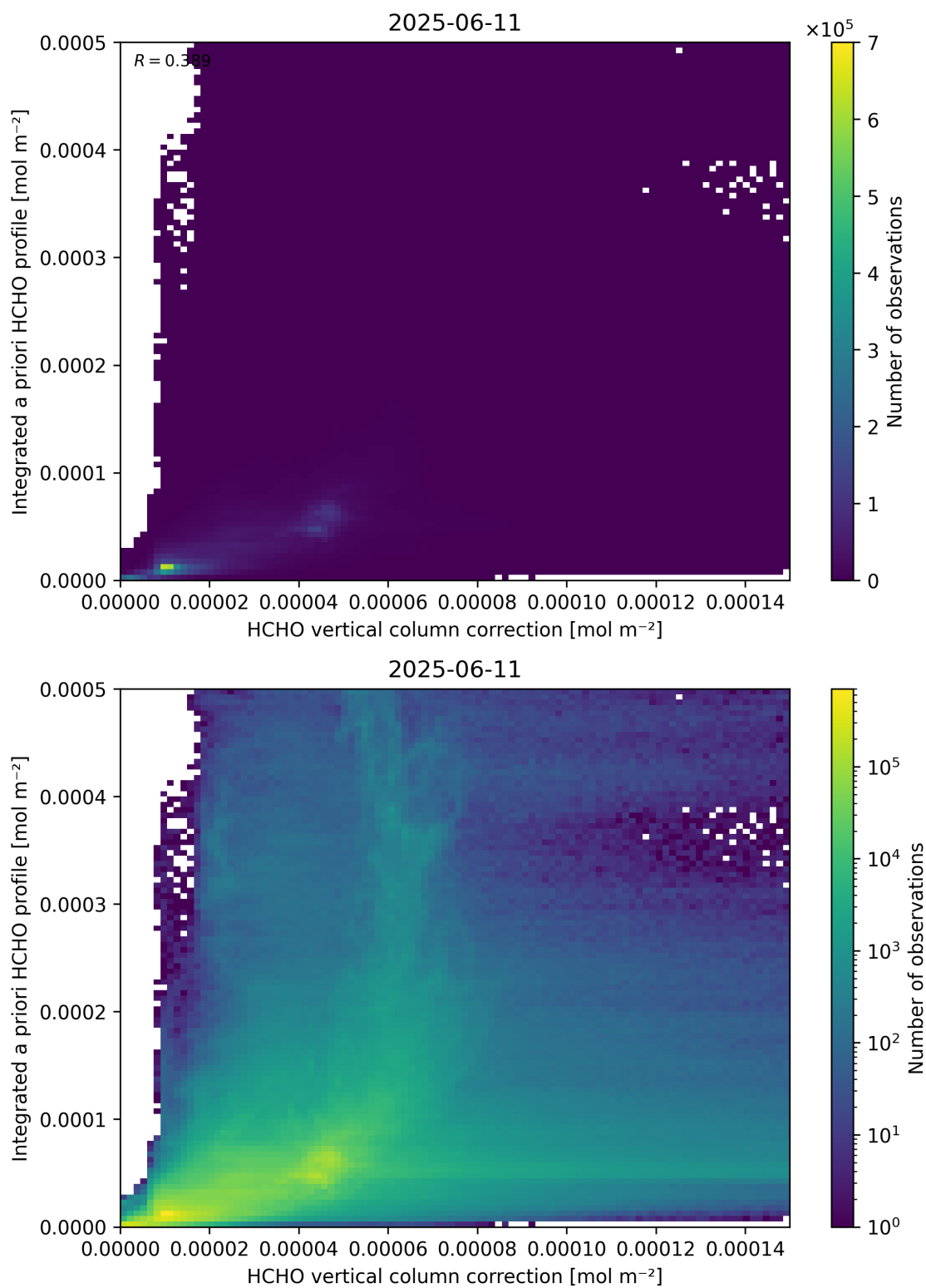
Figure 122: Scatter density plot of “HCHO vertical column correction” against “Integrated a priori HCHO profile” for 2025-06-11 to 2025-06-12.
