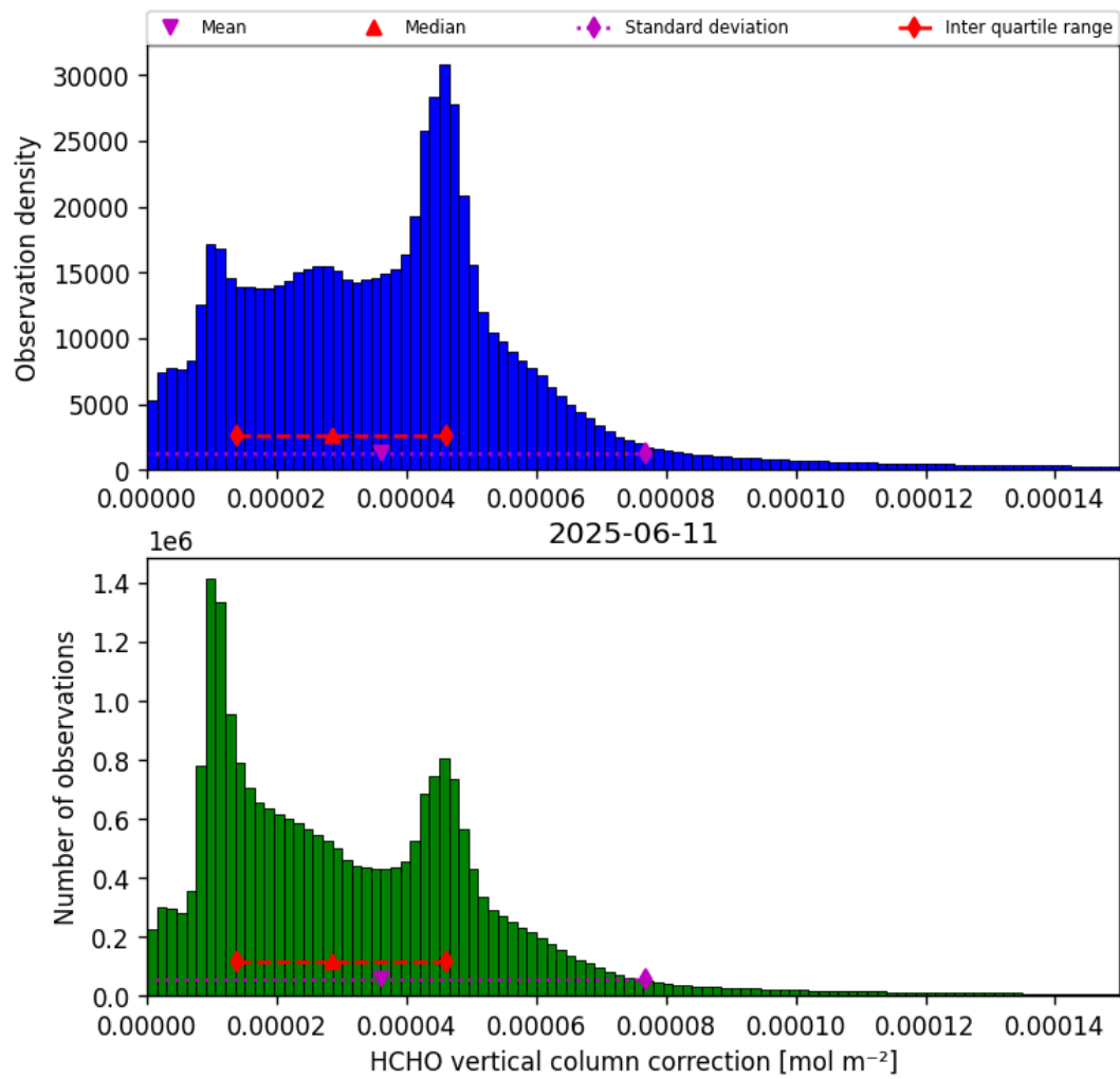
Figure 37: Histogram of “HCHO vertical column correction” for 2025-06-11 to 2025-06-12
