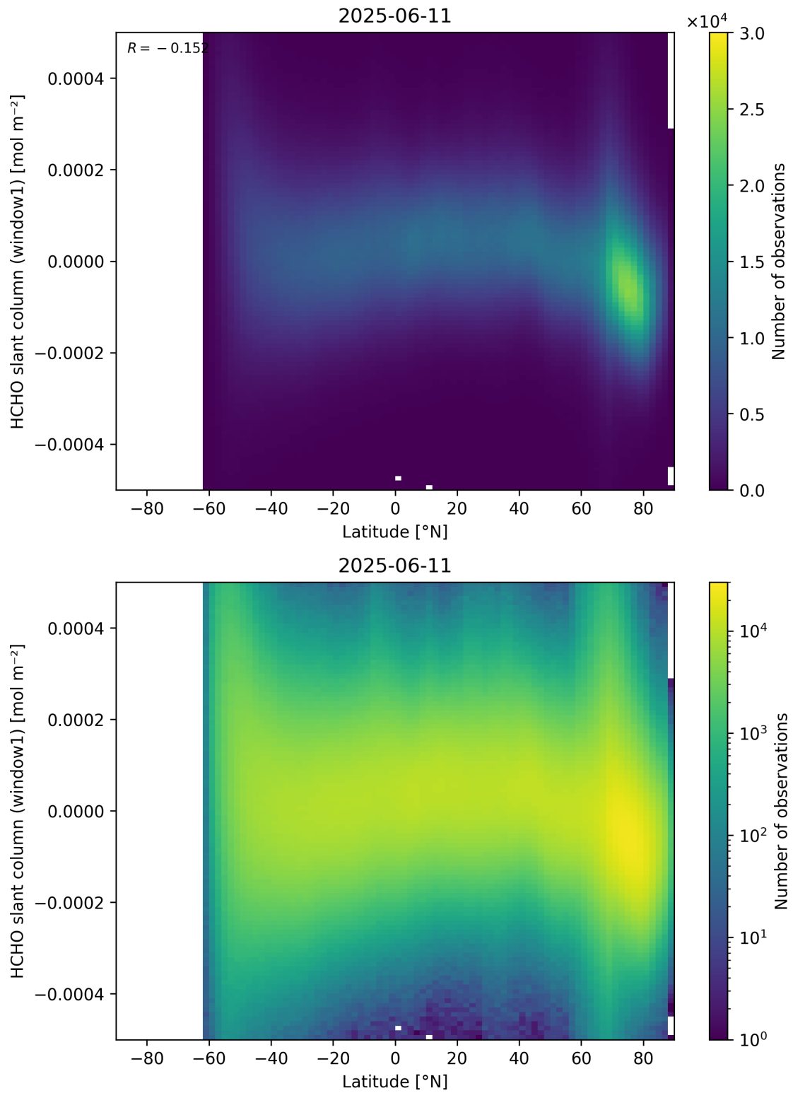
Figure 159: Scatter density plot of “Latitude” against “HCHO slant column (window1)” for 2025-06-11 to 2025-06-12.
