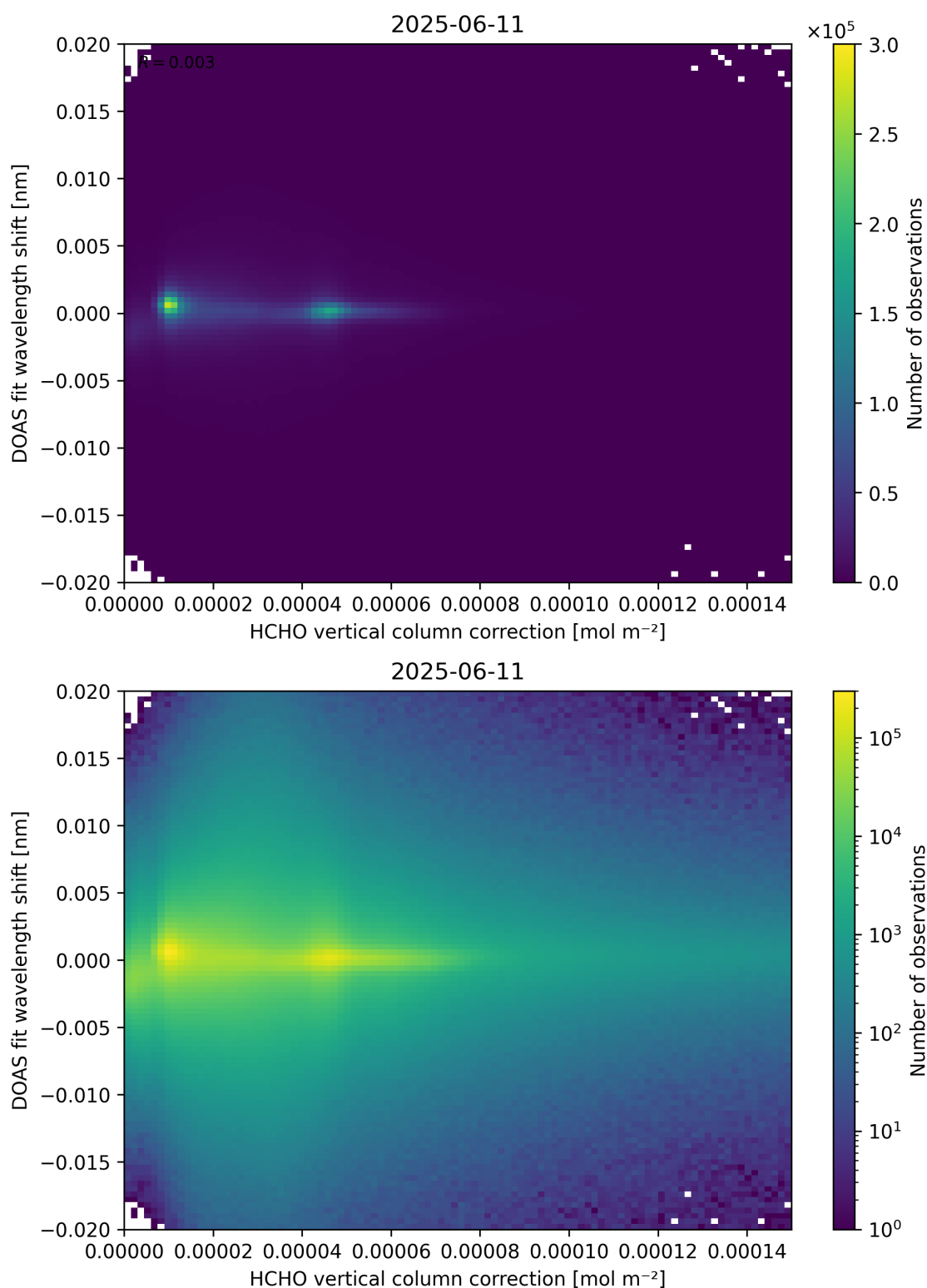
Figure 113: Scatter density plot of “HCHO vertical column correction” against “DOAS fit wavelength shift” for 2025-06-11 to 2025-06-12.
