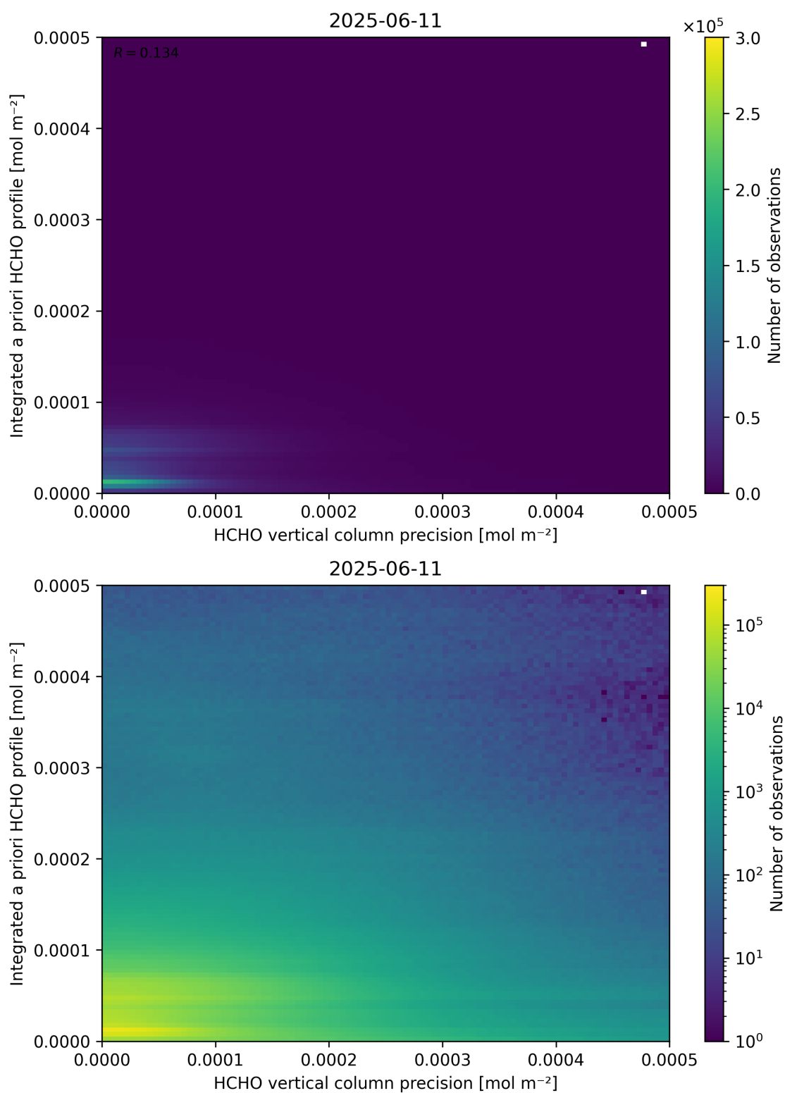
Figure 147: Scatter density plot of “HCHO vertical column precision” against “Integrated a priori HCHO profile” for 2025-06-11 to 2025-06-12.
