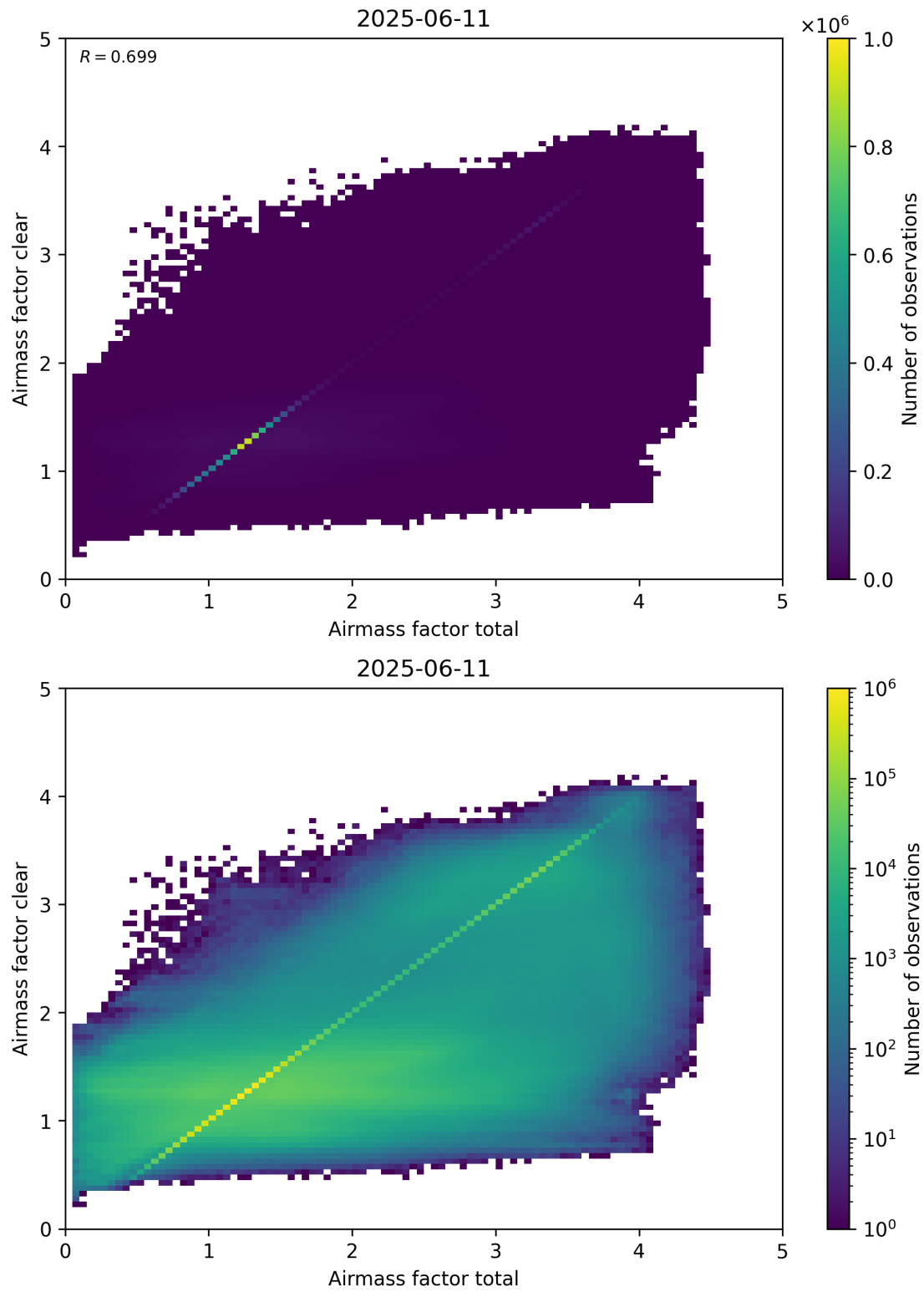
Figure 100: Scatter density plot of “Airmass factor total” against “Airmass factor clear” for 2025-06-11 to 2025-06-12.
