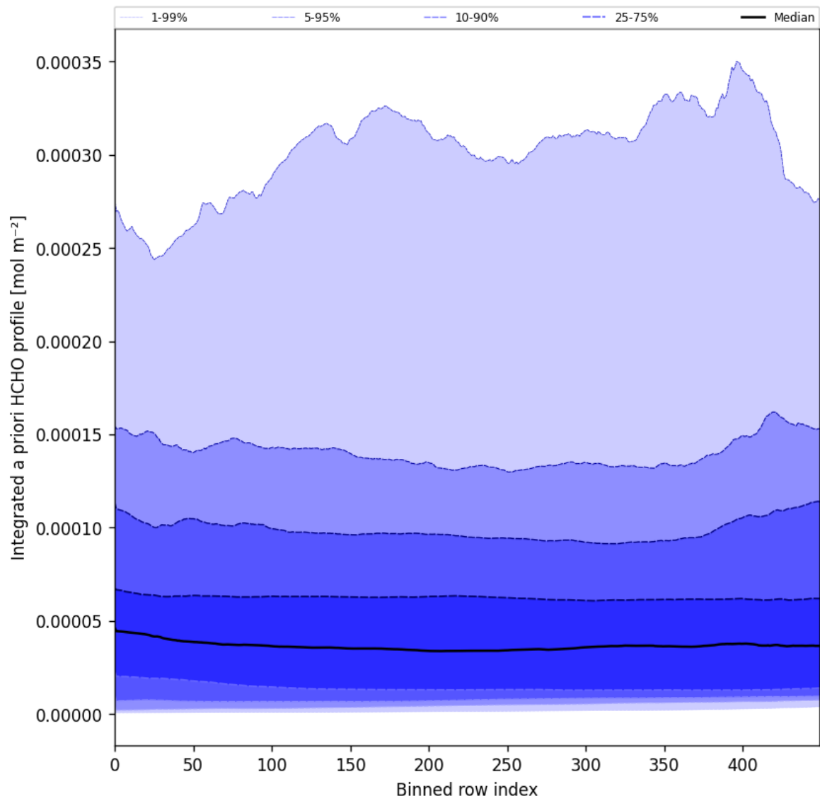
Figure 57: Along track statistics of “Integrated a priori HCHO profile” for 2025-06-11 to 2025-06-12
