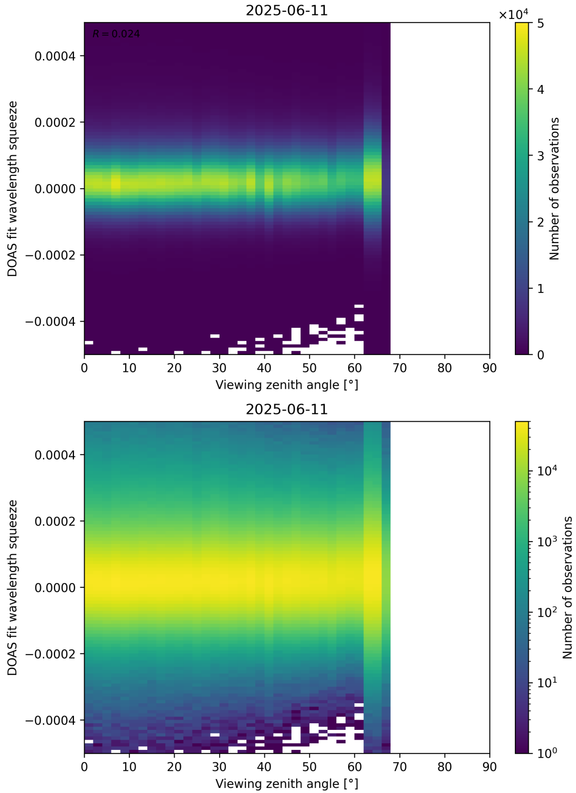
Figure 184: Scatter density plot of “Viewing zenith angle” against “DOAS fit wavelength squeeze” for 2025-06-11 to 2025-06-12.
