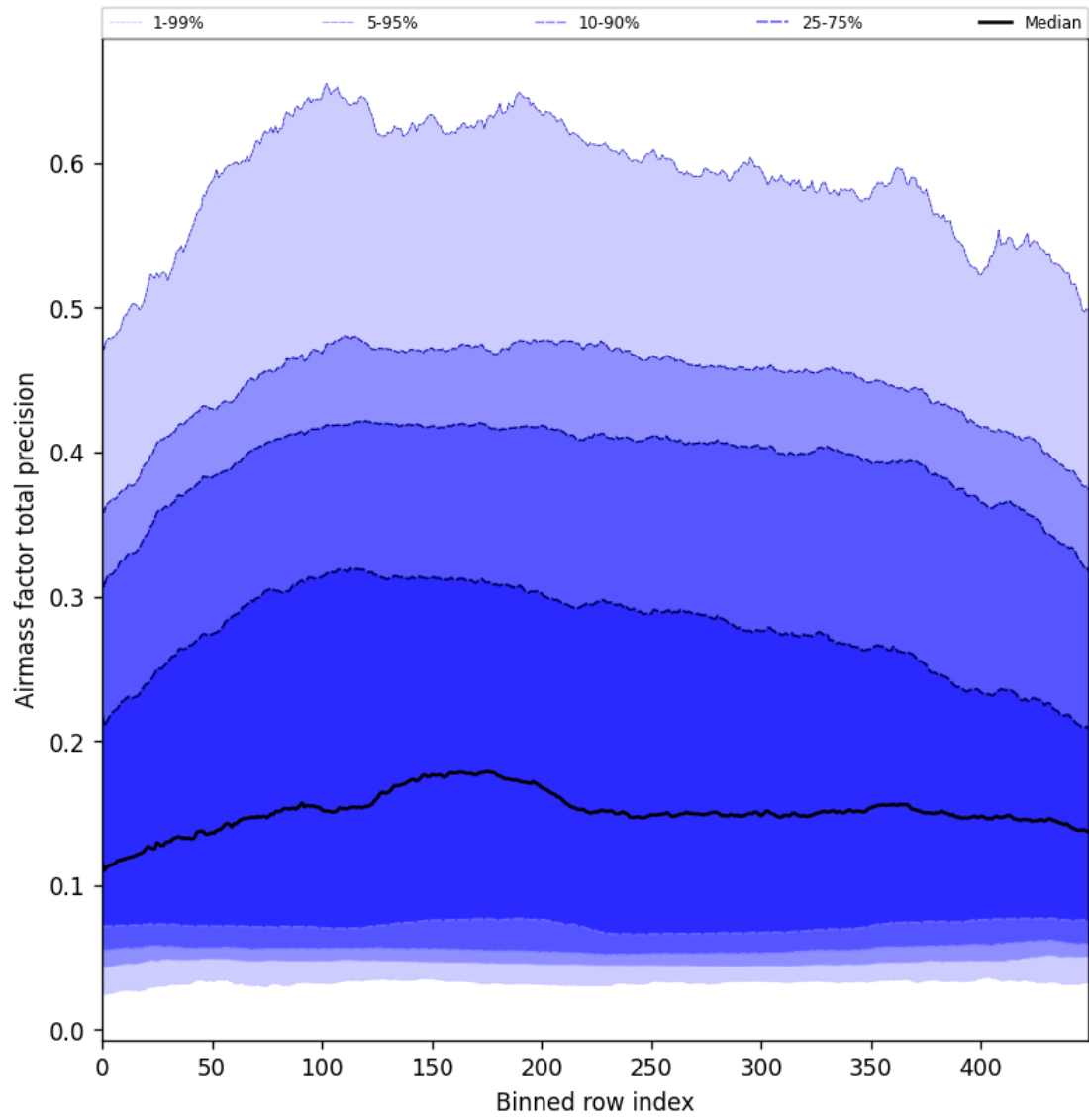
Figure 55: Along track statistics of “Airmass factor total precision” for 2025-06-11 to 2025-06-12
