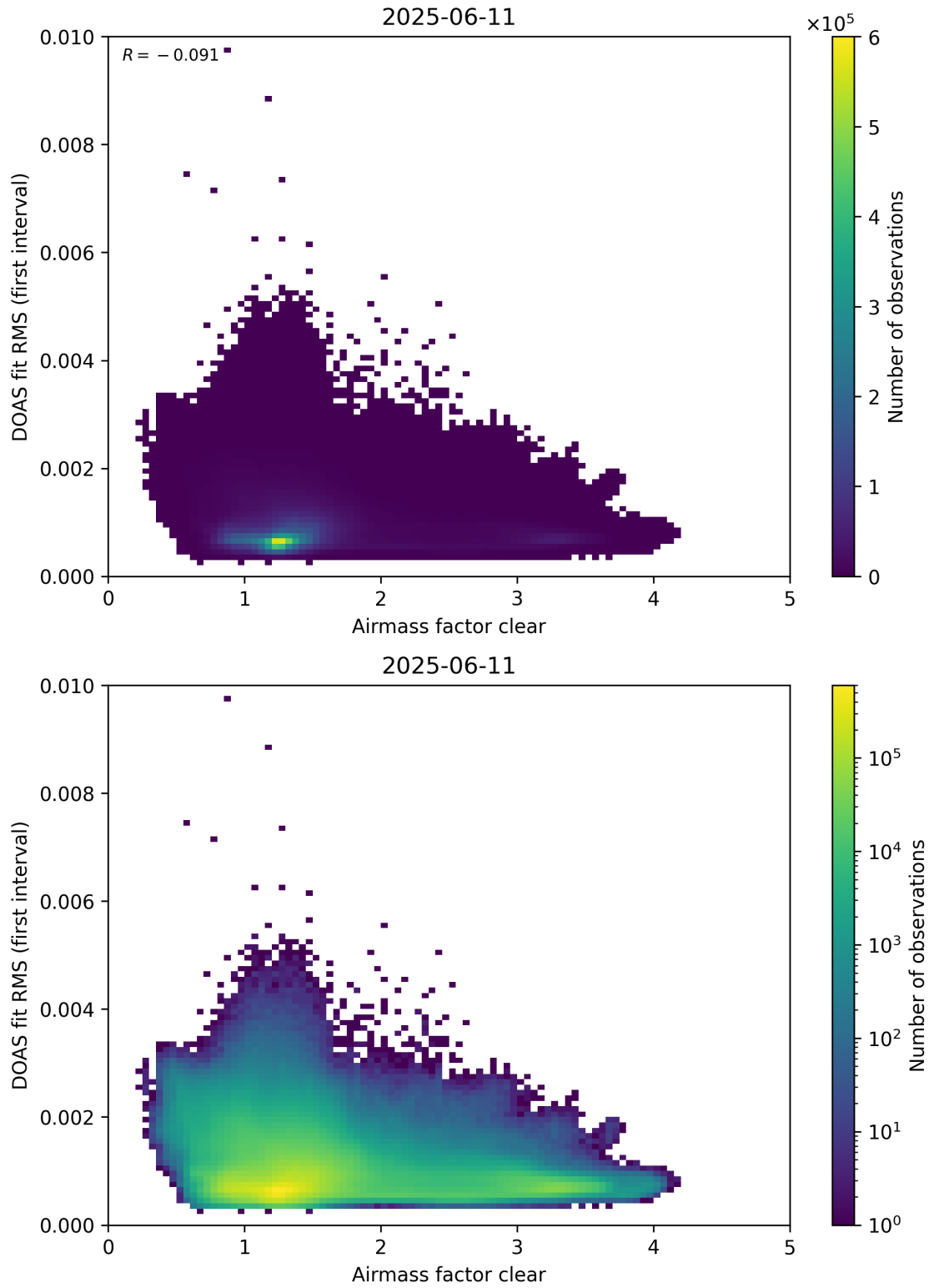
Figure 71: Scatter density plot of “Airmass factor clear” against “DOAS fit RMS (first interval)” for 2025-06-11 to 2025-06-12.
