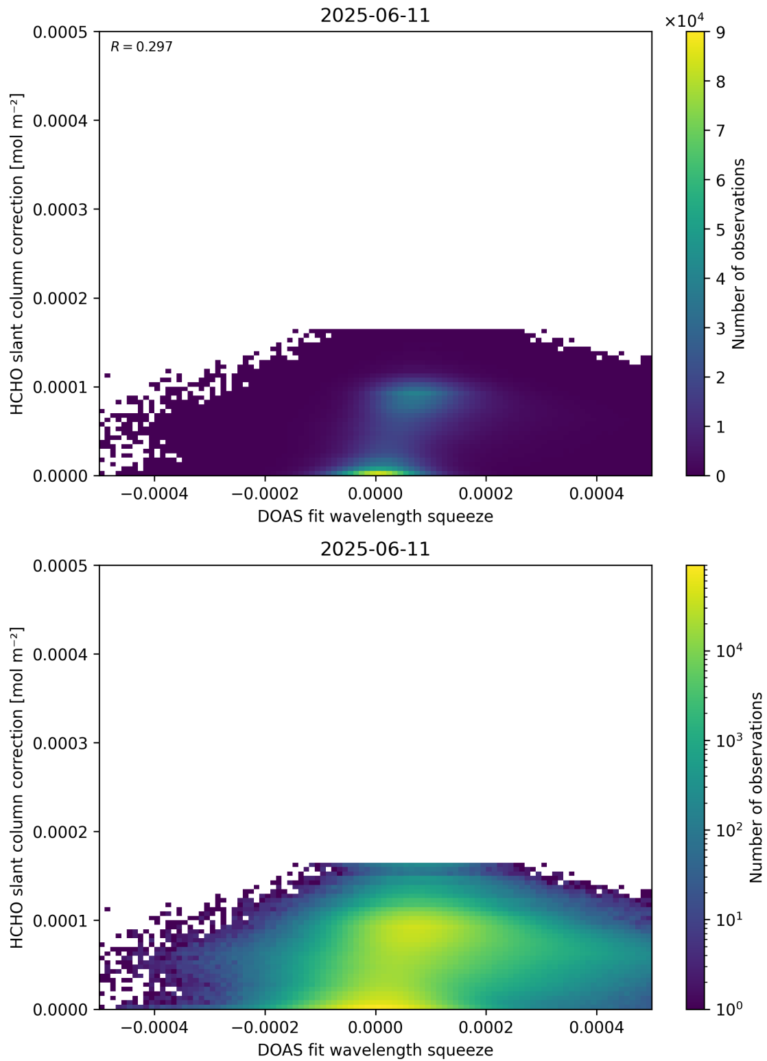
Figure 70: Scatter density plot of “DOAS fit wavelength squeeze” against “HCHO slant column correction” for 2025-06-11 to 2025-06-12.
