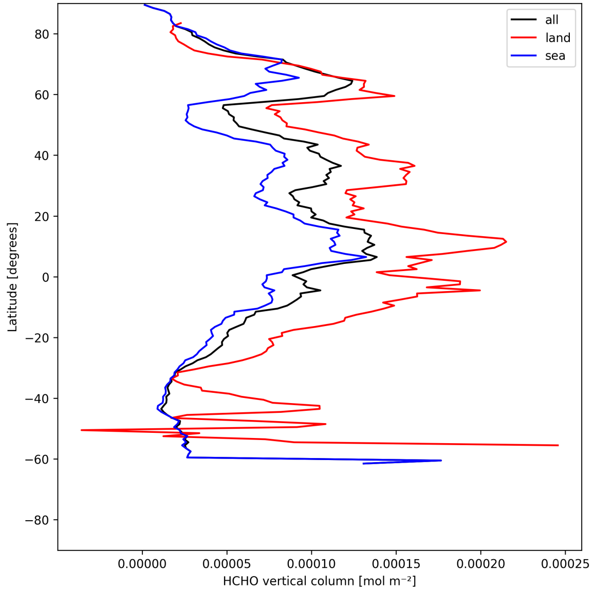
Figure 21: Zonal average of “HCHO vertical column” for 2025-06-11 to 2025-06-12.
