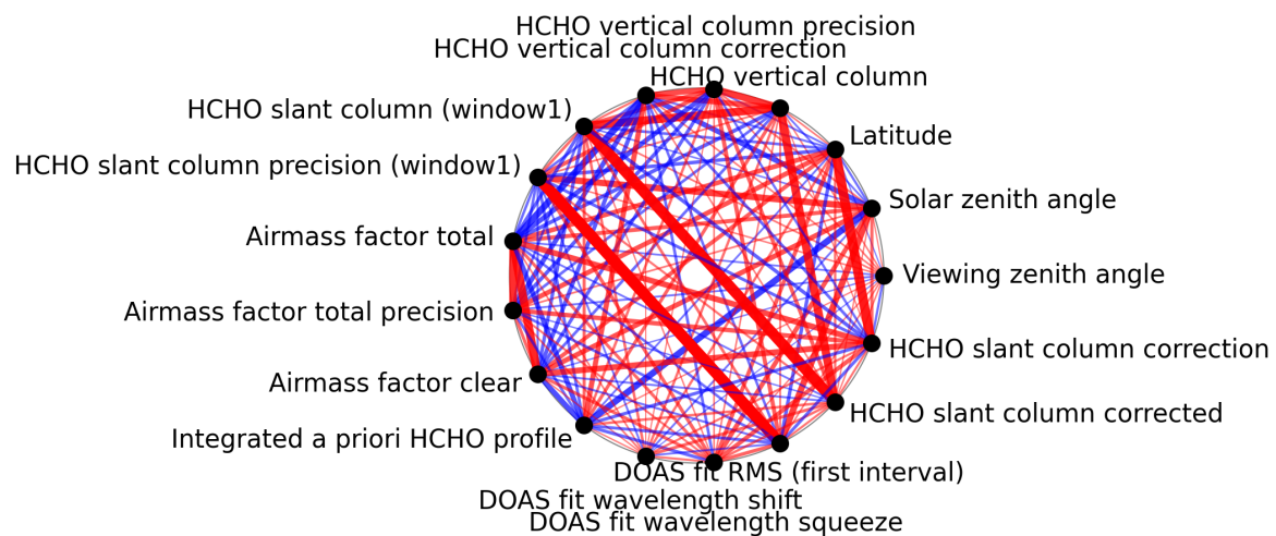
Figure 1: Map of correlation graph for 2025-06-11 to 2025-06-12.
