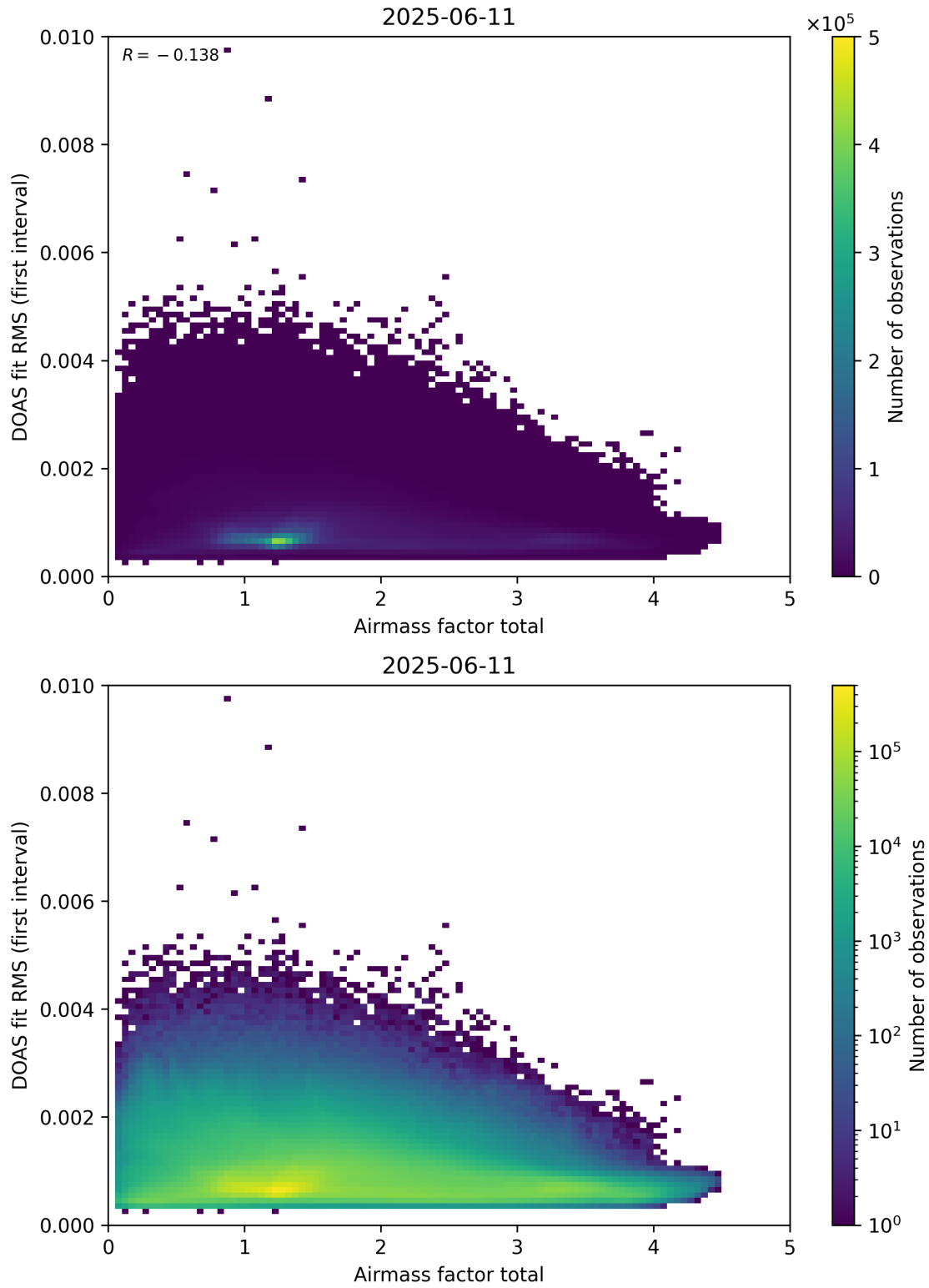
Figure 97: Scatter density plot of “Airmass factor total” against “DOAS fit RMS (first interval)” for 2025-06-11 to 2025-06-12.
