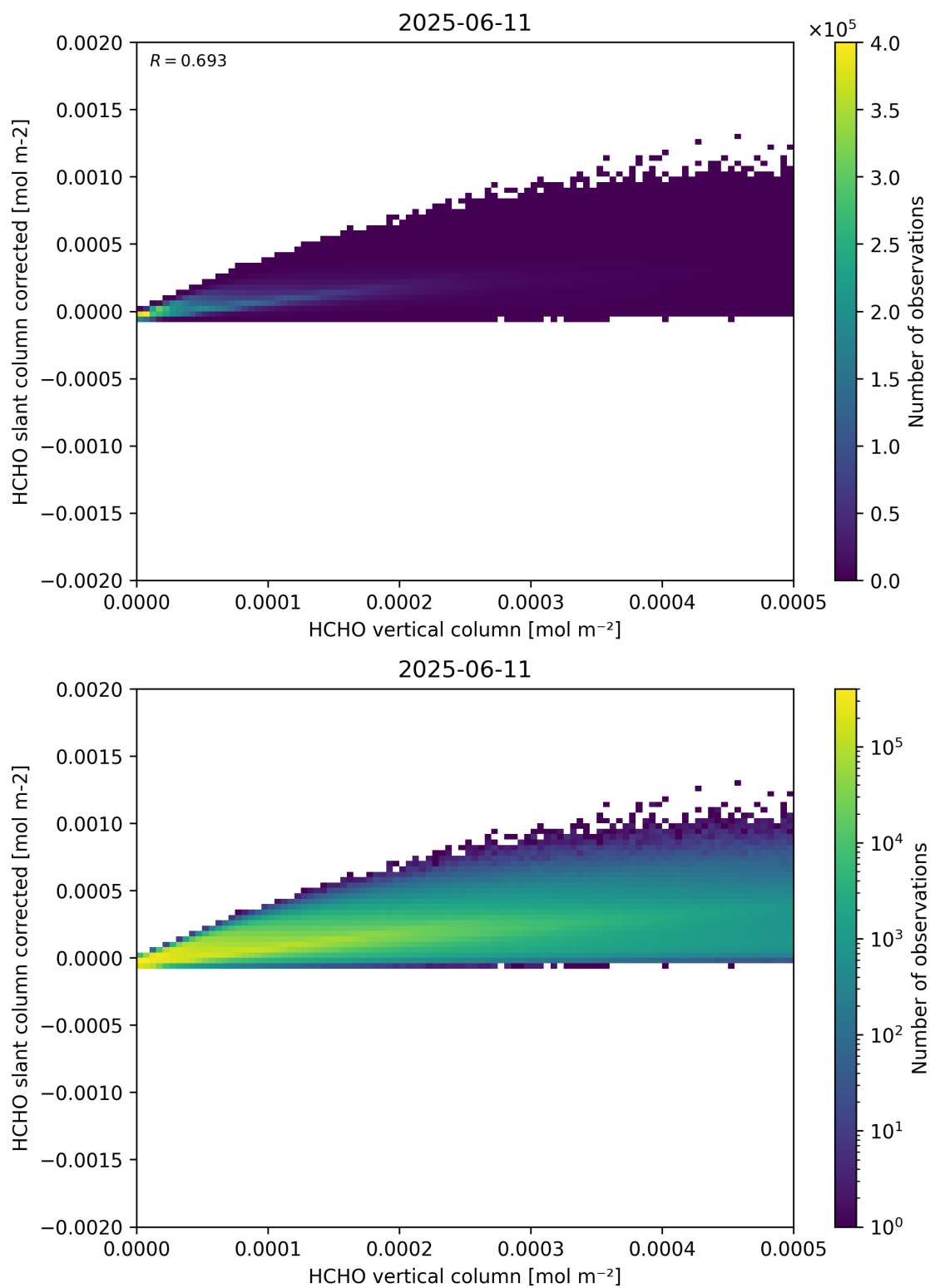
Figure 127: Scatter density plot of “HCHO vertical column” against “HCHO slant column corrected” for 2025-06-11 to 2025-06-12.
