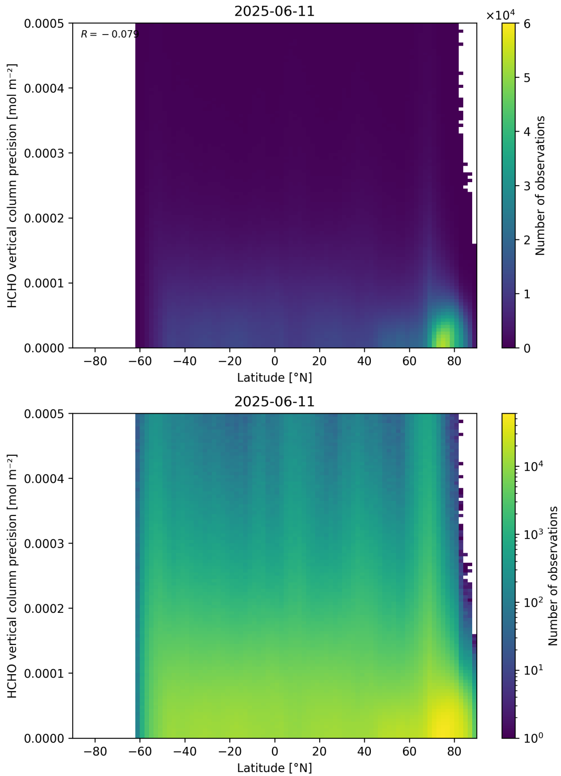
Figure 165: Scatter density plot of “Latitude” against “HCHO vertical column precision” for 2025-06-11 to 2025-06-12.
