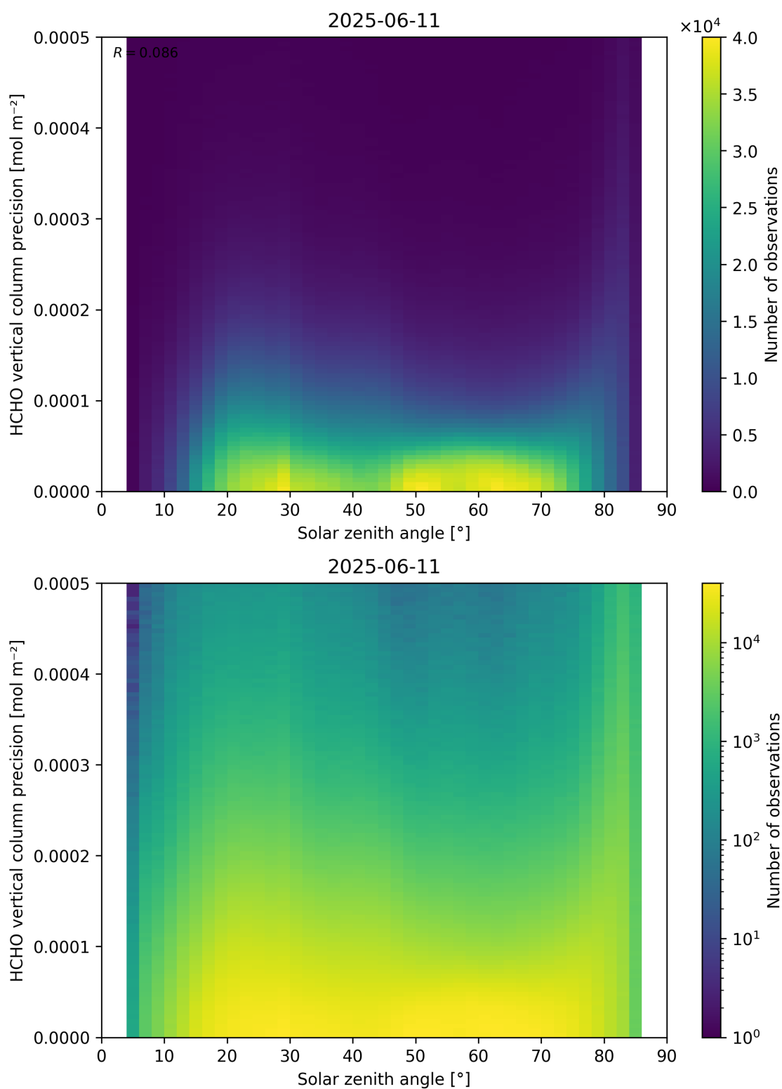
Figure 179: Scatter density plot of “Solar zenith angle” against “HCHO vertical column precision” for 2025-06-11 to 2025-06-12.
