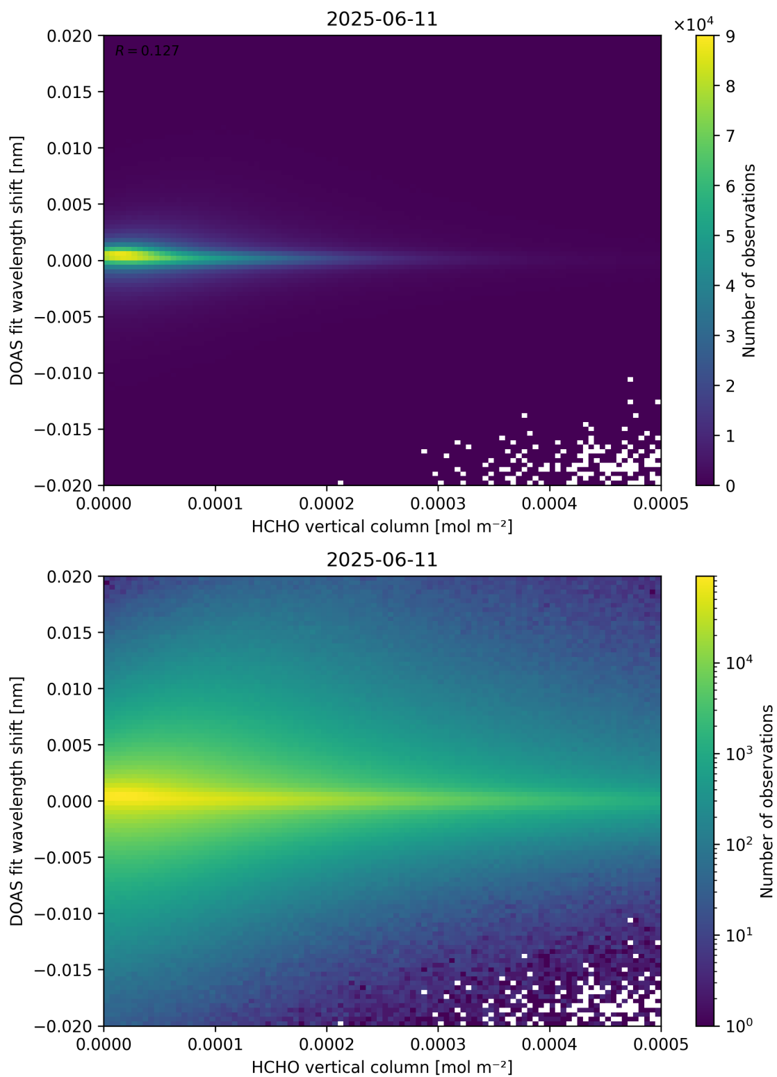
Figure 124: Scatter density plot of “HCHO vertical column” against “DOAS fit wavelength shift” for 2025-06-11 to 2025-06-12.
