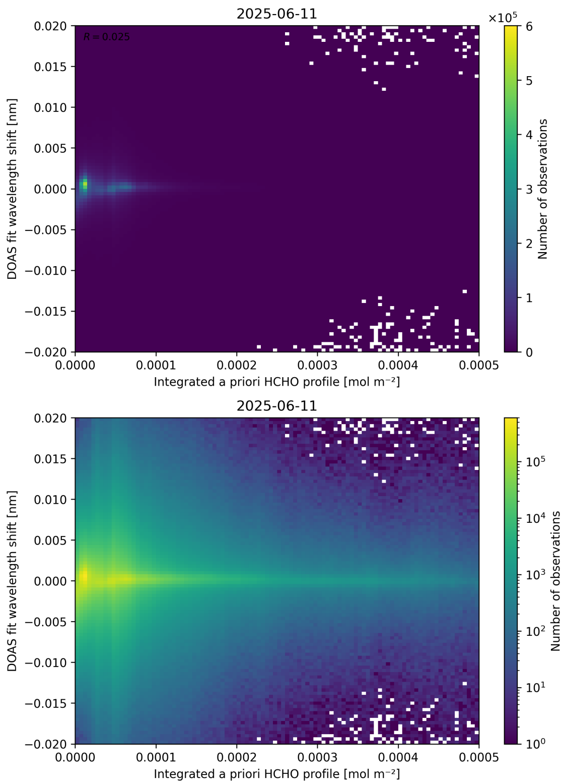
Figure 149: Scatter density plot of “Integrated a priori HCHO profile” against “DOAS fit wavelength shift” for 2025-06-11 to 2025-06-12.
