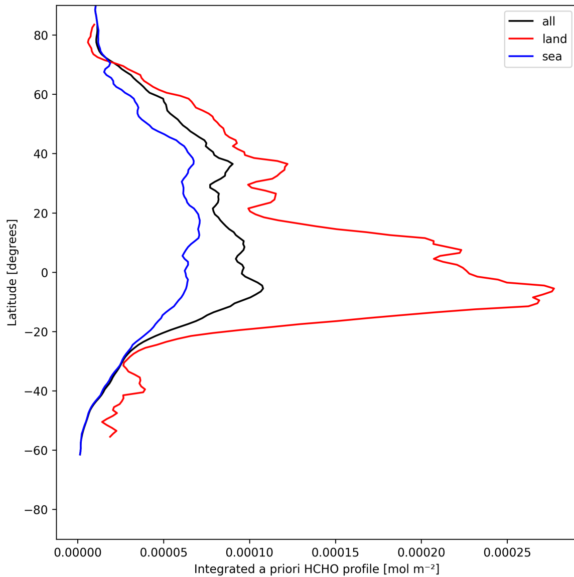
Figure 29: Zonal average of “Integrated a priori HCHO profile” for 2025-06-11 to 2025-06-12.
