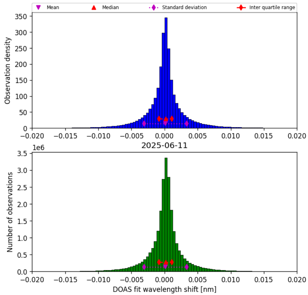
Figure 44: Histogram of “DOAS fit wavelength shift” for 2025-06-11 to 2025-06-12
