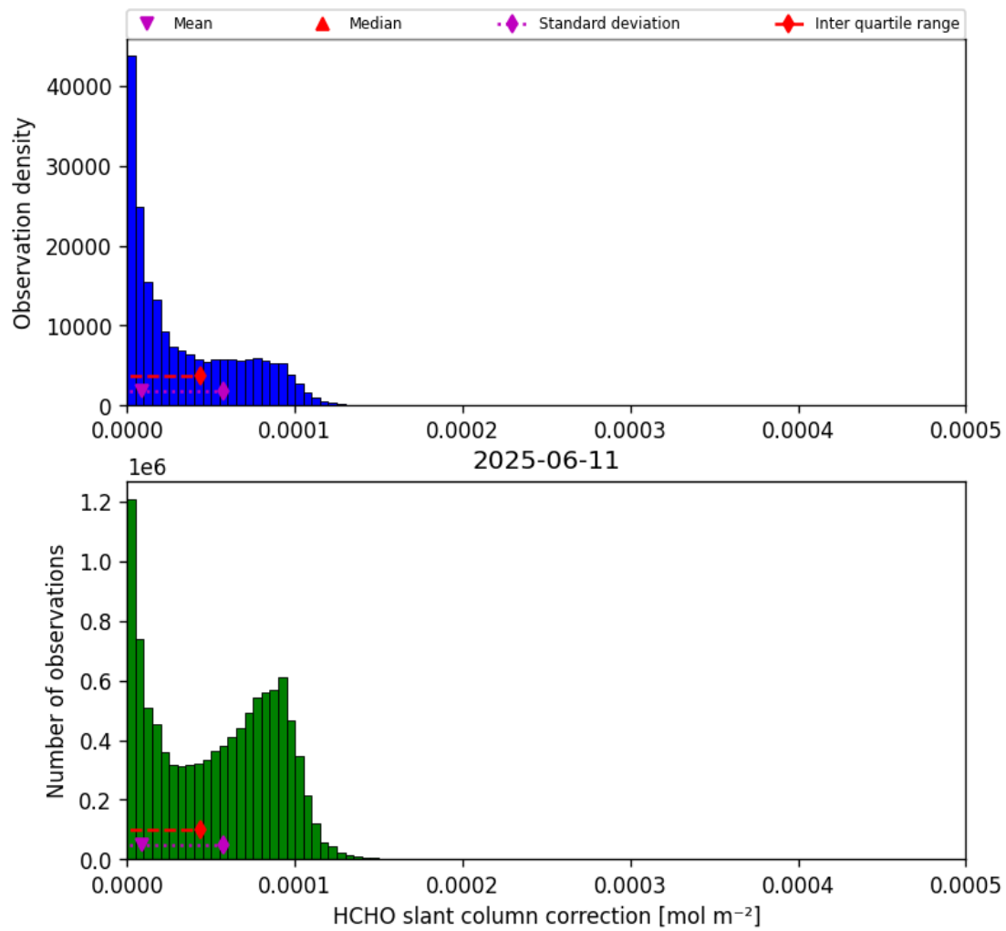
Figure 47: Histogram of “HCHO slant column correction” for 2025-06-11 to 2025-06-12
