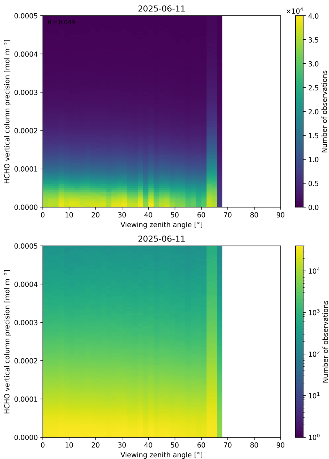
Figure 194: Scatter density plot of “Viewing zenith angle” against “HCHO vertical column precision” for 2025-06-11 to 2025-06-12.
