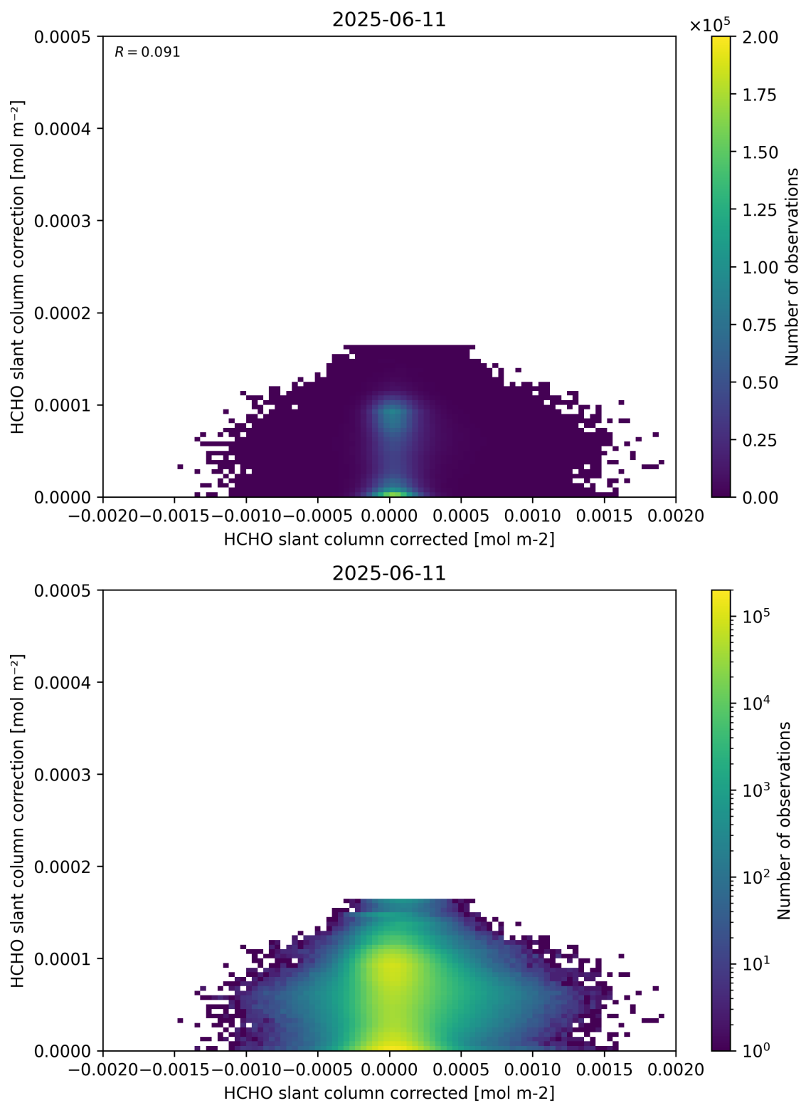
Figure 77: Scatter density plot of “HCHO slant column corrected” against “HCHO slant column correction” for 2025-06-11 to 2025-06-12.
