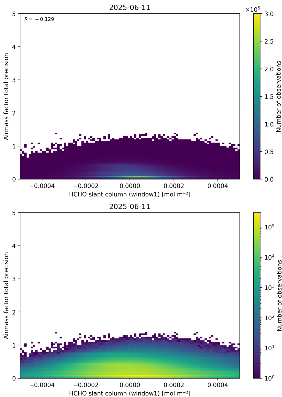
Figure 86: Scatter density plot of “HCHO slant column (window1)” against “Airmass factor total precision” for 2025-06-11 to 2025-06-12.
