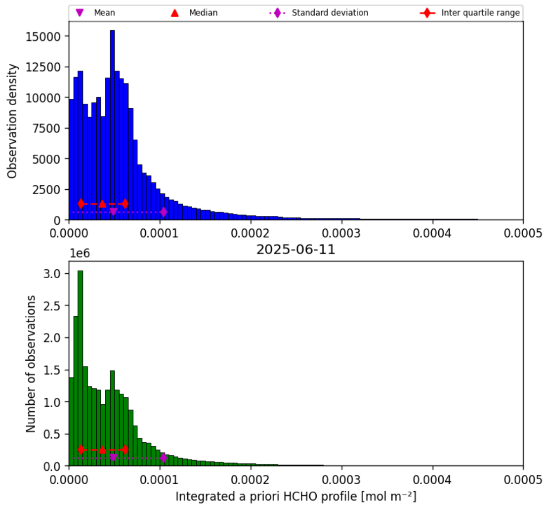
Figure 43: Histogram of “Integrated a priori HCHO profile” for 2025-06-11 to 2025-06-12
