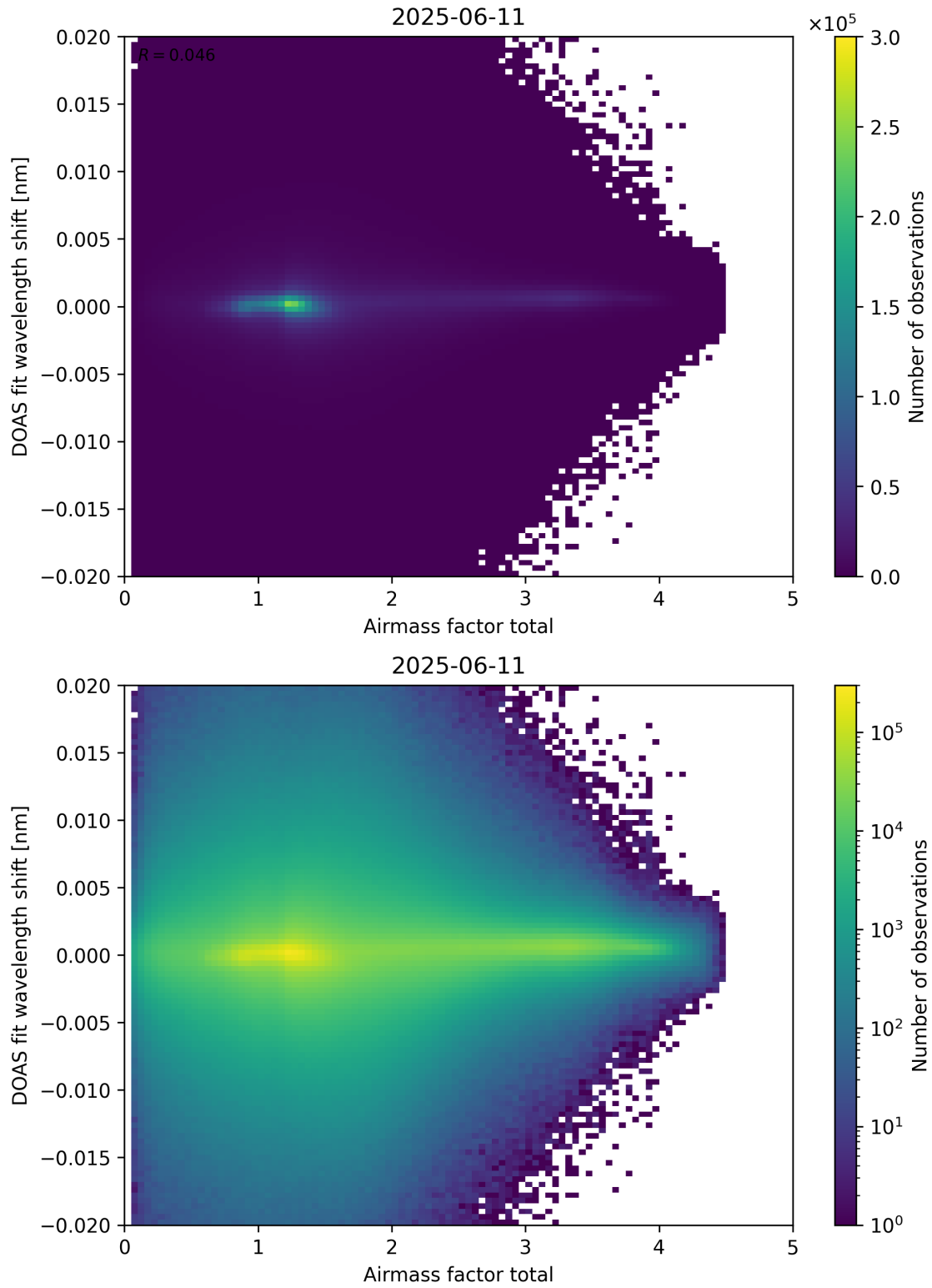
Figure 98: Scatter density plot of “Airmass factor total” against “DOAS fit wavelength shift” for 2025-06-11 to 2025-06-12.
