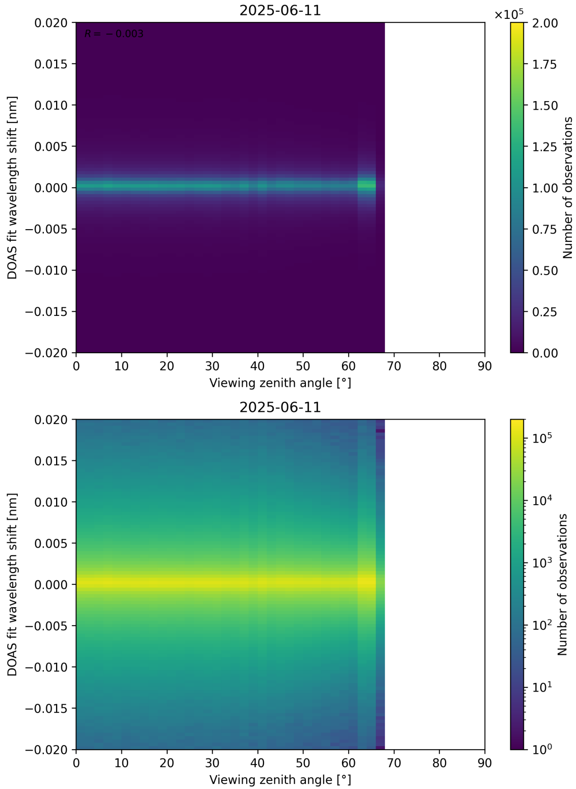
Figure 183: Scatter density plot of “Viewing zenith angle” against “DOAS fit wavelength shift” for 2025-06-11 to 2025-06-12.
