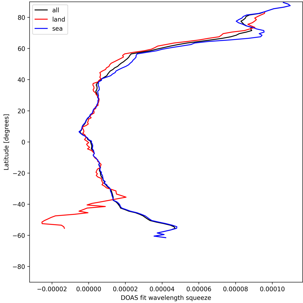
Figure 31: Zonal average of “DOAS fit wavelength squeeze” for 2025-06-11 to 2025-06-12.
