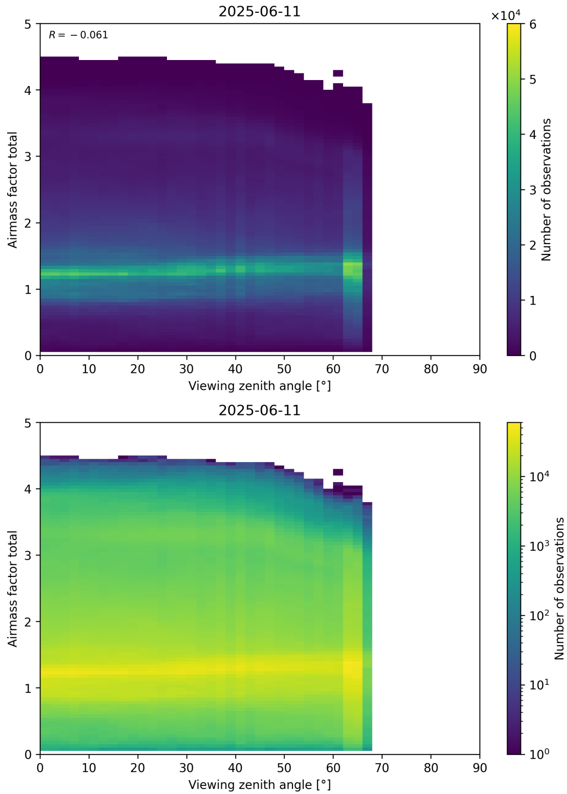
Figure 190: Scatter density plot of “Viewing zenith angle” against “Airmass factor total” for 2025-06-11 to 2025-06-12.
