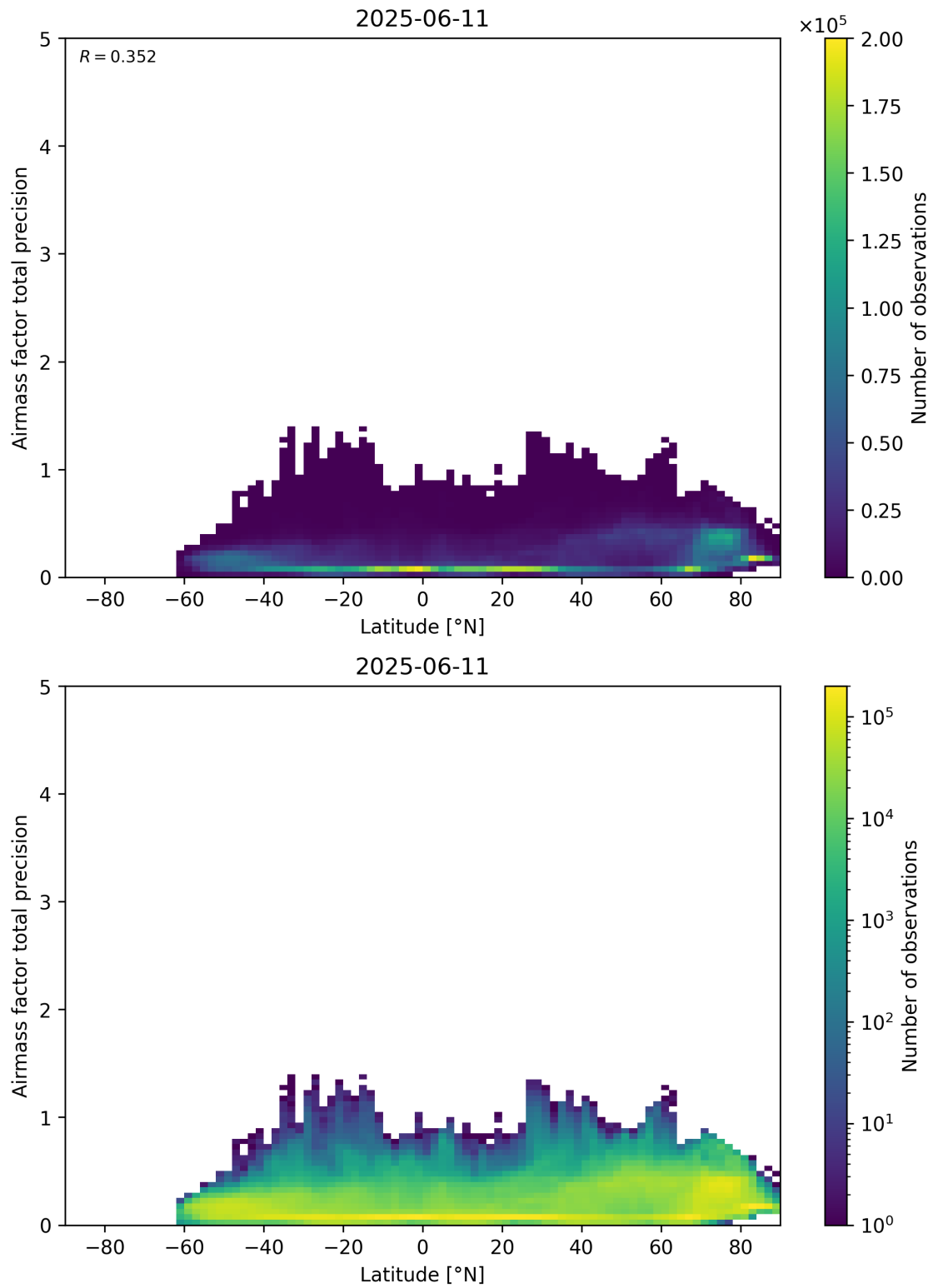
Figure 162: Scatter density plot of “Latitude” against “Airmass factor total precision” for 2025-06-11 to 2025-06-12.
