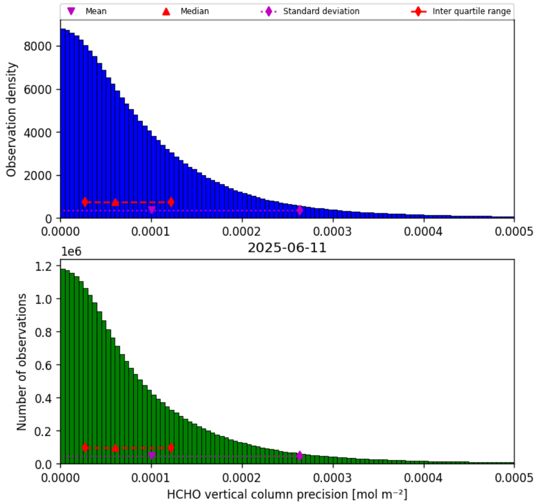
Figure 36: Histogram of “HCHO vertical column precision” for 2025-06-11 to 2025-06-12
