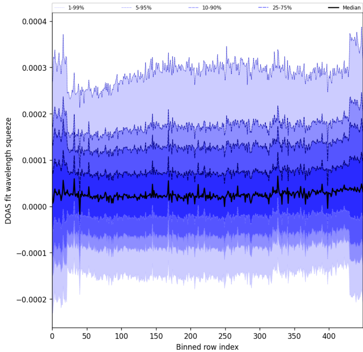
Figure 59: Along track statistics of “DOAS fit wavelength squeeze” for 2025-06-11 to 2025-06-12
