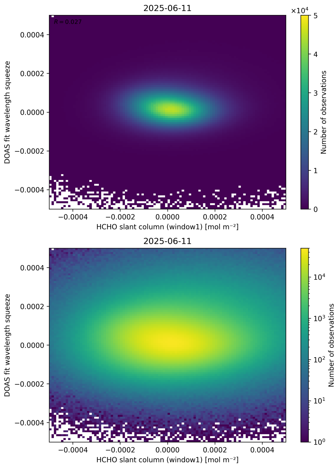
Figure 80: Scatter density plot of “HCHO slant column (window1)” against “DOAS fit wavelength squeeze” for 2025-06-11 to 2025-06-12.
