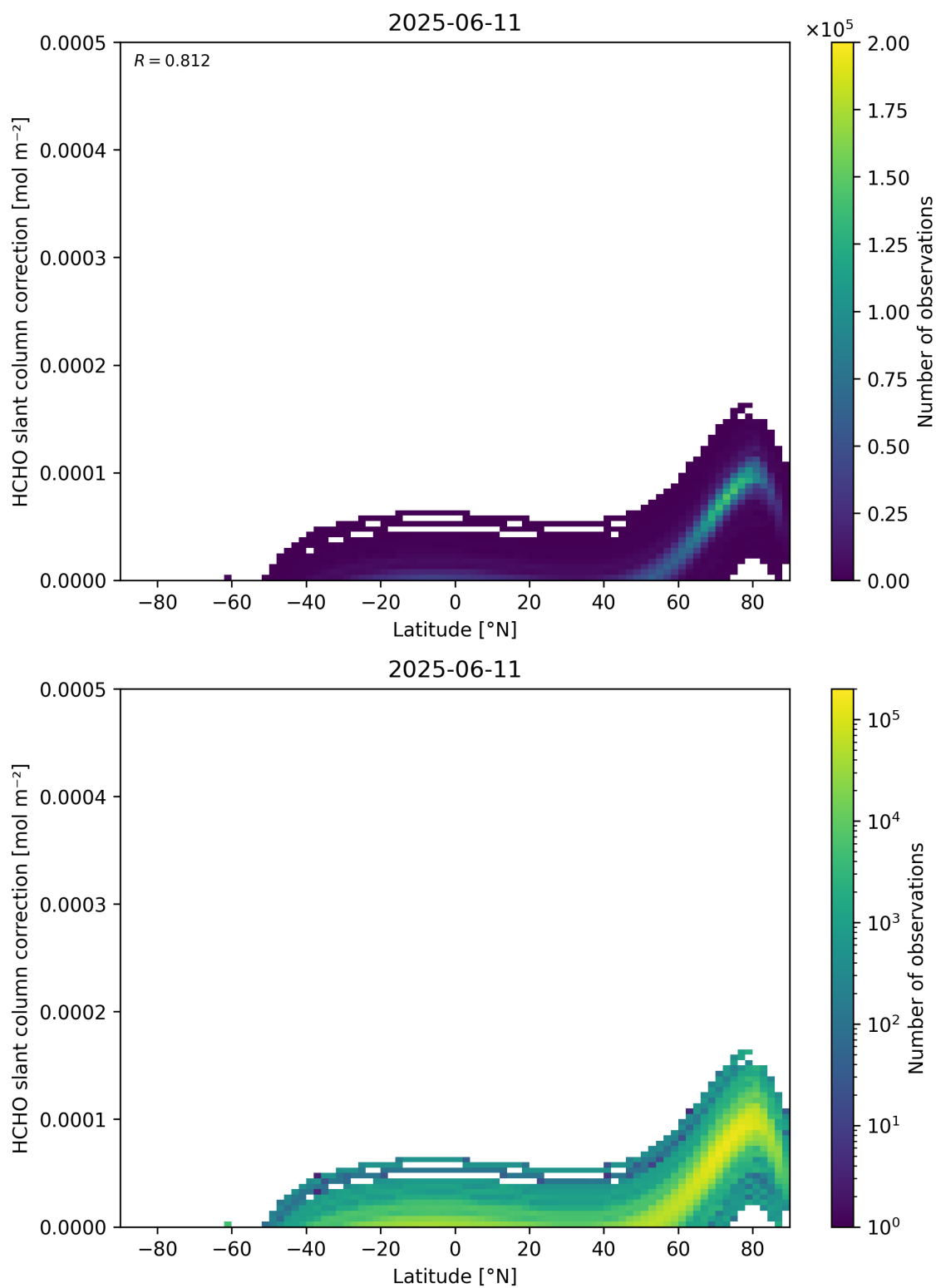
Figure 158: Scatter density plot of “Latitude” against “HCHO slant column correction” for 2025-06-11 to 2025-06-12.
