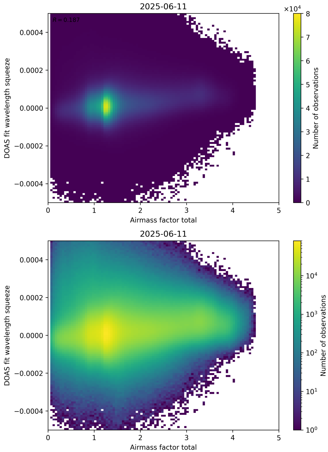
Figure 99: Scatter density plot of “Airmass factor total” against “DOAS fit wavelength squeeze” for 2025-06-11 to 2025-06-12.
