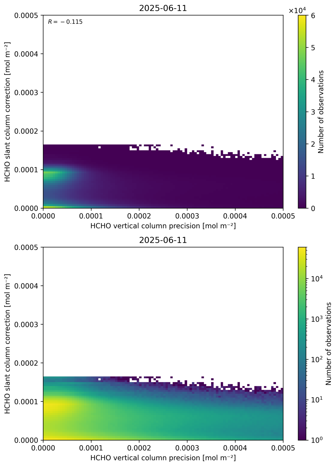
Figure 141: Scatter density plot of “HCHO vertical column precision” against “HCHO slant column correction” for 2025-06-11 to 2025-06-12.
