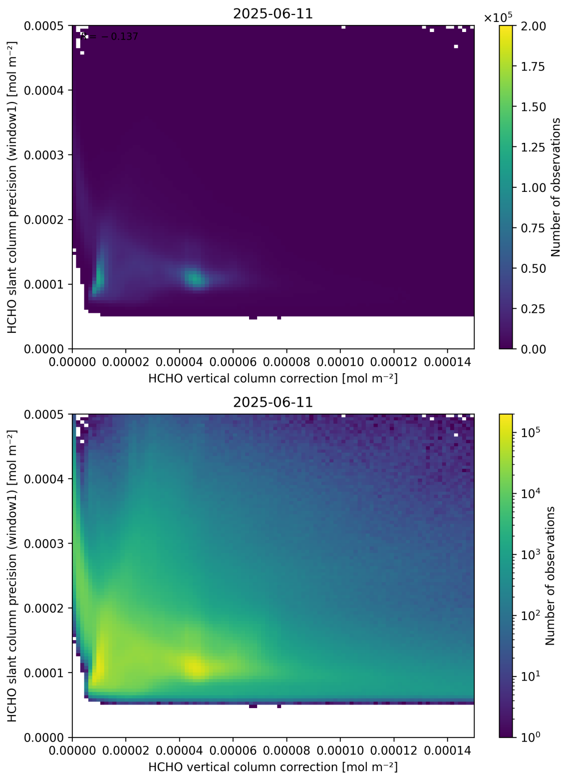
Figure 119: Scatter density plot of “HCHO vertical column correction” against “HCHO slant column precision (window1)” for 2025-06-11 to 2025-06-12.
