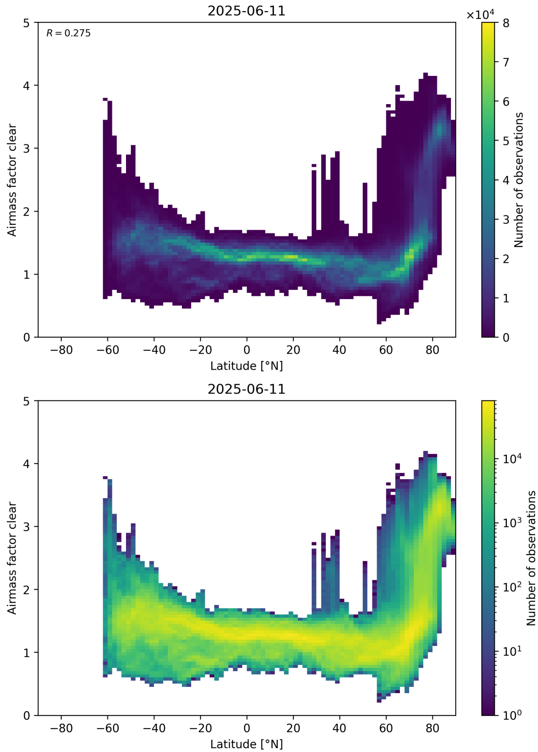
Figure 156: Scatter density plot of “Latitude” against “Airmass factor clear” for 2025-06-11 to 2025-06-12.
