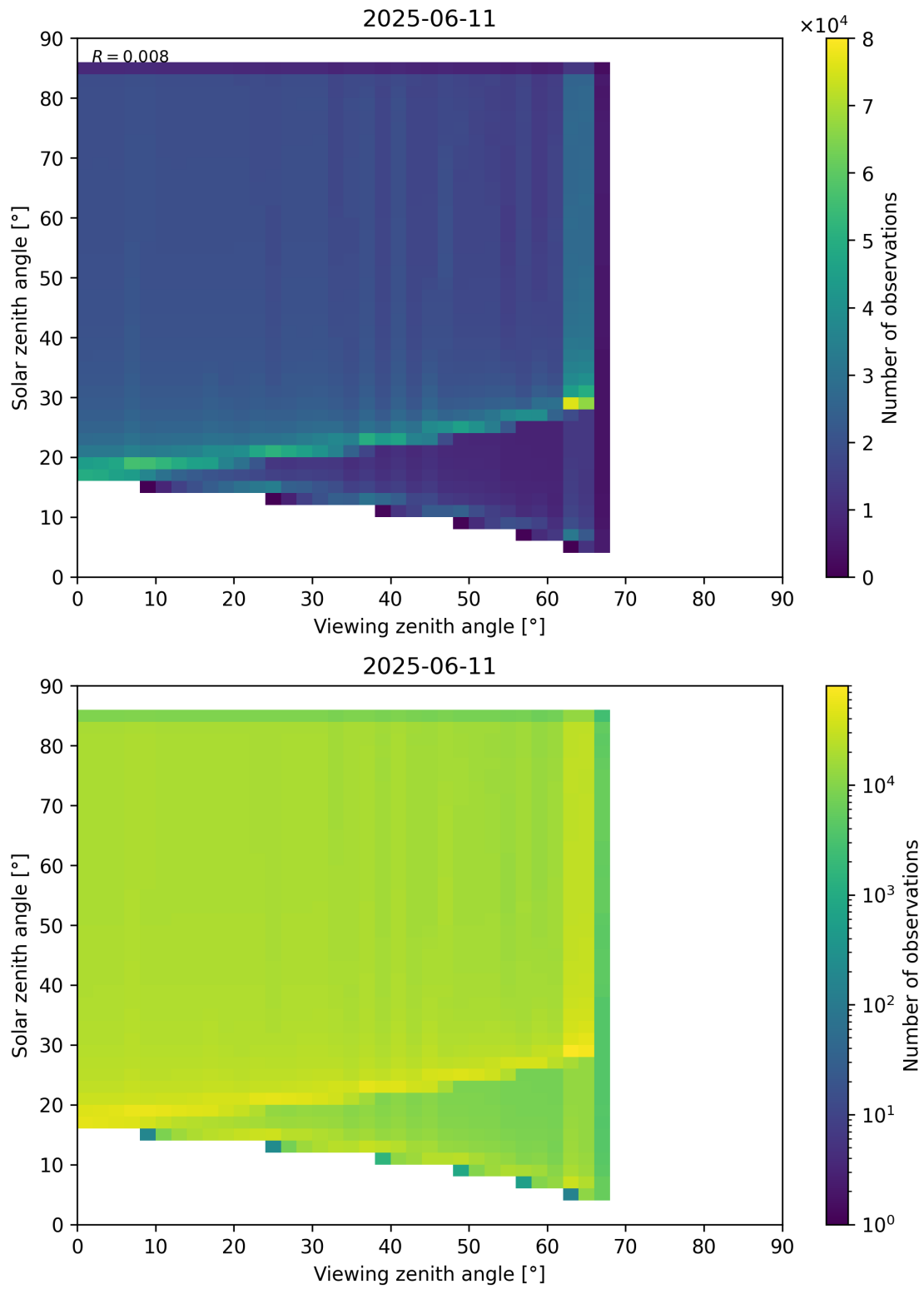
Figure 197: Scatter density plot of “Viewing zenith angle” against “Solar zenith angle” for 2025-06-11 to 2025-06-12.
