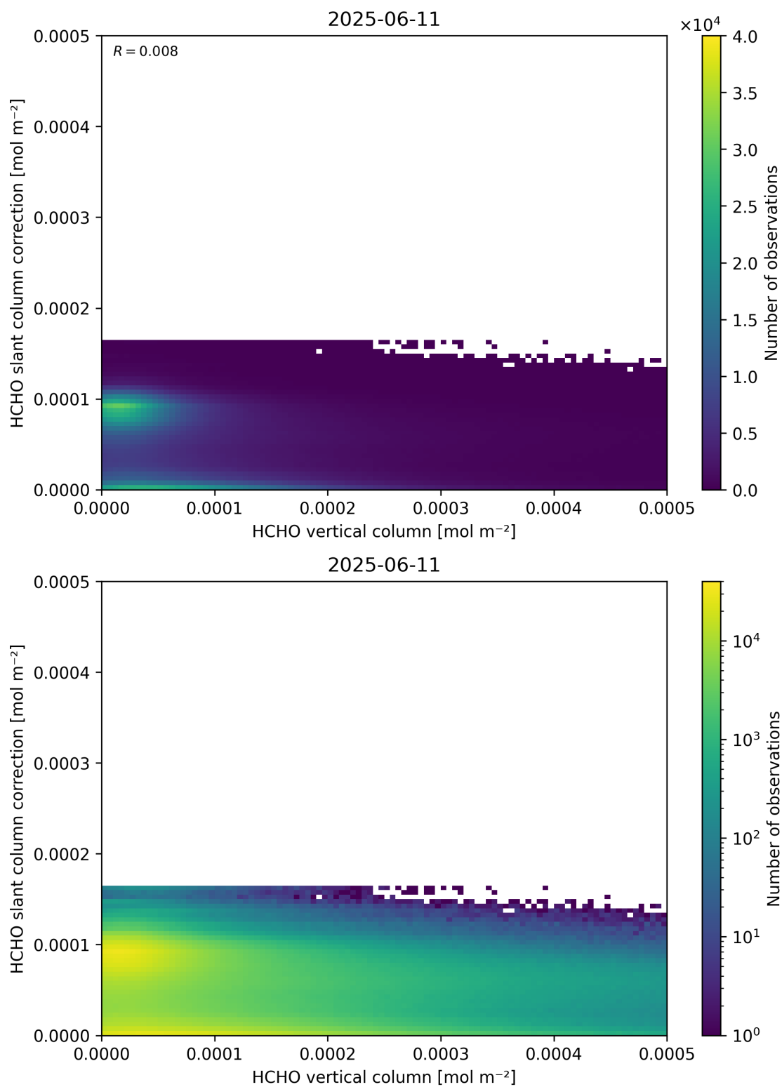
Figure 128: Scatter density plot of “HCHO vertical column” against “HCHO slant column correction” for 2025-06-11 to 2025-06-12.
