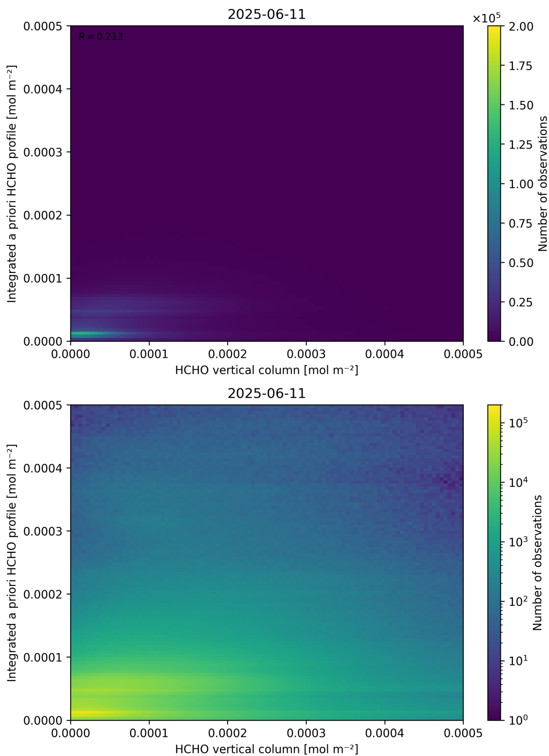
Figure 135: Scatter density plot of “HCHO vertical column” against “Integrated a priori HCHO profile” for 2025-06-11 to 2025-06-12.
