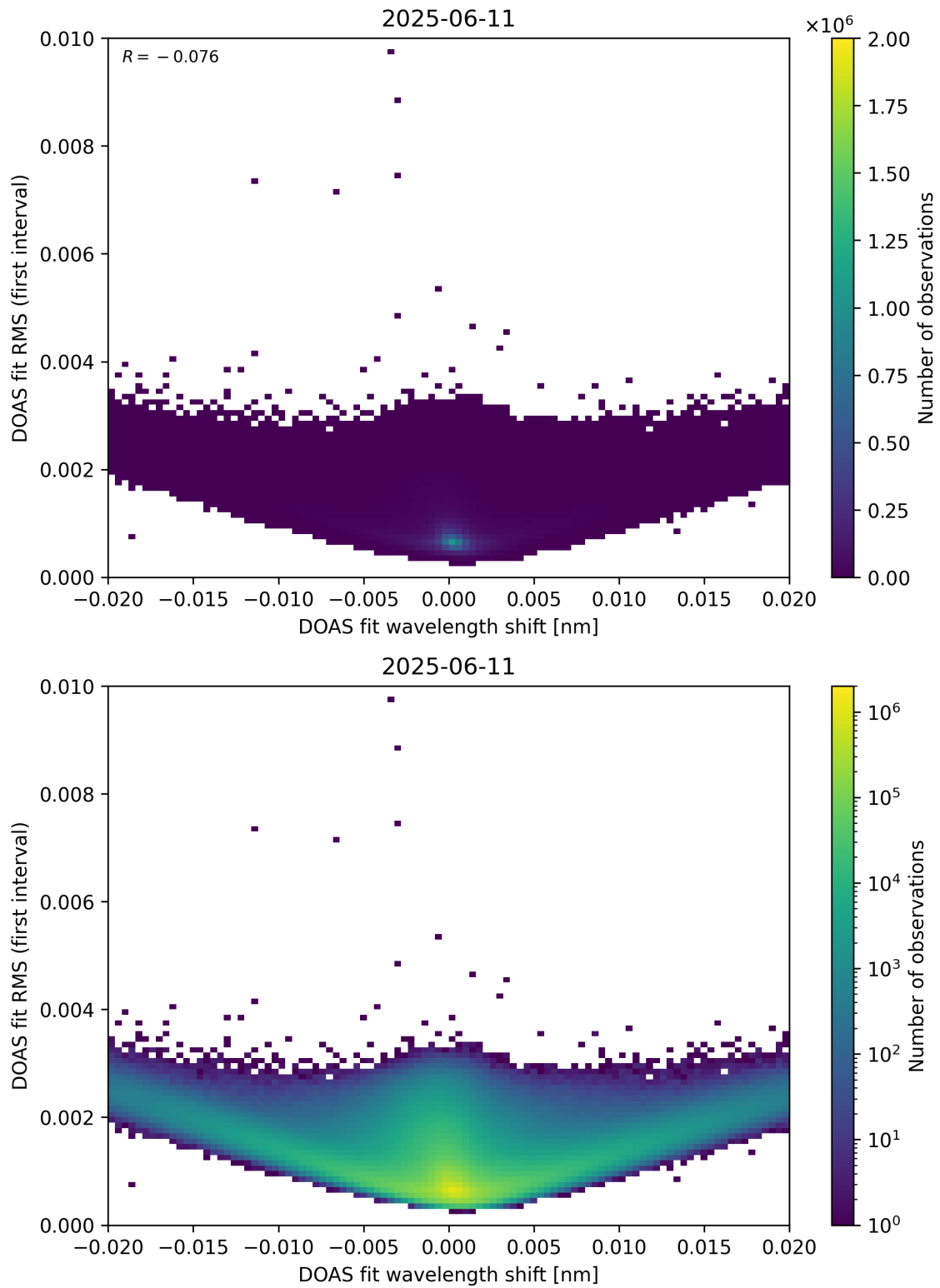
Figure 64: Scatter density plot of “DOAS fit wavelength shift” against “DOAS fit RMS (first interval)” for 2025-06-11 to 2025-06-12.
