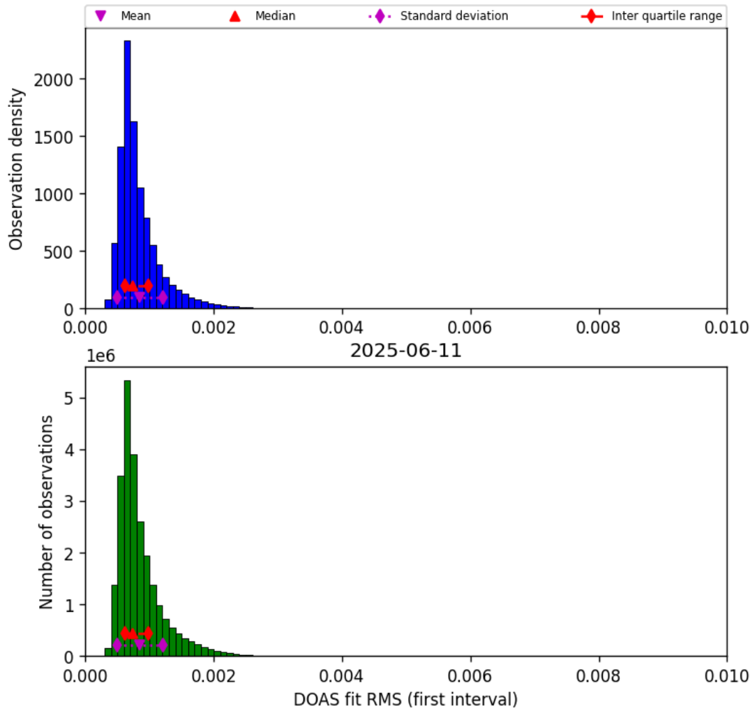
Figure 46: Histogram of “DOAS fit RMS (first interval)” for 2025-06-11 to 2025-06-12
