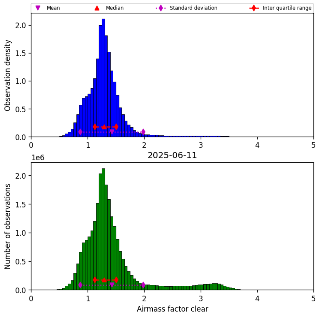
Figure 42: Histogram of “Airmass factor clear” for 2025-06-11 to 2025-06-12
