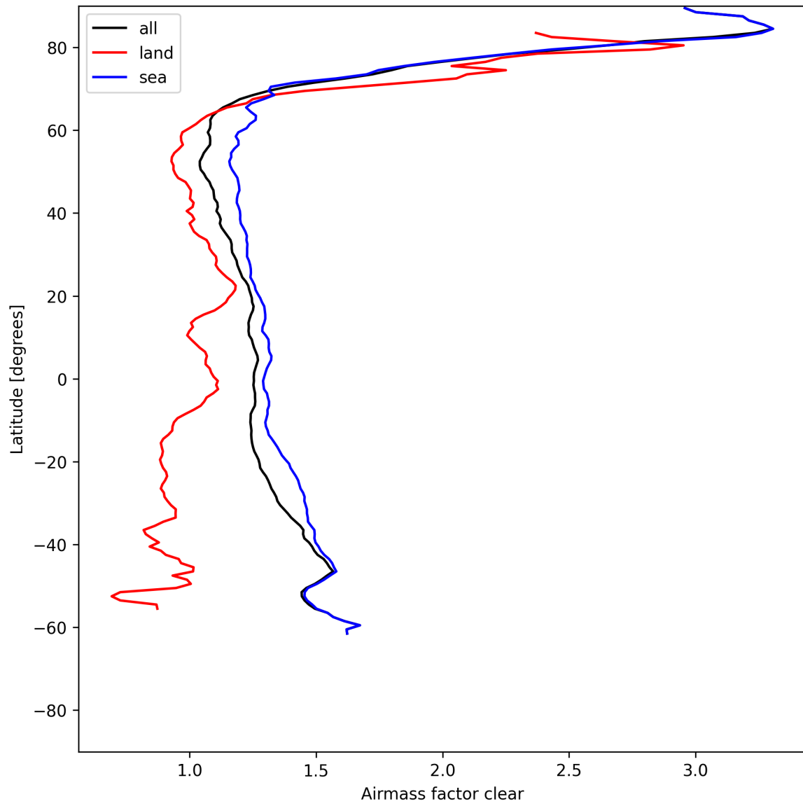
Figure 28: Zonal average of “Airmass factor clear” for 2025-06-11 to 2025-06-12.
