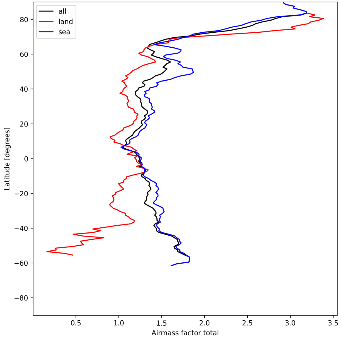
Figure 26: Zonal average of “Airmass factor total” for 2025-06-11 to 2025-06-12.
