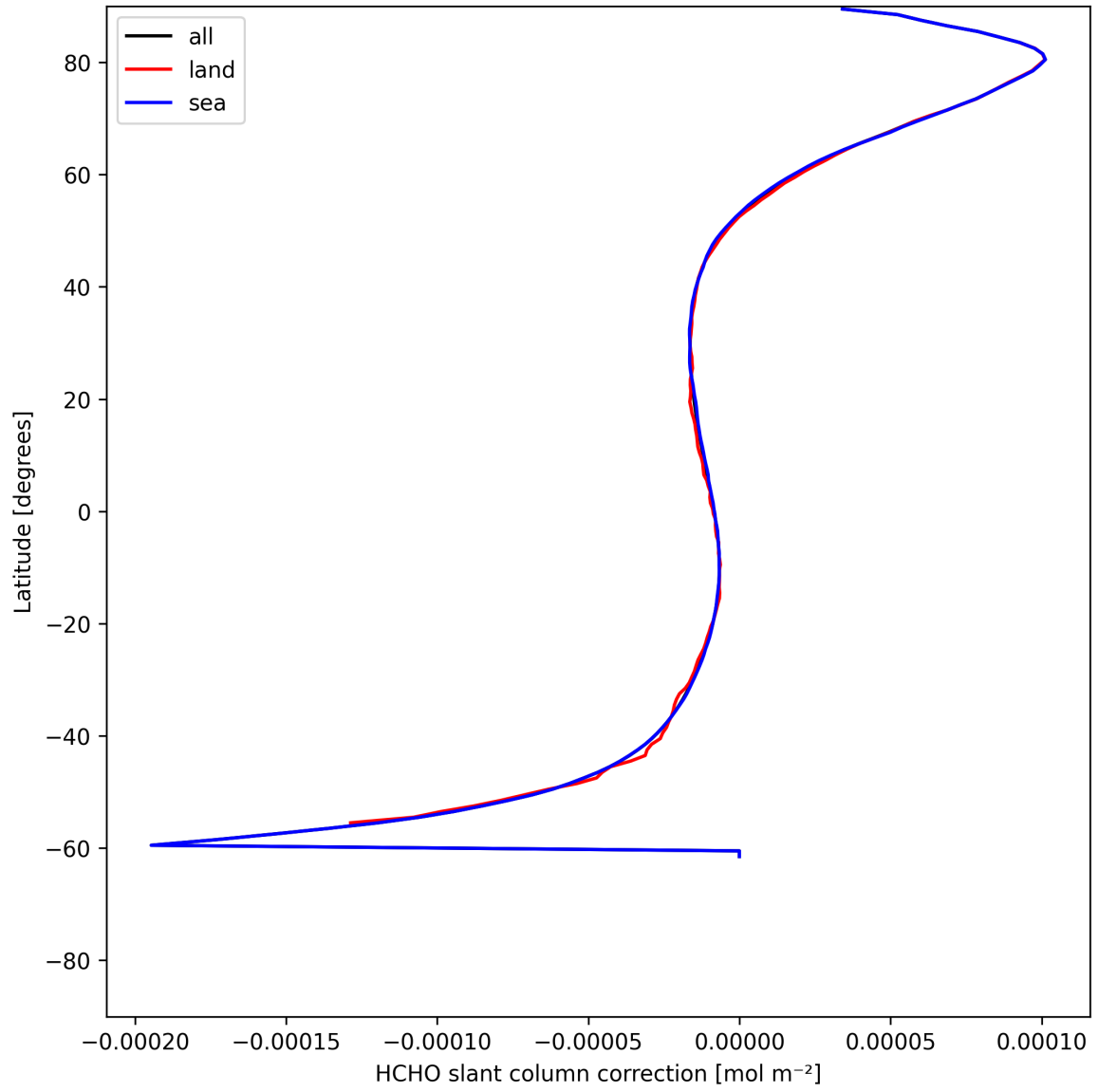
Figure 33: Zonal average of “HCHO slant column correction” for 2025-06-11 to 2025-06-13.
