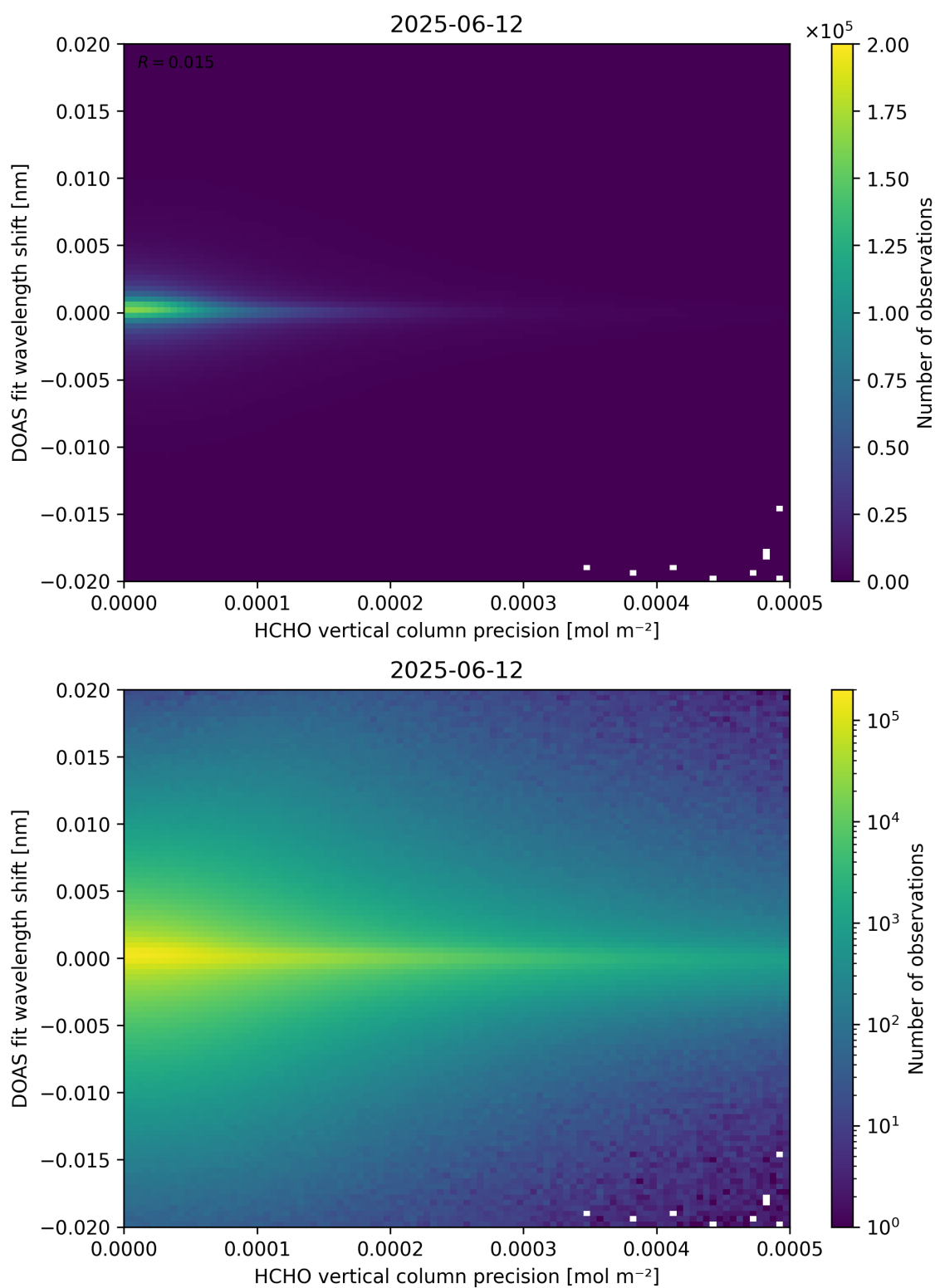
Figure 137: Scatter density plot of “HCHO vertical column precision” against “DOAS fit wavelength shift” for 2025-06-11 to 2025-06-13.
