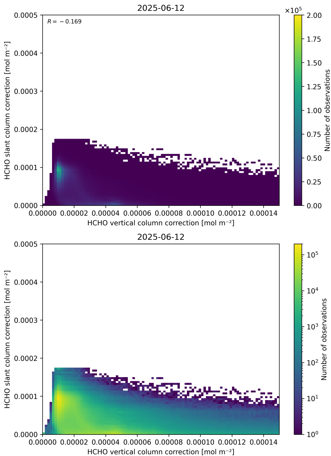
Figure 117: Scatter density plot of “HCHO vertical column correction” against “HCHO slant column correction” for 2025-06-11 to 2025-06-13.
