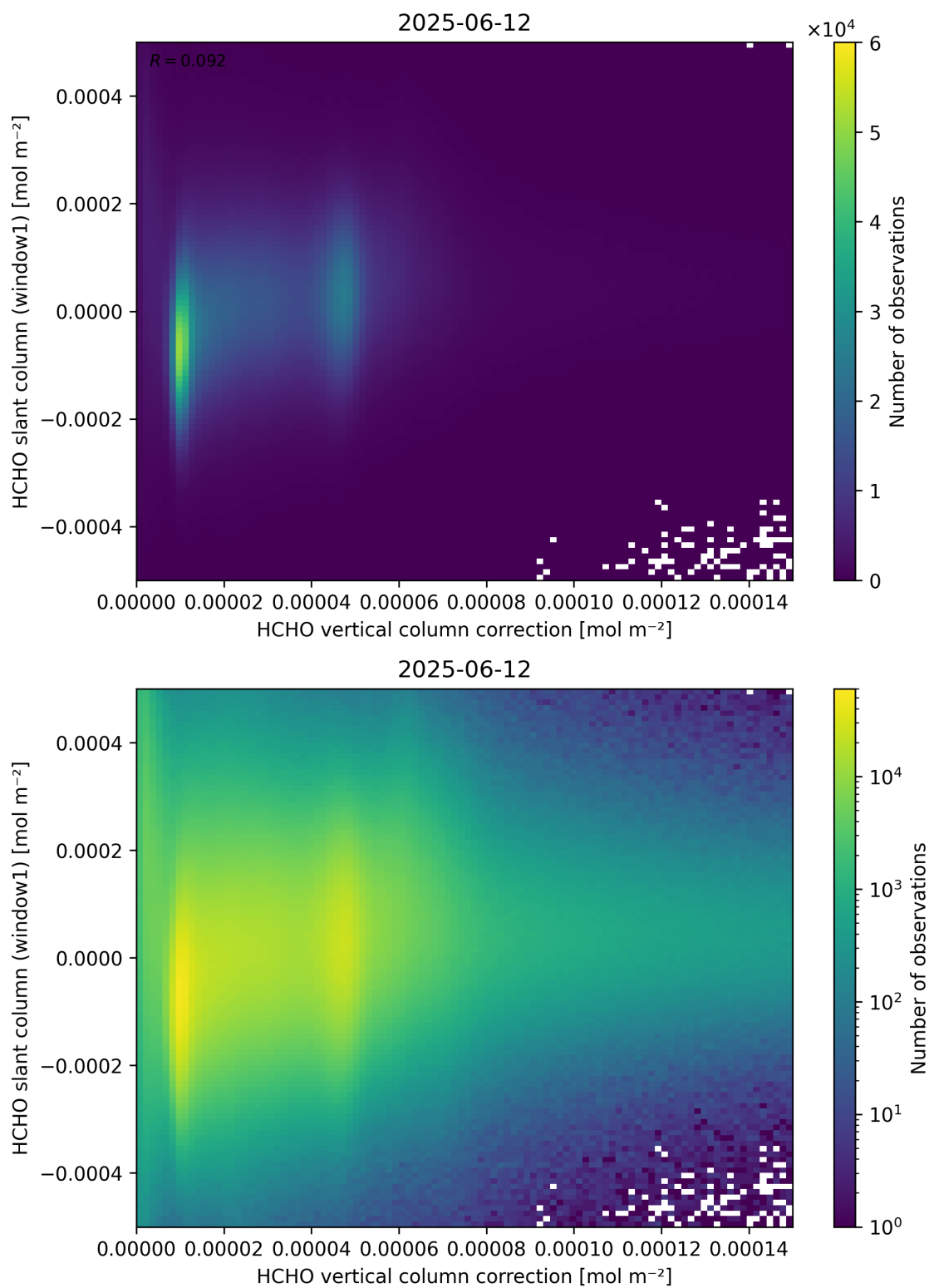
Figure 118: Scatter density plot of “HCHO vertical column correction” against “HCHO slant column (window1)” for 2025-06-11 to 2025-06-13.
