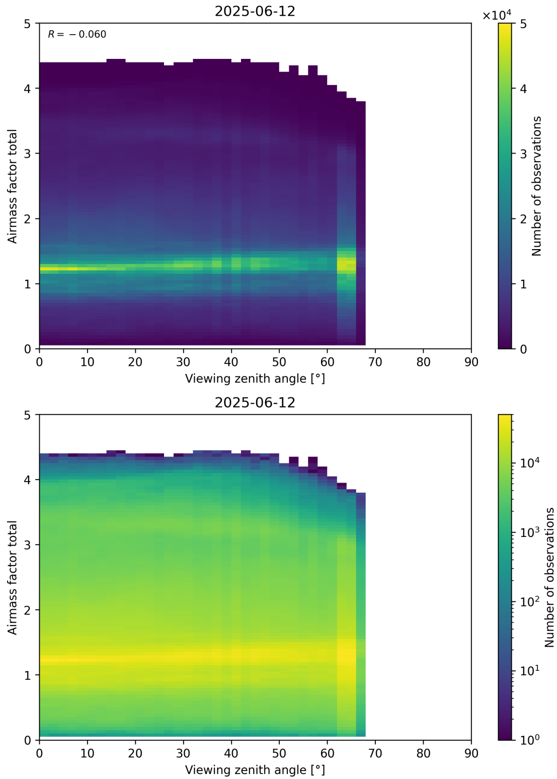
Figure 190: Scatter density plot of “Viewing zenith angle” against “Airmass factor total” for 2025-06-11 to 2025-06-13.
