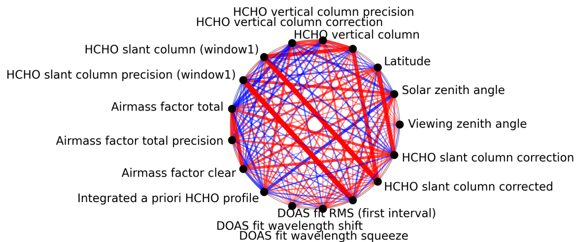
Figure 1: Map of correlation graph for 2025-06-11 to 2025-06-13.
