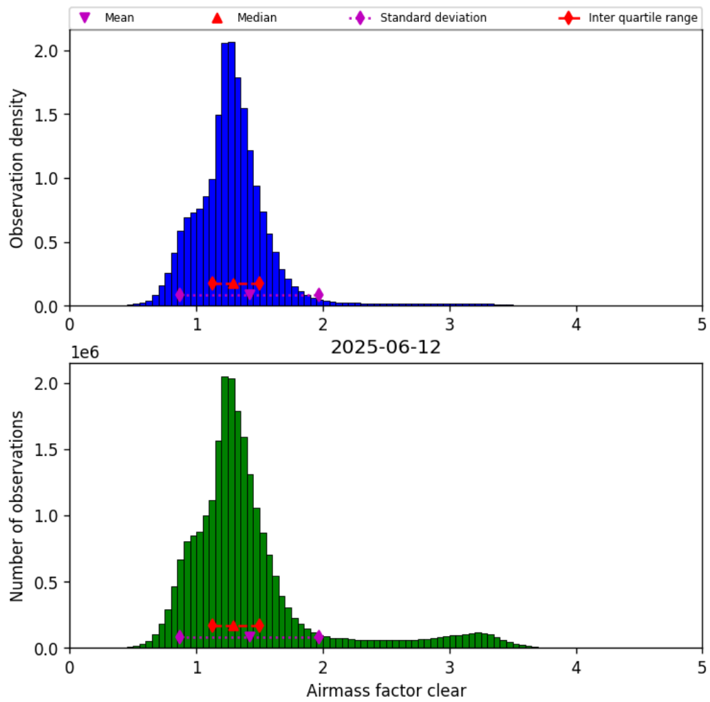
Figure 42: Histogram of “Airmass factor clear” for 2025-06-11 to 2025-06-13
