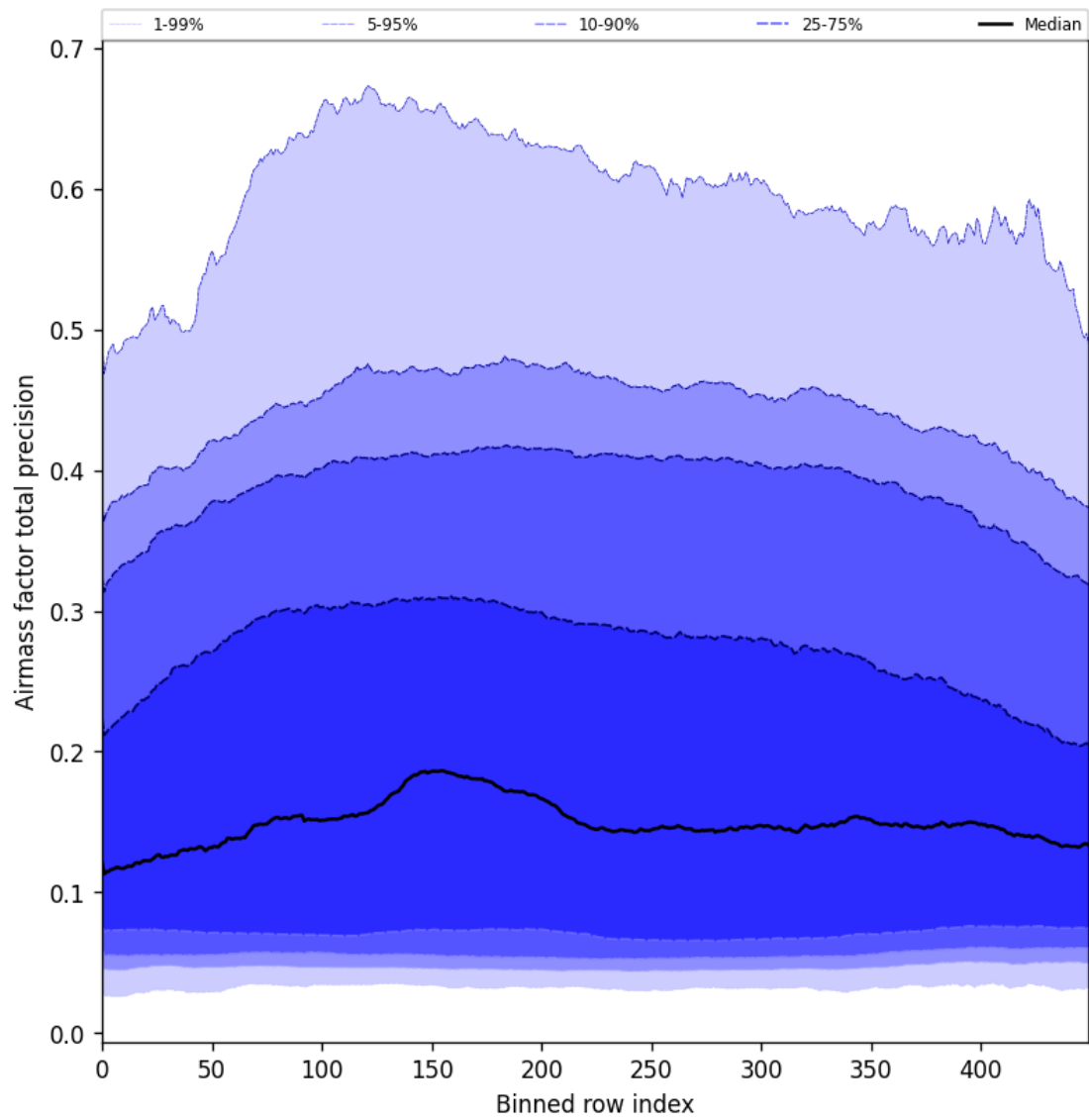
Figure 55: Along track statistics of “Airmass factor total precision” for 2025-06-11 to 2025-06-13
