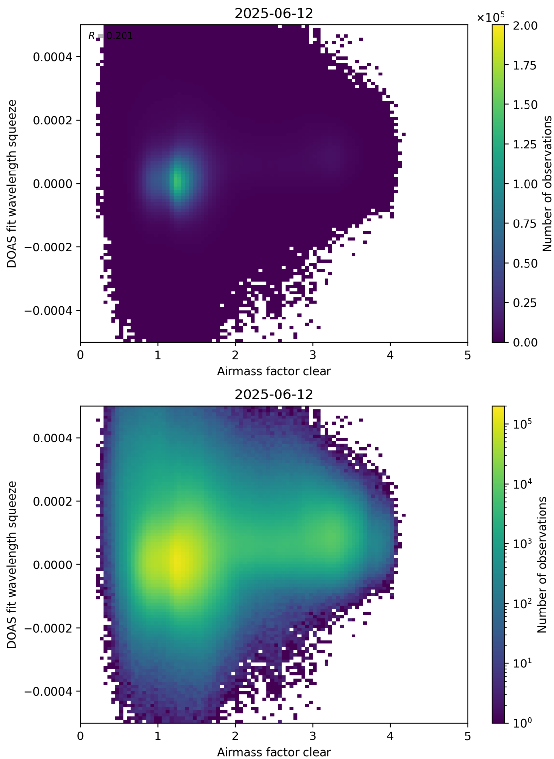
Figure 73: Scatter density plot of “Airmass factor clear” against “DOAS fit wavelength squeeze” for 2025-06-11 to 2025-06-13.
