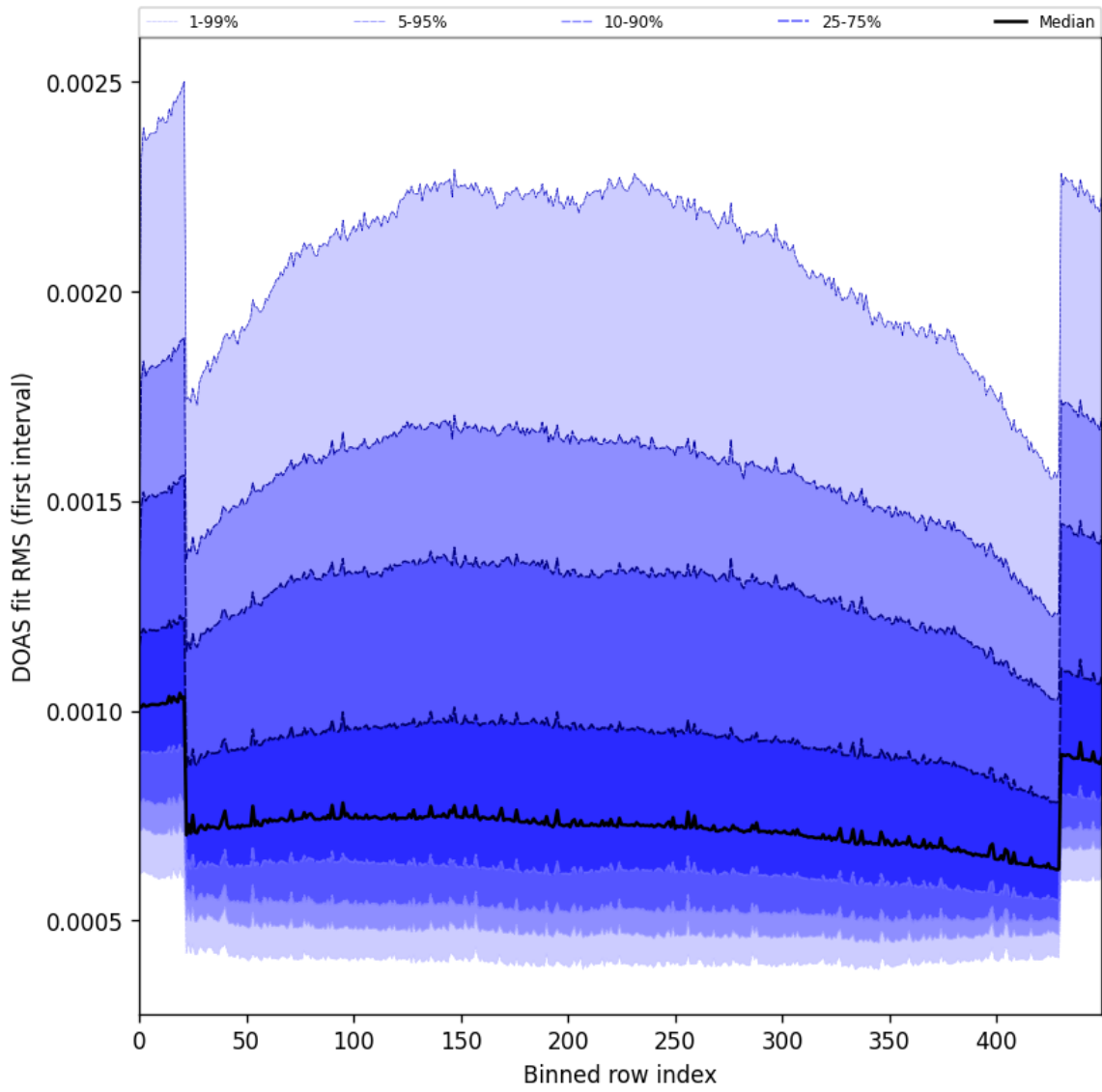
Figure 60: Along track statistics of “DOAS fit RMS (first interval)” for 2025-06-11 to 2025-06-13
