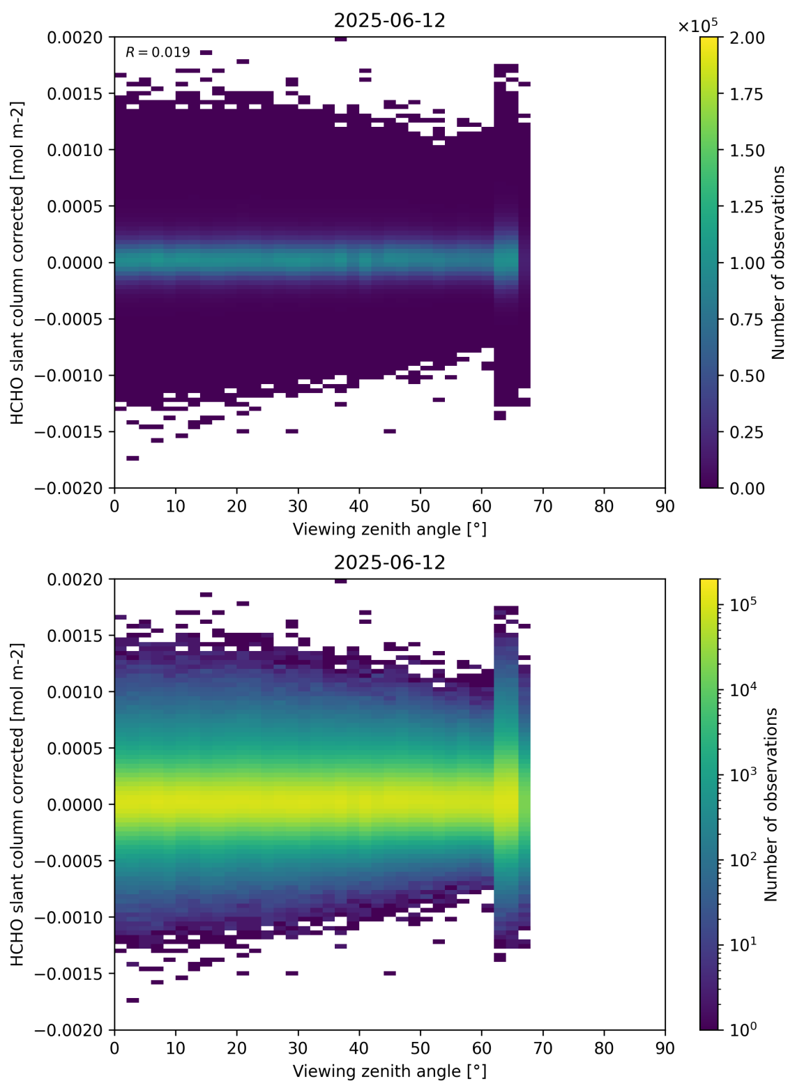
Figure 186: Scatter density plot of “Viewing zenith angle” against “HCHO slant column corrected” for 2025-06-11 to 2025-06-13.
