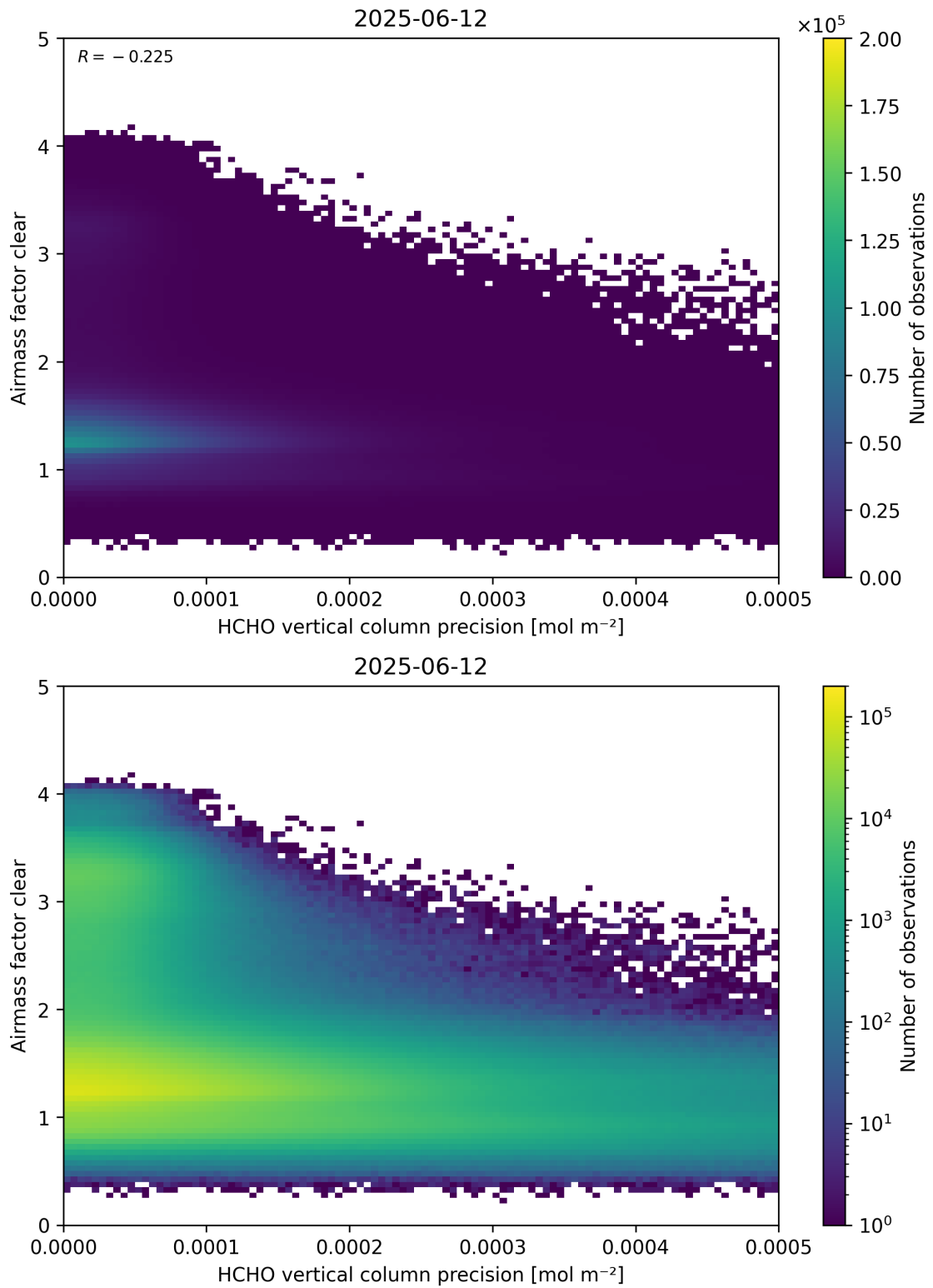
Figure 139: Scatter density plot of “HCHO vertical column precision” against “Airmass factor clear” for 2025-06-11 to 2025-06-13.
