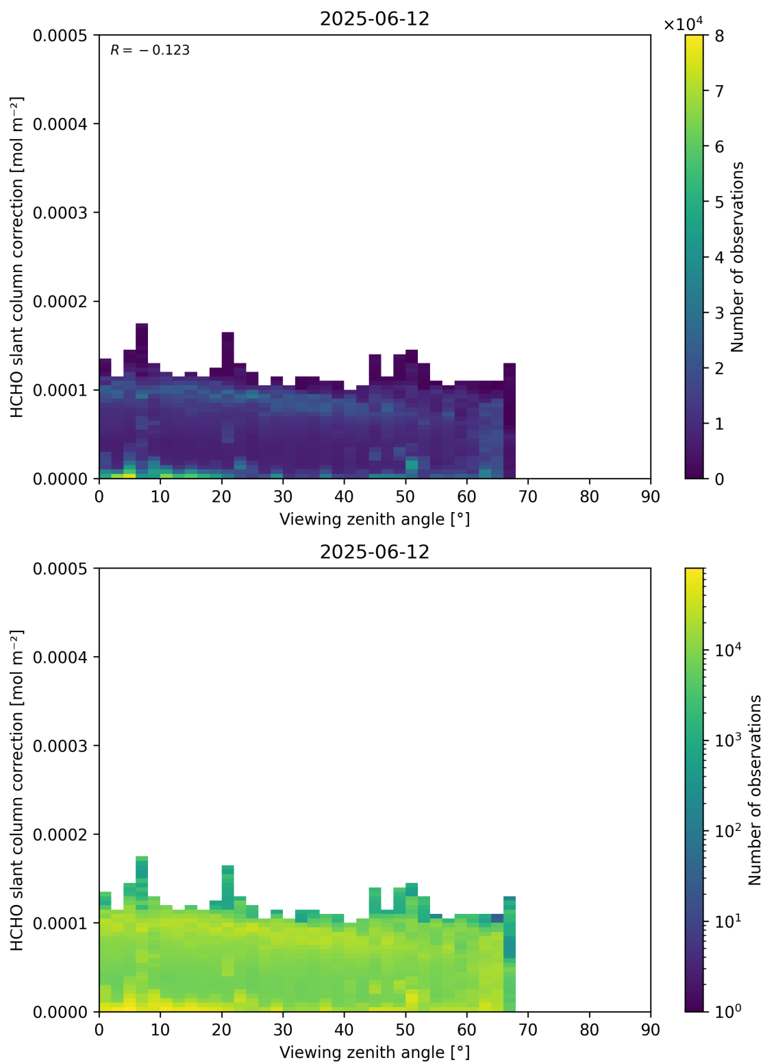
Figure 187: Scatter density plot of “Viewing zenith angle” against “HCHO slant column correction” for 2025-06-11 to 2025-06-13.
