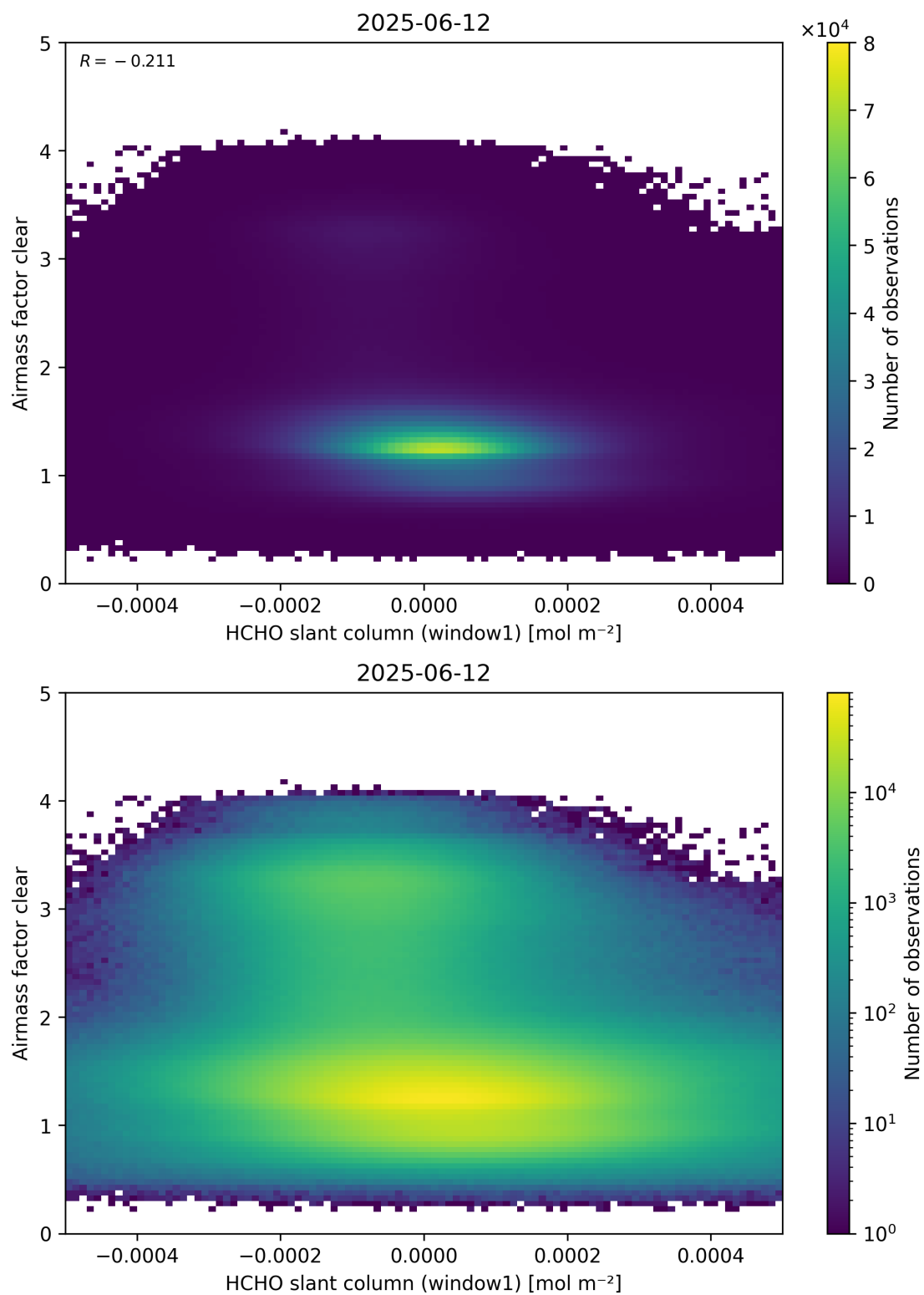
Figure 81: Scatter density plot of “HCHO slant column (window1)” against “Airmass factor clear” for 2025-06-11 to 2025-06-13.
