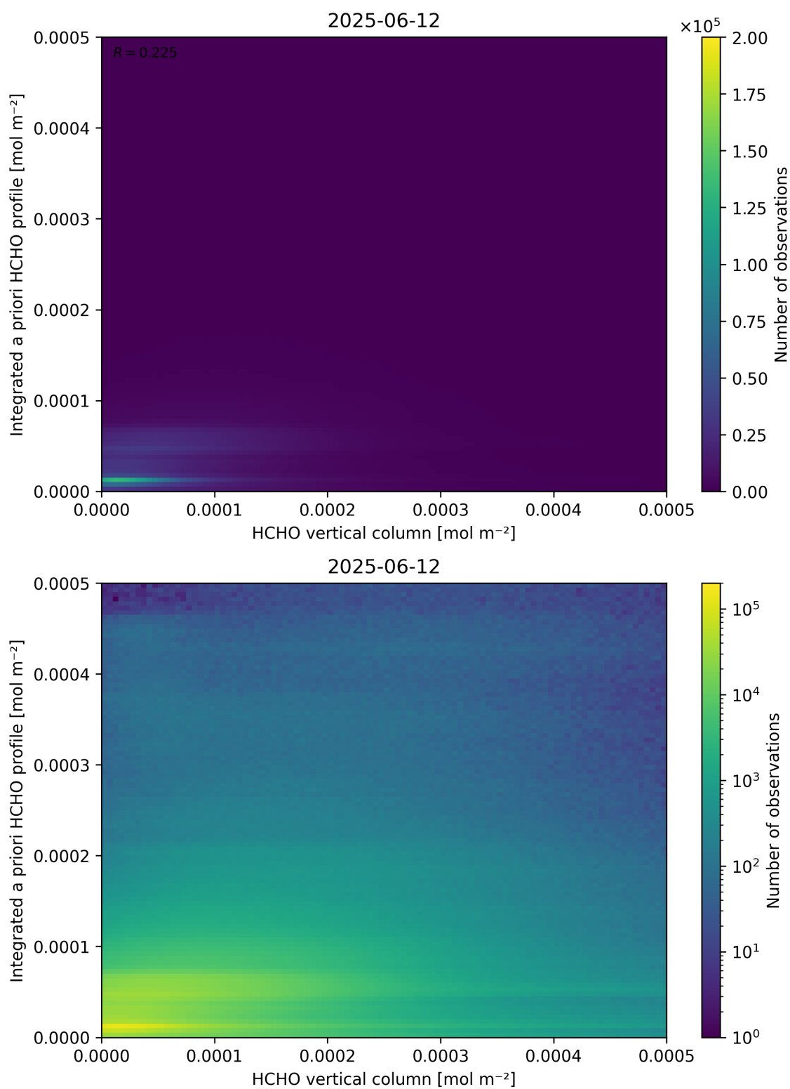
Figure 135: Scatter density plot of “HCHO vertical column” against “Integrated a priori HCHO profile” for 2025-06-11 to 2025-06-13.
