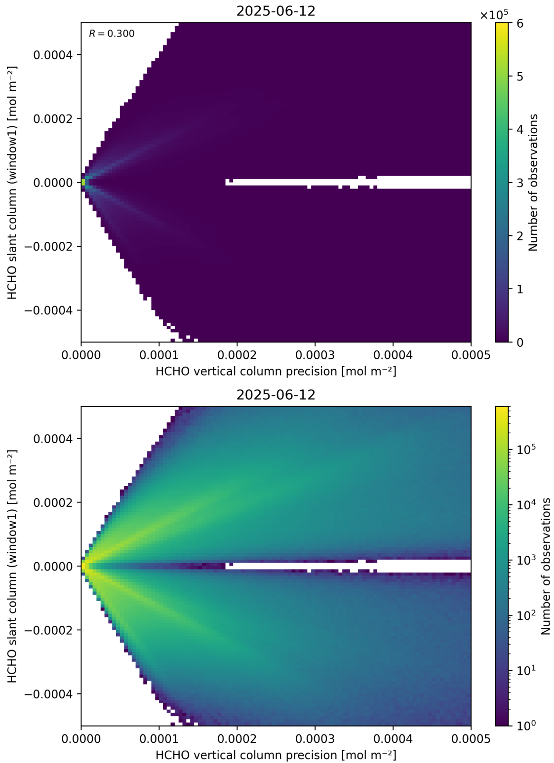
Figure 142: Scatter density plot of “HCHO vertical column precision” against “HCHO slant column (window1)” for 2025-06-11 to 2025-06-13.
