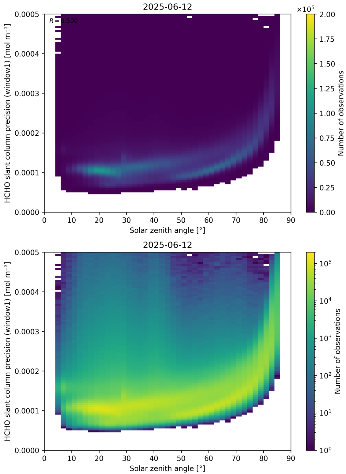
Figure 174: Scatter density plot of “Solar zenith angle” against “HCHO slant column precision (window1)” for 2025-06-11 to 2025-06-13.
