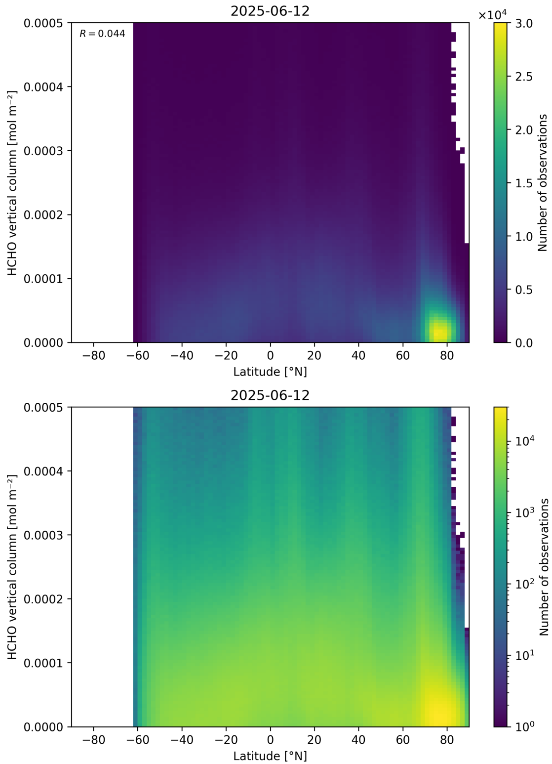
Figure 163: Scatter density plot of “Latitude” against “HCHO vertical column” for 2025-06-11 to 2025-06-13.
