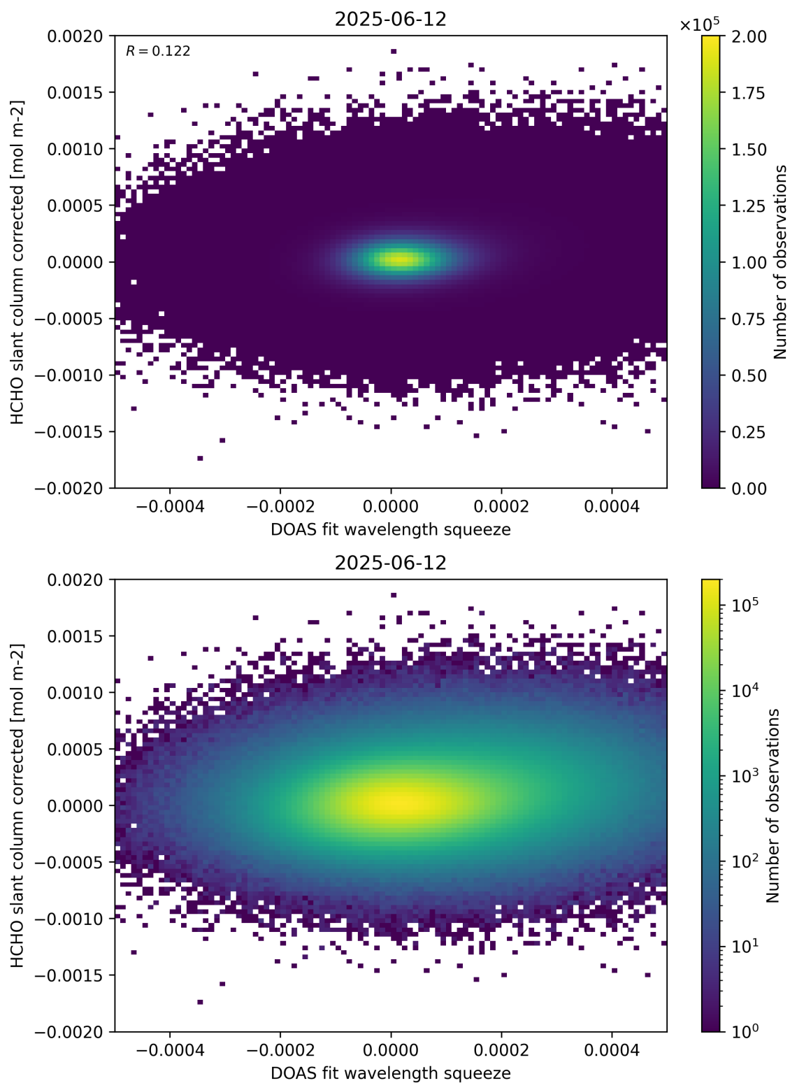
Figure 69: Scatter density plot of “DOAS fit wavelength squeeze” against “HCHO slant column corrected” for 2025-06-11 to 2025-06-13.
