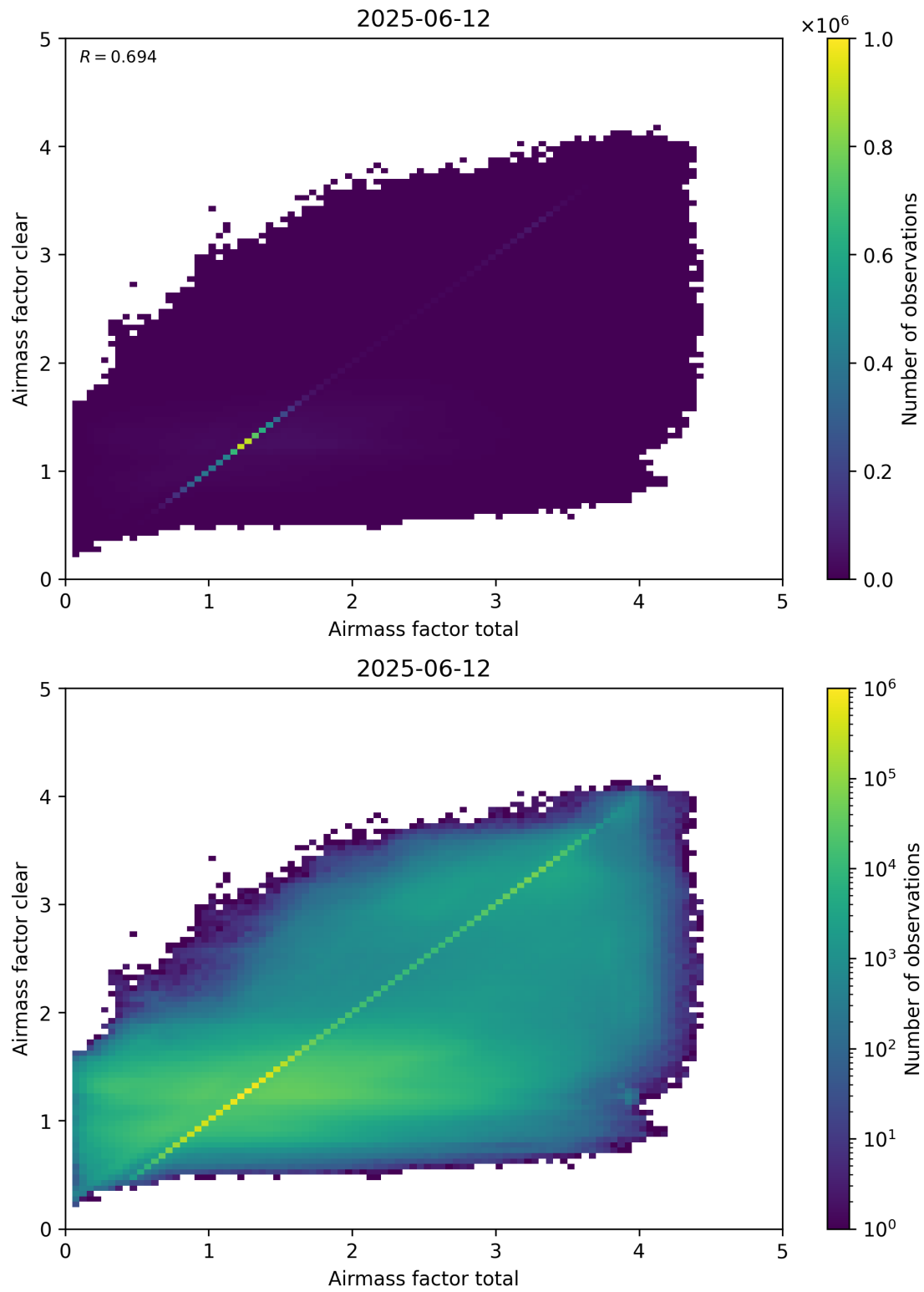
Figure 100: Scatter density plot of “Airmass factor total” against “Airmass factor clear” for 2025-06-11 to 2025-06-13.
