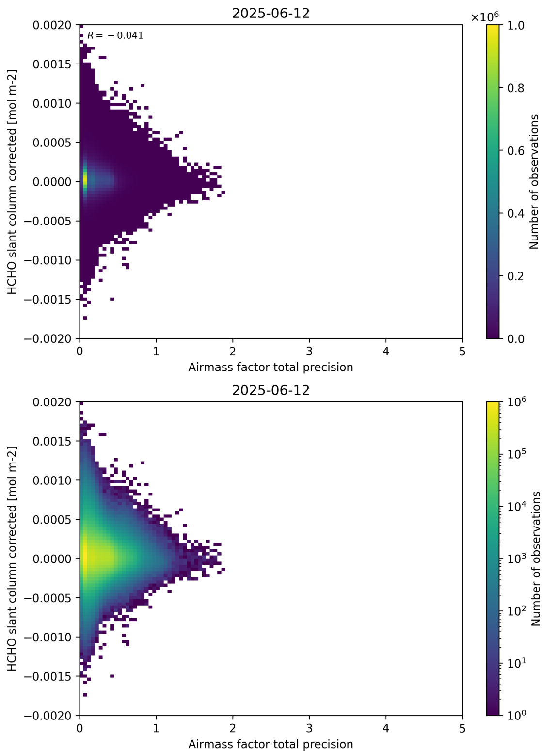
Figure 109: Scatter density plot of “Airmass factor total precision” against “HCHO slant column corrected” for 2025-06-11 to 2025-06-13.
