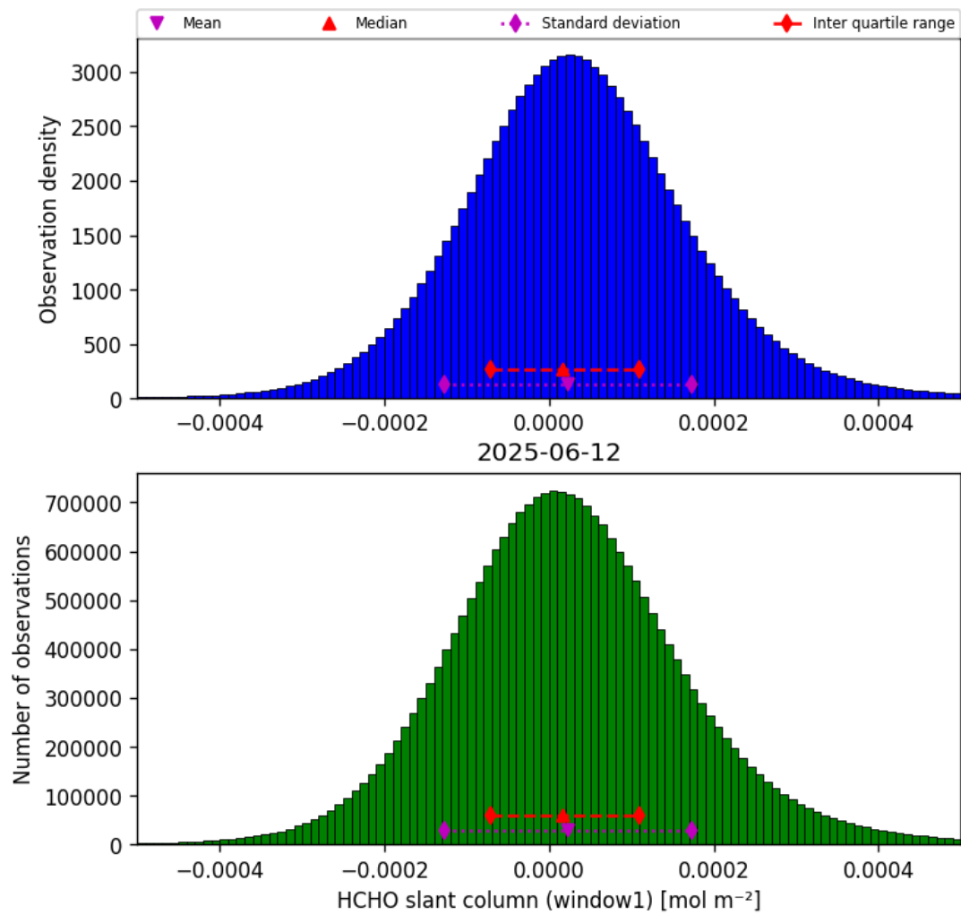
Figure 38: Histogram of “HCHO slant column (window1)” for 2025-06-11 to 2025-06-13
