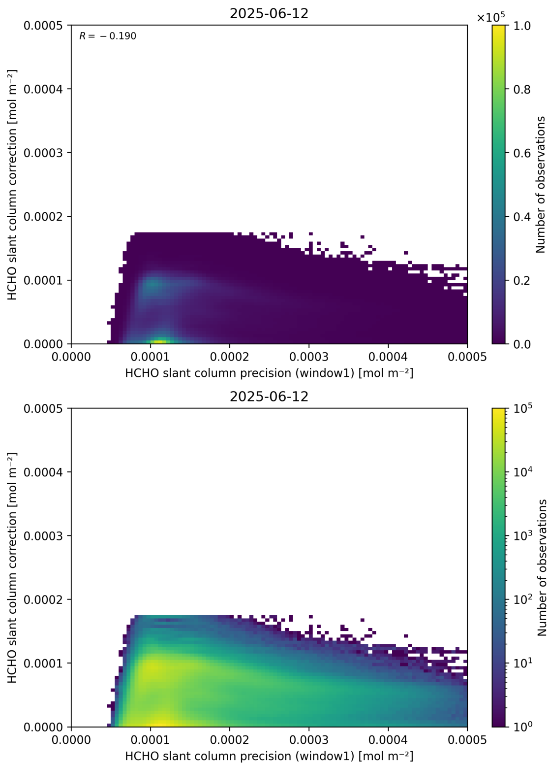
Figure 93: Scatter density plot of “HCHO slant column precision (window1)” against “HCHO slant column correction” for 2025-06-11 to 2025-06-13.
