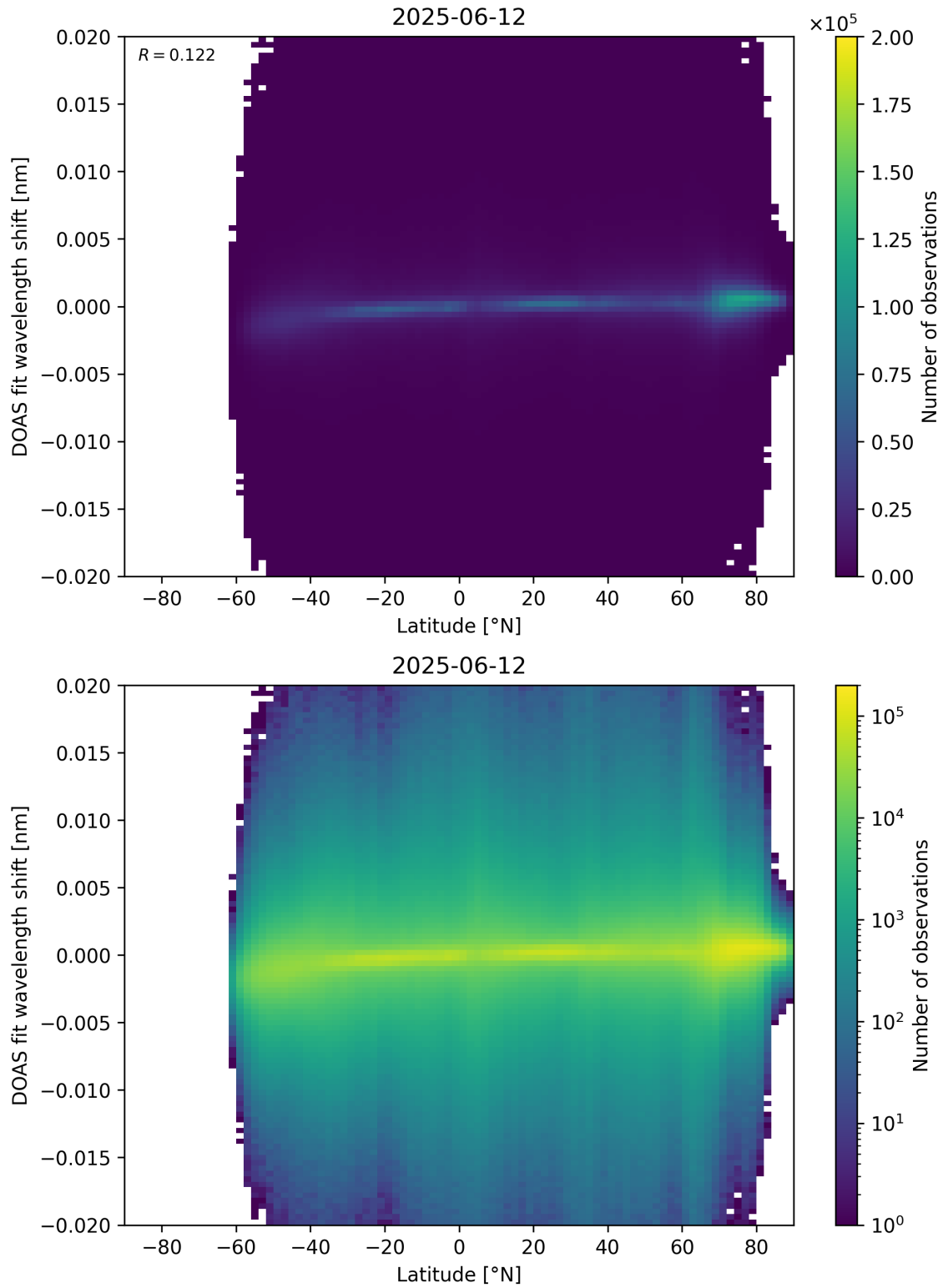
Figure 154: Scatter density plot of “Latitude” against “DOAS fit wavelength shift” for 2025-06-11 to 2025-06-13.
