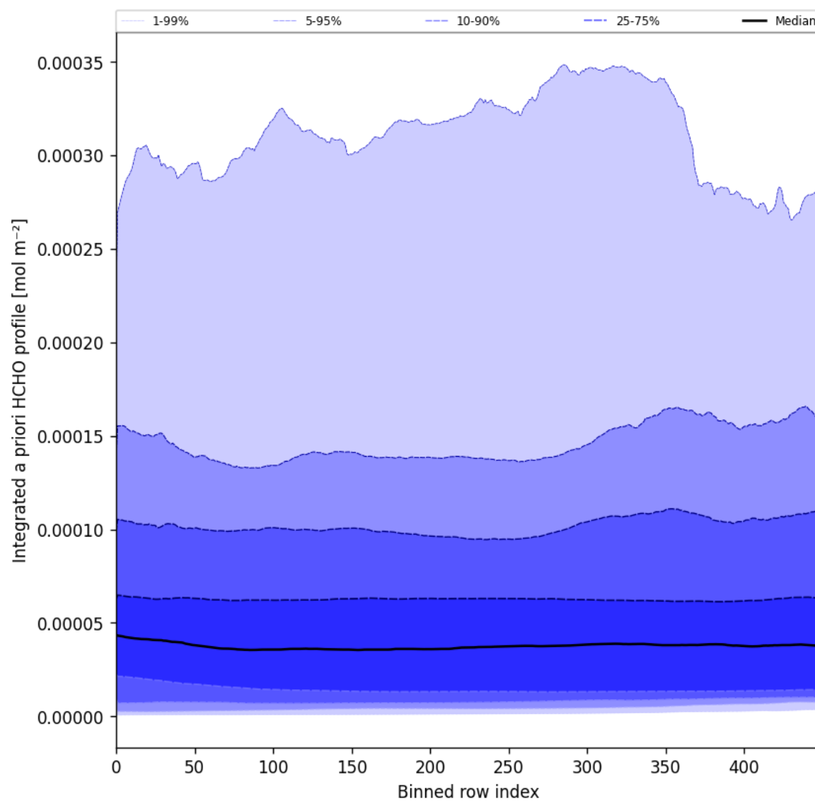
Figure 57: Along track statistics of “Integrated a priori HCHO profile” for 2025-06-11 to 2025-06-13
