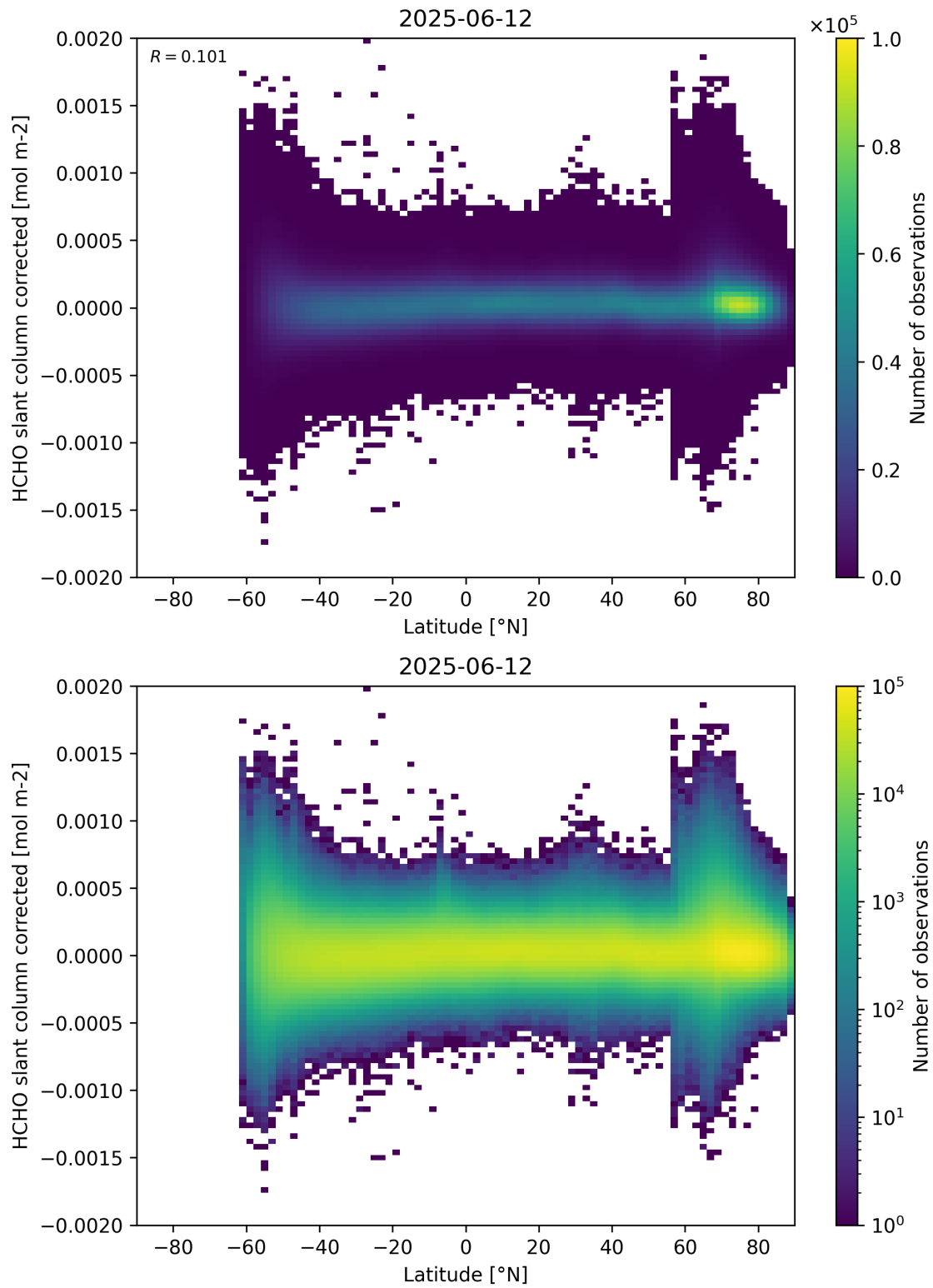
Figure 157: Scatter density plot of “Latitude” against “HCHO slant column corrected” for 2025-06-11 to 2025-06-13.
