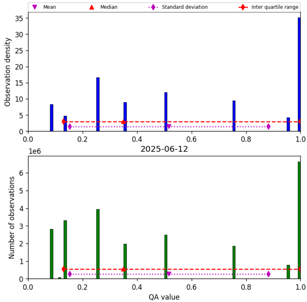
Figure 34: Histogram of “QA value” for 2025-06-11 to 2025-06-13
