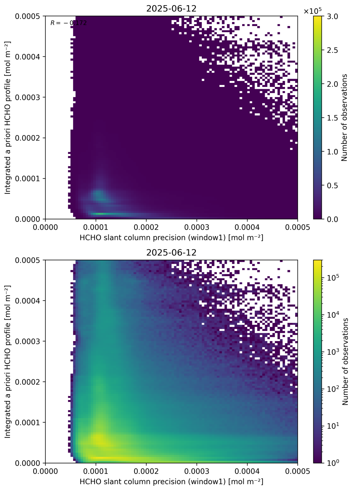
Figure 96: Scatter density plot of “HCHO slant column precision (window1)” against “Integrated a priori HCHO profile” for 2025-06-11 to 2025-06-13.
