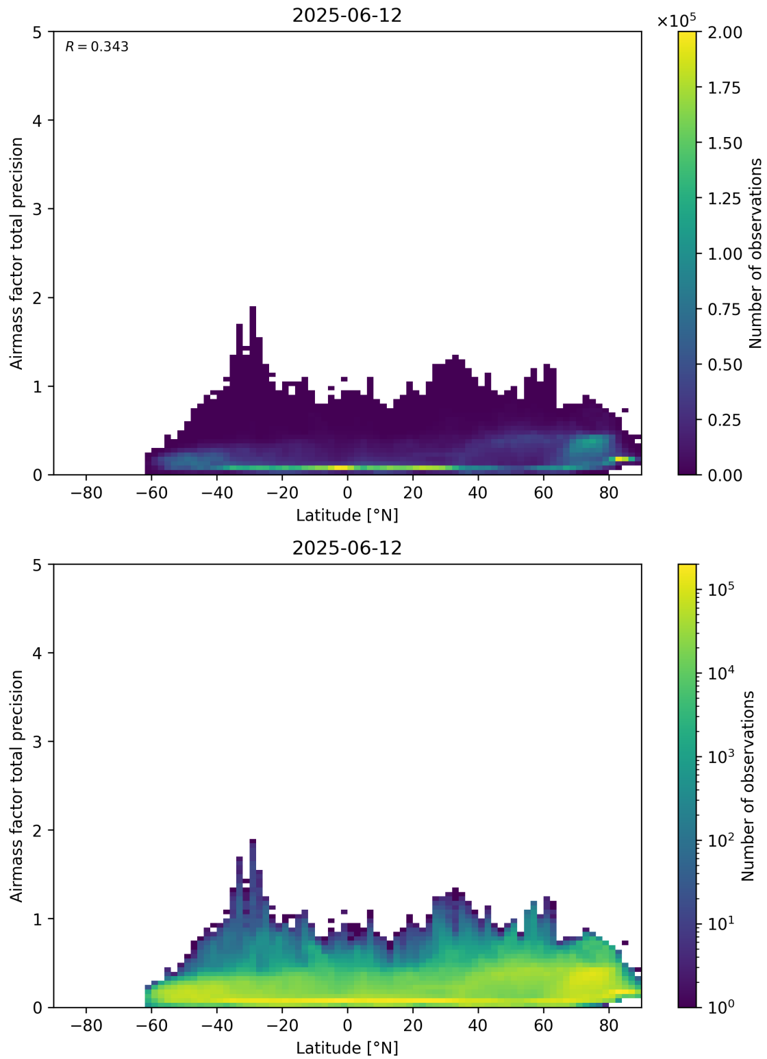
Figure 162: Scatter density plot of “Latitude” against “Airmass factor total precision” for 2025-06-11 to 2025-06-13.
