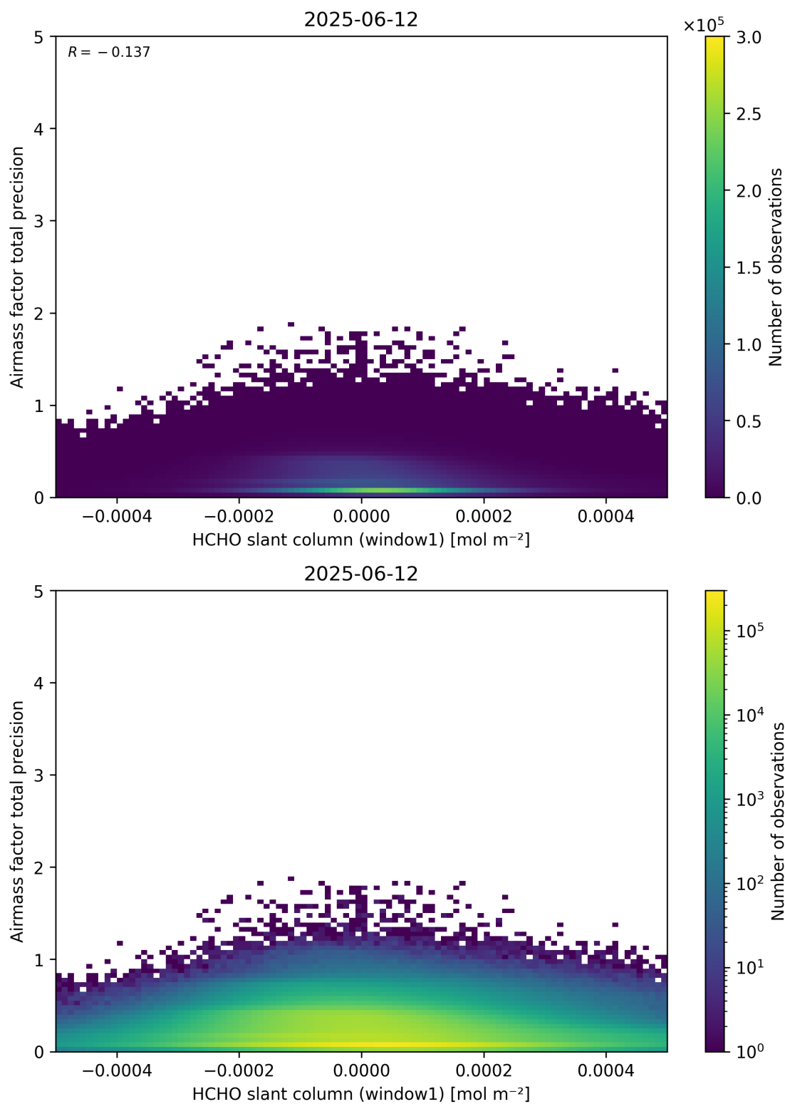
Figure 86: Scatter density plot of “HCHO slant column (window1)” against “Airmass factor total precision” for 2025-06-11 to 2025-06-13.
