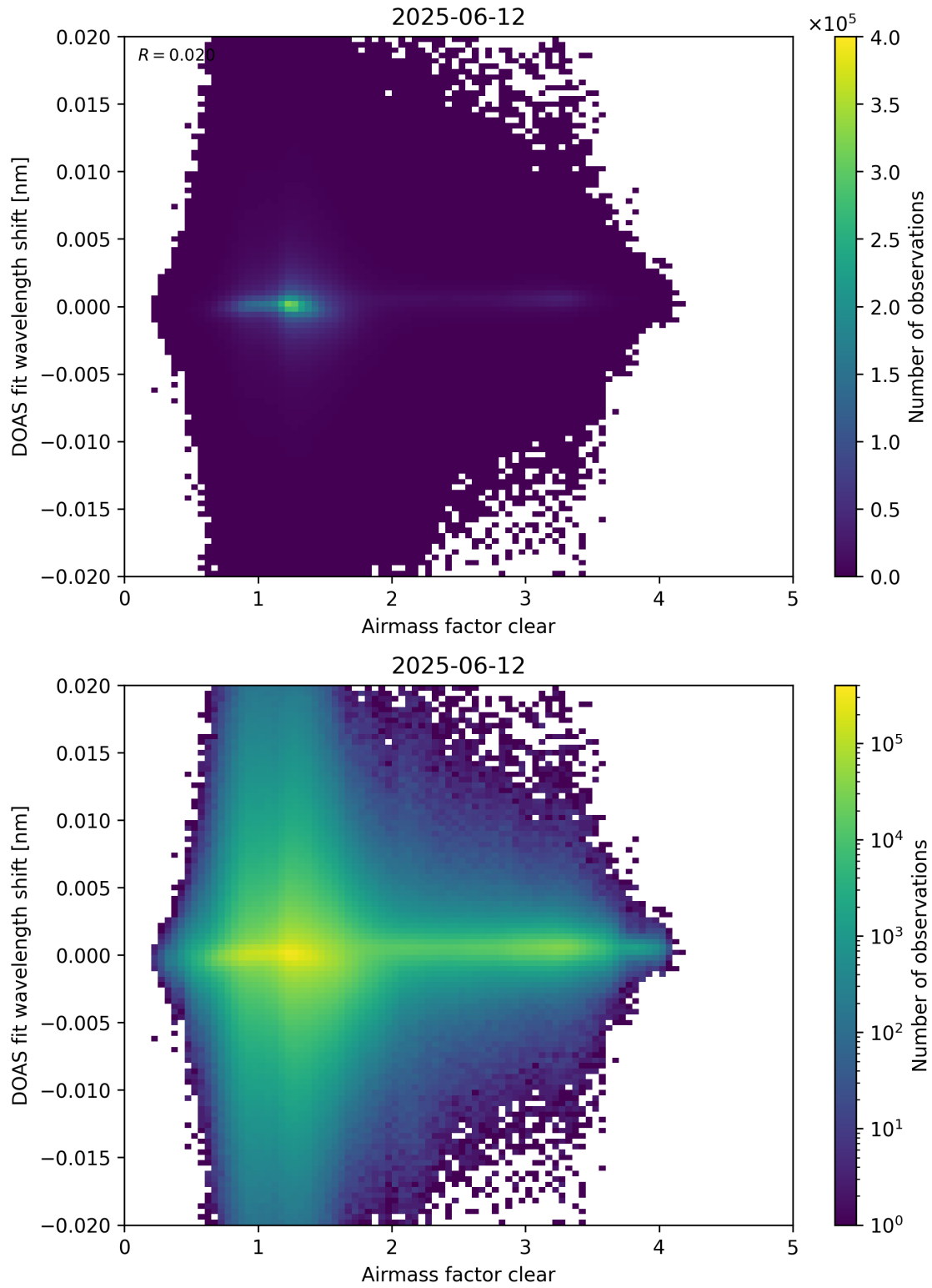
Figure 72: Scatter density plot of “Airmass factor clear” against “DOAS fit wavelength shift” for 2025-06-11 to 2025-06-13.
