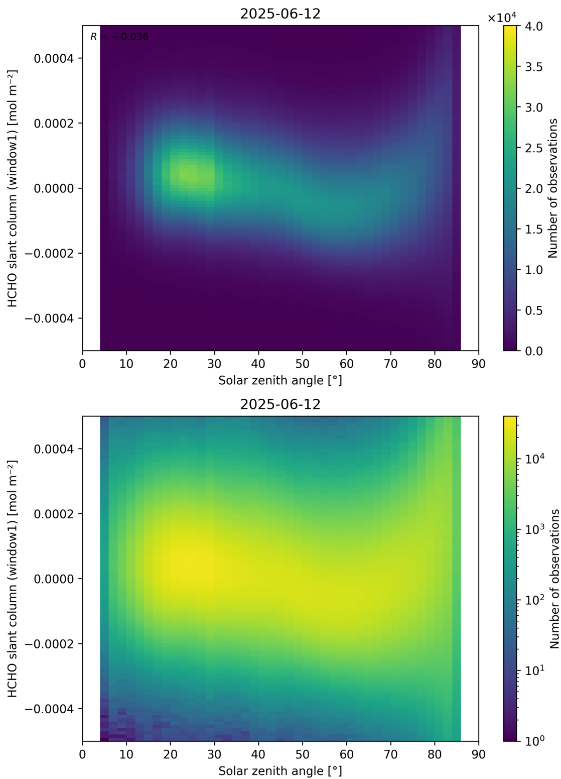
Figure 173: Scatter density plot of “Solar zenith angle” against “HCHO slant column (window1)” for 2025-06-11 to 2025-06-13.
