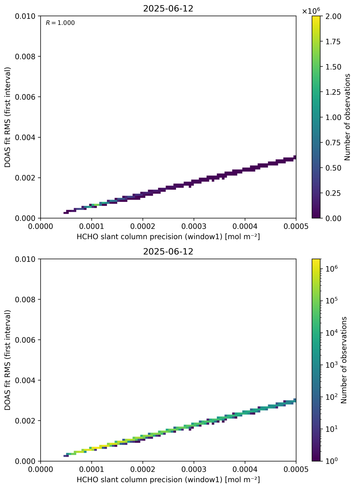
Figure 88: Scatter density plot of “HCHO slant column precision (window1)” against “DOAS fit RMS (first interval)” for 2025-06-11 to 2025-06-13.
