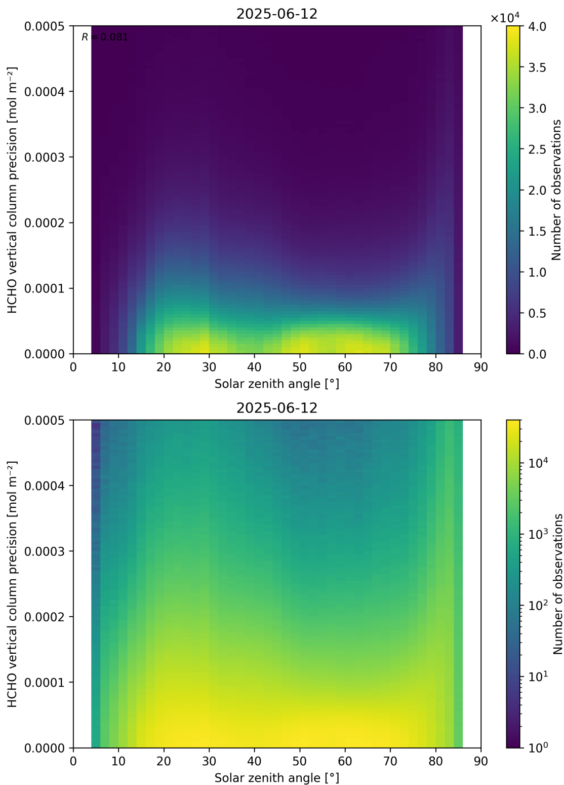
Figure 179: Scatter density plot of “Solar zenith angle” against “HCHO vertical column precision” for 2025-06-11 to 2025-06-13.
