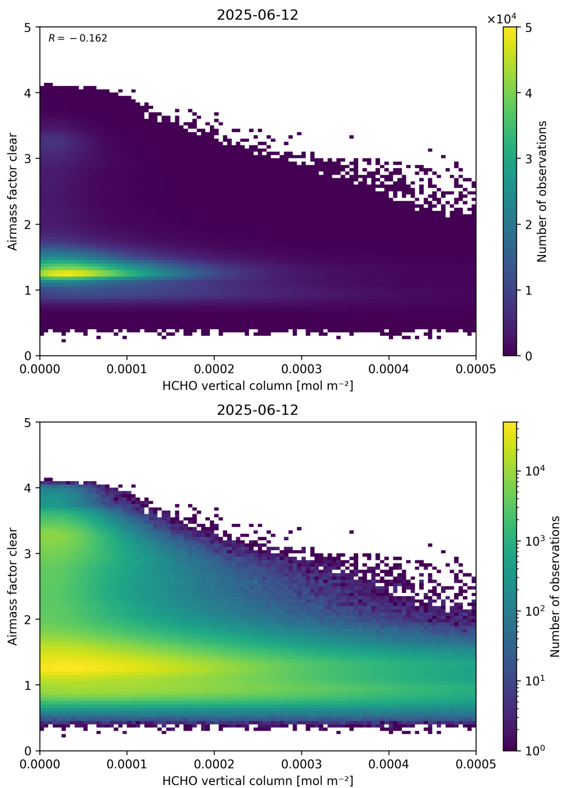
Figure 126: Scatter density plot of “HCHO vertical column” against “Airmass factor clear” for 2025-06-11 to 2025-06-13.
