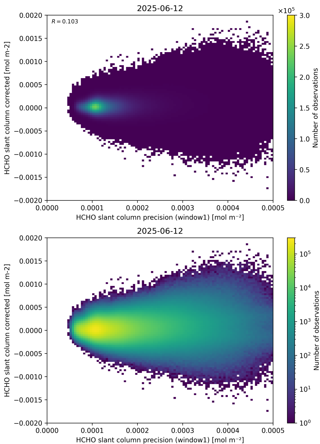
Figure 92: Scatter density plot of “HCHO slant column precision (window1)” against “HCHO slant column corrected” for 2025-06-11 to 2025-06-13.
