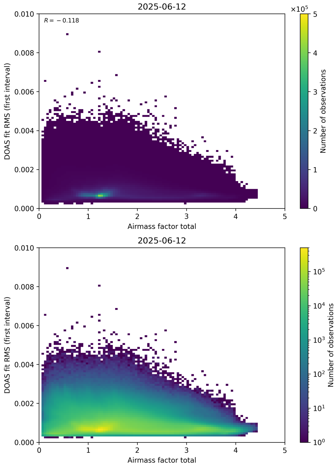
Figure 97: Scatter density plot of “Airmass factor total” against “DOAS fit RMS (first interval)” for 2025-06-11 to 2025-06-13.
