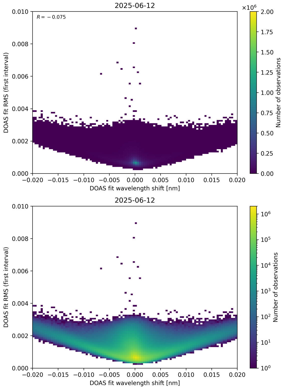
Figure 64: Scatter density plot of “DOAS fit wavelength shift” against “DOAS fit RMS (first interval)” for 2025-06-11 to 2025-06-13.
