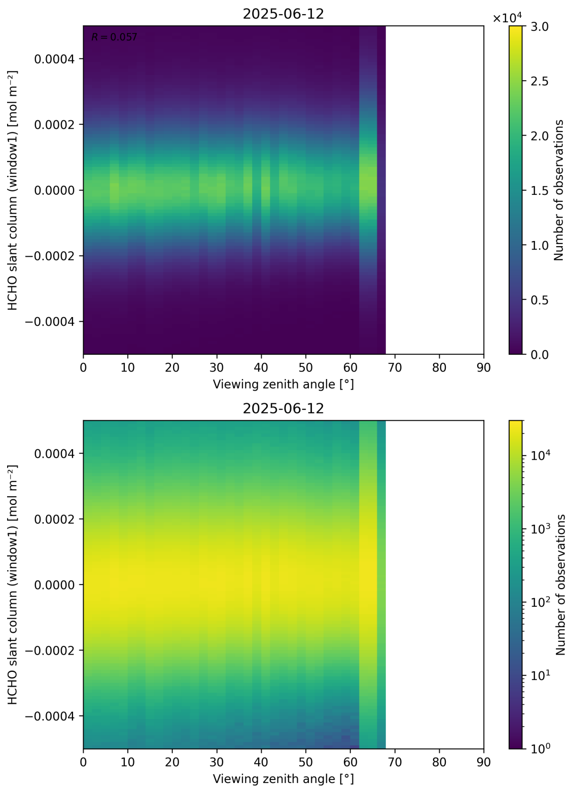
Figure 188: Scatter density plot of “Viewing zenith angle” against “HCHO slant column (window1)” for 2025-06-11 to 2025-06-13.
