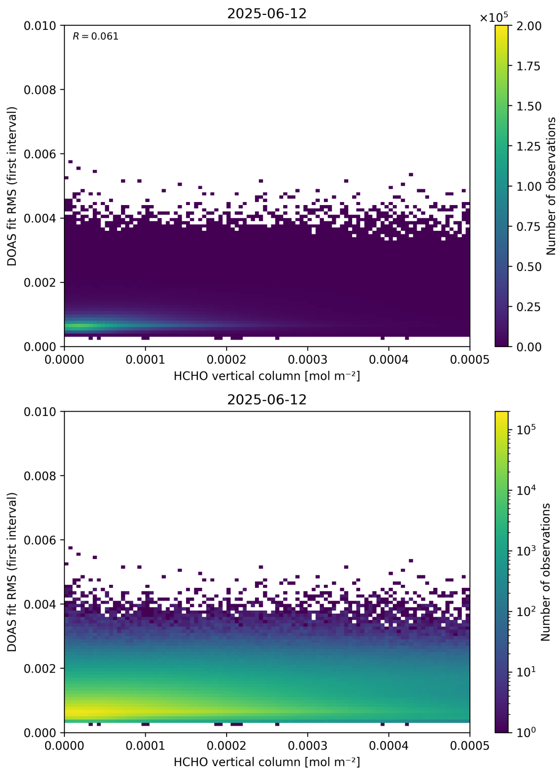
Figure 123: Scatter density plot of “HCHO vertical column” against “DOAS fit RMS (first interval)” for 2025-06-11 to 2025-06-13.
