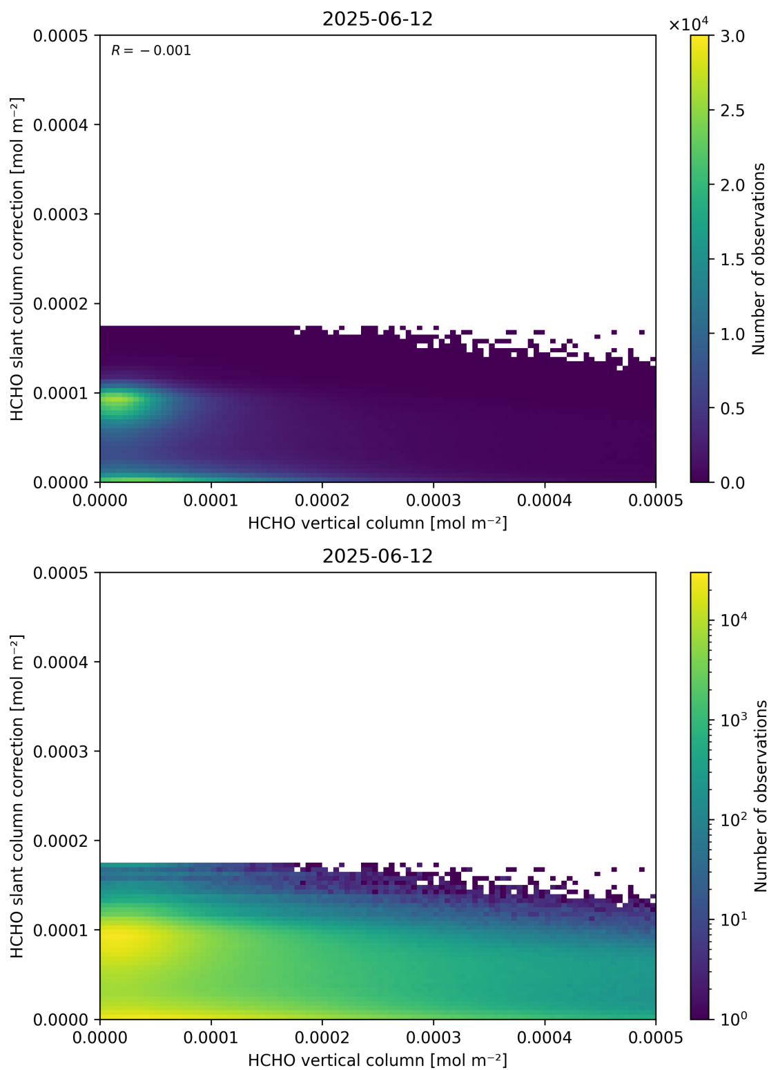
Figure 128: Scatter density plot of “HCHO vertical column” against “HCHO slant column correction” for 2025-06-11 to 2025-06-13.
