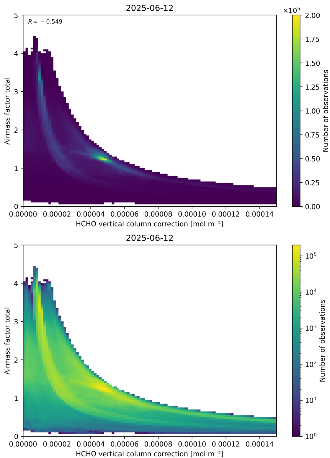
Figure 120: Scatter density plot of “HCHO vertical column correction” against “Airmass factor total” for 2025-06-11 to 2025-06-13.
