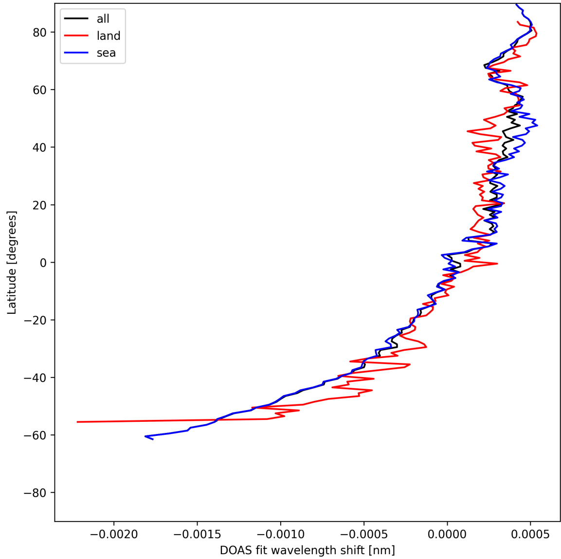
Figure 30: Zonal average of “DOAS fit wavelength shift” for 2025-06-11 to 2025-06-13.
