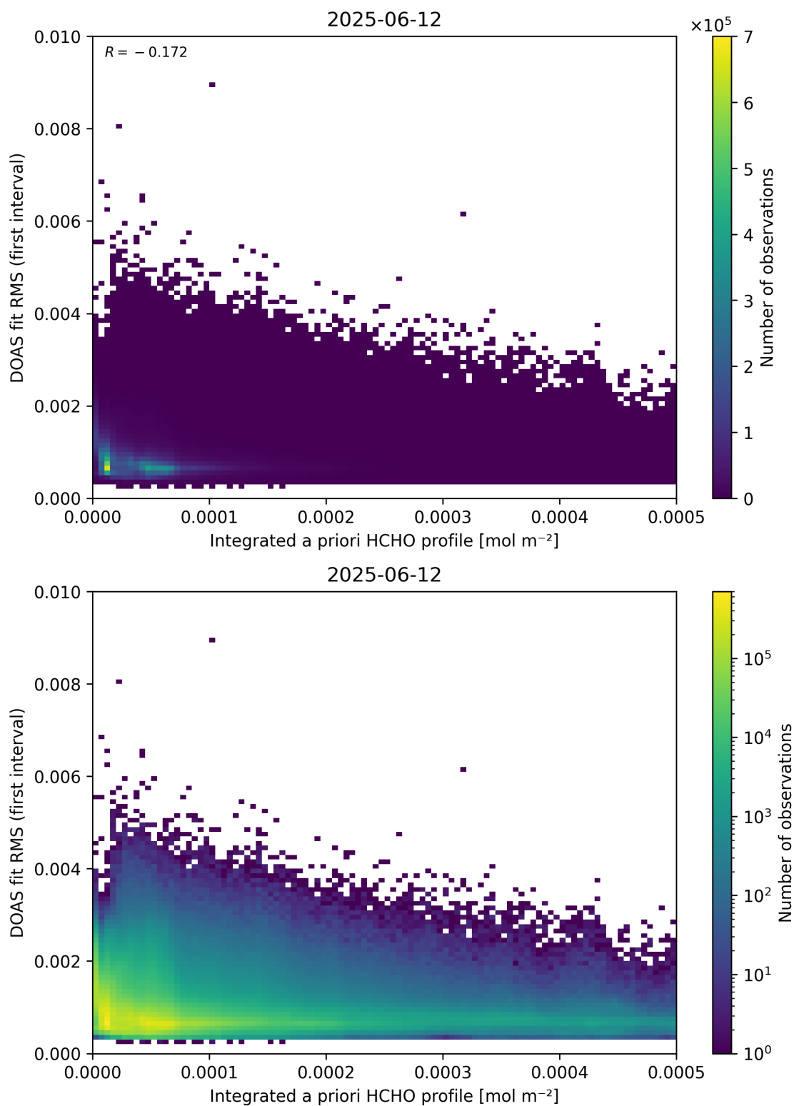
Figure 148: Scatter density plot of “Integrated a priori HCHO profile” against “DOAS fit RMS (first interval)” for 2025-06-11 to 2025-06-13.
