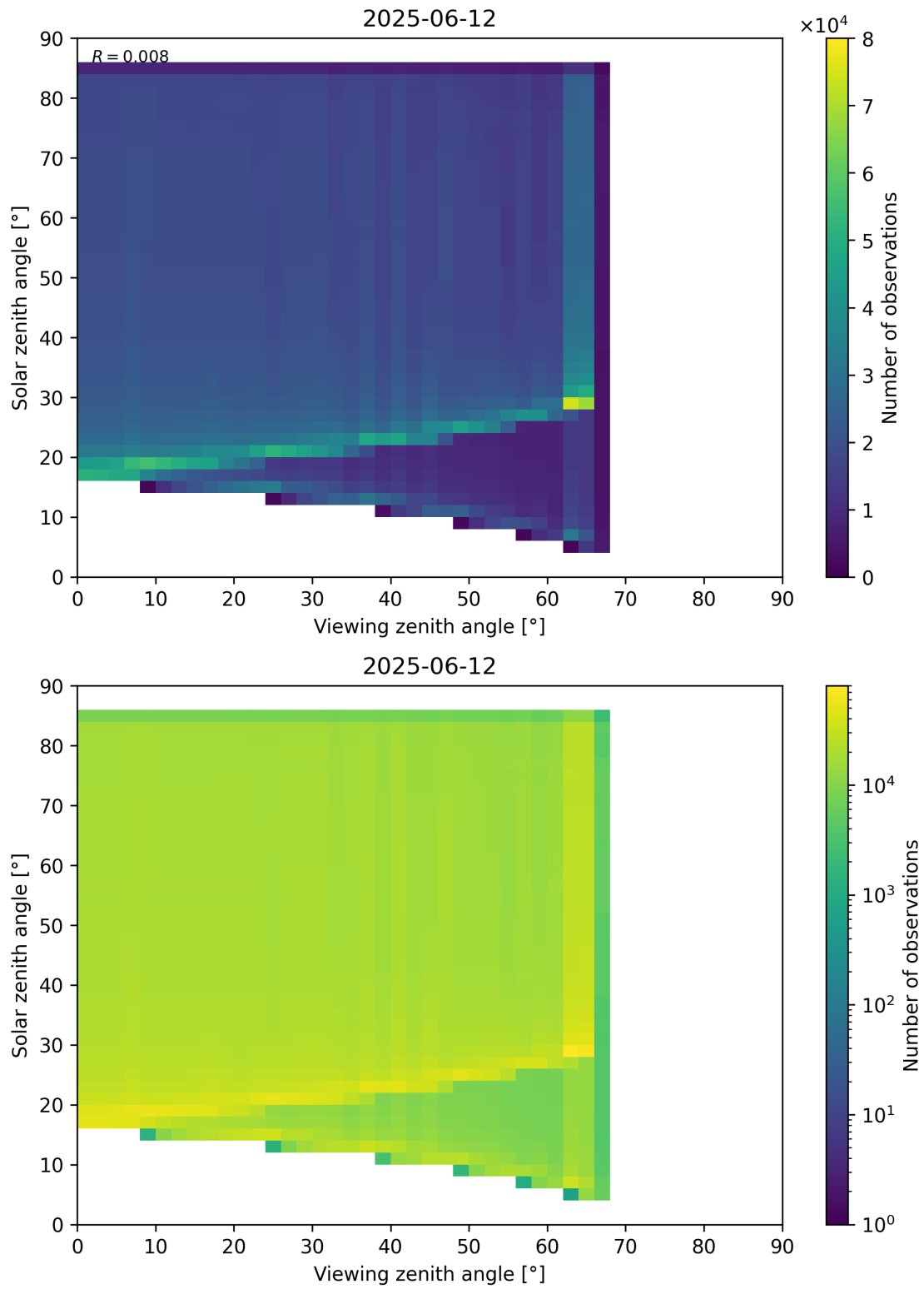
Figure 197: Scatter density plot of “Viewing zenith angle” against “Solar zenith angle” for 2025-06-11 to 2025-06-13.
