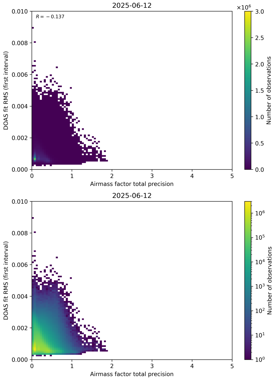
Figure 105: Scatter density plot of “Airmass factor total precision” against “DOAS fit RMS (first interval)” for 2025-06-11 to 2025-06-13.
