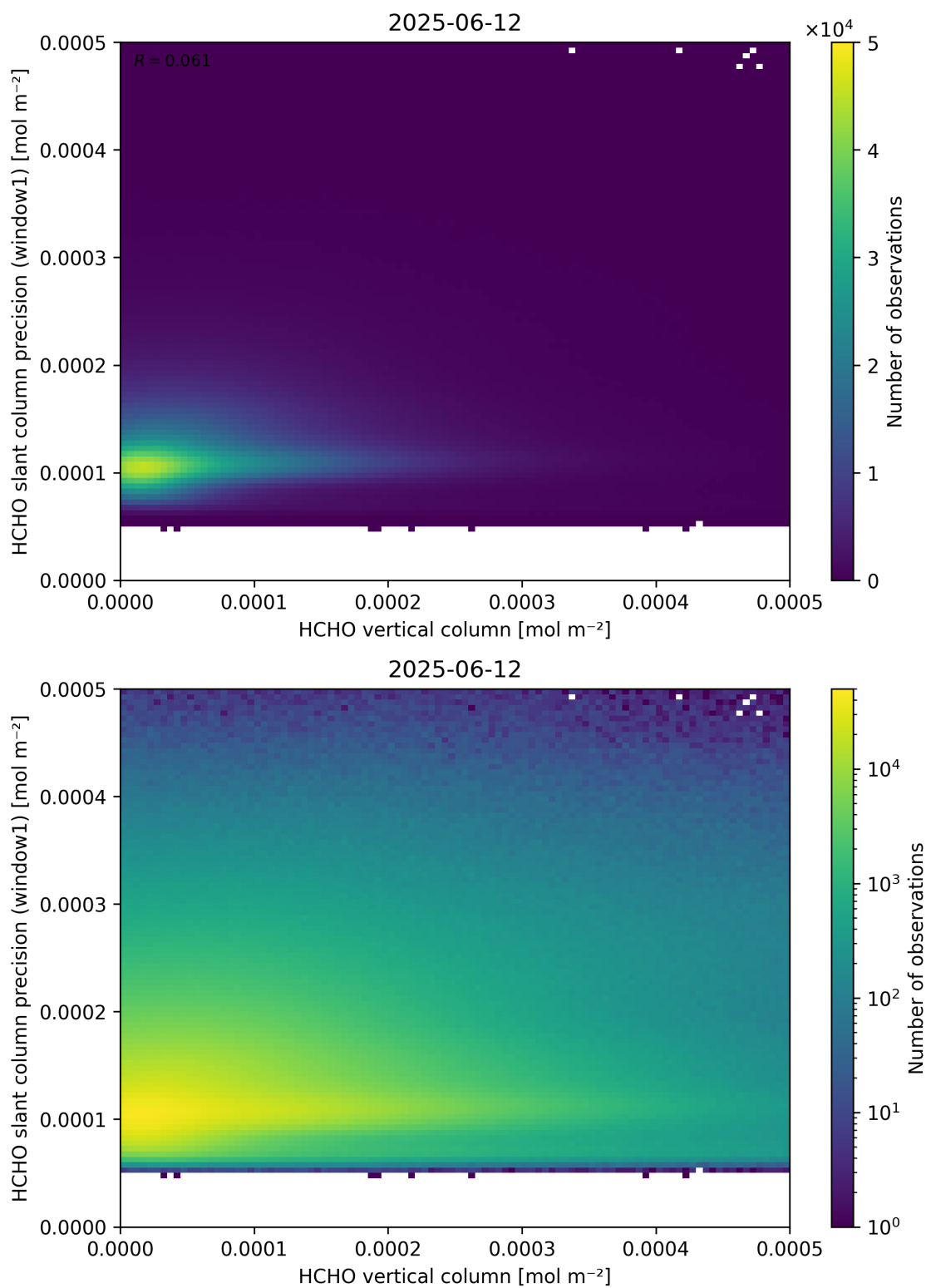
Figure 130: Scatter density plot of “HCHO vertical column” against “HCHO slant column precision (window1)” for 2025-06-11 to 2025-06-13.
