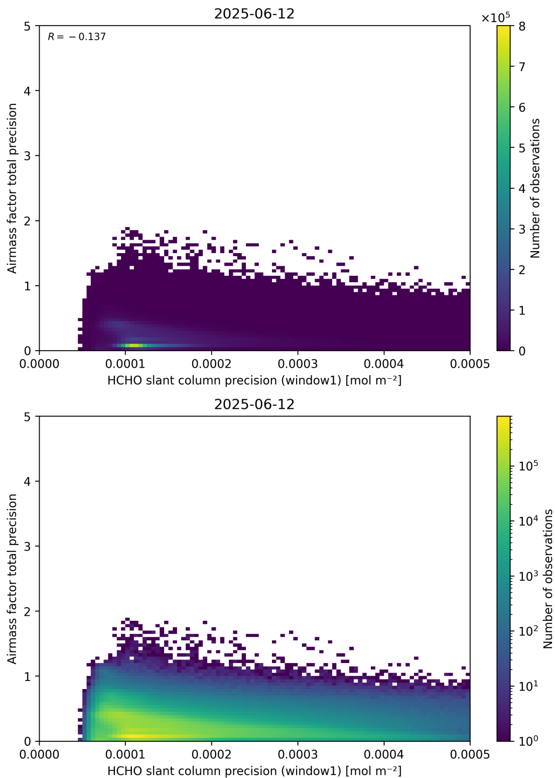
Figure 95: Scatter density plot of “HCHO slant column precision (window1)” against “Airmass factor total precision” for 2025-06-11 to 2025-06-13.
