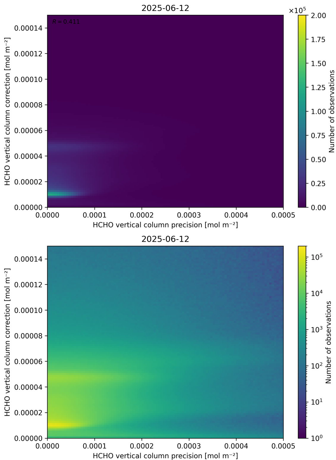
Figure 146: Scatter density plot of “HCHO vertical column precision” against “HCHO vertical column correction” for 2025-06-11 to 2025-06-13.
