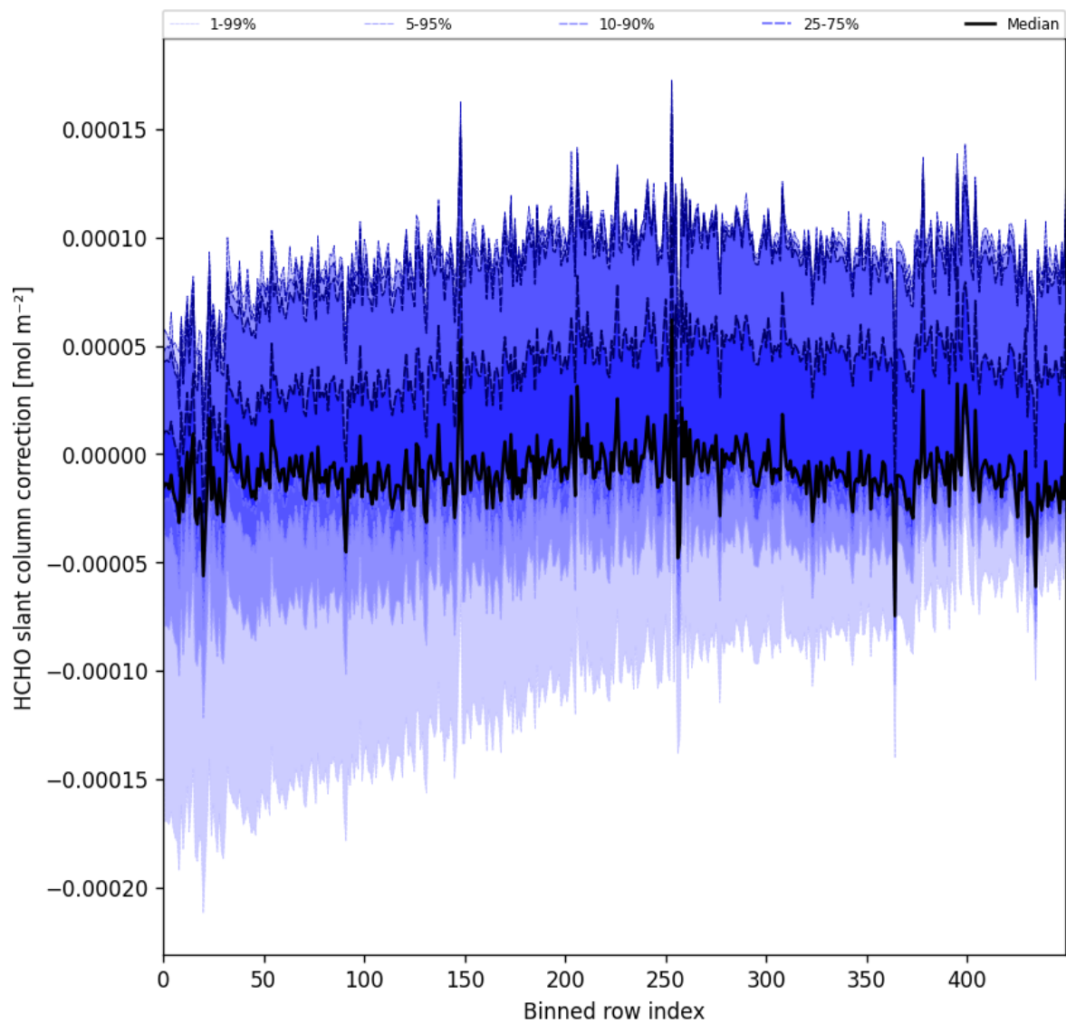
Figure 61: Along track statistics of “HCHO slant column correction” for 2025-06-11 to 2025-06-13
