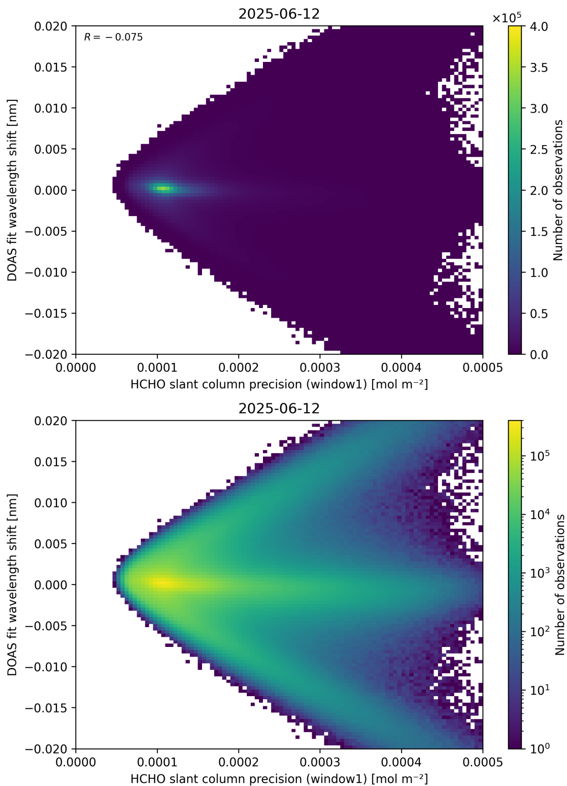
Figure 89: Scatter density plot of “HCHO slant column precision (window1)” against “DOAS fit wavelength shift” for 2025-06-11 to 2025-06-13.
