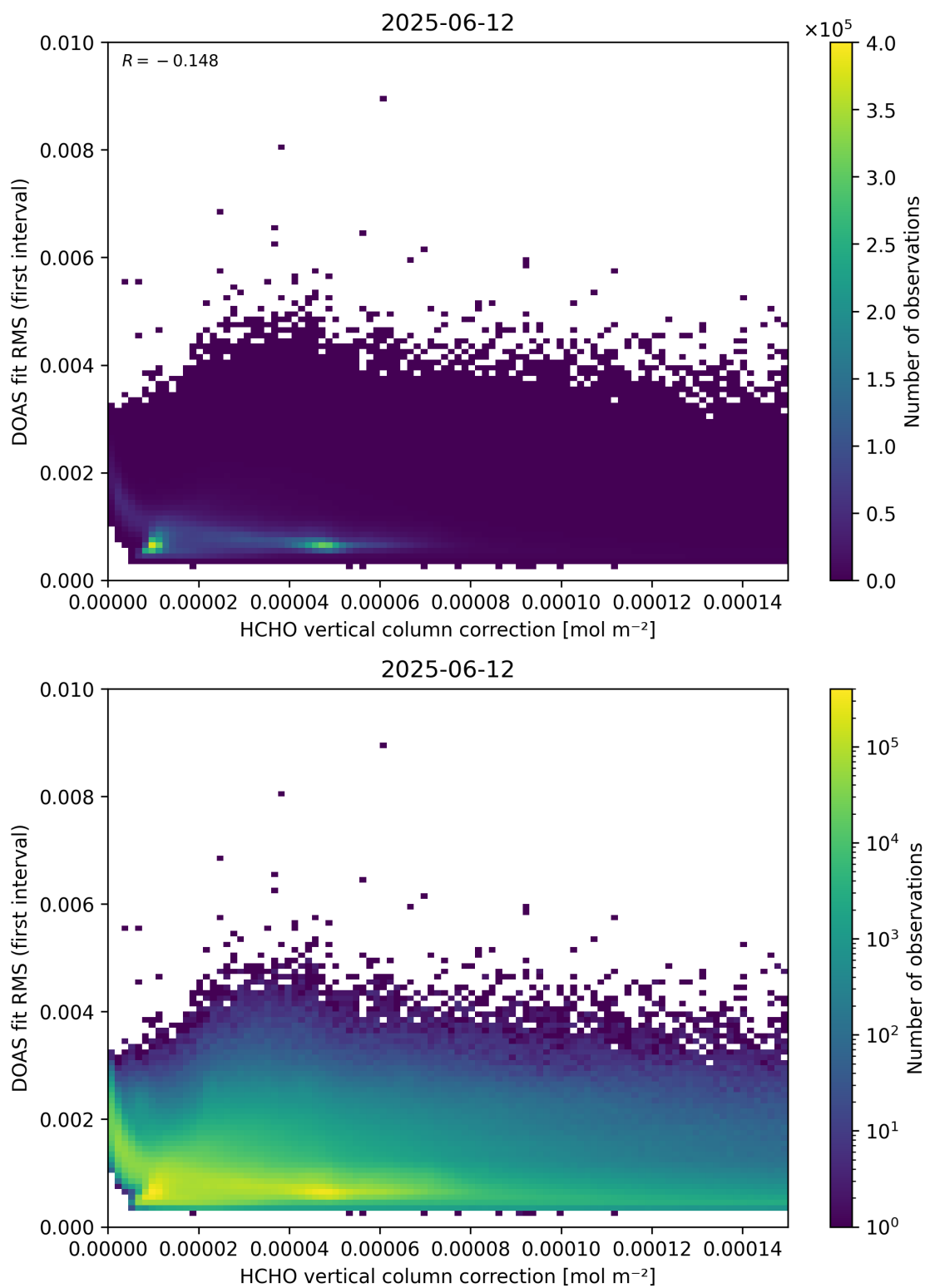
Figure 112: Scatter density plot of “HCHO vertical column correction” against “DOAS fit RMS (first interval)” for 2025-06-11 to 2025-06-13.
