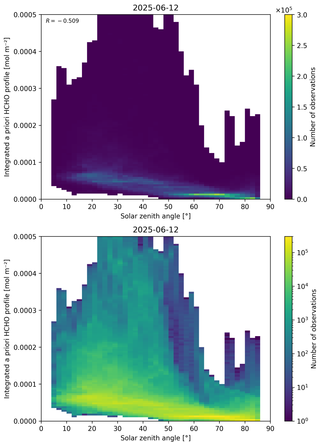
Figure 180: Scatter density plot of “Solar zenith angle” against “Integrated a priori HCHO profile” for 2025-06-11 to 2025-06-13.
