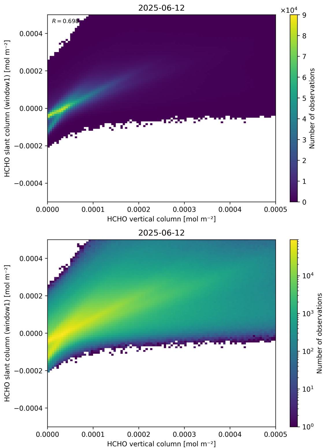
Figure 129: Scatter density plot of “HCHO vertical column” against “HCHO slant column (window1)” for 2025-06-11 to 2025-06-13.
