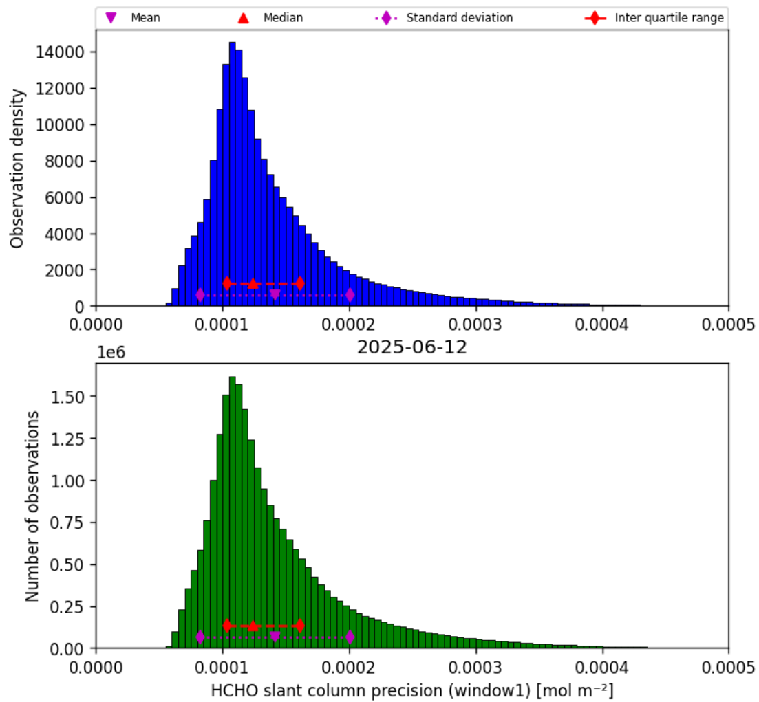
Figure 39: Histogram of “HCHO slant column precision (window1)” for 2025-06-11 to 2025-06-13
