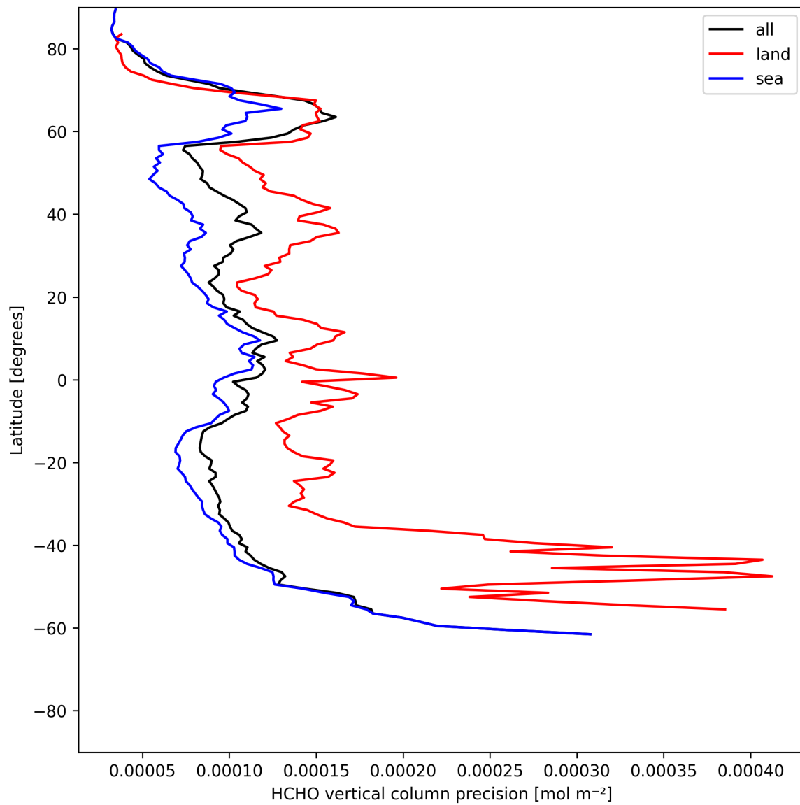
Figure 22: Zonal average of “HCHO vertical column precision” for 2025-06-11 to 2025-06-13.
