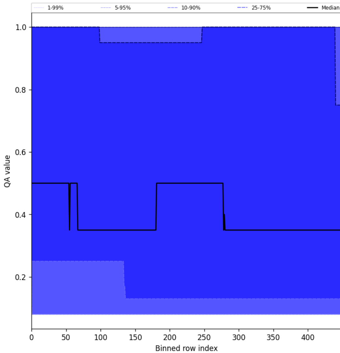
Figure 48: Along track statistics of “QA value” for 2025-06-11 to 2025-06-13
