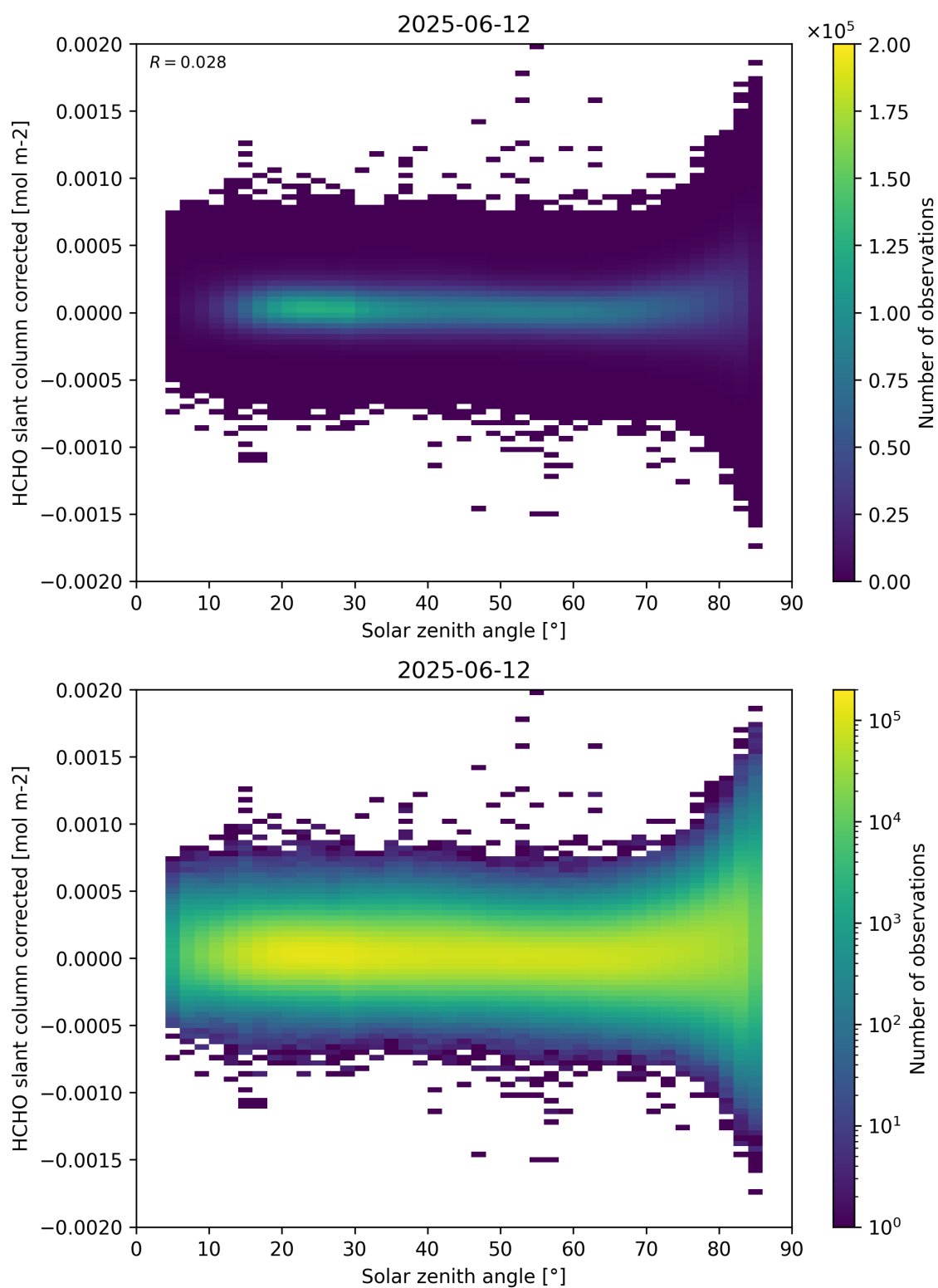
Figure 171: Scatter density plot of “Solar zenith angle” against “HCHO slant column corrected” for 2025-06-11 to 2025-06-13.
