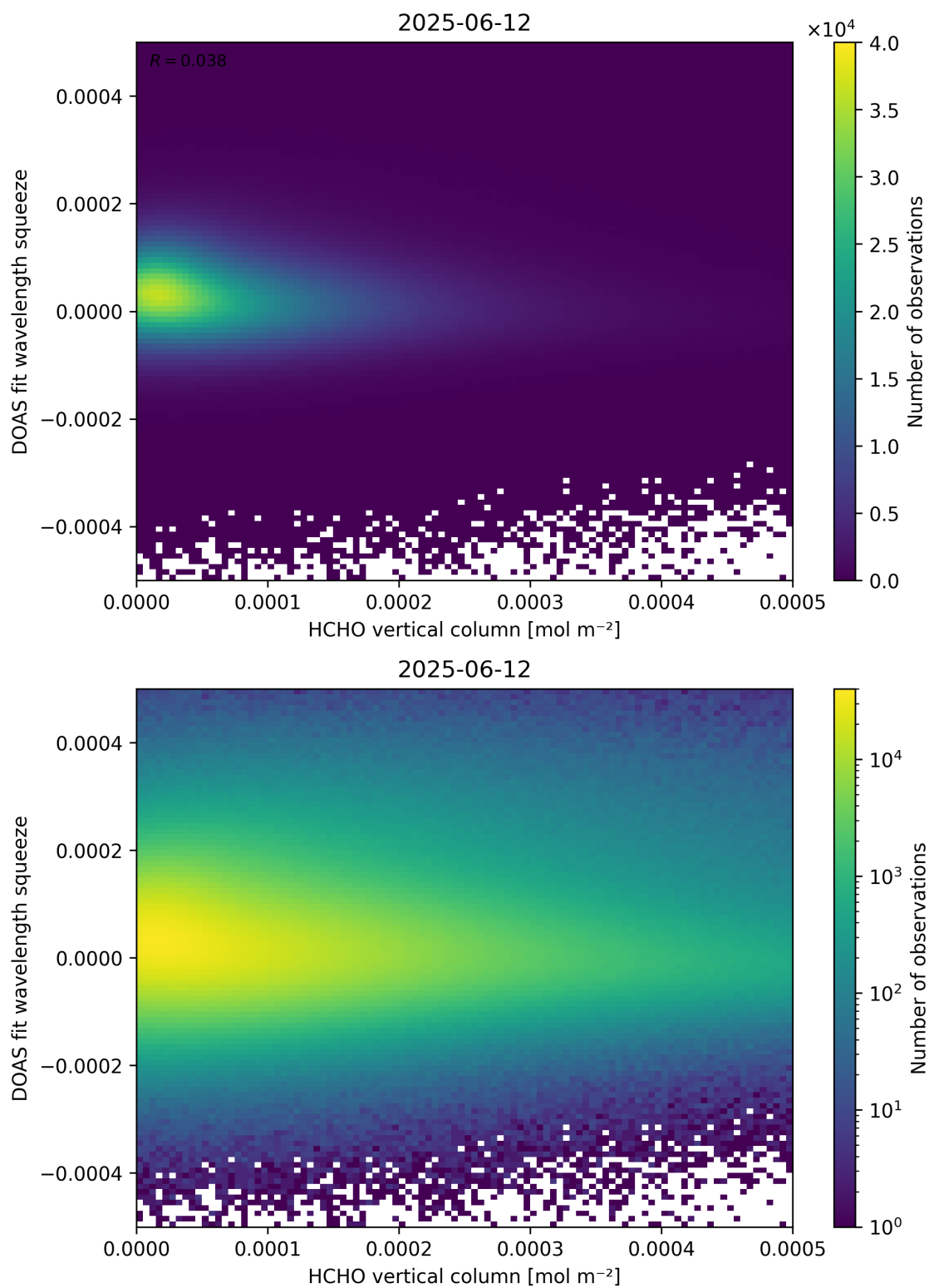
Figure 125: Scatter density plot of “HCHO vertical column” against “DOAS fit wavelength squeeze” for 2025-06-11 to 2025-06-13.
