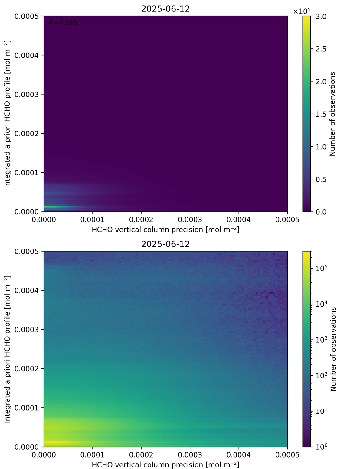
Figure 147: Scatter density plot of “HCHO vertical column precision” against “Integrated a priori HCHO profile” for 2025-06-11 to 2025-06-13.
