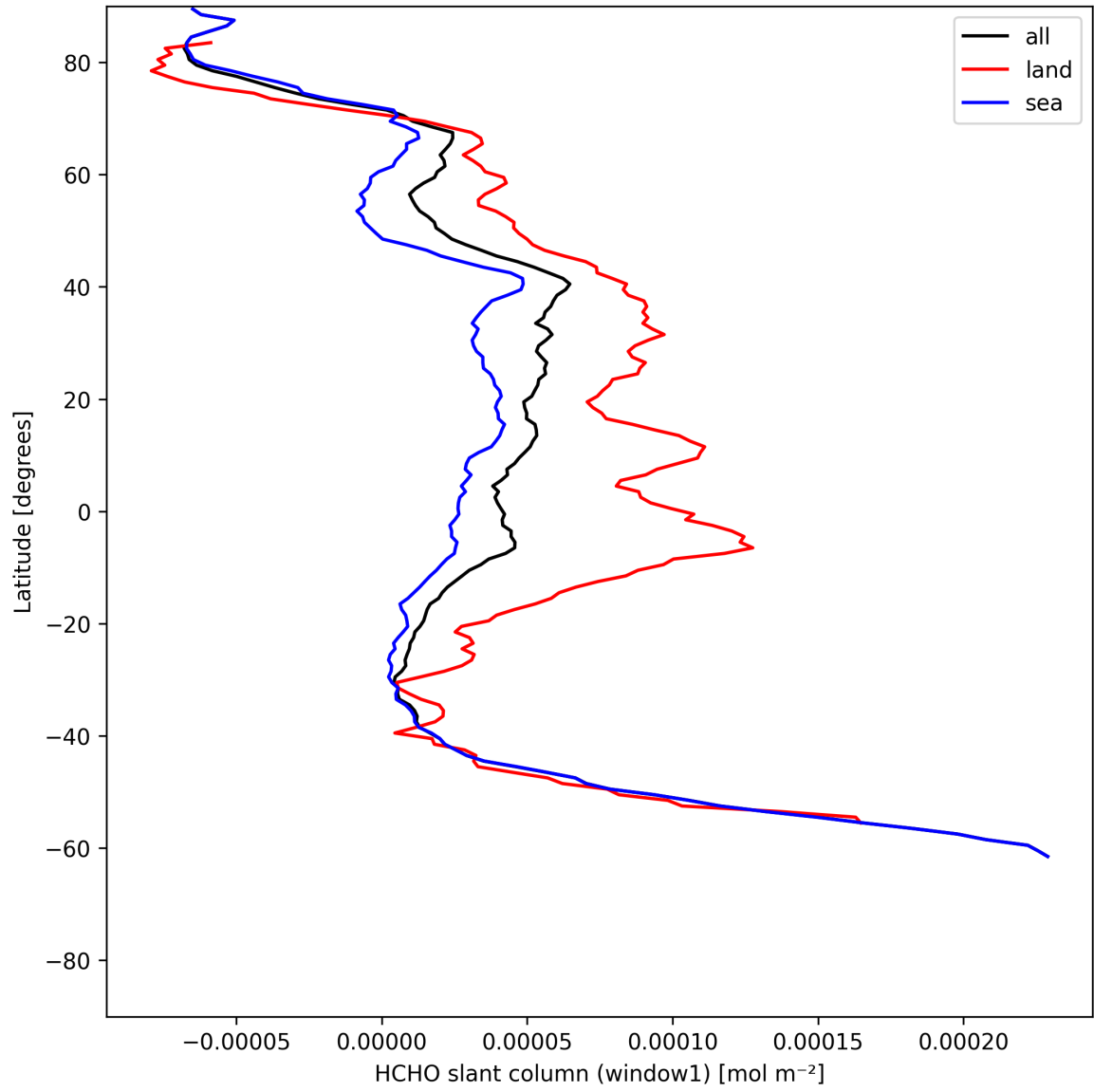
Figure 24: Zonal average of “HCHO slant column (window1)” for 2025-06-11 to 2025-06-13.
