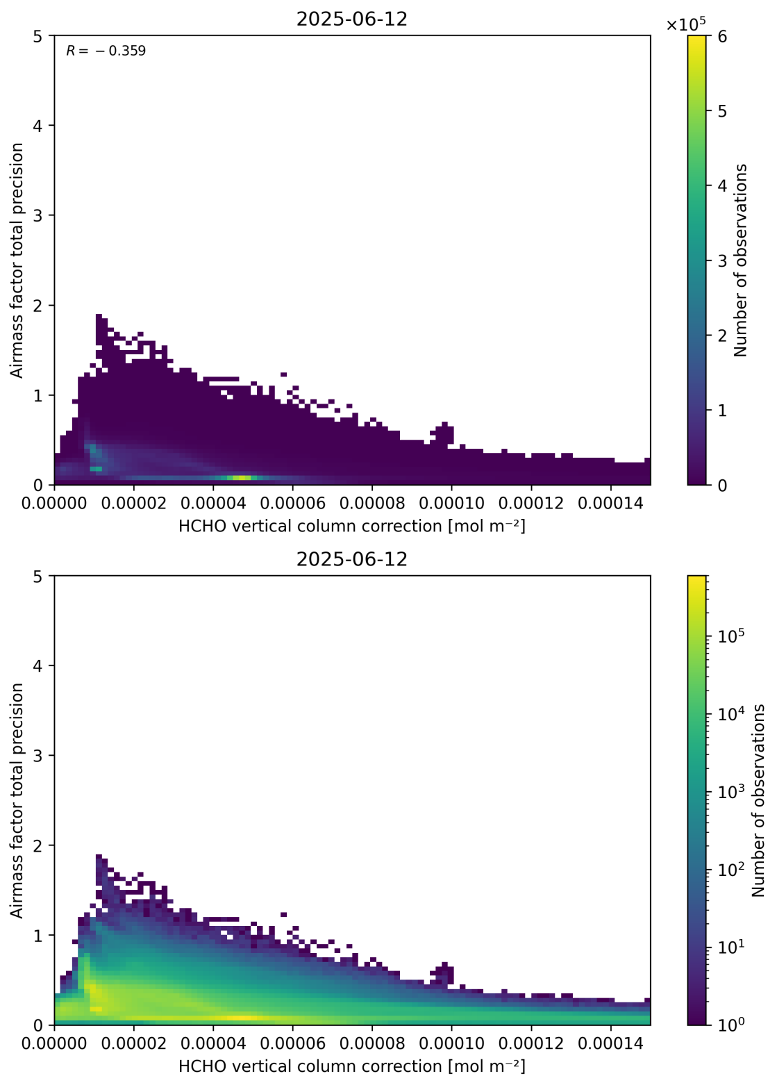
Figure 121: Scatter density plot of “HCHO vertical column correction” against “Airmass factor total precision” for 2025-06-11 to 2025-06-13.
