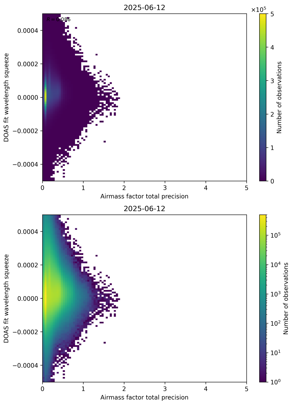
Figure 107: Scatter density plot of “Airmass factor total precision” against “DOAS fit wavelength squeeze” for 2025-06-11 to 2025-06-13.
