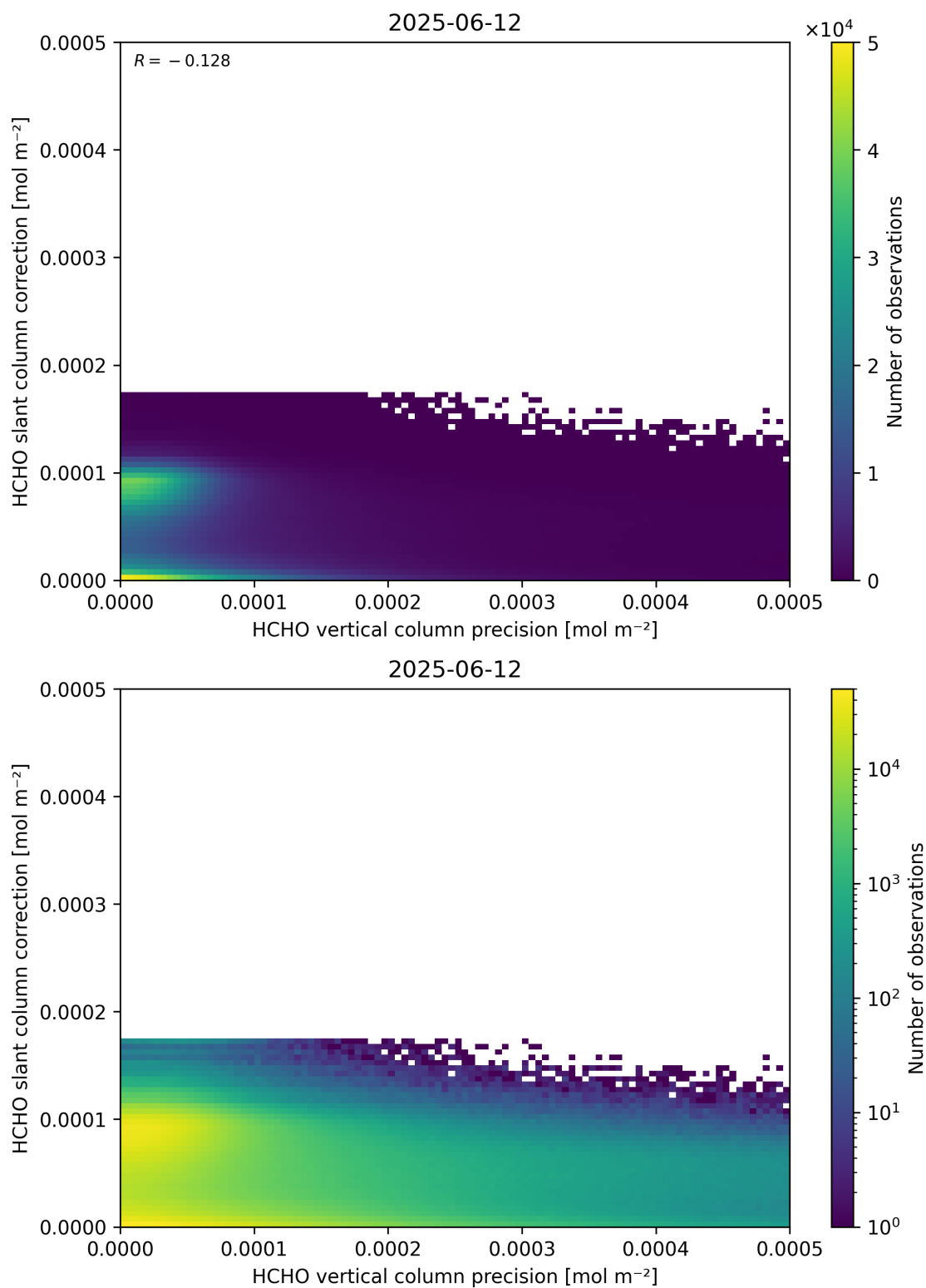
Figure 141: Scatter density plot of “HCHO vertical column precision” against “HCHO slant column correction” for 2025-06-11 to 2025-06-13.
