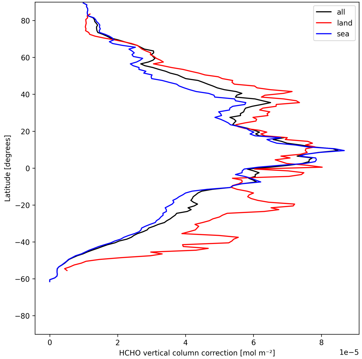
Figure 23: Zonal average of “HCHO vertical column correction” for 2025-06-11 to 2025-06-13.
