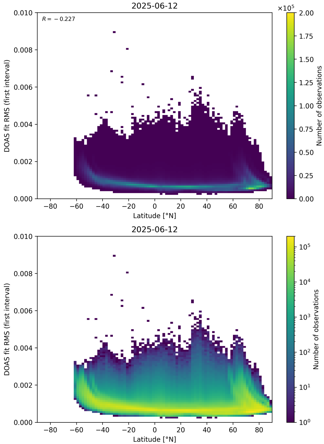
Figure 153: Scatter density plot of “Latitude” against “DOAS fit RMS (first interval)” for 2025-06-11 to 2025-06-13.
