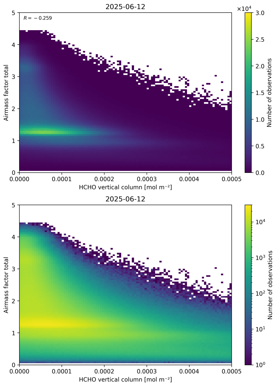
Figure 131: Scatter density plot of “HCHO vertical column” against “Airmass factor total” for 2025-06-11 to 2025-06-13.
