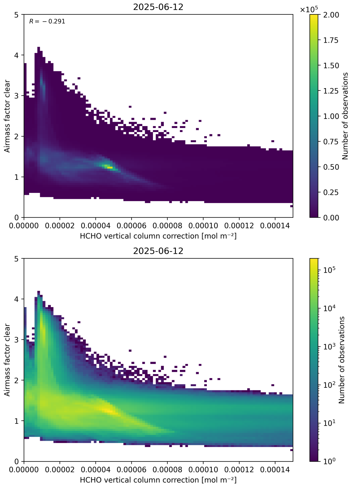
Figure 115: Scatter density plot of “HCHO vertical column correction” against “Airmass factor clear” for 2025-06-11 to 2025-06-13.
