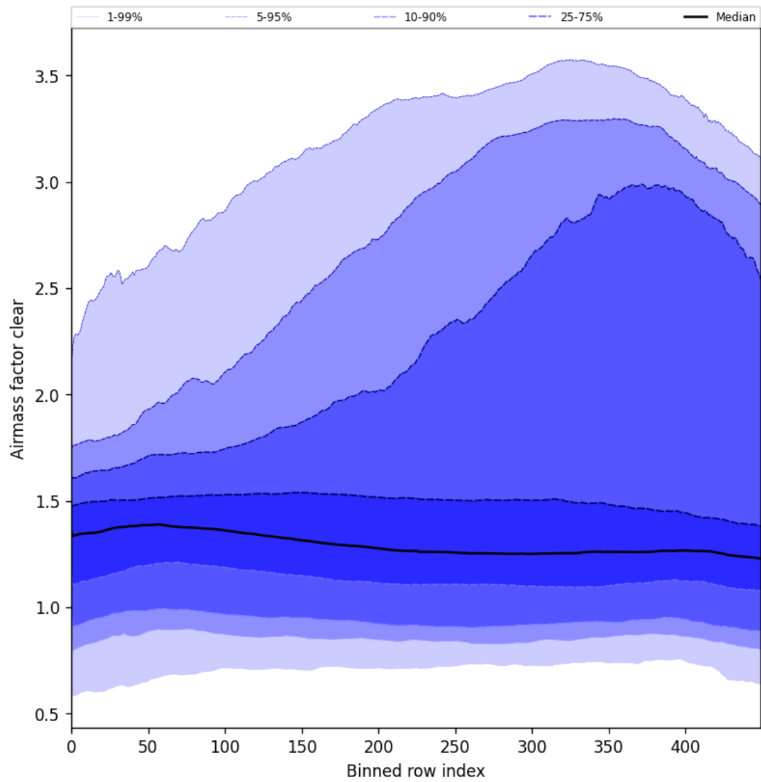
Figure 56: Along track statistics of “Airmass factor clear” for 2025-06-11 to 2025-06-13
