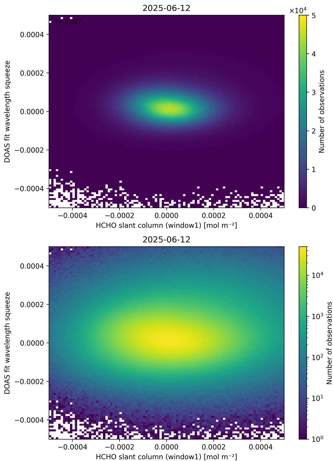
Figure 80: Scatter density plot of “HCHO slant column (window1)” against “DOAS fit wavelength squeeze” for 2025-06-11 to 2025-06-13.
