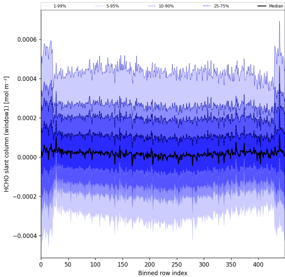
Figure 52: Along track statistics of “HCHO slant column (window1)” for 2025-06-11 to 2025-06-13
