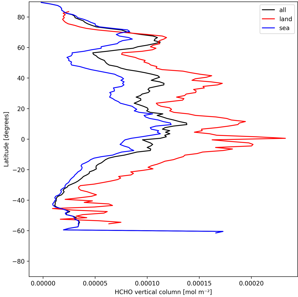
Figure 21: Zonal average of “HCHO vertical column” for 2025-06-11 to 2025-06-13.
