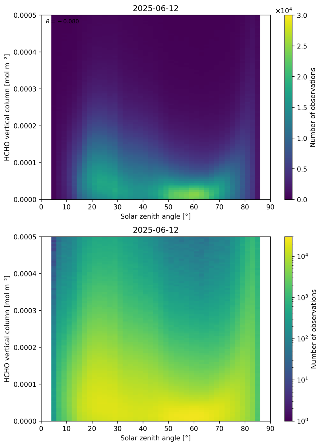
Figure 177: Scatter density plot of “Solar zenith angle” against “HCHO vertical column” for 2025-06-11 to 2025-06-13.
