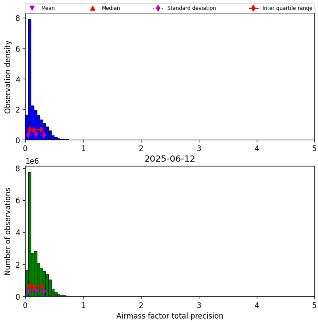
Figure 41: Histogram of “Airmass factor total precision” for 2025-06-11 to 2025-06-13
