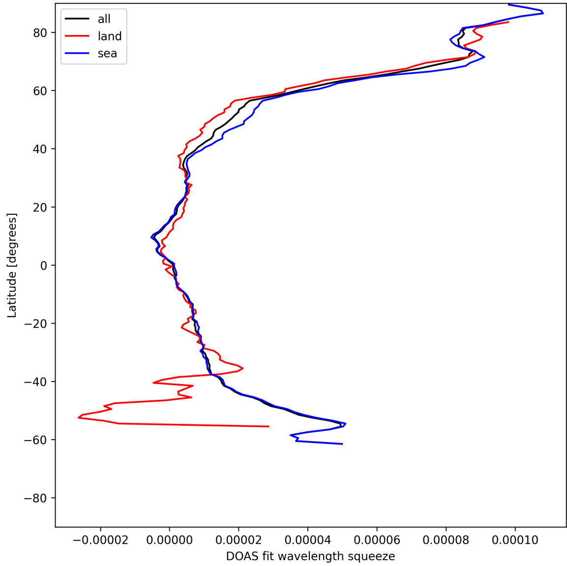
Figure 31: Zonal average of “DOAS fit wavelength squeeze” for 2025-06-11 to 2025-06-13.
