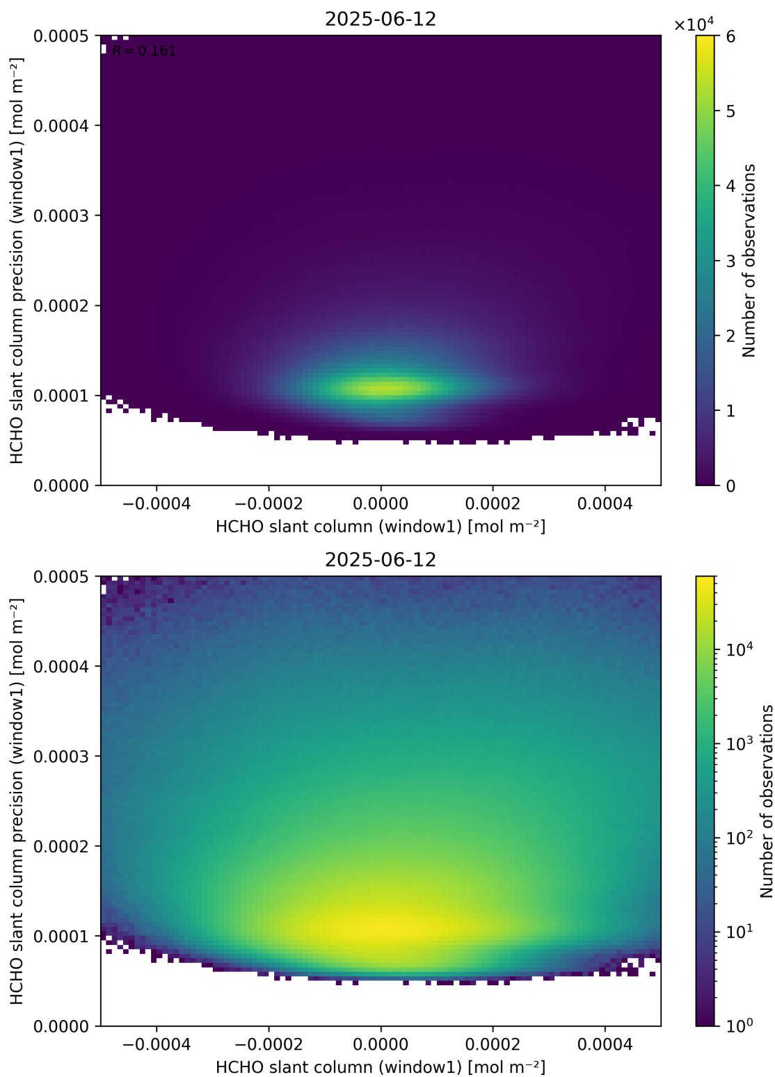
Figure 84: Scatter density plot of “HCHO slant column (window1)” against “HCHO slant column precision (window1)” for 2025-06-11 to 2025-06-13.
