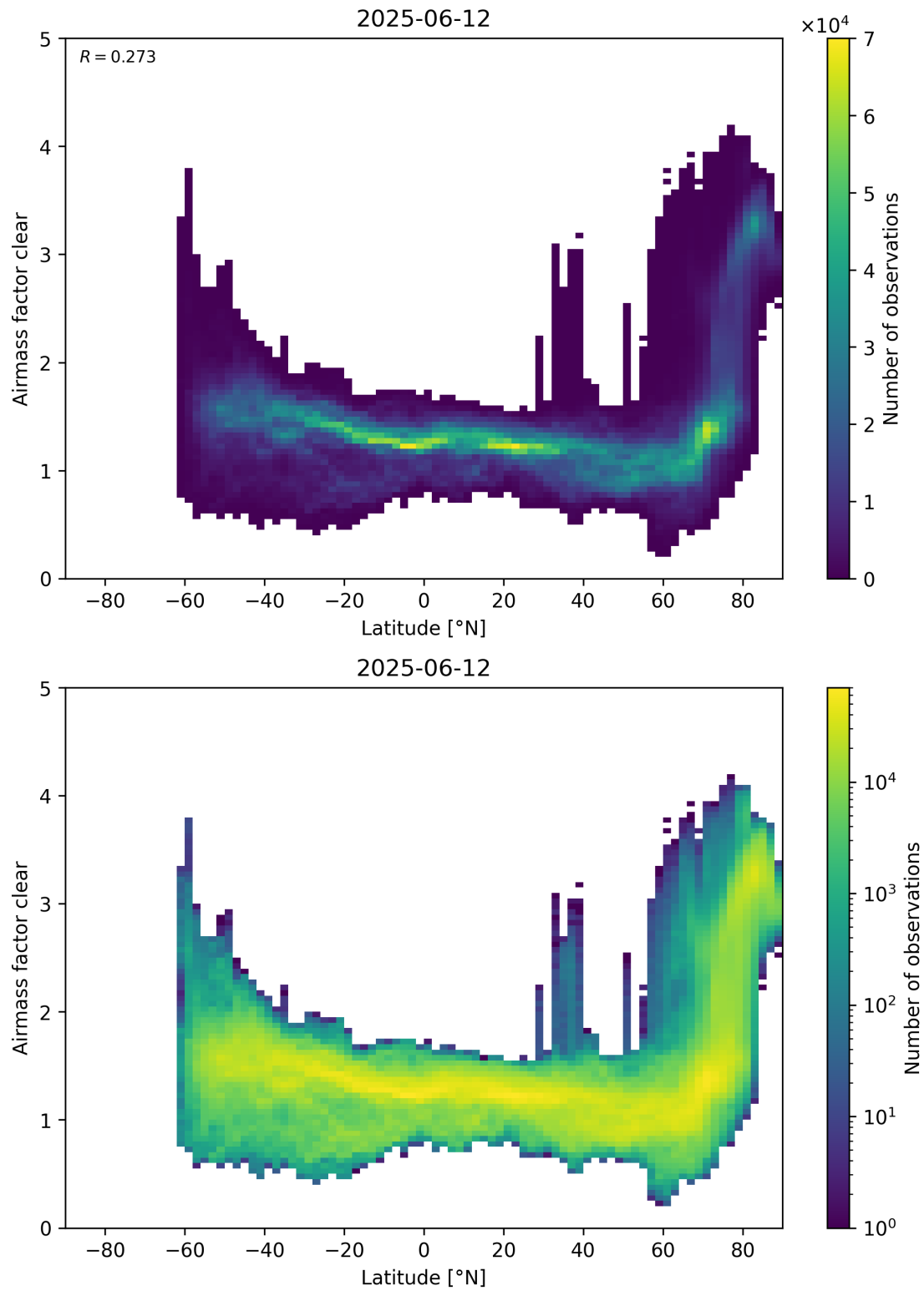
Figure 156: Scatter density plot of “Latitude” against “Airmass factor clear” for 2025-06-11 to 2025-06-13.
