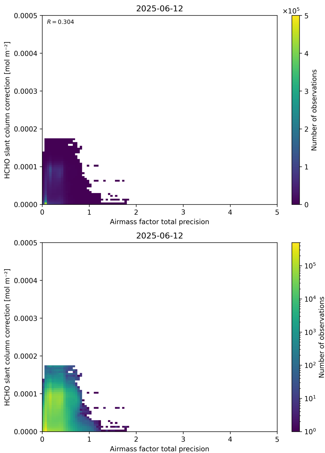
Figure 110: Scatter density plot of “Airmass factor total precision” against “HCHO slant column correction” for 2025-06-11 to 2025-06-13.
