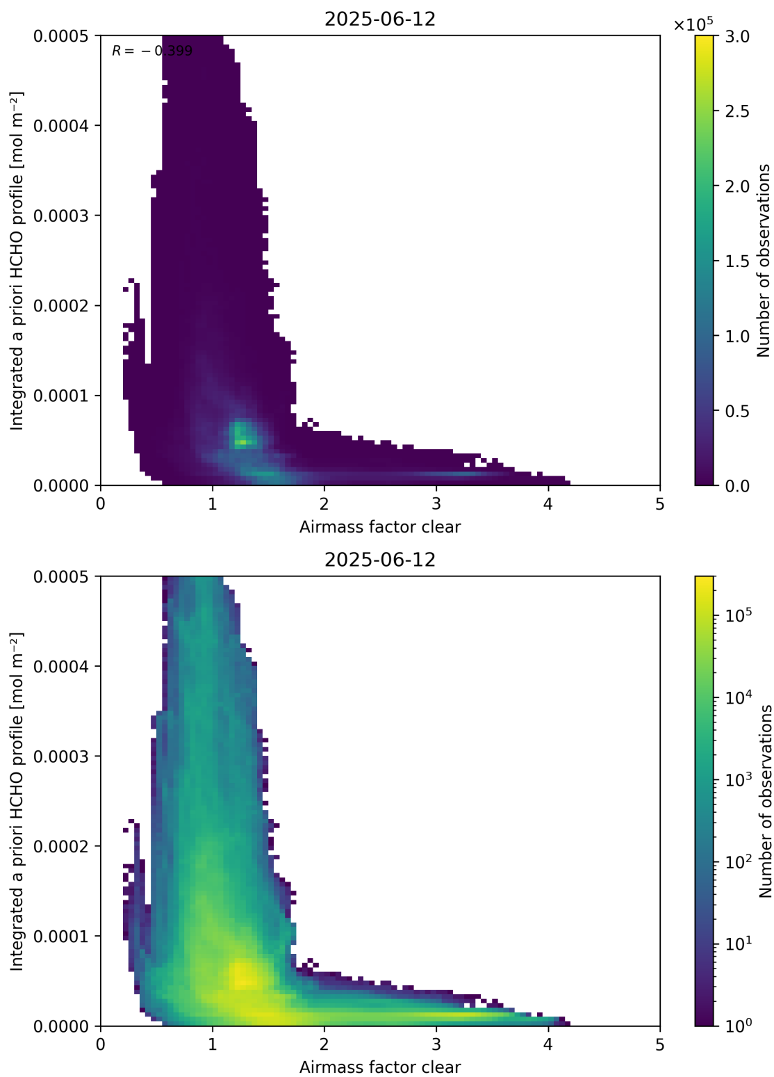
Figure 76: Scatter density plot of “Airmass factor clear” against “Integrated a priori HCHO profile” for 2025-06-11 to 2025-06-13.
