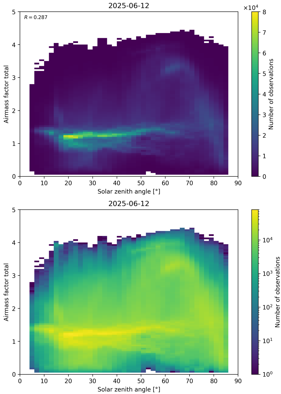
Figure 175: Scatter density plot of “Solar zenith angle” against “Airmass factor total” for 2025-06-11 to 2025-06-13.
