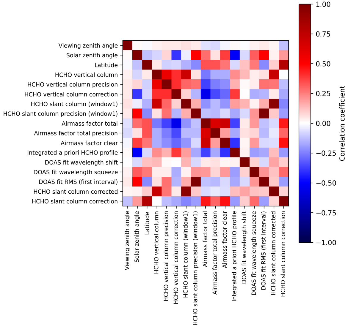
Figure 2: Map of correlation matrix for 2025-06-11 to 2025-06-13.
