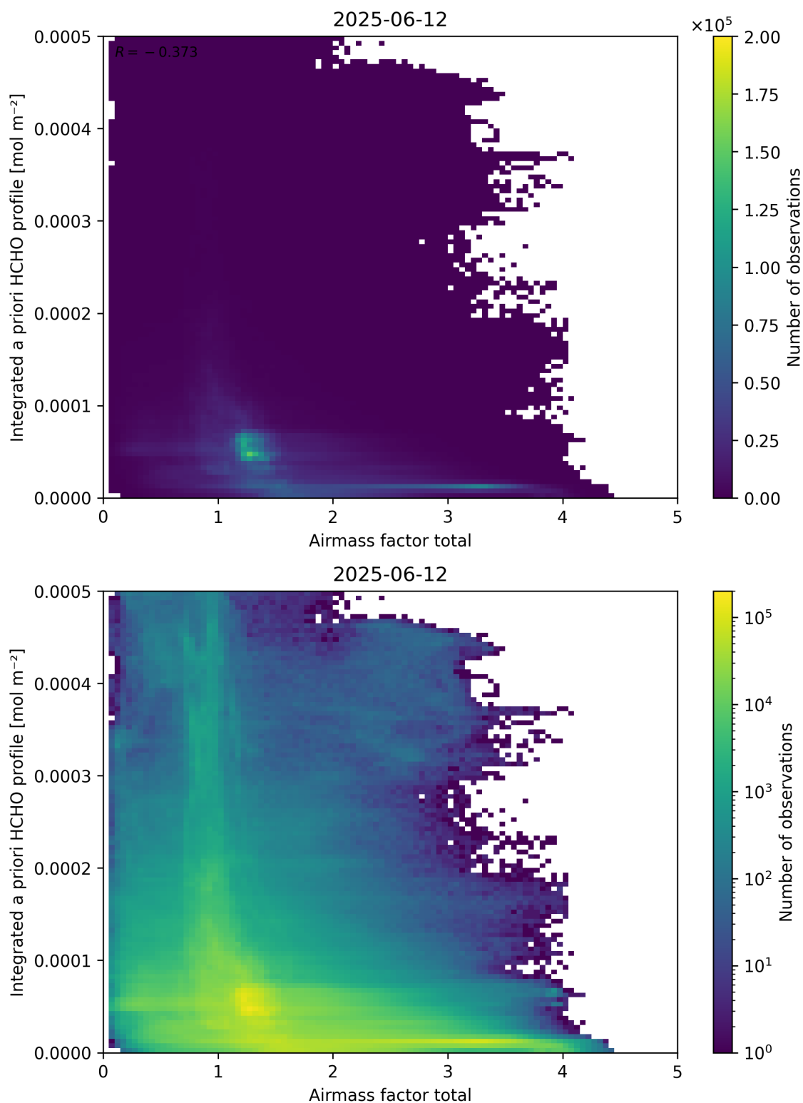
Figure 104: Scatter density plot of “Airmass factor total” against “Integrated a priori HCHO profile” for 2025-06-11 to 2025-06-13.
