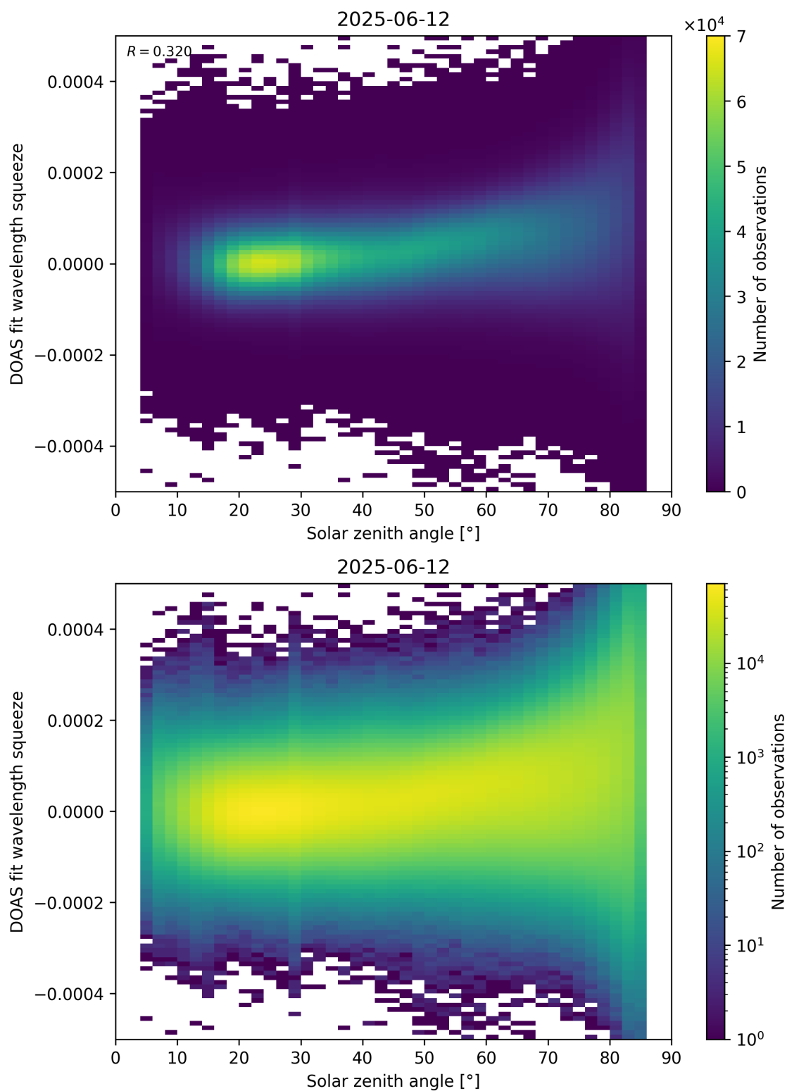
Figure 169: Scatter density plot of “Solar zenith angle” against “DOAS fit wavelength squeeze” for 2025-06-11 to 2025-06-13.
