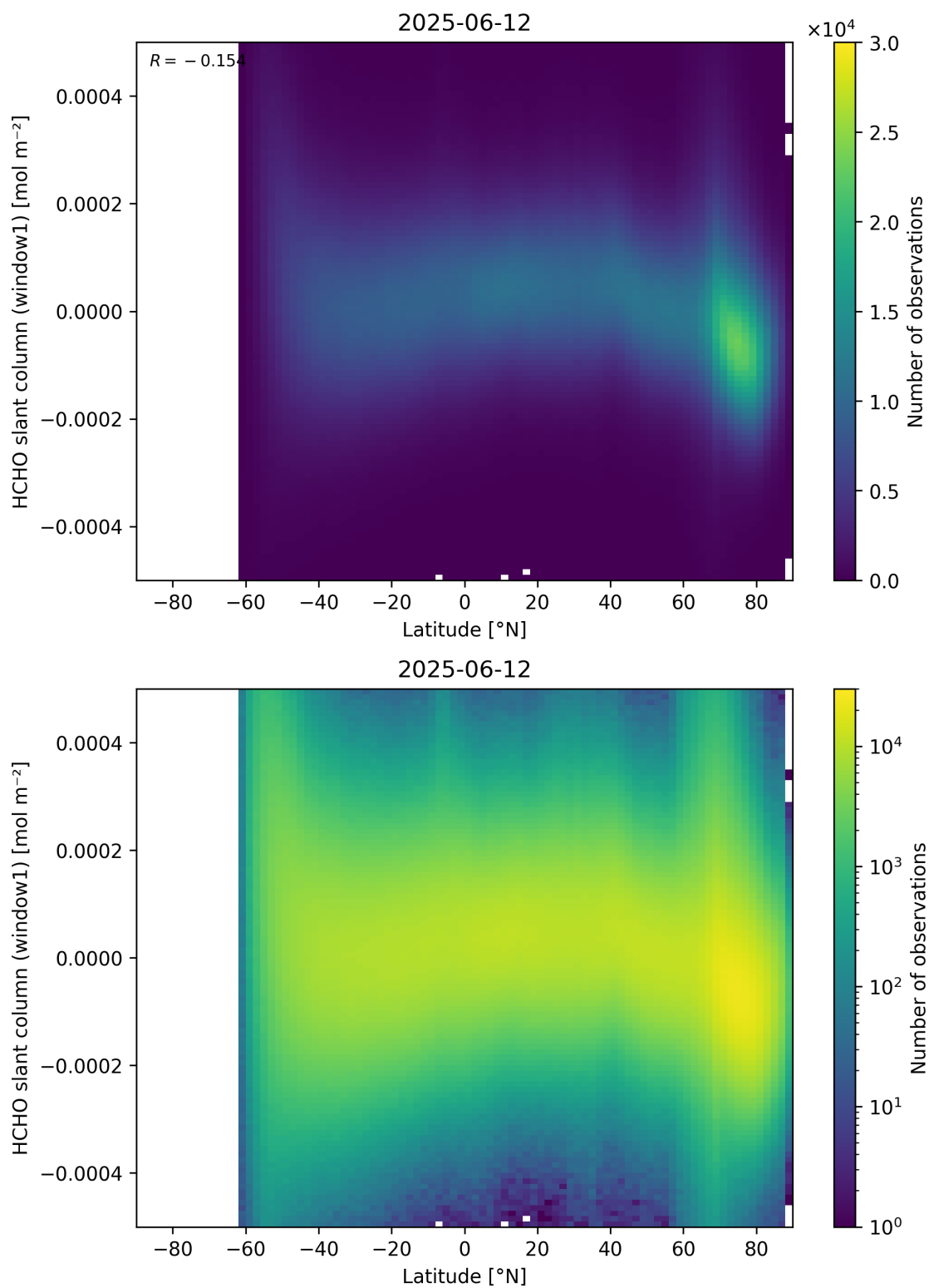
Figure 159: Scatter density plot of “Latitude” against “HCHO slant column (window1)” for 2025-06-11 to 2025-06-13.
