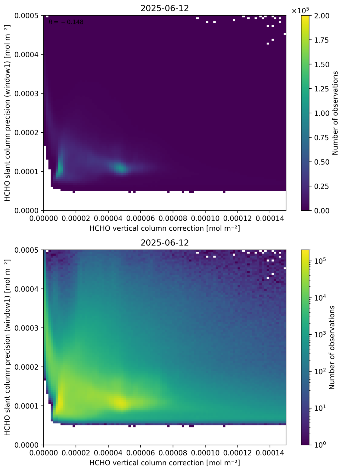
Figure 119: Scatter density plot of “HCHO vertical column correction” against “HCHO slant column precision (window1)” for 2025-06-11 to 2025-06-13.
