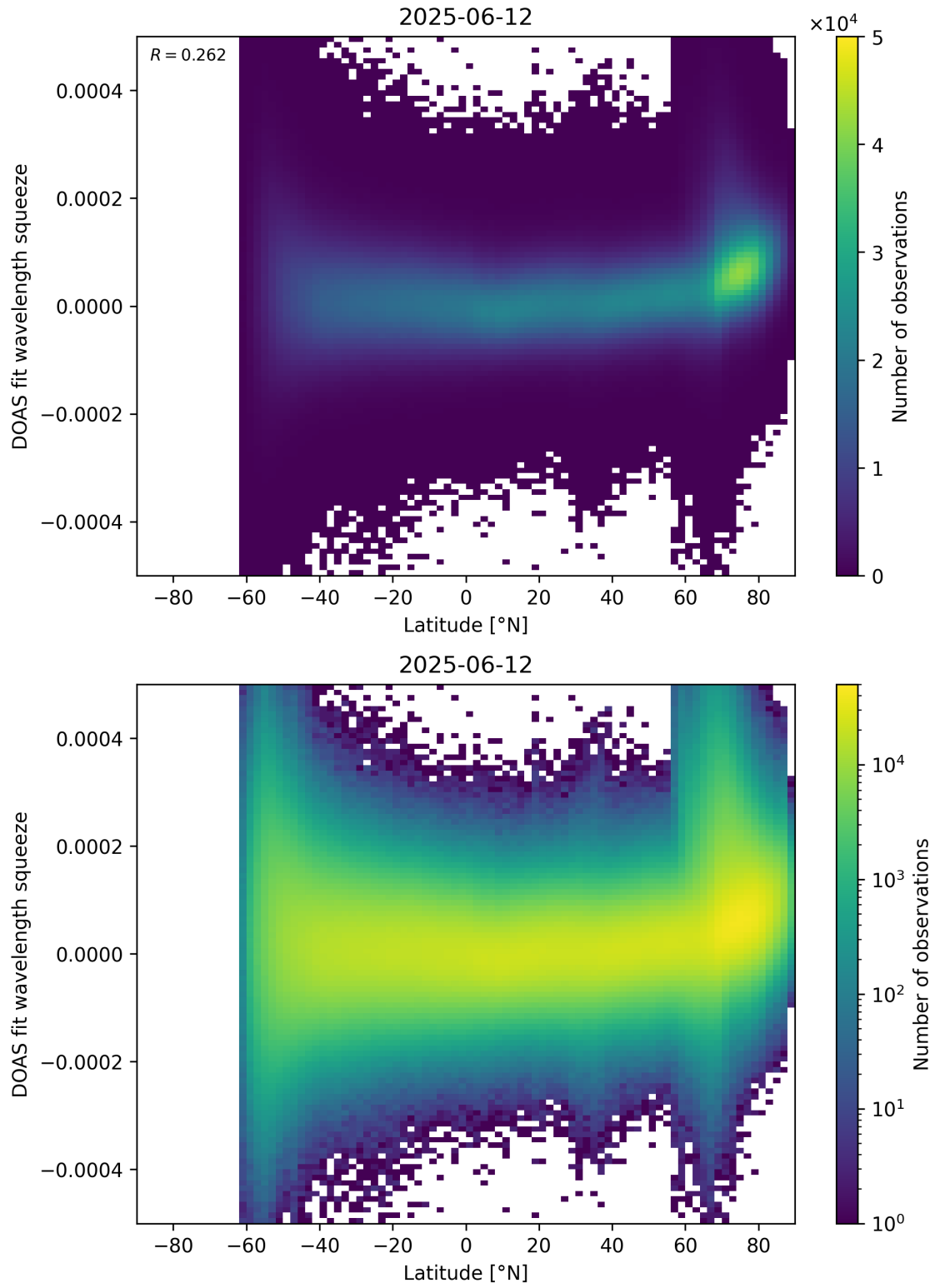
Figure 155: Scatter density plot of “Latitude” against “DOAS fit wavelength squeeze” for 2025-06-11 to 2025-06-13.
