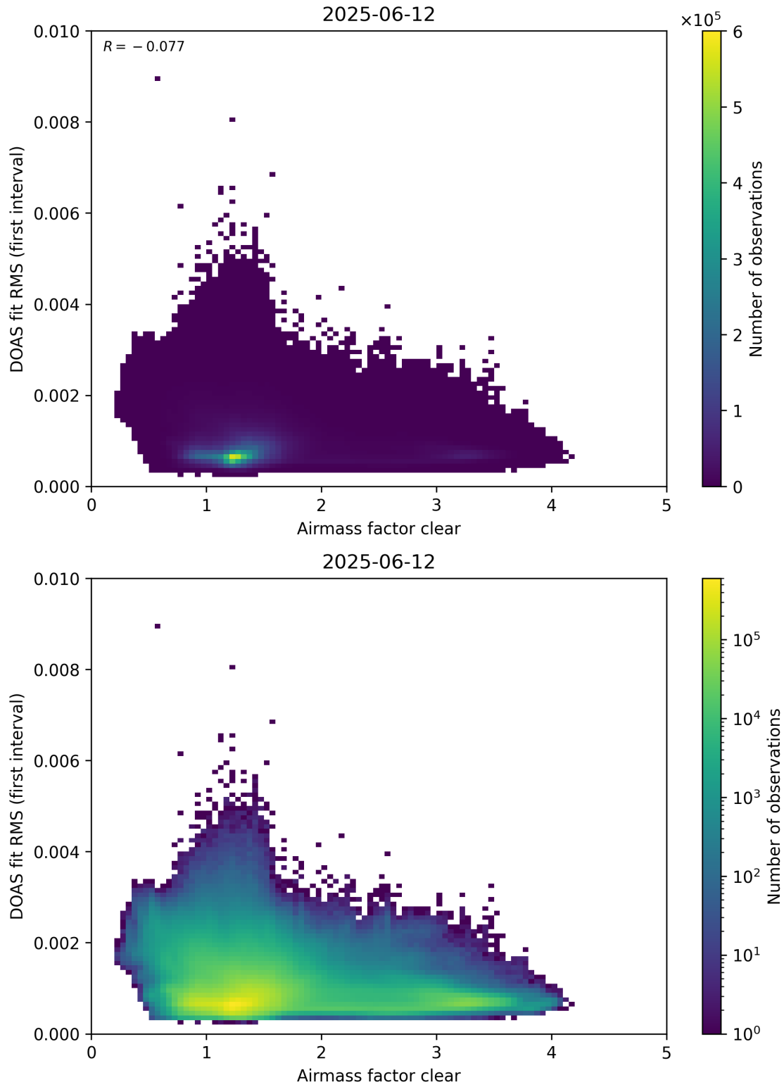
Figure 71: Scatter density plot of “Airmass factor clear” against “DOAS fit RMS (first interval)” for 2025-06-11 to 2025-06-13.
