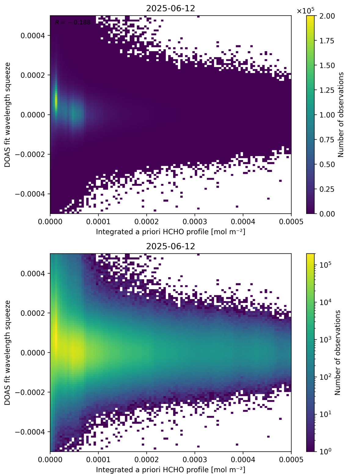
Figure 150: Scatter density plot of “Integrated a priori HCHO profile” against “DOAS fit wavelength squeeze” for 2025-06-11 to 2025-06-13.
