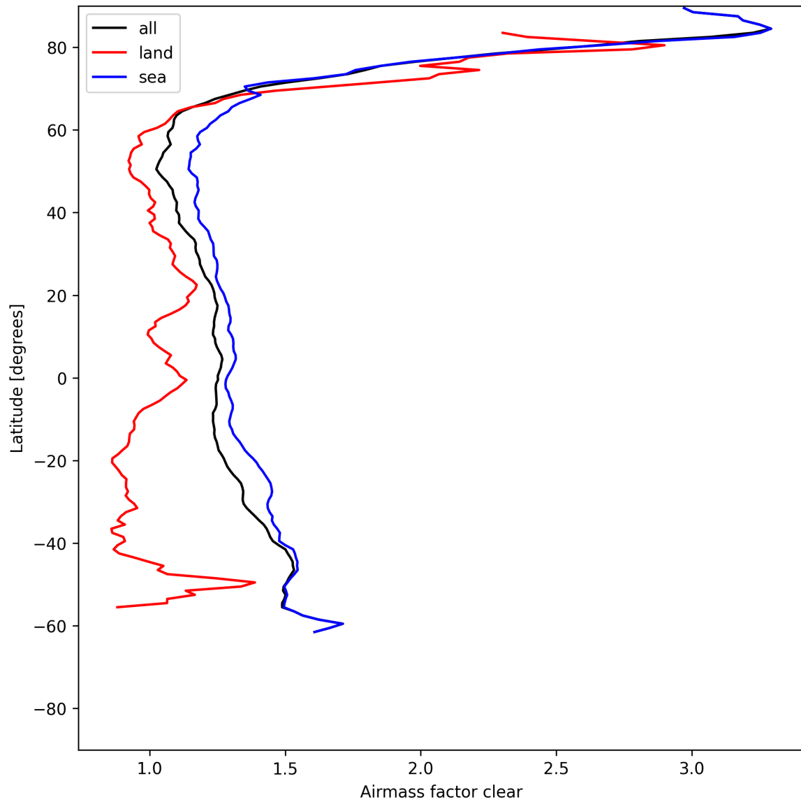
Figure 28: Zonal average of “Airmass factor clear” for 2025-06-11 to 2025-06-13.
