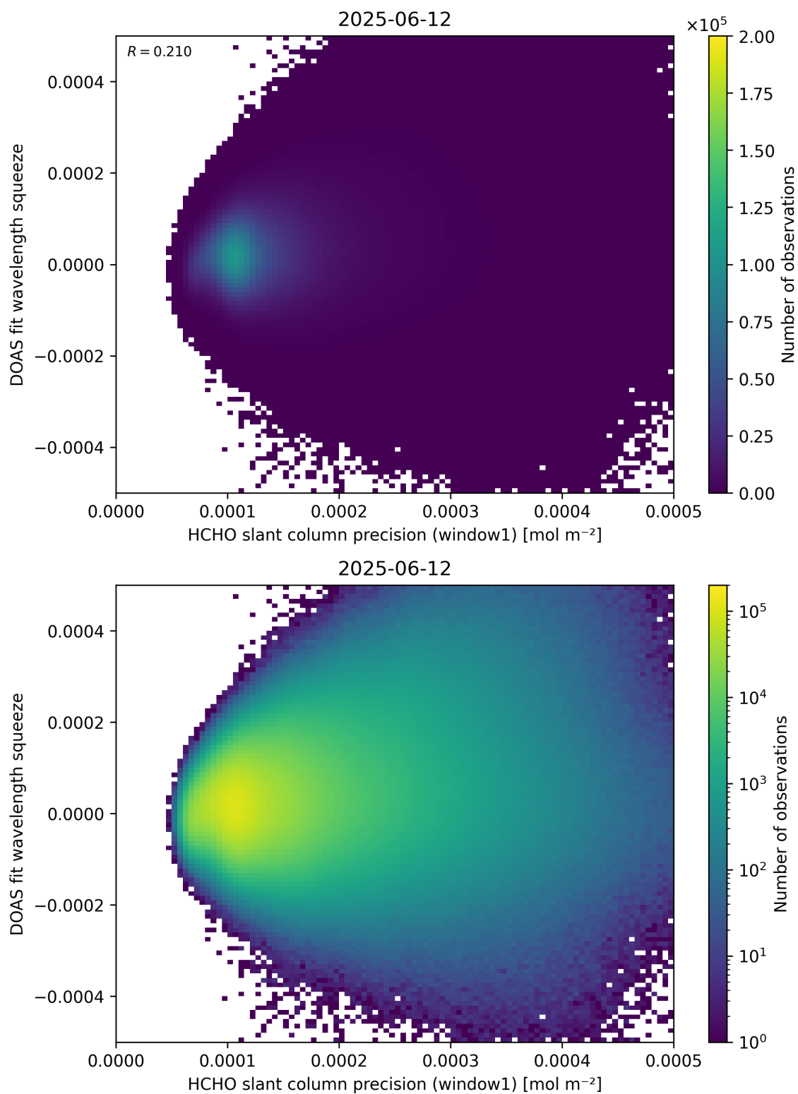
Figure 90: Scatter density plot of “HCHO slant column precision (window1)” against “DOAS fit wavelength squeeze” for 2025-06-11 to 2025-06-13.
