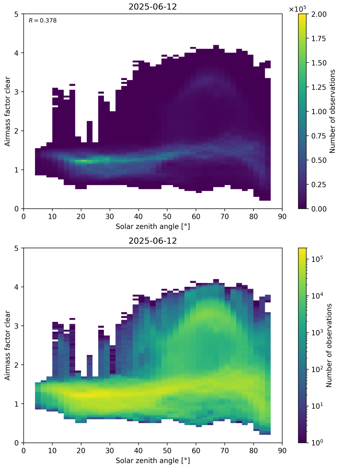
Figure 170: Scatter density plot of “Solar zenith angle” against “Airmass factor clear” for 2025-06-11 to 2025-06-13.
