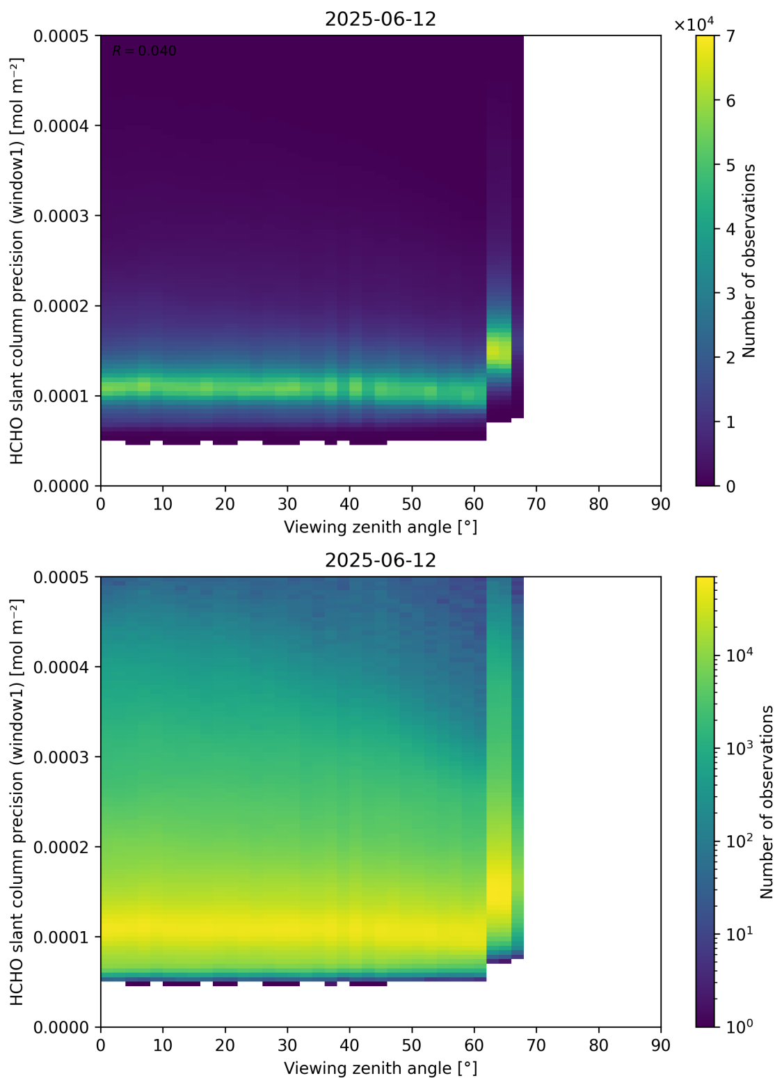
Figure 189: Scatter density plot of “Viewing zenith angle” against “HCHO slant column precision (window1)” for 2025-06-11 to 2025-06-13.
