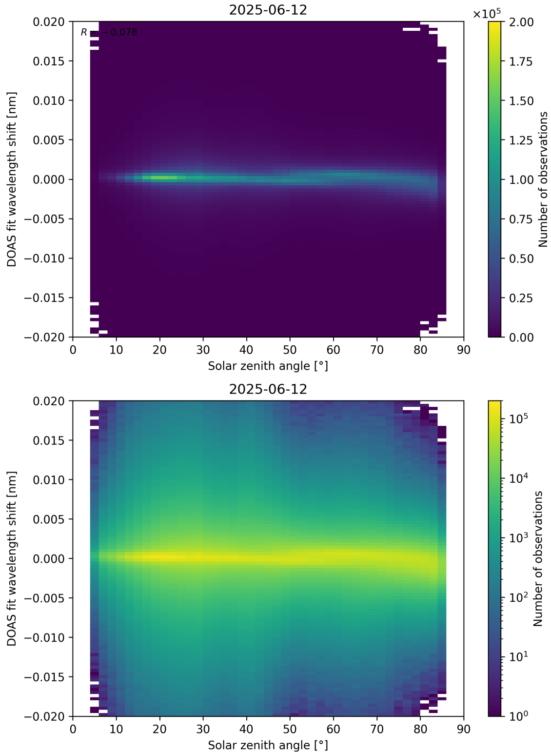
Figure 168: Scatter density plot of “Solar zenith angle” against “DOAS fit wavelength shift” for 2025-06-11 to 2025-06-13.
