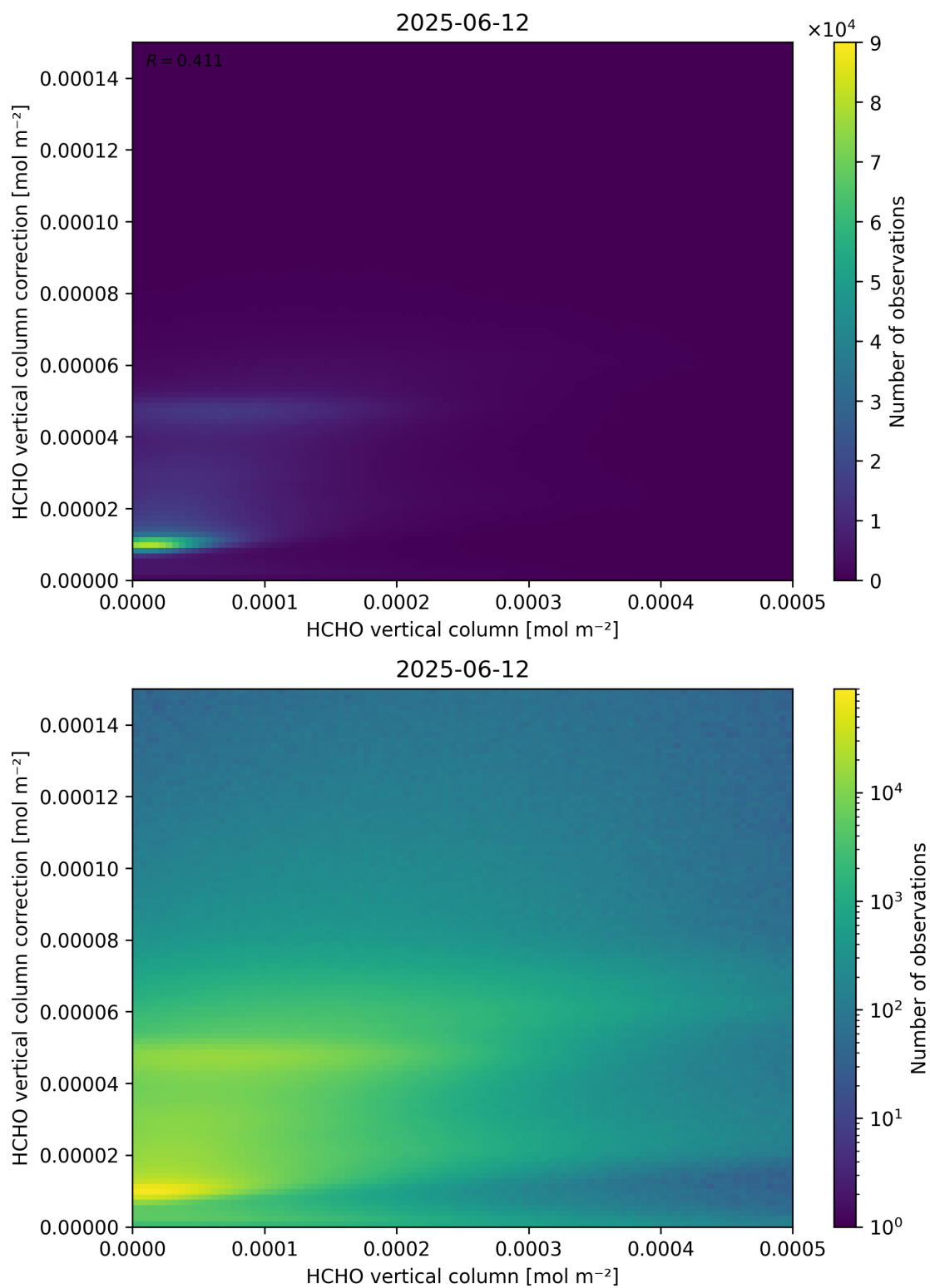
Figure 133: Scatter density plot of “HCHO vertical column” against “HCHO vertical column correction” for 2025-06-11 to 2025-06-13.
