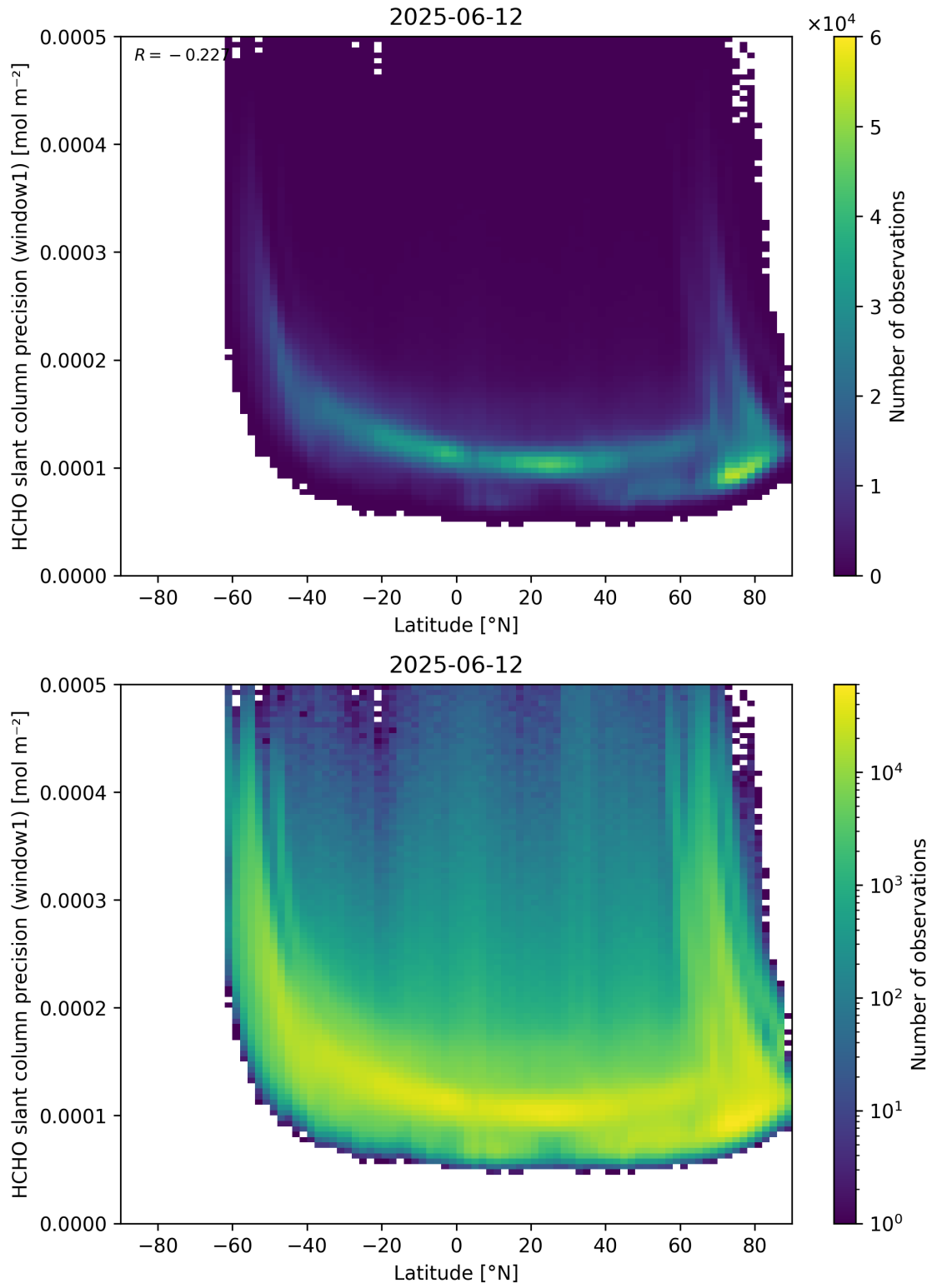
Figure 160: Scatter density plot of “Latitude” against “HCHO slant column precision (window1)” for 2025-06-11 to 2025-06-13.
