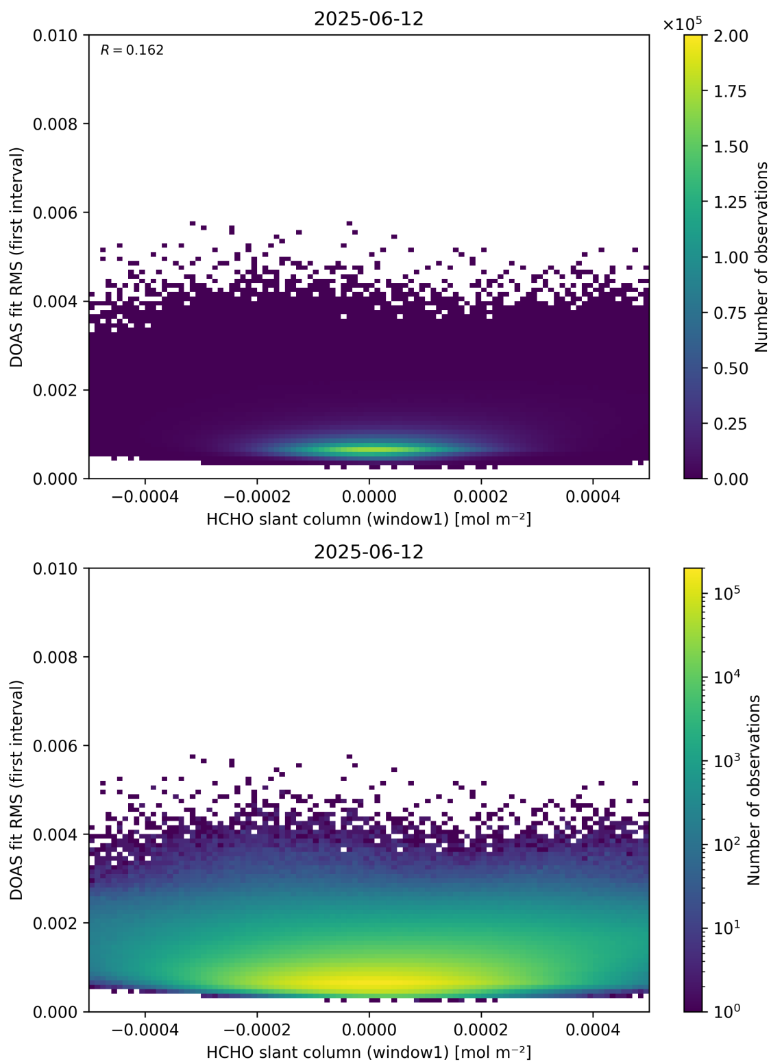
Figure 78: Scatter density plot of “HCHO slant column (window1)” against “DOAS fit RMS (first interval)” for 2025-06-11 to 2025-06-13.
