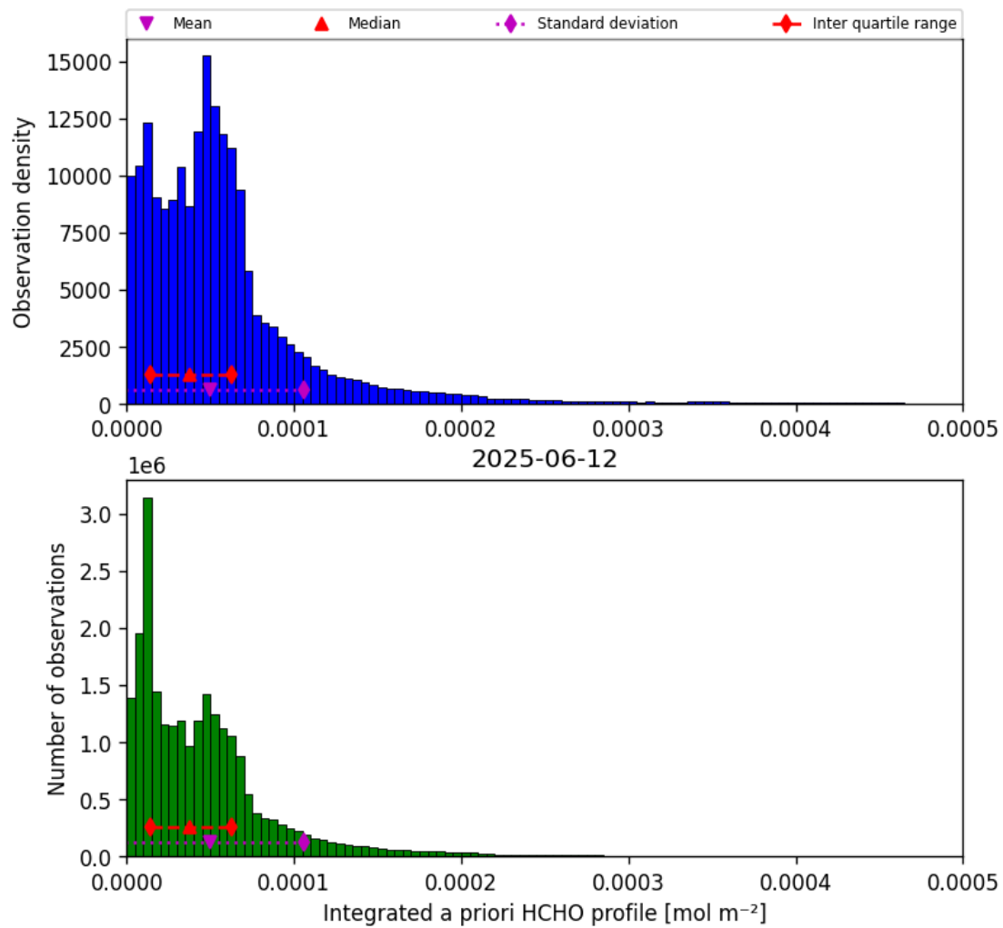
Figure 43: Histogram of “Integrated a priori HCHO profile” for 2025-06-11 to 2025-06-13
