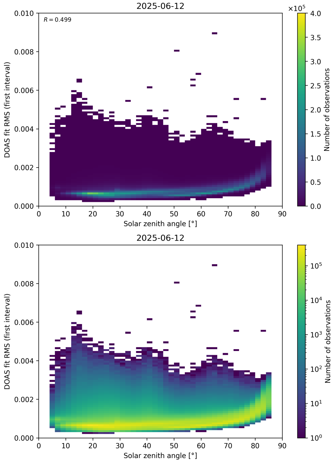
Figure 167: Scatter density plot of “Solar zenith angle” against “DOAS fit RMS (first interval)” for 2025-06-11 to 2025-06-13.
