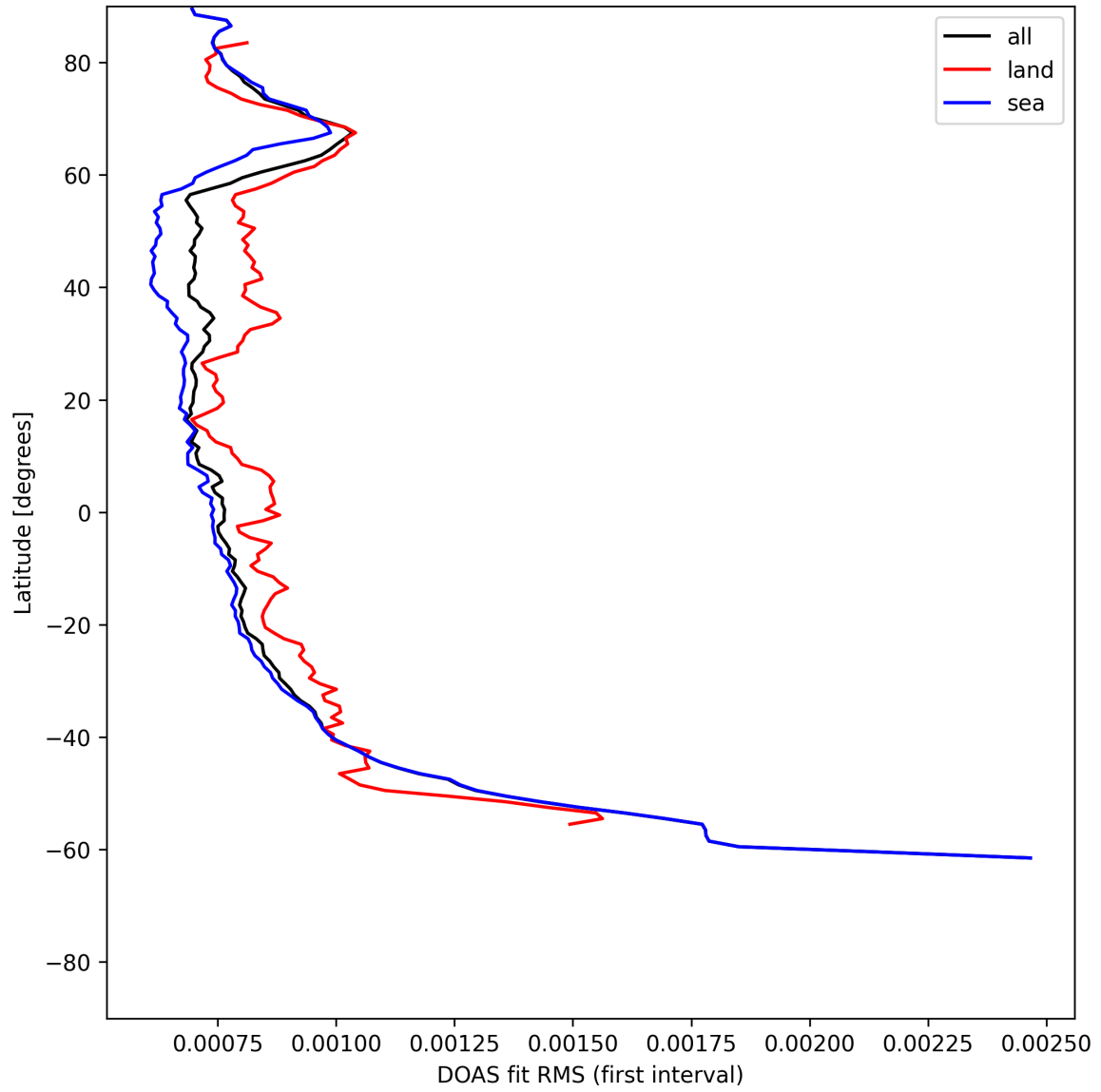
Figure 32: Zonal average of “DOAS fit RMS (first interval)” for 2025-06-11 to 2025-06-13.
