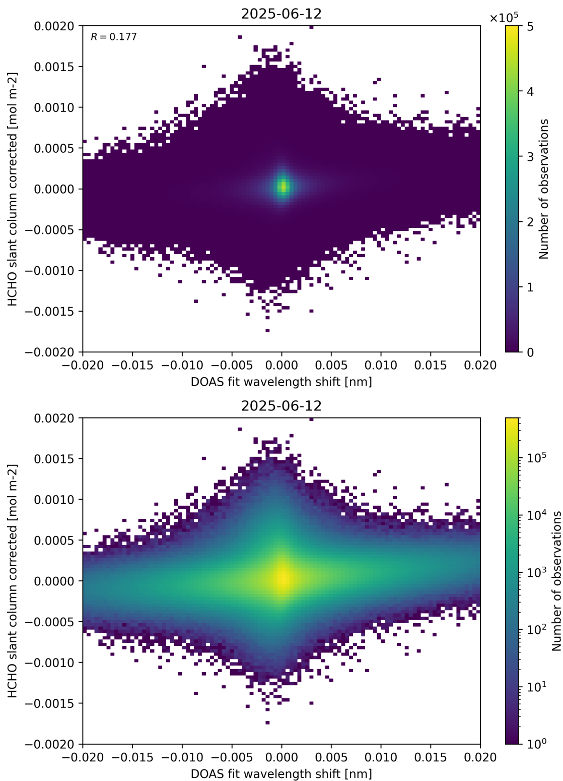
Figure 66: Scatter density plot of “DOAS fit wavelength shift” against “HCHO slant column corrected” for 2025-06-11 to 2025-06-13.
