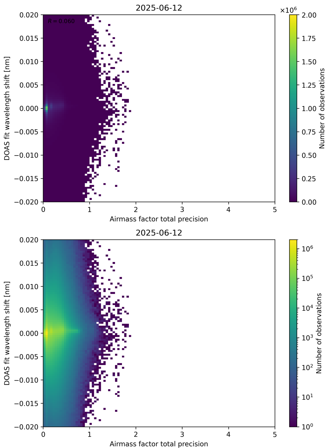
Figure 106: Scatter density plot of “Airmass factor total precision” against “DOAS fit wavelength shift” for 2025-06-11 to 2025-06-13.
