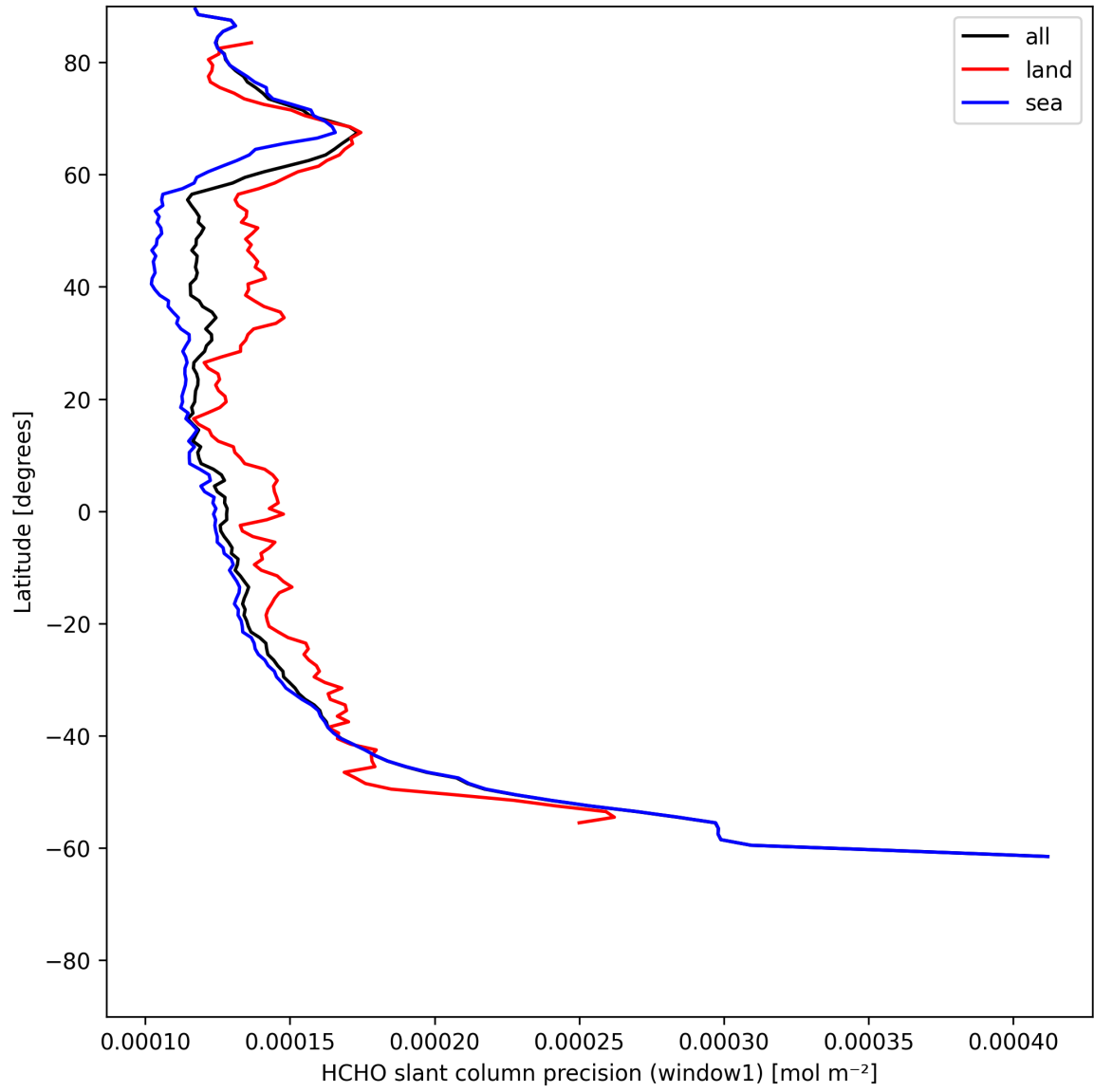
Figure 25: Zonal average of "HCHO slant column precision (window1)" for 2025-06-11 to 2025-06-13.
