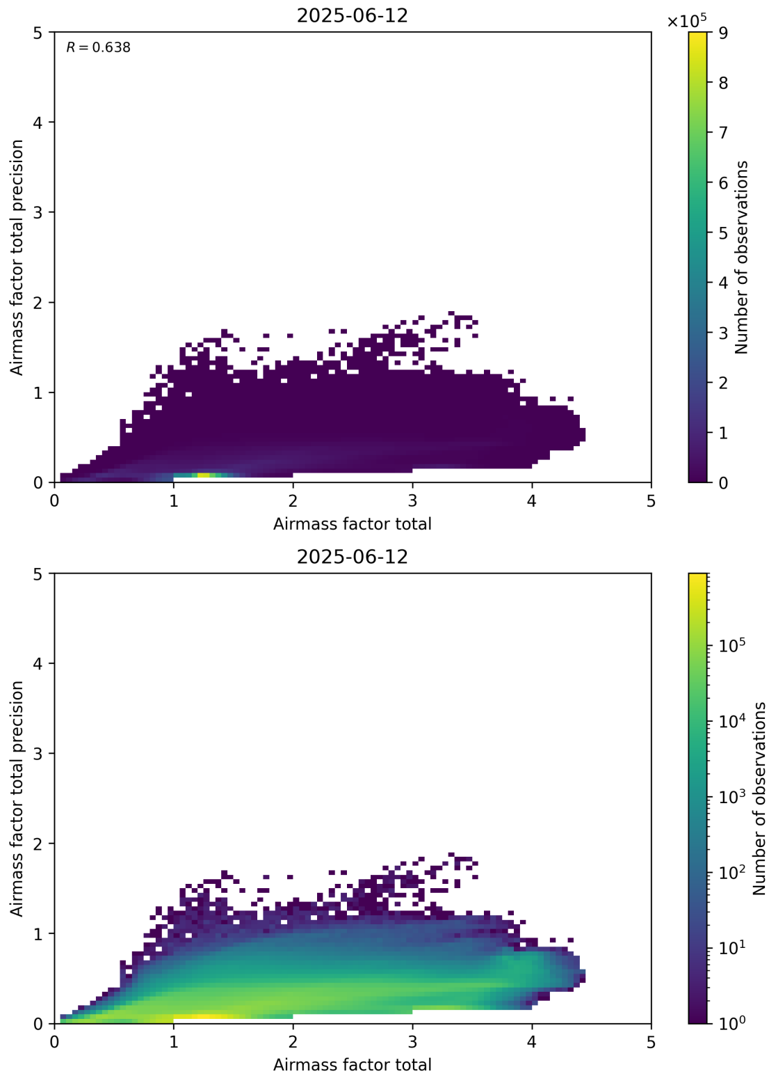
Figure 103: Scatter density plot of “Airmass factor total” against “Airmass factor total precision” for 2025-06-11 to 2025-06-13.
