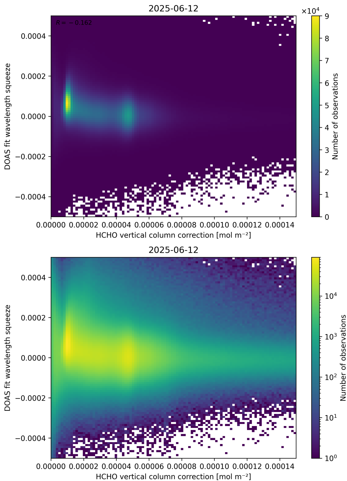
Figure 114: Scatter density plot of “HCHO vertical column correction” against “DOAS fit wavelength squeeze” for 2025-06-11 to 2025-06-13.
