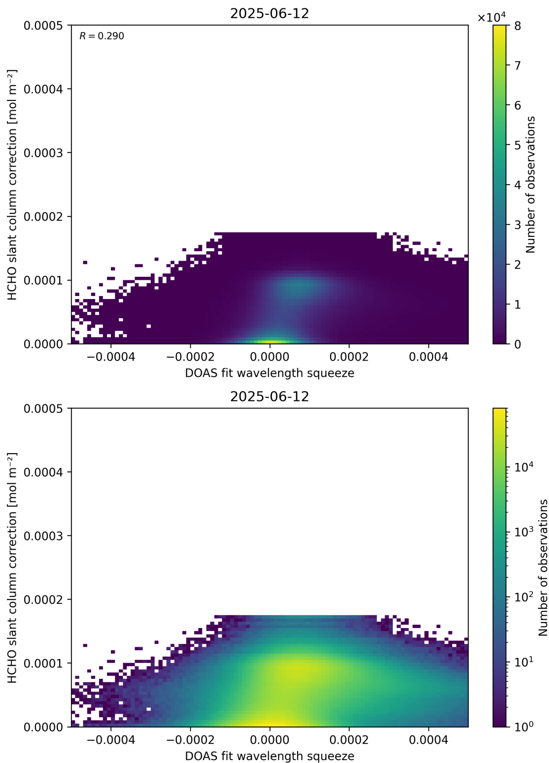
Figure 70: Scatter density plot of “DOAS fit wavelength squeeze” against “HCHO slant column correction” for 2025-06-11 to 2025-06-13.
