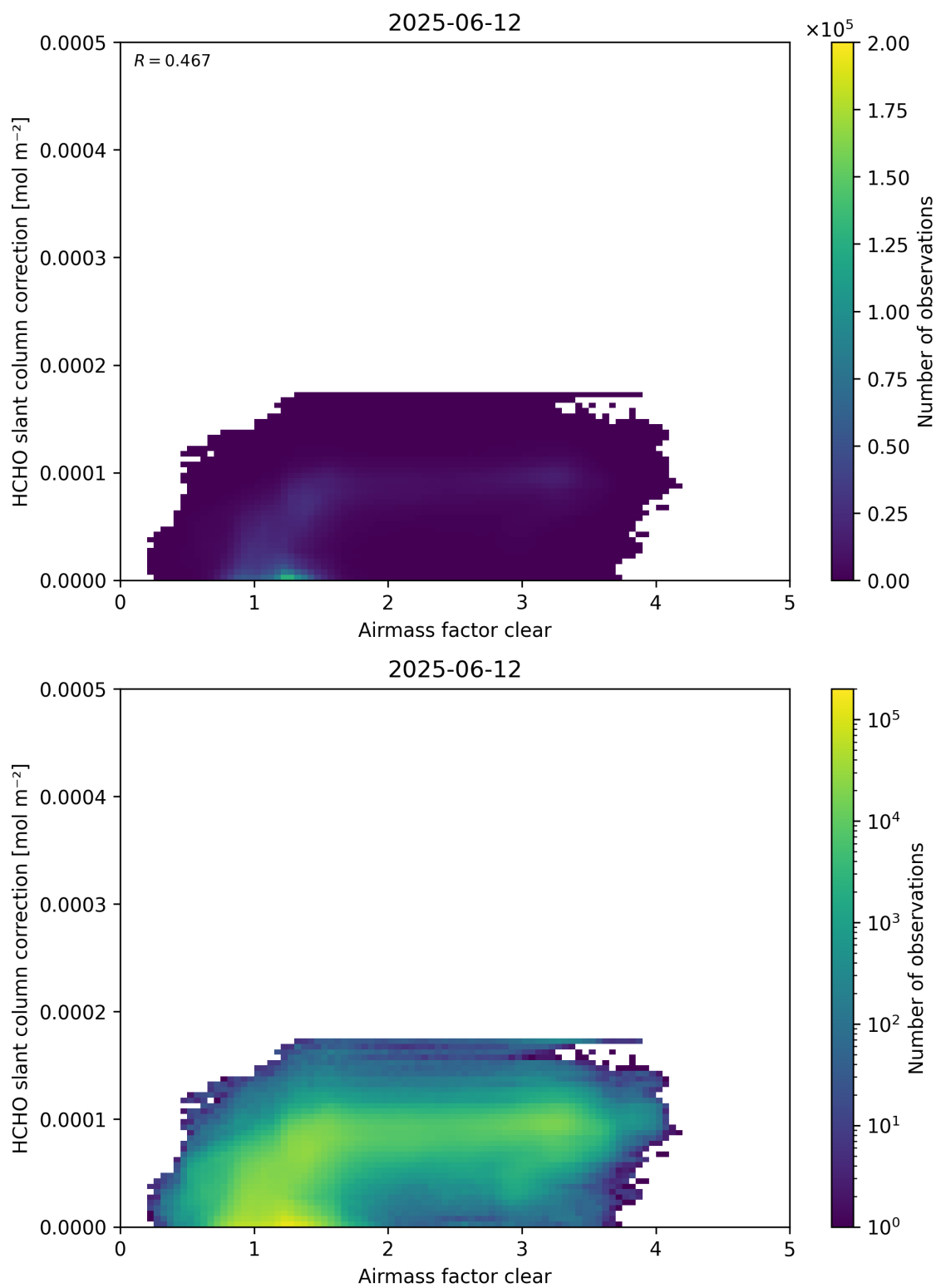
Figure 75: Scatter density plot of “Airmass factor clear” against “HCHO slant column correction” for 2025-06-11 to 2025-06-13.
