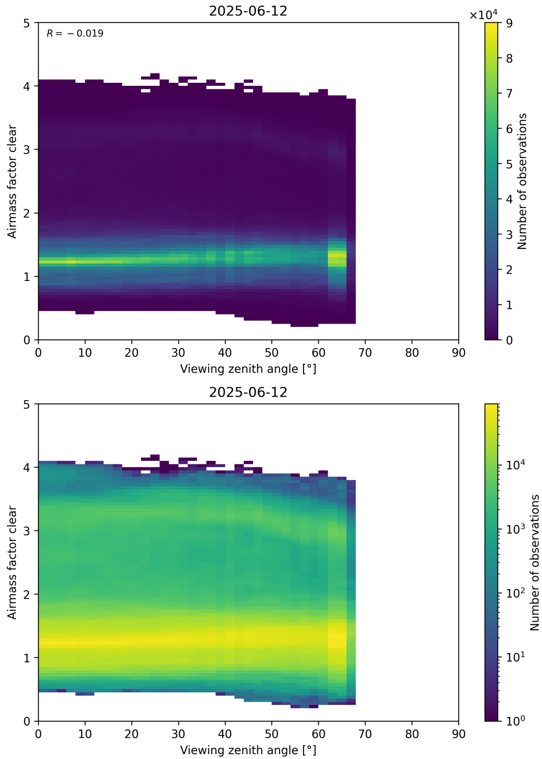
Figure 185: Scatter density plot of “Viewing zenith angle” against “Airmass factor clear” for 2025-06-11 to 2025-06-13.
