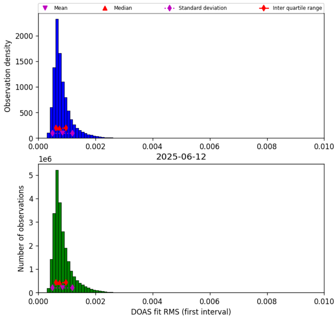
Figure 46: Histogram of “DOAS fit RMS (first interval)” for 2025-06-11 to 2025-06-13
