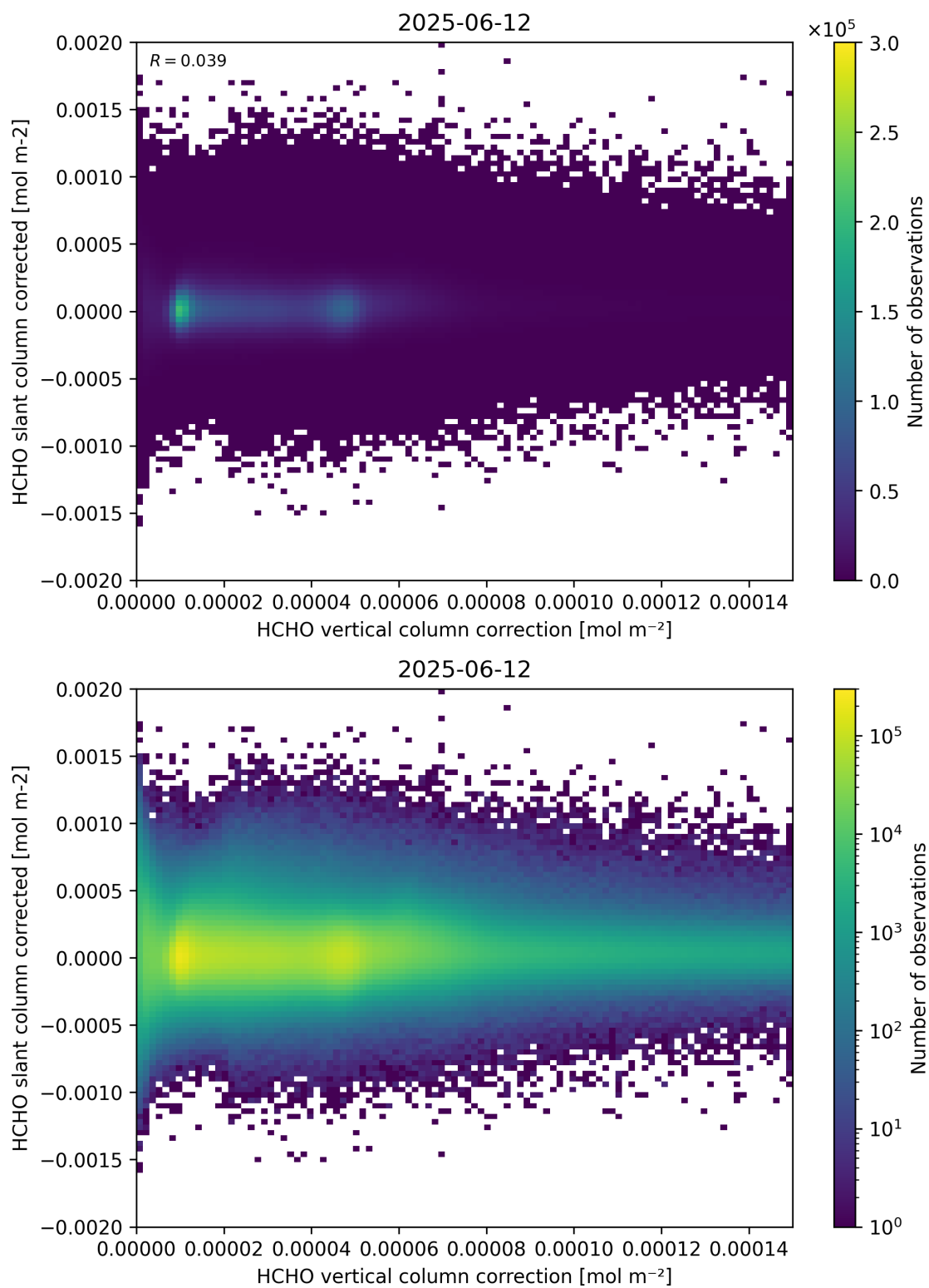
Figure 116: Scatter density plot of “HCHO vertical column correction” against “HCHO slant column corrected” for 2025-06-11 to 2025-06-13.
