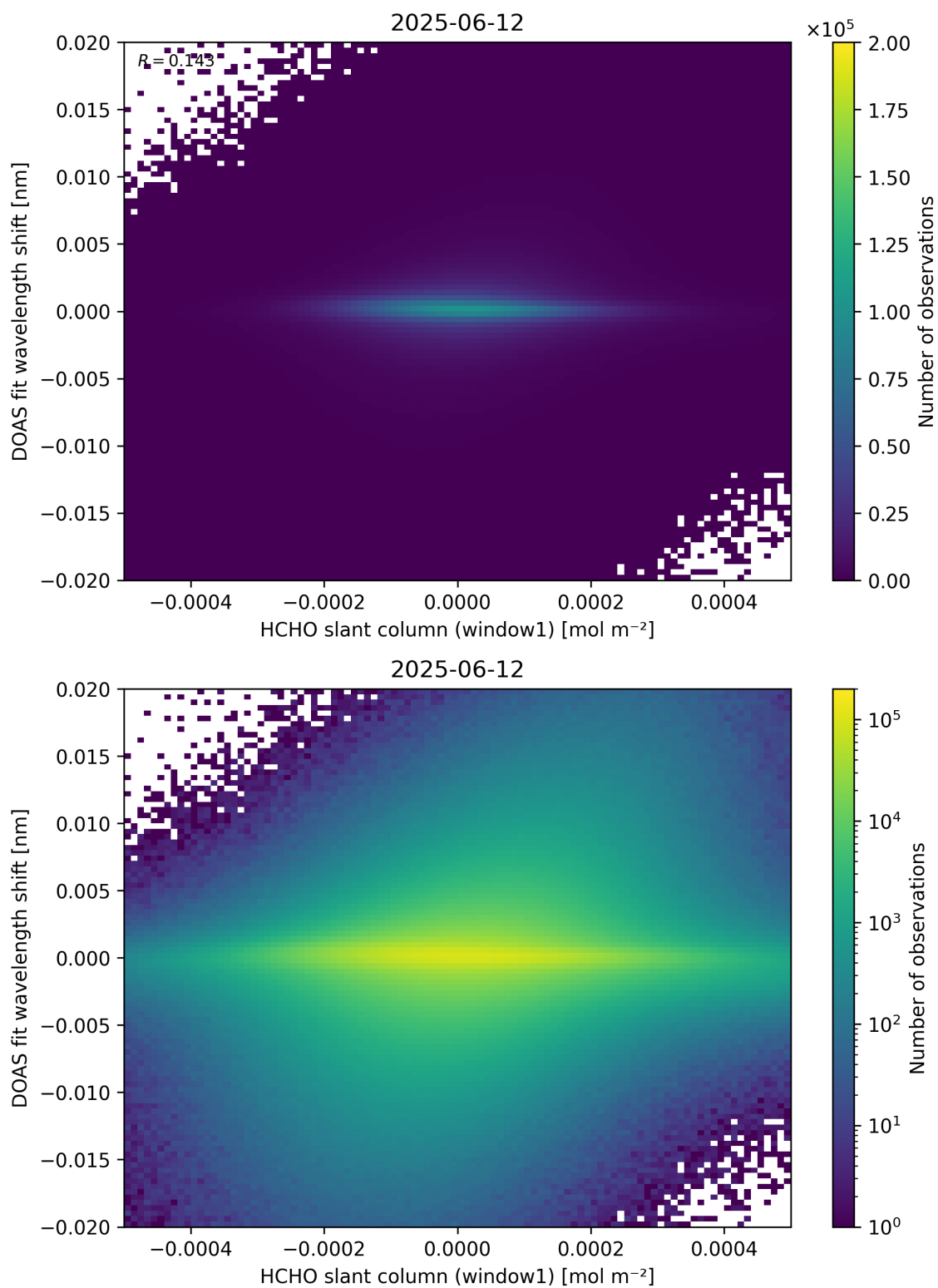
Figure 79: Scatter density plot of “HCHO slant column (window1)” against “DOAS fit wavelength shift” for 2025-06-11 to 2025-06-13.
