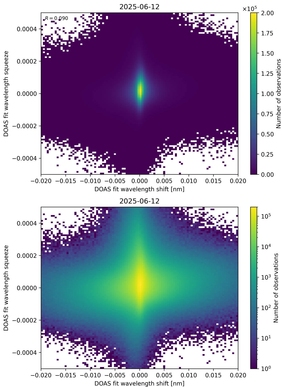
Figure 65: Scatter density plot of “DOAS fit wavelength shift” against “DOAS fit wavelength squeeze” for 2025-06-11 to 2025-06-13.
