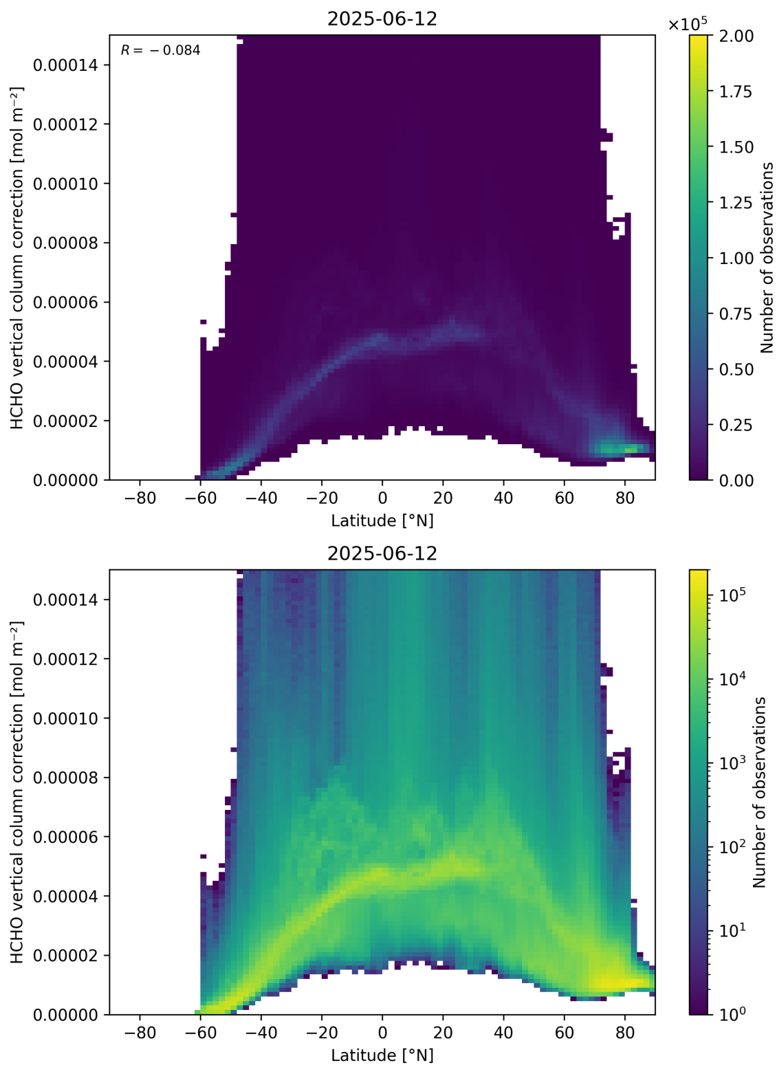
Figure 164: Scatter density plot of “Latitude” against “HCHO vertical column correction” for 2025-06-11 to 2025-06-13.
