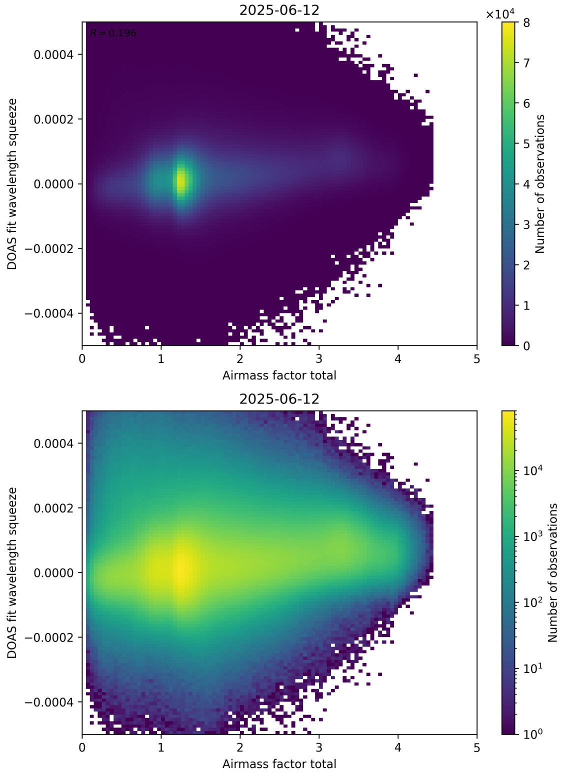
Figure 99: Scatter density plot of “Airmass factor total” against “DOAS fit wavelength squeeze” for 2025-06-11 to 2025-06-13.
