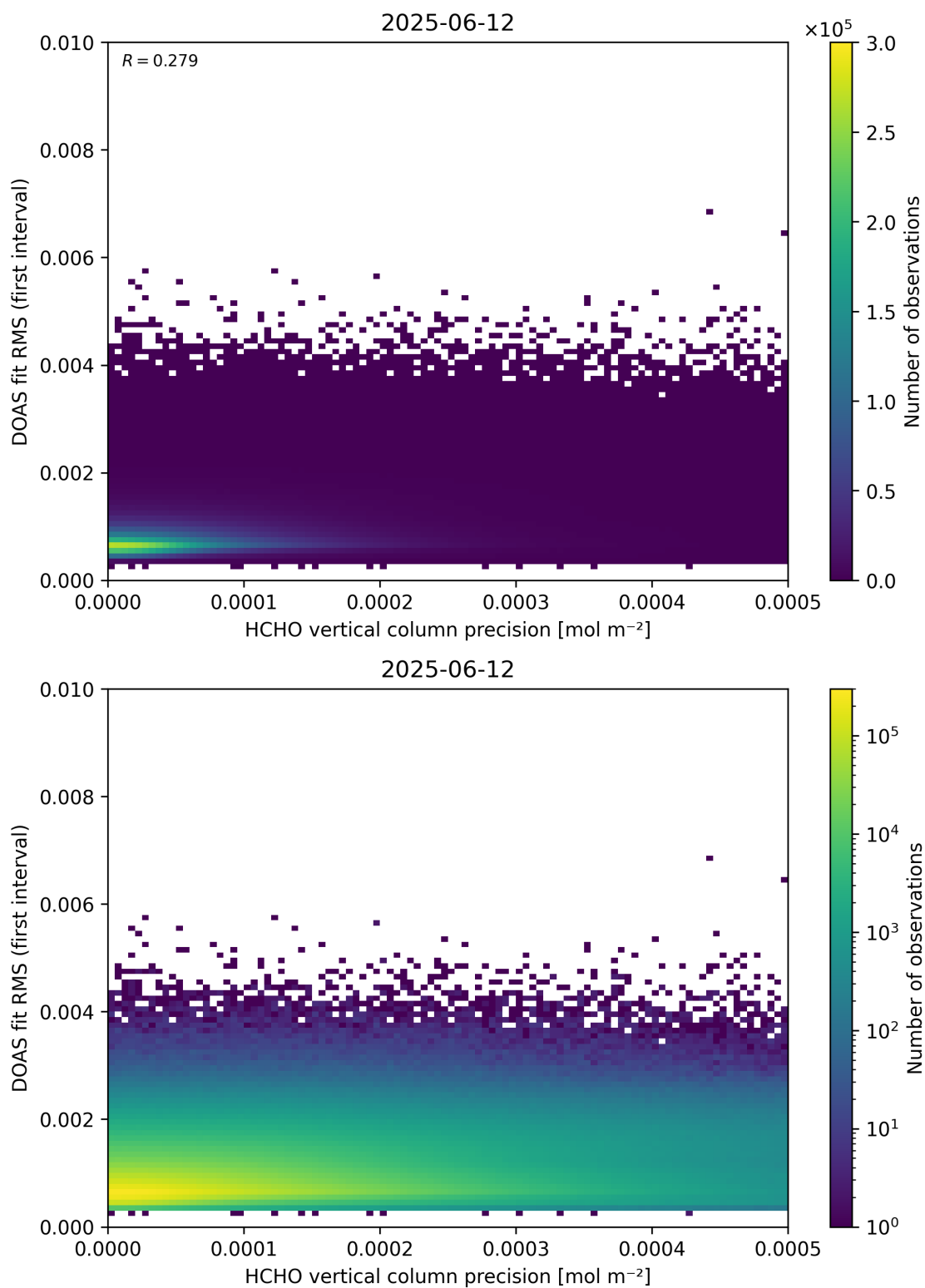
Figure 136: Scatter density plot of “HCHO vertical column precision” against “DOAS fit RMS (first interval)” for 2025-06-11 to 2025-06-13.
