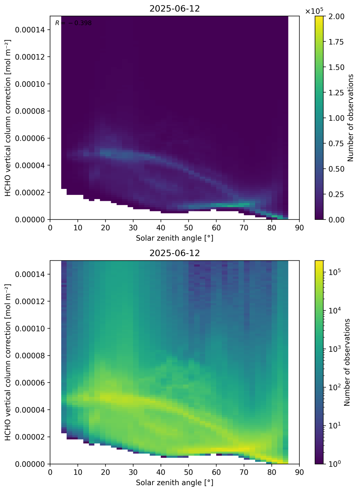
Figure 178: Scatter density plot of “Solar zenith angle” against “HCHO vertical column correction” for 2025-06-11 to 2025-06-13.
