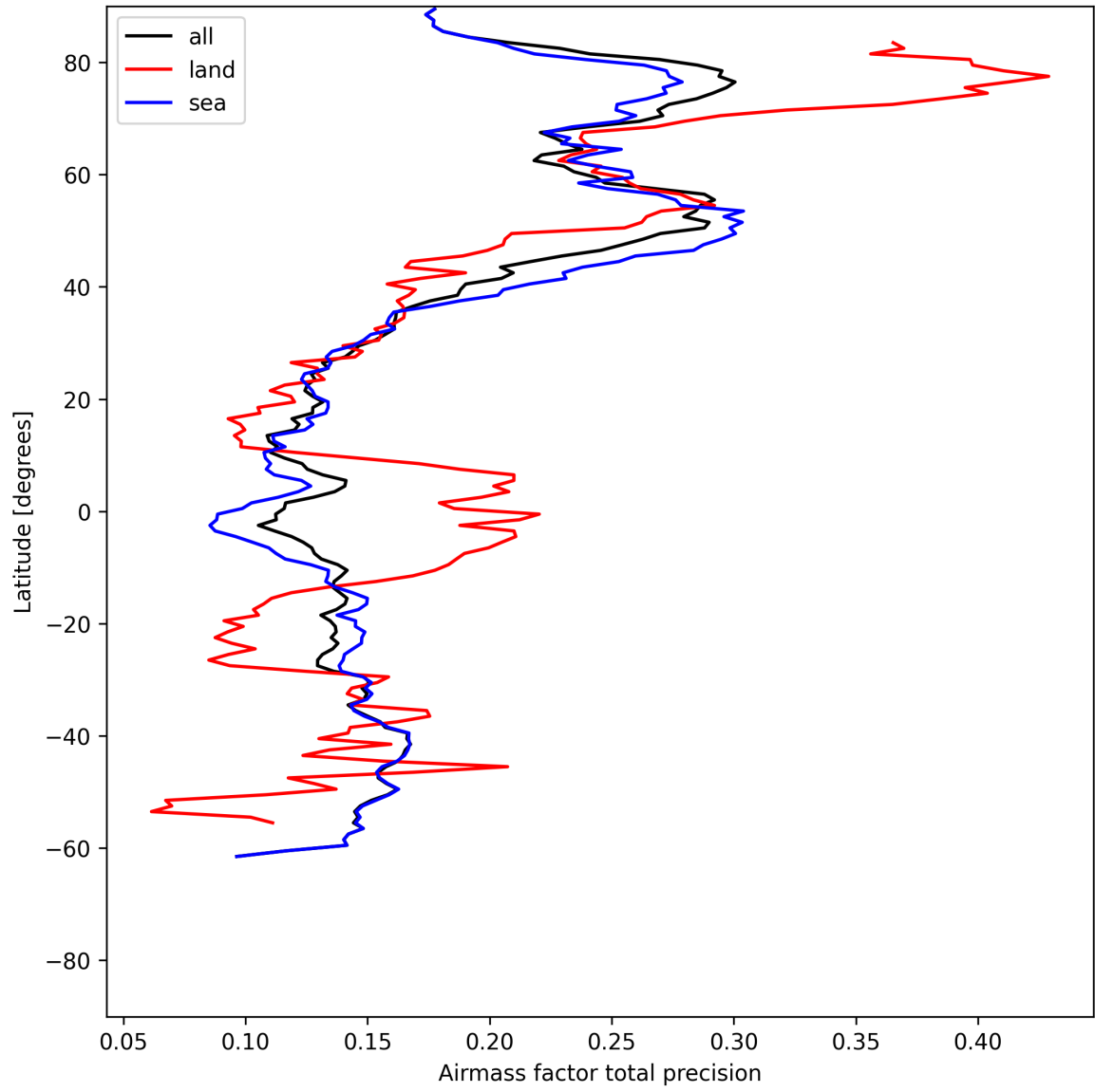
Figure 27: Zonal average of “Airmass factor total precision” for 2025-06-11 to 2025-06-13.
