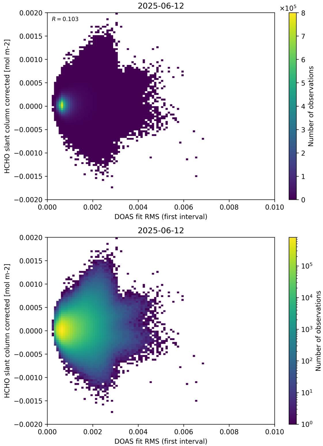
Figure 62: Scatter density plot of “DOAS fit RMS (first interval)” against “HCHO slant column corrected” for 2025-06-11 to 2025-06-13.
