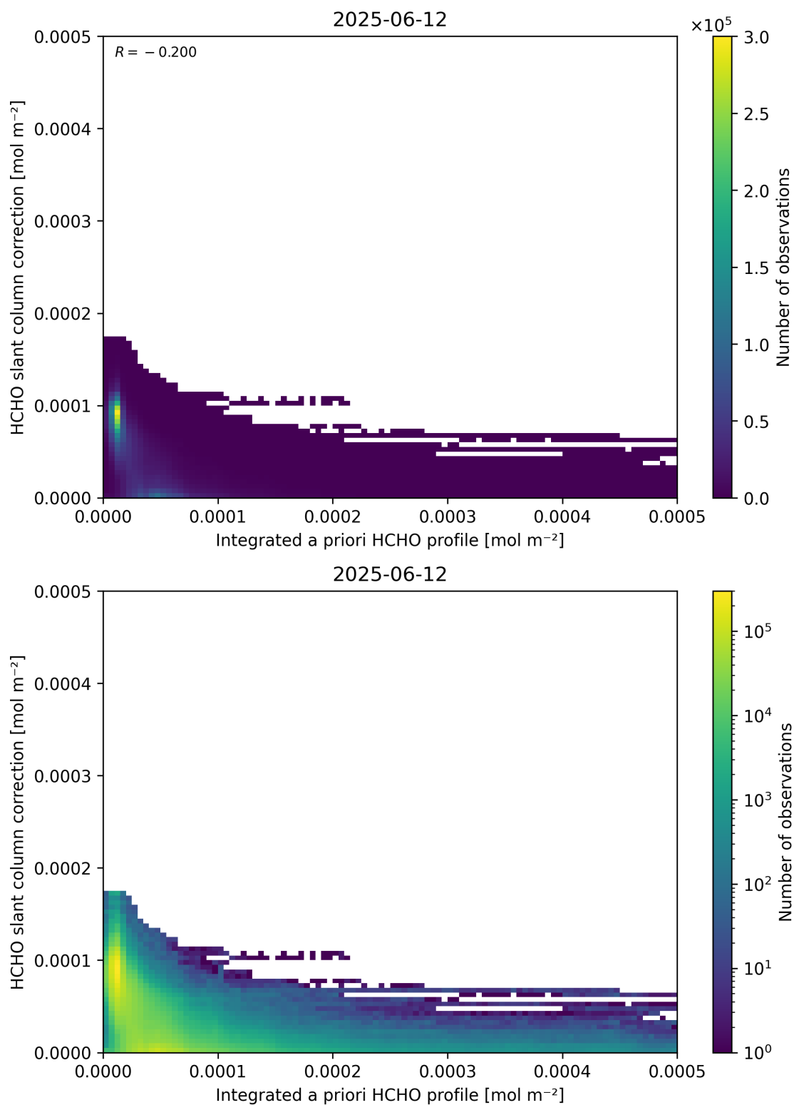
Figure 152: Scatter density plot of “Integrated a priori HCHO profile” against “HCHO slant column correction” for 2025-06-11 to 2025-06-13.
