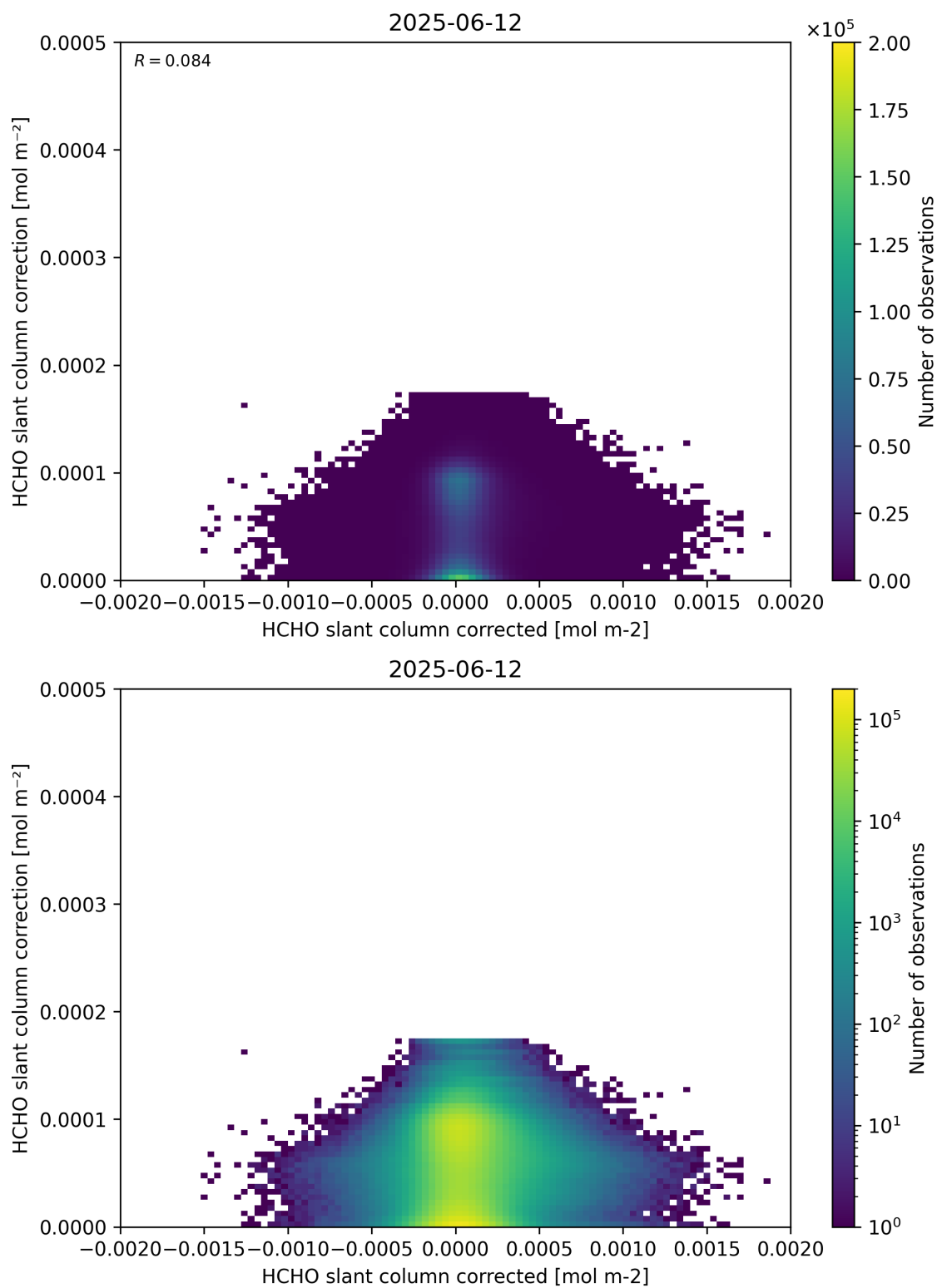
Figure 77: Scatter density plot of “HCHO slant column corrected” against “HCHO slant column correction” for 2025-06-11 to 2025-06-13.
