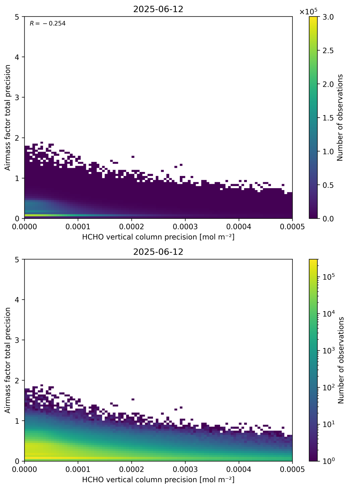
Figure 145: Scatter density plot of “HCHO vertical column precision” against “Airmass factor total precision” for 2025-06-11 to 2025-06-13.
