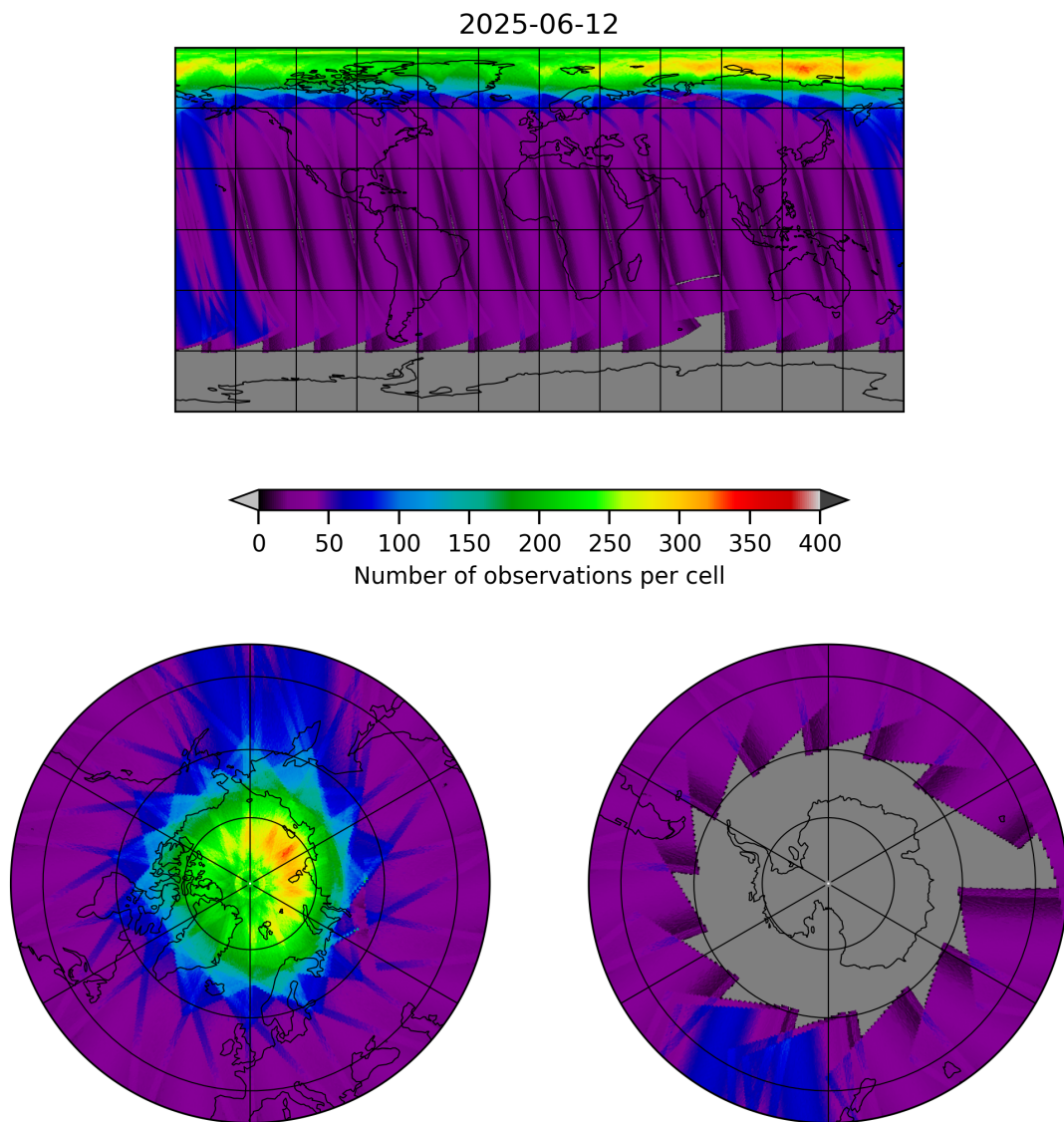
Figure 19: Map of the number of observations for 2025-06-11 to 2025-06-13
