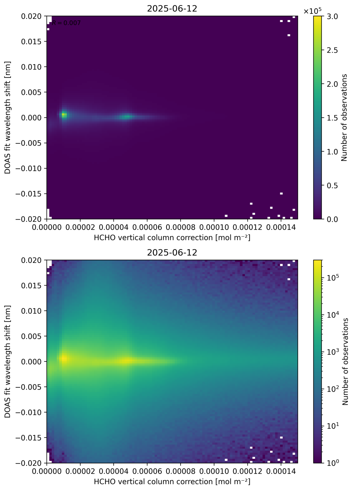
Figure 113: Scatter density plot of “HCHO vertical column correction” against “DOAS fit wavelength shift” for 2025-06-11 to 2025-06-13.
