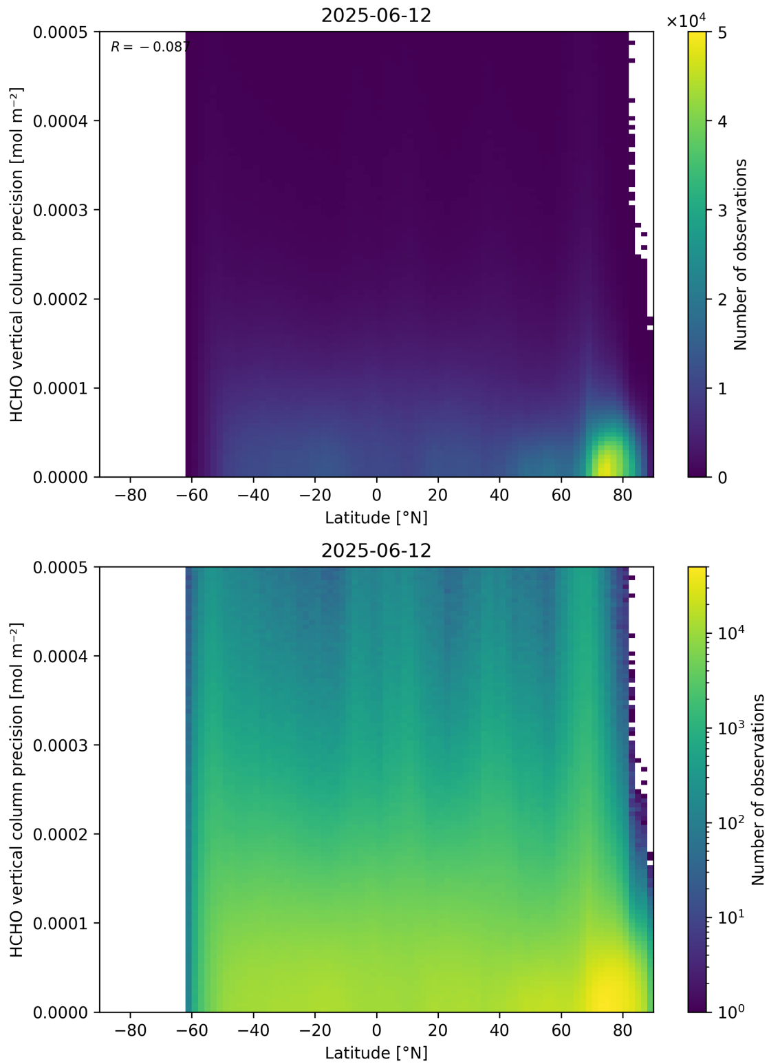
Figure 165: Scatter density plot of “Latitude” against “HCHO vertical column precision” for 2025-06-11 to 2025-06-13.
