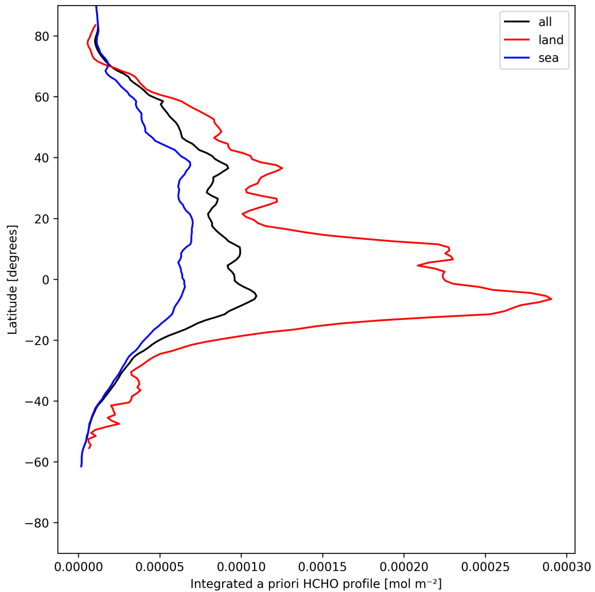
Figure 29: Zonal average of “Integrated a priori HCHO profile” for 2025-06-11 to 2025-06-13.
