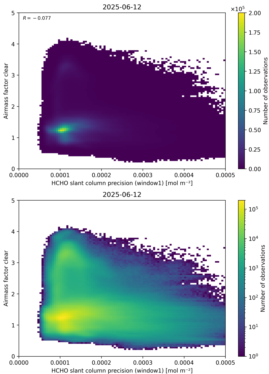
Figure 91: Scatter density plot of “HCHO slant column precision (window1)” against “Airmass factor clear” for 2025-06-11 to 2025-06-13.
