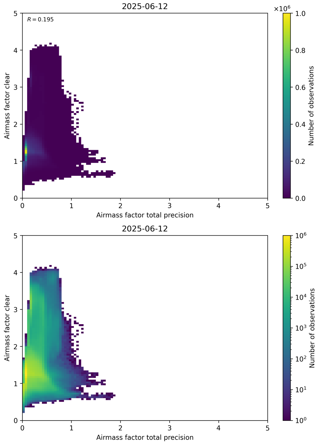
Figure 108: Scatter density plot of “Airmass factor total precision” against “Airmass factor clear” for 2025-06-11 to 2025-06-13.
