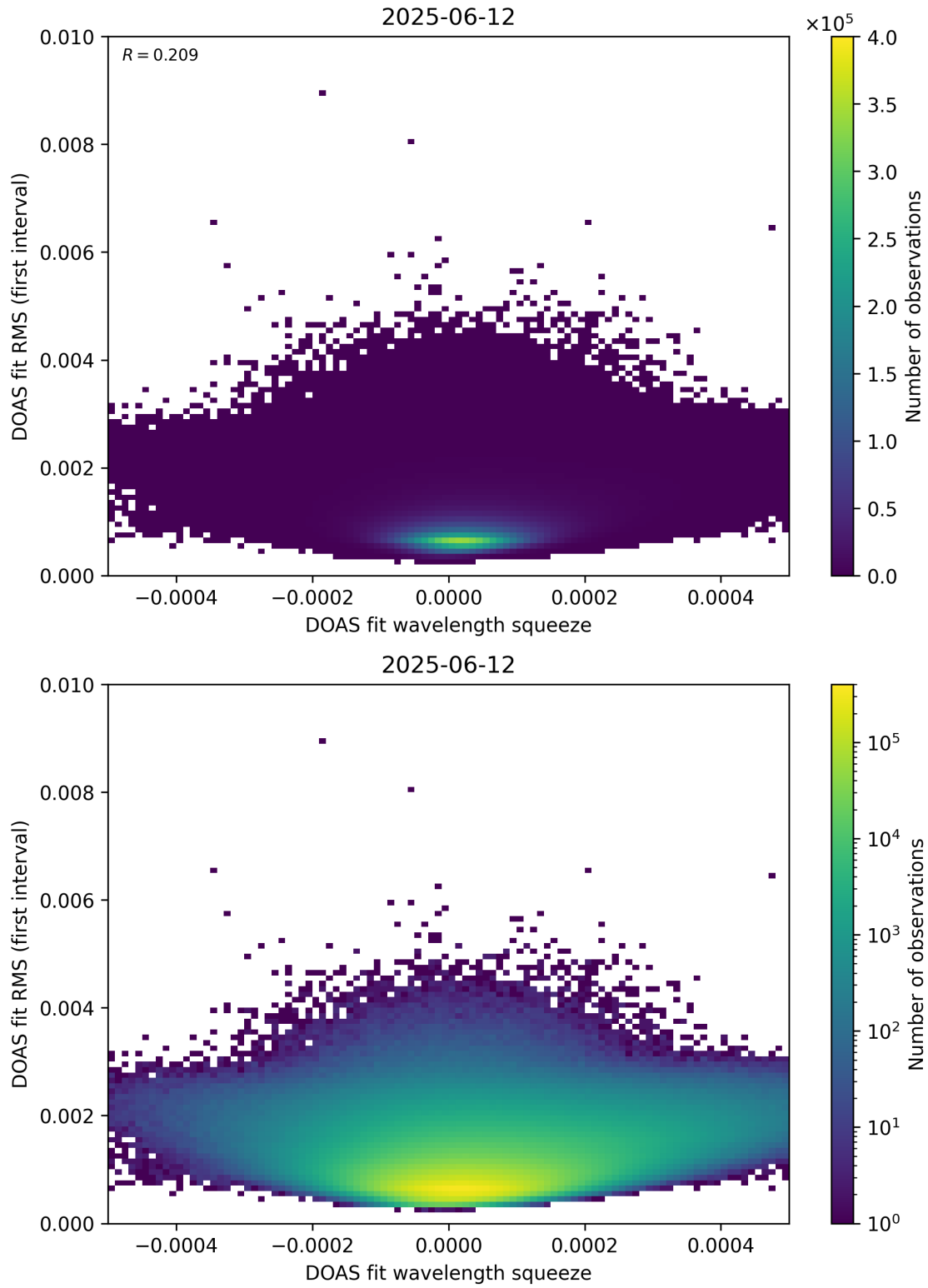
Figure 68: Scatter density plot of “DOAS fit wavelength squeeze” against “DOAS fit RMS (first interval)” for 2025-06-11 to 2025-06-13.
