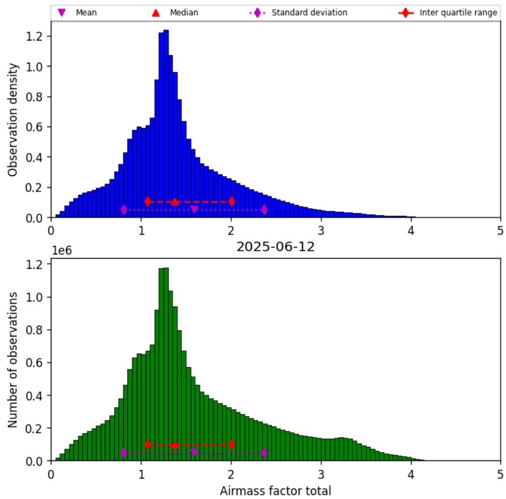
Figure 40: Histogram of “Airmass factor total” for 2025-06-11 to 2025-06-13
