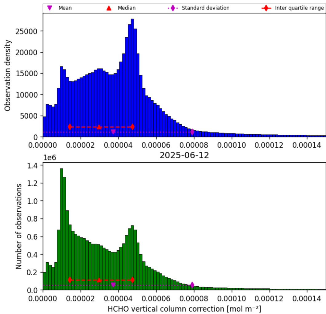
Figure 37: Histogram of “HCHO vertical column correction” for 2025-06-11 to 2025-06-13
