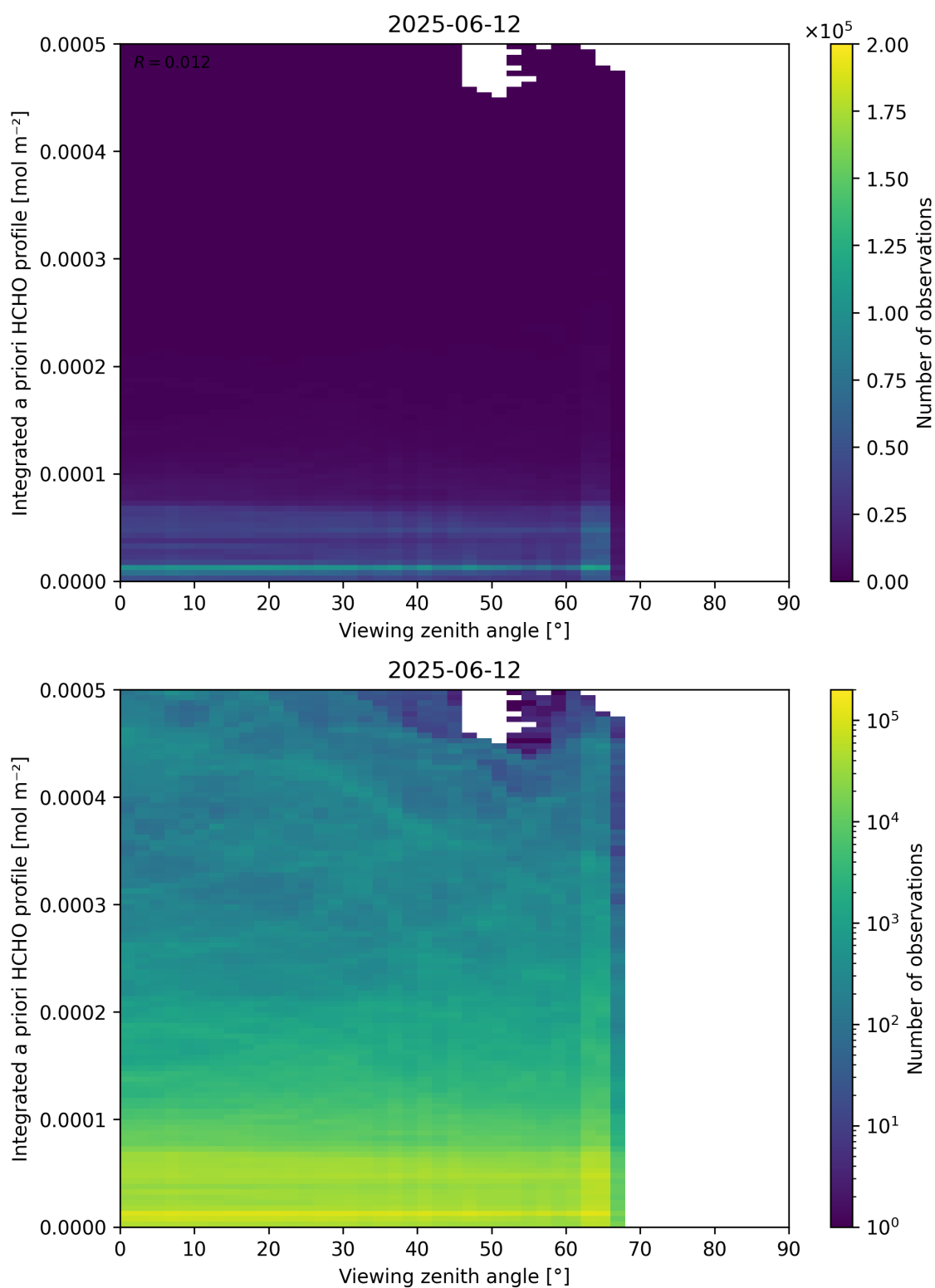
Figure 195: Scatter density plot of “Viewing zenith angle” against “Integrated a priori HCHO profile” for 2025-06-11 to 2025-06-13.
