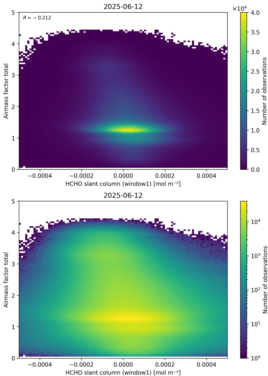
Figure 85: Scatter density plot of “HCHO slant column (window1)” against “Airmass factor total” for 2025-06-11 to 2025-06-13.
