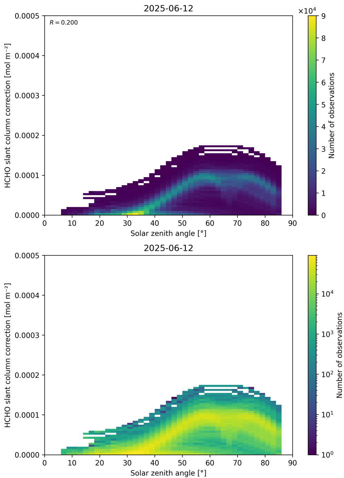
Figure 172: Scatter density plot of “Solar zenith angle” against “HCHO slant column correction” for 2025-06-11 to 2025-06-13.
