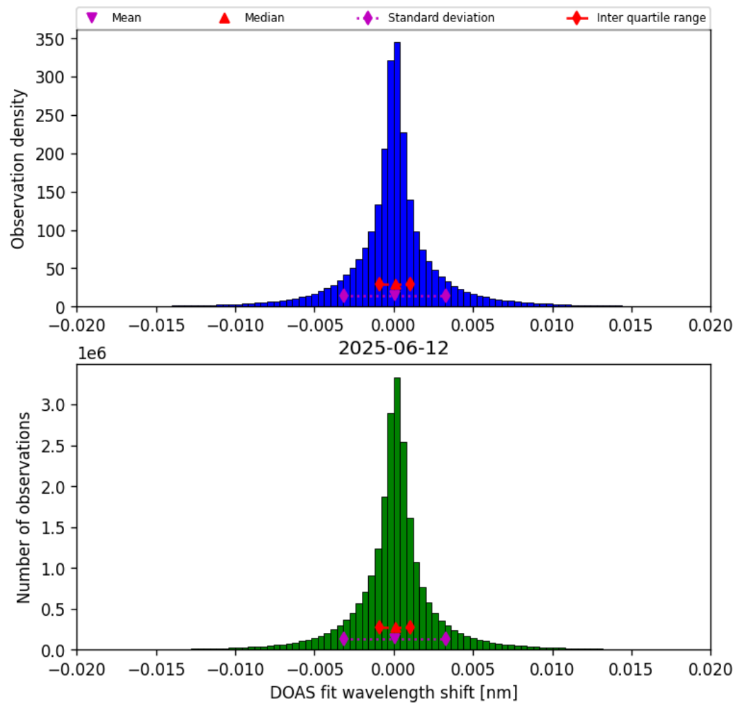
Figure 44: Histogram of “DOAS fit wavelength shift” for 2025-06-11 to 2025-06-13
