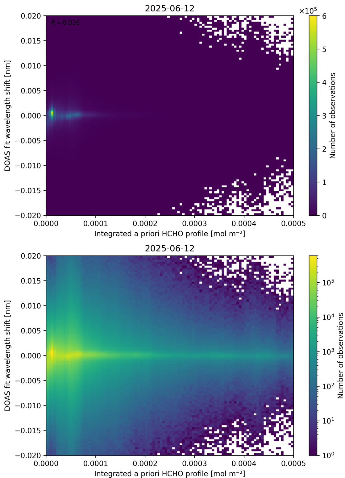
Figure 149: Scatter density plot of “Integrated a priori HCHO profile” against “DOAS fit wavelength shift” for 2025-06-11 to 2025-06-13.
