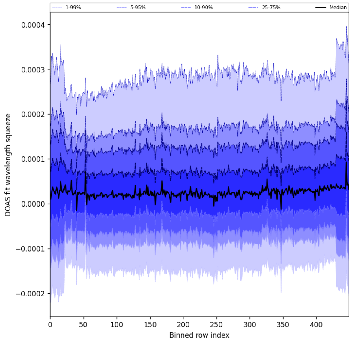
Figure 59: Along track statistics of “DOAS fit wavelength squeeze” for 2025-06-11 to 2025-06-13
