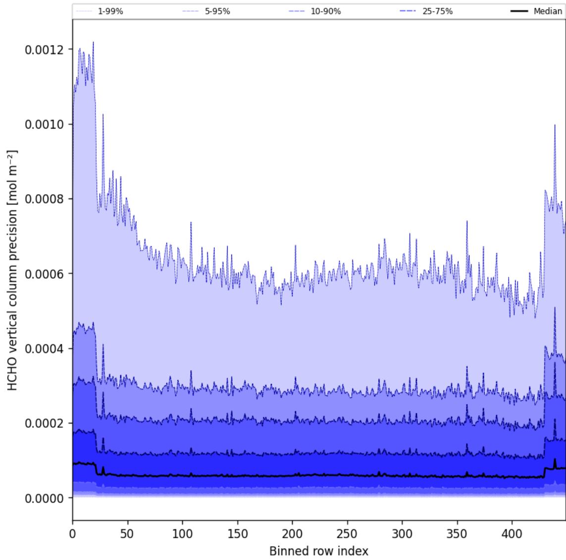
Figure 50: Along track statistics of “HCHO vertical column precision” for 2025-06-11 to 2025-06-13
