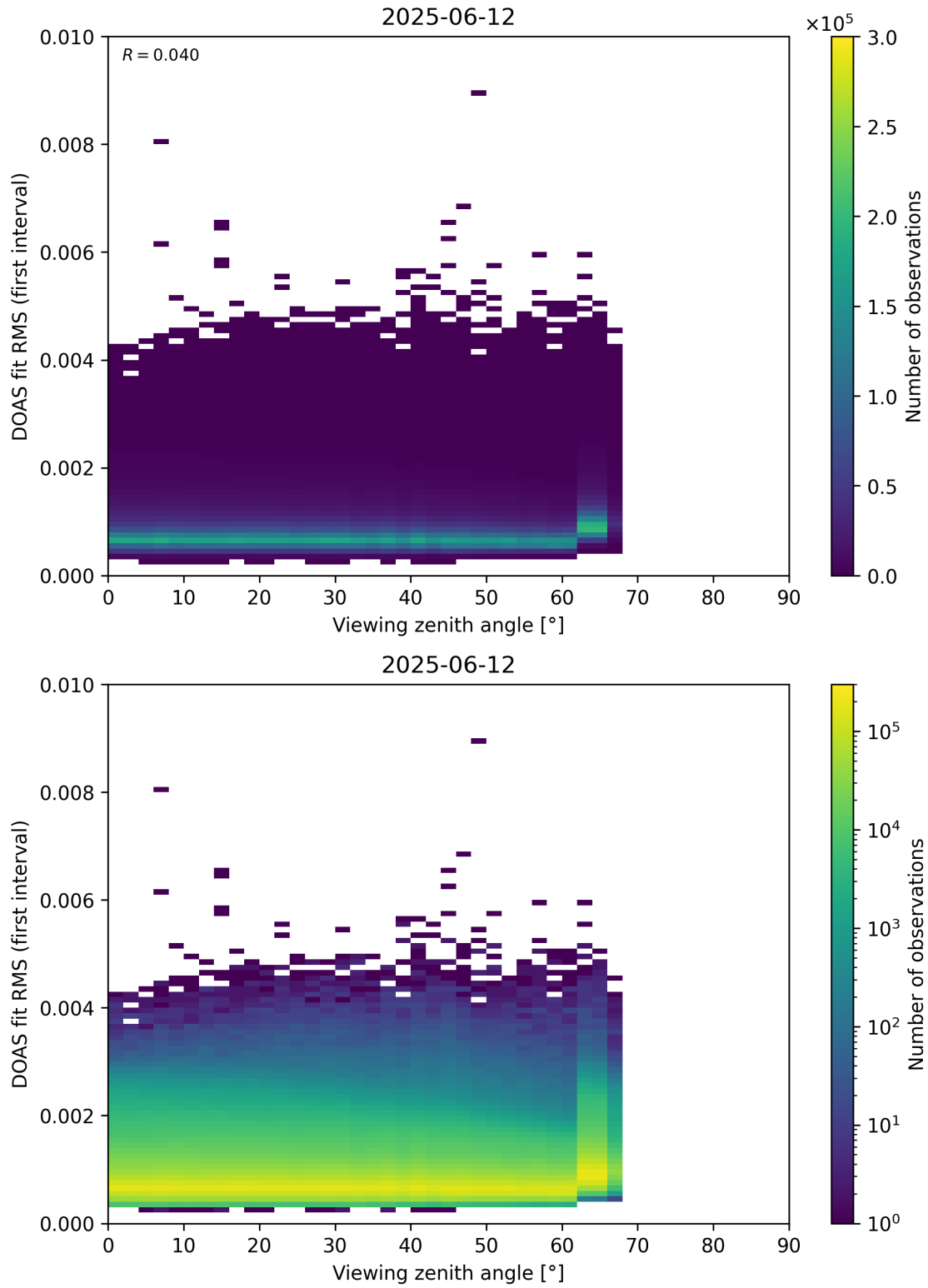
Figure 182: Scatter density plot of “Viewing zenith angle” against “DOAS fit RMS (first interval)” for 2025-06-11 to 2025-06-13.
