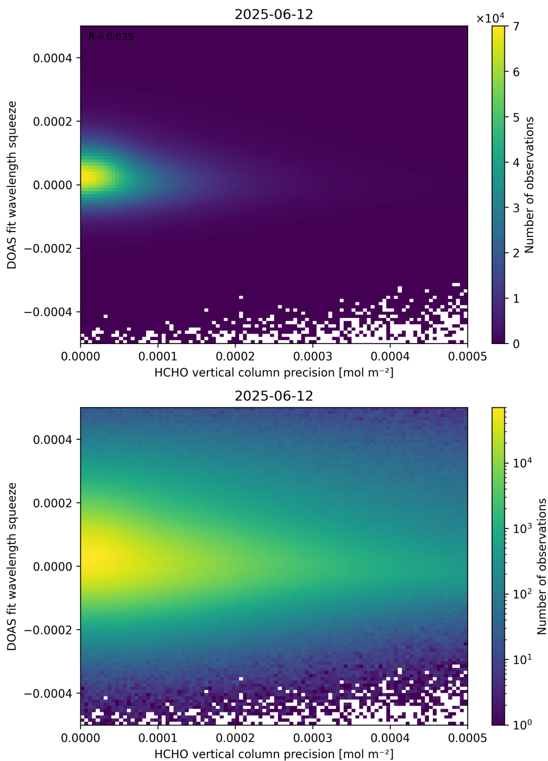
Figure 138: Scatter density plot of “HCHO vertical column precision” against “DOAS fit wavelength squeeze” for 2025-06-11 to 2025-06-13.
