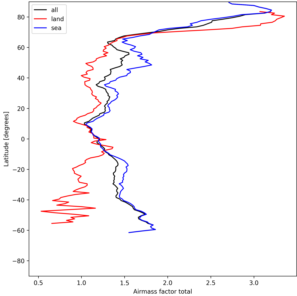
Figure 26: Zonal average of “Airmass factor total” for 2025-06-11 to 2025-06-13.
