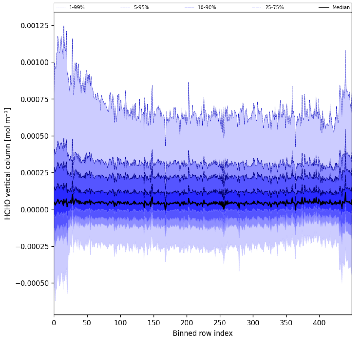
Figure 49: Along track statistics of “HCHO vertical column” for 2025-06-11 to 2025-06-13
