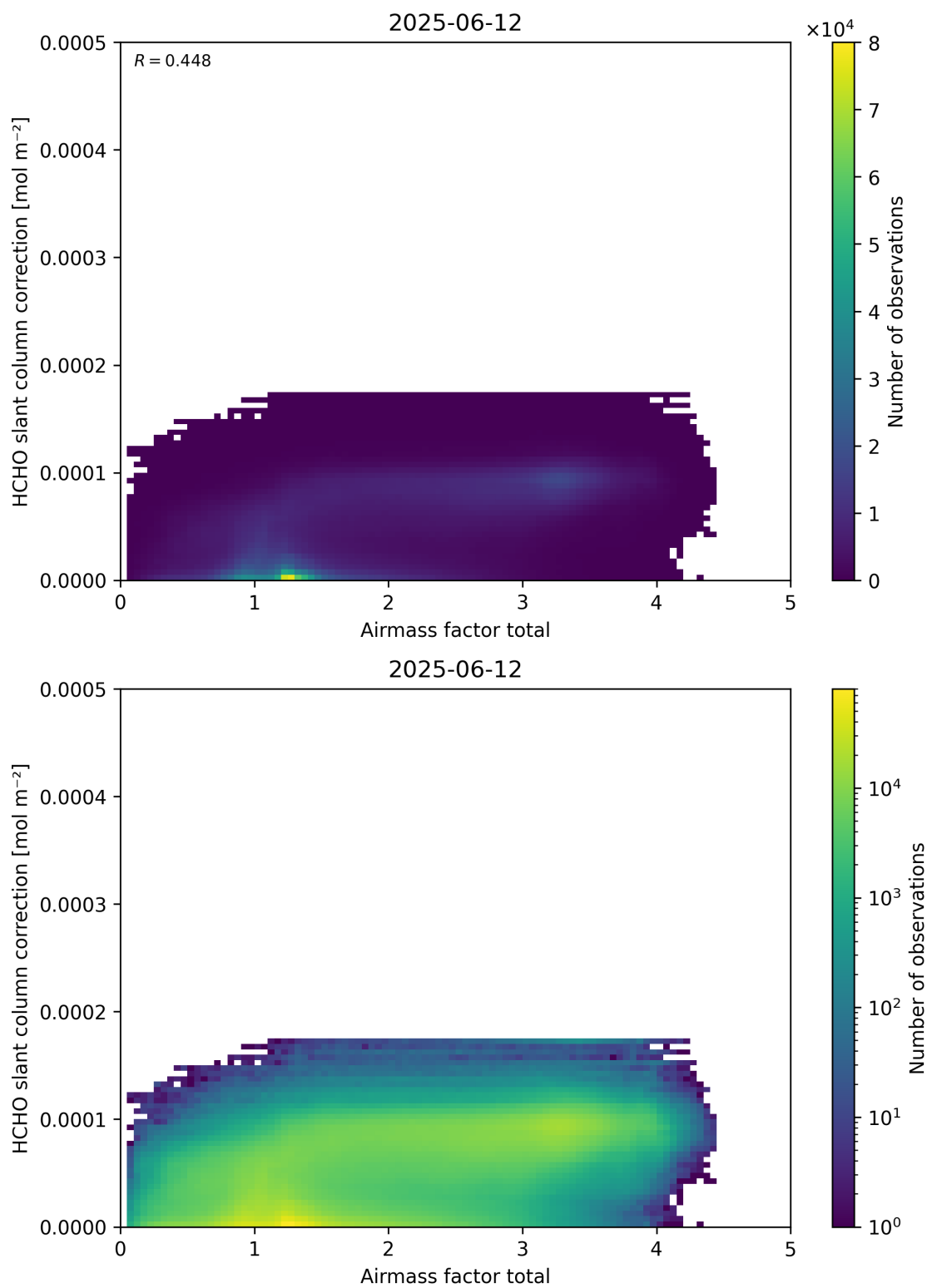
Figure 102: Scatter density plot of “Airmass factor total” against “HCHO slant column correction” for 2025-06-11 to 2025-06-13.
