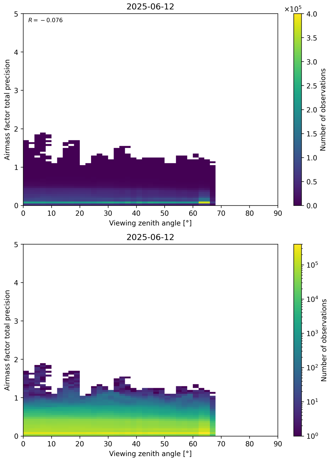
Figure 191: Scatter density plot of “Viewing zenith angle” against “Airmass factor total precision” for 2025-06-11 to 2025-06-13.
