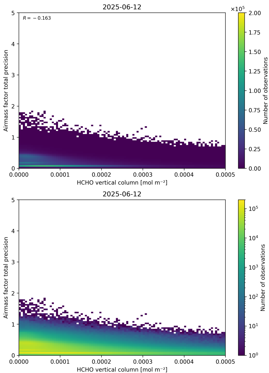
Figure 132: Scatter density plot of “HCHO vertical column” against “Airmass factor total precision” for 2025-06-11 to 2025-06-13.
