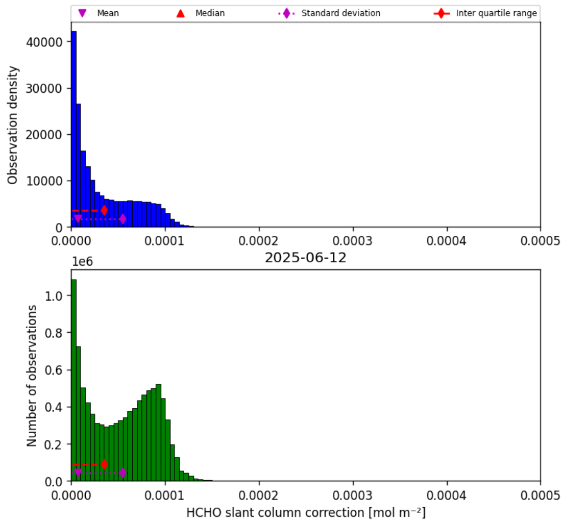
Figure 47: Histogram of “HCHO slant column correction” for 2025-06-11 to 2025-06-13
