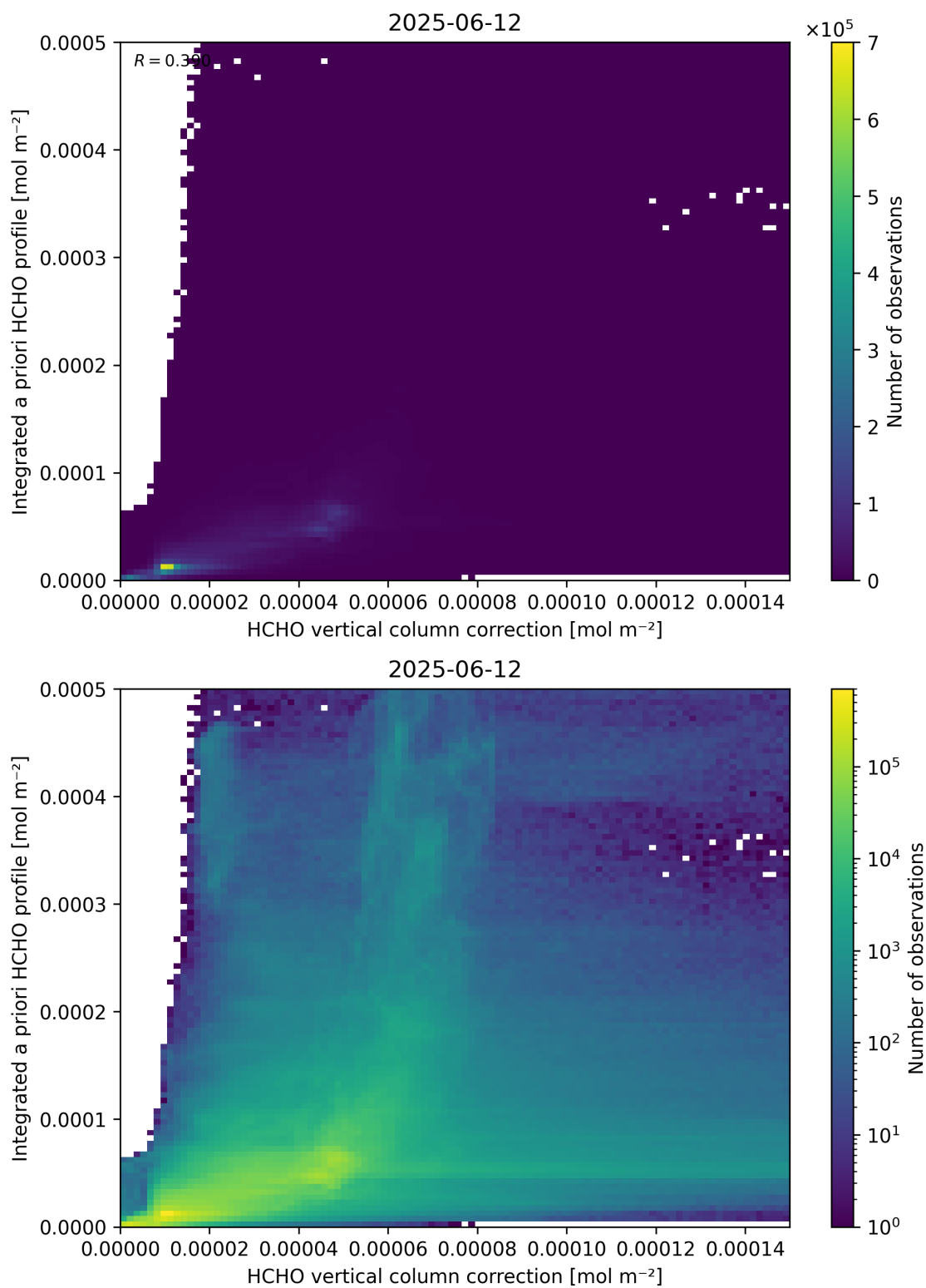
Figure 122: Scatter density plot of “HCHO vertical column correction” against “Integrated a priori HCHO profile” for 2025-06-11 to 2025-06-13.
