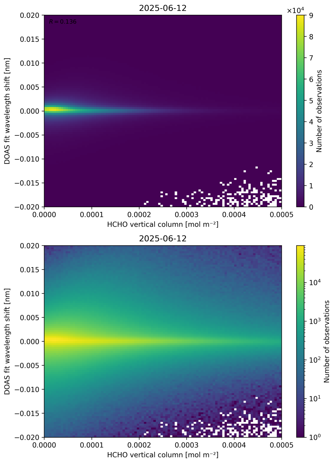
Figure 124: Scatter density plot of “HCHO vertical column” against “DOAS fit wavelength shift” for 2025-06-11 to 2025-06-13.
