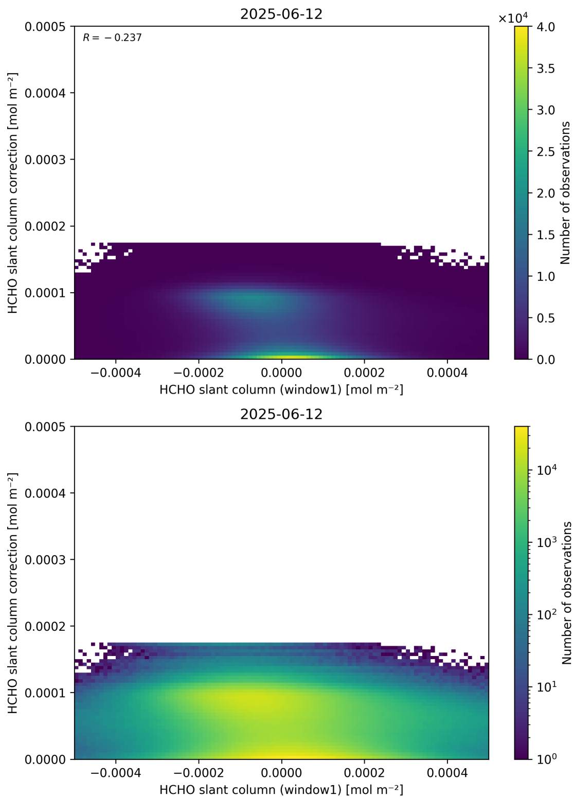
Figure 83: Scatter density plot of “HCHO slant column (window1)” against “HCHO slant column correction” for 2025-06-11 to 2025-06-13.
