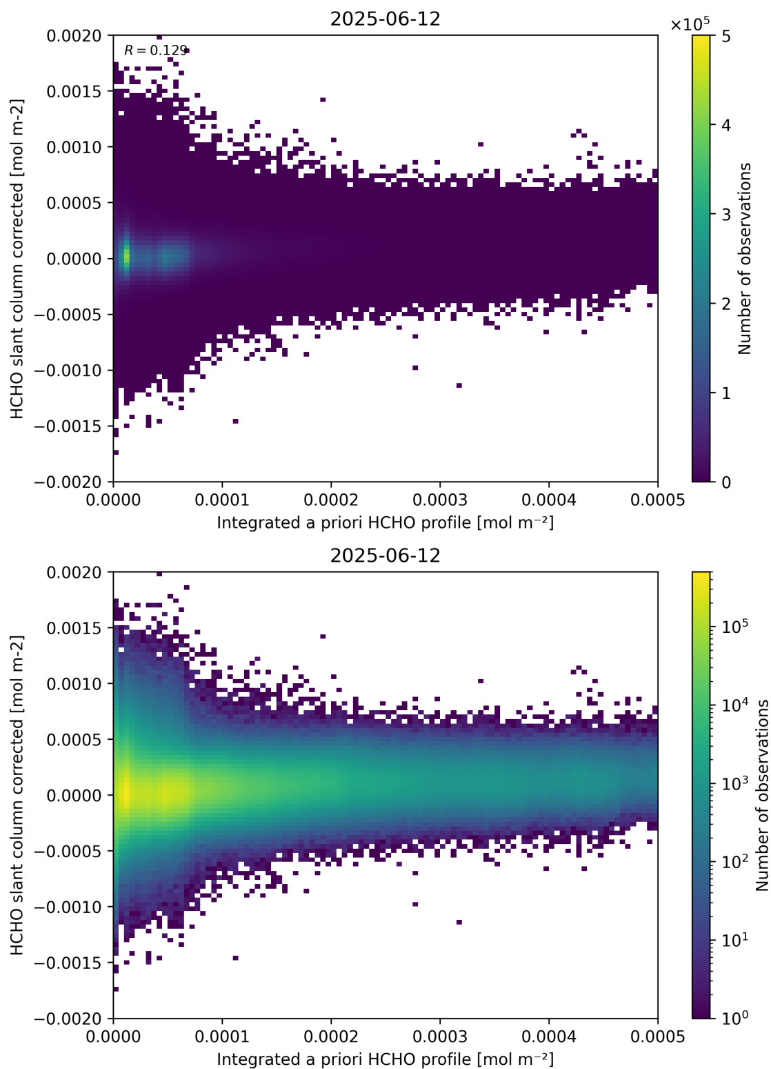
Figure 151: Scatter density plot of “Integrated a priori HCHO profile” against “HCHO slant column corrected” for 2025-06-11 to 2025-06-13.
