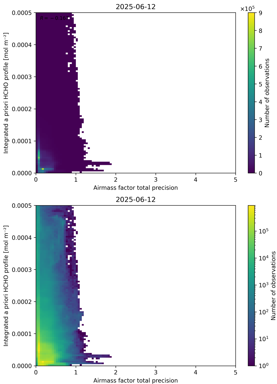
Figure 111: Scatter density plot of “Airmass factor total precision” against “Integrated a priori HCHO profile” for 2025-06-11 to 2025-06-13.
