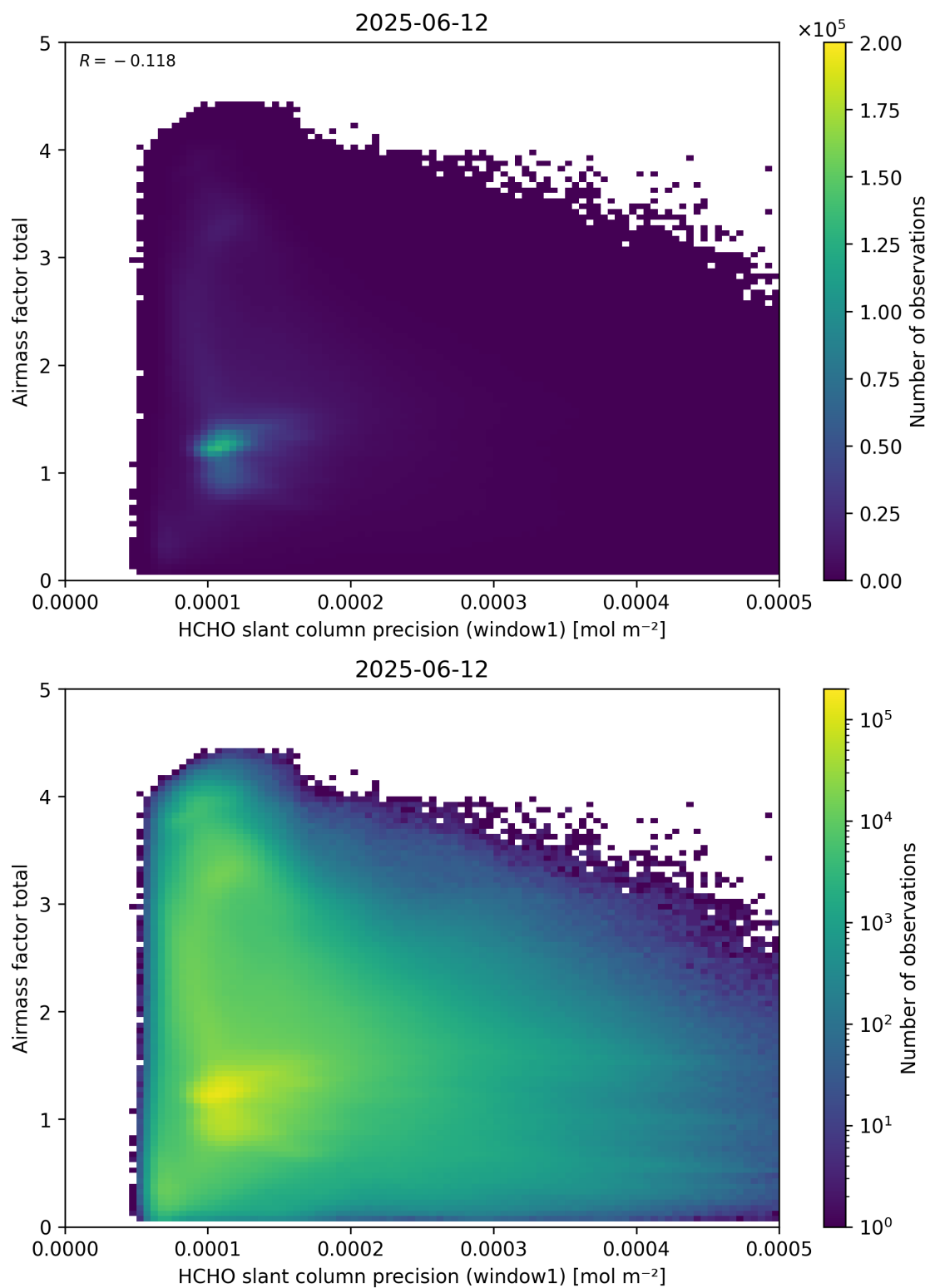
Figure 94: Scatter density plot of “HCHO slant column precision (window1)” against “Airmass factor total” for 2025-06-11 to 2025-06-13.
