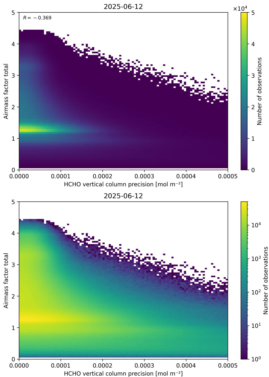
Figure 144: Scatter density plot of “HCHO vertical column precision” against “Airmass factor total” for 2025-06-11 to 2025-06-13.
