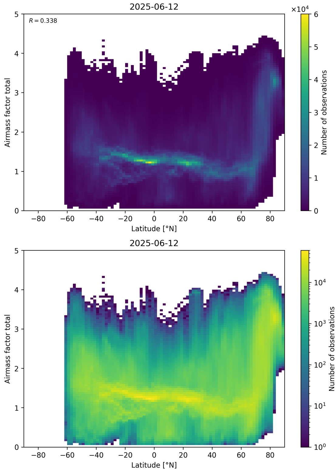
Figure 161: Scatter density plot of “Latitude” against “Airmass factor total” for 2025-06-11 to 2025-06-13.
