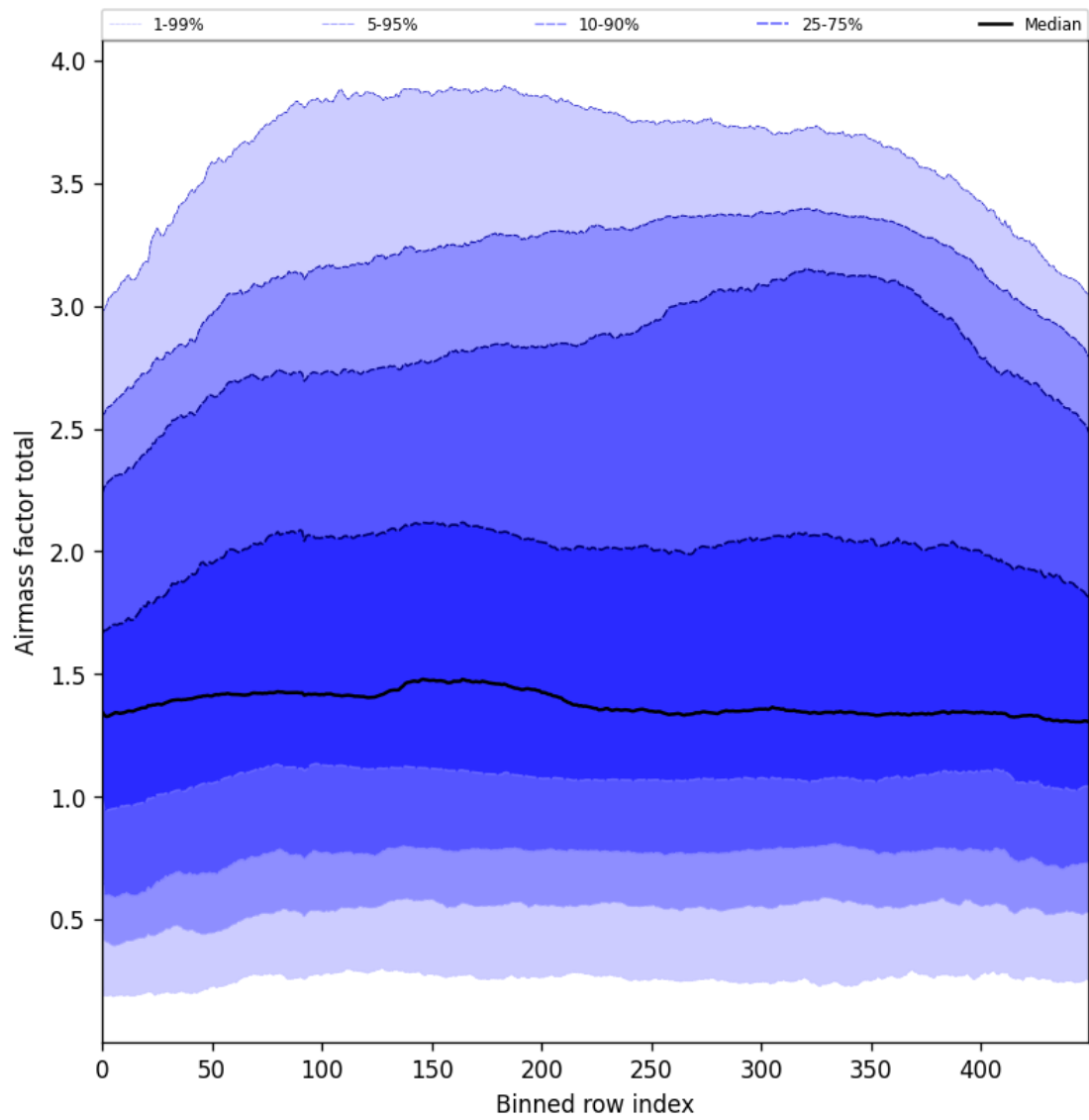
Figure 54: Along track statistics of “Airmass factor total” for 2025-06-11 to 2025-06-13
