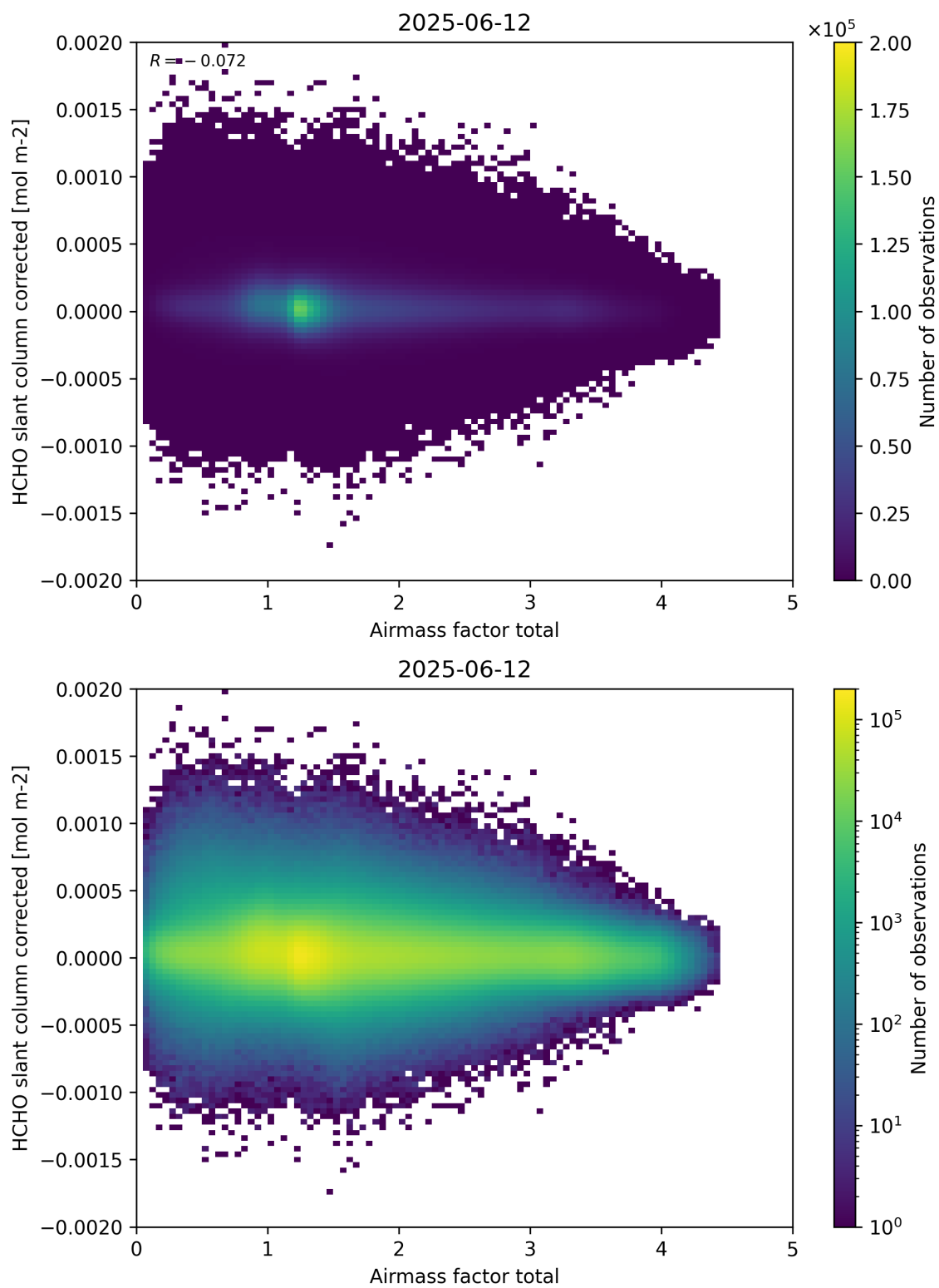
Figure 101: Scatter density plot of “Airmass factor total” against “HCHO slant column corrected” for 2025-06-11 to 2025-06-13.
