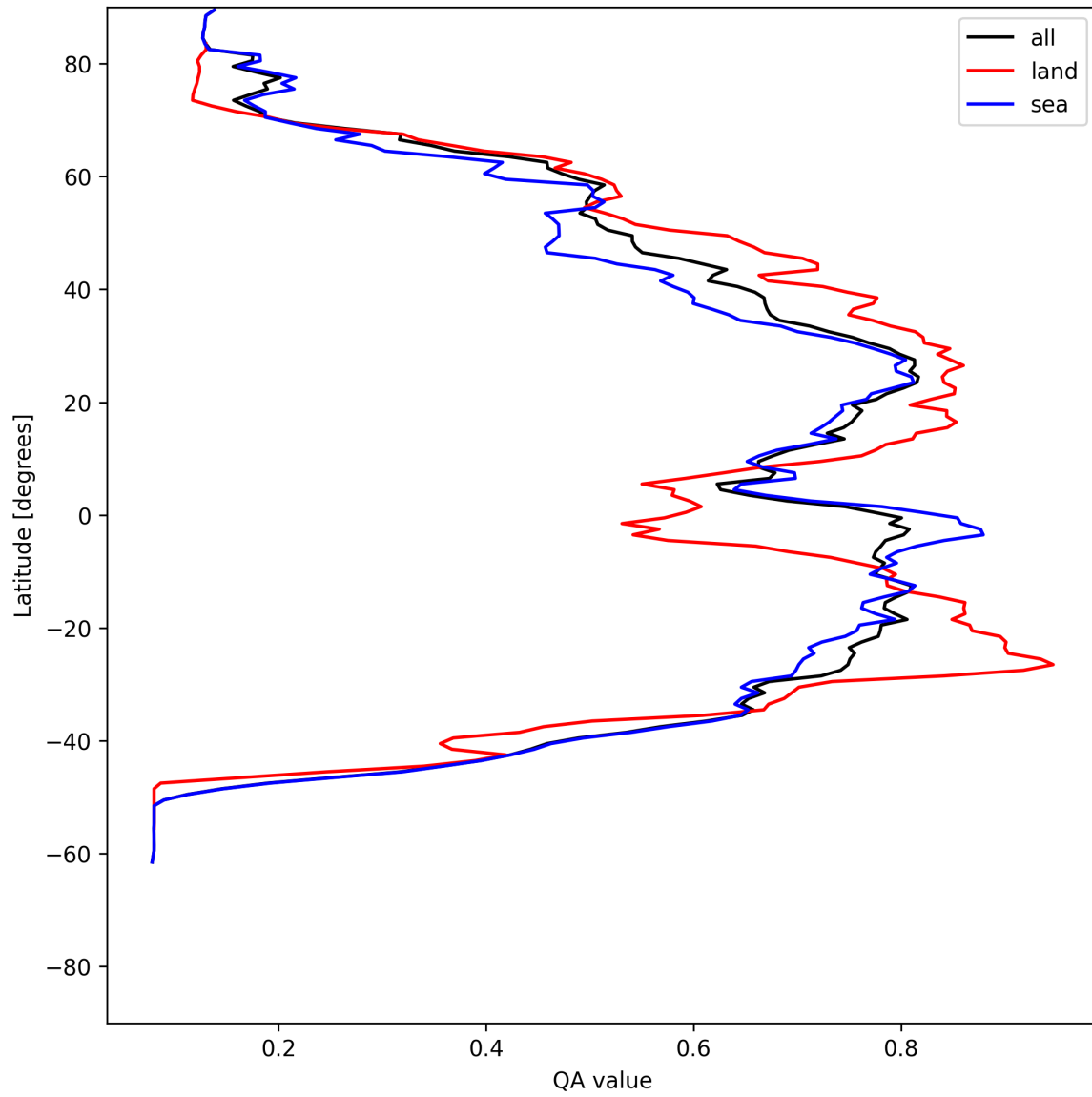
Figure 20: Zonal average of “QA value” for 2025-06-11 to 2025-06-13.
