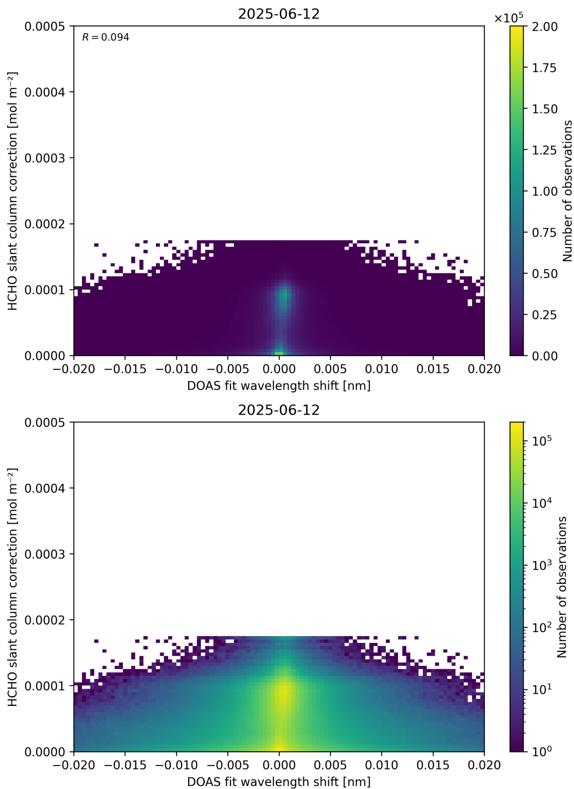
Figure 67: Scatter density plot of “DOAS fit wavelength shift” against “HCHO slant column correction” for 2025-06-11 to 2025-06-13.
