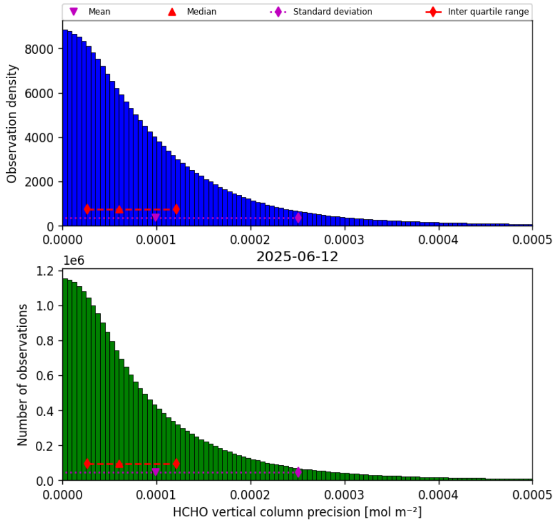
Figure 36: Histogram of “HCHO vertical column precision” for 2025-06-11 to 2025-06-13
