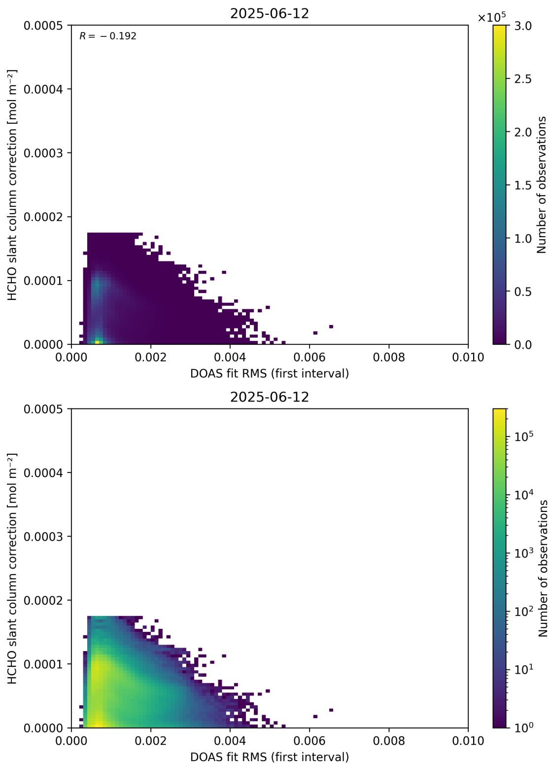
Figure 63: Scatter density plot of “DOAS fit RMS (first interval)” against “HCHO slant column correction” for 2025-06-11 to 2025-06-13.
