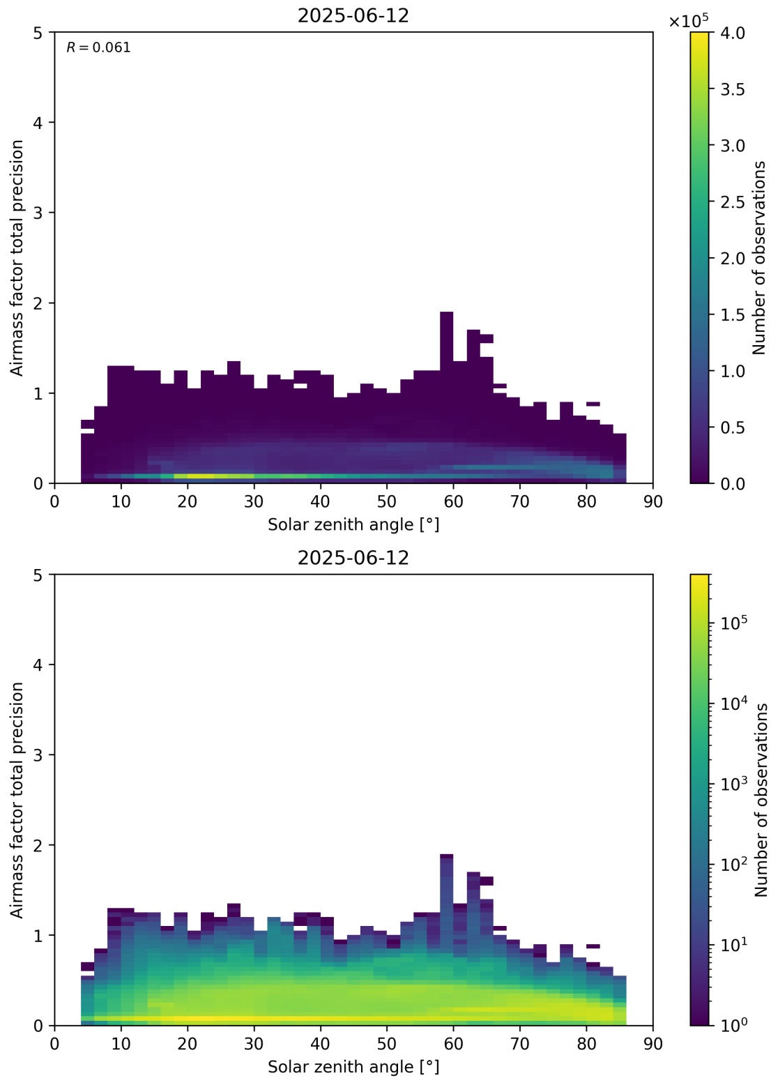
Figure 176: Scatter density plot of “Solar zenith angle” against “Airmass factor total precision” for 2025-06-11 to 2025-06-13.
