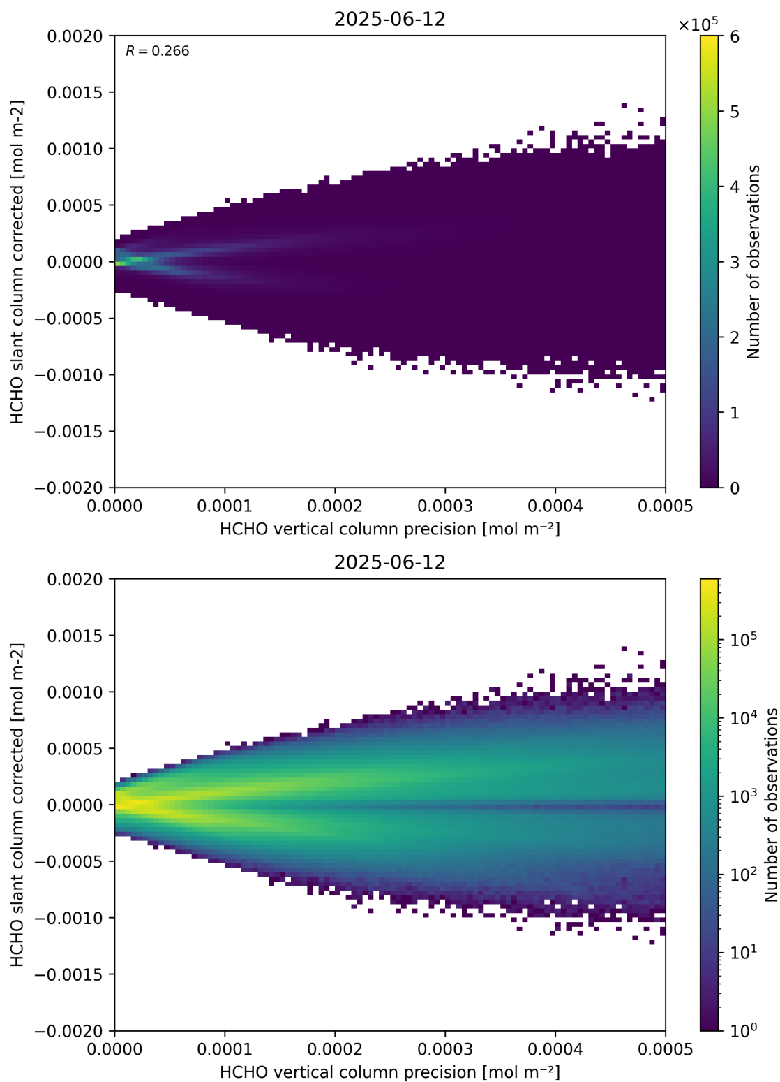
Figure 140: Scatter density plot of “HCHO vertical column precision” against “HCHO slant column corrected” for 2025-06-11 to 2025-06-13.
