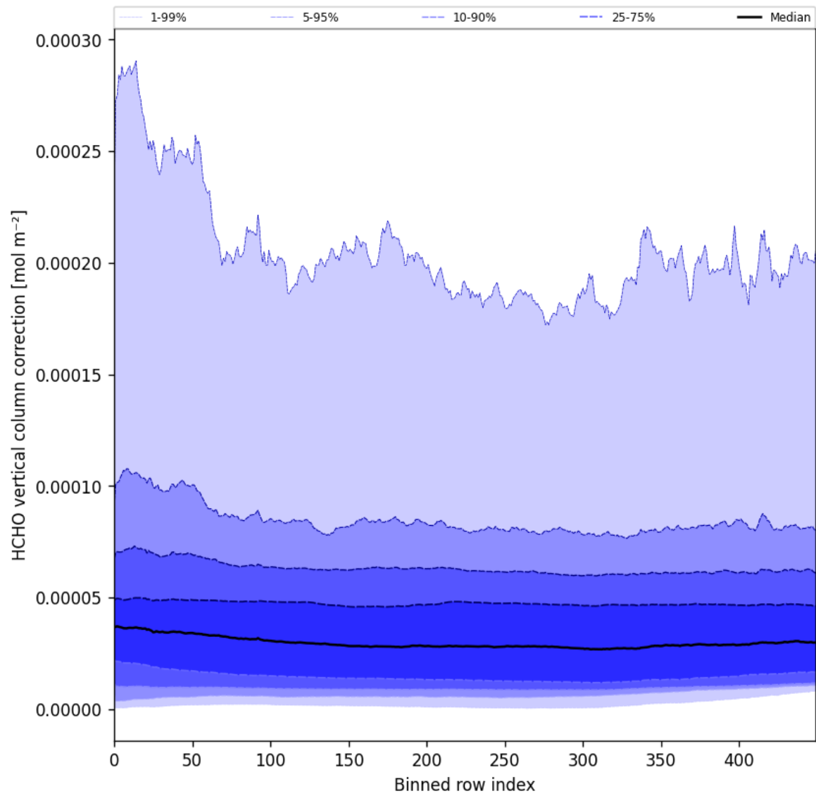
Figure 51: Along track statistics of “HCHO vertical column correction” for 2025-06-11 to 2025-06-13
