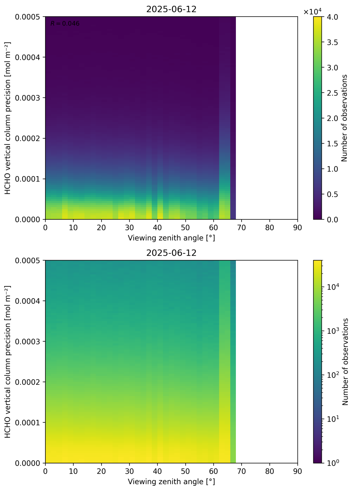
Figure 194: Scatter density plot of “Viewing zenith angle” against “HCHO vertical column precision” for 2025-06-11 to 2025-06-13.
