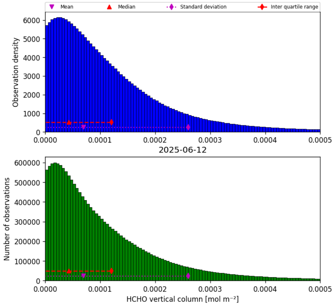
Figure 35: Histogram of “HCHO vertical column” for 2025-06-11 to 2025-06-13
