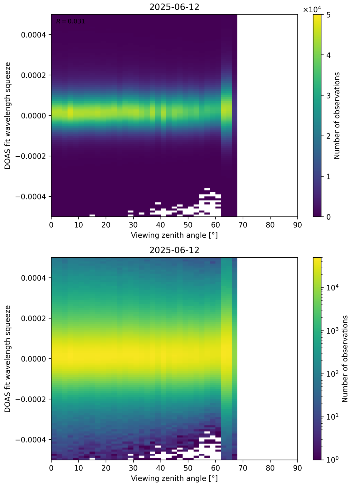
Figure 184: Scatter density plot of “Viewing zenith angle” against “DOAS fit wavelength squeeze” for 2025-06-11 to 2025-06-13.
