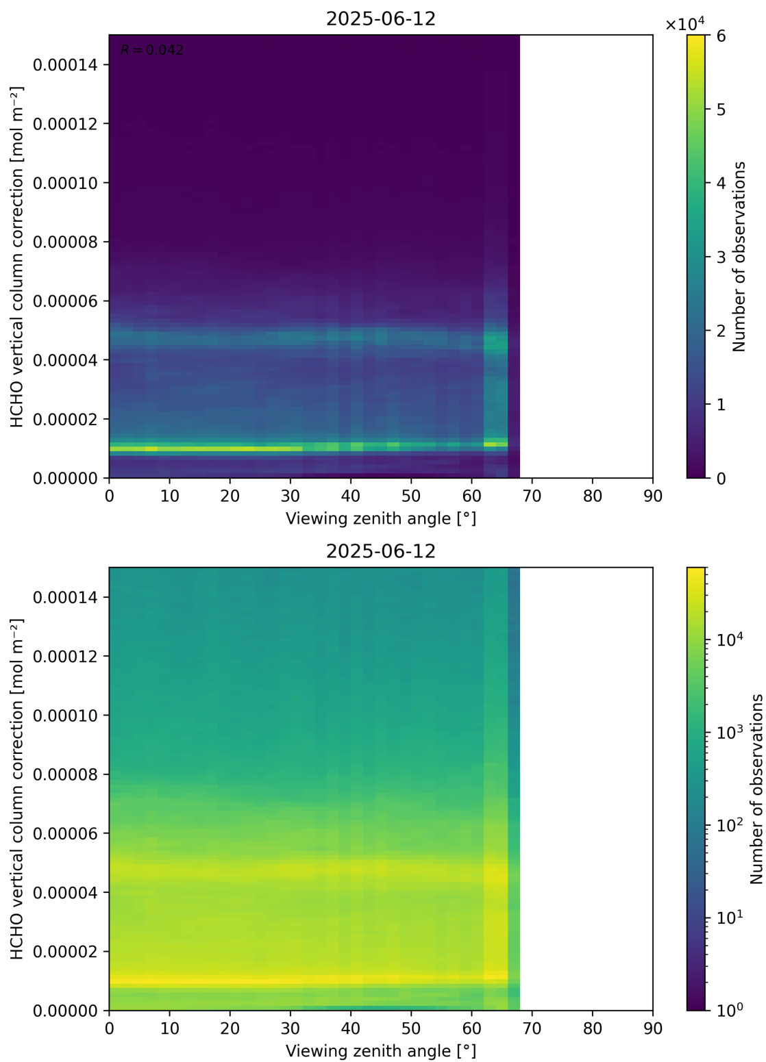
Figure 193: Scatter density plot of “Viewing zenith angle” against “HCHO vertical column correction” for 2025-06-11 to 2025-06-13.
