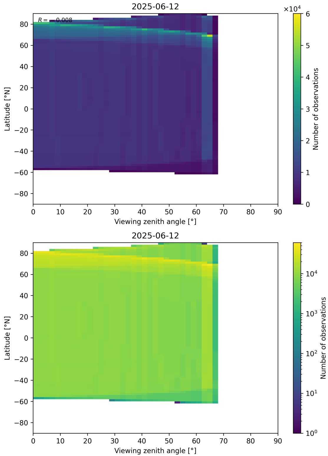
Figure 196: Scatter density plot of “Viewing zenith angle” against “Latitude” for 2025-06-11 to 2025-06-13.
