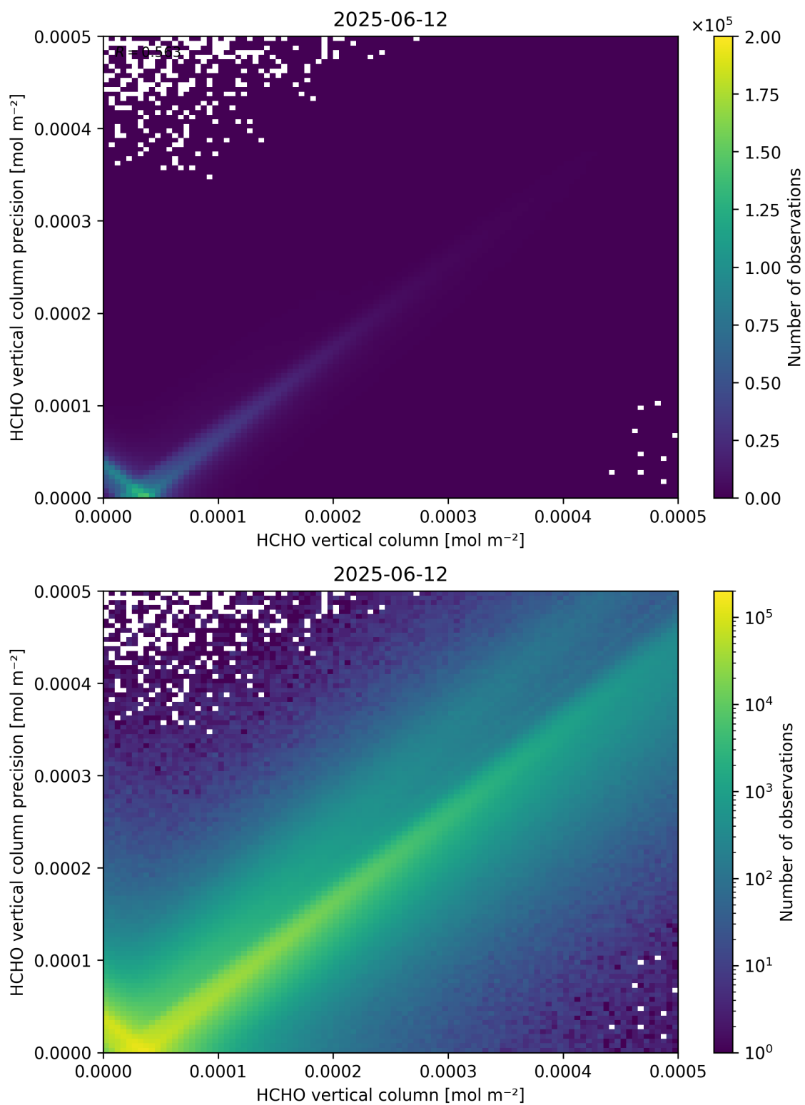
Figure 134: Scatter density plot of “HCHO vertical column” against “HCHO vertical column precision” for 2025-06-11 to 2025-06-13.
