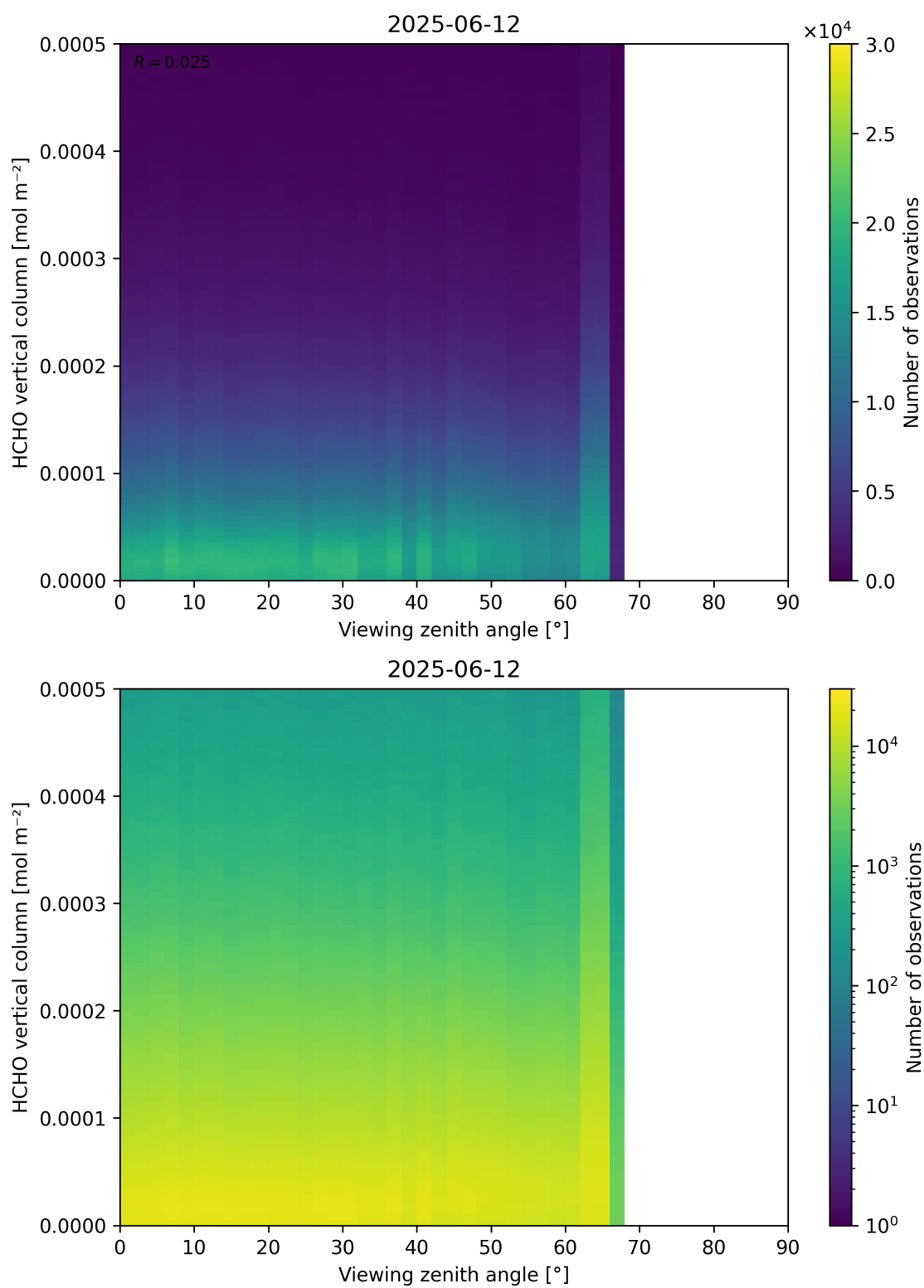
Figure 192: Scatter density plot of “Viewing zenith angle” against “HCHO vertical column” for 2025-06-11 to 2025-06-13.
