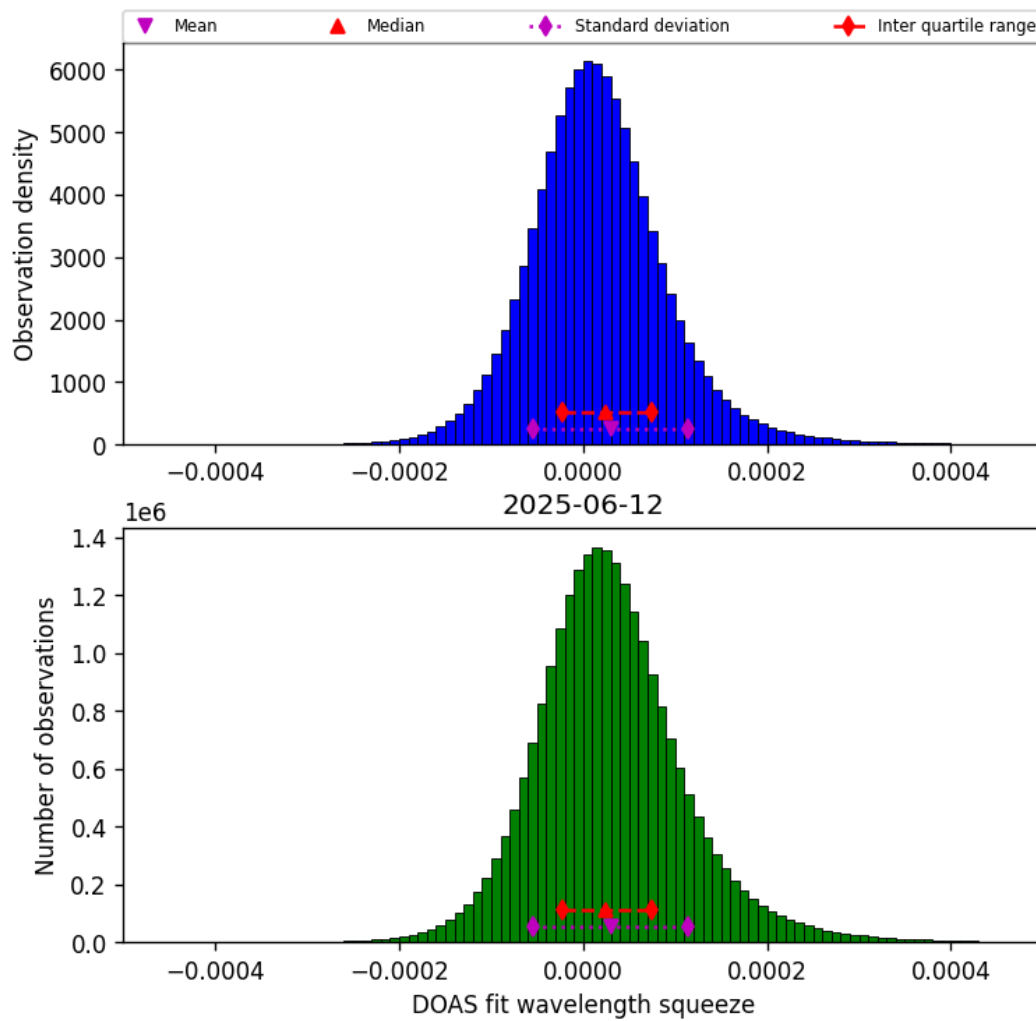
Figure 45: Histogram of “DOAS fit wavelength squeeze” for 2025-06-11 to 2025-06-13
