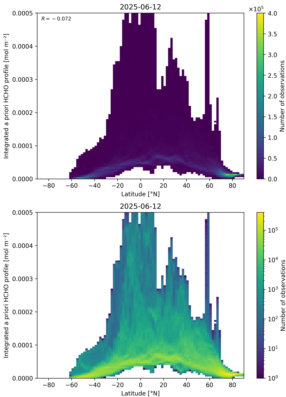
Figure 166: Scatter density plot of “Latitude” against “Integrated a priori HCHO profile” for 2025-06-11 to 2025-06-13.
