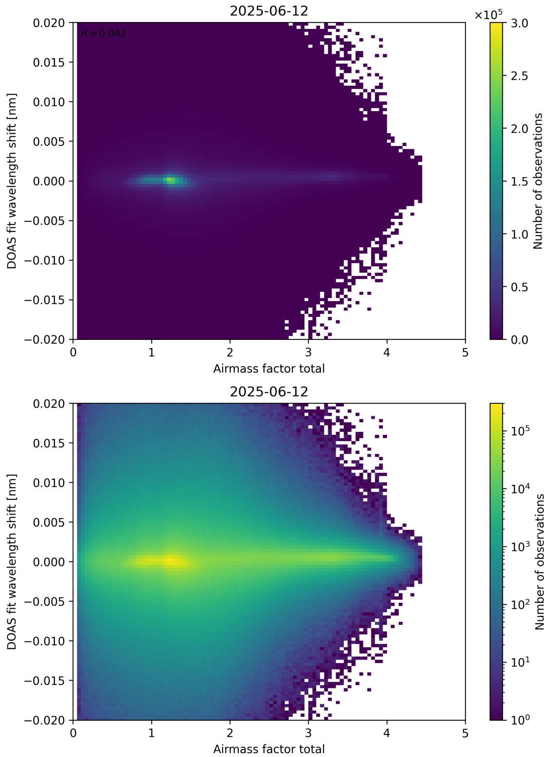
Figure 98: Scatter density plot of “Airmass factor total” against “DOAS fit wavelength shift” for 2025-06-11 to 2025-06-13.
