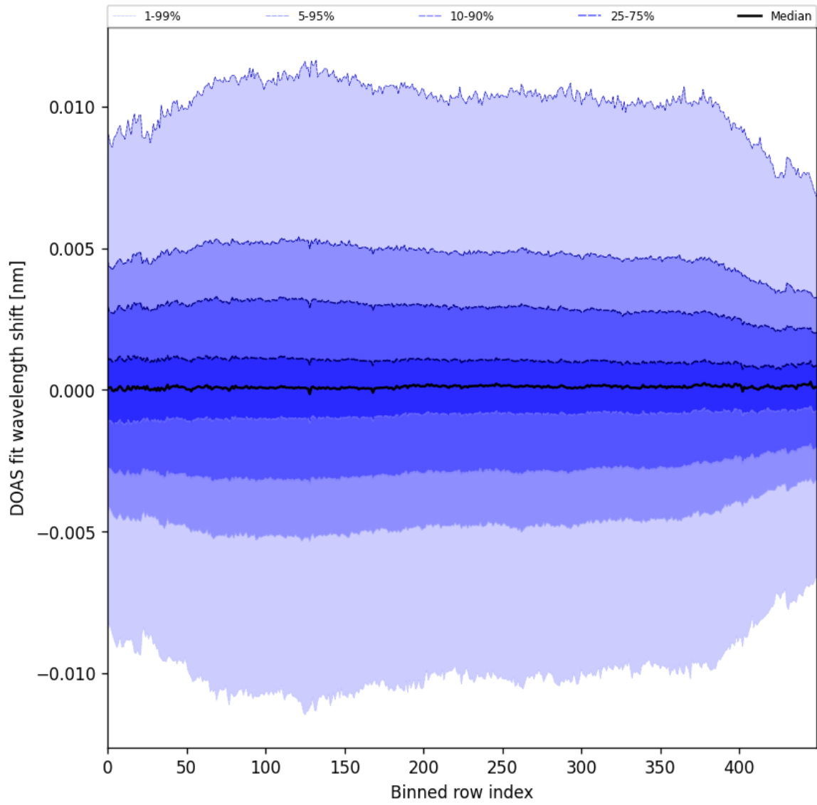
Figure 58: Along track statistics of “DOAS fit wavelength shift” for 2025-06-11 to 2025-06-13
