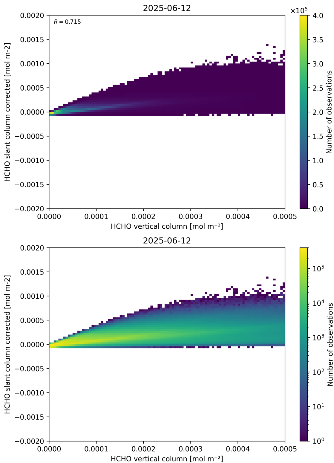
Figure 127: Scatter density plot of “HCHO vertical column” against “HCHO slant column corrected” for 2025-06-11 to 2025-06-13.
