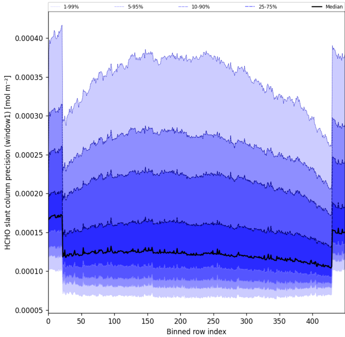
Figure 53: Along track statistics of “HCHO slant column precision (window1)” for 2025-06-11 to 2025-06-13
