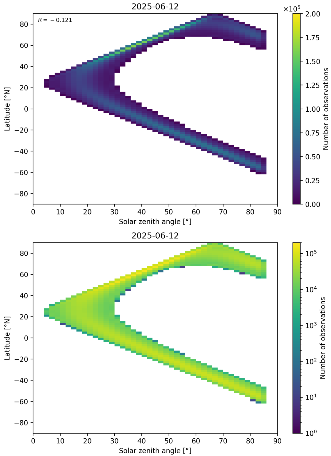
Figure 181: Scatter density plot of “Solar zenith angle” against “Latitude” for 2025-06-11 to 2025-06-13.
