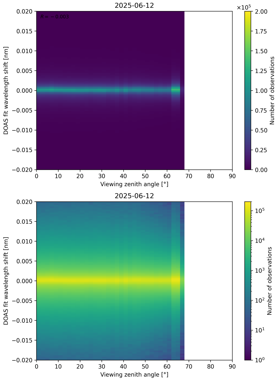
Figure 183: Scatter density plot of “Viewing zenith angle” against “DOAS fit wavelength shift” for 2025-06-11 to 2025-06-13.
