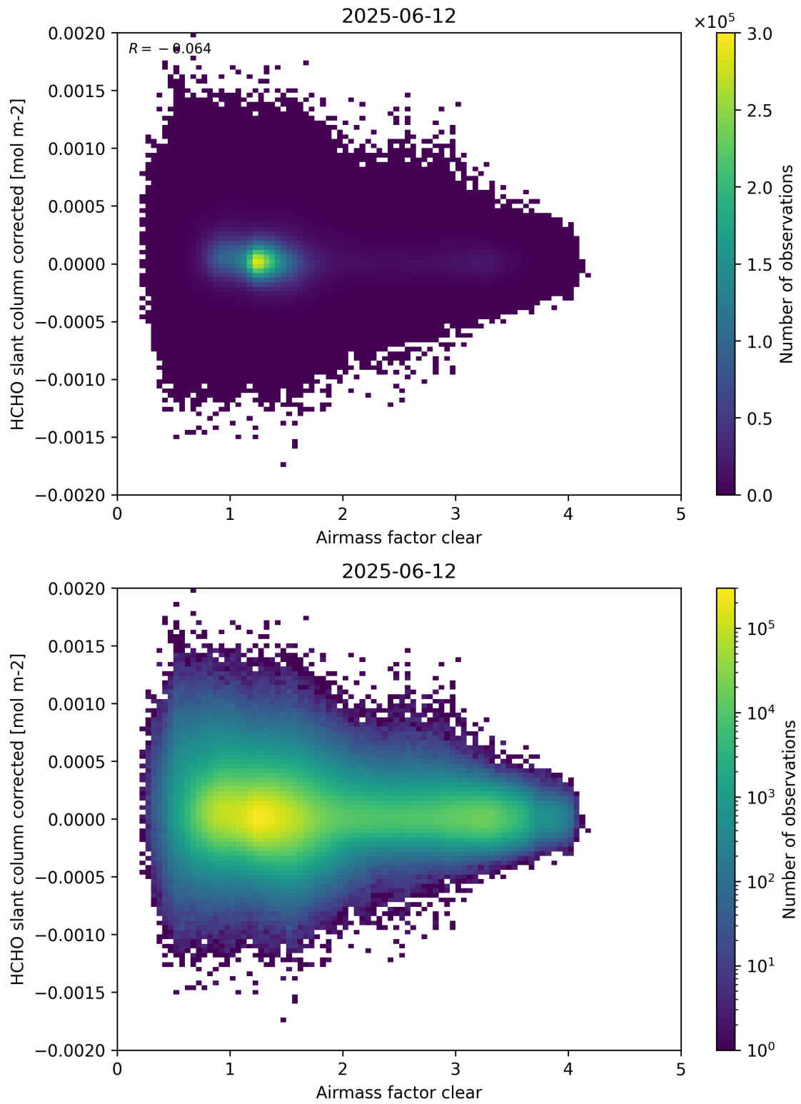
Figure 74: Scatter density plot of “Airmass factor clear” against “HCHO slant column corrected” for 2025-06-11 to 2025-06-13.
