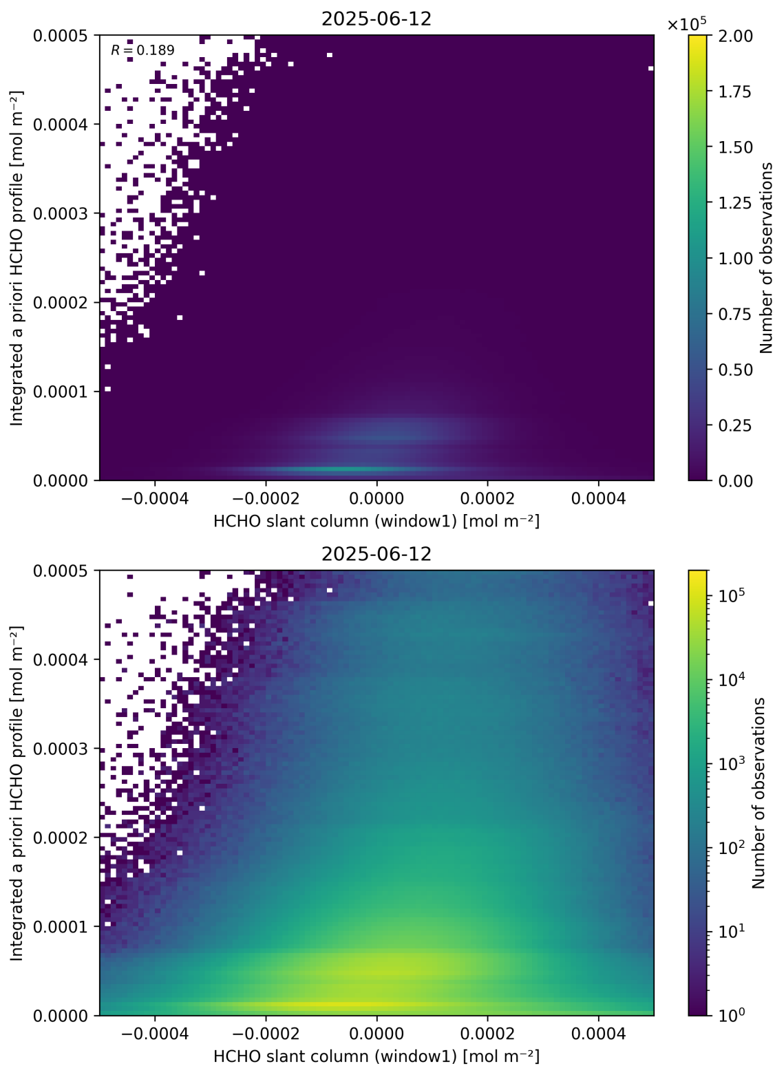
Figure 87: Scatter density plot of “HCHO slant column (window1)” against “Integrated a priori HCHO profile” for 2025-06-11 to 2025-06-13.
