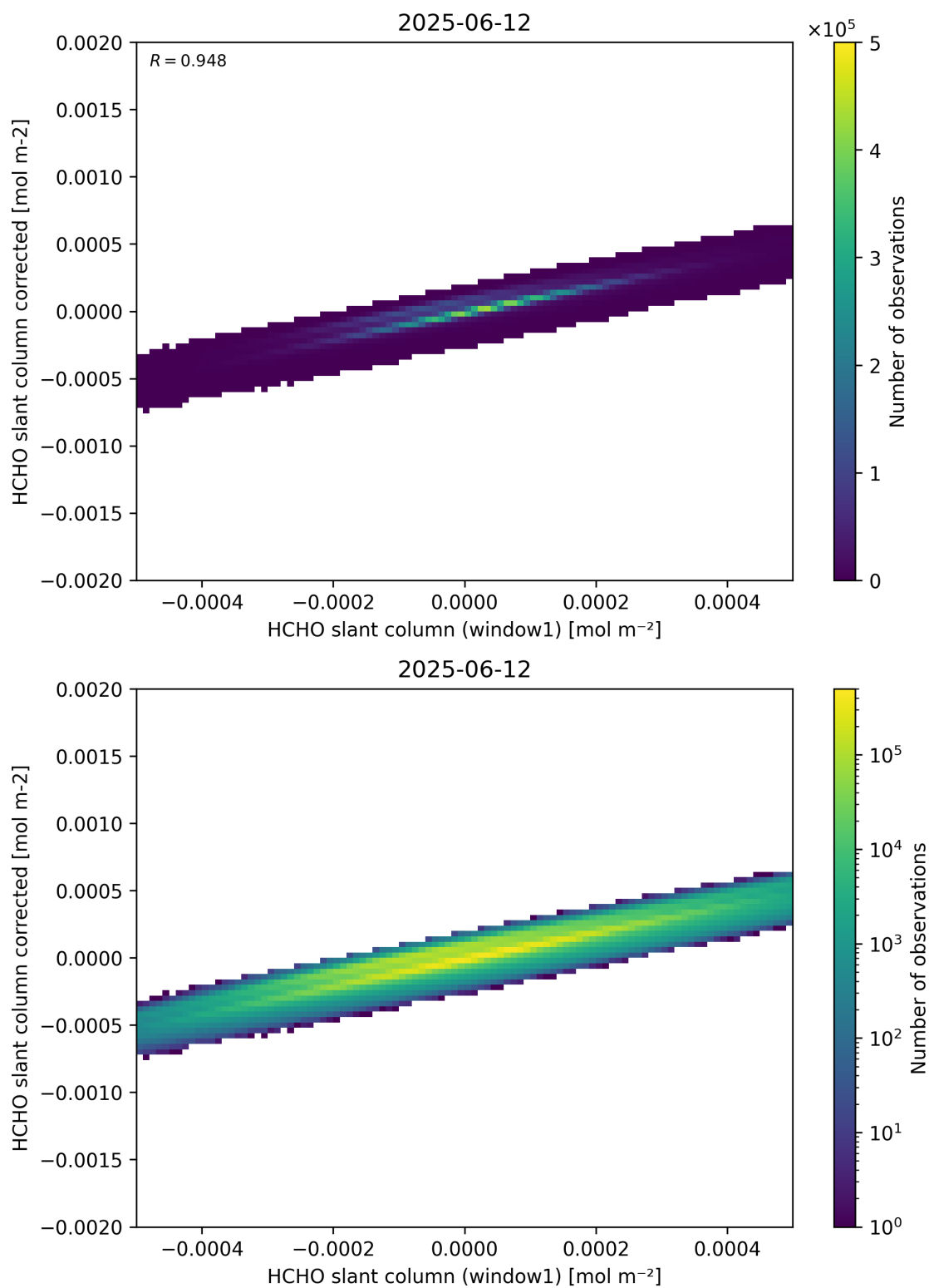
Figure 82: Scatter density plot of “HCHO slant column (window1)” against “HCHO slant column corrected” for 2025-06-11 to 2025-06-13.
