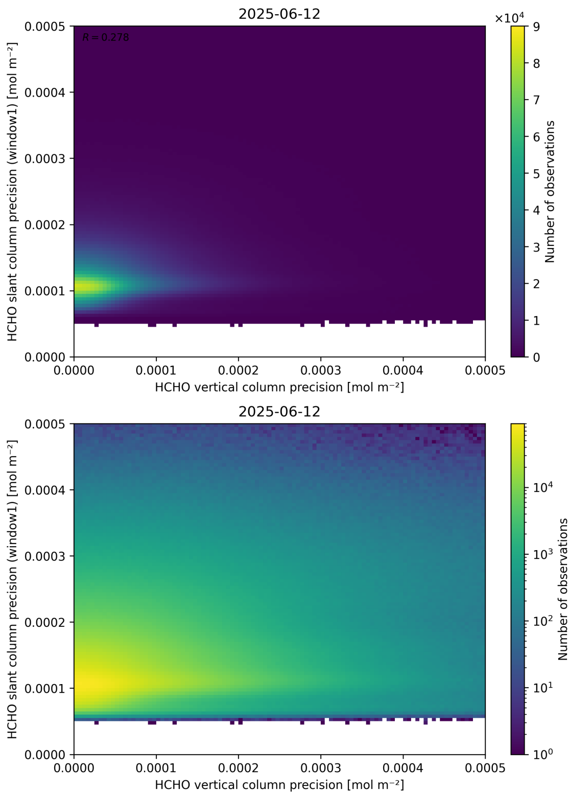
Figure 143: Scatter density plot of “HCHO vertical column precision” against “HCHO slant column precision (window1)” for 2025-06-11 to 2025-06-13.
