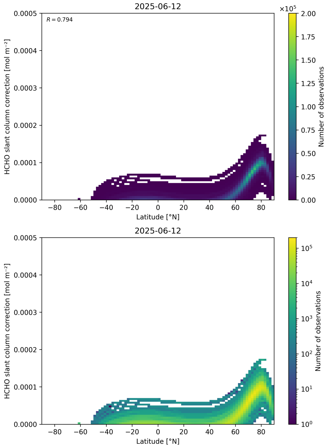
Figure 158: Scatter density plot of “Latitude” against “HCHO slant column correction” for 2025-06-11 to 2025-06-13.
