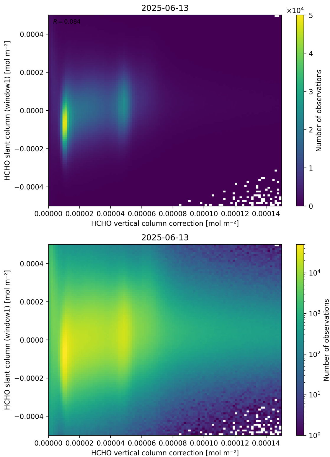
Figure 118: Scatter density plot of “HCHO vertical column correction” against “HCHO slant column (window1)” for 2025-06-12 to 2025-06-14.
