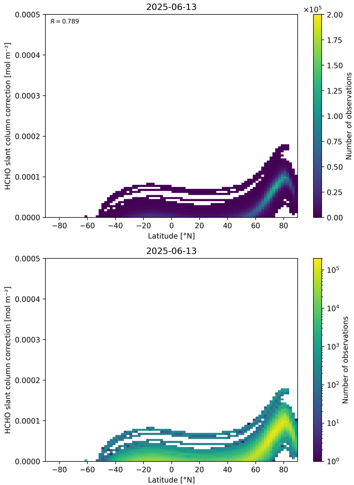
Figure 158: Scatter density plot of “Latitude” against “HCHO slant column correction” for 2025-06-12 to 2025-06-14.
