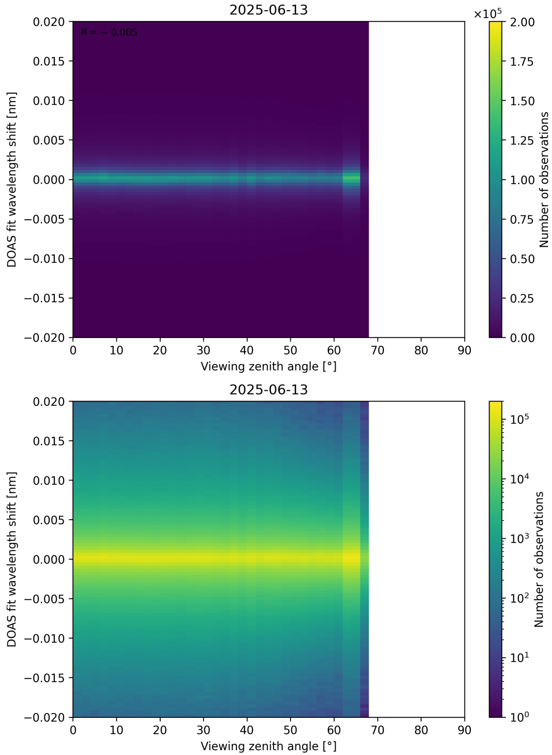
Figure 183: Scatter density plot of “Viewing zenith angle” against “DOAS fit wavelength shift” for 2025-06-12 to 2025-06-14.
