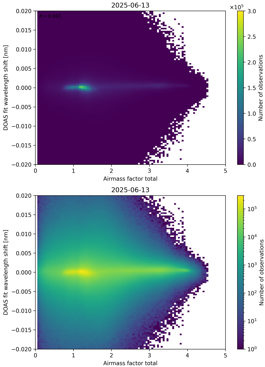
Figure 98: Scatter density plot of “Airmass factor total” against “DOAS fit wavelength shift” for 2025-06-12 to 2025-06-14.
