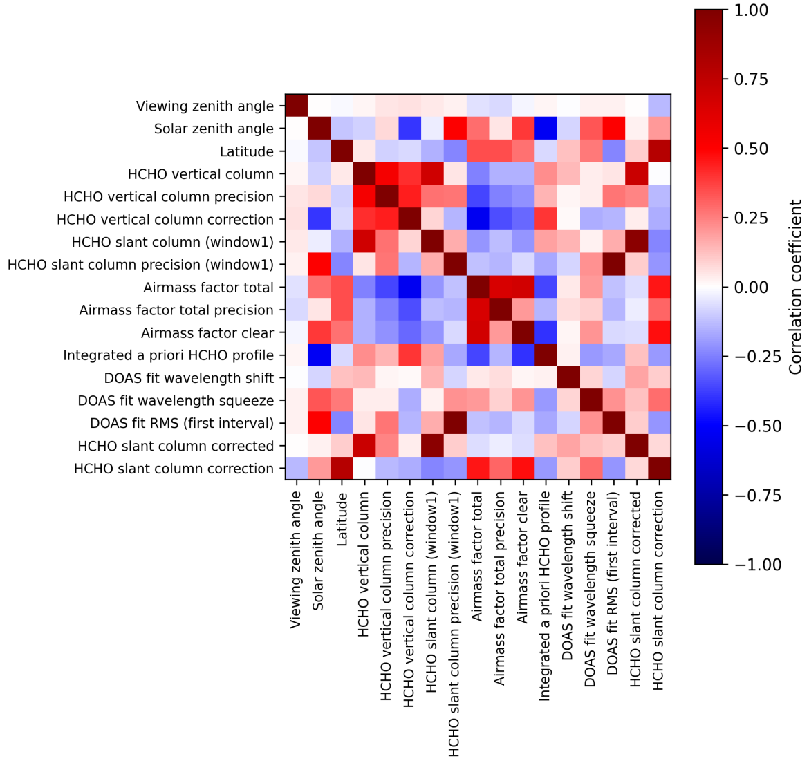
Figure 2: Map of correlation matrix for 2025-06-12 to 2025-06-14.
