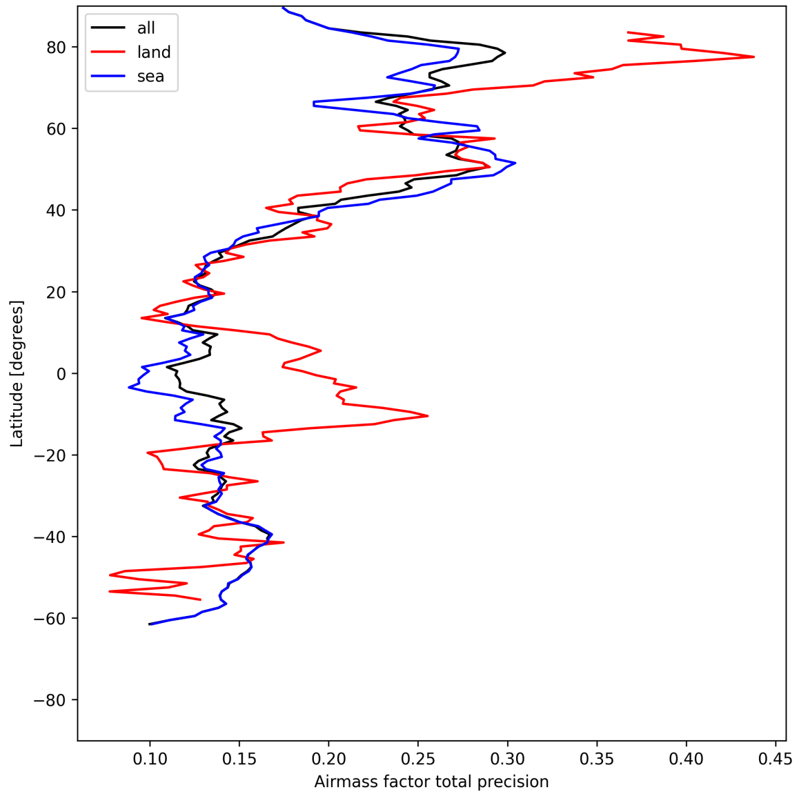
Figure 27: Zonal average of “Airmass factor total precision” for 2025-06-12 to 2025-06-14.
