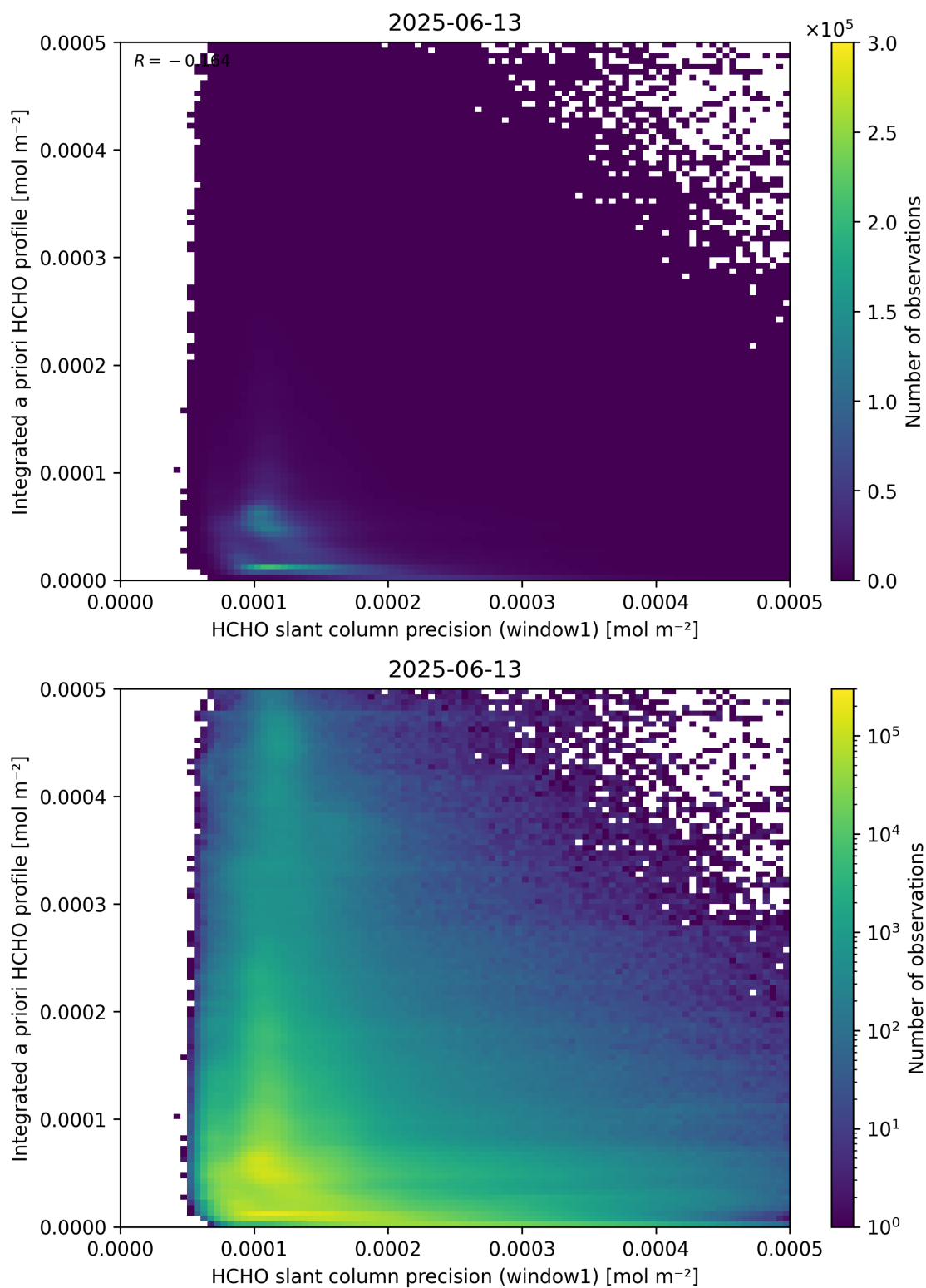
Figure 96: Scatter density plot of “HCHO slant column precision (window1)” against “Integrated a priori HCHO profile” for 2025-06-12 to 2025-06-14.
