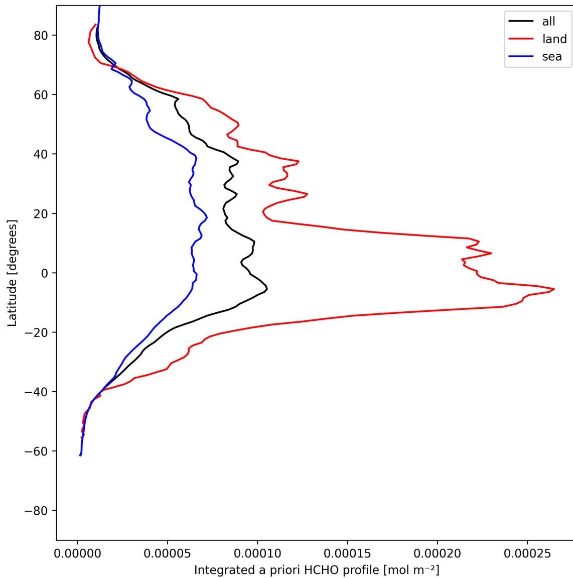
Figure 29: Zonal average of “Integrated a priori HCHO profile” for 2025-06-12 to 2025-06-14.
