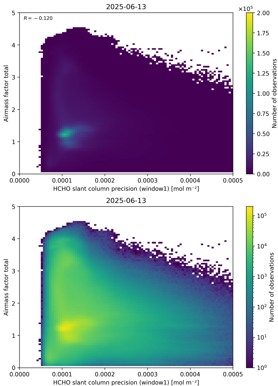
Figure 94: Scatter density plot of “HCHO slant column precision (window1)” against “Airmass factor total” for 2025-06-12 to 2025-06-14.
