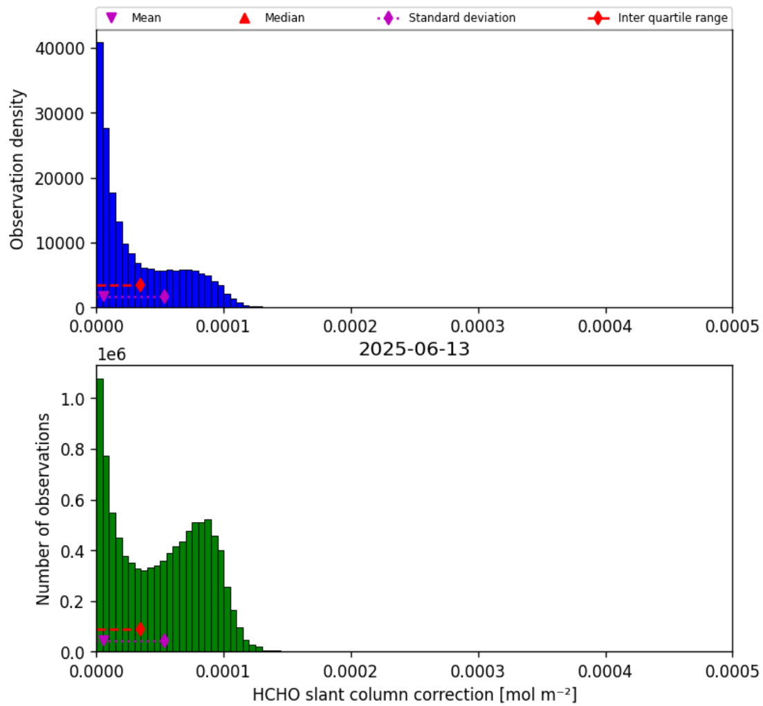
Figure 47: Histogram of “HCHO slant column correction” for 2025-06-12 to 2025-06-14
