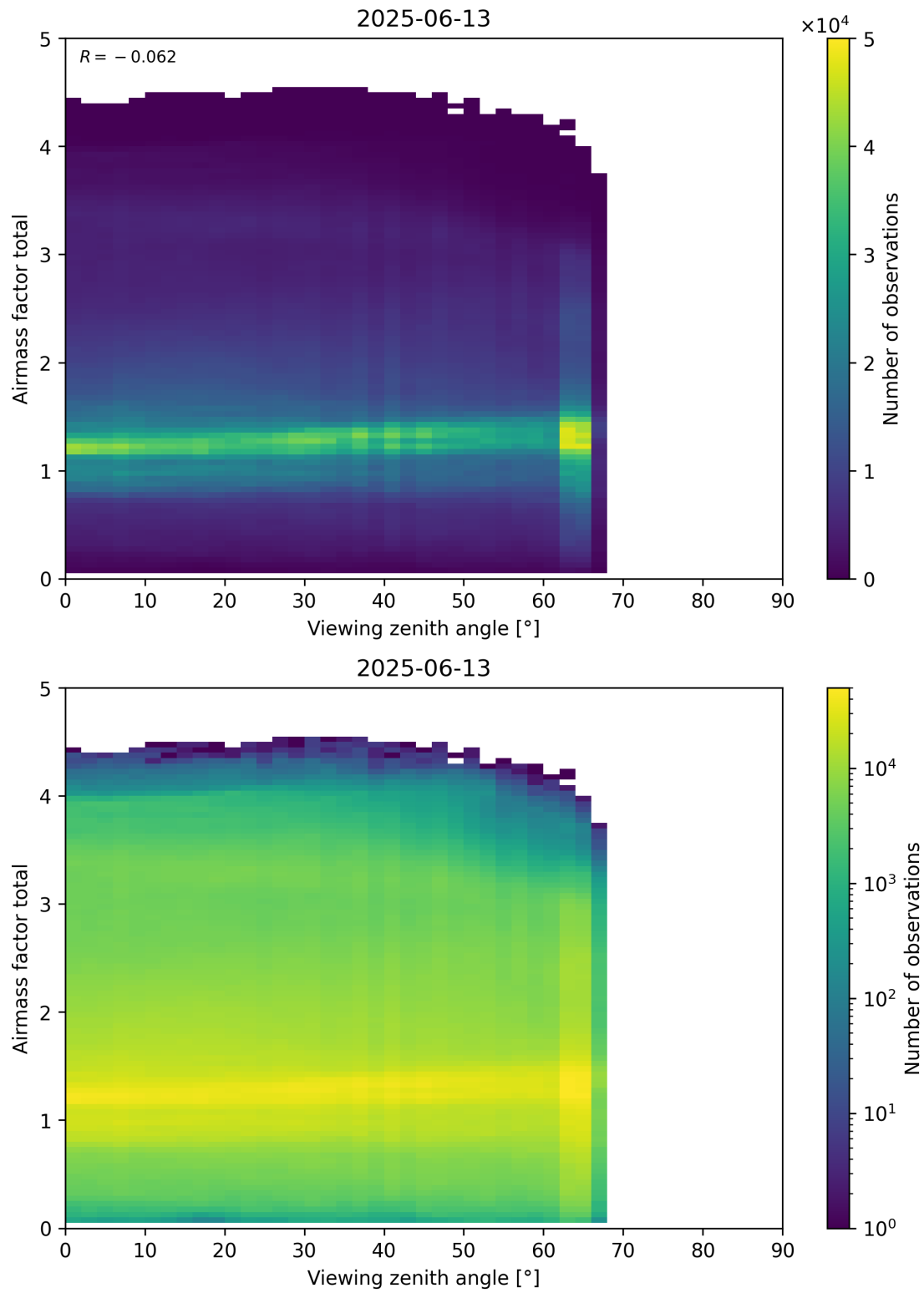
Figure 190: Scatter density plot of “Viewing zenith angle” against “Airmass factor total” for 2025-06-12 to 2025-06-14.
