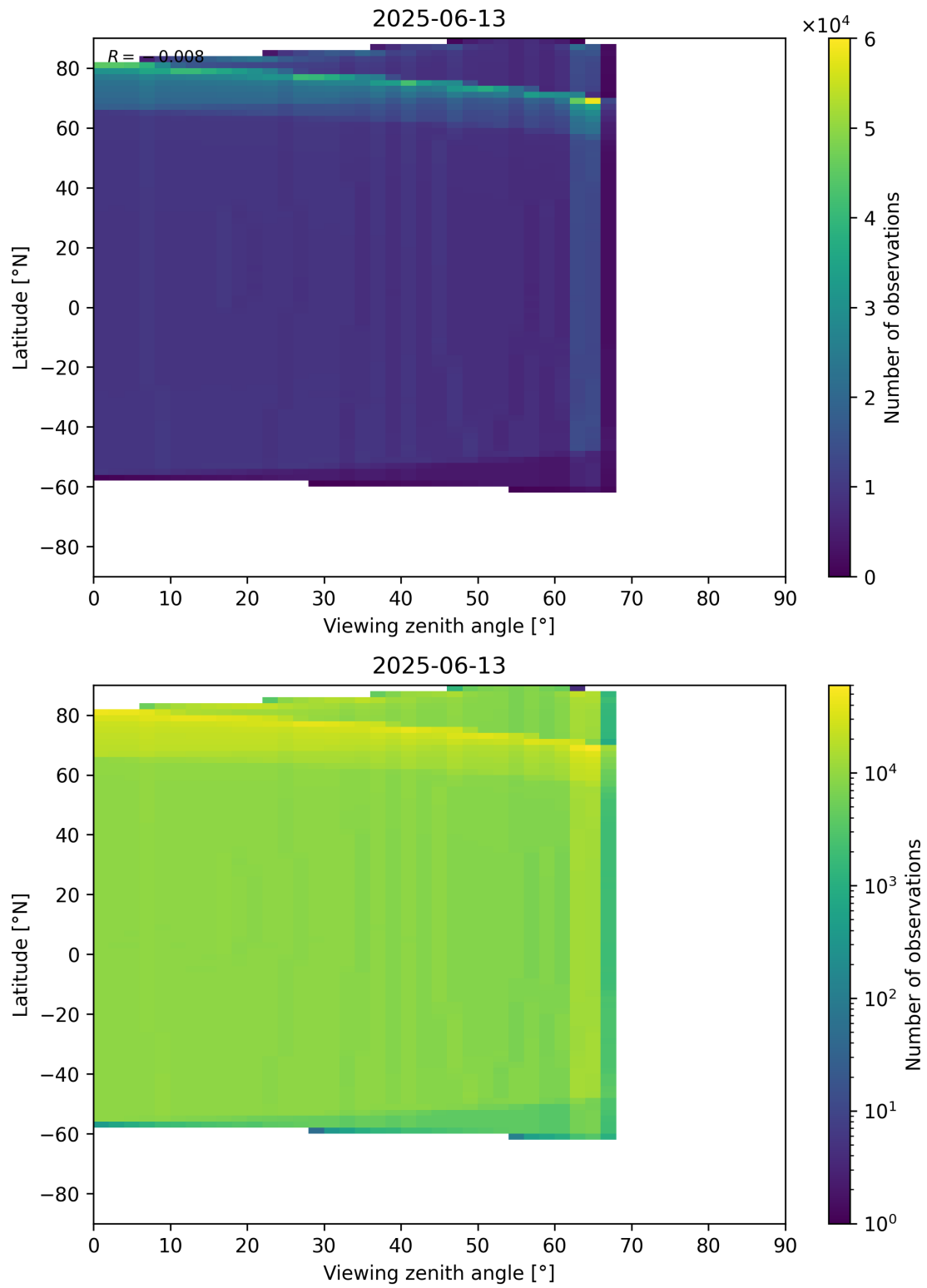
Figure 196: Scatter density plot of “Viewing zenith angle” against “Latitude” for 2025-06-12 to 2025-06-14.
