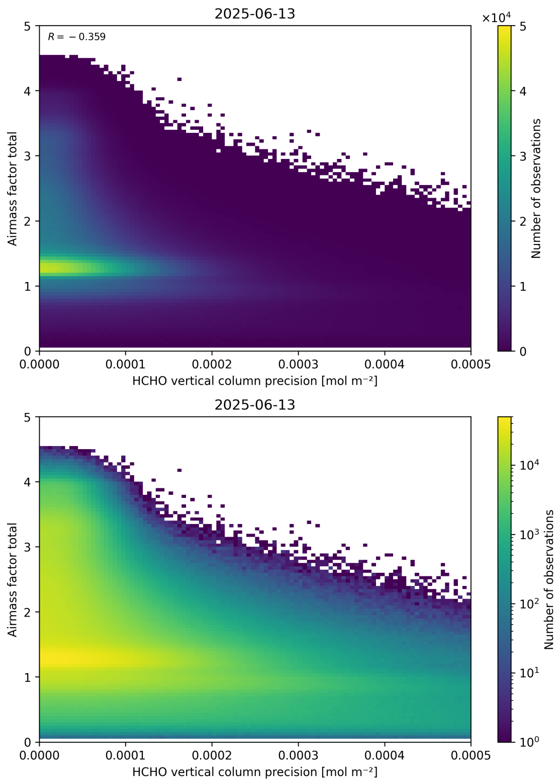
Figure 144: Scatter density plot of “HCHO vertical column precision” against “Airmass factor total” for 2025-06-12 to 2025-06-14.
