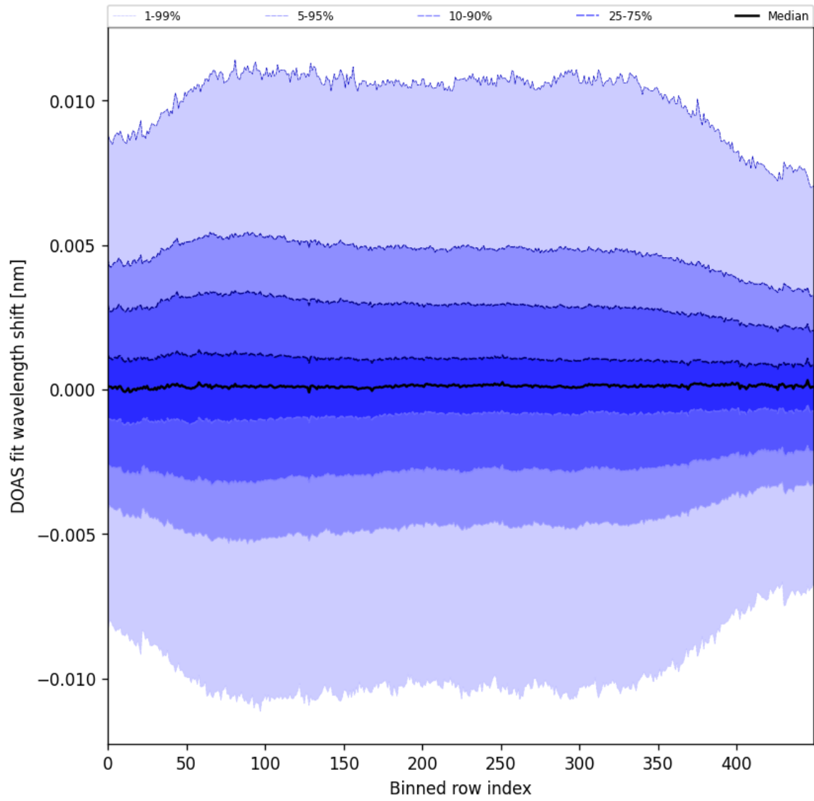
Figure 58: Along track statistics of “DOAS fit wavelength shift” for 2025-06-12 to 2025-06-14
