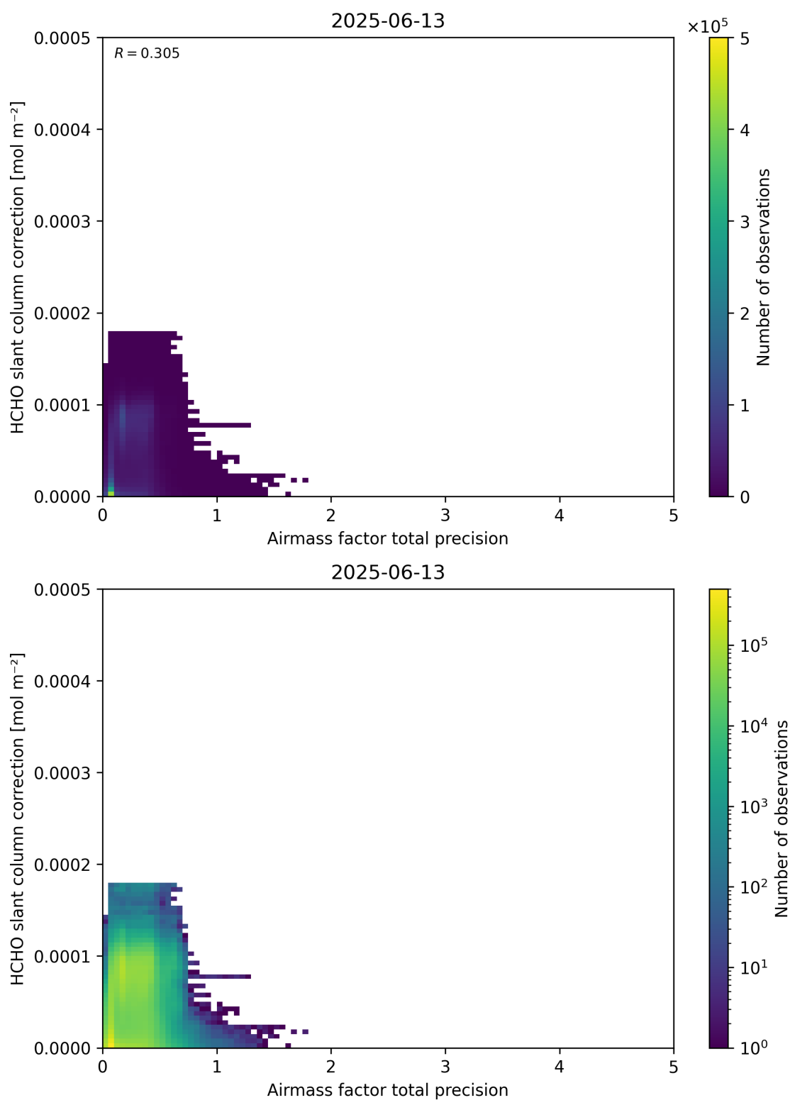
Figure 110: Scatter density plot of “Airmass factor total precision” against “HCHO slant column correction” for 2025-06-12 to 2025-06-14.
