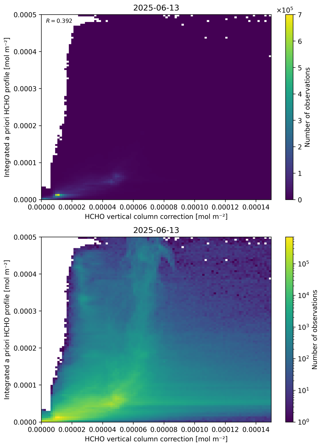
Figure 122: Scatter density plot of “HCHO vertical column correction” against “Integrated a priori HCHO profile” for 2025-06-12 to 2025-06-14.
