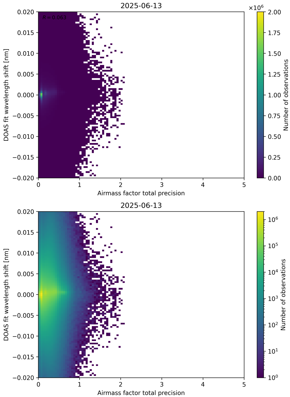
Figure 106: Scatter density plot of “Airmass factor total precision” against “DOAS fit wavelength shift” for 2025-06-12 to 2025-06-14.
