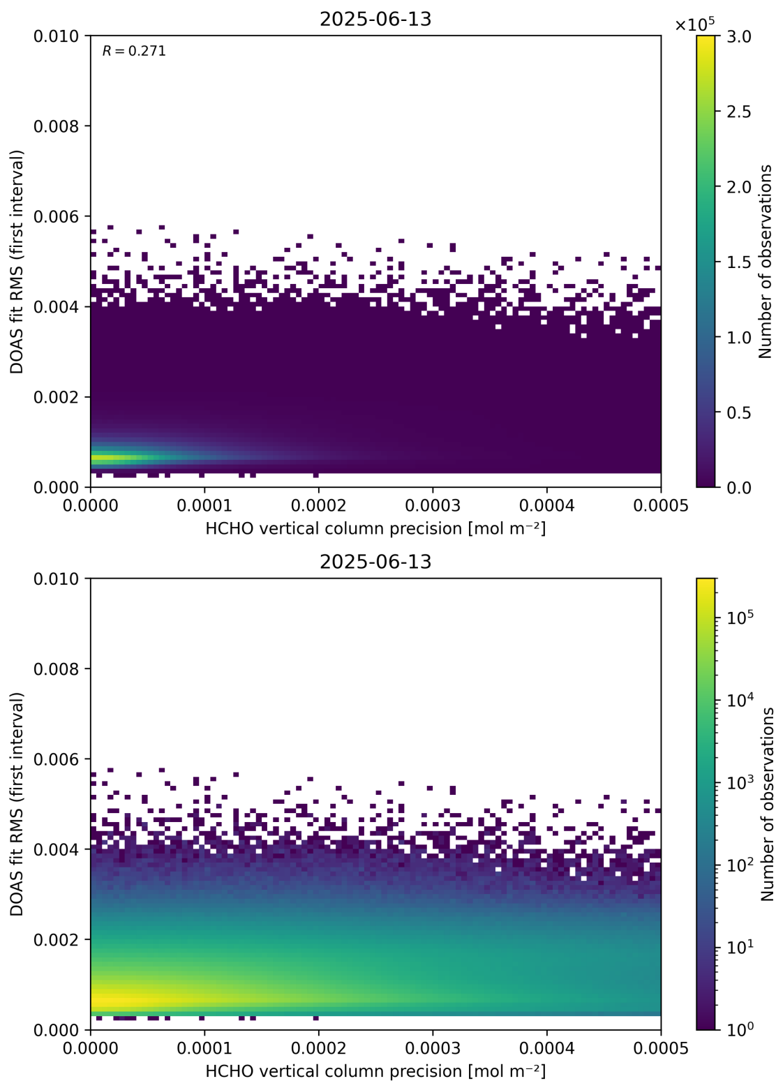
Figure 136: Scatter density plot of “HCHO vertical column precision” against “DOAS fit RMS (first interval)” for 2025-06-12 to 2025-06-14.
