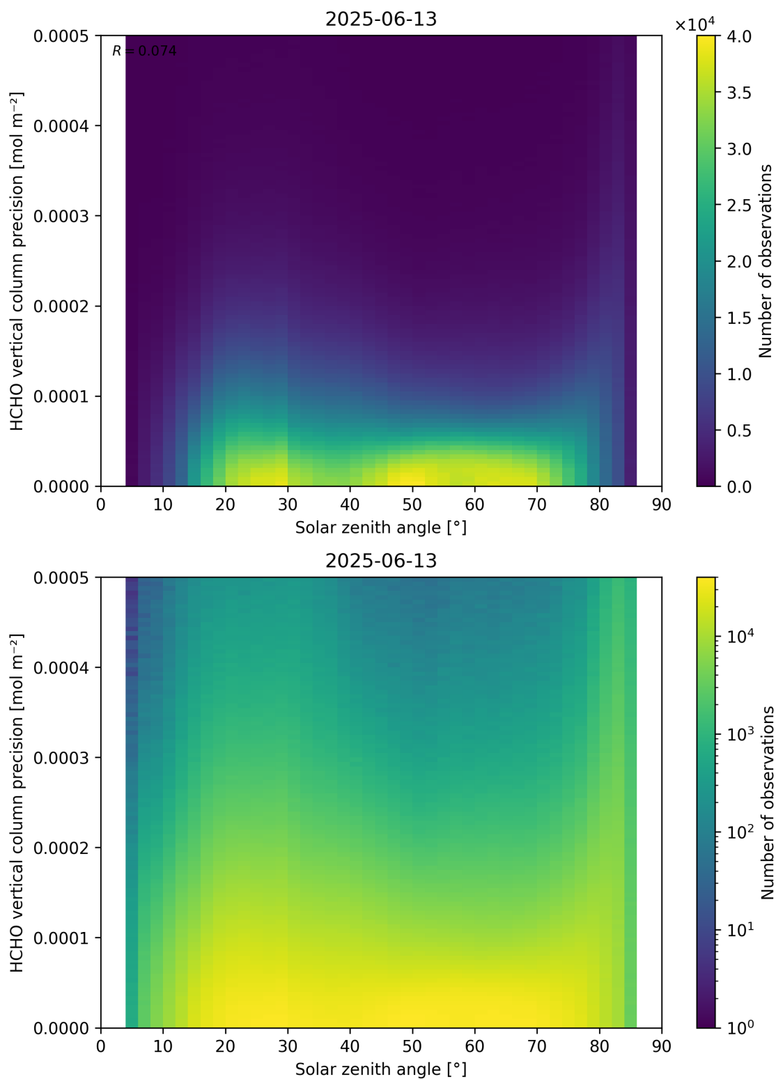
Figure 179: Scatter density plot of “Solar zenith angle” against “HCHO vertical column precision” for 2025-06-12 to 2025-06-14.
