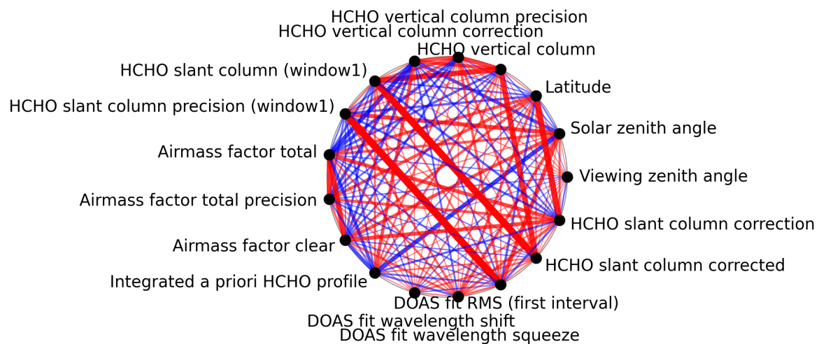
Figure 1: Map of correlation graph for 2025-06-12 to 2025-06-14.
