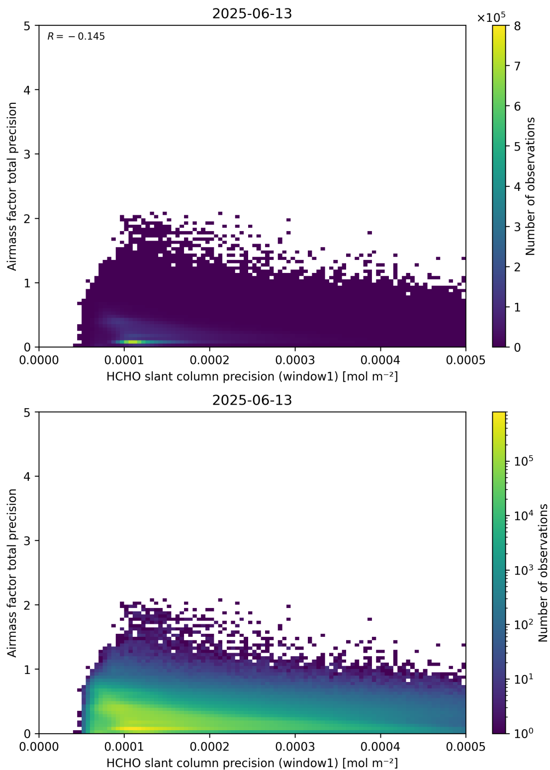
Figure 95: Scatter density plot of “HCHO slant column precision (window1)” against “Airmass factor total precision” for 2025-06-12 to 2025-06-14.
