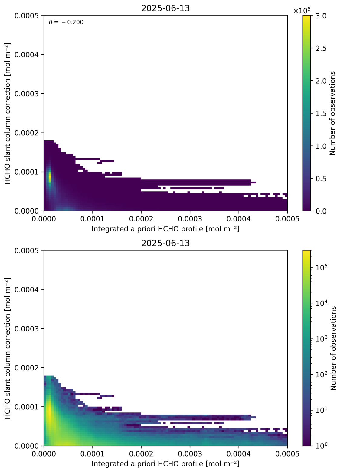
Figure 152: Scatter density plot of “Integrated a priori HCHO profile” against “HCHO slant column correction” for 2025-06-12 to 2025-06-14.
