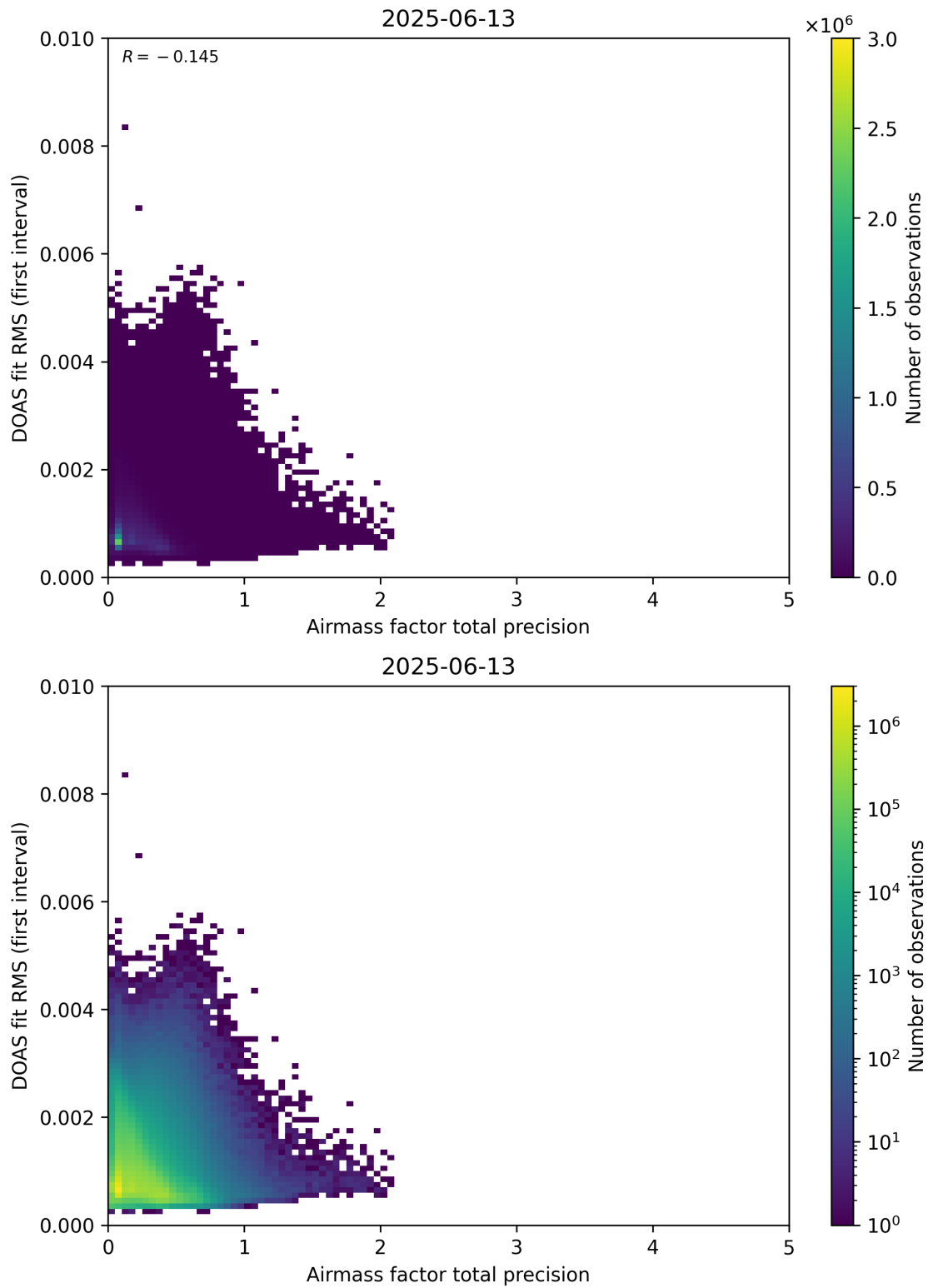
Figure 105: Scatter density plot of “Airmass factor total precision” against “DOAS fit RMS (first interval)” for 2025-06-12 to 2025-06-14.
