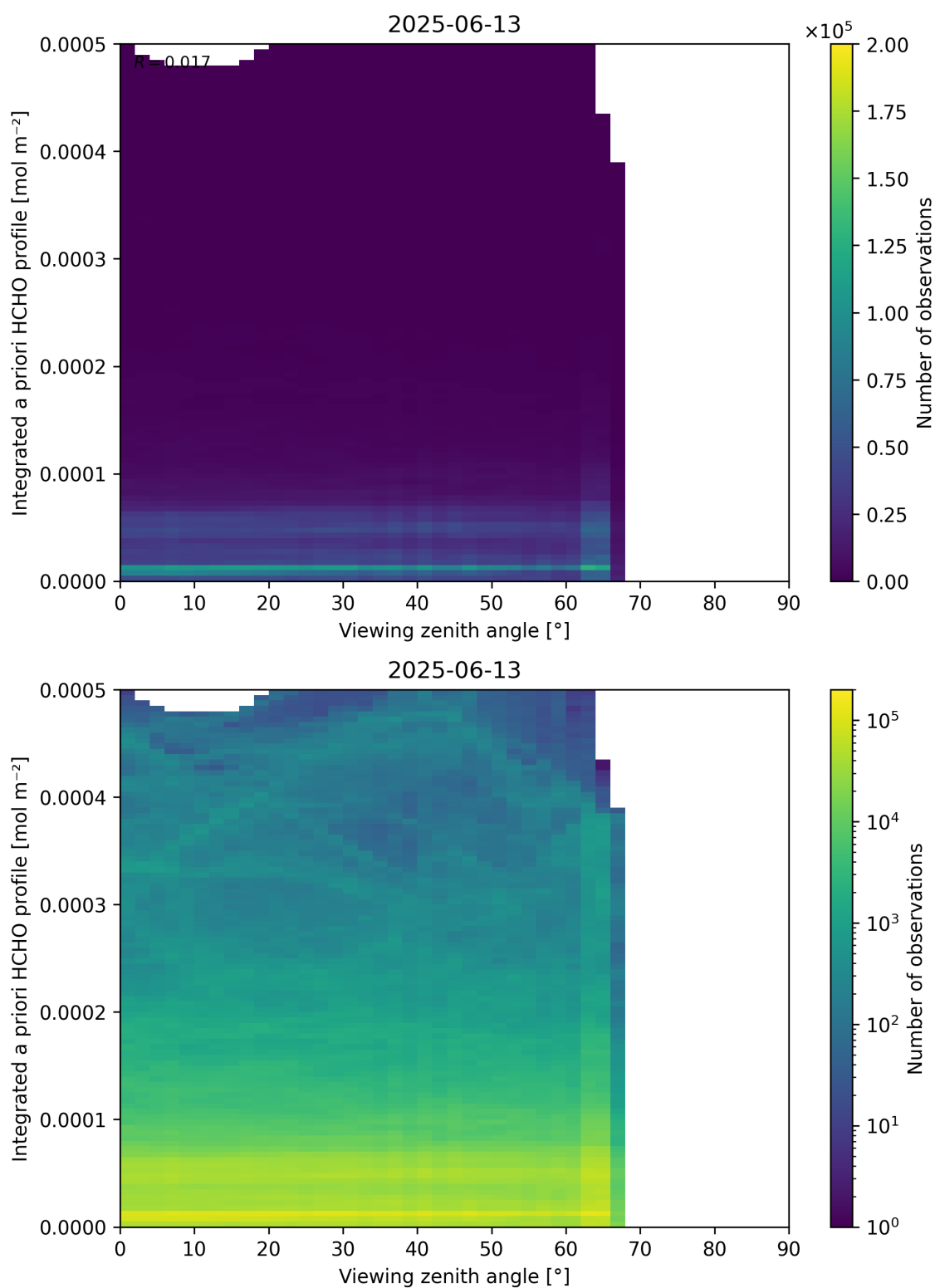
Figure 195: Scatter density plot of “Viewing zenith angle” against “Integrated a priori HCHO profile” for 2025-06-12 to 2025-06-14.
