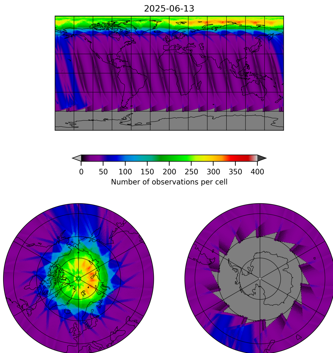
Figure 19: Map of the number of observations for 2025-06-12 to 2025-06-14
