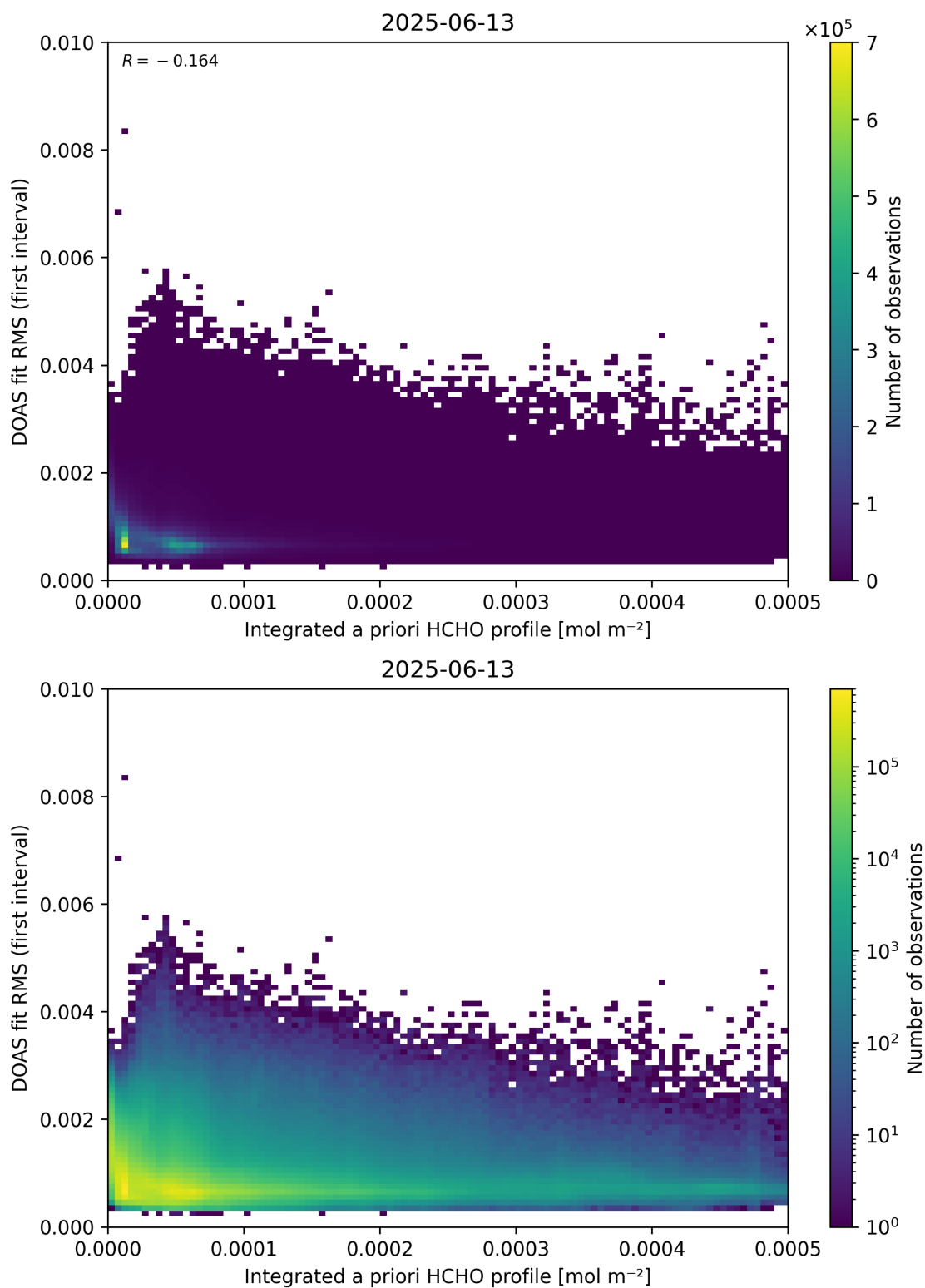
Figure 148: Scatter density plot of “Integrated a priori HCHO profile” against “DOAS fit RMS (first interval)” for 2025-06-12 to 2025-06-14.
