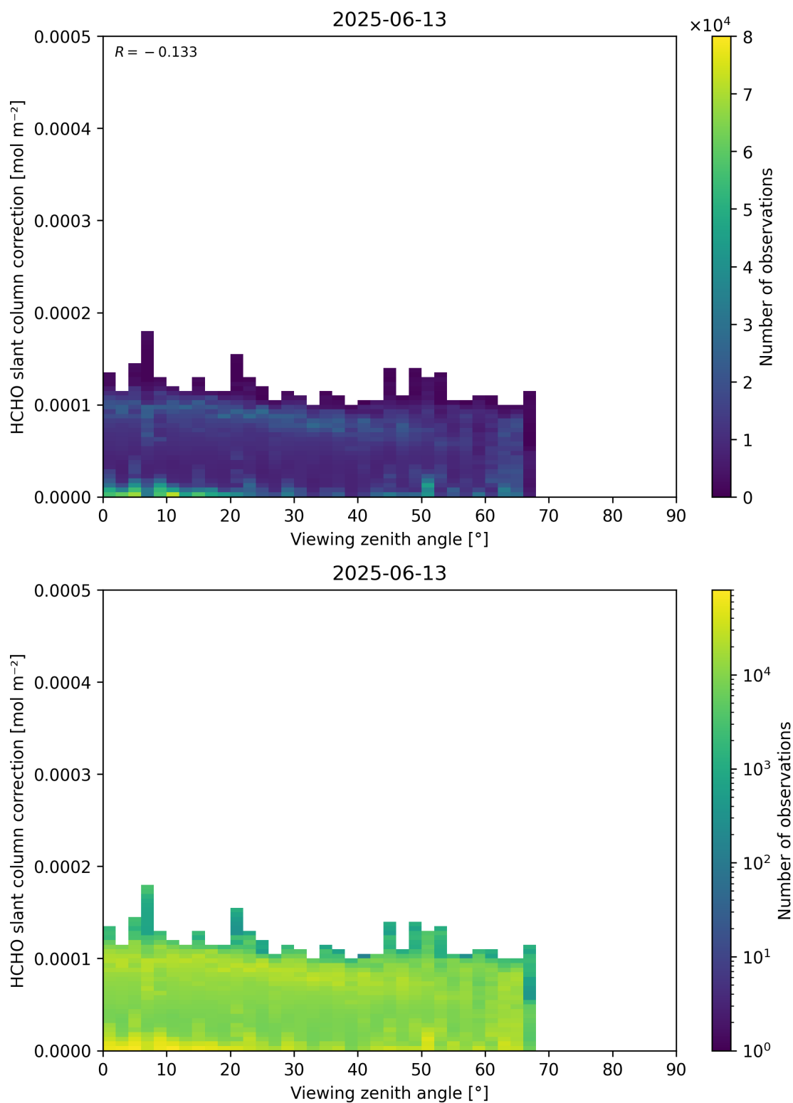
Figure 187: Scatter density plot of “Viewing zenith angle” against “HCHO slant column correction” for 2025-06-12 to 2025-06-14.
