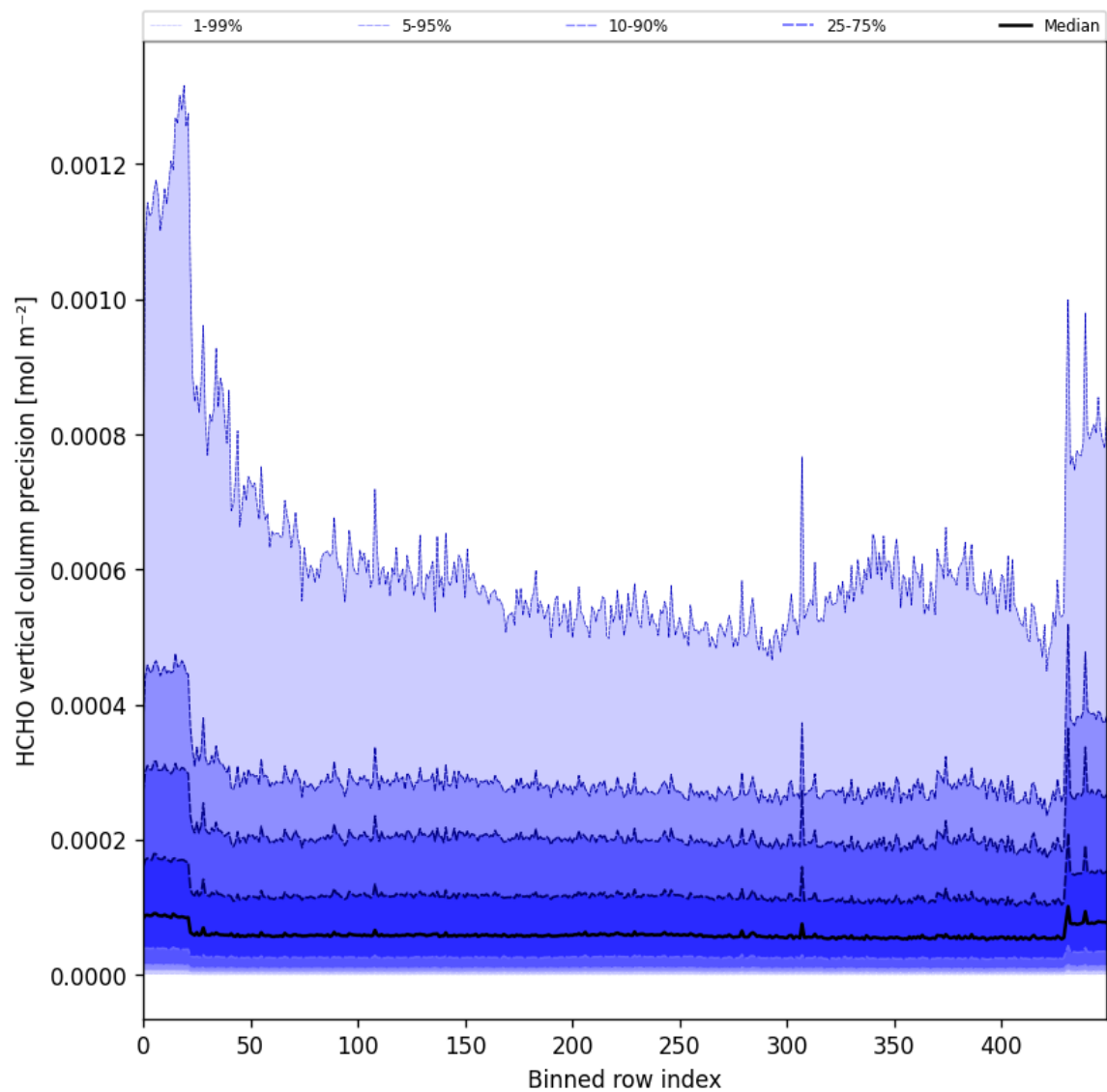
Figure 50: Along track statistics of “HCHO vertical column precision” for 2025-06-12 to 2025-06-14
