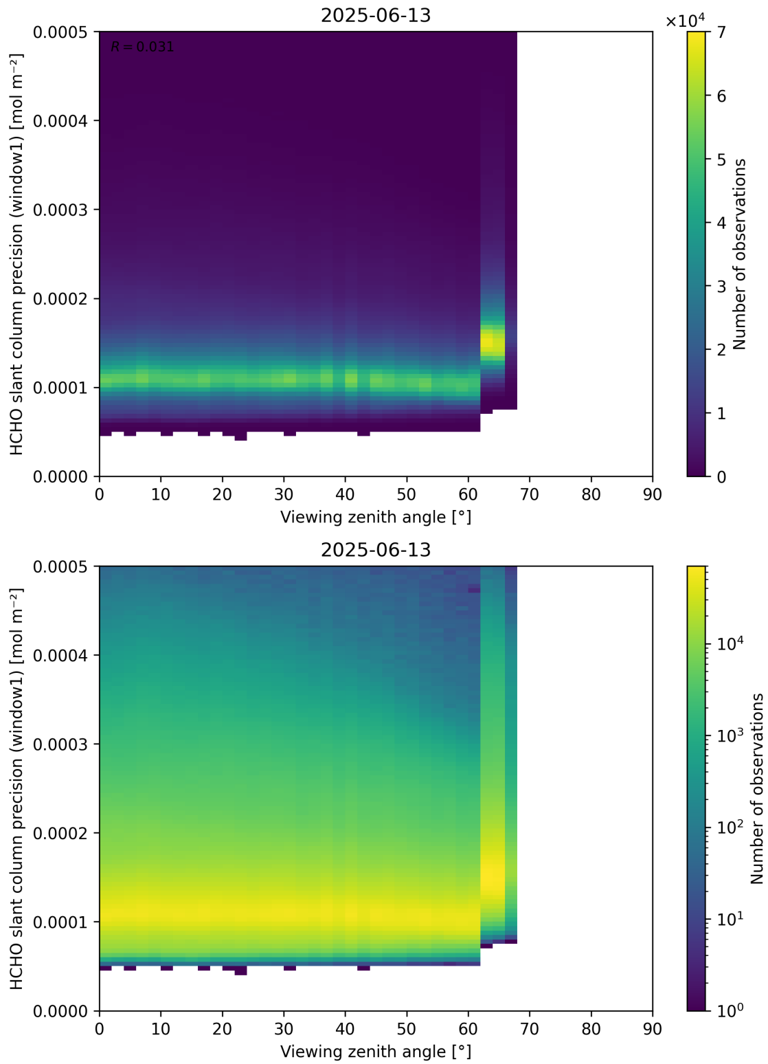
Figure 189: Scatter density plot of “Viewing zenith angle” against “HCHO slant column precision (window1)” for 2025-06-12 to 2025-06-14.
