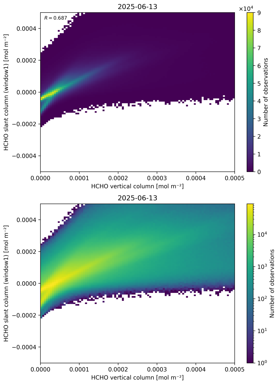
Figure 129: Scatter density plot of “HCHO vertical column” against “HCHO slant column (window1)” for 2025-06-12 to 2025-06-14.
