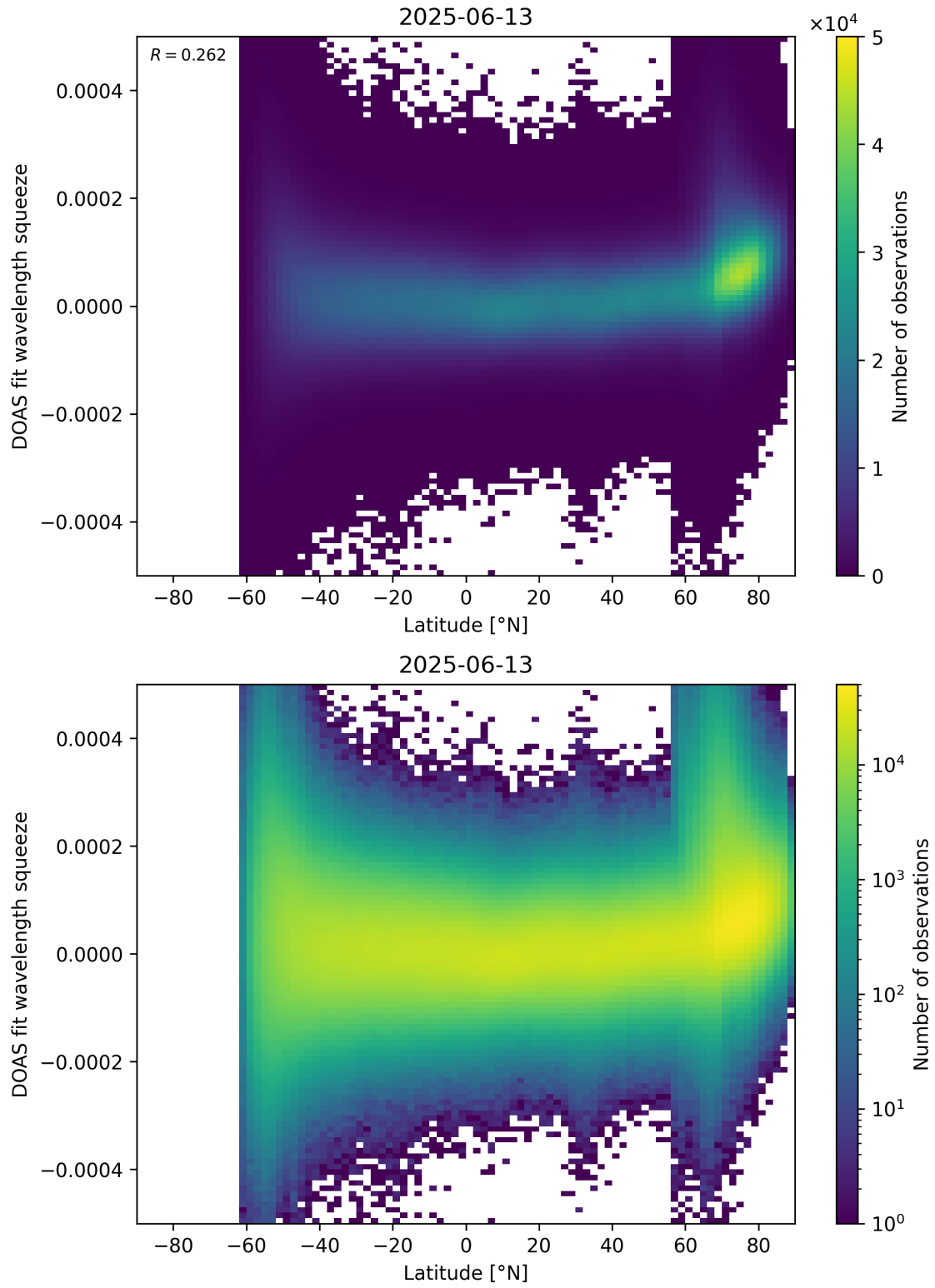
Figure 155: Scatter density plot of “Latitude” against “DOAS fit wavelength squeeze” for 2025-06-12 to 2025-06-14.
