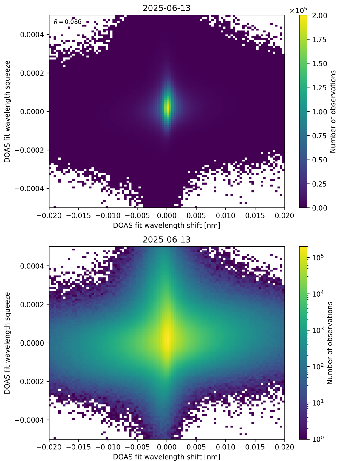
Figure 65: Scatter density plot of “DOAS fit wavelength shift” against “DOAS fit wavelength squeeze” for 2025-06-12 to 2025-06-14.
