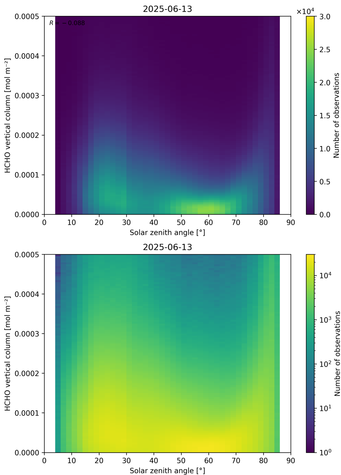
Figure 177: Scatter density plot of “Solar zenith angle” against “HCHO vertical column” for 2025-06-12 to 2025-06-14.
