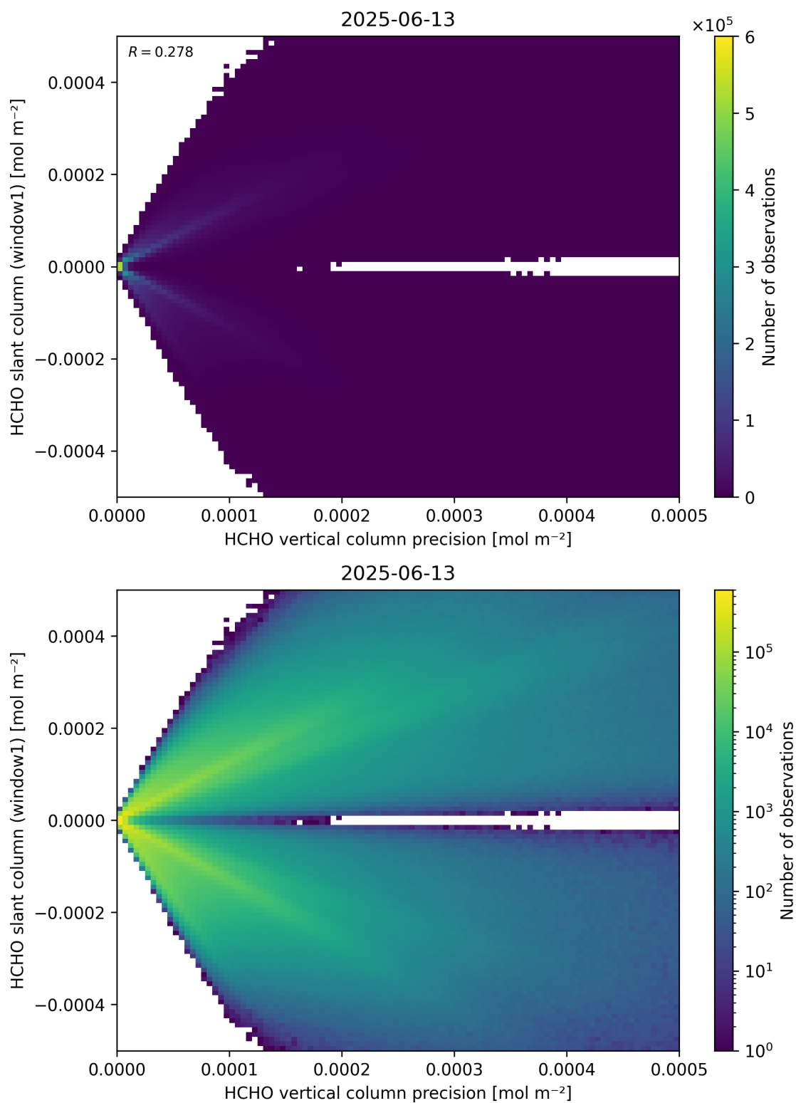
Figure 142: Scatter density plot of “HCHO vertical column precision” against “HCHO slant column (window1)” for 2025-06-12 to 2025-06-14.
