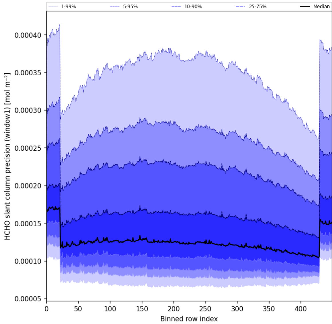
Figure 53: Along track statistics of “HCHO slant column precision (window1)” for 2025-06-12 to 2025-06-14
