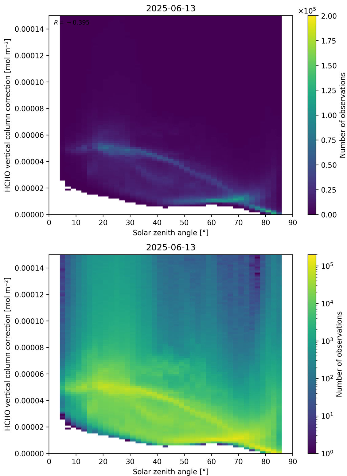
Figure 178: Scatter density plot of “Solar zenith angle” against “HCHO vertical column correction” for 2025-06-12 to 2025-06-14.
