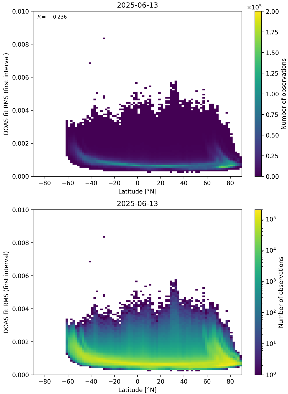
Figure 153: Scatter density plot of “Latitude” against “DOAS fit RMS (first interval)” for 2025-06-12 to 2025-06-14.
