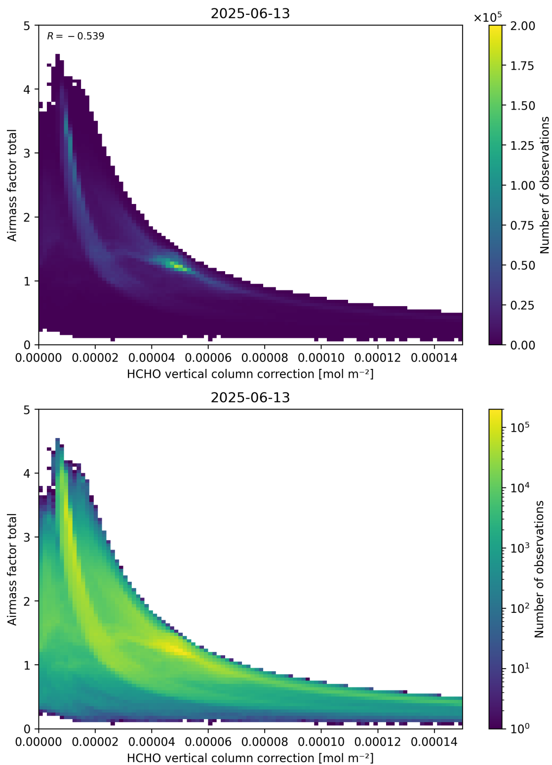
Figure 120: Scatter density plot of “HCHO vertical column correction” against “Airmass factor total” for 2025-06-12 to 2025-06-14.
