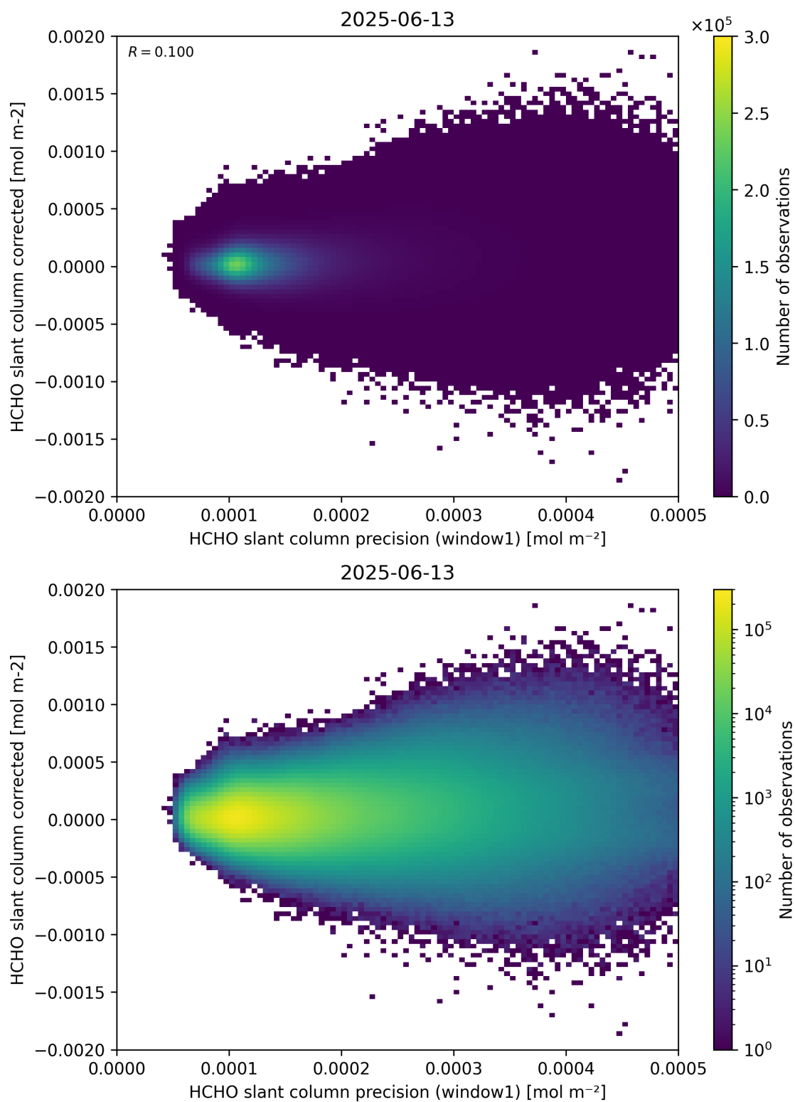
Figure 92: Scatter density plot of “HCHO slant column precision (window1)” against “HCHO slant column corrected” for 2025-06-12 to 2025-06-14.
