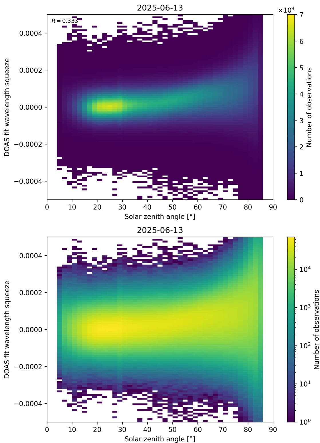
Figure 169: Scatter density plot of “Solar zenith angle” against “DOAS fit wavelength squeeze” for 2025-06-12 to 2025-06-14.
