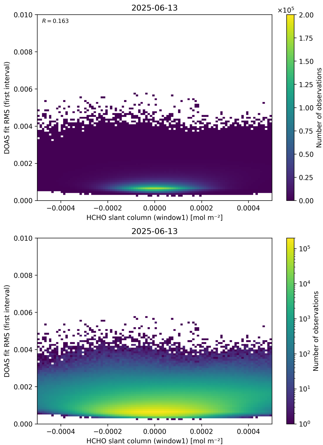
Figure 78: Scatter density plot of “HCHO slant column (window1)” against “DOAS fit RMS (first interval)” for 2025-06-12 to 2025-06-14.
