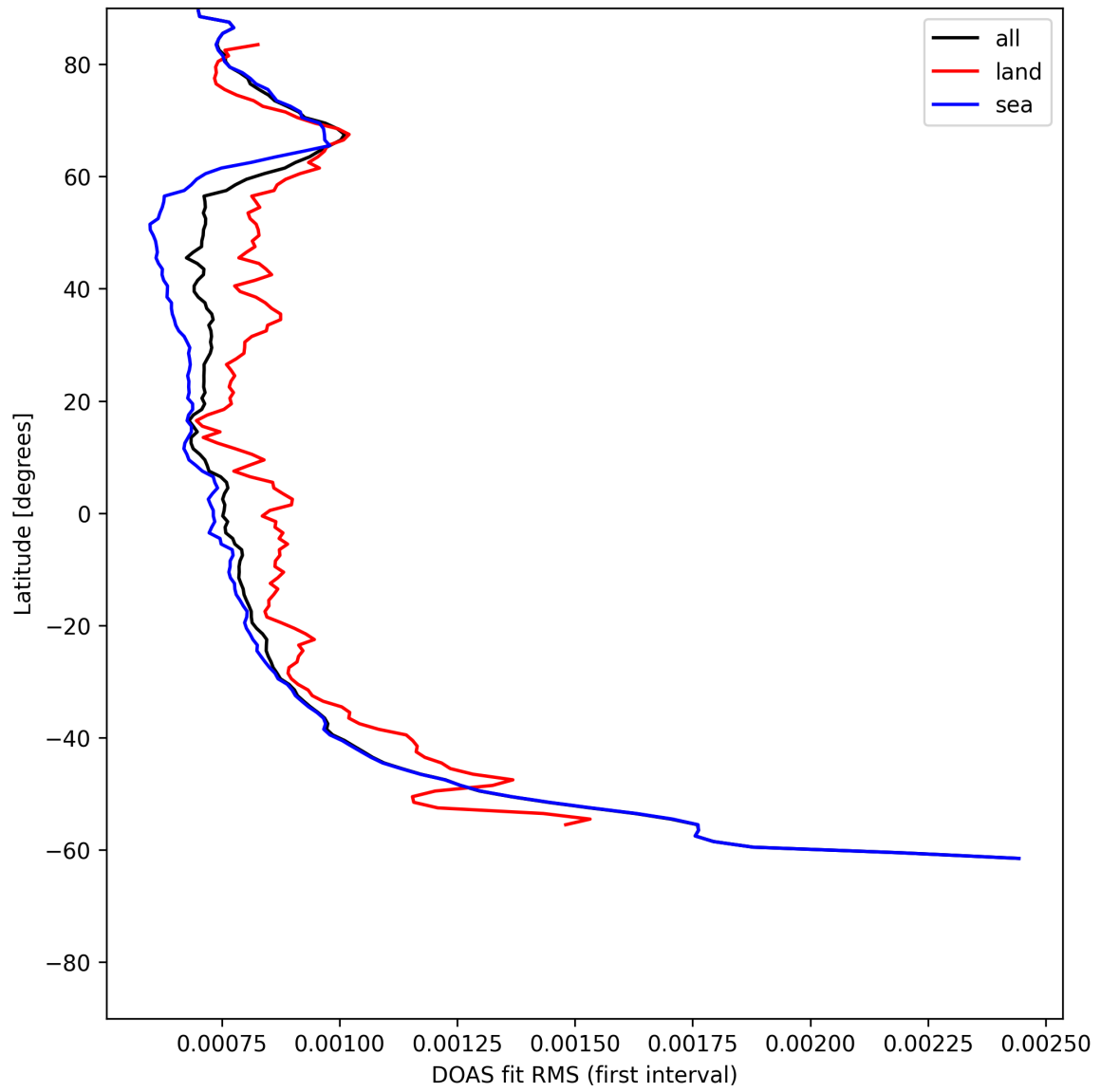
Figure 32: Zonal average of “DOAS fit RMS (first interval)” for 2025-06-12 to 2025-06-14.
