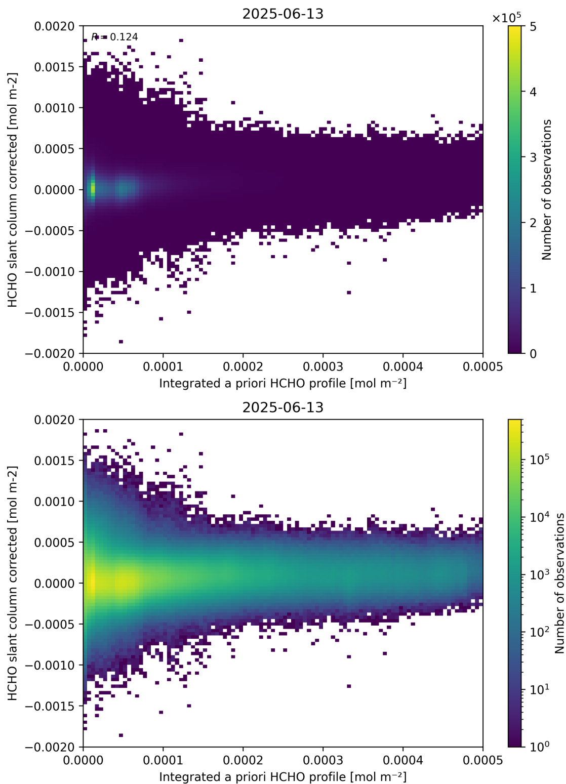
Figure 151: Scatter density plot of “Integrated a priori HCHO profile” against “HCHO slant column corrected” for 2025-06-12 to 2025-06-14.
