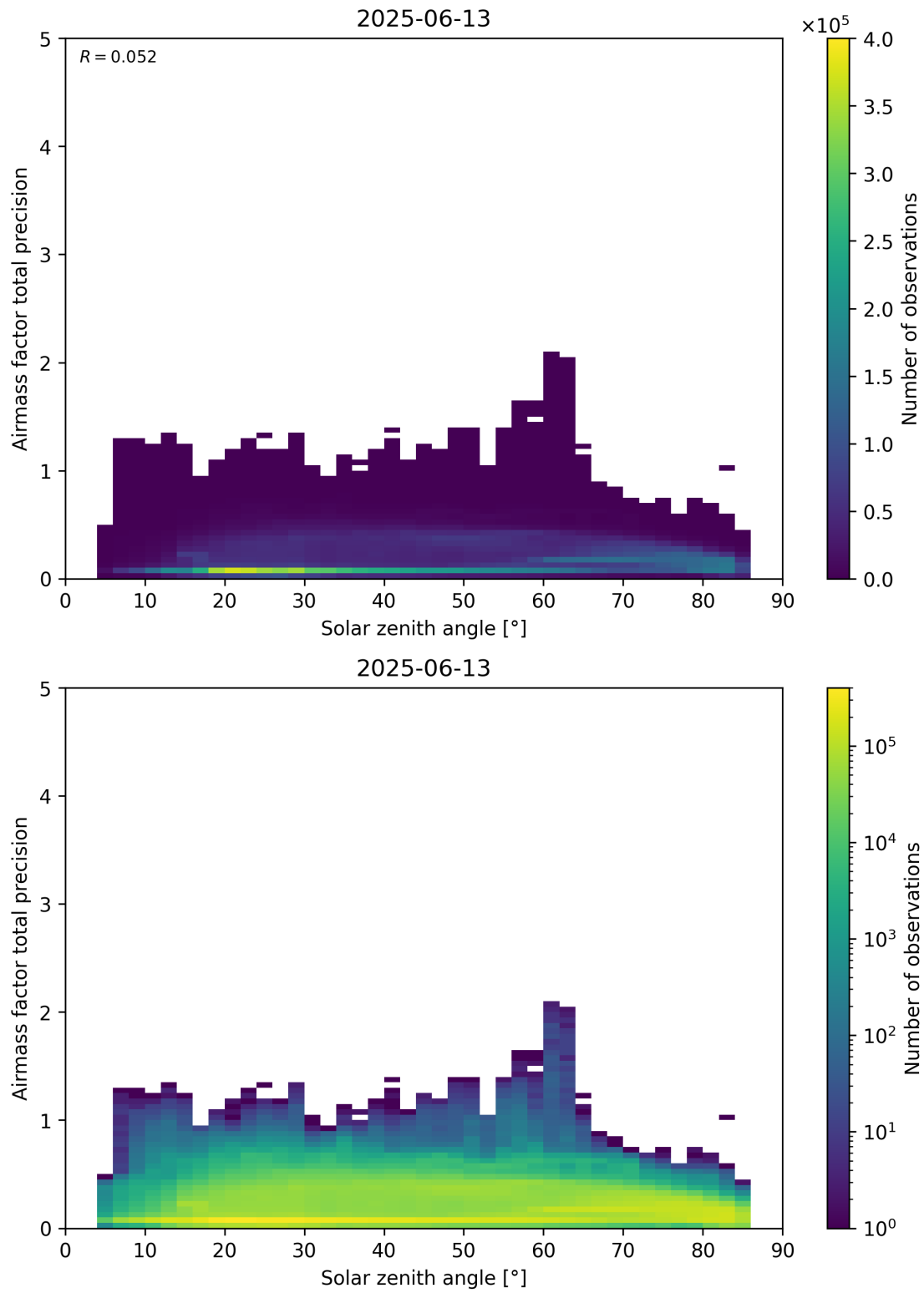
Figure 176: Scatter density plot of “Solar zenith angle” against “Airmass factor total precision” for 2025-06-12 to 2025-06-14.
