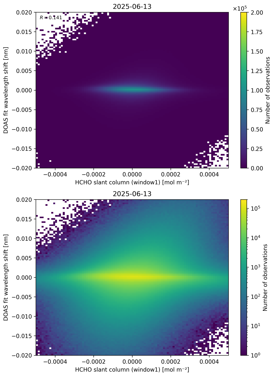
Figure 79: Scatter density plot of “HCHO slant column (window1)” against “DOAS fit wavelength shift” for 2025-06-12 to 2025-06-14.
