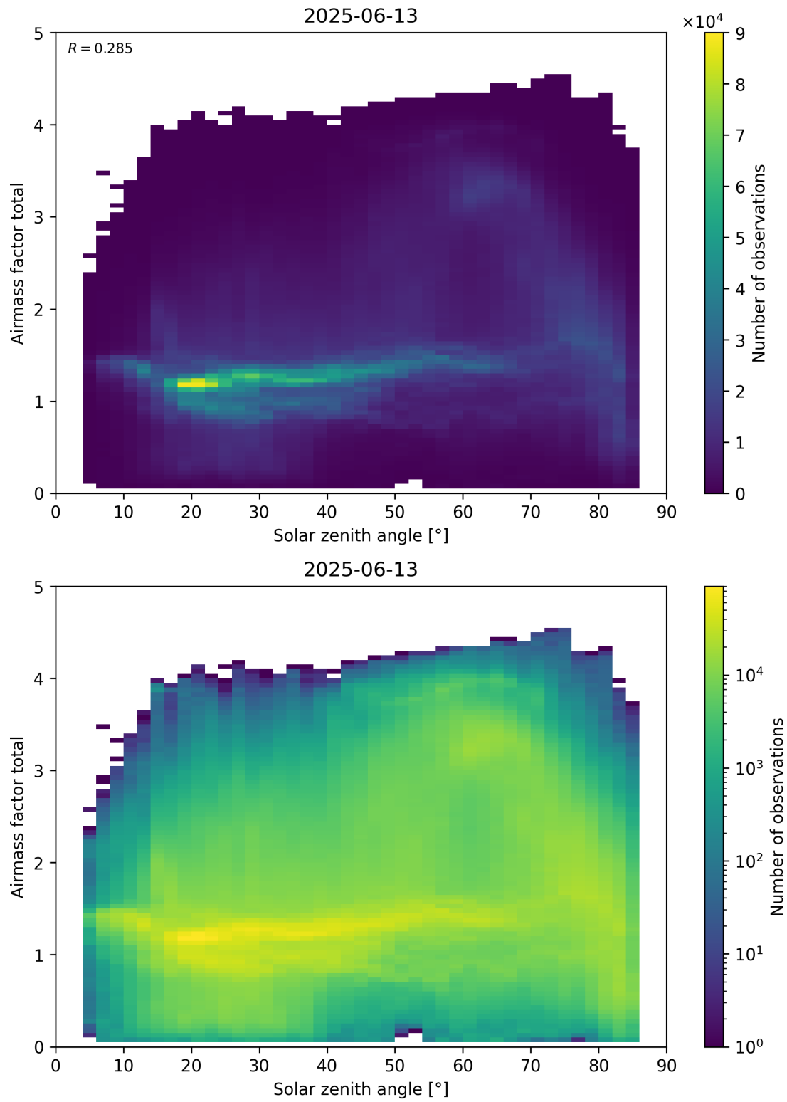
Figure 175: Scatter density plot of “Solar zenith angle” against “Airmass factor total” for 2025-06-12 to 2025-06-14.
