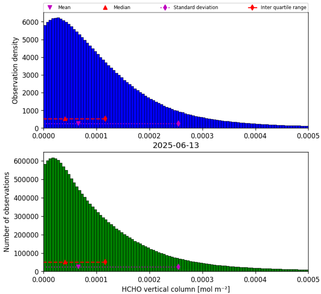
Figure 35: Histogram of “HCHO vertical column” for 2025-06-12 to 2025-06-14
