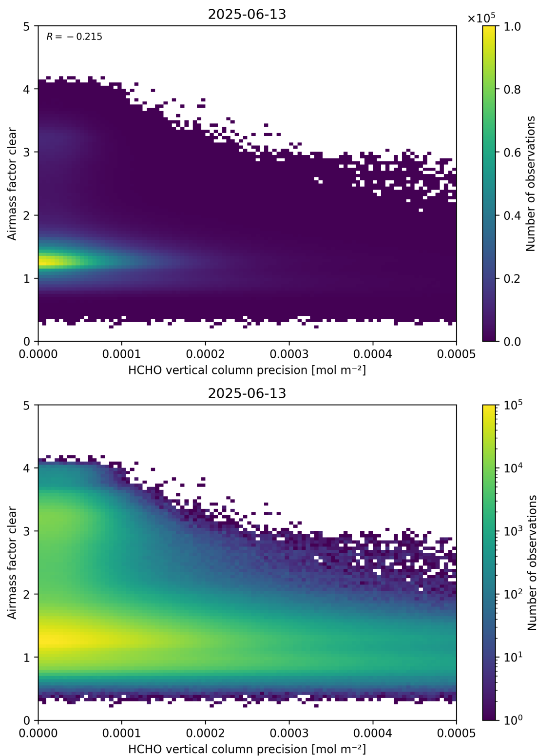
Figure 139: Scatter density plot of “HCHO vertical column precision” against “Airmass factor clear” for 2025-06-12 to 2025-06-14.
