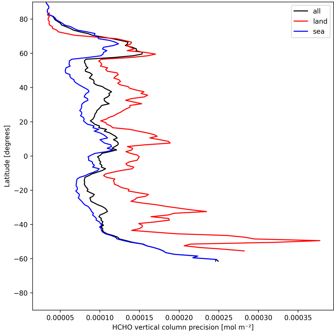
Figure 22: Zonal average of “HCHO vertical column precision” for 2025-06-12 to 2025-06-14.
