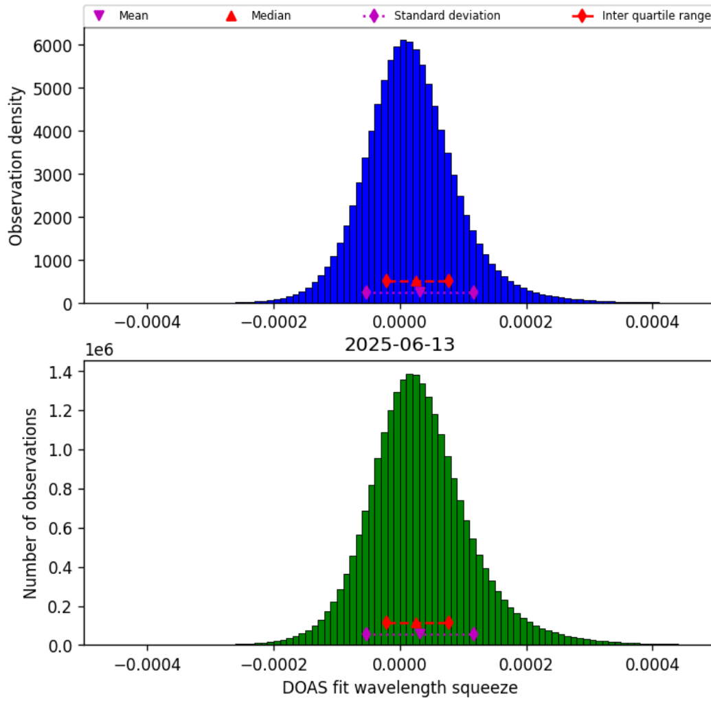
Figure 45: Histogram of “DOAS fit wavelength squeeze” for 2025-06-12 to 2025-06-14
