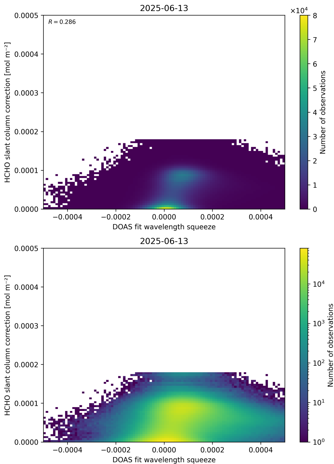
Figure 70: Scatter density plot of “DOAS fit wavelength squeeze” against “HCHO slant column correction” for 2025-06-12 to 2025-06-14.
