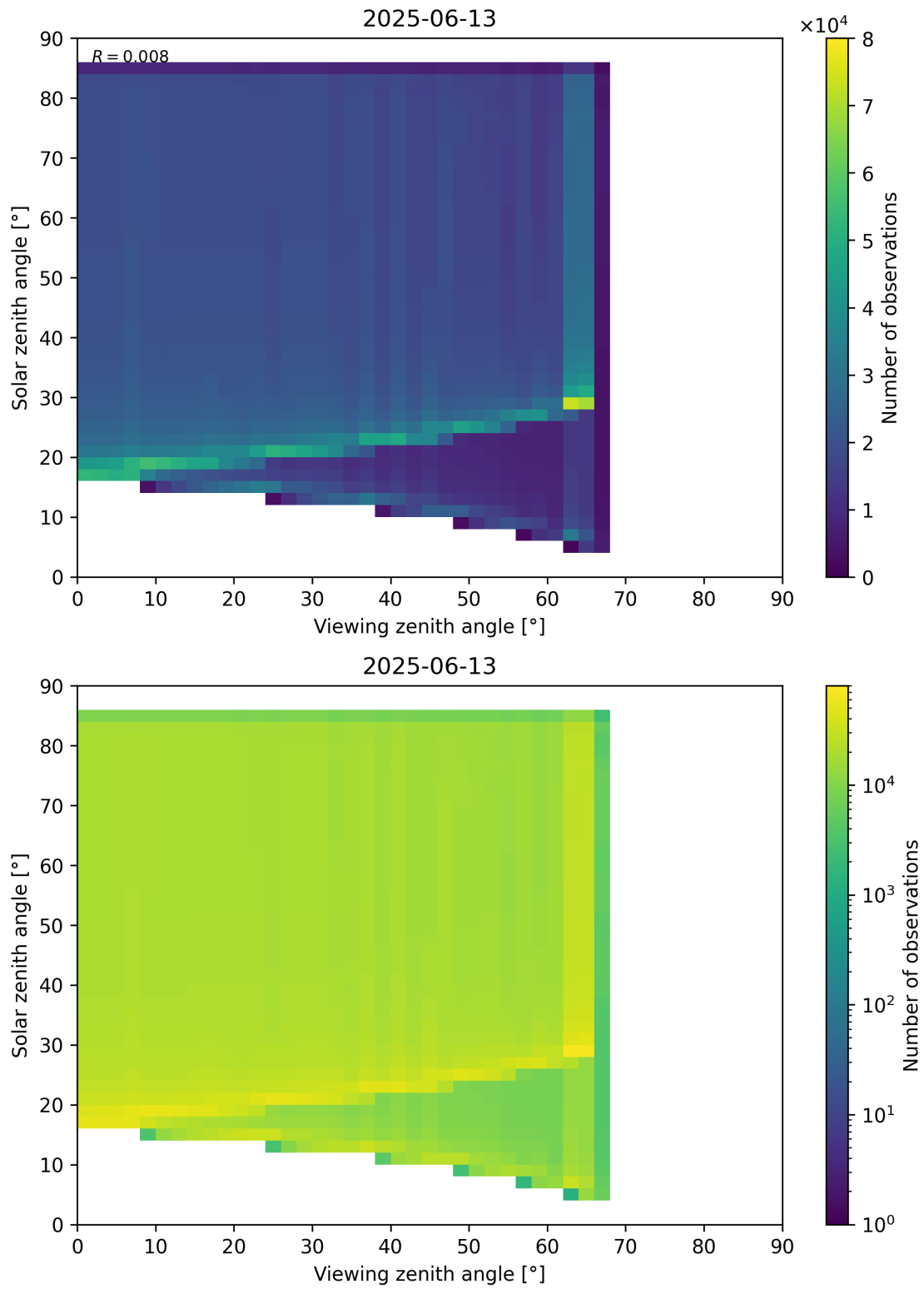
Figure 197: Scatter density plot of “Viewing zenith angle” against “Solar zenith angle” for 2025-06-12 to 2025-06-14.
