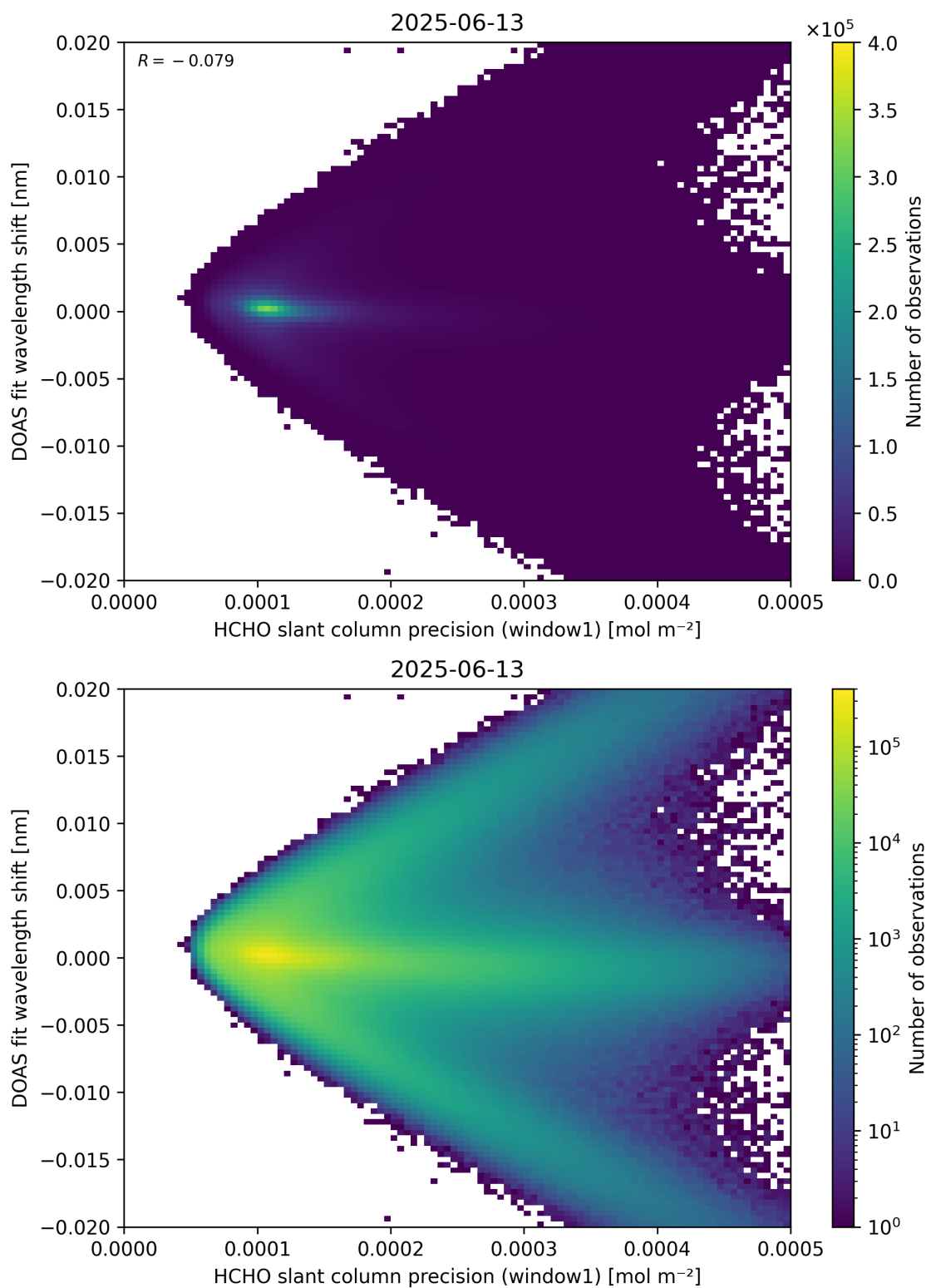
Figure 89: Scatter density plot of “HCHO slant column precision (window1)” against “DOAS fit wavelength shift” for 2025-06-12 to 2025-06-14.
