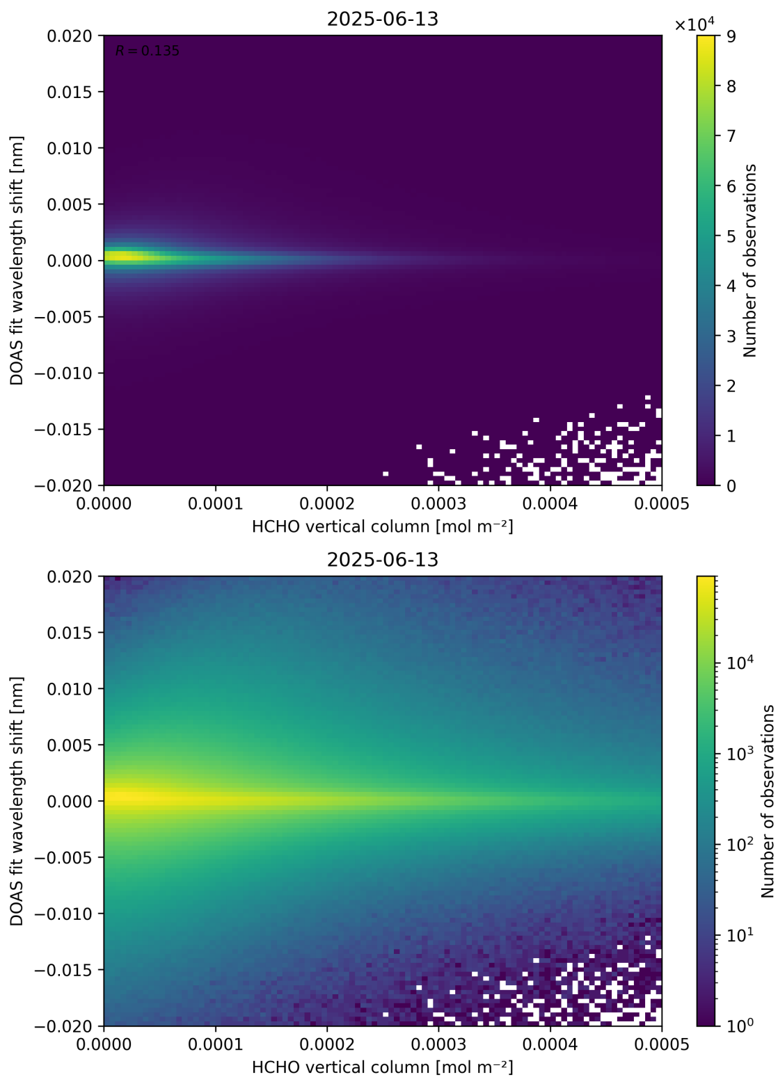
Figure 124: Scatter density plot of “HCHO vertical column” against “DOAS fit wavelength shift” for 2025-06-12 to 2025-06-14.
