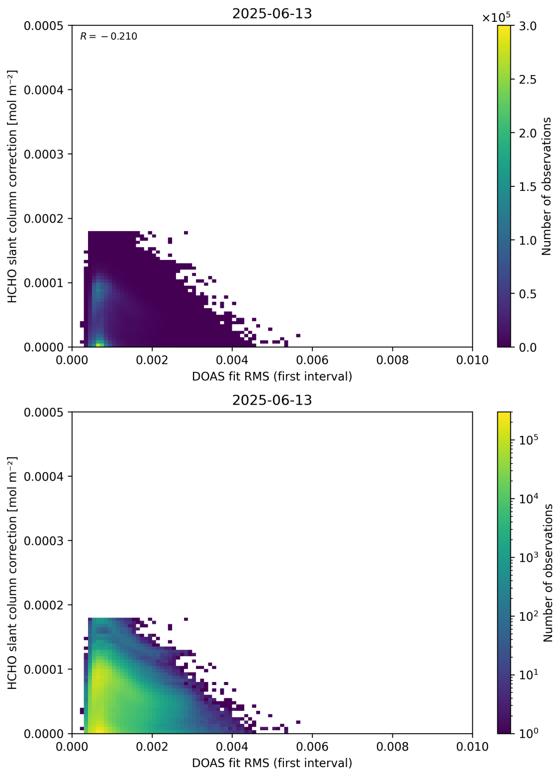
Figure 63: Scatter density plot of “DOAS fit RMS (first interval)” against “HCHO slant column correction” for 2025-06-12 to 2025-06-14.
