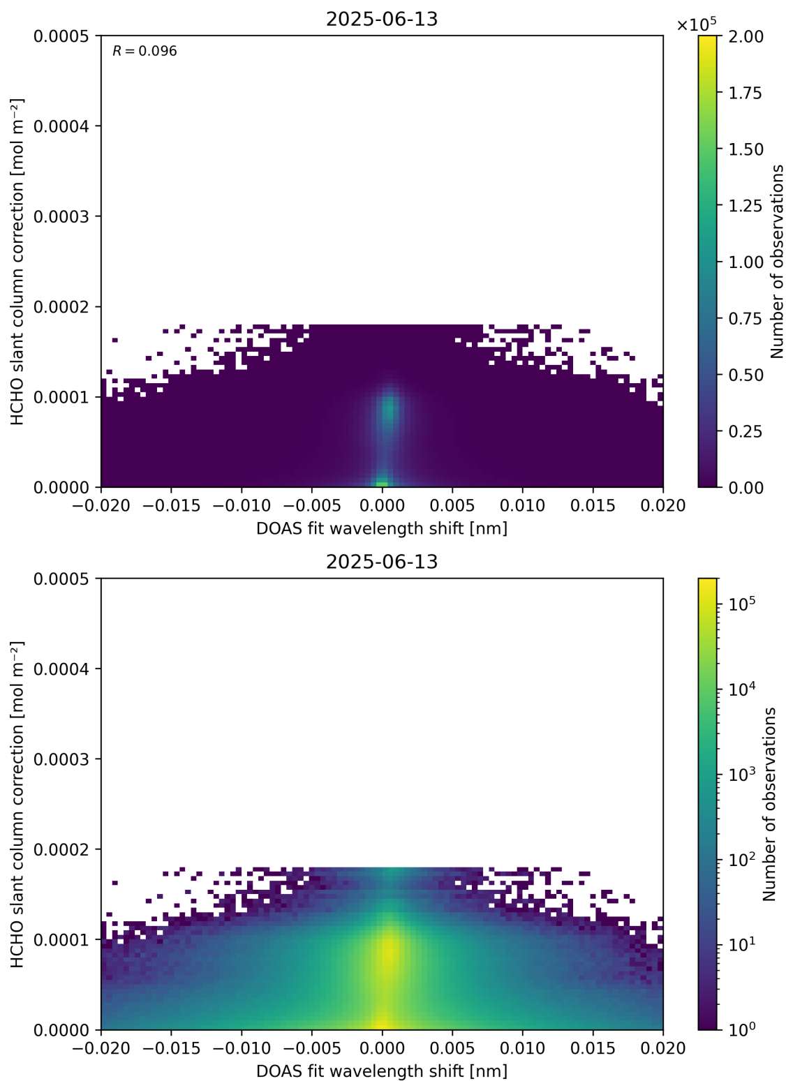
Figure 67: Scatter density plot of “DOAS fit wavelength shift” against “HCHO slant column correction” for 2025-06-12 to 2025-06-14.
