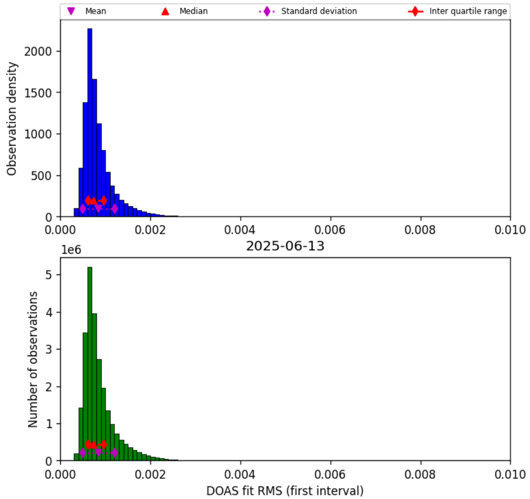
Figure 46: Histogram of “DOAS fit RMS (first interval)” for 2025-06-12 to 2025-06-14
