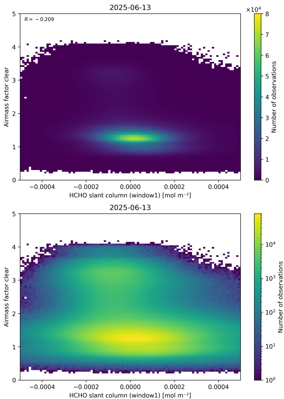
Figure 81: Scatter density plot of “HCHO slant column (window1)” against “Airmass factor clear” for 2025-06-12 to 2025-06-14.
