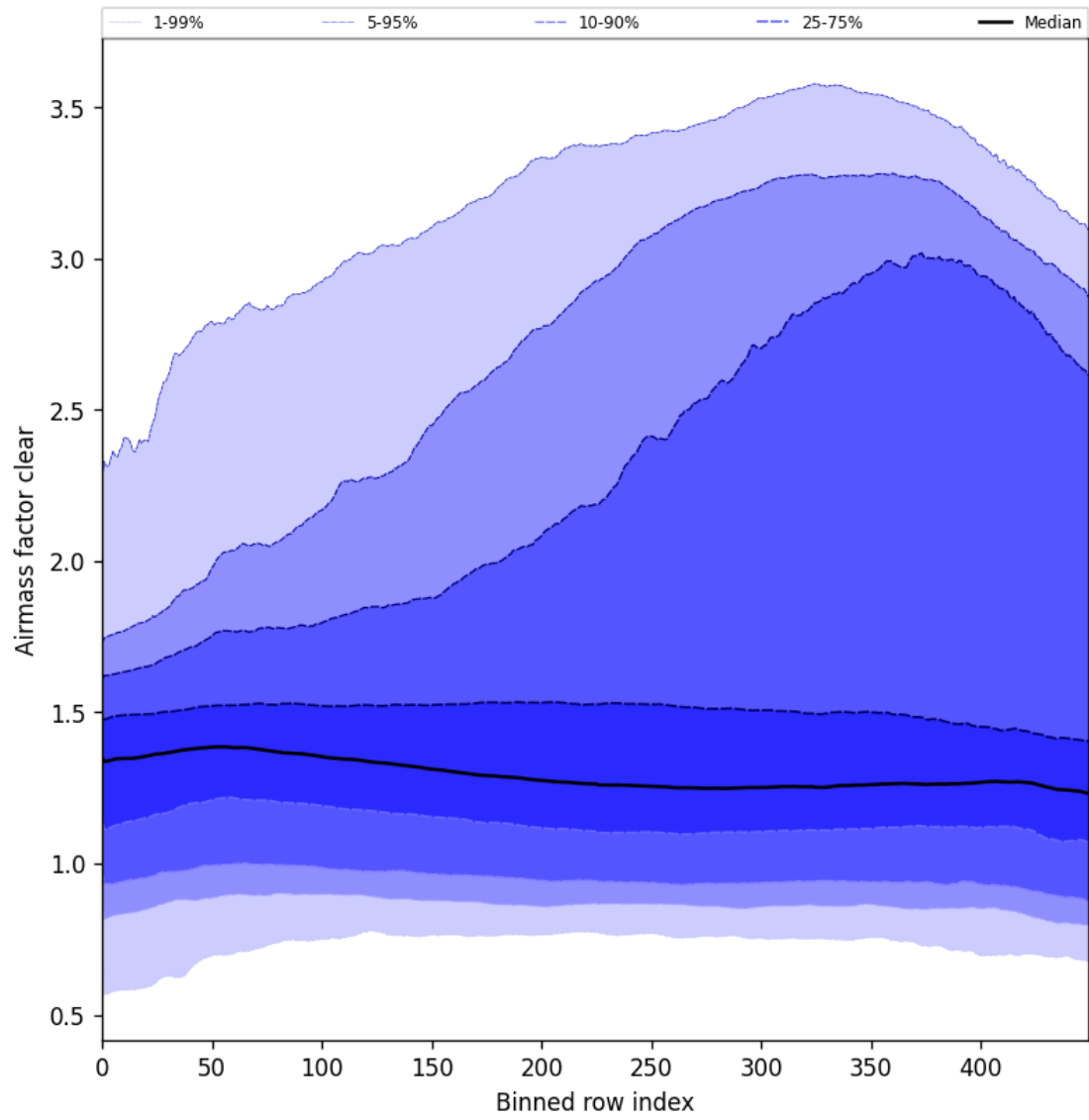
Figure 56: Along track statistics of “Air mass factor clear” for 2025-06-12 to 2025-06-14
