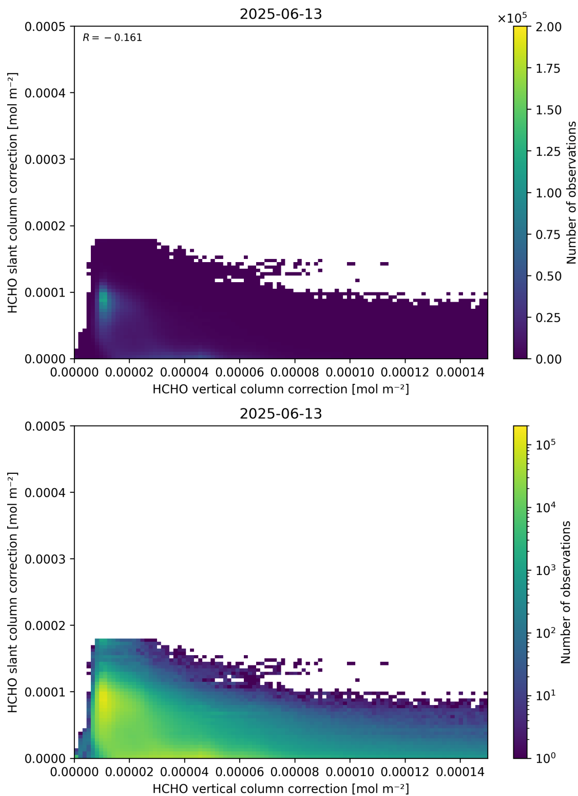
Figure 117: Scatter density plot of “HCHO vertical column correction” against “HCHO slant column correction” for 2025-06-12 to 2025-06-14.
