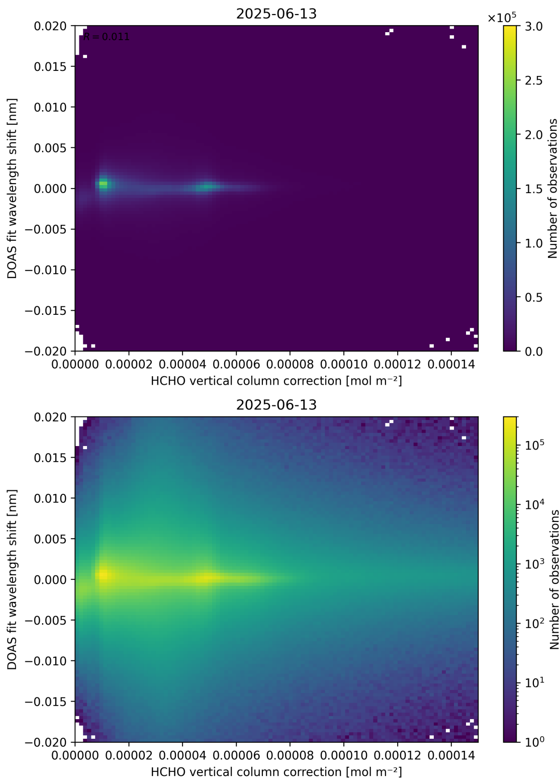
Figure 113: Scatter density plot of “HCHO vertical column correction” against “DOAS fit wavelength shift” for 2025-06-12 to 2025-06-14.
