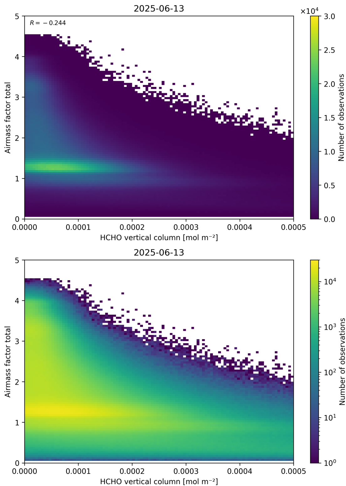
Figure 131: Scatter density plot of “HCHO vertical column” against “Airmass factor total” for 2025-06-12 to 2025-06-14.
