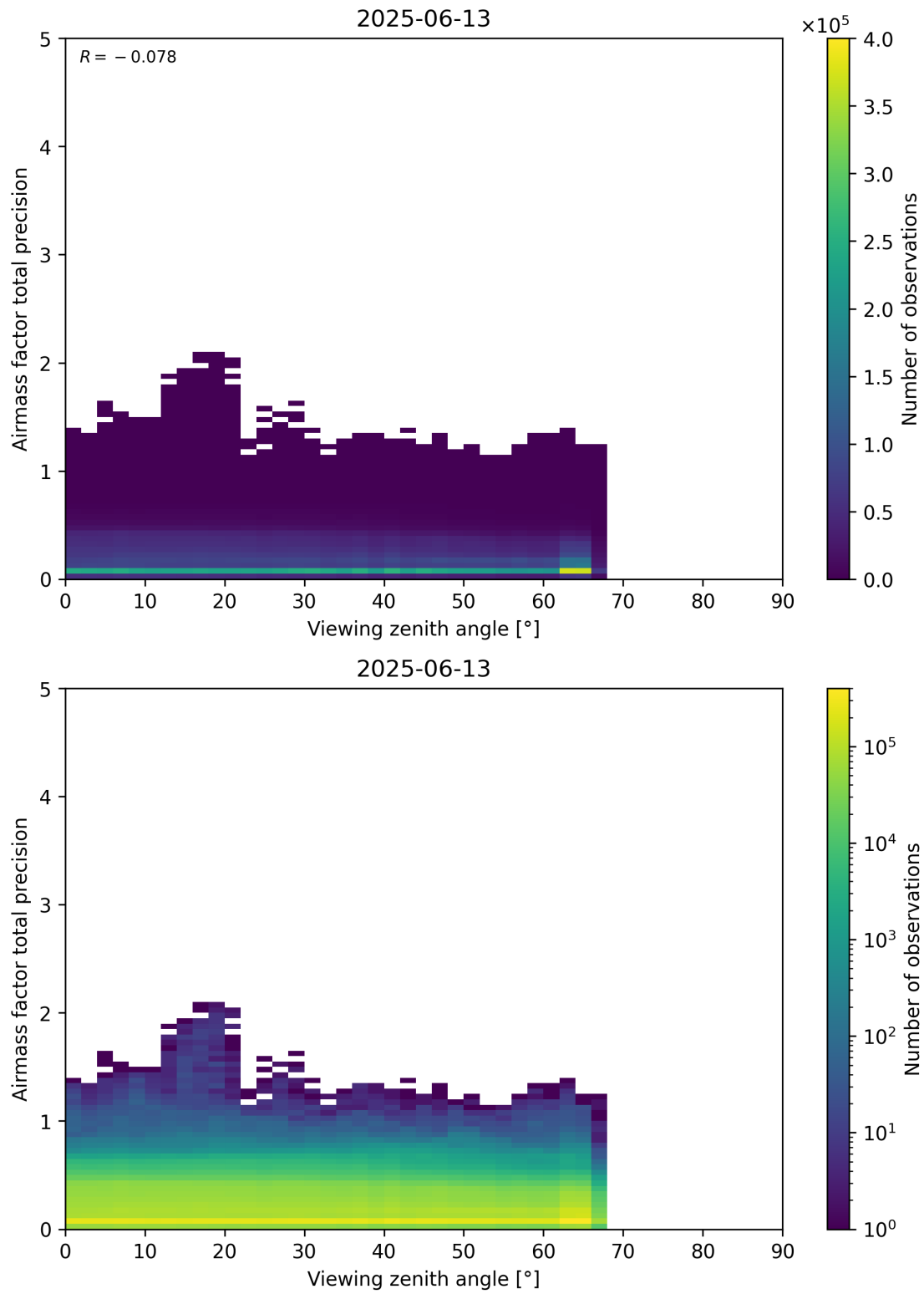
Figure 191: Scatter density plot of “Viewing zenith angle” against “Airmass factor total precision” for 2025-06-12 to 2025-06-14.
