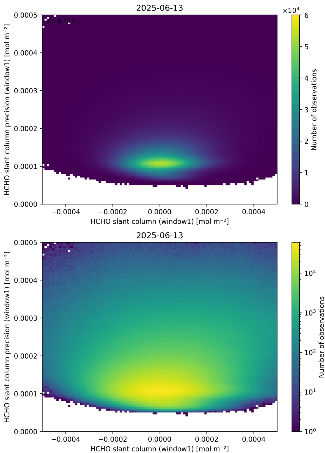
Figure 84: Scatter density plot of “HCHO slant column (window1)” against “HCHO slant column precision (window1)” for 2025-06-12 to 2025-06-14.
