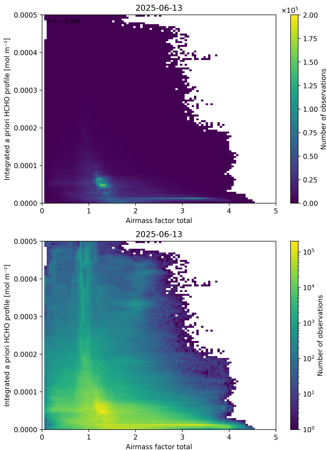
Figure 104: Scatter density plot of “Airmass factor total” against “Integrated a priori HCHO profile” for 2025-06-12 to 2025-06-14.
