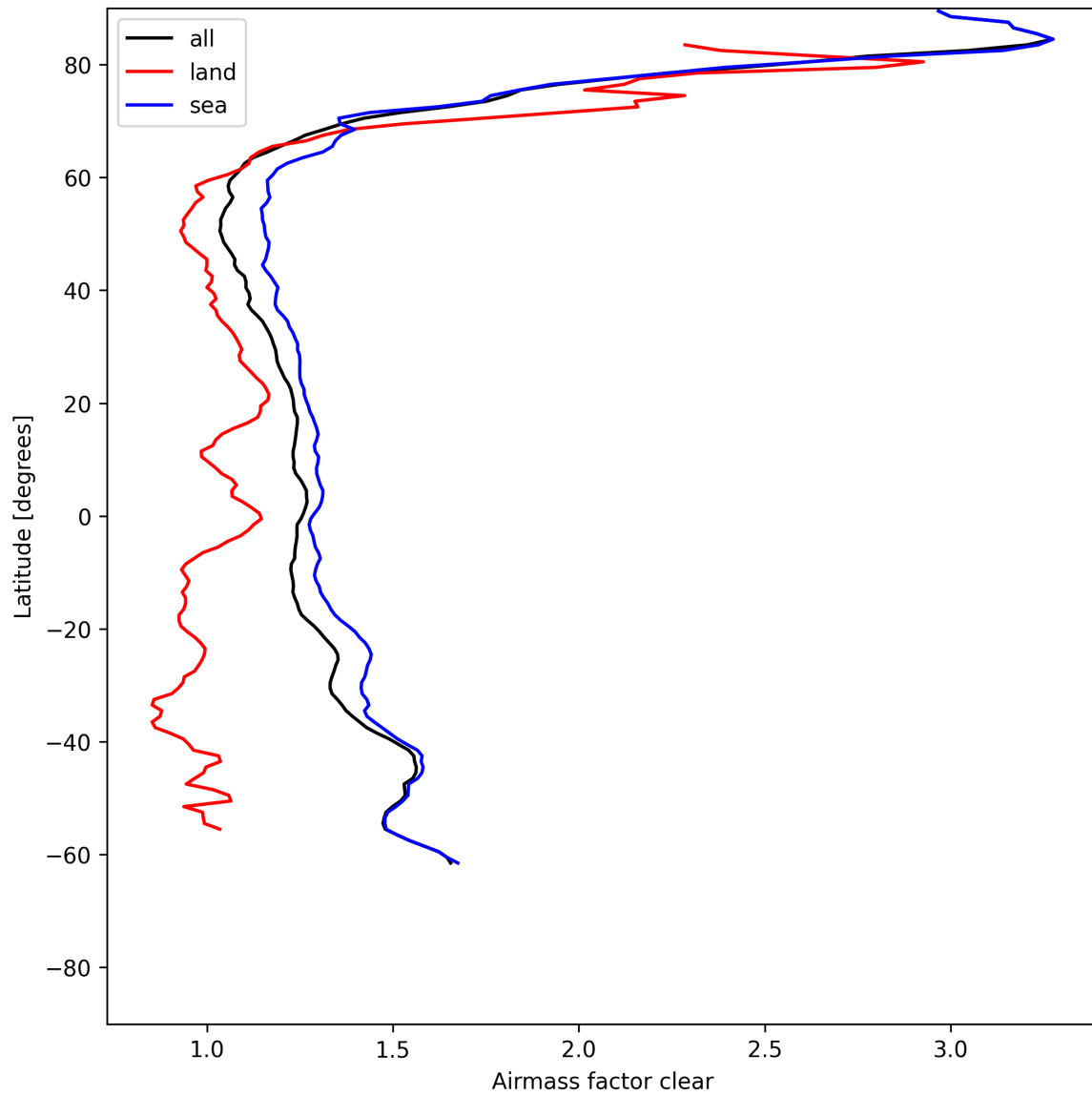
Figure 28: Zonal average of “Airmass factor clear” for 2025-06-12 to 2025-06-14.
