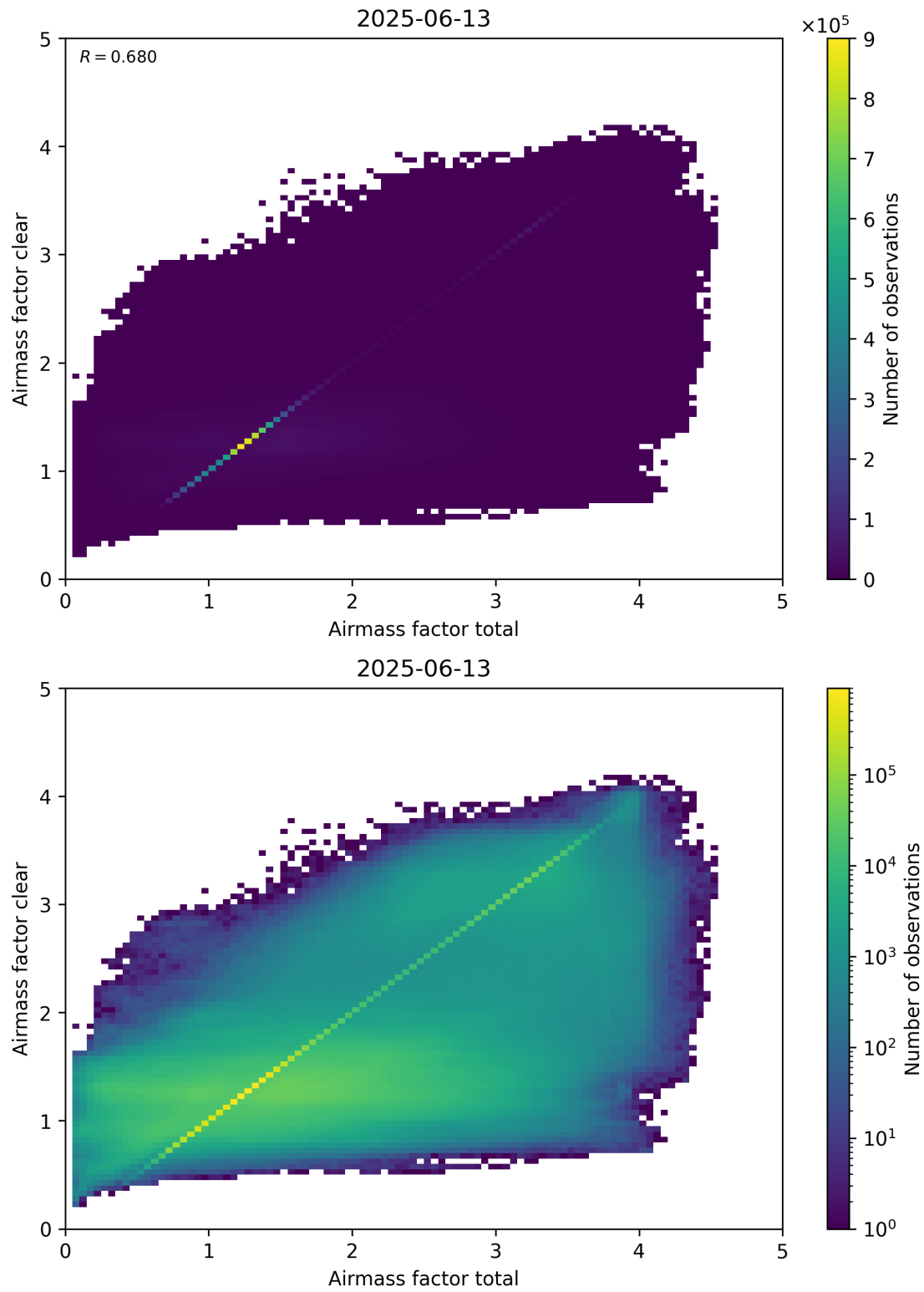
Figure 100: Scatter density plot of “Airmass factor total” against “Airmass factor clear” for 2025-06-12 to 2025-06-14.
