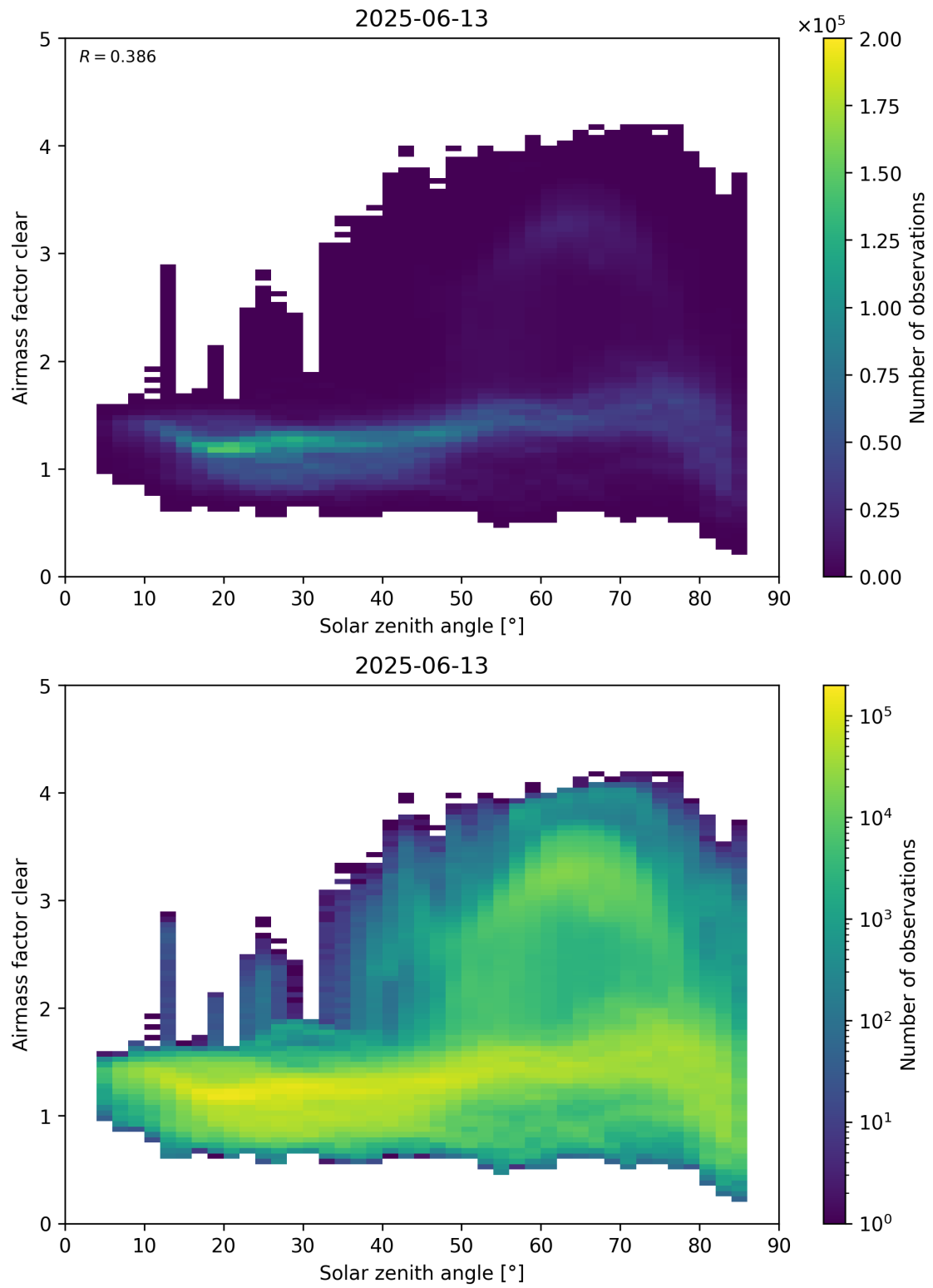
Figure 170: Scatter density plot of “Solar zenith angle” against “Airmass factor clear” for 2025-06-12 to 2025-06-14.
