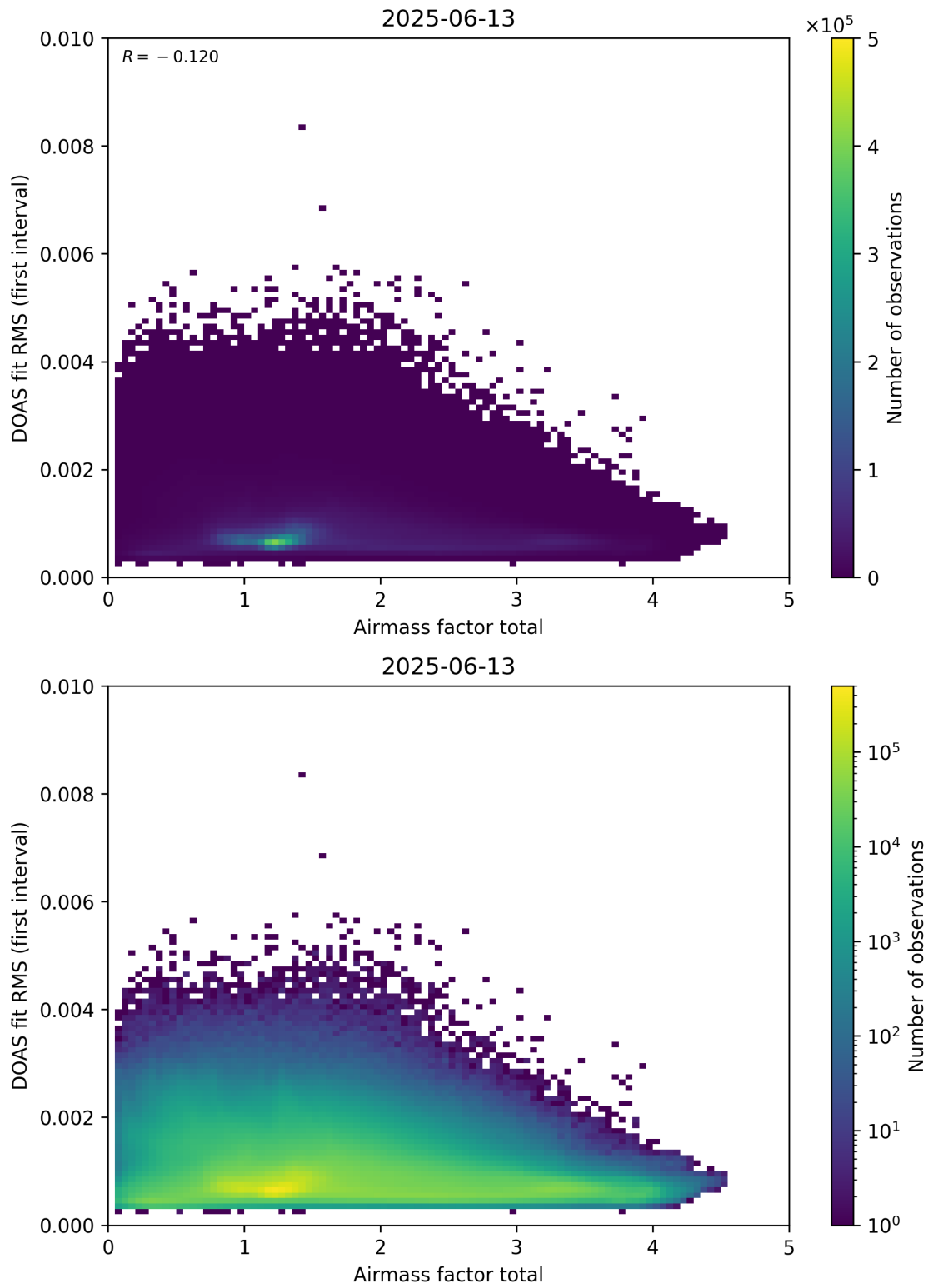
Figure 97: Scatter density plot of “Airmass factor total” against “DOAS fit RMS (first interval)” for 2025-06-12 to 2025-06-14.
