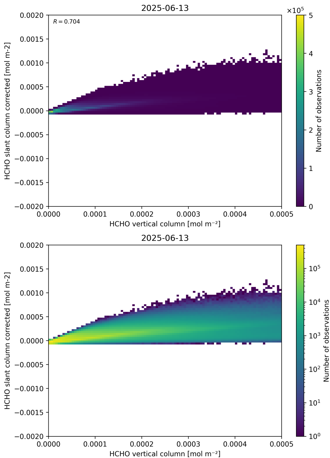
Figure 127: Scatter density plot of “HCHO vertical column” against “HCHO slant column corrected” for 2025-06-12 to 2025-06-14.
