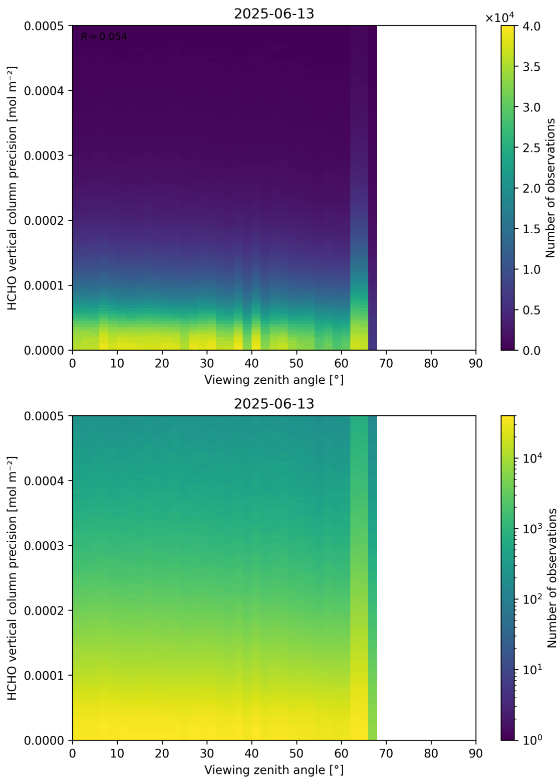
Figure 194: Scatter density plot of “Viewing zenith angle” against “HCHO vertical column precision” for 2025-06-12 to 2025-06-14.
