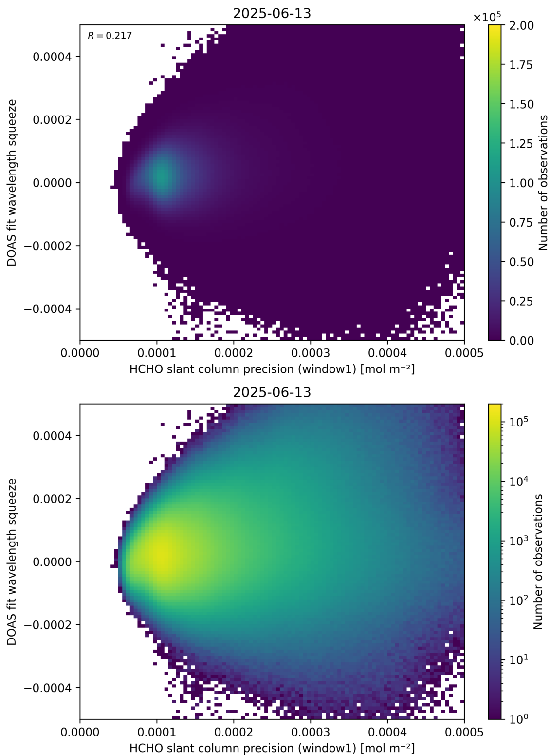
Figure 90: Scatter density plot of “HCHO slant column precision (window1)” against “DOAS fit wavelength squeeze” for 2025-06-12 to 2025-06-14.
