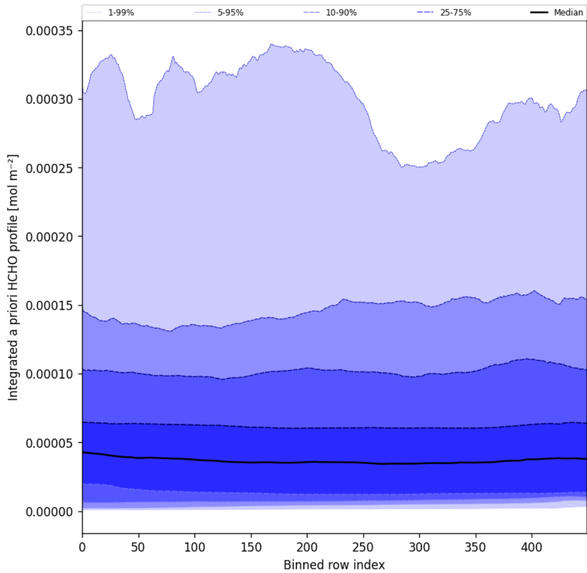
Figure 57: Along track statistics of “Integrated a priori HCHO profile” for 2025-06-12 to 2025-06-14
