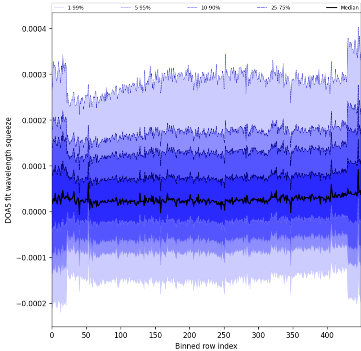
Figure 59: Along track statistics of “DOAS fit wavelength squeeze” for 2025-06-12 to 2025-06-14
