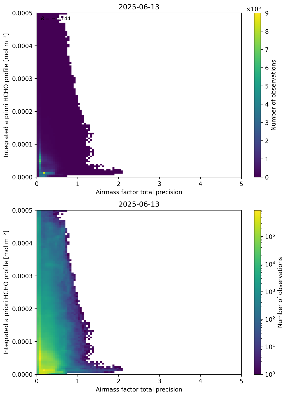
Figure 111: Scatter density plot of “Airmass factor total precision” against “Integrated a priori HCHO profile” for 2025-06-12 to 2025-06-14.
