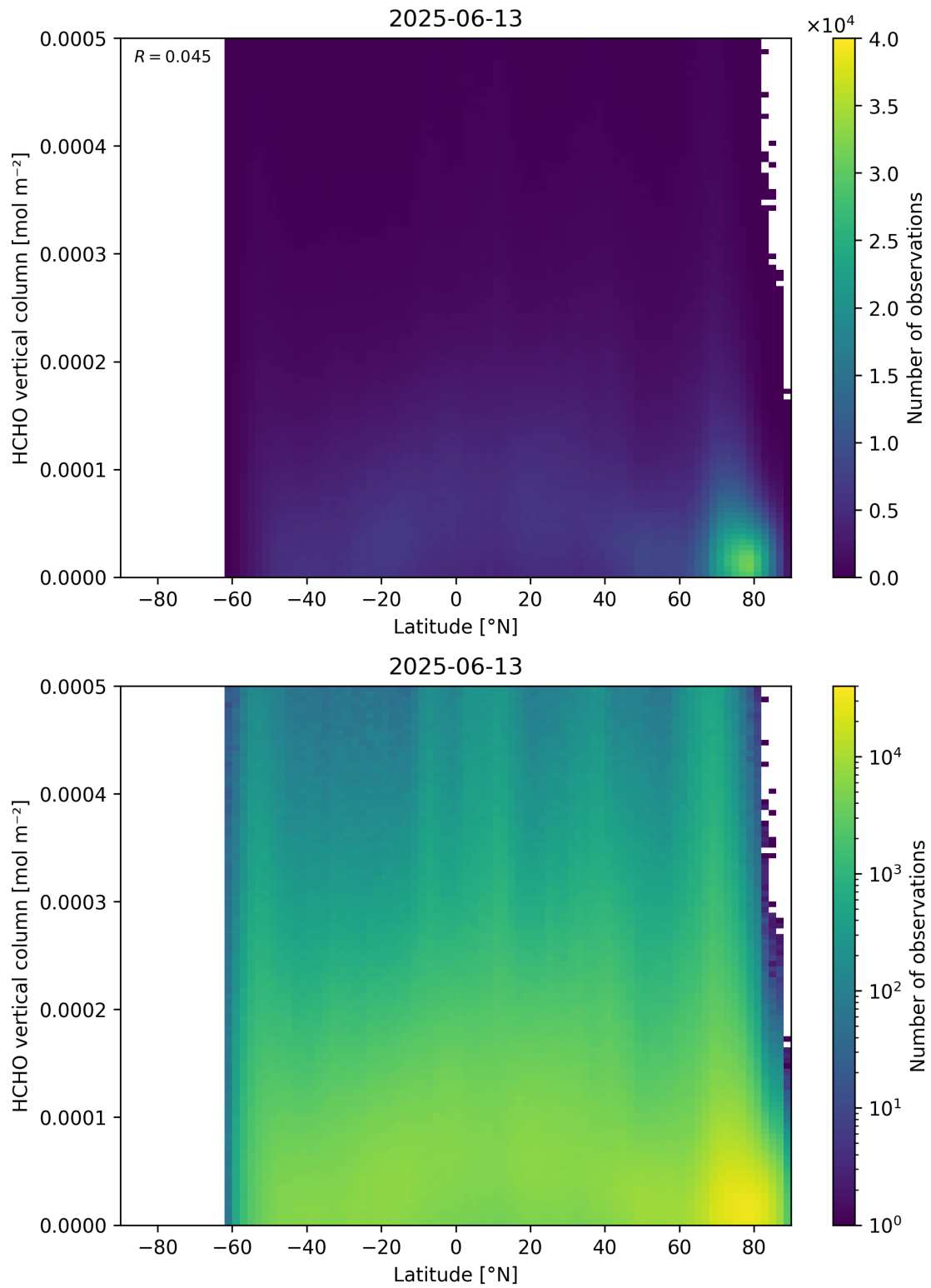
Figure 163: Scatter density plot of “Latitude” against “HCHO vertical column” for 2025-06-12 to 2025-06-14.
