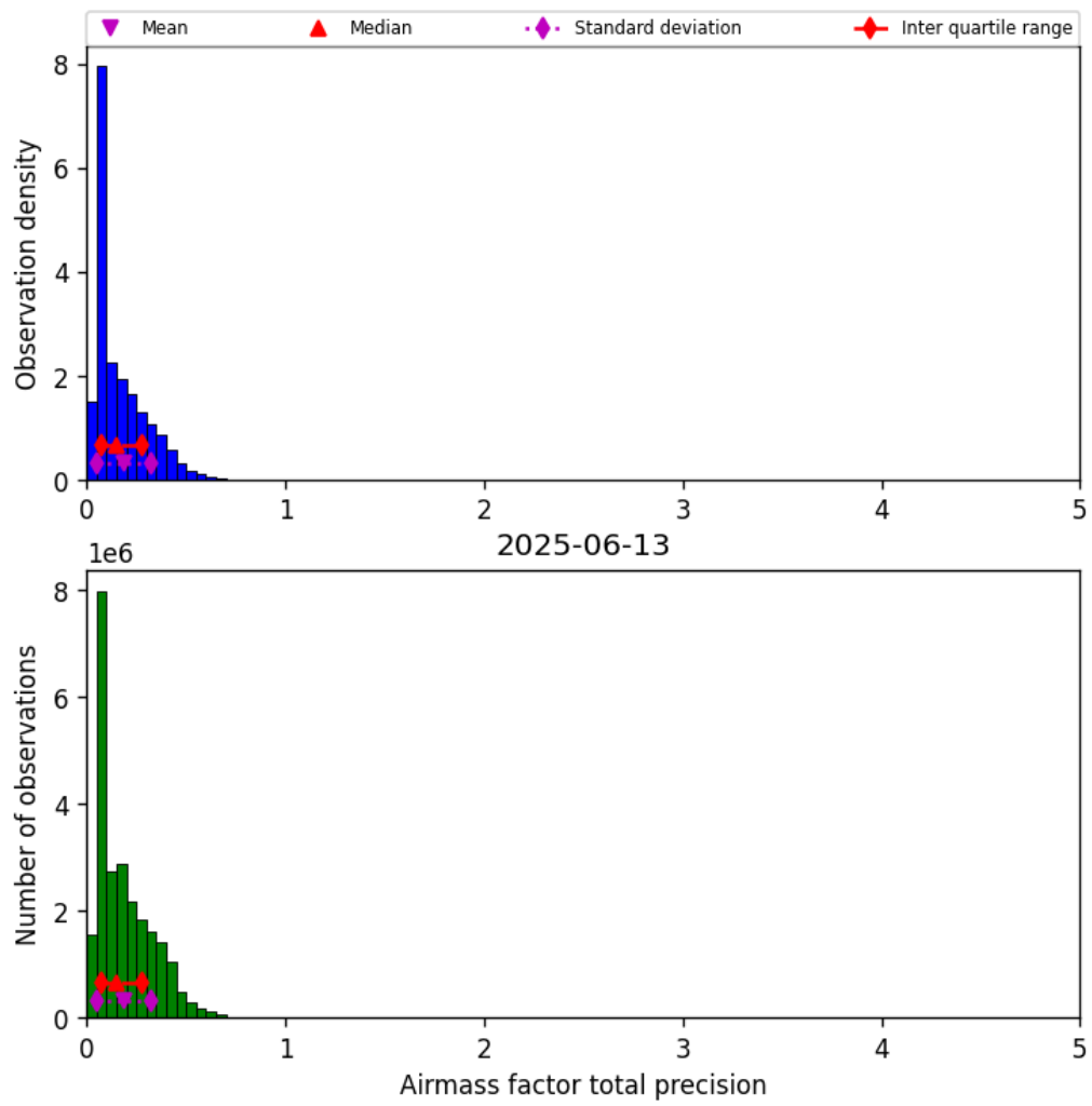
Figure 41: Histogram of “Airmass factor total precision” for 2025-06-12 to 2025-06-14
