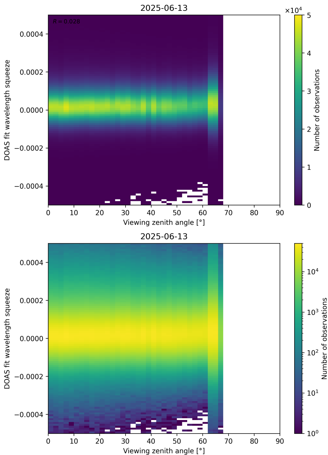
Figure 184: Scatter density plot of “Viewing zenith angle” against “DOAS fit wavelength squeeze” for 2025-06-12 to 2025-06-14.
