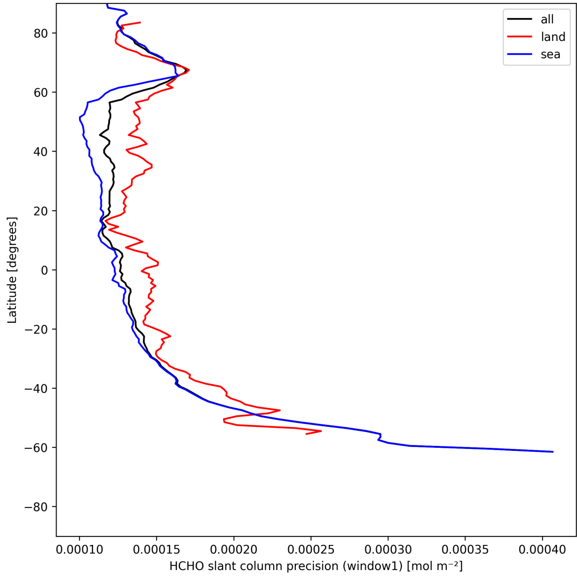
Figure 25: Zonal average of “HCHO slant column precision (window1)” for 2025-06-12 to 2025-06-14.
