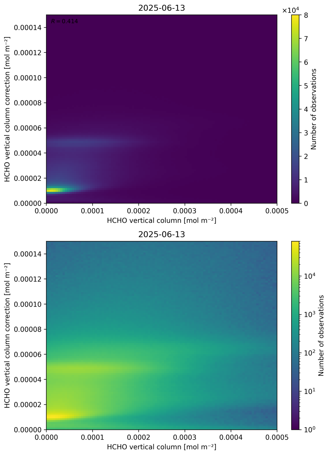
Figure 133: Scatter density plot of “HCHO vertical column” against “HCHO vertical column correction” for 2025-06-12 to 2025-06-14.
