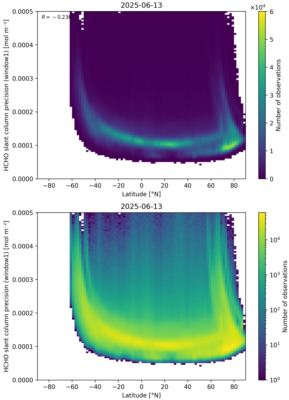
Figure 160: Scatter density plot of “Latitude” against “HCHO slant column precision (window1)” for 2025-06-12 to 2025-06-14.
