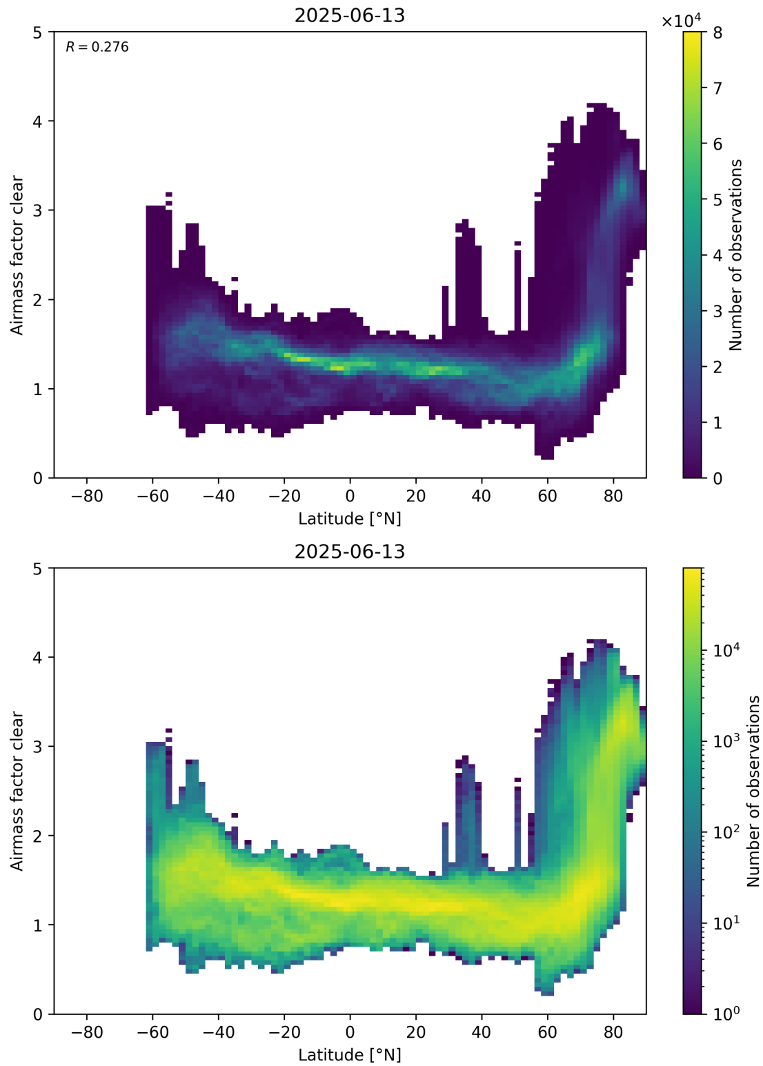
Figure 156: Scatter density plot of “Latitude” against “Airmass factor clear” for 2025-06-12 to 2025-06-14.
