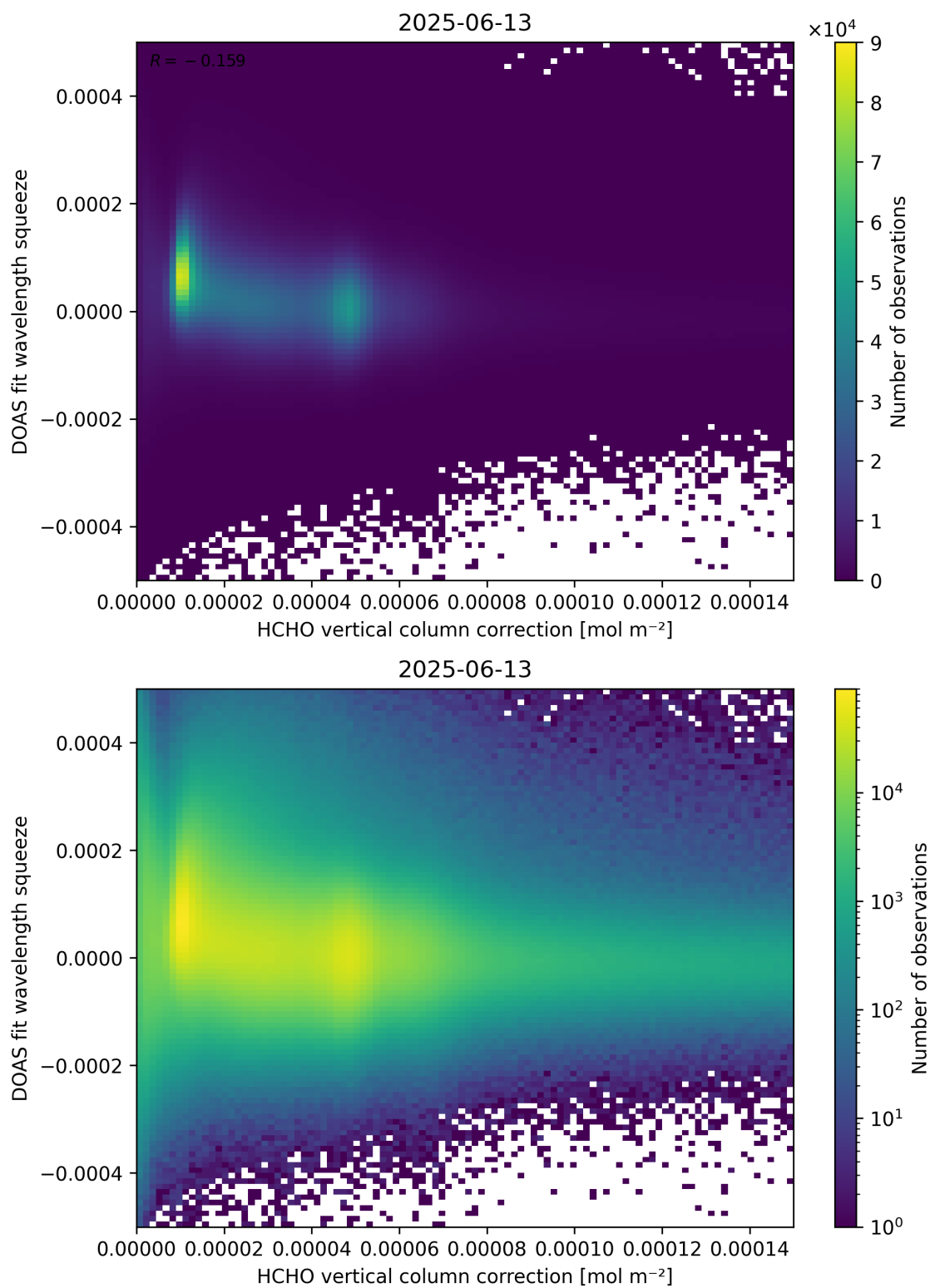
Figure 114: Scatter density plot of “HCHO vertical column correction” against “DOAS fit wavelength squeeze” for 2025-06-12 to 2025-06-14.
