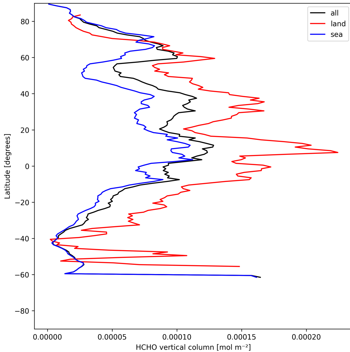
Figure 21: Zonal average of “HCHO vertical column” for 2025-06-12 to 2025-06-14.
