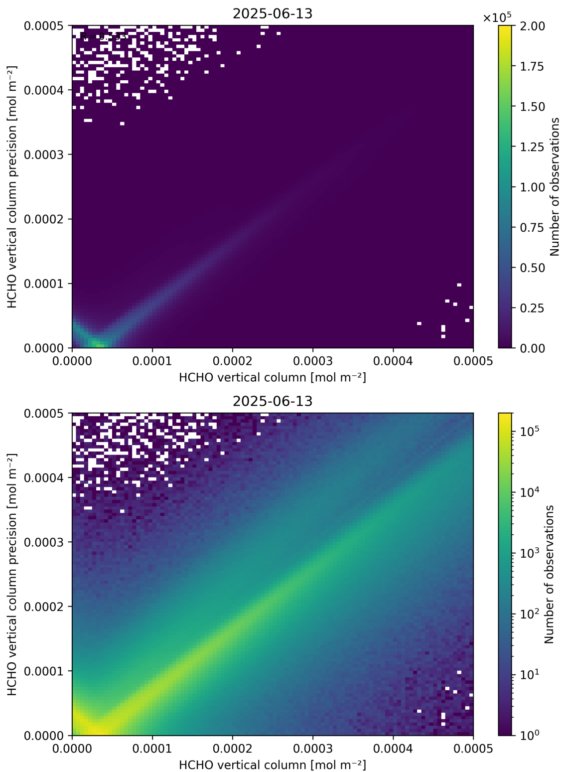
Figure 134: Scatter density plot of “HCHO vertical column” against “HCHO vertical column precision” for 2025-06-12 to 2025-06-14.
