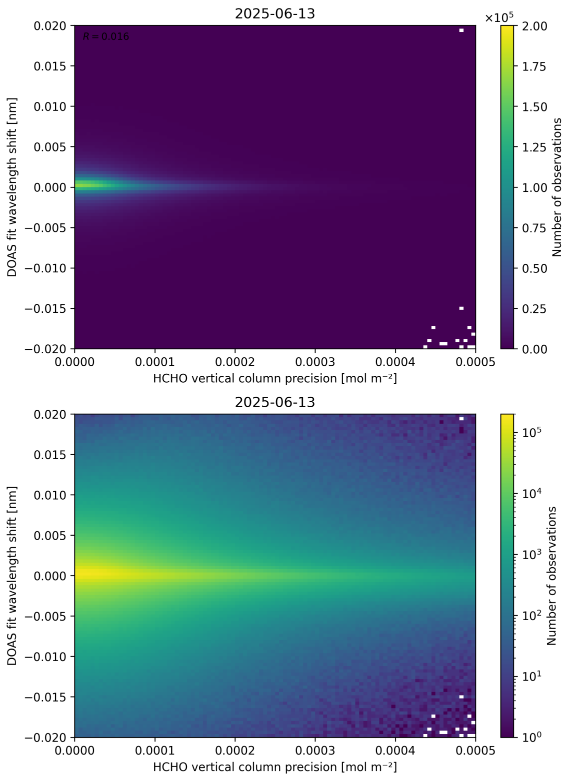
Figure 137: Scatter density plot of “HCHO vertical column precision” against “DOAS fit wavelength shift” for 2025-06-12 to 2025-06-14.
