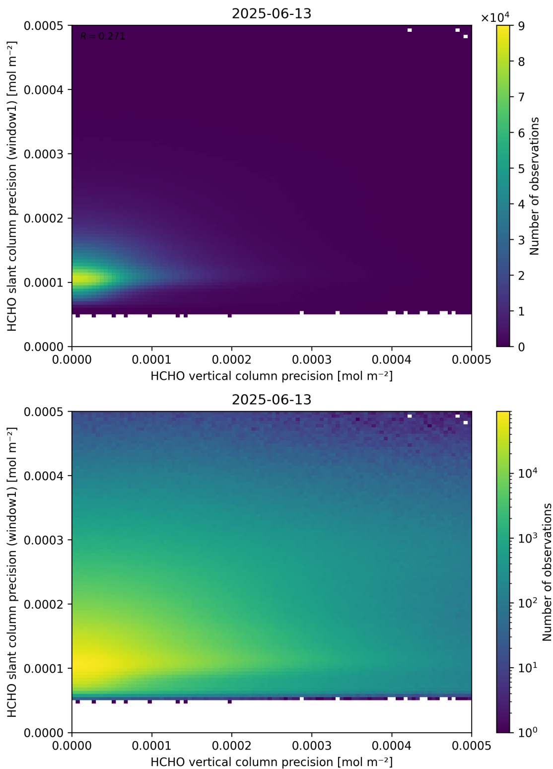
Figure 143: Scatter density plot of “HCHO vertical column precision” against “HCHO slant column precision (window1)” for 2025-06-12 to 2025-06-14.
