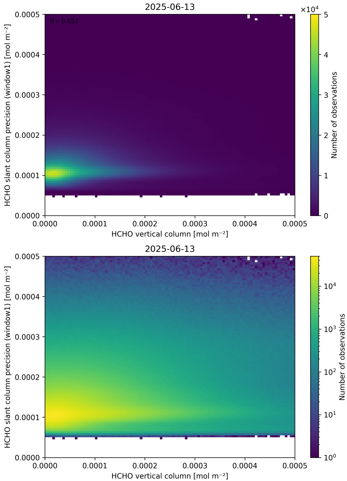
Figure 130: Scatter density plot of “HCHO vertical column” against “HCHO slant column precision (window1)” for 2025-06-12 to 2025-06-14.
