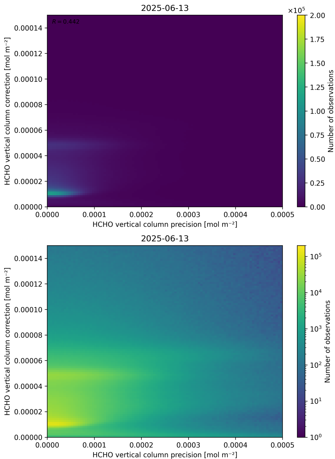
Figure 146: Scatter density plot of “HCHO vertical column precision” against “HCHO vertical column correction” for 2025-06-12 to 2025-06-14.
