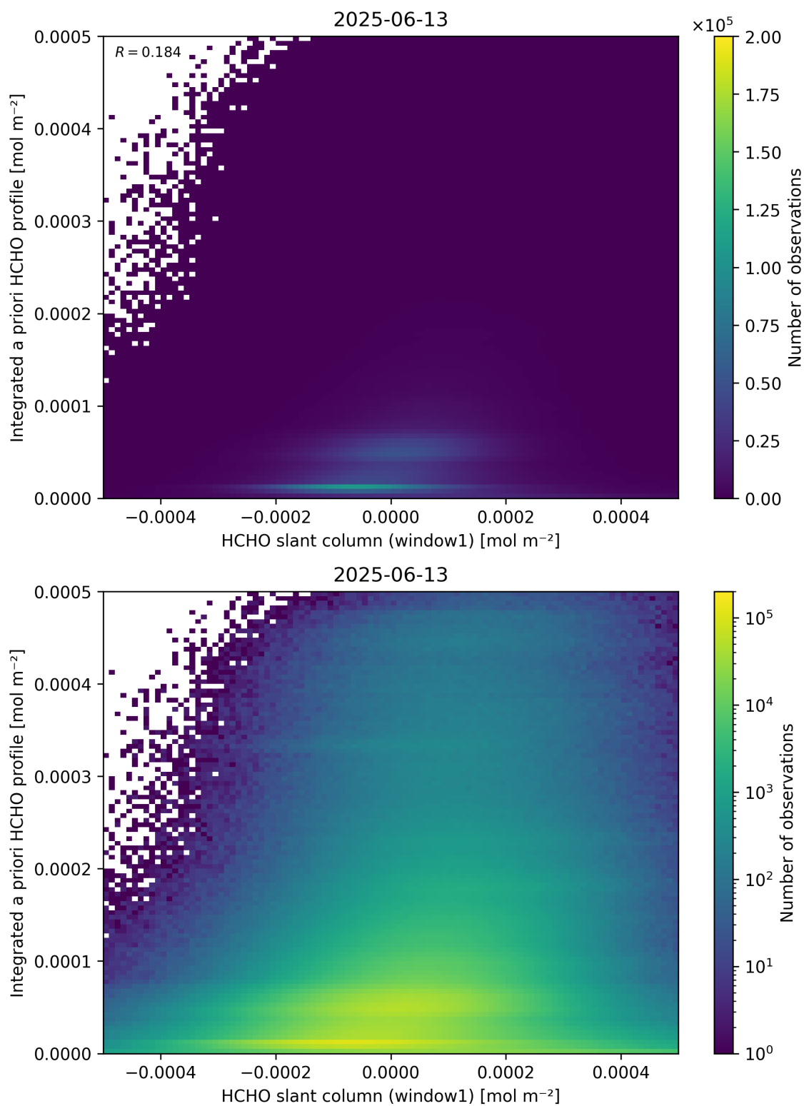
Figure 87: Scatter density plot of “HCHO slant column (window1)” against “Integrated a priori HCHO profile” for 2025-06-12 to 2025-06-14.
