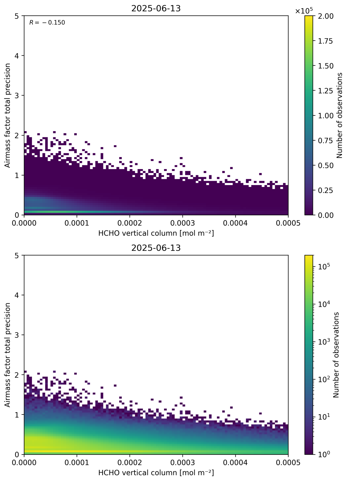
Figure 132: Scatter density plot of “HCHO vertical column” against “Airmass factor total precision” for 2025-06-12 to 2025-06-14.
