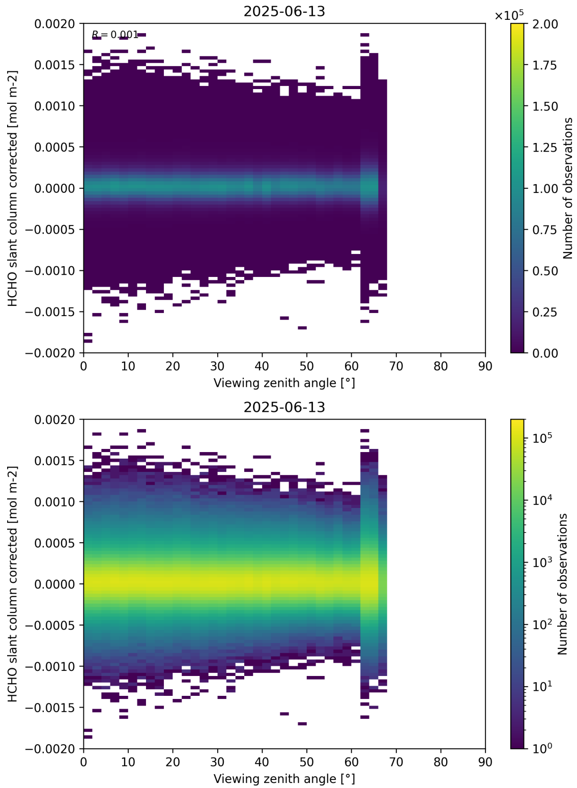
Figure 186: Scatter density plot of “Viewing zenith angle” against “HCHO slant column corrected” for 2025-06-12 to 2025-06-14.
