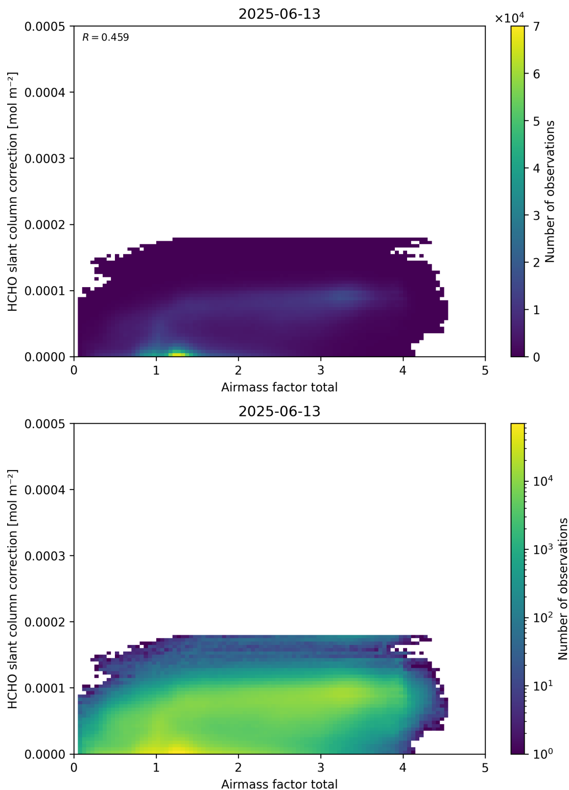
Figure 102: Scatter density plot of “Airmass factor total” against “HCHO slant column correction” for 2025-06-12 to 2025-06-14.
