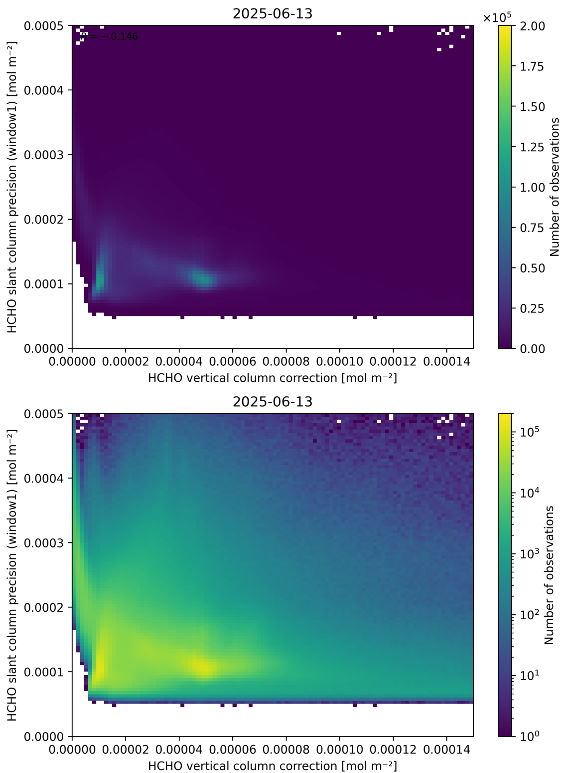
Figure 119: Scatter density plot of “HCHO vertical column correction” against “HCHO slant column precision (window1)” for 2025-06-12 to 2025-06-14.
