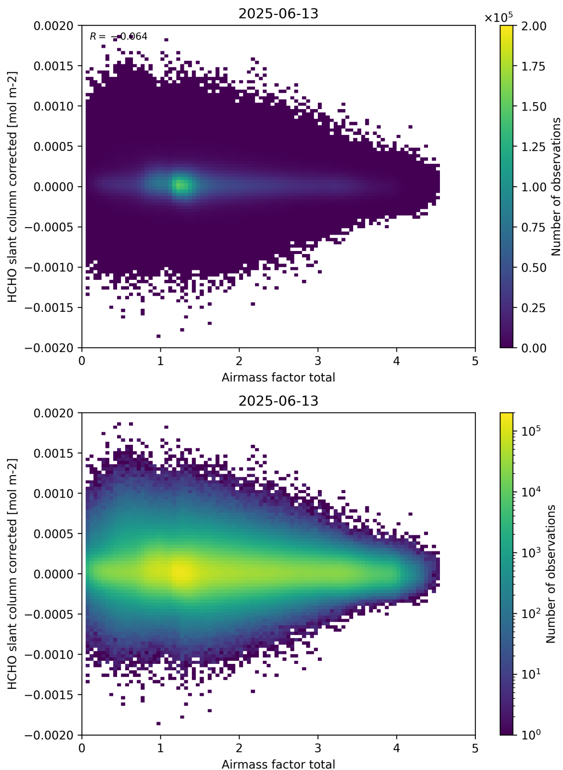
Figure 101: Scatter density plot of “Airmass factor total” against “HCHO slant column corrected” for 2025-06-12 to 2025-06-14.
