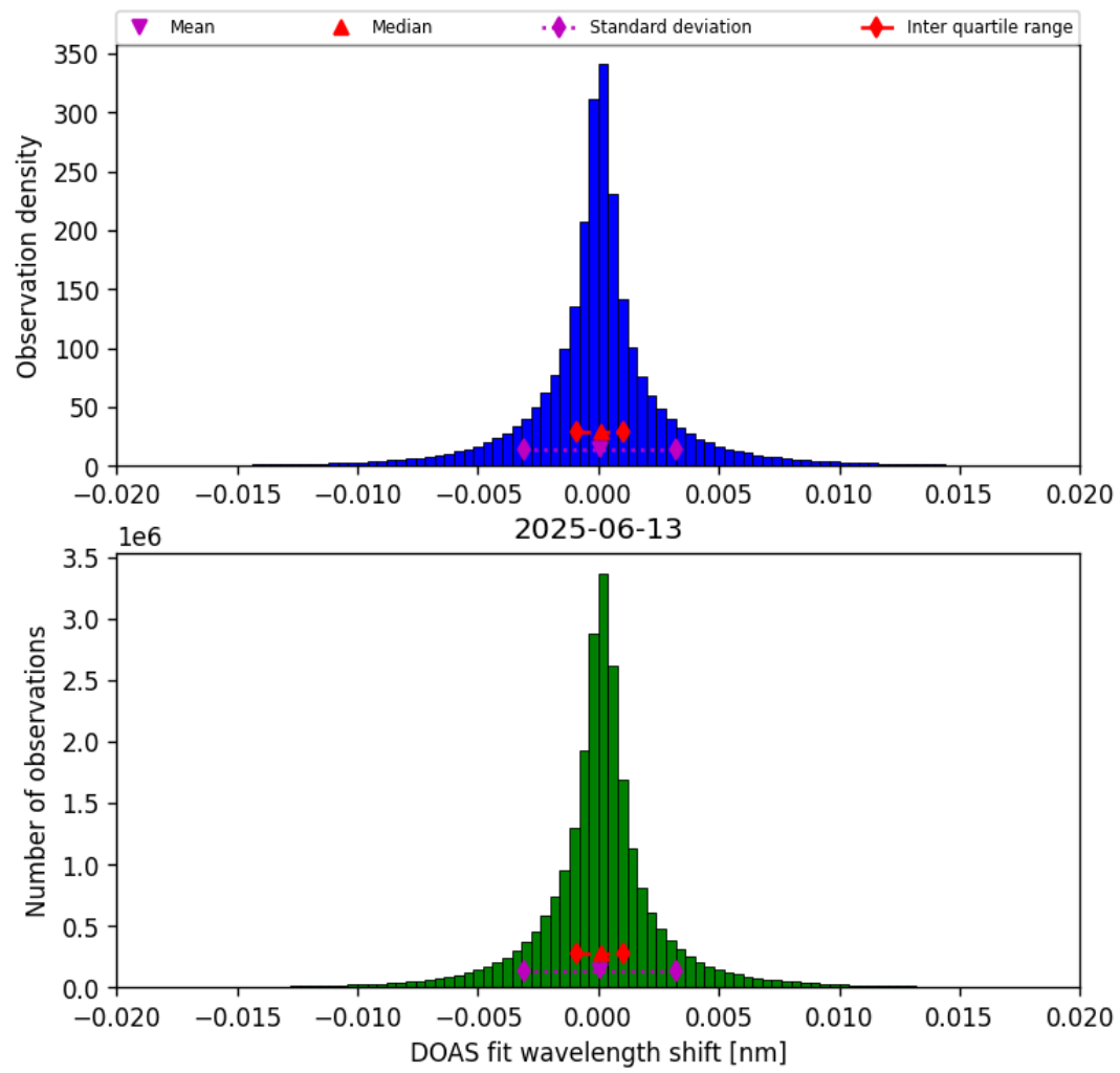
Figure 44: Histogram of “DOAS fit wavelength shift” for 2025-06-12 to 2025-06-14
