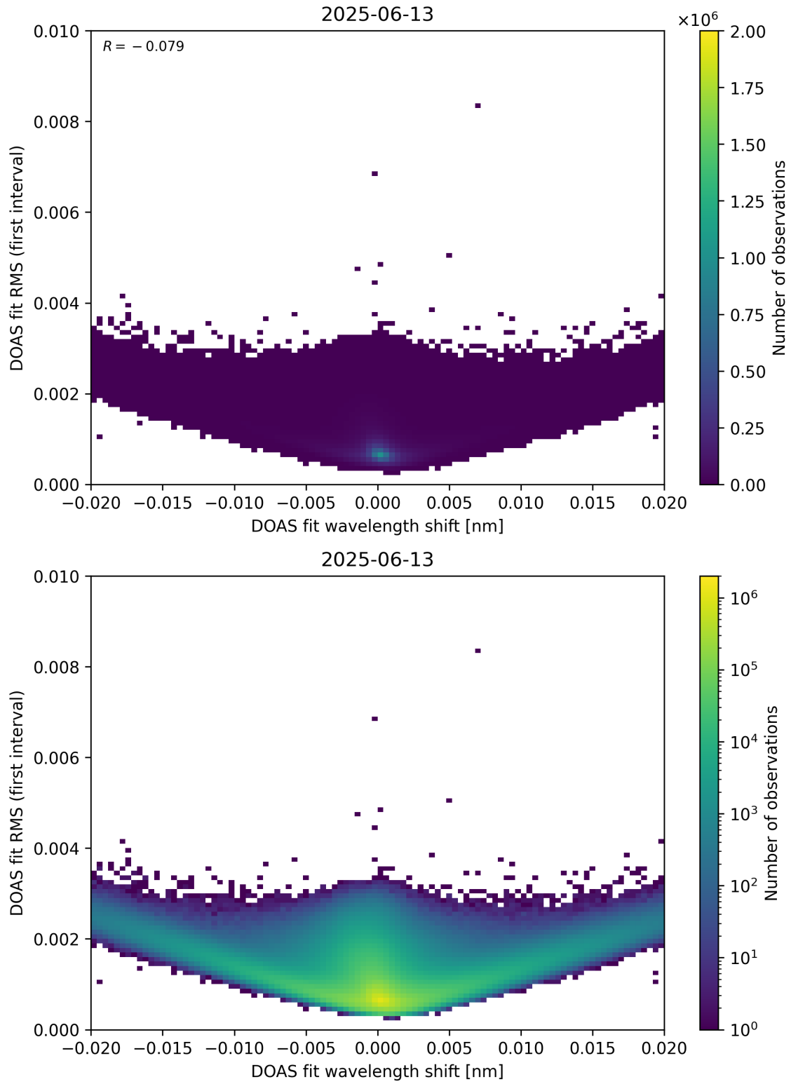
Figure 64: Scatter density plot of “DOAS fit wavelength shift” against “DOAS fit RMS (first interval)” for 2025-06-12 to 2025-06-14.
