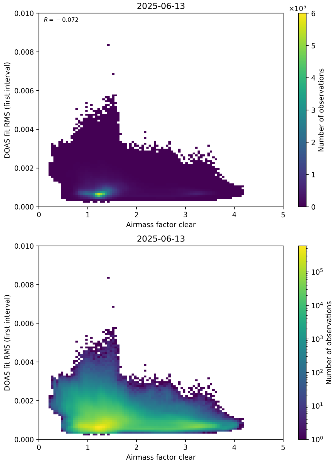
Figure 71: Scatter density plot of “Airmass factor clear” against “DOAS fit RMS (first interval)” for 2025-06-12 to 2025-06-14.
