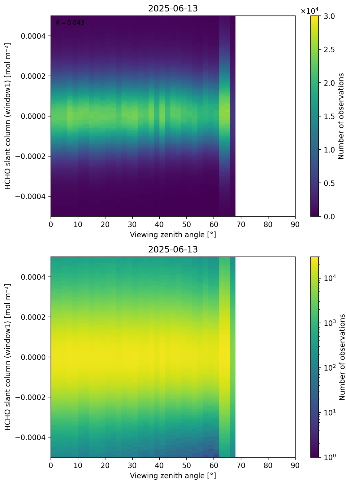
Figure 188: Scatter density plot of “Viewing zenith angle” against “HCHO slant column (window1)” for 2025-06-12 to 2025-06-14.
