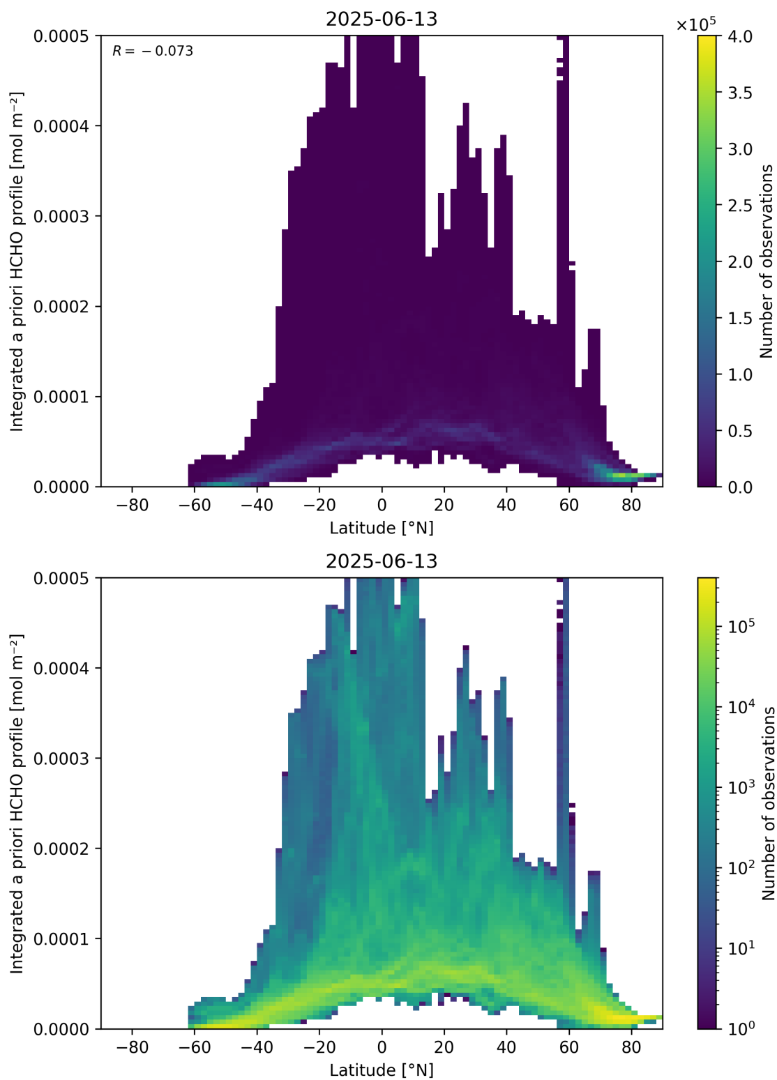
Figure 166: Scatter density plot of “Latitude” against “Integrated a priori HCHO profile” for 2025-06-12 to 2025-06-14.
