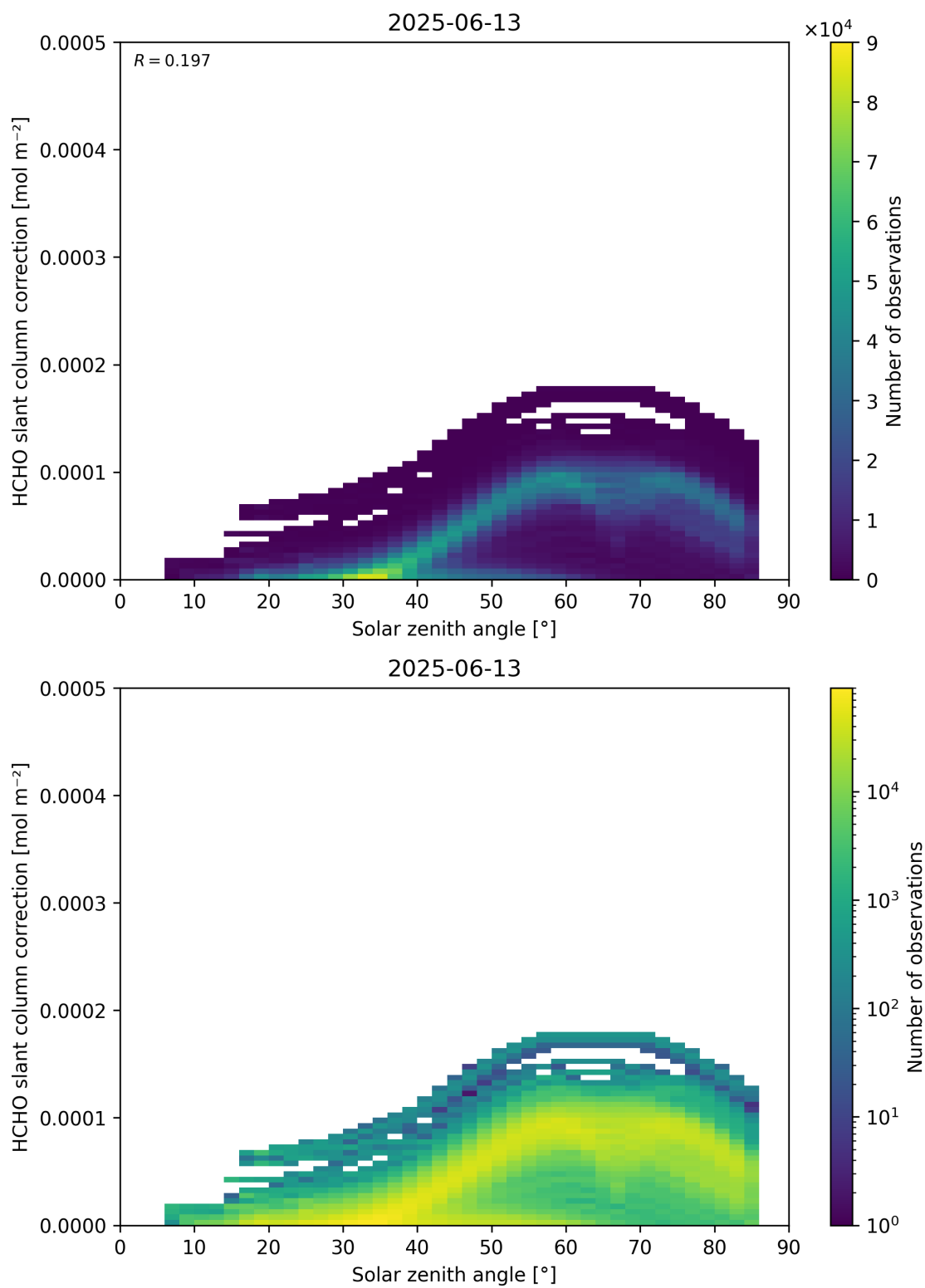
Figure 172: Scatter density plot of “Solar zenith angle” against “HCHO slant column correction” for 2025-06-12 to 2025-06-14.
