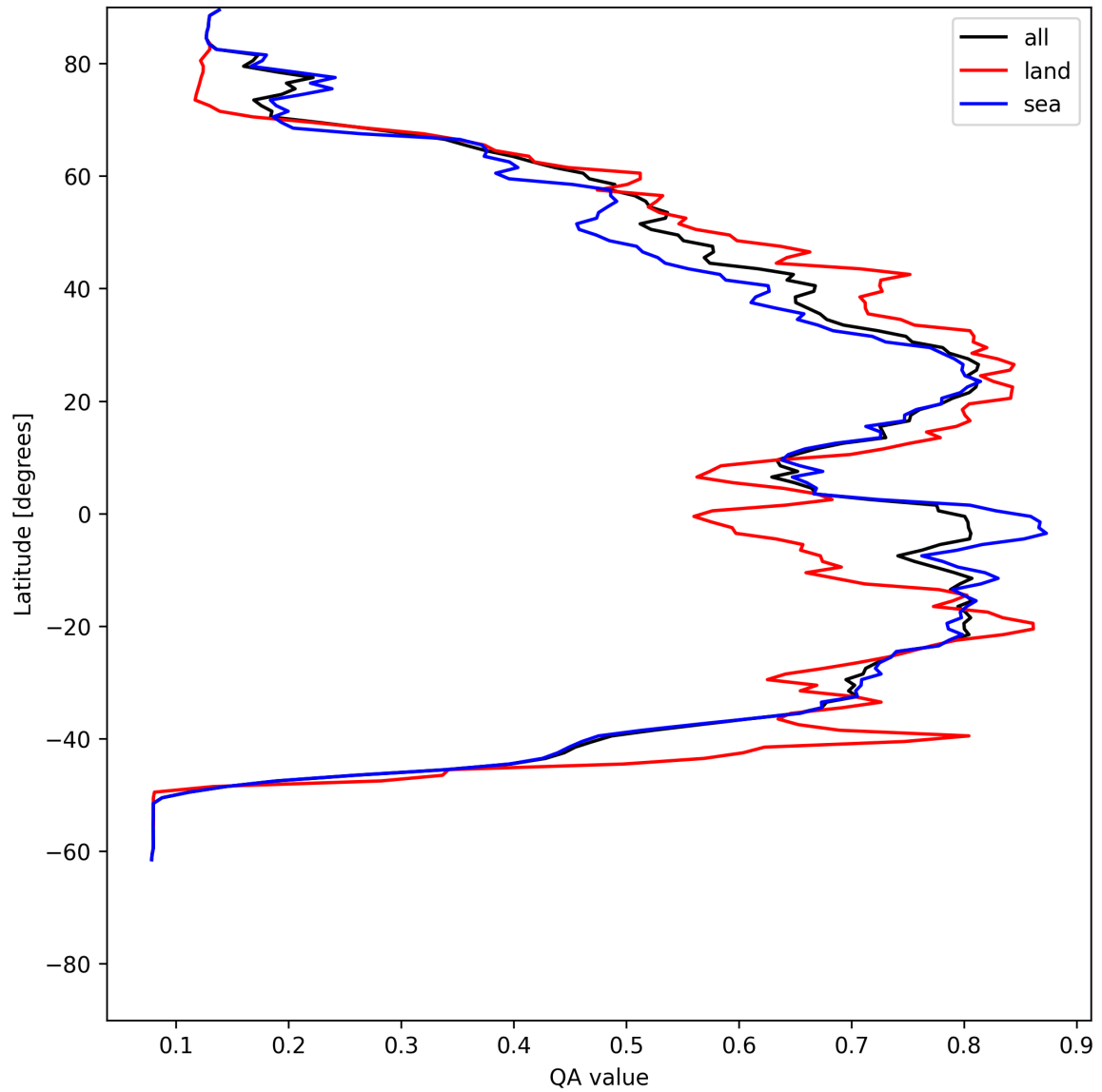
Figure 20: Zonal average of “QA value” for 2025-06-12 to 2025-06-14.
