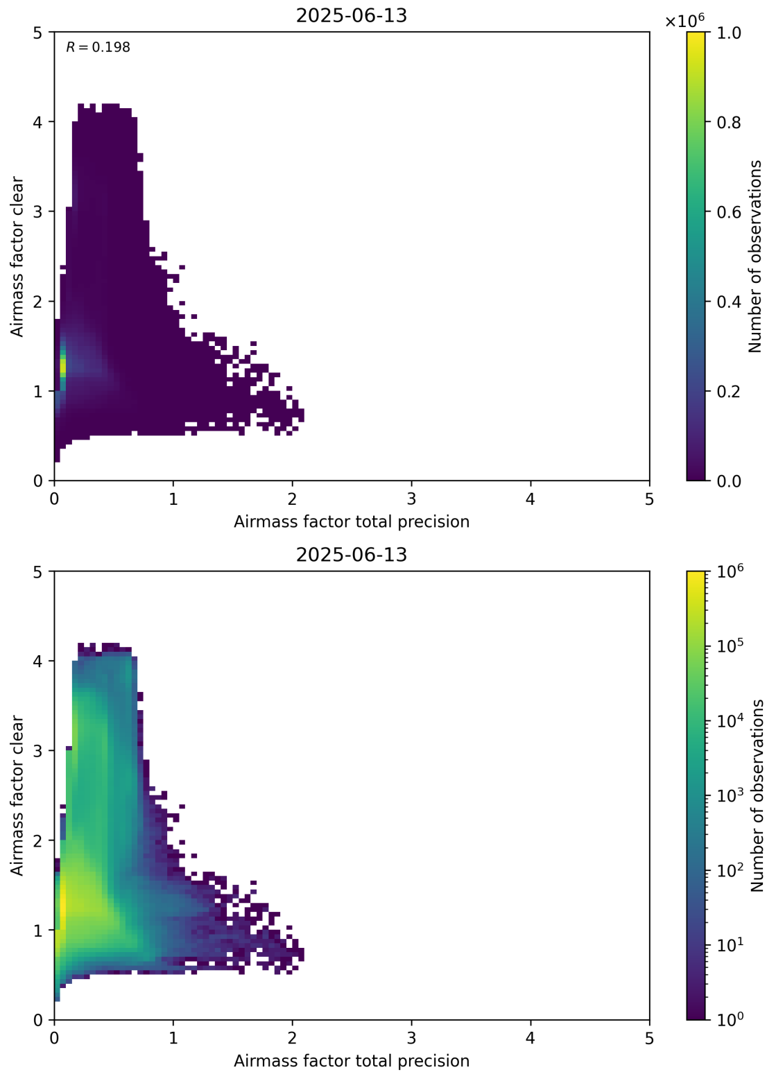
Figure 108: Scatter density plot of “Airmass factor total precision” against “Airmass factor clear” for 2025-06-12 to 2025-06-14.
