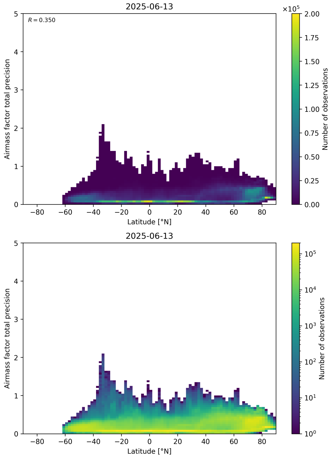
Figure 162: Scatter density plot of “Latitude” against “Airmass factor total precision” for 2025-06-12 to 2025-06-14.
