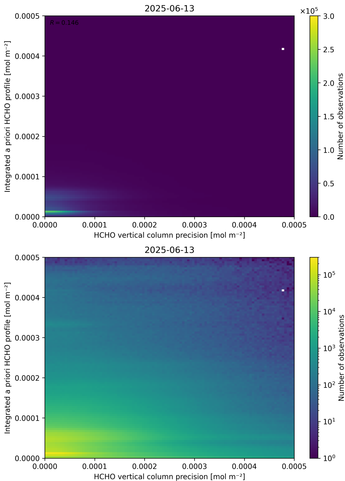
Figure 147: Scatter density plot of “HCHO vertical column precision” against “Integrated a priori HCHO profile” for 2025-06-12 to 2025-06-14.
