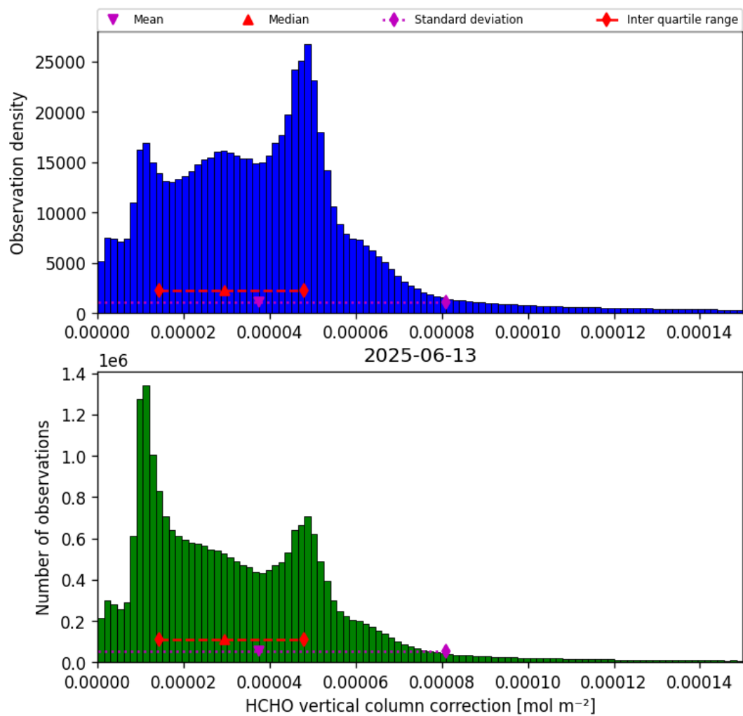
Figure 37: Histogram of “HCHO vertical column correction” for 2025-06-12 to 2025-06-14
