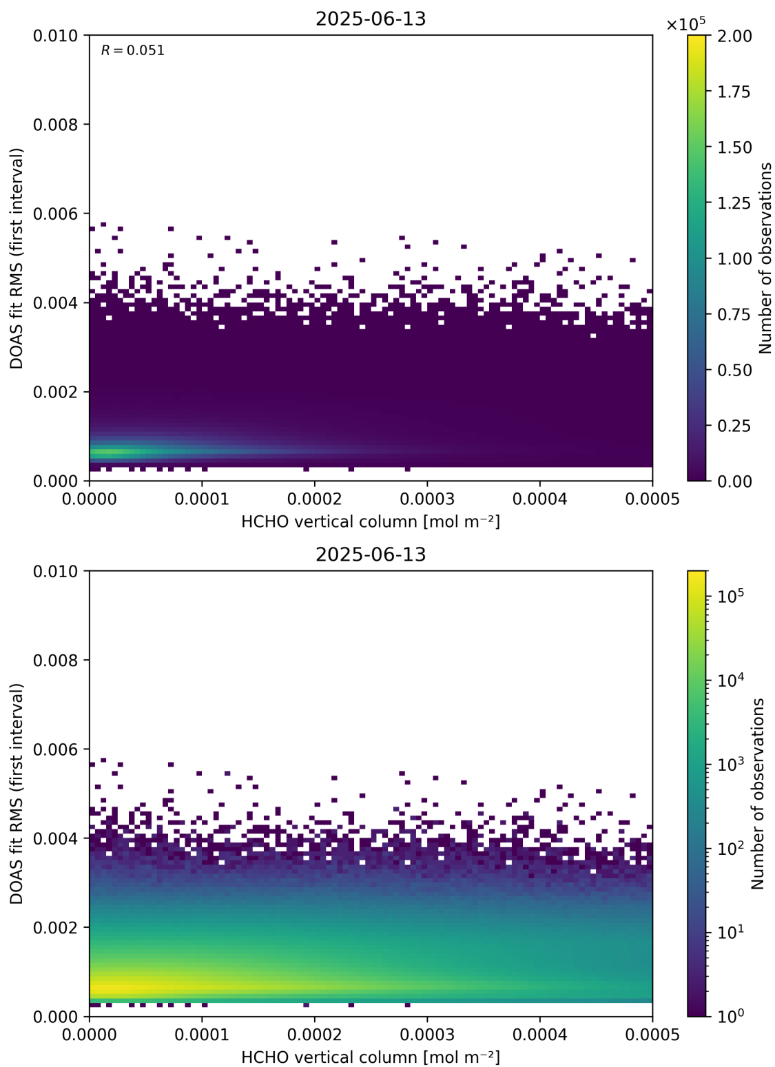
Figure 123: Scatter density plot of “HCHO vertical column” against “DOAS fit RMS (first interval)” for 2025-06-12 to 2025-06-14.
