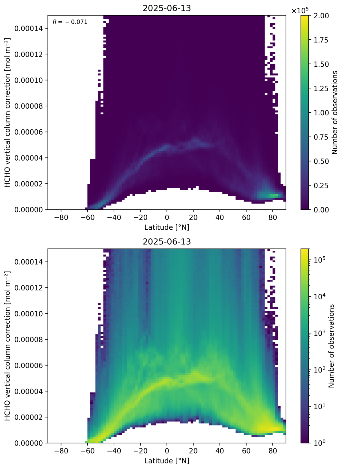
Figure 164: Scatter density plot of “Latitude” against “HCHO vertical column correction” for 2025-06-12 to 2025-06-14.
