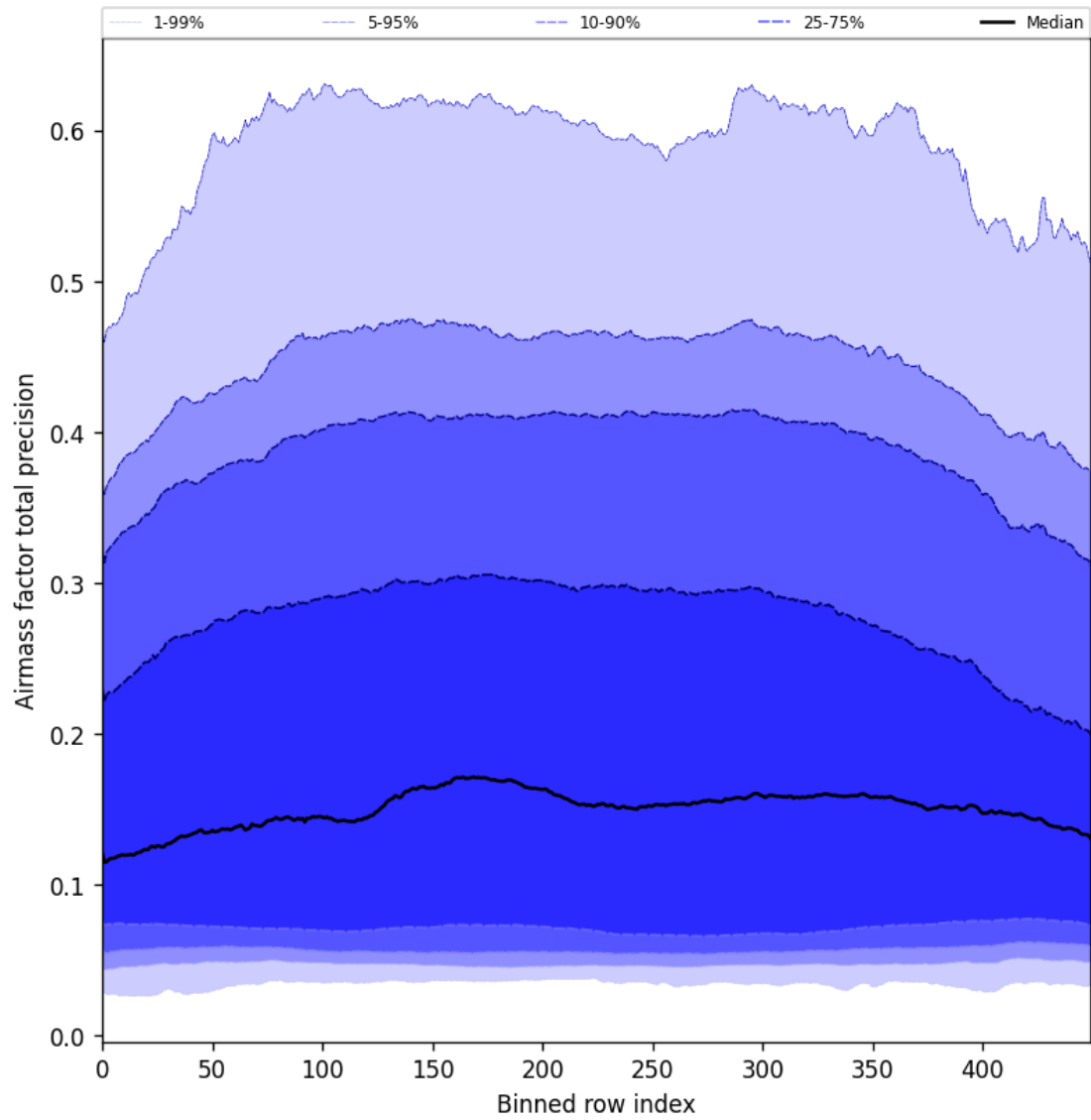
Figure 55: Along track statistics of “Airmass factor total precision” for 2025-06-12 to 2025-06-14
