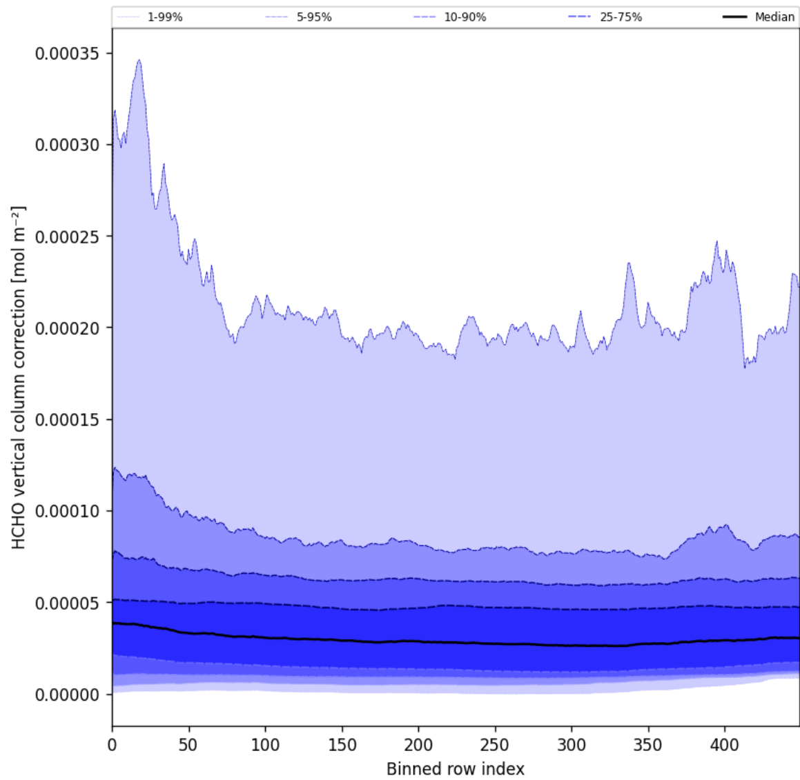
Figure 51: Along track statistics of “HCHO vertical column correction” for 2025-06-12 to 2025-06-14
