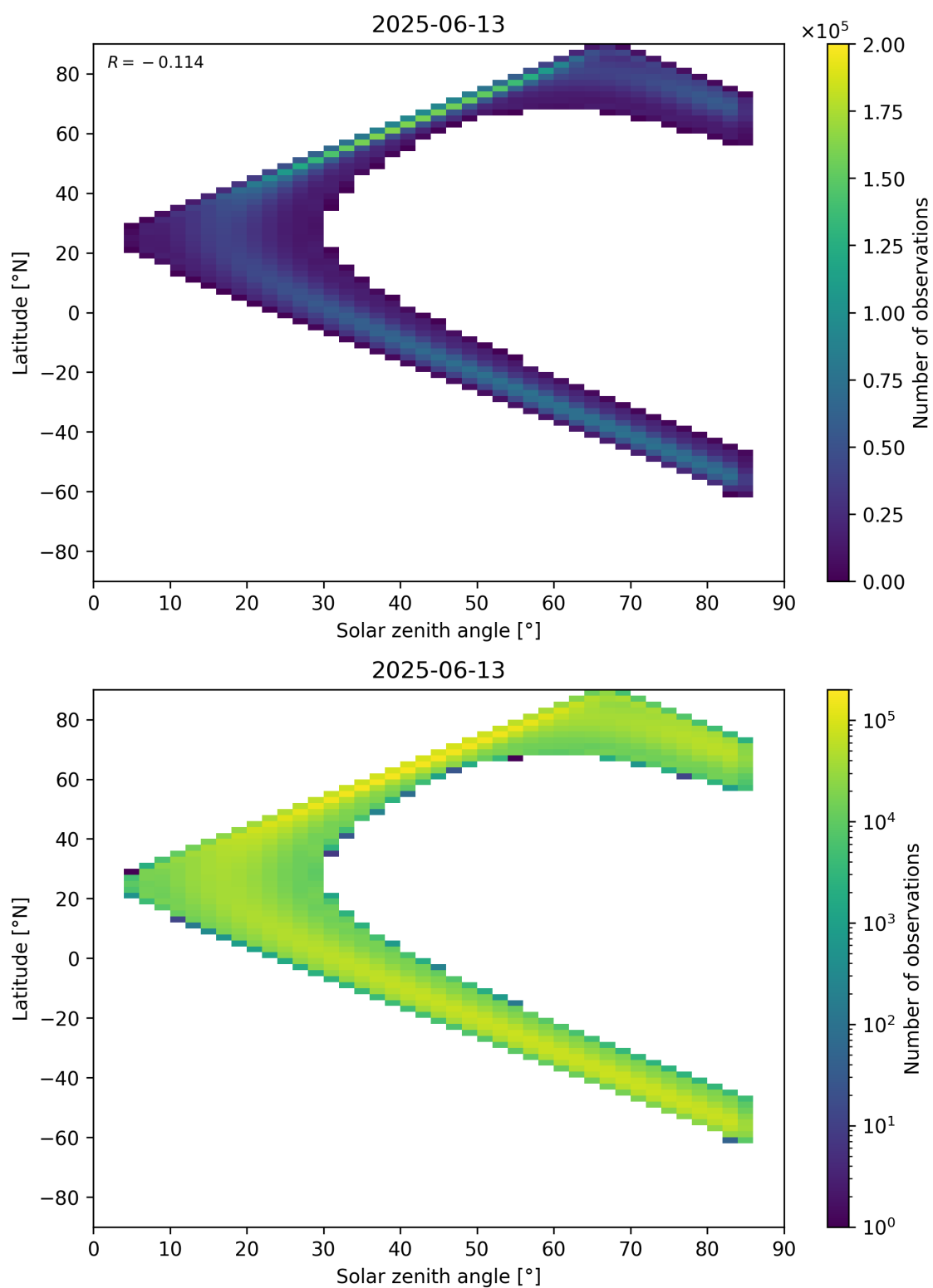
Figure 181: Scatter density plot of “Solar zenith angle” against “Latitude” for 2025-06-12 to 2025-06-14.
