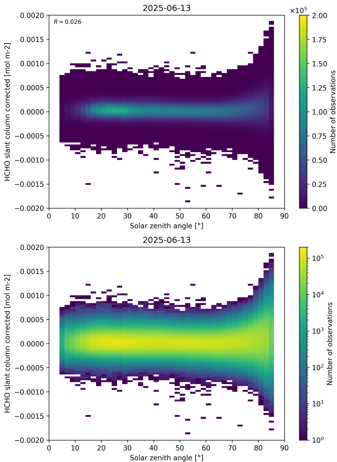
Figure 171: Scatter density plot of “Solar zenith angle” against “HCHO slant column corrected” for 2025-06-12 to 2025-06-14.
