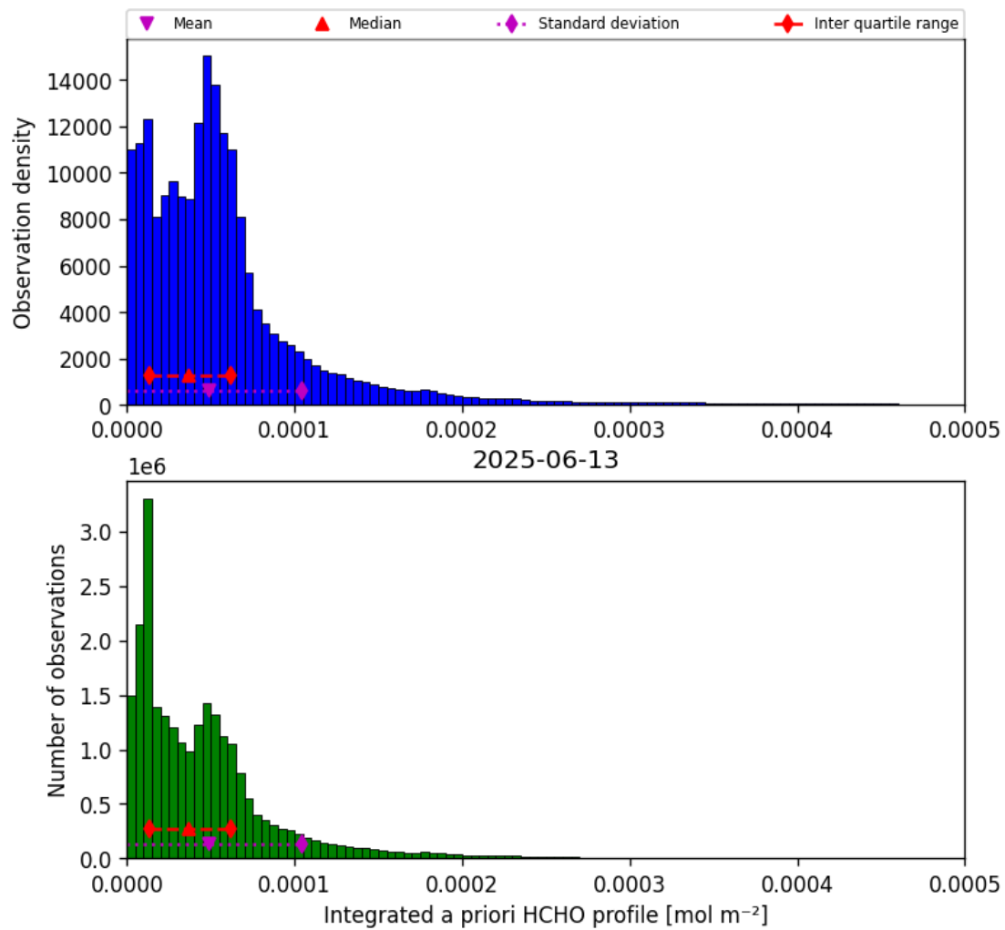
Figure 43: Histogram of “Integrated a priori HCHO profile” for 2025-06-12 to 2025-06-14
