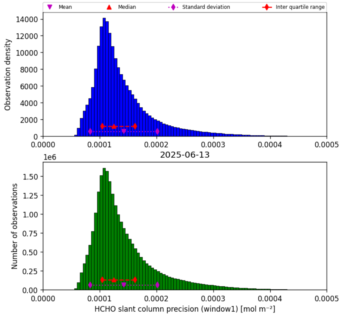
Figure 39: Histogram of “HCHO slant column precision (window1)” for 2025-06-12 to 2025-06-14
