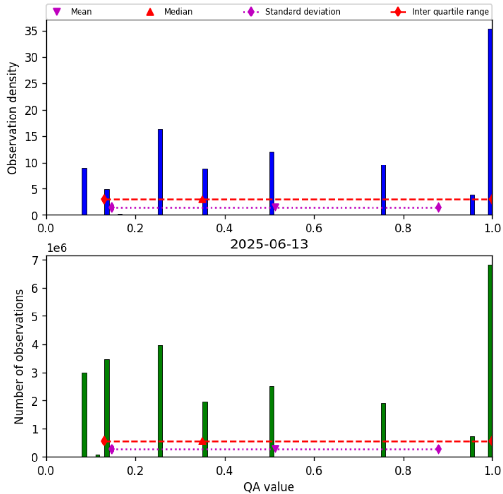
Figure 34: Histogram of “QA value” for 2025-06-12 to 2025-06-14
