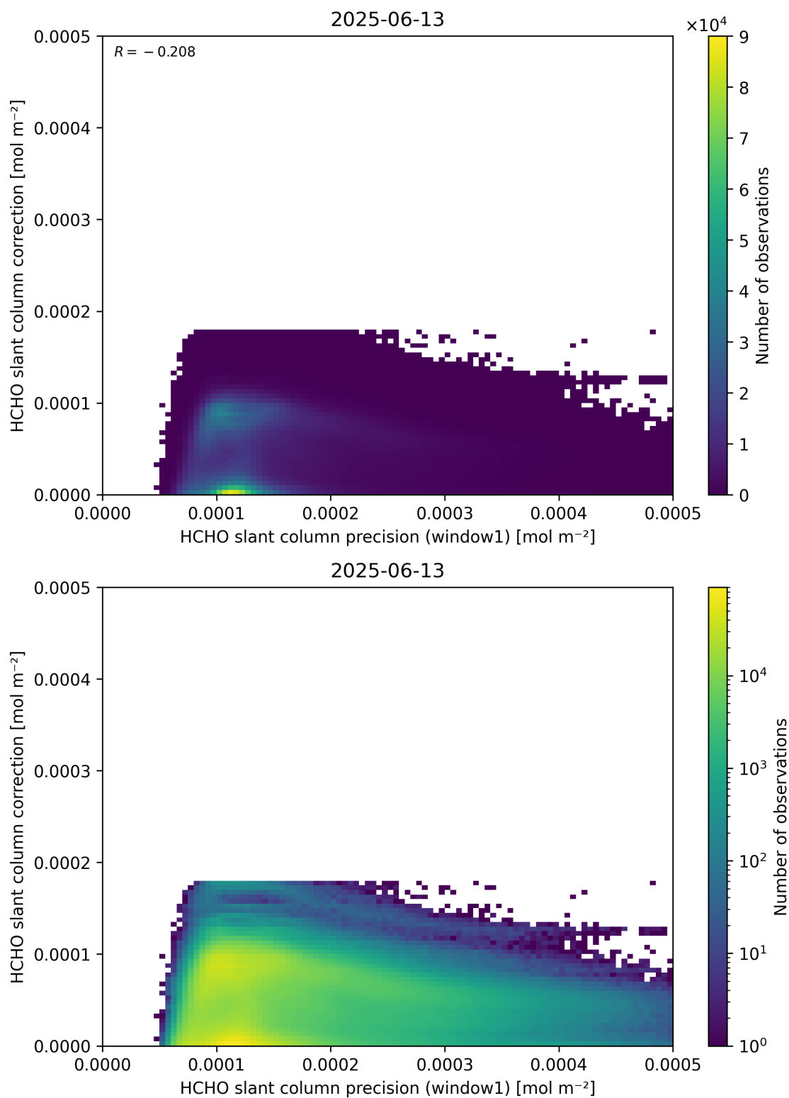
Figure 93: Scatter density plot of “HCHO slant column precision (window1)” against “HCHO slant column correction” for 2025-06-12 to 2025-06-14.
