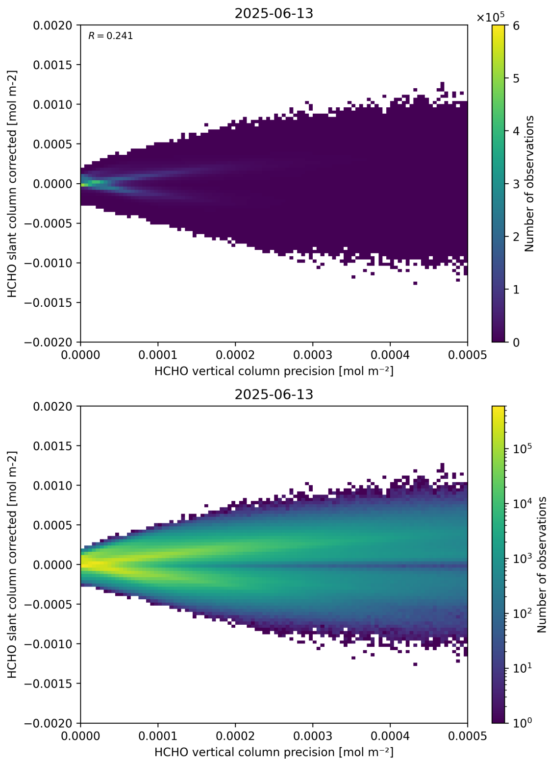
Figure 140: Scatter density plot of “HCHO vertical column precision” against “HCHO slant column corrected” for 2025-06-12 to 2025-06-14.
