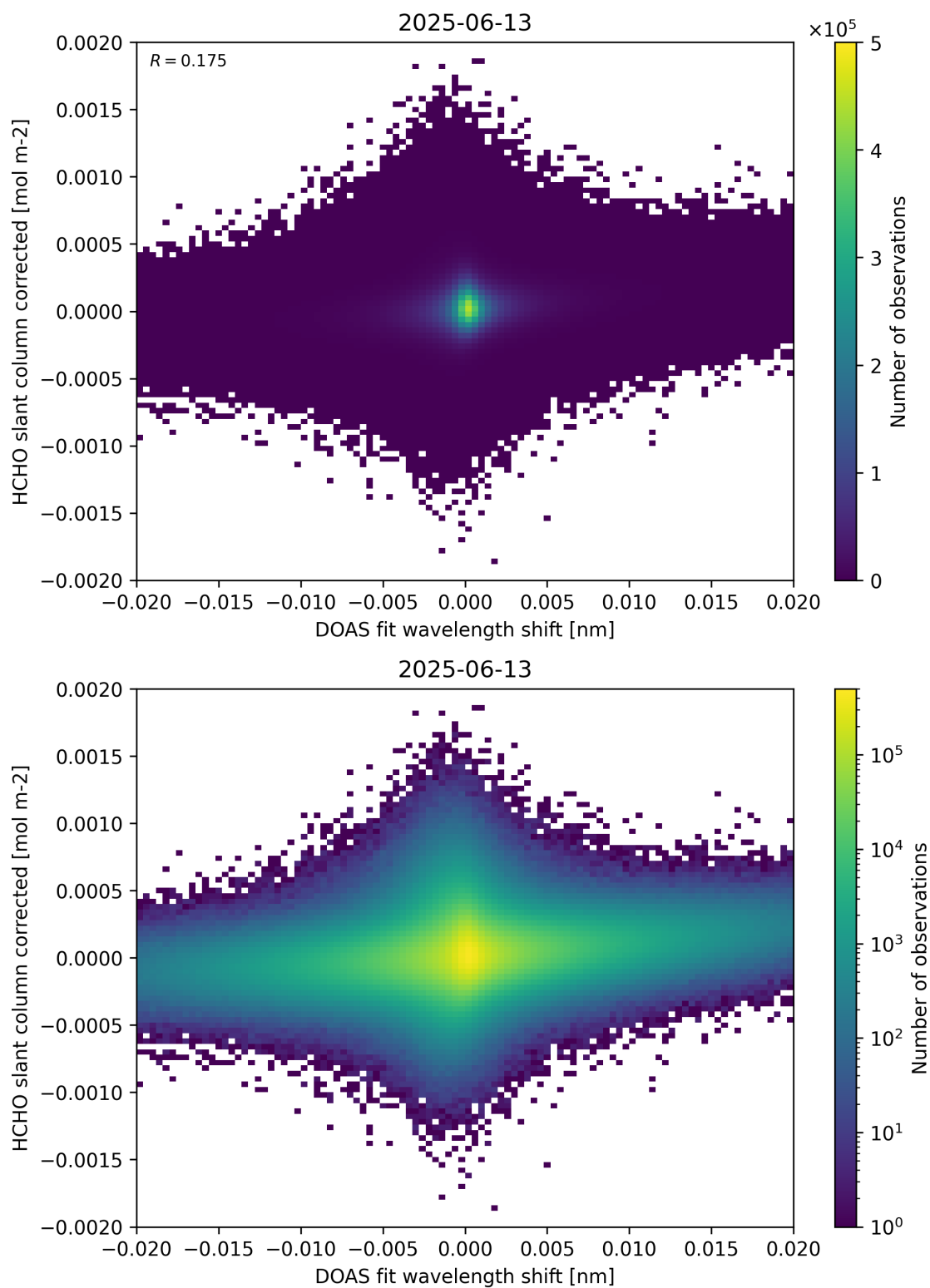
Figure 66: Scatter density plot of “DOAS fit wavelength shift” against “HCHO slant column corrected” for 2025-06-12 to 2025-06-14.
