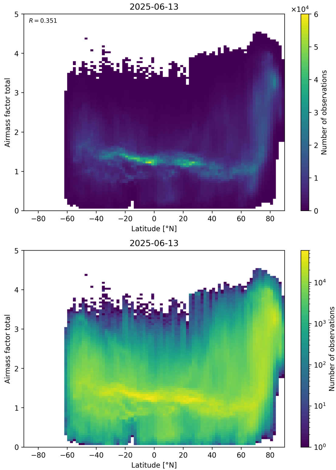
Figure 161: Scatter density plot of “Latitude” against “Airmass factor total” for 2025-06-12 to 2025-06-14.
