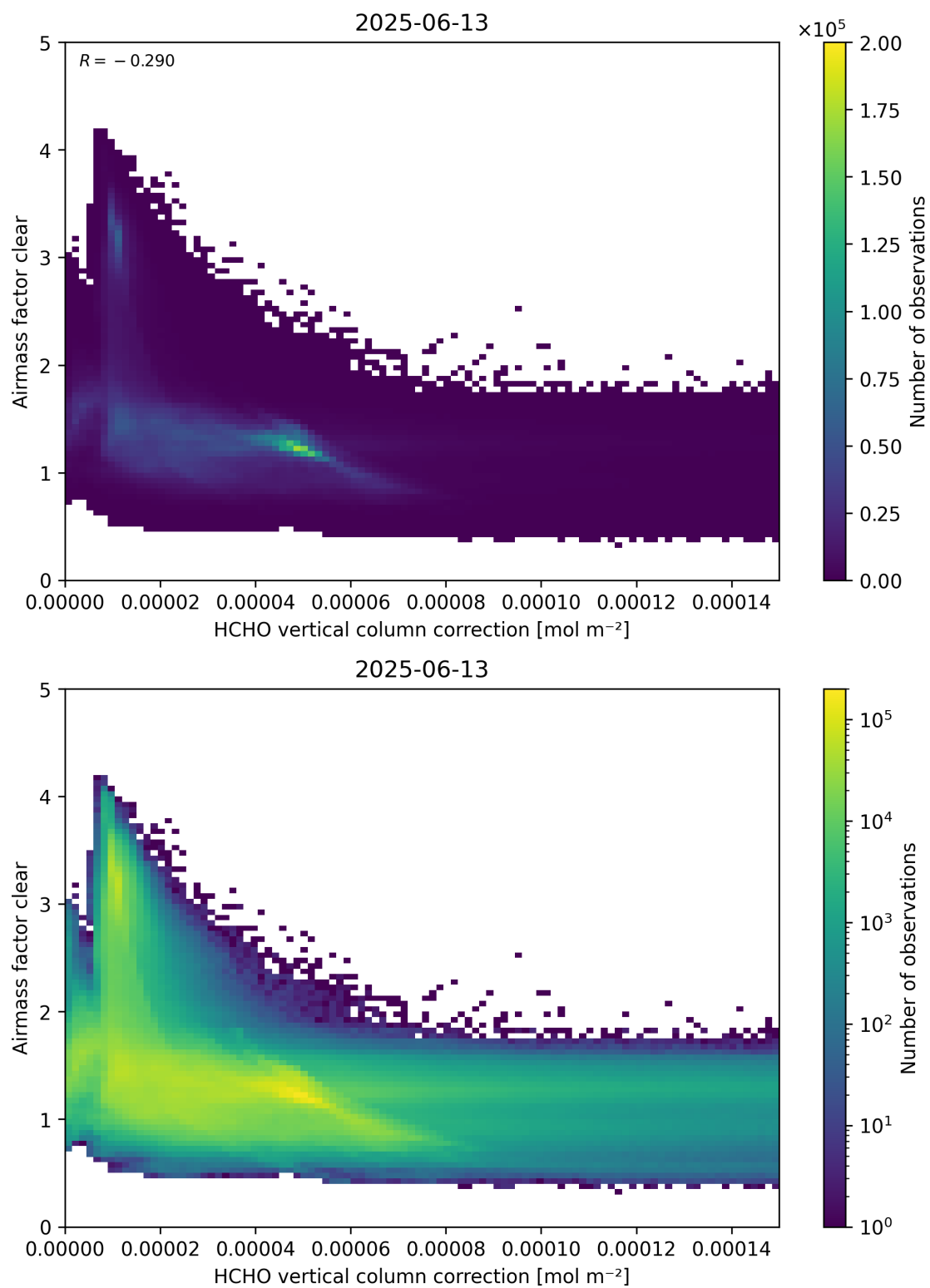
Figure 115: Scatter density plot of “HCHO vertical column correction” against “Airmass factor clear” for 2025-06-12 to 2025-06-14.
