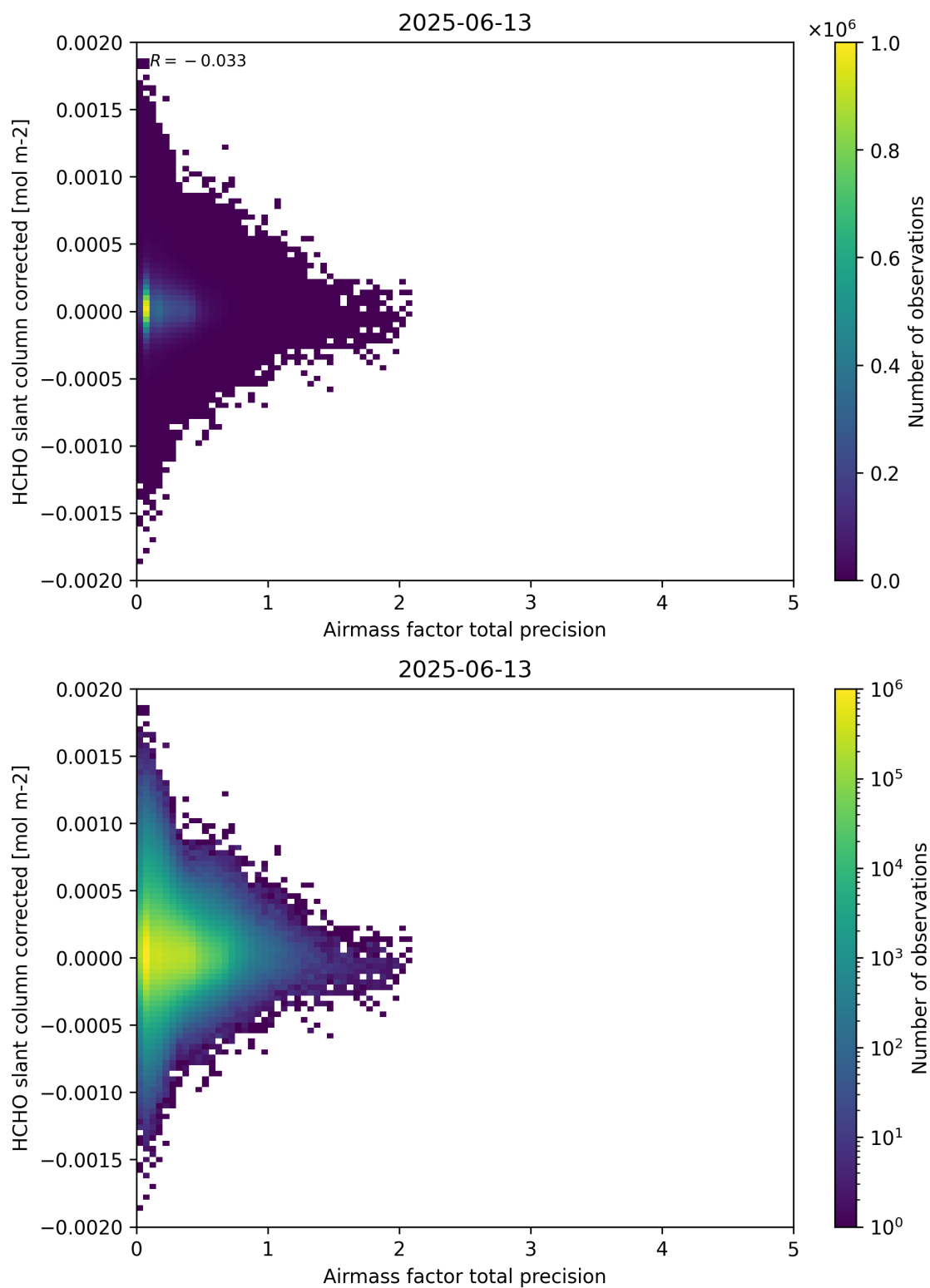
Figure 109: Scatter density plot of “Airmass factor total precision” against “HCHO slant column corrected” for 2025-06-12 to 2025-06-14.
