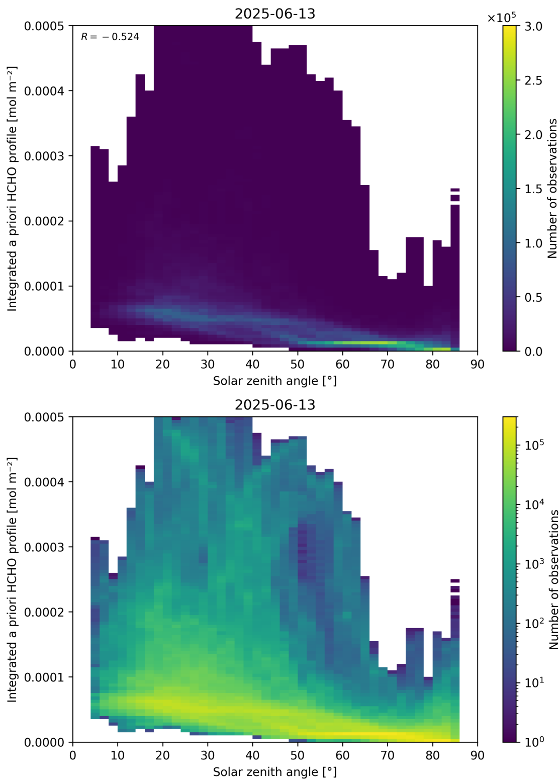
Figure 180: Scatter density plot of “Solar zenith angle” against “Integrated a priori HCHO profile” for 2025-06-12 to 2025-06-14.
