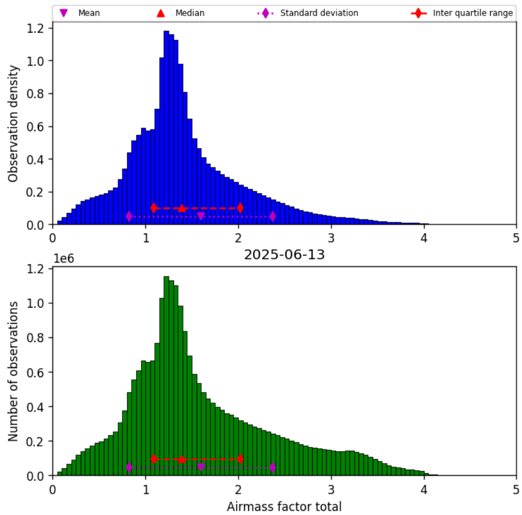
Figure 40: Histogram of “Airmass factor total” for 2025-06-12 to 2025-06-14
