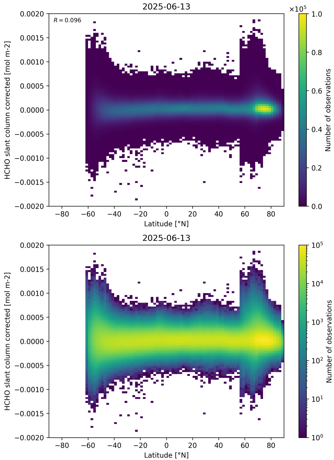
Figure 157: Scatter density plot of “Latitude” against “HCHO slant column corrected” for 2025-06-12 to 2025-06-14.
