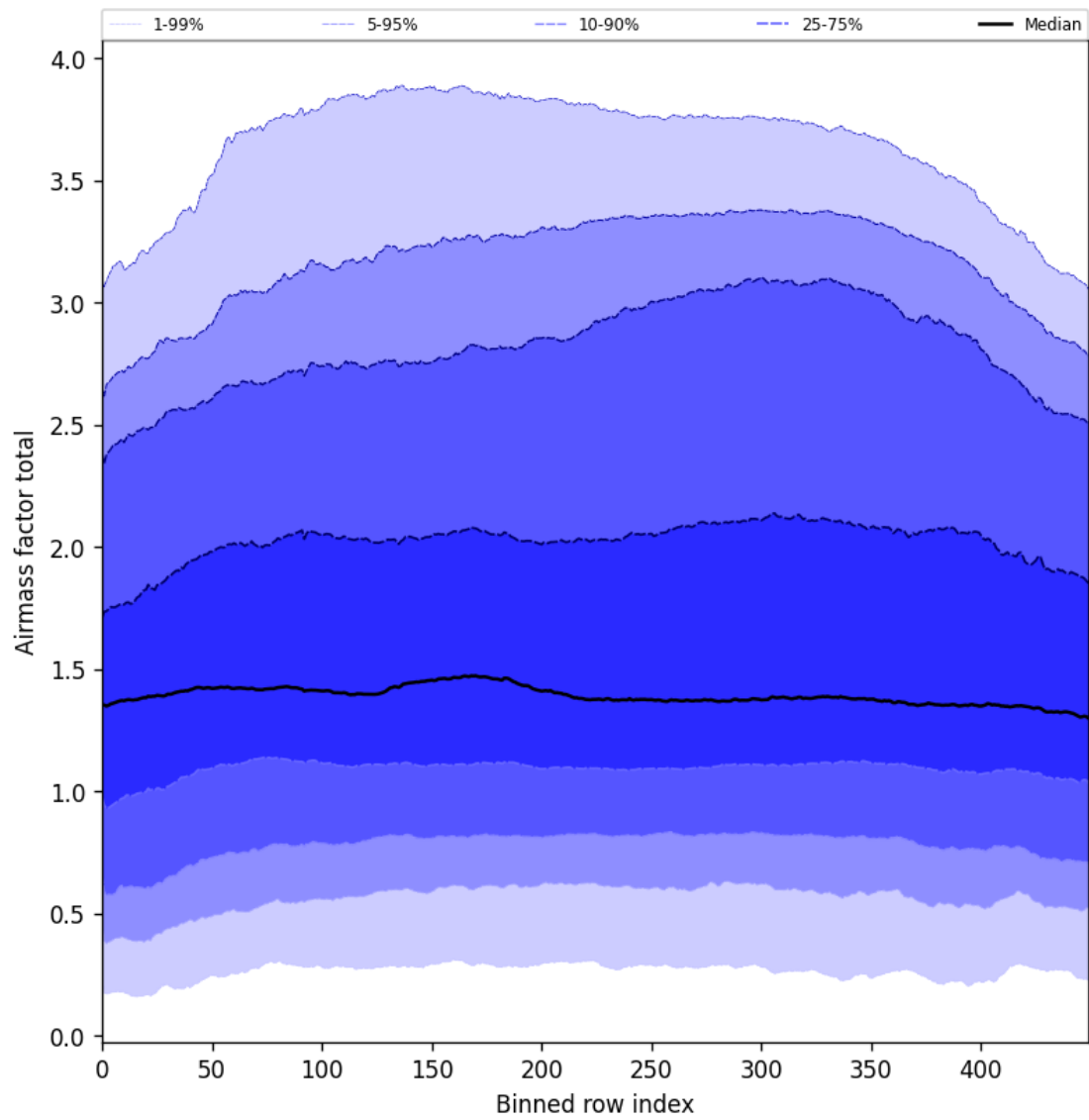
Figure 54: Along track statistics of “Airmass factor total” for 2025-06-12 to 2025-06-14
