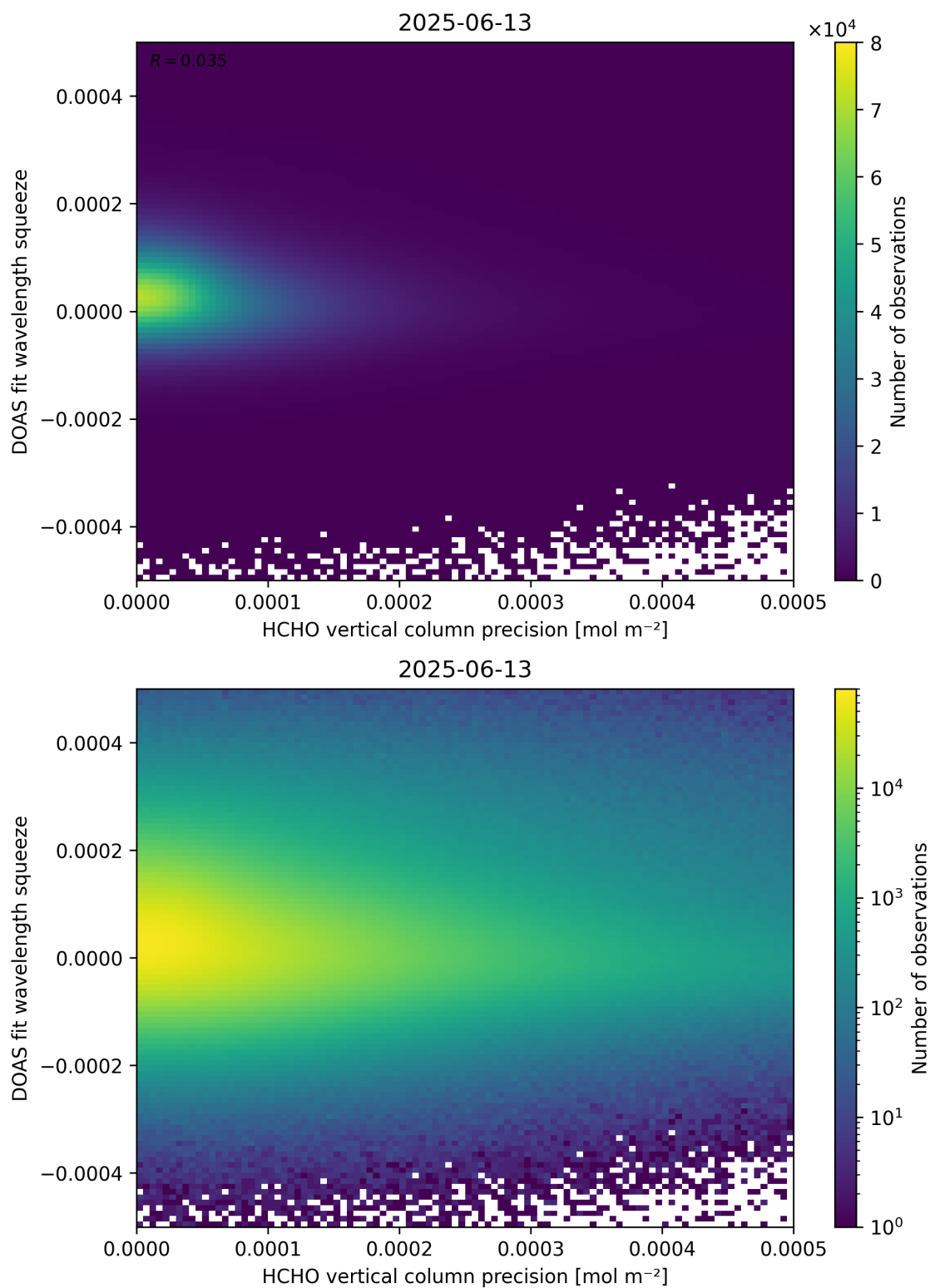
Figure 138: Scatter density plot of “HCHO vertical column precision” against “DOAS fit wavelength squeeze” for 2025-06-12 to 2025-06-14.
