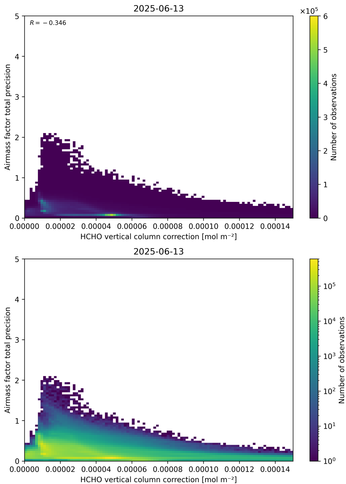
Figure 121: Scatter density plot of “HCHO vertical column correction” against “Airmass factor total precision” for 2025-06-12 to 2025-06-14.
