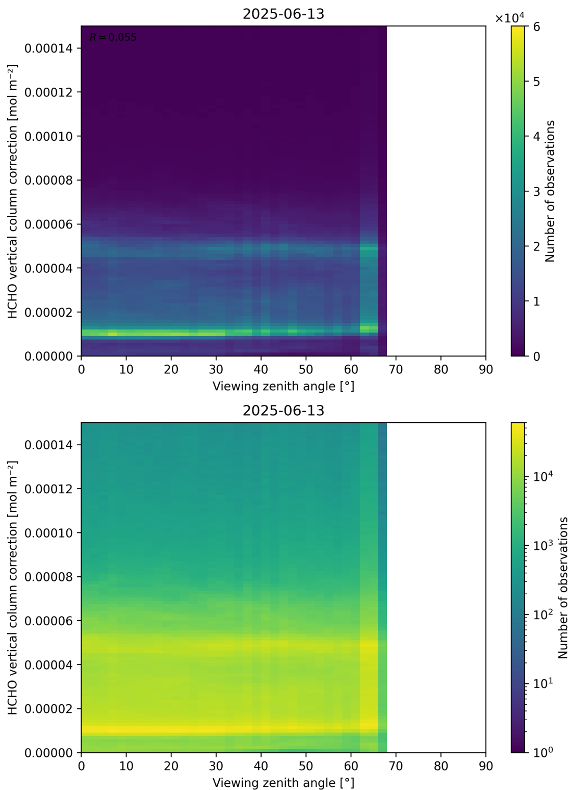
Figure 193: Scatter density plot of “Viewing zenith angle” against “HCHO vertical column correction” for 2025-06-12 to 2025-06-14.
