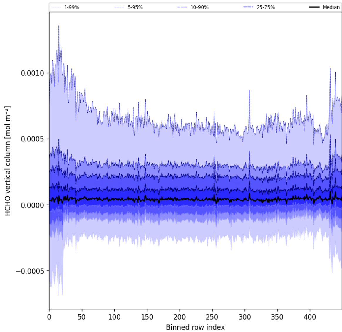
Figure 49: Along track statistics of “HCHO vertical column” for 2025-06-12 to 2025-06-14
