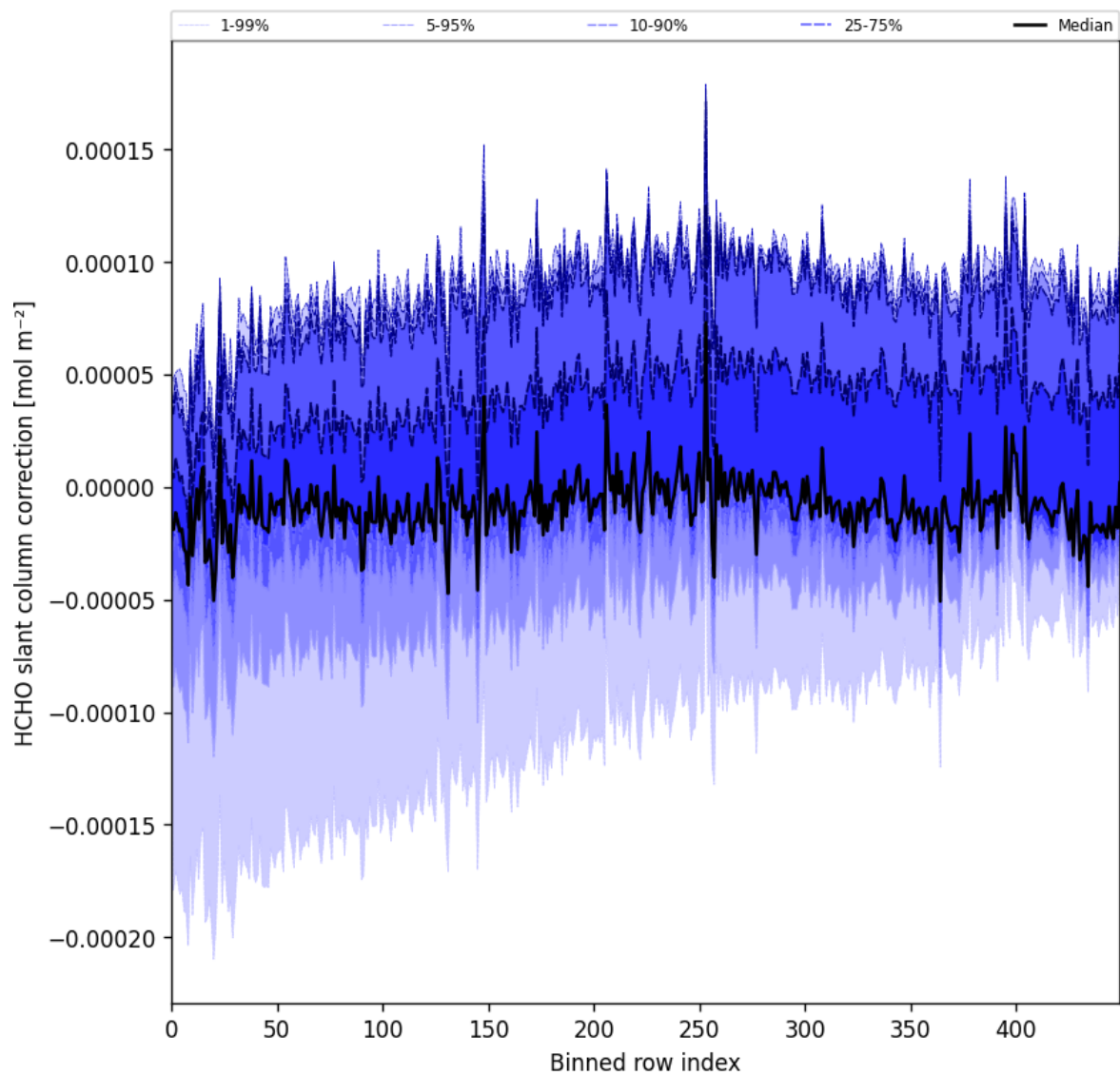
Figure 61: Along track statistics of “HCHO slant column correction” for 2025-06-12 to 2025-06-14
