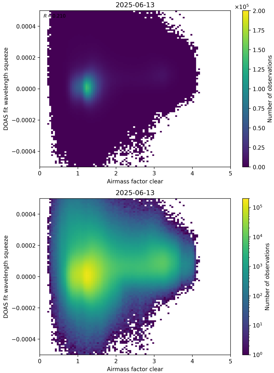
Figure 73: Scatter density plot of “Airmass factor clear” against “DOAS fit wavelength squeeze” for 2025-06-12 to 2025-06-14.
