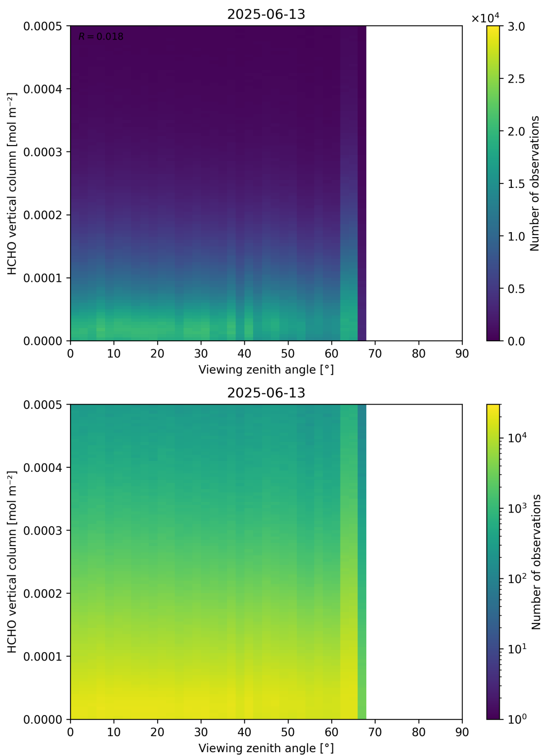
Figure 192: Scatter density plot of “Viewing zenith angle” against “HCHO vertical column” for 2025-06-12 to 2025-06-14.
