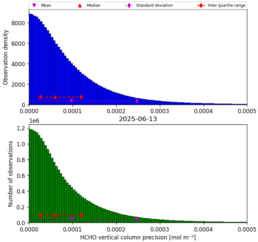
Figure 36: Histogram of “HCHO vertical column precision” for 2025-06-12 to 2025-06-14
