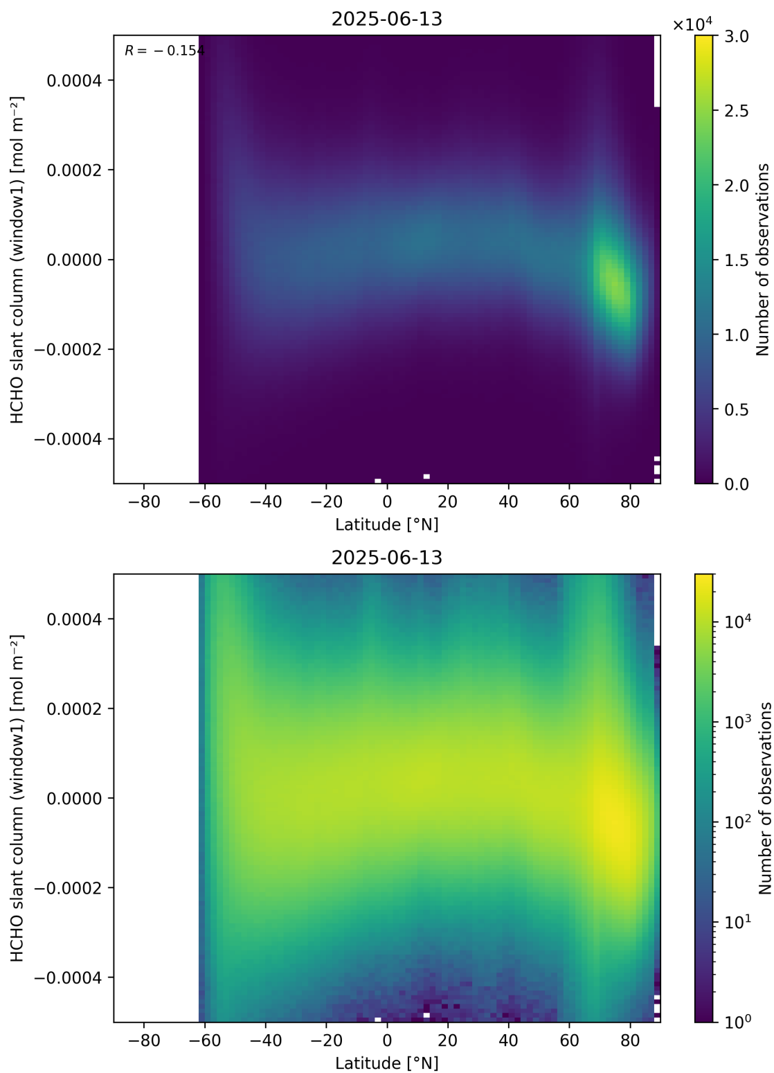
Figure 159: Scatter density plot of “Latitude” against “HCHO slant column (window1)” for 2025-06-12 to 2025-06-14.
