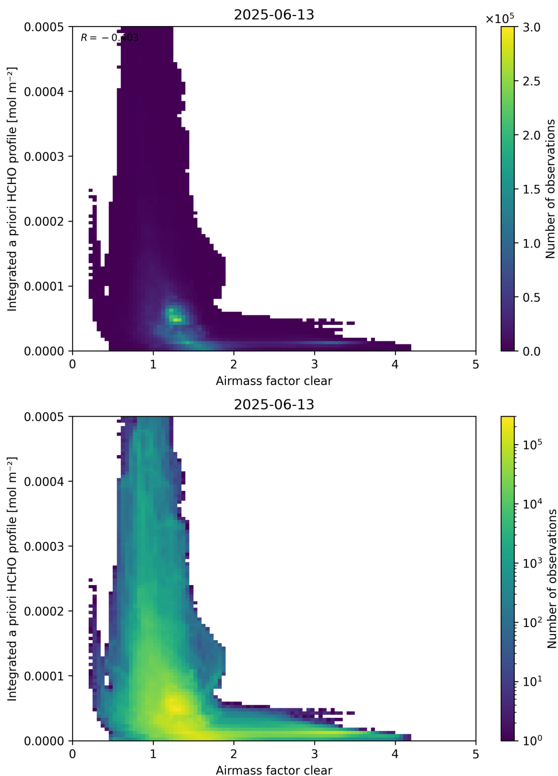
Figure 76: Scatter density plot of “Airmass factor clear” against “Integrated a priori HCHO profile” for 2025-06-12 to 2025-06-14.
