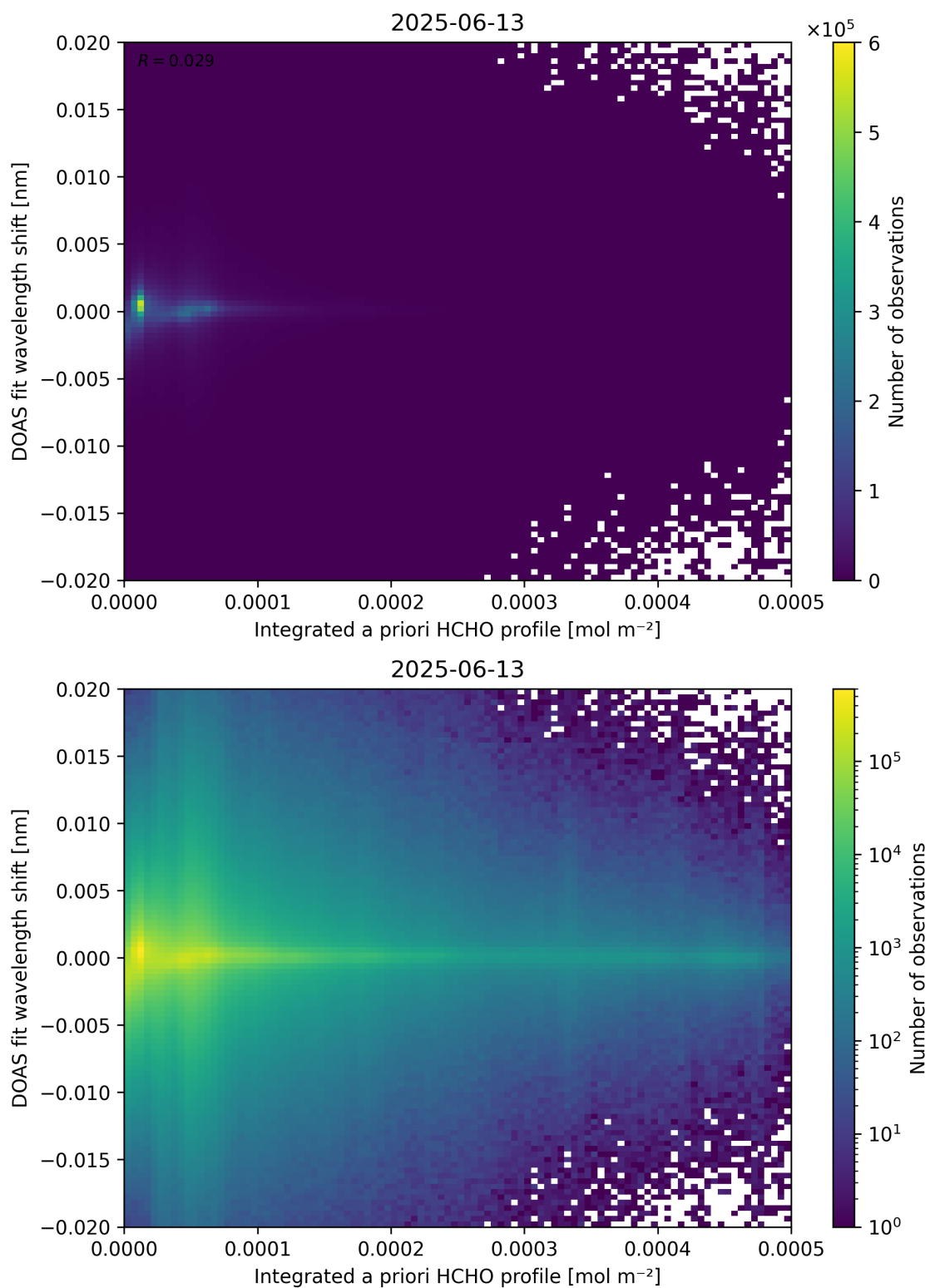
Figure 149: Scatter density plot of “Integrated a priori HCHO profile” against “DOAS fit wavelength shift” for 2025-06-12 to 2025-06-14.
