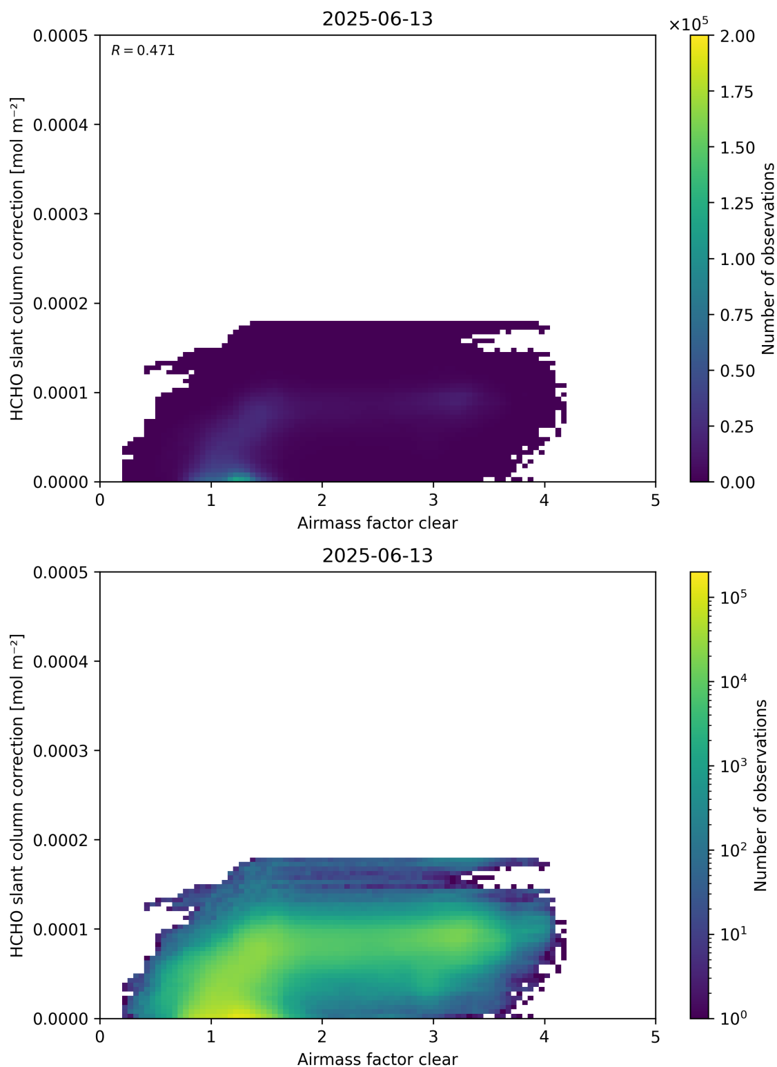
Figure 75: Scatter density plot of “Airmass factor clear” against “HCHO slant column correction” for 2025-06-12 to 2025-06-14.
