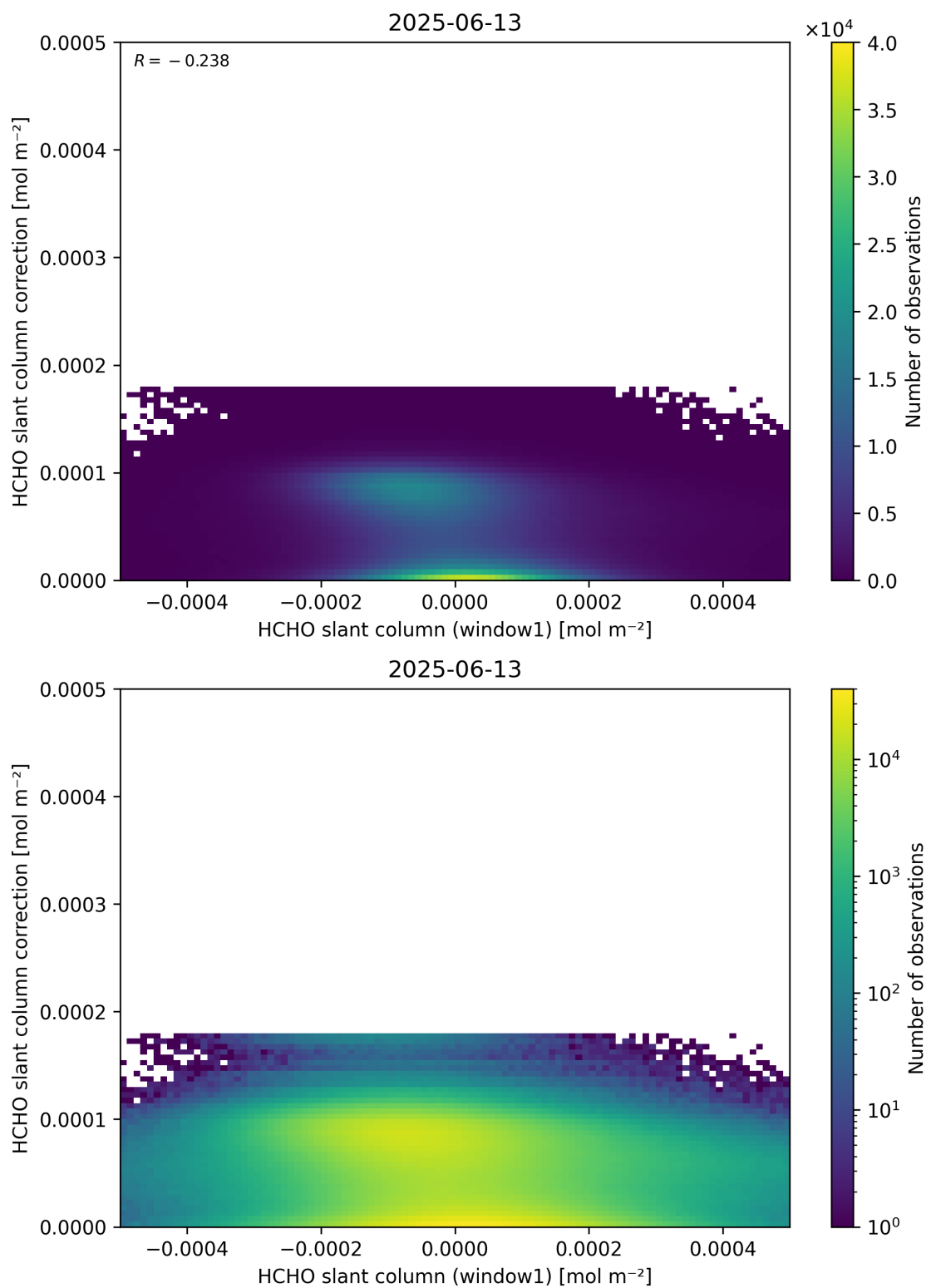
Figure 83: Scatter density plot of “HCHO slant column (window1)” against “HCHO slant column correction” for 2025-06-12 to 2025-06-14.
