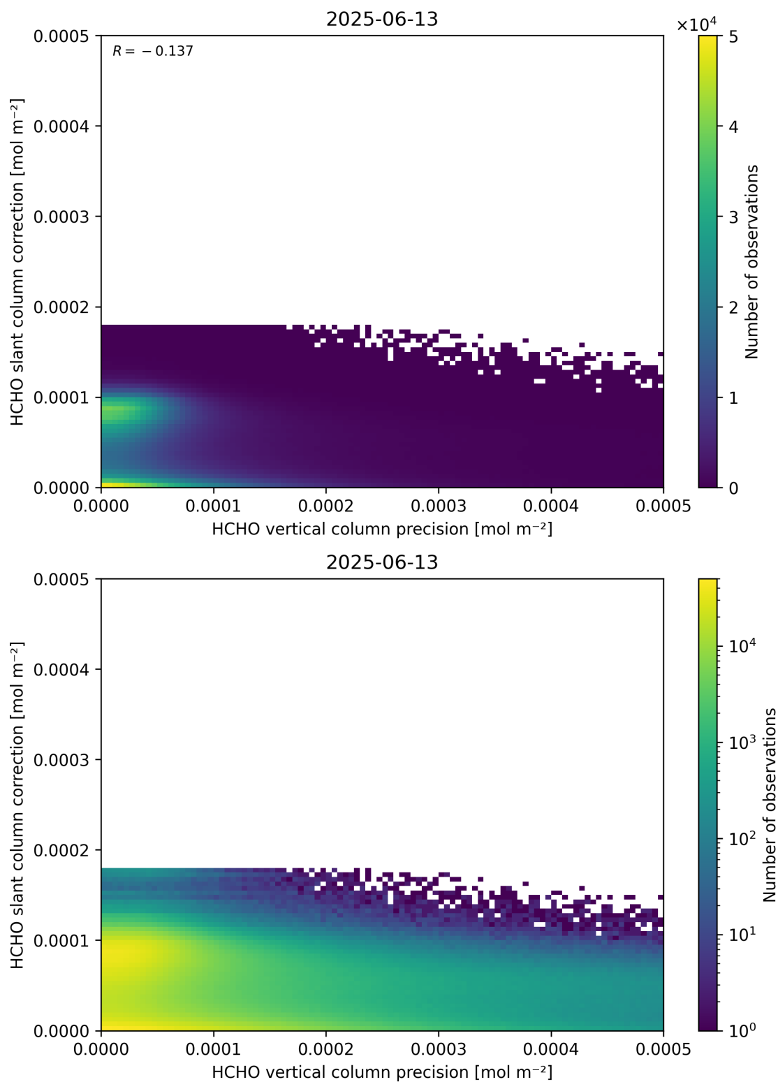
Figure 141: Scatter density plot of “HCHO vertical column precision” against “HCHO slant column correction” for 2025-06-12 to 2025-06-14.
