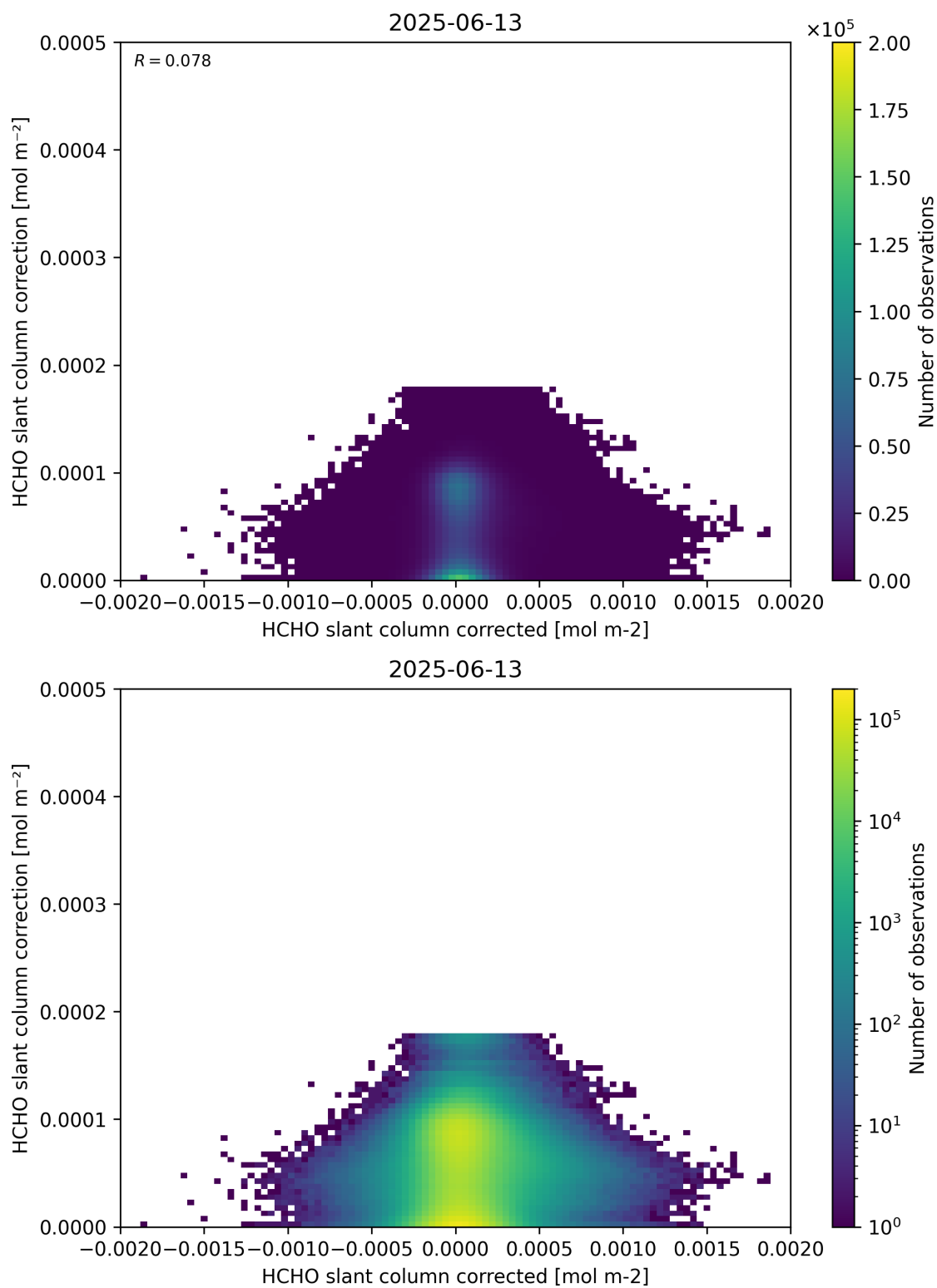
Figure 77: Scatter density plot of “HCHO slant column corrected” against “HCHO slant column correction” for 2025-06-12 to 2025-06-14.
