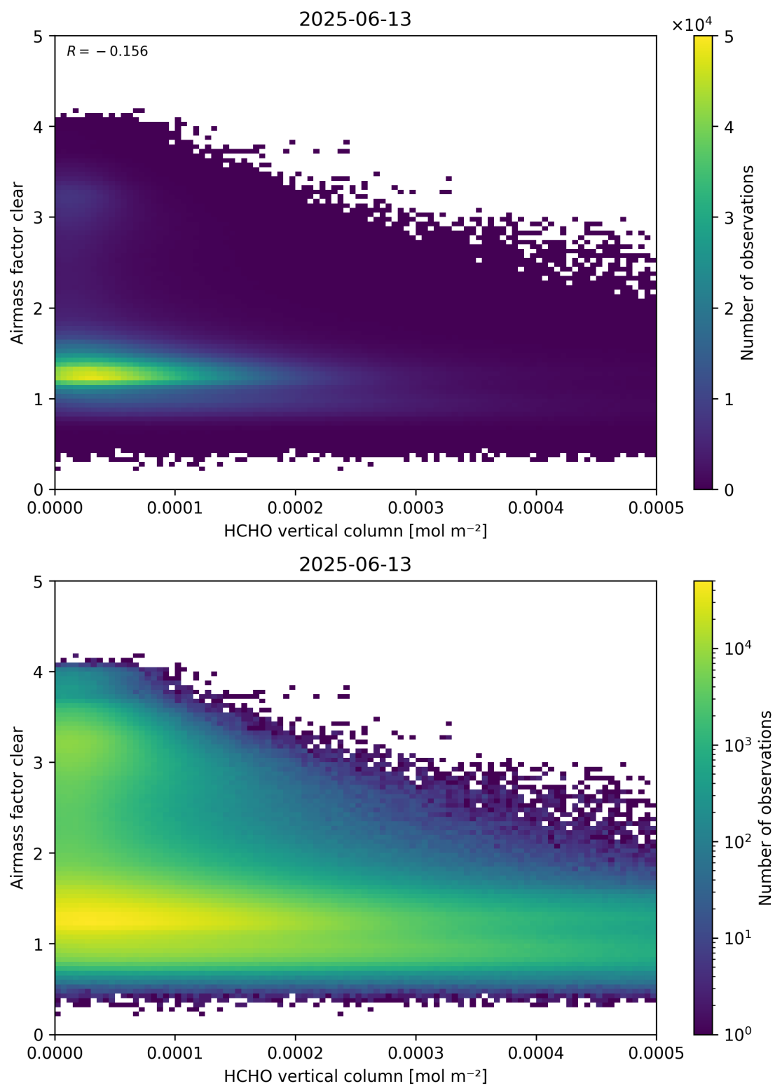
Figure 126: Scatter density plot of “HCHO vertical column” against “Airmass factor clear” for 2025-06-12 to 2025-06-14.
