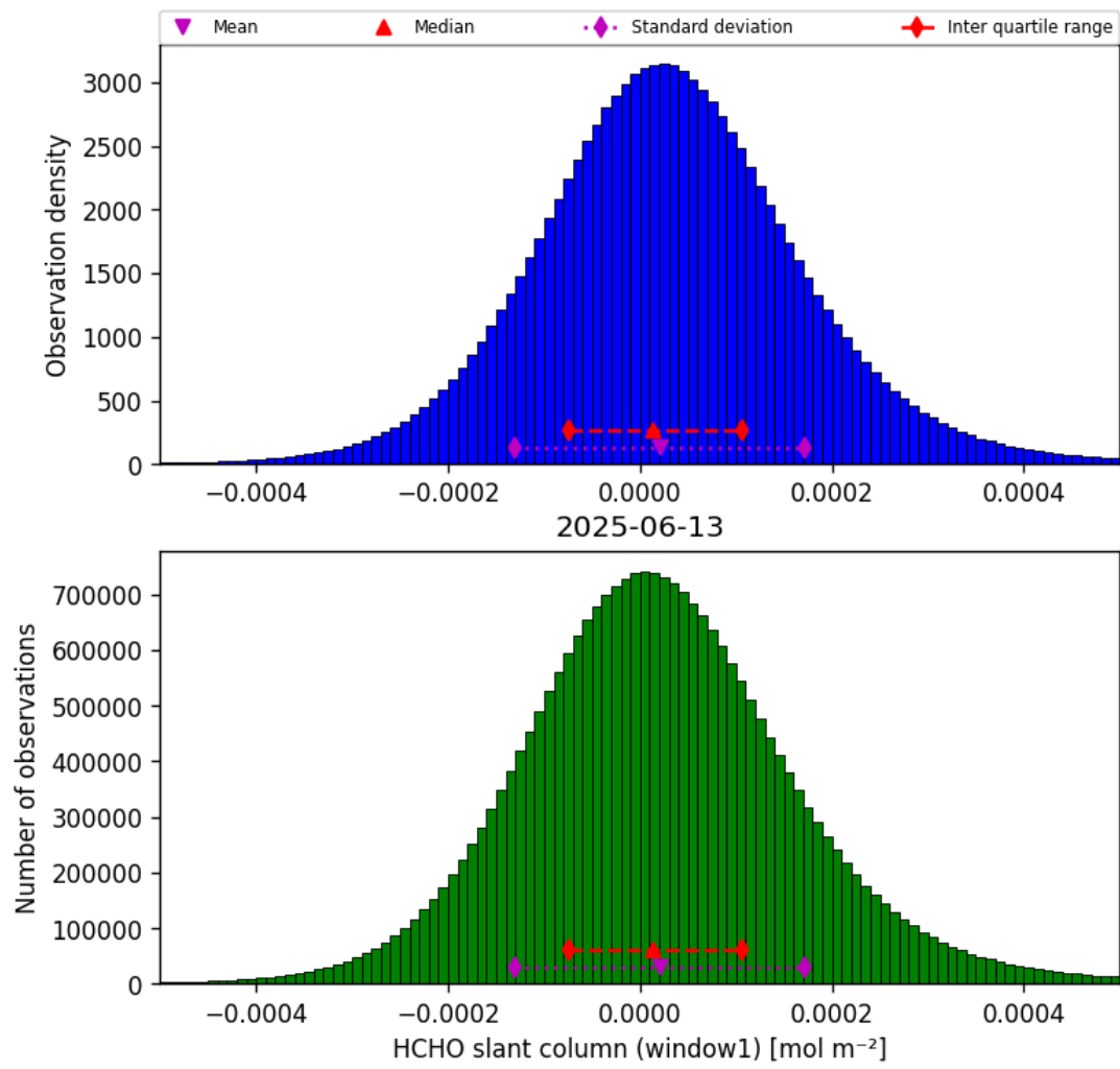
Figure 38: Histogram of “HCHO slant column (window1)” for 2025-06-12 to 2025-06-14
