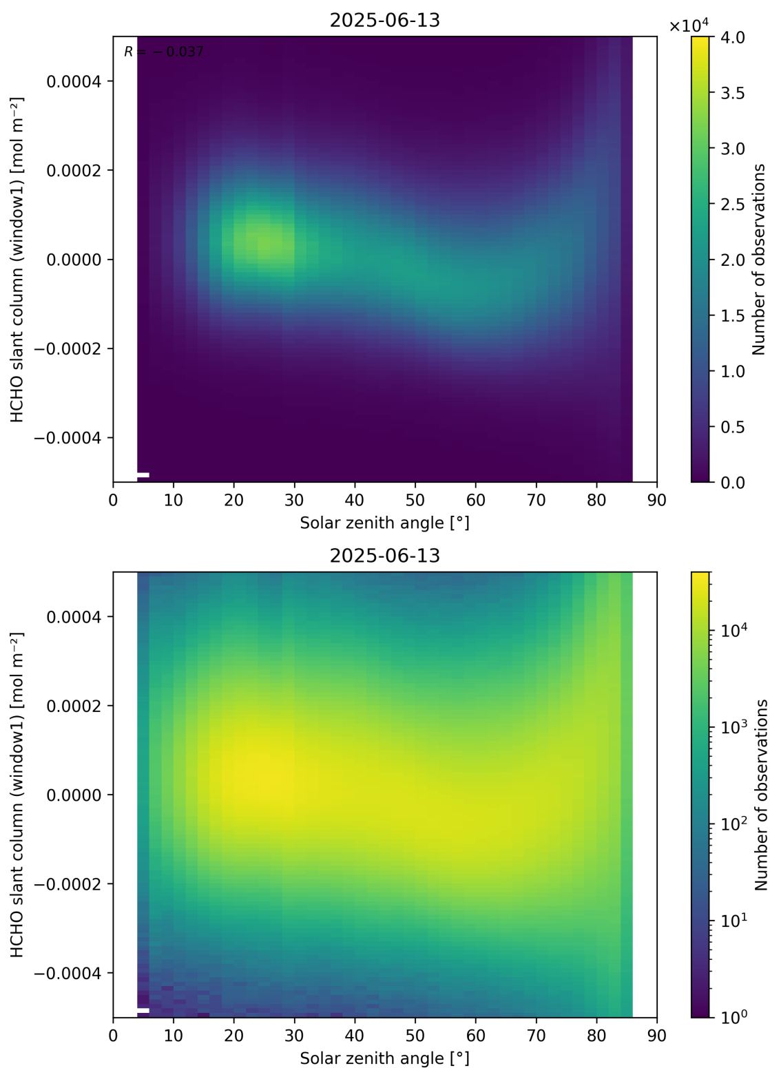
Figure 173: Scatter density plot of “Solar zenith angle” against “HCHO slant column (window1)” for 2025-06-12 to 2025-06-14.
