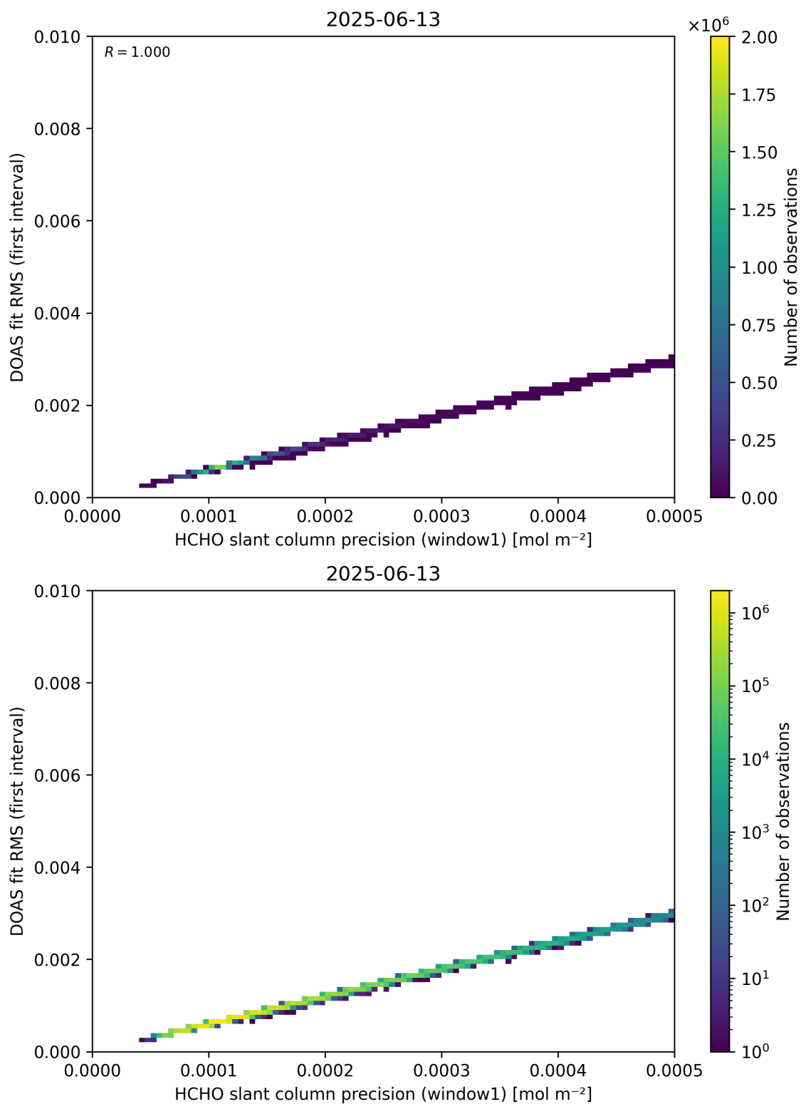
Figure 88: Scatter density plot of “HCHO slant column precision (window1)” against “DOAS fit RMS (first interval)” for 2025-06-12 to 2025-06-14.
