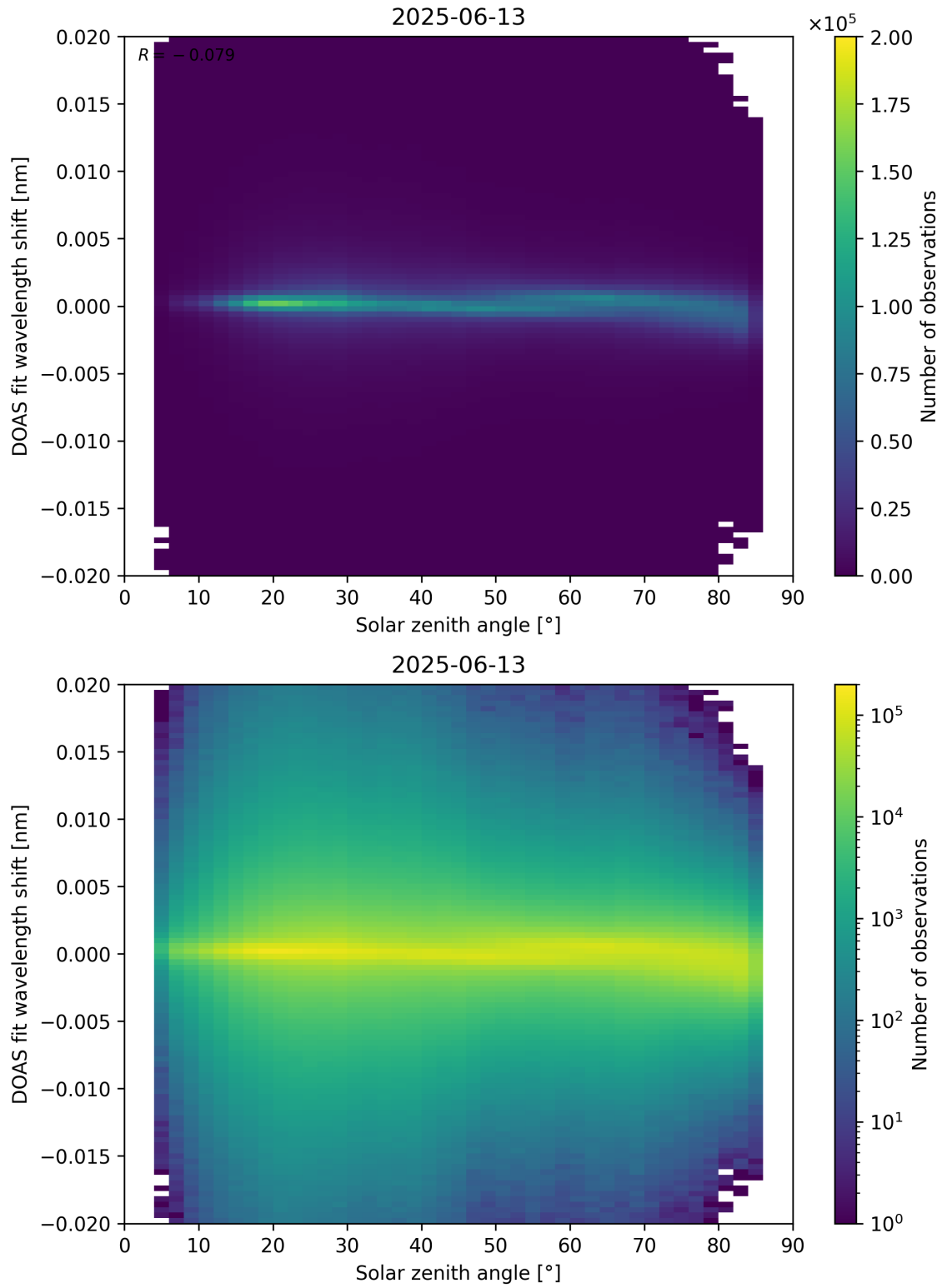
Figure 168: Scatter density plot of “Solar zenith angle” against “DOAS fit wavelength shift” for 2025-06-12 to 2025-06-14.
