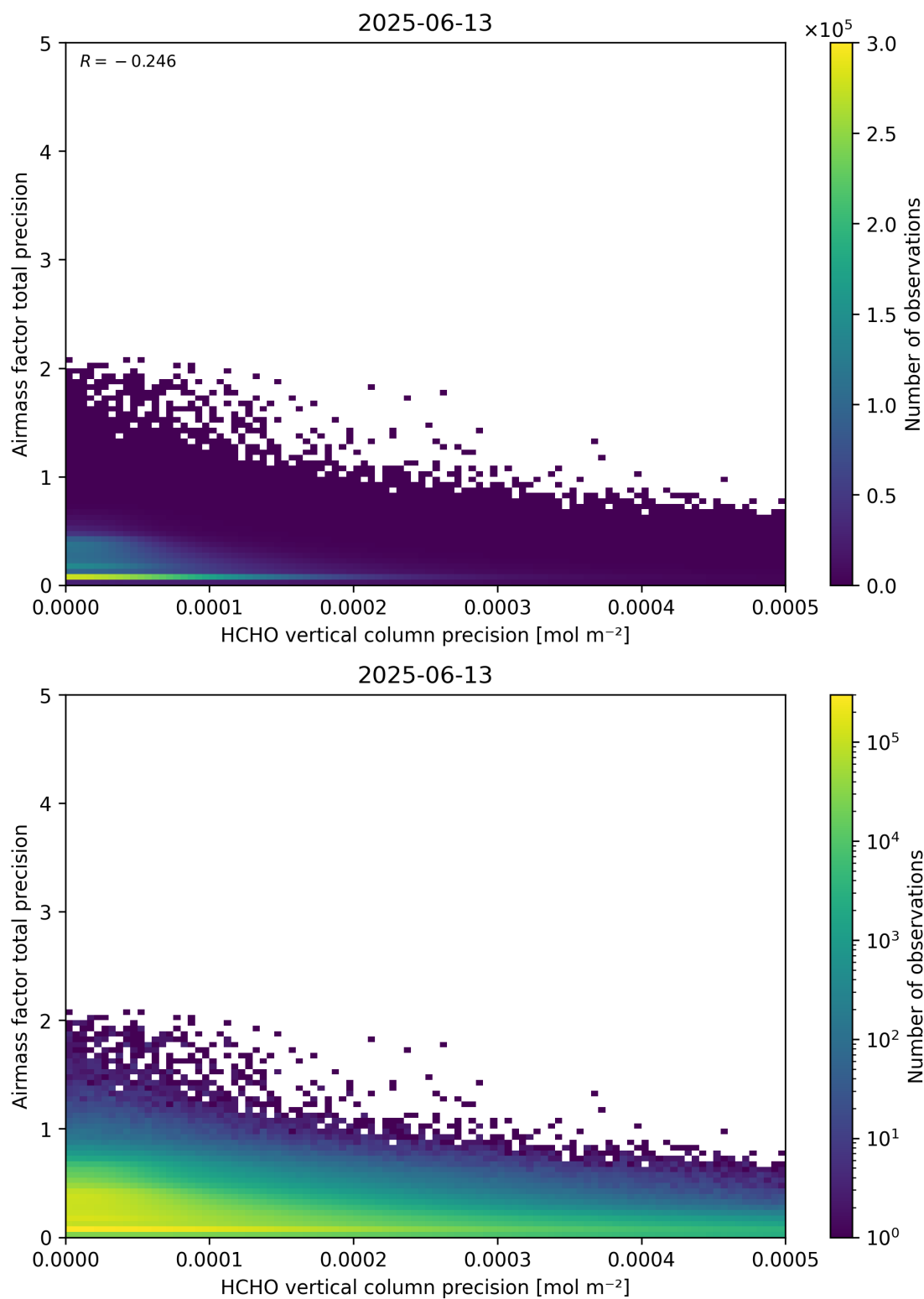
Figure 145: Scatter density plot of “HCHO vertical column precision” against “Airmass factor total precision” for 2025-06-12 to 2025-06-14.
