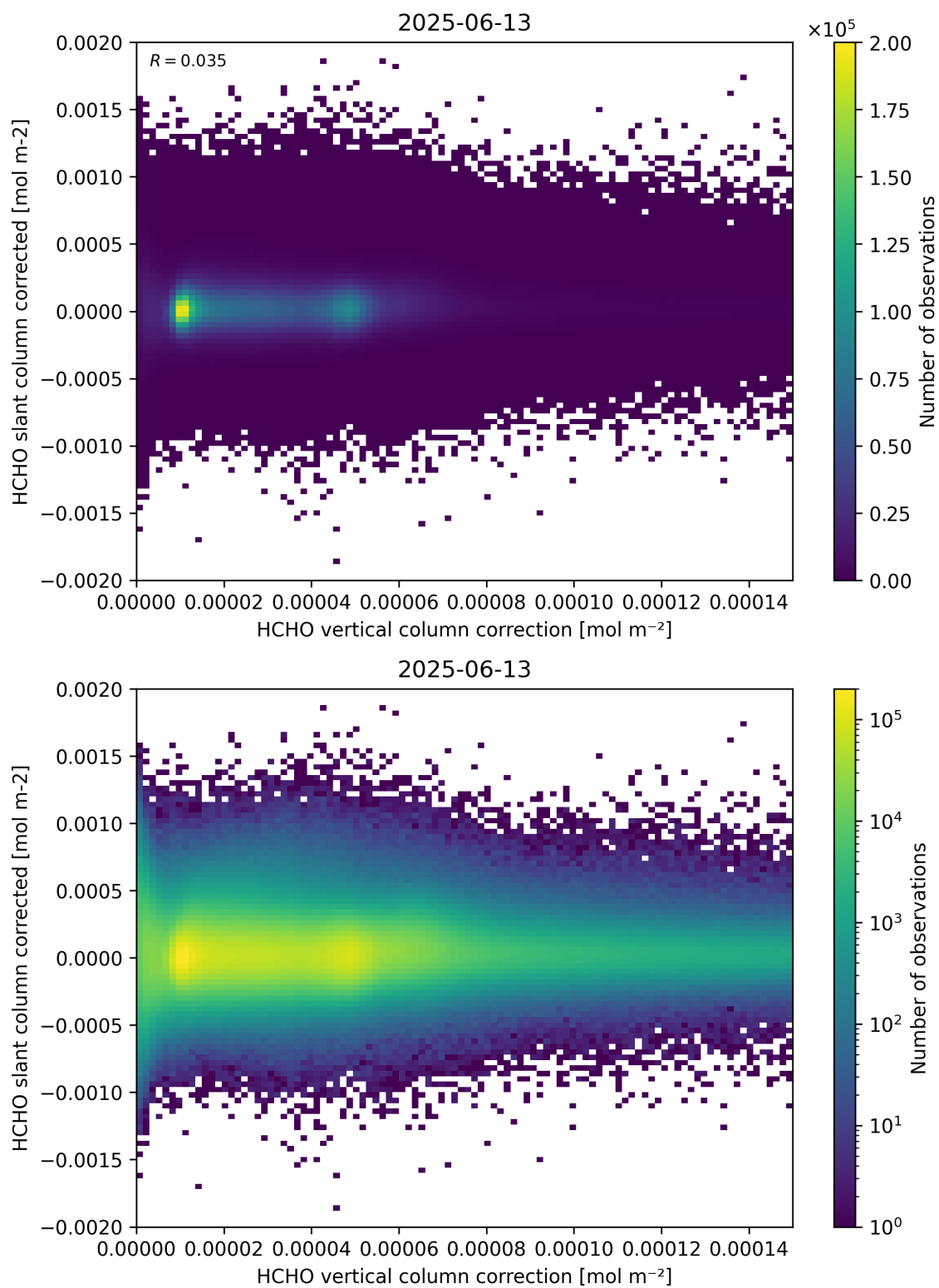
Figure 116: Scatter density plot of “HCHO vertical column correction” against “HCHO slant column corrected” for 2025-06-12 to 2025-06-14.
