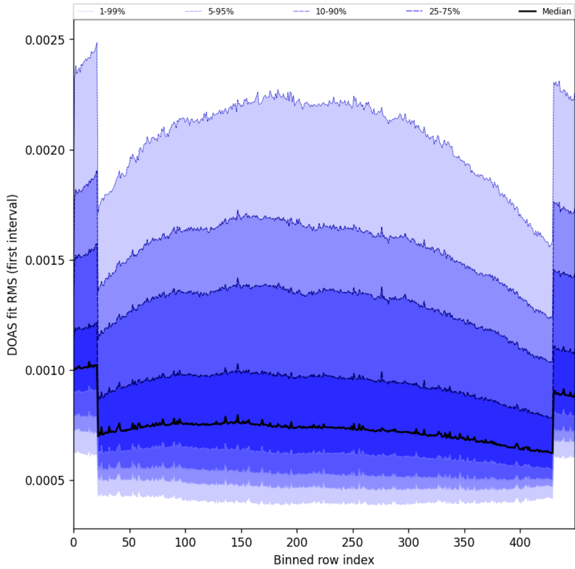
Figure 60: Along track statistics of “DOAS fit RMS (first interval)” for 2025-06-12 to 2025-06-14
