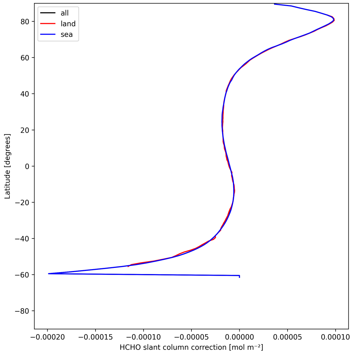
Figure 33: Zonal average of “HCHO slant column correction” for 2025-06-12 to 2025-06-14.
