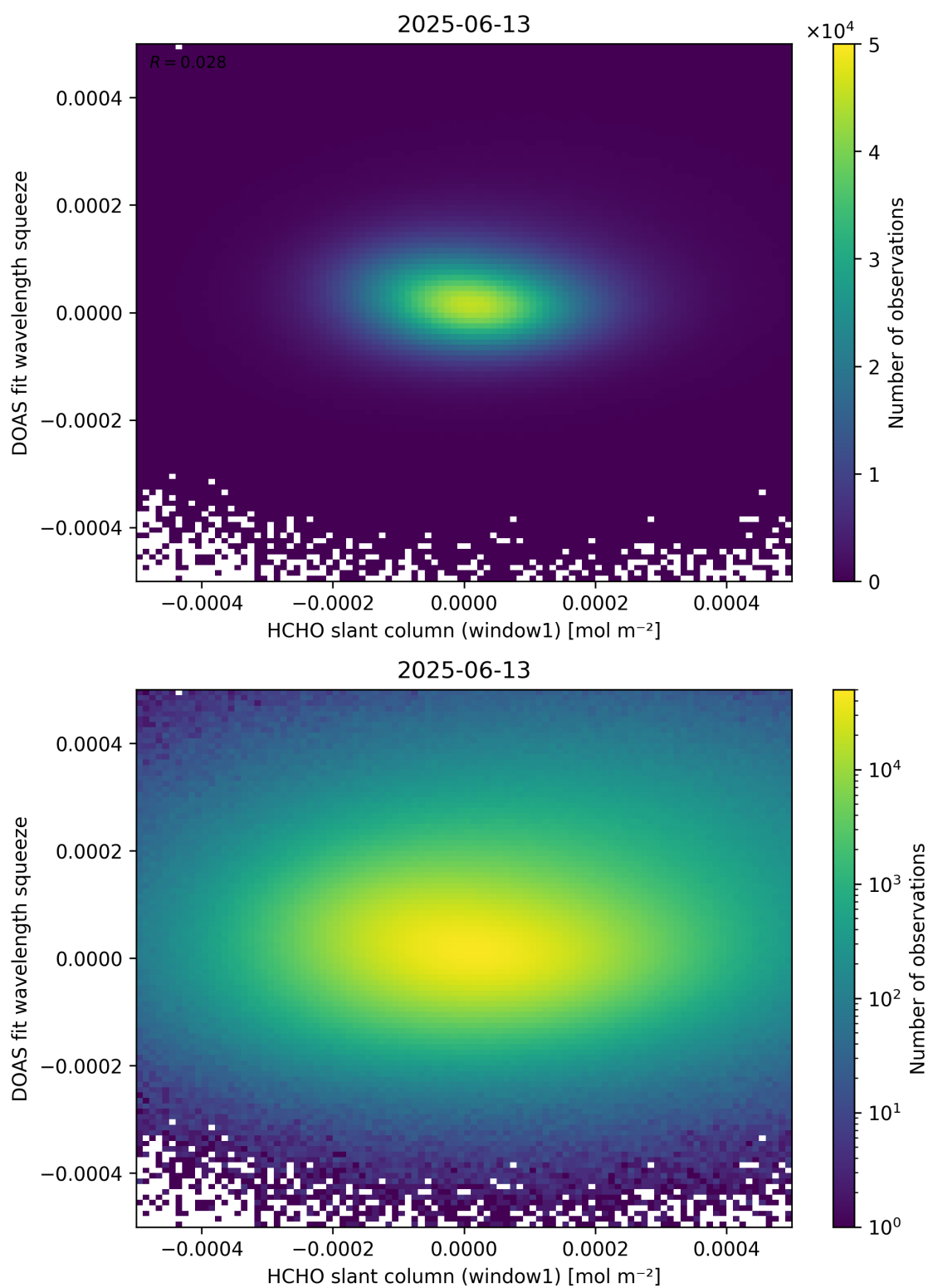
Figure 80: Scatter density plot of “HCHO slant column (window1)” against “DOAS fit wavelength squeeze” for 2025-06-12 to 2025-06-14.
