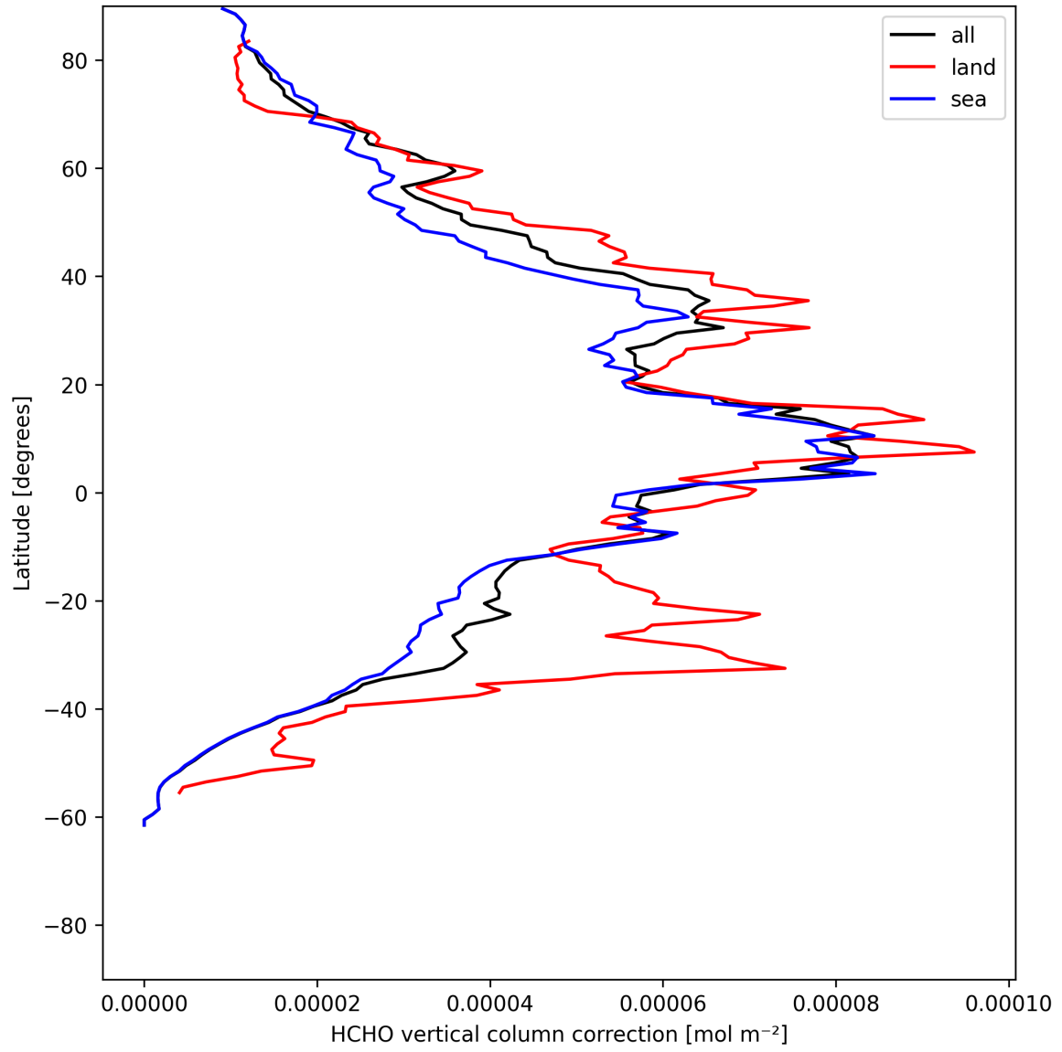
Figure 23: Zonal average of “HCHO vertical column correction” for 2025-06-12 to 2025-06-14.
