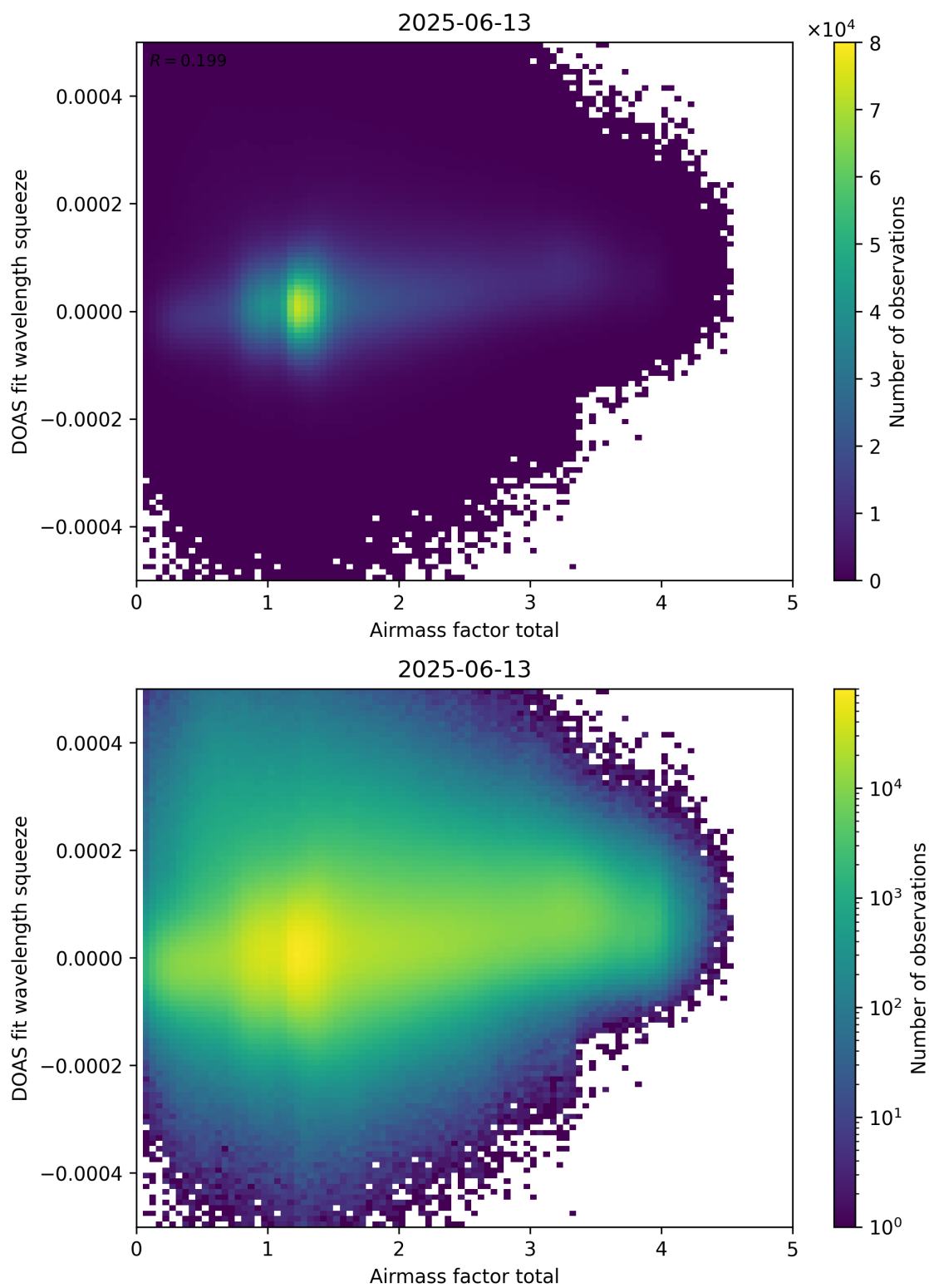
Figure 99: Scatter density plot of “Airmass factor total” against “DOAS fit wavelength squeeze” for 2025-06-12 to 2025-06-14.
