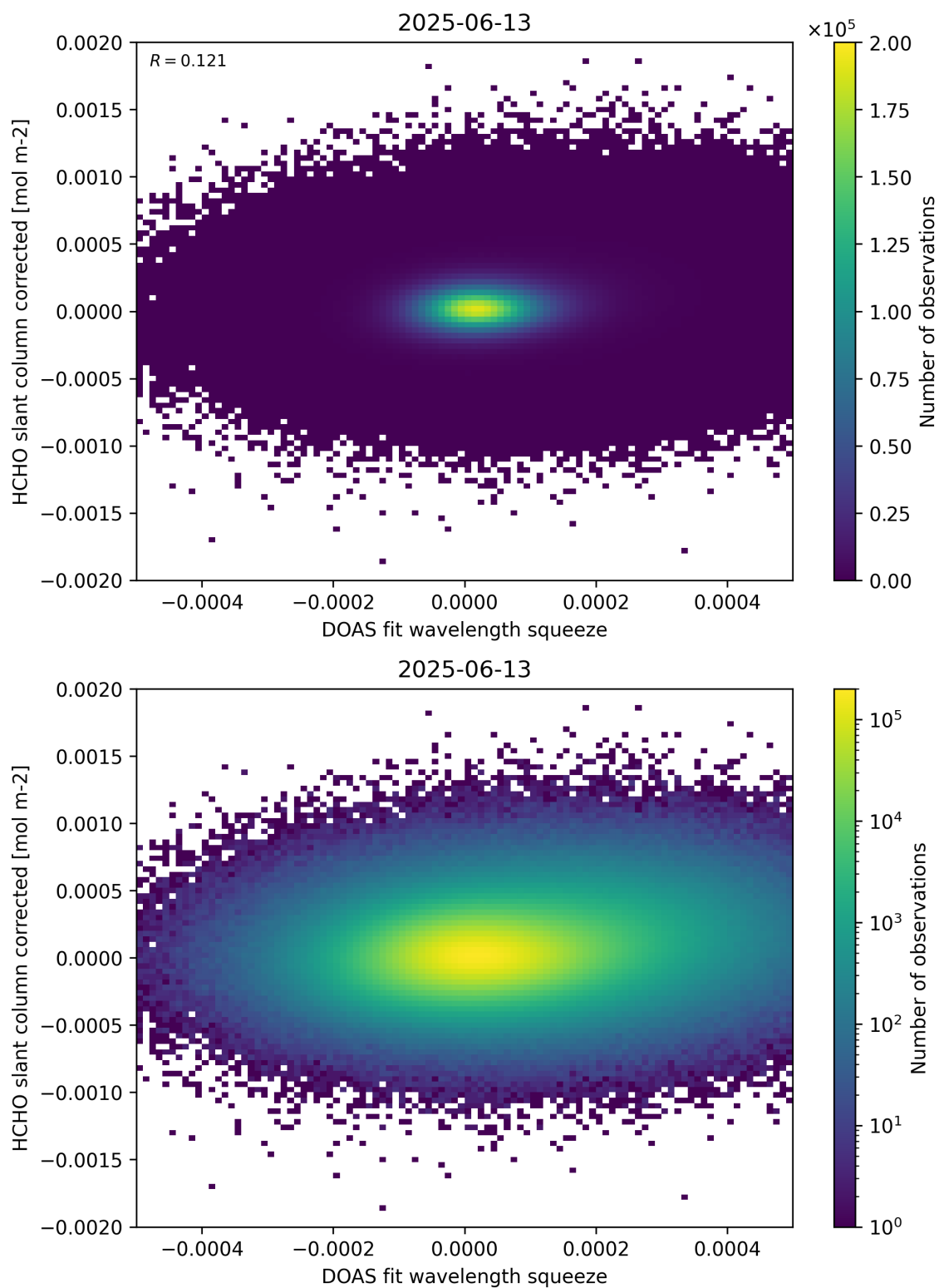
Figure 69: Scatter density plot of “DOAS fit wavelength squeeze” against “HCHO slant column corrected” for 2025-06-12 to 2025-06-14.
