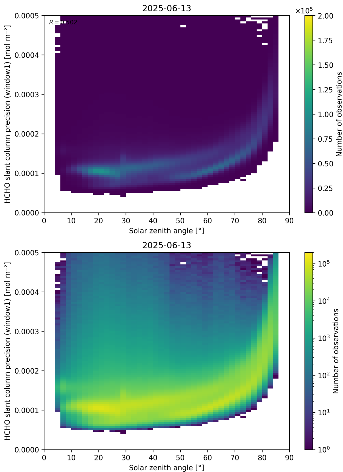
Figure 174: Scatter density plot of “Solar zenith angle” against “HCHO slant column precision (window1)” for 2025-06-12 to 2025-06-14.
