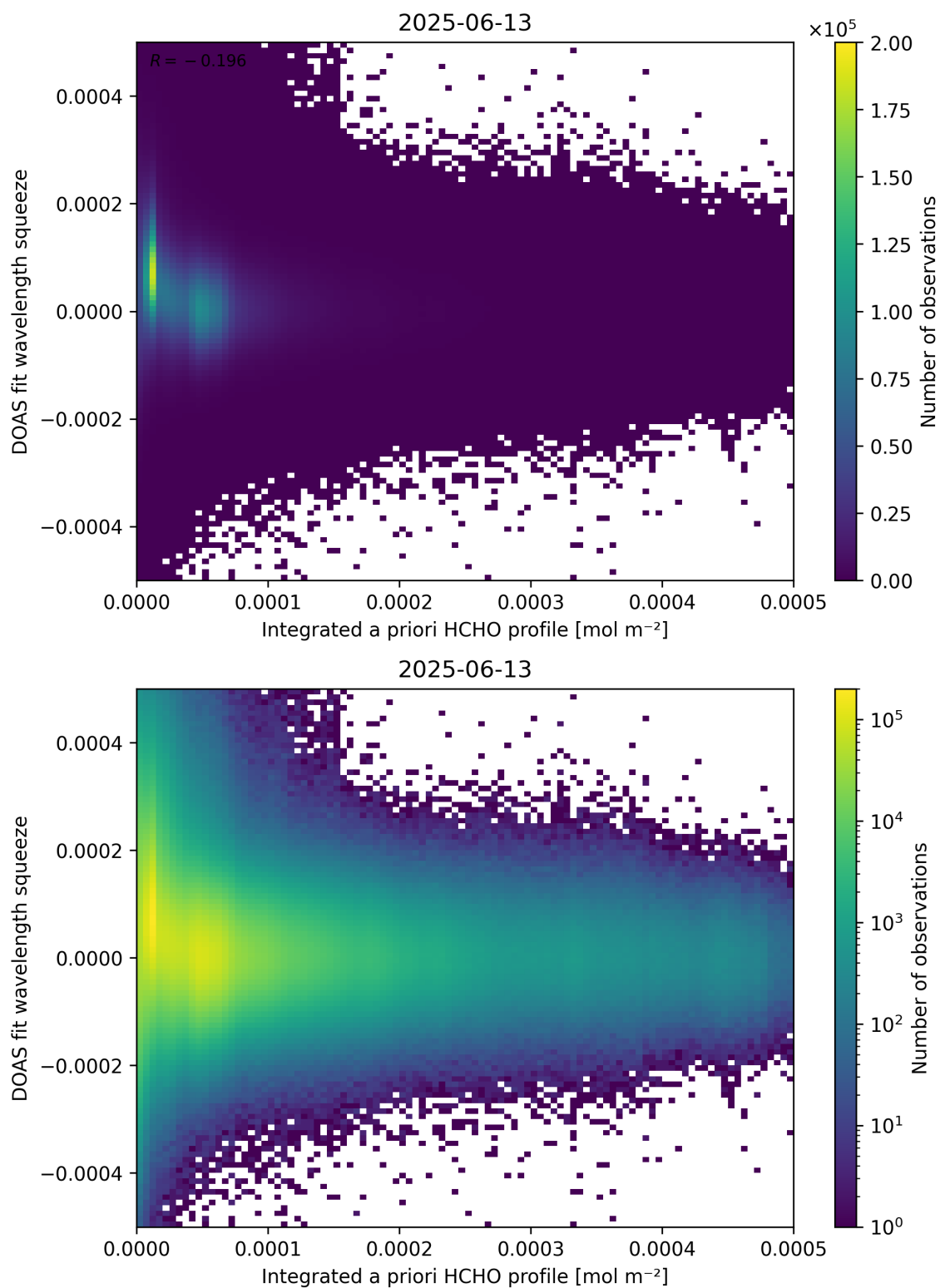
Figure 150: Scatter density plot of “Integrated a priori HCHO profile” against “DOAS fit wavelength squeeze” for 2025-06-12 to 2025-06-14.
