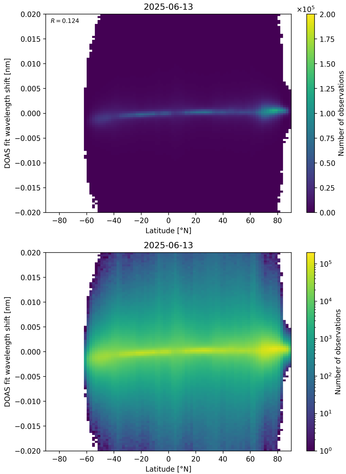
Figure 154: Scatter density plot of “Latitude” against “DOAS fit wavelength shift” for 2025-06-12 to 2025-06-14.
