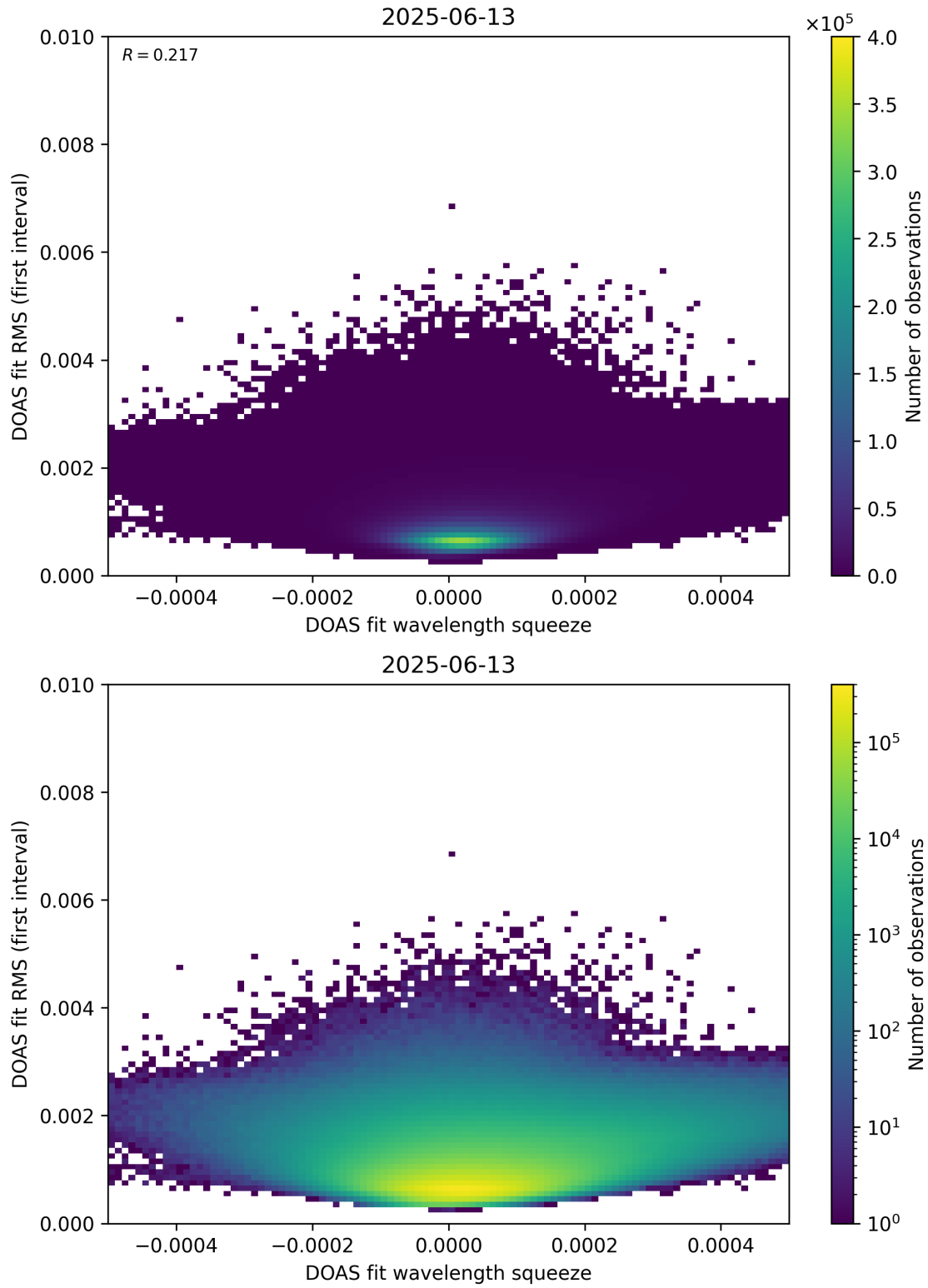
Figure 68: Scatter density plot of “DOAS fit wavelength squeeze” against “DOAS fit RMS (first interval)” for 2025-06-12 to 2025-06-14.
