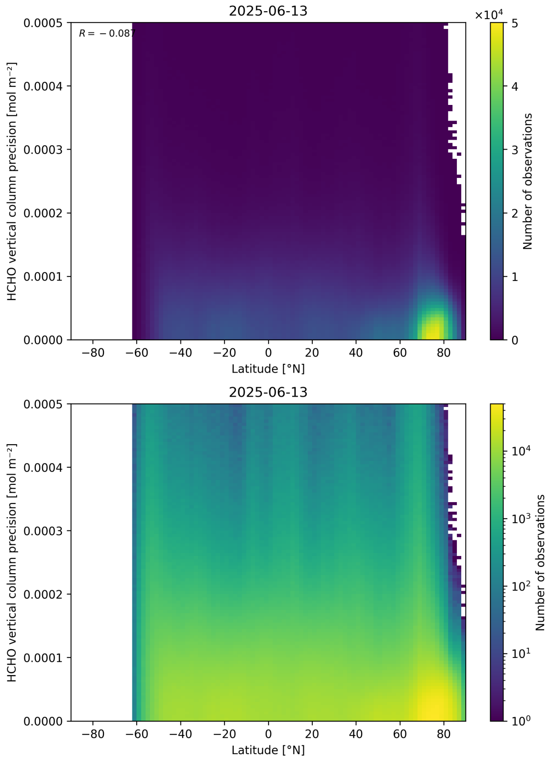
Figure 165: Scatter density plot of “Latitude” against “HCHO vertical column precision” for 2025-06-12 to 2025-06-14.
