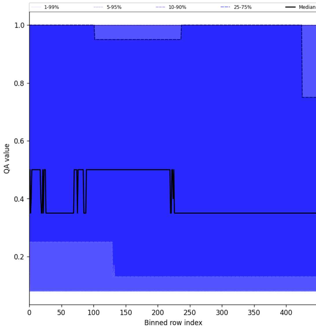
Figure 48: Along track statistics of “QA value” for 2025-06-12 to 2025-06-14
