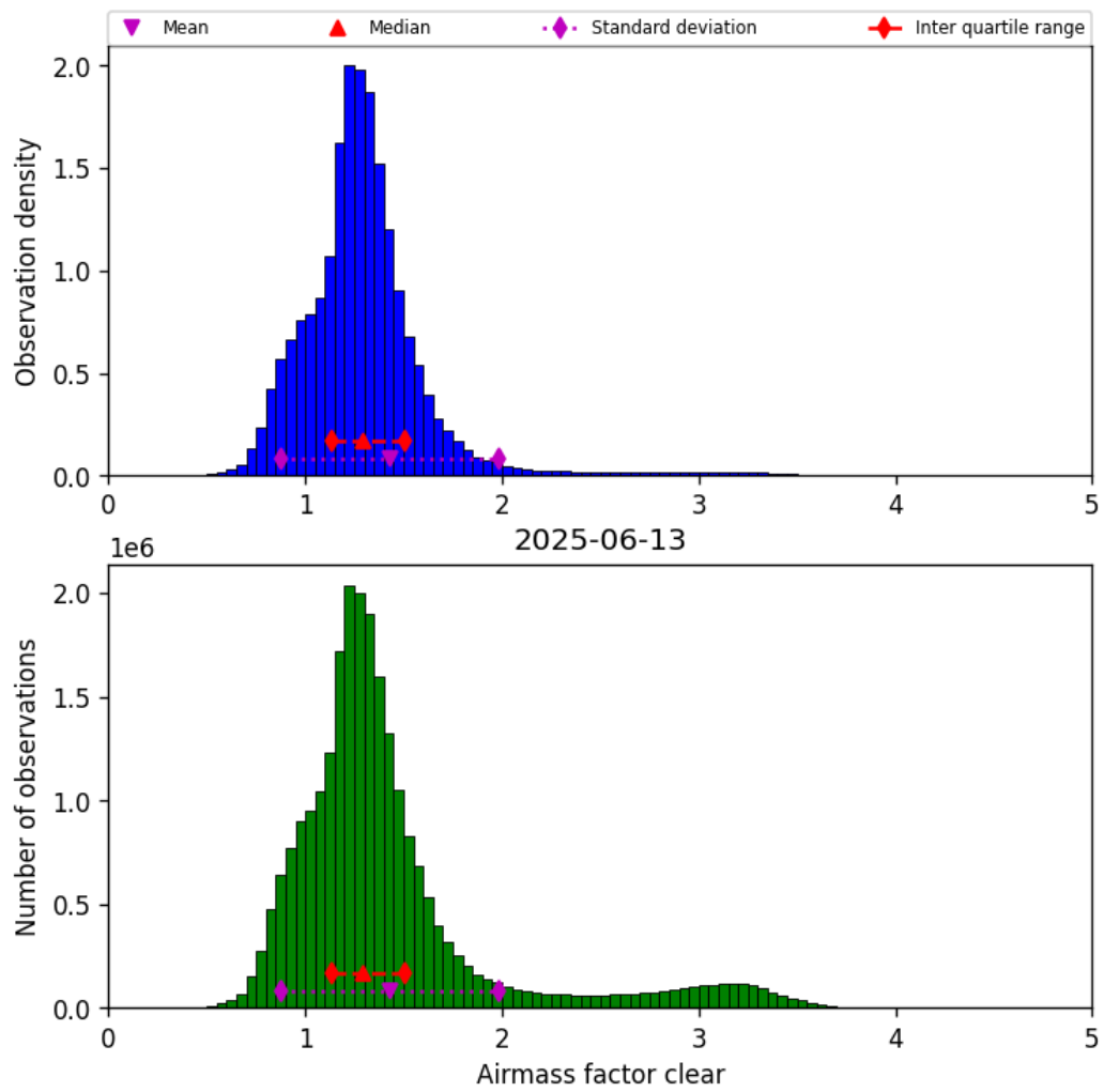
Figure 42: Histogram of “Airmass factor clear” for 2025-06-12 to 2025-06-14
