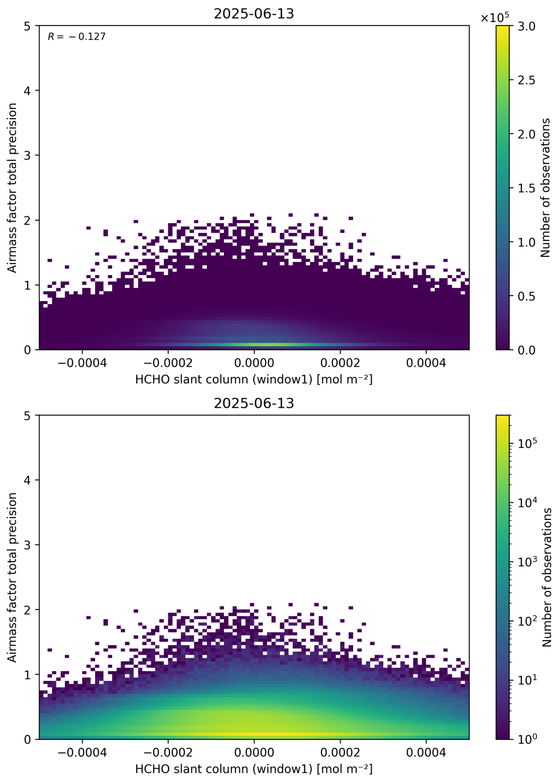
Figure 86: Scatter density plot of “HCHO slant column (window1)” against “Airmass factor total precision” for 2025-06-12 to 2025-06-14.
