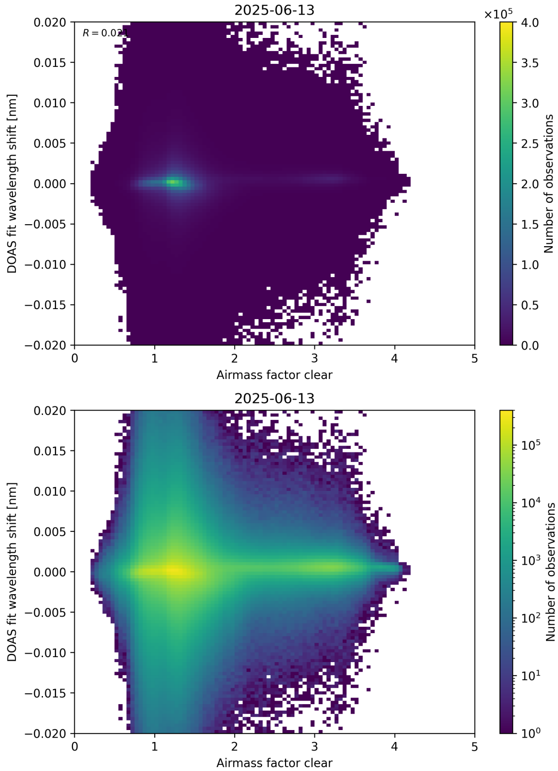
Figure 72: Scatter density plot of “Airmass factor clear” against “DOAS fit wavelength shift” for 2025-06-12 to 2025-06-14.
