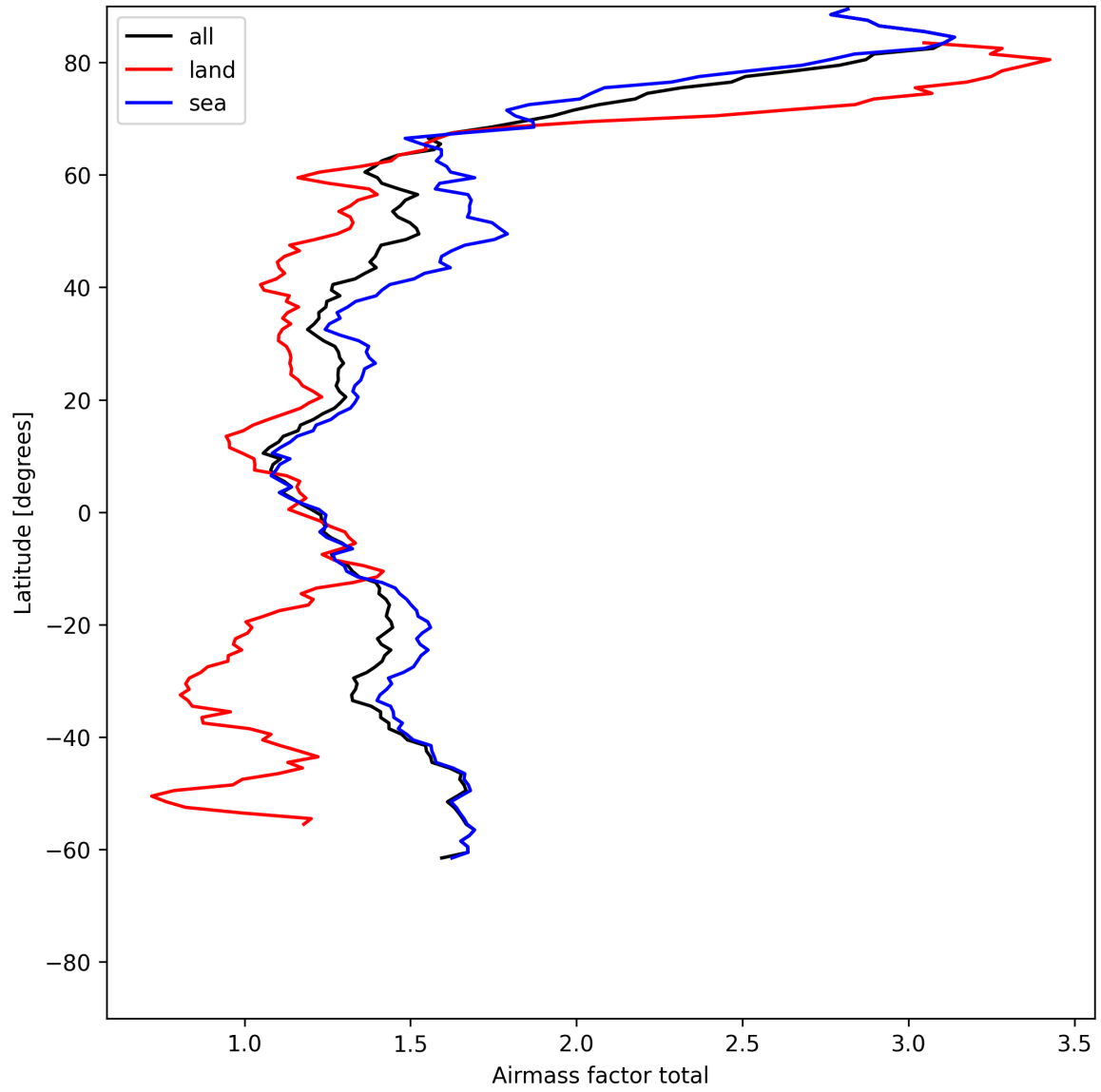
Figure 26: Zonal average of “Airmass factor total” for 2025-06-12 to 2025-06-14.
