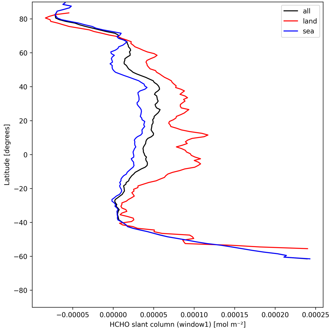
Figure 24: Zonal average of “HCHO slant column (window1)” for 2025-06-12 to 2025-06-14.
