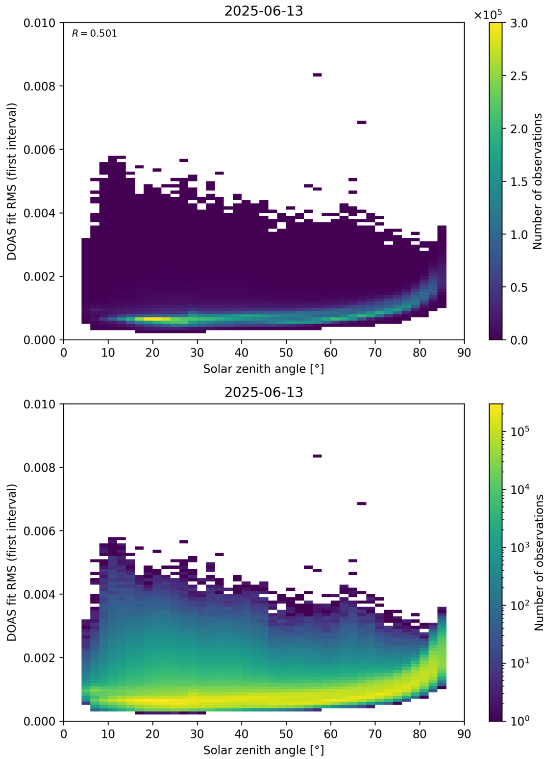
Figure 167: Scatter density plot of “Solar zenith angle” against “DOAS fit RMS (first interval)” for 2025-06-12 to 2025-06-14.
