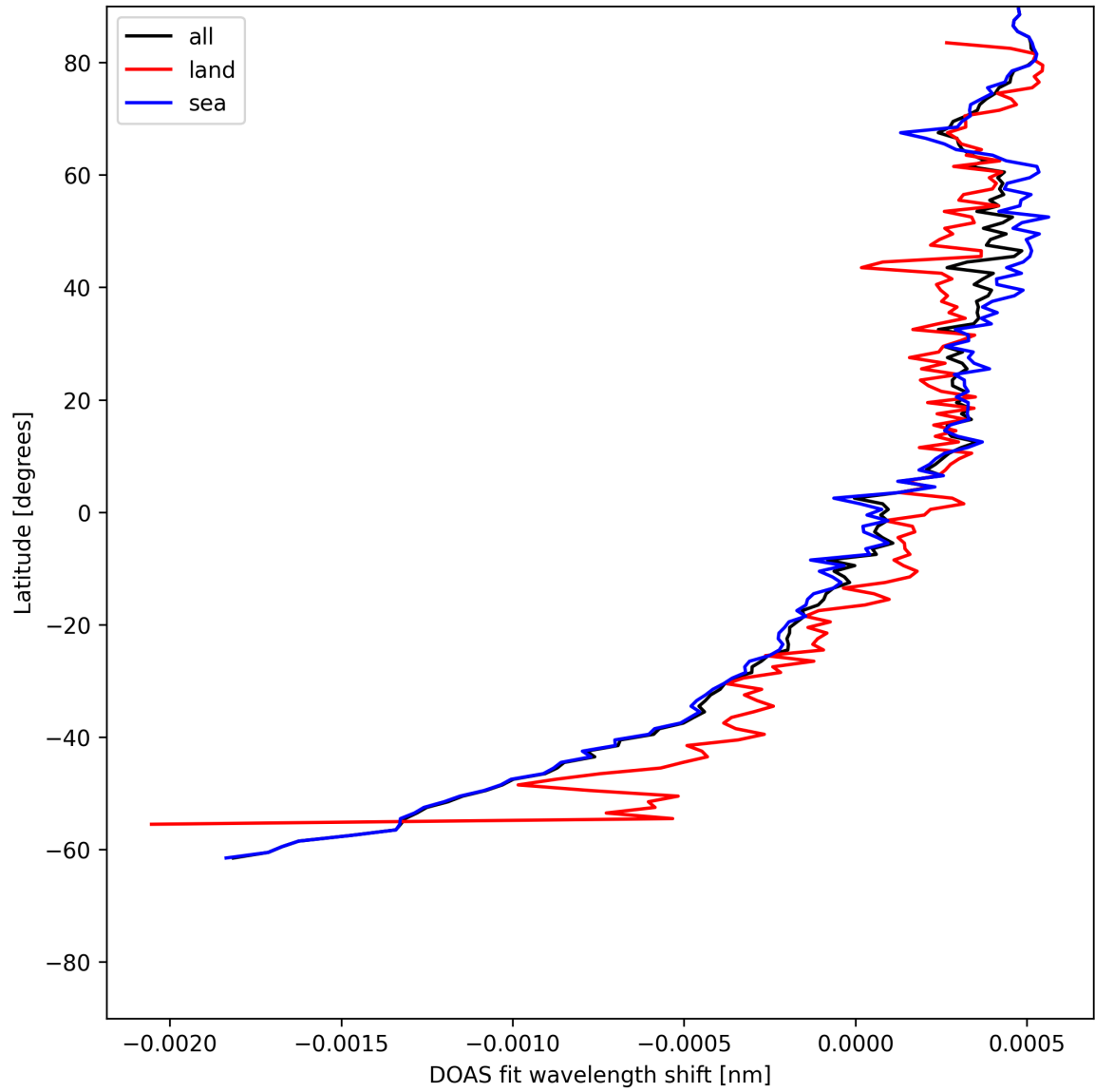
Figure 30: Zonal average of “DOAS fit wavelength shift” for 2025-06-12 to 2025-06-14.
