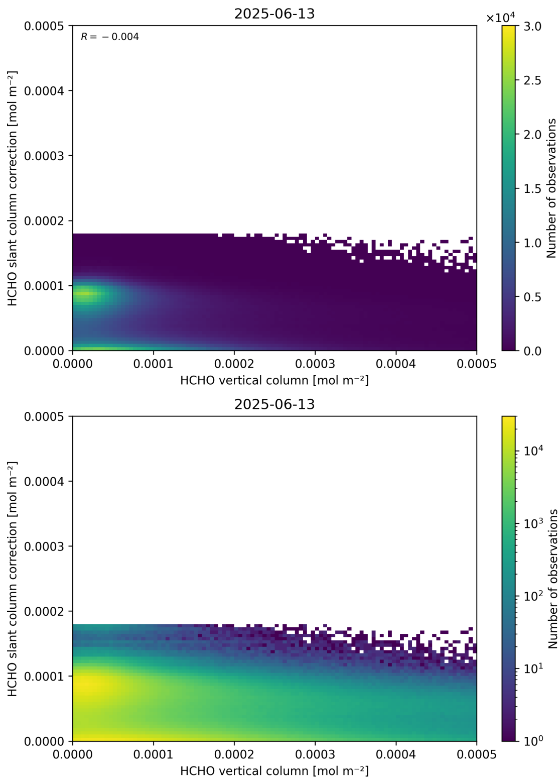
Figure 128: Scatter density plot of “HCHO vertical column” against “HCHO slant column correction” for 2025-06-12 to 2025-06-14.
