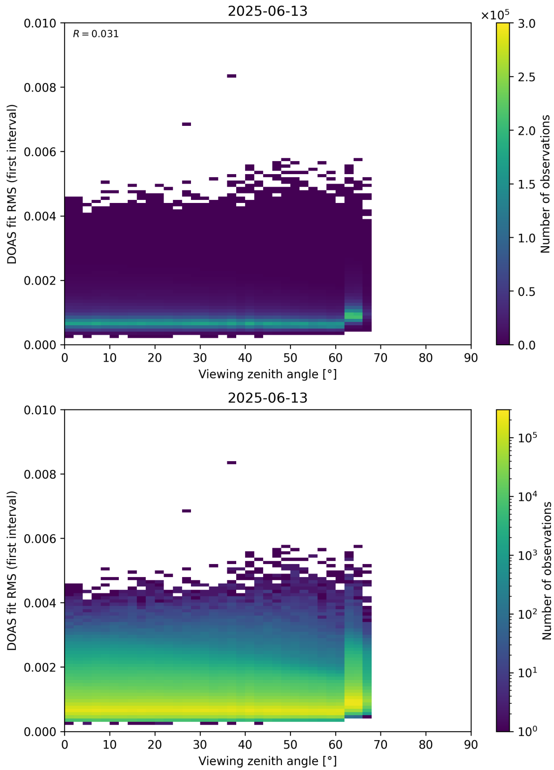
Figure 182: Scatter density plot of “Viewing zenith angle” against “DOAS fit RMS (first interval)” for 2025-06-12 to 2025-06-14.
