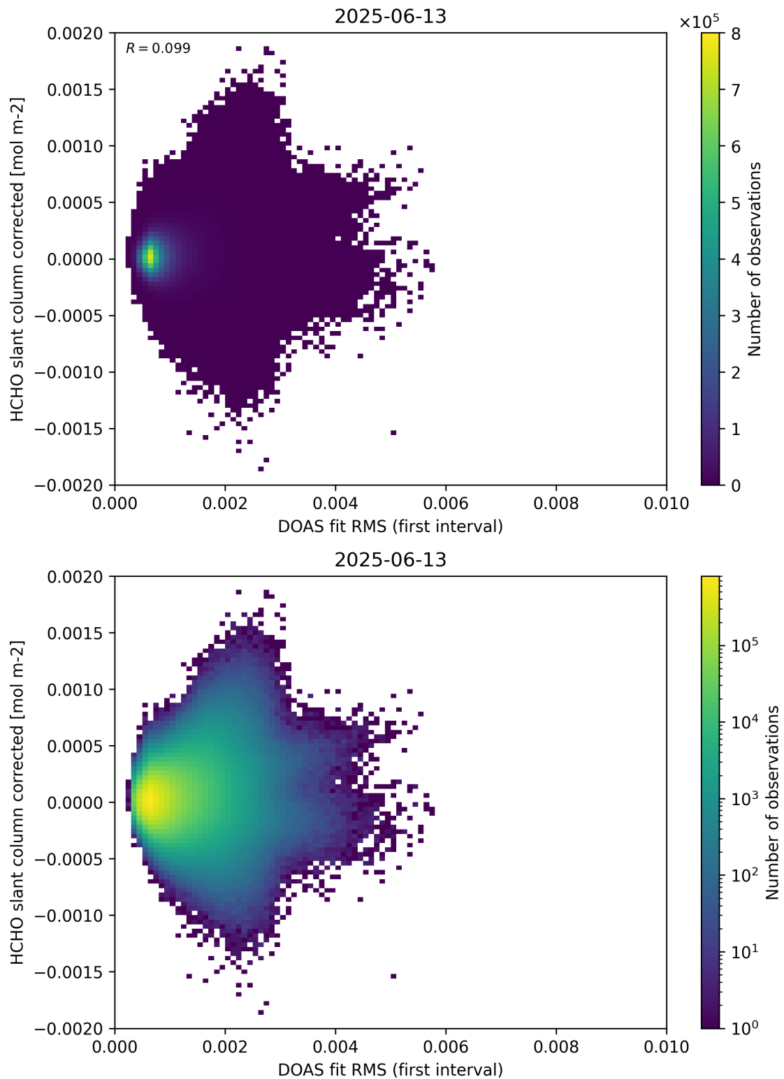
Figure 62: Scatter density plot of “DOAS fit RMS (first interval)” against “HCHO slant column corrected” for 2025-06-12 to 2025-06-14.
