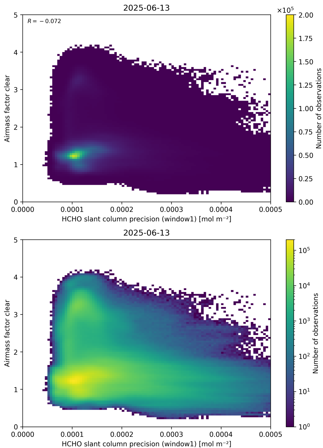
Figure 91: Scatter density plot of “HCHO slant column precision (window1)” against “Airmass factor clear” for 2025-06-12 to 2025-06-14.
