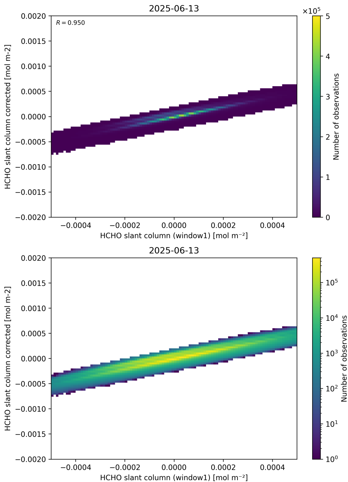
Figure 82: Scatter density plot of “HCHO slant column (window1)” against “HCHO slant column corrected” for 2025-06-12 to 2025-06-14.
