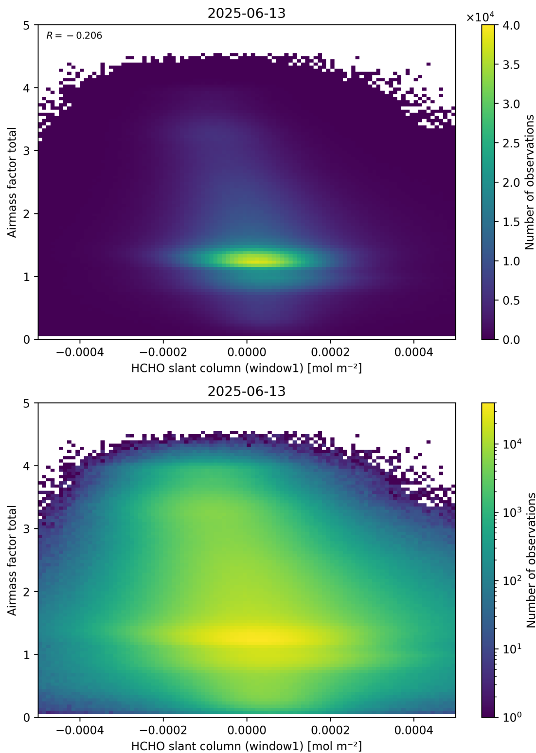
Figure 85: Scatter density plot of “HCHO slant column (window1)” against “Airmass factor total” for 2025-06-12 to 2025-06-14.
