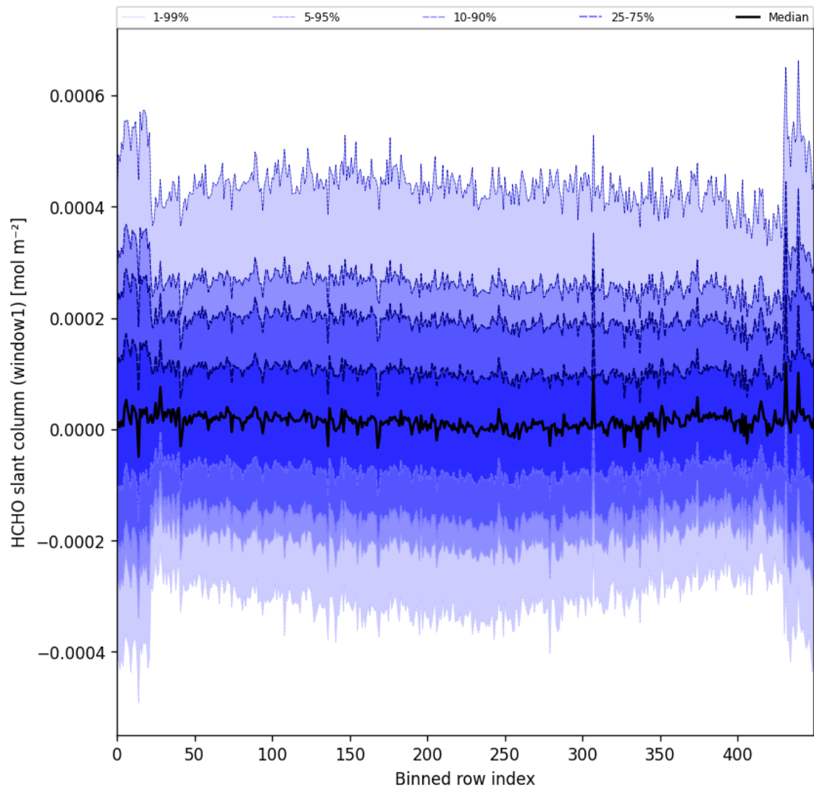
Figure 52: Along track statistics of “HCHO slant column (window1)” for 2025-06-12 to 2025-06-14
