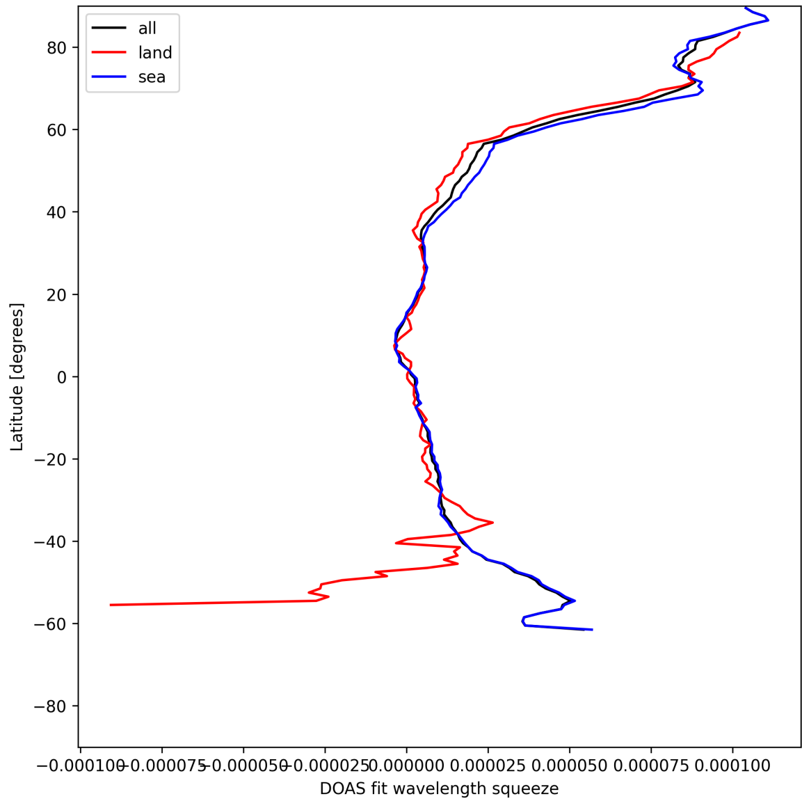
Figure 31: Zonal average of “DOAS fit wavelength squeeze” for 2025-06-12 to 2025-06-14.
