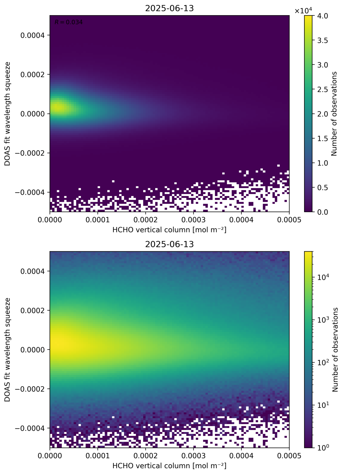
Figure 125: Scatter density plot of “HCHO vertical column” against “DOAS fit wavelength squeeze” for 2025-06-12 to 2025-06-14.
