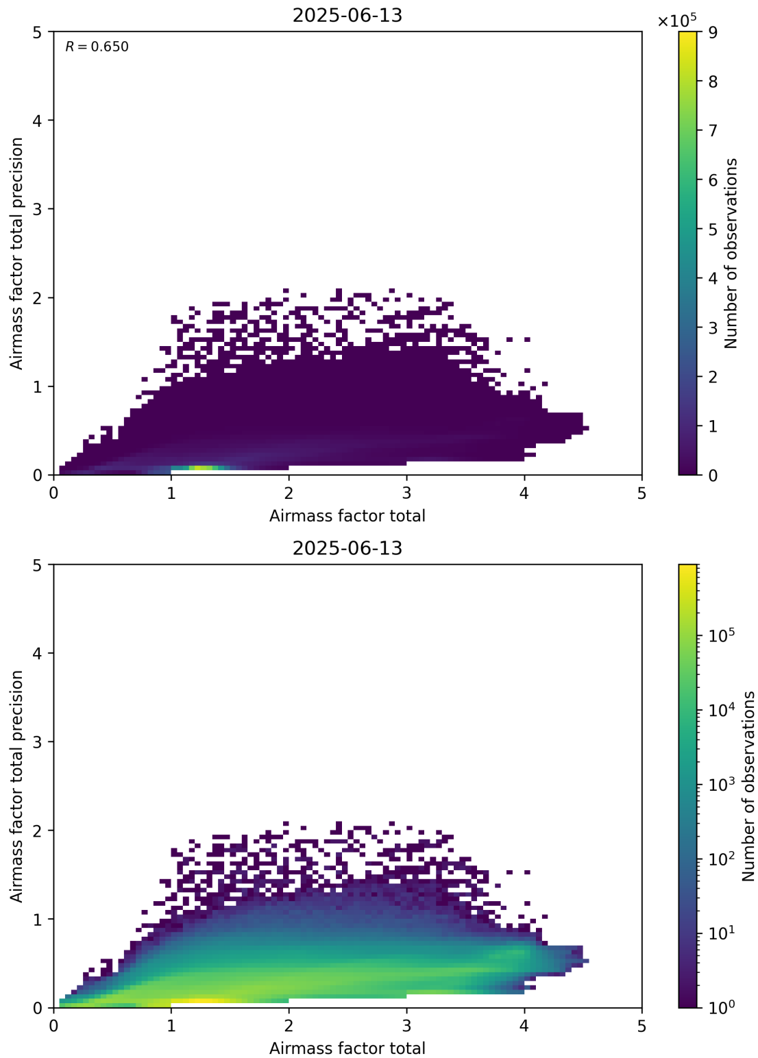
Figure 103: Scatter density plot of “Airmass factor total” against “Airmass factor total precision” for 2025-06-12 to 2025-06-14.
