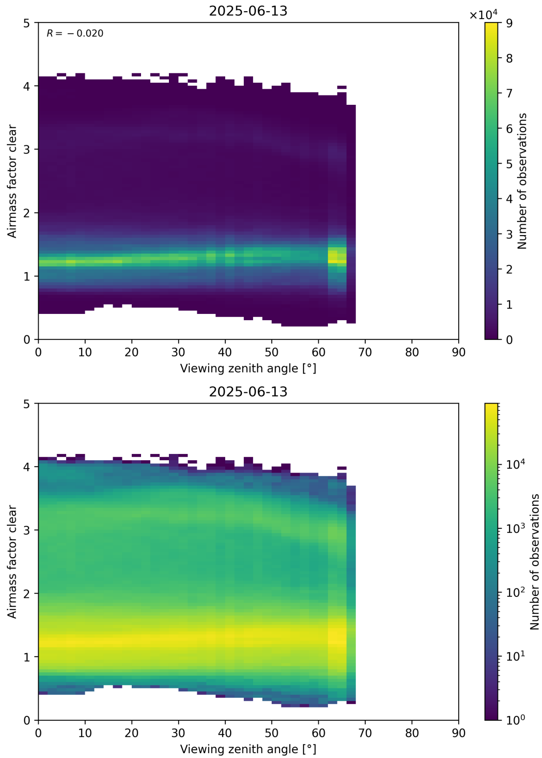
Figure 185: Scatter density plot of “Viewing zenith angle” against “Airmass factor clear” for 2025-06-12 to 2025-06-14.
