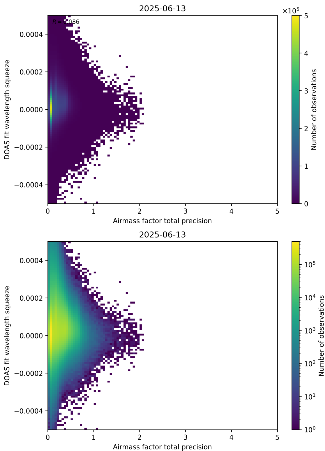
Figure 107: Scatter density plot of “Airmass factor total precision” against “DOAS fit wavelength squeeze” for 2025-06-12 to 2025-06-14.
