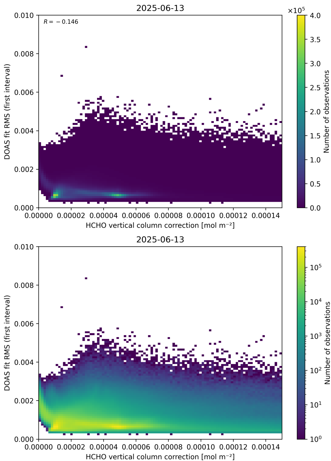
Figure 112: Scatter density plot of “HCHO vertical column correction” against “DOAS fit RMS (first interval)” for 2025-06-12 to 2025-06-14.
