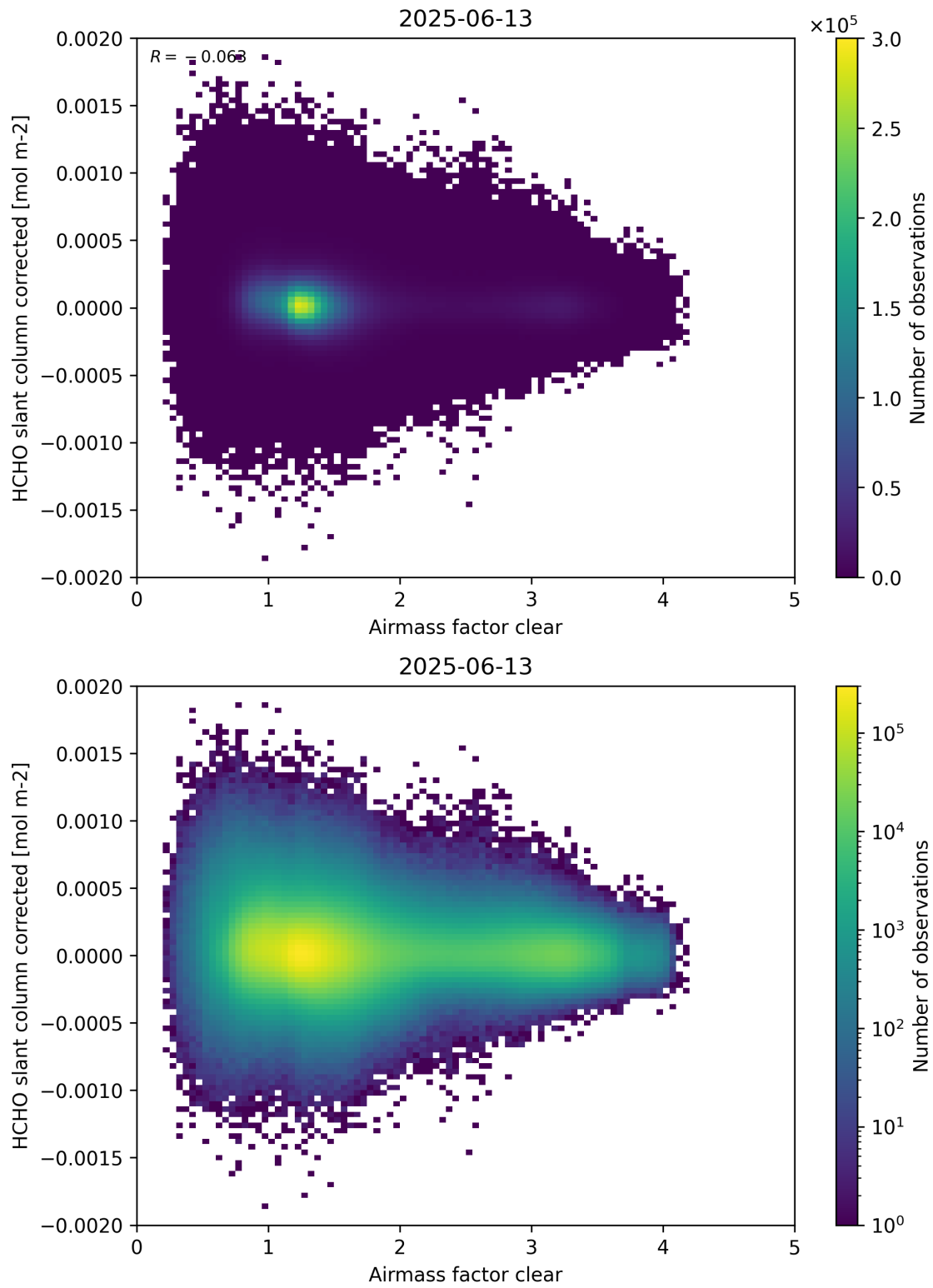
Figure 74: Scatter density plot of “Airmass factor clear” against “HCHO slant column corrected” for 2025-06-12 to 2025-06-14.
