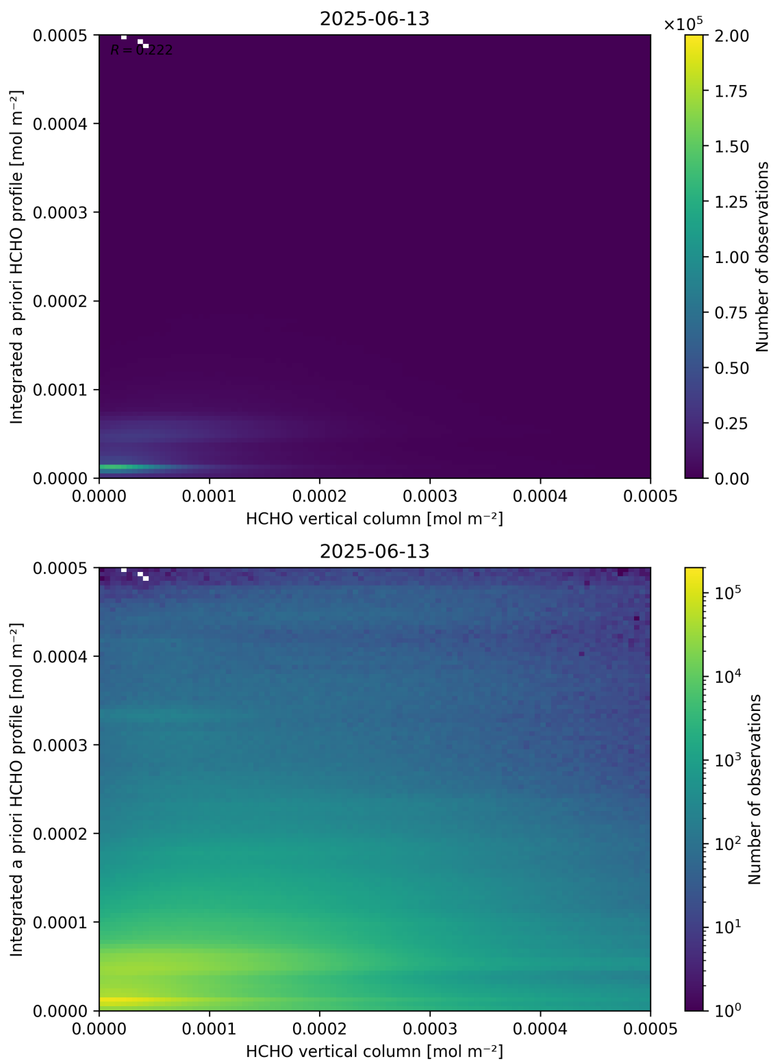
Figure 135: Scatter density plot of “HCHO vertical column” against “Integrated a priori HCHO profile” for 2025-06-12 to 2025-06-14.
