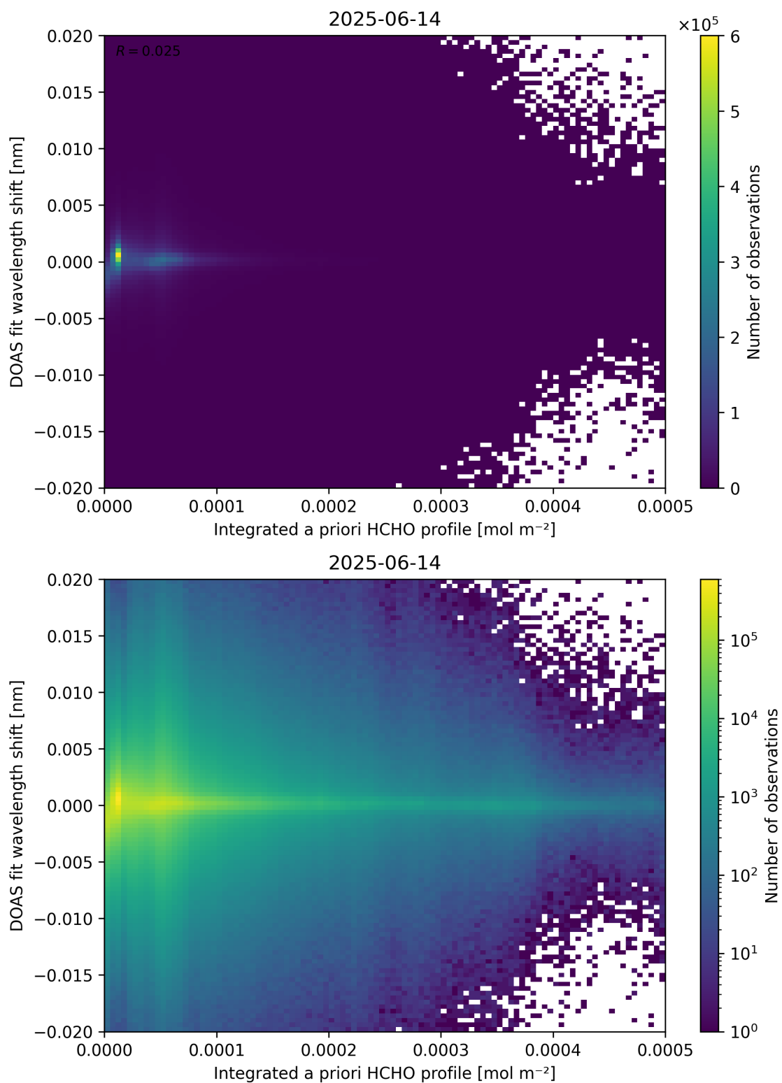
Figure 149: Scatter density plot of “Integrated a priori HCHO profile” against “DOAS fit wavelength shift” for 2025-06-13 to 2025-06-15.
