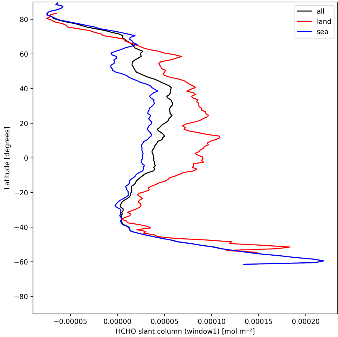
Figure 24: Zonal average of “HCHO slant column (window1)” for 2025-06-13 to 2025-06-15.
