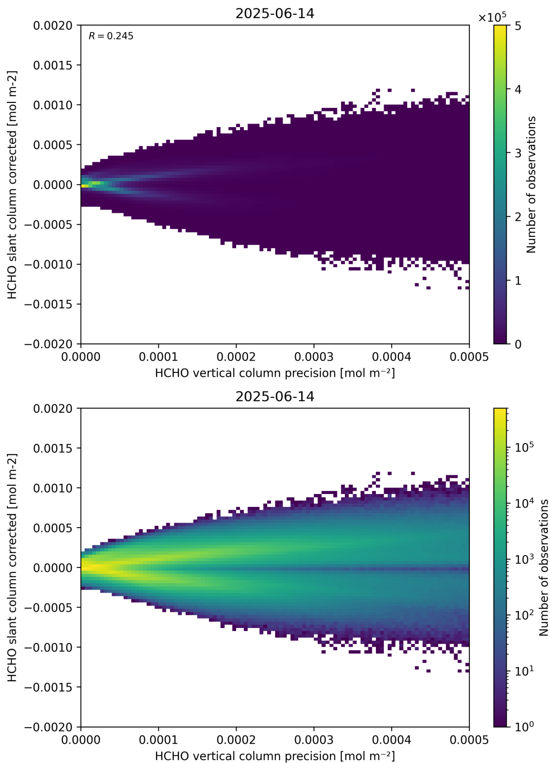
Figure 140: Scatter density plot of “HCHO vertical column precision” against “HCHO slant column corrected” for 2025-06-13 to 2025-06-15.
