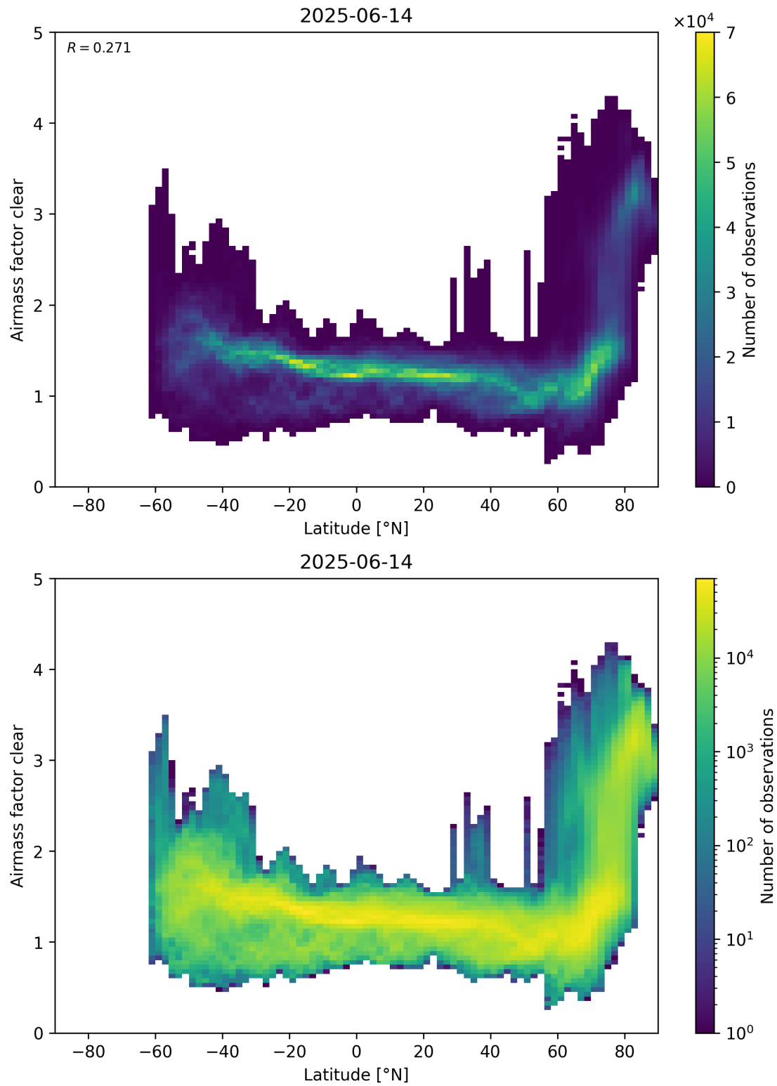
Figure 156: Scatter density plot of “Latitude” against “Airmass factor clear” for 2025-06-13 to 2025-06-15.
