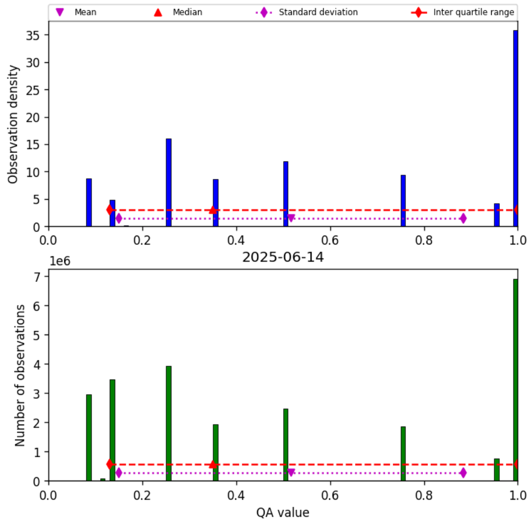
Figure 34: Histogram of “QA value” for 2025-06-13 to 2025-06-15
