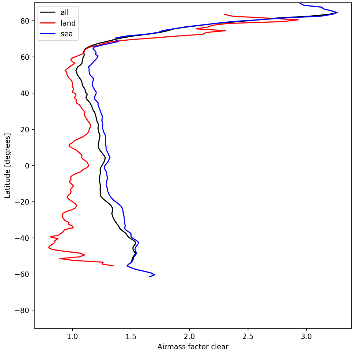
Figure 28: Zonal average of “Airmass factor clear” for 2025-06-13 to 2025-06-15.
