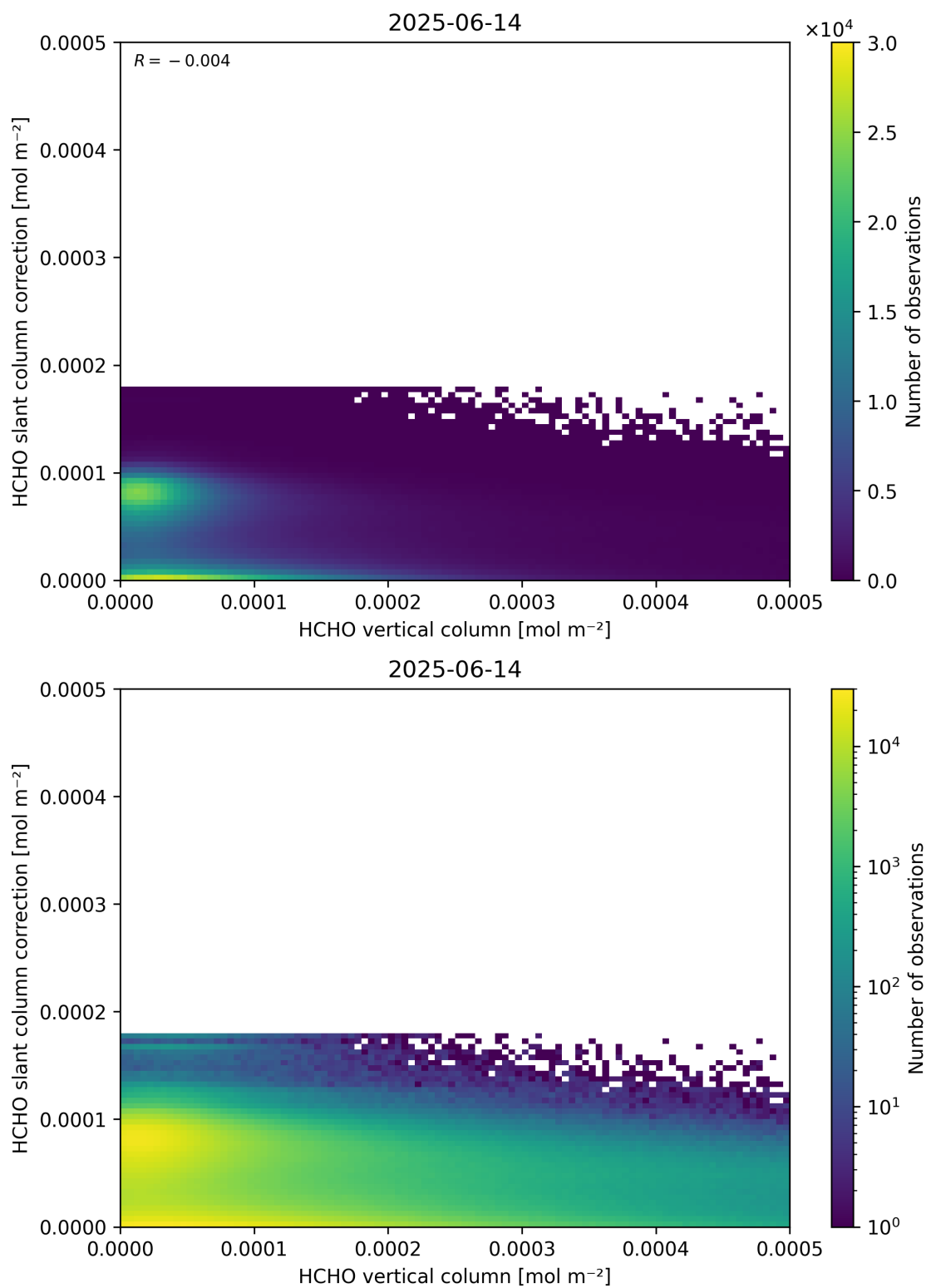
Figure 128: Scatter density plot of “HCHO vertical column” against “HCHO slant column correction” for 2025-06-13 to 2025-06-15.
