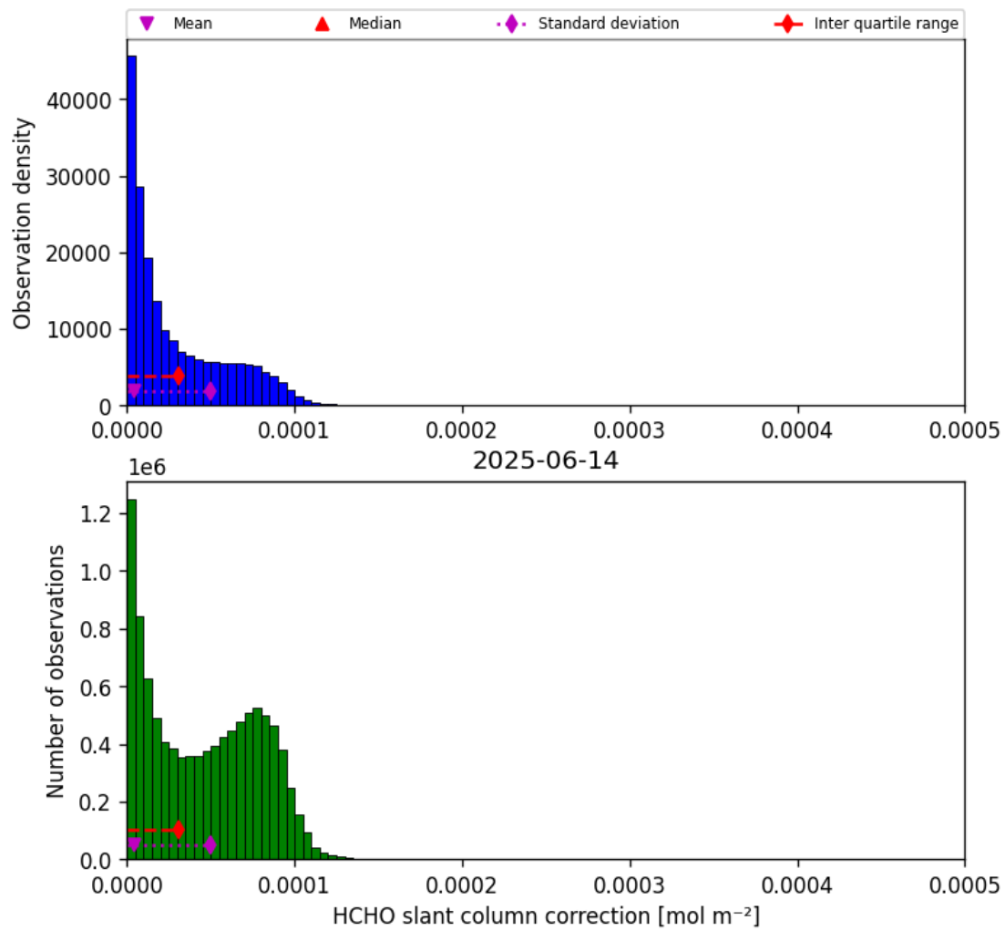
Figure 47: Histogram of “HCHO slant column correction” for 2025-06-13 to 2025-06-15
