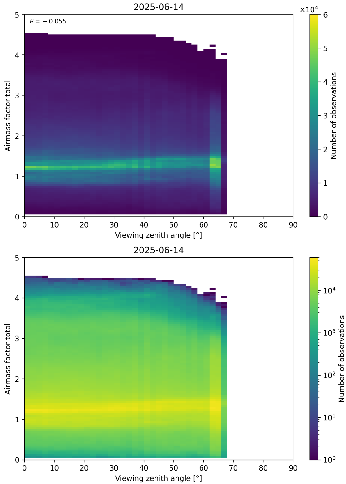
Figure 190: Scatter density plot of “Viewing zenith angle” against “Airmass factor total” for 2025-06-13 to 2025-06-15.
