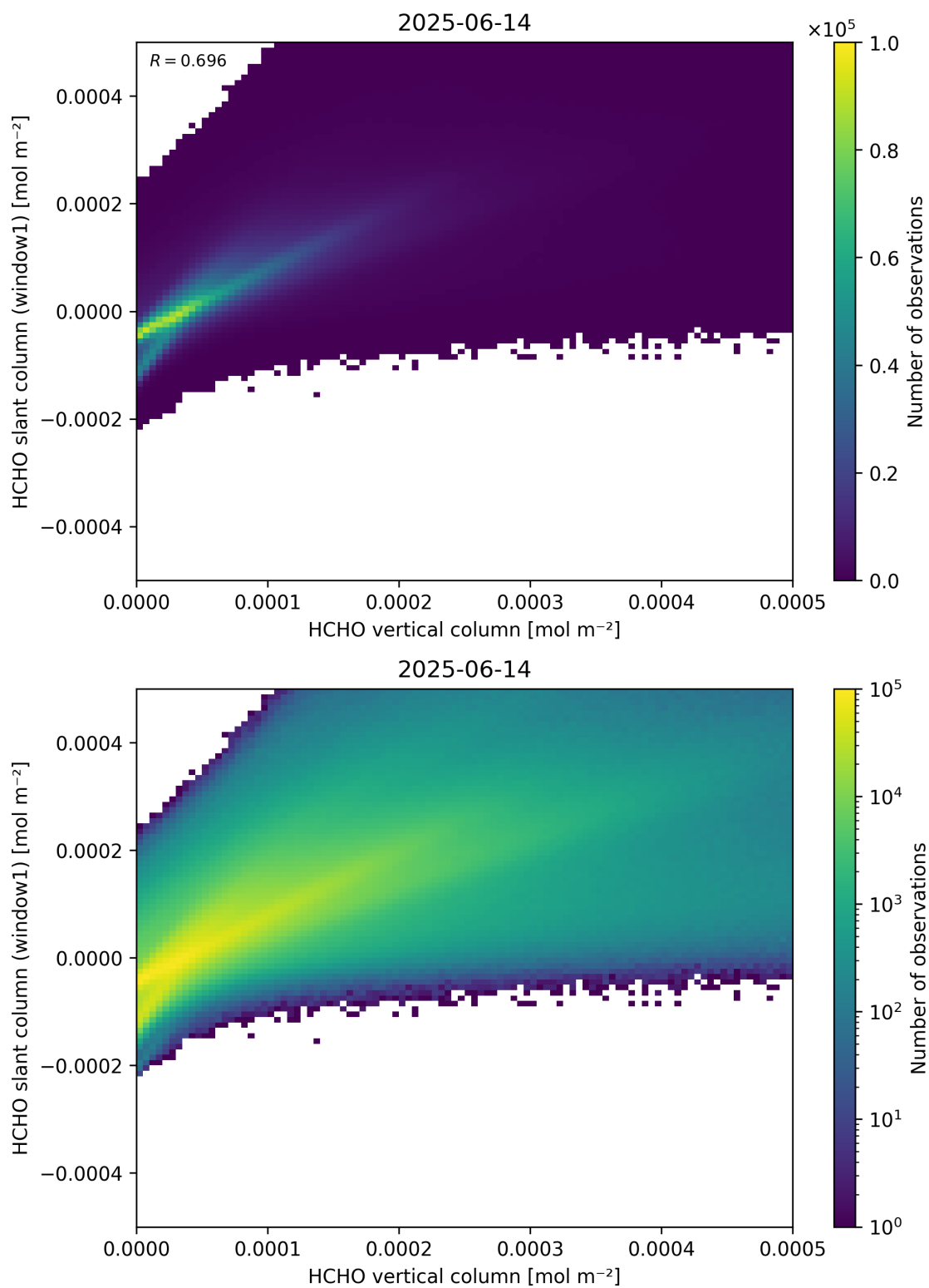
Figure 129: Scatter density plot of “HCHO vertical column” against “HCHO slant column (window1)” for 2025-06-13 to 2025-06-15.
