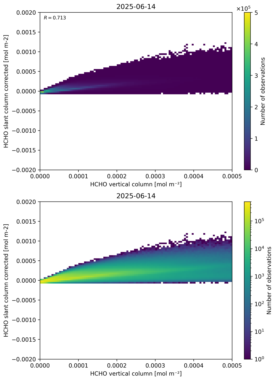
Figure 127: Scatter density plot of “HCHO vertical column” against “HCHO slant column corrected” for 2025-06-13 to 2025-06-15.
