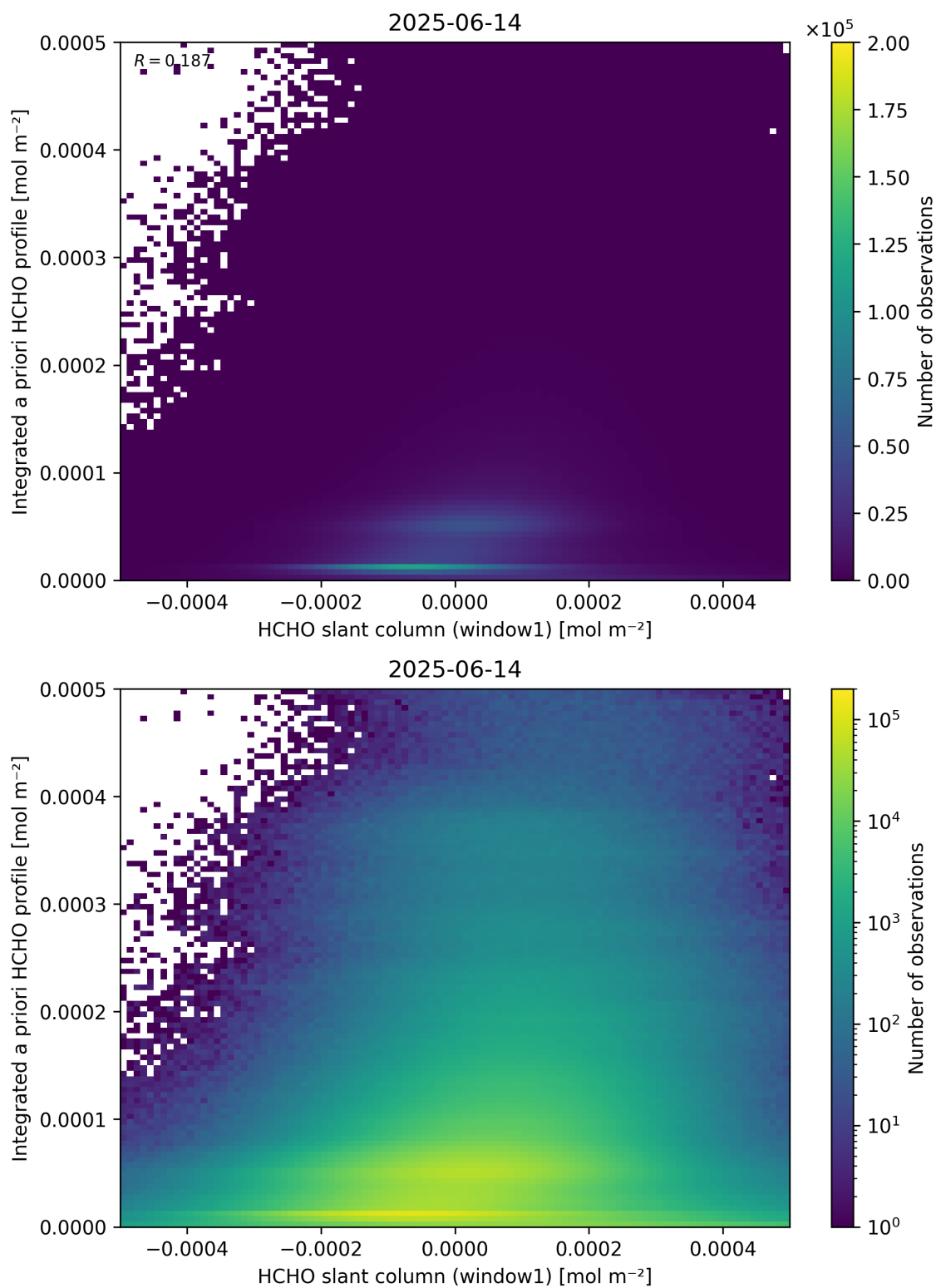
Figure 87: Scatter density plot of “HCHO slant column (window1)” against “Integrated a priori HCHO profile” for 2025-06-13 to 2025-06-15.
