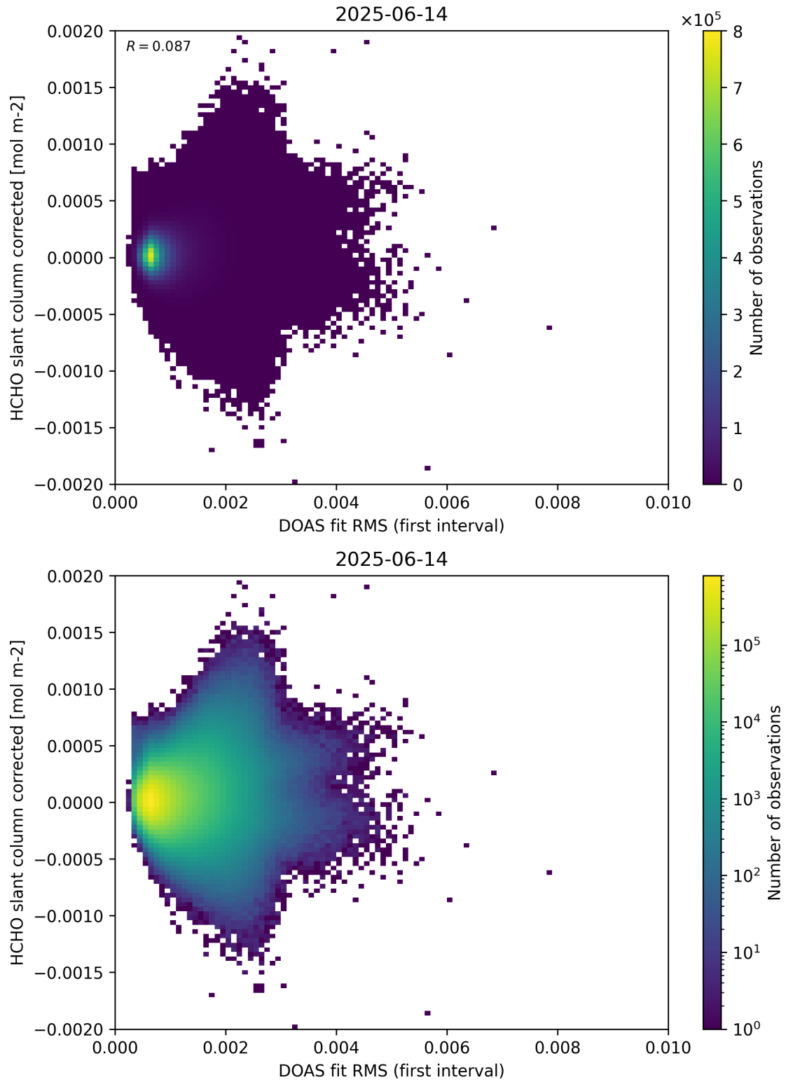
Figure 62: Scatter density plot of “DOAS fit RMS (first interval)” against “HCHO slant column corrected” for 2025-06-13 to 2025-06-15.
