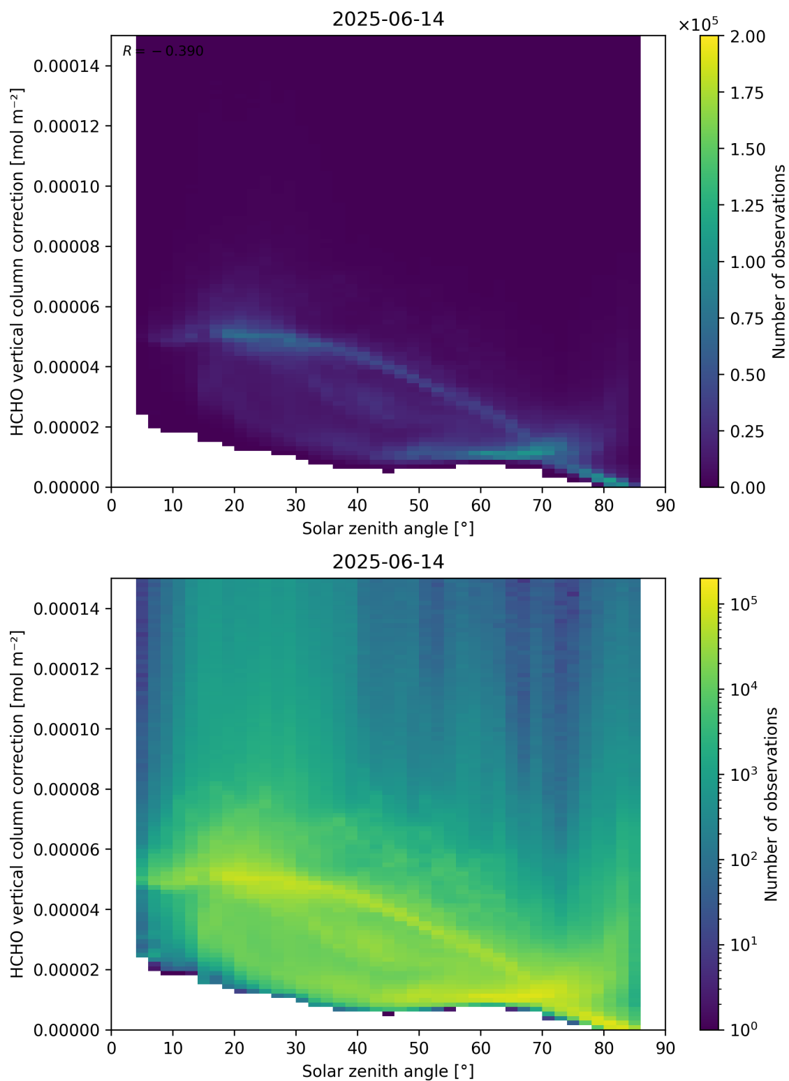
Figure 178: Scatter density plot of “Solar zenith angle” against “HCHO vertical column correction” for 2025-06-13 to 2025-06-15.
