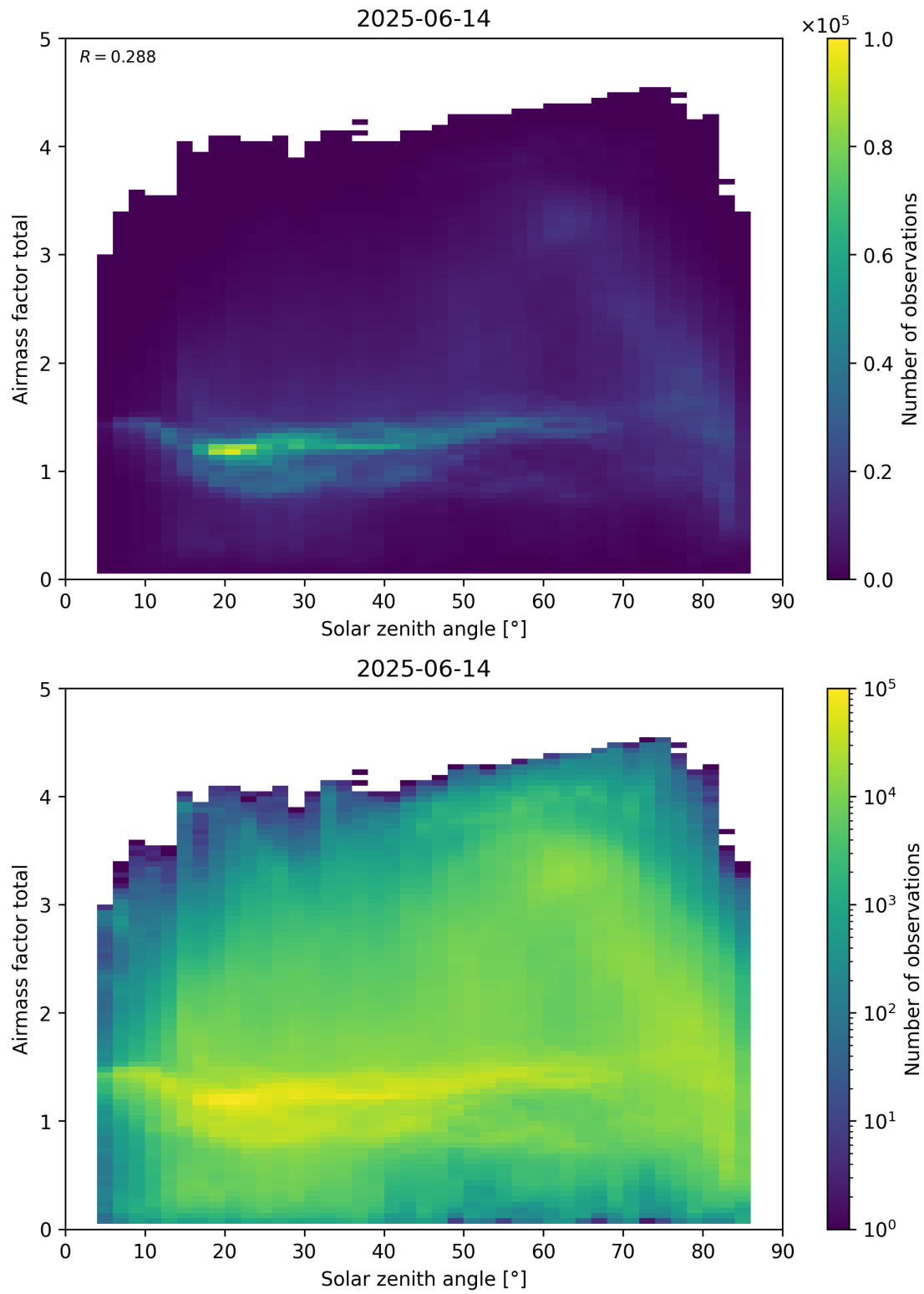
Figure 175: Scatter density plot of “Solar zenith angle” against “Airmass factor total” for 2025-06-13 to 2025-06-15.
