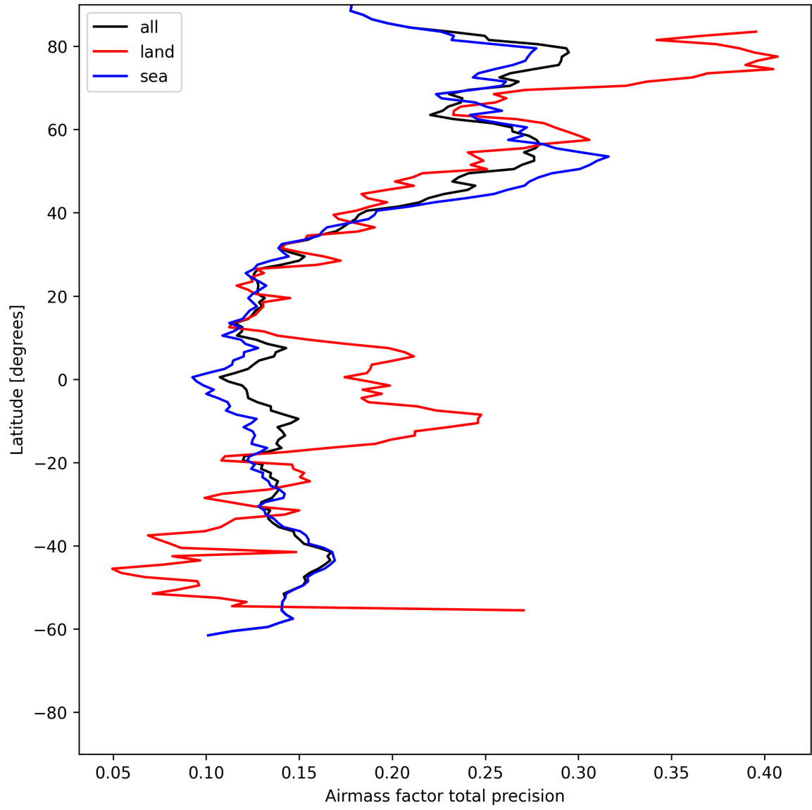
Figure 27: Zonal average of “Airmass factor total precision” for 2025-06-13 to 2025-06-15.
