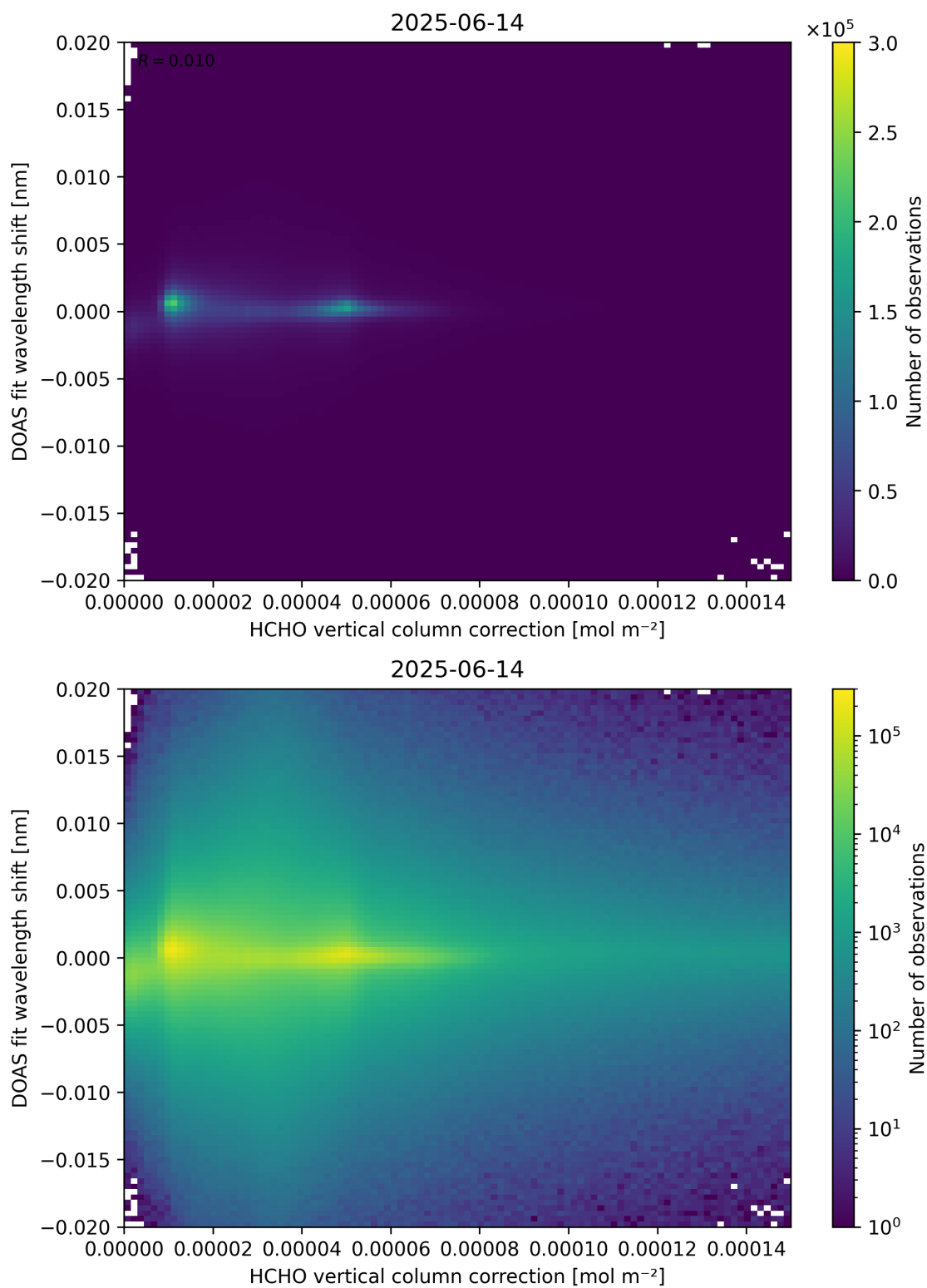
Figure 113: Scatter density plot of “HCHO vertical column correction” against “DOAS fit wavelength shift” for 2025-06-13 to 2025-06-15.
