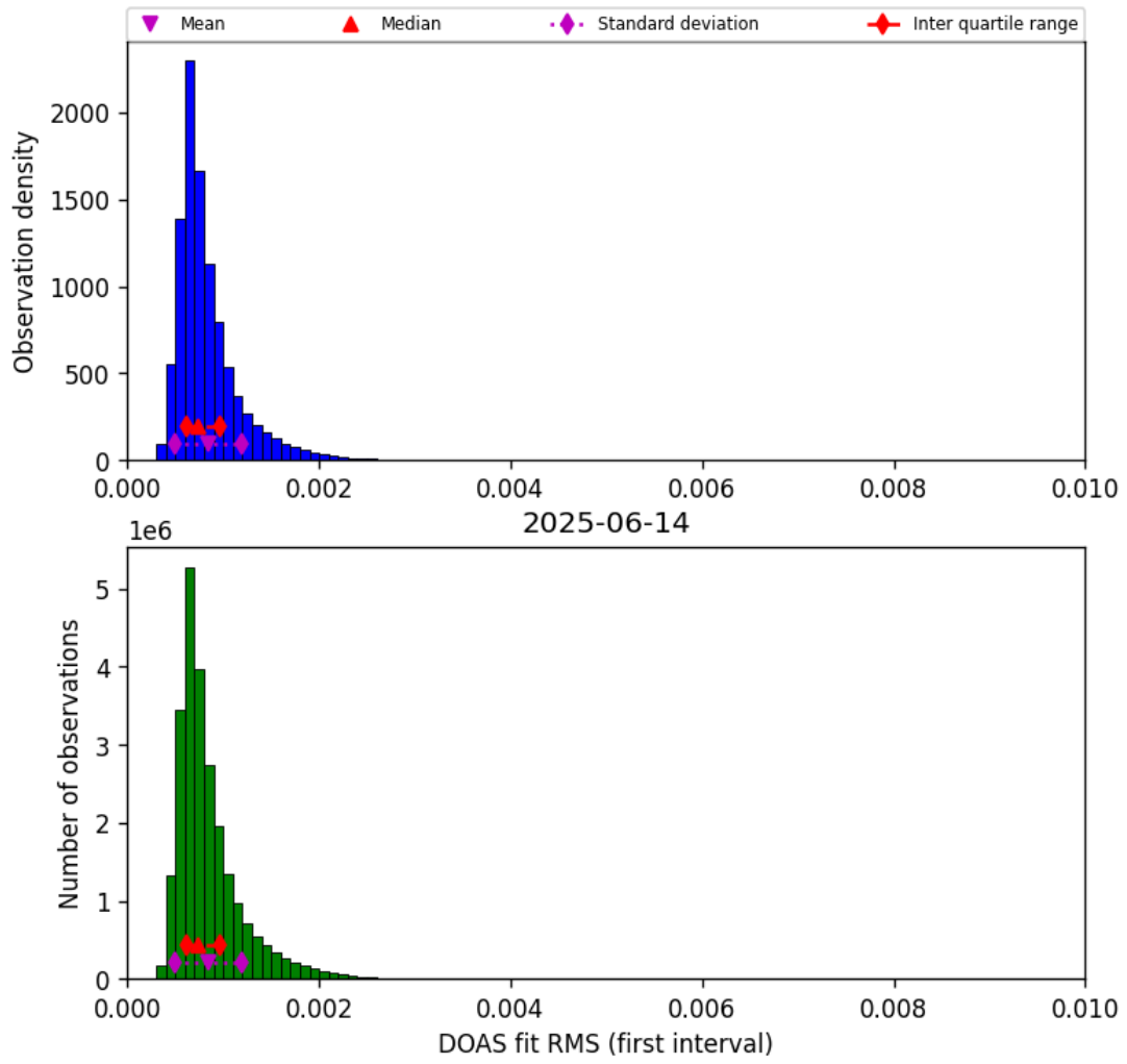
Figure 46: Histogram of “DOAS fit RMS (first interval)” for 2025-06-13 to 2025-06-15
