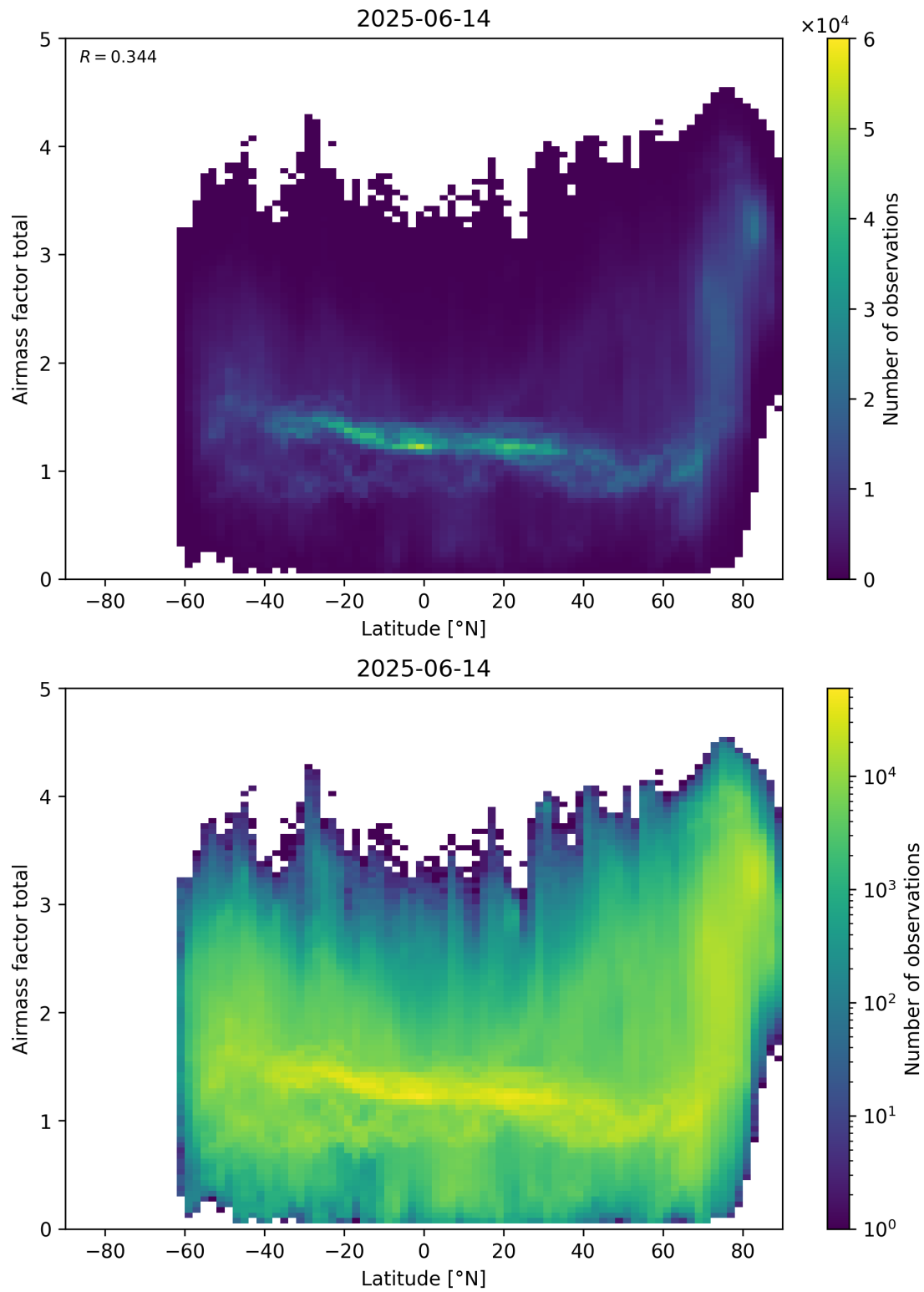
Figure 161: Scatter density plot of “Latitude” against “Airmass factor total” for 2025-06-13 to 2025-06-15.
