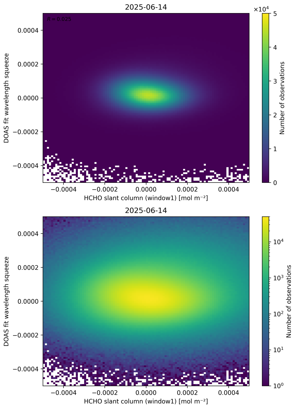
Figure 80: Scatter density plot of “HCHO slant column (window1)” against “DOAS fit wavelength squeeze” for 2025-06-13 to 2025-06-15.
