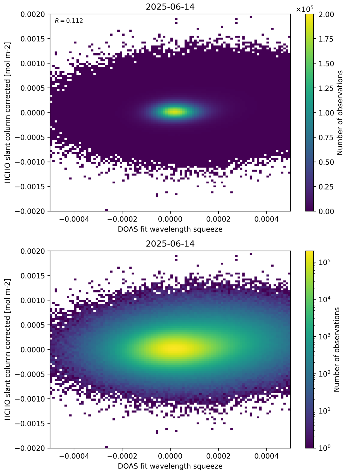
Figure 69: Scatter density plot of “DOAS fit wavelength squeeze” against “HCHO slant column corrected” for 2025-06-13 to 2025-06-15.
