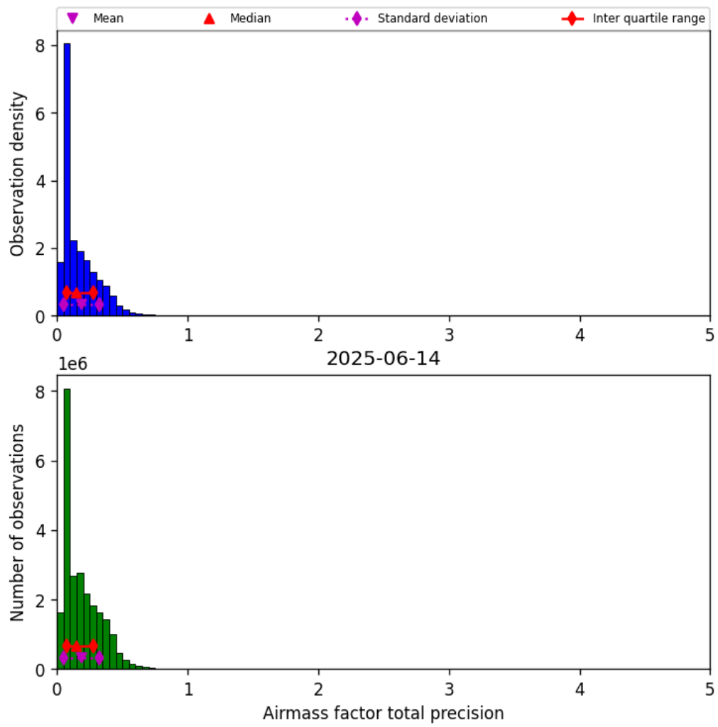
Figure 41: Histogram of “Airmass factor total precision” for 2025-06-13 to 2025-06-15
