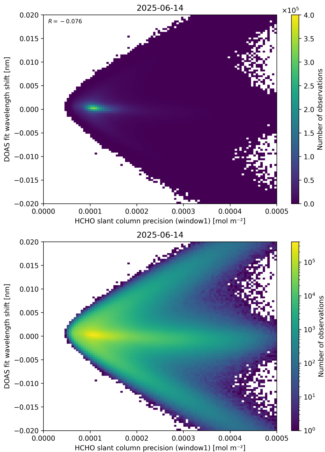
Figure 89: Scatter density plot of “HCHO slant column precision (window1)” against “DOAS fit wavelength shift” for 2025-06-13 to 2025-06-15.
