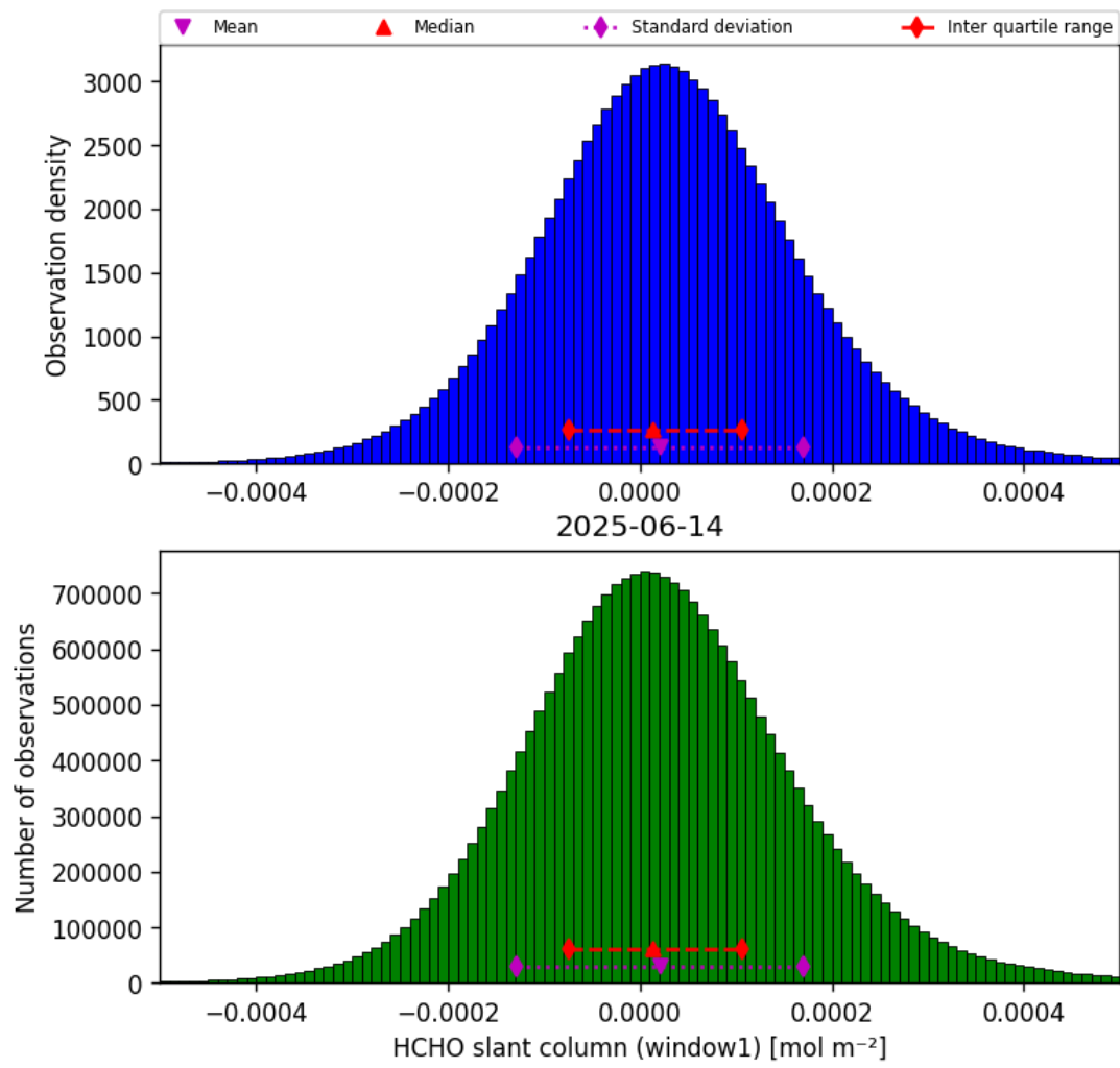
Figure 38: Histogram of “HCHO slant column (window1)” for 2025-06-13 to 2025-06-15
