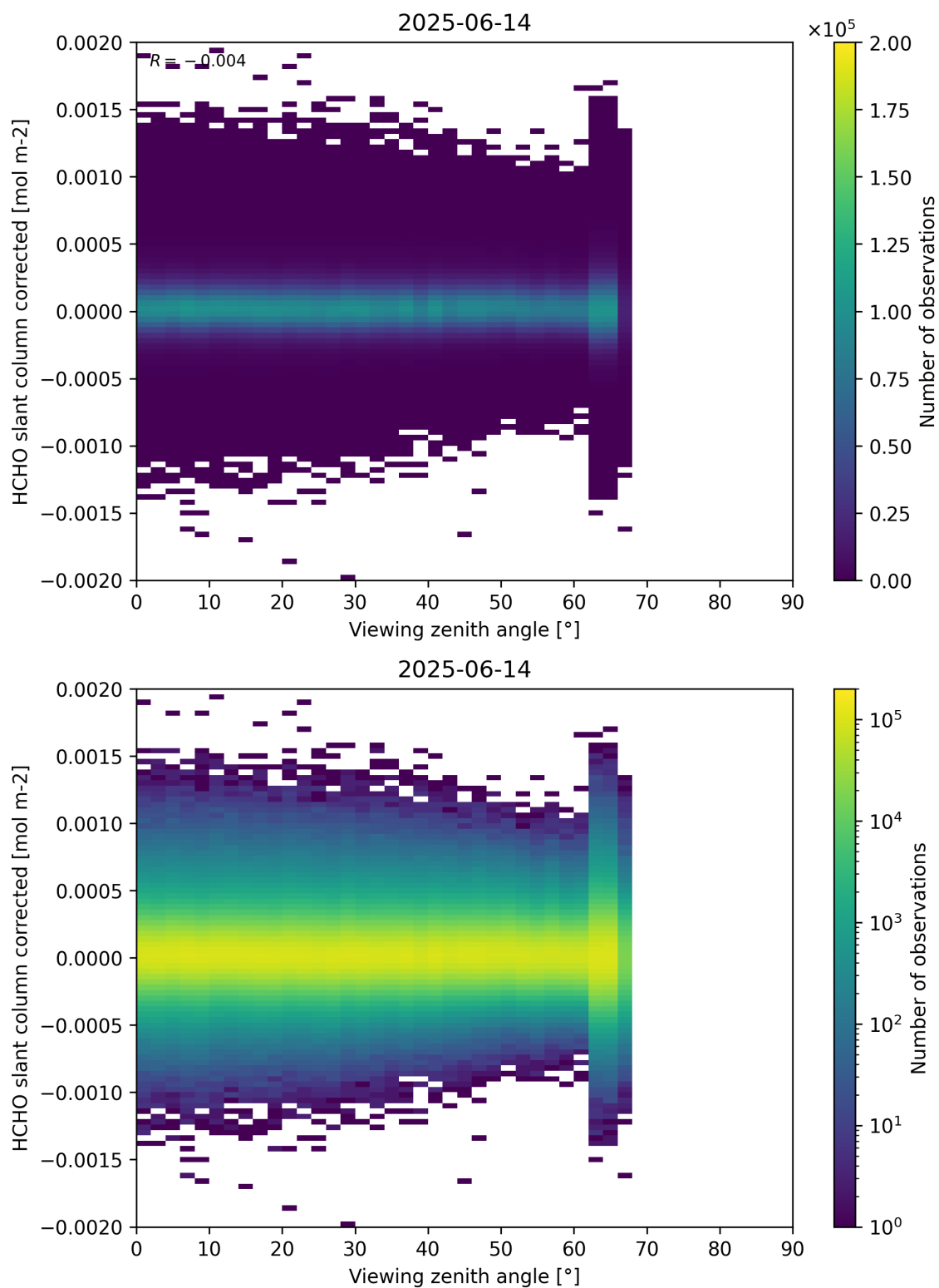
Figure 186: Scatter density plot of “Viewing zenith angle” against “HCHO slant column corrected” for 2025-06-13 to 2025-06-15.
