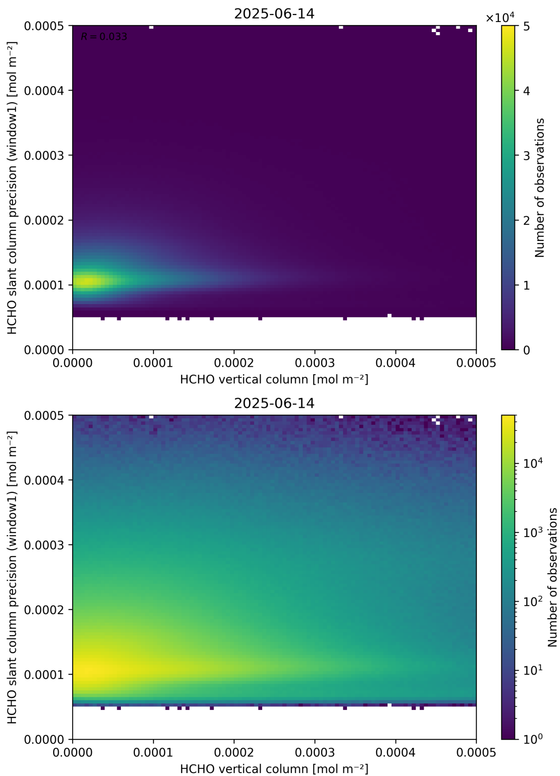
Figure 130: Scatter density plot of “HCHO vertical column” against “HCHO slant column precision (window1)” for 2025-06-13 to 2025-06-15.
