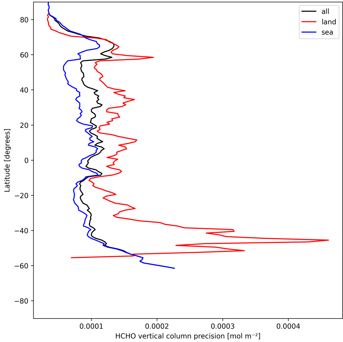
Figure 22: Zonal average of “HCHO vertical column precision” for 2025-06-13 to 2025-06-15.
