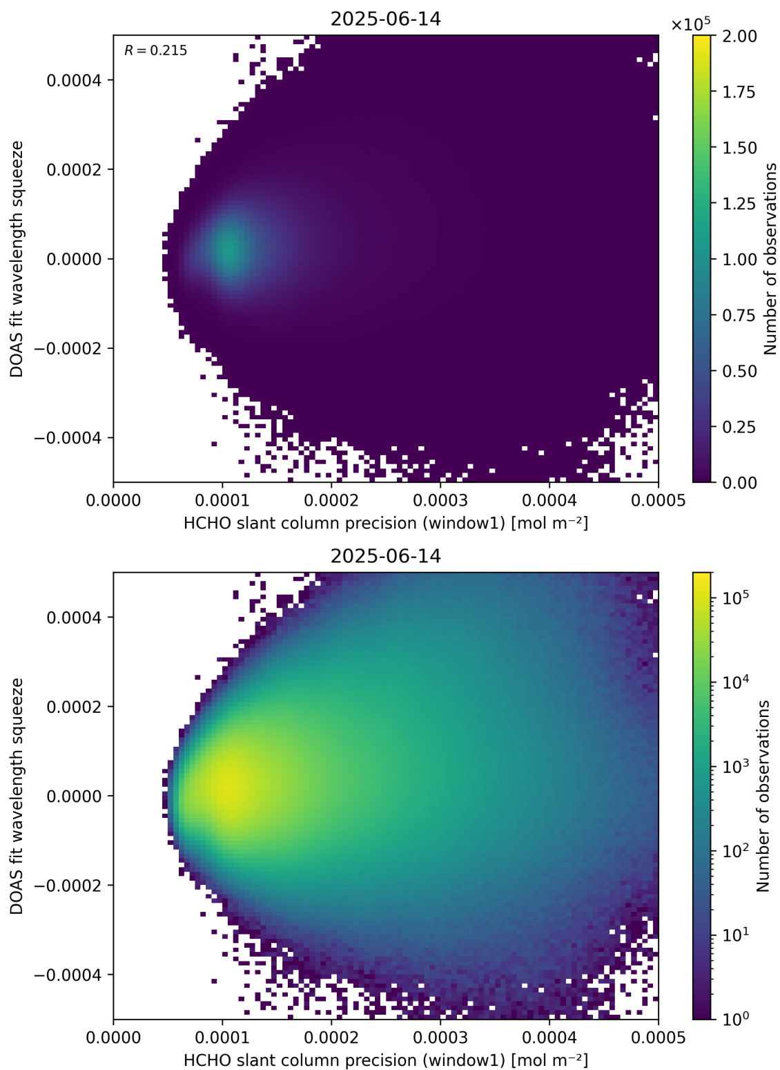
Figure 90: Scatter density plot of “HCHO slant column precision (window1)” against “DOAS fit wavelength squeeze” for 2025-06-13 to 2025-06-15.
