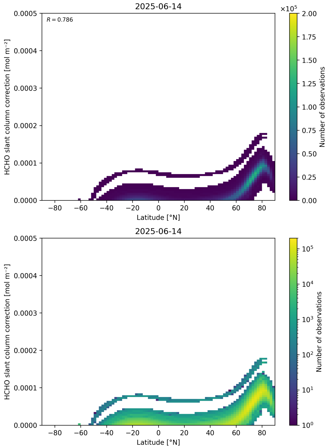
Figure 158: Scatter density plot of “Latitude” against “HCHO slant column correction” for 2025-06-13 to 2025-06-15.
