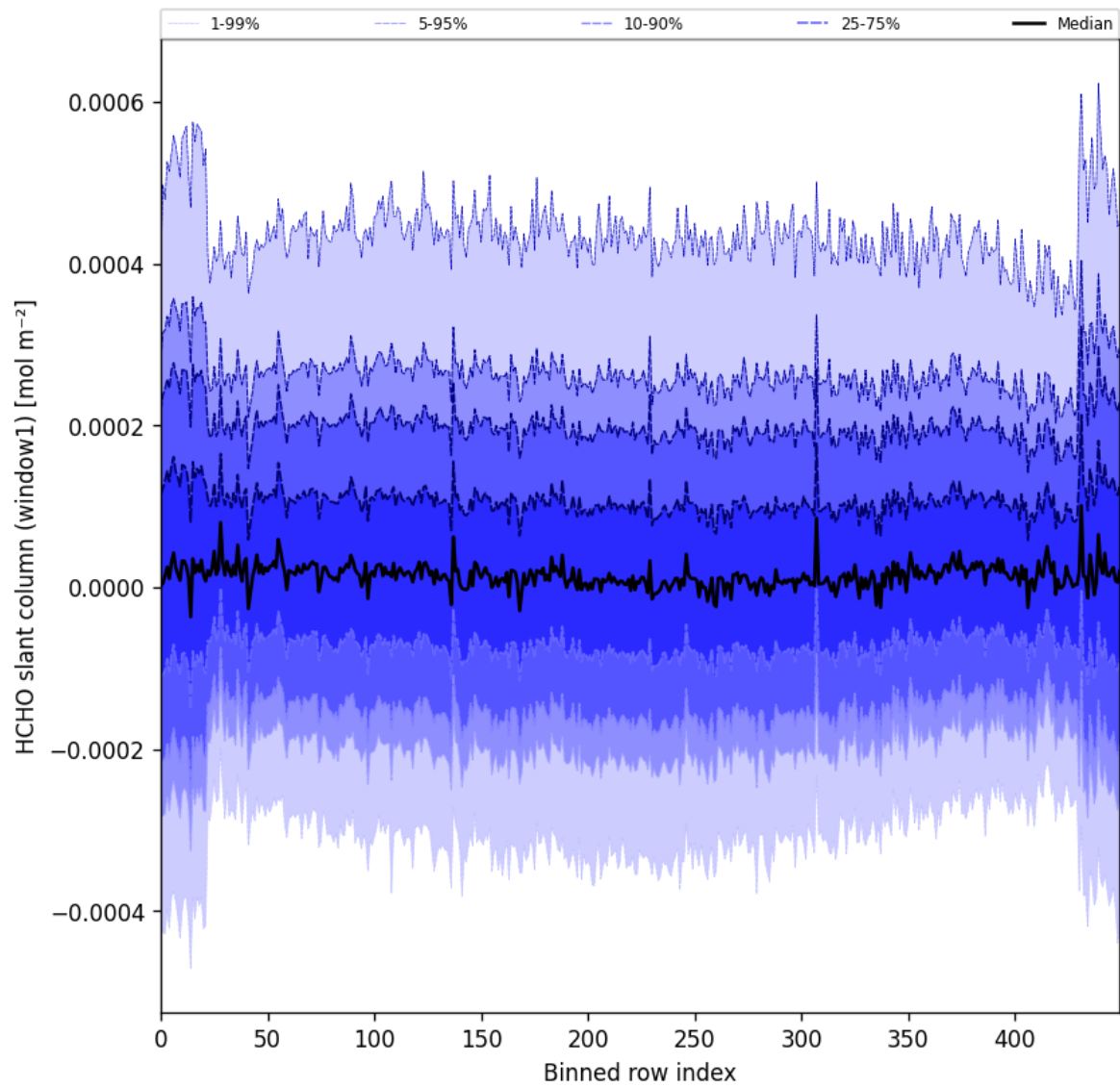
Figure 52: Along track statistics of “HCHO slant column (window1)” for 2025-06-13 to 2025-06-15
