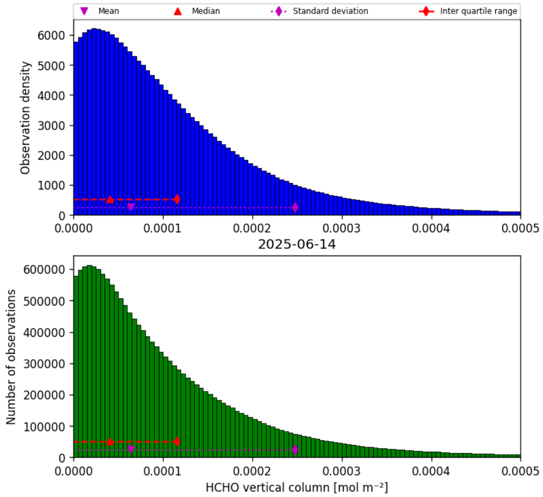
Figure 35: Histogram of “HCHO vertical column” for 2025-06-13 to 2025-06-15
