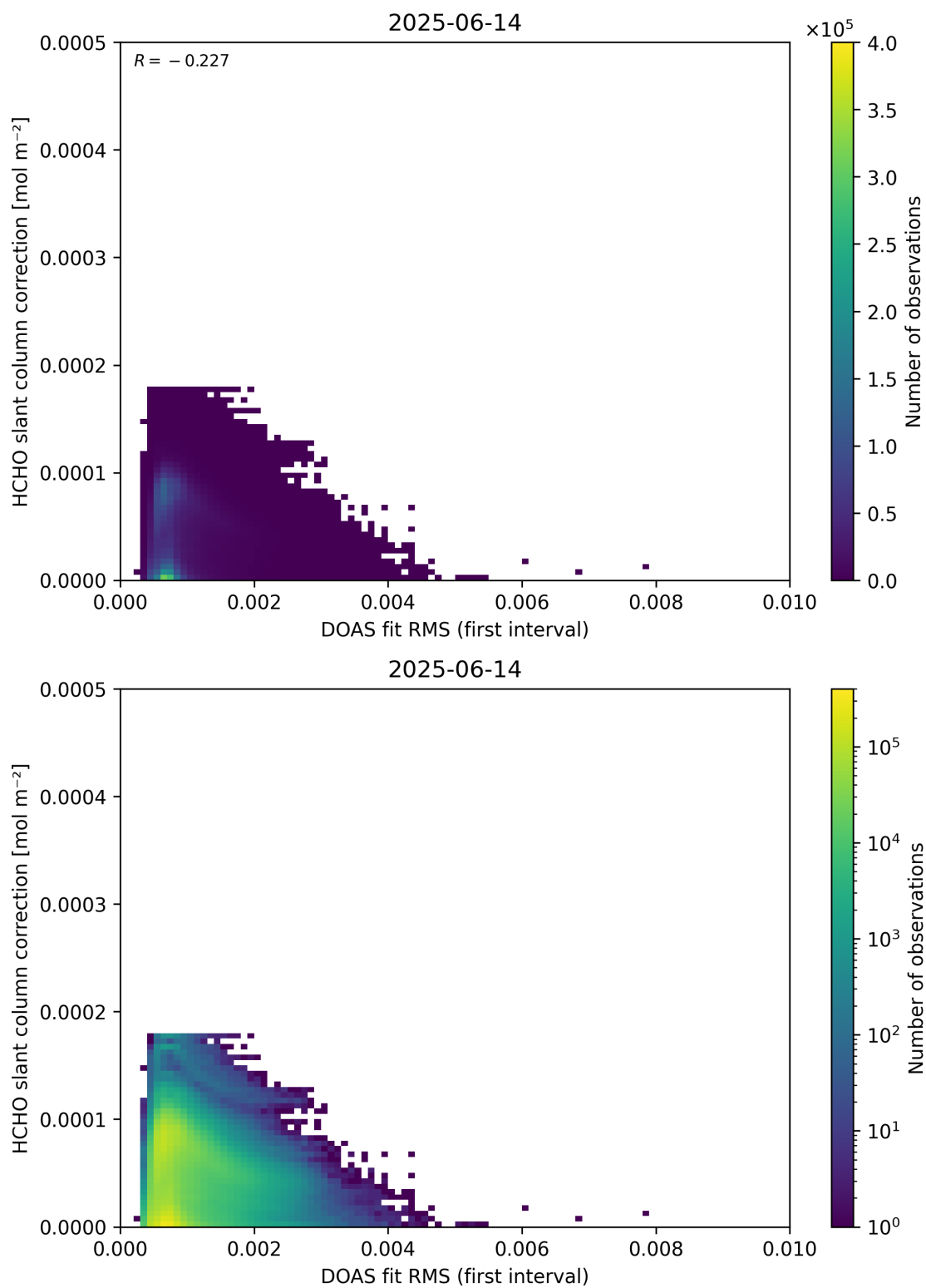
Figure 63: Scatter density plot of “DOAS fit RMS (first interval)” against “HCHO slant column correction” for 2025-06-13 to 2025-06-15.
