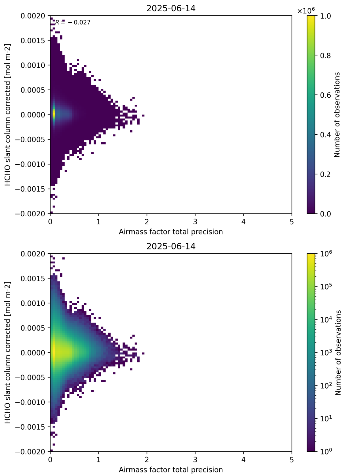
Figure 109: Scatter density plot of “Airmass factor total precision” against “HCHO slant column corrected” for 2025-06-13 to 2025-06-15.
