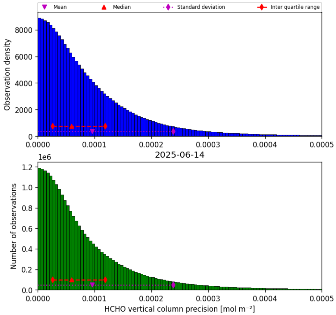
Figure 36: Histogram of “HCHO vertical column precision” for 2025-06-13 to 2025-06-15
