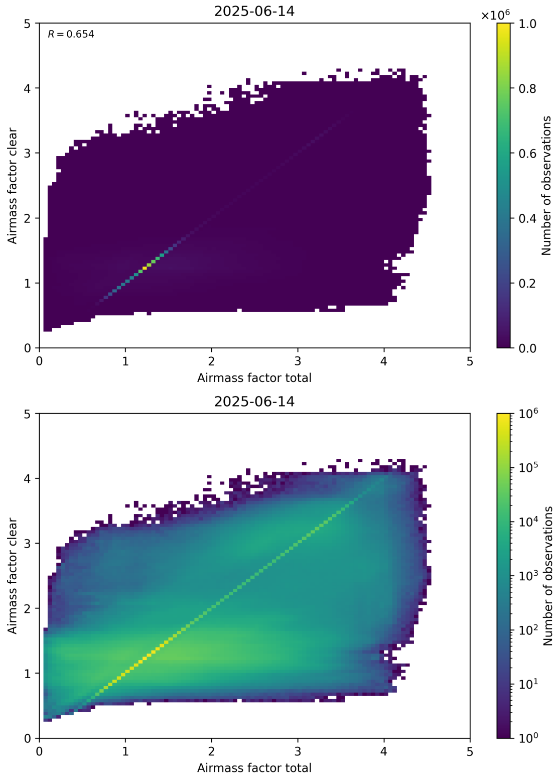
Figure 100: Scatter density plot of “Airmass factor total” against “Airmass factor clear” for 2025-06-13 to 2025-06-15.
