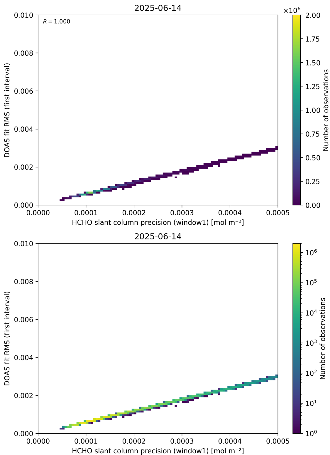
Figure 88: Scatter density plot of “HCHO slant column precision (window1)” against “DOAS fit RMS (first interval)” for 2025-06-13 to 2025-06-15.
