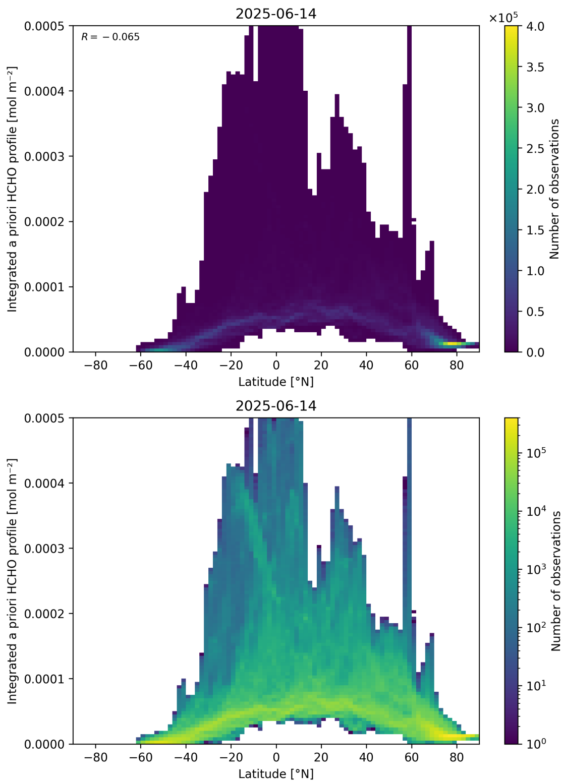
Figure 166: Scatter density plot of “Latitude” against “Integrated a priori HCHO profile” for 2025-06-13 to 2025-06-15.
