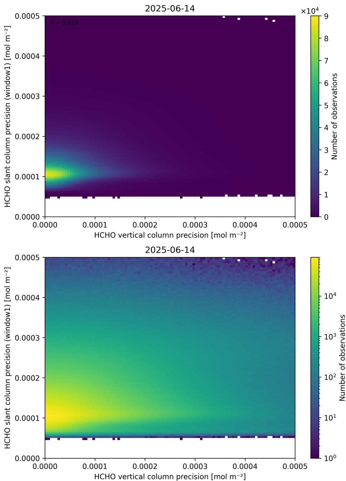
Figure 143: Scatter density plot of “HCHO vertical column precision” against “HCHO slant column precision (window1)” for 2025-06-13 to 2025-06-15.
