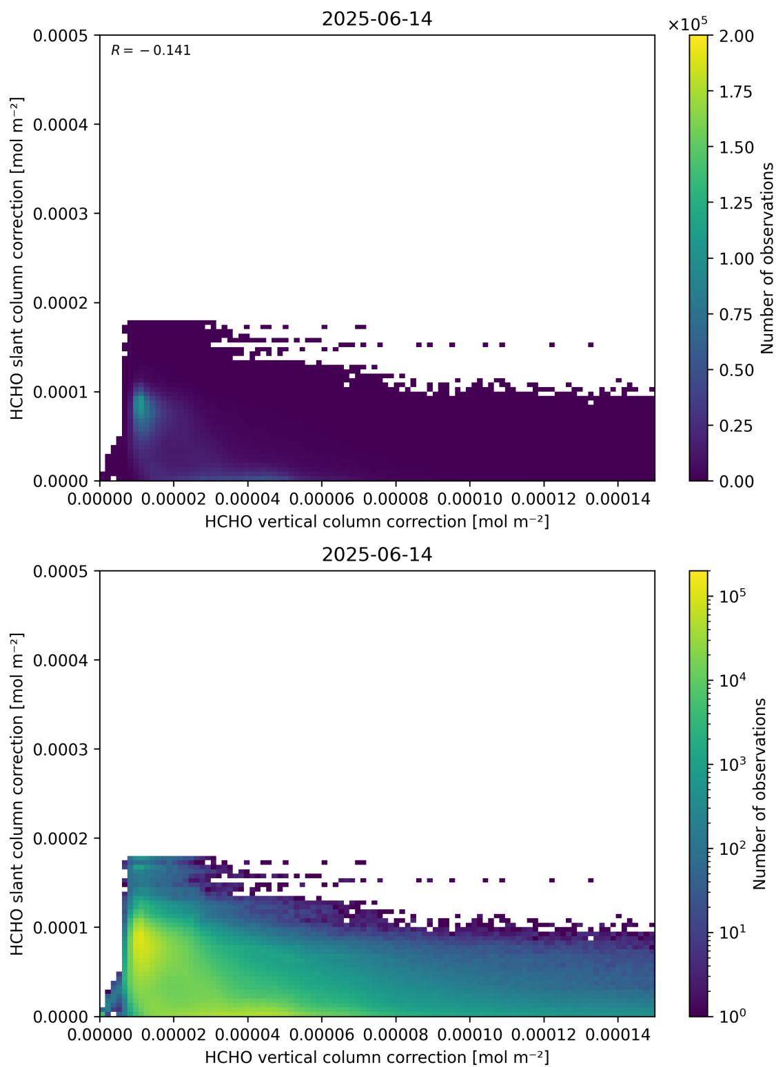
Figure 117: Scatter density plot of “HCHO vertical column correction” against “HCHO slant column correction” for 2025-06-13 to 2025-06-15.
