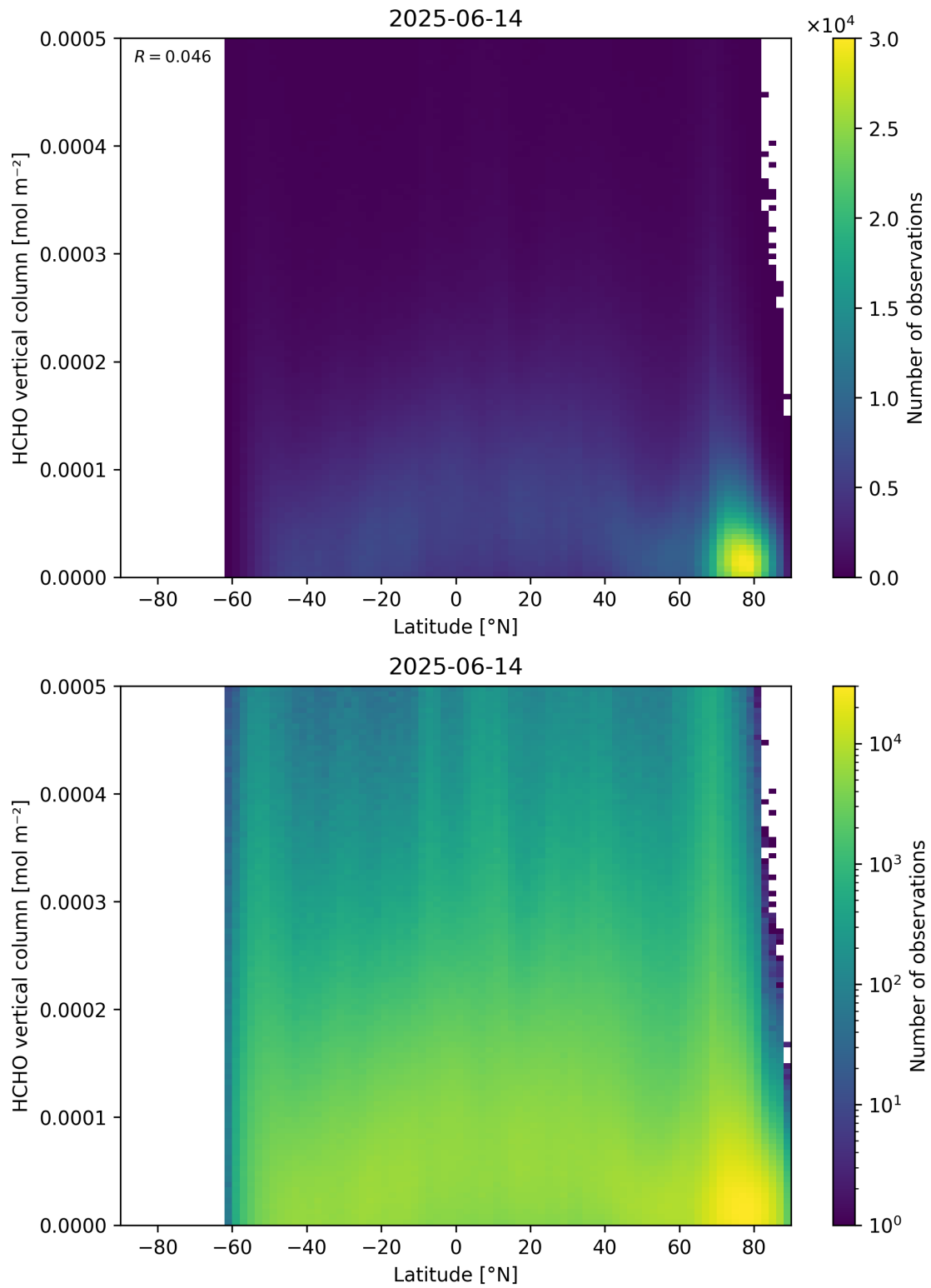
Figure 163: Scatter density plot of “Latitude” against “HCHO vertical column” for 2025-06-13 to 2025-06-15.
