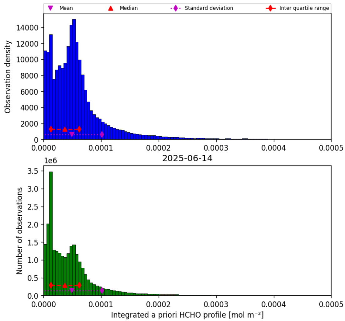
Figure 43: Histogram of “Integrated a priori HCHO profile” for 2025-06-13 to 2025-06-15
