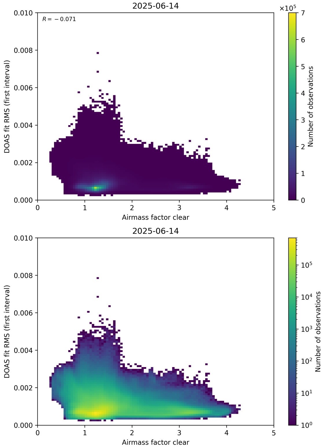
Figure 71: Scatter density plot of “Airmass factor clear” against “DOAS fit RMS (first interval)” for 2025-06-13 to 2025-06-15.
