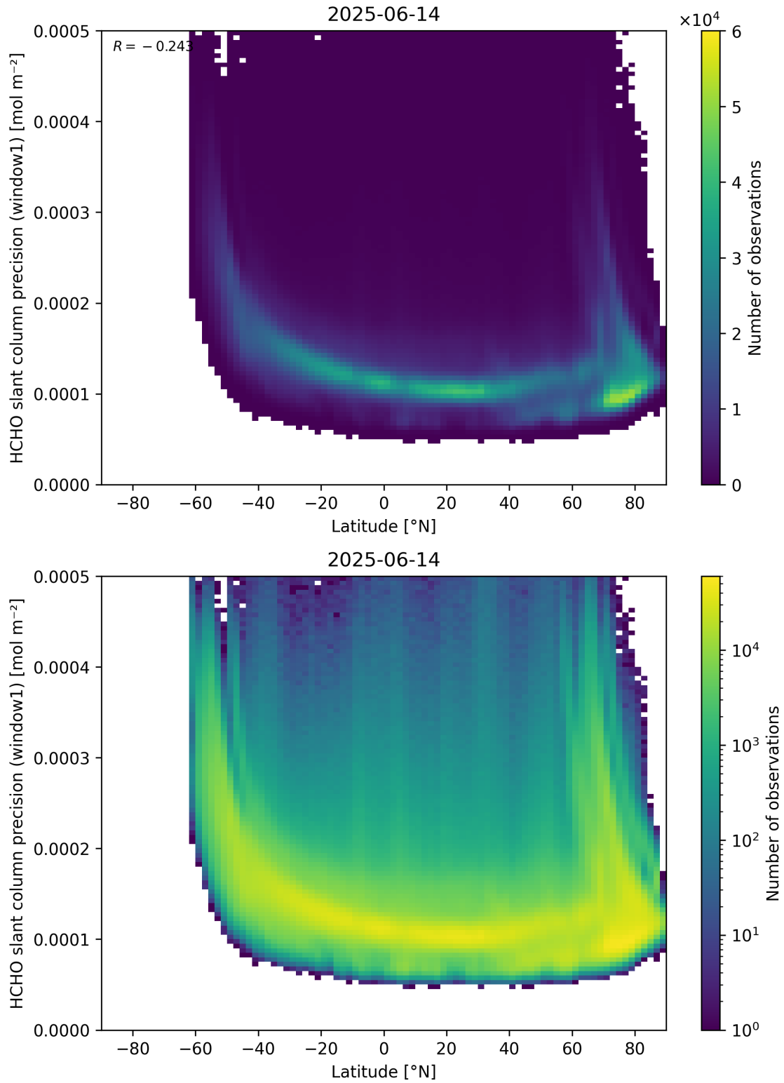
Figure 160: Scatter density plot of “Latitude” against “HCHO slant column precision (window1)” for 2025-06-13 to 2025-06-15.
