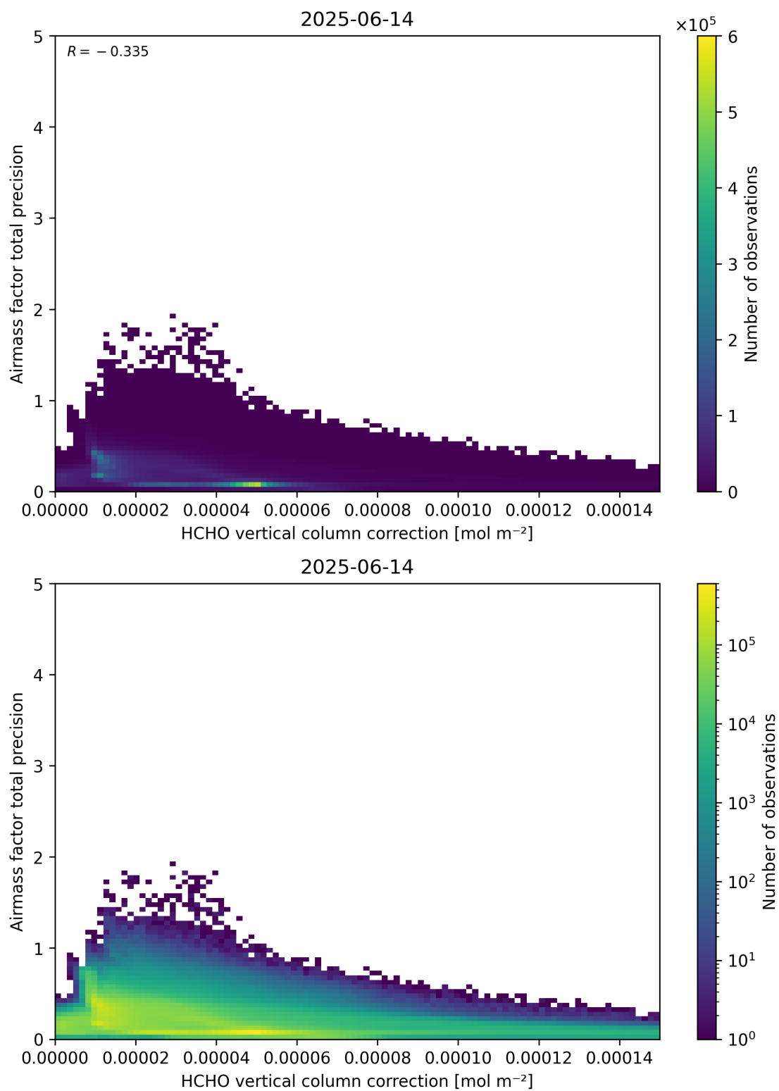
Figure 121: Scatter density plot of “HCHO vertical column correction” against “Airmass factor total precision” for 2025-06-13 to 2025-06-15.
