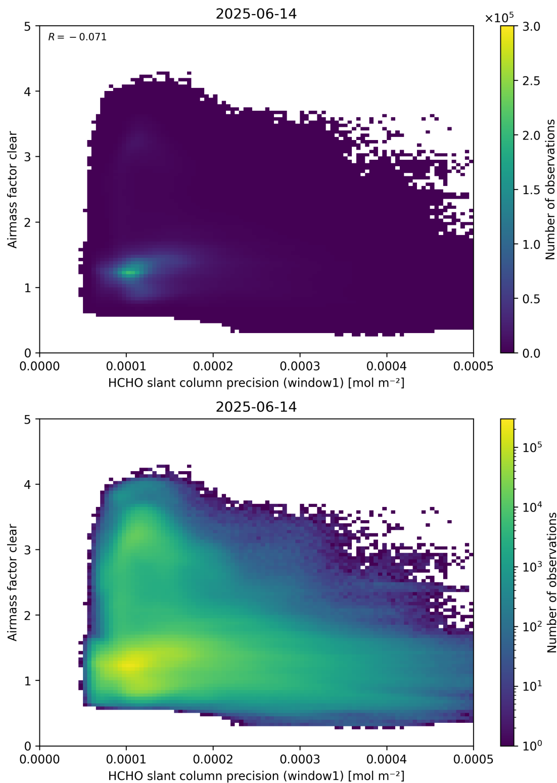
Figure 91: Scatter density plot of “HCHO slant column precision (window1)” against “Airmass factor clear” for 2025-06-13 to 2025-06-15.
