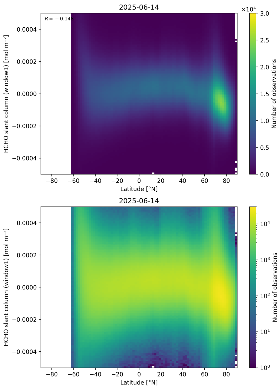
Figure 159: Scatter density plot of “Latitude” against “HCHO slant column (window1)” for 2025-06-13 to 2025-06-15.
