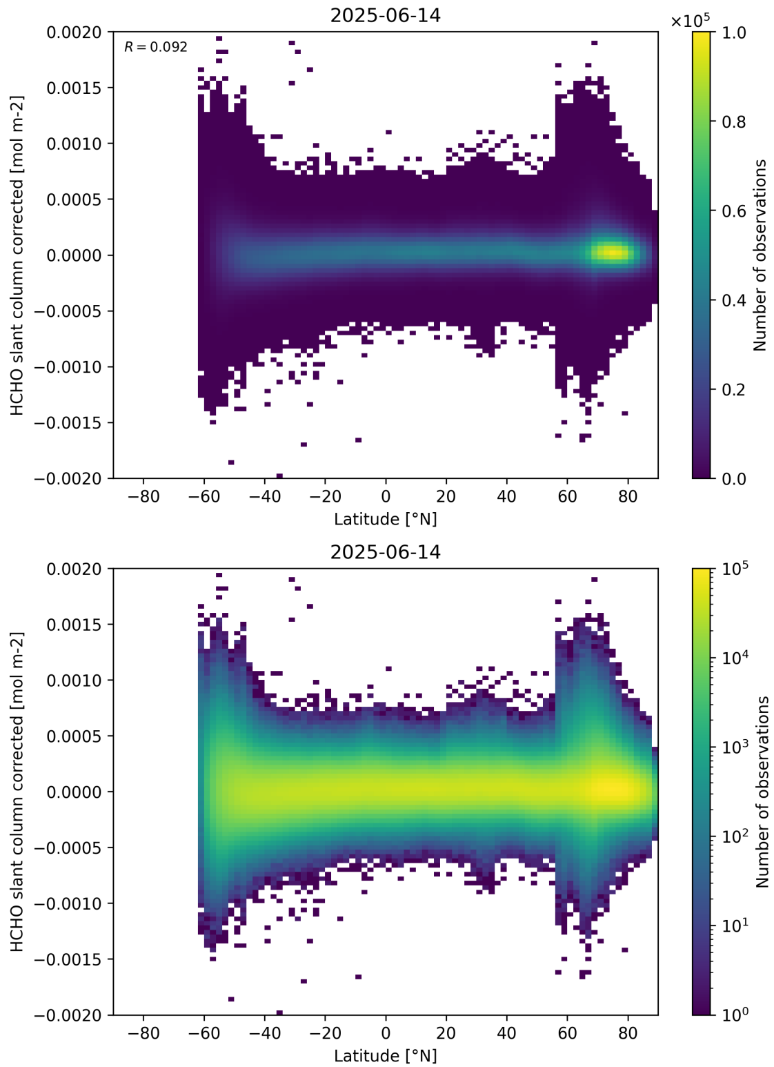
Figure 157: Scatter density plot of “Latitude” against “HCHO slant column corrected” for 2025-06-13 to 2025-06-15.
