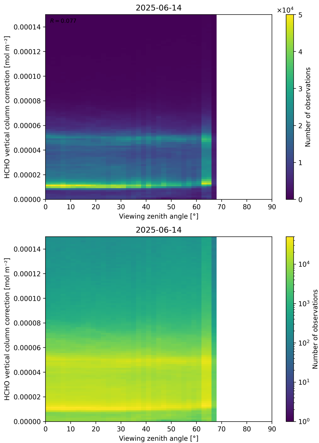
Figure 193: Scatter density plot of “Viewing zenith angle” against “HCHO vertical column correction” for 2025-06-13 to 2025-06-15.
