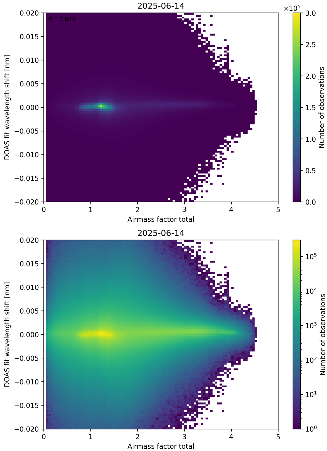
Figure 98: Scatter density plot of “Airmass factor total” against “DOAS fit wavelength shift” for 2025-06-13 to 2025-06-15.
