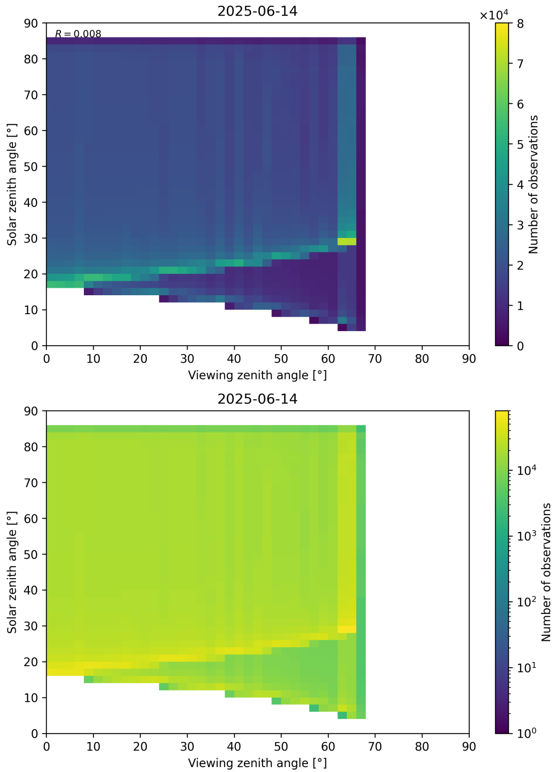
Figure 197: Scatter density plot of “Viewing zenith angle” against “Solar zenith angle” for 2025-06-13 to 2025-06-15.
