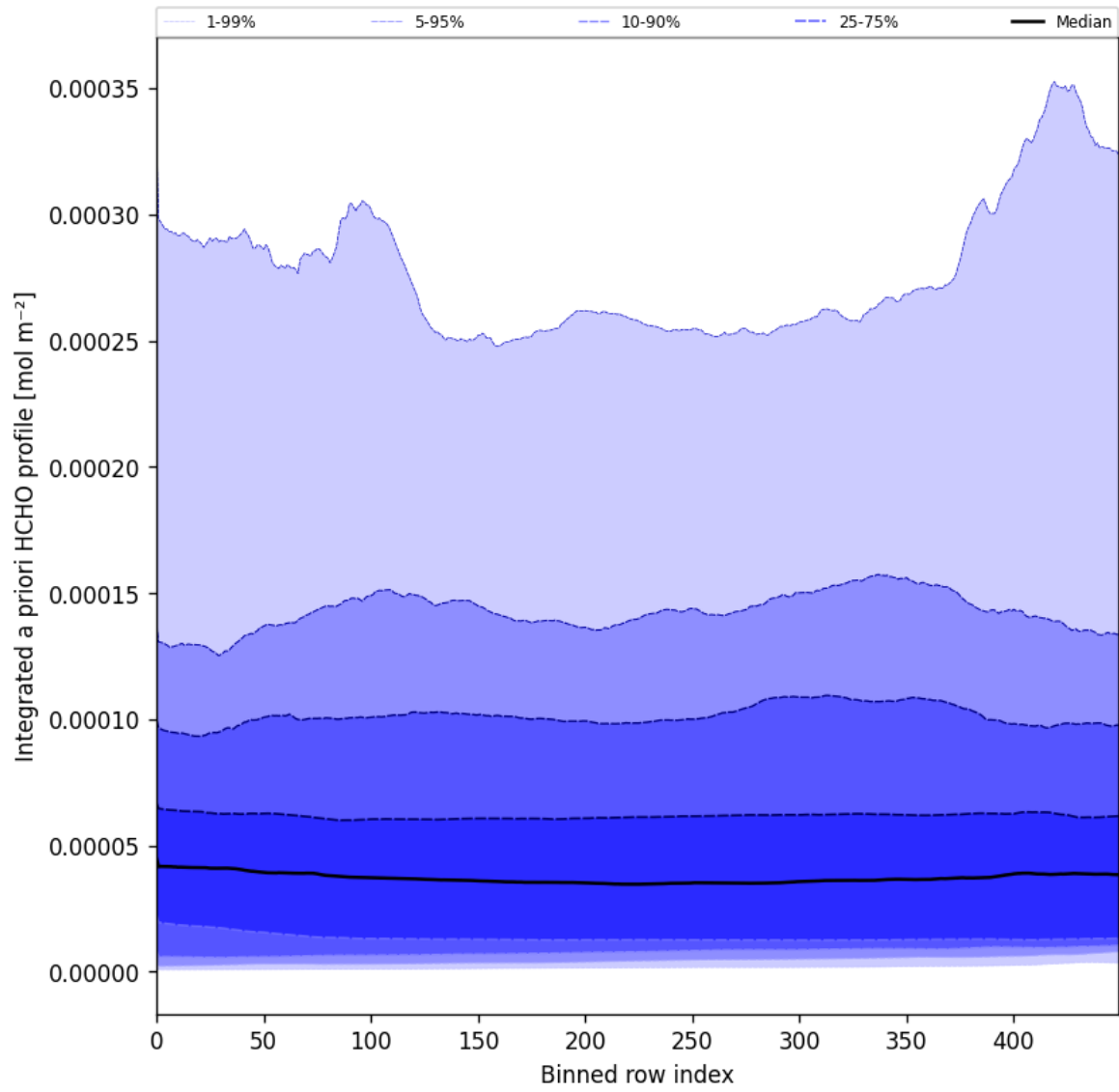
Figure 57: Along track statistics of “Integrated a priori HCHO profile” for 2025-06-13 to 2025-06-15
