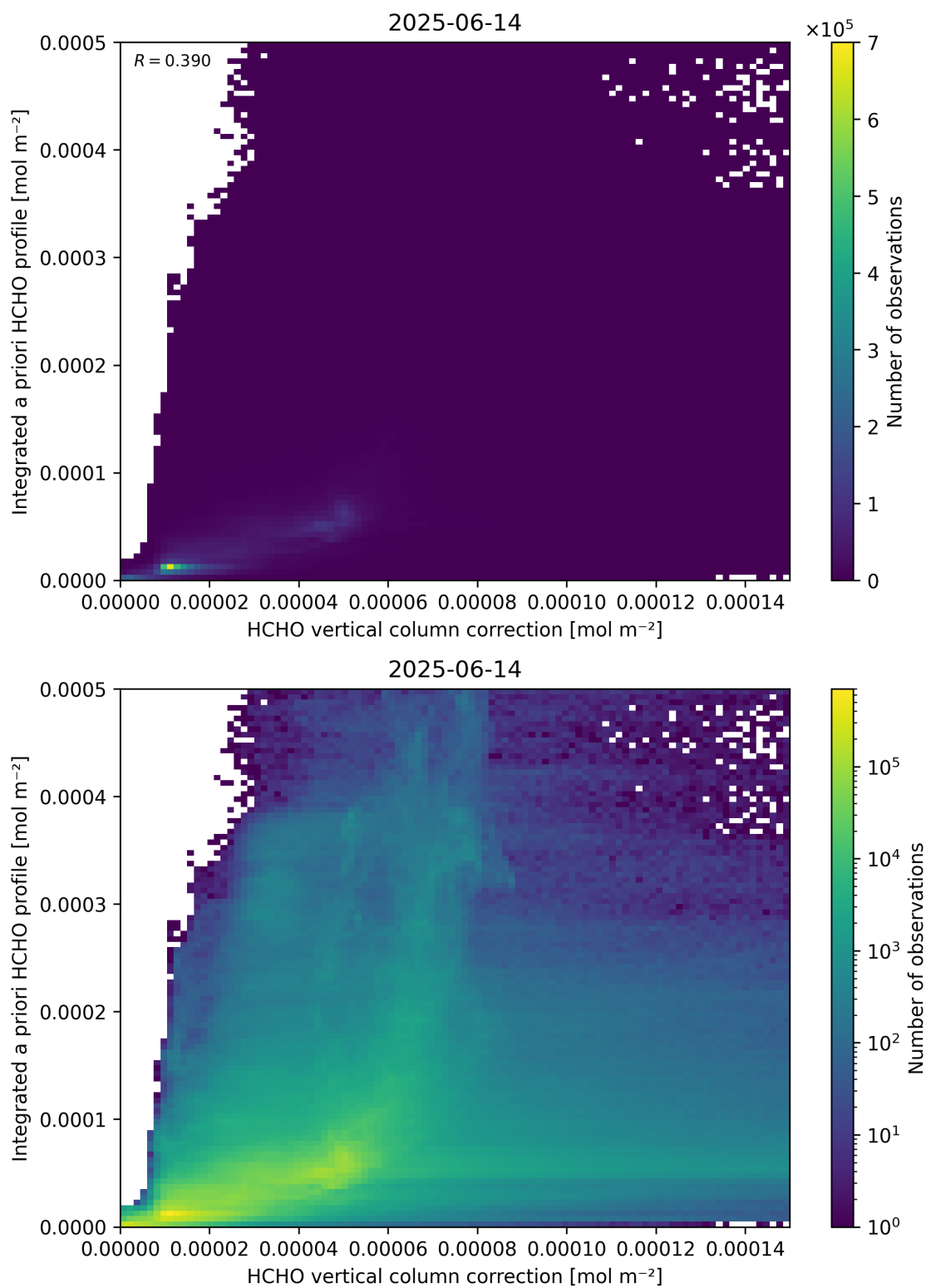
Figure 122: Scatter density plot of “HCHO vertical column correction” against “Integrated a priori HCHO profile” for 2025-06-13 to 2025-06-15.
