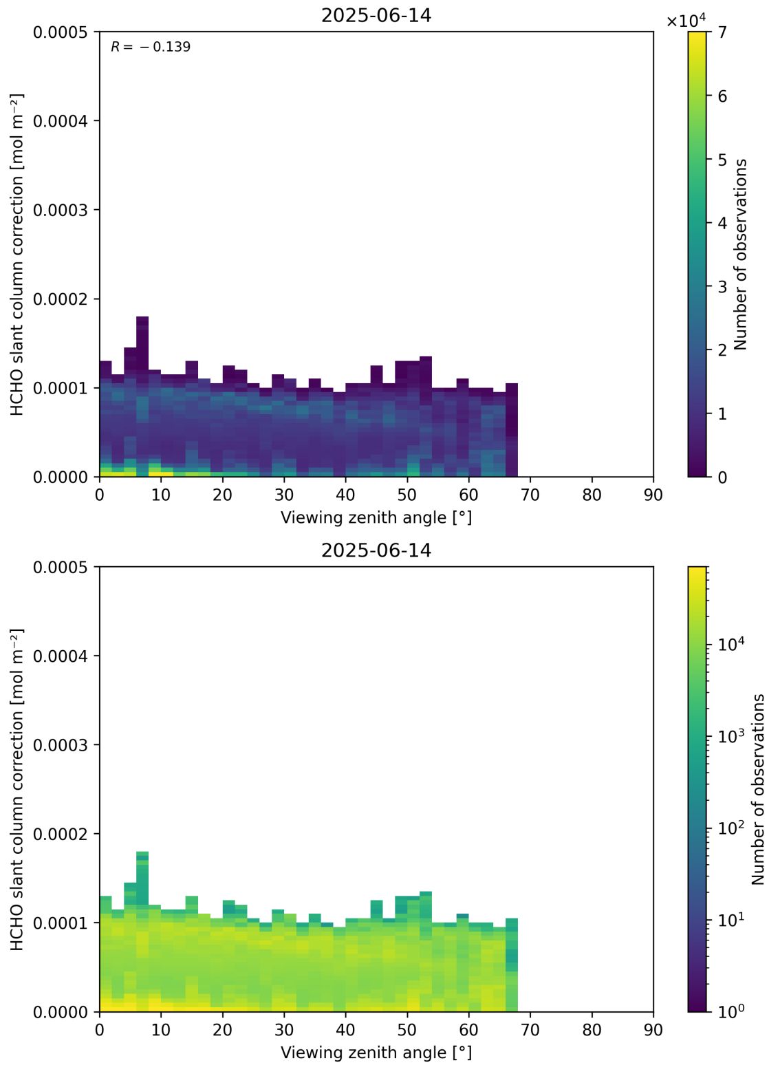
Figure 187: Scatter density plot of “Viewing zenith angle” against “HCHO slant column correction” for 2025-06-13 to 2025-06-15.
