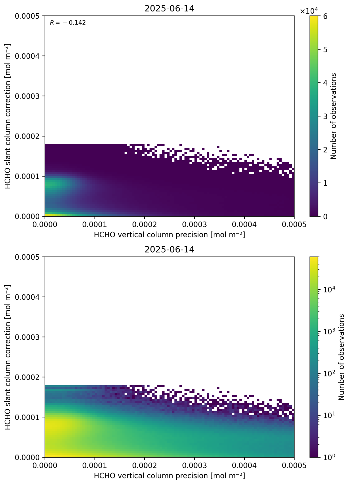
Figure 141: Scatter density plot of “HCHO vertical column precision” against “HCHO slant column correction” for 2025-06-13 to 2025-06-15.
