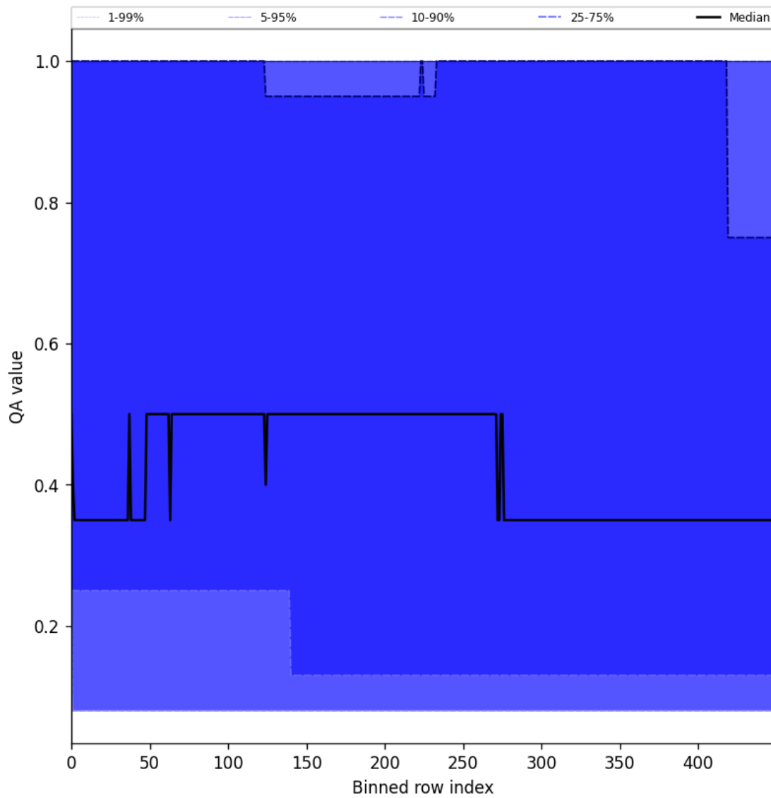
Figure 48: Along track statistics of “QA value” for 2025-06-13 to 2025-06-15
