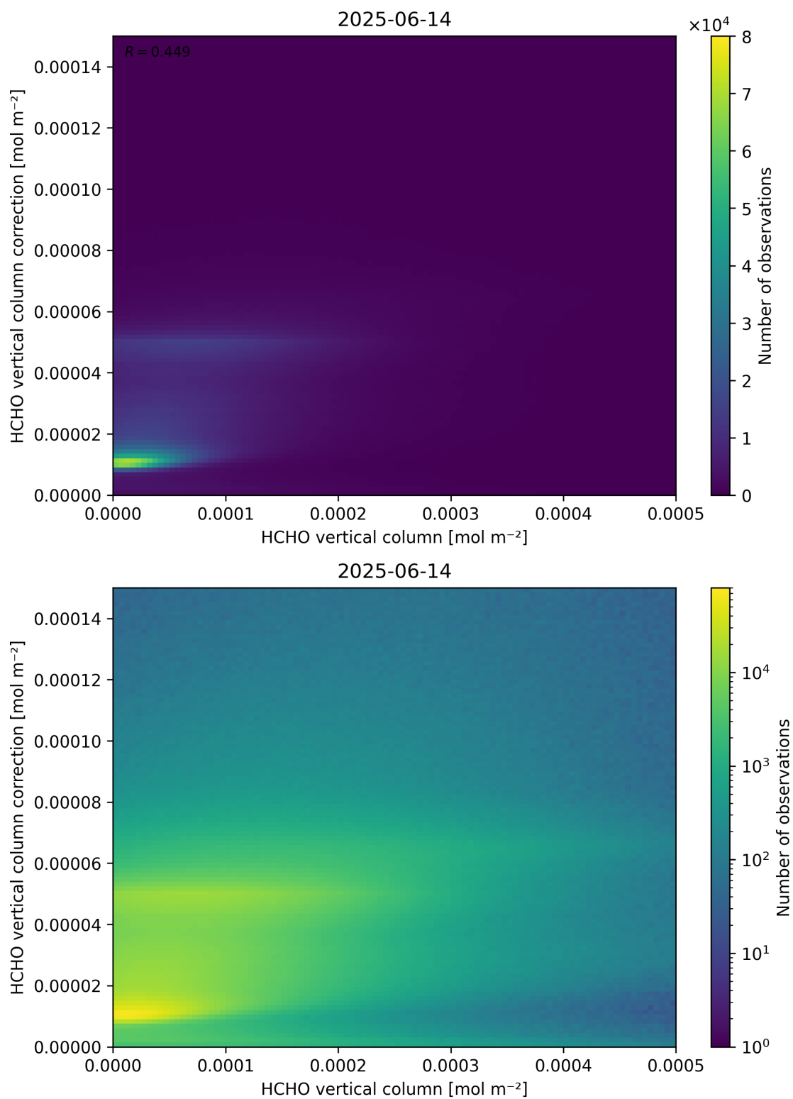
Figure 133: Scatter density plot of “HCHO vertical column” against “HCHO vertical column correction” for 2025-06-13 to 2025-06-15.
