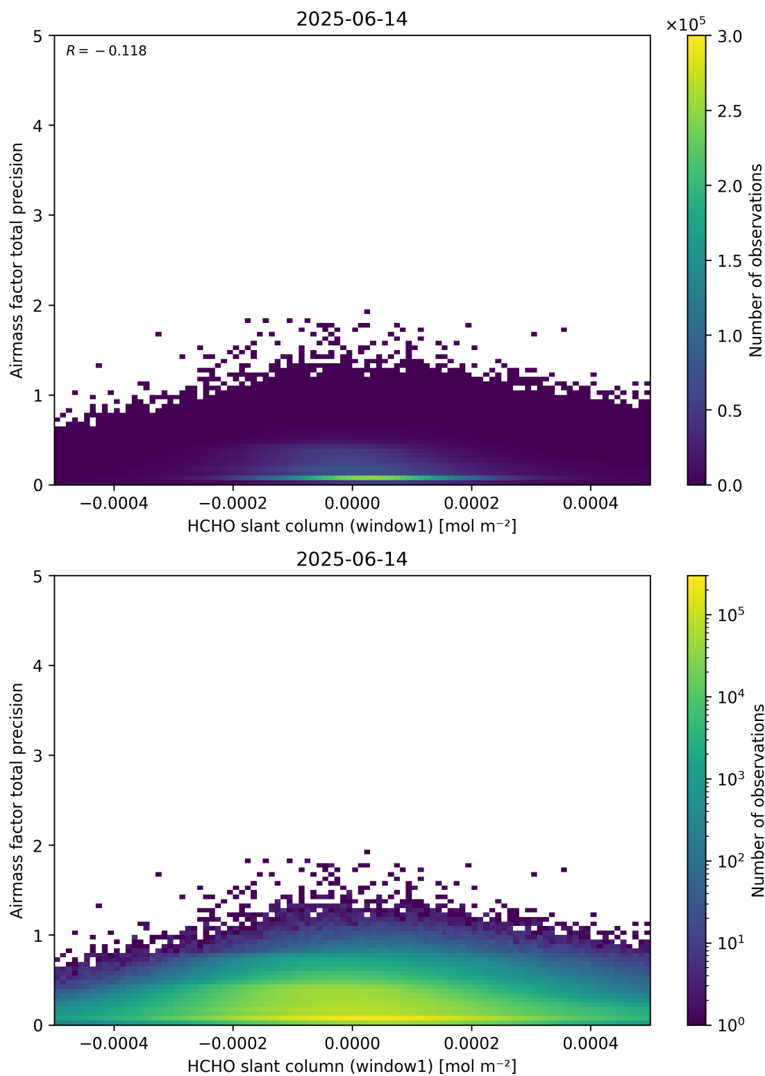
Figure 86: Scatter density plot of “HCHO slant column (window1)” against “Airmass factor total precision” for 2025-06-13 to 2025-06-15.
