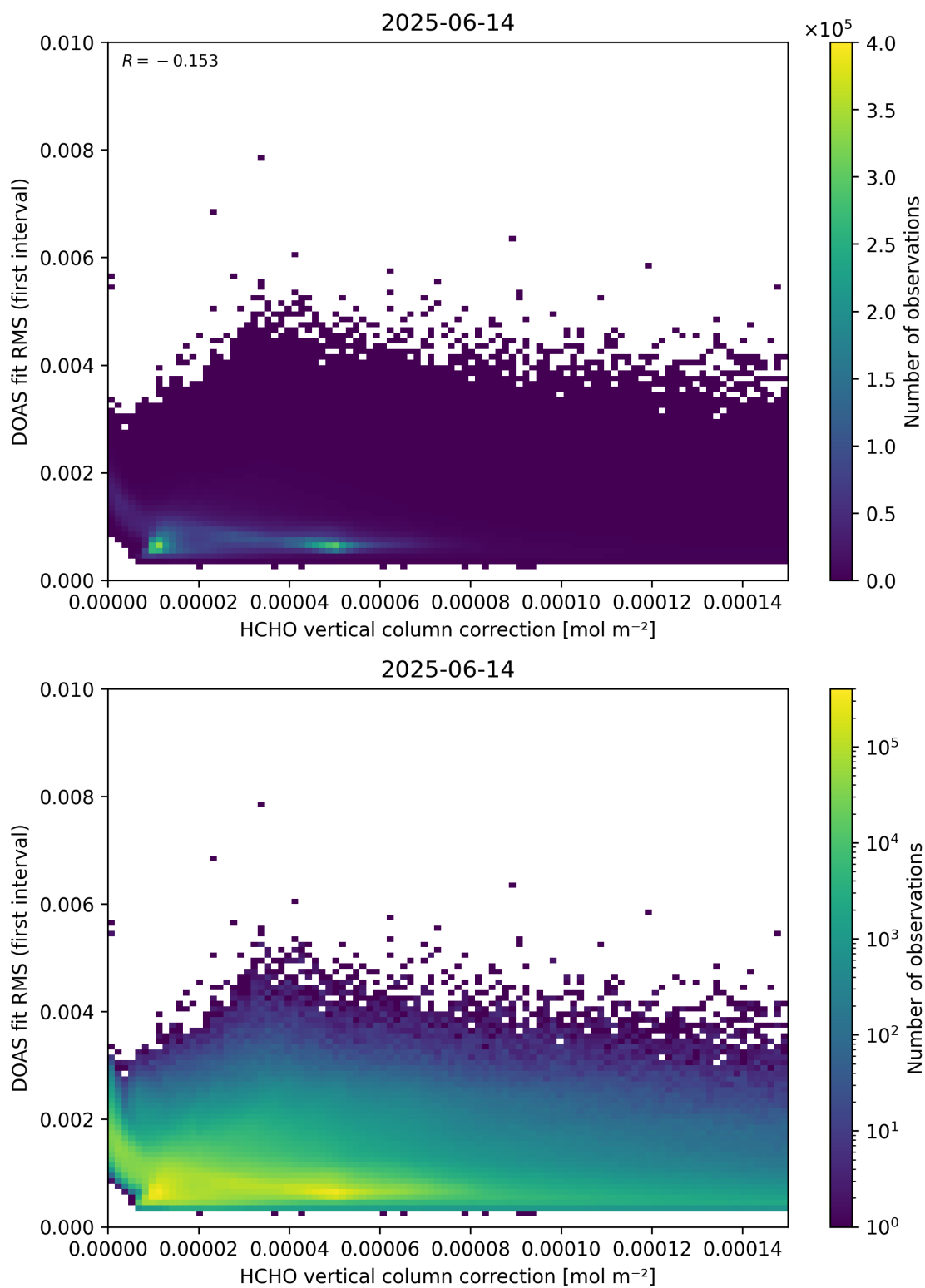
Figure 112: Scatter density plot of “HCHO vertical column correction” against “DOAS fit RMS (first interval)” for 2025-06-13 to 2025-06-15.
