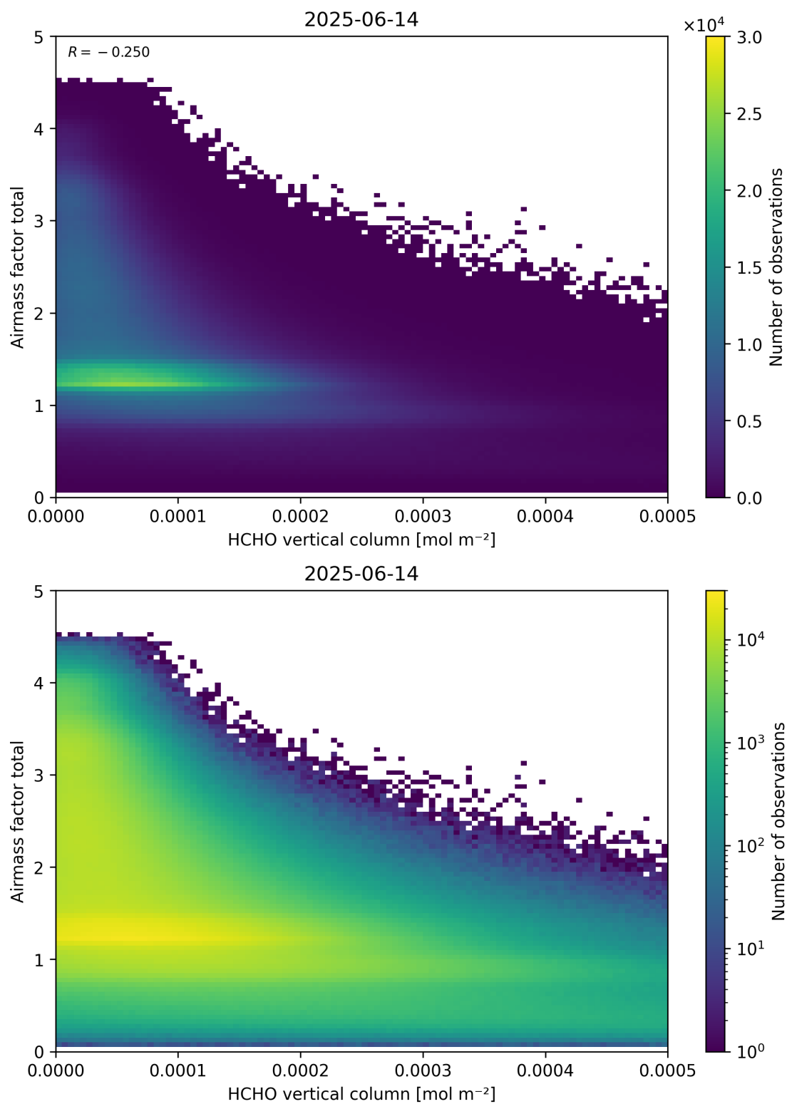
Figure 131: Scatter density plot of “HCHO vertical column” against “Airmass factor total” for 2025-06-13 to 2025-06-15.
