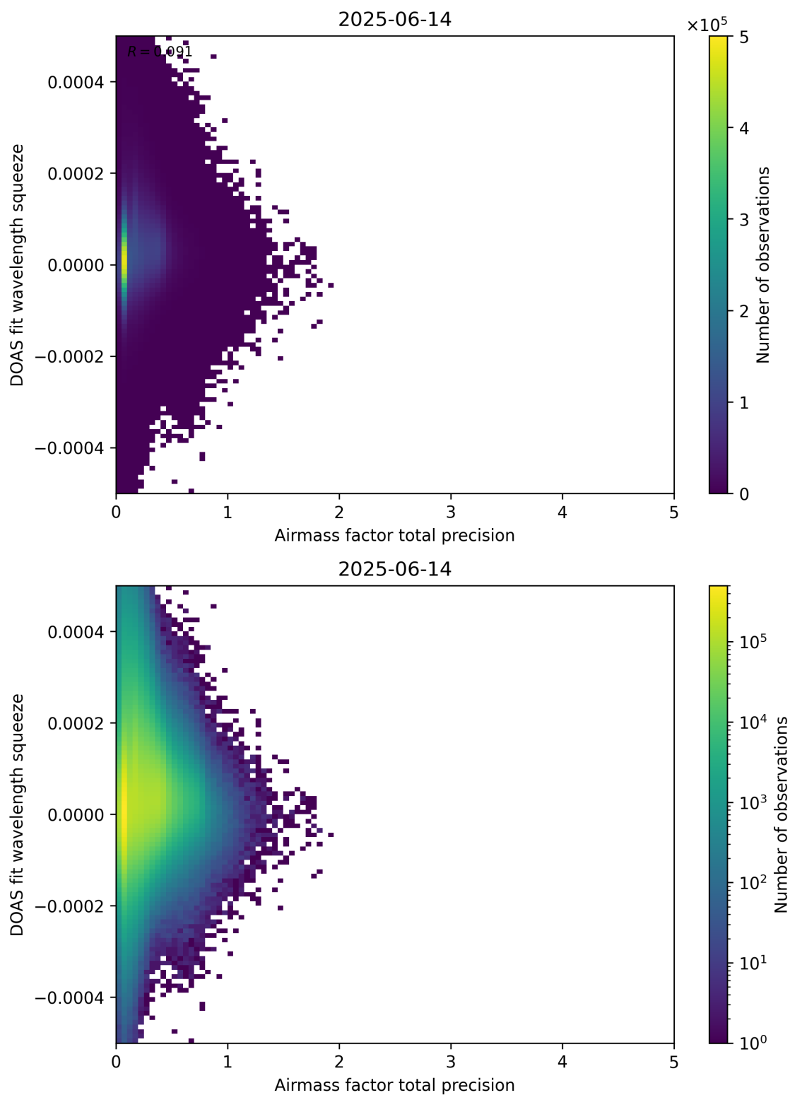
Figure 107: Scatter density plot of “Airmass factor total precision” against “DOAS fit wavelength squeeze” for 2025-06-13 to 2025-06-15.
