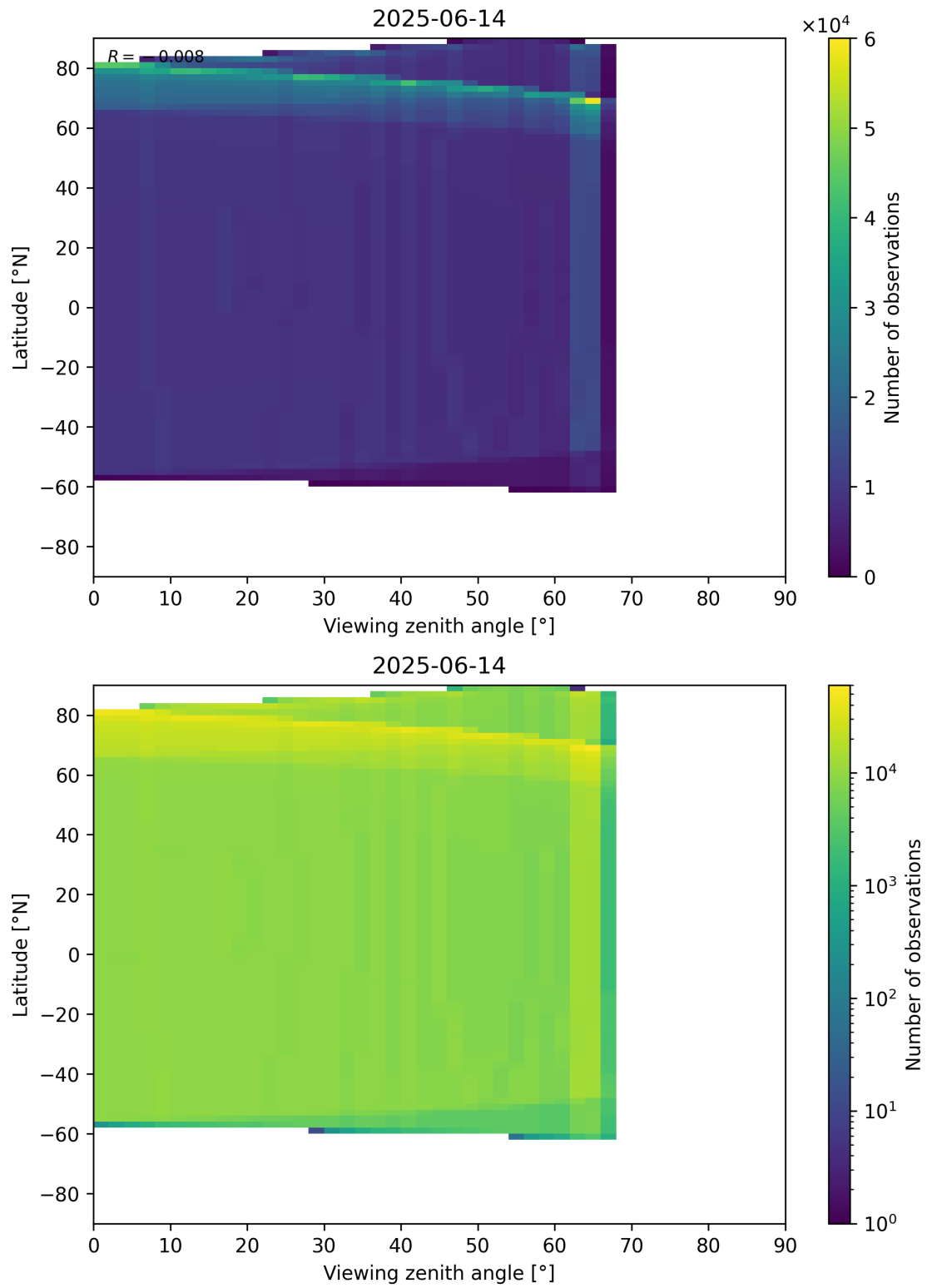
Figure 196: Scatter density plot of “Viewing zenith angle” against “Latitude” for 2025-06-13 to 2025-06-15.
