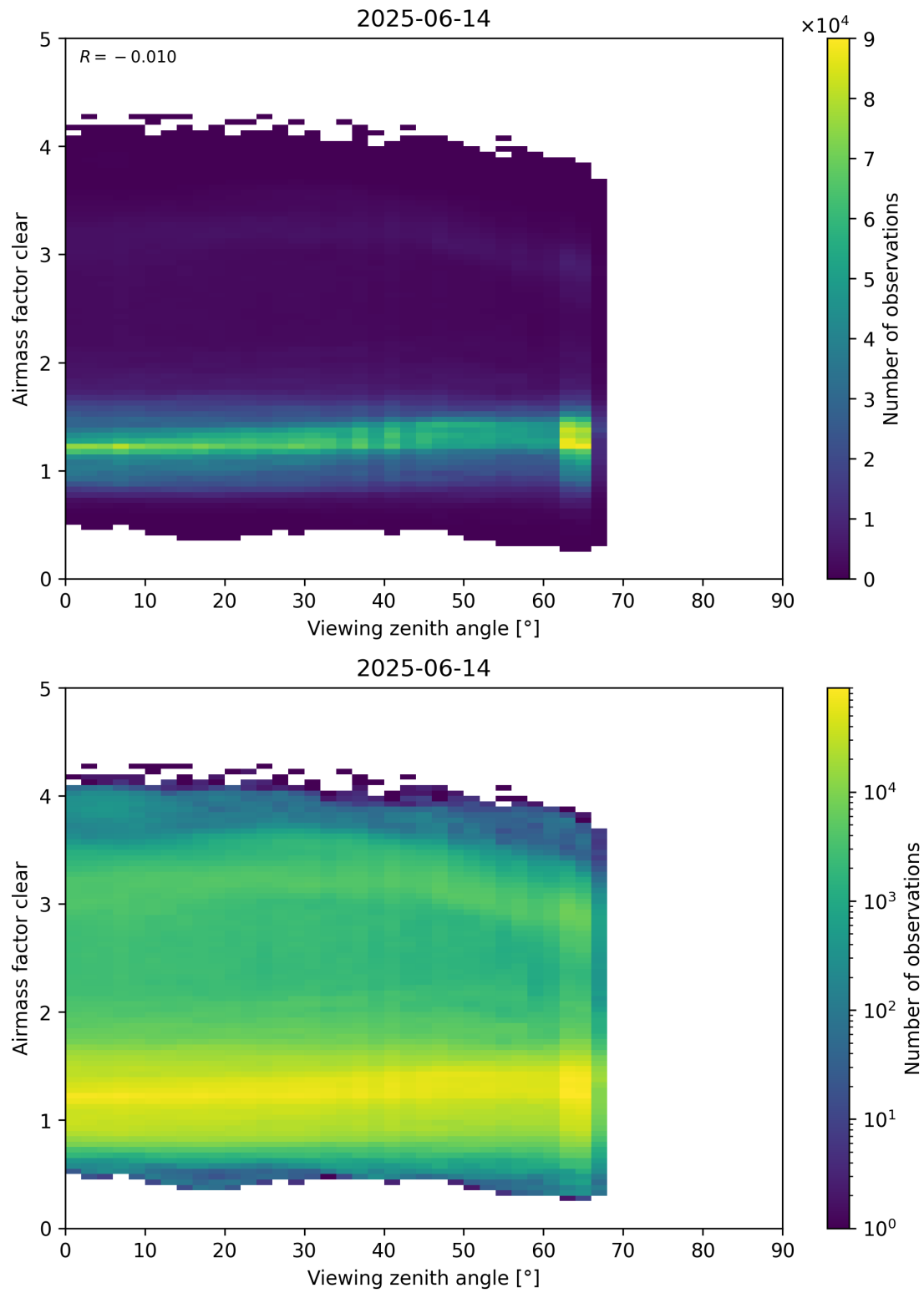
Figure 185: Scatter density plot of “Viewing zenith angle” against “Airmass factor clear” for 2025-06-13 to 2025-06-15.
