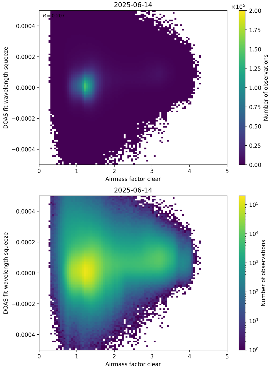
Figure 73: Scatter density plot of “Airmass factor clear” against “DOAS fit wavelength squeeze” for 2025-06-13 to 2025-06-15.
