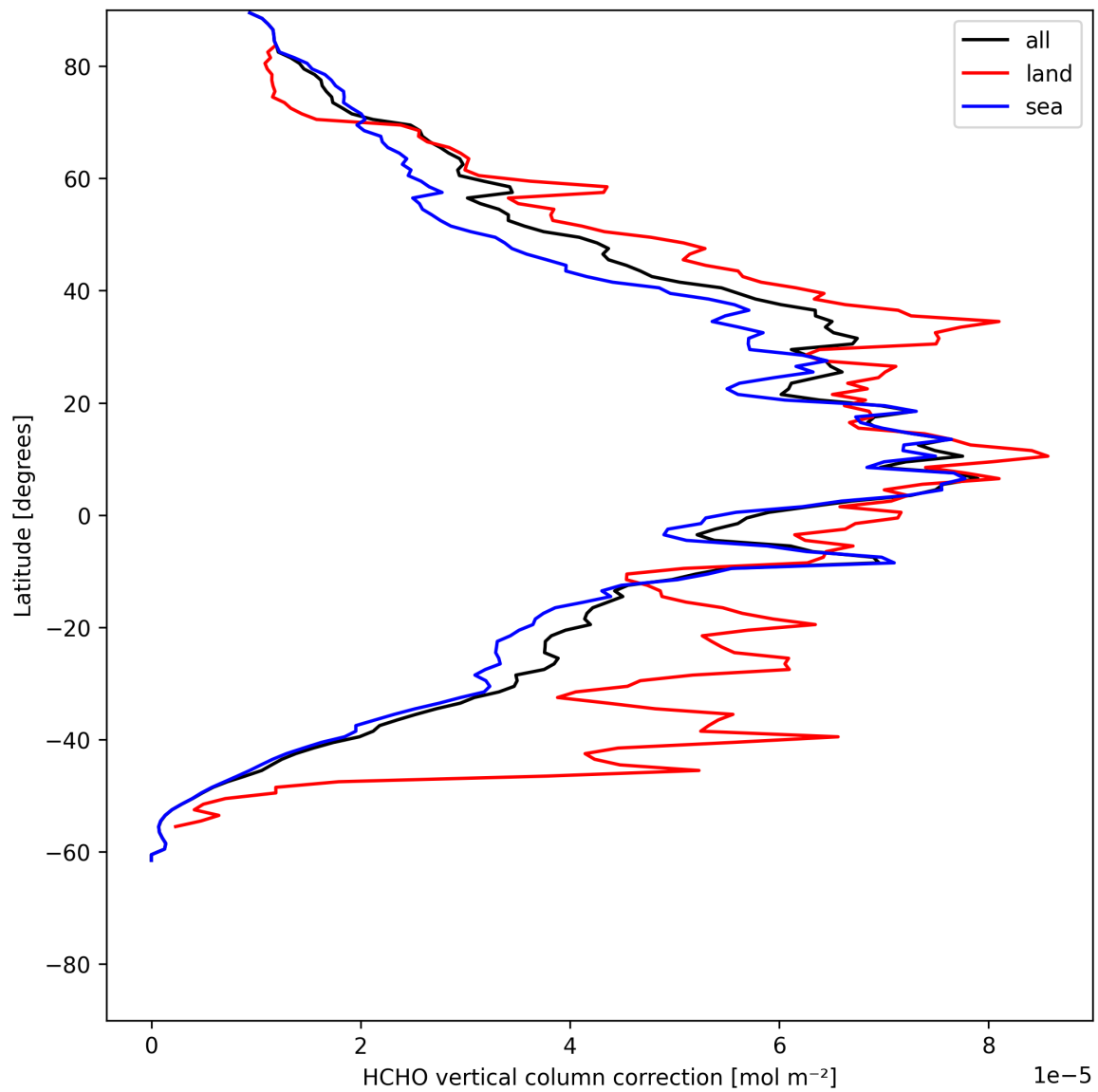
Figure 23: Zonal average of “HCHO vertical column correction” for 2025-06-13 to 2025-06-15.
