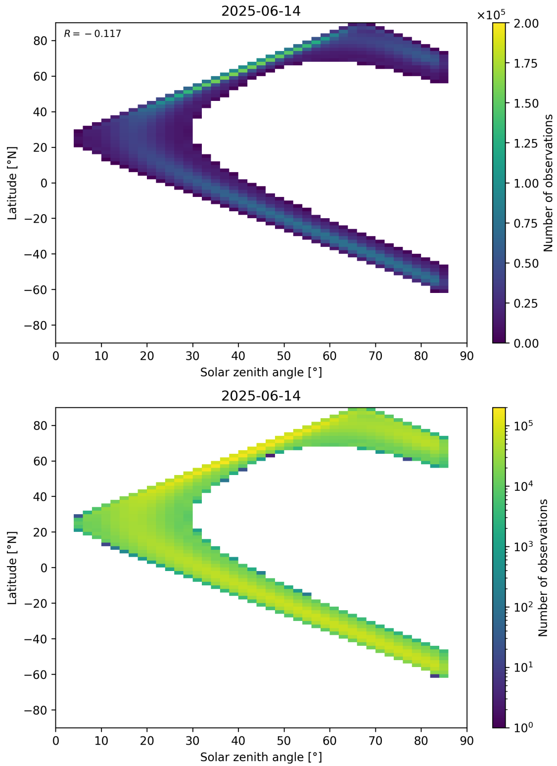
Figure 181: Scatter density plot of “Solar zenith angle” against “Latitude” for 2025-06-13 to 2025-06-15.
