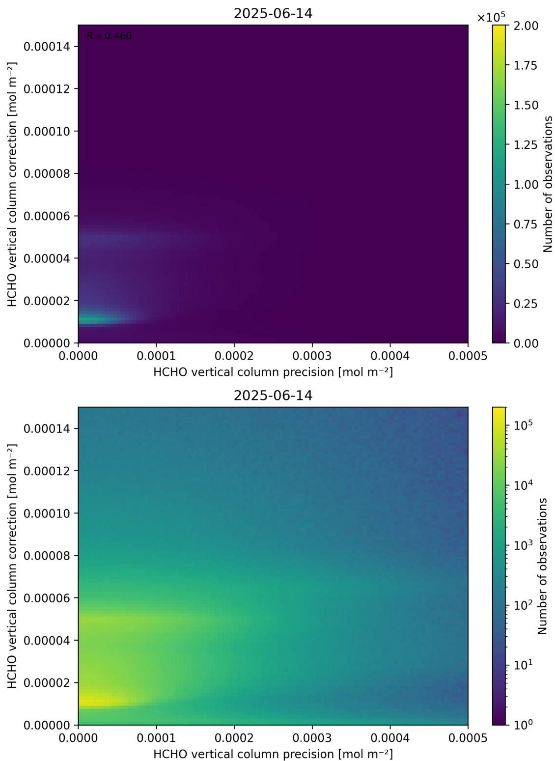
Figure 146: Scatter density plot of “HCHO vertical column precision” against “HCHO vertical column correction” for 2025-06-13 to 2025-06-15.
