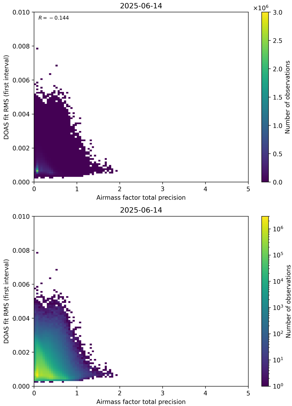
Figure 105: Scatter density plot of “Airmass factor total precision” against “DOAS fit RMS (first interval)” for 2025-06-13 to 2025-06-15.
