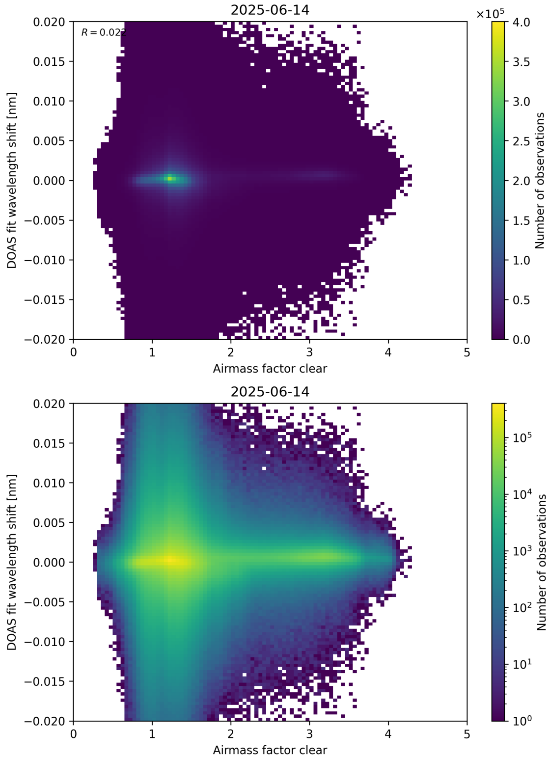
Figure 72: Scatter density plot of “Airmass factor clear” against “DOAS fit wavelength shift” for 2025-06-13 to 2025-06-15.
