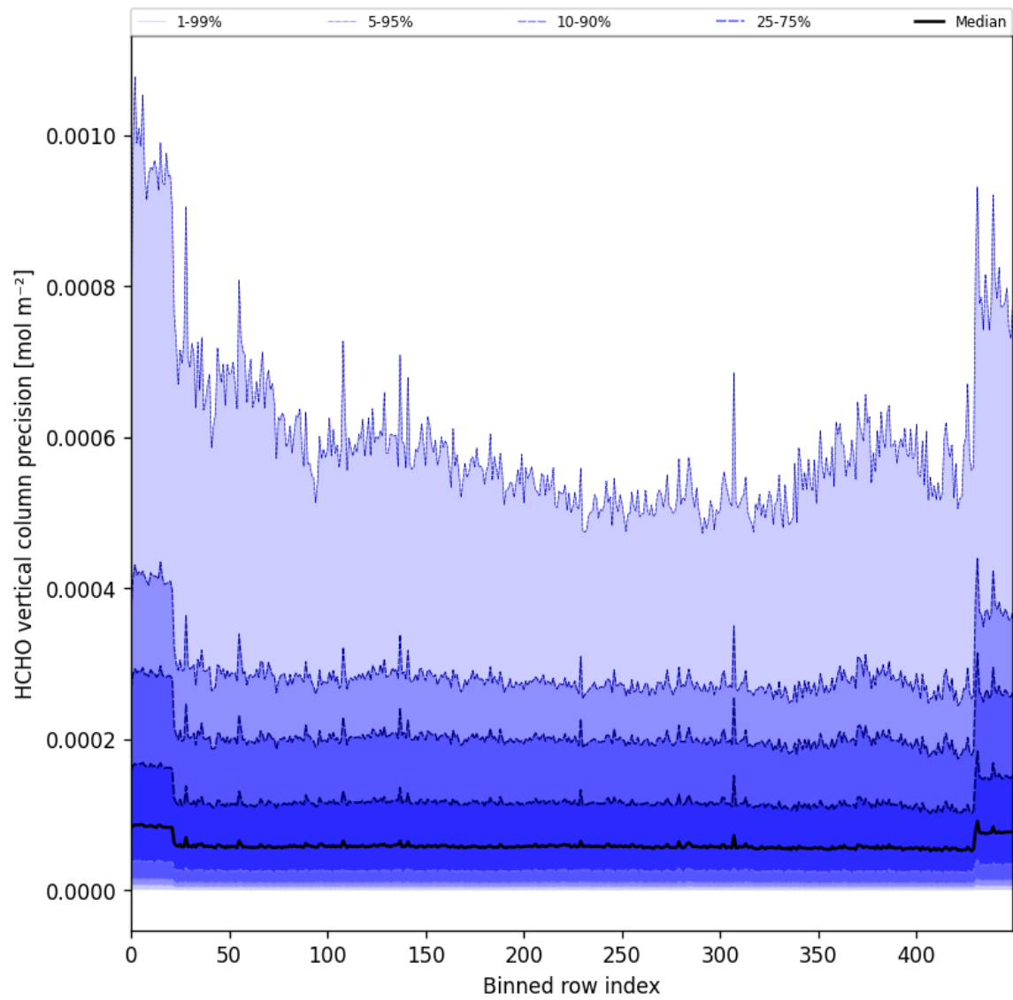
Figure 50: Along track statistics of “HCHO vertical column precision” for 2025-06-13 to 2025-06-15
