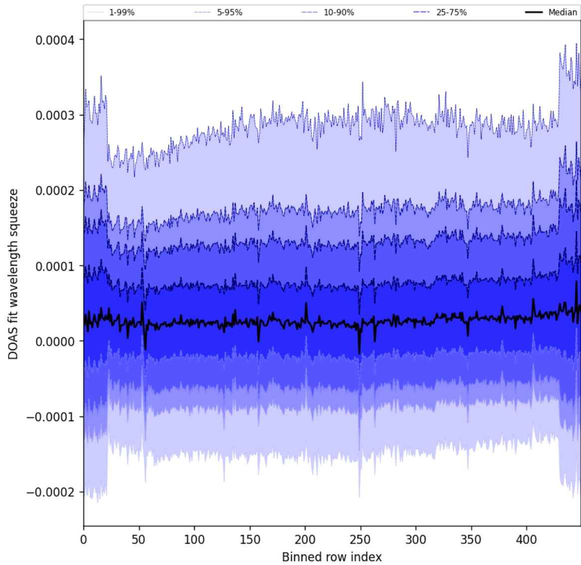
Figure 59: Along track statistics of “DOAS fit wavelength squeeze” for 2025-06-13 to 2025-06-15
