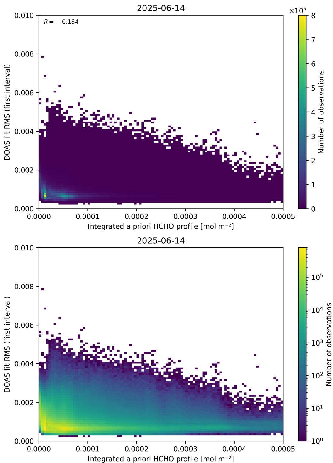
Figure 148: Scatter density plot of “Integrated a priori HCHO profile” against “DOAS fit RMS (first interval)” for 2025-06-13 to 2025-06-15.
