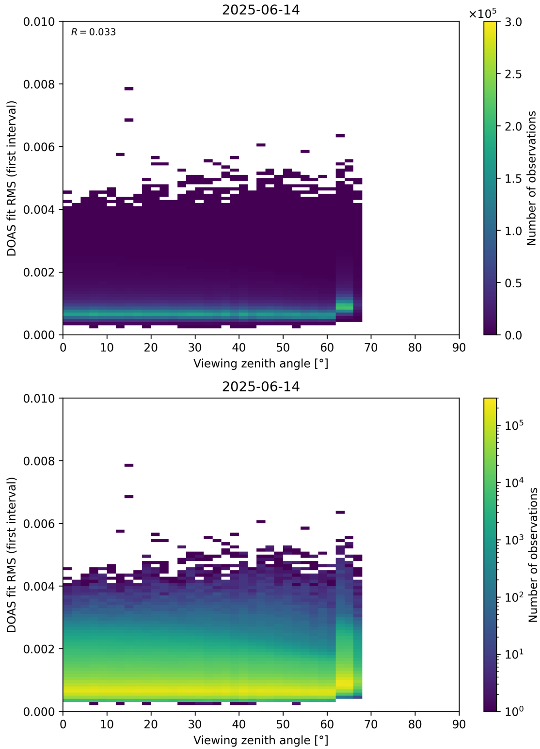
Figure 182: Scatter density plot of “Viewing zenith angle” against “DOAS fit RMS (first interval)” for 2025-06-13 to 2025-06-15.
