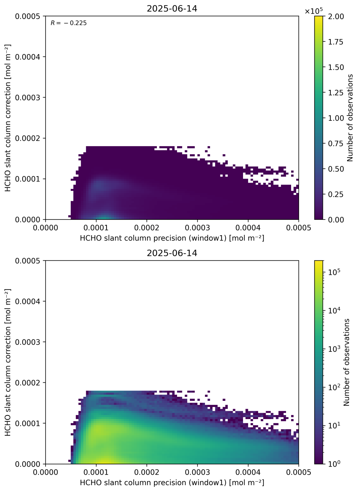
Figure 93: Scatter density plot of “HCHO slant column precision (window1)” against “HCHO slant column correction” for 2025-06-13 to 2025-06-15.
