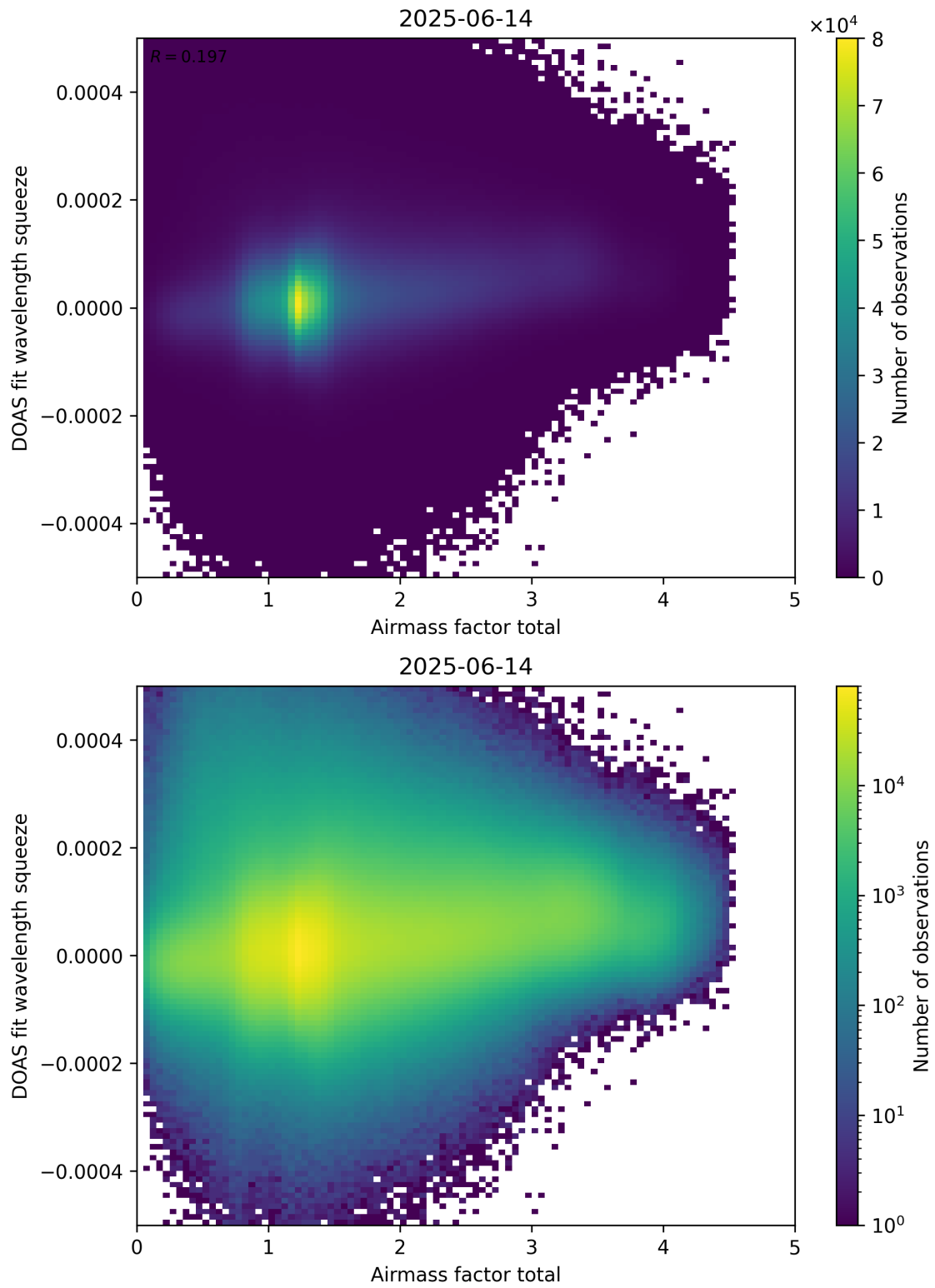
Figure 99: Scatter density plot of “Airmass factor total” against “DOAS fit wavelength squeeze” for 2025-06-13 to 2025-06-15.
