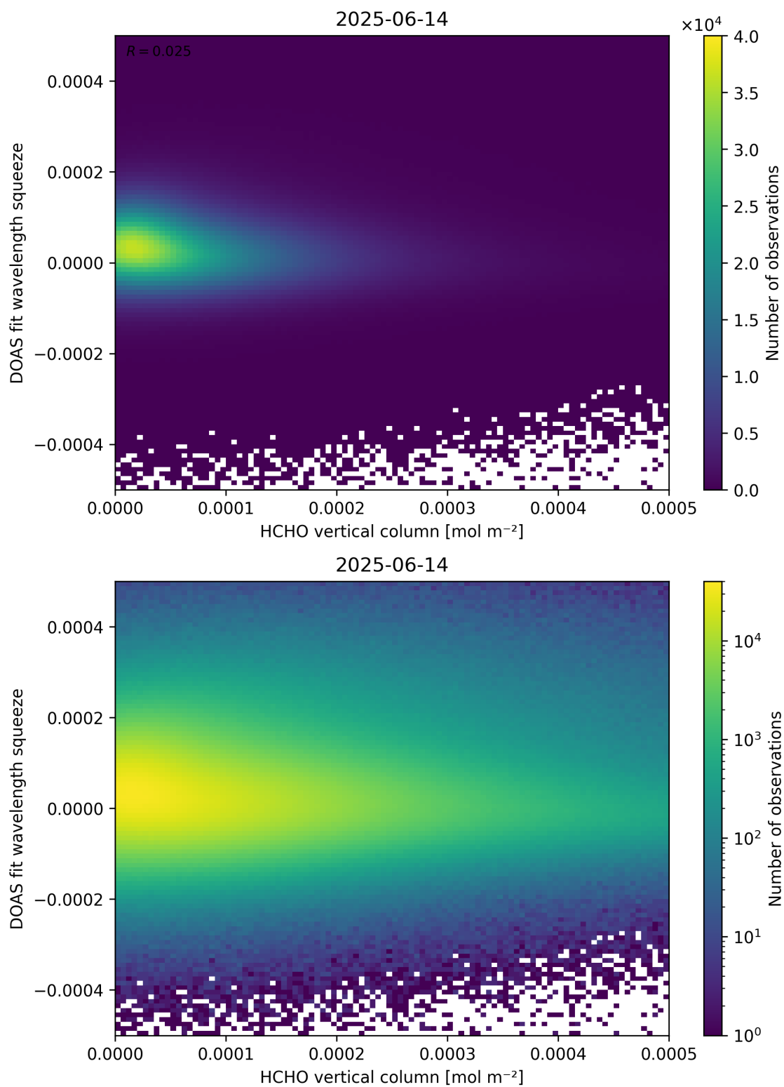
Figure 125: Scatter density plot of “HCHO vertical column” against “DOAS fit wavelength squeeze” for 2025-06-13 to 2025-06-15.
