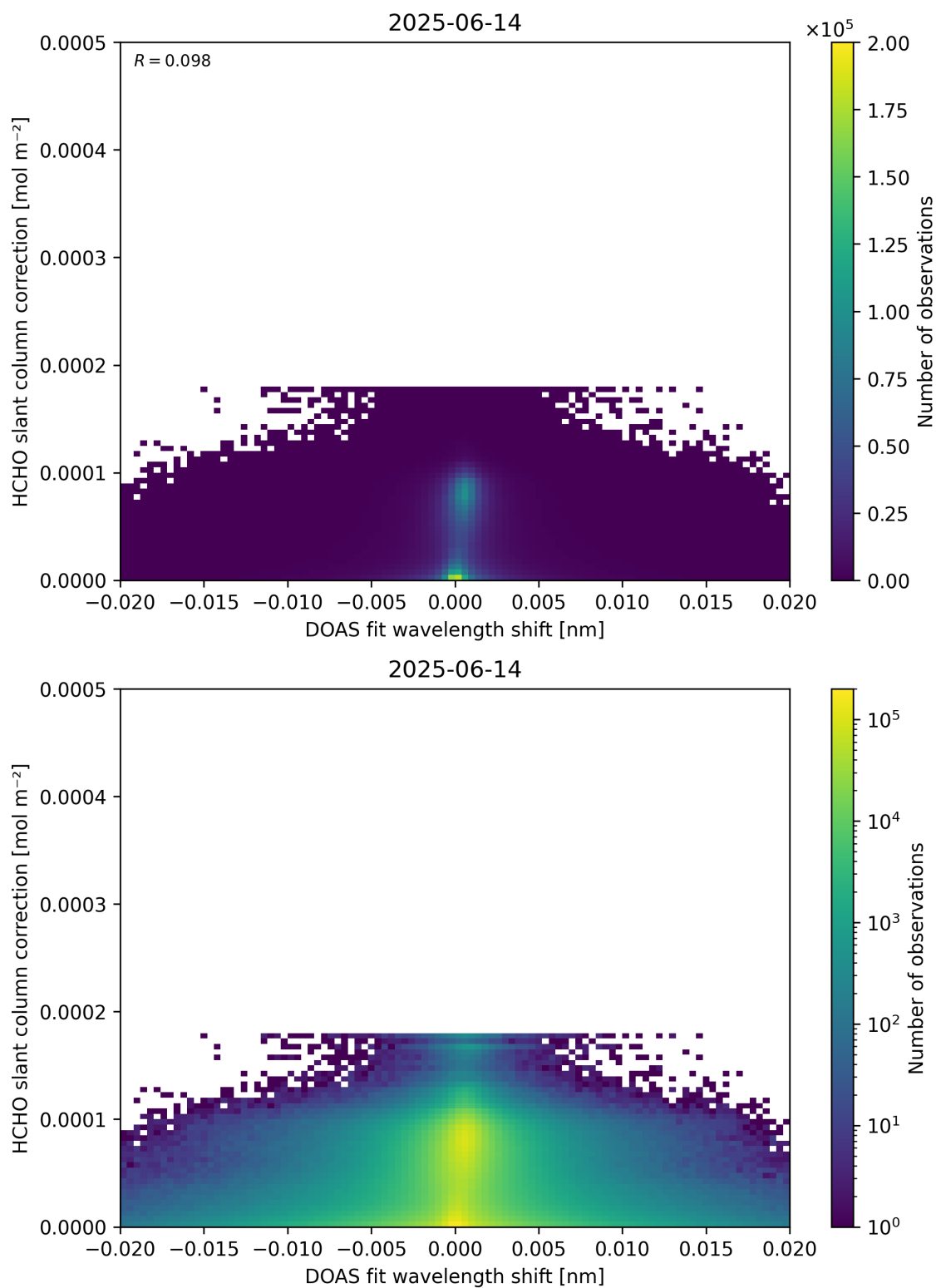
Figure 67: Scatter density plot of “DOAS fit wavelength shift” against “HCHO slant column correction” for 2025-06-13 to 2025-06-15.
