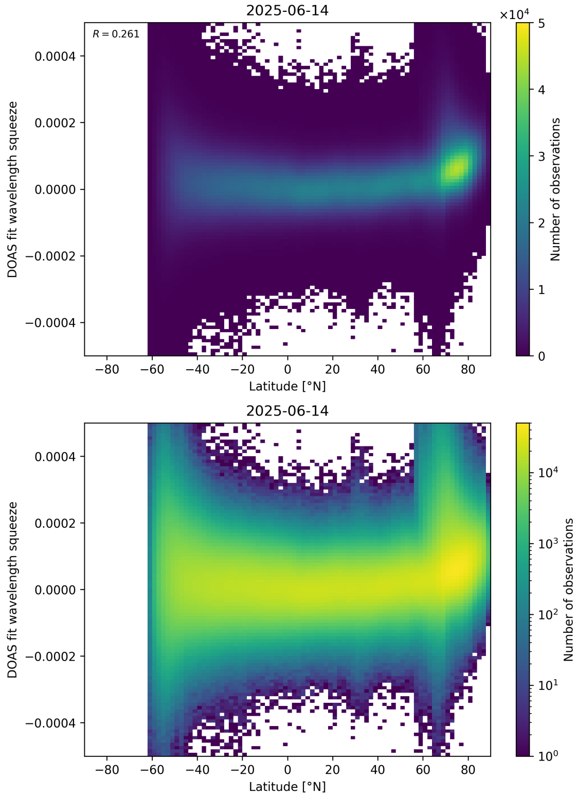
Figure 155: Scatter density plot of “Latitude” against “DOAS fit wavelength squeeze” for 2025-06-13 to 2025-06-15.
