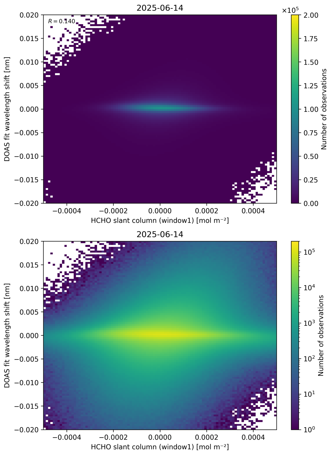
Figure 79: Scatter density plot of “HCHO slant column (window1)” against “DOAS fit wavelength shift” for 2025-06-13 to 2025-06-15.
