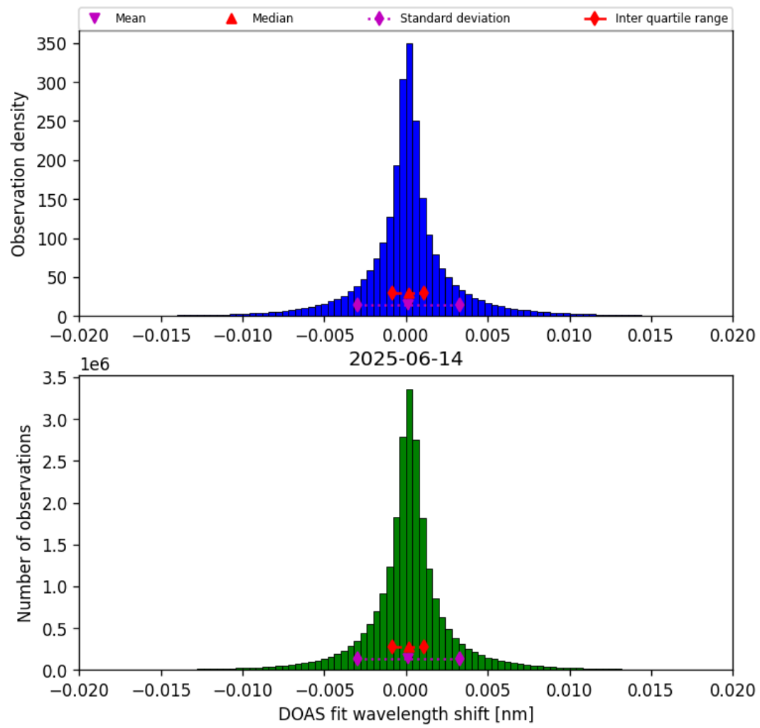
Figure 44: Histogram of “DOAS fit wavelength shift” for 2025-06-13 to 2025-06-15
