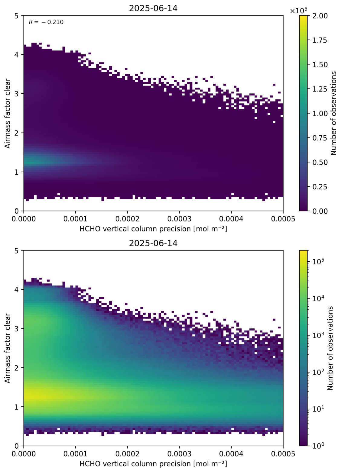
Figure 139: Scatter density plot of “HCHO vertical column precision” against “Airmass factor clear” for 2025-06-13 to 2025-06-15.
