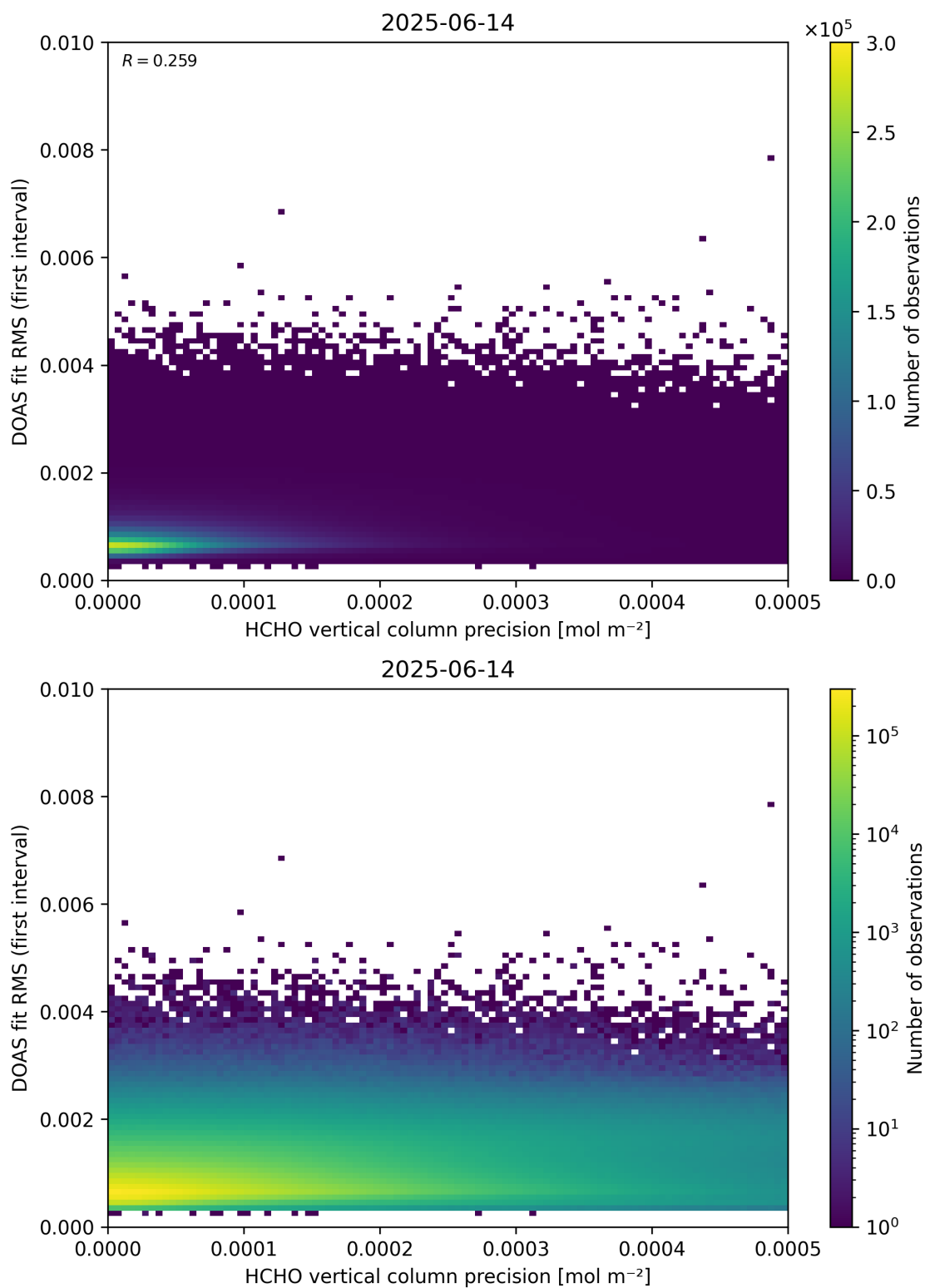
Figure 136: Scatter density plot of “HCHO vertical column precision” against “DOAS fit RMS (first interval)” for 2025-06-13 to 2025-06-15.
