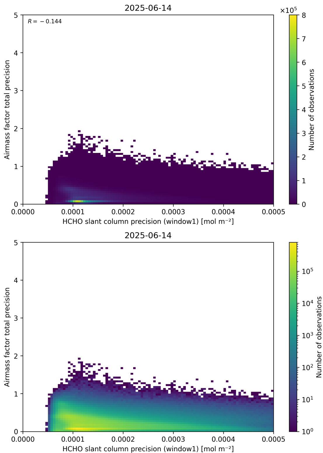
Figure 95: Scatter density plot of “HCHO slant column precision (window1)” against “Airmass factor total precision” for 2025-06-13 to 2025-06-15.
