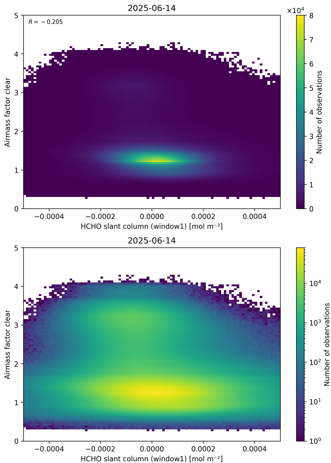
Figure 81: Scatter density plot of “HCHO slant column (window1)” against “Airmass factor clear” for 2025-06-13 to 2025-06-15.
