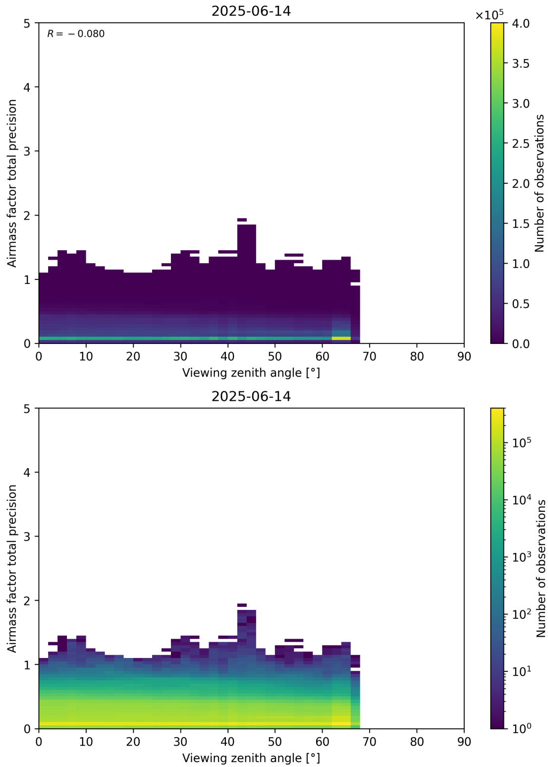
Figure 191: Scatter density plot of “Viewing zenith angle” against “Airmass factor total precision” for 2025-06-13 to 2025-06-15.
