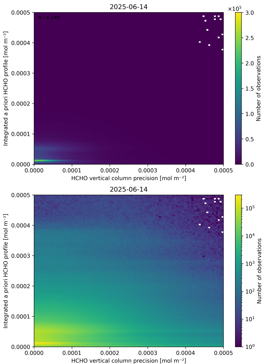
Figure 147: Scatter density plot of “HCHO vertical column precision” against “Integrated a priori HCHO profile” for 2025-06-13 to 2025-06-15.
