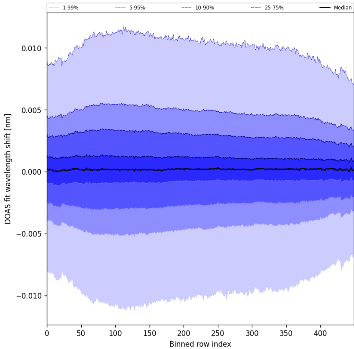
Figure 58: Along track statistics of “DOAS fit wavelength shift” for 2025-06-13 to 2025-06-15
