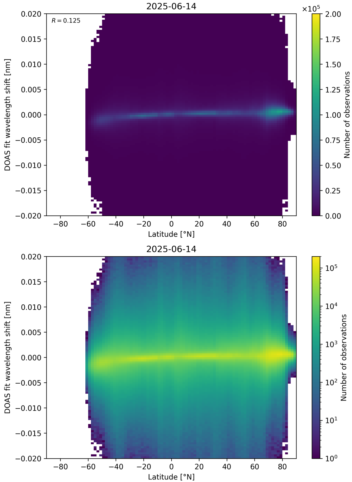
Figure 154: Scatter density plot of “Latitude” against “DOAS fit wavelength shift” for 2025-06-13 to 2025-06-15.
