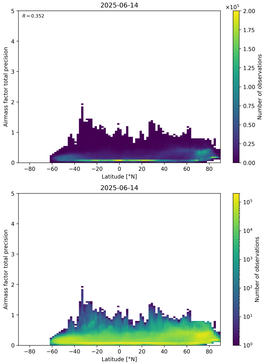
Figure 162: Scatter density plot of “Latitude” against “Airmass factor total precision” for 2025-06-13 to 2025-06-15.
