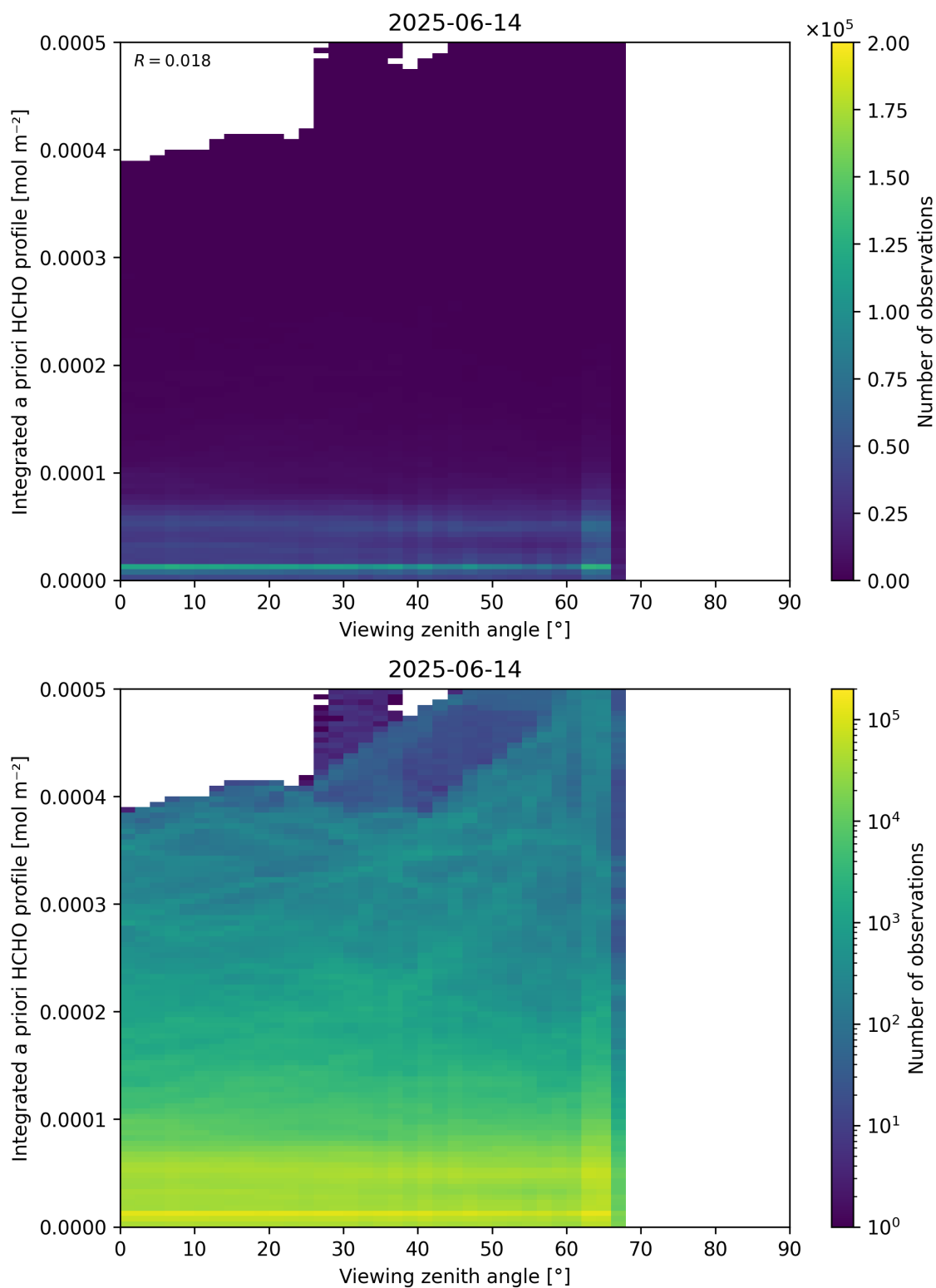
Figure 195: Scatter density plot of “Viewing zenith angle” against “Integrated a priori HCHO profile” for 2025-06-13 to 2025-06-15.
