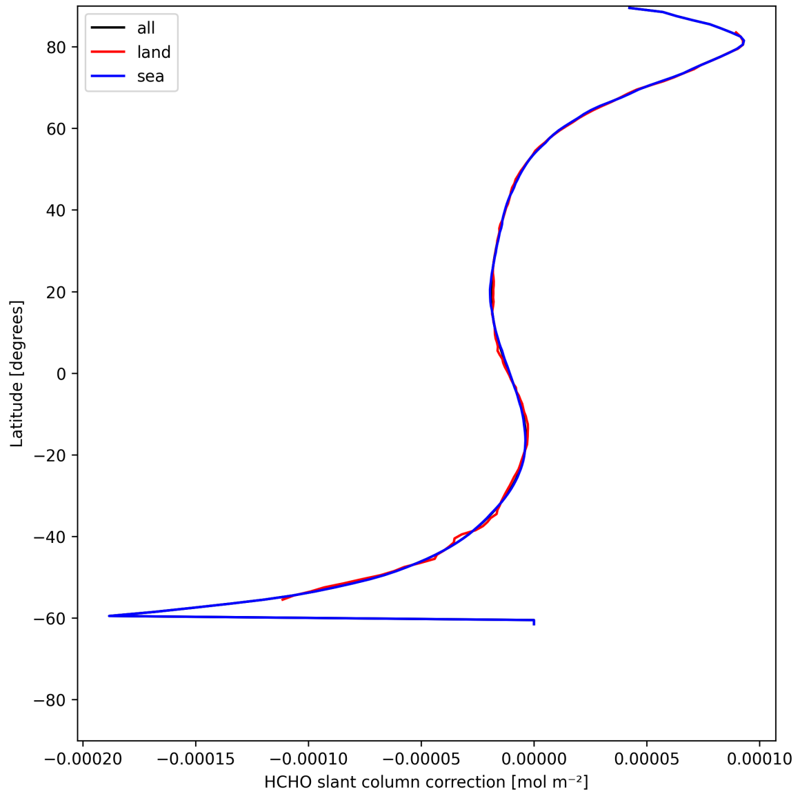
Figure 33: Zonal average of “HCHO slant column correction” for 2025-06-13 to 2025-06-15.
