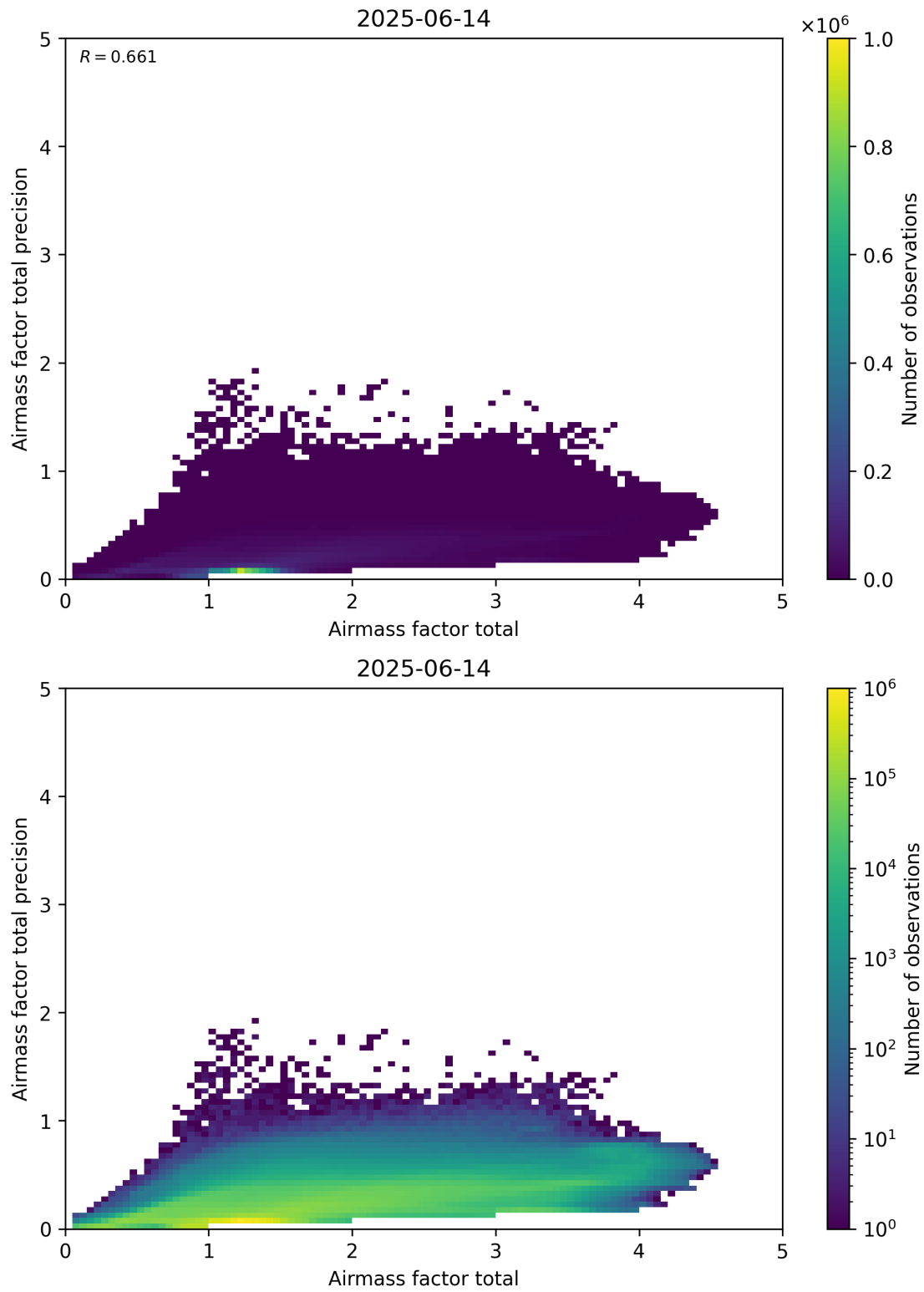
Figure 103: Scatter density plot of “Airmass factor total” against “Airmass factor total precision” for 2025-06-13 to 2025-06-15.
