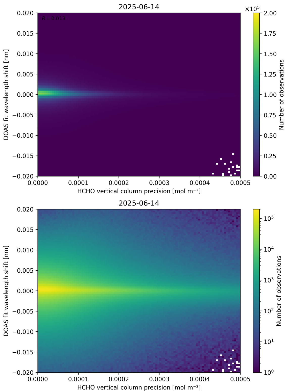
Figure 137: Scatter density plot of “HCHO vertical column precision” against “DOAS fit wavelength shift” for 2025-06-13 to 2025-06-15.
