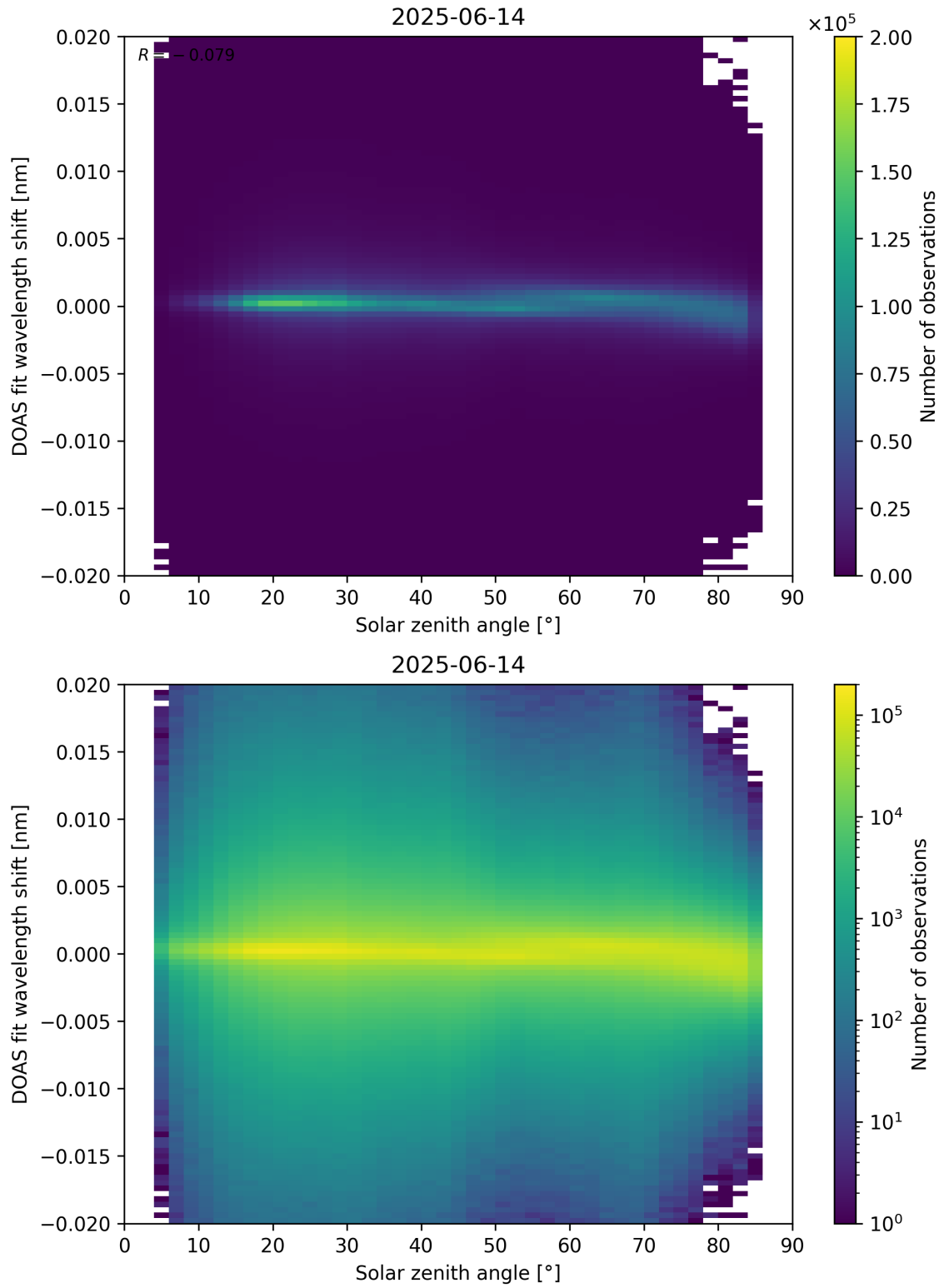
Figure 168: Scatter density plot of “Solar zenith angle” against “DOAS fit wavelength shift” for 2025-06-13 to 2025-06-15.
