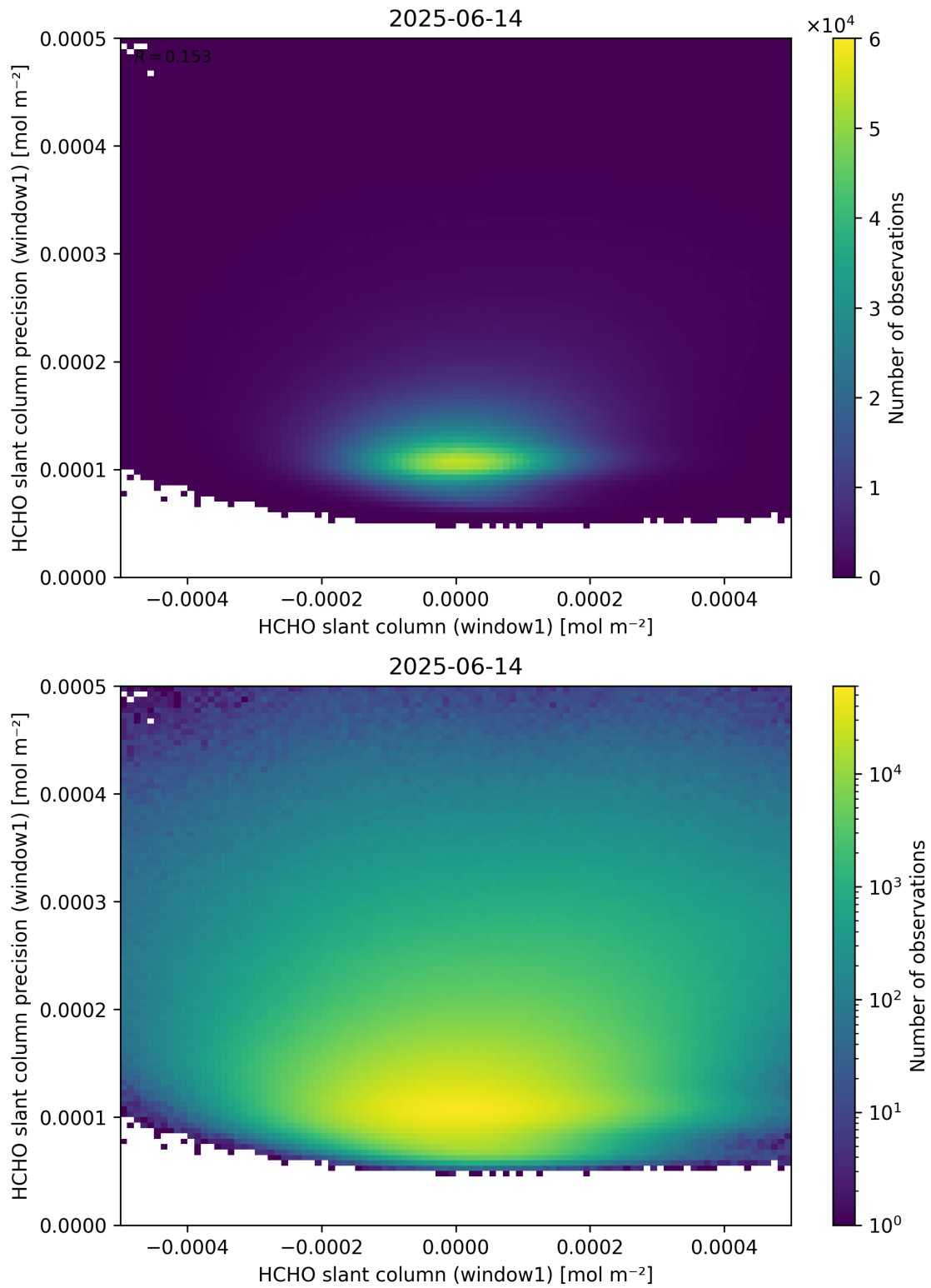
Figure 84: Scatter density plot of “HCHO slant column (window1)” against “HCHO slant column precision (window1)” for 2025-06-13 to 2025-06-15.
