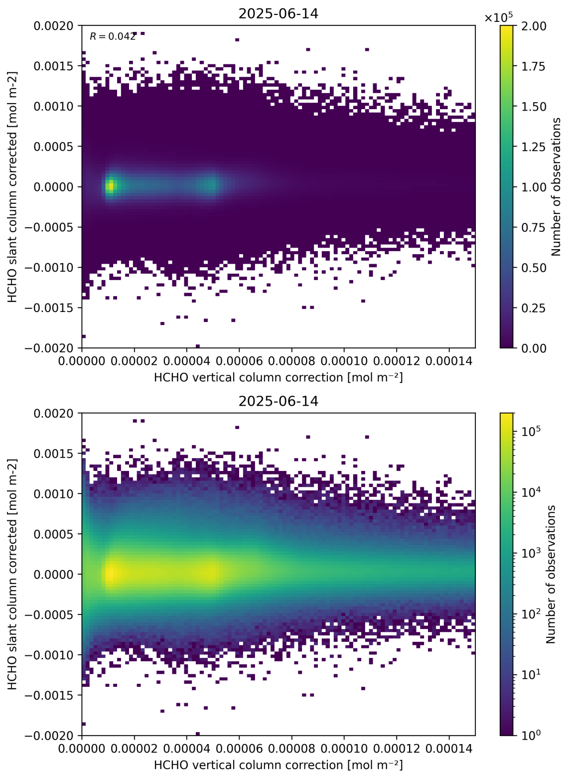
Figure 116: Scatter density plot of “HCHO vertical column correction” against “HCHO slant column corrected” for 2025-06-13 to 2025-06-15.
