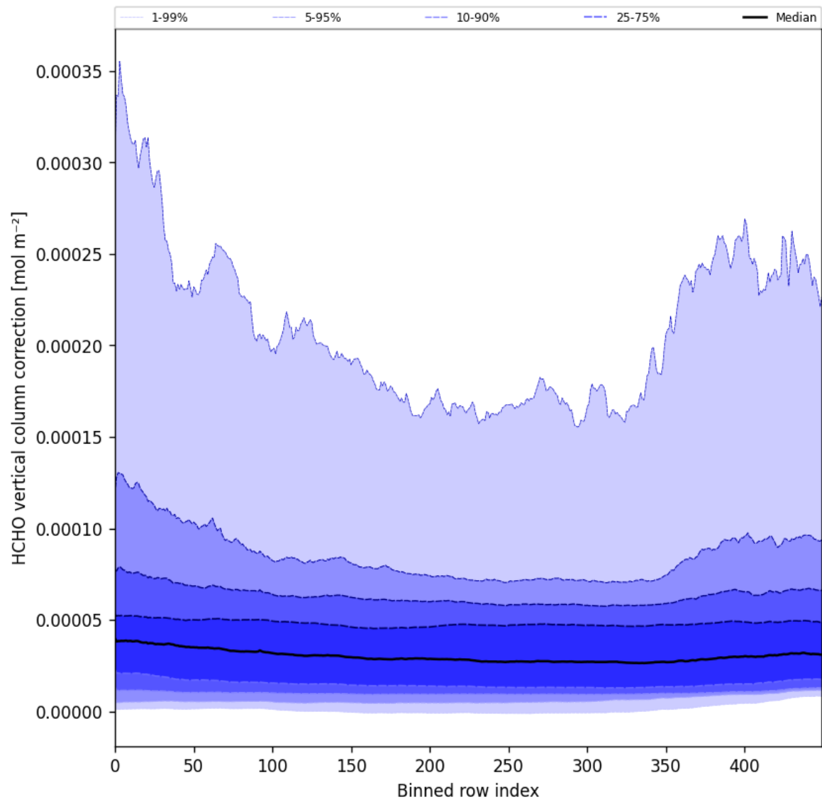
Figure 51: Along track statistics of “HCHO vertical column correction” for 2025-06-13 to 2025-06-15
