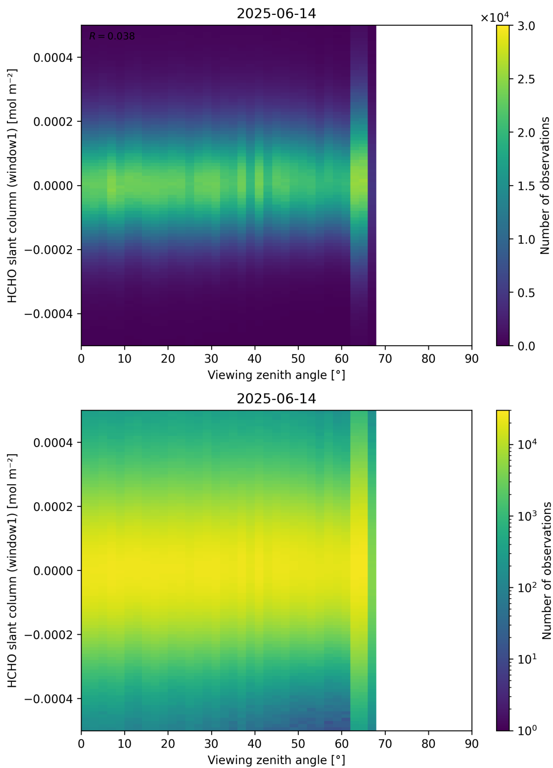
Figure 188: Scatter density plot of “Viewing zenith angle” against “HCHO slant column (window1)” for 2025-06-13 to 2025-06-15.
