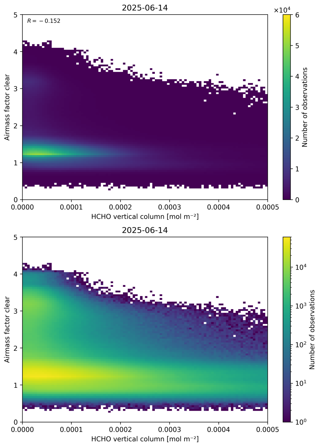
Figure 126: Scatter density plot of “HCHO vertical column” against “Airmass factor clear” for 2025-06-13 to 2025-06-15.
