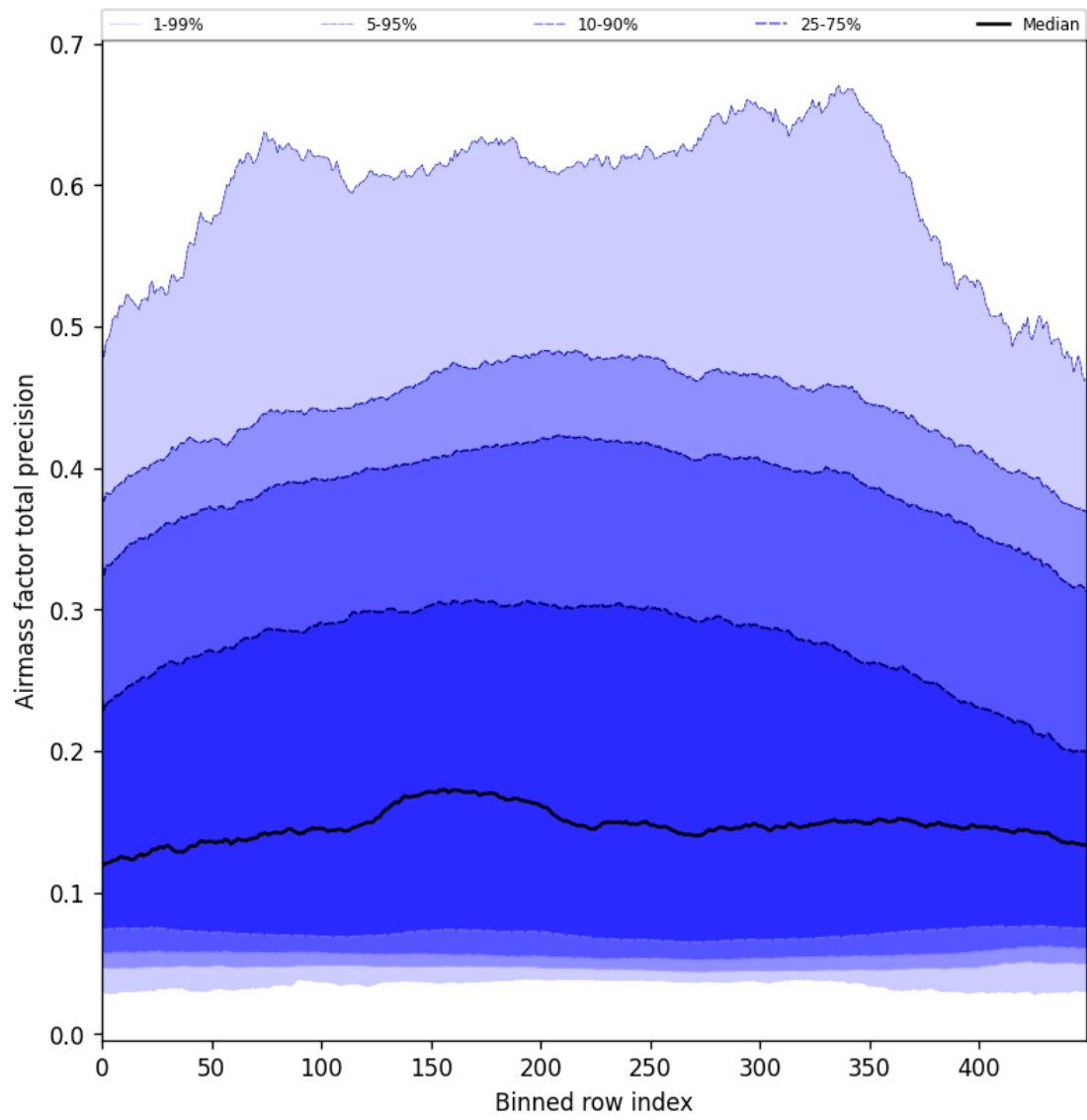
Figure 55: Along track statistics of “Airmass factor total precision” for 2025-06-13 to 2025-06-15
