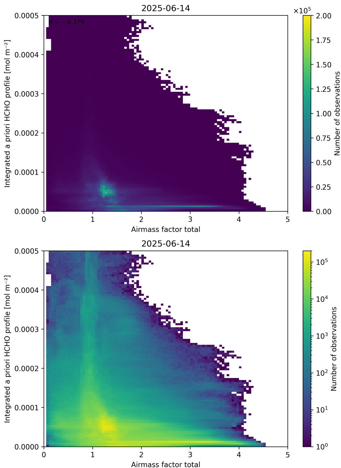
Figure 104: Scatter density plot of “Airmass factor total” against “Integrated a priori HCHO profile” for 2025-06-13 to 2025-06-15.
