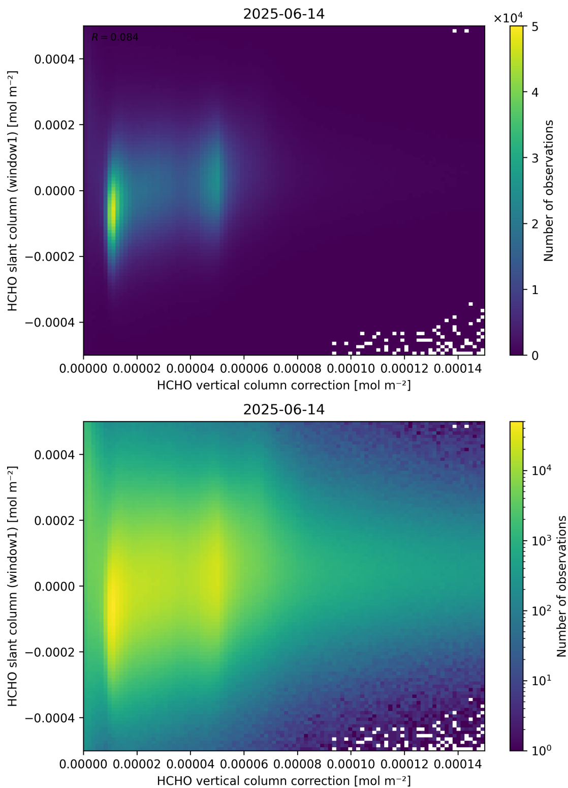
Figure 118: Scatter density plot of “HCHO vertical column correction” against “HCHO slant column (window1)” for 2025-06-13 to 2025-06-15.
