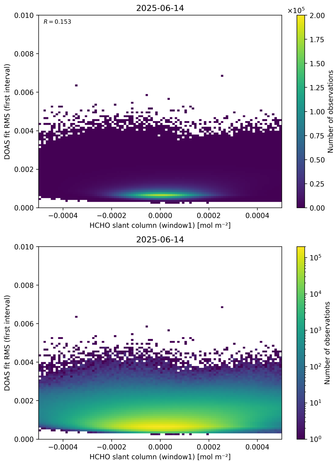
Figure 78: Scatter density plot of “HCHO slant column (window1)” against “DOAS fit RMS (first interval)” for 2025-06-13 to 2025-06-15.
