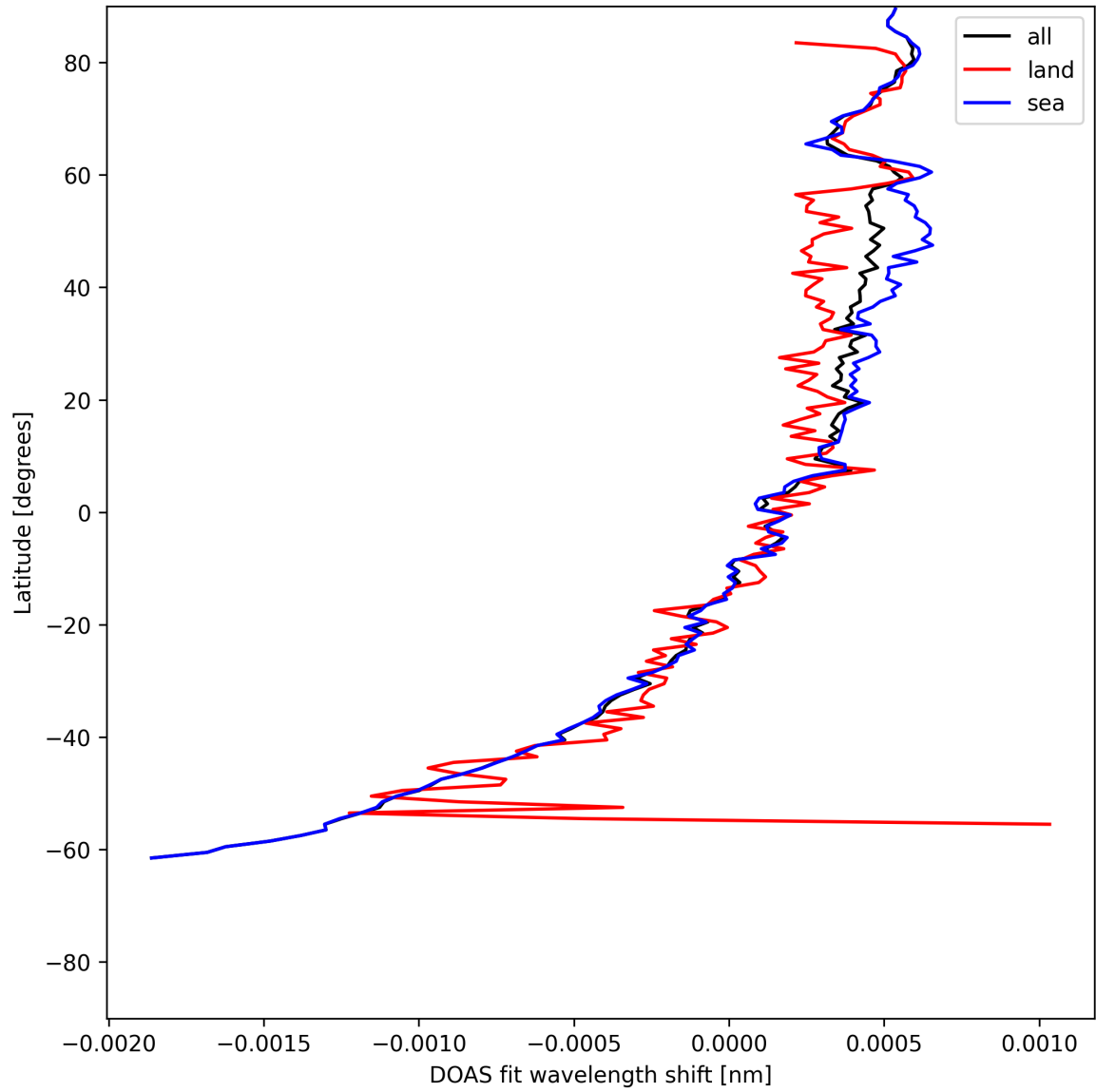
Figure 30: Zonal average of “DOAS fit wavelength shift” for 2025-06-13 to 2025-06-15.
