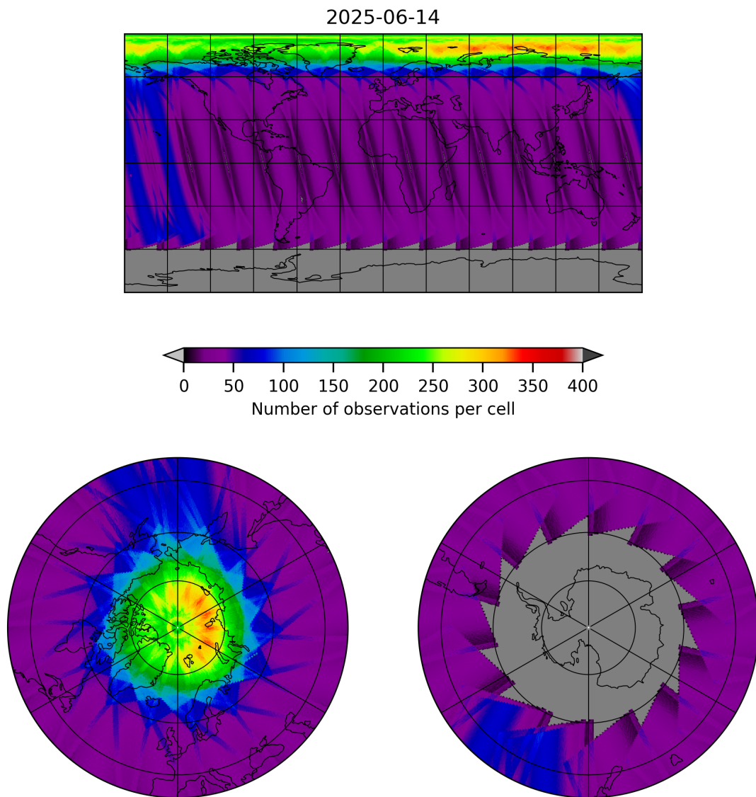
Figure 19: Map of the number of observations for 2025-06-13 to 2025-06-15
