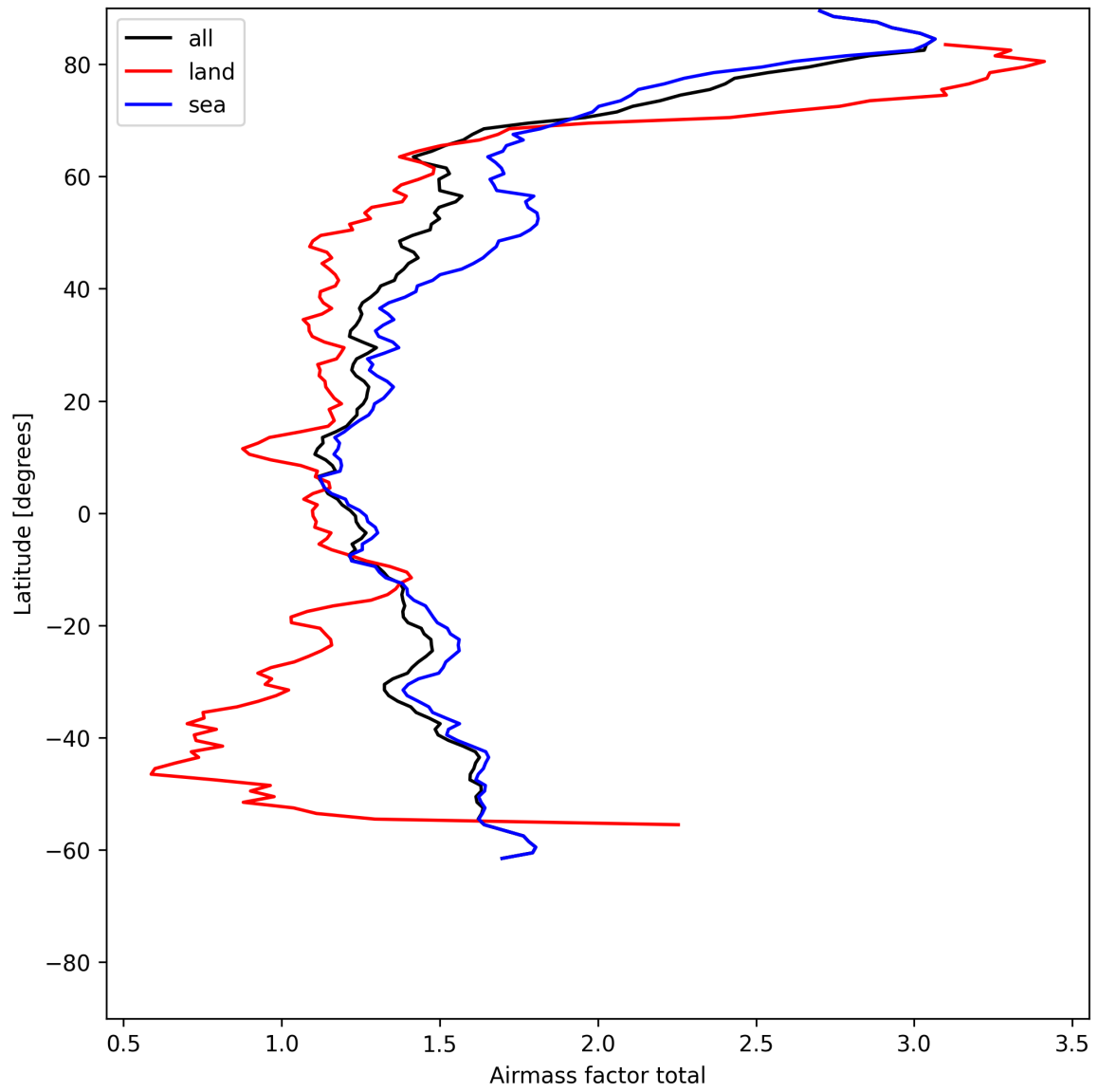
Figure 26: Zonal average of “Airmass factor total” for 2025-06-13 to 2025-06-15.
