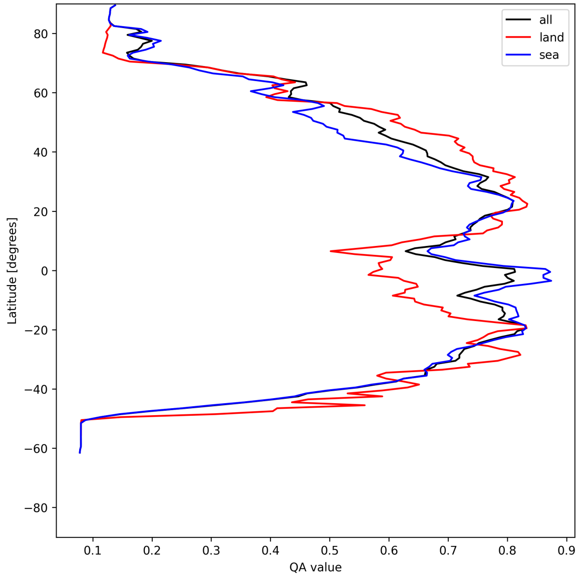
Figure 20: Zonal average of “QA value” for 2025-06-13 to 2025-06-15.
