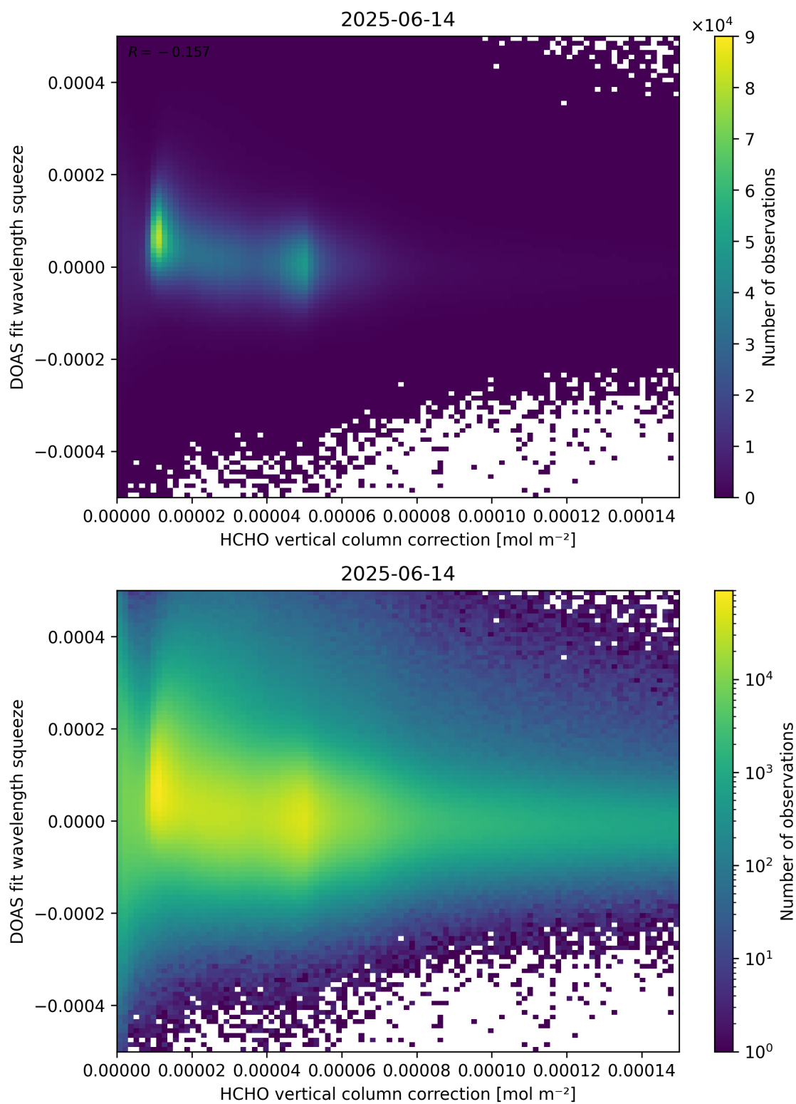
Figure 114: Scatter density plot of “HCHO vertical column correction” against “DOAS fit wavelength squeeze” for 2025-06-13 to 2025-06-15.
