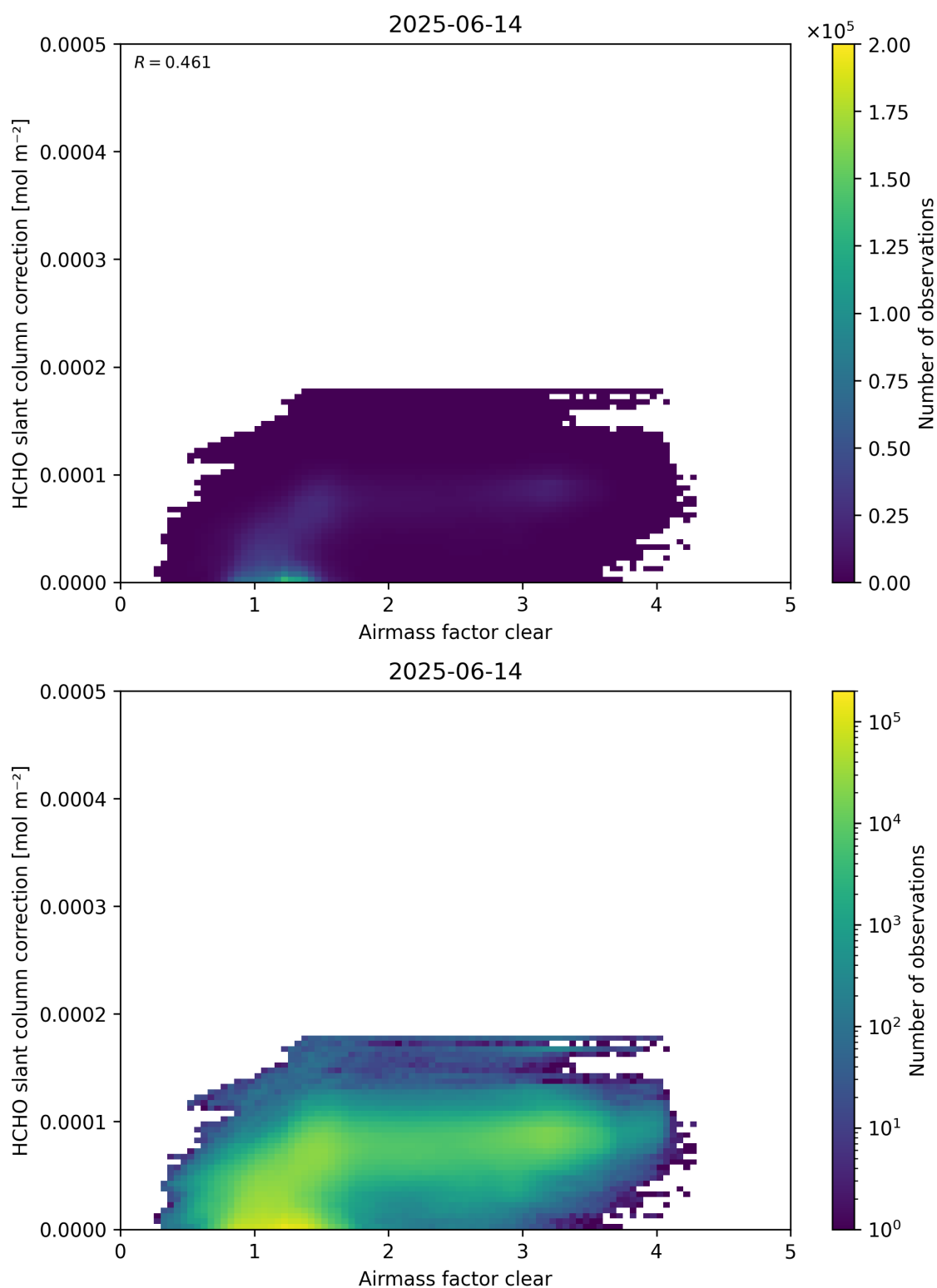
Figure 75: Scatter density plot of “Airmass factor clear” against “HCHO slant column correction” for 2025-06-13 to 2025-06-15.
