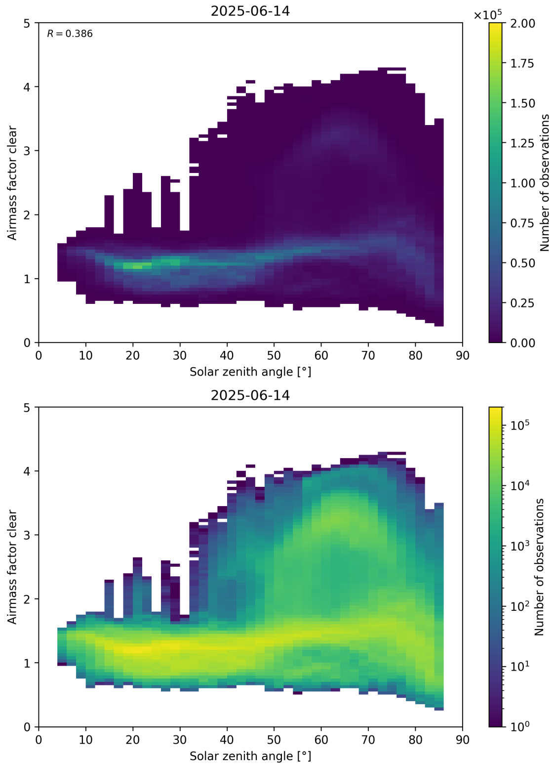
Figure 170: Scatter density plot of “Solar zenith angle” against “Airmass factor clear” for 2025-06-13 to 2025-06-15.
