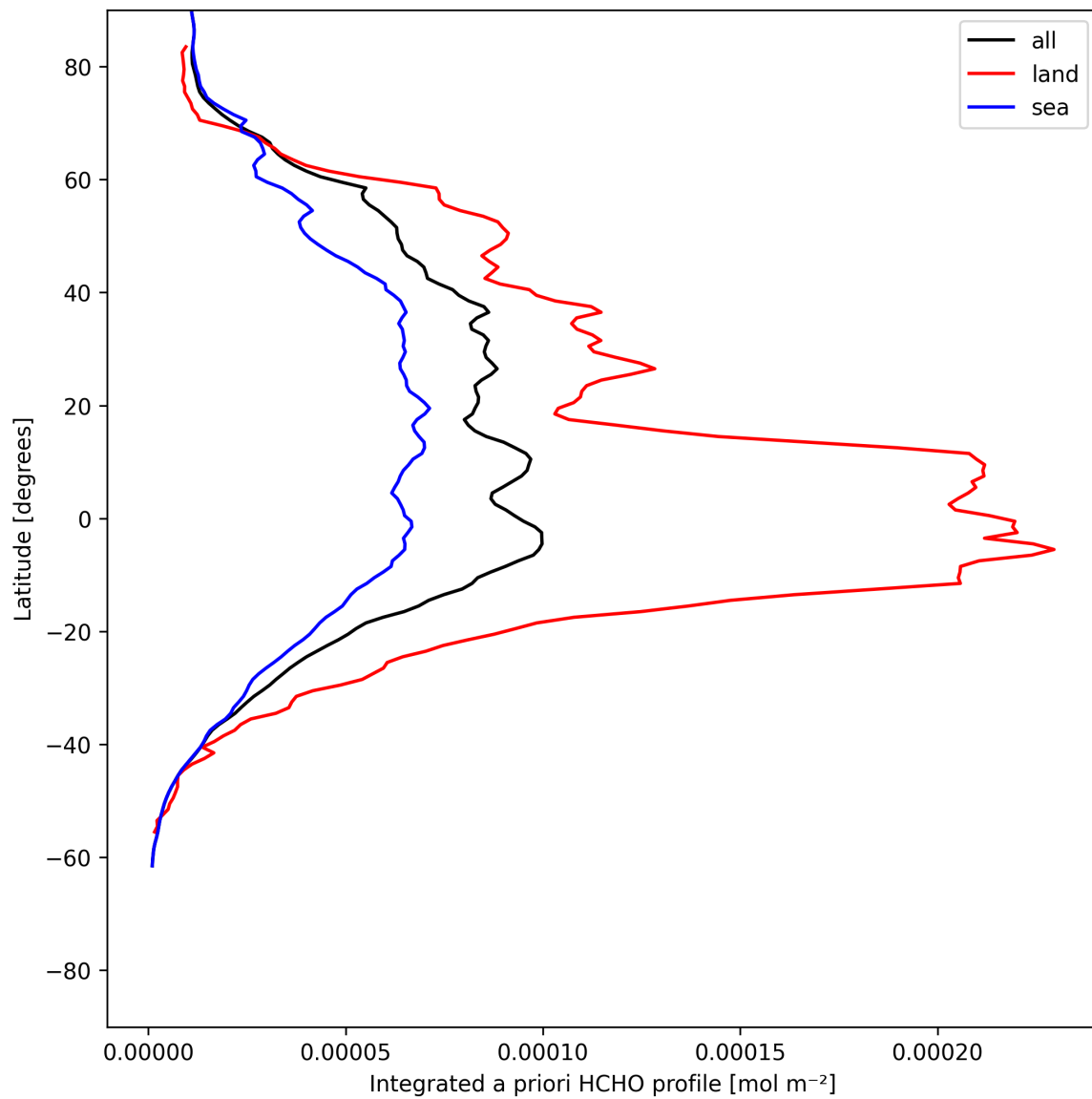
Figure 29: Zonal average of “Integrated a priori HCHO profile” for 2025-06-13 to 2025-06-15.
