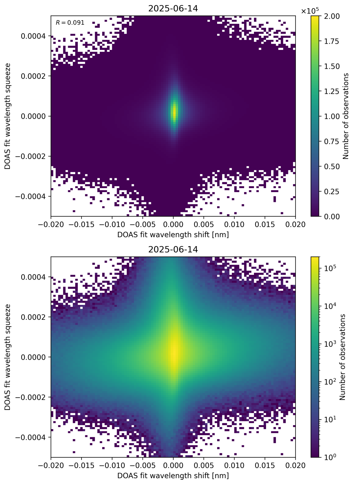
Figure 65: Scatter density plot of “DOAS fit wavelength shift” against “DOAS fit wavelength squeeze” for 2025-06-13 to 2025-06-15.
