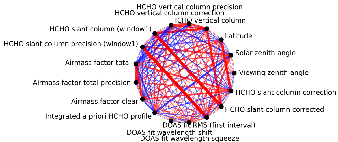
Figure 1: Map of correlation graph for 2025-06-13 to 2025-06-15.
