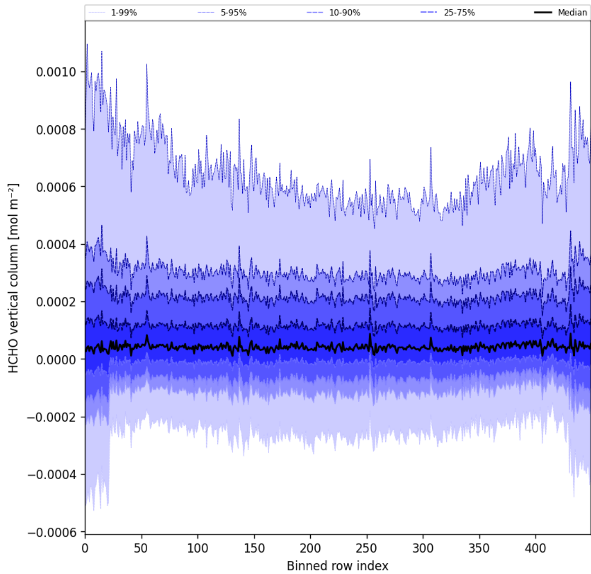
Figure 49: Along track statistics of “HCHO vertical column” for 2025-06-13 to 2025-06-15
