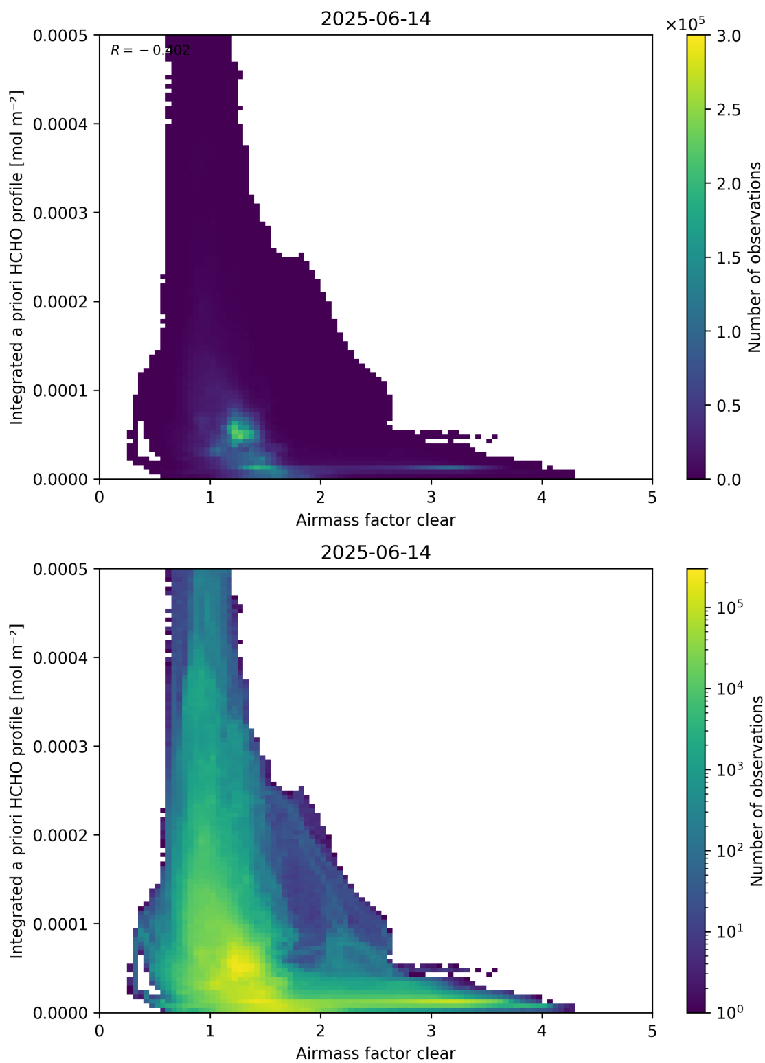
Figure 76: Scatter density plot of “Airmass factor clear” against “Integrated a priori HCHO profile” for 2025-06-13 to 2025-06-15.
