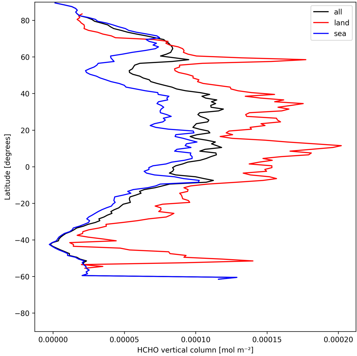
Figure 21: Zonal average of “HCHO vertical column” for 2025-06-13 to 2025-06-15.
