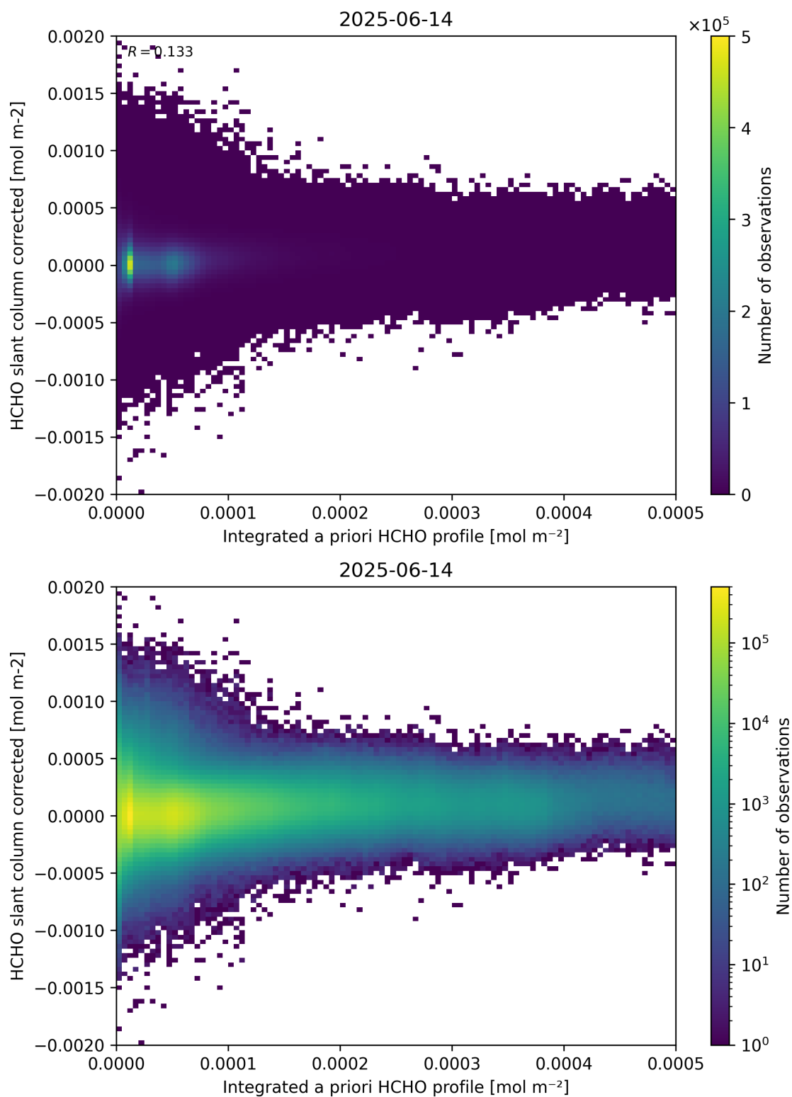
Figure 151: Scatter density plot of “Integrated a priori HCHO profile” against “HCHO slant column corrected” for 2025-06-13 to 2025-06-15.
