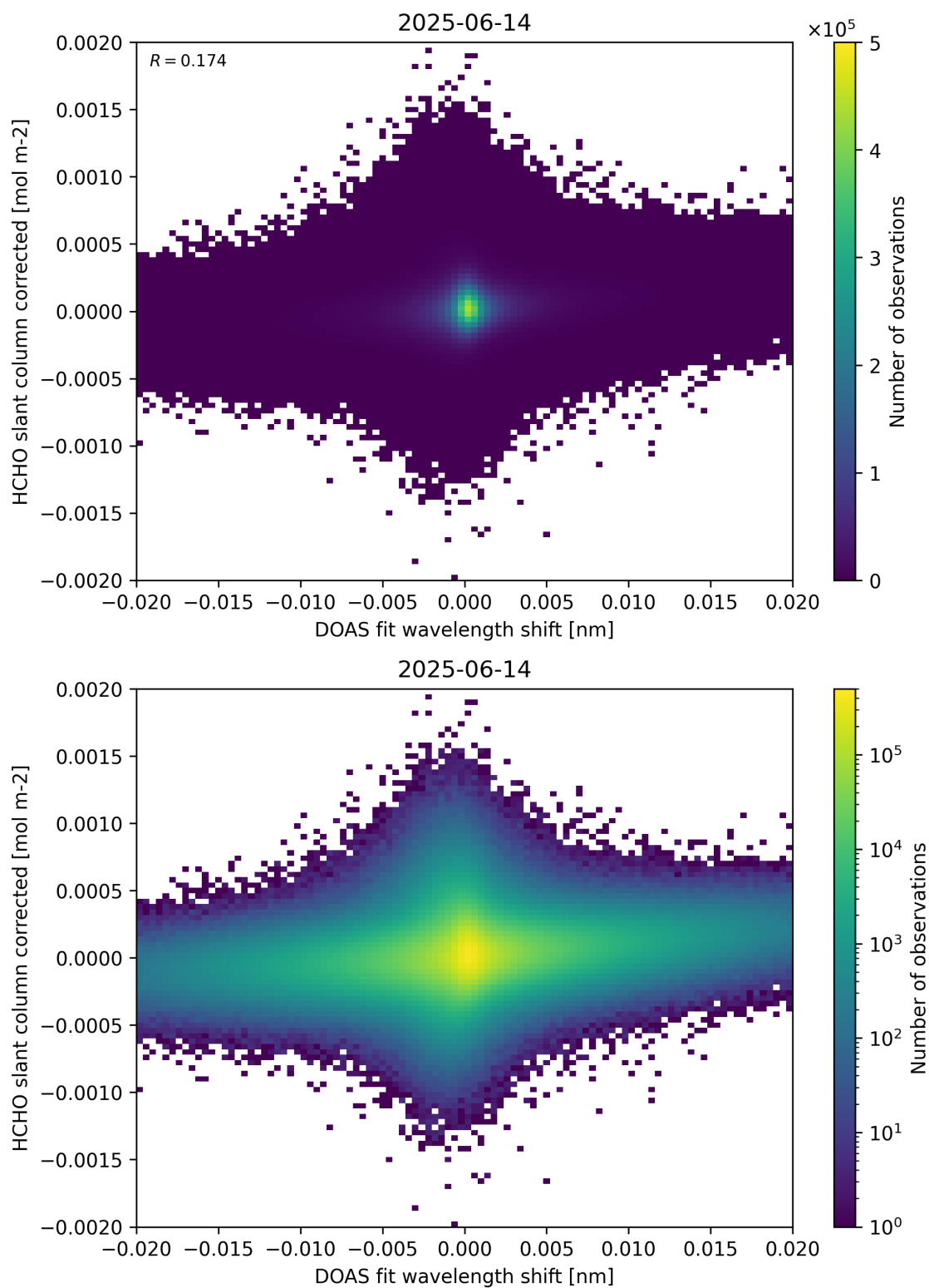
Figure 66: Scatter density plot of “DOAS fit wavelength shift” against “HCHO slant column corrected” for 2025-06-13 to 2025-06-15.
