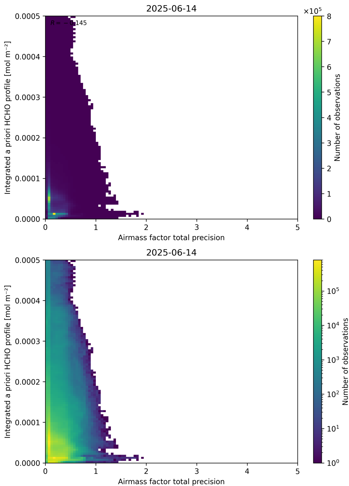
Figure 111: Scatter density plot of “Airmass factor total precision” against “Integrated a priori HCHO profile” for 2025-06-13 to 2025-06-15.
