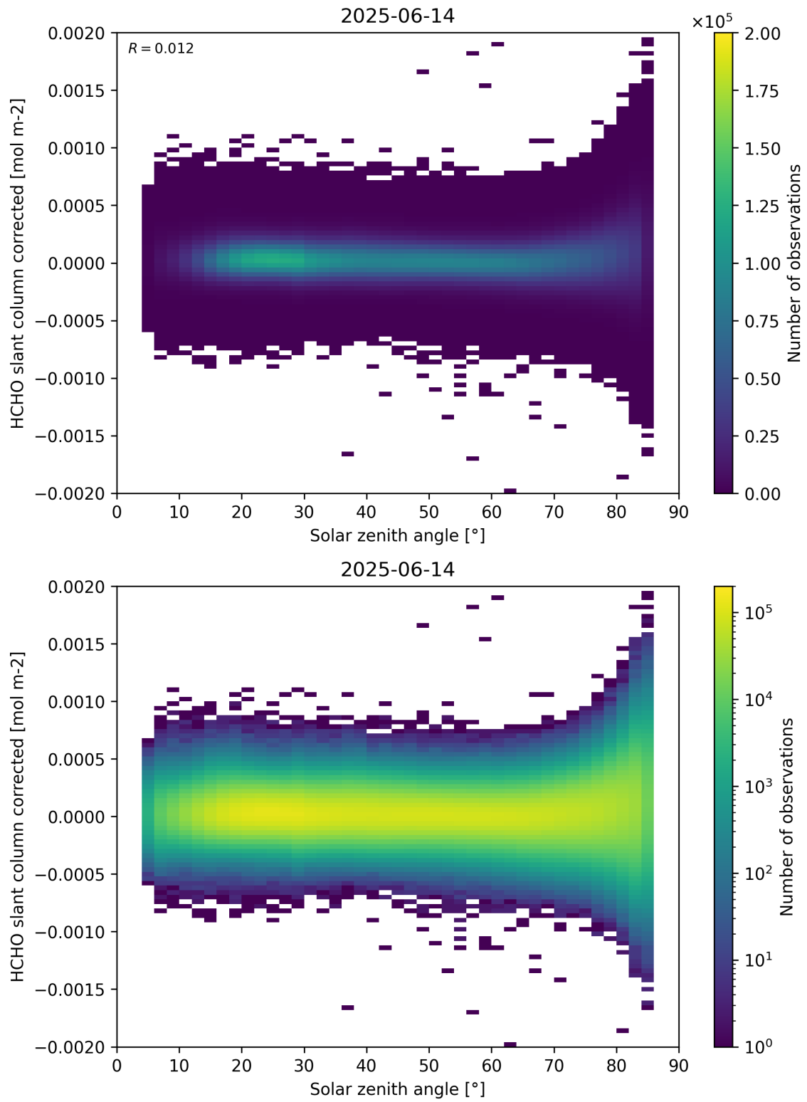
Figure 171: Scatter density plot of “Solar zenith angle” against “HCHO slant column corrected” for 2025-06-13 to 2025-06-15.
