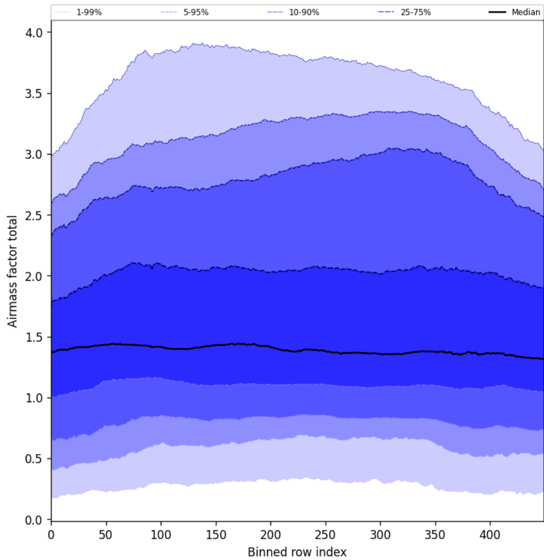
Figure 54: Along track statistics of “Airmass factor total” for 2025-06-13 to 2025-06-15
