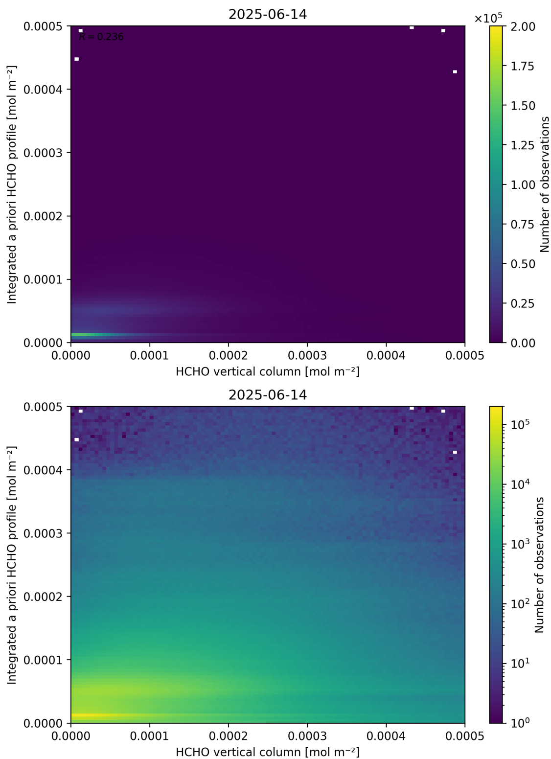
Figure 135: Scatter density plot of “HCHO vertical column” against “Integrated a priori HCHO profile” for 2025-06-13 to 2025-06-15.
