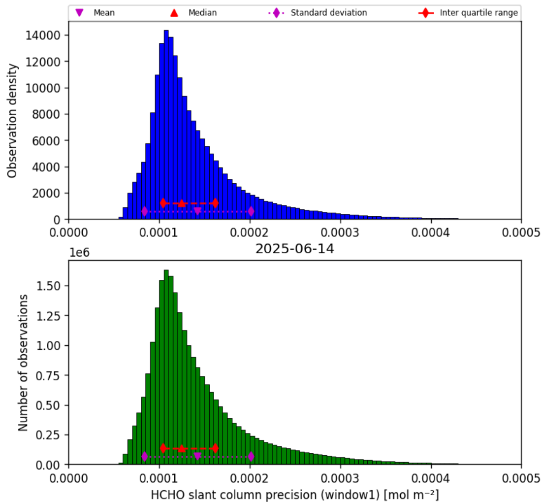
Figure 39: Histogram of “HCHO slant column precision (window1)” for 2025-06-13 to 2025-06-15
