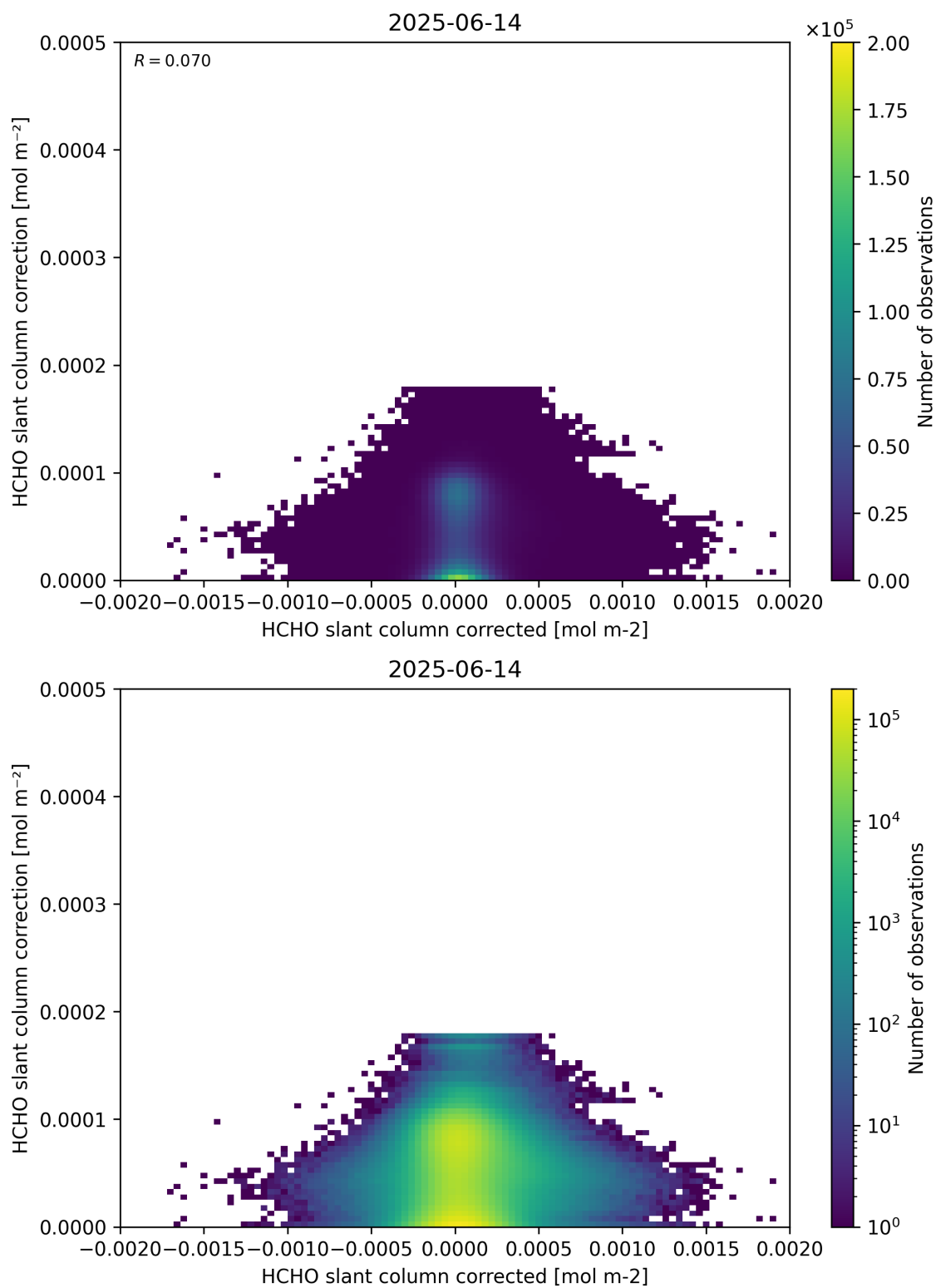
Figure 77: Scatter density plot of “HCHO slant column corrected” against “HCHO slant column correction” for 2025-06-13 to 2025-06-15.
