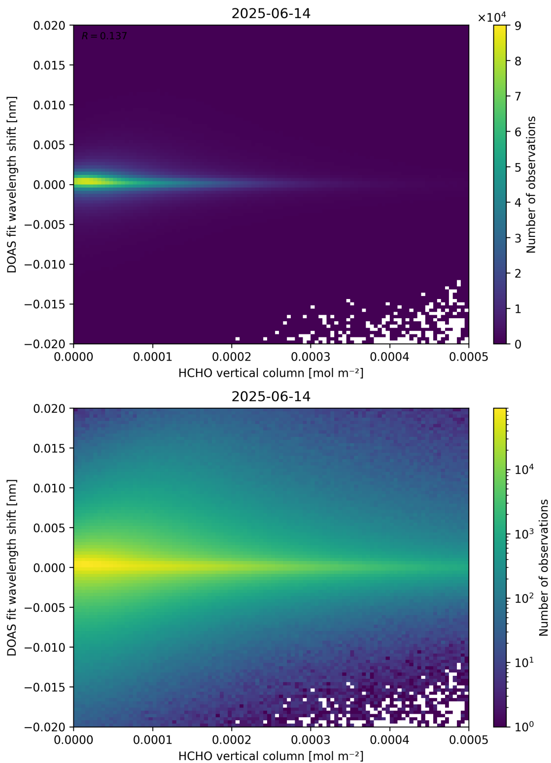
Figure 124: Scatter density plot of “HCHO vertical column” against “DOAS fit wavelength shift” for 2025-06-13 to 2025-06-15.
