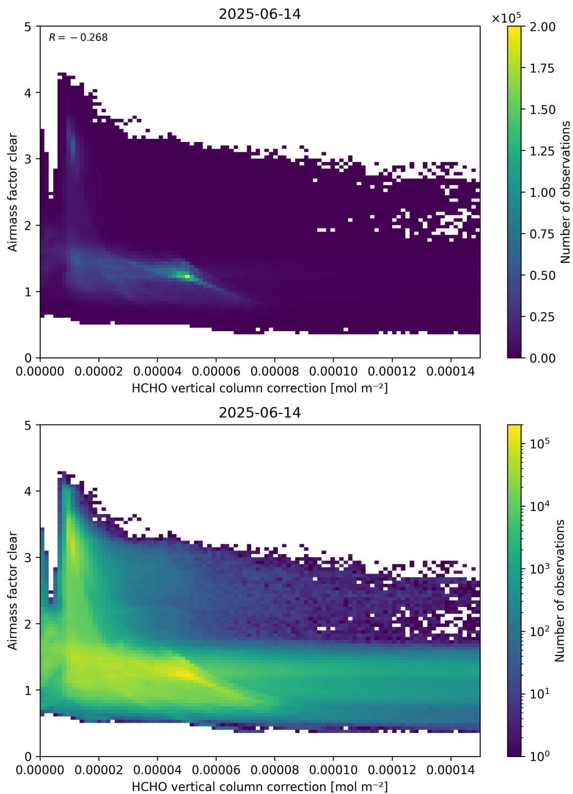
Figure 115: Scatter density plot of “HCHO vertical column correction” against “Airmass factor clear” for 2025-06-13 to 2025-06-15.
