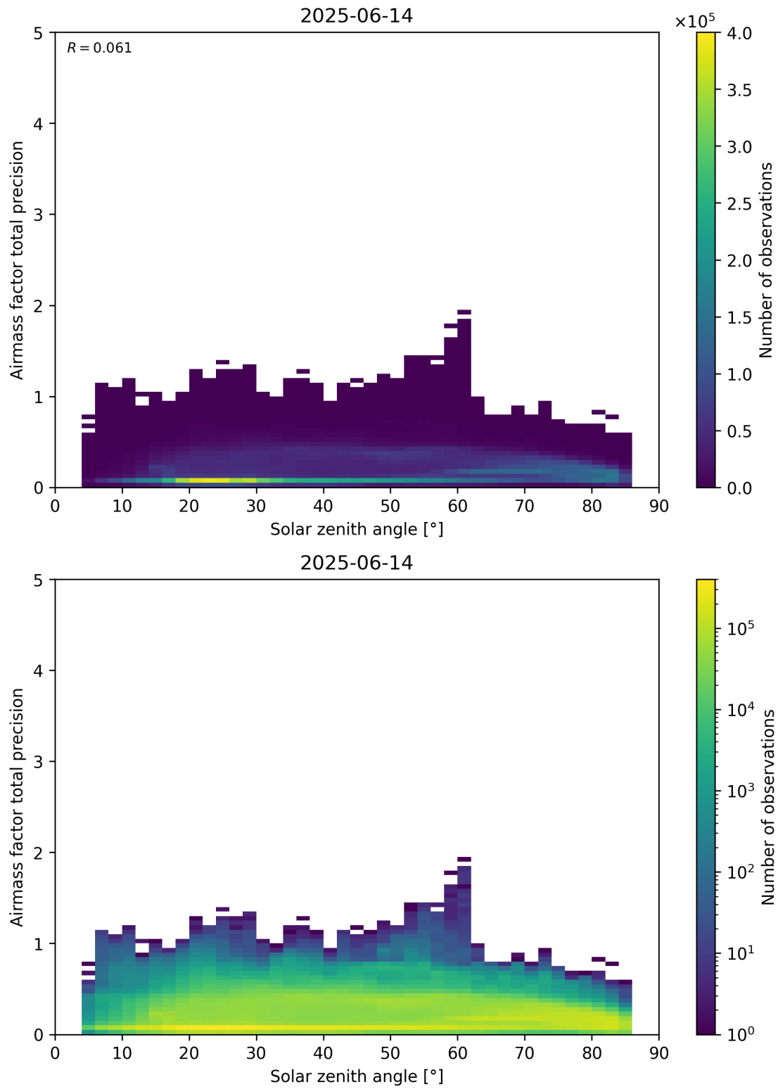
Figure 176: Scatter density plot of “Solar zenith angle” against “Airmass factor total precision” for 2025-06-13 to 2025-06-15.
