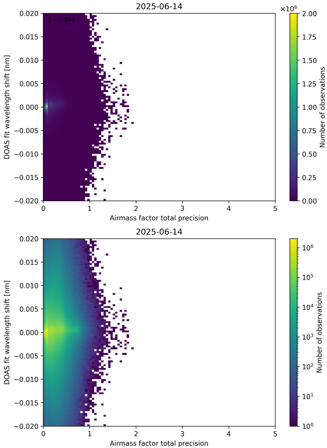
Figure 106: Scatter density plot of “Airmass factor total precision” against “DOAS fit wavelength shift” for 2025-06-13 to 2025-06-15.
