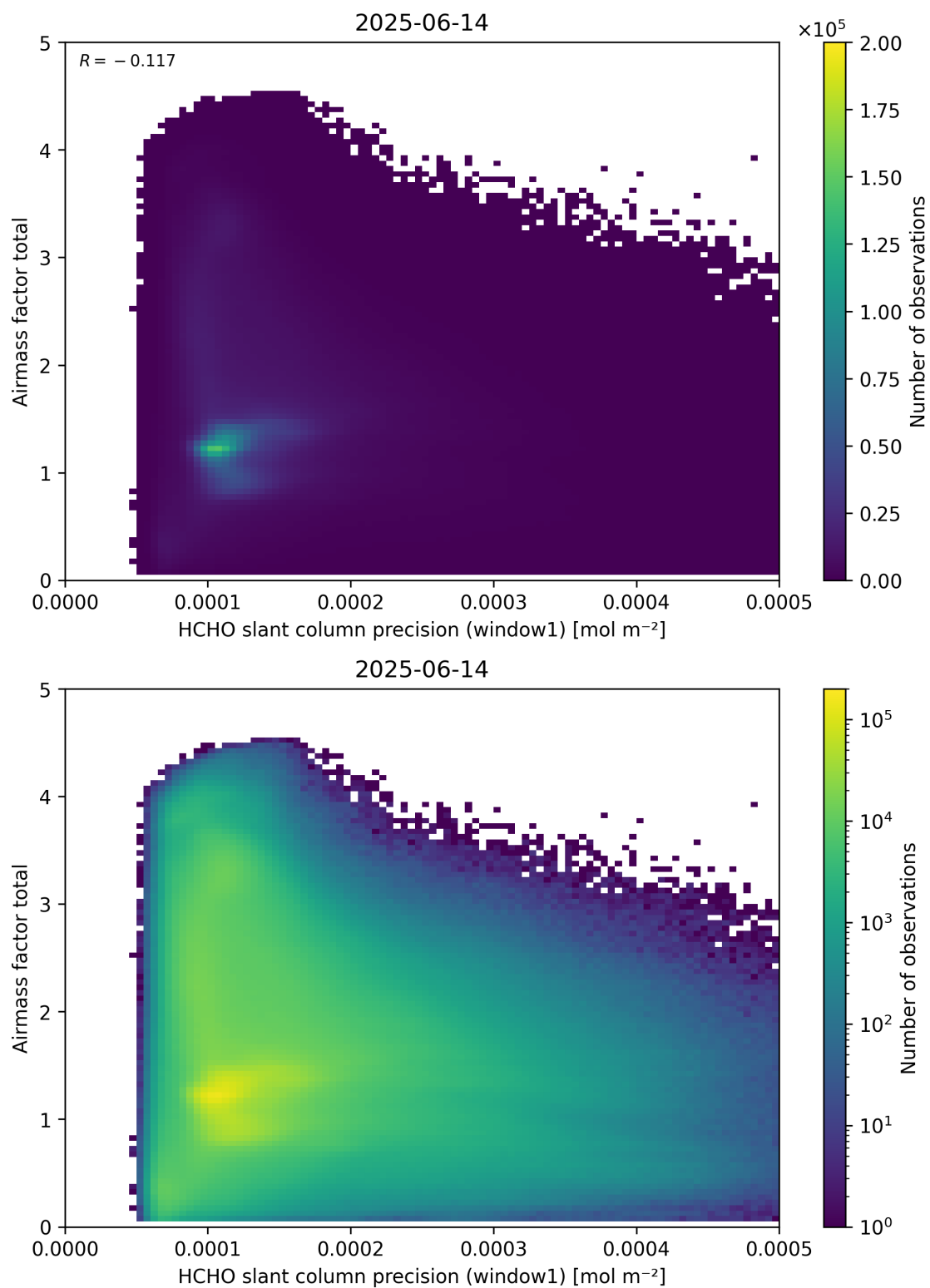
Figure 94: Scatter density plot of “HCHO slant column precision (window1)” against “Airmass factor total” for 2025-06-13 to 2025-06-15.
