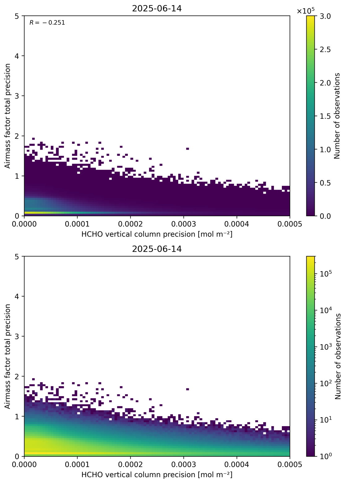
Figure 145: Scatter density plot of “HCHO vertical column precision” against “Airmass factor total precision” for 2025-06-13 to 2025-06-15.
