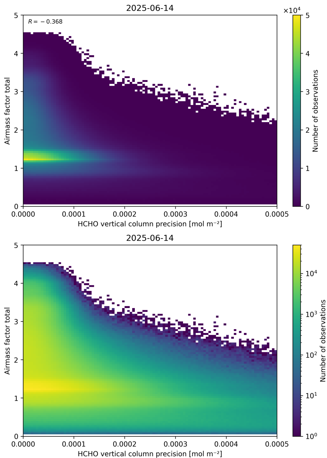
Figure 144: Scatter density plot of “HCHO vertical column precision” against “Airmass factor total” for 2025-06-13 to 2025-06-15.
