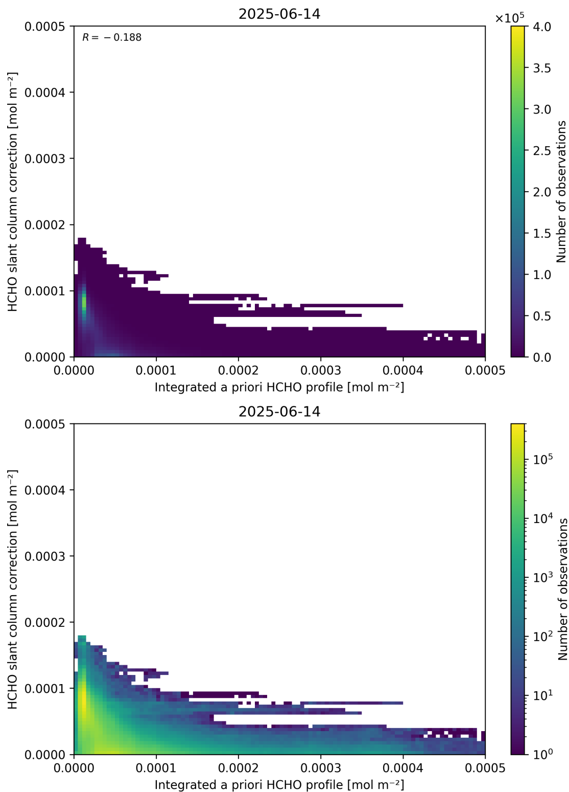
Figure 152: Scatter density plot of “Integrated a priori HCHO profile” against “HCHO slant column correction” for 2025-06-13 to 2025-06-15.
