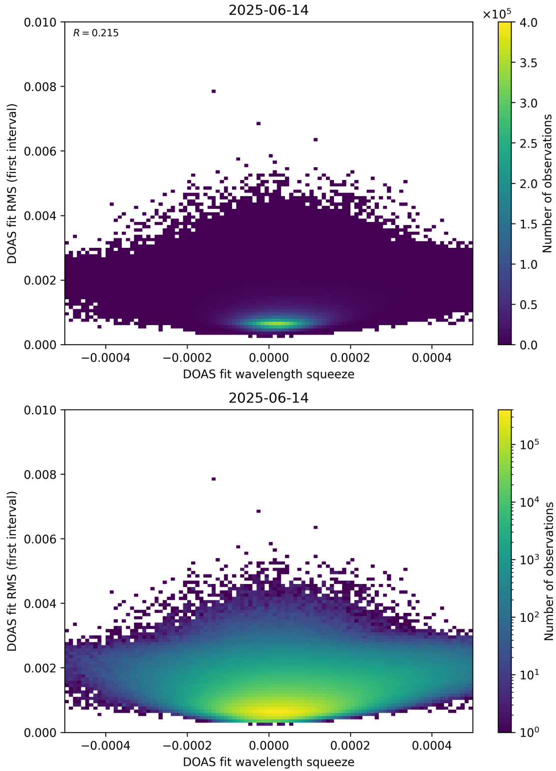
Figure 68: Scatter density plot of “DOAS fit wavelength squeeze” against “DOAS fit RMS (first interval)” for 2025-06-13 to 2025-06-15.
