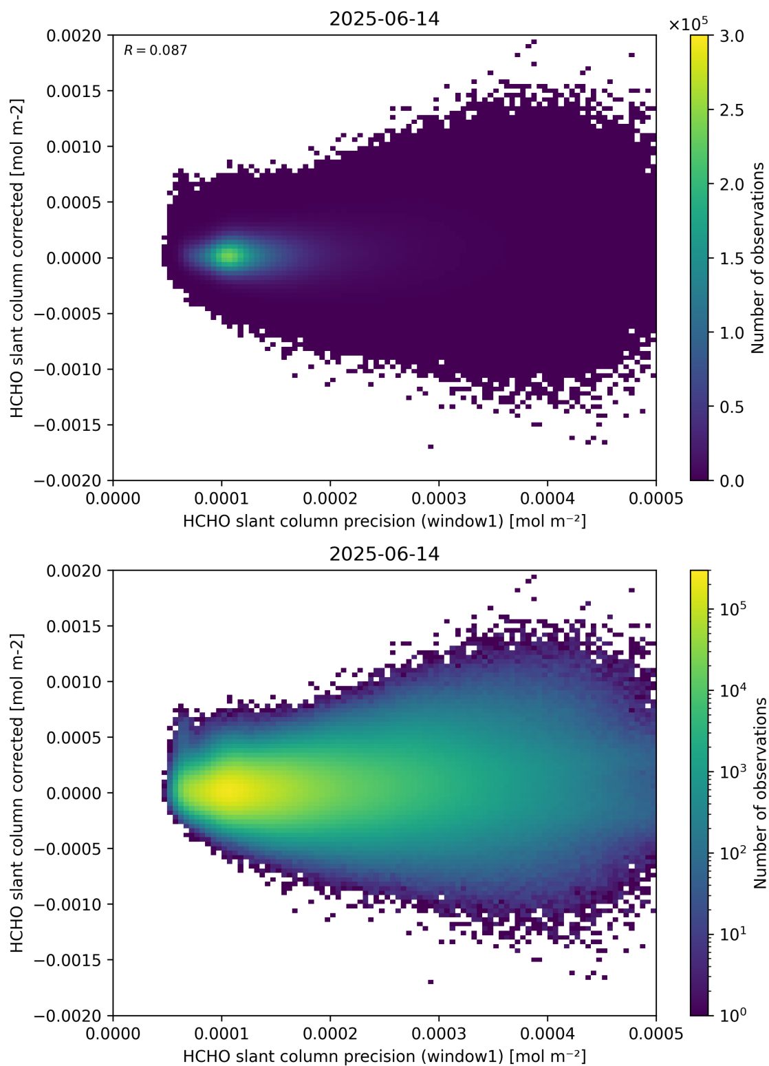
Figure 92: Scatter density plot of “HCHO slant column precision (window1)” against “HCHO slant column corrected” for 2025-06-13 to 2025-06-15.
