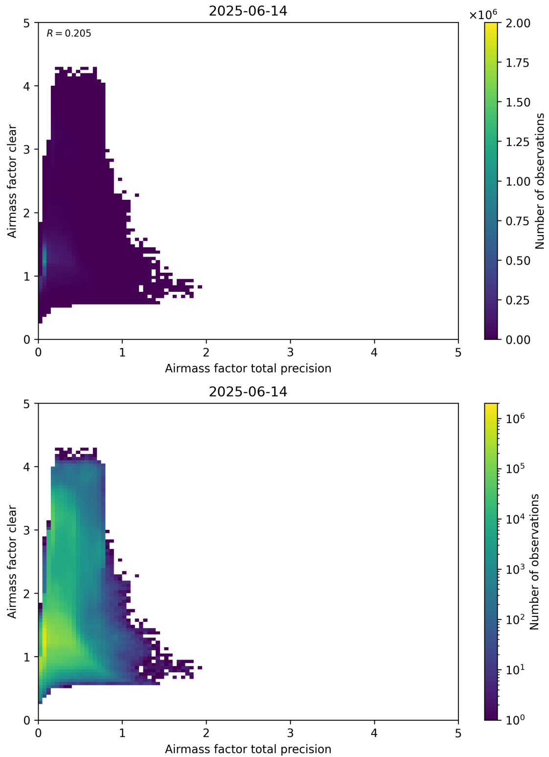
Figure 108: Scatter density plot of “Airmass factor total precision” against “Airmass factor clear” for 2025-06-13 to 2025-06-15.
