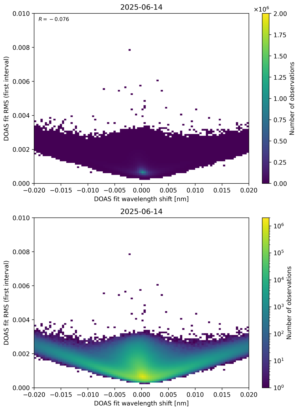
Figure 64: Scatter density plot of “DOAS fit wavelength shift” against “DOAS fit RMS (first interval)” for 2025-06-13 to 2025-06-15.
