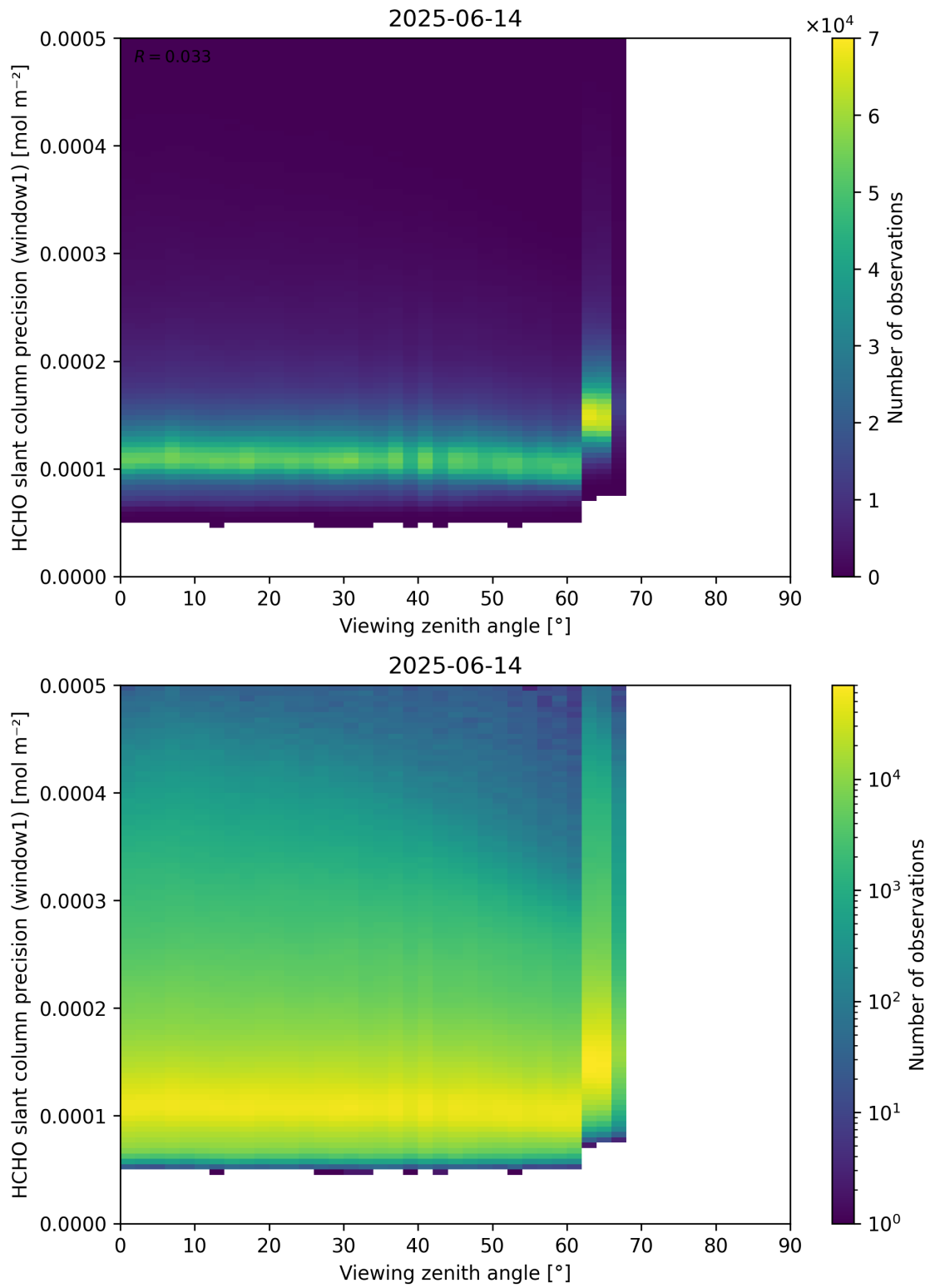
Figure 189: Scatter density plot of “Viewing zenith angle” against “HCHO slant column precision (window1)” for 2025-06-13 to 2025-06-15.
