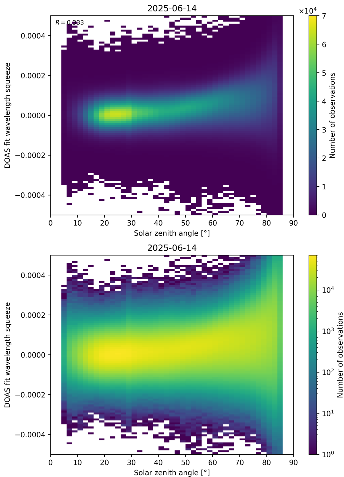
Figure 169: Scatter density plot of “Solar zenith angle” against “DOAS fit wavelength squeeze” for 2025-06-13 to 2025-06-15.
