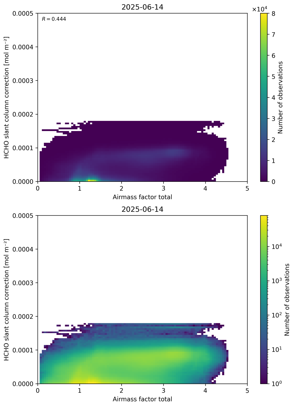
Figure 102: Scatter density plot of “Airmass factor total” against “HCHO slant column correction” for 2025-06-13 to 2025-06-15.
