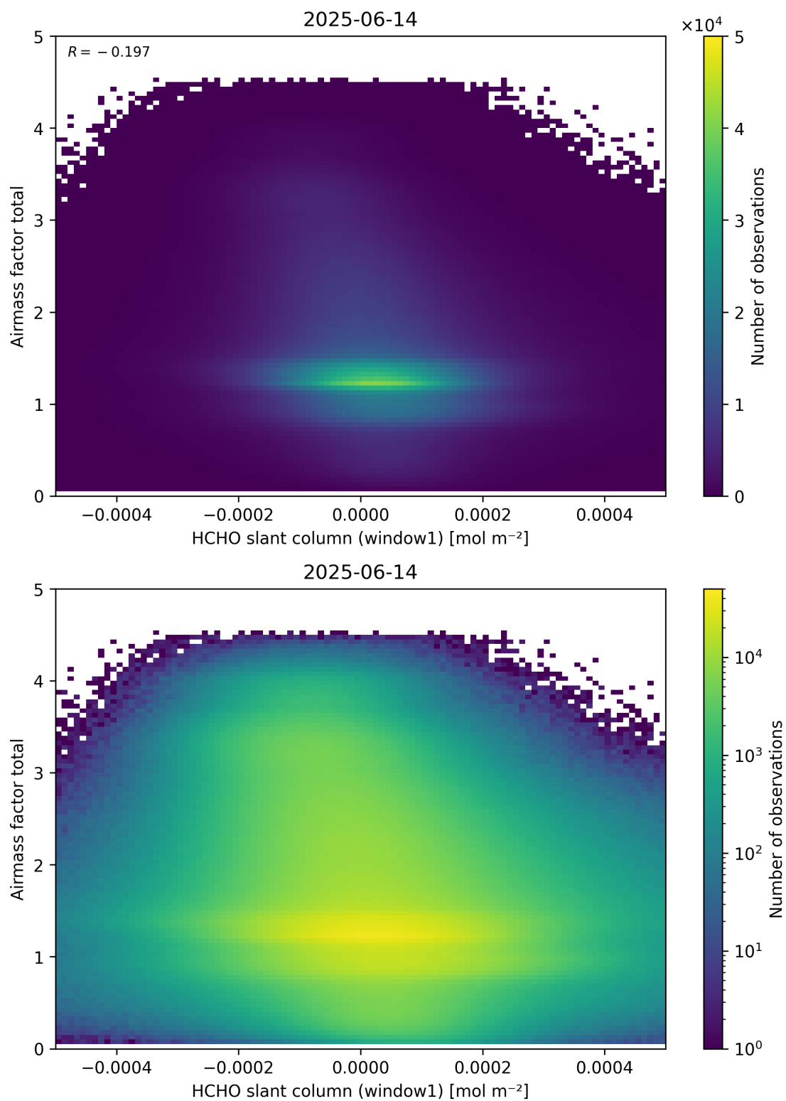
Figure 85: Scatter density plot of “HCHO slant column (window1)” against “Airmass factor total” for 2025-06-13 to 2025-06-15.
