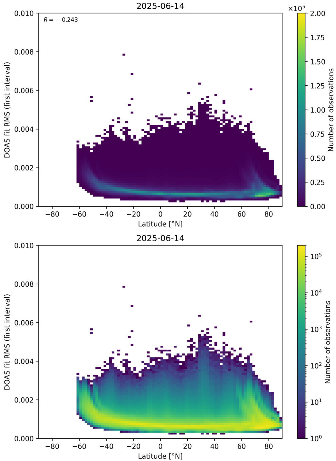
Figure 153: Scatter density plot of “Latitude” against “DOAS fit RMS (first interval)” for 2025-06-13 to 2025-06-15.
