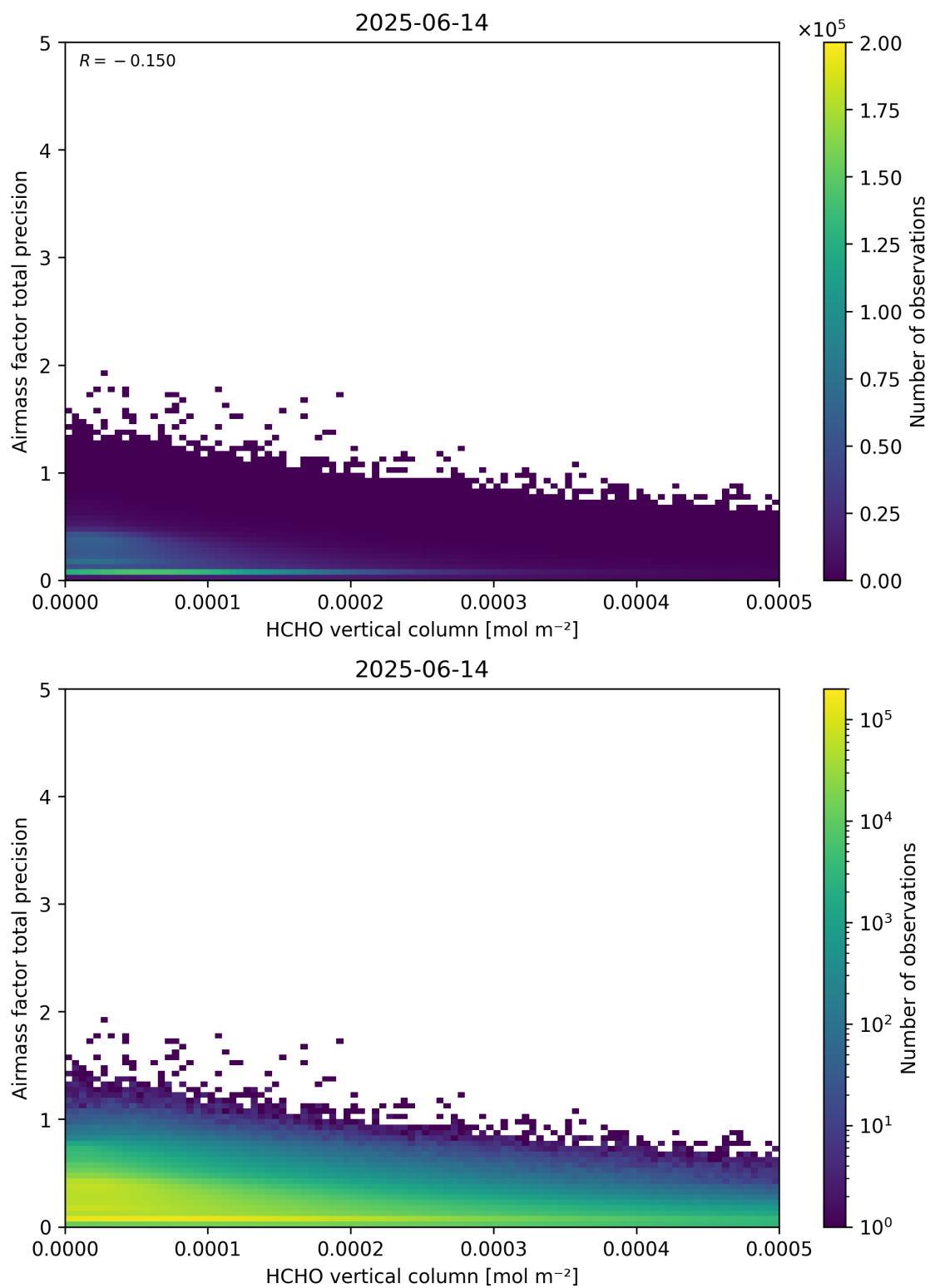
Figure 132: Scatter density plot of “HCHO vertical column” against “Airmass factor total precision” for 2025-06-13 to 2025-06-15.
