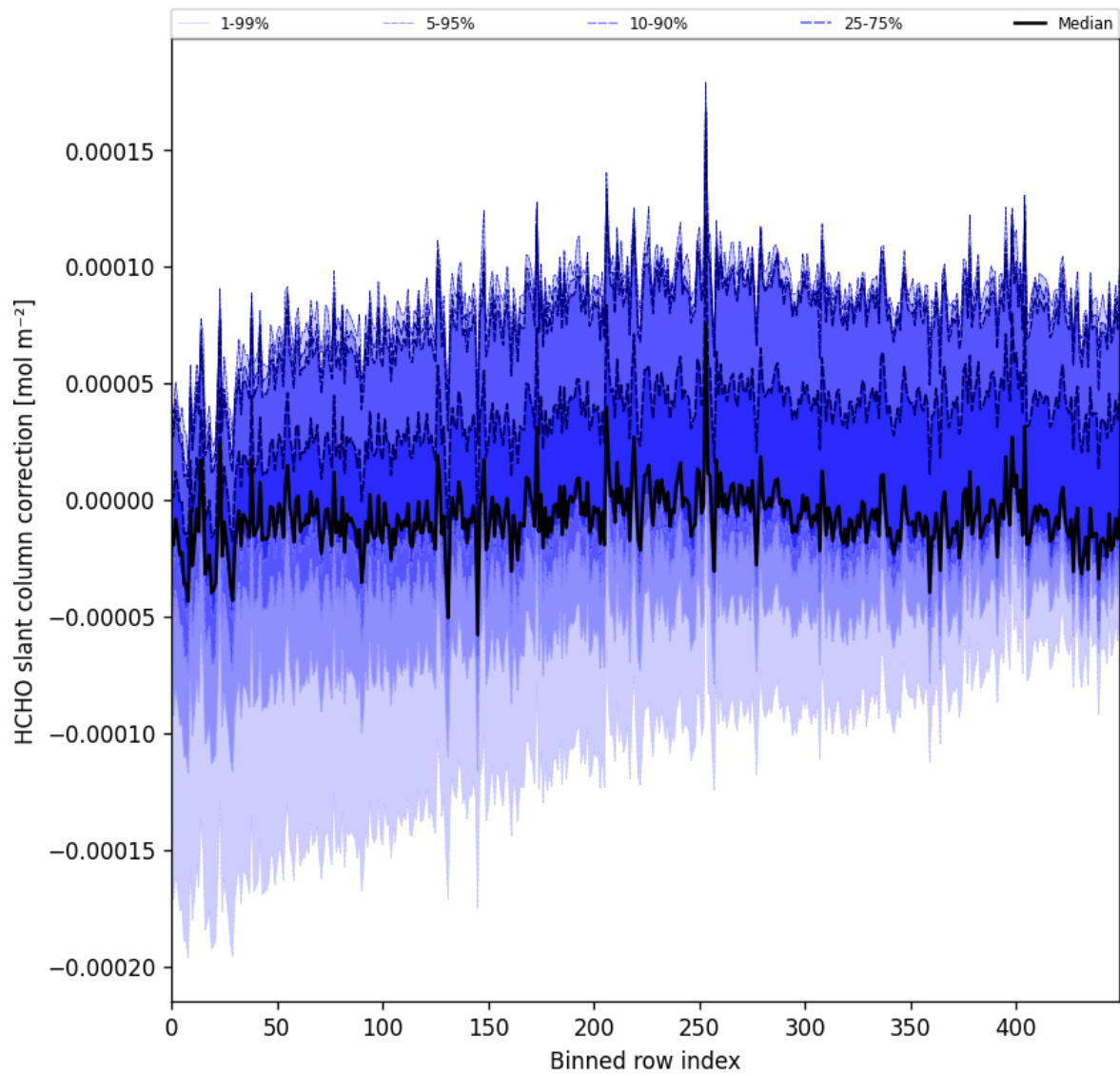
Figure 61: Along track statistics of “HCHO slant column correction” for 2025-06-13 to 2025-06-15
