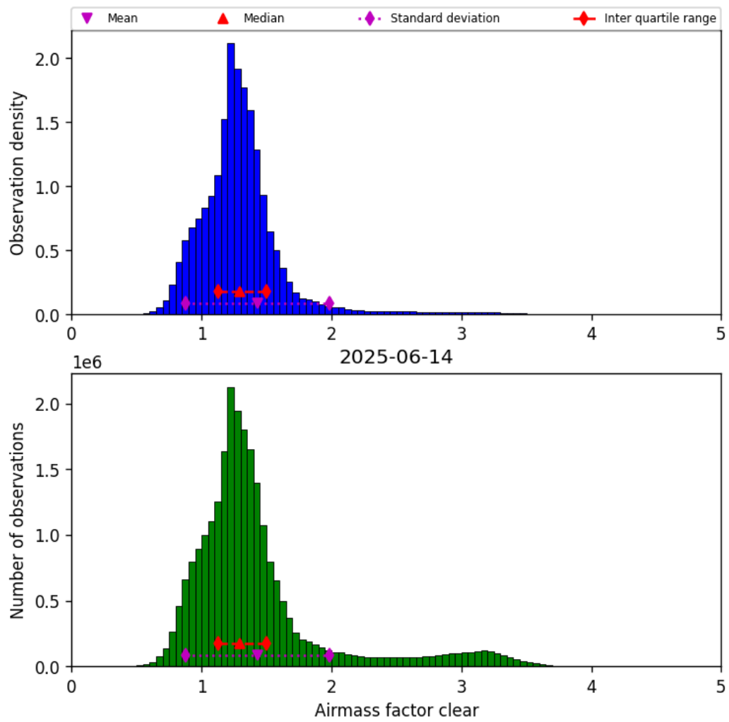
Figure 42: Histogram of “Airmass factor clear” for 2025-06-13 to 2025-06-15
