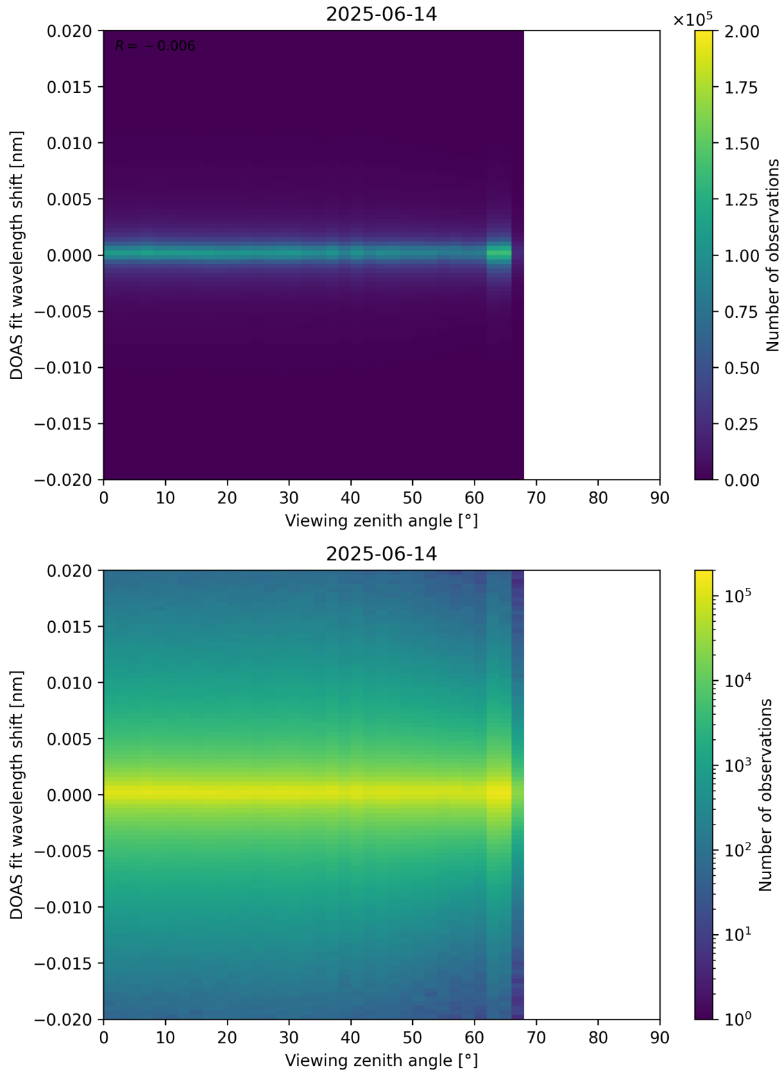
Figure 183: Scatter density plot of “Viewing zenith angle” against “DOAS fit wavelength shift” for 2025-06-13 to 2025-06-15.
