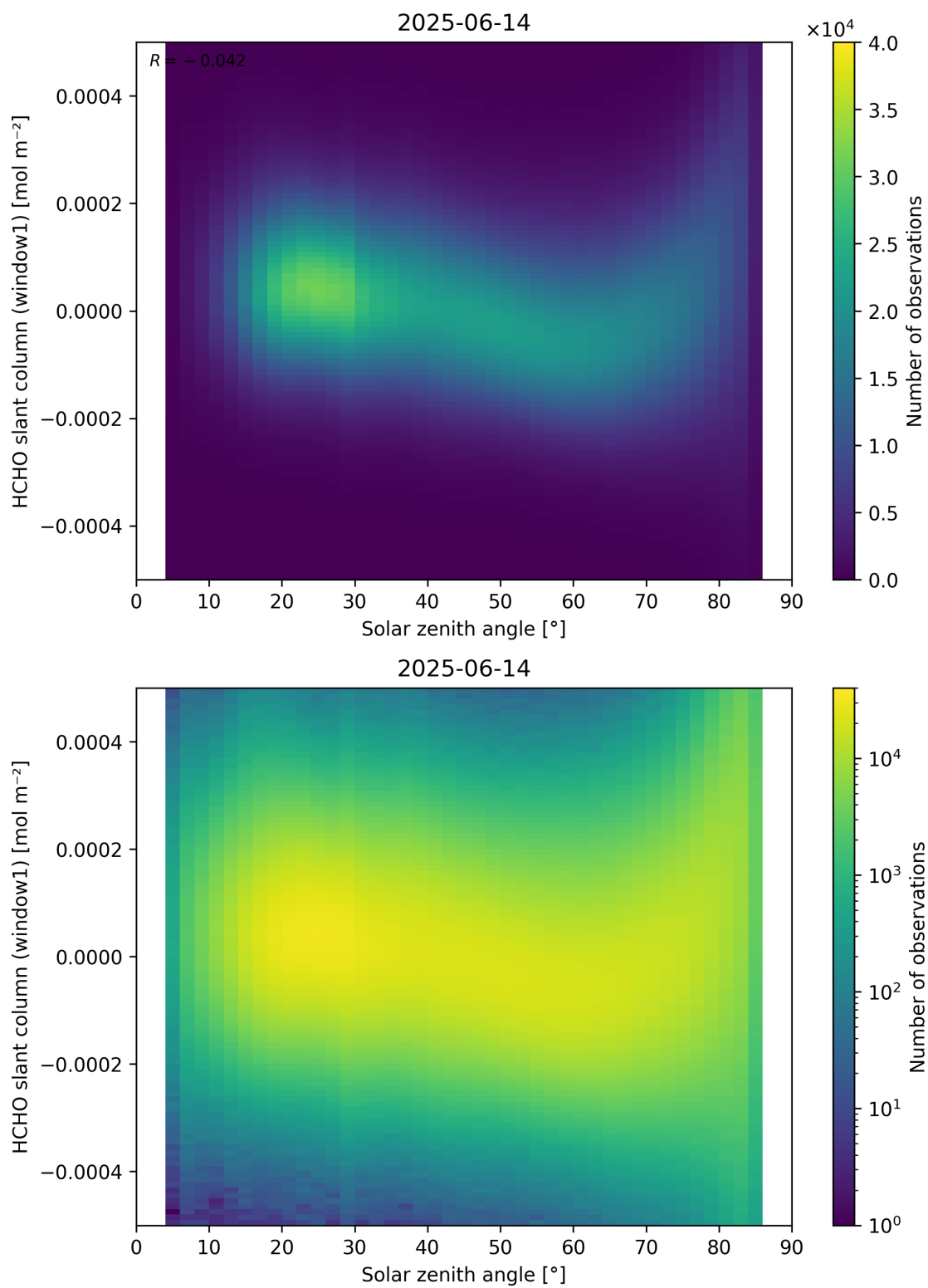
Figure 173: Scatter density plot of “Solar zenith angle” against “HCHO slant column (window1)” for 2025-06-13 to 2025-06-15.
