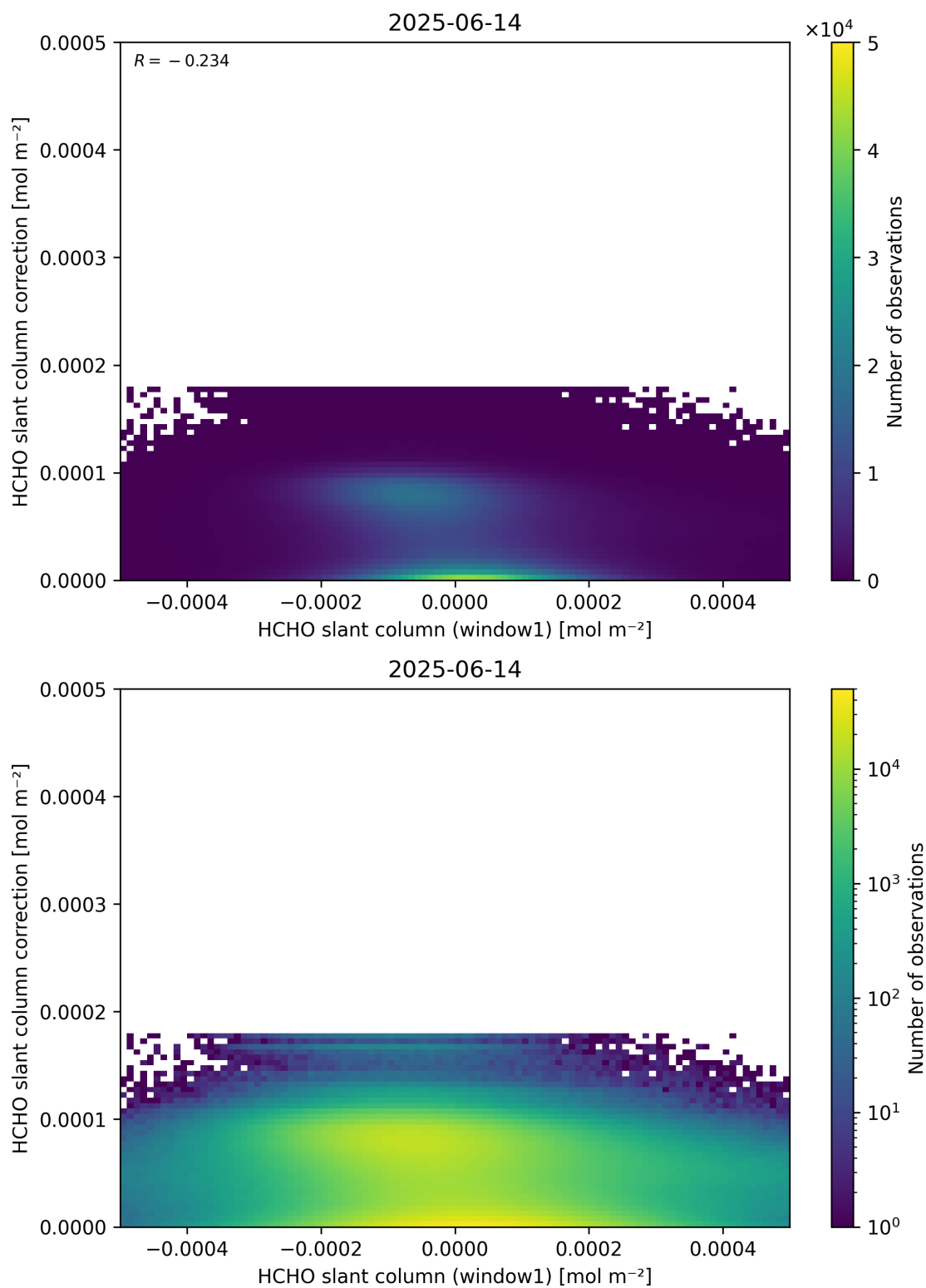
Figure 83: Scatter density plot of “HCHO slant column (window1)” against “HCHO slant column correction” for 2025-06-13 to 2025-06-15.
