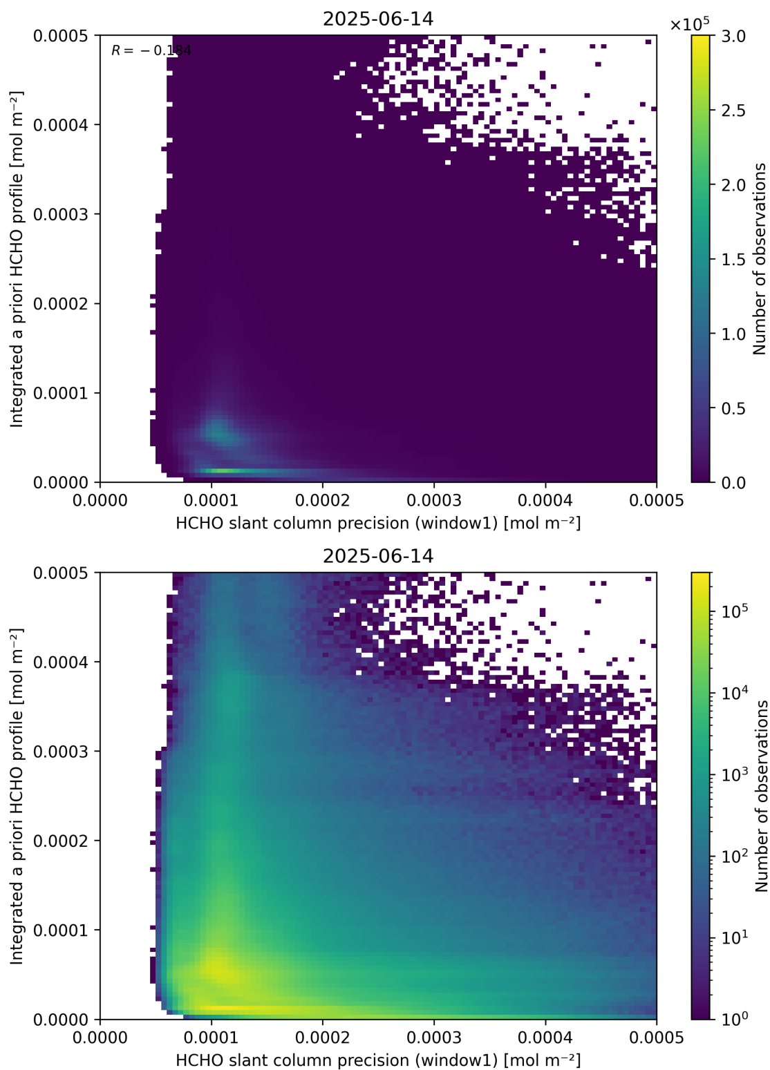
Figure 96: Scatter density plot of “HCHO slant column precision (window1)” against “Integrated a priori HCHO profile” for 2025-06-13 to 2025-06-15.
