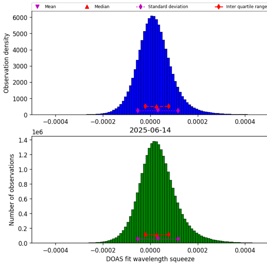
Figure 45: Histogram of “DOAS fit wavelength squeeze” for 2025-06-13 to 2025-06-15
