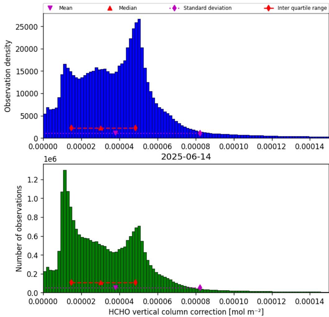
Figure 37: Histogram of “HCHO vertical column correction” for 2025-06-13 to 2025-06-15
