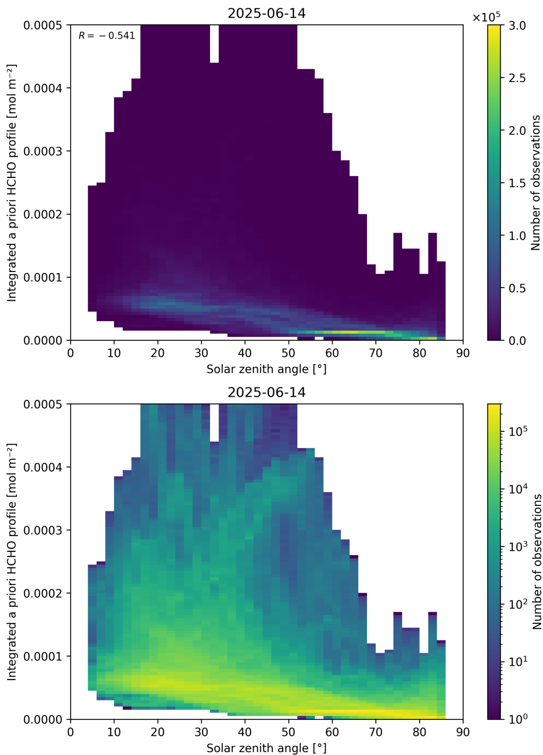
Figure 180: Scatter density plot of “Solar zenith angle” against “Integrated a priori HCHO profile” for 2025-06-13 to 2025-06-15.
