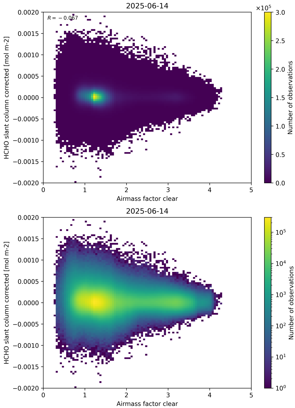
Figure 74: Scatter density plot of “Airmass factor clear” against “HCHO slant column corrected” for 2025-06-13 to 2025-06-15.
