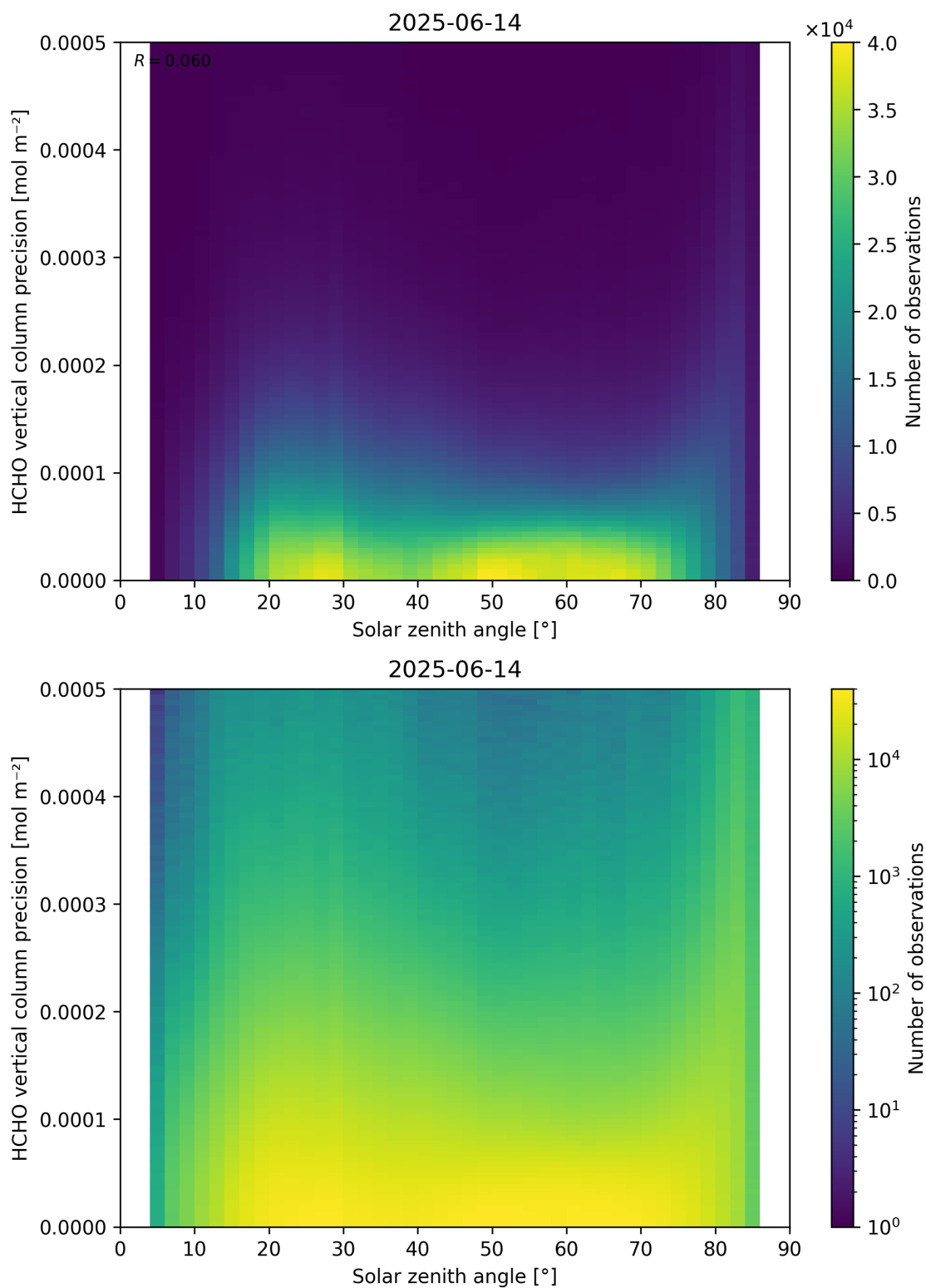
Figure 179: Scatter density plot of “Solar zenith angle” against “HCHO vertical column precision” for 2025-06-13 to 2025-06-15.
