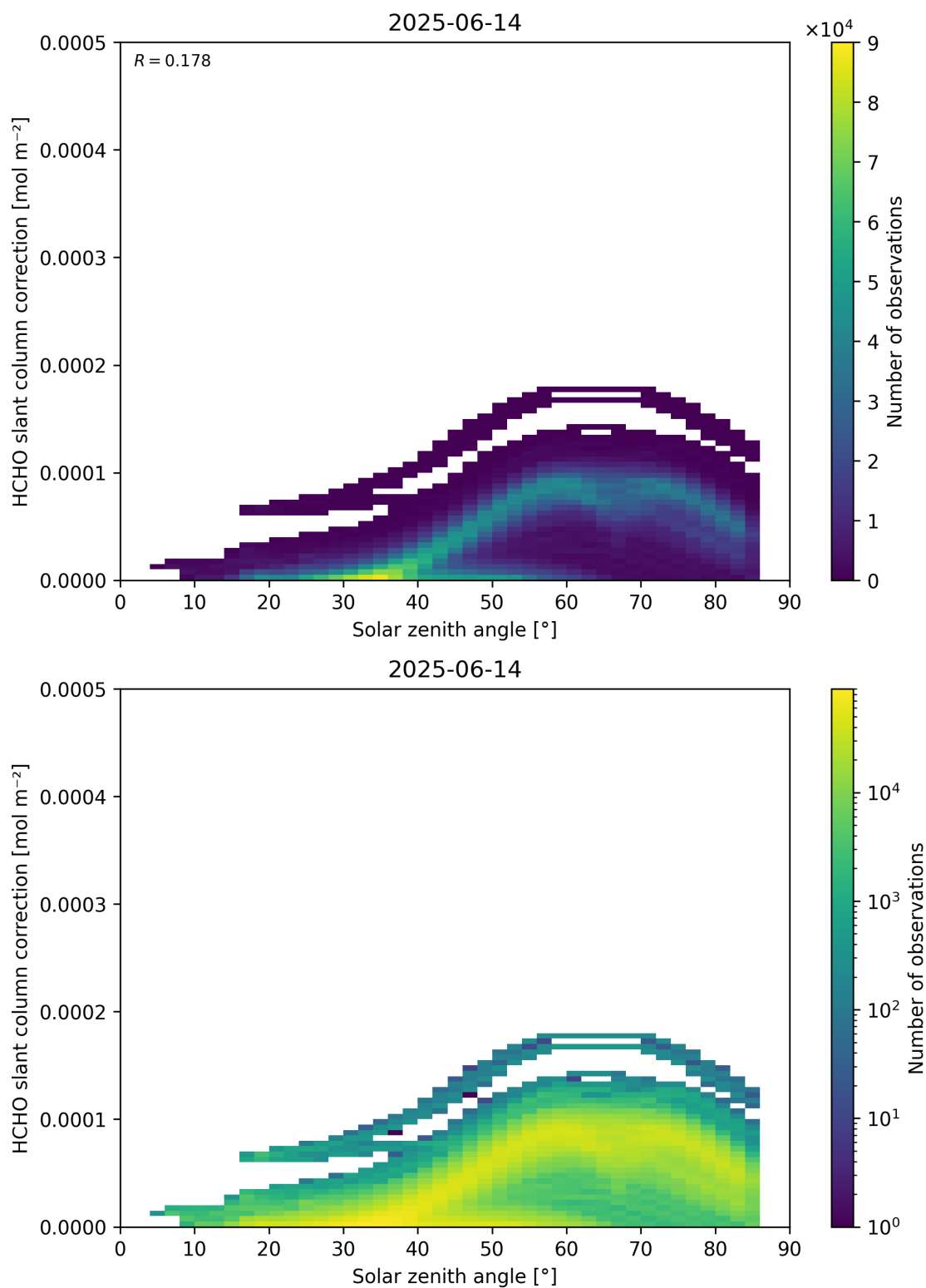
Figure 172: Scatter density plot of “Solar zenith angle” against “HCHO slant column correction” for 2025-06-13 to 2025-06-15.
