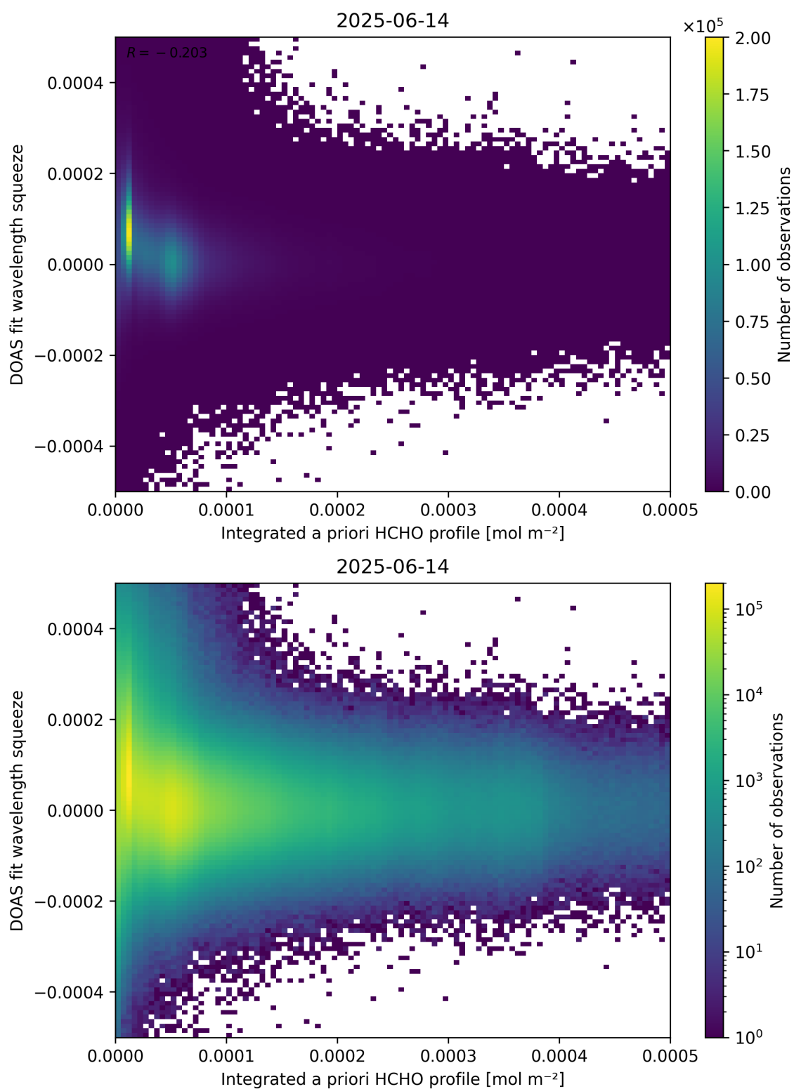
Figure 150: Scatter density plot of “Integrated a priori HCHO profile” against “DOAS fit wavelength squeeze” for 2025-06-13 to 2025-06-15.
