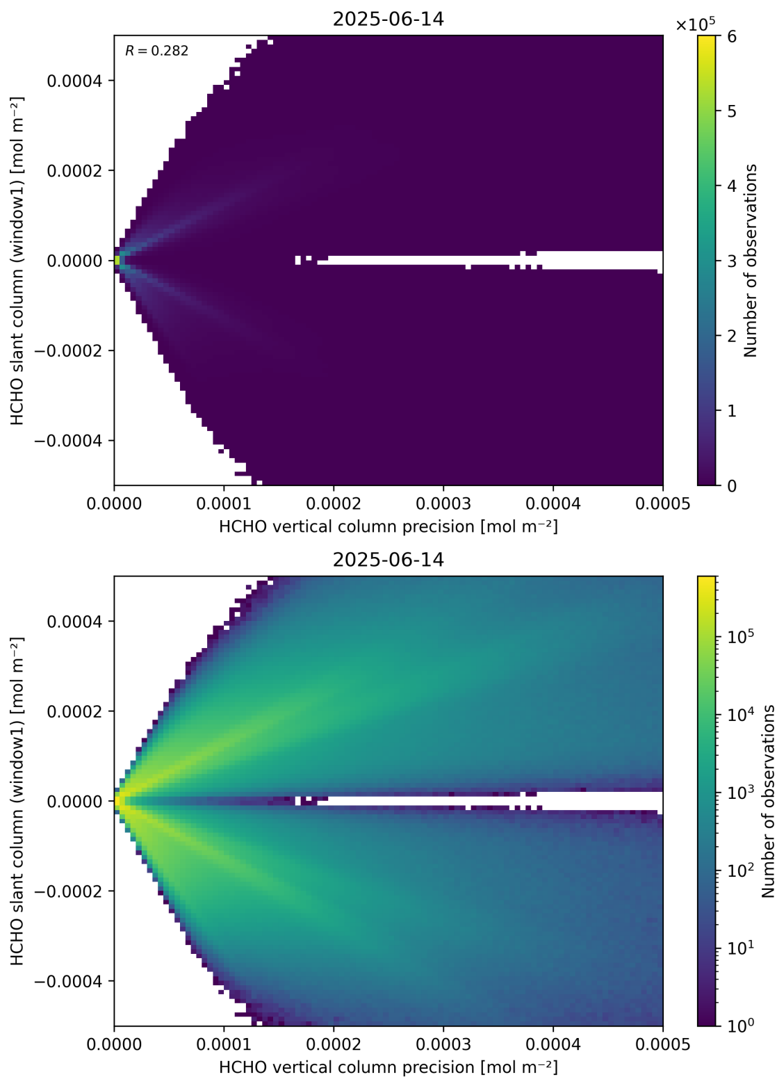
Figure 142: Scatter density plot of “HCHO vertical column precision” against “HCHO slant column (window1)” for 2025-06-13 to 2025-06-15.
