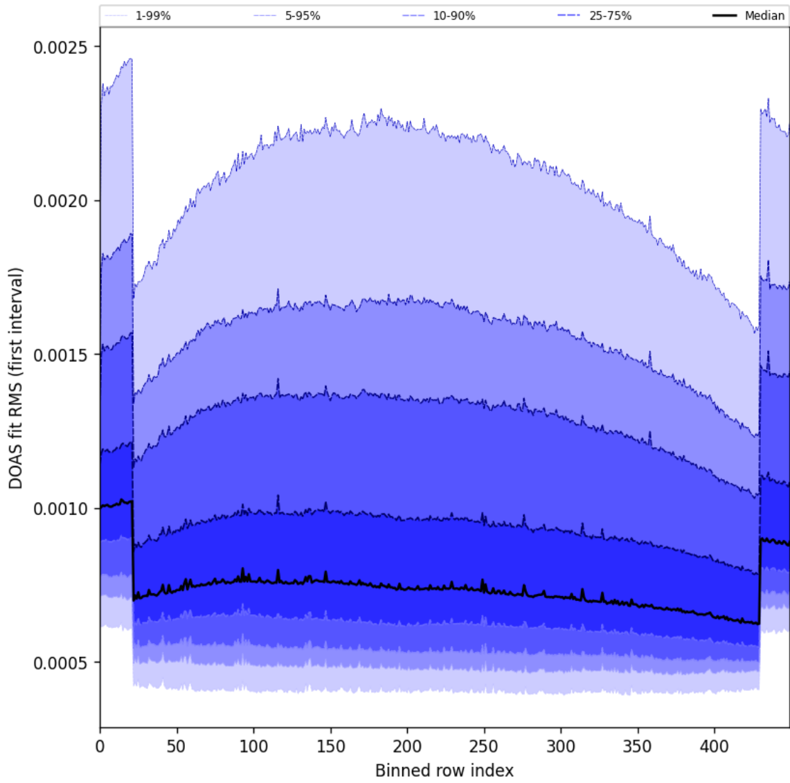
Figure 60: Along track statistics of “DOAS fit RMS (first interval)” for 2025-06-13 to 2025-06-15
