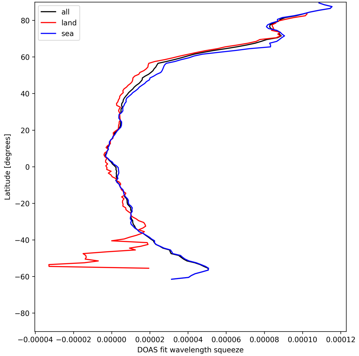
Figure 31: Zonal average of “DOAS fit wavelength squeeze” for 2025-06-13 to 2025-06-15.
