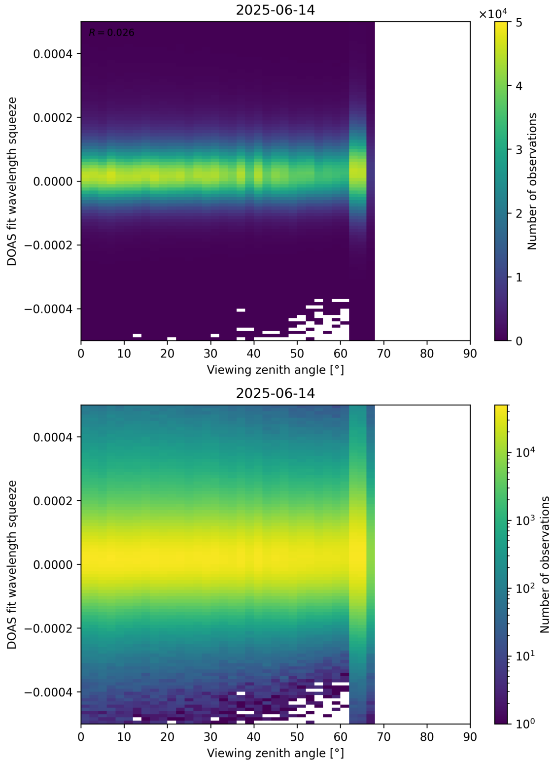
Figure 184: Scatter density plot of “Viewing zenith angle” against “DOAS fit wavelength squeeze” for 2025-06-13 to 2025-06-15.
