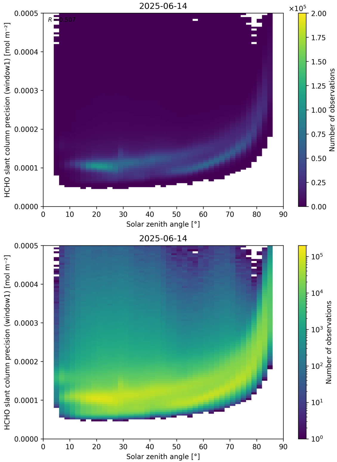
Figure 174: Scatter density plot of “Solar zenith angle” against “HCHO slant column precision (window1)” for 2025-06-13 to 2025-06-15.
