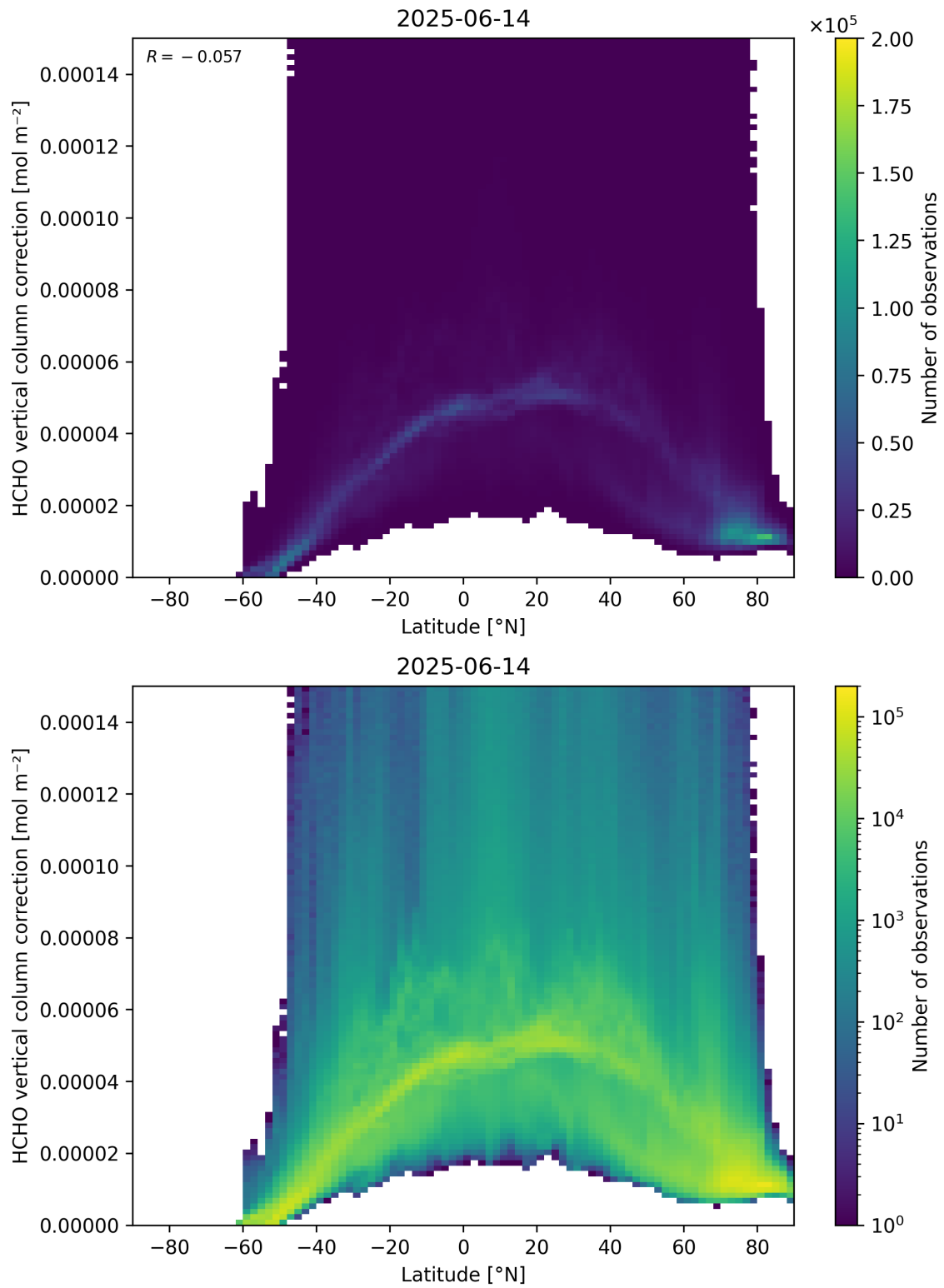
Figure 164: Scatter density plot of “Latitude” against “HCHO vertical column correction” for 2025-06-13 to 2025-06-15.
