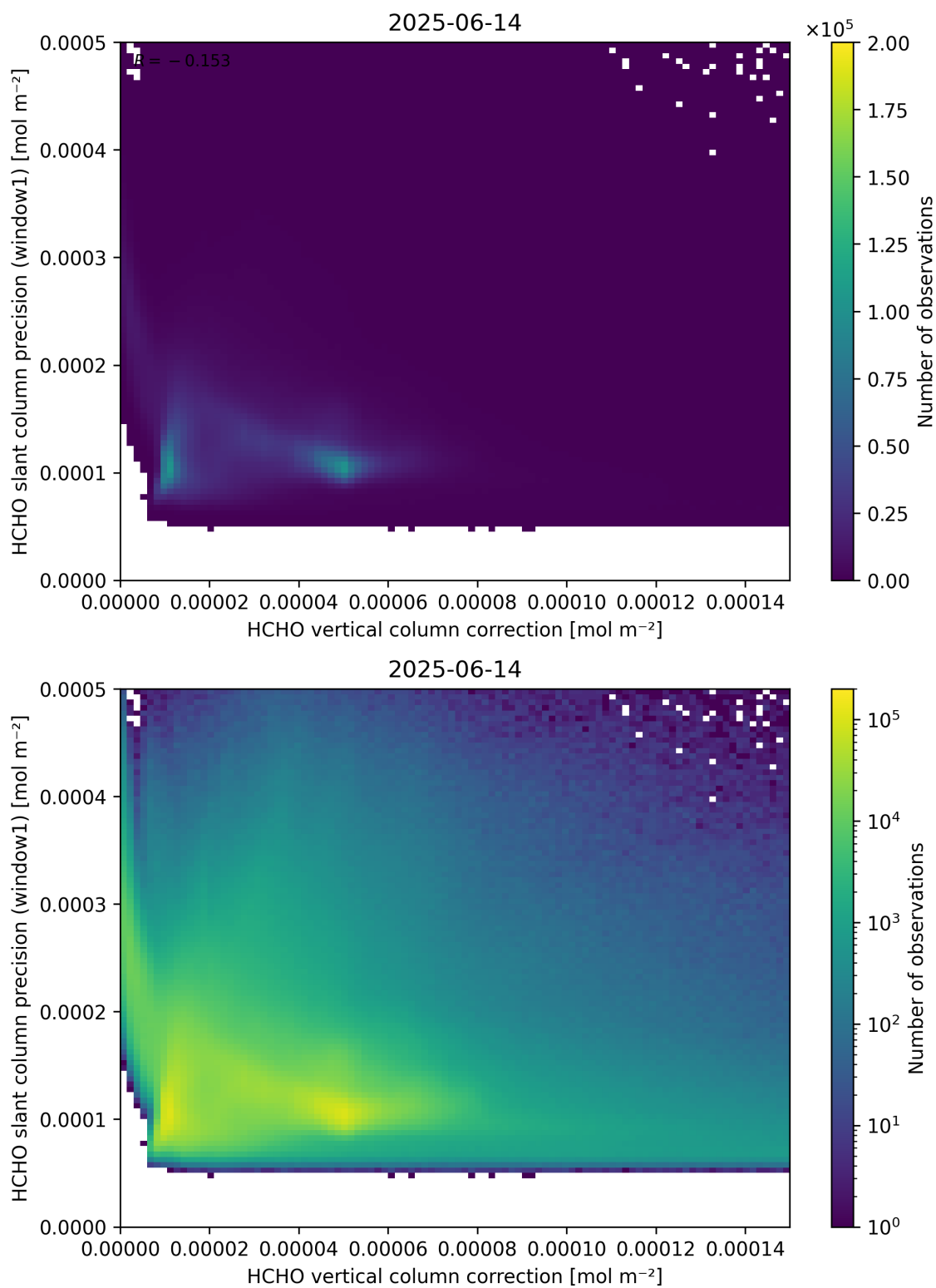
Figure 119: Scatter density plot of “HCHO vertical column correction” against “HCHO slant column precision (window1)” for 2025-06-13 to 2025-06-15.
