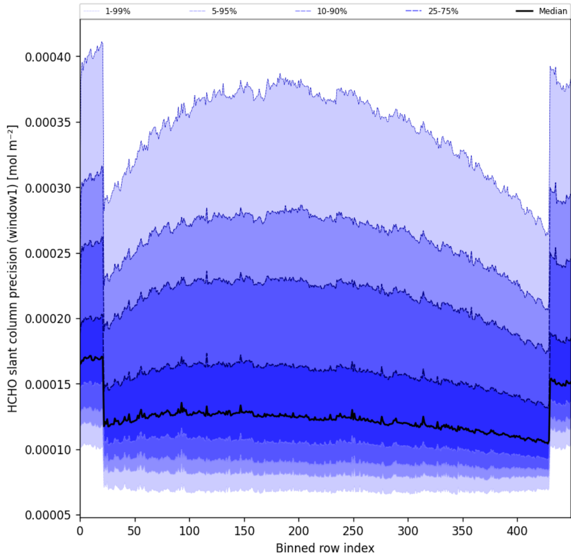
Figure 53: Along track statistics of “HCHO slant column precision (window1)” for 2025-06-13 to 2025-06-15
