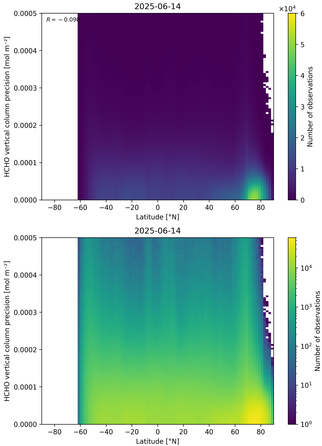
Figure 165: Scatter density plot of “Latitude” against “HCHO vertical column precision” for 2025-06-13 to 2025-06-15.
