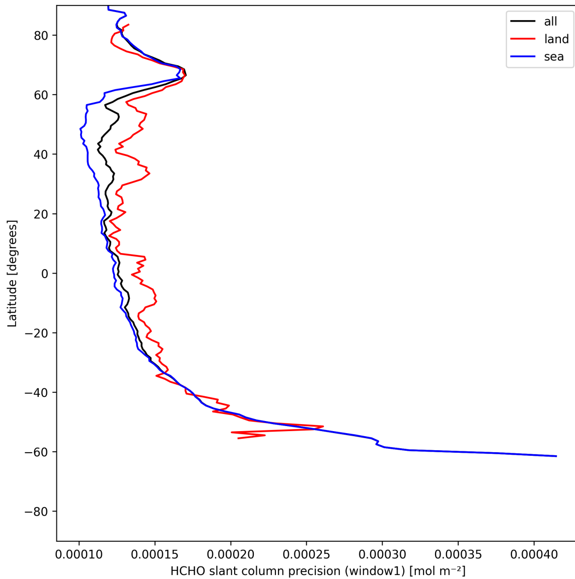
Figure 25: Zonal average of “HCHO slant column precision (window1)” for 2025-06-13 to 2025-06-15.
