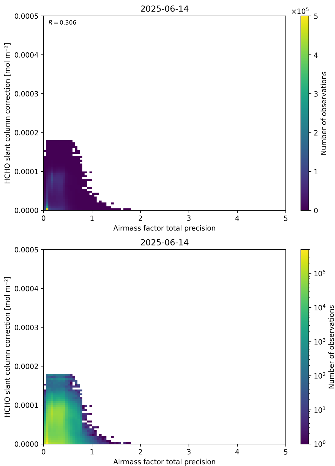
Figure 110: Scatter density plot of “Airmass factor total precision” against “HCHO slant column correction” for 2025-06-13 to 2025-06-15.
