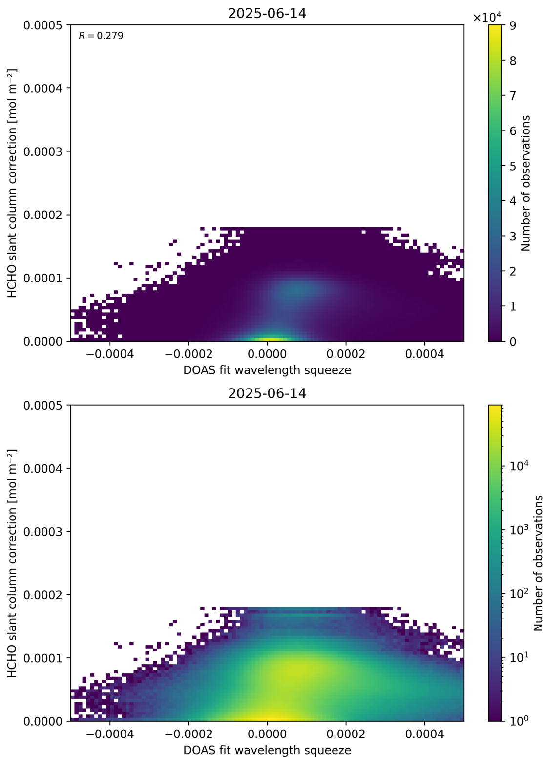
Figure 70: Scatter density plot of “DOAS fit wavelength squeeze” against “HCHO slant column correction” for 2025-06-13 to 2025-06-15.
