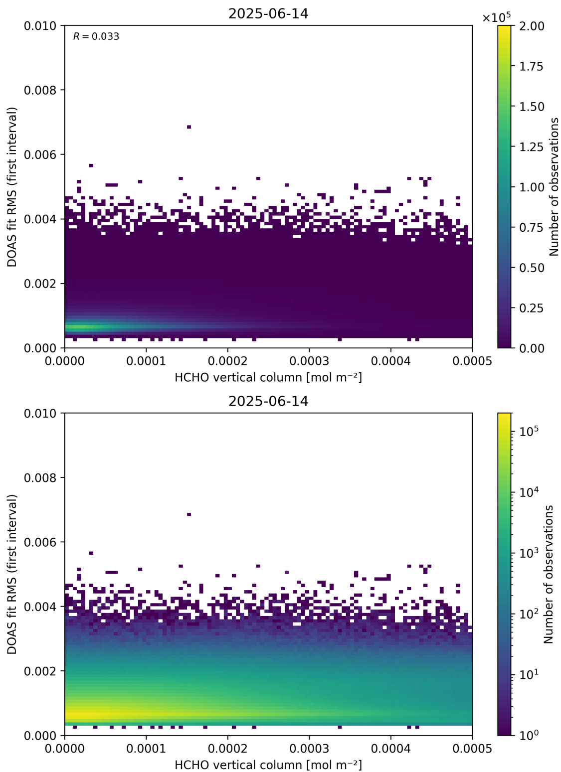
Figure 123: Scatter density plot of “HCHO vertical column” against “DOAS fit RMS (first interval)” for 2025-06-13 to 2025-06-15.
