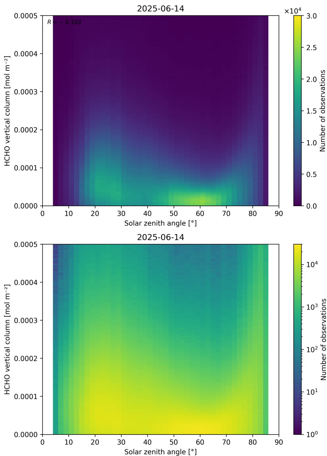
Figure 177: Scatter density plot of “Solar zenith angle” against “HCHO vertical column” for 2025-06-13 to 2025-06-15.
