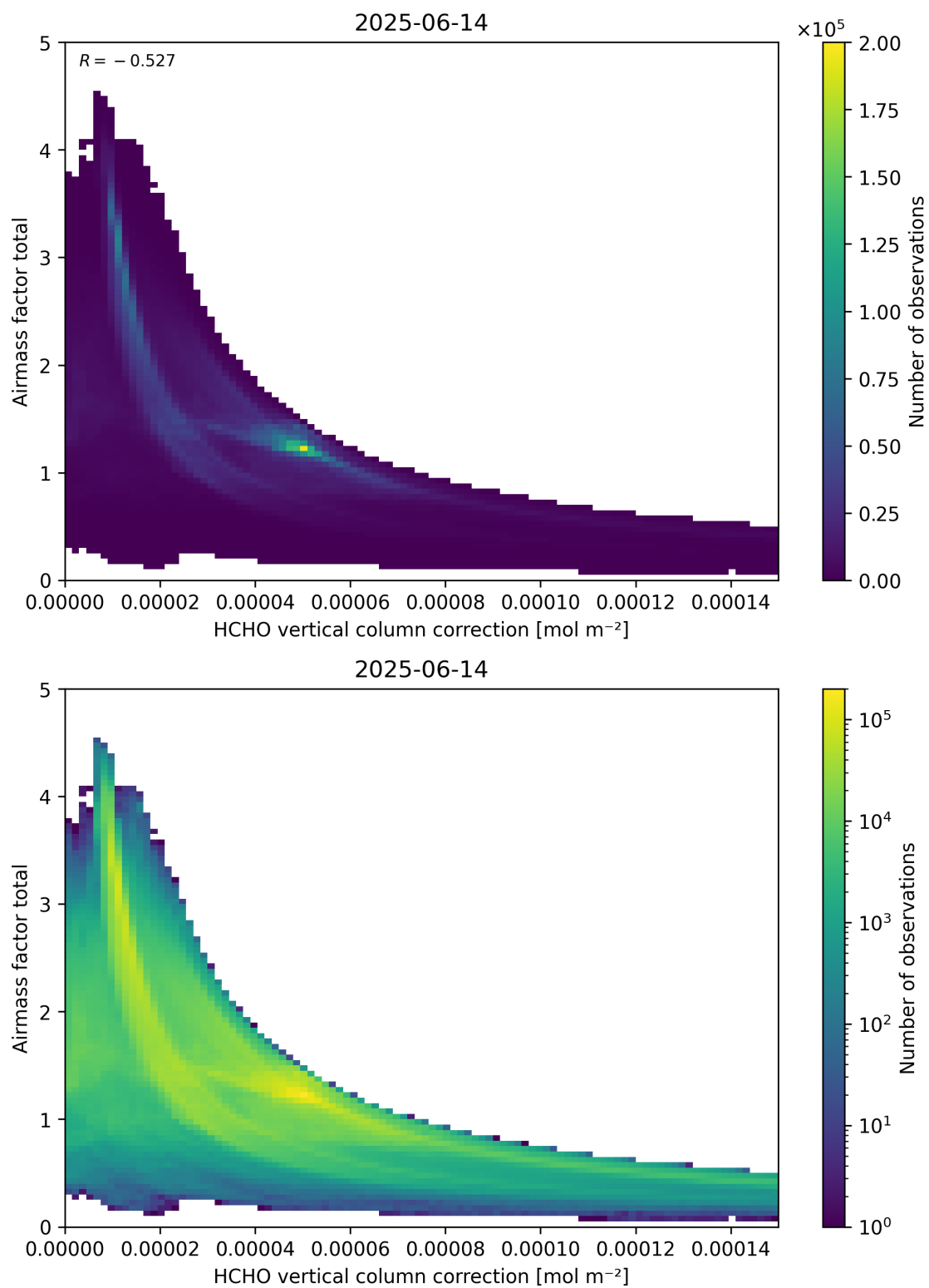
Figure 120: Scatter density plot of “HCHO vertical column correction” against “Airmass factor total” for 2025-06-13 to 2025-06-15.
