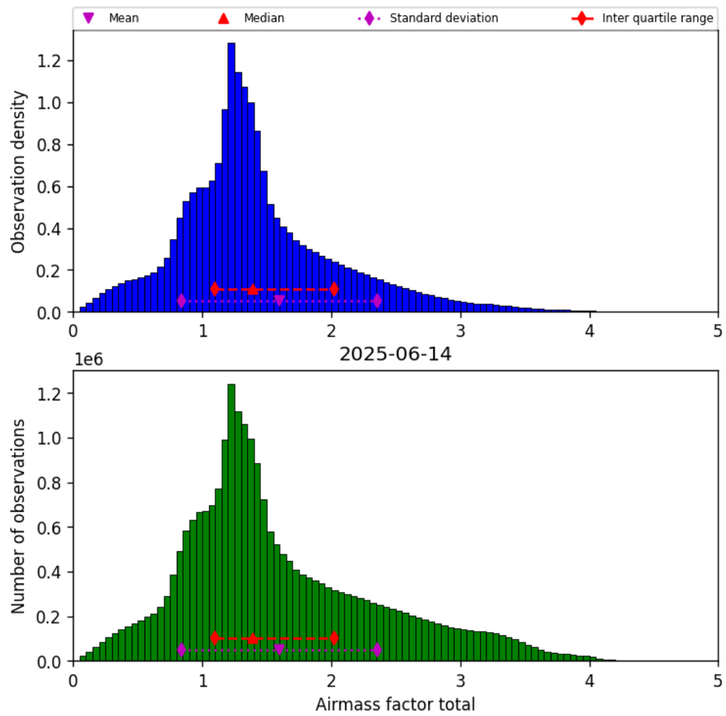
Figure 40: Histogram of “Airmass factor total” for 2025-06-13 to 2025-06-15
