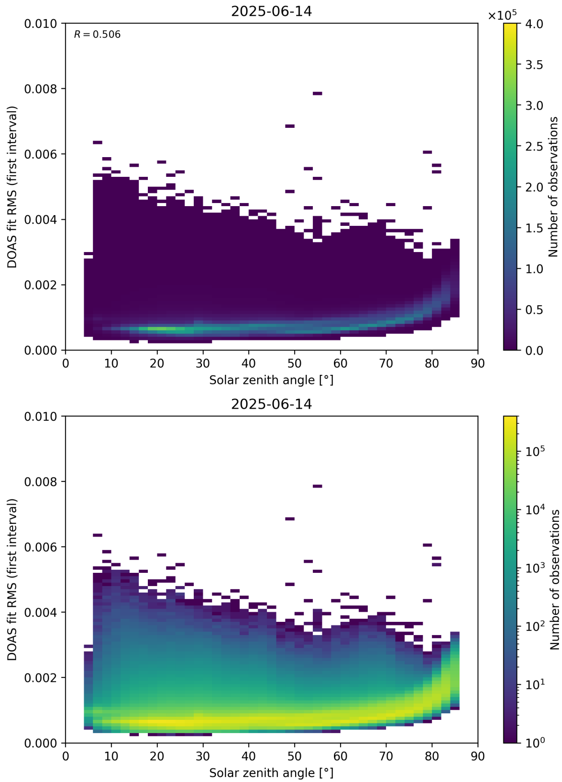
Figure 167: Scatter density plot of “Solar zenith angle” against “DOAS fit RMS (first interval)” for 2025-06-13 to 2025-06-15.
