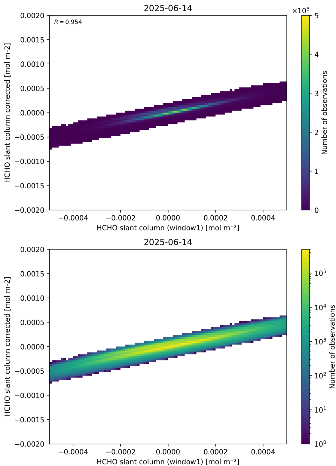
Figure 82: Scatter density plot of “HCHO slant column (window1)” against “HCHO slant column corrected” for 2025-06-13 to 2025-06-15.
