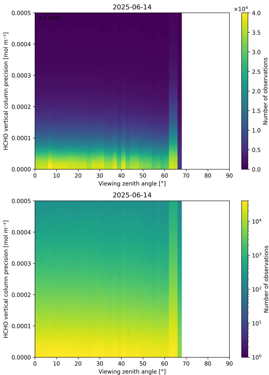
Figure 194: Scatter density plot of “Viewing zenith angle” against “HCHO vertical column precision” for 2025-06-13 to 2025-06-15.
