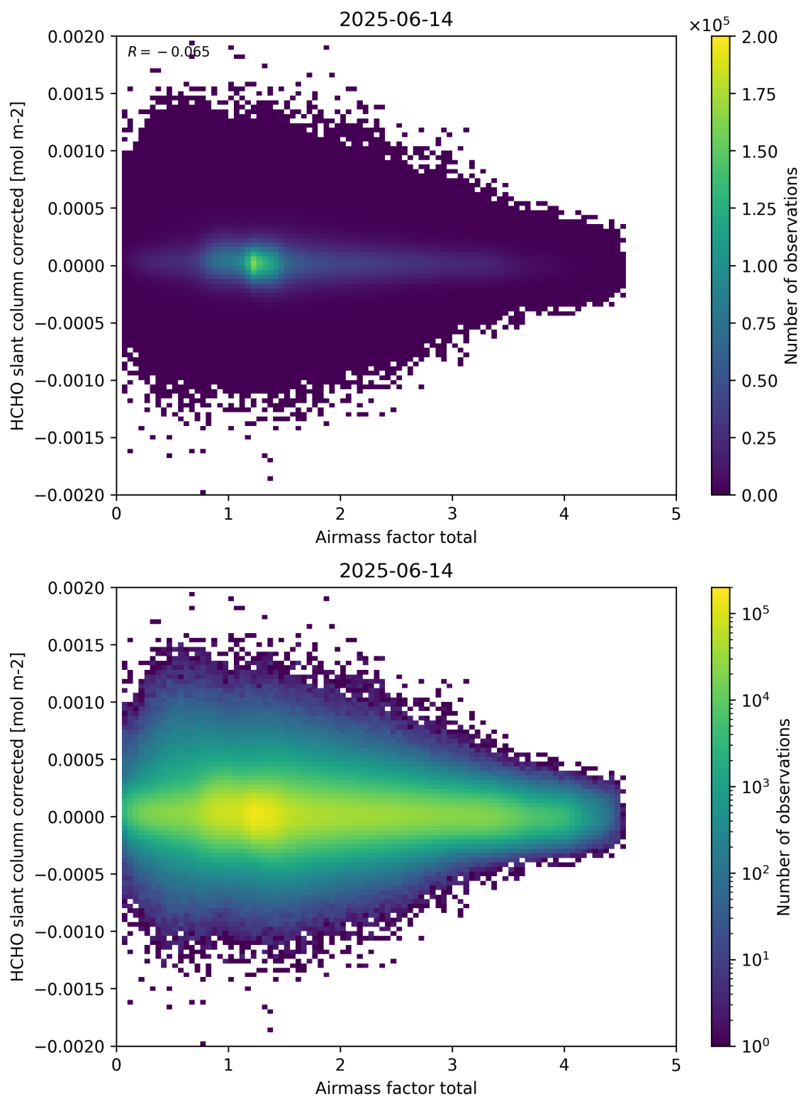
Figure 101: Scatter density plot of “Airmass factor total” against “HCHO slant column corrected” for 2025-06-13 to 2025-06-15.
