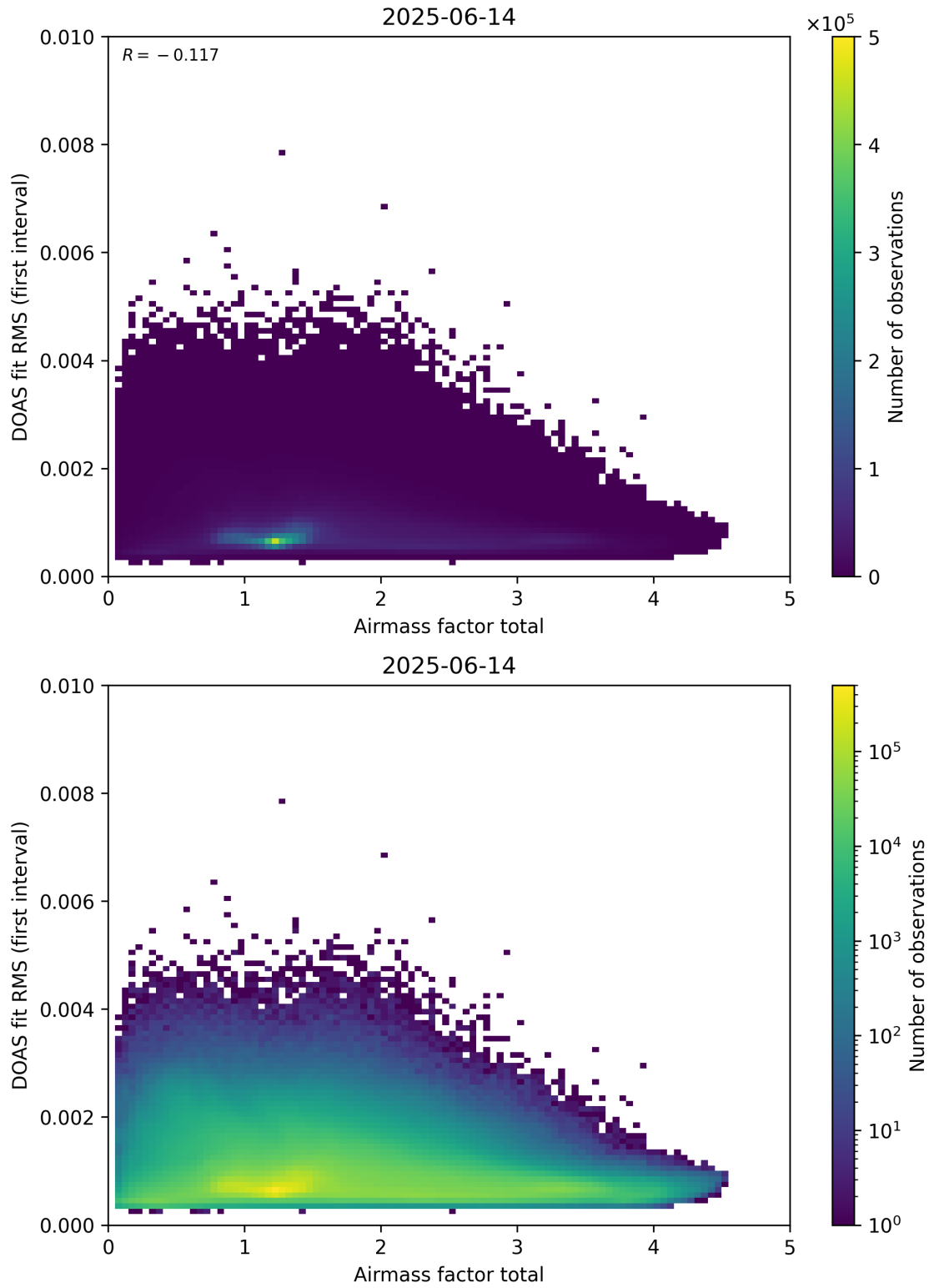
Figure 97: Scatter density plot of “Airmass factor total” against “DOAS fit RMS (first interval)” for 2025-06-13 to 2025-06-15.
