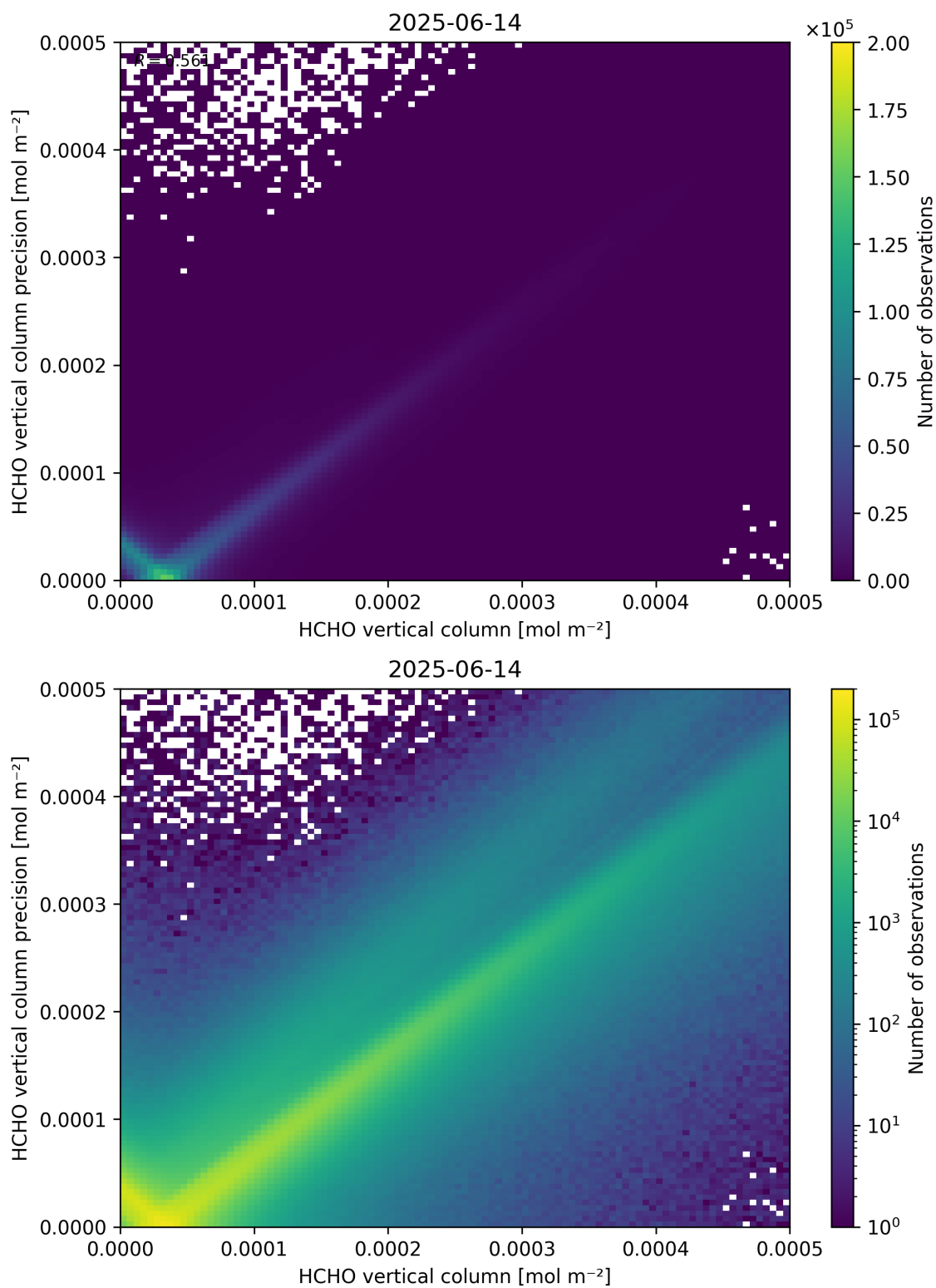
Figure 134: Scatter density plot of “HCHO vertical column” against “HCHO vertical column precision” for 2025-06-13 to 2025-06-15.
