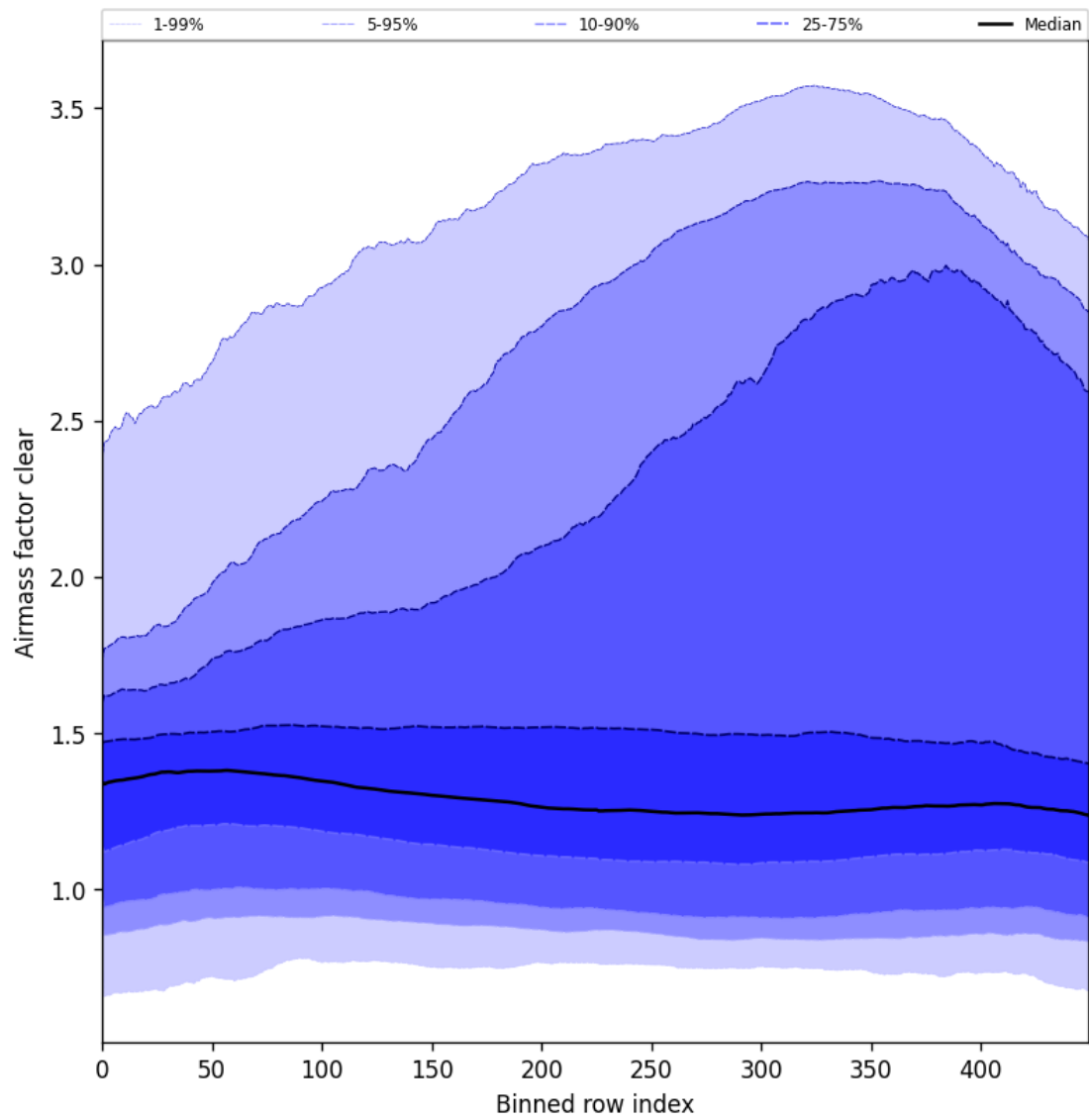
Figure 56: Along track statistics of “Airmass factor clear” for 2025-06-13 to 2025-06-15
