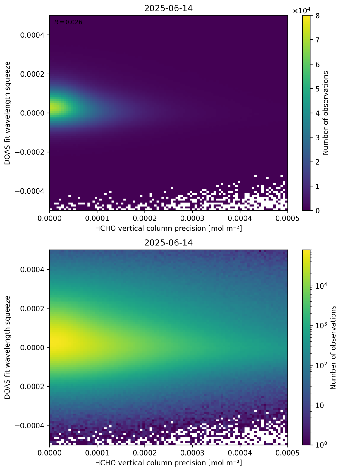
Figure 138: Scatter density plot of “HCHO vertical column precision” against “DOAS fit wavelength squeeze” for 2025-06-13 to 2025-06-15.
