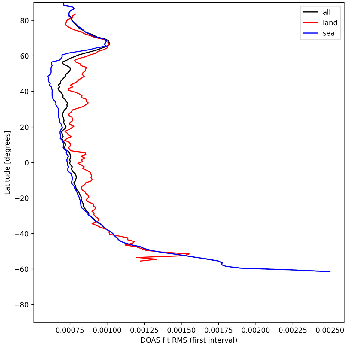
Figure 32: Zonal average of “DOAS fit RMS (first interval)” for 2025-06-13 to 2025-06-15.
