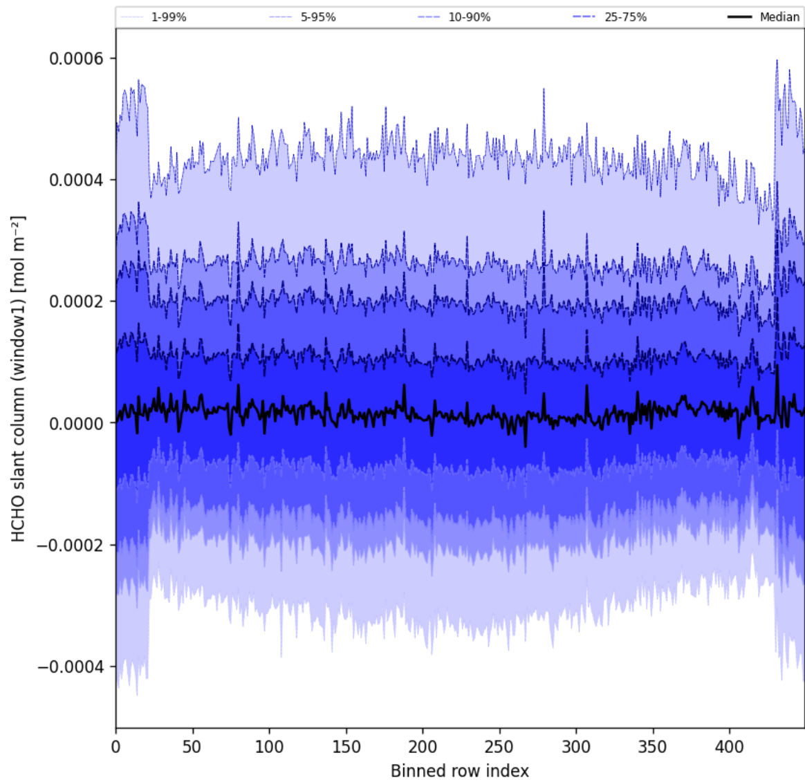
Figure 52: Along track statistics of “HCHO slant column (window1)” for 2025-06-14 to 2025-06-16
