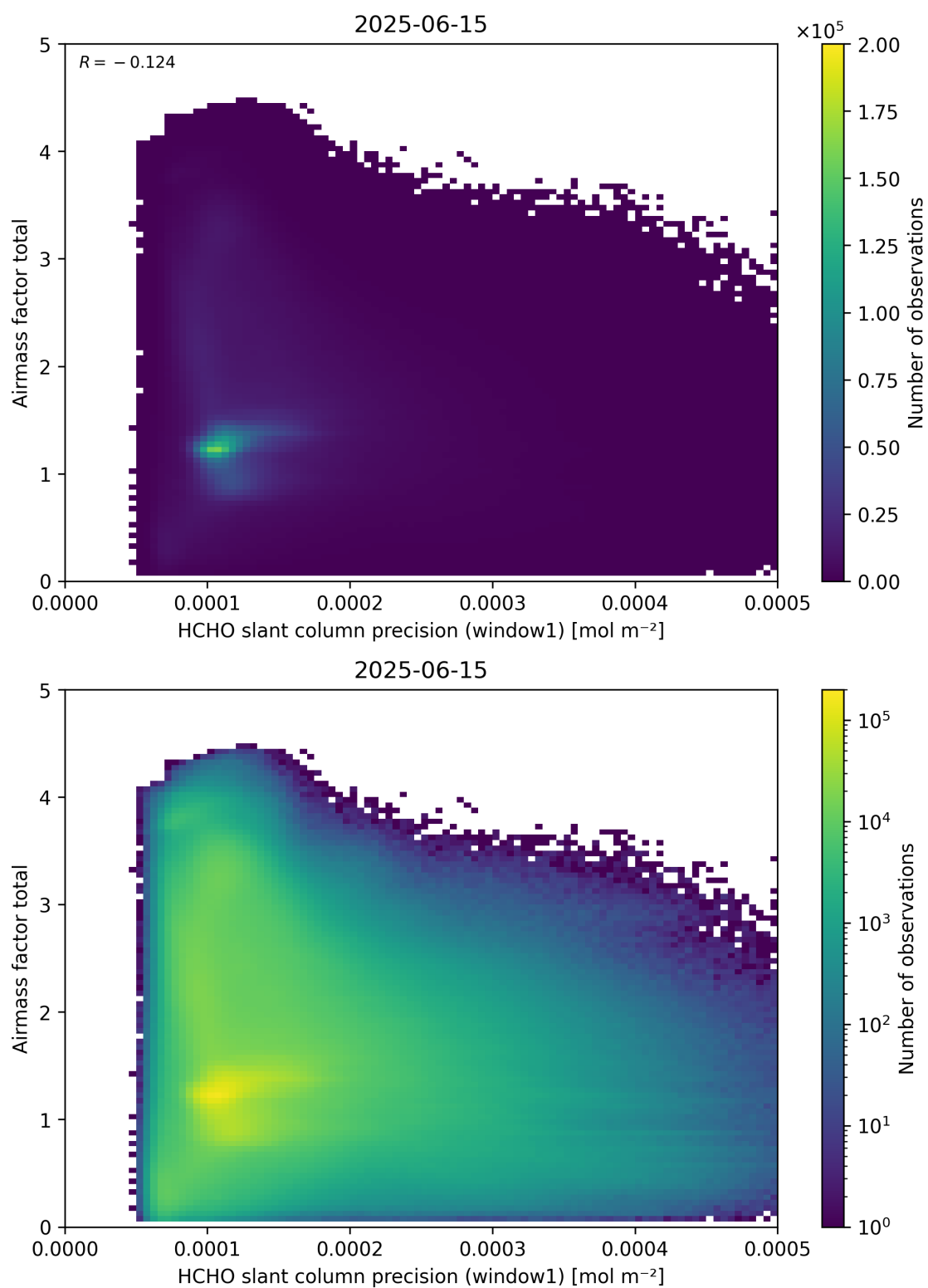
Figure 94: Scatter density plot of “HCHO slant column precision (window1)” against “Airmass factor total” for 2025-06-14 to 2025-06-16.
