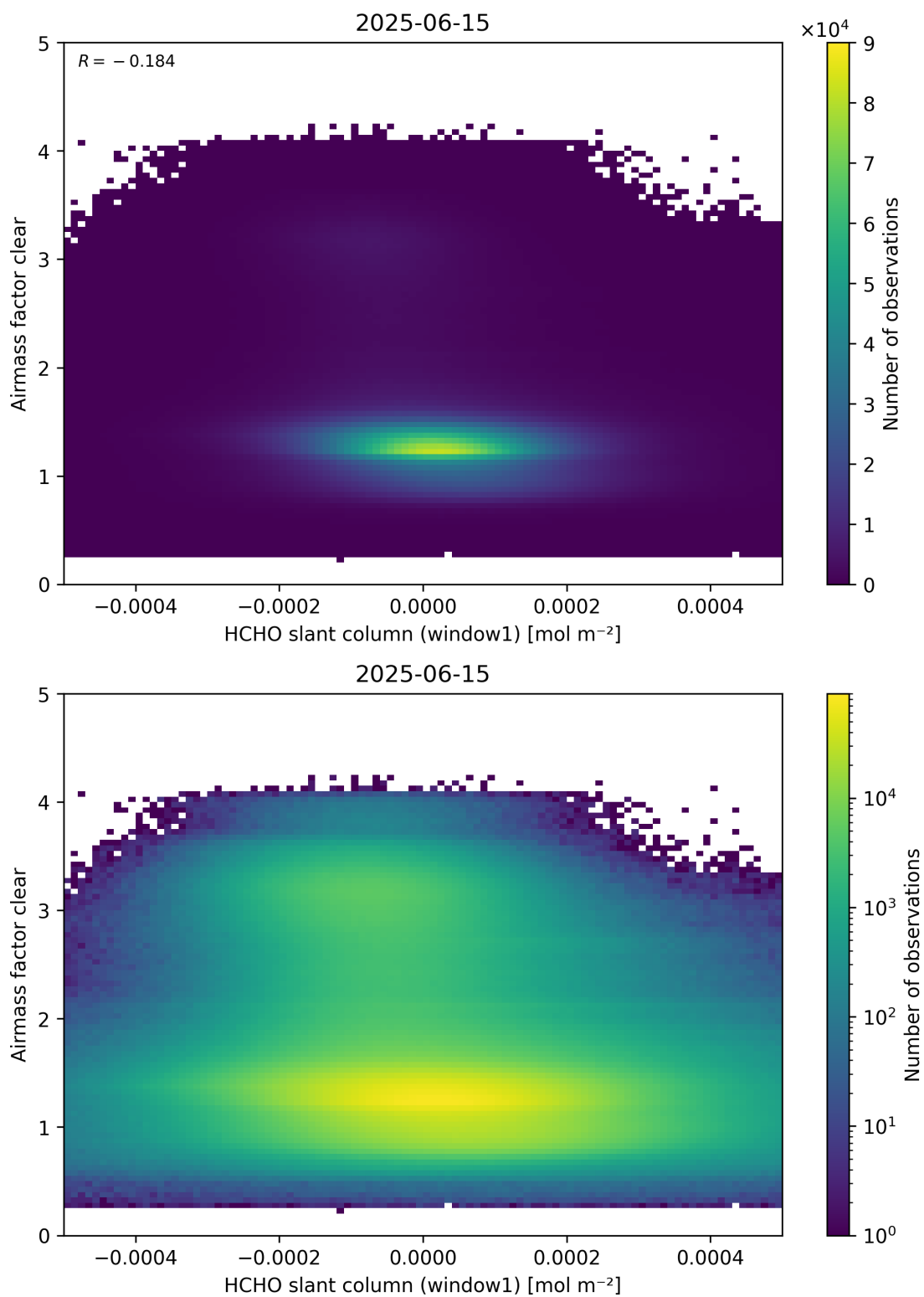
Figure 81: Scatter density plot of “HCHO slant column (window1)” against “Airmass factor clear” for 2025-06-14 to 2025-06-16.
