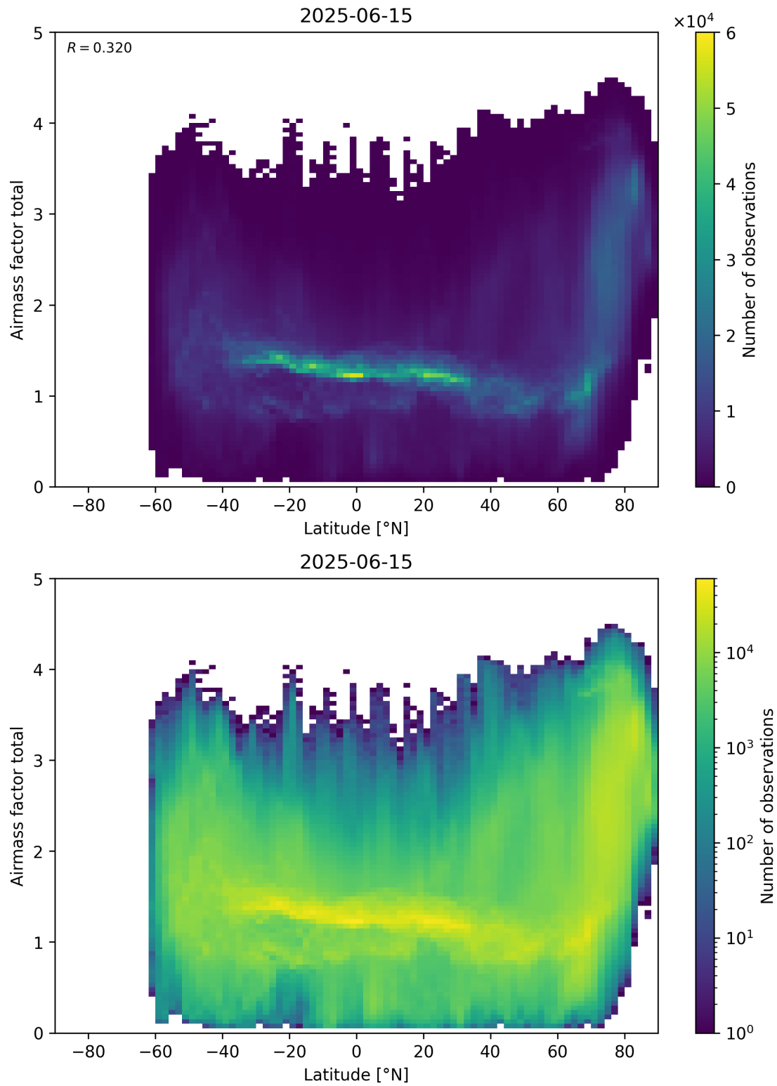
Figure 161: Scatter density plot of “Latitude” against “Airmass factor total” for 2025-06-14 to 2025-06-16.
