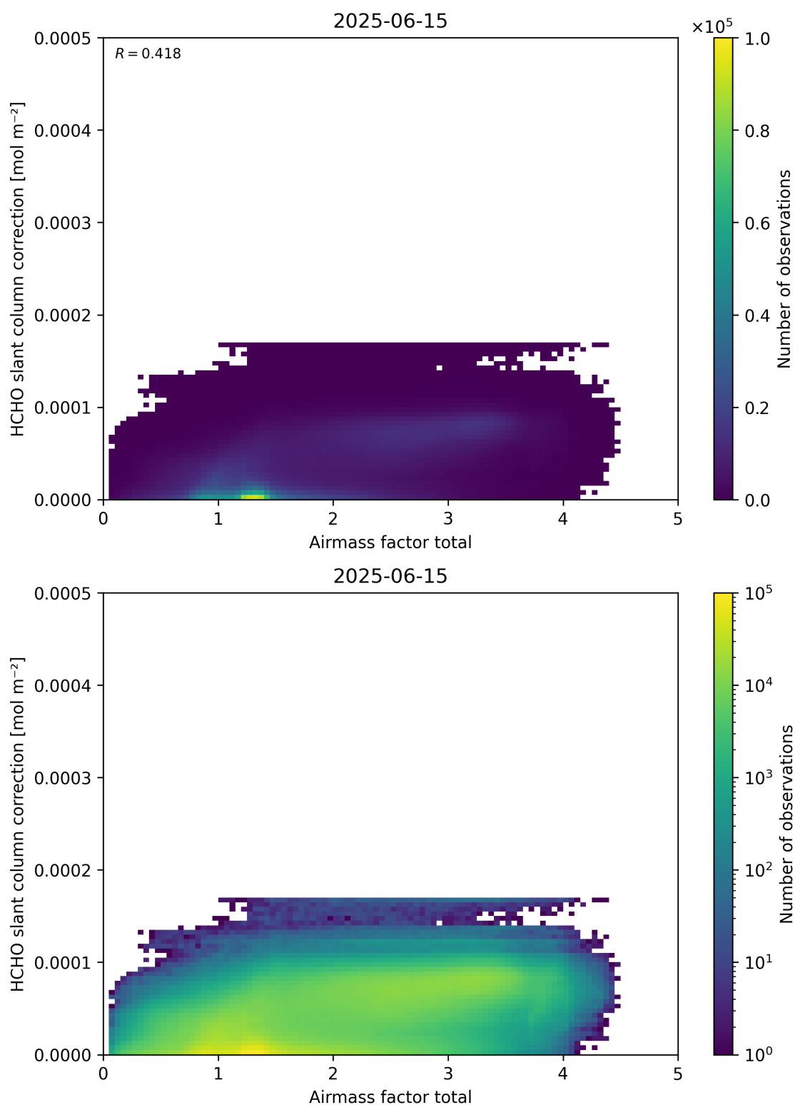
Figure 102: Scatter density plot of “Airmass factor total” against “HCHO slant column correction” for 2025-06-14 to 2025-06-16.
