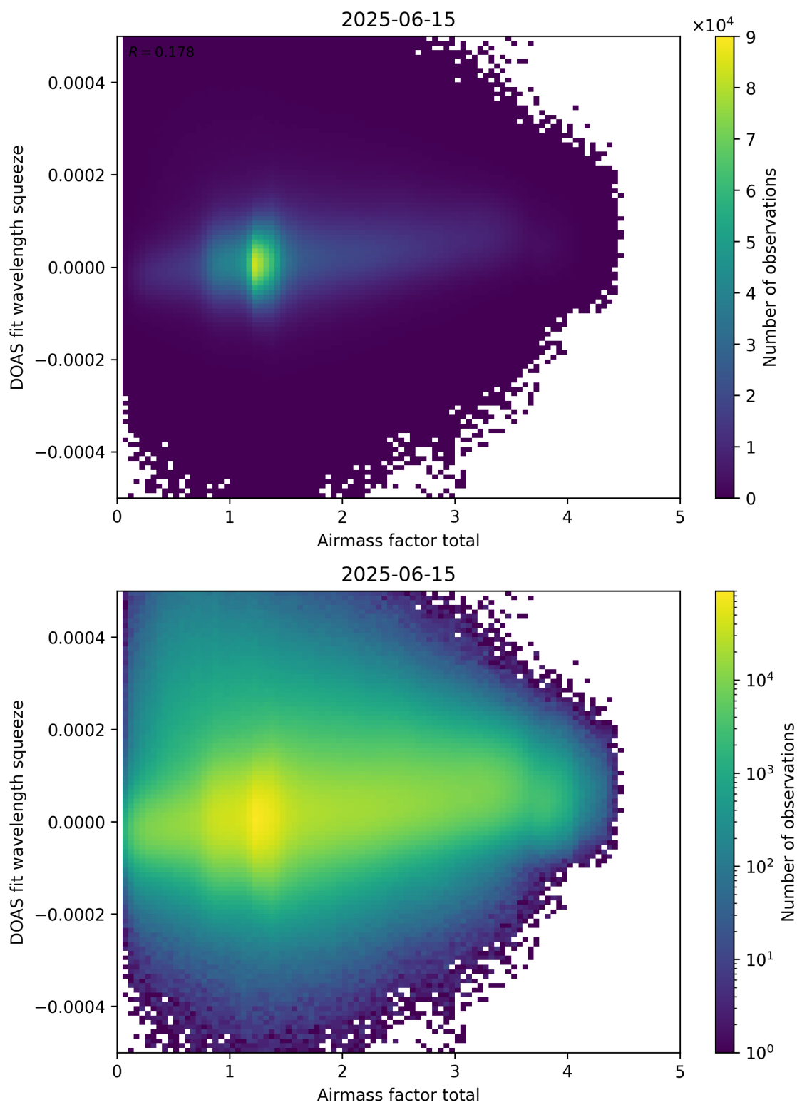
Figure 99: Scatter density plot of “Airmass factor total” against “DOAS fit wavelength squeeze” for 2025-06-14 to 2025-06-16.
