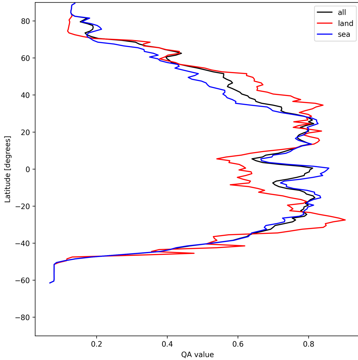
Figure 20: Zonal average of “QA value” for 2025-06-14 to 2025-06-16.
