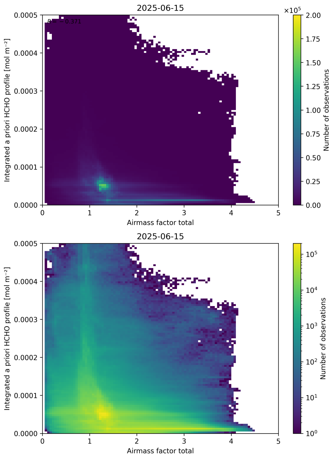
Figure 104: Scatter density plot of “Airmass factor total” against “Integrated a priori HCHO profile” for 2025-06-14 to 2025-06-16.
