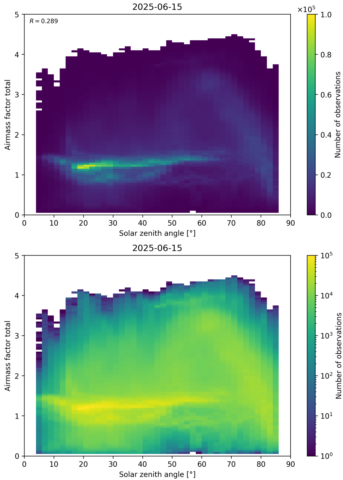
Figure 175: Scatter density plot of “Solar zenith angle” against “Airmass factor total” for 2025-06-14 to 2025-06-16.
