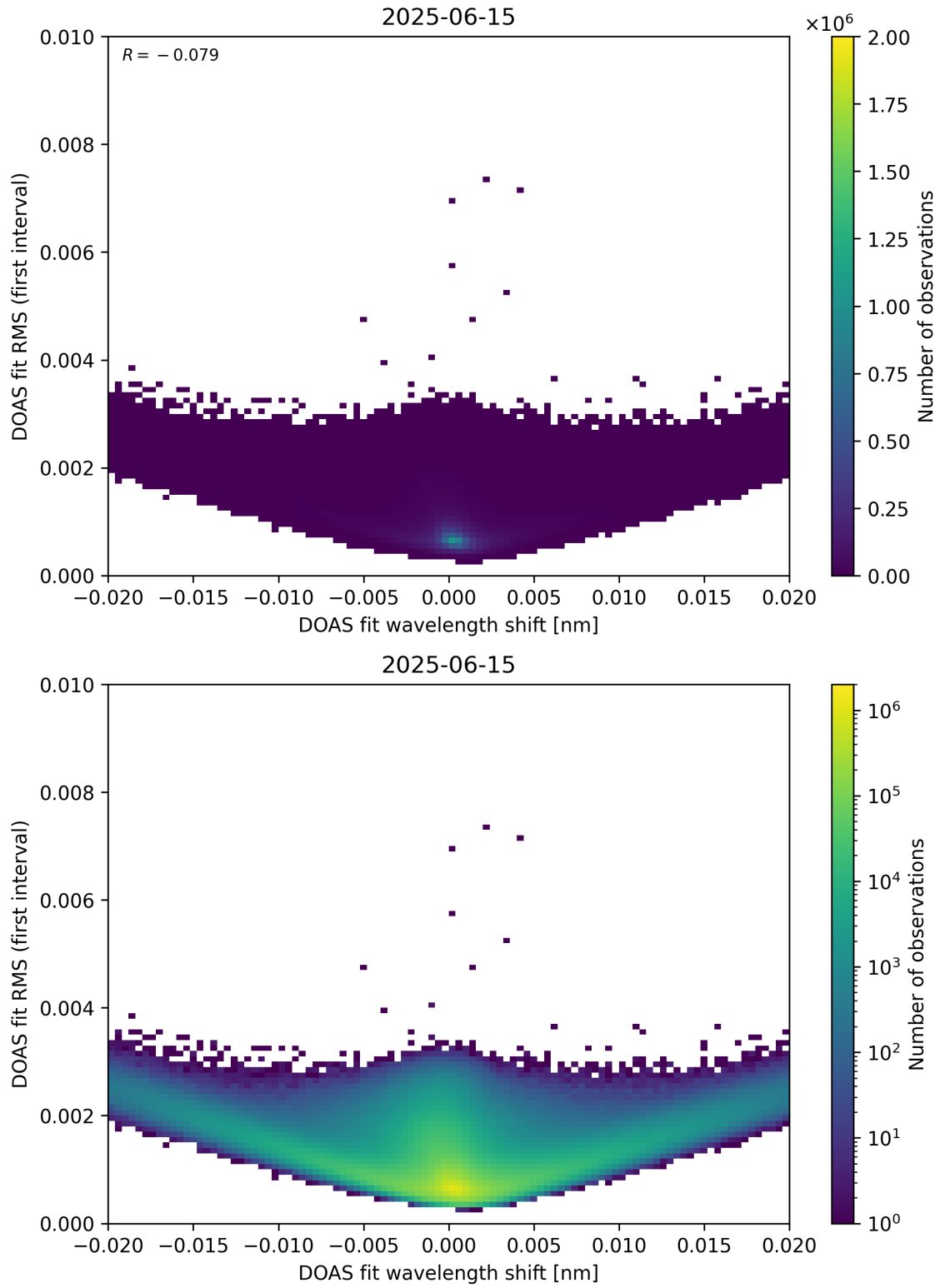
Figure 64: Scatter density plot of “DOAS fit wavelength shift” against “DOAS fit RMS (first interval)” for 2025-06-14 to 2025-06-16.
