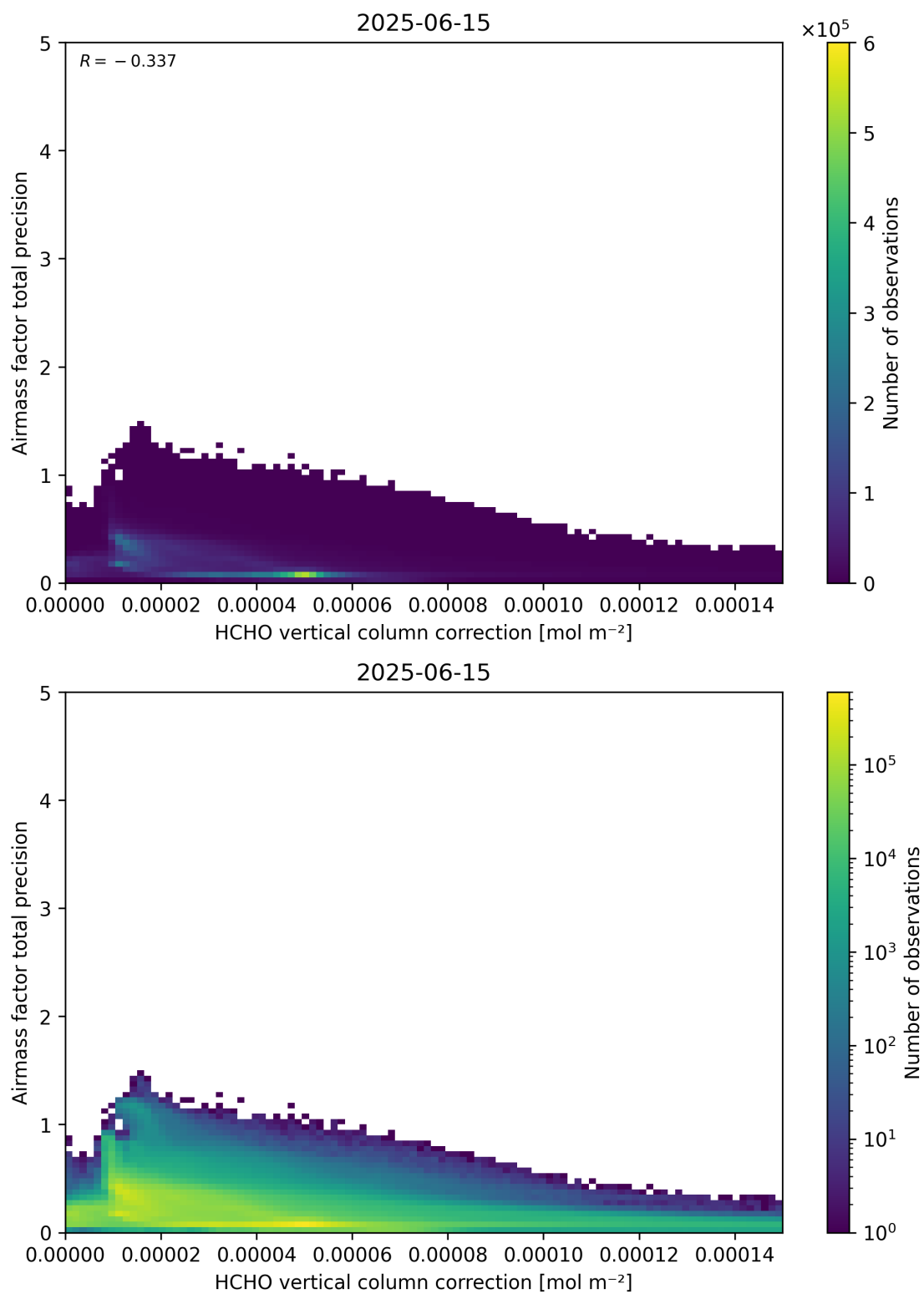
Figure 121: Scatter density plot of “HCHO vertical column correction” against “Airmass factor total precision” for 2025-06-14 to 2025-06-16.
