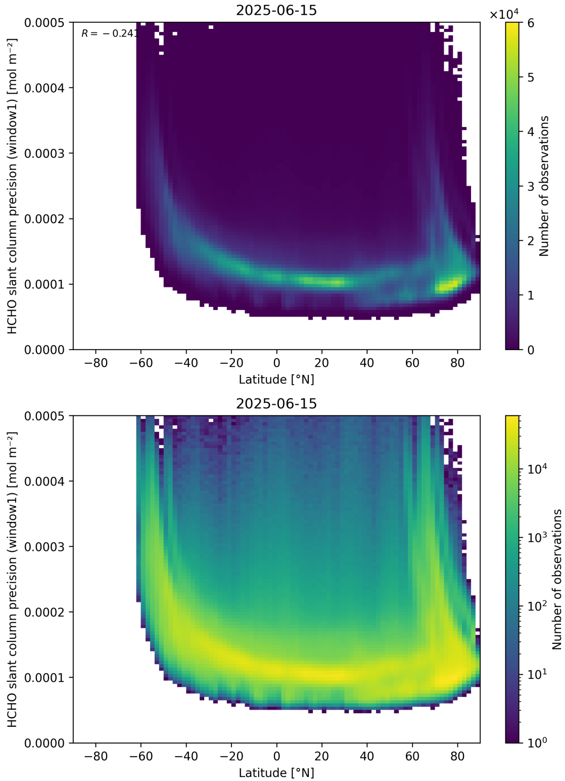
Figure 160: Scatter density plot of “Latitude” against “HCHO slant column precision (window1)” for 2025-06-14 to 2025-06-16.
