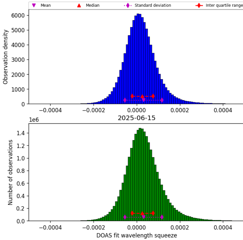
Figure 45: Histogram of “DOAS fit wavelength squeeze” for 2025-06-14 to 2025-06-16
