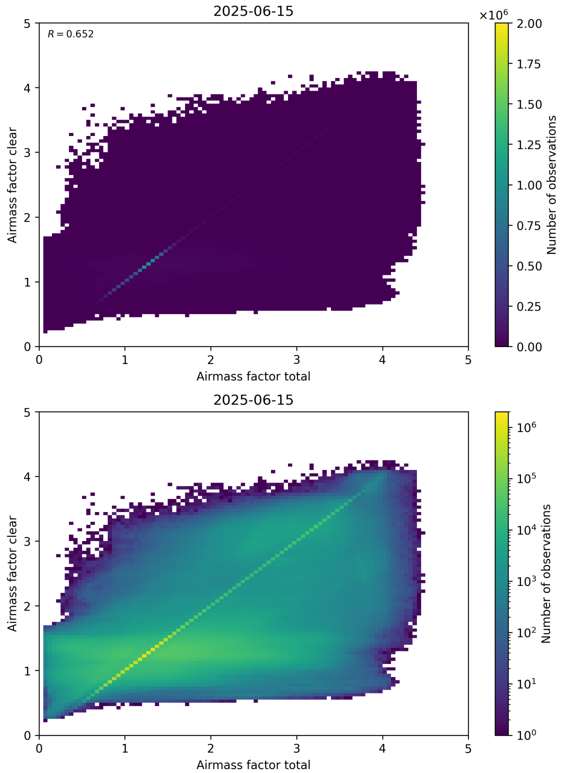
Figure 100: Scatter density plot of “Airmass factor total” against “Airmass factor clear” for 2025-06-14 to 2025-06-16.
