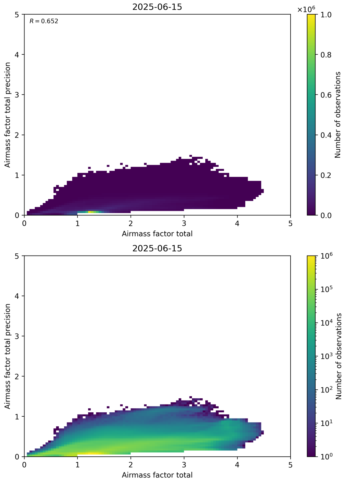
Figure 103: Scatter density plot of “Airmass factor total” against “Airmass factor total precision” for 2025-06-14 to 2025-06-16.
