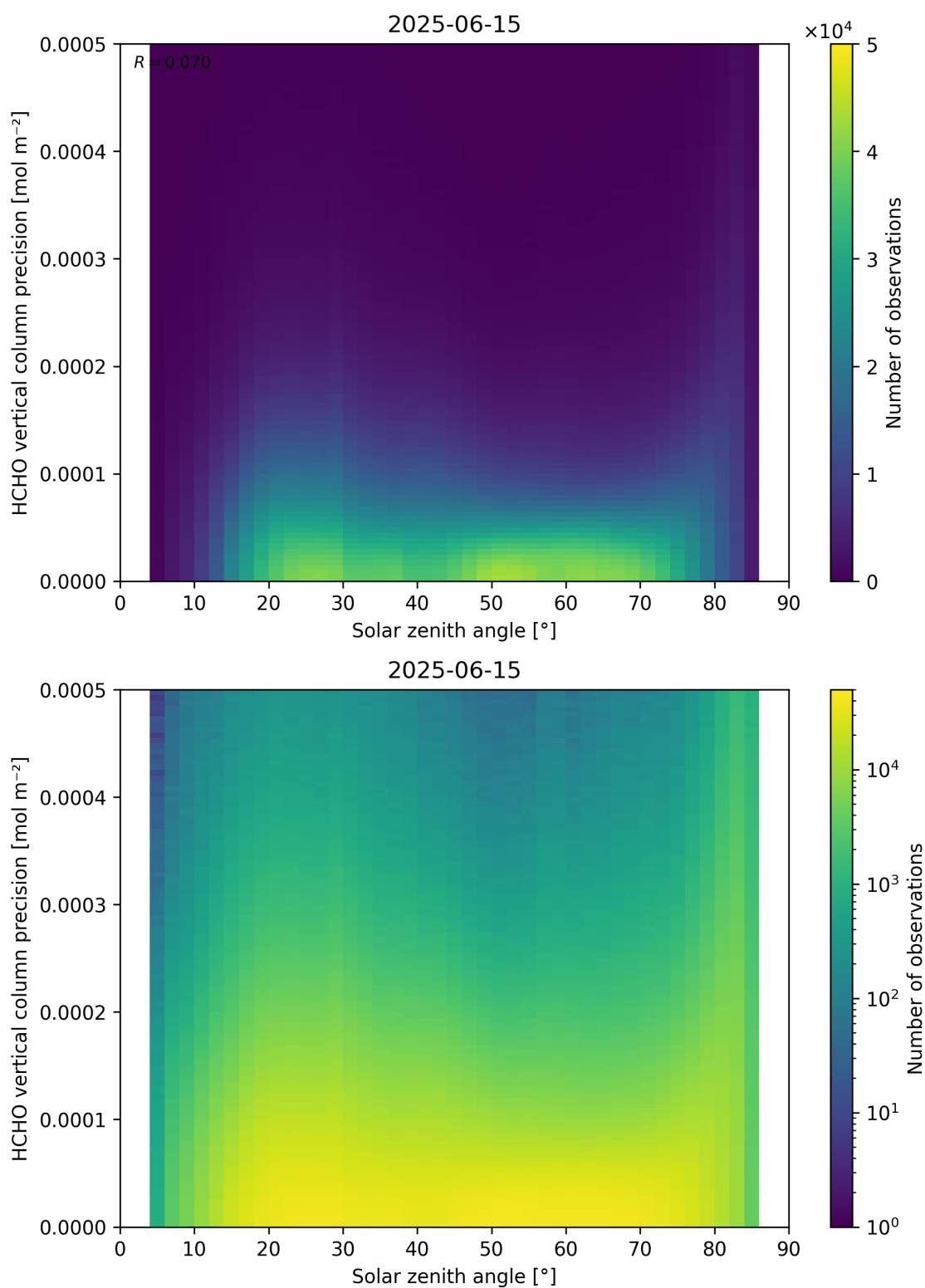
Figure 179: Scatter density plot of “Solar zenith angle” against “HCHO vertical column precision” for 2025-06-14 to 2025-06-16.
