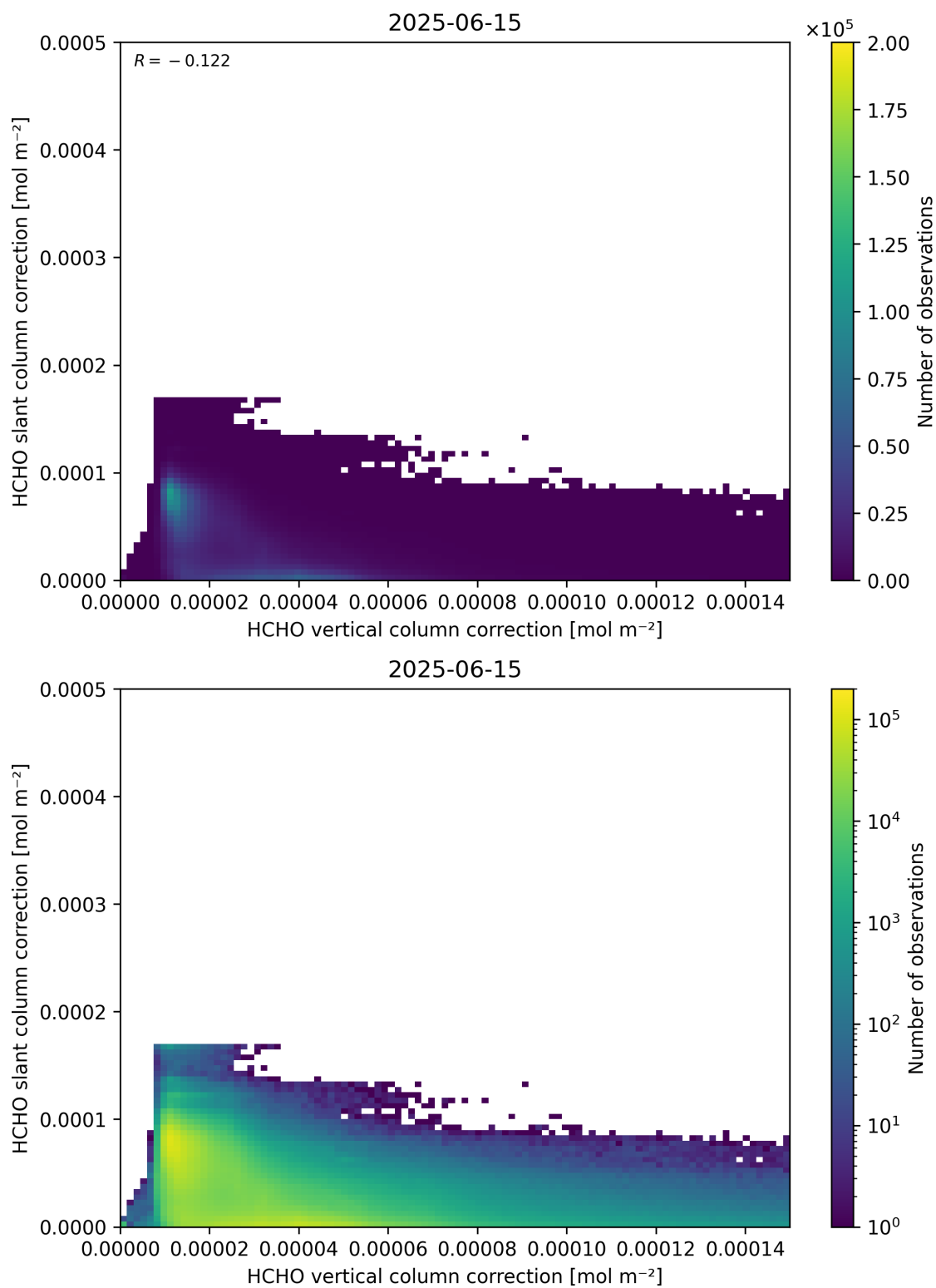
Figure 117: Scatter density plot of “HCHO vertical column correction” against “HCHO slant column correction” for 2025-06-14 to 2025-06-16.
