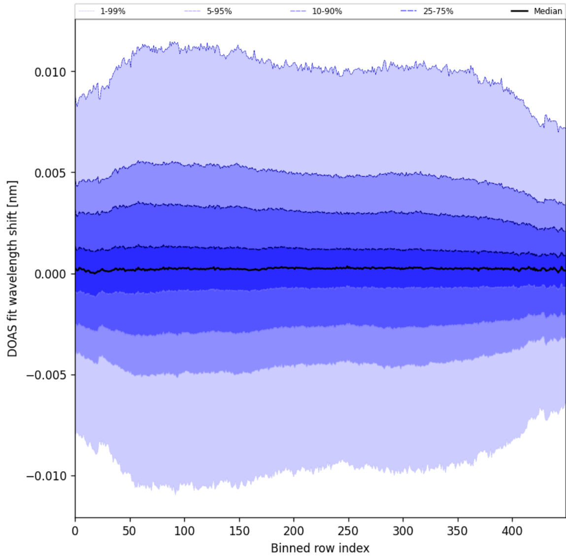
Figure 58: Along track statistics of “DOAS fit wavelength shift” for 2025-06-14 to 2025-06-16
