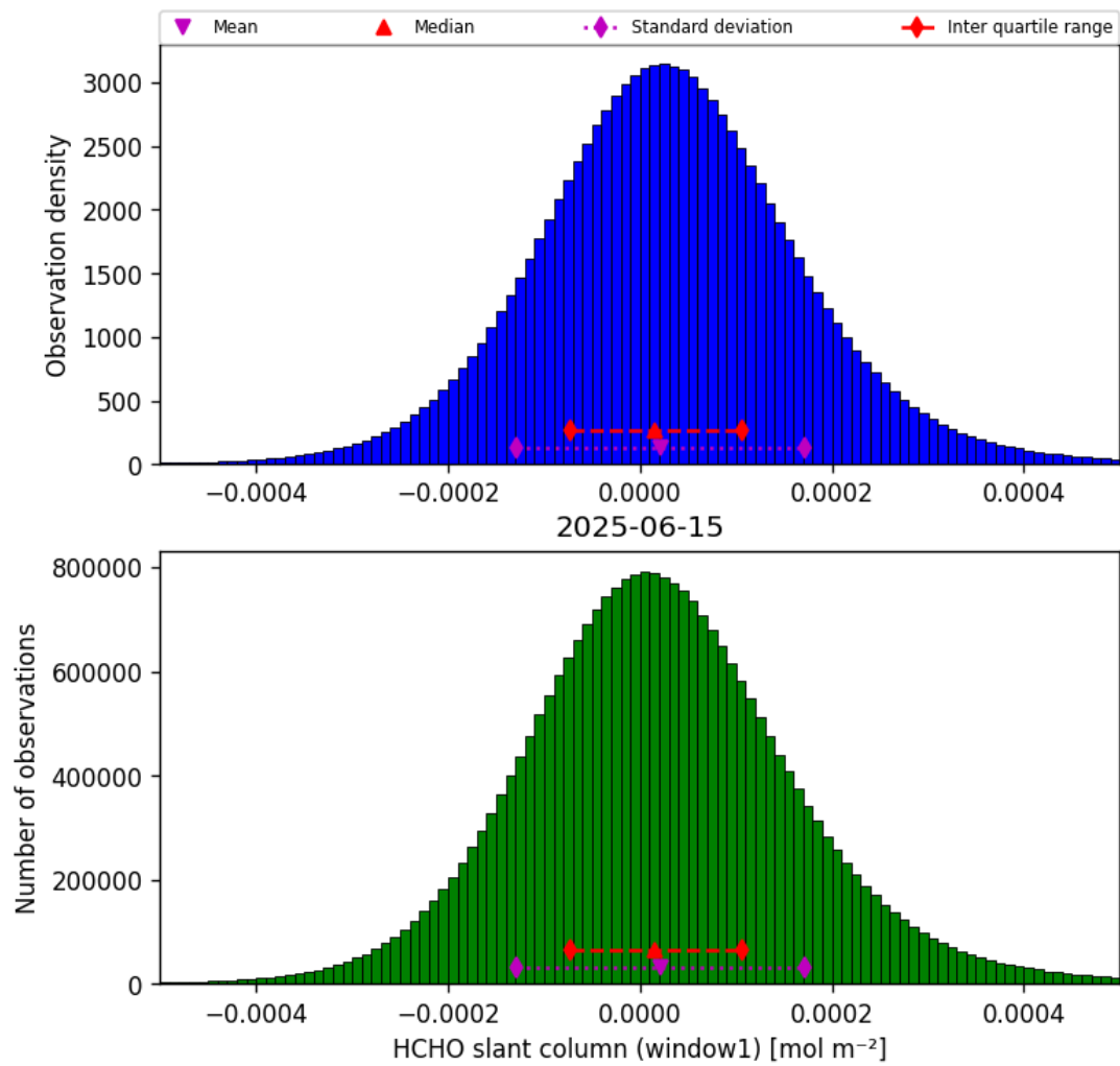
Figure 38: Histogram of “HCHO slant column (window1)” for 2025-06-14 to 2025-06-16
