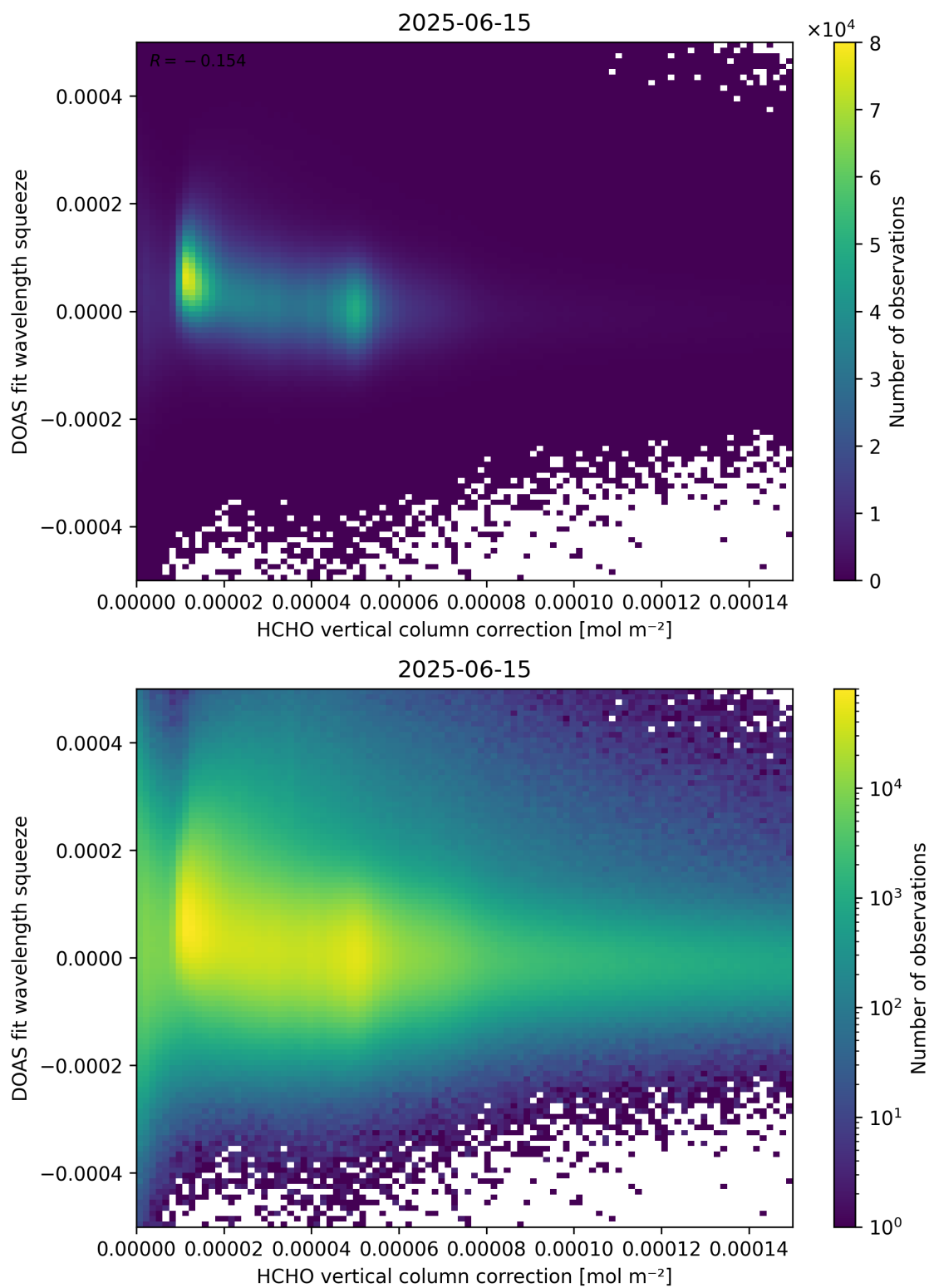
Figure 114: Scatter density plot of “HCHO vertical column correction” against “DOAS fit wavelength squeeze” for 2025-06-14 to 2025-06-16.
