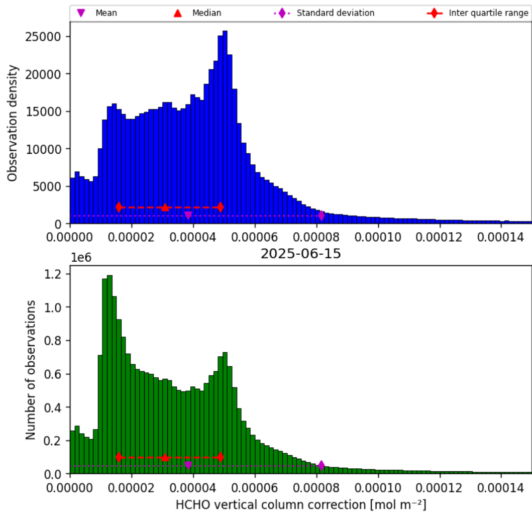
Figure 37: Histogram of “HCHO vertical column correction” for 2025-06-14 to 2025-06-16
