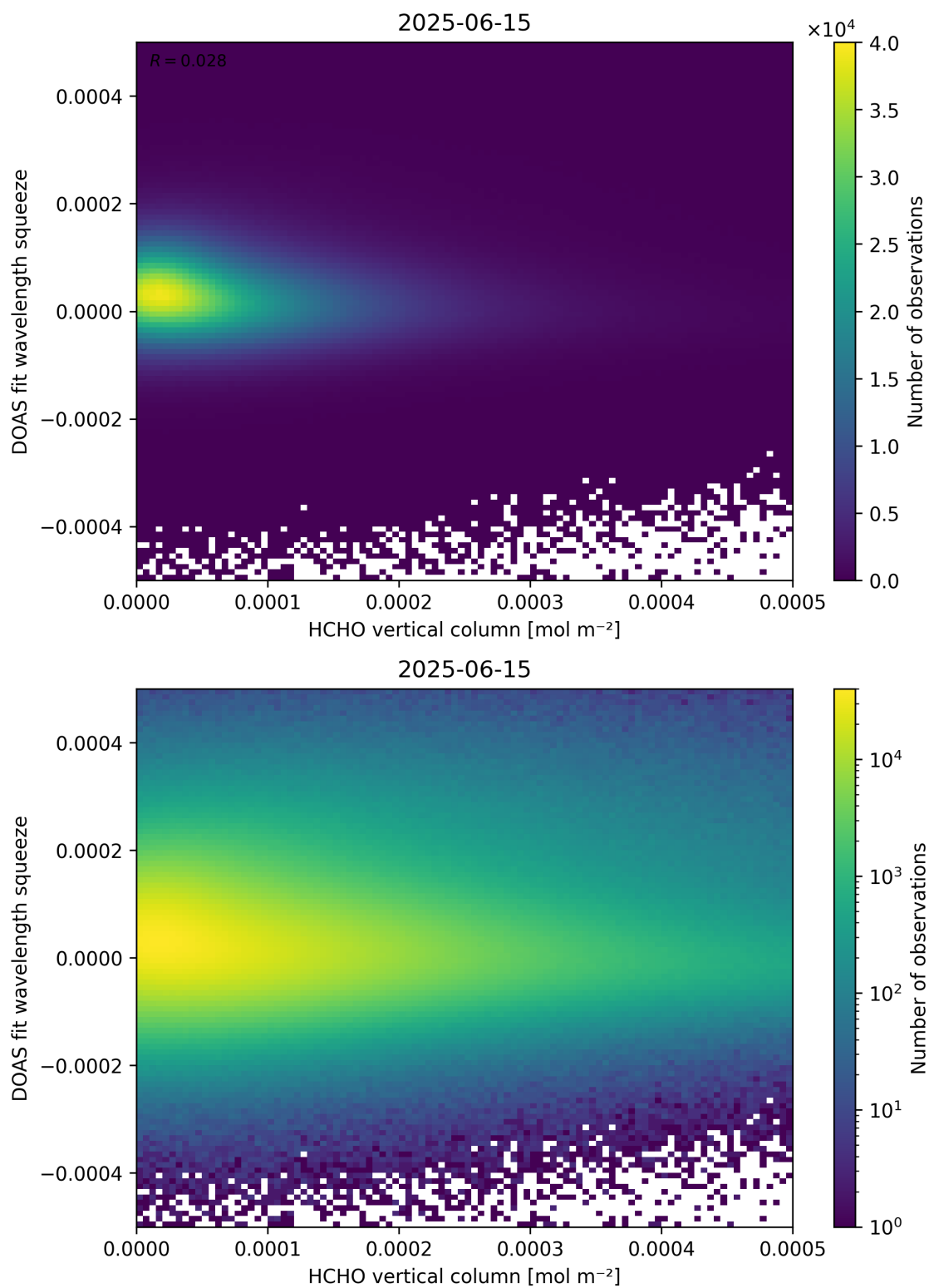
Figure 125: Scatter density plot of “HCHO vertical column” against “DOAS fit wavelength squeeze” for 2025-06-14 to 2025-06-16.
