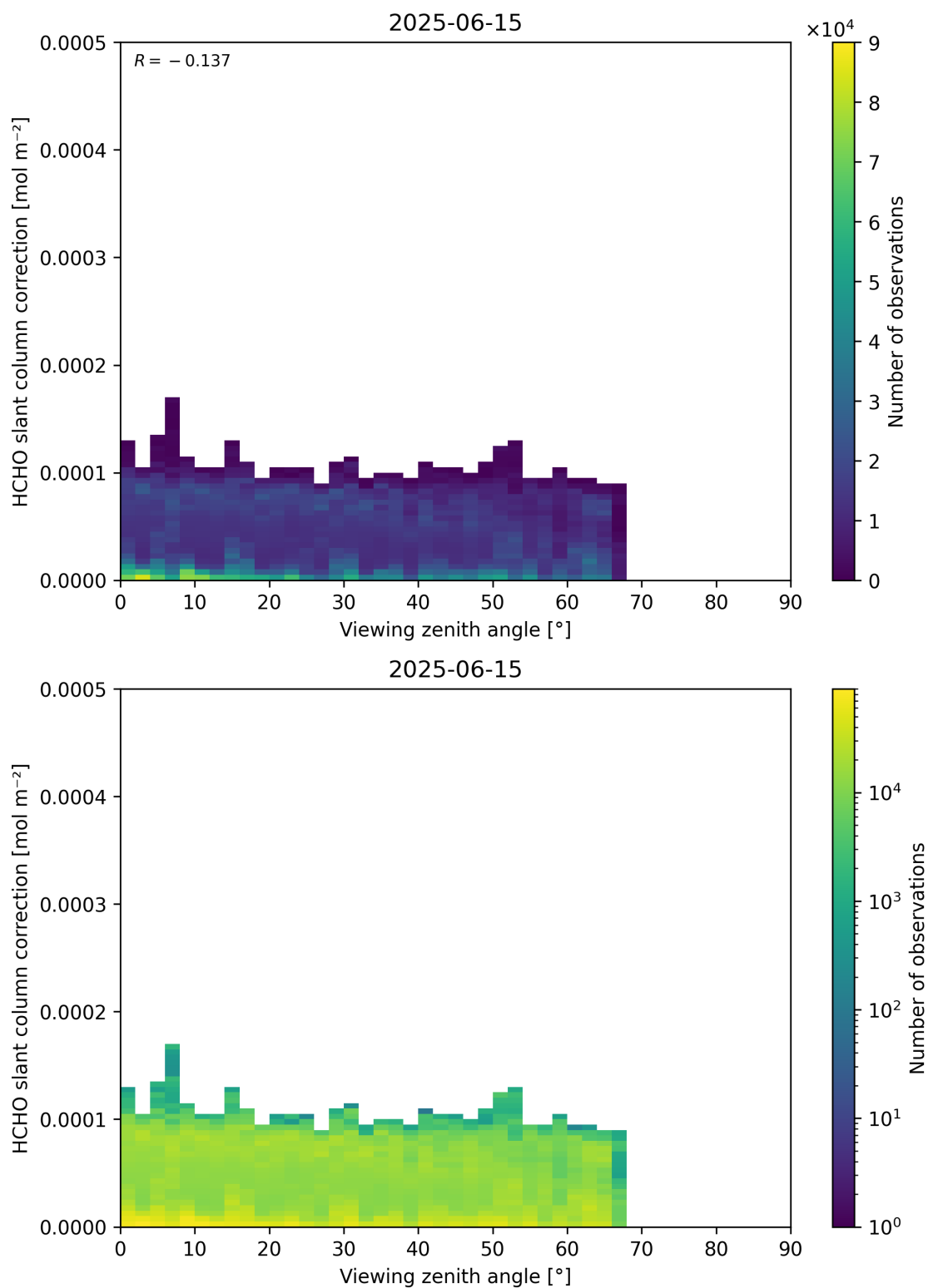
Figure 187: Scatter density plot of “Viewing zenith angle” against “HCHO slant column correction” for 2025-06-14 to 2025-06-16.
