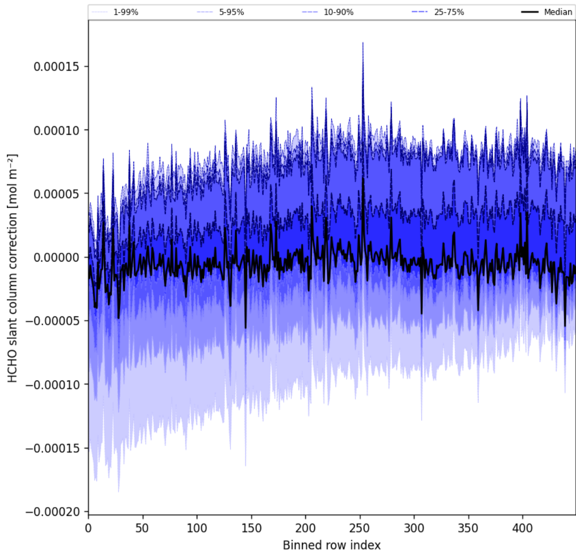
Figure 61: Along track statistics of “HCHO slant column correction” for 2025-06-14 to 2025-06-16
