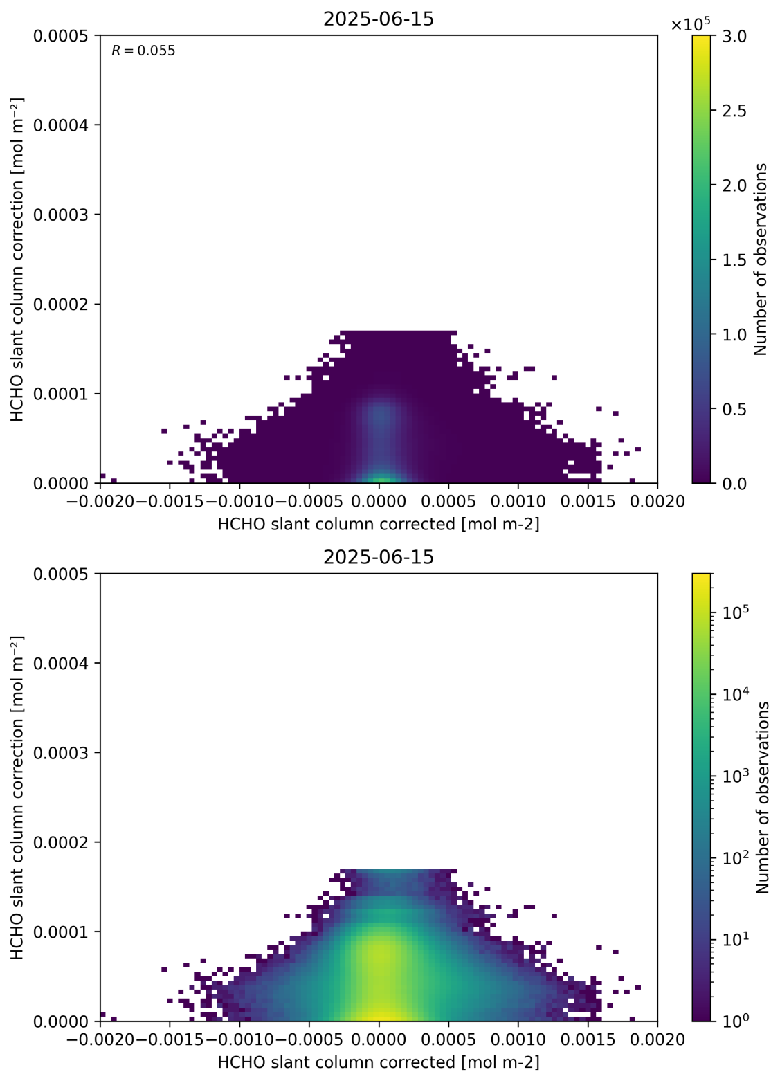
Figure 77: Scatter density plot of “HCHO slant column corrected” against “HCHO slant column correction” for 2025-06-14 to 2025-06-16.
