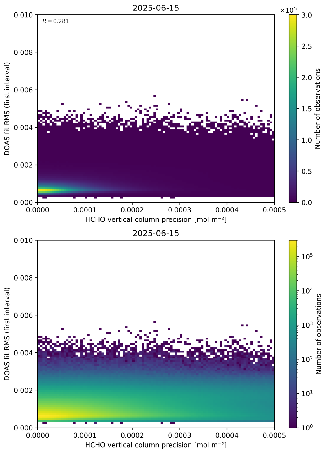
Figure 136: Scatter density plot of “HCHO vertical column precision” against “DOAS fit RMS (first interval)” for 2025-06-14 to 2025-06-16.
