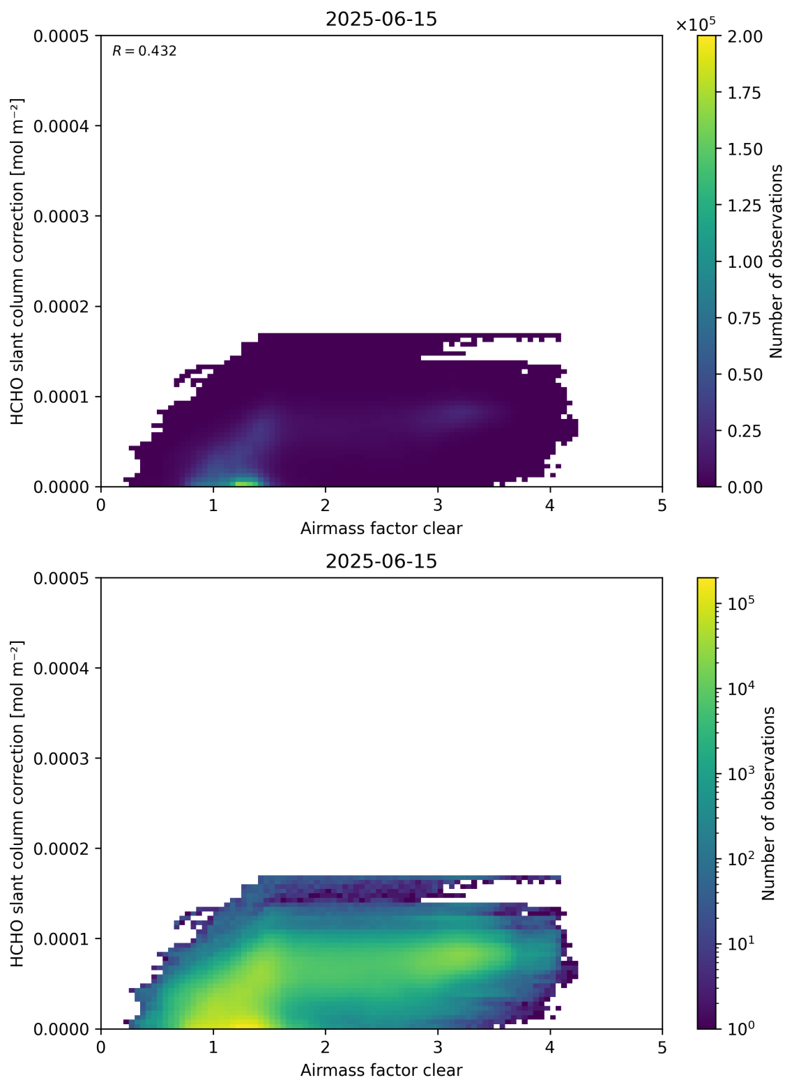
Figure 75: Scatter density plot of “Airmass factor clear” against “HCHO slant column correction” for 2025-06-14 to 2025-06-16.
