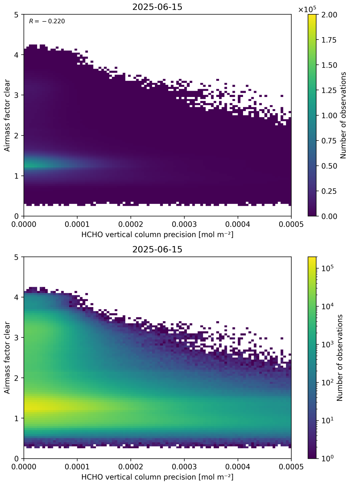
Figure 139: Scatter density plot of “HCHO vertical column precision” against “Airmass factor clear” for 2025-06-14 to 2025-06-16.
