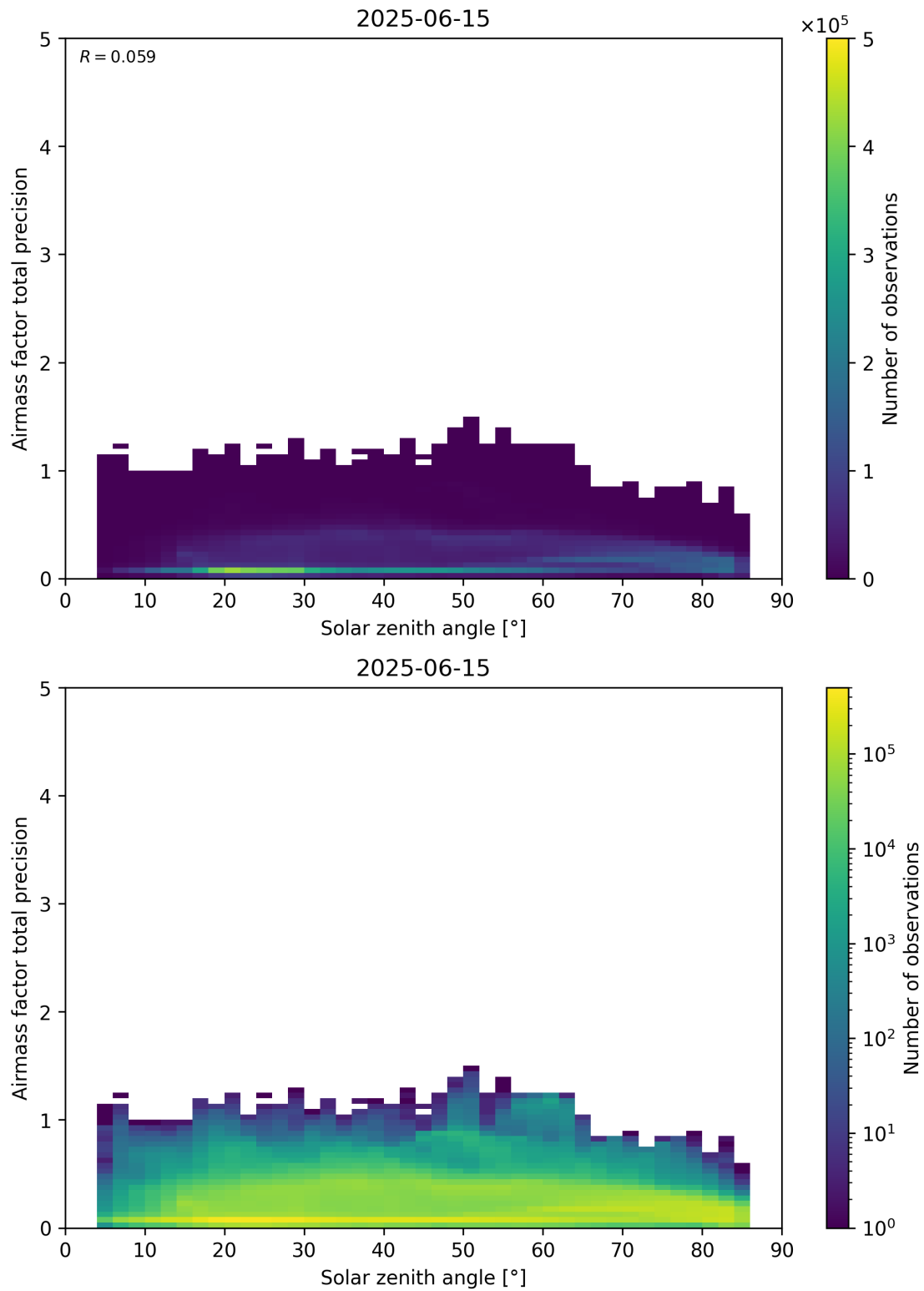
Figure 176: Scatter density plot of “Solar zenith angle” against “Airmass factor total precision” for 2025-06-14 to 2025-06-16.
