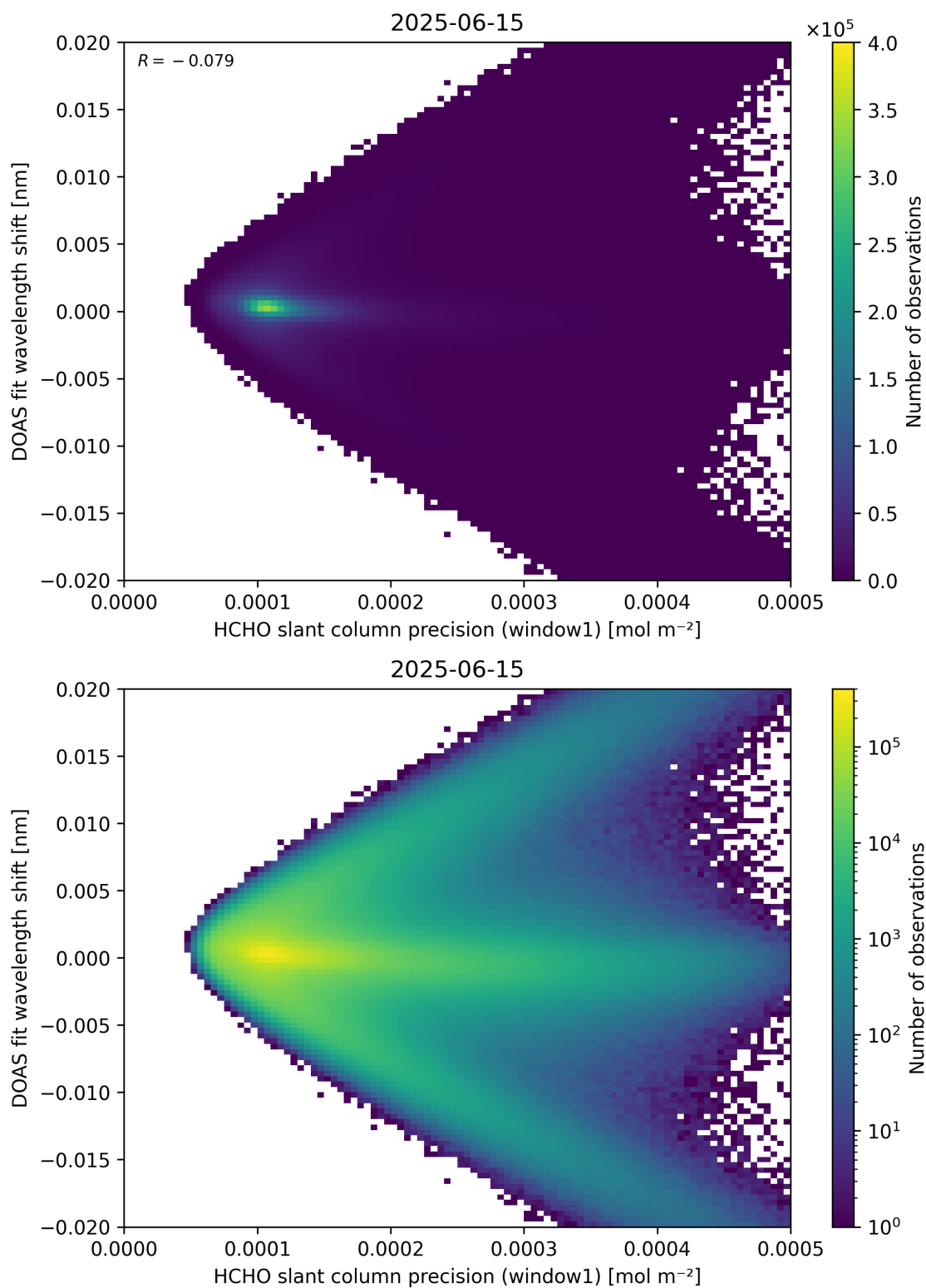
Figure 89: Scatter density plot of “HCHO slant column precision (window1)” against “DOAS fit wavelength shift” for 2025-06-14 to 2025-06-16.
