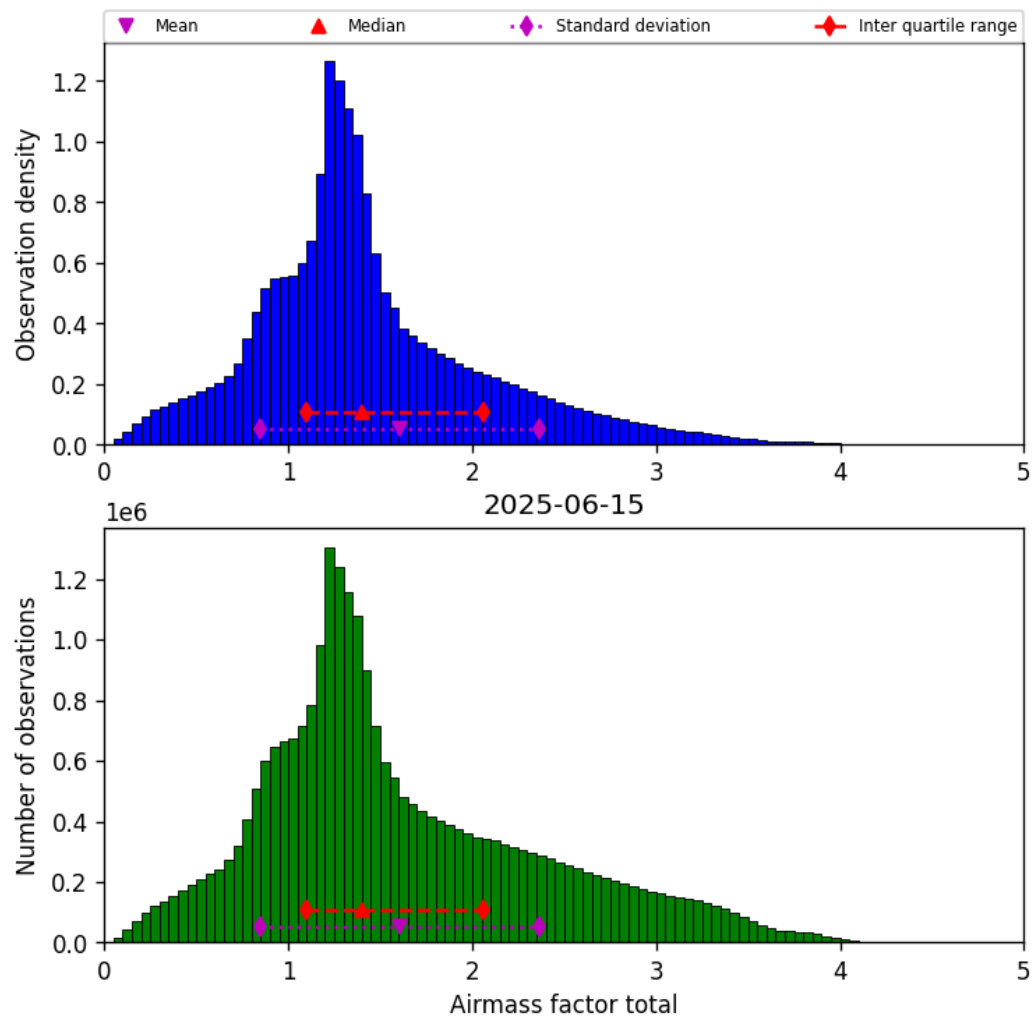
Figure 40: Histogram of “Airmass factor total” for 2025-06-14 to 2025-06-16
