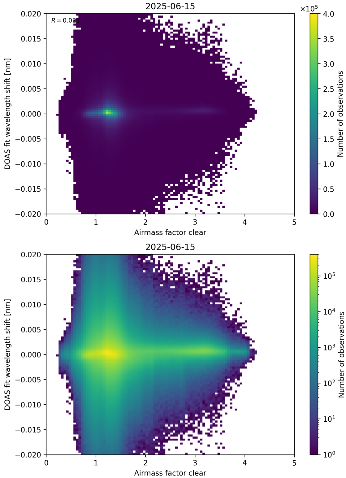
Figure 72: Scatter density plot of “Airmass factor clear” against “DOAS fit wavelength shift” for 2025-06-14 to 2025-06-16.
