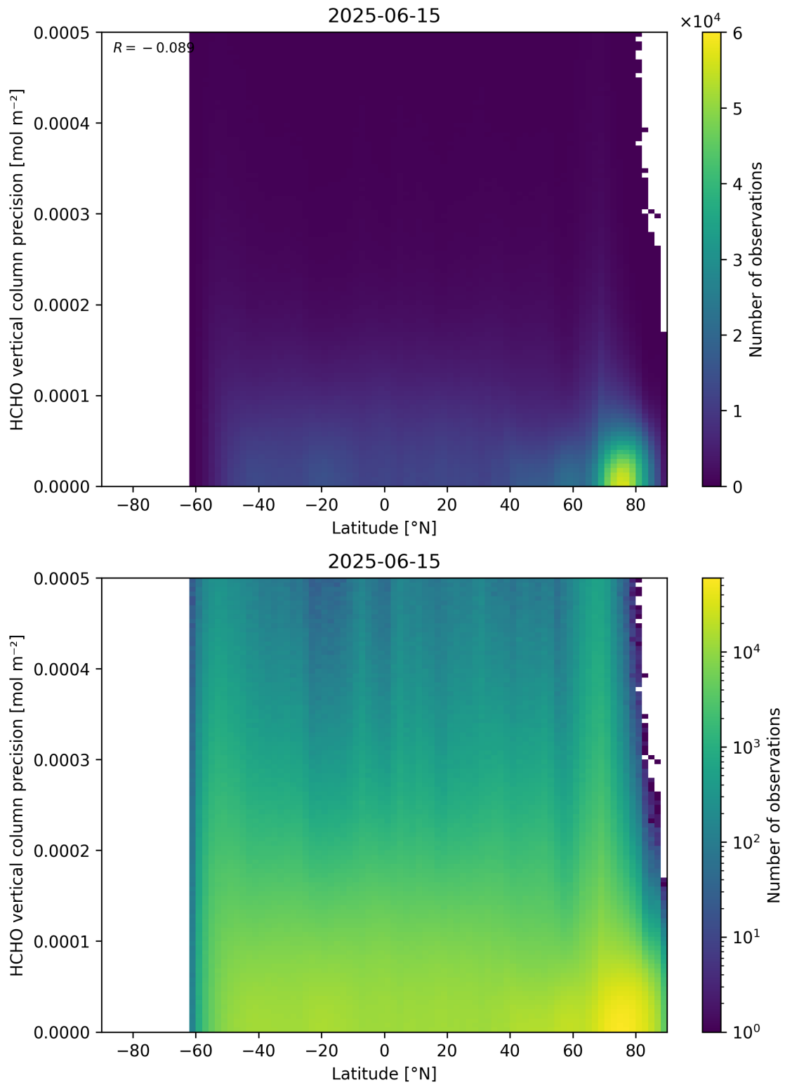
Figure 165: Scatter density plot of “Latitude” against “HCHO vertical column precision” for 2025-06-14 to 2025-06-16.
