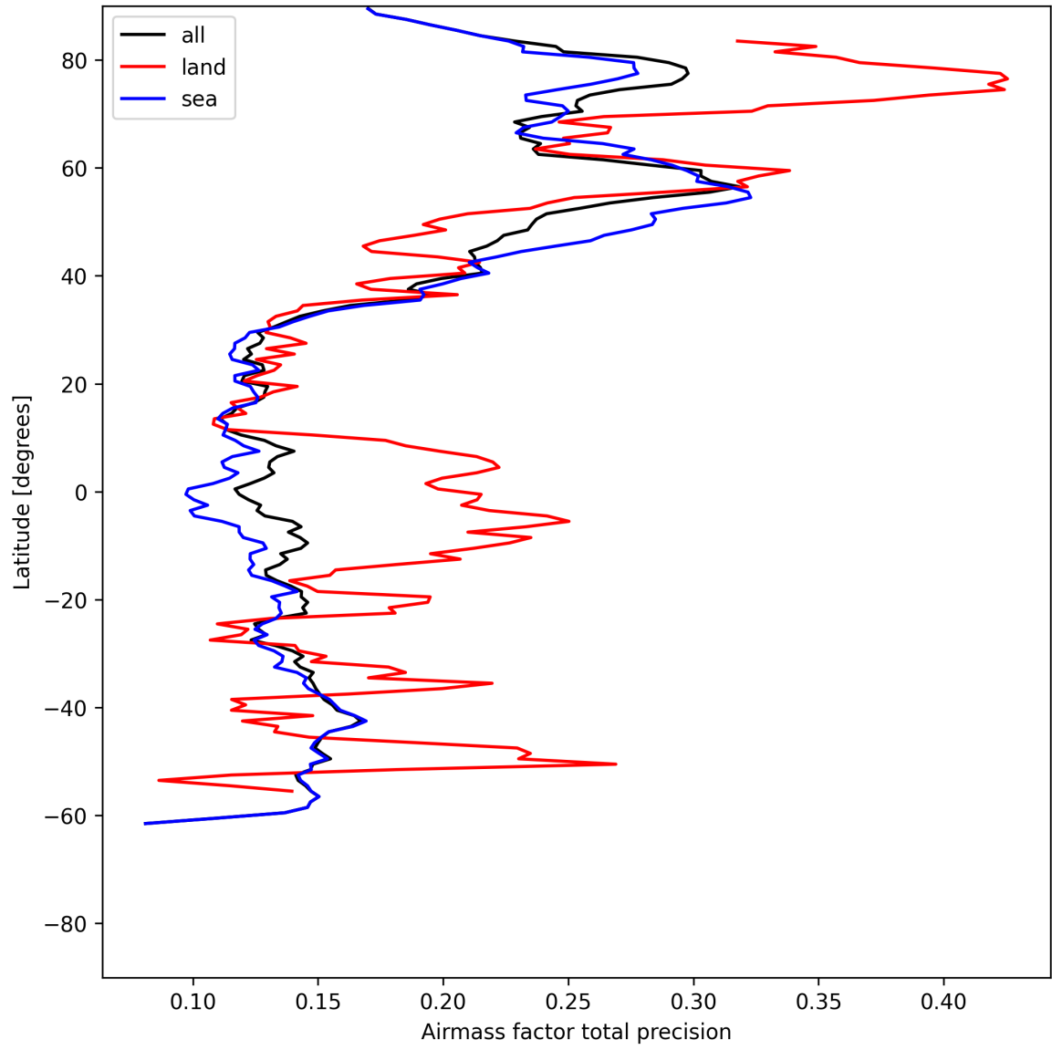
Figure 27: Zonal average of “Airmass factor total precision” for 2025-06-14 to 2025-06-16.
