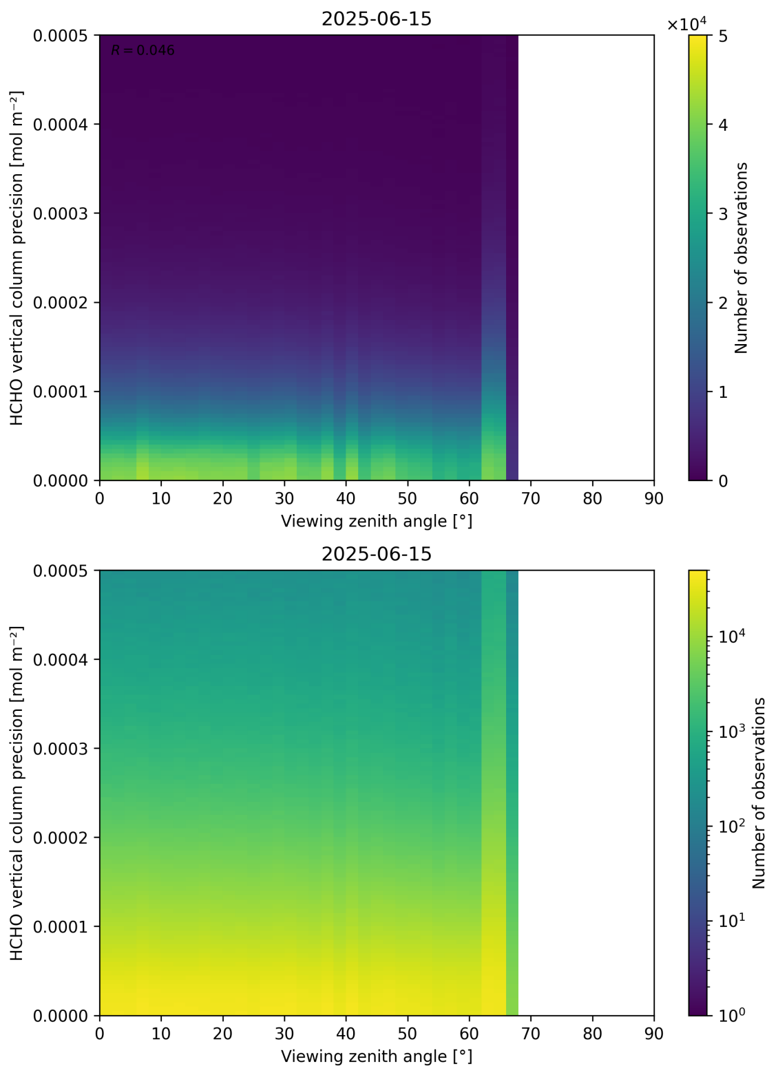
Figure 194: Scatter density plot of “Viewing zenith angle” against “HCHO vertical column precision” for 2025-06-14 to 2025-06-16.
