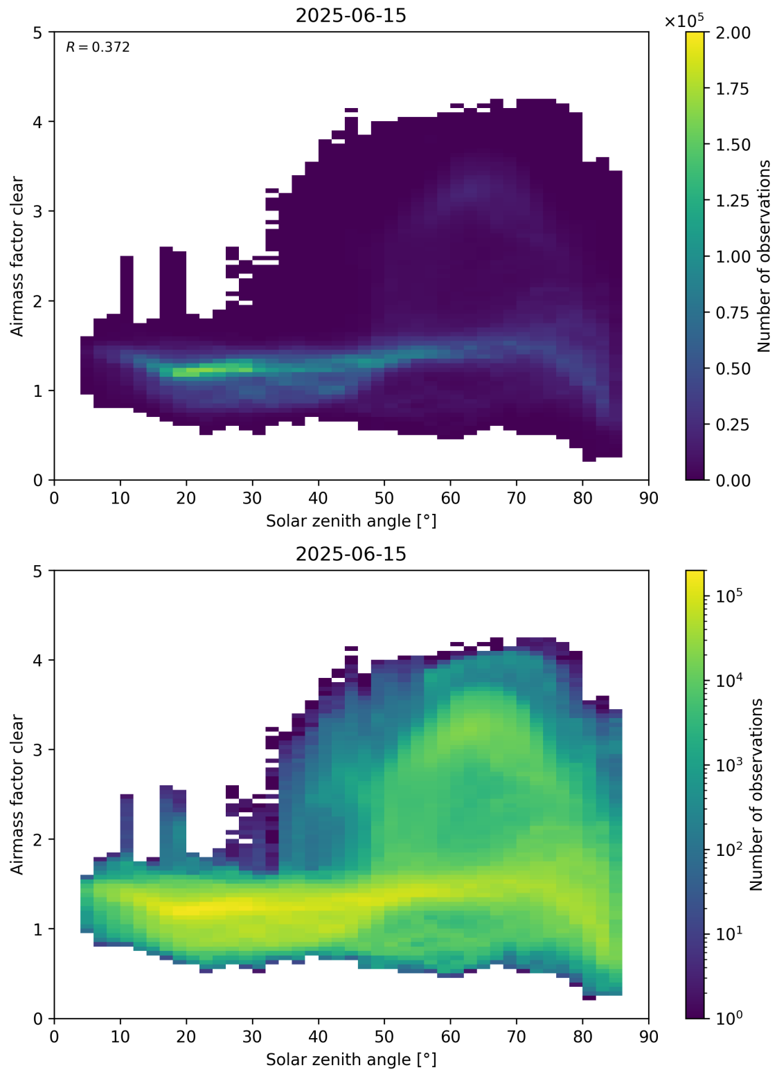
Figure 170: Scatter density plot of “Solar zenith angle” against “Airmass factor clear” for 2025-06-14 to 2025-06-16.
