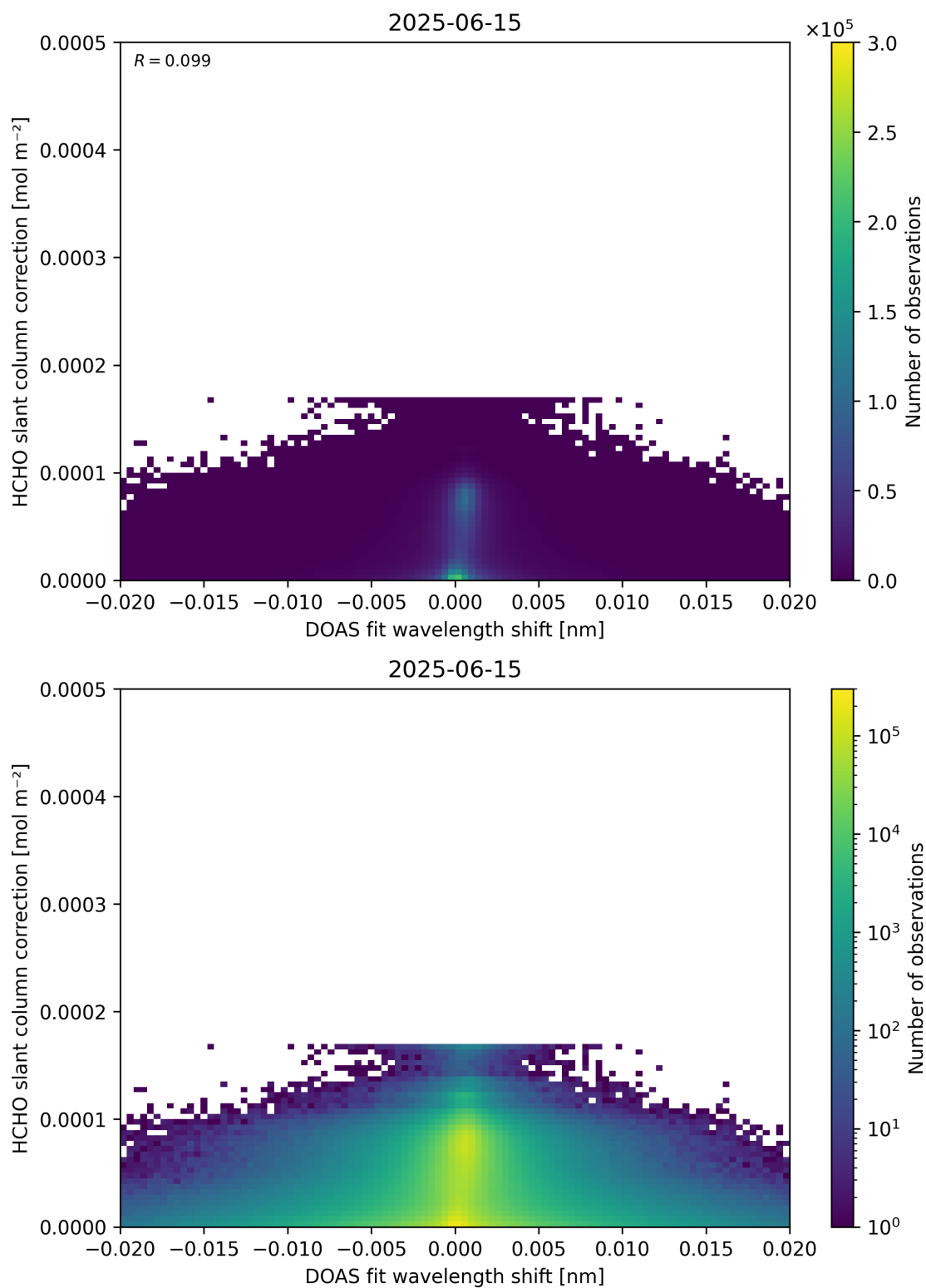
Figure 67: Scatter density plot of “DOAS fit wavelength shift” against “HCHO slant column correction” for 2025-06-14 to 2025-06-16.
