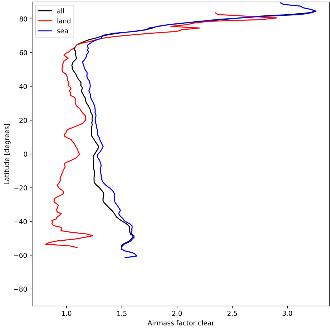
Figure 28: Zonal average of “Airmass factor clear” for 2025-06-14 to 2025-06-16.
