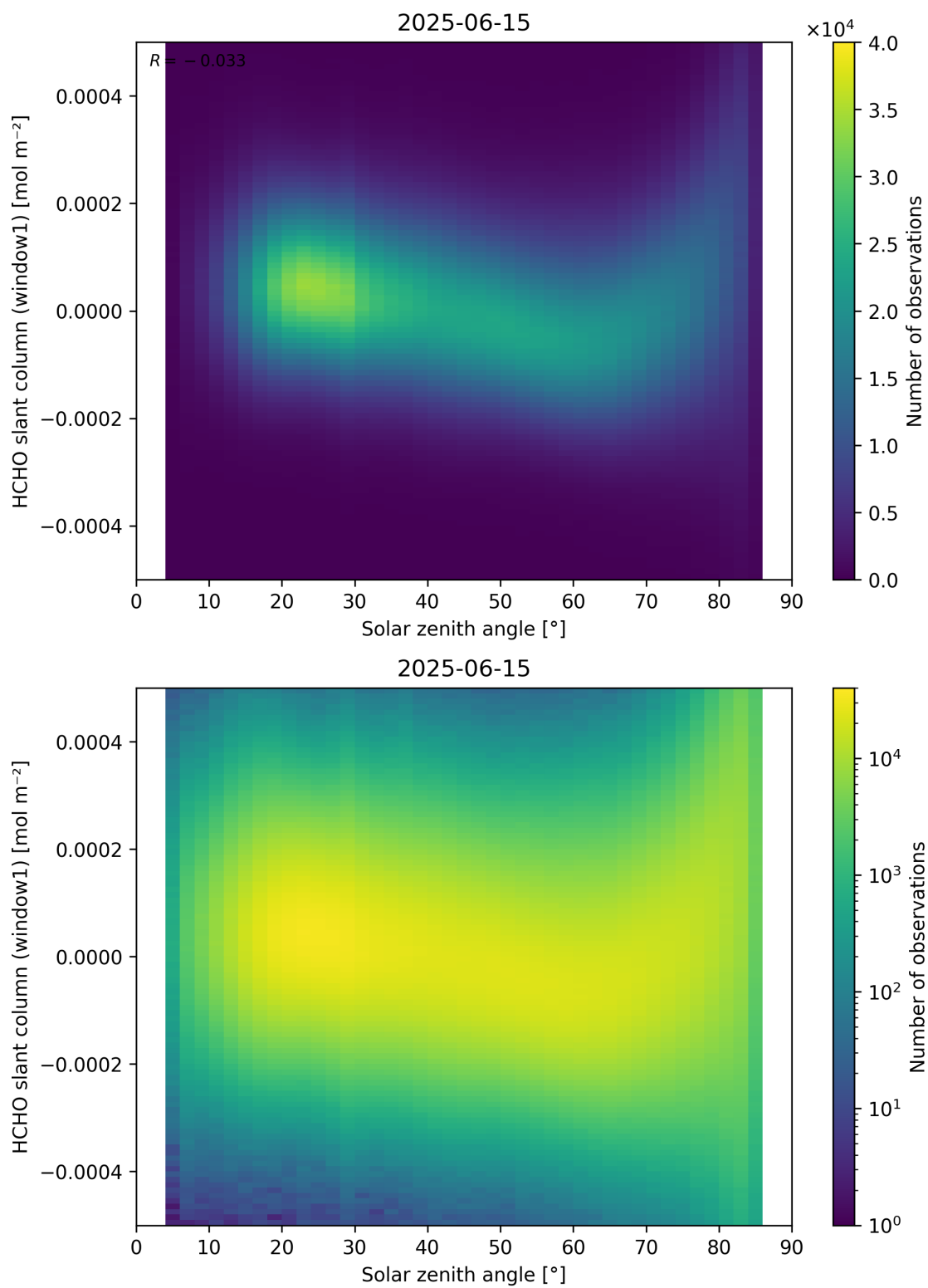
Figure 173: Scatter density plot of “Solar zenith angle” against “HCHO slant column (window1)” for 2025-06-14 to 2025-06-16.
