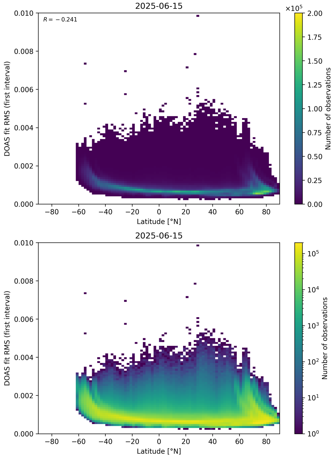
Figure 153: Scatter density plot of “Latitude” against “DOAS fit RMS (first interval)” for 2025-06-14 to 2025-06-16.
