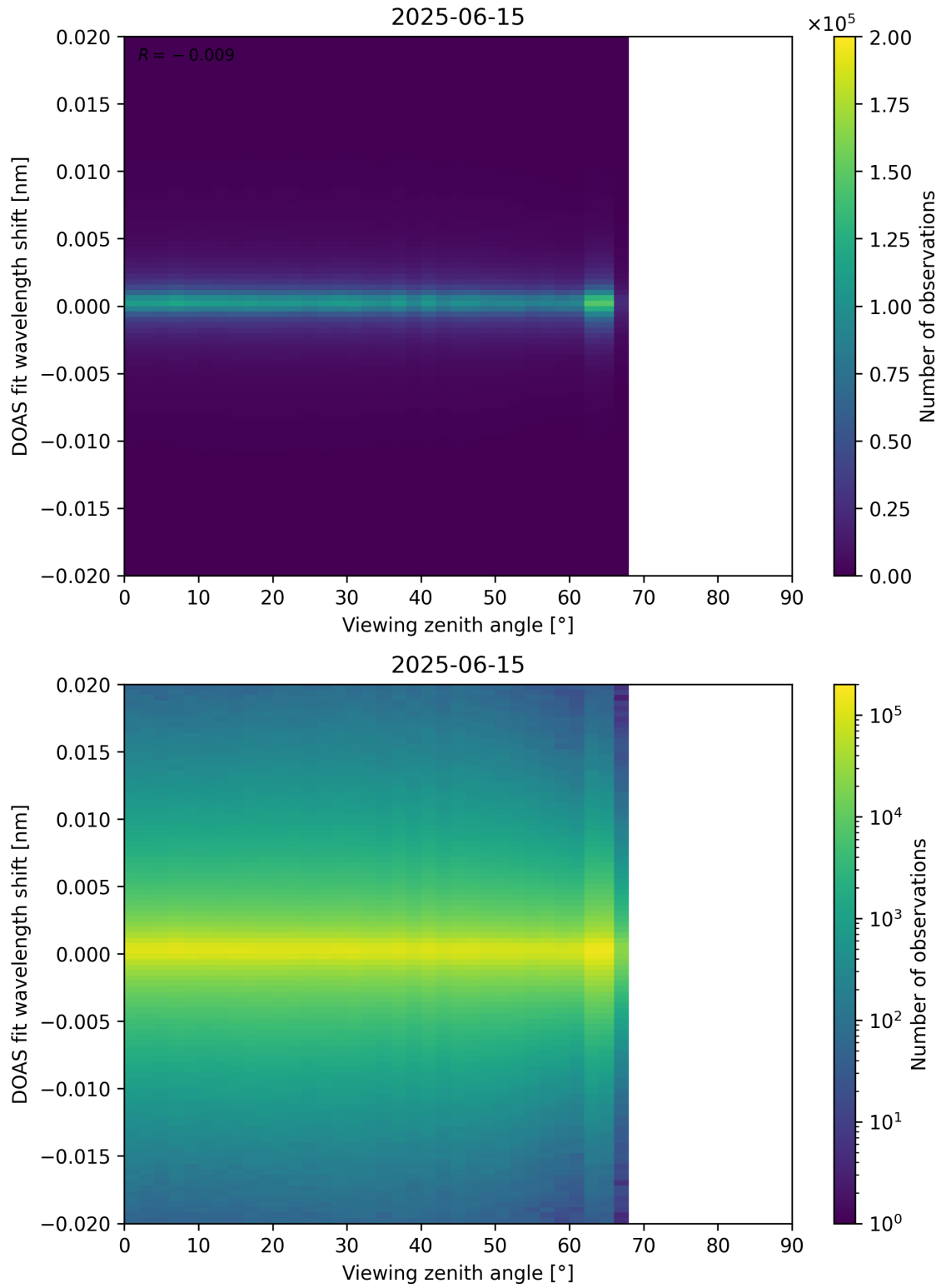
Figure 183: Scatter density plot of “Viewing zenith angle” against “DOAS fit wavelength shift” for 2025-06-14 to 2025-06-16.
