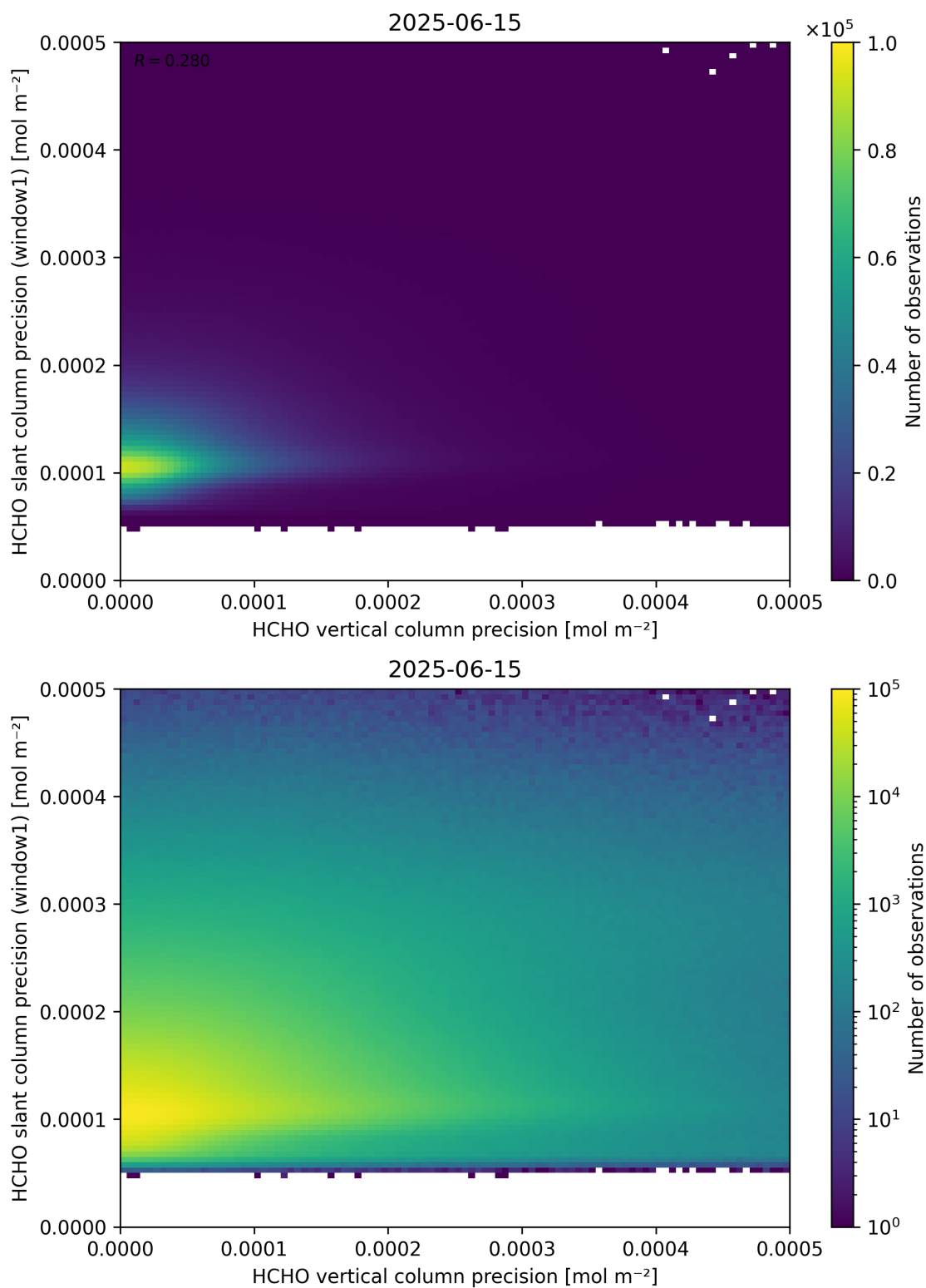
Figure 143: Scatter density plot of “HCHO vertical column precision” against “HCHO slant column precision (window1)” for 2025-06-14 to 2025-06-16.
