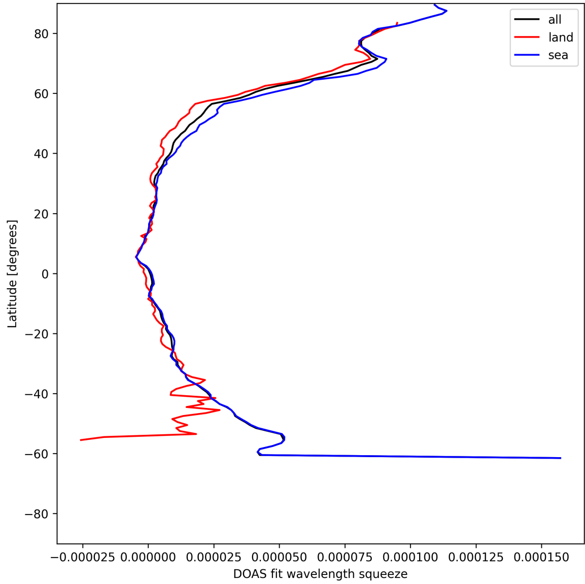
Figure 31: Zonal average of “DOAS fit wavelength squeeze” for 2025-06-14 to 2025-06-16.
