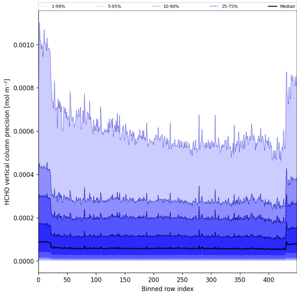
Figure 50: Along track statistics of “HCHO vertical column precision” for 2025-06-14 to 2025-06-16
