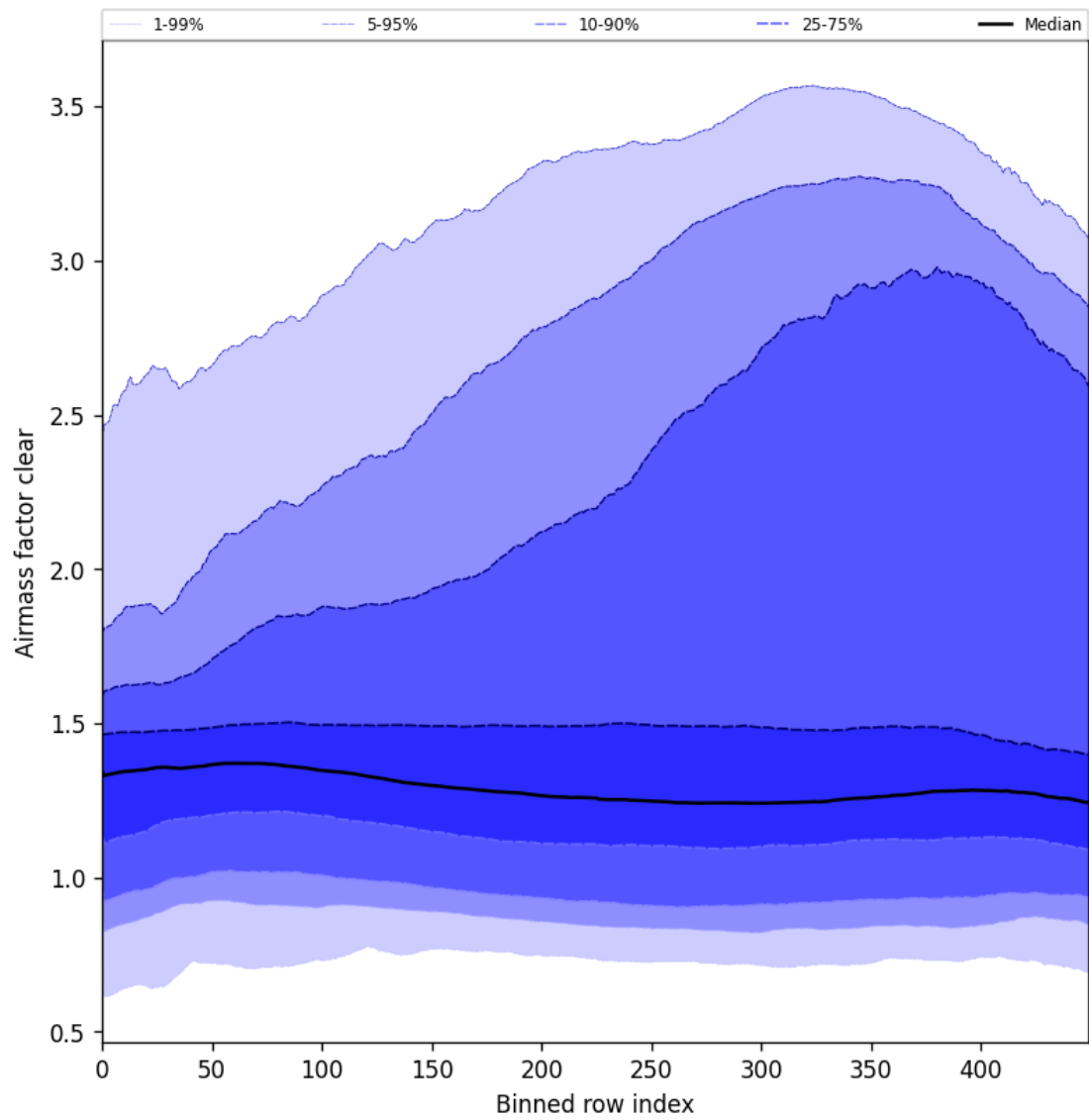
Figure 56: Along track statistics of “Air mass factor clear” for 2025-06-14 to 2025-06-16
