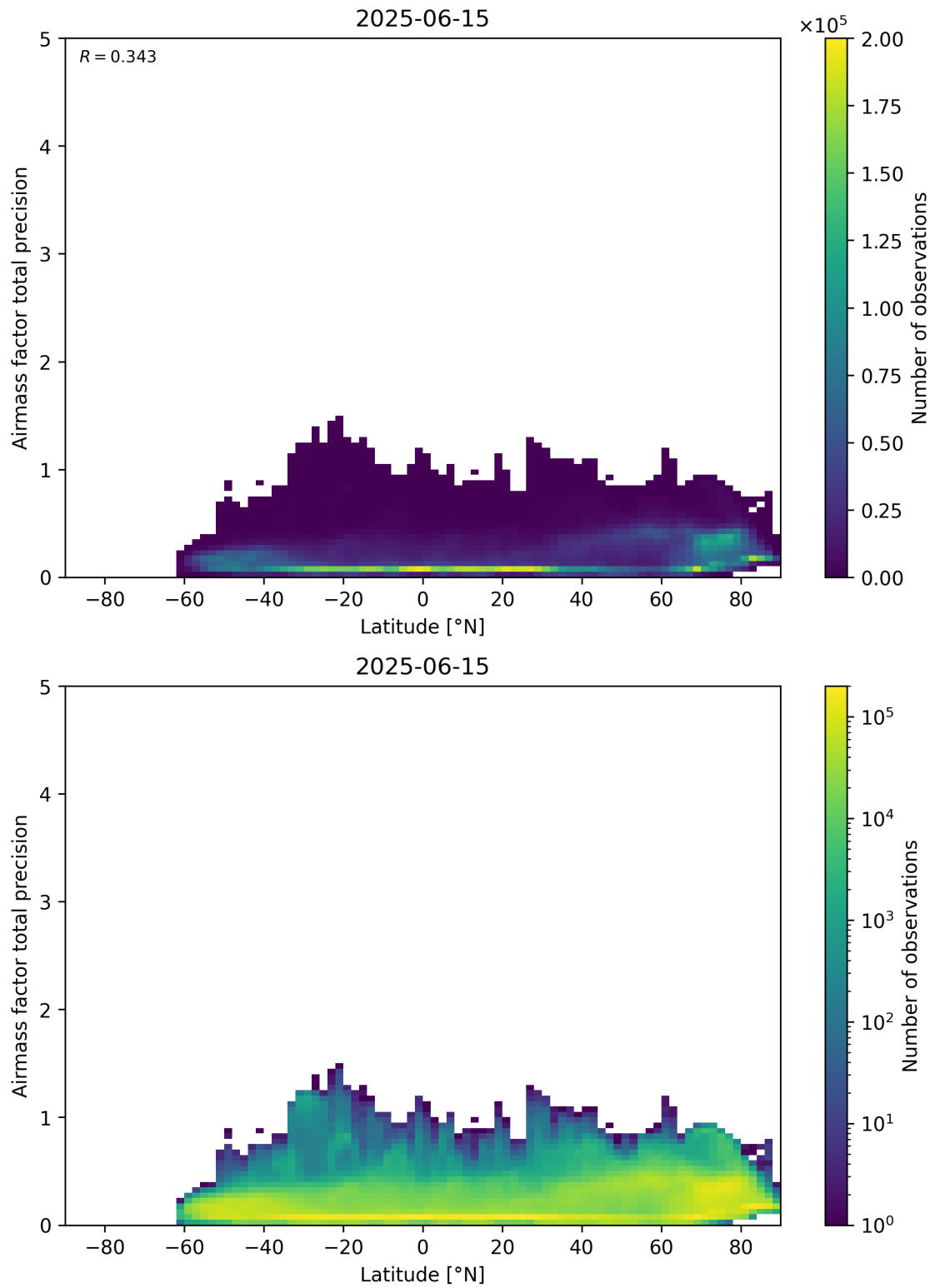
Figure 162: Scatter density plot of “Latitude” against “Airmass factor total precision” for 2025-06-14 to 2025-06-16.
