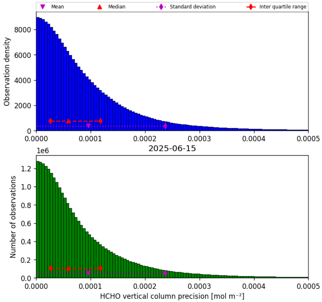
Figure 36: Histogram of “HCHO vertical column precision” for 2025-06-14 to 2025-06-16
