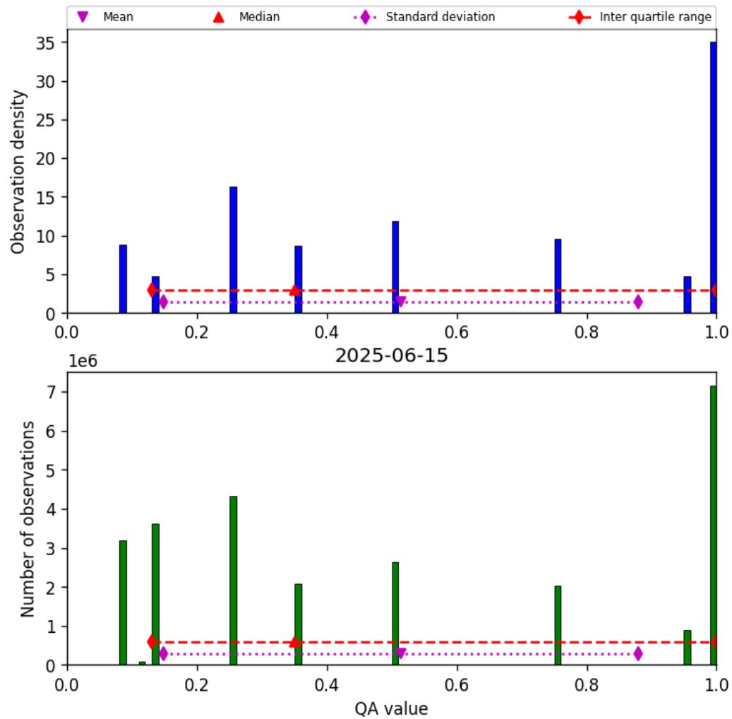
Figure 34: Histogram of “QA value” for 2025-06-14 to 2025-06-16
