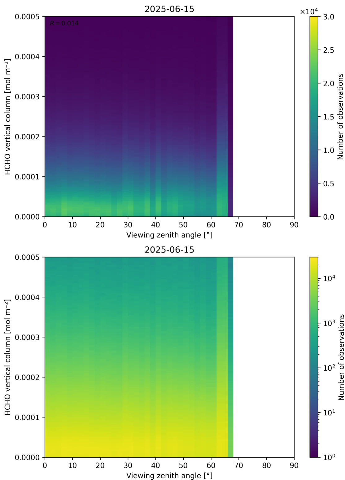
Figure 192: Scatter density plot of “Viewing zenith angle” against “HCHO vertical column” for 2025-06-14 to 2025-06-16.
