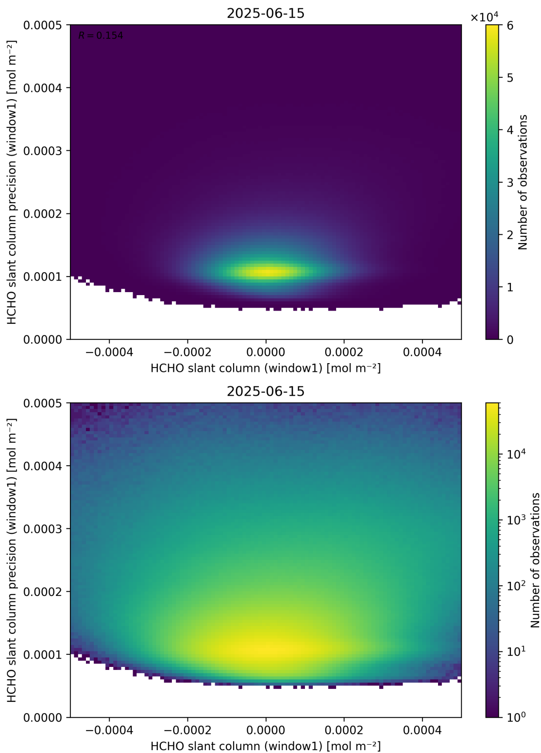
Figure 84: Scatter density plot of “HCHO slant column (window1)” against “HCHO slant column precision (window1)” for 2025-06-14 to 2025-06-16.
