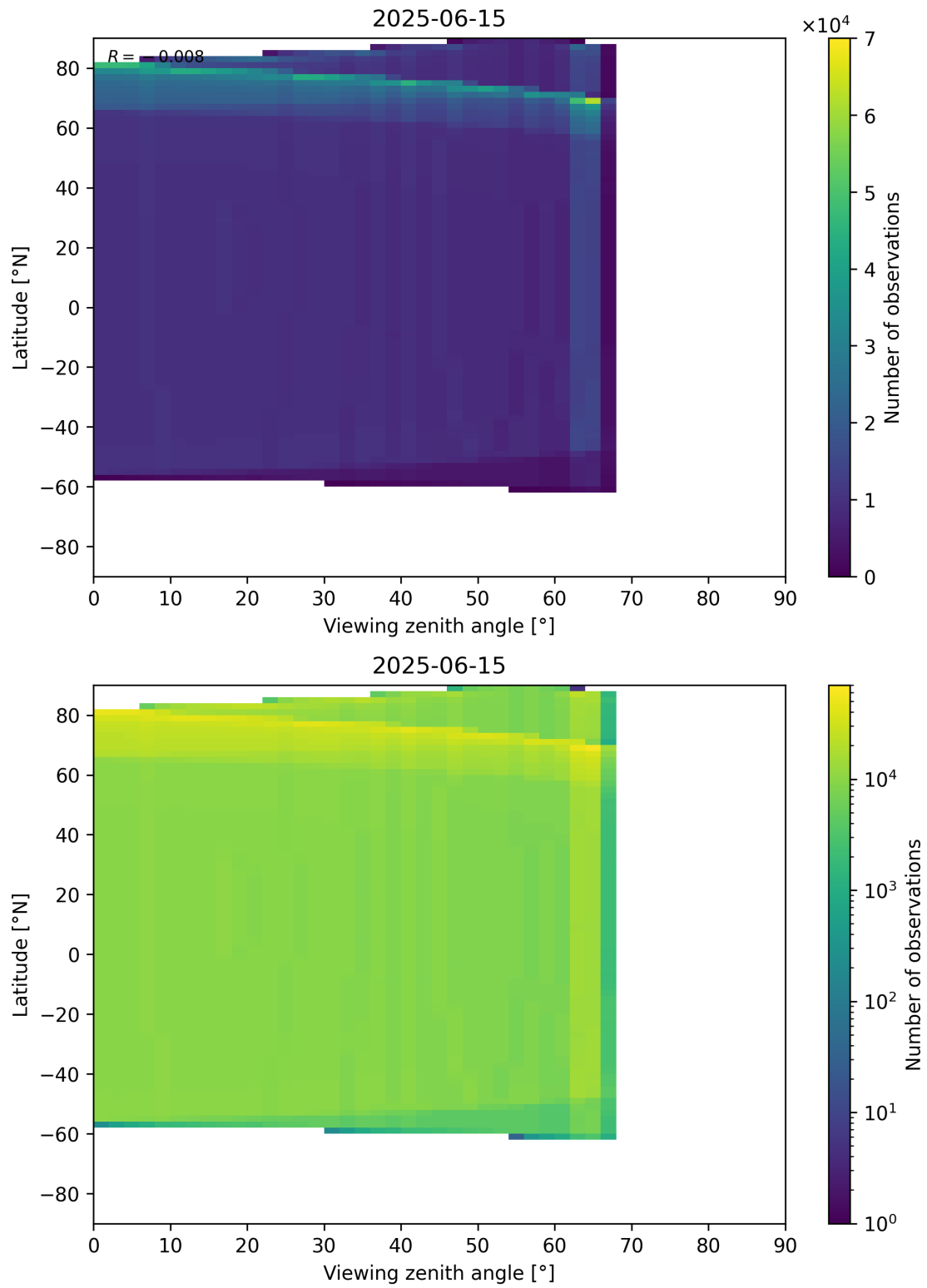
Figure 196: Scatter density plot of “Viewing zenith angle” against “Latitude” for 2025-06-14 to 2025-06-16.
