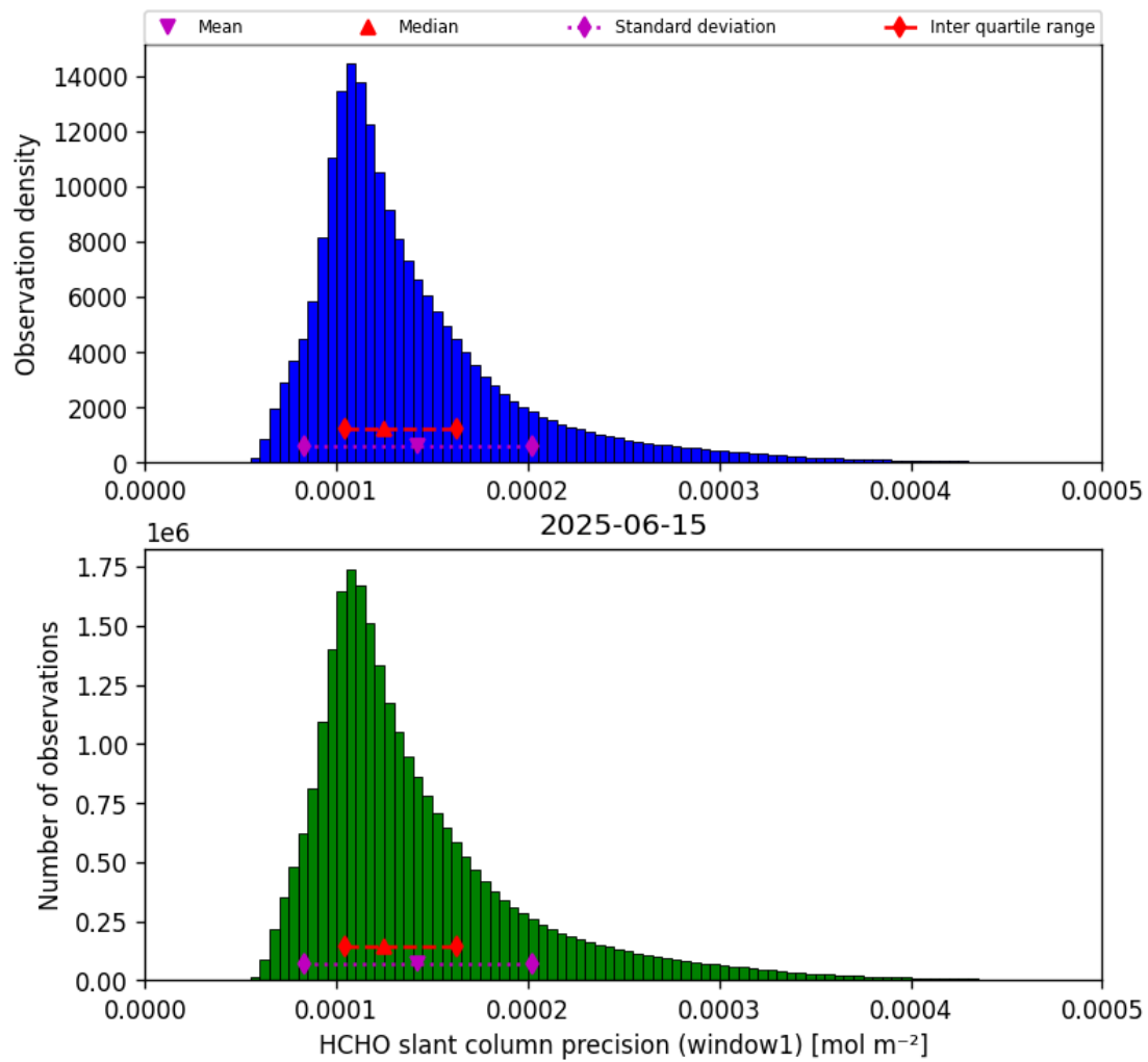
Figure 39: Histogram of “HCHO slant column precision (window1)” for 2025-06-14 to 2025-06-16
