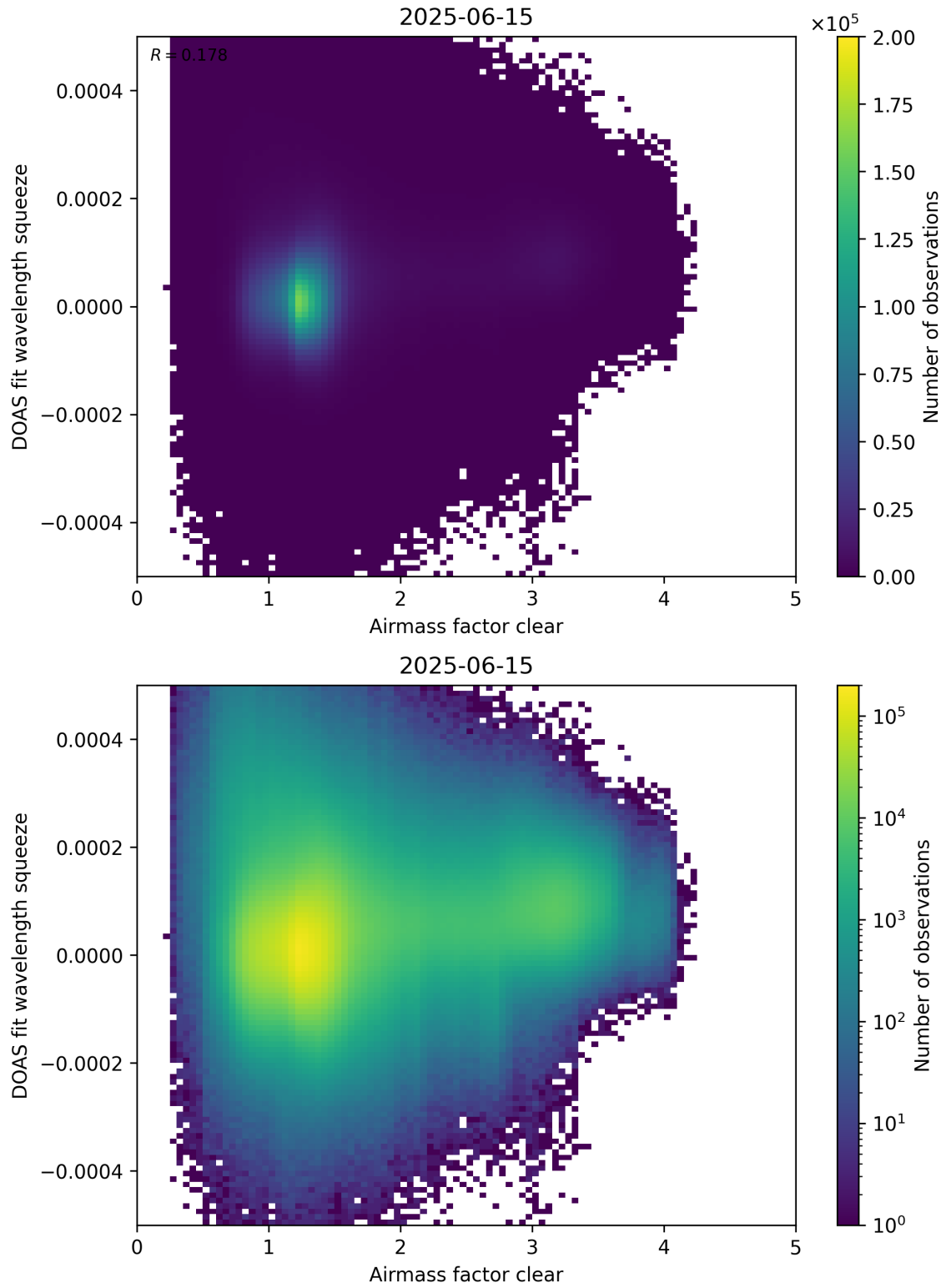
Figure 73: Scatter density plot of “Airmass factor clear” against “DOAS fit wavelength squeeze” for 2025-06-14 to 2025-06-16.
