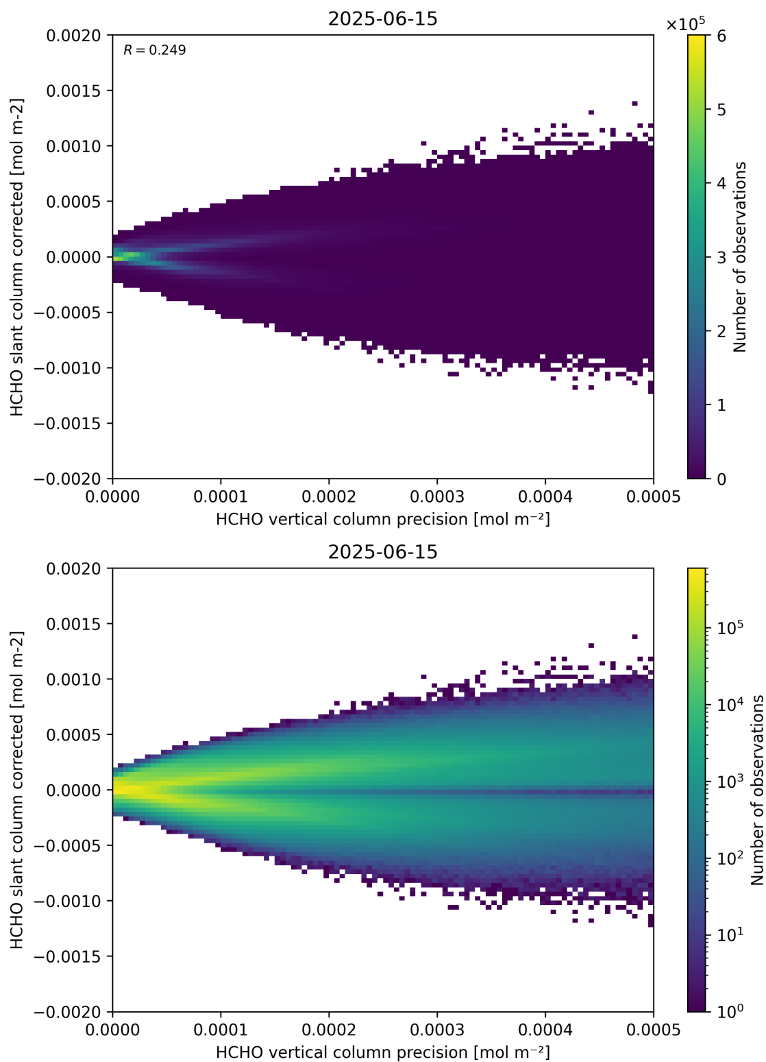
Figure 140: Scatter density plot of “HCHO vertical column precision” against “HCHO slant column corrected” for 2025-06-14 to 2025-06-16.
