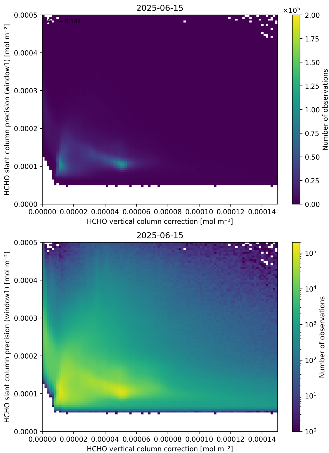
Figure 119: Scatter density plot of “HCHO vertical column correction” against “HCHO slant column precision (window1)” for 2025-06-14 to 2025-06-16.
