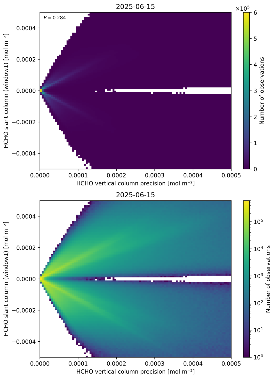
Figure 142: Scatter density plot of “HCHO vertical column precision” against “HCHO slant column (window1)” for 2025-06-14 to 2025-06-16.
