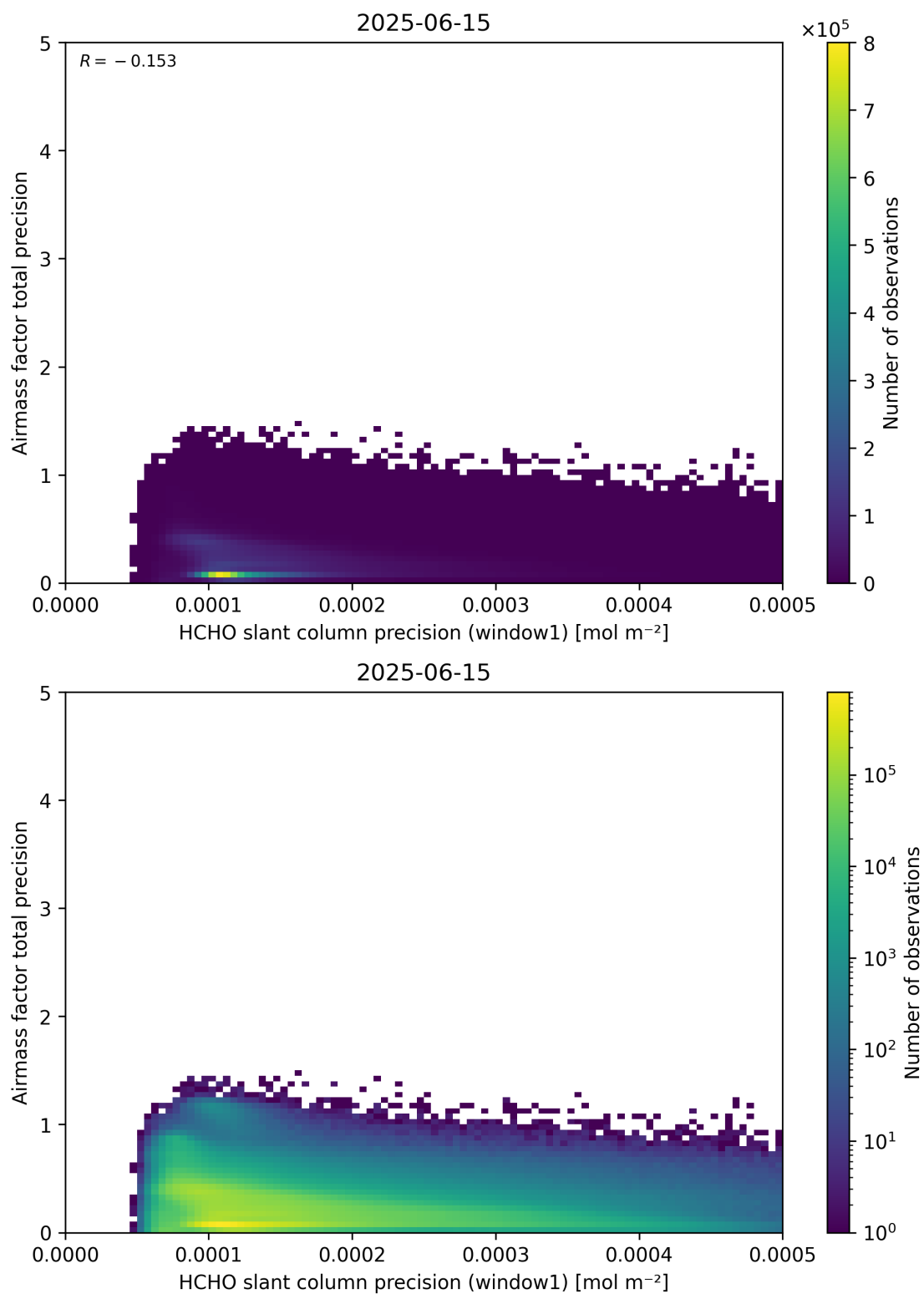
Figure 95: Scatter density plot of “HCHO slant column precision (window1)” against “Airmass factor total precision” for 2025-06-14 to 2025-06-16.
