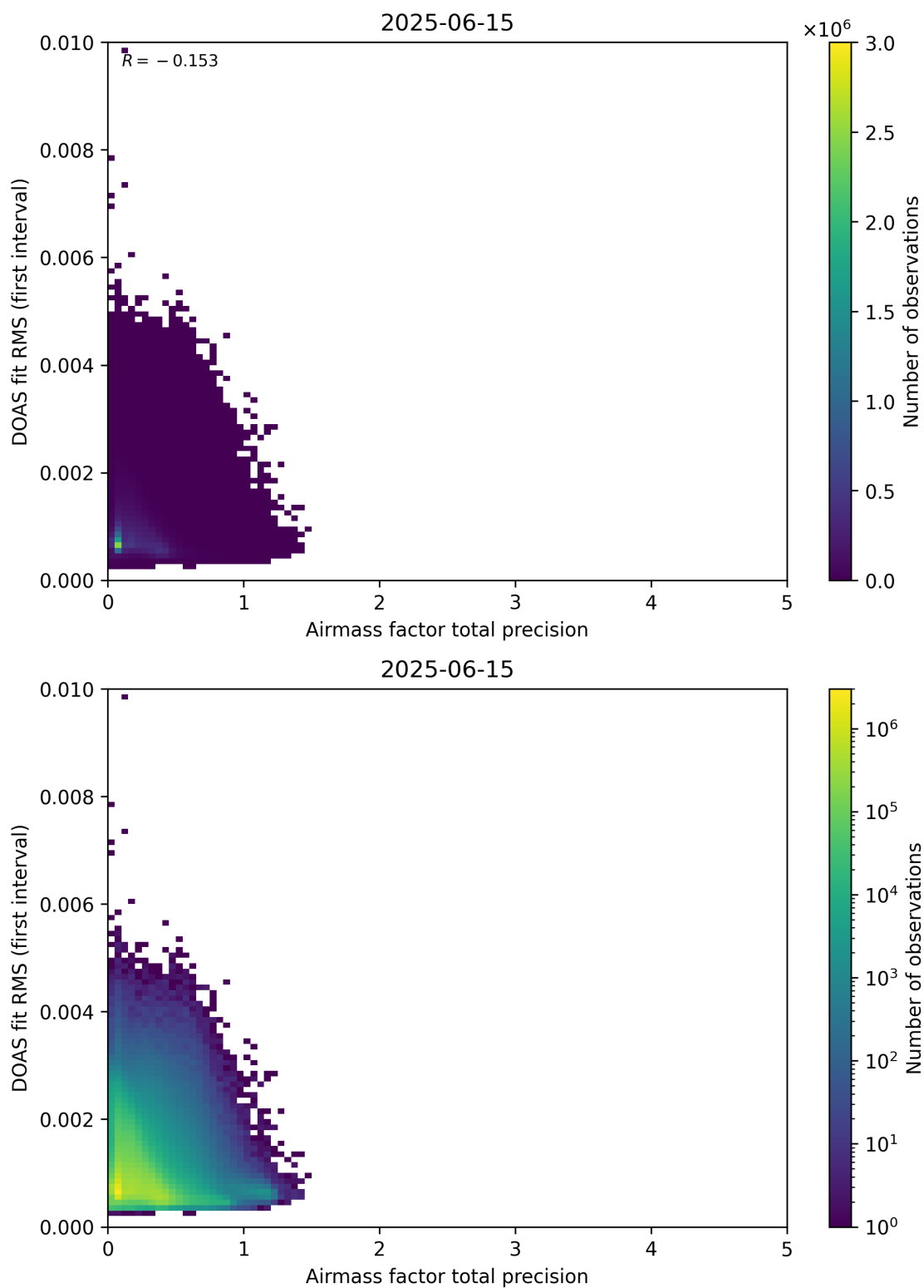
Figure 105: Scatter density plot of “Airmass factor total precision” against “DOAS fit RMS (first interval)” for 2025-06-14 to 2025-06-16.
