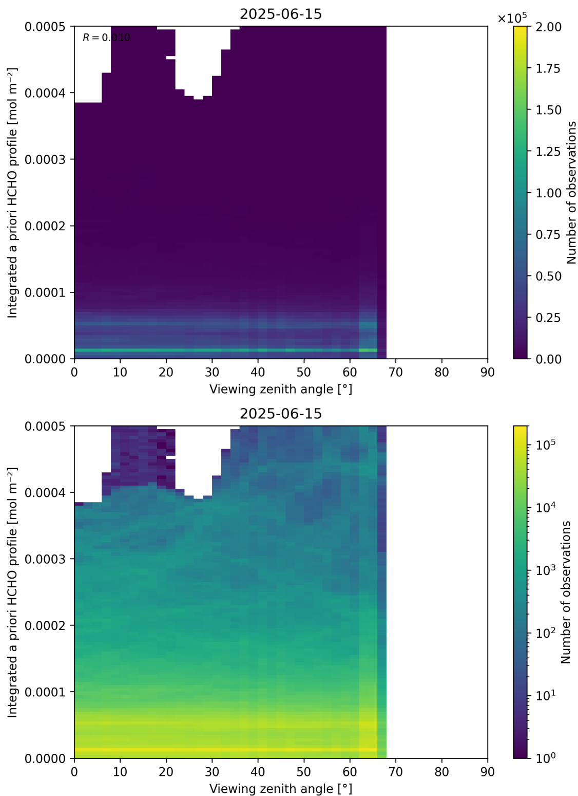
Figure 195: Scatter density plot of “Viewing zenith angle” against “Integrated a priori HCHO profile” for 2025-06-14 to 2025-06-16.
