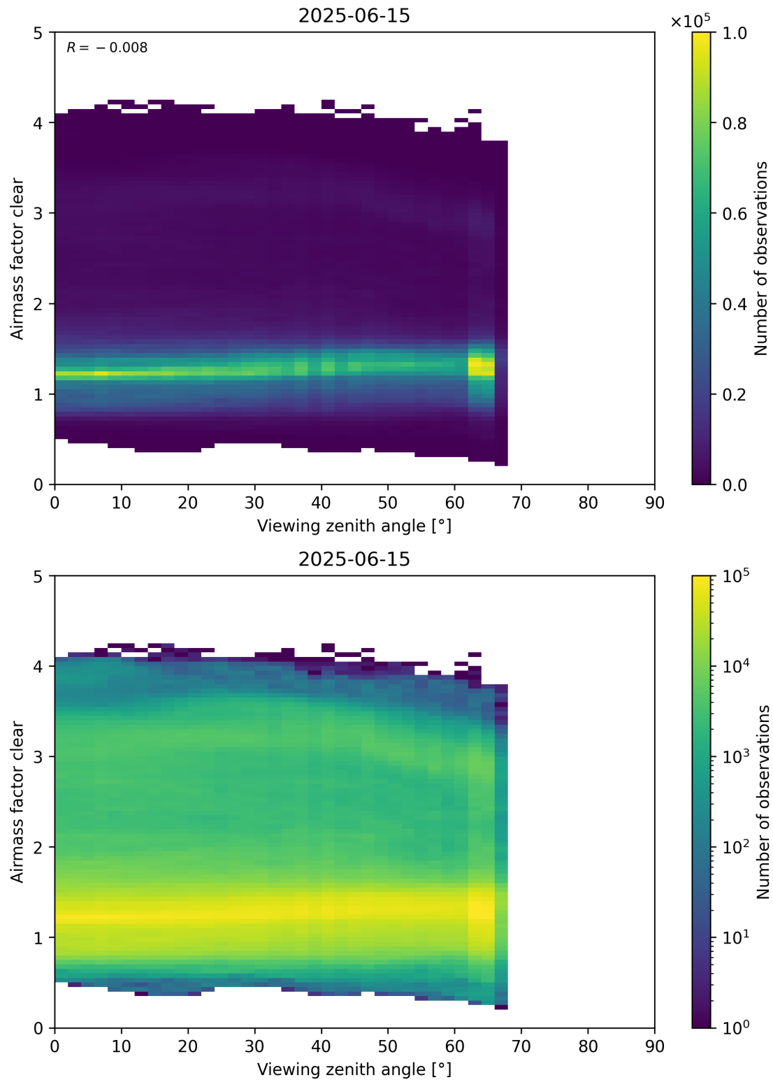
Figure 185: Scatter density plot of “Viewing zenith angle” against “Airmass factor clear” for 2025-06-14 to 2025-06-16.
