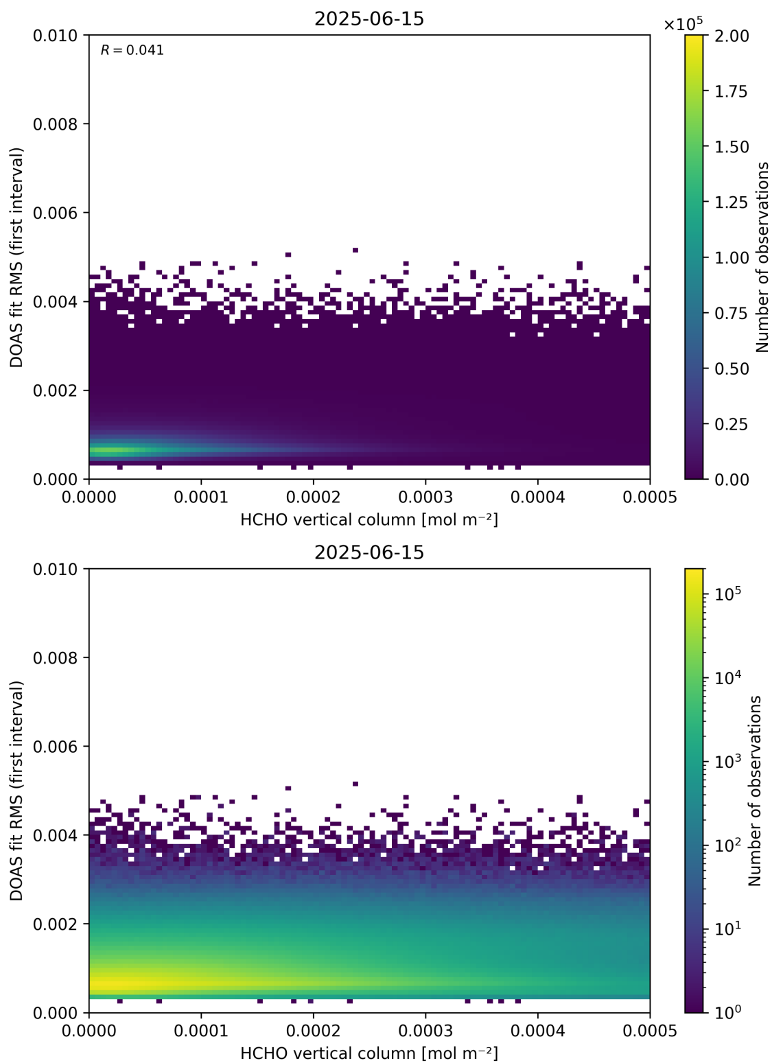
Figure 123: Scatter density plot of “HCHO vertical column” against “DOAS fit RMS (first interval)” for 2025-06-14 to 2025-06-16.
