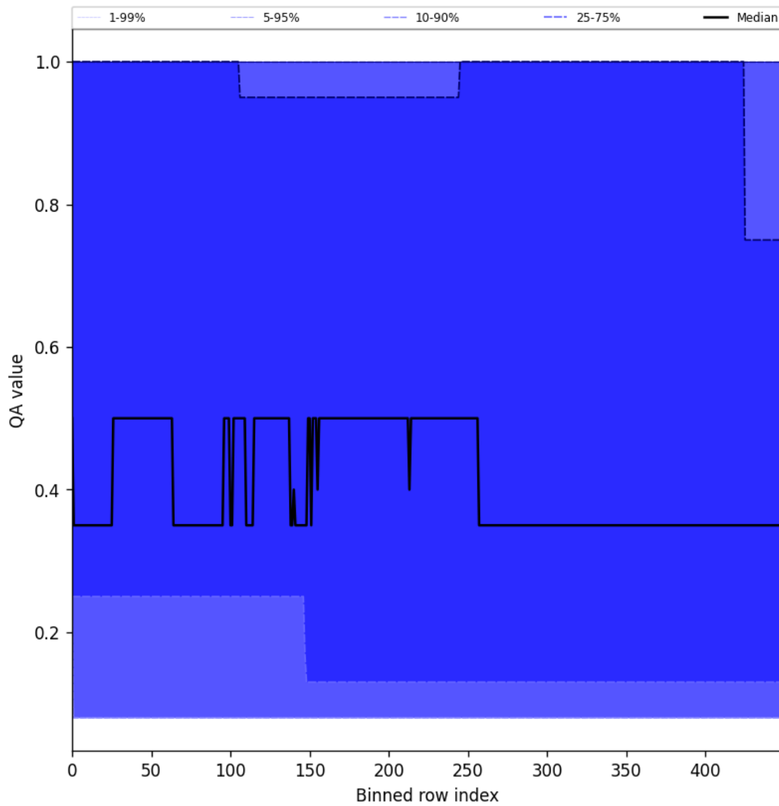
Figure 48: Along track statistics of “QA value” for 2025-06-14 to 2025-06-16
