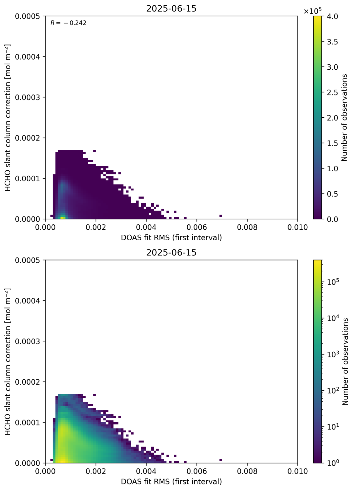
Figure 63: Scatter density plot of “DOAS fit RMS (first interval)” against “HCHO slant column correction” for 2025-06-14 to 2025-06-16.
