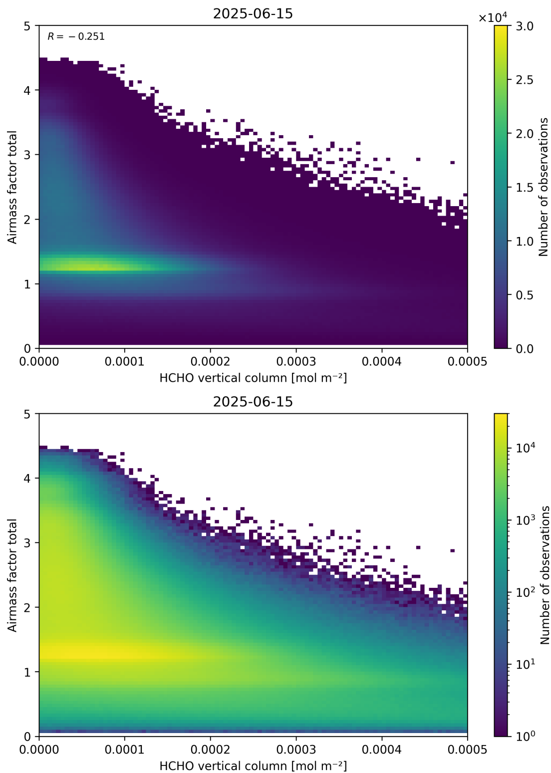
Figure 131: Scatter density plot of “HCHO vertical column” against “Airmass factor total” for 2025-06-14 to 2025-06-16.
