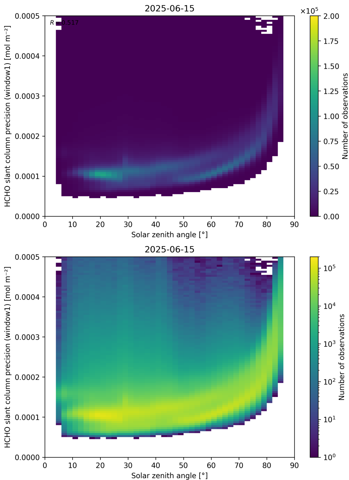
Figure 174: Scatter density plot of “Solar zenith angle” against “HCHO slant column precision (window1)” for 2025-06-14 to 2025-06-16.
