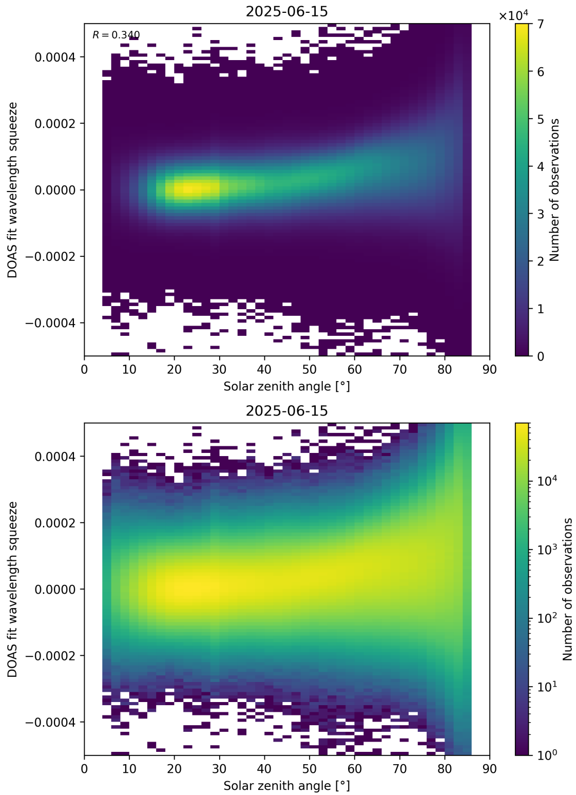
Figure 169: Scatter density plot of “Solar zenith angle” against “DOAS fit wavelength squeeze” for 2025-06-14 to 2025-06-16.
