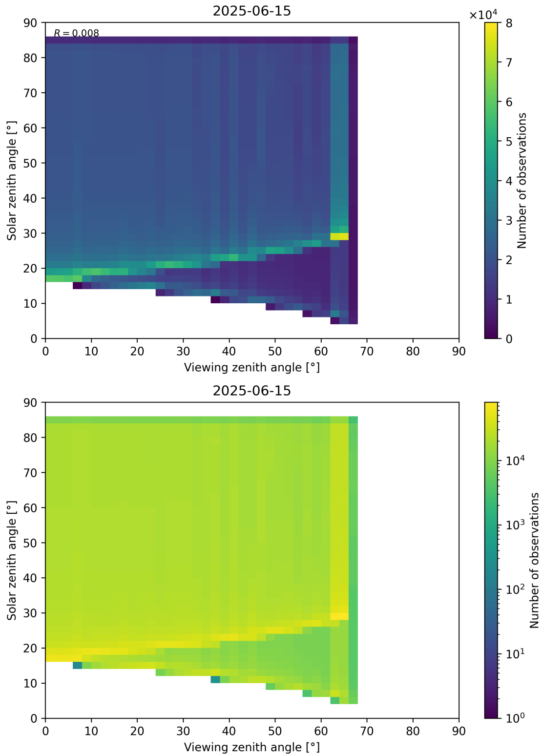
Figure 197: Scatter density plot of “Viewing zenith angle” against “Solar zenith angle” for 2025-06-14 to 2025-06-16.
