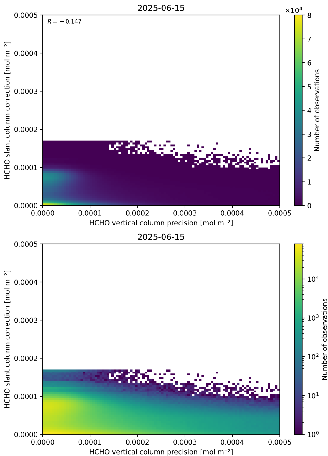
Figure 141: Scatter density plot of “HCHO vertical column precision” against “HCHO slant column correction” for 2025-06-14 to 2025-06-16.
