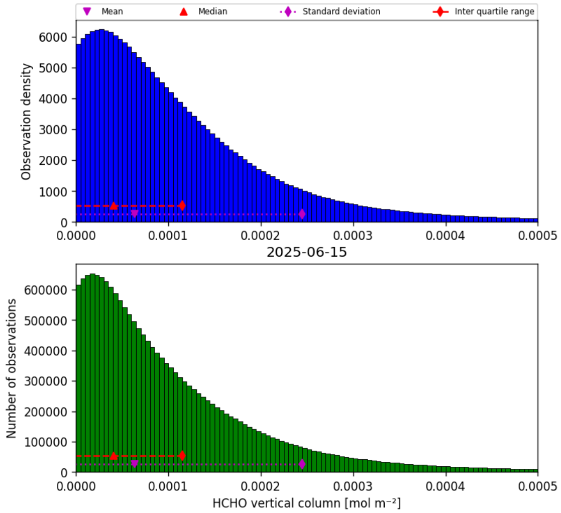
Figure 35: Histogram of “HCHO vertical column” for 2025-06-14 to 2025-06-16
