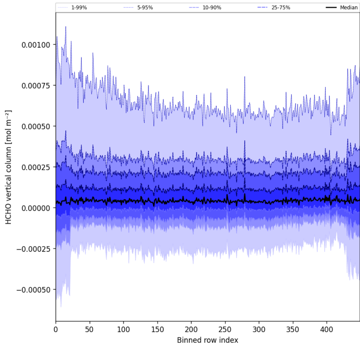
Figure 49: Along track statistics of “HCHO vertical column” for 2025-06-14 to 2025-06-16
