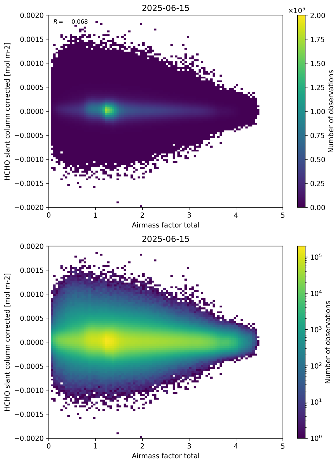
Figure 101: Scatter density plot of “Airmass factor total” against “HCHO slant column corrected” for 2025-06-14 to 2025-06-16.
