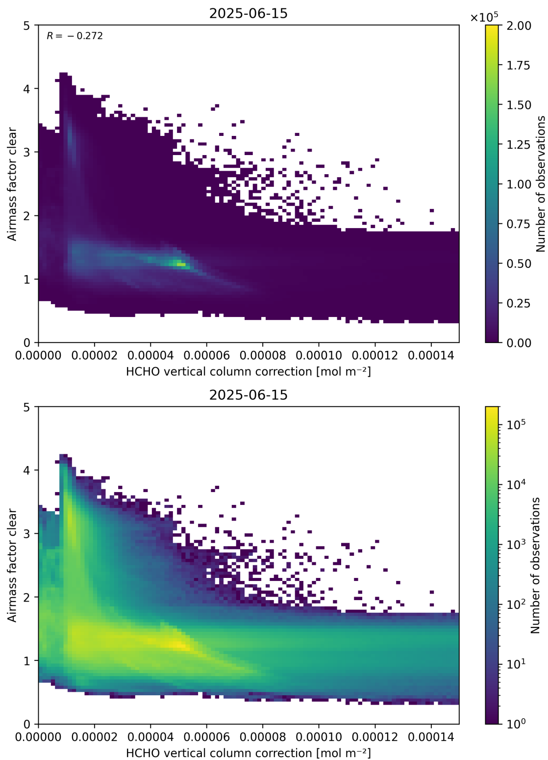
Figure 115: Scatter density plot of “HCHO vertical column correction” against “Airmass factor clear” for 2025-06-14 to 2025-06-16.
