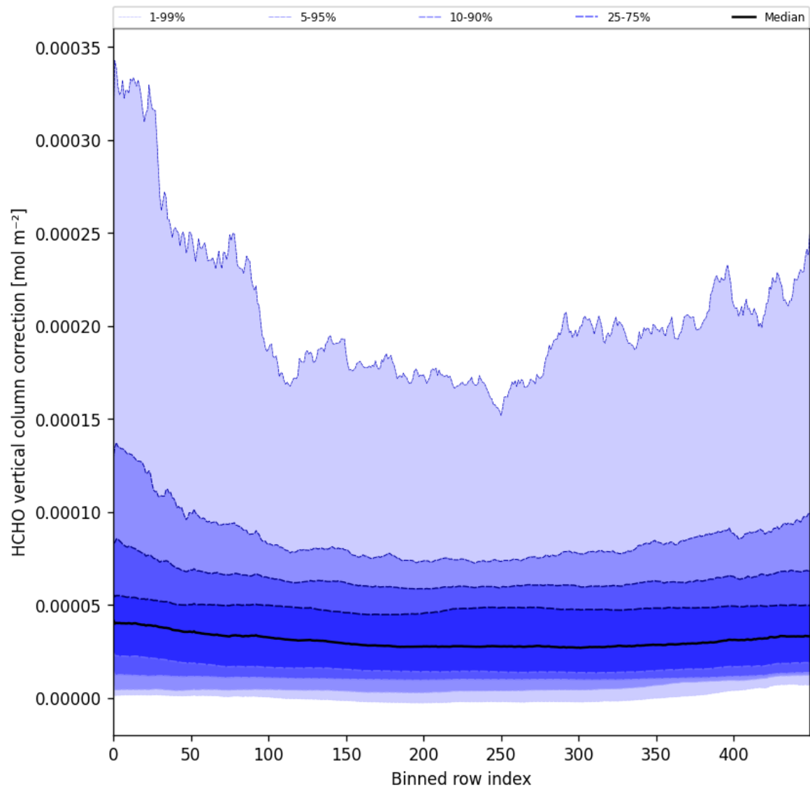
Figure 51: Along track statistics of “HCHO vertical column correction” for 2025-06-14 to 2025-06-16
