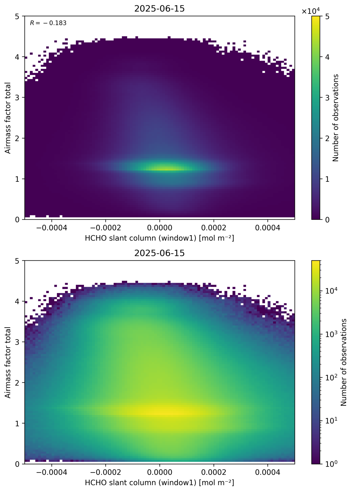
Figure 85: Scatter density plot of “HCHO slant column (window1)” against “Airmass factor total” for 2025-06-14 to 2025-06-16.
