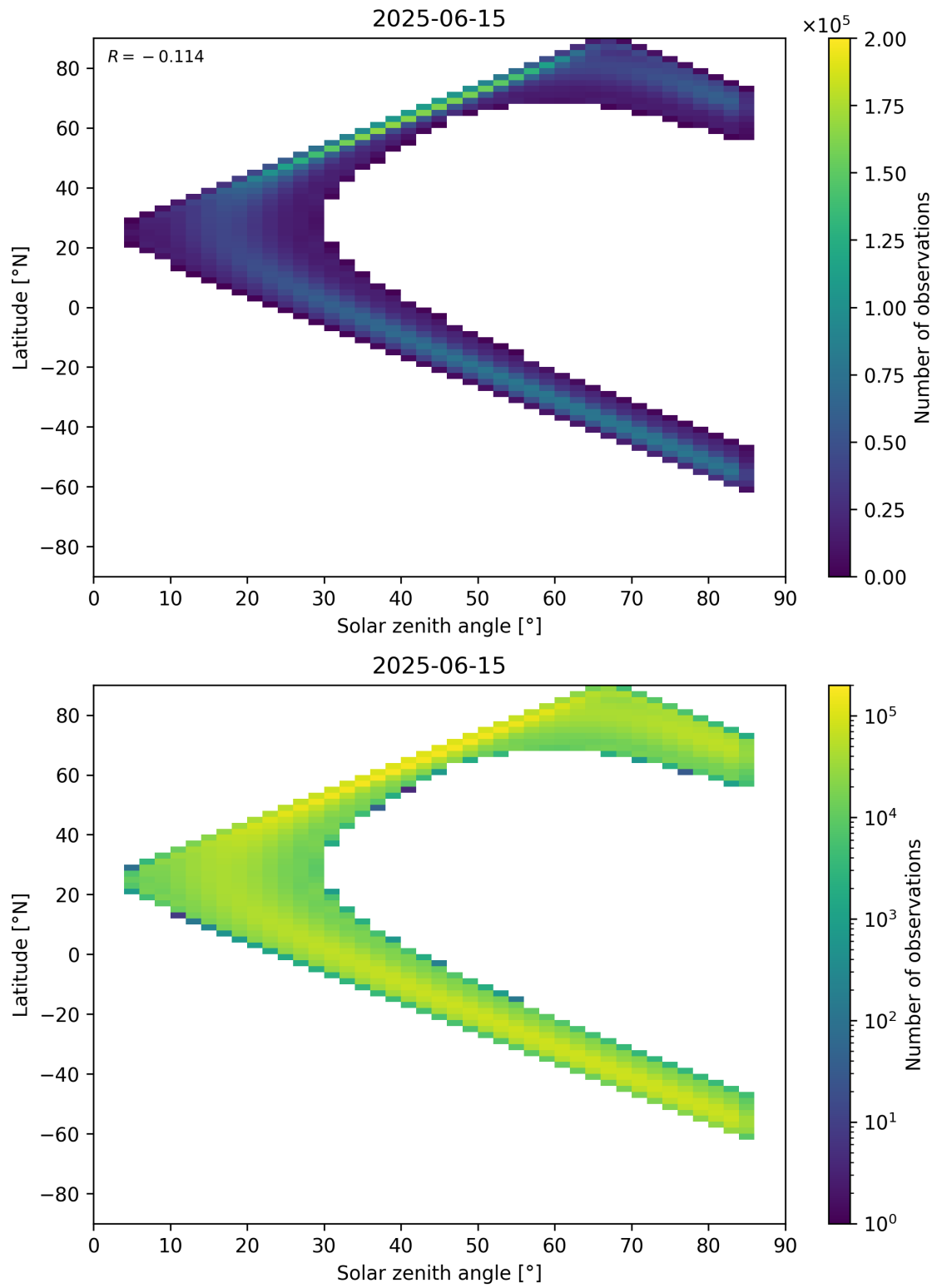
Figure 181: Scatter density plot of “Solar zenith angle” against “Latitude” for 2025-06-14 to 2025-06-16.
