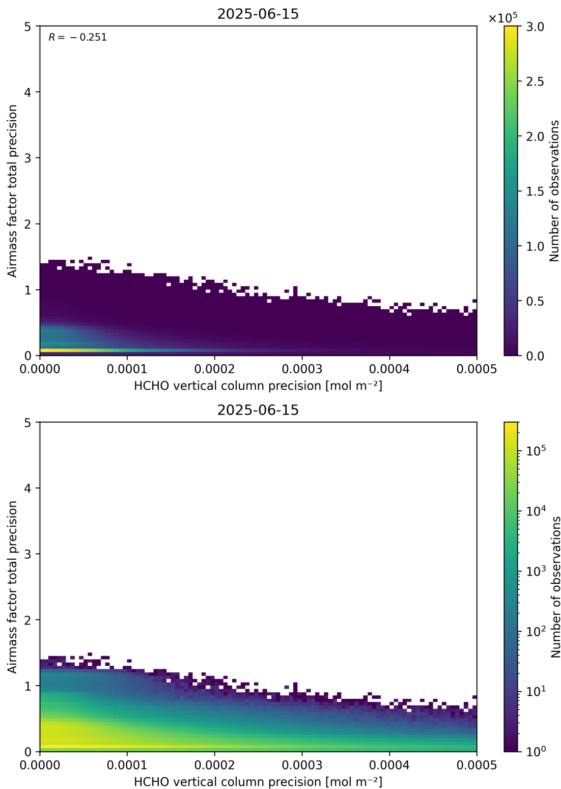
Figure 145: Scatter density plot of “HCHO vertical column precision” against “Airmass factor total precision” for 2025-06-14 to 2025-06-16.
