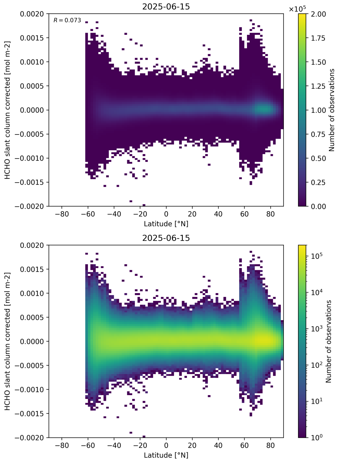
Figure 157: Scatter density plot of “Latitude” against “HCHO slant column corrected” for 2025-06-14 to 2025-06-16.
