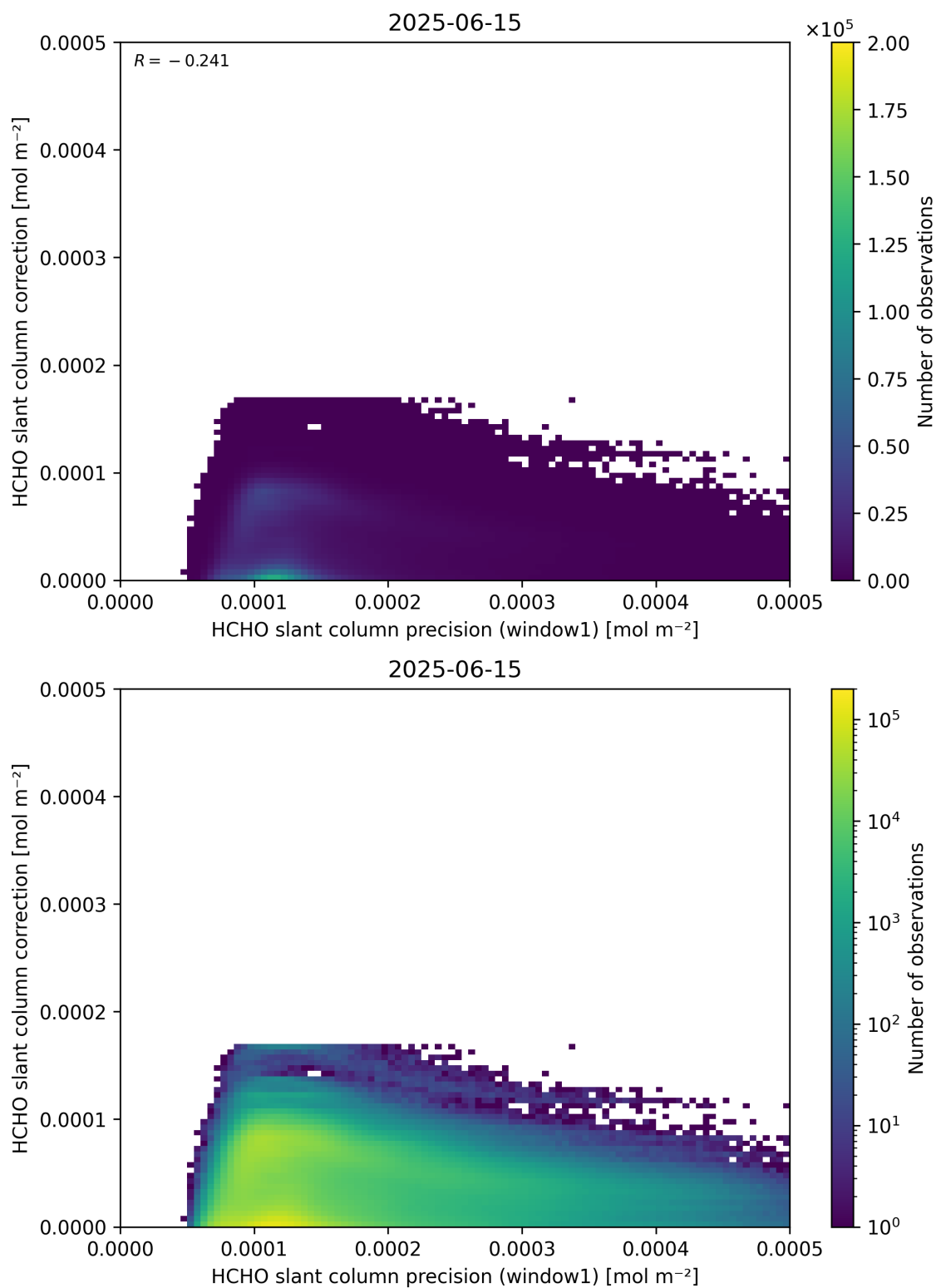
Figure 93: Scatter density plot of “HCHO slant column precision (window1)” against “HCHO slant column correction” for 2025-06-14 to 2025-06-16.
