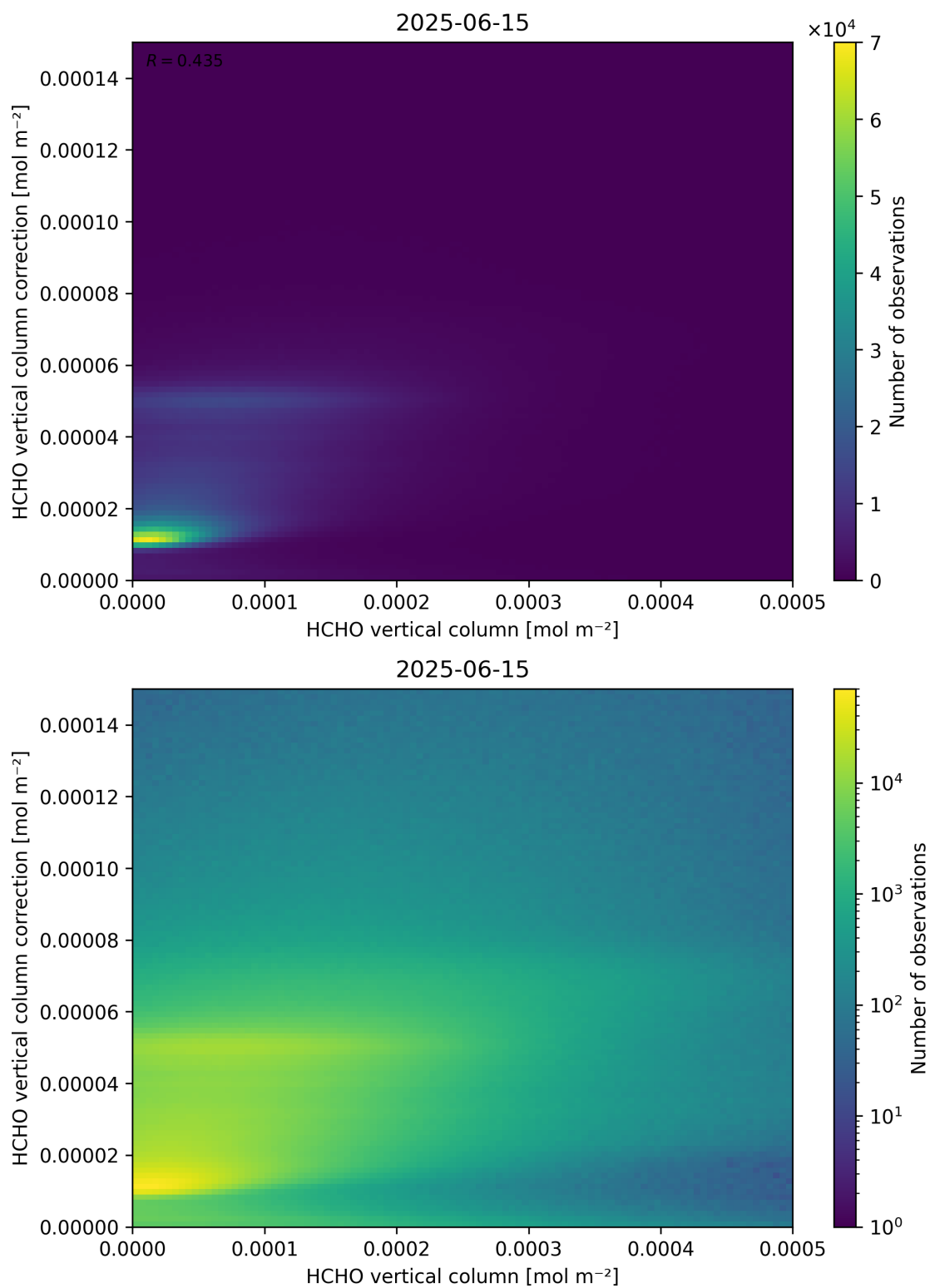
Figure 133: Scatter density plot of “HCHO vertical column” against “HCHO vertical column correction” for 2025-06-14 to 2025-06-16.
