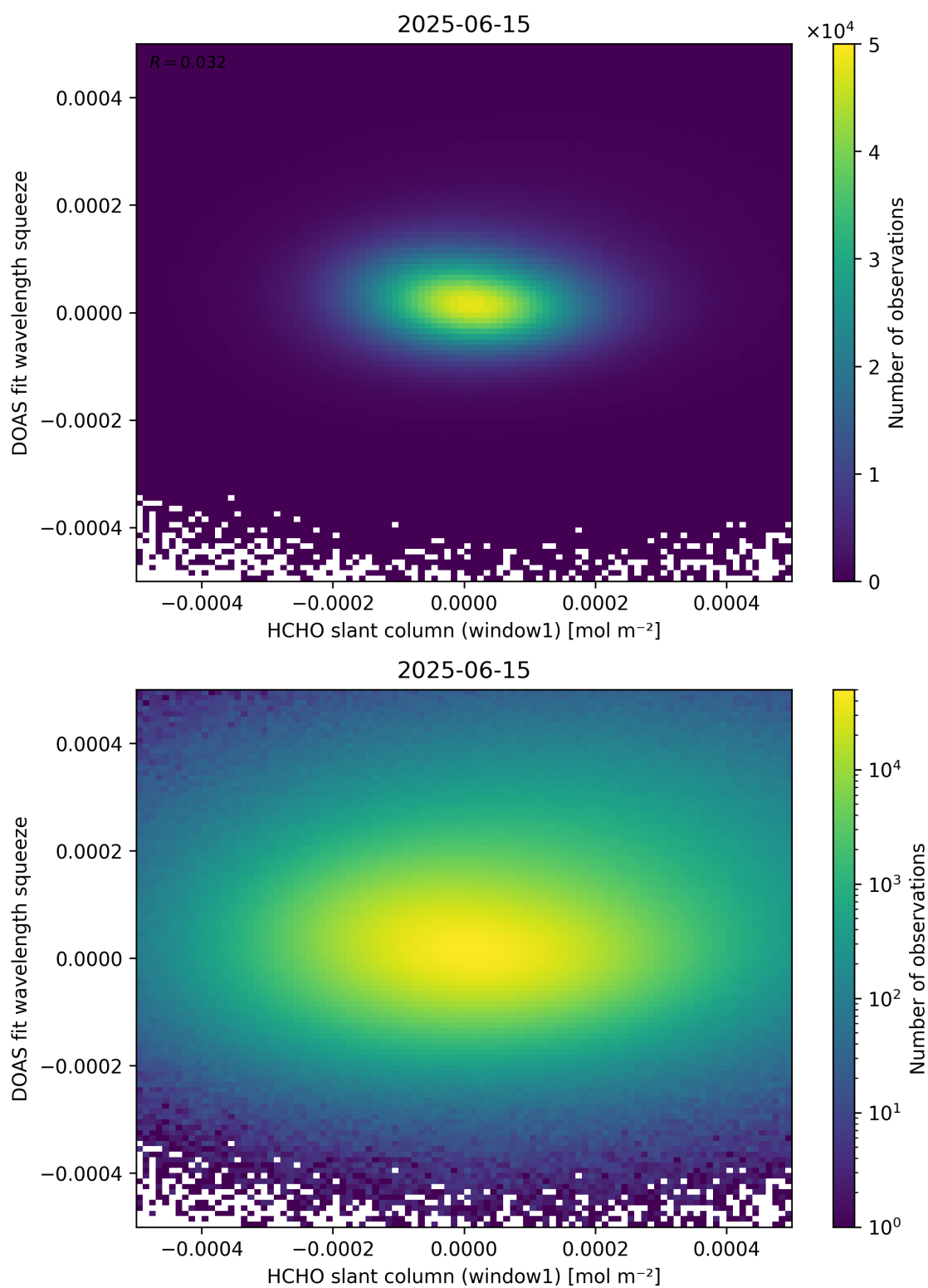
Figure 80: Scatter density plot of “HCHO slant column (window1)” against “DOAS fit wavelength squeeze” for 2025-06-14 to 2025-06-16.
