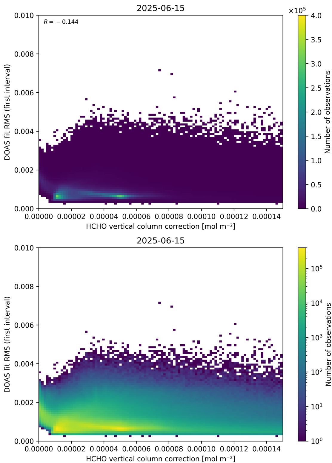
Figure 112: Scatter density plot of “HCHO vertical column correction” against “DOAS fit RMS (first interval)” for 2025-06-14 to 2025-06-16.
