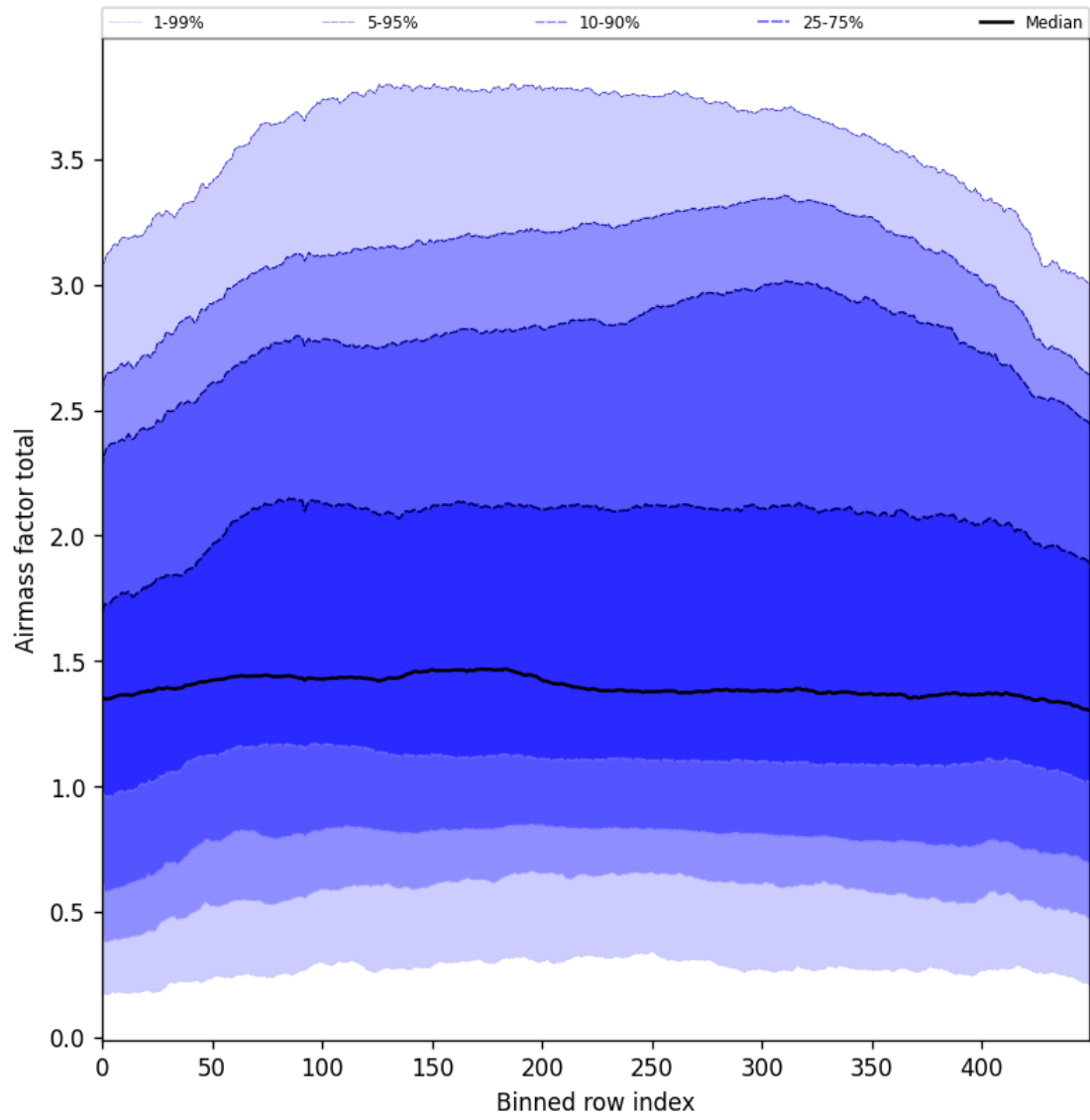
Figure 54: Along track statistics of “Airmass factor total” for 2025-06-14 to 2025-06-16
