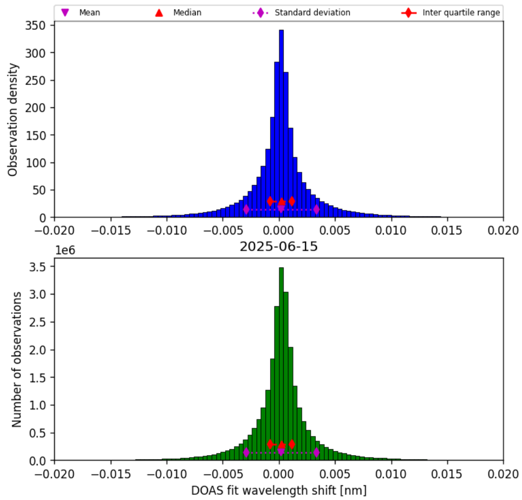
Figure 44: Histogram of “DOAS fit wavelength shift” for 2025-06-14 to 2025-06-16
