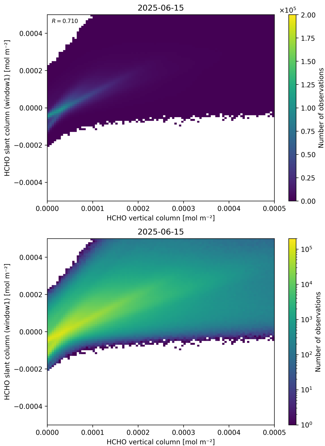
Figure 129: Scatter density plot of “HCHO vertical column” against “HCHO slant column (window1)” for 2025-06-14 to 2025-06-16.
