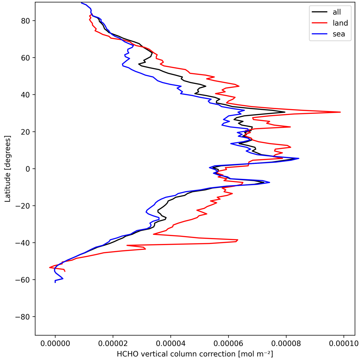
Figure 23: Zonal average of “HCHO vertical column correction” for 2025-06-14 to 2025-06-16.
