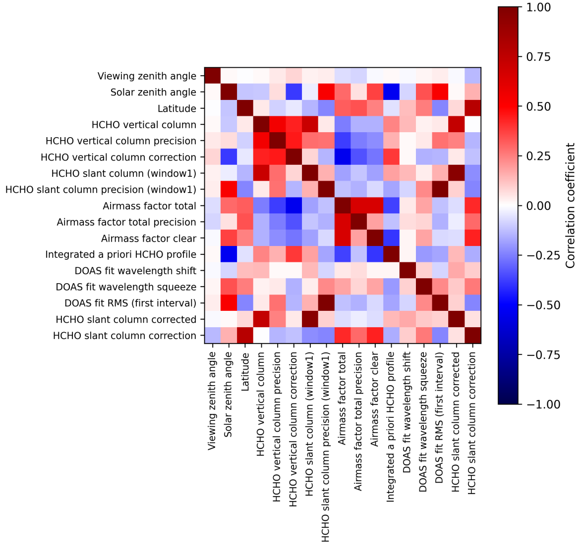
Figure 2: Map of correlation matrix for 2025-06-14 to 2025-06-16.
