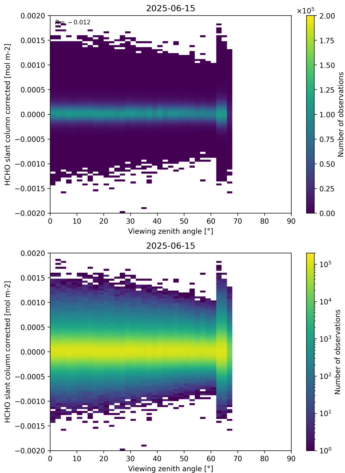
Figure 186: Scatter density plot of “Viewing zenith angle” against “HCHO slant column corrected” for 2025-06-14 to 2025-06-16.
