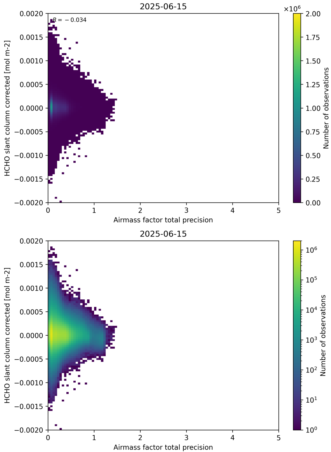
Figure 109: Scatter density plot of “Airmass factor total precision” against “HCHO slant column corrected” for 2025-06-14 to 2025-06-16.
