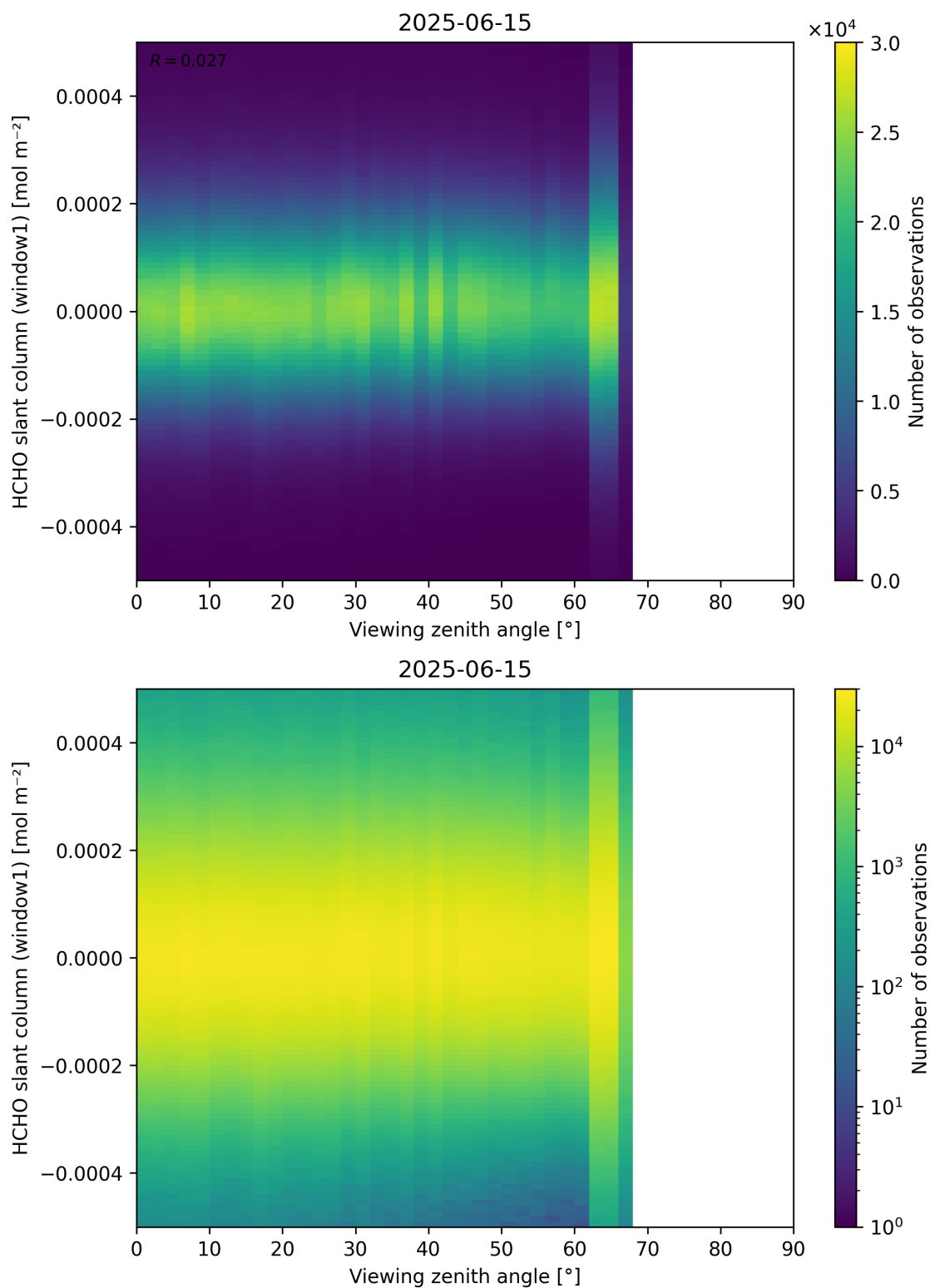
Figure 188: Scatter density plot of “Viewing zenith angle” against “HCHO slant column (window1)” for 2025-06-14 to 2025-06-16.
