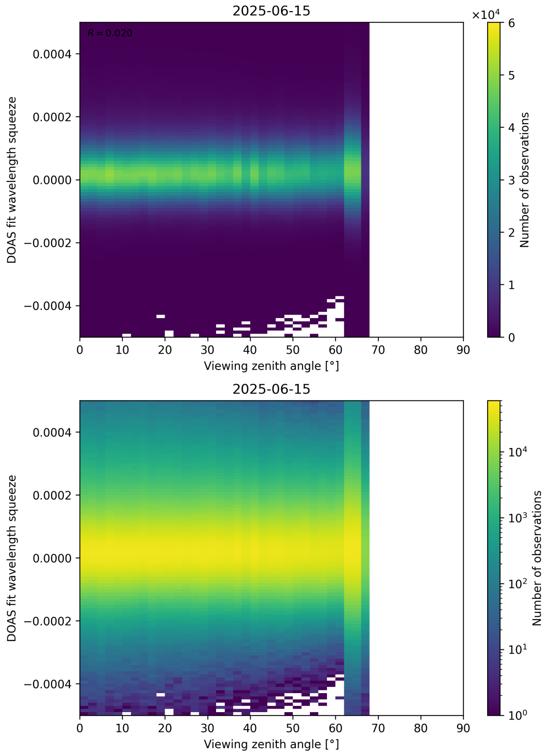
Figure 184: Scatter density plot of “Viewing zenith angle” against “DOAS fit wavelength squeeze” for 2025-06-14 to 2025-06-16.
