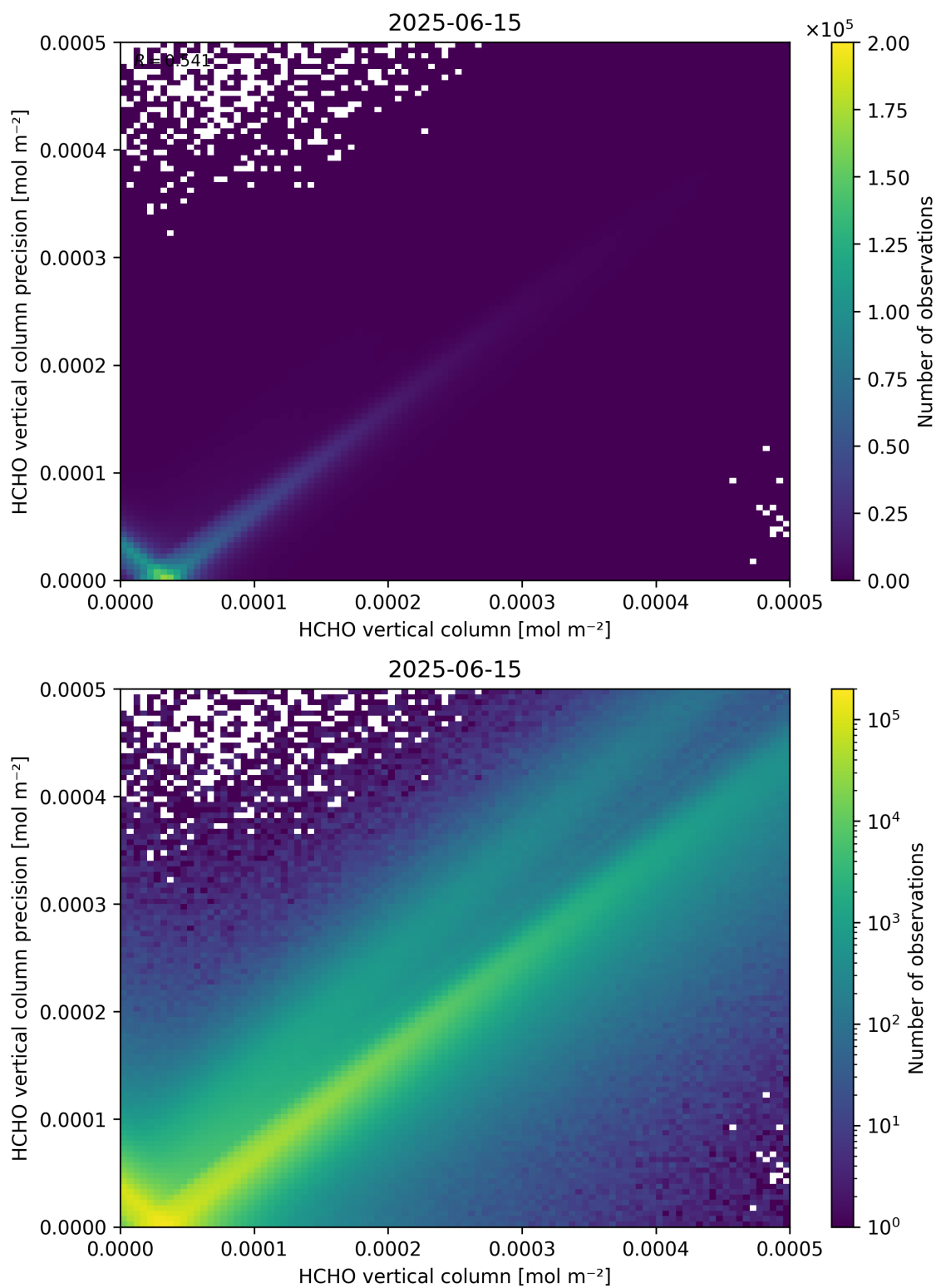
Figure 134: Scatter density plot of “HCHO vertical column” against “HCHO vertical column precision” for 2025-06-14 to 2025-06-16.
