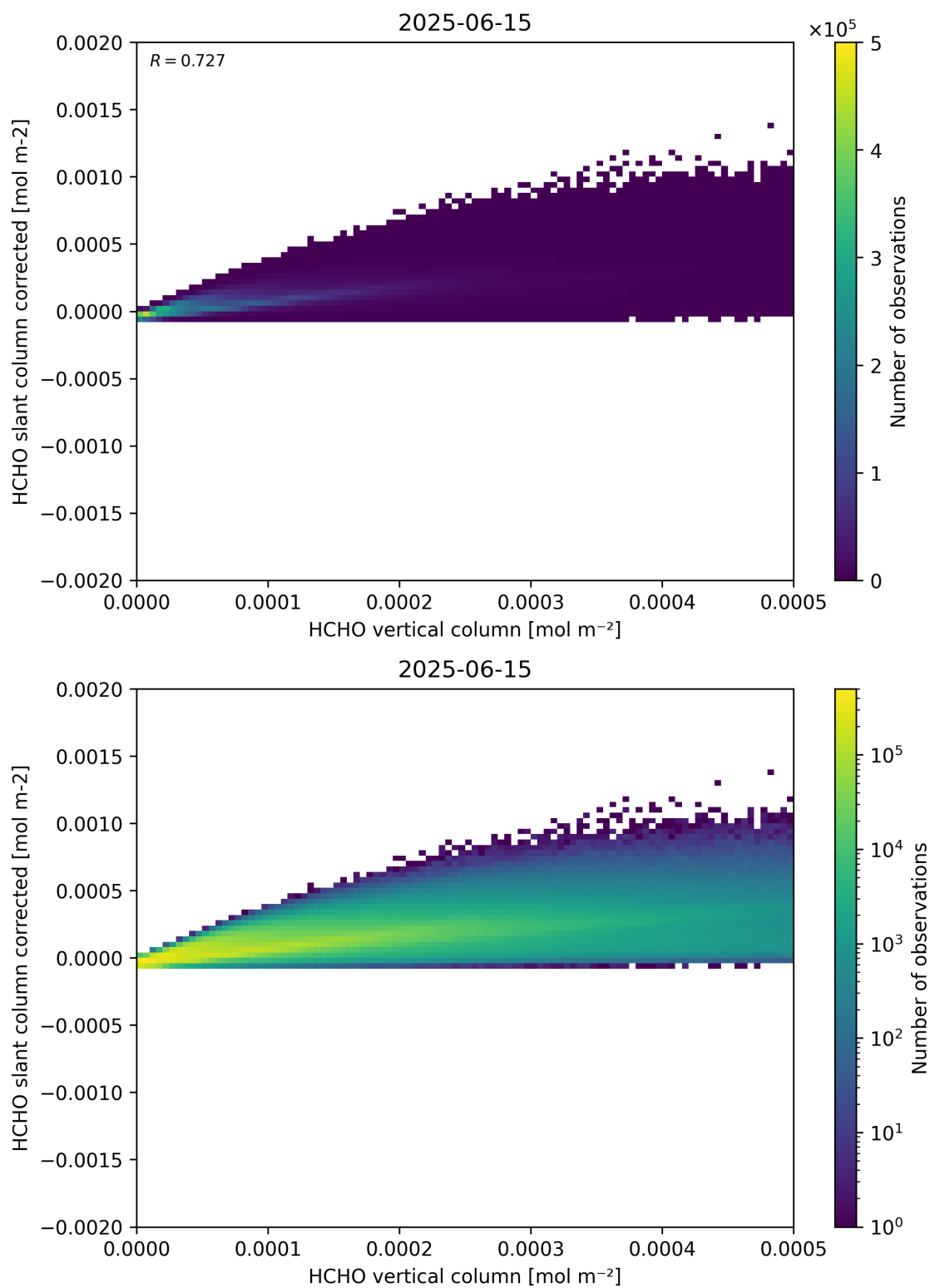
Figure 127: Scatter density plot of “HCHO vertical column” against “HCHO slant column corrected” for 2025-06-14 to 2025-06-16.
