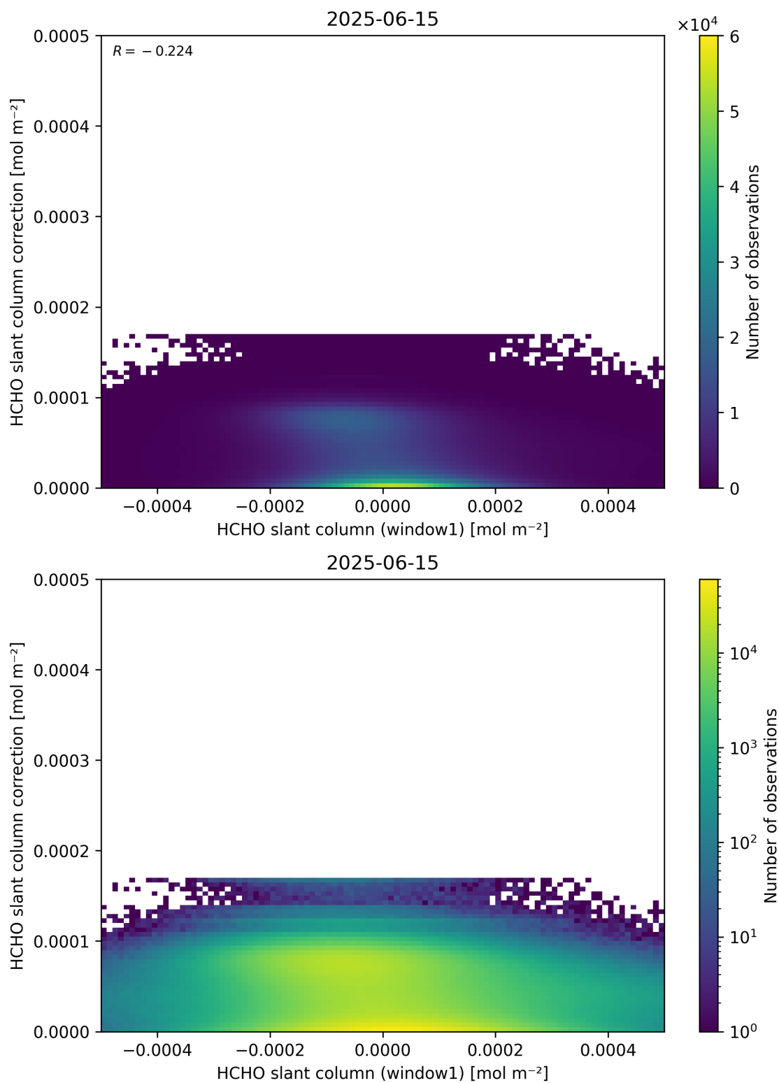
Figure 83: Scatter density plot of “HCHO slant column (window1)” against “HCHO slant column correction” for 2025-06-14 to 2025-06-16.
