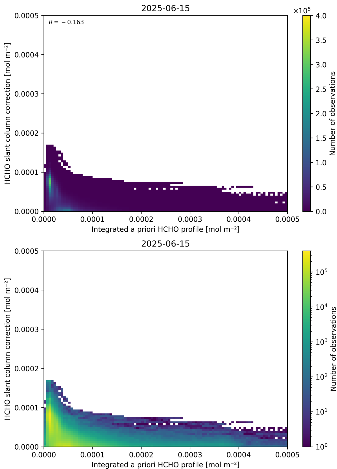
Figure 152: Scatter density plot of “Integrated a priori HCHO profile” against “HCHO slant column correction” for 2025-06-14 to 2025-06-16.
