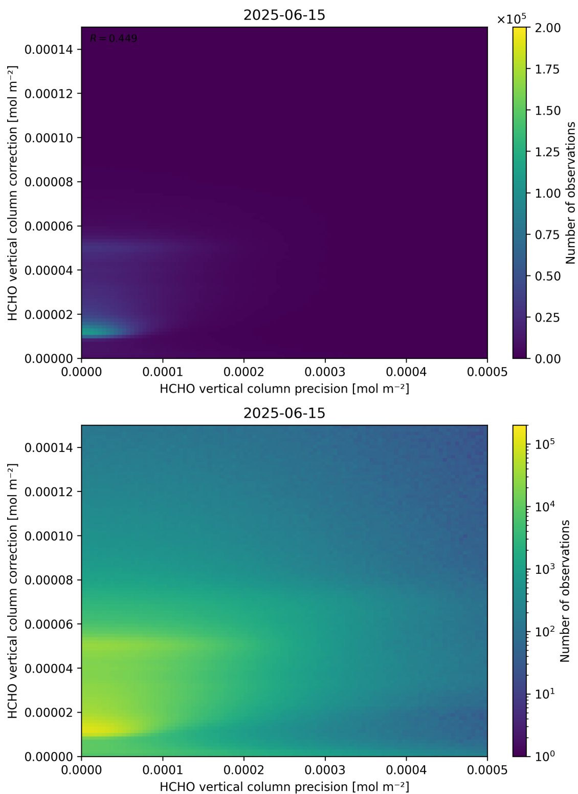
Figure 146: Scatter density plot of “HCHO vertical column precision” against “HCHO vertical column correction” for 2025-06-14 to 2025-06-16.
