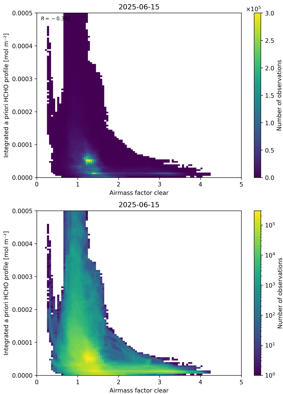
Figure 76: Scatter density plot of “Airmass factor clear” against “Integrated a priori HCHO profile” for 2025-06-14 to 2025-06-16.
