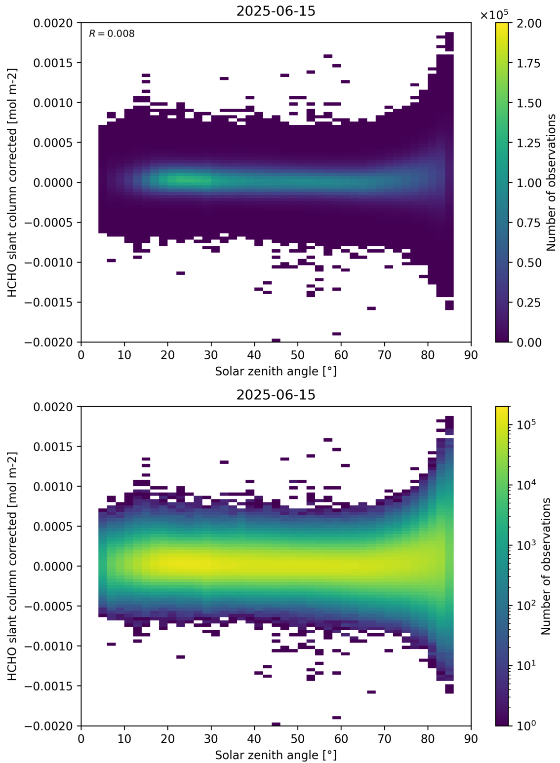
Figure 171: Scatter density plot of “Solar zenith angle” against “HCHO slant column corrected” for 2025-06-14 to 2025-06-16.
