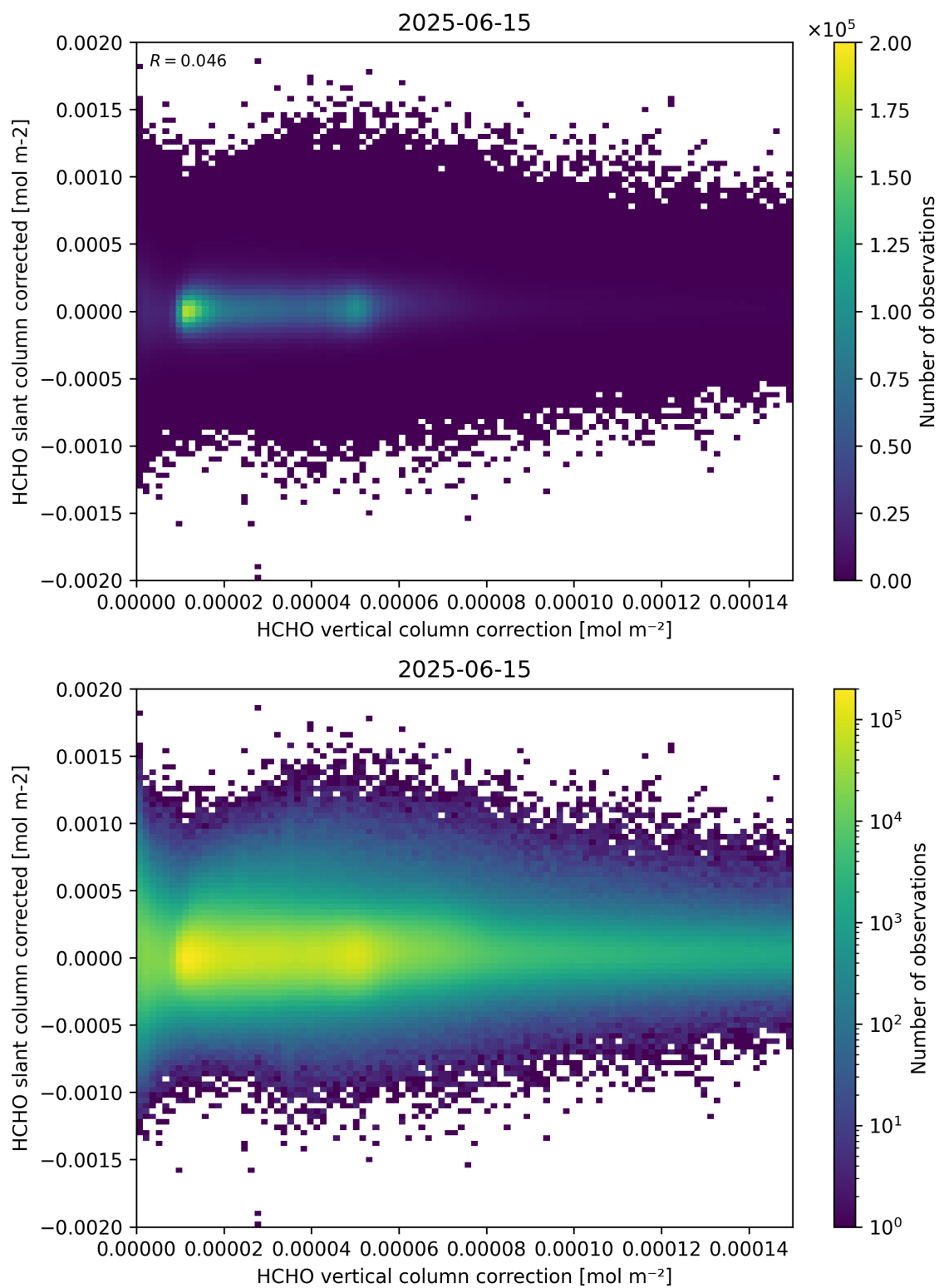
Figure 116: Scatter density plot of “HCHO vertical column correction” against “HCHO slant column corrected” for 2025-06-14 to 2025-06-16.
