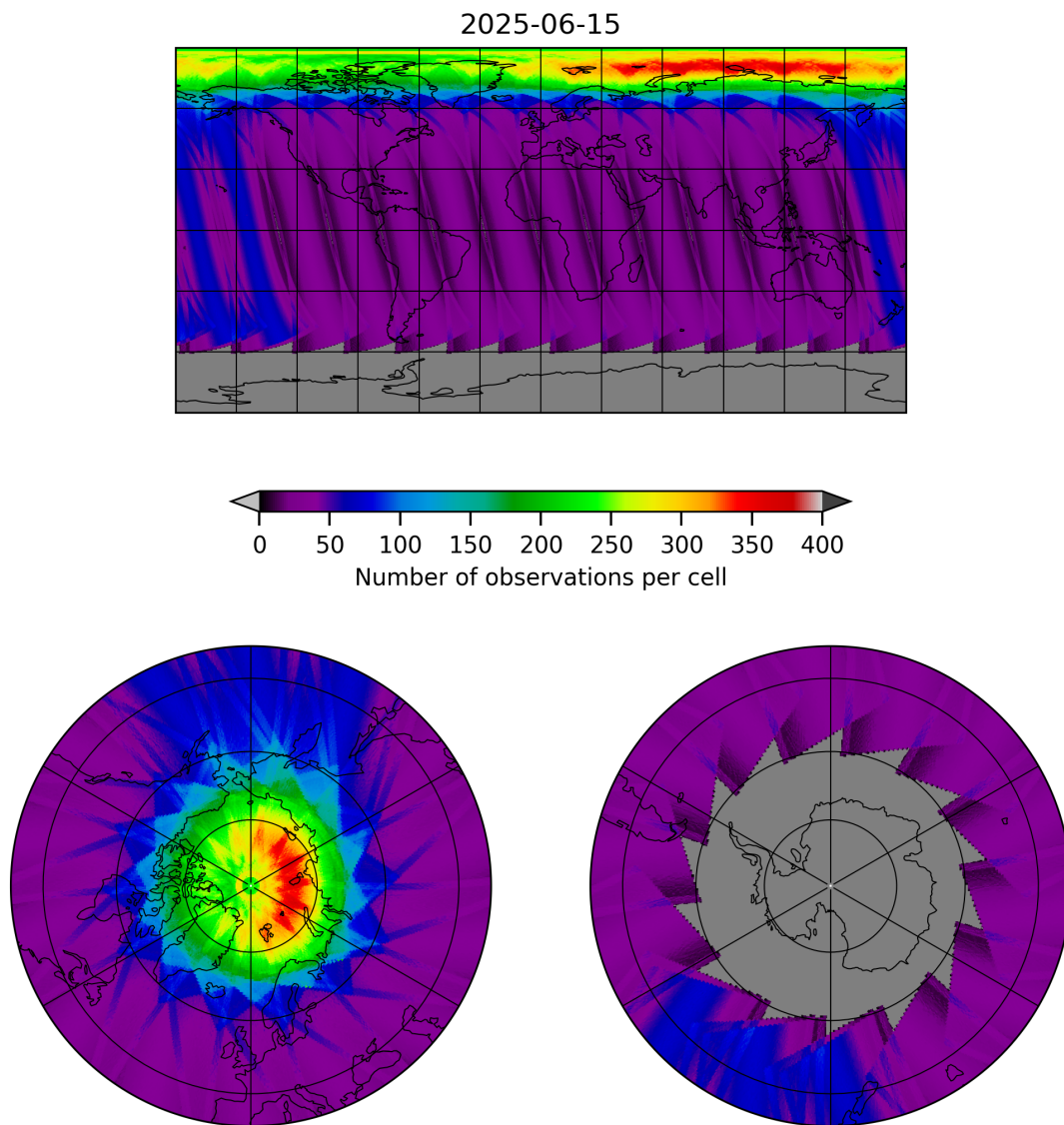
Figure 19: Map of the number of observations for 2025-06-14 to 2025-06-16
