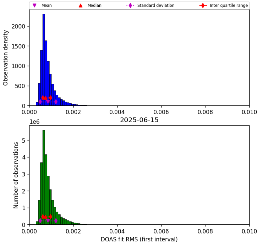
Figure 46: Histogram of “DOAS fit RMS (first interval)” for 2025-06-14 to 2025-06-16
