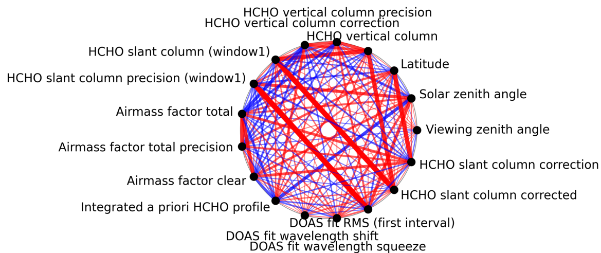
Figure 1: Map of correlation graph for 2025-06-14 to 2025-06-16.
