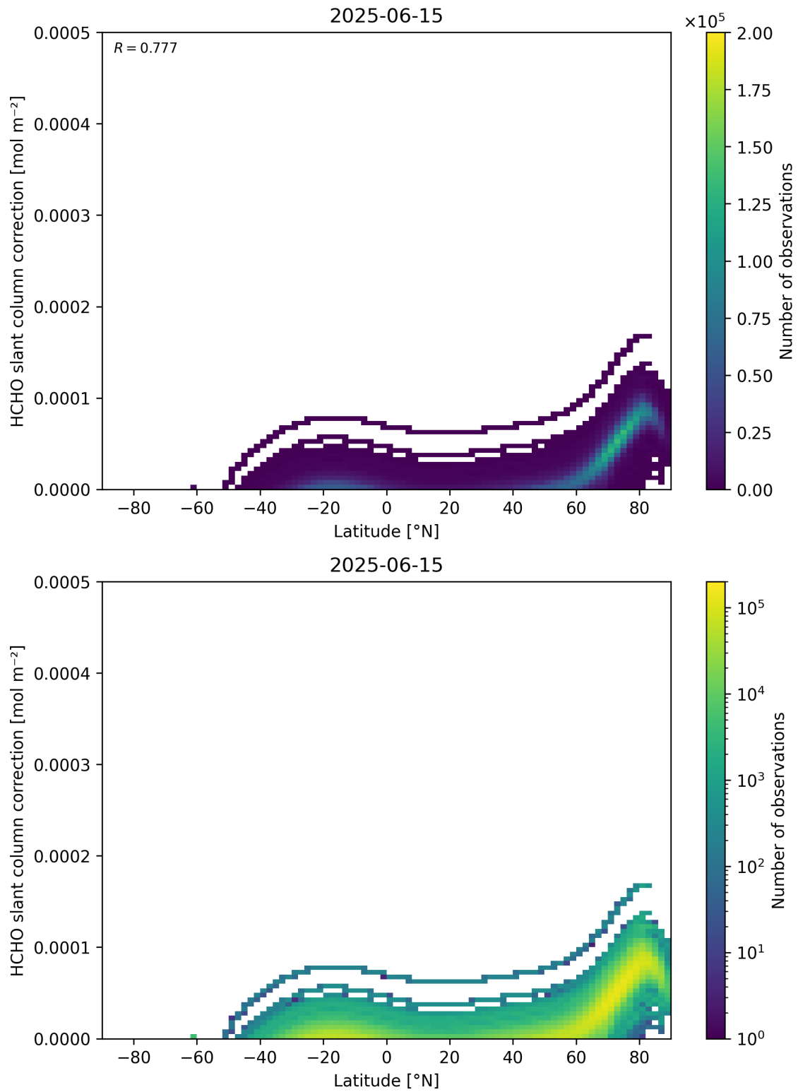
Figure 158: Scatter density plot of “Latitude” against “HCHO slant column correction” for 2025-06-14 to 2025-06-16.
