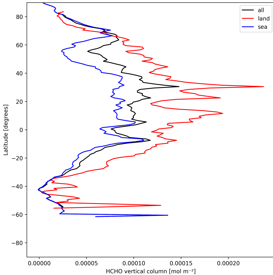
Figure 21: Zonal average of “HCHO vertical column” for 2025-06-14 to 2025-06-16.
