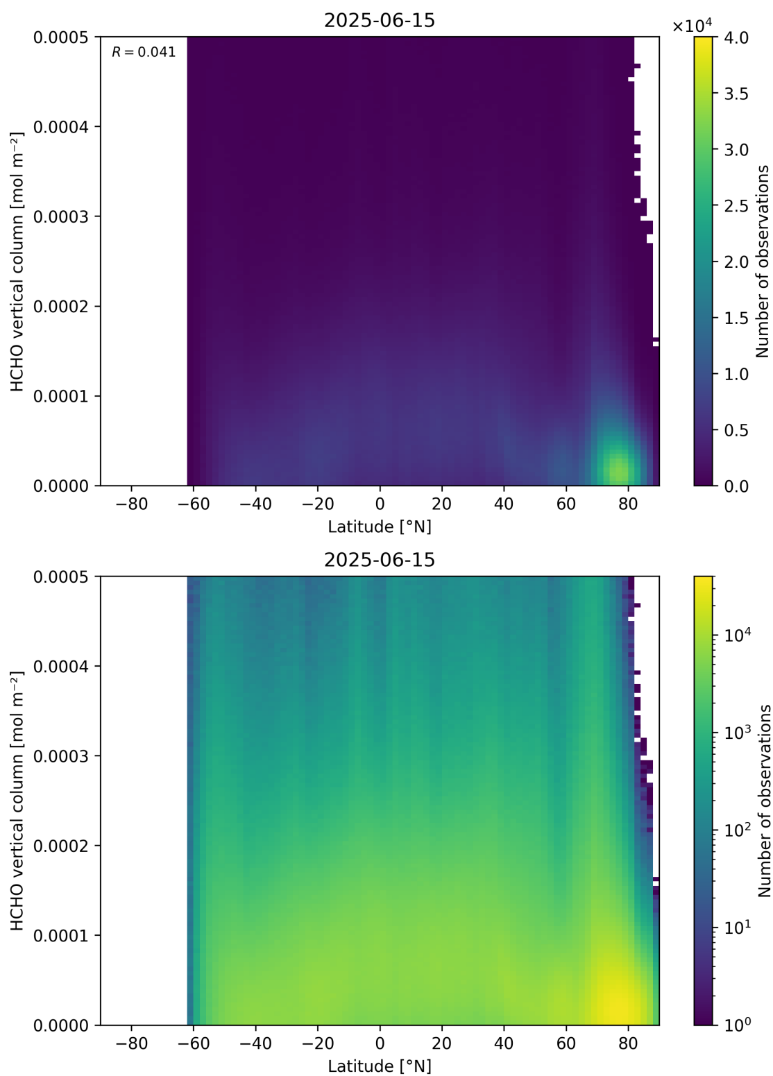
Figure 163: Scatter density plot of “Latitude” against “HCHO vertical column” for 2025-06-14 to 2025-06-16.
