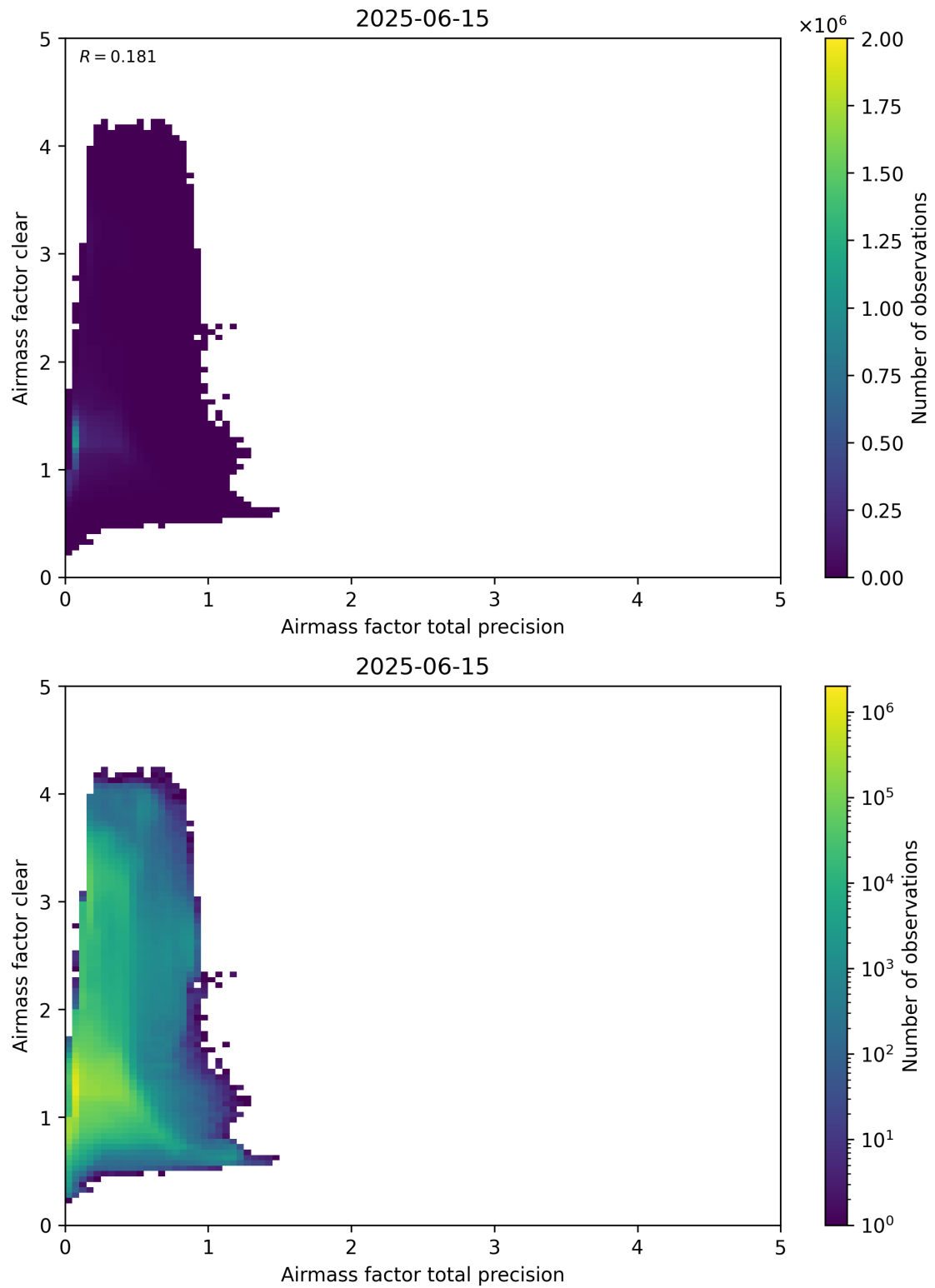
Figure 108: Scatter density plot of “Airmass factor total precision” against “Airmass factor clear” for 2025-06-14 to 2025-06-16.
