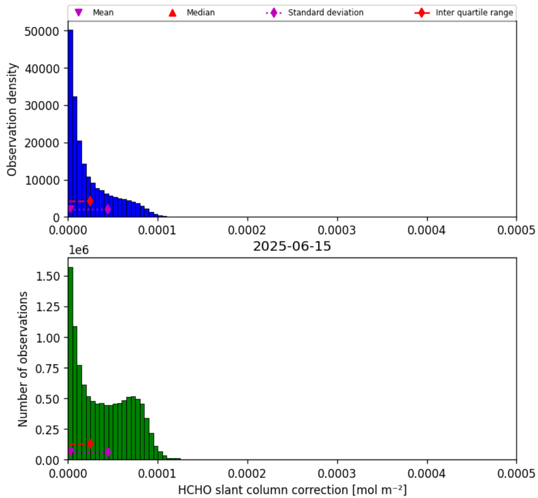
Figure 47: Histogram of “HCHO slant column correction” for 2025-06-14 to 2025-06-16
