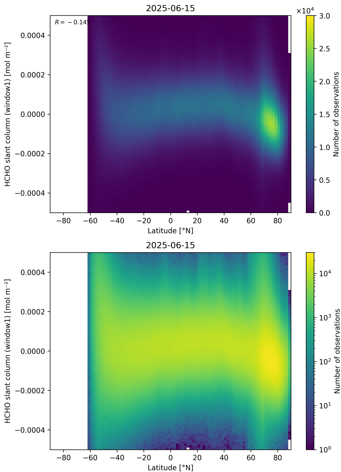
Figure 159: Scatter density plot of “Latitude” against “HCHO slant column (window1)” for 2025-06-14 to 2025-06-16.
