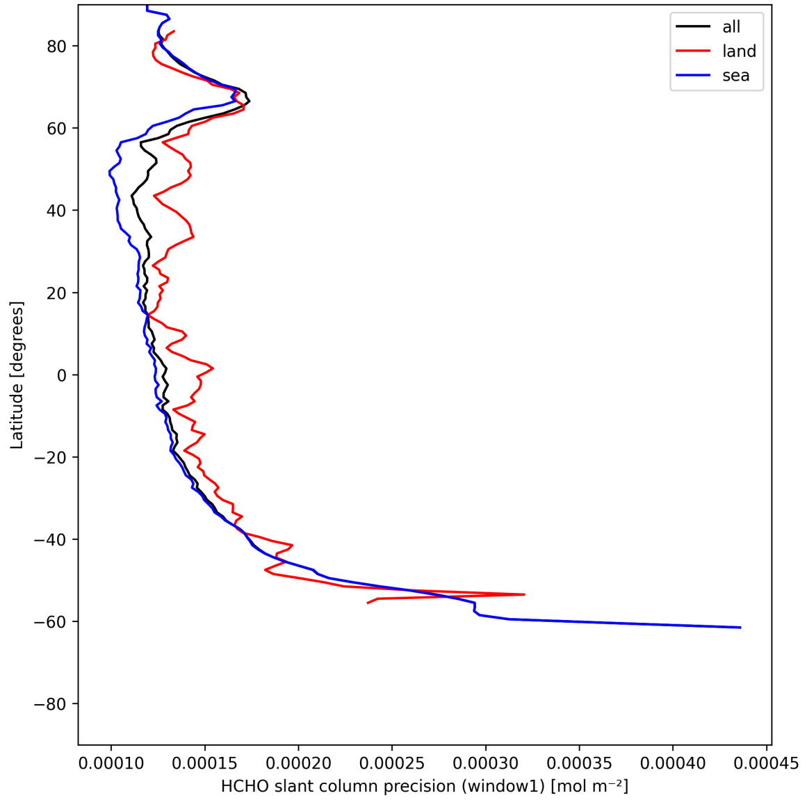
Figure 25: Zonal average of “HCHO slant column precision (window1)” for 2025-06-14 to 2025-06-16.
