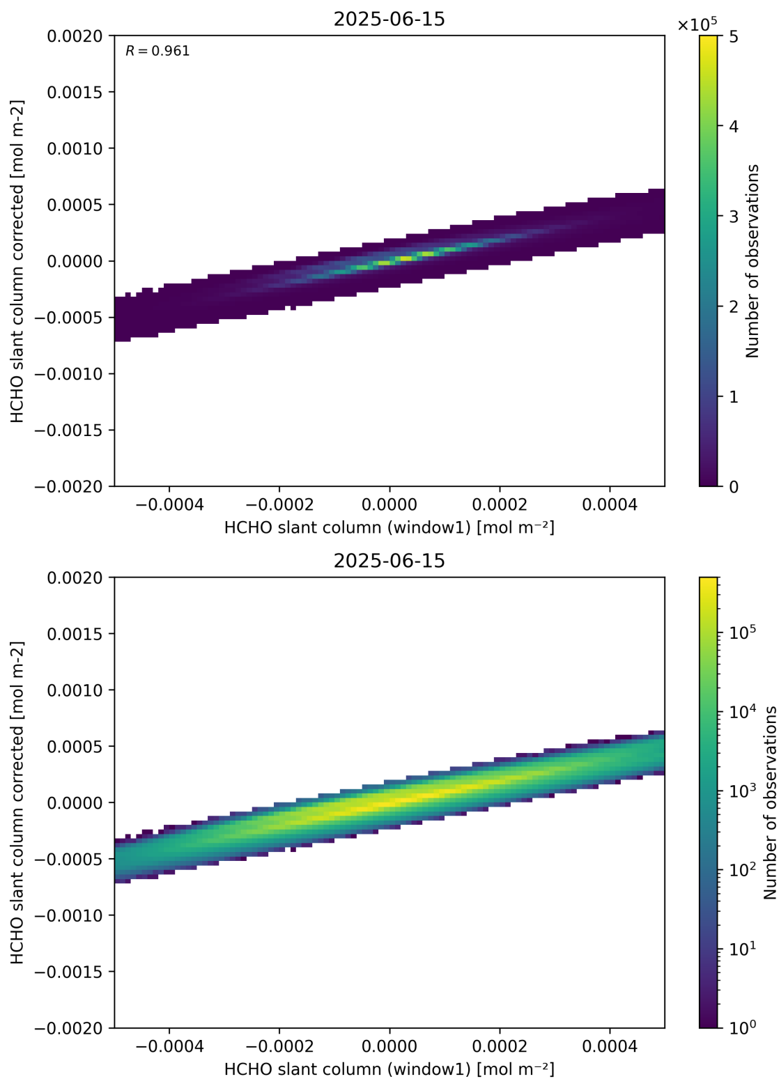
Figure 82: Scatter density plot of “HCHO slant column (window1)” against “HCHO slant column corrected” for 2025-06-14 to 2025-06-16.
