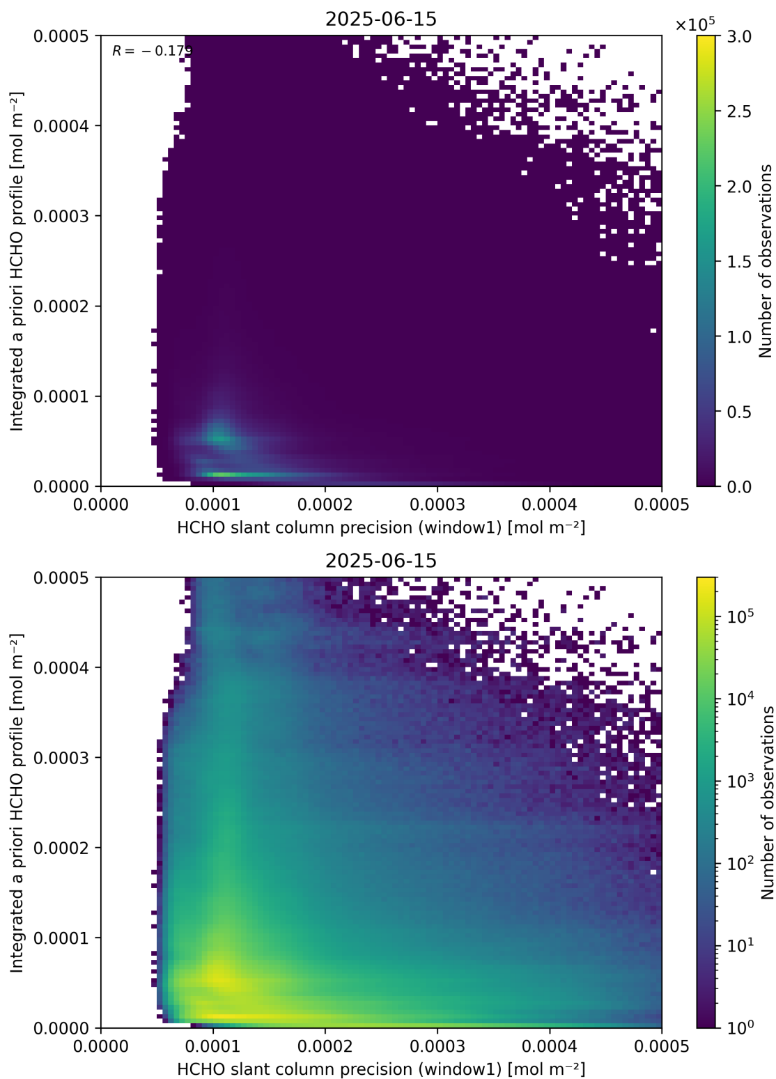
Figure 96: Scatter density plot of “HCHO slant column precision (window1)” against “Integrated a priori HCHO profile” for 2025-06-14 to 2025-06-16.
