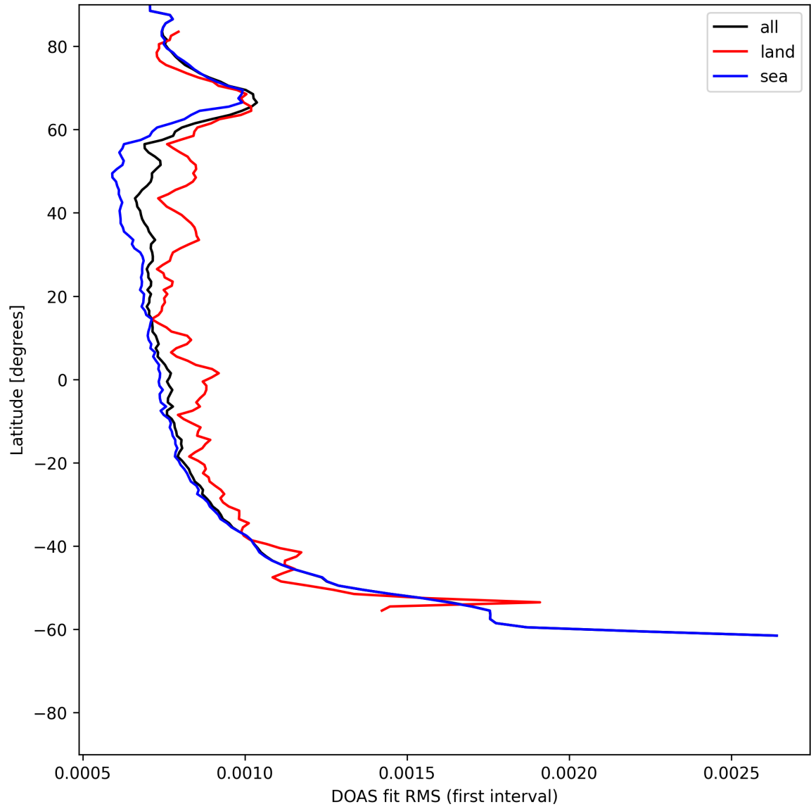
Figure 32: Zonal average of "DOAS fit RMS (first interval)" for 2025-06-14 to 2025-06-16.
