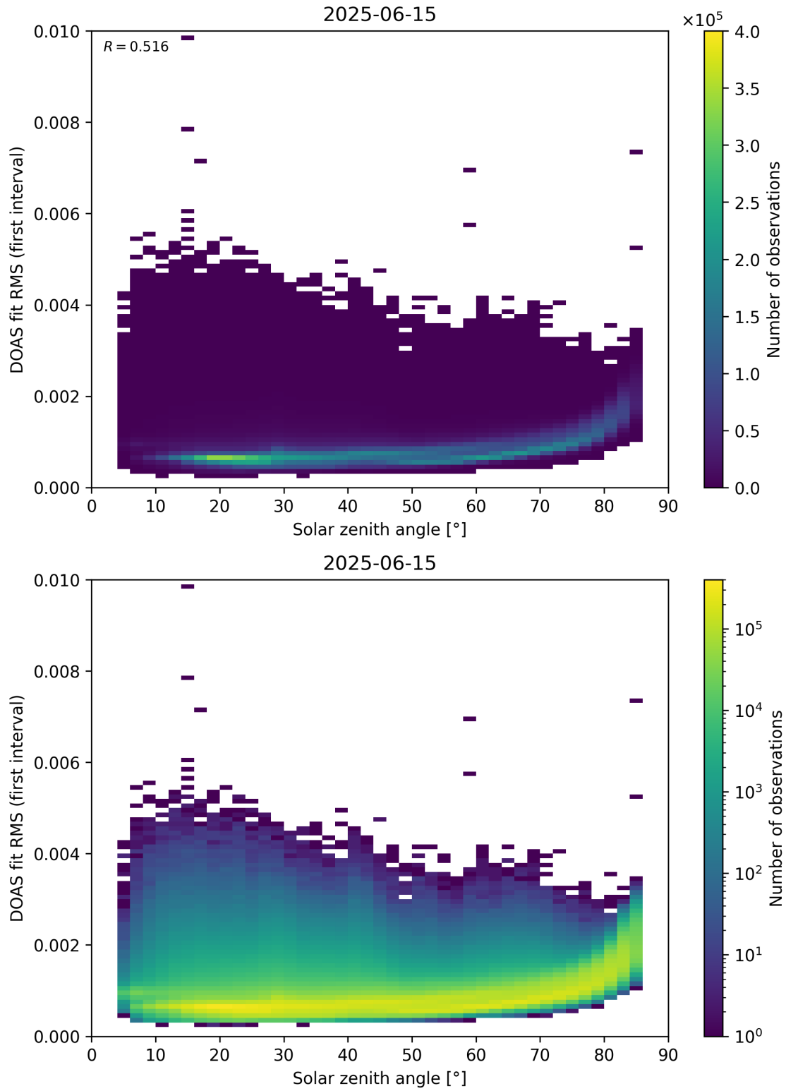
Figure 167: Scatter density plot of “Solar zenith angle” against “DOAS fit RMS (first interval)” for 2025-06-14 to 2025-06-16.
