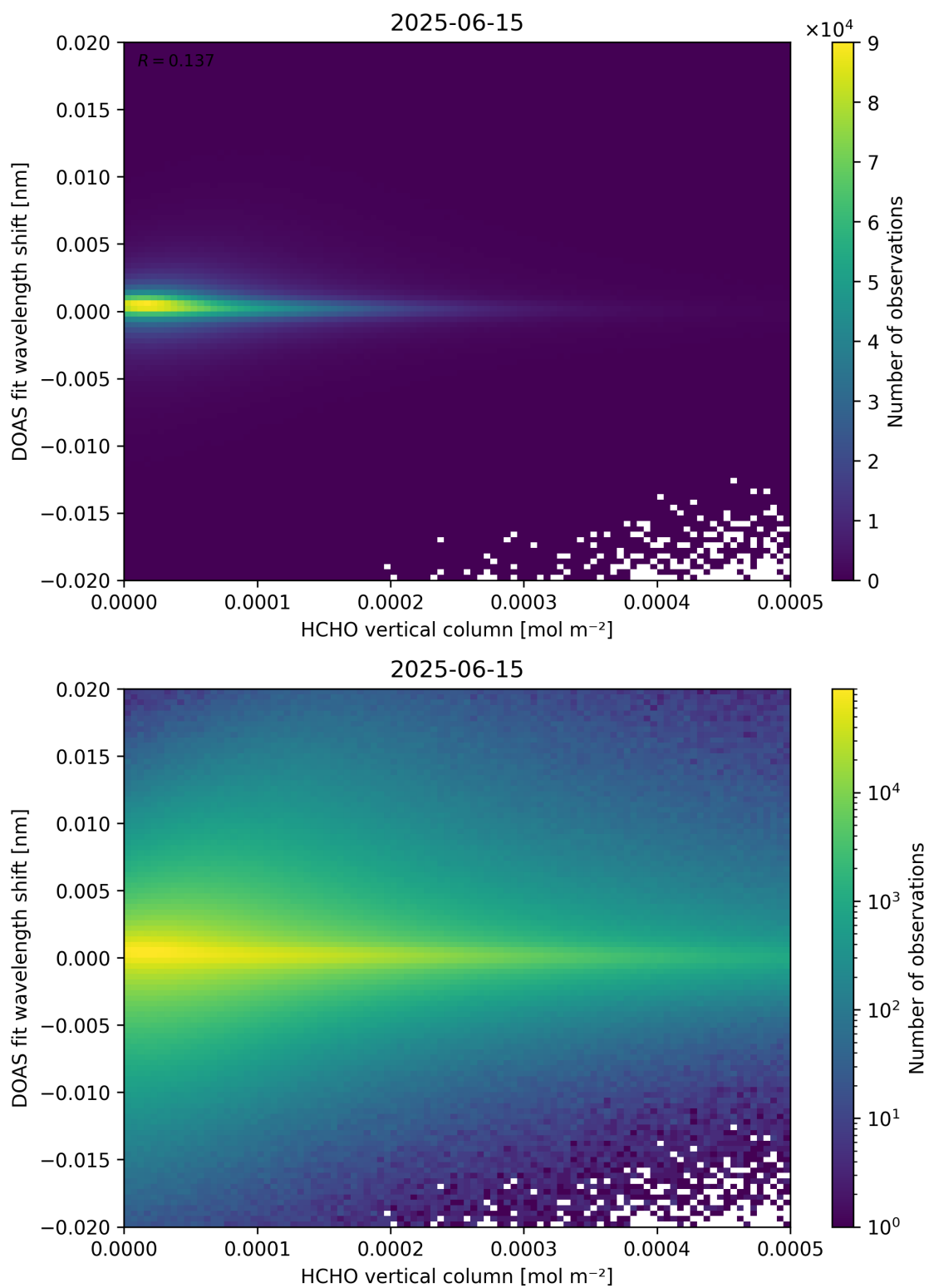
Figure 124: Scatter density plot of “HCHO vertical column” against “DOAS fit wavelength shift” for 2025-06-14 to 2025-06-16.
