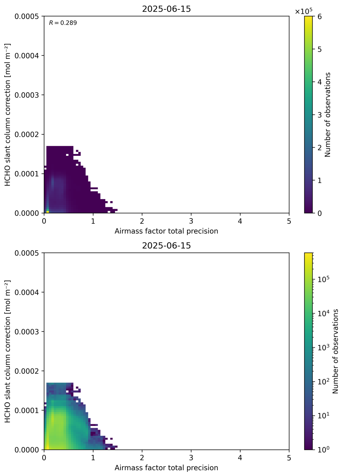
Figure 110: Scatter density plot of “Airmass factor total precision” against “HCHO slant column correction” for 2025-06-14 to 2025-06-16.
