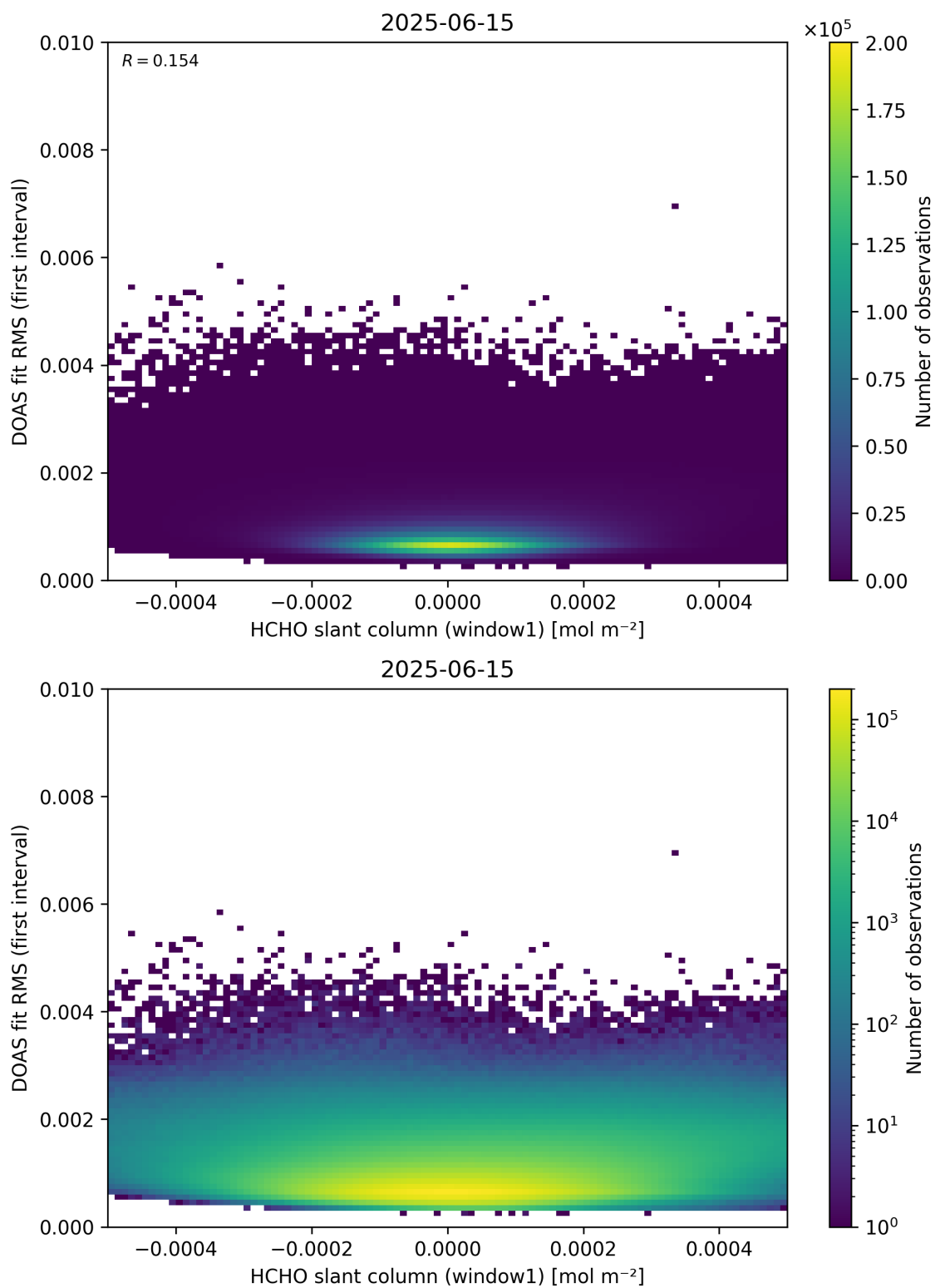
Figure 78: Scatter density plot of “HCHO slant column (window1)” against “DOAS fit RMS (first interval)” for 2025-06-14 to 2025-06-16.
