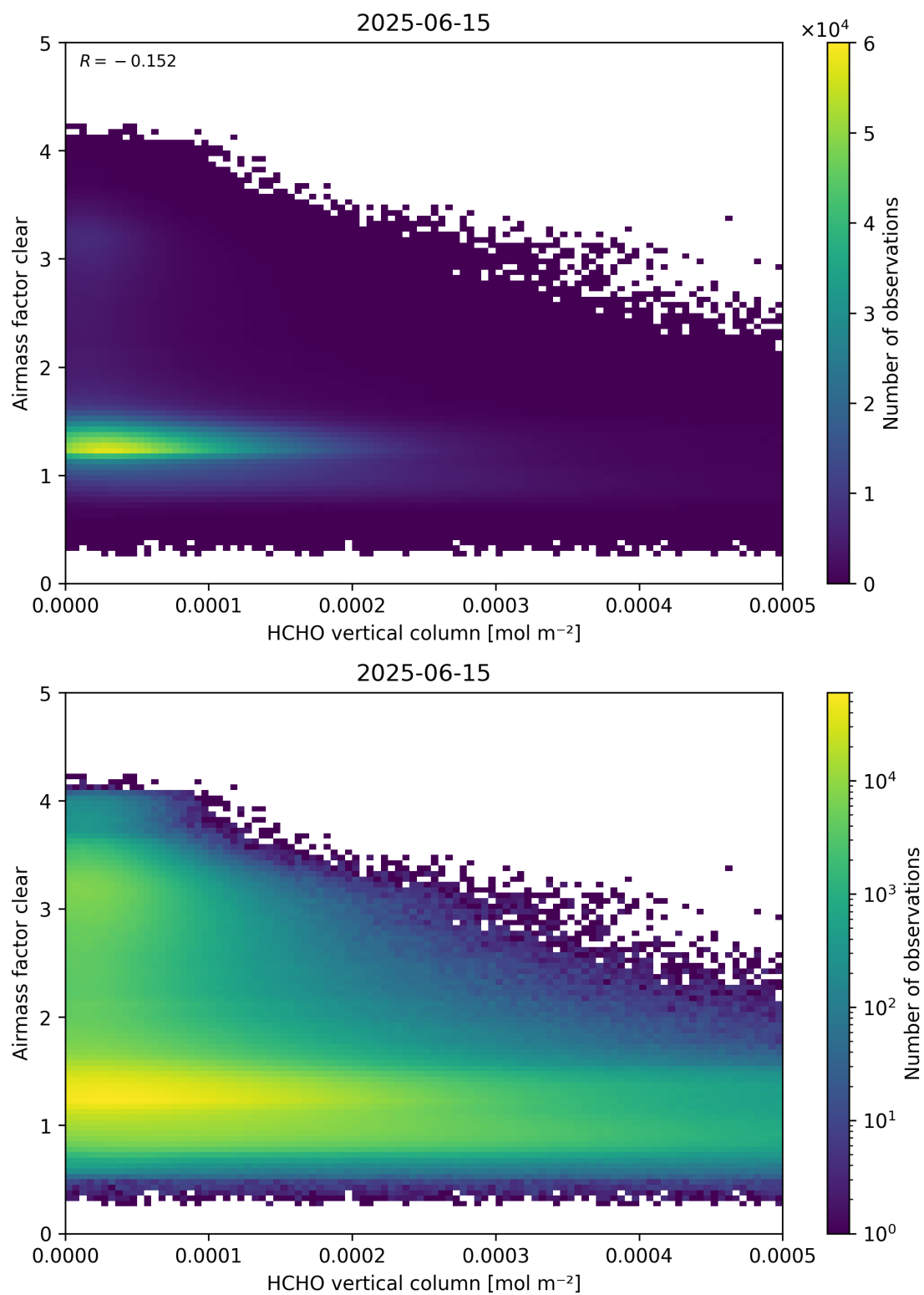
Figure 126: Scatter density plot of “HCHO vertical column” against “Airmass factor clear” for 2025-06-14 to 2025-06-16.
