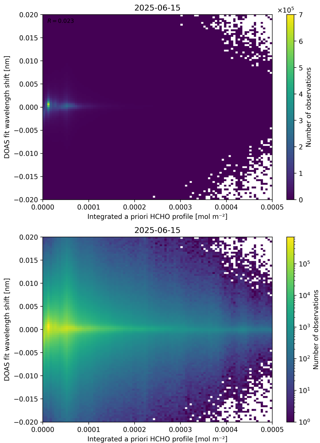
Figure 149: Scatter density plot of “Integrated a priori HCHO profile” against “DOAS fit wavelength shift” for 2025-06-14 to 2025-06-16.
