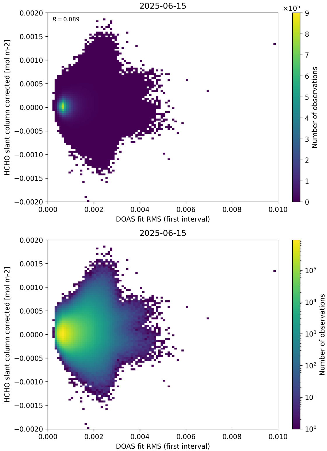
Figure 62: Scatter density plot of “DOAS fit RMS (first interval)” against “HCHO slant column corrected” for 2025-06-14 to 2025-06-16.
