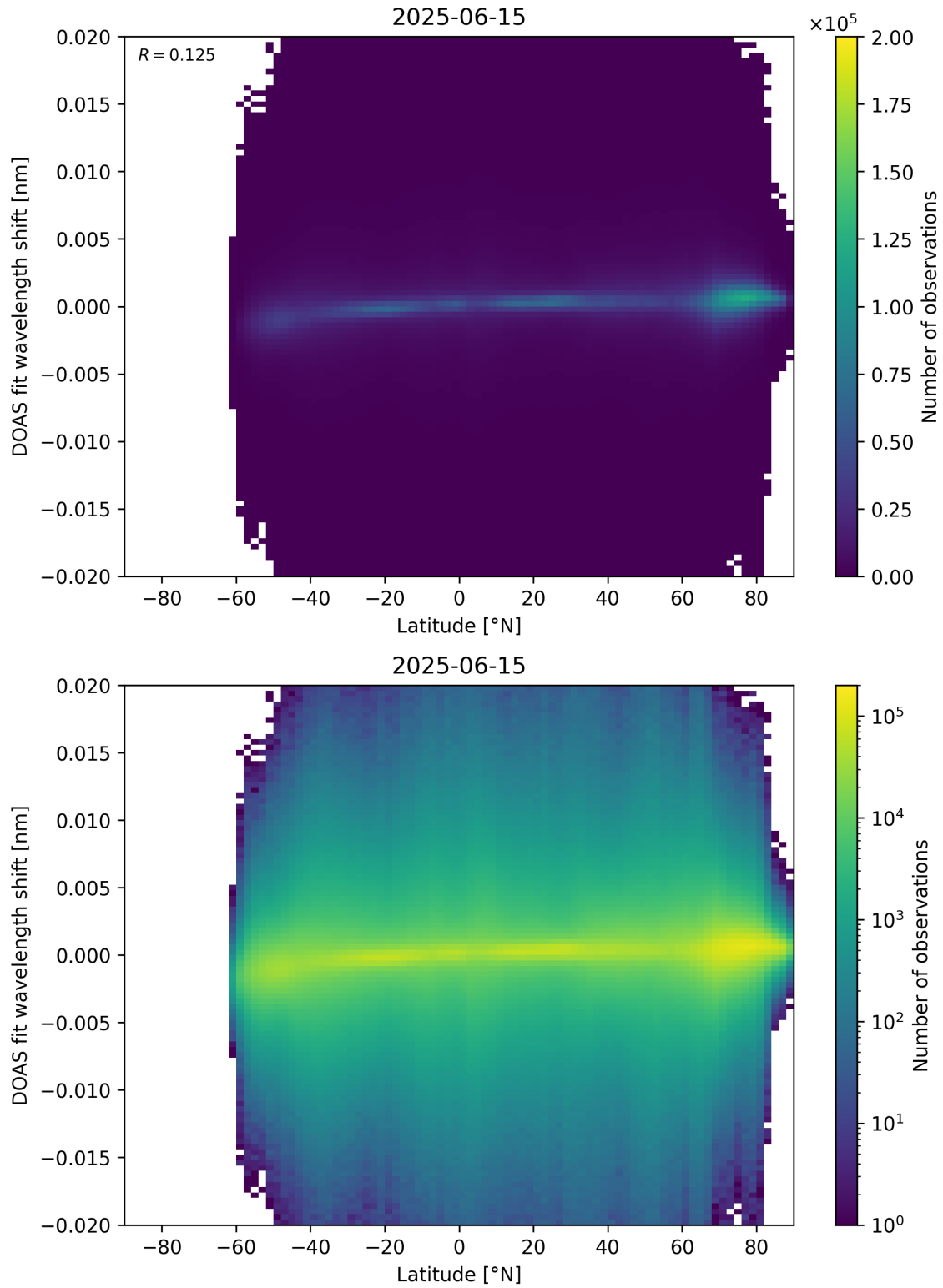
Figure 154: Scatter density plot of “Latitude” against “DOAS fit wavelength shift” for 2025-06-14 to 2025-06-16.
