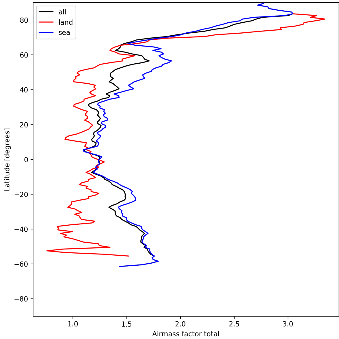
Figure 26: Zonal average of “Airmass factor total” for 2025-06-14 to 2025-06-16.
