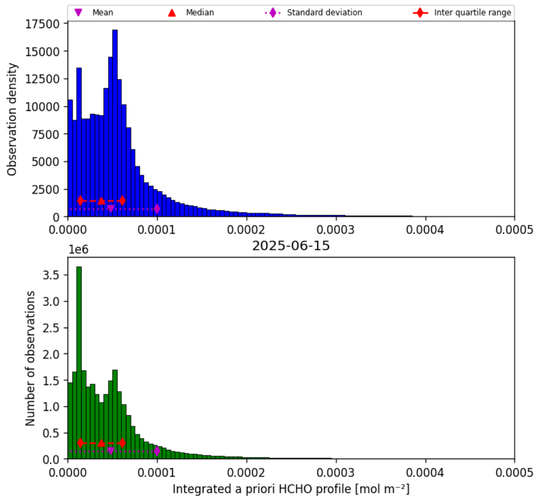
Figure 43: Histogram of “Integrated a priori HCHO profile” for 2025-06-14 to 2025-06-16
