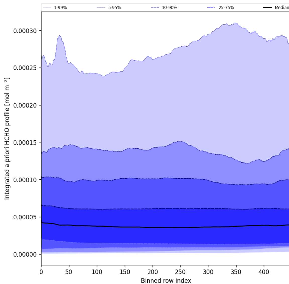
Figure 57: Along track statistics of “Integrated a priori HCHO profile” for 2025-06-14 to 2025-06-16
