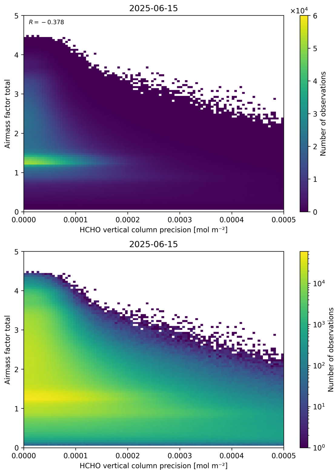
Figure 144: Scatter density plot of “HCHO vertical column precision” against “Airmass factor total” for 2025-06-14 to 2025-06-16.
