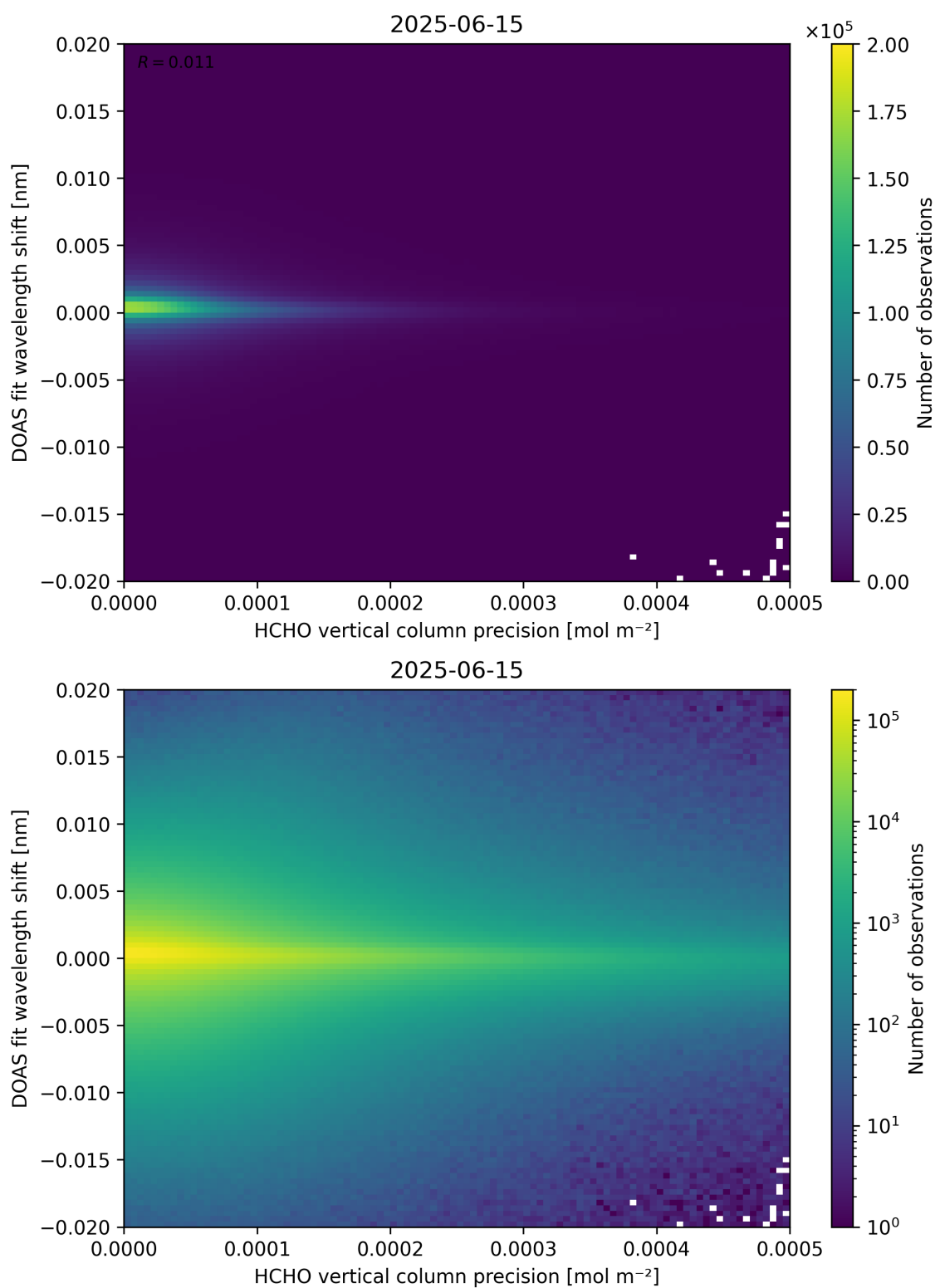
Figure 137: Scatter density plot of “HCHO vertical column precision” against “DOAS fit wavelength shift” for 2025-06-14 to 2025-06-16.
