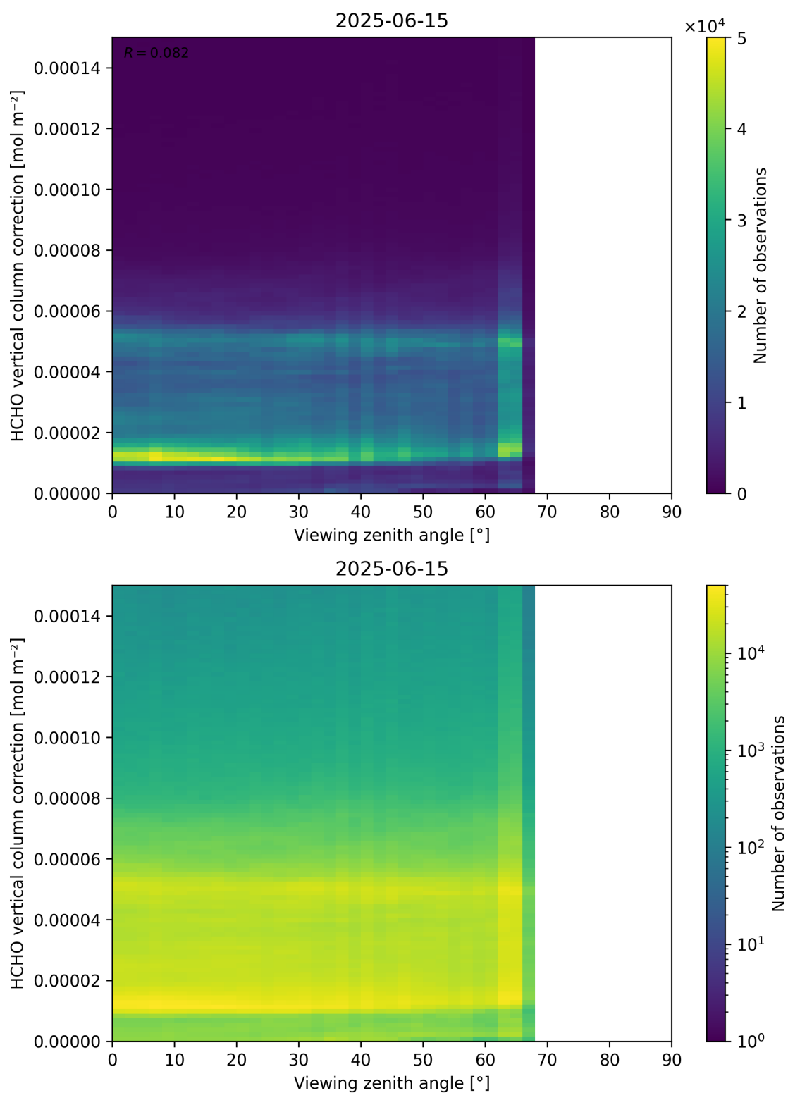
Figure 193: Scatter density plot of “Viewing zenith angle” against “HCHO vertical column correction” for 2025-06-14 to 2025-06-16.
