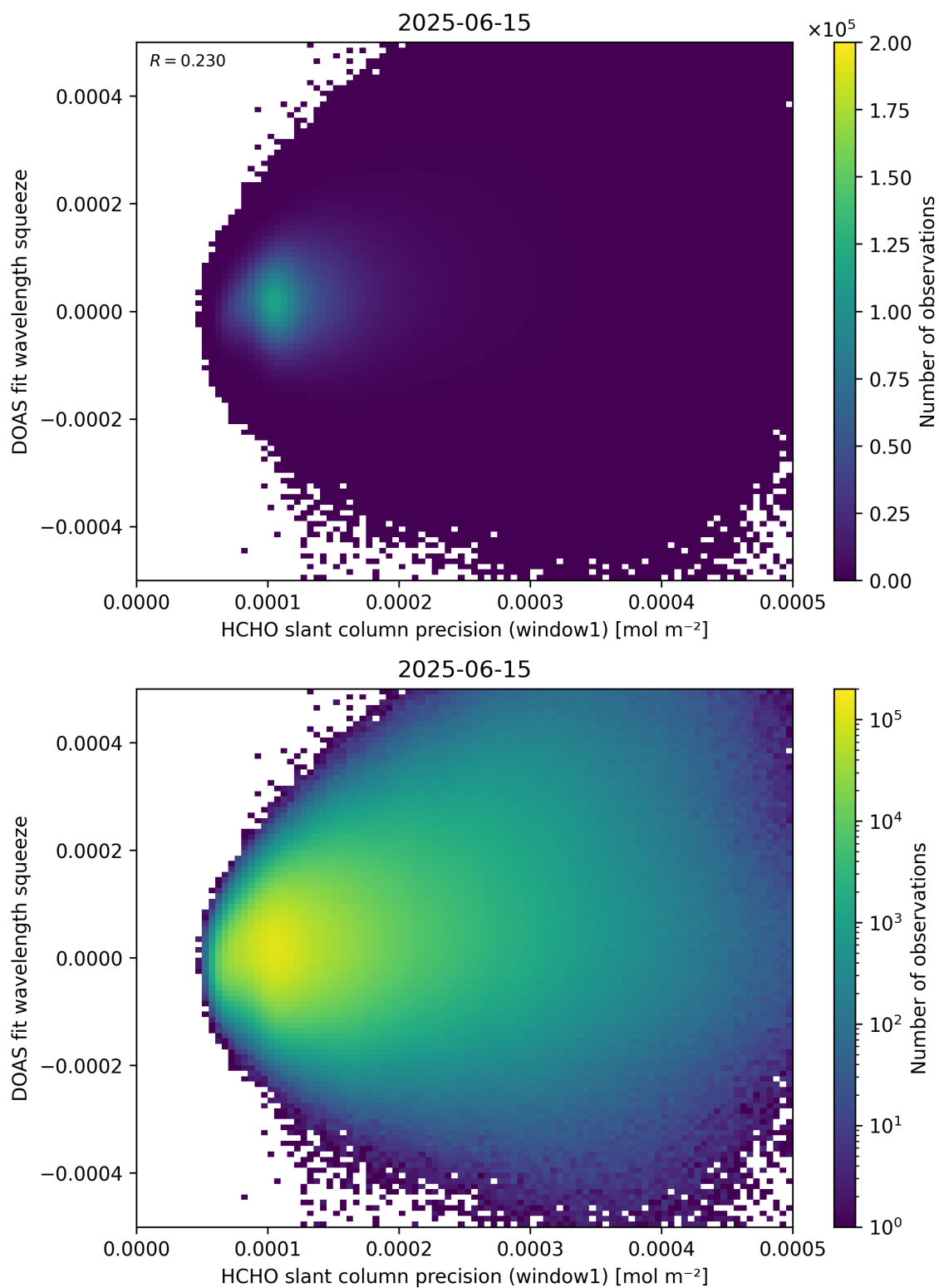
Figure 90: Scatter density plot of “HCHO slant column precision (window1)” against “DOAS fit wavelength squeeze” for 2025-06-14 to 2025-06-16.
