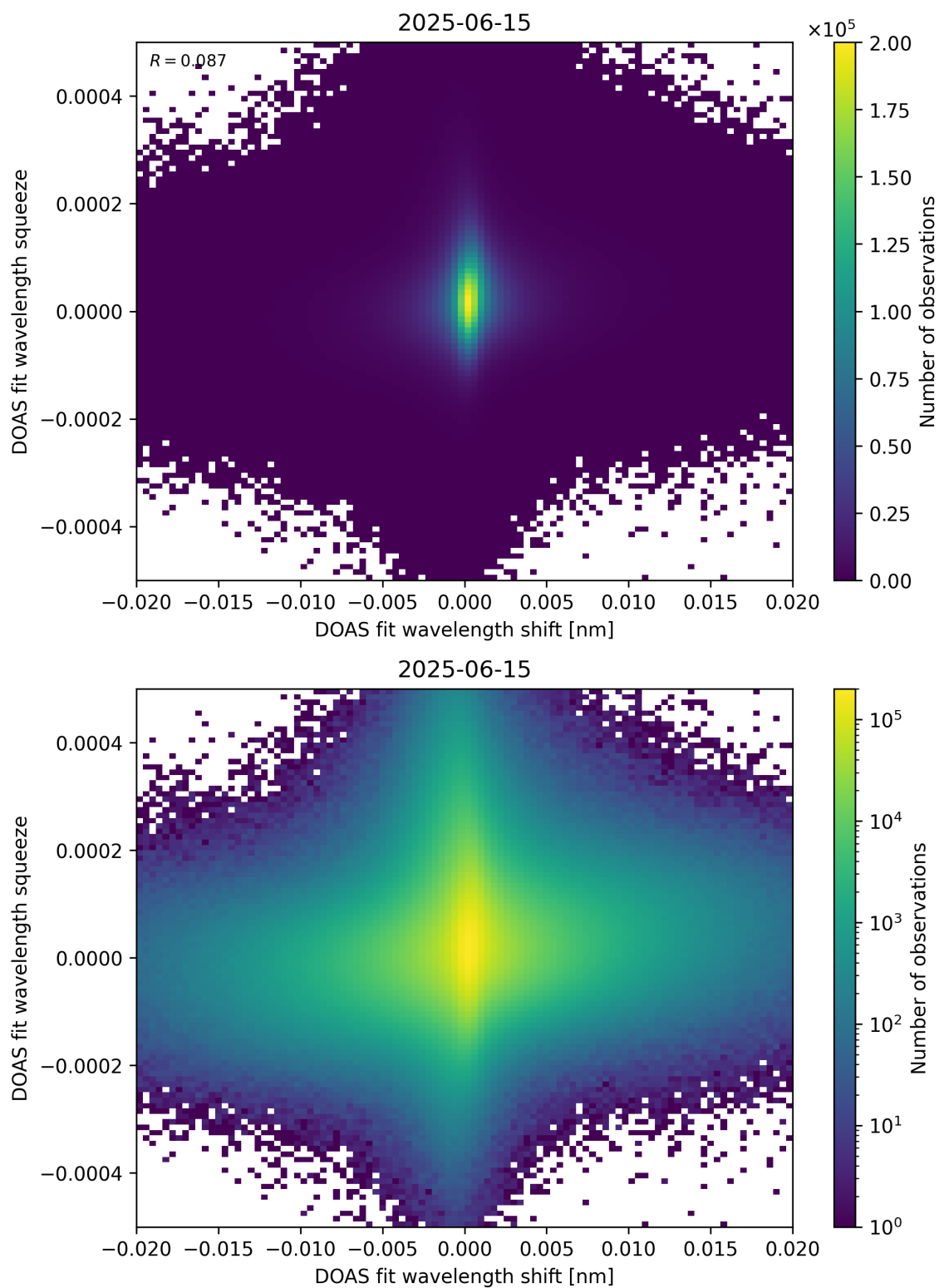
Figure 65: Scatter density plot of “DOAS fit wavelength shift” against “DOAS fit wavelength squeeze” for 2025-06-14 to 2025-06-16.
