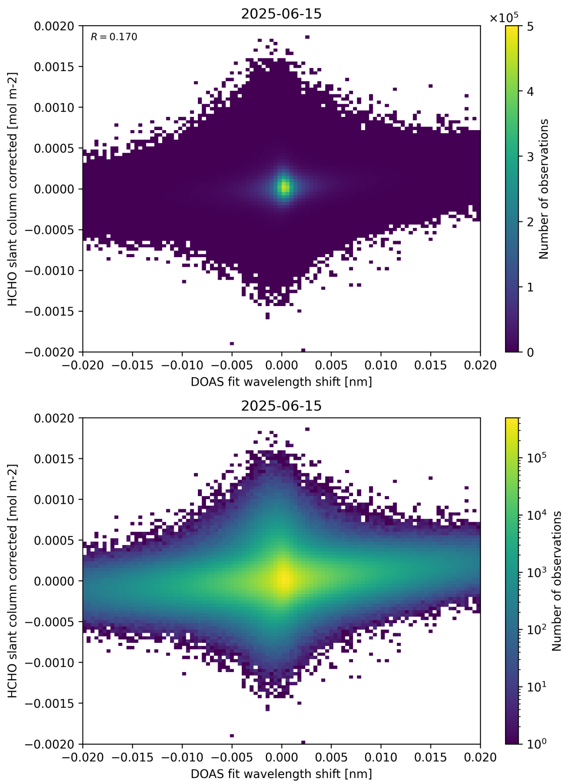
Figure 66: Scatter density plot of “DOAS fit wavelength shift” against “HCHO slant column corrected” for 2025-06-14 to 2025-06-16.
