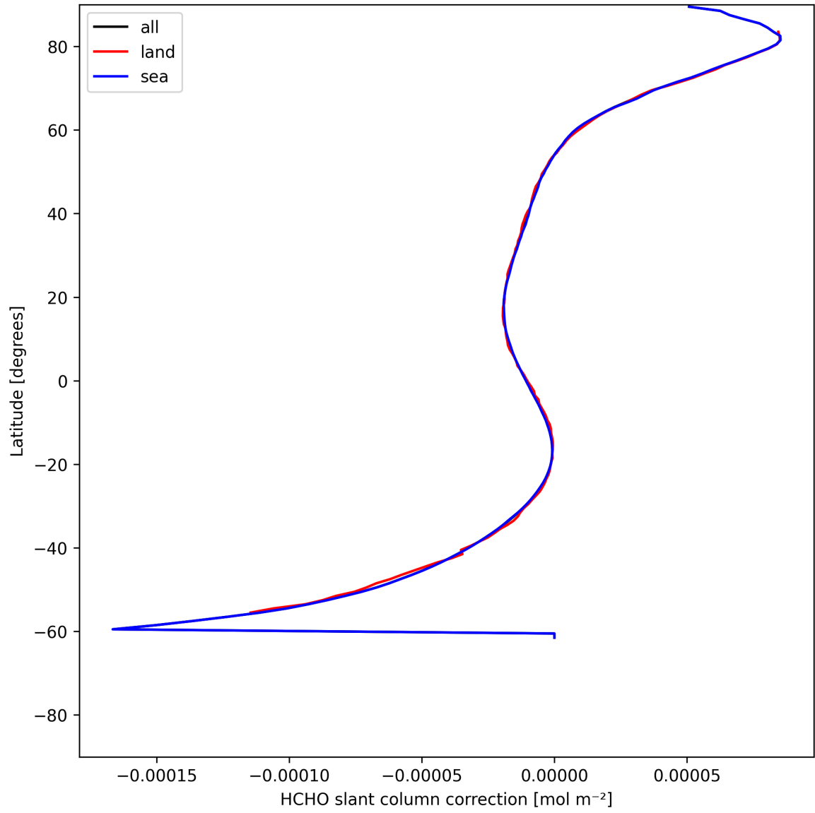
Figure 33: Zonal average of “HCHO slant column correction” for 2025-06-14 to 2025-06-16.
