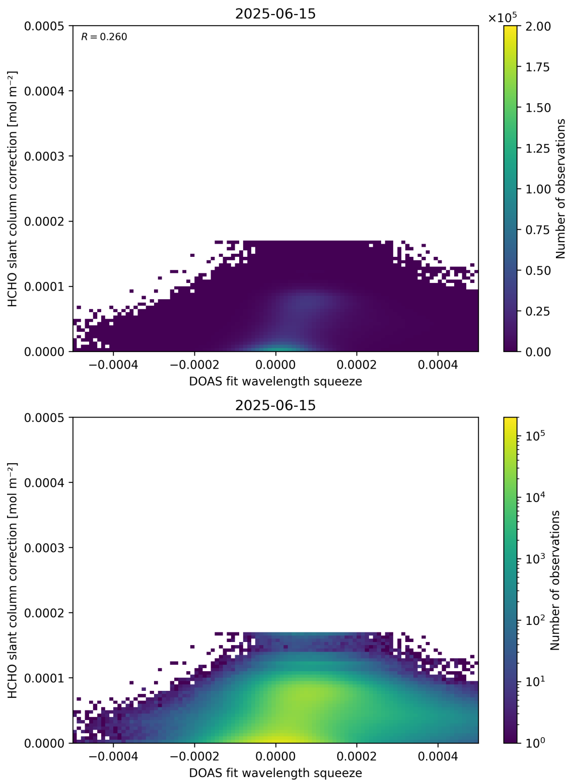
Figure 70: Scatter density plot of “DOAS fit wavelength squeeze” against “HCHO slant column correction” for 2025-06-14 to 2025-06-16.
