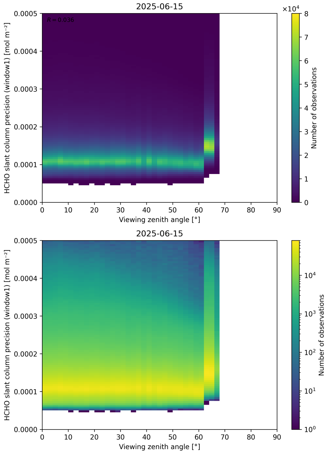
Figure 189: Scatter density plot of “Viewing zenith angle” against “HCHO slant column precision (window1)” for 2025-06-14 to 2025-06-16.
