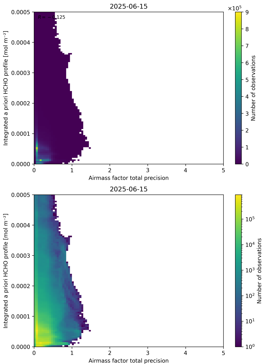
Figure 111: Scatter density plot of “Airmass factor total precision” against “Integrated a priori HCHO profile” for 2025-06-14 to 2025-06-16.
