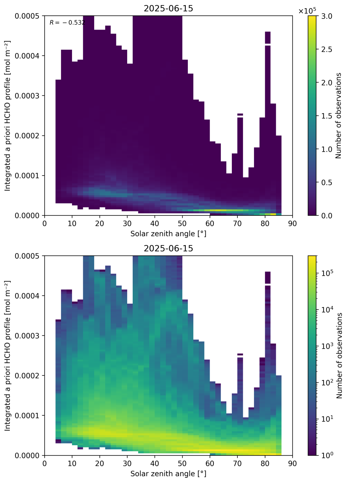
Figure 180: Scatter density plot of “Solar zenith angle” against “Integrated a priori HCHO profile” for 2025-06-14 to 2025-06-16.
