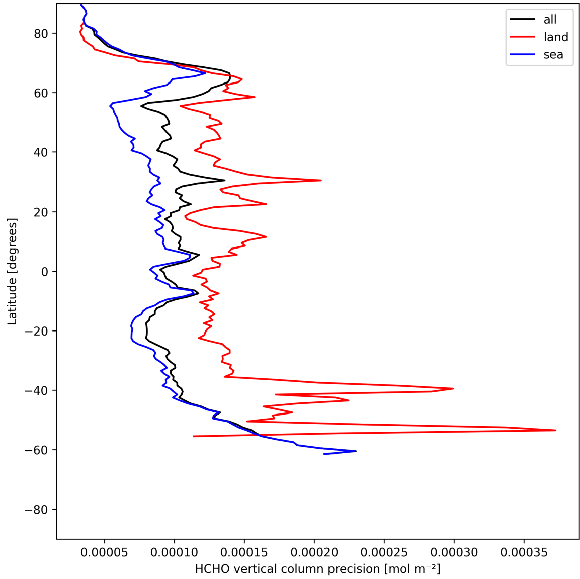
Figure 22: Zonal average of “HCHO vertical column precision” for 2025-06-14 to 2025-06-16.
