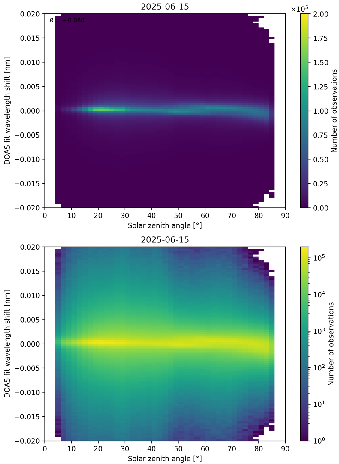
Figure 168: Scatter density plot of “Solar zenith angle” against “DOAS fit wavelength shift” for 2025-06-14 to 2025-06-16.
