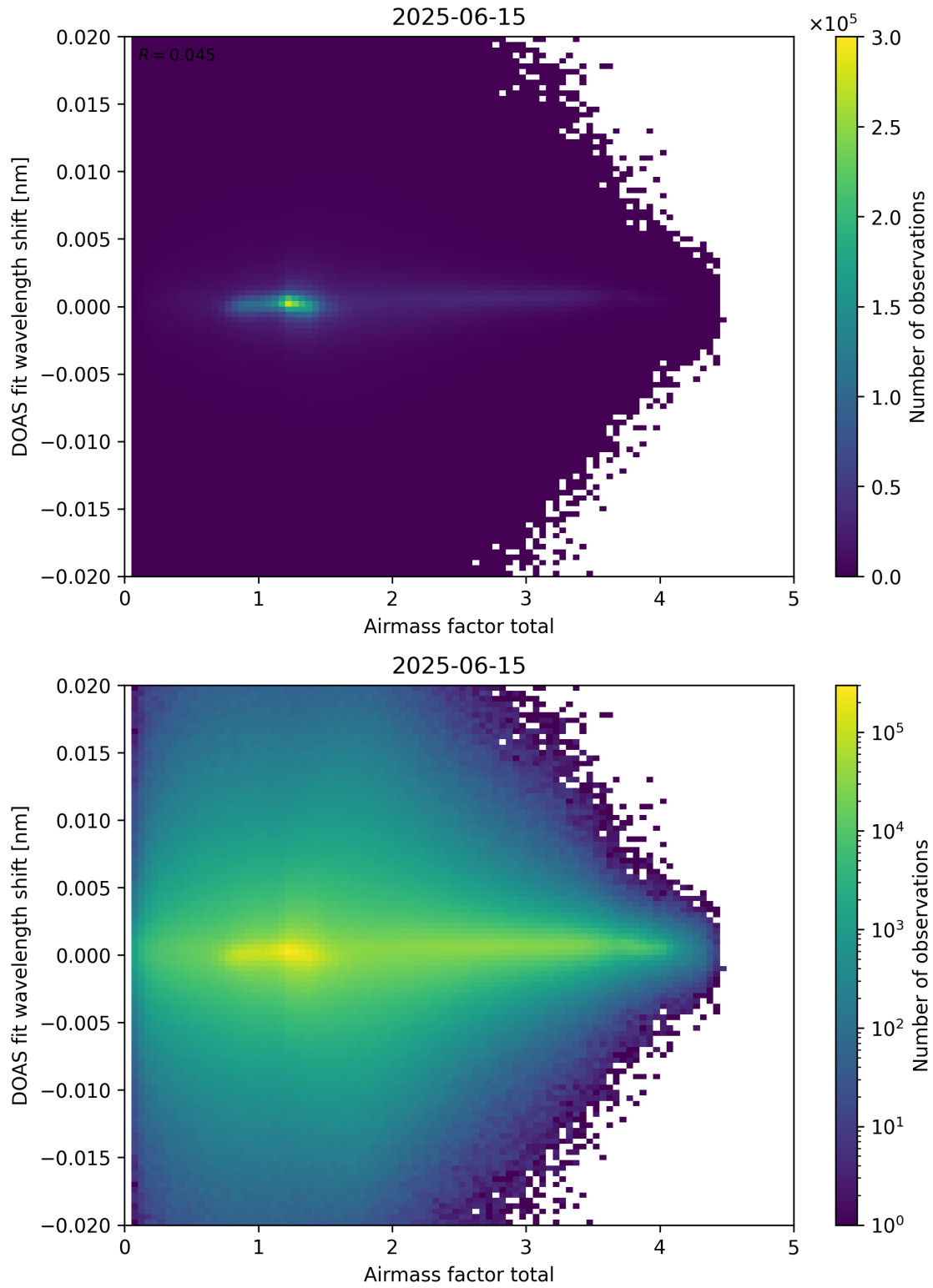
Figure 98: Scatter density plot of “Airmass factor total” against “DOAS fit wavelength shift” for 2025-06-14 to 2025-06-16.
