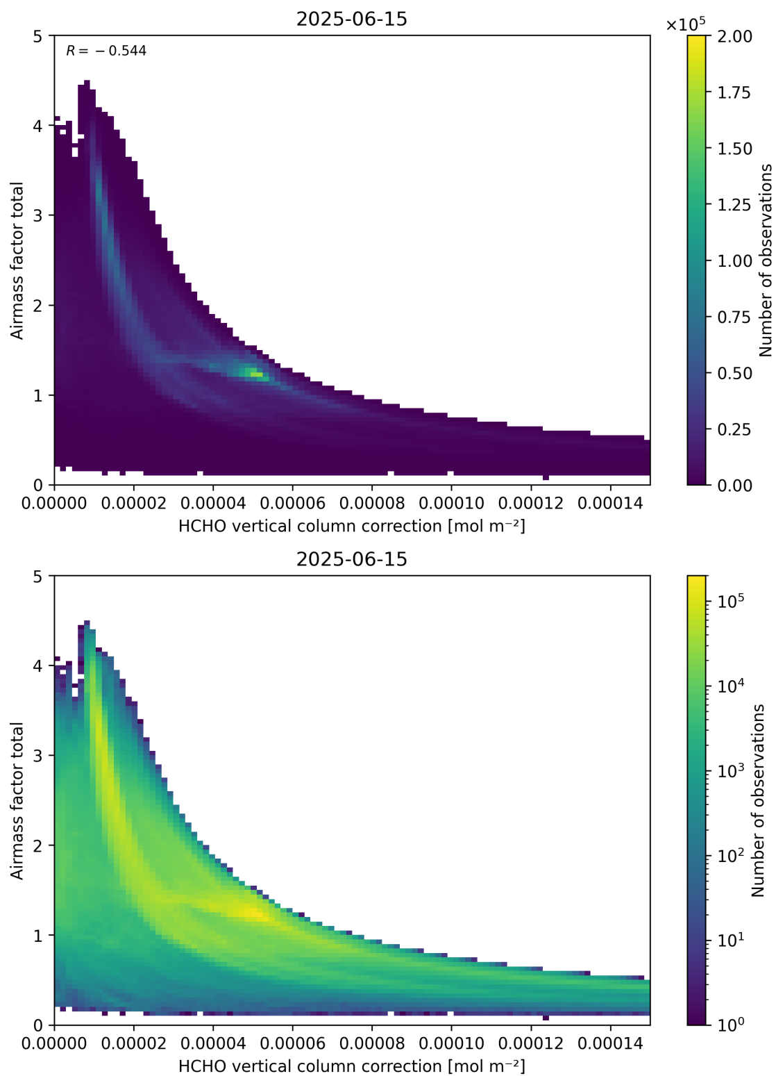
Figure 120: Scatter density plot of “HCHO vertical column correction” against “Airmass factor total” for 2025-06-14 to 2025-06-16.
