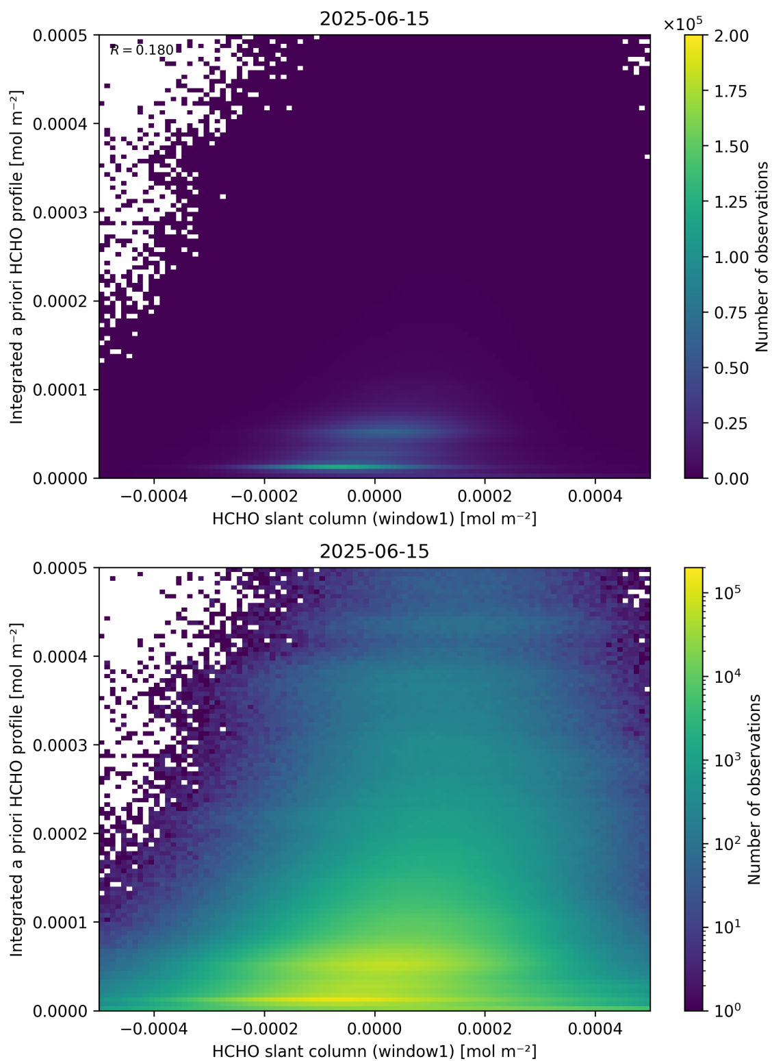
Figure 87: Scatter density plot of “HCHO slant column (window1)” against “Integrated a priori HCHO profile” for 2025-06-14 to 2025-06-16.
