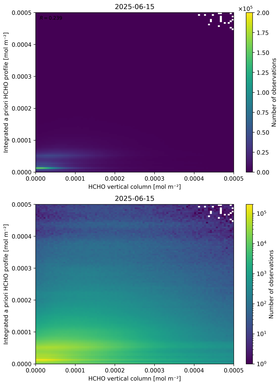
Figure 135: Scatter density plot of “HCHO vertical column” against “Integrated a priori HCHO profile” for 2025-06-14 to 2025-06-16.
