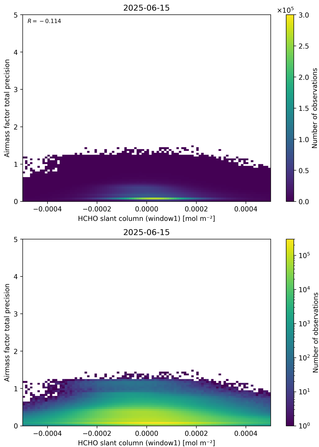
Figure 86: Scatter density plot of “HCHO slant column (window1)” against “Air mass factor total precision” for 2025-06-14 to 2025-06-16.
