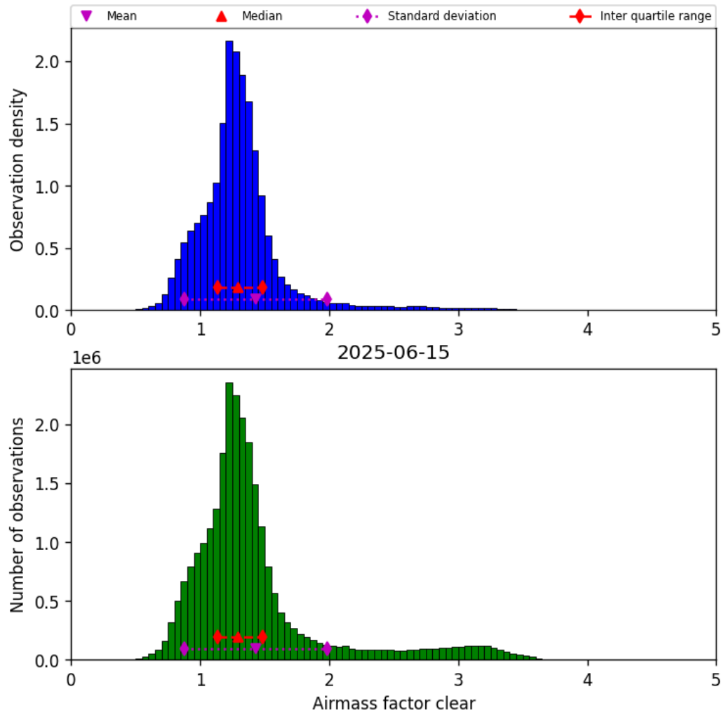
Figure 42: Histogram of “Airmass factor clear” for 2025-06-14 to 2025-06-16
