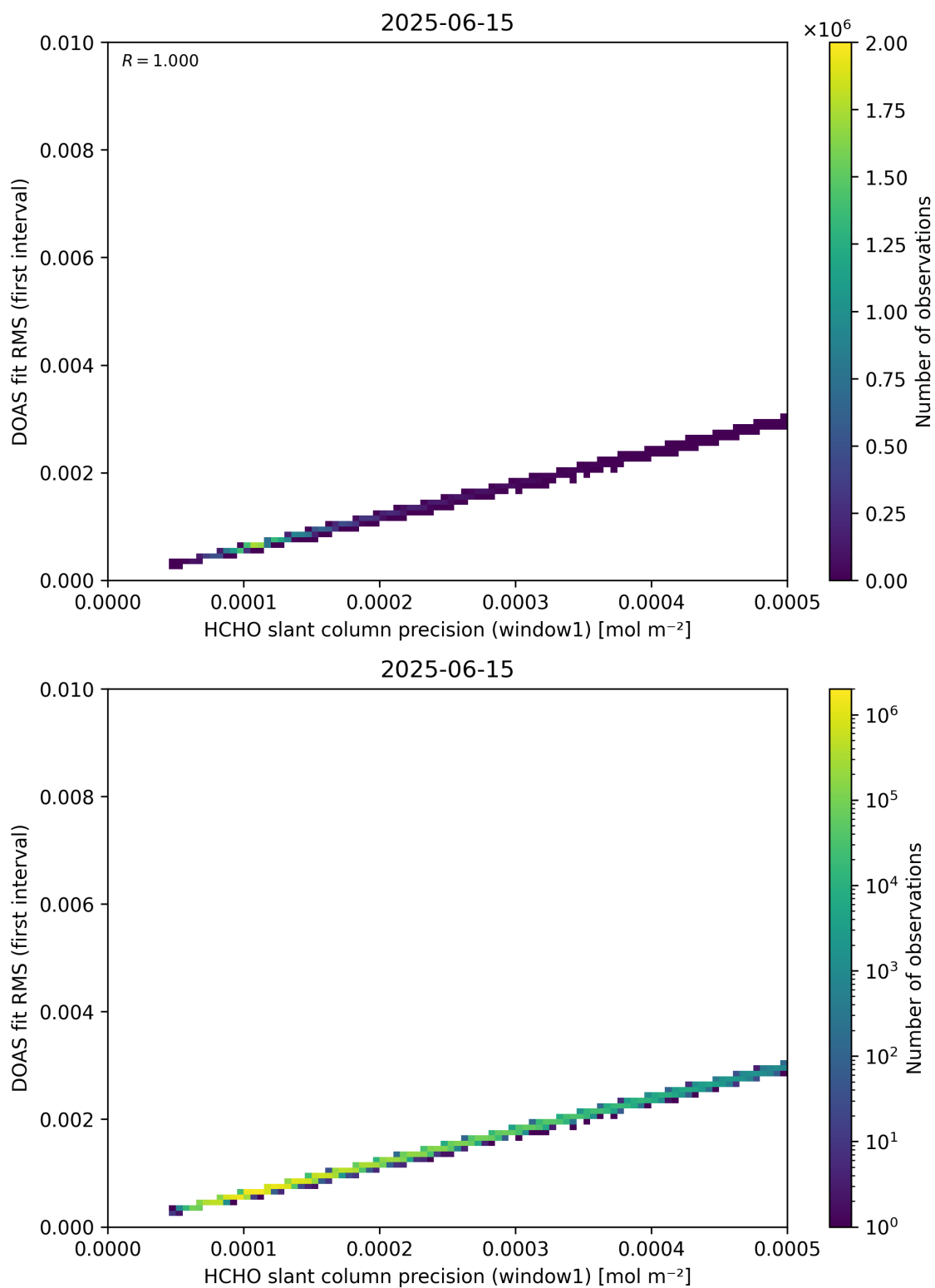
Figure 88: Scatter density plot of “HCHO slant column precision (window1)” against “DOAS fit RMS (first interval)” for 2025-06-14 to 2025-06-16.
