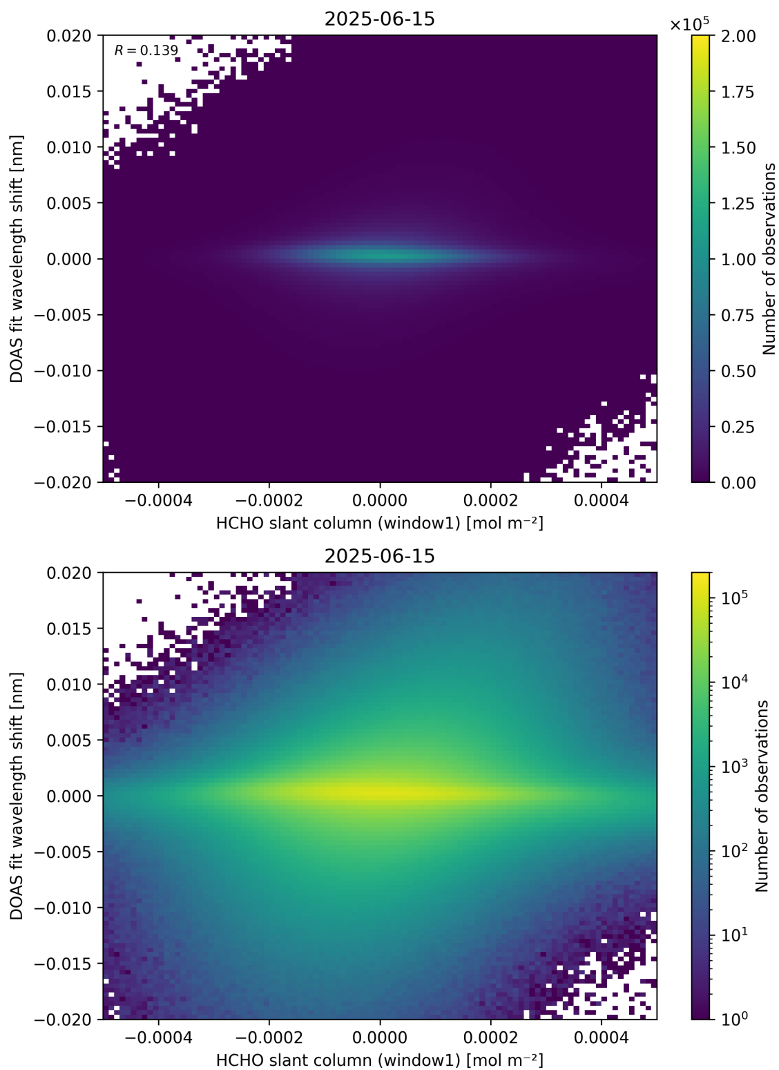
Figure 79: Scatter density plot of “HCHO slant column (window1)” against “DOAS fit wavelength shift” for 2025-06-14 to 2025-06-16.
