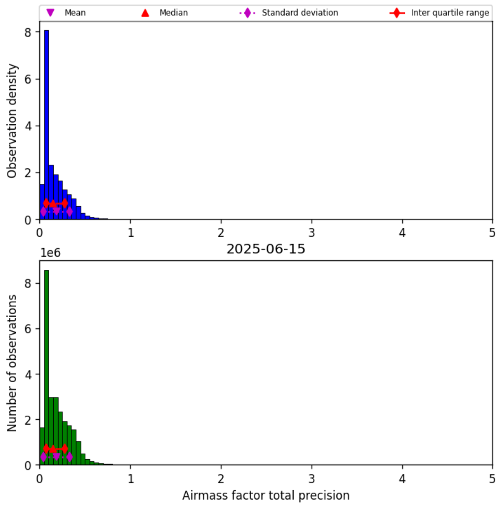
Figure 41: Histogram of “Airmass factor total precision” for 2025-06-14 to 2025-06-16
