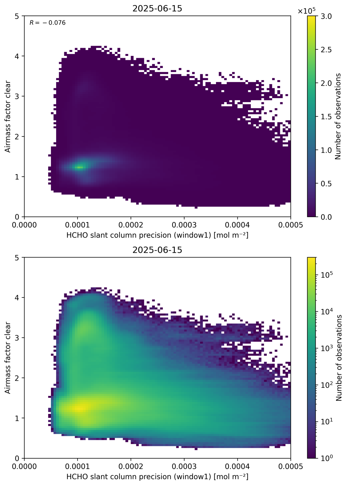
Figure 91: Scatter density plot of “HCHO slant column precision (window1)” against “Airmass factor clear” for 2025-06-14 to 2025-06-16.
