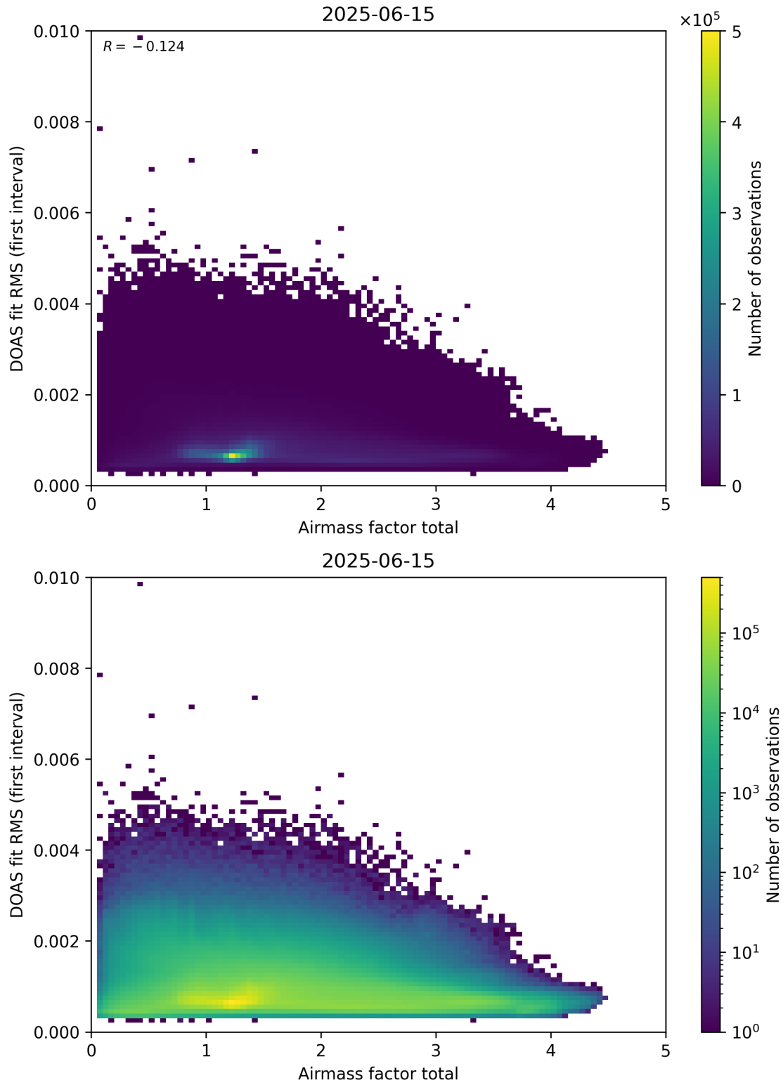
Figure 97: Scatter density plot of “Airmass factor total” against “DOAS fit RMS (first interval)” for 2025-06-14 to 2025-06-16.
