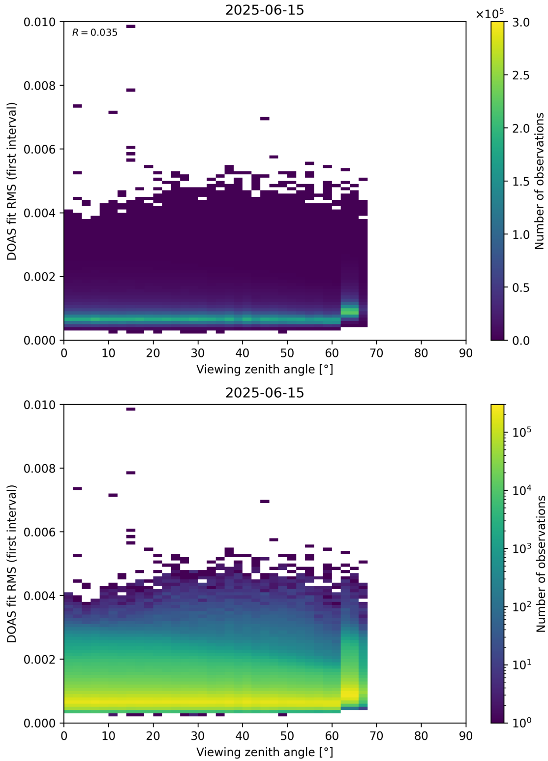
Figure 182: Scatter density plot of “Viewing zenith angle” against “DOAS fit RMS (first interval)” for 2025-06-14 to 2025-06-16.
