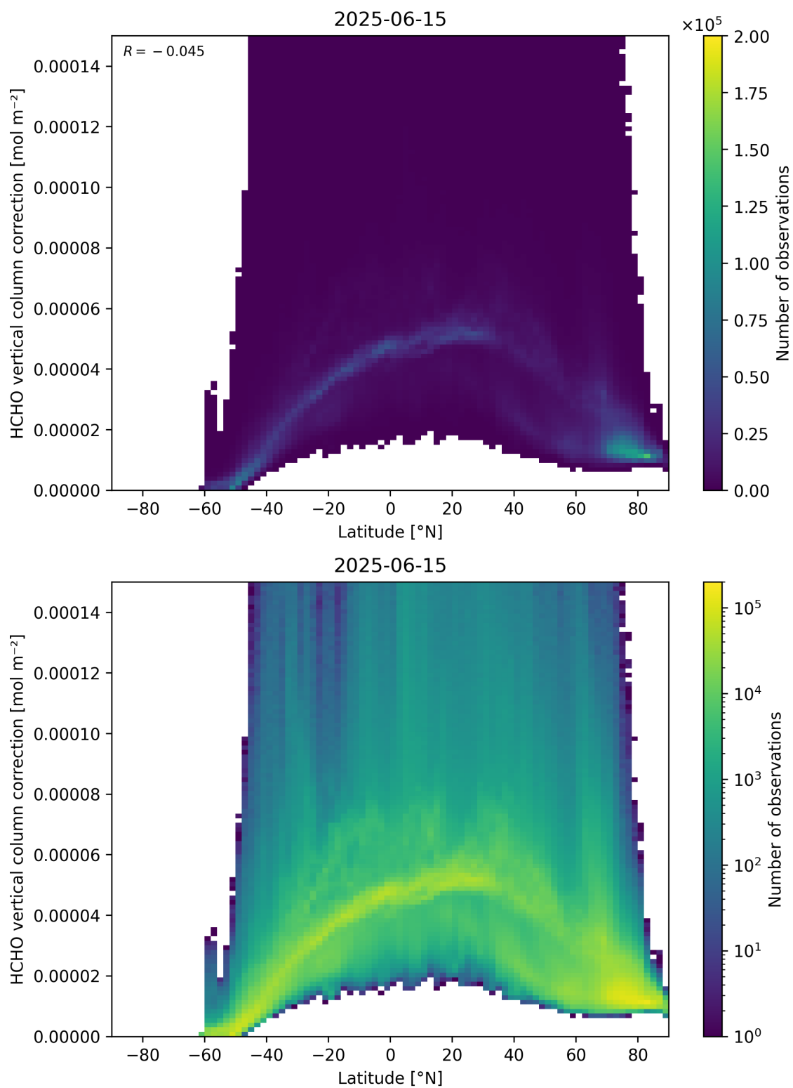
Figure 164: Scatter density plot of “Latitude” against “HCHO vertical column correction” for 2025-06-14 to 2025-06-16.
