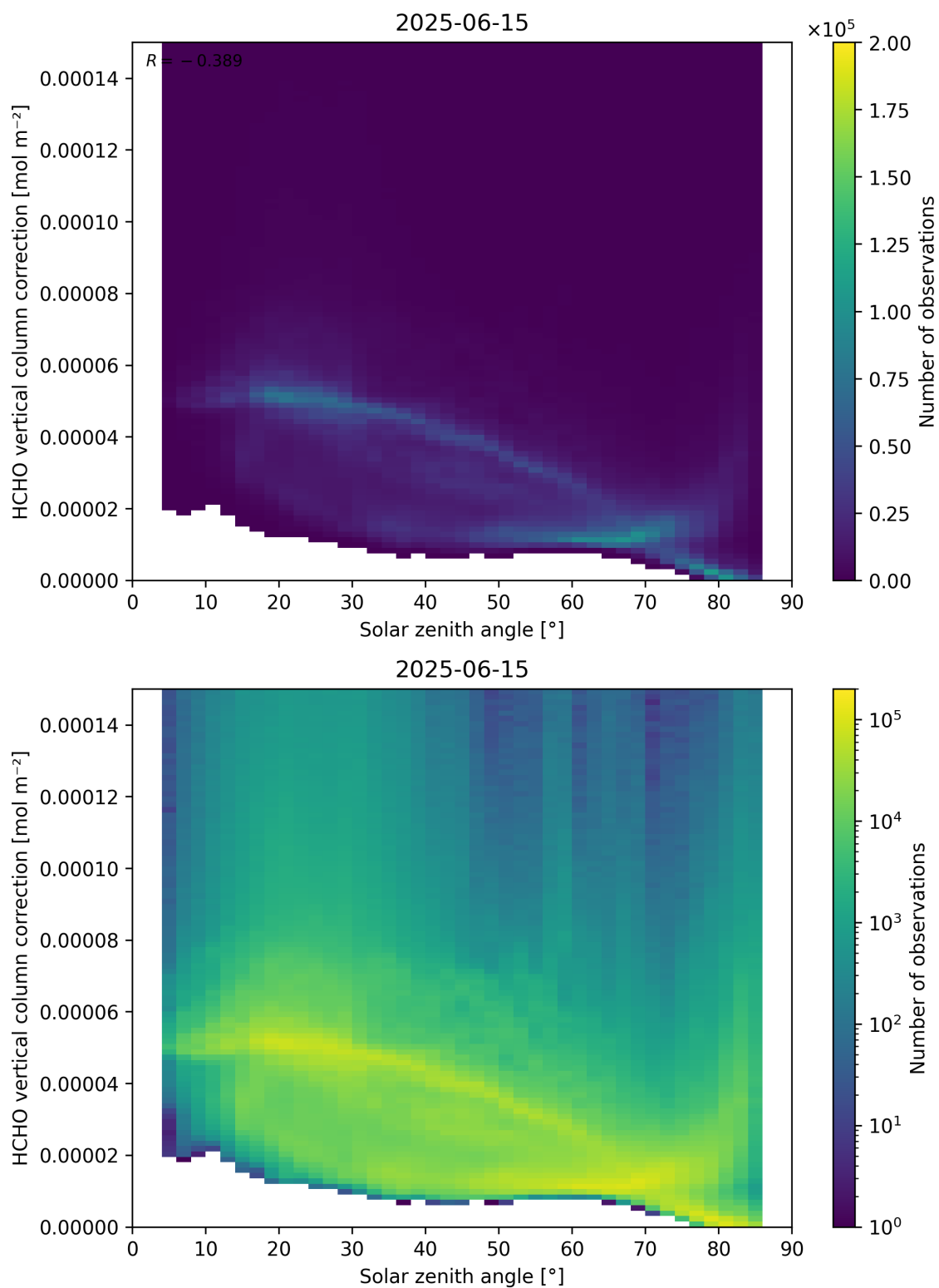
Figure 178: Scatter density plot of “Solar zenith angle” against “HCHO vertical column correction” for 2025-06-14 to 2025-06-16.
