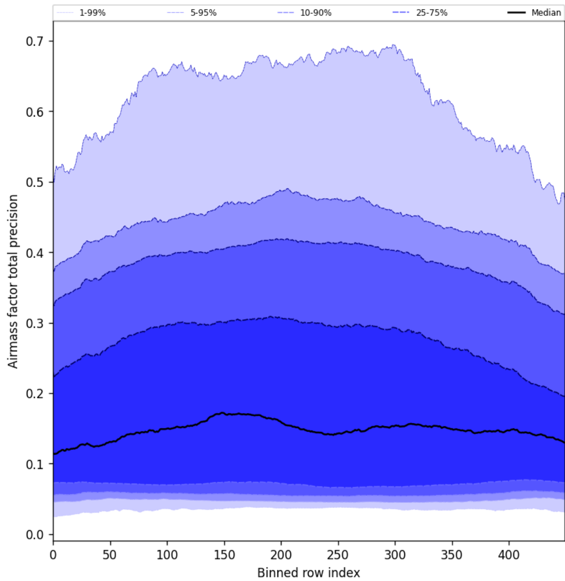
Figure 55: Along track statistics of “Airmass factor total precision” for 2025-06-14 to 2025-06-16
