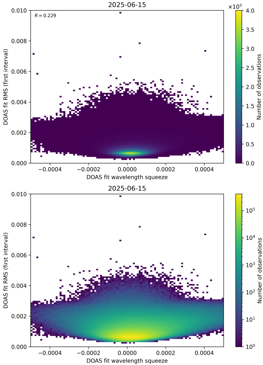
Figure 68: Scatter density plot of “DOAS fit wavelength squeeze” against “DOAS fit RMS (first interval)” for 2025-06-14 to 2025-06-16.
