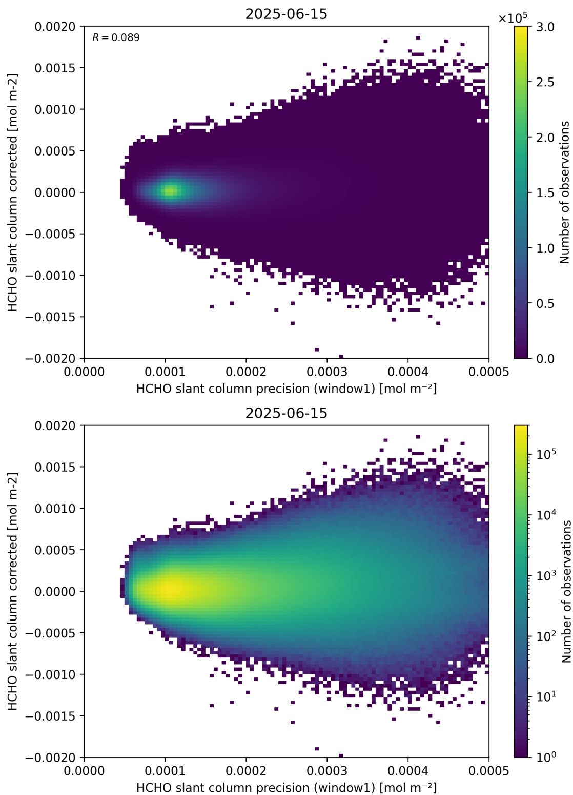
Figure 92: Scatter density plot of “HCHO slant column precision (window1)” against “HCHO slant column corrected” for 2025-06-14 to 2025-06-16.
