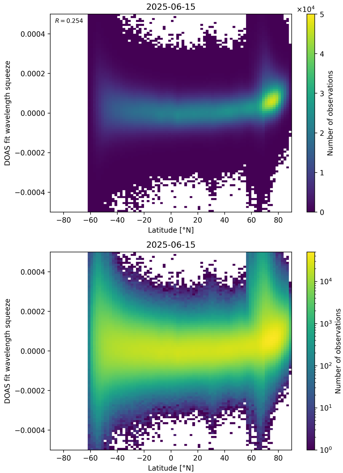
Figure 155: Scatter density plot of “Latitude” against “DOAS fit wavelength squeeze” for 2025-06-14 to 2025-06-16.
