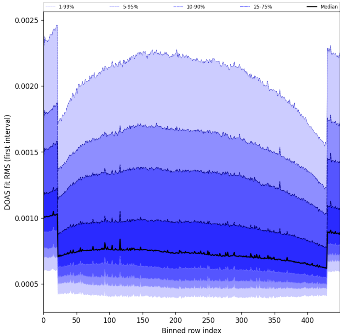
Figure 60: Along track statistics of “DOAS fit RMS (first interval)” for 2025-06-14 to 2025-06-16
