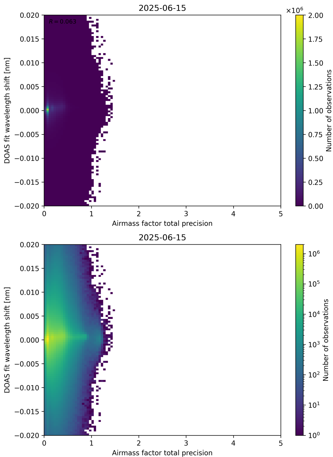
Figure 106: Scatter density plot of “Airmass factor total precision” against “DOAS fit wavelength shift” for 2025-06-14 to 2025-06-16.
