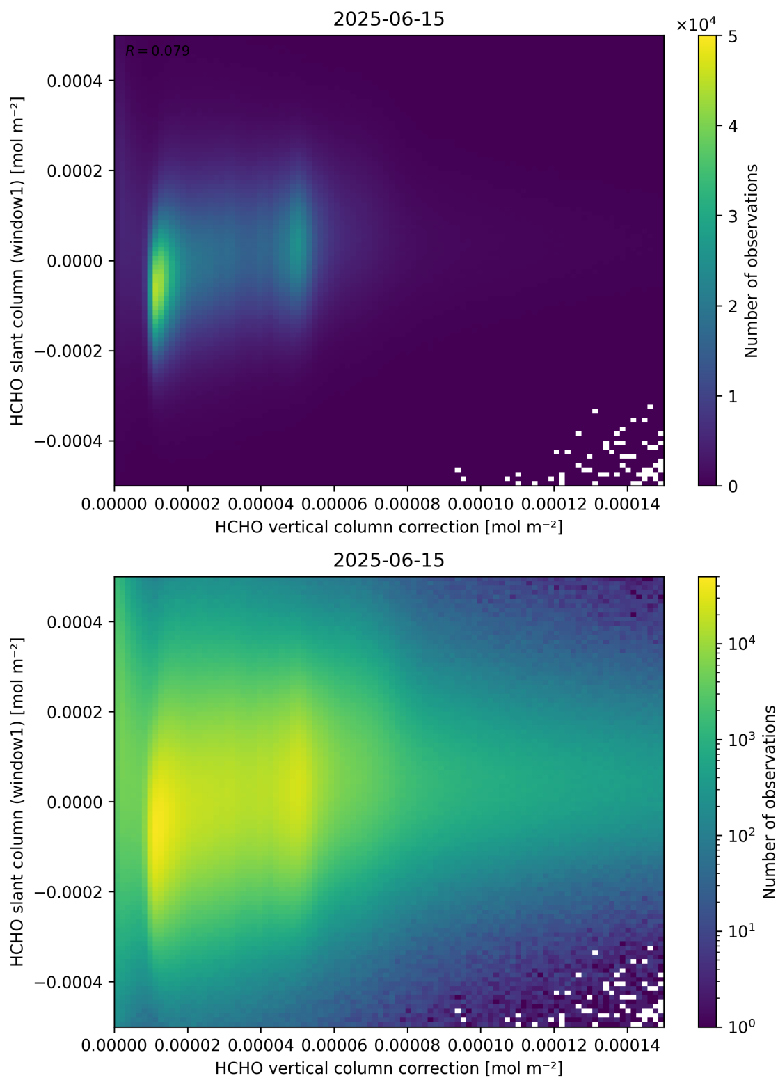
Figure 118: Scatter density plot of “HCHO vertical column correction” against “HCHO slant column (window1)” for 2025-06-14 to 2025-06-16.
