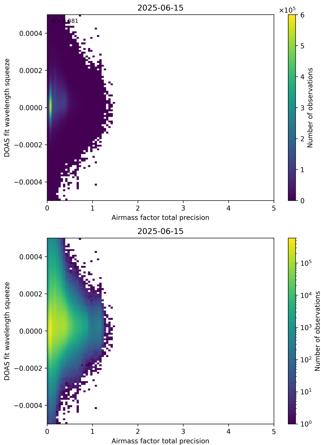
Figure 107: Scatter density plot of “Airmass factor total precision” against “DOAS fit wavelength squeeze” for 2025-06-14 to 2025-06-16.
