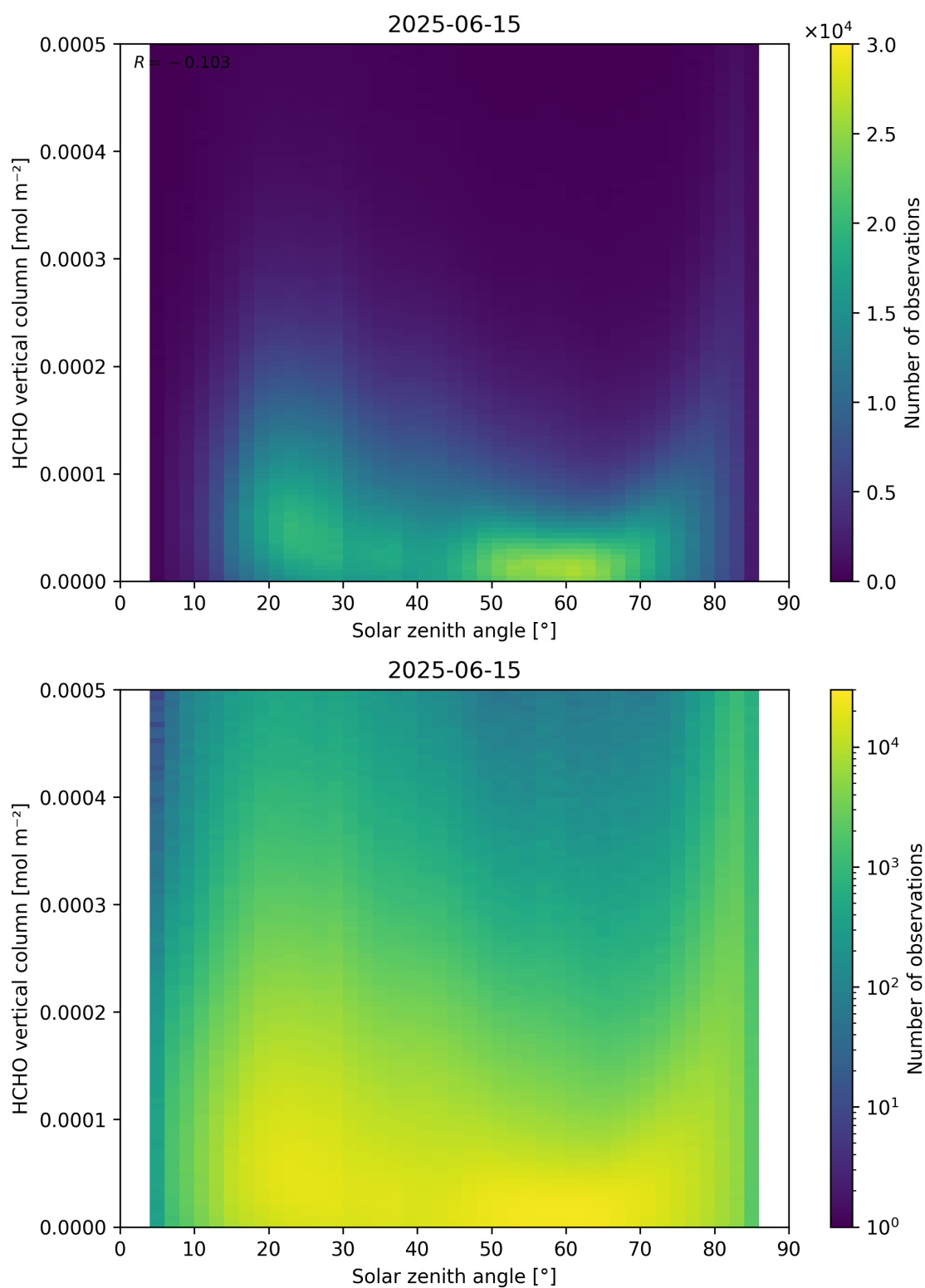
Figure 177: Scatter density plot of “Solar zenith angle” against “HCHO vertical column” for 2025-06-14 to 2025-06-16.
