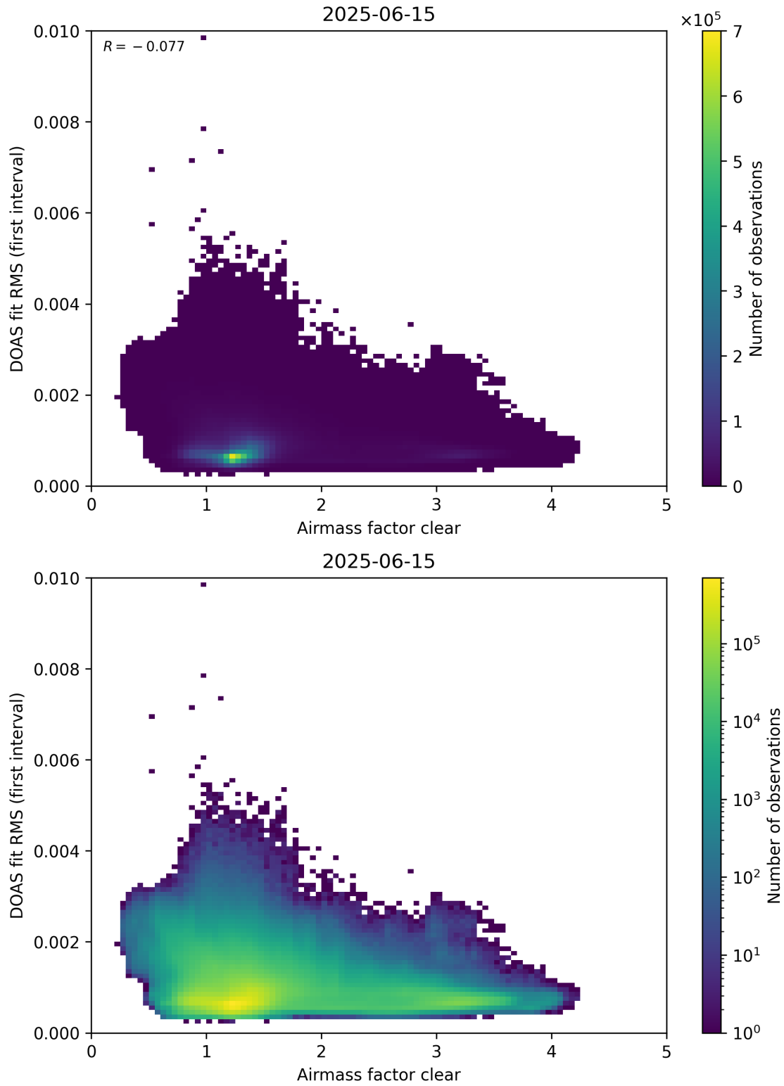
Figure 71: Scatter density plot of “Airmass factor clear” against “DOAS fit RMS (first interval)” for 2025-06-14 to 2025-06-16.
