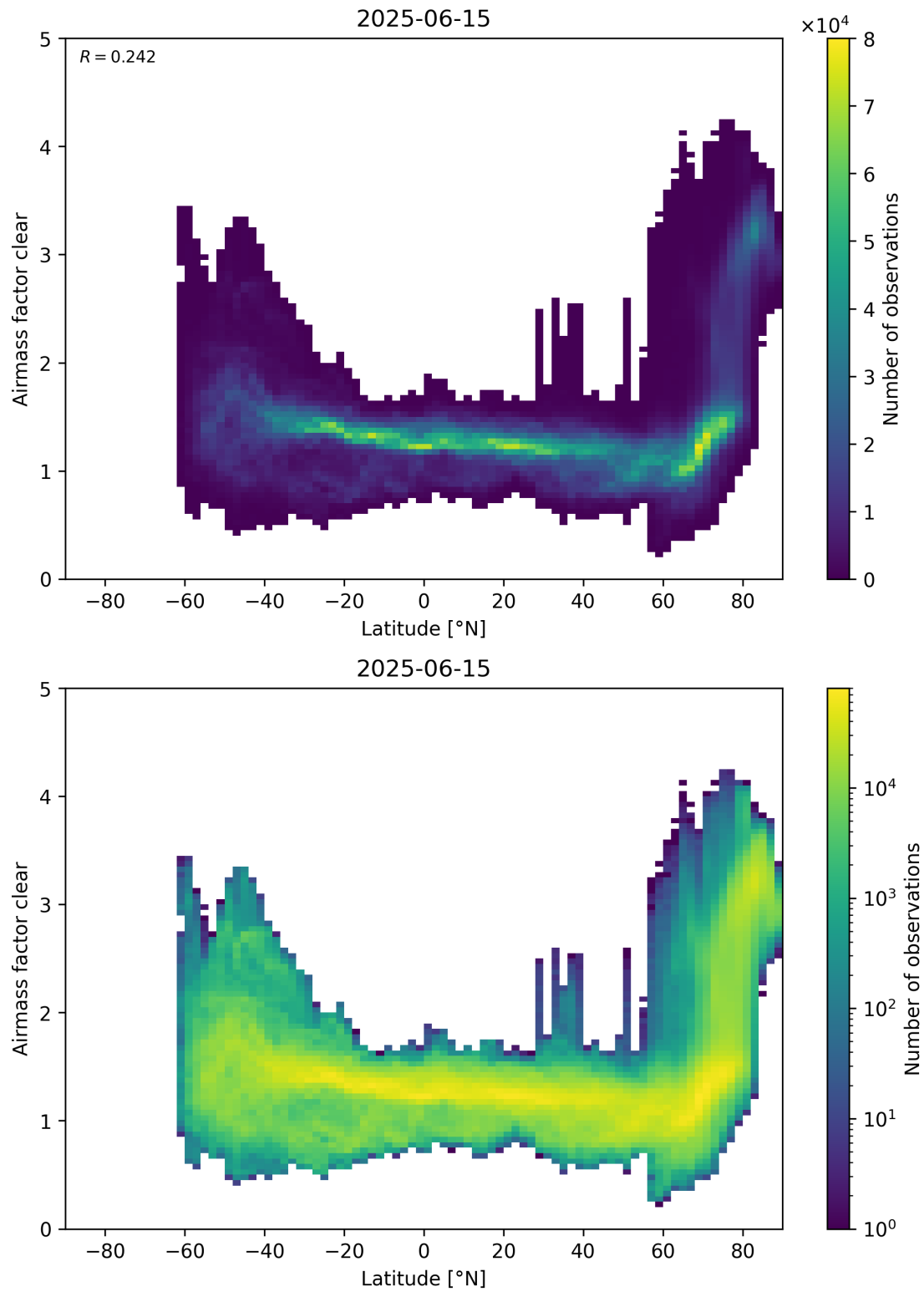
Figure 156: Scatter density plot of “Latitude” against “Airmass factor clear” for 2025-06-14 to 2025-06-16.
