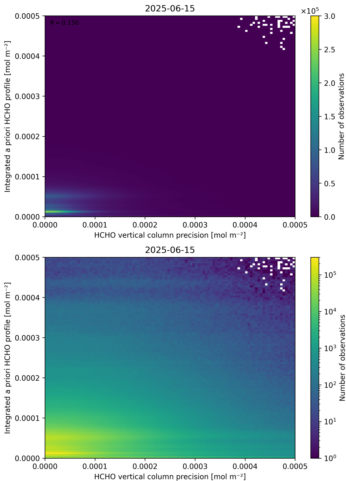
Figure 147: Scatter density plot of “HCHO vertical column precision” against “Integrated a priori HCHO profile” for 2025-06-14 to 2025-06-16.
