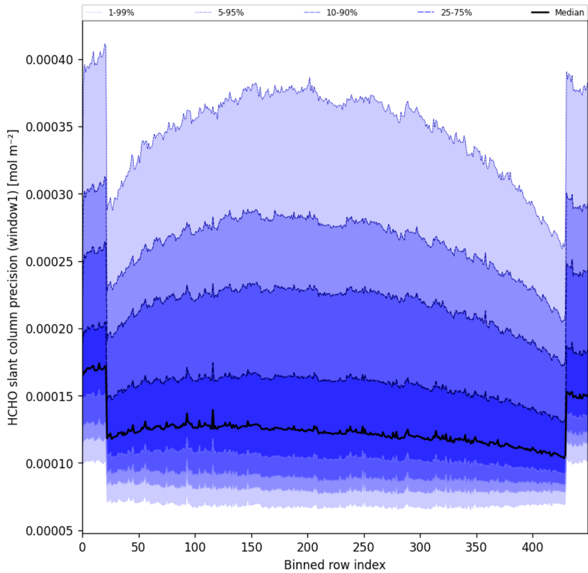
Figure 53: Along track statistics of “HCHO slant column precision (window1)” for 2025-06-14 to 2025-06-16
