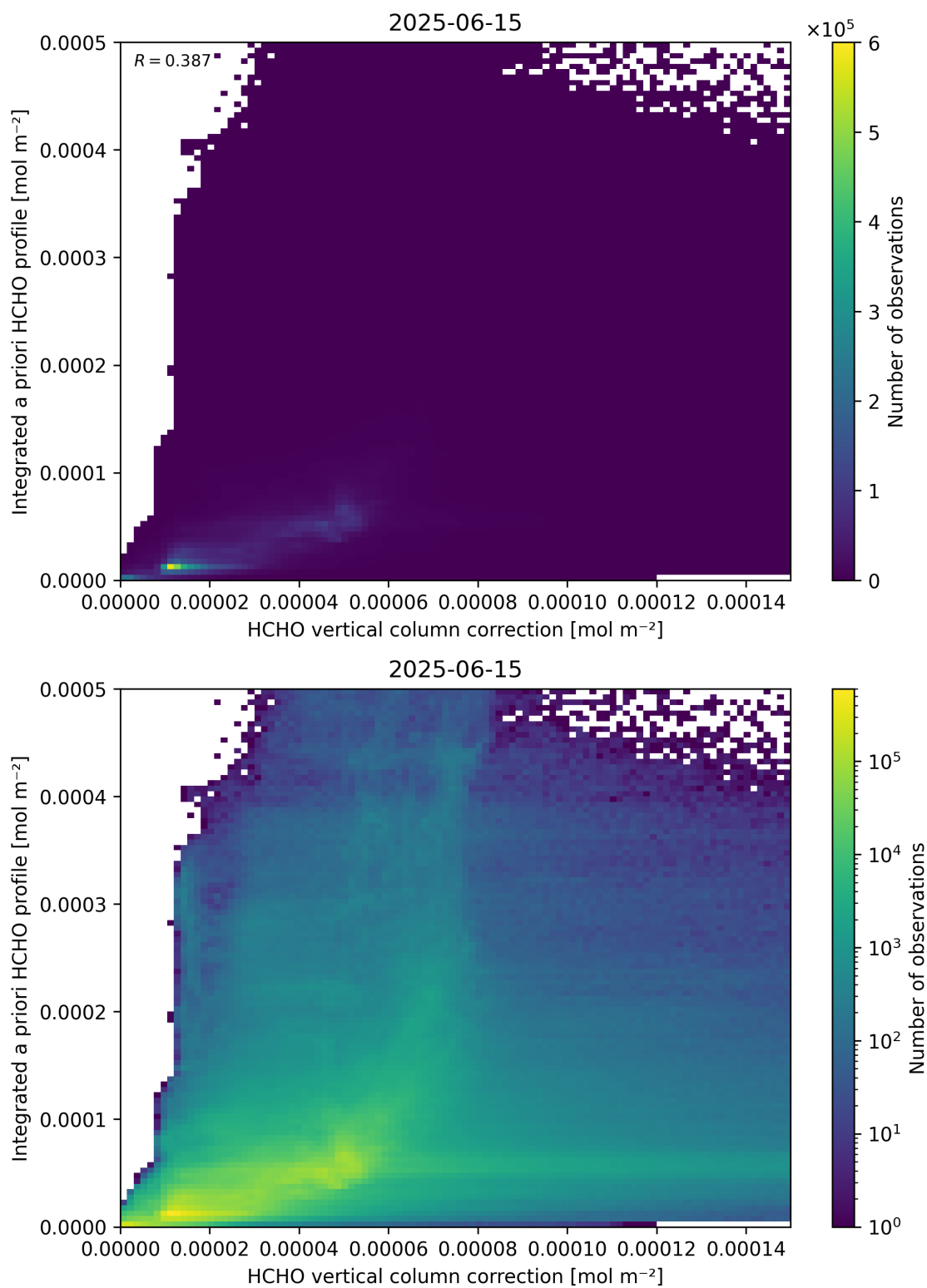
Figure 122: Scatter density plot of “HCHO vertical column correction” against “Integrated a priori HCHO profile” for 2025-06-14 to 2025-06-16.
