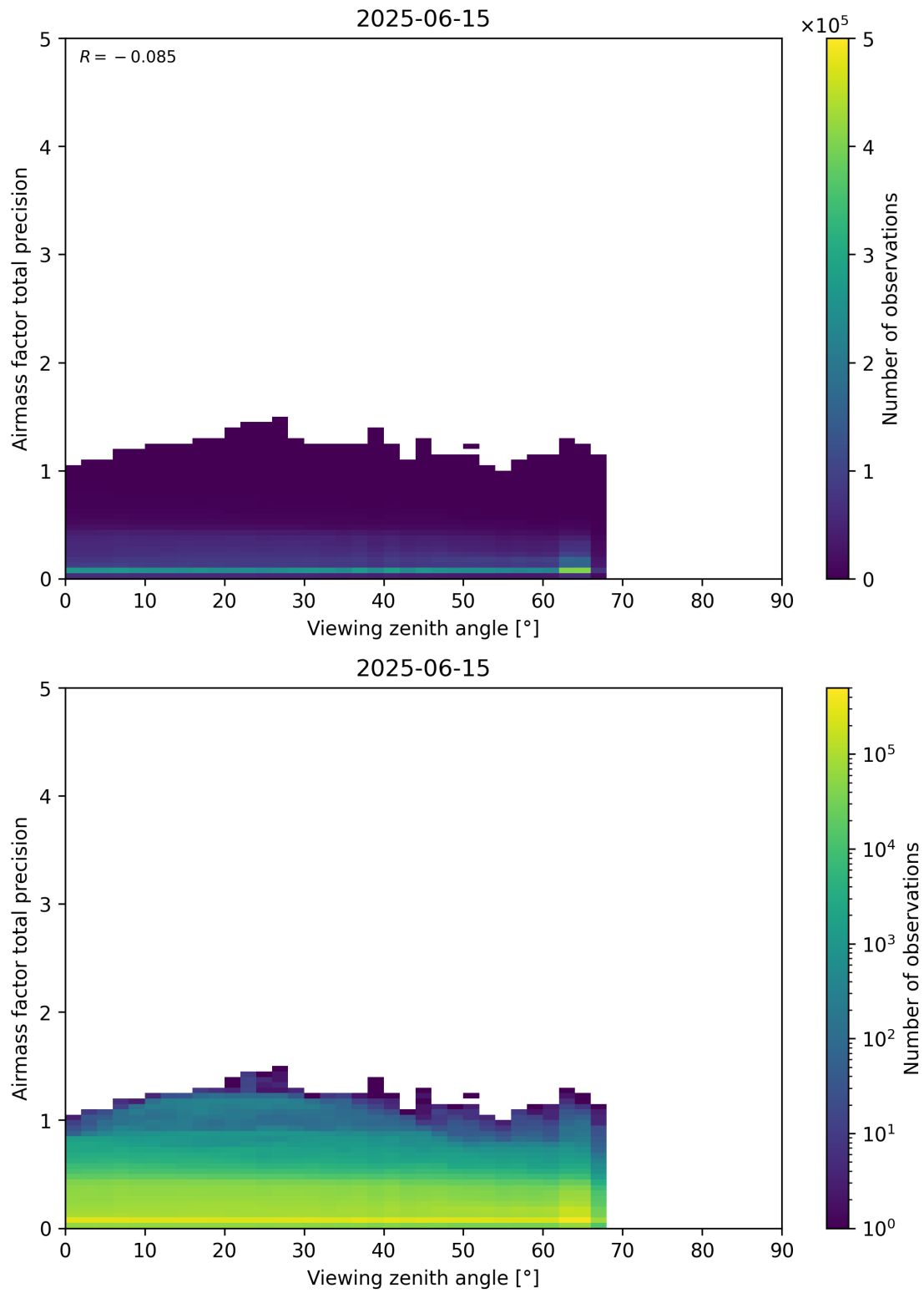
Figure 191: Scatter density plot of “Viewing zenith angle” against “Airmass factor total precision” for 2025-06-14 to 2025-06-16.
