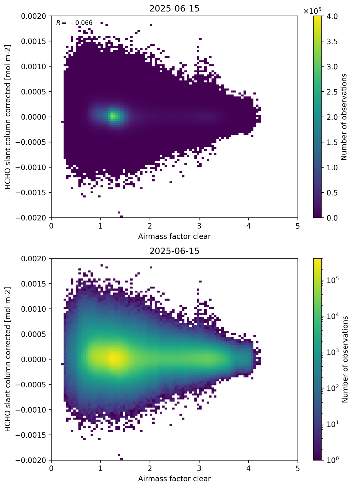
Figure 74: Scatter density plot of “Airmass factor clear” against “HCHO slant column corrected” for 2025-06-14 to 2025-06-16.
