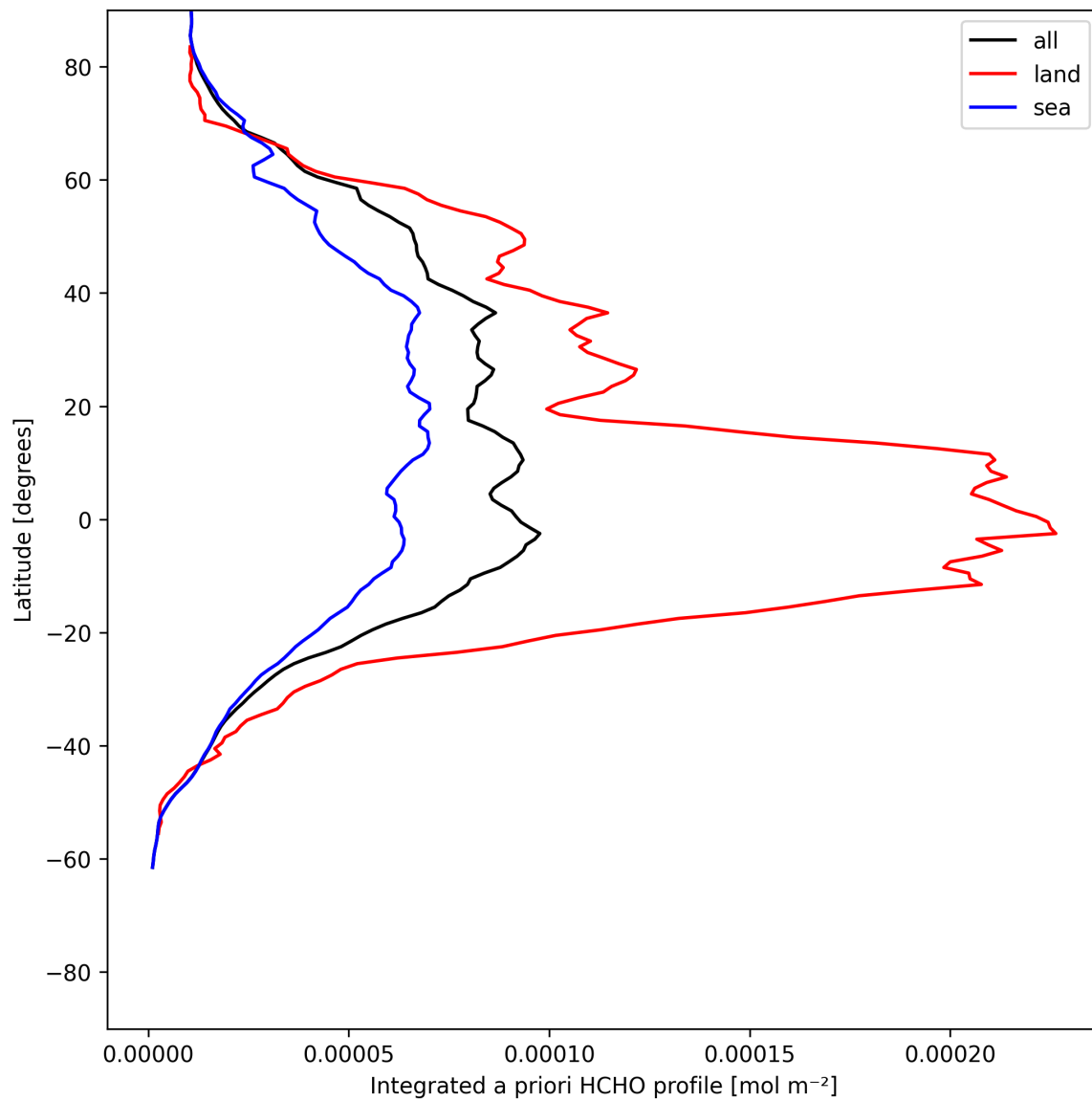
Figure 29: Zonal average of “Integrated a priori HCHO profile” for 2025-06-14 to 2025-06-16.
