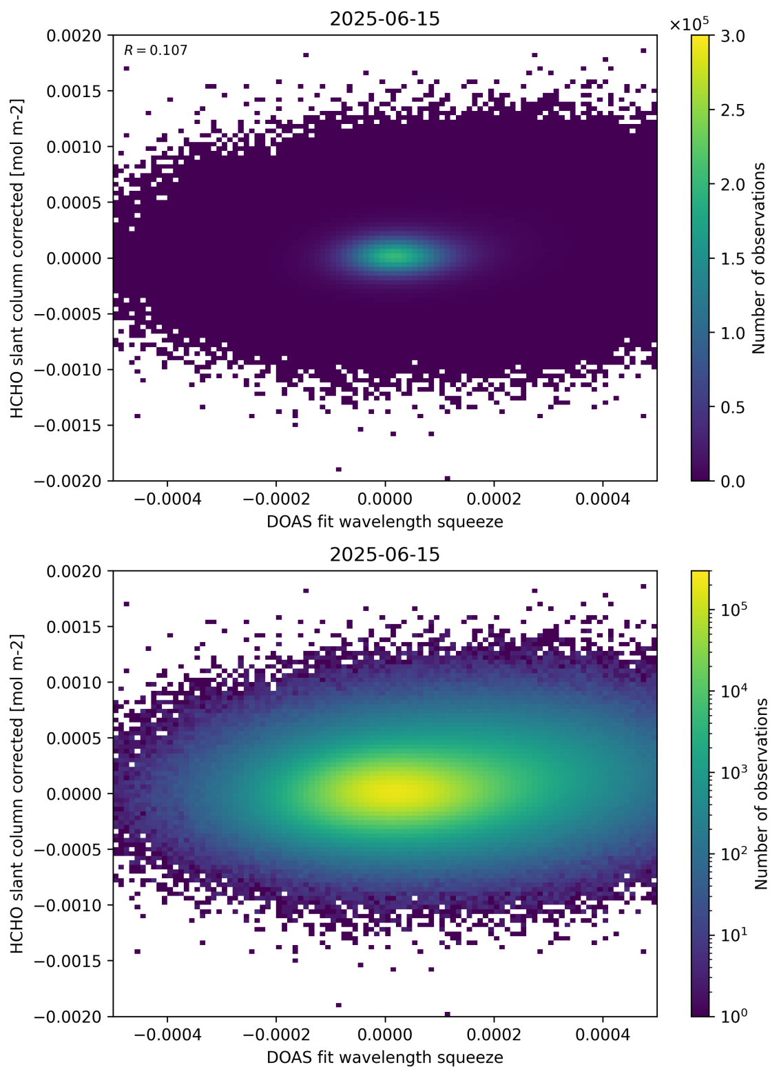
Figure 69: Scatter density plot of “DOAS fit wavelength squeeze” against “HCHO slant column corrected” for 2025-06-14 to 2025-06-16.
