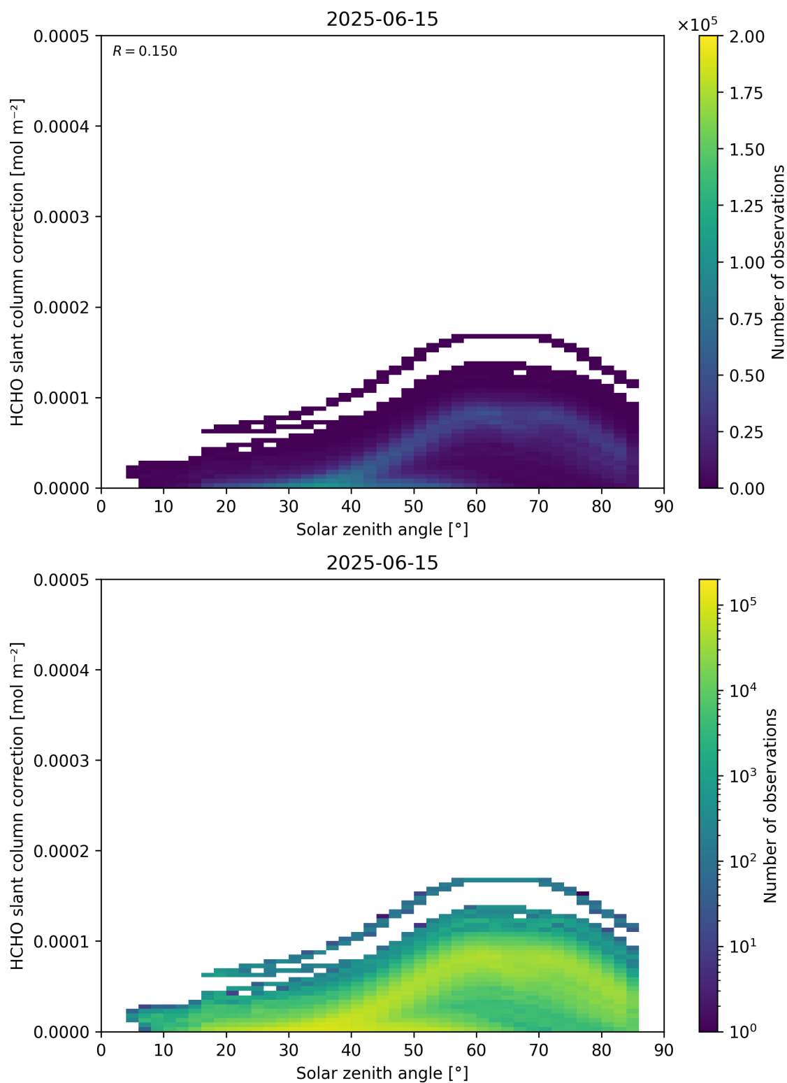
Figure 172: Scatter density plot of “Solar zenith angle” against “HCHO slant column correction” for 2025-06-14 to 2025-06-16.
