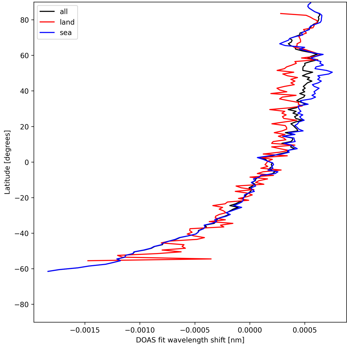
Figure 30: Zonal average of “DOAS fit wavelength shift” for 2025-06-14 to 2025-06-16.
