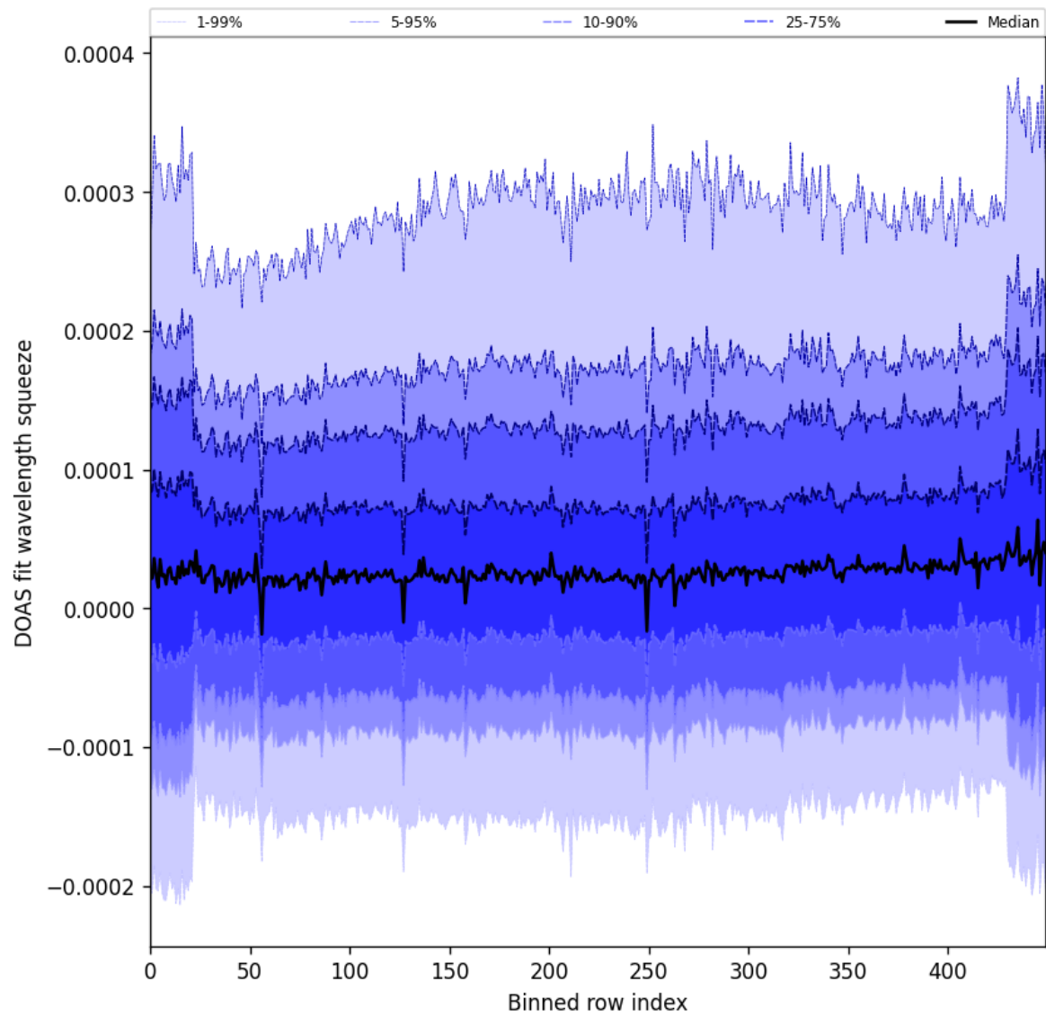
Figure 59: Along track statistics of “DOAS fit wavelength squeeze” for 2025-06-14 to 2025-06-16
