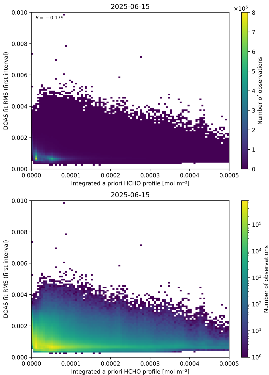
Figure 148: Scatter density plot of “Integrated a priori HCHO profile” against “DOAS fit RMS (first interval)” for 2025-06-14 to 2025-06-16.
