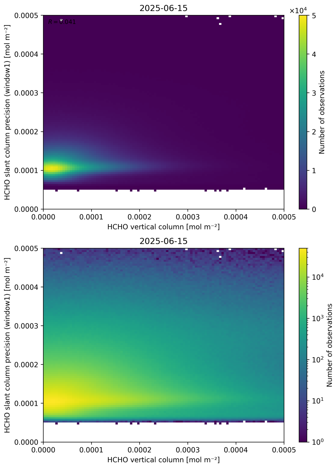
Figure 130: Scatter density plot of “HCHO vertical column” against “HCHO slant column precision (window1)” for 2025-06-14 to 2025-06-16.
