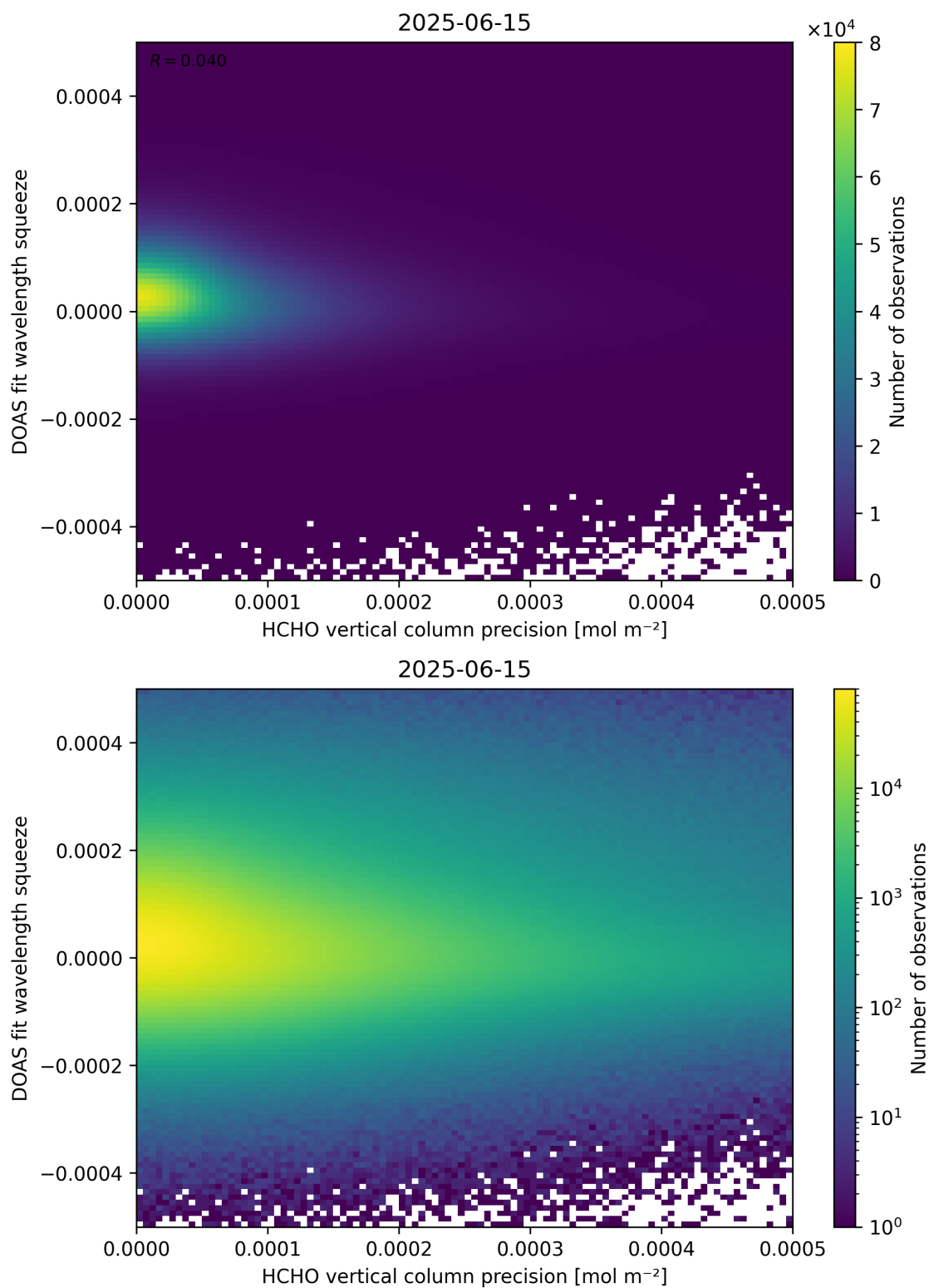
Figure 138: Scatter density plot of “HCHO vertical column precision” against “DOAS fit wavelength squeeze” for 2025-06-14 to 2025-06-16.
