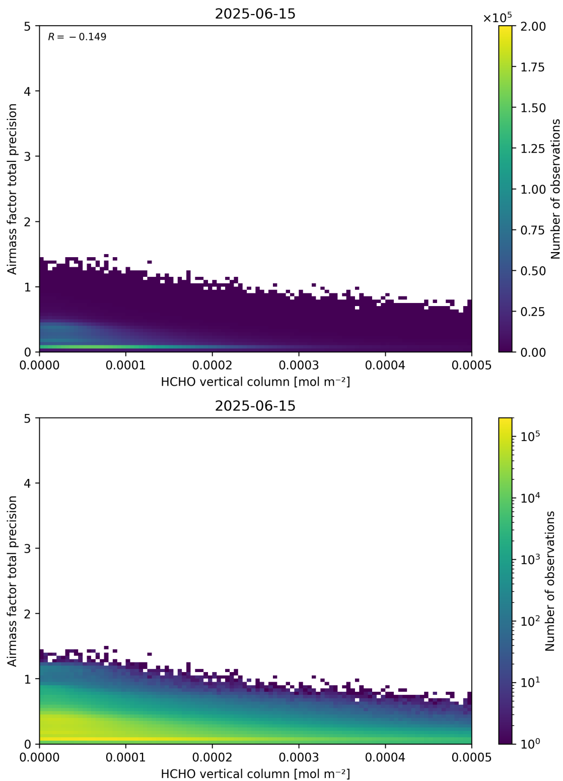
Figure 132: Scatter density plot of “HCHO vertical column” against “Airmass factor total precision” for 2025-06-14 to 2025-06-16.
