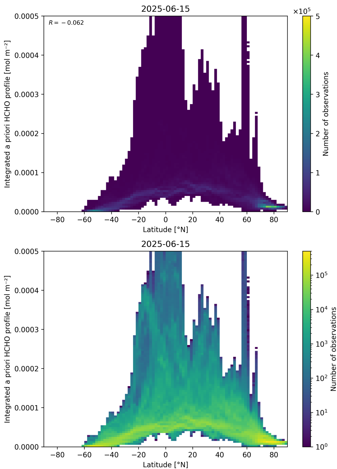
Figure 166: Scatter density plot of “Latitude” against “Integrated a priori HCHO profile” for 2025-06-14 to 2025-06-16.
