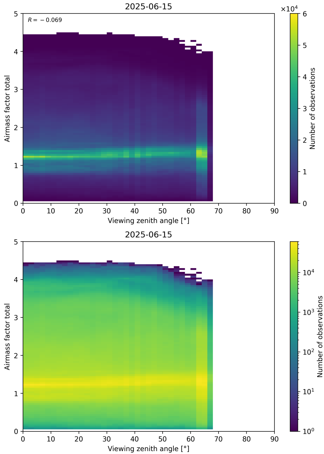
Figure 190: Scatter density plot of “Viewing zenith angle” against “Airmass factor total” for 2025-06-14 to 2025-06-16.
