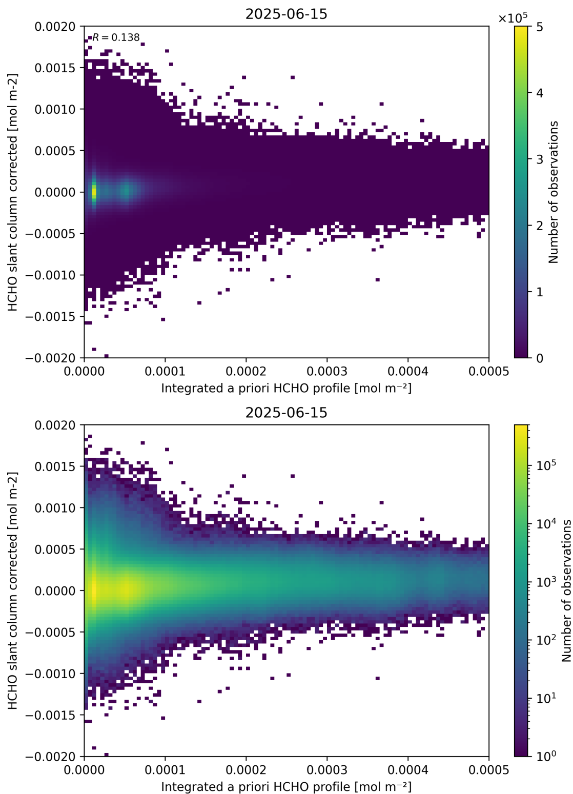
Figure 151: Scatter density plot of “Integrated a priori HCHO profile” against “HCHO slant column corrected” for 2025-06-14 to 2025-06-16.
