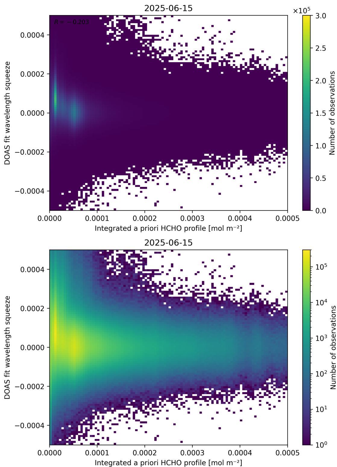
Figure 150: Scatter density plot of “Integrated a priori HCHO profile” against “DOAS fit wavelength squeeze” for 2025-06-14 to 2025-06-16.
