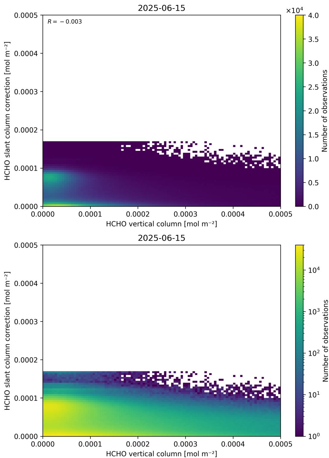
Figure 128: Scatter density plot of “HCHO vertical column” against “HCHO slant column correction” for 2025-06-14 to 2025-06-16.
