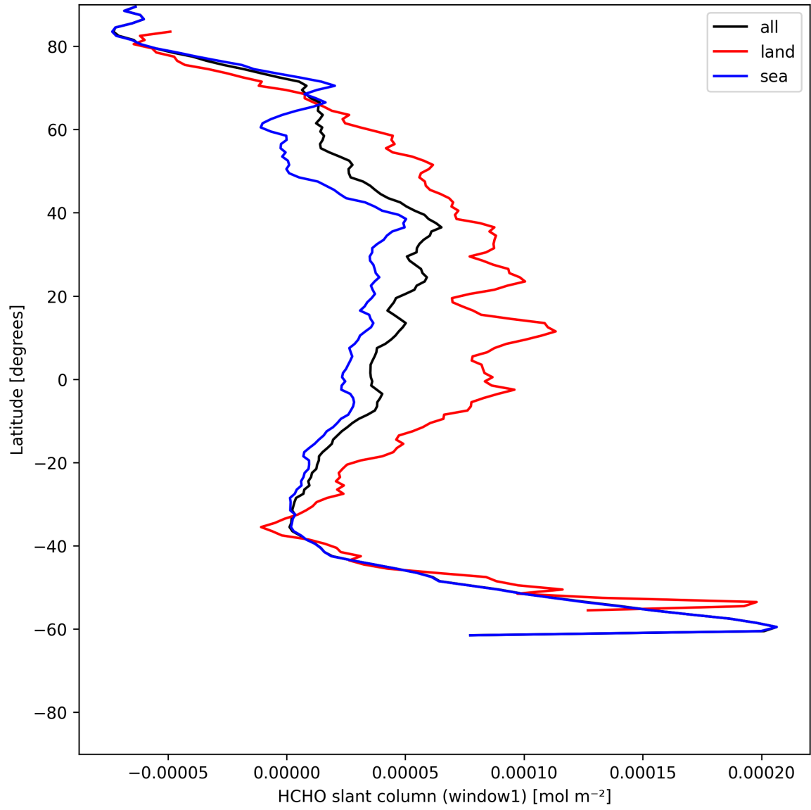
Figure 24: Zonal average of “HCHO slant column (window1)” for 2025-06-14 to 2025-06-16.
