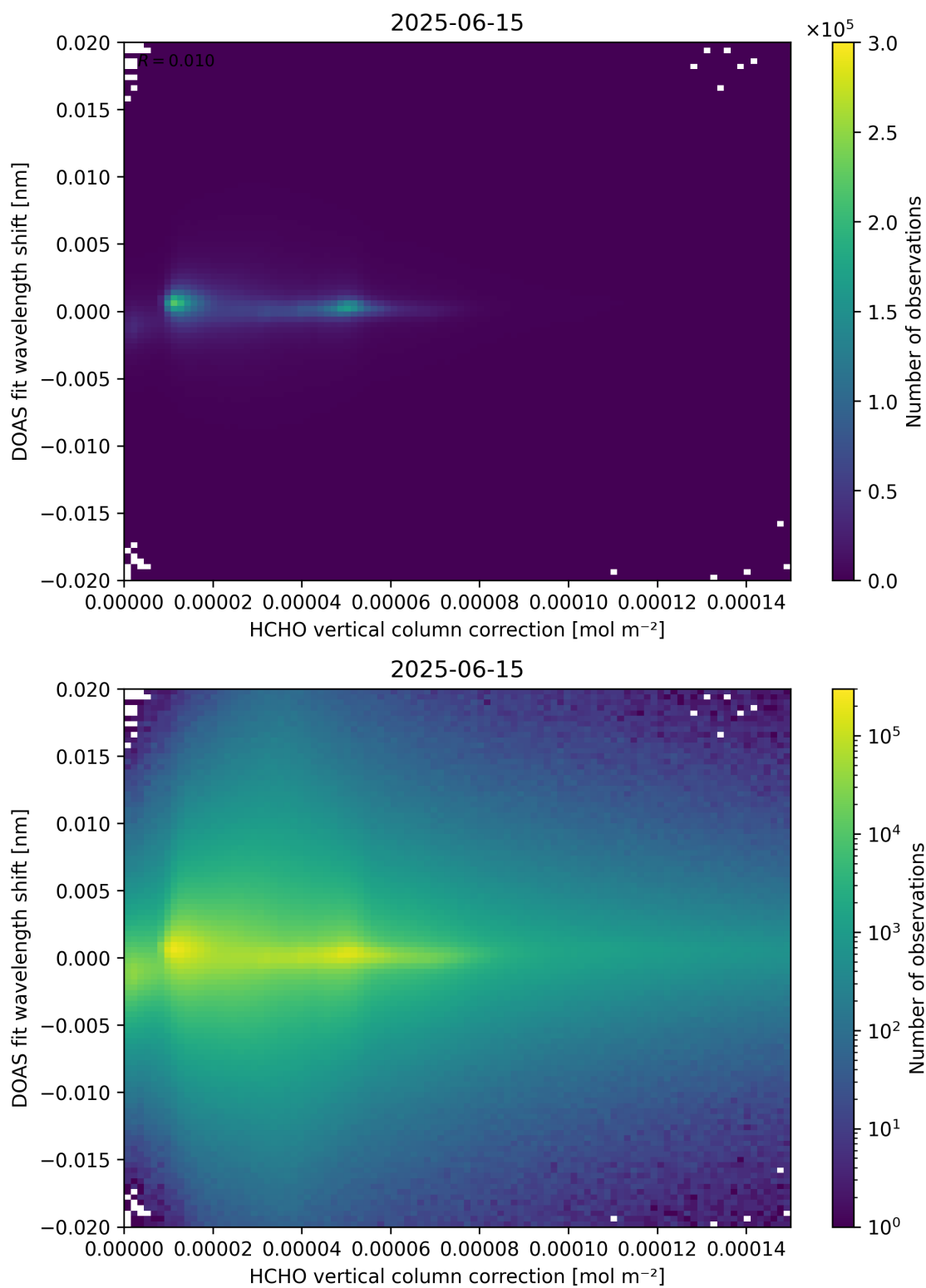
Figure 113: Scatter density plot of “HCHO vertical column correction” against “DOAS fit wavelength shift” for 2025-06-14 to 2025-06-16.
