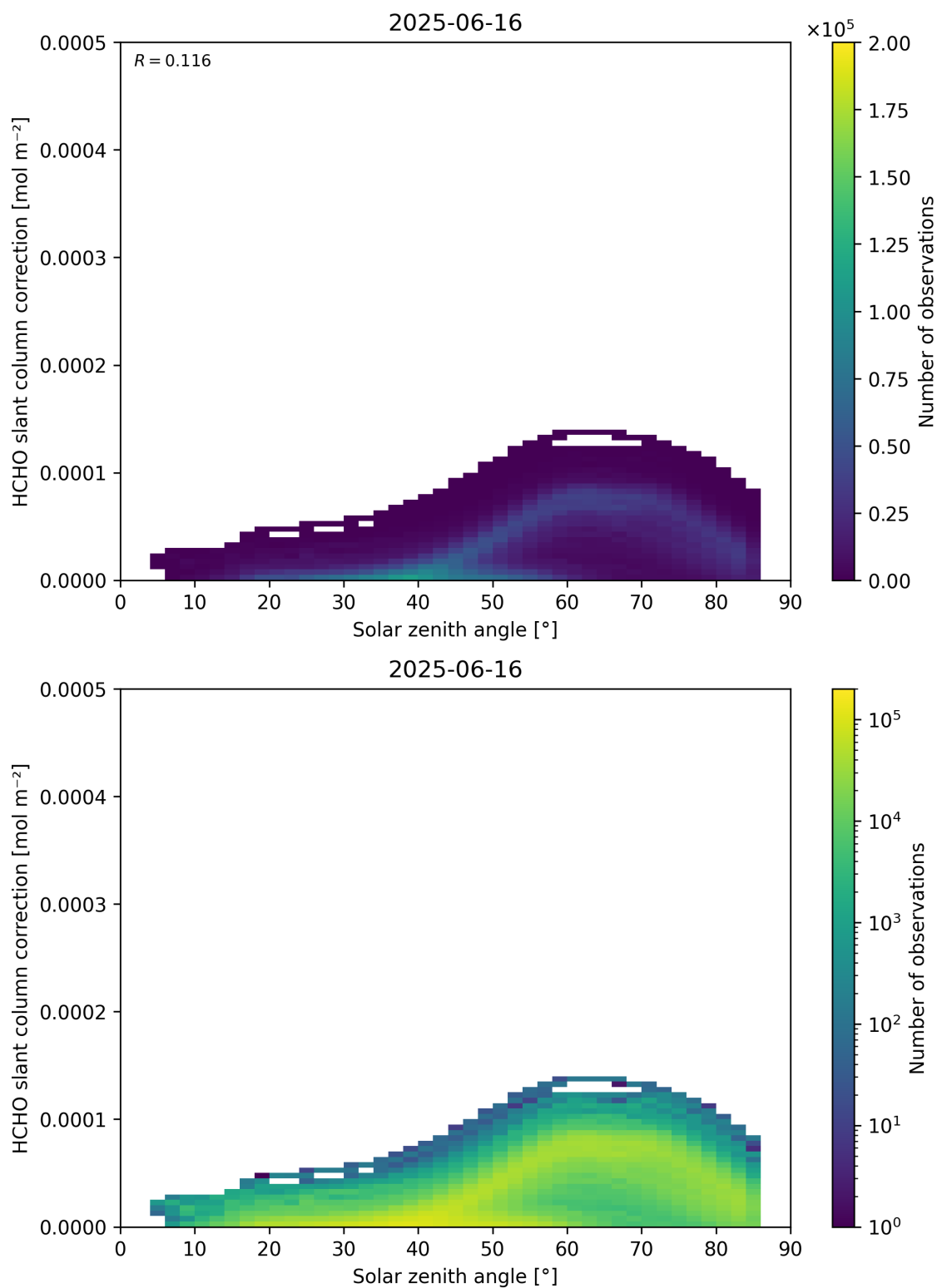
Figure 172: Scatter density plot of “Solar zenith angle” against “HCHO slant column correction” for 2025-06-16 to 2025-06-17.
