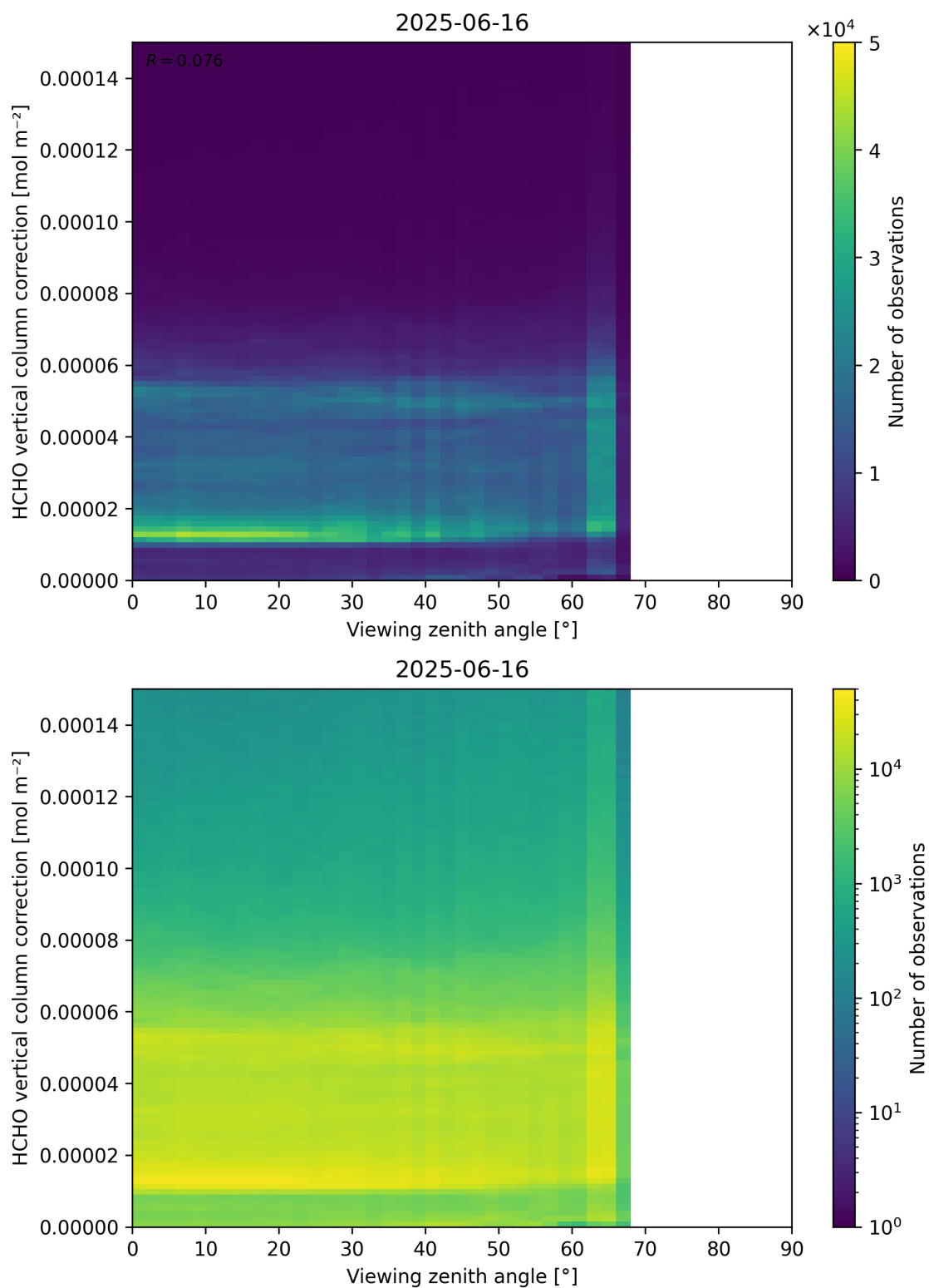
Figure 193: Scatter density plot of “Viewing zenith angle” against “HCHO vertical column correction” for 2025-06-16 to 2025-06-17.
