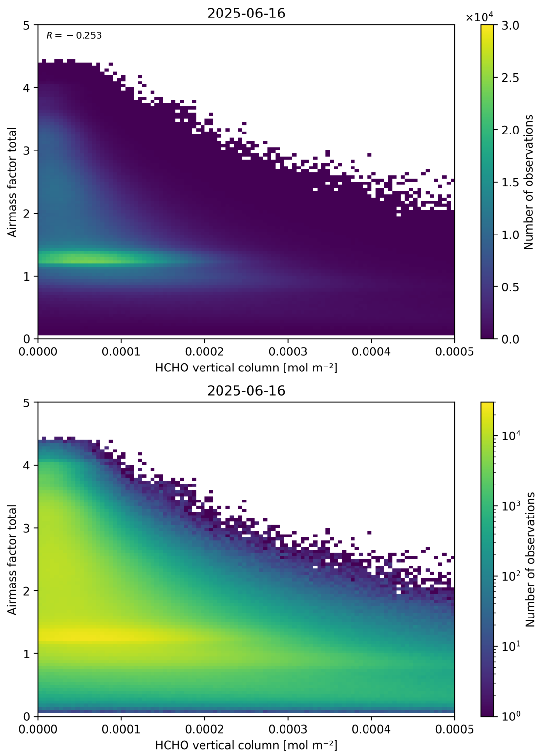
Figure 131: Scatter density plot of “HCHO vertical column” against “Airmass factor total” for 2025-06-16 to 2025-06-17.
