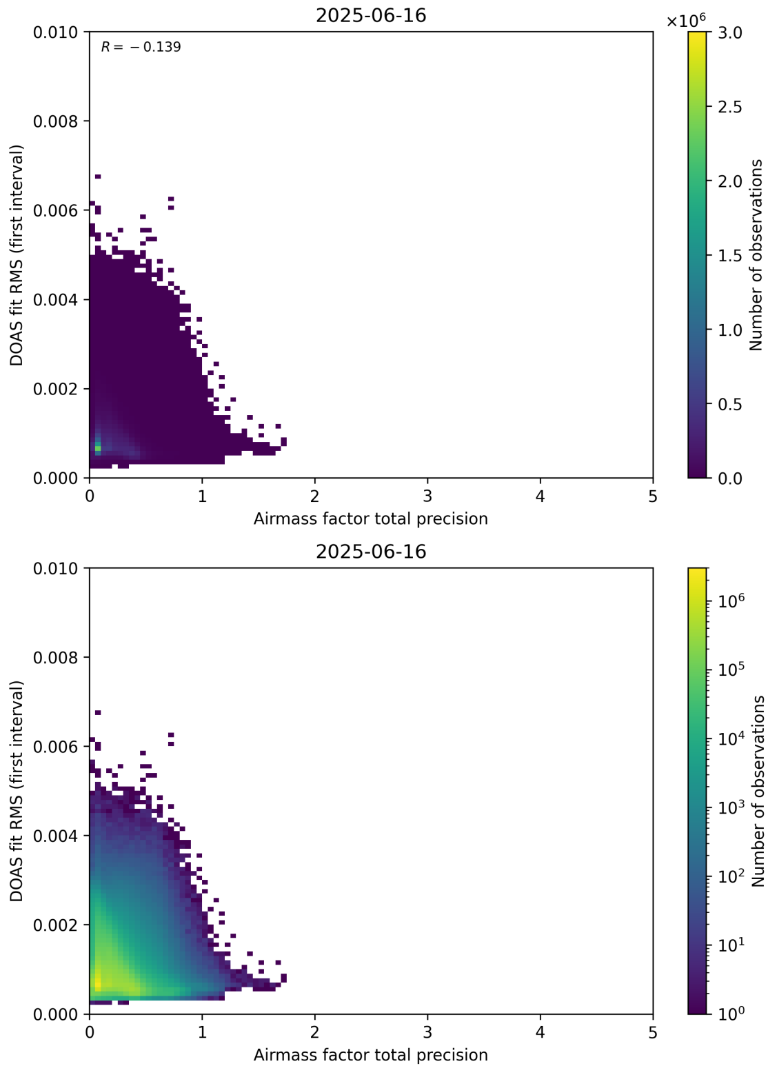
Figure 105: Scatter density plot of “Airmass factor total precision” against “DOAS fit RMS (first interval)” for 2025-06-16 to 2025-06-17.
