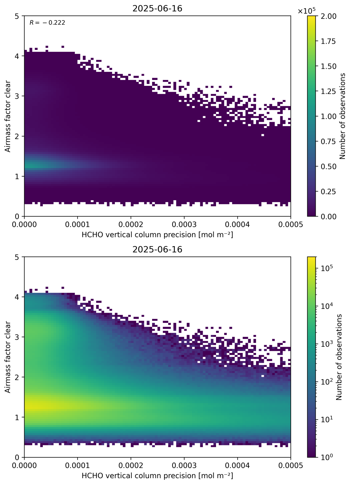
Figure 139: Scatter density plot of “HCHO vertical column precision” against “Airmass factor clear” for 2025-06-16 to 2025-06-17.
