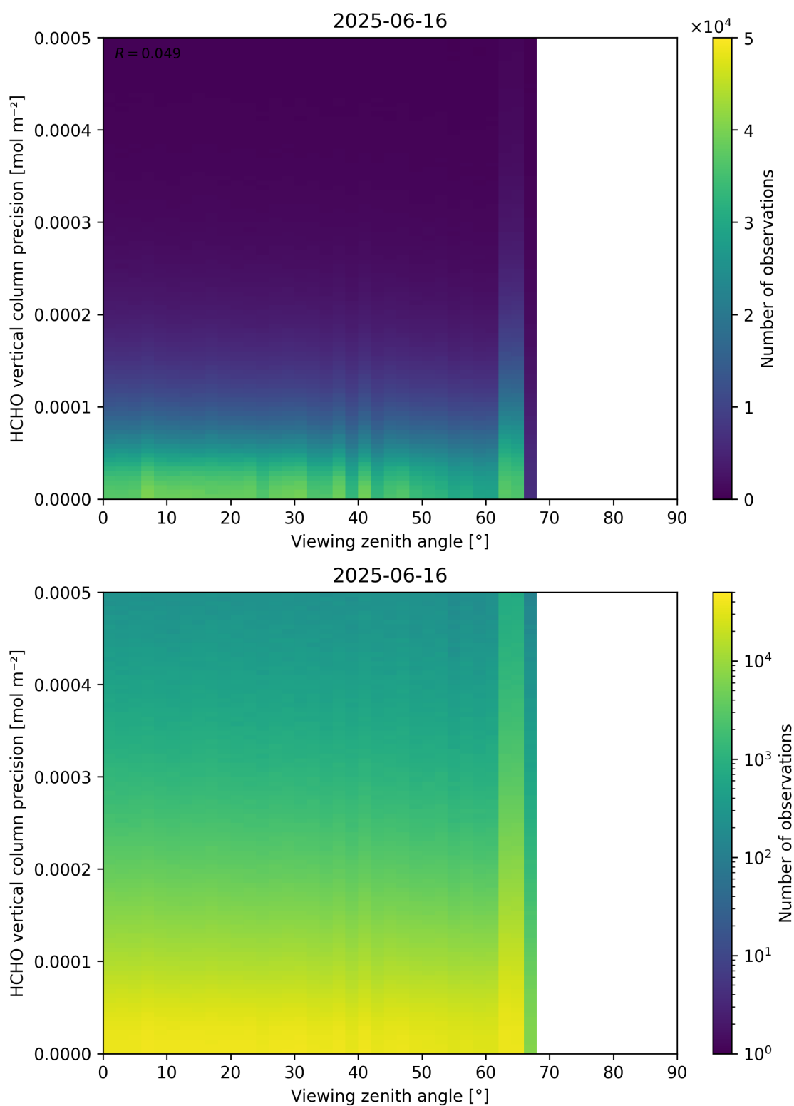
Figure 194: Scatter density plot of “Viewing zenith angle” against “HCHO vertical column precision” for 2025-06-16 to 2025-06-17.
