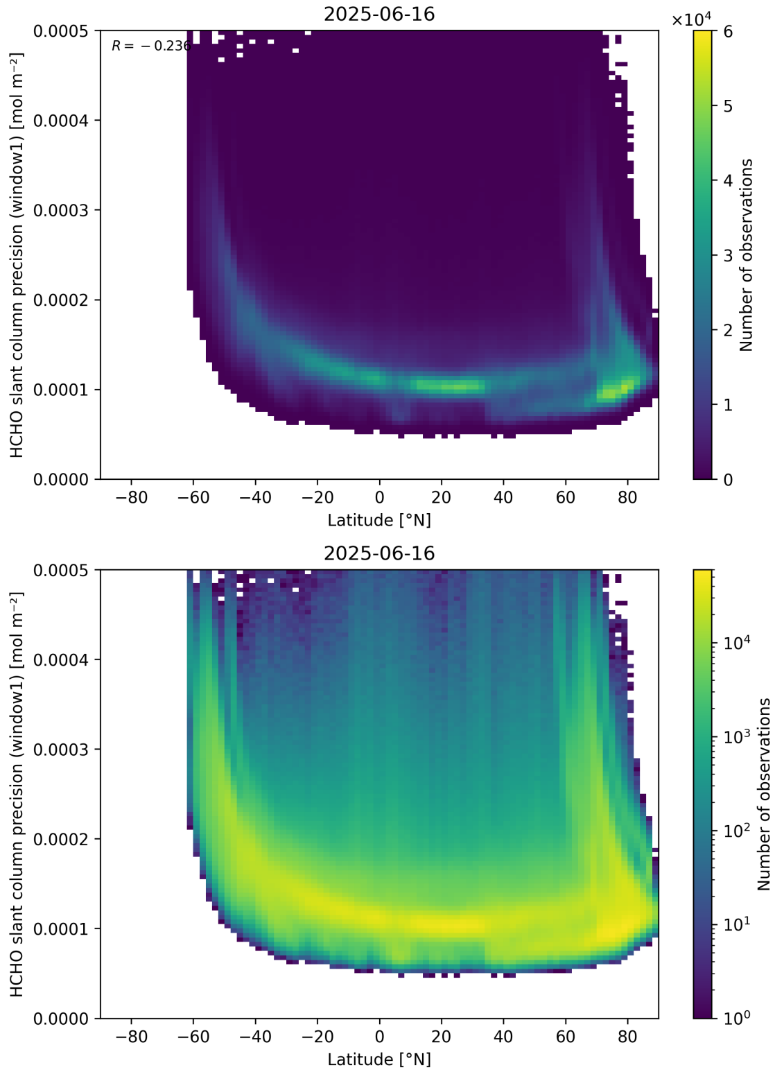
Figure 160: Scatter density plot of “Latitude” against “HCHO slant column precision (window1)” for 2025-06-16 to 2025-06-17.
