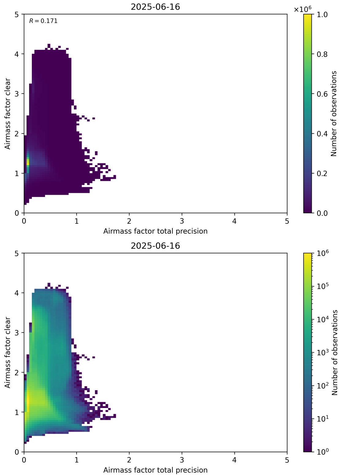
Figure 108: Scatter density plot of “Airmass factor total precision” against “Airmass factor clear” for 2025-06-16 to 2025-06-17.
