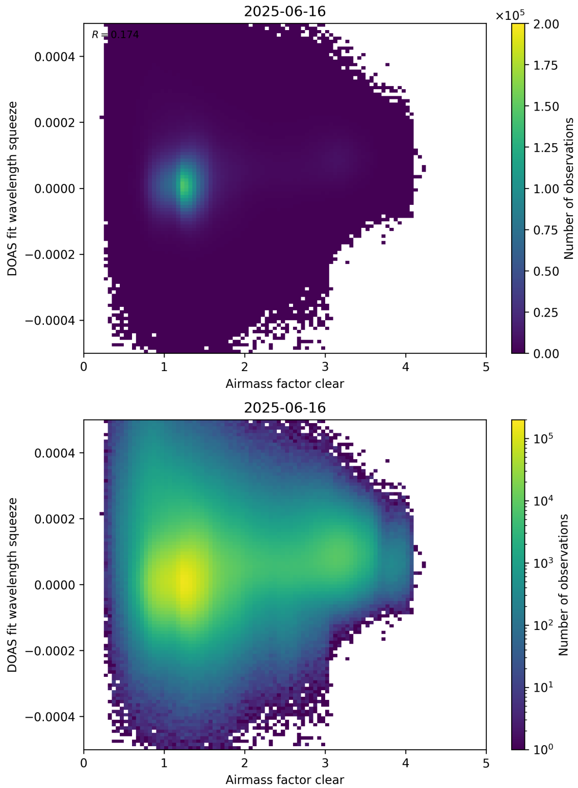
Figure 73: Scatter density plot of “Airmass factor clear” against “DOAS fit wavelength squeeze” for 2025-06-16 to 2025-06-17.
