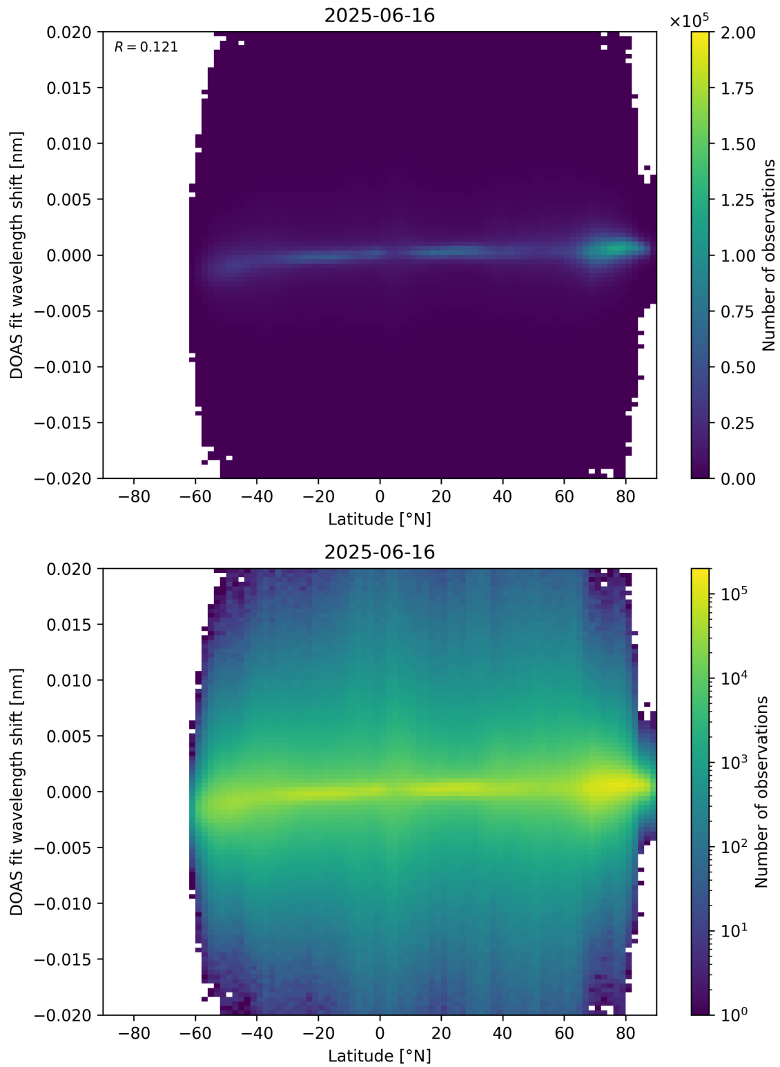
Figure 154: Scatter density plot of “Latitude” against “DOAS fit wavelength shift” for 2025-06-16 to 2025-06-17.
