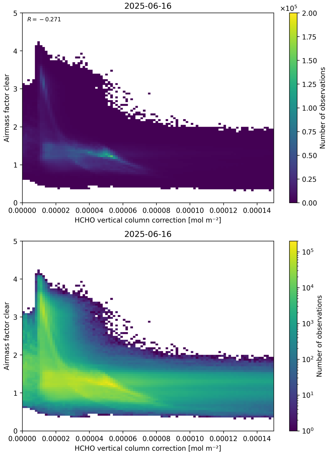
Figure 115: Scatter density plot of “HCHO vertical column correction” against “Airmass factor clear” for 2025-06-16 to 2025-06-17.
