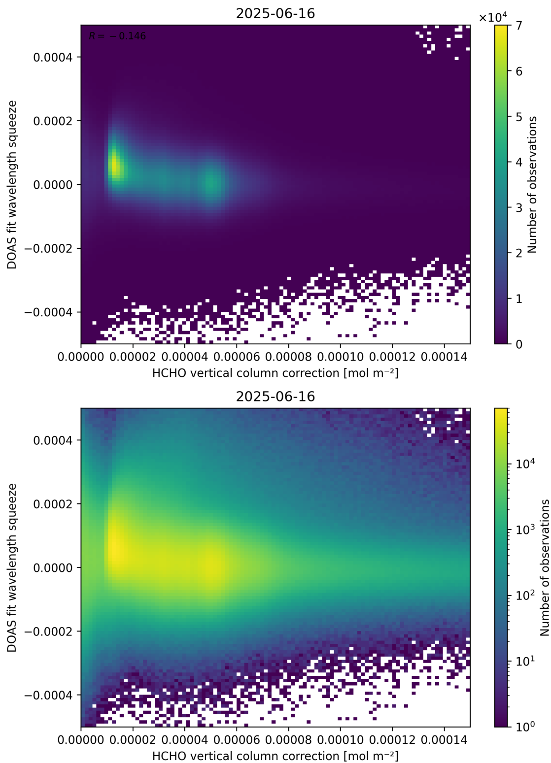
Figure 114: Scatter density plot of “HCHO vertical column correction” against “DOAS fit wavelength squeeze” for 2025-06-16 to 2025-06-17.
