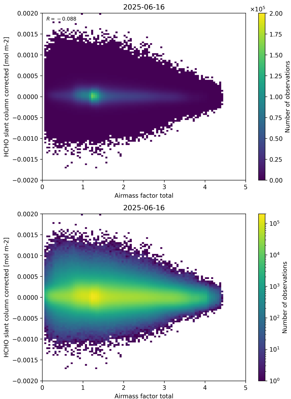
Figure 101: Scatter density plot of “Airmass factor total” against “HCHO slant column corrected” for 2025-06-16 to 2025-06-17.
