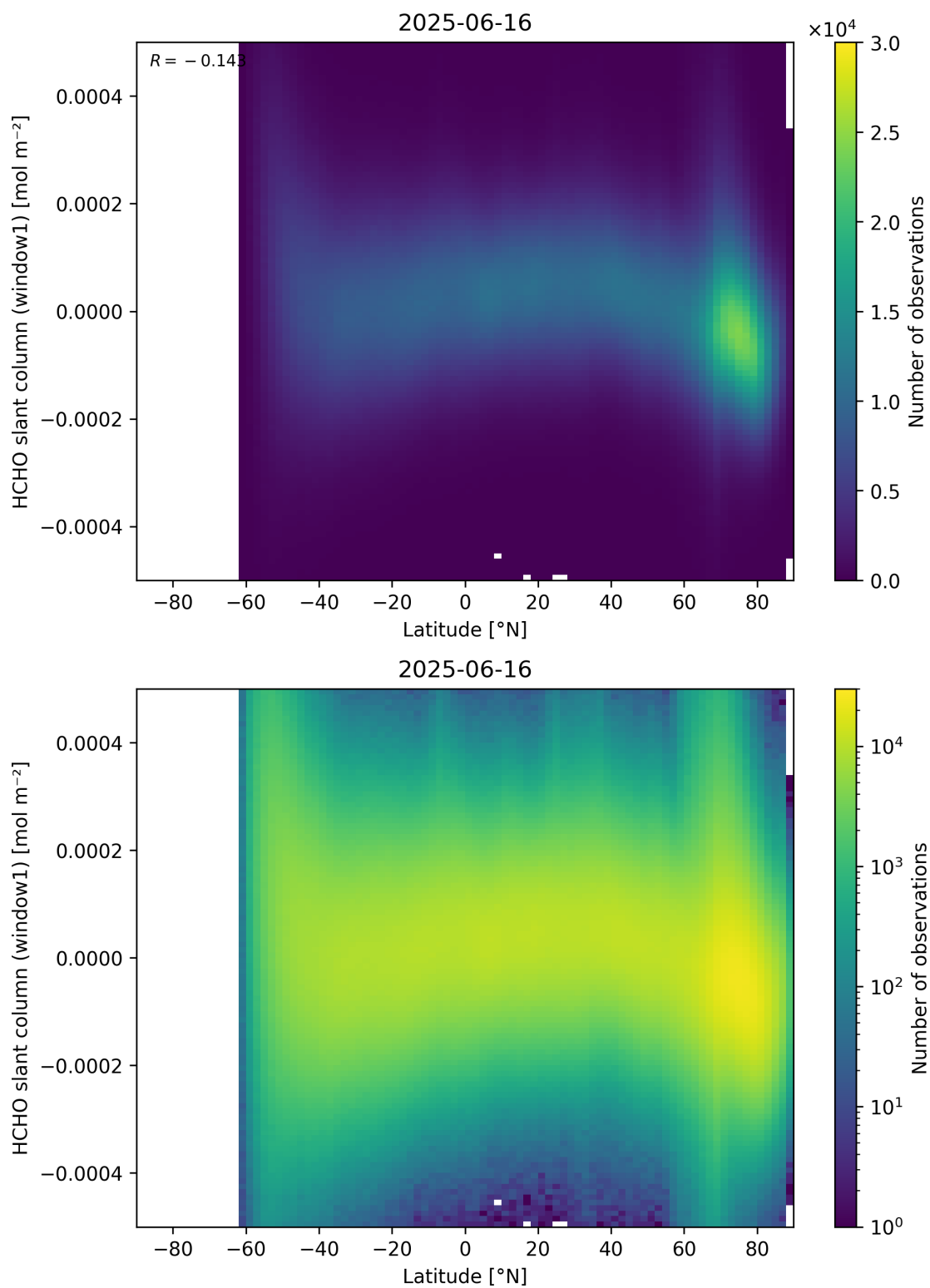
Figure 159: Scatter density plot of “Latitude” against “HCHO slant column (window1)” for 2025-06-16 to 2025-06-17.
