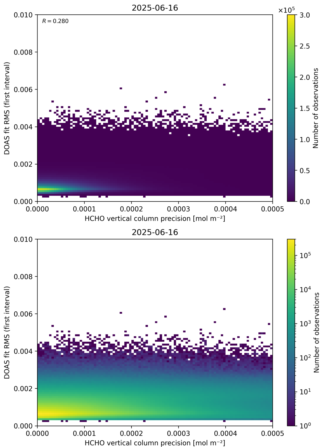
Figure 136: Scatter density plot of “HCHO vertical column precision” against “DOAS fit RMS (first interval)” for 2025-06-16 to 2025-06-17.
