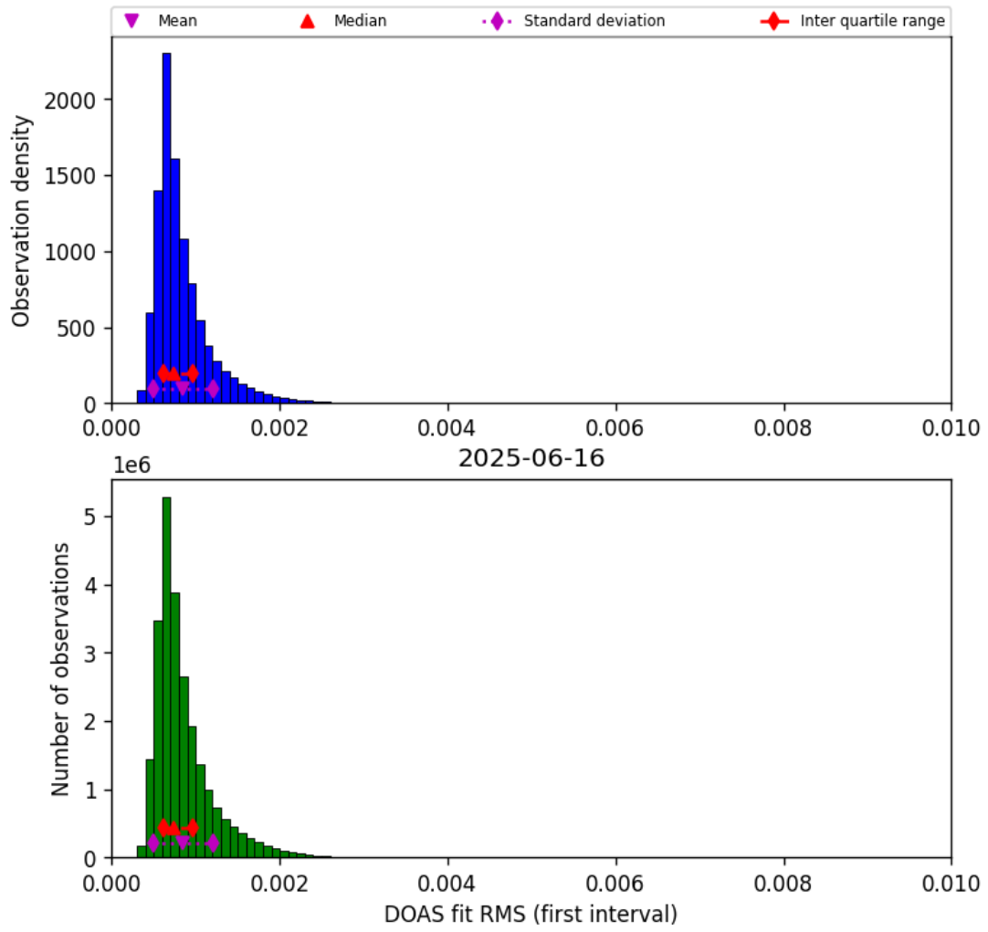
Figure 46: Histogram of “DOAS fit RMS (first interval)” for 2025-06-16 to 2025-06-17
