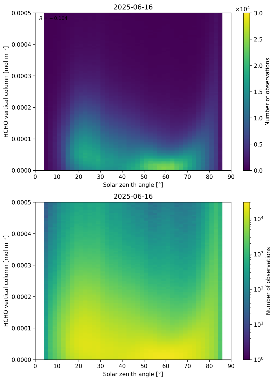
Figure 177: Scatter density plot of “Solar zenith angle” against “HCHO vertical column” for 2025-06-16 to 2025-06-17.
