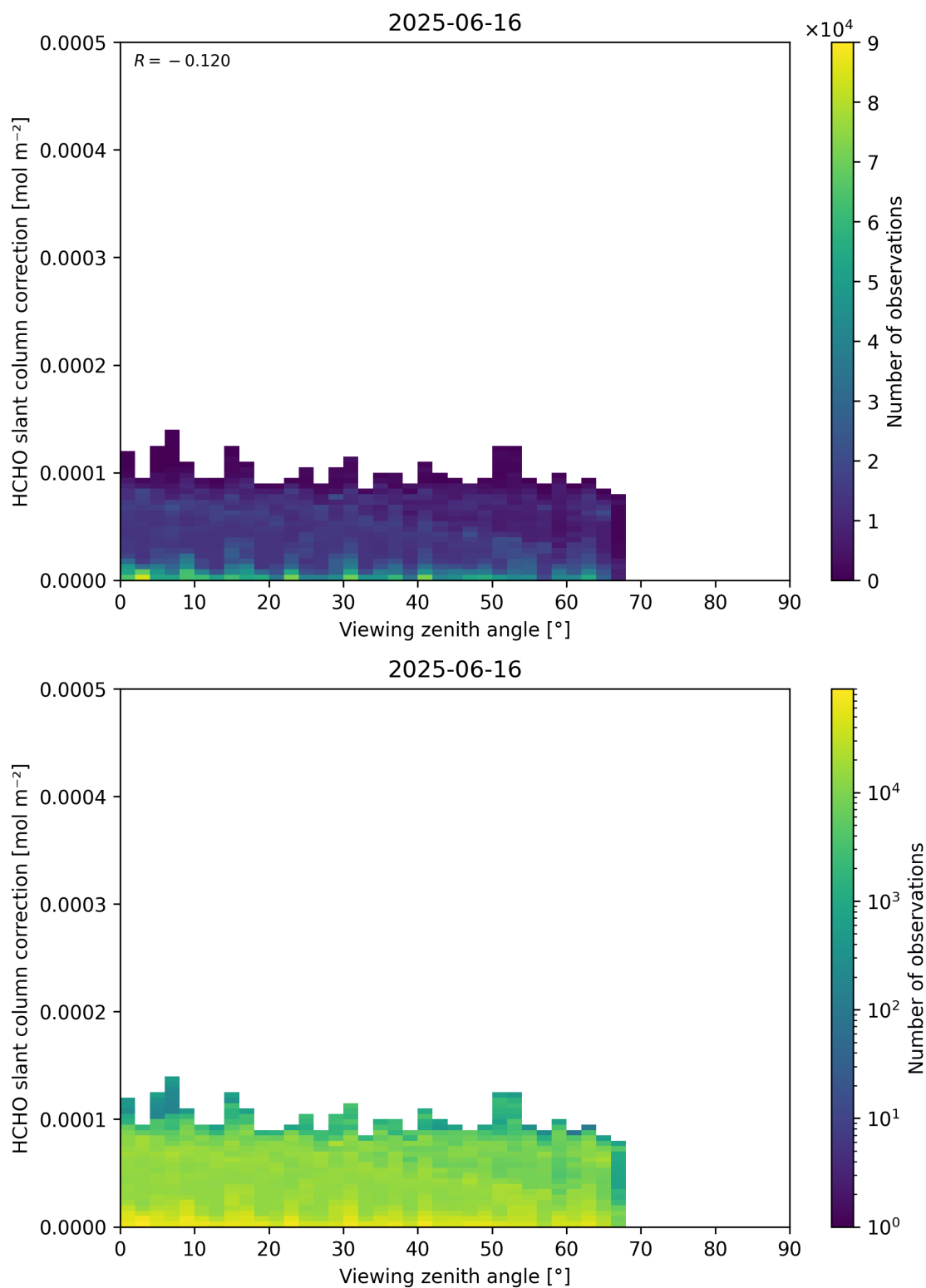
Figure 187: Scatter density plot of “Viewing zenith angle” against “HCHO slant column correction” for 2025-06-16 to 2025-06-17.
