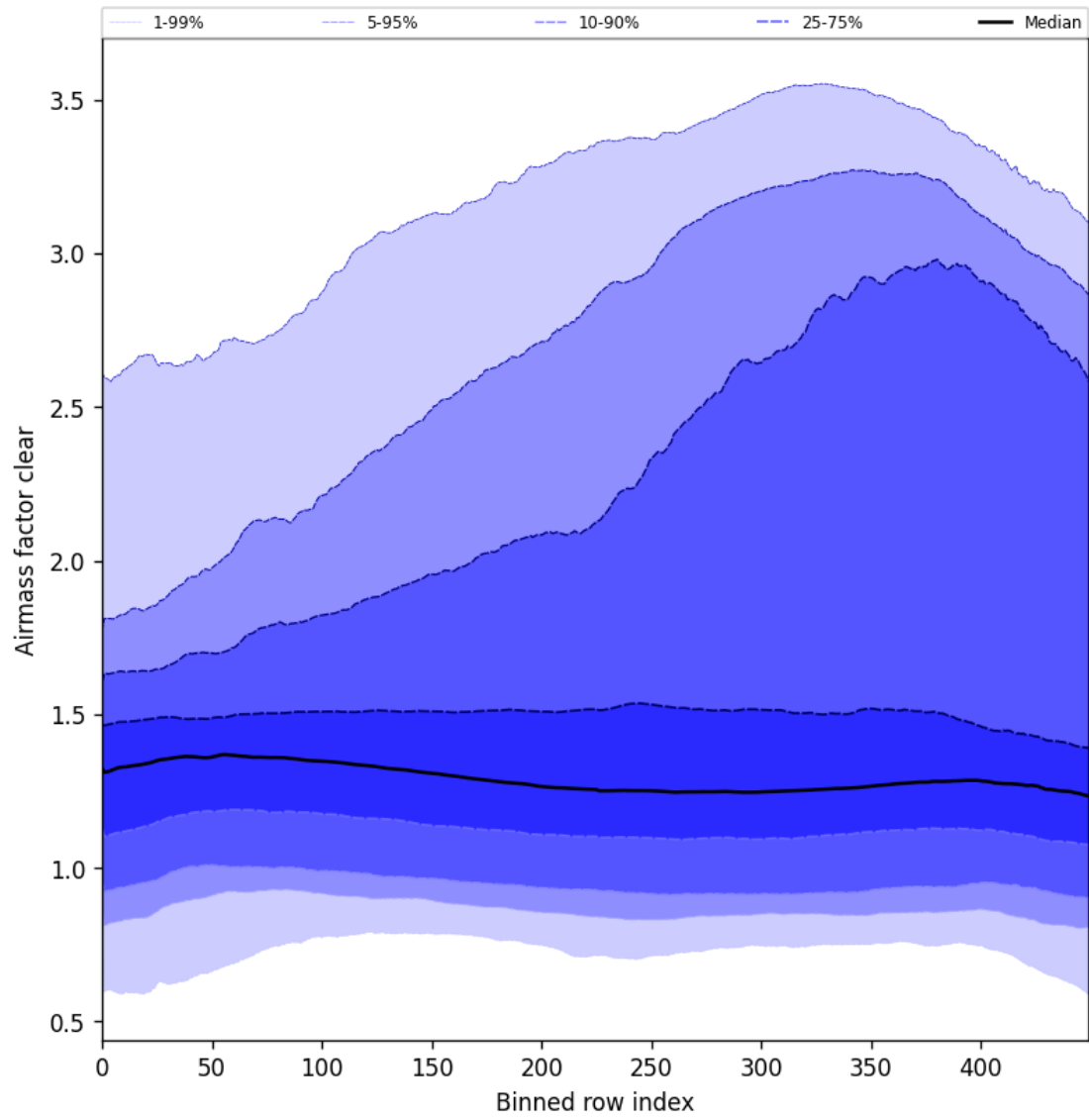
Figure 56: Along track statistics of “Air mass factor clear” for 2025-06-16 to 2025-06-17
