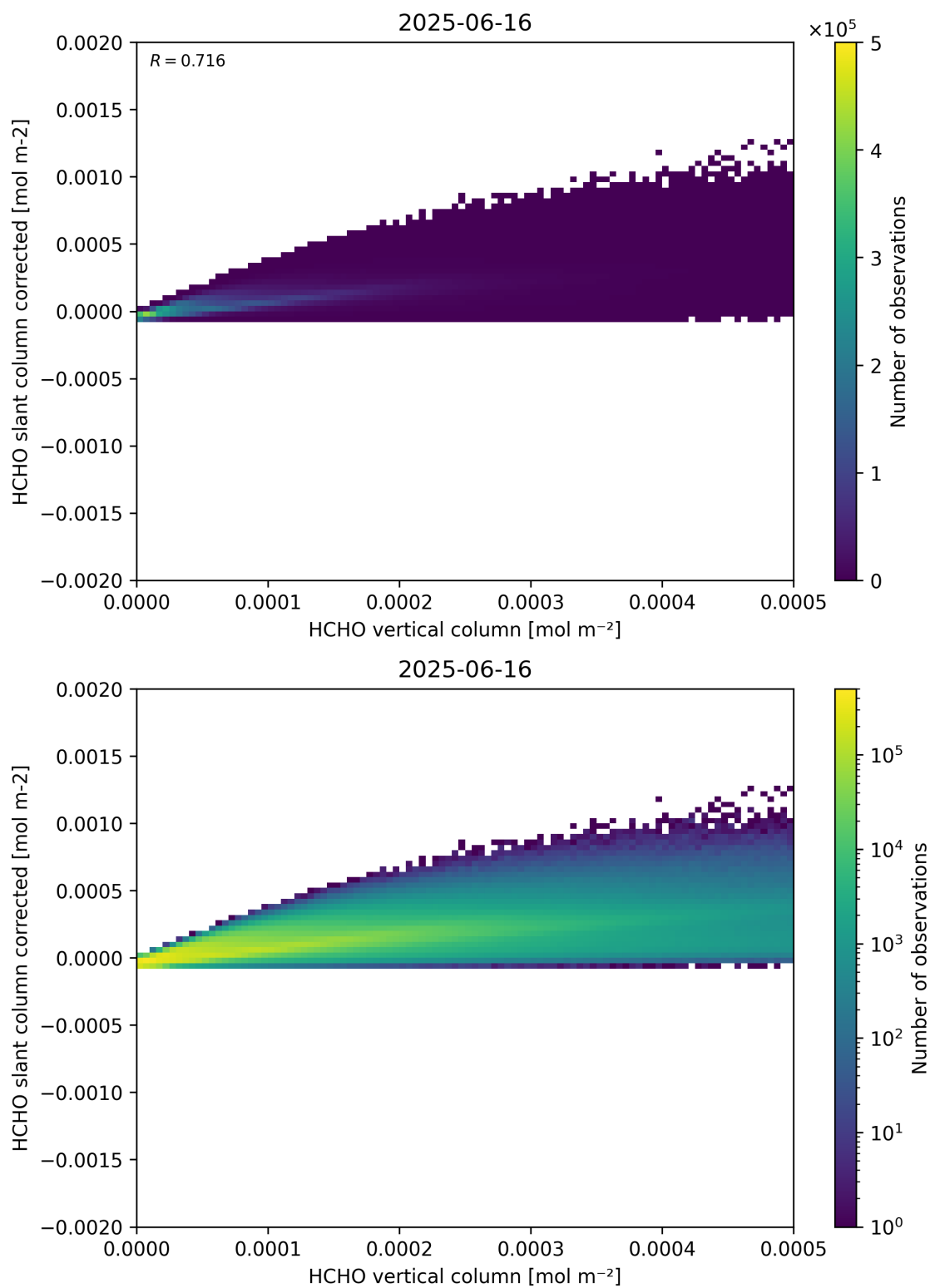
Figure 127: Scatter density plot of “HCHO vertical column” against “HCHO slant column corrected” for 2025-06-16 to 2025-06-17.
