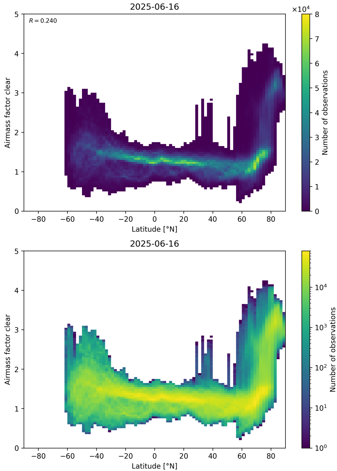
Figure 156: Scatter density plot of “Latitude” against “Airmass factor clear” for 2025-06-16 to 2025-06-17.
