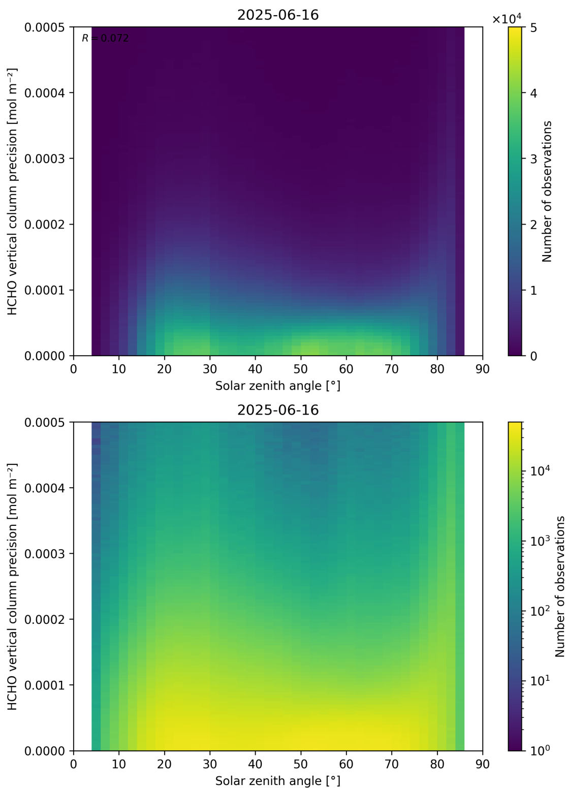
Figure 179: Scatter density plot of “Solar zenith angle” against “HCHO vertical column precision” for 2025-06-16 to 2025-06-17.
