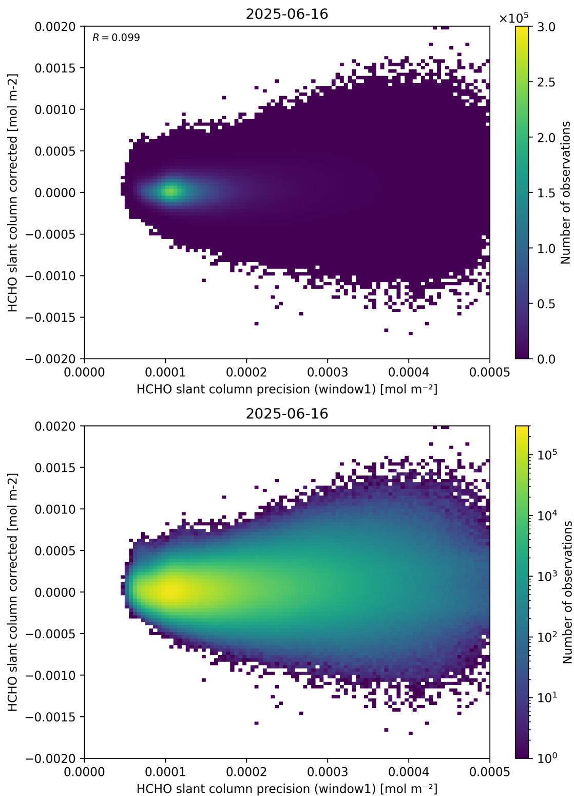
Figure 92: Scatter density plot of “HCHO slant column precision (window1)” against “HCHO slant column corrected” for 2025-06-16 to 2025-06-17.
