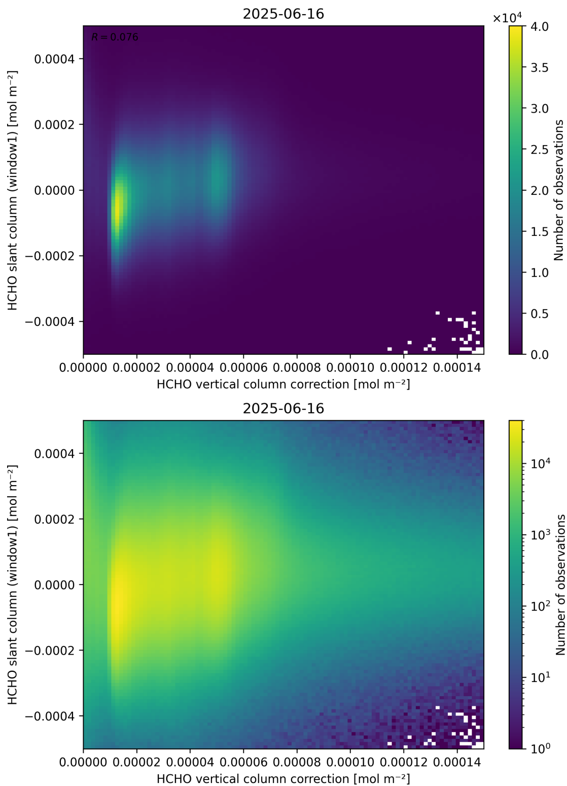
Figure 118: Scatter density plot of “HCHO vertical column correction” against “HCHO slant column (window1)” for 2025-06-16 to 2025-06-17.
