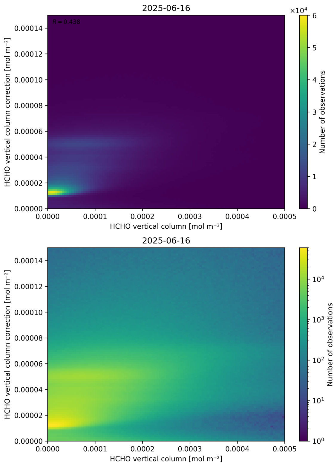
Figure 133: Scatter density plot of “HCHO vertical column” against “HCHO vertical column correction” for 2025-06-16 to 2025-06-17.
