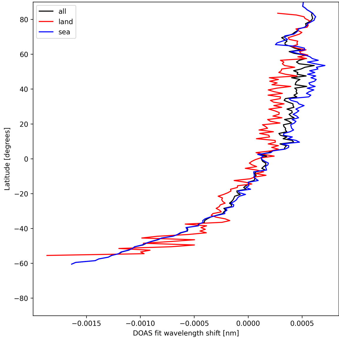
Figure 30: Zonal average of “DOAS fit wavelength shift” for 2025-06-16 to 2025-06-17.
