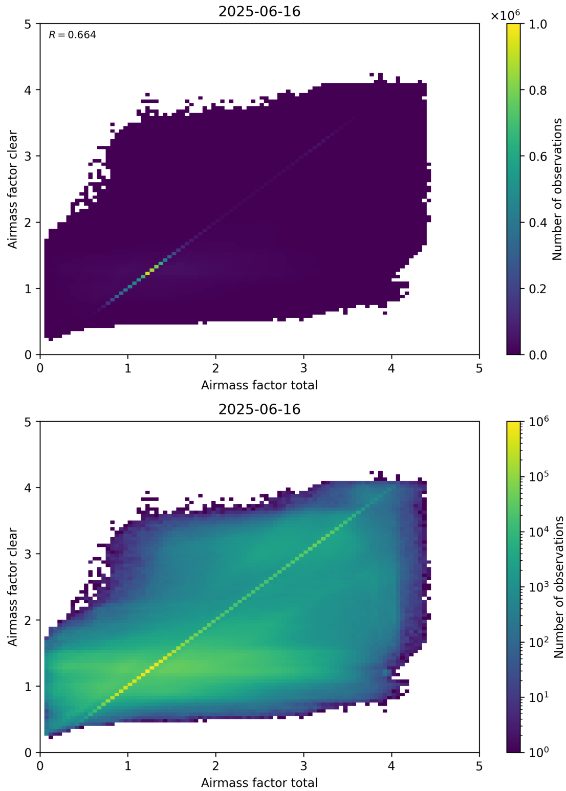
Figure 100: Scatter density plot of “Airmass factor total” against “Airmass factor clear” for 2025-06-16 to 2025-06-17.
