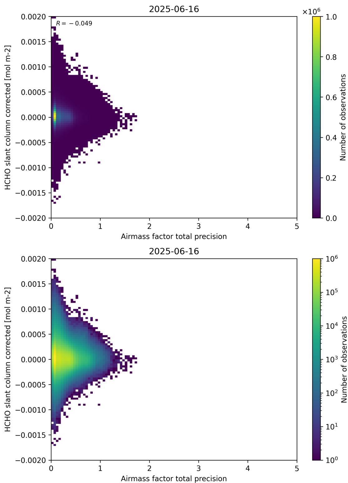
Figure 109: Scatter density plot of “Airmass factor total precision” against “HCHO slant column corrected” for 2025-06-16 to 2025-06-17.
