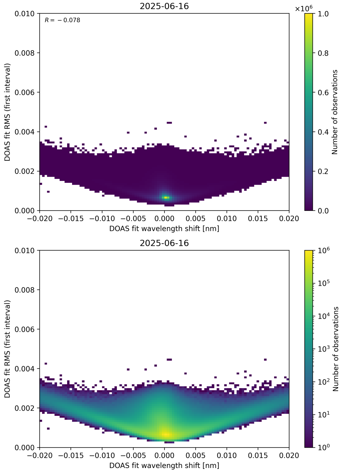
Figure 64: Scatter density plot of “DOAS fit wavelength shift” against “DOAS fit RMS (first interval)” for 2025-06-16 to 2025-06-17.
