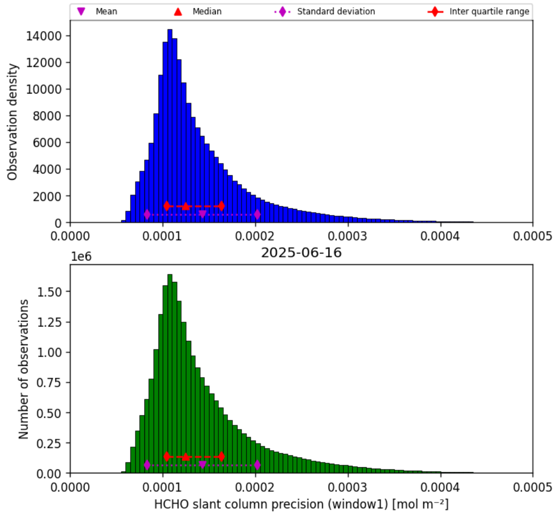
Figure 39: Histogram of “HCHO slant column precision (window1)” for 2025-06-16 to 2025-06-17
