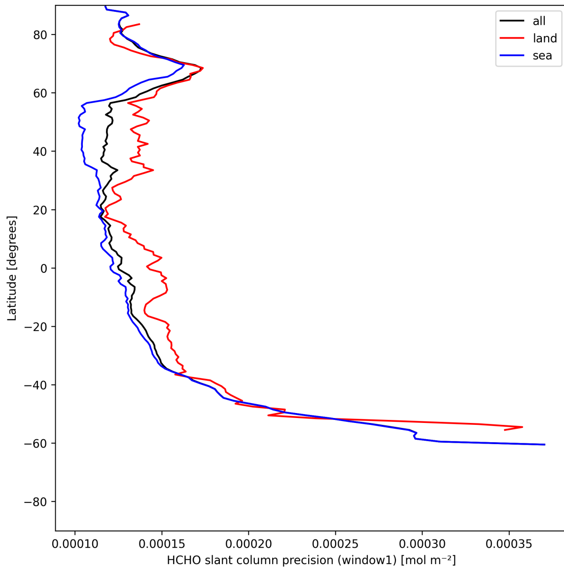
Figure 25: Zonal average of “HCHO slant column precision (window1)” for 2025-06-16 to 2025-06-17.
