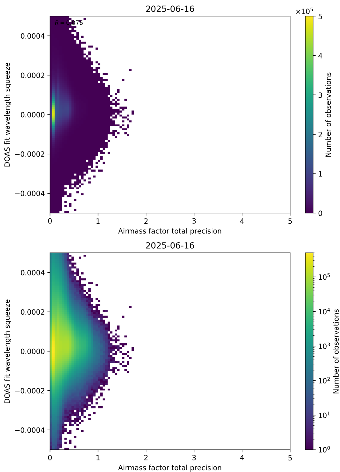
Figure 107: Scatter density plot of “Airmass factor total precision” against “DOAS fit wavelength squeeze” for 2025-06-16 to 2025-06-17.
