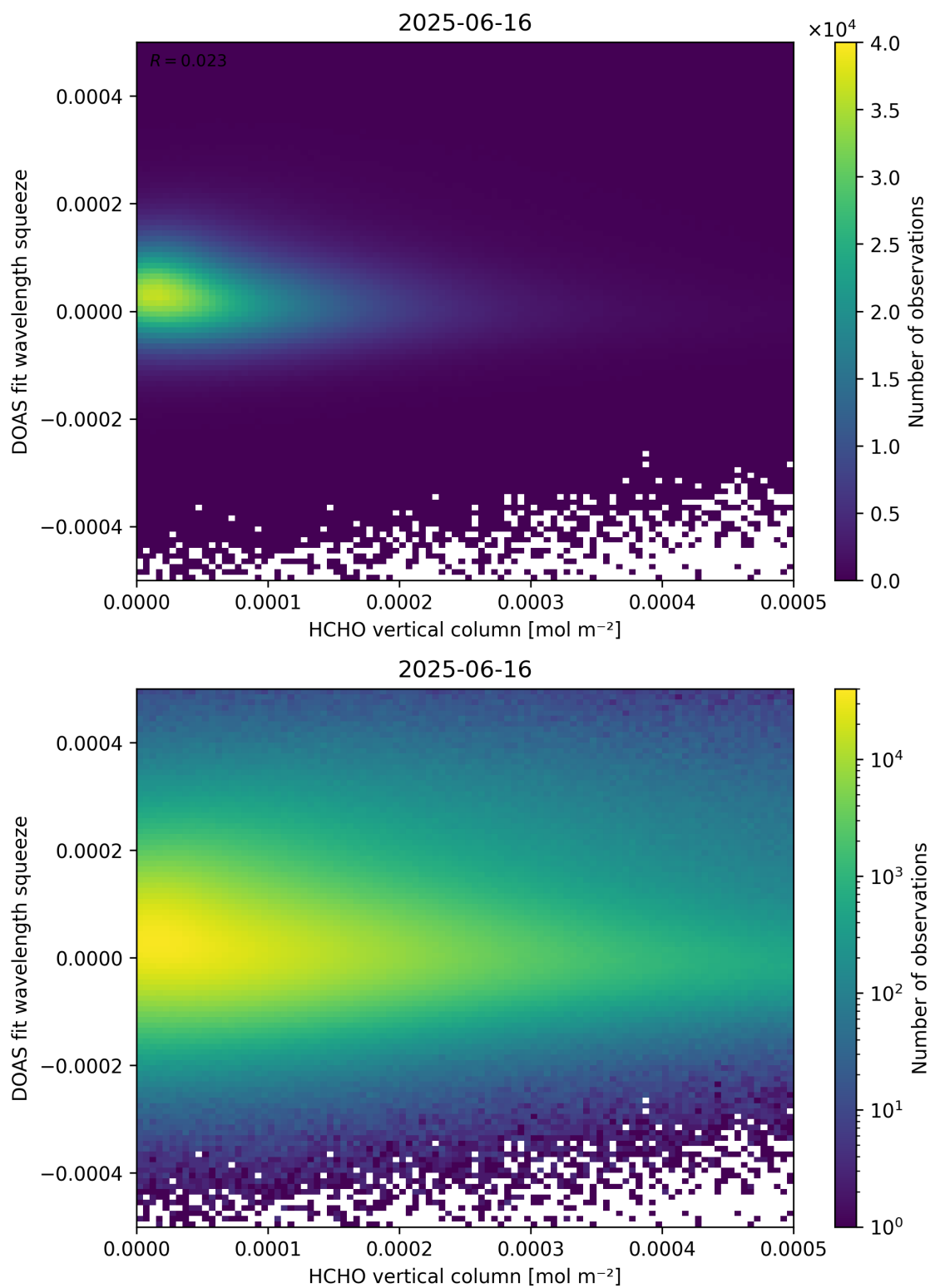
Figure 125: Scatter density plot of “HCHO vertical column” against “DOAS fit wavelength squeeze” for 2025-06-16 to 2025-06-17.
