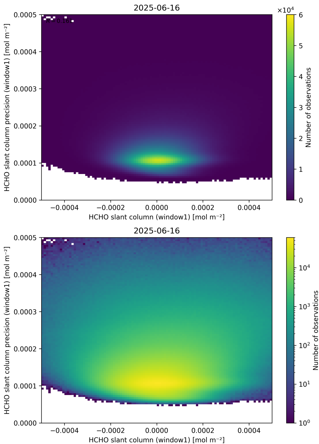
Figure 84: Scatter density plot of “HCHO slant column (window1)” against “HCHO slant column precision (window1)” for 2025-06-16 to 2025-06-17.
