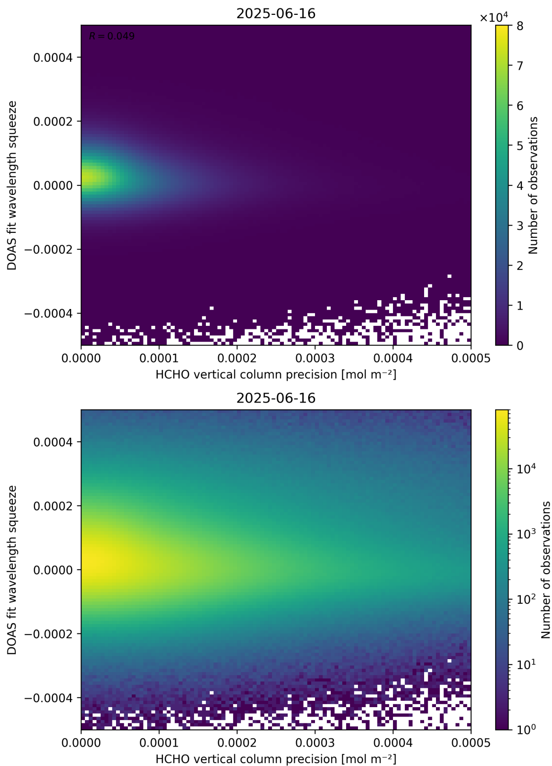
Figure 138: Scatter density plot of “HCHO vertical column precision” against “DOAS fit wavelength squeeze” for 2025-06-16 to 2025-06-17.
