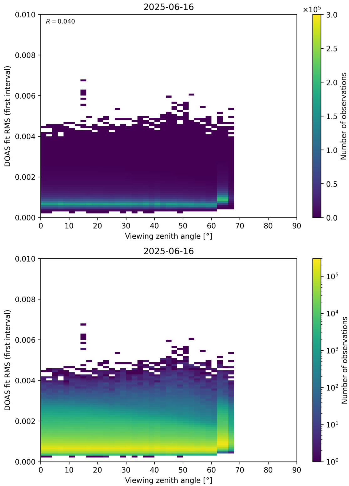
Figure 182: Scatter density plot of “Viewing zenith angle” against “DOAS fit RMS (first interval)” for 2025-06-16 to 2025-06-17.
