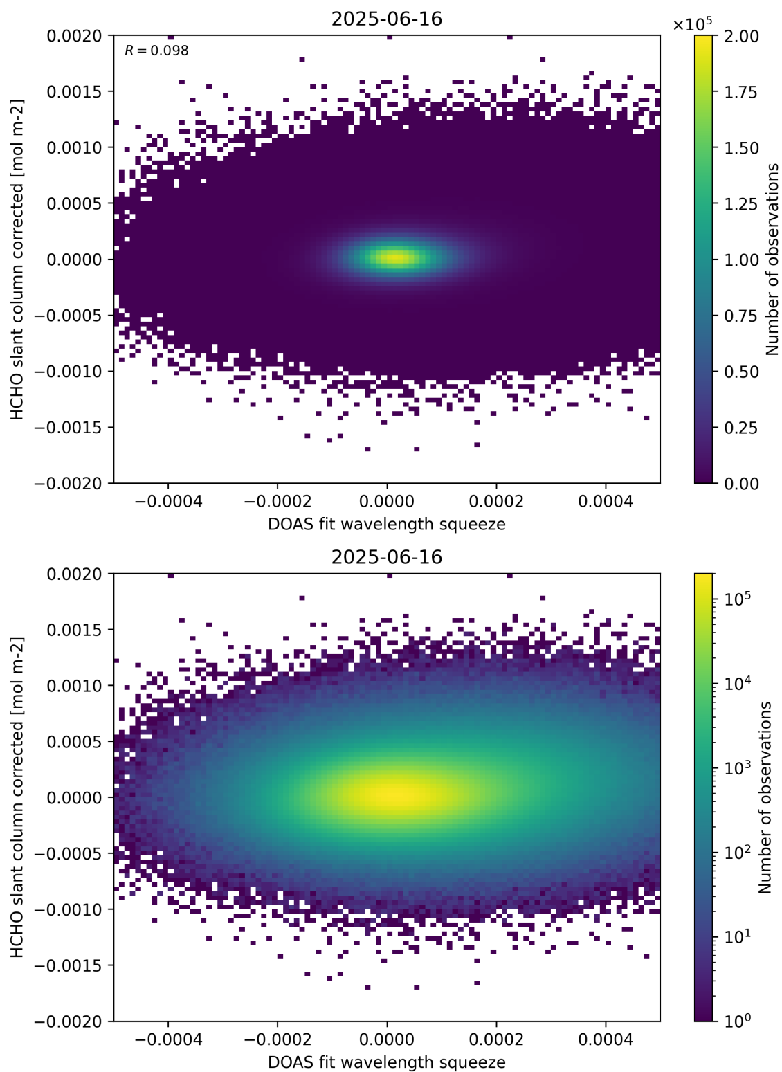
Figure 69: Scatter density plot of “DOAS fit wavelength squeeze” against “HCHO slant column corrected” for 2025-06-16 to 2025-06-17.
