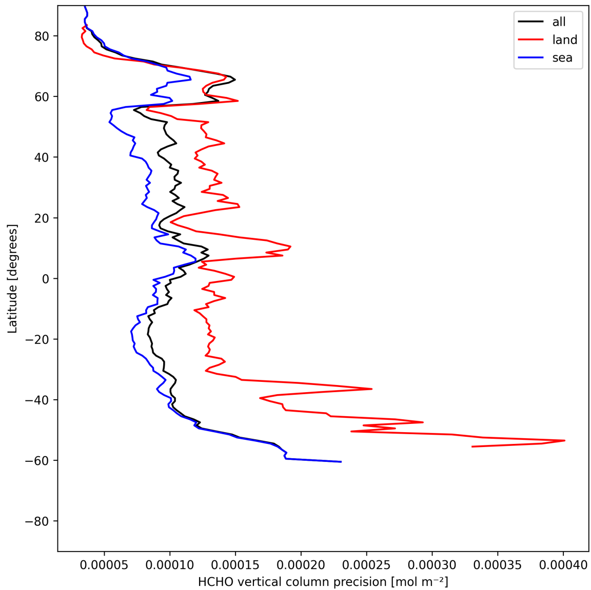
Figure 22: Zonal average of “HCHO vertical column precision” for 2025-06-16 to 2025-06-17.
