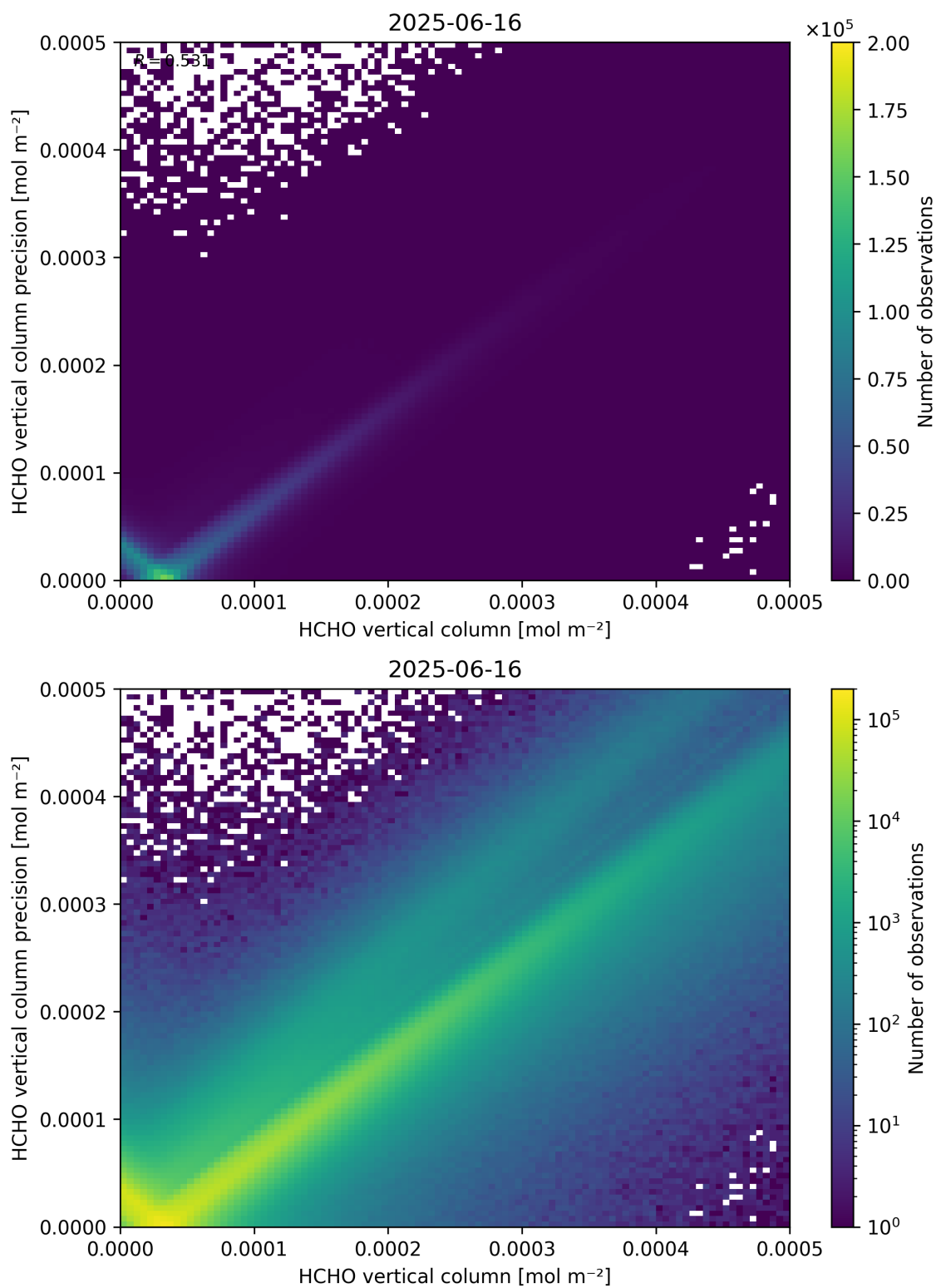
Figure 134: Scatter density plot of “HCHO vertical column” against “HCHO vertical column precision” for 2025-06-16 to 2025-06-17.
