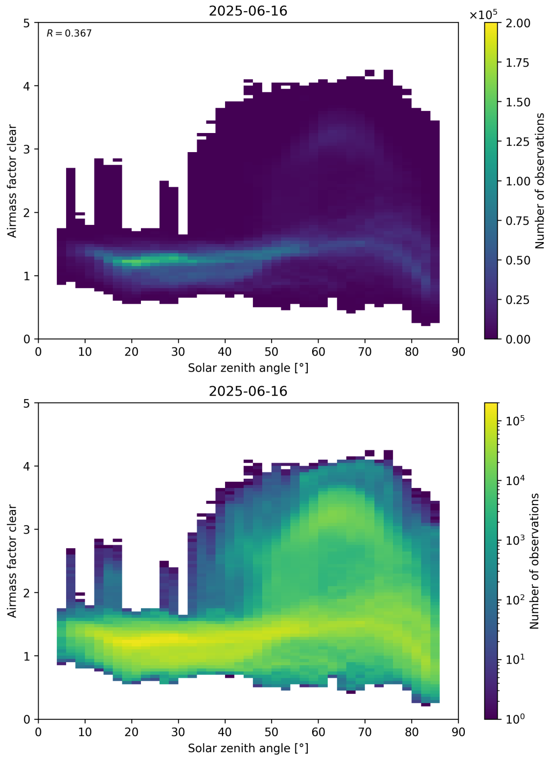
Figure 170: Scatter density plot of “Solar zenith angle” against “Airmass factor clear” for 2025-06-16 to 2025-06-17.
