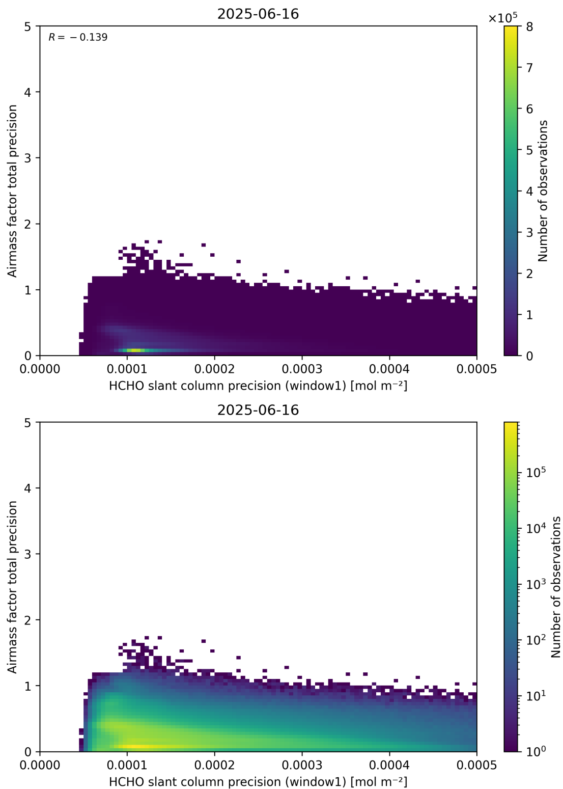
Figure 95: Scatter density plot of “HCHO slant column precision (window1)” against “Airmass factor total precision” for 2025-06-16 to 2025-06-17.
