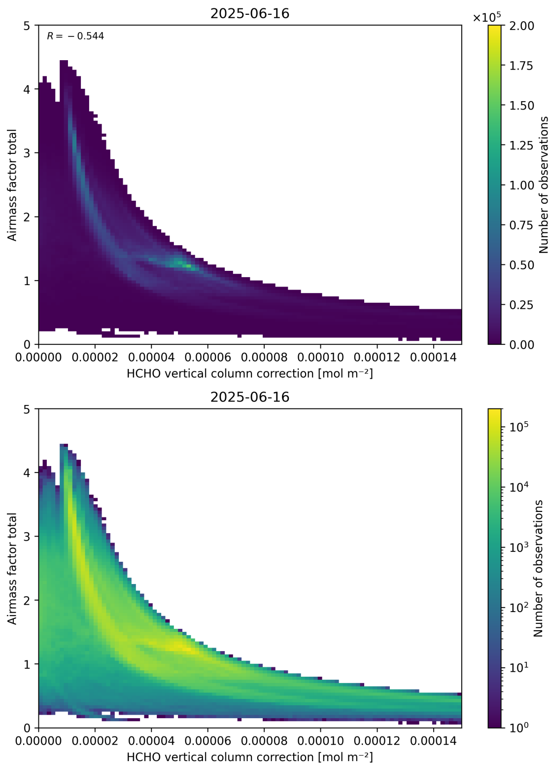
Figure 120: Scatter density plot of “HCHO vertical column correction” against “Airmass factor total” for 2025-06-16 to 2025-06-17.
