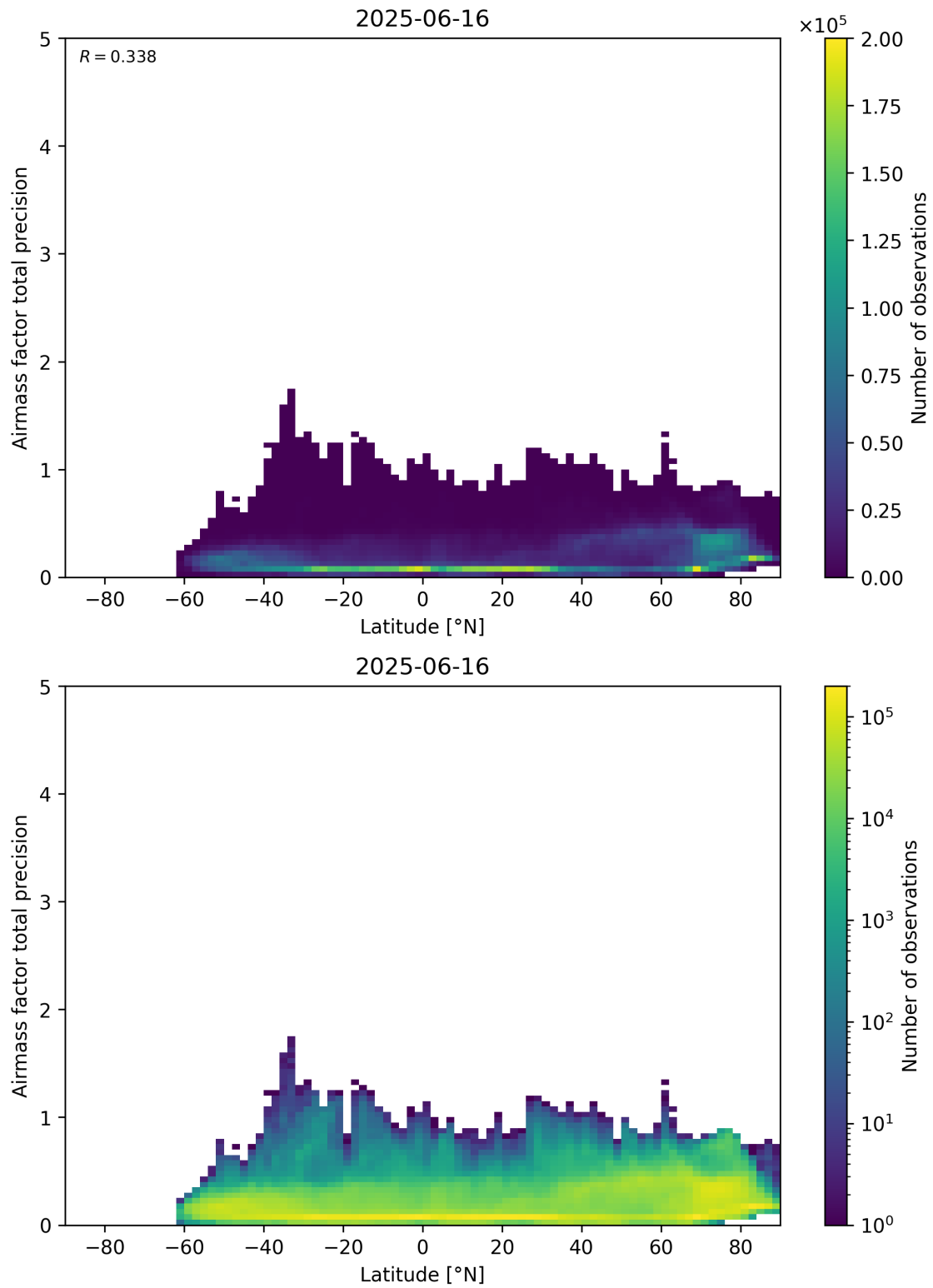
Figure 162: Scatter density plot of “Latitude” against “Airmass factor total precision” for 2025-06-16 to 2025-06-17.
