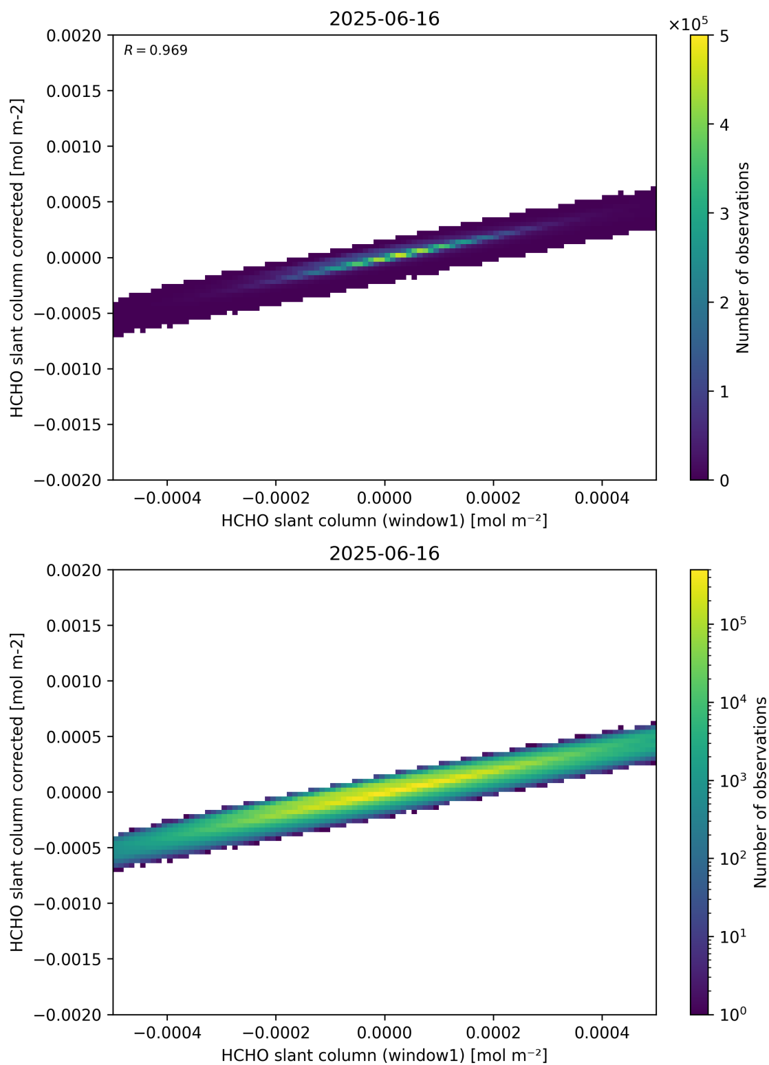
Figure 82: Scatter density plot of “HCHO slant column (window1)” against “HCHO slant column corrected” for 2025-06-16 to 2025-06-17.
