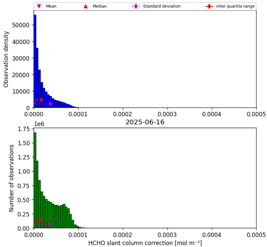
Figure 47: Histogram of “HCHO slant column correction” for 2025-06-16 to 2025-06-17
