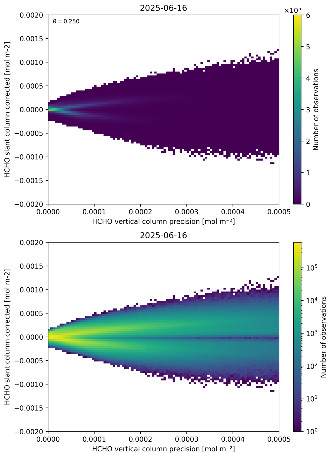
Figure 140: Scatter density plot of “HCHO vertical column precision” against “HCHO slant column corrected” for 2025-06-16 to 2025-06-17.
