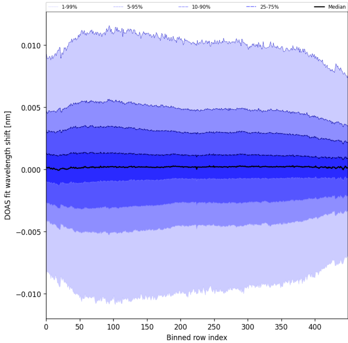
Figure 58: Along track statistics of “DOAS fit wavelength shift” for 2025-06-16 to 2025-06-17
