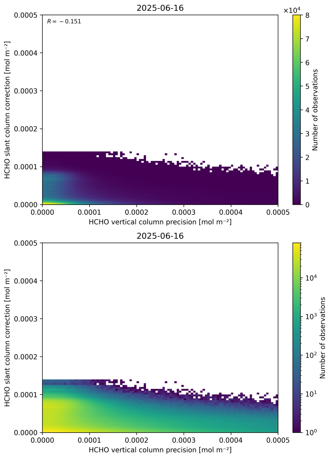
Figure 141: Scatter density plot of “HCHO vertical column precision” against “HCHO slant column correction” for 2025-06-16 to 2025-06-17.
