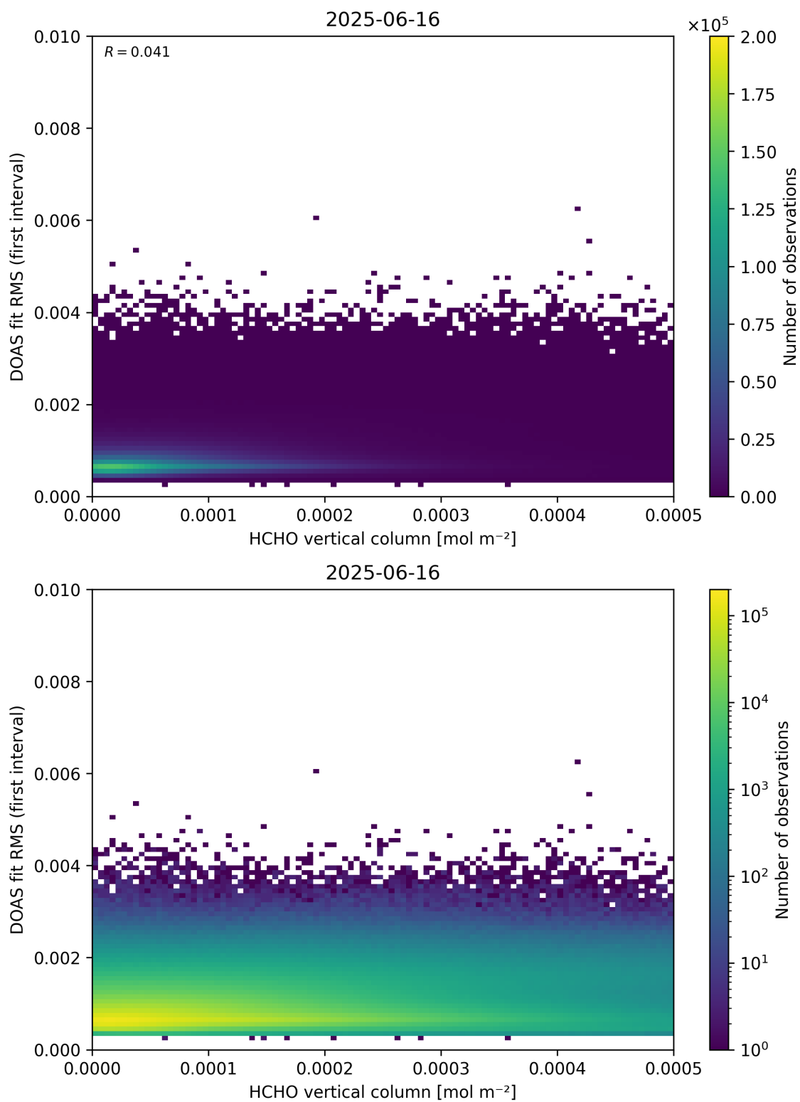
Figure 123: Scatter density plot of “HCHO vertical column” against “DOAS fit RMS (first interval)” for 2025-06-16 to 2025-06-17.
