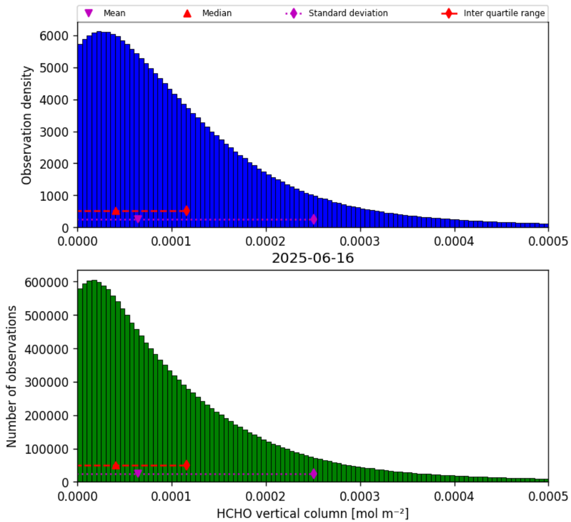
Figure 35: Histogram of “HCHO vertical column” for 2025-06-16 to 2025-06-17
