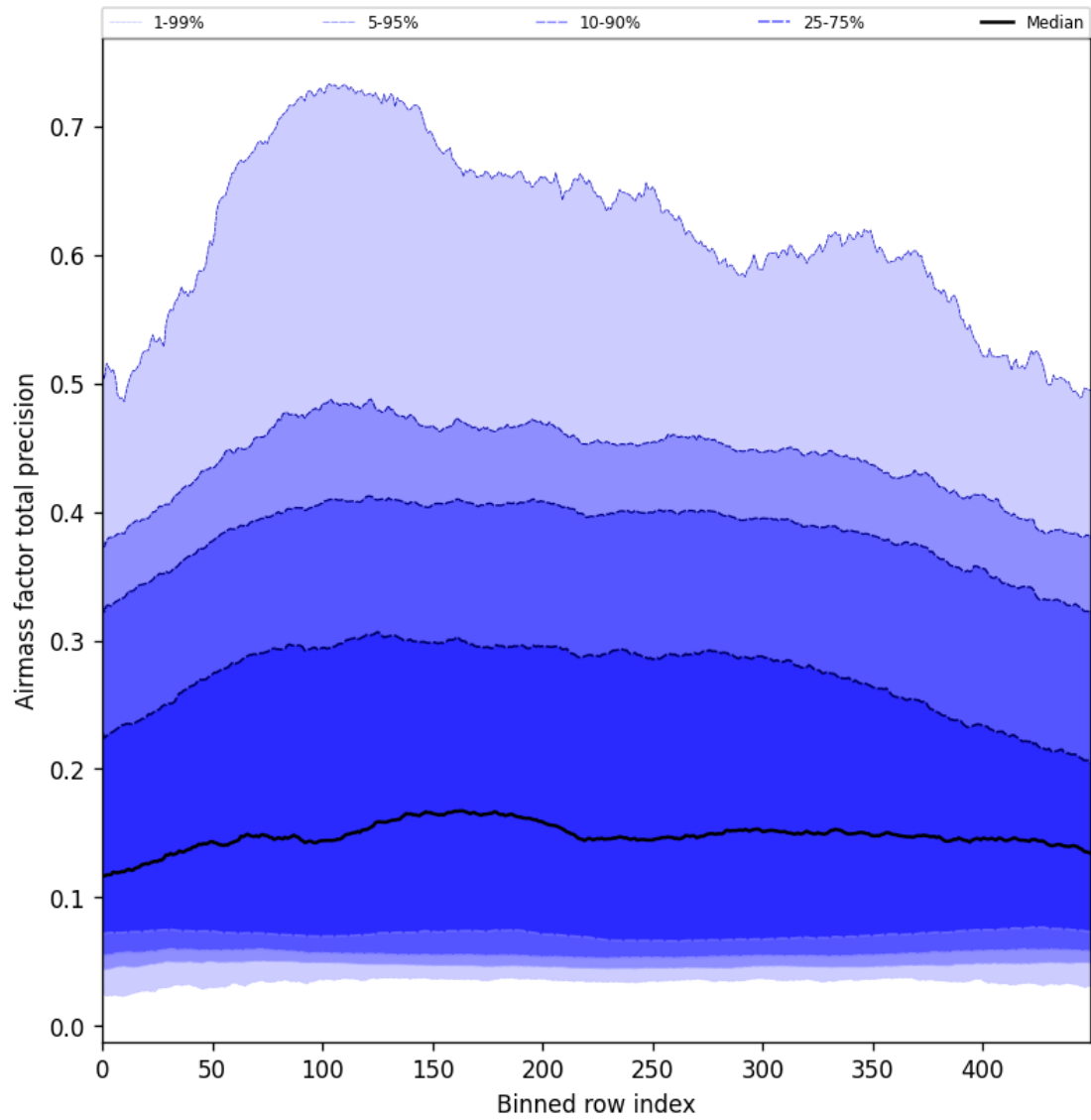
Figure 55: Along track statistics of “Airmass factor total precision” for 2025-06-16 to 2025-06-17
