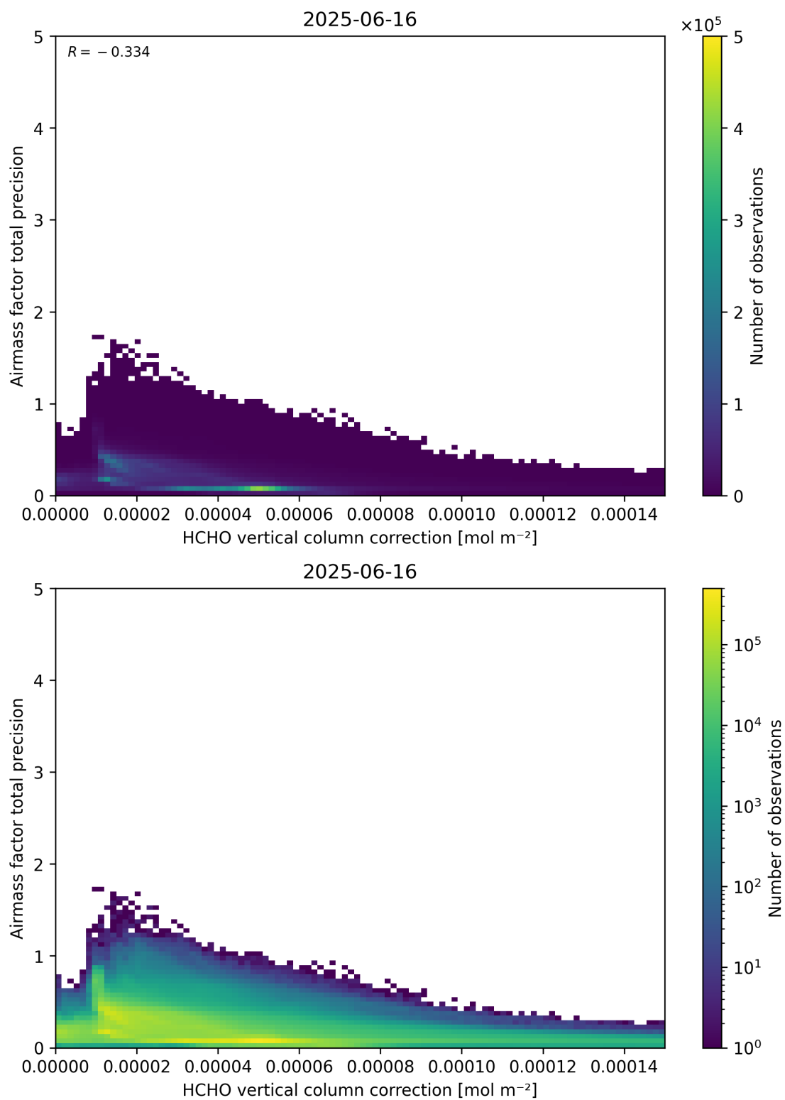
Figure 121: Scatter density plot of “HCHO vertical column correction” against “Airmass factor total precision” for 2025-06-16 to 2025-06-17.
