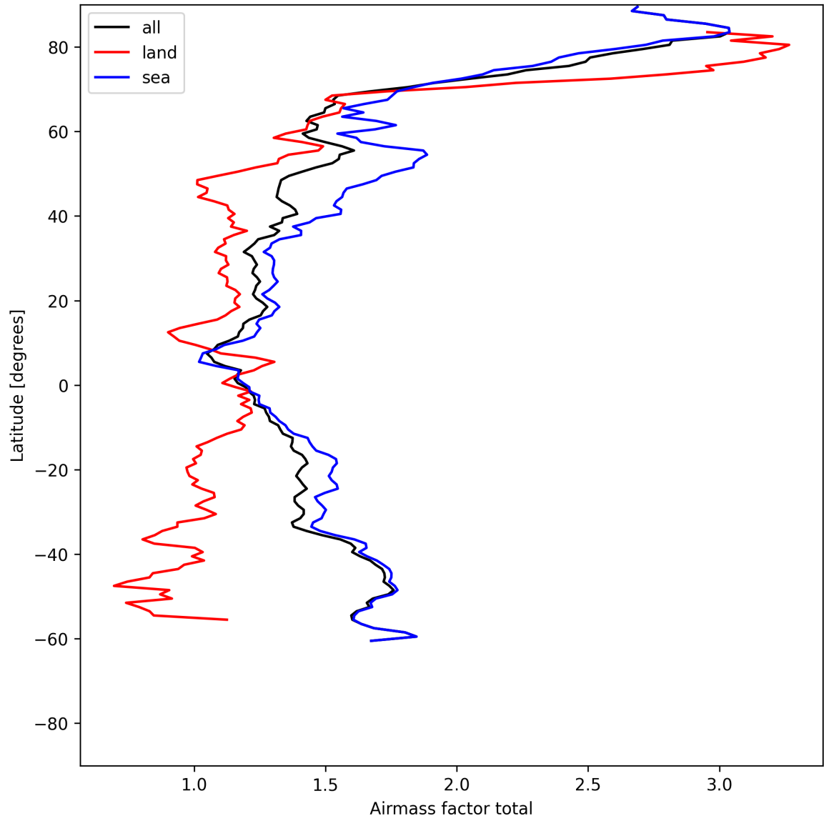
Figure 26: Zonal average of “Airmass factor total” for 2025-06-16 to 2025-06-17.
