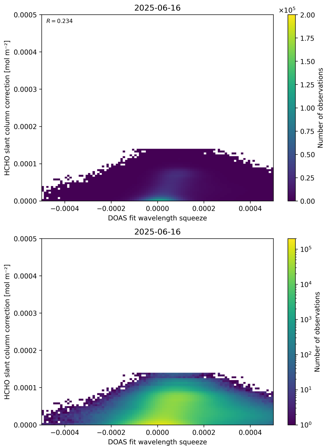
Figure 70: Scatter density plot of “DOAS fit wavelength squeeze” against “HCHO slant column correction” for 2025-06-16 to 2025-06-17.
