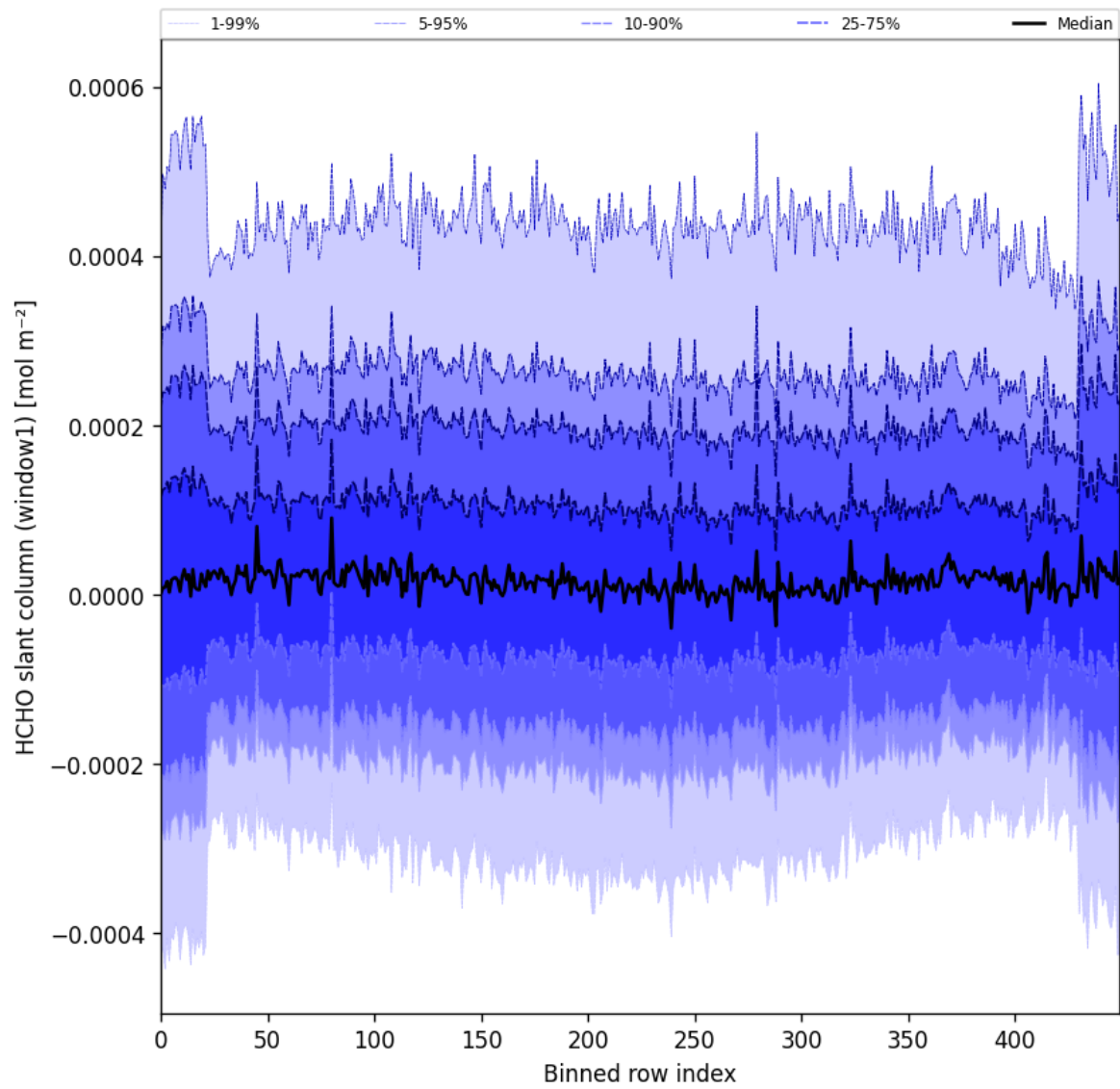
Figure 52: Along track statistics of “HCHO slant column (window1)” for 2025-06-16 to 2025-06-17
