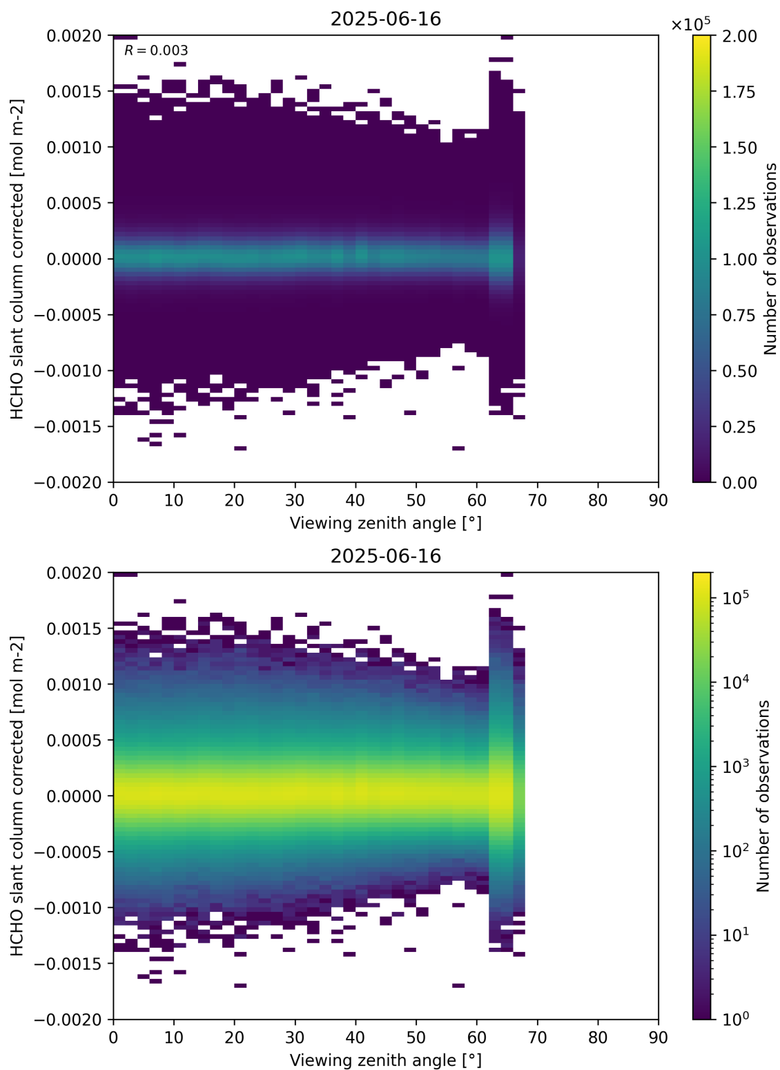
Figure 186: Scatter density plot of “Viewing zenith angle” against “HCHO slant column corrected” for 2025-06-16 to 2025-06-17.
