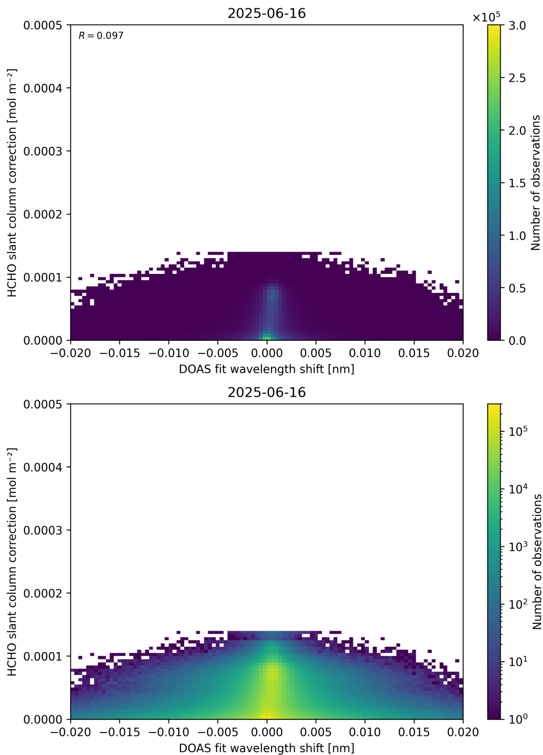
Figure 67: Scatter density plot of “DOAS fit wavelength shift” against “HCHO slant column correction” for 2025-06-16 to 2025-06-17.
