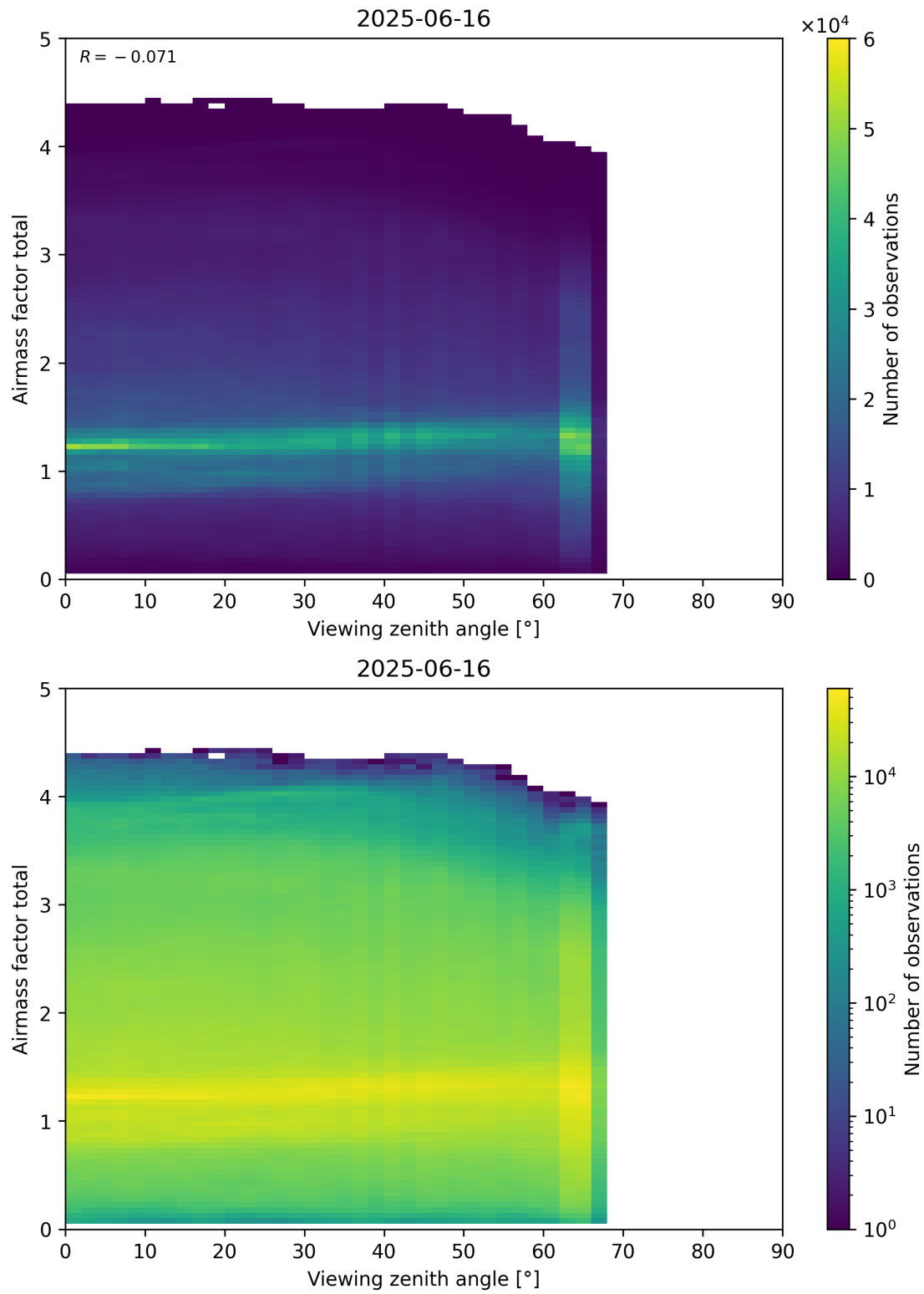
Figure 190: Scatter density plot of “Viewing zenith angle” against “Airmass factor total” for 2025-06-16 to 2025-06-17.
