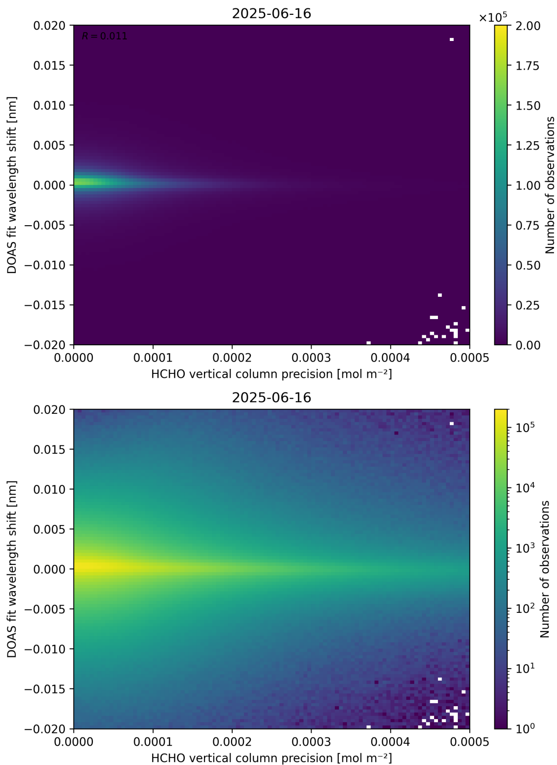
Figure 137: Scatter density plot of “HCHO vertical column precision” against “DOAS fit wavelength shift” for 2025-06-16 to 2025-06-17.
