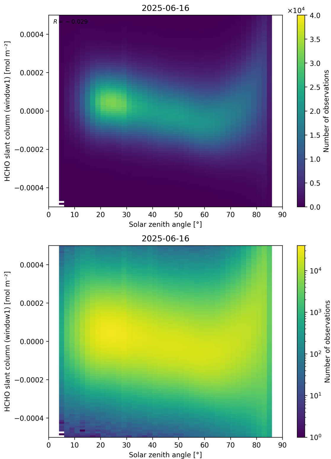
Figure 173: Scatter density plot of “Solar zenith angle” against “HCHO slant column (window1)” for 2025-06-16 to 2025-06-17.
