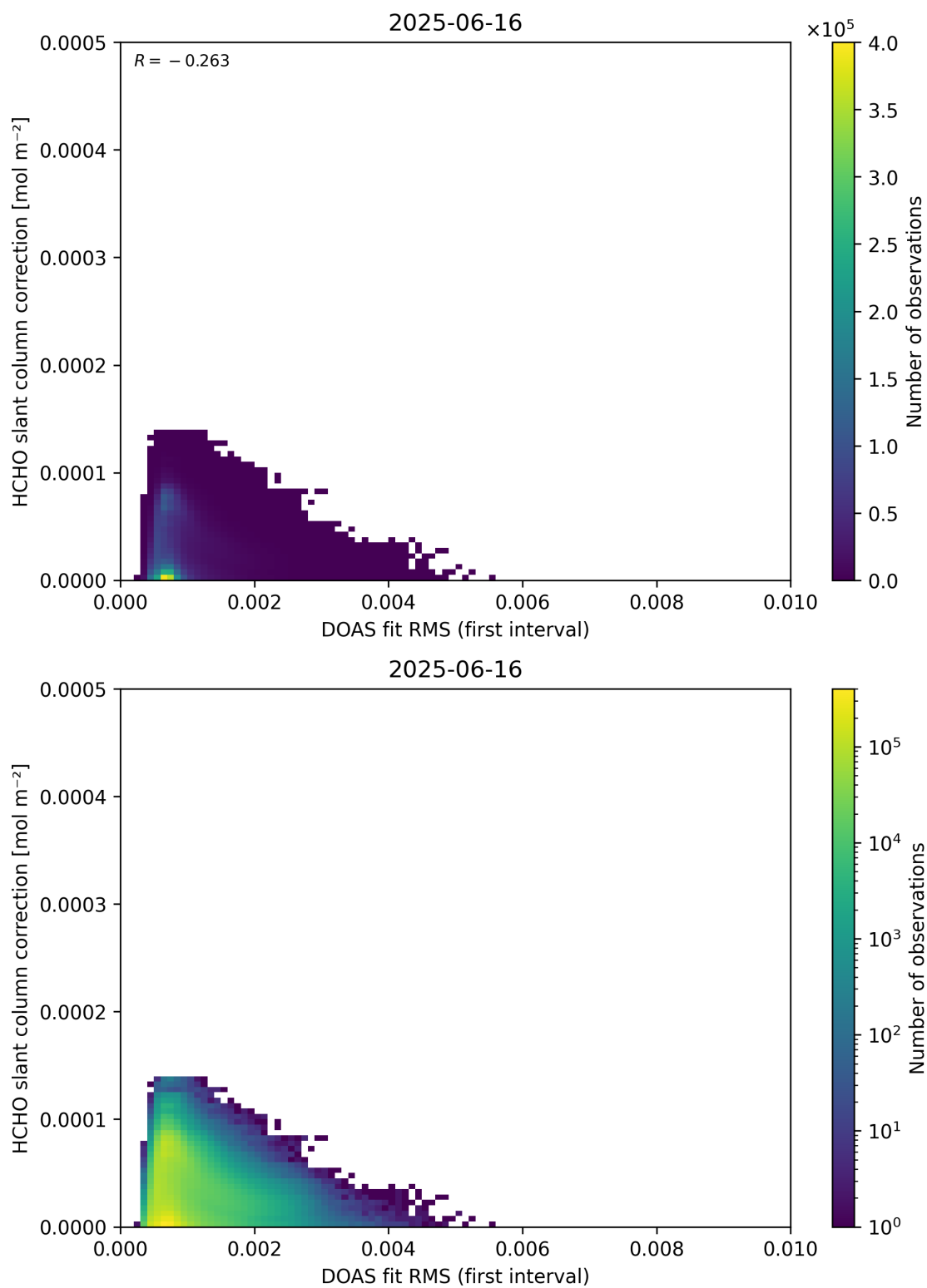
Figure 63: Scatter density plot of “DOAS fit RMS (first interval)” against “HCHO slant column correction” for 2025-06-16 to 2025-06-17.
