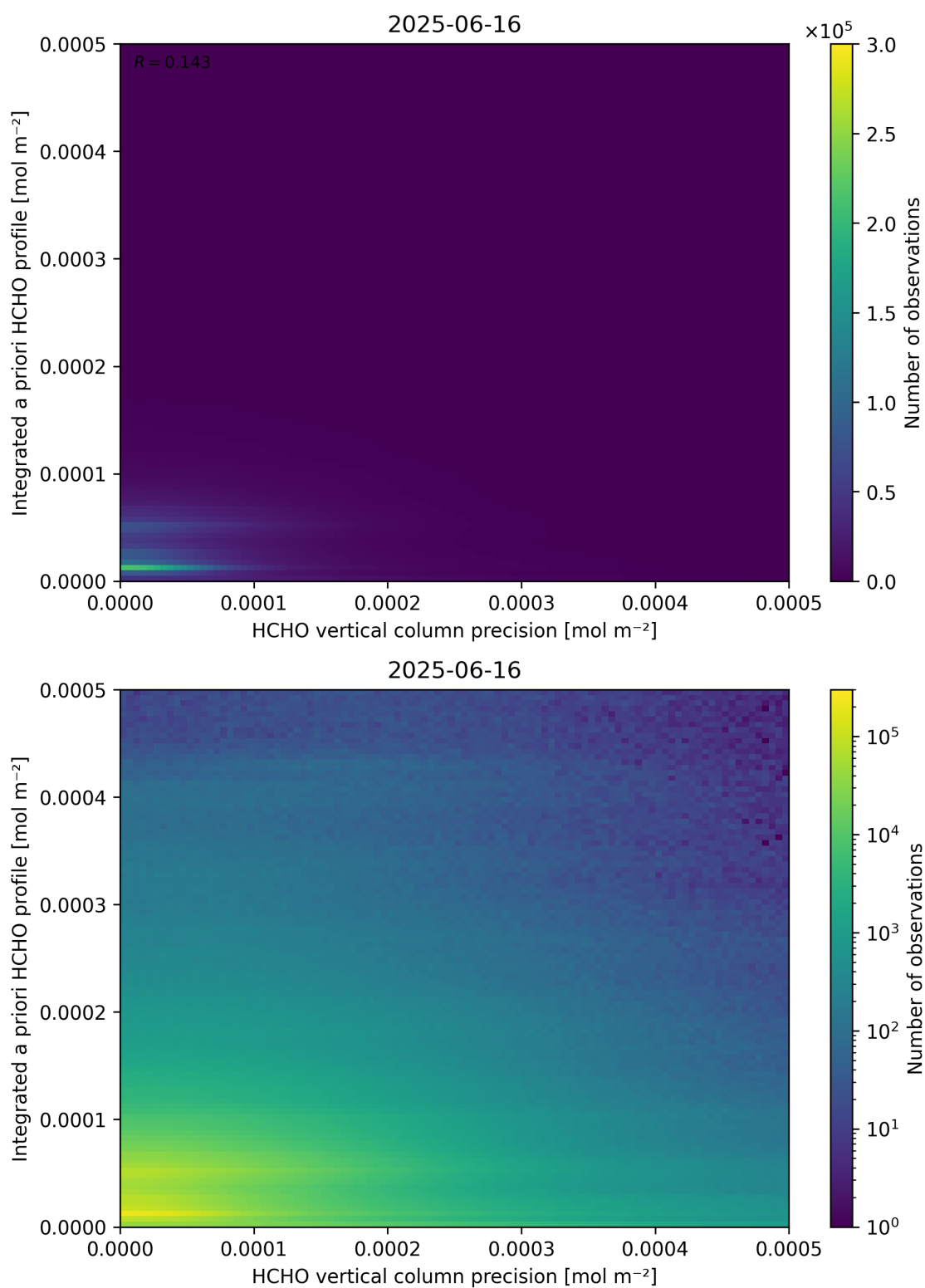
Figure 147: Scatter density plot of “HCHO vertical column precision” against “Integrated a priori HCHO profile” for 2025-06-16 to 2025-06-17.
