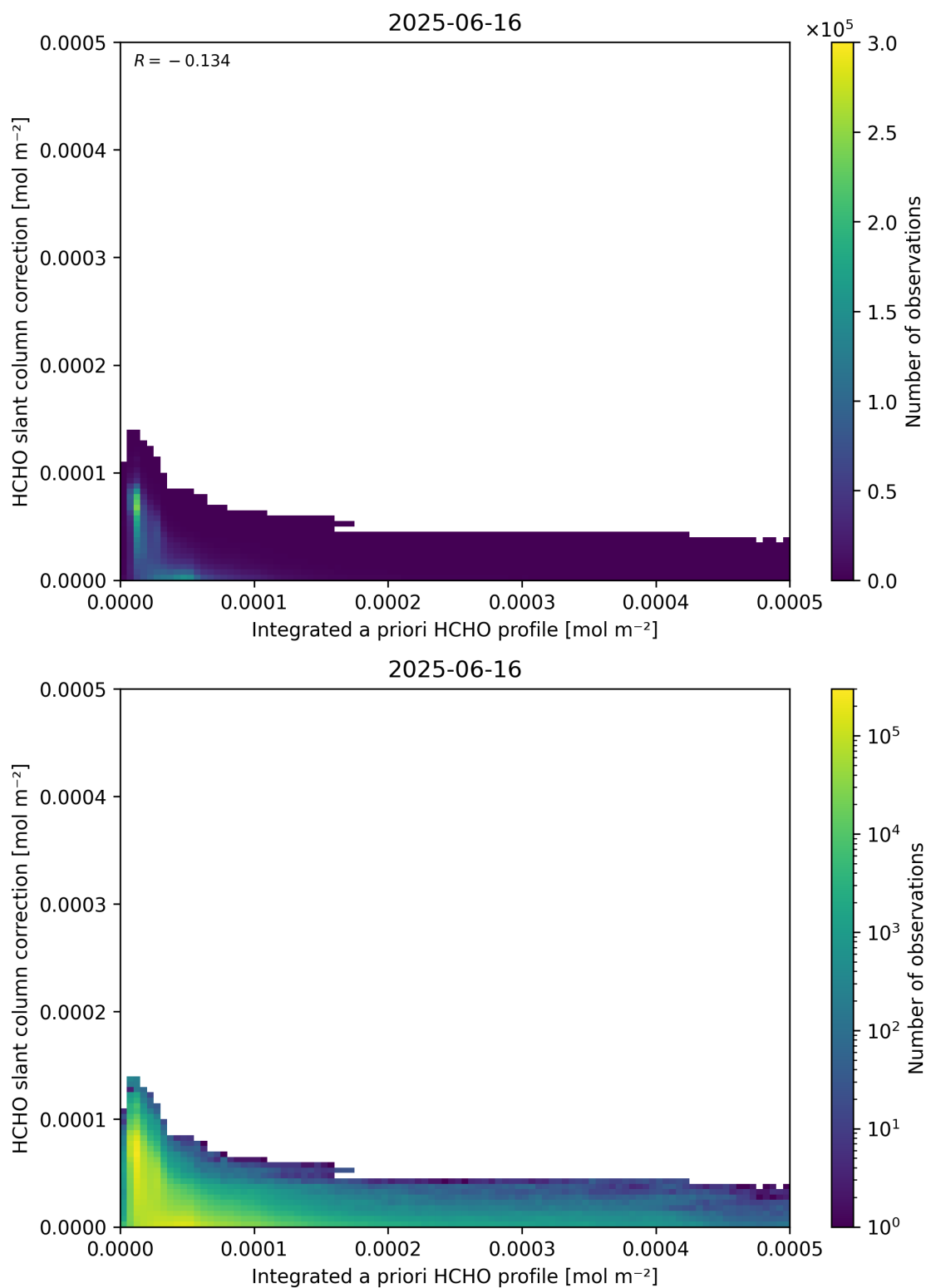
Figure 152: Scatter density plot of “Integrated a priori HCHO profile” against “HCHO slant column correction” for 2025-06-16 to 2025-06-17.
