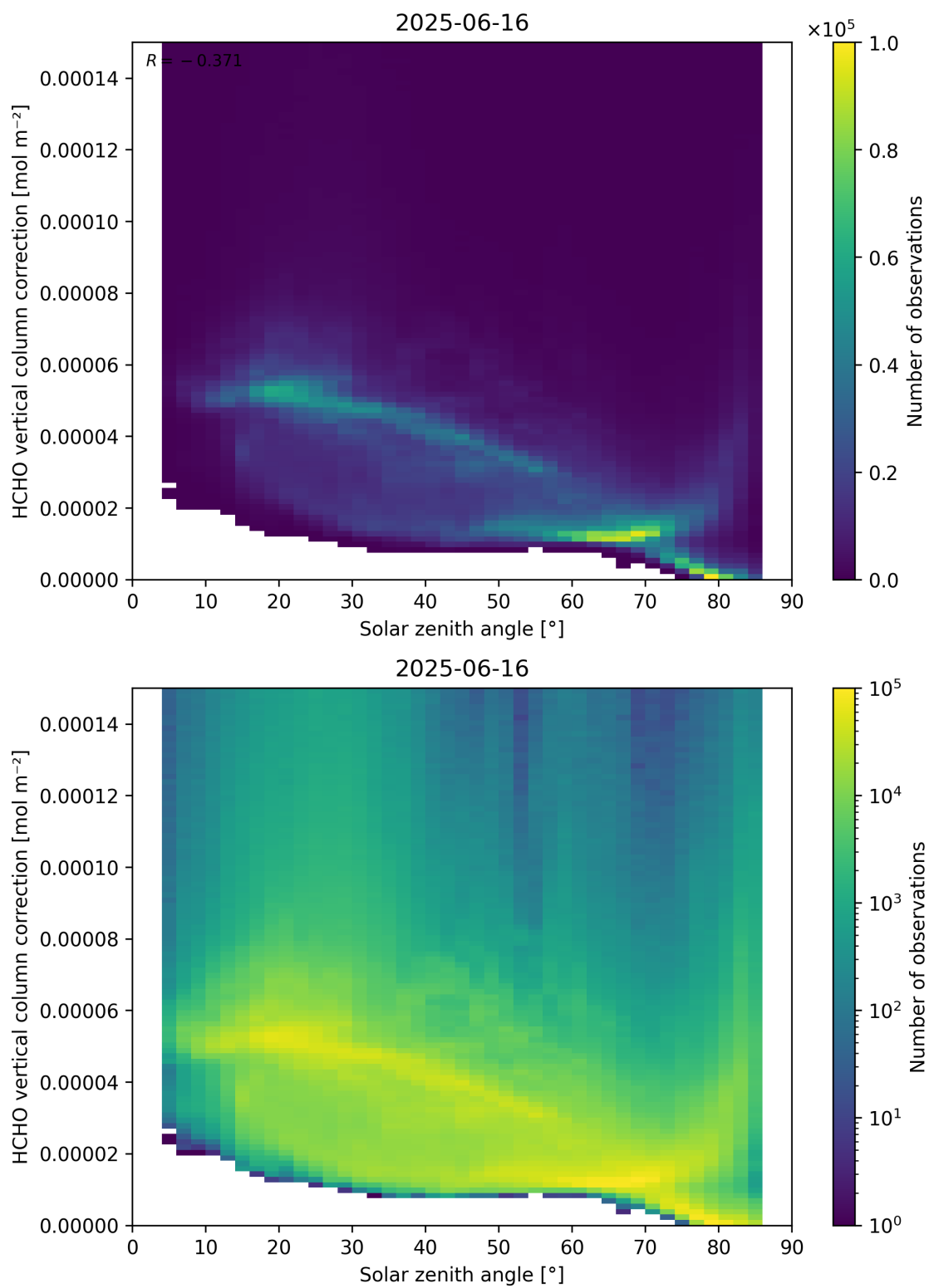
Figure 178: Scatter density plot of “Solar zenith angle” against “HCHO vertical column correction” for 2025-06-16 to 2025-06-17.
