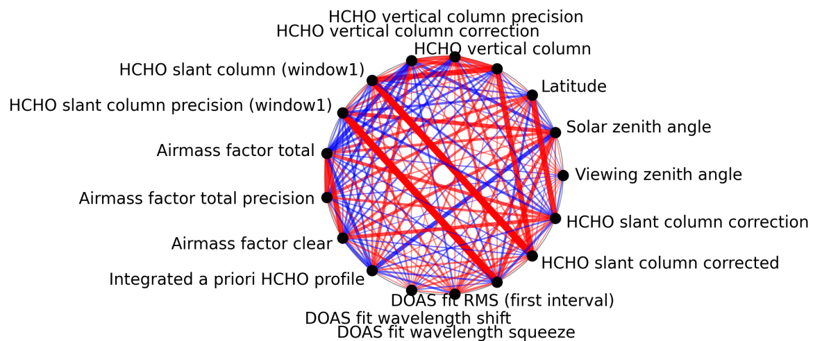
Figure 1: Map of correlation graph for 2025-06-16 to 2025-06-17.
