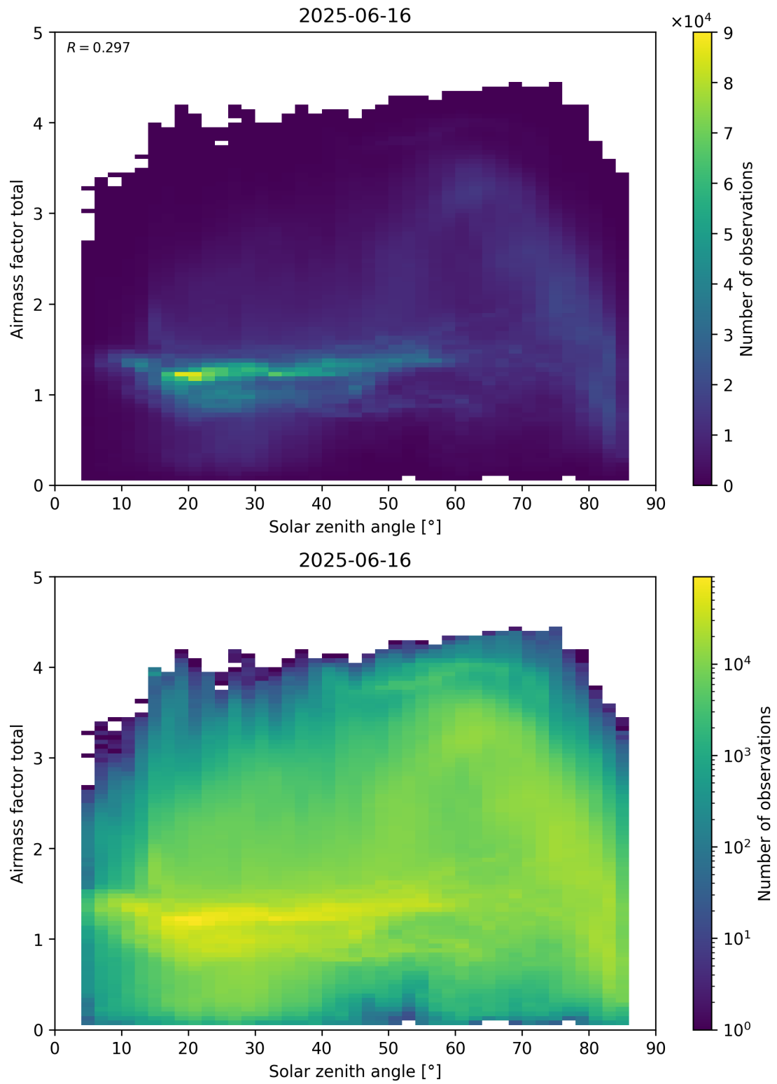
Figure 175: Scatter density plot of “Solar zenith angle” against “Airmass factor total” for 2025-06-16 to 2025-06-17.
