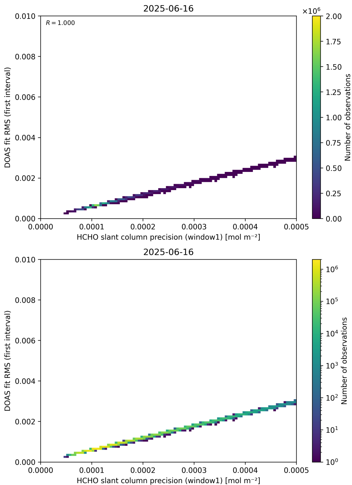
Figure 88: Scatter density plot of “HCHO slant column precision (window1)” against “DOAS fit RMS (first interval)” for 2025-06-16 to 2025-06-17.
