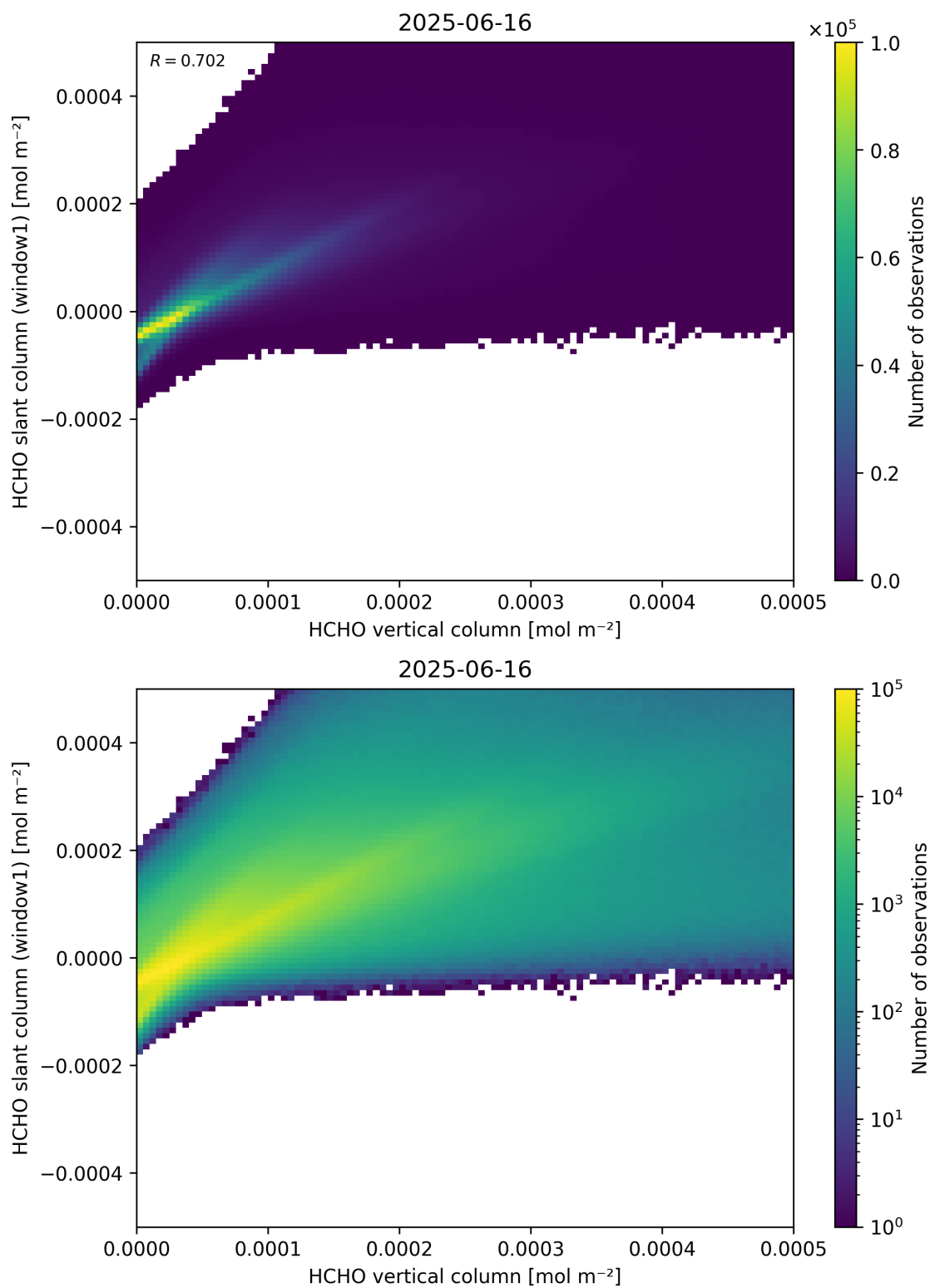
Figure 129: Scatter density plot of “HCHO vertical column” against “HCHO slant column (window1)” for 2025-06-16 to 2025-06-17.
