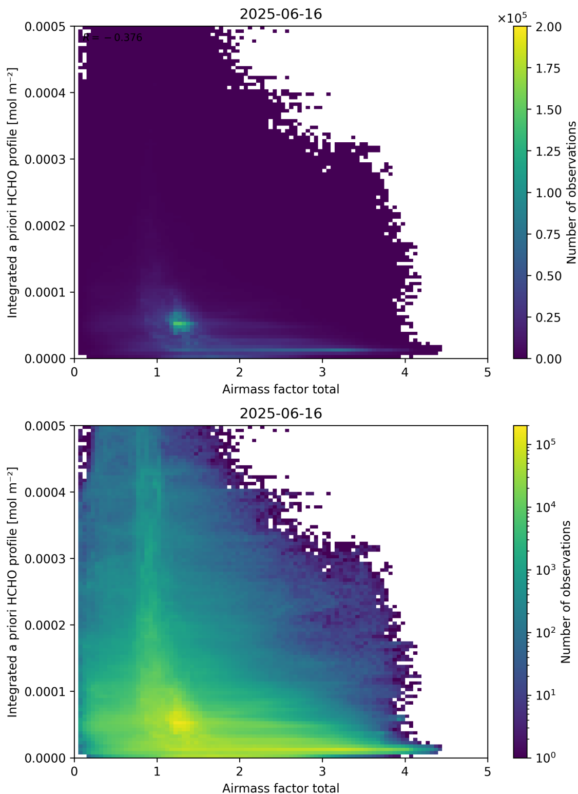
Figure 104: Scatter density plot of “Airmass factor total” against “Integrated a priori HCHO profile” for 2025-06-16 to 2025-06-17.
