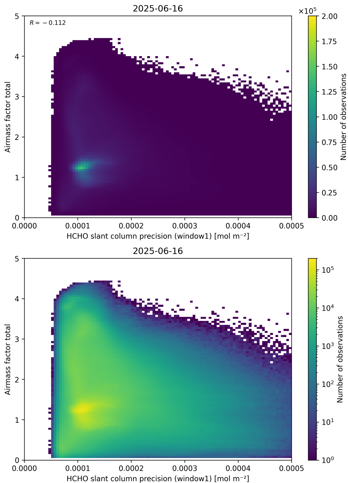
Figure 94: Scatter density plot of “HCHO slant column precision (window1)” against “Airmass factor total” for 2025-06-16 to 2025-06-17.
