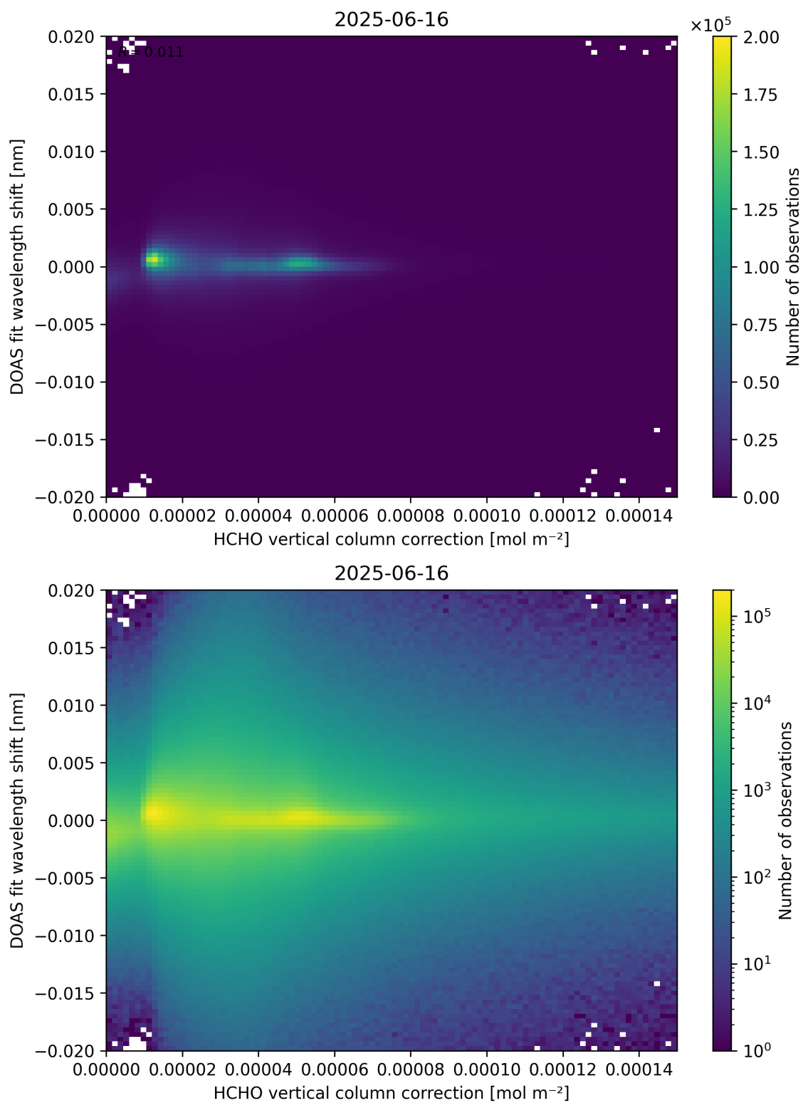
Figure 113: Scatter density plot of “HCHO vertical column correction” against “DOAS fit wavelength shift” for 2025-06-16 to 2025-06-17.
