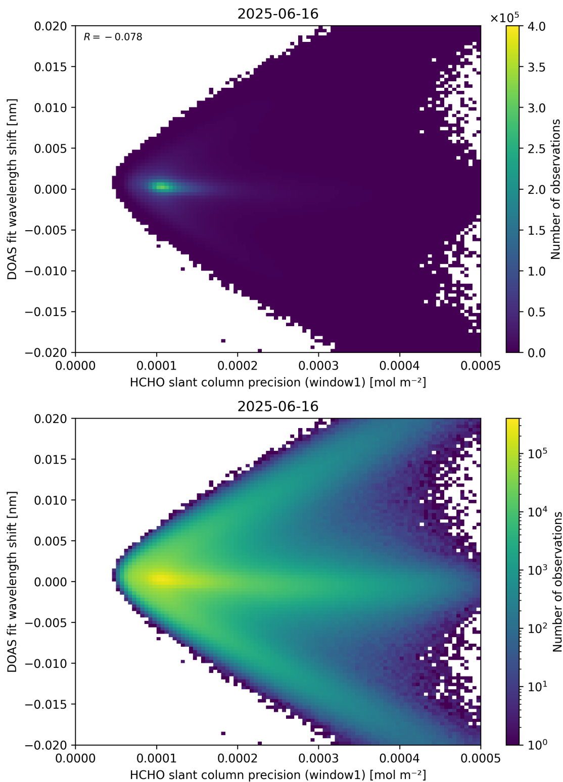
Figure 89: Scatter density plot of “HCHO slant column precision (window1)” against “DOAS fit wavelength shift” for 2025-06-16 to 2025-06-17.
