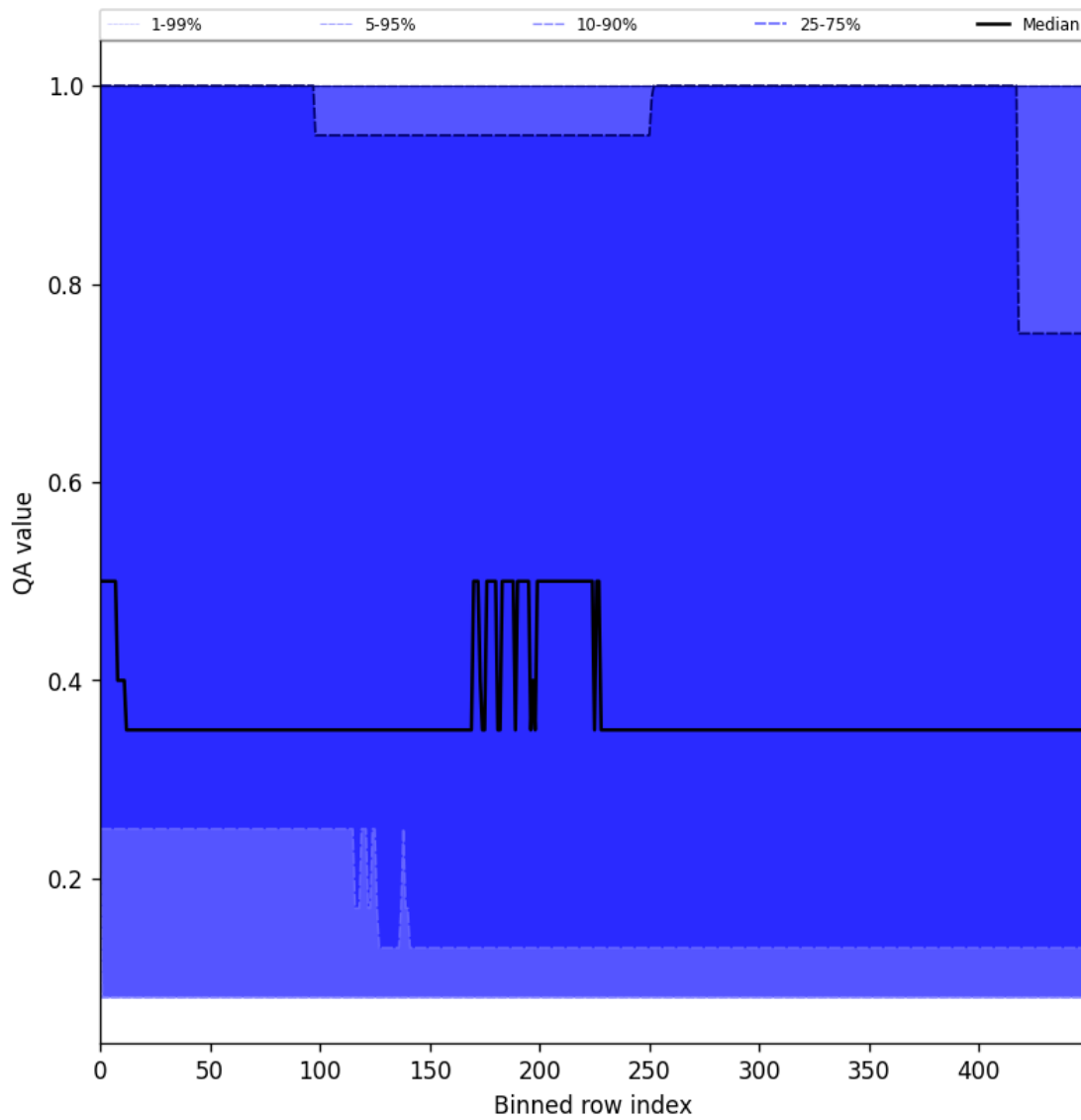
Figure 48: Along track statistics of “QA value” for 2025-06-16 to 2025-06-17
