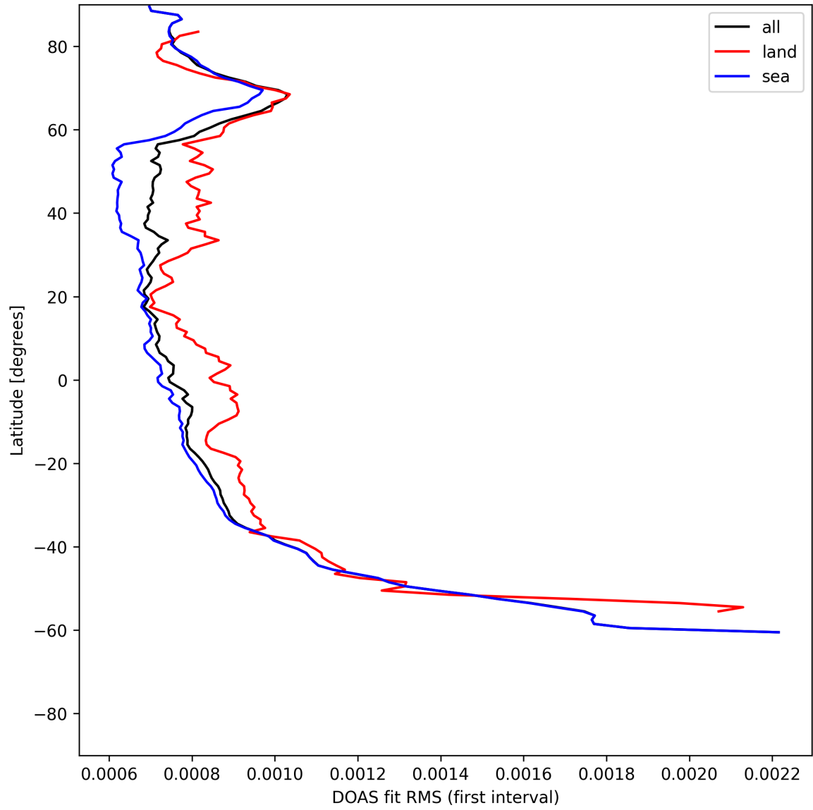
Figure 32: Zonal average of “DOAS fit RMS (first interval)” for 2025-06-16 to 2025-06-17.
