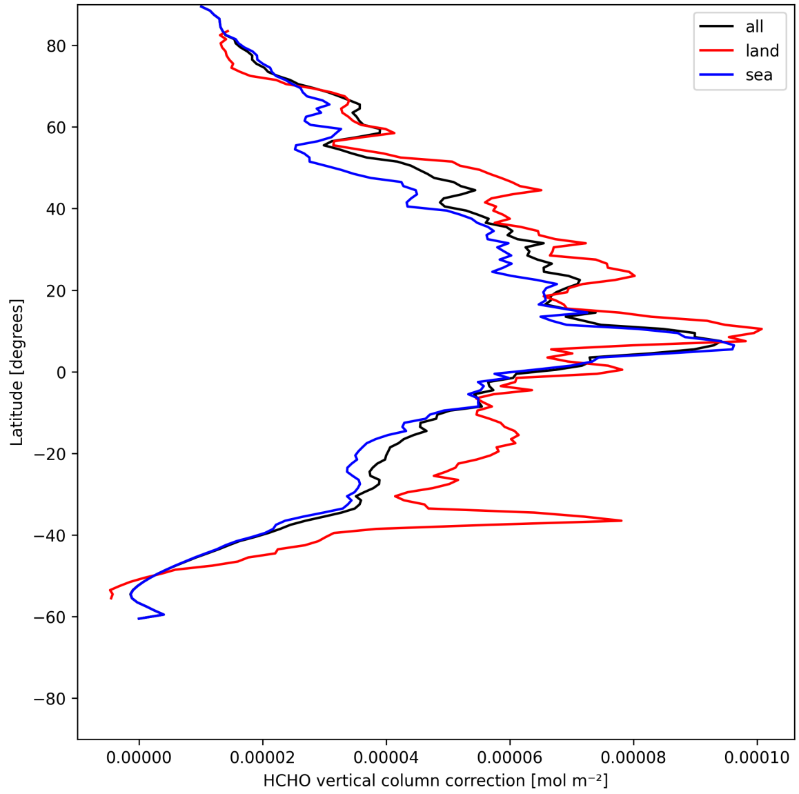
Figure 23: Zonal average of “HCHO vertical column correction” for 2025-06-16 to 2025-06-17.
