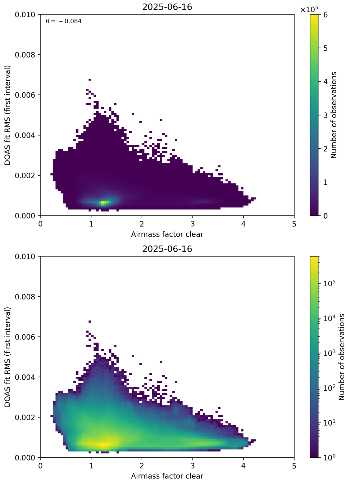
Figure 71: Scatter density plot of “Airmass factor clear” against “DOAS fit RMS (first interval)” for 2025-06-16 to 2025-06-17.
