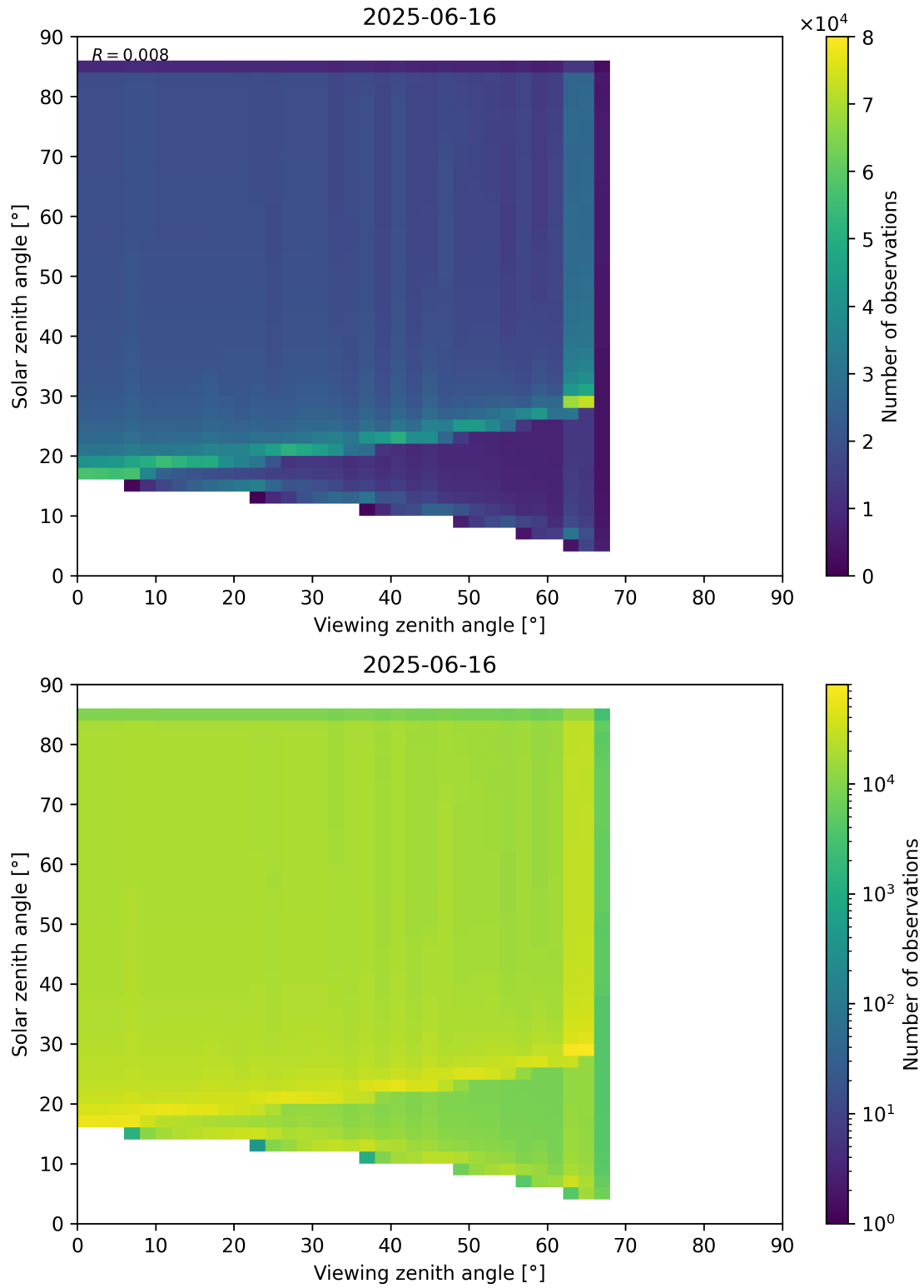
Figure 197: Scatter density plot of “Viewing zenith angle” against “Solar zenith angle” for 2025-06-16 to 2025-06-17.
