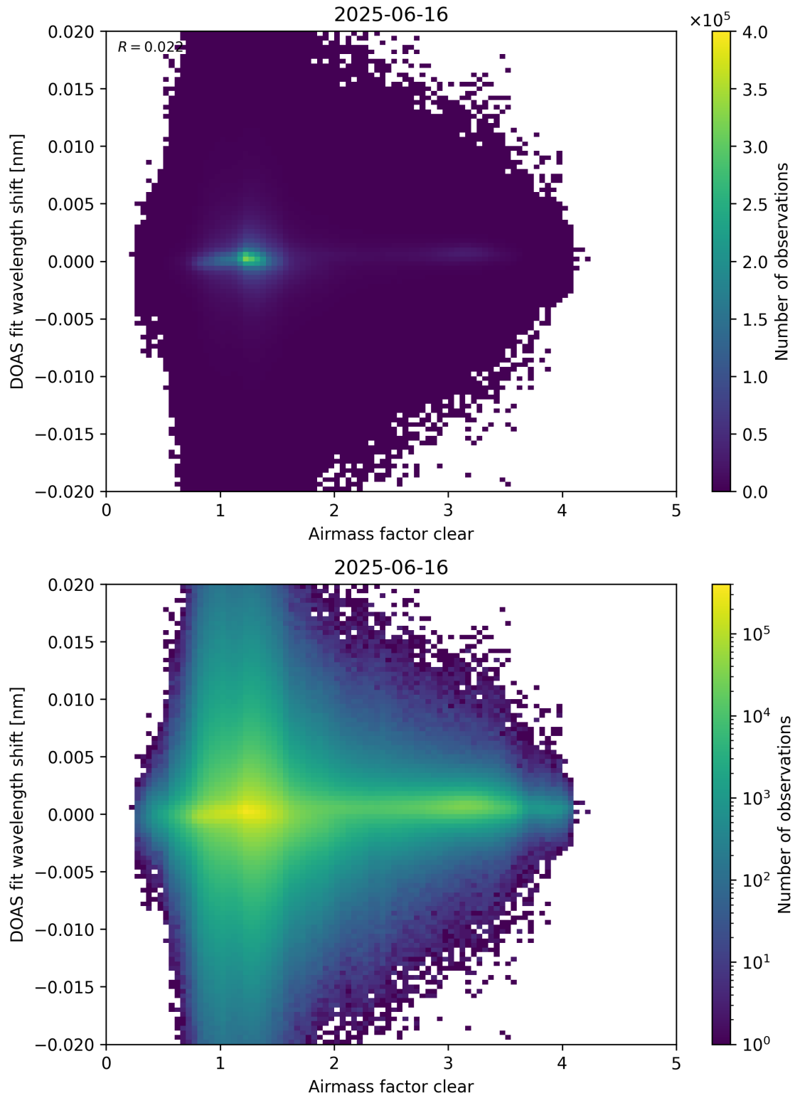
Figure 72: Scatter density plot of “Airmass factor clear” against “DOAS fit wavelength shift” for 2025-06-16 to 2025-06-17.
