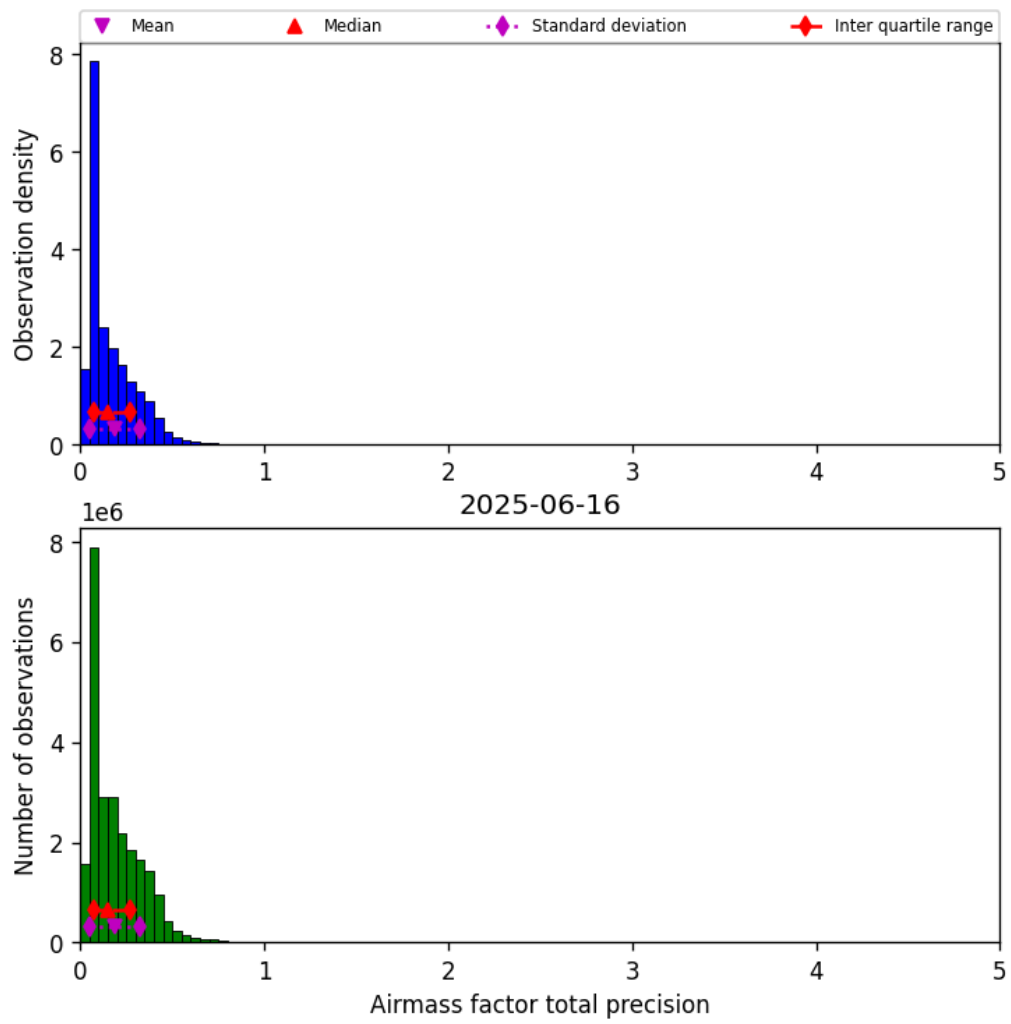
Figure 41: Histogram of “Airmass factor total precision” for 2025-06-16 to 2025-06-17
