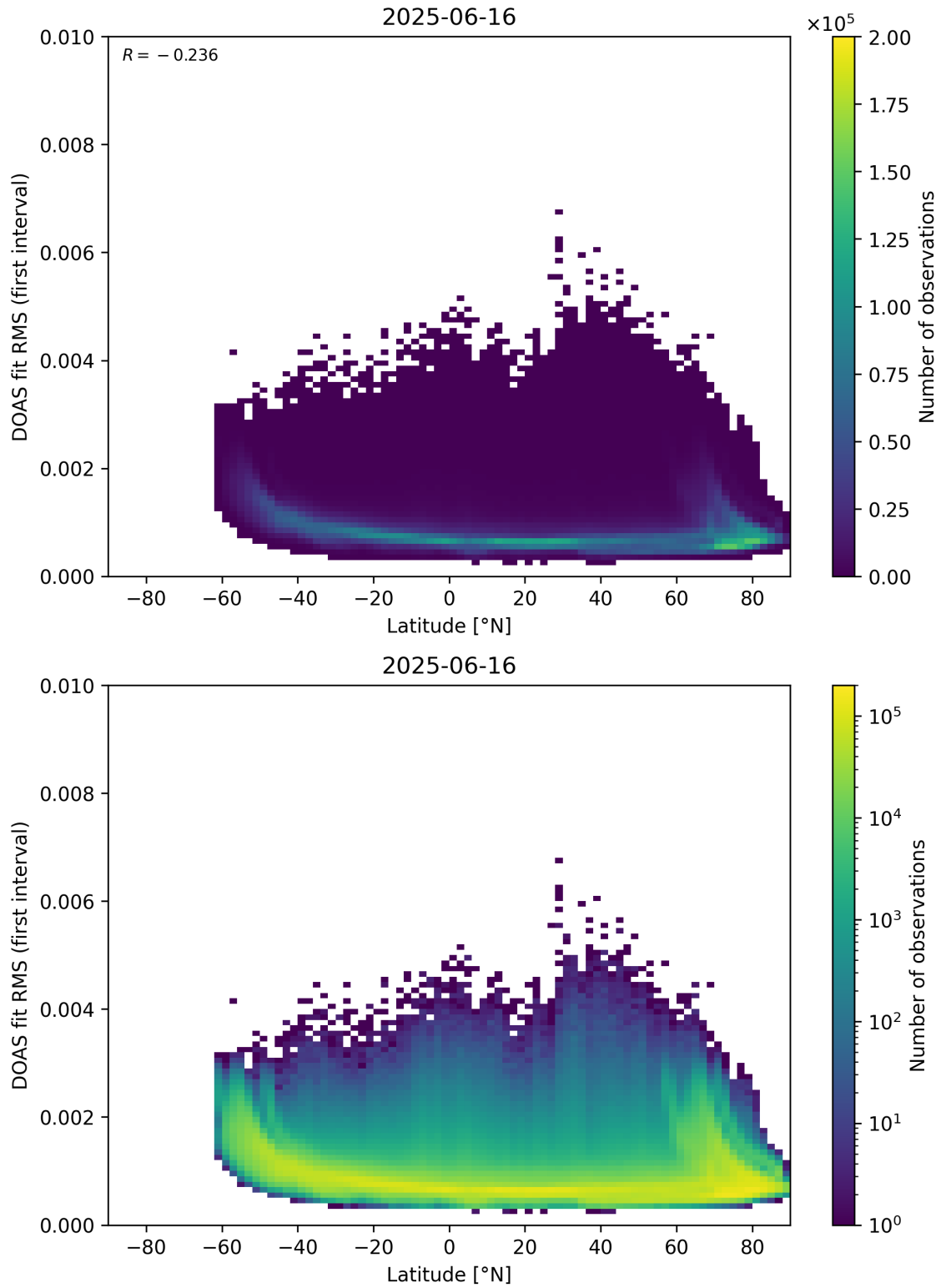
Figure 153: Scatter density plot of “Latitude” against “DOAS fit RMS (first interval)” for 2025-06-16 to 2025-06-17.
