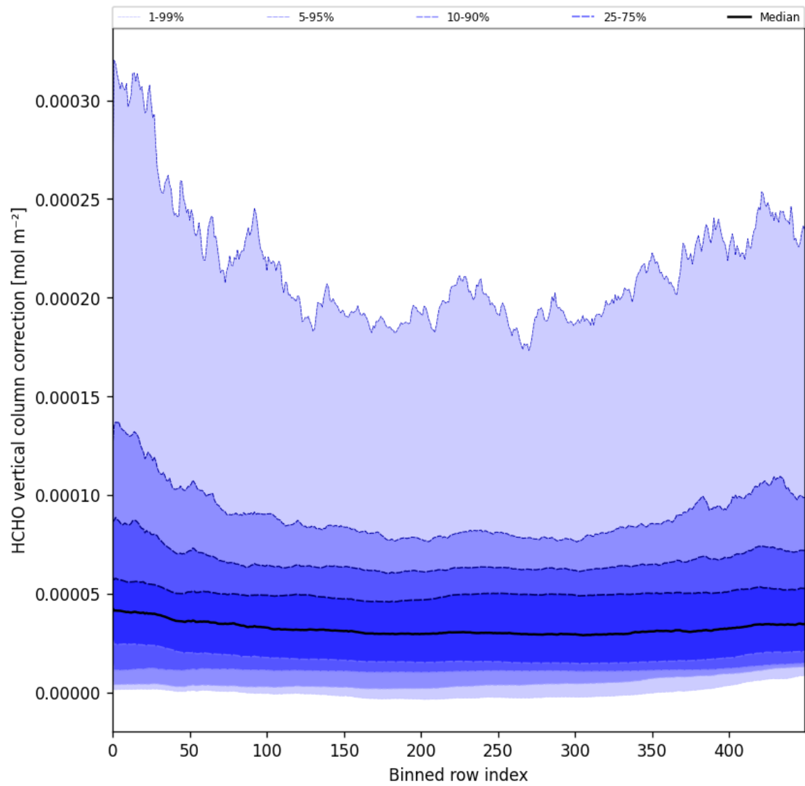
Figure 51: Along track statistics of “HCHO vertical column correction” for 2025-06-16 to 2025-06-17
