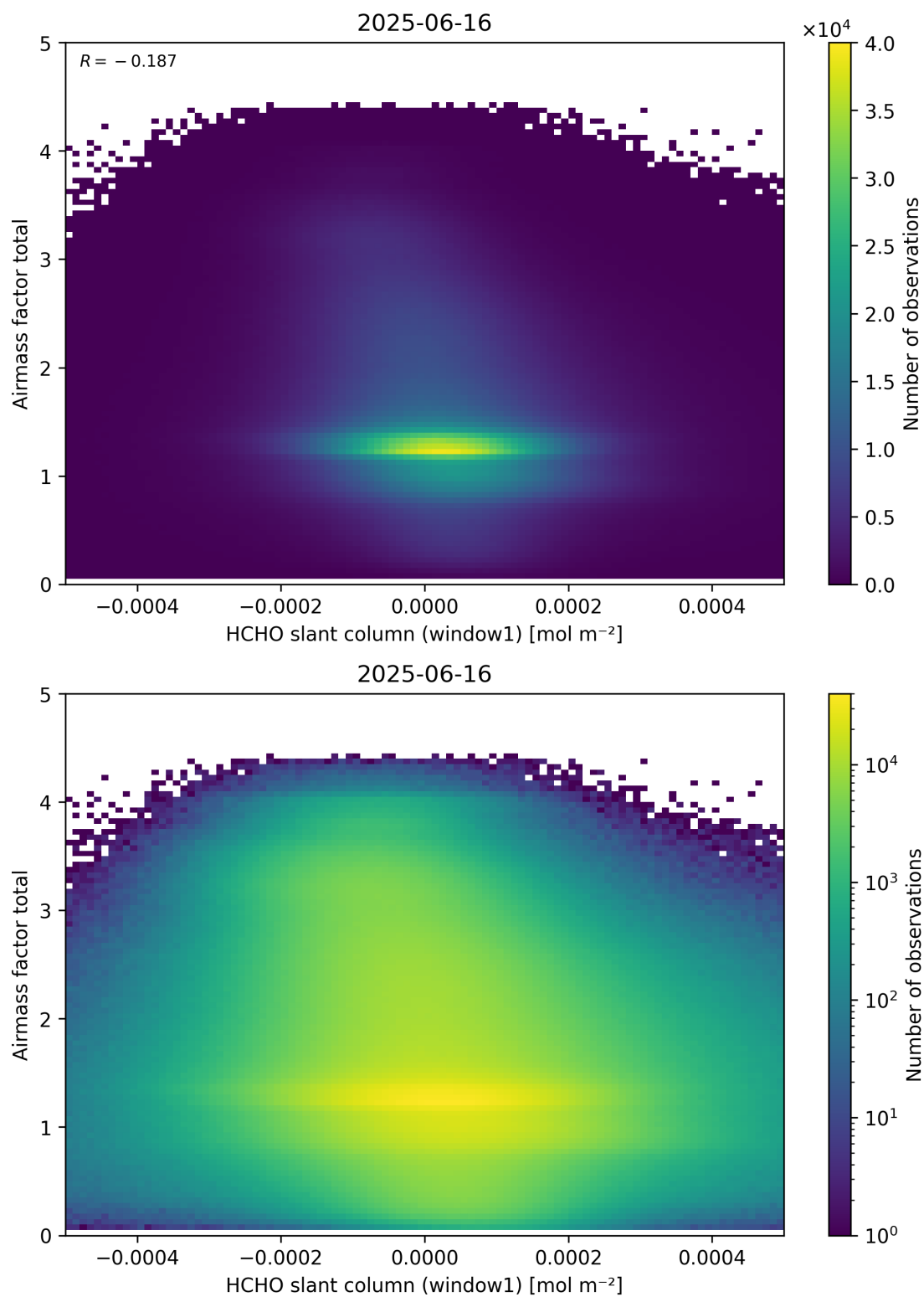
Figure 85: Scatter density plot of “HCHO slant column (window1)” against “Airmass factor total” for 2025-06-16 to 2025-06-17.
