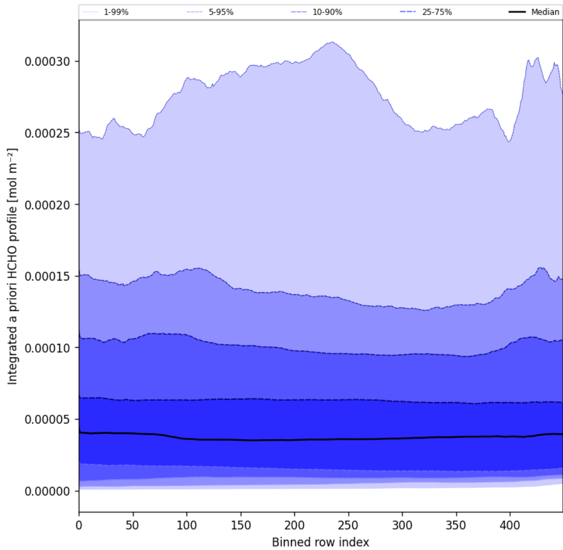
Figure 57: Along track statistics of “Integrated a priori HCHO profile” for 2025-06-16 to 2025-06-17
