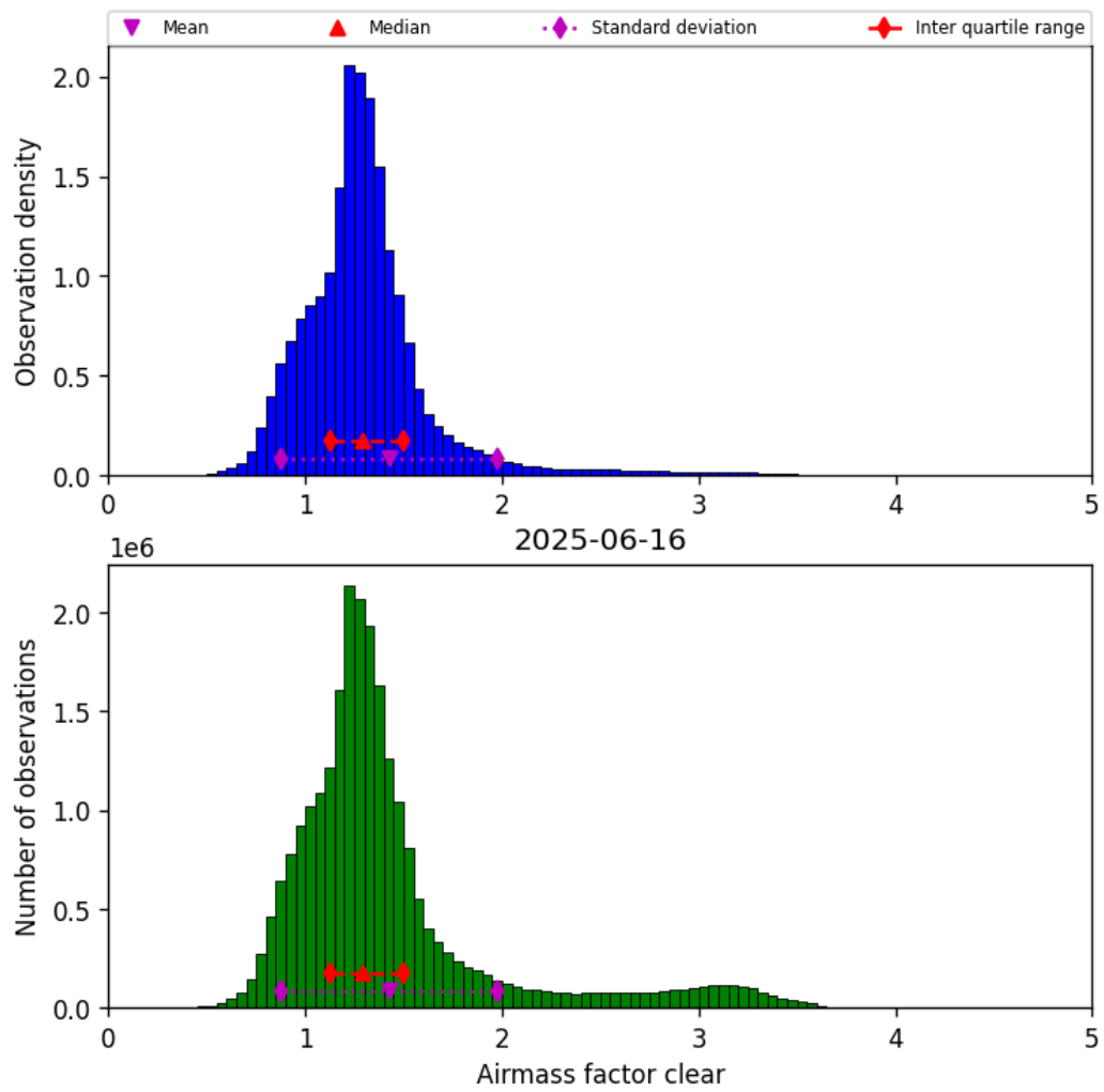
Figure 42: Histogram of “Airmass factor clear” for 2025-06-16 to 2025-06-17
