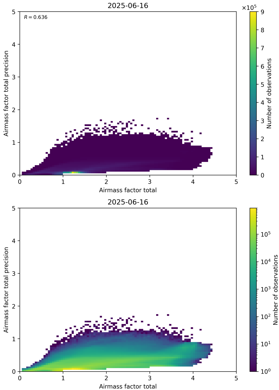
Figure 103: Scatter density plot of “Airmass factor total” against “Airmass factor total precision” for 2025-06-16 to 2025-06-17.
