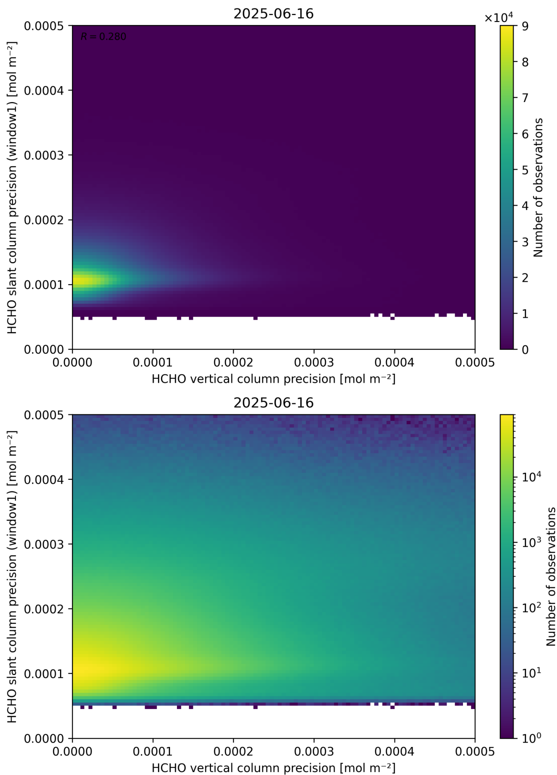
Figure 143: Scatter density plot of “HCHO vertical column precision” against “HCHO slant column precision (window1)” for 2025-06-16 to 2025-06-17.
