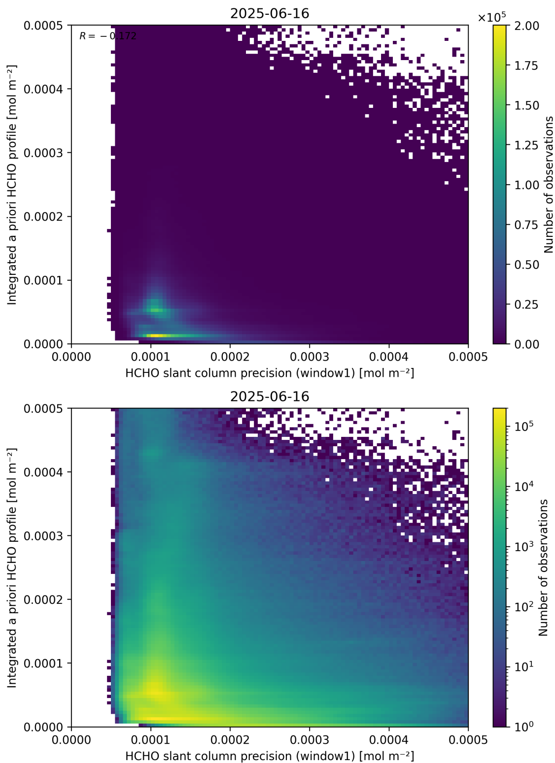
Figure 96: Scatter density plot of “HCHO slant column precision (window1)” against “Integrated a priori HCHO profile” for 2025-06-16 to 2025-06-17.
