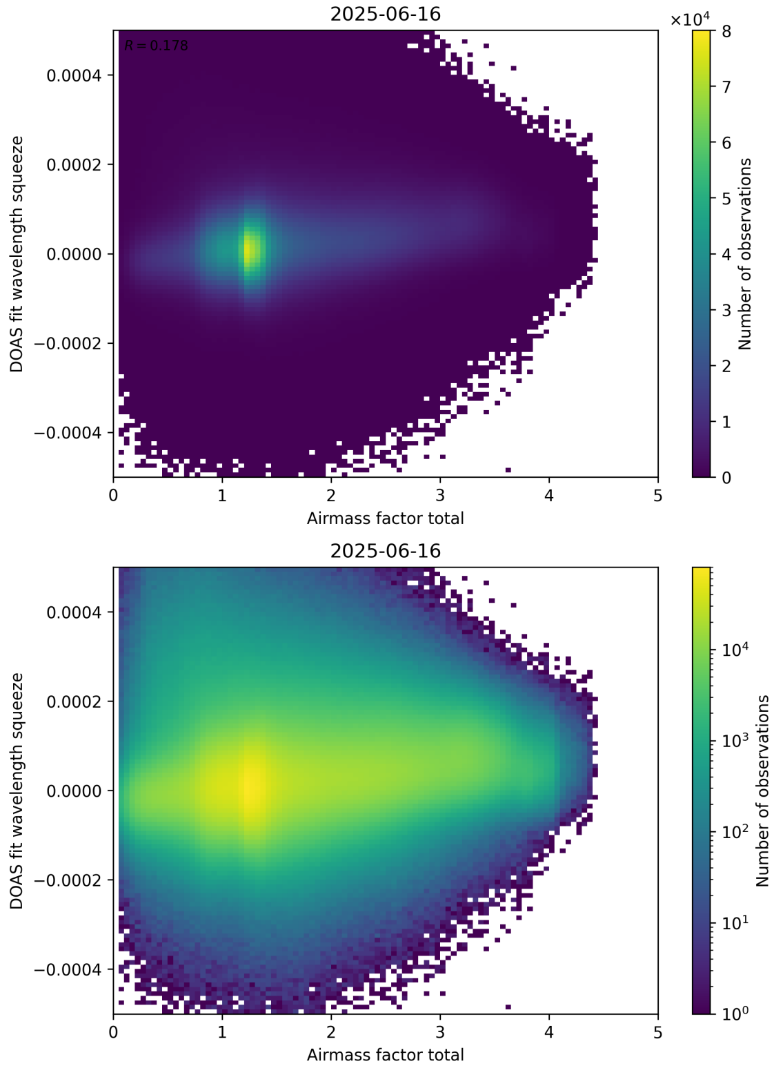
Figure 99: Scatter density plot of “Airmass factor total” against “DOAS fit wavelength squeeze” for 2025-06-16 to 2025-06-17.
