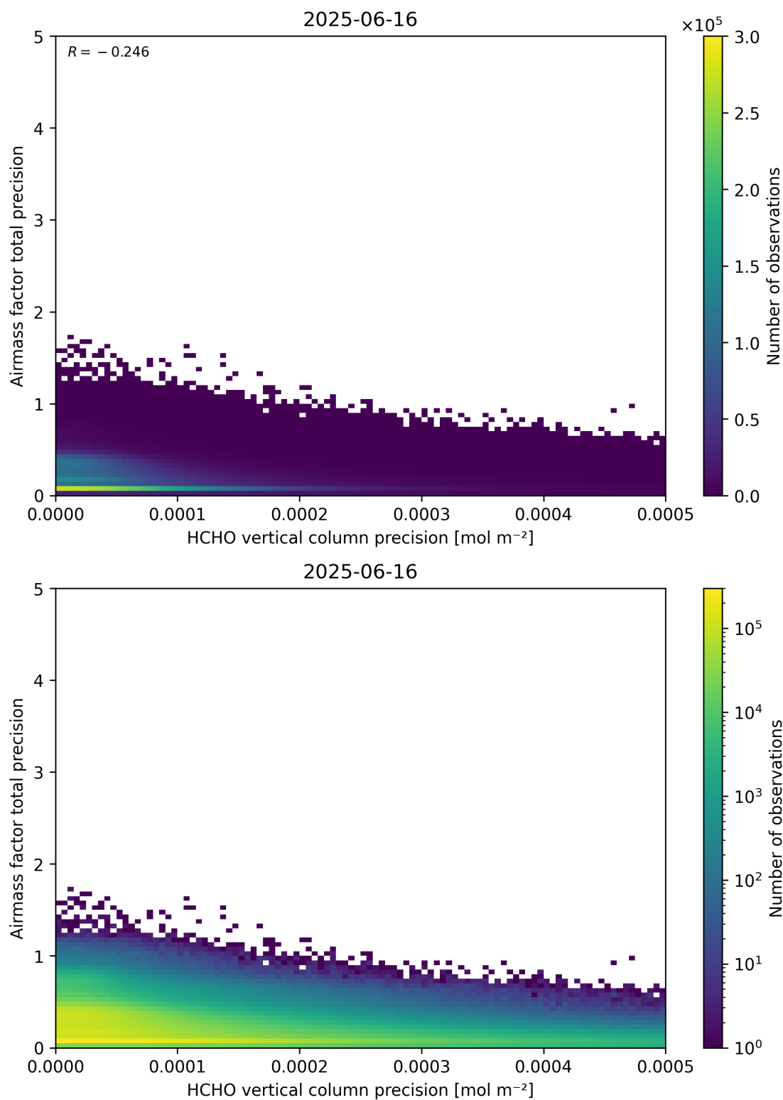
Figure 145: Scatter density plot of “HCHO vertical column precision” against “Airmass factor total precision” for 2025-06-16 to 2025-06-17.
