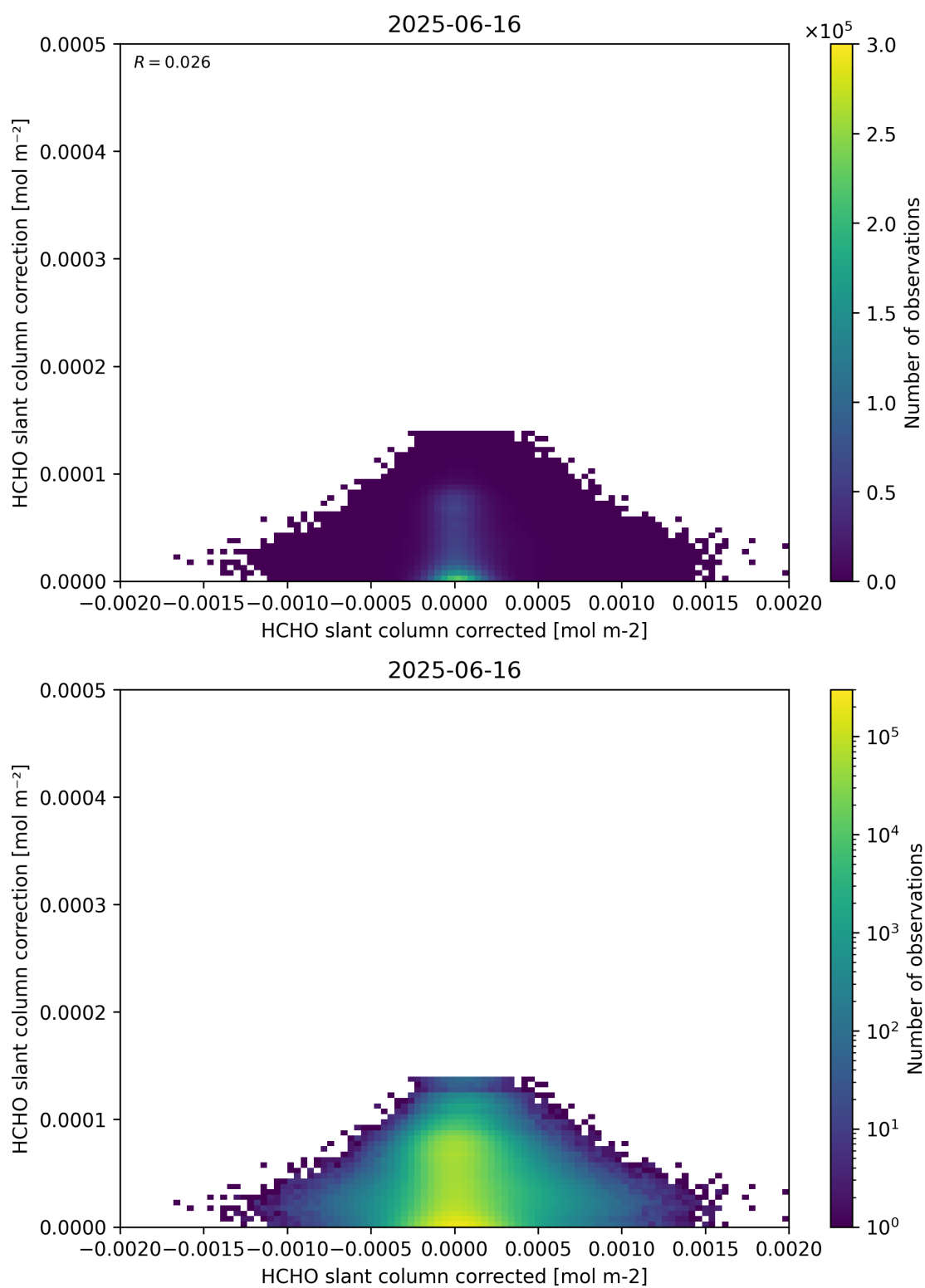
Figure 77: Scatter density plot of “HCHO slant column corrected” against “HCHO slant column correction” for 2025-06-16 to 2025-06-17.
