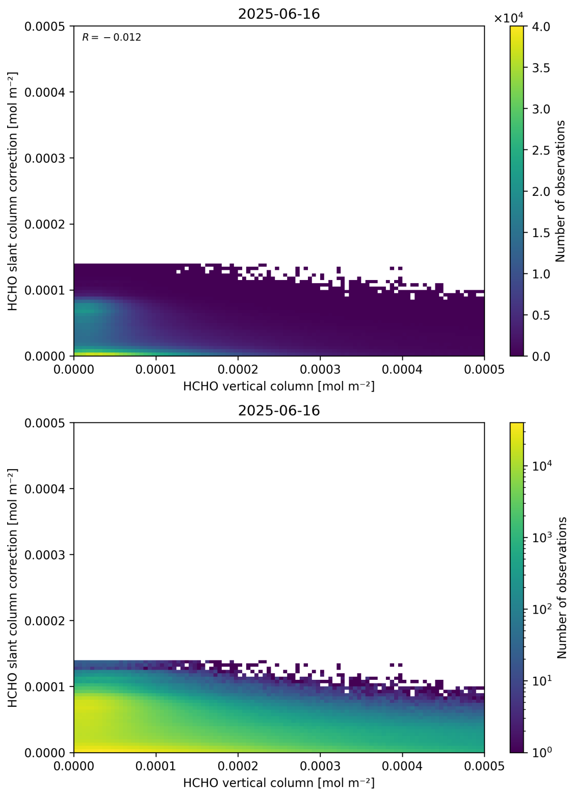
Figure 128: Scatter density plot of “HCHO vertical column” against “HCHO slant column correction” for 2025-06-16 to 2025-06-17.
