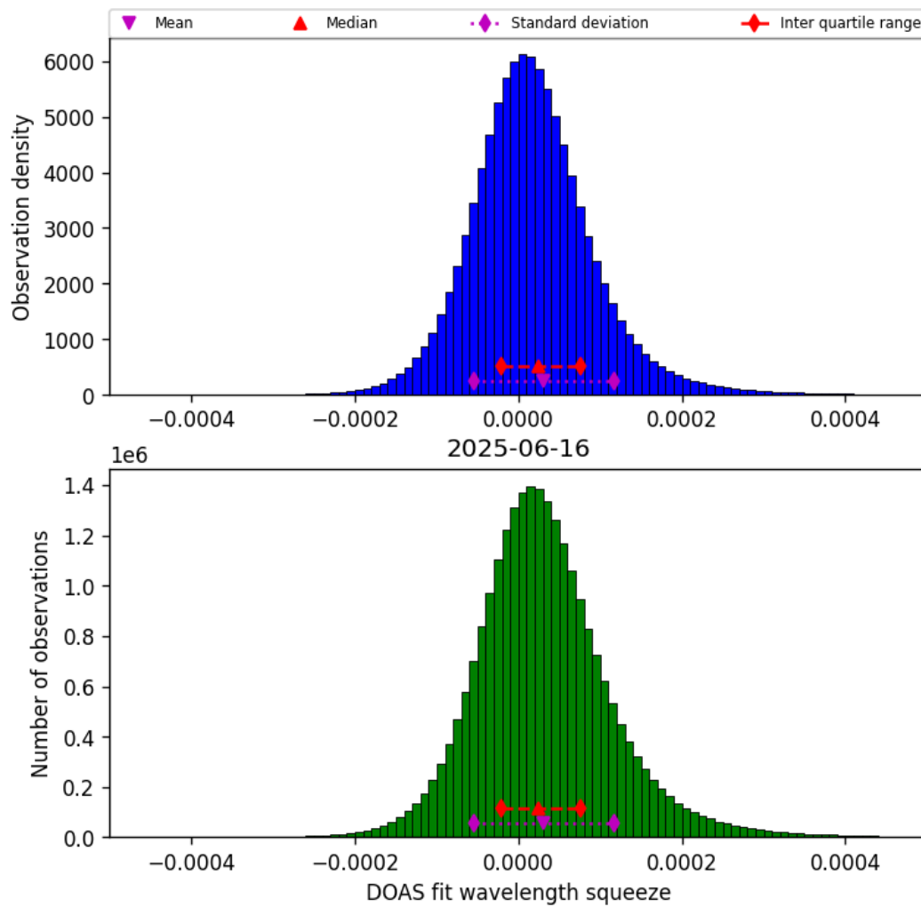
Figure 45: Histogram of “DOAS fit wavelength squeeze” for 2025-06-16 to 2025-06-17
