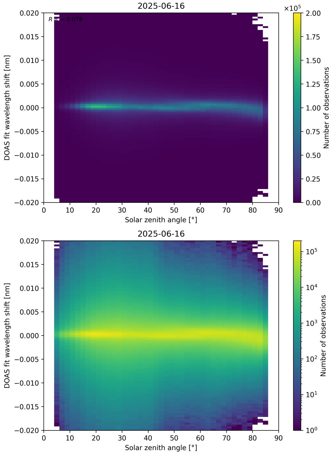
Figure 168: Scatter density plot of “Solar zenith angle” against “DOAS fit wavelength shift” for 2025-06-16 to 2025-06-17.
