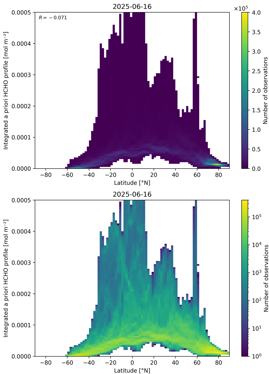
Figure 166: Scatter density plot of “Latitude” against “Integrated a priori HCHO profile” for 2025-06-16 to 2025-06-17.
