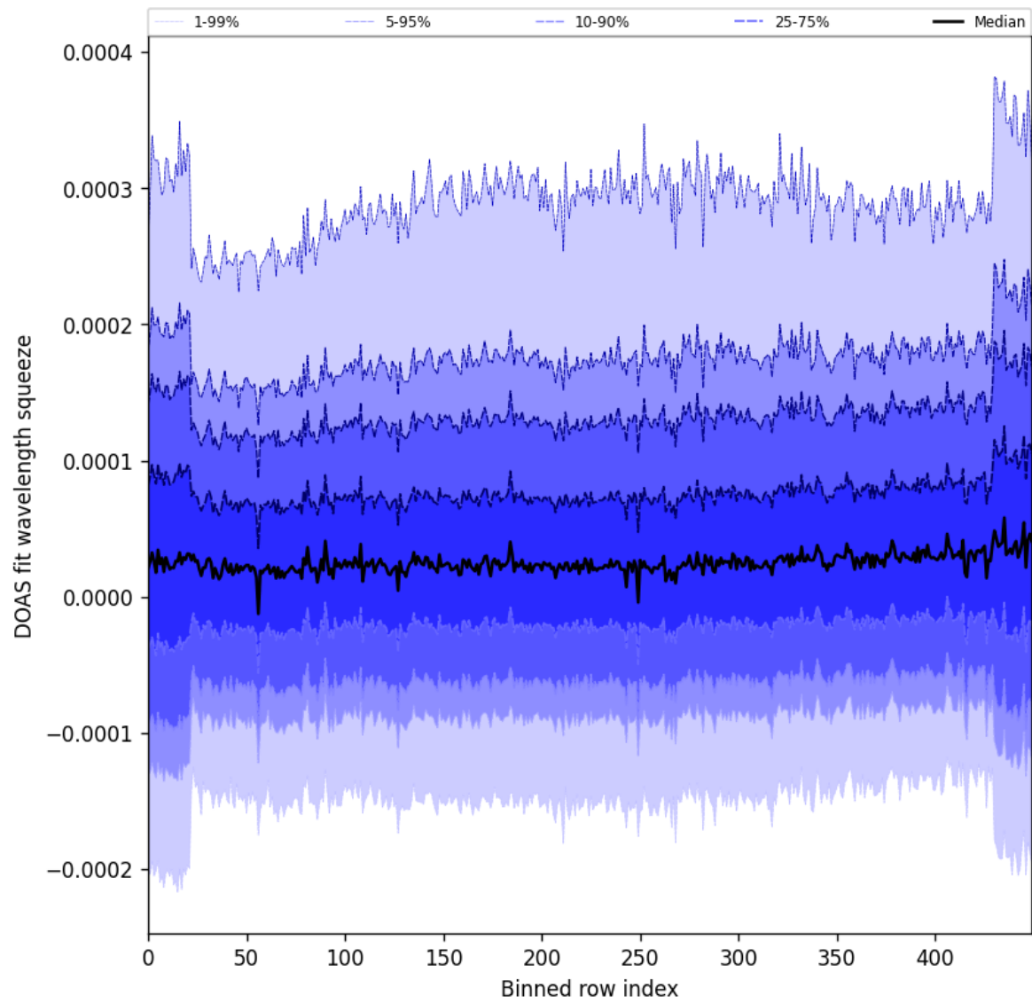
Figure 59: Along track statistics of “DOAS fit wavelength squeeze” for 2025-06-16 to 2025-06-17
