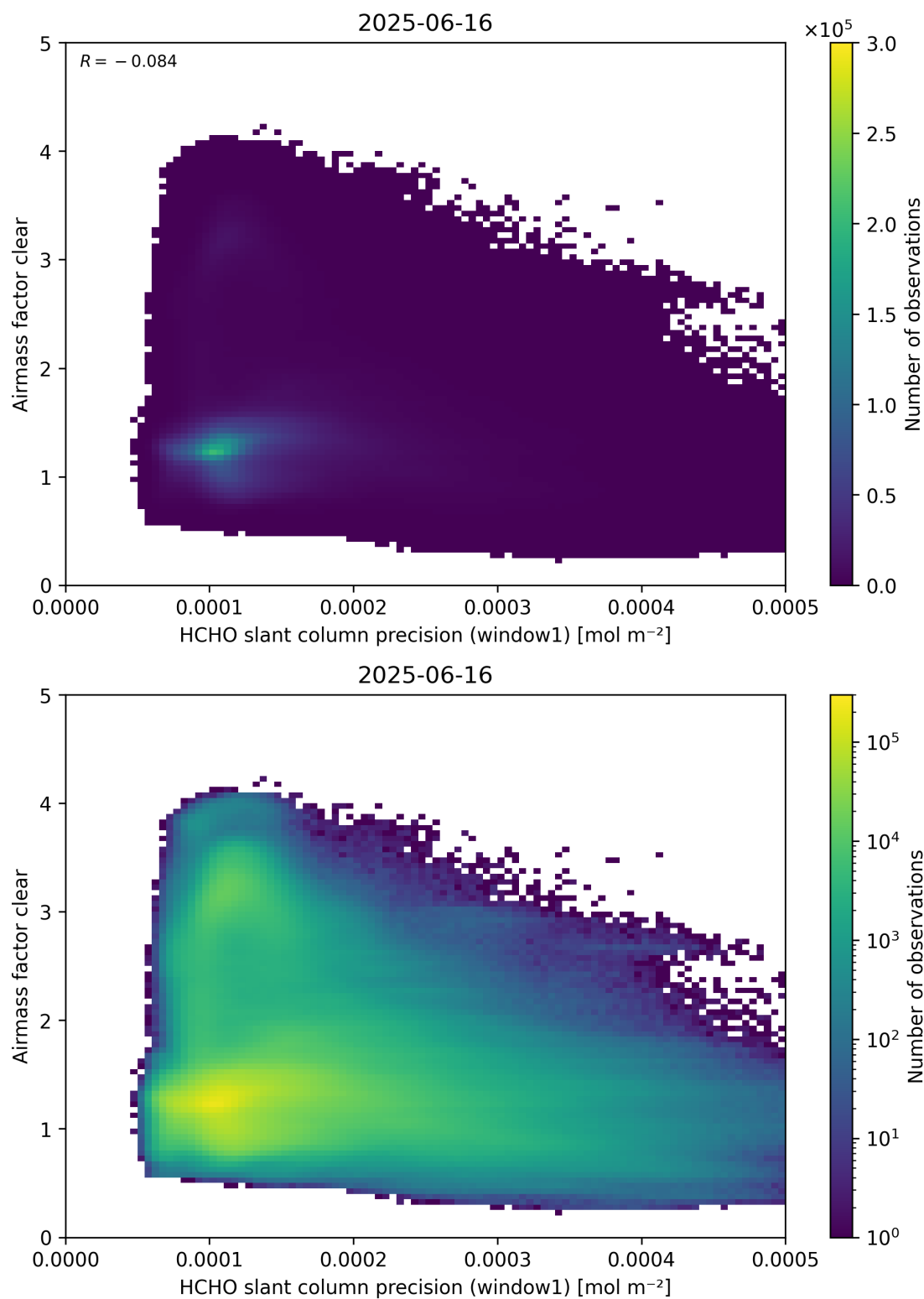
Figure 91: Scatter density plot of “HCHO slant column precision (window1)” against “Airmass factor clear” for 2025-06-16 to 2025-06-17.
