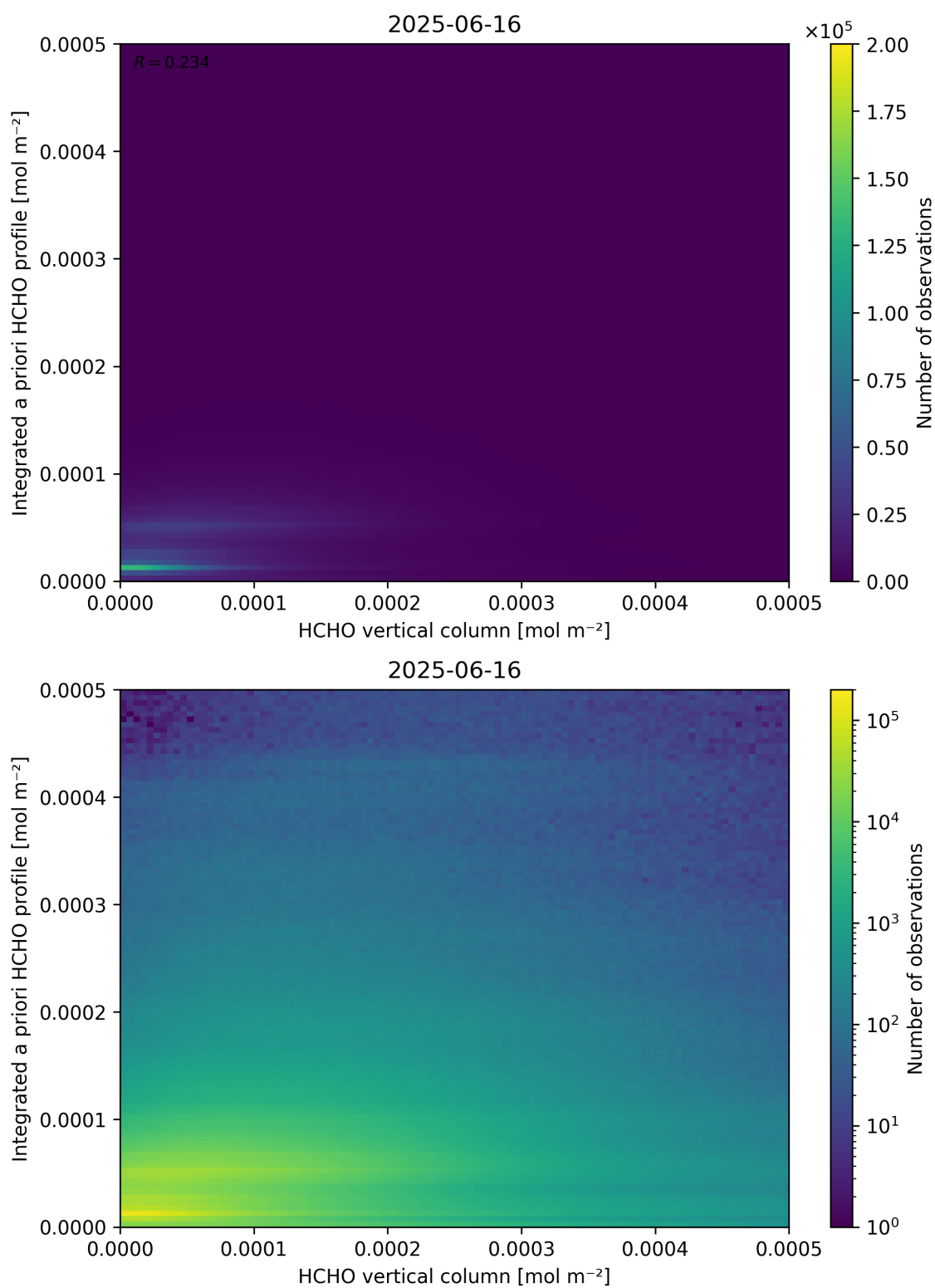
Figure 135: Scatter density plot of “HCHO vertical column” against “Integrated a priori HCHO profile” for 2025-06-16 to 2025-06-17.
