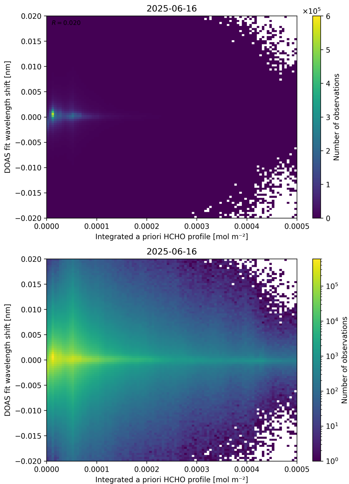
Figure 149: Scatter density plot of “Integrated a priori HCHO profile” against “DOAS fit wavelength shift” for 2025-06-16 to 2025-06-17.
