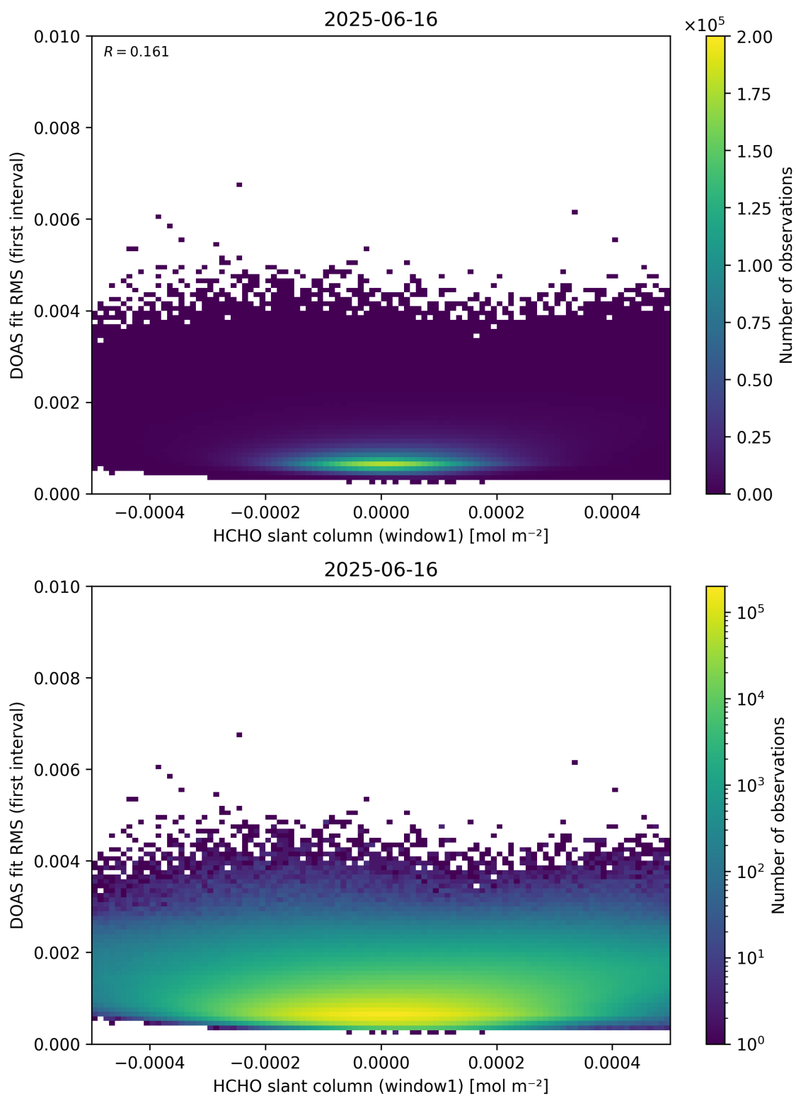
Figure 78: Scatter density plot of “HCHO slant column (window1)” against “DOAS fit RMS (first interval)” for 2025-06-16 to 2025-06-17.
