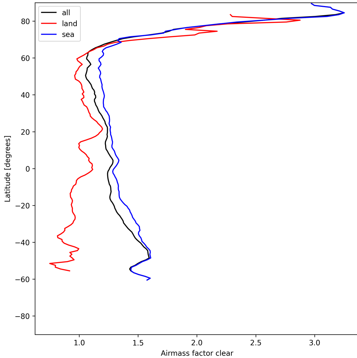
Figure 28: Zonal average of “Airmass factor clear” for 2025-06-16 to 2025-06-17.
