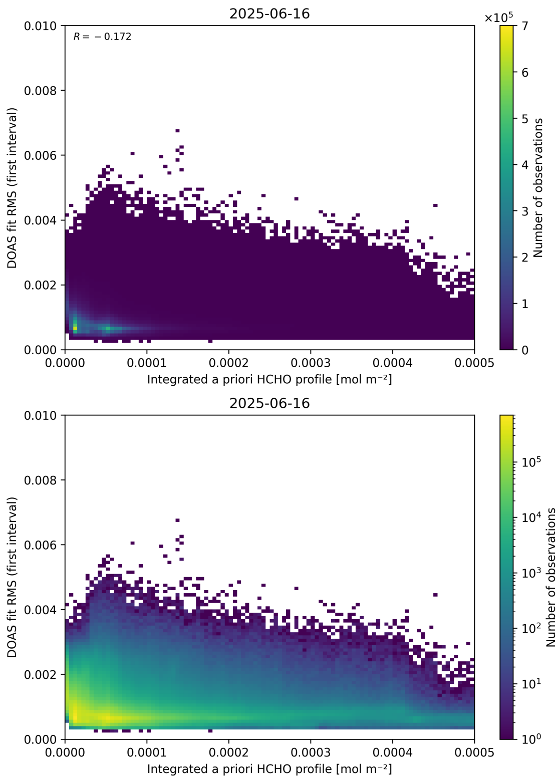
Figure 148: Scatter density plot of “Integrated a priori HCHO profile” against “DOAS fit RMS (first interval)” for 2025-06-16 to 2025-06-17.
