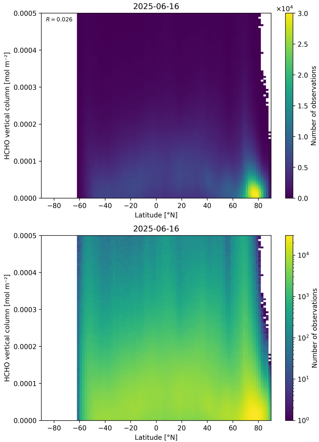
Figure 163: Scatter density plot of “Latitude” against “HCHO vertical column” for 2025-06-16 to 2025-06-17.
