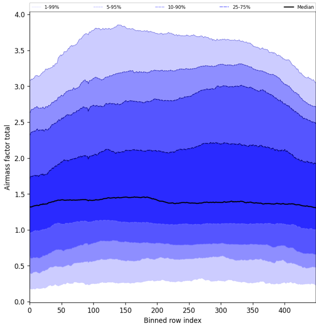
Figure 54: Along track statistics of “Airmass factor total” for 2025-06-16 to 2025-06-17
