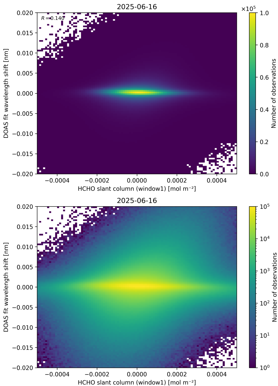
Figure 79: Scatter density plot of “HCHO slant column (window1)” against “DOAS fit wavelength shift” for 2025-06-16 to 2025-06-17.
