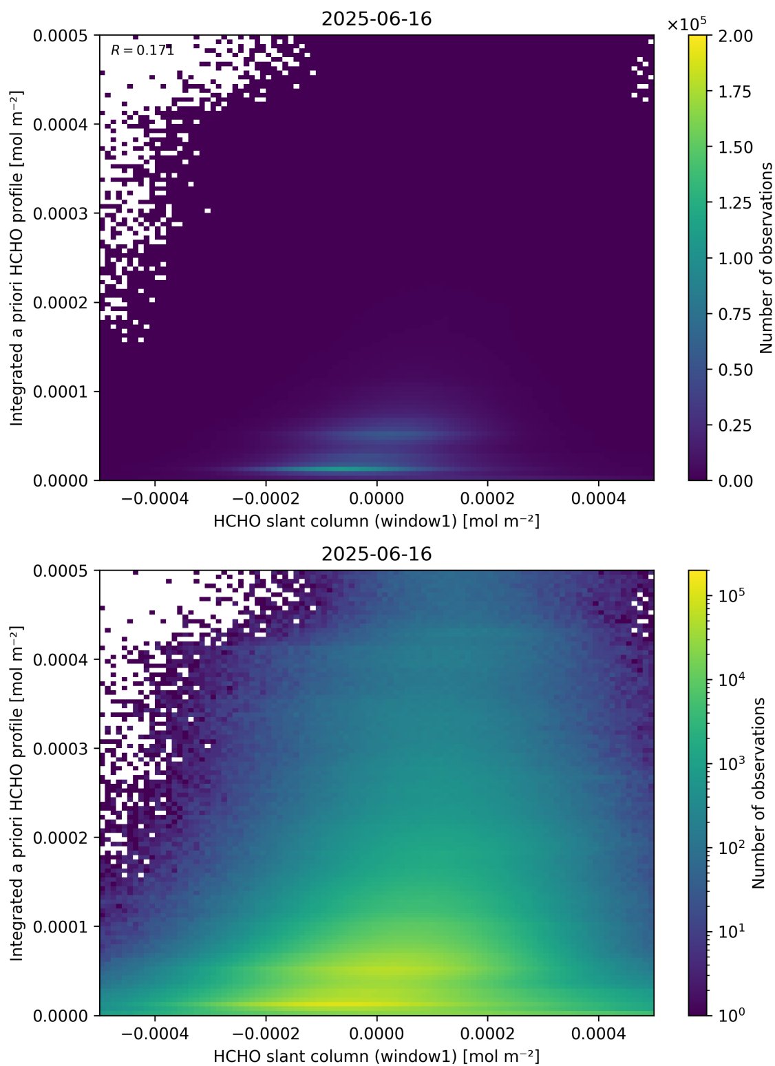
Figure 87: Scatter density plot of “HCHO slant column (window1)” against “Integrated a priori HCHO profile” for 2025-06-16 to 2025-06-17.
