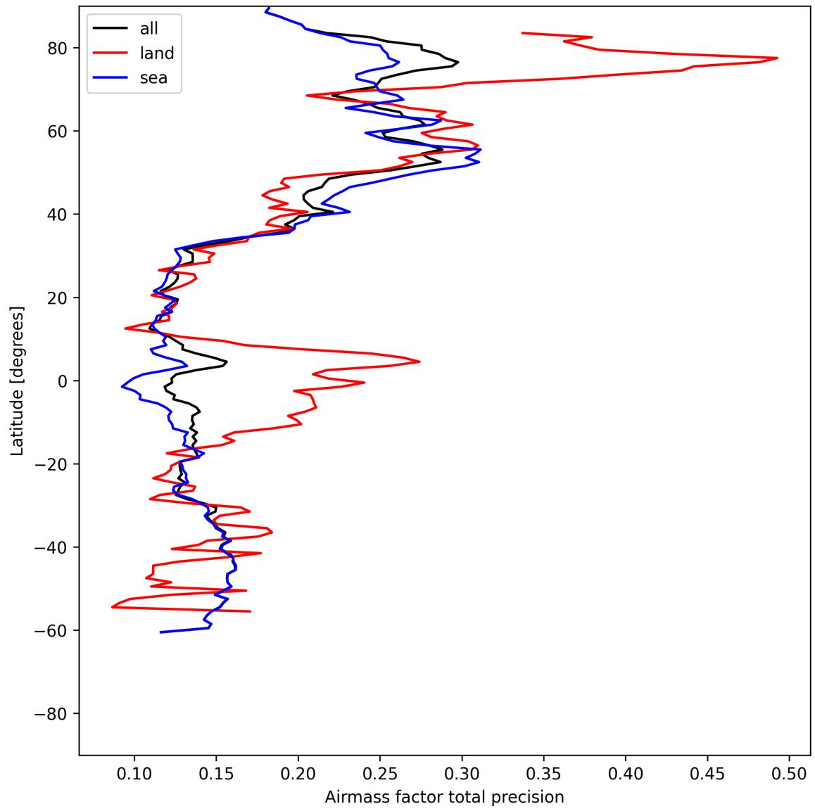
Figure 27: Zonal average of “Airmass factor total precision” for 2025-06-16 to 2025-06-17.
