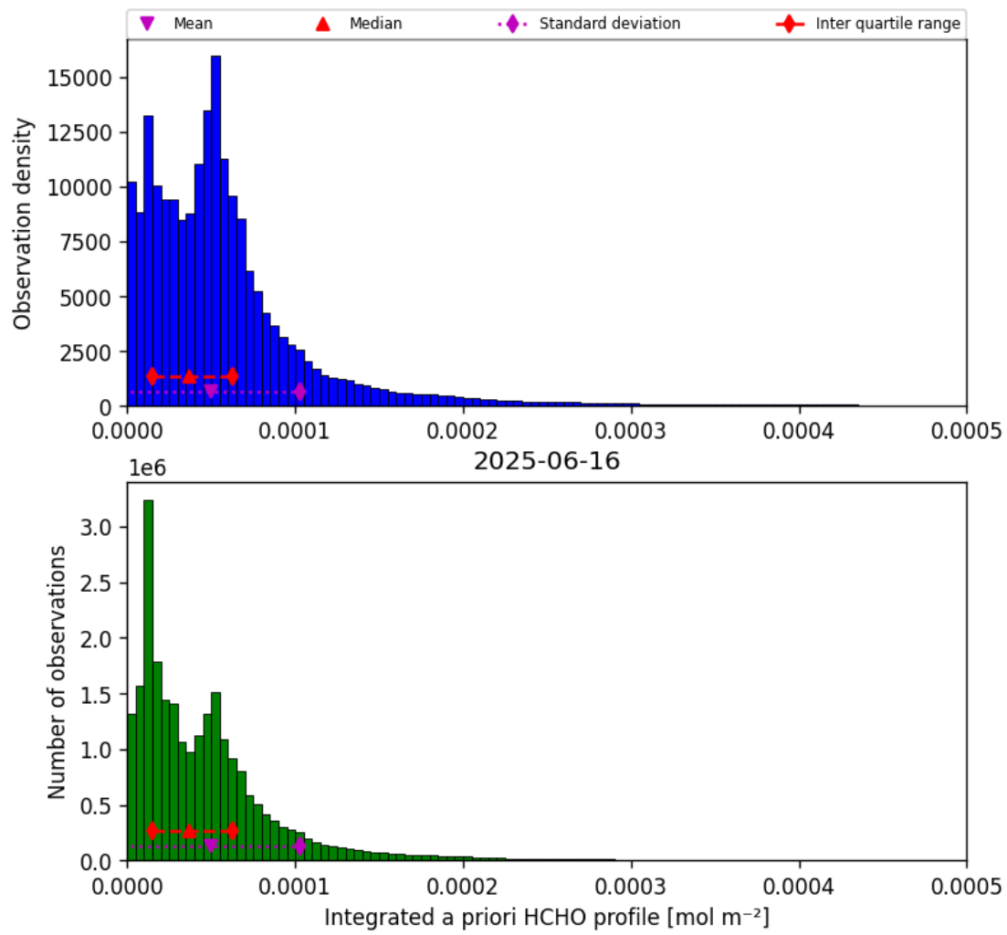
Figure 43: Histogram of “Integrated a priori HCHO profile” for 2025-06-16 to 2025-06-17
