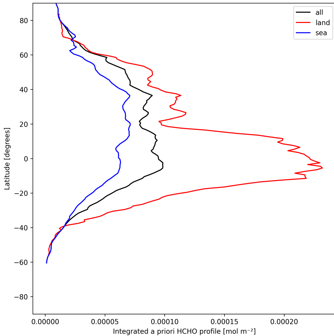
Figure 29: Zonal average of “Integrated a priori HCHO profile” for 2025-06-16 to 2025-06-17.
