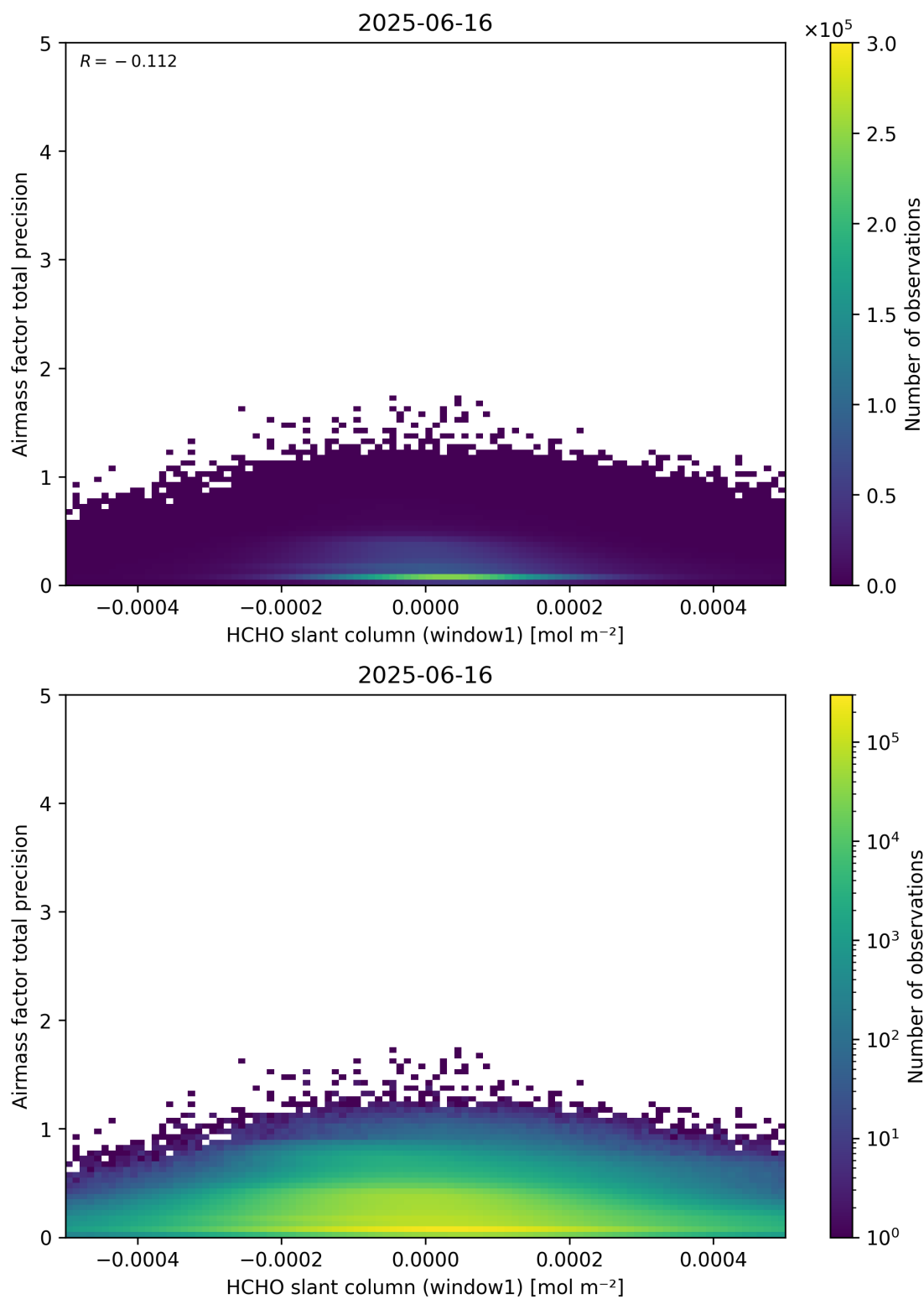
Figure 86: Scatter density plot of “HCHO slant column (window1)” against “Airmass factor total precision” for 2025-06-16 to 2025-06-17.
