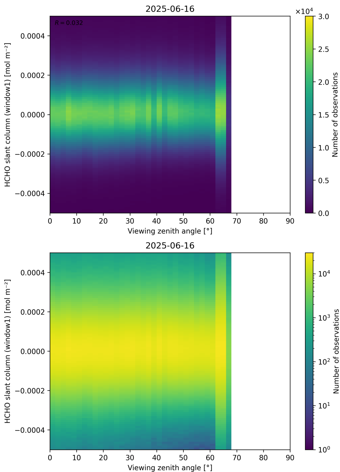
Figure 188: Scatter density plot of “Viewing zenith angle” against “HCHO slant column (window1)” for 2025-06-16 to 2025-06-17.
