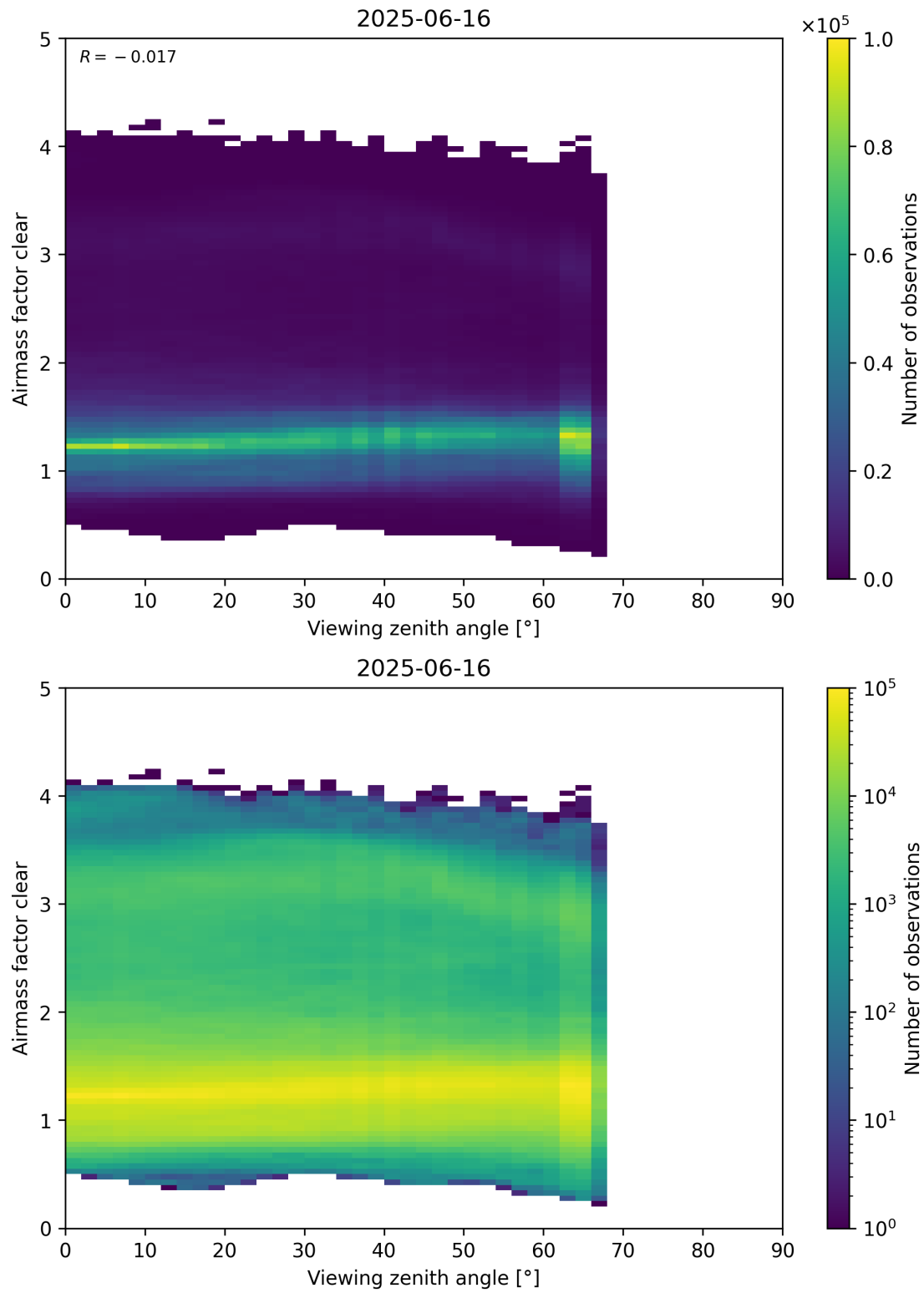
Figure 185: Scatter density plot of “Viewing zenith angle” against “Airmass factor clear” for 2025-06-16 to 2025-06-17.
