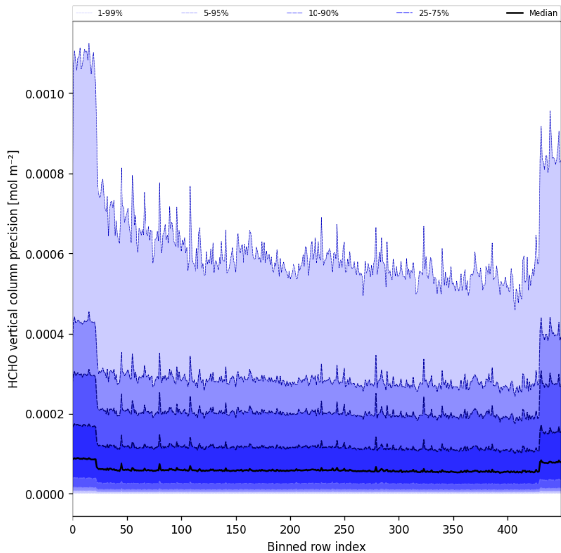
Figure 50: Along track statistics of “HCHO vertical column precision” for 2025-06-16 to 2025-06-17
