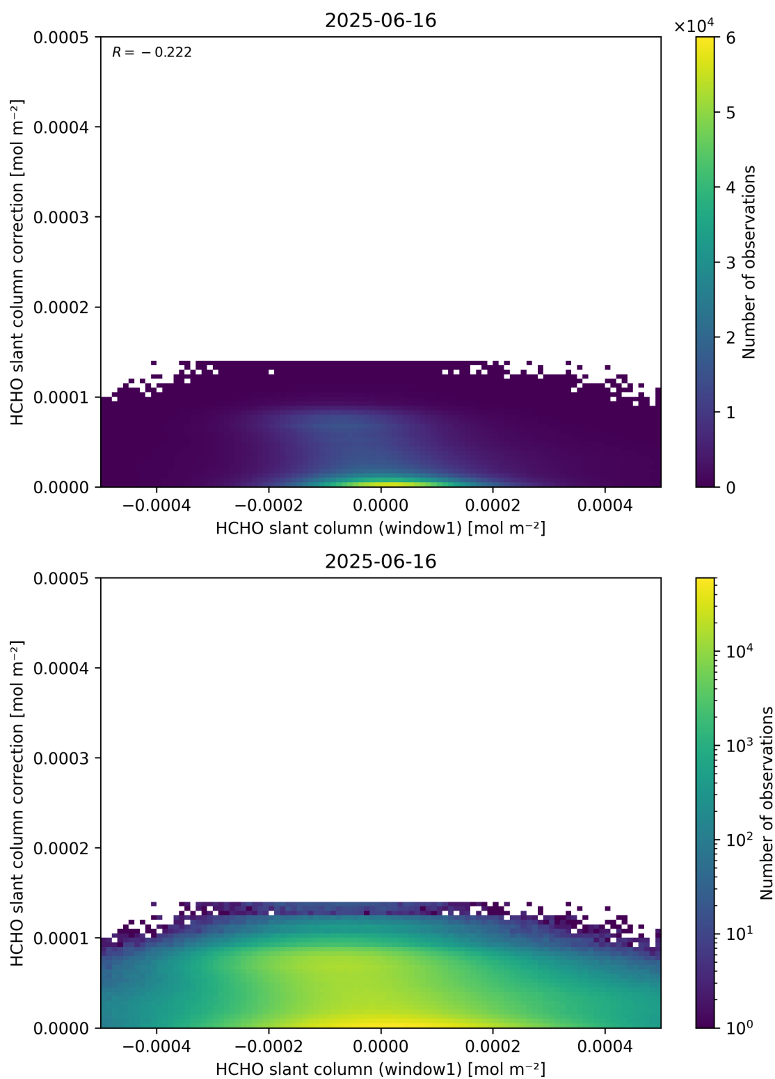
Figure 83: Scatter density plot of “HCHO slant column (window1)” against “HCHO slant column correction” for 2025-06-16 to 2025-06-17.
