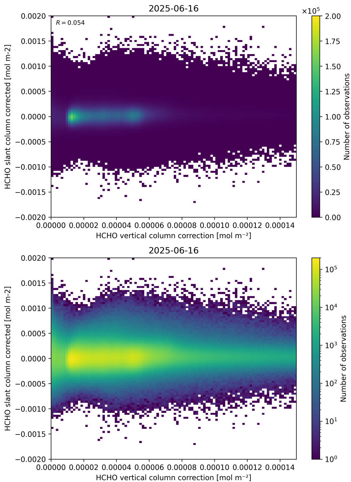
Figure 116: Scatter density plot of “HCHO vertical column correction” against “HCHO slant column corrected” for 2025-06-16 to 2025-06-17.
