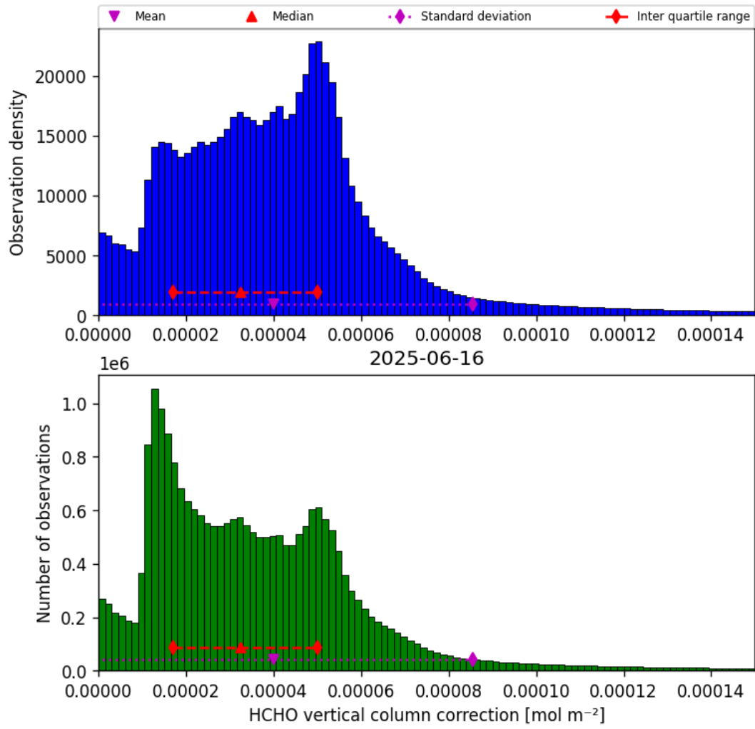
Figure 37: Histogram of “HCHO vertical column correction” for 2025-06-16 to 2025-06-17
