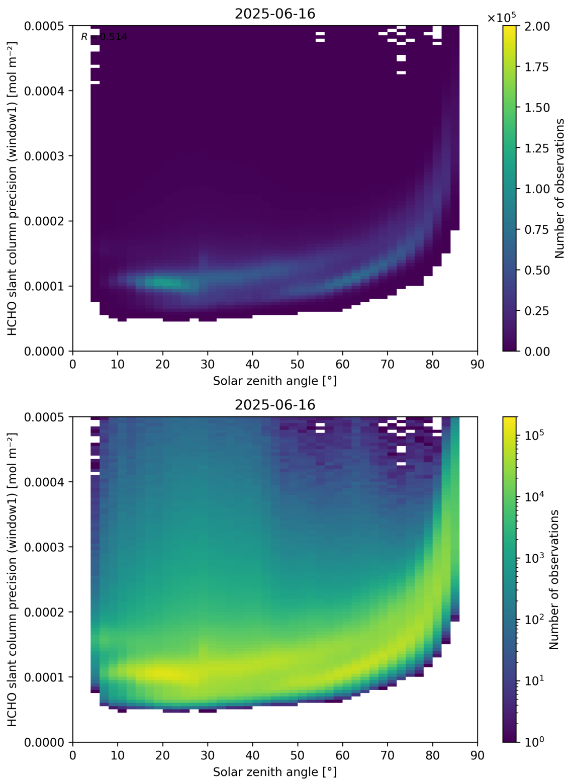
Figure 174: Scatter density plot of “Solar zenith angle” against “HCHO slant column precision (window1)” for 2025-06-16 to 2025-06-17.
