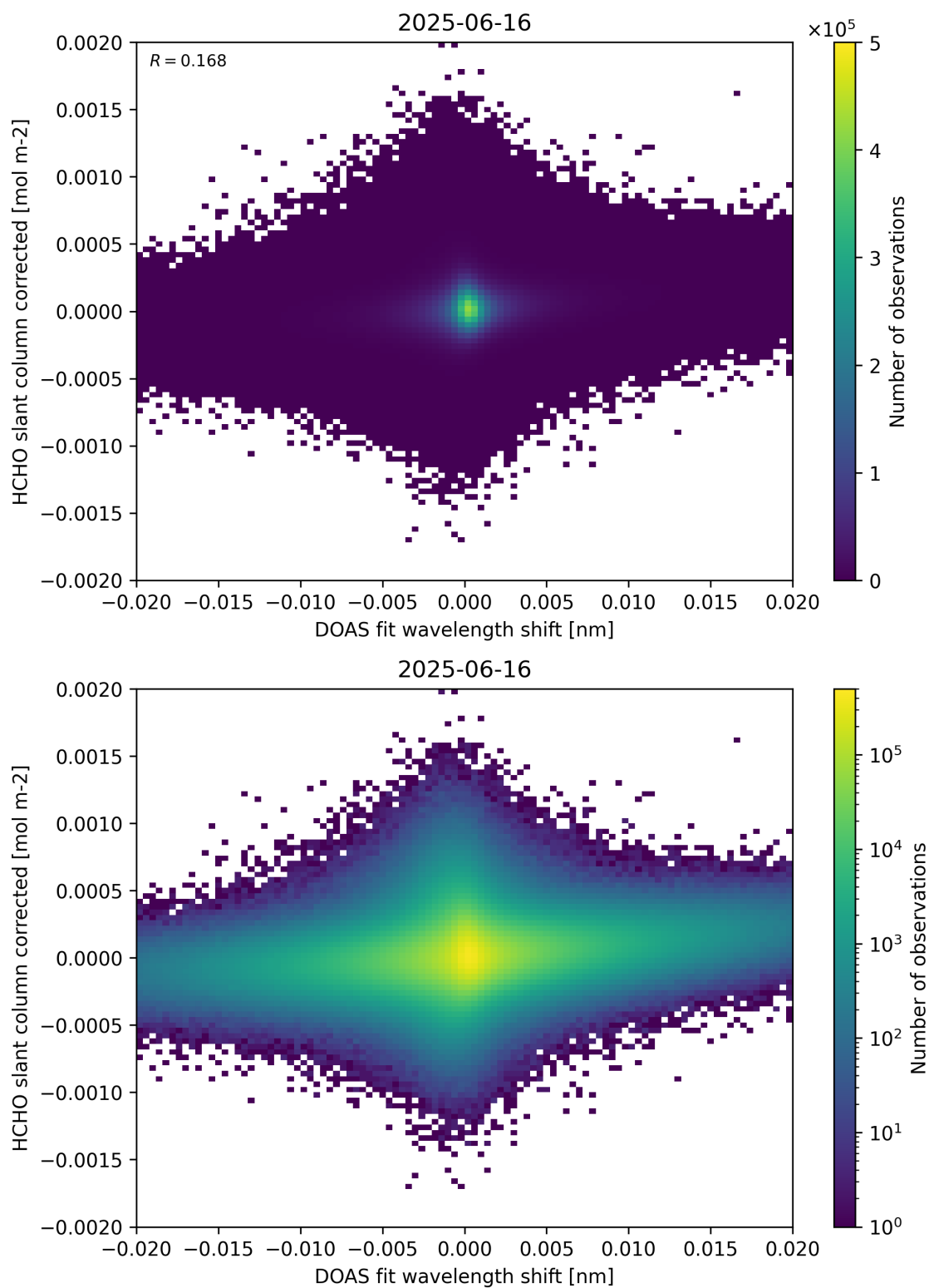
Figure 66: Scatter density plot of “DOAS fit wavelength shift” against “HCHO slant column corrected” for 2025-06-16 to 2025-06-17.
