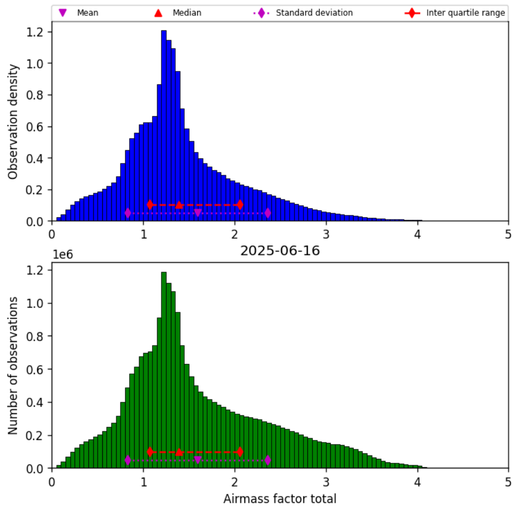
Figure 40: Histogram of “Airmass factor total” for 2025-06-16 to 2025-06-17
