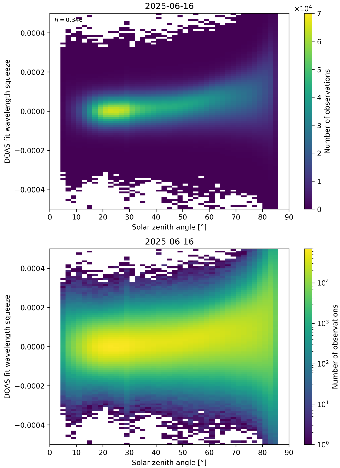
Figure 169: Scatter density plot of “Solar zenith angle” against “DOAS fit wavelength squeeze” for 2025-06-16 to 2025-06-17.
