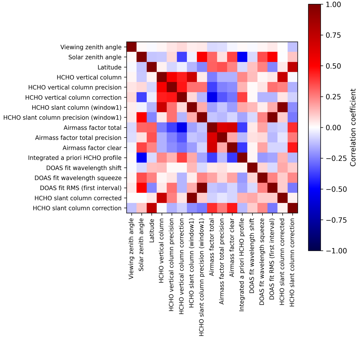
Figure 2: Map of correlation matrix for 2025-06-16 to 2025-06-17.
