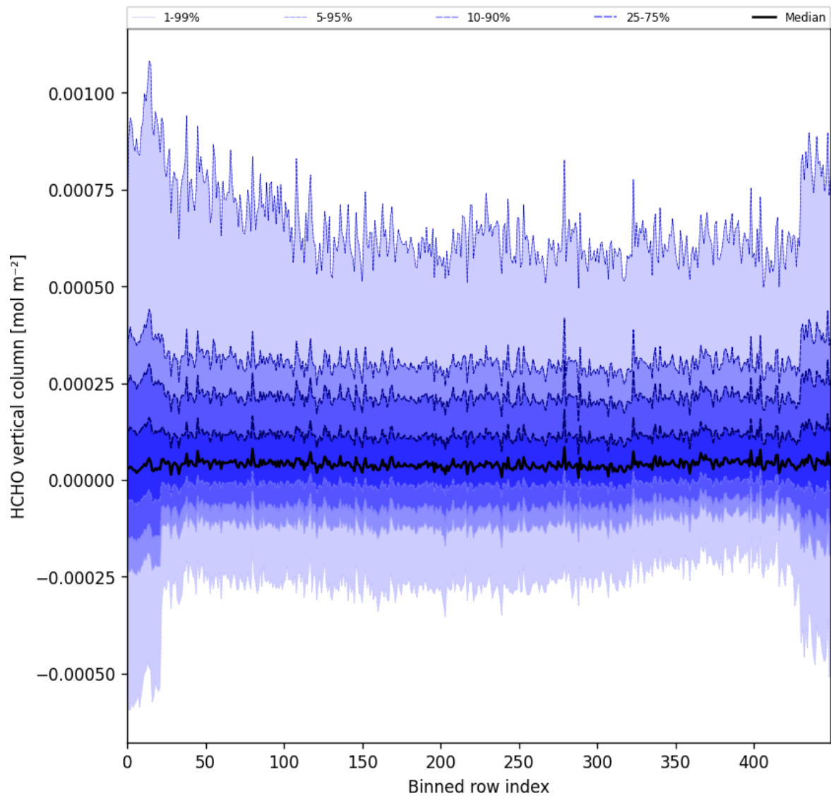
Figure 49: Along track statistics of “HCHO vertical column” for 2025-06-16 to 2025-06-17
