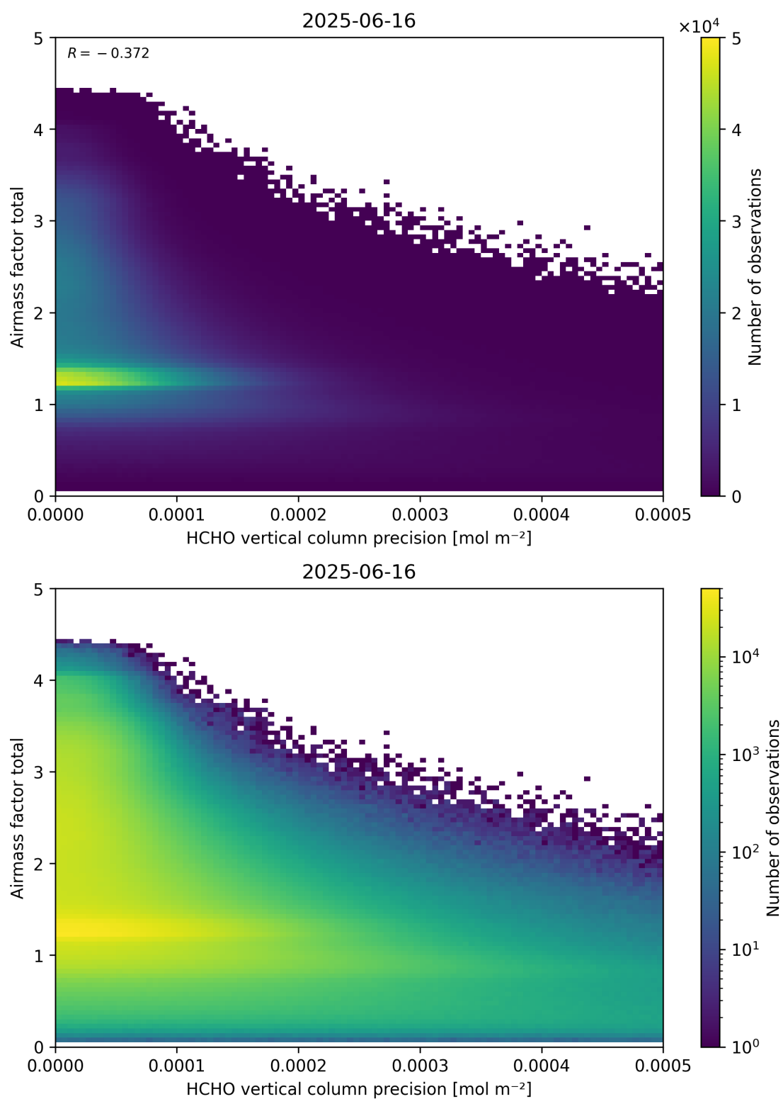
Figure 144: Scatter density plot of “HCHO vertical column precision” against “Airmass factor total” for 2025-06-16 to 2025-06-17.
