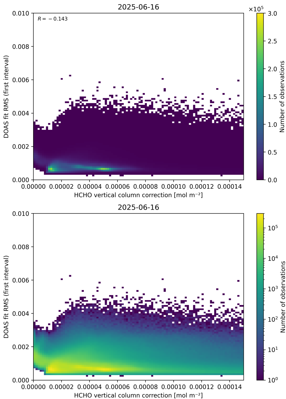
Figure 112: Scatter density plot of “HCHO vertical column correction” against “DOAS fit RMS (first interval)” for 2025-06-16 to 2025-06-17.
