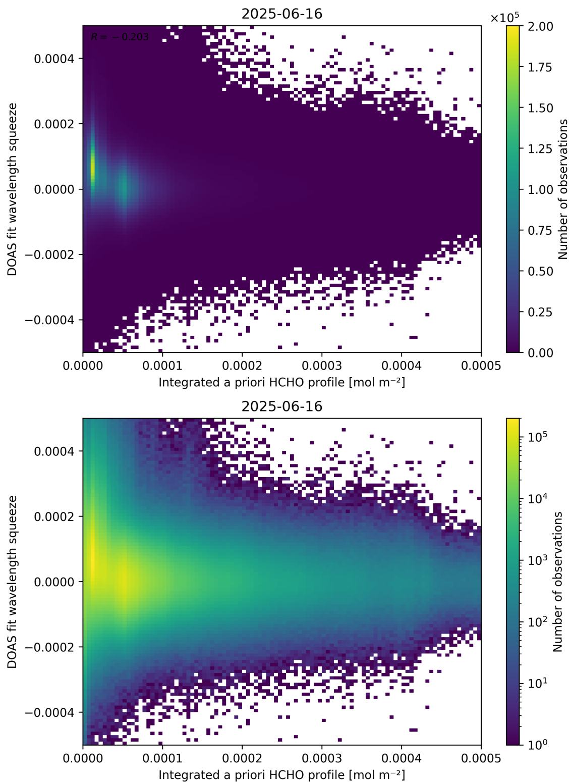
Figure 150: Scatter density plot of “Integrated a priori HCHO profile” against “DOAS fit wavelength squeeze” for 2025-06-16 to 2025-06-17.
