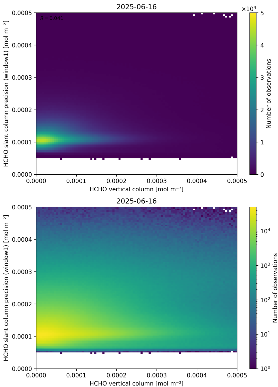
Figure 130: Scatter density plot of “HCHO vertical column” against “HCHO slant column precision (window1)” for 2025-06-16 to 2025-06-17.
