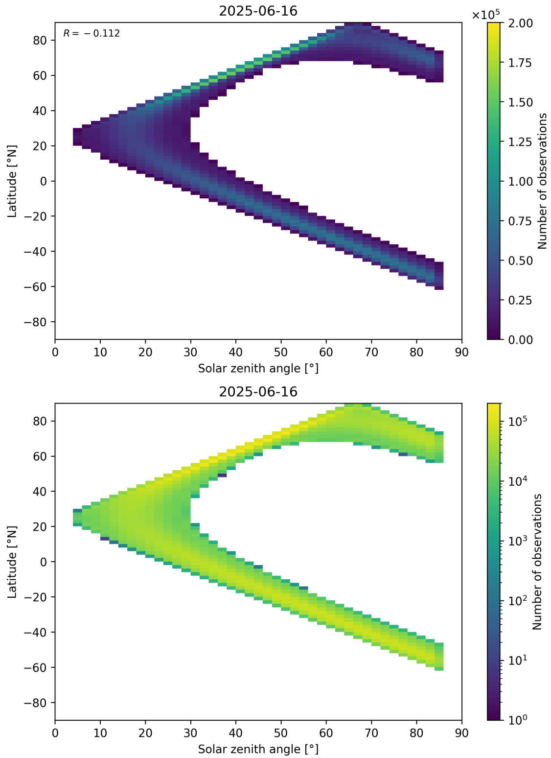
Figure 181: Scatter density plot of “Solar zenith angle” against “Latitude” for 2025-06-16 to 2025-06-17.
