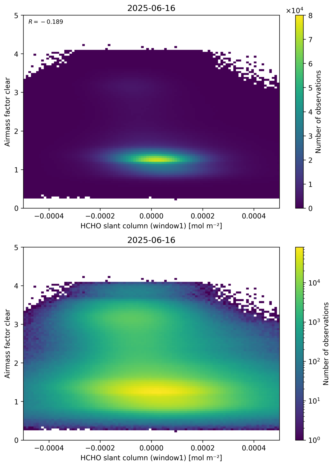
Figure 81: Scatter density plot of “HCHO slant column (window1)” against “Airmass factor clear” for 2025-06-16 to 2025-06-17.
