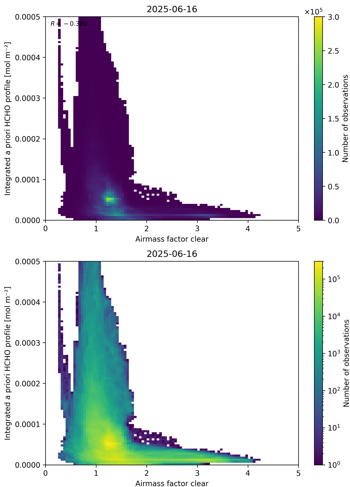
Figure 76: Scatter density plot of “Airmass factor clear” against “Integrated a priori HCHO profile” for 2025-06-16 to 2025-06-17.
