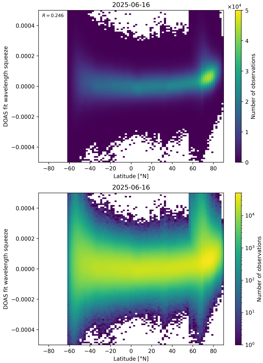
Figure 155: Scatter density plot of “Latitude” against “DOAS fit wavelength squeeze” for 2025-06-16 to 2025-06-17.
