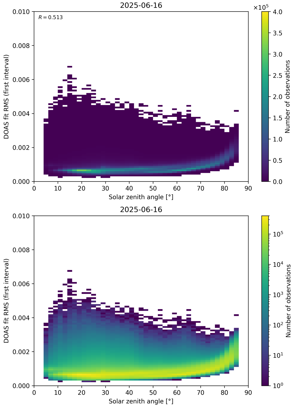
Figure 167: Scatter density plot of “Solar zenith angle” against “DOAS fit RMS (first interval)” for 2025-06-16 to 2025-06-17.
