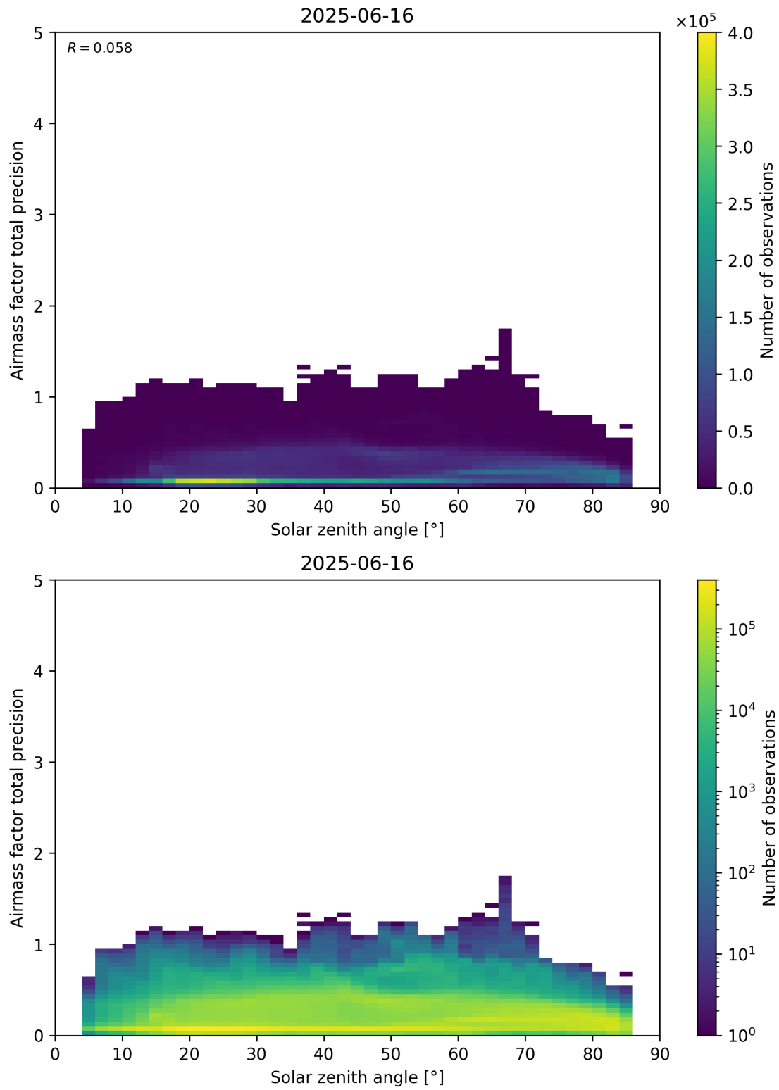
Figure 176: Scatter density plot of “Solar zenith angle” against “Airmass factor total precision” for 2025-06-16 to 2025-06-17.
