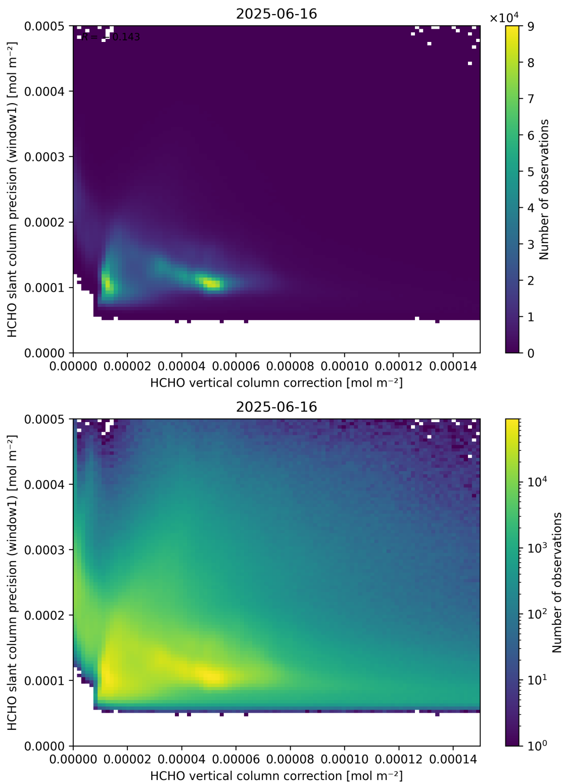
Figure 119: Scatter density plot of “HCHO vertical column correction” against “HCHO slant column precision (window1)” for 2025-06-16 to 2025-06-17.
