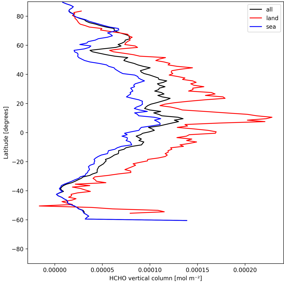
Figure 21: Zonal average of “HCHO vertical column” for 2025-06-16 to 2025-06-17.
