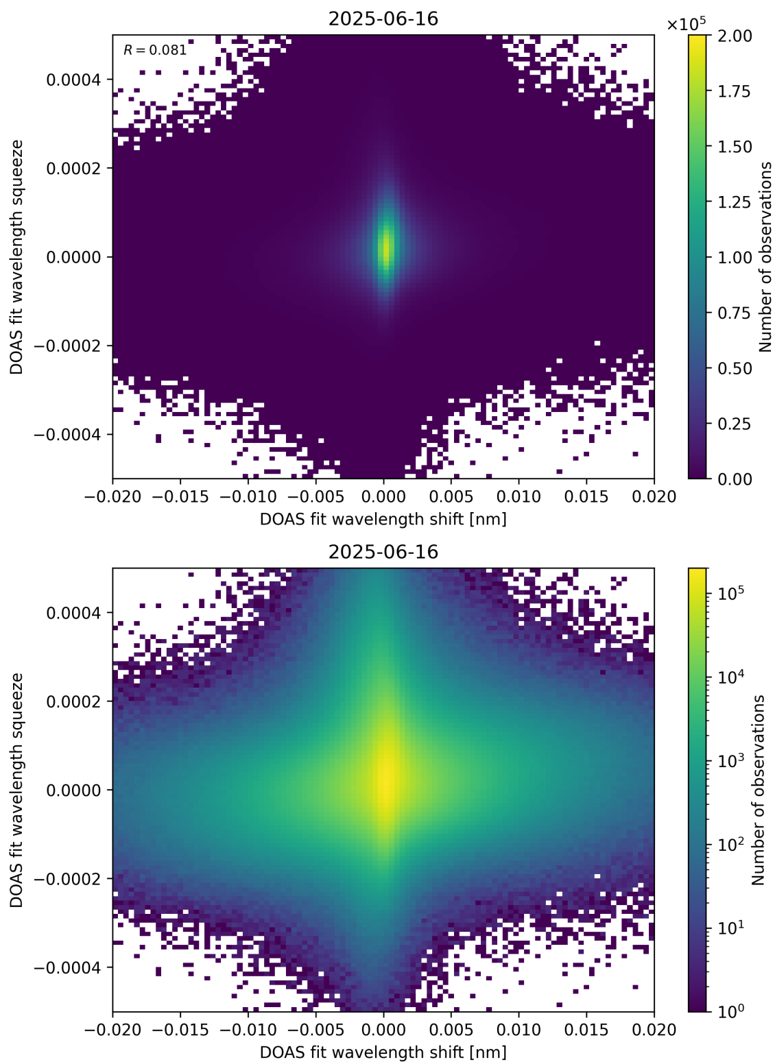
Figure 65: Scatter density plot of “DOAS fit wavelength shift” against “DOAS fit wavelength squeeze” for 2025-06-16 to 2025-06-17.
