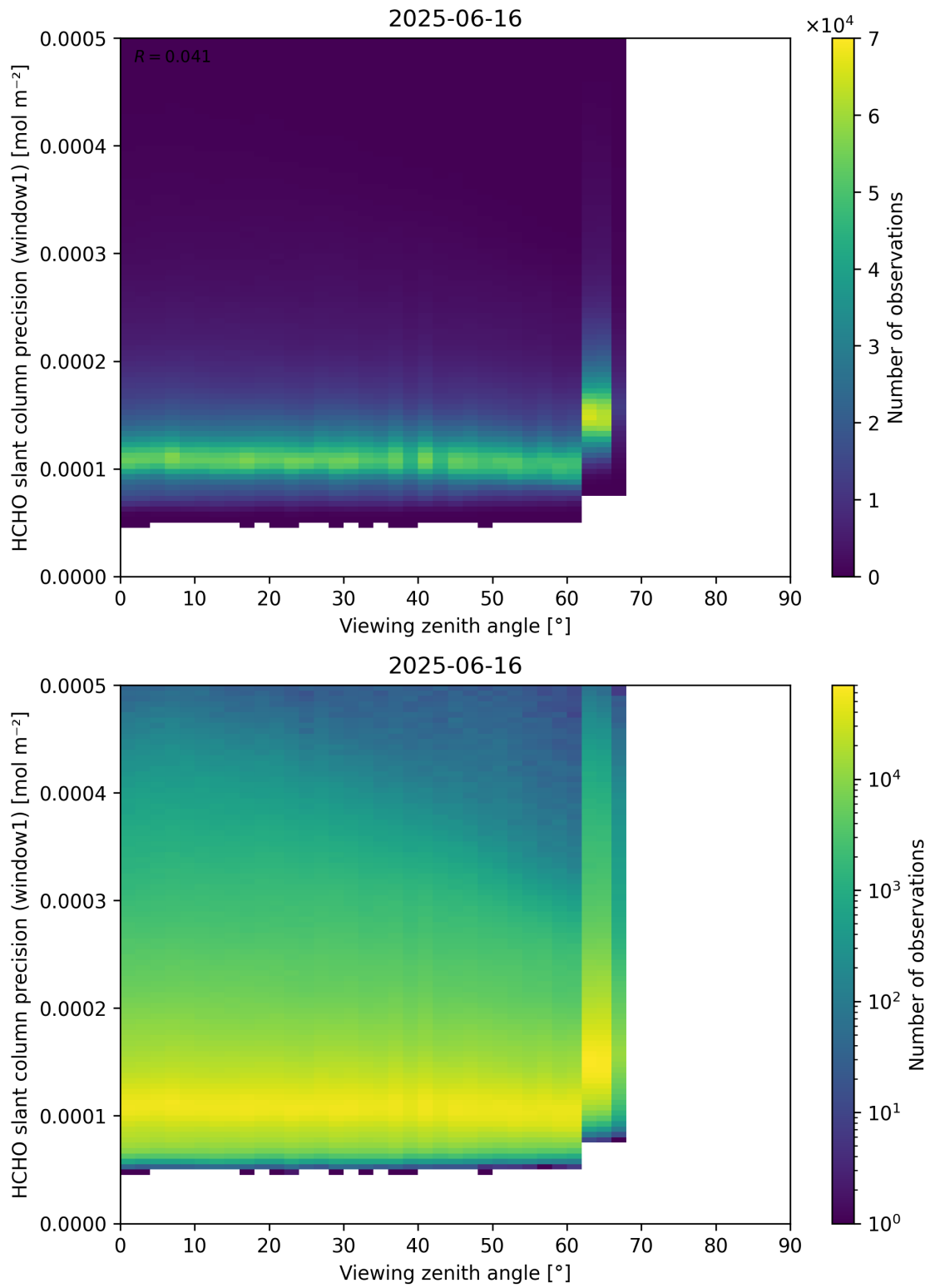
Figure 189: Scatter density plot of “Viewing zenith angle” against “HCHO slant column precision (window1)” for 2025-06-16 to 2025-06-17.
