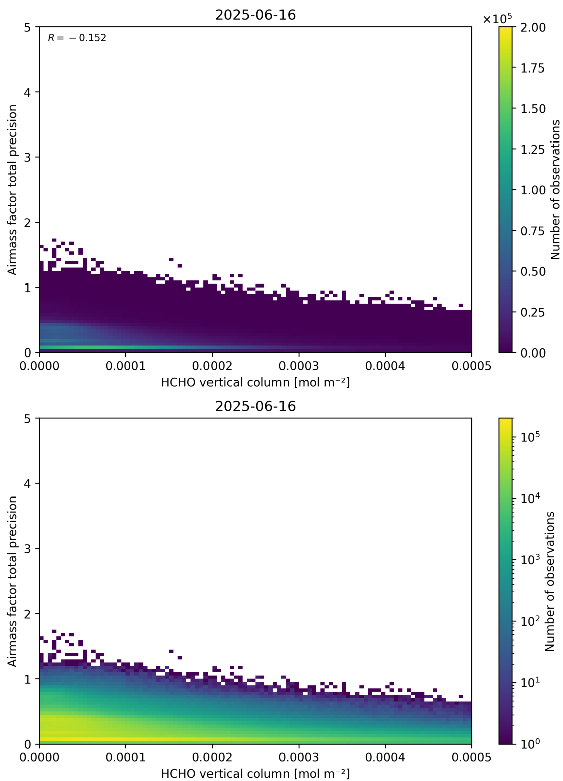
Figure 132: Scatter density plot of “HCHO vertical column” against “Airmass factor total precision” for 2025-06-16 to 2025-06-17.
