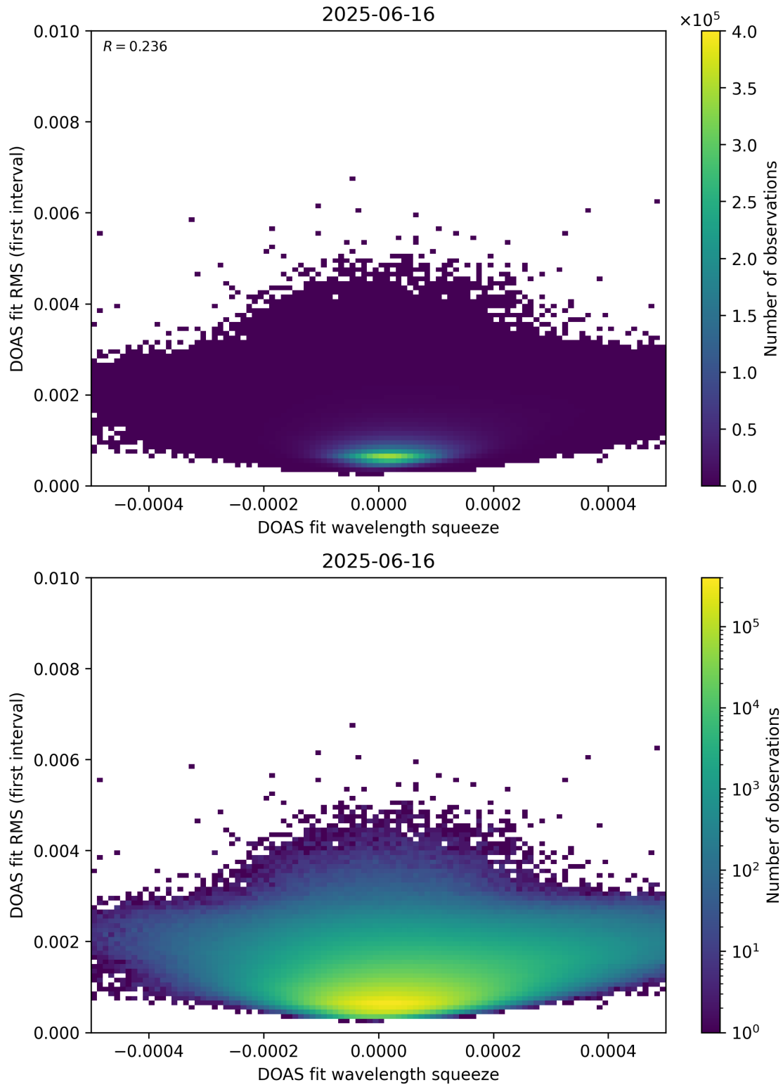
Figure 68: Scatter density plot of “DOAS fit wavelength squeeze” against “DOAS fit RMS (first interval)” for 2025-06-16 to 2025-06-17.
