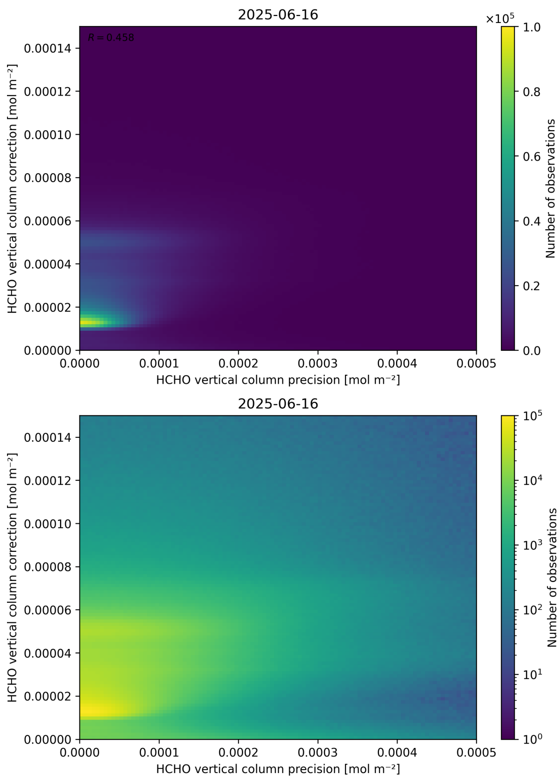
Figure 146: Scatter density plot of “HCHO vertical column precision” against “HCHO vertical column correction” for 2025-06-16 to 2025-06-17.
