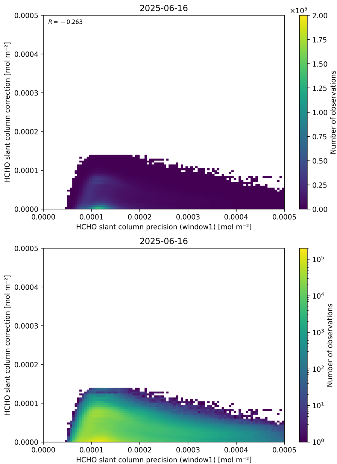
Figure 93: Scatter density plot of “HCHO slant column precision (window1)” against “HCHO slant column correction” for 2025-06-16 to 2025-06-17.
