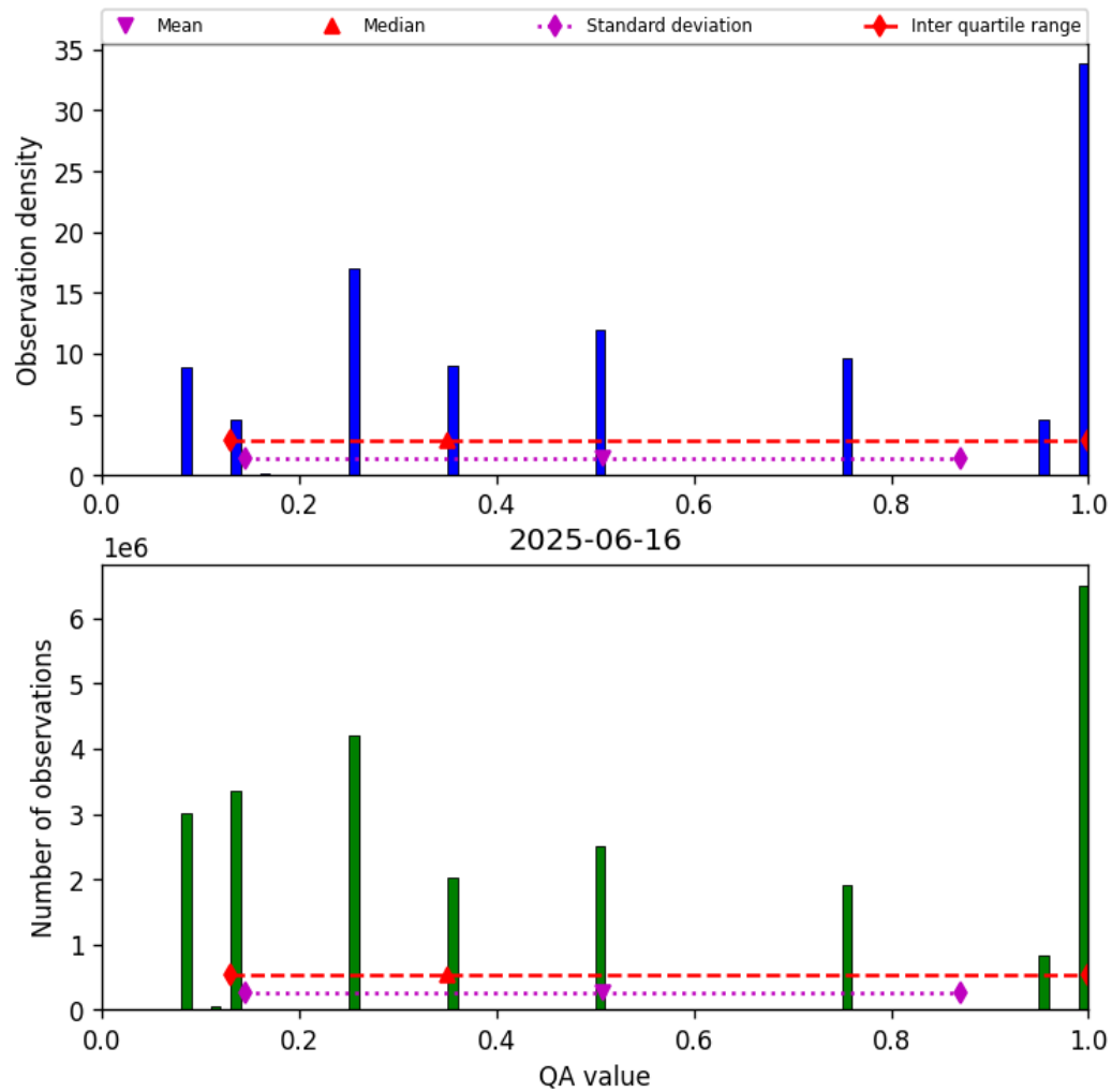
Figure 34: Histogram of “QA value” for 2025-06-16 to 2025-06-17
