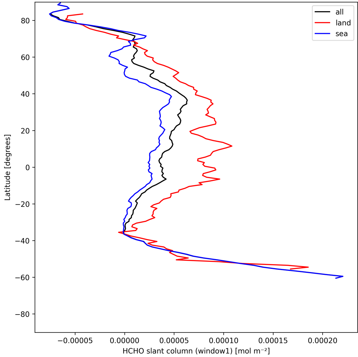
Figure 24: Zonal average of “HCHO slant column (window1)” for 2025-06-16 to 2025-06-17.
