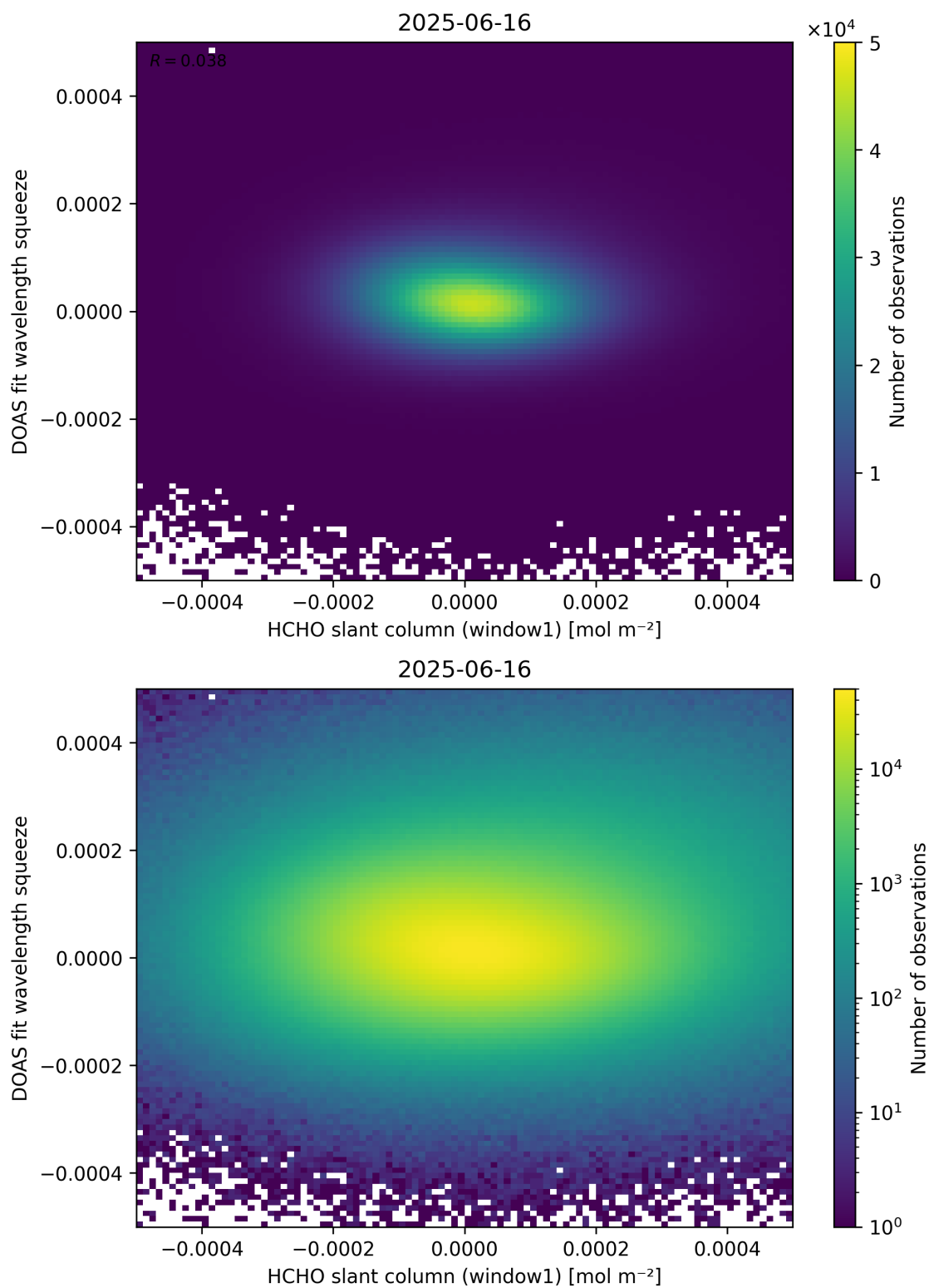
Figure 80: Scatter density plot of “HCHO slant column (window1)” against “DOAS fit wavelength squeeze” for 2025-06-16 to 2025-06-17.
