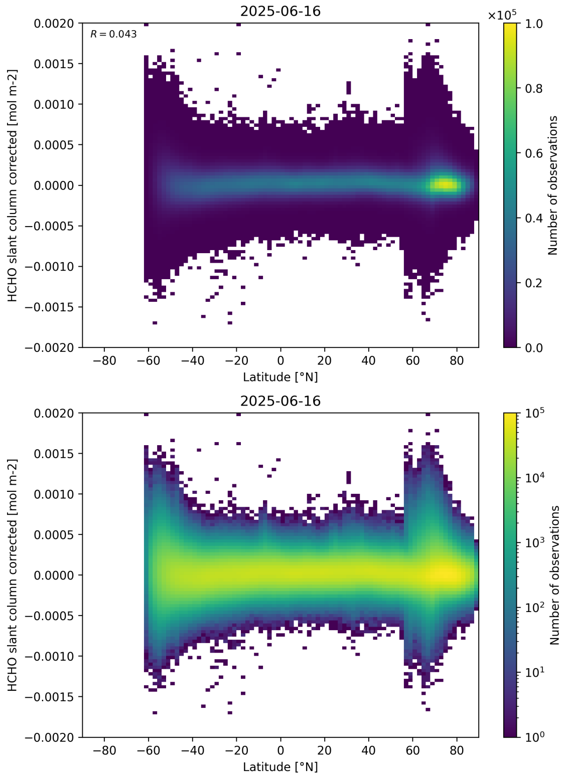
Figure 157: Scatter density plot of “Latitude” against “HCHO slant column corrected” for 2025-06-16 to 2025-06-17.
