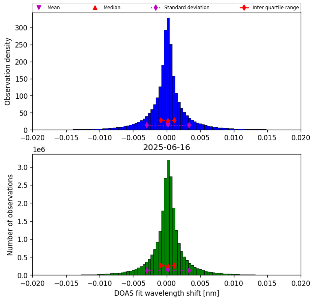
Figure 44: Histogram of “DOAS fit wavelength shift” for 2025-06-16 to 2025-06-17
