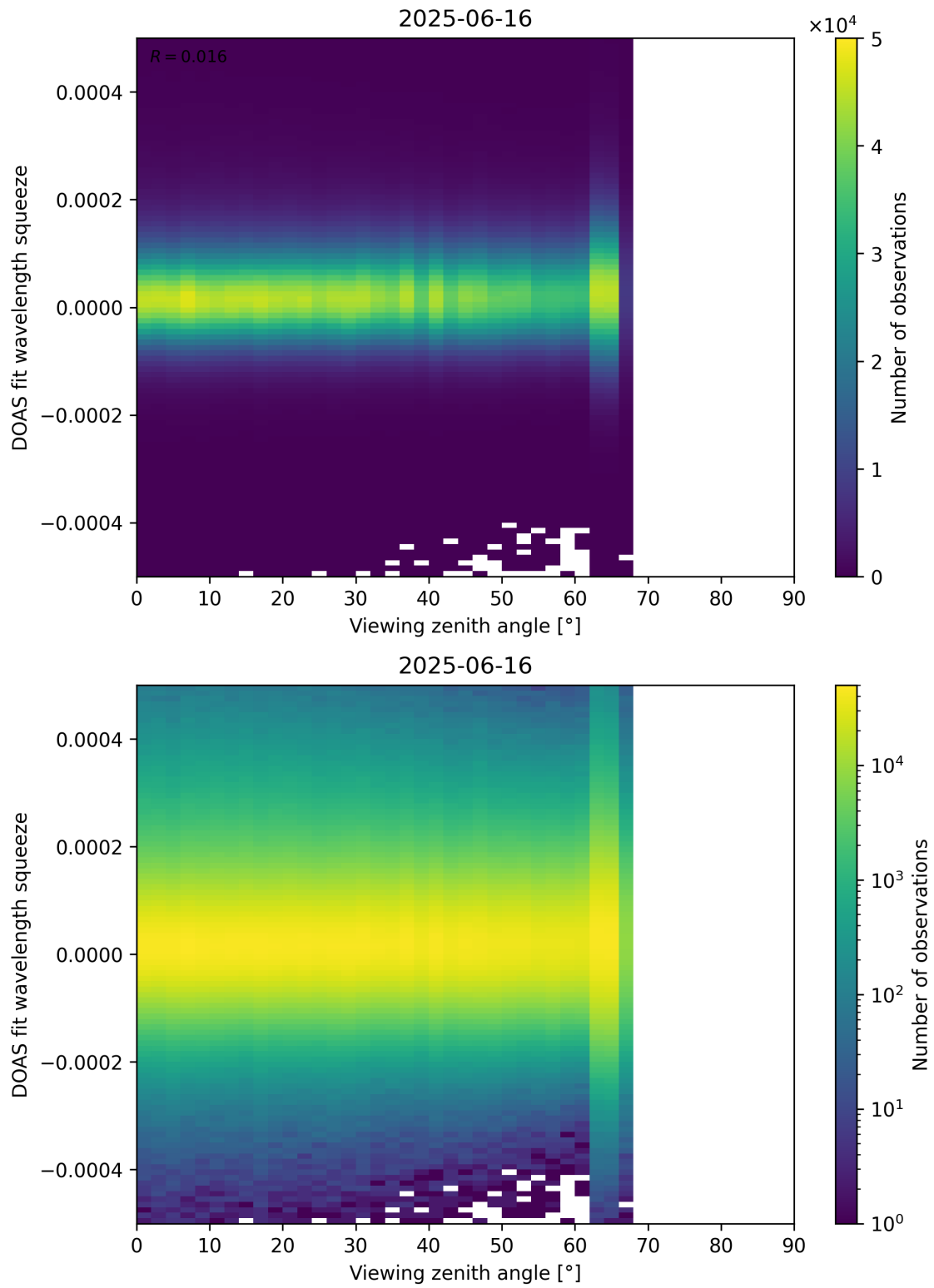
Figure 184: Scatter density plot of “Viewing zenith angle” against “DOAS fit wavelength squeeze” for 2025-06-16 to 2025-06-17.
