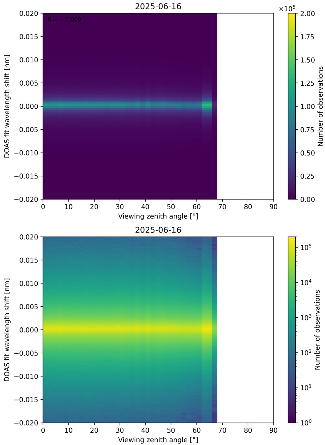
Figure 183: Scatter density plot of “Viewing zenith angle” against “DOAS fit wavelength shift” for 2025-06-16 to 2025-06-17.
