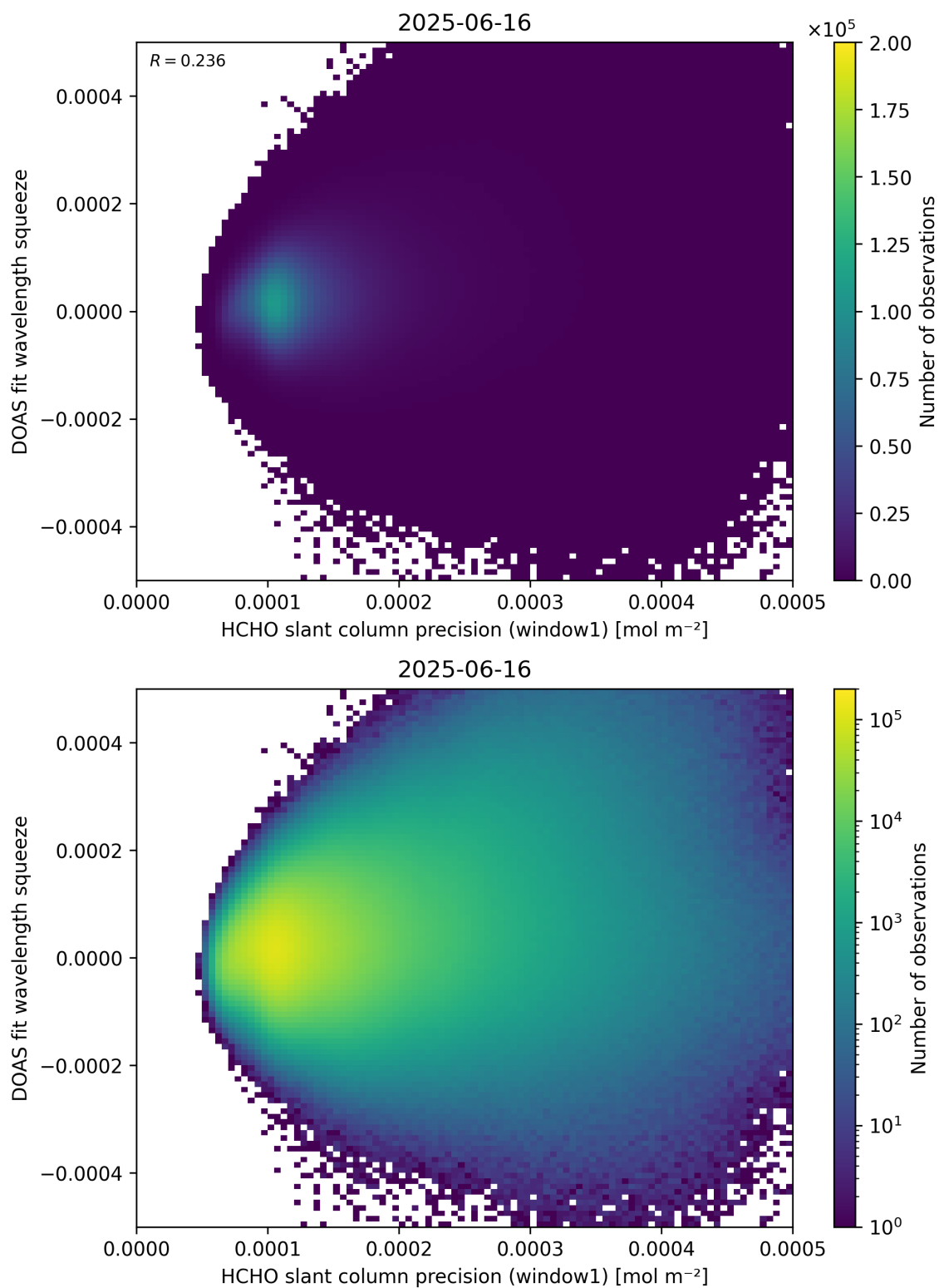
Figure 90: Scatter density plot of “HCHO slant column precision (window1)” against “DOAS fit wavelength squeeze” for 2025-06-16 to 2025-06-17.
