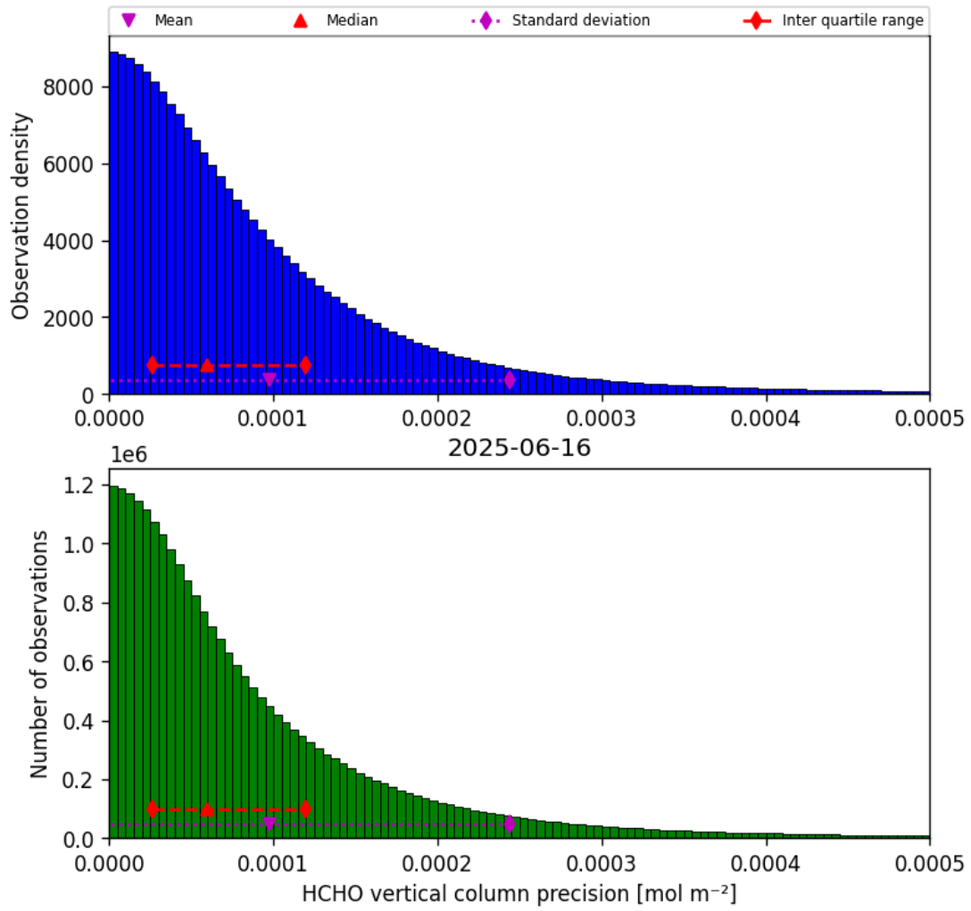
Figure 36: Histogram of “HCHO vertical column precision” for 2025-06-16 to 2025-06-17
