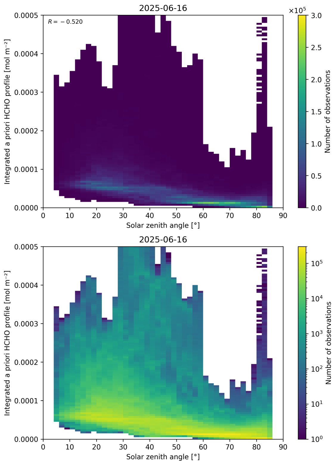
Figure 180: Scatter density plot of “Solar zenith angle” against “Integrated a priori HCHO profile” for 2025-06-16 to 2025-06-17.
