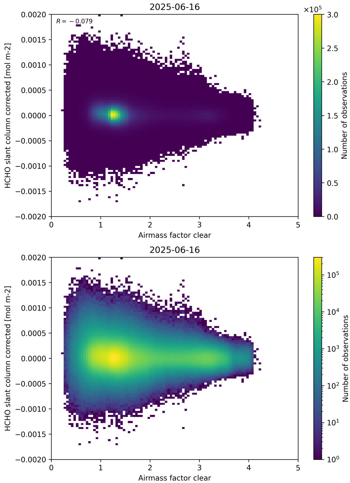
Figure 74: Scatter density plot of “Airmass factor clear” against “HCHO slant column corrected” for 2025-06-16 to 2025-06-17.
