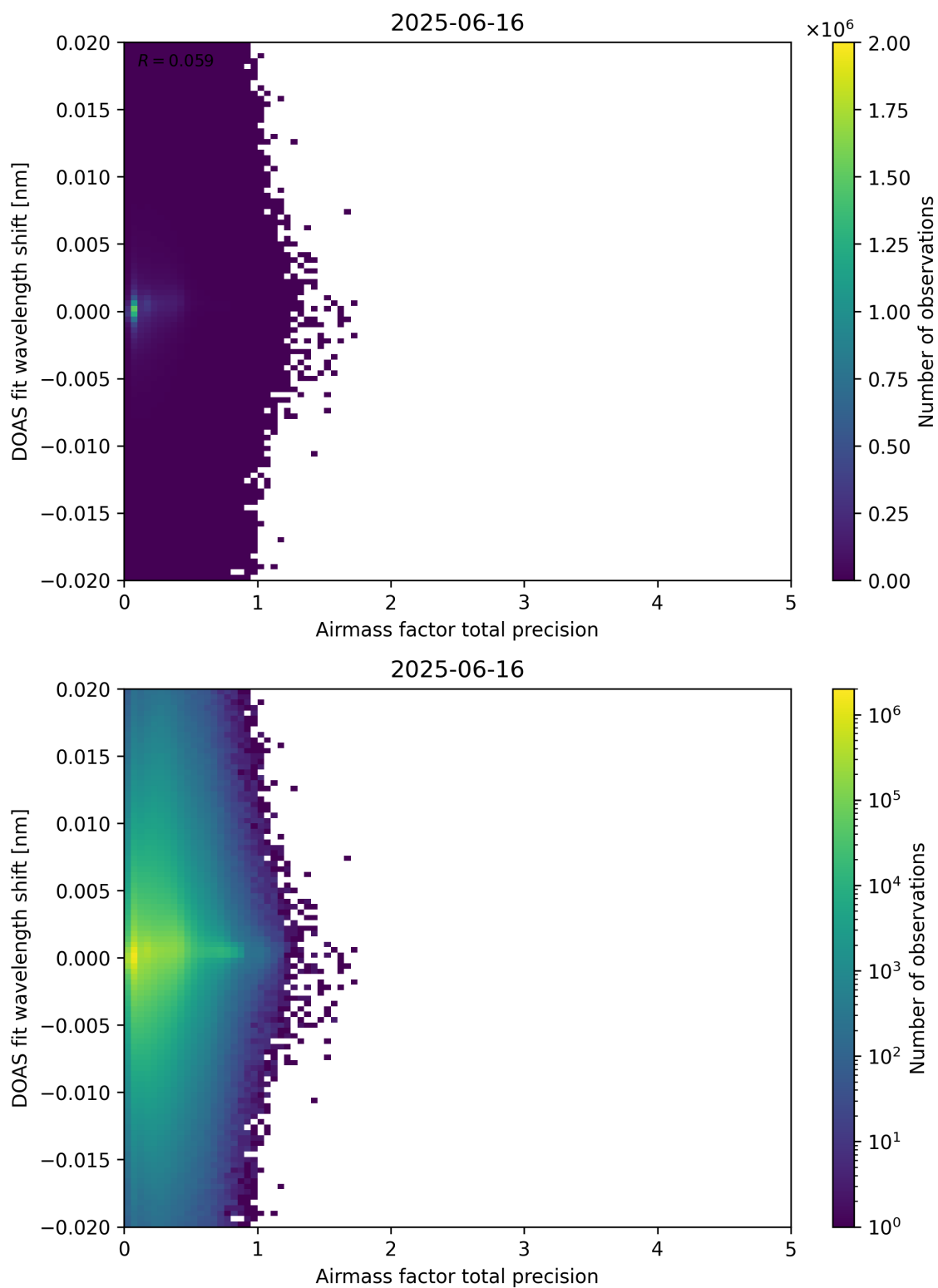
Figure 106: Scatter density plot of “Airmass factor total precision” against “DOAS fit wavelength shift” for 2025-06-16 to 2025-06-17.
