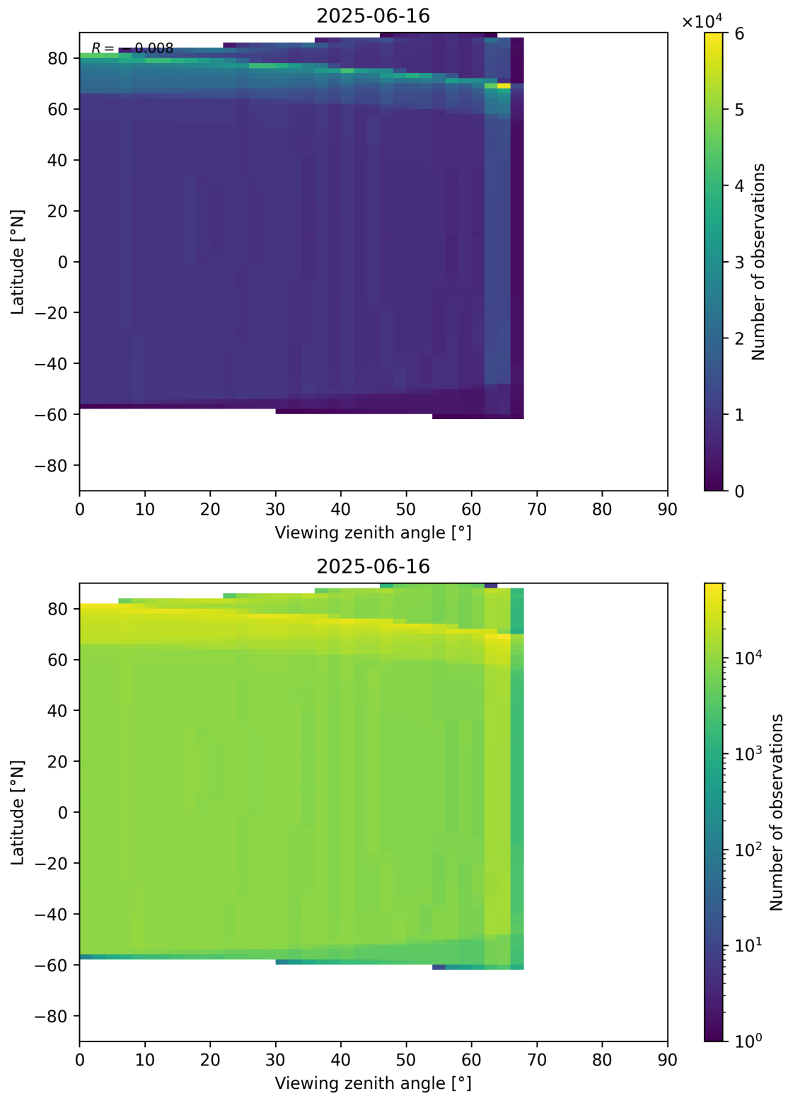
Figure 196: Scatter density plot of “Viewing zenith angle” against “Latitude” for 2025-06-16 to 2025-06-17.
