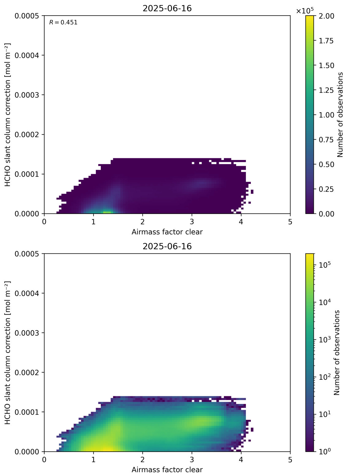
Figure 75: Scatter density plot of “Airmass factor clear” against “HCHO slant column correction” for 2025-06-16 to 2025-06-17.
