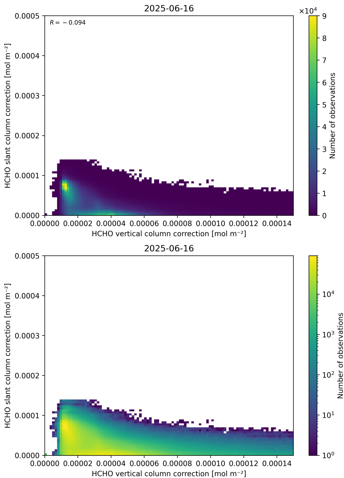
Figure 117: Scatter density plot of “HCHO vertical column correction” against “HCHO slant column correction” for 2025-06-16 to 2025-06-17.
