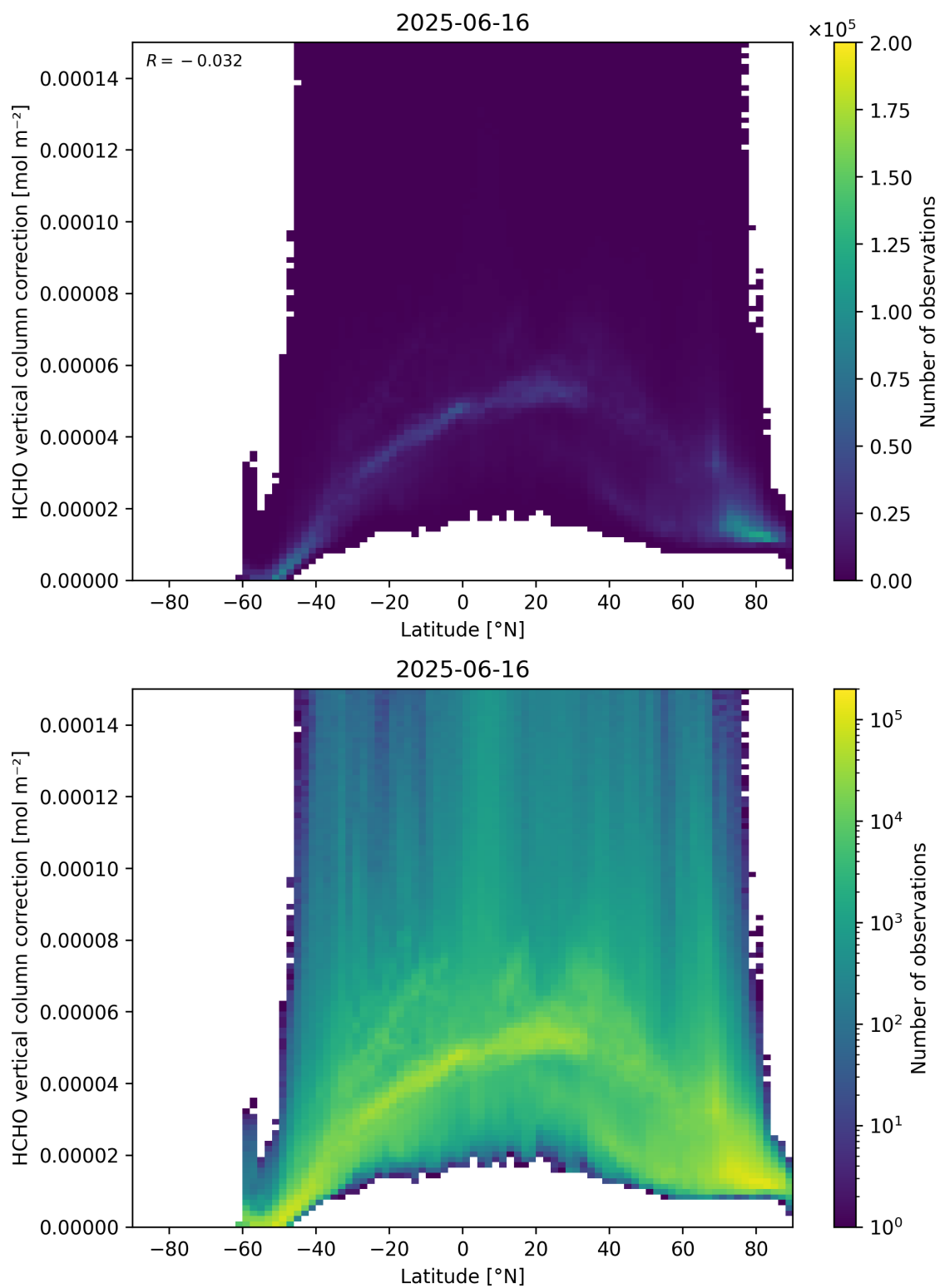
Figure 164: Scatter density plot of “Latitude” against “HCHO vertical column correction” for 2025-06-16 to 2025-06-17.
