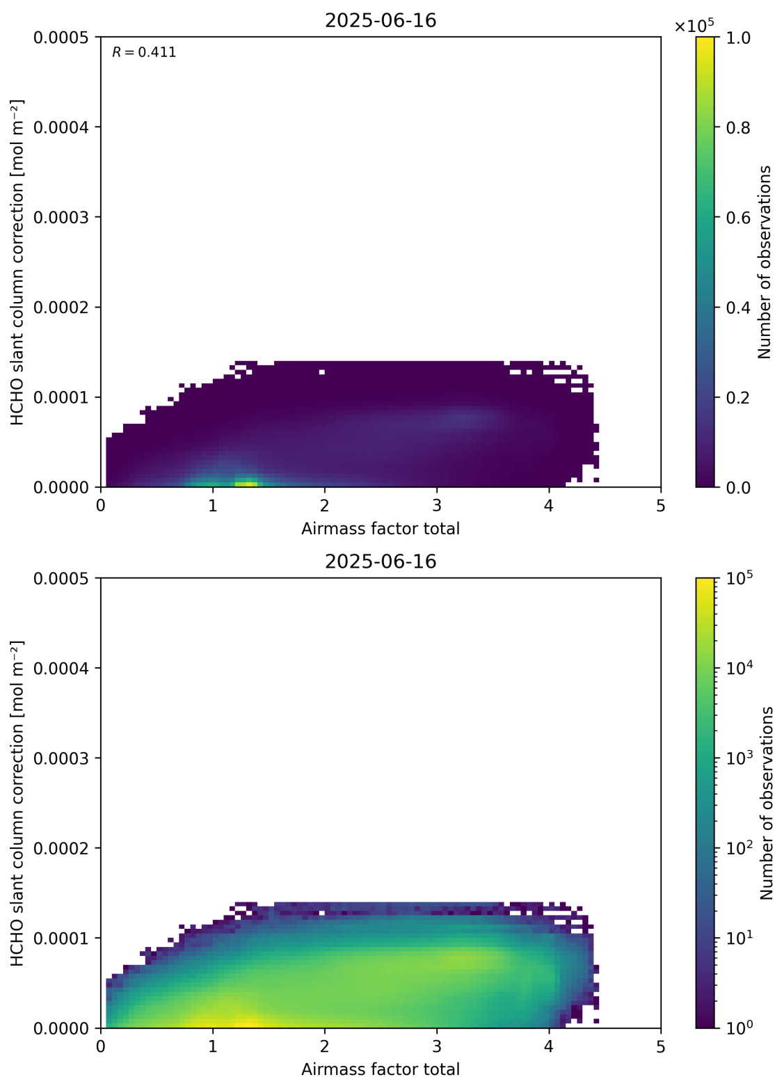
Figure 102: Scatter density plot of “Airmass factor total” against “HCHO slant column correction” for 2025-06-16 to 2025-06-17.
