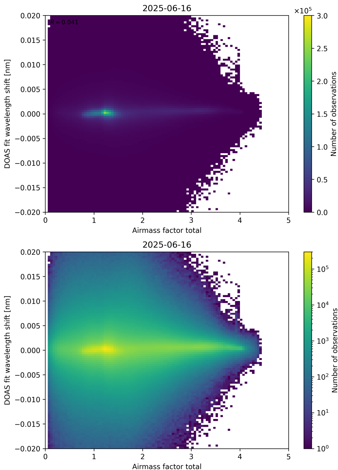
Figure 98: Scatter density plot of “Airmass factor total” against “DOAS fit wavelength shift” for 2025-06-16 to 2025-06-17.
