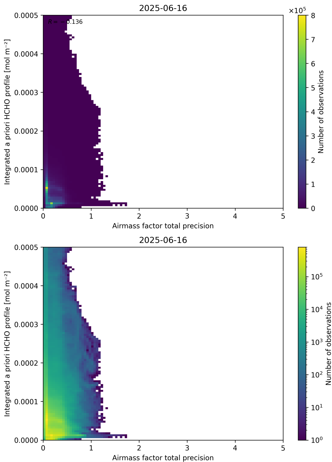
Figure 111: Scatter density plot of “Airmass factor total precision” against “Integrated a priori HCHO profile” for 2025-06-16 to 2025-06-17.
