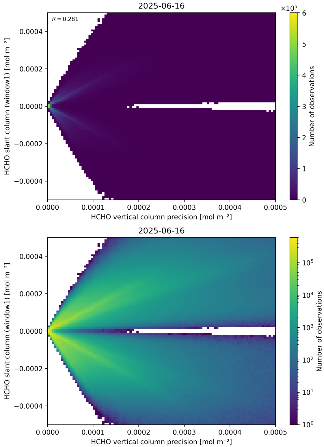
Figure 142: Scatter density plot of “HCHO vertical column precision” against “HCHO slant column (window1)” for 2025-06-16 to 2025-06-17.
