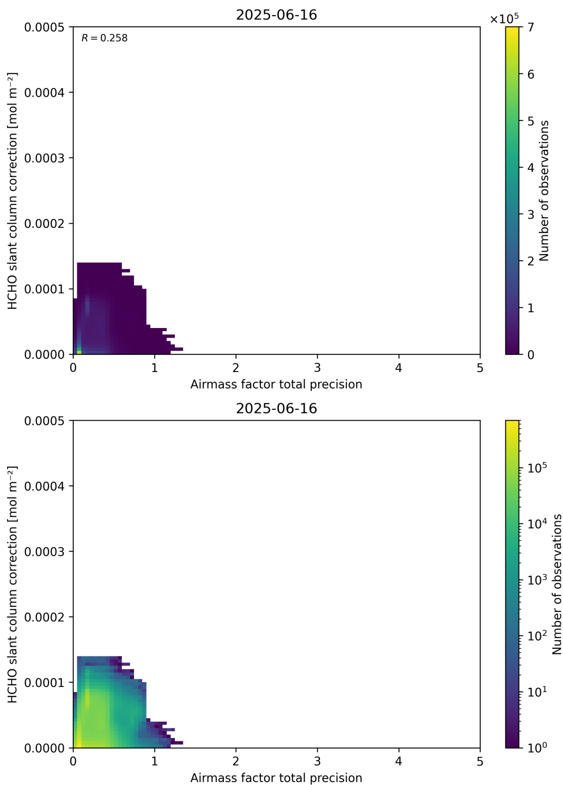
Figure 110: Scatter density plot of “Airmass factor total precision” against “HCHO slant column correction” for 2025-06-16 to 2025-06-17.
