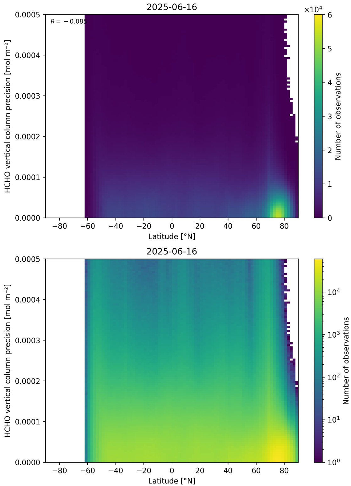
Figure 165: Scatter density plot of “Latitude” against “HCHO vertical column precision” for 2025-06-16 to 2025-06-17.
