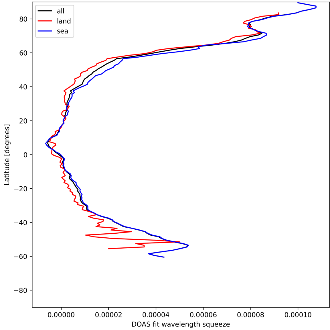
Figure 31: Zonal average of “DOAS fit wavelength squeeze” for 2025-06-16 to 2025-06-17.
