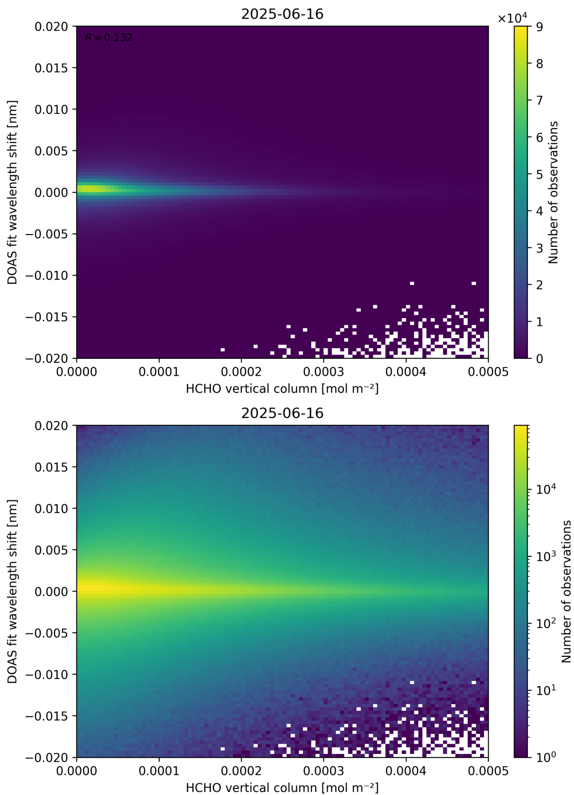
Figure 124: Scatter density plot of “HCHO vertical column” against “DOAS fit wavelength shift” for 2025-06-16 to 2025-06-17.
