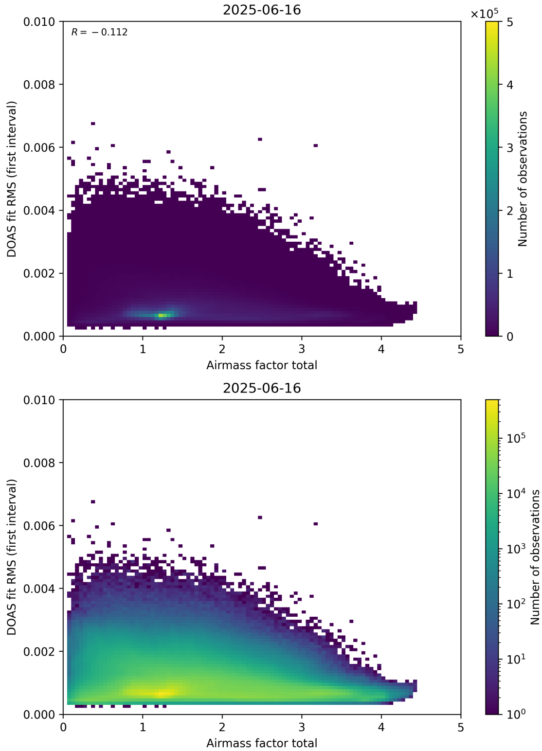
Figure 97: Scatter density plot of “Airmass factor total” against “DOAS fit RMS (first interval)” for 2025-06-16 to 2025-06-17.
