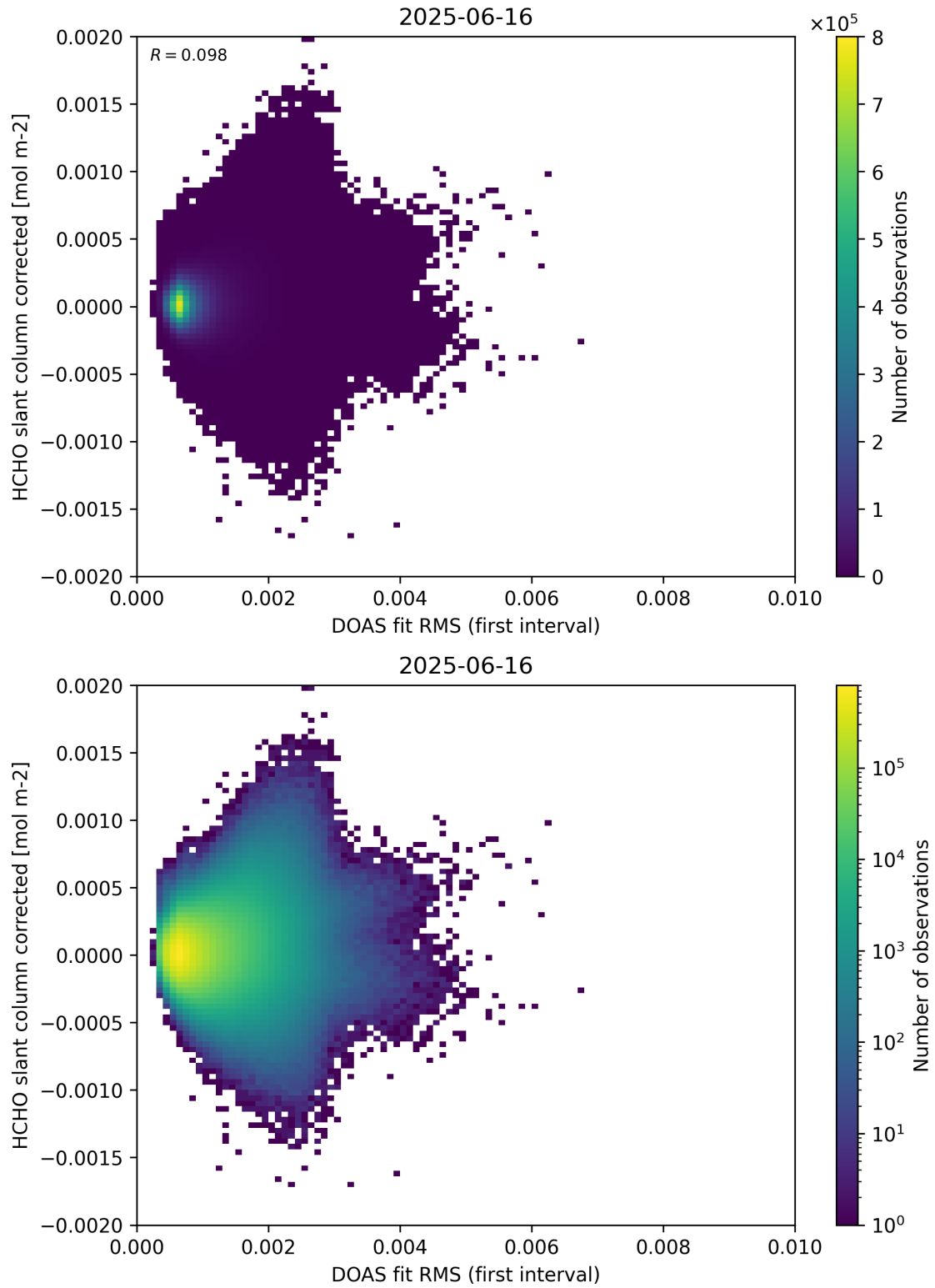
Figure 62: Scatter density plot of “DOAS fit RMS (first interval)” against “HCHO slant column corrected” for 2025-06-16 to 2025-06-17.
