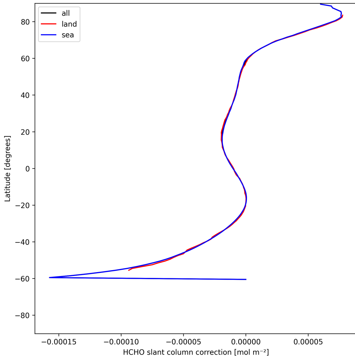
Figure 33: Zonal average of “HCHO slant column correction” for 2025-06-16 to 2025-06-17.
