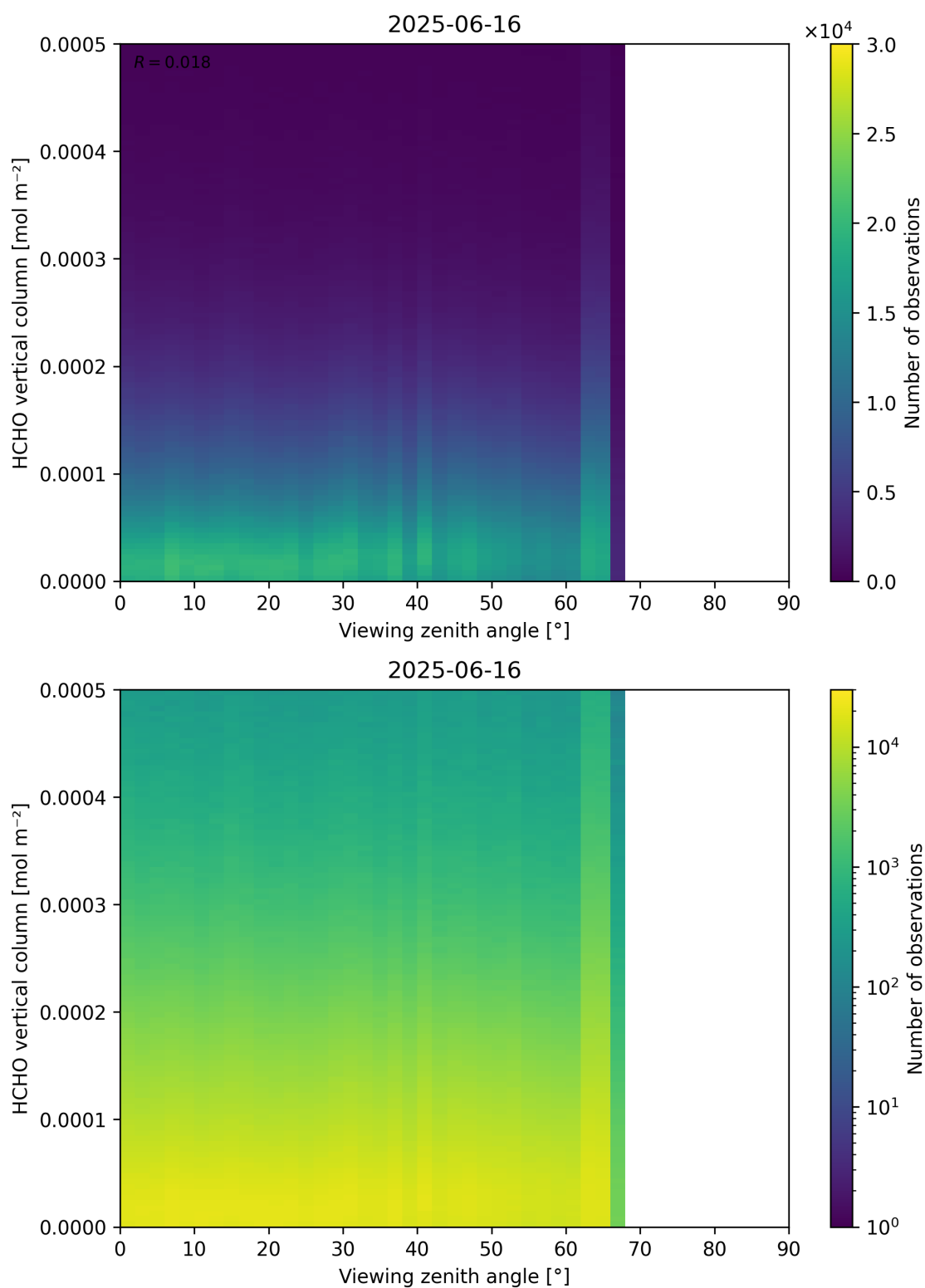
Figure 192: Scatter density plot of “Viewing zenith angle” against “HCHO vertical column” for 2025-06-16 to 2025-06-17.
