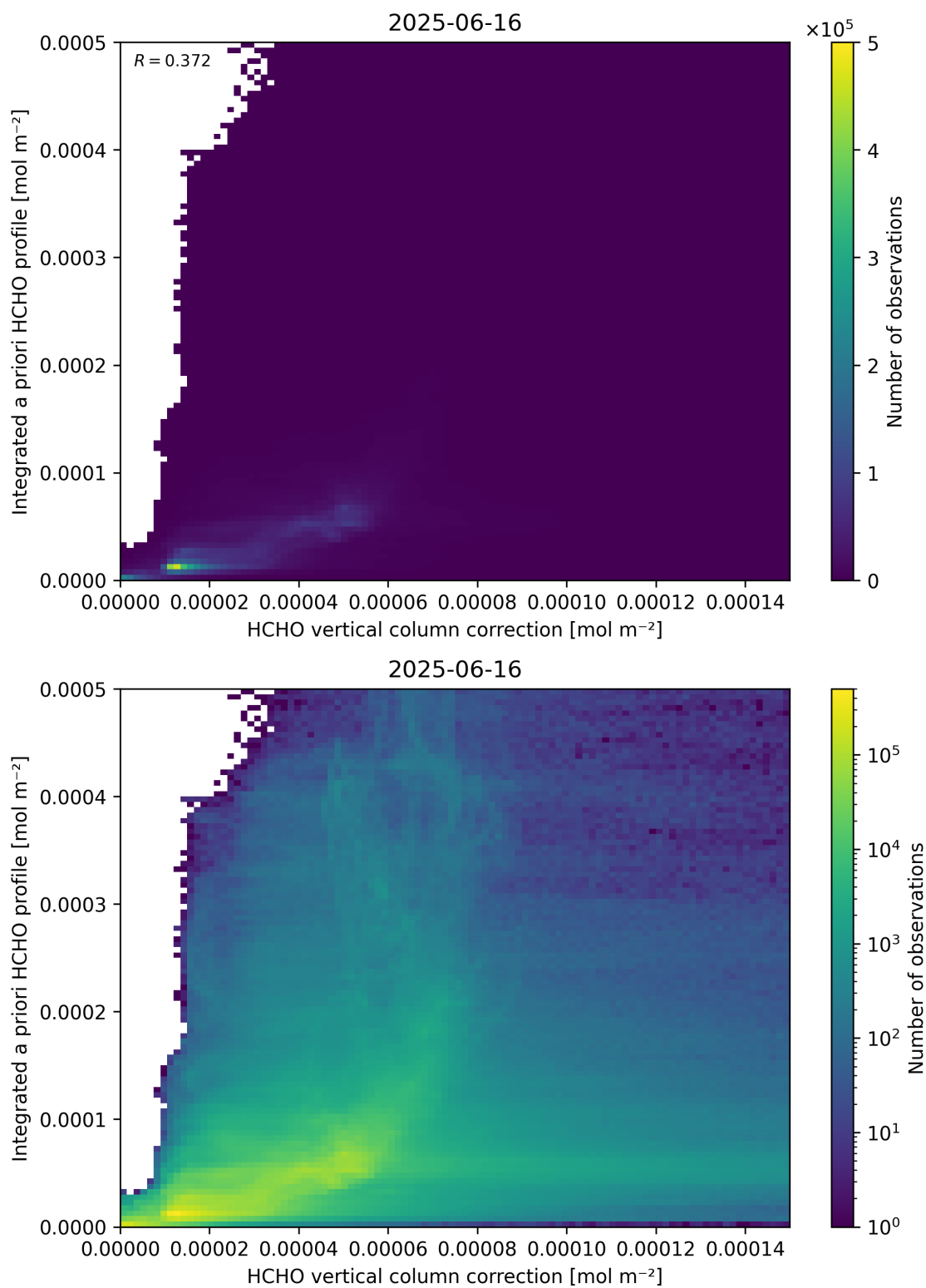
Figure 122: Scatter density plot of “HCHO vertical column correction” against “Integrated a priori HCHO profile” for 2025-06-16 to 2025-06-17.
