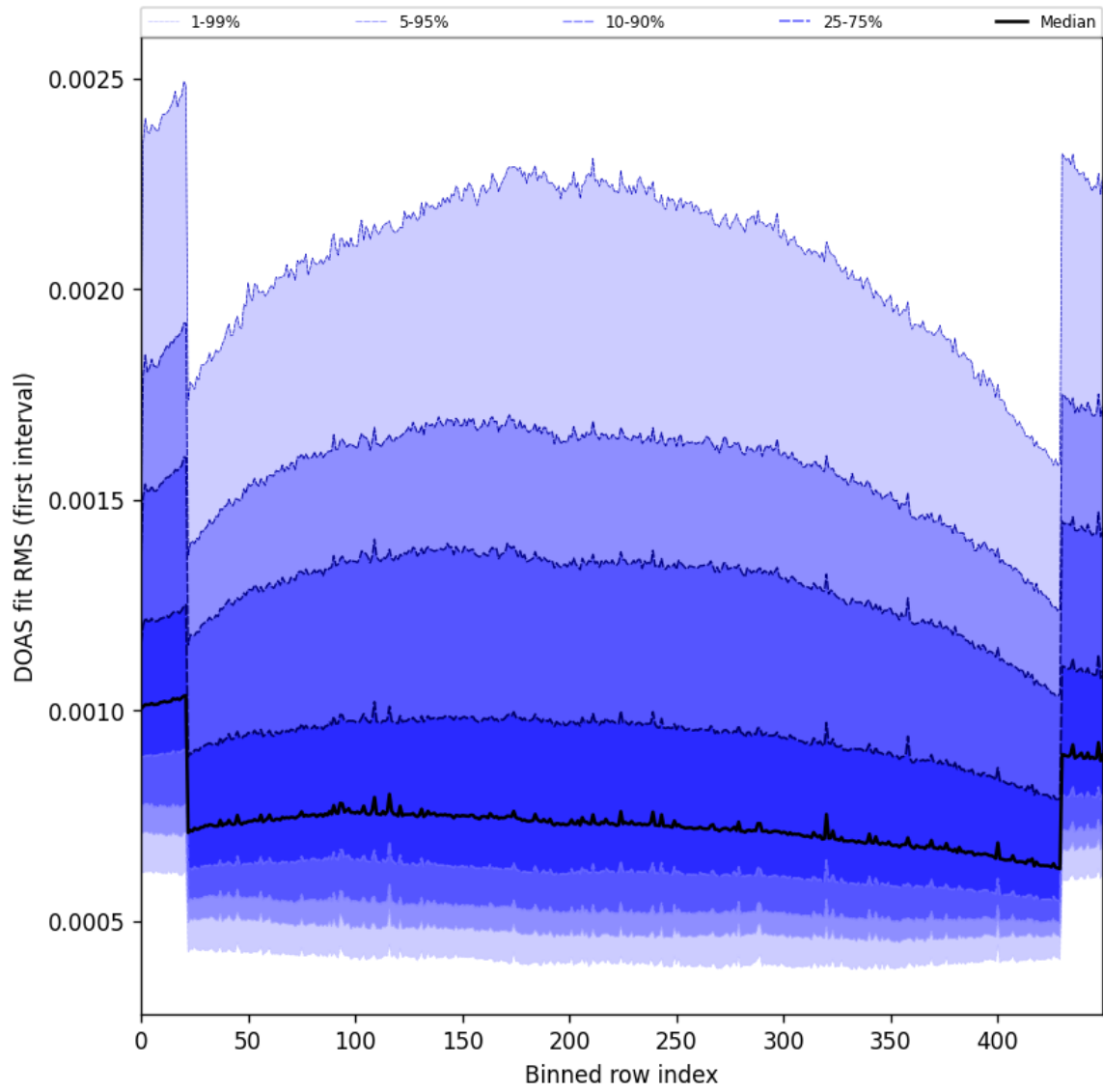
Figure 60: Along track statistics of “DOAS fit RMS (first interval)” for 2025-06-16 to 2025-06-17
