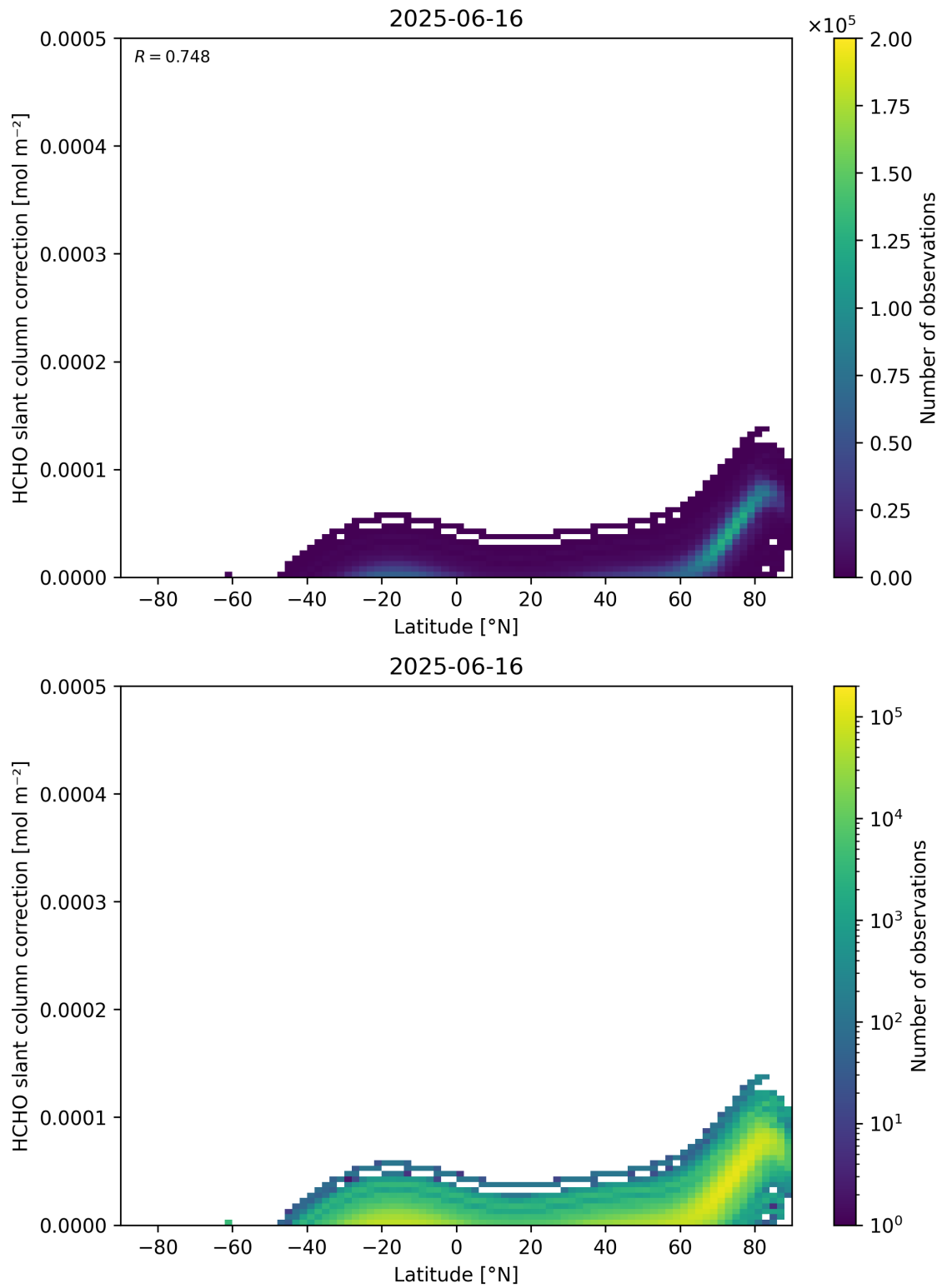
Figure 158: Scatter density plot of “Latitude” against “HCHO slant column correction” for 2025-06-16 to 2025-06-17.
