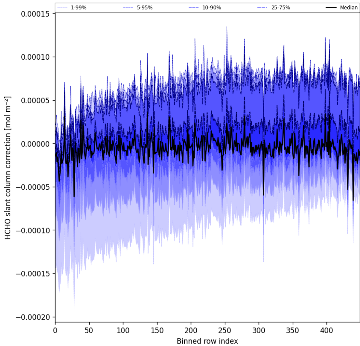
Figure 61: Along track statistics of “HCHO slant column correction” for 2025-06-16 to 2025-06-17
