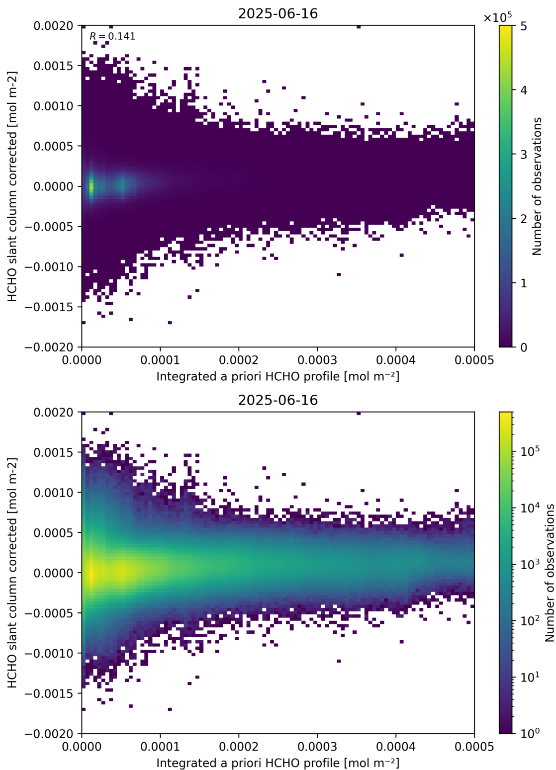
Figure 151: Scatter density plot of “Integrated a priori HCHO profile” against “HCHO slant column corrected” for 2025-06-16 to 2025-06-17.
