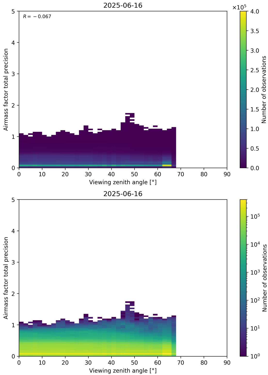
Figure 191: Scatter density plot of “Viewing zenith angle” against “Airmass factor total precision” for 2025-06-16 to 2025-06-17.
