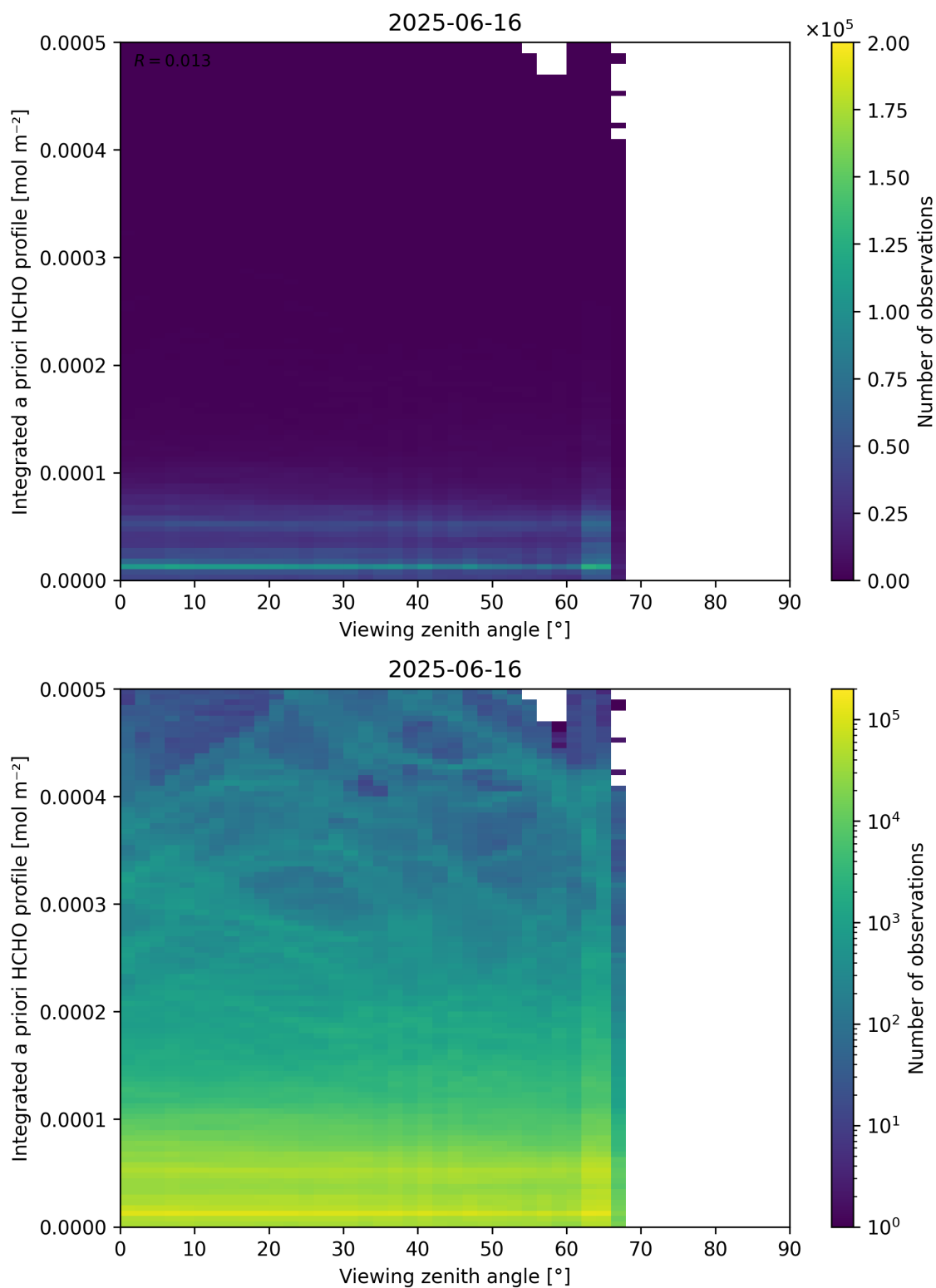
Figure 195: Scatter density plot of “Viewing zenith angle” against “Integrated a priori HCHO profile” for 2025-06-16 to 2025-06-17.
