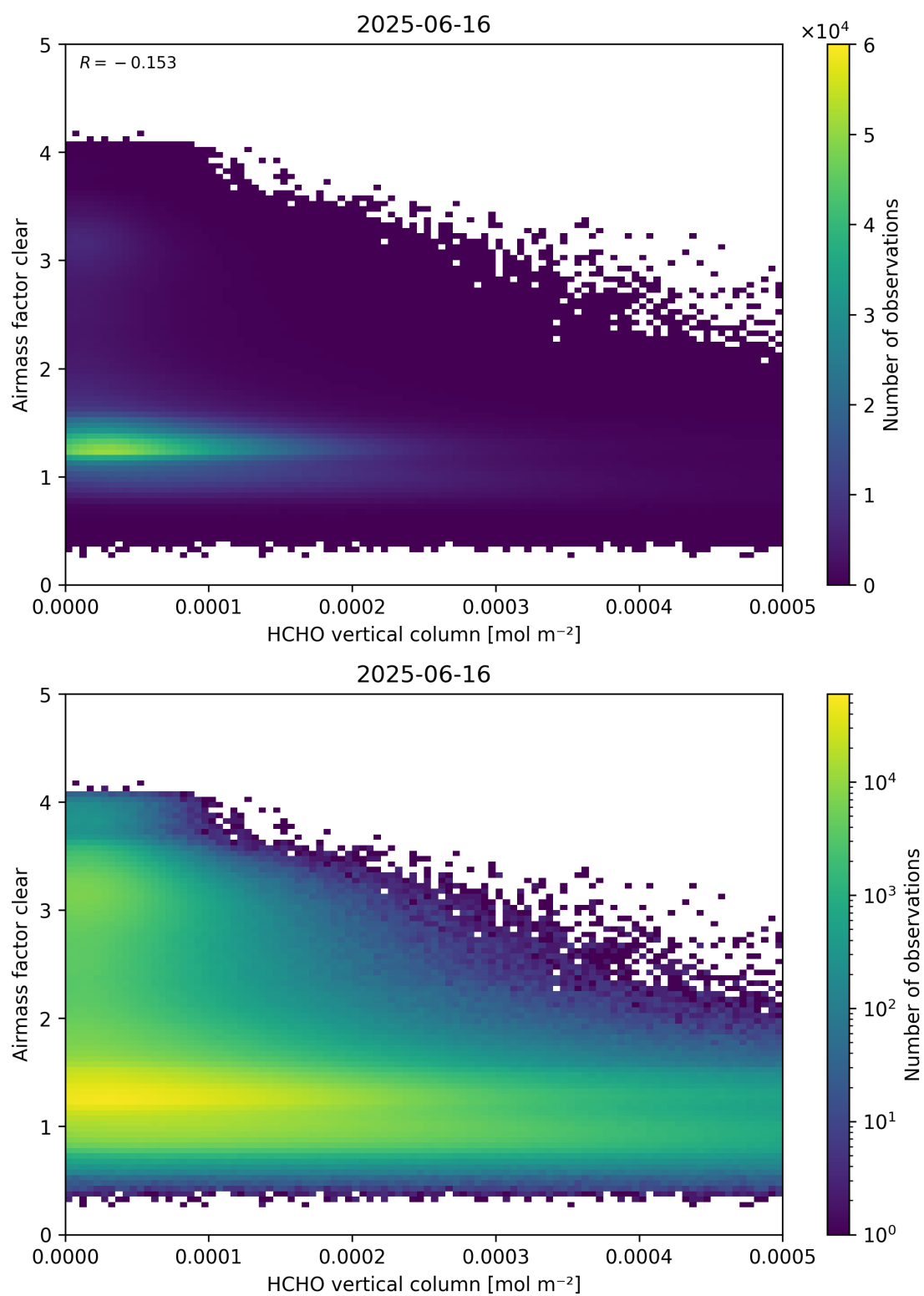
Figure 126: Scatter density plot of “HCHO vertical column” against “Airmass factor clear” for 2025-06-16 to 2025-06-17.
