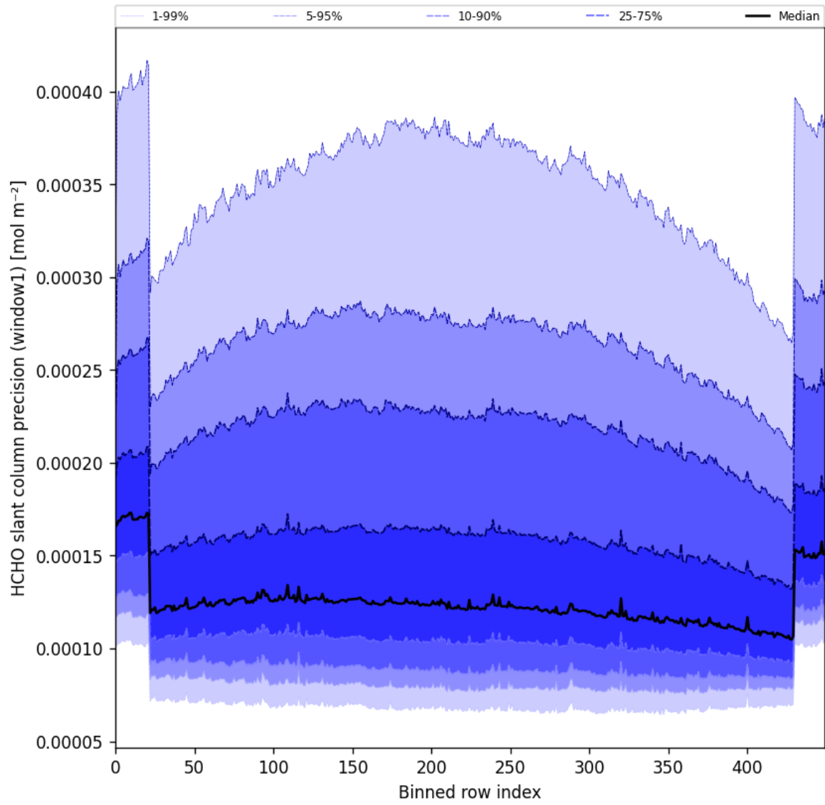
Figure 53: Along track statistics of “HCHO slant column precision (window1)” for 2025-06-16 to 2025-06-17
