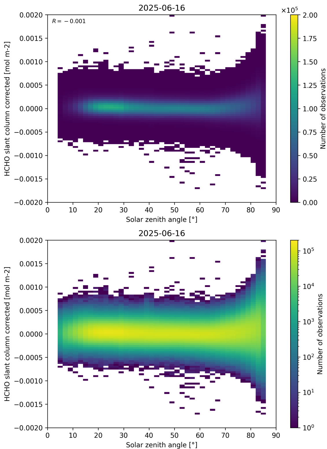
Figure 171: Scatter density plot of “Solar zenith angle” against “HCHO slant column corrected” for 2025-06-16 to 2025-06-17.
