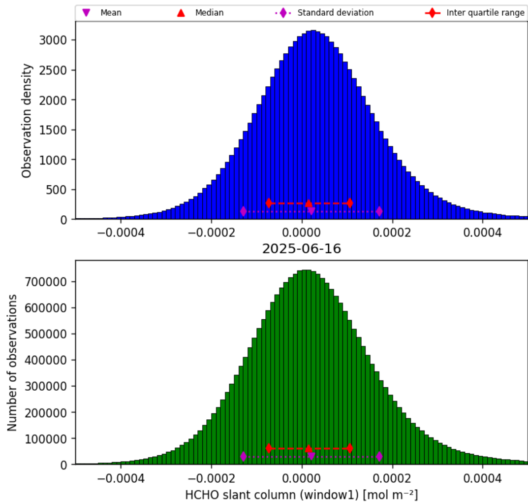
Figure 38: Histogram of “HCHO slant column (window1)” for 2025-06-16 to 2025-06-17
