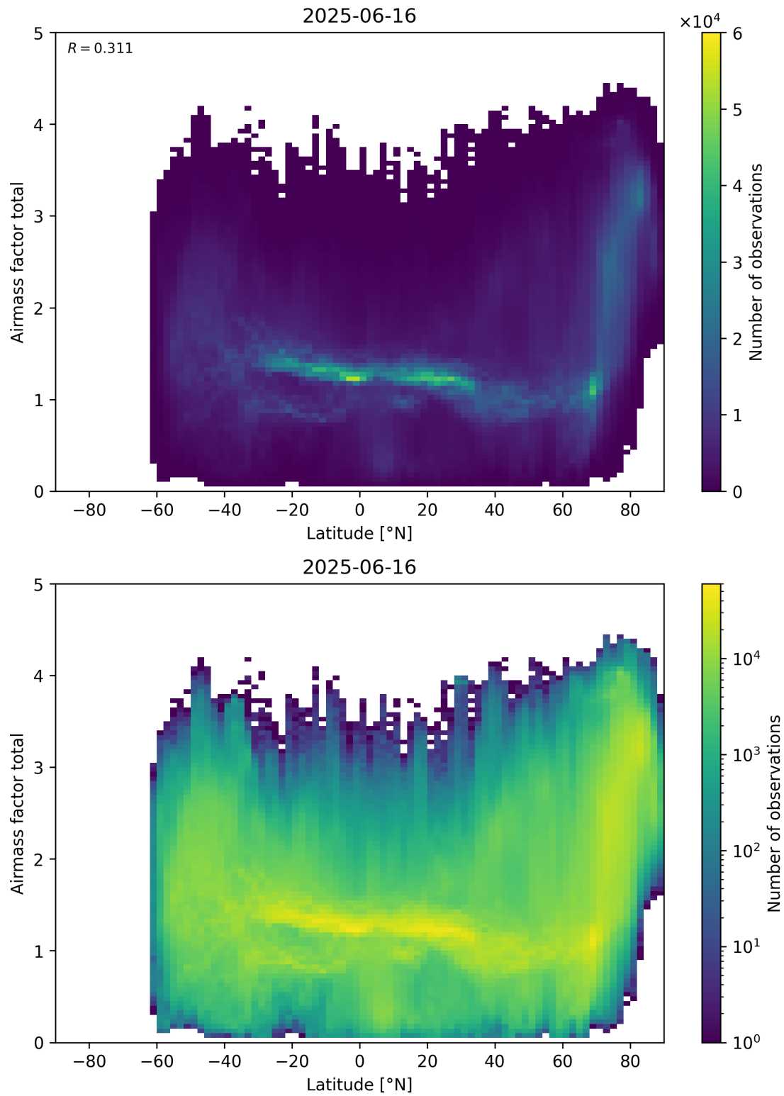
Figure 161: Scatter density plot of “Latitude” against “Airmass factor total” for 2025-06-16 to 2025-06-17.
