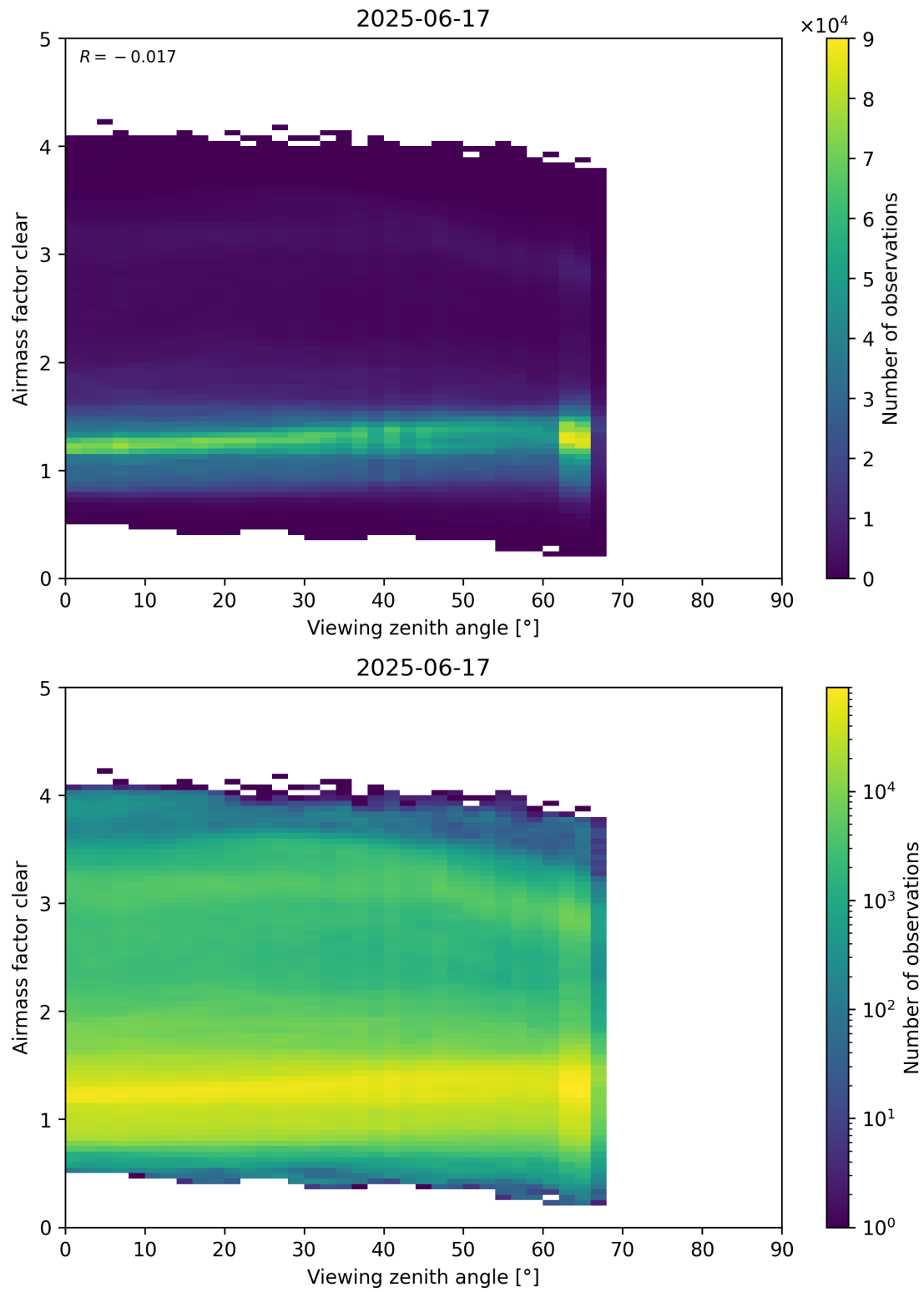
Figure 185: Scatter density plot of “Viewing zenith angle” against “Airmass factor clear” for 2025-06-17 to 2025-06-18.
