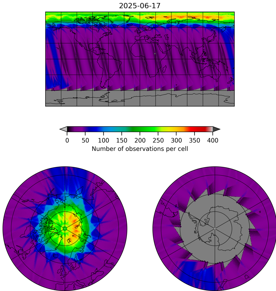
Figure 19: Map of the number of observations for 2025-06-17 to 2025-06-18
