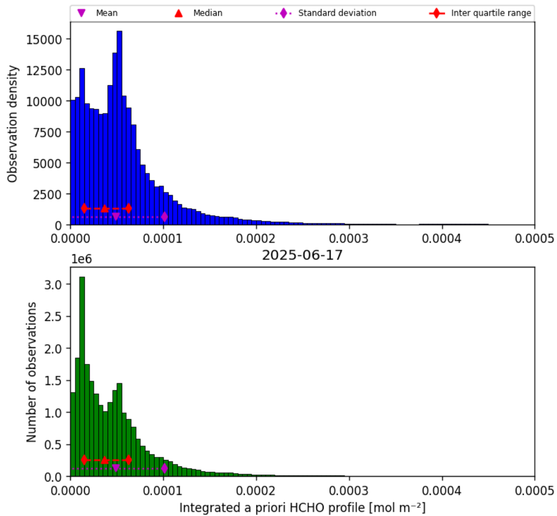
Figure 43: Histogram of “Integrated a priori HCHO profile” for 2025-06-17 to 2025-06-18
