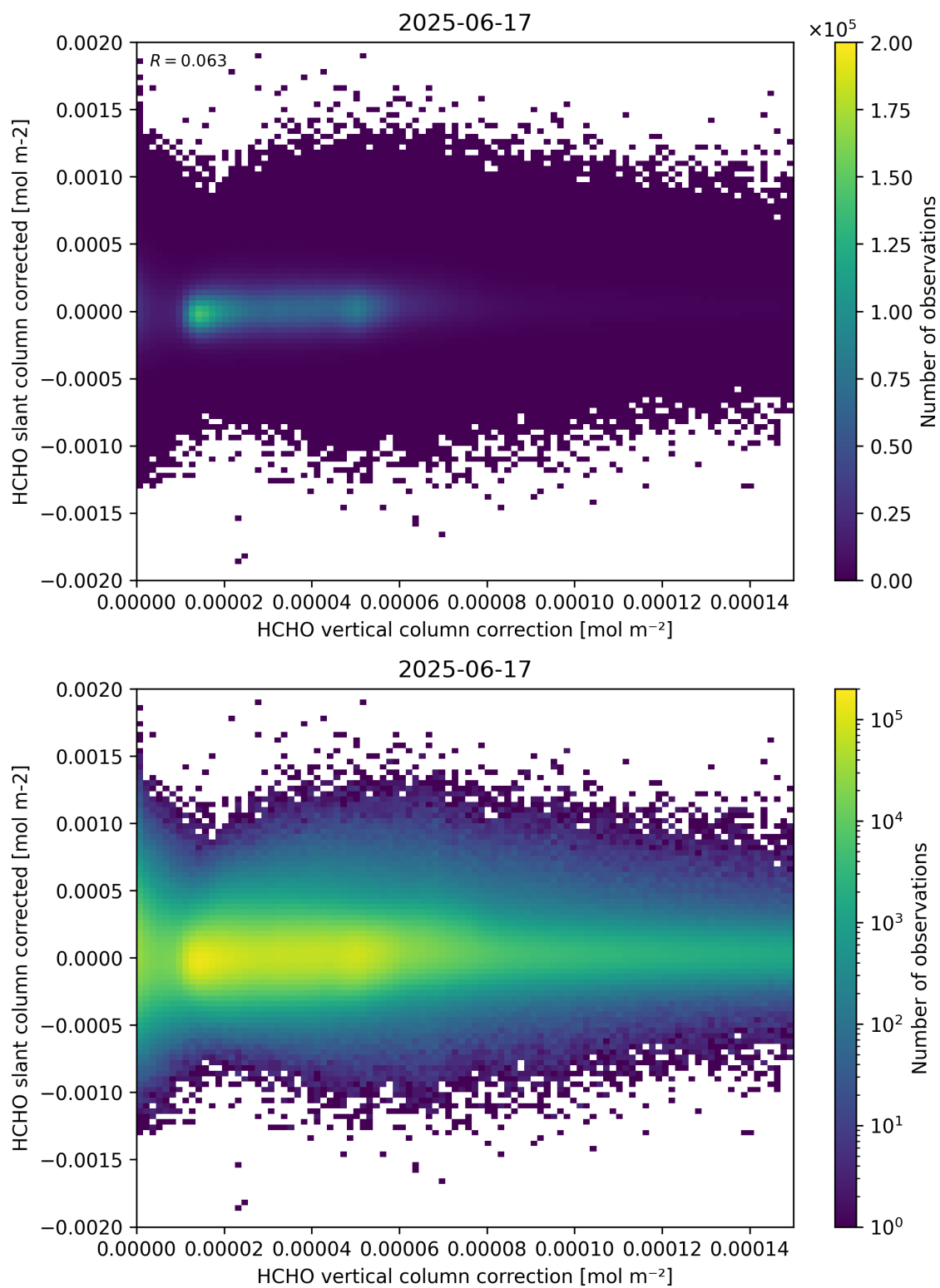
Figure 116: Scatter density plot of “HCHO vertical column correction” against “HCHO slant column corrected” for 2025-06-17 to 2025-06-18.
