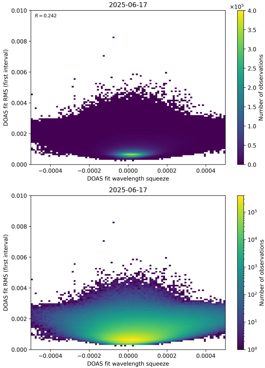
Figure 68: Scatter density plot of “DOAS fit wavelength squeeze” against “DOAS fit RMS (first interval)” for 2025-06-17 to 2025-06-18.
