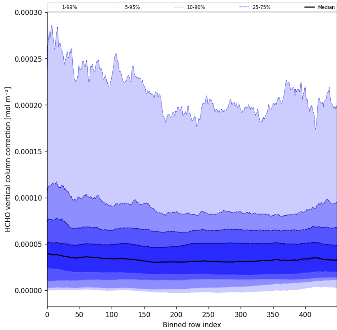
Figure 51: Along track statistics of “HCHO vertical column correction” for 2025-06-17 to 2025-06-18
