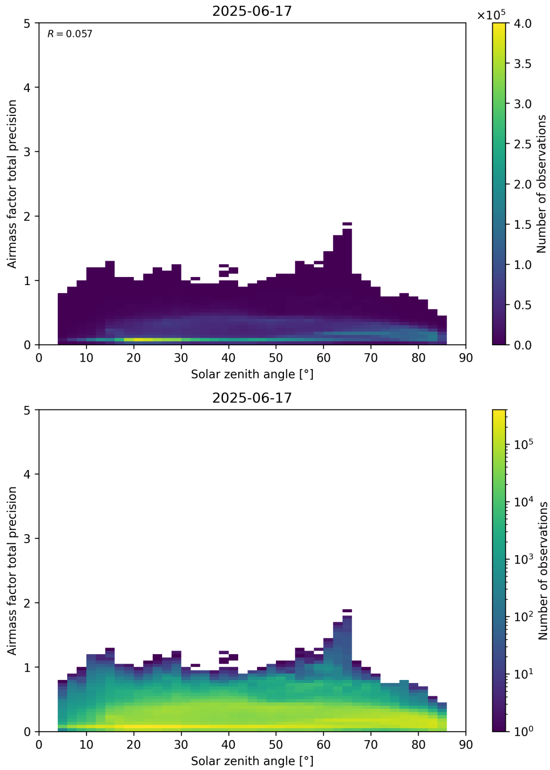
Figure 176: Scatter density plot of “Solar zenith angle” against “Airmass factor total precision” for 2025-06-17 to 2025-06-18.
