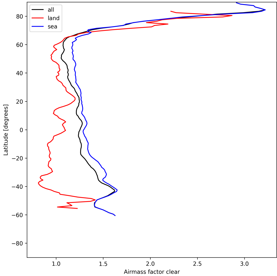
Figure 28: Zonal average of “Airmass factor clear” for 2025-06-17 to 2025-06-18.
