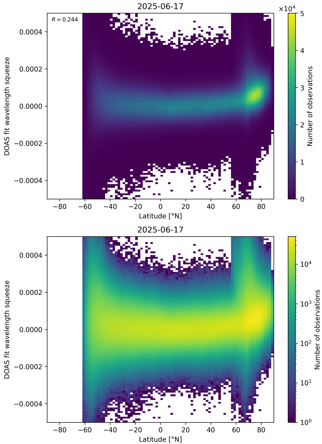
Figure 155: Scatter density plot of “Latitude” against “DOAS fit wavelength squeeze” for 2025-06-17 to 2025-06-18.
