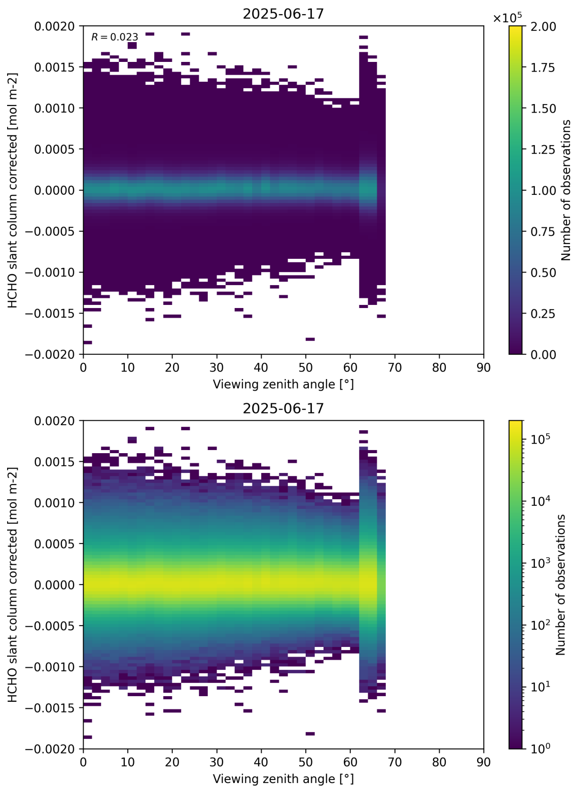
Figure 186: Scatter density plot of “Viewing zenith angle” against “HCHO slant column corrected” for 2025-06-17 to 2025-06-18.
