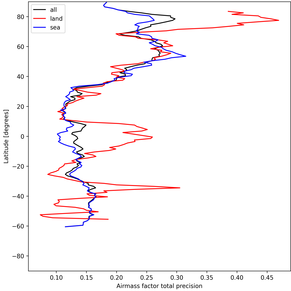
Figure 27: Zonal average of “Airmass factor total precision” for 2025-06-17 to 2025-06-18.
