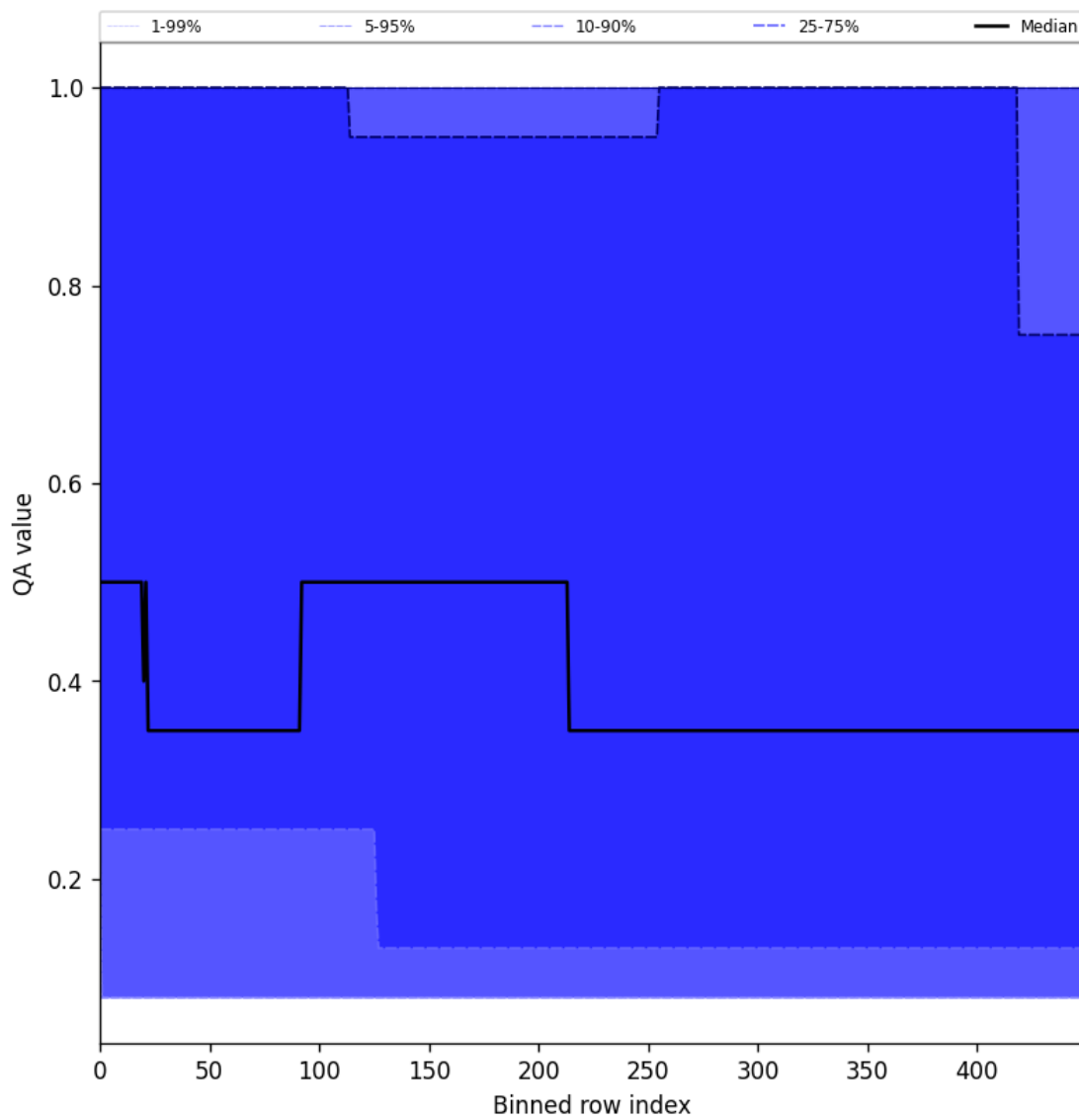
Figure 48: Along track statistics of “QA value” for 2025-06-17 to 2025-06-18
