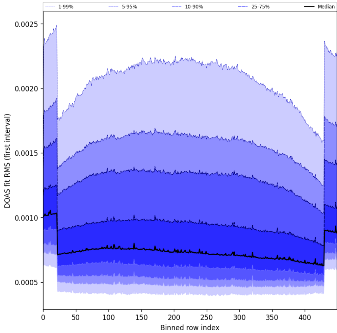
Figure 60: Along track statistics of “DOAS fit RMS (first interval)” for 2025-06-17 to 2025-06-18
