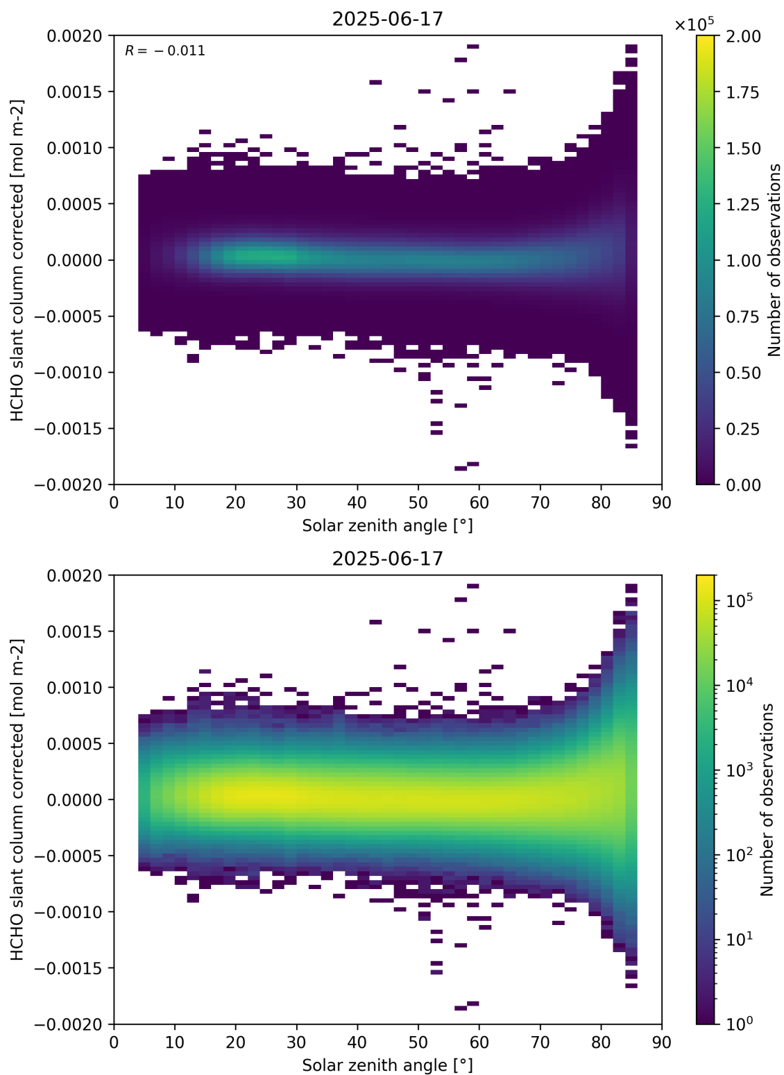
Figure 171: Scatter density plot of “Solar zenith angle” against “HCHO slant column corrected” for 2025-06-17 to 2025-06-18.
