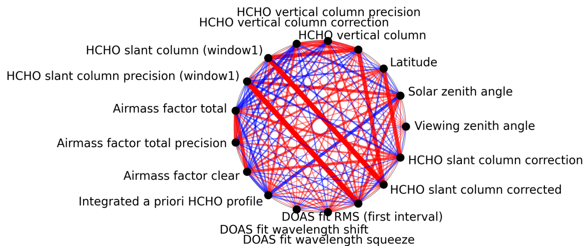
Figure 1: Map of correlation graph for 2025-06-17 to 2025-06-18.
