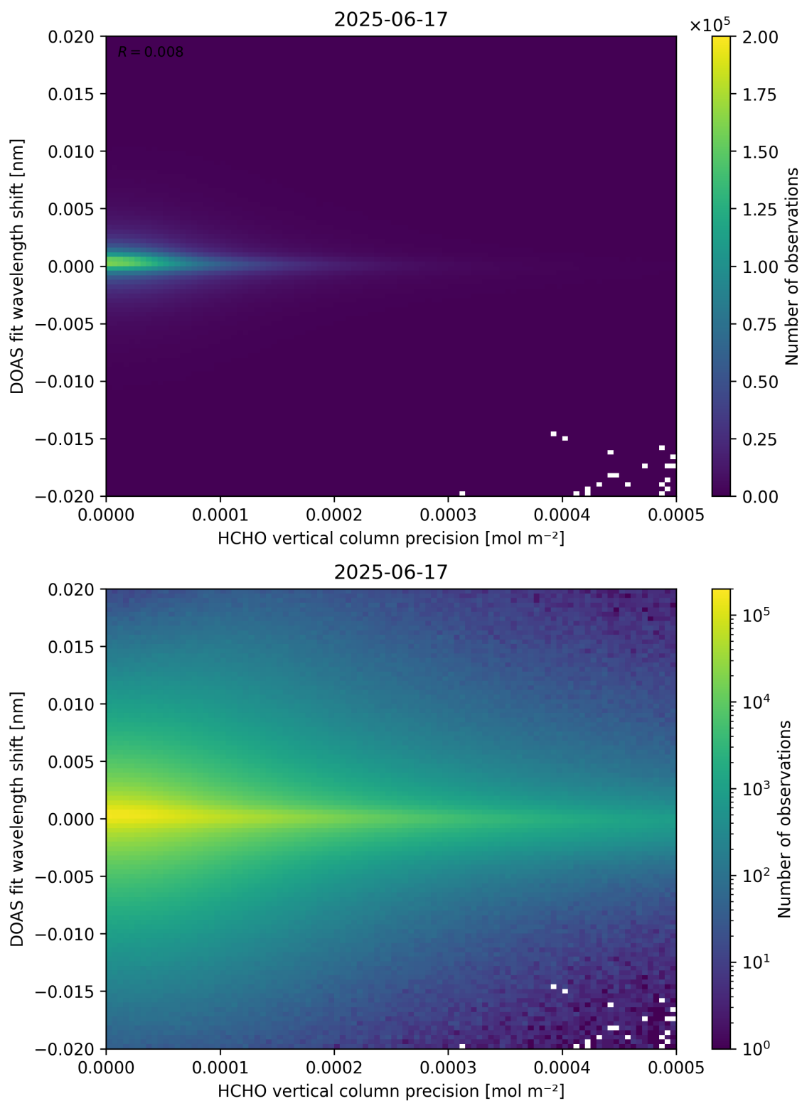
Figure 137: Scatter density plot of “HCHO vertical column precision” against “DOAS fit wavelength shift” for 2025-06-17 to 2025-06-18.
