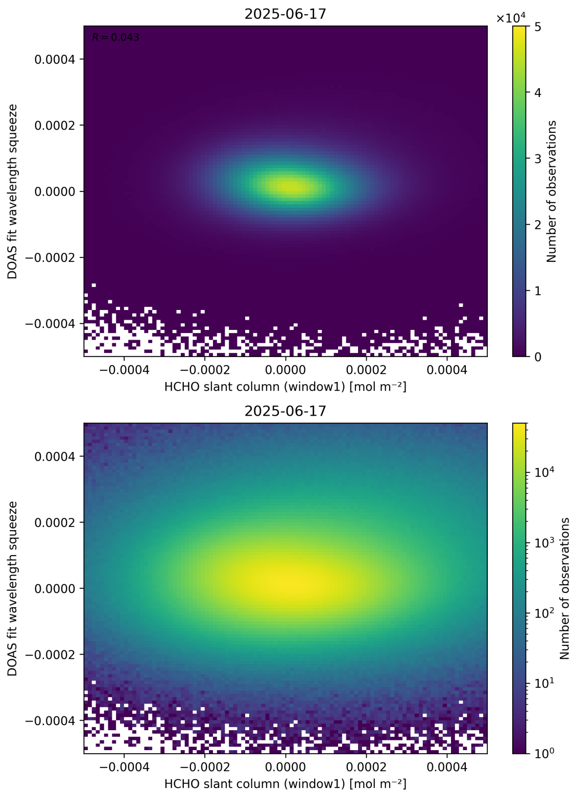
Figure 80: Scatter density plot of “HCHO slant column (window1)” against “DOAS fit wavelength squeeze” for 2025-06-17 to 2025-06-18.
