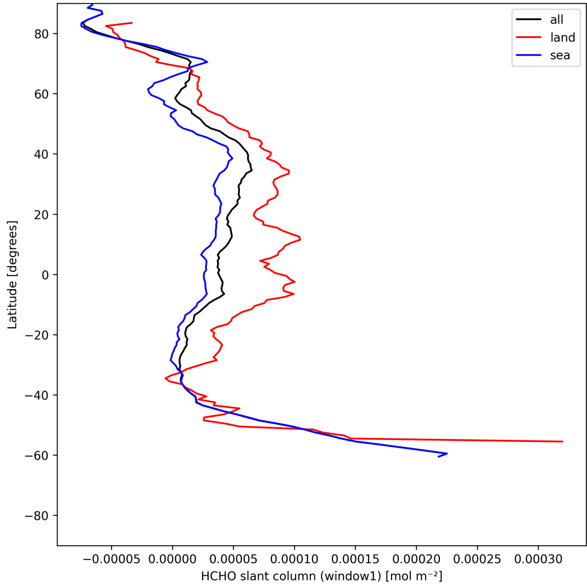
Figure 24: Zonal average of “HCHO slant column (window1)” for 2025-06-17 to 2025-06-18.
