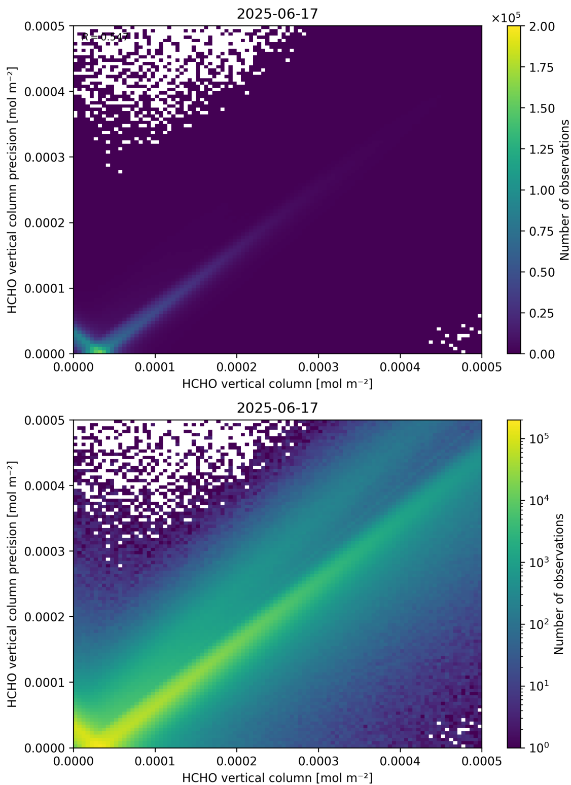
Figure 134: Scatter density plot of “HCHO vertical column” against “HCHO vertical column precision” for 2025-06-17 to 2025-06-18.
