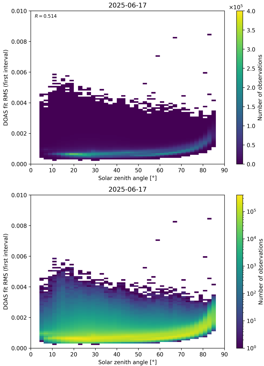
Figure 167: Scatter density plot of “Solar zenith angle” against “DOAS fit RMS (first interval)” for 2025-06-17 to 2025-06-18.
