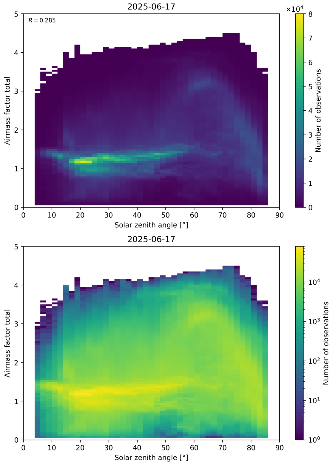
Figure 175: Scatter density plot of “Solar zenith angle” against “Airmass factor total” for 2025-06-17 to 2025-06-18.
