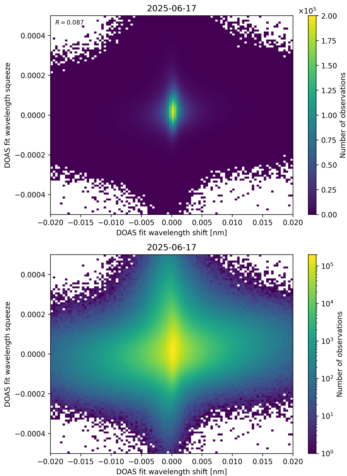
Figure 65: Scatter density plot of “DOAS fit wavelength shift” against “DOAS fit wavelength squeeze” for 2025-06-17 to 2025-06-18.
