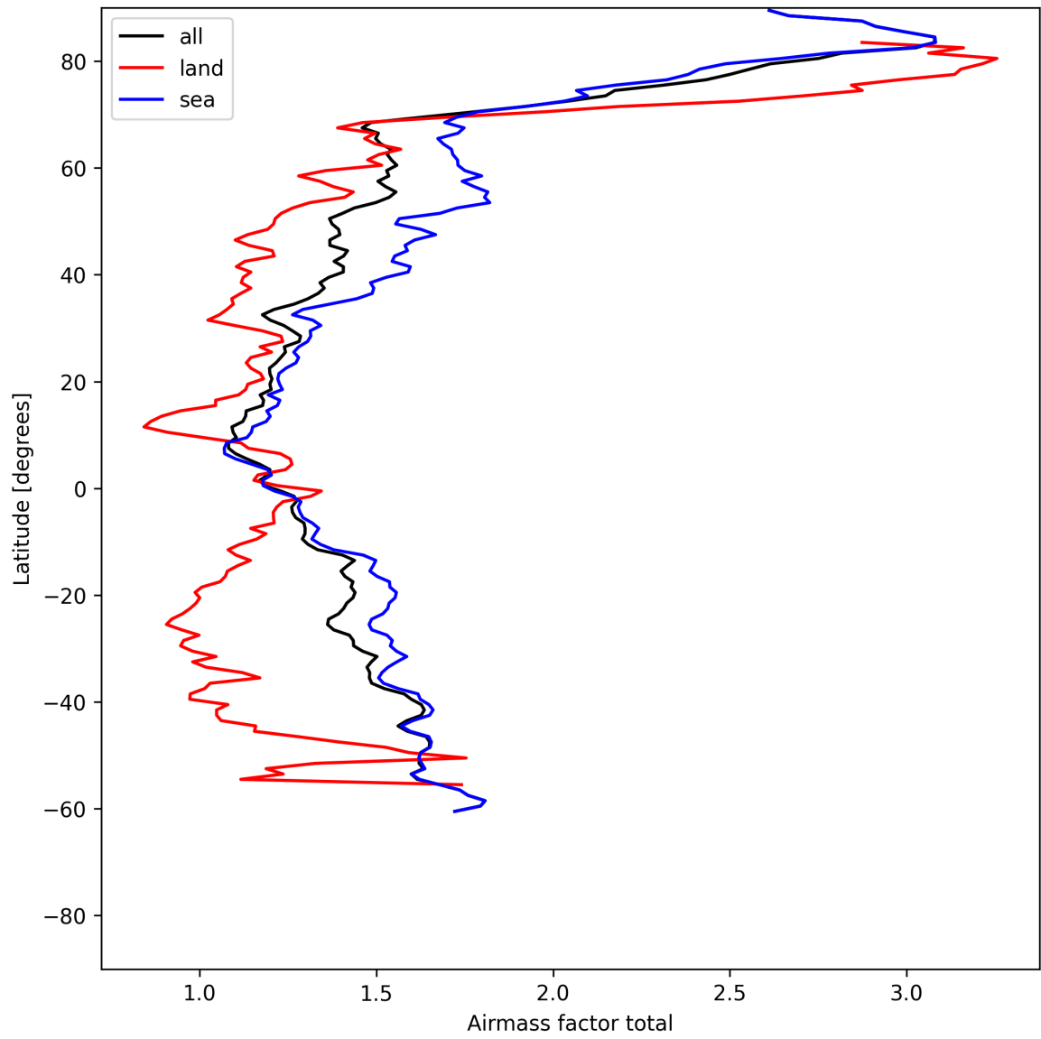
Figure 26: Zonal average of “Airmass factor total” for 2025-06-17 to 2025-06-18.
