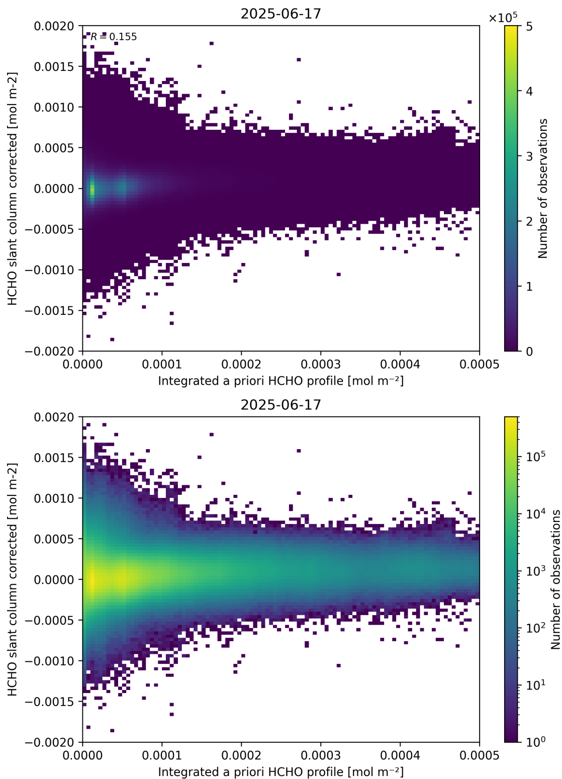
Figure 151: Scatter density plot of “Integrated a priori HCHO profile” against “HCHO slant column corrected” for 2025-06-17 to 2025-06-18.
