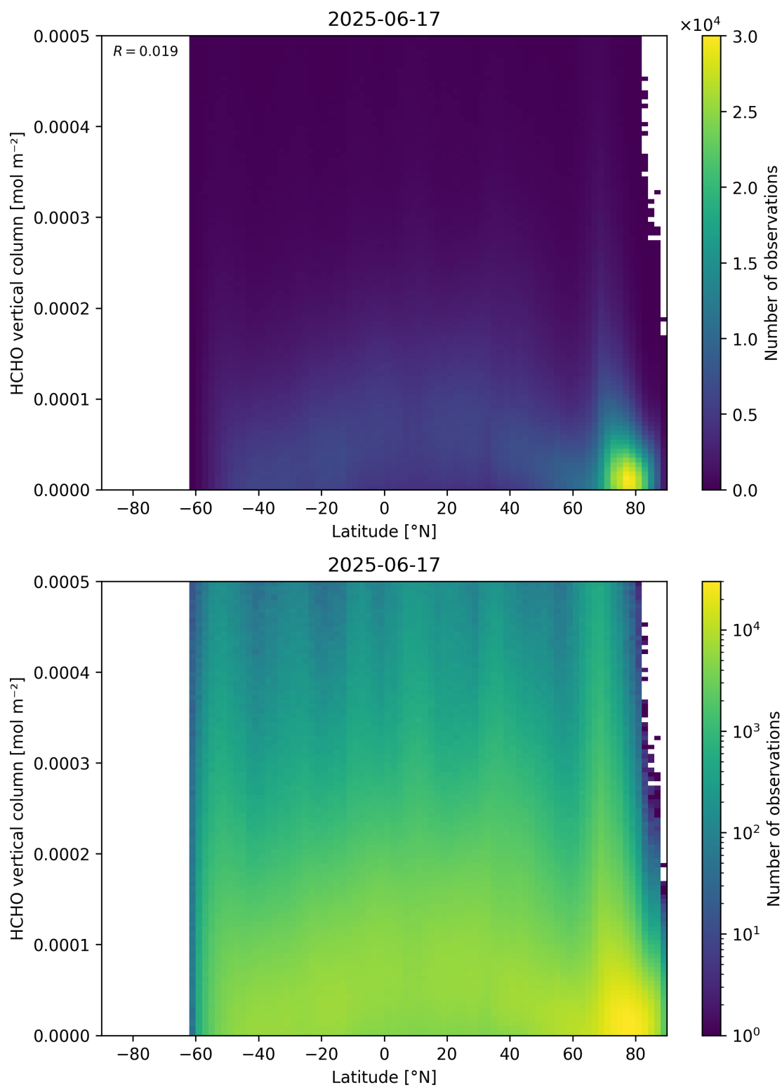
Figure 163: Scatter density plot of “Latitude” against “HCHO vertical column” for 2025-06-17 to 2025-06-18.
