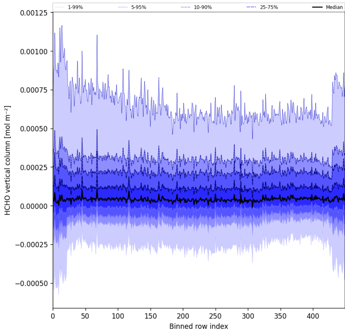
Figure 49: Along track statistics of “HCHO vertical column” for 2025-06-17 to 2025-06-18
