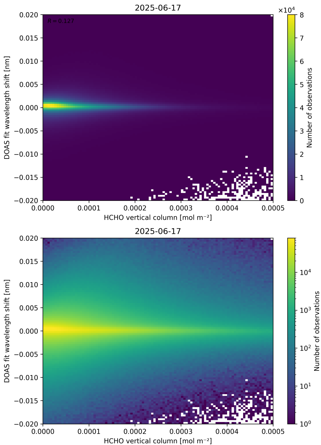
Figure 124: Scatter density plot of “HCHO vertical column” against “DOAS fit wavelength shift” for 2025-06-17 to 2025-06-18.
