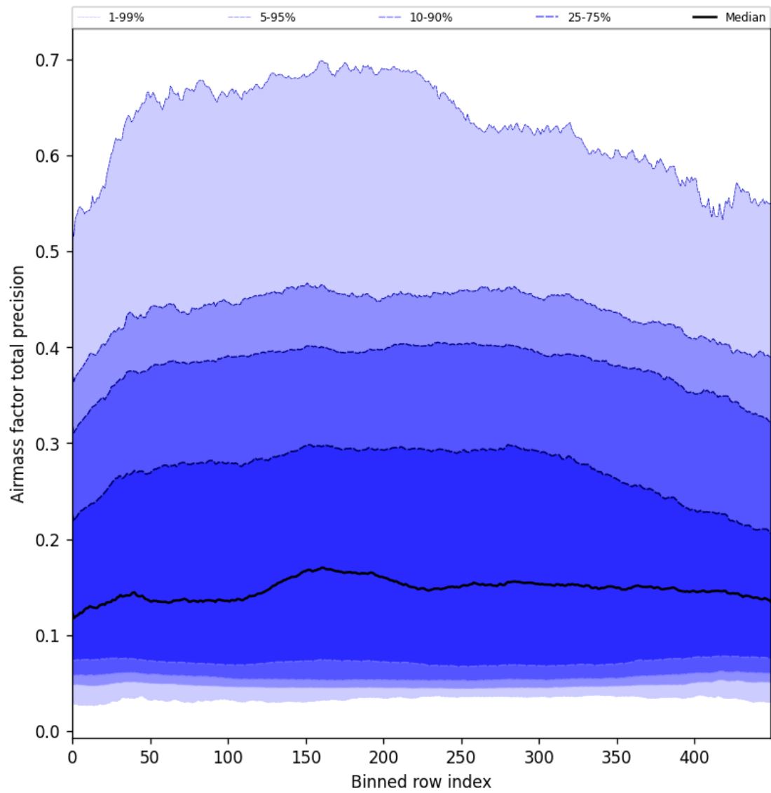
Figure 55: Along track statistics of “Airmass factor total precision” for 2025-06-17 to 2025-06-18
