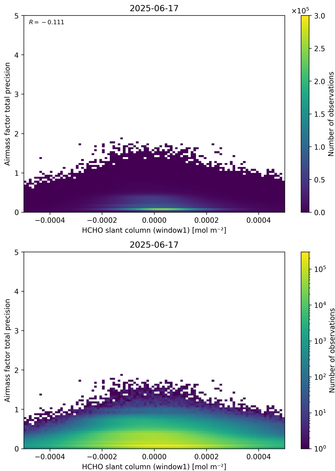
Figure 86: Scatter density plot of “HCHO slant column (window1)” against “Airmass factor total precision” for 2025-06-17 to 2025-06-18.
