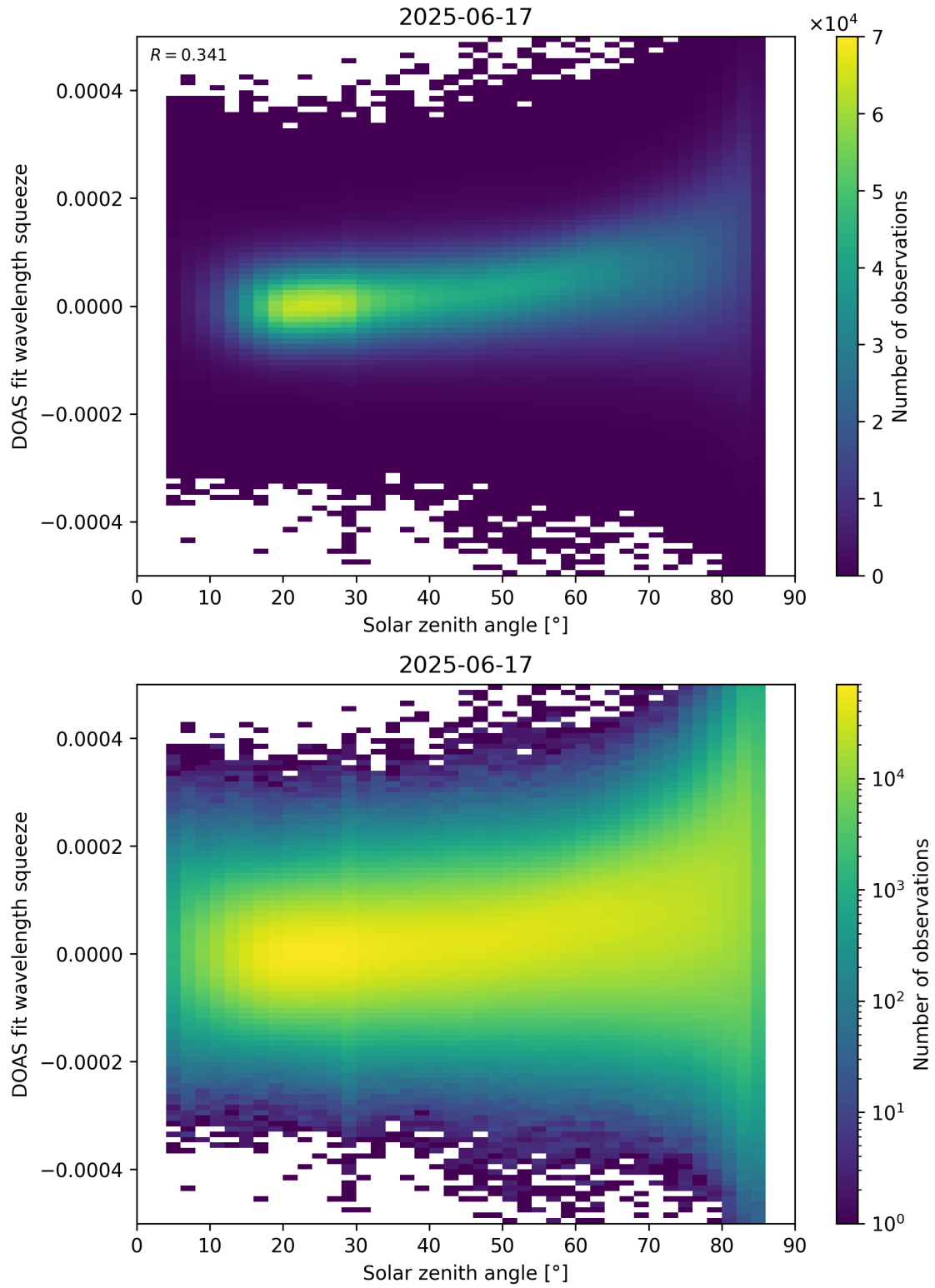
Figure 169: Scatter density plot of “Solar zenith angle” against “DOAS fit wavelength squeeze” for 2025-06-17 to 2025-06-18.
