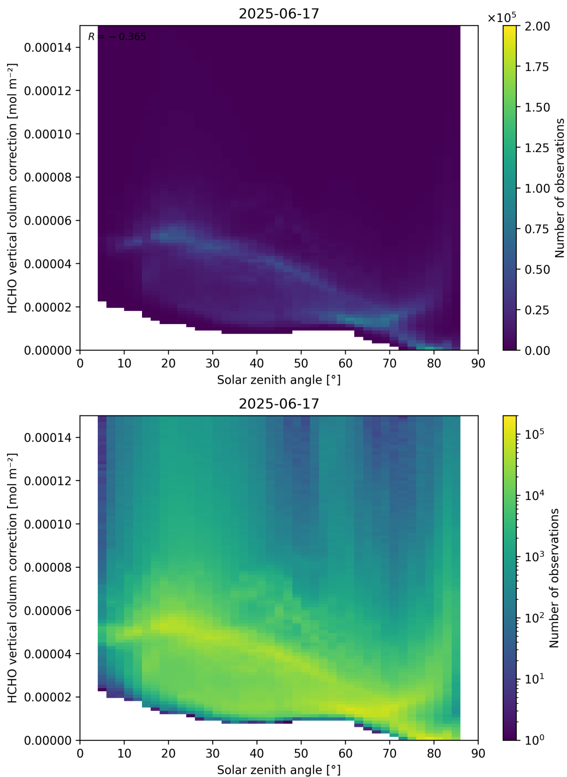
Figure 178: Scatter density plot of “Solar zenith angle” against “HCHO vertical column correction” for 2025-06-17 to 2025-06-18.
