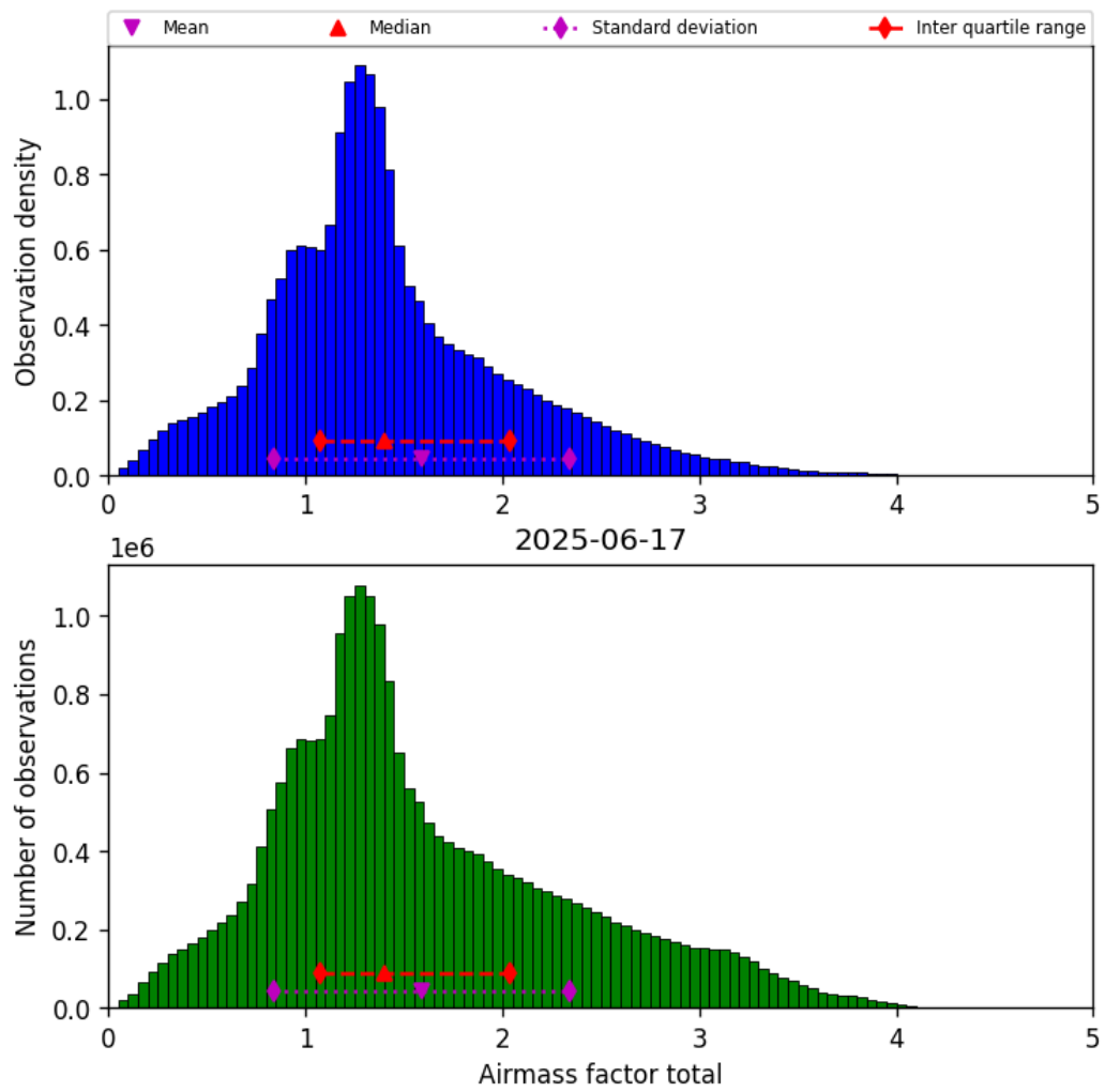
Figure 40: Histogram of “Airmass factor total” for 2025-06-17 to 2025-06-18
