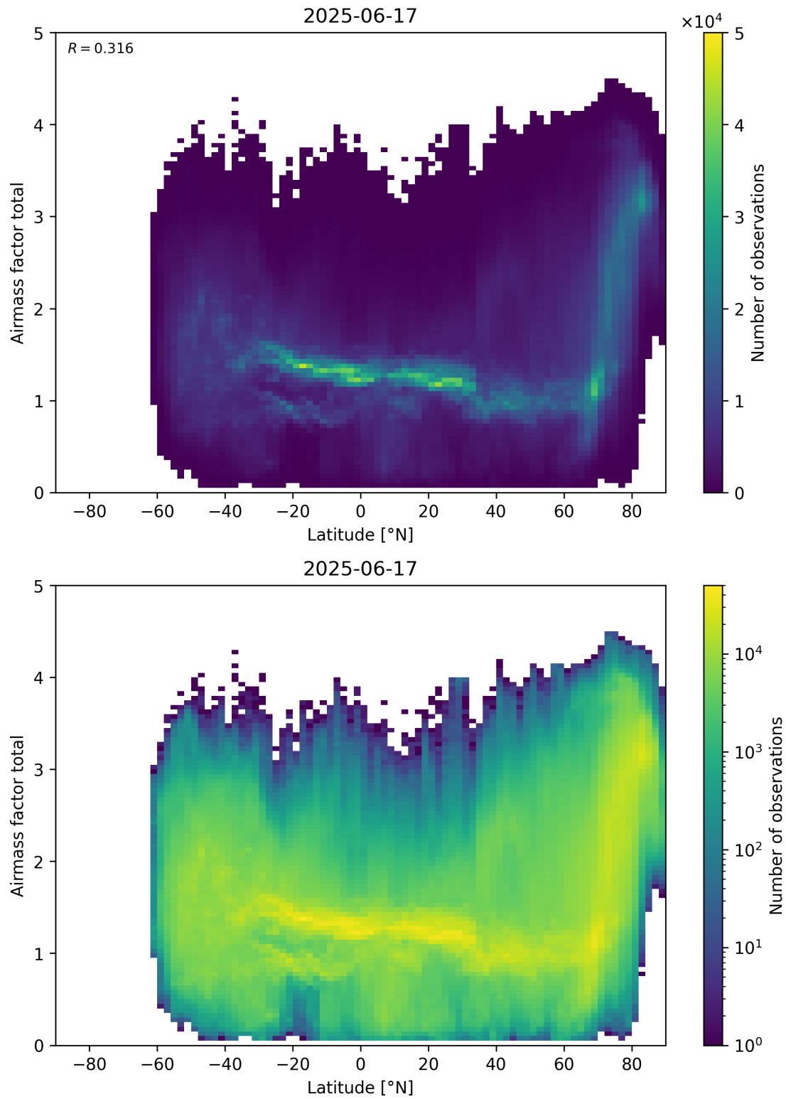
Figure 161: Scatter density plot of “Latitude” against “Airmass factor total” for 2025-06-17 to 2025-06-18.
