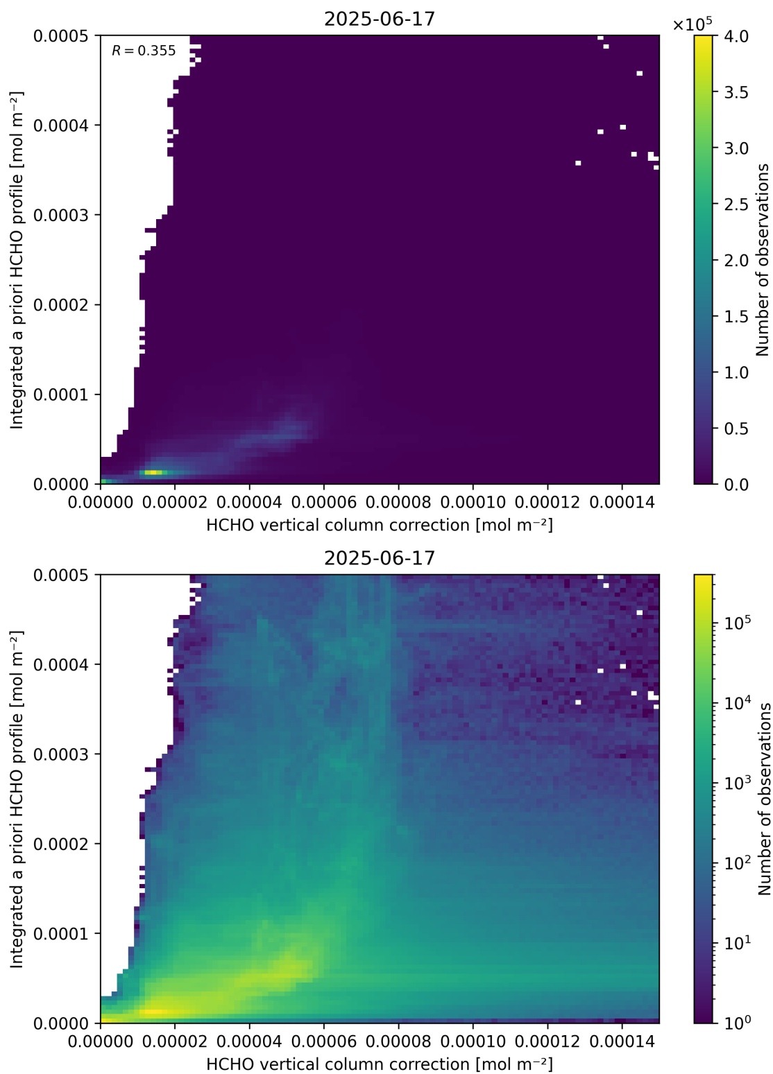
Figure 122: Scatter density plot of “HCHO vertical column correction” against “Integrated a priori HCHO profile” for 2025-06-17 to 2025-06-18.
