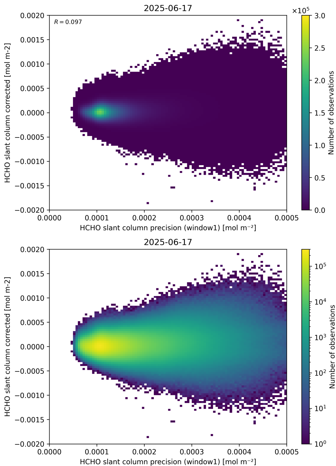
Figure 92: Scatter density plot of “HCHO slant column precision (window1)” against “HCHO slant column corrected” for 2025-06-17 to 2025-06-18.
