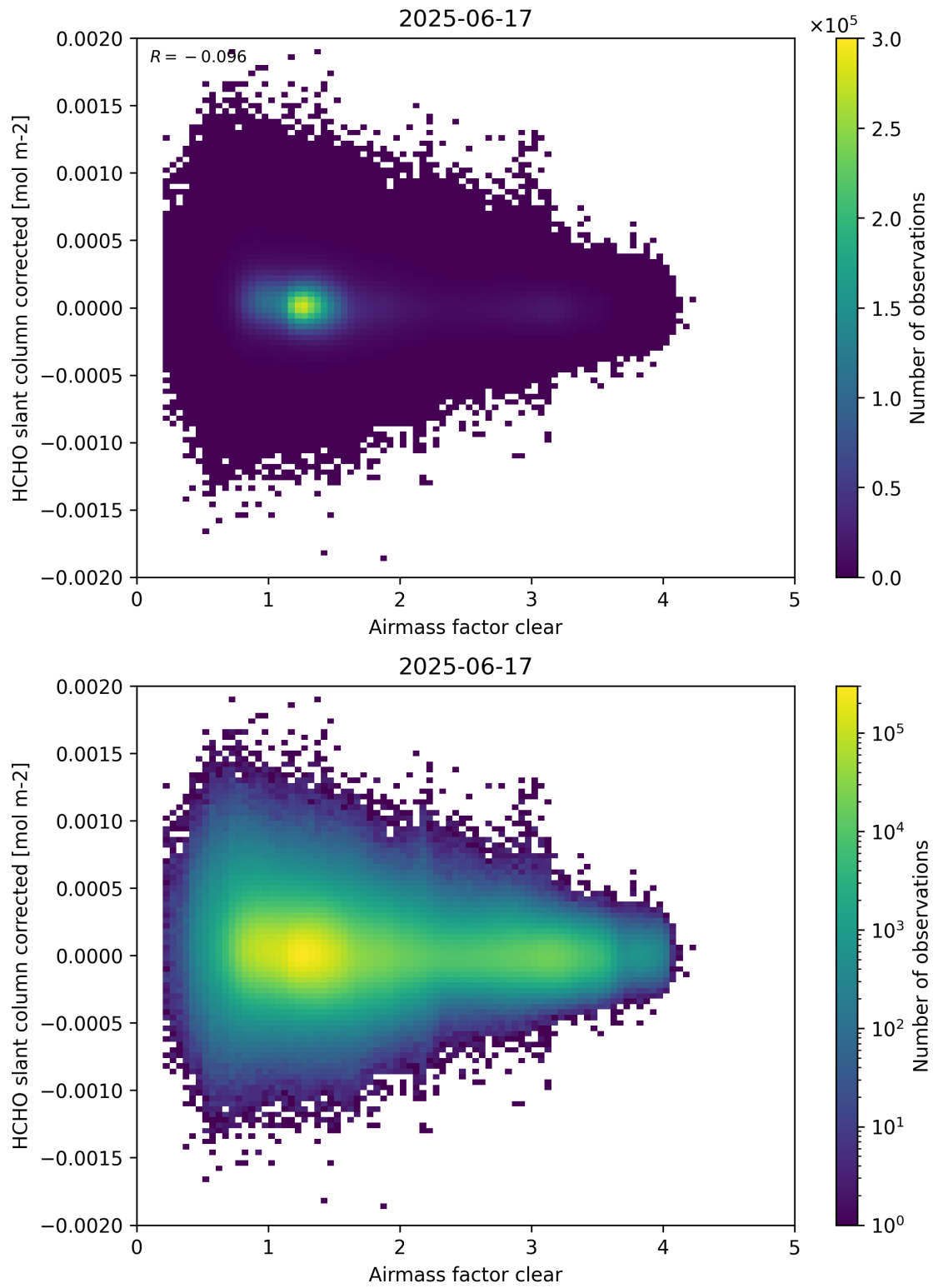
Figure 74: Scatter density plot of “Airmass factor clear” against “HCHO slant column corrected” for 2025-06-17 to 2025-06-18.
