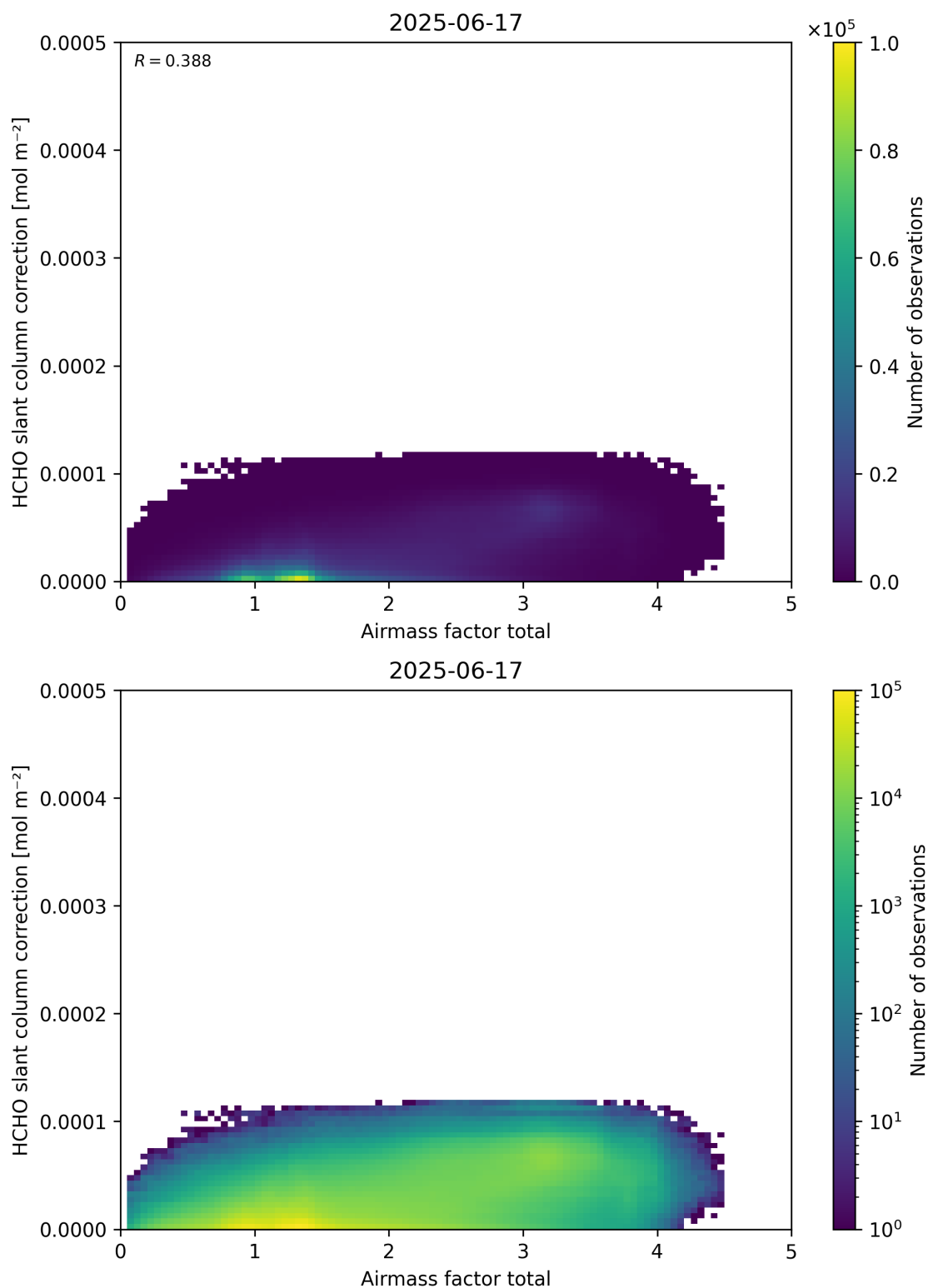
Figure 102: Scatter density plot of “Airmass factor total” against “HCHO slant column correction” for 2025-06-17 to 2025-06-18.
