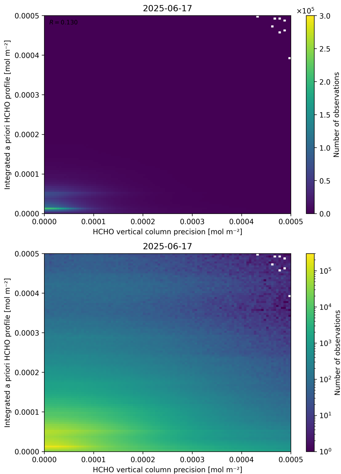
Figure 147: Scatter density plot of “HCHO vertical column precision” against “Integrated a priori HCHO profile” for 2025-06-17 to 2025-06-18.
