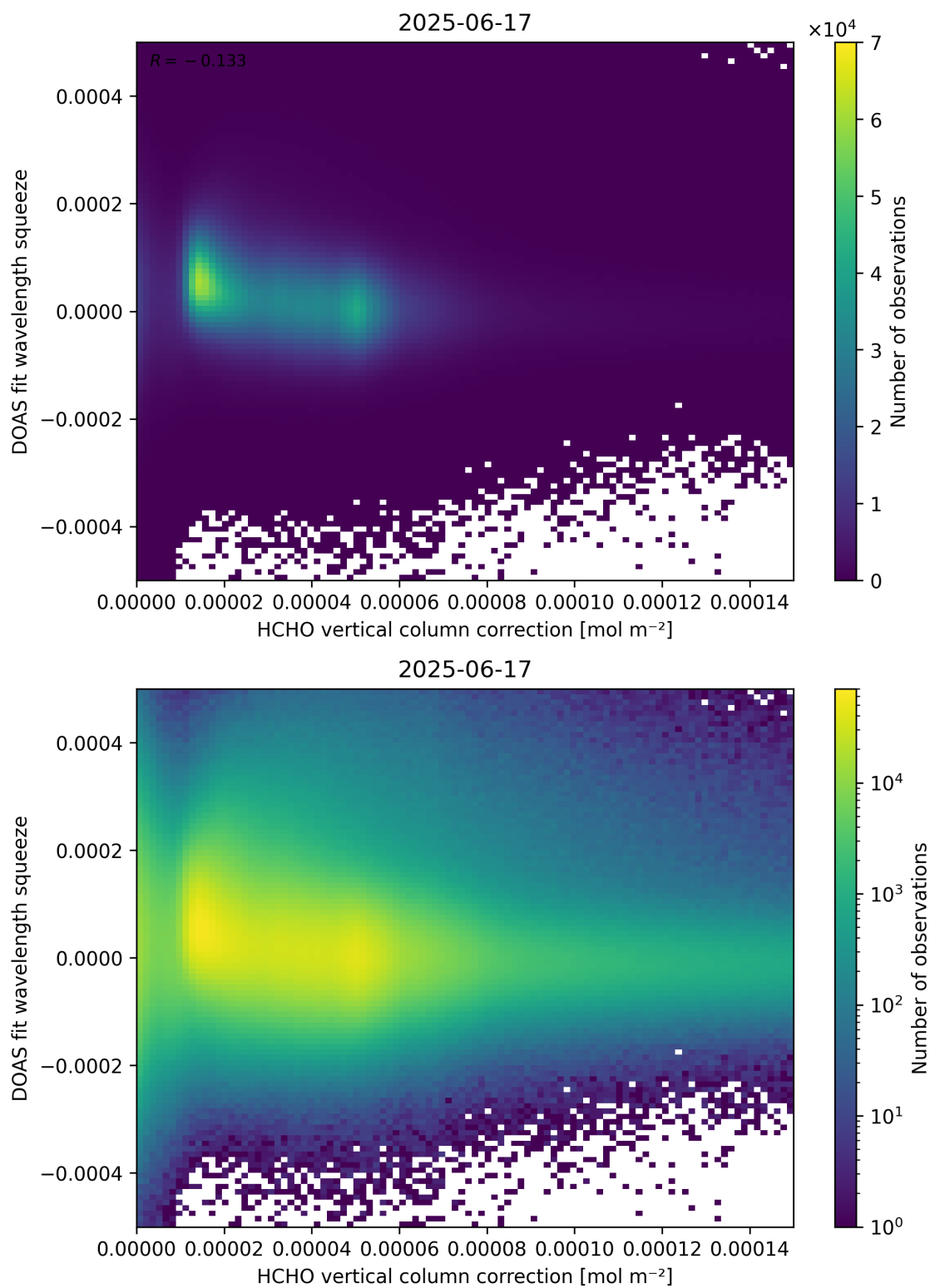
Figure 114: Scatter density plot of “HCHO vertical column correction” against “DOAS fit wavelength squeeze” for 2025-06-17 to 2025-06-18.
