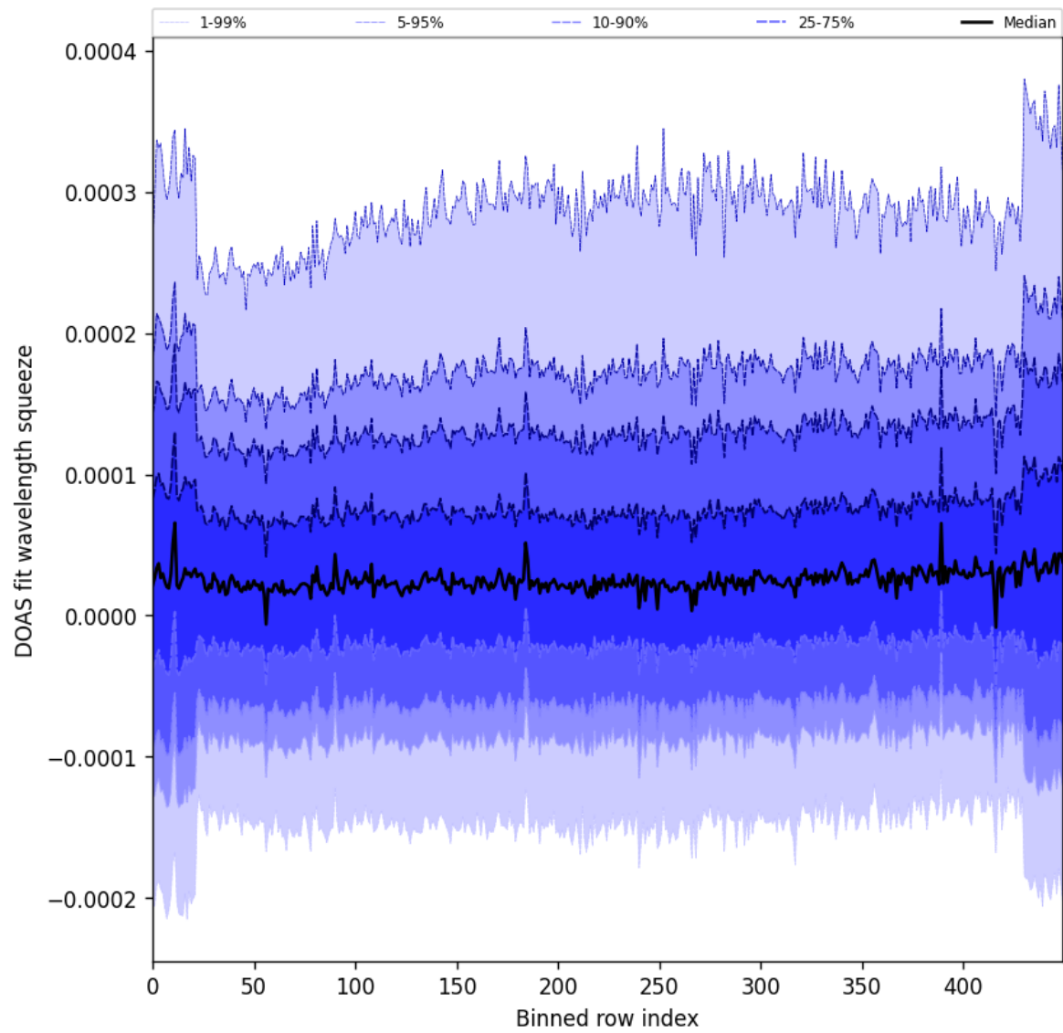
Figure 59: Along track statistics of “DOAS fit wavelength squeeze” for 2025-06-17 to 2025-06-18
