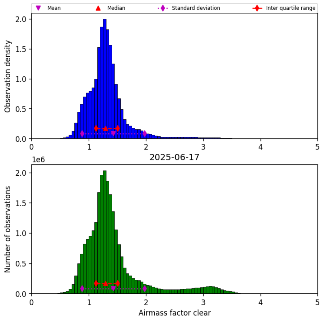
Figure 42: Histogram of “Airmass factor clear” for 2025-06-17 to 2025-06-18
