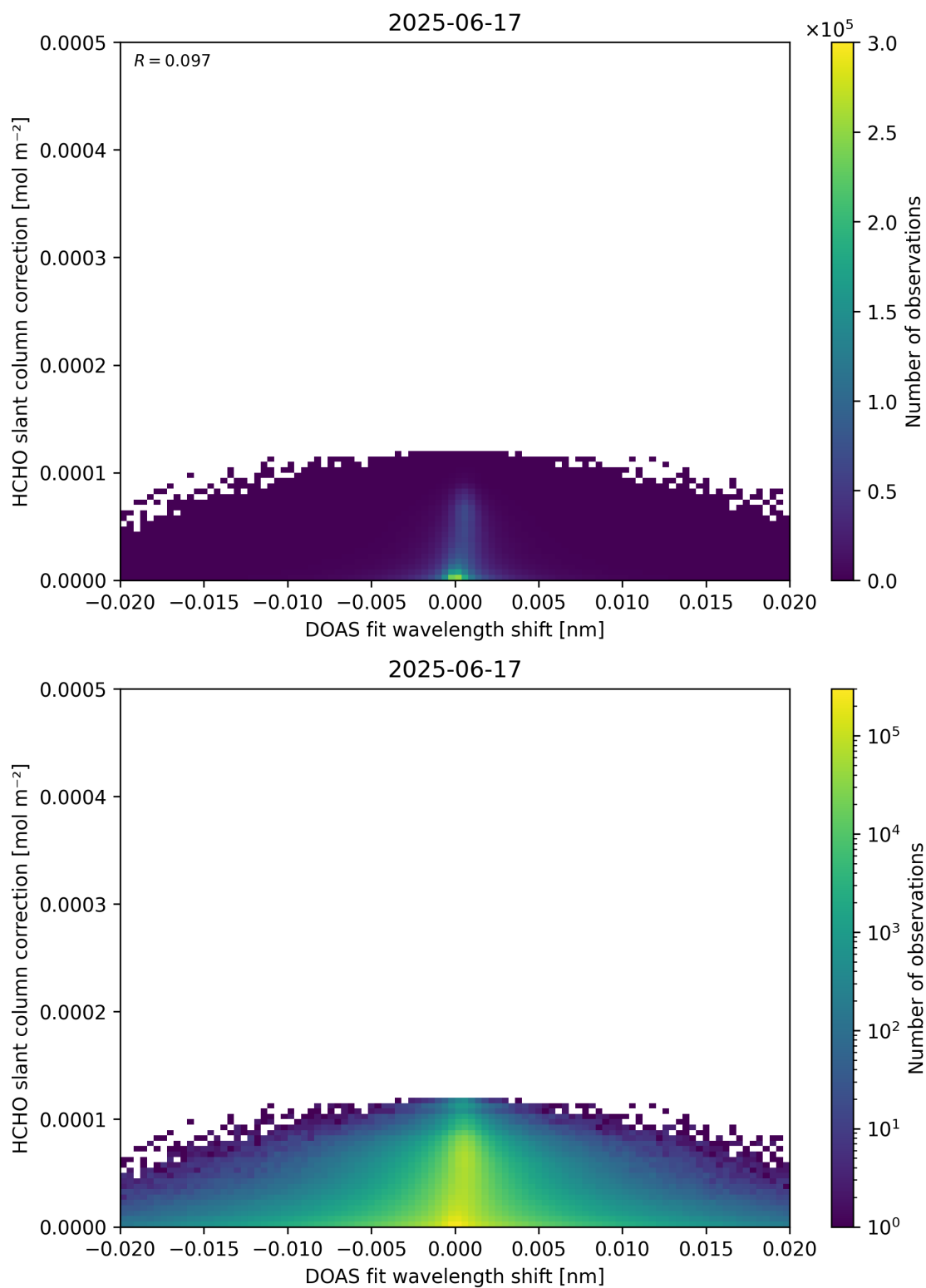
Figure 67: Scatter density plot of “DOAS fit wavelength shift” against “HCHO slant column correction” for 2025-06-17 to 2025-06-18.
