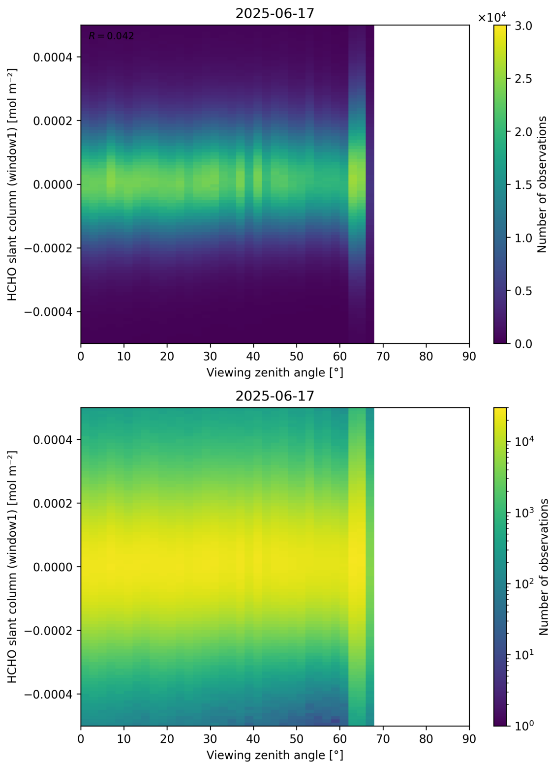
Figure 188: Scatter density plot of “Viewing zenith angle” against “HCHO slant column (window1)” for 2025-06-17 to 2025-06-18.
