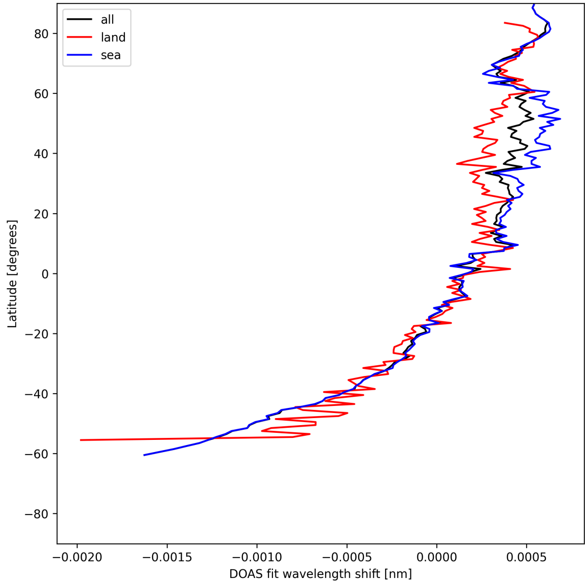
Figure 30: Zonal average of “DOAS fit wavelength shift” for 2025-06-17 to 2025-06-18.
