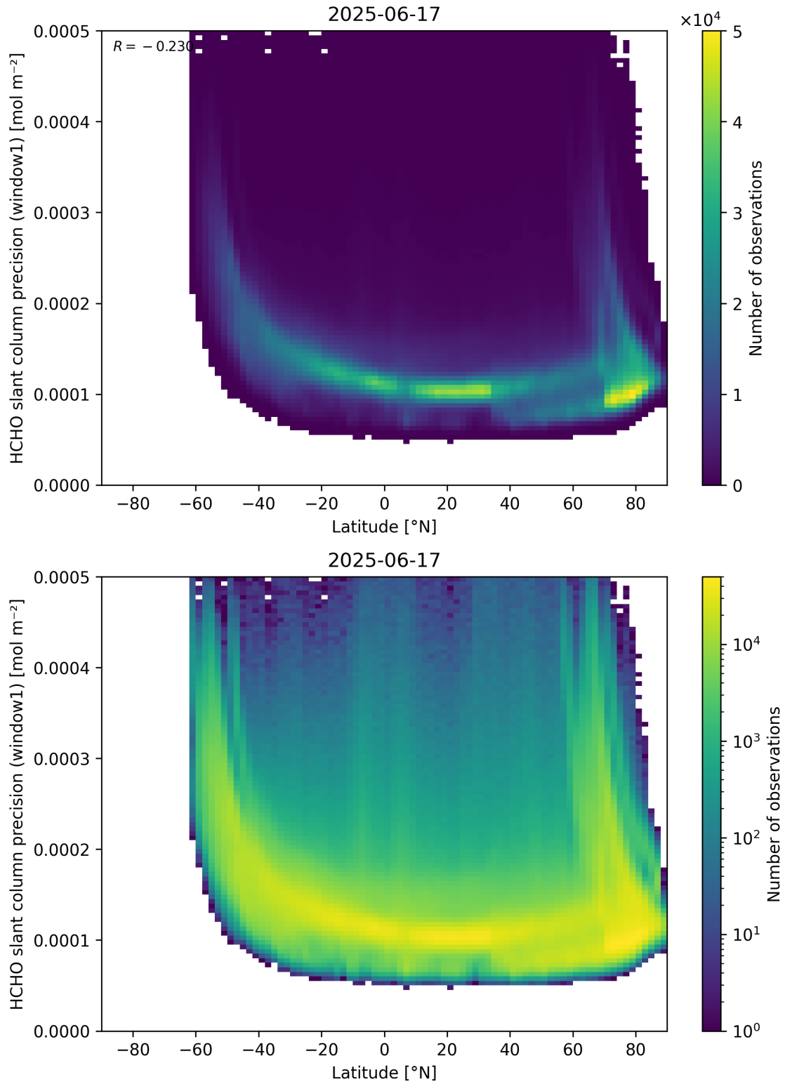
Figure 160: Scatter density plot of “Latitude” against “HCHO slant column precision (window1)” for 2025-06-17 to 2025-06-18.
