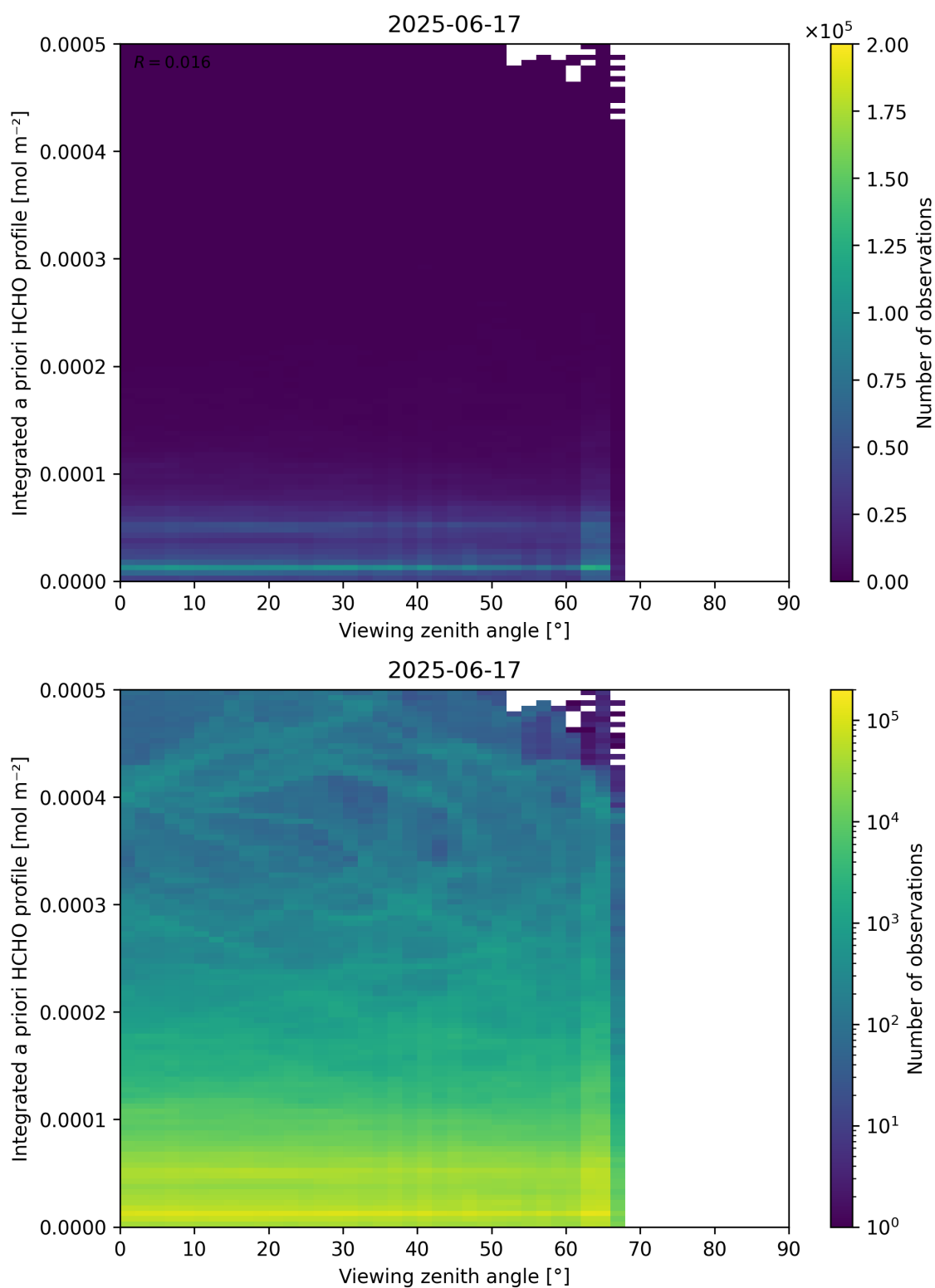
Figure 195: Scatter density plot of “Viewing zenith angle” against “Integrated a priori HCHO profile” for 2025-06-17 to 2025-06-18.
