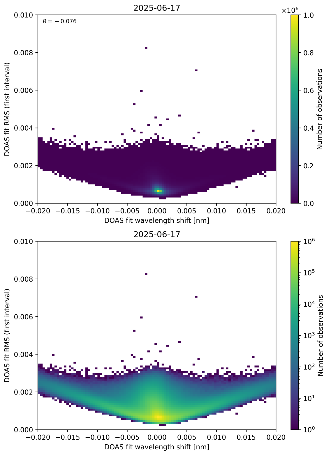
Figure 64: Scatter density plot of “DOAS fit wavelength shift” against “DOAS fit RMS (first interval)” for 2025-06-17 to 2025-06-18.
