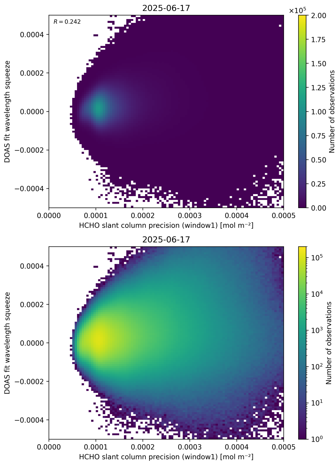
Figure 90: Scatter density plot of “HCHO slant column precision (window1)” against “DOAS fit wavelength squeeze” for 2025-06-17 to 2025-06-18.
