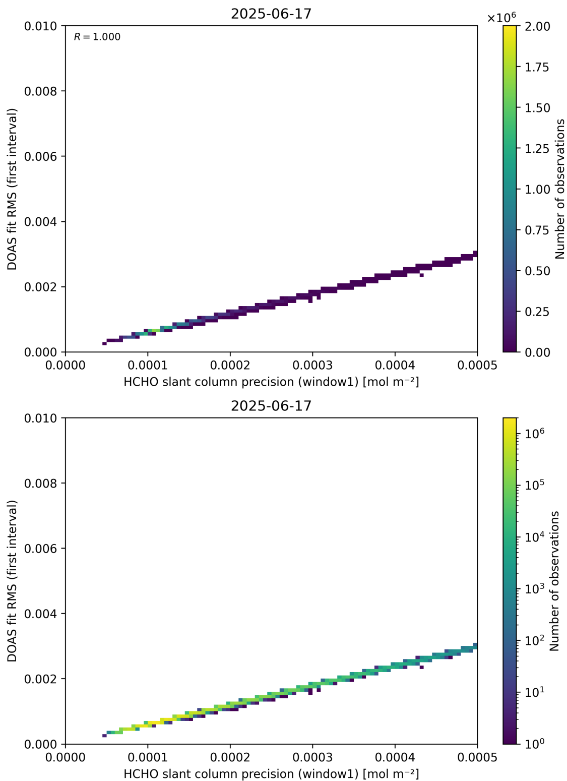
Figure 88: Scatter density plot of “HCHO slant column precision (window1)” against “DOAS fit RMS (first interval)” for 2025-06-17 to 2025-06-18.
