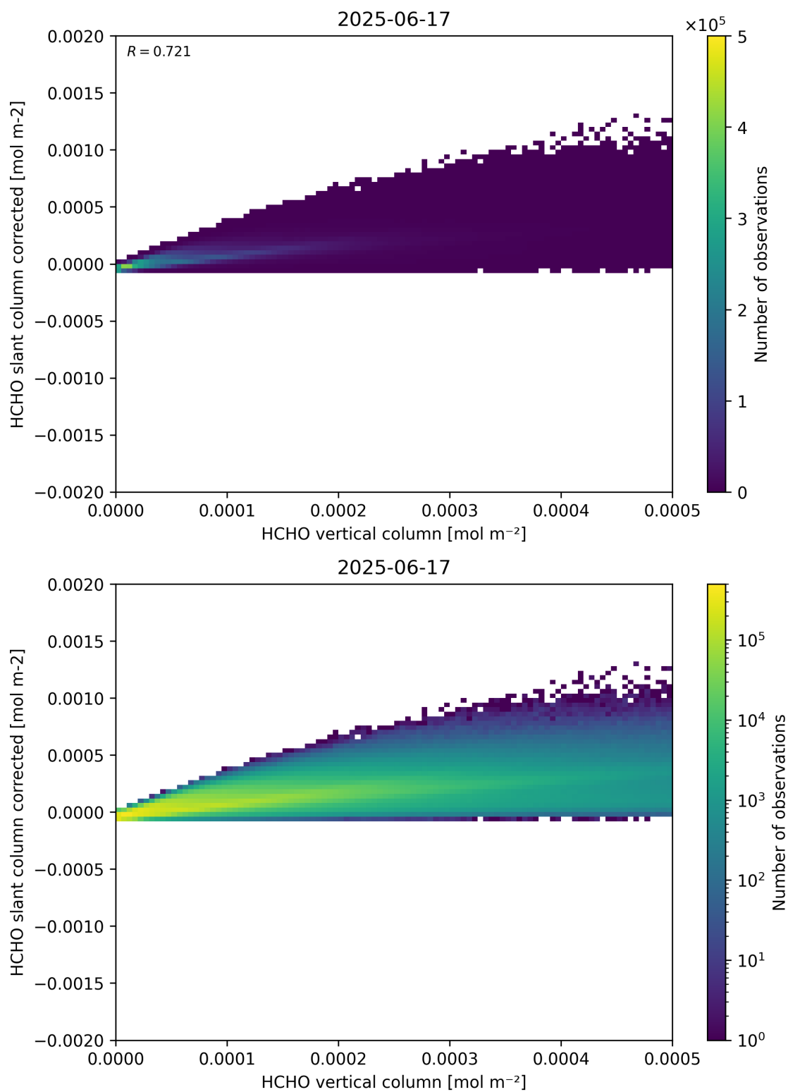
Figure 127: Scatter density plot of “HCHO vertical column” against “HCHO slant column corrected” for 2025-06-17 to 2025-06-18.
