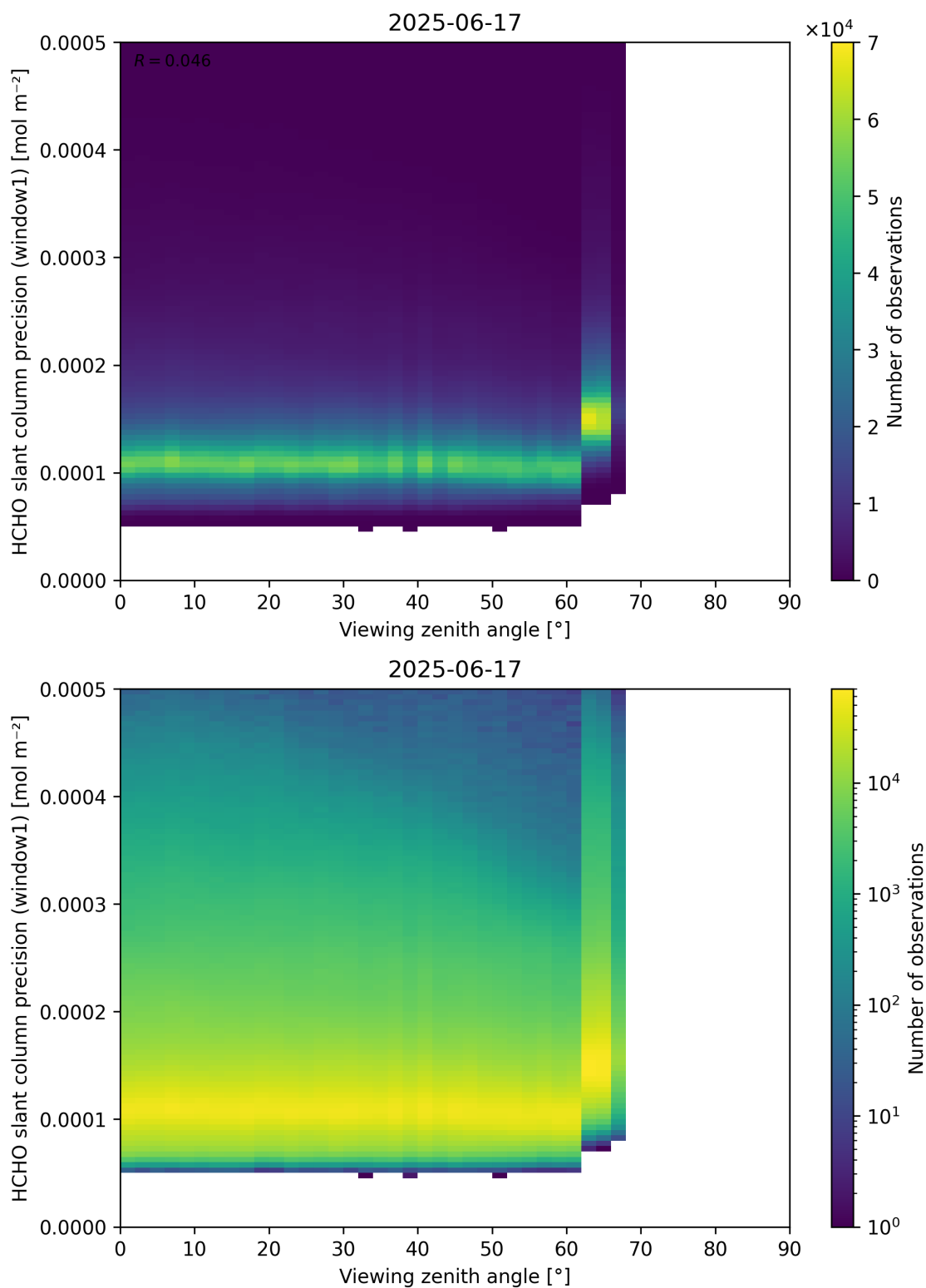
Figure 189: Scatter density plot of “Viewing zenith angle” against “HCHO slant column precision (window1)” for 2025-06-17 to 2025-06-18.
