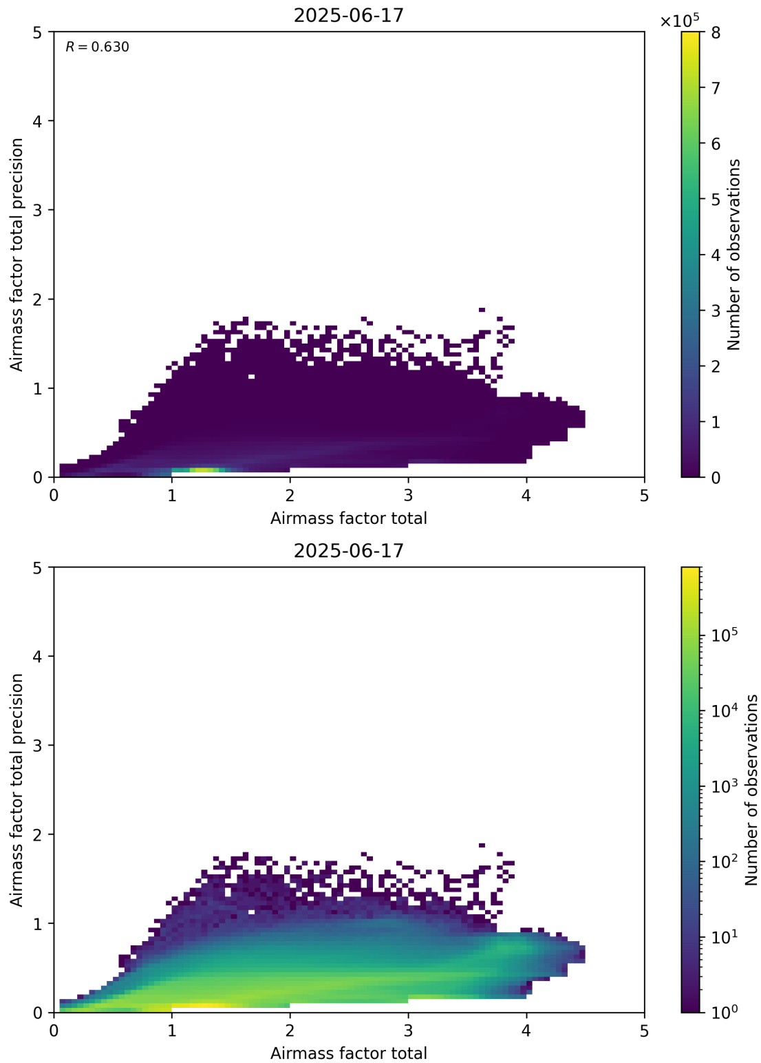
Figure 103: Scatter density plot of “Airmass factor total” against “Airmass factor total precision” for 2025-06-17 to 2025-06-18.
