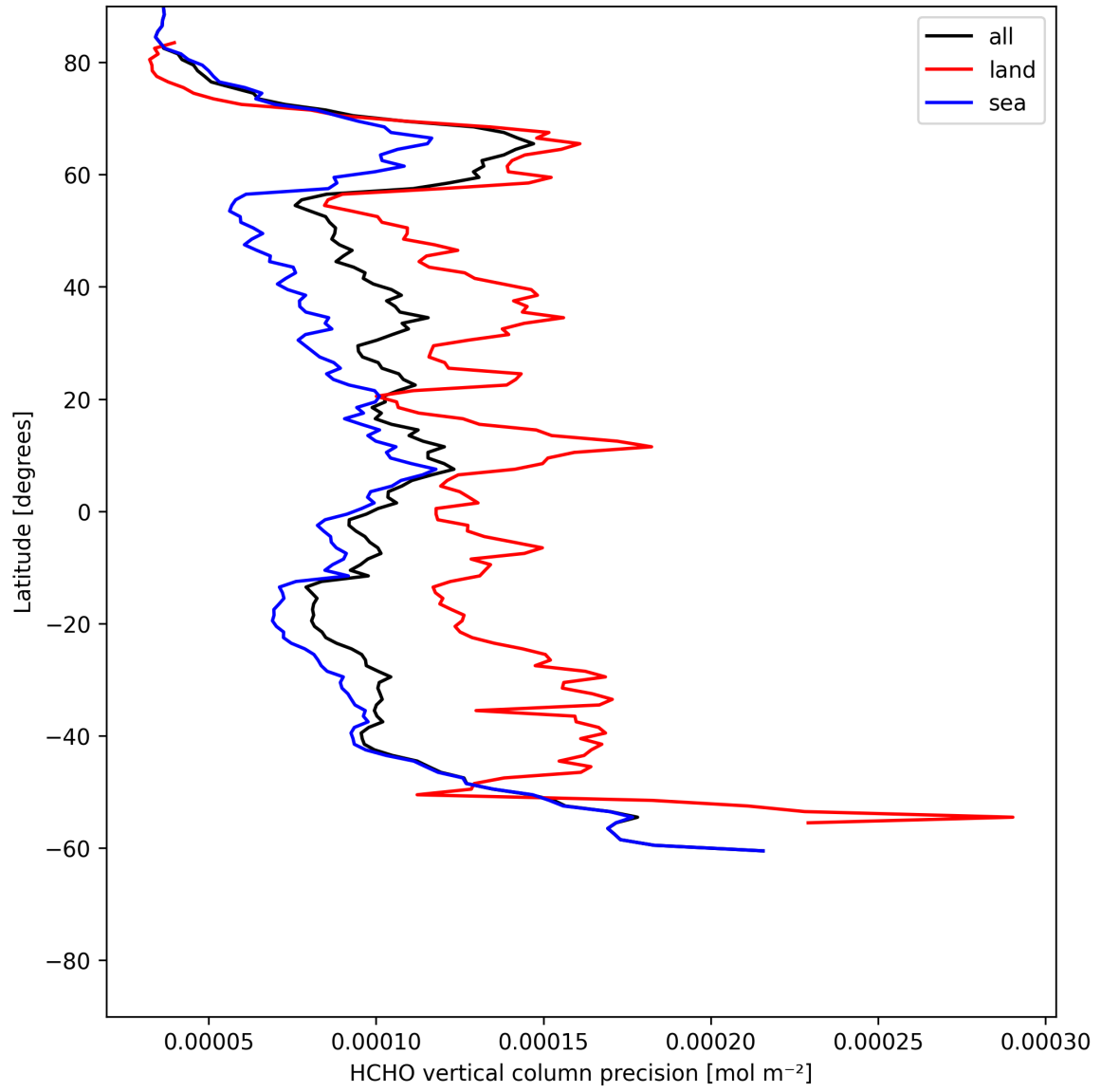
Figure 22: Zonal average of “HCHO vertical column precision” for 2025-06-17 to 2025-06-18.
