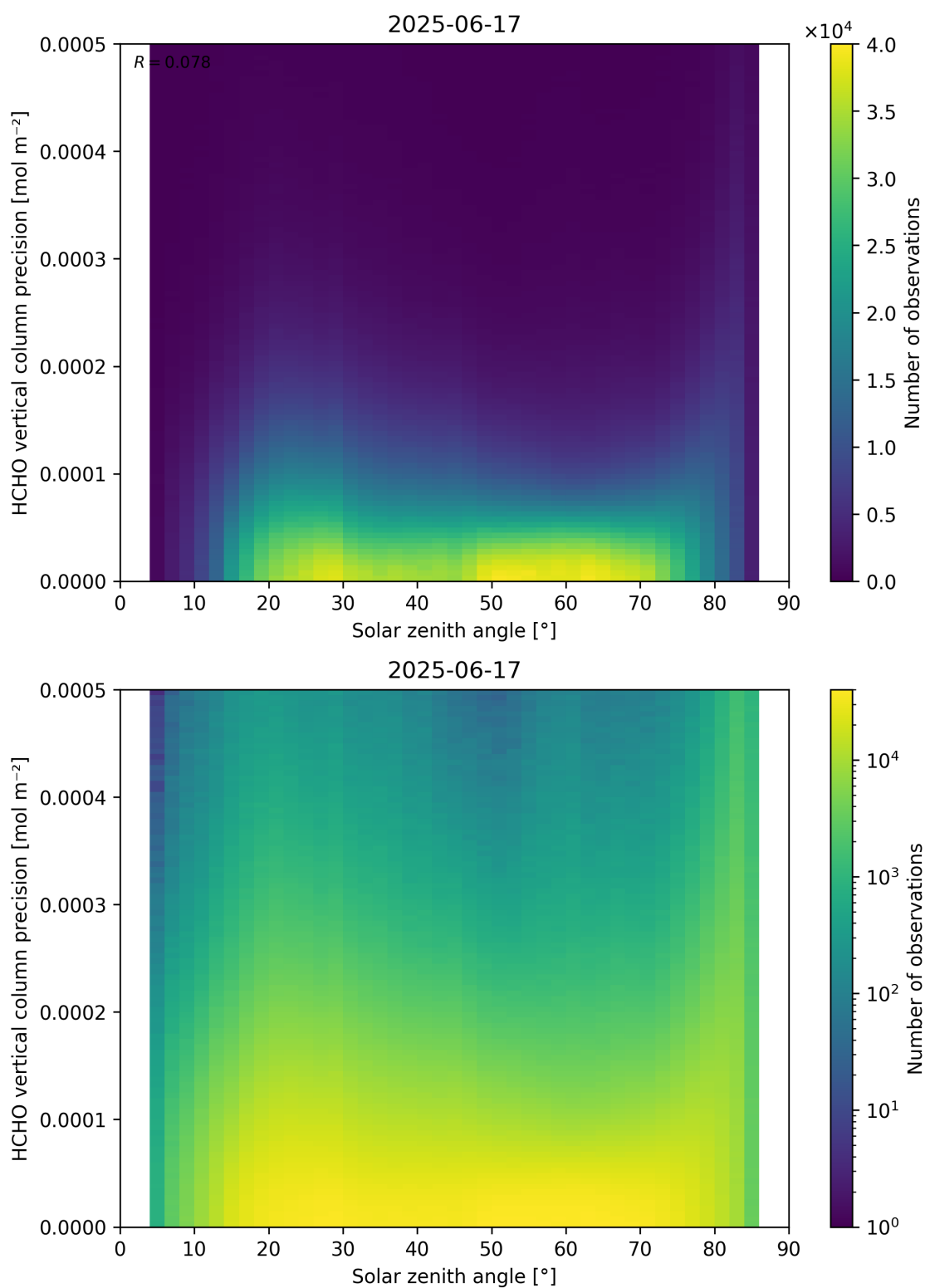
Figure 179: Scatter density plot of “Solar zenith angle” against “HCHO vertical column precision” for 2025-06-17 to 2025-06-18.
