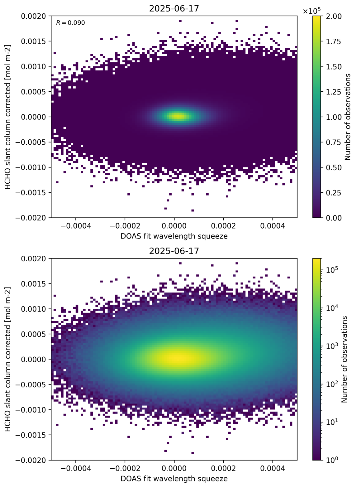
Figure 69: Scatter density plot of “DOAS fit wavelength squeeze” against “HCHO slant column corrected” for 2025-06-17 to 2025-06-18.
