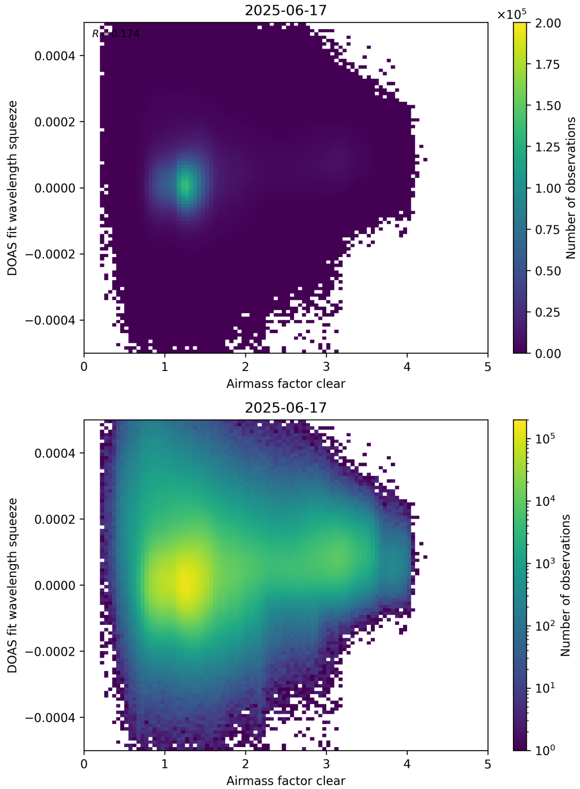
Figure 73: Scatter density plot of “Airmass factor clear” against “DOAS fit wavelength squeeze” for 2025-06-17 to 2025-06-18.
