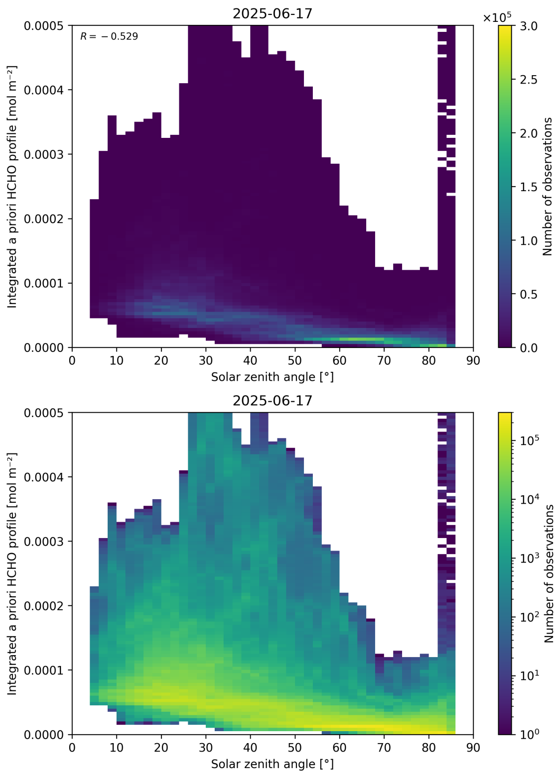
Figure 180: Scatter density plot of “Solar zenith angle” against “Integrated a priori HCHO profile” for 2025-06-17 to 2025-06-18.
