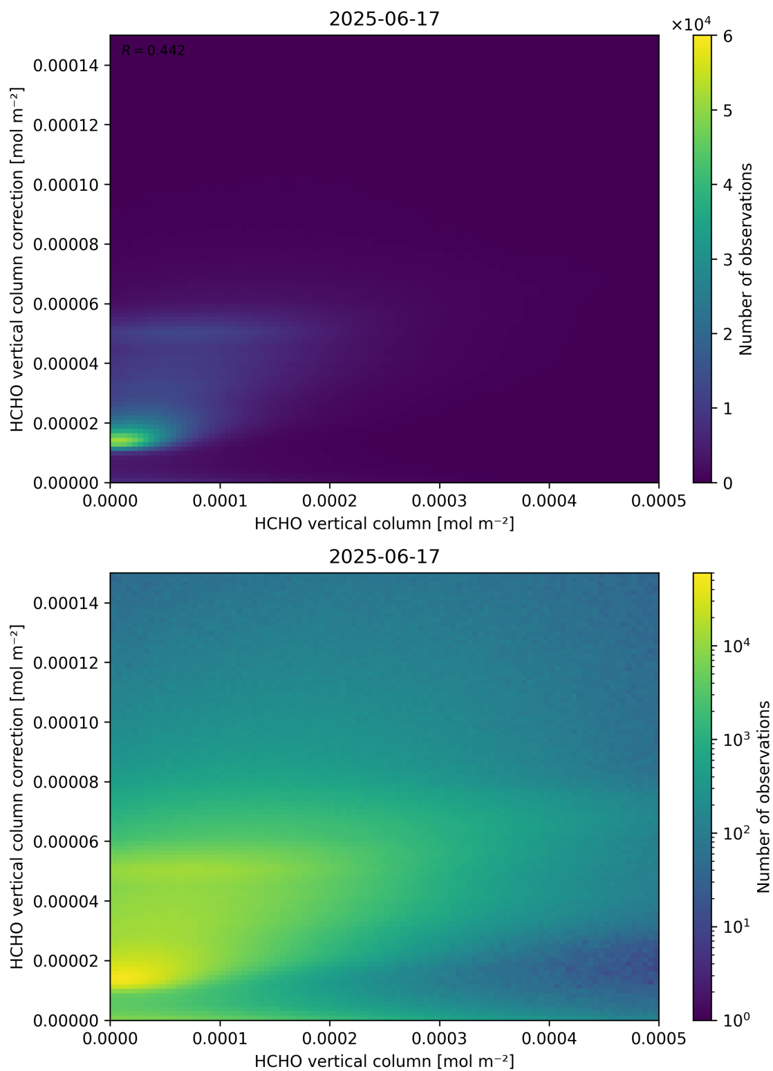
Figure 133: Scatter density plot of “HCHO vertical column” against “HCHO vertical column correction” for 2025-06-17 to 2025-06-18.
