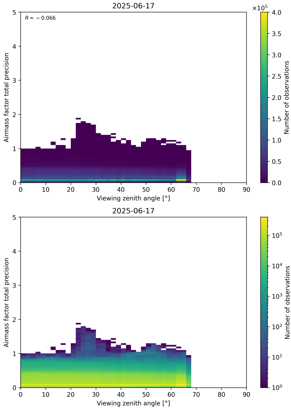
Figure 191: Scatter density plot of “Viewing zenith angle” against “Airmass factor total precision” for 2025-06-17 to 2025-06-18.
