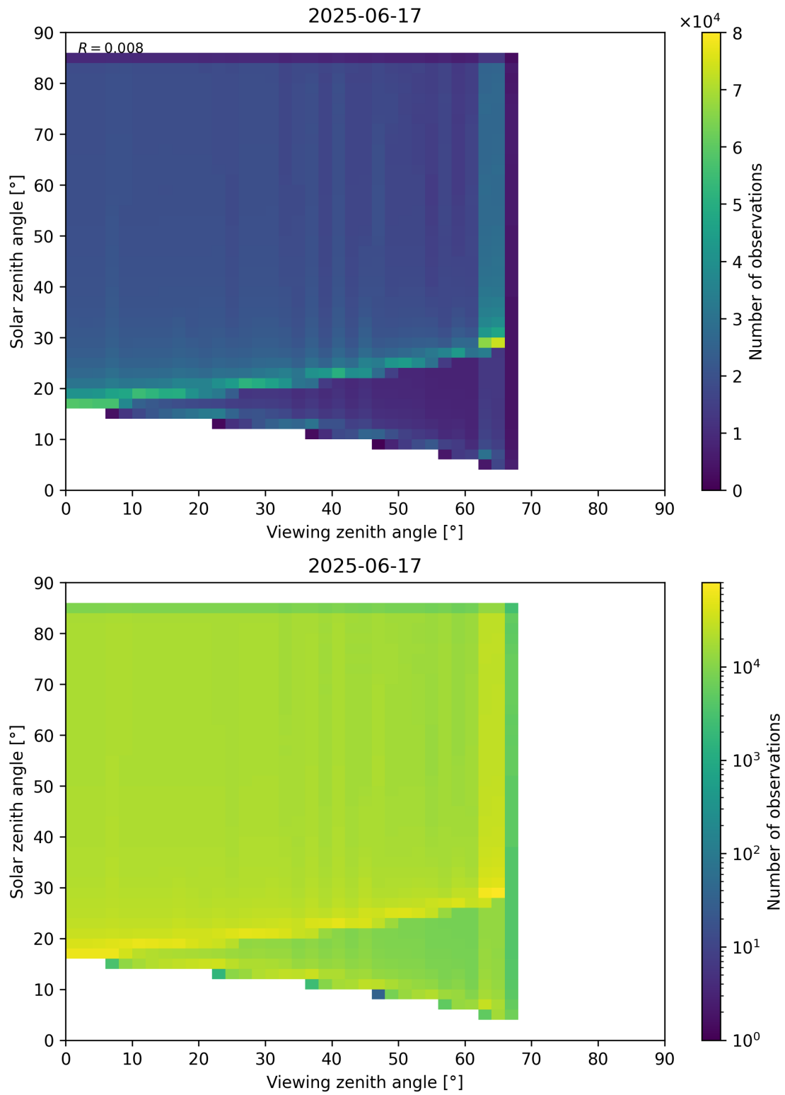
Figure 197: Scatter density plot of “Viewing zenith angle” against “Solar zenith angle” for 2025-06-17 to 2025-06-18.
