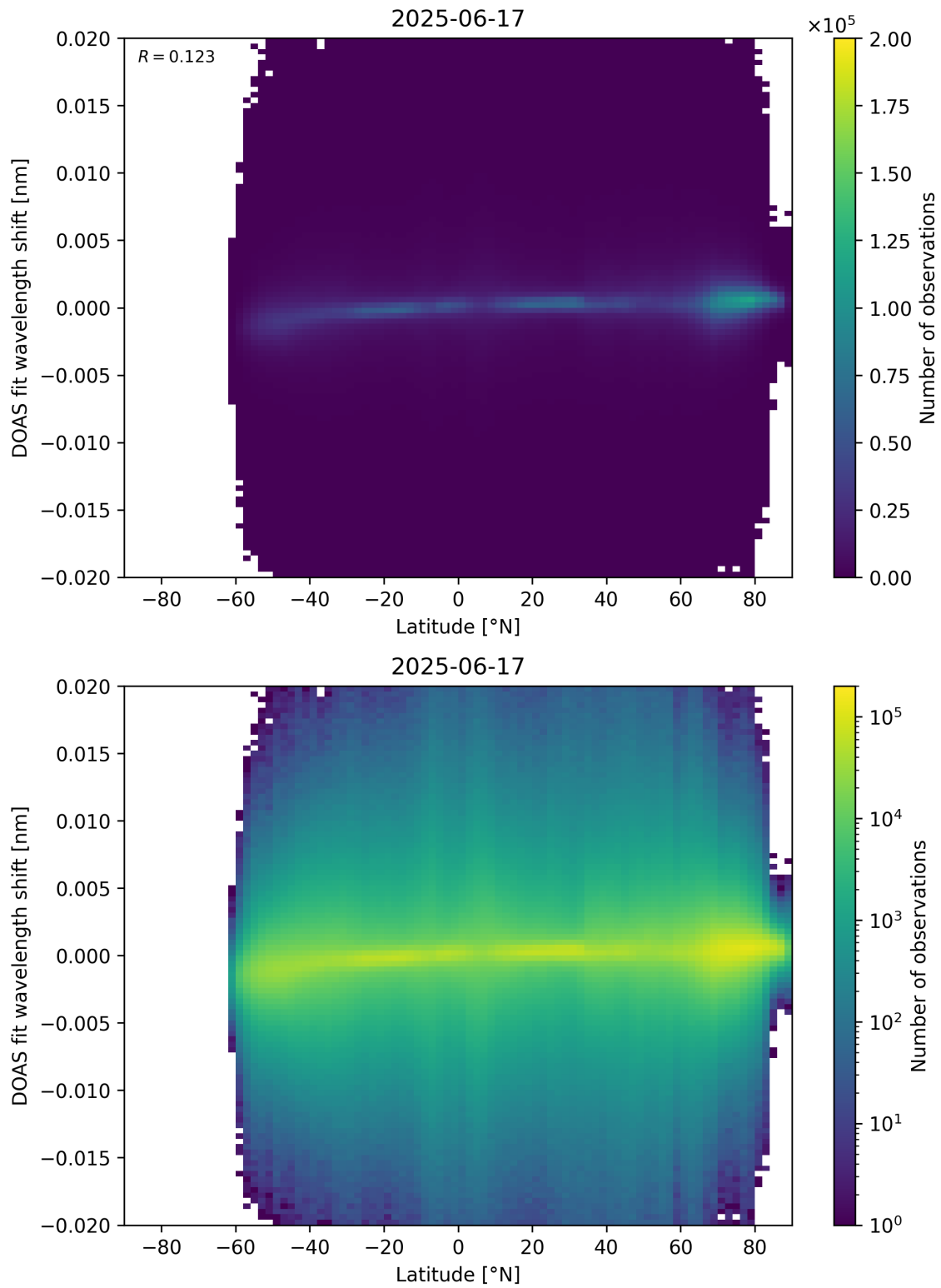
Figure 154: Scatter density plot of “Latitude” against “DOAS fit wavelength shift” for 2025-06-17 to 2025-06-18.
