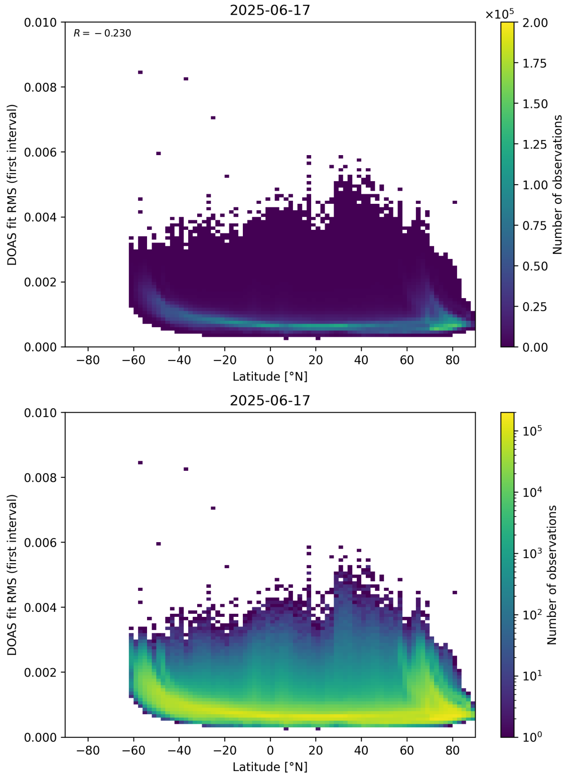
Figure 153: Scatter density plot of “Latitude” against “DOAS fit RMS (first interval)” for 2025-06-17 to 2025-06-18.
