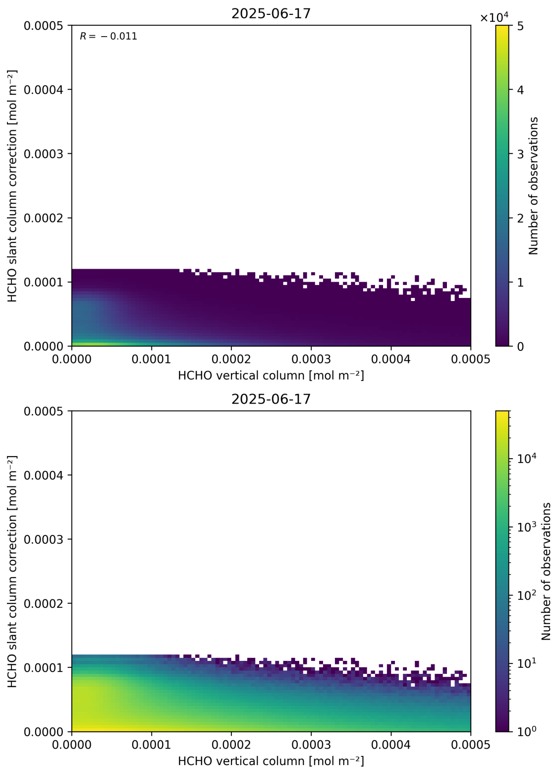
Figure 128: Scatter density plot of “HCHO vertical column” against “HCHO slant column correction” for 2025-06-17 to 2025-06-18.
