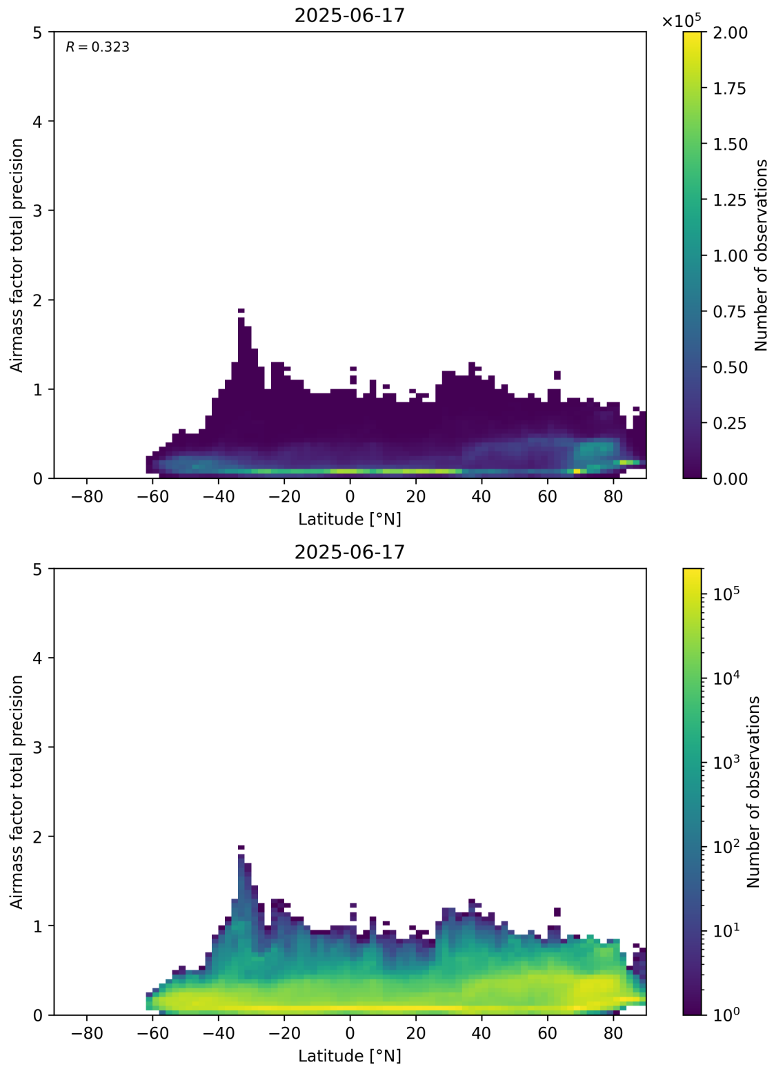
Figure 162: Scatter density plot of “Latitude” against “Airmass factor total precision” for 2025-06-17 to 2025-06-18.
