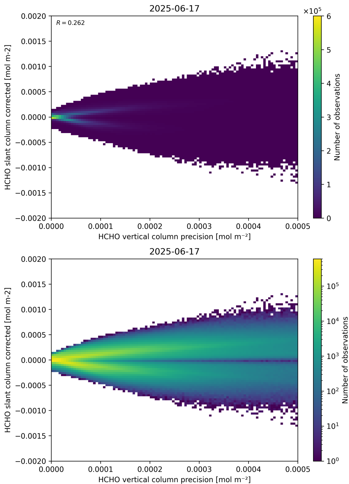
Figure 140: Scatter density plot of “HCHO vertical column precision” against “HCHO slant column corrected” for 2025-06-17 to 2025-06-18.
