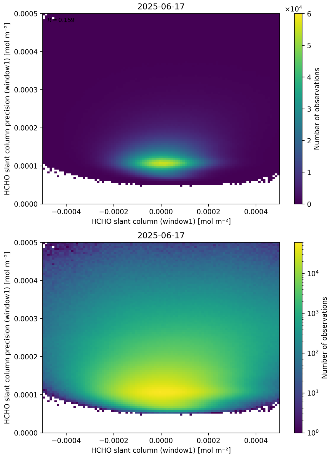
Figure 84: Scatter density plot of “HCHO slant column (window1)” against “HCHO slant column precision (window1)” for 2025-06-17 to 2025-06-18.
