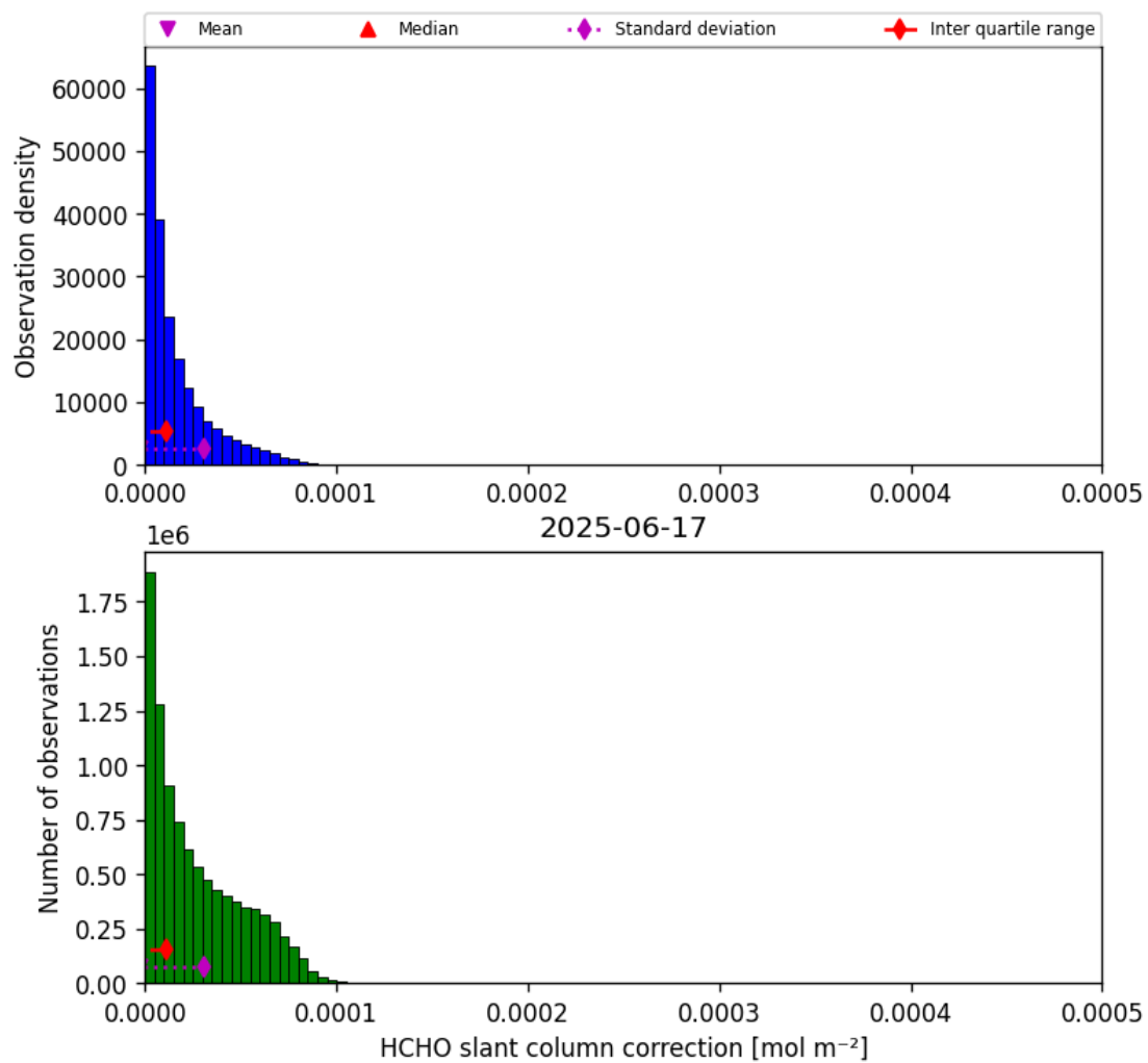
Figure 47: Histogram of “HCHO slant column correction” for 2025-06-17 to 2025-06-18
