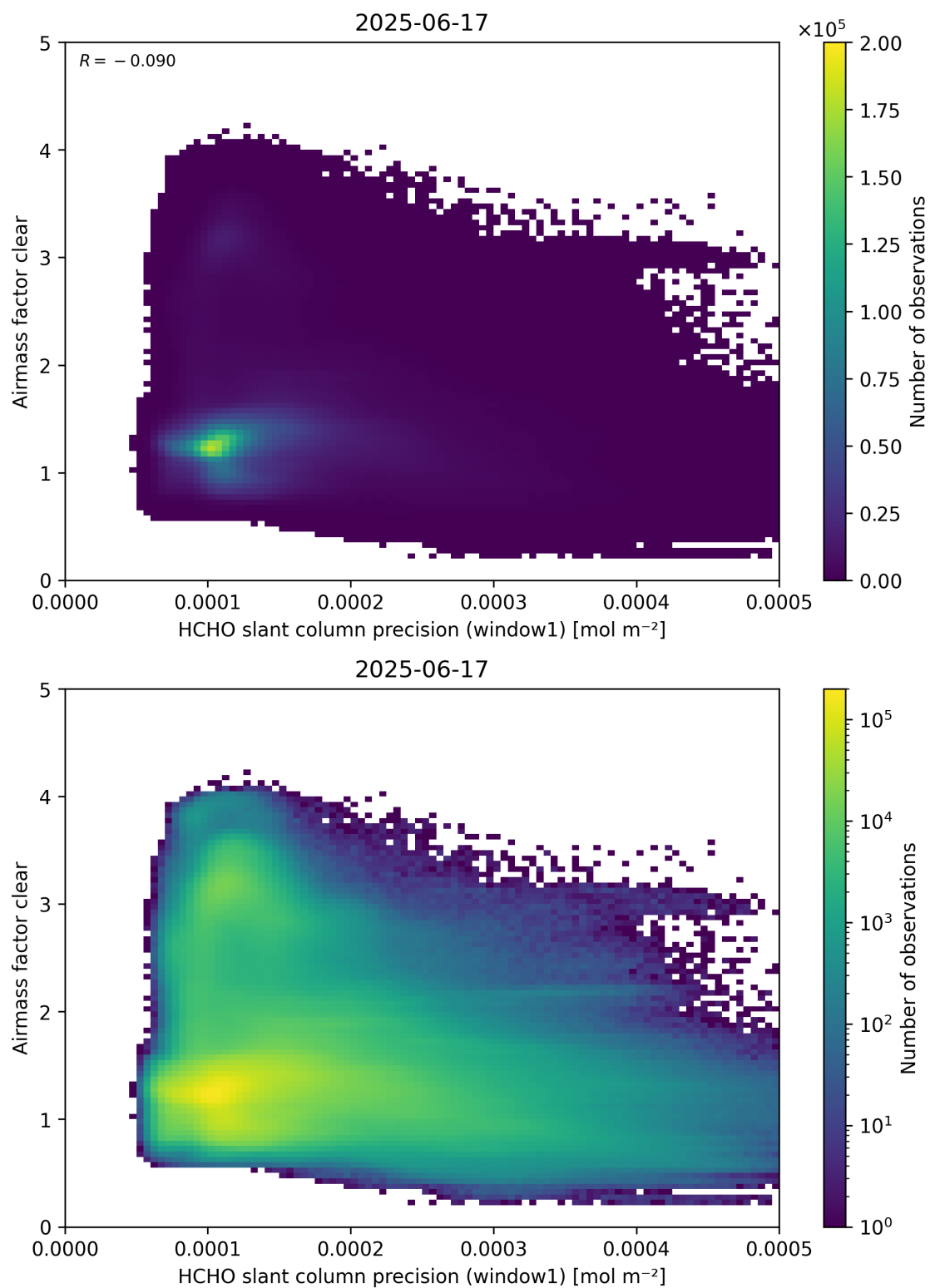
Figure 91: Scatter density plot of “HCHO slant column precision (window1)” against “Airmass factor clear” for 2025-06-17 to 2025-06-18.
