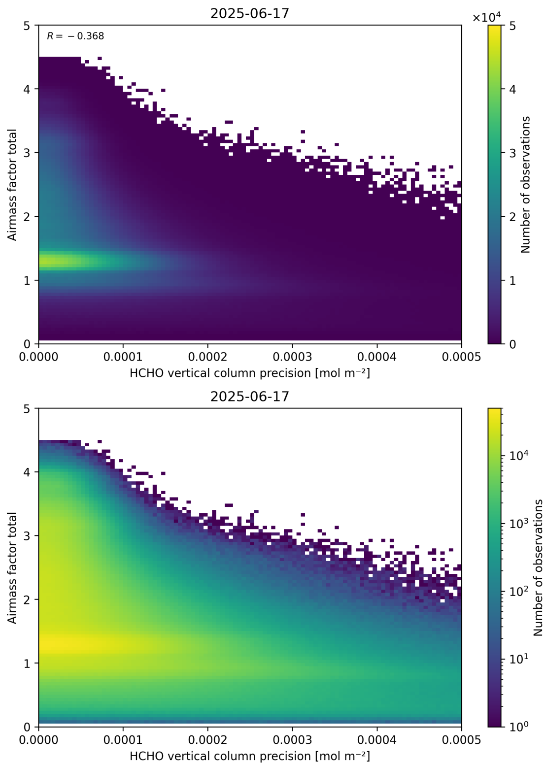
Figure 144: Scatter density plot of “HCHO vertical column precision” against “Airmass factor total” for 2025-06-17 to 2025-06-18.
