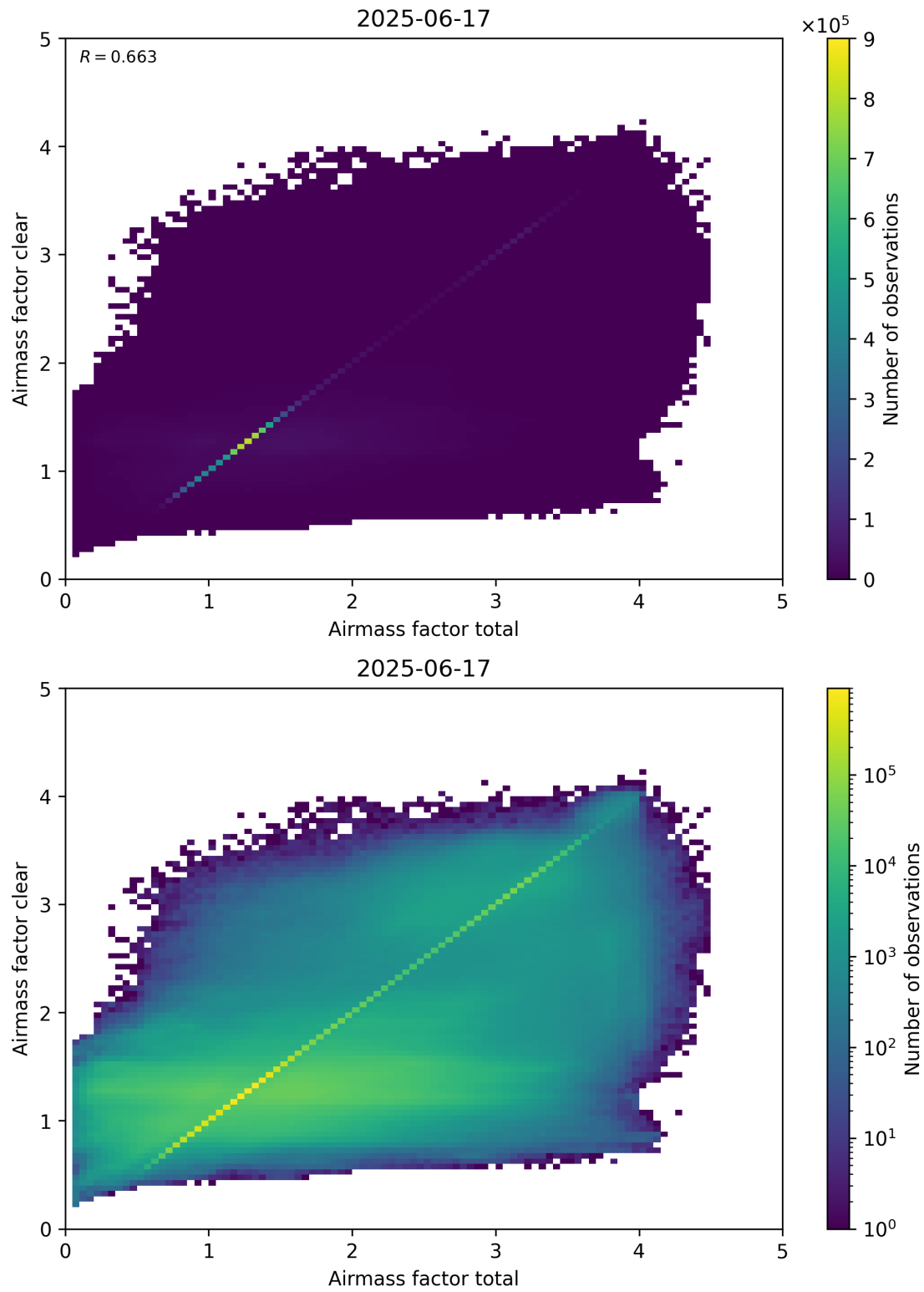
Figure 100: Scatter density plot of “Airmass factor total” against “Airmass factor clear” for 2025-06-17 to 2025-06-18.
