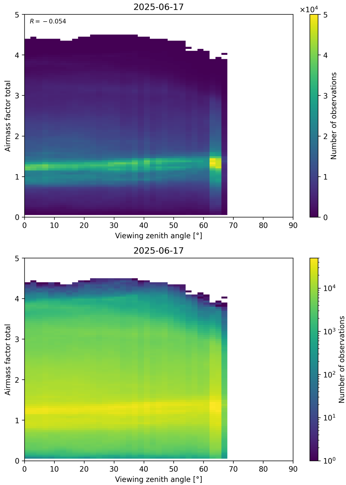
Figure 190: Scatter density plot of “Viewing zenith angle” against “Airmass factor total” for 2025-06-17 to 2025-06-18.
