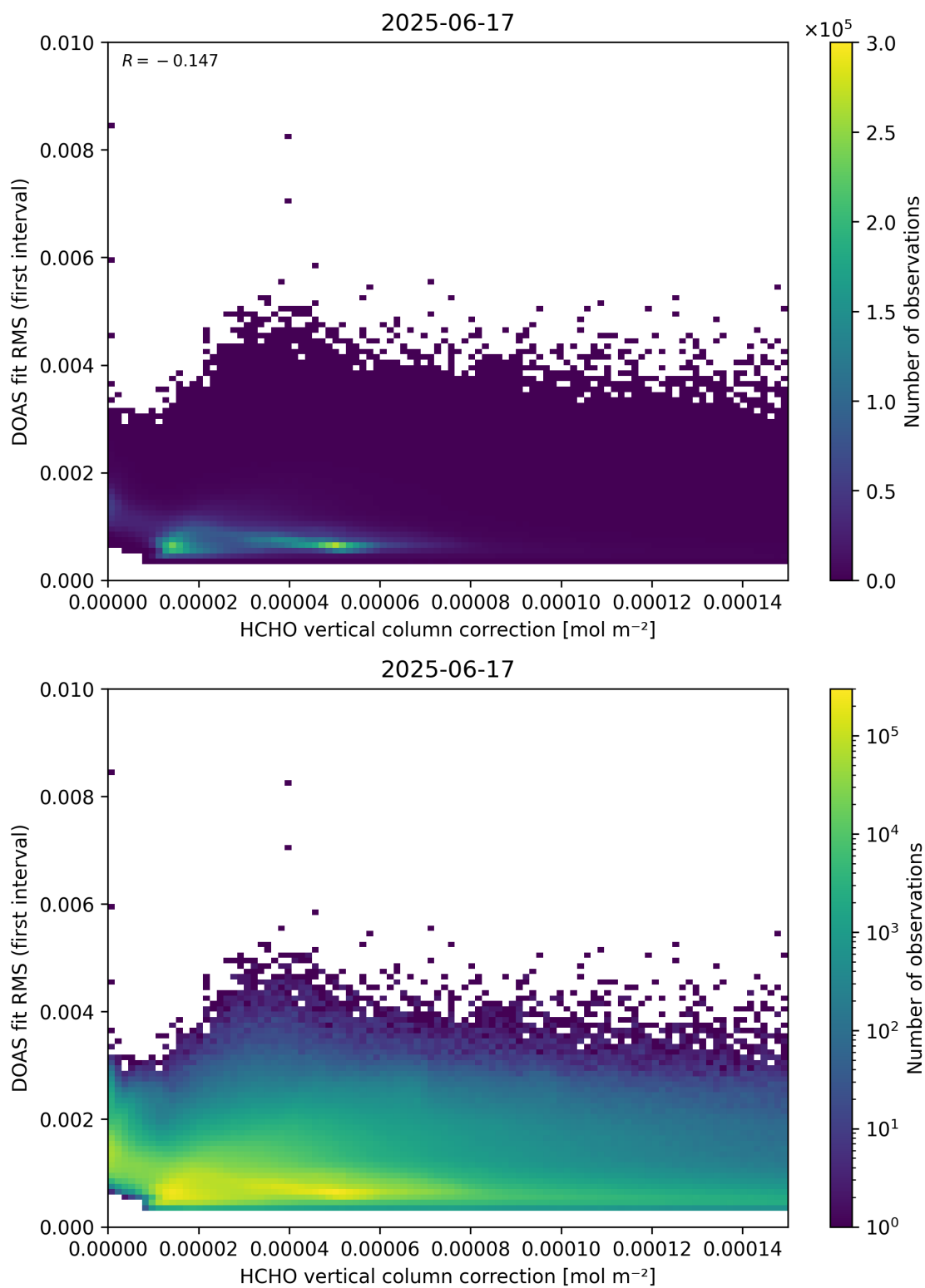
Figure 112: Scatter density plot of “HCHO vertical column correction” against “DOAS fit RMS (first interval)” for 2025-06-17 to 2025-06-18.
