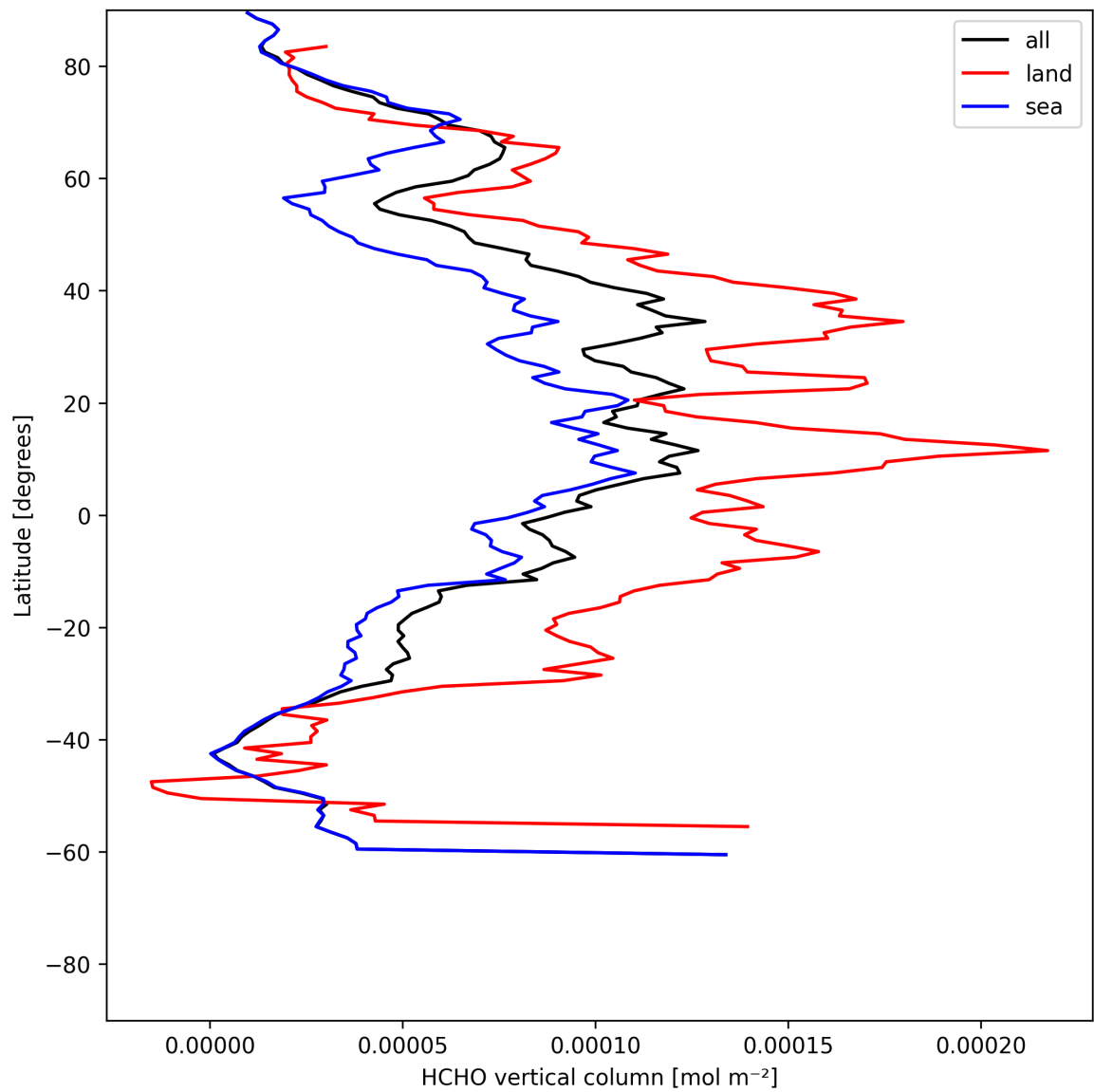
Figure 21: Zonal average of “HCHO vertical column” for 2025-06-17 to 2025-06-18.
