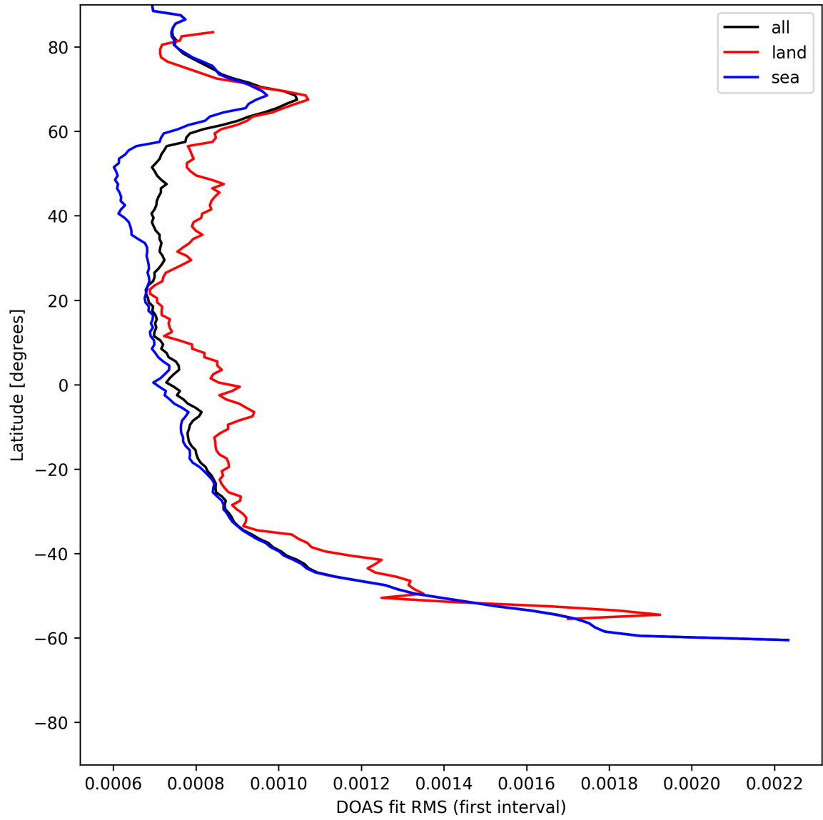
Figure 32: Zonal average of “DOAS fit RMS (first interval)” for 2025-06-17 to 2025-06-18.
