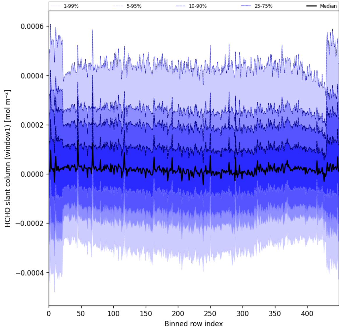
Figure 52: Along track statistics of “HCHO slant column (window1)” for 2025-06-17 to 2025-06-18
