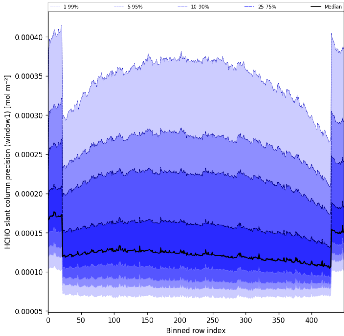
Figure 53: Along track statistics of “HCHO slant column precision (window1)” for 2025-06-17 to 2025-06-18
