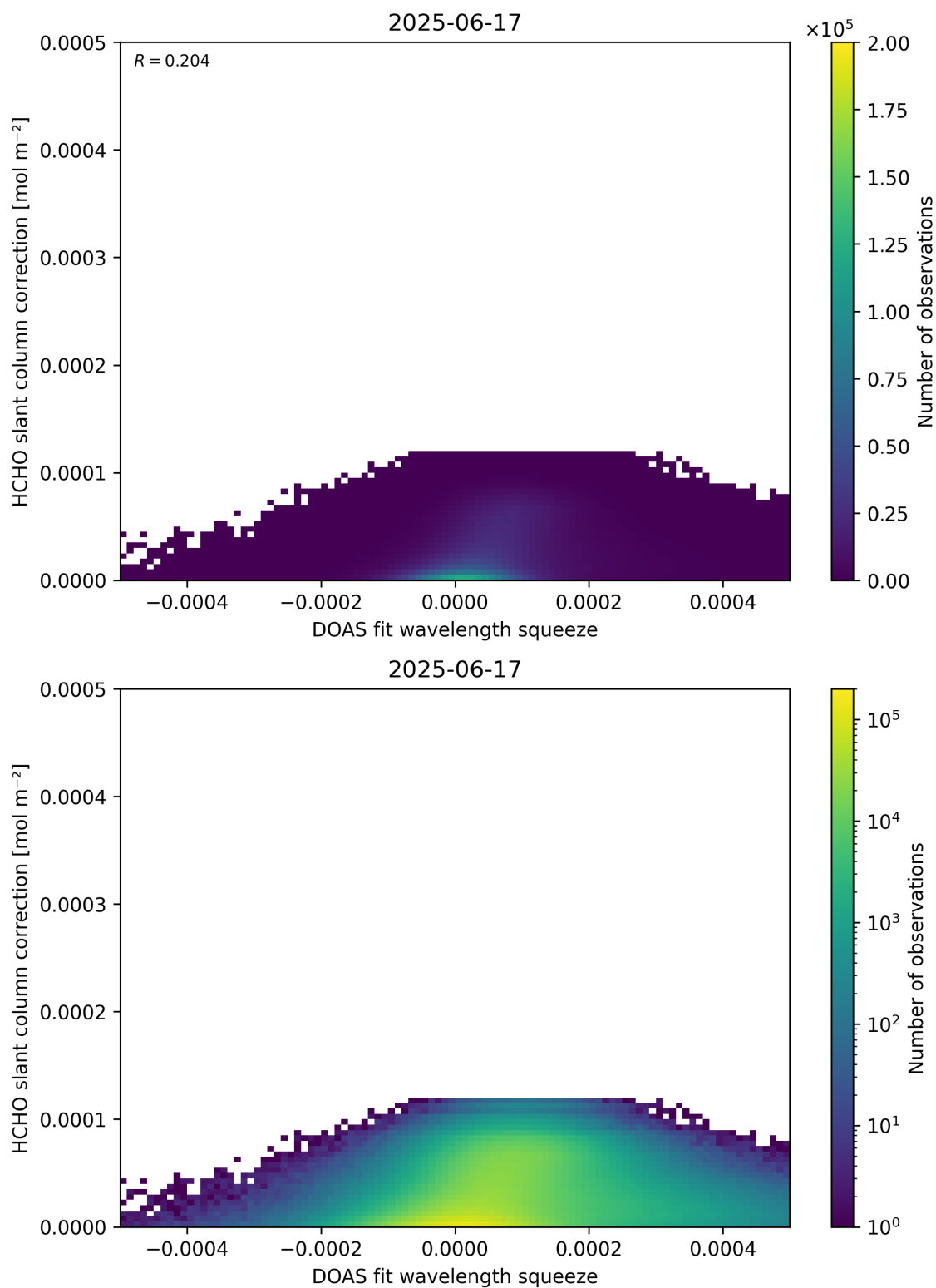
Figure 70: Scatter density plot of “DOAS fit wavelength squeeze” against “HCHO slant column correction” for 2025-06-17 to 2025-06-18.
