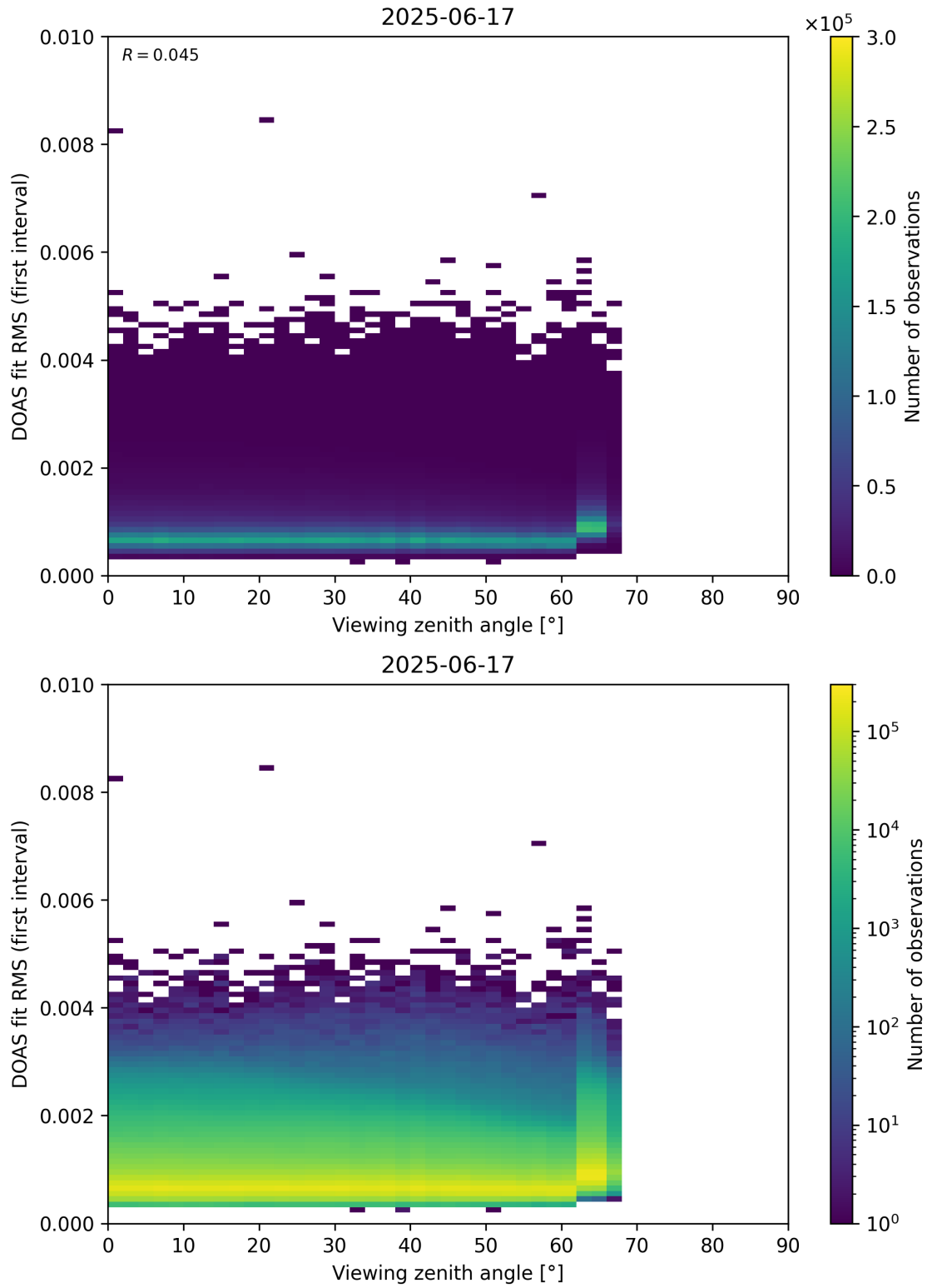
Figure 182: Scatter density plot of “Viewing zenith angle” against “DOAS fit RMS (first interval)” for 2025-06-17 to 2025-06-18.
