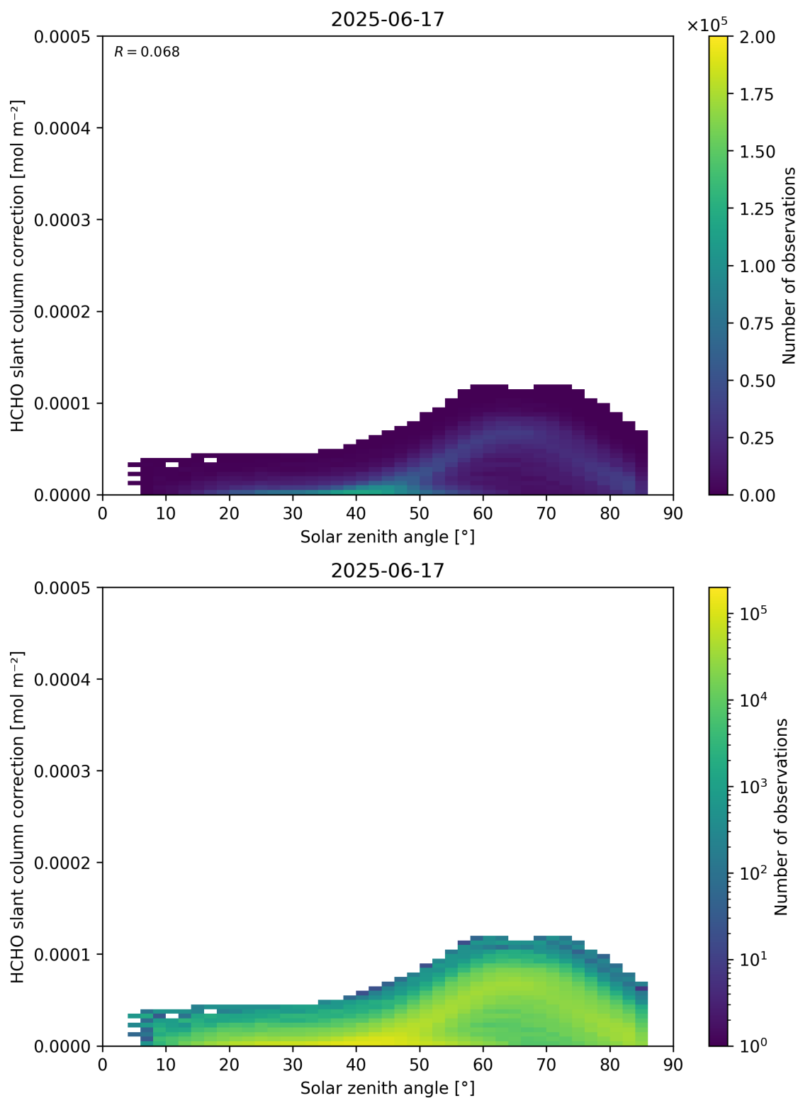
Figure 172: Scatter density plot of “Solar zenith angle” against “HCHO slant column correction” for 2025-06-17 to 2025-06-18.
