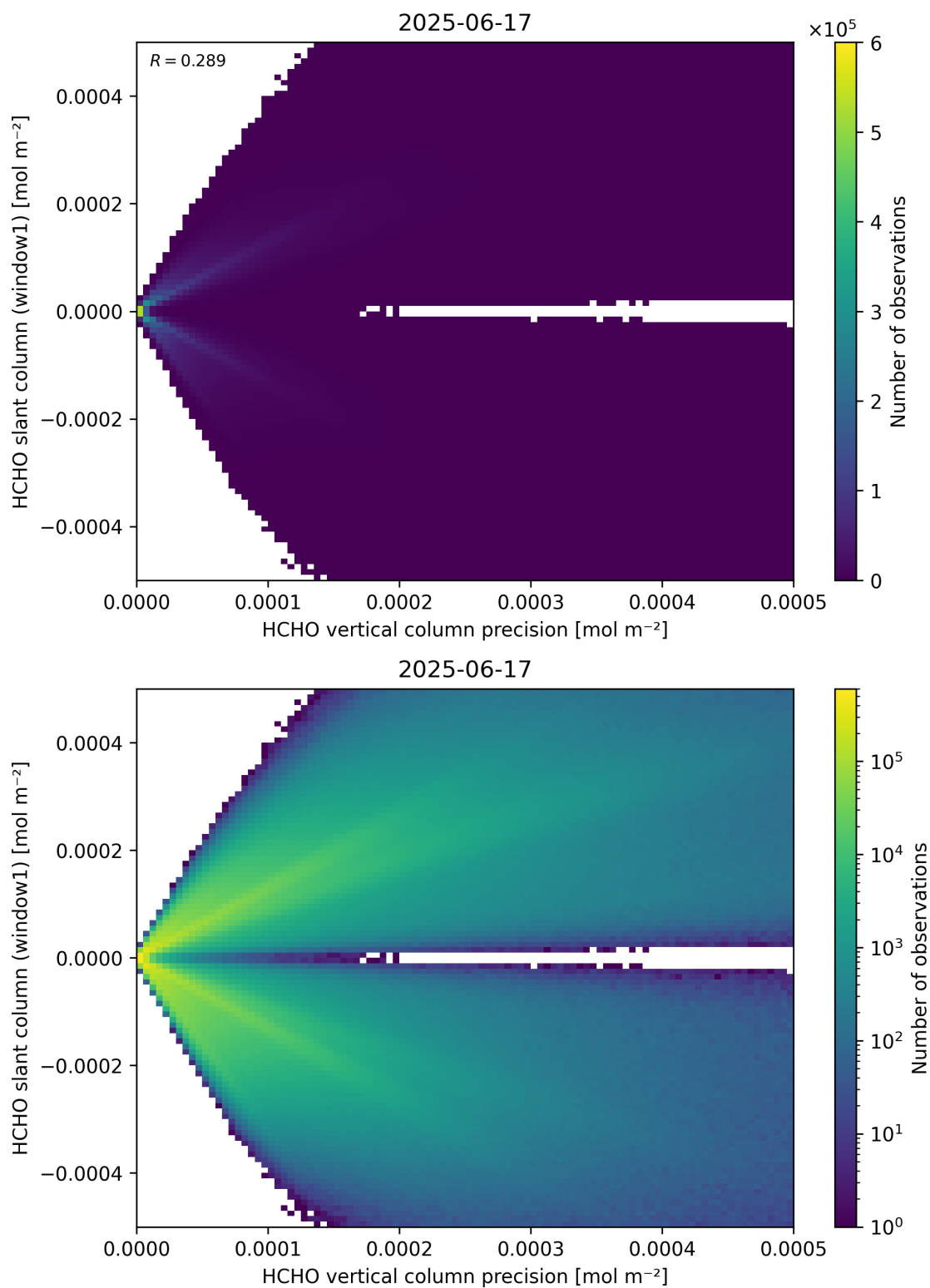
Figure 142: Scatter density plot of “HCHO vertical column precision” against “HCHO slant column (window1)” for 2025-06-17 to 2025-06-18.
