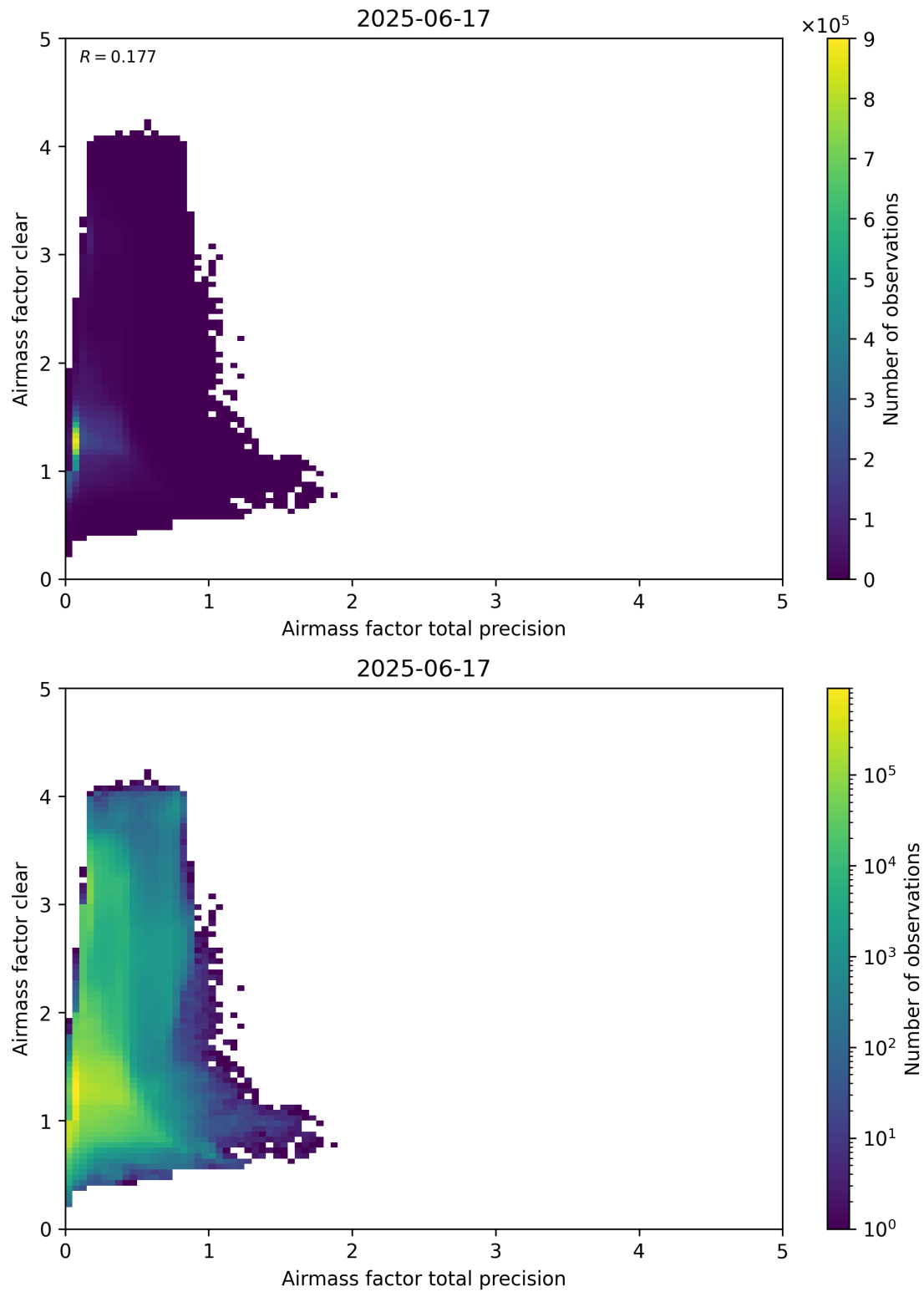
Figure 108: Scatter density plot of “Airmass factor total precision” against “Airmass factor clear” for 2025-06-17 to 2025-06-18.
