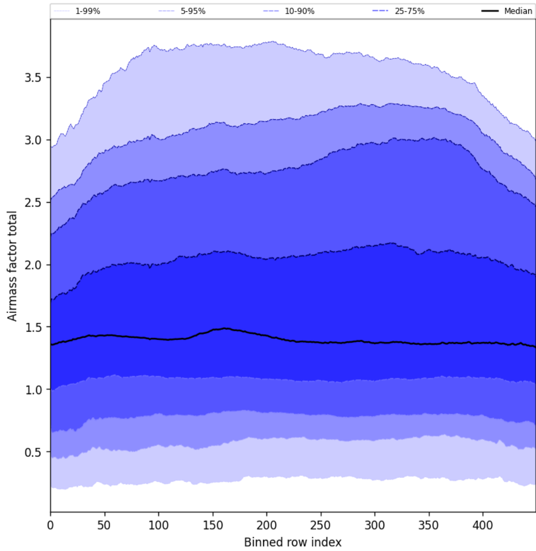
Figure 54: Along track statistics of “Airmass factor total” for 2025-06-17 to 2025-06-18
