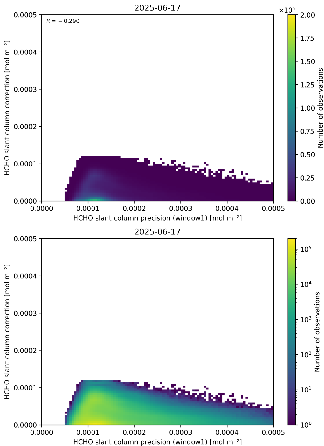
Figure 93: Scatter density plot of “HCHO slant column precision (window1)” against “HCHO slant column correction” for 2025-06-17 to 2025-06-18.
