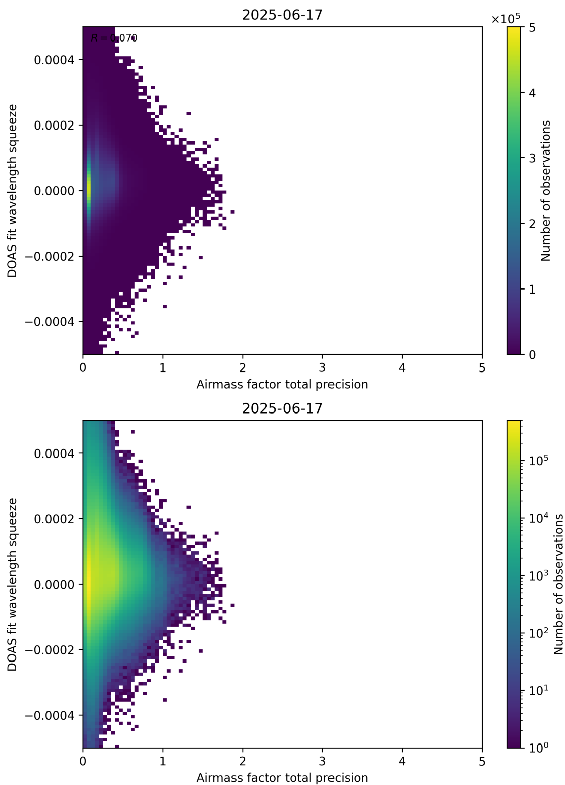
Figure 107: Scatter density plot of “Airmass factor total precision” against “DOAS fit wavelength squeeze” for 2025-06-17 to 2025-06-18.
