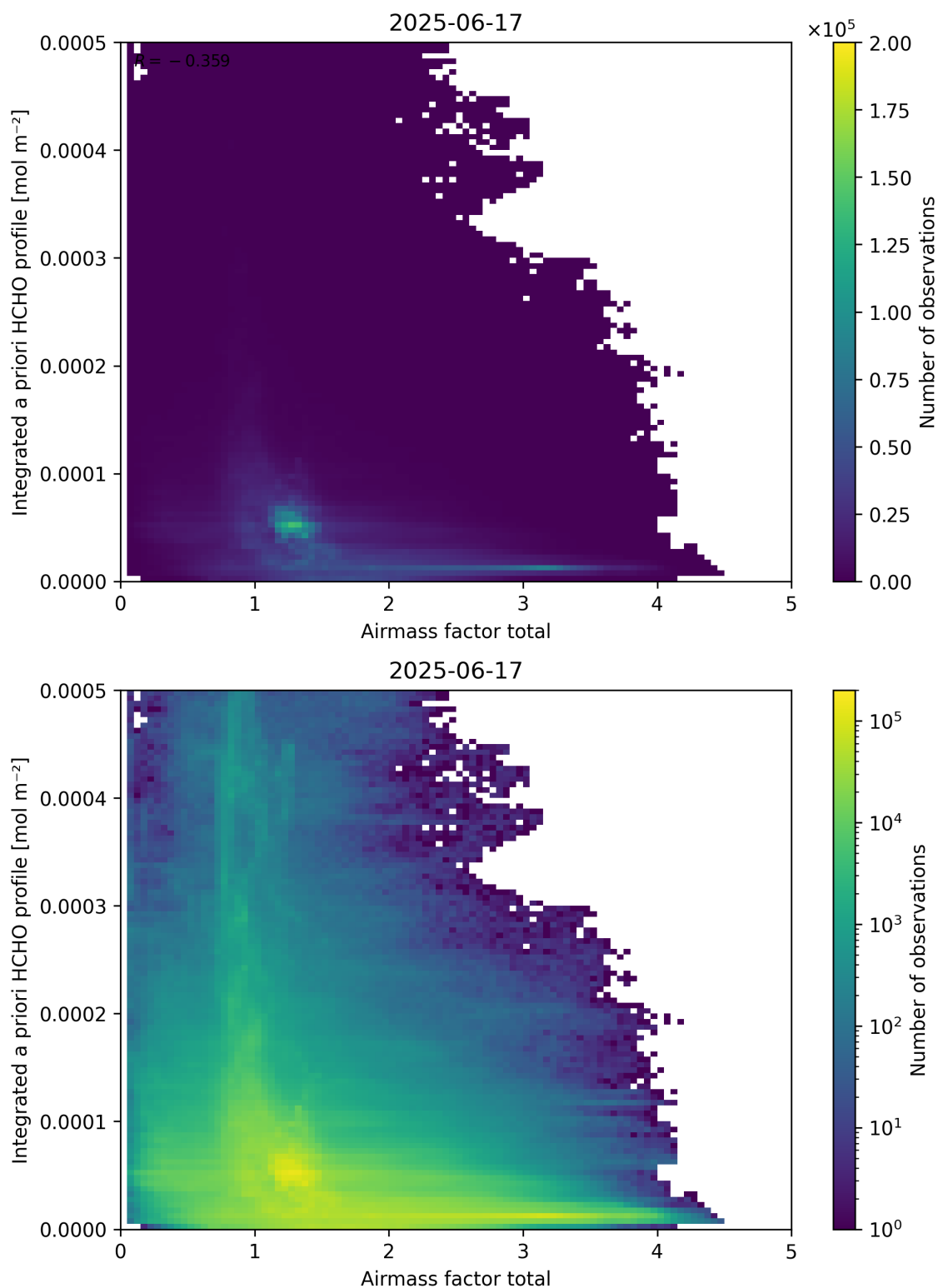
Figure 104: Scatter density plot of “Airmass factor total” against “Integrated a priori HCHO profile” for 2025-06-17 to 2025-06-18.
