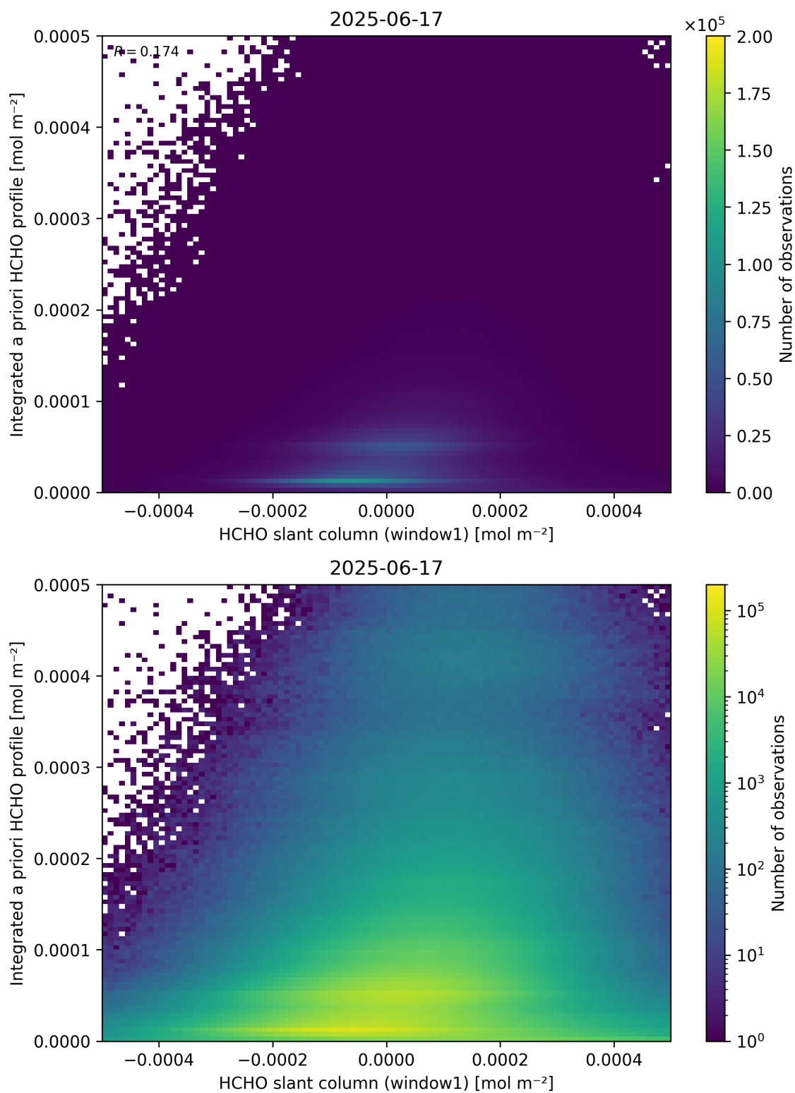
Figure 87: Scatter density plot of “HCHO slant column (window1)” against “Integrated a priori HCHO profile” for 2025-06-17 to 2025-06-18.
