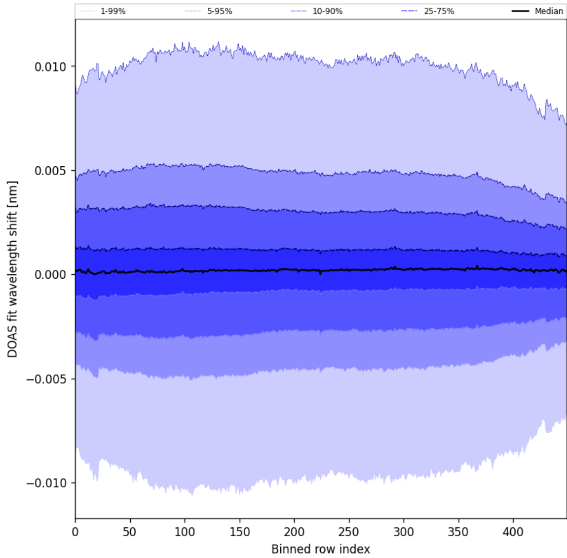
Figure 58: Along track statistics of “DOAS fit wavelength shift” for 2025-06-17 to 2025-06-18
