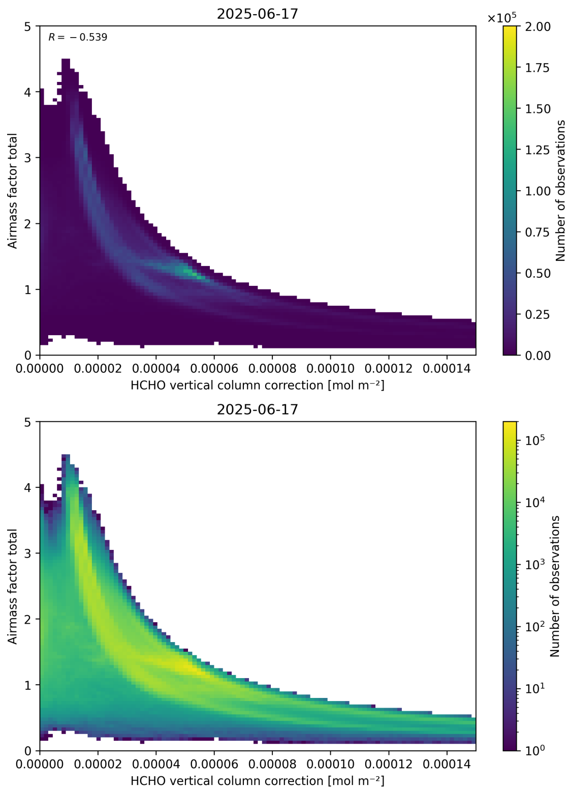
Figure 120: Scatter density plot of “HCHO vertical column correction” against “Airmass factor total” for 2025-06-17 to 2025-06-18.
