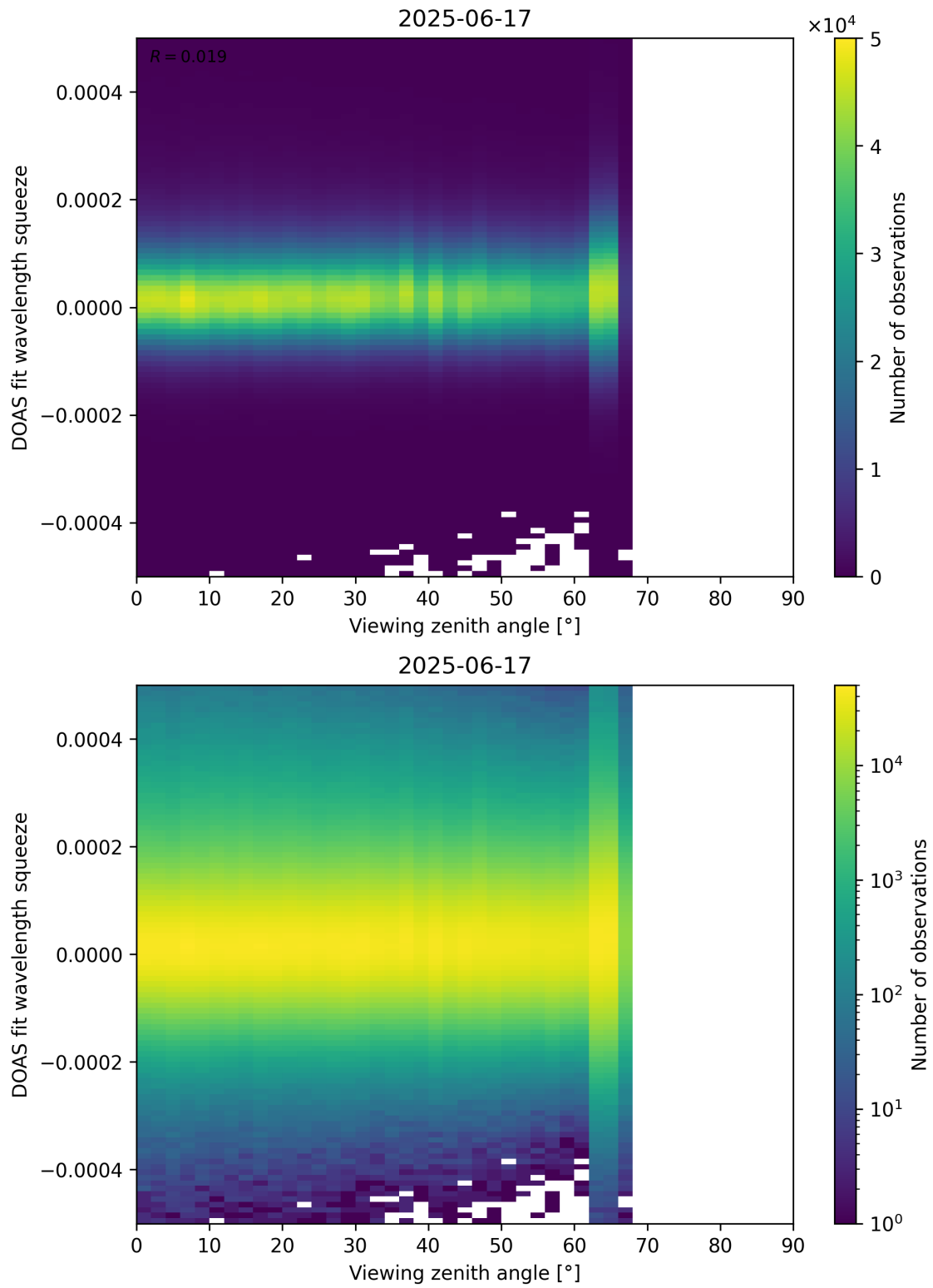
Figure 184: Scatter density plot of “Viewing zenith angle” against “DOAS fit wavelength squeeze” for 2025-06-17 to 2025-06-18.
