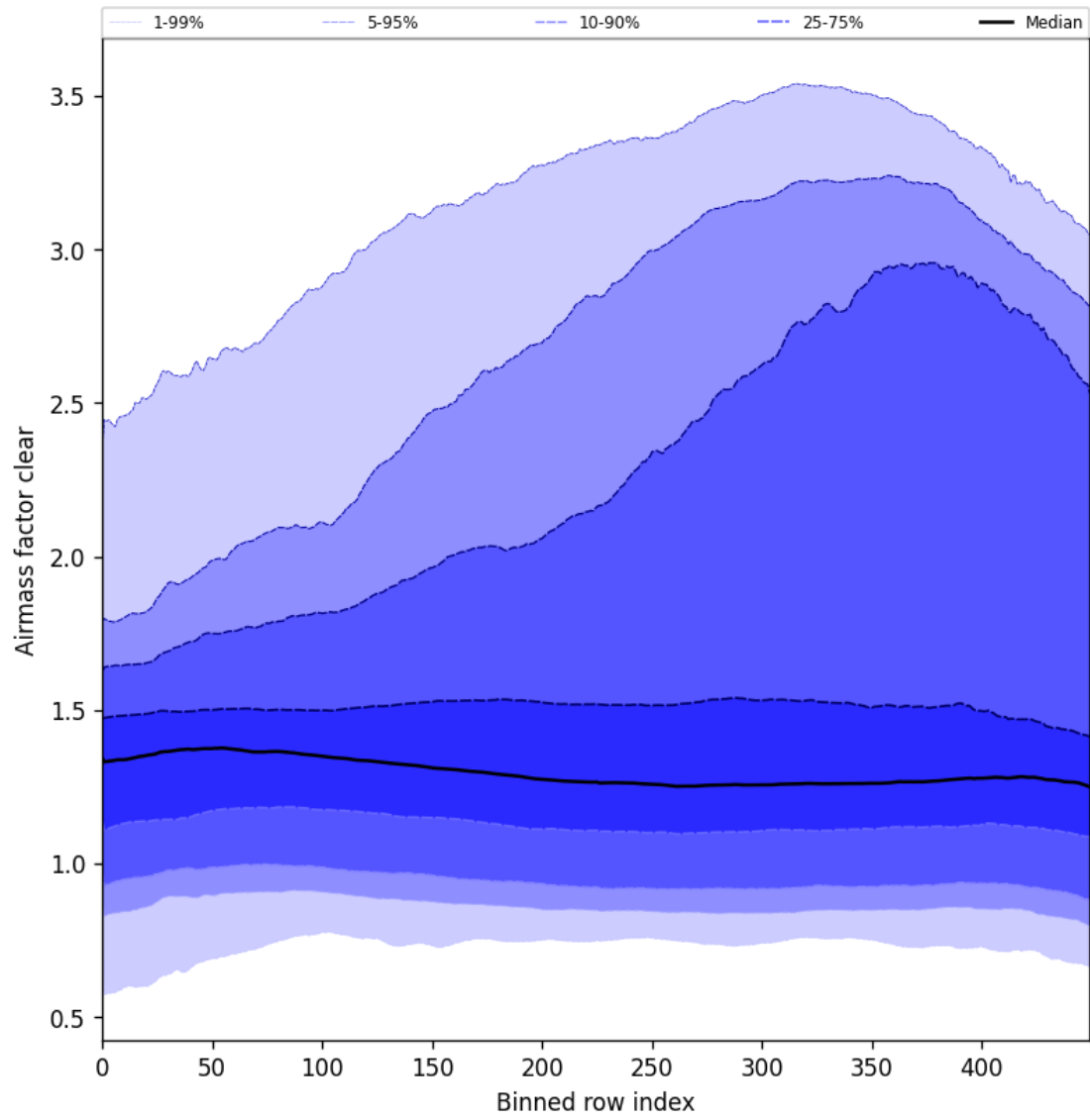
Figure 56: Along track statistics of “Air mass factor clear” for 2025-06-17 to 2025-06-18
