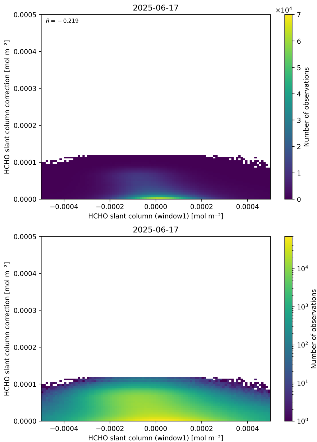
Figure 83: Scatter density plot of “HCHO slant column (window1)” against “HCHO slant column correction” for 2025-06-17 to 2025-06-18.
