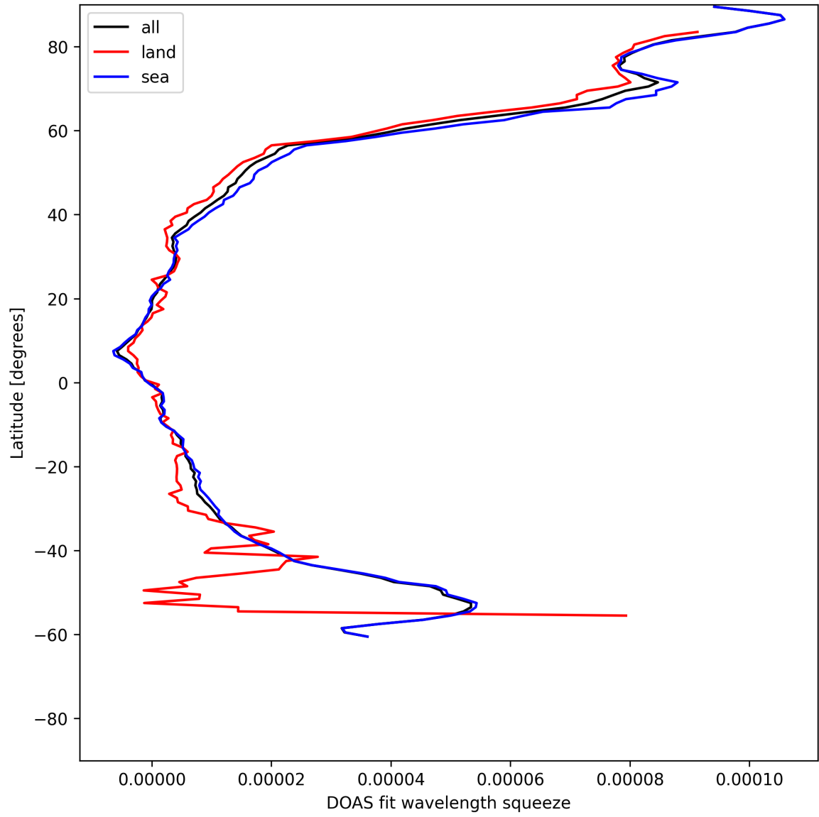
Figure 31: Zonal average of “DOAS fit wavelength squeeze” for 2025-06-17 to 2025-06-18.
