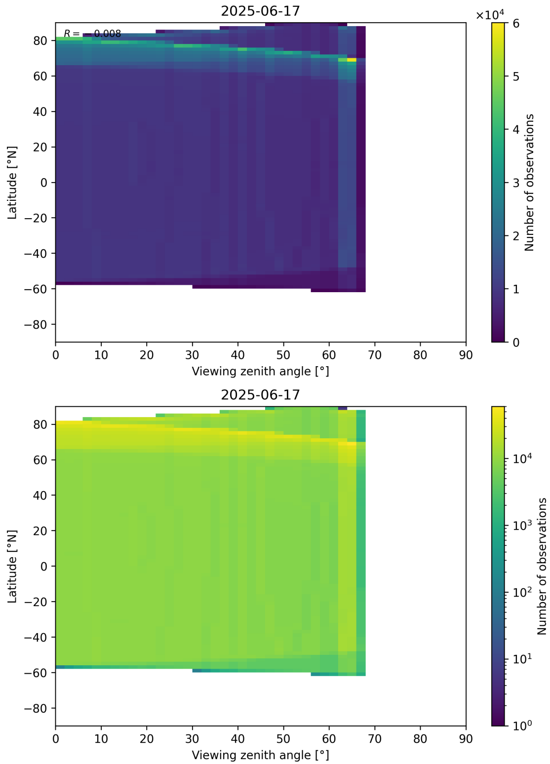
Figure 196: Scatter density plot of “Viewing zenith angle” against “Latitude” for 2025-06-17 to 2025-06-18.
