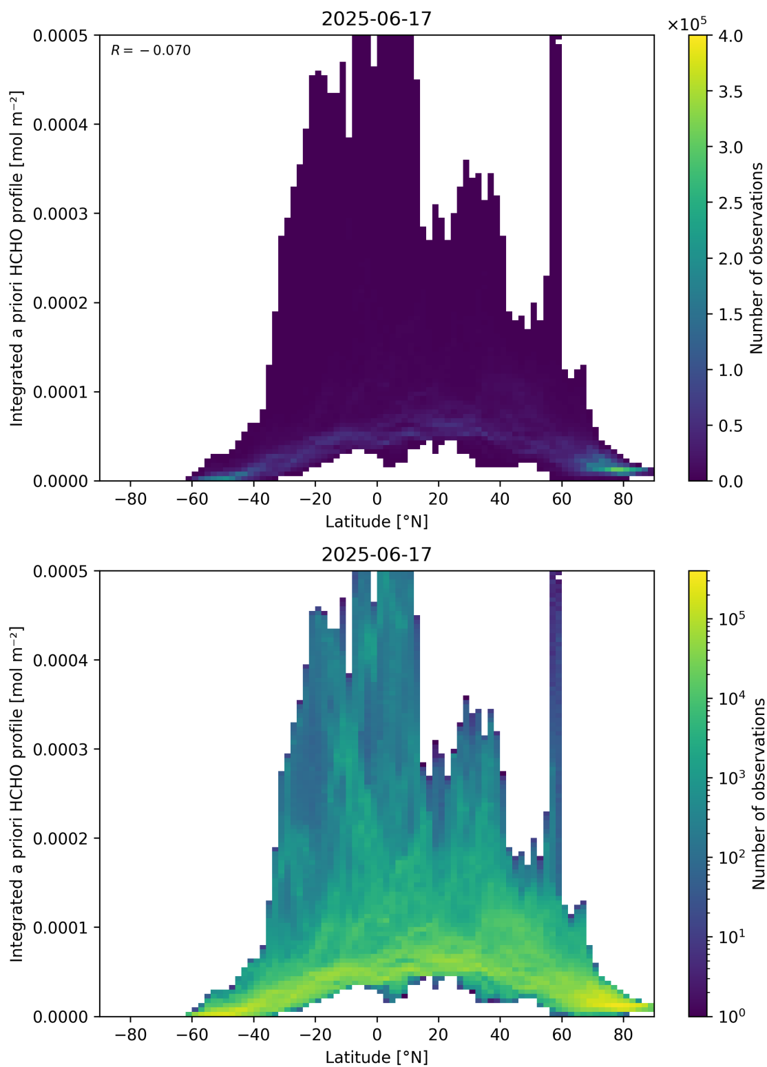
Figure 166: Scatter density plot of “Latitude” against “Integrated a priori HCHO profile” for 2025-06-17 to 2025-06-18.
