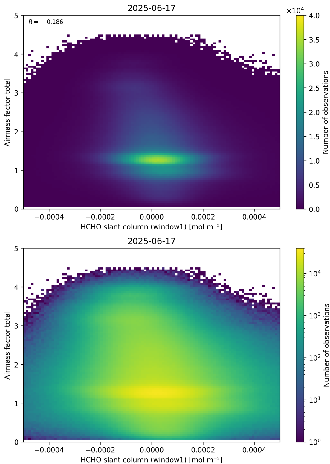
Figure 85: Scatter density plot of “HCHO slant column (window1)” against “Airmass factor total” for 2025-06-17 to 2025-06-18.
