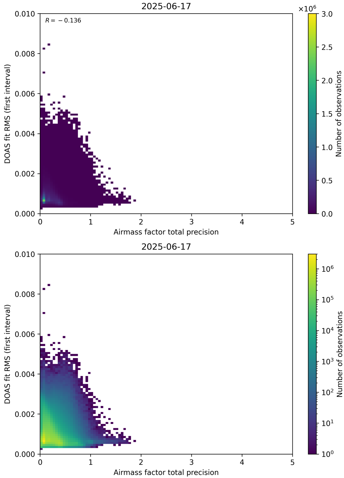
Figure 105: Scatter density plot of “Airmass factor total precision” against “DOAS fit RMS (first interval)” for 2025-06-17 to 2025-06-18.
