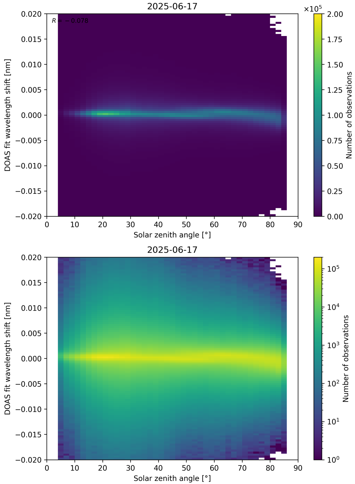
Figure 168: Scatter density plot of “Solar zenith angle” against “DOAS fit wavelength shift” for 2025-06-17 to 2025-06-18.
