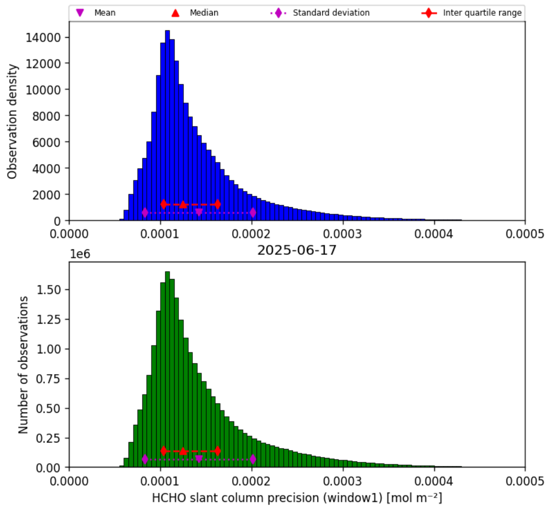
Figure 39: Histogram of “HCHO slant column precision (window1)” for 2025-06-17 to 2025-06-18
