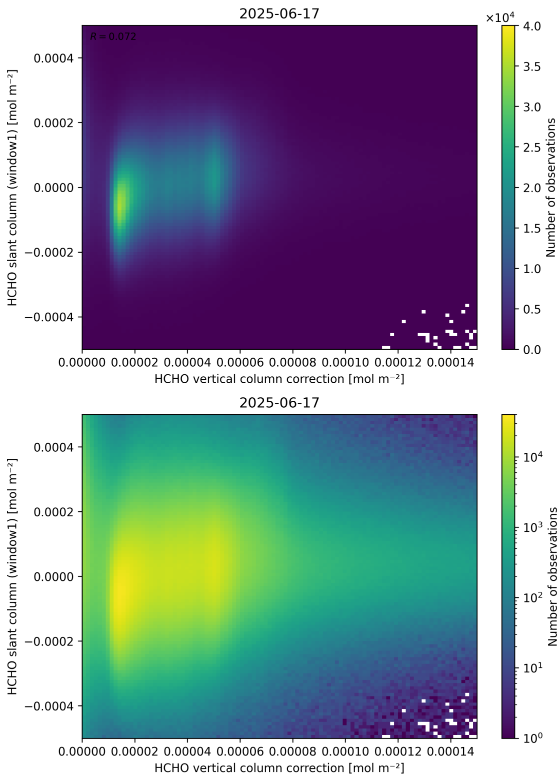
Figure 118: Scatter density plot of “HCHO vertical column correction” against “HCHO slant column (window1)” for 2025-06-17 to 2025-06-18.
