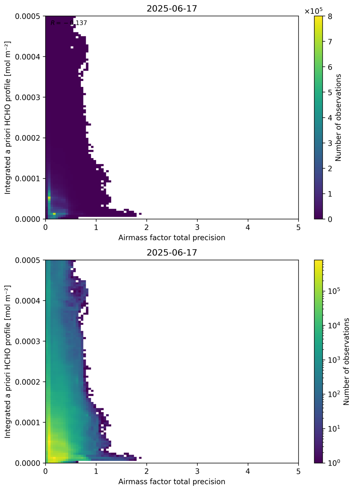
Figure 111: Scatter density plot of “Airmass factor total precision” against “Integrated a priori HCHO profile” for 2025-06-17 to 2025-06-18.
