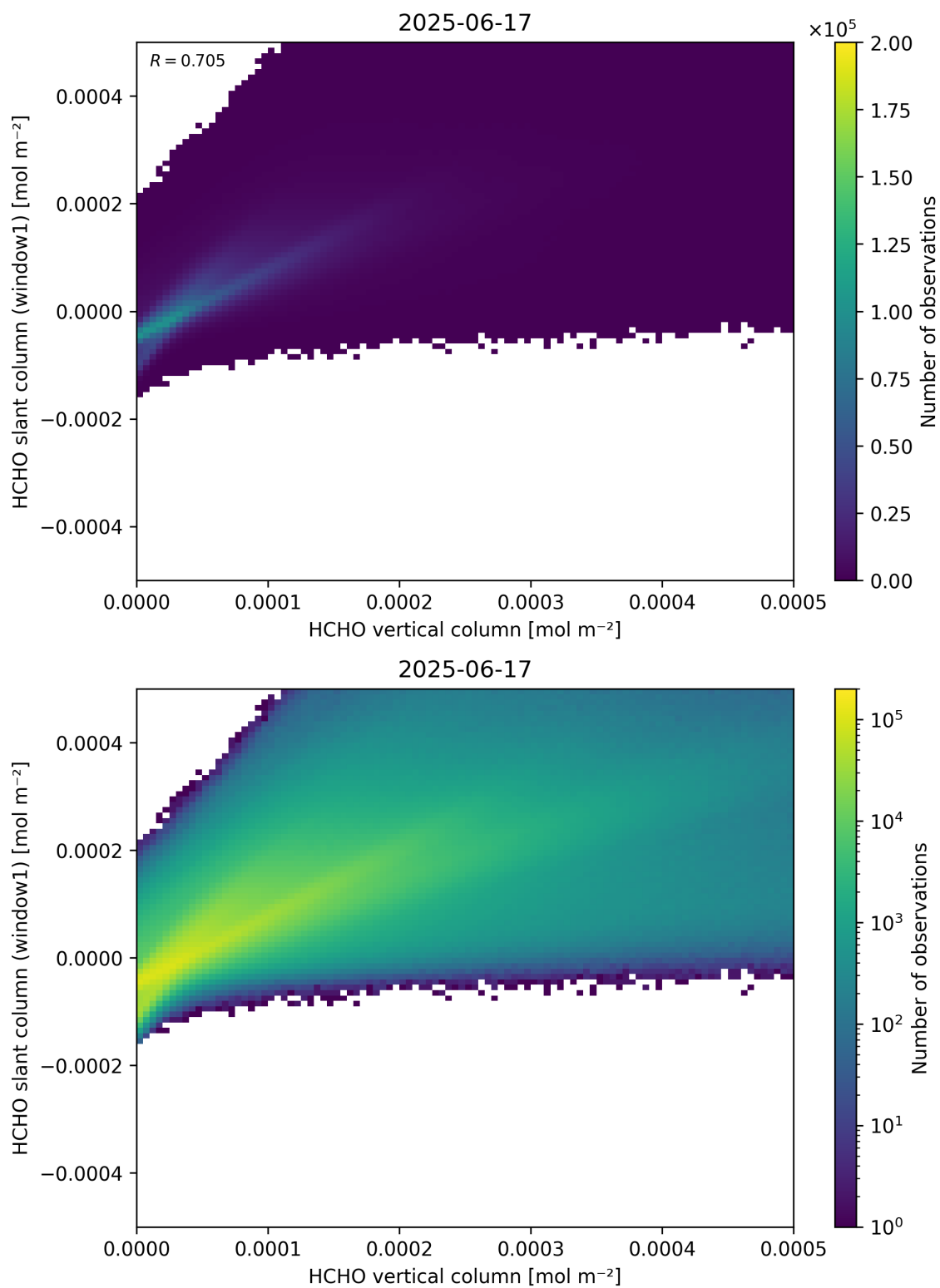
Figure 129: Scatter density plot of “HCHO vertical column” against “HCHO slant column (window1)” for 2025-06-17 to 2025-06-18.
