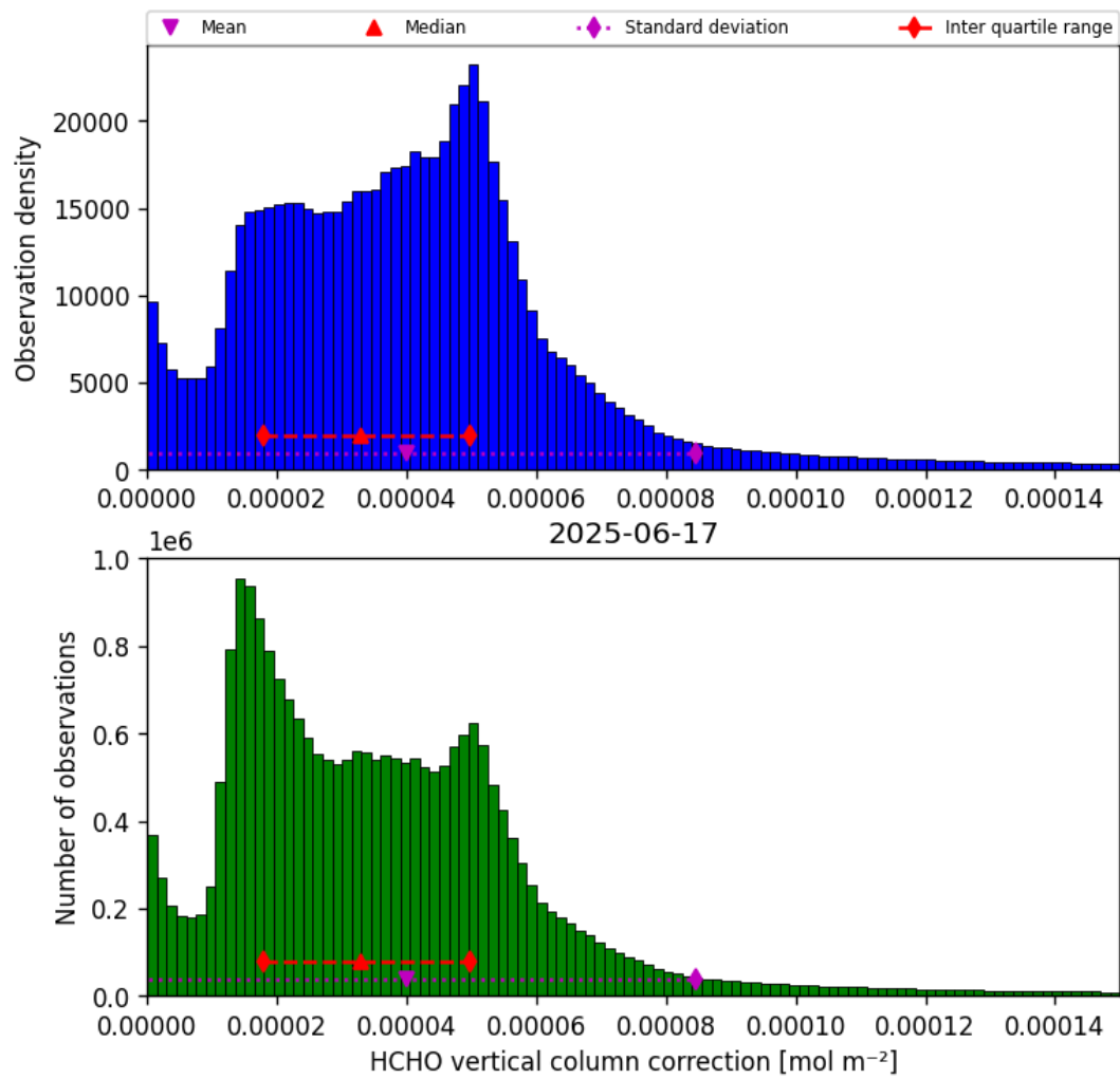
Figure 37: Histogram of “HCHO vertical column correction” for 2025-06-17 to 2025-06-18
