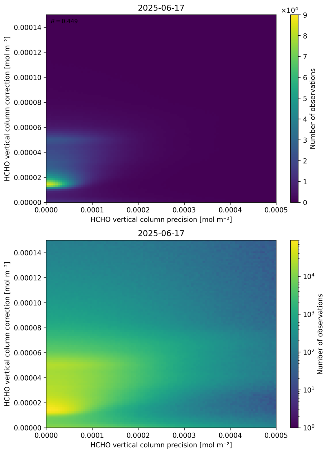
Figure 146: Scatter density plot of “HCHO vertical column precision” against “HCHO vertical column correction” for 2025-06-17 to 2025-06-18.
