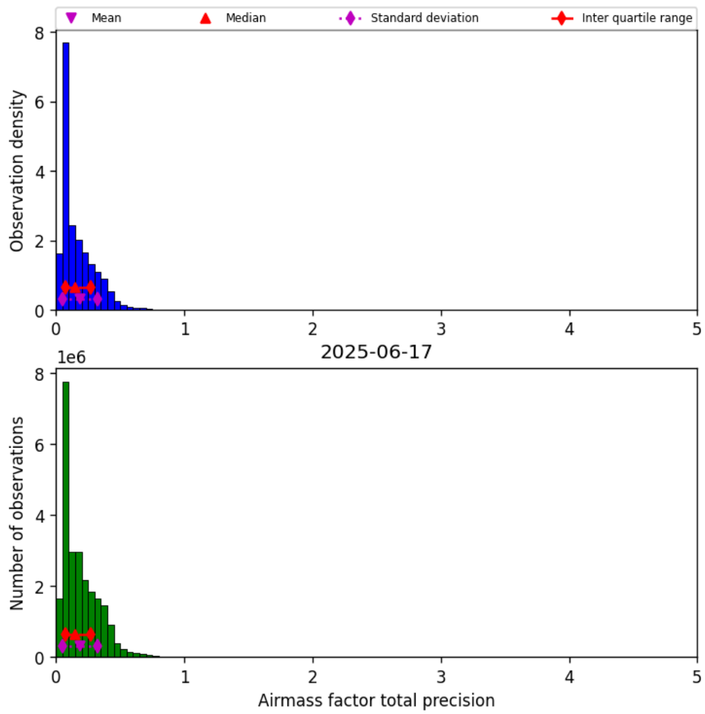
Figure 41: Histogram of “Airmass factor total precision” for 2025-06-17 to 2025-06-18
