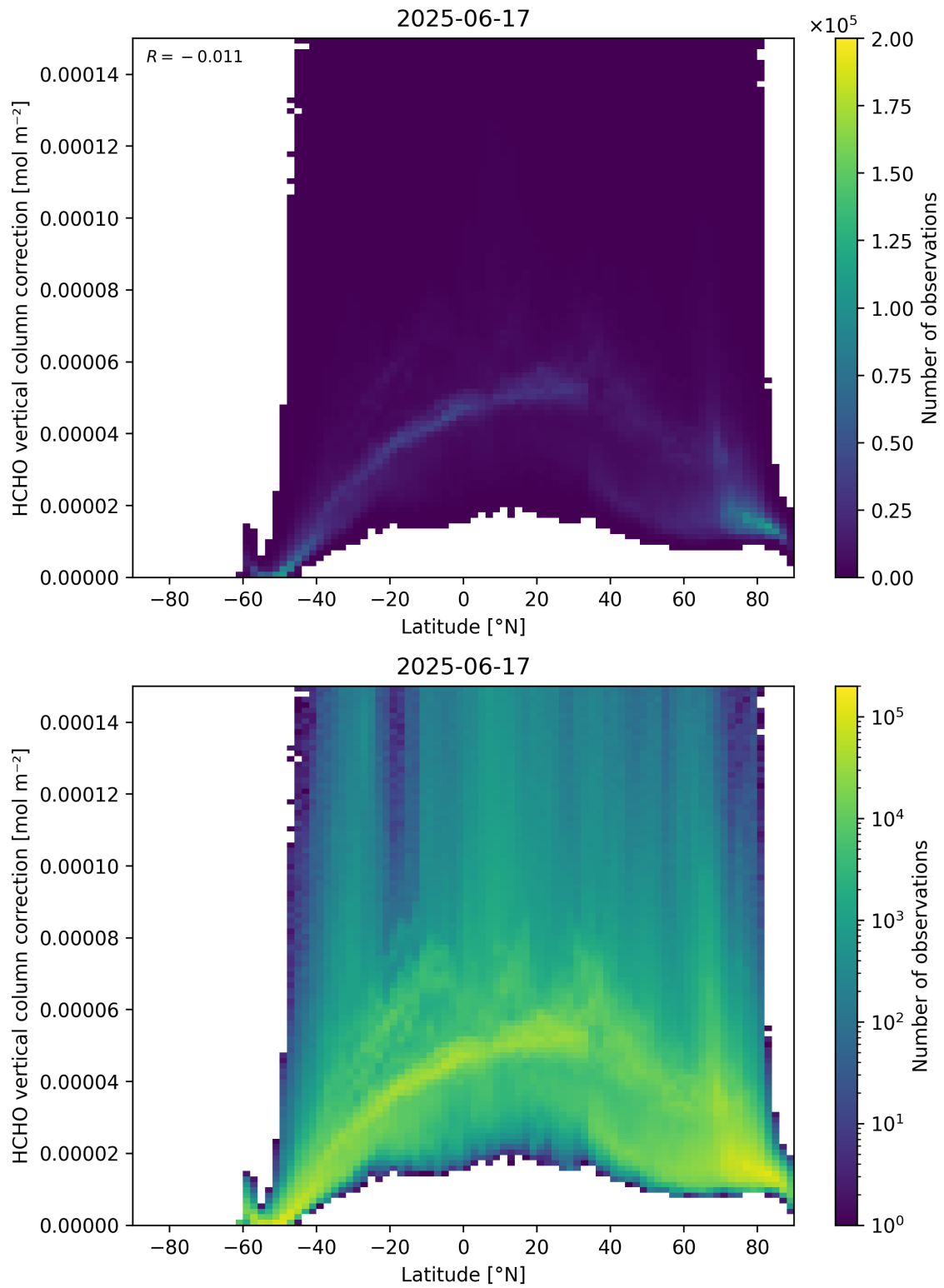
Figure 164: Scatter density plot of “Latitude” against “HCHO vertical column correction” for 2025-06-17 to 2025-06-18.
