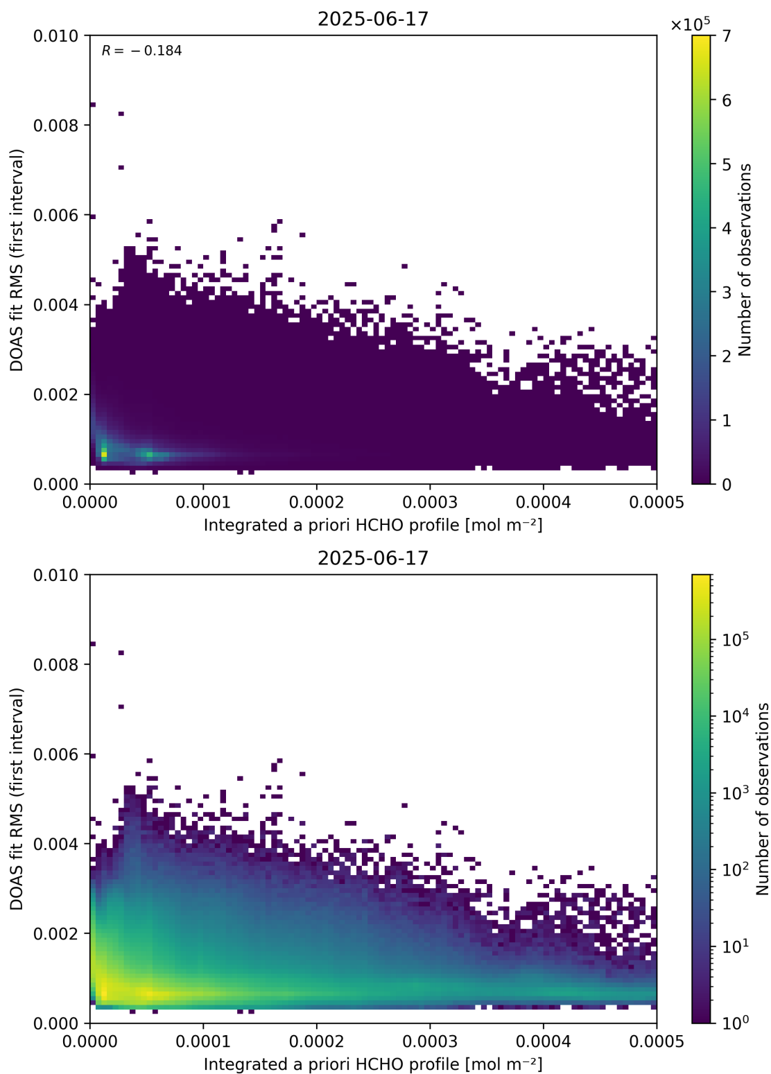
Figure 148: Scatter density plot of “Integrated a priori HCHO profile” against “DOAS fit RMS (first interval)” for 2025-06-17 to 2025-06-18.
