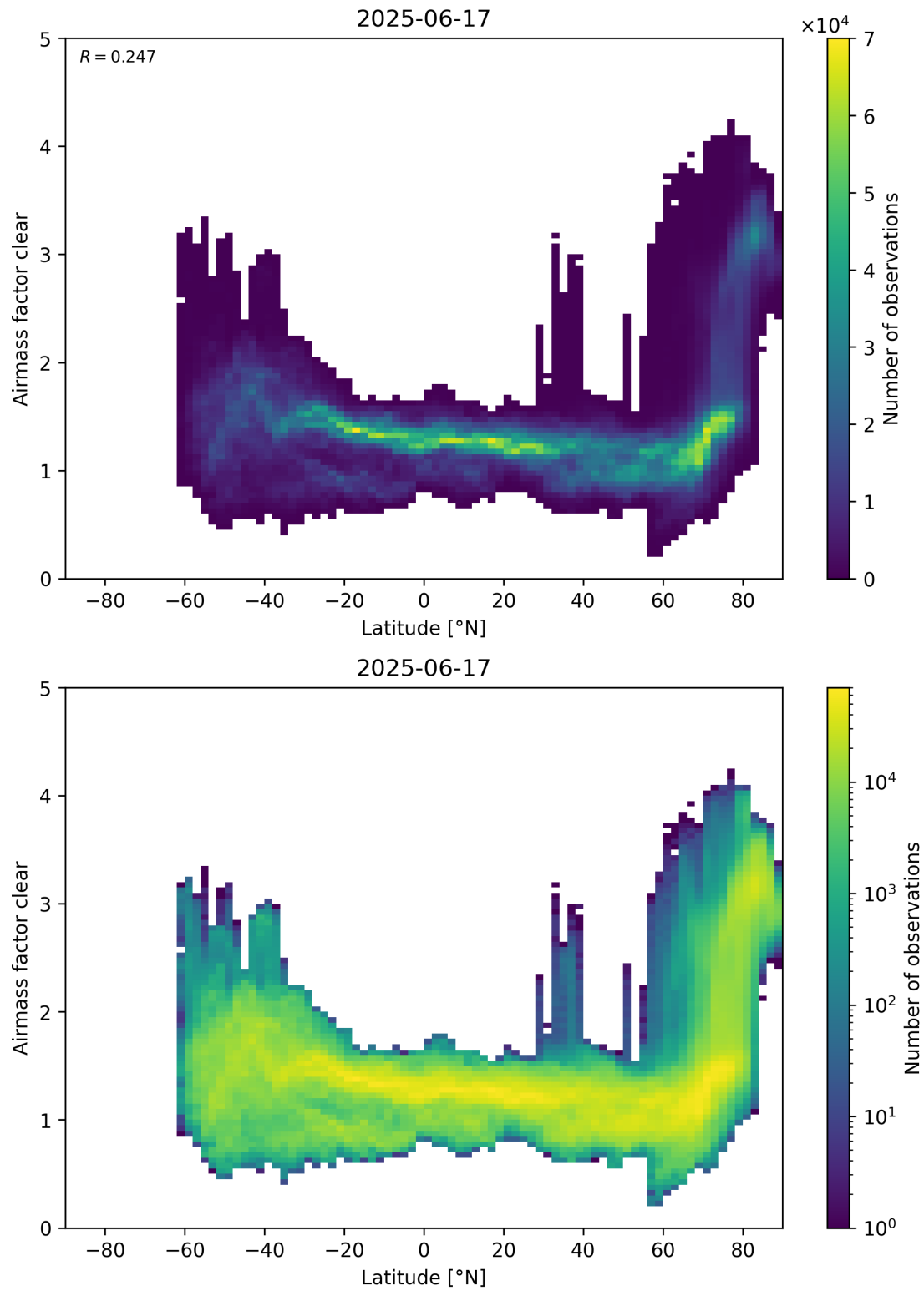
Figure 156: Scatter density plot of “Latitude” against “Airmass factor clear” for 2025-06-17 to 2025-06-18.
