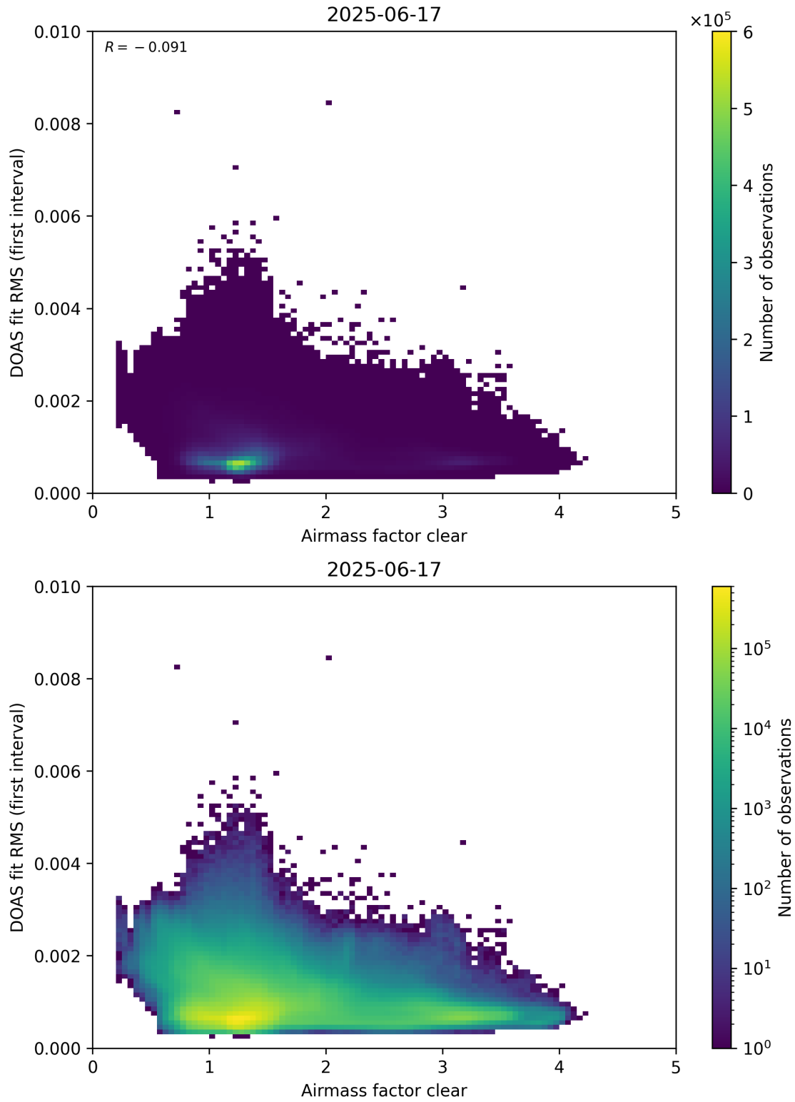
Figure 71: Scatter density plot of “Airmass factor clear” against “DOAS fit RMS (first interval)” for 2025-06-17 to 2025-06-18.
