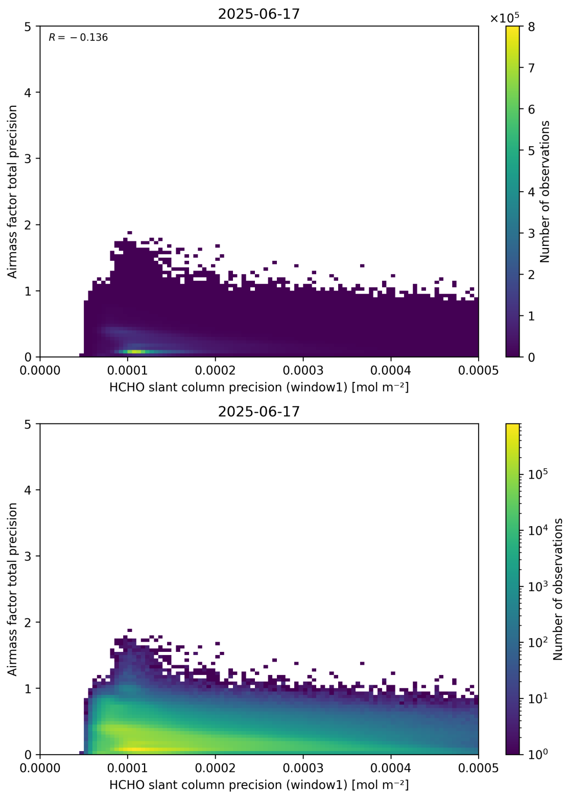
Figure 95: Scatter density plot of “HCHO slant column precision (window1)” against “Airmass factor total precision” for 2025-06-17 to 2025-06-18.
