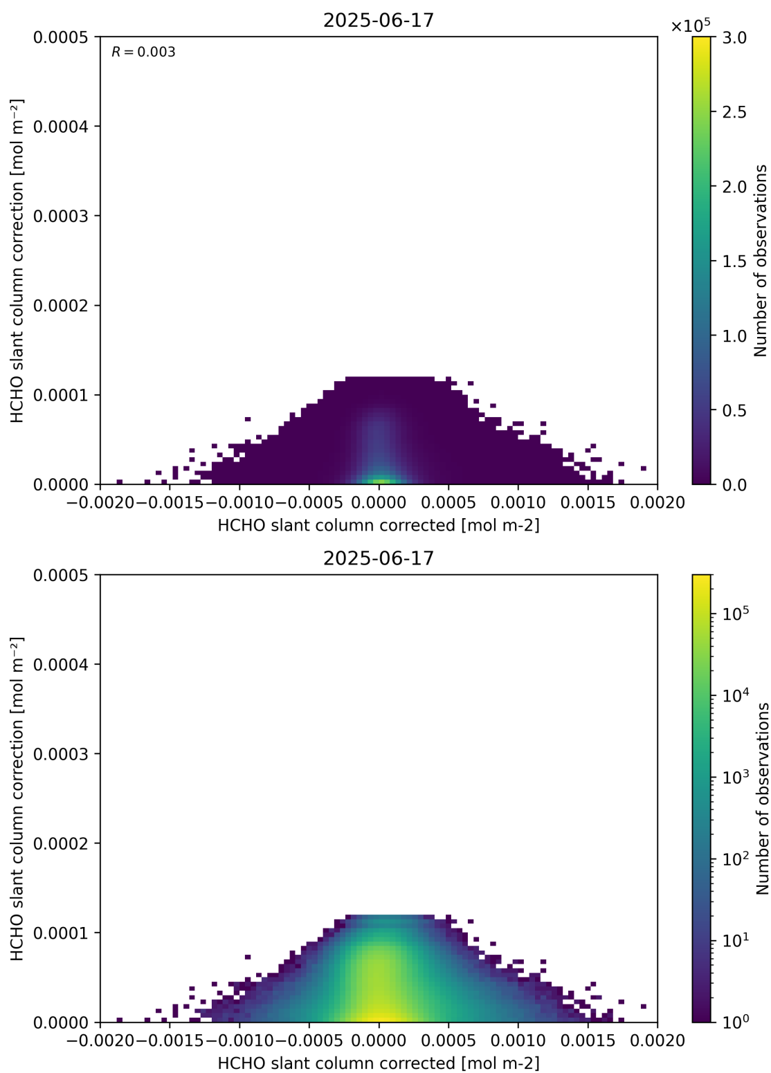
Figure 77: Scatter density plot of “HCHO slant column corrected” against “HCHO slant column correction” for 2025-06-17 to 2025-06-18.
