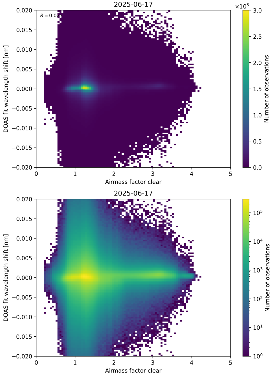
Figure 72: Scatter density plot of “Airmass factor clear” against “DOAS fit wavelength shift” for 2025-06-17 to 2025-06-18.
