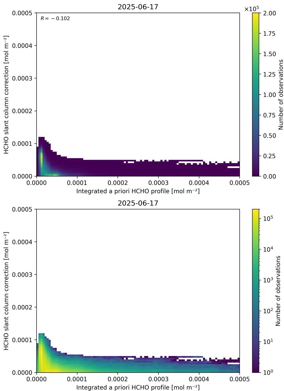
Figure 152: Scatter density plot of “Integrated a priori HCHO profile” against “HCHO slant column correction” for 2025-06-17 to 2025-06-18.
