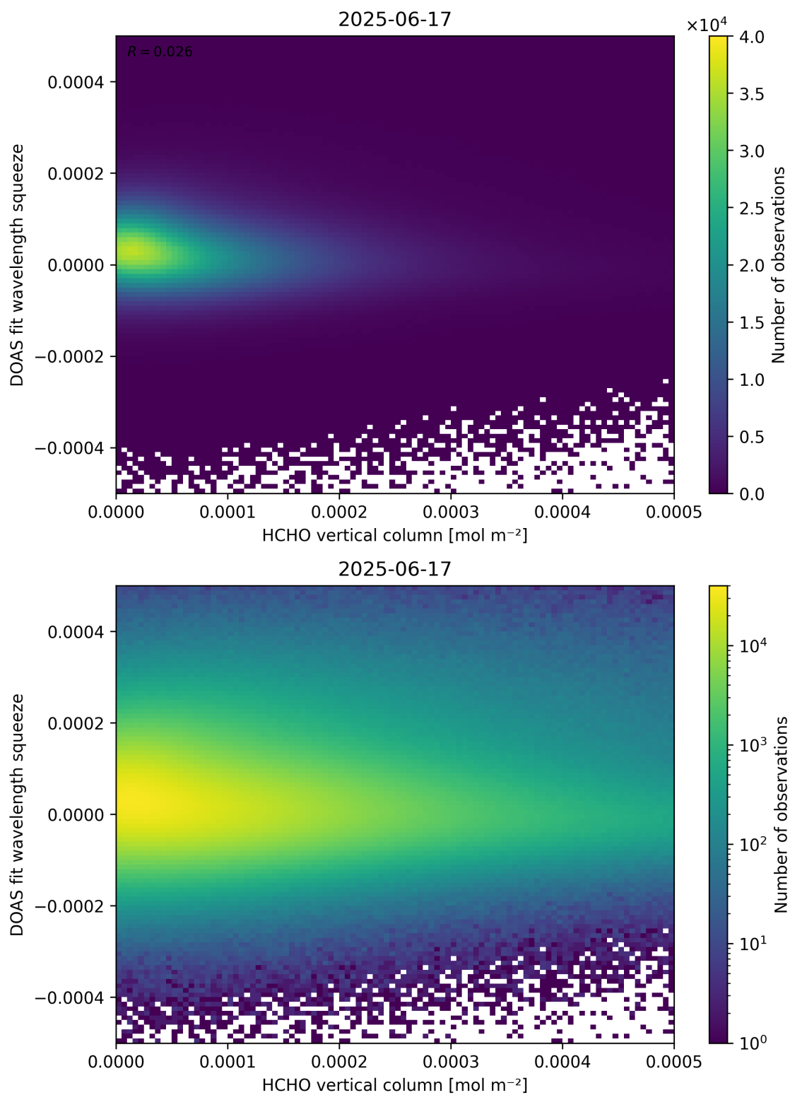
Figure 125: Scatter density plot of “HCHO vertical column” against “DOAS fit wavelength squeeze” for 2025-06-17 to 2025-06-18.
