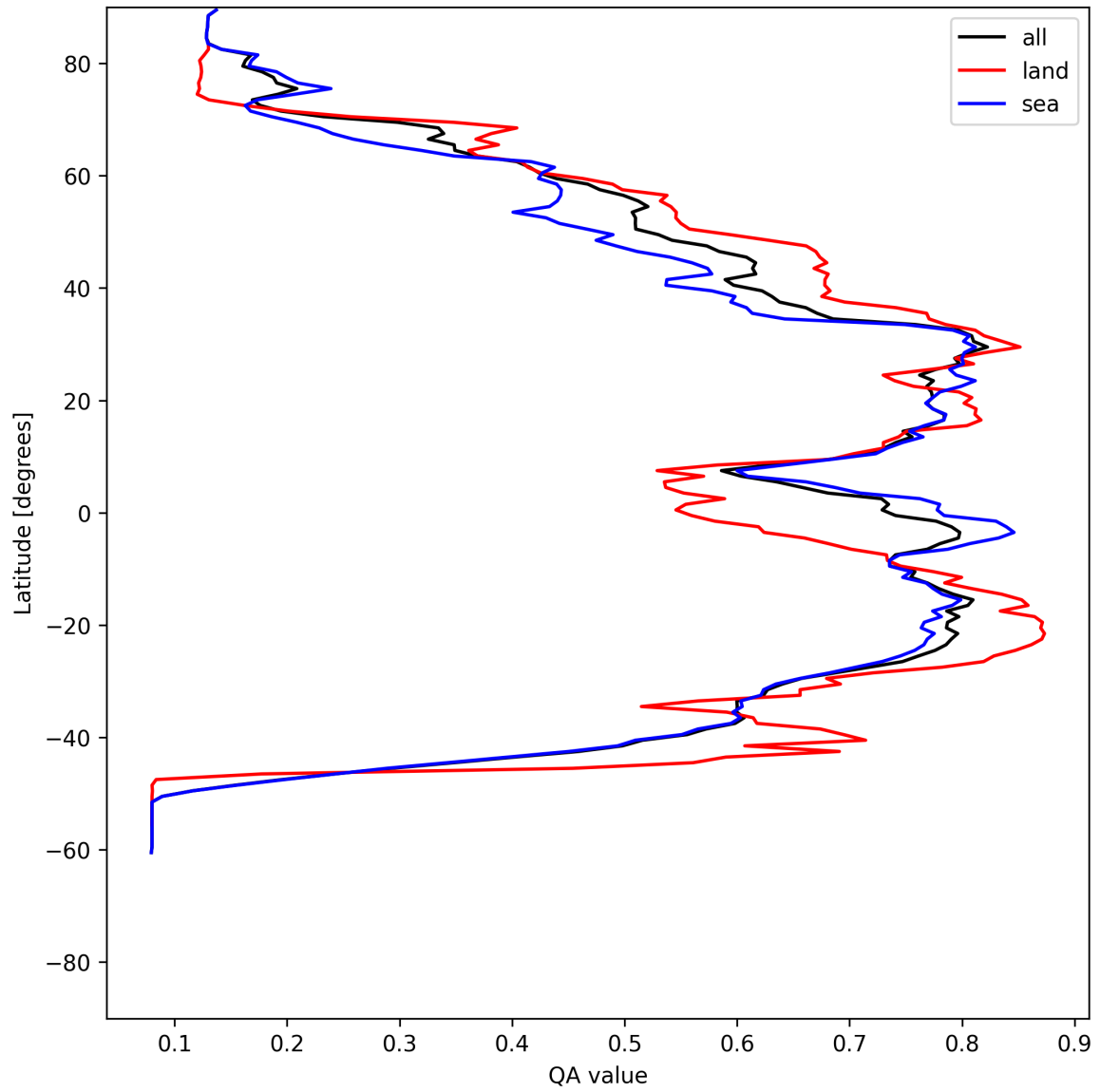
Figure 20: Zonal average of “QA value” for 2025-06-17 to 2025-06-18.
