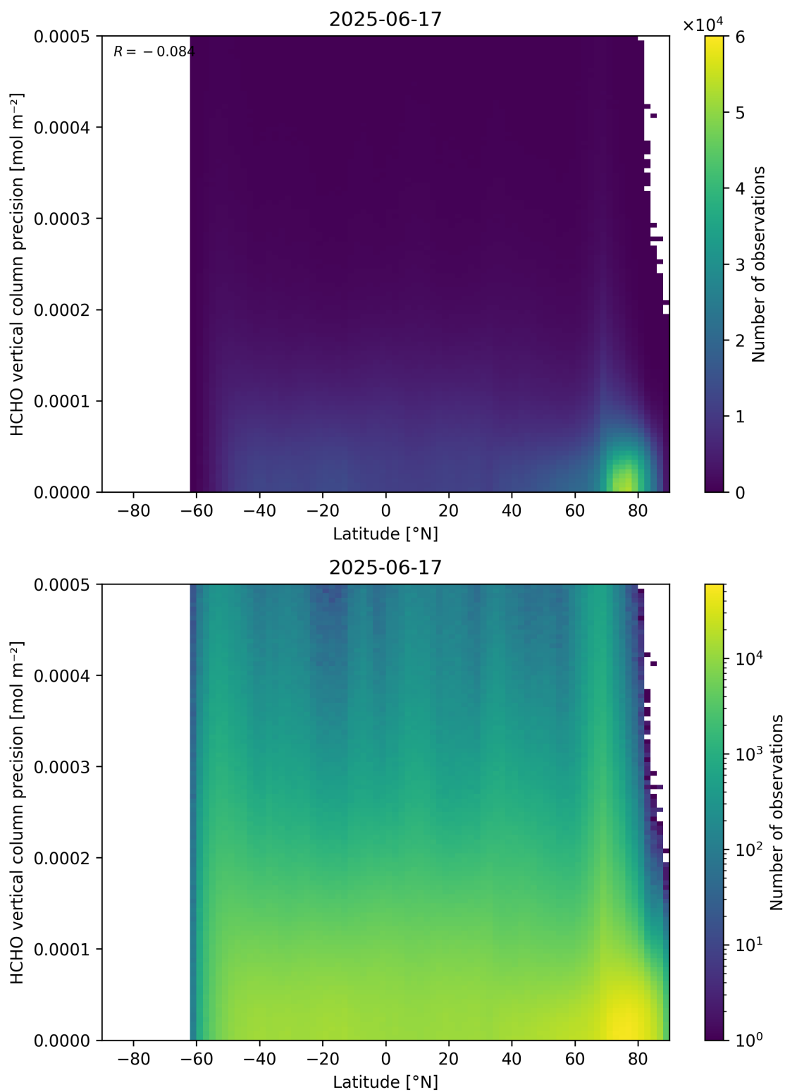
Figure 165: Scatter density plot of “Latitude” against “HCHO vertical column precision” for 2025-06-17 to 2025-06-18.
