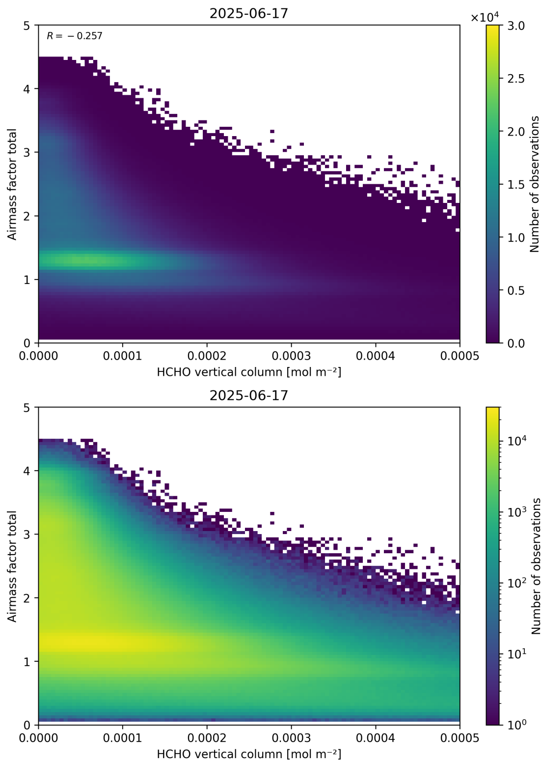
Figure 131: Scatter density plot of “HCHO vertical column” against “Airmass factor total” for 2025-06-17 to 2025-06-18.
