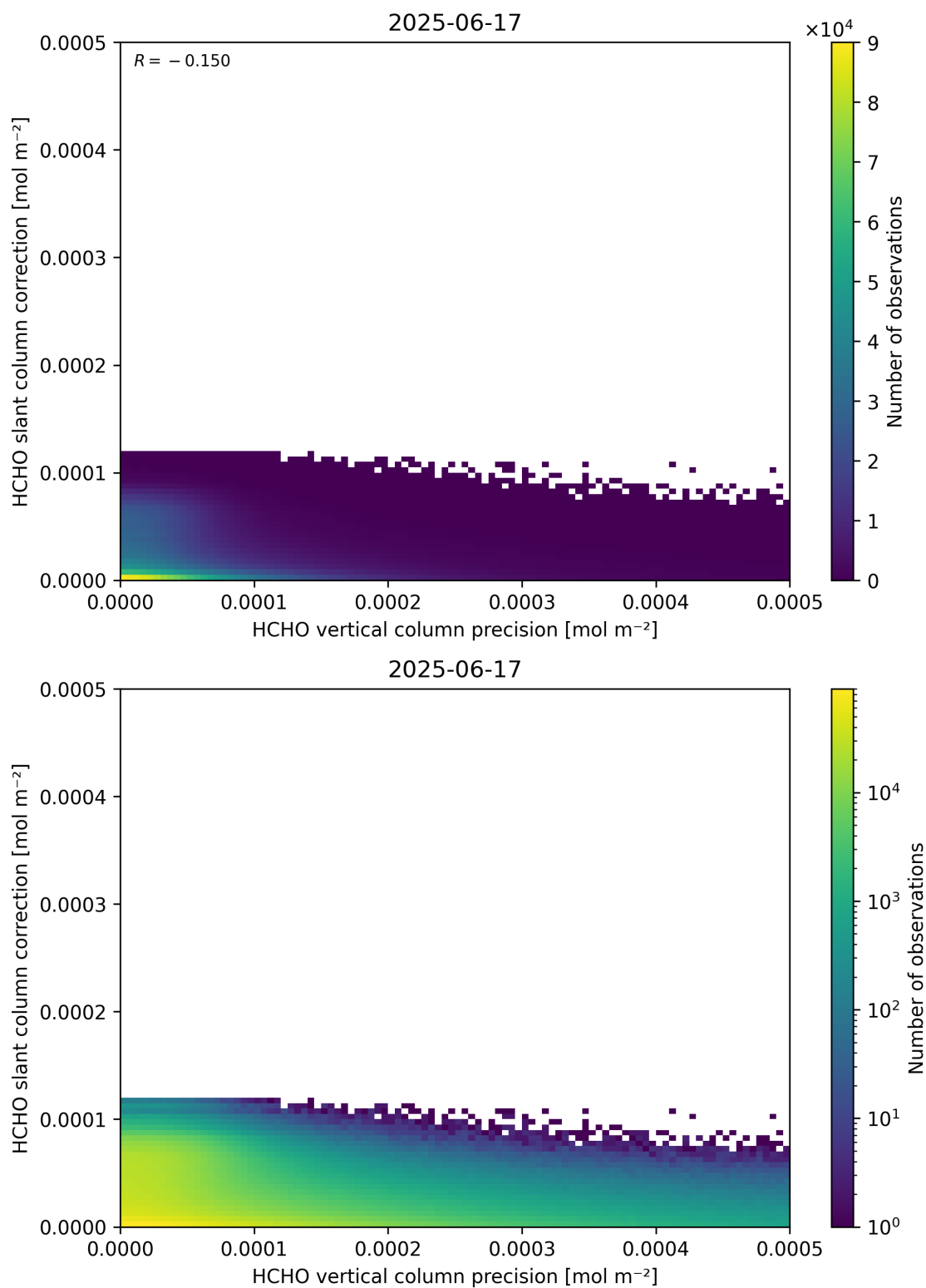
Figure 141: Scatter density plot of “HCHO vertical column precision” against “HCHO slant column correction” for 2025-06-17 to 2025-06-18.
