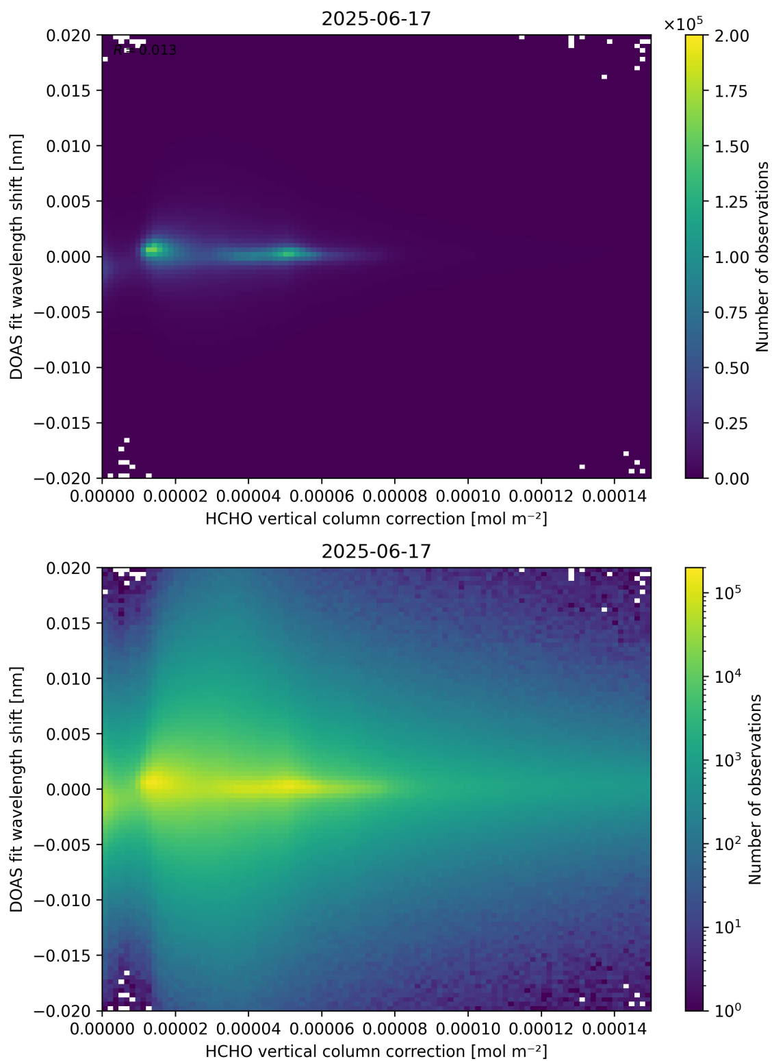
Figure 113: Scatter density plot of “HCHO vertical column correction” against “DOAS fit wavelength shift” for 2025-06-17 to 2025-06-18.
