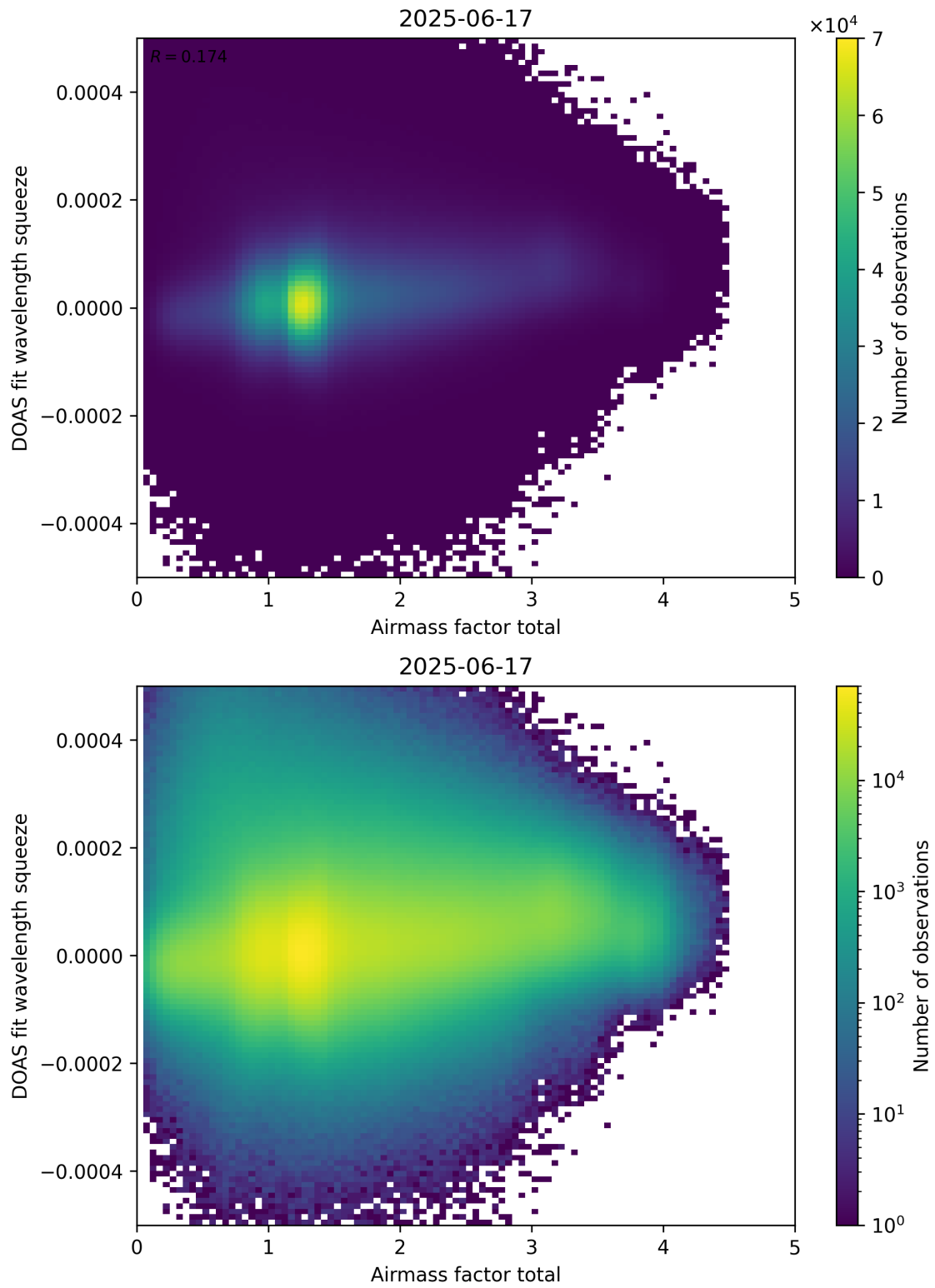
Figure 99: Scatter density plot of “Airmass factor total” against “DOAS fit wavelength squeeze” for 2025-06-17 to 2025-06-18.
