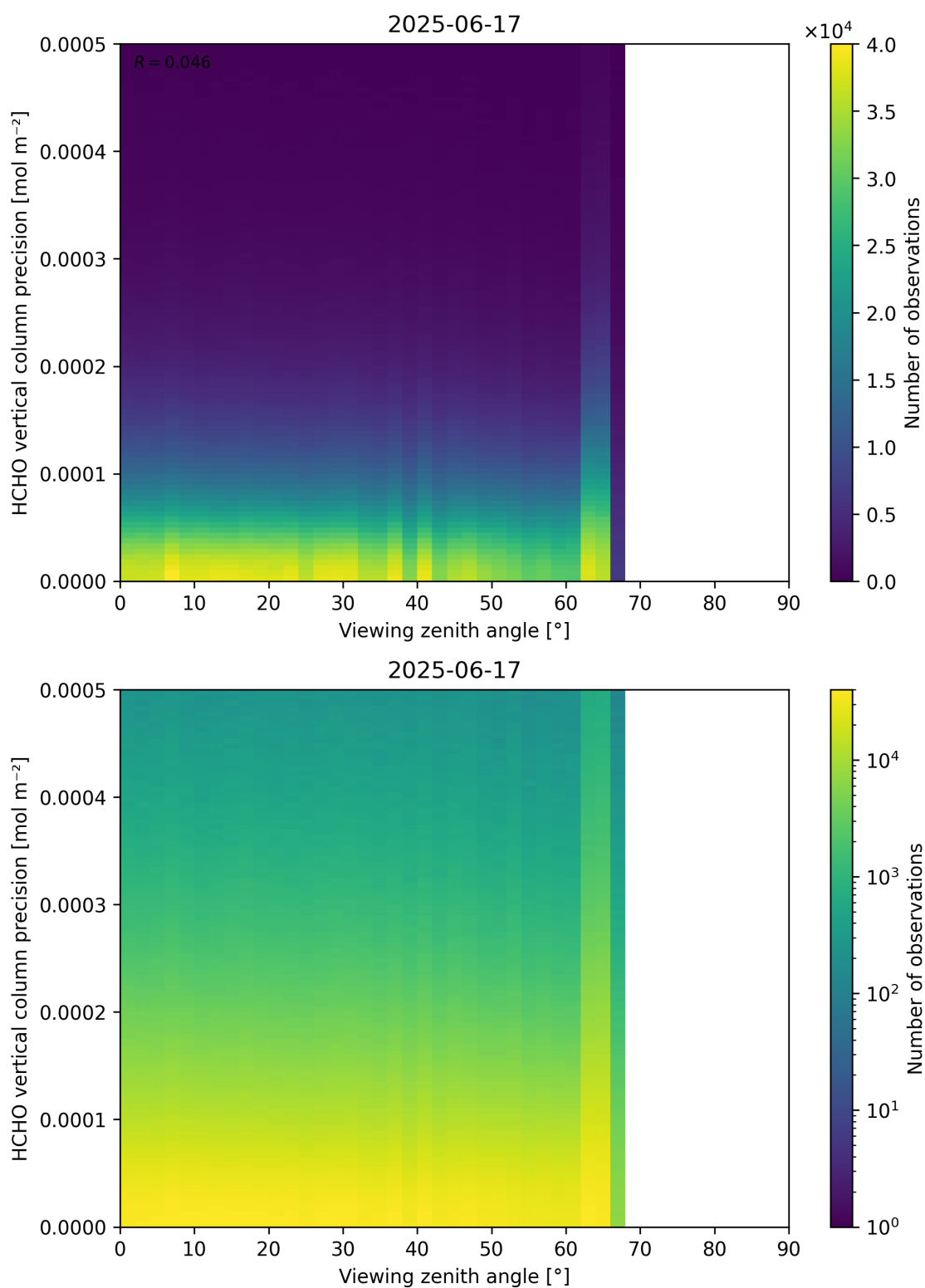
Figure 194: Scatter density plot of “Viewing zenith angle” against “HCHO vertical column precision” for 2025-06-17 to 2025-06-18.
