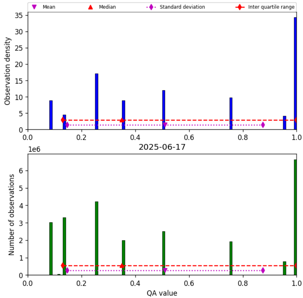
Figure 34: Histogram of “QA value” for 2025-06-17 to 2025-06-18
