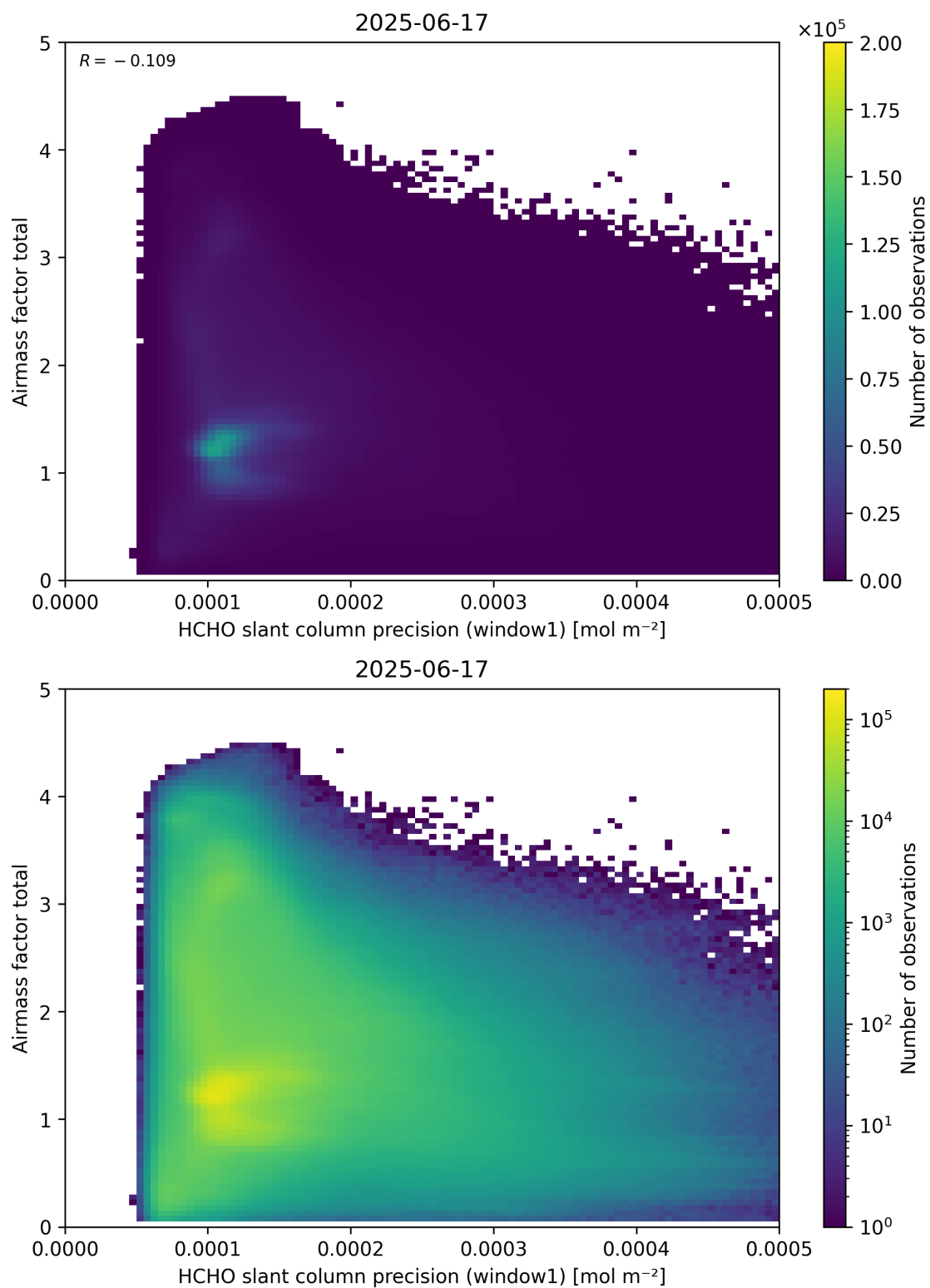
Figure 94: Scatter density plot of “HCHO slant column precision (window1)” against “Airmass factor total” for 2025-06-17 to 2025-06-18.
