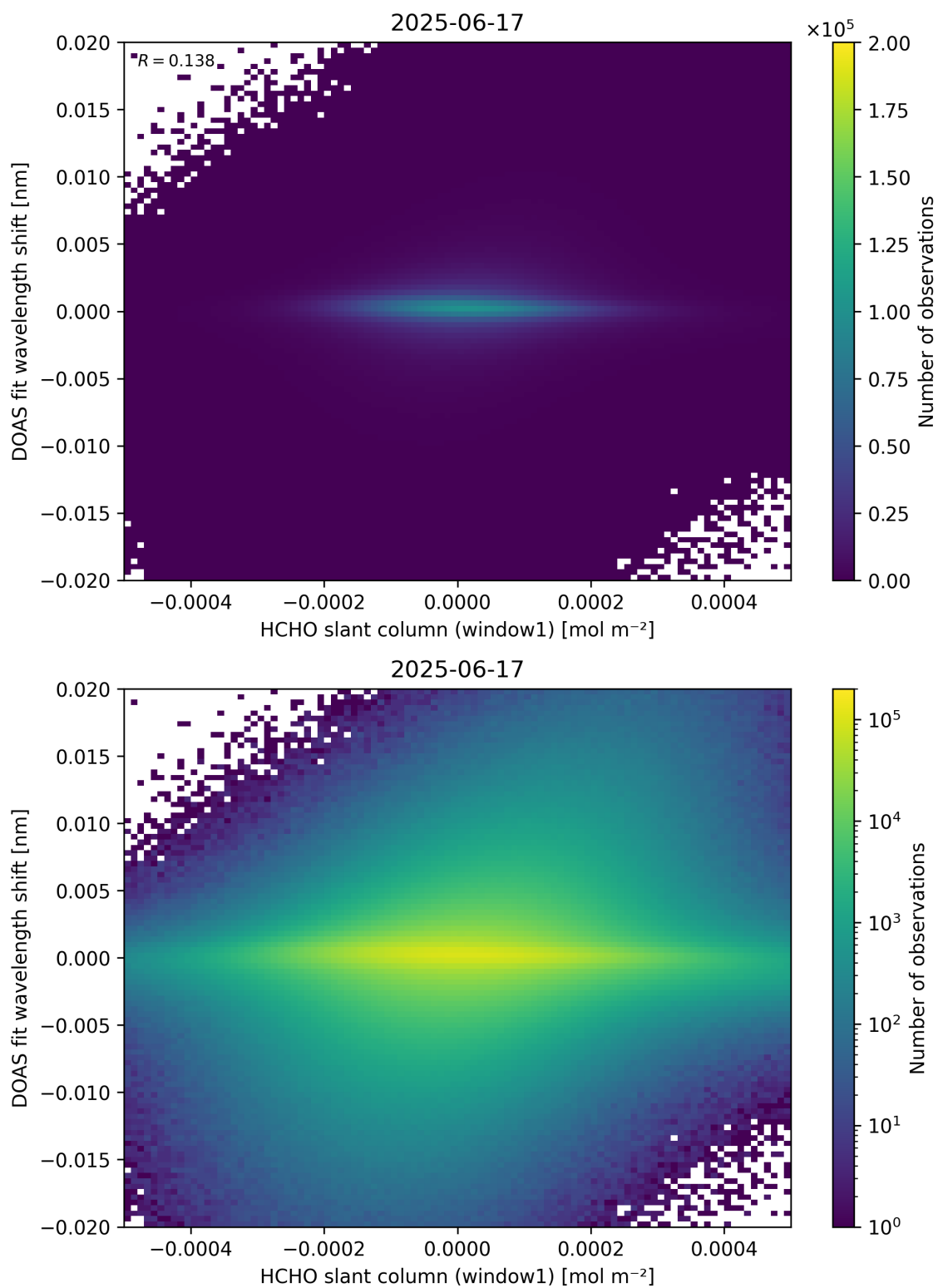
Figure 79: Scatter density plot of “HCHO slant column (window1)” against “DOAS fit wavelength shift” for 2025-06-17 to 2025-06-18.
