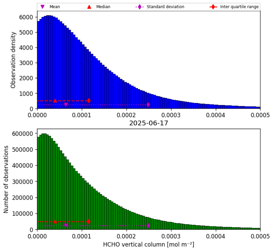
Figure 35: Histogram of “HCHO vertical column” for 2025-06-17 to 2025-06-18
