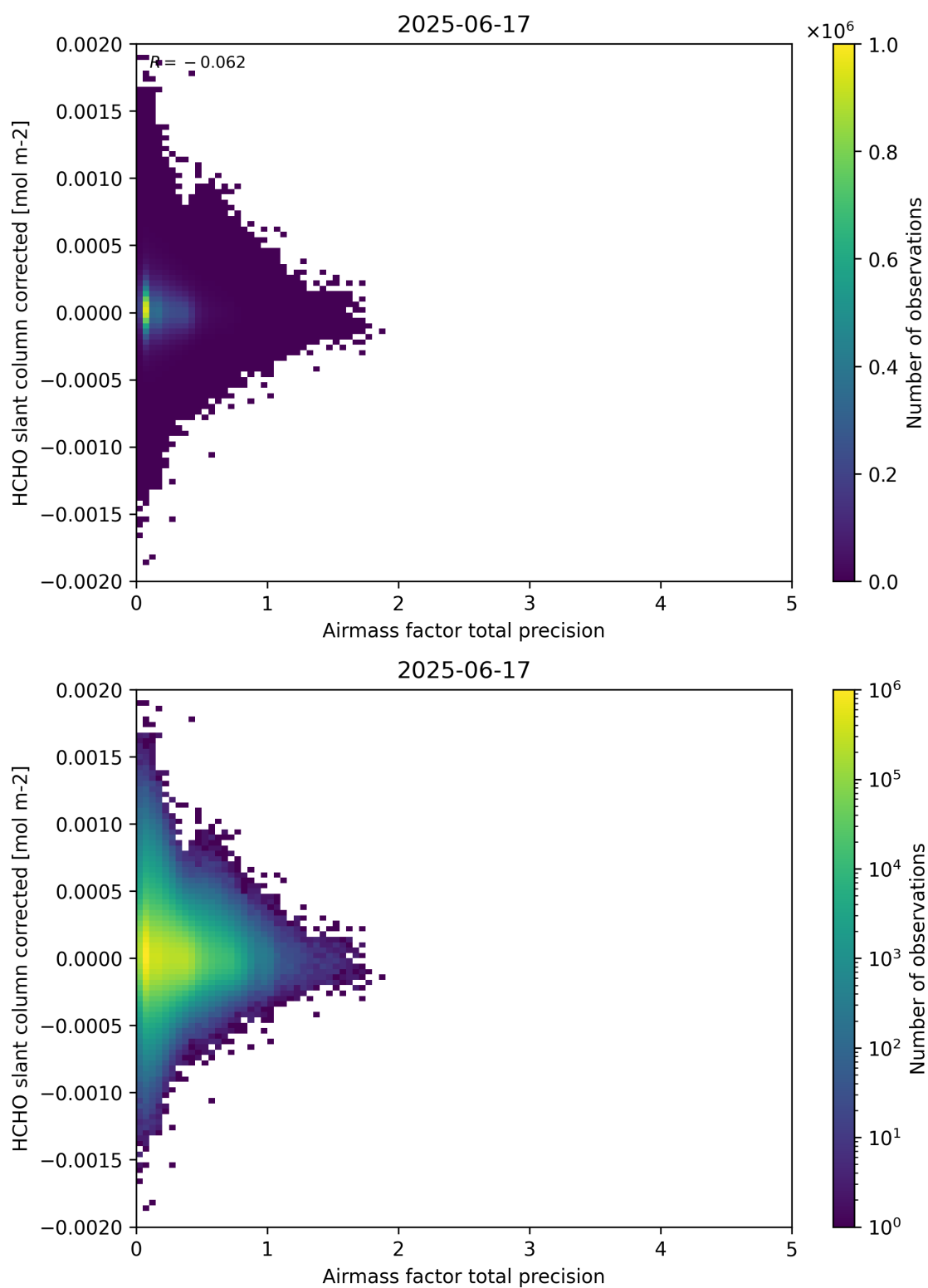
Figure 109: Scatter density plot of “Airmass factor total precision” against “HCHO slant column corrected” for 2025-06-17 to 2025-06-18.
