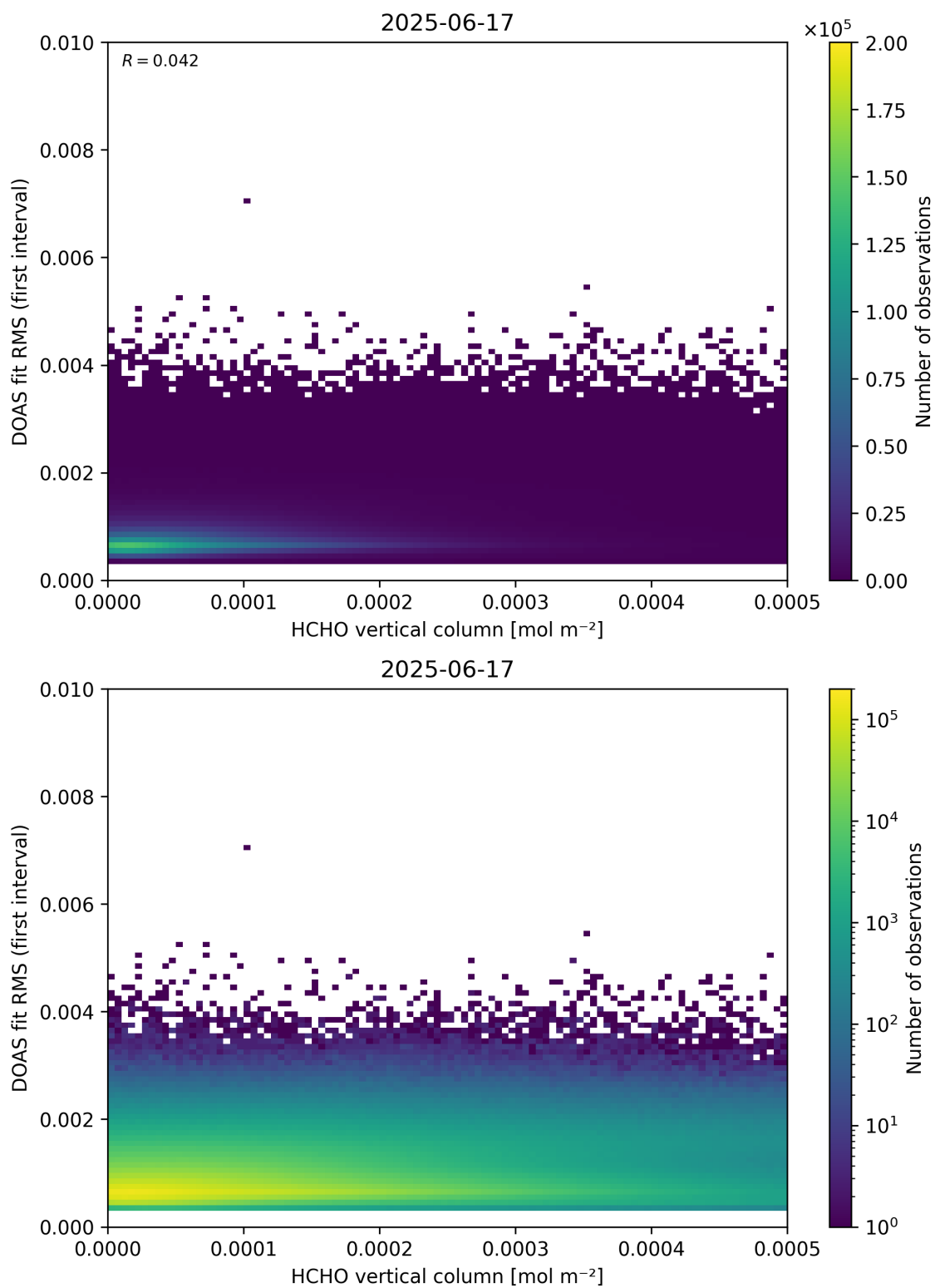
Figure 123: Scatter density plot of “HCHO vertical column” against “DOAS fit RMS (first interval)” for 2025-06-17 to 2025-06-18.
