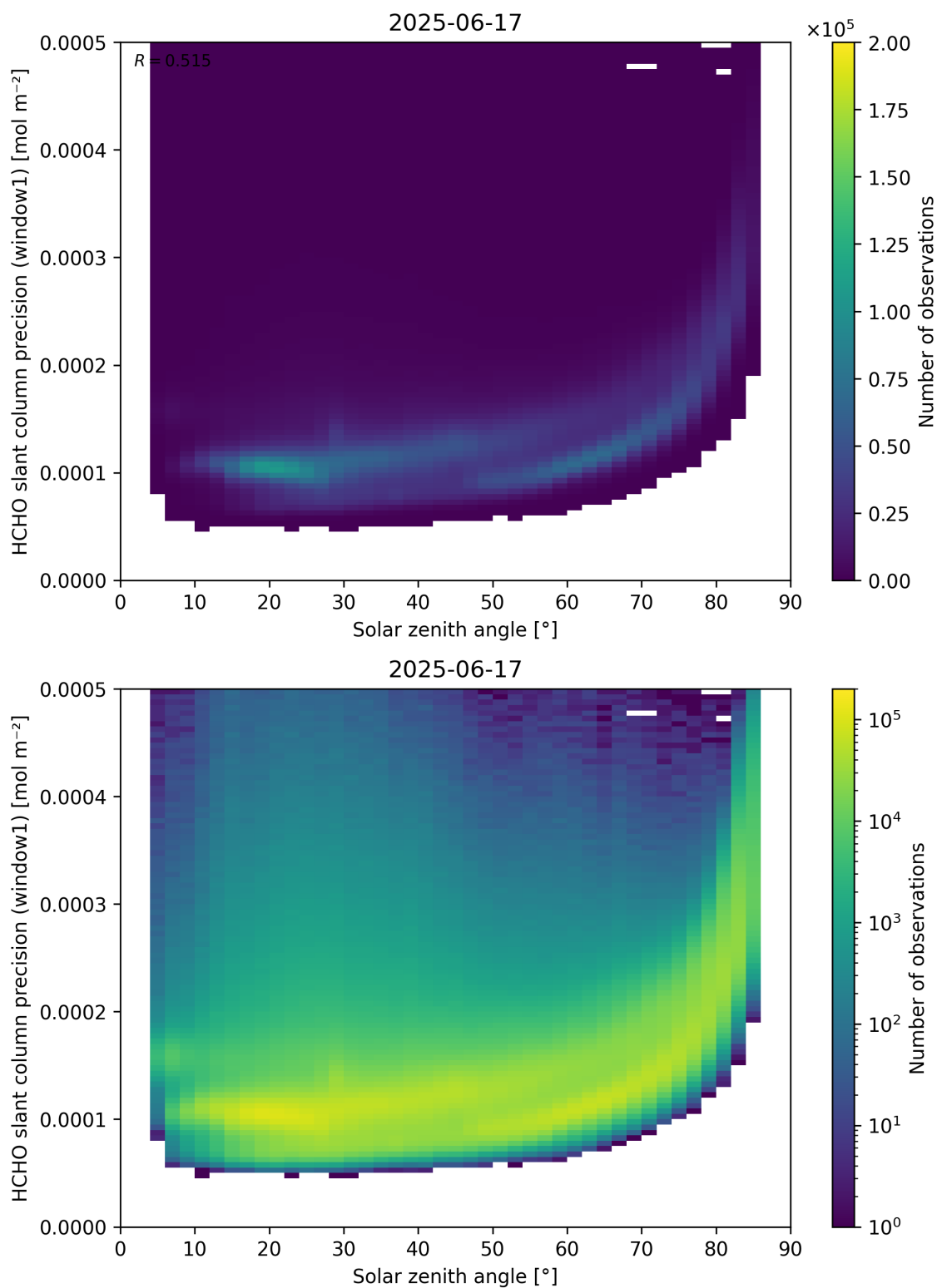
Figure 174: Scatter density plot of “Solar zenith angle” against “HCHO slant column precision (window1)” for 2025-06-17 to 2025-06-18.
