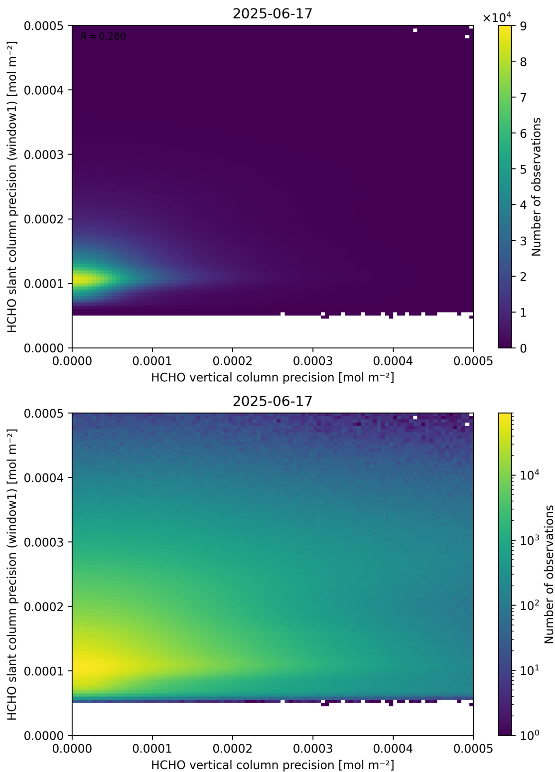
Figure 143: Scatter density plot of “HCHO vertical column precision” against “HCHO slant column precision (window1)” for 2025-06-17 to 2025-06-18.
