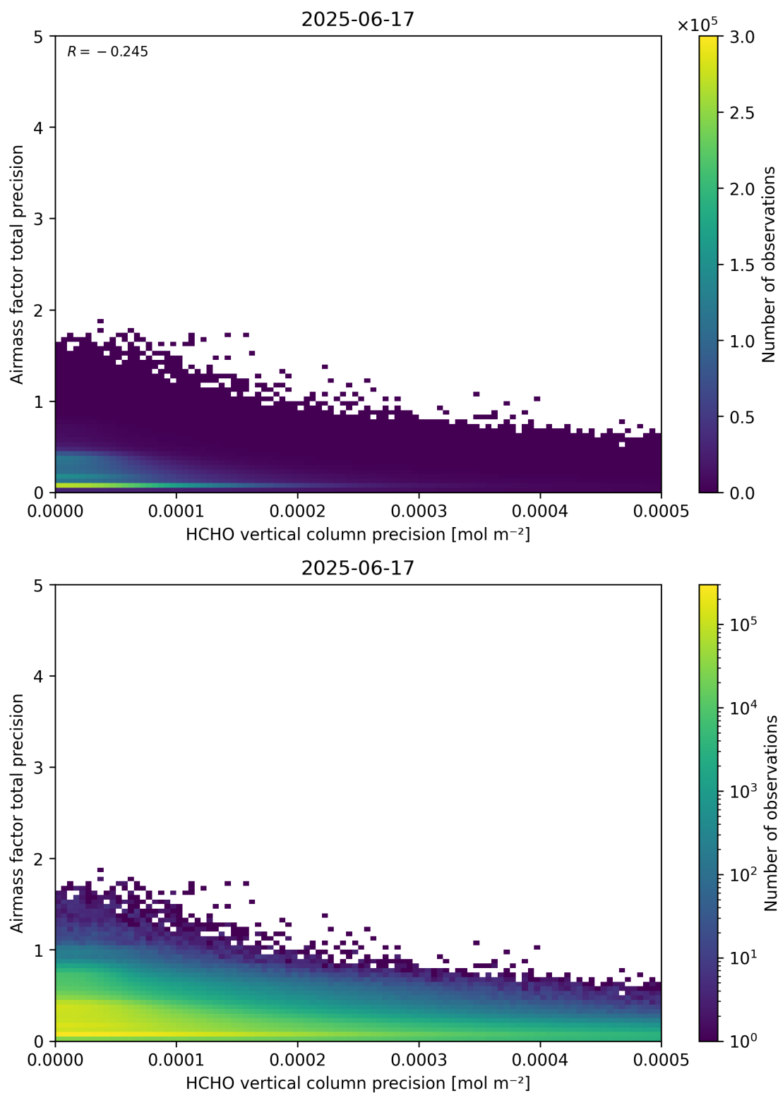
Figure 145: Scatter density plot of “HCHO vertical column precision” against “Airmass factor total precision” for 2025-06-17 to 2025-06-18.
