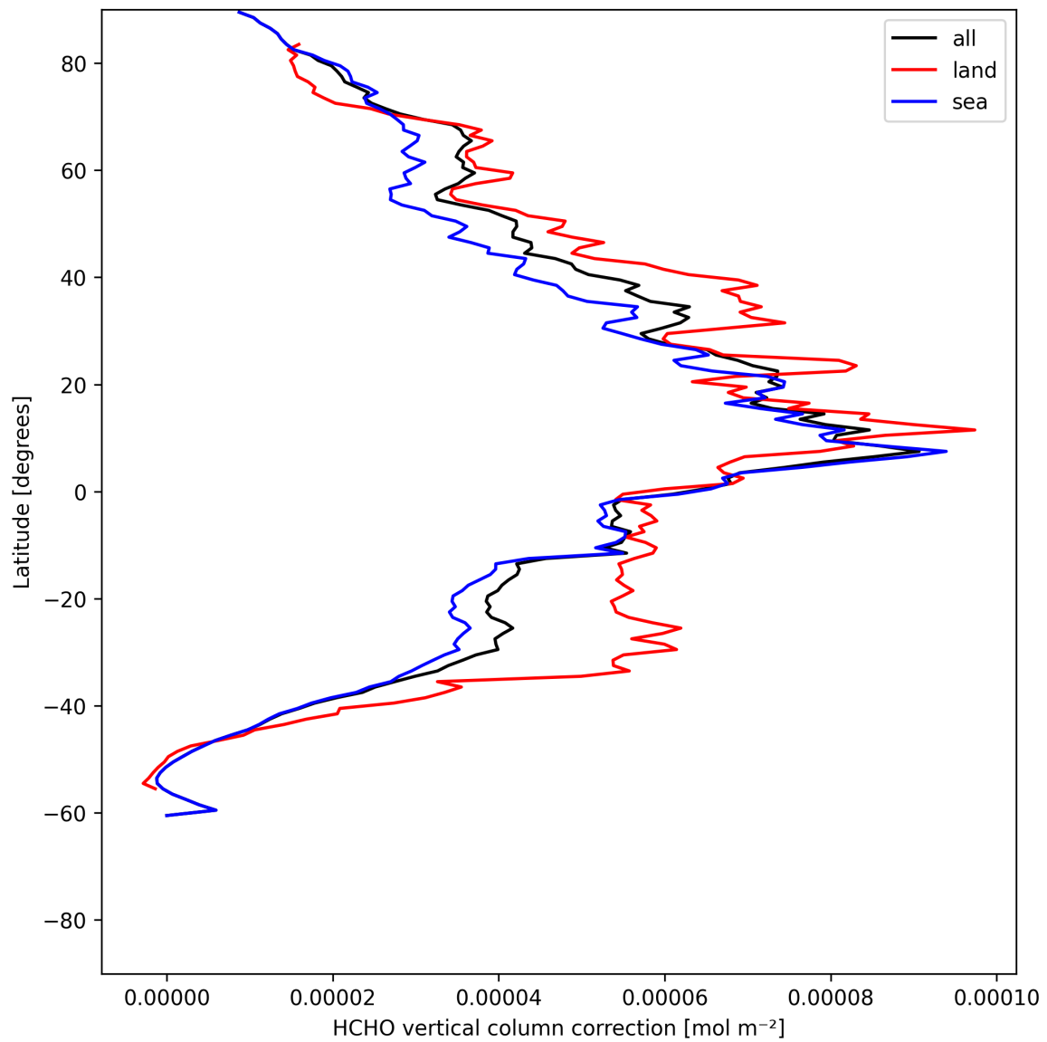
Figure 23: Zonal average of “HCHO vertical column correction” for 2025-06-17 to 2025-06-18.
