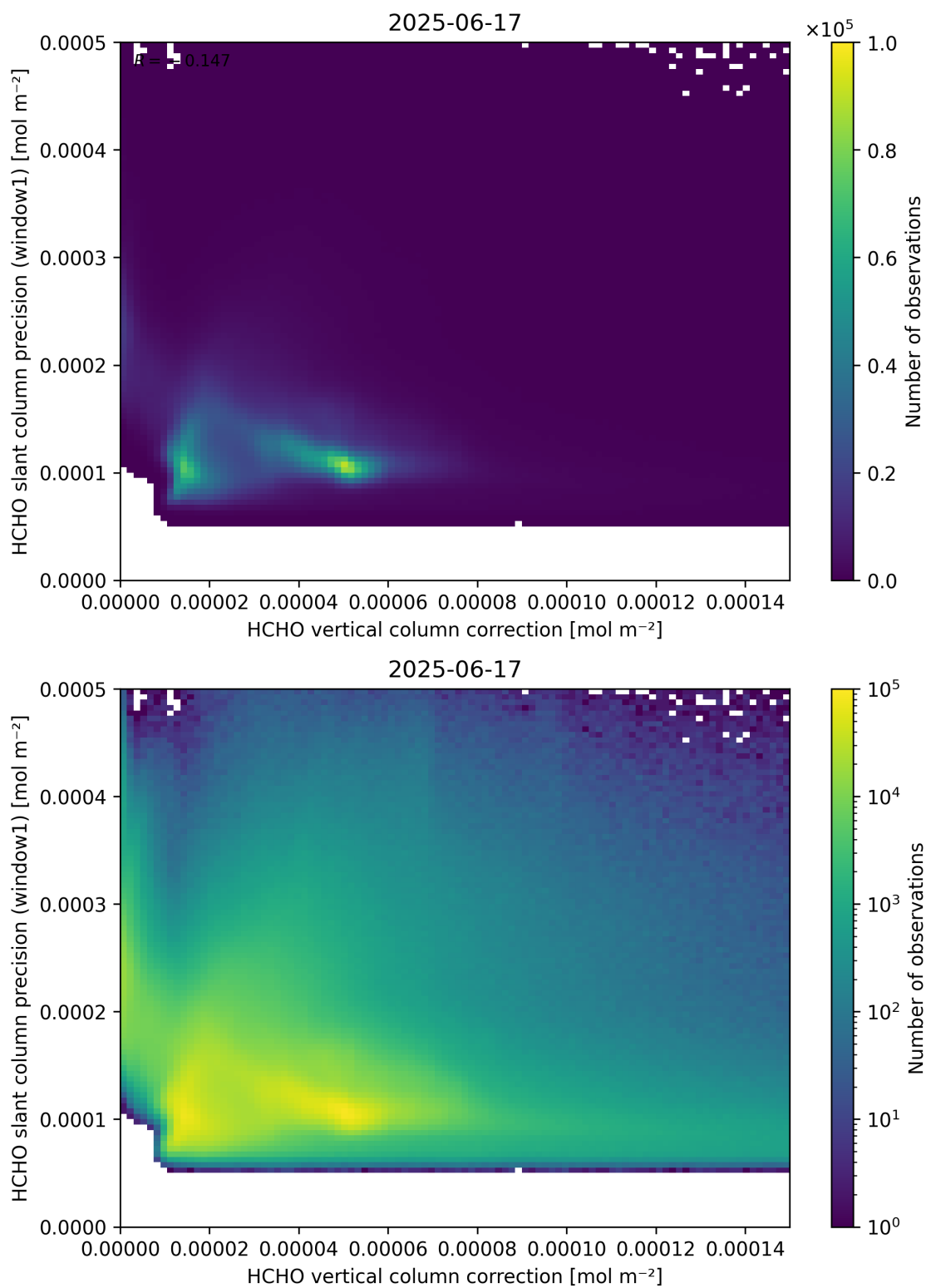
Figure 119: Scatter density plot of “HCHO vertical column correction” against “HCHO slant column precision (window1)” for 2025-06-17 to 2025-06-18.
