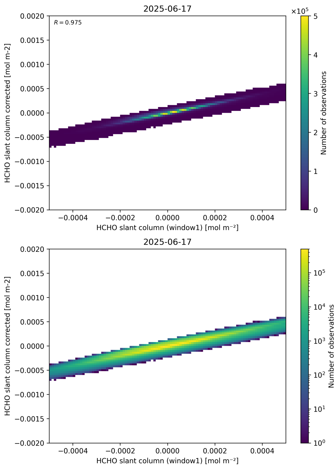
Figure 82: Scatter density plot of “HCHO slant column (window1)” against “HCHO slant column corrected” for 2025-06-17 to 2025-06-18.
