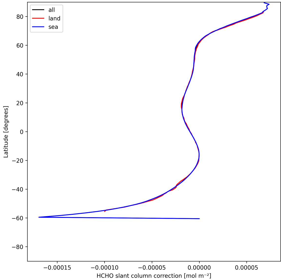
Figure 33: Zonal average of “HCHO slant column correction” for 2025-06-17 to 2025-06-18.
