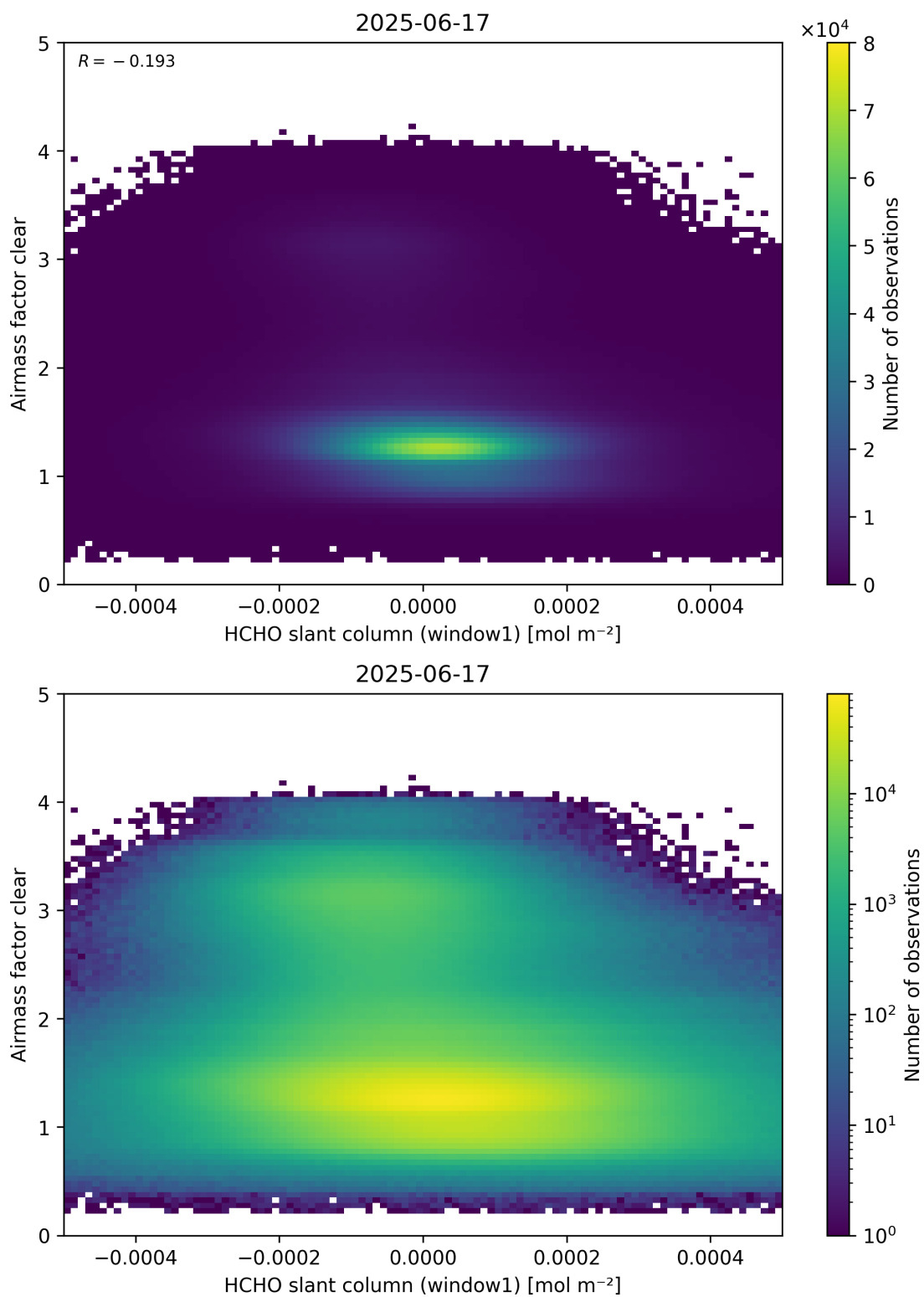
Figure 81: Scatter density plot of “HCHO slant column (window1)” against “Airmass factor clear” for 2025-06-17 to 2025-06-18.
