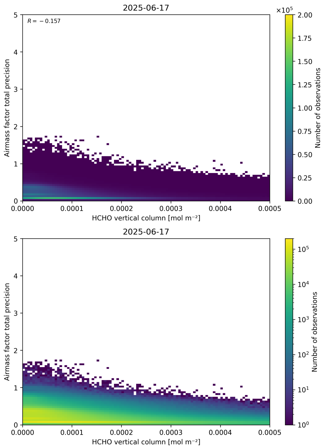
Figure 132: Scatter density plot of “HCHO vertical column” against “Airmass factor total precision” for 2025-06-17 to 2025-06-18.
