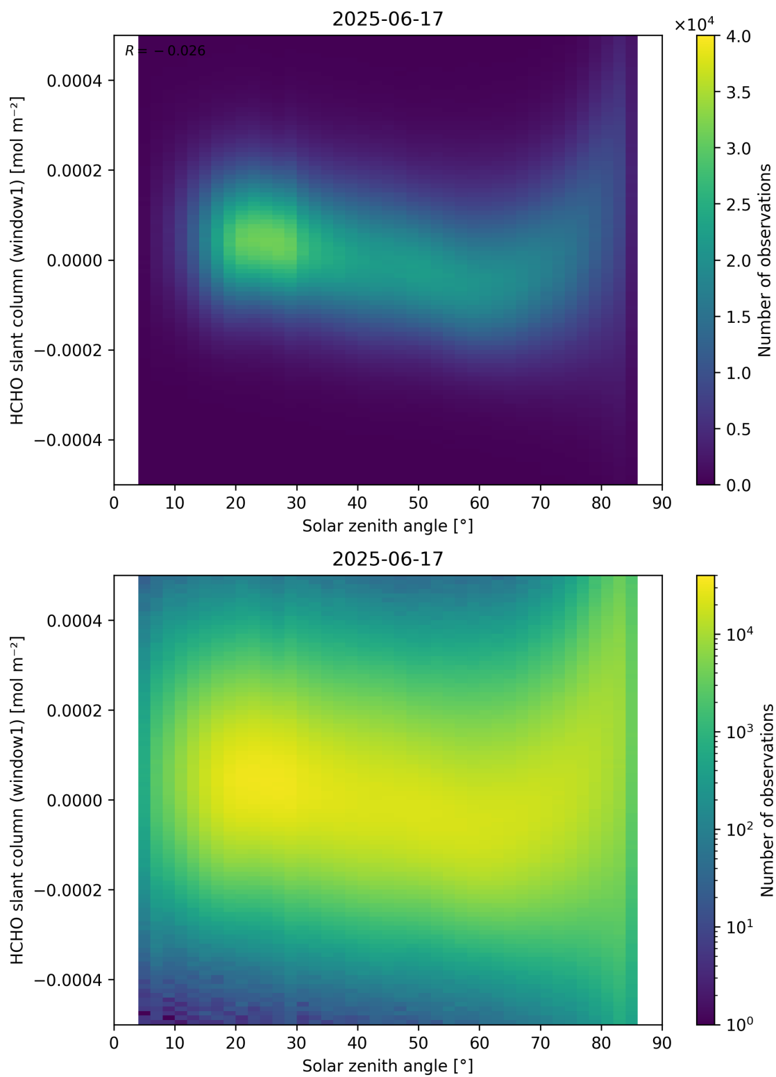
Figure 173: Scatter density plot of “Solar zenith angle” against “HCHO slant column (window1)” for 2025-06-17 to 2025-06-18.
