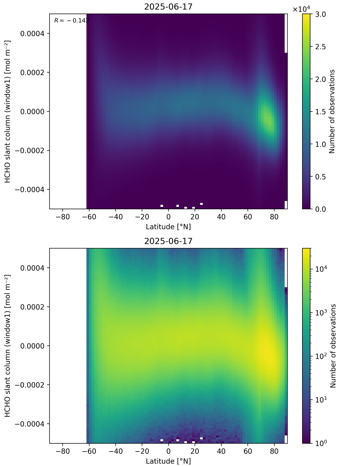
Figure 159: Scatter density plot of “Latitude” against “HCHO slant column (window1)” for 2025-06-17 to 2025-06-18.
