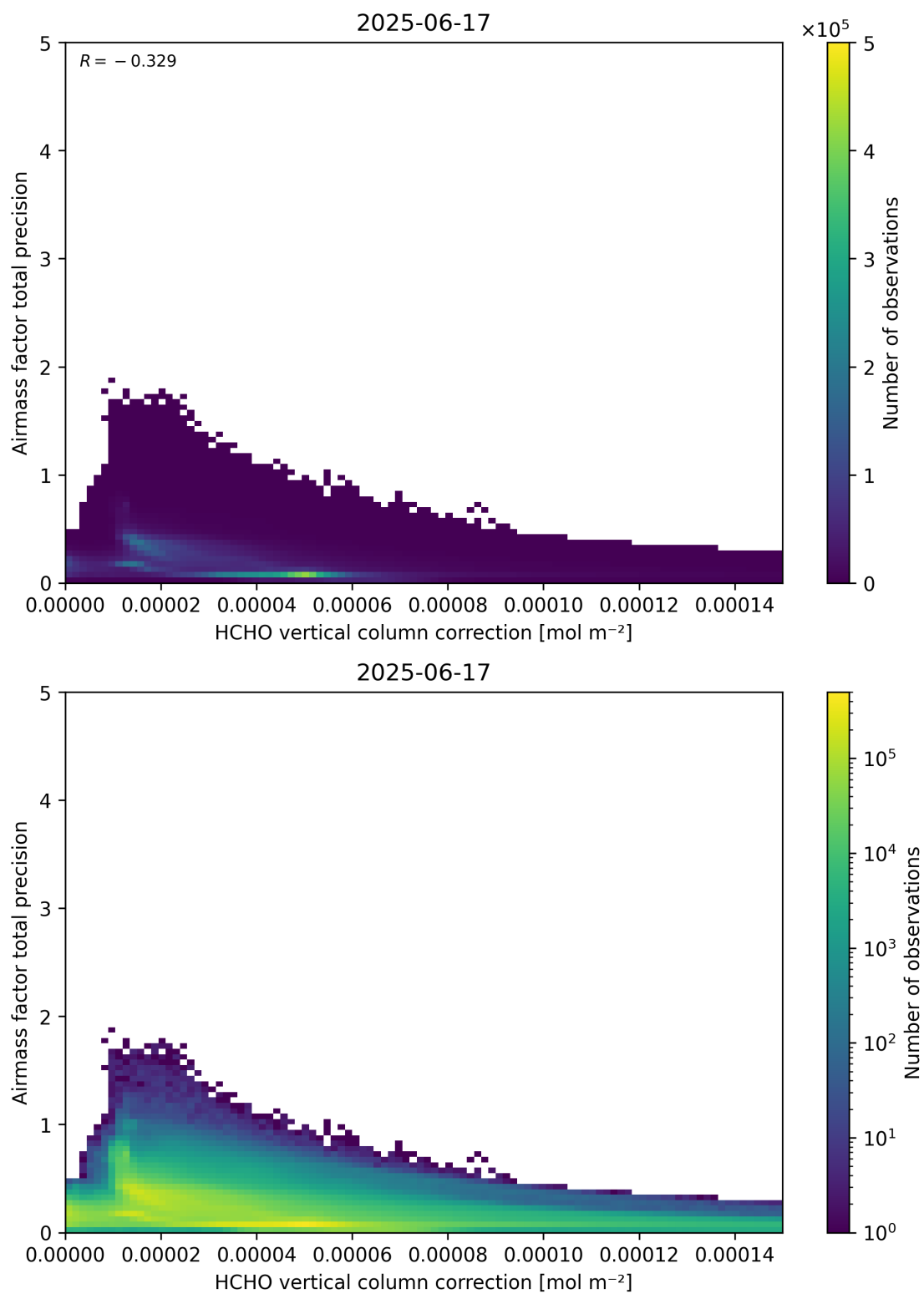
Figure 121: Scatter density plot of “HCHO vertical column correction” against “Airmass factor total precision” for 2025-06-17 to 2025-06-18.
