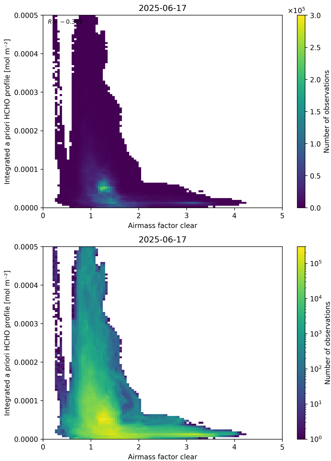
Figure 76: Scatter density plot of “Airmass factor clear” against “Integrated a priori HCHO profile” for 2025-06-17 to 2025-06-18.
