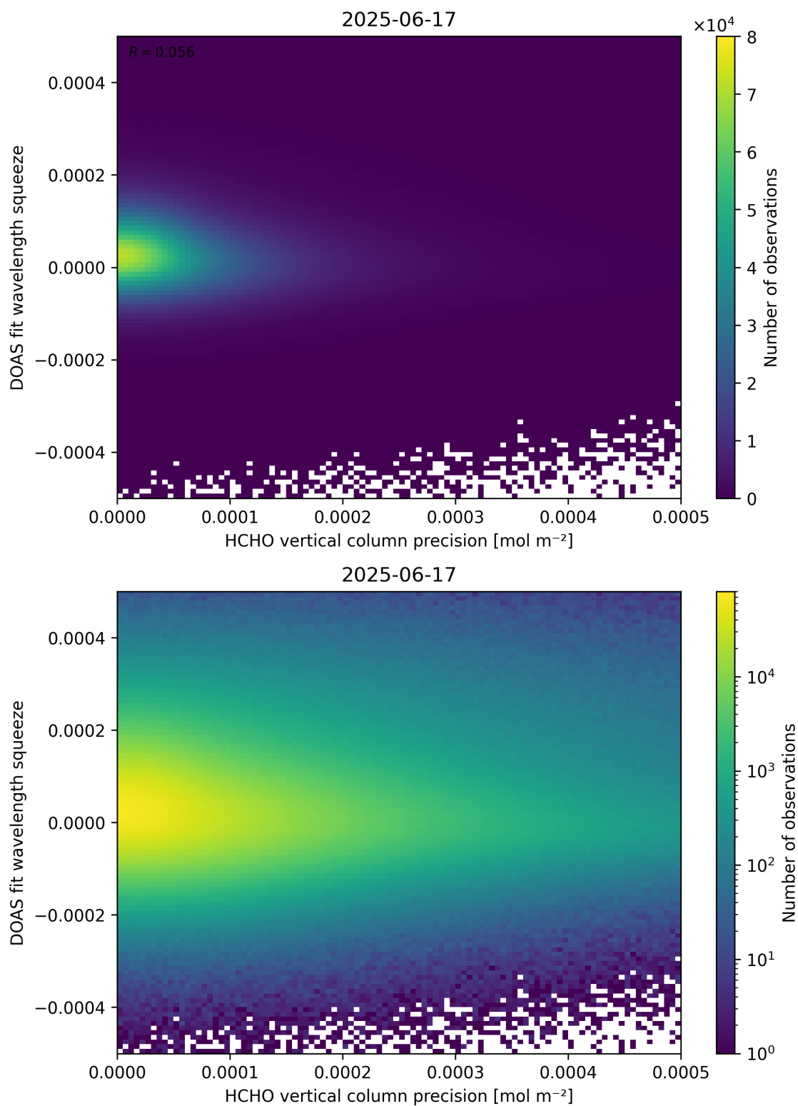
Figure 138: Scatter density plot of “HCHO vertical column precision” against “DOAS fit wavelength squeeze” for 2025-06-17 to 2025-06-18.
