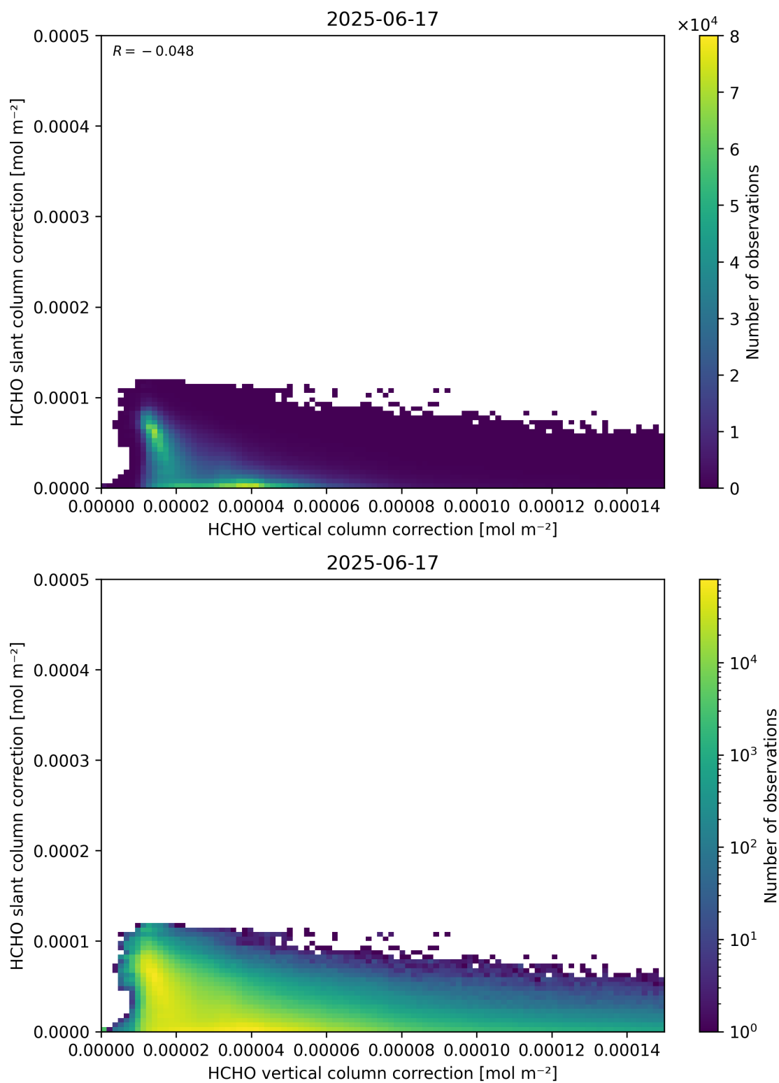
Figure 117: Scatter density plot of “HCHO vertical column correction” against “HCHO slant column correction” for 2025-06-17 to 2025-06-18.
