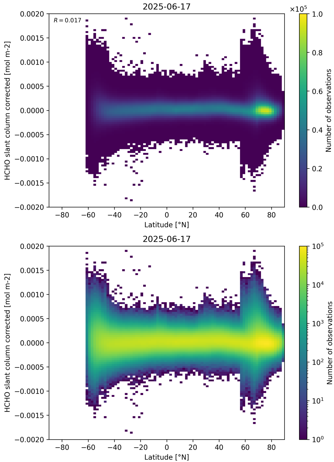
Figure 157: Scatter density plot of “Latitude” against “HCHO slant column corrected” for 2025-06-17 to 2025-06-18.
