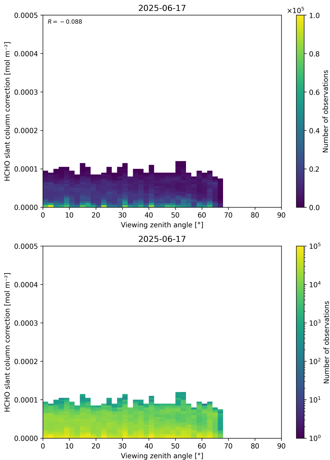
Figure 187: Scatter density plot of “Viewing zenith angle” against “HCHO slant column correction” for 2025-06-17 to 2025-06-18.
