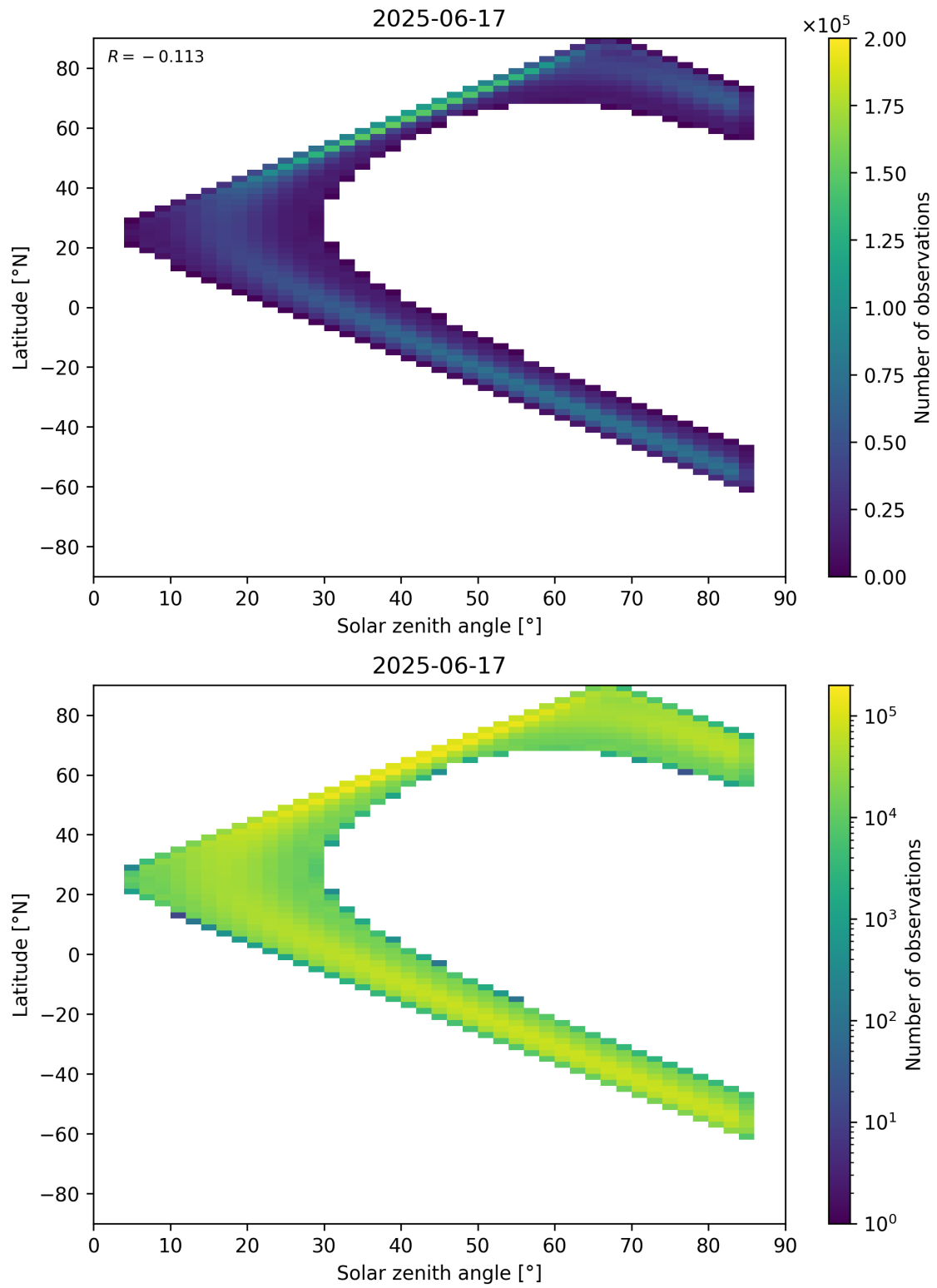
Figure 181: Scatter density plot of “Solar zenith angle” against “Latitude” for 2025-06-17 to 2025-06-18.
