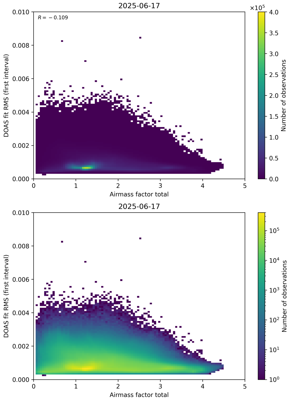
Figure 97: Scatter density plot of “Airmass factor total” against “DOAS fit RMS (first interval)” for 2025-06-17 to 2025-06-18.
