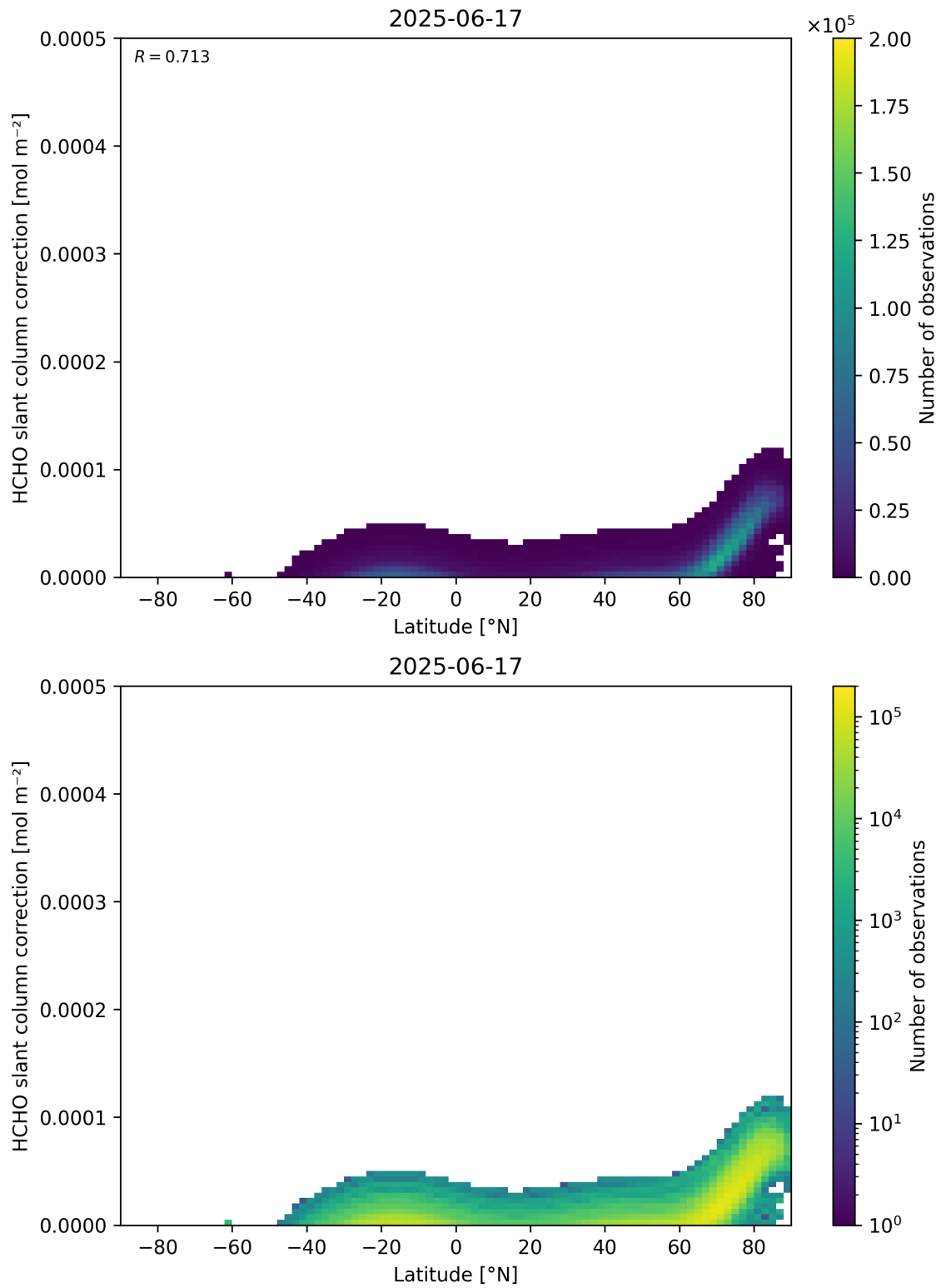
Figure 158: Scatter density plot of “Latitude” against “HCHO slant column correction” for 2025-06-17 to 2025-06-18.
