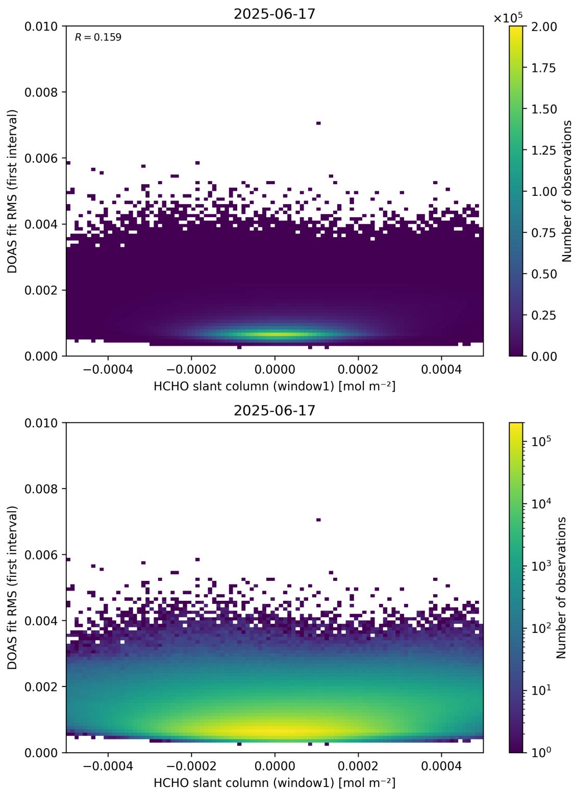
Figure 78: Scatter density plot of “HCHO slant column (window1)” against “DOAS fit RMS (first interval)” for 2025-06-17 to 2025-06-18.
