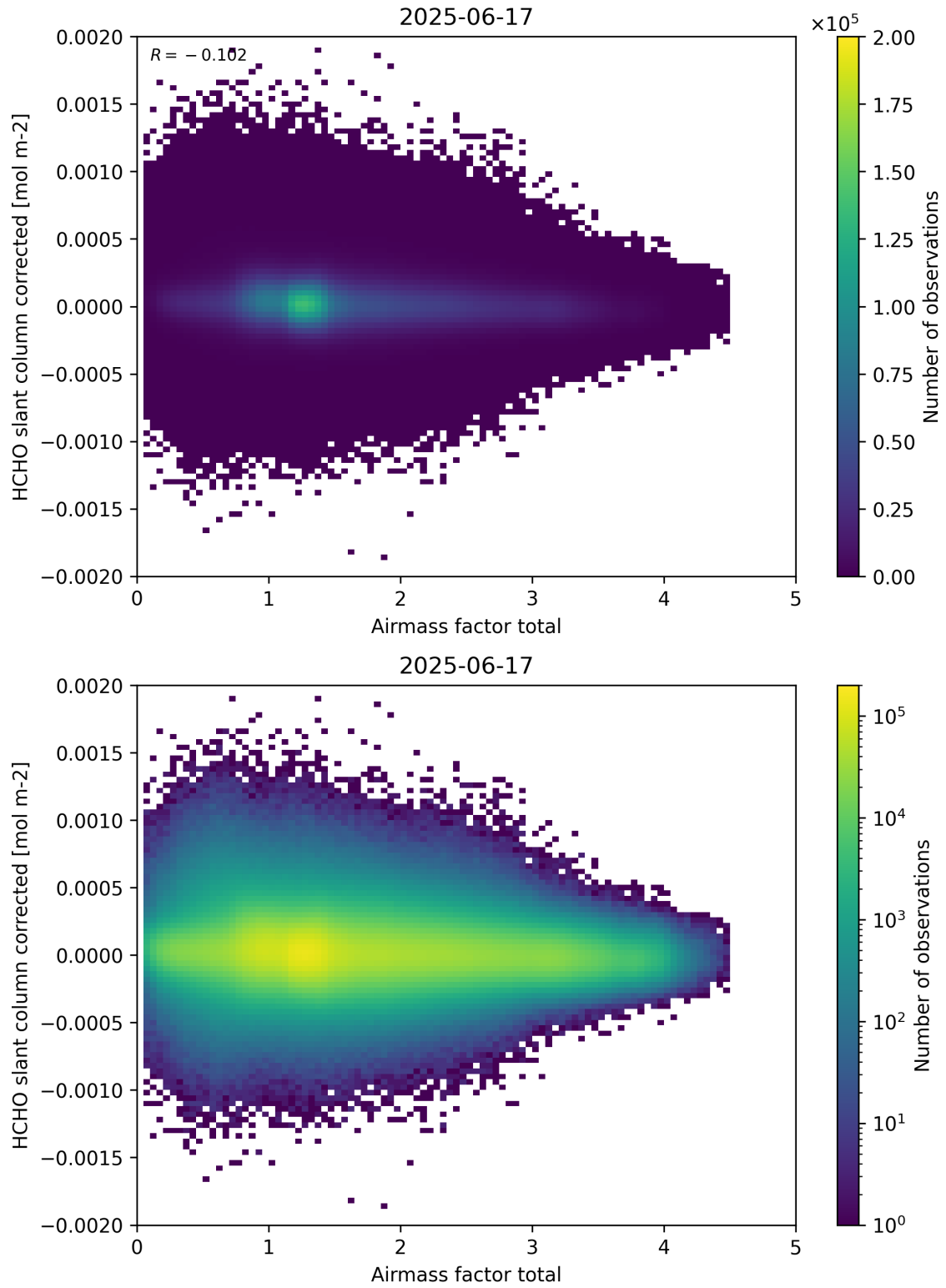
Figure 101: Scatter density plot of “Airmass factor total” against “HCHO slant column corrected” for 2025-06-17 to 2025-06-18.
