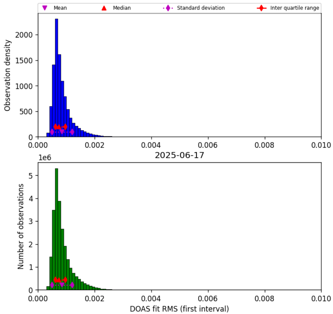
Figure 46: Histogram of “DOAS fit RMS (first interval)” for 2025-06-17 to 2025-06-18
