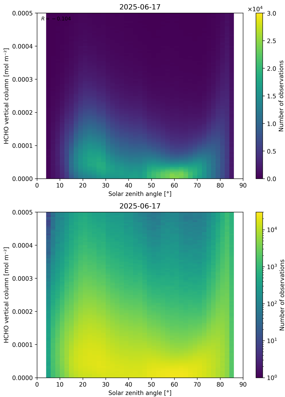
Figure 177: Scatter density plot of “Solar zenith angle” against “HCHO vertical column” for 2025-06-17 to 2025-06-18.
