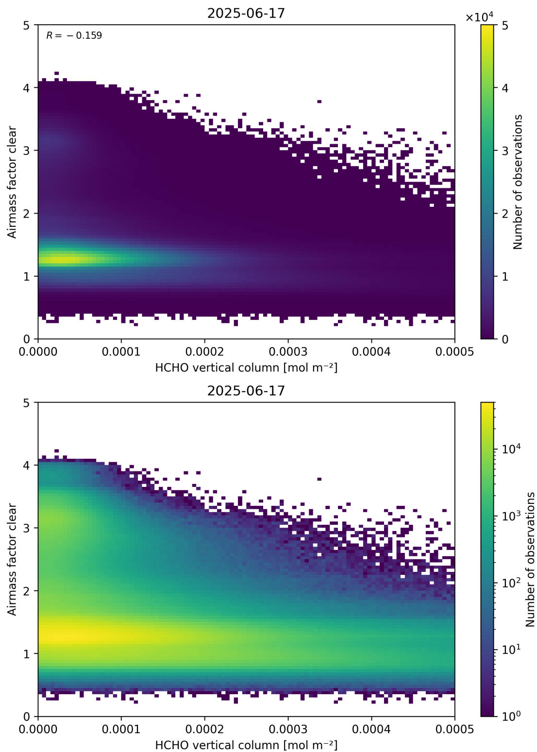
Figure 126: Scatter density plot of “HCHO vertical column” against “Airmass factor clear” for 2025-06-17 to 2025-06-18.
