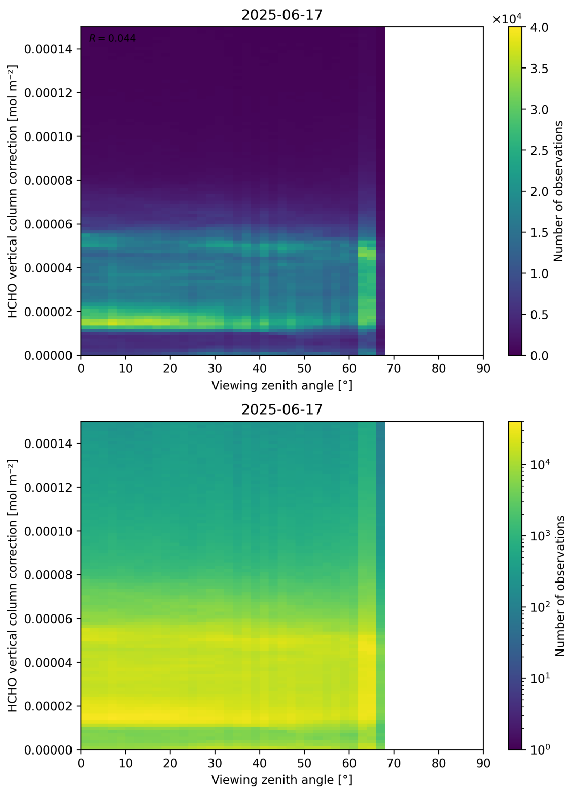
Figure 193: Scatter density plot of “Viewing zenith angle” against “HCHO vertical column correction” for 2025-06-17 to 2025-06-18.
