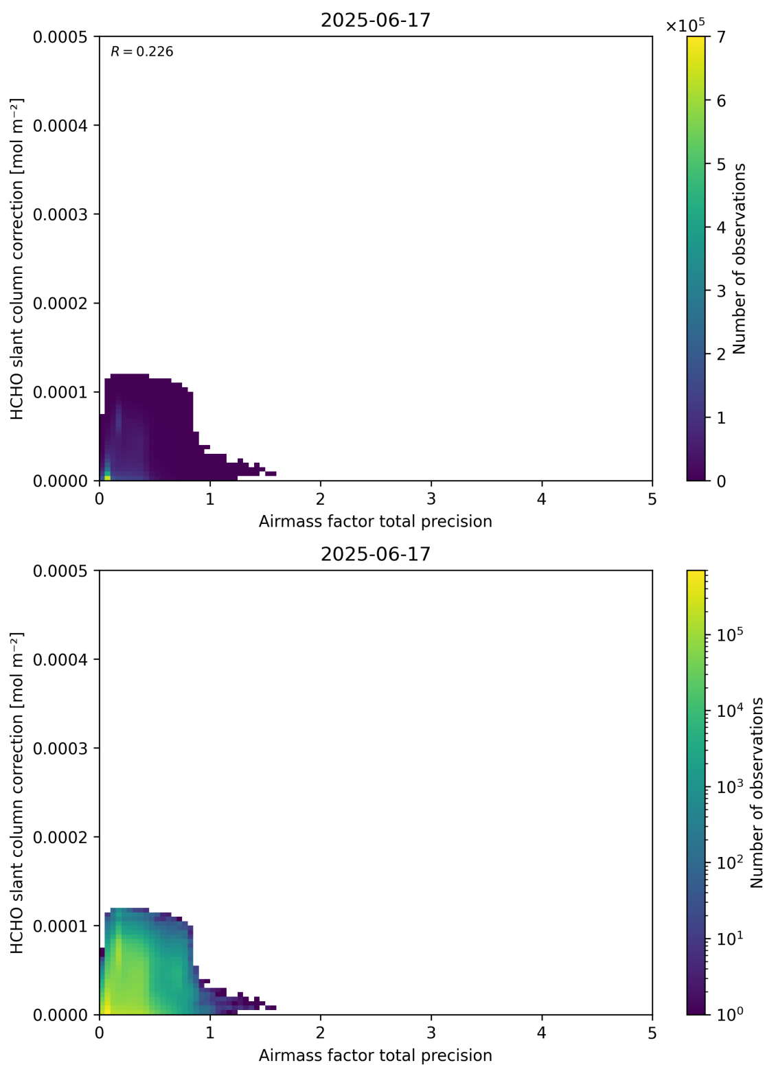
Figure 110: Scatter density plot of “Airmass factor total precision” against “HCHO slant column correction” for 2025-06-17 to 2025-06-18.
