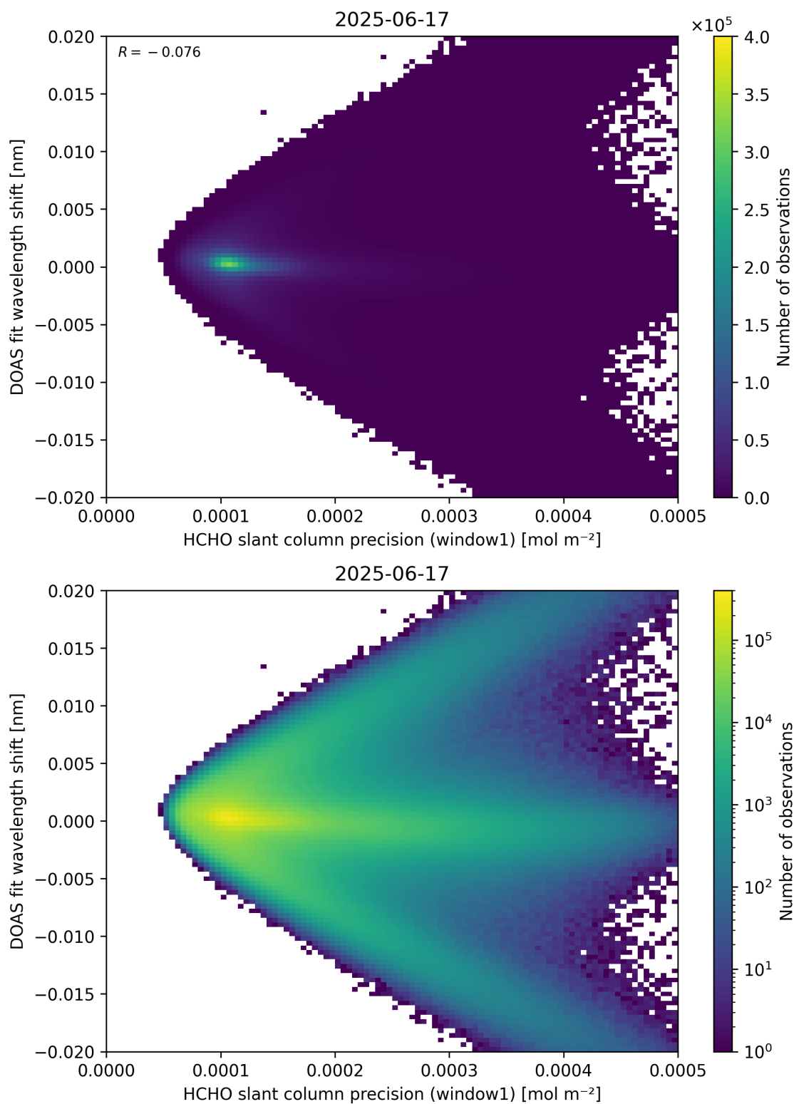
Figure 89: Scatter density plot of “HCHO slant column precision (window1)” against “DOAS fit wavelength shift” for 2025-06-17 to 2025-06-18.
