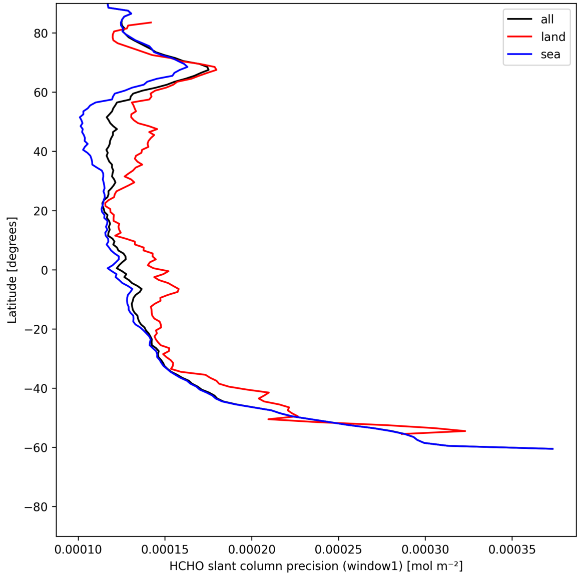
Figure 25: Zonal average of "HCHO slant column precision (window1)" for 2025-06-17 to 2025-06-18.
