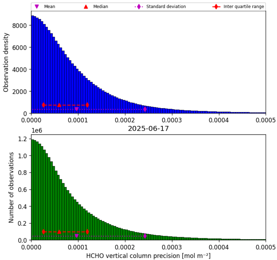
Figure 36: Histogram of “HCHO vertical column precision” for 2025-06-17 to 2025-06-18
