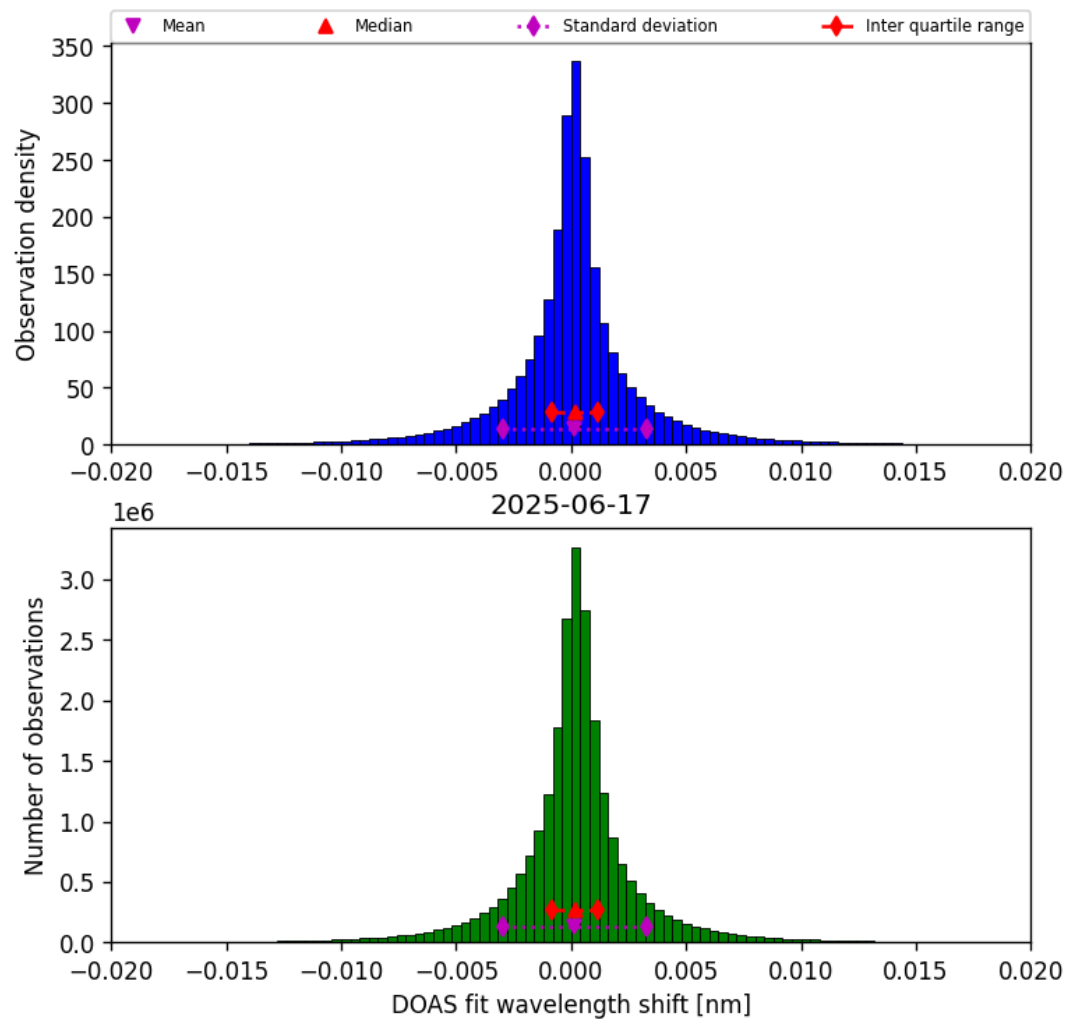
Figure 44: Histogram of “DOAS fit wavelength shift” for 2025-06-17 to 2025-06-18
