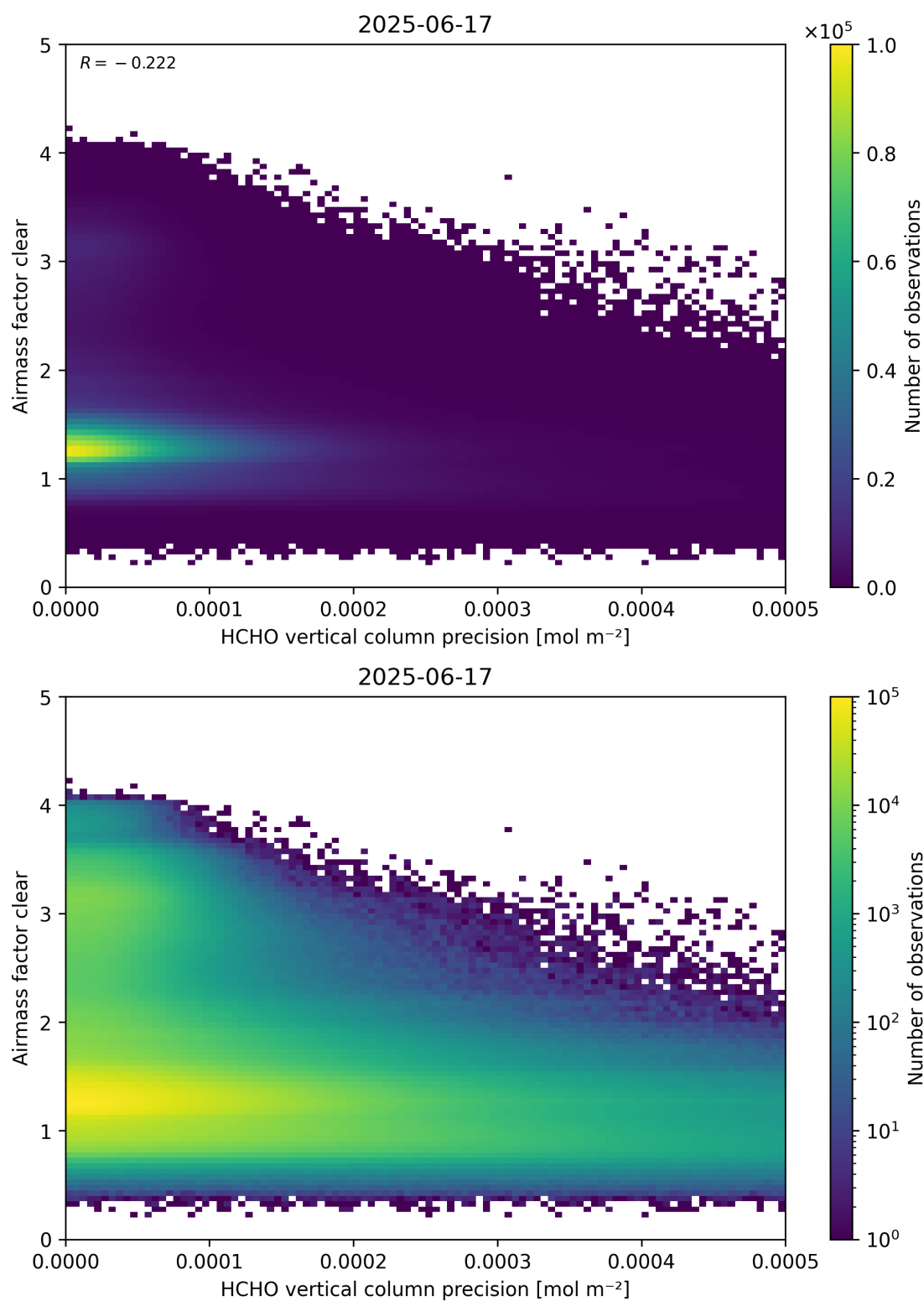
Figure 139: Scatter density plot of “HCHO vertical column precision” against “Airmass factor clear” for 2025-06-17 to 2025-06-18.
