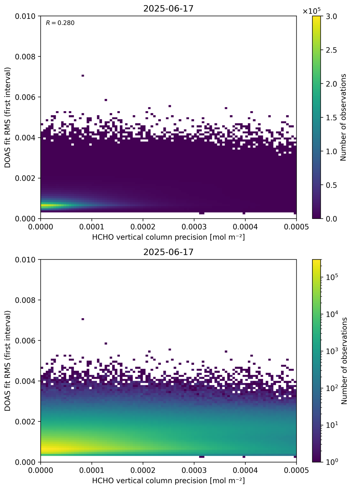
Figure 136: Scatter density plot of “HCHO vertical column precision” against “DOAS fit RMS (first interval)” for 2025-06-17 to 2025-06-18.
