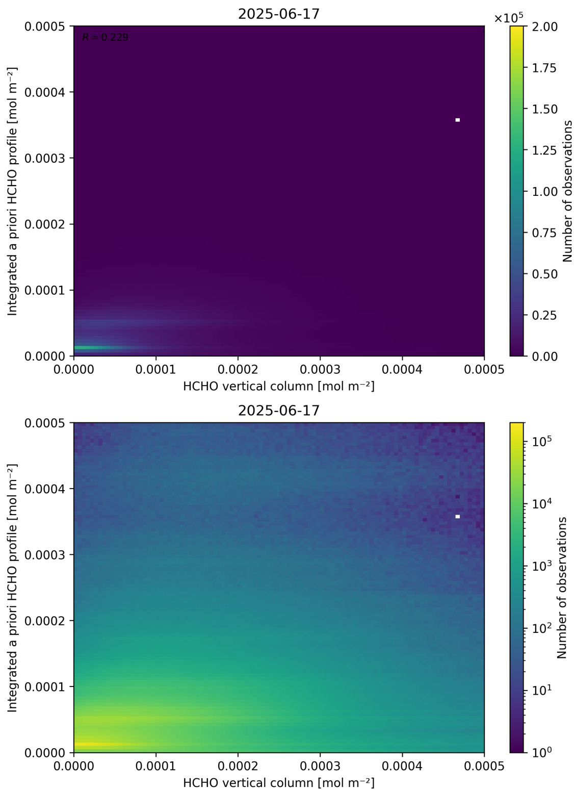
Figure 135: Scatter density plot of “HCHO vertical column” against “Integrated a priori HCHO profile” for 2025-06-17 to 2025-06-18.
