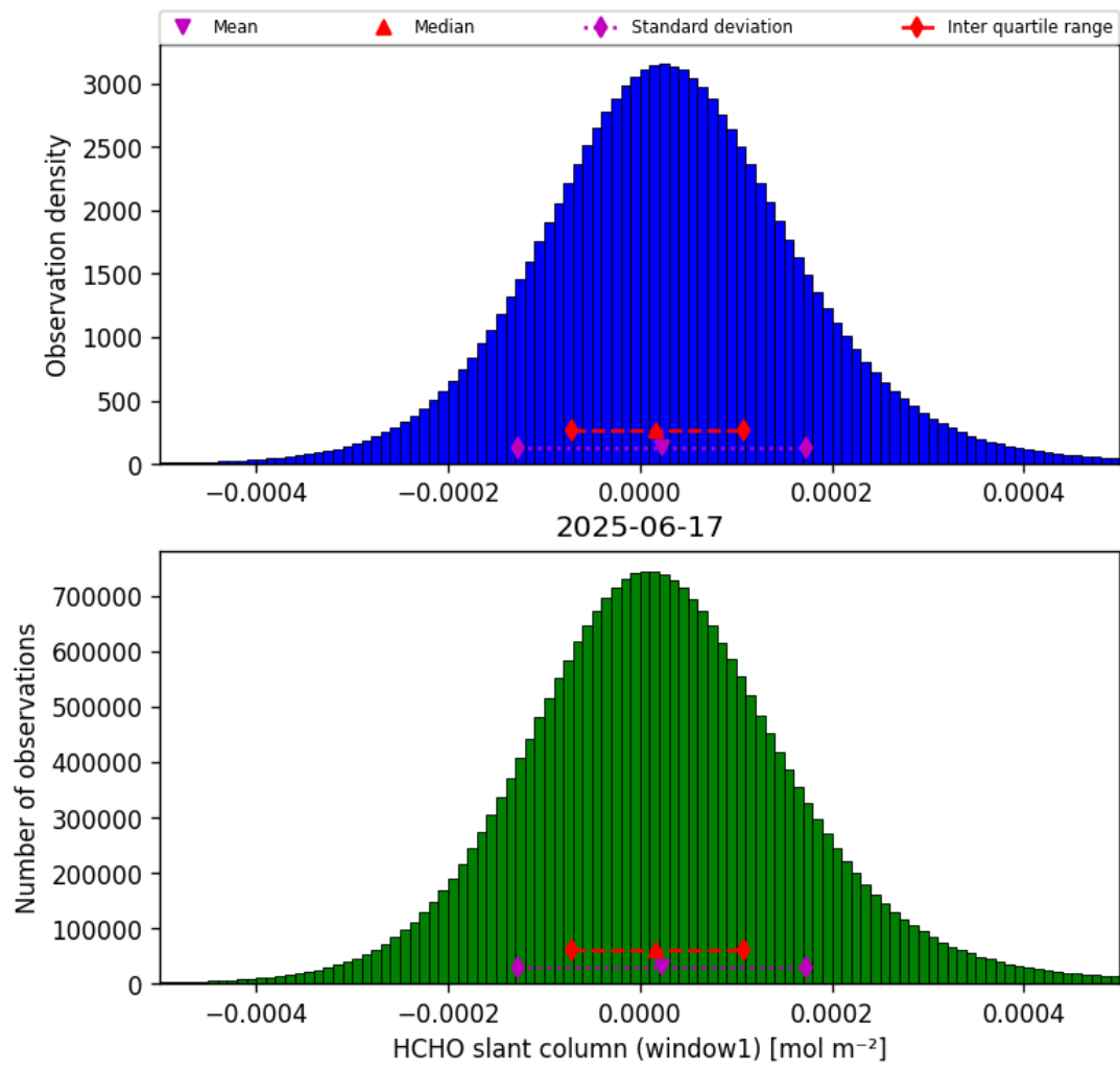
Figure 38: Histogram of “HCHO slant column (window1)” for 2025-06-17 to 2025-06-18
