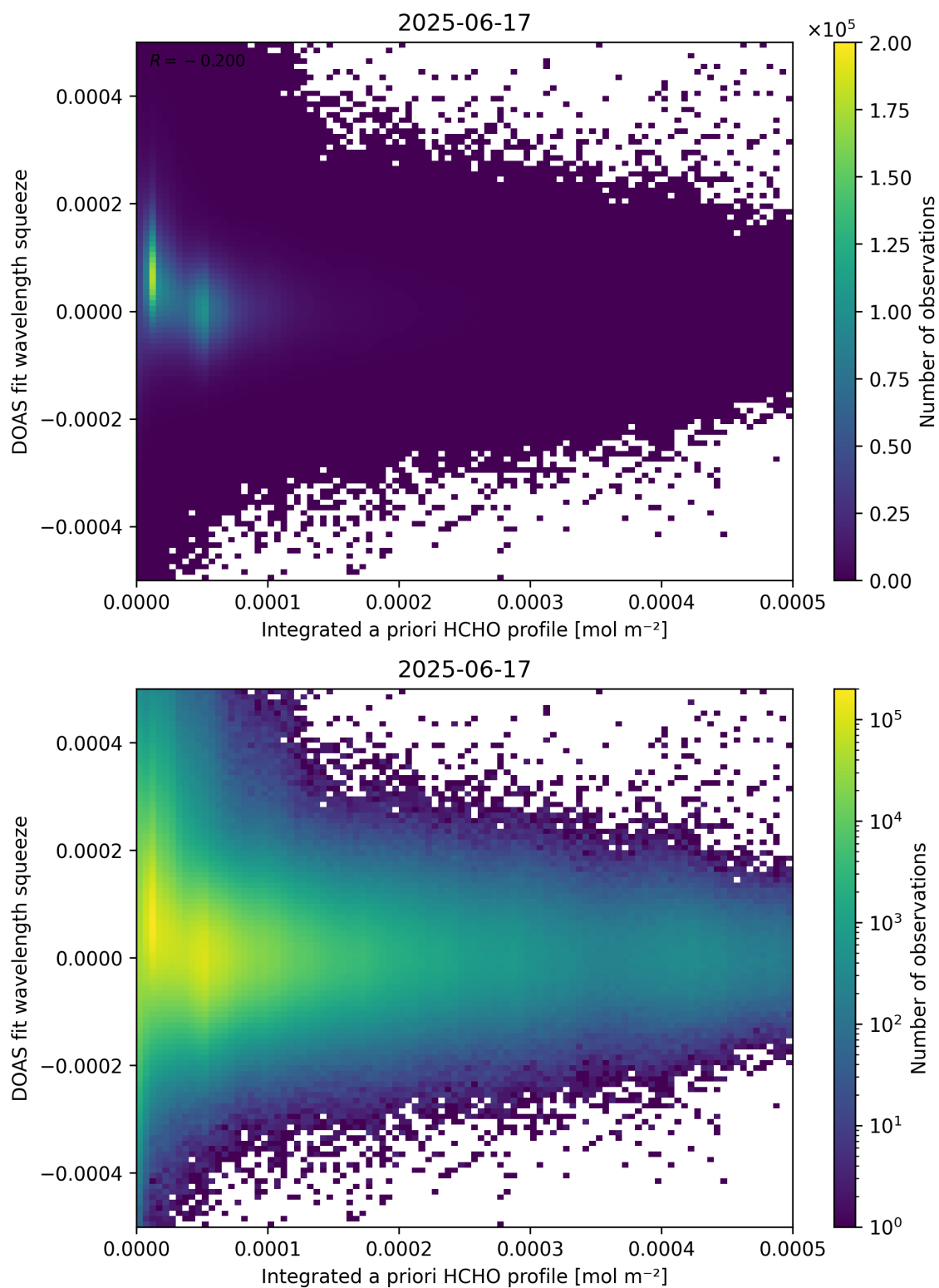
Figure 150: Scatter density plot of “Integrated a priori HCHO profile” against “DOAS fit wavelength squeeze” for 2025-06-17 to 2025-06-18.
