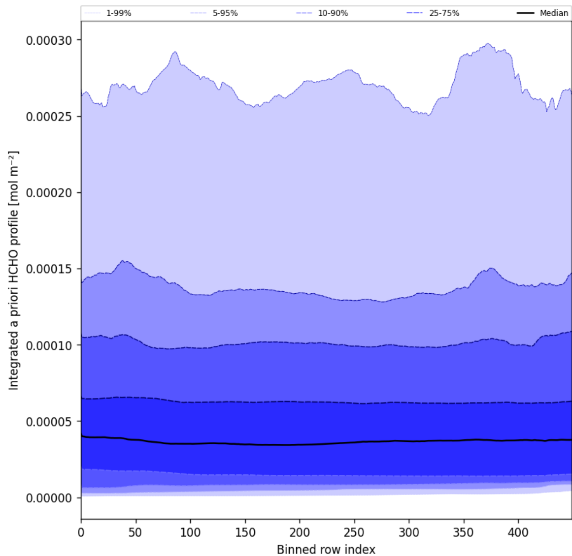
Figure 57: Along track statistics of "Integrated a priori HCHO profile" for 2025-06-17 to 2025-06-18
