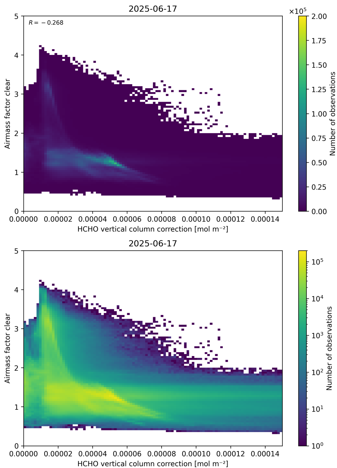
Figure 115: Scatter density plot of “HCHO vertical column correction” against “Airmass factor clear” for 2025-06-17 to 2025-06-18.
