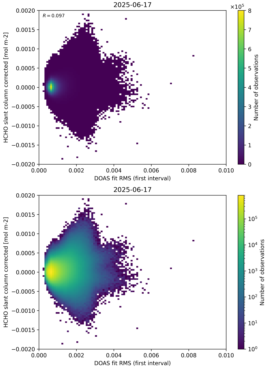
Figure 62: Scatter density plot of “DOAS fit RMS (first interval)” against “HCHO slant column corrected” for 2025-06-17 to 2025-06-18.
