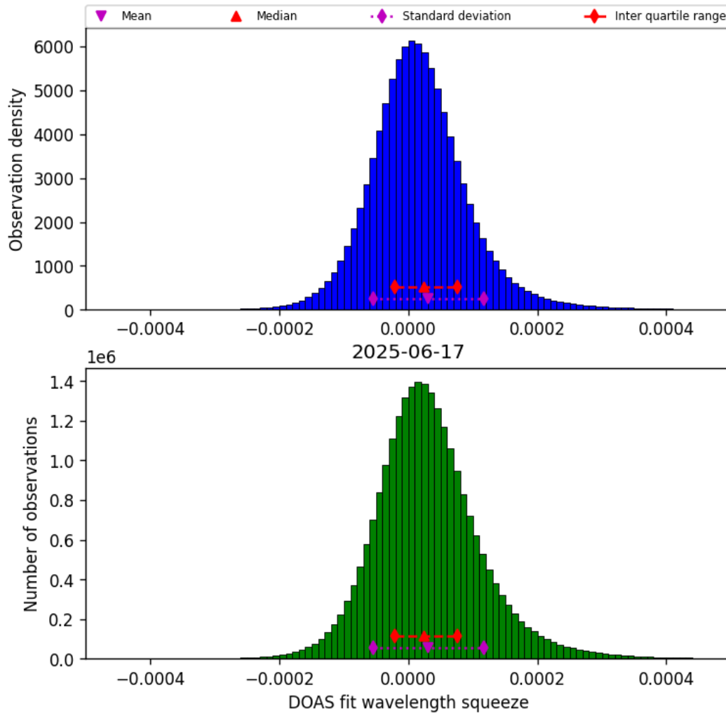
Figure 45: Histogram of “DOAS fit wavelength squeeze” for 2025-06-17 to 2025-06-18
