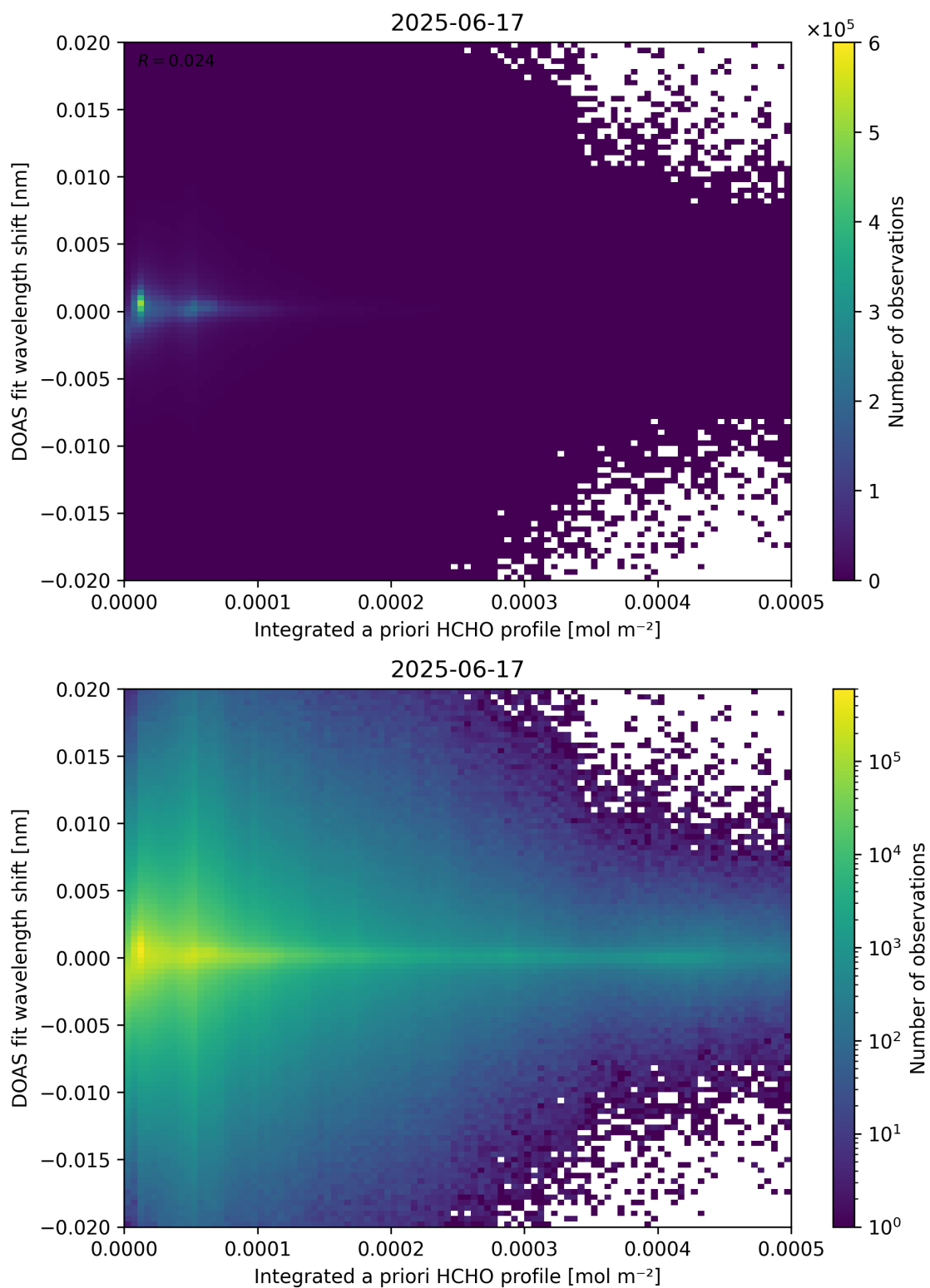
Figure 149: Scatter density plot of “Integrated a priori HCHO profile” against “DOAS fit wavelength shift” for 2025-06-17 to 2025-06-18.
