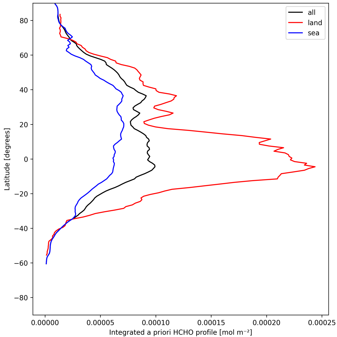
Figure 29: Zonal average of “Integrated a priori HCHO profile” for 2025-06-17 to 2025-06-18.
