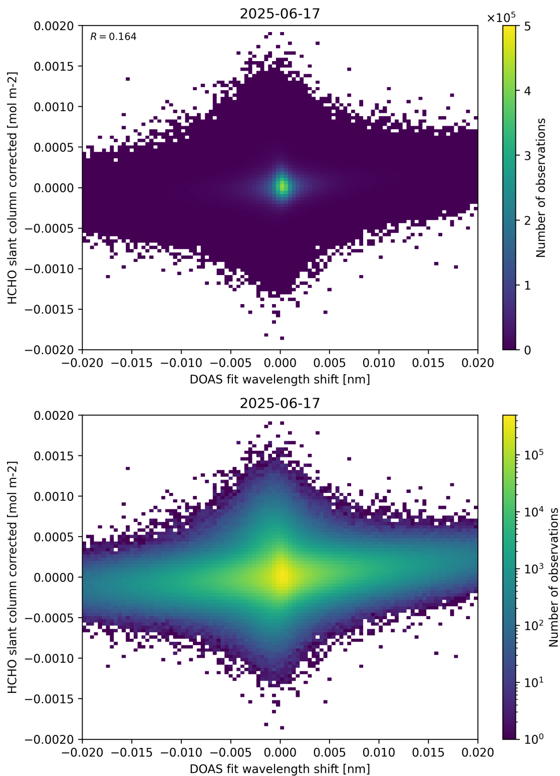
Figure 66: Scatter density plot of “DOAS fit wavelength shift” against “HCHO slant column corrected” for 2025-06-17 to 2025-06-18.
