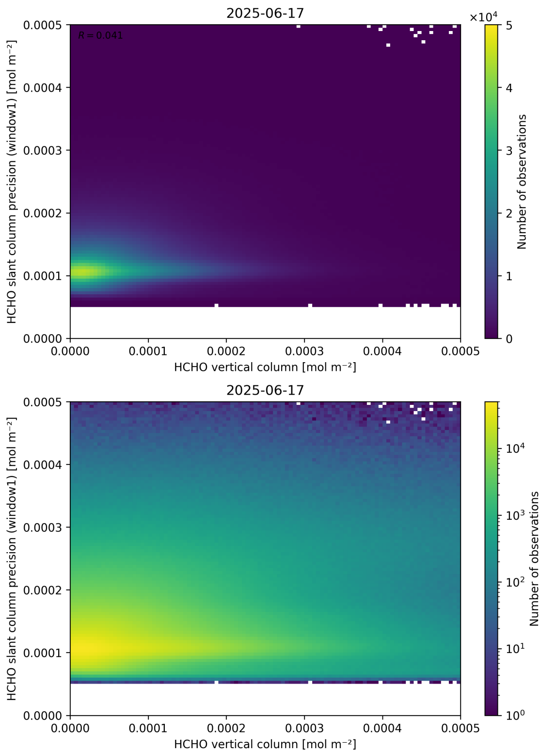
Figure 130: Scatter density plot of “HCHO vertical column” against “HCHO slant column precision (window1)” for 2025-06-17 to 2025-06-18.
