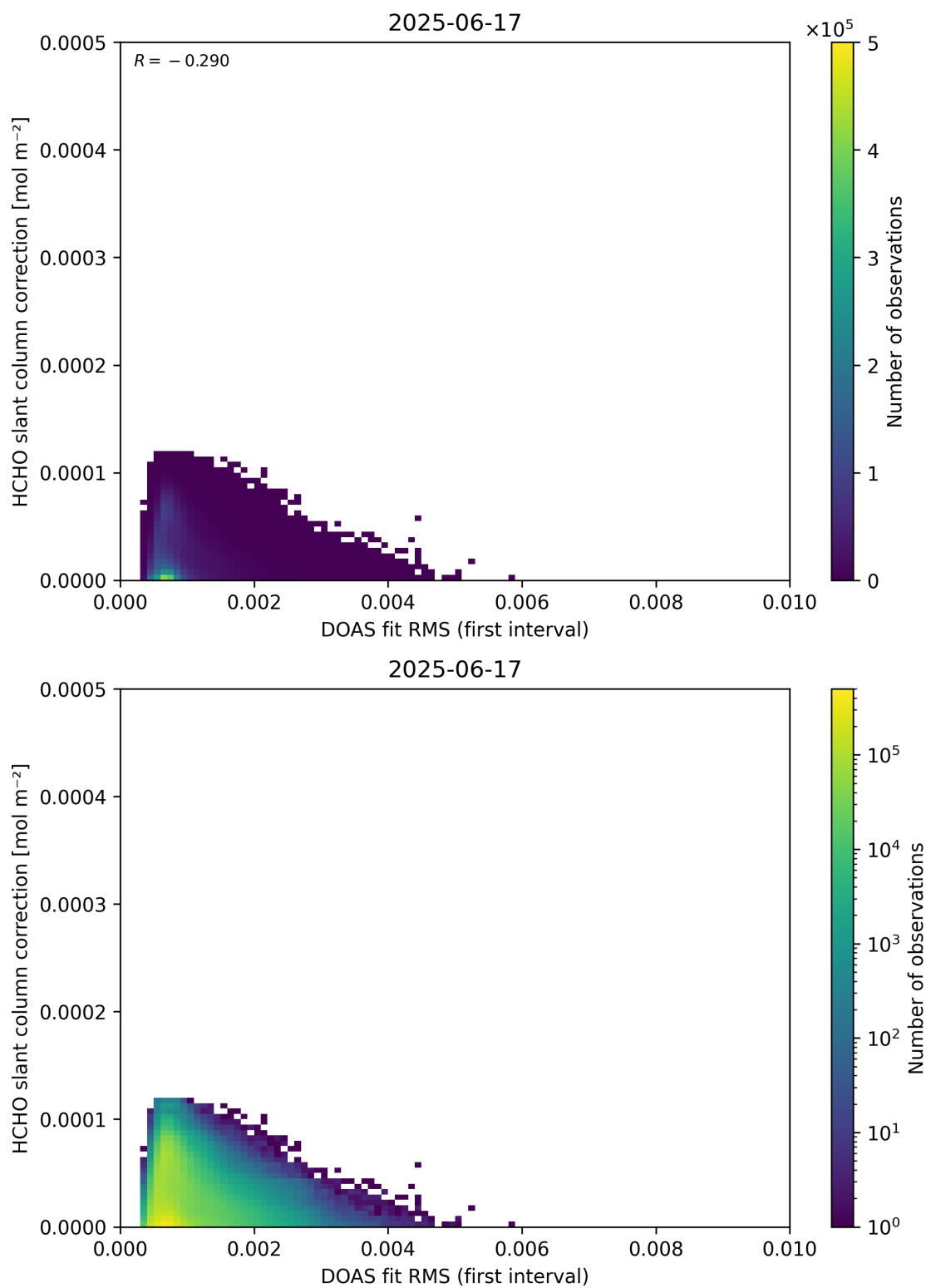
Figure 63: Scatter density plot of “DOAS fit RMS (first interval)” against “HCHO slant column correction” for 2025-06-17 to 2025-06-18.
