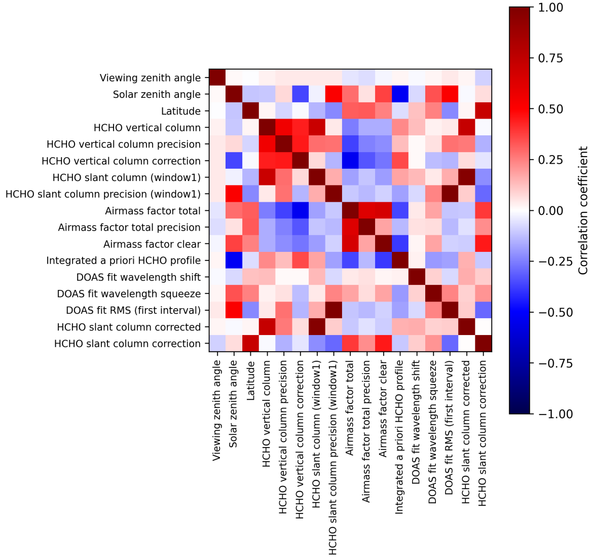
Figure 2: Map of correlation matrix for 2025-06-17 to 2025-06-18.
