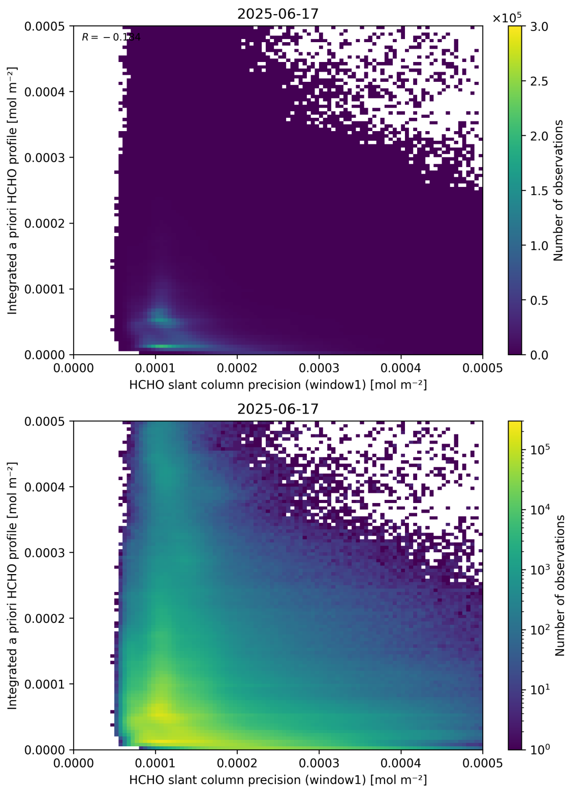
Figure 96: Scatter density plot of “HCHO slant column precision (window1)” against “Integrated a priori HCHO profile” for 2025-06-17 to 2025-06-18.
