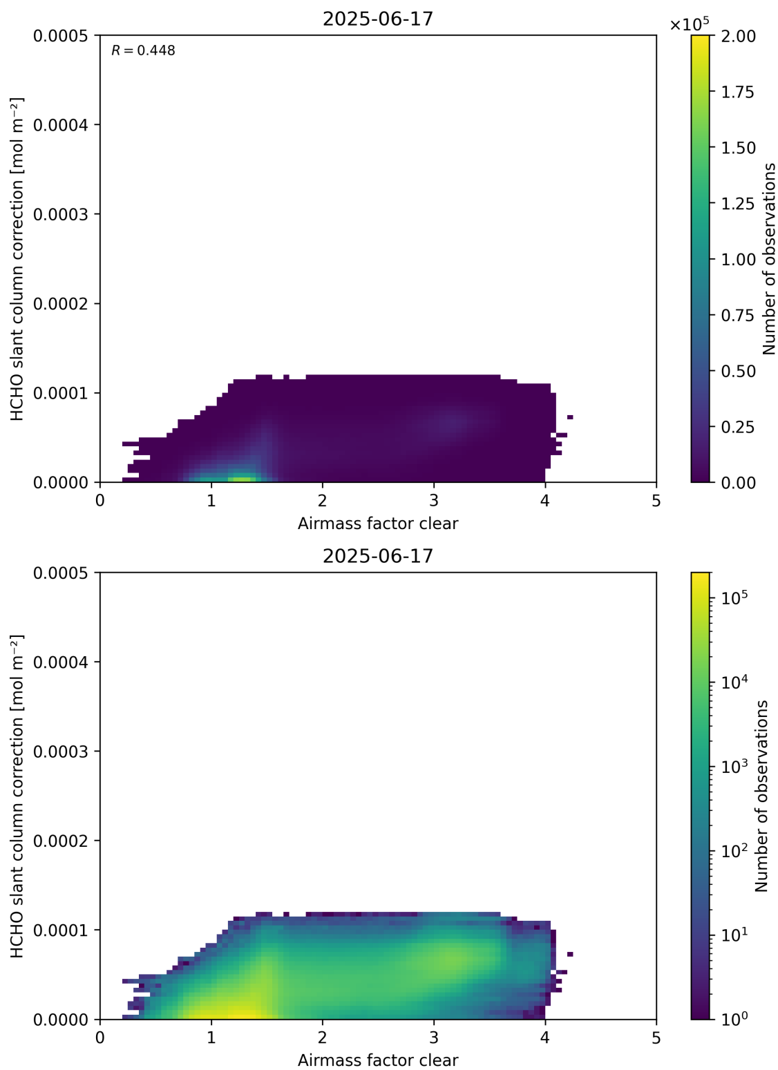
Figure 75: Scatter density plot of “Airmass factor clear” against “HCHO slant column correction” for 2025-06-17 to 2025-06-18.
