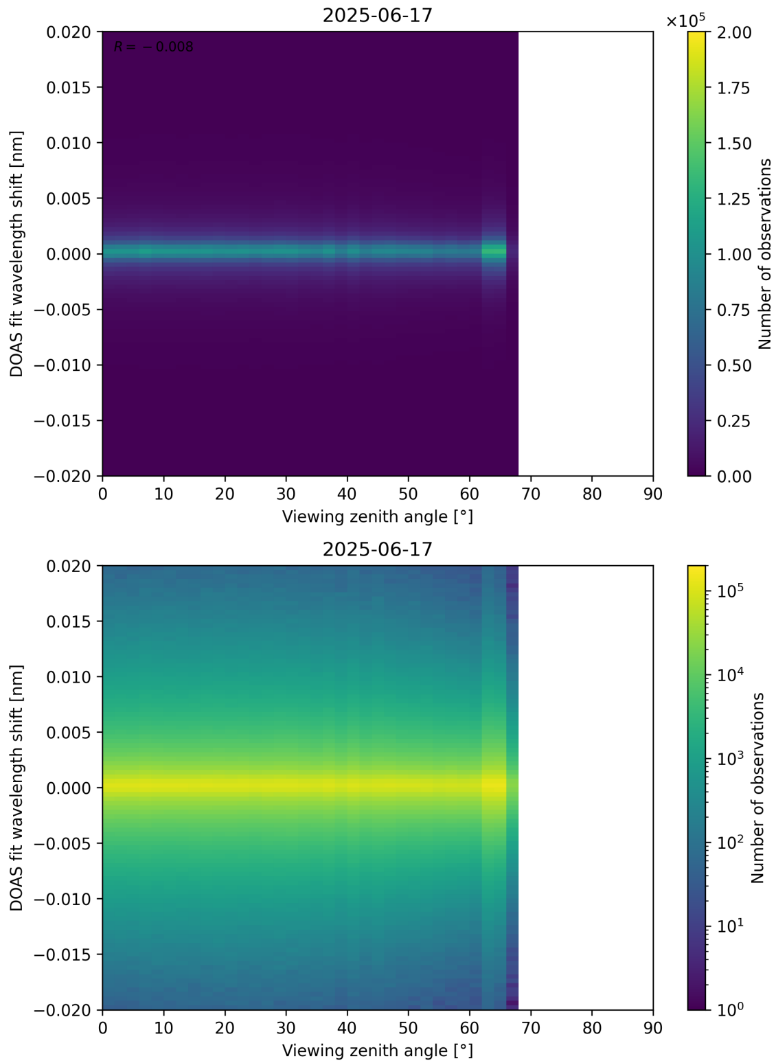
Figure 183: Scatter density plot of “Viewing zenith angle” against “DOAS fit wavelength shift” for 2025-06-17 to 2025-06-18.
