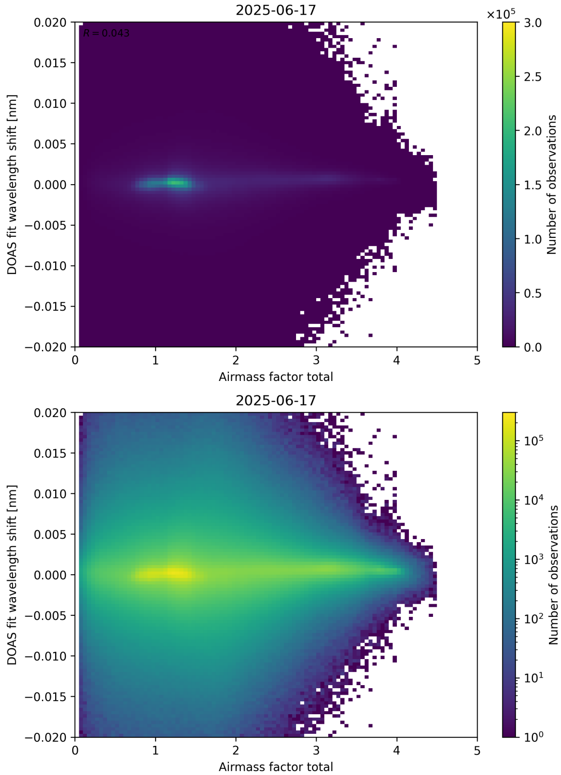
Figure 98: Scatter density plot of “Airmass factor total” against “DOAS fit wavelength shift” for 2025-06-17 to 2025-06-18.
