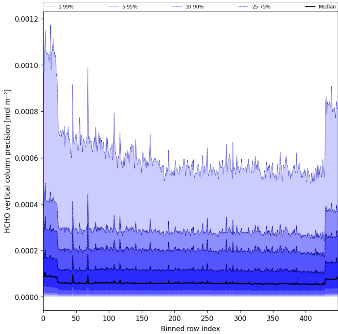
Figure 50: Along track statistics of “HCHO vertical column precision” for 2025-06-17 to 2025-06-18
