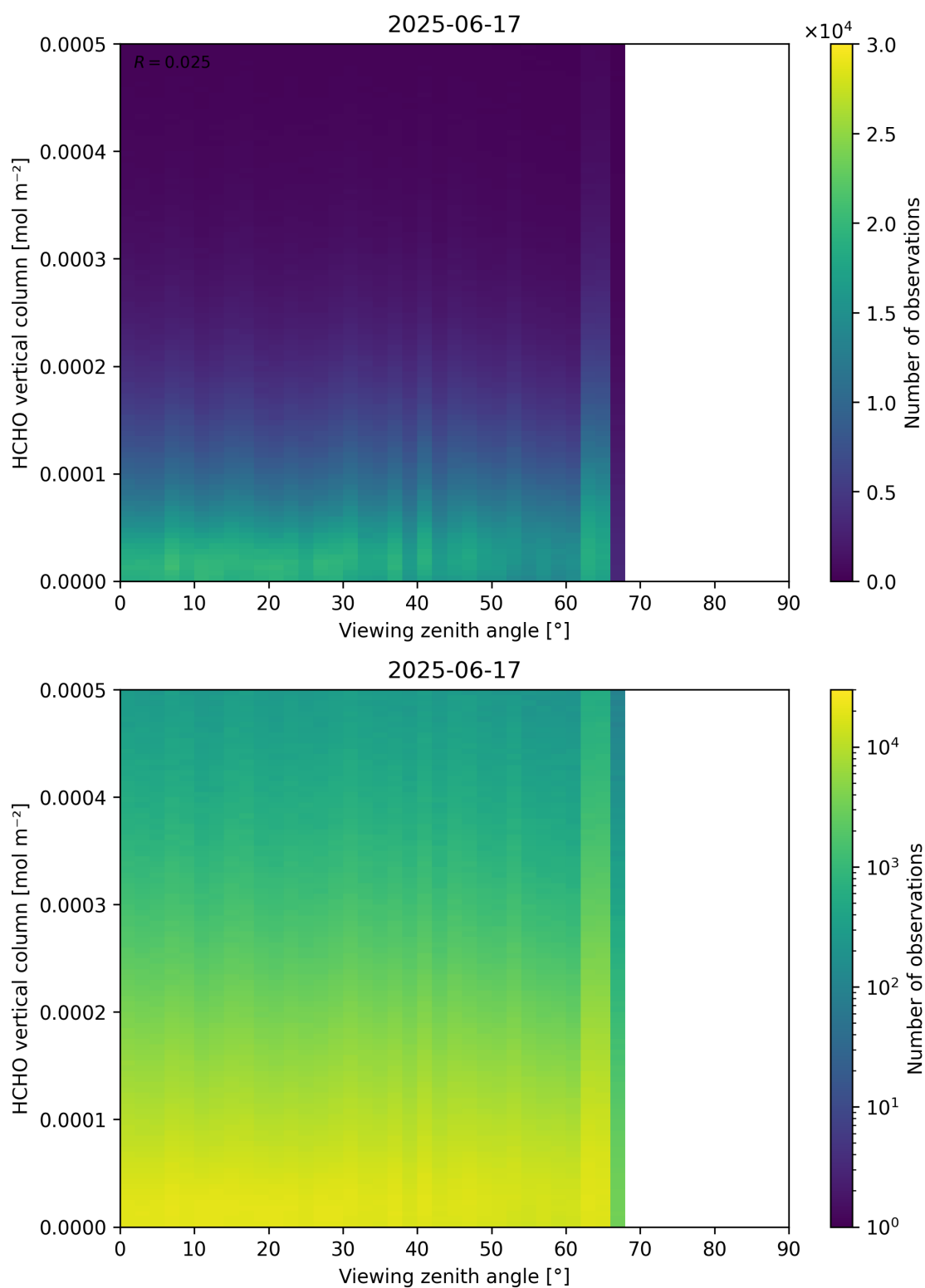
Figure 192: Scatter density plot of “Viewing zenith angle” against “HCHO vertical column” for 2025-06-17 to 2025-06-18.
