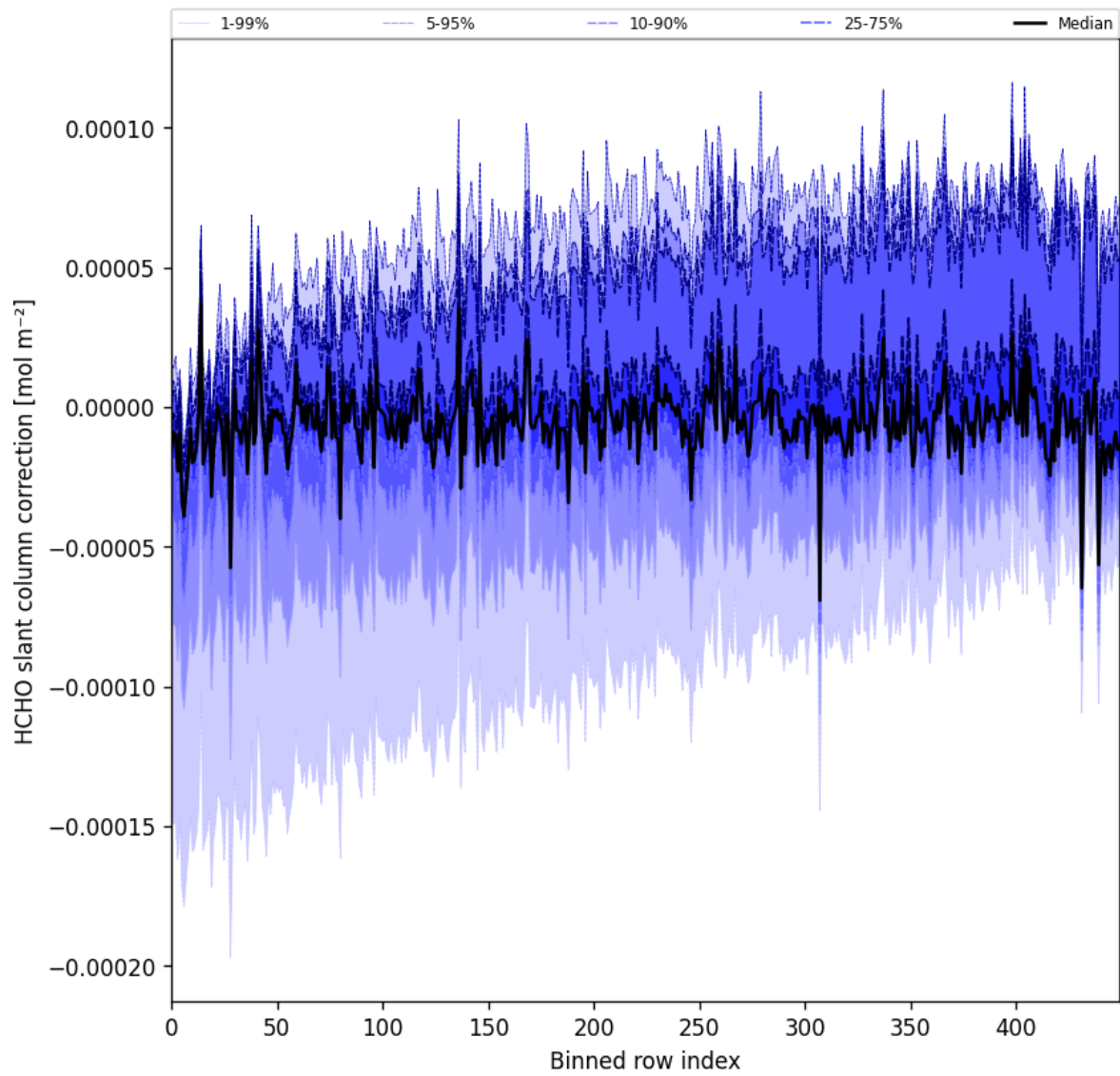
Figure 61: Along track statistics of “HCHO slant column correction” for 2025-06-17 to 2025-06-18
