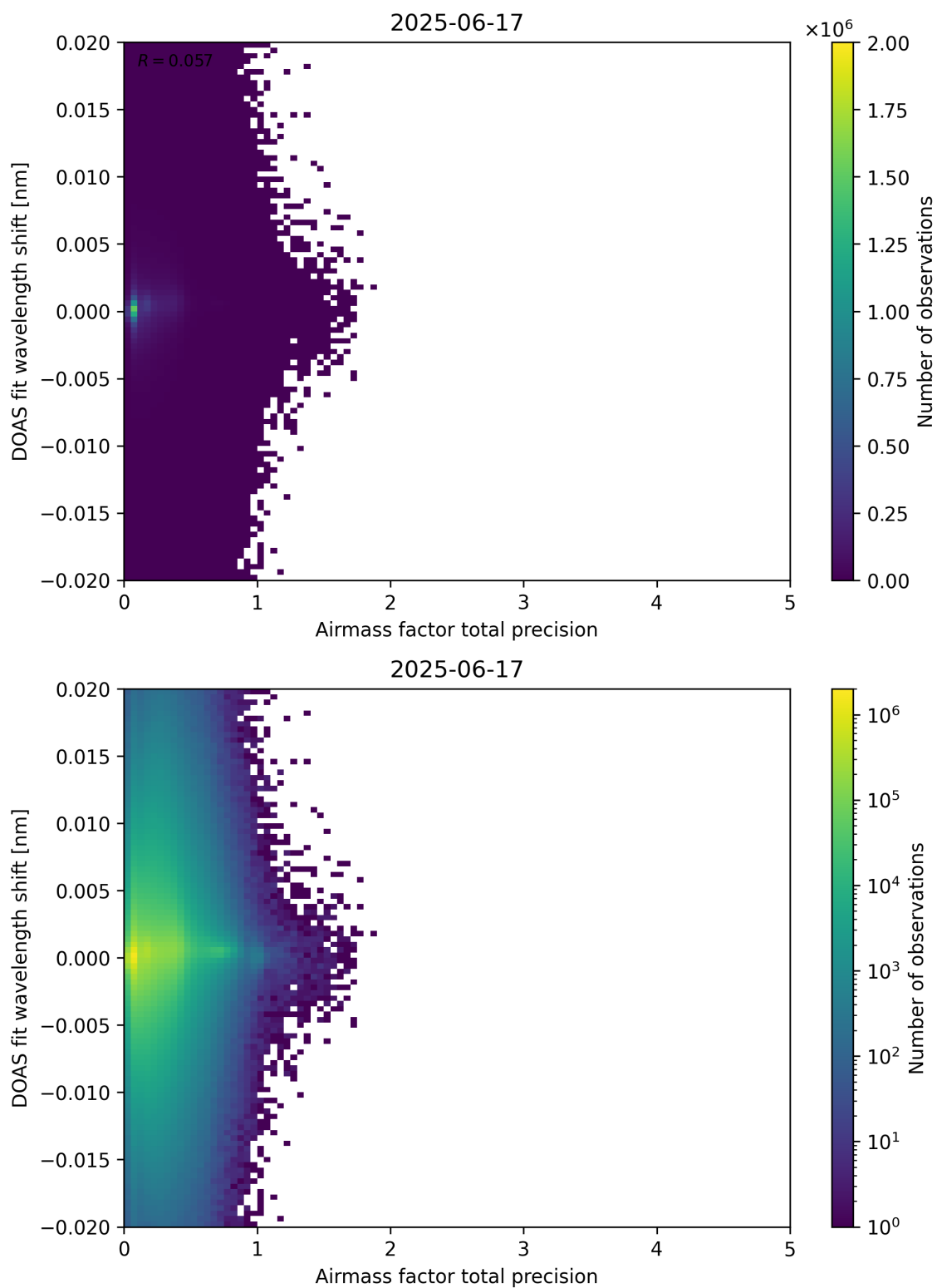
Figure 106: Scatter density plot of “Airmass factor total precision” against “DOAS fit wavelength shift” for 2025-06-17 to 2025-06-18.
