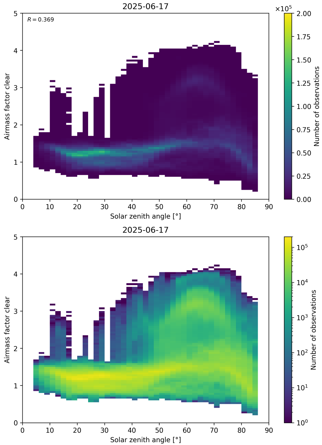
Figure 170: Scatter density plot of “Solar zenith angle” against “Airmass factor clear” for 2025-06-17 to 2025-06-18.
