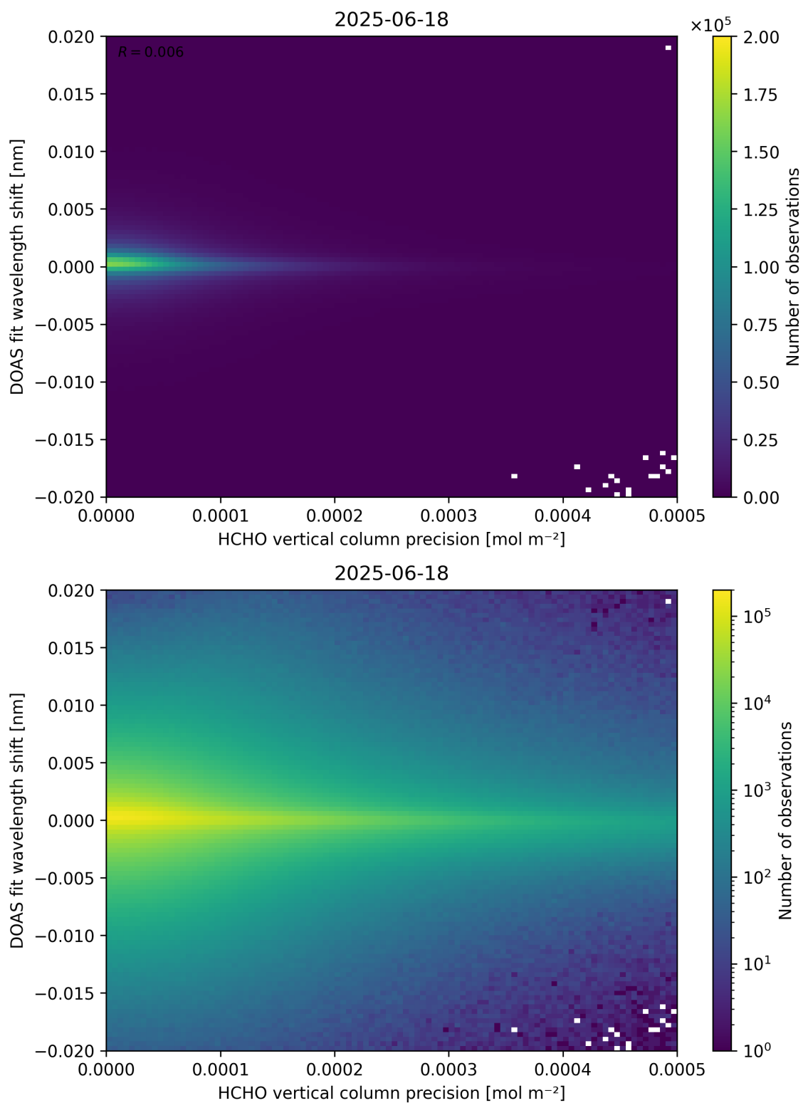
Figure 137: Scatter density plot of “HCHO vertical column precision” against “DOAS fit wavelength shift” for 2025-06-17 to 2025-06-19.
