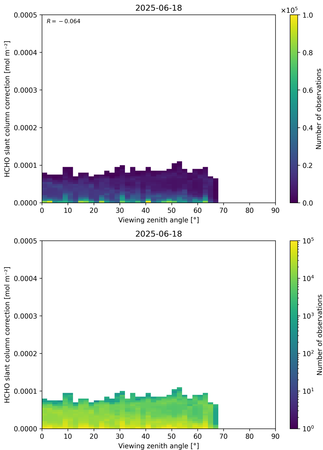
Figure 187: Scatter density plot of “Viewing zenith angle” against “HCHO slant column correction” for 2025-06-17 to 2025-06-19.
