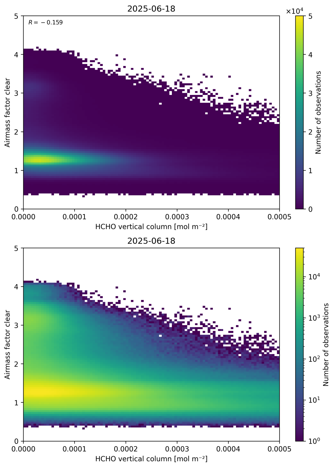
Figure 126: Scatter density plot of “HCHO vertical column” against “Airmass factor clear” for 2025-06-17 to 2025-06-19.
