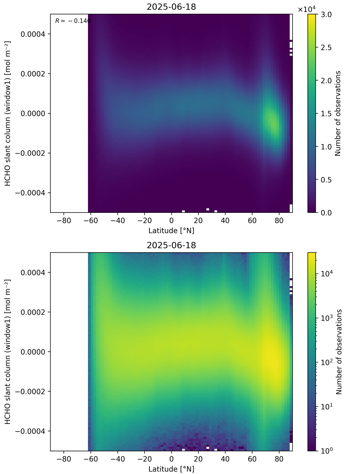
Figure 159: Scatter density plot of “Latitude” against “HCHO slant column (window1)” for 2025-06-17 to 2025-06-19.
