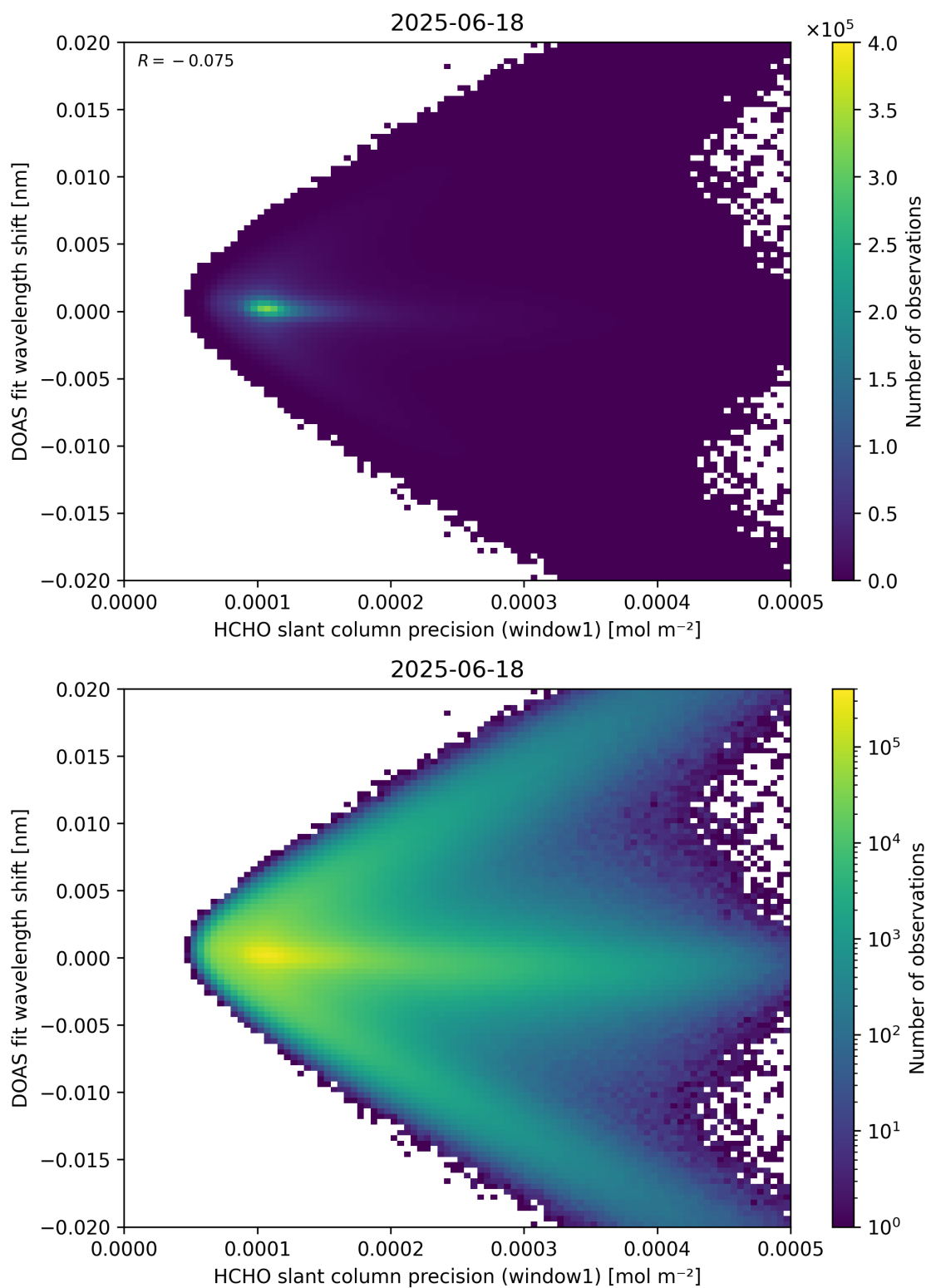
Figure 89: Scatter density plot of “HCHO slant column precision (window1)” against “DOAS fit wavelength shift” for 2025-06-17 to 2025-06-19.
