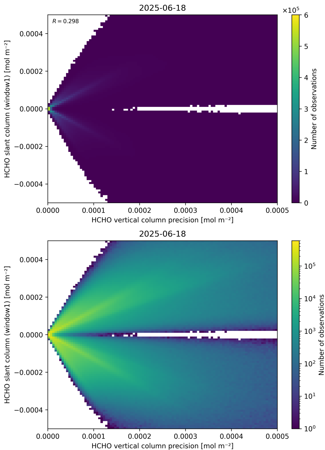
Figure 142: Scatter density plot of “HCHO vertical column precision” against “HCHO slant column (window1)” for 2025-06-17 to 2025-06-19.
