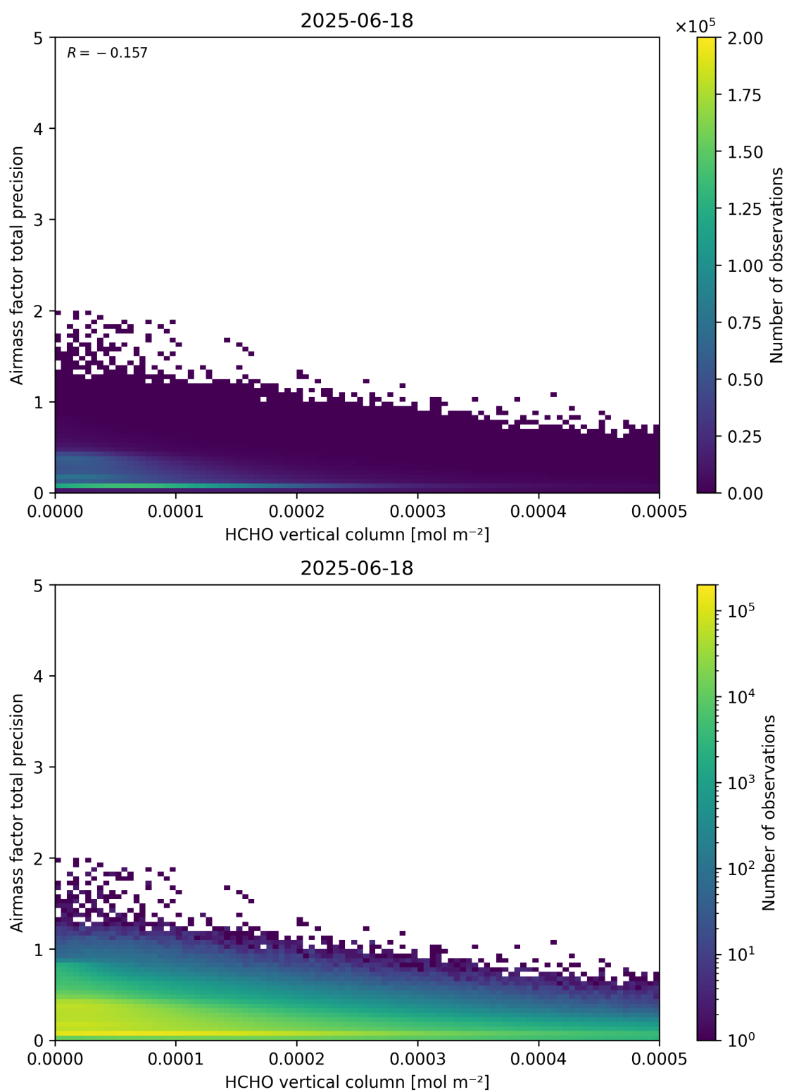
Figure 132: Scatter density plot of “HCHO vertical column” against “Airmass factor total precision” for 2025-06-17 to 2025-06-19.
