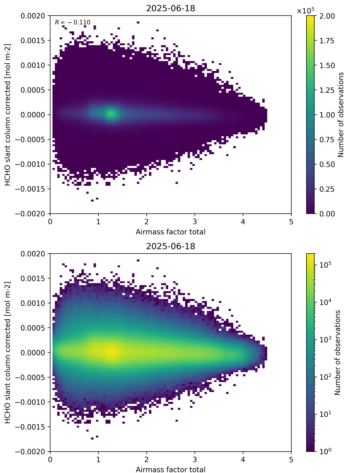
Figure 101: Scatter density plot of “Airmass factor total” against “HCHO slant column corrected” for 2025-06-17 to 2025-06-19.
