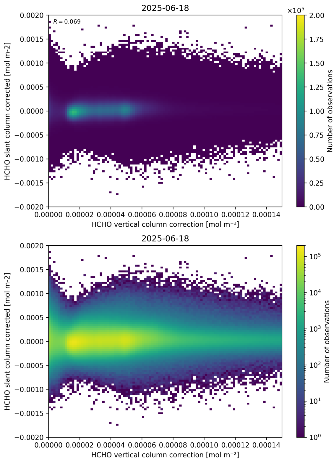
Figure 116: Scatter density plot of “HCHO vertical column correction” against “HCHO slant column corrected” for 2025-06-17 to 2025-06-19.
