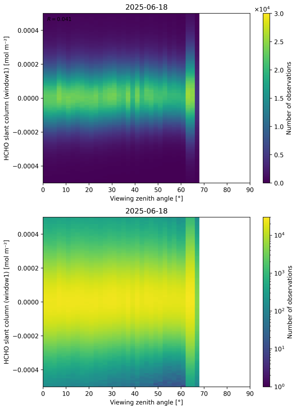
Figure 188: Scatter density plot of “Viewing zenith angle” against “HCHO slant column (window1)” for 2025-06-17 to 2025-06-19.
