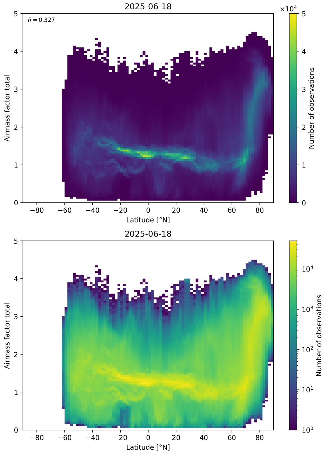
Figure 161: Scatter density plot of “Latitude” against “Airmass factor total” for 2025-06-17 to 2025-06-19.
