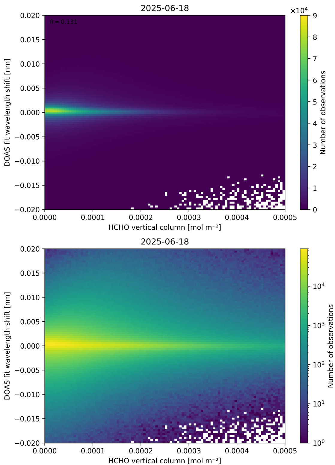
Figure 124: Scatter density plot of “HCHO vertical column” against “DOAS fit wavelength shift” for 2025-06-17 to 2025-06-19.
