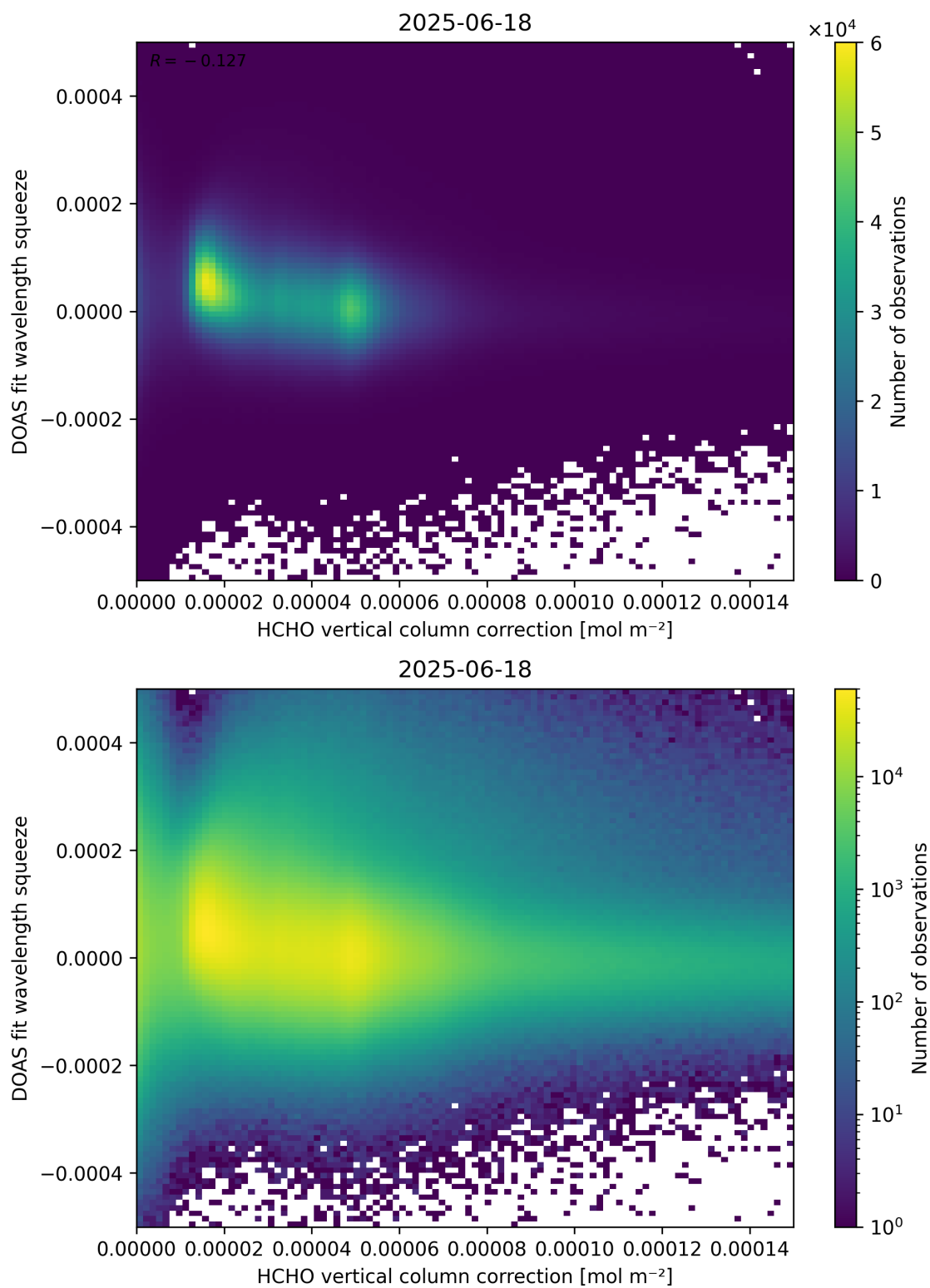
Figure 114: Scatter density plot of “HCHO vertical column correction” against “DOAS fit wavelength squeeze” for 2025-06-17 to 2025-06-19.
