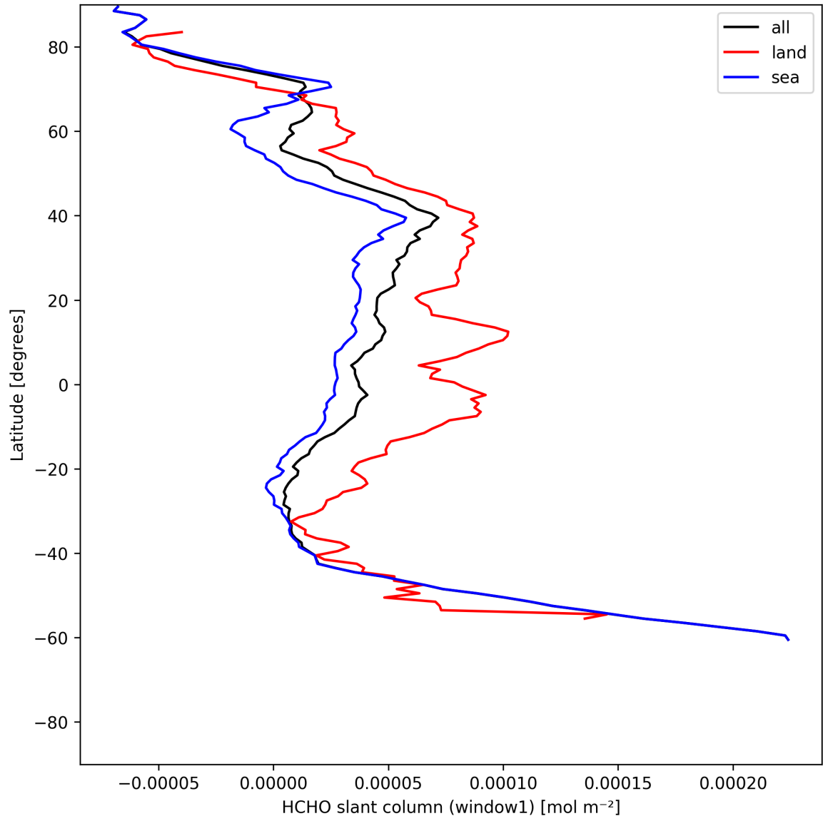
Figure 24: Zonal average of “HCHO slant column (window1)” for 2025-06-17 to 2025-06-19.
