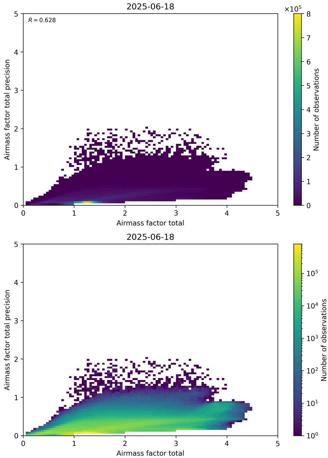
Figure 103: Scatter density plot of “Airmass factor total” against “Airmass factor total precision” for 2025-06-17 to 2025-06-19.
