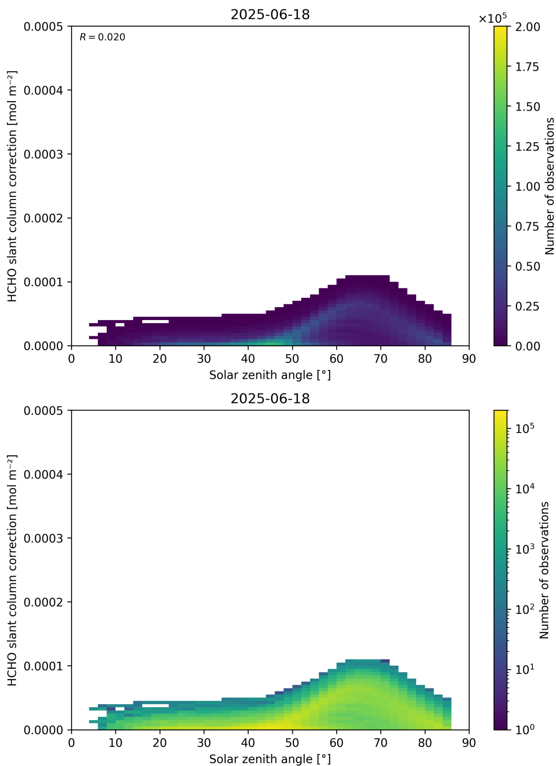
Figure 172: Scatter density plot of “Solar zenith angle” against “HCHO slant column correction” for 2025-06-17 to 2025-06-19.
