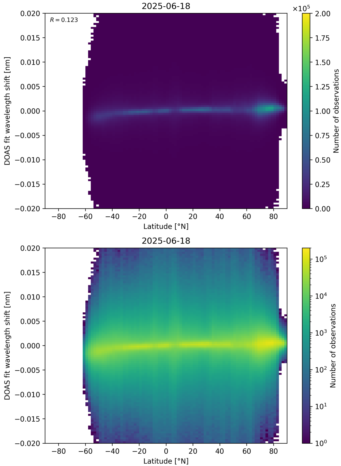
Figure 154: Scatter density plot of “Latitude” against “DOAS fit wavelength shift” for 2025-06-17 to 2025-06-19.
