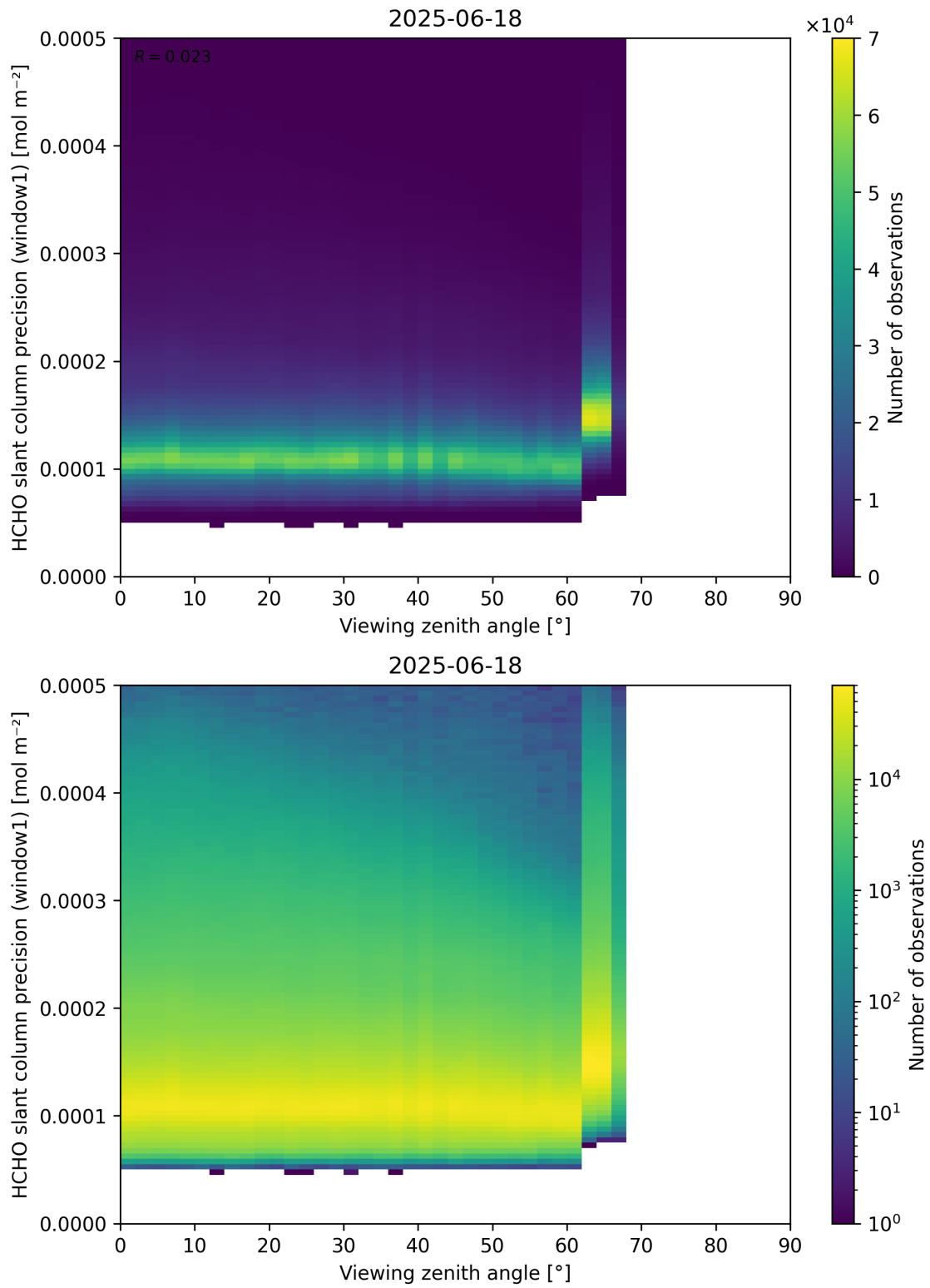
Figure 189: Scatter density plot of “Viewing zenith angle” against “HCHO slant column precision (window1)” for 2025-06-17 to 2025-06-19.
