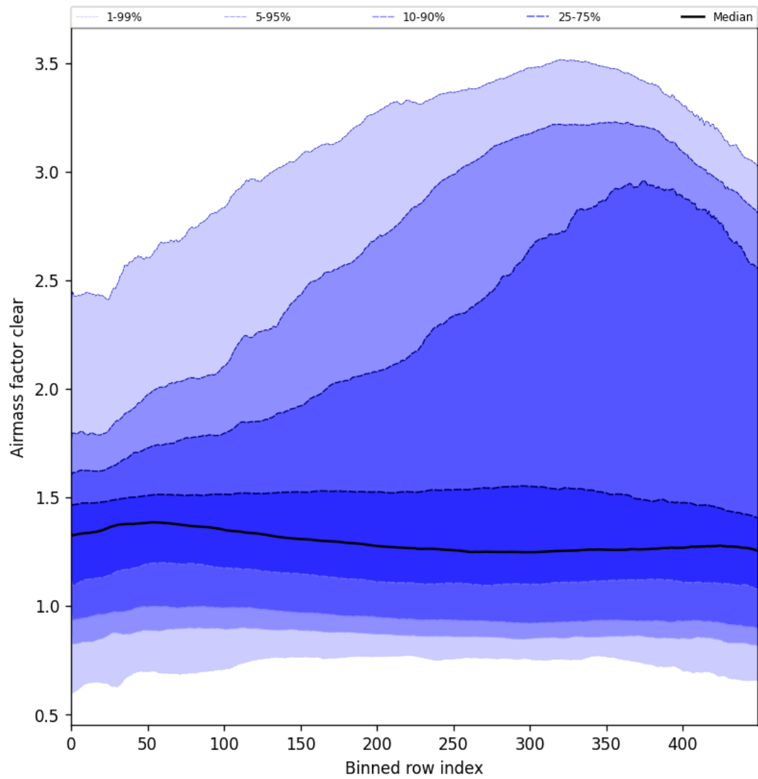
Figure 56: Along track statistics of “Airmass factor clear” for 2025-06-17 to 2025-06-19
