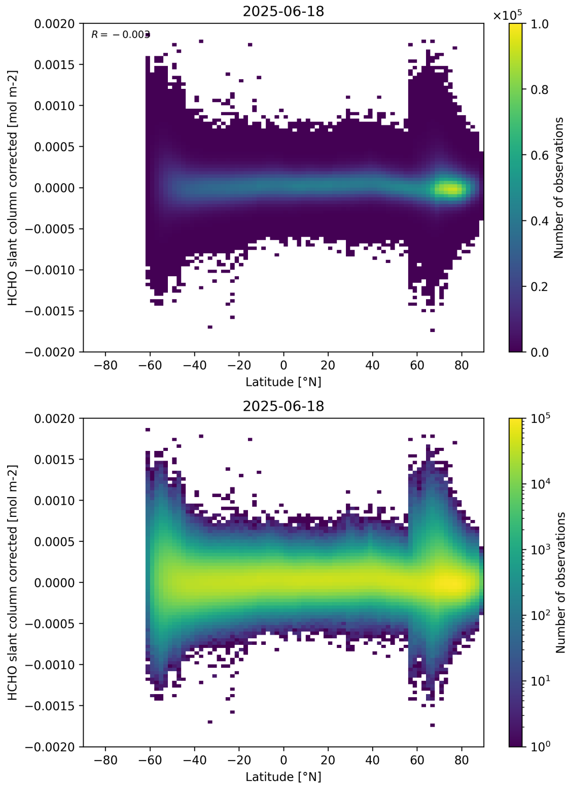
Figure 157: Scatter density plot of “Latitude” against “HCHO slant column corrected” for 2025-06-17 to 2025-06-19.
