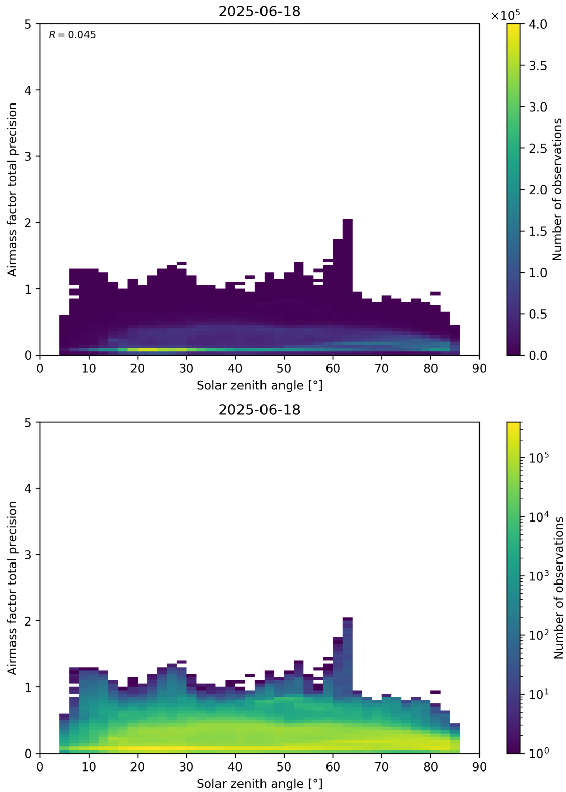
Figure 176: Scatter density plot of “Solar zenith angle” against “Airmass factor total precision” for 2025-06-17 to 2025-06-19.
