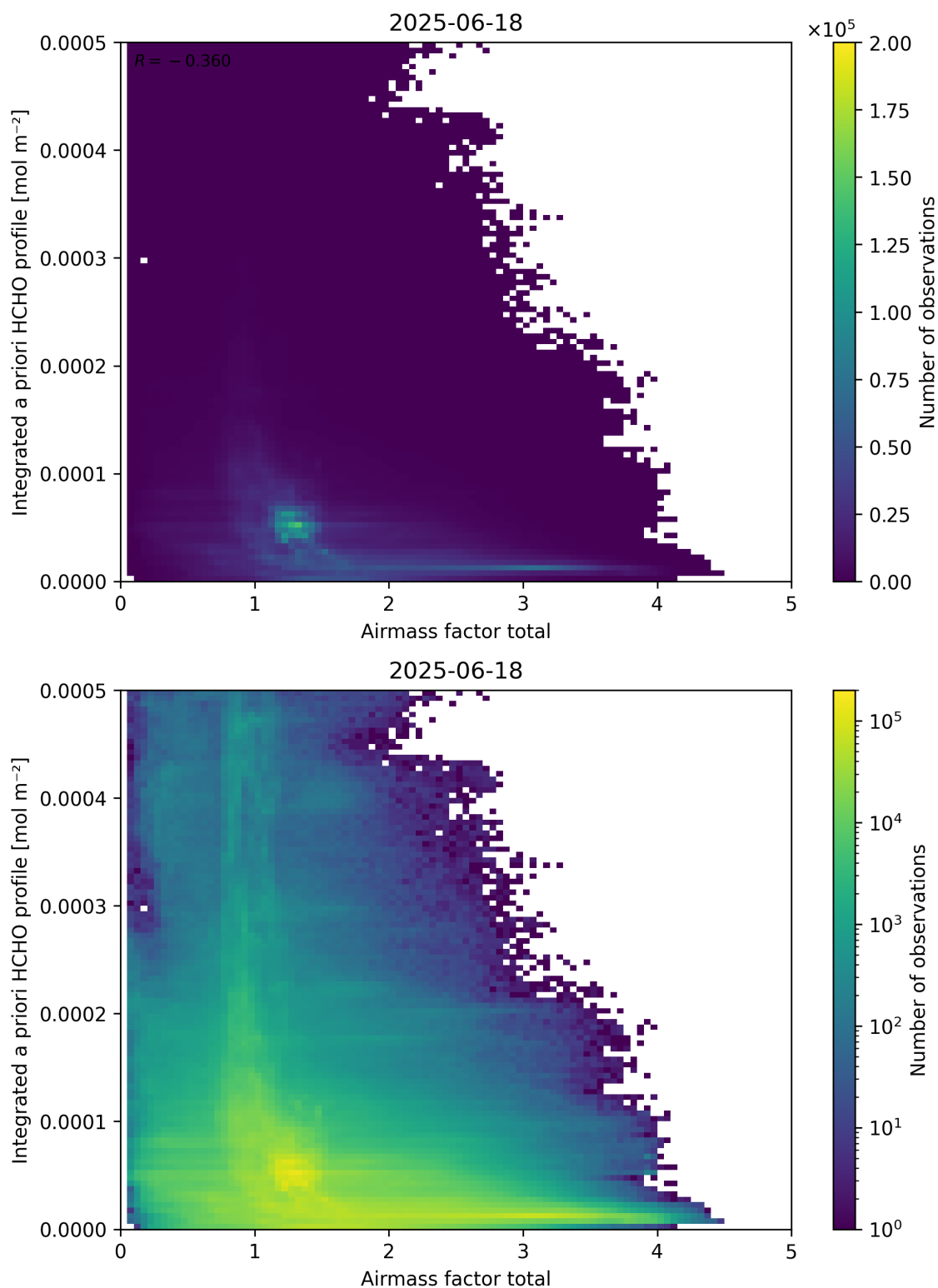
Figure 104: Scatter density plot of “Airmass factor total” against “Integrated a priori HCHO profile” for 2025-06-17 to 2025-06-19.
