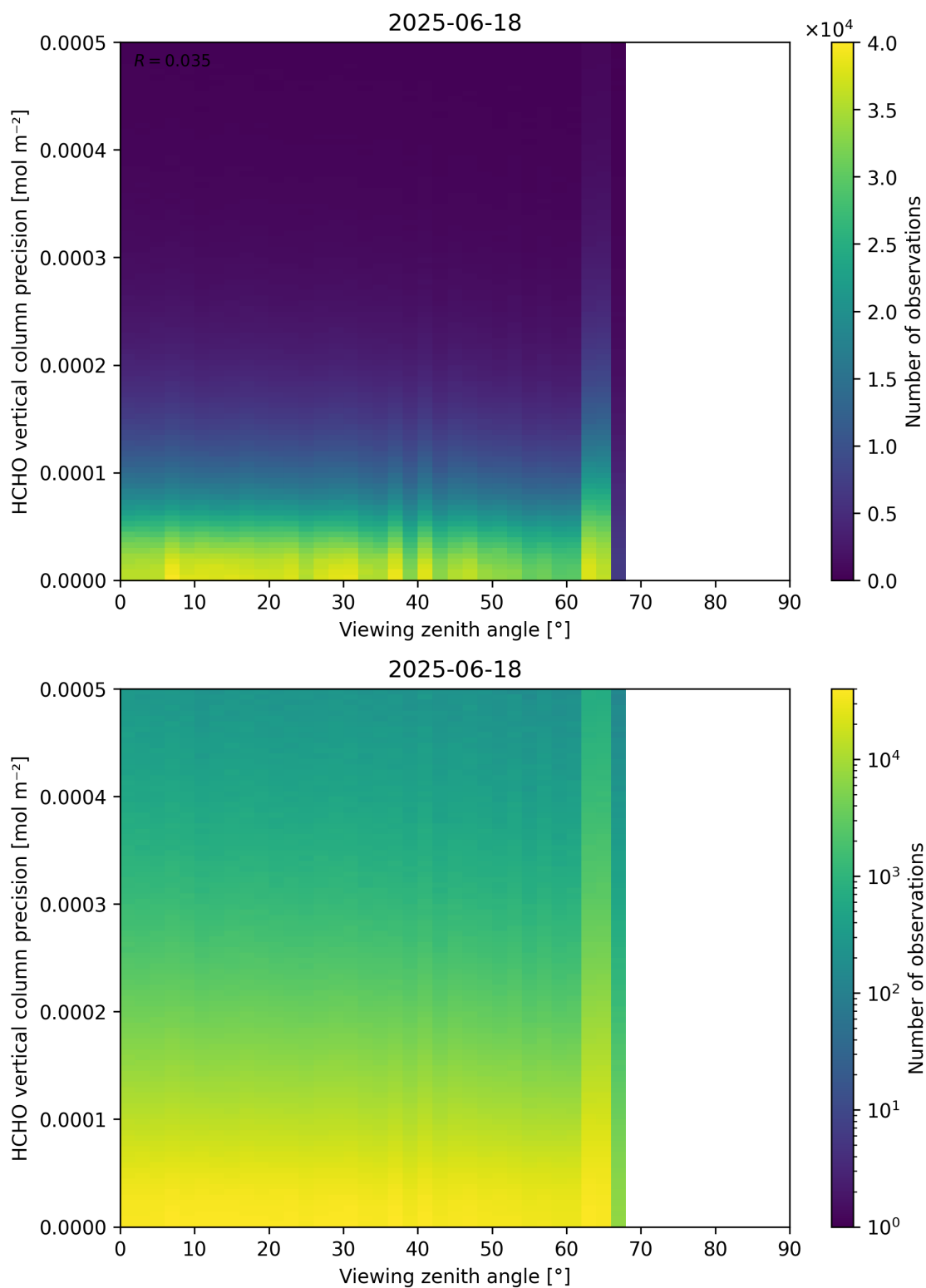
Figure 194: Scatter density plot of “Viewing zenith angle” against “HCHO vertical column precision” for 2025-06-17 to 2025-06-19.
