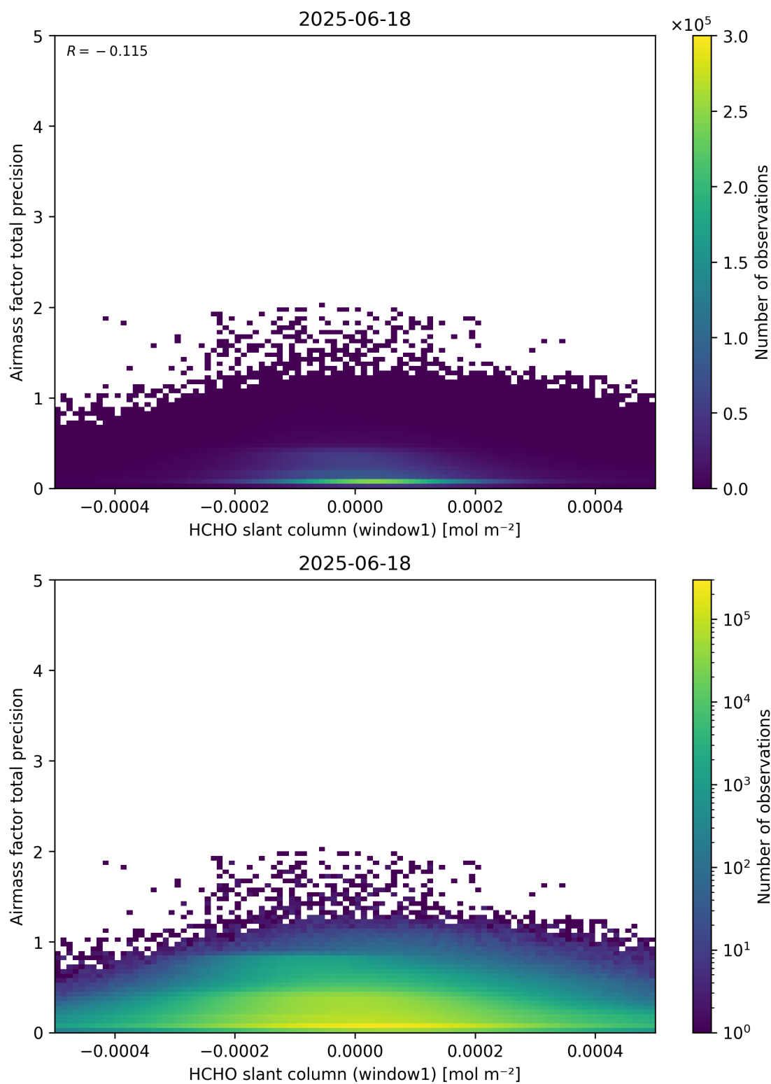
Figure 86: Scatter density plot of “HCHO slant column (window1)” against “Airmass factor total precision” for 2025-06-17 to 2025-06-19.
