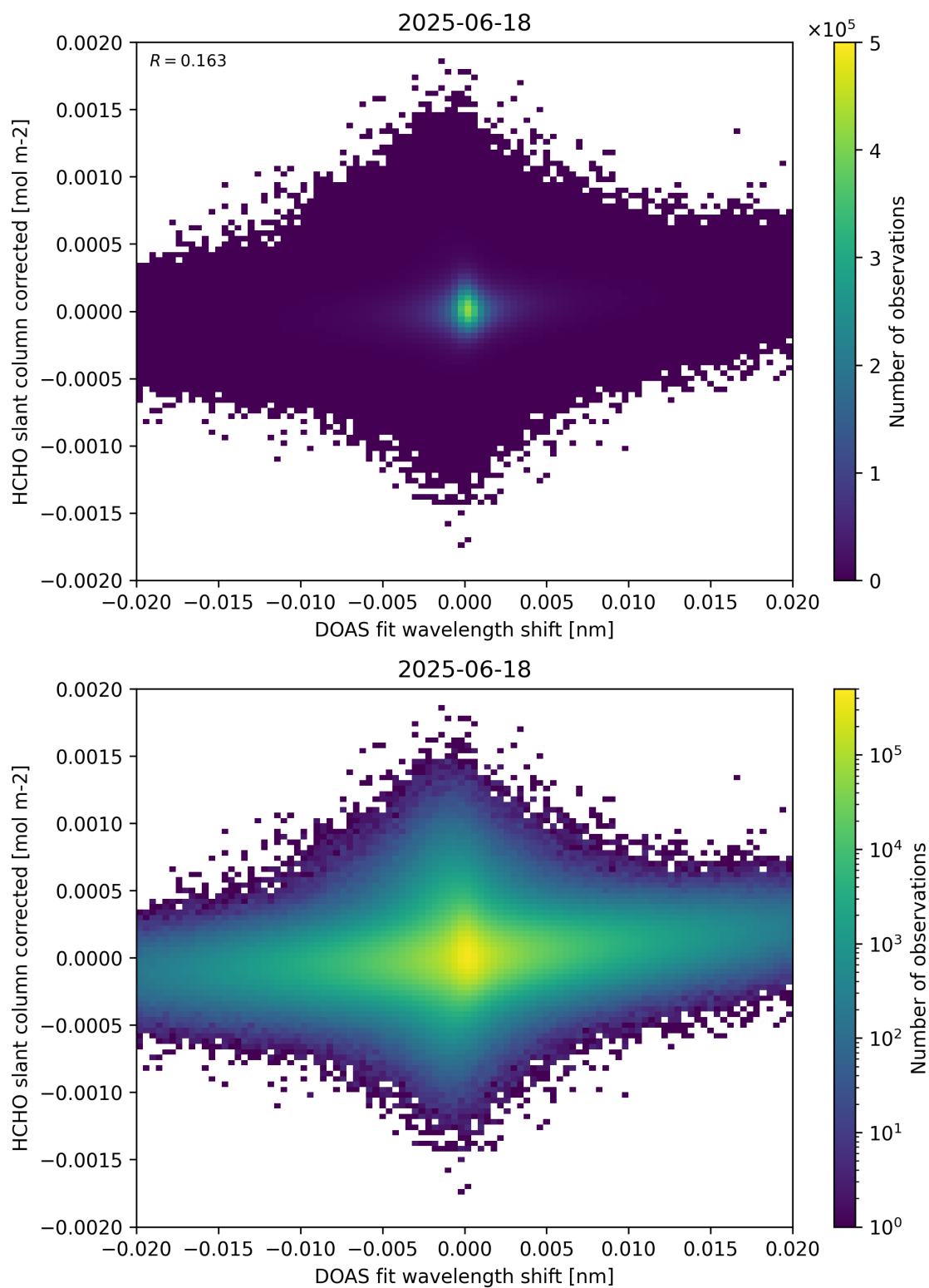
Figure 66: Scatter density plot of “DOAS fit wavelength shift” against “HCHO slant column corrected” for 2025-06-17 to 2025-06-19.
