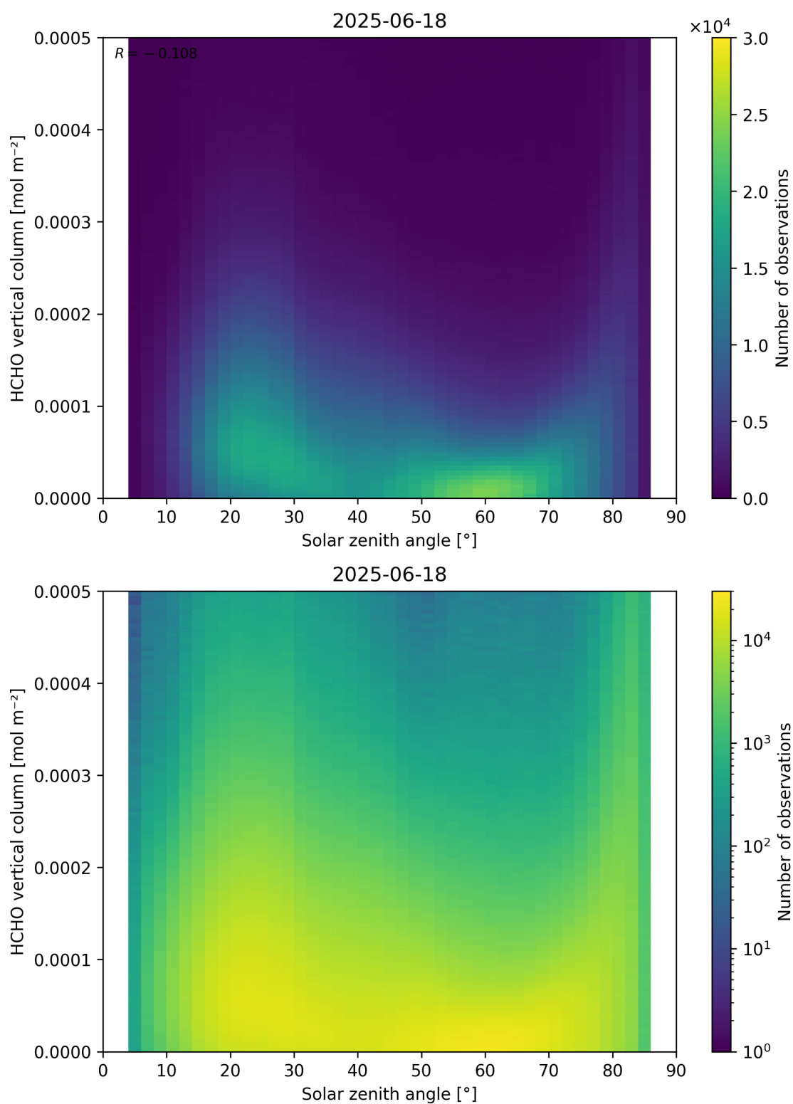
Figure 177: Scatter density plot of “Solar zenith angle” against “HCHO vertical column” for 2025-06-17 to 2025-06-19.
