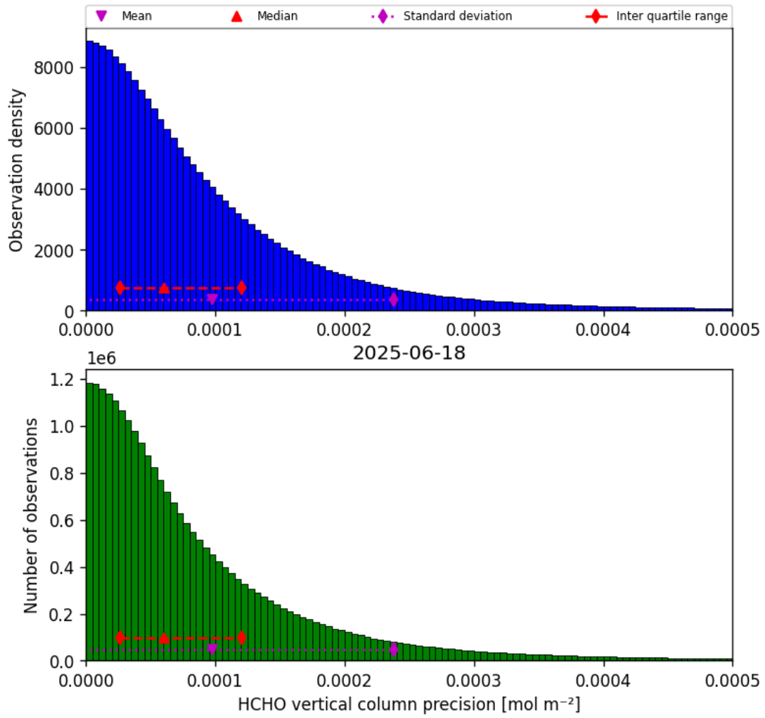
Figure 36: Histogram of “HCHO vertical column precision” for 2025-06-17 to 2025-06-19
