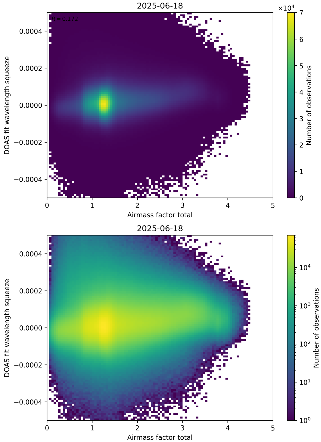
Figure 99: Scatter density plot of “Airmass factor total” against “DOAS fit wavelength squeeze” for 2025-06-17 to 2025-06-19.
