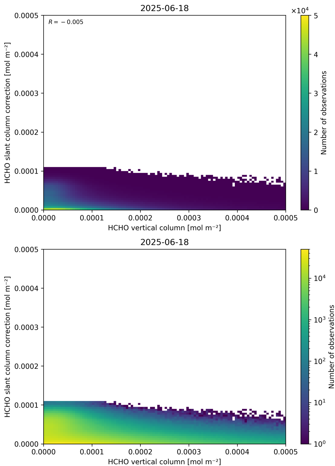
Figure 128: Scatter density plot of “HCHO vertical column” against “HCHO slant column correction” for 2025-06-17 to 2025-06-19.
