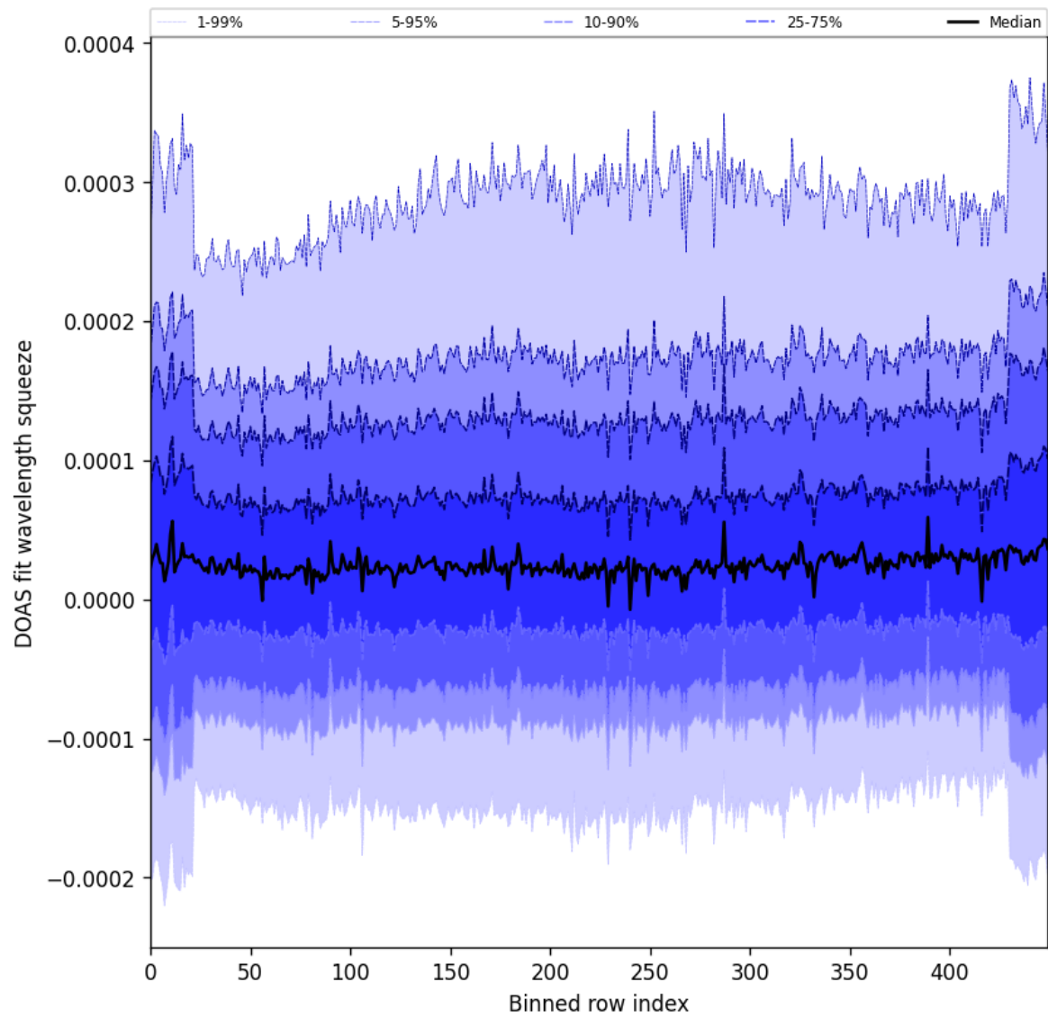
Figure 59: Along track statistics of “DOAS fit wavelength squeeze” for 2025-06-17 to 2025-06-19
