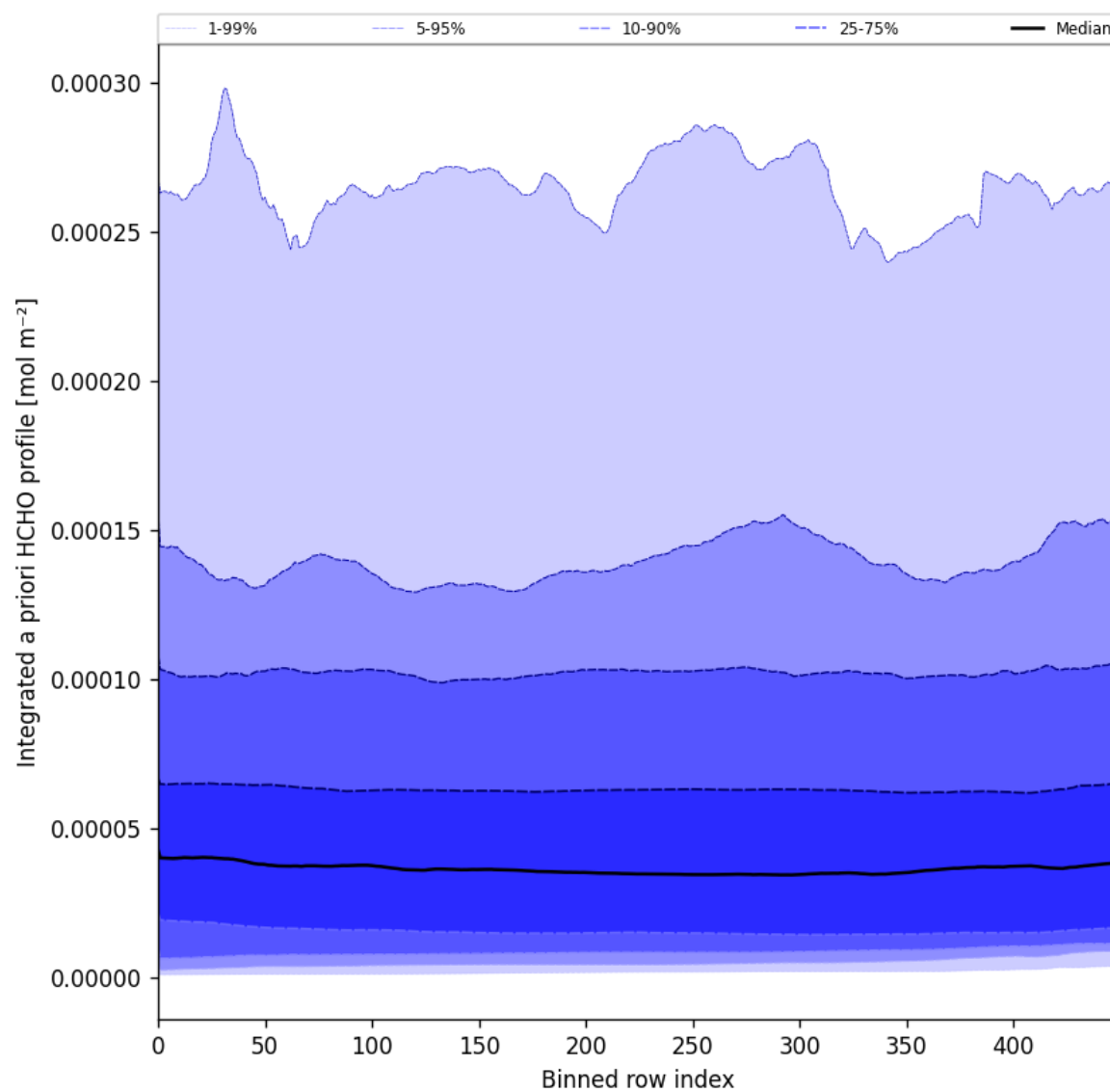
Figure 57: Along track statistics of "Integrated a priori HCHO profile" for 2025-06-17 to 2025-06-19
