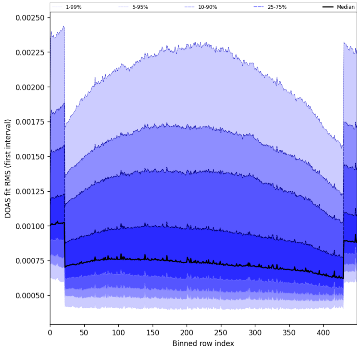
Figure 60: Along track statistics of “DOAS fit RMS (first interval)” for 2025-06-17 to 2025-06-19
