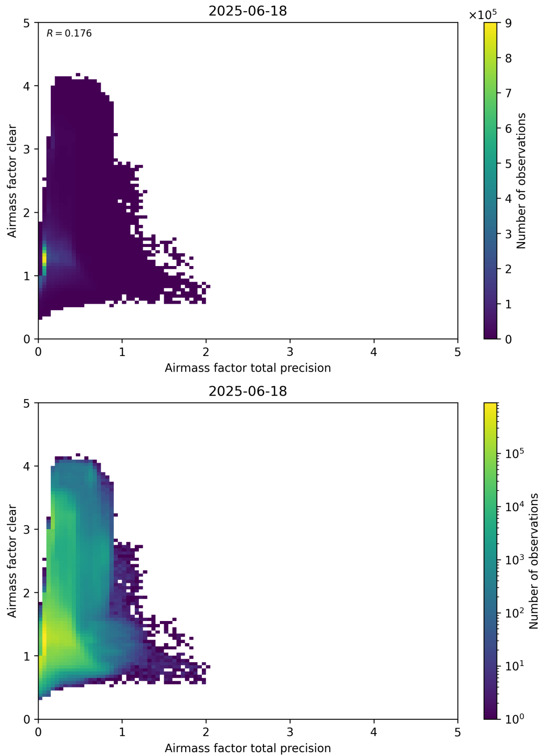
Figure 108: Scatter density plot of “Airmass factor total precision” against “Airmass factor clear” for 2025-06-17 to 2025-06-19.
