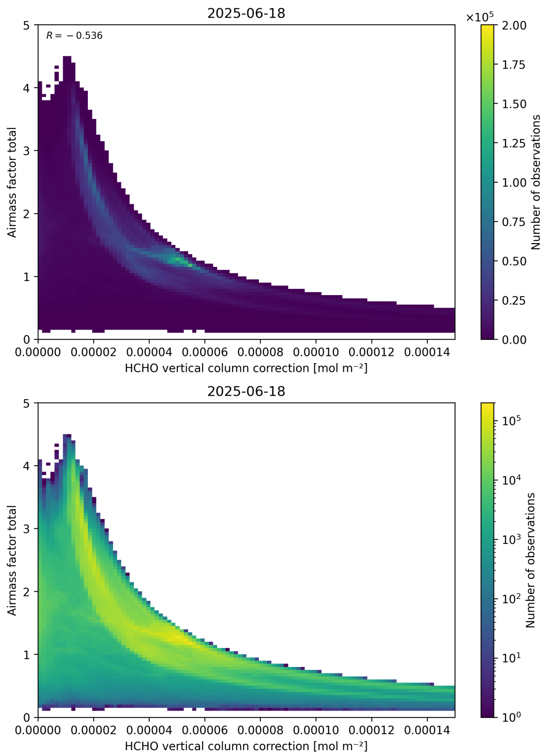
Figure 120: Scatter density plot of “HCHO vertical column correction” against “Airmass factor total” for 2025-06-17 to 2025-06-19.
