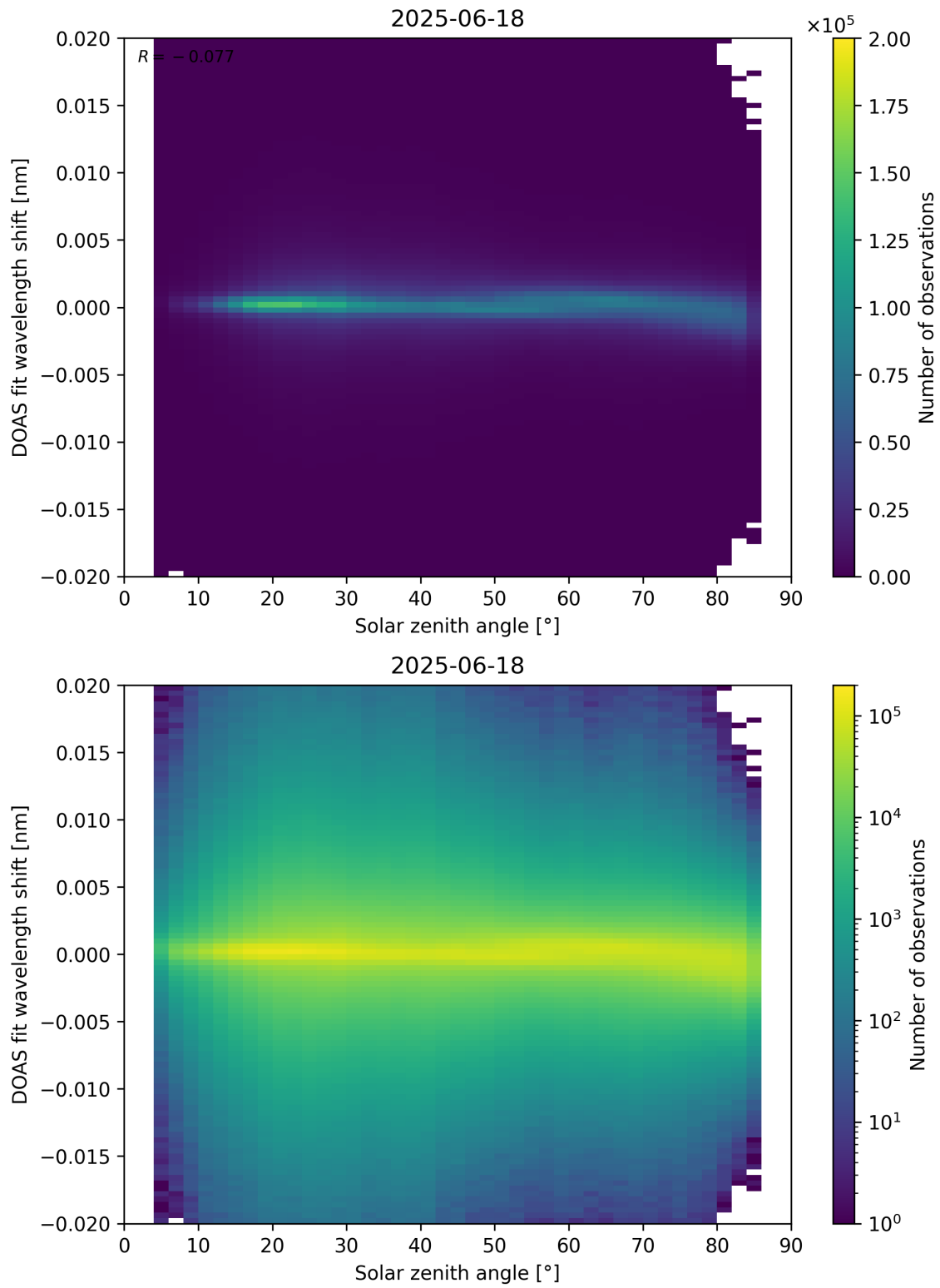
Figure 168: Scatter density plot of “Solar zenith angle” against “DOAS fit wavelength shift” for 2025-06-17 to 2025-06-19.
