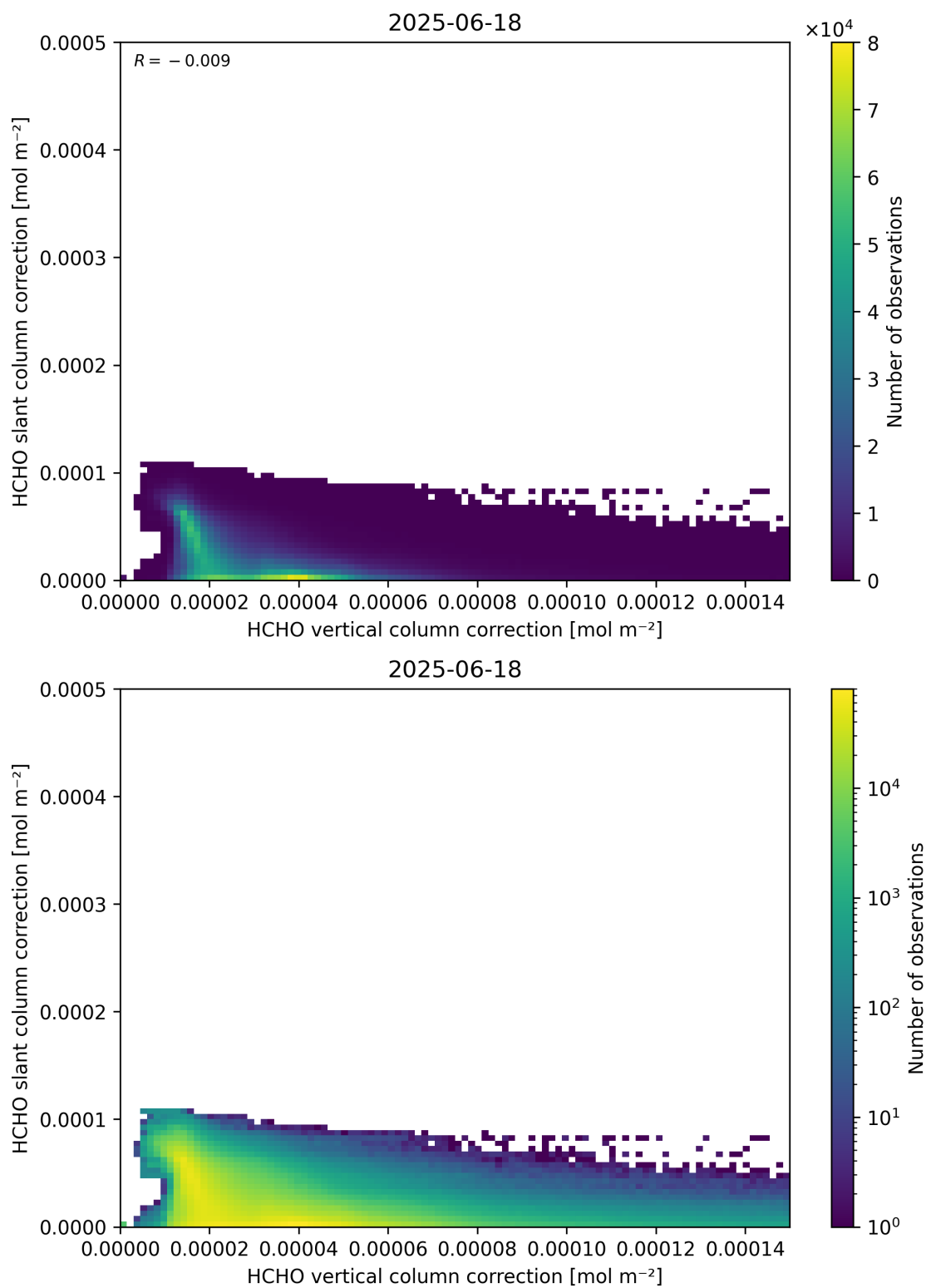
Figure 117: Scatter density plot of “HCHO vertical column correction” against “HCHO slant column correction” for 2025-06-17 to 2025-06-19.
