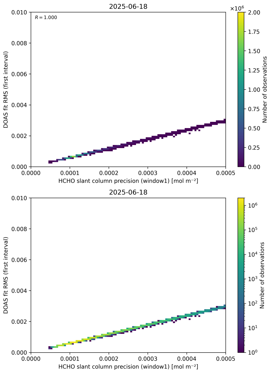
Figure 88: Scatter density plot of “HCHO slant column precision (window1)” against “DOAS fit RMS (first interval)” for 2025-06-17 to 2025-06-19.
