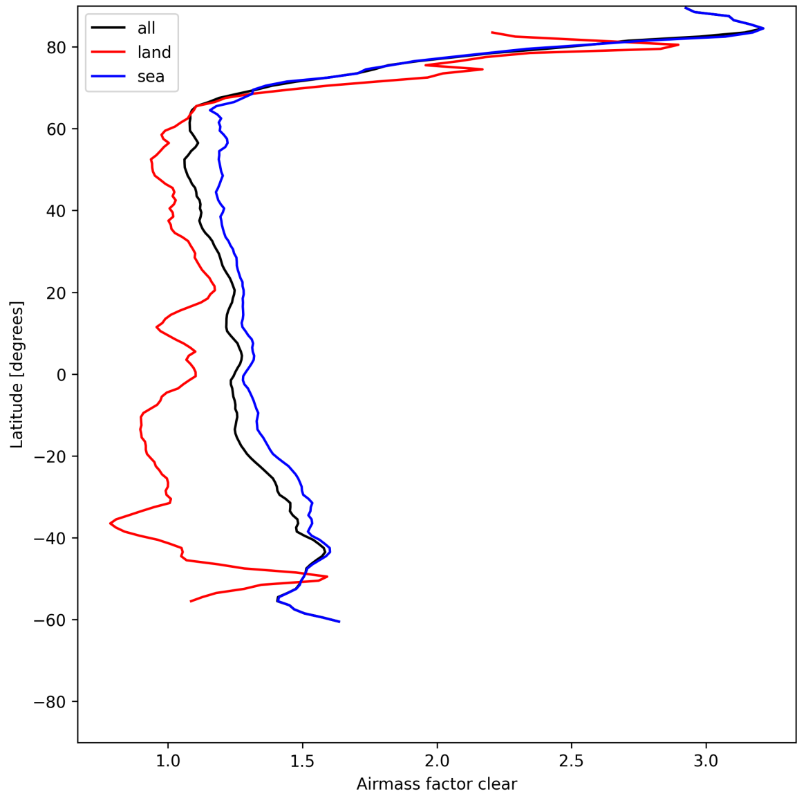
Figure 28: Zonal average of “Airmass factor clear” for 2025-06-17 to 2025-06-19.
