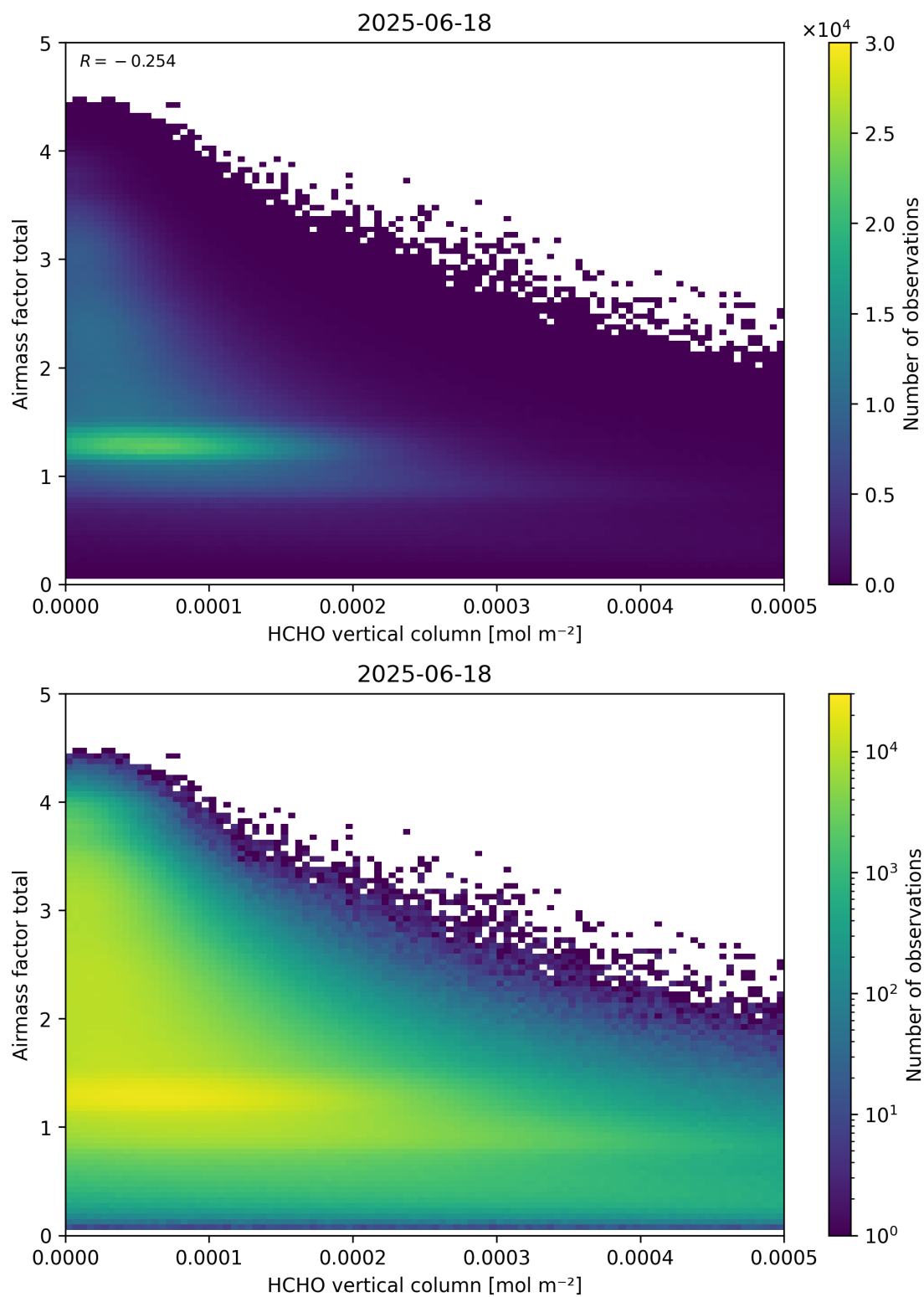
Figure 131: Scatter density plot of “HCHO vertical column” against “Airmass factor total” for 2025-06-17 to 2025-06-19.
