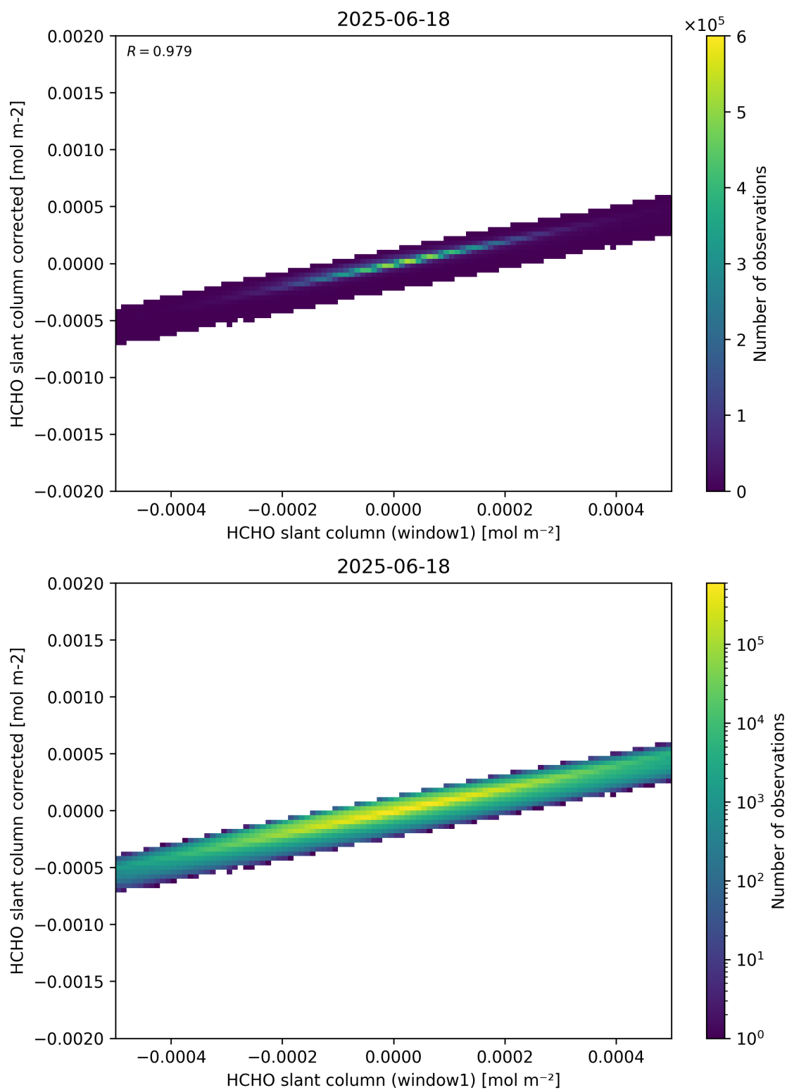
Figure 82: Scatter density plot of “HCHO slant column (window1)” against “HCHO slant column corrected” for 2025-06-17 to 2025-06-19.
