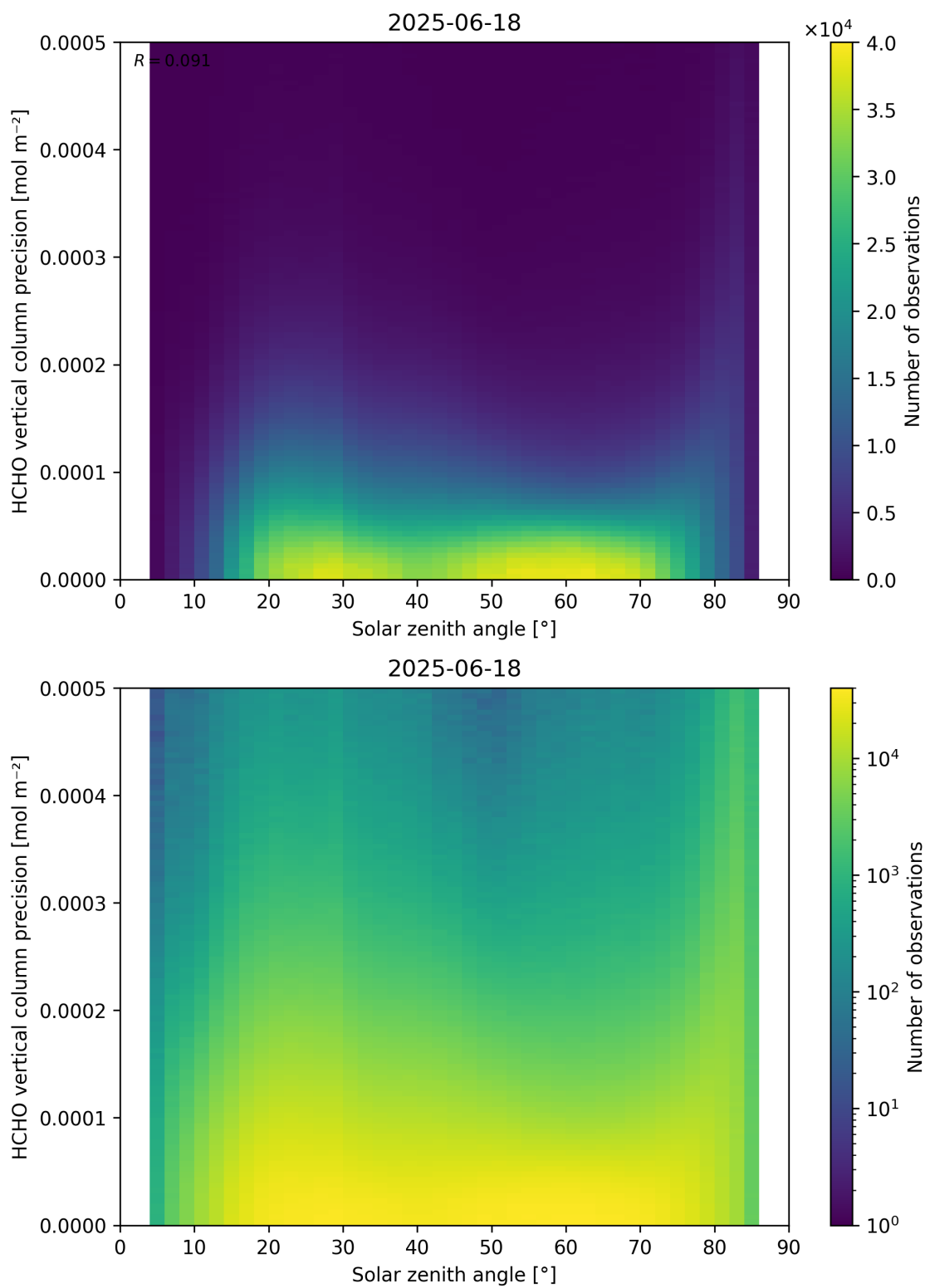
Figure 179: Scatter density plot of “Solar zenith angle” against “HCHO vertical column precision” for 2025-06-17 to 2025-06-19.
