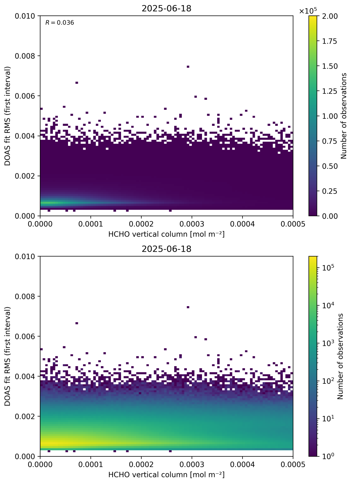
Figure 123: Scatter density plot of “HCHO vertical column” against “DOAS fit RMS (first interval)” for 2025-06-17 to 2025-06-19.
