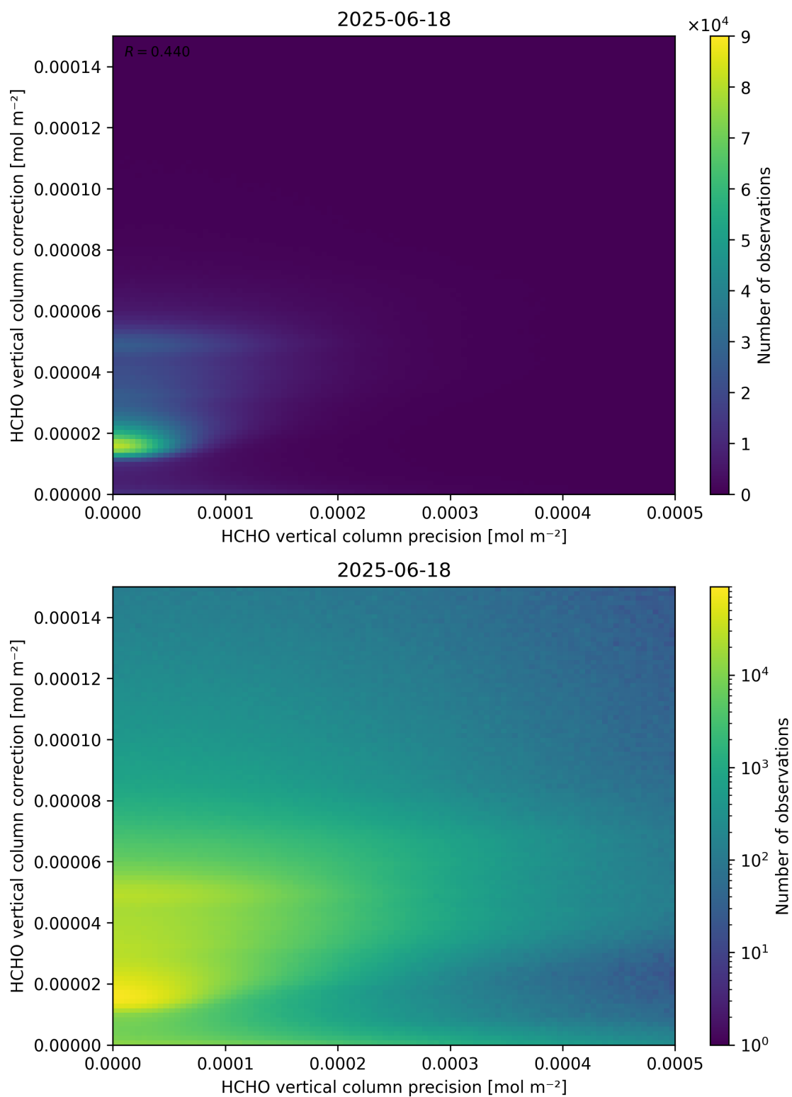
Figure 146: Scatter density plot of “HCHO vertical column precision” against “HCHO vertical column correction” for 2025-06-17 to 2025-06-19.
