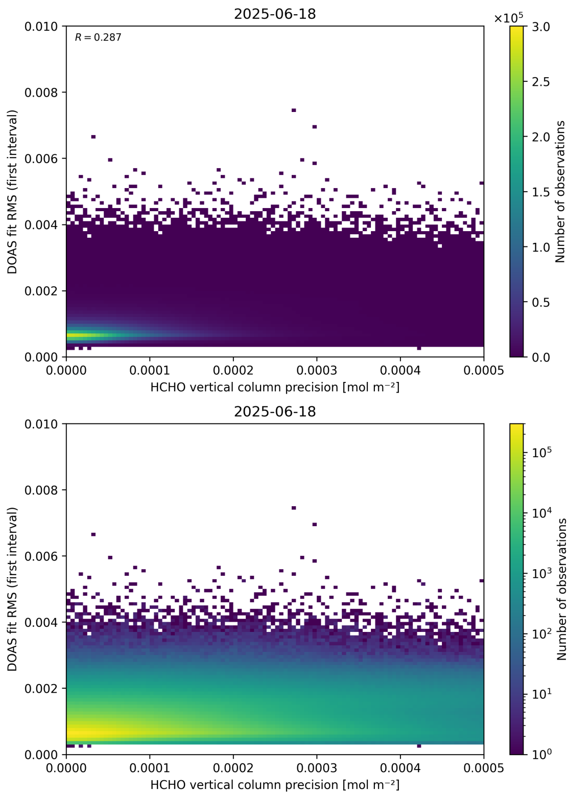
Figure 136: Scatter density plot of “HCHO vertical column precision” against “DOAS fit RMS (first interval)” for 2025-06-17 to 2025-06-19.
