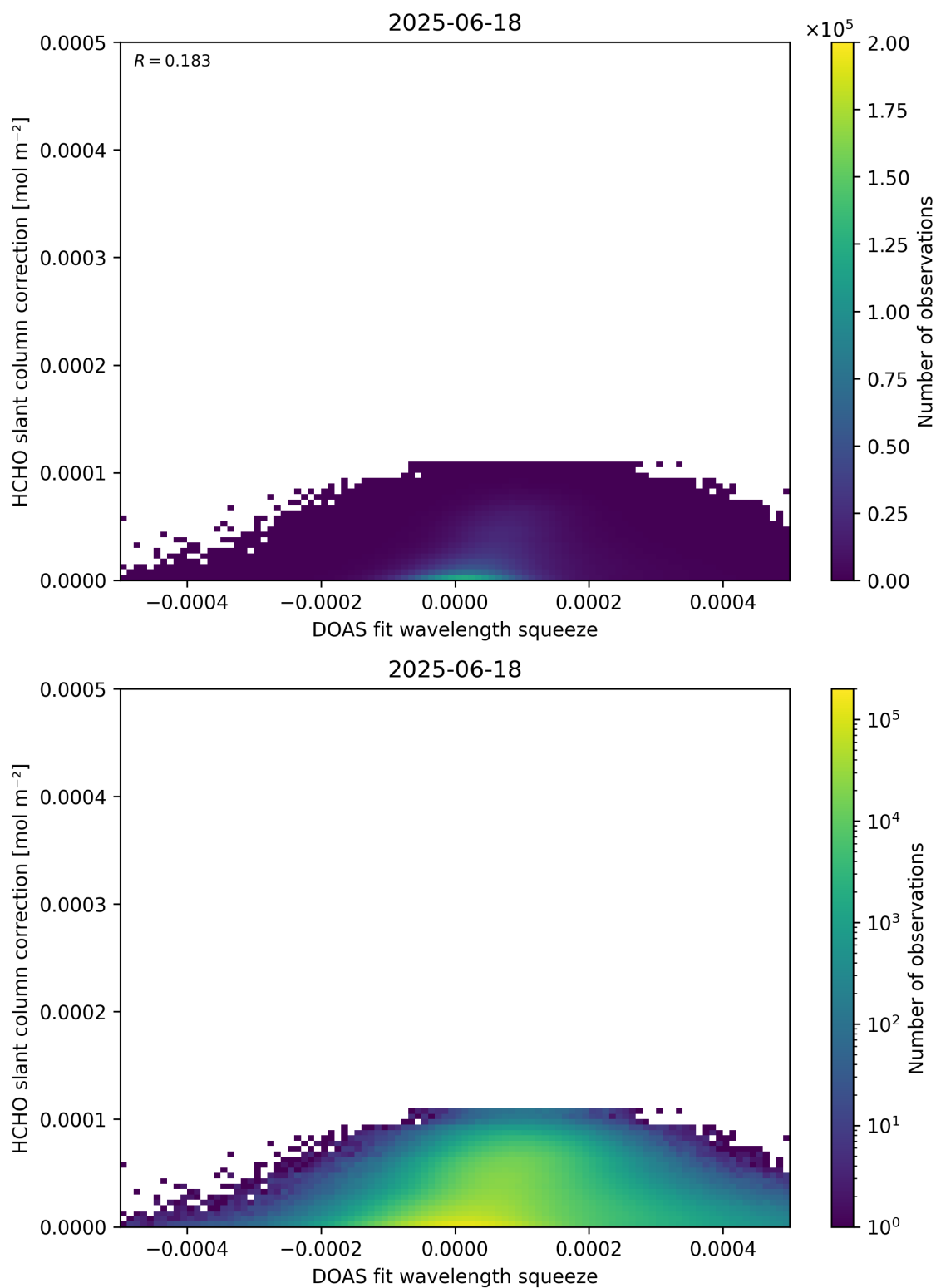
Figure 70: Scatter density plot of “DOAS fit wavelength squeeze” against “HCHO slant column correction” for 2025-06-17 to 2025-06-19.
