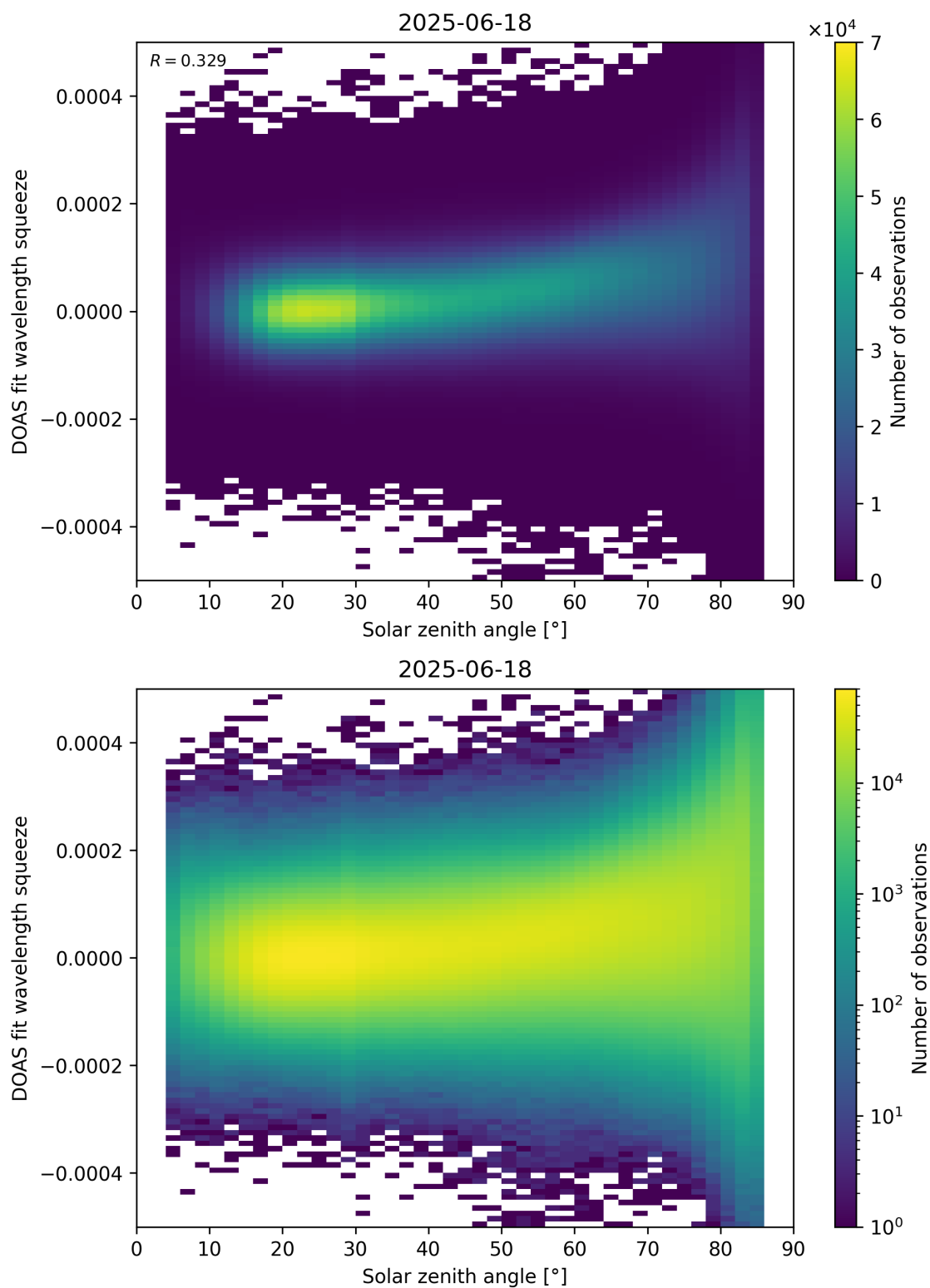
Figure 169: Scatter density plot of “Solar zenith angle” against “DOAS fit wavelength squeeze” for 2025-06-17 to 2025-06-19.
