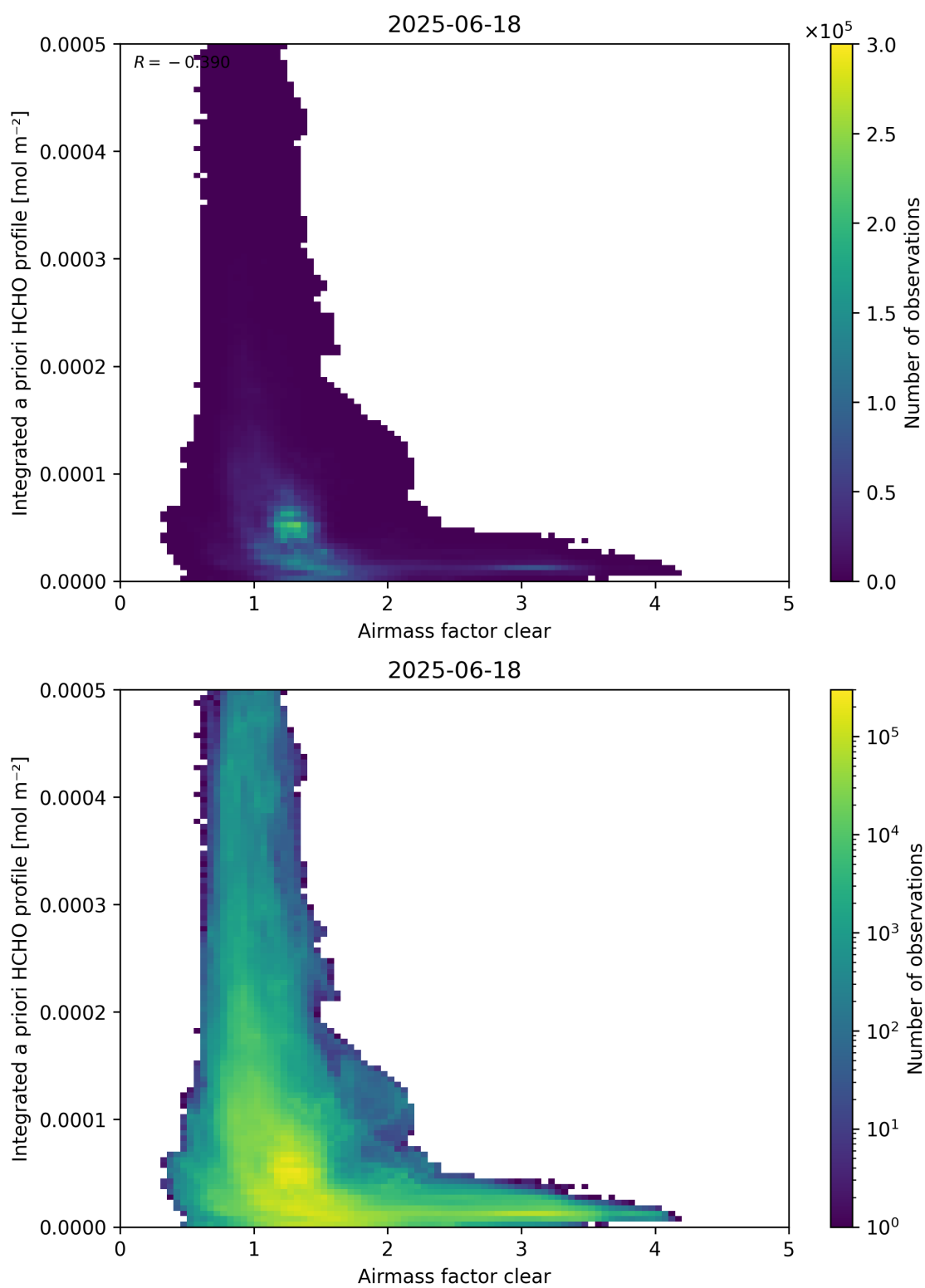
Figure 76: Scatter density plot of “Airmass factor clear” against “Integrated a priori HCHO profile” for 2025-06-17 to 2025-06-19.
