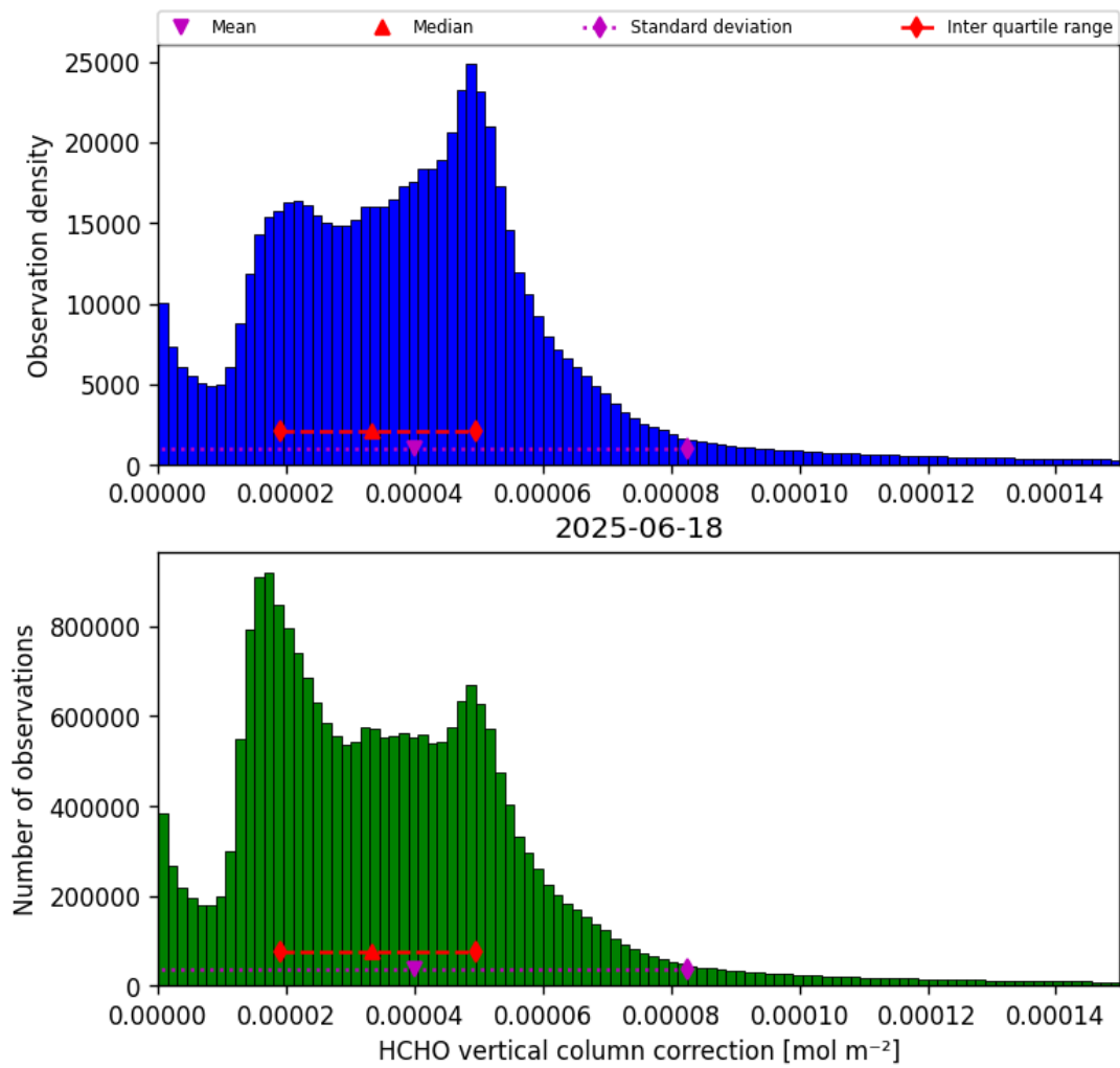
Figure 37: Histogram of “HCHO vertical column correction” for 2025-06-17 to 2025-06-19
