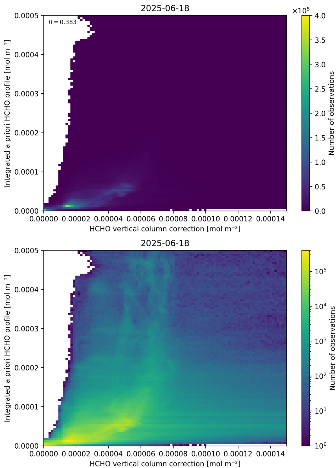
Figure 122: Scatter density plot of “HCHO vertical column correction” against “Integrated a priori HCHO profile” for 2025-06-17 to 2025-06-19.
