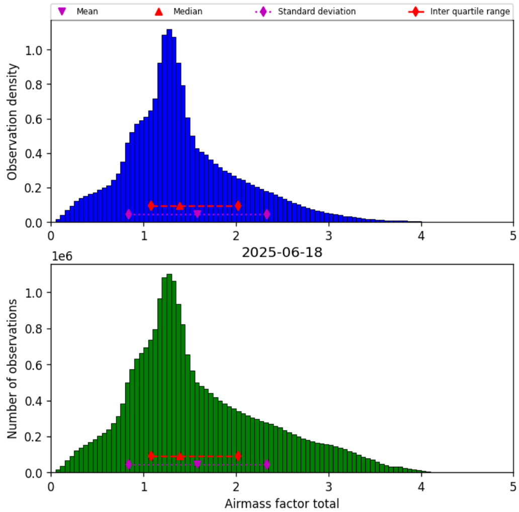
Figure 40: Histogram of “Airmass factor total” for 2025-06-17 to 2025-06-19
