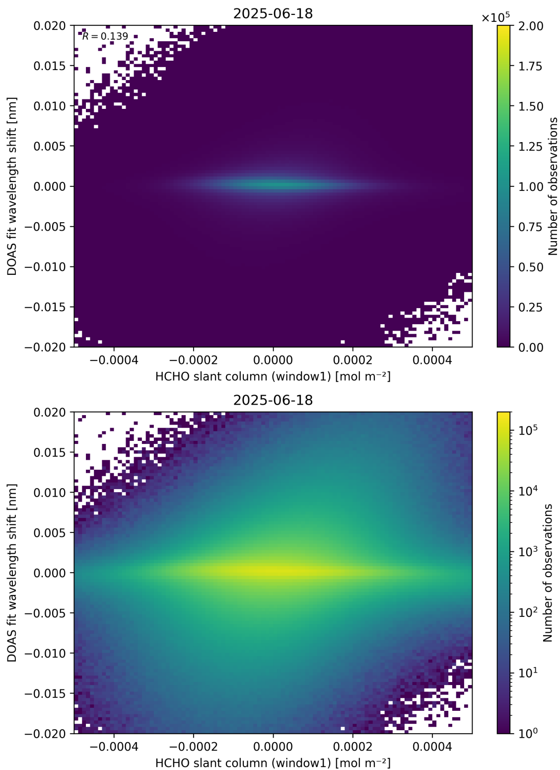
Figure 79: Scatter density plot of “HCHO slant column (window1)” against “DOAS fit wavelength shift” for 2025-06-17 to 2025-06-19.
