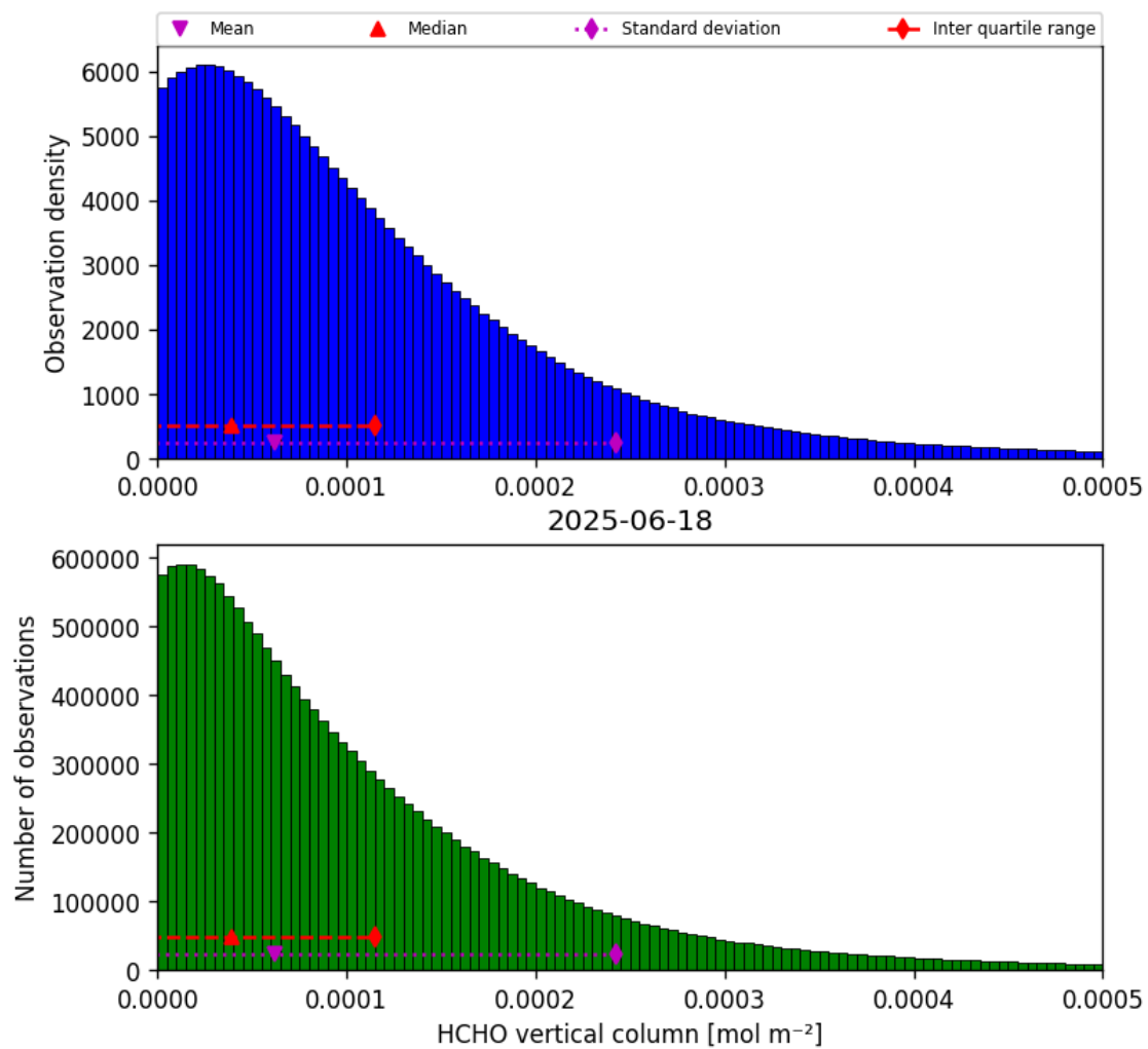
Figure 35: Histogram of “HCHO vertical column” for 2025-06-17 to 2025-06-19
