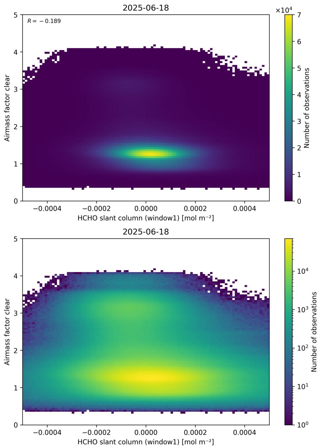
Figure 81: Scatter density plot of “HCHO slant column (window1)” against “Airmass factor clear” for 2025-06-17 to 2025-06-19.
