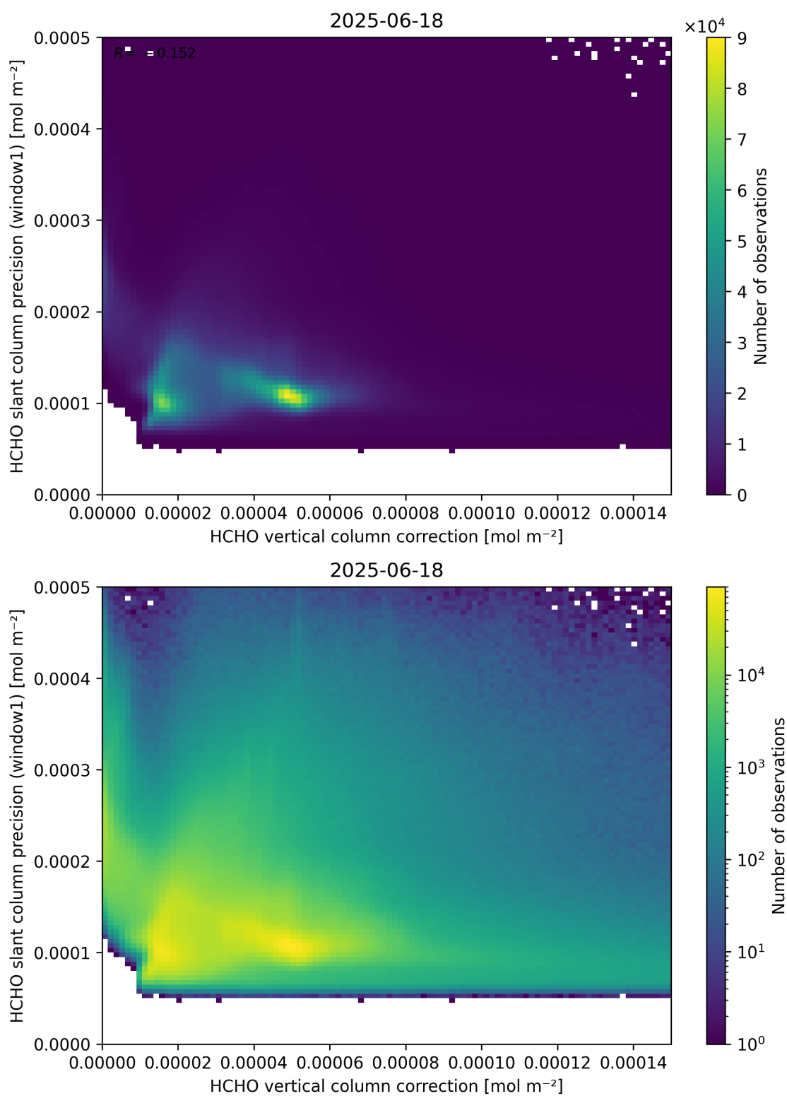
Figure 119: Scatter density plot of “HCHO vertical column correction” against “HCHO slant column precision (window1)” for 2025-06-17 to 2025-06-19.
