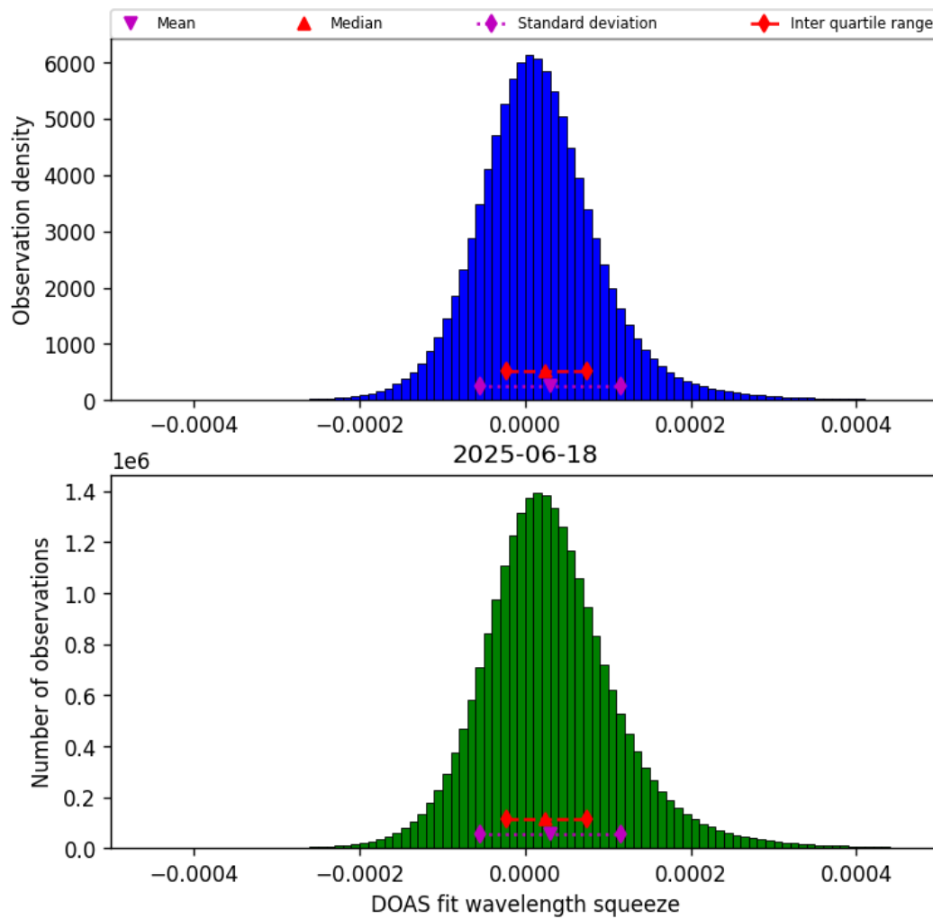
Figure 45: Histogram of “DOAS fit wavelength squeeze” for 2025-06-17 to 2025-06-19
