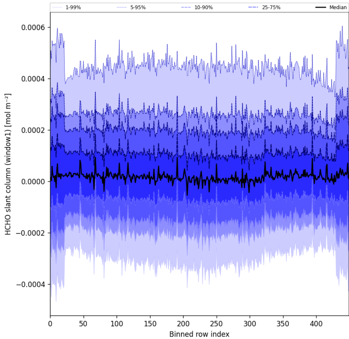
Figure 52: Along track statistics of “HCHO slant column (window1)” for 2025-06-17 to 2025-06-19
