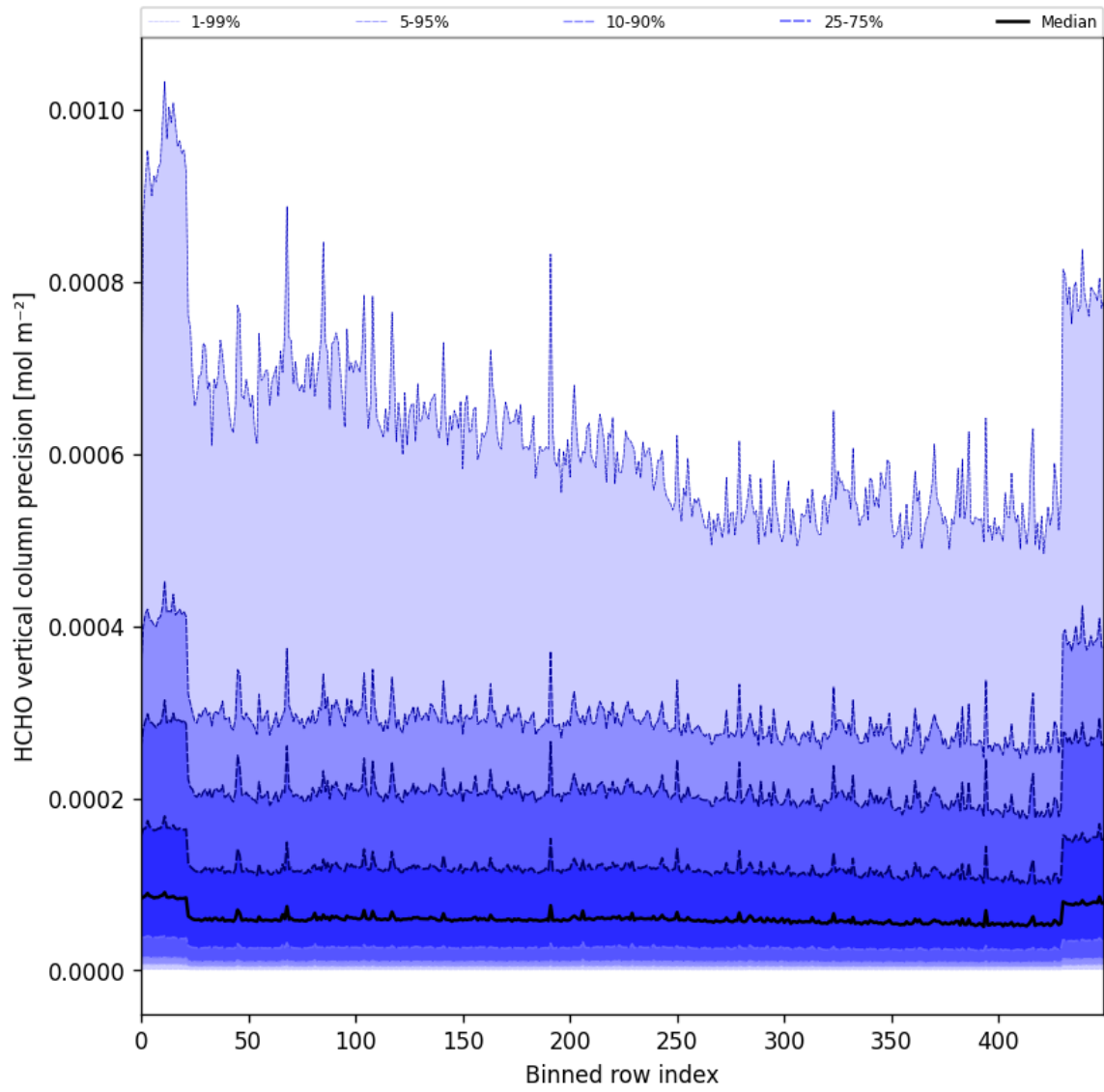
Figure 50: Along track statistics of “HCHO vertical column precision” for 2025-06-17 to 2025-06-19
