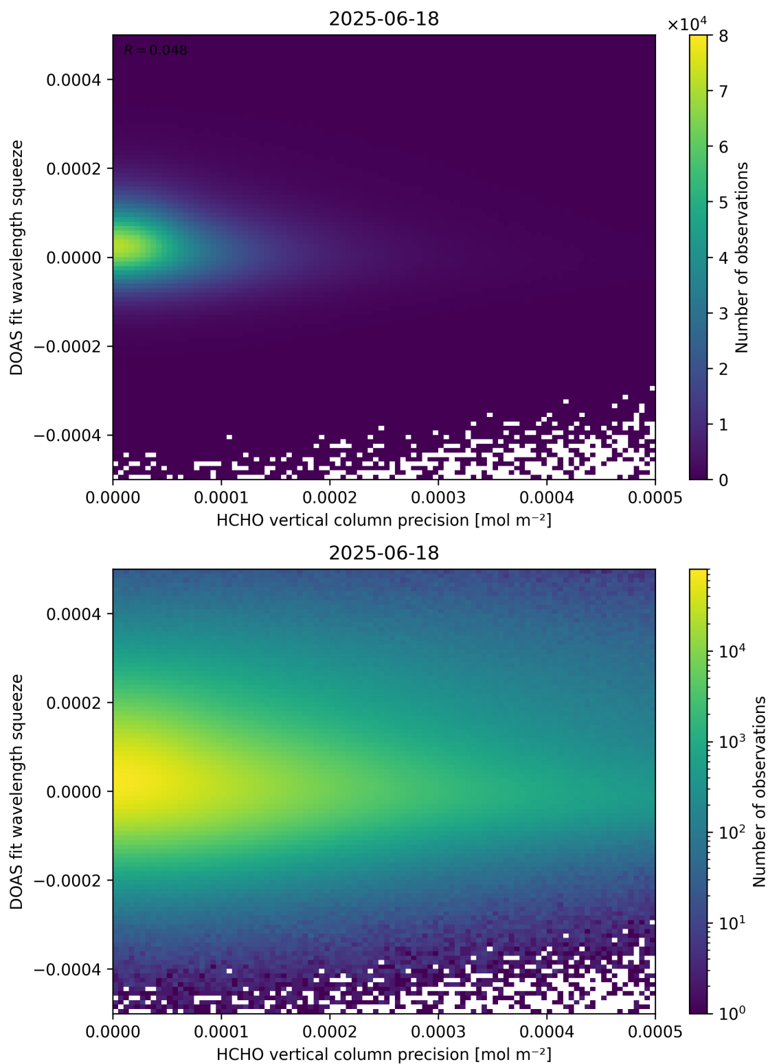
Figure 138: Scatter density plot of “HCHO vertical column precision” against “DOAS fit wavelength squeeze” for 2025-06-17 to 2025-06-19.
