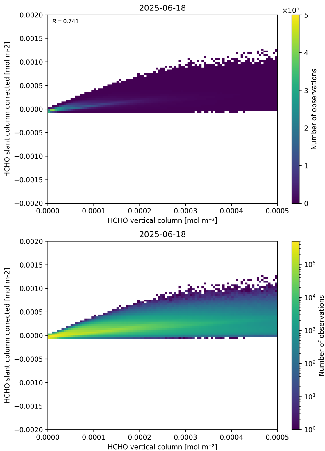
Figure 127: Scatter density plot of “HCHO vertical column” against “HCHO slant column corrected” for 2025-06-17 to 2025-06-19.
