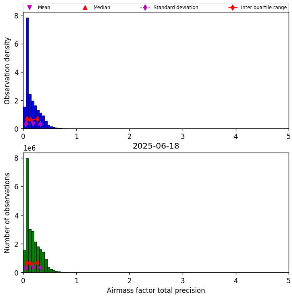
Figure 41: Histogram of “Airmass factor total precision” for 2025-06-17 to 2025-06-19
