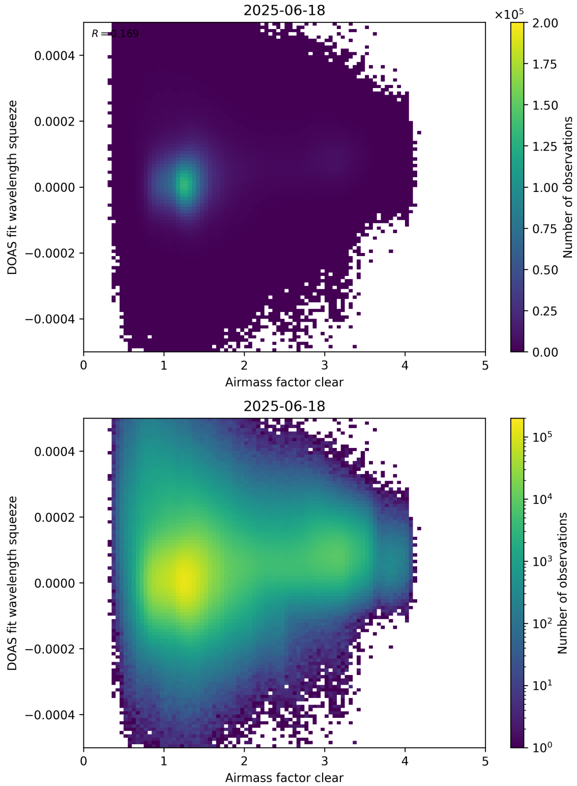
Figure 73: Scatter density plot of “Airmass factor clear” against “DOAS fit wavelength squeeze” for 2025-06-17 to 2025-06-19.
