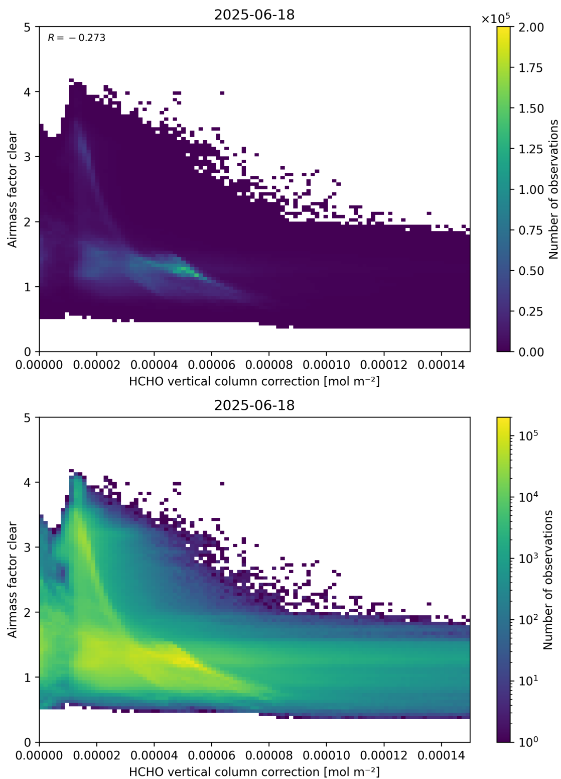
Figure 115: Scatter density plot of “HCHO vertical column correction” against “Airmass factor clear” for 2025-06-17 to 2025-06-19.
