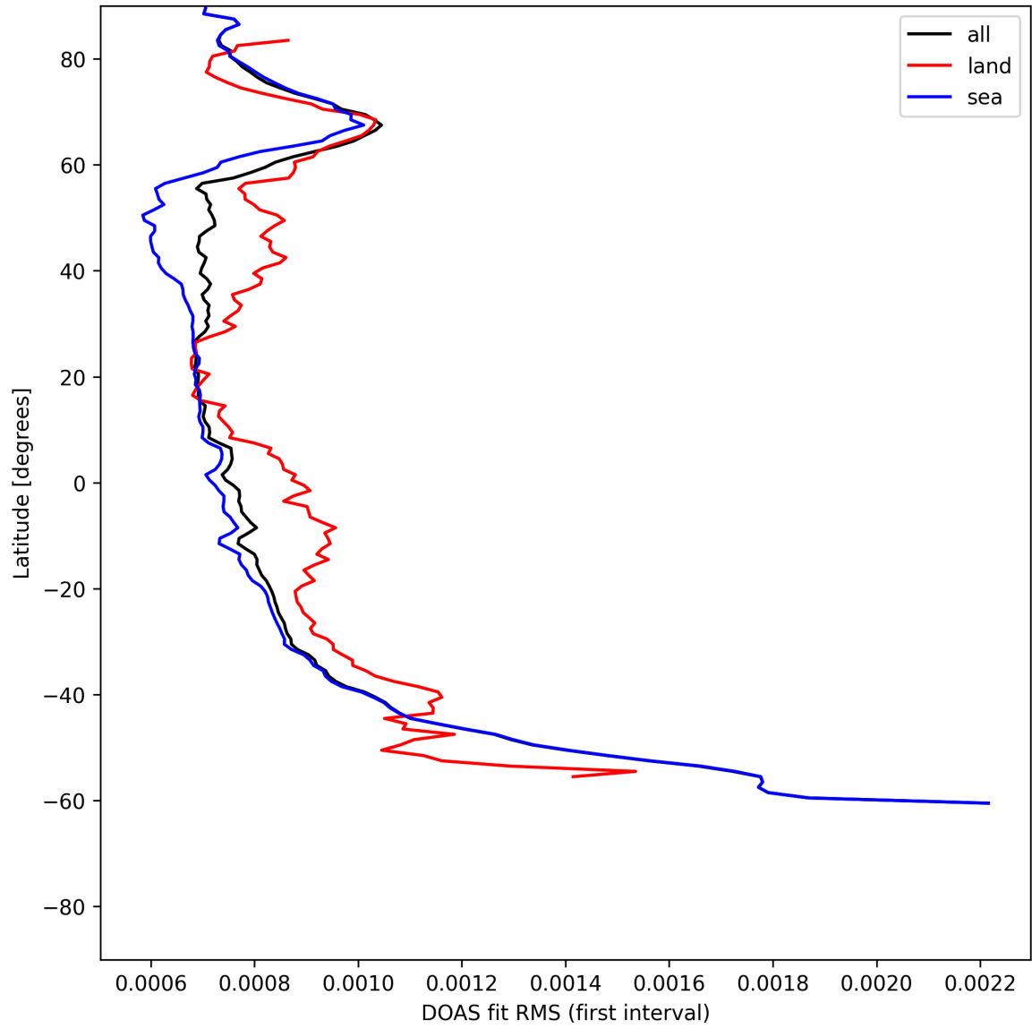
Figure 32: Zonal average of “DOAS fit RMS (first interval)” for 2025-06-17 to 2025-06-19.
