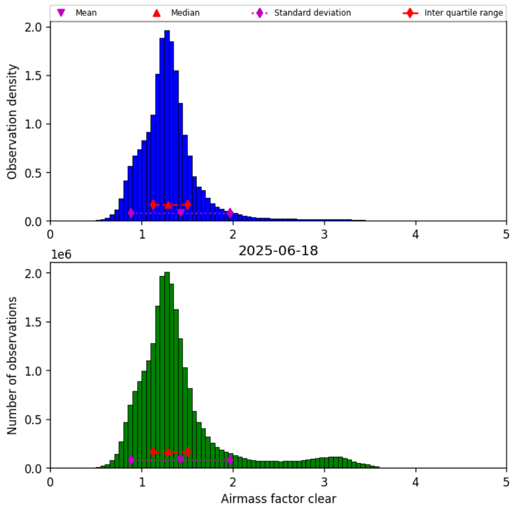
Figure 42: Histogram of “Airmass factor clear” for 2025-06-17 to 2025-06-19
