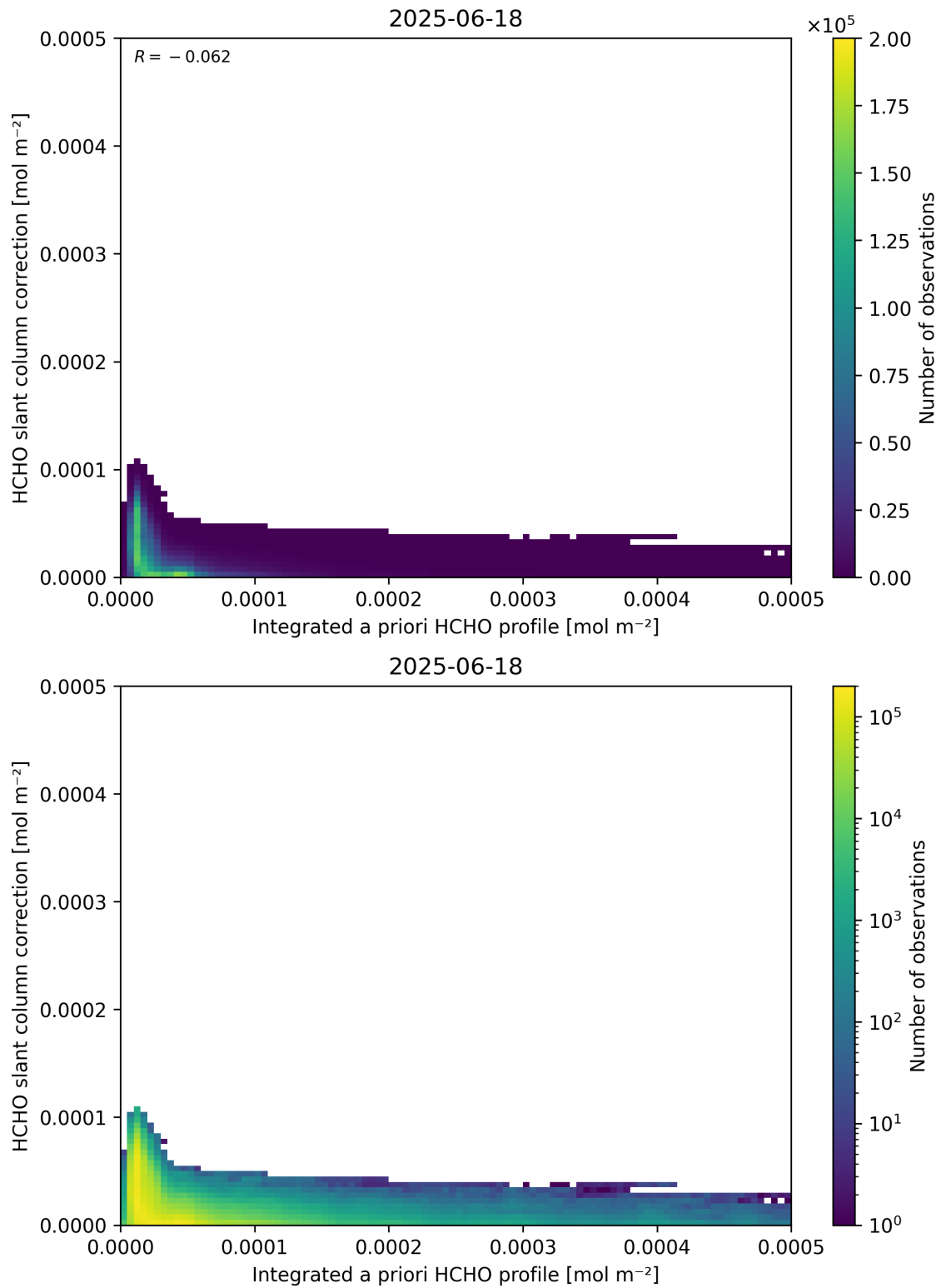
Figure 152: Scatter density plot of “Integrated a priori HCHO profile” against “HCHO slant column correction” for 2025-06-17 to 2025-06-19.
