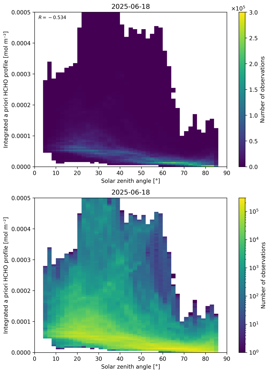
Figure 180: Scatter density plot of “Solar zenith angle” against “Integrated a priori HCHO profile” for 2025-06-17 to 2025-06-19.
