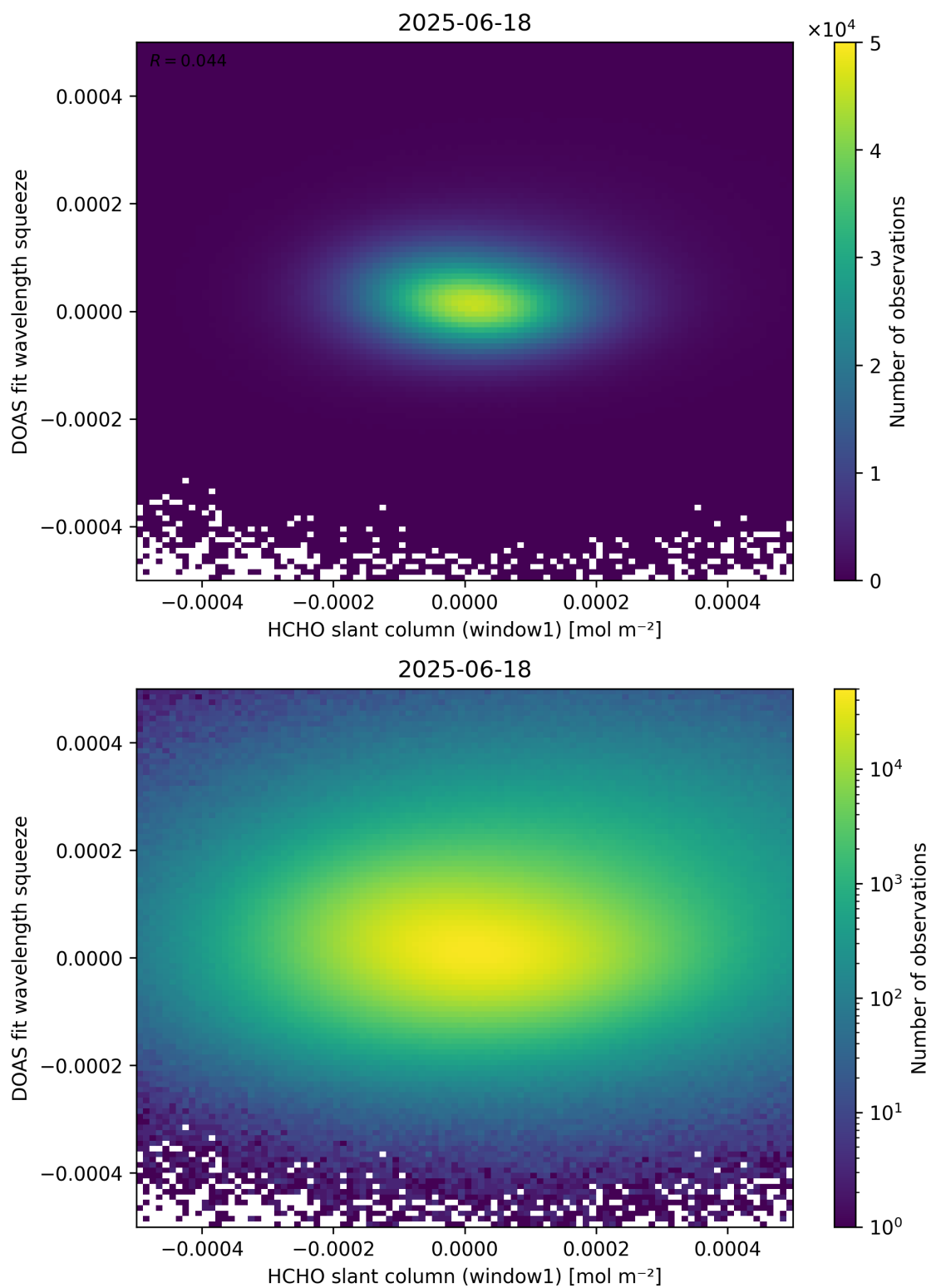
Figure 80: Scatter density plot of “HCHO slant column (window1)” against “DOAS fit wavelength squeeze” for 2025-06-17 to 2025-06-19.
