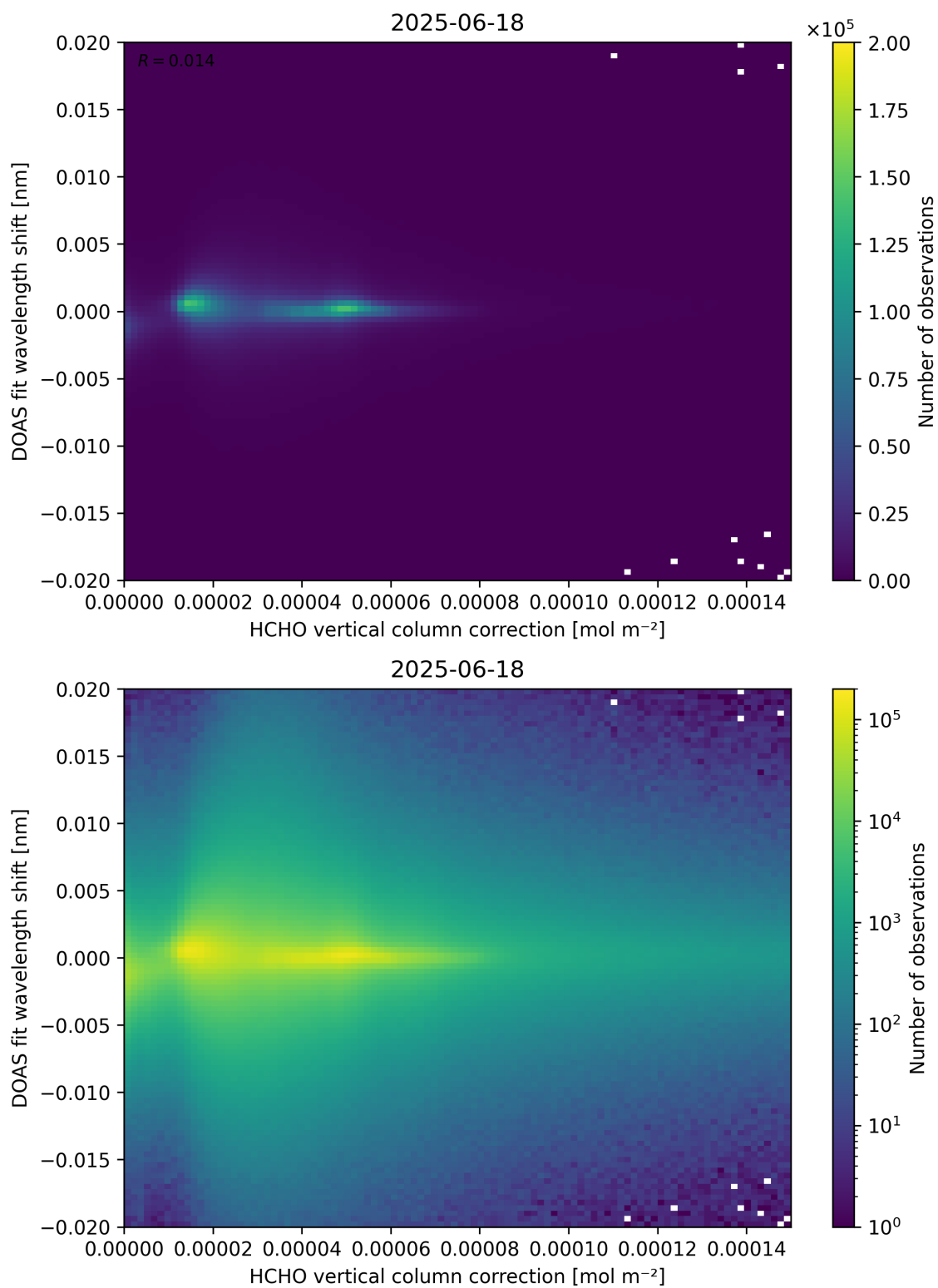
Figure 113: Scatter density plot of “HCHO vertical column correction” against “DOAS fit wavelength shift” for 2025-06-17 to 2025-06-19.
