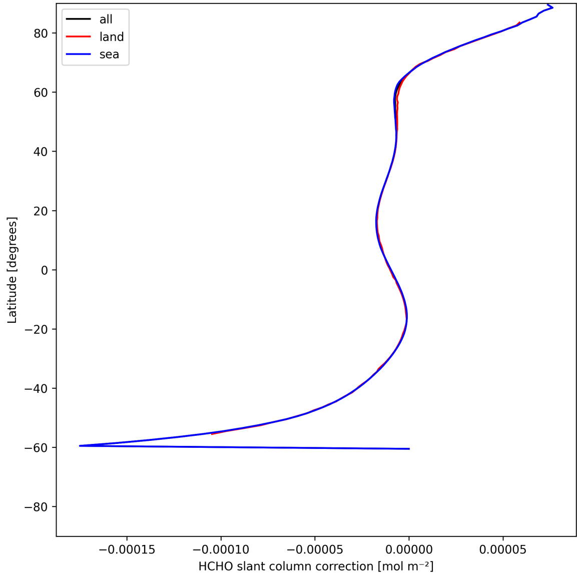
Figure 33: Zonal average of “HCHO slant column correction” for 2025-06-17 to 2025-06-19.
