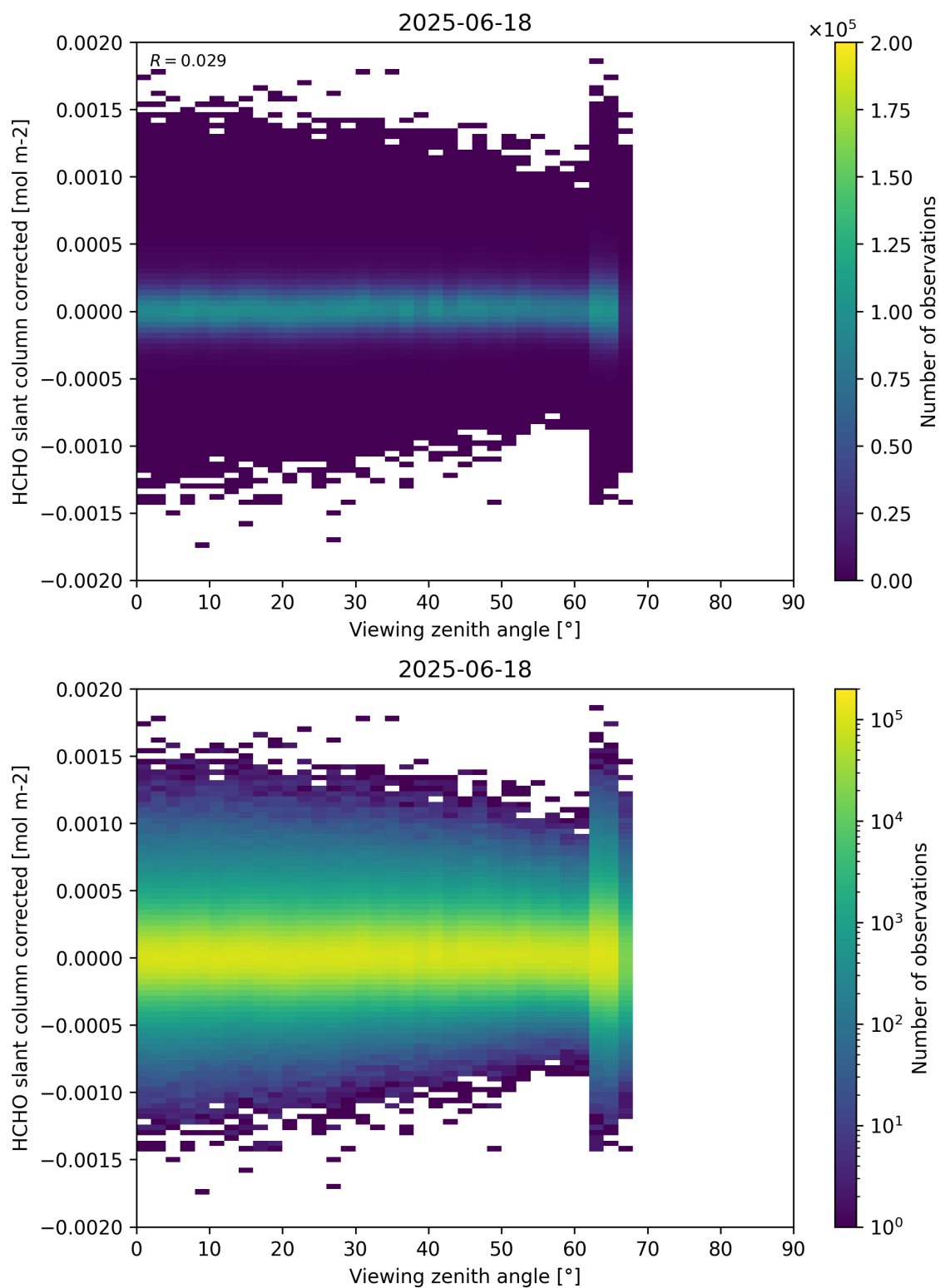
Figure 186: Scatter density plot of “Viewing zenith angle” against “HCHO slant column corrected” for 2025-06-17 to 2025-06-19.
