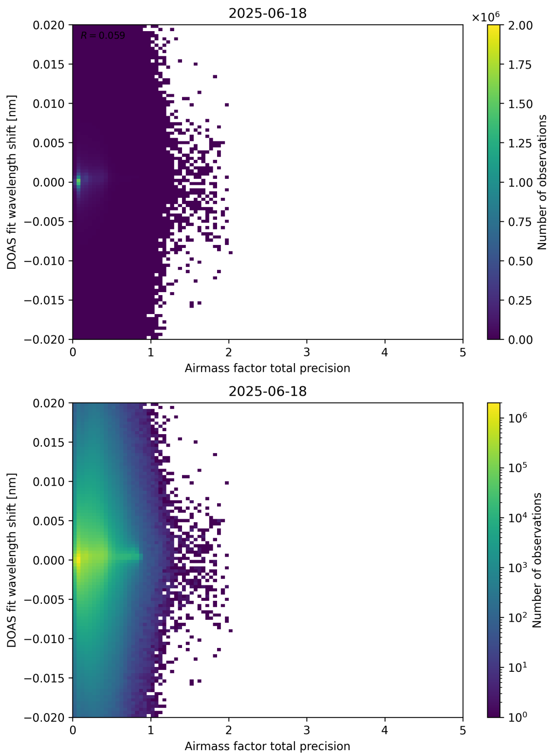
Figure 106: Scatter density plot of “Airmass factor total precision” against “DOAS fit wavelength shift” for 2025-06-17 to 2025-06-19.
