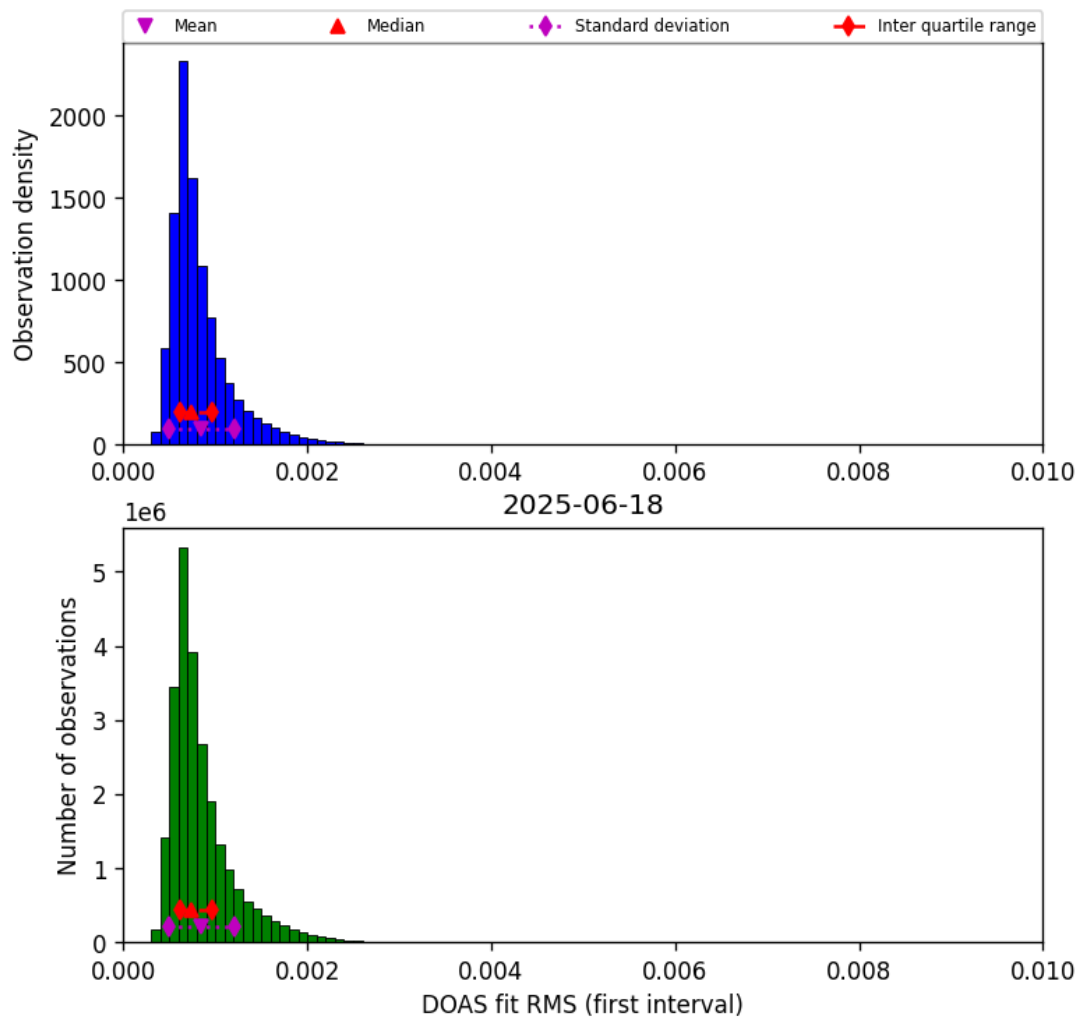
Figure 46: Histogram of “DOAS fit RMS (first interval)” for 2025-06-17 to 2025-06-19
