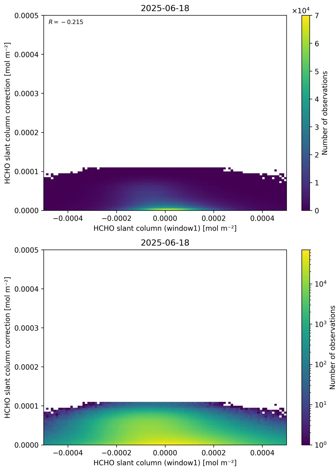
Figure 83: Scatter density plot of “HCHO slant column (window1)” against “HCHO slant column correction” for 2025-06-17 to 2025-06-19.
