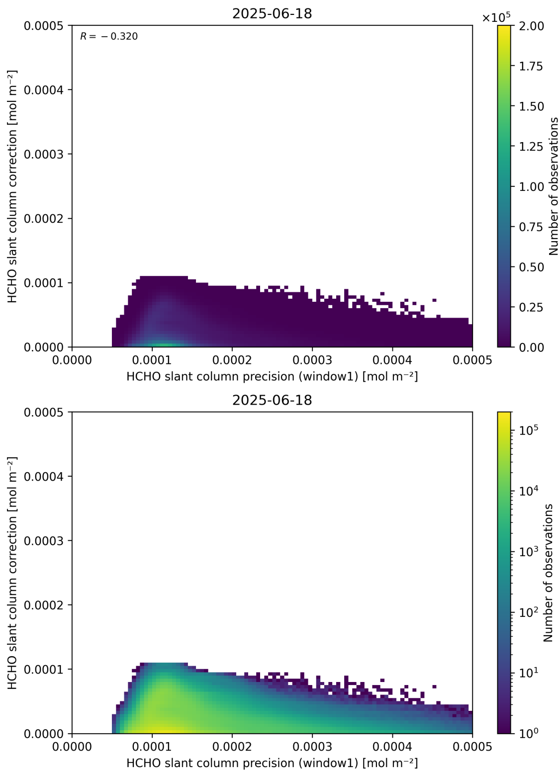
Figure 93: Scatter density plot of “HCHO slant column precision (window1)” against “HCHO slant column correction” for 2025-06-17 to 2025-06-19.
