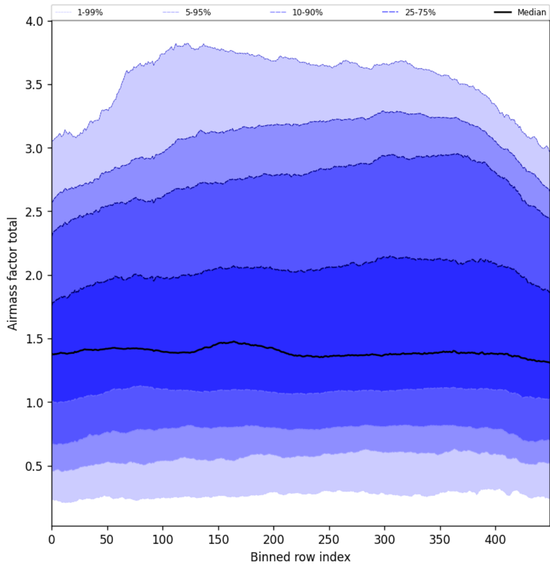
Figure 54: Along track statistics of “Airmass factor total” for 2025-06-17 to 2025-06-19
