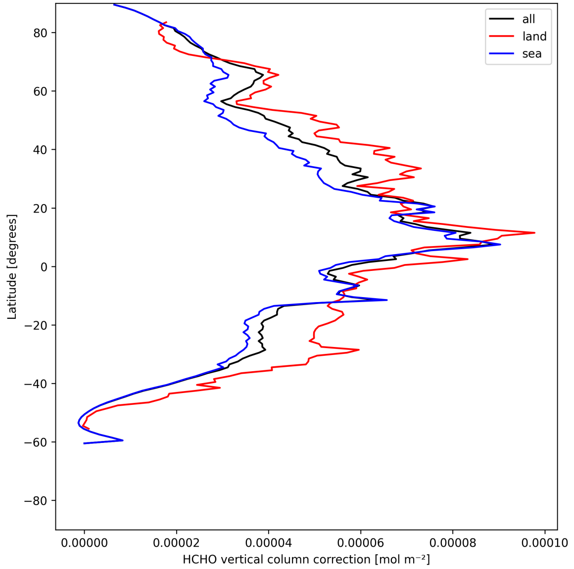
Figure 23: Zonal average of “HCHO vertical column correction” for 2025-06-17 to 2025-06-19.
