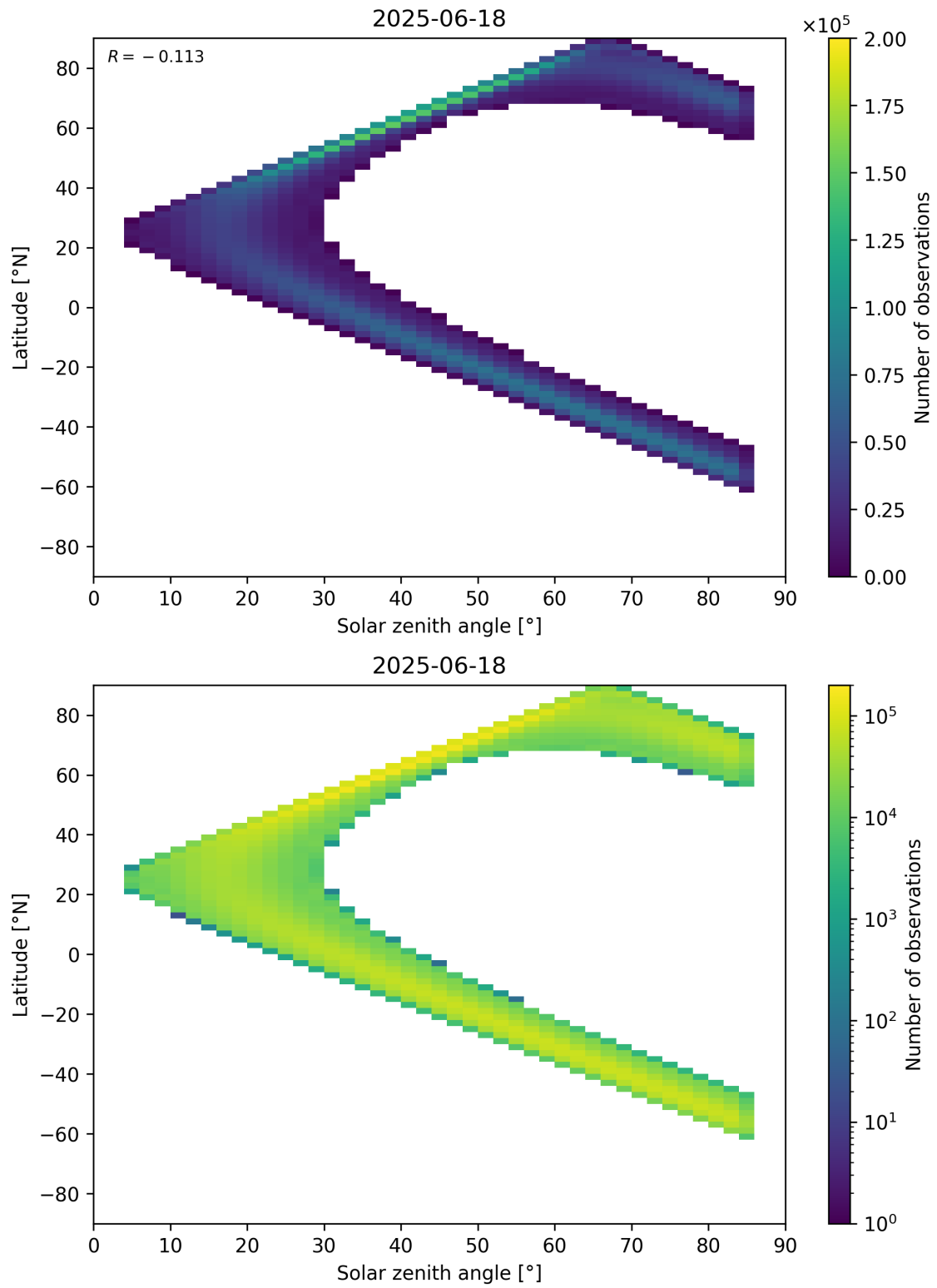
Figure 181: Scatter density plot of “Solar zenith angle” against “Latitude” for 2025-06-17 to 2025-06-19.
