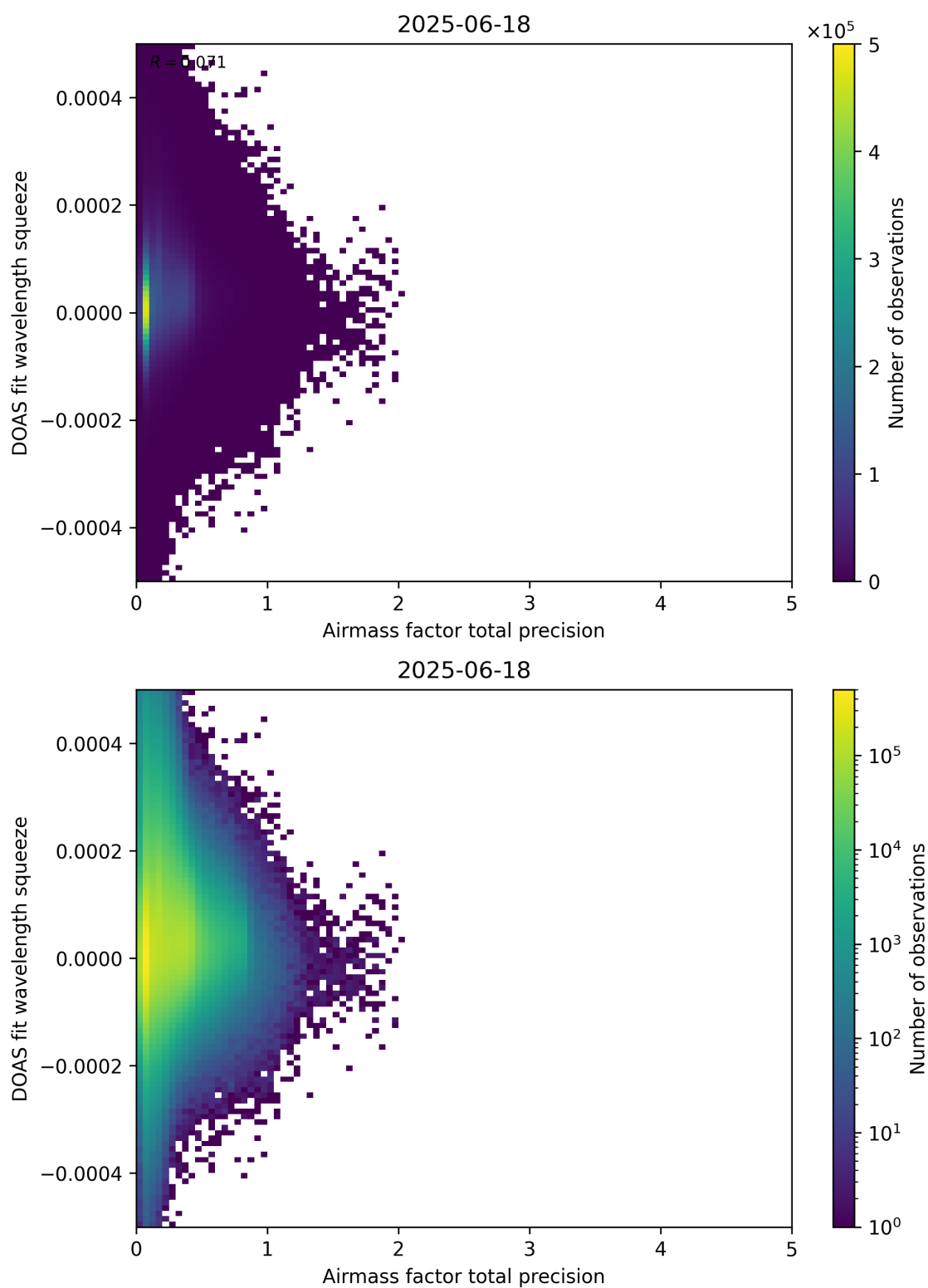
Figure 107: Scatter density plot of “Airmass factor total precision” against “DOAS fit wavelength squeeze” for 2025-06-17 to 2025-06-19.
