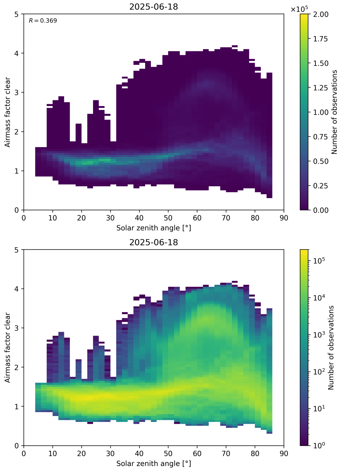
Figure 170: Scatter density plot of “Solar zenith angle” against “Airmass factor clear” for 2025-06-17 to 2025-06-19.
