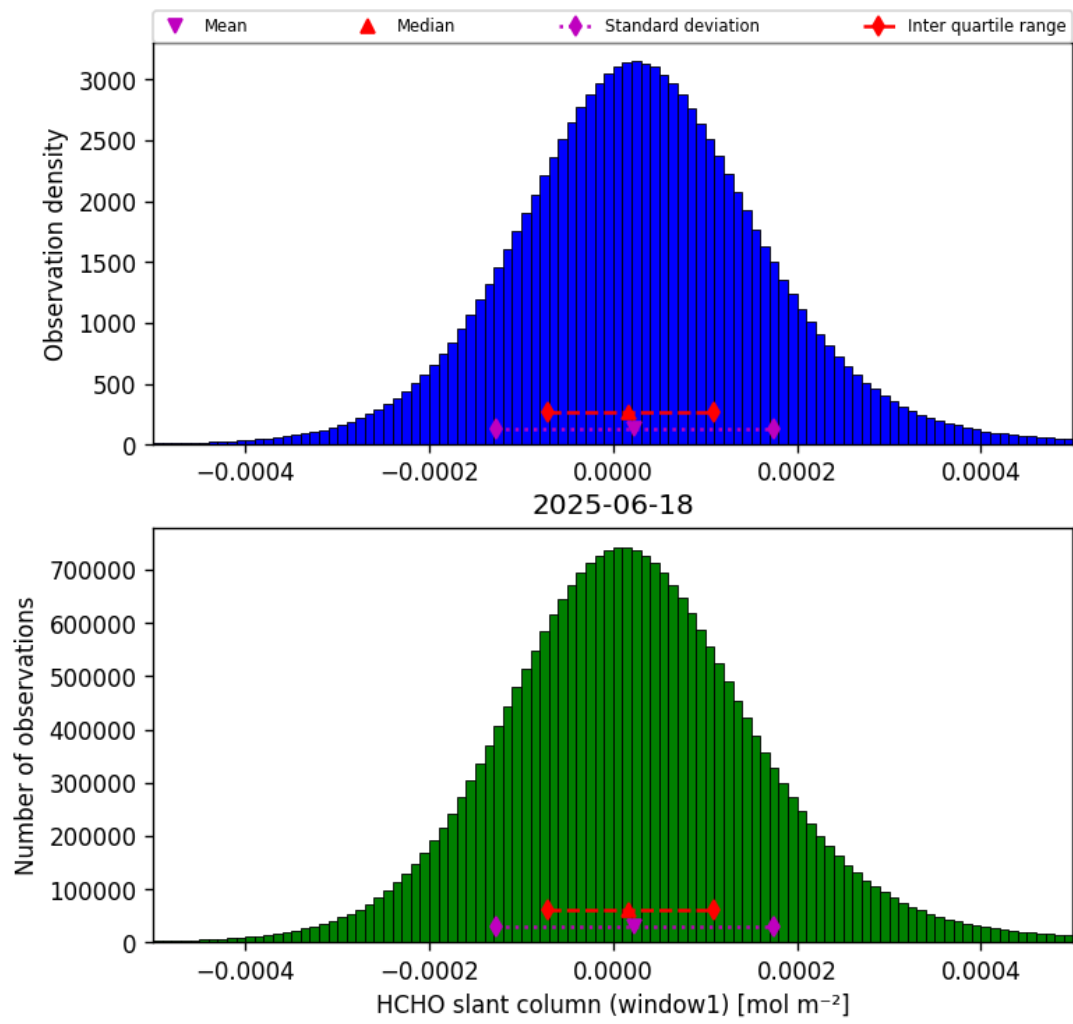
Figure 38: Histogram of “HCHO slant column (window1)” for 2025-06-17 to 2025-06-19
