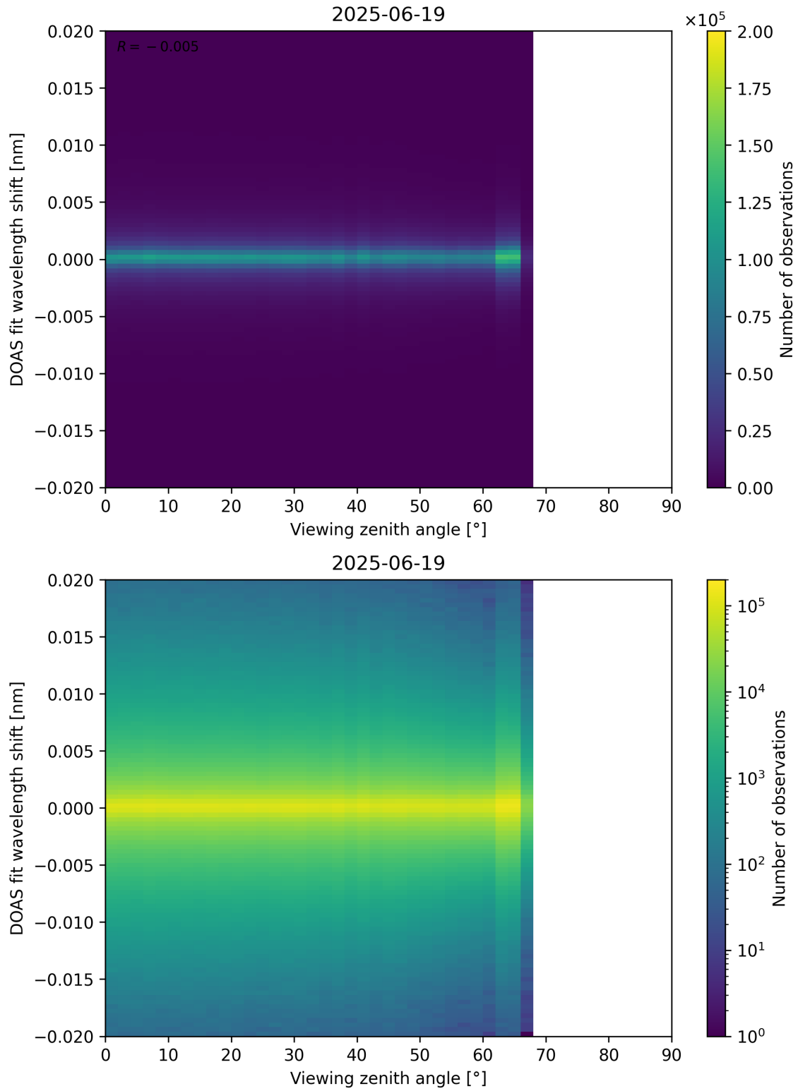
Figure 183: Scatter density plot of “Viewing zenith angle” against “DOAS fit wavelength shift” for 2025-06-18 to 2025-06-20.
