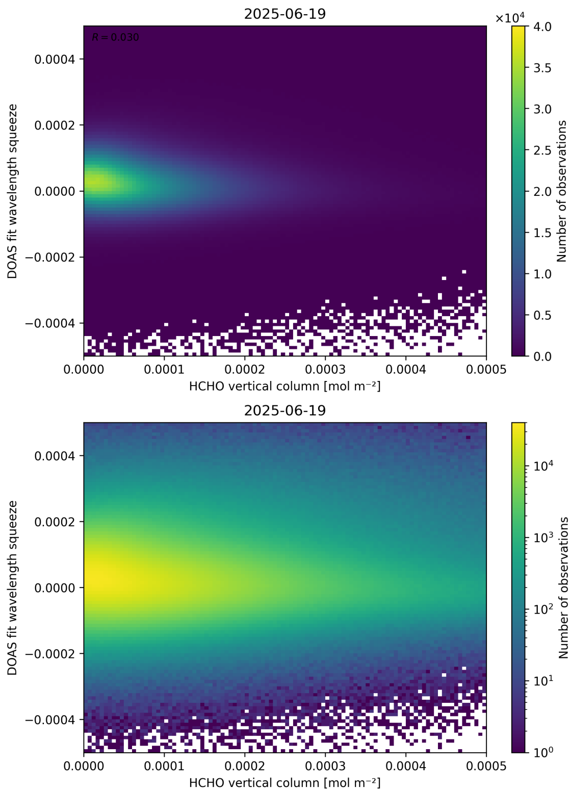
Figure 125: Scatter density plot of “HCHO vertical column” against “DOAS fit wavelength squeeze” for 2025-06-18 to 2025-06-20.
