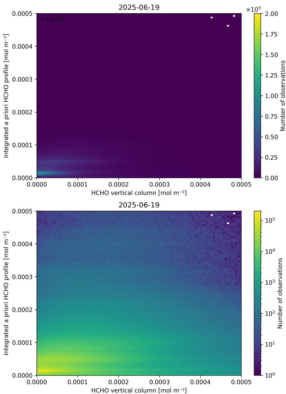
Figure 135: Scatter density plot of “HCHO vertical column” against “Integrated a priori HCHO profile” for 2025-06-18 to 2025-06-20.
