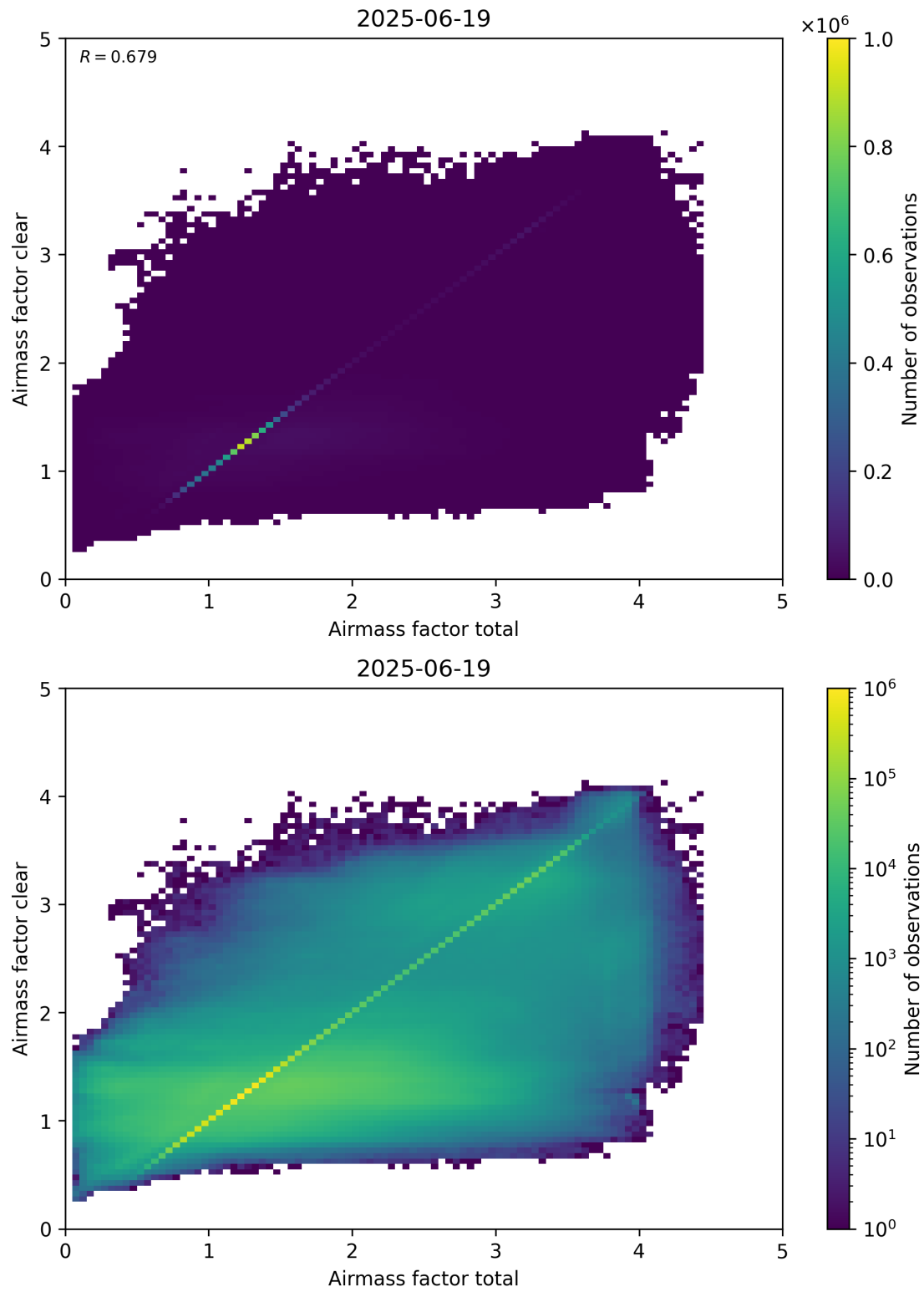
Figure 100: Scatter density plot of “Airmass factor total” against “Airmass factor clear” for 2025-06-18 to 2025-06-20.
