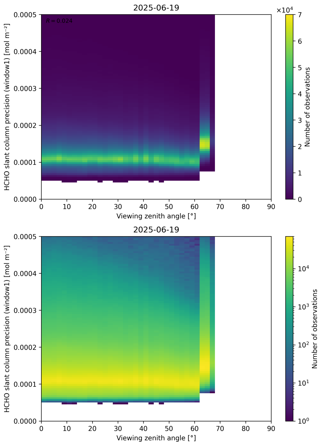
Figure 189: Scatter density plot of “Viewing zenith angle” against “HCHO slant column precision (window1)” for 2025-06-18 to 2025-06-20.
