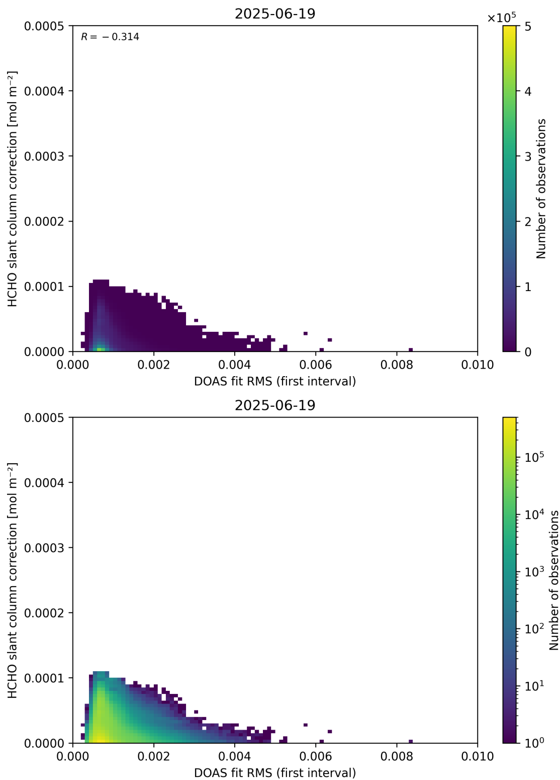
Figure 63: Scatter density plot of “DOAS fit RMS (first interval)” against “HCHO slant column correction” for 2025-06-18 to 2025-06-20.
