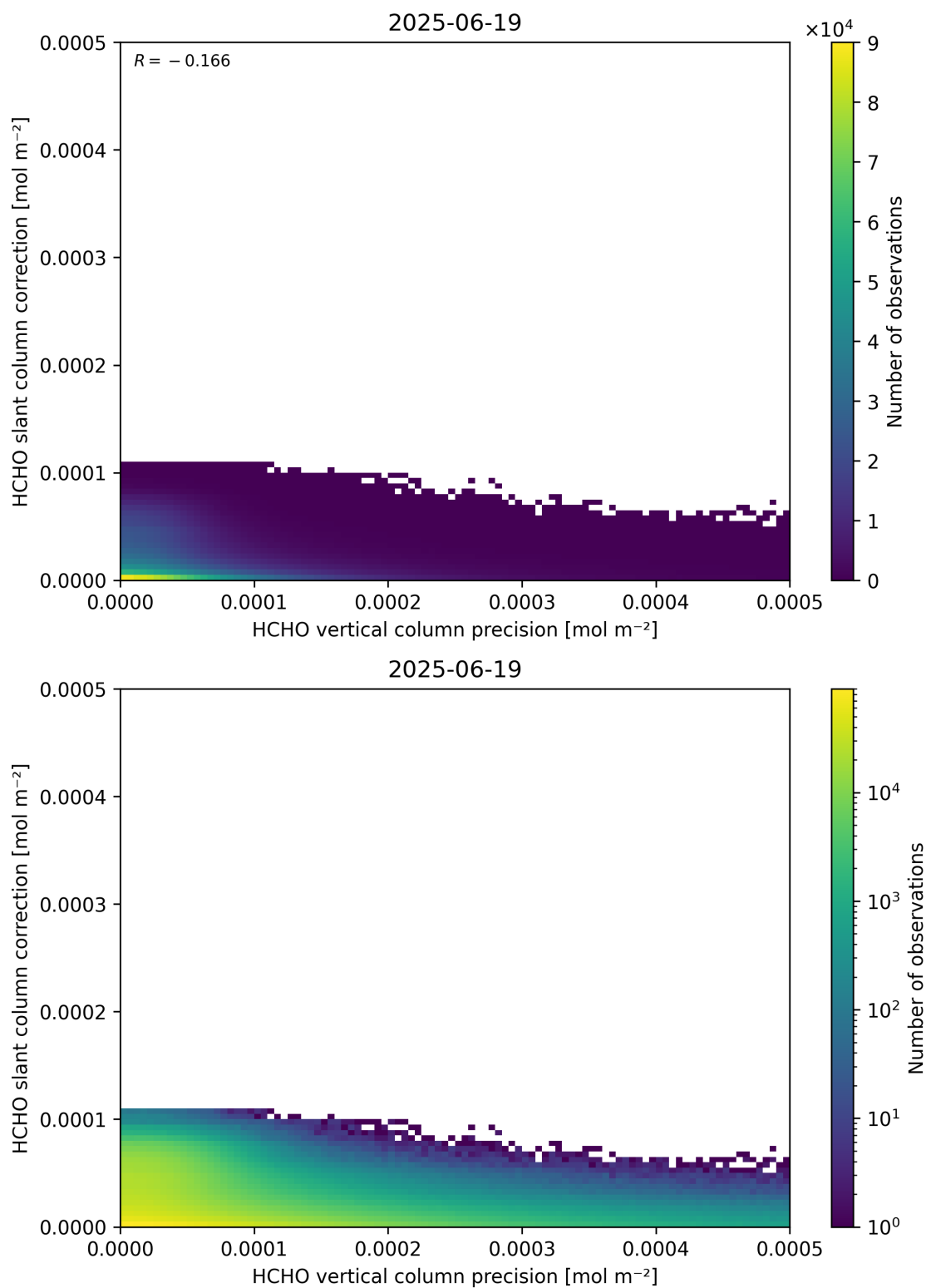
Figure 141: Scatter density plot of “HCHO vertical column precision” against “HCHO slant column correction” for 2025-06-18 to 2025-06-20.
