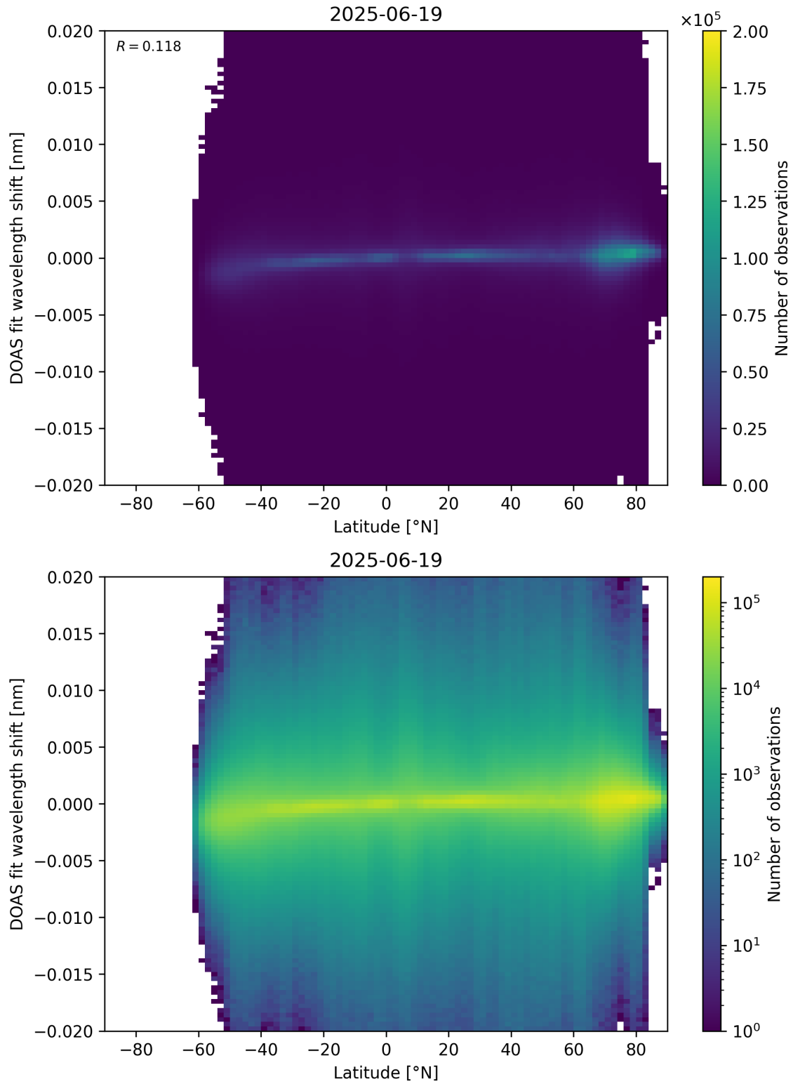
Figure 154: Scatter density plot of “Latitude” against “DOAS fit wavelength shift” for 2025-06-18 to 2025-06-20.
