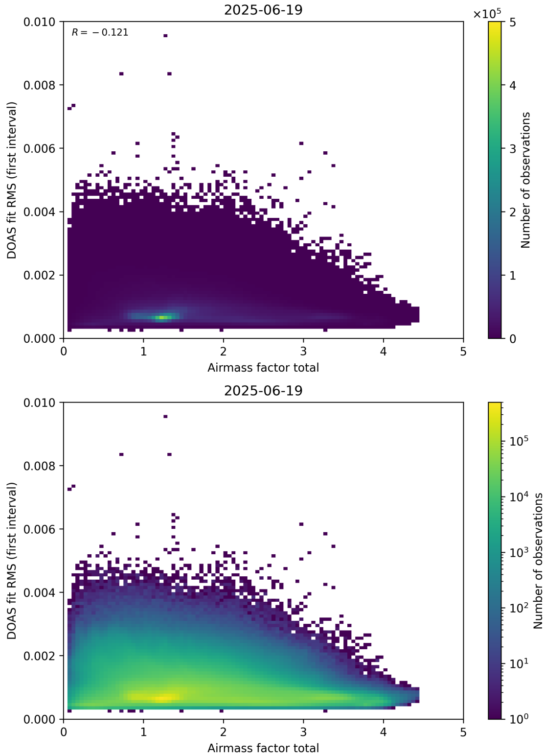
Figure 97: Scatter density plot of “Airmass factor total” against “DOAS fit RMS (first interval)” for 2025-06-18 to 2025-06-20.
