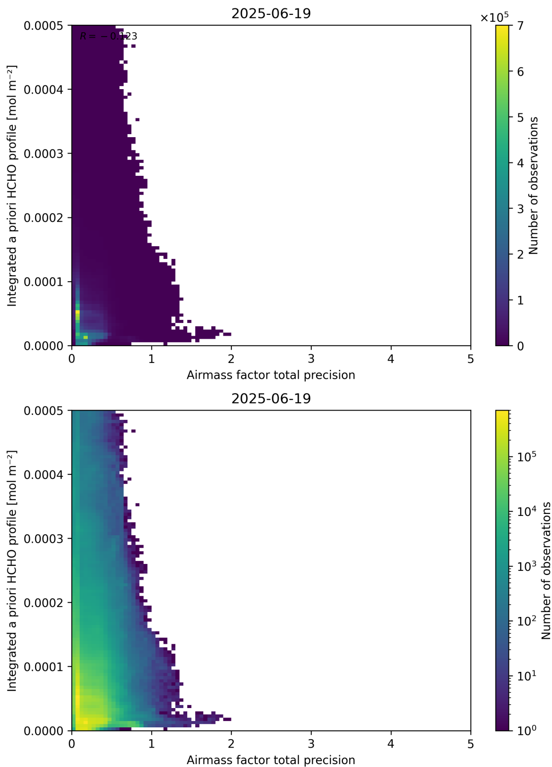
Figure 111: Scatter density plot of “Airmass factor total precision” against “Integrated a priori HCHO profile” for 2025-06-18 to 2025-06-20.
