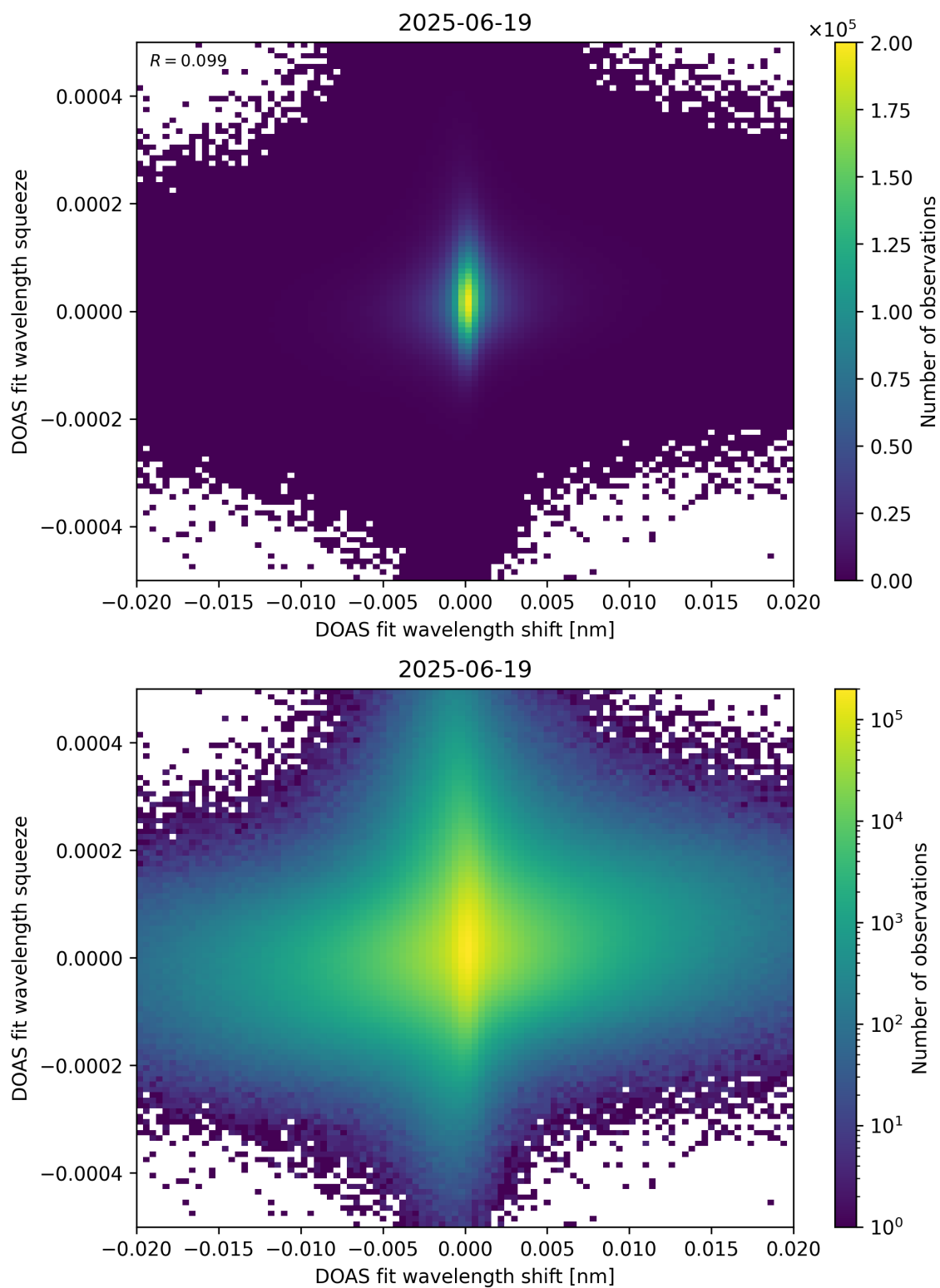
Figure 65: Scatter density plot of “DOAS fit wavelength shift” against “DOAS fit wavelength squeeze” for 2025-06-18 to 2025-06-20.
