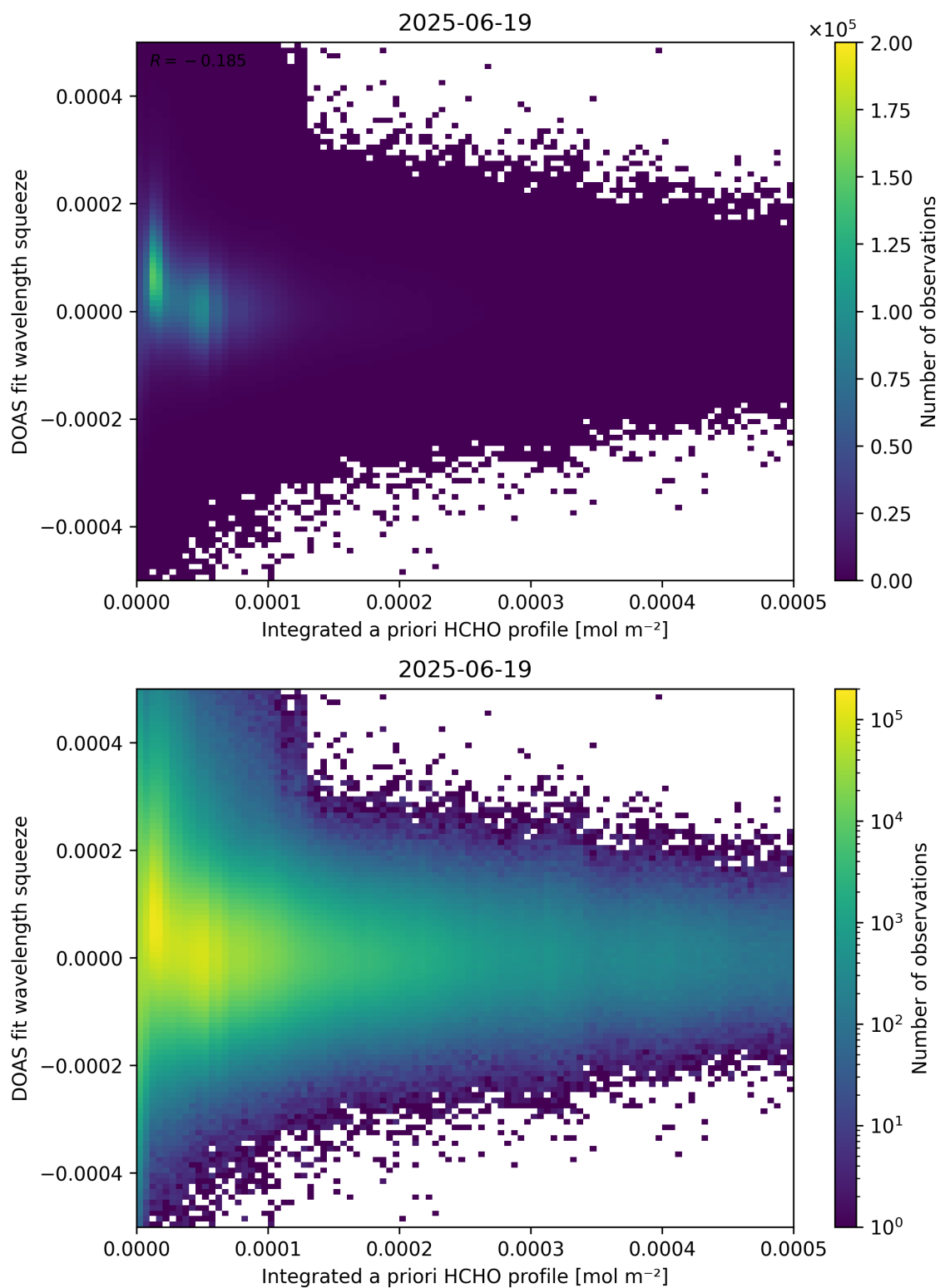
Figure 150: Scatter density plot of “Integrated a priori HCHO profile” against “DOAS fit wavelength squeeze” for 2025-06-18 to 2025-06-20.
