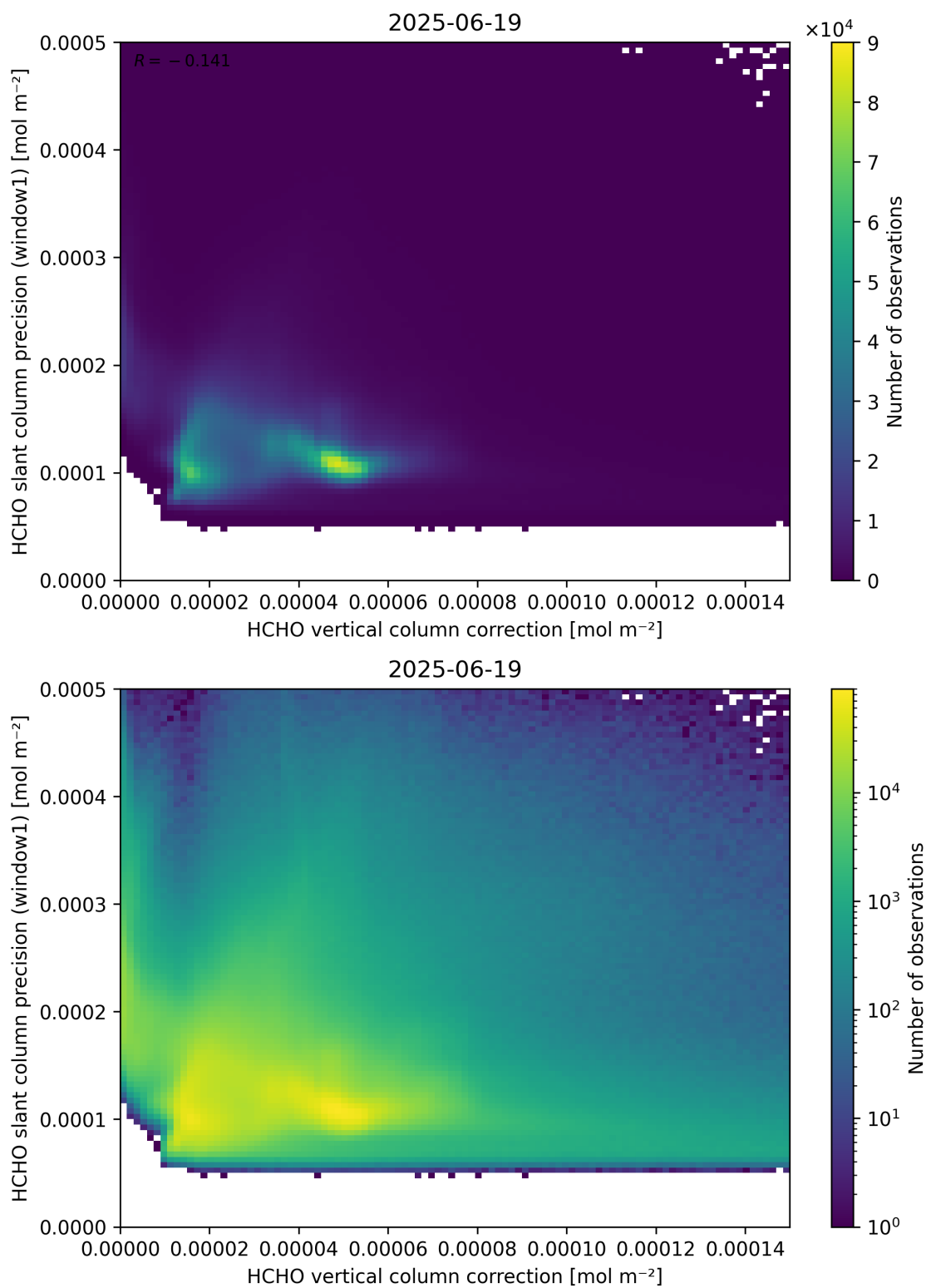
Figure 119: Scatter density plot of “HCHO vertical column correction” against “HCHO slant column precision (window1)” for 2025-06-18 to 2025-06-20.
