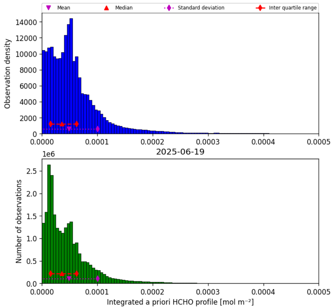
Figure 43: Histogram of “Integrated a priori HCHO profile” for 2025-06-18 to 2025-06-20
