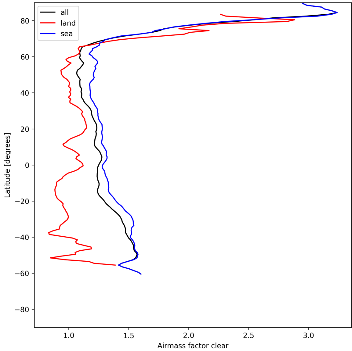
Figure 28: Zonal average of “Airmass factor clear” for 2025-06-18 to 2025-06-20.
