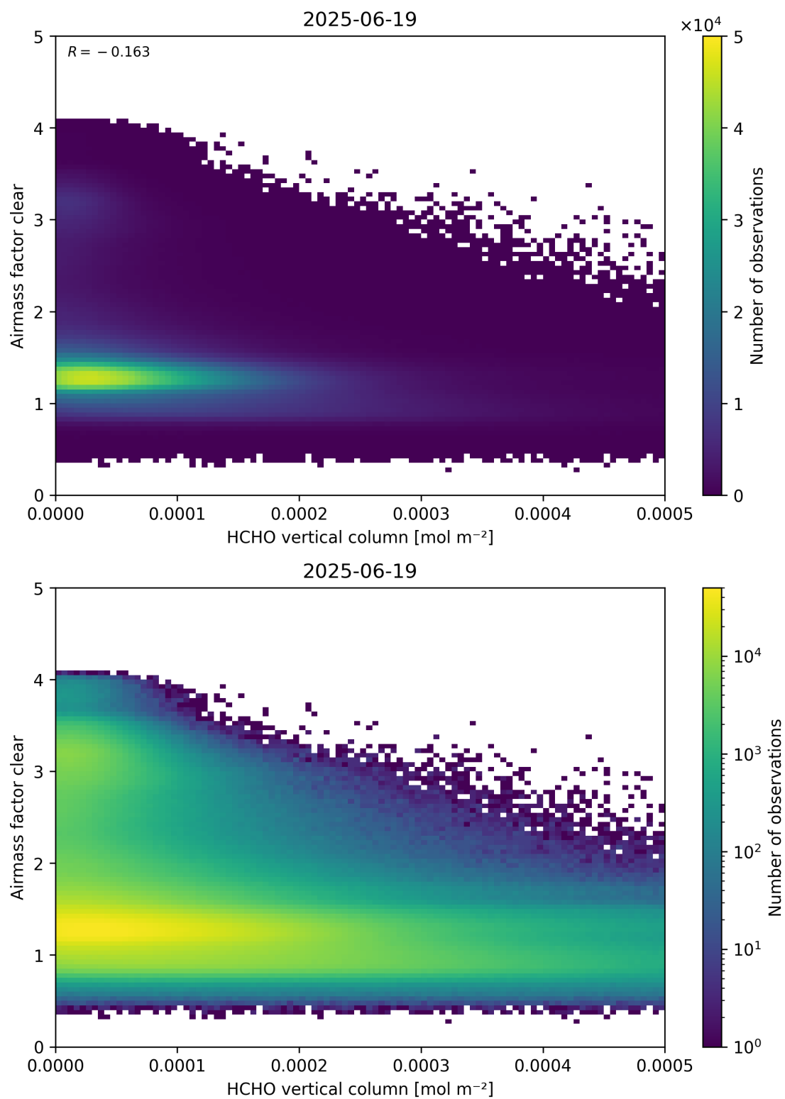
Figure 126: Scatter density plot of “HCHO vertical column” against “Airmass factor clear” for 2025-06-18 to 2025-06-20.
