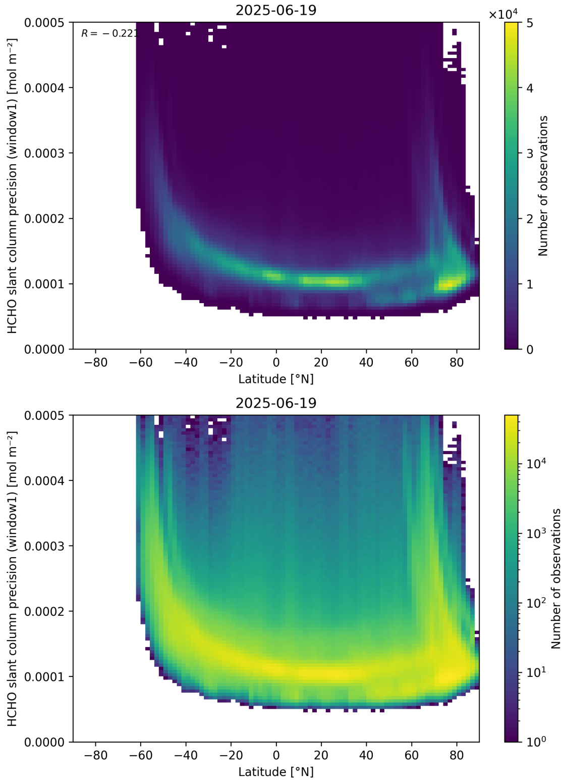
Figure 160: Scatter density plot of “Latitude” against “HCHO slant column precision (window1)” for 2025-06-18 to 2025-06-20.
