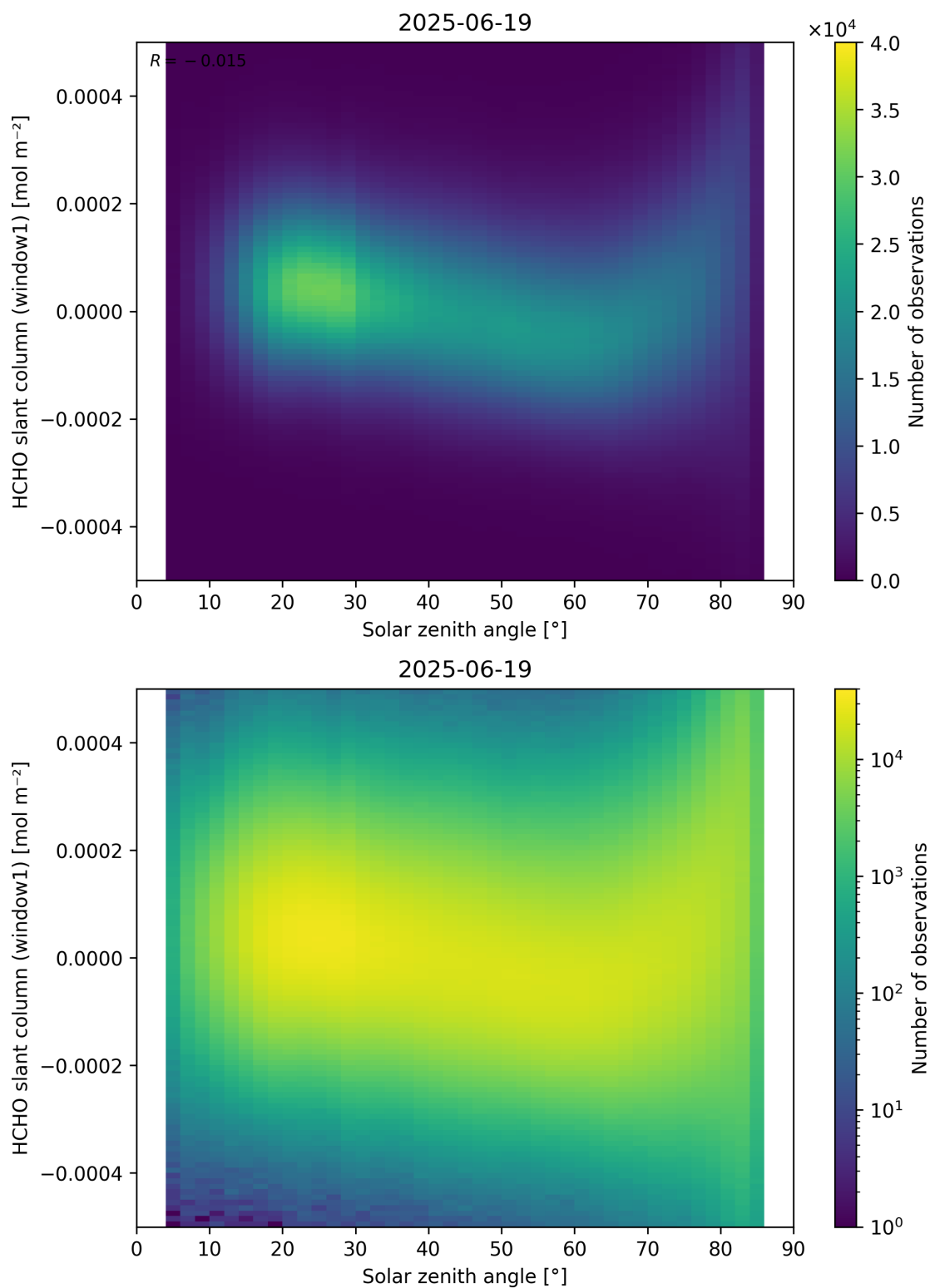
Figure 173: Scatter density plot of “Solar zenith angle” against “HCHO slant column (window1)” for 2025-06-18 to 2025-06-20.
