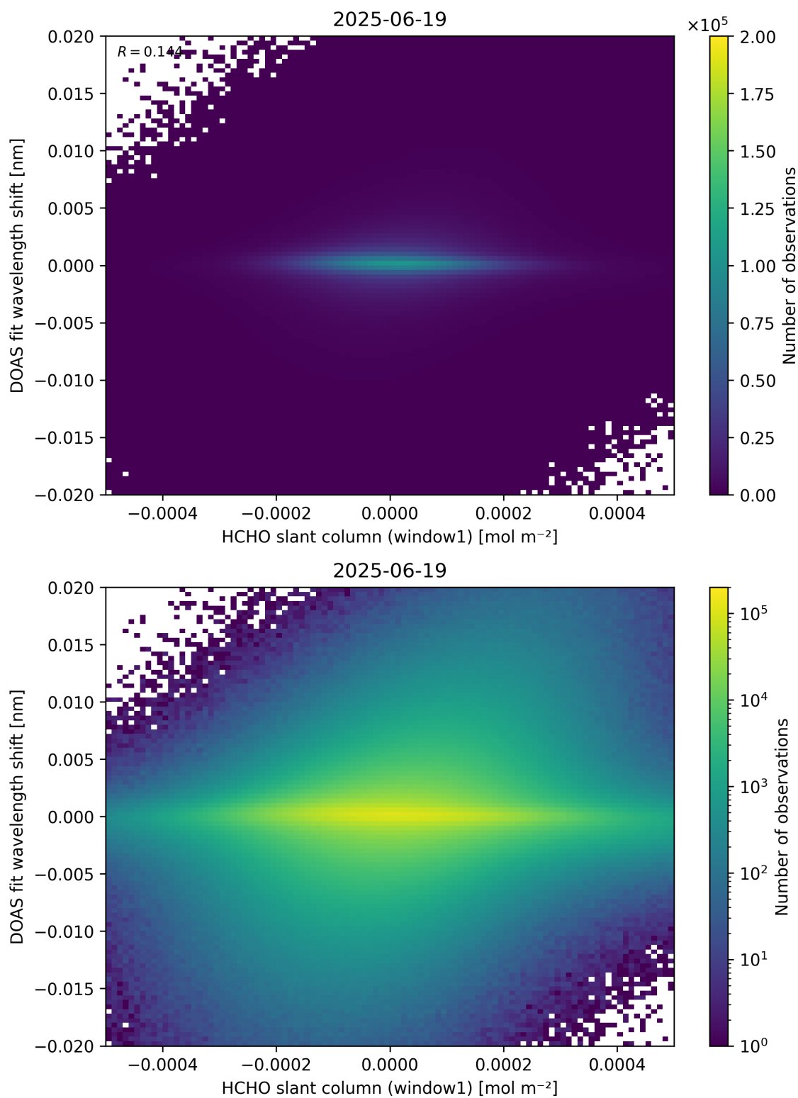
Figure 79: Scatter density plot of “HCHO slant column (window1)” against “DOAS fit wavelength shift” for 2025-06-18 to 2025-06-20.
