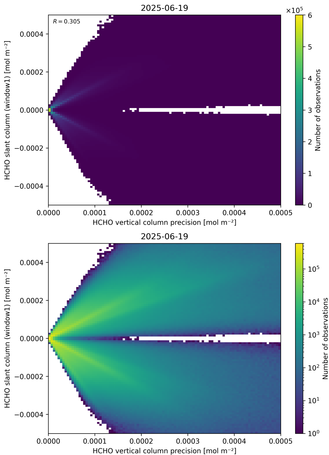
Figure 142: Scatter density plot of “HCHO vertical column precision” against “HCHO slant column (window1)” for 2025-06-18 to 2025-06-20.
