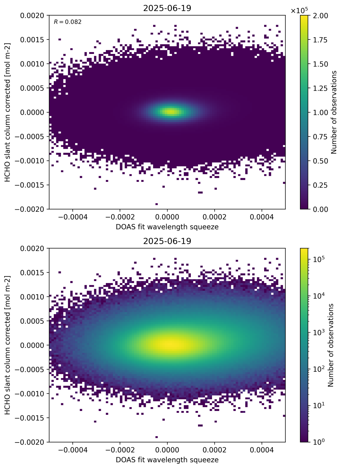
Figure 69: Scatter density plot of “DOAS fit wavelength squeeze” against “HCHO slant column corrected” for 2025-06-18 to 2025-06-20.
