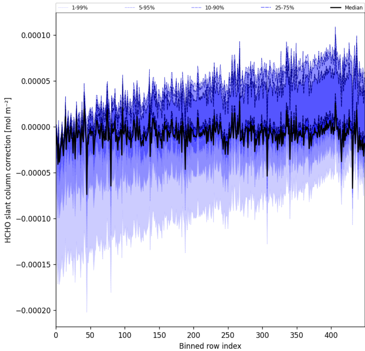
Figure 61: Along track statistics of “HCHO slant column correction” for 2025-06-18 to 2025-06-20
