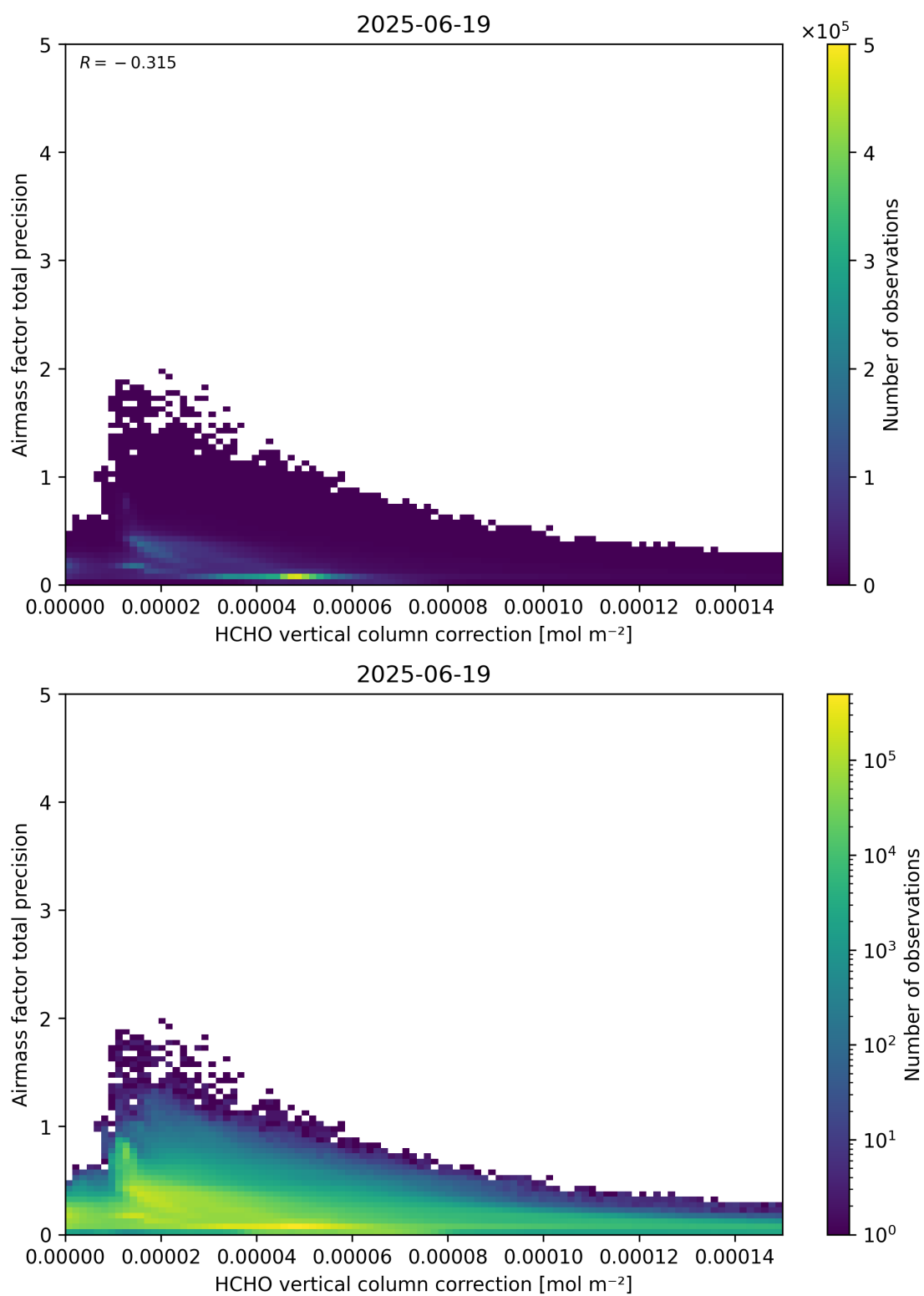
Figure 121: Scatter density plot of “HCHO vertical column correction” against “Airmass factor total precision” for 2025-06-18 to 2025-06-20.
