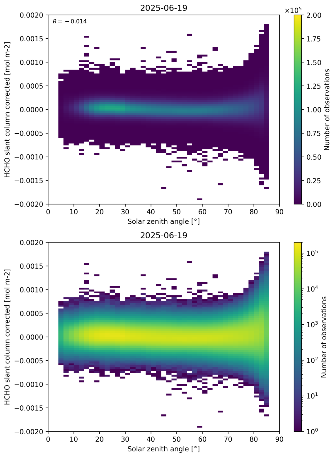
Figure 171: Scatter density plot of “Solar zenith angle” against “HCHO slant column corrected” for 2025-06-18 to 2025-06-20.
