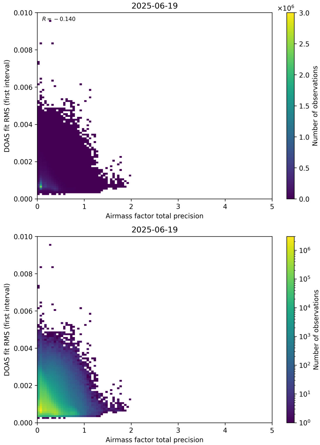
Figure 105: Scatter density plot of “Airmass factor total precision” against “DOAS fit RMS (first interval)” for 2025-06-18 to 2025-06-20.
