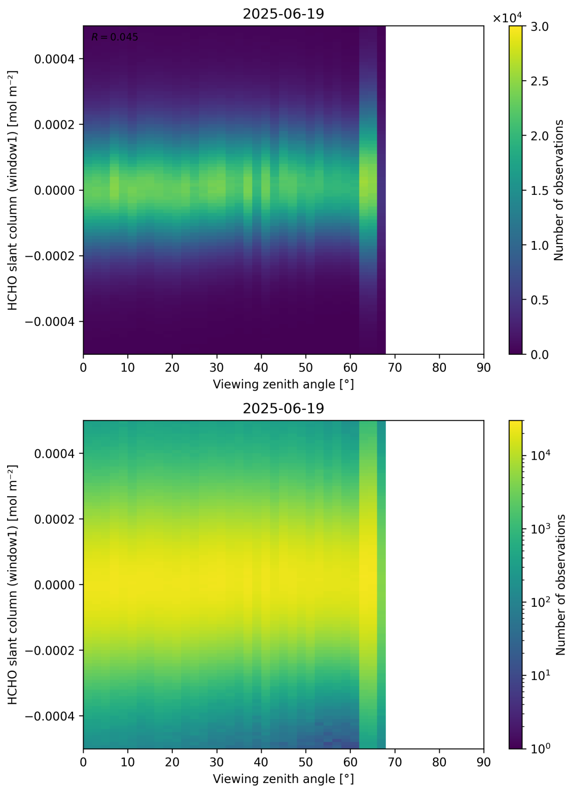
Figure 188: Scatter density plot of “Viewing zenith angle” against “HCHO slant column (window1)” for 2025-06-18 to 2025-06-20.
