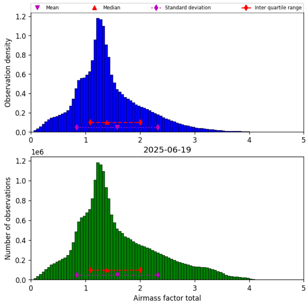
Figure 40: Histogram of “Airmass factor total” for 2025-06-18 to 2025-06-20
