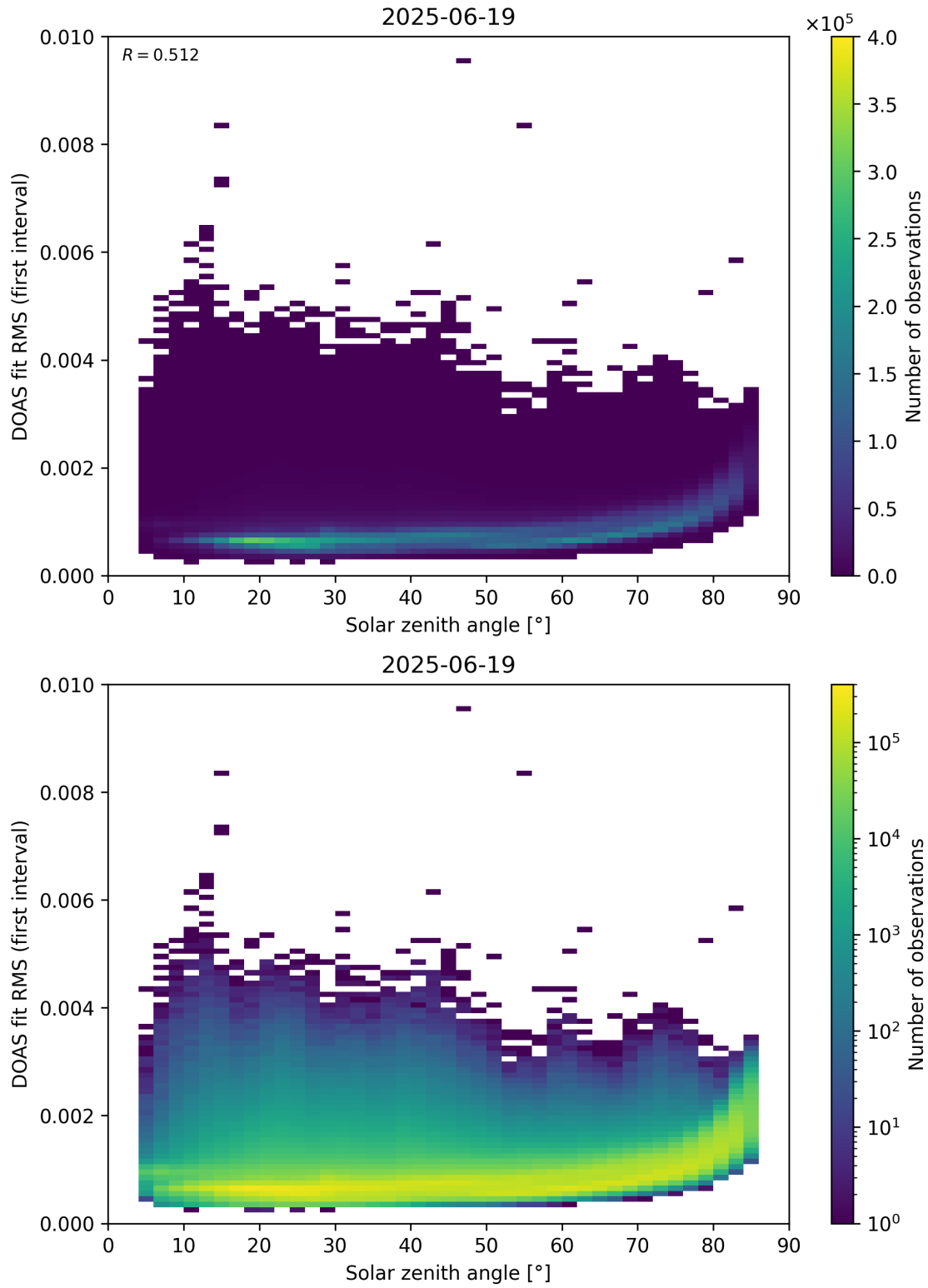
Figure 167: Scatter density plot of “Solar zenith angle” against “DOAS fit RMS (first interval)” for 2025-06-18 to 2025-06-20.
