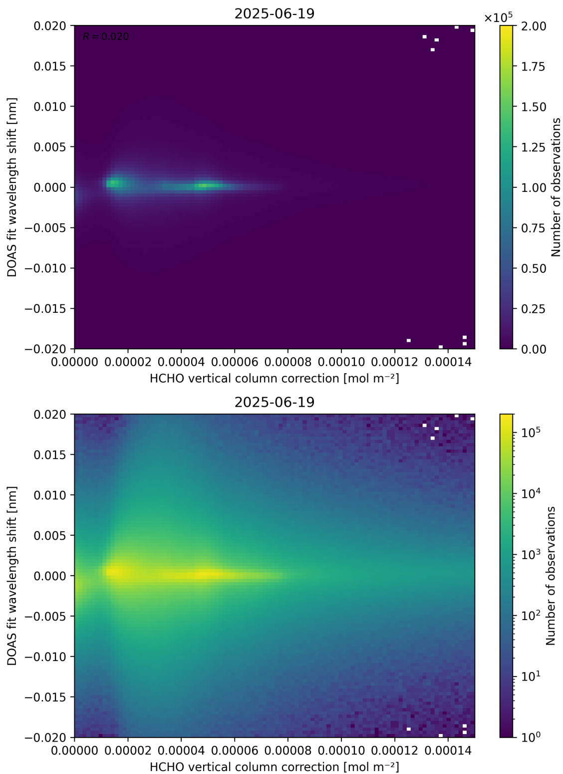
Figure 113: Scatter density plot of “HCHO vertical column correction” against “DOAS fit wavelength shift” for 2025-06-18 to 2025-06-20.
