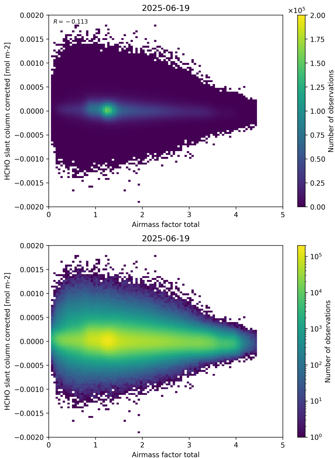
Figure 101: Scatter density plot of “Airmass factor total” against “HCHO slant column corrected” for 2025-06-18 to 2025-06-20.
