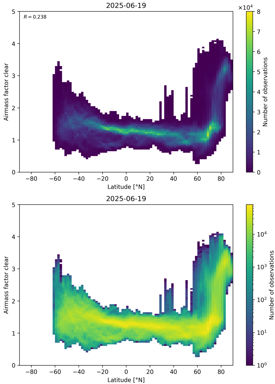
Figure 156: Scatter density plot of “Latitude” against “Airmass factor clear” for 2025-06-18 to 2025-06-20.
