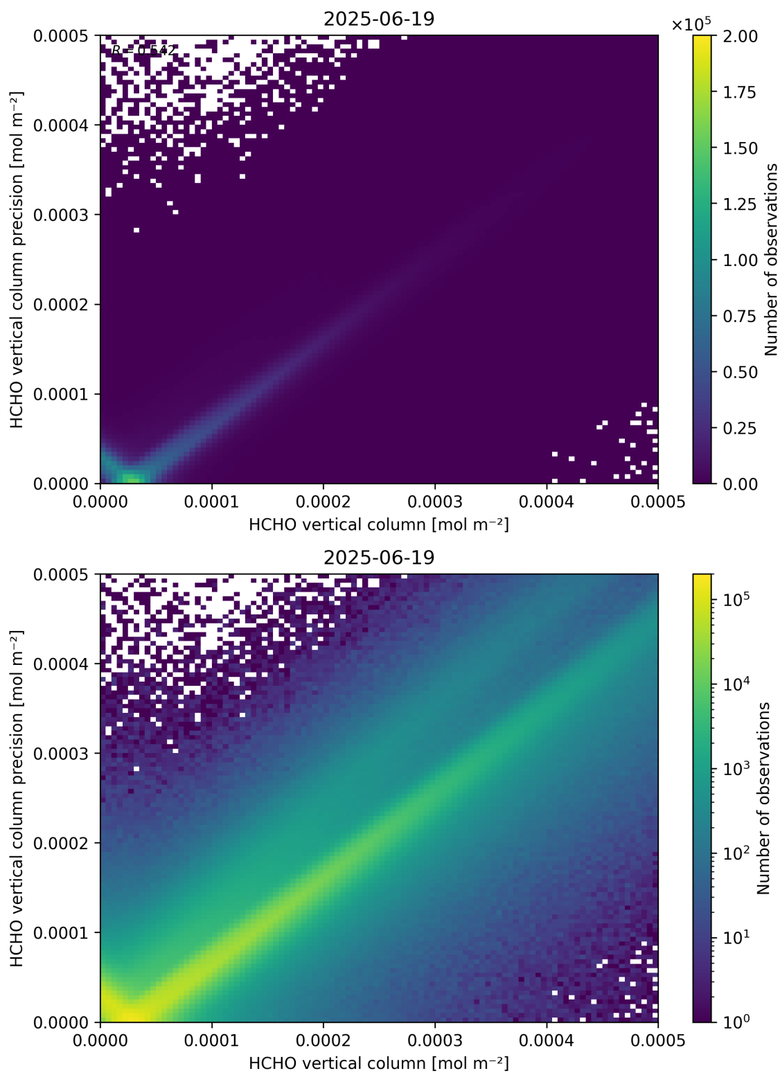
Figure 134: Scatter density plot of “HCHO vertical column” against “HCHO vertical column precision” for 2025-06-18 to 2025-06-20.
