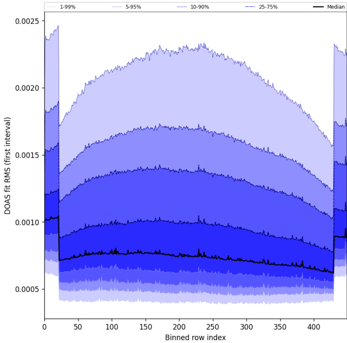
Figure 60: Along track statistics of “DOAS fit RMS (first interval)” for 2025-06-18 to 2025-06-20
