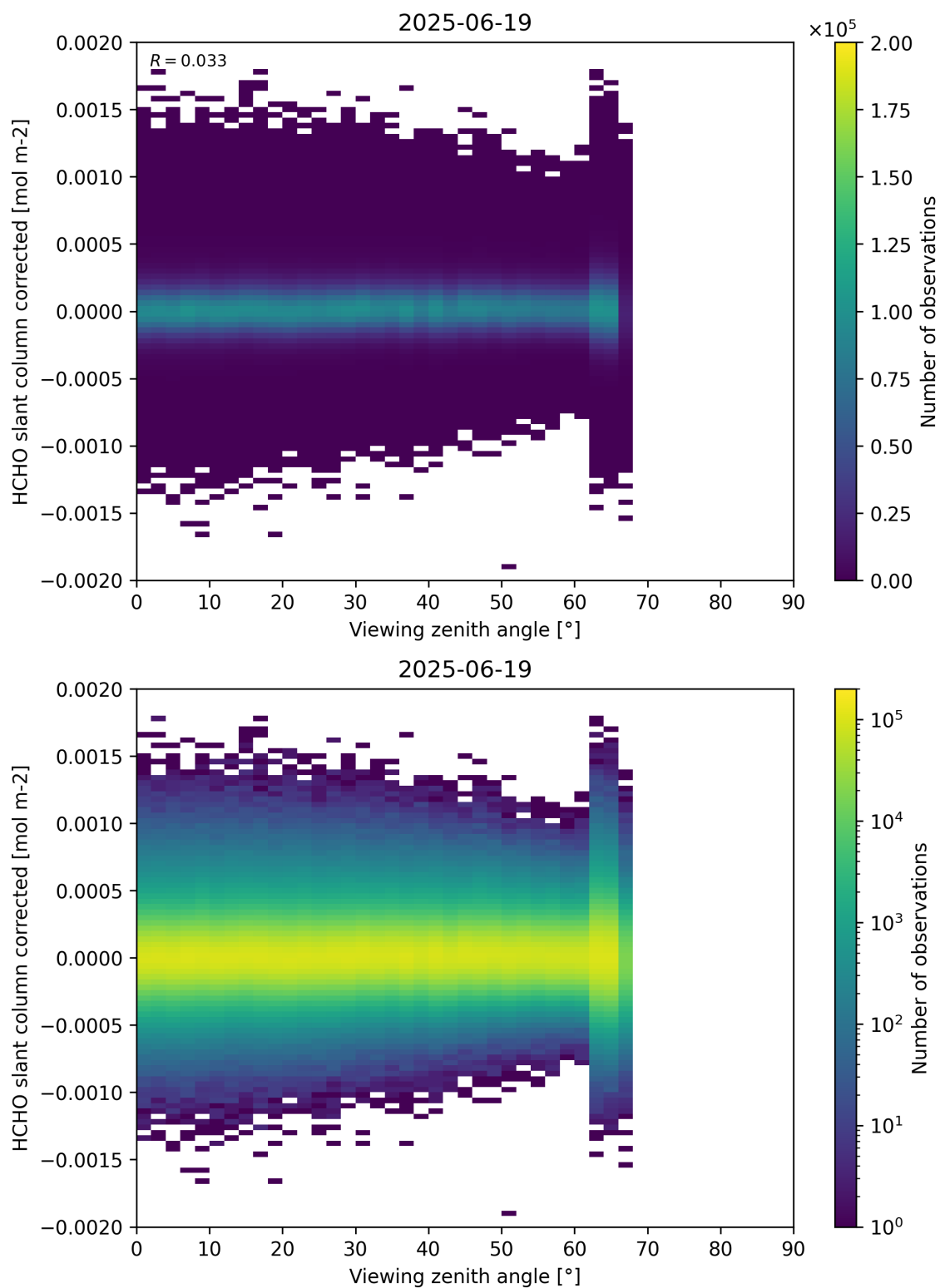
Figure 186: Scatter density plot of “Viewing zenith angle” against “HCHO slant column corrected” for 2025-06-18 to 2025-06-20.
