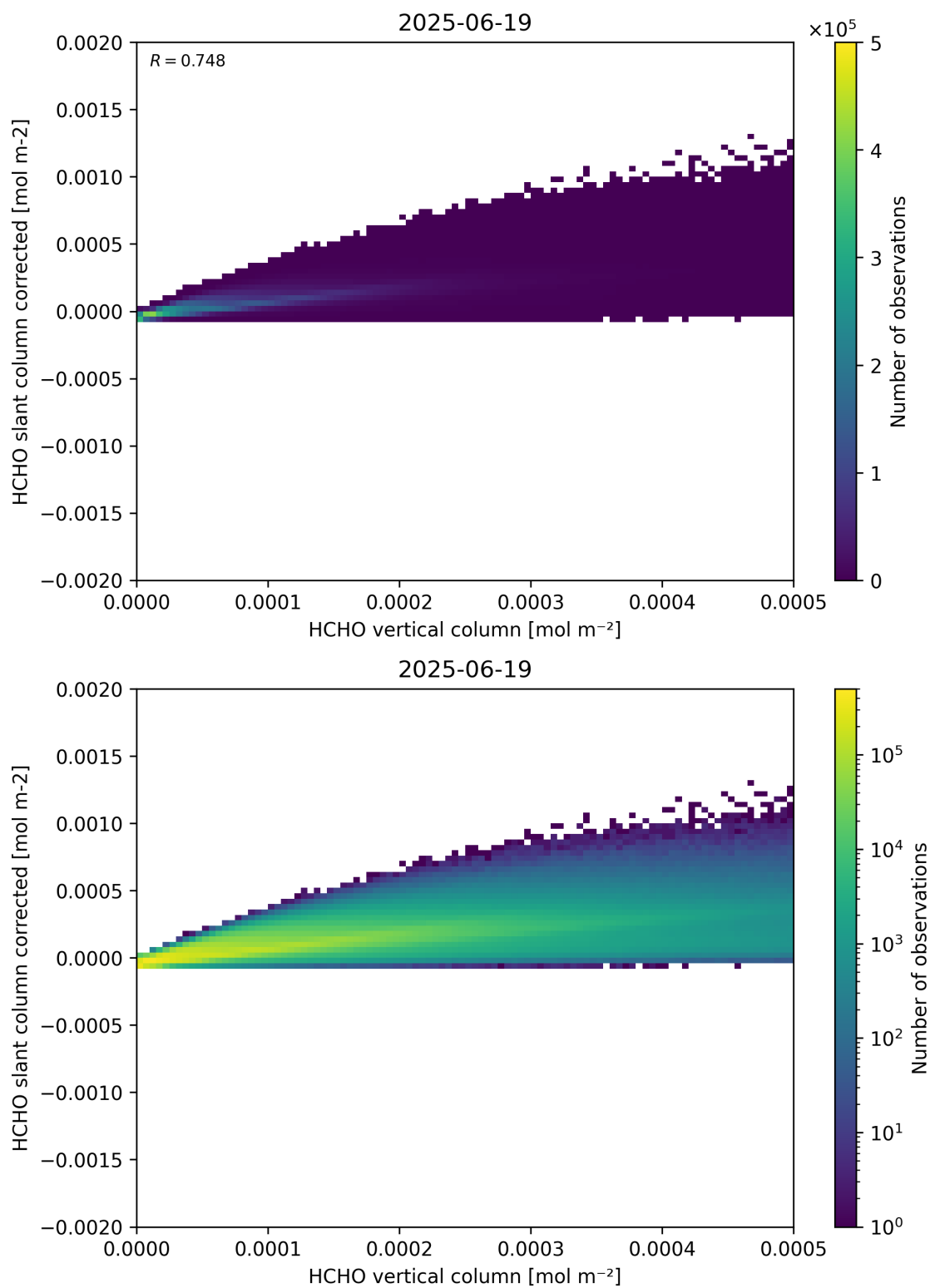
Figure 127: Scatter density plot of “HCHO vertical column” against “HCHO slant column corrected” for 2025-06-18 to 2025-06-20.
