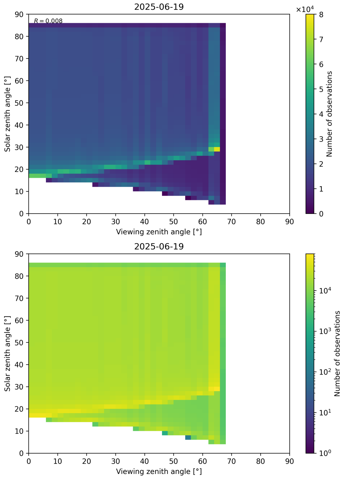
Figure 197: Scatter density plot of “Viewing zenith angle” against “Solar zenith angle” for 2025-06-18 to 2025-06-20.
