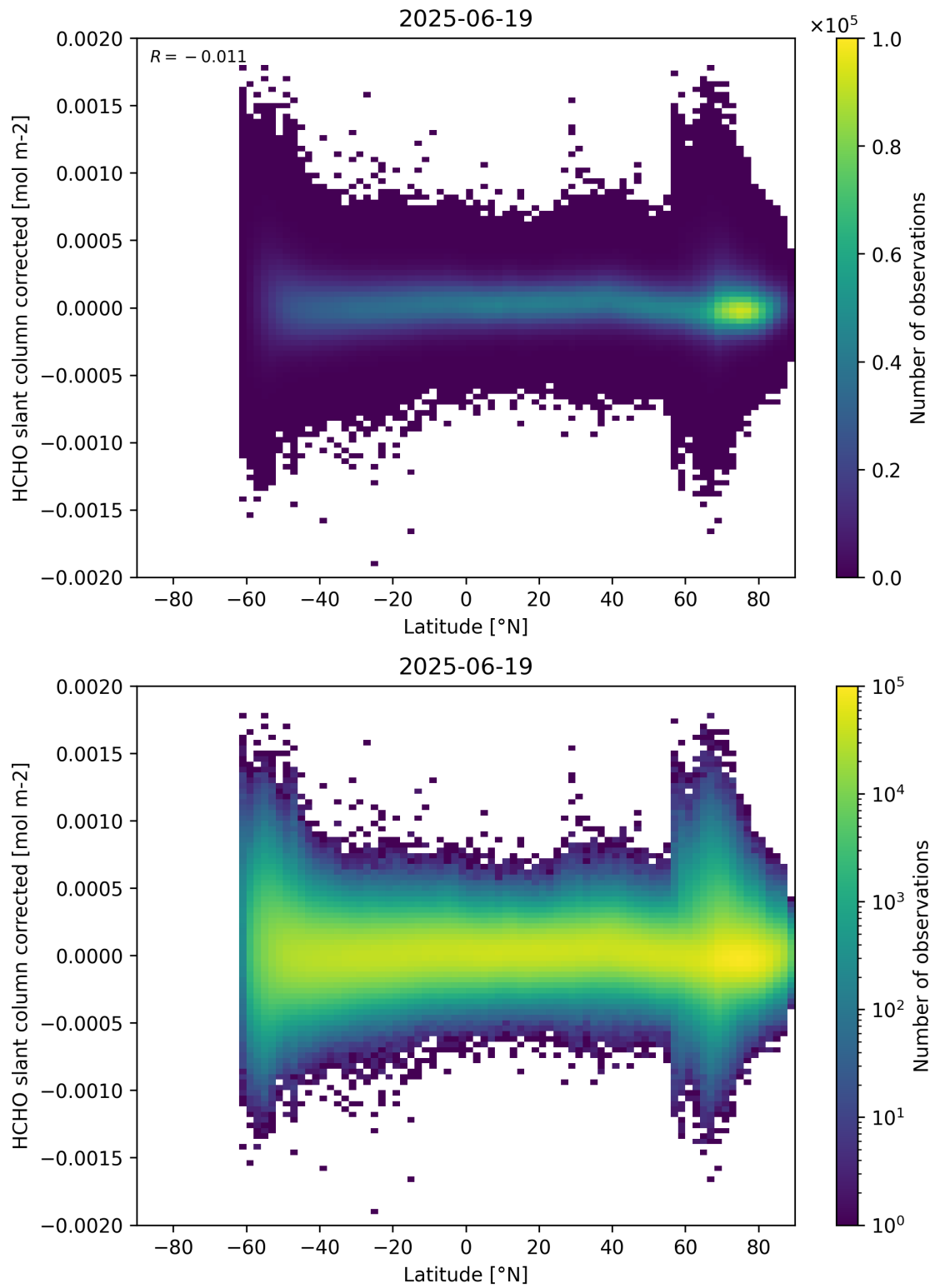
Figure 157: Scatter density plot of “Latitude” against “HCHO slant column corrected” for 2025-06-18 to 2025-06-20.
