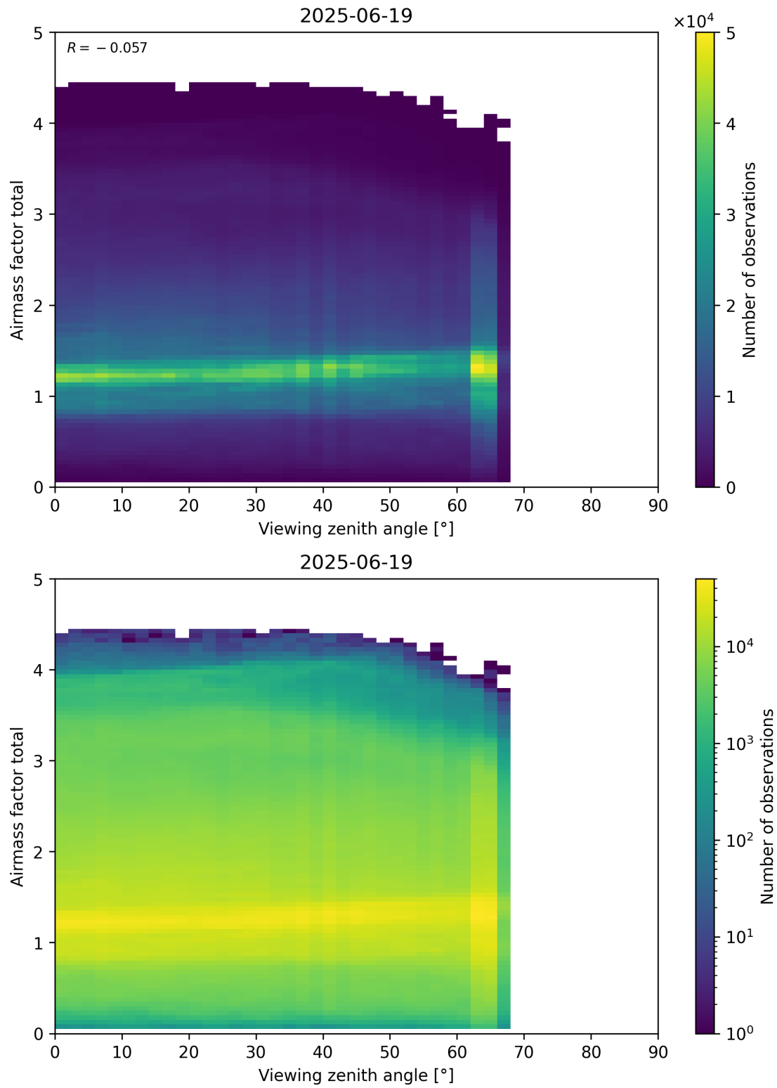
Figure 190: Scatter density plot of “Viewing zenith angle” against “Airmass factor total” for 2025-06-18 to 2025-06-20.
