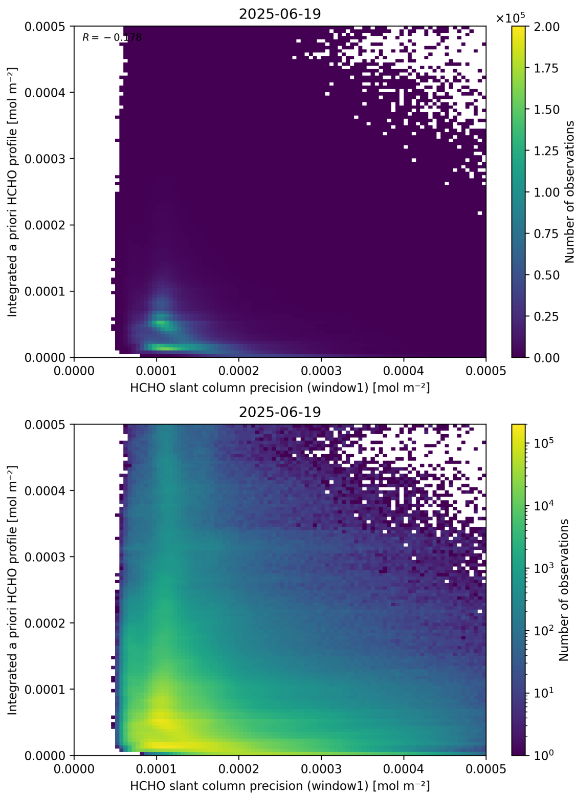
Figure 96: Scatter density plot of “HCHO slant column precision (window1)” against “Integrated a priori HCHO profile” for 2025-06-18 to 2025-06-20.
