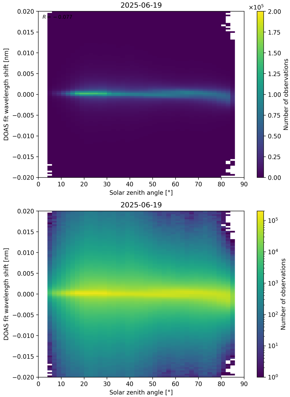
Figure 168: Scatter density plot of “Solar zenith angle” against “DOAS fit wavelength shift” for 2025-06-18 to 2025-06-20.
