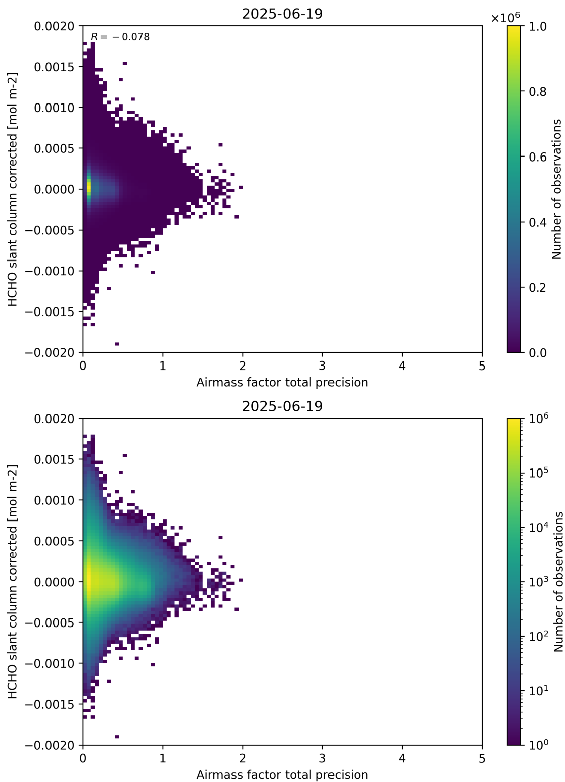
Figure 109: Scatter density plot of “Airmass factor total precision” against “HCHO slant column corrected” for 2025-06-18 to 2025-06-20.
