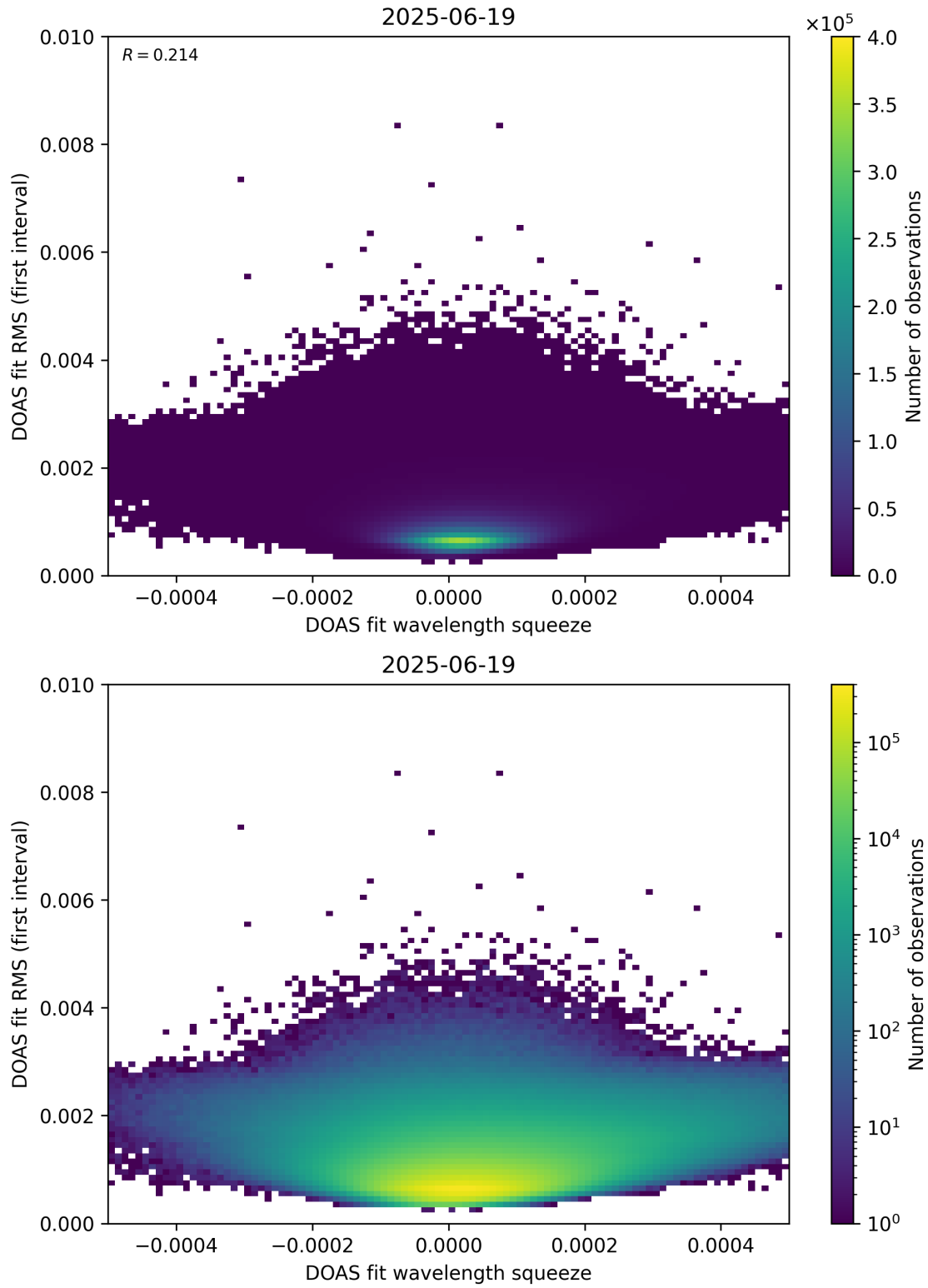
Figure 68: Scatter density plot of “DOAS fit wavelength squeeze” against “DOAS fit RMS (first interval)” for 2025-06-18 to 2025-06-20.
