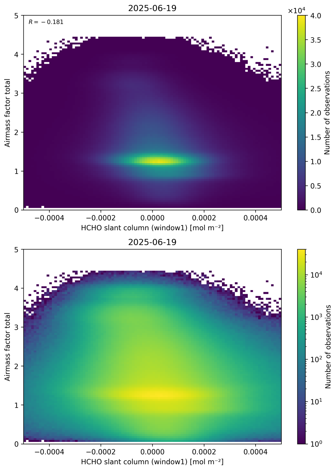
Figure 85: Scatter density plot of “HCHO slant column (window1)” against “Airmass factor total” for 2025-06-18 to 2025-06-20.
