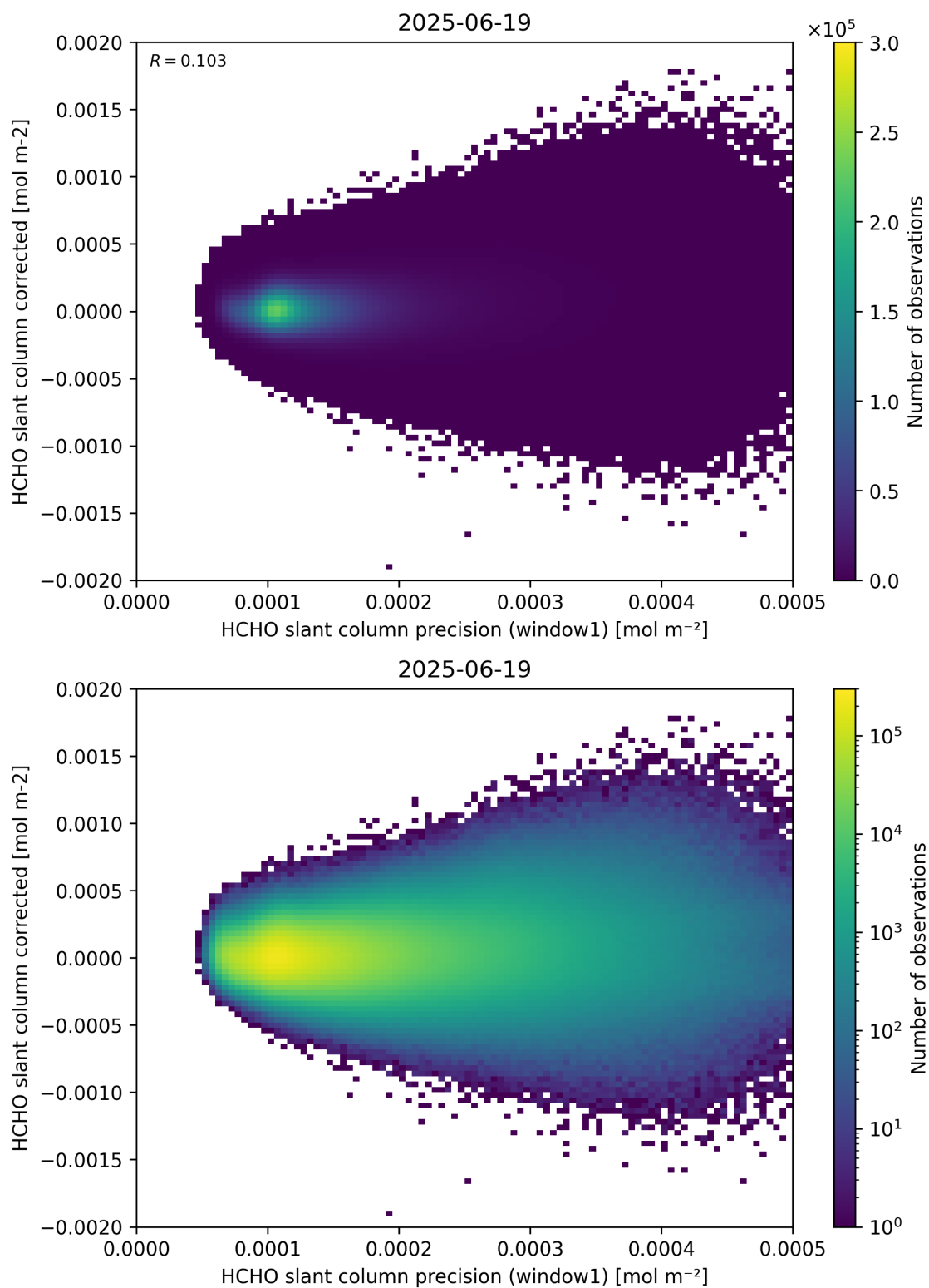
Figure 92: Scatter density plot of “HCHO slant column precision (window1)” against “HCHO slant column corrected” for 2025-06-18 to 2025-06-20.
