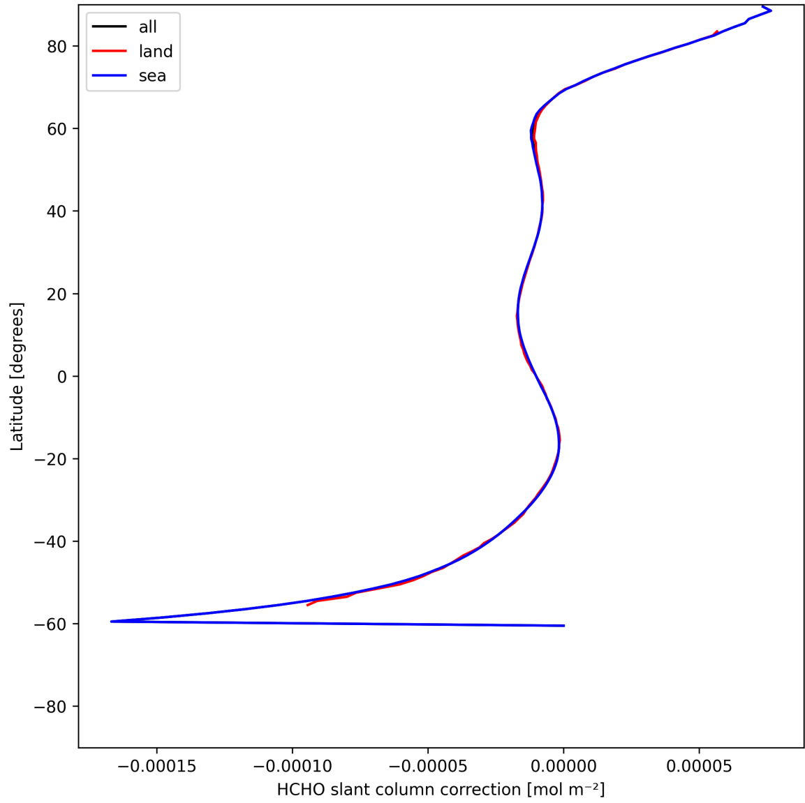
Figure 33: Zonal average of “HCHO slant column correction” for 2025-06-18 to 2025-06-20.
