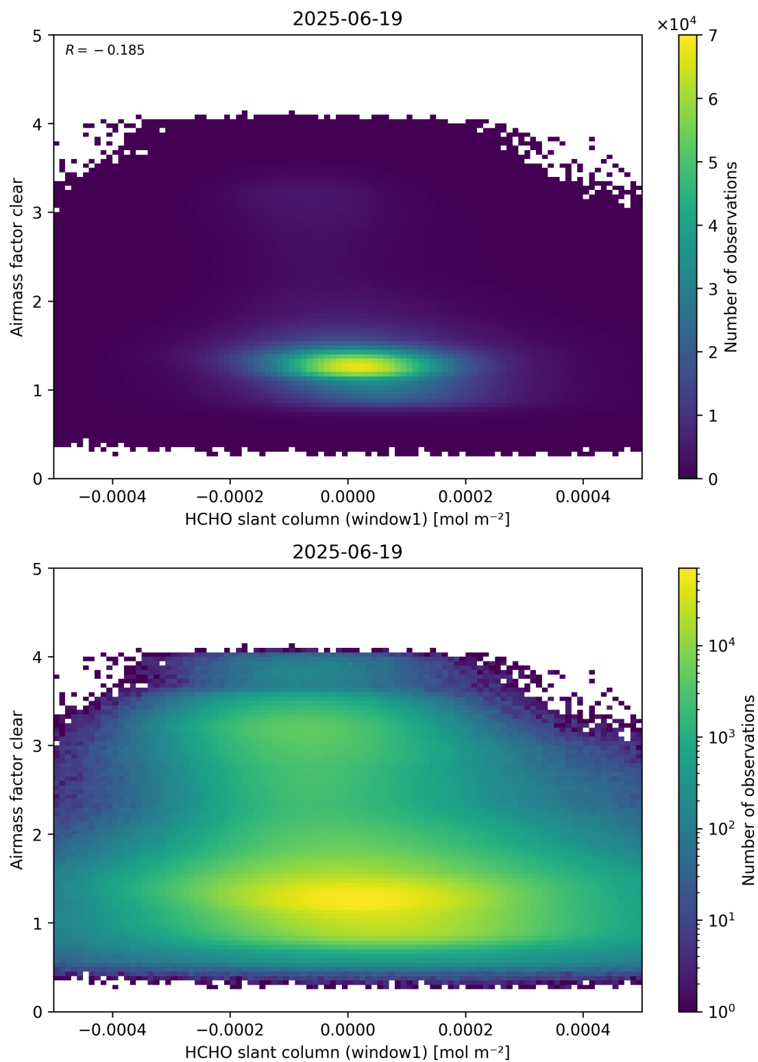
Figure 81: Scatter density plot of “HCHO slant column (window1)” against “Airmass factor clear” for 2025-06-18 to 2025-06-20.
