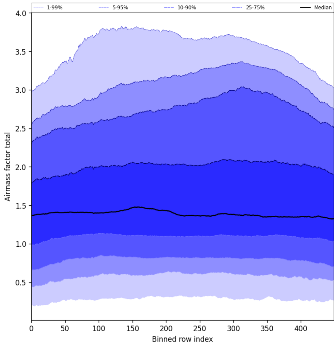
Figure 54: Along track statistics of “Airmass factor total” for 2025-06-18 to 2025-06-20
