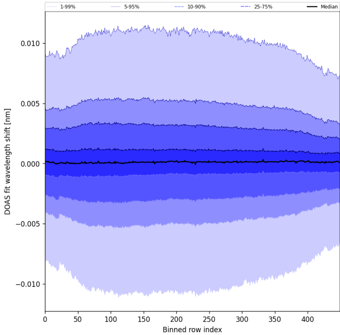
Figure 58: Along track statistics of “DOAS fit wavelength shift” for 2025-06-18 to 2025-06-20
