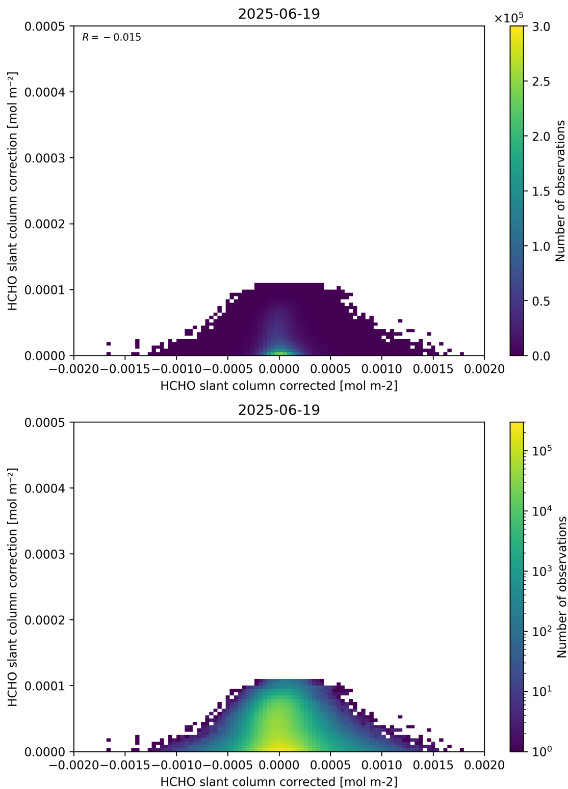
Figure 77: Scatter density plot of “HCHO slant column corrected” against “HCHO slant column correction” for 2025-06-18 to 2025-06-20.
