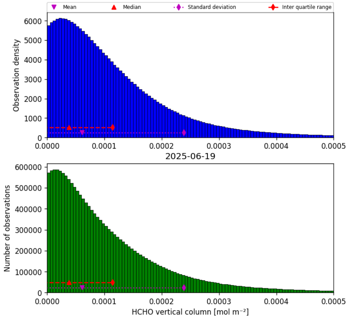
Figure 35: Histogram of “HCHO vertical column” for 2025-06-18 to 2025-06-20
