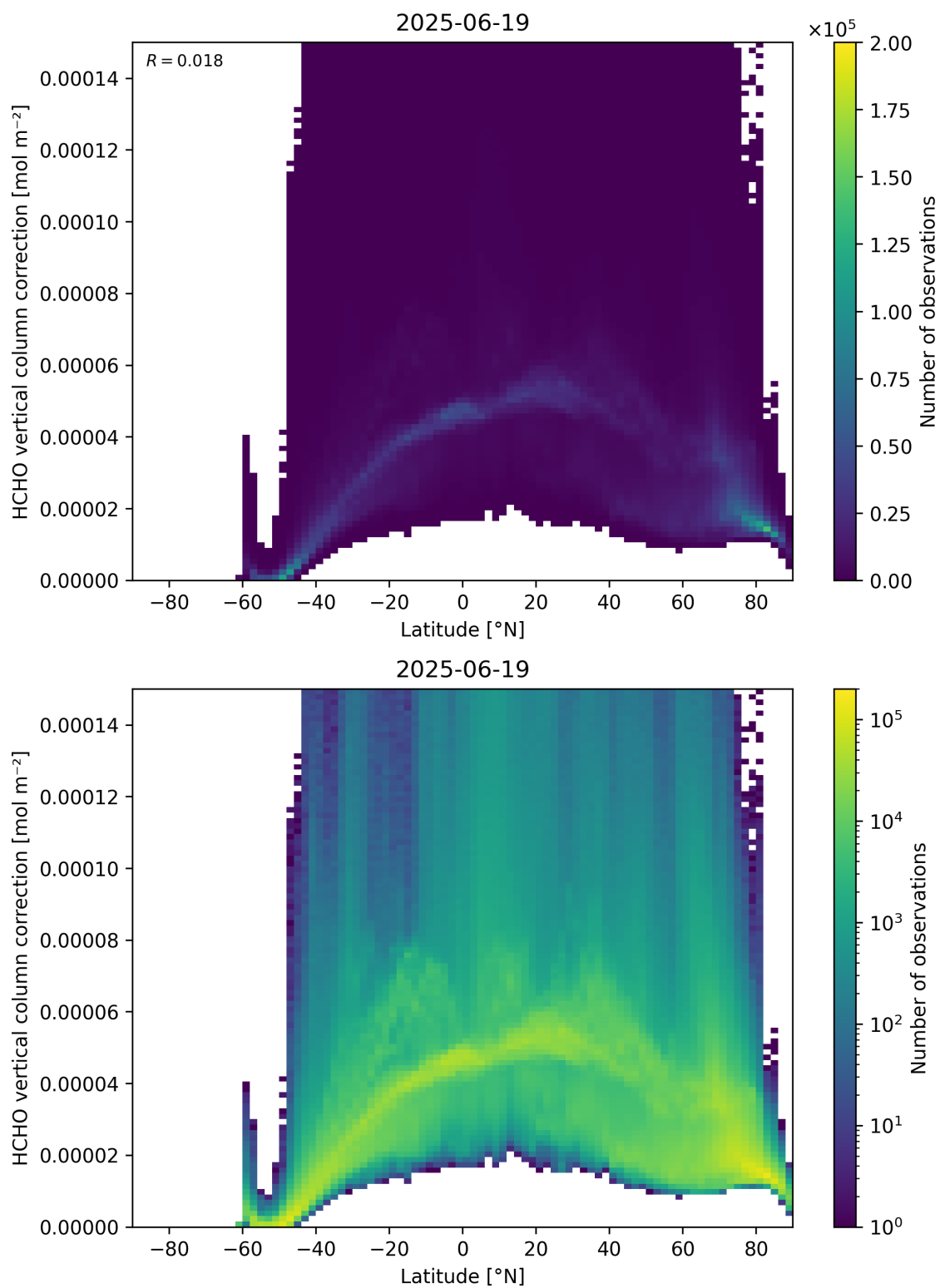
Figure 164: Scatter density plot of “Latitude” against “HCHO vertical column correction” for 2025-06-18 to 2025-06-20.
