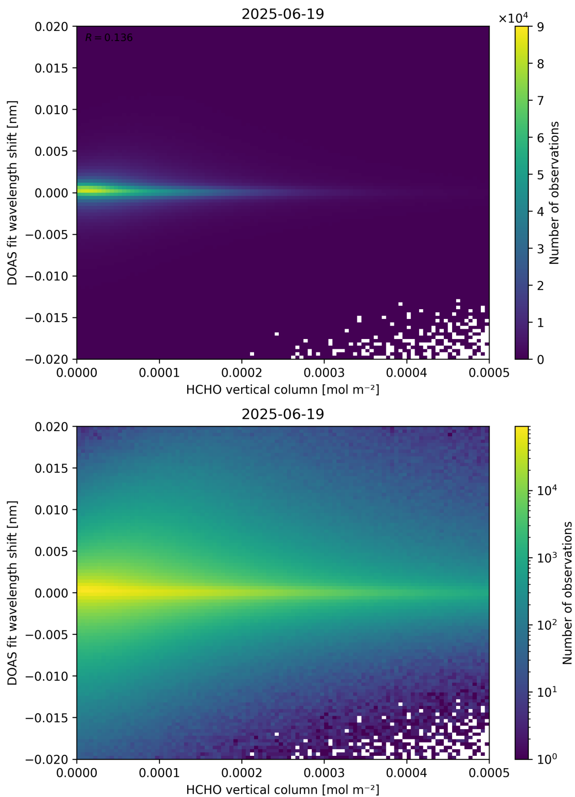
Figure 124: Scatter density plot of “HCHO vertical column” against “DOAS fit wavelength shift” for 2025-06-18 to 2025-06-20.
