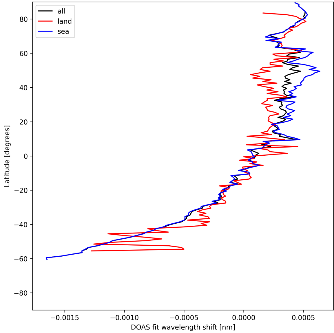
Figure 30: Zonal average of “DOAS fit wavelength shift” for 2025-06-18 to 2025-06-20.
