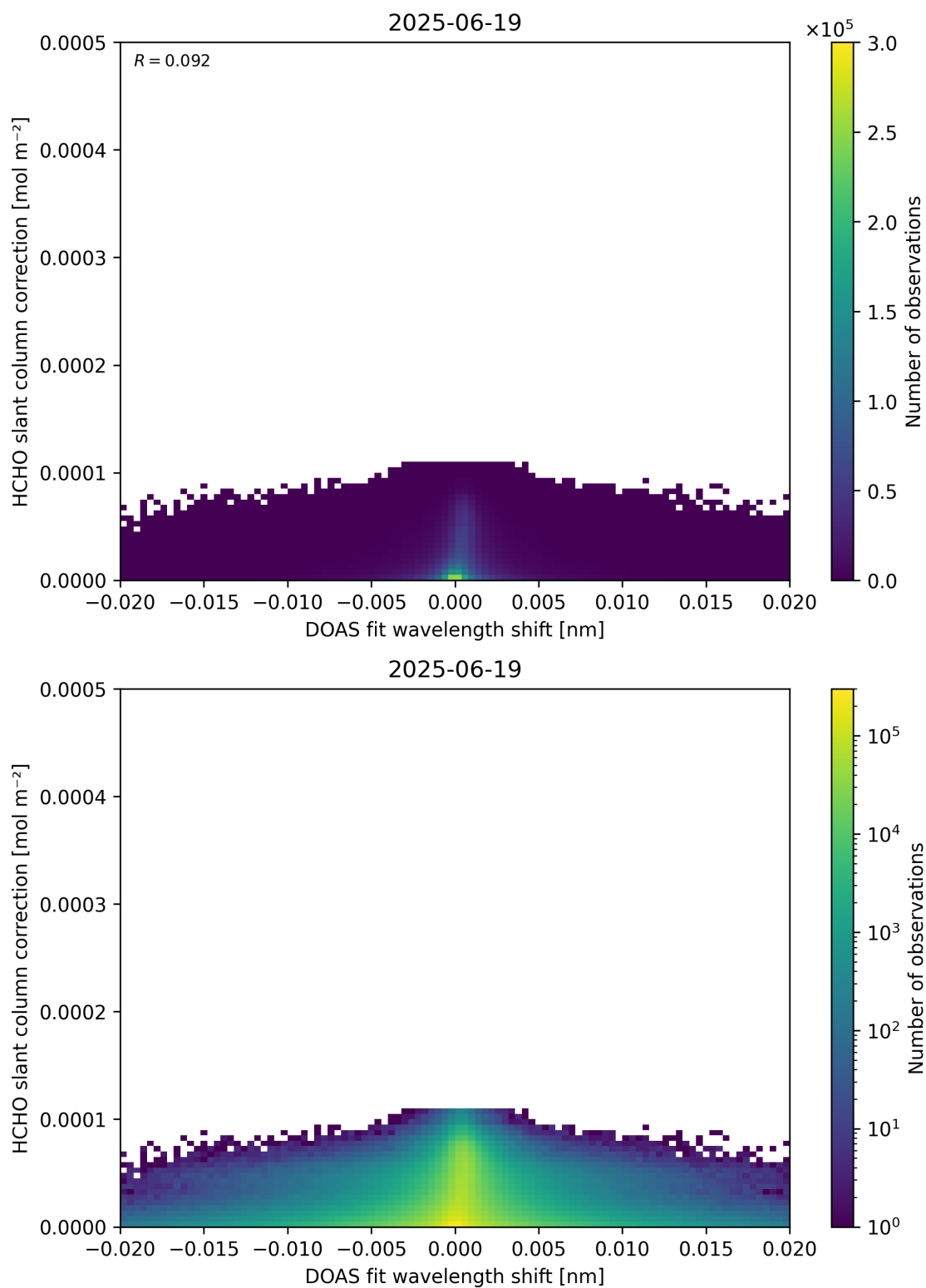
Figure 67: Scatter density plot of “DOAS fit wavelength shift” against “HCHO slant column correction” for 2025-06-18 to 2025-06-20.
