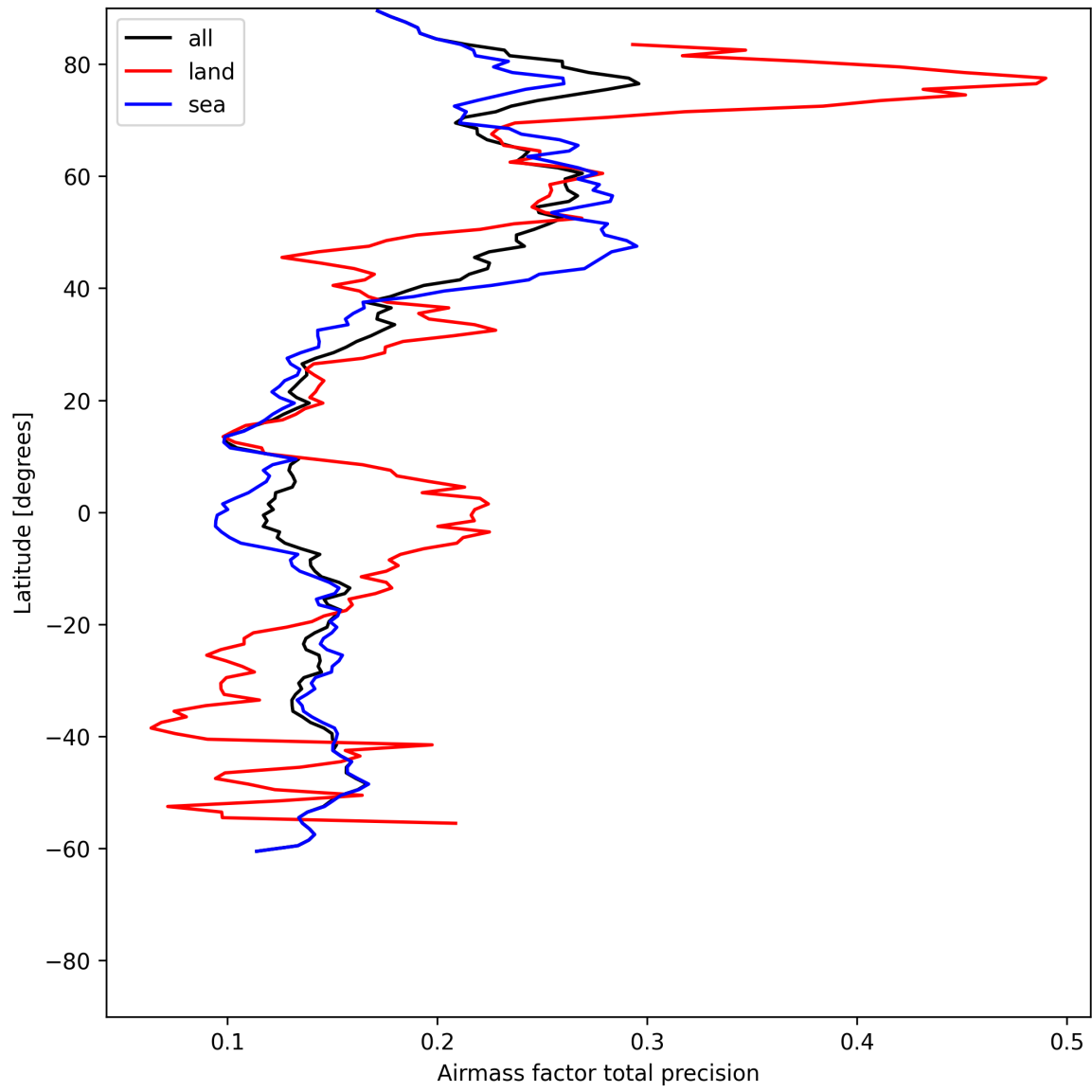
Figure 27: Zonal average of “Airmass factor total precision” for 2025-06-18 to 2025-06-20.
