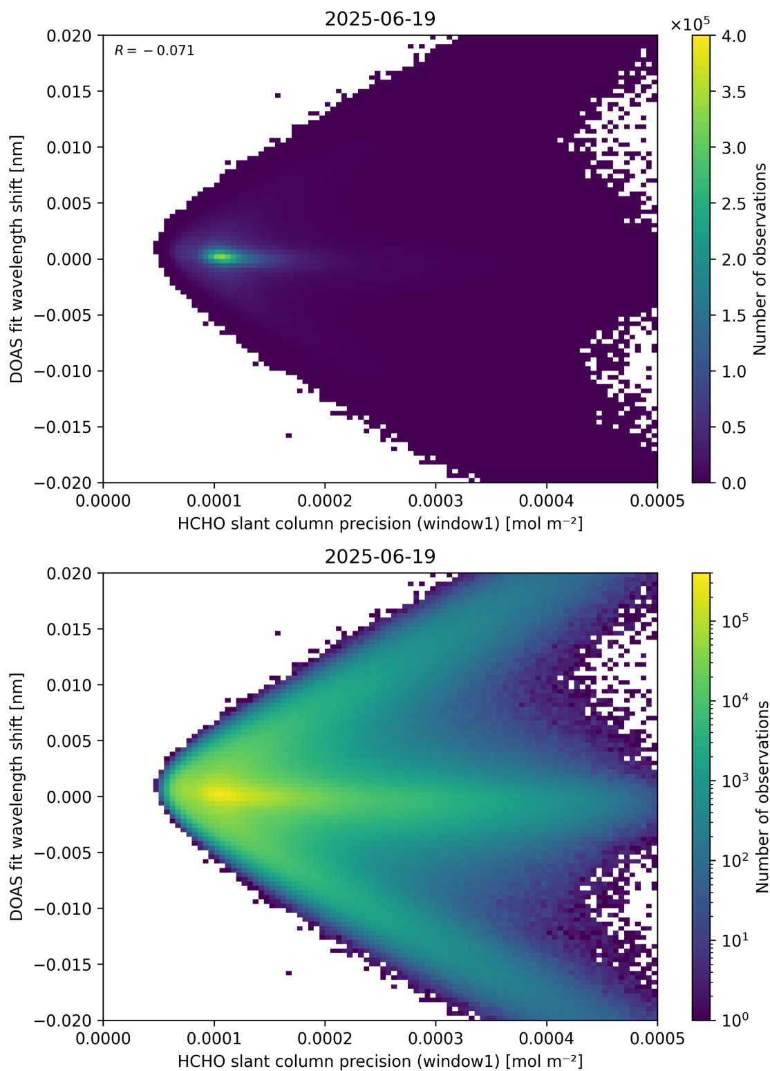
Figure 89: Scatter density plot of “HCHO slant column precision (window1)” against “DOAS fit wavelength shift” for 2025-06-18 to 2025-06-20.
