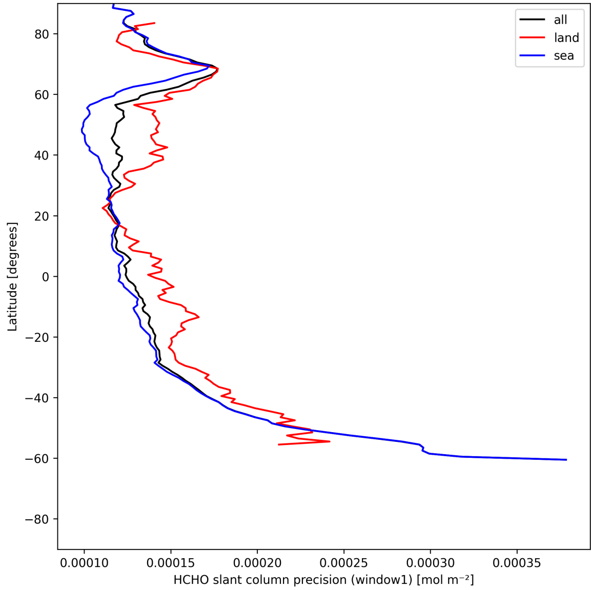
Figure 25: Zonal average of “HCHO slant column precision (window1)” for 2025-06-18 to 2025-06-20.
