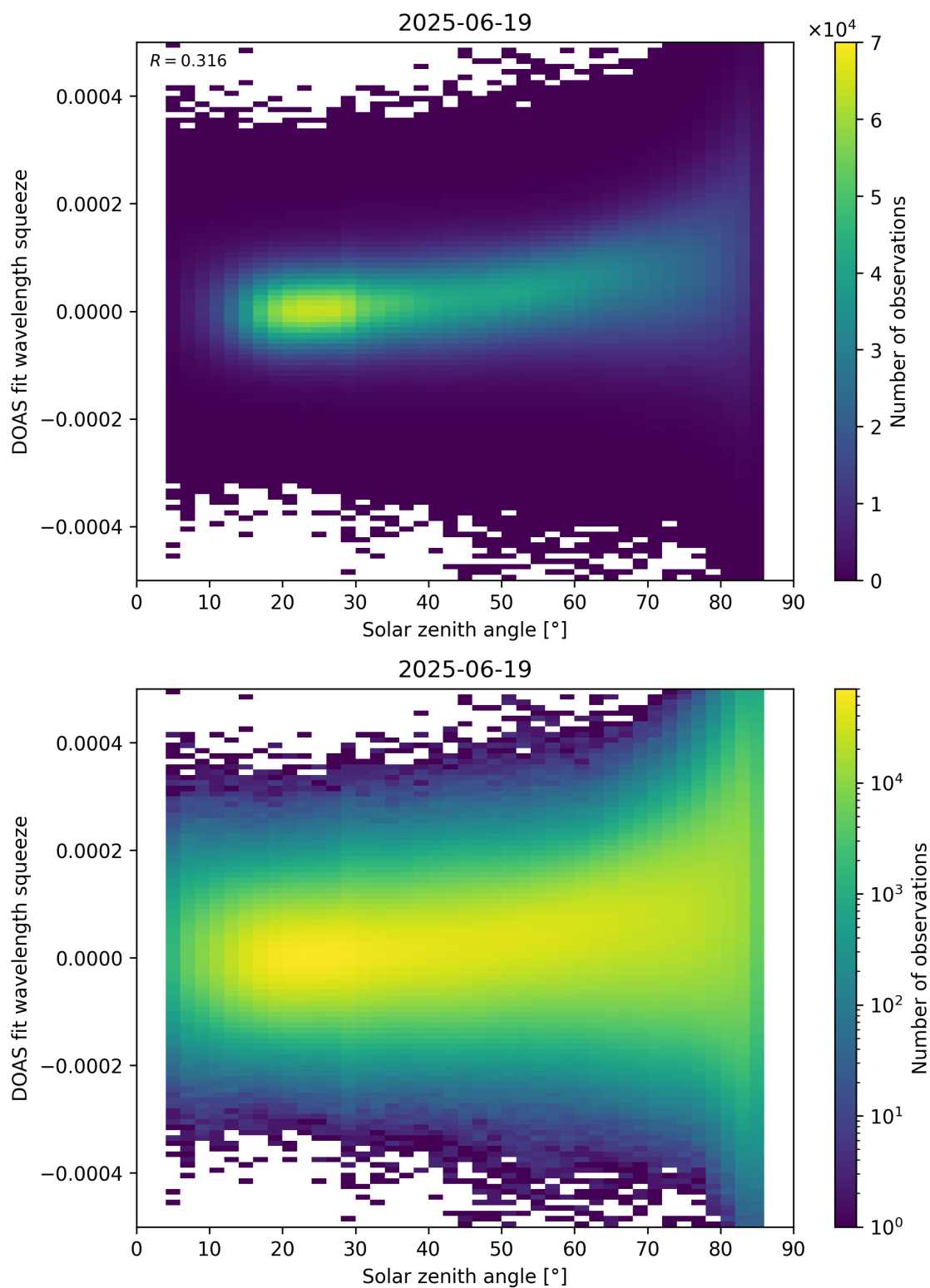
Figure 169: Scatter density plot of “Solar zenith angle” against “DOAS fit wavelength squeeze” for 2025-06-18 to 2025-06-20.
