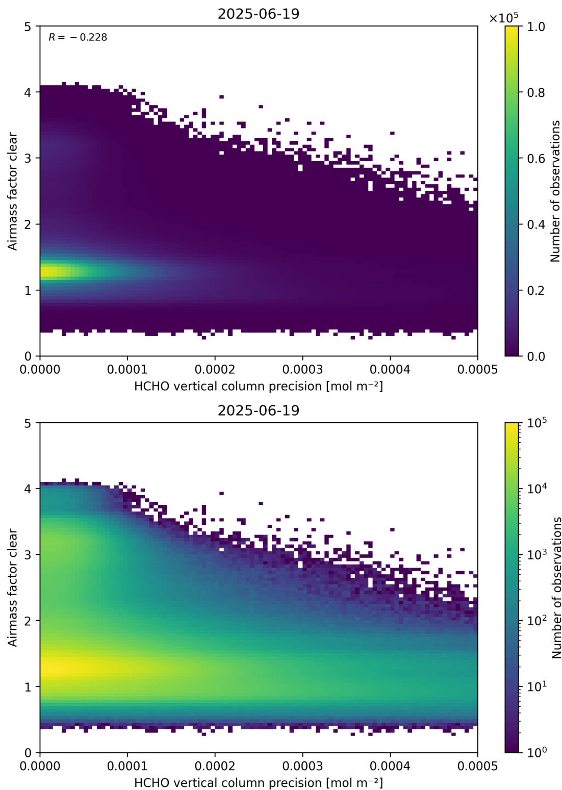
Figure 139: Scatter density plot of “HCHO vertical column precision” against “Airmass factor clear” for 2025-06-18 to 2025-06-20.
