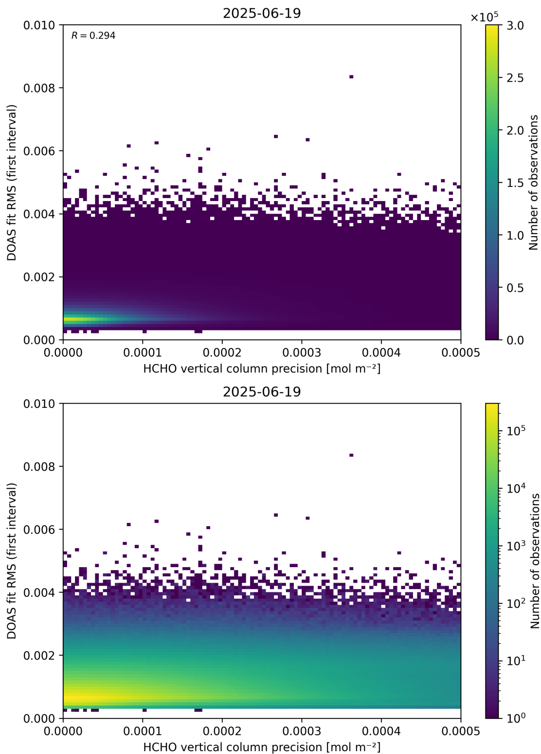
Figure 136: Scatter density plot of “HCHO vertical column precision” against “DOAS fit RMS (first interval)” for 2025-06-18 to 2025-06-20.
