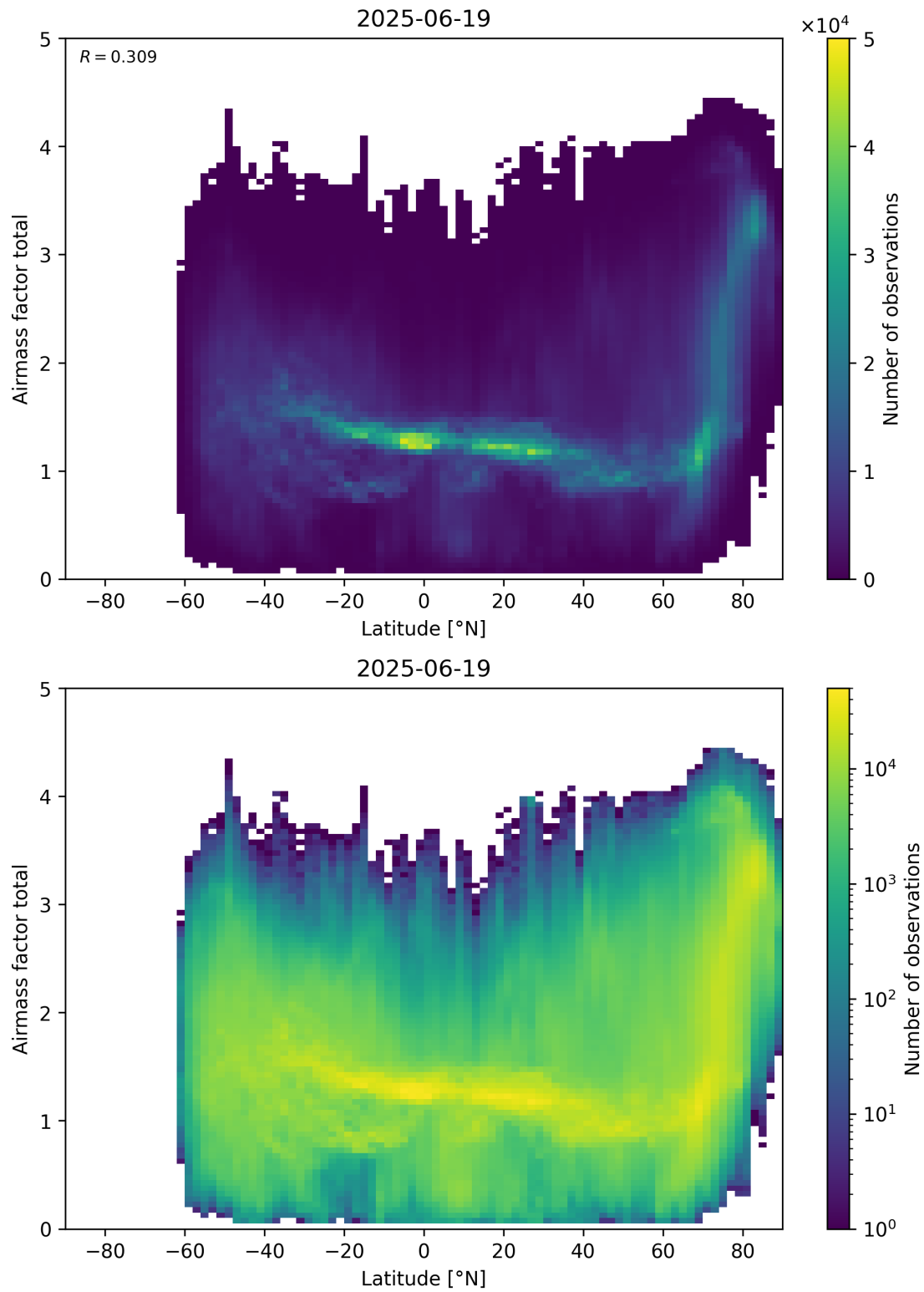
Figure 161: Scatter density plot of “Latitude” against “Airmass factor total” for 2025-06-18 to 2025-06-20.
