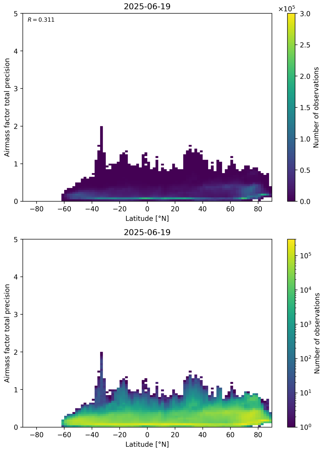
Figure 162: Scatter density plot of “Latitude” against “Airmass factor total precision” for 2025-06-18 to 2025-06-20.
