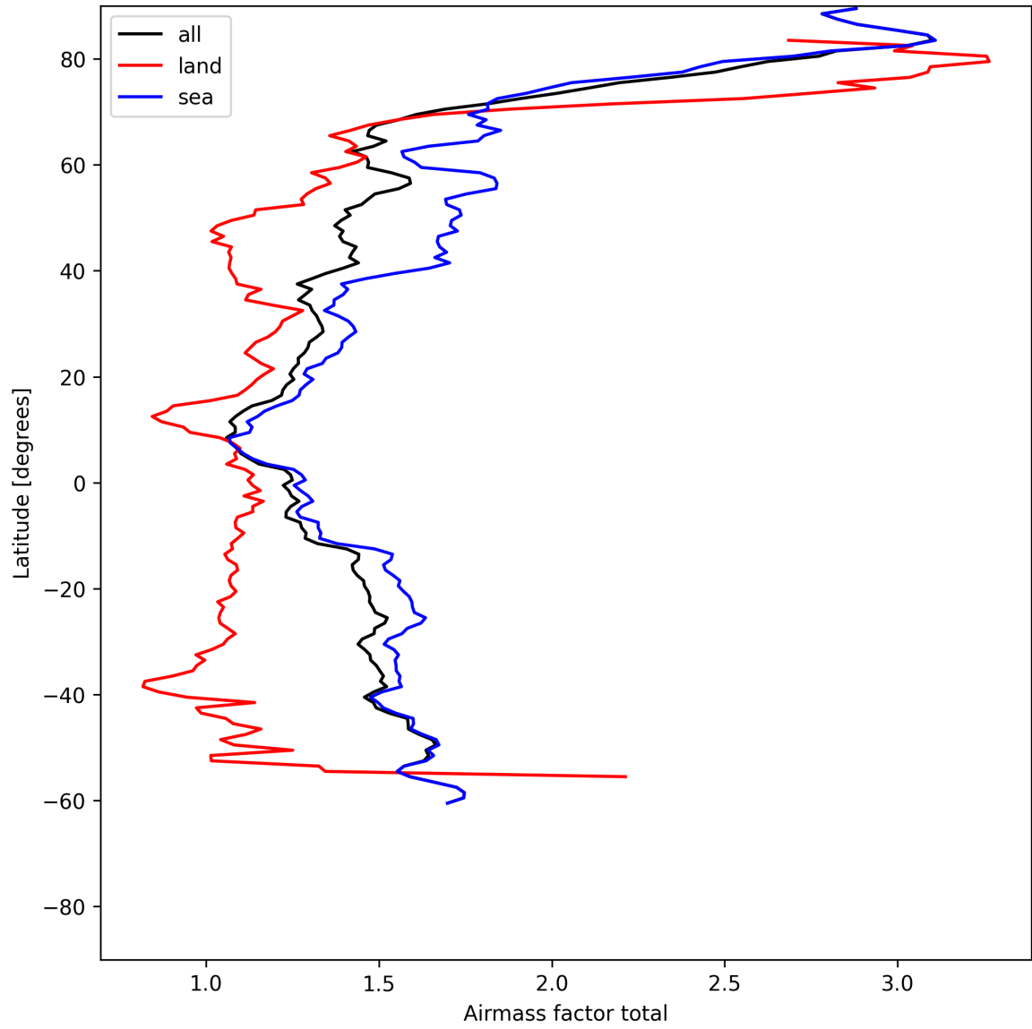
Figure 26: Zonal average of “Airmass factor total” for 2025-06-18 to 2025-06-20.
