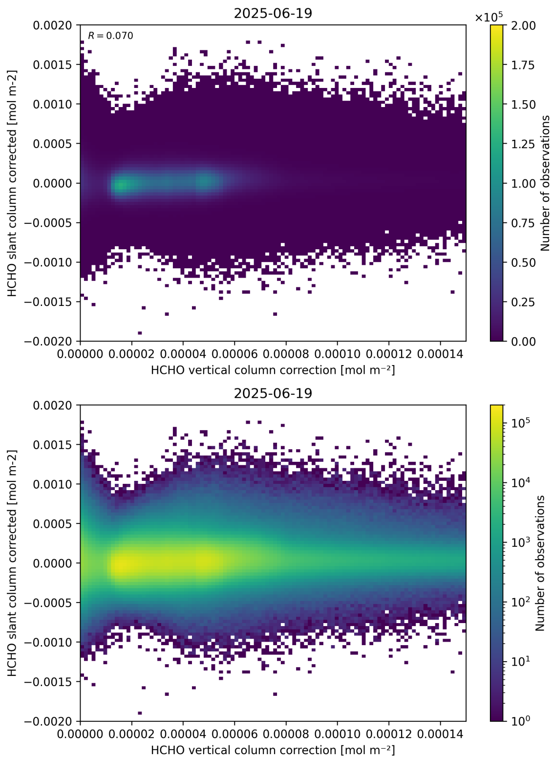
Figure 116: Scatter density plot of “HCHO vertical column correction” against “HCHO slant column corrected” for 2025-06-18 to 2025-06-20.
