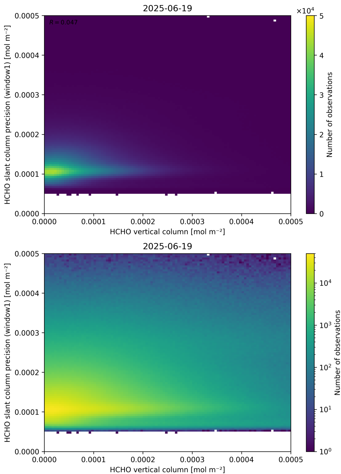
Figure 130: Scatter density plot of “HCHO vertical column” against “HCHO slant column precision (window1)” for 2025-06-18 to 2025-06-20.
