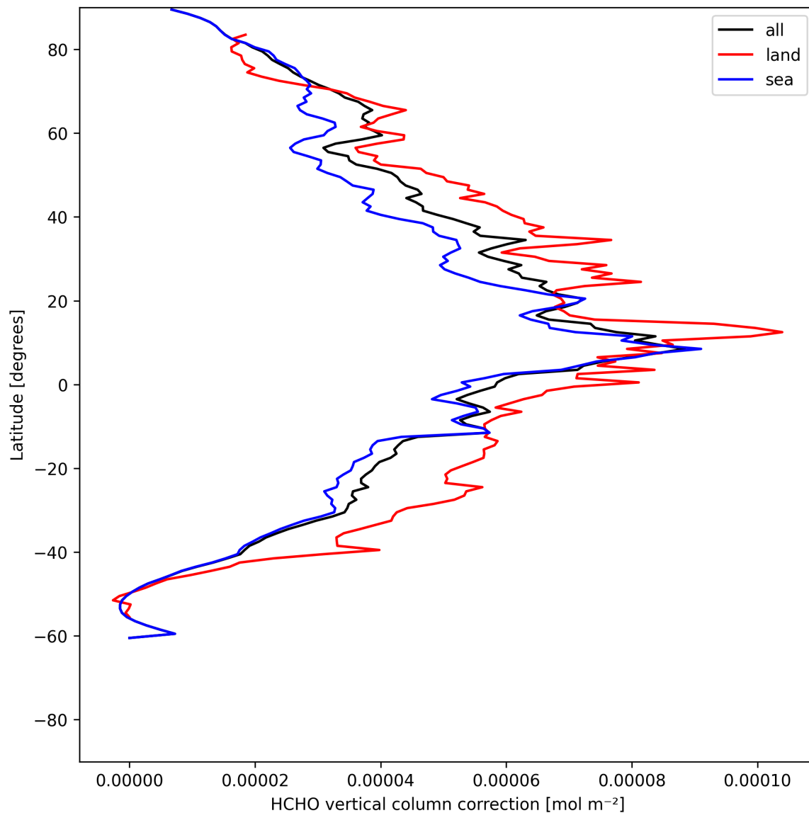
Figure 23: Zonal average of “HCHO vertical column correction” for 2025-06-18 to 2025-06-20.
