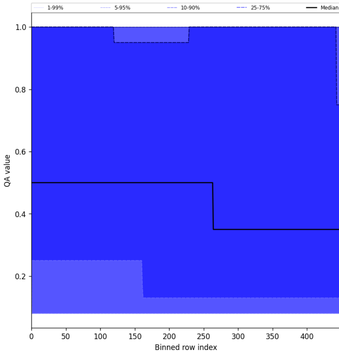
Figure 48: Along track statistics of “QA value” for 2025-06-18 to 2025-06-20
