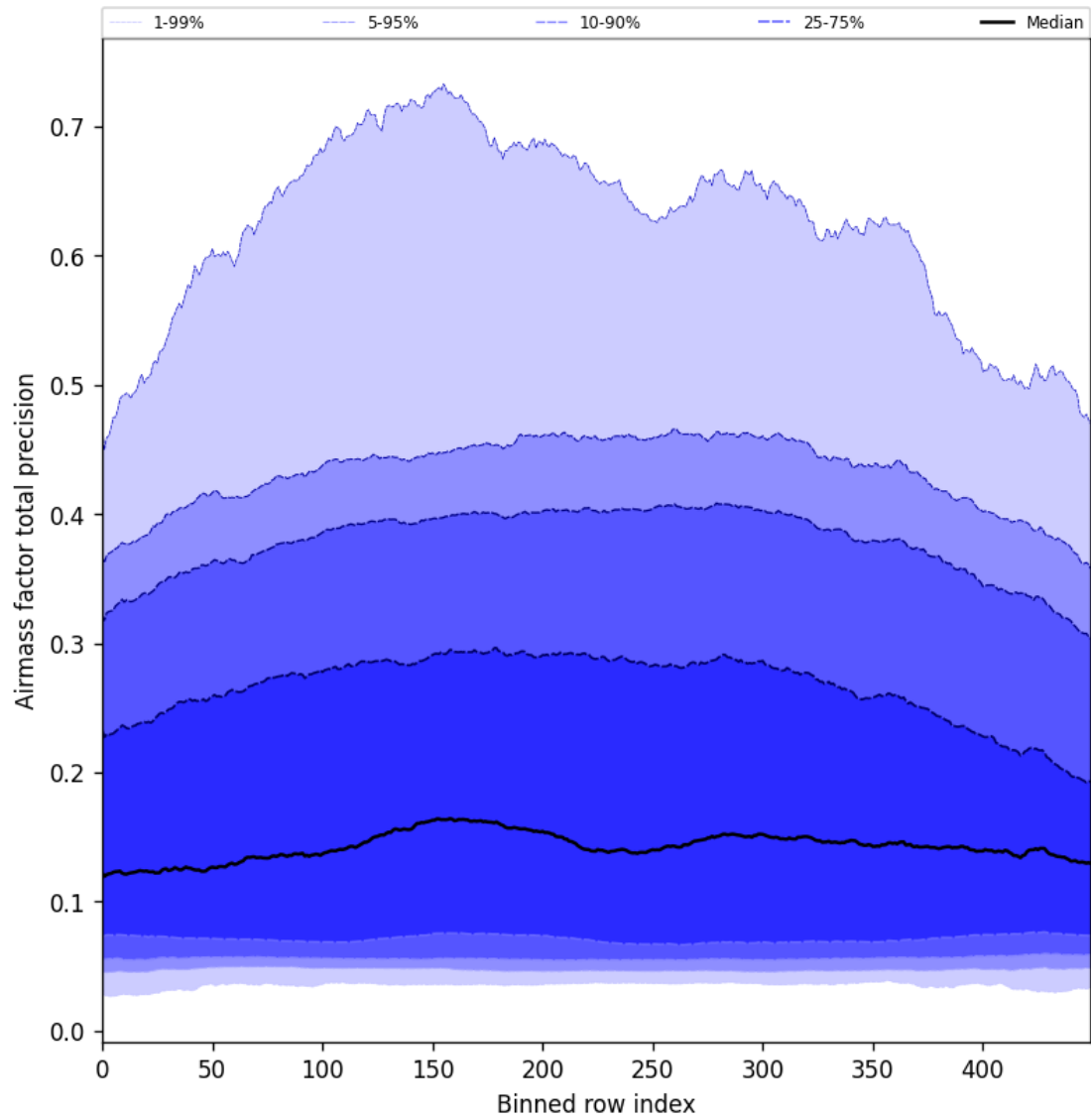
Figure 55: Along track statistics of “Airmass factor total precision” for 2025-06-18 to 2025-06-20
