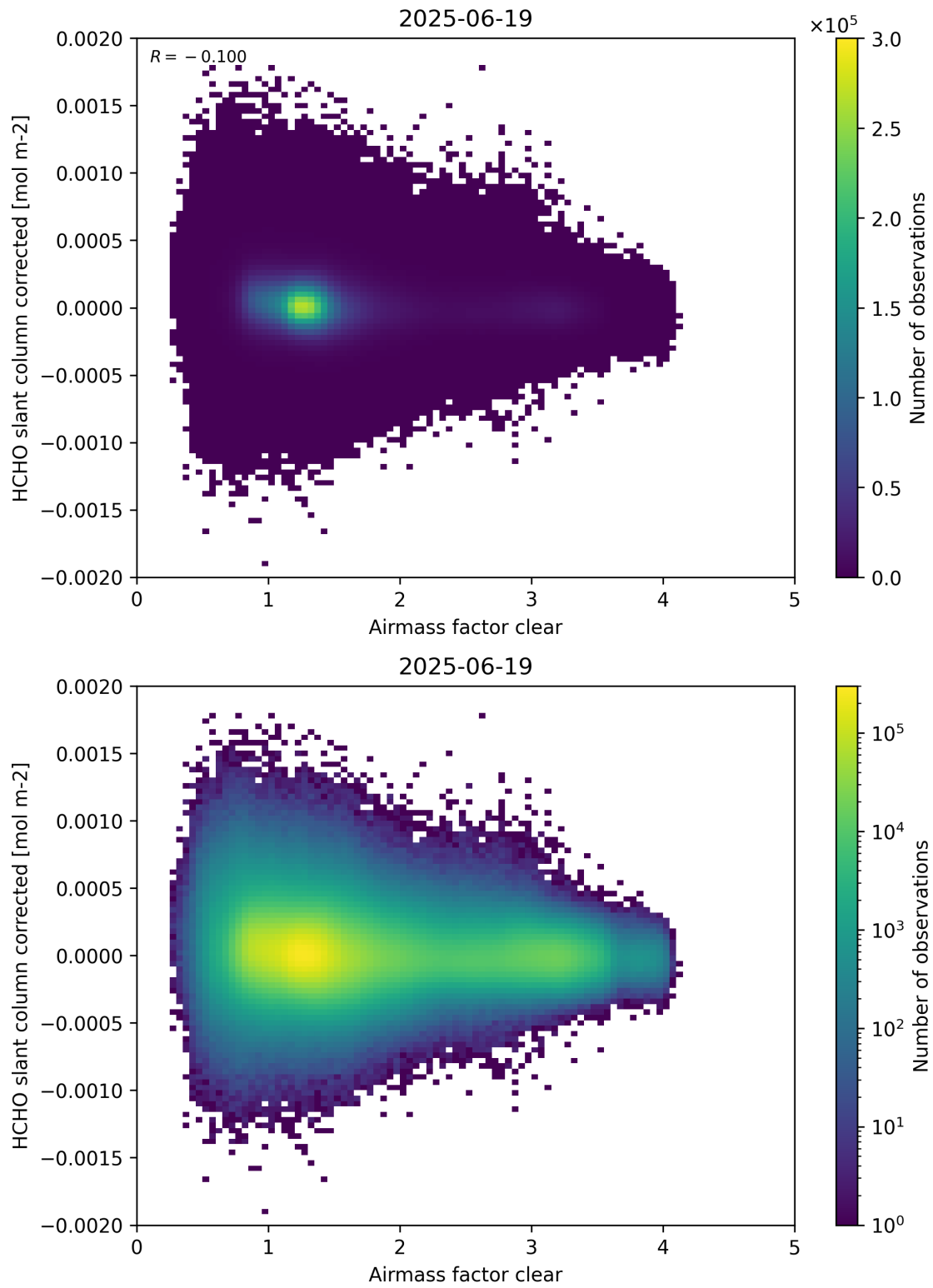
Figure 74: Scatter density plot of “Airmass factor clear” against “HCHO slant column corrected” for 2025-06-18 to 2025-06-20.
