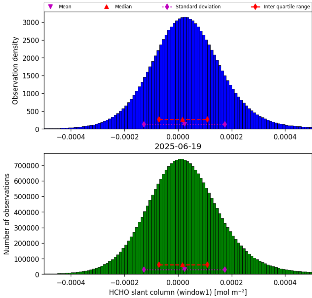
Figure 38: Histogram of “HCHO slant column (window1)” for 2025-06-18 to 2025-06-20
