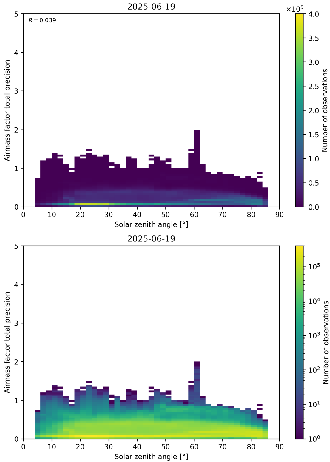
Figure 176: Scatter density plot of “Solar zenith angle” against “Airmass factor total precision” for 2025-06-18 to 2025-06-20.
