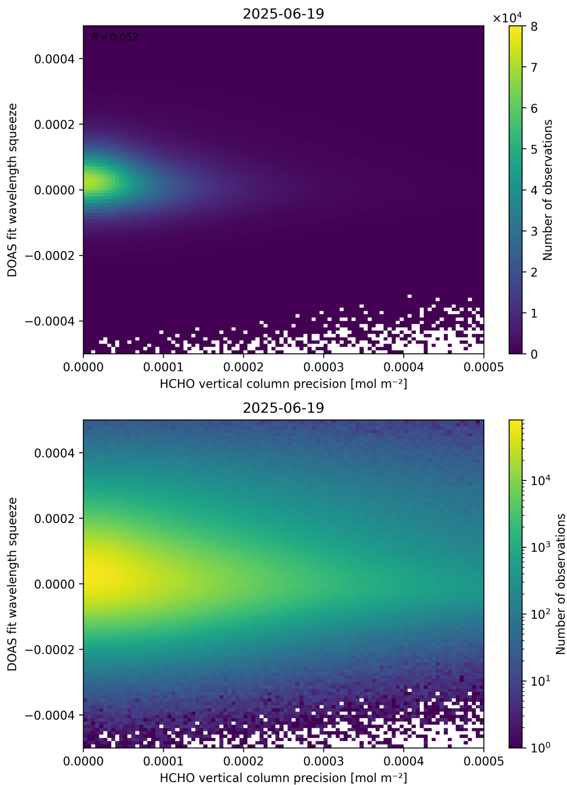
Figure 138: Scatter density plot of “HCHO vertical column precision” against “DOAS fit wavelength squeeze” for 2025-06-18 to 2025-06-20.
