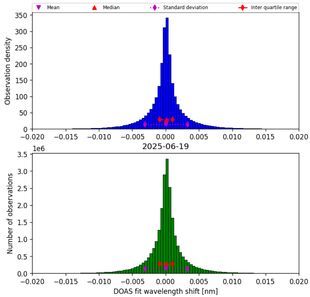
Figure 44: Histogram of “DOAS fit wavelength shift” for 2025-06-18 to 2025-06-20
