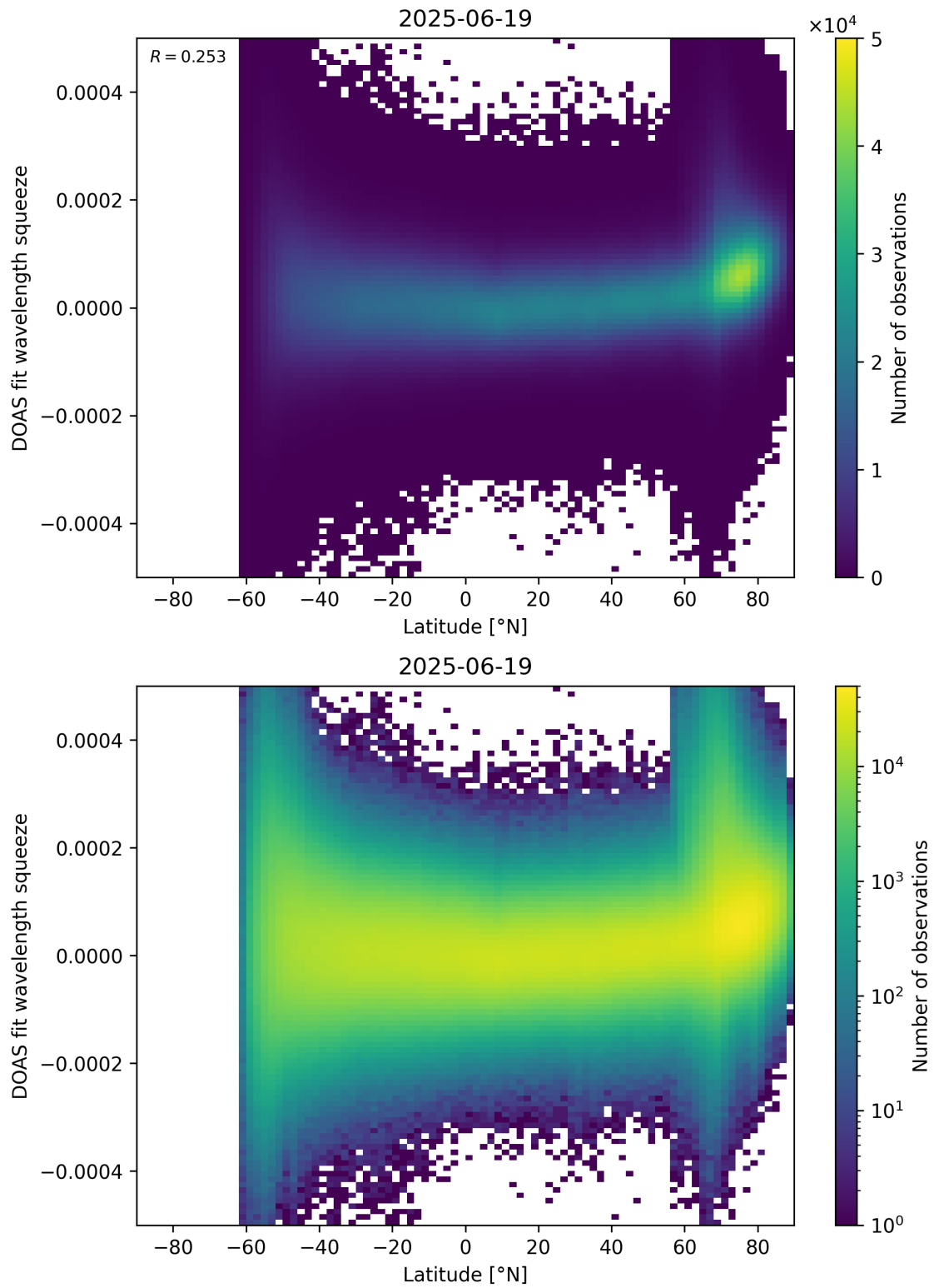
Figure 155: Scatter density plot of “Latitude” against “DOAS fit wavelength squeeze” for 2025-06-18 to 2025-06-20.
