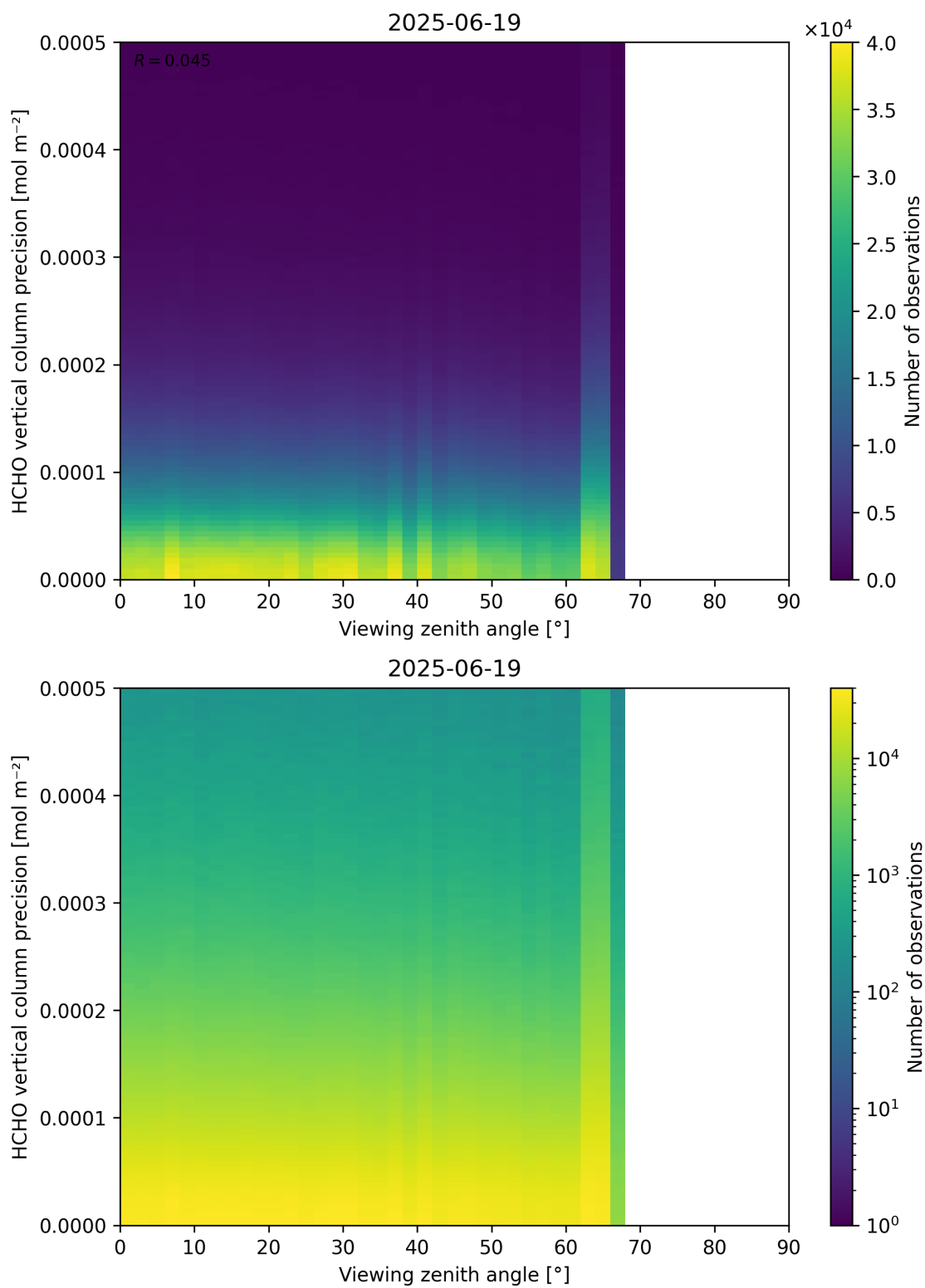
Figure 194: Scatter density plot of “Viewing zenith angle” against “HCHO vertical column precision” for 2025-06-18 to 2025-06-20.
