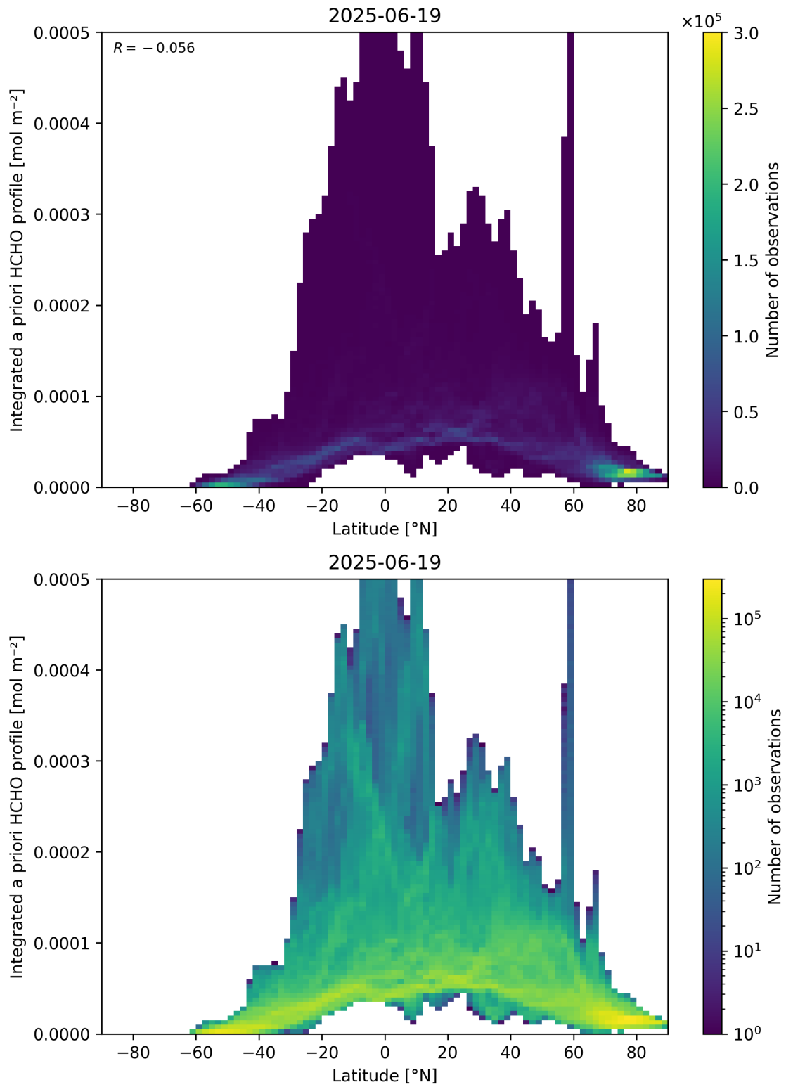
Figure 166: Scatter density plot of “Latitude” against “Integrated a priori HCHO profile” for 2025-06-18 to 2025-06-20.
