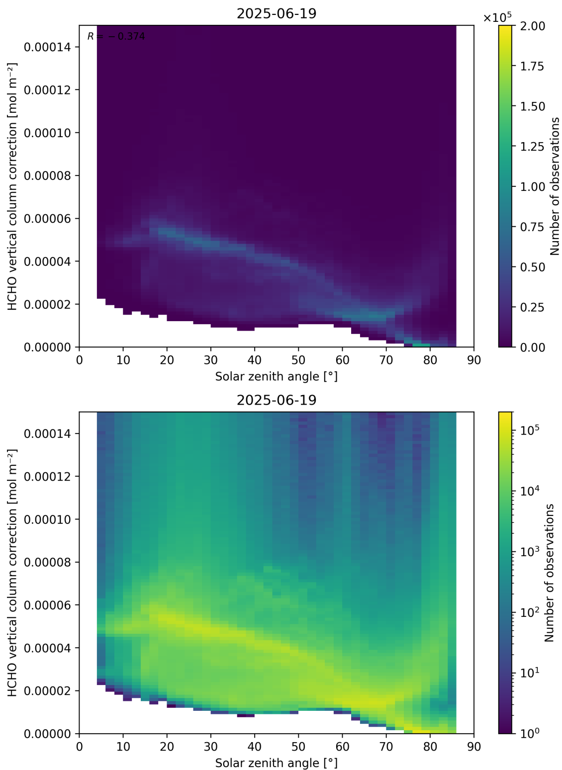
Figure 178: Scatter density plot of “Solar zenith angle” against “HCHO vertical column correction” for 2025-06-18 to 2025-06-20.
