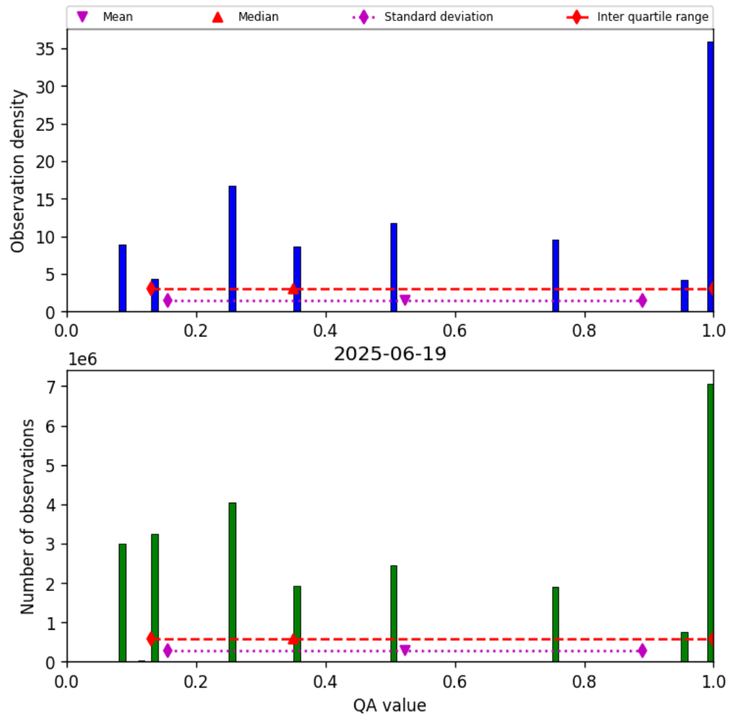
Figure 34: Histogram of “QA value” for 2025-06-18 to 2025-06-20
