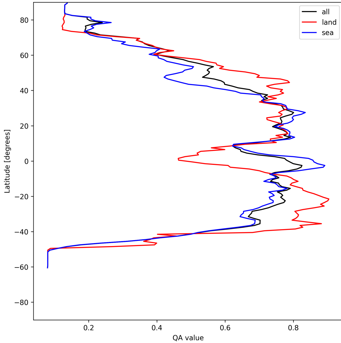
Figure 20: Zonal average of “QA value” for 2025-06-18 to 2025-06-20.
