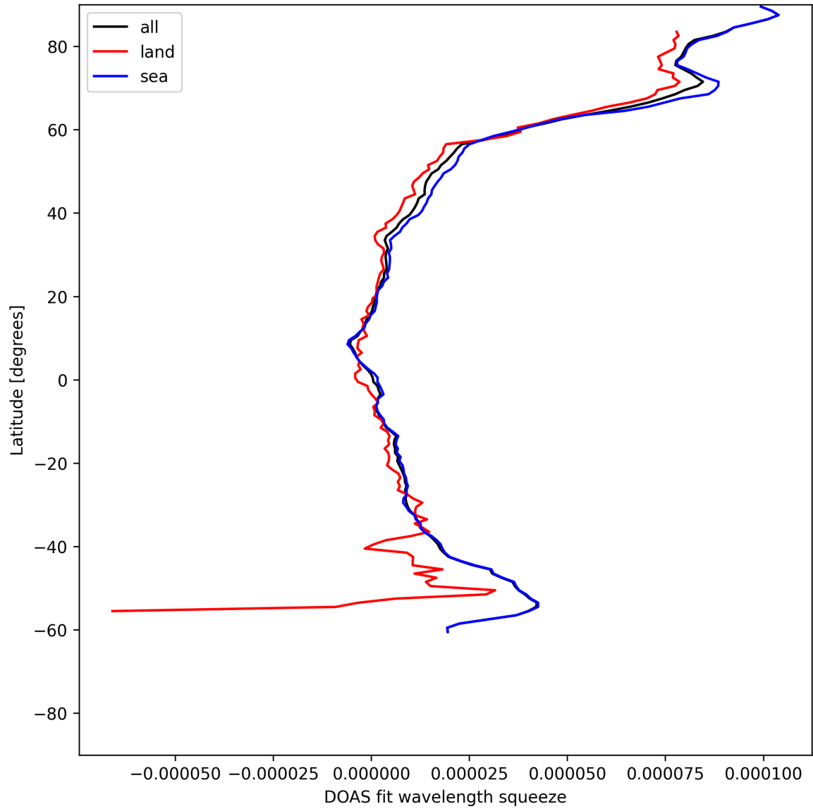
Figure 31: Zonal average of “DOAS fit wavelength squeeze” for 2025-06-18 to 2025-06-20.
