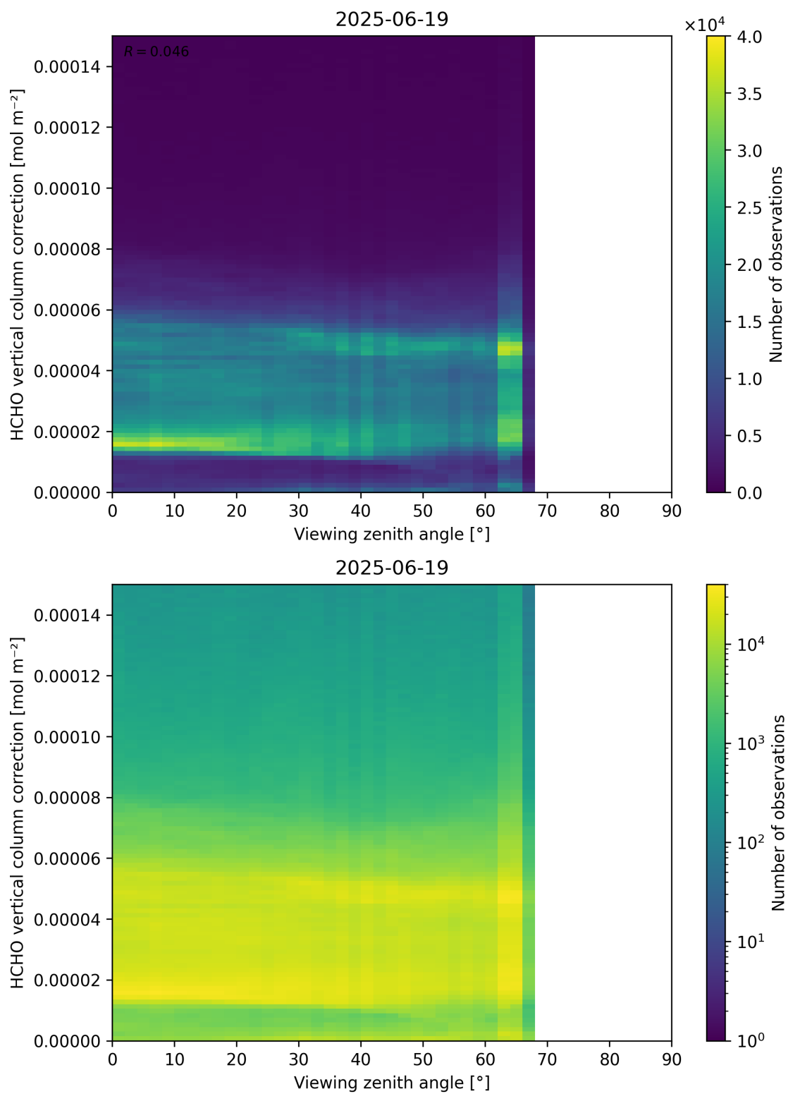
Figure 193: Scatter density plot of “Viewing zenith angle” against “HCHO vertical column correction” for 2025-06-18 to 2025-06-20.
