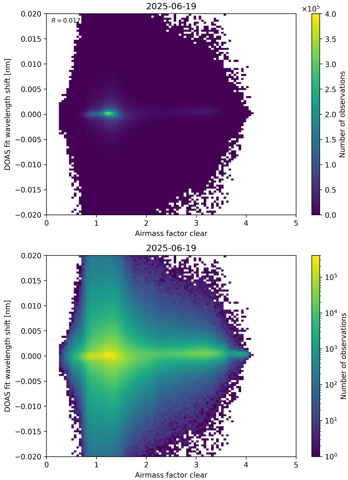
Figure 72: Scatter density plot of “Airmass factor clear” against “DOAS fit wavelength shift” for 2025-06-18 to 2025-06-20.
