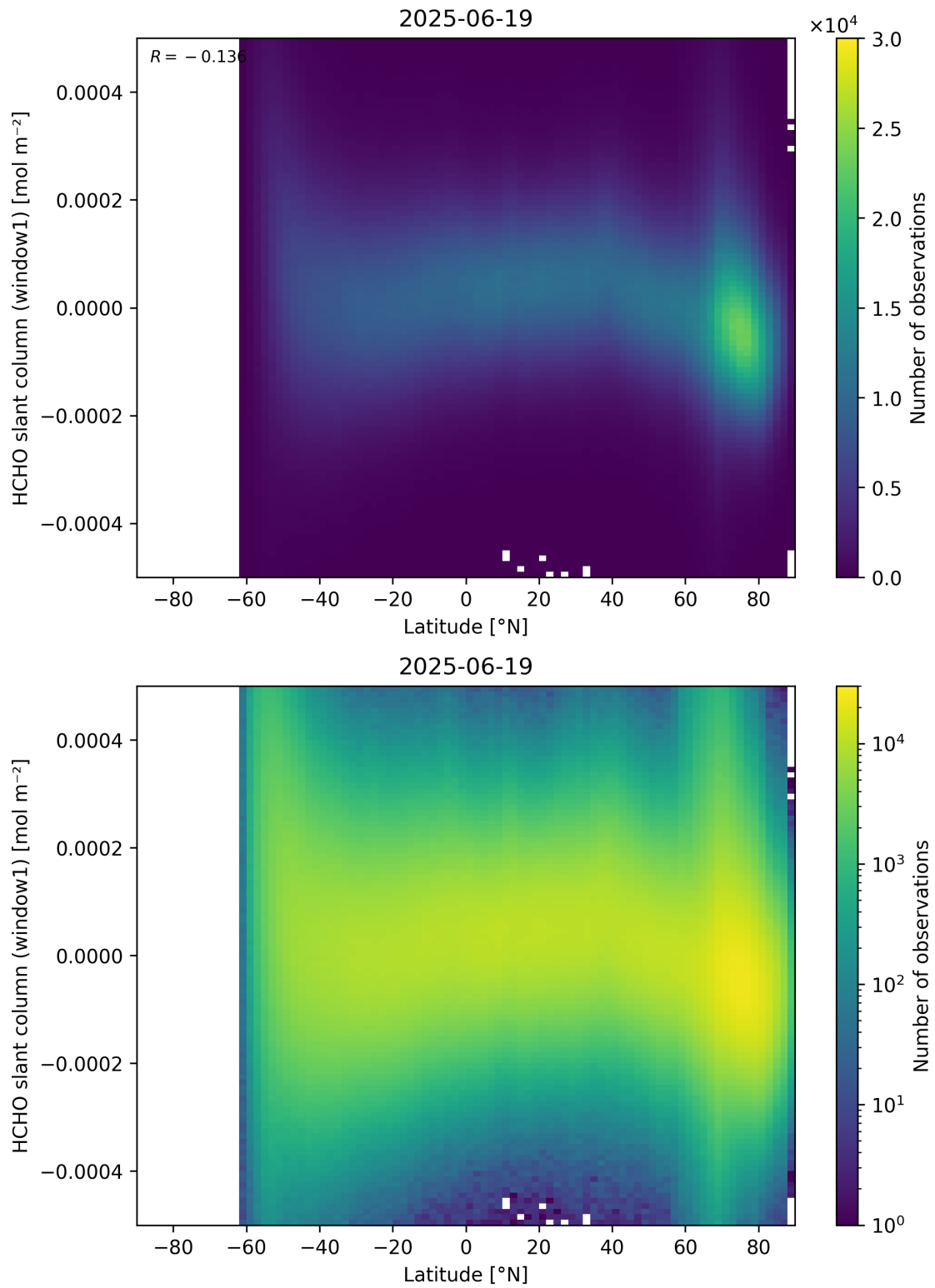
Figure 159: Scatter density plot of “Latitude” against “HCHO slant column (window1)” for 2025-06-18 to 2025-06-20.
