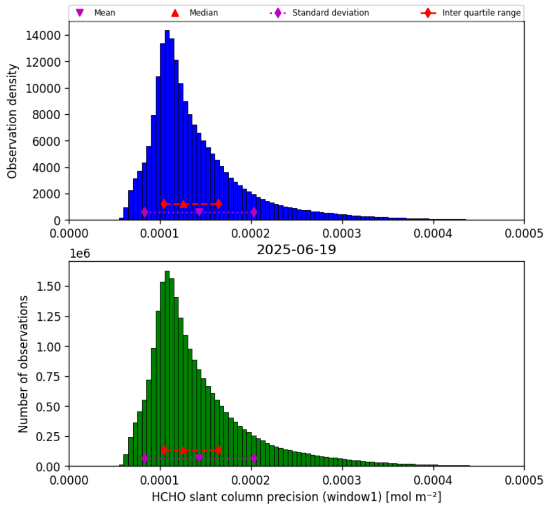
Figure 39: Histogram of “HCHO slant column precision (window1)” for 2025-06-18 to 2025-06-20
