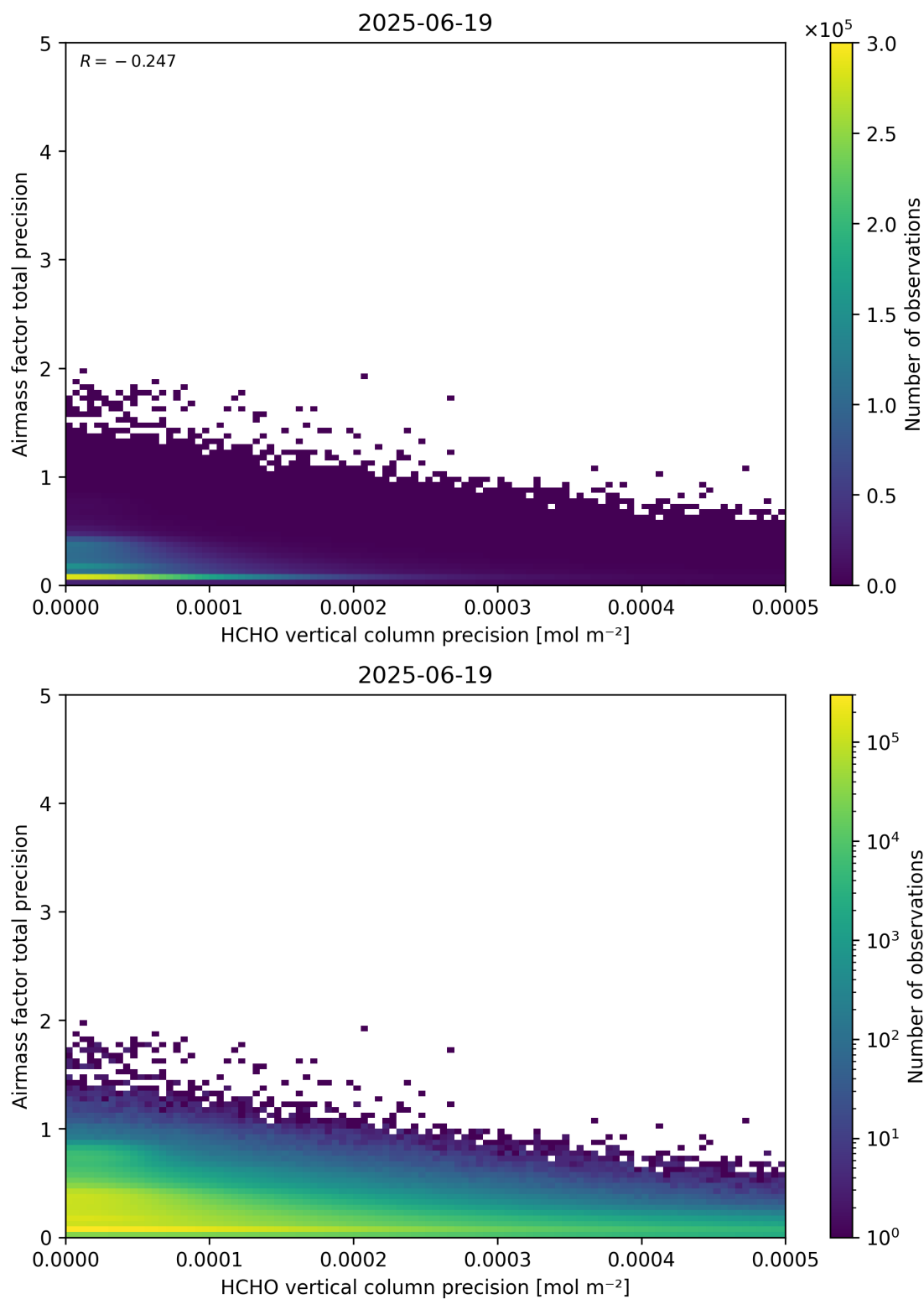
Figure 145: Scatter density plot of “HCHO vertical column precision” against “Airmass factor total precision” for 2025-06-18 to 2025-06-20.
