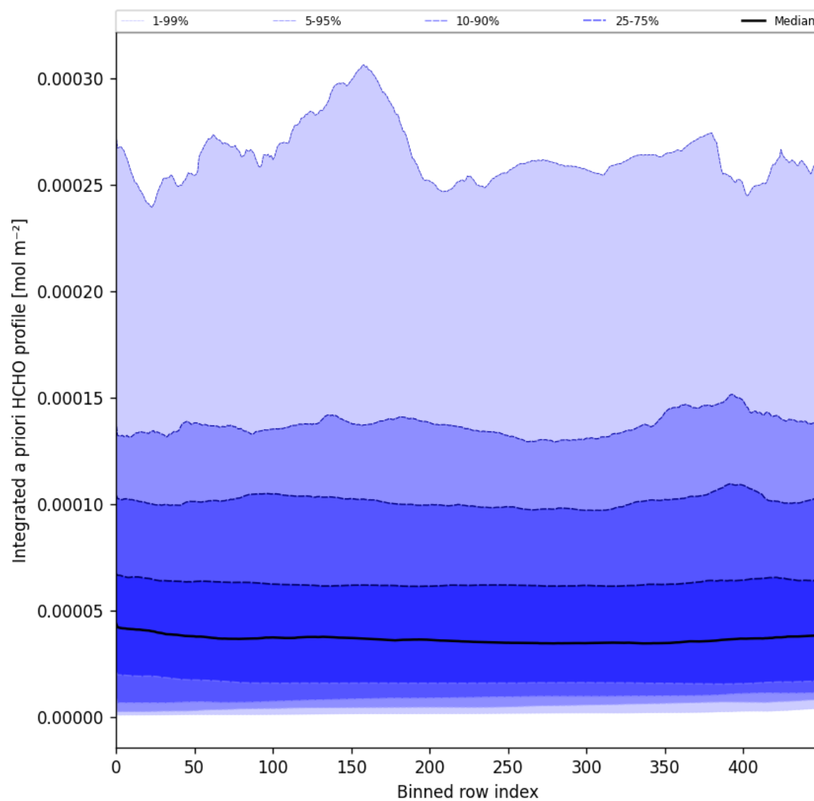
Figure 57: Along track statistics of “Integrated a priori HCHO profile” for 2025-06-18 to 2025-06-20
