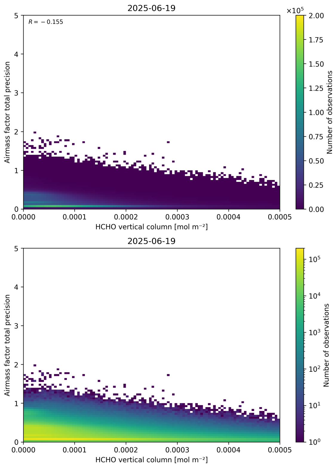
Figure 132: Scatter density plot of “HCHO vertical column” against “Airmass factor total precision” for 2025-06-18 to 2025-06-20.
