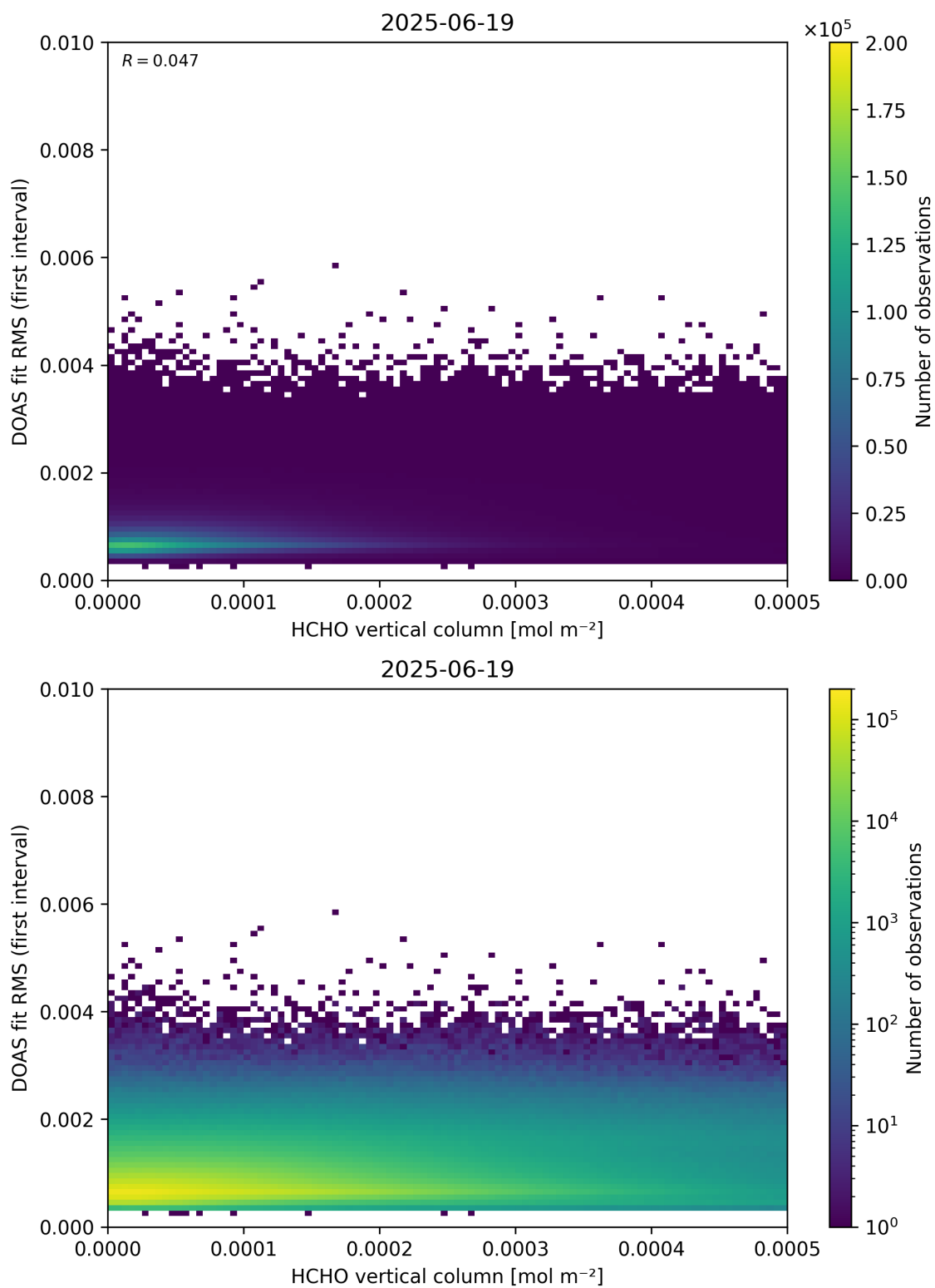
Figure 123: Scatter density plot of “HCHO vertical column” against “DOAS fit RMS (first interval)” for 2025-06-18 to 2025-06-20.
