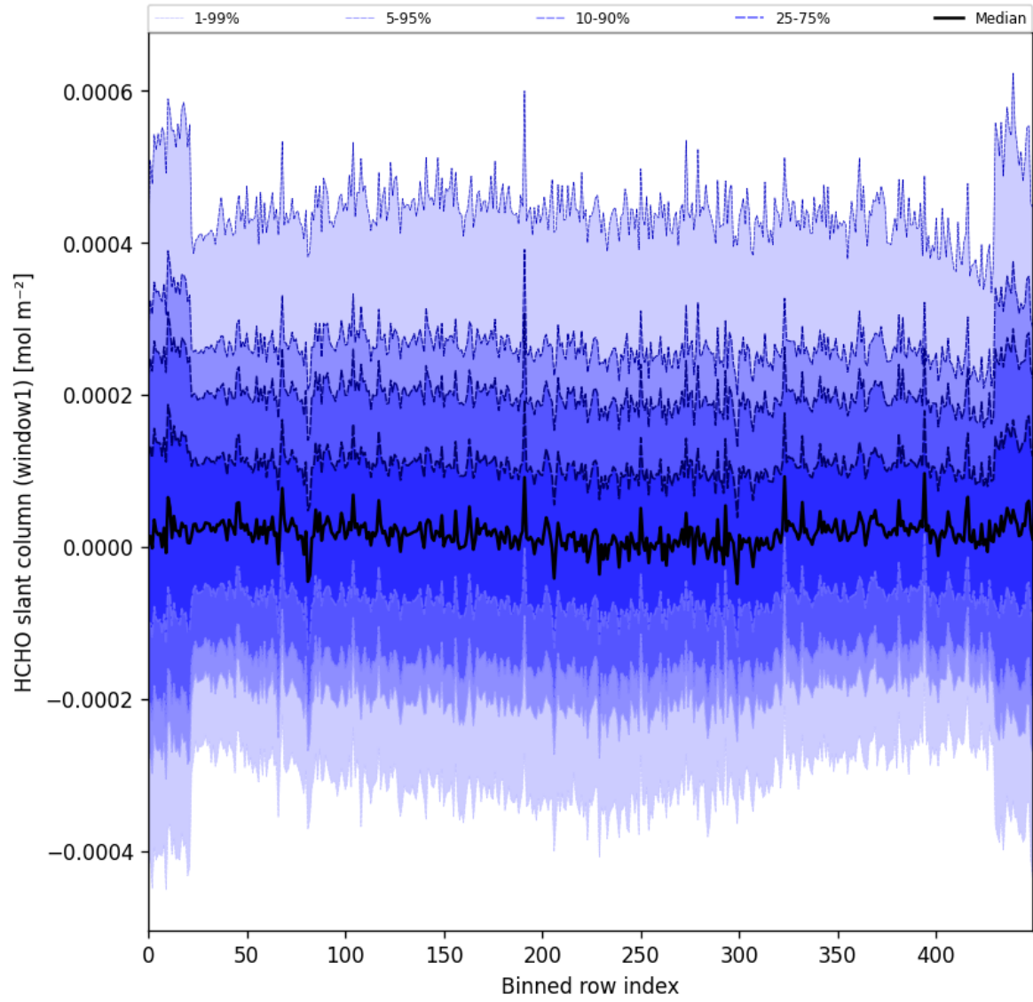
Figure 52: Along track statistics of “HCHO slant column (window1)” for 2025-06-18 to 2025-06-20
