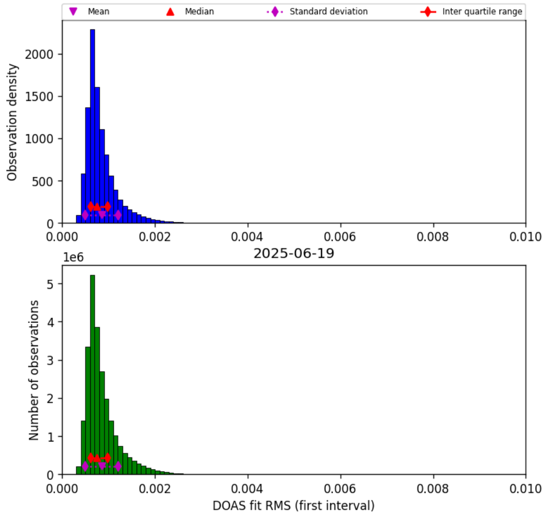
Figure 46: Histogram of “DOAS fit RMS (first interval)” for 2025-06-18 to 2025-06-20
