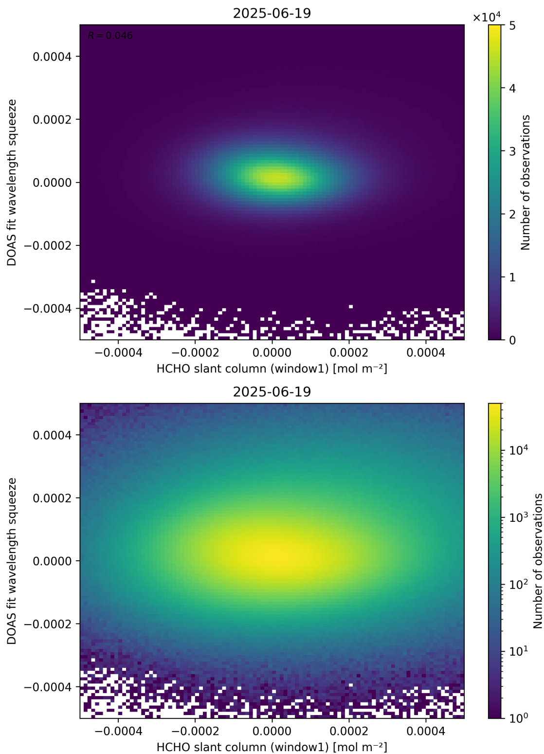
Figure 80: Scatter density plot of “HCHO slant column (window1)” against “DOAS fit wavelength squeeze” for 2025-06-18 to 2025-06-20.
