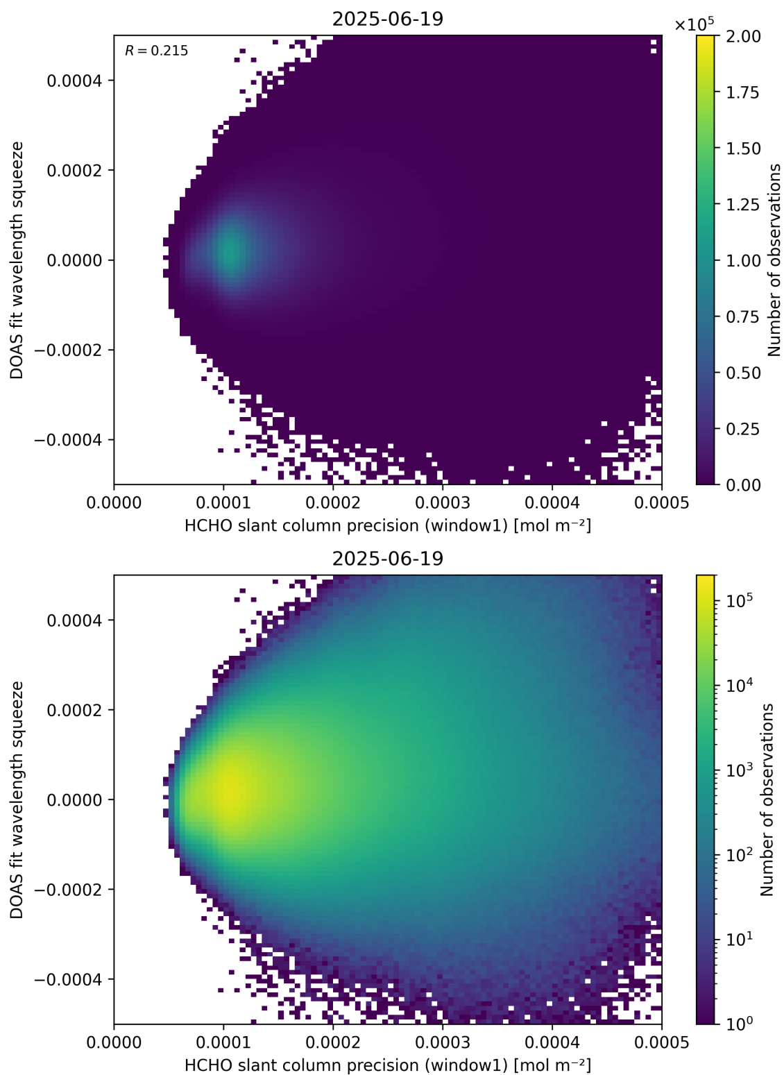
Figure 90: Scatter density plot of “HCHO slant column precision (window1)” against “DOAS fit wavelength squeeze” for 2025-06-18 to 2025-06-20.
