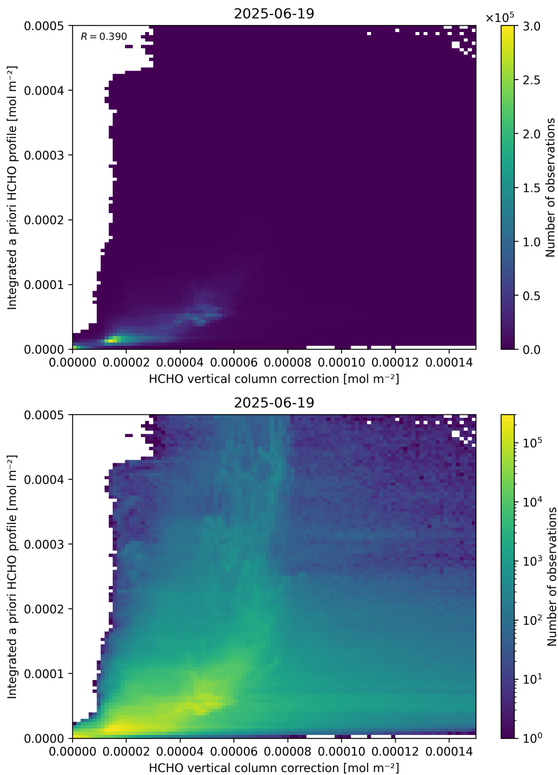
Figure 122: Scatter density plot of “HCHO vertical column correction” against “Integrated a priori HCHO profile” for 2025-06-18 to 2025-06-20.
