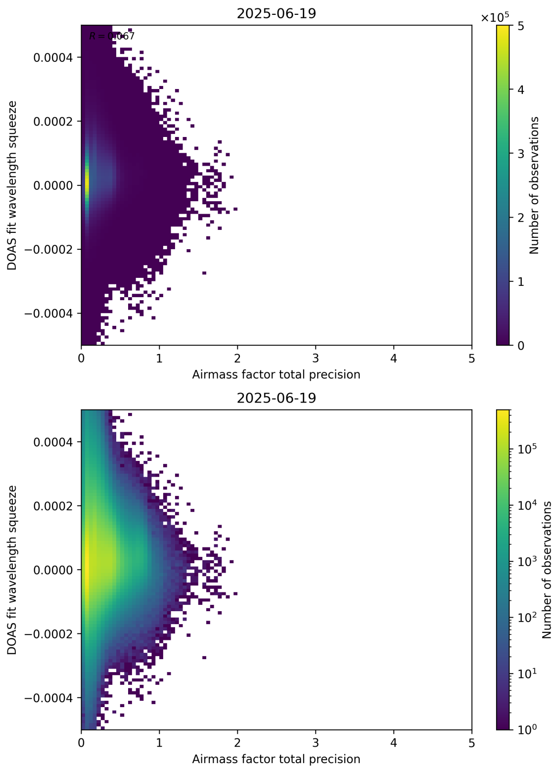
Figure 107: Scatter density plot of “Airmass factor total precision” against “DOAS fit wavelength squeeze” for 2025-06-18 to 2025-06-20.
