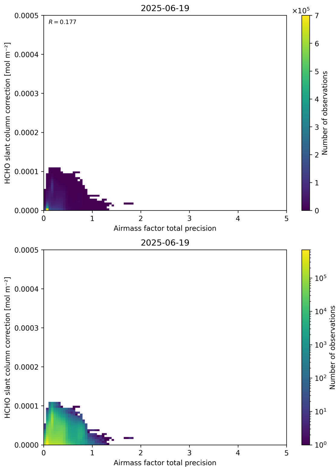
Figure 110: Scatter density plot of “Airmass factor total precision” against “HCHO slant column correction” for 2025-06-18 to 2025-06-20.
