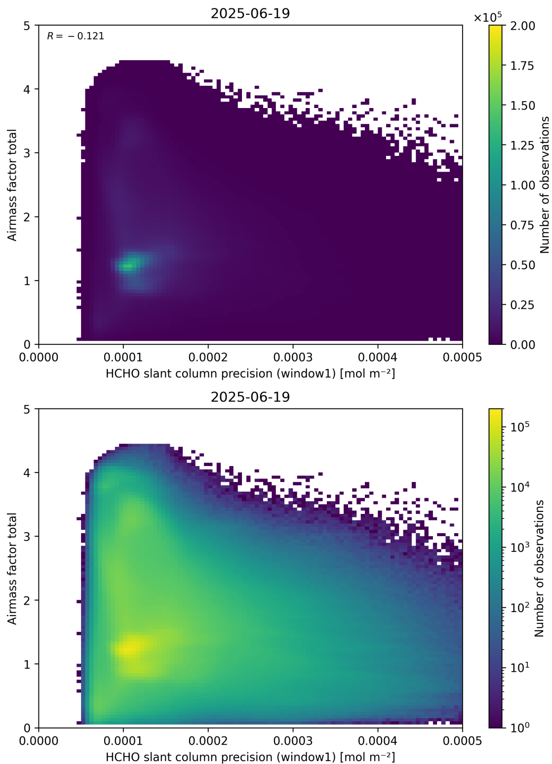
Figure 94: Scatter density plot of “HCHO slant column precision (window1)” against “Airmass factor total” for 2025-06-18 to 2025-06-20.
