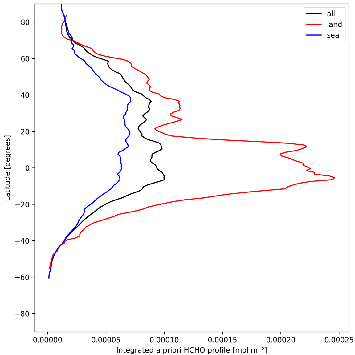
Figure 29: Zonal average of “Integrated a priori HCHO profile” for 2025-06-18 to 2025-06-20.
