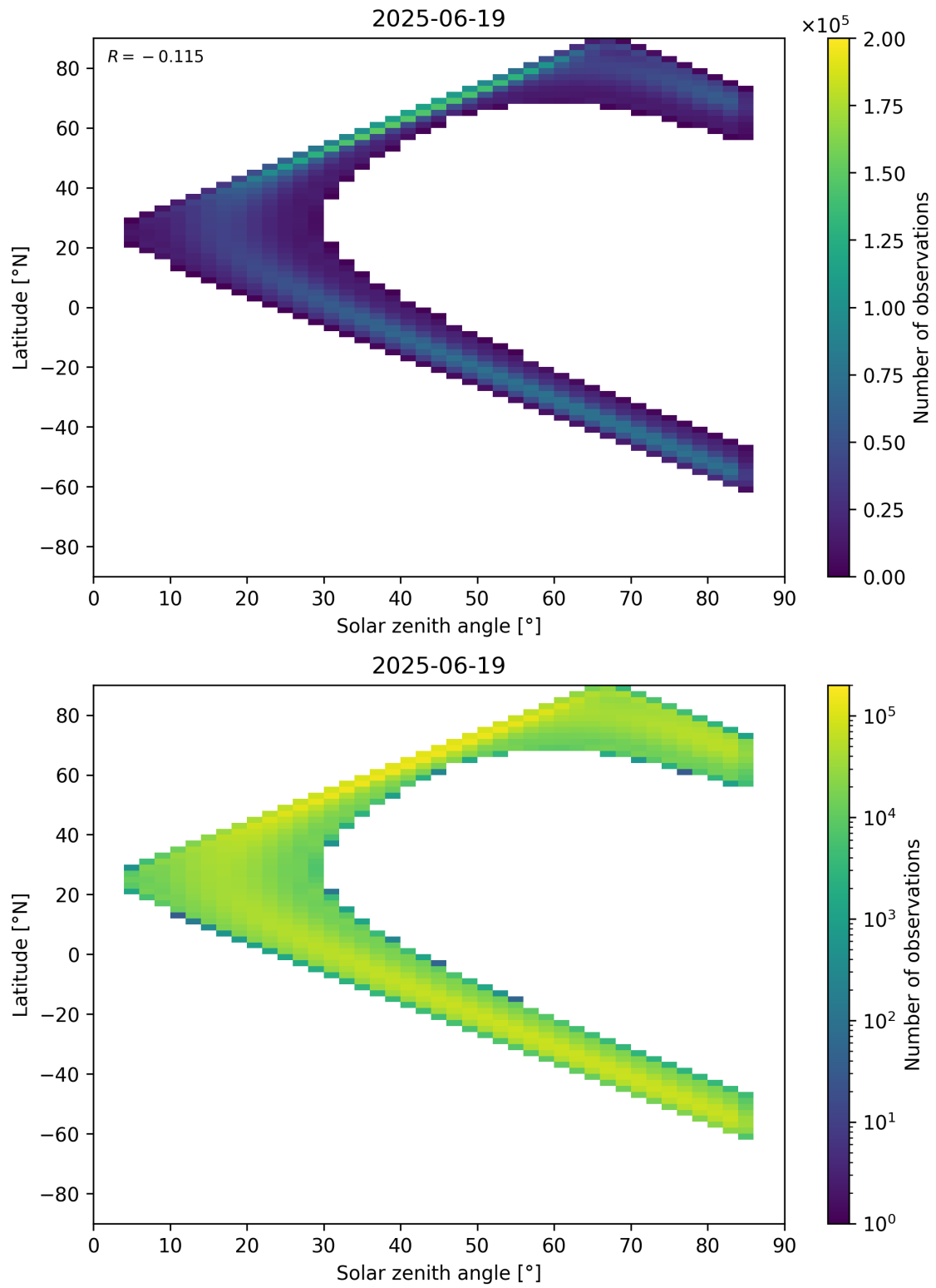
Figure 181: Scatter density plot of “Solar zenith angle” against “Latitude” for 2025-06-18 to 2025-06-20.
