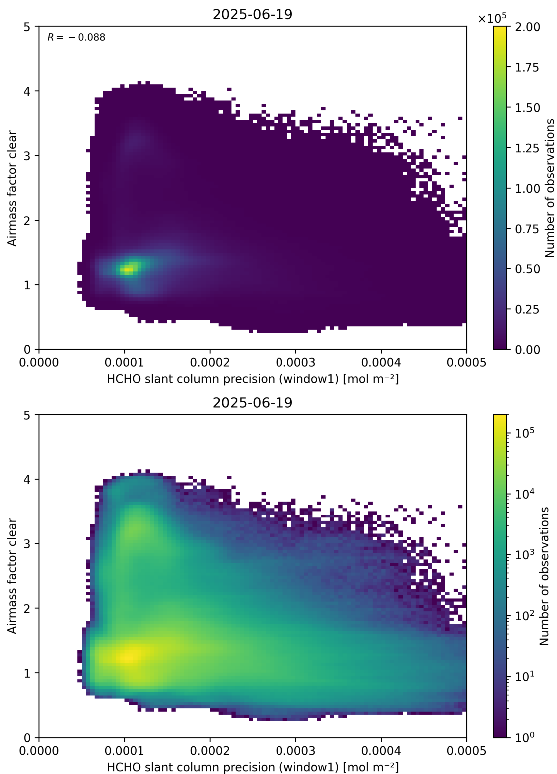
Figure 91: Scatter density plot of “HCHO slant column precision (window1)” against “Airmass factor clear” for 2025-06-18 to 2025-06-20.
