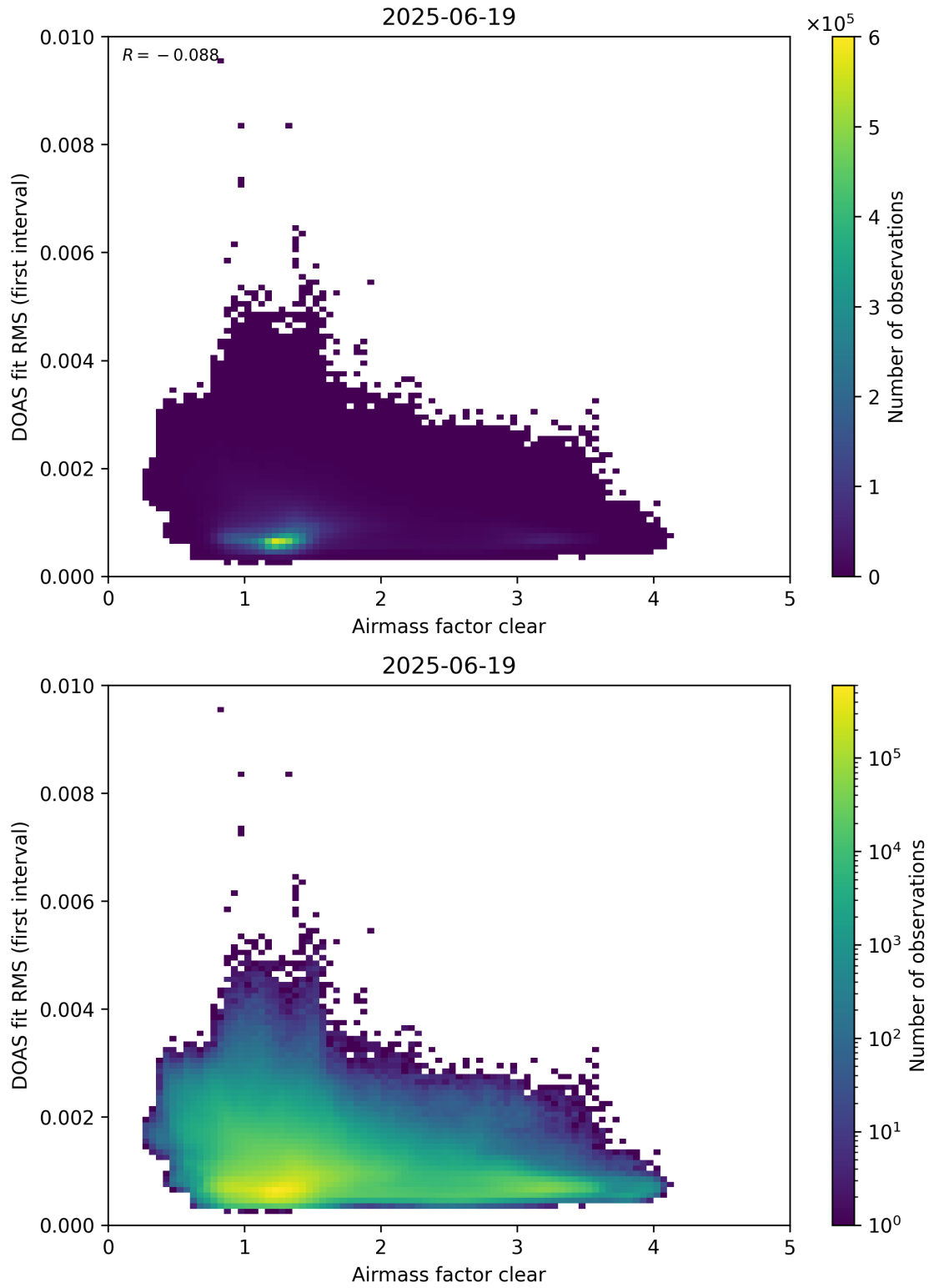
Figure 71: Scatter density plot of “Airmass factor clear” against “DOAS fit RMS (first interval)” for 2025-06-18 to 2025-06-20.
