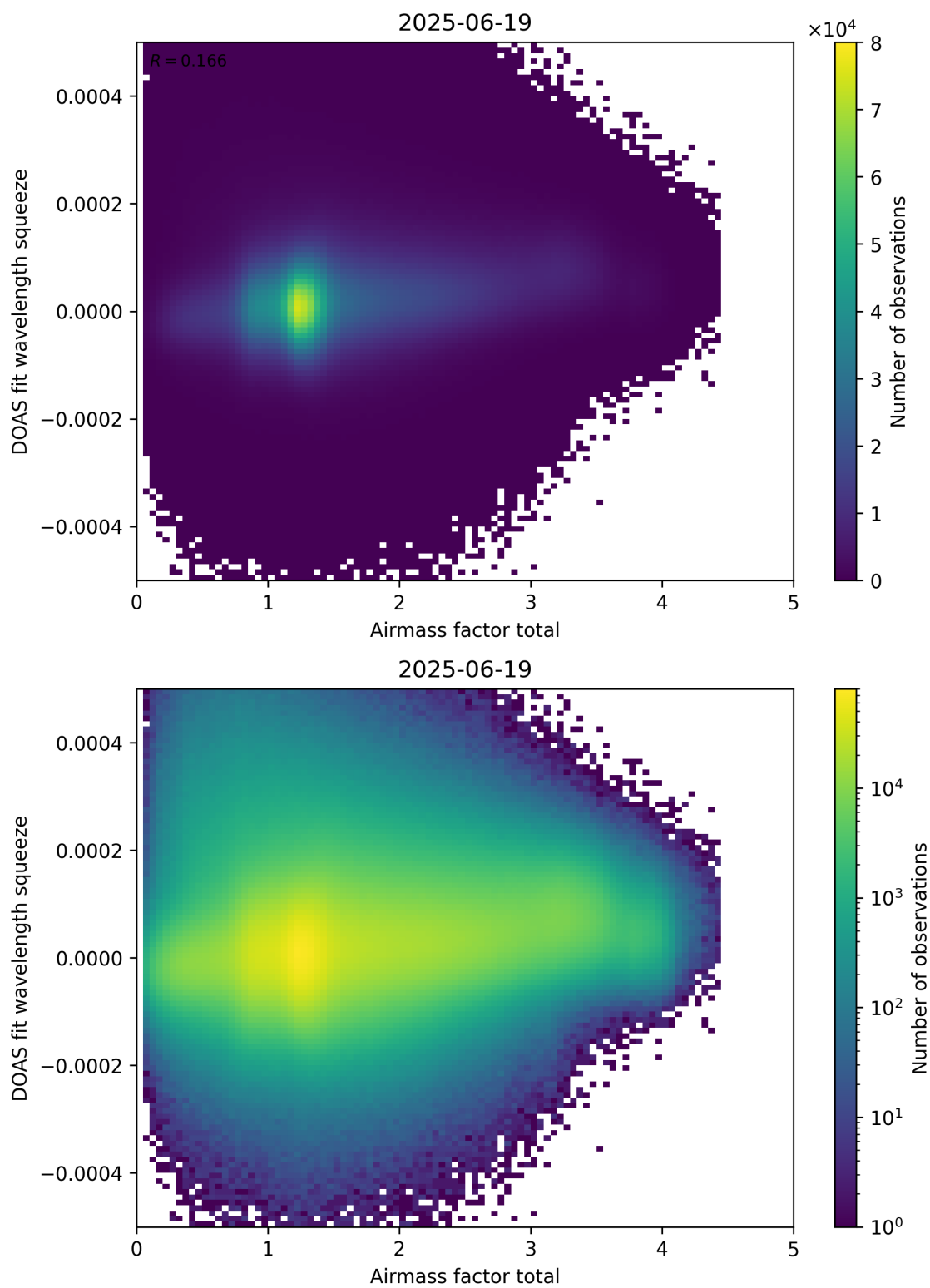
Figure 99: Scatter density plot of “Airmass factor total” against “DOAS fit wavelength squeeze” for 2025-06-18 to 2025-06-20.
