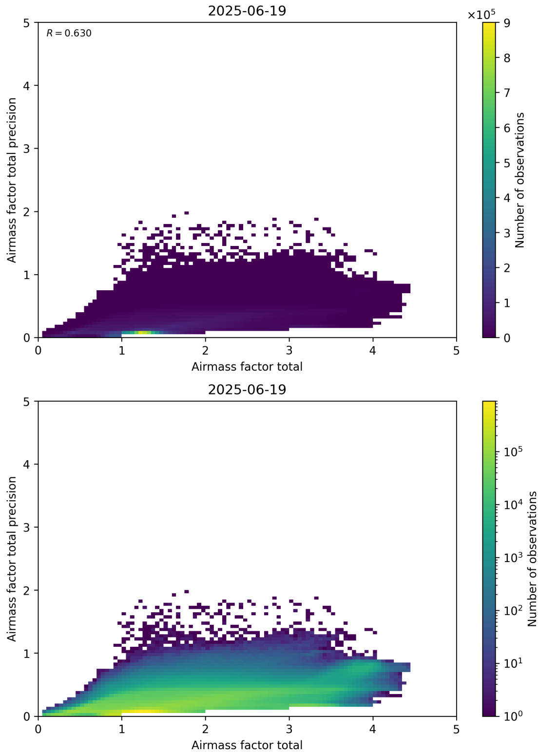
Figure 103: Scatter density plot of “Airmass factor total” against “Airmass factor total precision” for 2025-06-18 to 2025-06-20.
