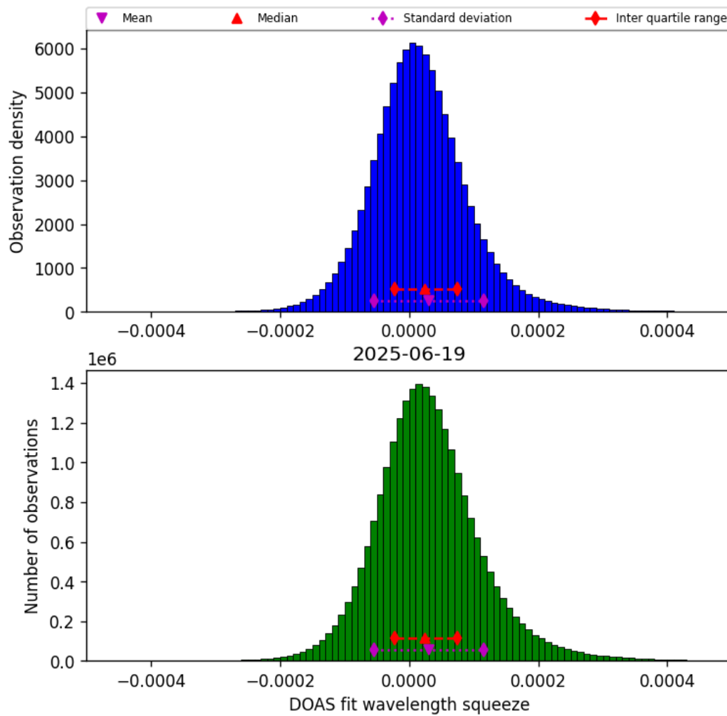
Figure 45: Histogram of “DOAS fit wavelength squeeze” for 2025-06-18 to 2025-06-20
