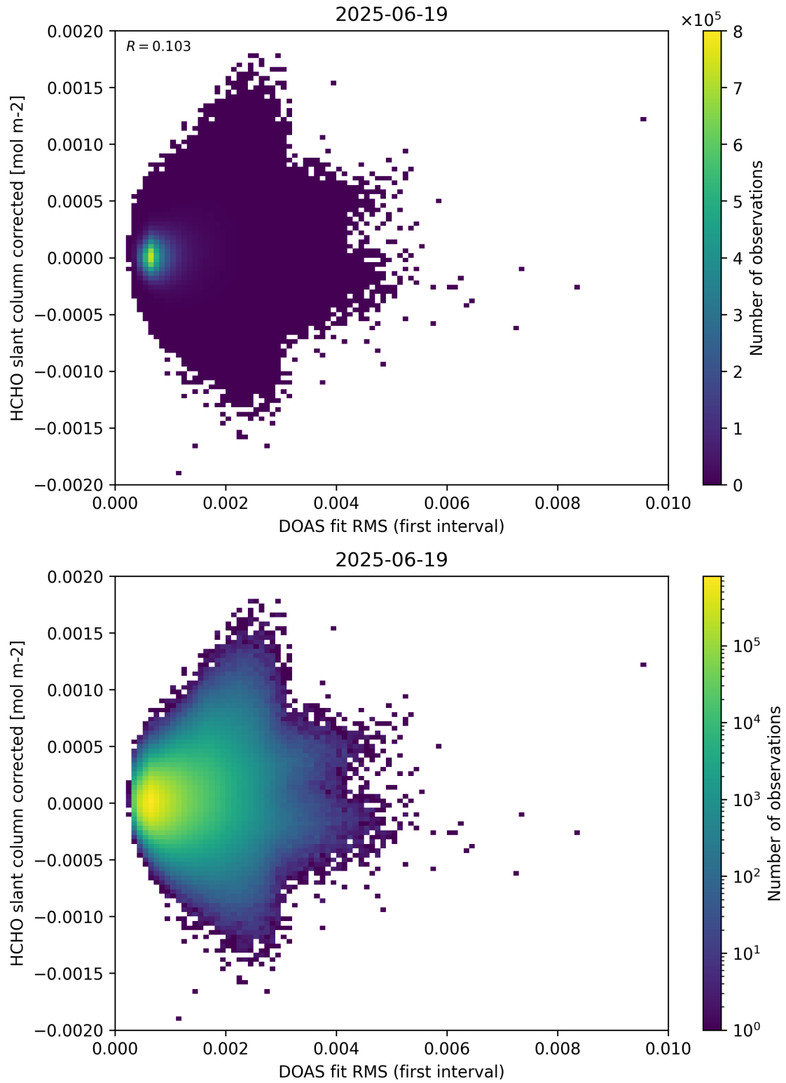
Figure 62: Scatter density plot of “DOAS fit RMS (first interval)” against “HCHO slant column corrected” for 2025-06-18 to 2025-06-20.
