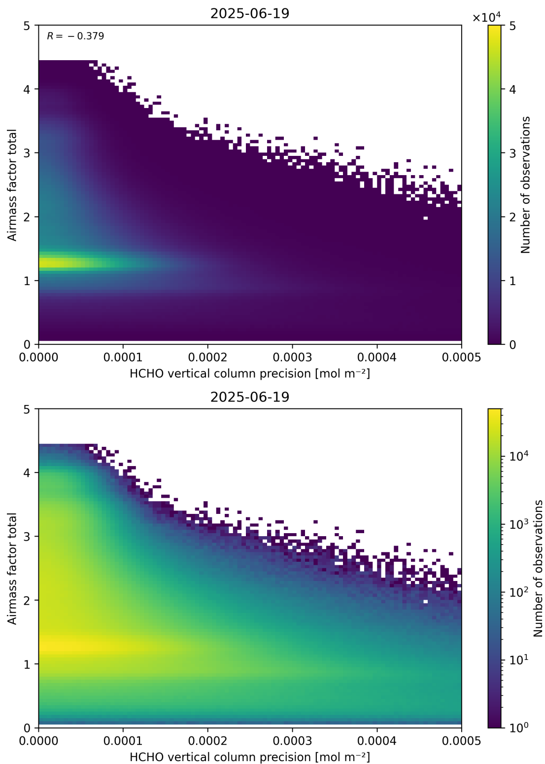
Figure 144: Scatter density plot of “HCHO vertical column precision” against “Airmass factor total” for 2025-06-18 to 2025-06-20.
