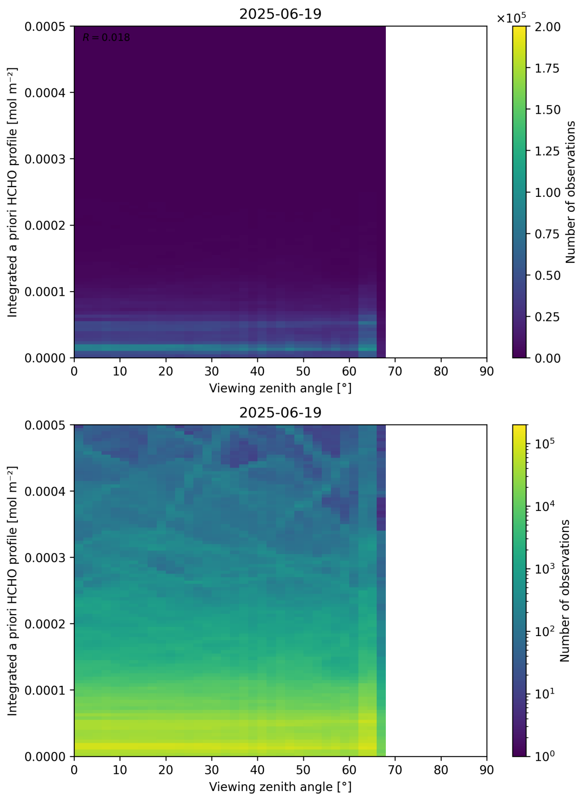
Figure 195: Scatter density plot of “Viewing zenith angle” against “Integrated a priori HCHO profile” for 2025-06-18 to 2025-06-20.
