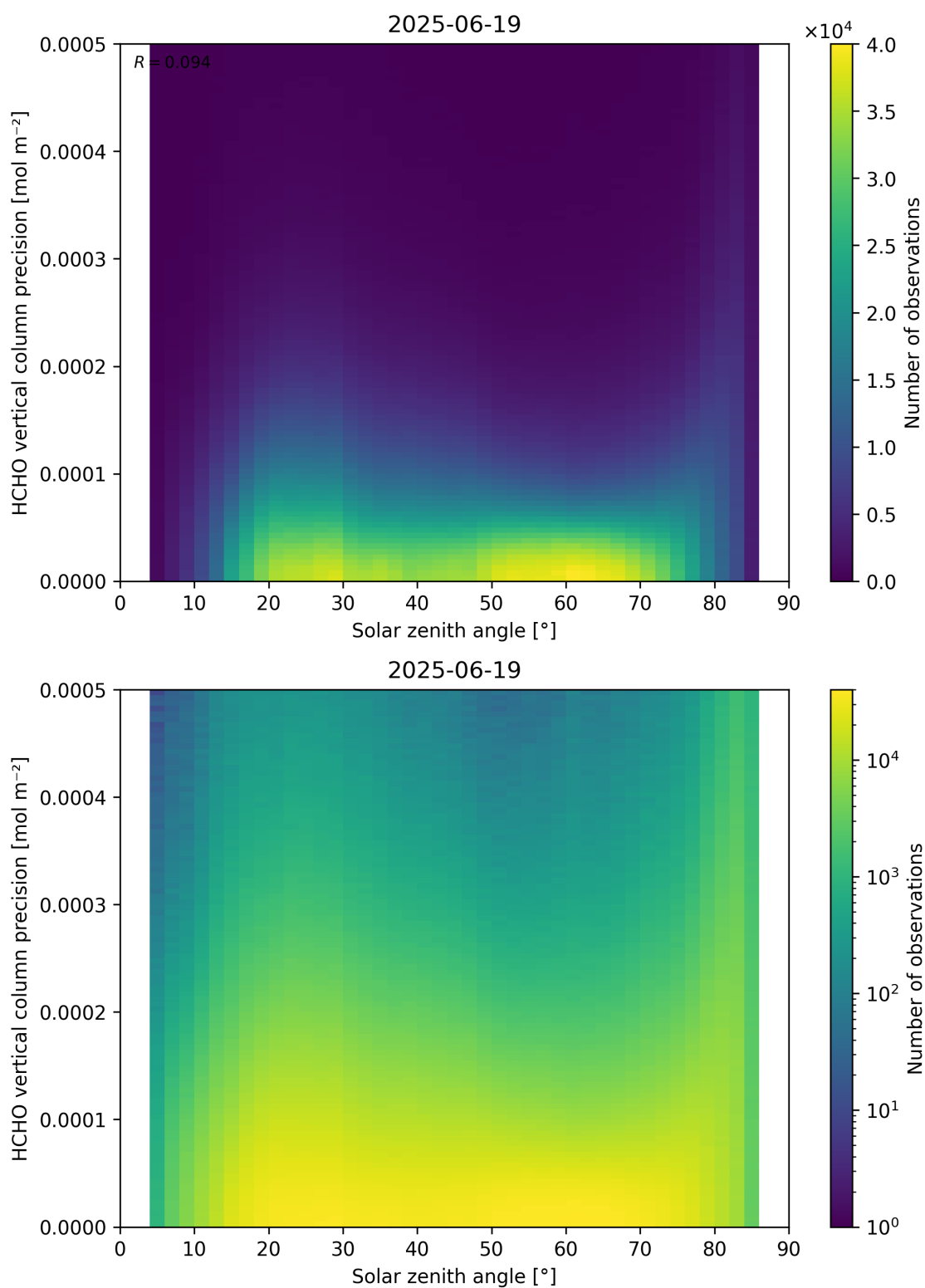
Figure 179: Scatter density plot of “Solar zenith angle” against “HCHO vertical column precision” for 2025-06-18 to 2025-06-20.
