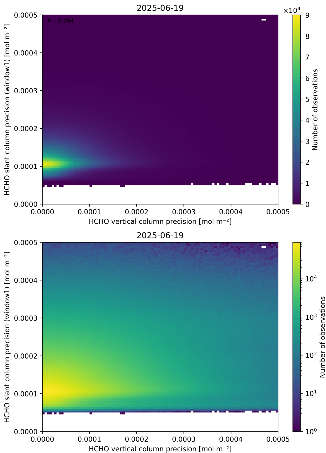
Figure 143: Scatter density plot of “HCHO vertical column precision” against “HCHO slant column precision (window1)” for 2025-06-18 to 2025-06-20.
