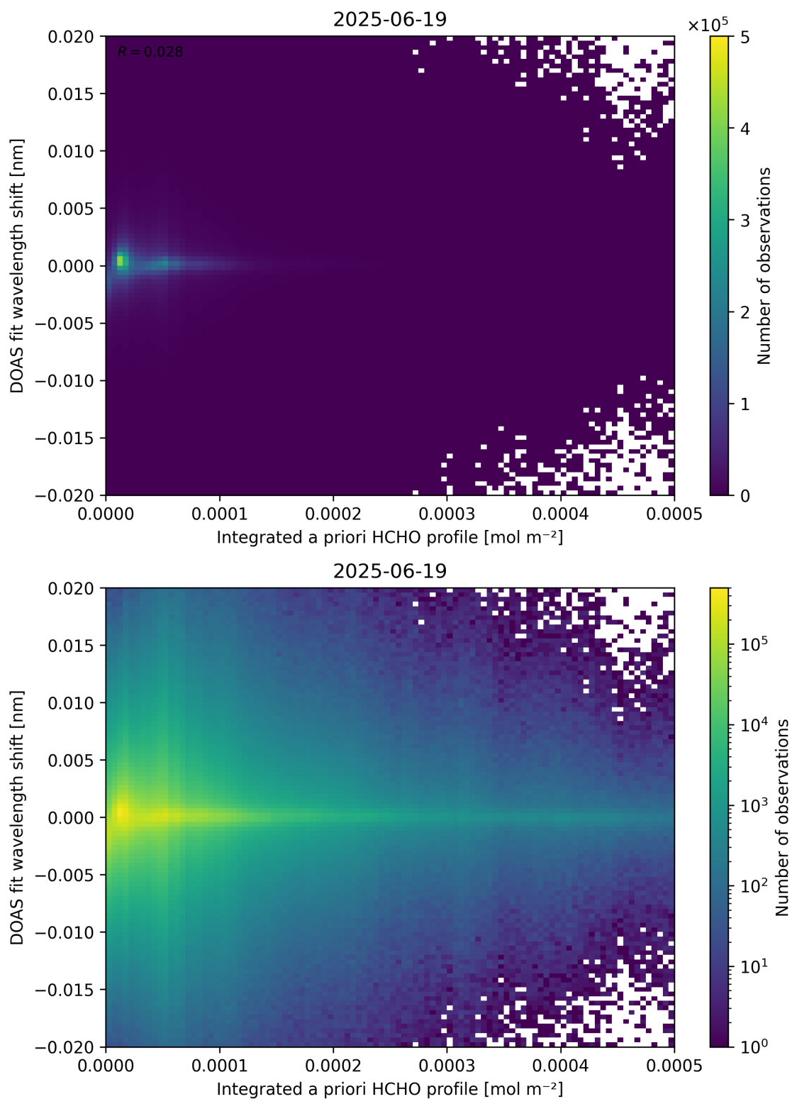
Figure 149: Scatter density plot of “Integrated a priori HCHO profile” against “DOAS fit wavelength shift” for 2025-06-18 to 2025-06-20.
