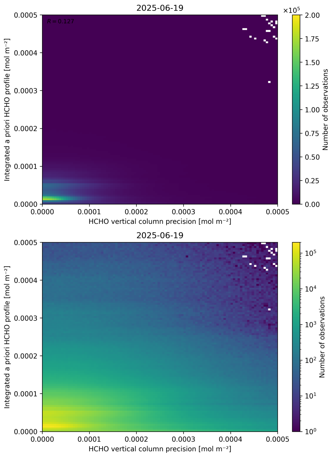
Figure 147: Scatter density plot of “HCHO vertical column precision” against “Integrated a priori HCHO profile” for 2025-06-18 to 2025-06-20.
