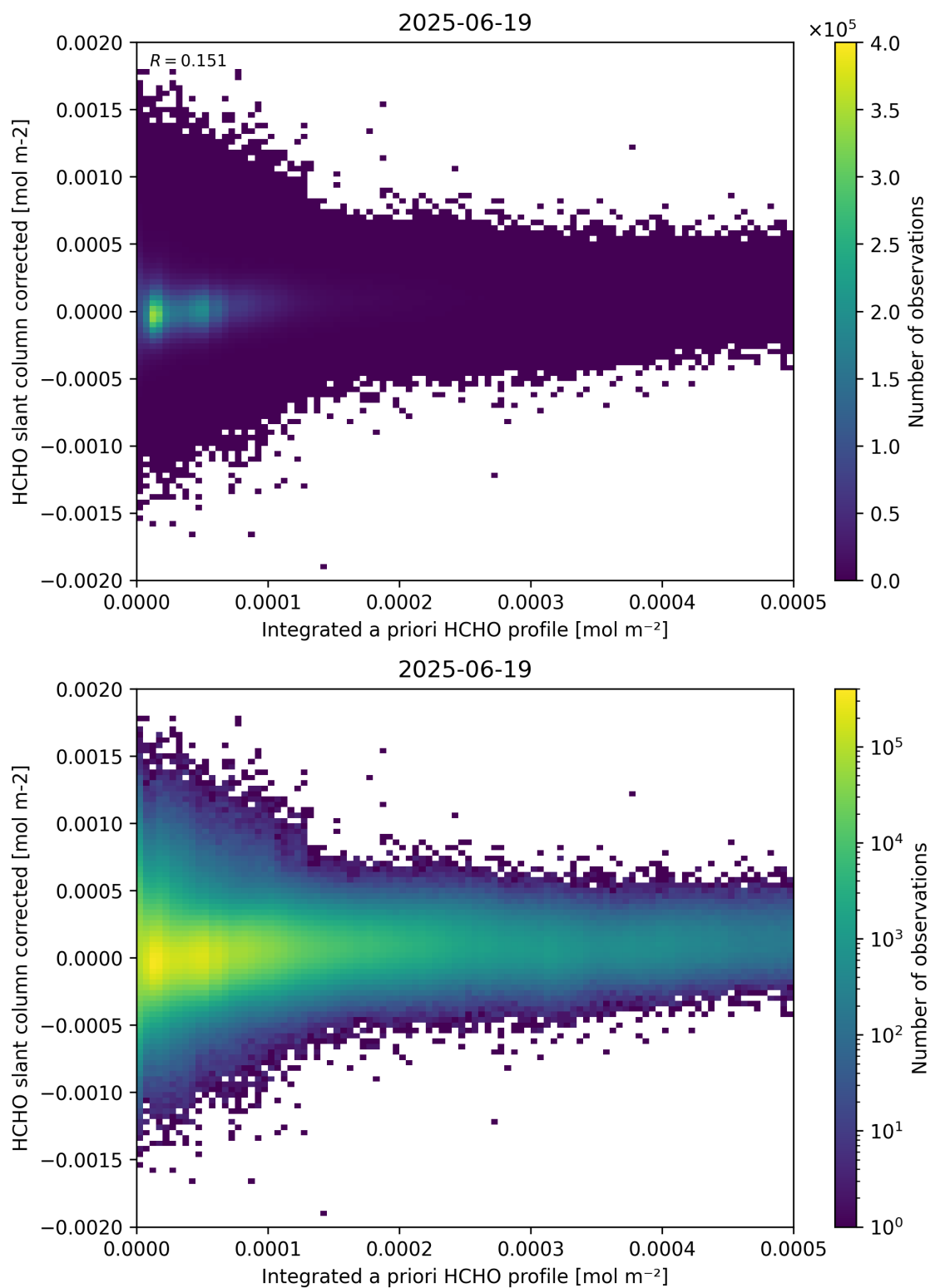
Figure 151: Scatter density plot of “Integrated a priori HCHO profile” against “HCHO slant column corrected” for 2025-06-18 to 2025-06-20.
