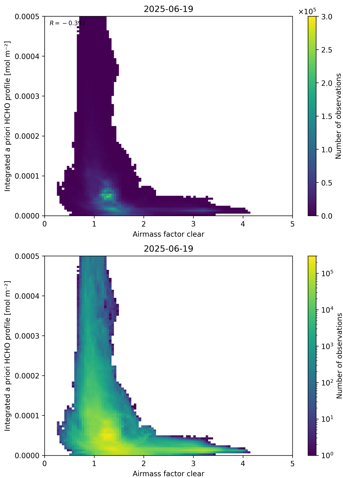
Figure 76: Scatter density plot of “Airmass factor clear” against “Integrated a priori HCHO profile” for 2025-06-18 to 2025-06-20.
