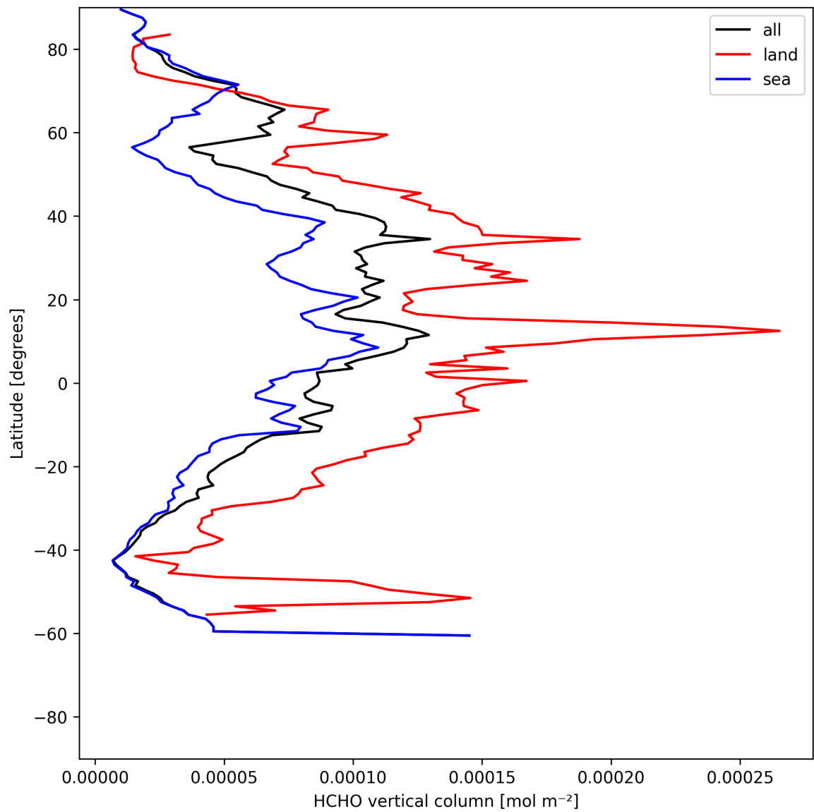
Figure 21: Zonal average of “HCHO vertical column” for 2025-06-18 to 2025-06-20.
