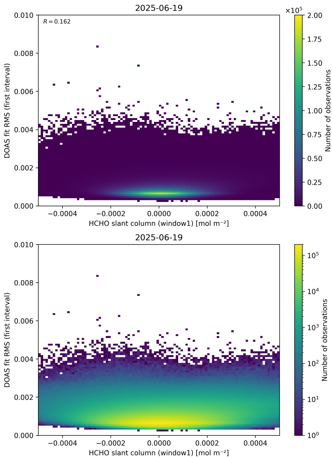
Figure 78: Scatter density plot of “HCHO slant column (window1)” against “DOAS fit RMS (first interval)” for 2025-06-18 to 2025-06-20.
