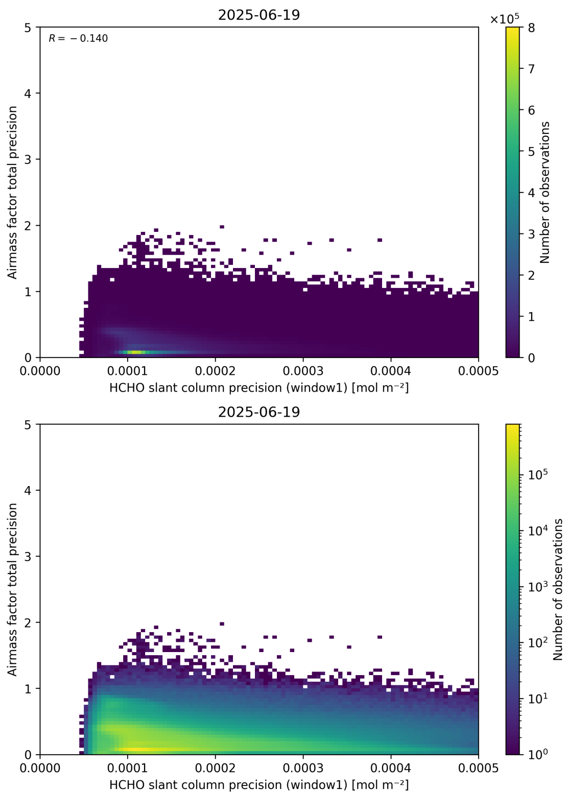
Figure 95: Scatter density plot of “HCHO slant column precision (window1)” against “Airmass factor total precision” for 2025-06-18 to 2025-06-20.
