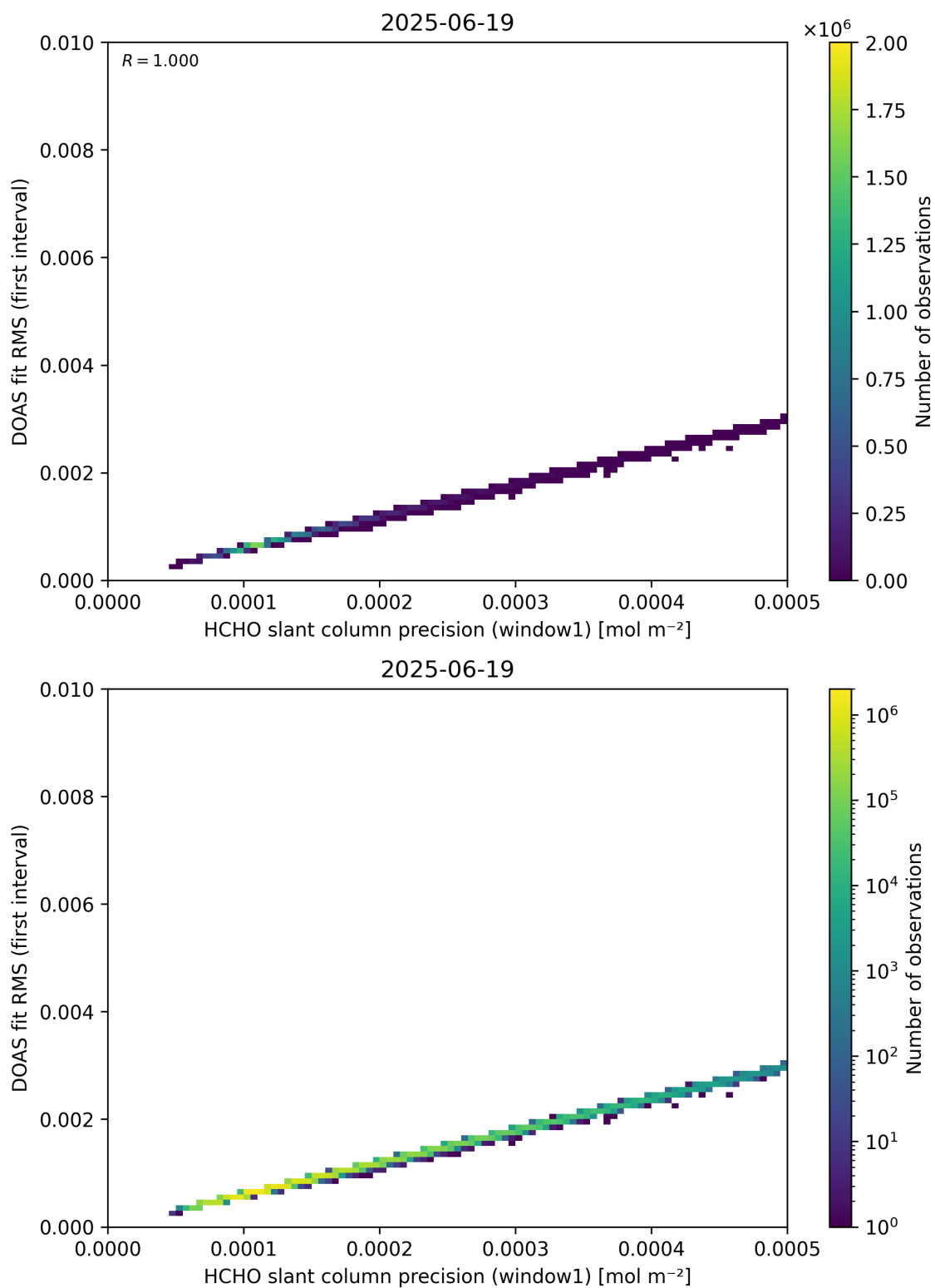
Figure 88: Scatter density plot of “HCHO slant column precision (window1)” against “DOAS fit RMS (first interval)” for 2025-06-18 to 2025-06-20.
