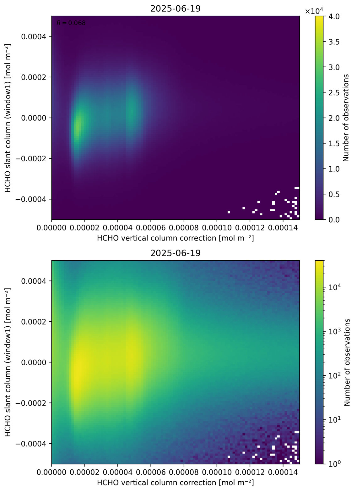
Figure 118: Scatter density plot of “HCHO vertical column correction” against “HCHO slant column (window1)” for 2025-06-18 to 2025-06-20.
