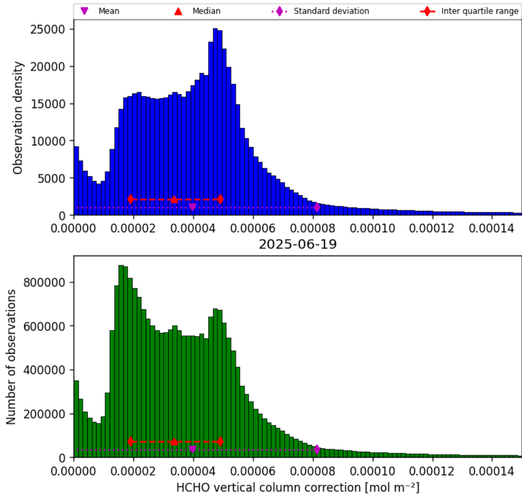
Figure 37: Histogram of “HCHO vertical column correction” for 2025-06-18 to 2025-06-20
