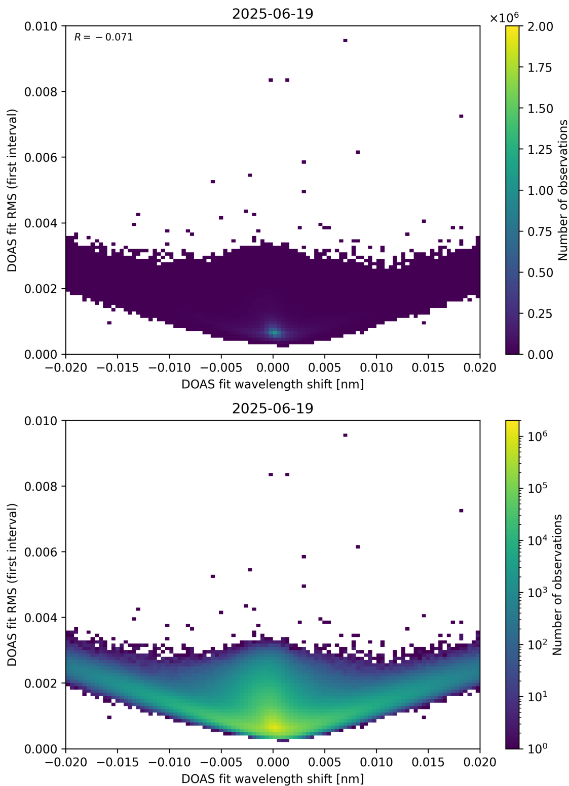
Figure 64: Scatter density plot of “DOAS fit wavelength shift” against “DOAS fit RMS (first interval)” for 2025-06-18 to 2025-06-20.
