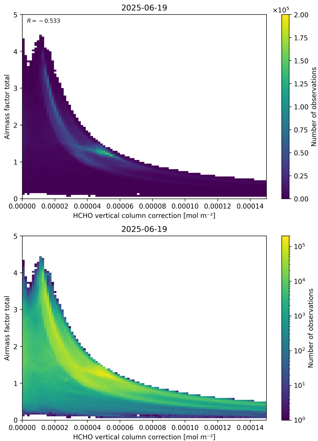
Figure 120: Scatter density plot of “HCHO vertical column correction” against “Airmass factor total” for 2025-06-18 to 2025-06-20.
