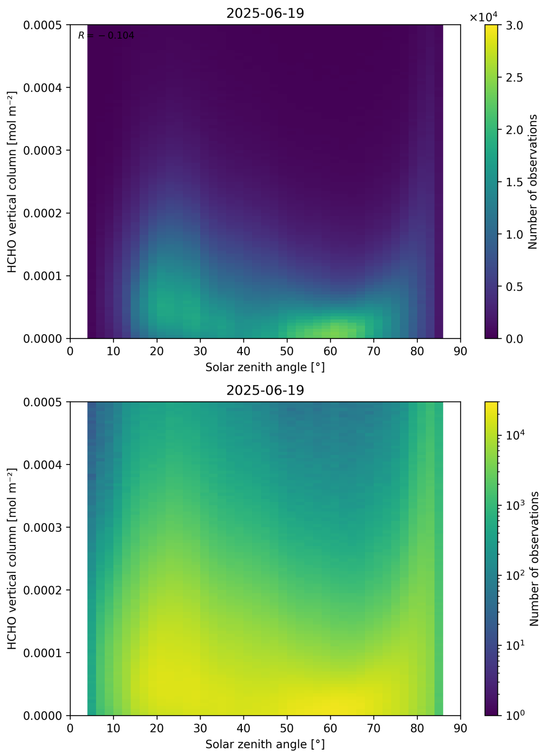
Figure 177: Scatter density plot of “Solar zenith angle” against “HCHO vertical column” for 2025-06-18 to 2025-06-20.
