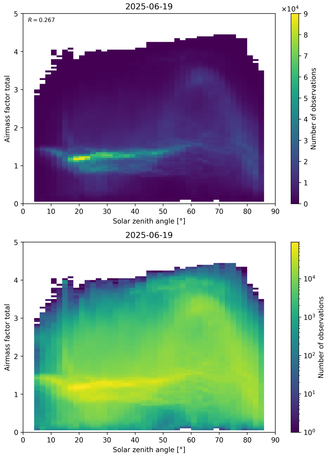
Figure 175: Scatter density plot of “Solar zenith angle” against “Airmass factor total” for 2025-06-18 to 2025-06-20.
