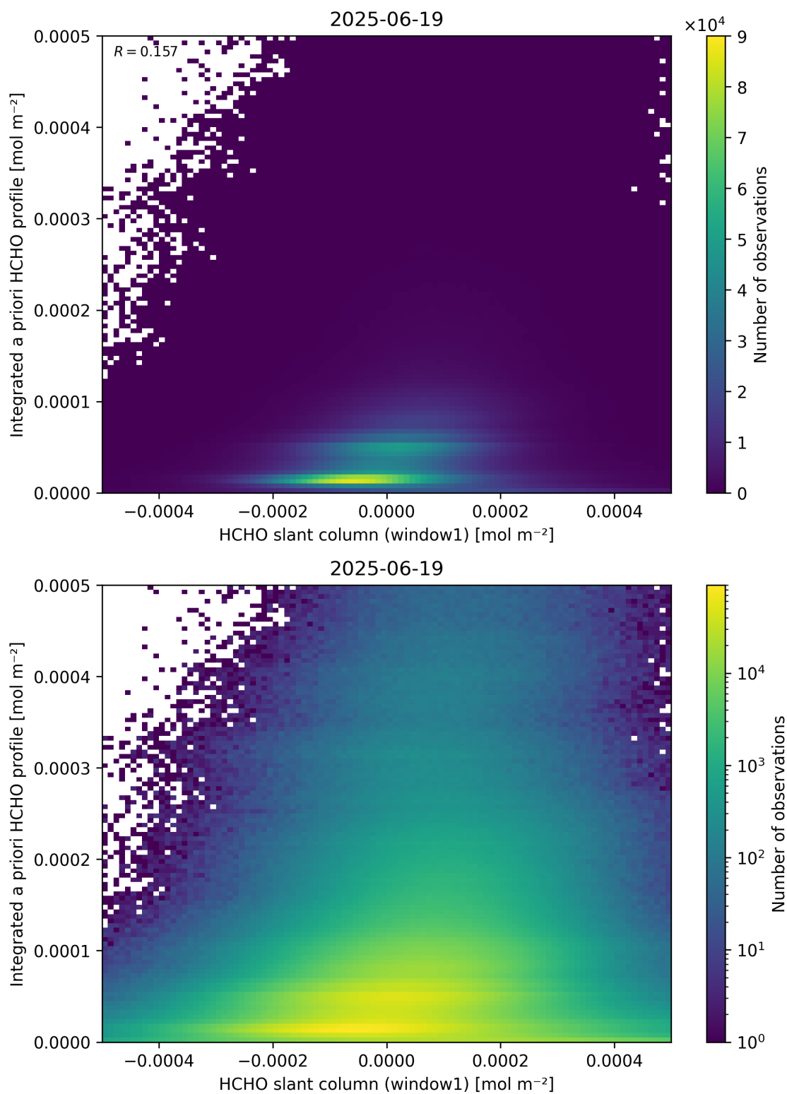
Figure 87: Scatter density plot of “HCHO slant column (window1)” against “Integrated a priori HCHO profile” for 2025-06-18 to 2025-06-20.
