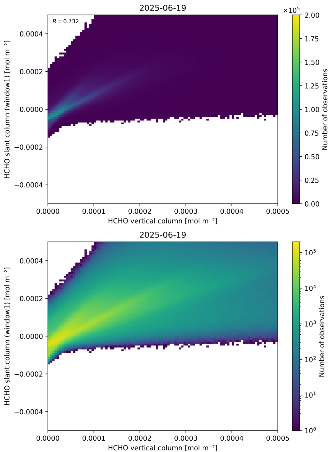
Figure 129: Scatter density plot of “HCHO vertical column” against “HCHO slant column (window1)” for 2025-06-18 to 2025-06-20.
