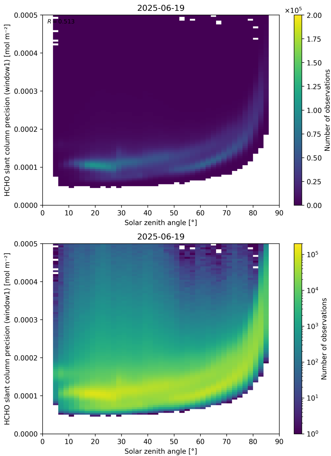
Figure 174: Scatter density plot of “Solar zenith angle” against “HCHO slant column precision (window1)” for 2025-06-18 to 2025-06-20.
