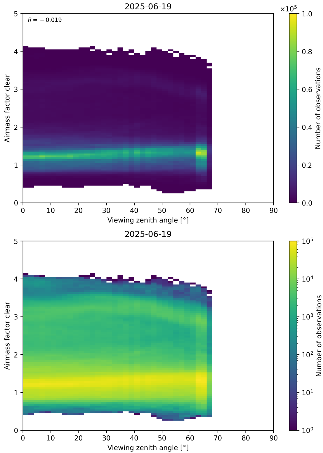
Figure 185: Scatter density plot of “Viewing zenith angle” against “Airmass factor clear” for 2025-06-18 to 2025-06-20.
