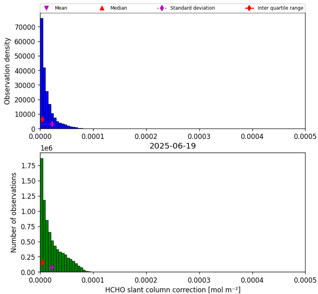
Figure 47: Histogram of “HCHO slant column correction” for 2025-06-18 to 2025-06-20
