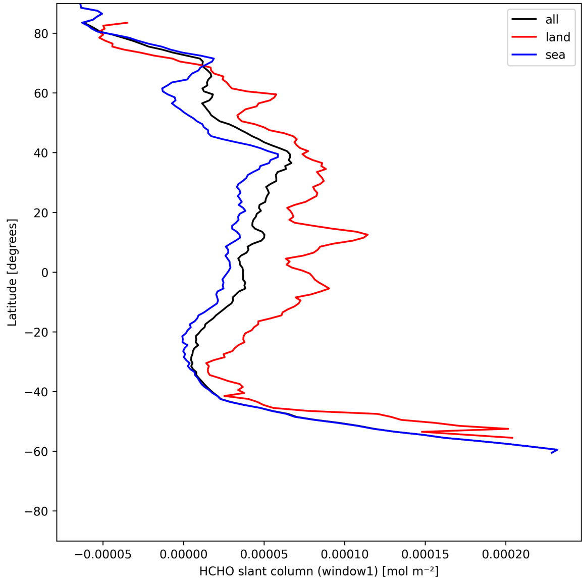
Figure 24: Zonal average of “HCHO slant column (window1)” for 2025-06-18 to 2025-06-20.
