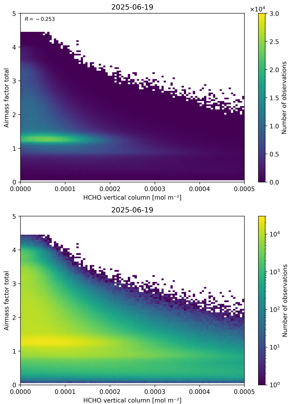
Figure 131: Scatter density plot of “HCHO vertical column” against “Airmass factor total” for 2025-06-18 to 2025-06-20.
