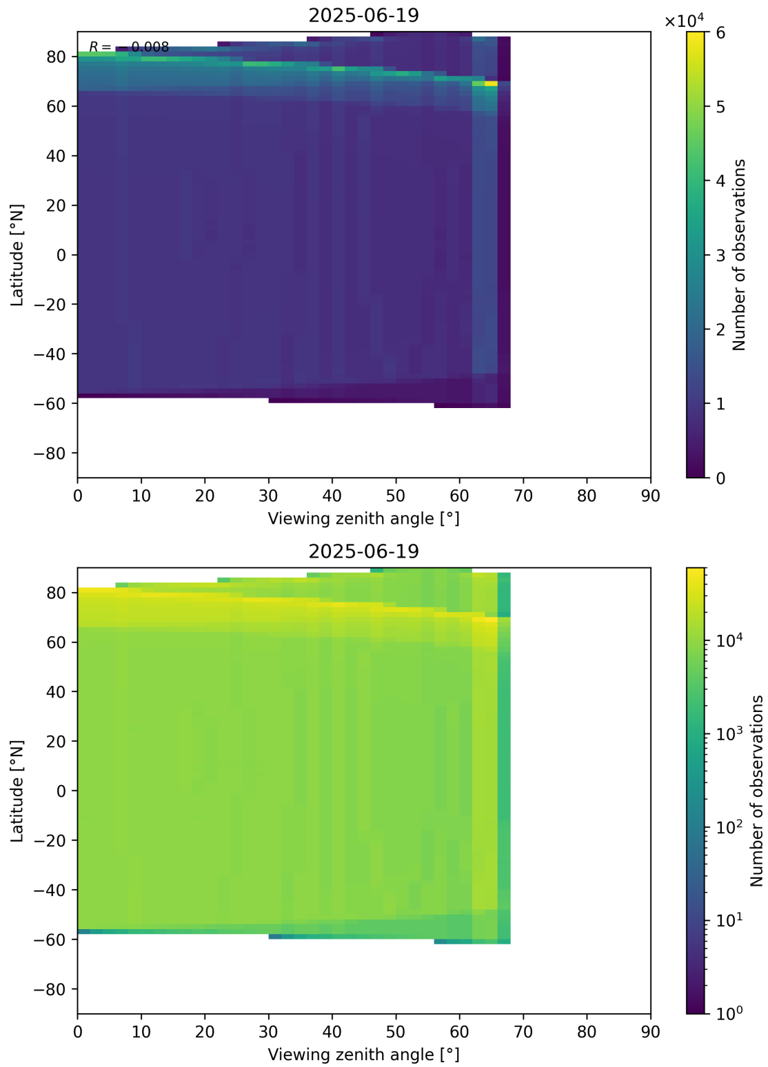
Figure 196: Scatter density plot of “Viewing zenith angle” against “Latitude” for 2025-06-18 to 2025-06-20.
