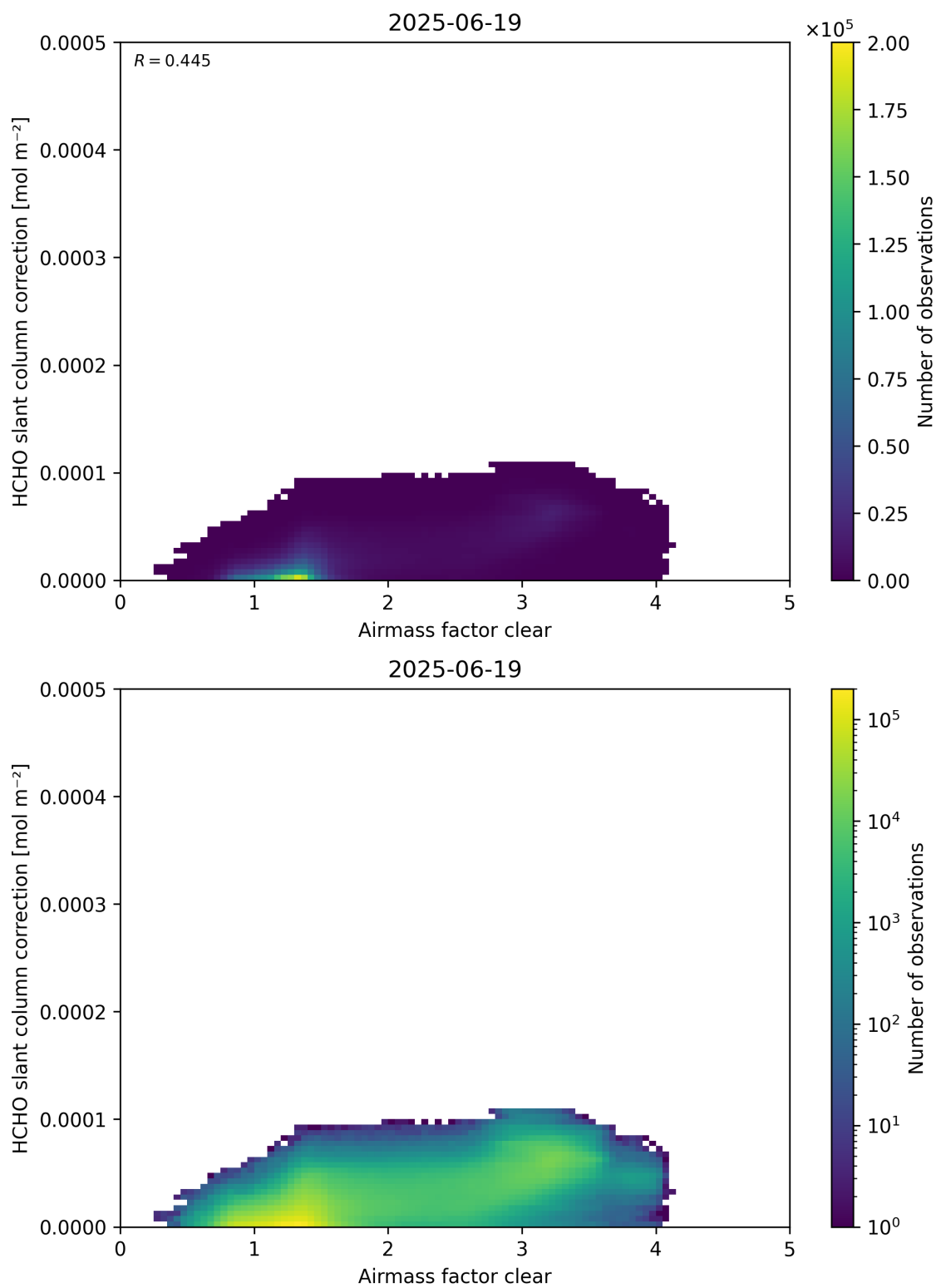
Figure 75: Scatter density plot of “Airmass factor clear” against “HCHO slant column correction” for 2025-06-18 to 2025-06-20.
