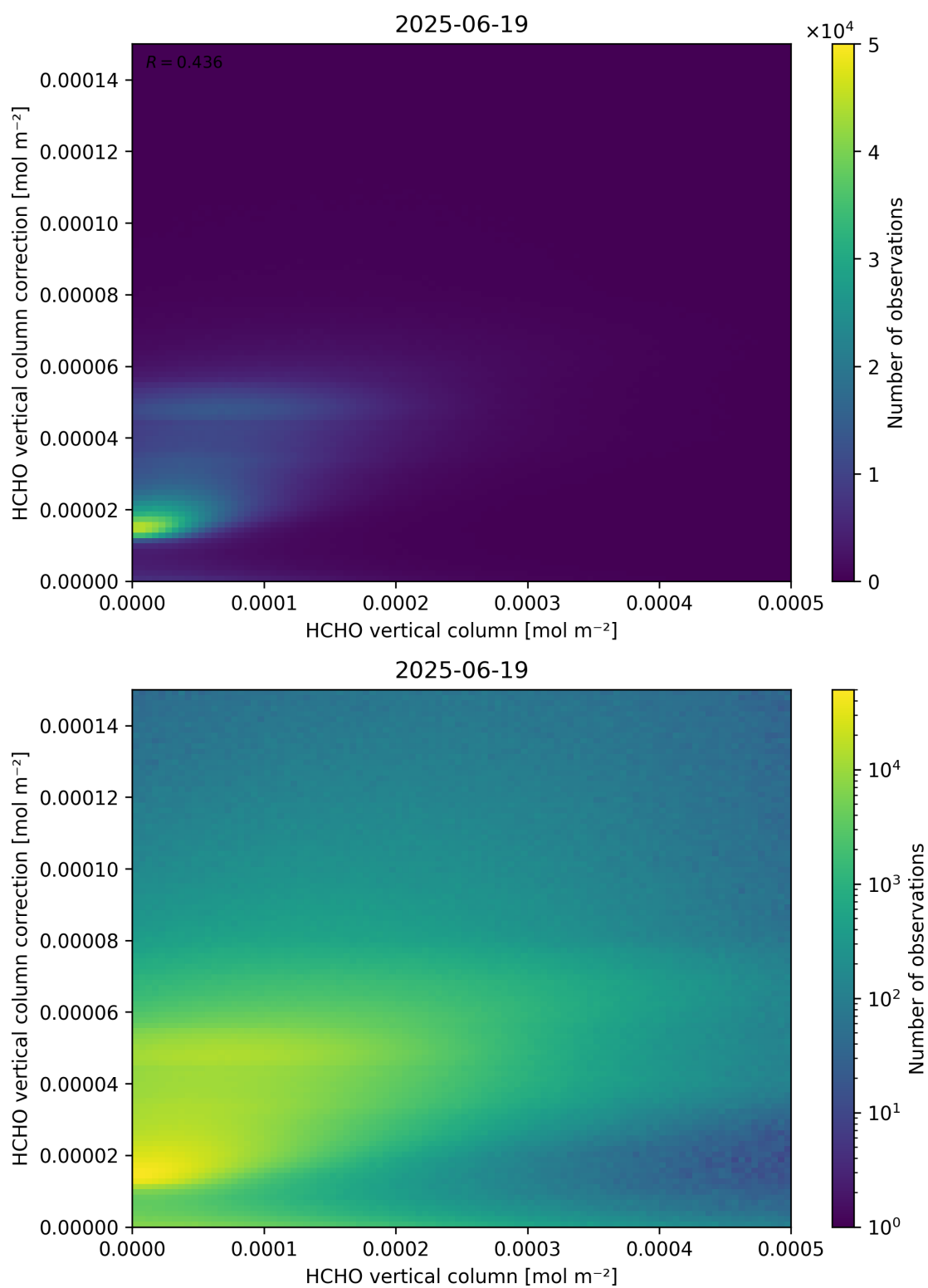
Figure 133: Scatter density plot of “HCHO vertical column” against “HCHO vertical column correction” for 2025-06-18 to 2025-06-20.
