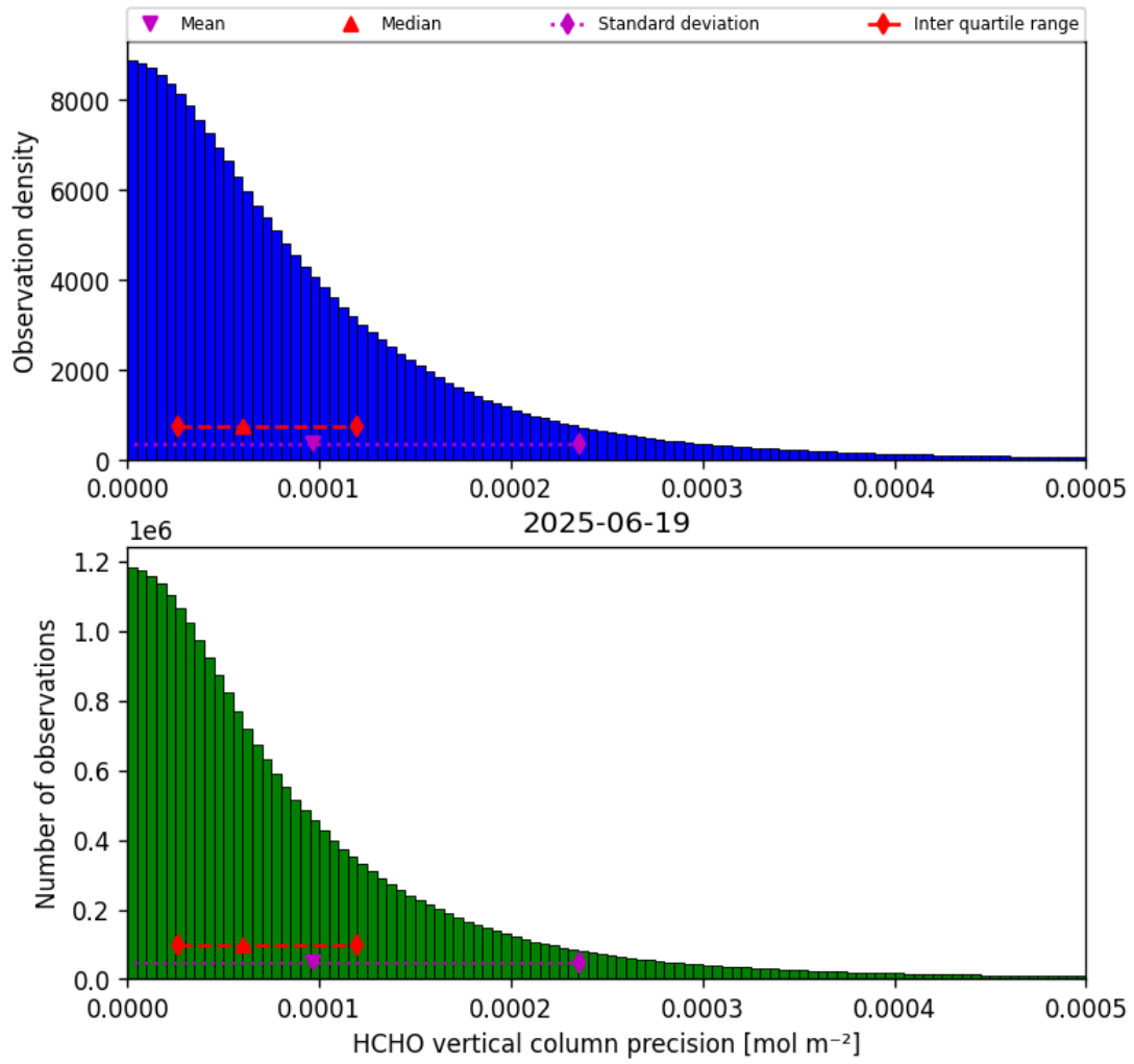
Figure 36: Histogram of “HCHO vertical column precision” for 2025-06-18 to 2025-06-20
