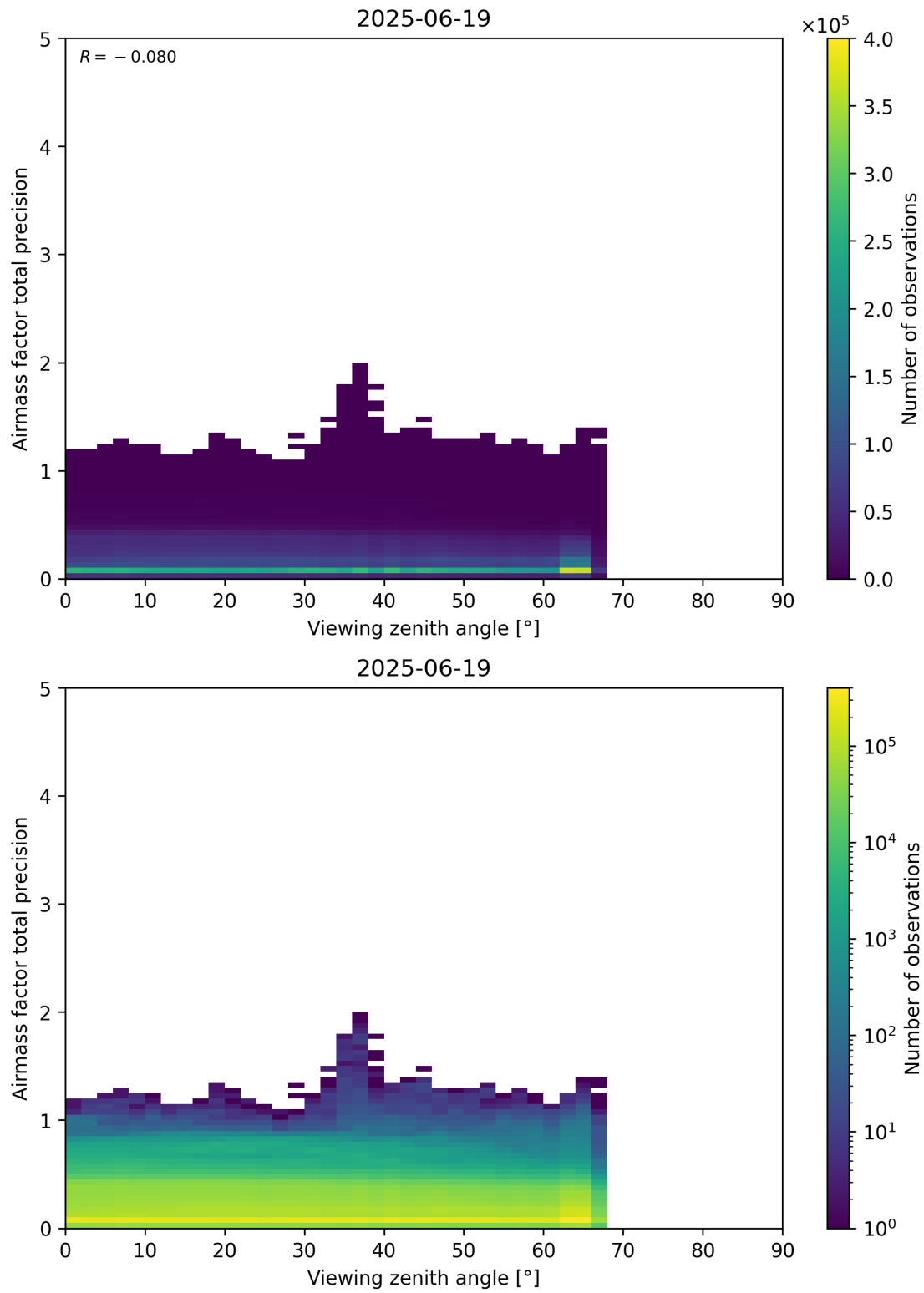
Figure 191: Scatter density plot of “Viewing zenith angle” against “Airmass factor total precision” for 2025-06-18 to 2025-06-20.
