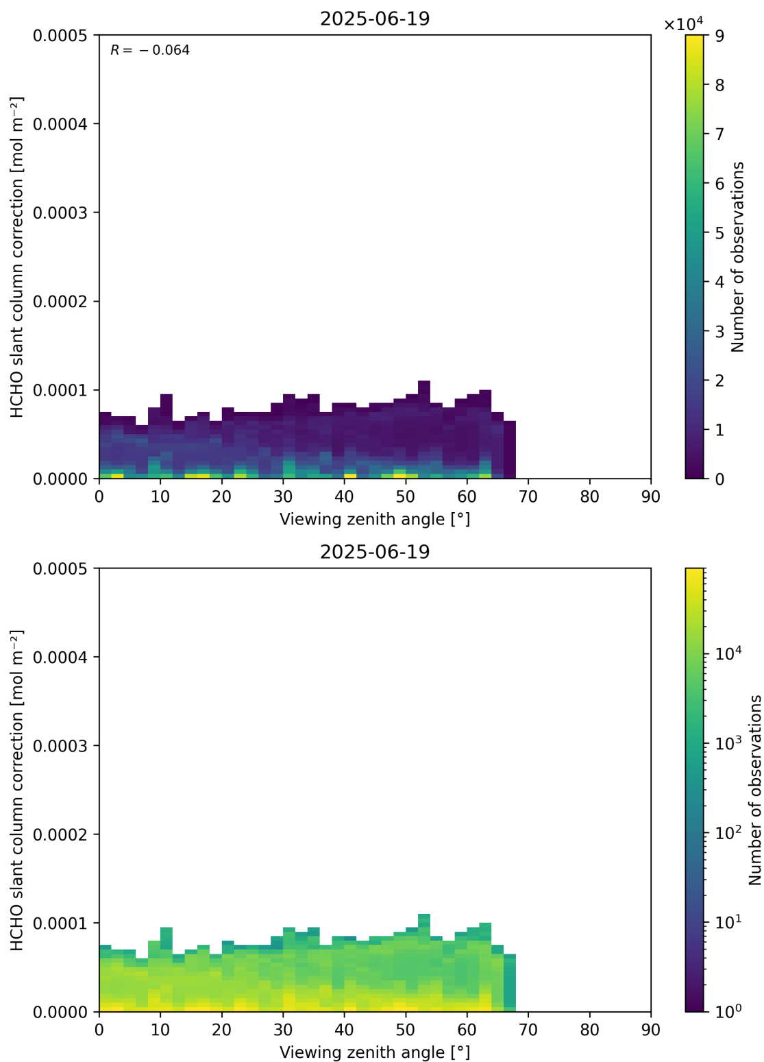
Figure 187: Scatter density plot of “Viewing zenith angle” against “HCHO slant column correction” for 2025-06-18 to 2025-06-20.
