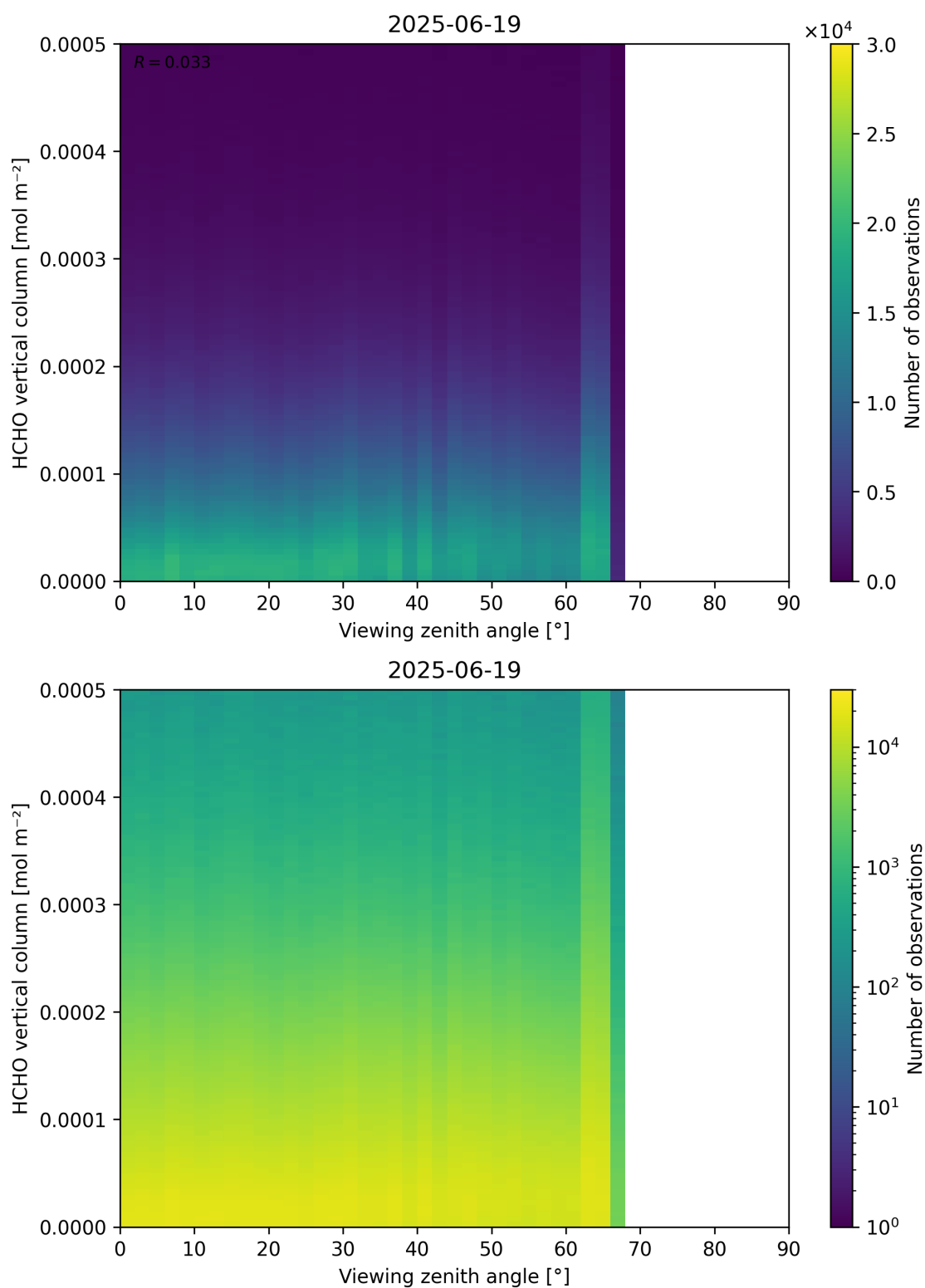
Figure 192: Scatter density plot of “Viewing zenith angle” against “HCHO vertical column” for 2025-06-18 to 2025-06-20.
