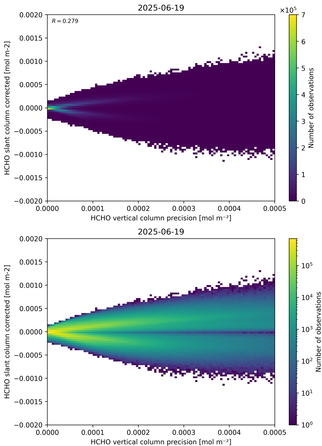
Figure 140: Scatter density plot of “HCHO vertical column precision” against “HCHO slant column corrected” for 2025-06-18 to 2025-06-20.
