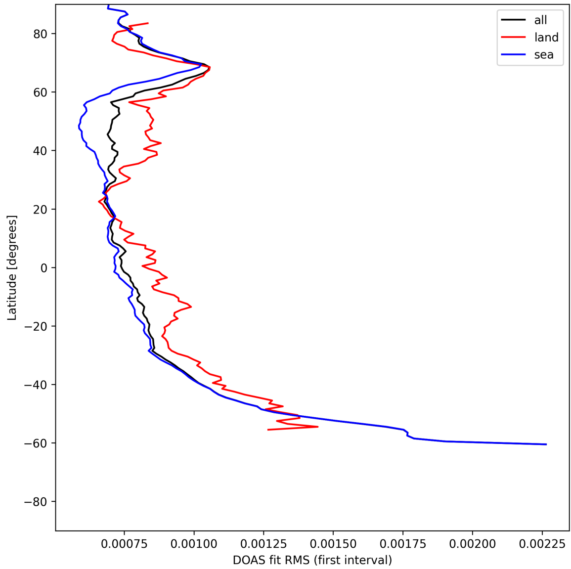
Figure 32: Zonal average of “DOAS fit RMS (first interval)” for 2025-06-18 to 2025-06-20.
