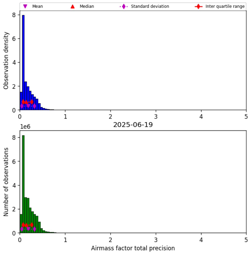
Figure 41: Histogram of “Airmass factor total precision” for 2025-06-18 to 2025-06-20
