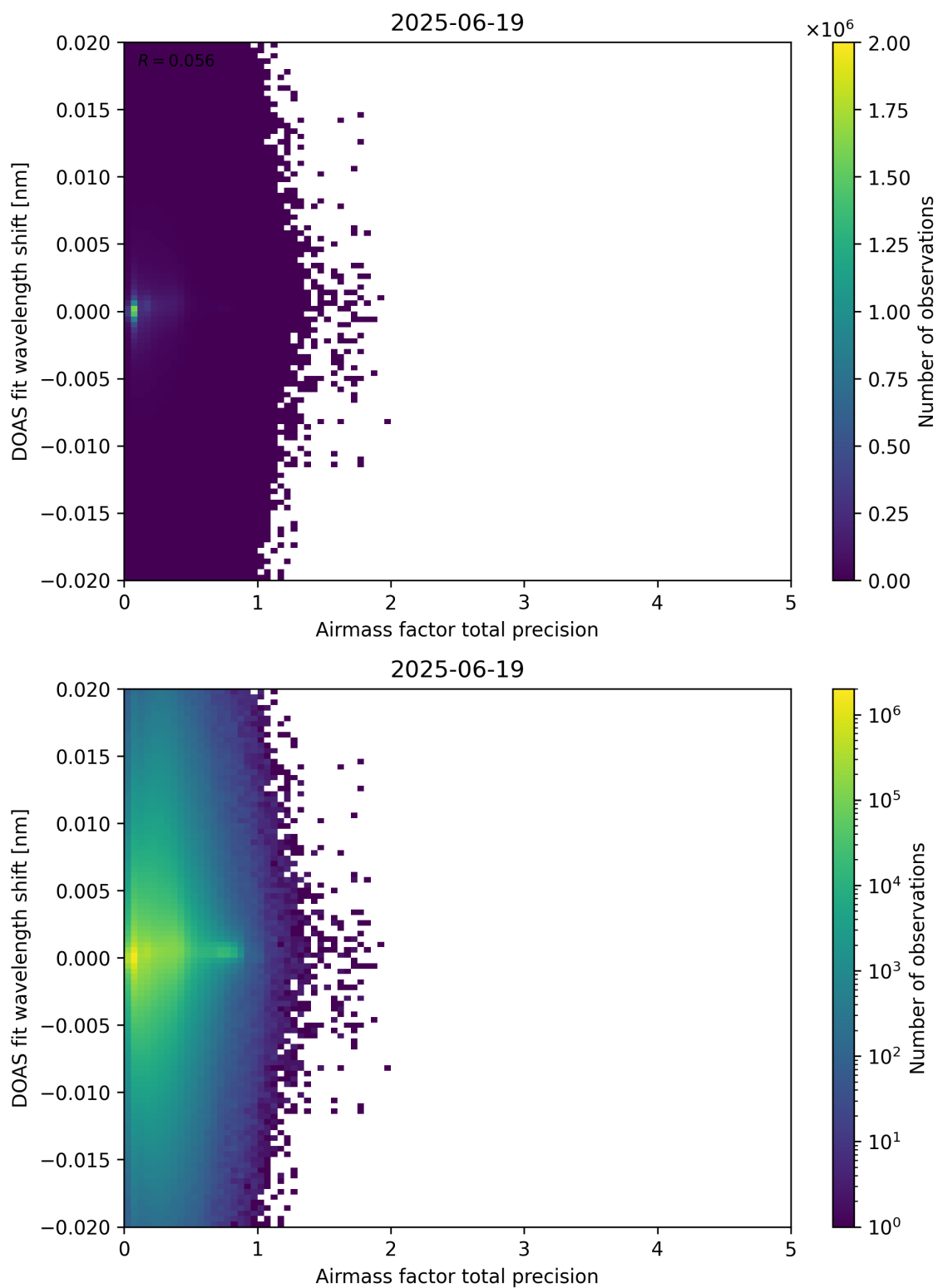
Figure 106: Scatter density plot of “Airmass factor total precision” against “DOAS fit wavelength shift” for 2025-06-18 to 2025-06-20.
