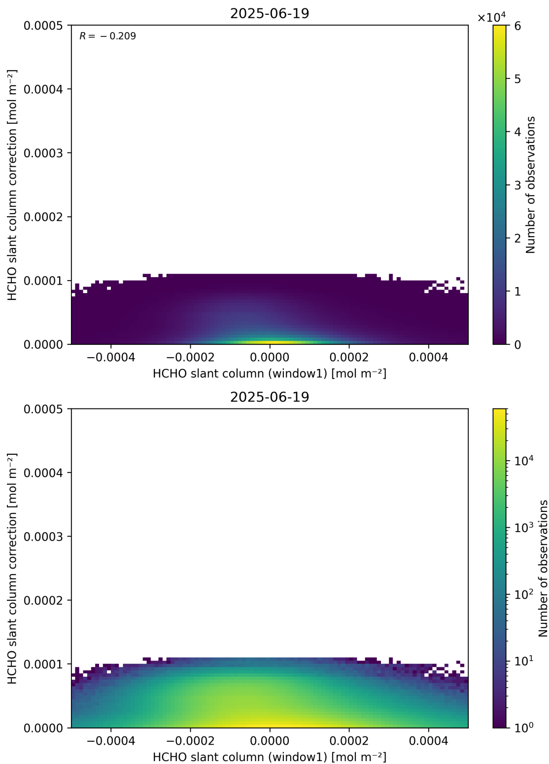
Figure 83: Scatter density plot of “HCHO slant column (window1)” against “HCHO slant column correction” for 2025-06-18 to 2025-06-20.
