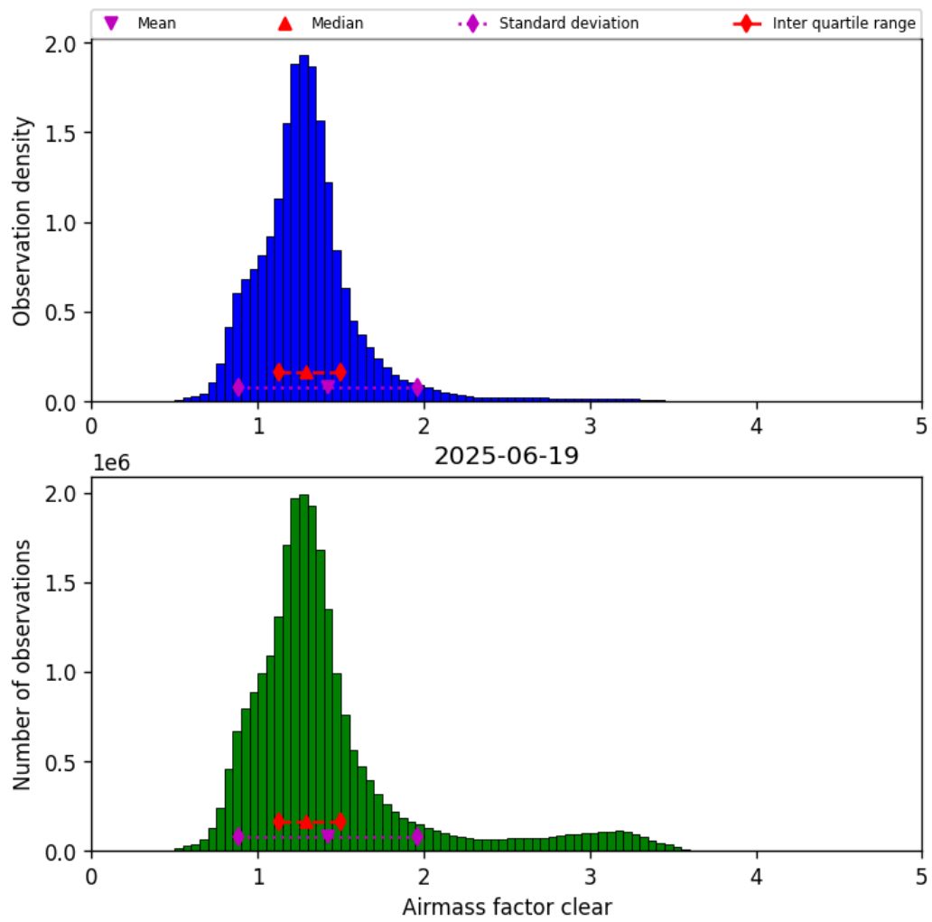
Figure 42: Histogram of “Airmass factor clear” for 2025-06-18 to 2025-06-20
