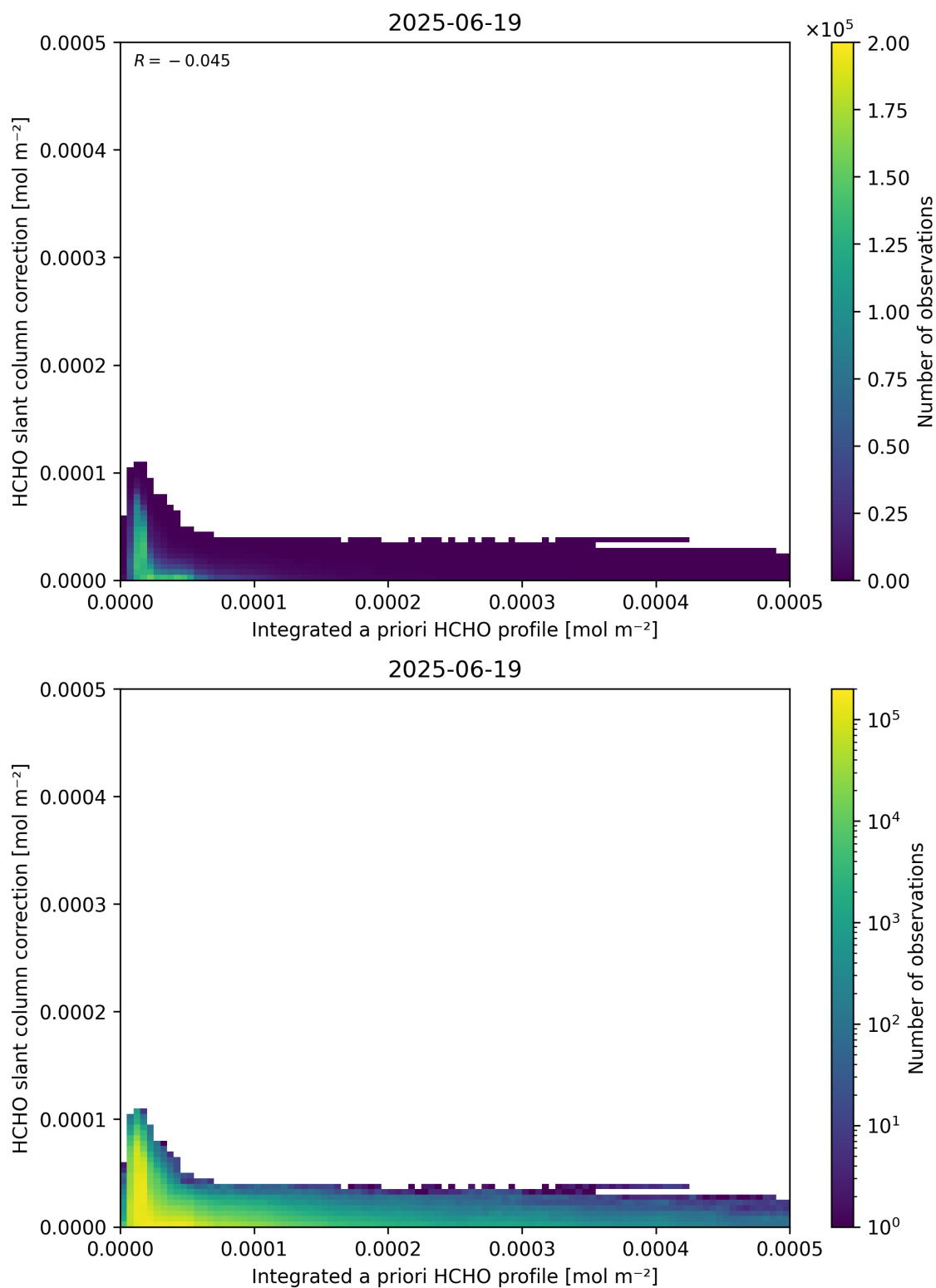
Figure 152: Scatter density plot of “Integrated a priori HCHO profile” against “HCHO slant column correction” for 2025-06-18 to 2025-06-20.
