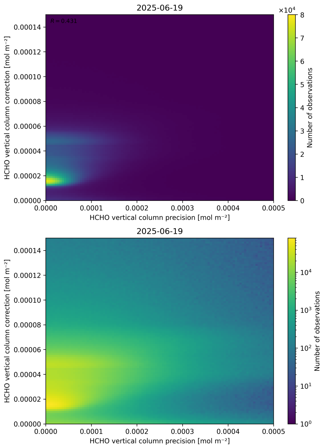
Figure 146: Scatter density plot of “HCHO vertical column precision” against “HCHO vertical column correction” for 2025-06-18 to 2025-06-20.
