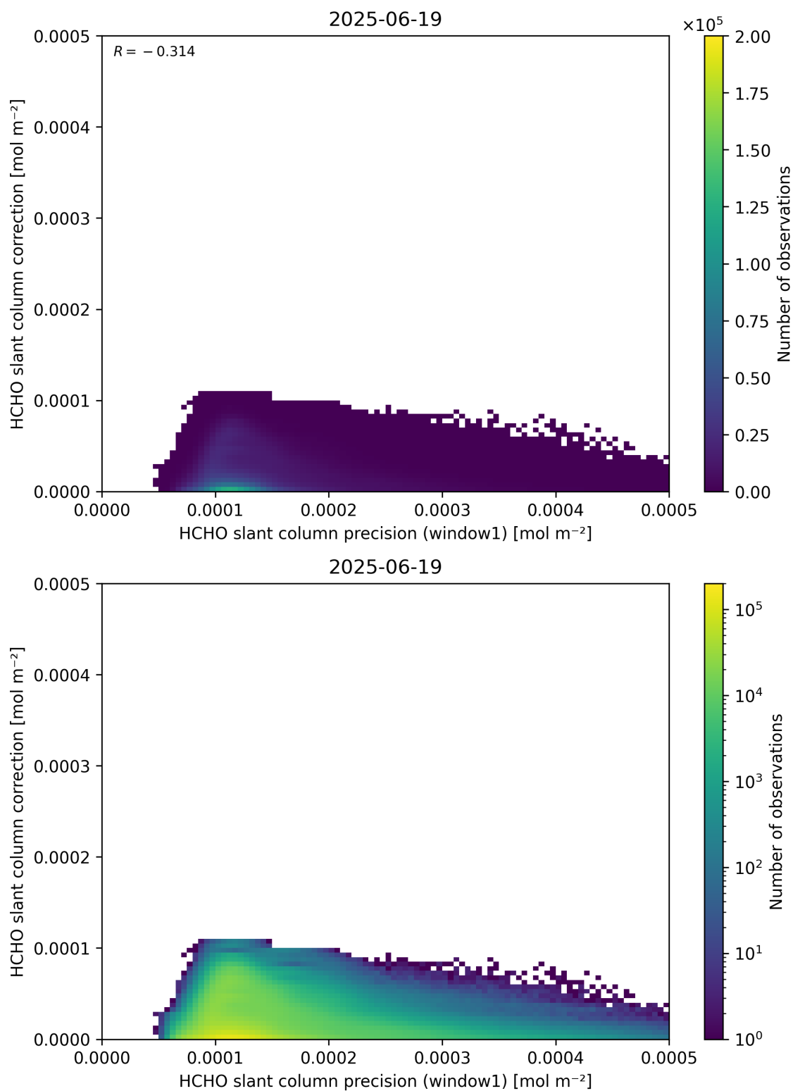
Figure 93: Scatter density plot of “HCHO slant column precision (window1)” against “HCHO slant column correction” for 2025-06-18 to 2025-06-20.
