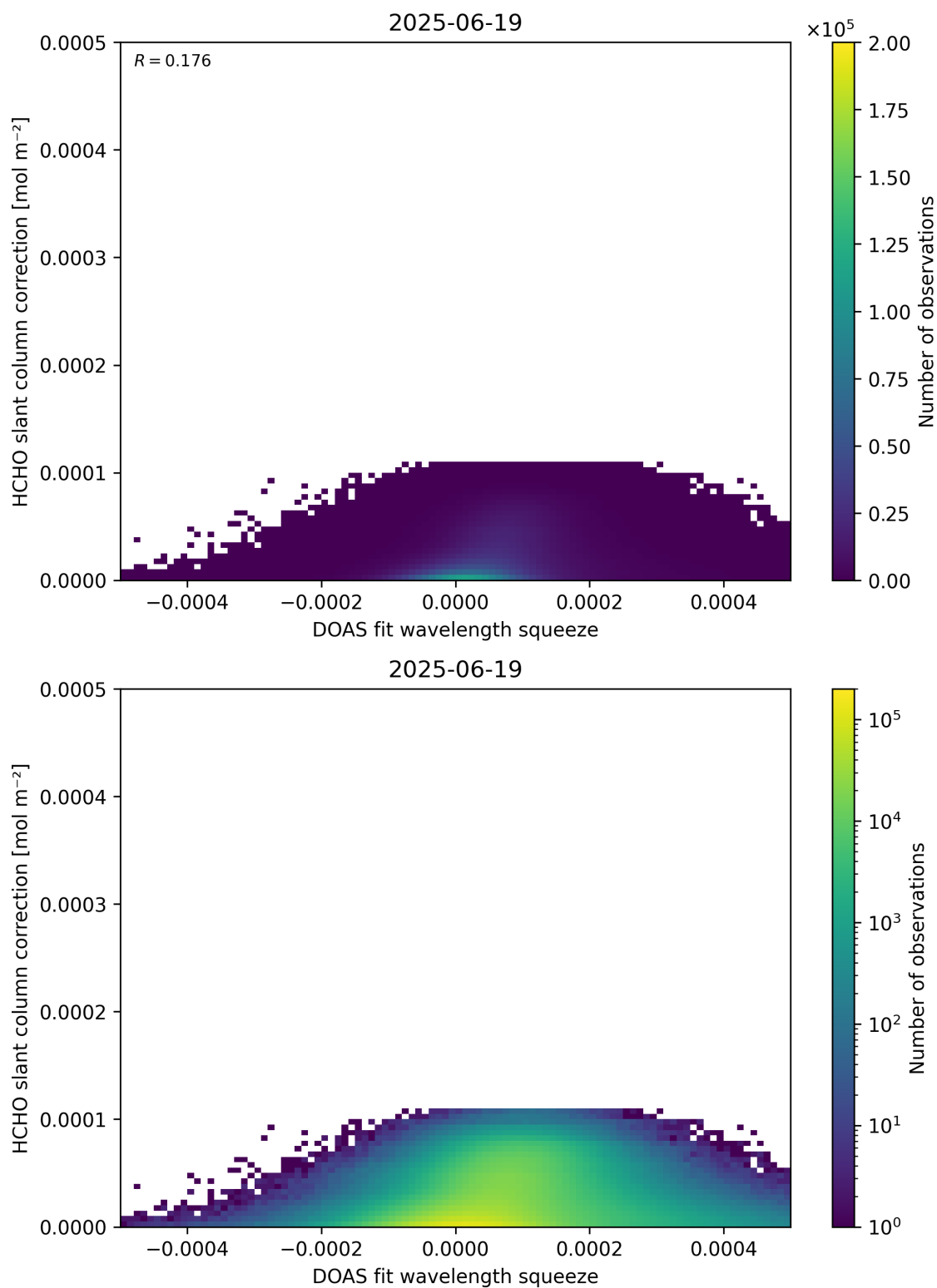
Figure 70: Scatter density plot of “DOAS fit wavelength squeeze” against “HCHO slant column correction” for 2025-06-18 to 2025-06-20.
