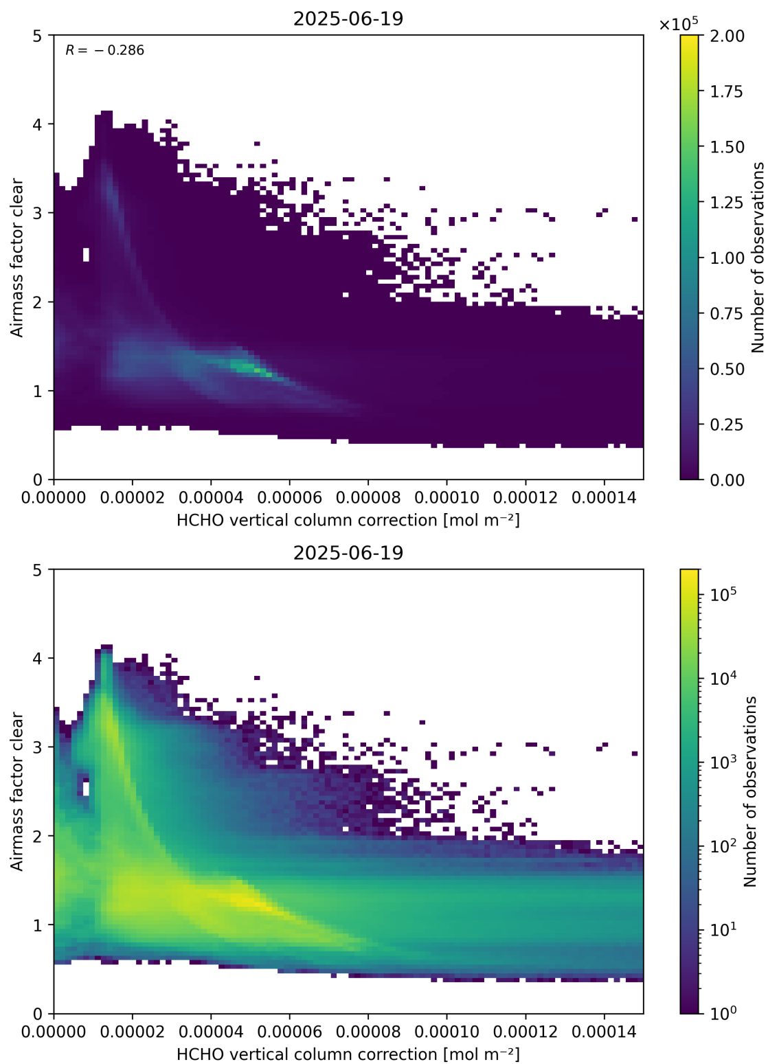
Figure 115: Scatter density plot of “HCHO vertical column correction” against “Airmass factor clear” for 2025-06-18 to 2025-06-20.
