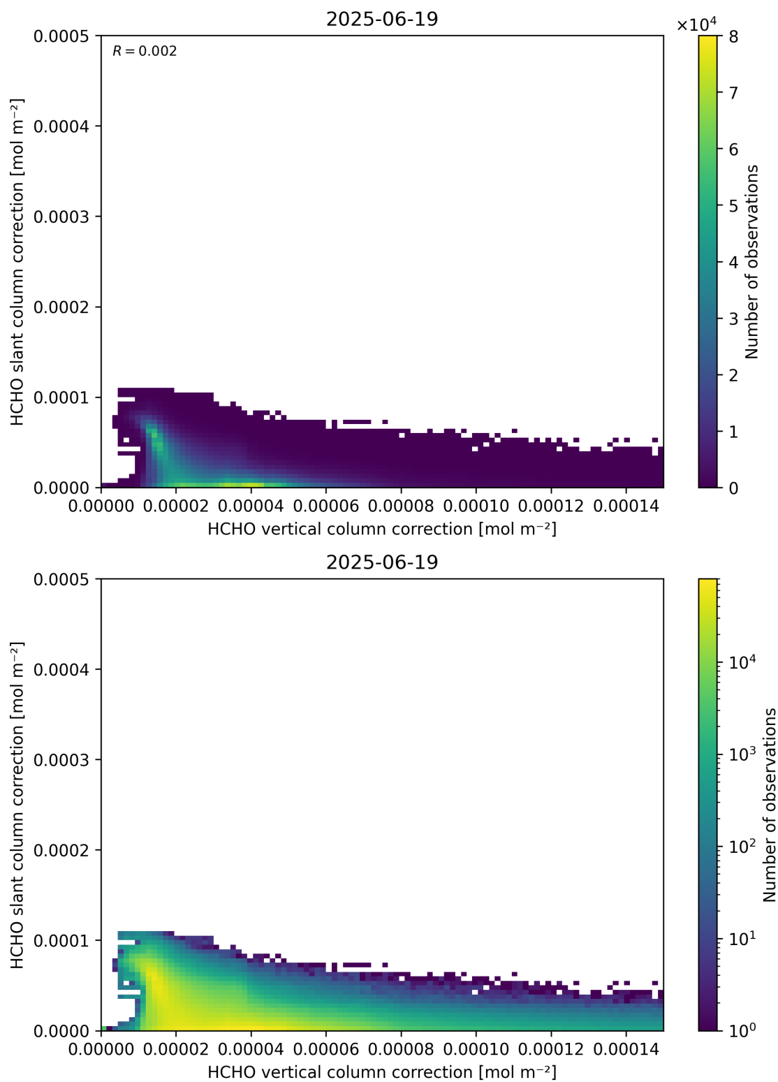
Figure 117: Scatter density plot of “HCHO vertical column correction” against “HCHO slant column correction” for 2025-06-18 to 2025-06-20.
