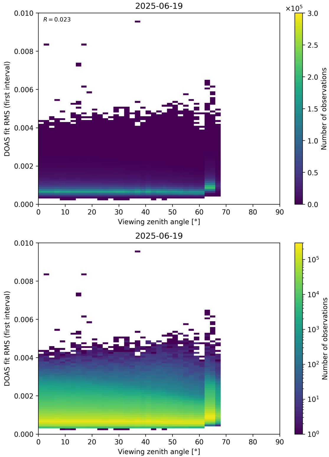
Figure 182: Scatter density plot of “Viewing zenith angle” against “DOAS fit RMS (first interval)” for 2025-06-18 to 2025-06-20.
