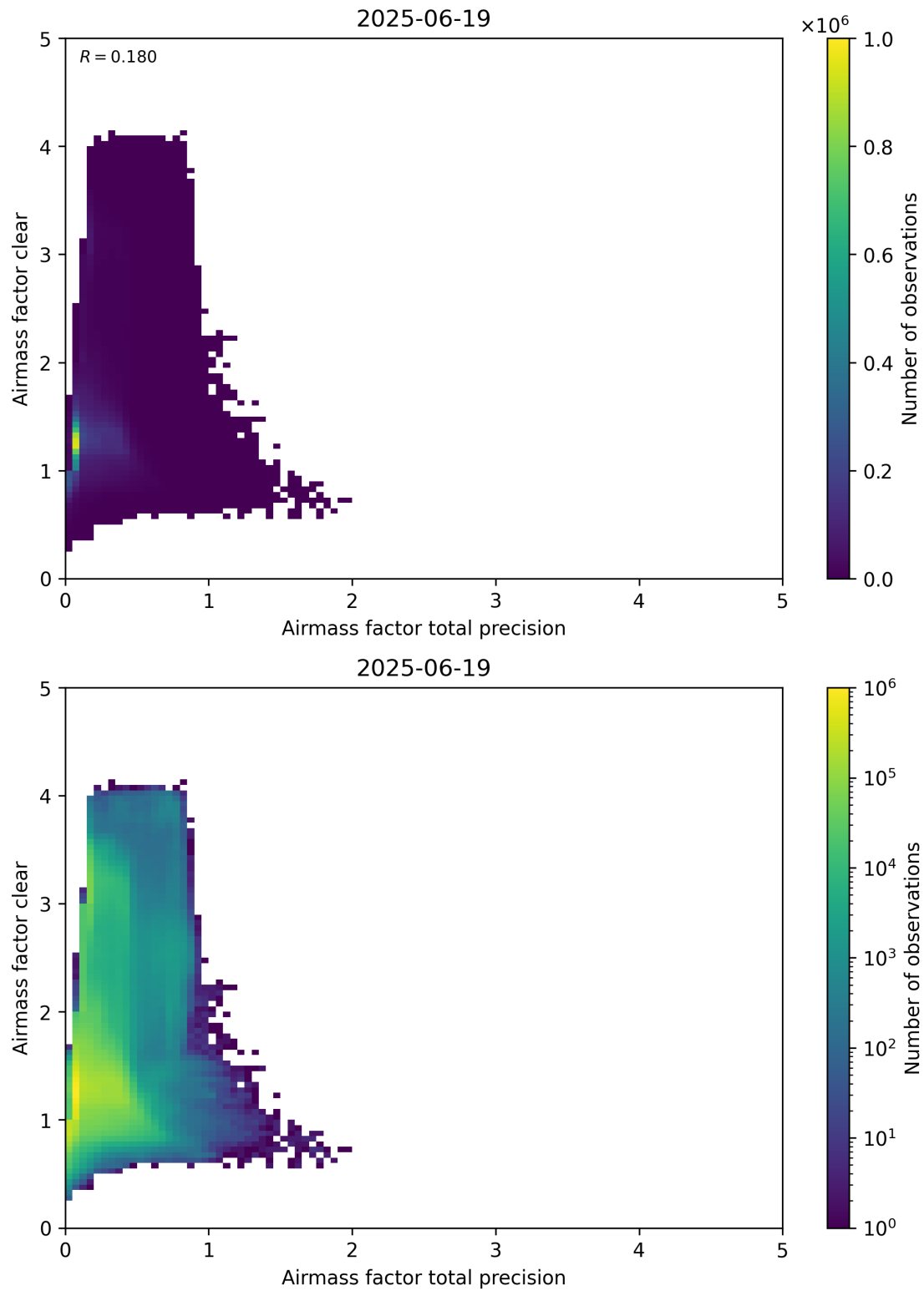
Figure 108: Scatter density plot of “Airmass factor total precision” against “Airmass factor clear” for 2025-06-18 to 2025-06-20.
