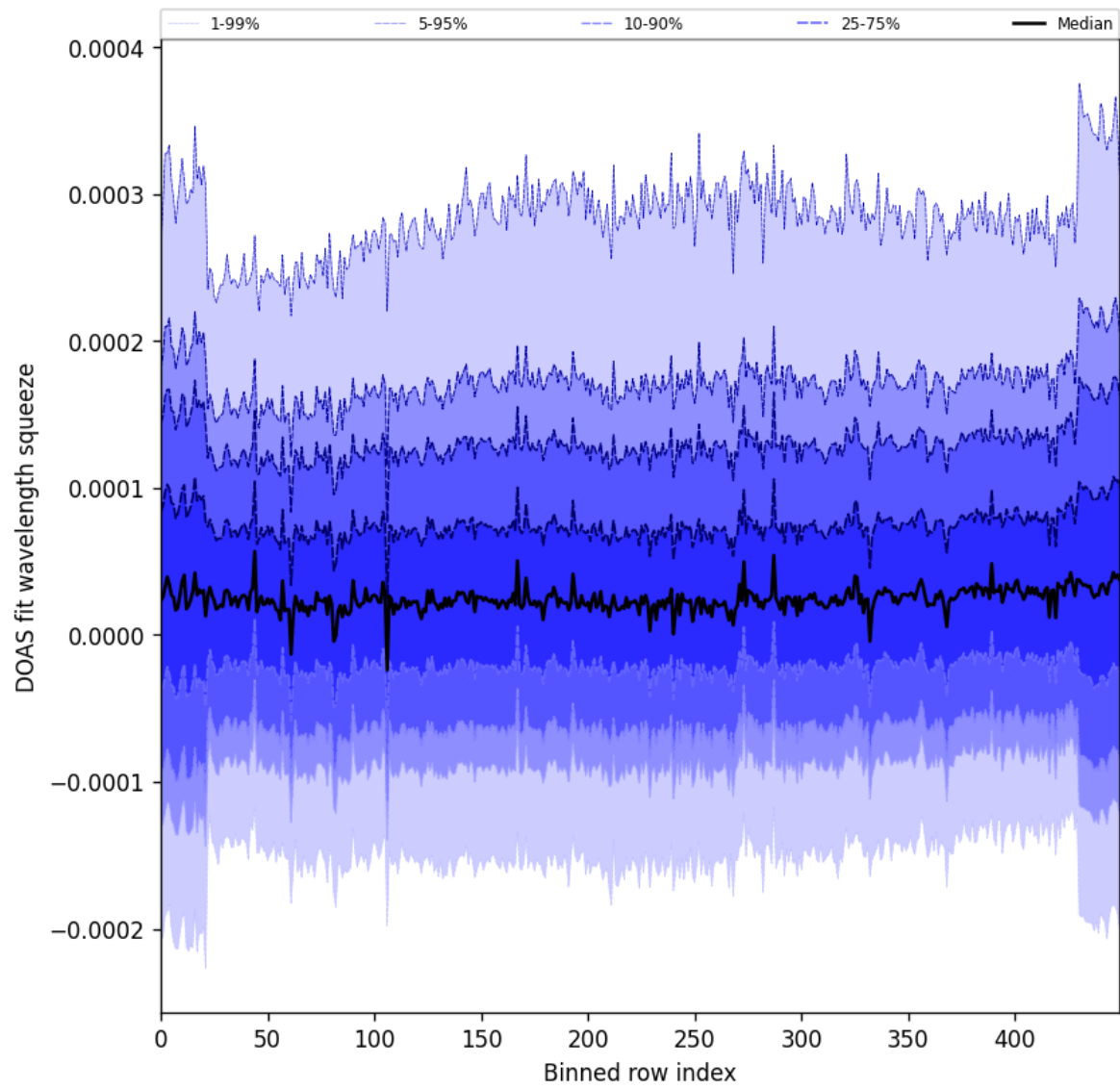
Figure 59: Along track statistics of “DOAS fit wavelength squeeze” for 2025-06-18 to 2025-06-20
