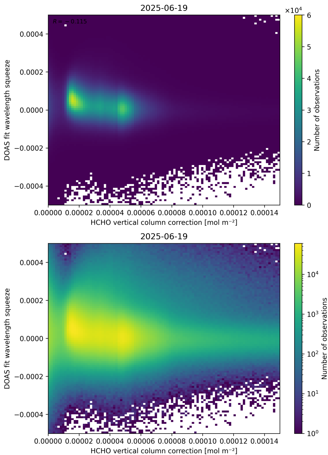
Figure 114: Scatter density plot of “HCHO vertical column correction” against “DOAS fit wavelength squeeze” for 2025-06-18 to 2025-06-20.
