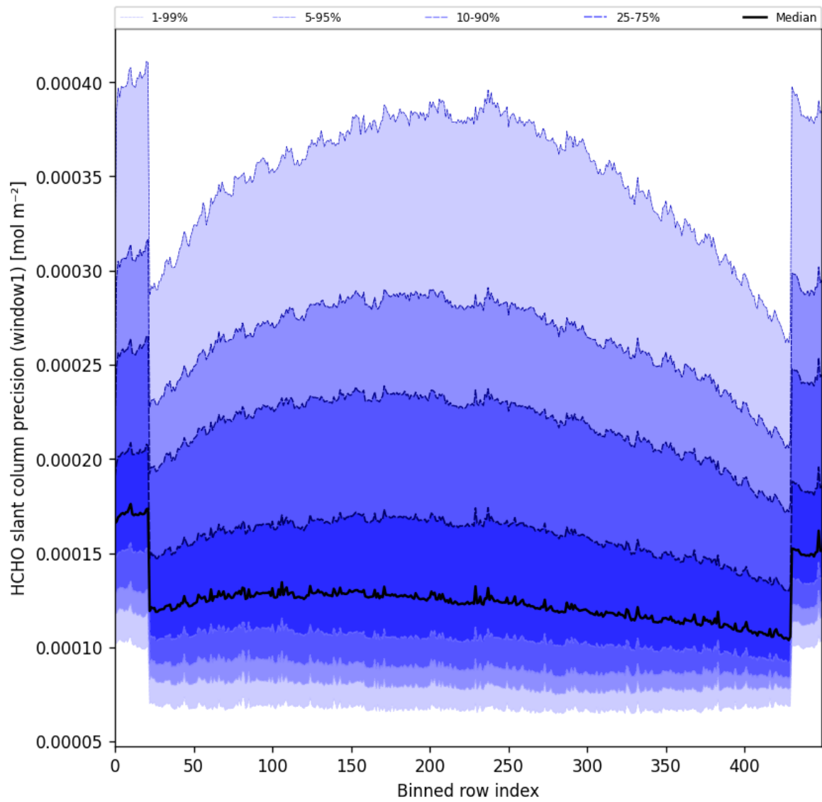
Figure 53: Along track statistics of “HCHO slant column precision (window1)” for 2025-06-18 to 2025-06-20
