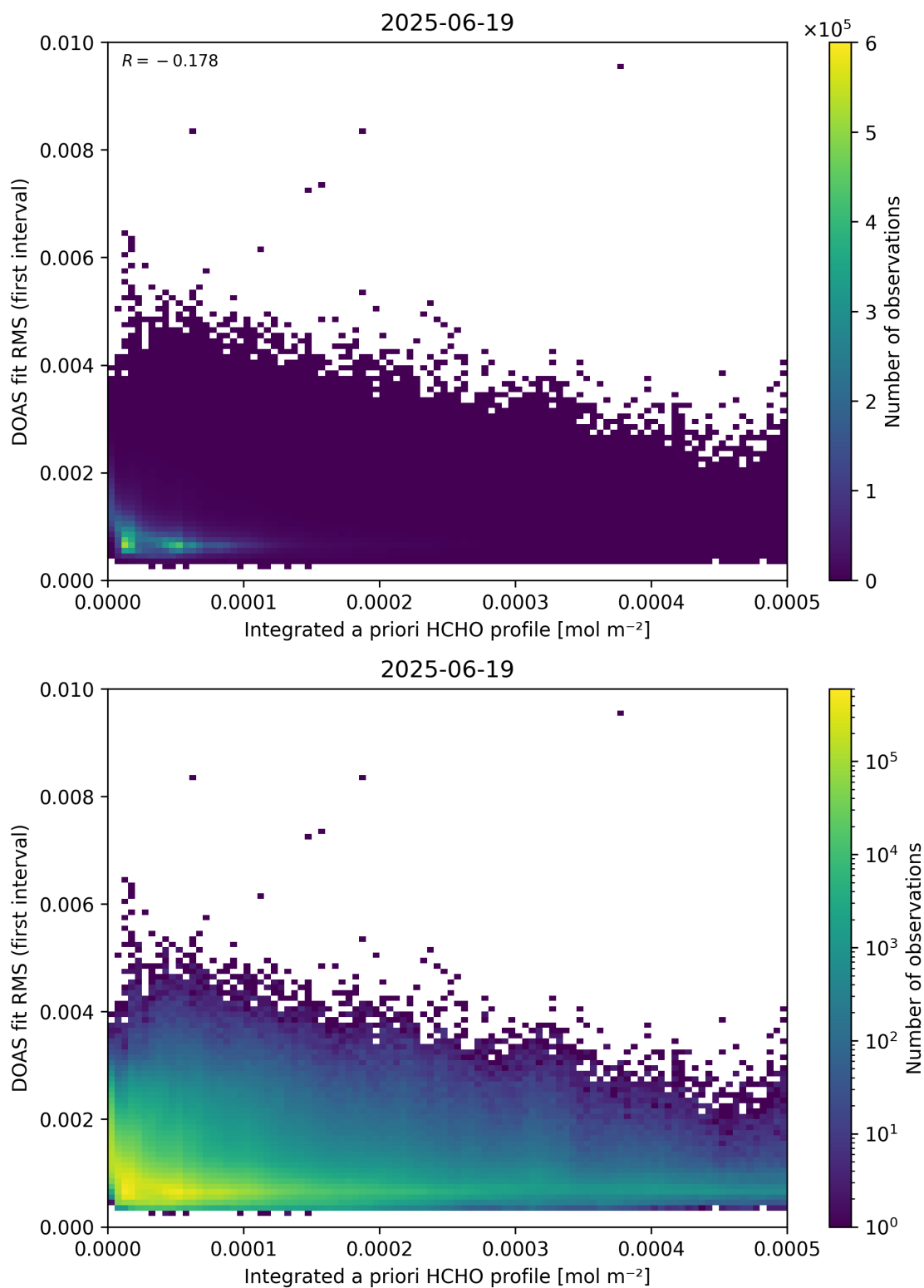
Figure 148: Scatter density plot of “Integrated a priori HCHO profile” against “DOAS fit RMS (first interval)” for 2025-06-18 to 2025-06-20.
