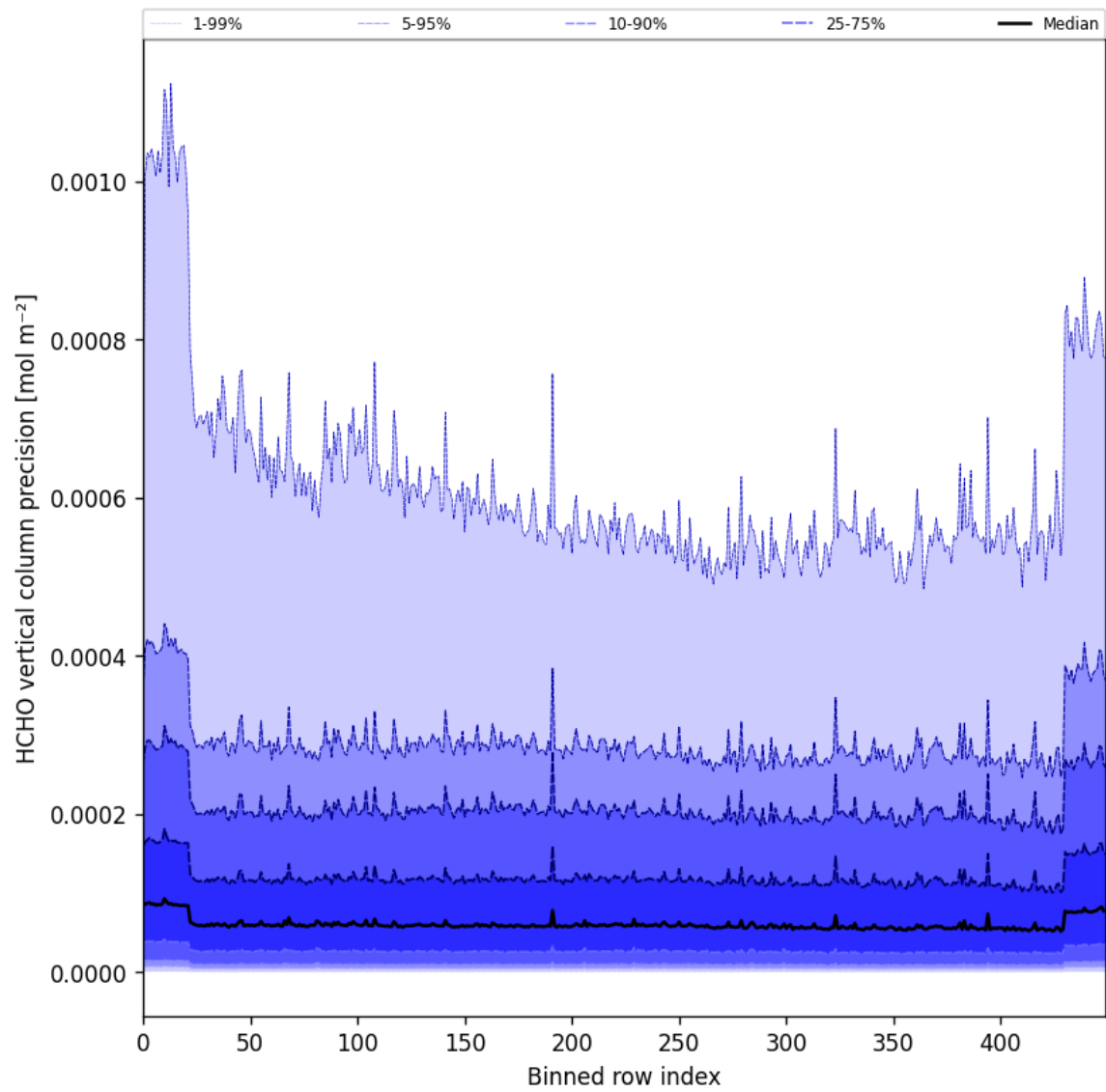
Figure 50: Along track statistics of “HCHO vertical column precision” for 2025-06-18 to 2025-06-20
