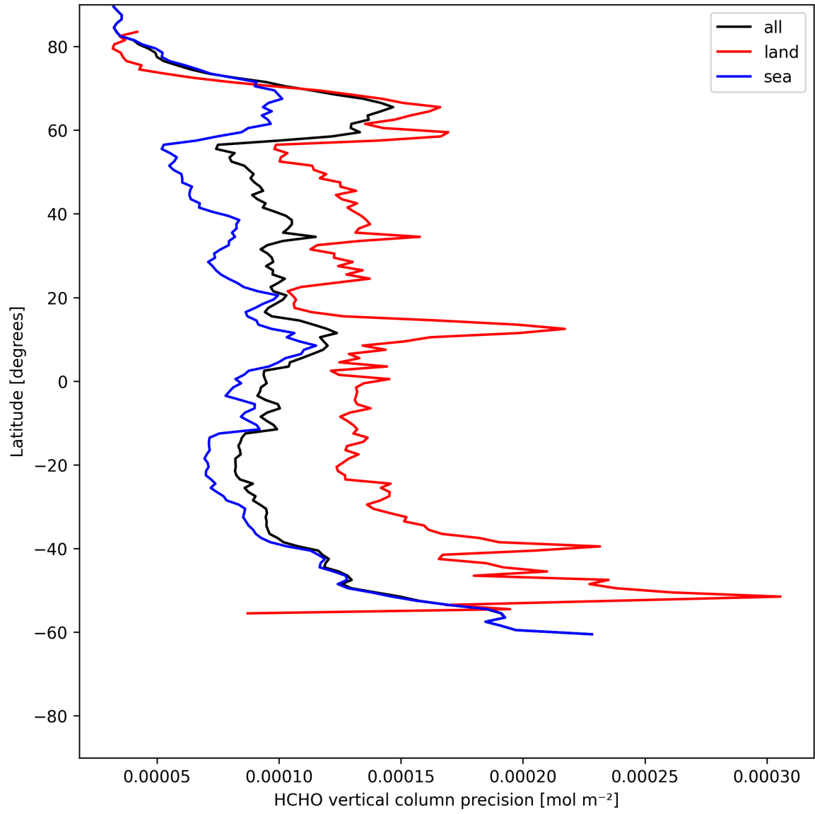
Figure 22: Zonal average of “HCHO vertical column precision” for 2025-06-18 to 2025-06-20.
