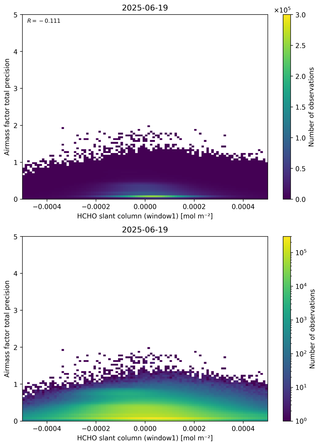
Figure 86: Scatter density plot of “HCHO slant column (window1)” against “Airmass factor total precision” for 2025-06-18 to 2025-06-20.
