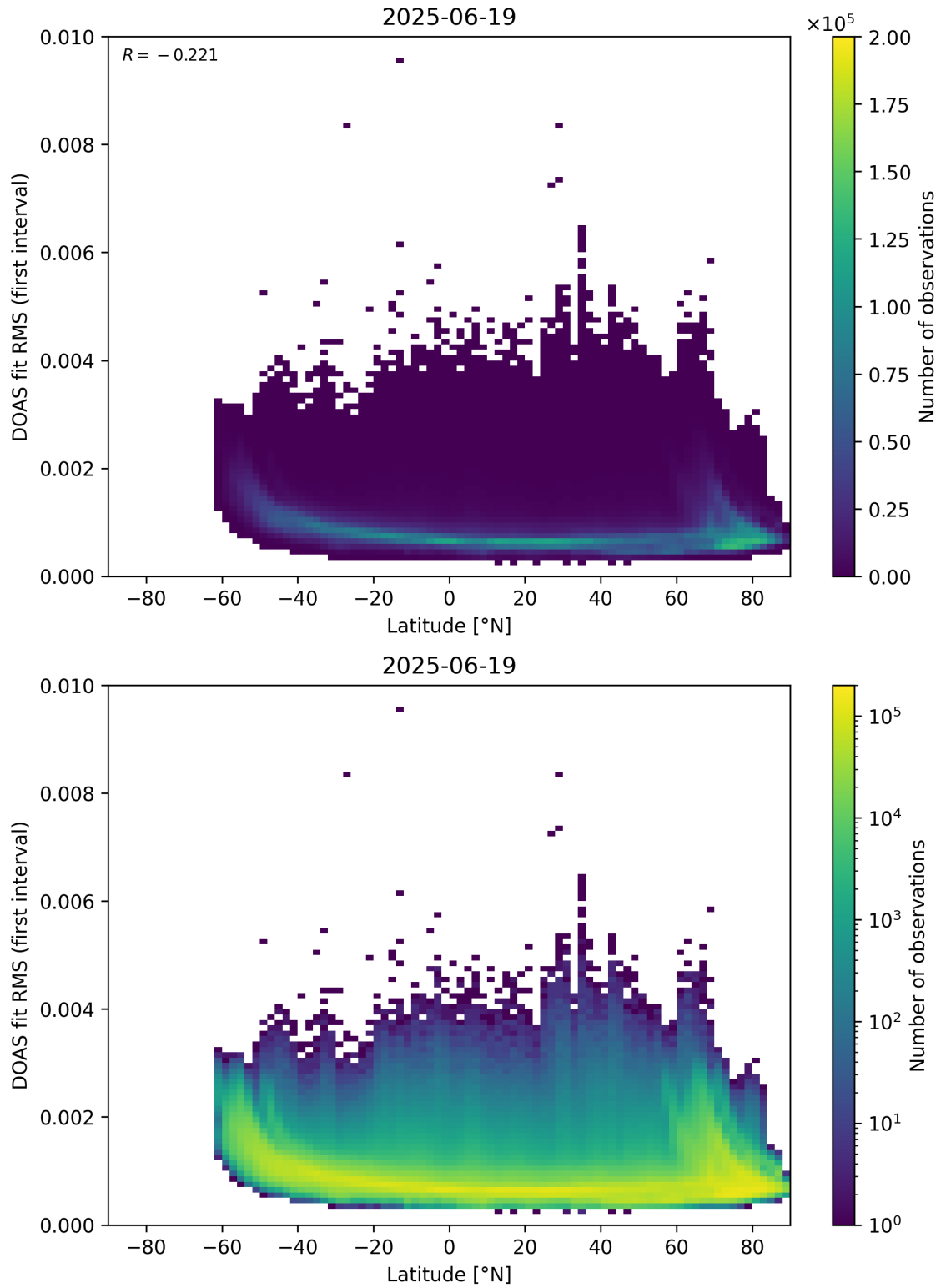
Figure 153: Scatter density plot of “Latitude” against “DOAS fit RMS (first interval)” for 2025-06-18 to 2025-06-20.
