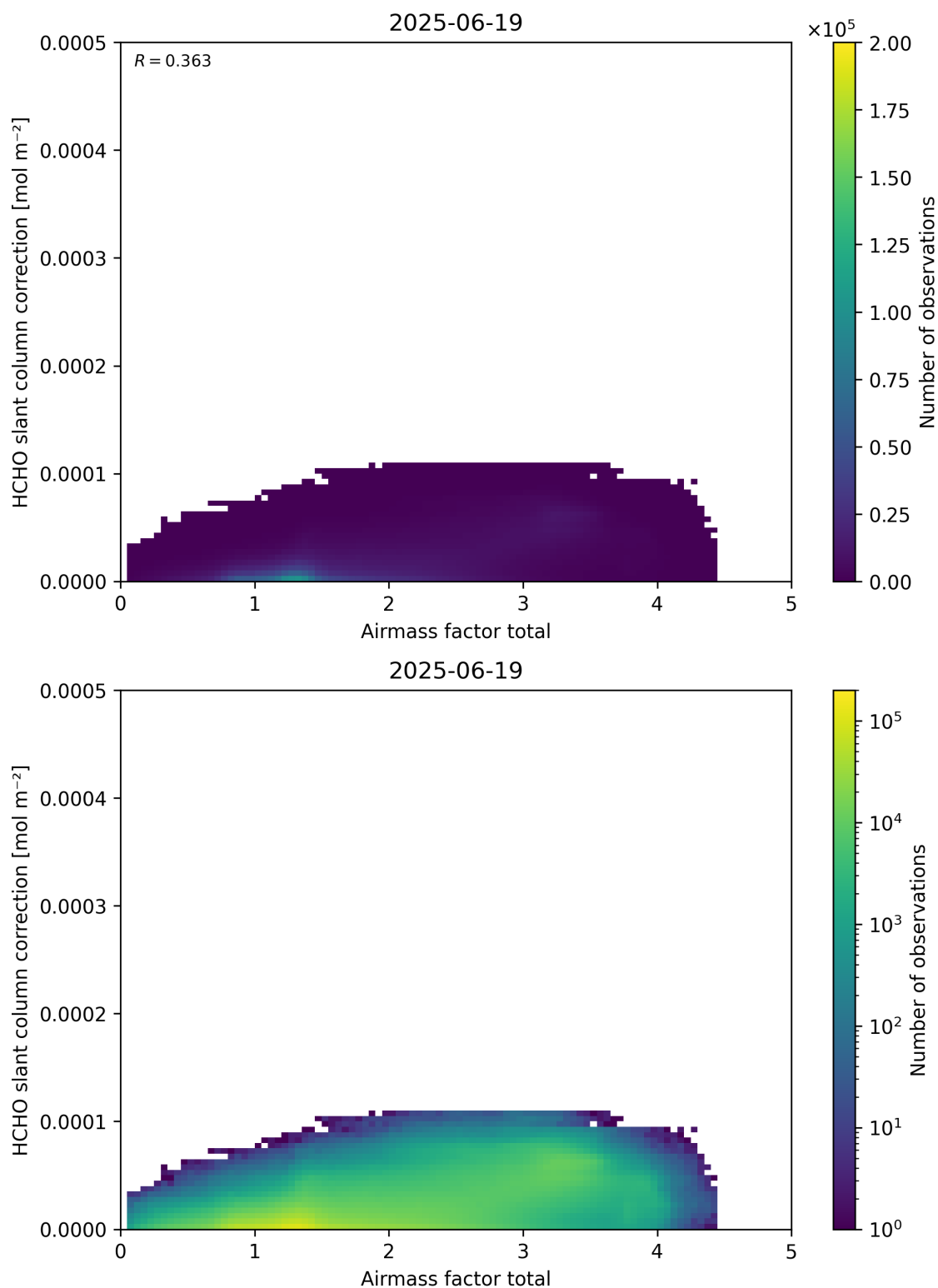
Figure 102: Scatter density plot of “Airmass factor total” against “HCHO slant column correction” for 2025-06-18 to 2025-06-20.
