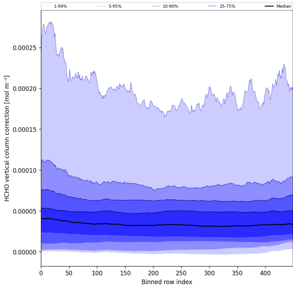
Figure 51: Along track statistics of “HCHO vertical column correction” for 2025-06-18 to 2025-06-20
