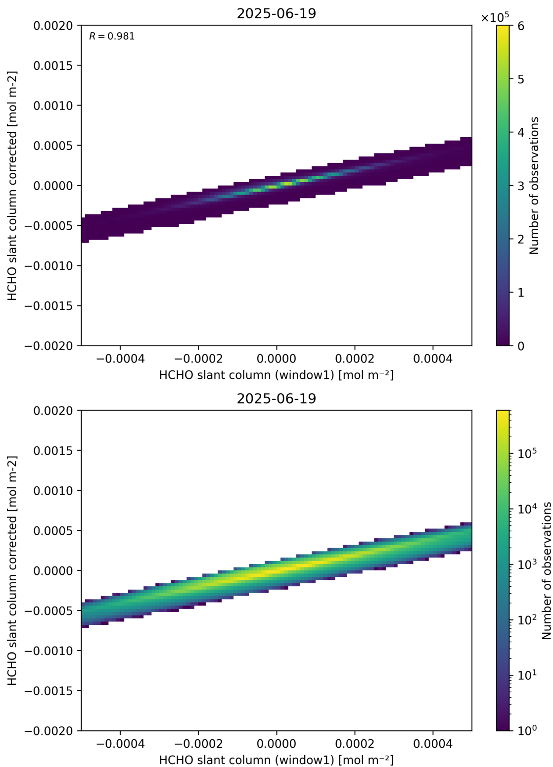
Figure 82: Scatter density plot of “HCHO slant column (window1)” against “HCHO slant column corrected” for 2025-06-18 to 2025-06-20.
