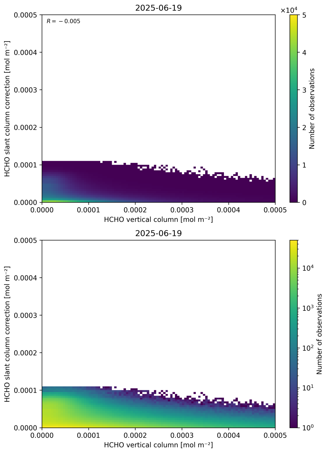
Figure 128: Scatter density plot of “HCHO vertical column” against “HCHO slant column correction” for 2025-06-18 to 2025-06-20.
