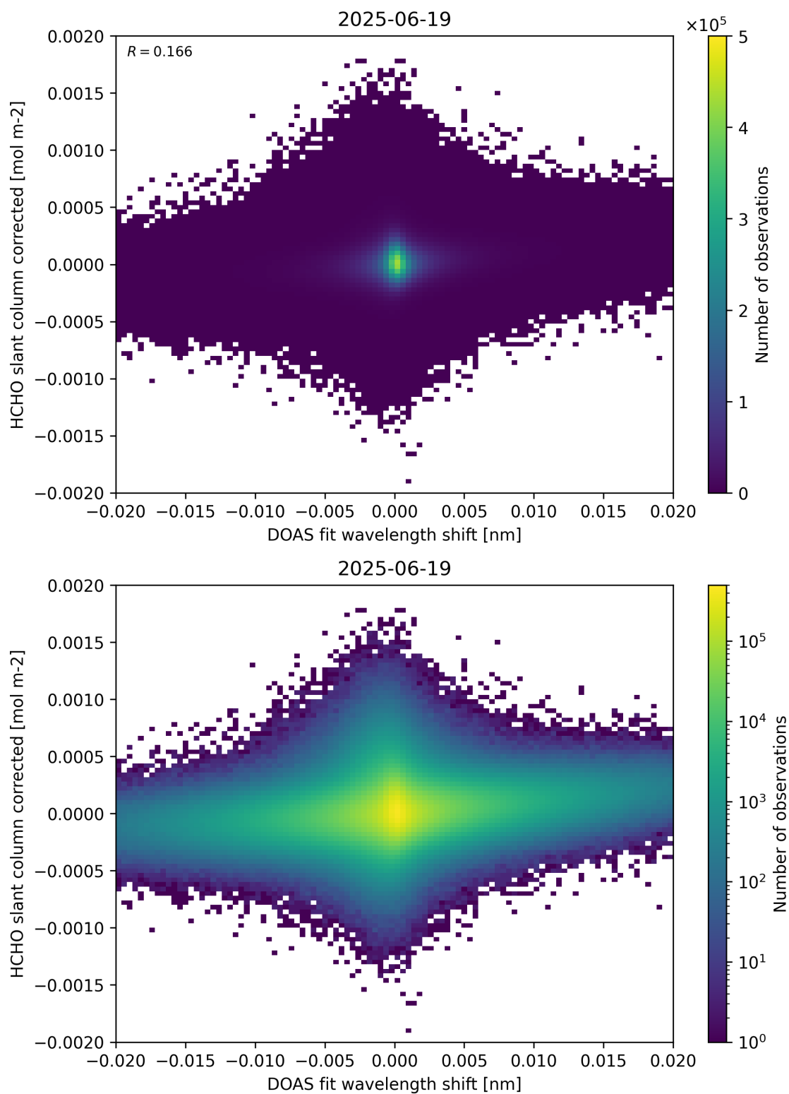
Figure 66: Scatter density plot of “DOAS fit wavelength shift” against “HCHO slant column corrected” for 2025-06-18 to 2025-06-20.
