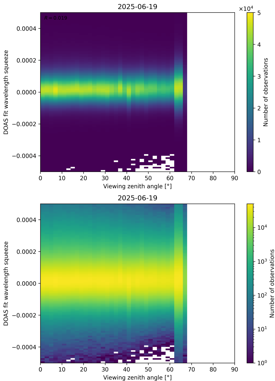
Figure 184: Scatter density plot of “Viewing zenith angle” against “DOAS fit wavelength squeeze” for 2025-06-18 to 2025-06-20.
