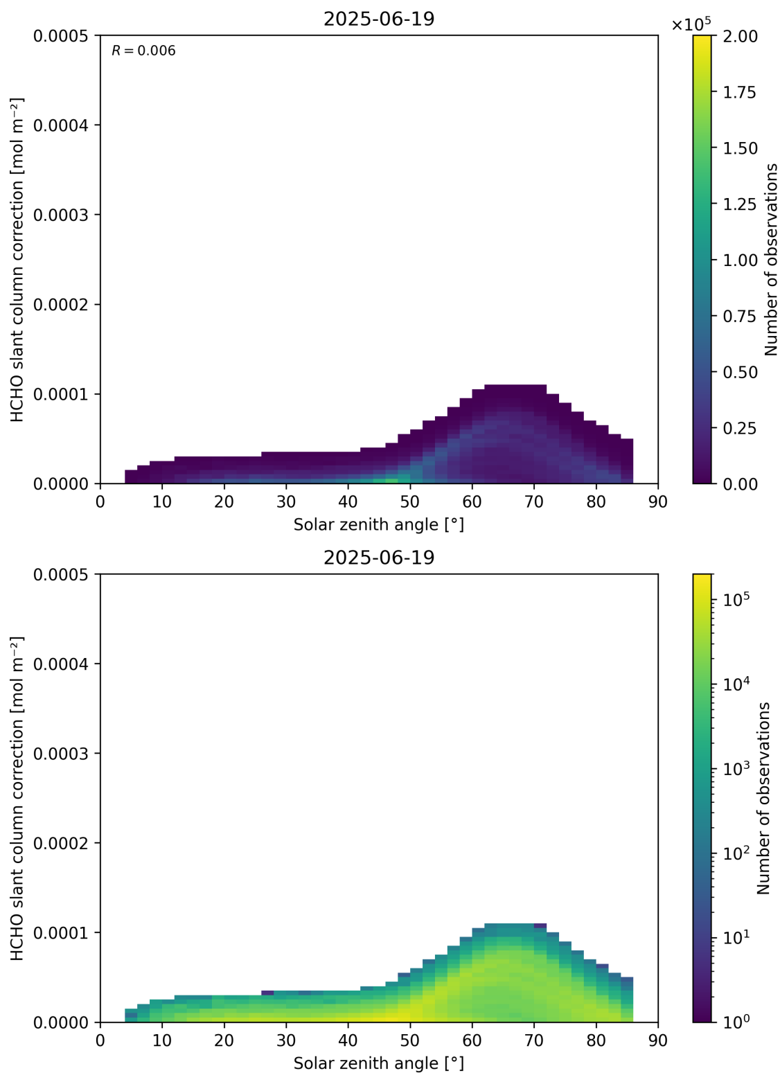
Figure 172: Scatter density plot of “Solar zenith angle” against “HCHO slant column correction” for 2025-06-18 to 2025-06-20.
