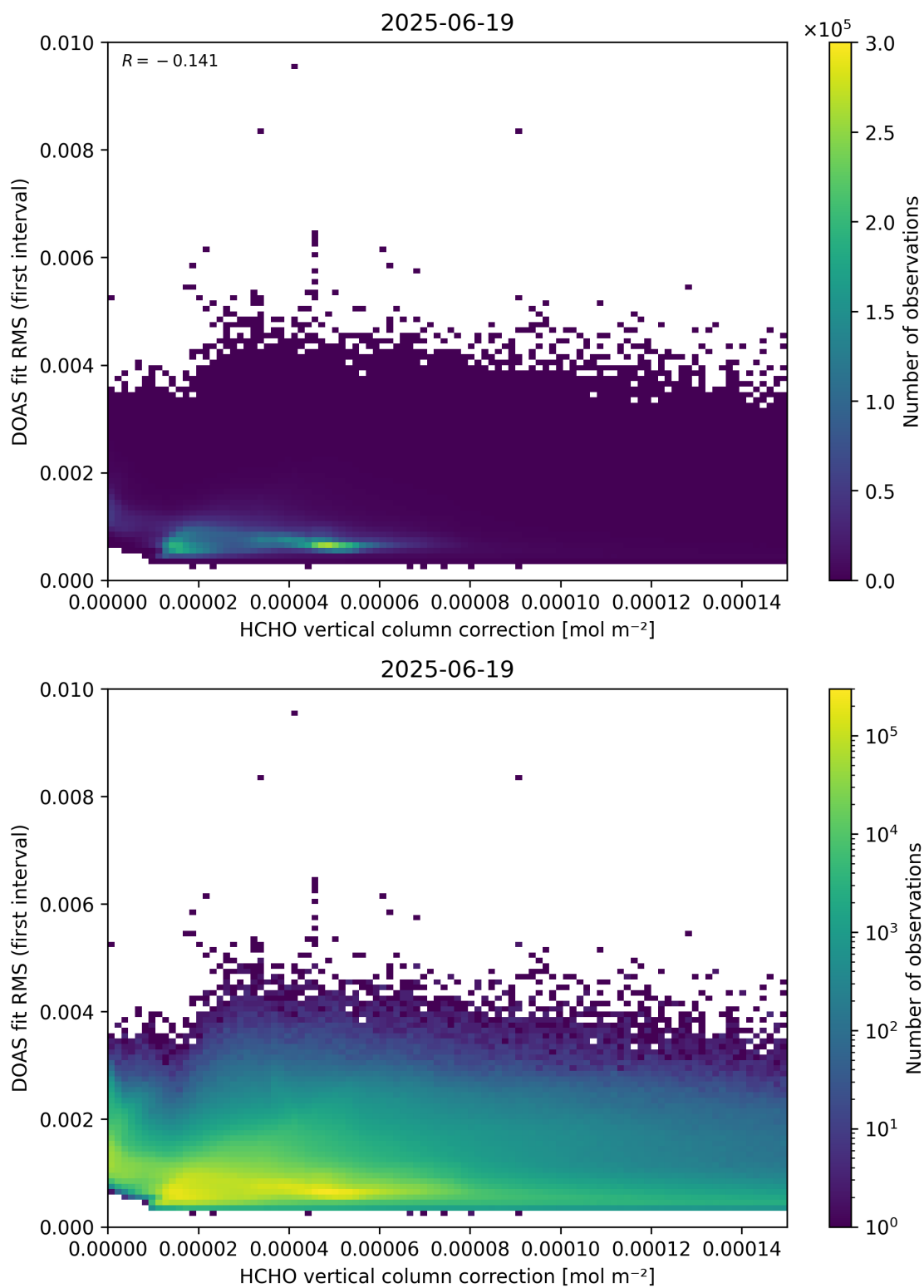
Figure 112: Scatter density plot of “HCHO vertical column correction” against “DOAS fit RMS (first interval)” for 2025-06-18 to 2025-06-20.
