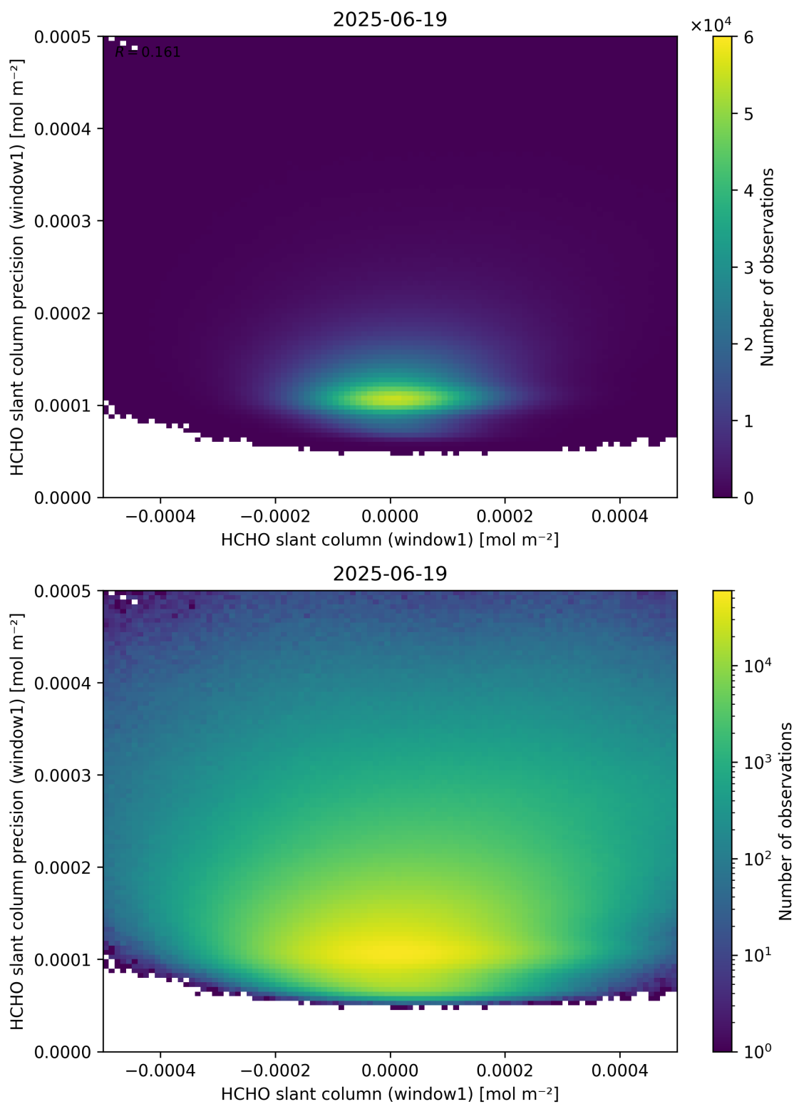
Figure 84: Scatter density plot of “HCHO slant column (window1)” against “HCHO slant column precision (window1)” for 2025-06-18 to 2025-06-20.
