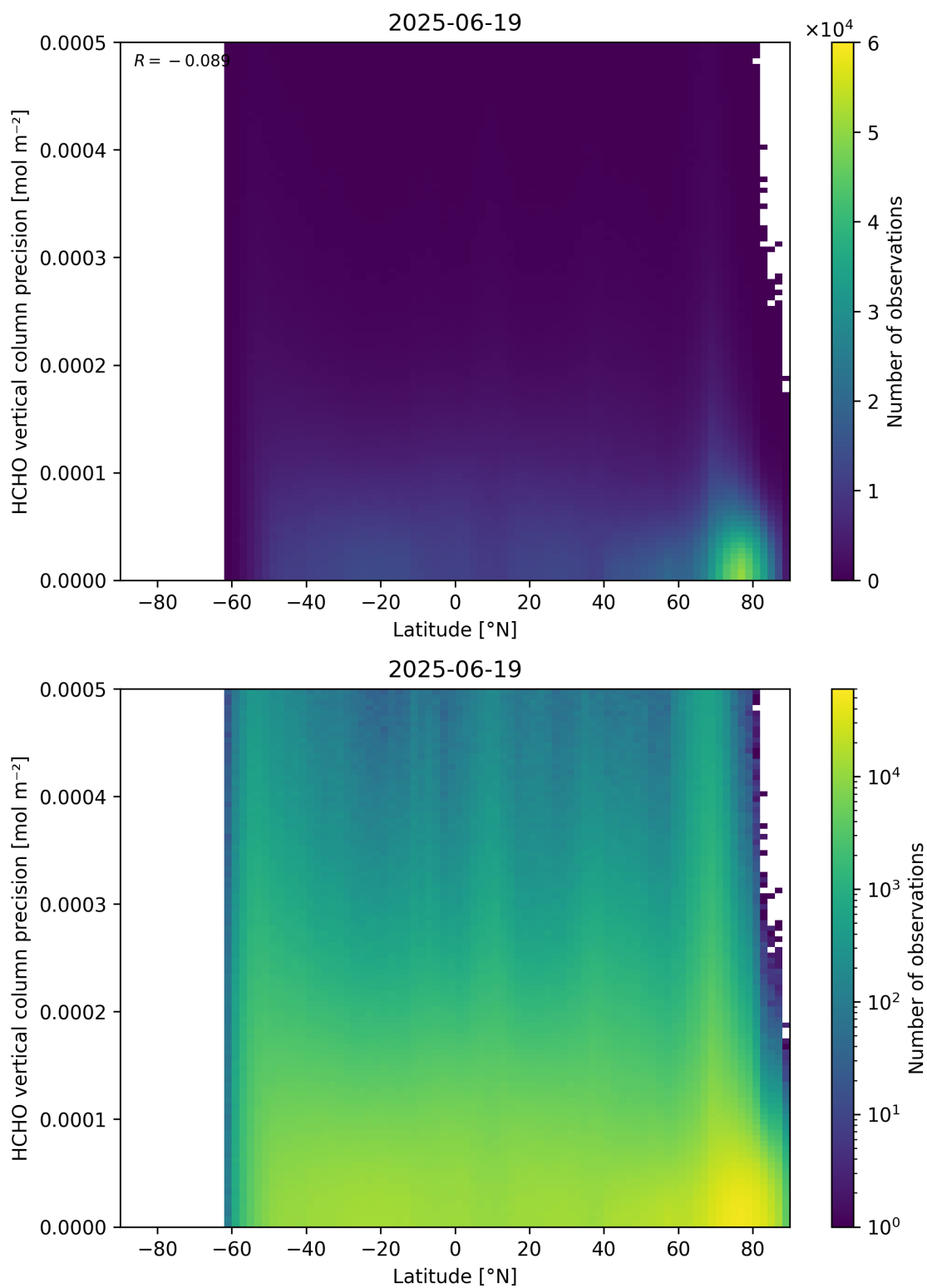
Figure 165: Scatter density plot of “Latitude” against “HCHO vertical column precision” for 2025-06-18 to 2025-06-20.
