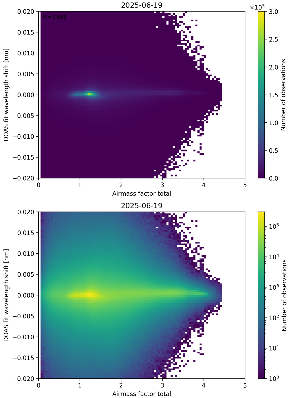
Figure 98: Scatter density plot of “Airmass factor total” against “DOAS fit wavelength shift” for 2025-06-18 to 2025-06-20.
