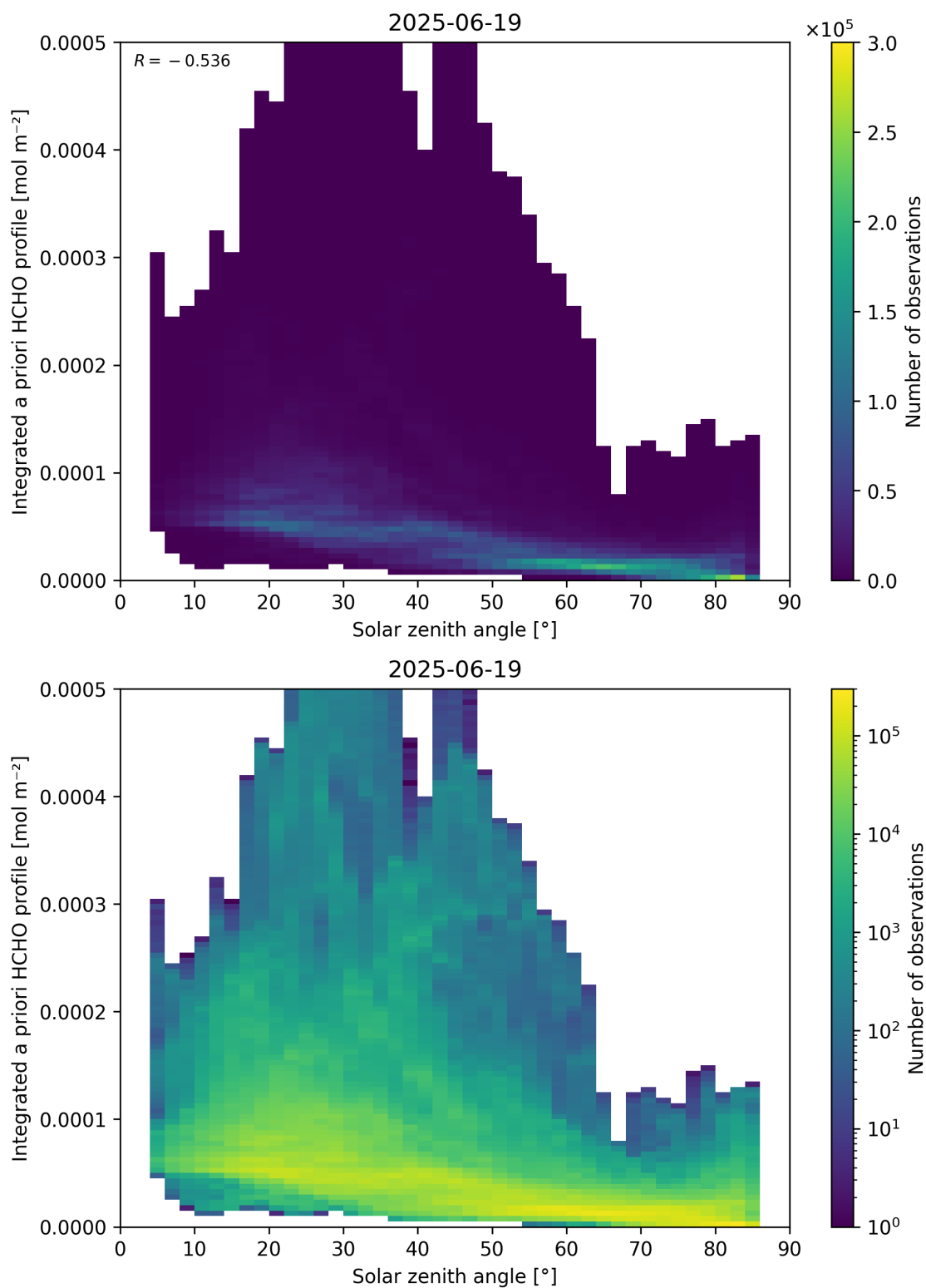
Figure 180: Scatter density plot of “Solar zenith angle” against “Integrated a priori HCHO profile” for 2025-06-18 to 2025-06-20.
