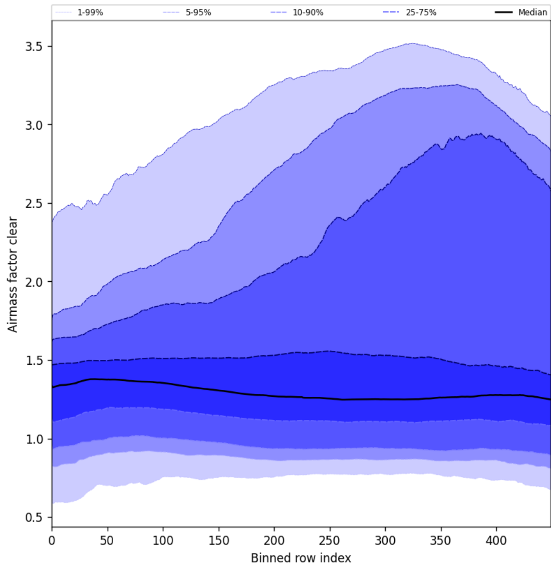
Figure 56: Along track statistics of “Airmass factor clear” for 2025-06-18 to 2025-06-20
