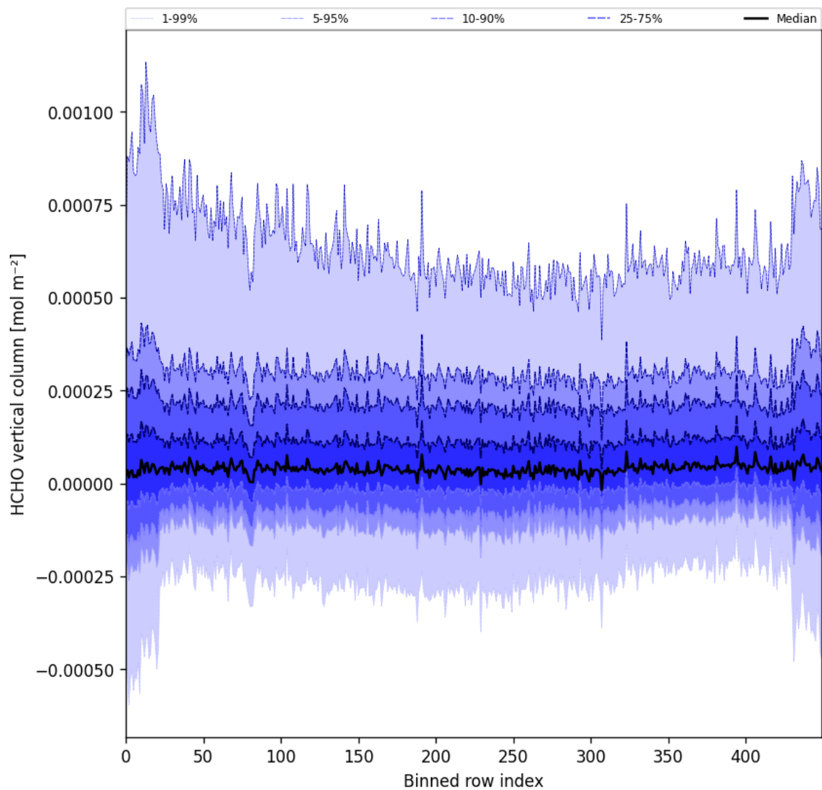
Figure 49: Along track statistics of “HCHO vertical column” for 2025-06-18 to 2025-06-20
