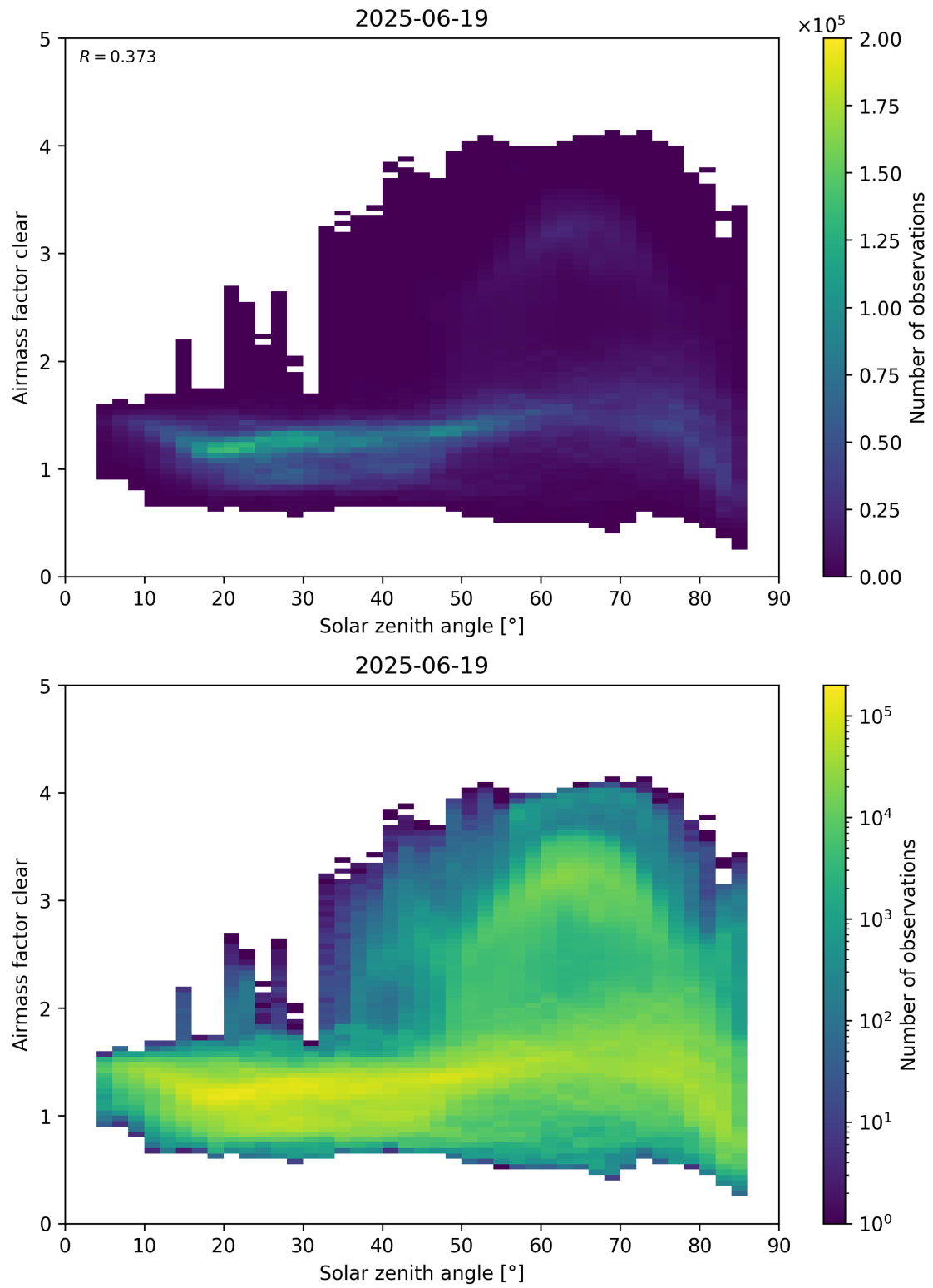
Figure 170: Scatter density plot of “Solar zenith angle” against “Airmass factor clear” for 2025-06-18 to 2025-06-20.
