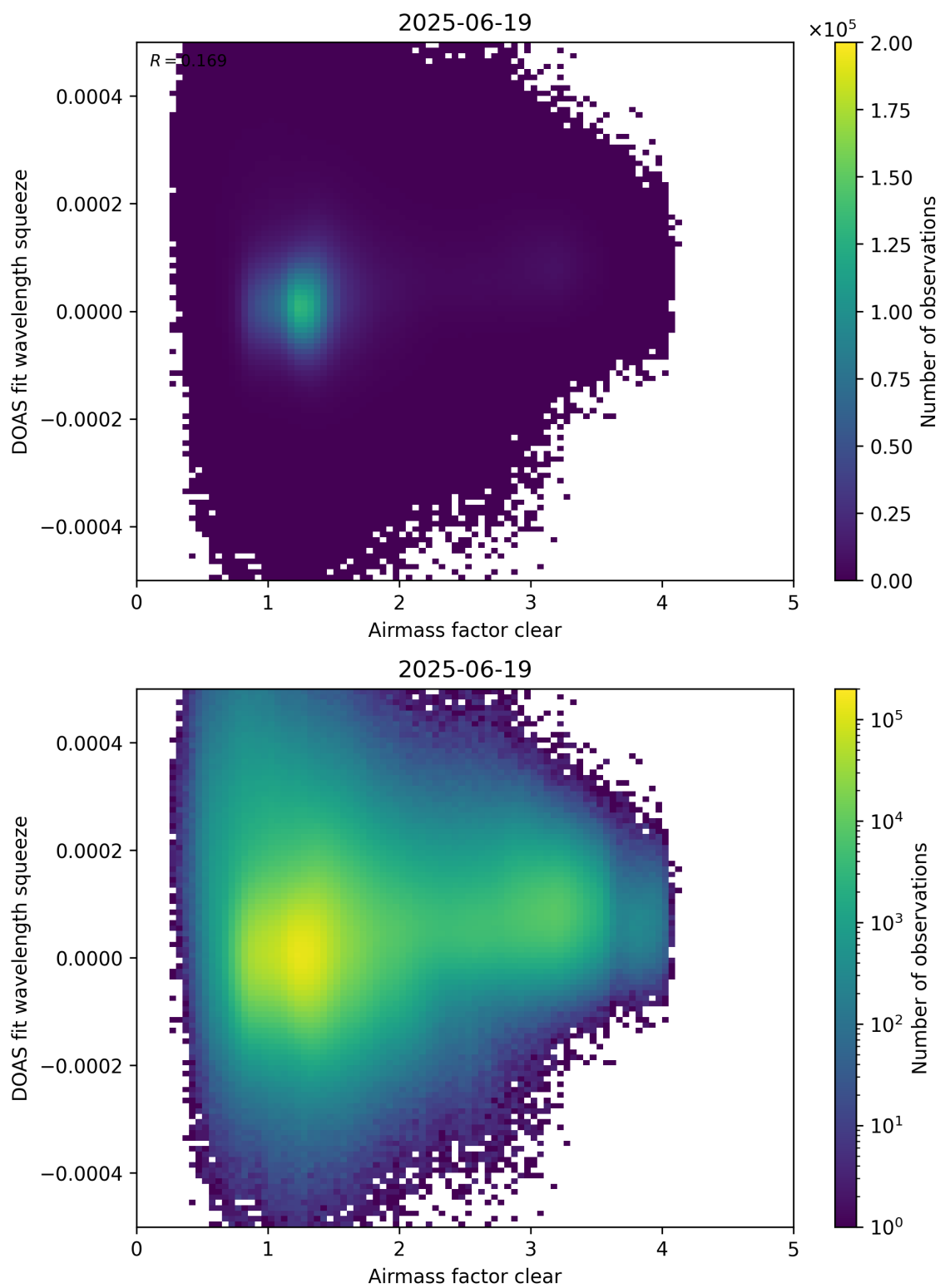
Figure 73: Scatter density plot of “Airmass factor clear” against “DOAS fit wavelength squeeze” for 2025-06-18 to 2025-06-20.
