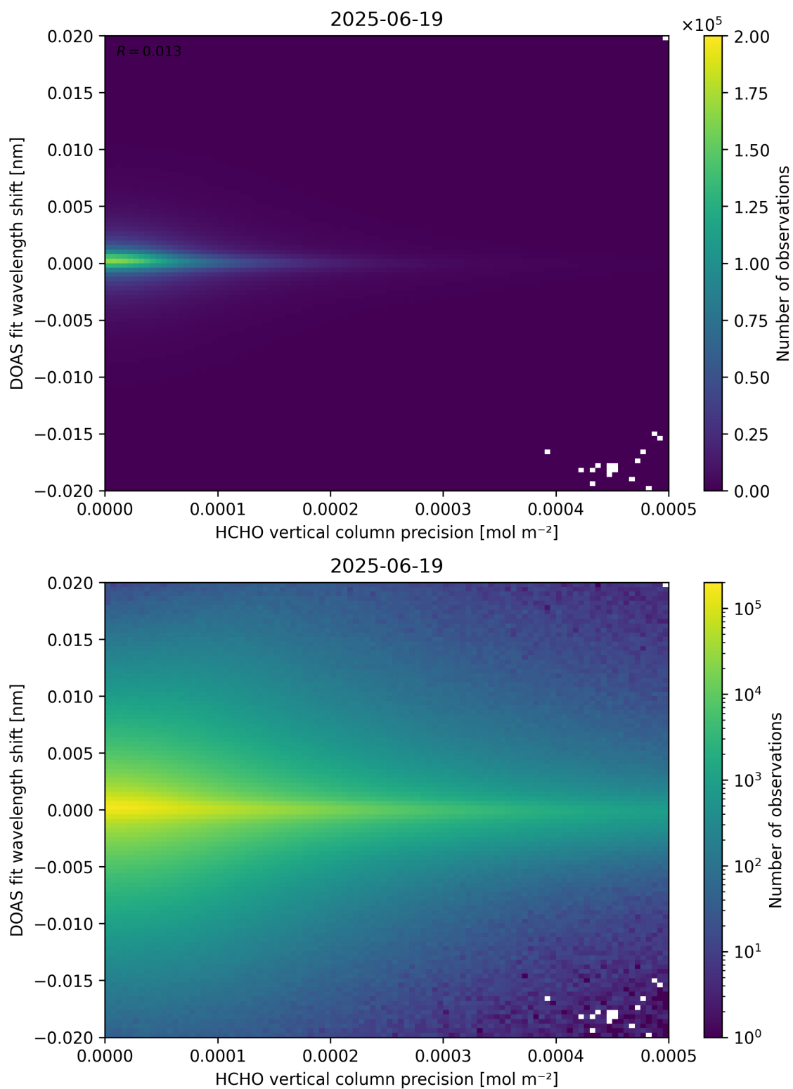
Figure 137: Scatter density plot of “HCHO vertical column precision” against “DOAS fit wavelength shift” for 2025-06-18 to 2025-06-20.
