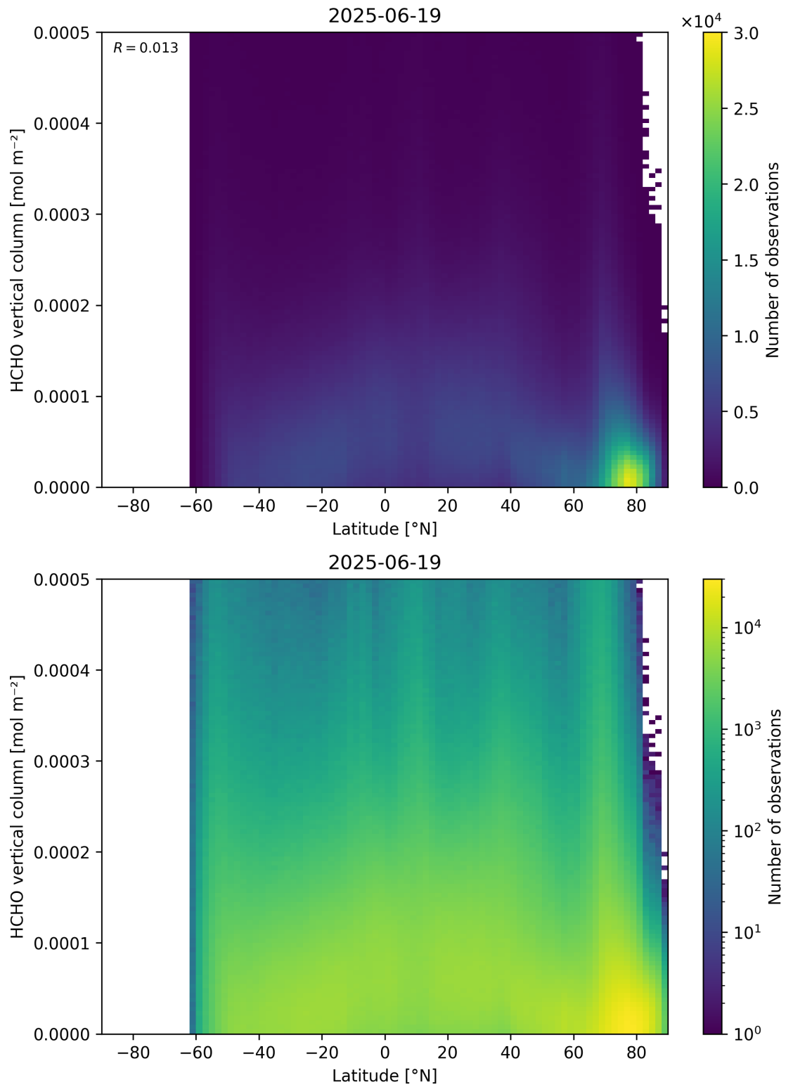
Figure 163: Scatter density plot of “Latitude” against “HCHO vertical column” for 2025-06-18 to 2025-06-20.
