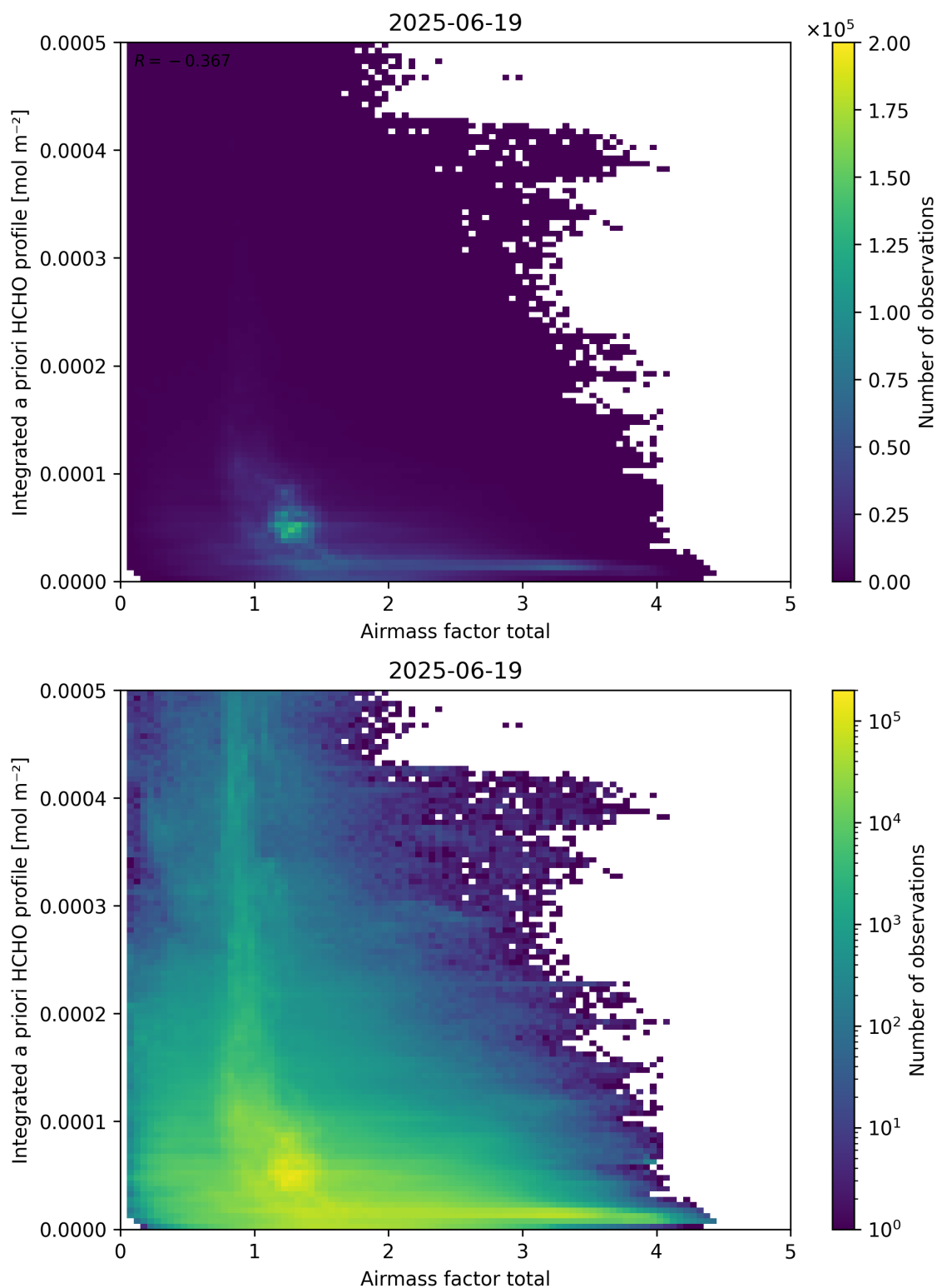
Figure 104: Scatter density plot of “Airmass factor total” against “Integrated a priori HCHO profile” for 2025-06-18 to 2025-06-20.
