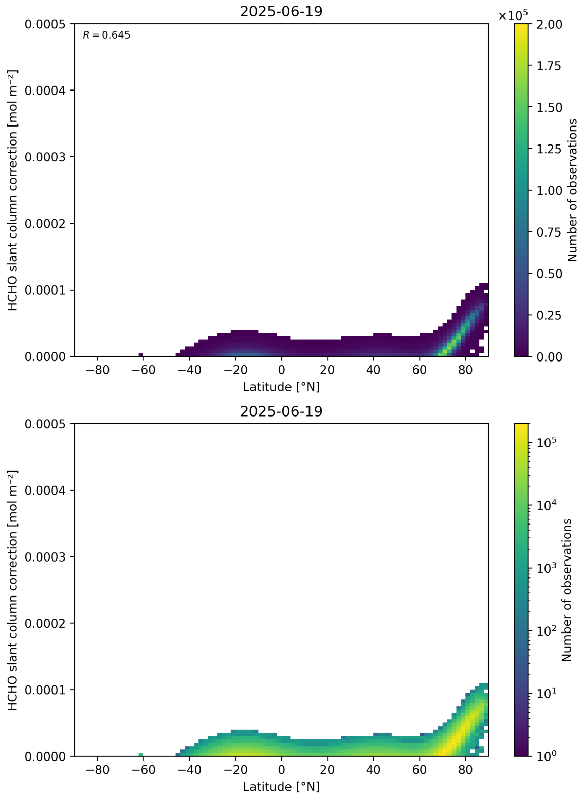
Figure 158: Scatter density plot of “Latitude” against “HCHO slant column correction” for 2025-06-18 to 2025-06-20.
