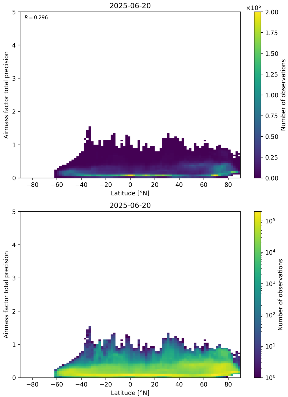
Figure 162: Scatter density plot of “Latitude” against “Airmass factor total precision” for 2025-06-19 to 2025-06-21.
