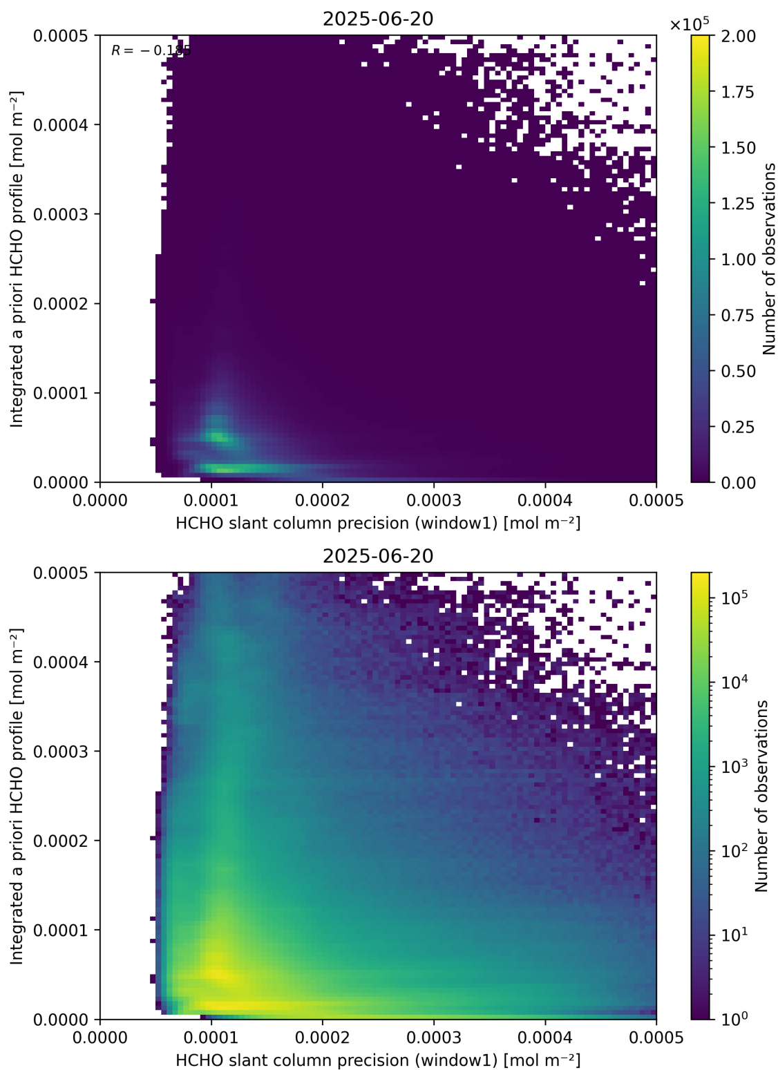
Figure 96: Scatter density plot of “HCHO slant column precision (window1)” against “Integrated a priori HCHO profile” for 2025-06-19 to 2025-06-21.
