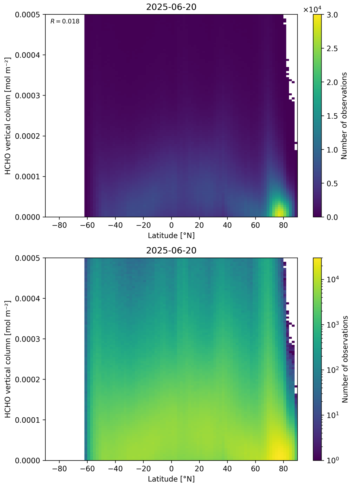
Figure 163: Scatter density plot of “Latitude” against “HCHO vertical column” for 2025-06-19 to 2025-06-21.
