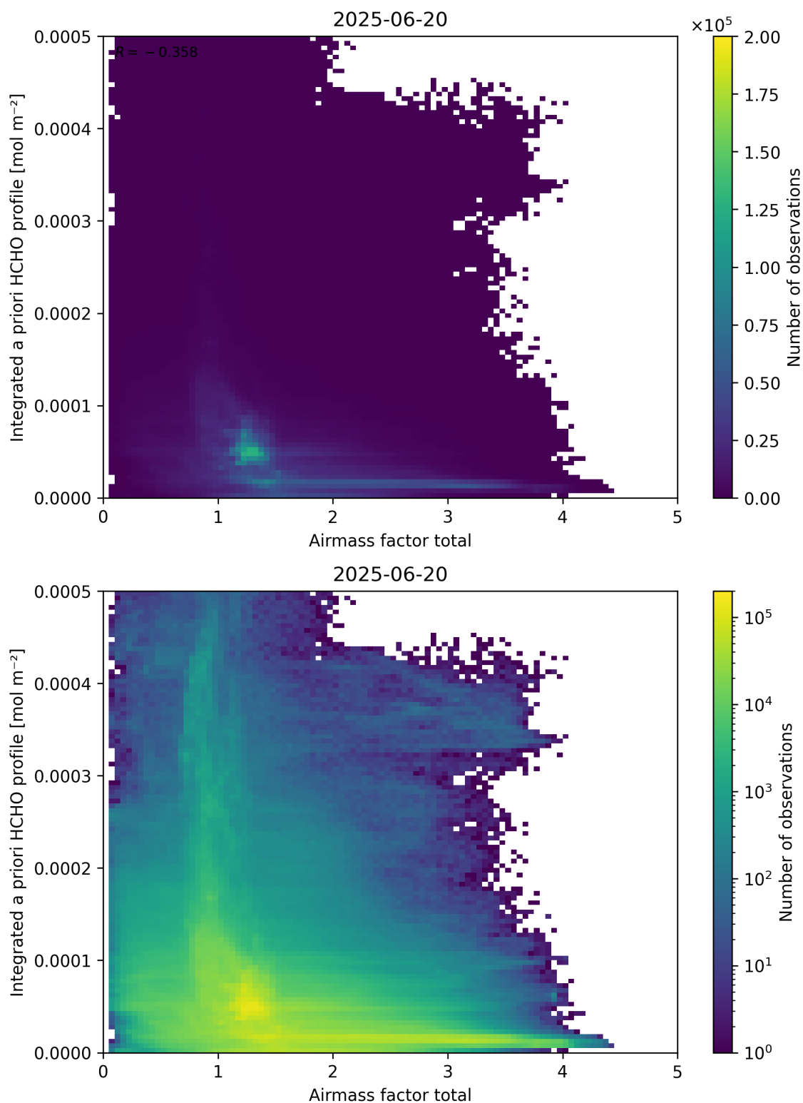
Figure 104: Scatter density plot of “Airmass factor total” against “Integrated a priori HCHO profile” for 2025-06-19 to 2025-06-21.
