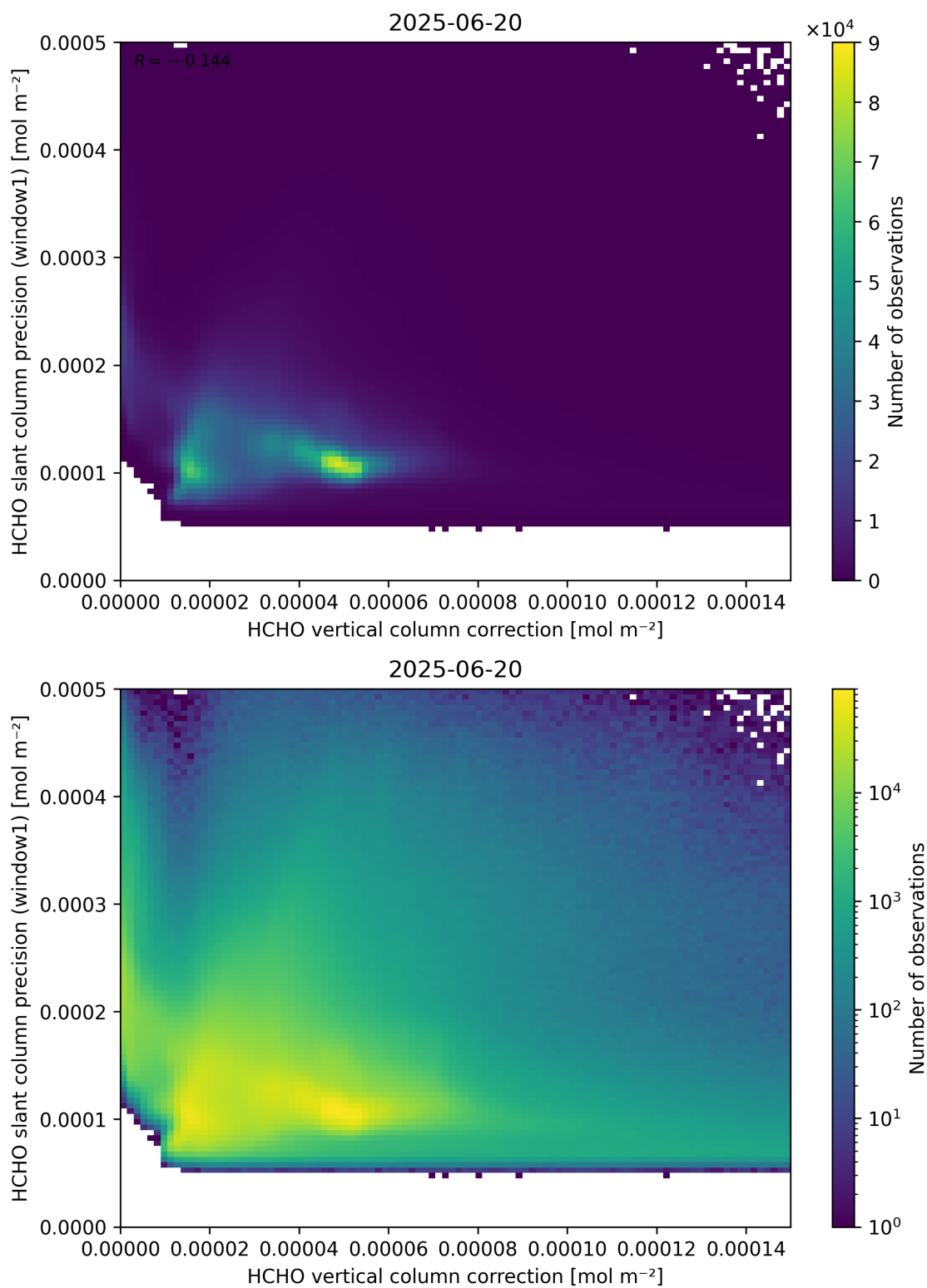
Figure 119: Scatter density plot of “HCHO vertical column correction” against “HCHO slant column precision (window1)” for 2025-06-19 to 2025-06-21.
