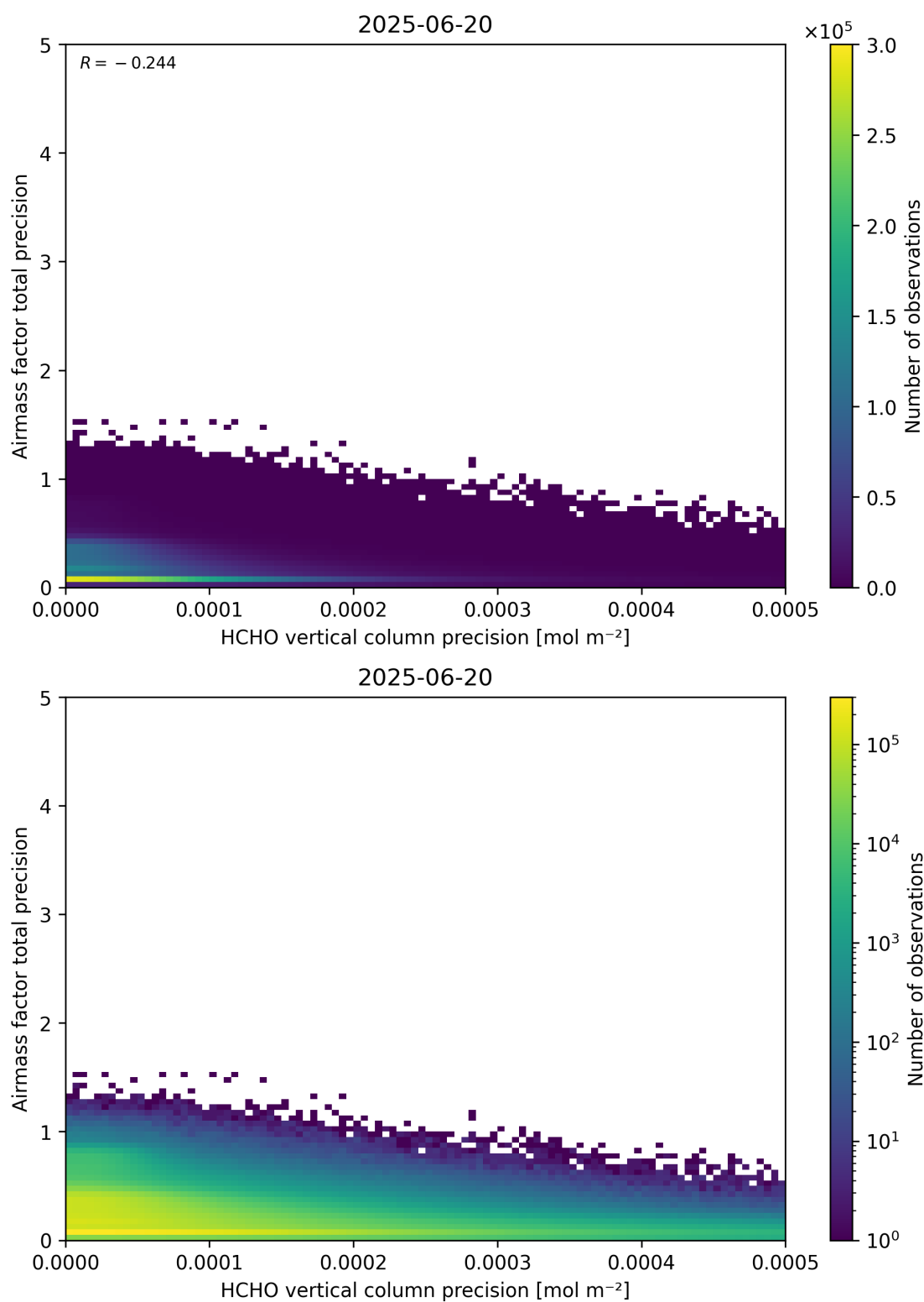
Figure 145: Scatter density plot of “HCHO vertical column precision” against “Airmass factor total precision” for 2025-06-19 to 2025-06-21.
