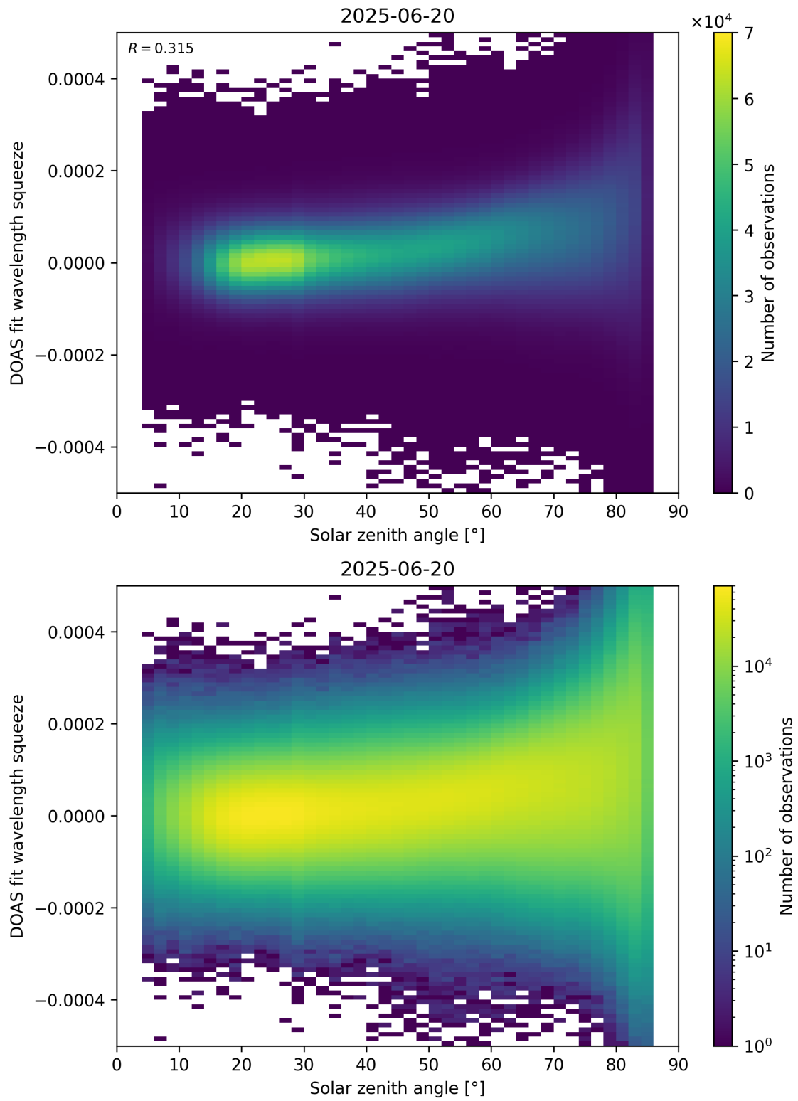
Figure 169: Scatter density plot of “Solar zenith angle” against “DOAS fit wavelength squeeze” for 2025-06-19 to 2025-06-21.
