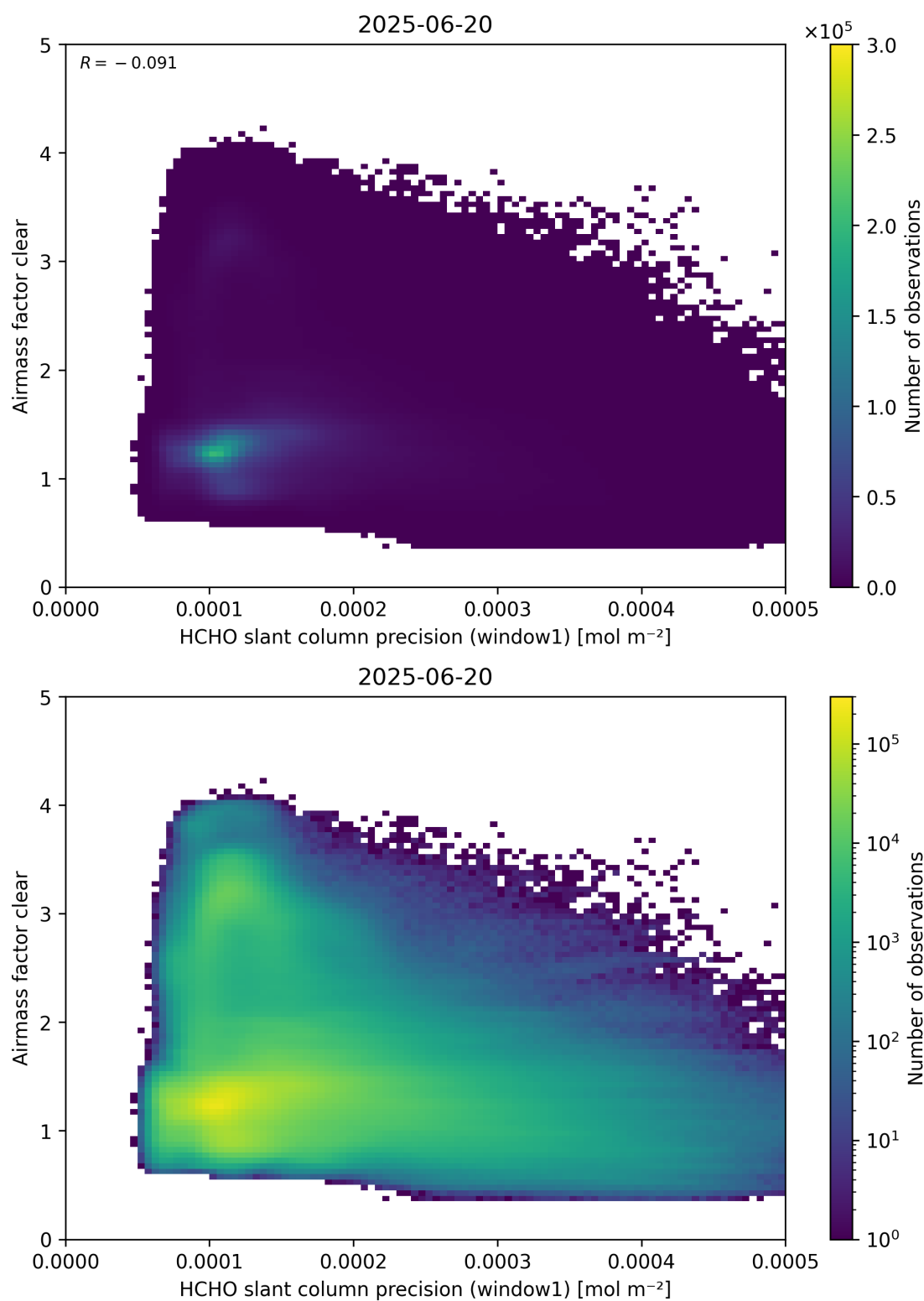
Figure 91: Scatter density plot of “HCHO slant column precision (window1)” against “Airmass factor clear” for 2025-06-19 to 2025-06-21.
