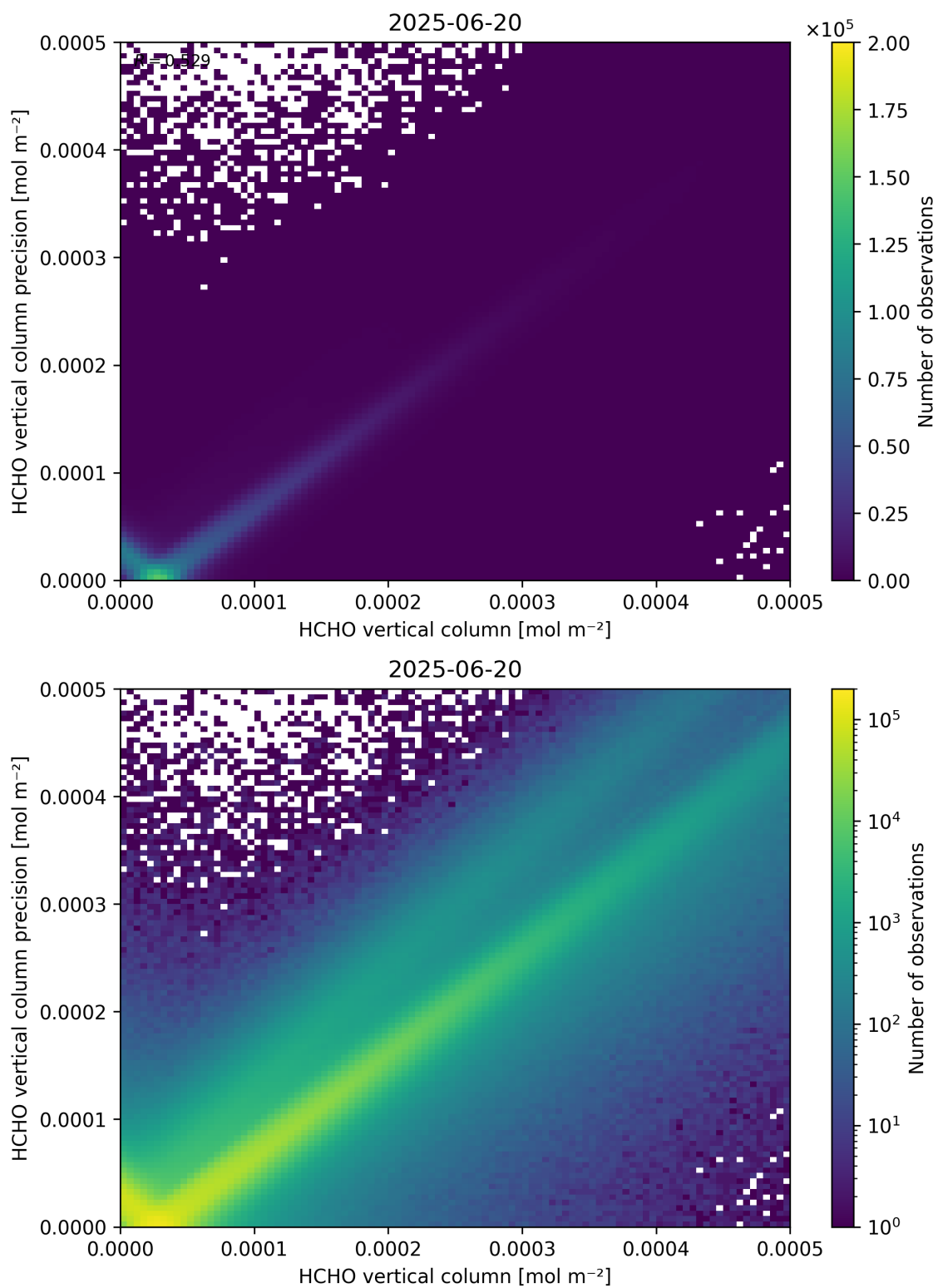
Figure 134: Scatter density plot of “HCHO vertical column” against “HCHO vertical column precision” for 2025-06-19 to 2025-06-21.
