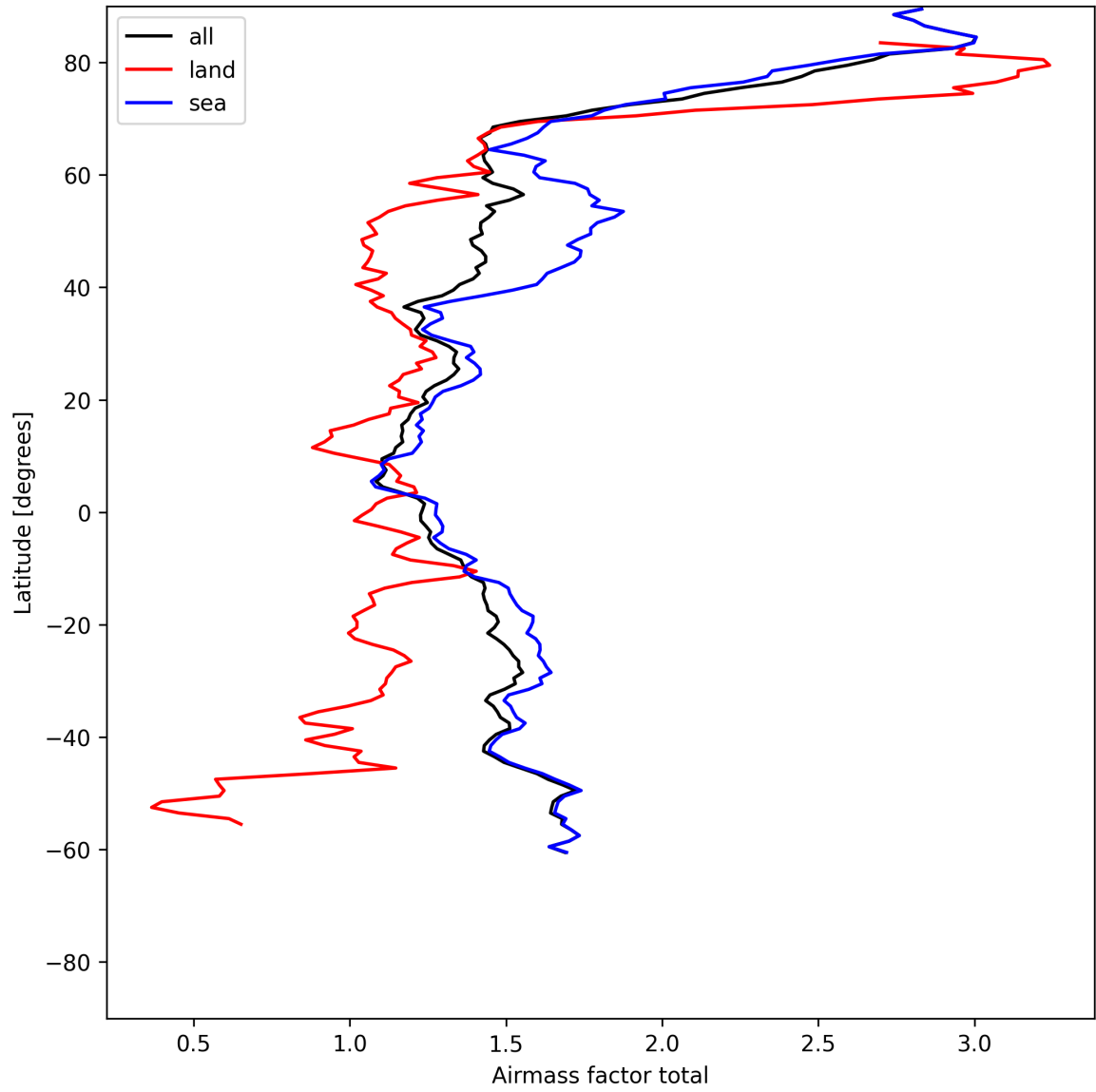
Figure 26: Zonal average of “Airmass factor total” for 2025-06-19 to 2025-06-21.
