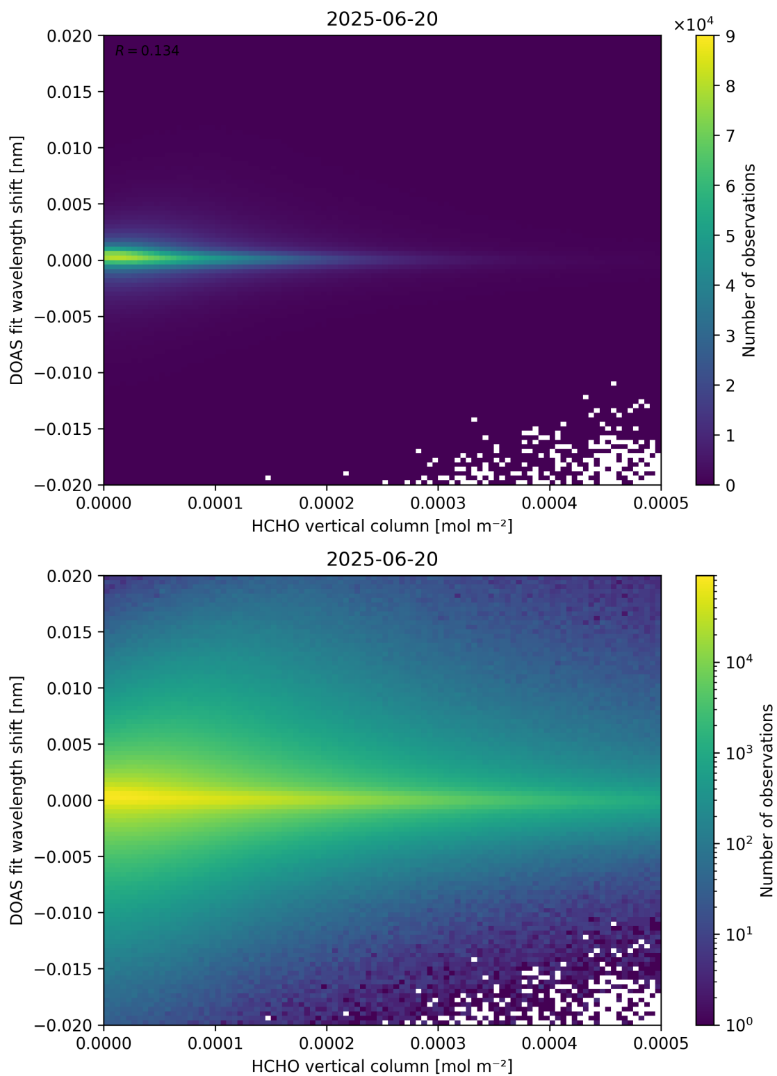
Figure 124: Scatter density plot of “HCHO vertical column” against “DOAS fit wavelength shift” for 2025-06-19 to 2025-06-21.
