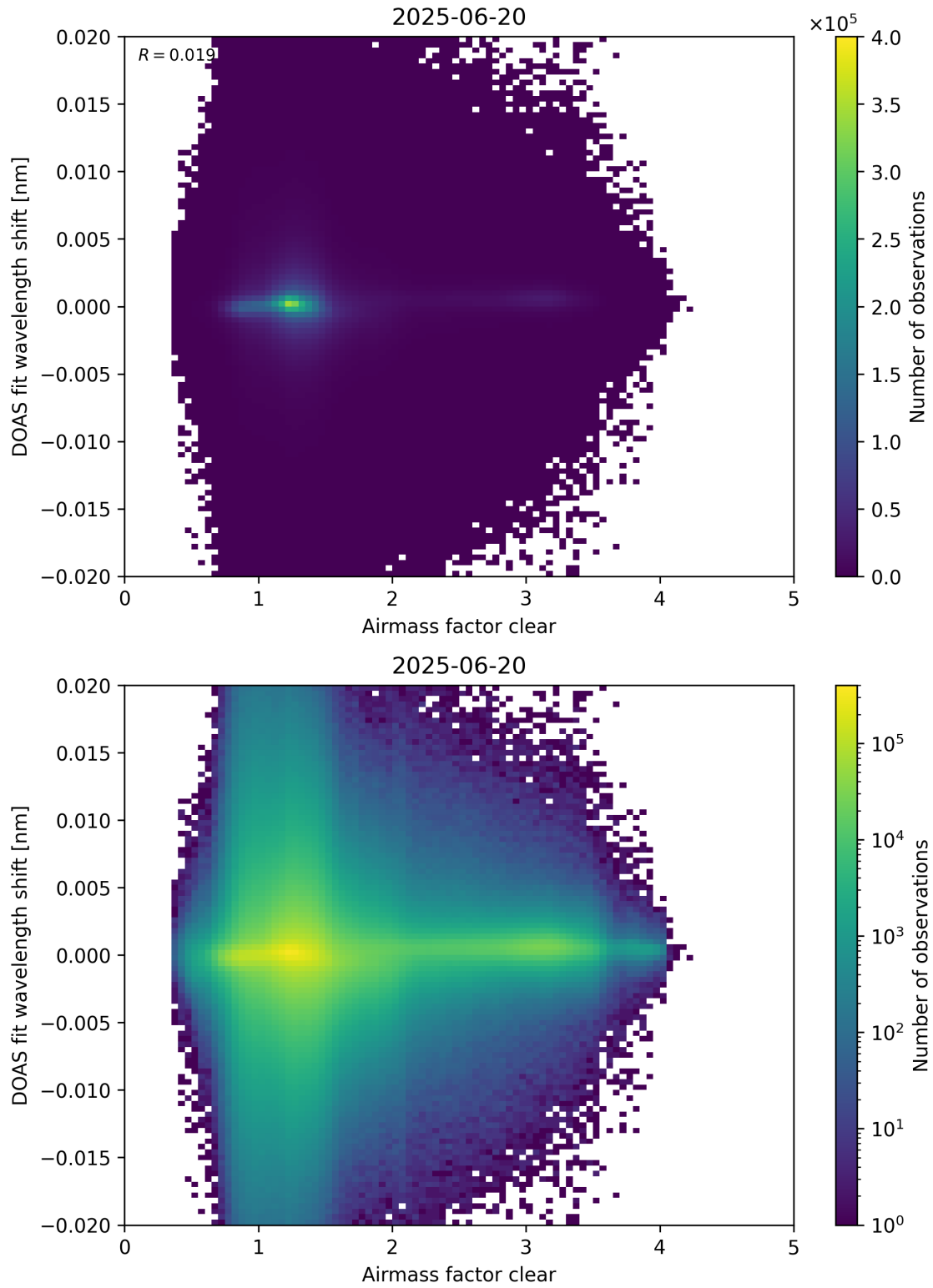
Figure 72: Scatter density plot of “Airmass factor clear” against “DOAS fit wavelength shift” for 2025-06-19 to 2025-06-21.
