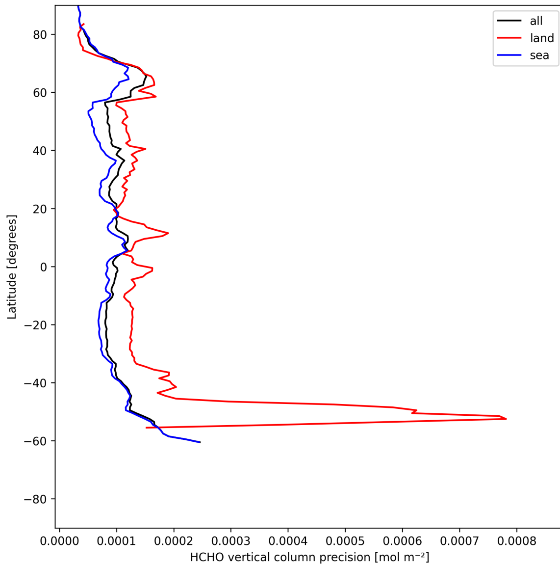
Figure 22: Zonal average of “HCHO vertical column precision” for 2025-06-19 to 2025-06-21.
