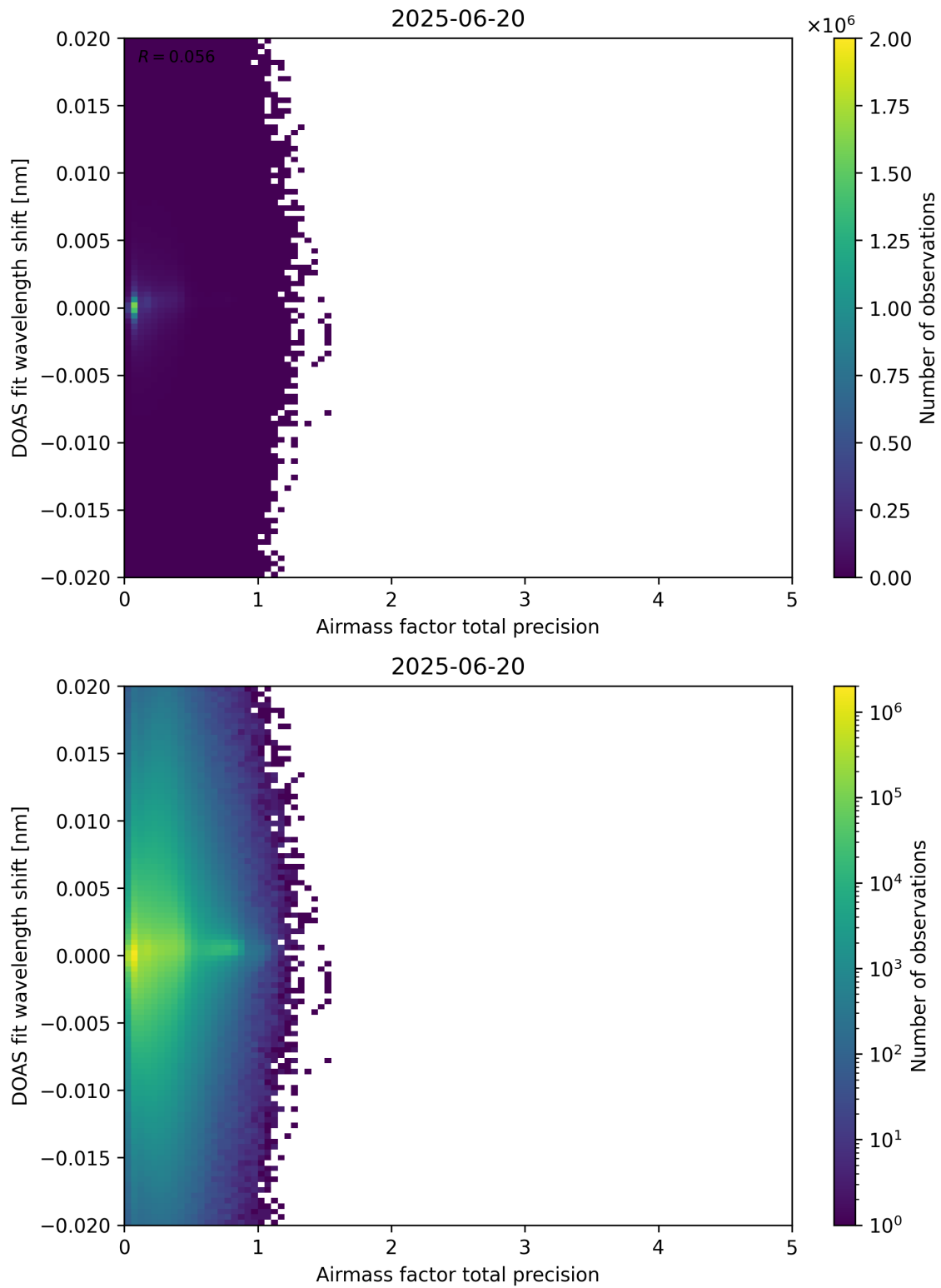
Figure 106: Scatter density plot of “Airmass factor total precision” against “DOAS fit wavelength shift” for 2025-06-19 to 2025-06-21.
