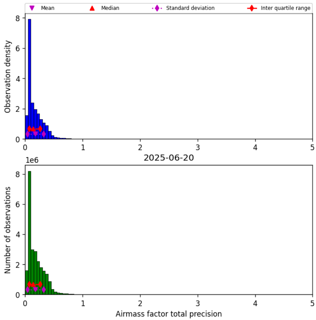
Figure 41: Histogram of “Airmass factor total precision” for 2025-06-19 to 2025-06-21
