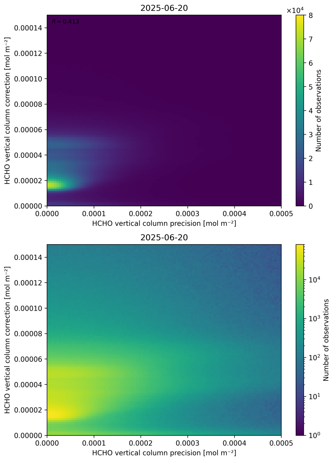
Figure 146: Scatter density plot of “HCHO vertical column precision” against “HCHO vertical column correction” for 2025-06-19 to 2025-06-21.
