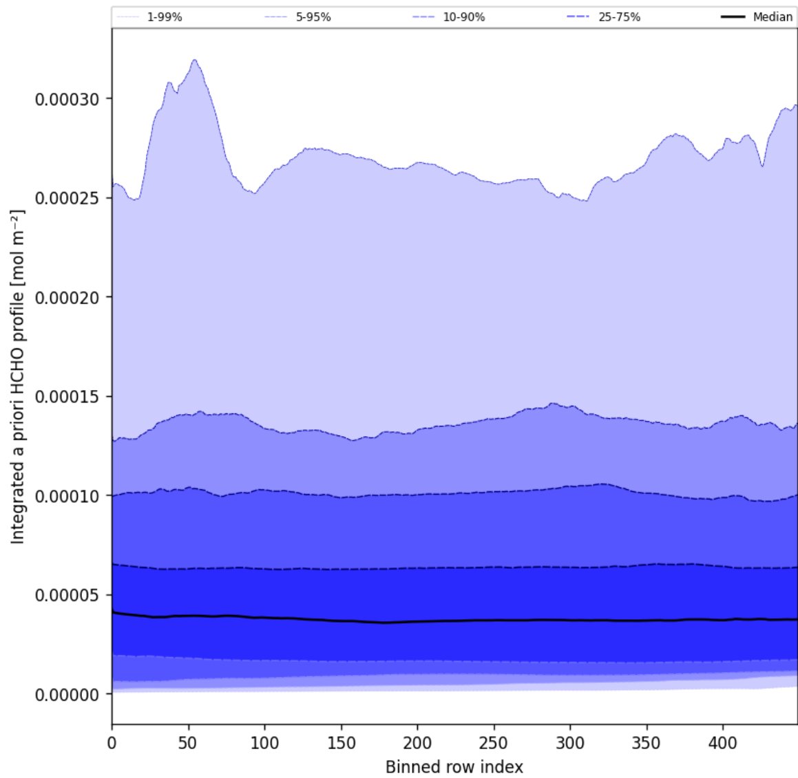
Figure 57: Along track statistics of “Integrated a priori HCHO profile” for 2025-06-19 to 2025-06-21
