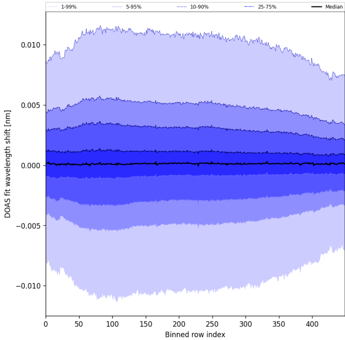
Figure 58: Along track statistics of “DOAS fit wavelength shift” for 2025-06-19 to 2025-06-21
