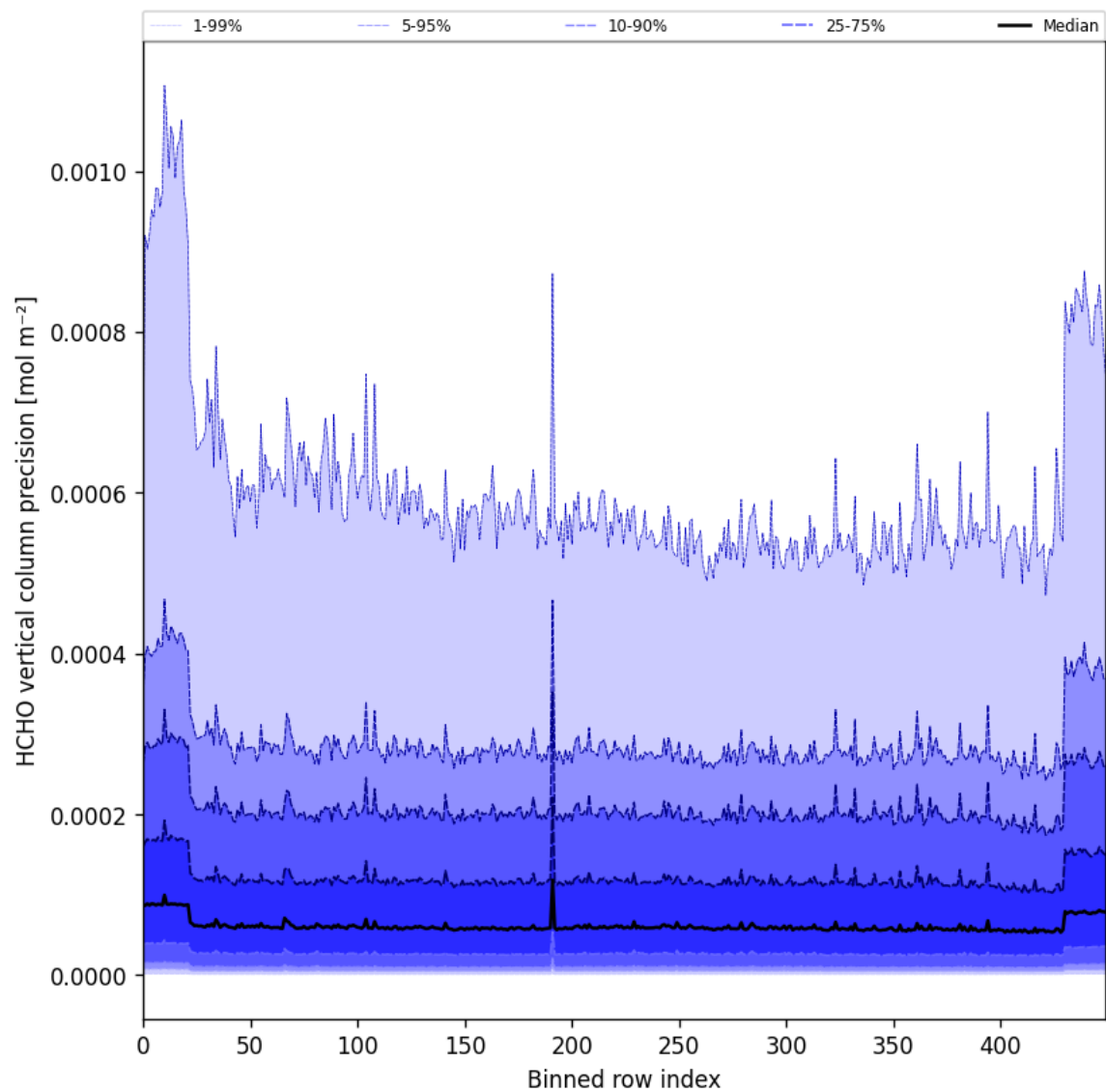
Figure 50: Along track statistics of “HCHO vertical column precision” for 2025-06-19 to 2025-06-21
