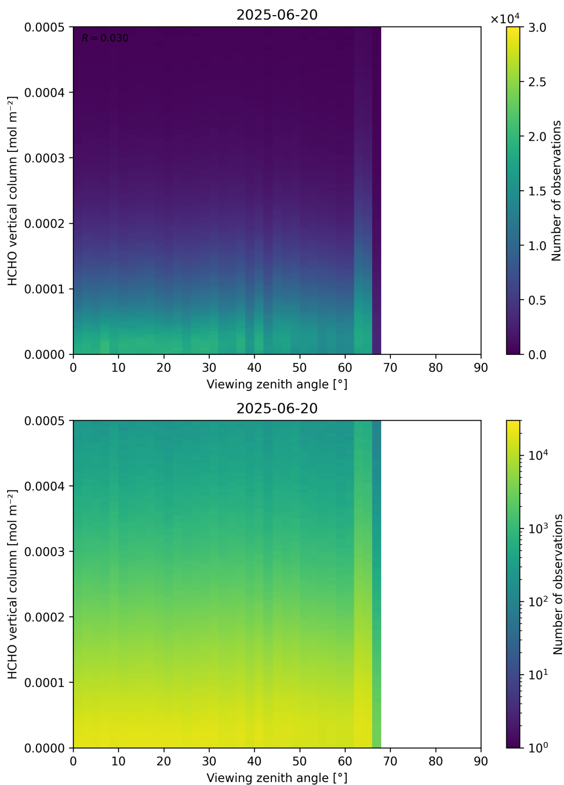
Figure 192: Scatter density plot of “Viewing zenith angle” against “HCHO vertical column” for 2025-06-19 to 2025-06-21.
