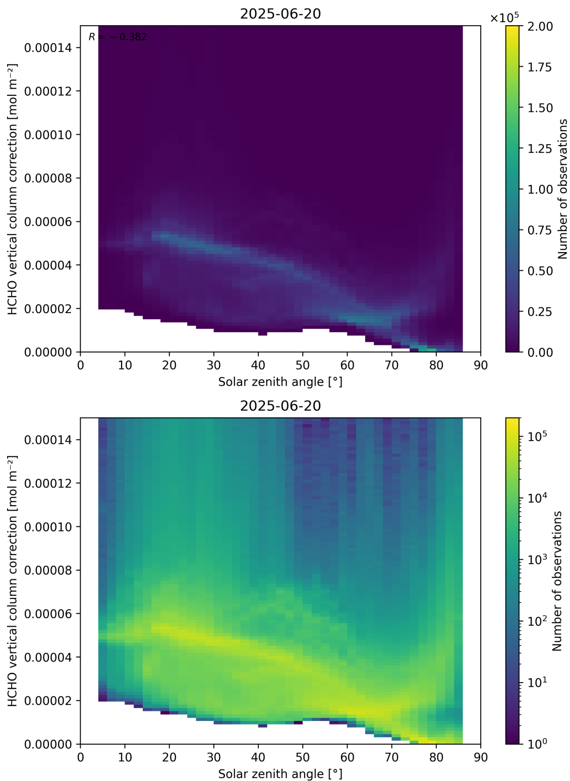
Figure 178: Scatter density plot of “Solar zenith angle” against “HCHO vertical column correction” for 2025-06-19 to 2025-06-21.
