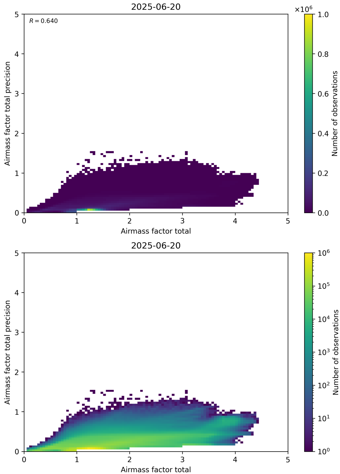
Figure 103: Scatter density plot of “Airmass factor total” against “Airmass factor total precision” for 2025-06-19 to 2025-06-21.
