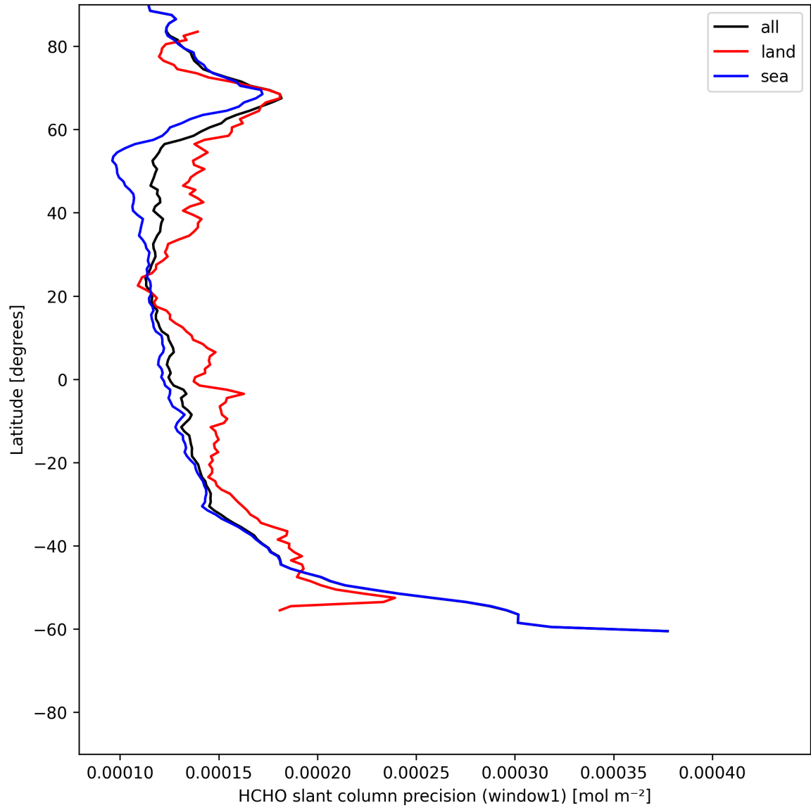
Figure 25: Zonal average of "HCHO slant column precision (window1)" for 2025-06-19 to 2025-06-21.
