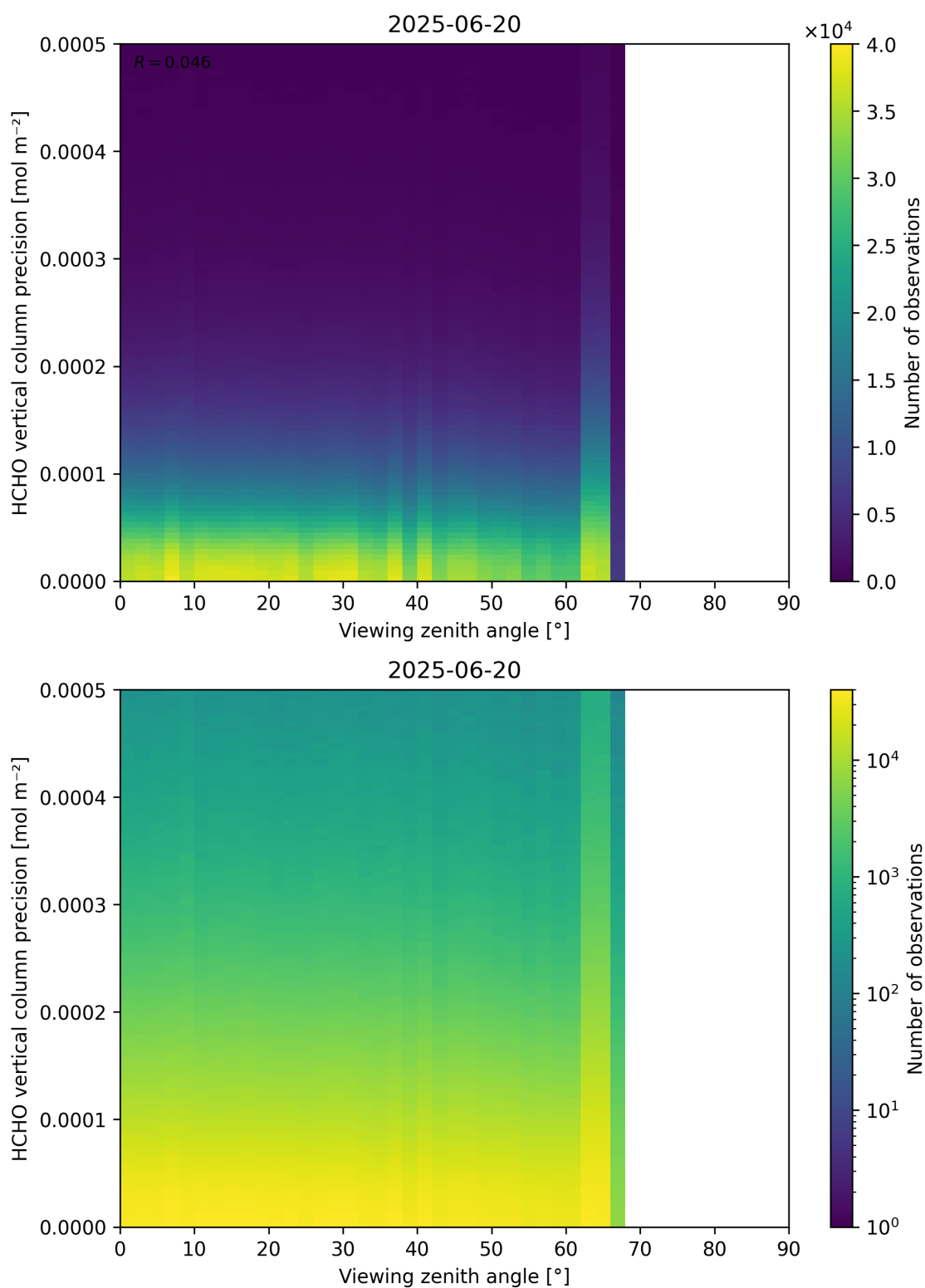
Figure 194: Scatter density plot of “Viewing zenith angle” against “HCHO vertical column precision” for 2025-06-19 to 2025-06-21.
