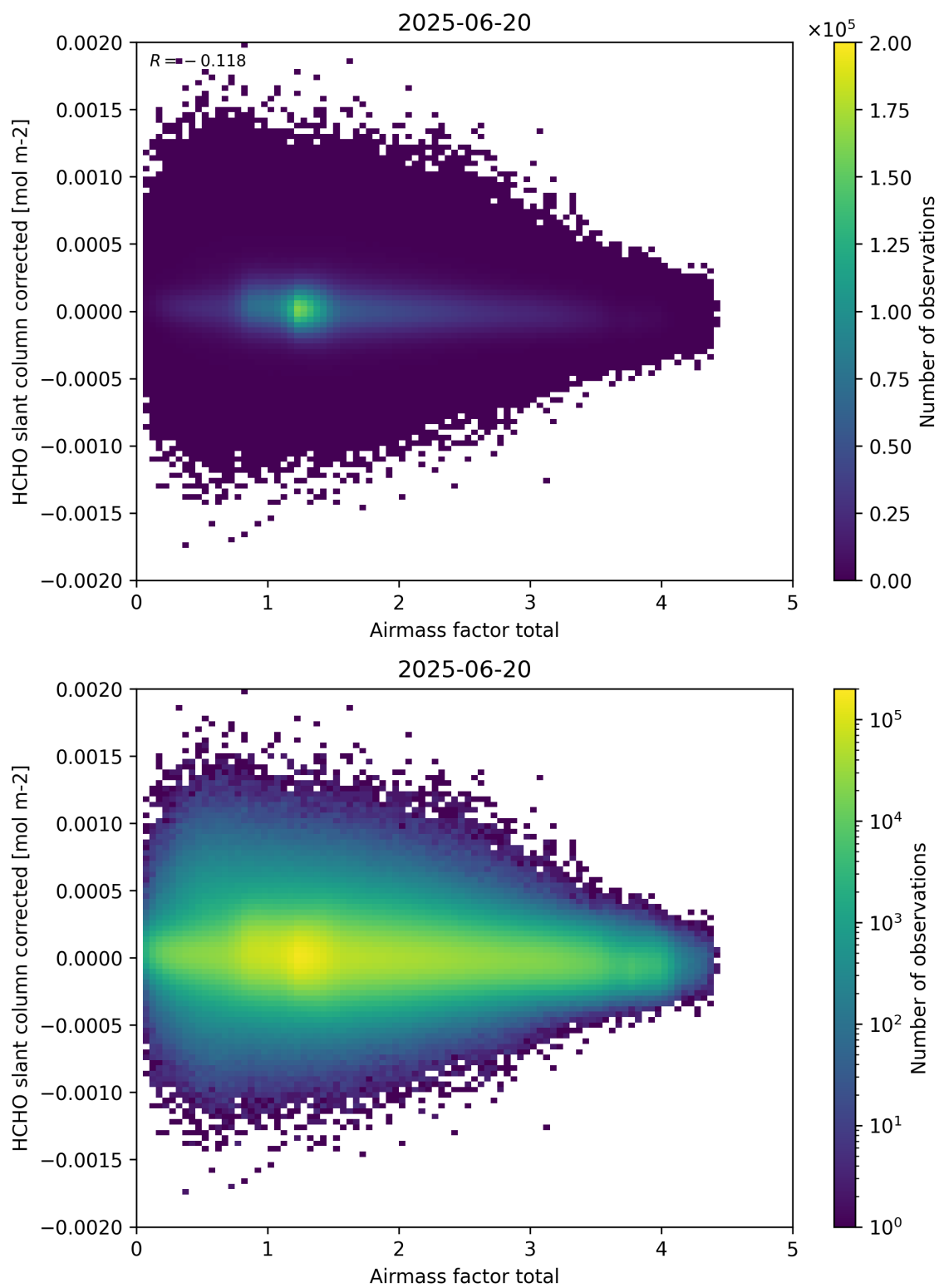
Figure 101: Scatter density plot of “Airmass factor total” against “HCHO slant column corrected” for 2025-06-19 to 2025-06-21.
