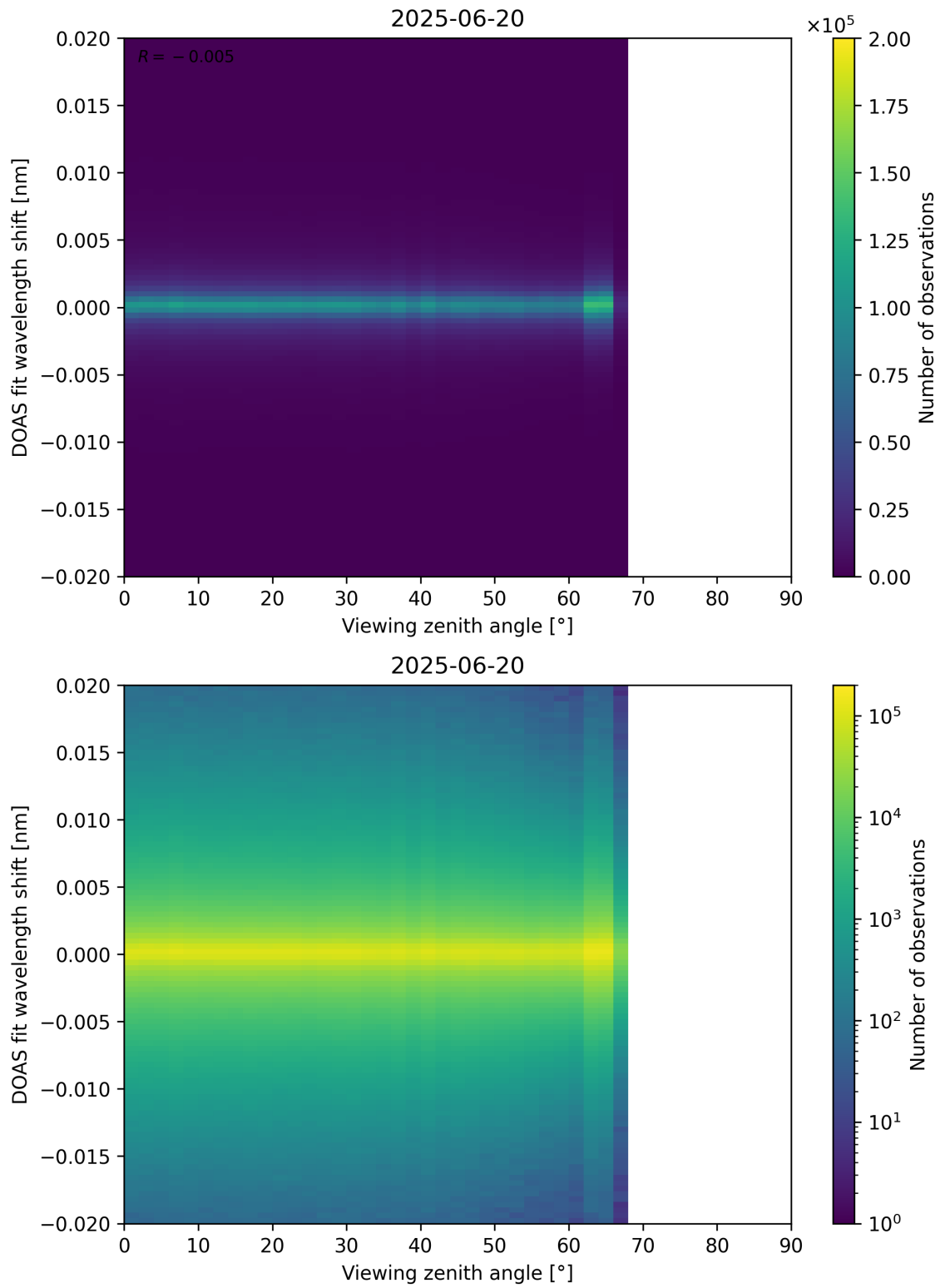
Figure 183: Scatter density plot of “Viewing zenith angle” against “DOAS fit wavelength shift” for 2025-06-19 to 2025-06-21.
