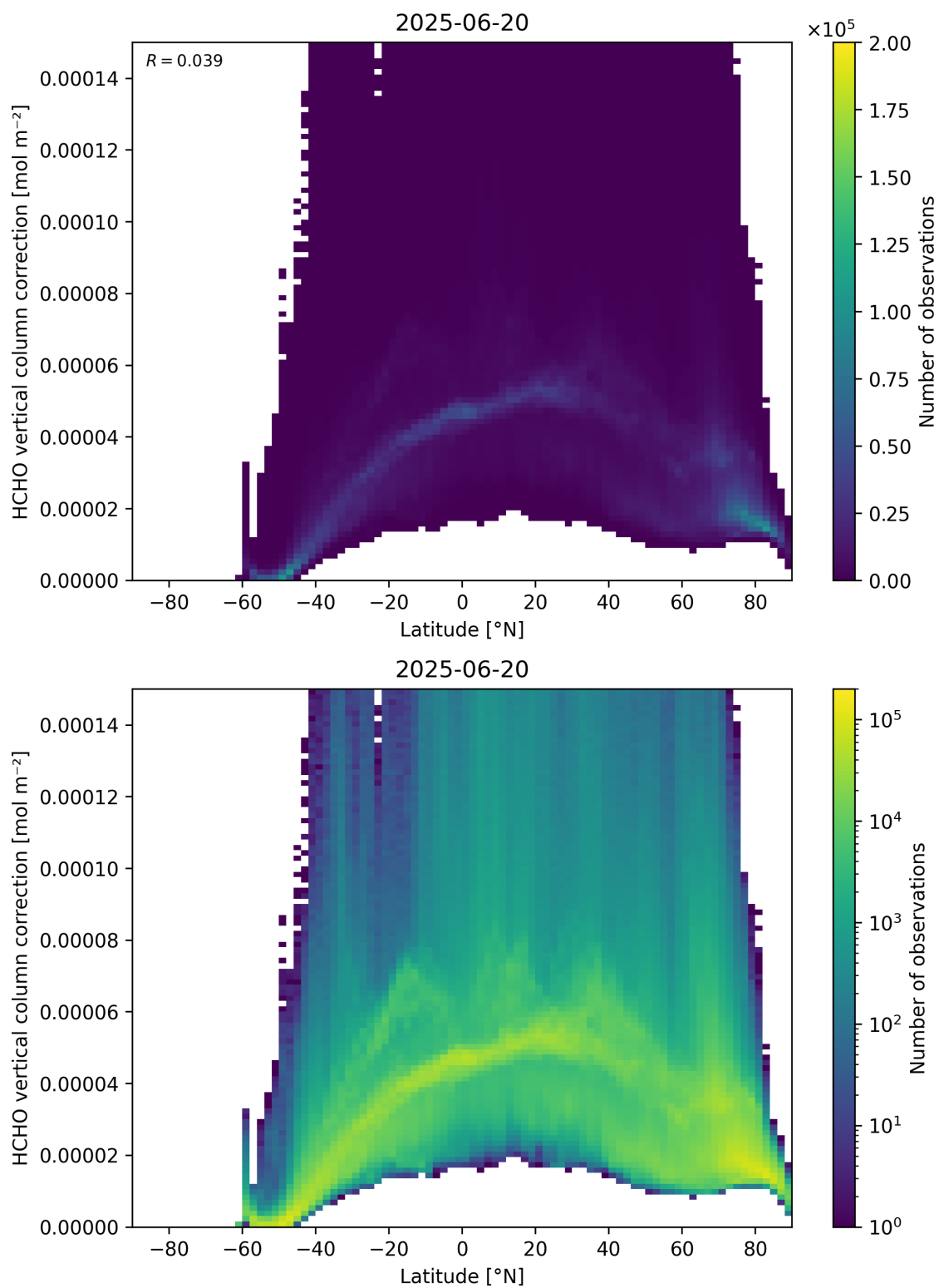
Figure 164: Scatter density plot of “Latitude” against “HCHO vertical column correction” for 2025-06-19 to 2025-06-21.
