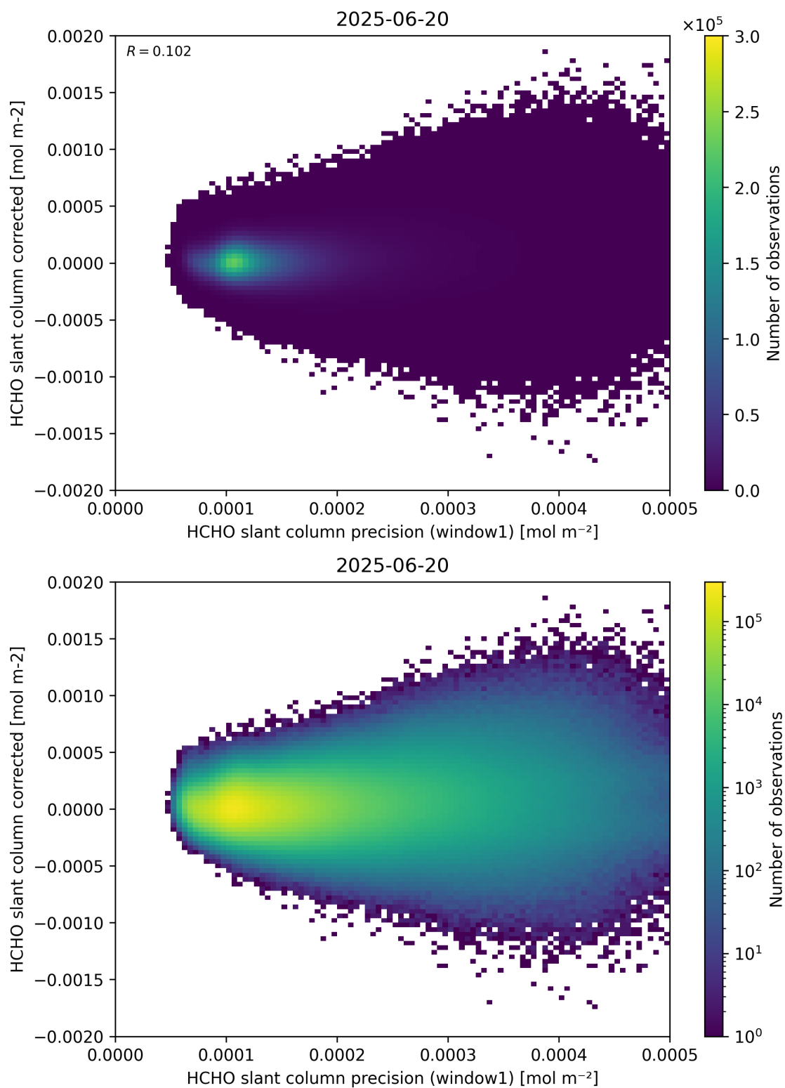
Figure 92: Scatter density plot of “HCHO slant column precision (window1)” against “HCHO slant column corrected” for 2025-06-19 to 2025-06-21.
