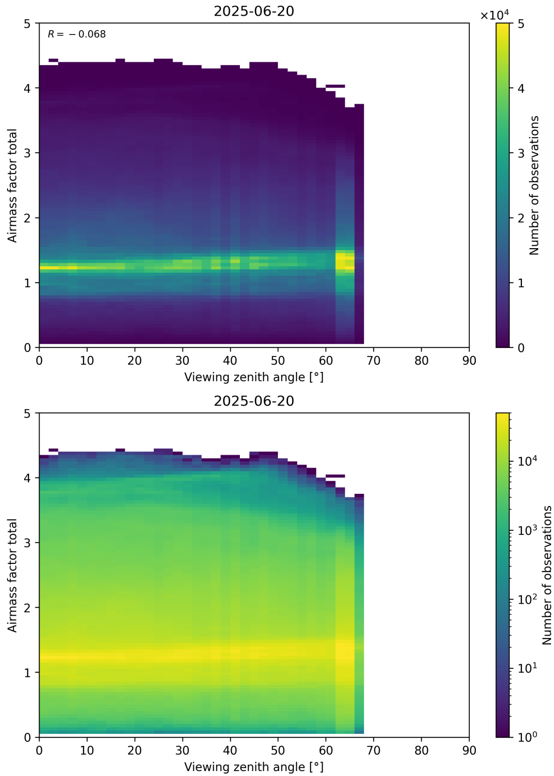
Figure 190: Scatter density plot of “Viewing zenith angle” against “Airmass factor total” for 2025-06-19 to 2025-06-21.
