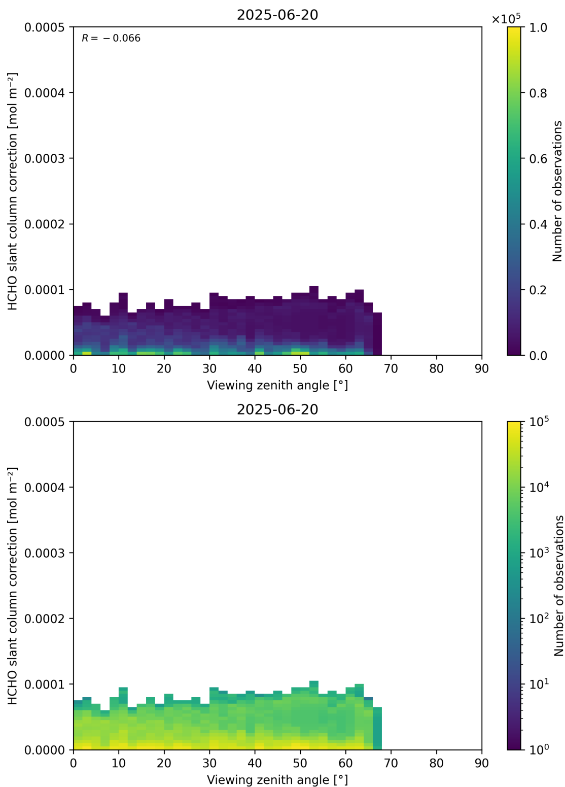
Figure 187: Scatter density plot of “Viewing zenith angle” against “HCHO slant column correction” for 2025-06-19 to 2025-06-21.
