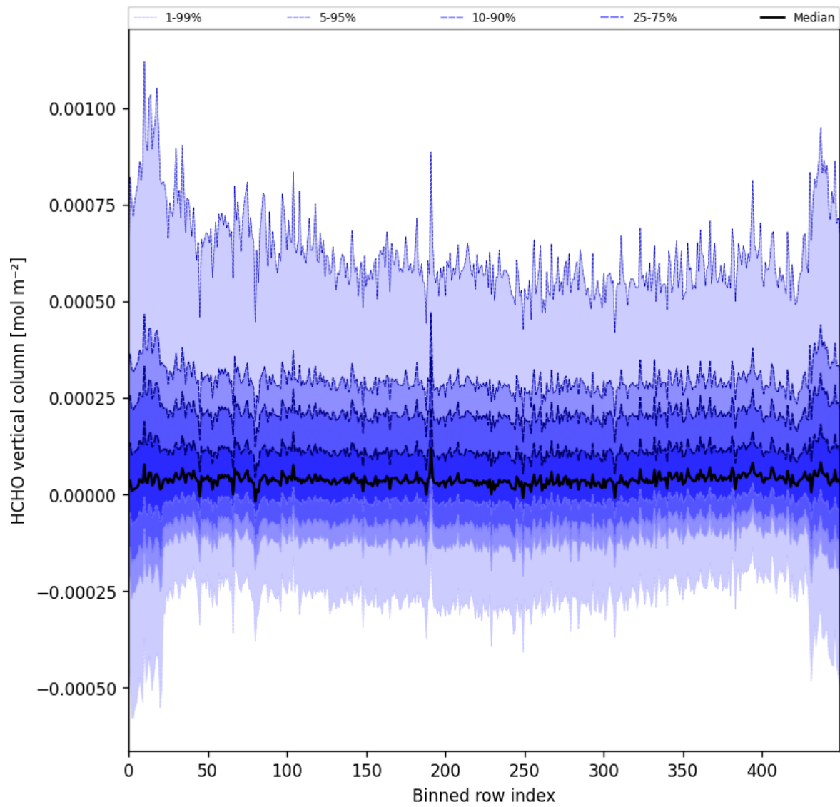
Figure 49: Along track statistics of “HCHO vertical column” for 2025-06-19 to 2025-06-21
