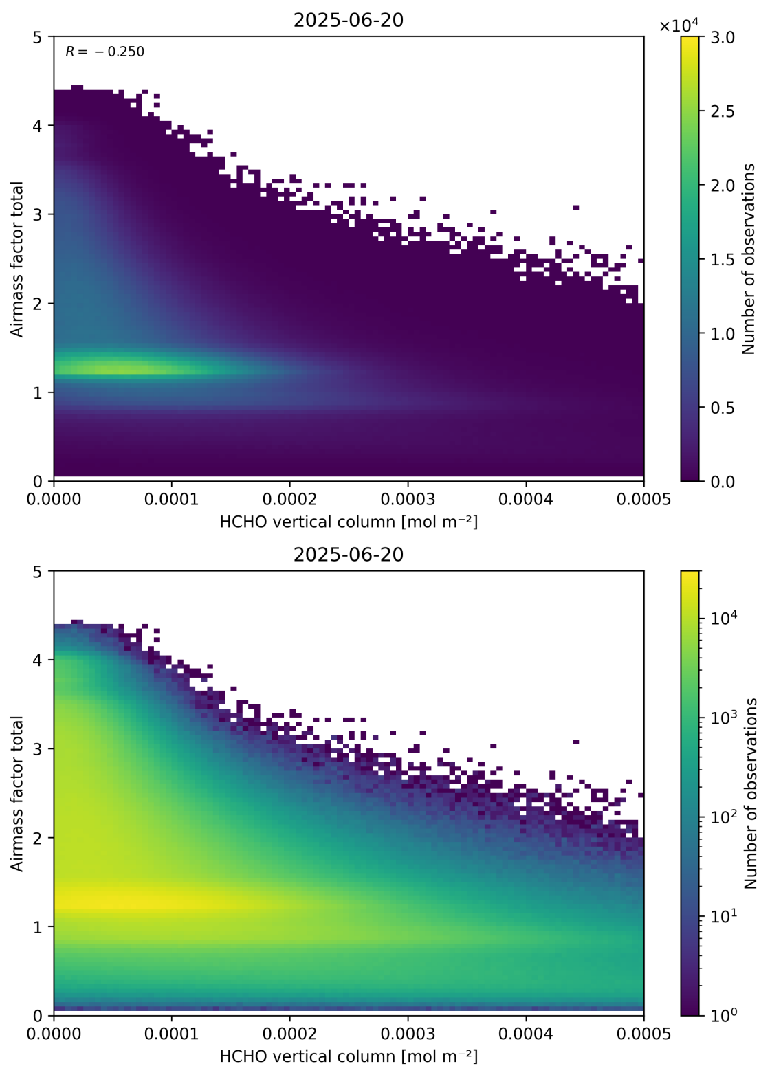
Figure 131: Scatter density plot of “HCHO vertical column” against “Airmass factor total” for 2025-06-19 to 2025-06-21.
