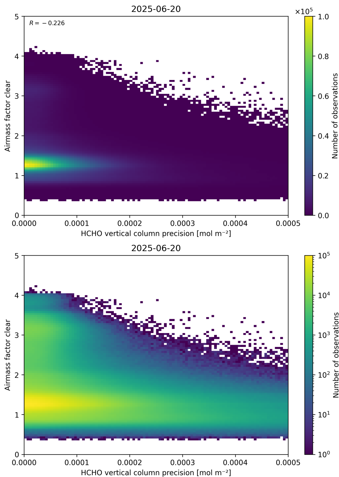
Figure 139: Scatter density plot of “HCHO vertical column precision” against “Airmass factor clear” for 2025-06-19 to 2025-06-21.
