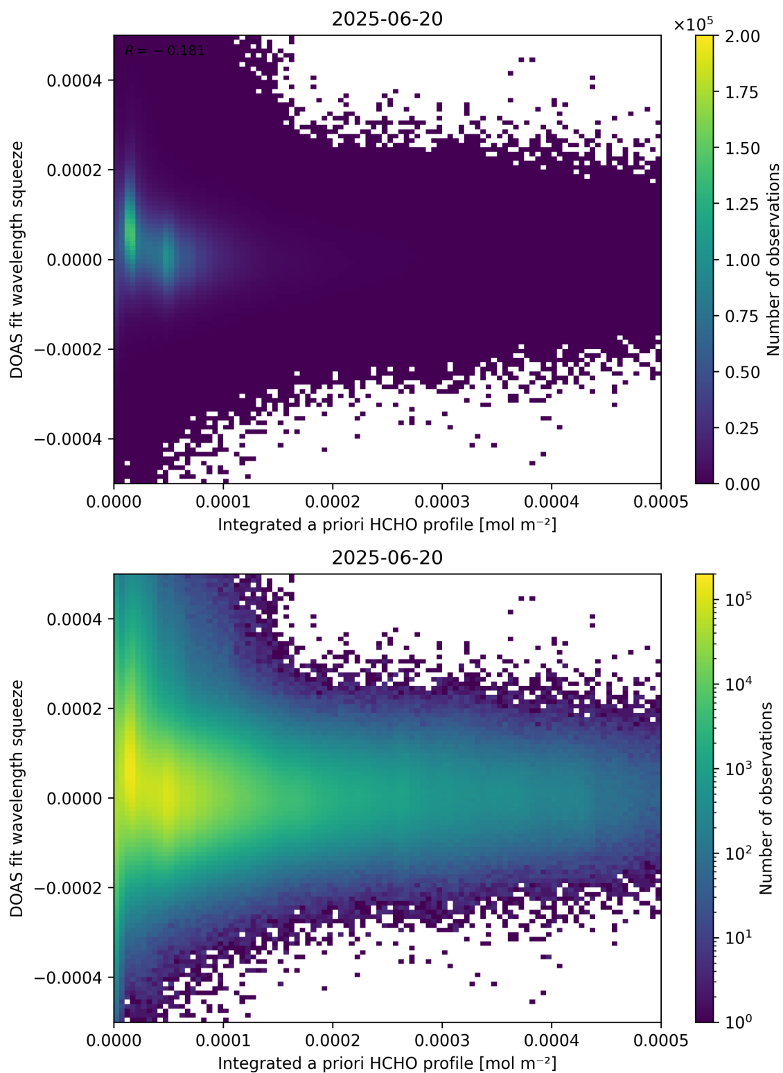
Figure 150: Scatter density plot of “Integrated a priori HCHO profile” against “DOAS fit wavelength squeeze” for 2025-06-19 to 2025-06-21.
