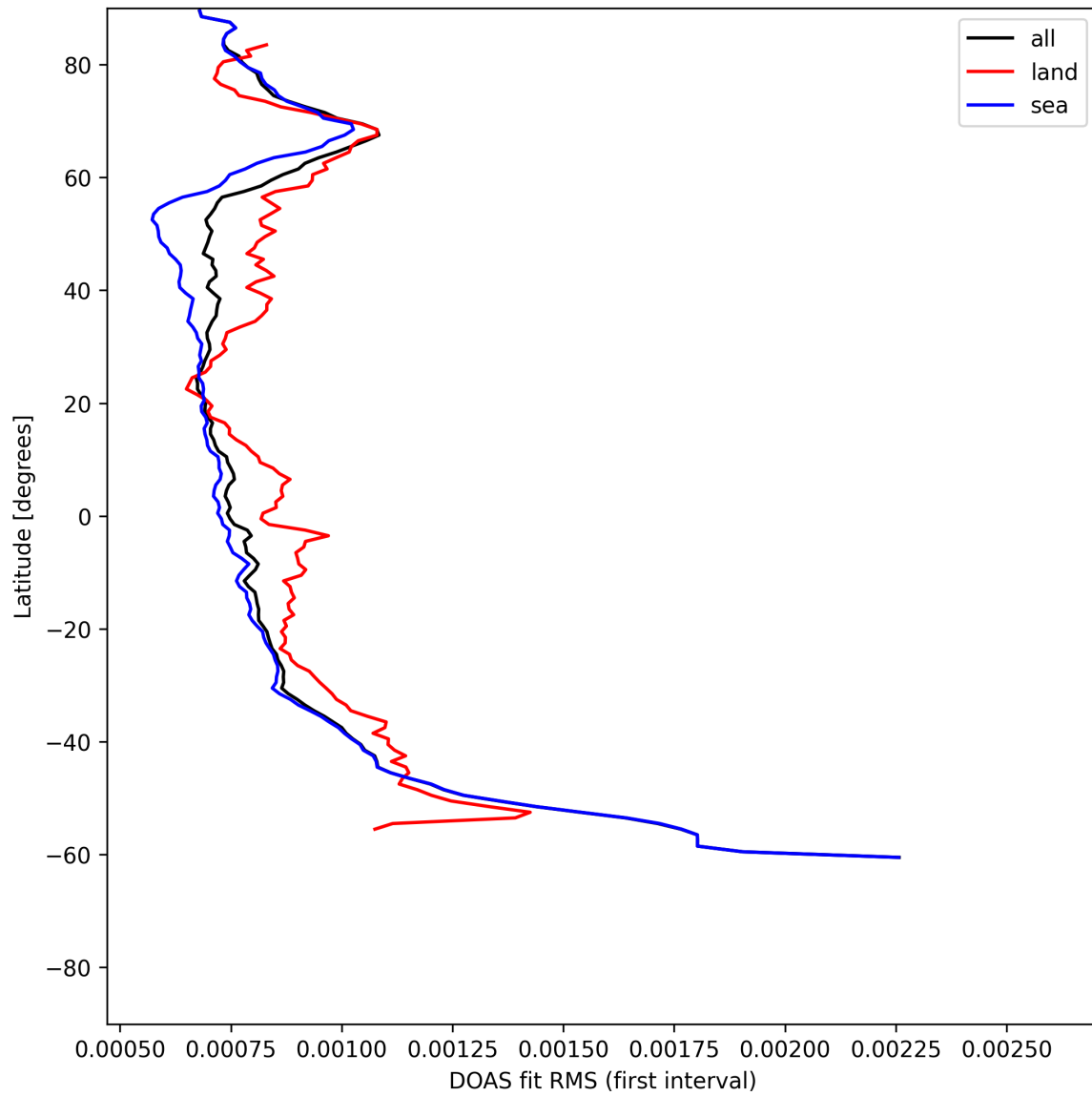
Figure 32: Zonal average of “DOAS fit RMS (first interval)” for 2025-06-19 to 2025-06-21.
