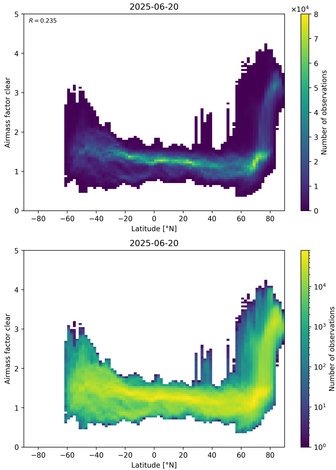
Figure 156: Scatter density plot of “Latitude” against “Airmass factor clear” for 2025-06-19 to 2025-06-21.
