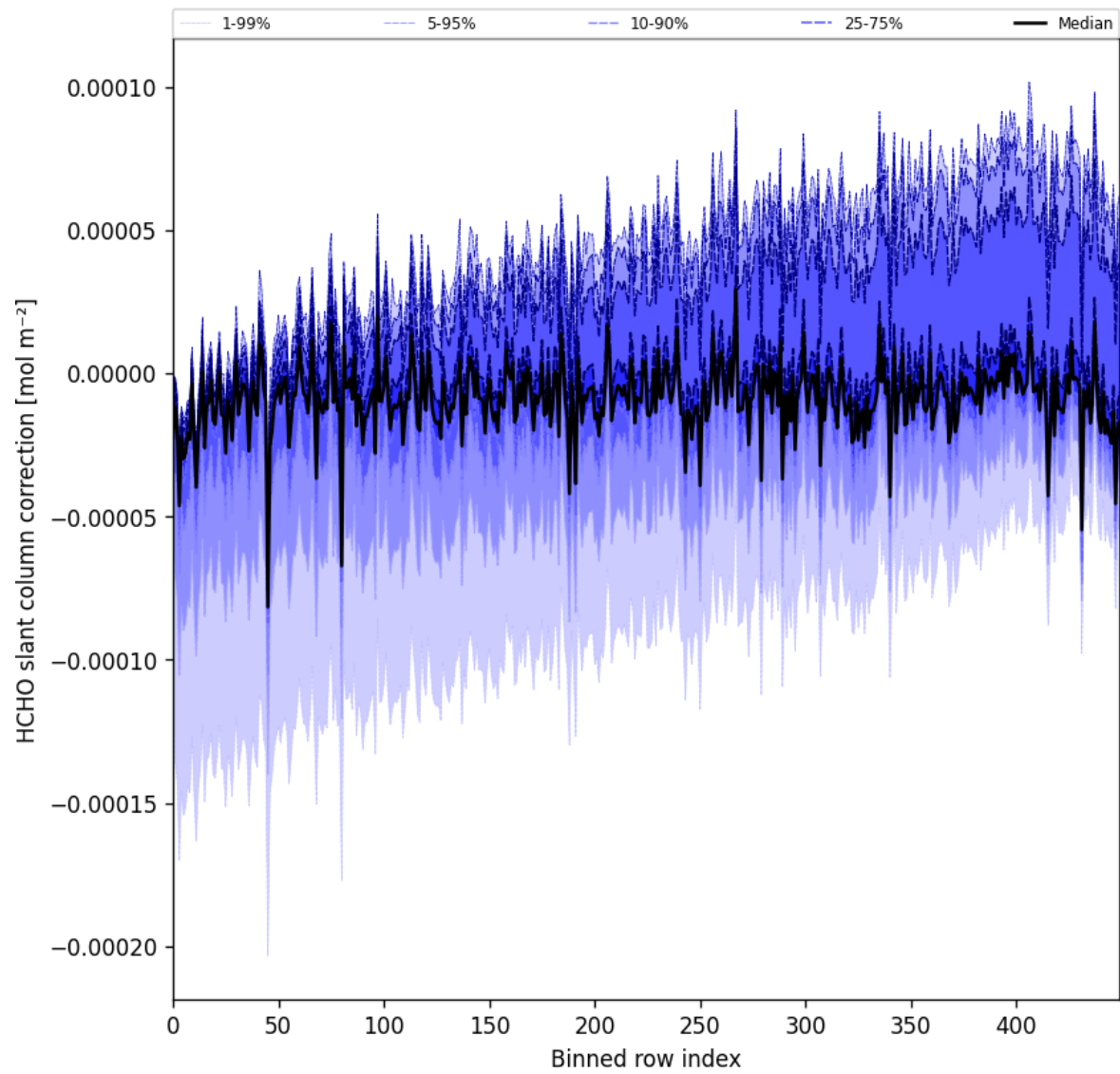
Figure 61: Along track statistics of “HCHO slant column correction” for 2025-06-19 to 2025-06-21
