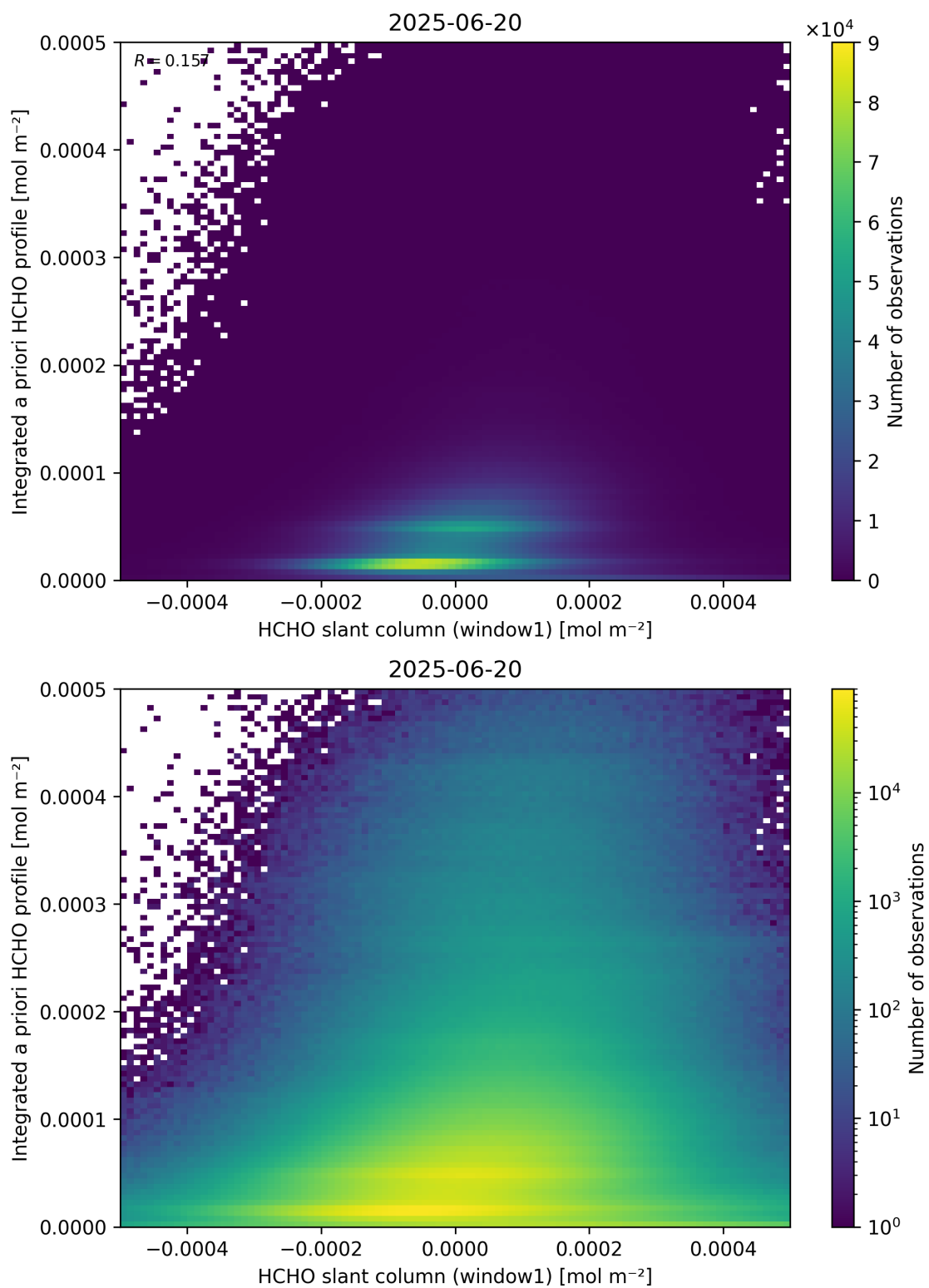
Figure 87: Scatter density plot of “HCHO slant column (window1)” against “Integrated a priori HCHO profile” for 2025-06-19 to 2025-06-21.
