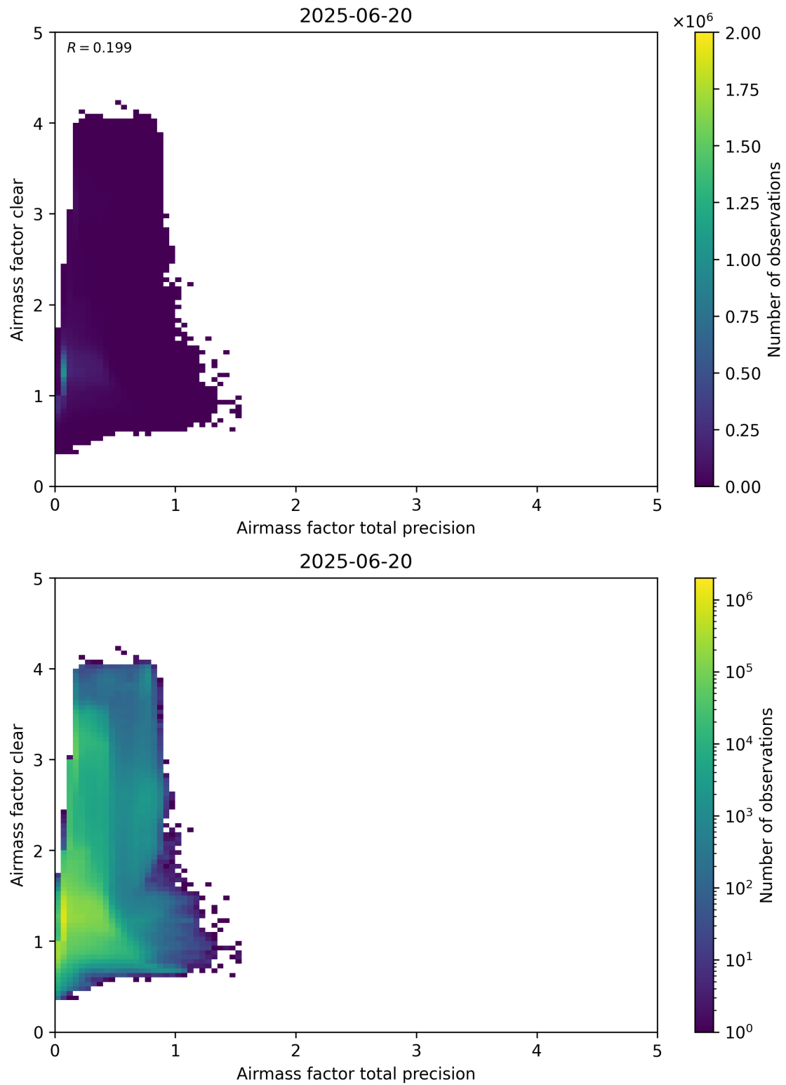
Figure 108: Scatter density plot of “Airmass factor total precision” against “Airmass factor clear” for 2025-06-19 to 2025-06-21.
