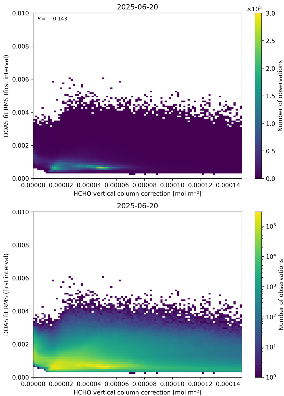
Figure 112: Scatter density plot of “HCHO vertical column correction” against “DOAS fit RMS (first interval)” for 2025-06-19 to 2025-06-21.
