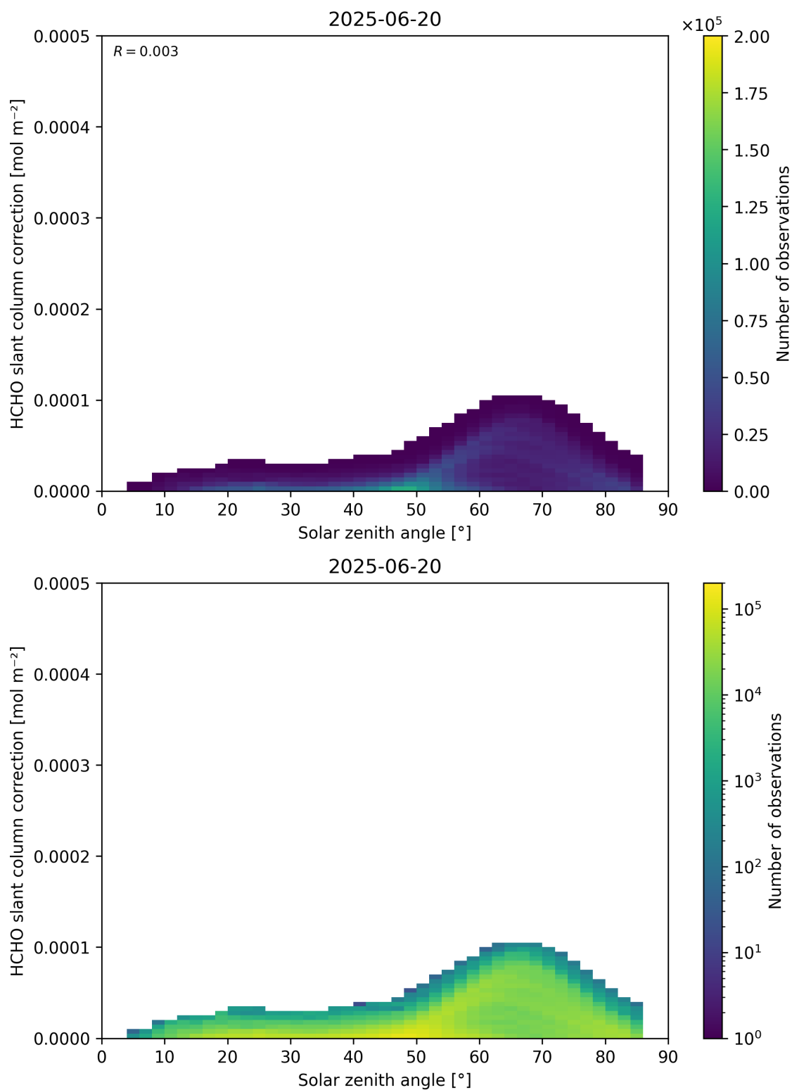
Figure 172: Scatter density plot of “Solar zenith angle” against “HCHO slant column correction” for 2025-06-19 to 2025-06-21.
