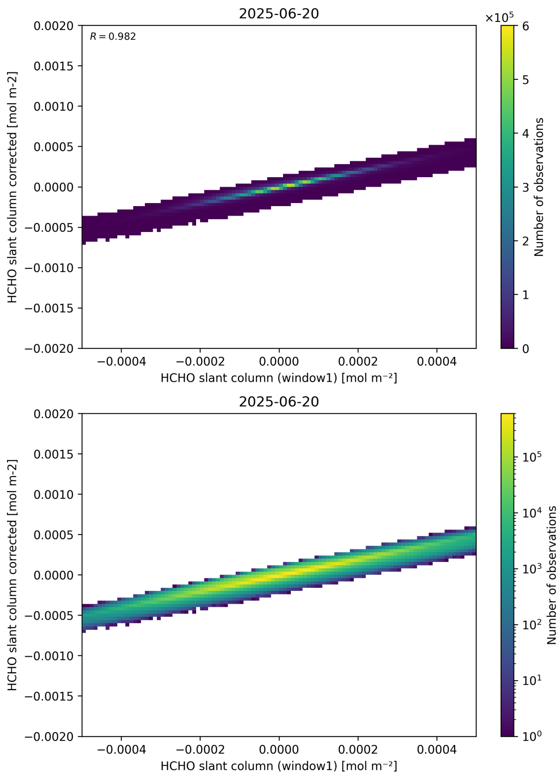
Figure 82: Scatter density plot of “HCHO slant column (window1)” against “HCHO slant column corrected” for 2025-06-19 to 2025-06-21.
