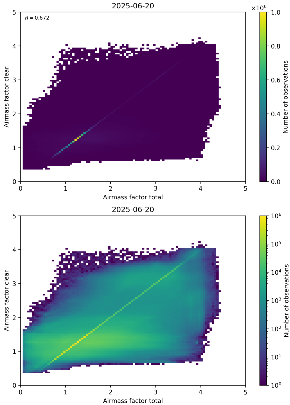
Figure 100: Scatter density plot of “Airmass factor total” against “Airmass factor clear” for 2025-06-19 to 2025-06-21.
