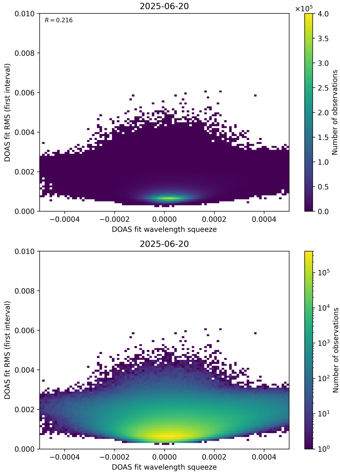
Figure 68: Scatter density plot of “DOAS fit wavelength squeeze” against “DOAS fit RMS (first interval)” for 2025-06-19 to 2025-06-21.
