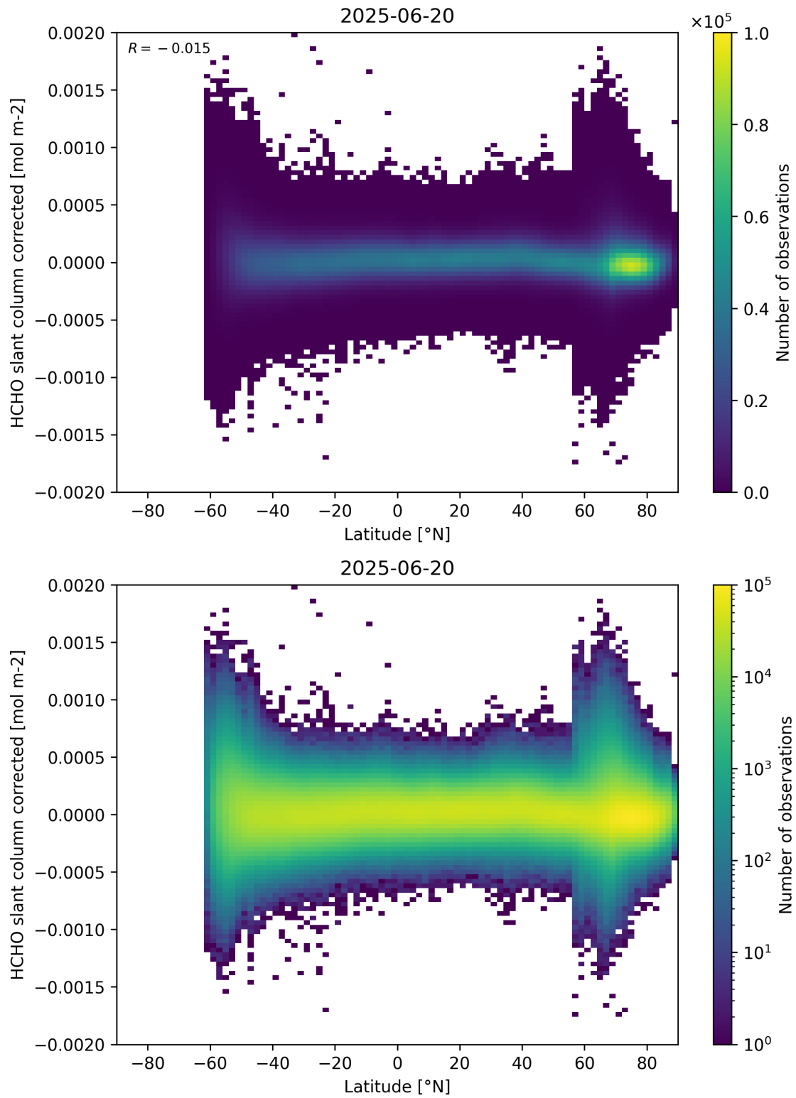
Figure 157: Scatter density plot of “Latitude” against “HCHO slant column corrected” for 2025-06-19 to 2025-06-21.
