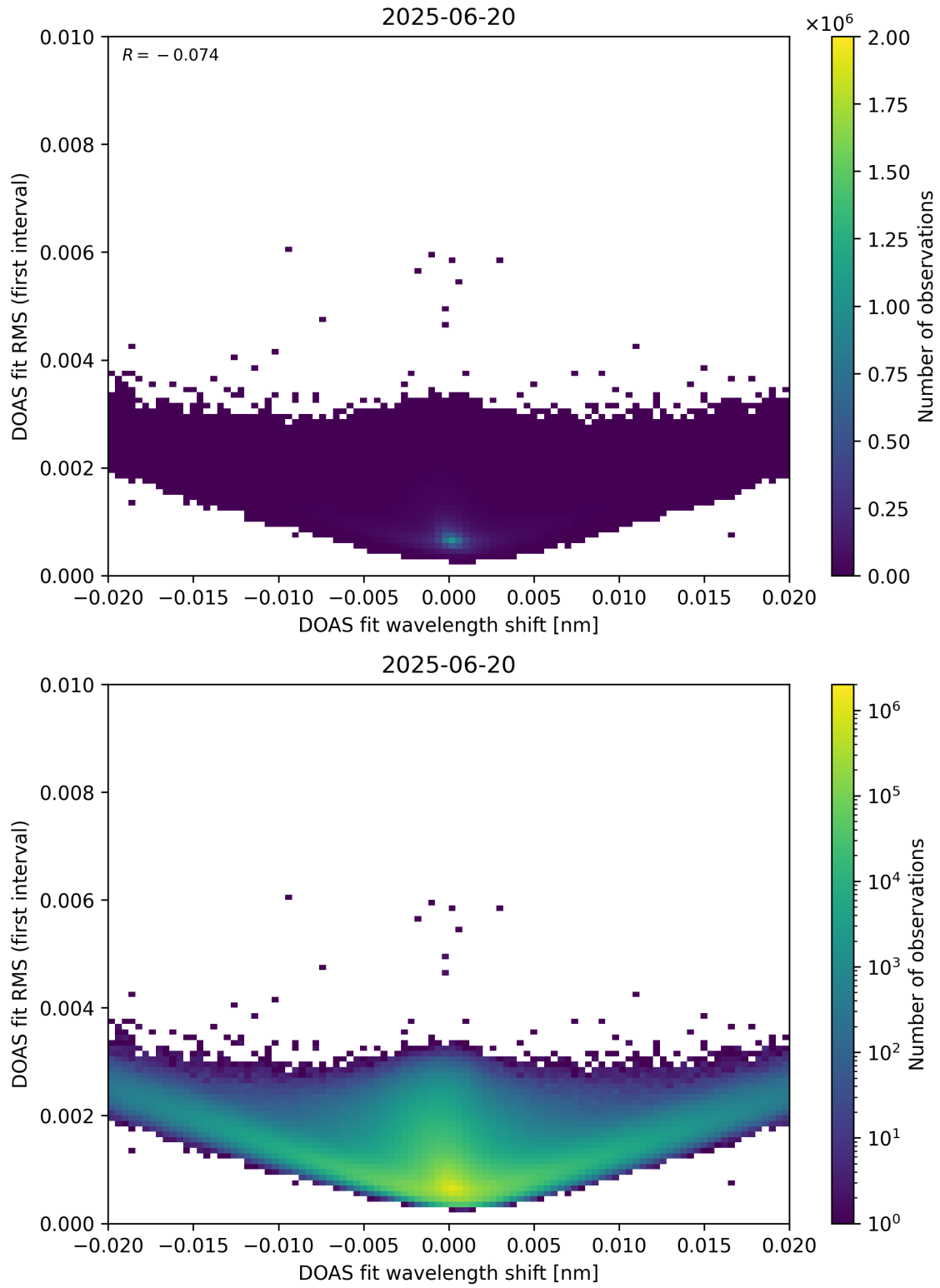
Figure 64: Scatter density plot of “DOAS fit wavelength shift” against “DOAS fit RMS (first interval)” for 2025-06-19 to 2025-06-21.
