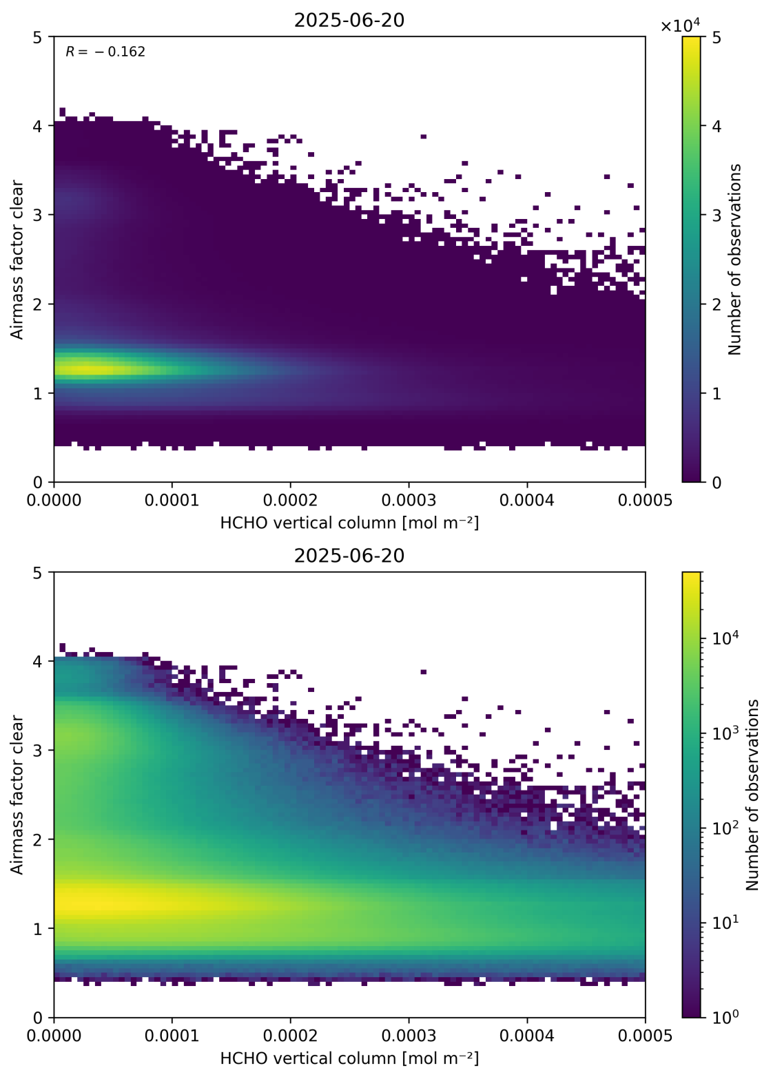
Figure 126: Scatter density plot of “HCHO vertical column” against “Airmass factor clear” for 2025-06-19 to 2025-06-21.
