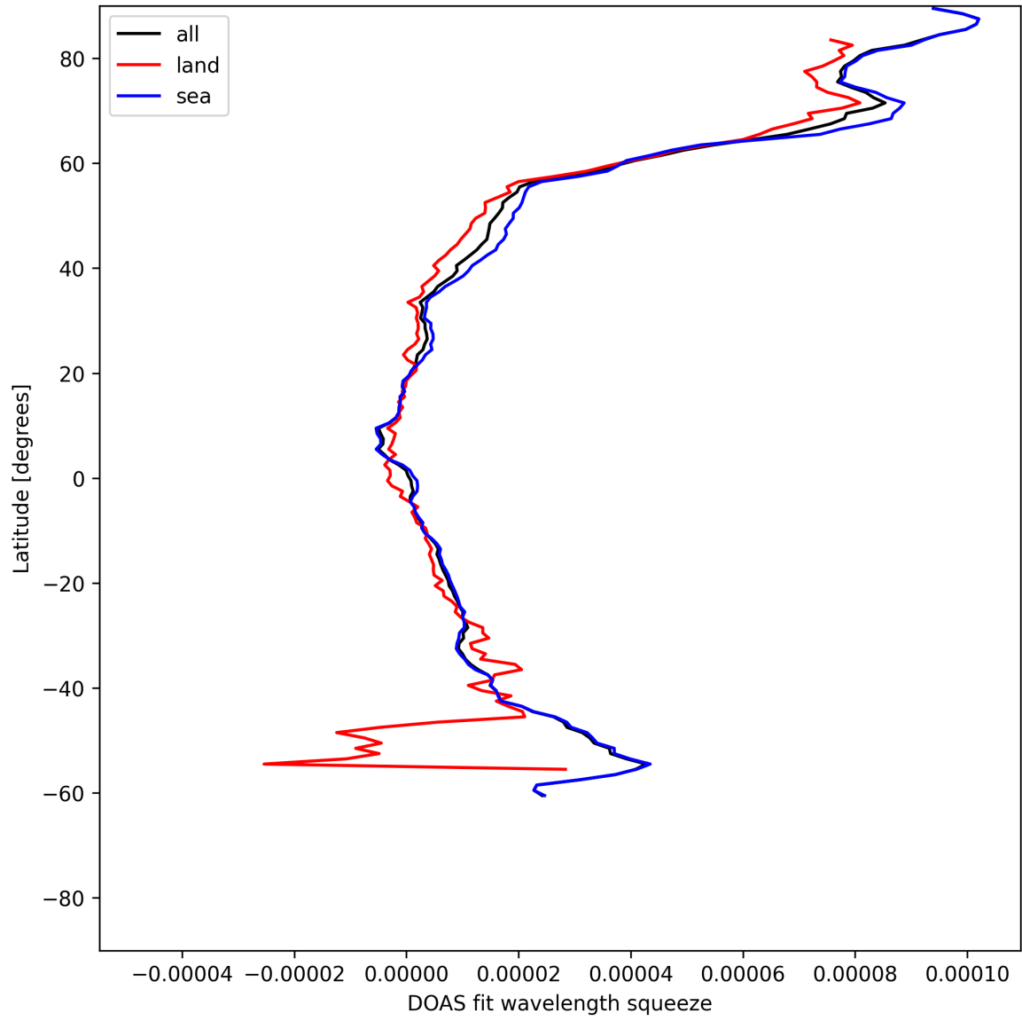
Figure 31: Zonal average of “DOAS fit wavelength squeeze” for 2025-06-19 to 2025-06-21.
