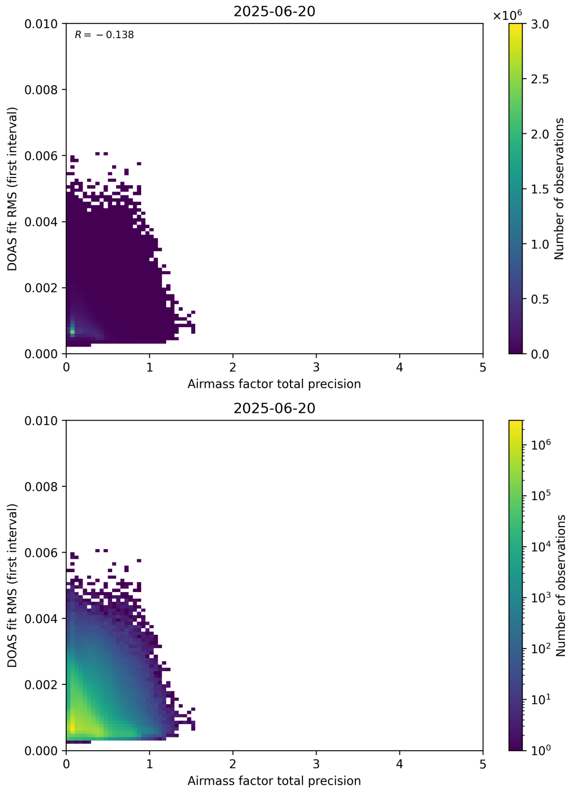
Figure 105: Scatter density plot of “Airmass factor total precision” against “DOAS fit RMS (first interval)” for 2025-06-19 to 2025-06-21.
