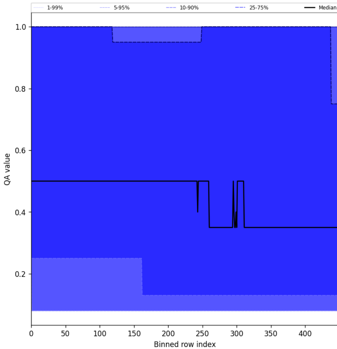
Figure 48: Along track statistics of “QA value” for 2025-06-19 to 2025-06-21
