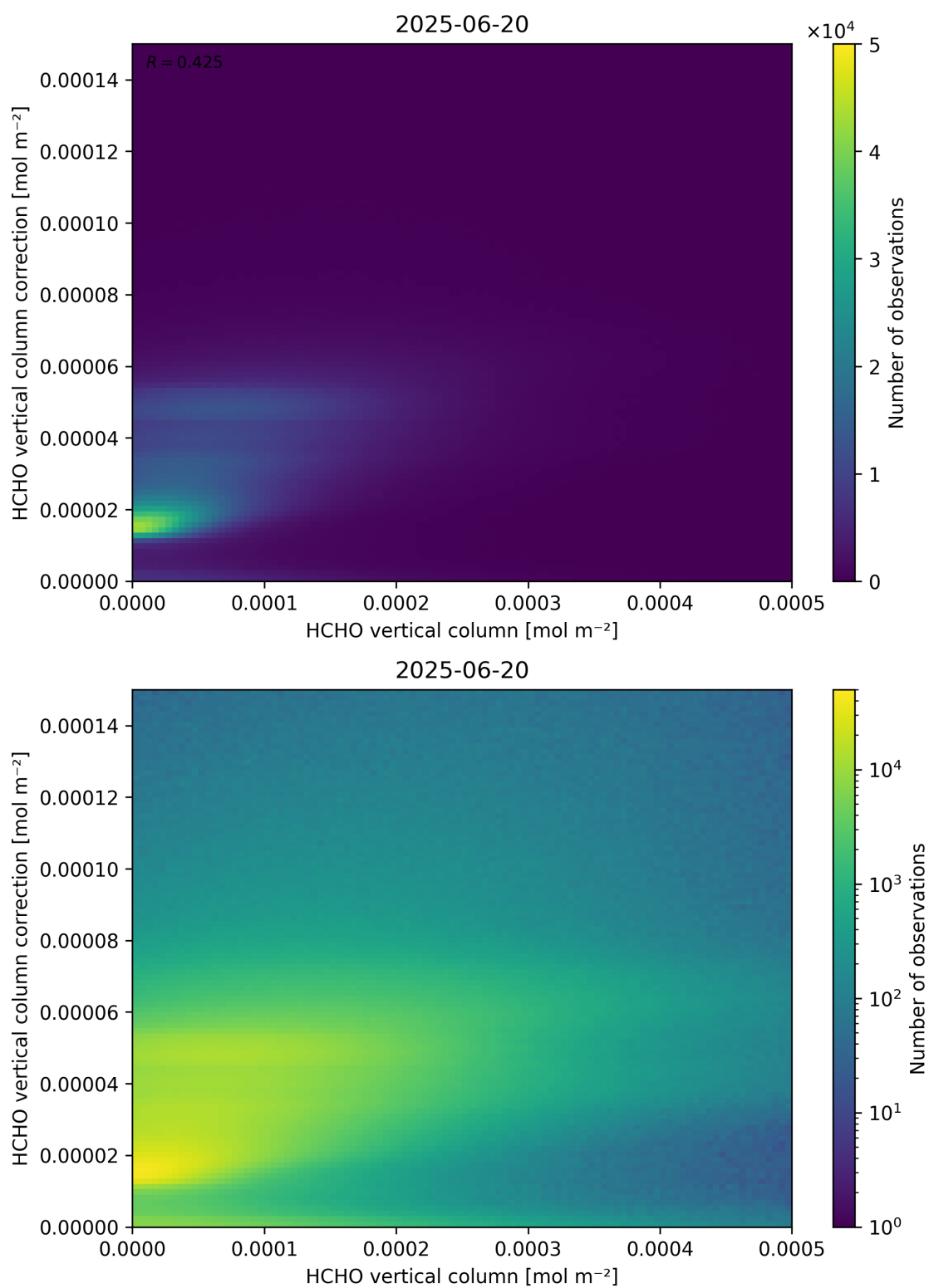
Figure 133: Scatter density plot of “HCHO vertical column” against “HCHO vertical column correction” for 2025-06-19 to 2025-06-21.
