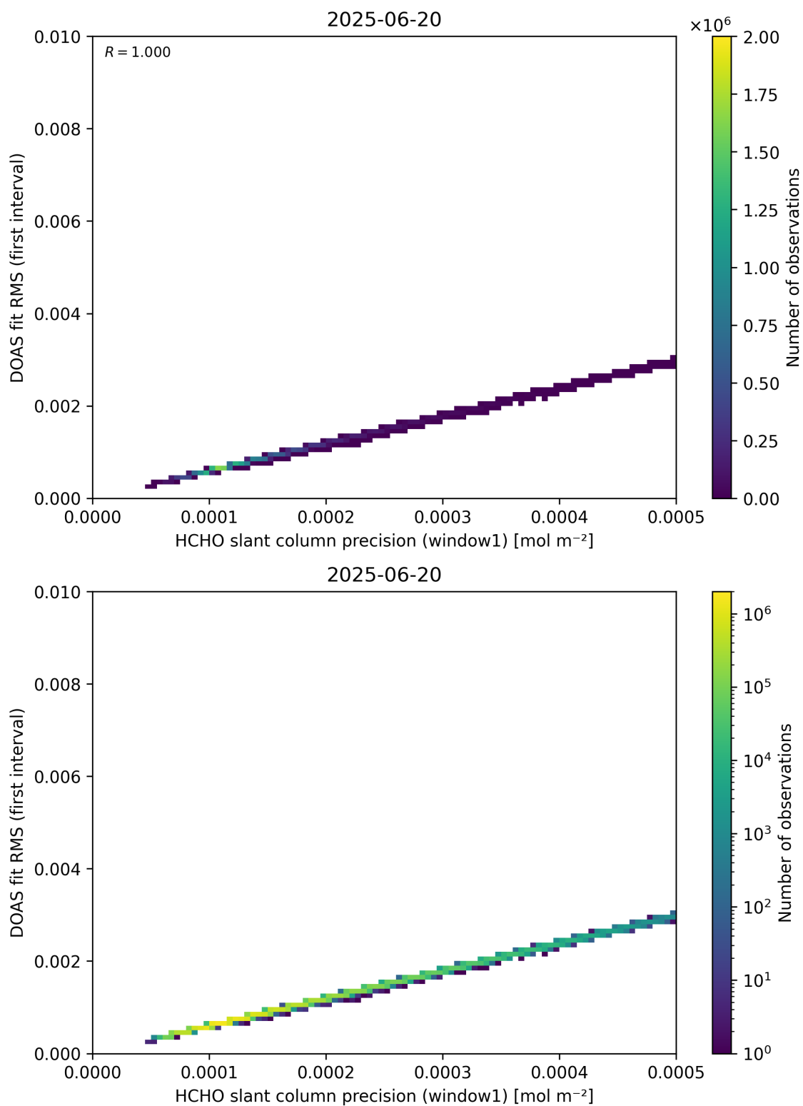
Figure 88: Scatter density plot of “HCHO slant column precision (window1)” against “DOAS fit RMS (first interval)” for 2025-06-19 to 2025-06-21.
