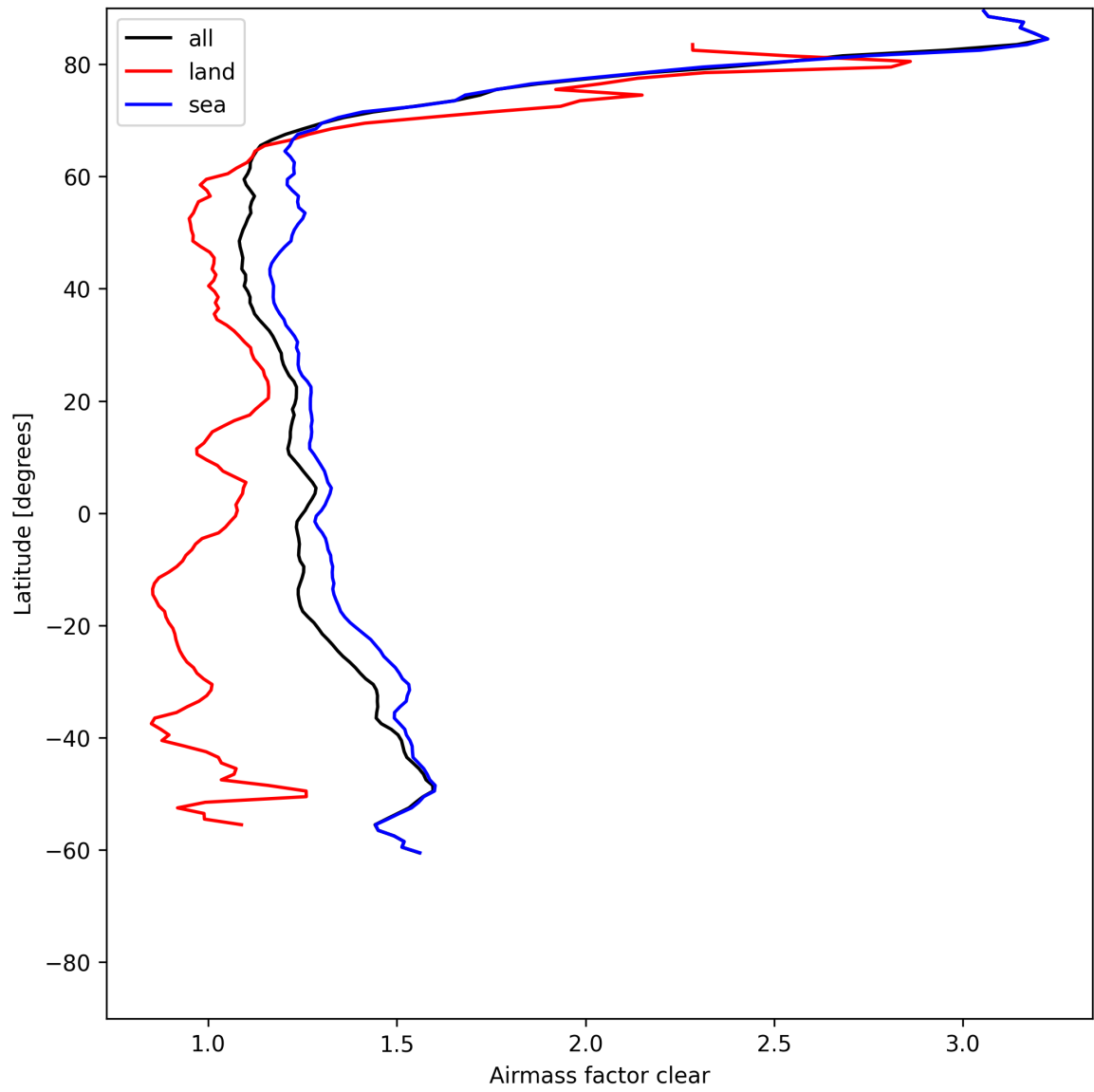
Figure 28: Zonal average of “Airmass factor clear” for 2025-06-19 to 2025-06-21.
