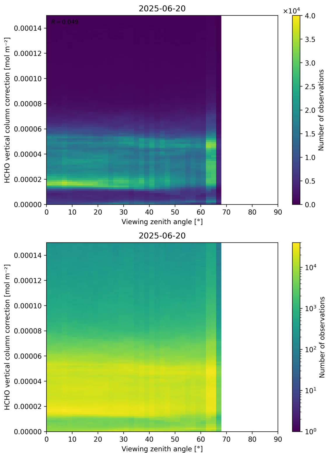
Figure 193: Scatter density plot of “Viewing zenith angle” against “HCHO vertical column correction” for 2025-06-19 to 2025-06-21.
