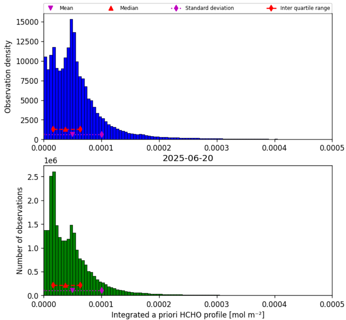
Figure 43: Histogram of “Integrated a priori HCHO profile” for 2025-06-19 to 2025-06-21
