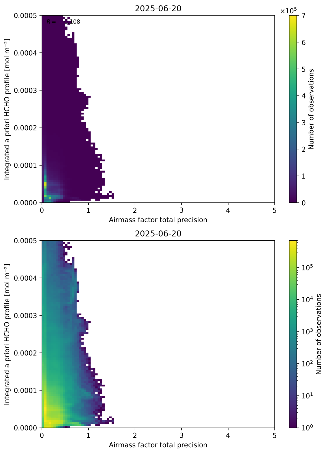
Figure 111: Scatter density plot of “Airmass factor total precision” against “Integrated a priori HCHO profile” for 2025-06-19 to 2025-06-21.
