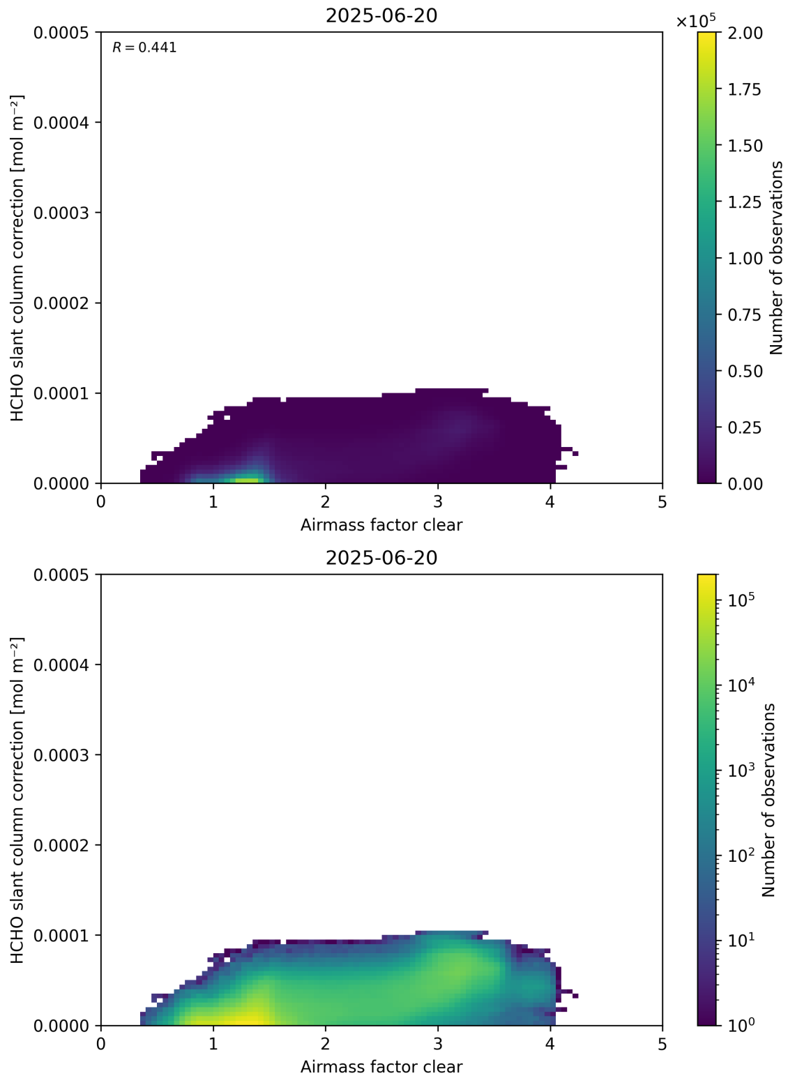
Figure 75: Scatter density plot of “Airmass factor clear” against “HCHO slant column correction” for 2025-06-19 to 2025-06-21.
