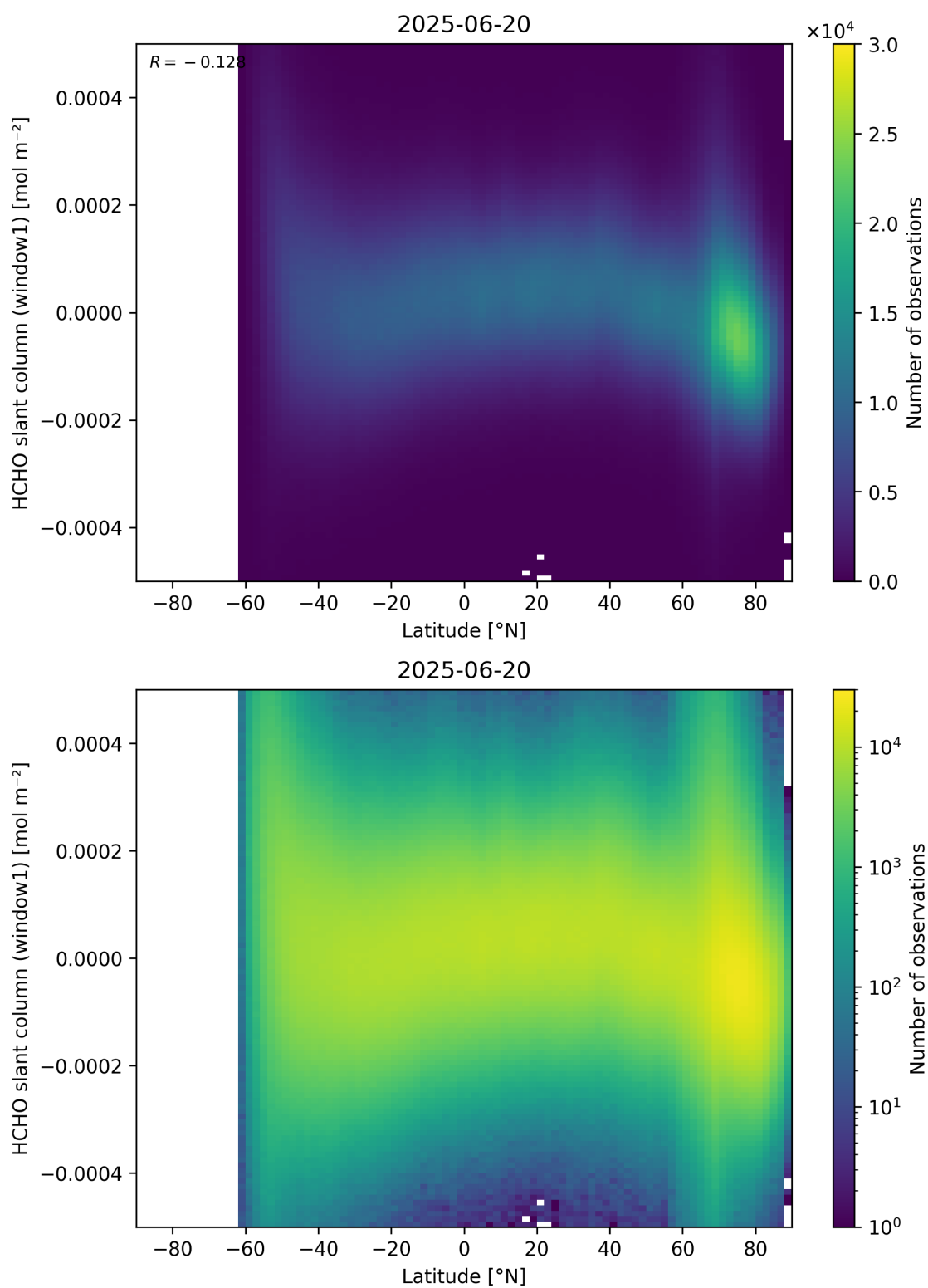
Figure 159: Scatter density plot of “Latitude” against “HCHO slant column (window1)” for 2025-06-19 to 2025-06-21.
