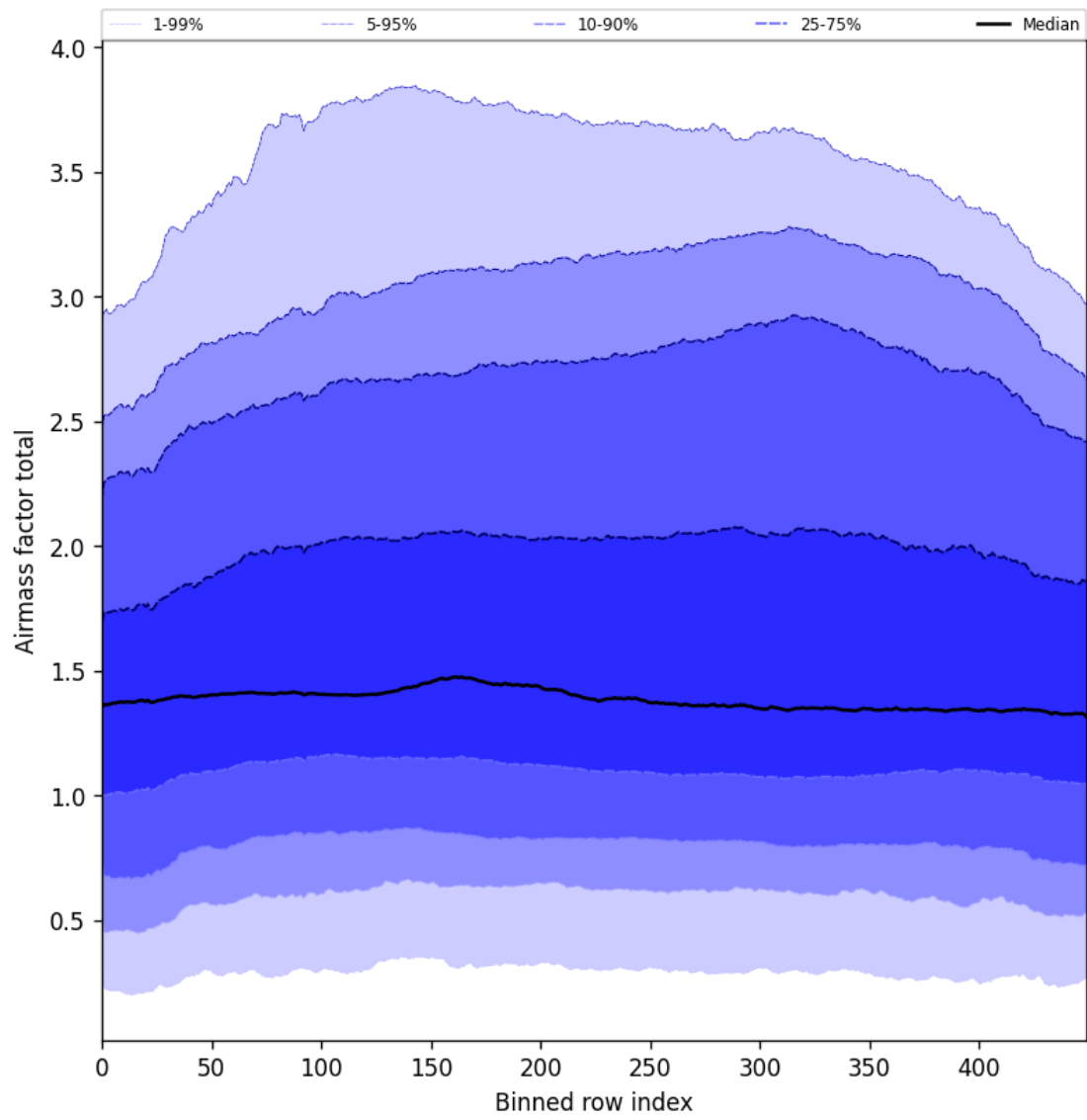
Figure 54: Along track statistics of “Airmass factor total” for 2025-06-19 to 2025-06-21
