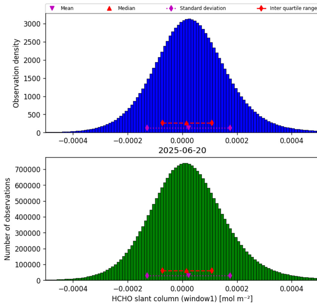
Figure 38: Histogram of “HCHO slant column (window1)” for 2025-06-19 to 2025-06-21
