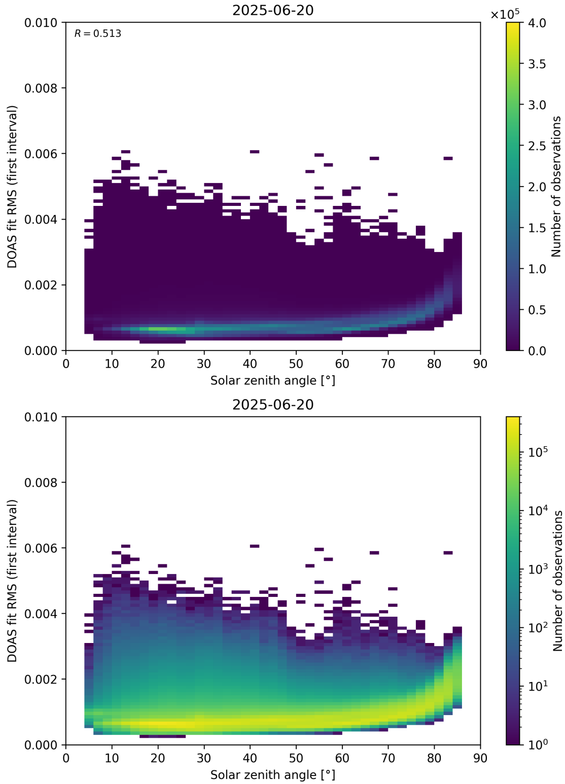
Figure 167: Scatter density plot of “Solar zenith angle” against “DOAS fit RMS (first interval)” for 2025-06-19 to 2025-06-21.
