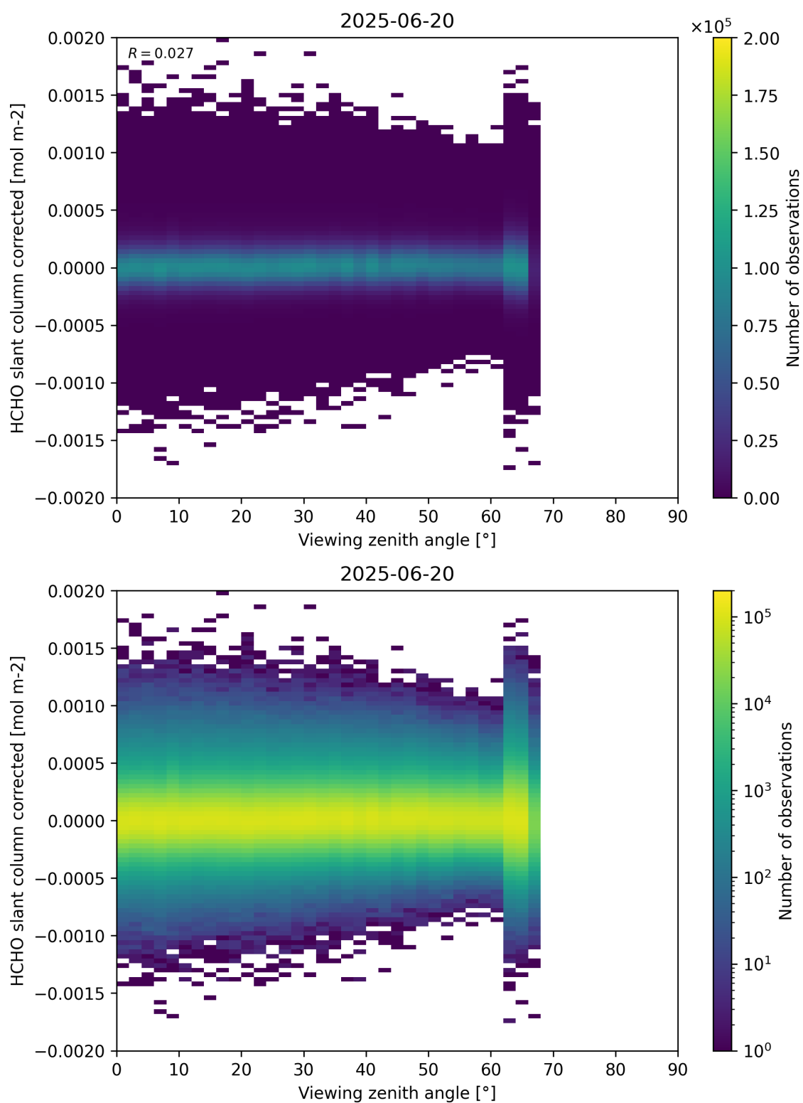
Figure 186: Scatter density plot of “Viewing zenith angle” against “HCHO slant column corrected” for 2025-06-19 to 2025-06-21.
