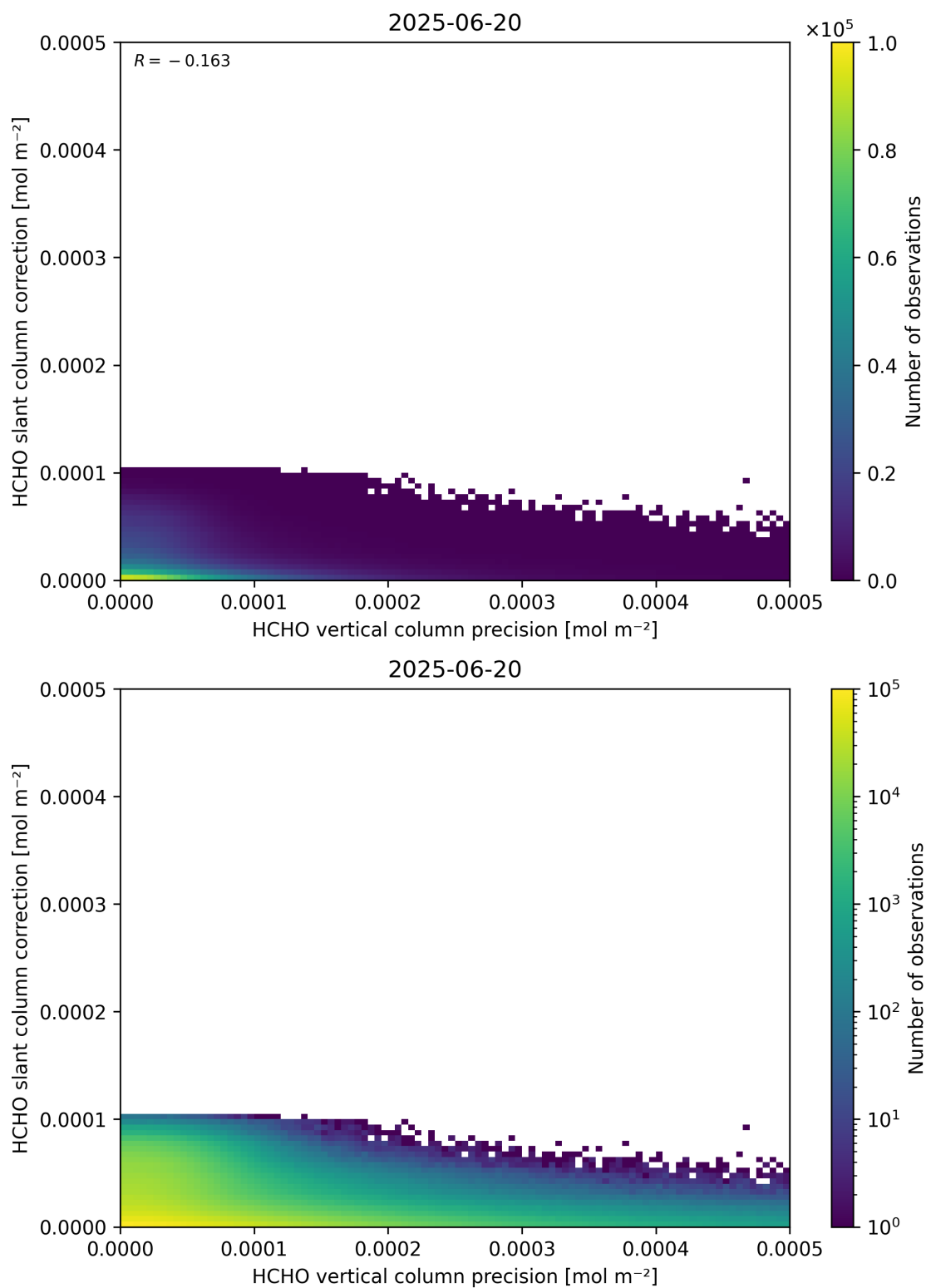
Figure 141: Scatter density plot of “HCHO vertical column precision” against “HCHO slant column correction” for 2025-06-19 to 2025-06-21.
