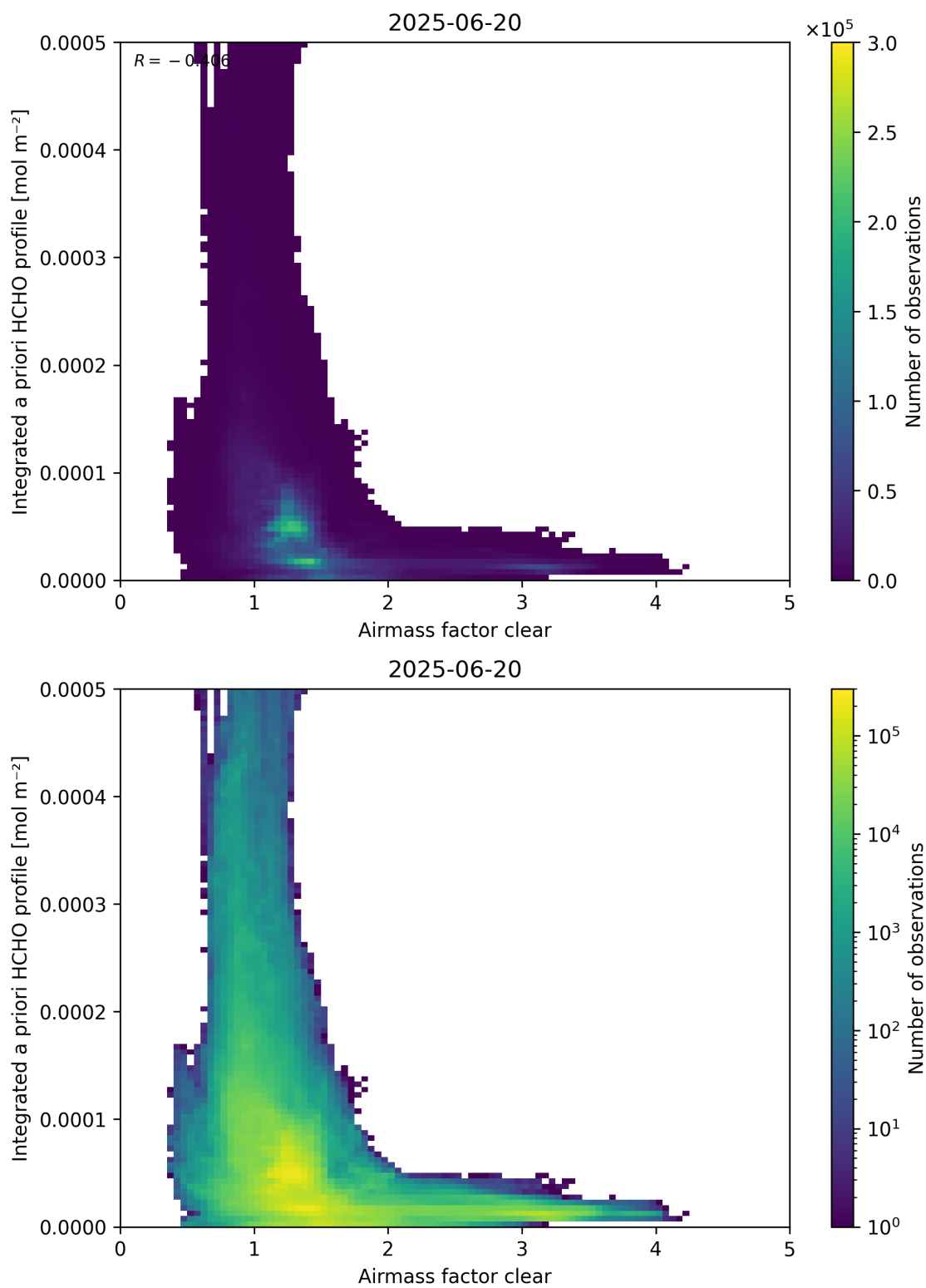
Figure 76: Scatter density plot of “Airmass factor clear” against “Integrated a priori HCHO profile” for 2025-06-19 to 2025-06-21.
