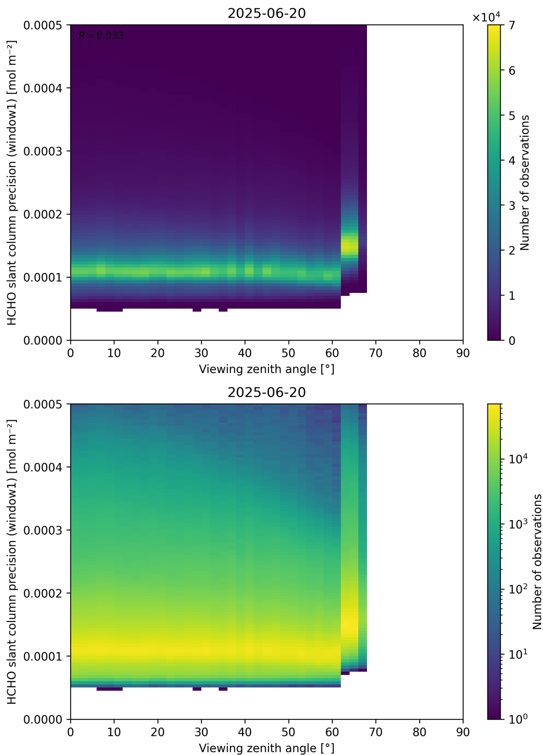
Figure 189: Scatter density plot of “Viewing zenith angle” against “HCHO slant column precision (window1)” for 2025-06-19 to 2025-06-21.
